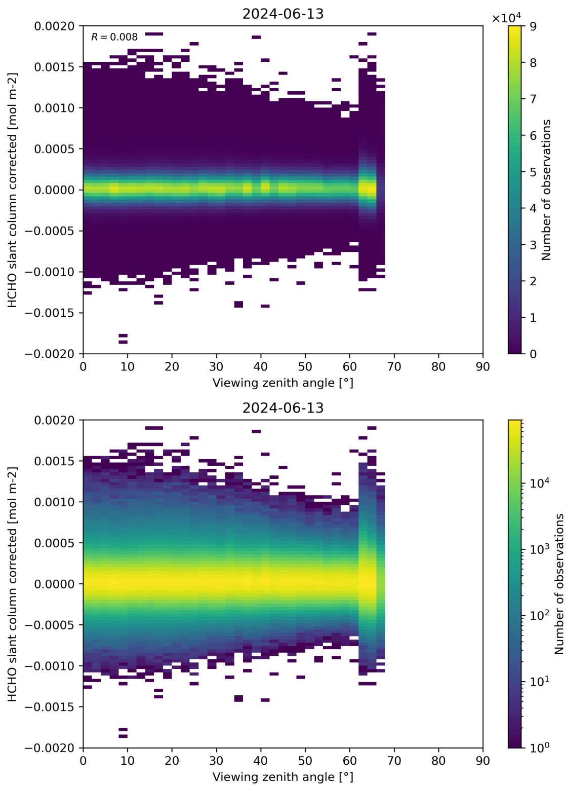
Figure 186: Scatter density plot of “Viewing zenith angle” against “HCHO slant column corrected” for 2024-06-13 to 2024-06-14.
