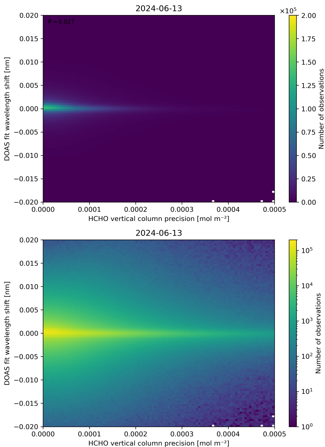
Figure 137: Scatter density plot of “HCHO vertical column precision” against “DOAS fit wavelength shift” for 2024-06-13 to 2024-06-14.
