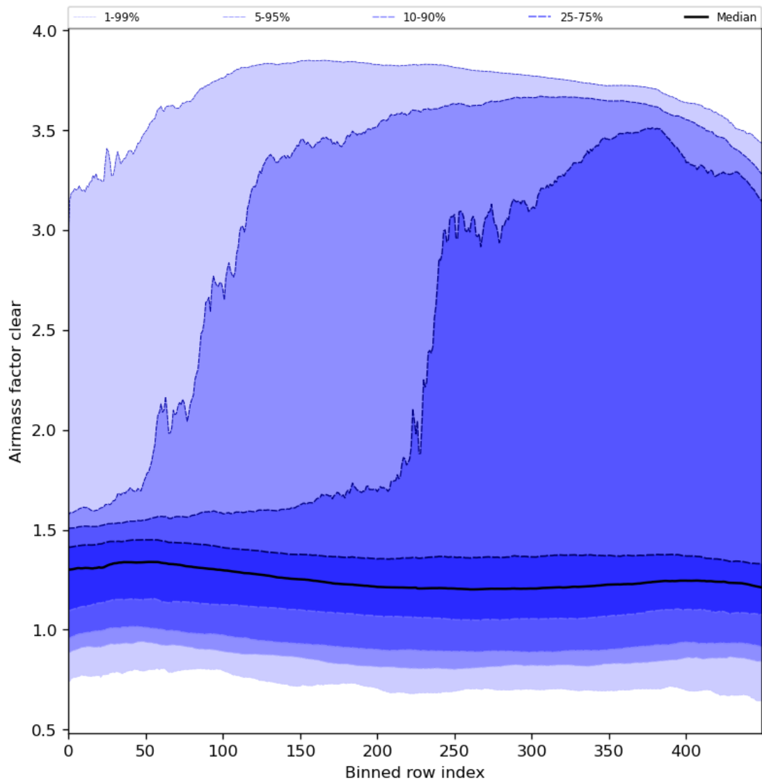
Figure 56: Along track statistics of “Airmass factor clear” for 2024-06-13 to 2024-06-14
