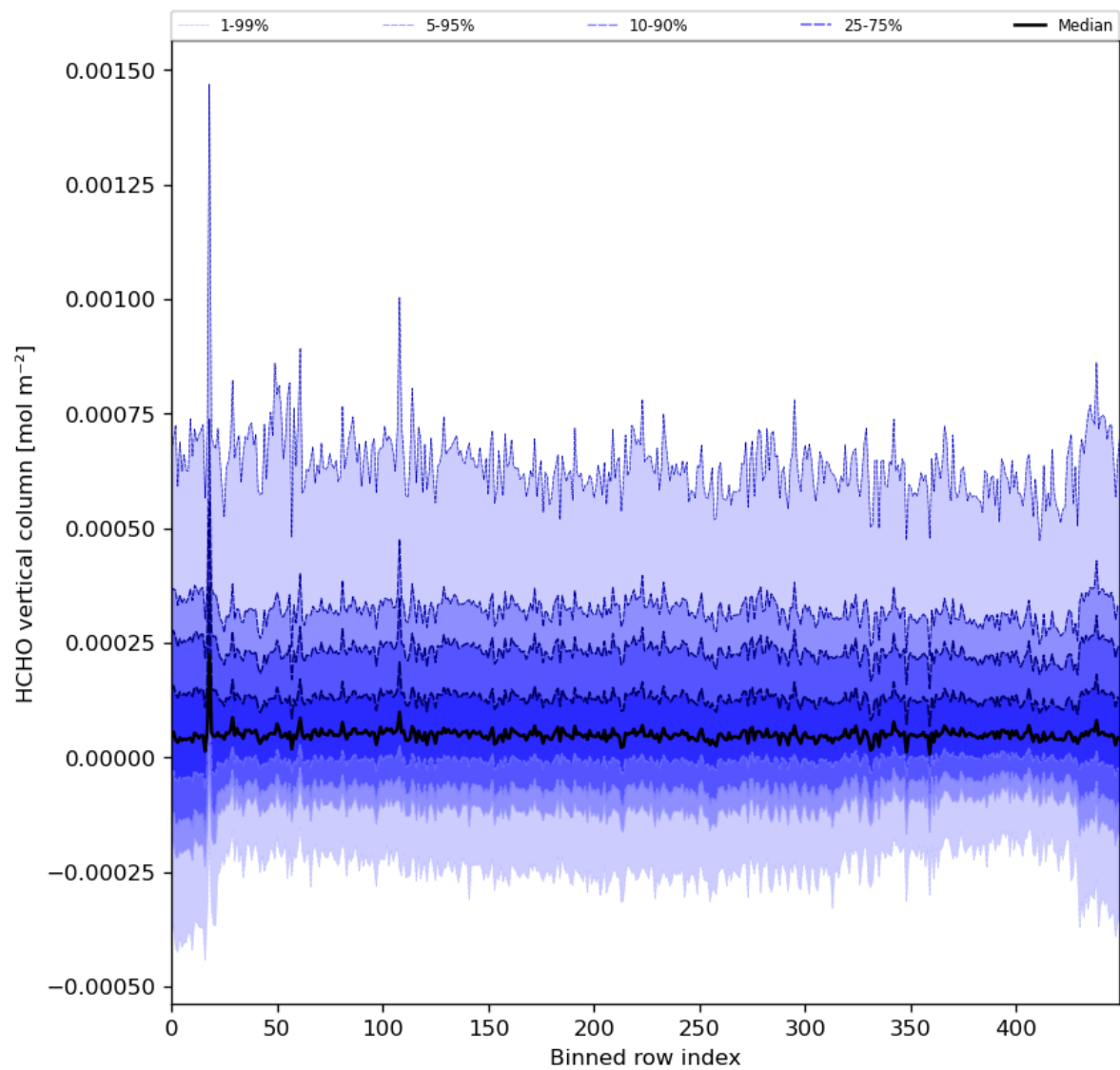
Figure 49: Along track statistics of “HCHO vertical column” for 2024-06-13 to 2024-06-14
