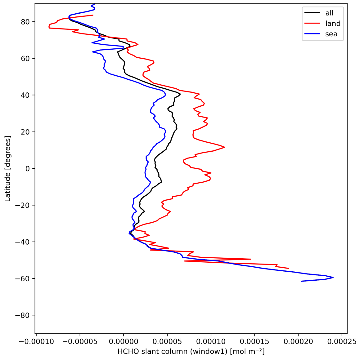
Figure 24: Zonal average of “HCHO slant column (window1)” for 2024-06-13 to 2024-06-14.
