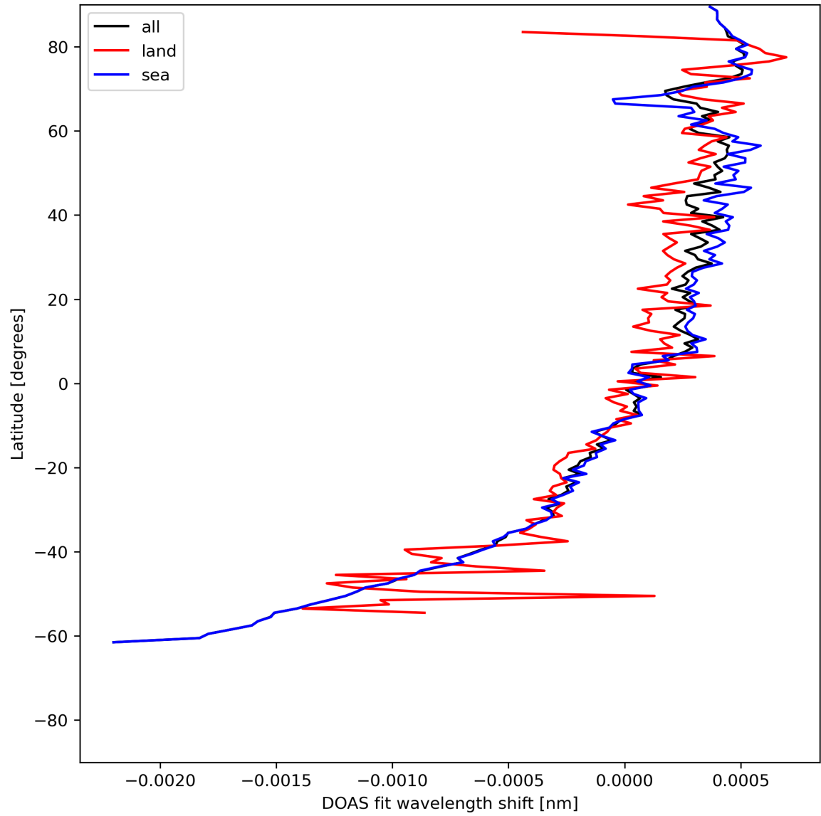
Figure 30: Zonal average of “DOAS fit wavelength shift” for 2024-06-13 to 2024-06-14.
