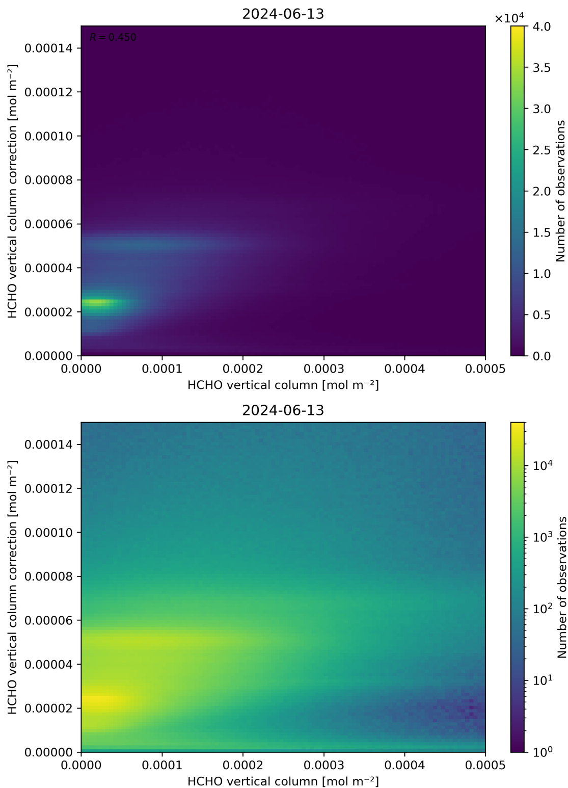
Figure 133: Scatter density plot of “HCHO vertical column” against “HCHO vertical column correction” for 2024-06-13 to 2024-06-14.
