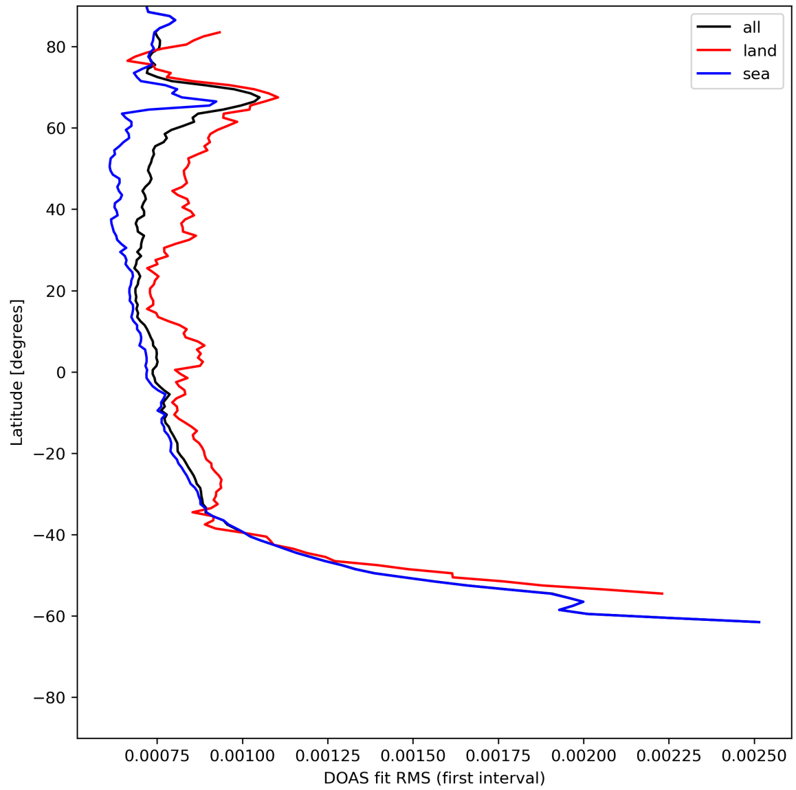
Figure 32: Zonal average of "DOAS fit RMS (first interval)" for 2024-06-13 to 2024-06-14.
