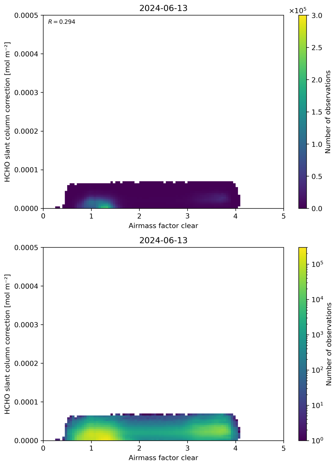
Figure 75: Scatter density plot of “Airmass factor clear” against “HCHO slant column correction” for 2024-06-13 to 2024-06-14.
