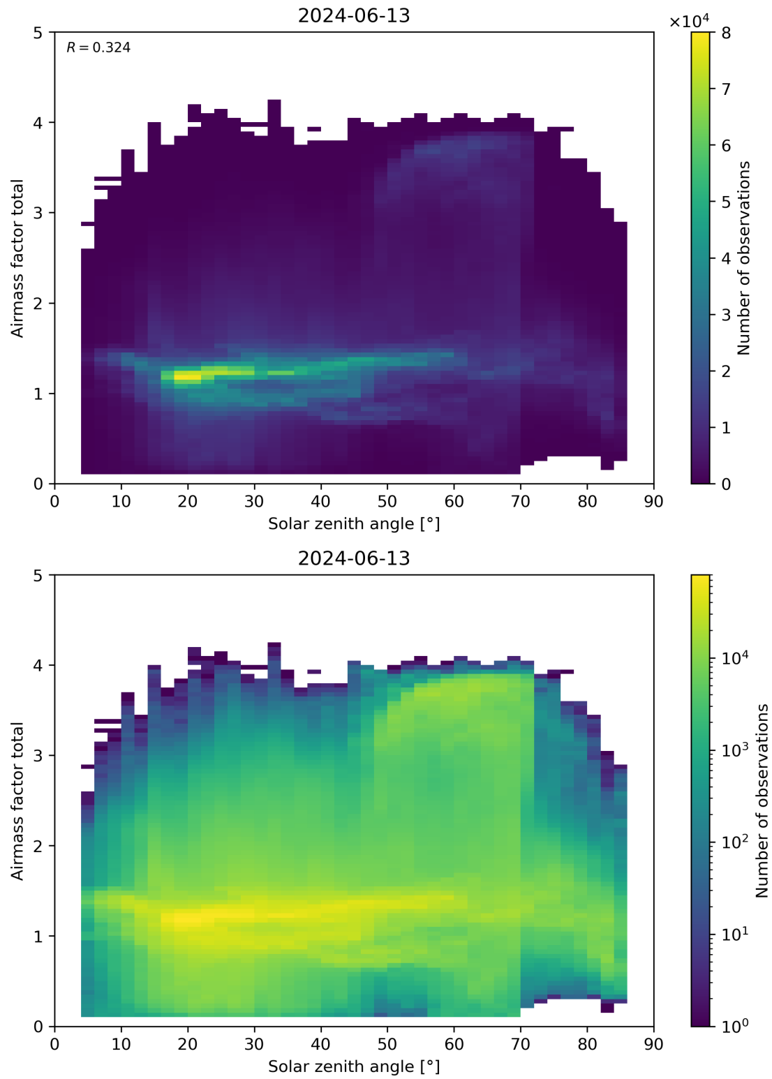
Figure 175: Scatter density plot of “Solar zenith angle” against “Airmass factor total” for 2024-06-13 to 2024-06-14.
