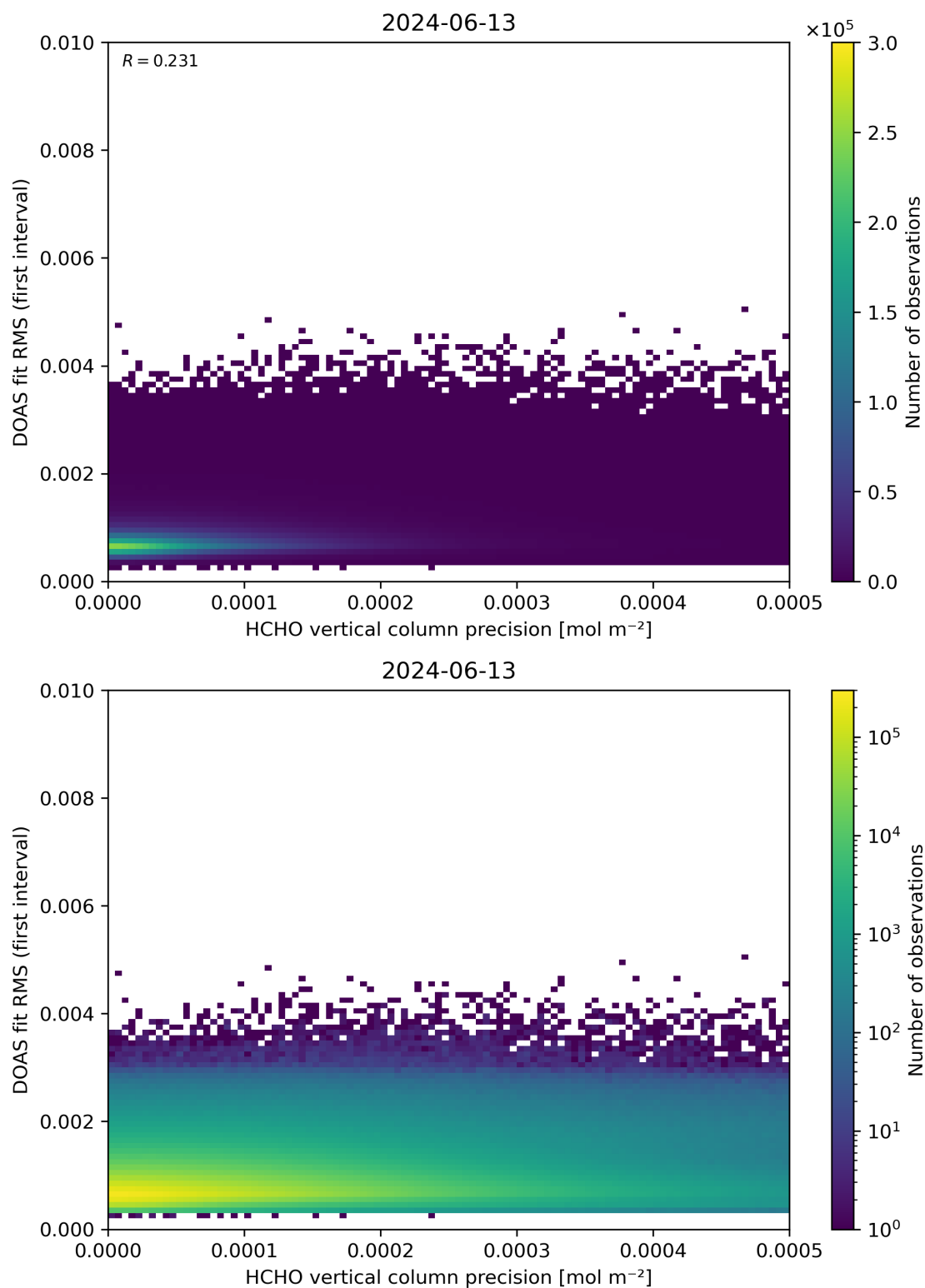
Figure 136: Scatter density plot of “HCHO vertical column precision” against “DOAS fit RMS (first interval)” for 2024-06-13 to 2024-06-14.
