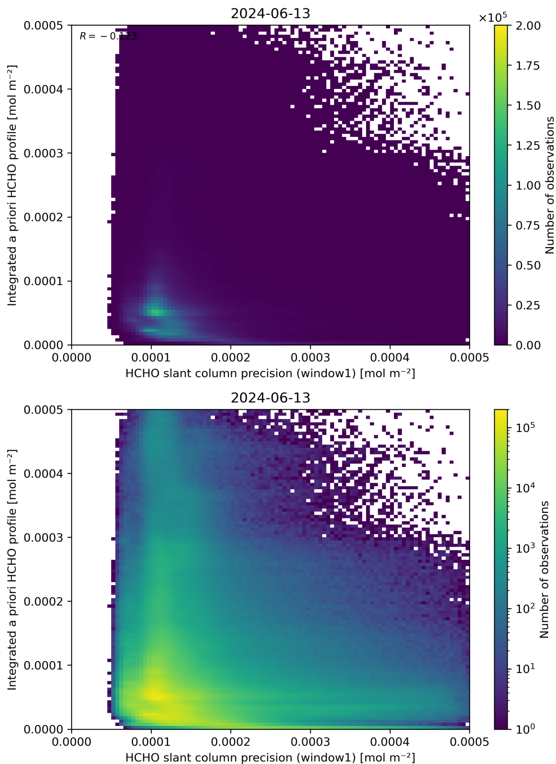
Figure 96: Scatter density plot of “HCHO slant column precision (window1)” against “Integrated a priori HCHO profile” for 2024-06-13 to 2024-06-14.
