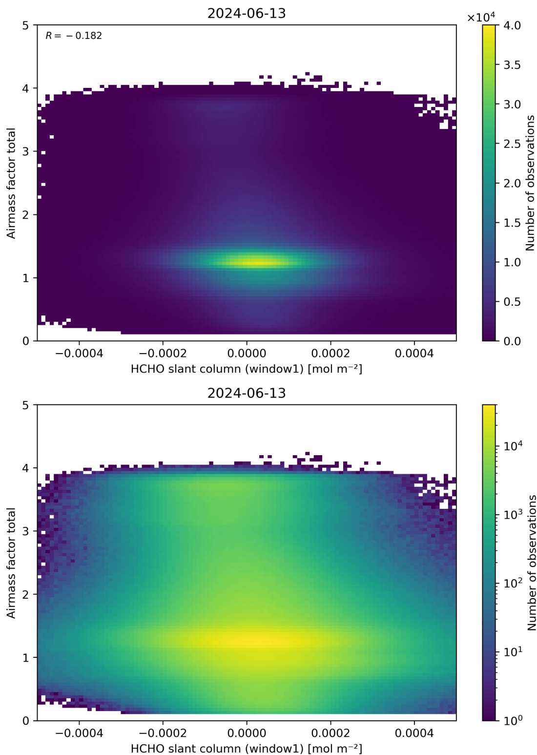
Figure 85: Scatter density plot of “HCHO slant column (window1)” against “Airmass factor total” for 2024-06-13 to 2024-06-14.
