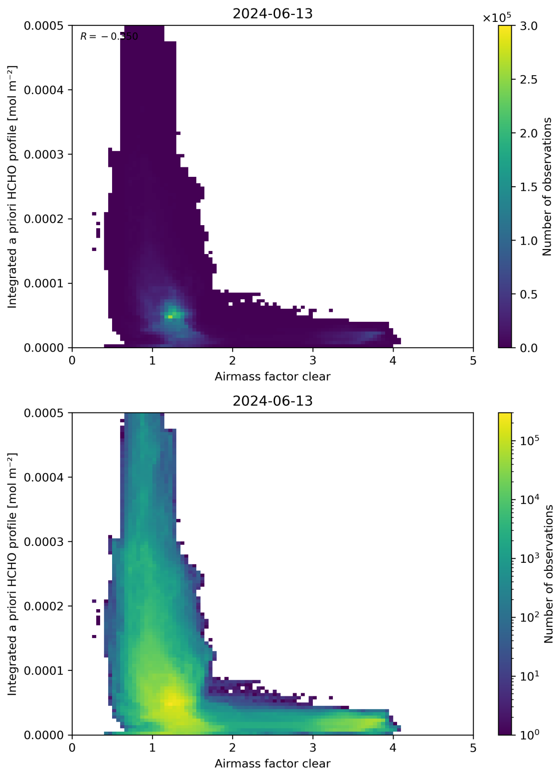
Figure 76: Scatter density plot of “Airmass factor clear” against “Integrated a priori HCHO profile” for 2024-06-13 to 2024-06-14.
