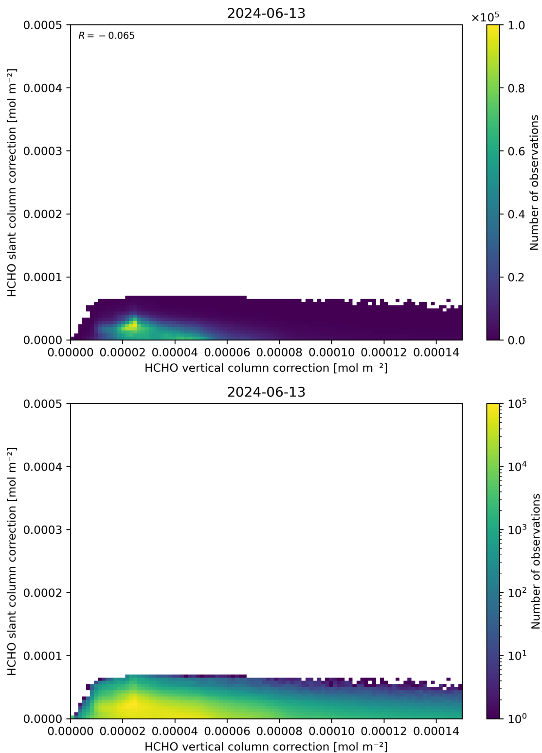
Figure 117: Scatter density plot of “HCHO vertical column correction” against “HCHO slant column correction” for 2024-06-13 to 2024-06-14.
