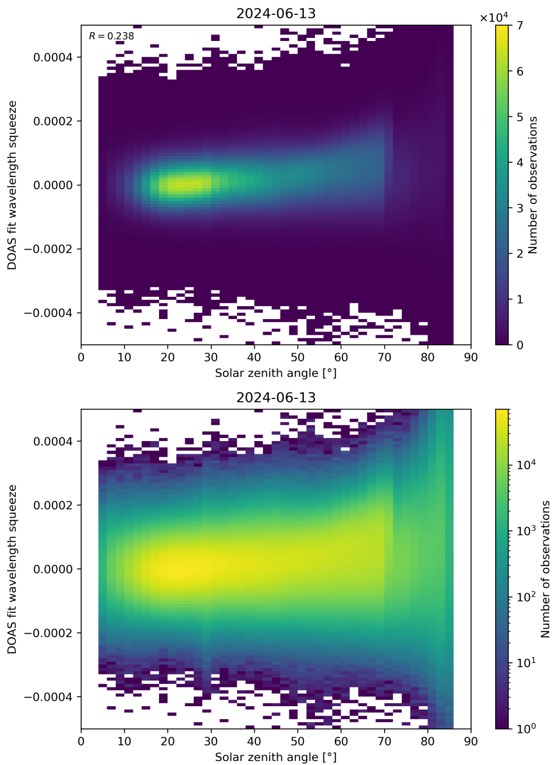
Figure 169: Scatter density plot of “Solar zenith angle” against “DOAS fit wavelength squeeze” for 2024-06-13 to 2024-06-14.
