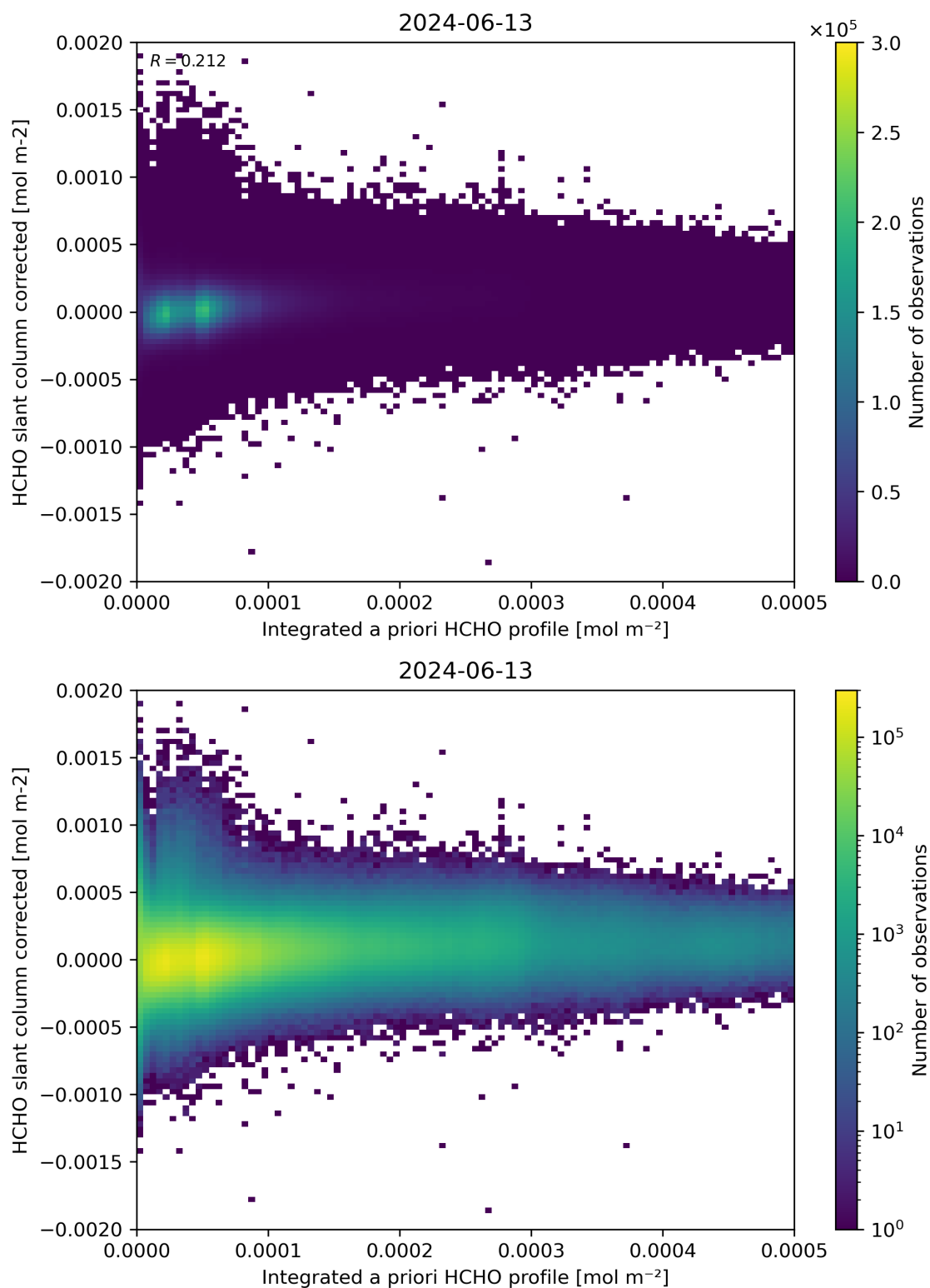
Figure 151: Scatter density plot of “Integrated a priori HCHO profile” against “HCHO slant column corrected” for 2024-06-13 to 2024-06-14.
