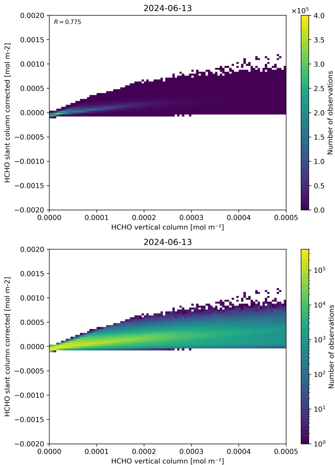
Figure 127: Scatter density plot of “HCHO vertical column” against “HCHO slant column corrected” for 2024-06-13 to 2024-06-14.
