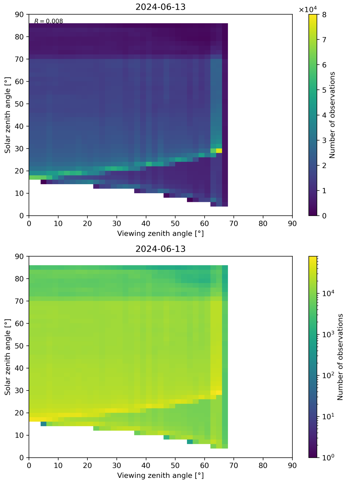
Figure 197: Scatter density plot of “Viewing zenith angle” against “Solar zenith angle” for 2024-06-13 to 2024-06-14.
