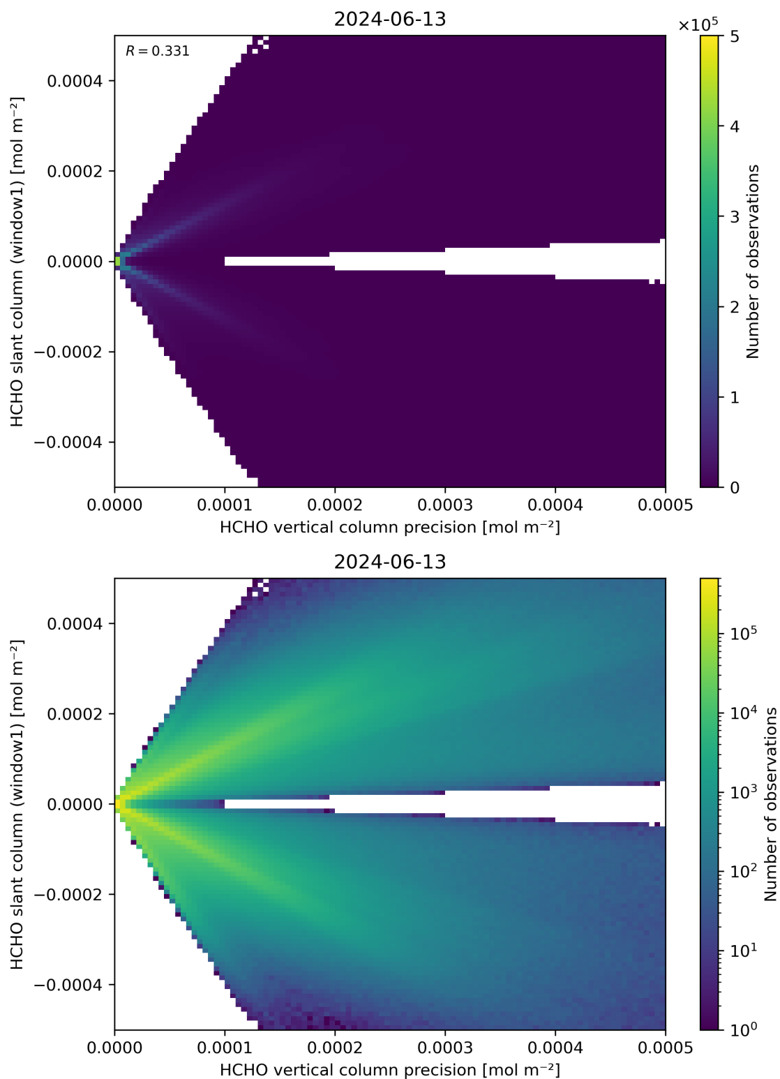
Figure 142: Scatter density plot of “HCHO vertical column precision” against “HCHO slant column (window1)” for 2024-06-13 to 2024-06-14.
