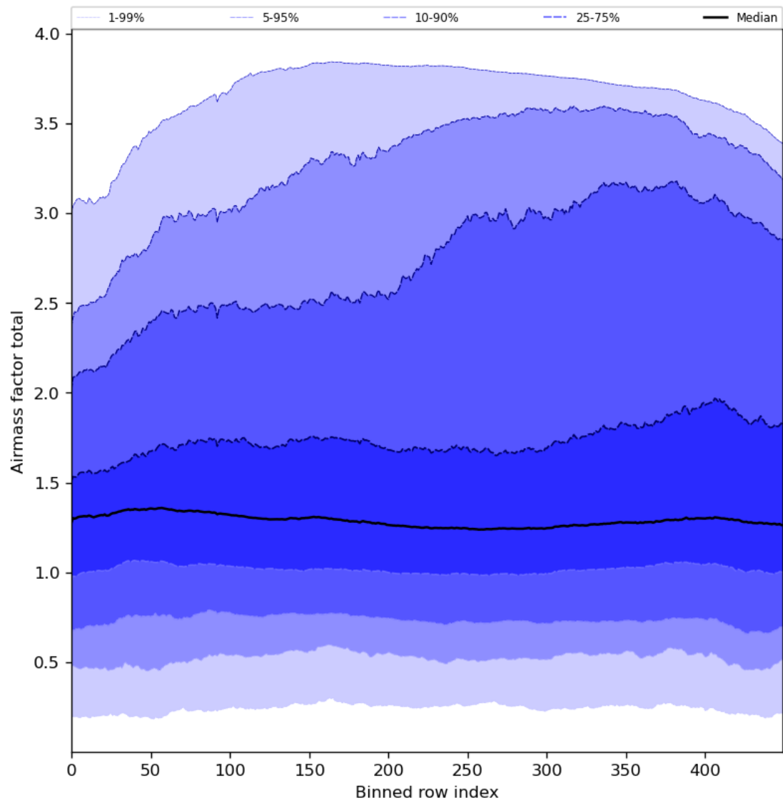
Figure 54: Along track statistics of “Airmass factor total” for 2024-06-13 to 2024-06-14
