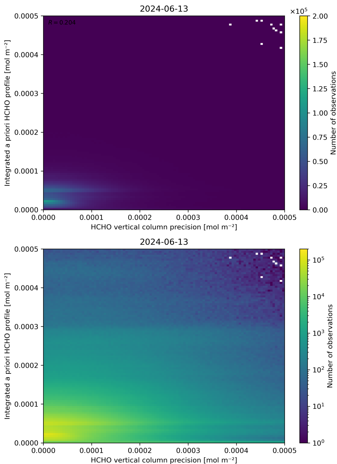
Figure 147: Scatter density plot of “HCHO vertical column precision” against “Integrated a priori HCHO profile” for 2024-06-13 to 2024-06-14.
