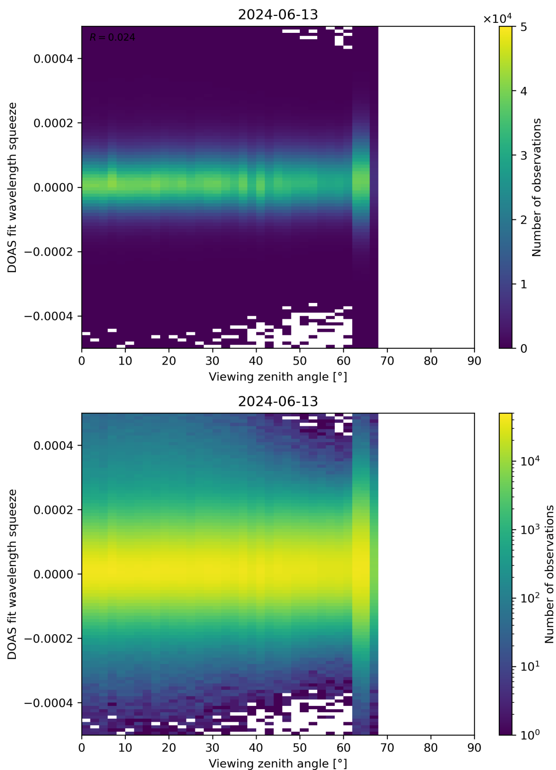
Figure 184: Scatter density plot of “Viewing zenith angle” against “DOAS fit wavelength squeeze” for 2024-06-13 to 2024-06-14.
