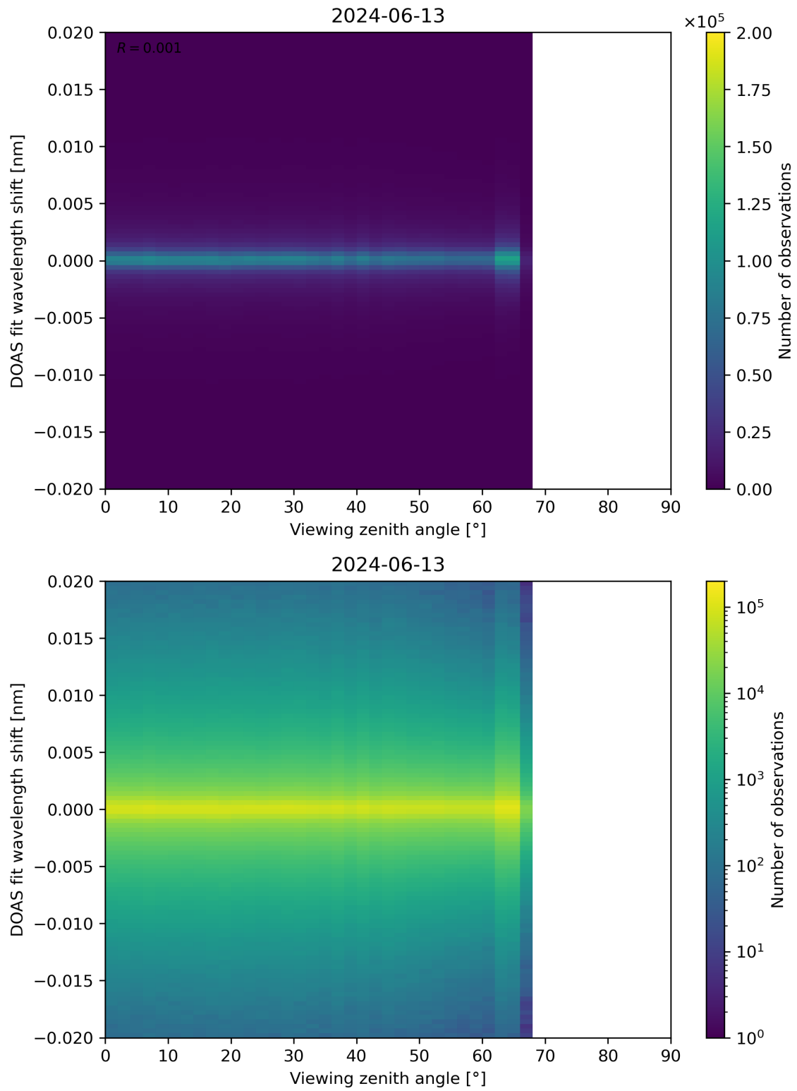
Figure 183: Scatter density plot of “Viewing zenith angle” against “DOAS fit wavelength shift” for 2024-06-13 to 2024-06-14.
