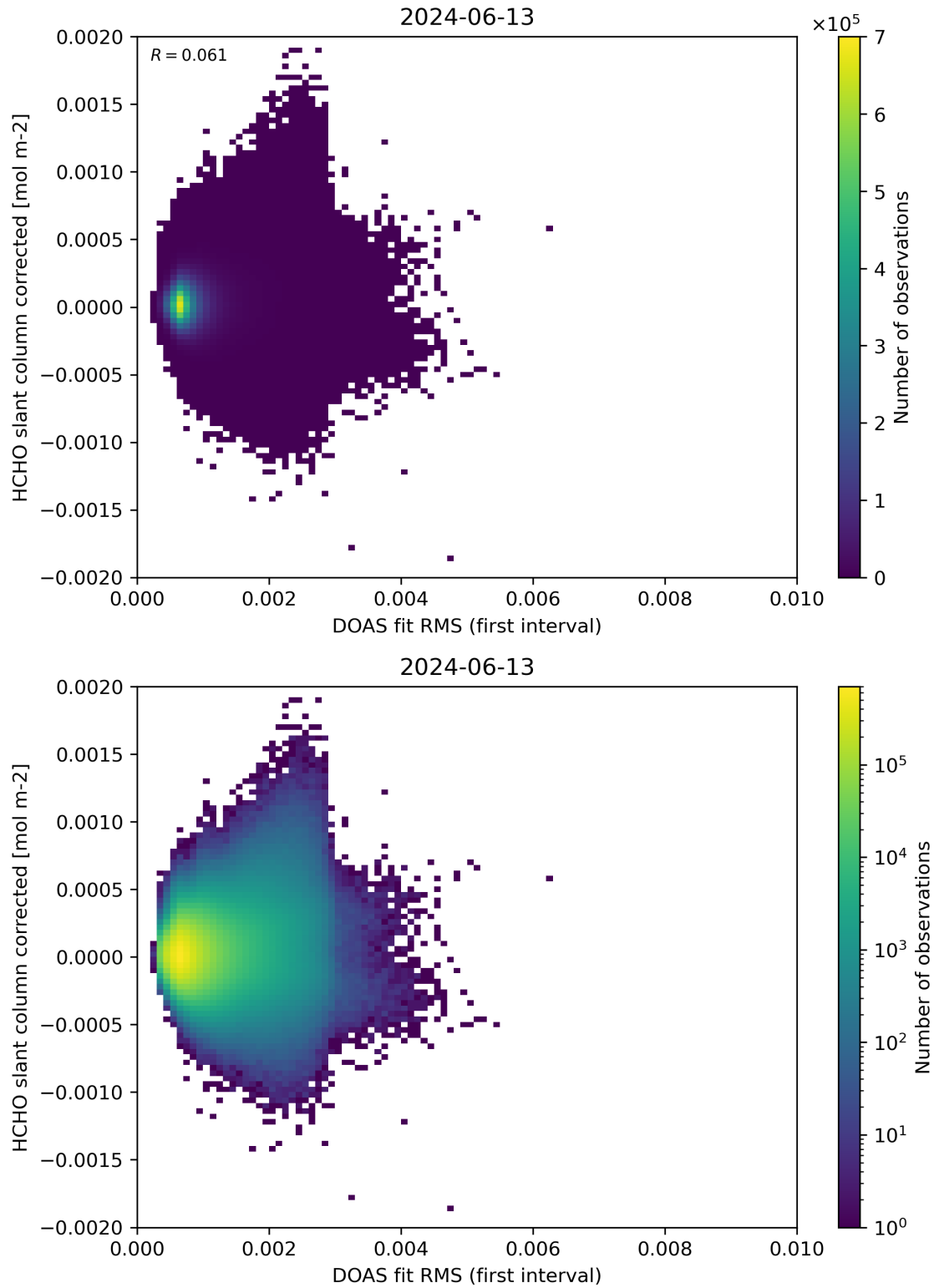
Figure 62: Scatter density plot of “DOAS fit RMS (first interval)” against “HCHO slant column corrected” for 2024-06-13 to 2024-06-14.
