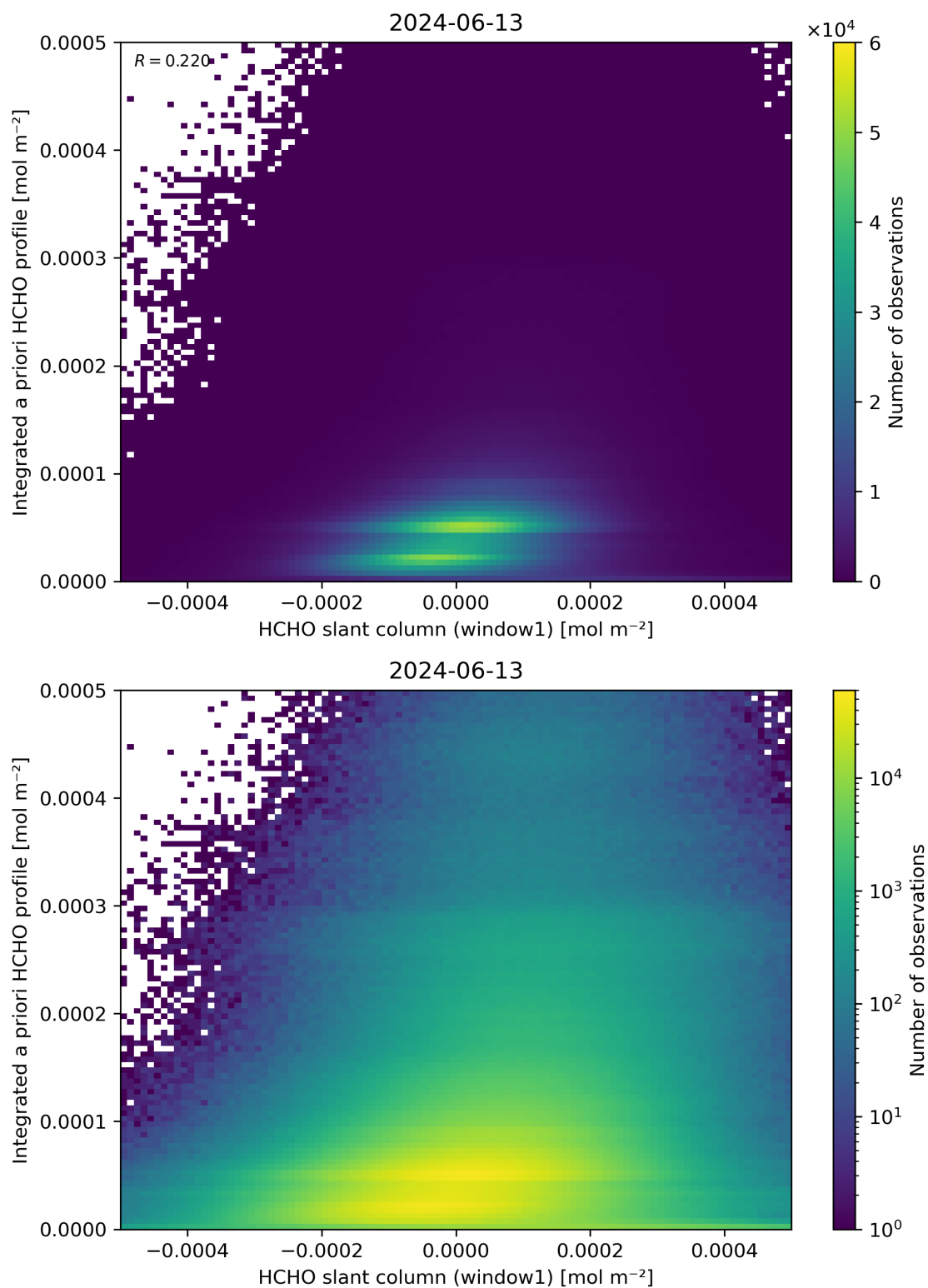
Figure 87: Scatter density plot of “HCHO slant column (window1)” against “Integrated a priori HCHO profile” for 2024-06-13 to 2024-06-14.
