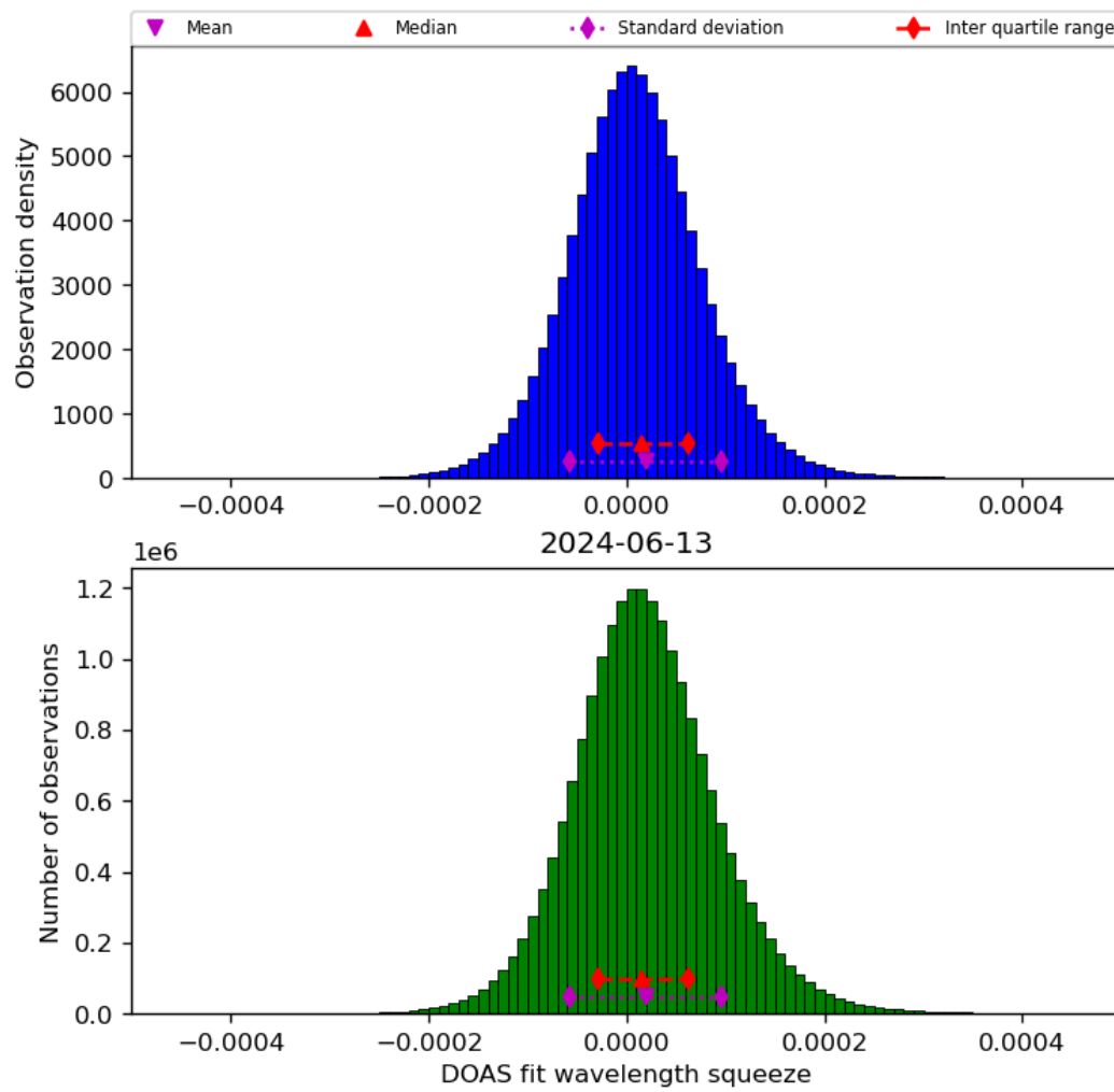
Figure 45: Histogram of “DOAS fit wavelength squeeze” for 2024-06-13 to 2024-06-14
