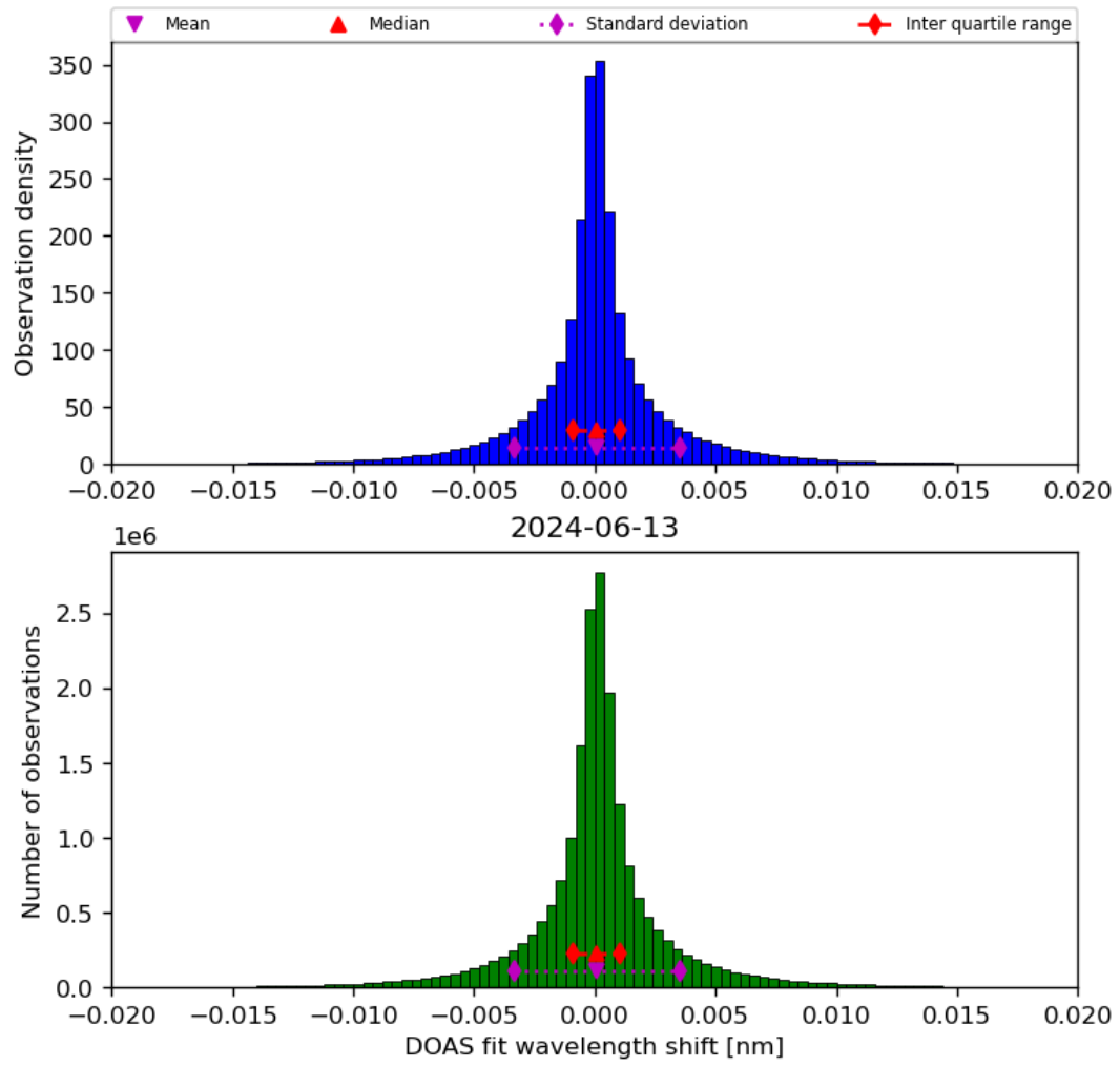
Figure 44: Histogram of “DOAS fit wavelength shift” for 2024-06-13 to 2024-06-14
