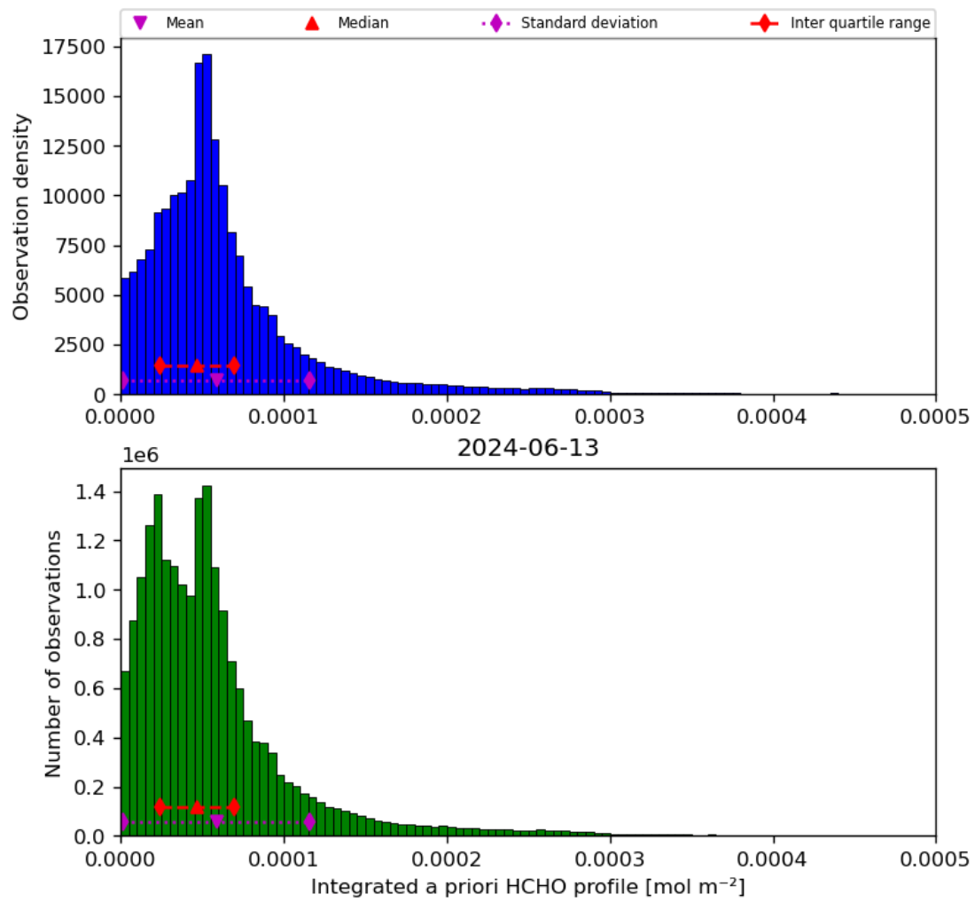
Figure 43: Histogram of “Integrated a priori HCHO profile” for 2024-06-13 to 2024-06-14
