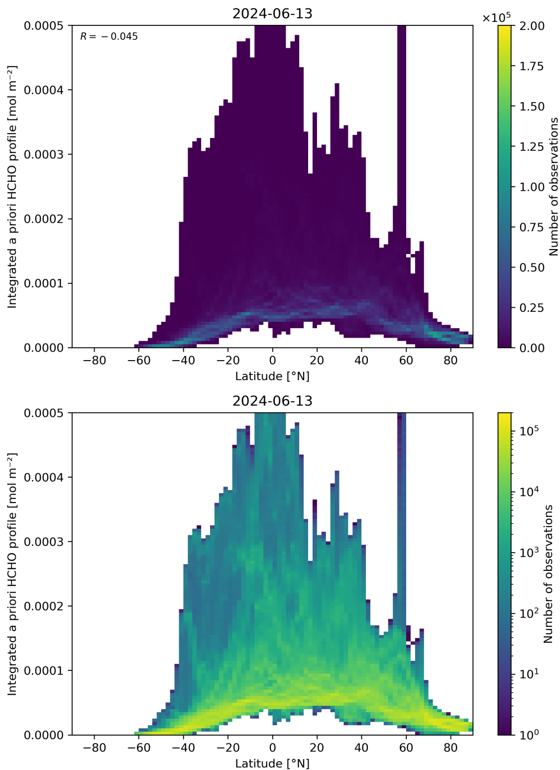
Figure 166: Scatter density plot of “Latitude” against “Integrated a priori HCHO profile” for 2024-06-13 to 2024-06-14.
