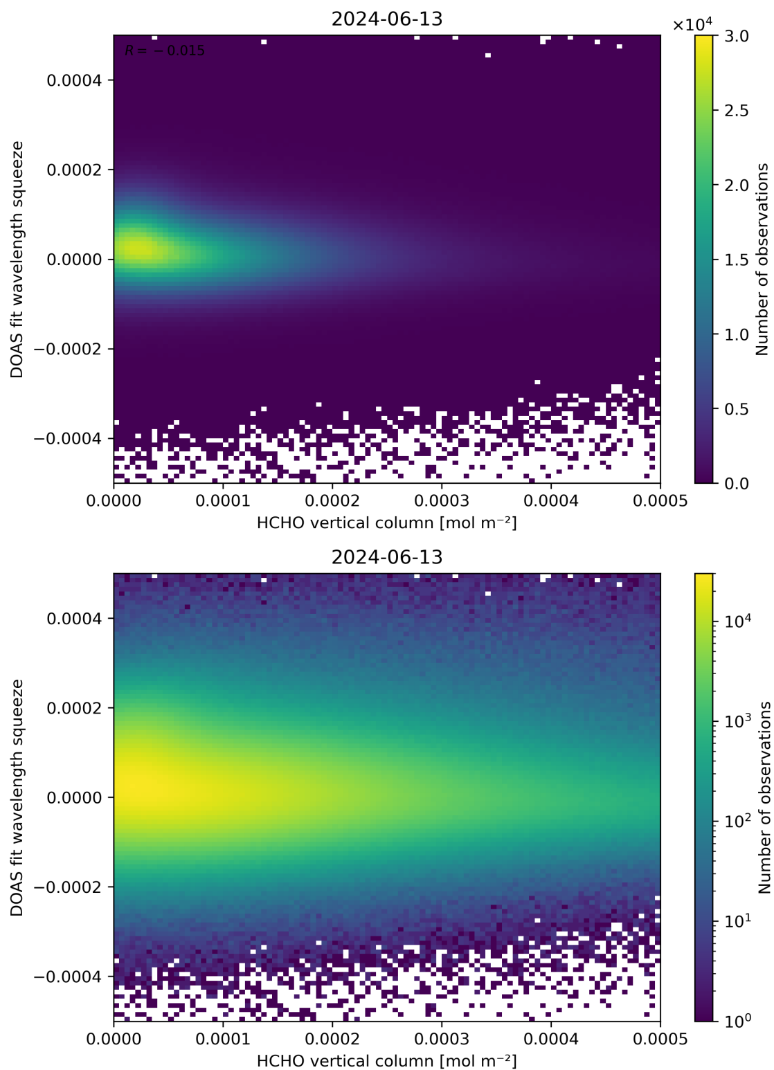
Figure 125: Scatter density plot of “HCHO vertical column” against “DOAS fit wavelength squeeze” for 2024-06-13 to 2024-06-14.
