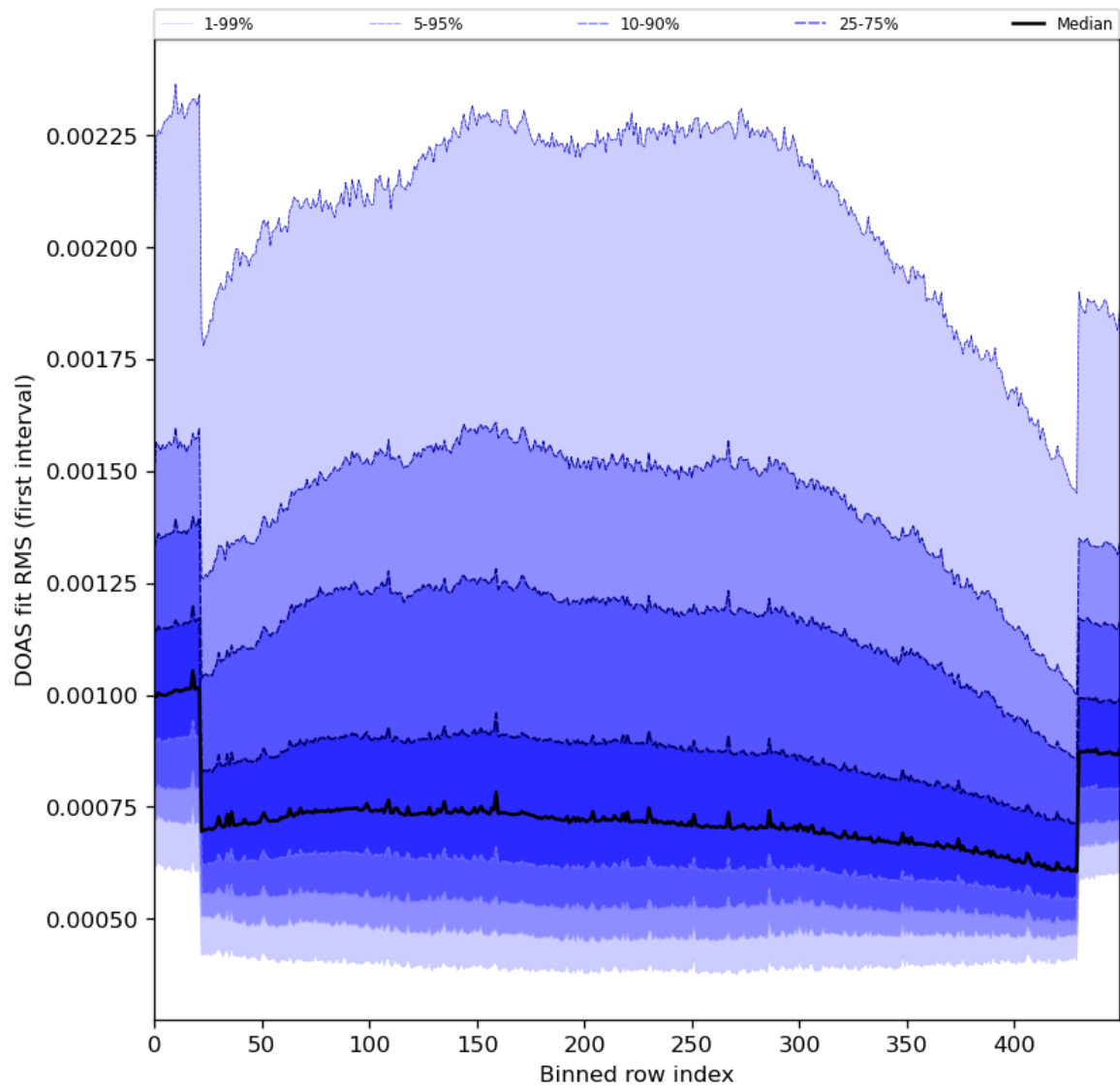
Figure 60: Along track statistics of “DOAS fit RMS (first interval)” for 2024-06-13 to 2024-06-14
