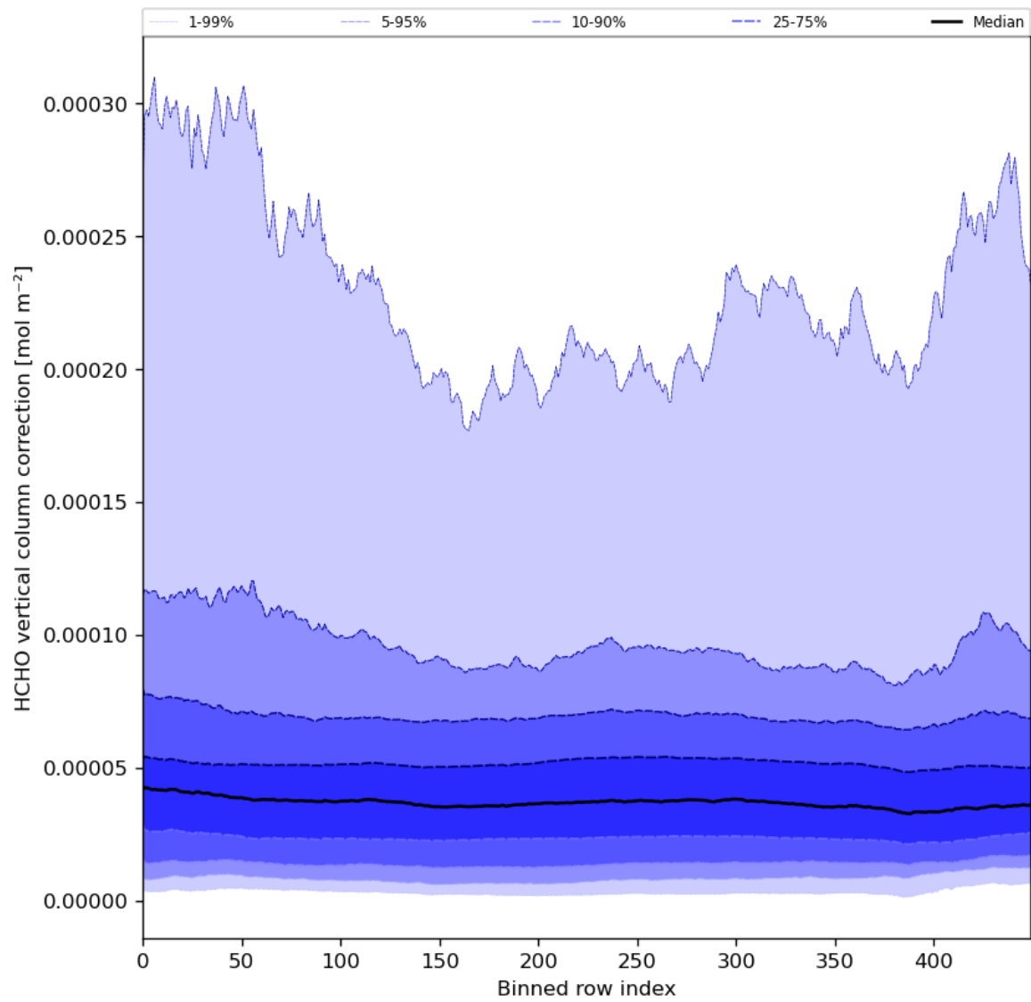
Figure 51: Along track statistics of “HCHO vertical column correction” for 2024-06-13 to 2024-06-14
