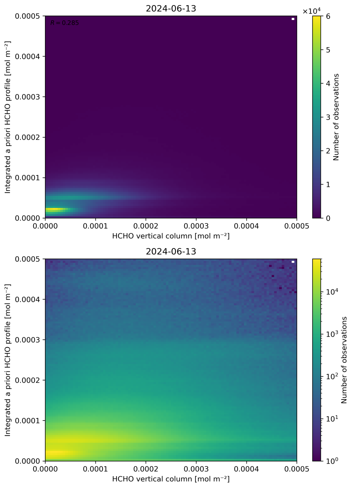
Figure 135: Scatter density plot of “HCHO vertical column” against “Integrated a priori HCHO profile” for 2024-06-13 to 2024-06-14.
