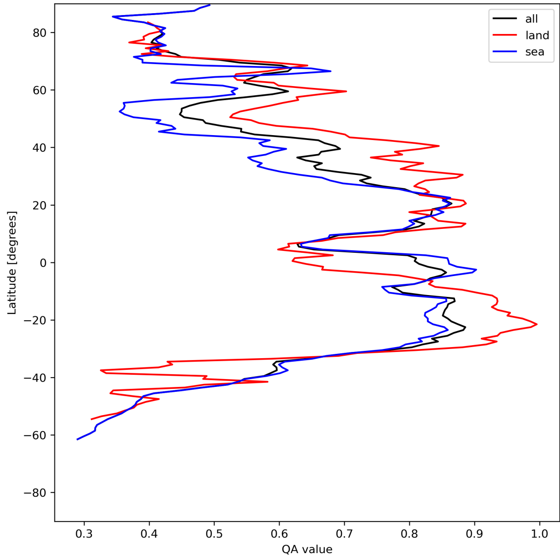
Figure 20: Zonal average of “QA value” for 2024-06-13 to 2024-06-14.
