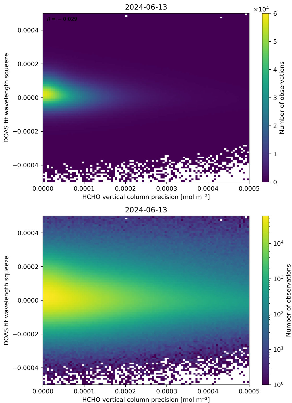
Figure 138: Scatter density plot of “HCHO vertical column precision” against “DOAS fit wavelength squeeze” for 2024-06-13 to 2024-06-14.
