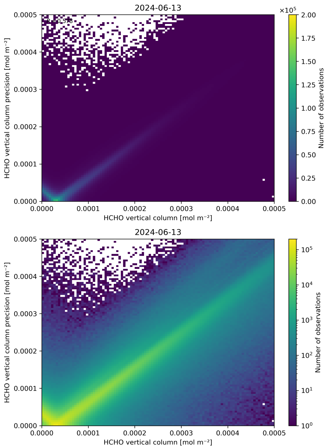
Figure 134: Scatter density plot of “HCHO vertical column” against “HCHO vertical column precision” for 2024-06-13 to 2024-06-14.
