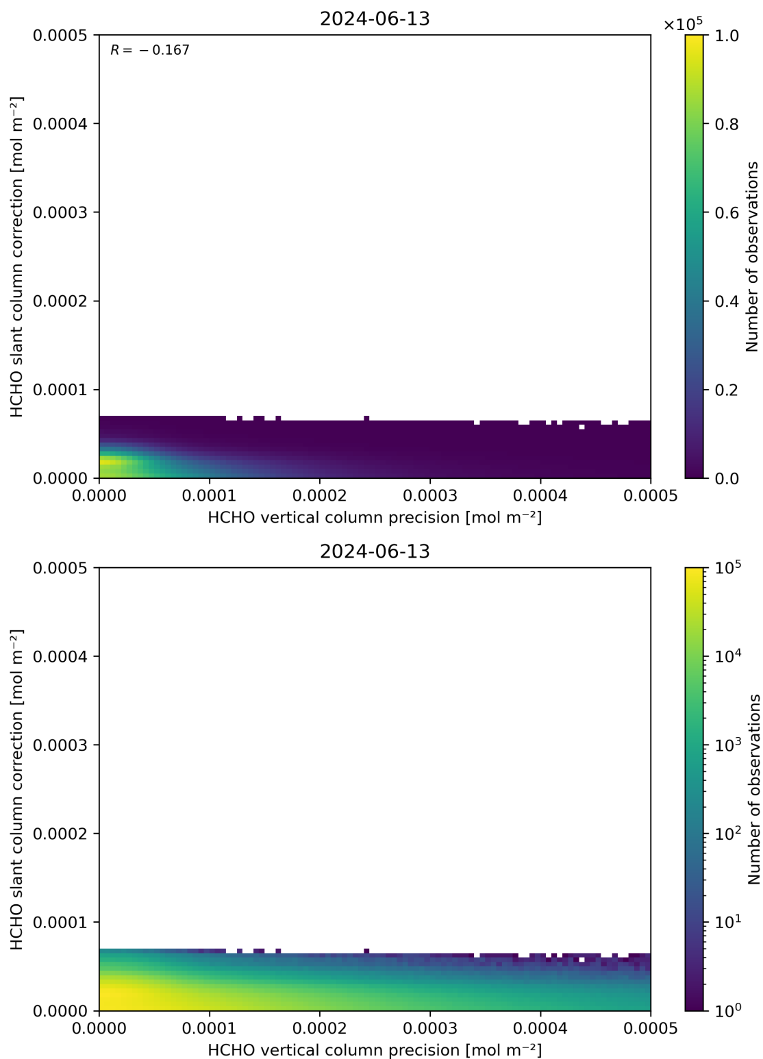
Figure 141: Scatter density plot of “HCHO vertical column precision” against “HCHO slant column correction” for 2024-06-13 to 2024-06-14.
