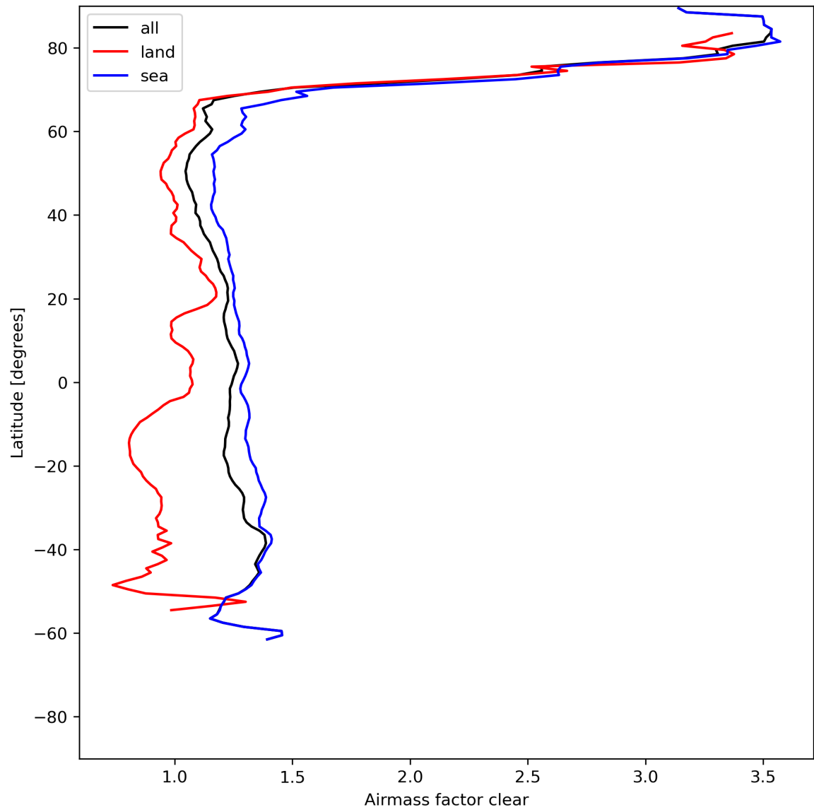
Figure 28: Zonal average of “Airmass factor clear” for 2024-06-13 to 2024-06-14.
