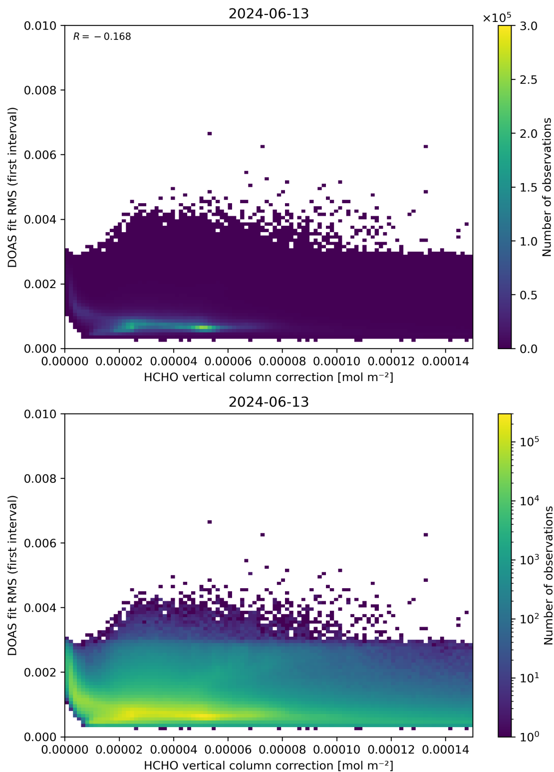
Figure 112: Scatter density plot of “HCHO vertical column correction” against “DOAS fit RMS (first interval)” for 2024-06-13 to 2024-06-14.
