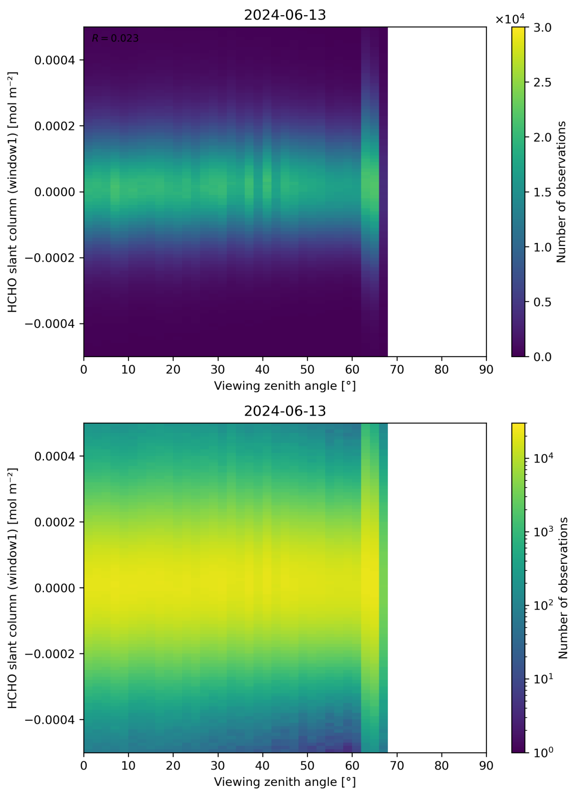
Figure 188: Scatter density plot of “Viewing zenith angle” against “HCHO slant column (window1)” for 2024-06-13 to 2024-06-14.
