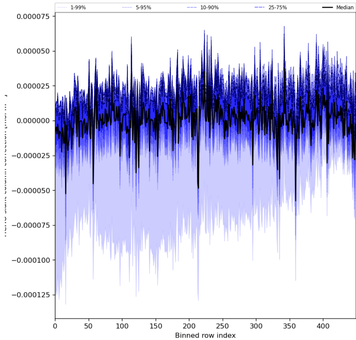
Figure 61: Along track statistics of “HCHO slant column correction” for 2024-06-13 to 2024-06-14
