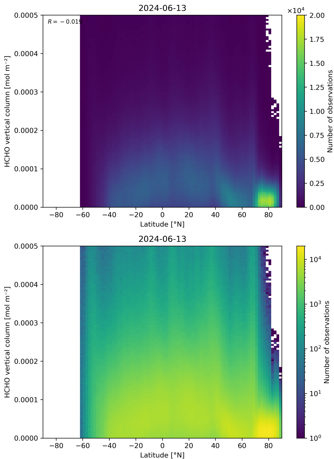
Figure 163: Scatter density plot of “Latitude” against “HCHO vertical column” for 2024-06-13 to 2024-06-14.
