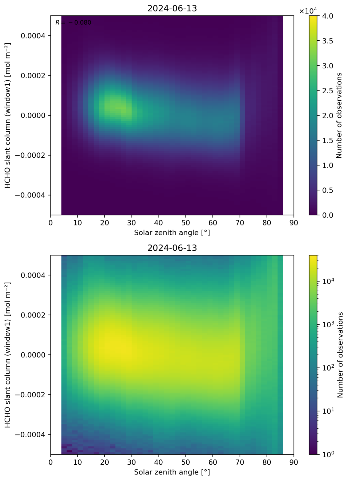
Figure 173: Scatter density plot of “Solar zenith angle” against “HCHO slant column (window1)” for 2024-06-13 to 2024-06-14.
