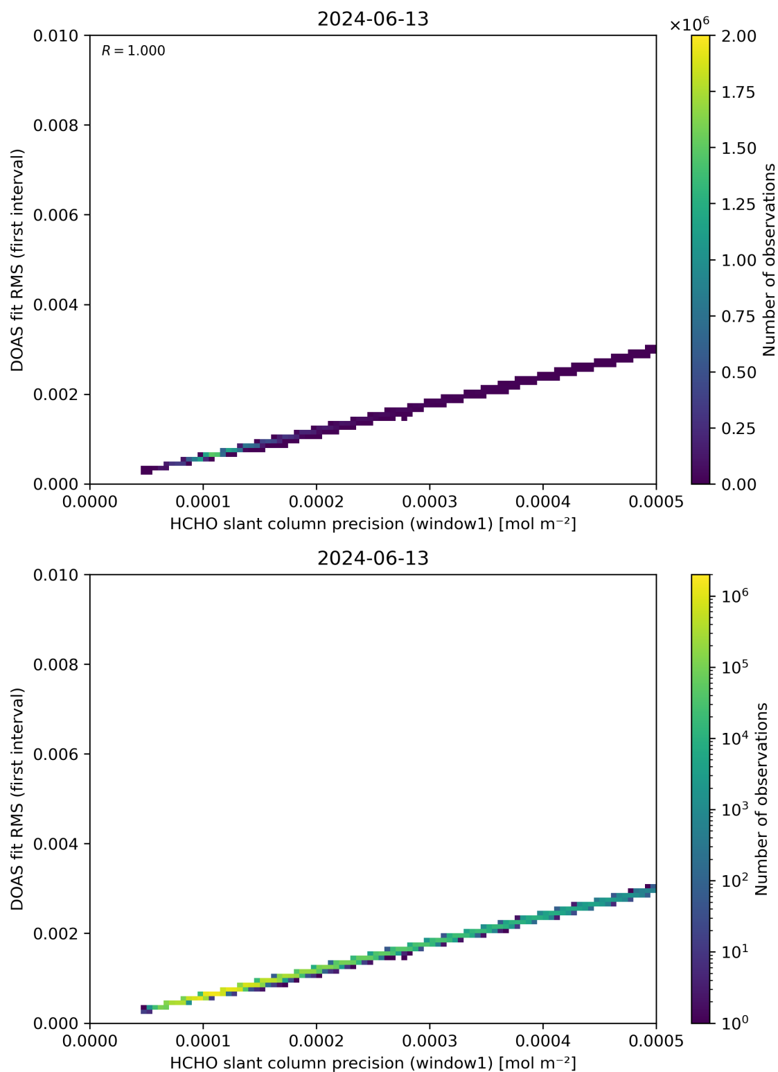
Figure 88: Scatter density plot of “HCHO slant column precision (window1)” against “DOAS fit RMS (first interval)” for 2024-06-13 to 2024-06-14.
