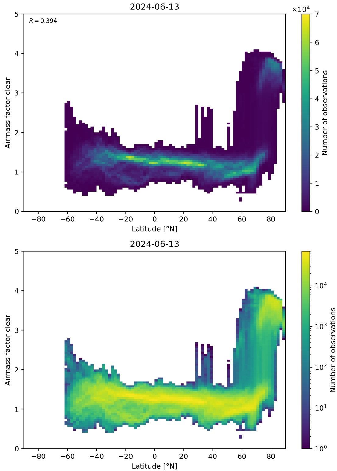
Figure 156: Scatter density plot of “Latitude” against “Airmass factor clear” for 2024-06-13 to 2024-06-14.
