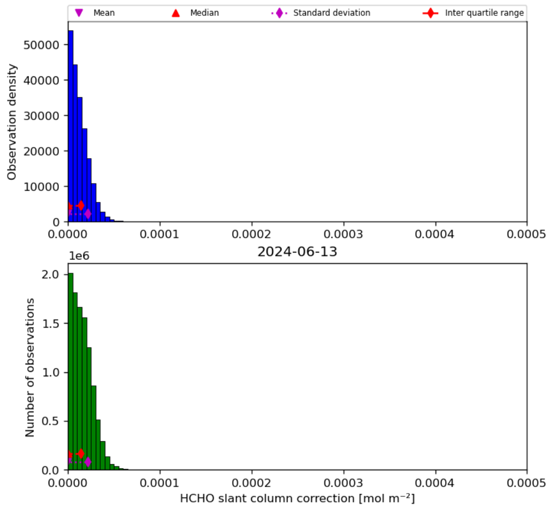
Figure 47: Histogram of “HCHO slant column correction” for 2024-06-13 to 2024-06-14
