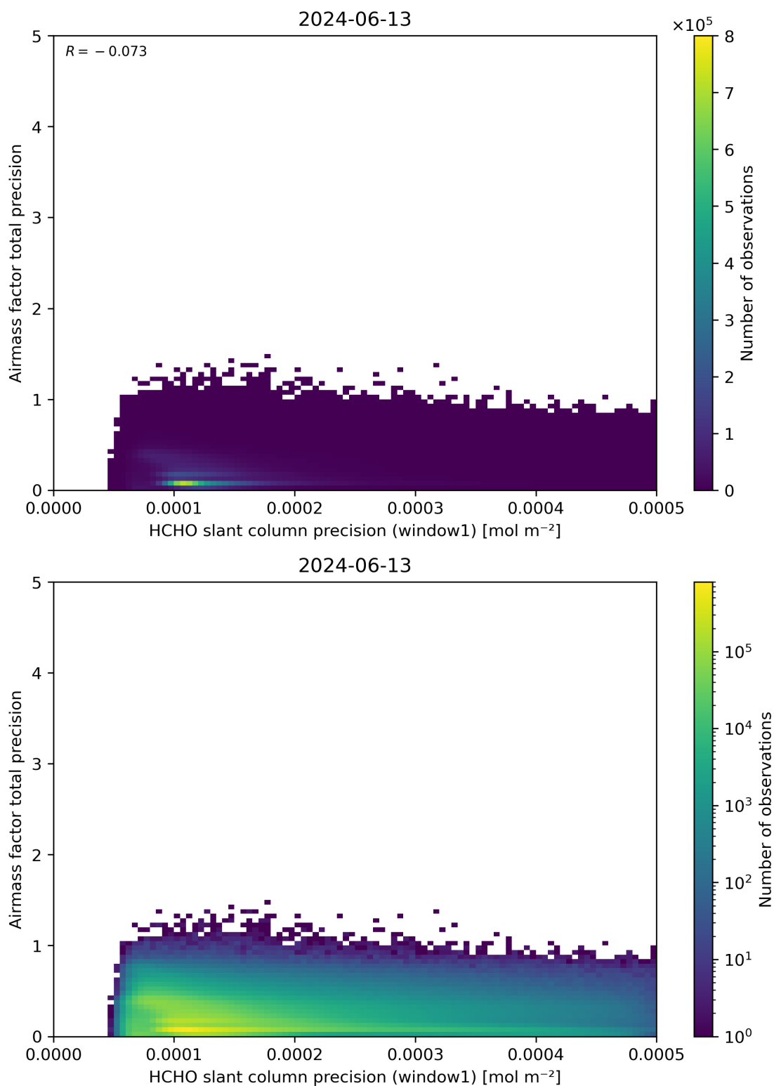
Figure 95: Scatter density plot of “HCHO slant column precision (window1)” against “Airmass factor total precision” for 2024-06-13 to 2024-06-14.
