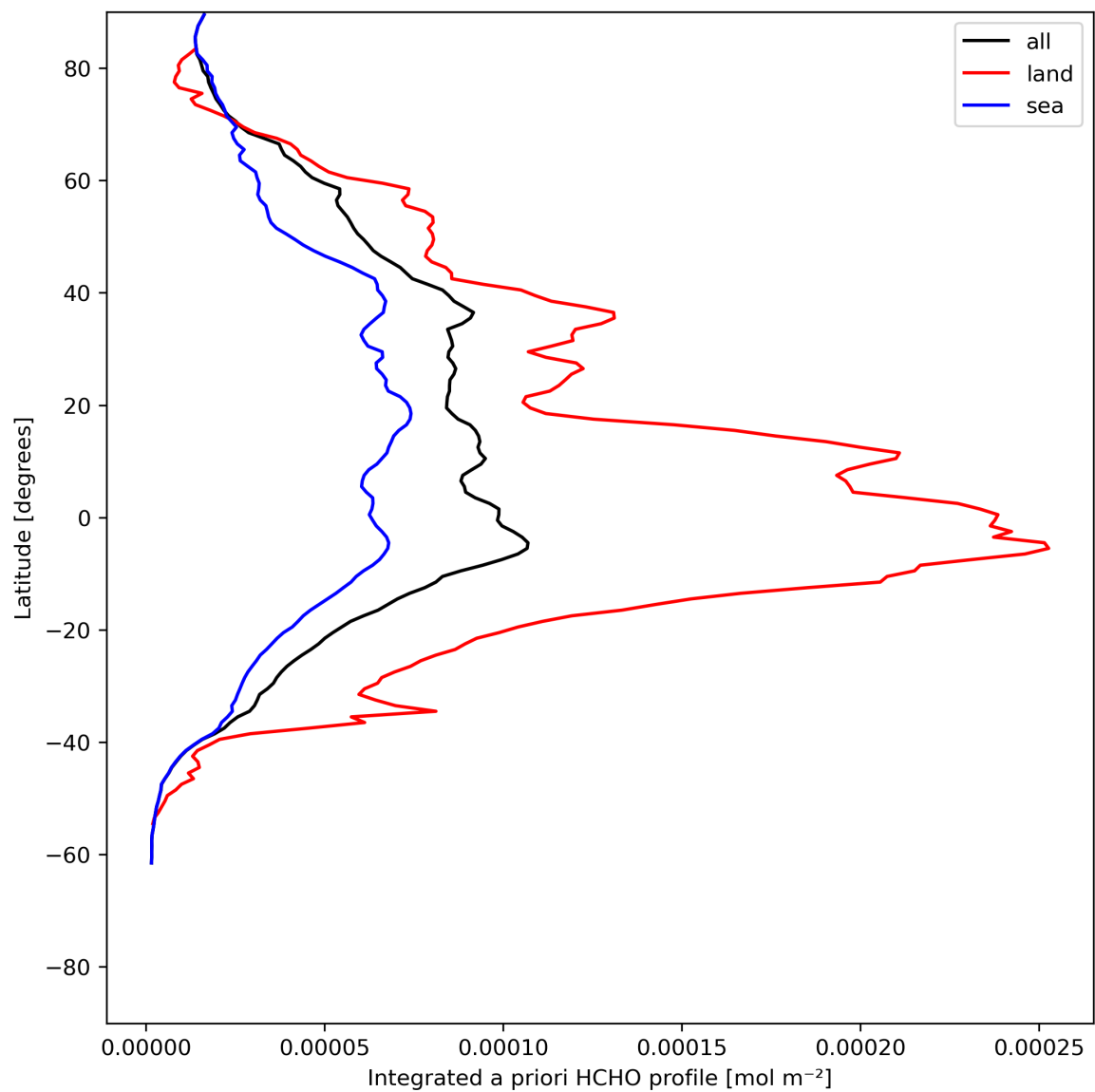
Figure 29: Zonal average of “Integrated a priori HCHO profile” for 2024-06-13 to 2024-06-14.
