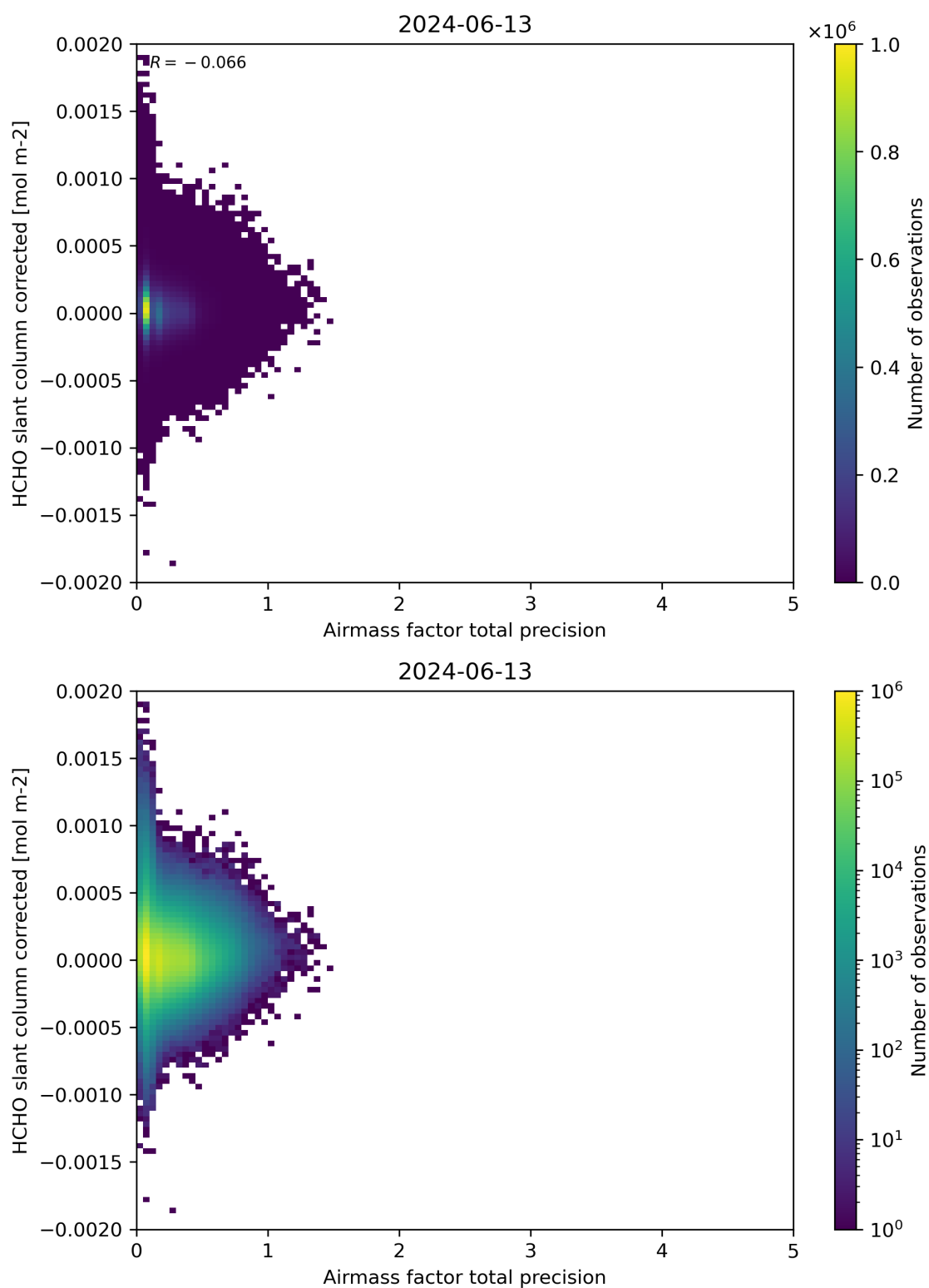
Figure 109: Scatter density plot of “Airmass factor total precision” against “HCHO slant column corrected” for 2024-06-13 to 2024-06-14.
