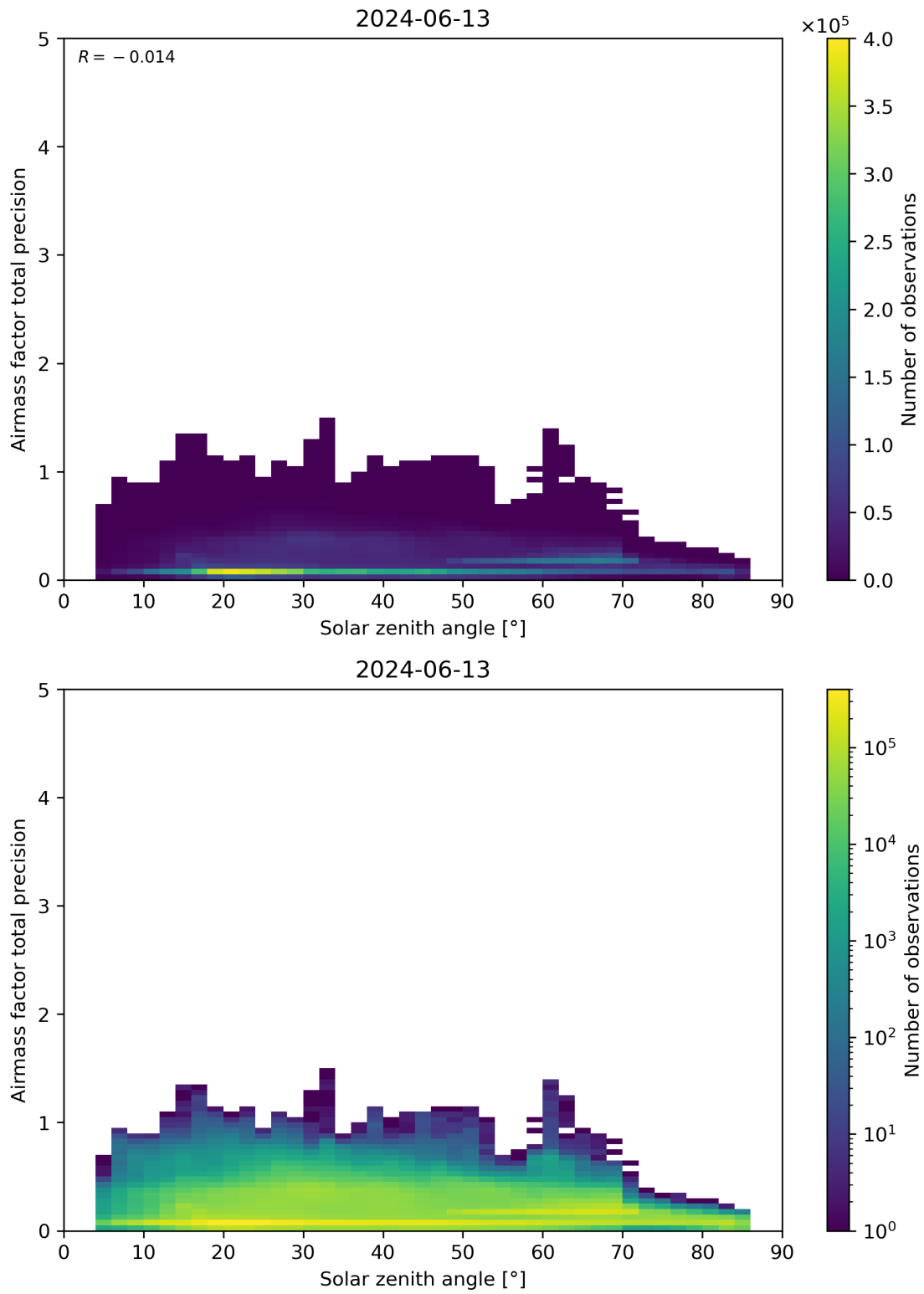
Figure 176: Scatter density plot of “Solar zenith angle” against “Airmass factor total precision” for 2024-06-13 to 2024-06-14.
