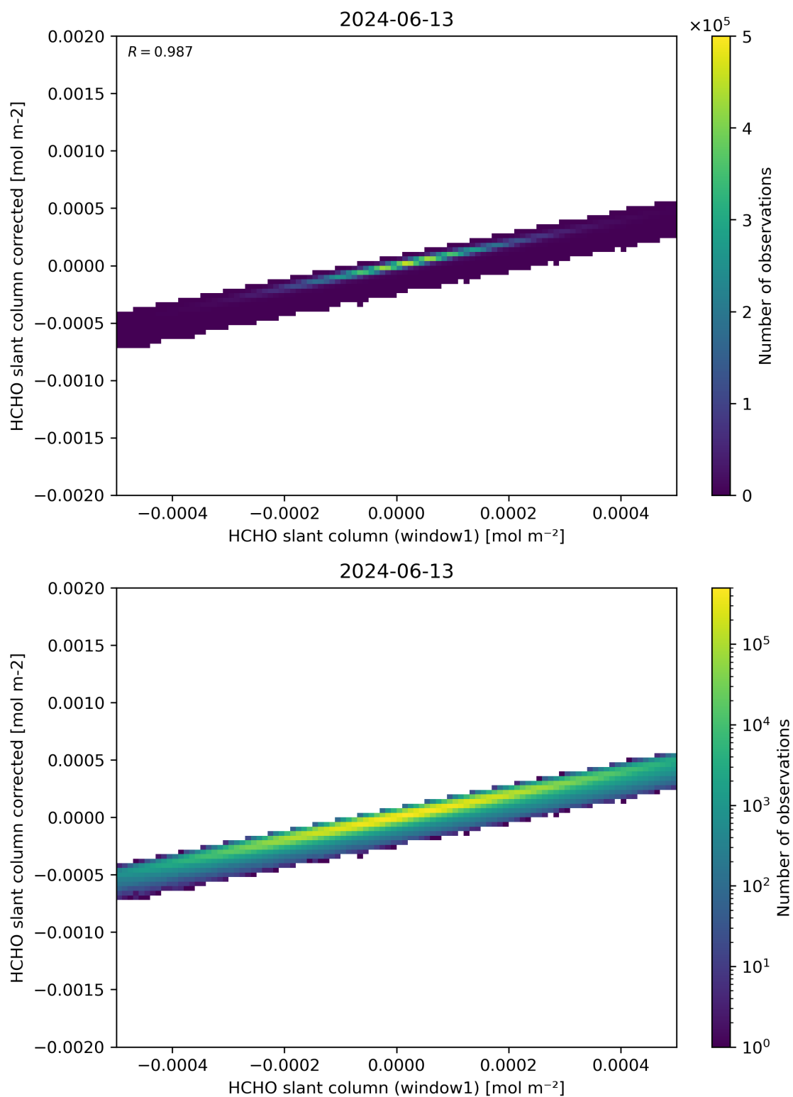
Figure 82: Scatter density plot of “HCHO slant column (window1)” against “HCHO slant column corrected” for 2024-06-13 to 2024-06-14.
