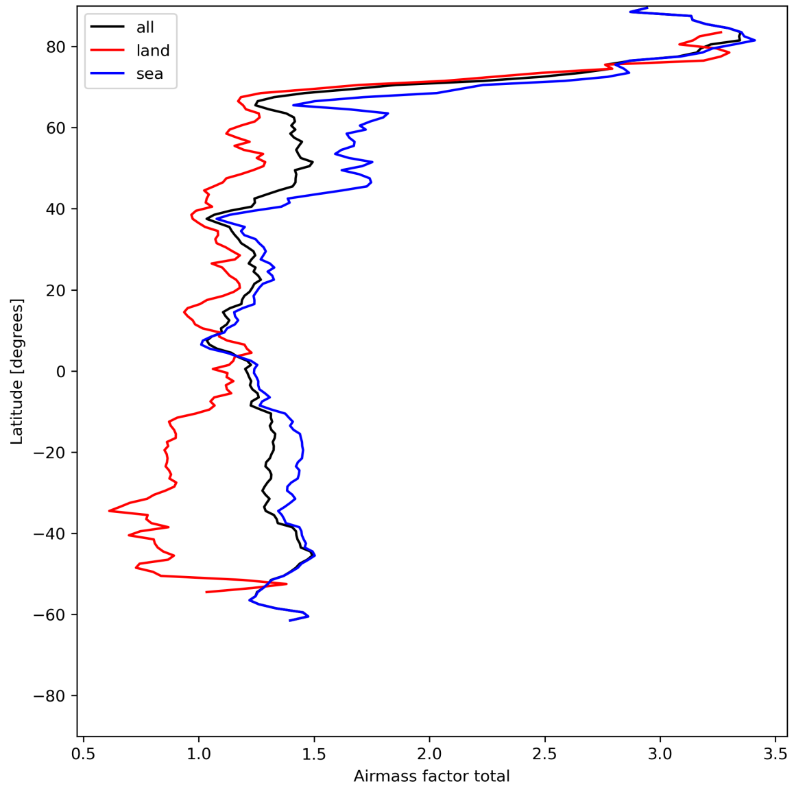
Figure 26: Zonal average of “Airmass factor total” for 2024-06-13 to 2024-06-14.
