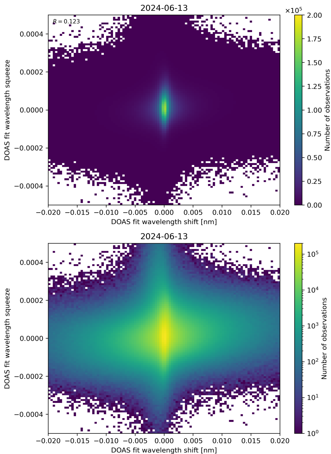
Figure 65: Scatter density plot of “DOAS fit wavelength shift” against “DOAS fit wavelength squeeze” for 2024-06-13 to 2024-06-14.
