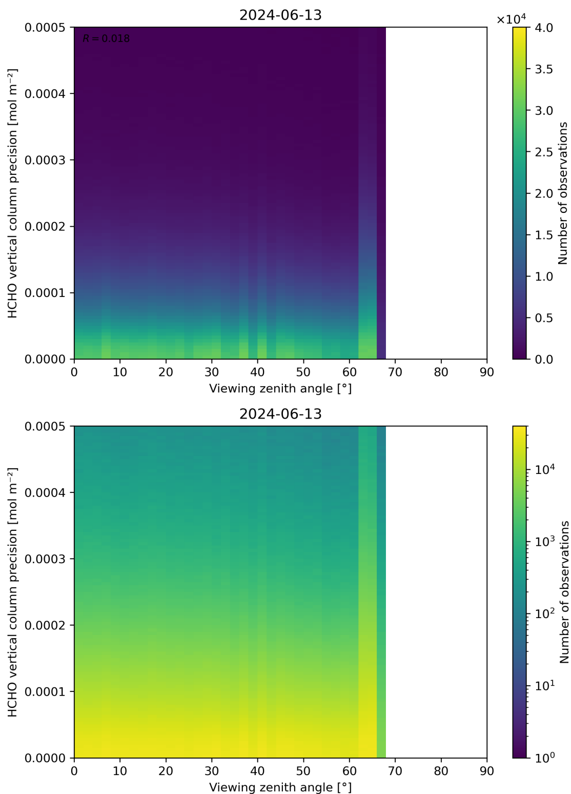
Figure 194: Scatter density plot of “Viewing zenith angle” against “HCHO vertical column precision” for 2024-06-13 to 2024-06-14.
