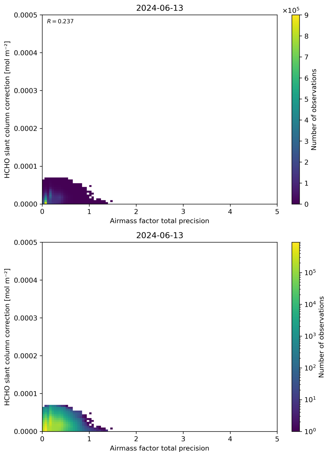
Figure 110: Scatter density plot of “Airmass factor total precision” against “HCHO slant column correction” for 2024-06-13 to 2024-06-14.
