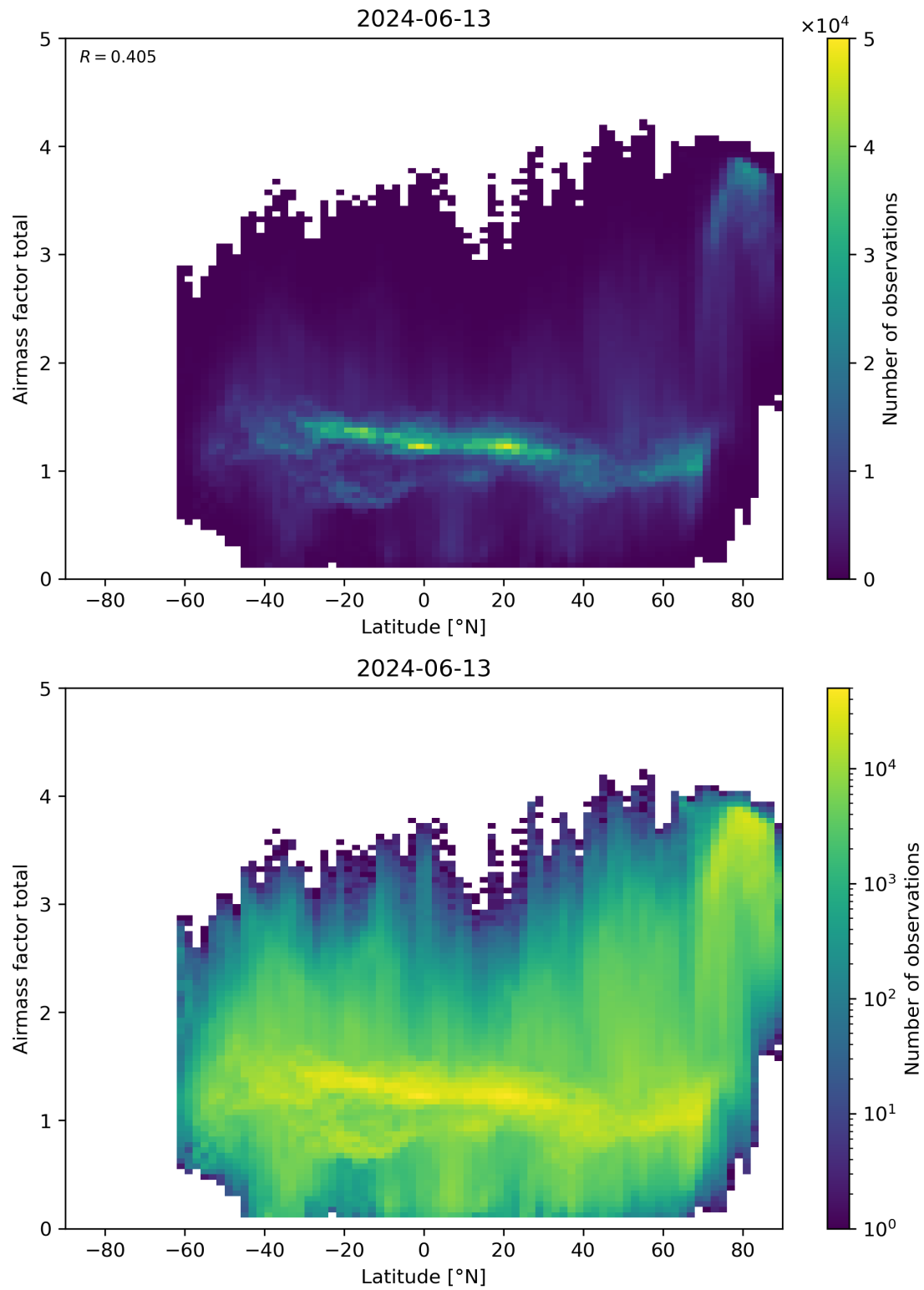
Figure 161: Scatter density plot of “Latitude” against “Airmass factor total” for 2024-06-13 to 2024-06-14.
