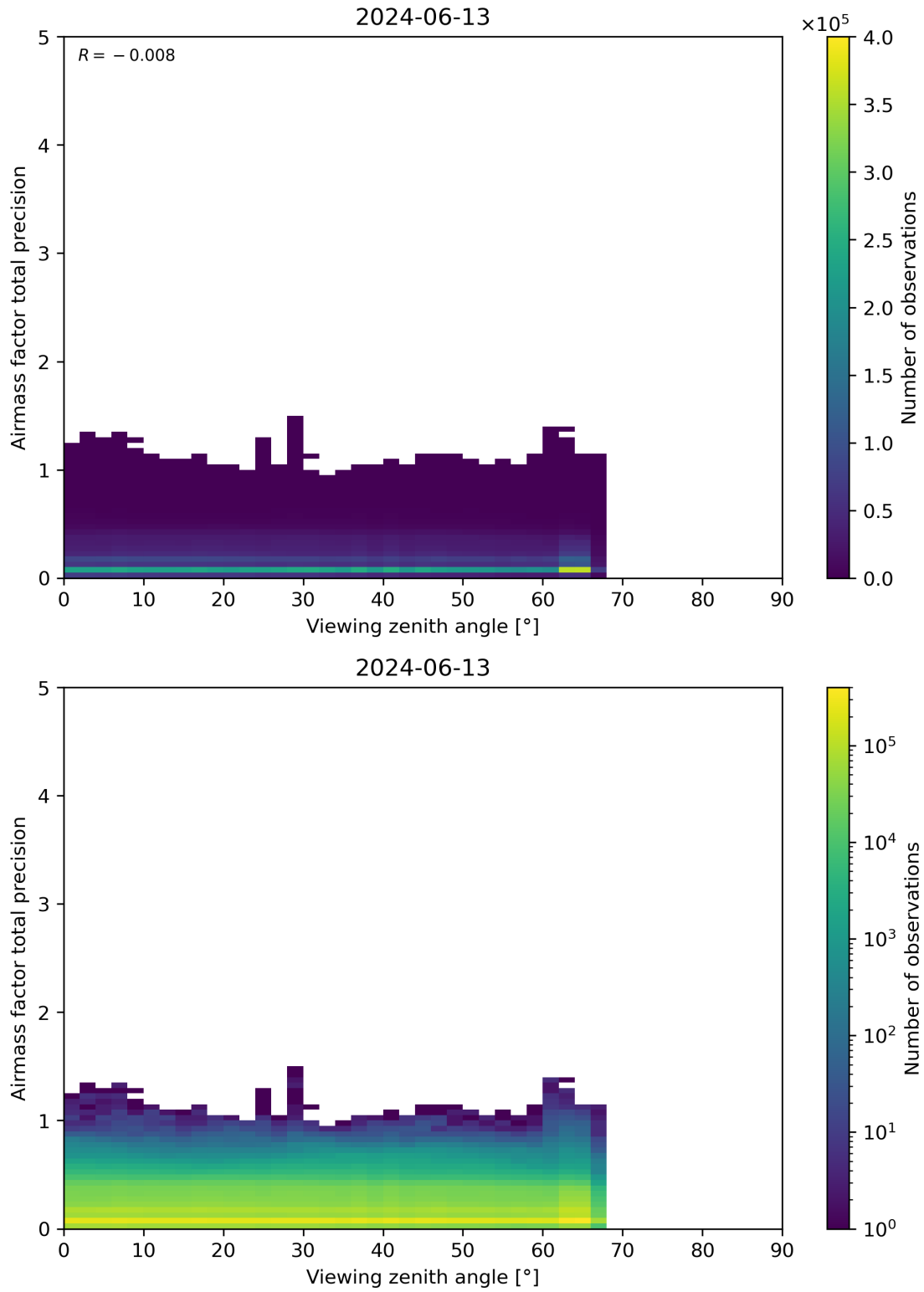
Figure 191: Scatter density plot of “Viewing zenith angle” against “Airmass factor total precision” for 2024-06-13 to 2024-06-14.
