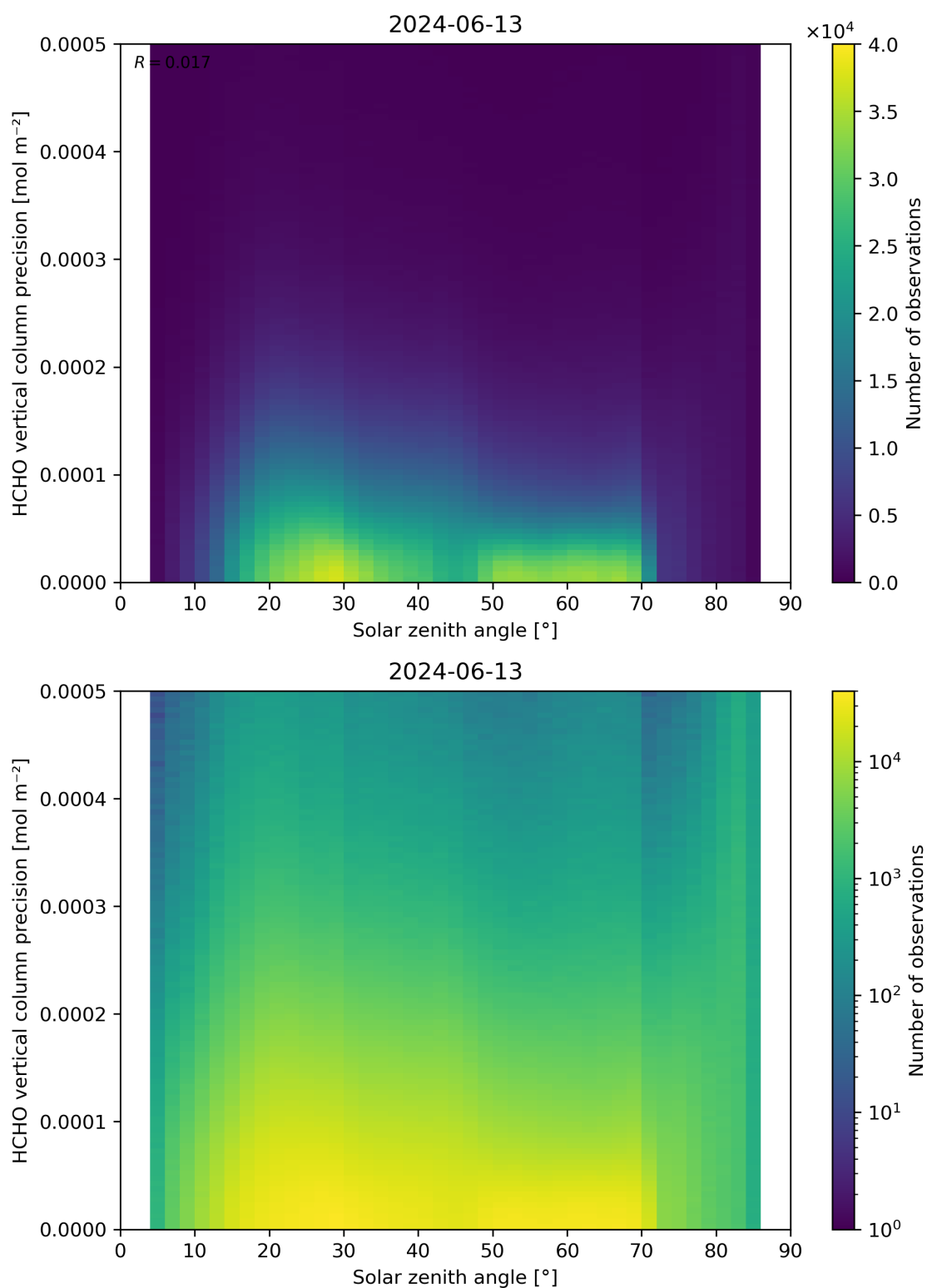
Figure 179: Scatter density plot of “Solar zenith angle” against “HCHO vertical column precision” for 2024-06-13 to 2024-06-14.
