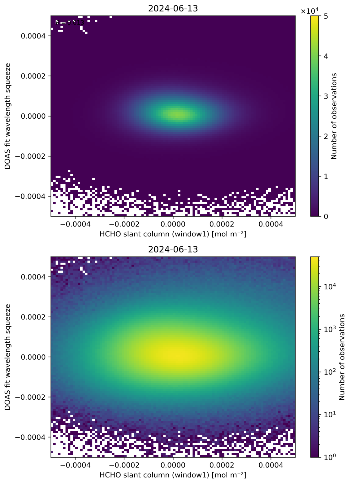
Figure 80: Scatter density plot of “HCHO slant column (window1)” against “DOAS fit wavelength squeeze” for 2024-06-13 to 2024-06-14.
