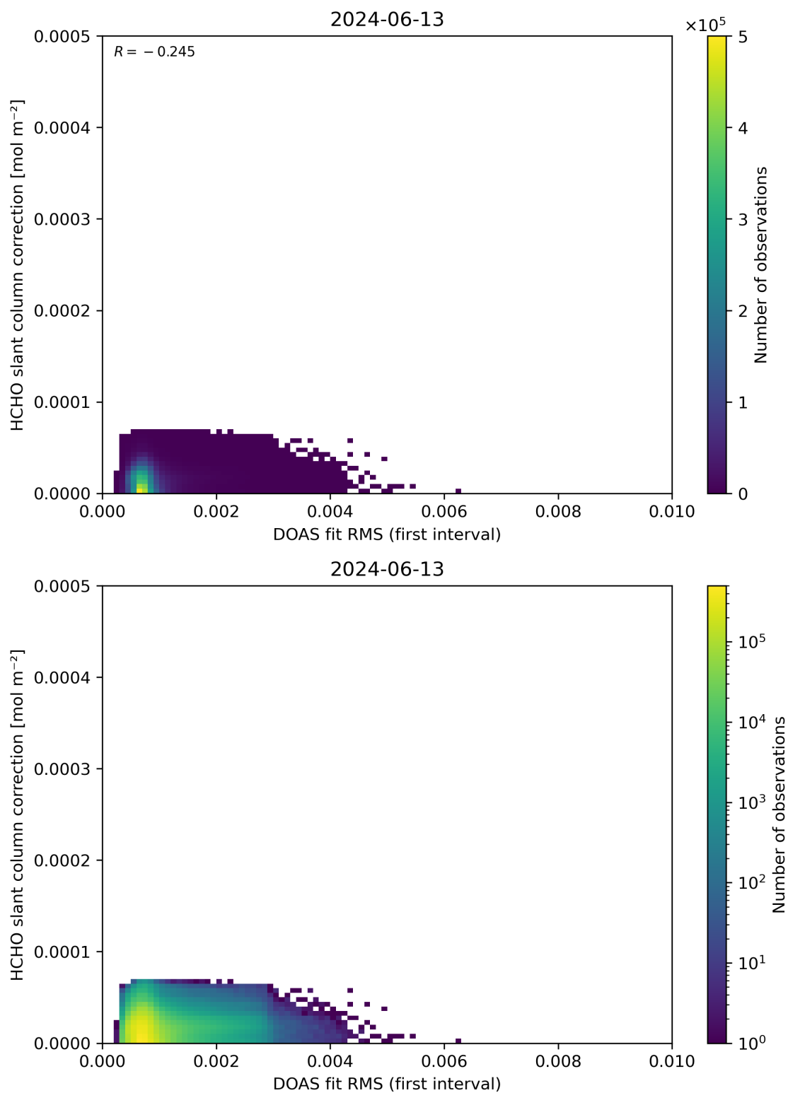
Figure 63: Scatter density plot of “DOAS fit RMS (first interval)” against “HCHO slant column correction” for 2024-06-13 to 2024-06-14.
