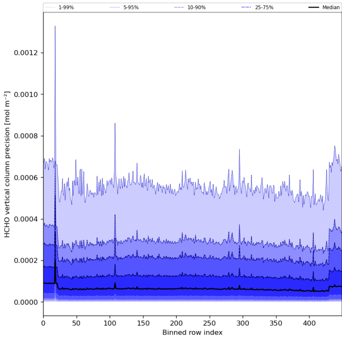
Figure 50: Along track statistics of “HCHO vertical column precision” for 2024-06-13 to 2024-06-14
