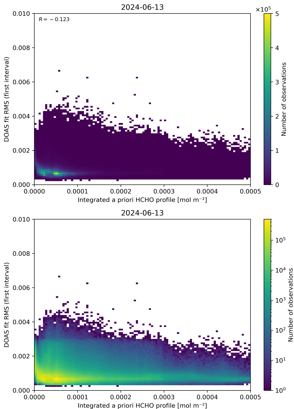
Figure 148: Scatter density plot of “Integrated a priori HCHO profile” against “DOAS fit RMS (first interval)” for 2024-06-13 to 2024-06-14.
