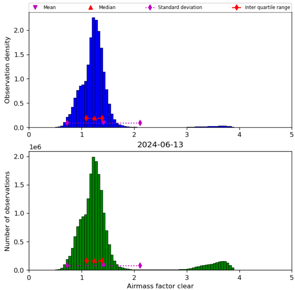
Figure 42: Histogram of “Airmass factor clear” for 2024-06-13 to 2024-06-14
