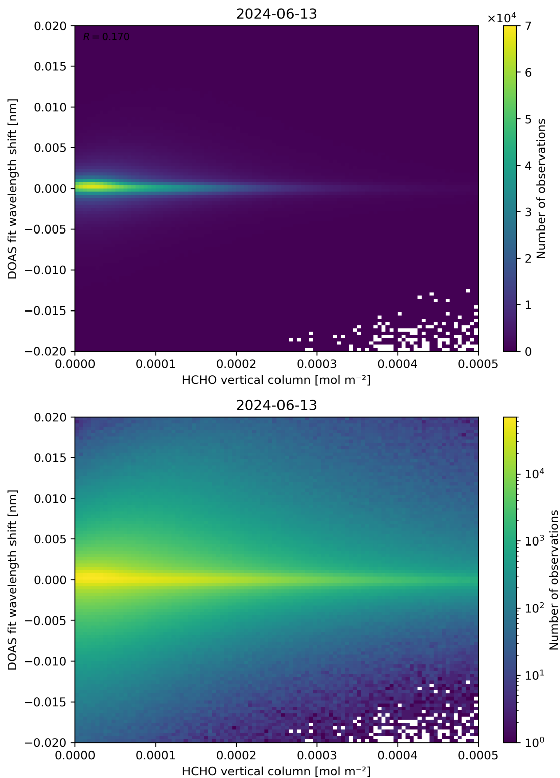
Figure 124: Scatter density plot of “HCHO vertical column” against “DOAS fit wavelength shift” for 2024-06-13 to 2024-06-14.
