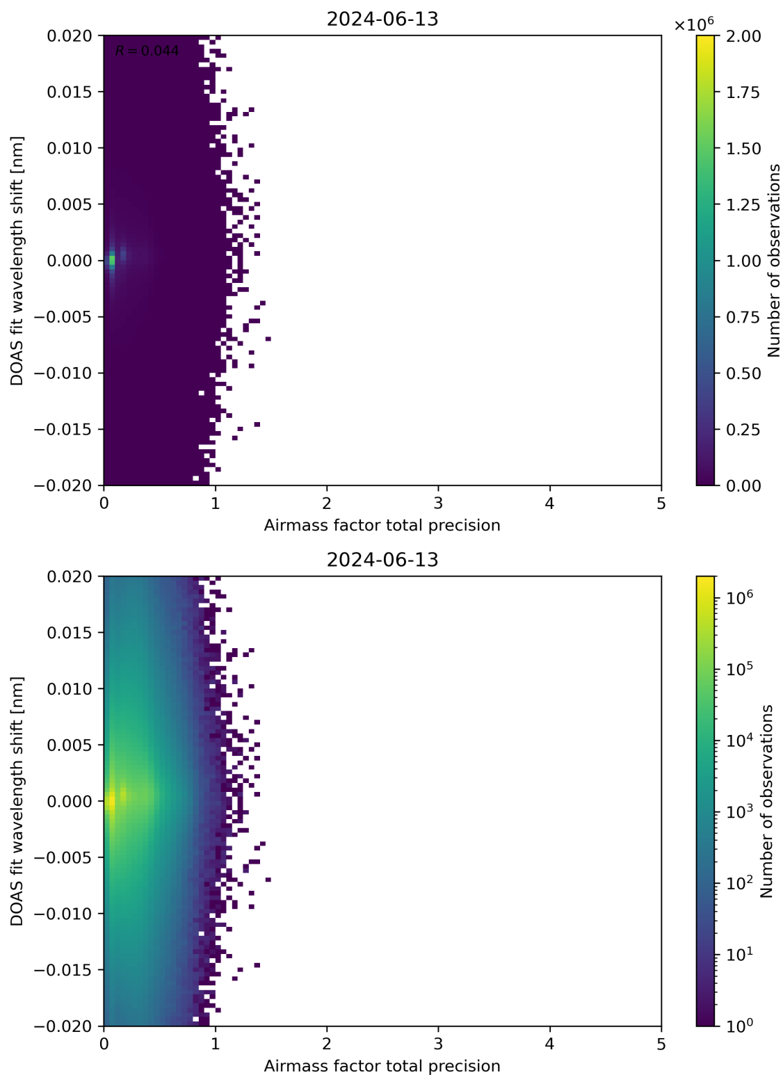
Figure 106: Scatter density plot of “Airmass factor total precision” against “DOAS fit wavelength shift” for 2024-06-13 to 2024-06-14.
