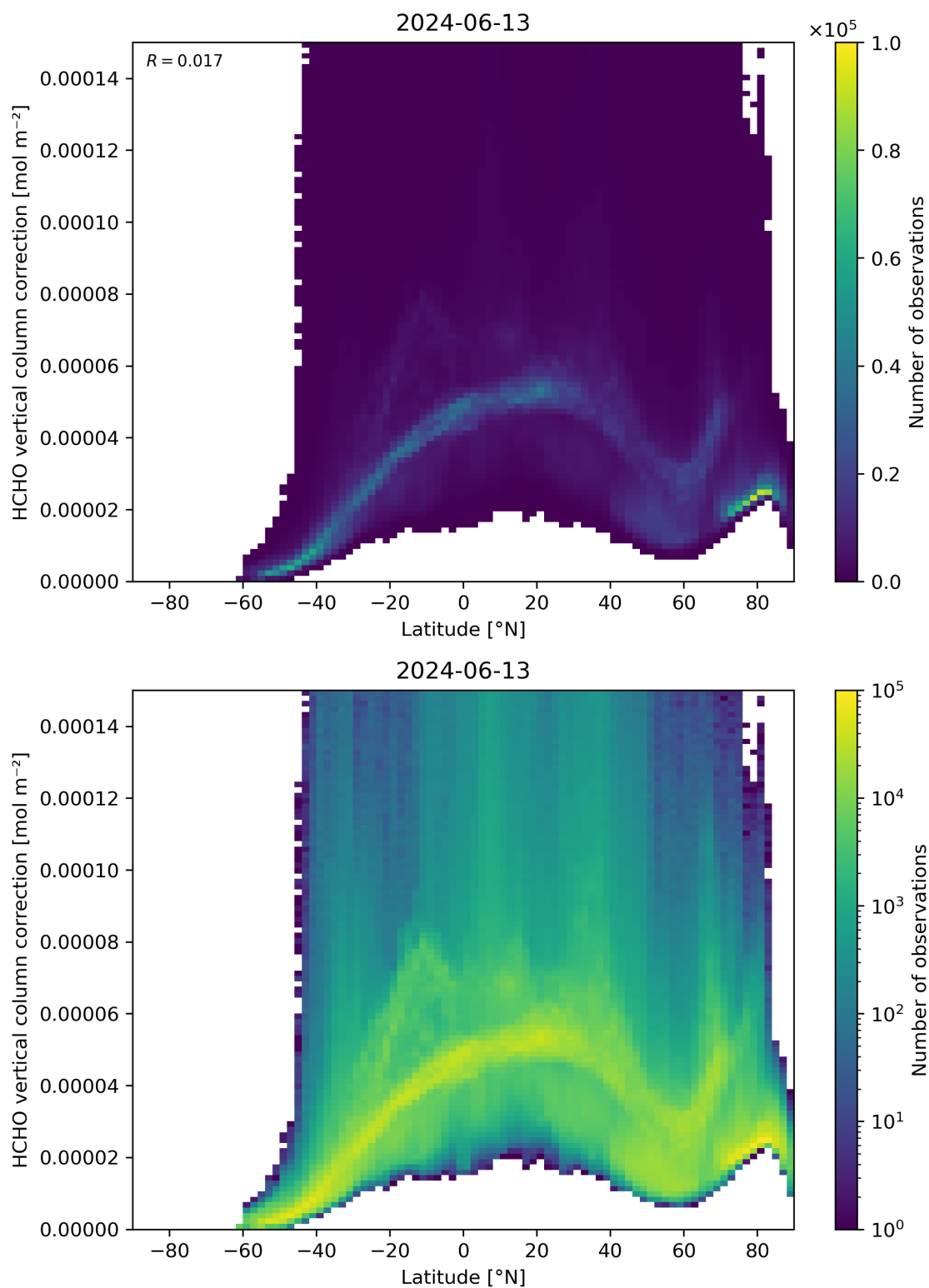
Figure 164: Scatter density plot of “Latitude” against “HCHO vertical column correction” for 2024-06-13 to 2024-06-14.
