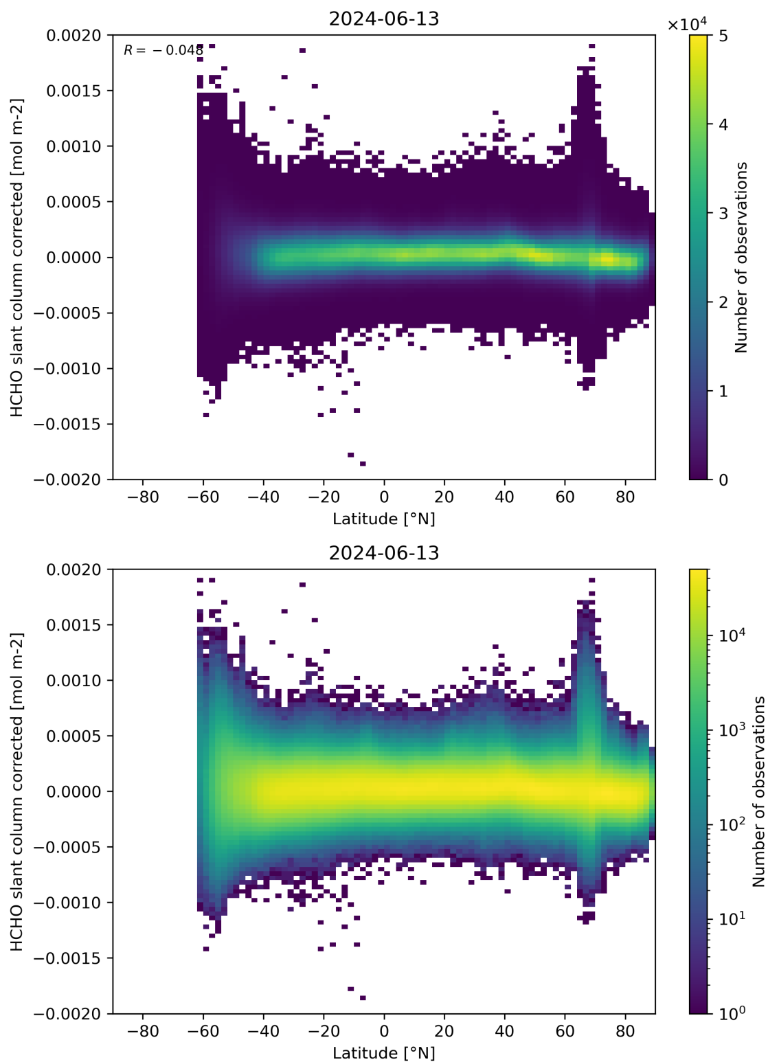
Figure 157: Scatter density plot of “Latitude” against “HCHO slant column corrected” for 2024-06-13 to 2024-06-14.
