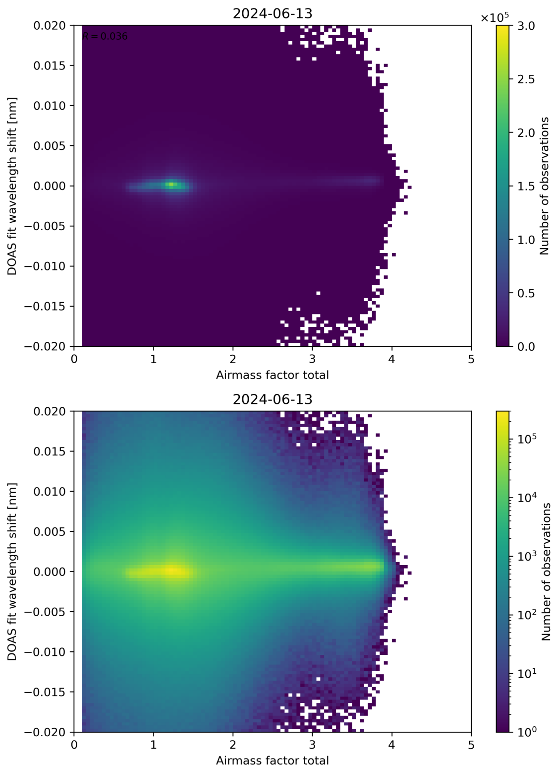
Figure 98: Scatter density plot of “Airmass factor total” against “DOAS fit wavelength shift” for 2024-06-13 to 2024-06-14.
