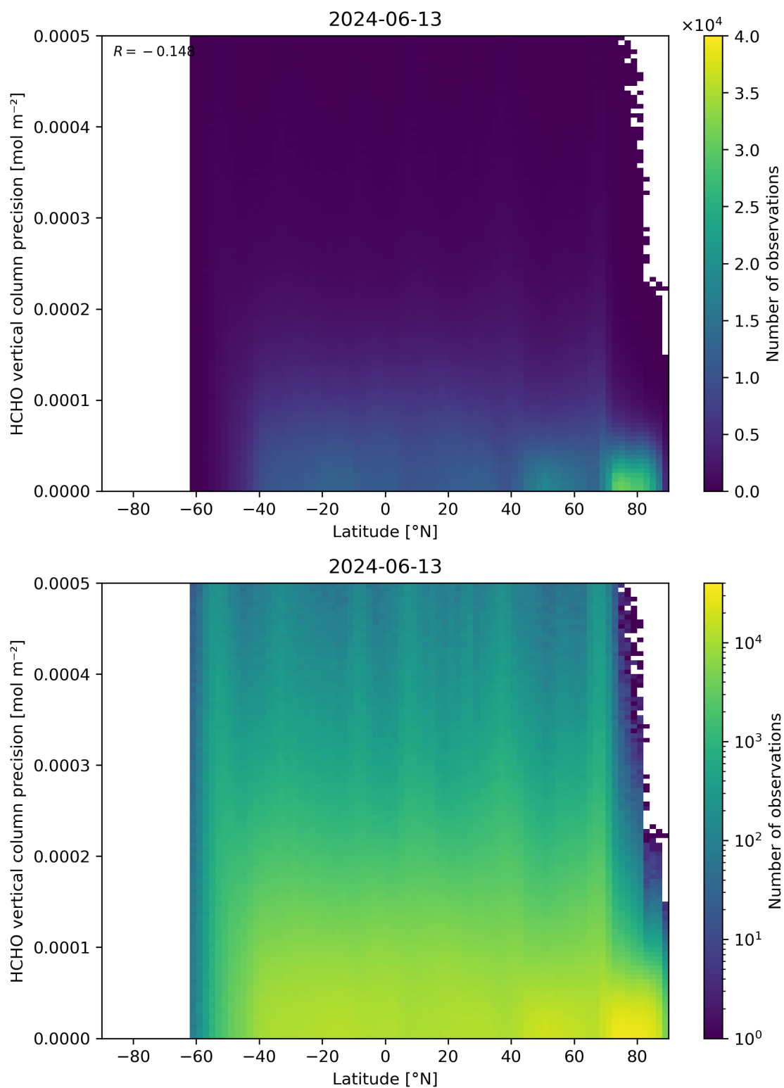
Figure 165: Scatter density plot of “Latitude” against “HCHO vertical column precision” for 2024-06-13 to 2024-06-14.
