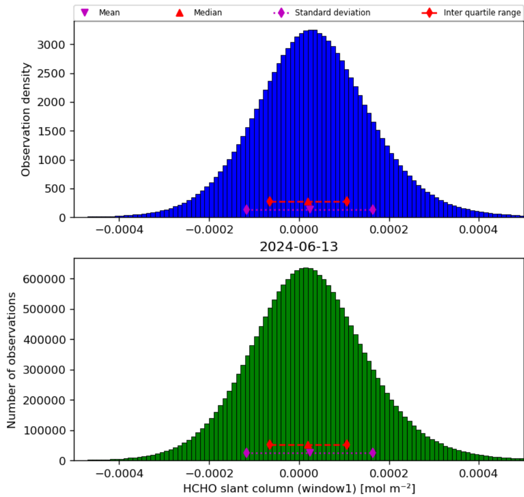
Figure 38: Histogram of “HCHO slant column (window1)” for 2024-06-13 to 2024-06-14
