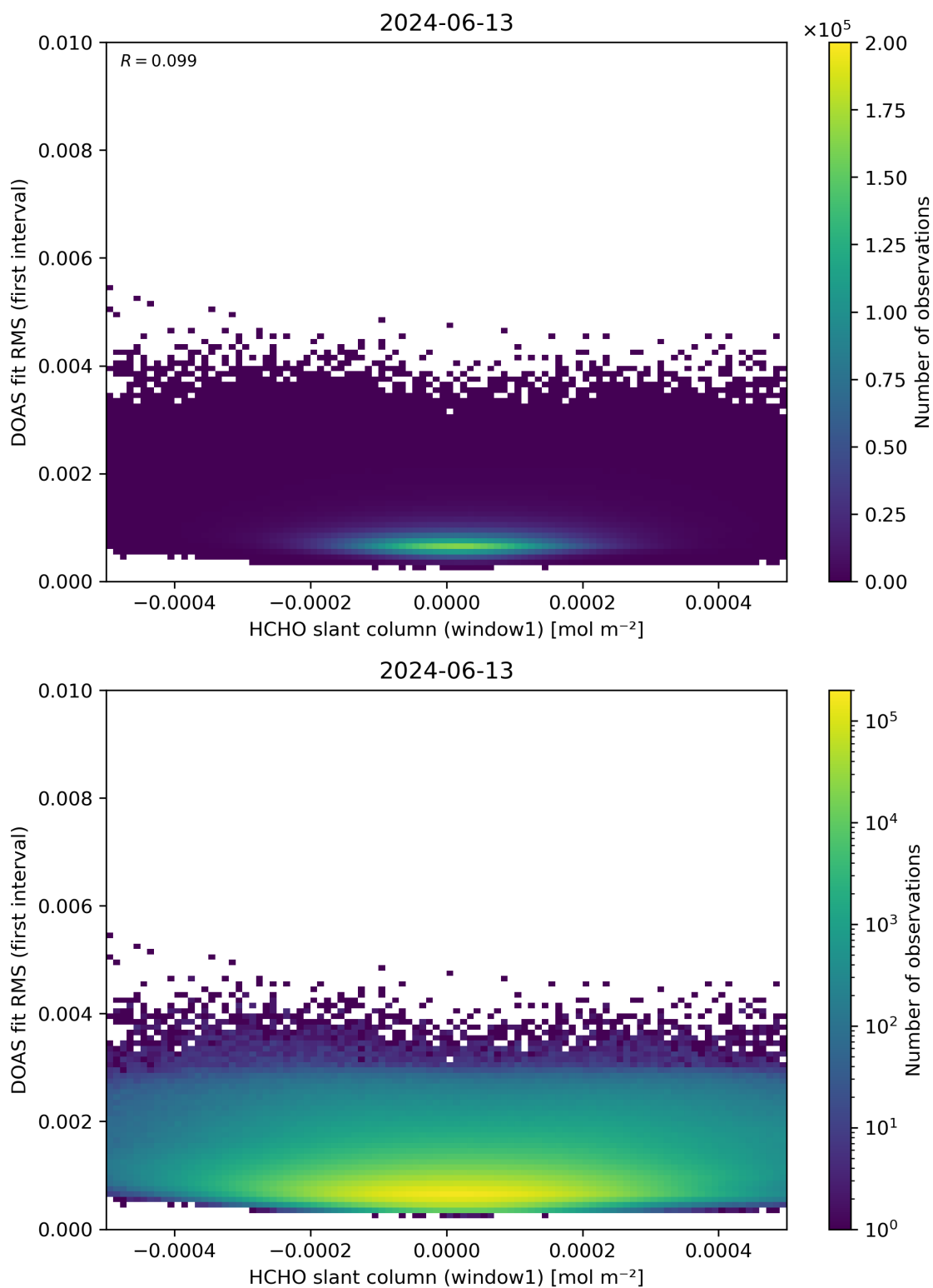
Figure 78: Scatter density plot of “HCHO slant column (window1)” against “DOAS fit RMS (first interval)” for 2024-06-13 to 2024-06-14.
