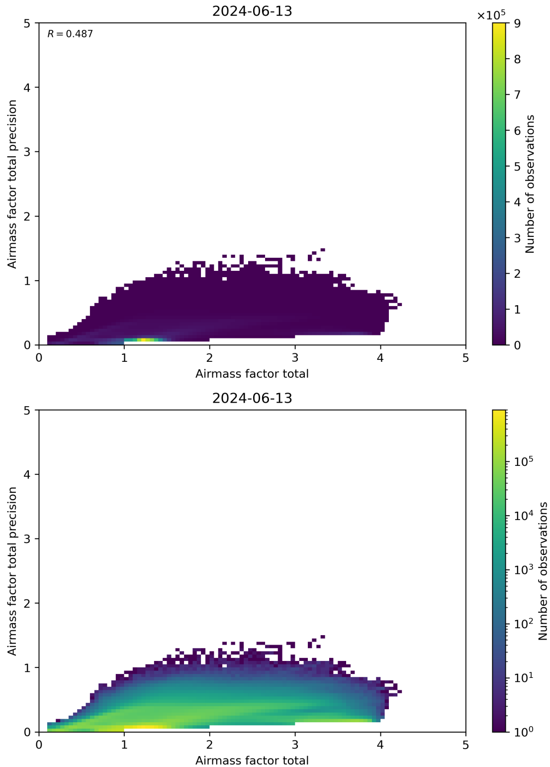
Figure 103: Scatter density plot of “Airmass factor total” against “Airmass factor total precision” for 2024-06-13 to 2024-06-14.
