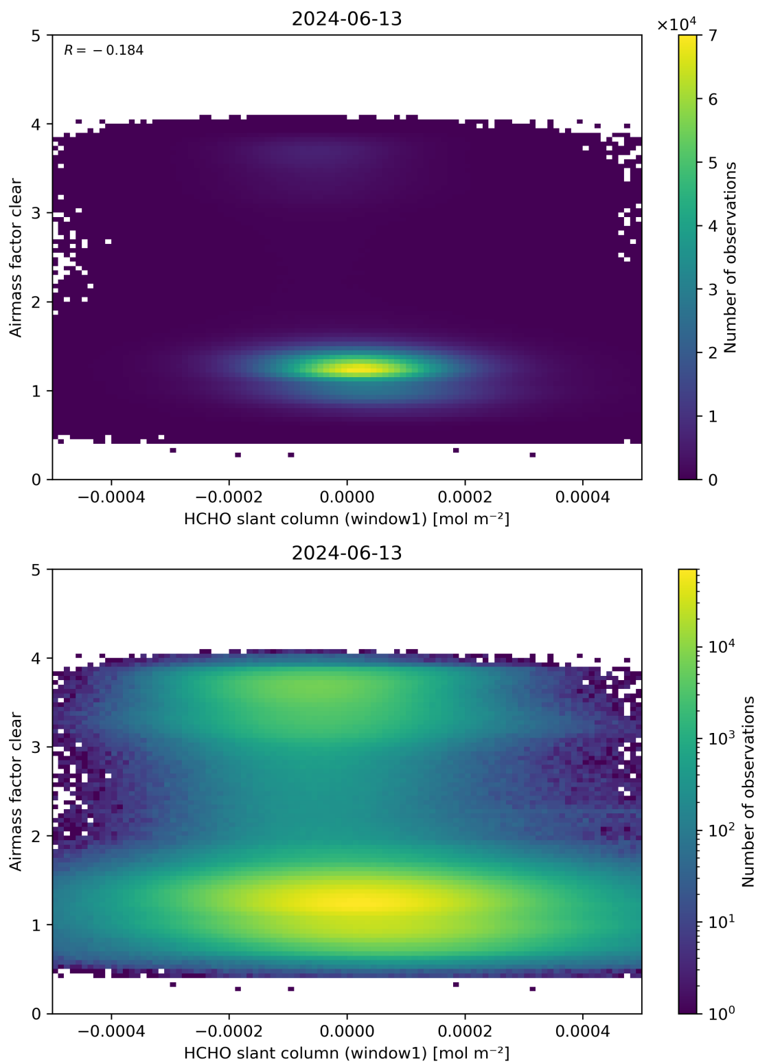
Figure 81: Scatter density plot of “HCHO slant column (window1)” against “Airmass factor clear” for 2024-06-13 to 2024-06-14.
