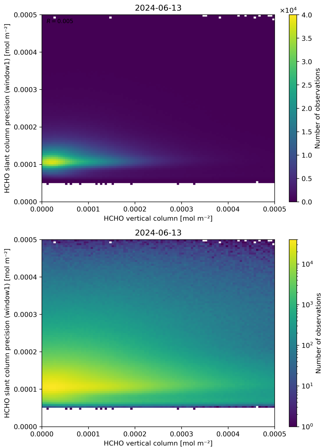
Figure 130: Scatter density plot of “HCHO vertical column” against “HCHO slant column precision (window1)” for 2024-06-13 to 2024-06-14.
