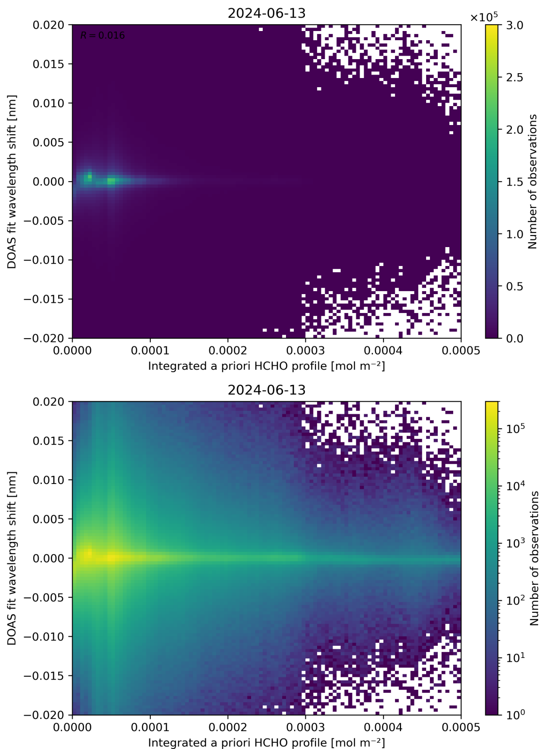
Figure 149: Scatter density plot of “Integrated a priori HCHO profile” against “DOAS fit wavelength shift” for 2024-06-13 to 2024-06-14.
