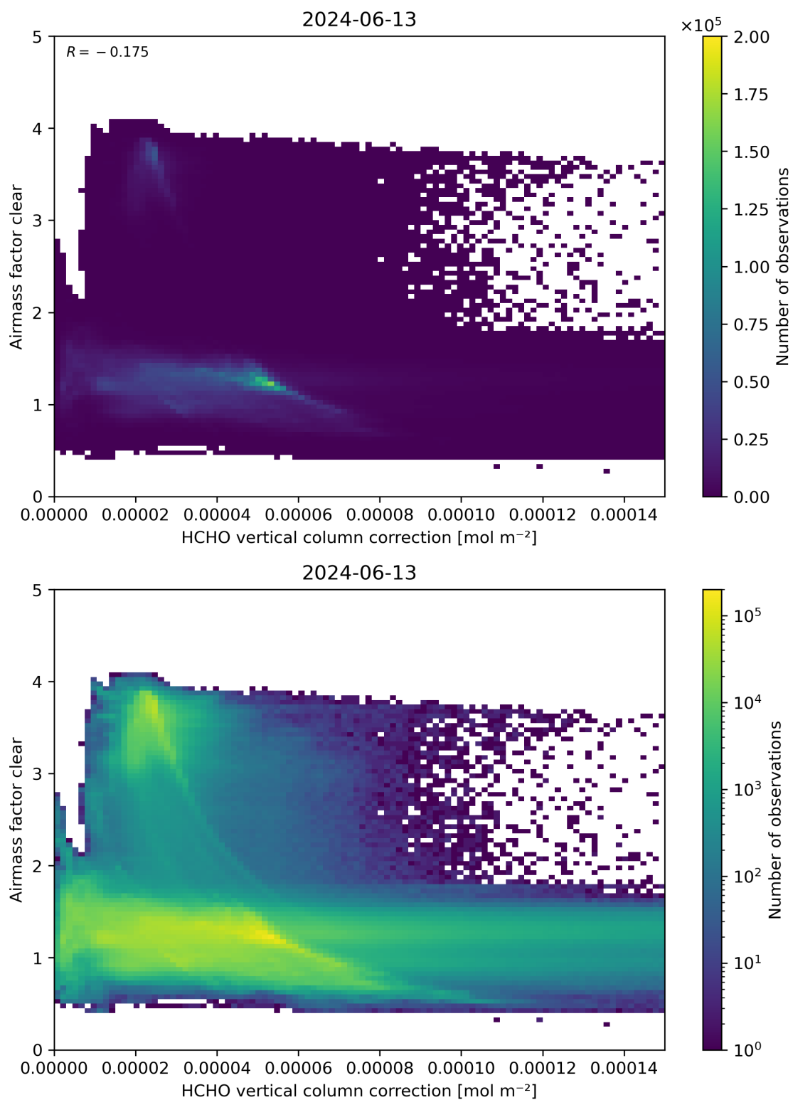
Figure 115: Scatter density plot of “HCHO vertical column correction” against “Airmass factor clear” for 2024-06-13 to 2024-06-14.
