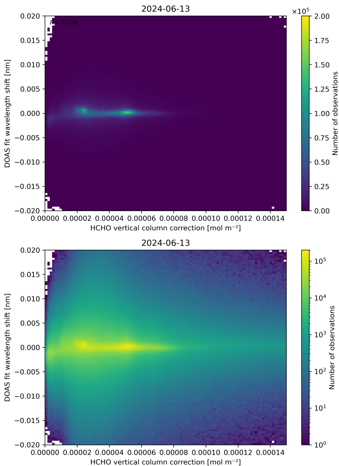
Figure 113: Scatter density plot of “HCHO vertical column correction” against “DOAS fit wavelength shift” for 2024-06-13 to 2024-06-14.
