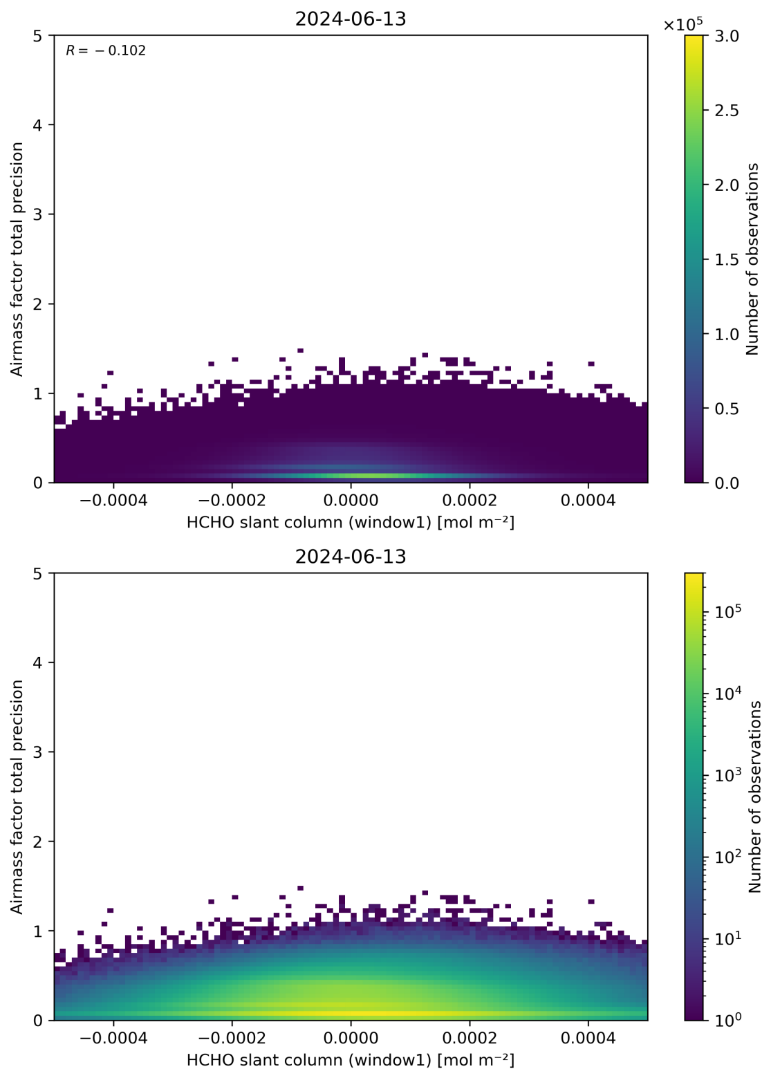
Figure 86: Scatter density plot of “HCHO slant column (window1)” against “Airmass factor total precision” for 2024-06-13 to 2024-06-14.
