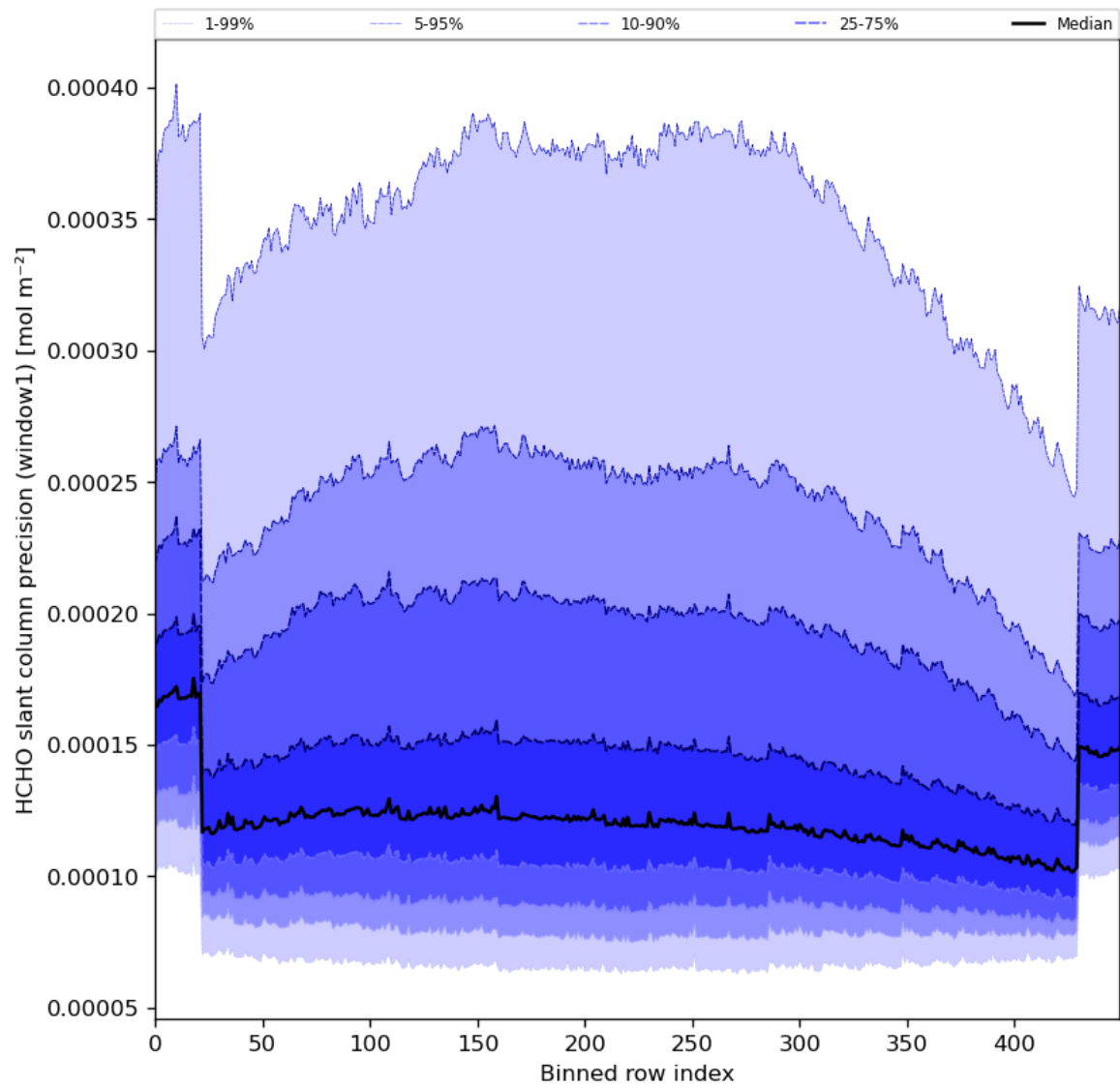
Figure 53: Along track statistics of “HCHO slant column precision (window1)” for 2024-06-13 to 2024-06-14
