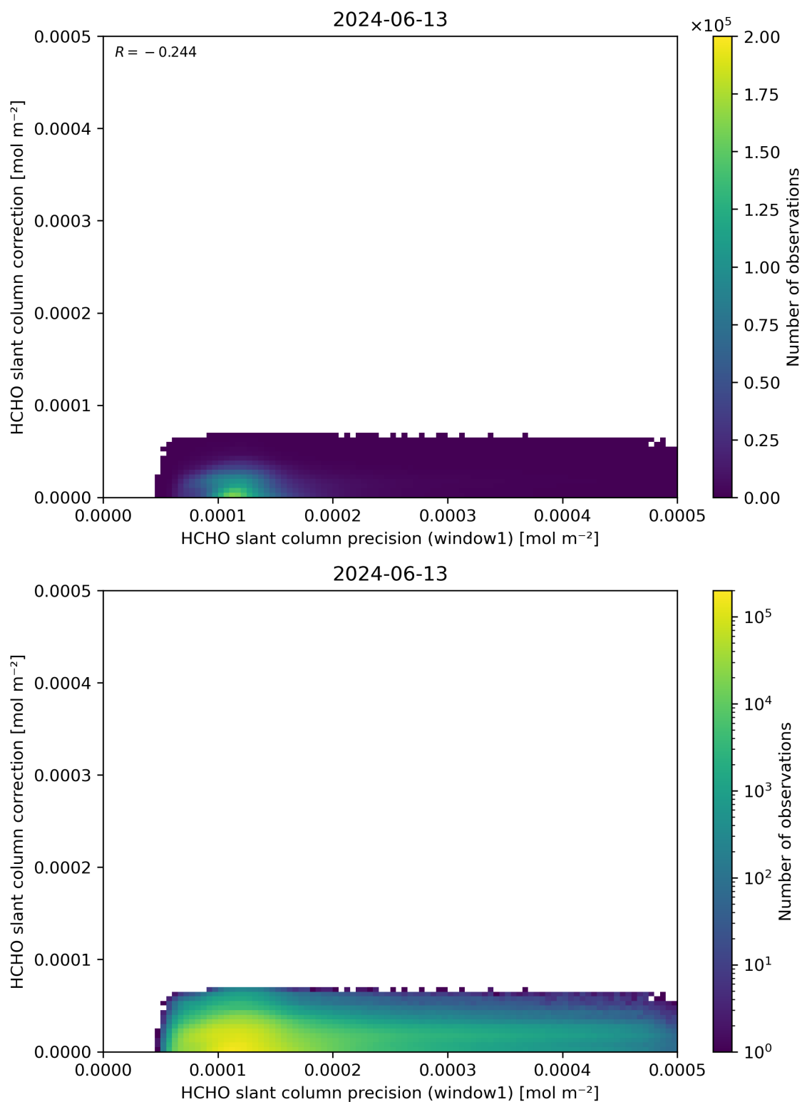
Figure 93: Scatter density plot of “HCHO slant column precision (window1)” against “HCHO slant column correction” for 2024-06-13 to 2024-06-14.
