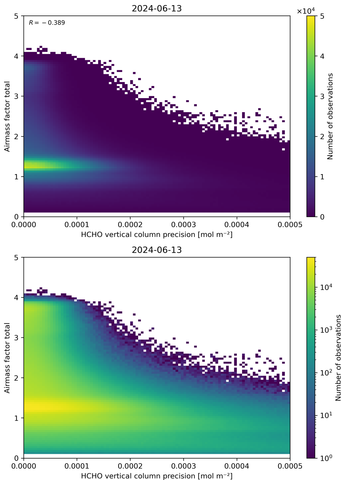
Figure 144: Scatter density plot of “HCHO vertical column precision” against “Airmass factor total” for 2024-06-13 to 2024-06-14.
