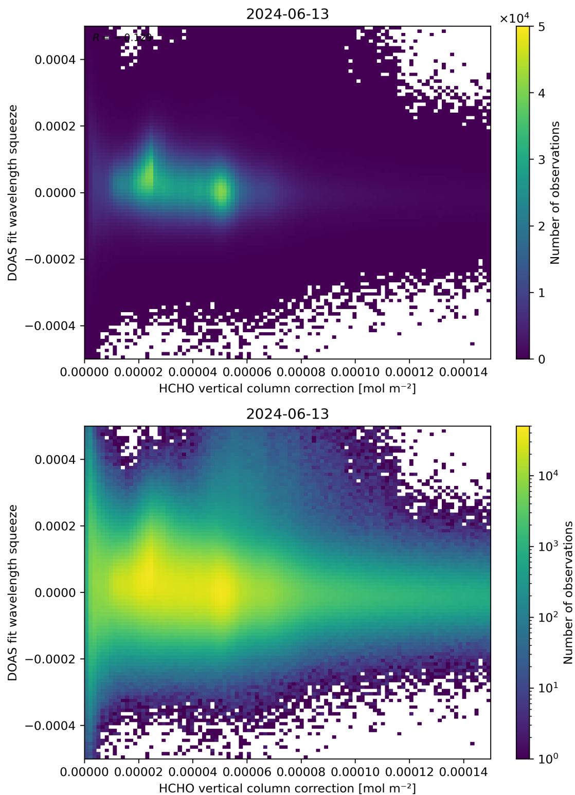
Figure 114: Scatter density plot of “HCHO vertical column correction” against “DOAS fit wavelength squeeze” for 2024-06-13 to 2024-06-14.
