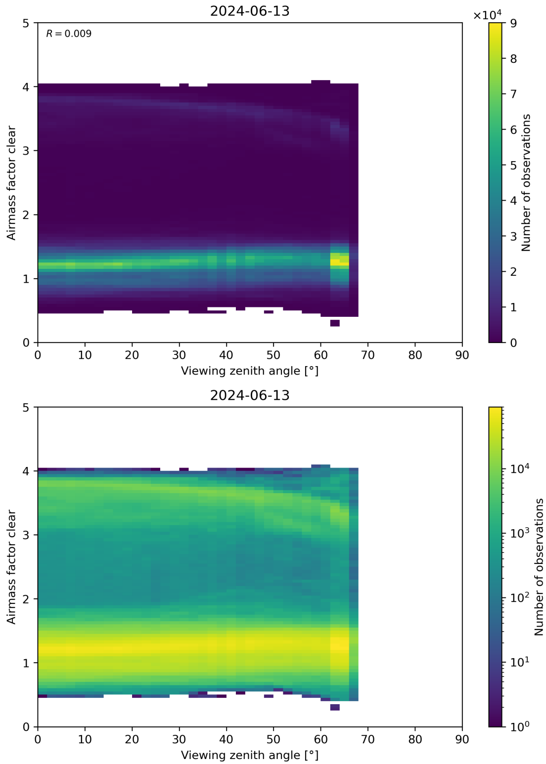
Figure 185: Scatter density plot of “Viewing zenith angle” against “Airmass factor clear” for 2024-06-13 to 2024-06-14.
