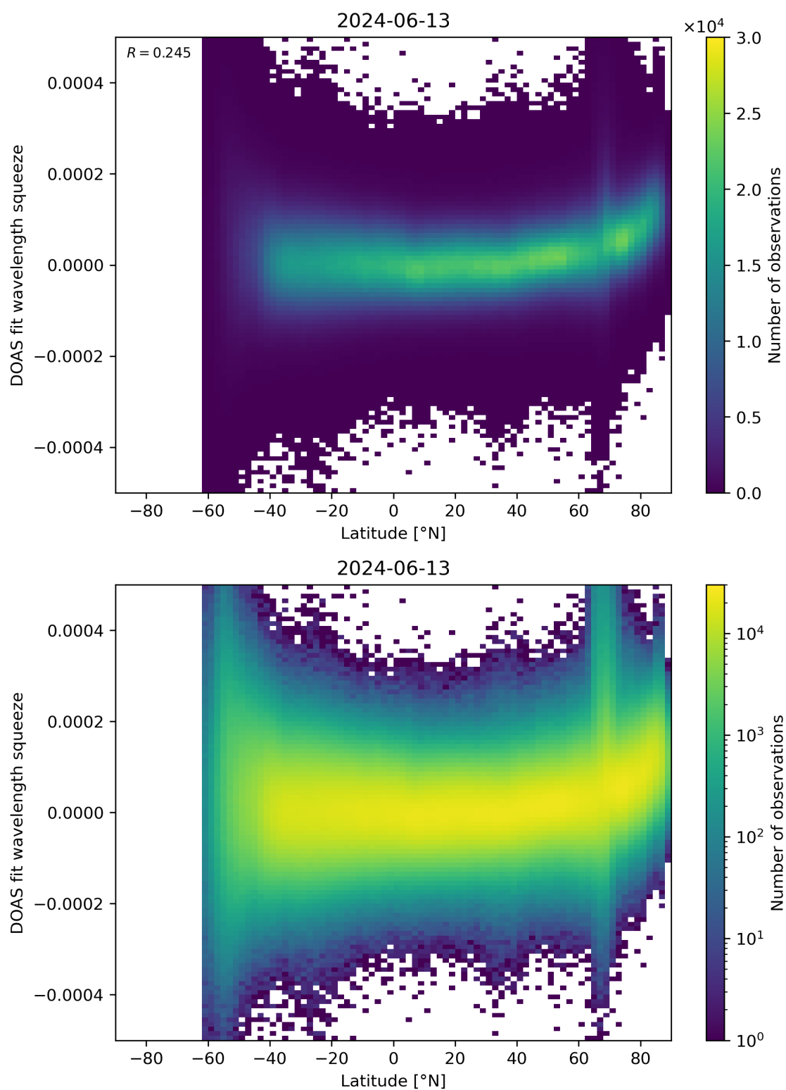
Figure 155: Scatter density plot of “Latitude” against “DOAS fit wavelength squeeze” for 2024-06-13 to 2024-06-14.
