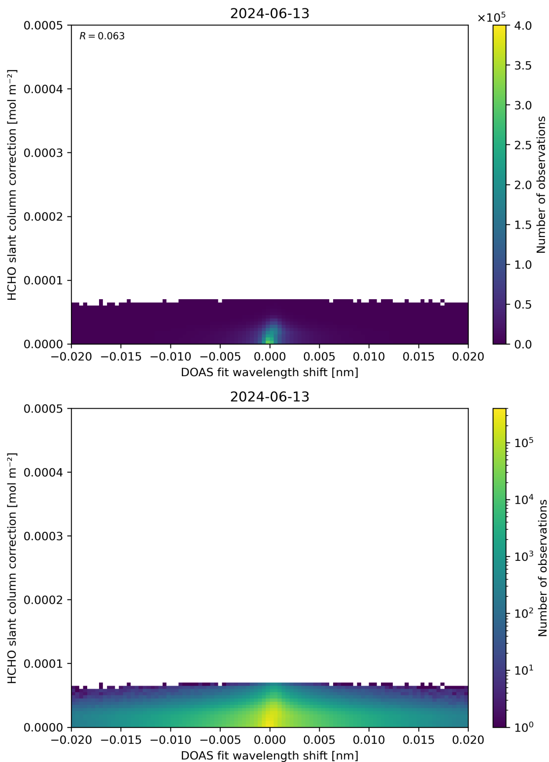
Figure 67: Scatter density plot of “DOAS fit wavelength shift” against “HCHO slant column correction” for 2024-06-13 to 2024-06-14.
