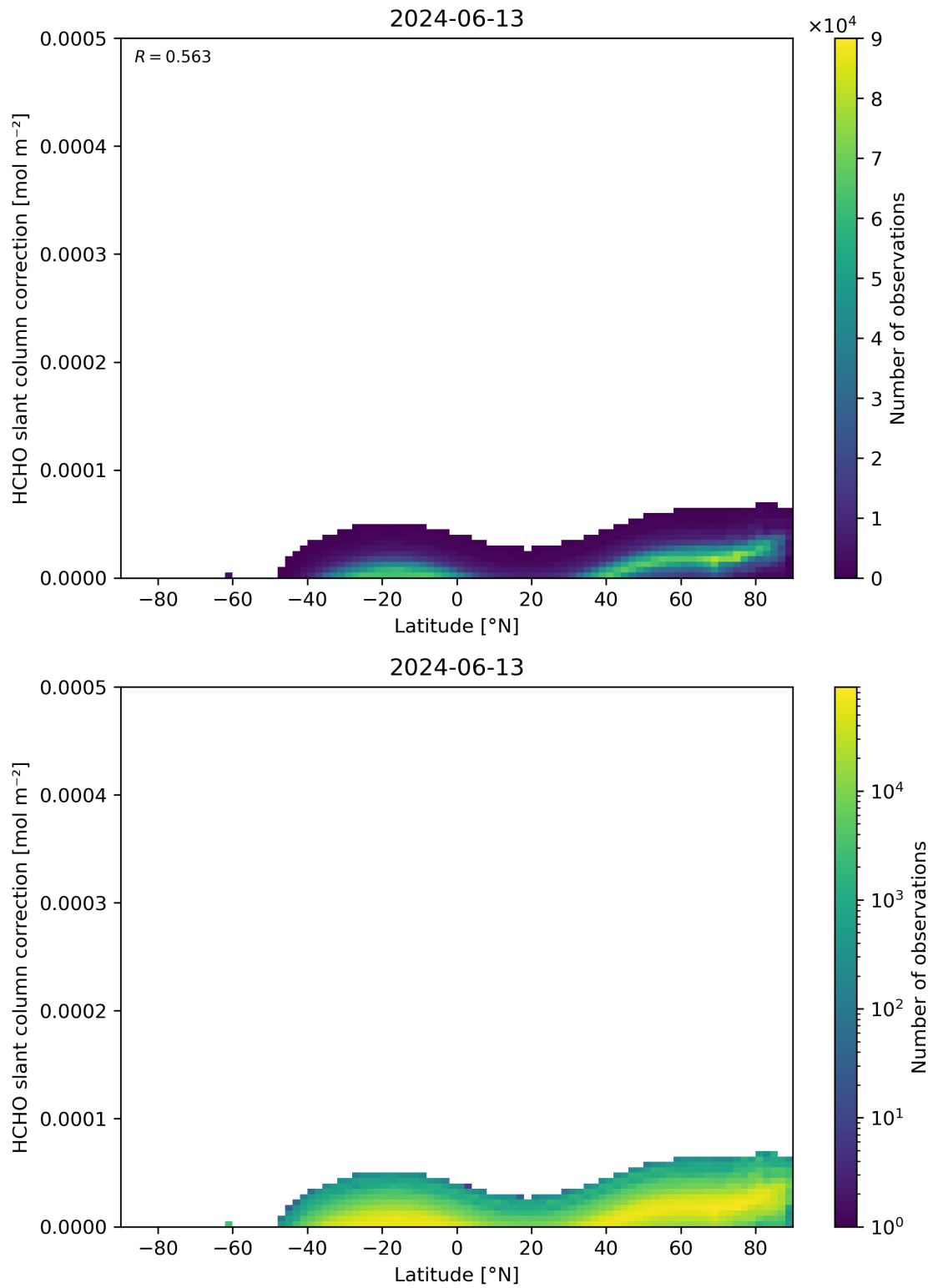
Figure 158: Scatter density plot of “Latitude” against “HCHO slant column correction” for 2024-06-13 to 2024-06-14.
