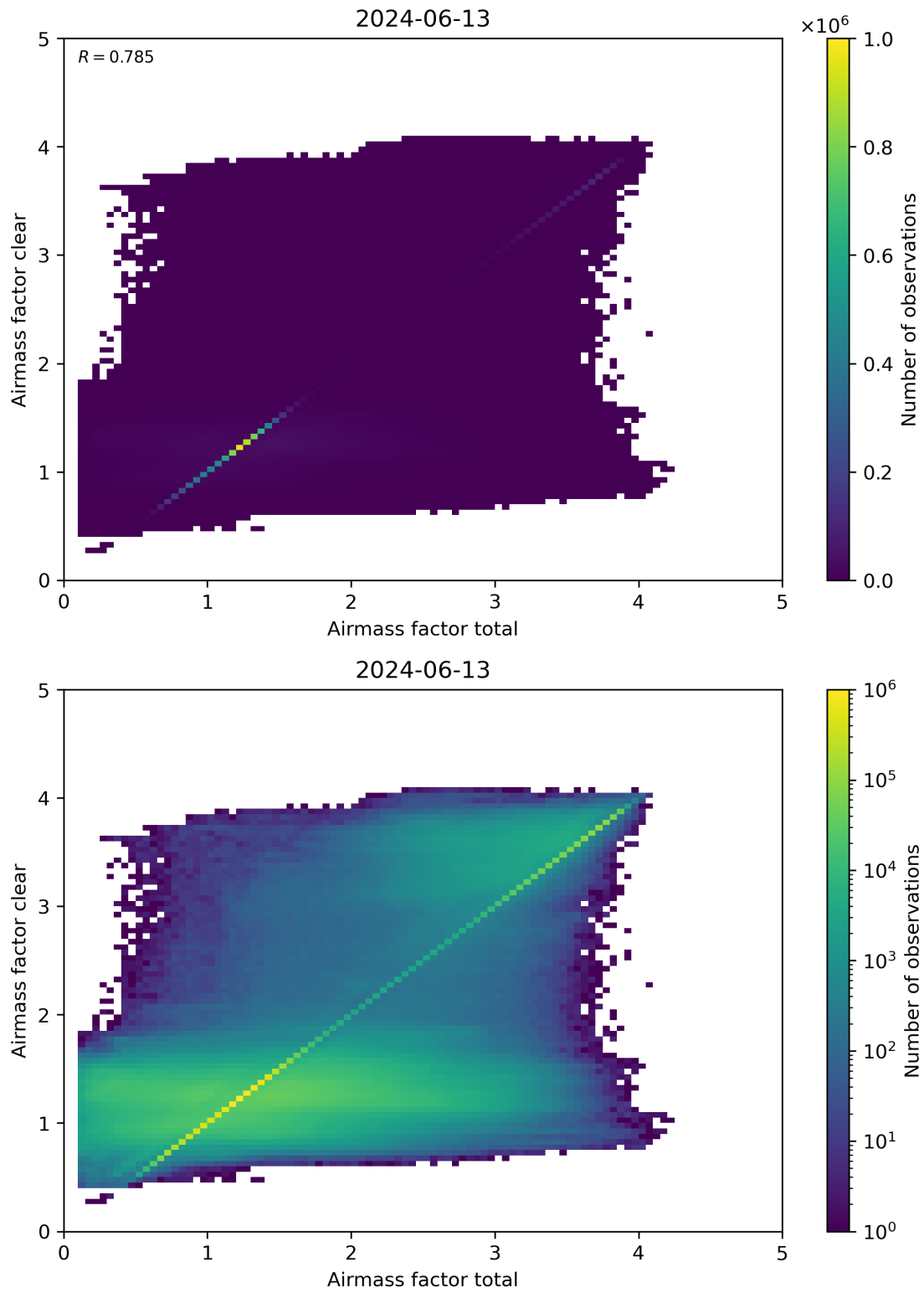
Figure 100: Scatter density plot of “Airmass factor total” against “Airmass factor clear” for 2024-06-13 to 2024-06-14.
