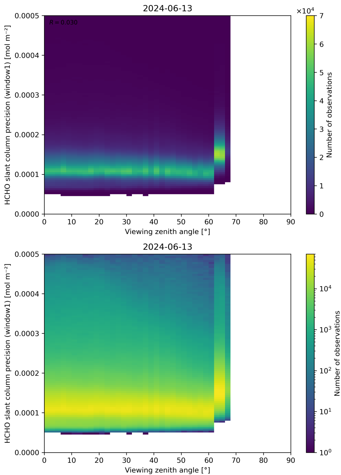
Figure 189: Scatter density plot of “Viewing zenith angle” against “HCHO slant column precision (window1)” for 2024-06-13 to 2024-06-14.
