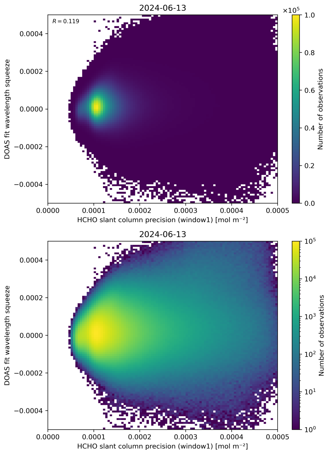
Figure 90: Scatter density plot of “HCHO slant column precision (window1)” against “DOAS fit wavelength squeeze” for 2024-06-13 to 2024-06-14.
