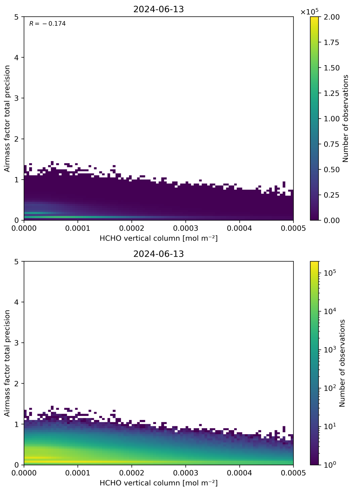
Figure 132: Scatter density plot of “HCHO vertical column” against “Airmass factor total precision” for 2024-06-13 to 2024-06-14.
