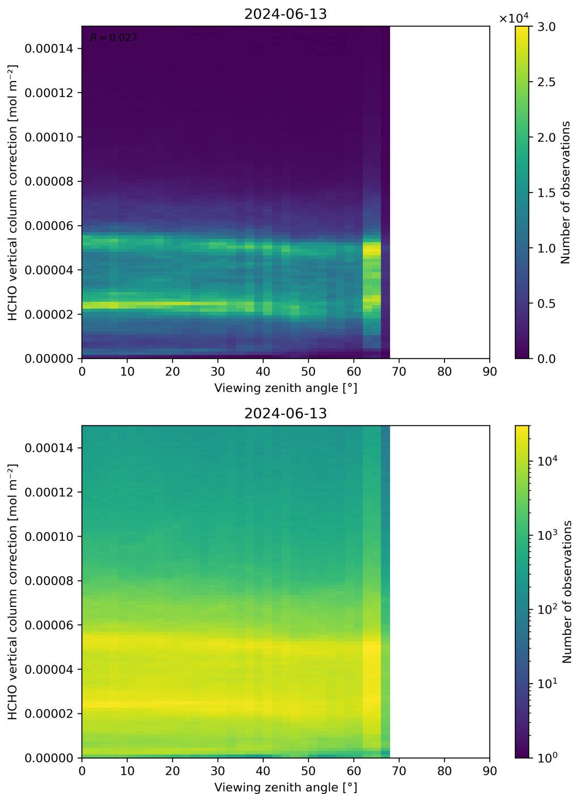
Figure 193: Scatter density plot of “Viewing zenith angle” against “HCHO vertical column correction” for 2024-06-13 to 2024-06-14.
