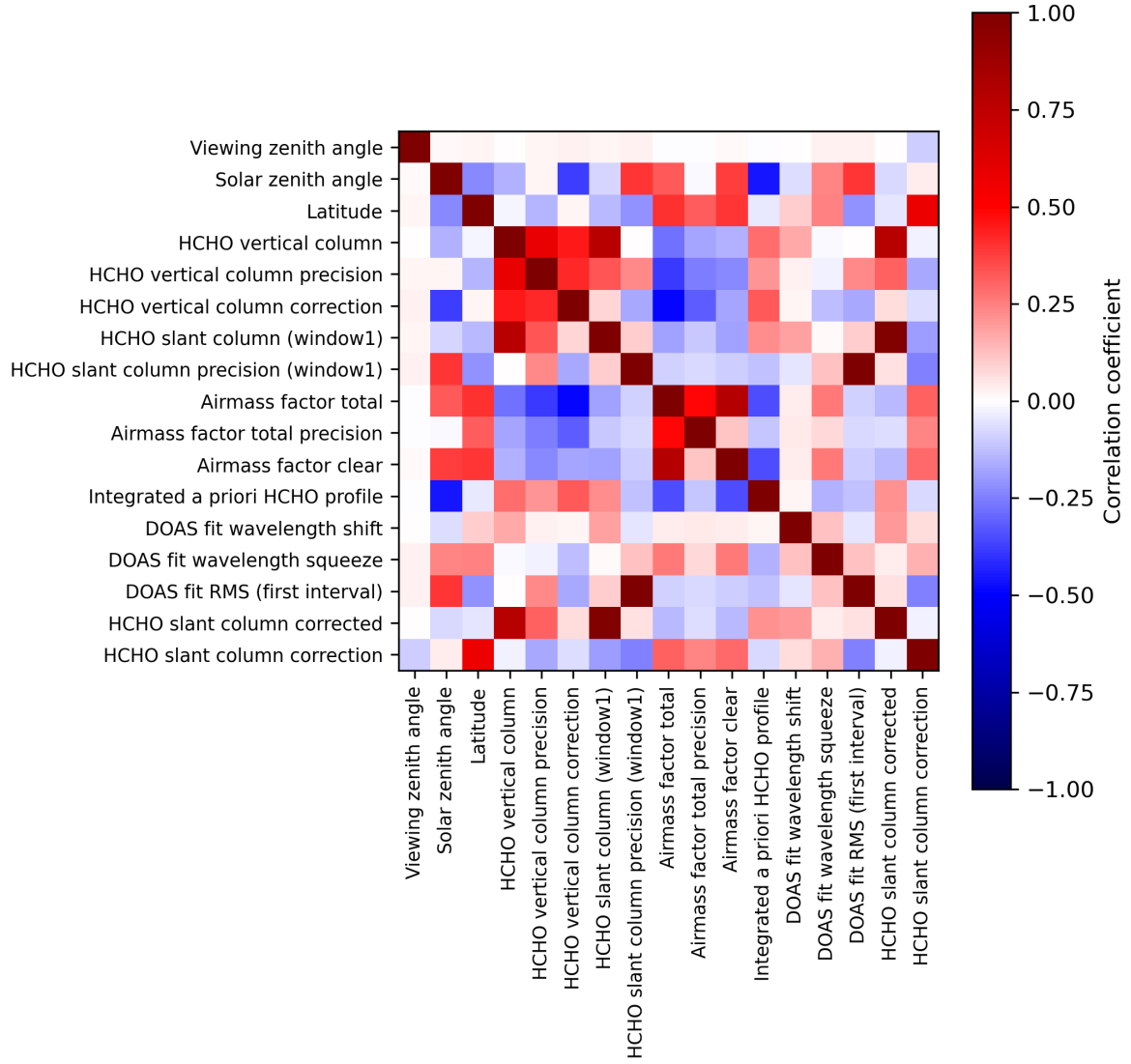
Figure 2: Map of correlation matrix for 2024-06-13 to 2024-06-14.
