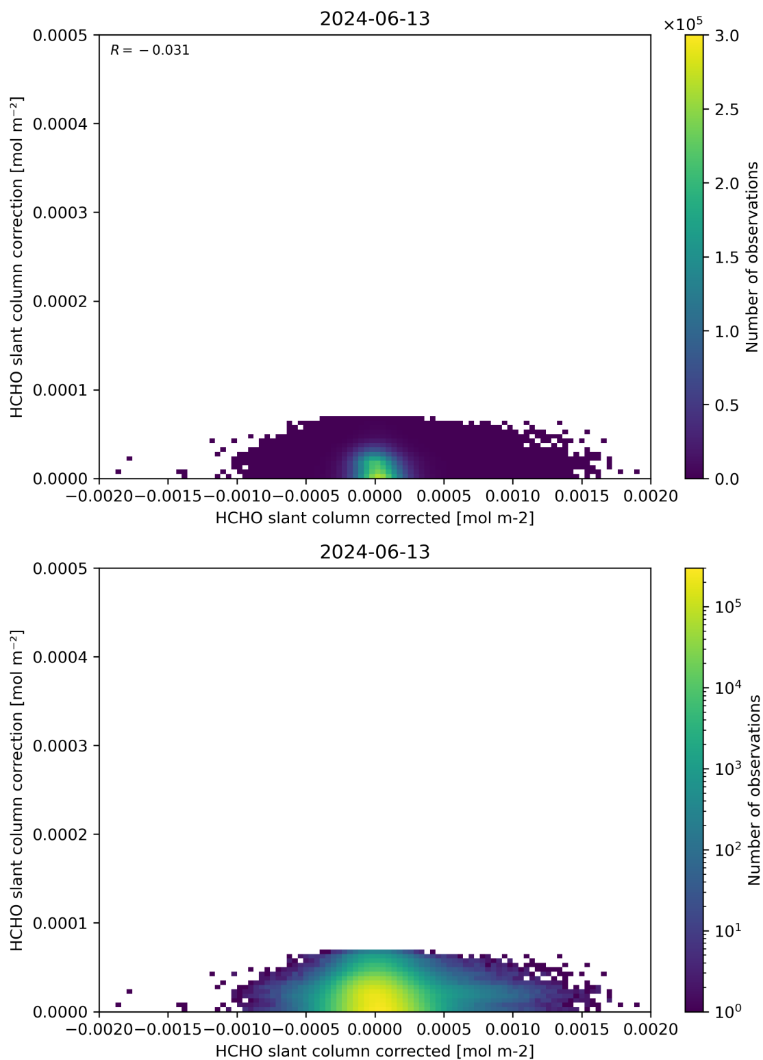
Figure 77: Scatter density plot of “HCHO slant column corrected” against “HCHO slant column correction” for 2024-06-13 to 2024-06-14.
