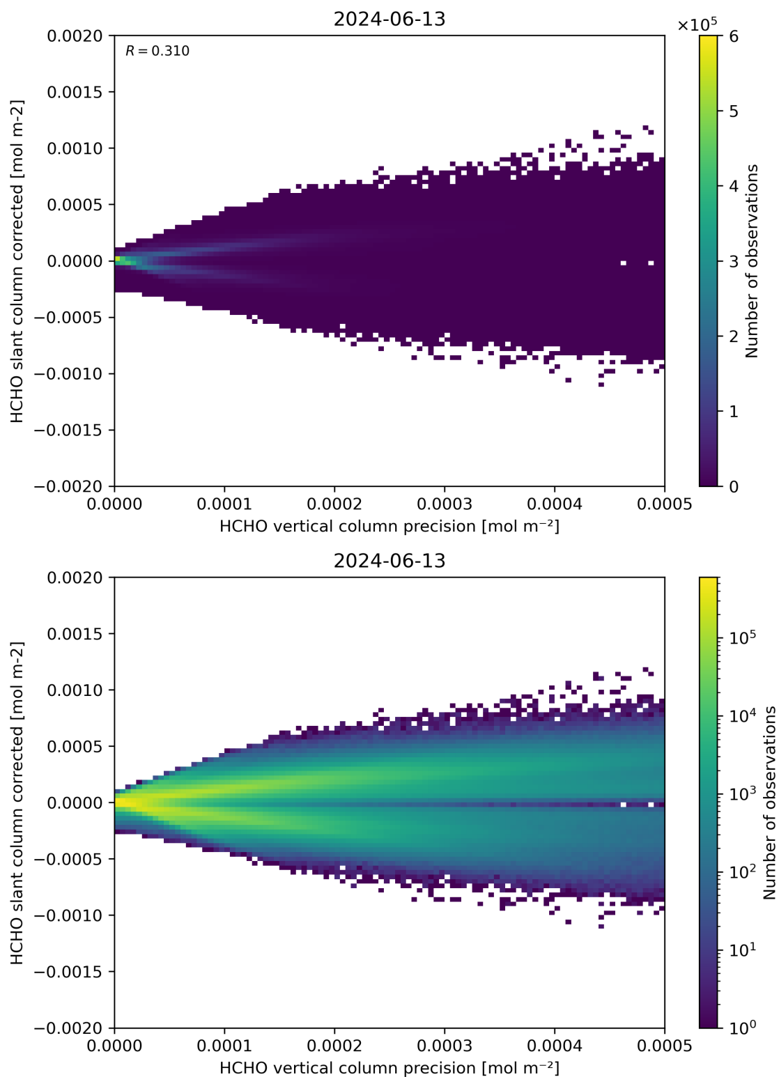
Figure 140: Scatter density plot of “HCHO vertical column precision” against “HCHO slant column corrected” for 2024-06-13 to 2024-06-14.
