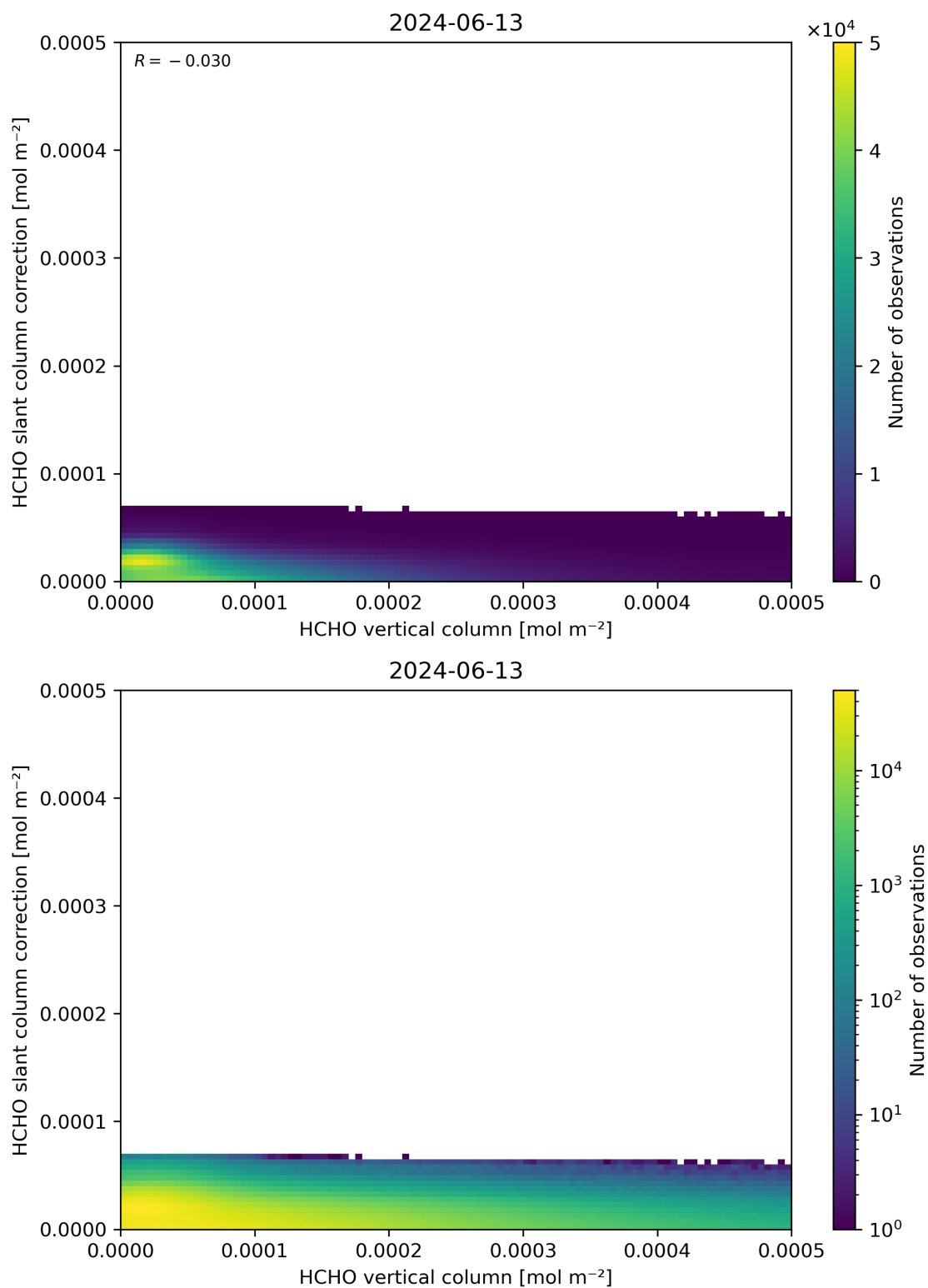
Figure 128: Scatter density plot of “HCHO vertical column” against “HCHO slant column correction” for 2024-06-13 to 2024-06-14.
