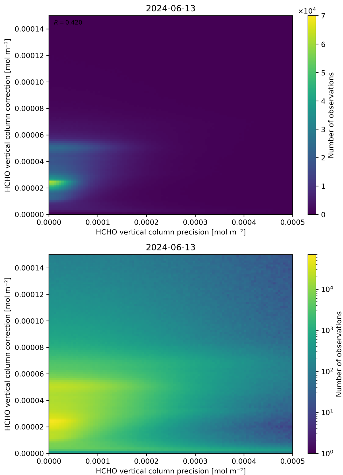
Figure 146: Scatter density plot of “HCHO vertical column precision” against “HCHO vertical column correction” for 2024-06-13 to 2024-06-14.
