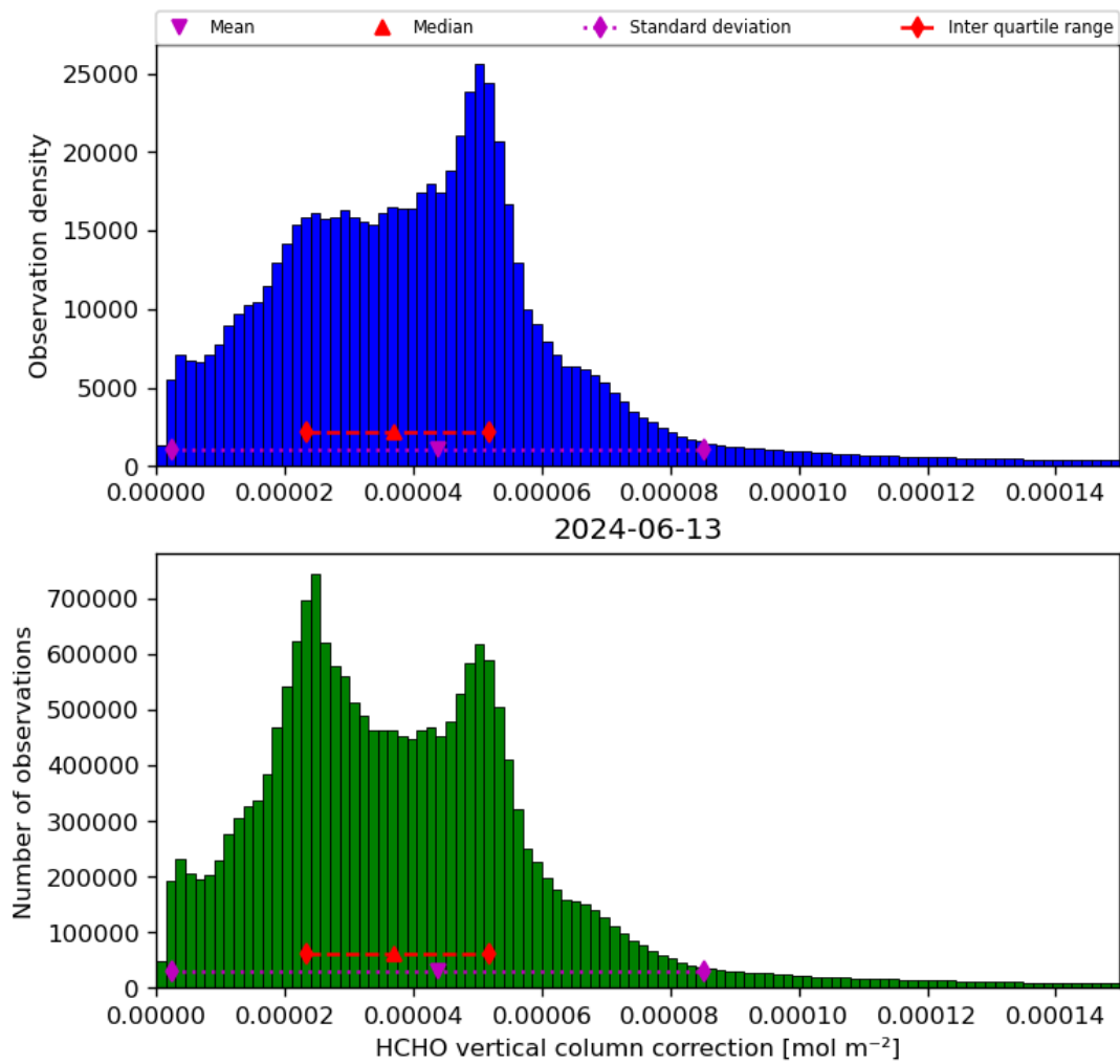
Figure 37: Histogram of “HCHO vertical column correction” for 2024-06-13 to 2024-06-14
