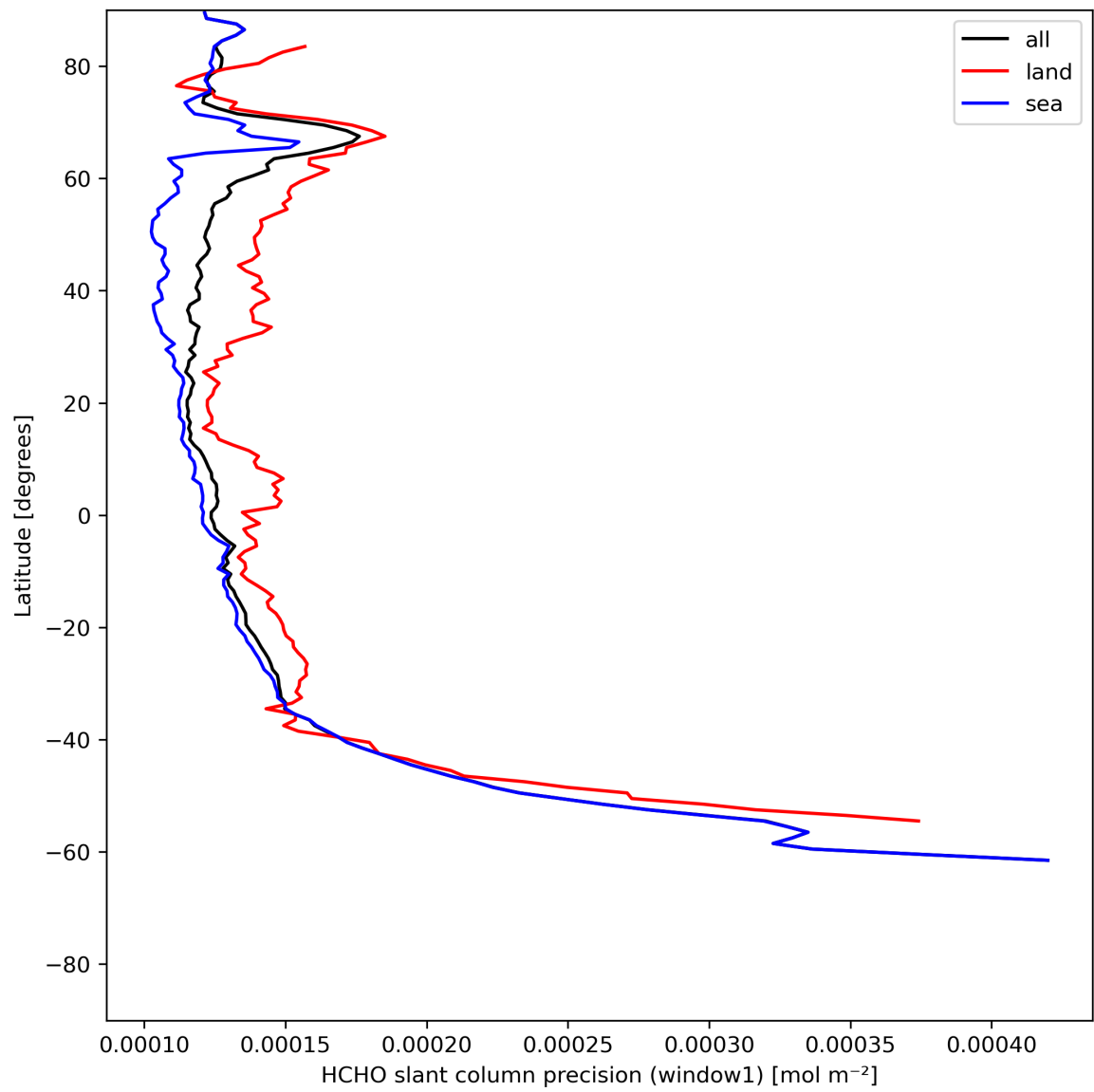
Figure 25: Zonal average of “HCHO slant column precision (window1)” for 2024-06-13 to 2024-06-14.
