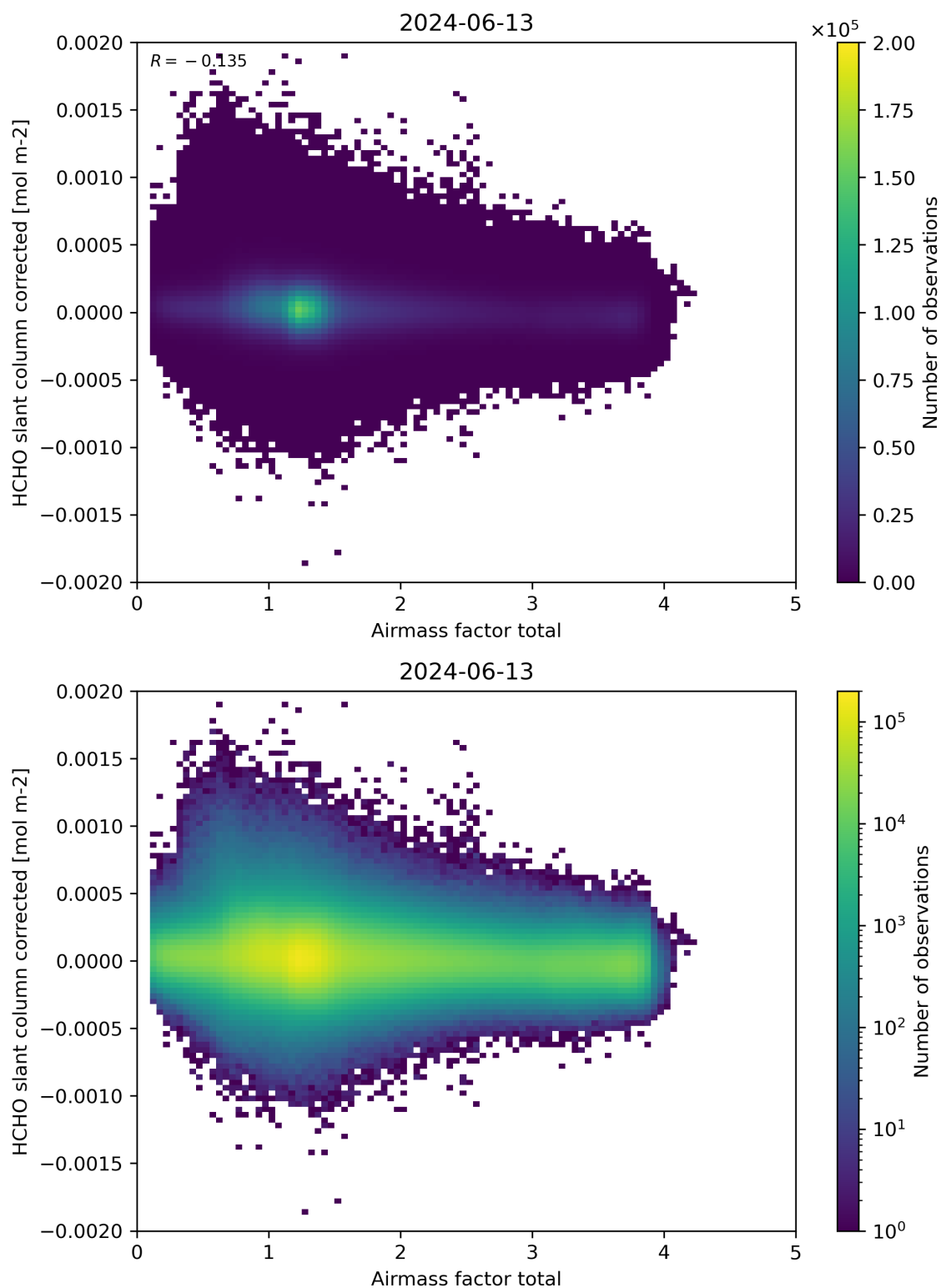
Figure 101: Scatter density plot of “Airmass factor total” against “HCHO slant column corrected” for 2024-06-13 to 2024-06-14.
