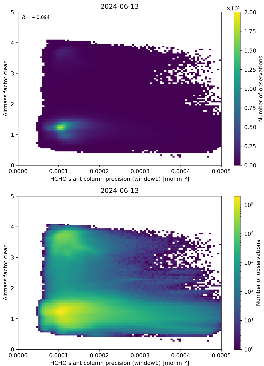
Figure 91: Scatter density plot of “HCHO slant column precision (window1)” against “Airmass factor clear” for 2024-06-13 to 2024-06-14.
