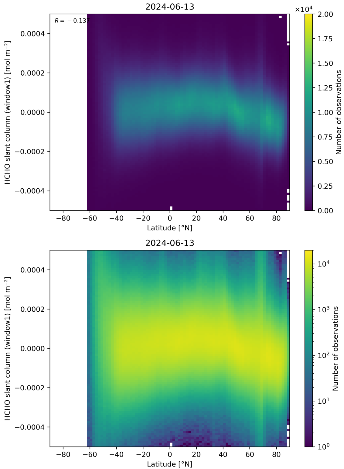
Figure 159: Scatter density plot of “Latitude” against “HCHO slant column (window1)” for 2024-06-13 to 2024-06-14.
