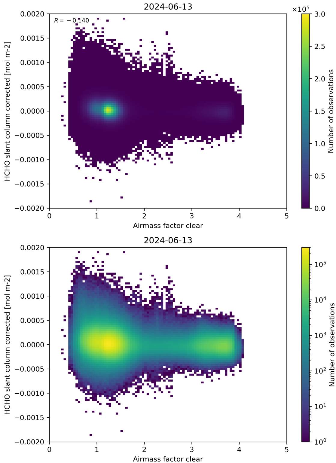
Figure 74: Scatter density plot of “Airmass factor clear” against “HCHO slant column corrected” for 2024-06-13 to 2024-06-14.
