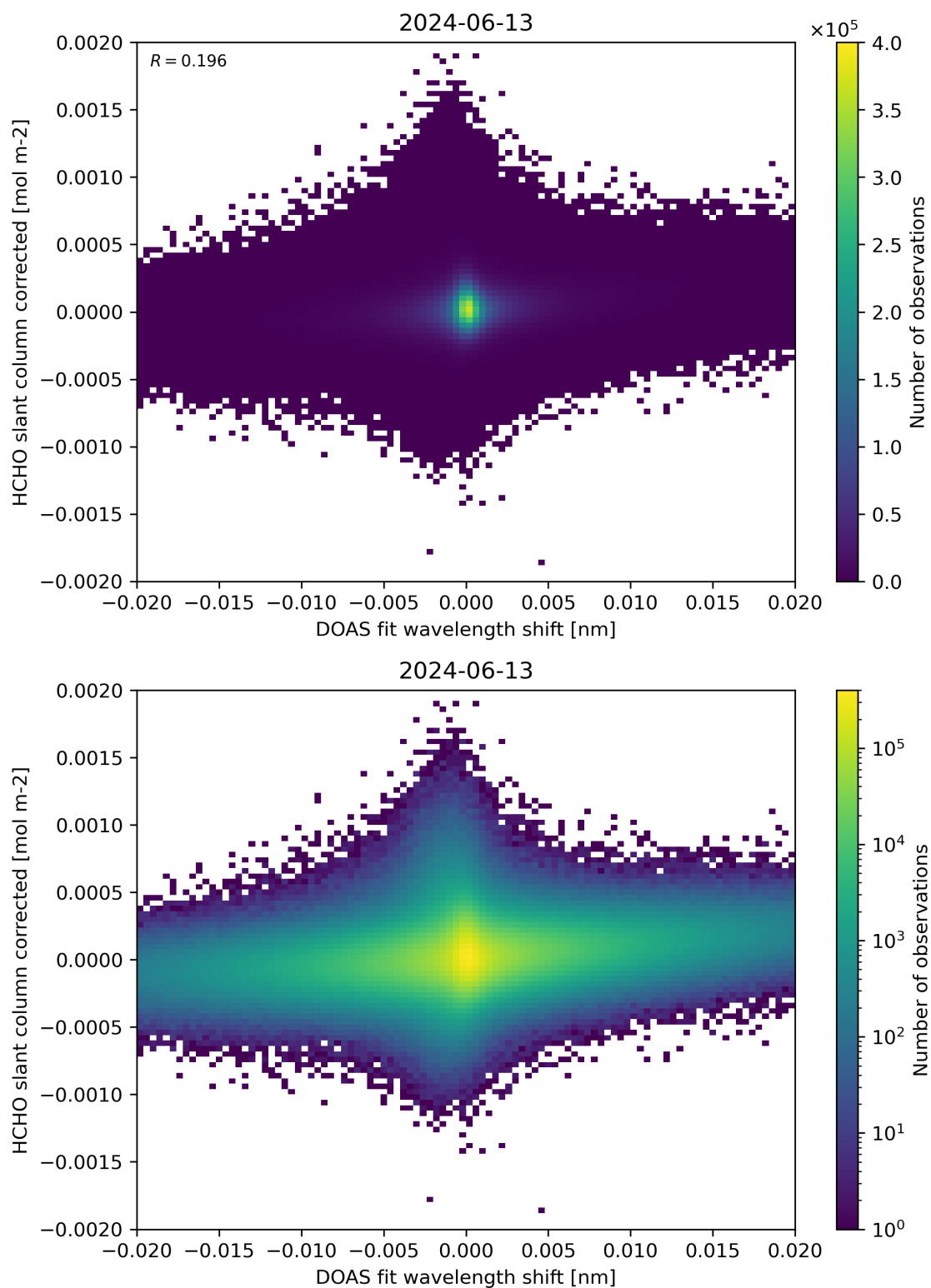
Figure 66: Scatter density plot of “DOAS fit wavelength shift” against “HCHO slant column corrected” for 2024-06-13 to 2024-06-14.
