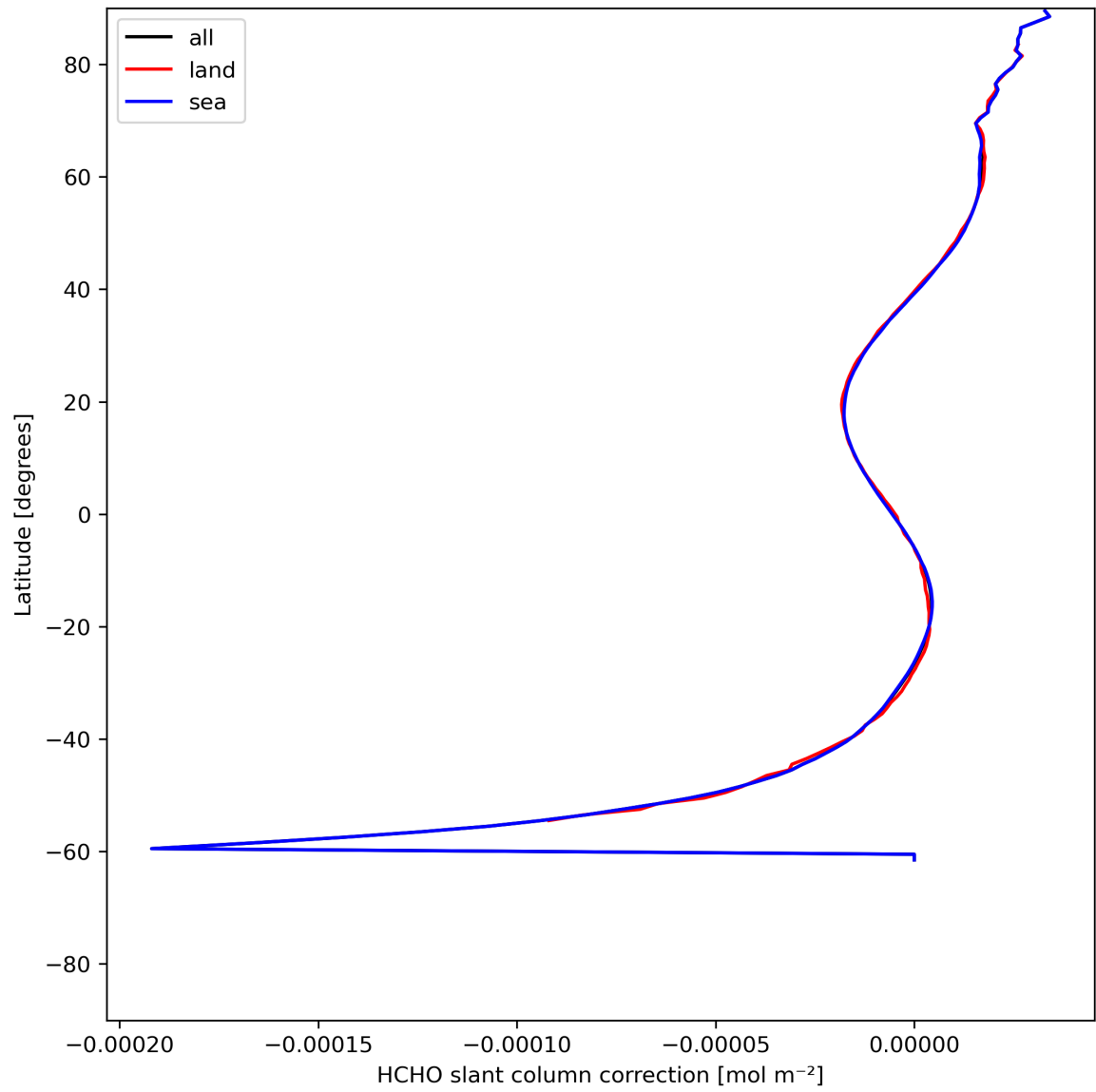
Figure 33: Zonal average of "HCHO slant column correction" for 2024-06-13 to 2024-06-14.
