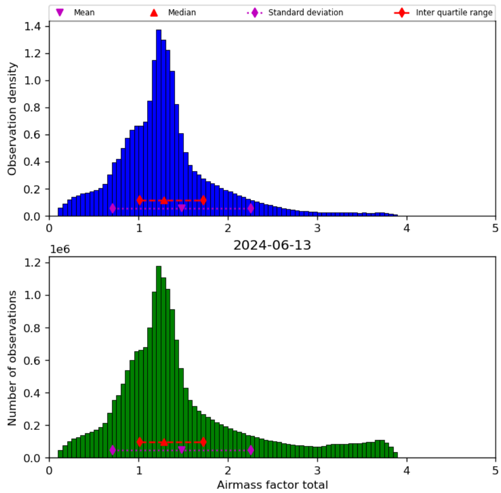
Figure 40: Histogram of “Airmass factor total” for 2024-06-13 to 2024-06-14
