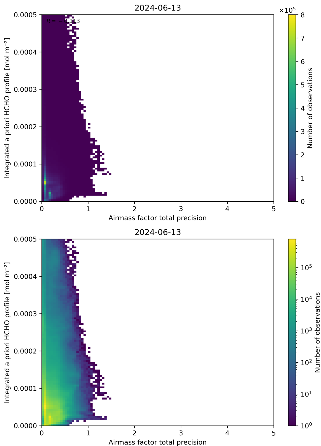
Figure 111: Scatter density plot of “Airmass factor total precision” against “Integrated a priori HCHO profile” for 2024-06-13 to 2024-06-14.
