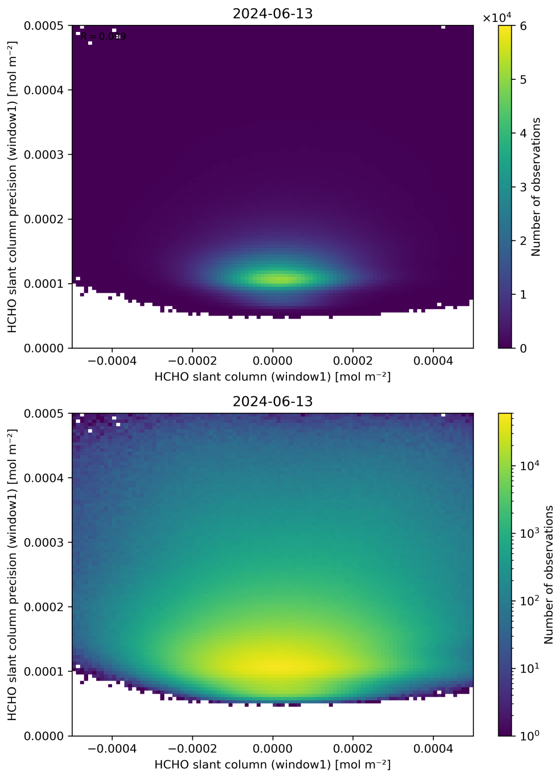
Figure 84: Scatter density plot of “HCHO slant column (window1)” against “HCHO slant column precision (window1)” for 2024-06-13 to 2024-06-14.
