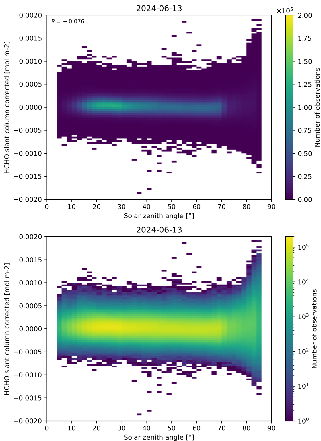
Figure 171: Scatter density plot of “Solar zenith angle” against “HCHO slant column corrected” for 2024-06-13 to 2024-06-14.
