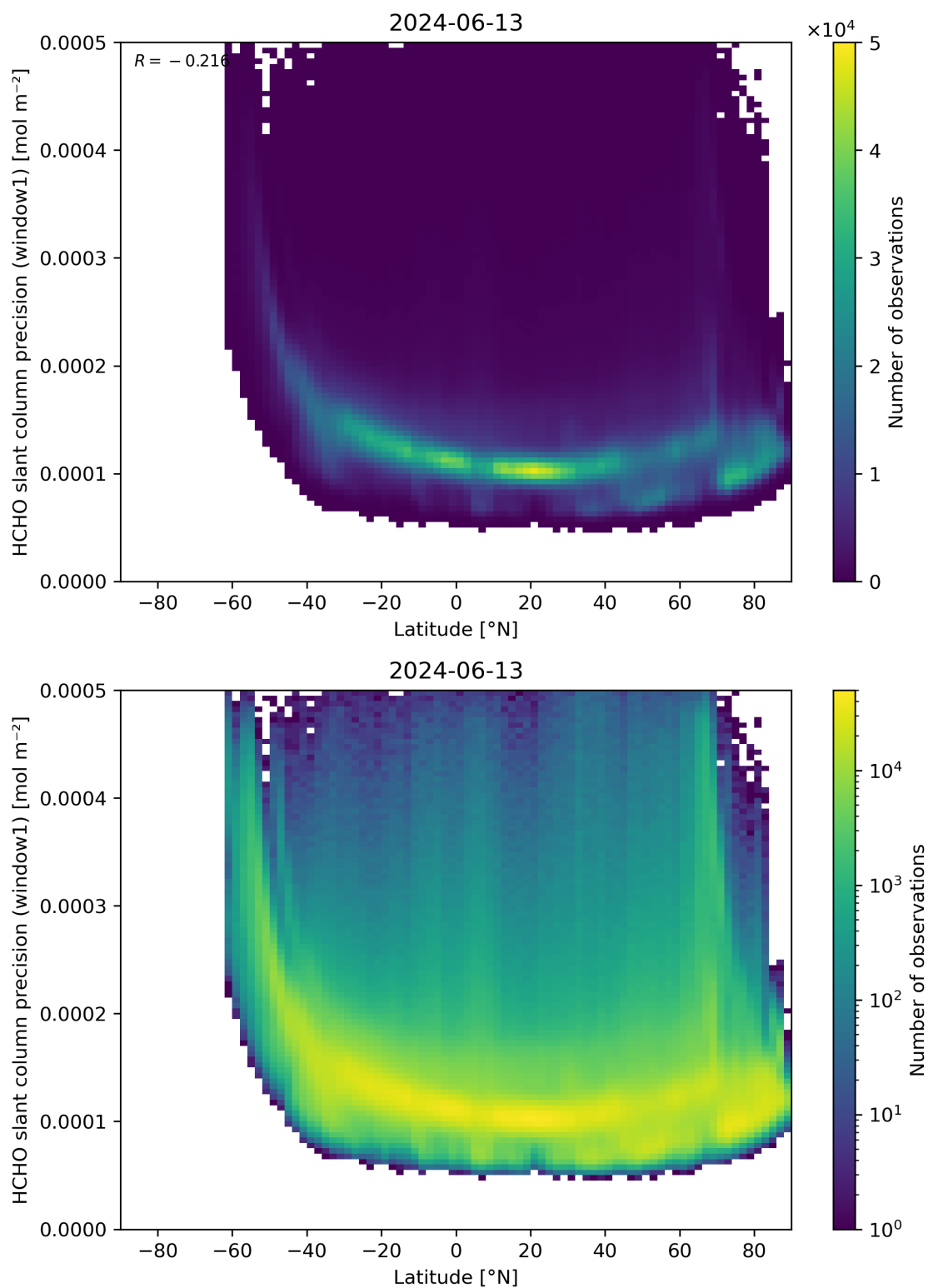
Figure 160: Scatter density plot of “Latitude” against “HCHO slant column precision (window1)” for 2024-06-13 to 2024-06-14.
