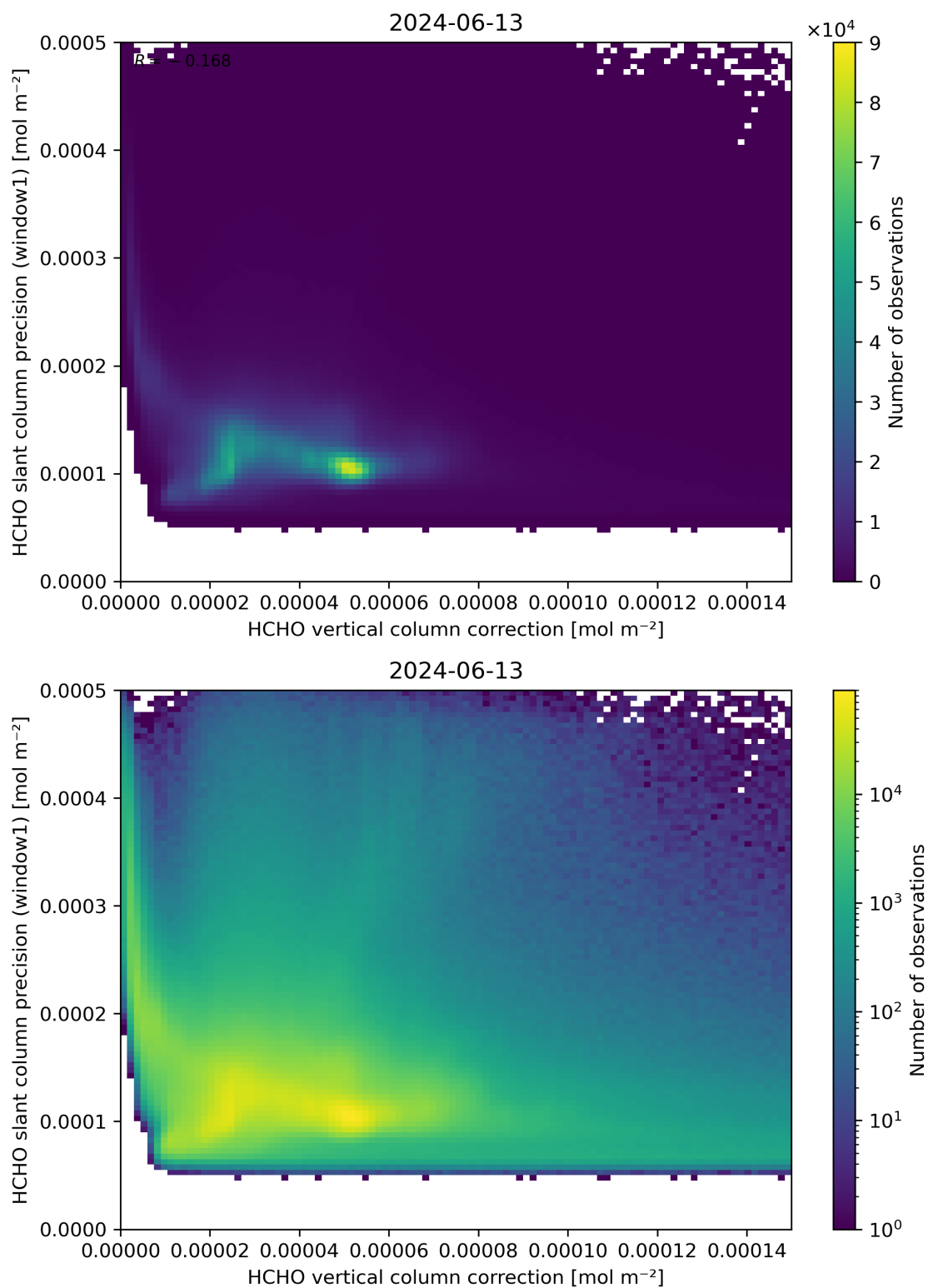
Figure 119: Scatter density plot of “HCHO vertical column correction” against “HCHO slant column precision (window1)” for 2024-06-13 to 2024-06-14.
