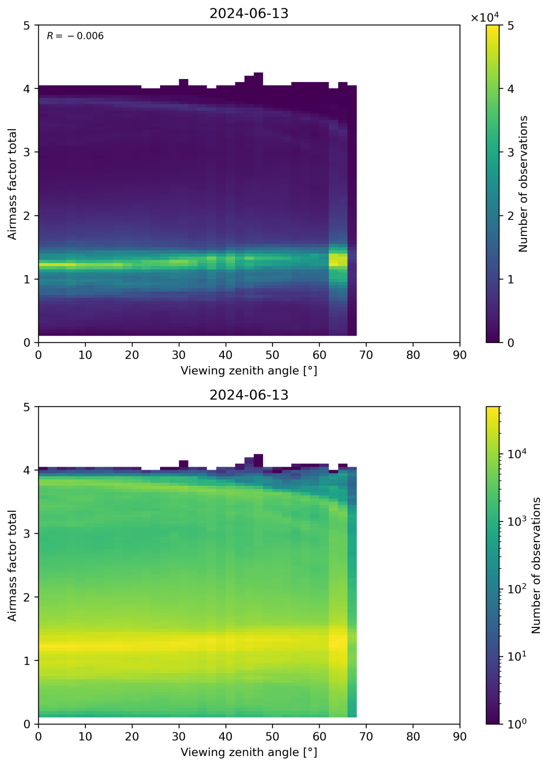
Figure 190: Scatter density plot of “Viewing zenith angle” against “Airmass factor total” for 2024-06-13 to 2024-06-14.
