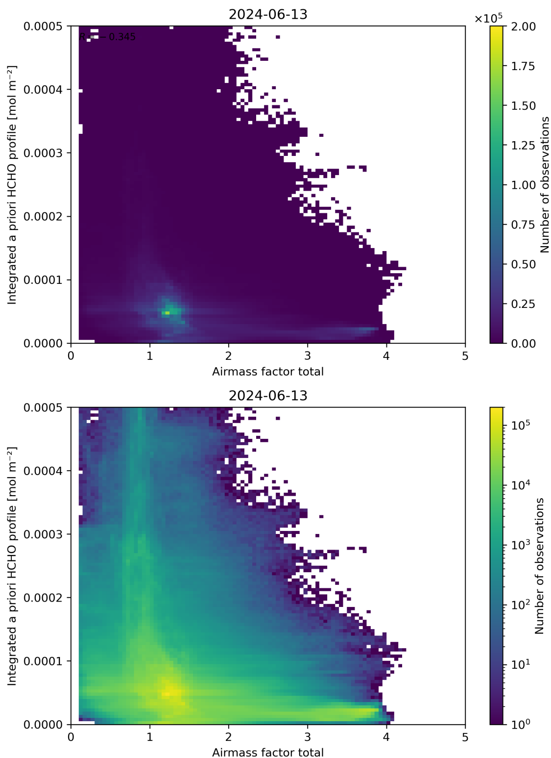
Figure 104: Scatter density plot of “Airmass factor total” against “Integrated a priori HCHO profile” for 2024-06-13 to 2024-06-14.
