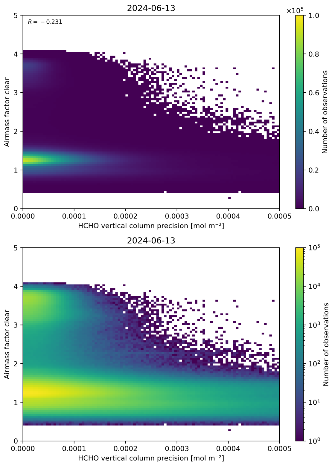
Figure 139: Scatter density plot of “HCHO vertical column precision” against “Airmass factor clear” for 2024-06-13 to 2024-06-14.
