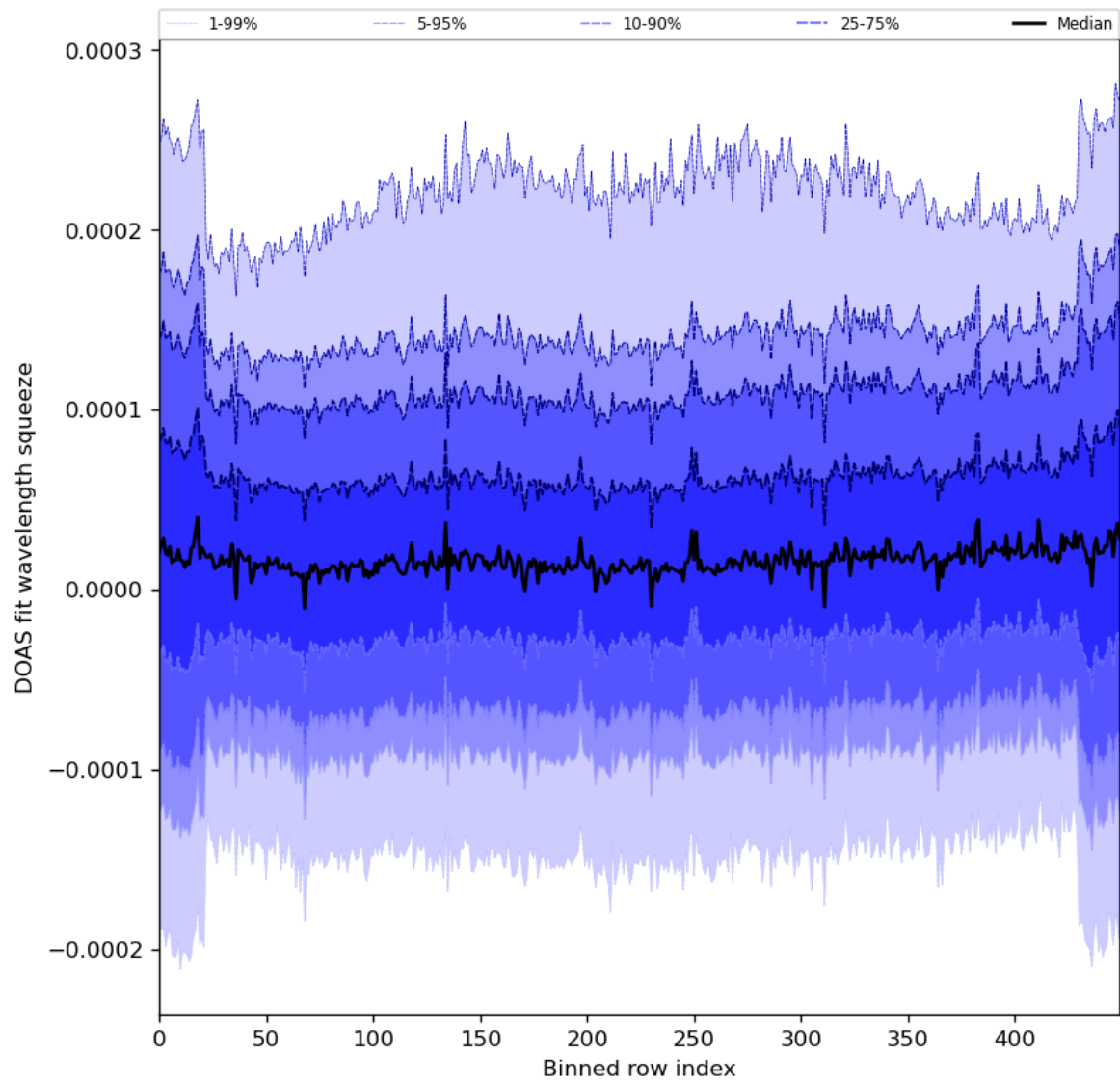
Figure 59: Along track statistics of “DOAS fit wavelength squeeze” for 2024-06-13 to 2024-06-14
