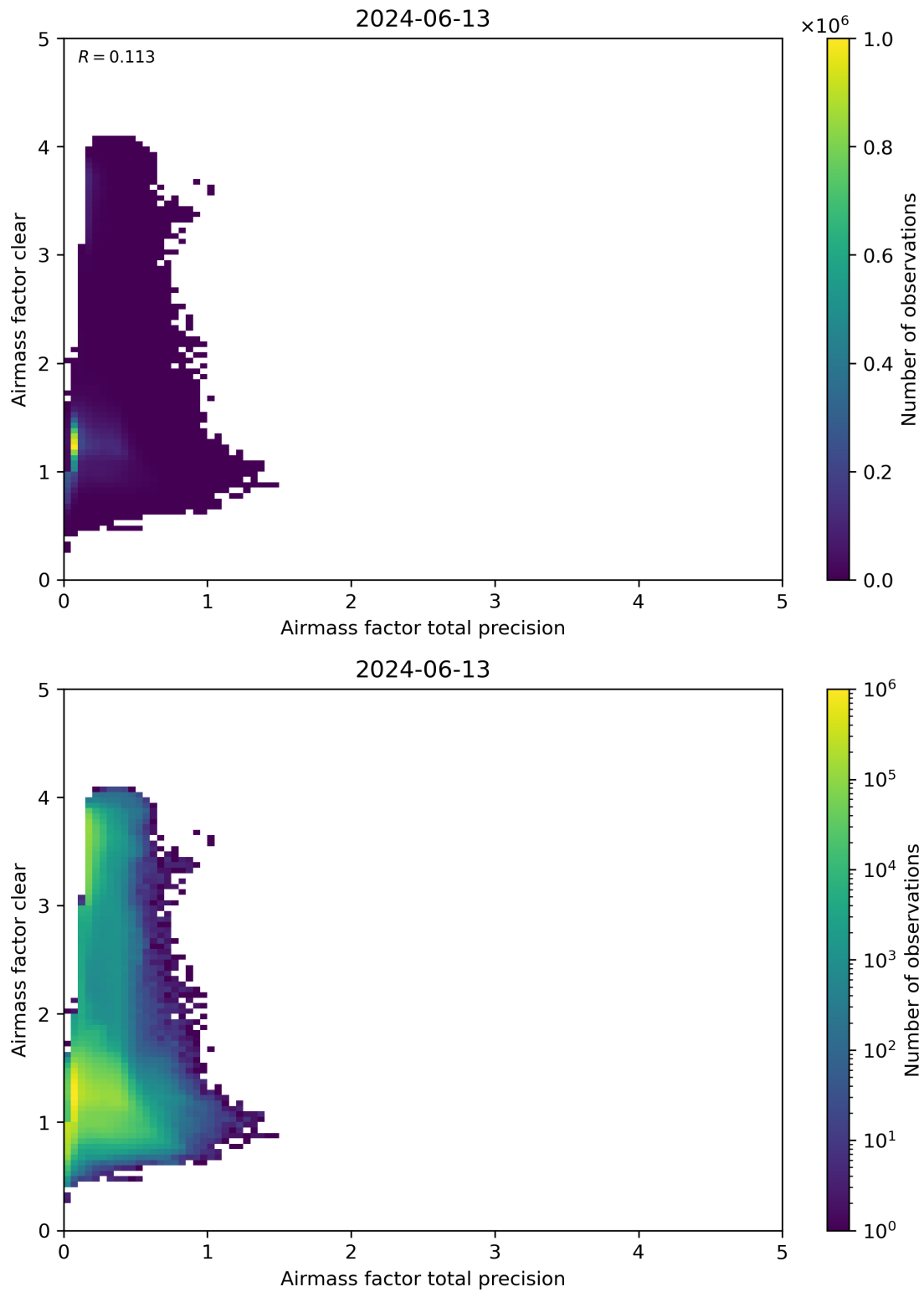
Figure 108: Scatter density plot of “Airmass factor total precision” against “Airmass factor clear” for 2024-06-13 to 2024-06-14.
