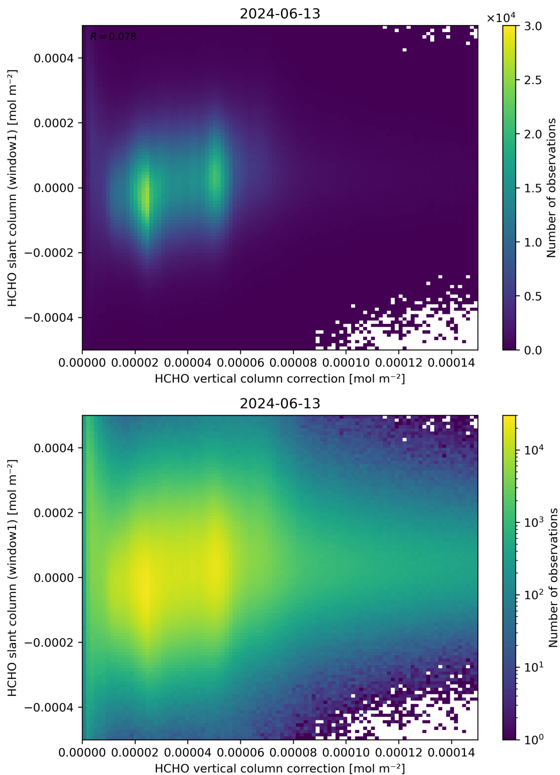
Figure 118: Scatter density plot of “HCHO vertical column correction” against “HCHO slant column (window1)” for 2024-06-13 to 2024-06-14.
