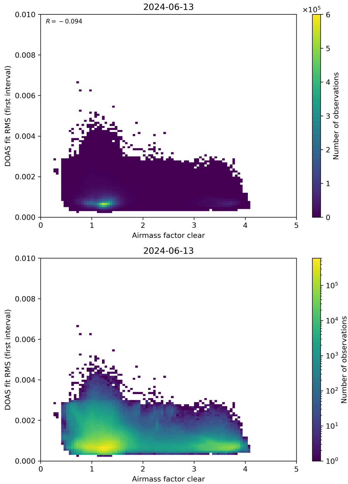
Figure 71: Scatter density plot of “Airmass factor clear” against “DOAS fit RMS (first interval)” for 2024-06-13 to 2024-06-14.
