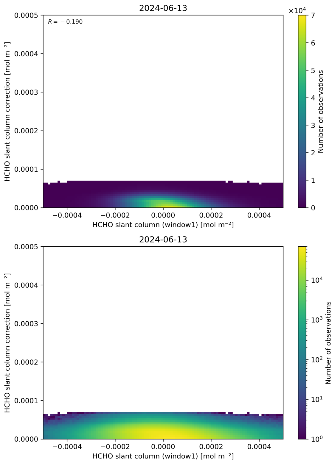
Figure 83: Scatter density plot of “HCHO slant column (window1)” against “HCHO slant column correction” for 2024-06-13 to 2024-06-14.
