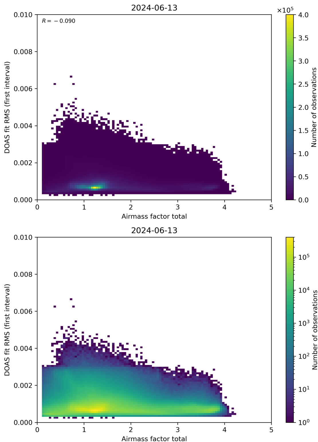
Figure 97: Scatter density plot of “Airmass factor total” against “DOAS fit RMS (first interval)” for 2024-06-13 to 2024-06-14.
