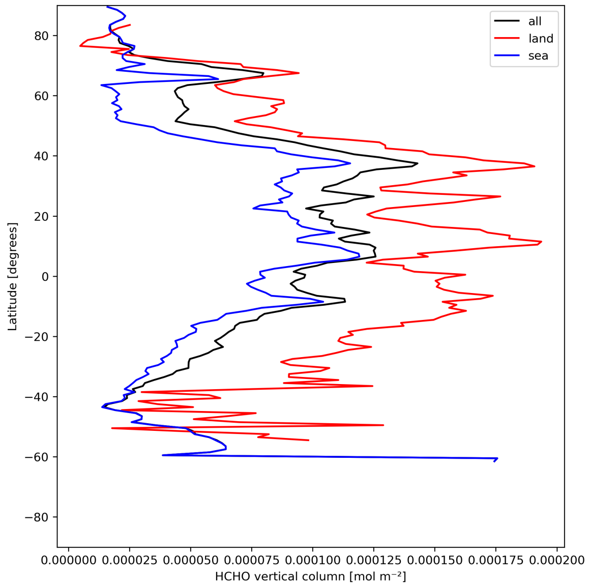
Figure 21: Zonal average of “HCHO vertical column” for 2024-06-13 to 2024-06-14.
