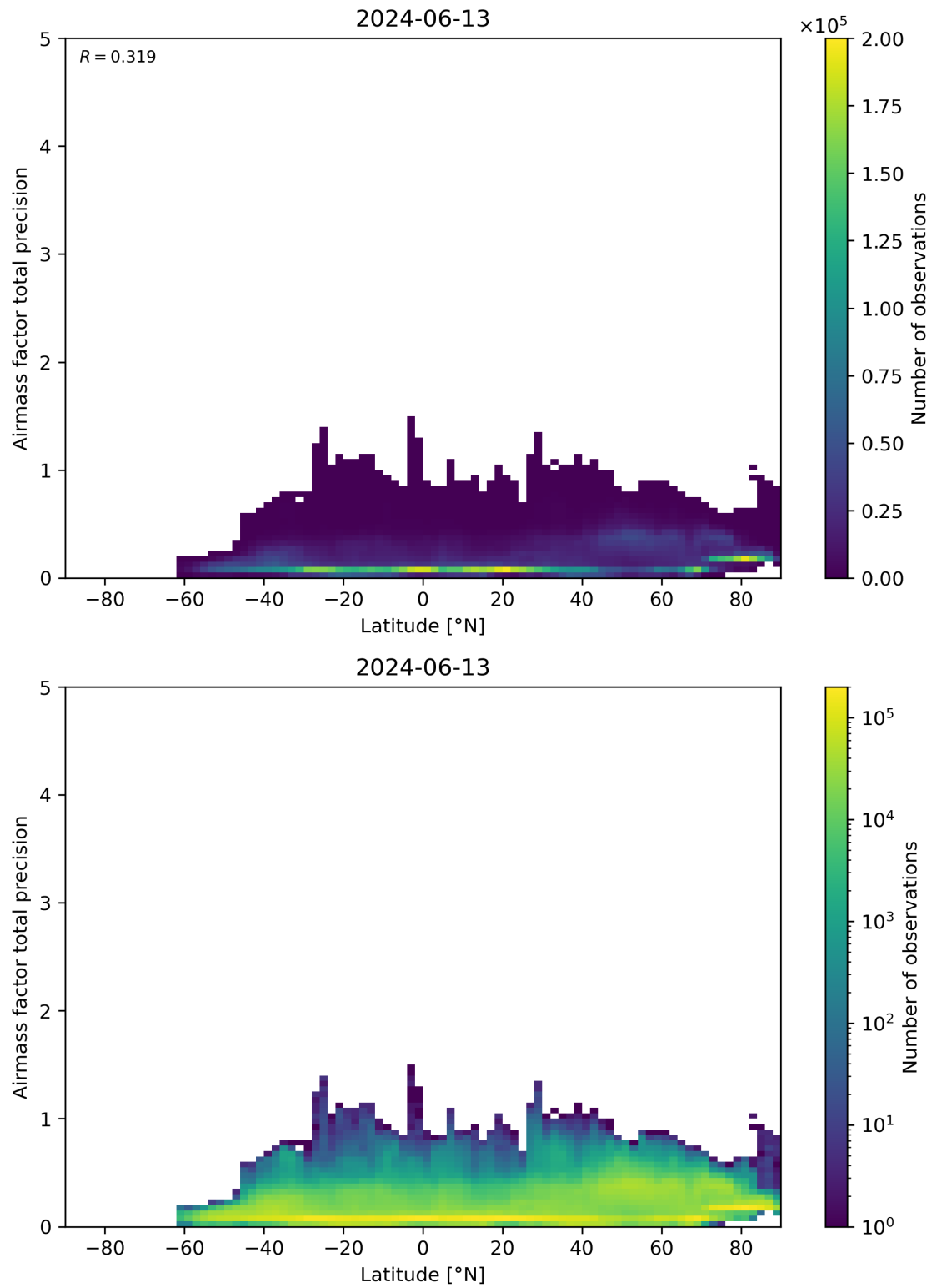
Figure 162: Scatter density plot of “Latitude” against “Airmass factor total precision” for 2024-06-13 to 2024-06-14.
