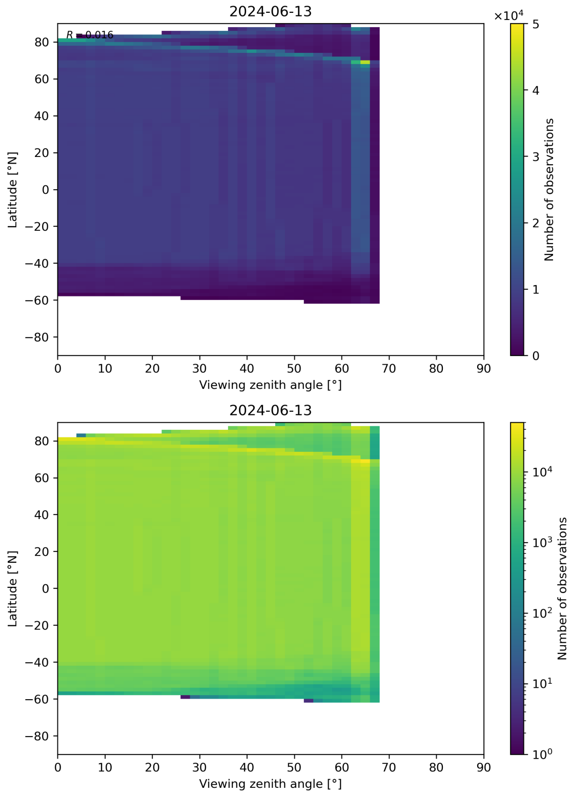
Figure 196: Scatter density plot of “Viewing zenith angle” against “Latitude” for 2024-06-13 to 2024-06-14.
