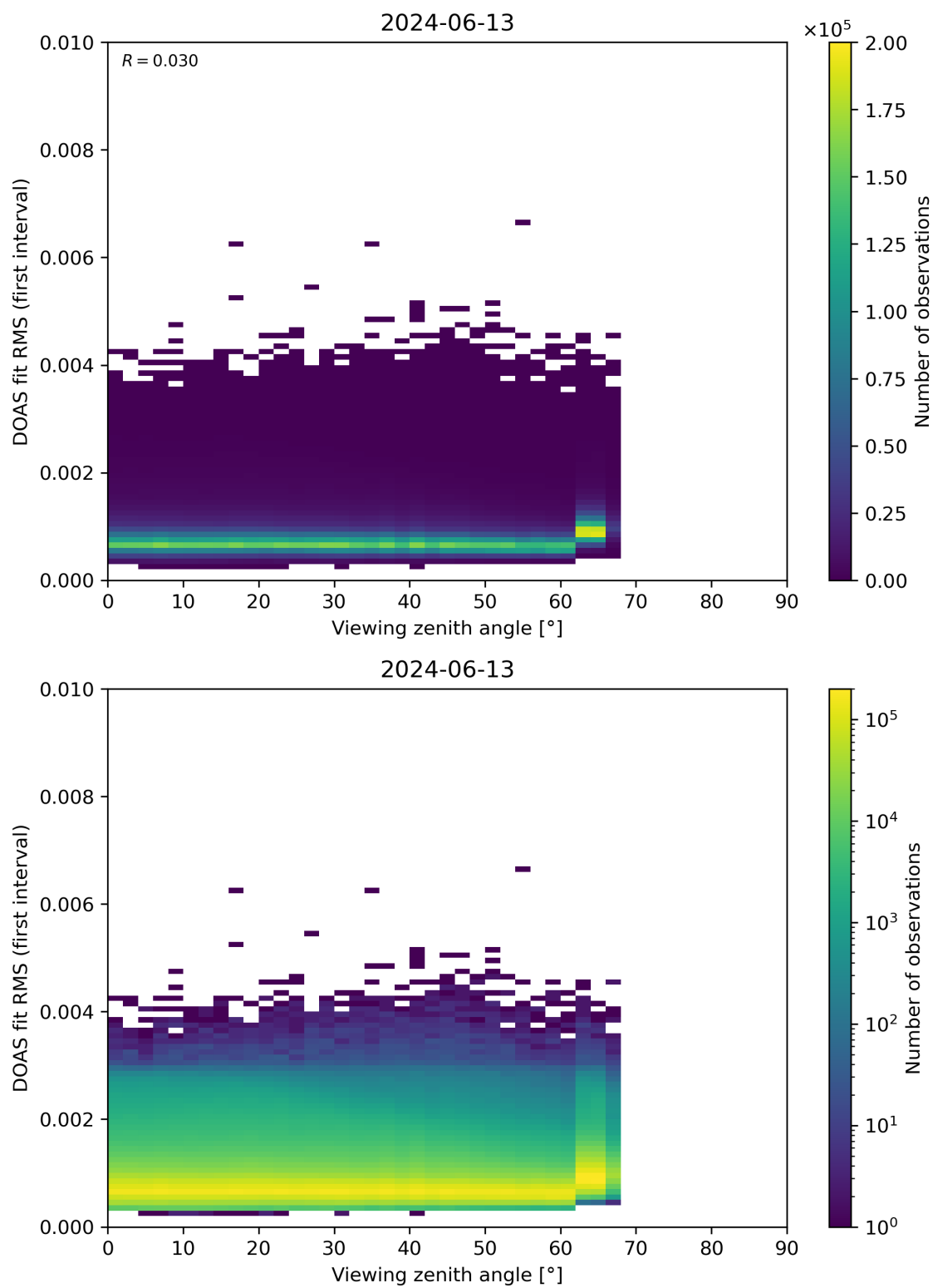
Figure 182: Scatter density plot of “Viewing zenith angle” against “DOAS fit RMS (first interval)” for 2024-06-13 to 2024-06-14.
