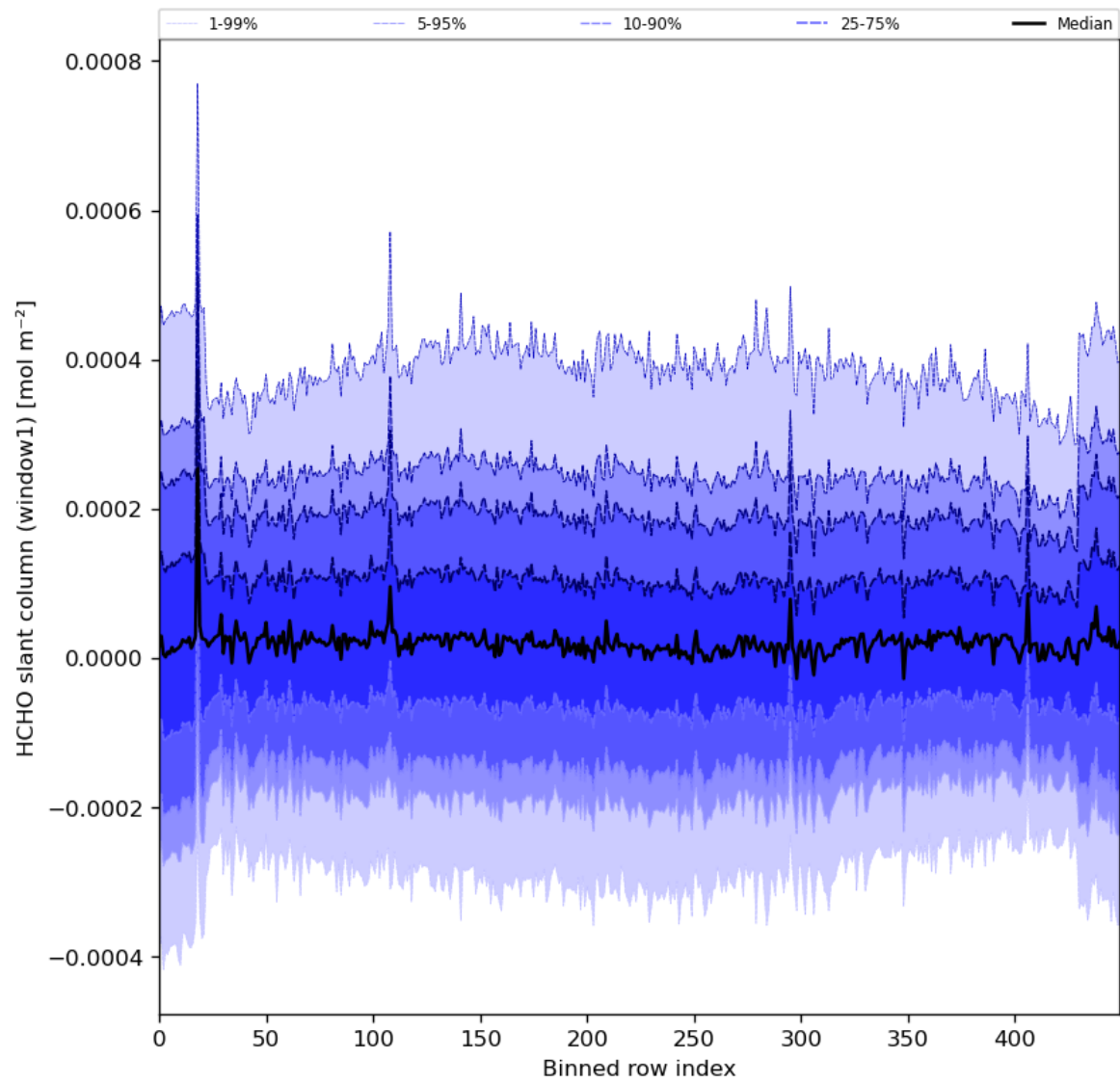
Figure 52: Along track statistics of “HCHO slant column (window1)” for 2024-06-13 to 2024-06-14
