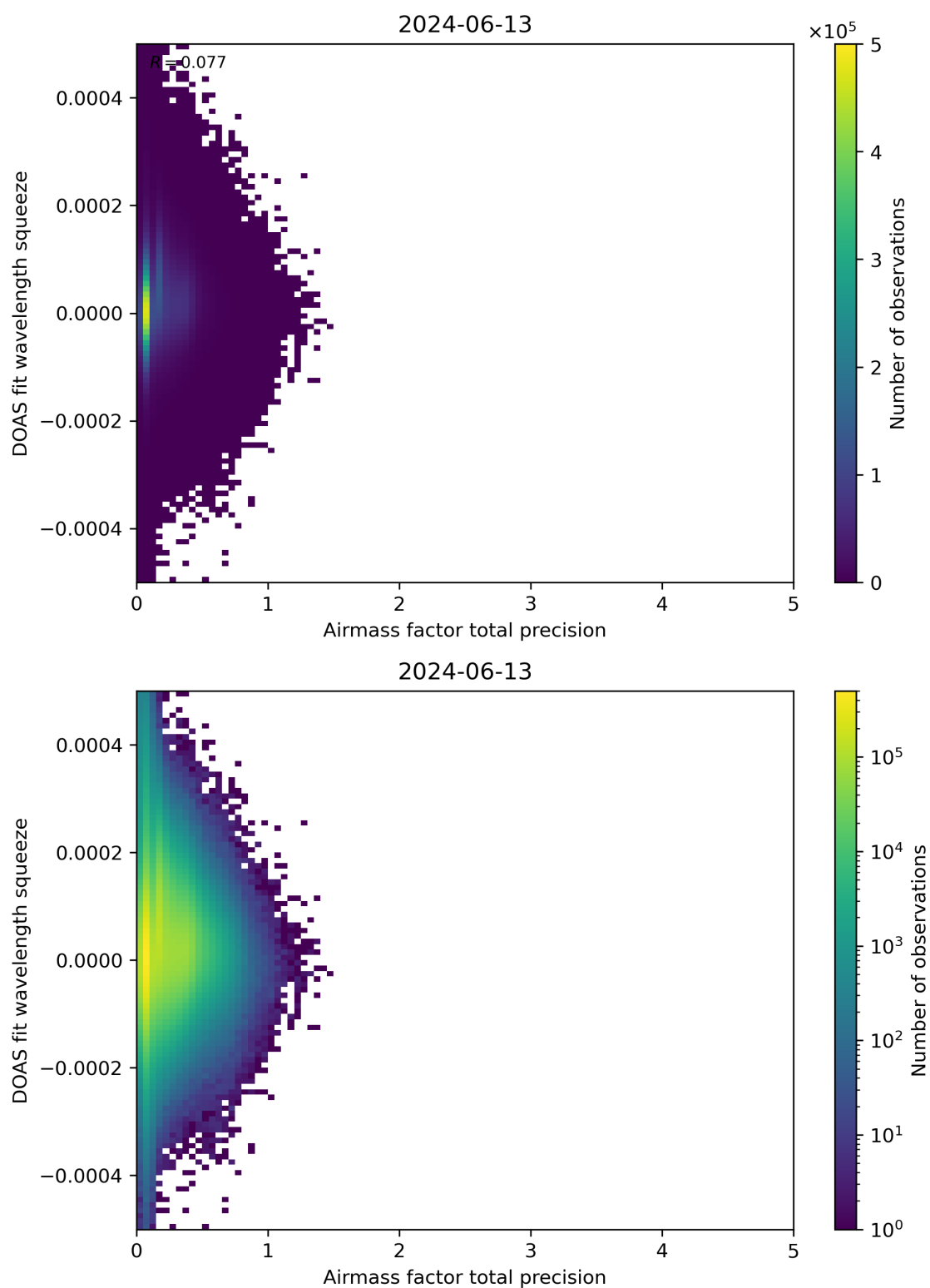
Figure 107: Scatter density plot of “Airmass factor total precision” against “DOAS fit wavelength squeeze” for 2024-06-13 to 2024-06-14.
