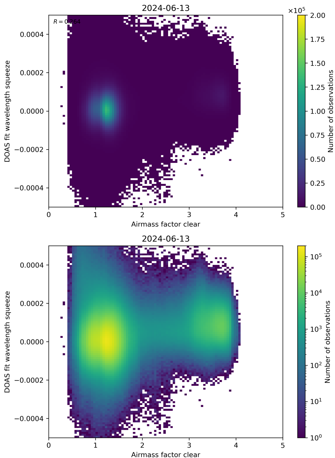
Figure 73: Scatter density plot of “Airmass factor clear” against “DOAS fit wavelength squeeze” for 2024-06-13 to 2024-06-14.
