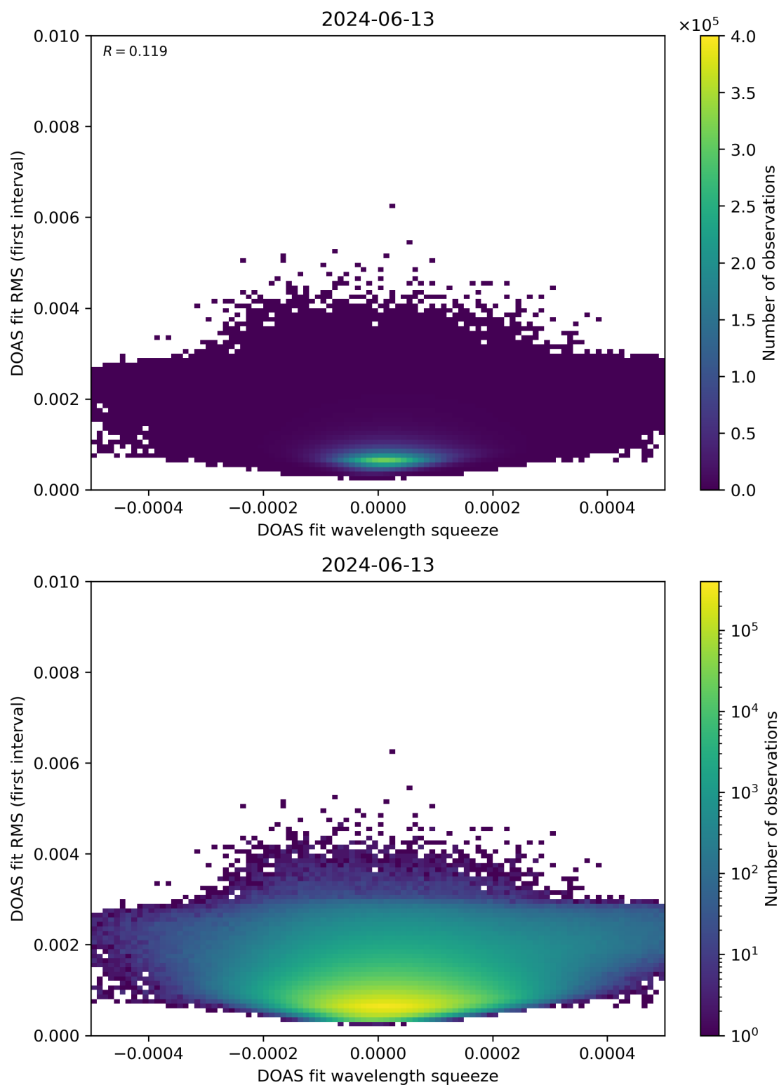
Figure 68: Scatter density plot of “DOAS fit wavelength squeeze” against “DOAS fit RMS (first interval)” for 2024-06-13 to 2024-06-14.
