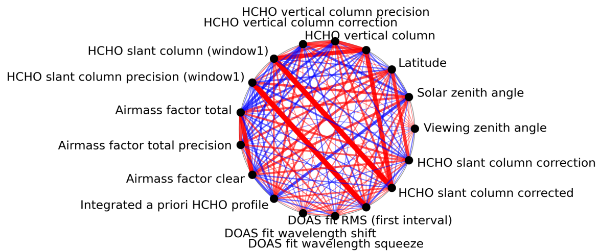
Figure 1: Map of correlation graph for 2024-06-13 to 2024-06-14.
