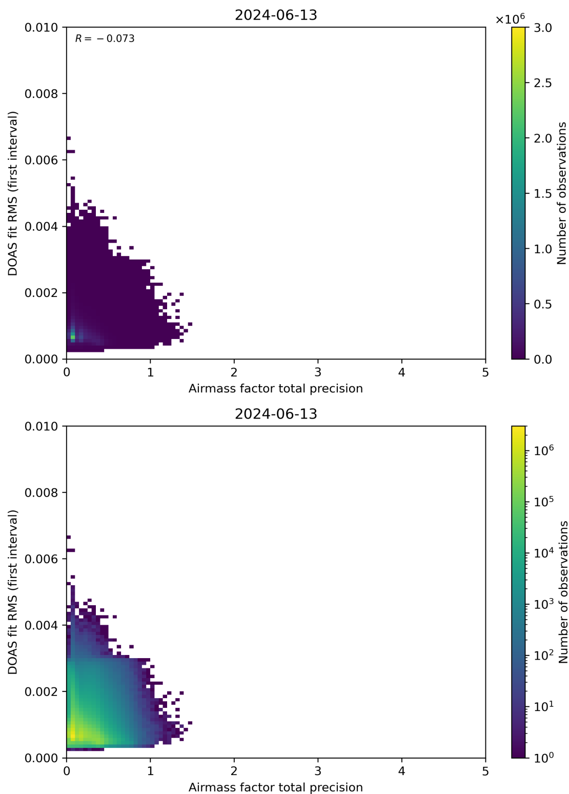
Figure 105: Scatter density plot of “Airmass factor total precision” against “DOAS fit RMS (first interval)” for 2024-06-13 to 2024-06-14.
