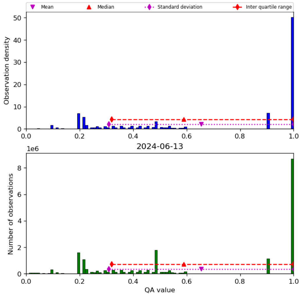
Figure 34: Histogram of “QA value” for 2024-06-13 to 2024-06-14
