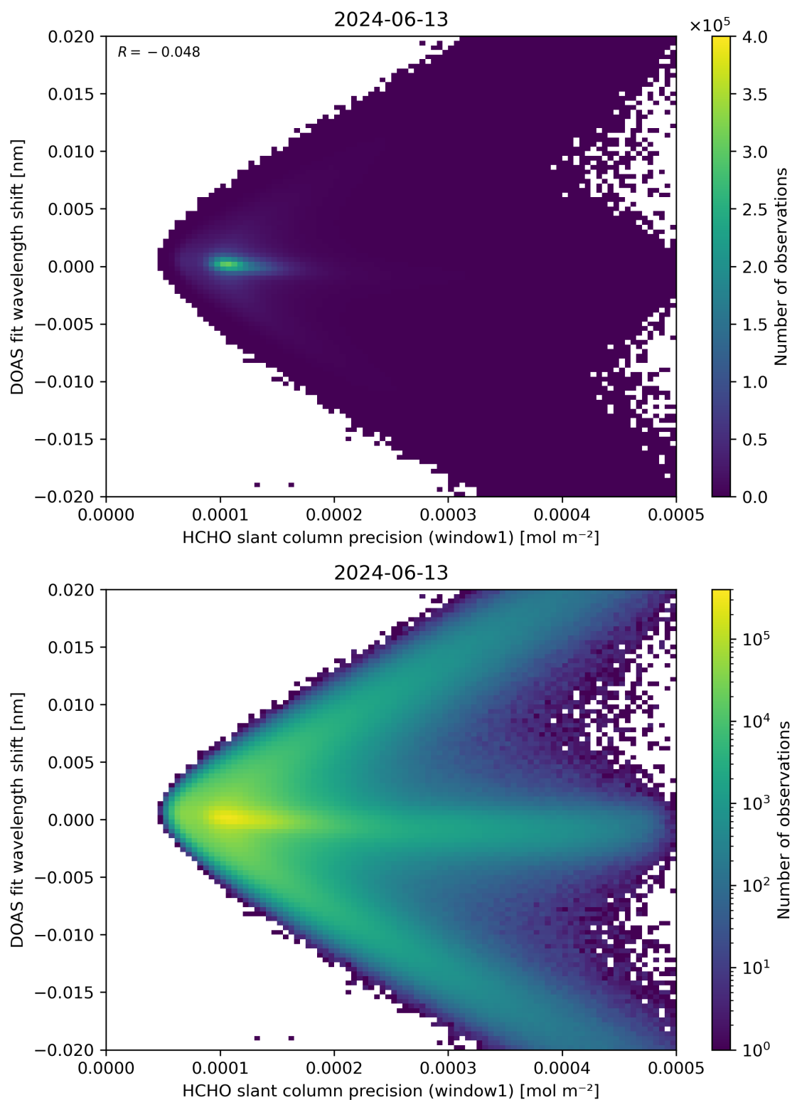
Figure 89: Scatter density plot of “HCHO slant column precision (window1)” against “DOAS fit wavelength shift” for 2024-06-13 to 2024-06-14.
