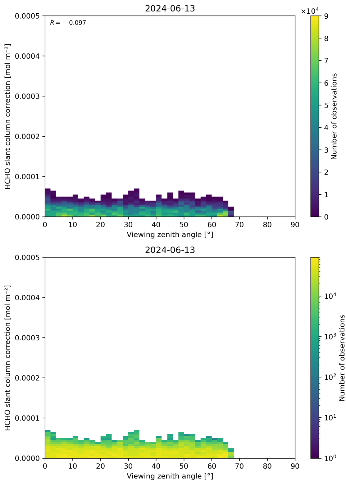
Figure 187: Scatter density plot of “Viewing zenith angle” against “HCHO slant column correction” for 2024-06-13 to 2024-06-14.
