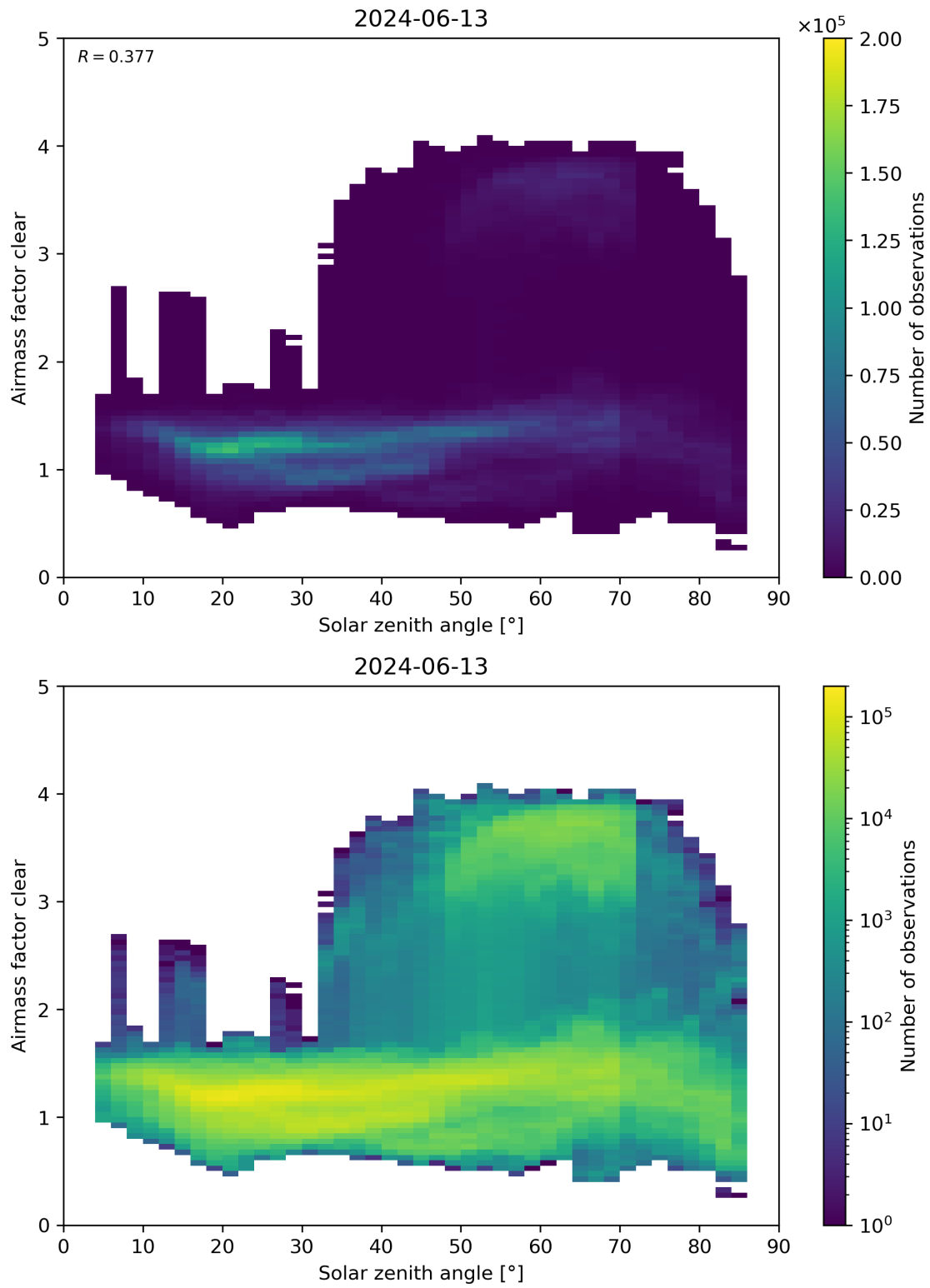
Figure 170: Scatter density plot of “Solar zenith angle” against “Airmass factor clear” for 2024-06-13 to 2024-06-14.
