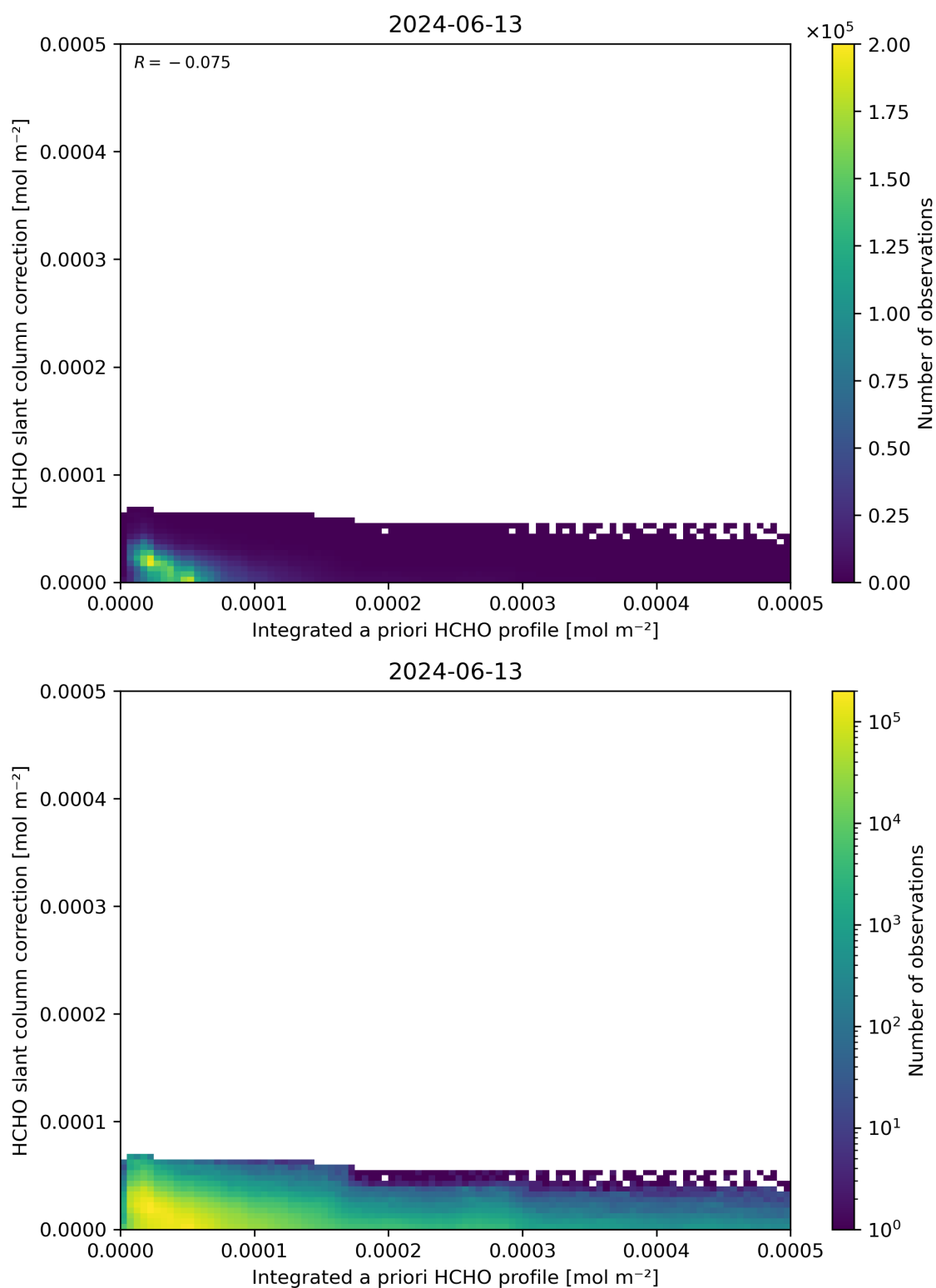
Figure 152: Scatter density plot of “Integrated a priori HCHO profile” against “HCHO slant column correction” for 2024-06-13 to 2024-06-14.
