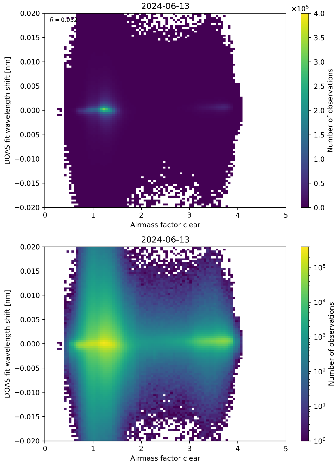
Figure 72: Scatter density plot of “Airmass factor clear” against “DOAS fit wavelength shift” for 2024-06-13 to 2024-06-14.
