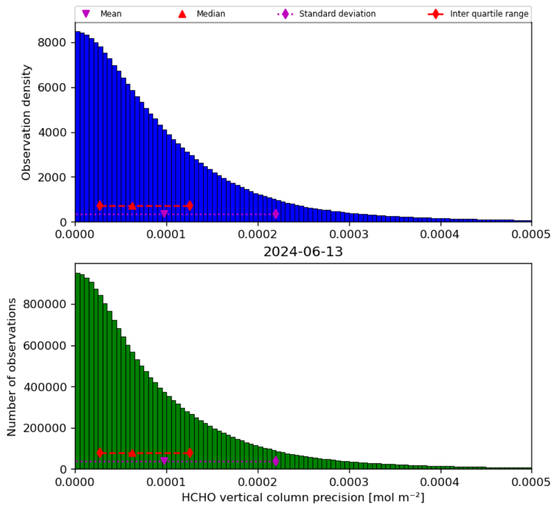
Figure 36: Histogram of “HCHO vertical column precision” for 2024-06-13 to 2024-06-14
