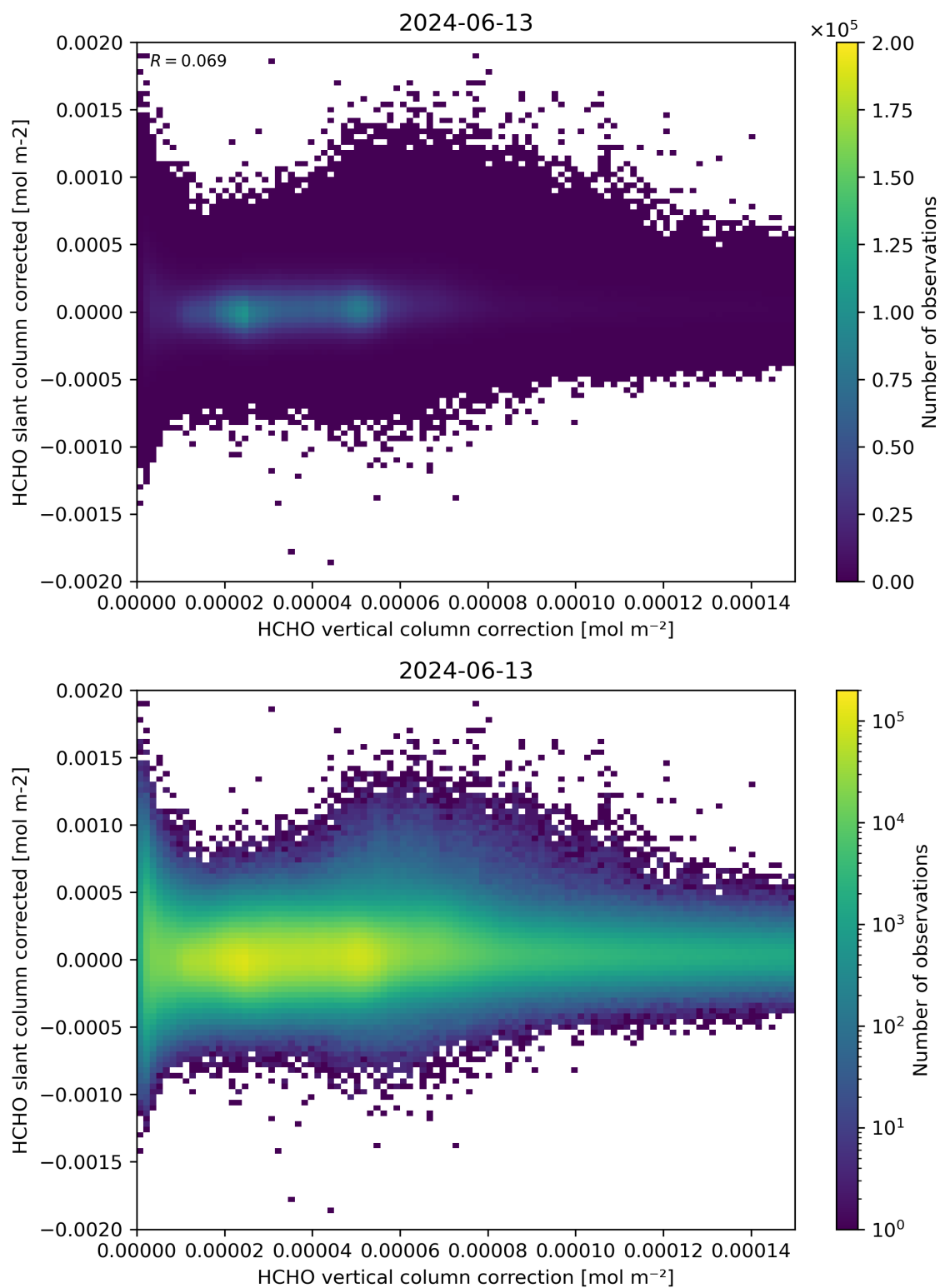
Figure 116: Scatter density plot of “HCHO vertical column correction” against “HCHO slant column corrected” for 2024-06-13 to 2024-06-14.
