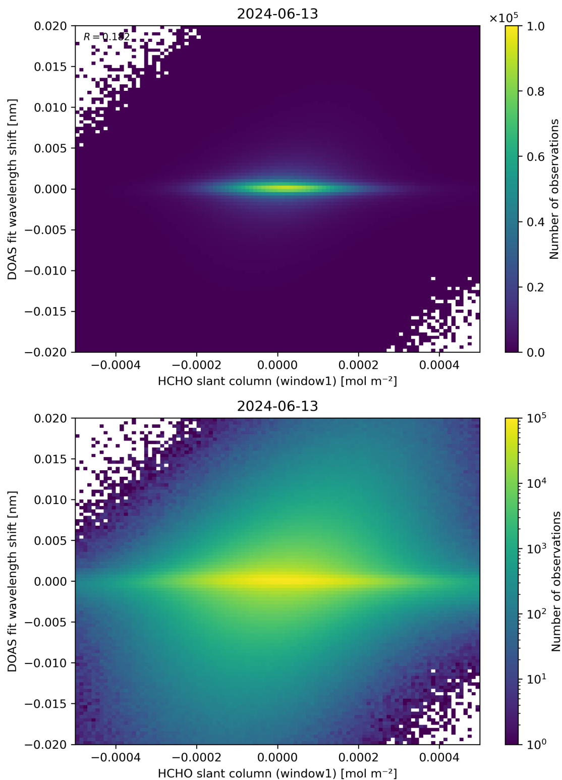
Figure 79: Scatter density plot of “HCHO slant column (window1)” against “DOAS fit wavelength shift” for 2024-06-13 to 2024-06-14.
