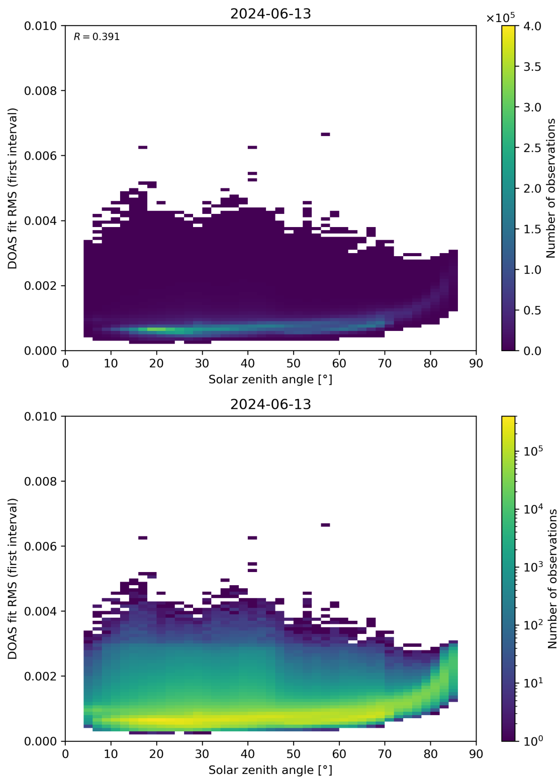
Figure 167: Scatter density plot of “Solar zenith angle” against “DOAS fit RMS (first interval)” for 2024-06-13 to 2024-06-14.
