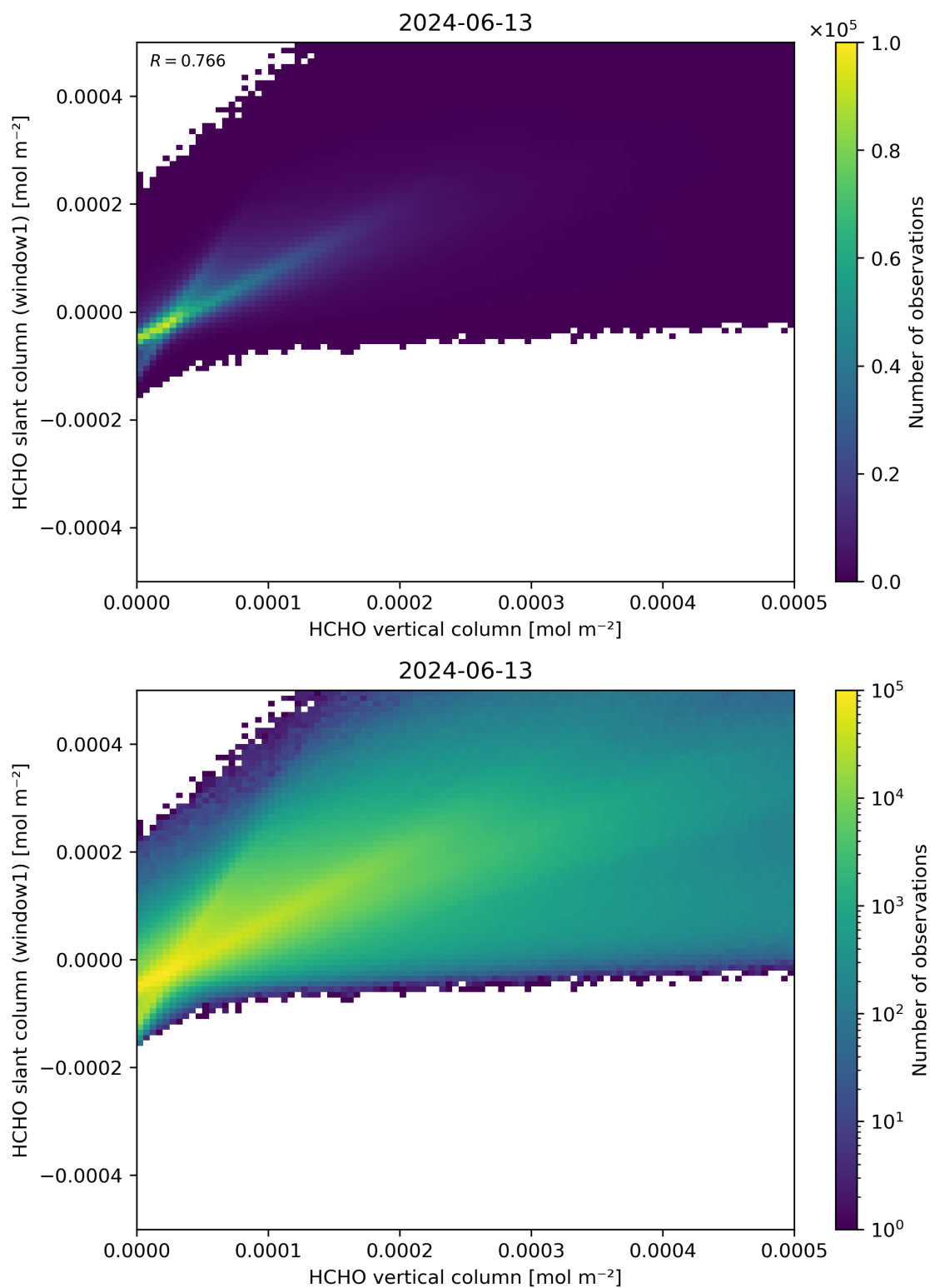
Figure 129: Scatter density plot of “HCHO vertical column” against “HCHO slant column (window1)” for 2024-06-13 to 2024-06-14.
