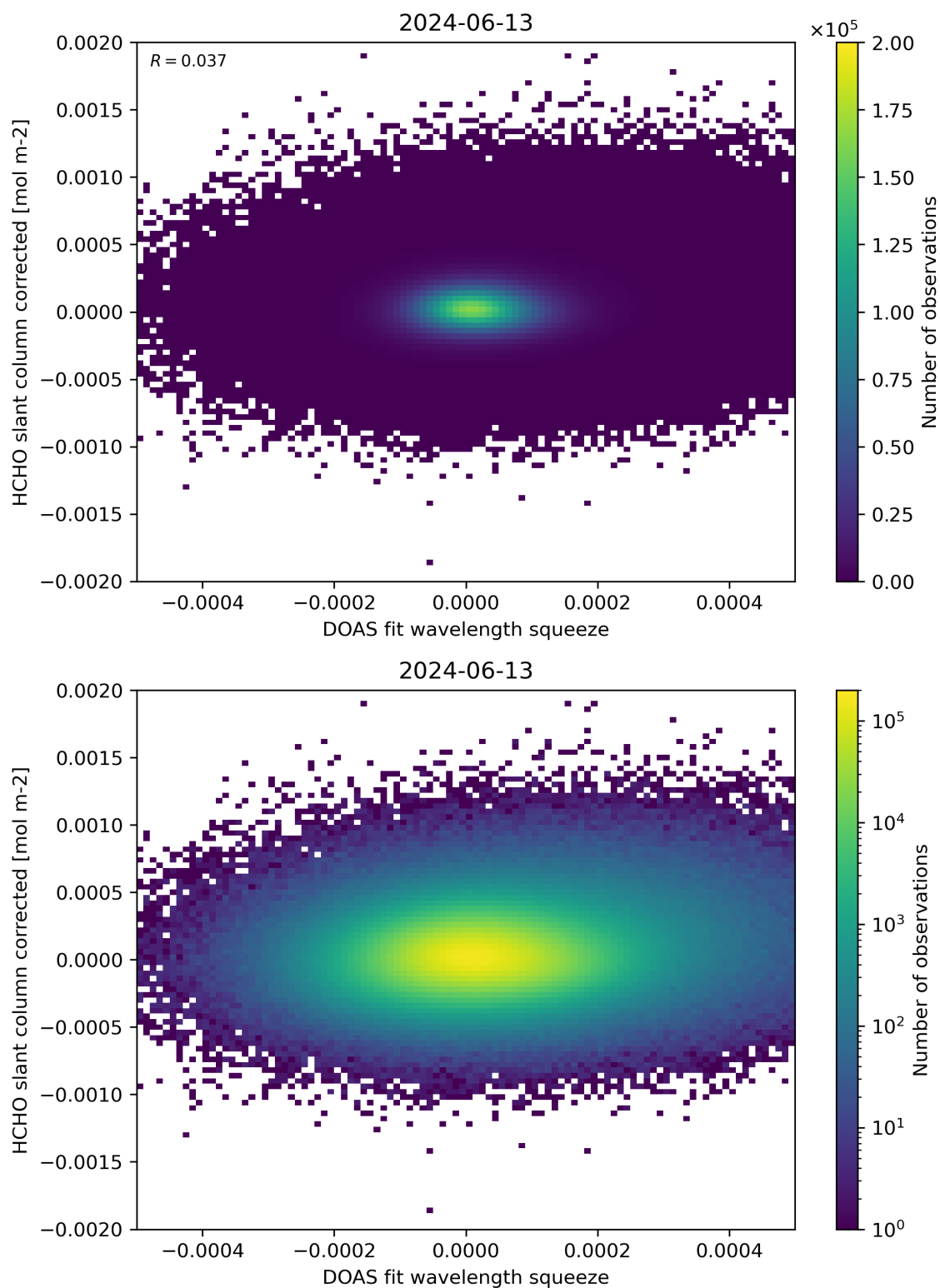
Figure 69: Scatter density plot of “DOAS fit wavelength squeeze” against “HCHO slant column corrected” for 2024-06-13 to 2024-06-14.
