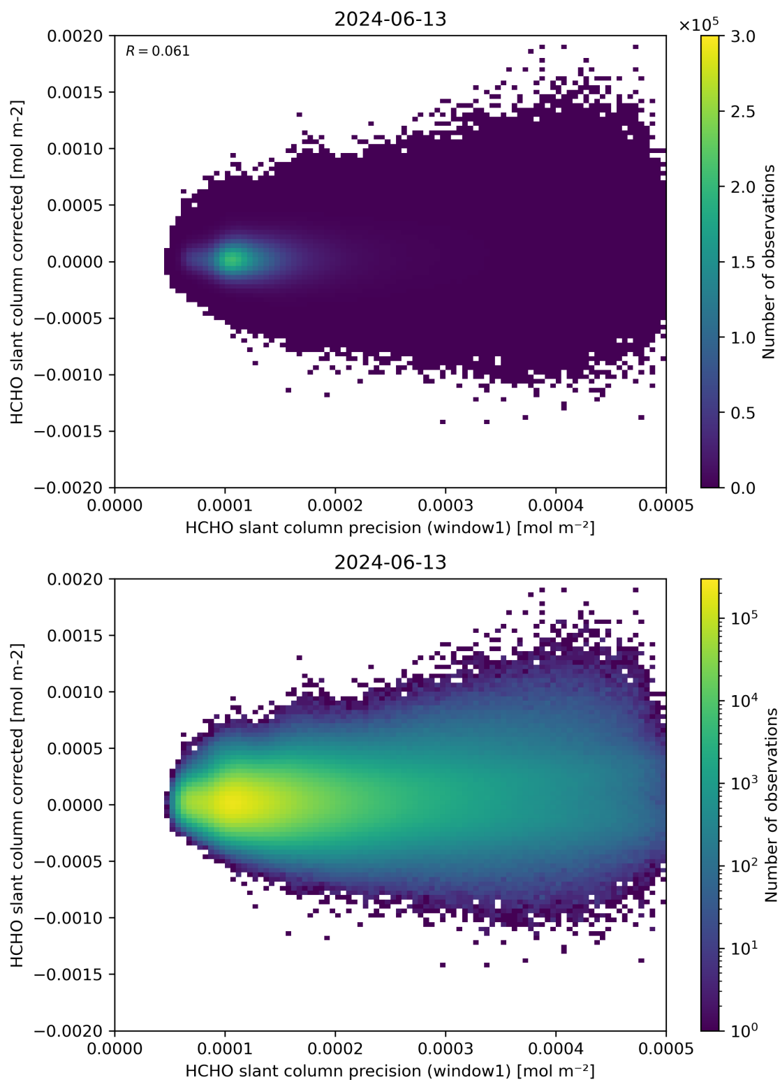
Figure 92: Scatter density plot of “HCHO slant column precision (window1)” against “HCHO slant column corrected” for 2024-06-13 to 2024-06-14.
