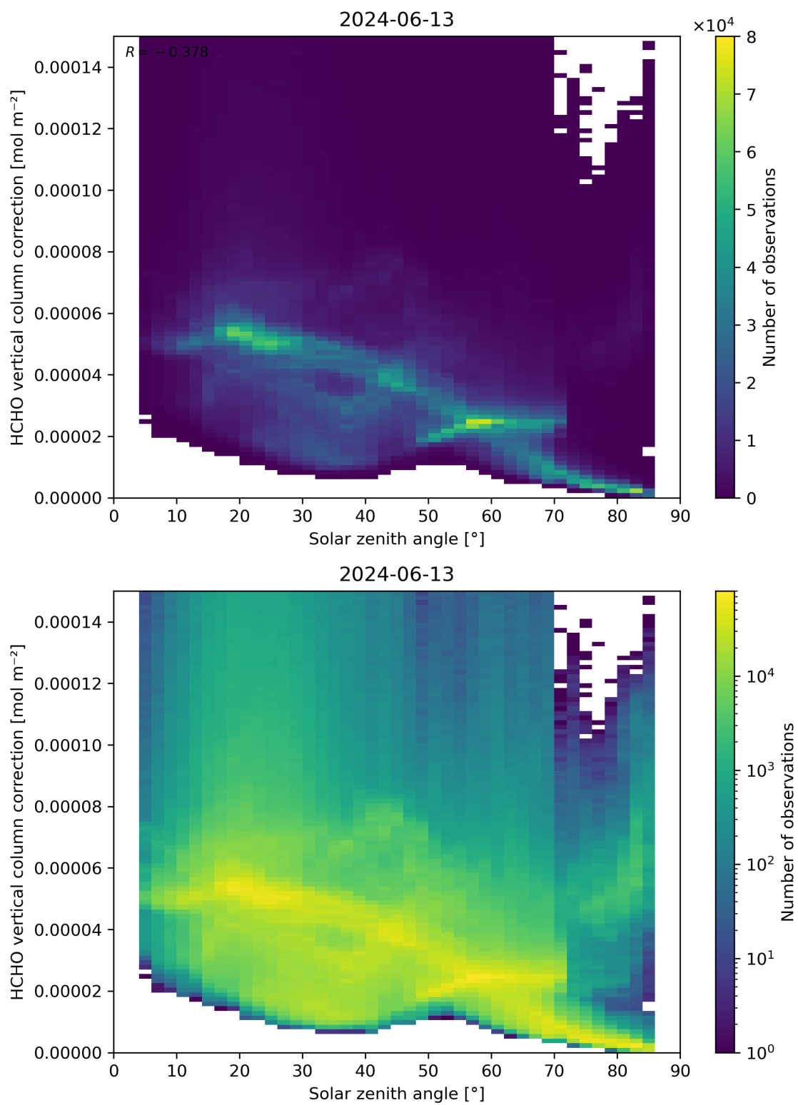
Figure 178: Scatter density plot of “Solar zenith angle” against “HCHO vertical column correction” for 2024-06-13 to 2024-06-14.
