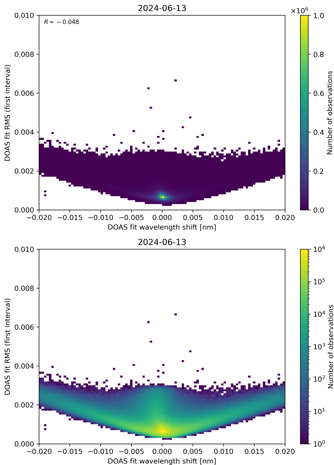
Figure 64: Scatter density plot of “DOAS fit wavelength shift” against “DOAS fit RMS (first interval)” for 2024-06-13 to 2024-06-14.
