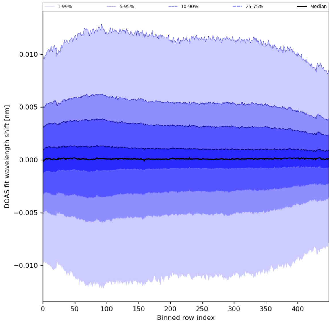
Figure 58: Along track statistics of “DOAS fit wavelength shift” for 2024-06-13 to 2024-06-14
