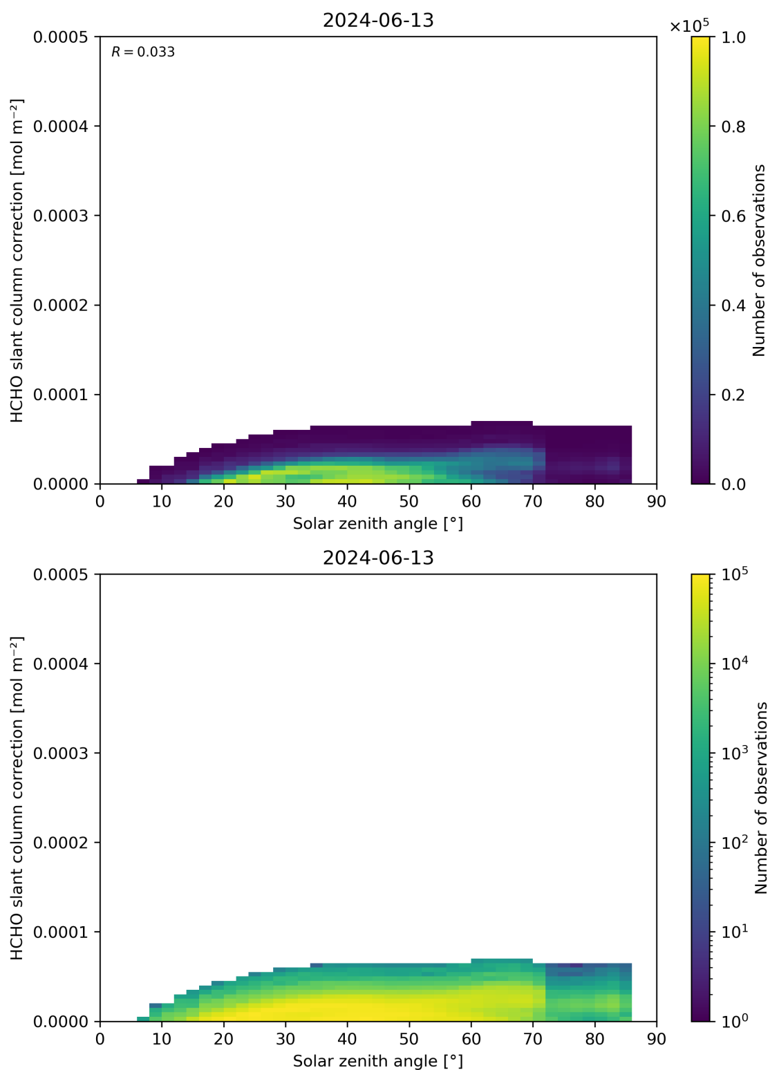
Figure 172: Scatter density plot of “Solar zenith angle” against “HCHO slant column correction” for 2024-06-13 to 2024-06-14.
