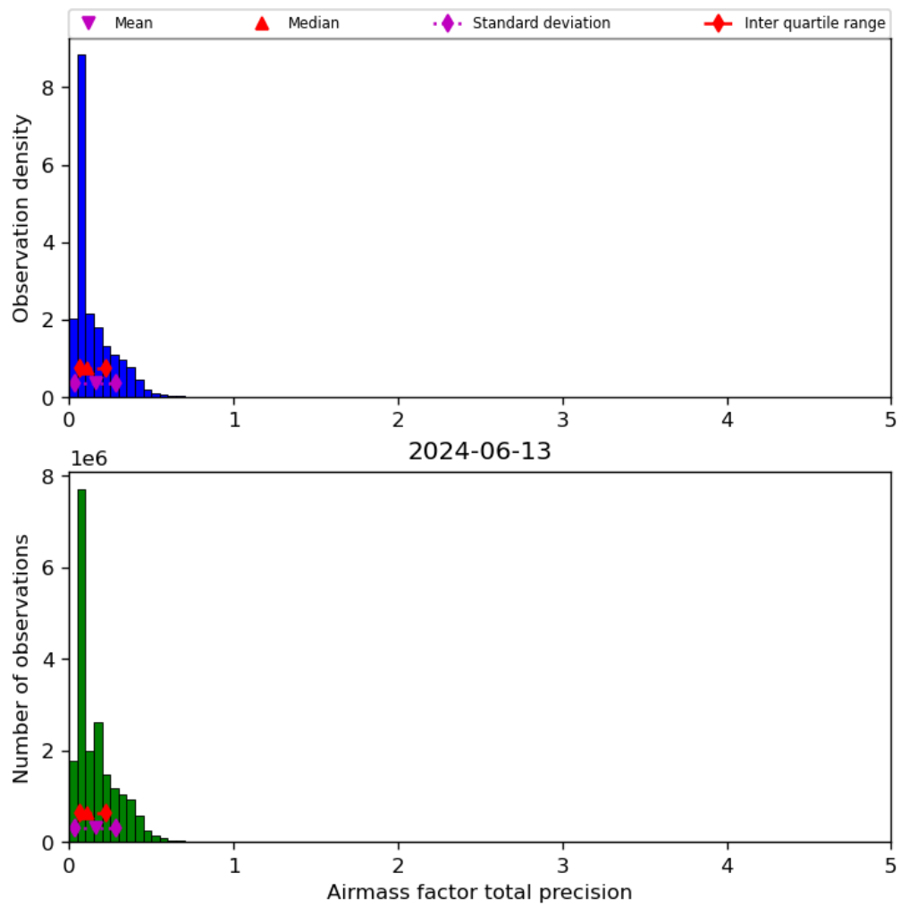
Figure 41: Histogram of “Airmass factor total precision” for 2024-06-13 to 2024-06-14
