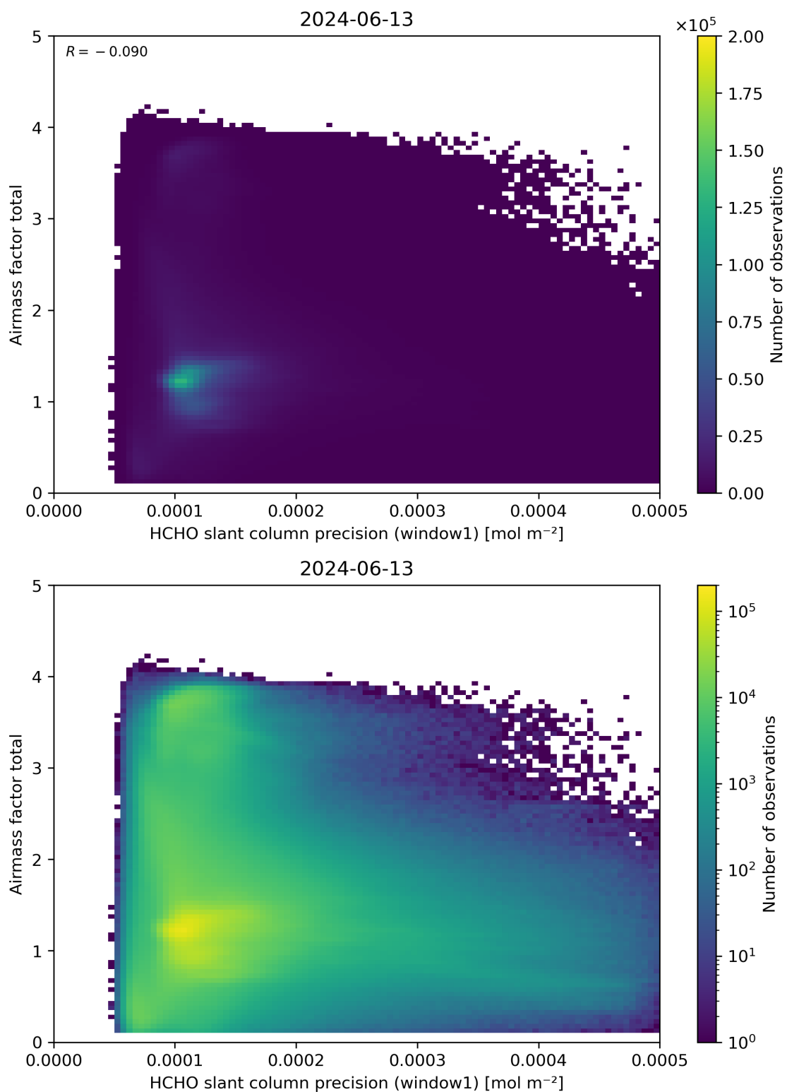
Figure 94: Scatter density plot of “HCHO slant column precision (window1)” against “Airmass factor total” for 2024-06-13 to 2024-06-14.
