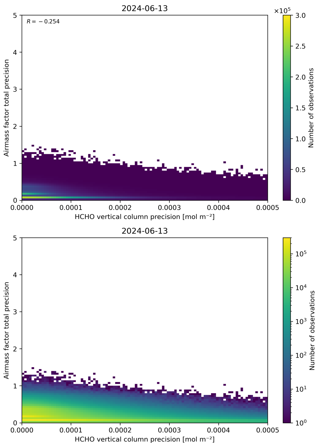
Figure 145: Scatter density plot of “HCHO vertical column precision” against “Airmass factor total precision” for 2024-06-13 to 2024-06-14.
