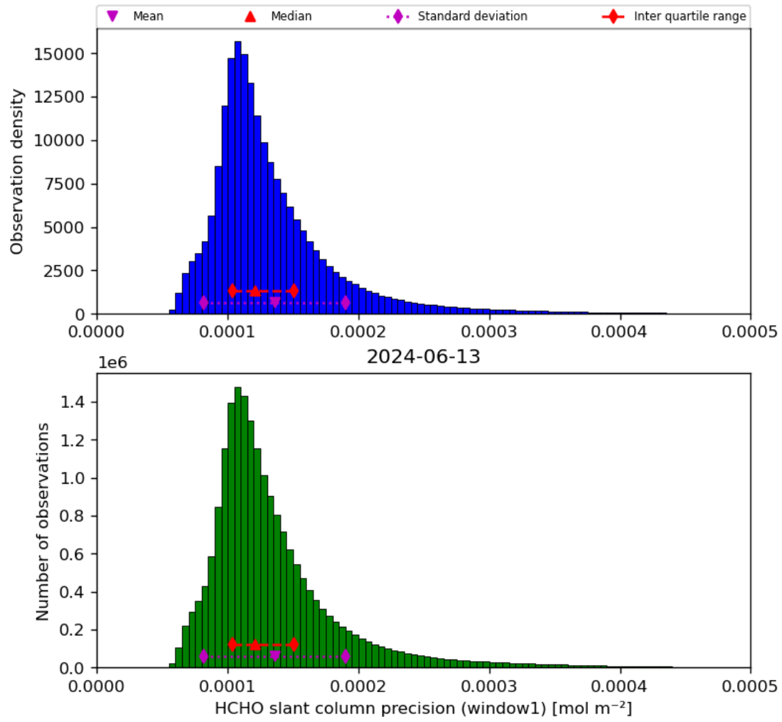
Figure 39: Histogram of “HCHO slant column precision (window1)” for 2024-06-13 to 2024-06-14
