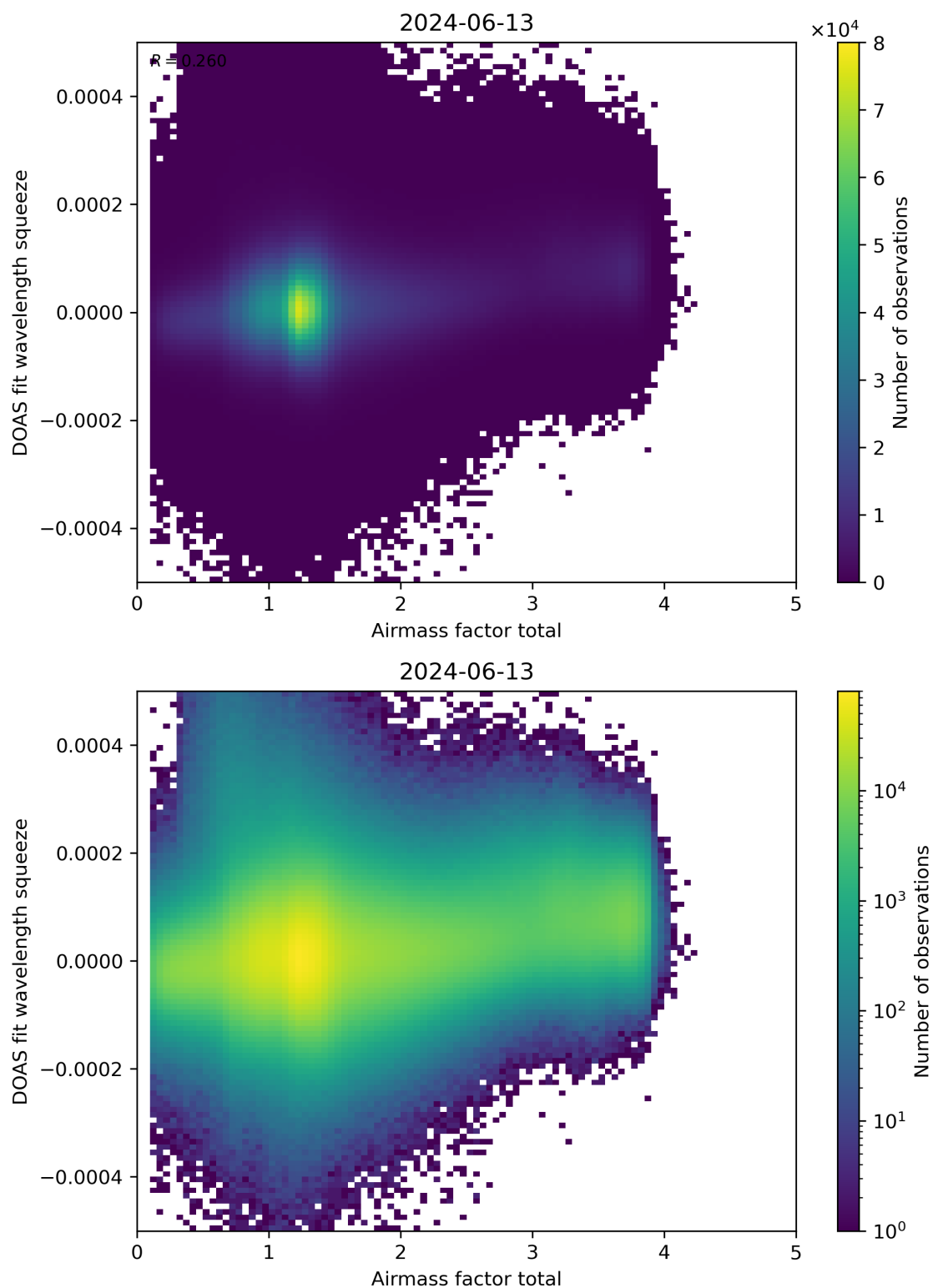
Figure 99: Scatter density plot of “Airmass factor total” against “DOAS fit wavelength squeeze” for 2024-06-13 to 2024-06-14.
