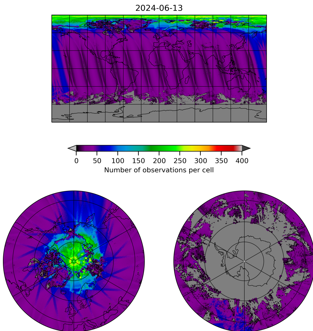
Figure 19: Map of the number of observations for 2024-06-13 to 2024-06-14
