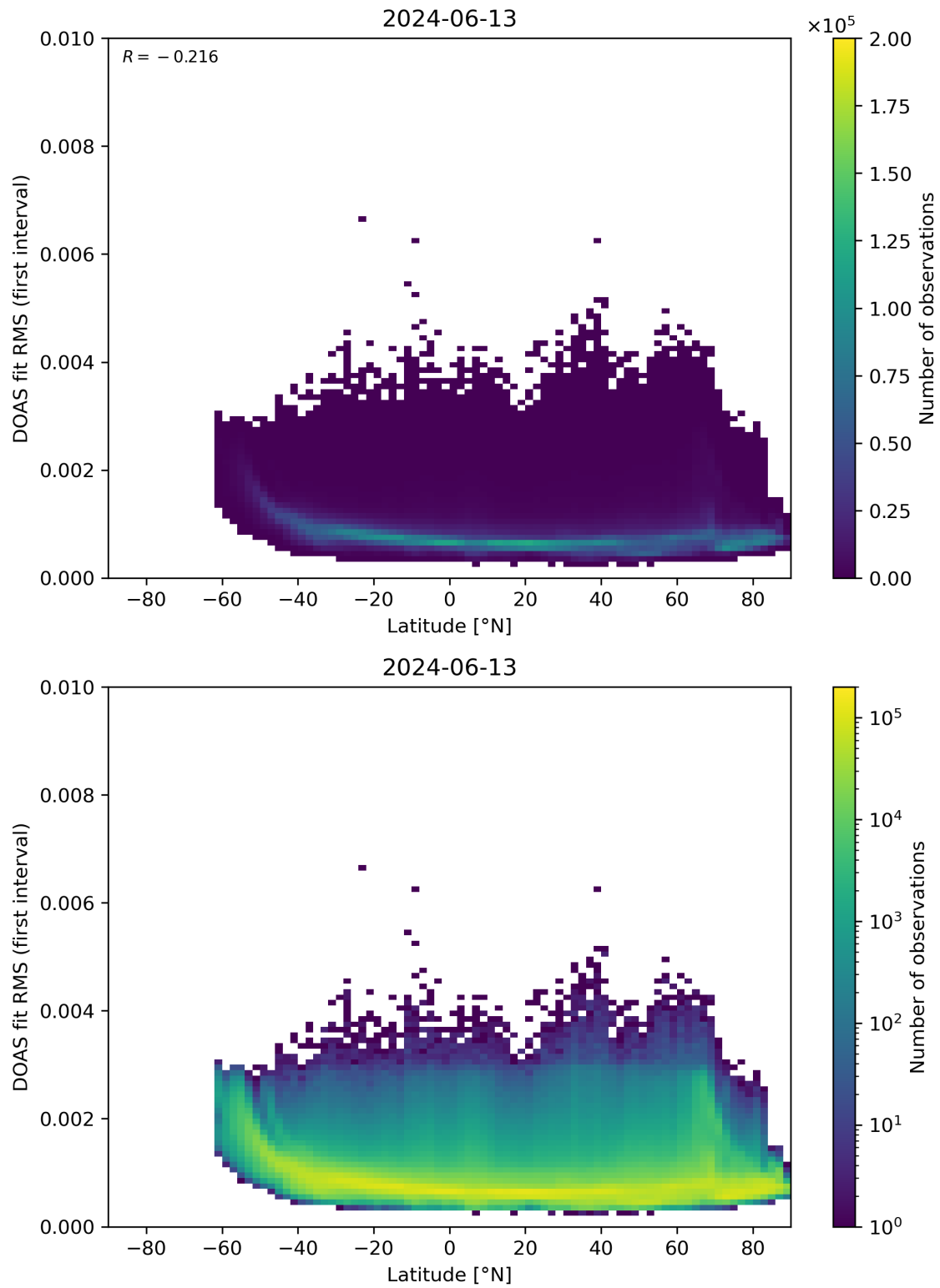
Figure 153: Scatter density plot of “Latitude” against “DOAS fit RMS (first interval)” for 2024-06-13 to 2024-06-14.
