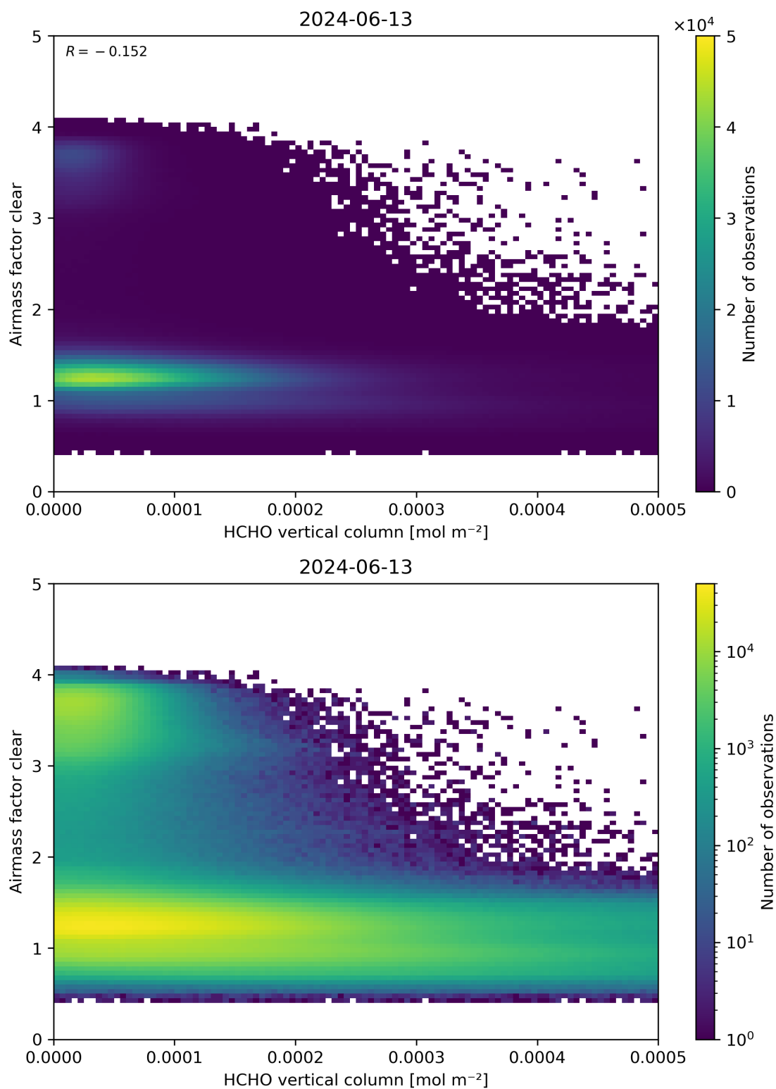
Figure 126: Scatter density plot of “HCHO vertical column” against “Airmass factor clear” for 2024-06-13 to 2024-06-14.
