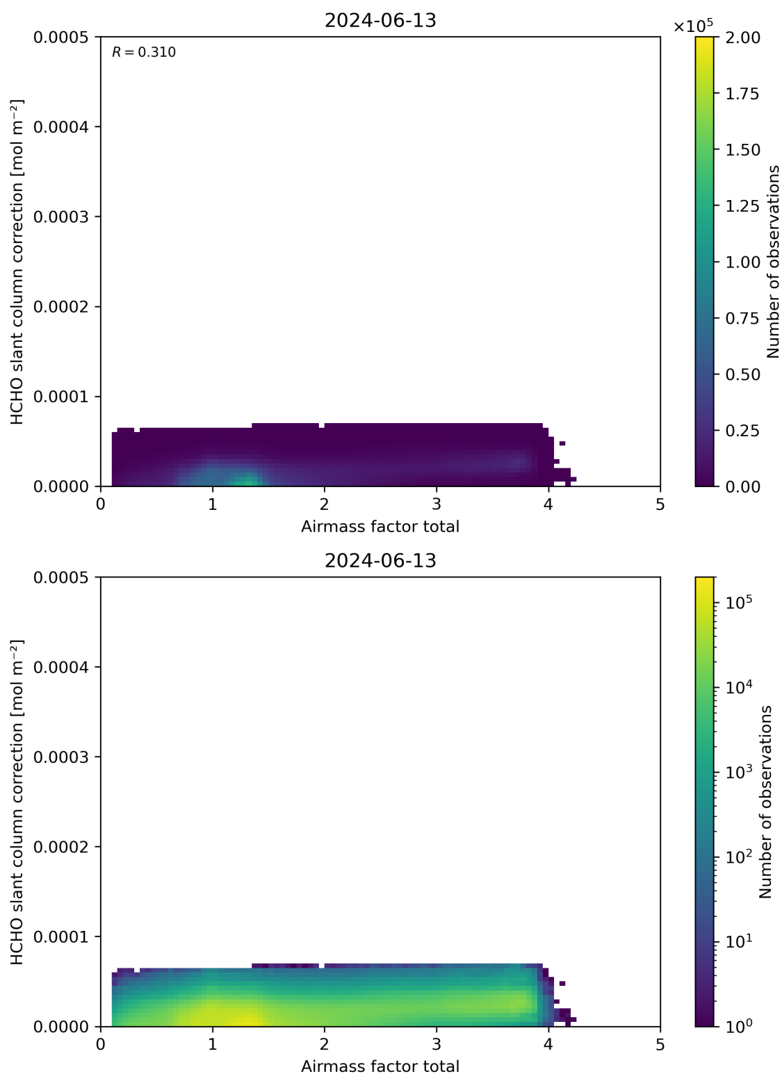
Figure 102: Scatter density plot of “Airmass factor total” against “HCHO slant column correction” for 2024-06-13 to 2024-06-14.
