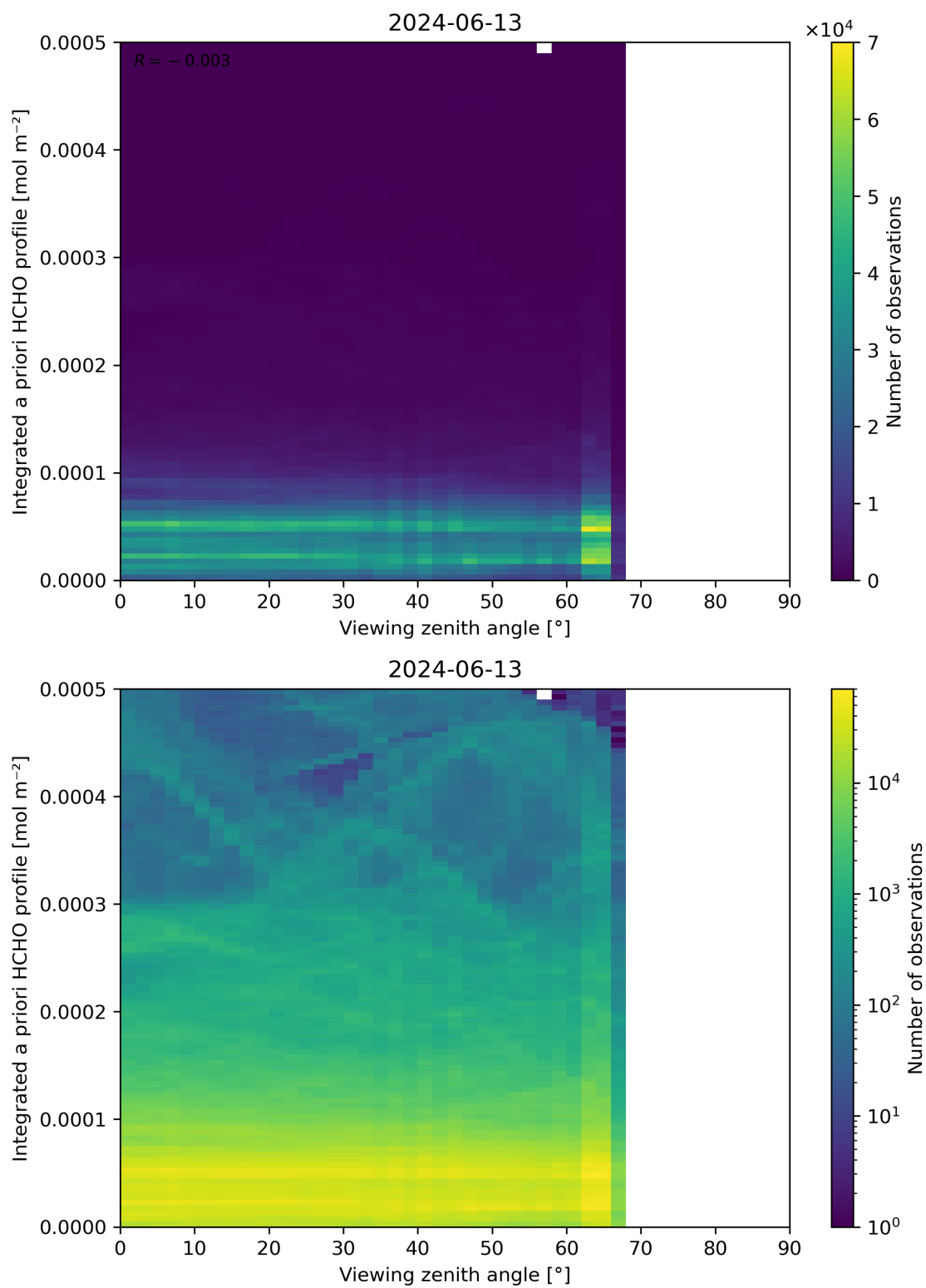
Figure 195: Scatter density plot of “Viewing zenith angle” against “Integrated a priori HCHO profile” for 2024-06-13 to 2024-06-14.
