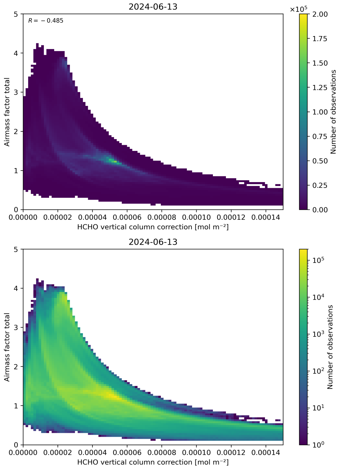
Figure 120: Scatter density plot of “HCHO vertical column correction” against “Airmass factor total” for 2024-06-13 to 2024-06-14.
