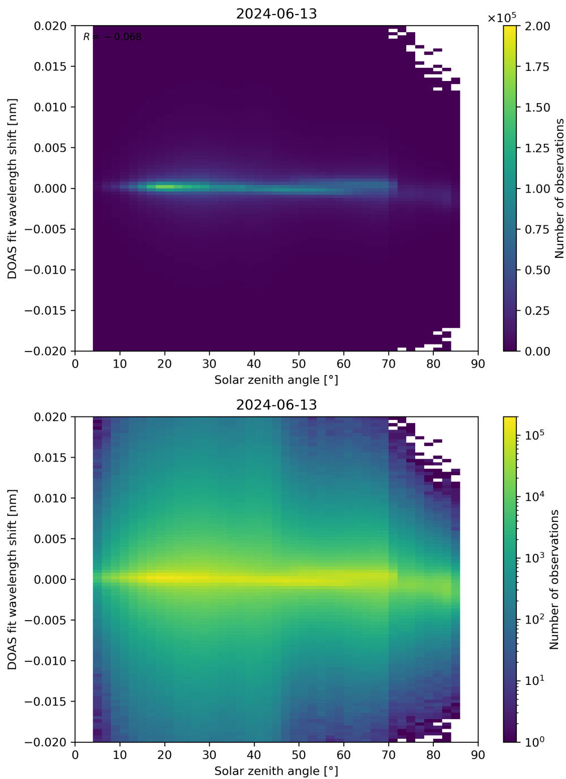
Figure 168: Scatter density plot of “Solar zenith angle” against “DOAS fit wavelength shift” for 2024-06-13 to 2024-06-14.
