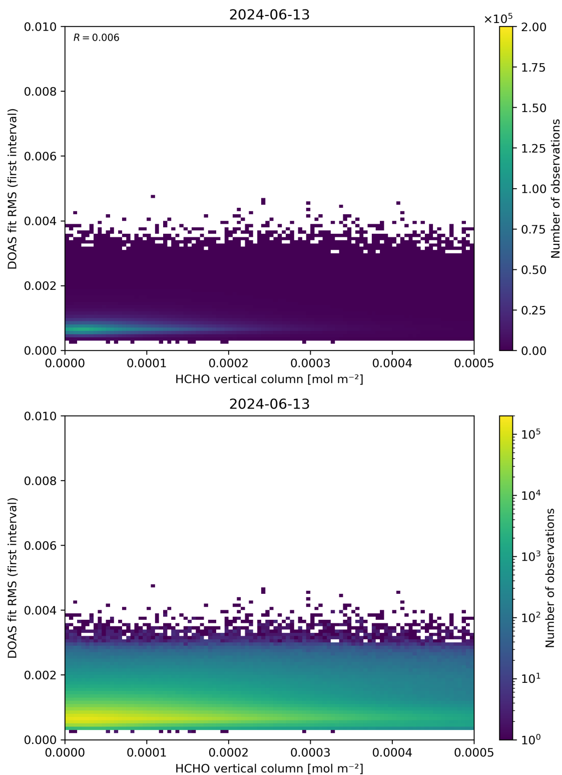
Figure 123: Scatter density plot of “HCHO vertical column” against “DOAS fit RMS (first interval)” for 2024-06-13 to 2024-06-14.
