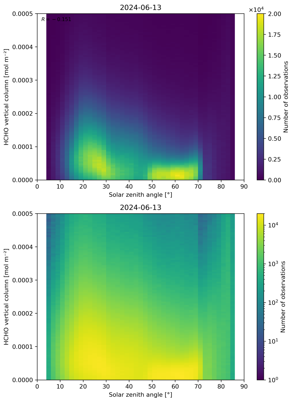
Figure 177: Scatter density plot of “Solar zenith angle” against “HCHO vertical column” for 2024-06-13 to 2024-06-14.
