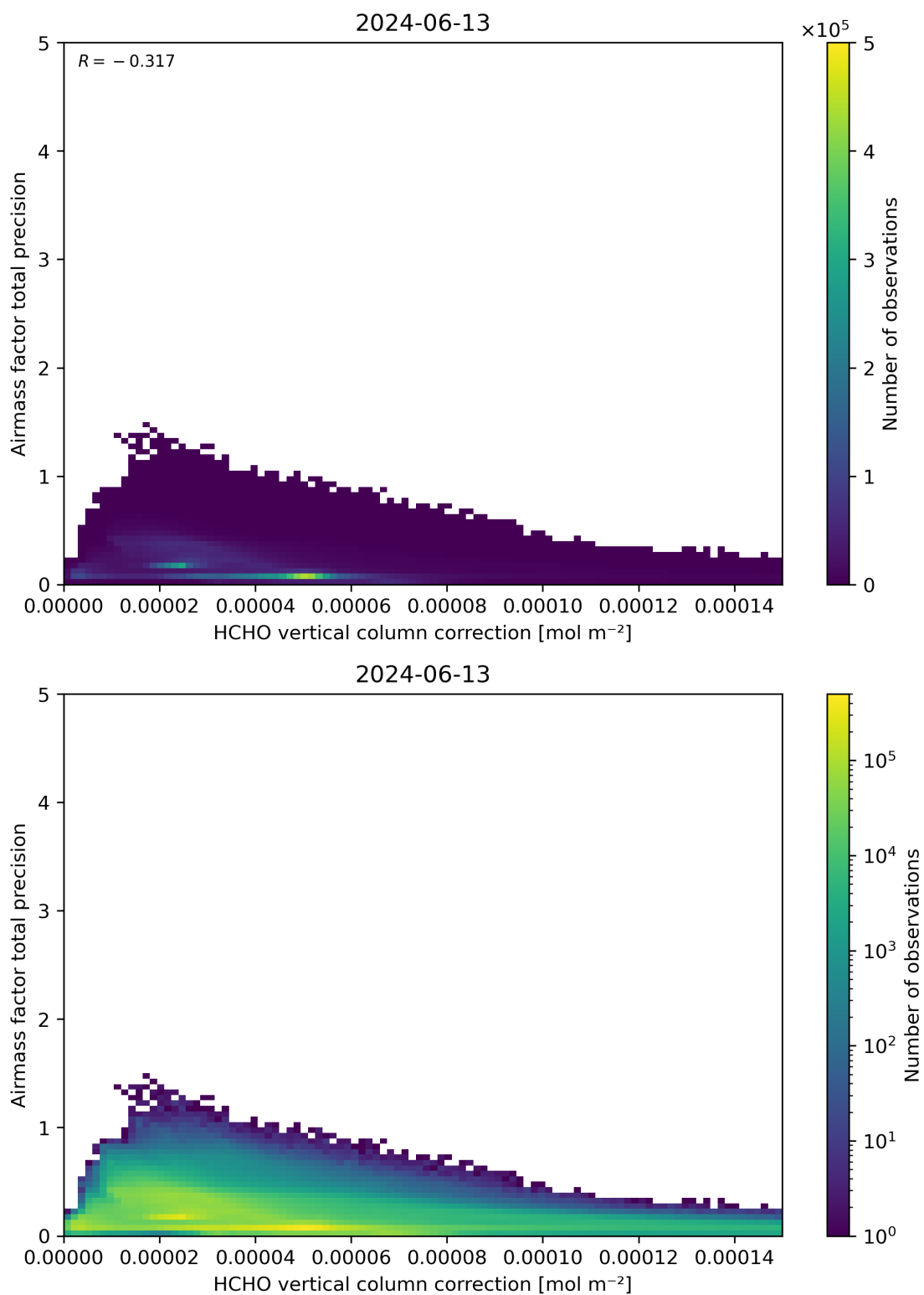
Figure 121: Scatter density plot of “HCHO vertical column correction” against “Airmass factor total precision” for 2024-06-13 to 2024-06-14.
