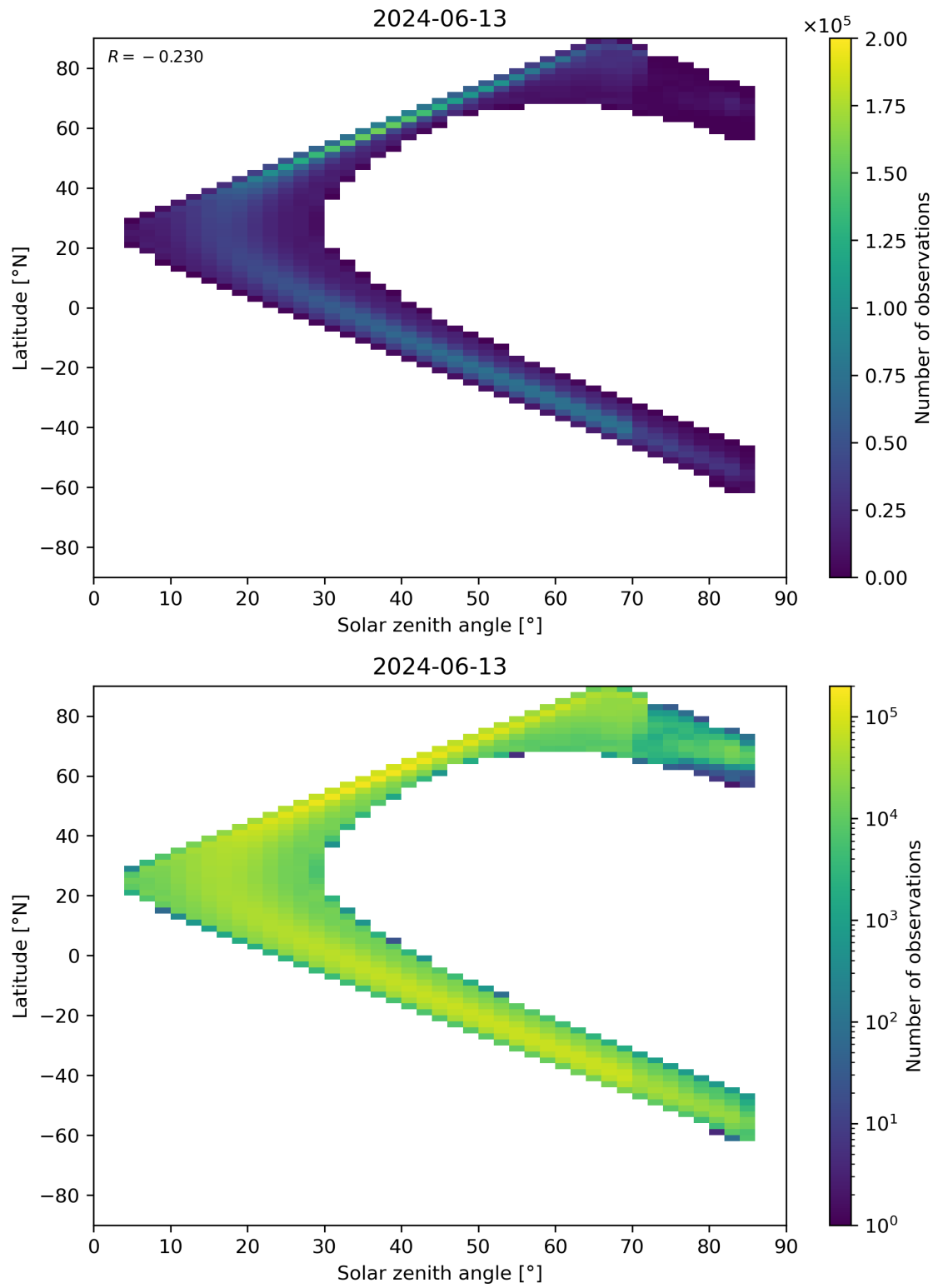
Figure 181: Scatter density plot of “Solar zenith angle” against “Latitude” for 2024-06-13 to 2024-06-14.
