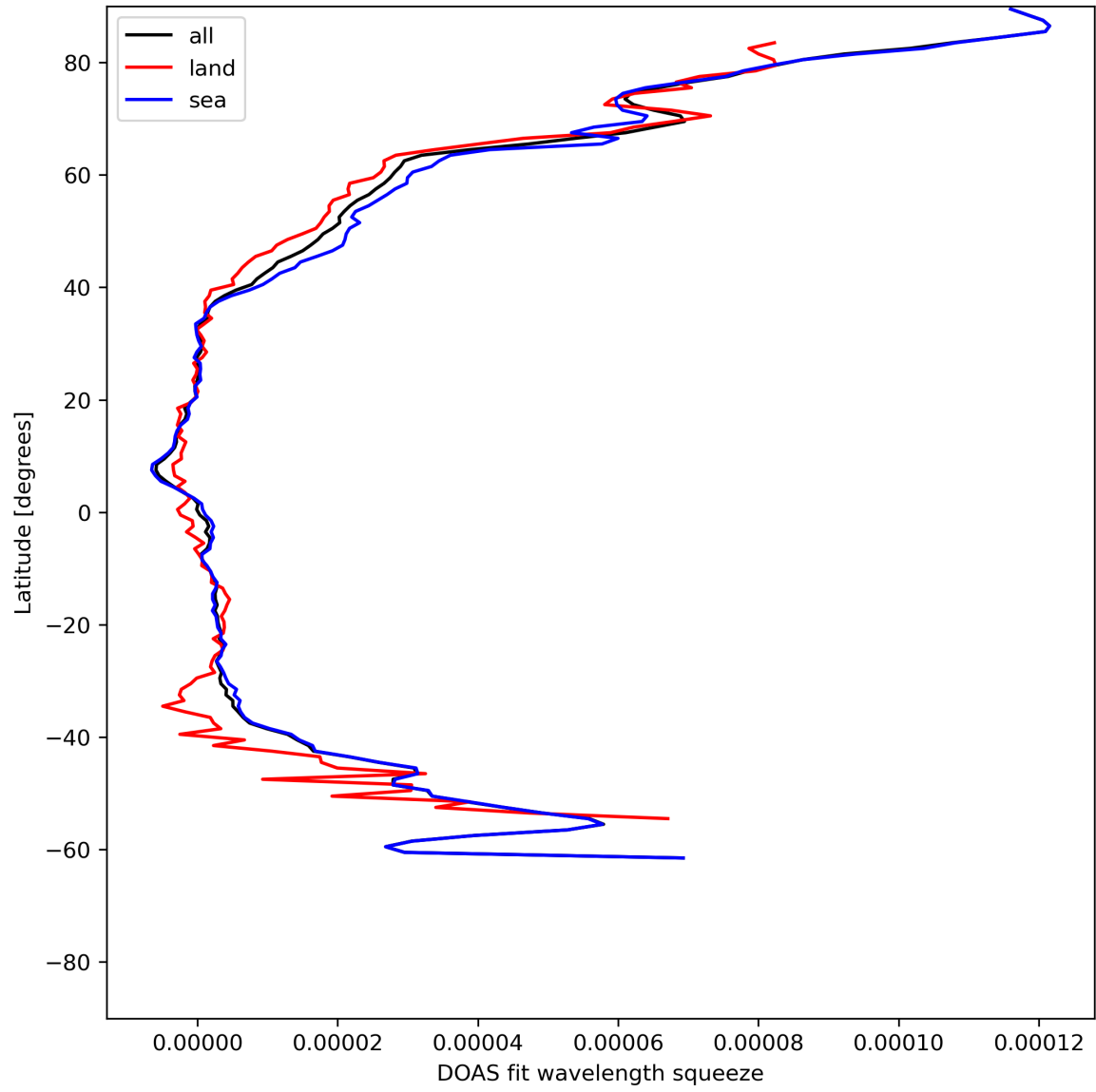
Figure 31: Zonal average of “DOAS fit wavelength squeeze” for 2024-06-13 to 2024-06-14.
