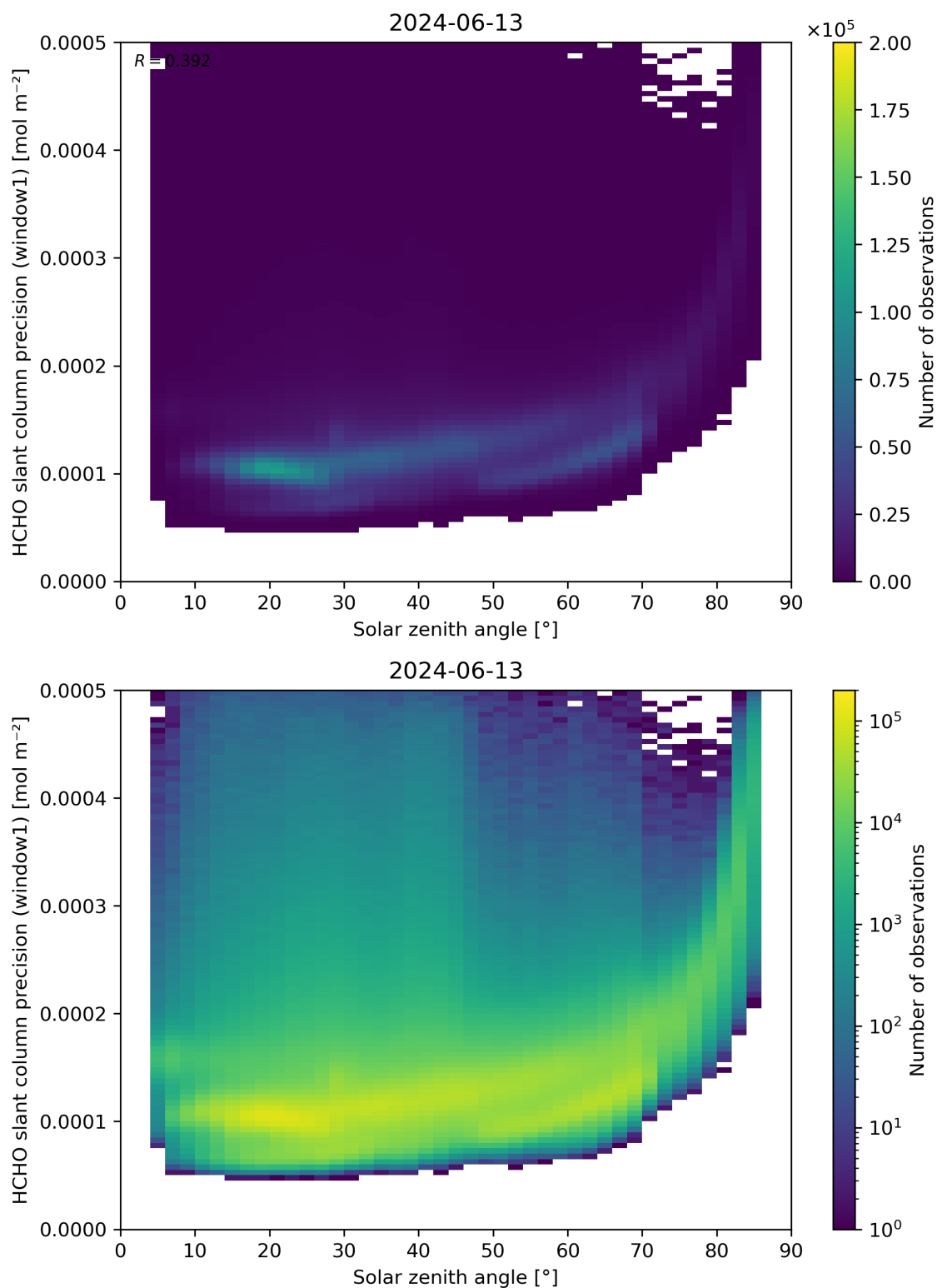
Figure 174: Scatter density plot of “Solar zenith angle” against “HCHO slant column precision (window1)” for 2024-06-13 to 2024-06-14.
