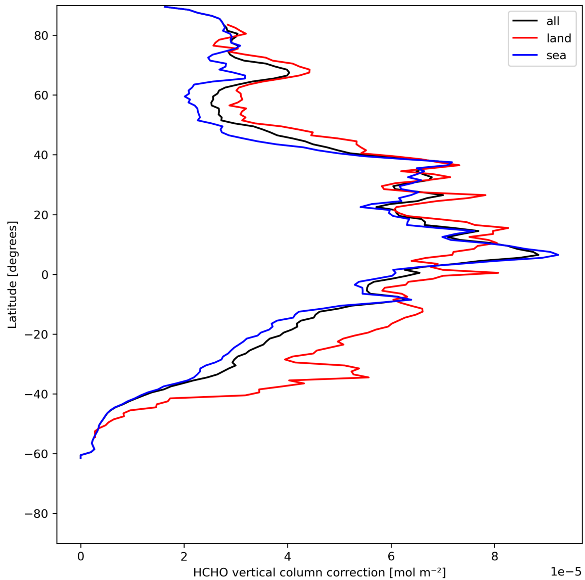
Figure 23: Zonal average of “HCHO vertical column correction” for 2024-06-13 to 2024-06-14.
