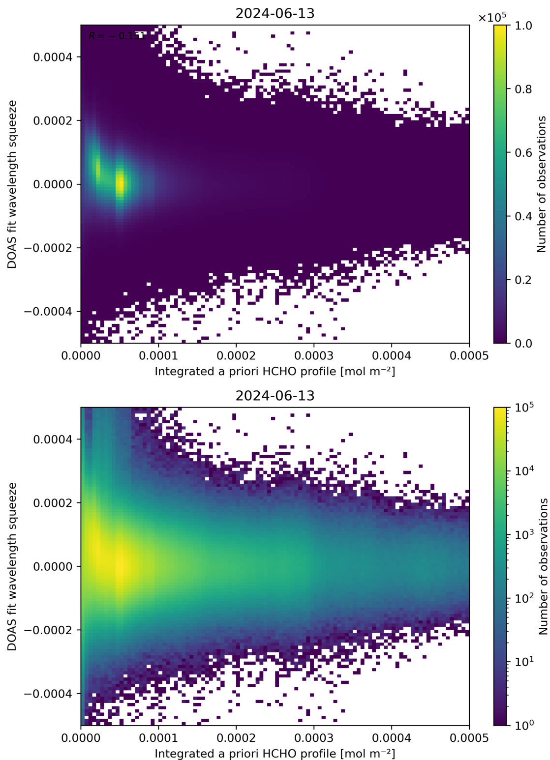
Figure 150: Scatter density plot of “Integrated a priori HCHO profile” against “DOAS fit wavelength squeeze” for 2024-06-13 to 2024-06-14.
