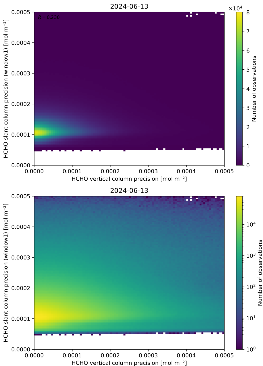
Figure 143: Scatter density plot of “HCHO vertical column precision” against “HCHO slant column precision (window1)” for 2024-06-13 to 2024-06-14.
