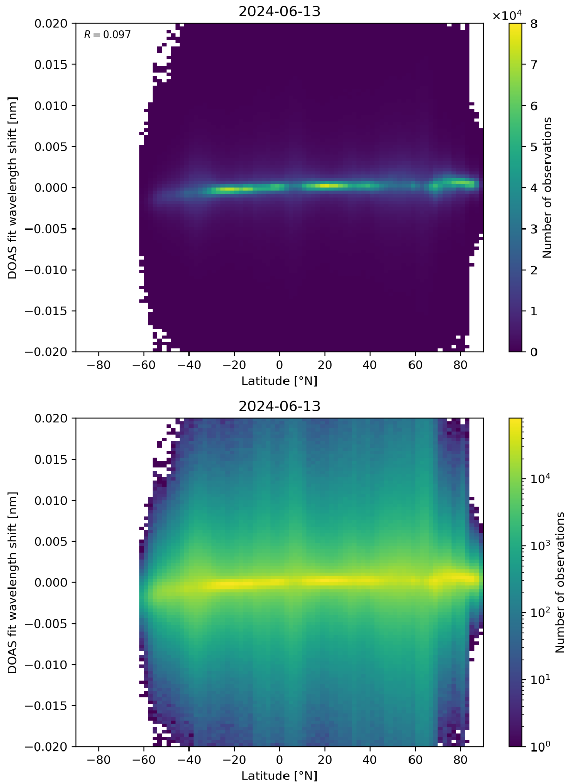
Figure 154: Scatter density plot of “Latitude” against “DOAS fit wavelength shift” for 2024-06-13 to 2024-06-14.
