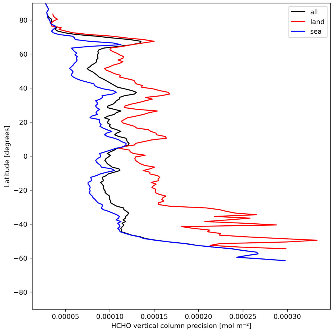
Figure 22: Zonal average of “HCHO vertical column precision” for 2024-06-13 to 2024-06-14.
