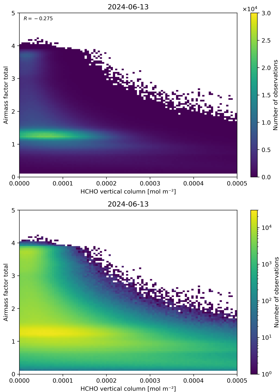
Figure 131: Scatter density plot of “HCHO vertical column” against “Airmass factor total” for 2024-06-13 to 2024-06-14.
