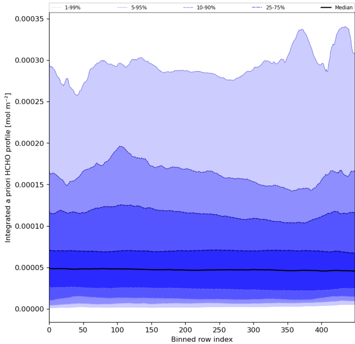
Figure 57: Along track statistics of “Integrated a priori HCHO profile” for 2024-06-13 to 2024-06-14
