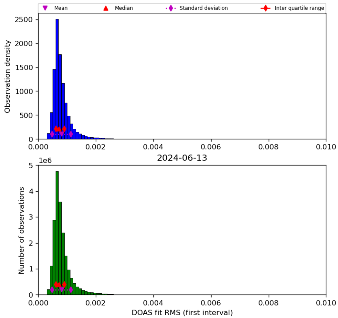
Figure 46: Histogram of “DOAS fit RMS (first interval)” for 2024-06-13 to 2024-06-14
