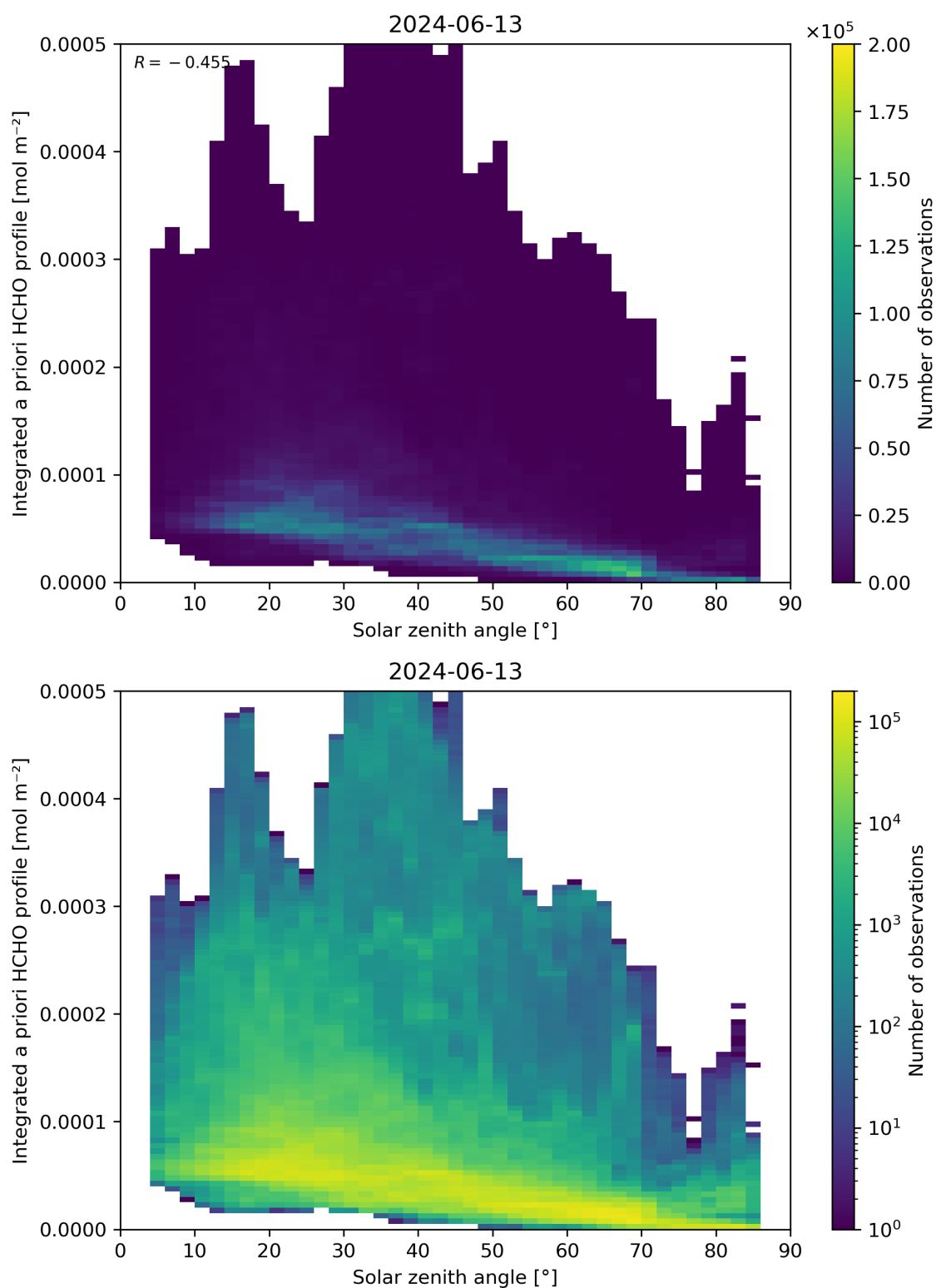
Figure 180: Scatter density plot of “Solar zenith angle” against “Integrated a priori HCHO profile” for 2024-06-13 to 2024-06-14.
