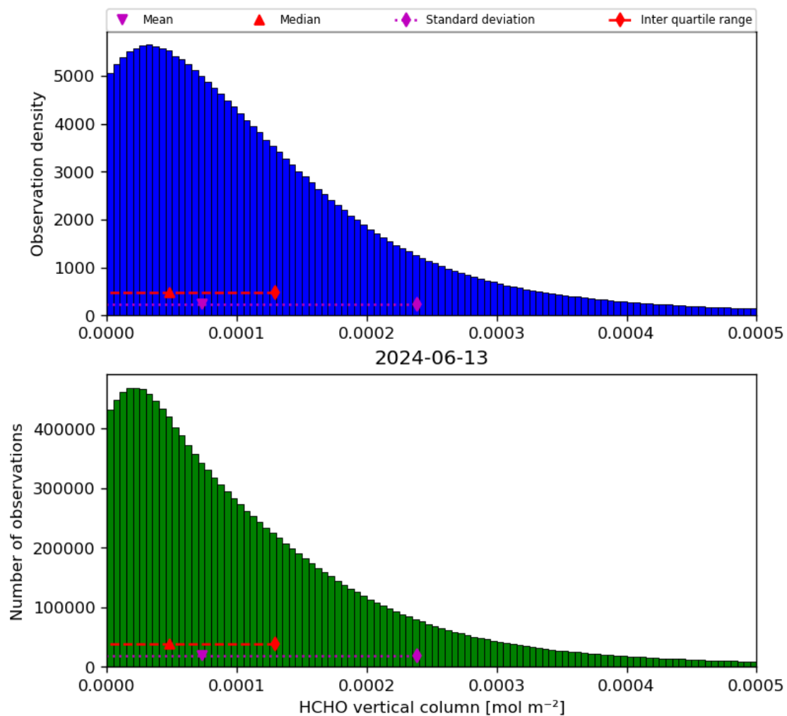
Figure 35: Histogram of “HCHO vertical column” for 2024-06-13 to 2024-06-14
