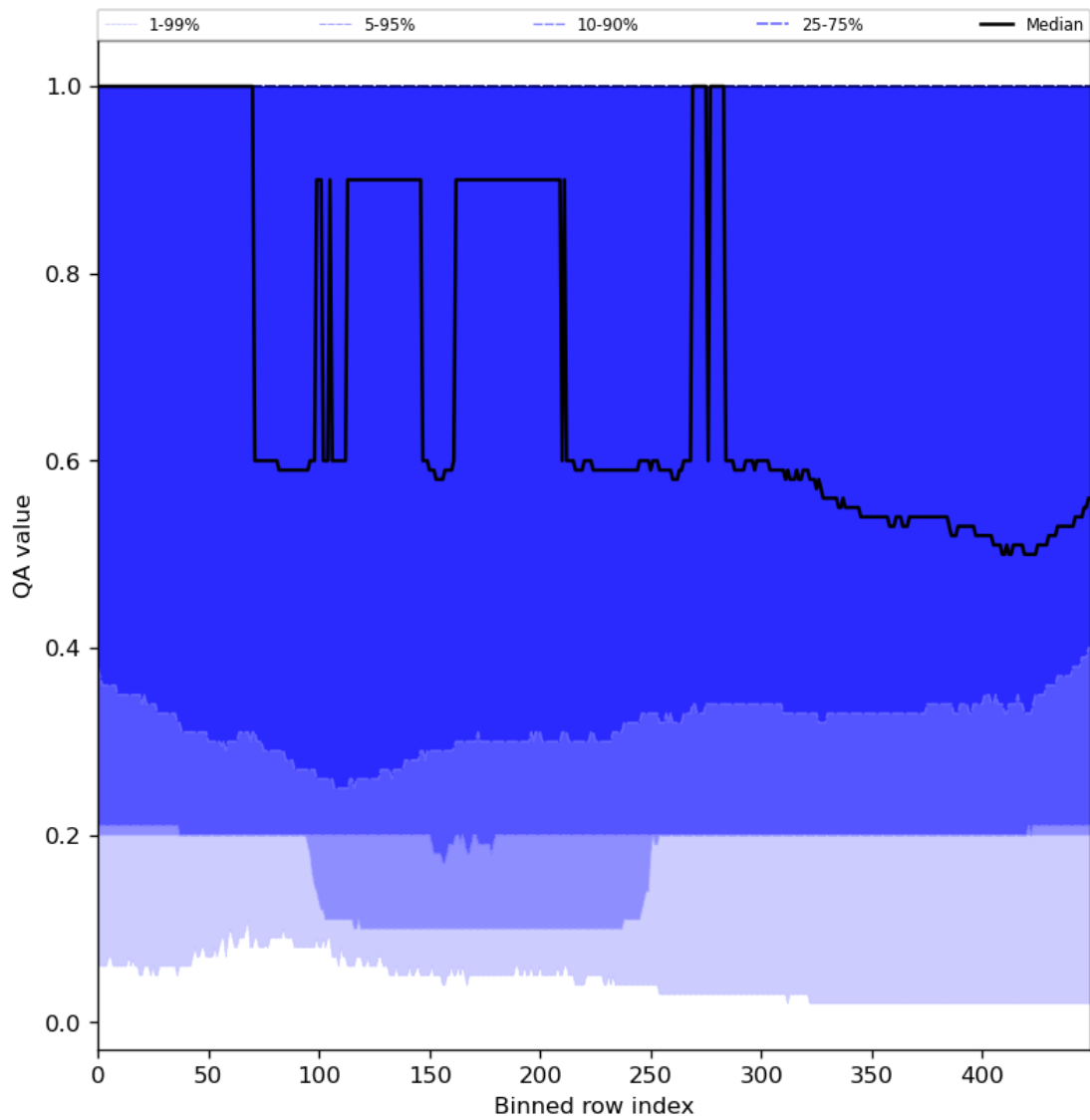
Figure 48: Along track statistics of “QA value” for 2024-06-13 to 2024-06-14
