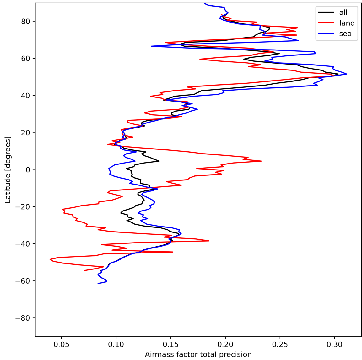
Figure 27: Zonal average of “Airmass factor total precision” for 2024-06-13 to 2024-06-14.
