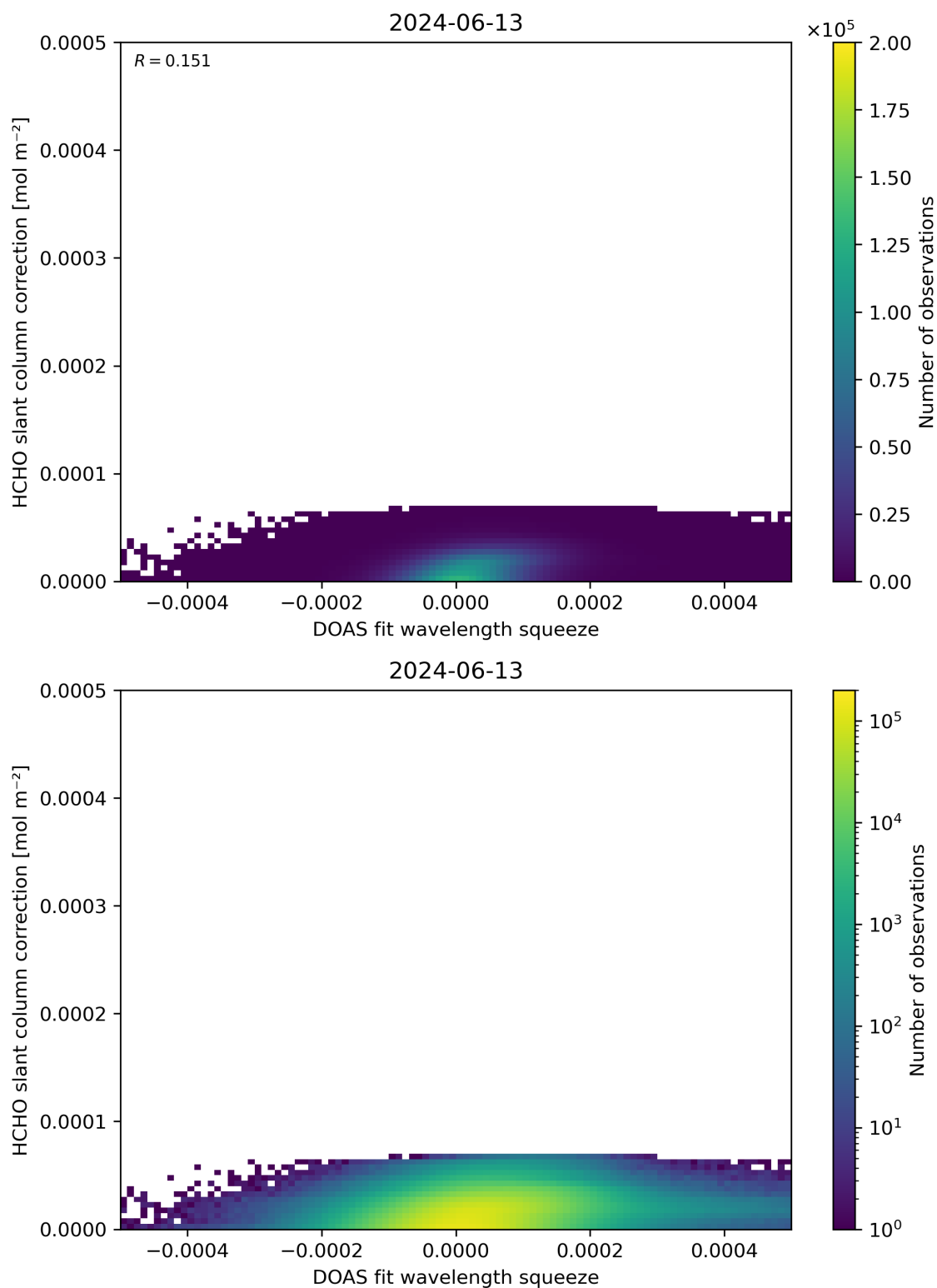
Figure 70: Scatter density plot of “DOAS fit wavelength squeeze” against “HCHO slant column correction” for 2024-06-13 to 2024-06-14.
