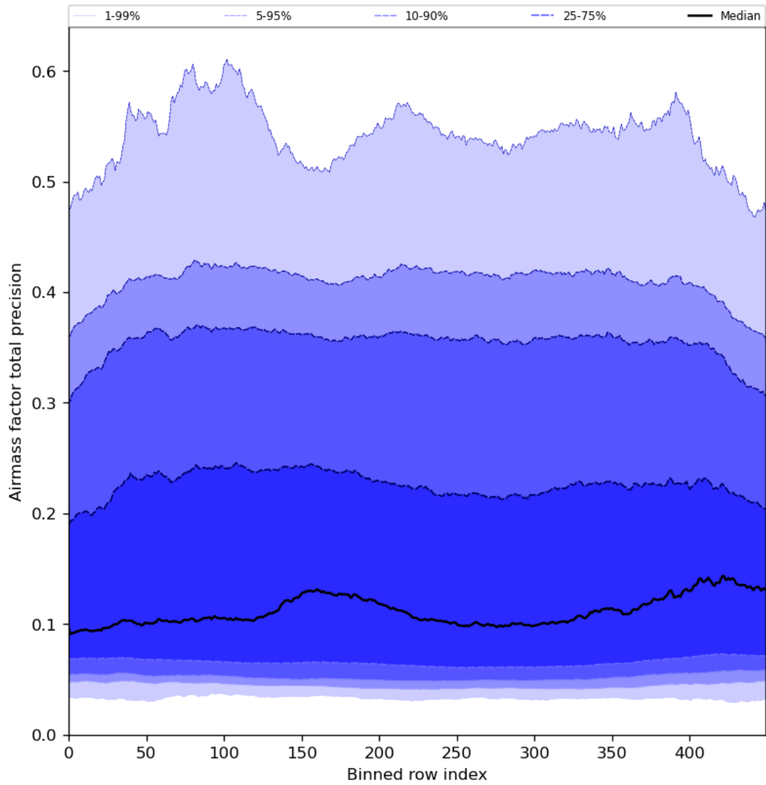
Figure 55: Along track statistics of “Airmass factor total precision” for 2024-06-13 to 2024-06-14
