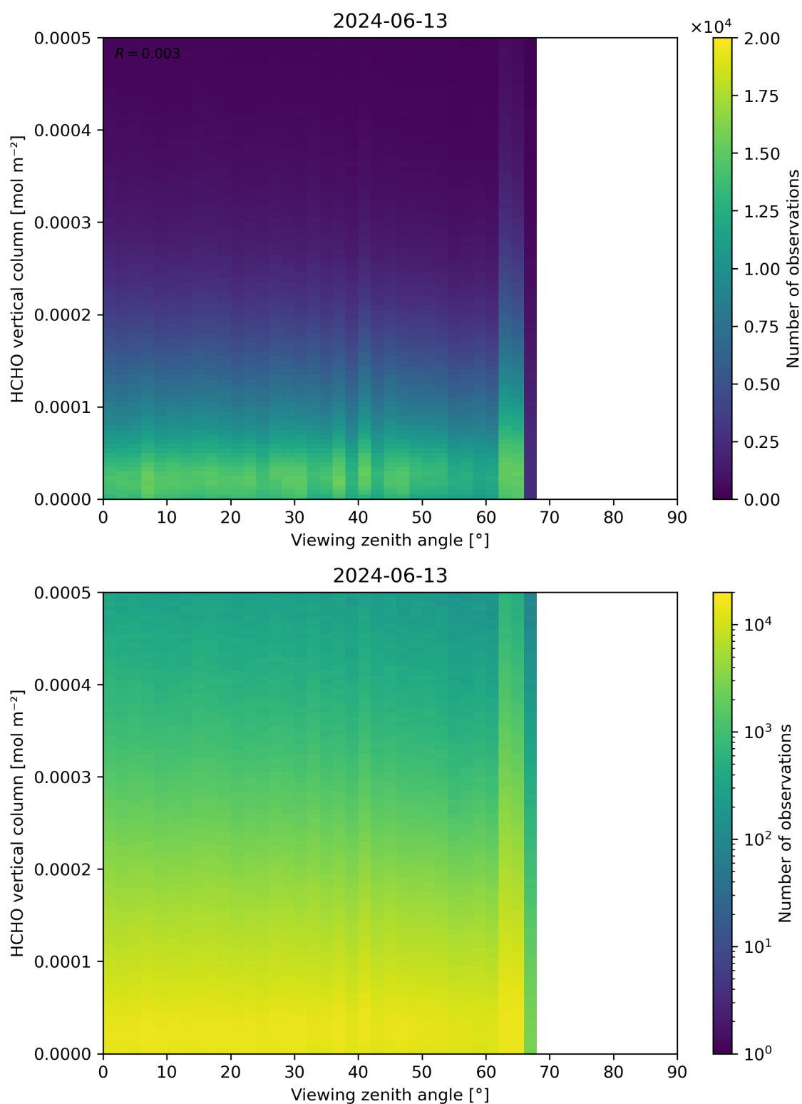
Figure 192: Scatter density plot of “Viewing zenith angle” against “HCHO vertical column” for 2024-06-13 to 2024-06-14.
