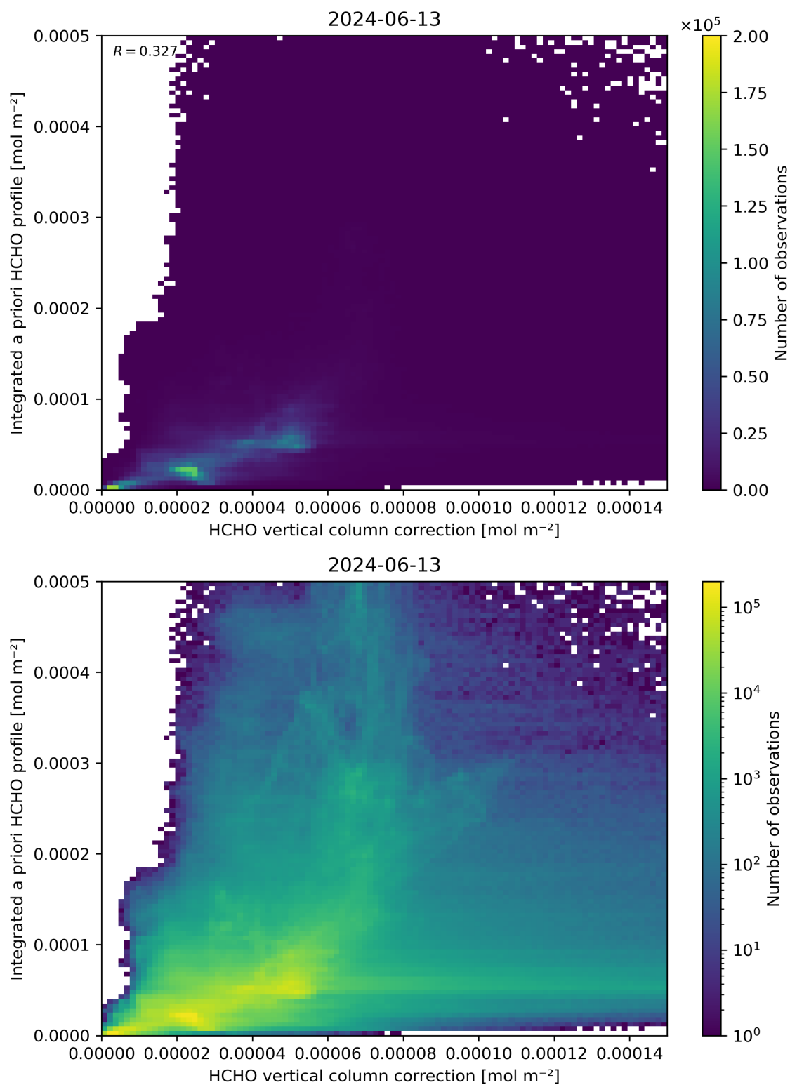
Figure 122: Scatter density plot of “HCHO vertical column correction” against “Integrated a priori HCHO profile” for 2024-06-13 to 2024-06-14.
