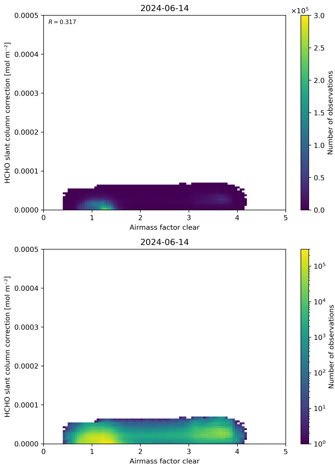
Figure 75: Scatter density plot of “Airmass factor clear” against “HCHO slant column correction” for 2024-06-13 to 2024-06-15.
