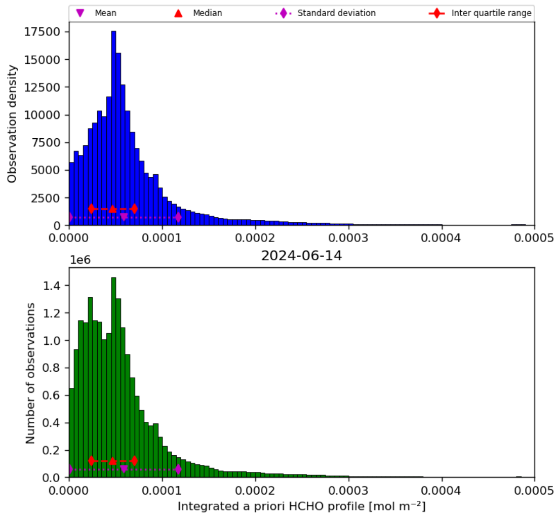
Figure 43: Histogram of “Integrated a priori HCHO profile” for 2024-06-13 to 2024-06-15
