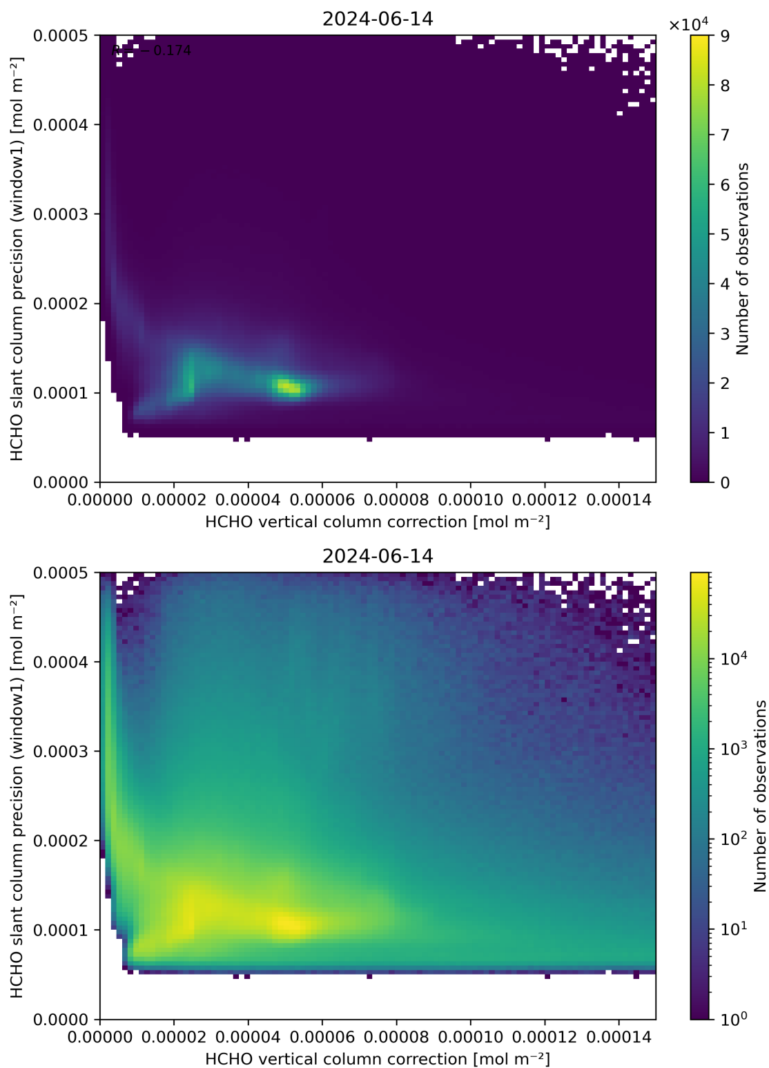
Figure 119: Scatter density plot of “HCHO vertical column correction” against “HCHO slant column precision (window1)” for 2024-06-13 to 2024-06-15.
