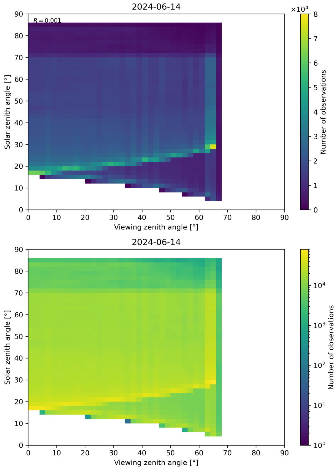
Figure 197: Scatter density plot of “Viewing zenith angle” against “Solar zenith angle” for 2024-06-13 to 2024-06-15.
