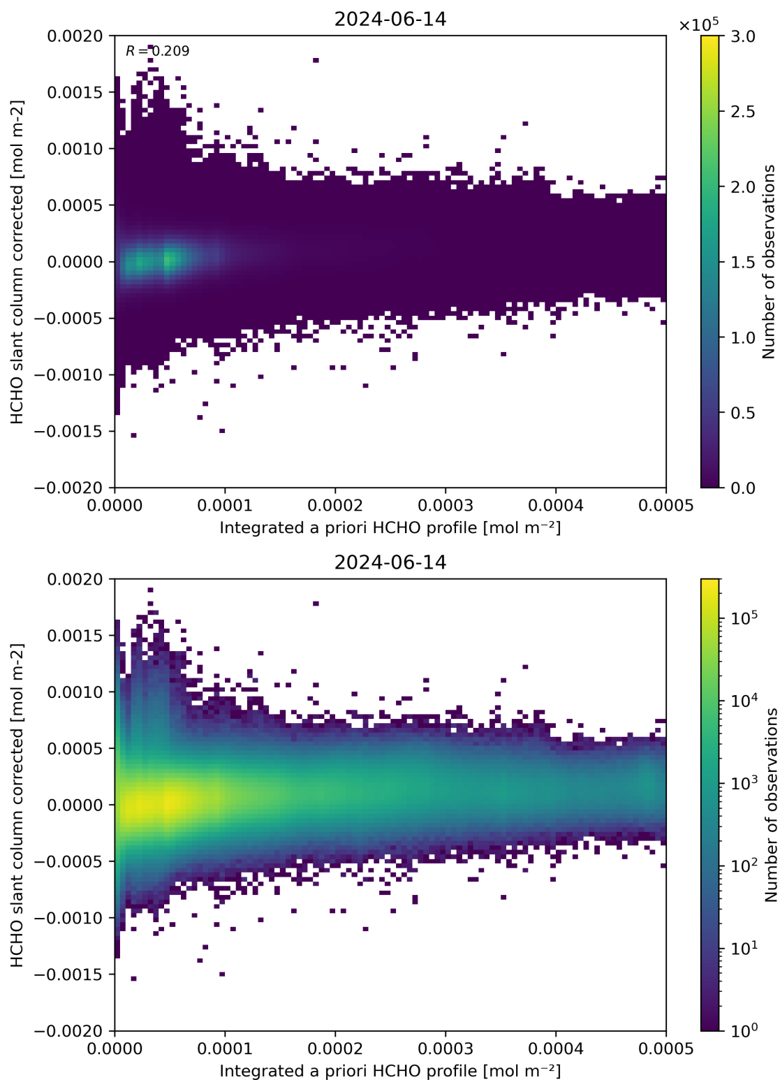
Figure 151: Scatter density plot of “Integrated a priori HCHO profile” against “HCHO slant column corrected” for 2024-06-13 to 2024-06-15.
