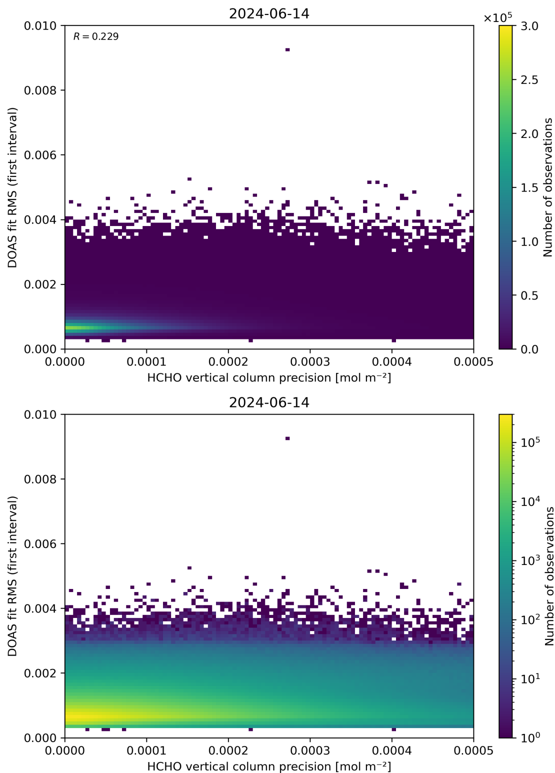
Figure 136: Scatter density plot of “HCHO vertical column precision” against “DOAS fit RMS (first interval)” for 2024-06-13 to 2024-06-15.
