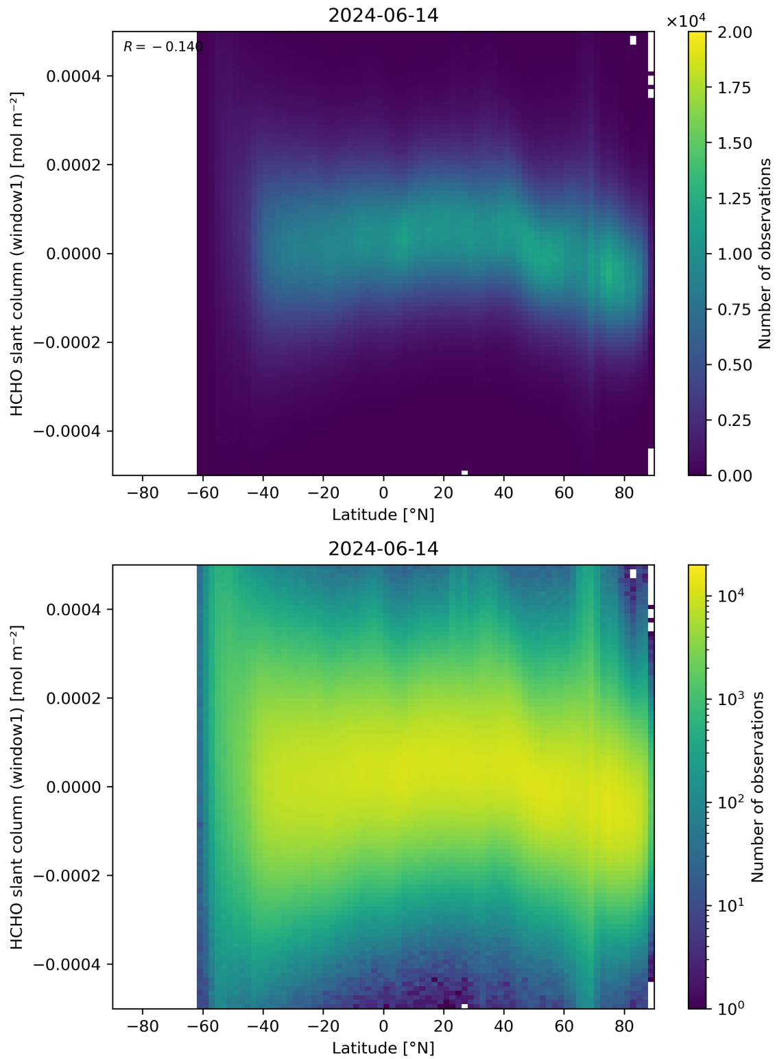
Figure 159: Scatter density plot of “Latitude” against “HCHO slant column (window1)” for 2024-06-13 to 2024-06-15.
