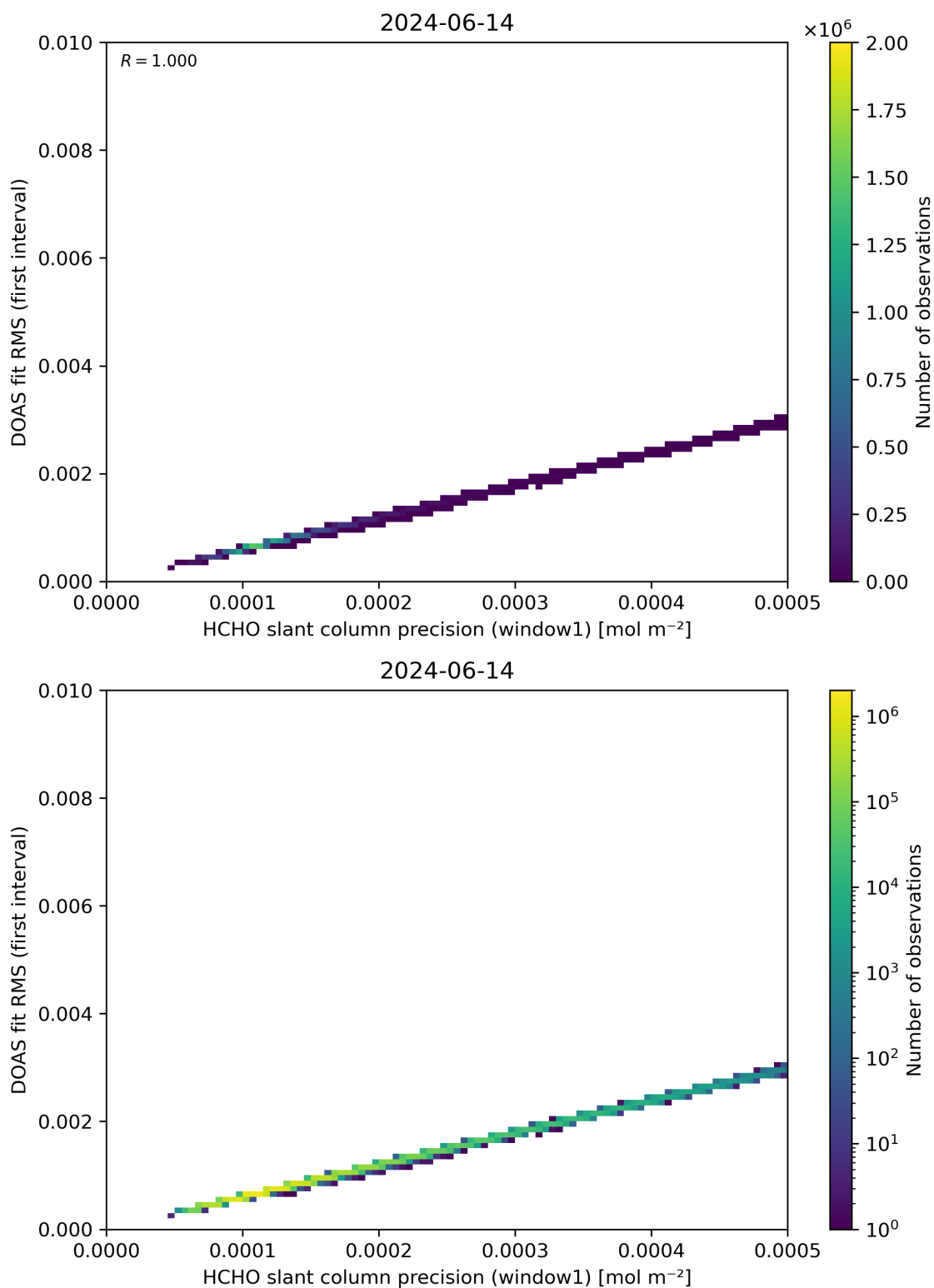
Figure 88: Scatter density plot of “HCHO slant column precision (window1)” against “DOAS fit RMS (first interval)” for 2024-06-13 to 2024-06-15.
