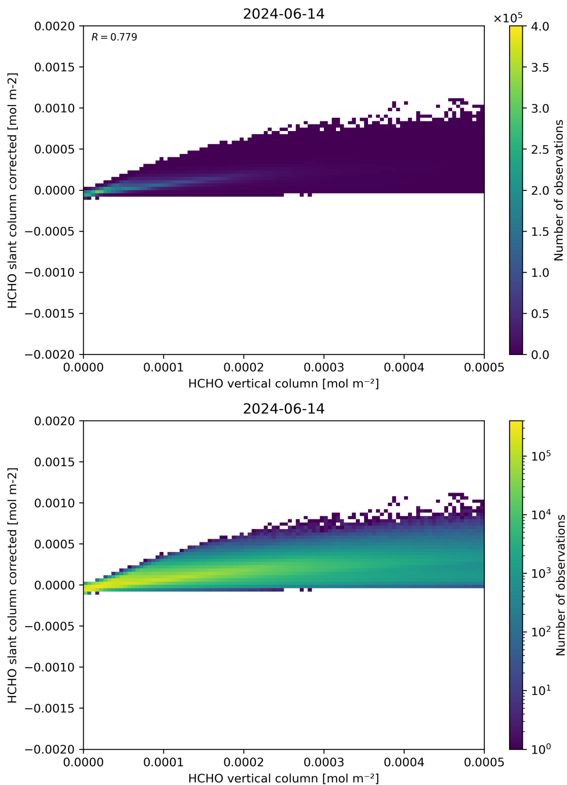
Figure 127: Scatter density plot of “HCHO vertical column” against “HCHO slant column corrected” for 2024-06-13 to 2024-06-15.
