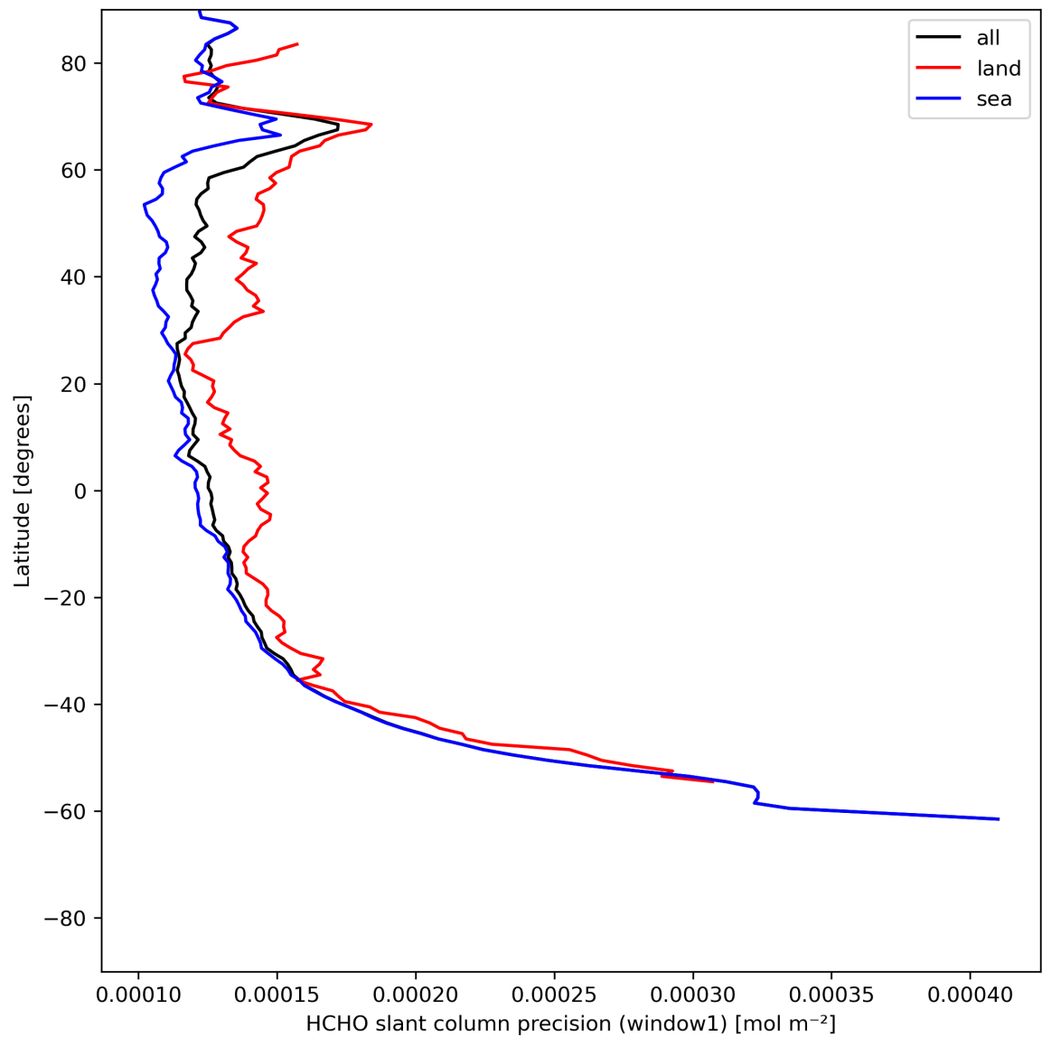
Figure 25: Zonal average of “HCHO slant column precision (window1)” for 2024-06-13 to 2024-06-15.
