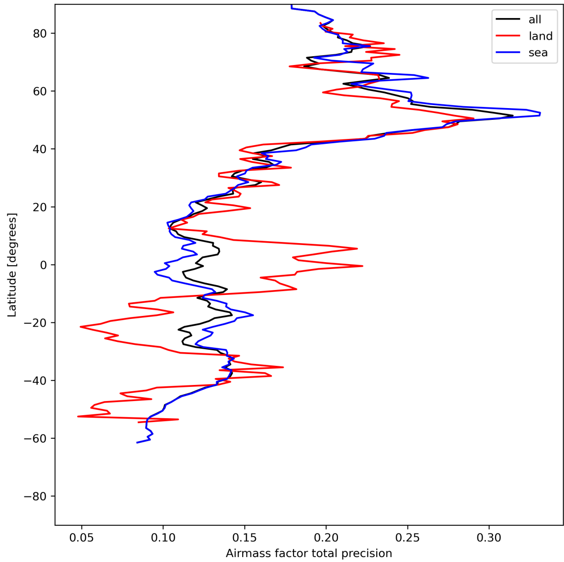
Figure 27: Zonal average of “Airmass factor total precision” for 2024-06-13 to 2024-06-15.
