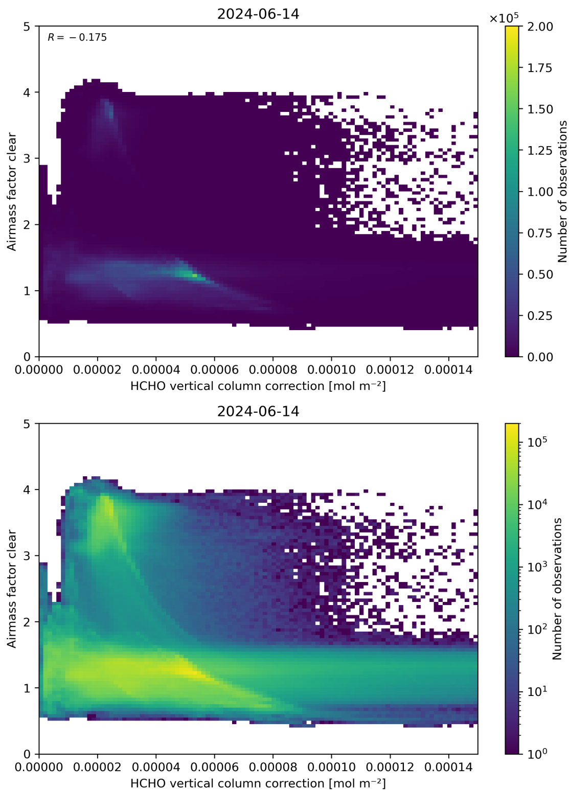
Figure 115: Scatter density plot of “HCHO vertical column correction” against “Airmass factor clear” for 2024-06-13 to 2024-06-15.
