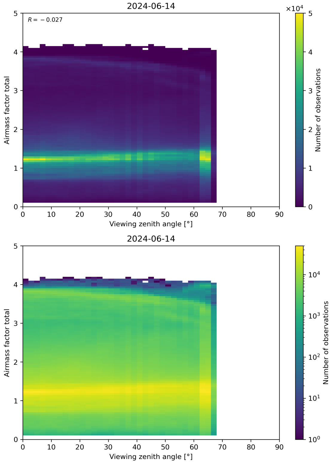
Figure 190: Scatter density plot of “Viewing zenith angle” against “Airmass factor total” for 2024-06-13 to 2024-06-15.
