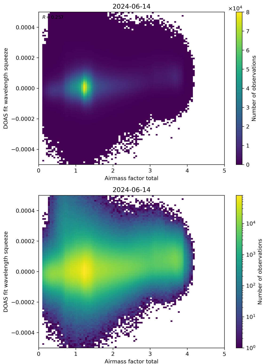
Figure 99: Scatter density plot of “Airmass factor total” against “DOAS fit wavelength squeeze” for 2024-06-13 to 2024-06-15.
