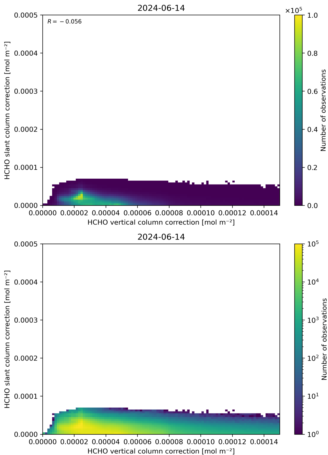
Figure 117: Scatter density plot of “HCHO vertical column correction” against “HCHO slant column correction” for 2024-06-13 to 2024-06-15.
