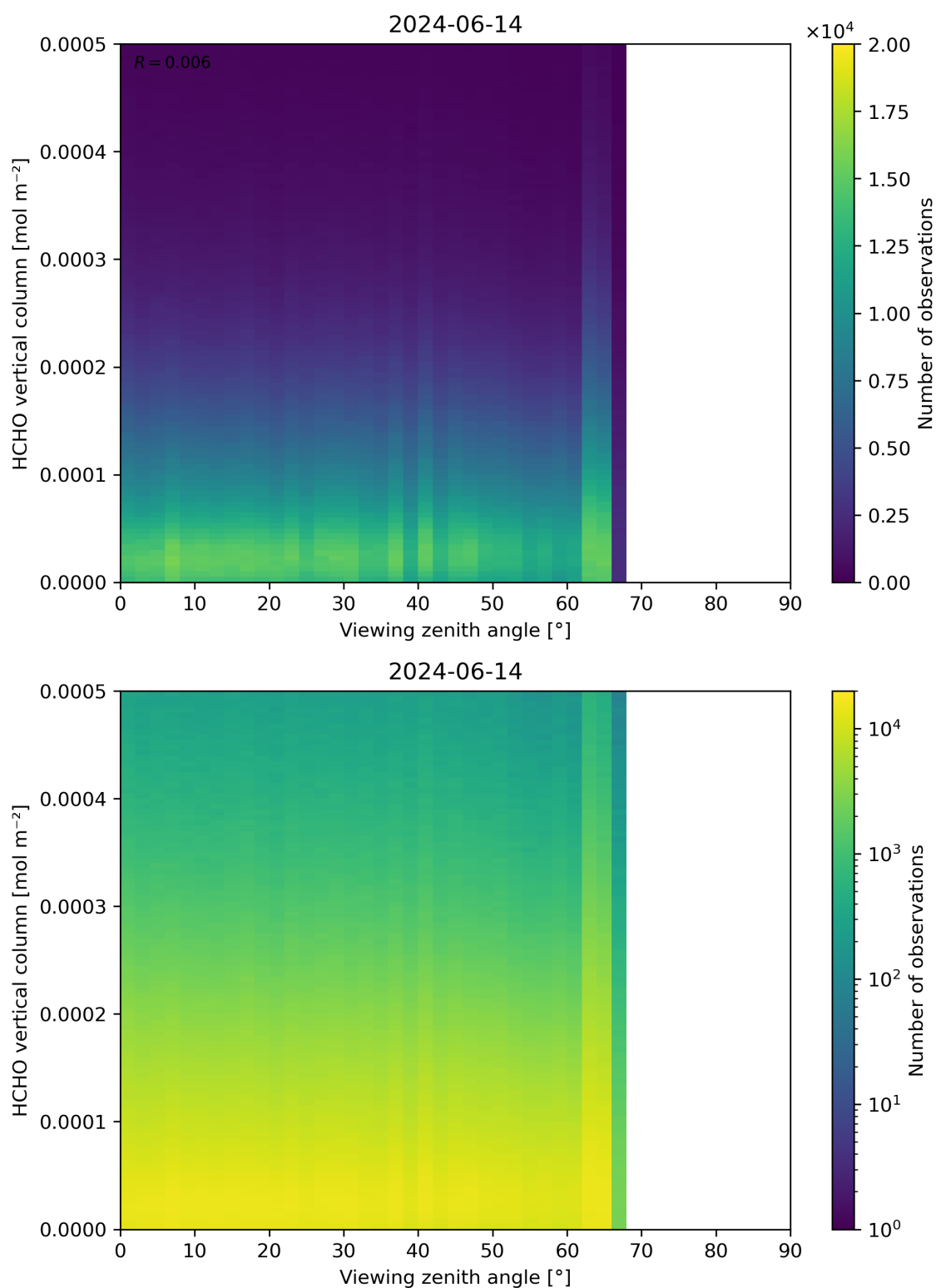
Figure 192: Scatter density plot of “Viewing zenith angle” against “HCHO vertical column” for 2024-06-13 to 2024-06-15.
