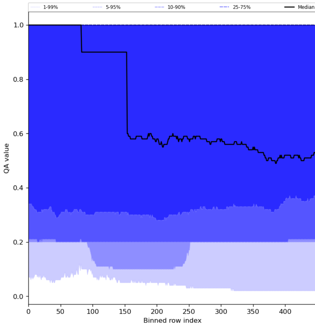
Figure 48: Along track statistics of “QA value” for 2024-06-13 to 2024-06-15
