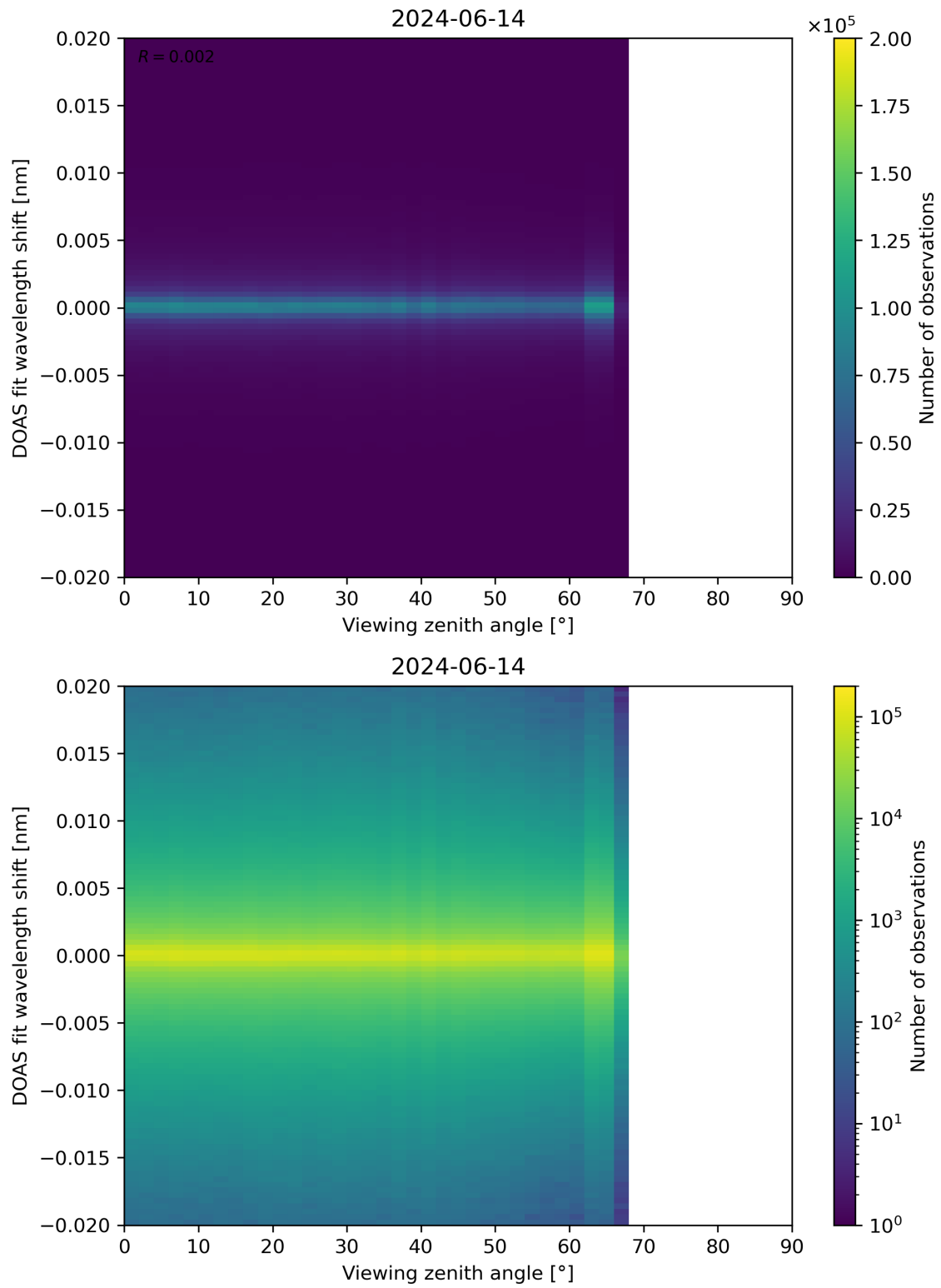
Figure 183: Scatter density plot of “Viewing zenith angle” against “DOAS fit wavelength shift” for 2024-06-13 to 2024-06-15.
