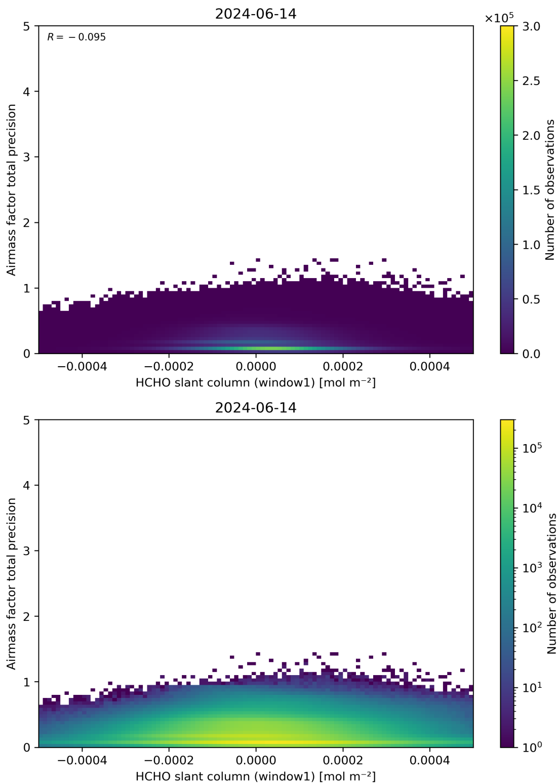
Figure 86: Scatter density plot of “HCHO slant column (window1)” against “Airmass factor total precision” for 2024-06-13 to 2024-06-15.
