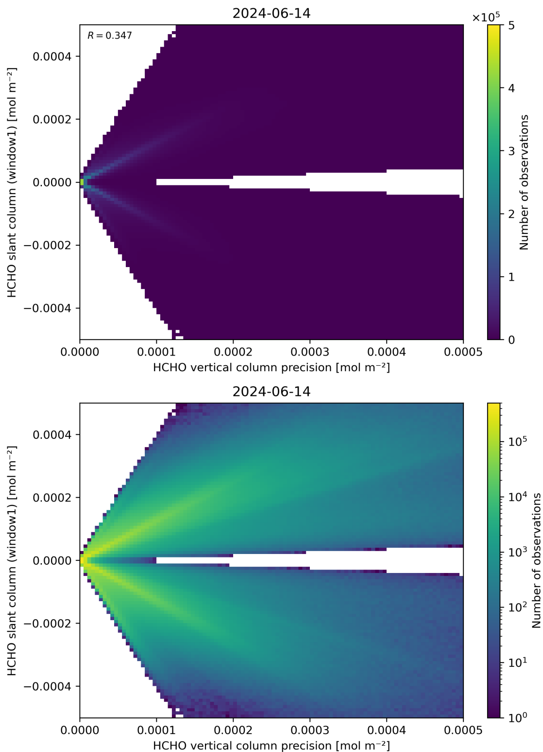
Figure 142: Scatter density plot of “HCHO vertical column precision” against “HCHO slant column (window1)” for 2024-06-13 to 2024-06-15.
