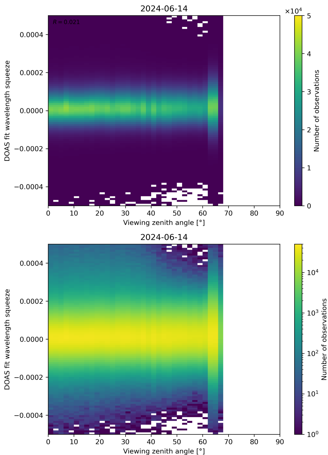
Figure 184: Scatter density plot of “Viewing zenith angle” against “DOAS fit wavelength squeeze” for 2024-06-13 to 2024-06-15.
