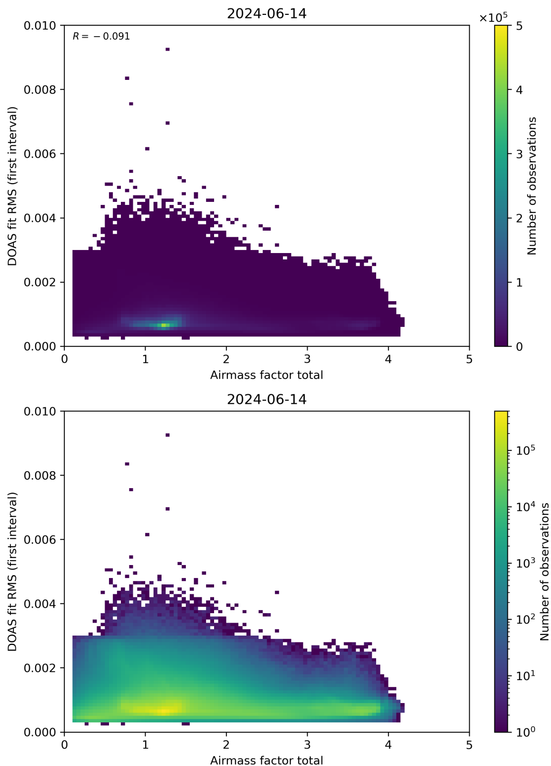
Figure 97: Scatter density plot of “Airmass factor total” against “DOAS fit RMS (first interval)” for 2024-06-13 to 2024-06-15.
