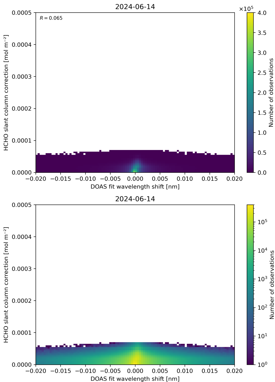
Figure 67: Scatter density plot of “DOAS fit wavelength shift” against “HCHO slant column correction” for 2024-06-13 to 2024-06-15.
