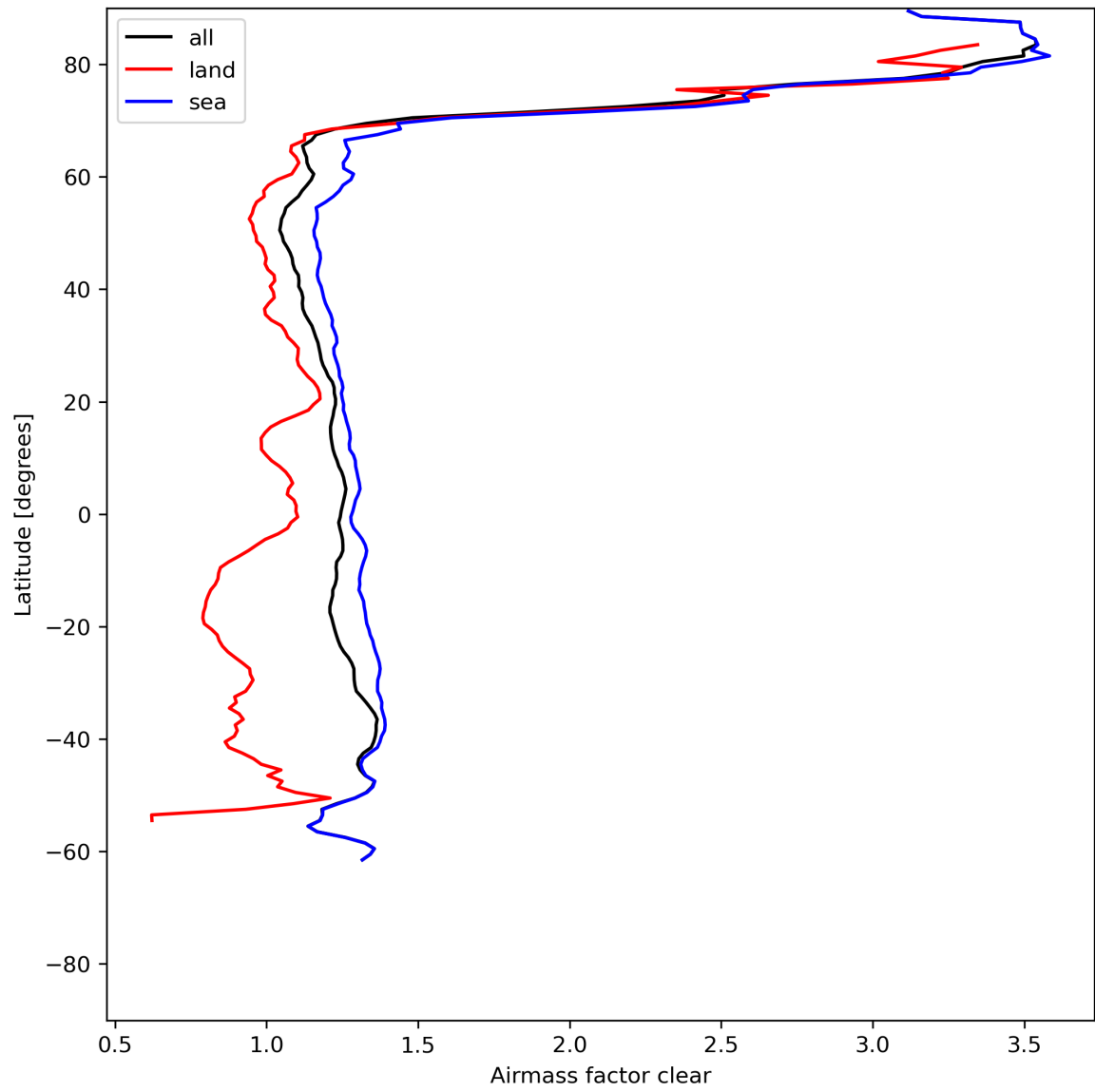
Figure 28: Zonal average of “Airmass factor clear” for 2024-06-13 to 2024-06-15.
