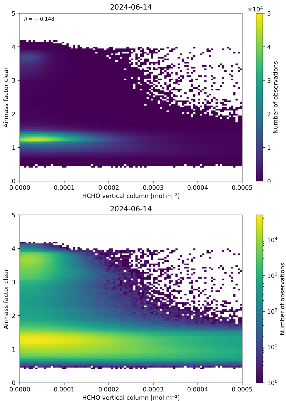
Figure 126: Scatter density plot of “HCHO vertical column” against “Airmass factor clear” for 2024-06-13 to 2024-06-15.
