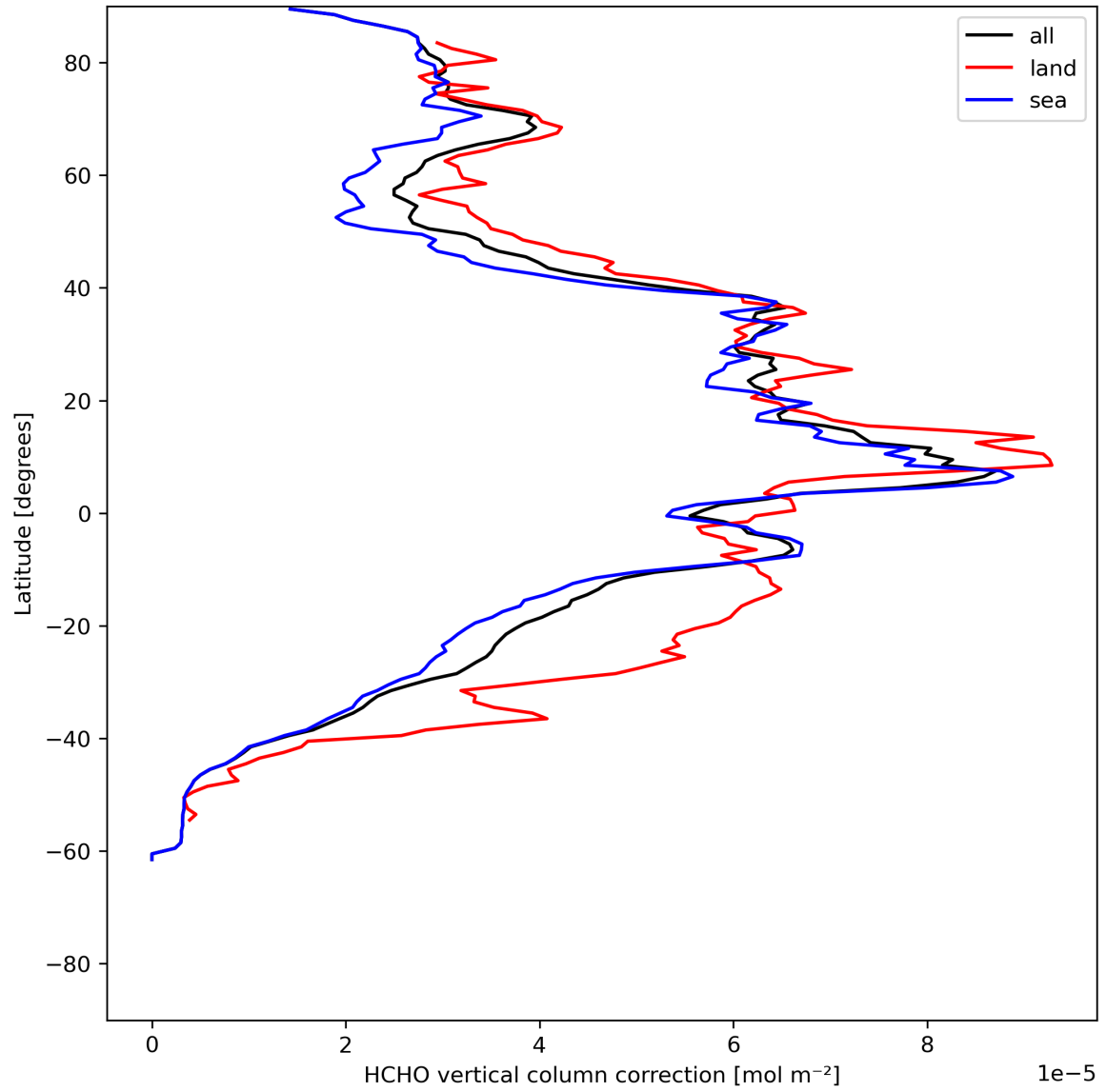
Figure 23: Zonal average of “HCHO vertical column correction” for 2024-06-13 to 2024-06-15.
