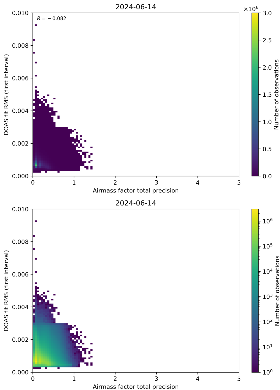
Figure 105: Scatter density plot of “Airmass factor total precision” against “DOAS fit RMS (first interval)” for 2024-06-13 to 2024-06-15.
