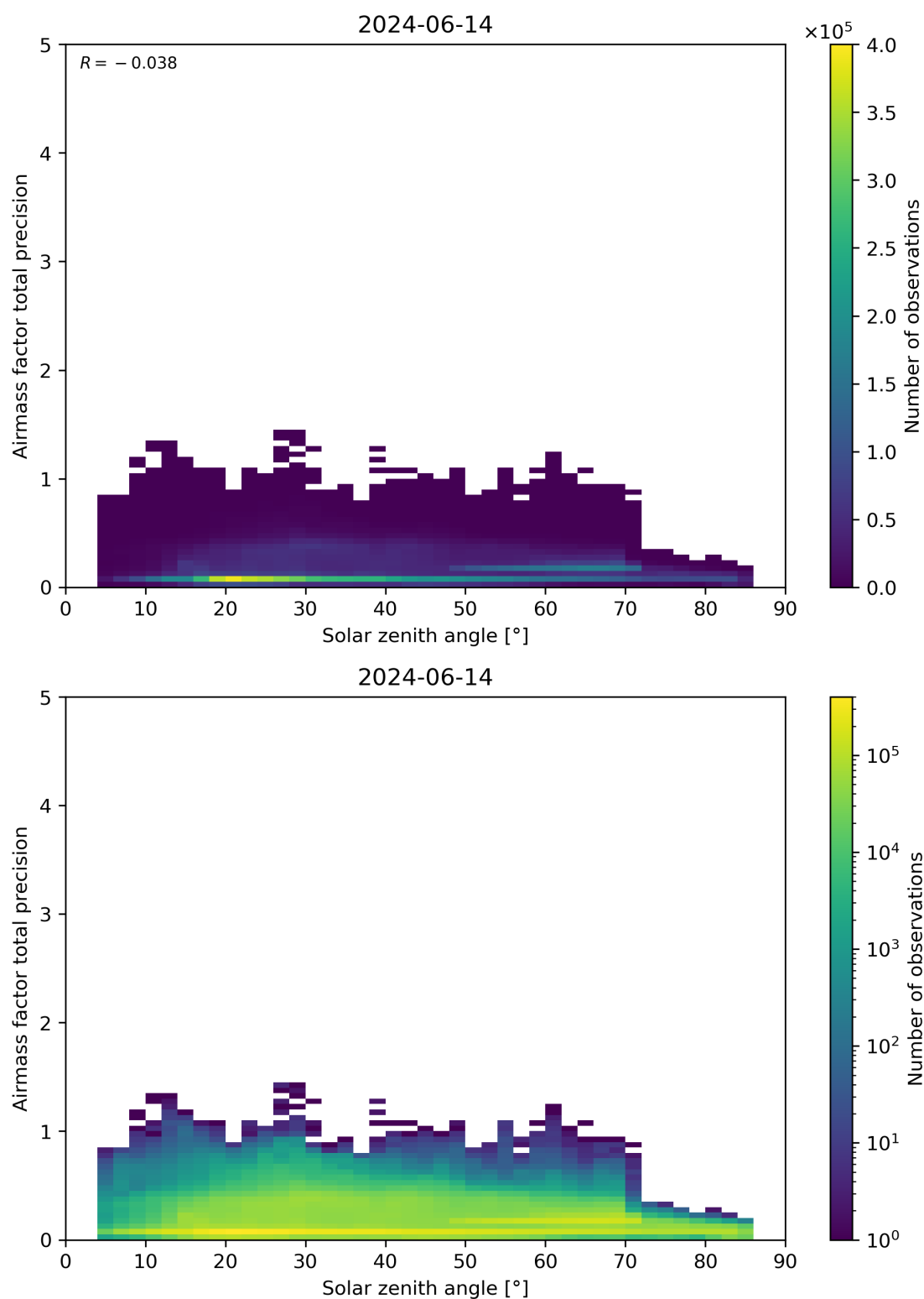
Figure 176: Scatter density plot of “Solar zenith angle” against “Airmass factor total precision” for 2024-06-13 to 2024-06-15.
