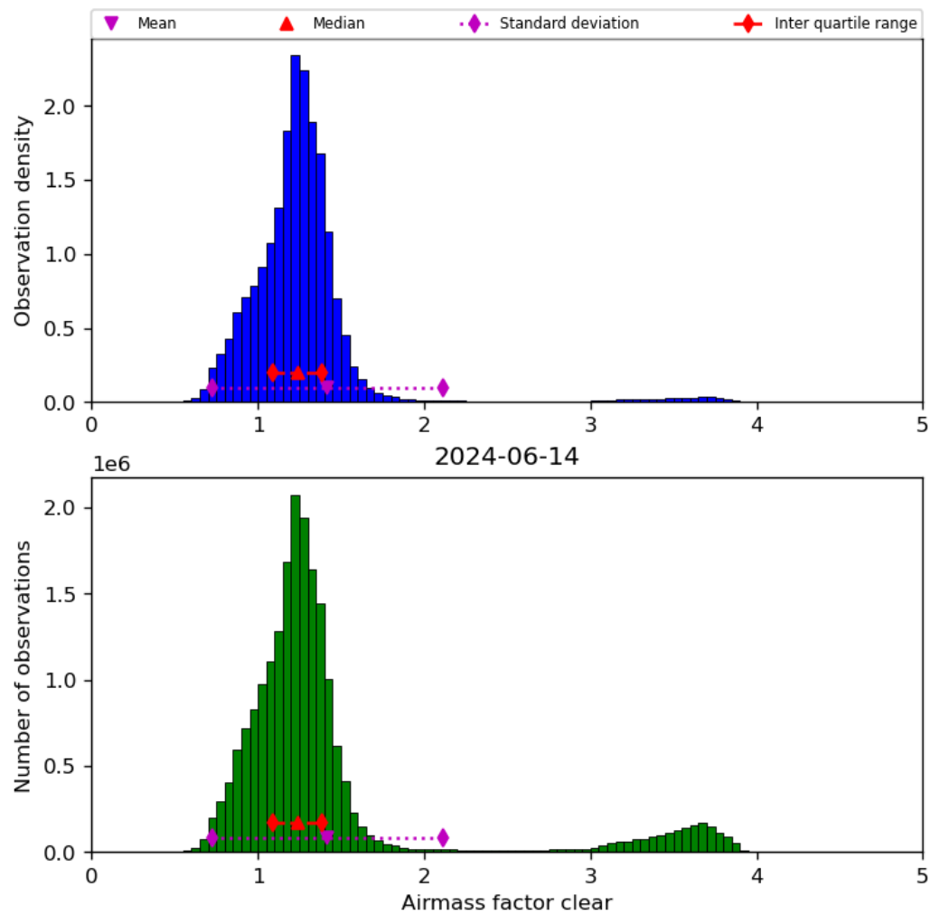
Figure 42: Histogram of “Airmass factor clear” for 2024-06-13 to 2024-06-15
