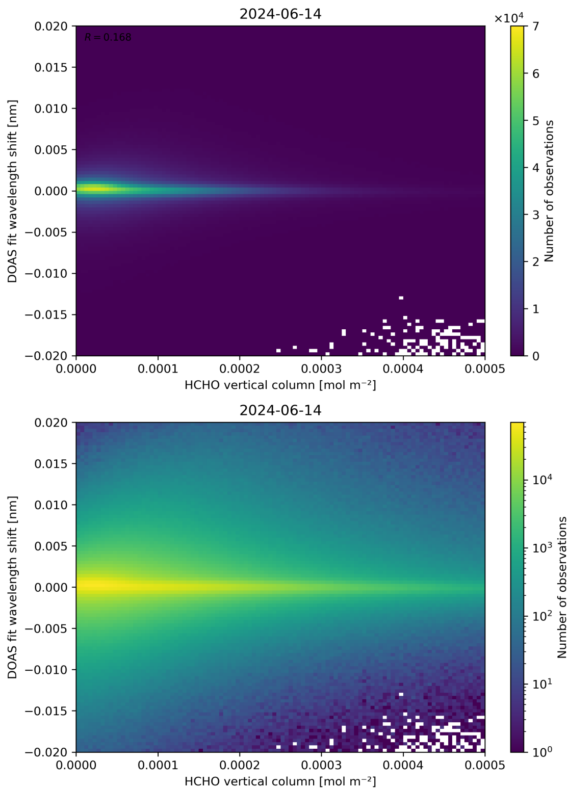
Figure 124: Scatter density plot of “HCHO vertical column” against “DOAS fit wavelength shift” for 2024-06-13 to 2024-06-15.
