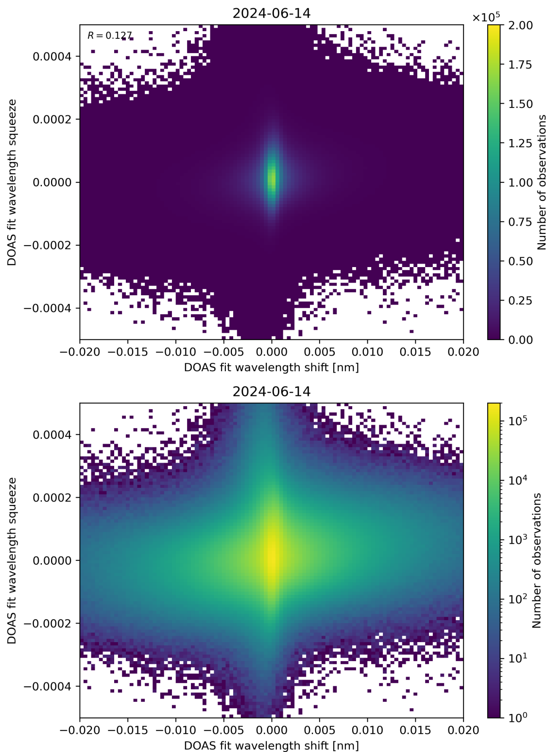
Figure 65: Scatter density plot of “DOAS fit wavelength shift” against “DOAS fit wavelength squeeze” for 2024-06-13 to 2024-06-15.
