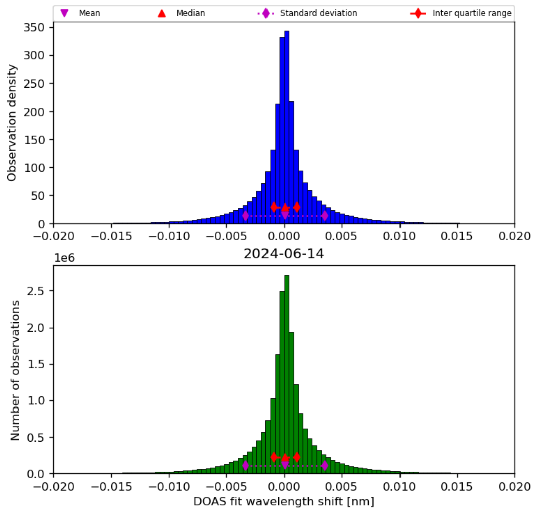
Figure 44: Histogram of “DOAS fit wavelength shift” for 2024-06-13 to 2024-06-15
