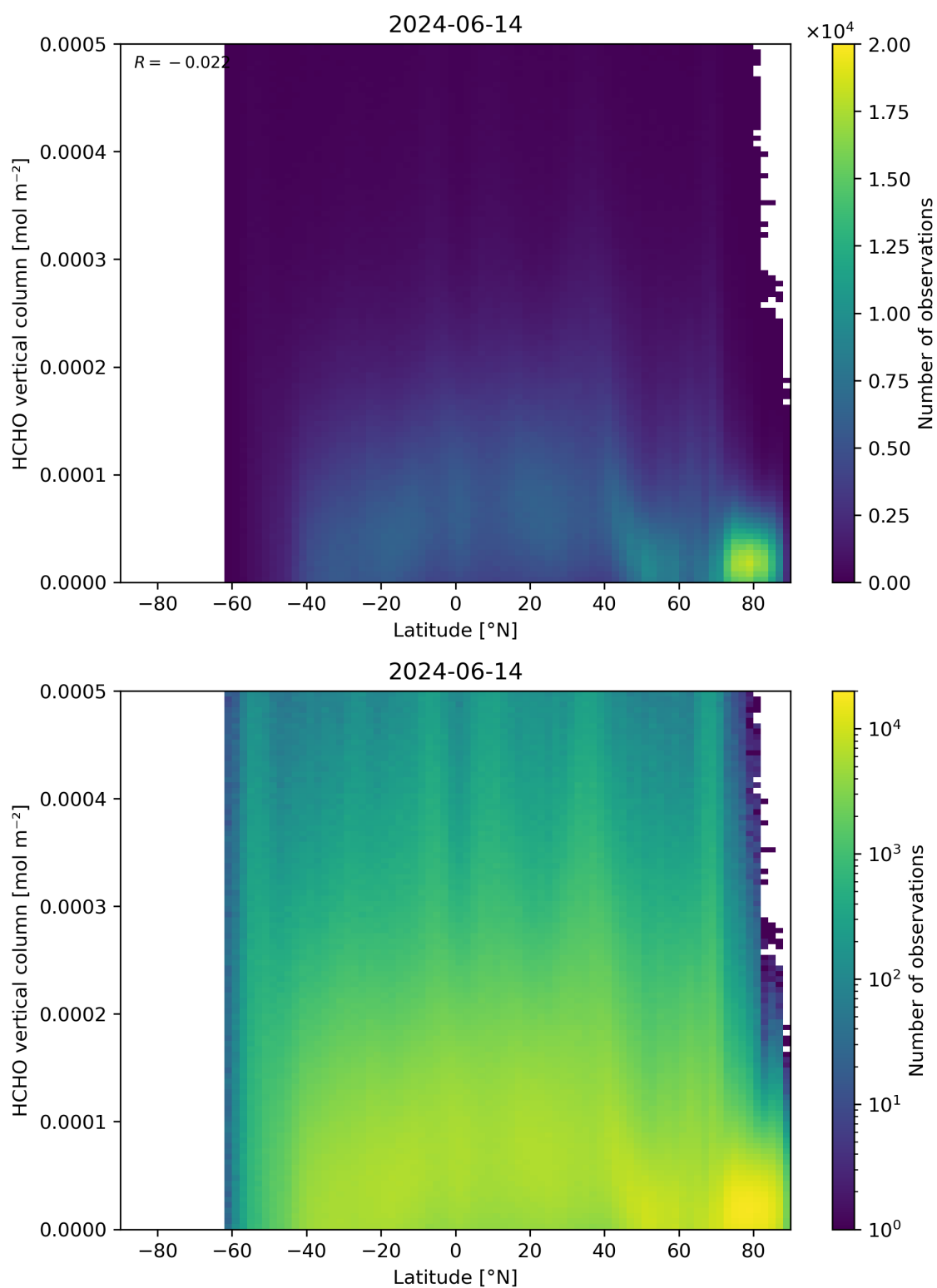
Figure 163: Scatter density plot of “Latitude” against “HCHO vertical column” for 2024-06-13 to 2024-06-15.
