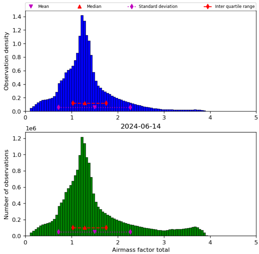
Figure 40: Histogram of “Airmass factor total” for 2024-06-13 to 2024-06-15
