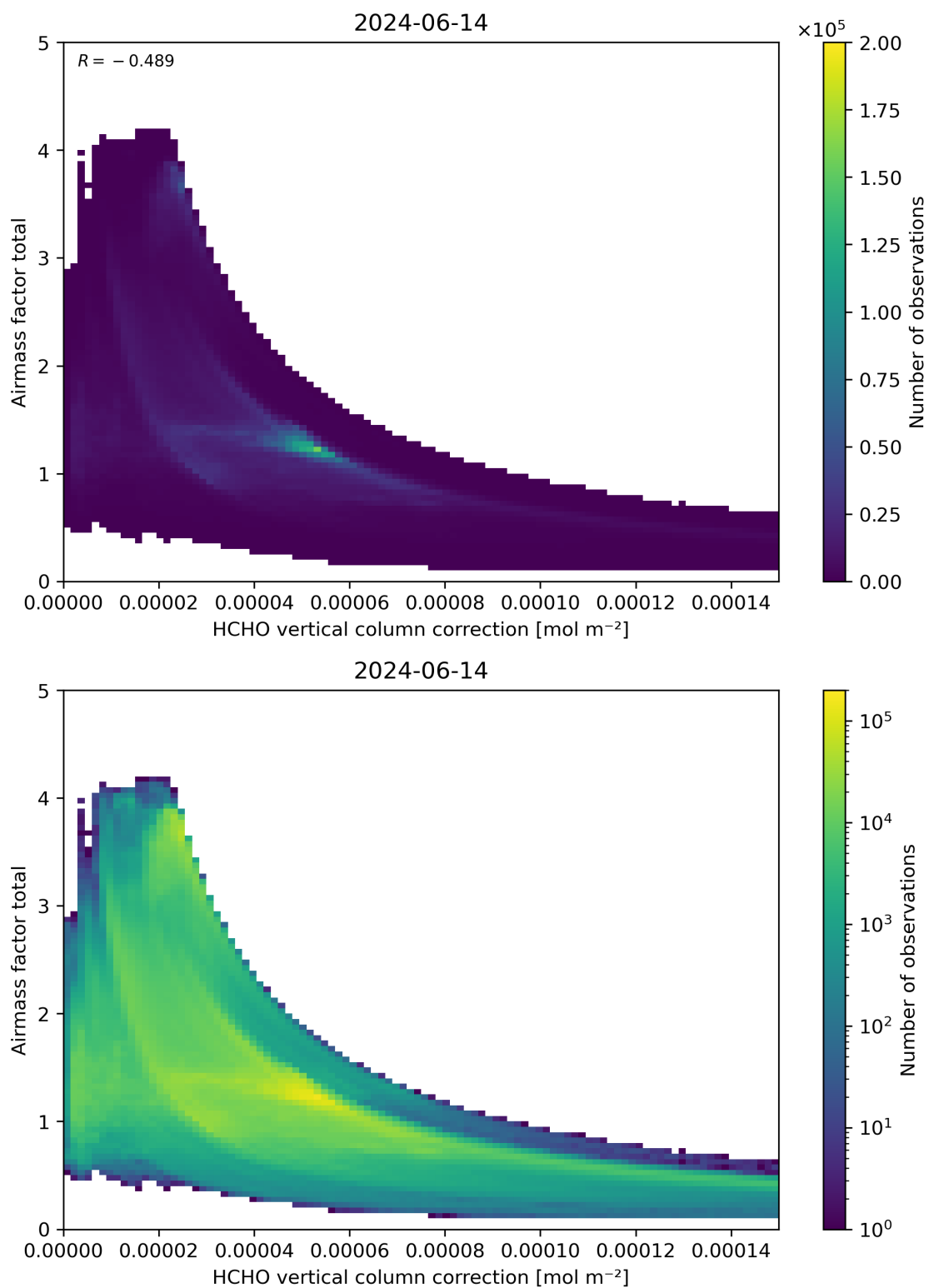
Figure 120: Scatter density plot of “HCHO vertical column correction” against “Airmass factor total” for 2024-06-13 to 2024-06-15.
