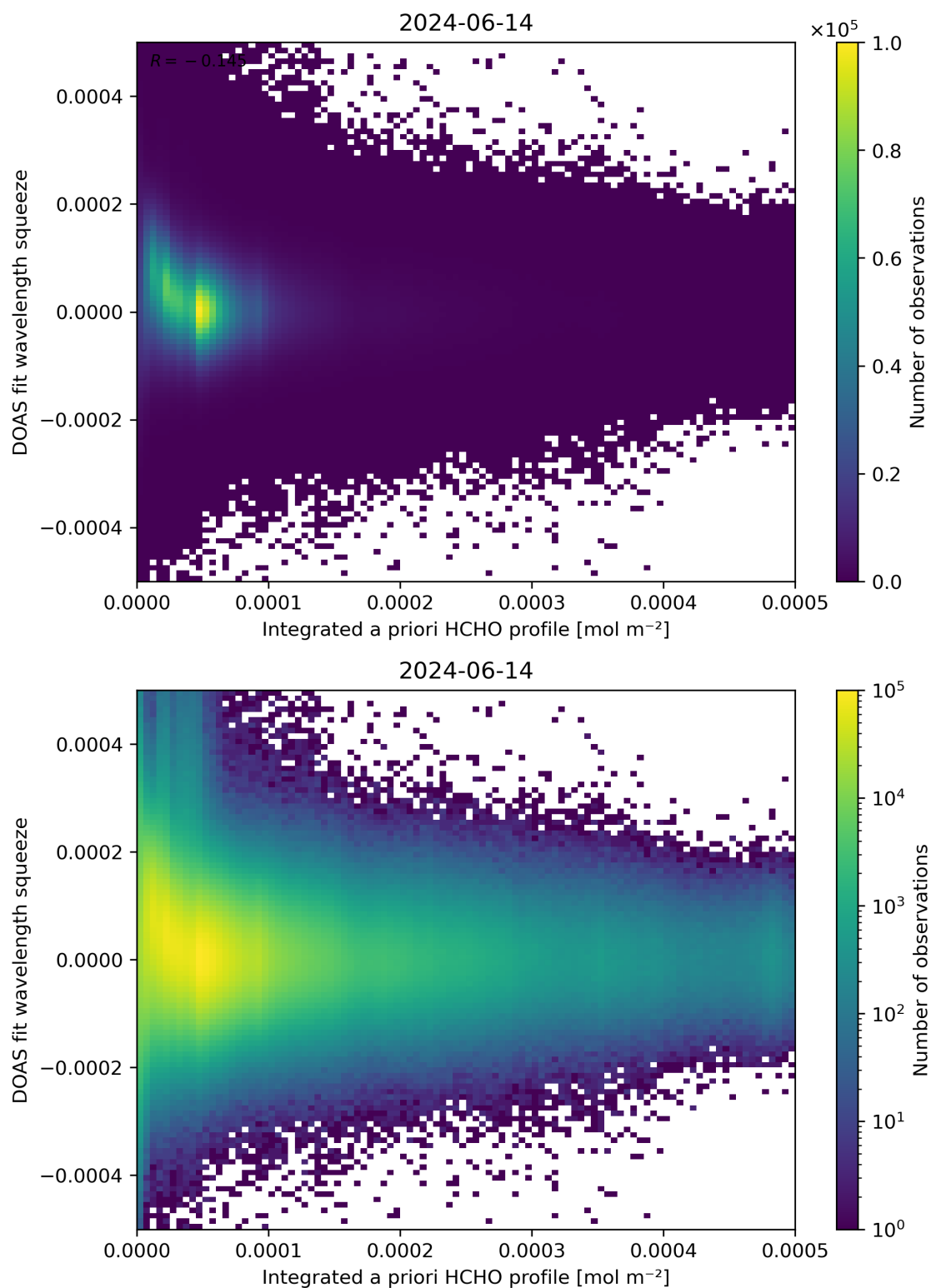
Figure 150: Scatter density plot of “Integrated a priori HCHO profile” against “DOAS fit wavelength squeeze” for 2024-06-13 to 2024-06-15.
