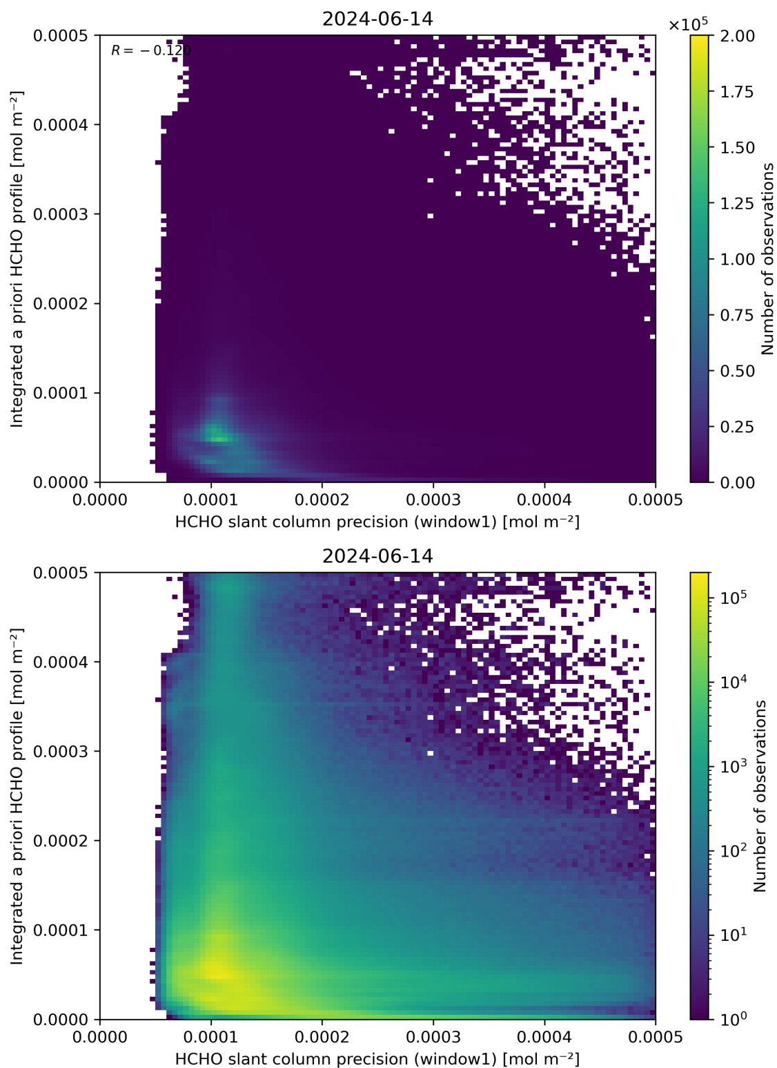
Figure 96: Scatter density plot of “HCHO slant column precision (window1)” against “Integrated a priori HCHO profile” for 2024-06-13 to 2024-06-15.
