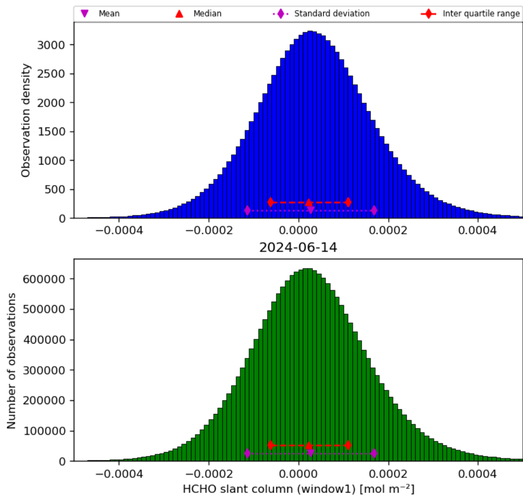
Figure 38: Histogram of “HCHO slant column (window1)” for 2024-06-13 to 2024-06-15
