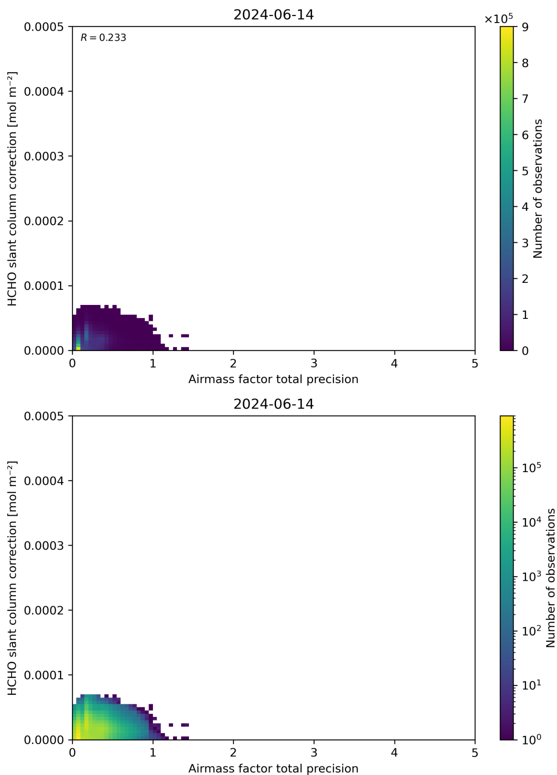
Figure 110: Scatter density plot of “Airmass factor total precision” against “HCHO slant column correction” for 2024-06-13 to 2024-06-15.
