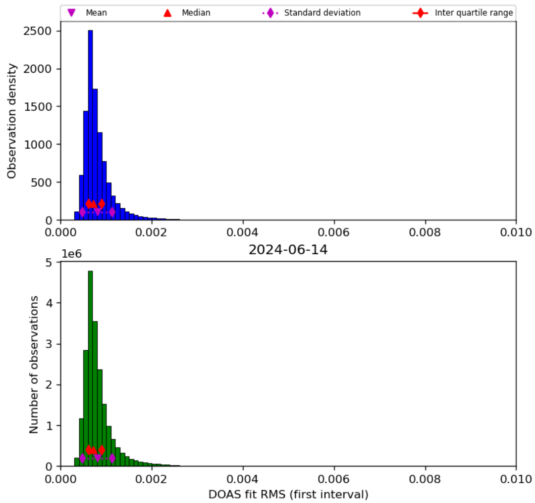
Figure 46: Histogram of “DOAS fit RMS (first interval)” for 2024-06-13 to 2024-06-15
