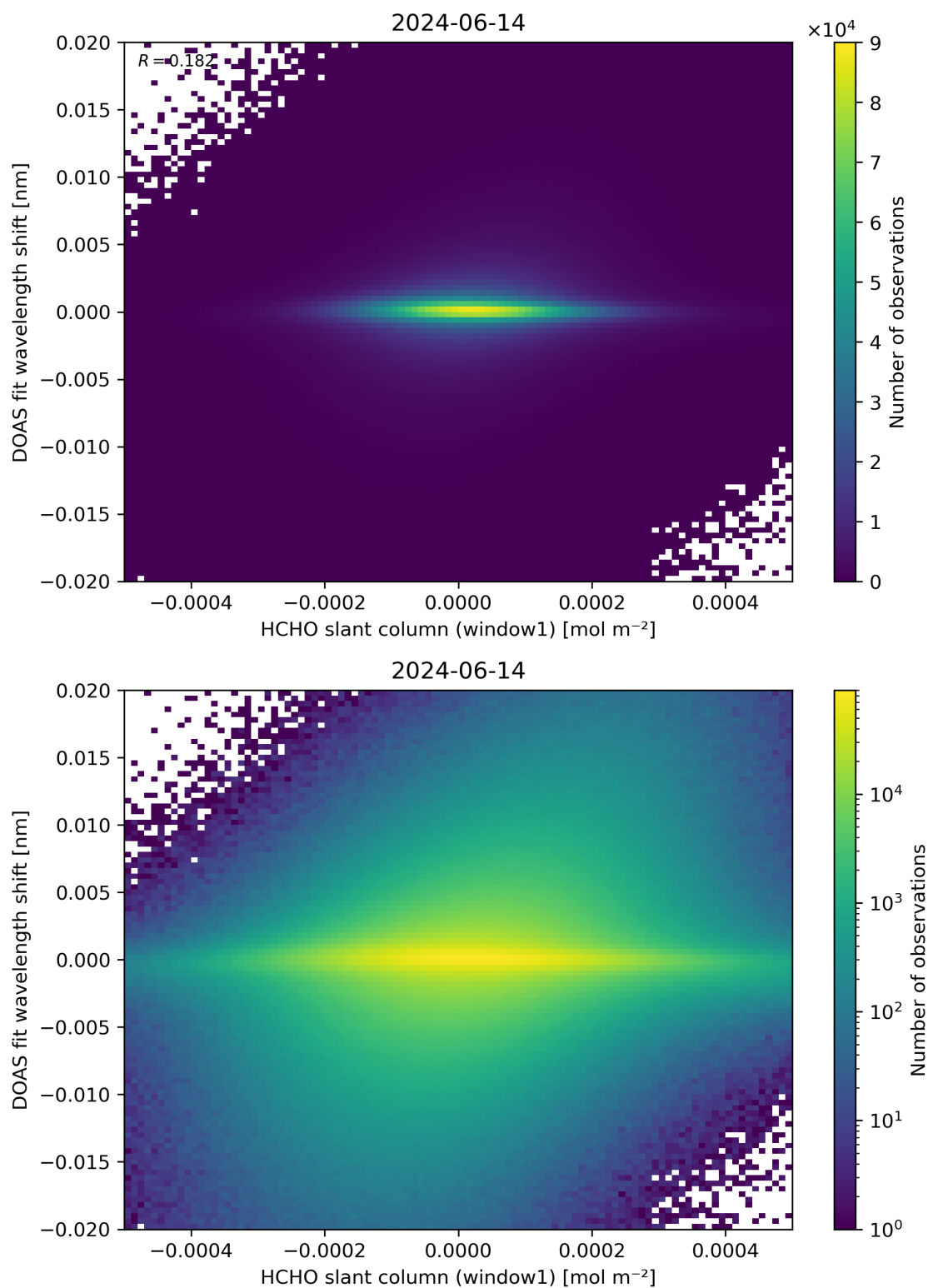
Figure 79: Scatter density plot of “HCHO slant column (window1)” against “DOAS fit wavelength shift” for 2024-06-13 to 2024-06-15.
