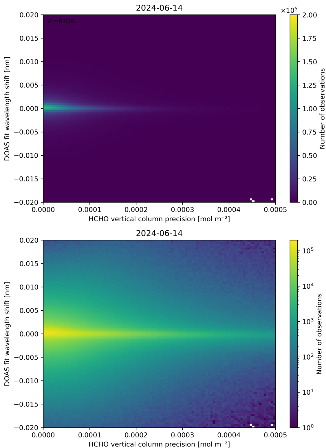
Figure 137: Scatter density plot of “HCHO vertical column precision” against “DOAS fit wavelength shift” for 2024-06-13 to 2024-06-15.
