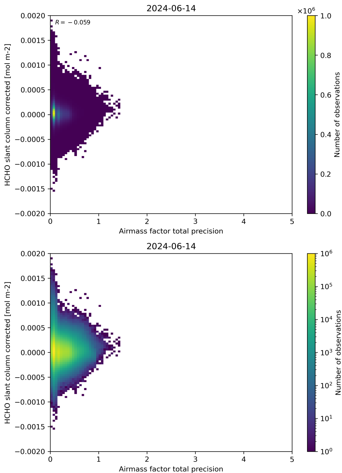
Figure 109: Scatter density plot of “Airmass factor total precision” against “HCHO slant column corrected” for 2024-06-13 to 2024-06-15.
