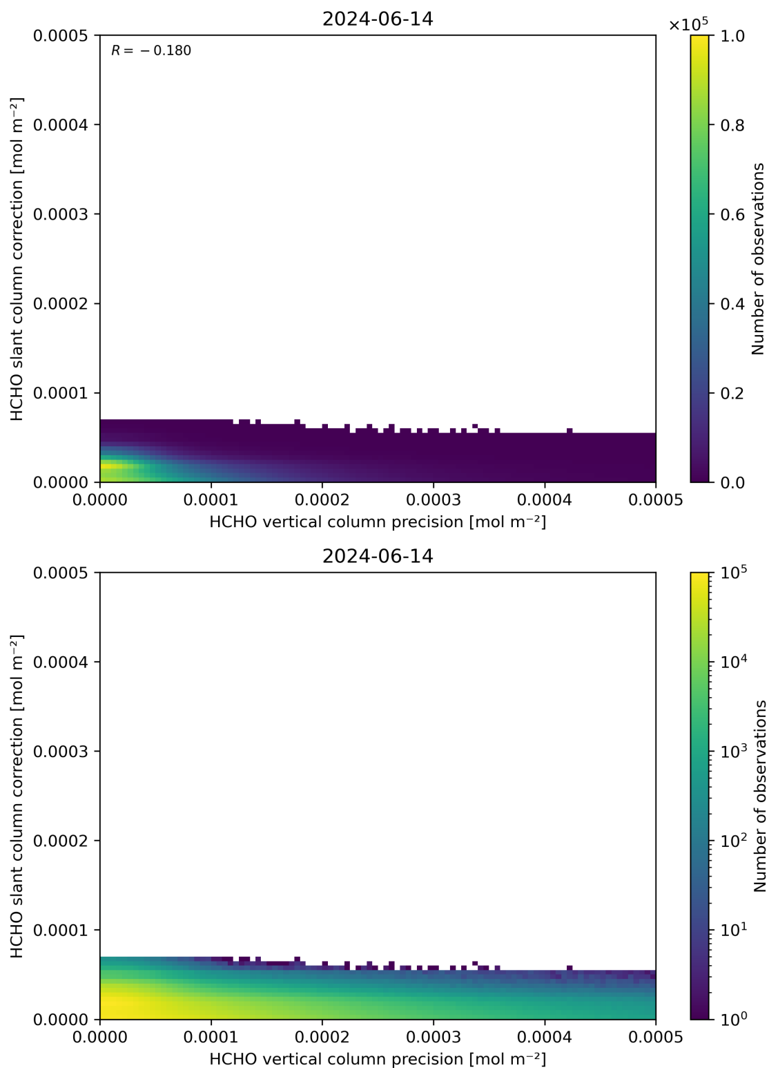
Figure 141: Scatter density plot of “HCHO vertical column precision” against “HCHO slant column correction” for 2024-06-13 to 2024-06-15.
