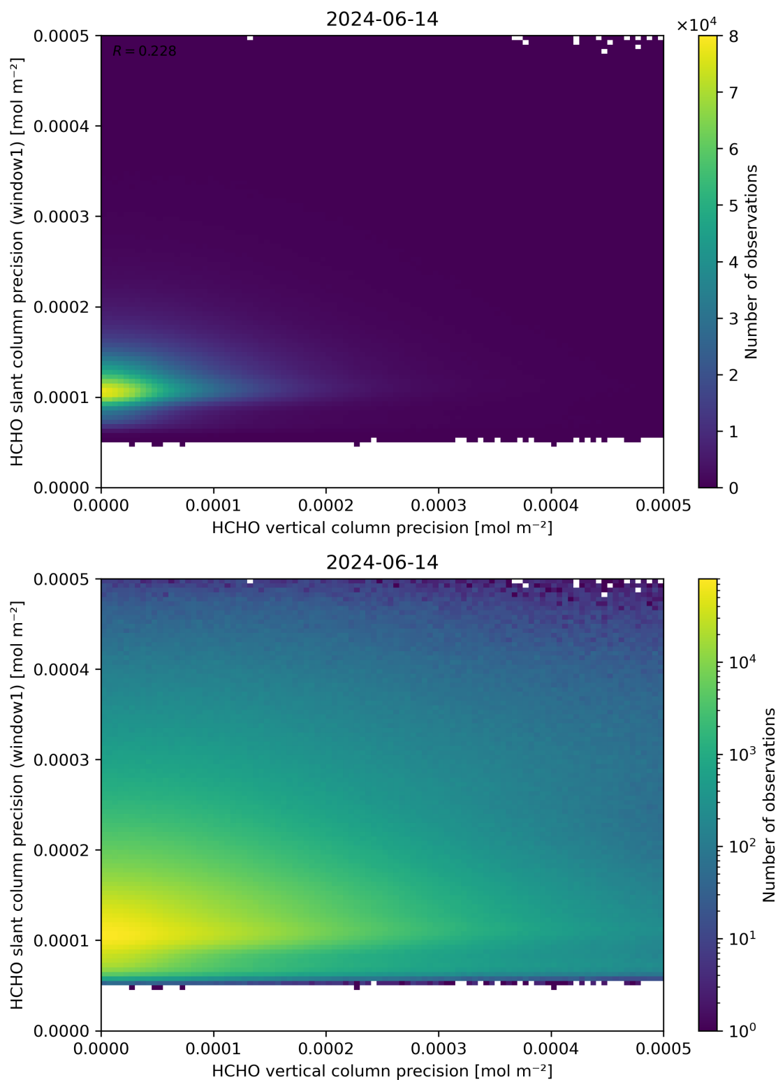
Figure 143: Scatter density plot of “HCHO vertical column precision” against “HCHO slant column precision (window1)” for 2024-06-13 to 2024-06-15.
