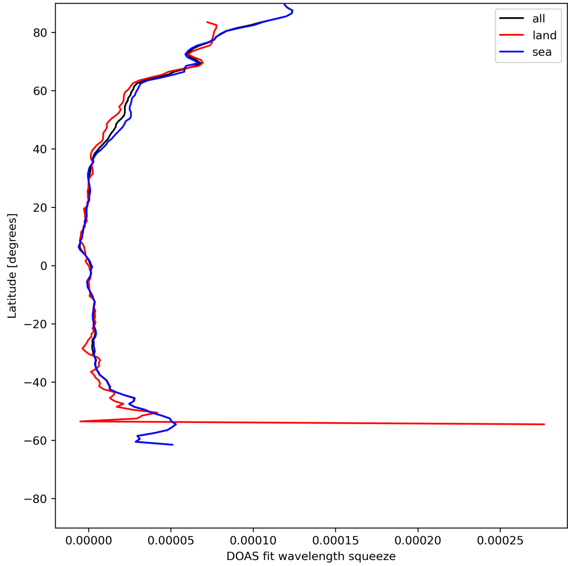
Figure 31: Zonal average of “DOAS fit wavelength squeeze” for 2024-06-13 to 2024-06-15.
