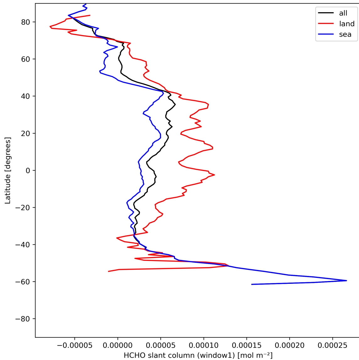
Figure 24: Zonal average of “HCHO slant column (window1)” for 2024-06-13 to 2024-06-15.
