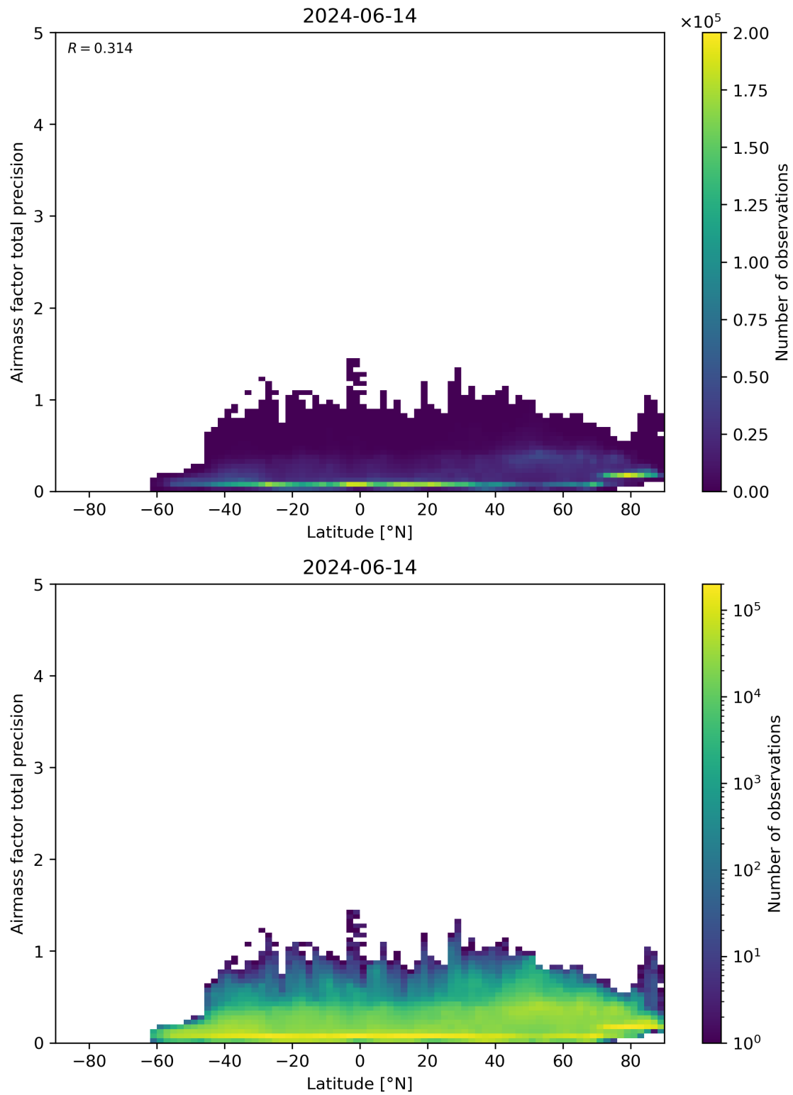
Figure 162: Scatter density plot of “Latitude” against “Airmass factor total precision” for 2024-06-13 to 2024-06-15.
