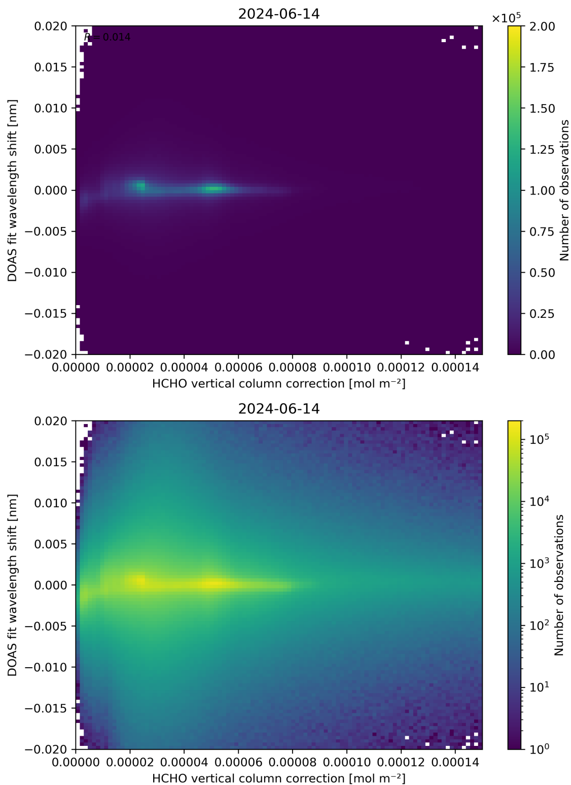
Figure 113: Scatter density plot of “HCHO vertical column correction” against “DOAS fit wavelength shift” for 2024-06-13 to 2024-06-15.
