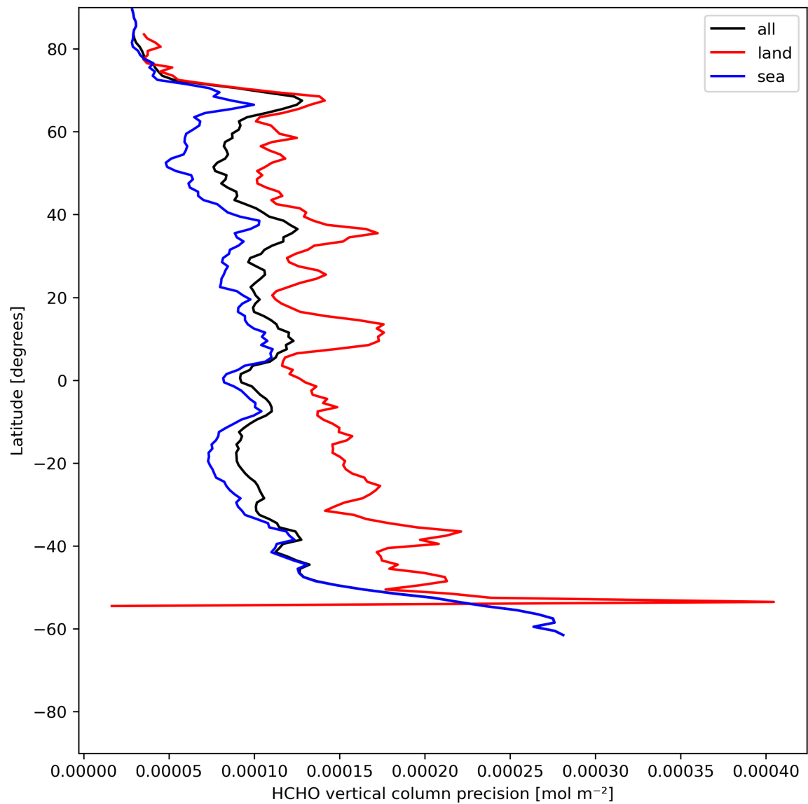
Figure 22: Zonal average of “HCHO vertical column precision” for 2024-06-13 to 2024-06-15.
