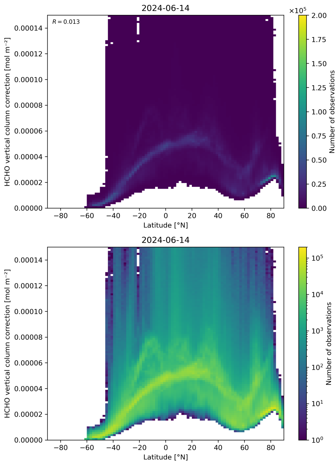
Figure 164: Scatter density plot of “Latitude” against “HCHO vertical column correction” for 2024-06-13 to 2024-06-15.
