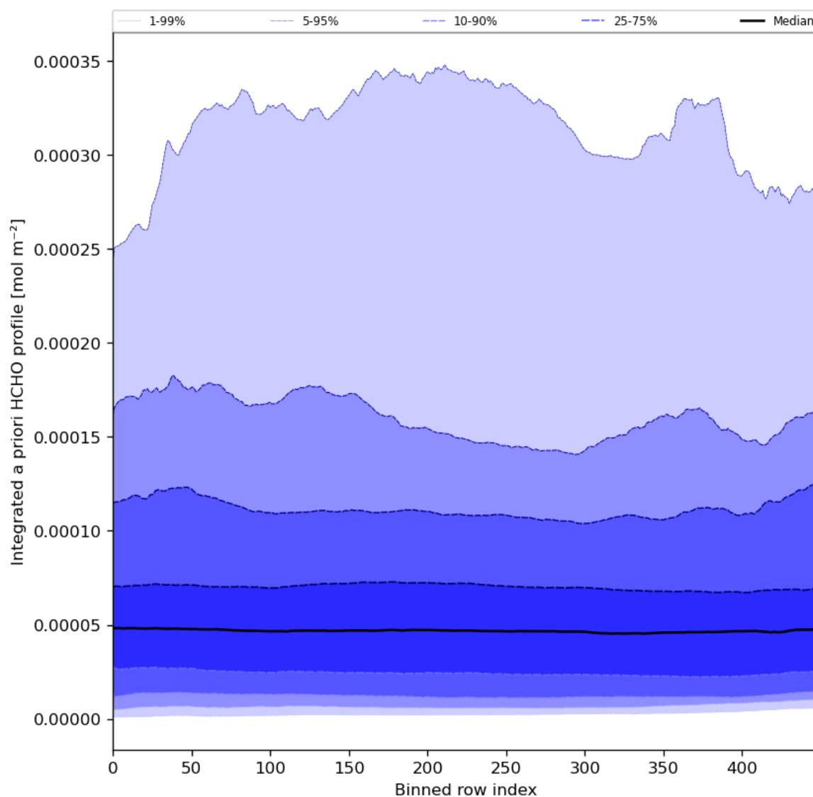
Figure 57: Along track statistics of “Integrated a priori HCHO profile” for 2024-06-13 to 2024-06-15
