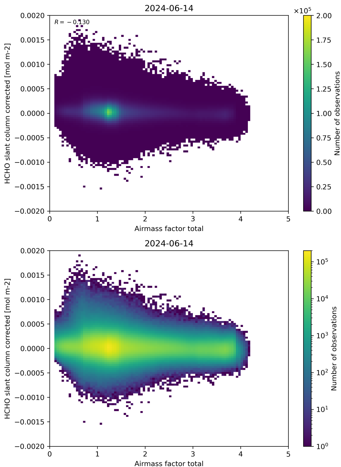
Figure 101: Scatter density plot of “Airmass factor total” against “HCHO slant column corrected” for 2024-06-13 to 2024-06-15.
