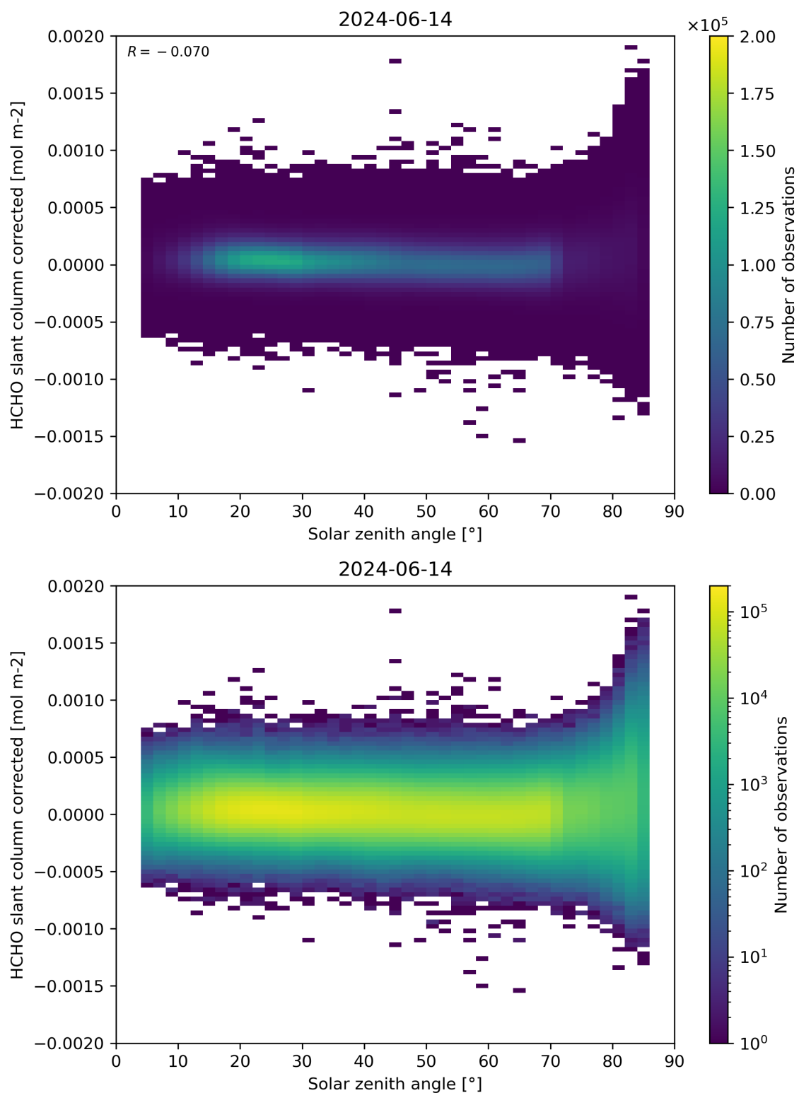
Figure 171: Scatter density plot of “Solar zenith angle” against “HCHO slant column corrected” for 2024-06-13 to 2024-06-15.
