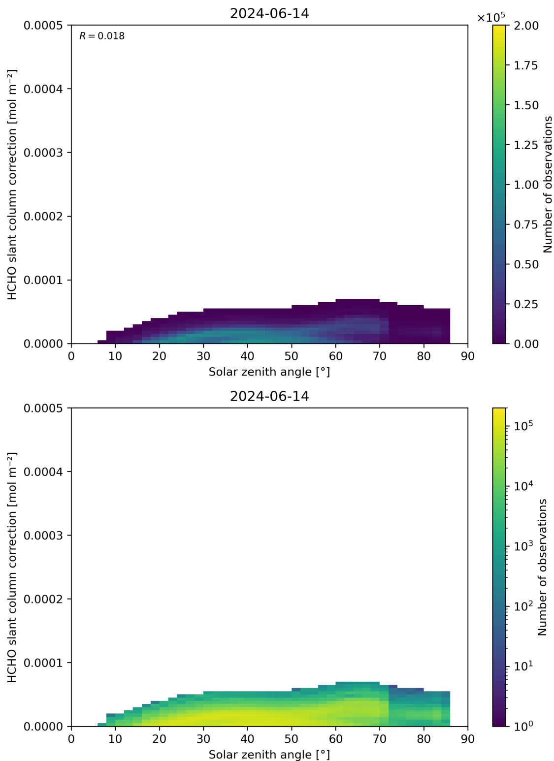
Figure 172: Scatter density plot of “Solar zenith angle” against “HCHO slant column correction” for 2024-06-13 to 2024-06-15.
