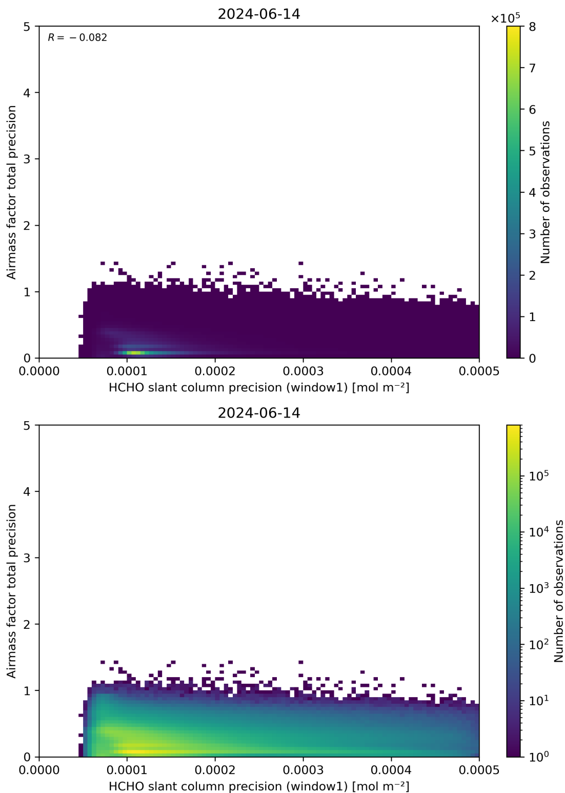
Figure 95: Scatter density plot of “HCHO slant column precision (window1)” against “Airmass factor total precision” for 2024-06-13 to 2024-06-15.
