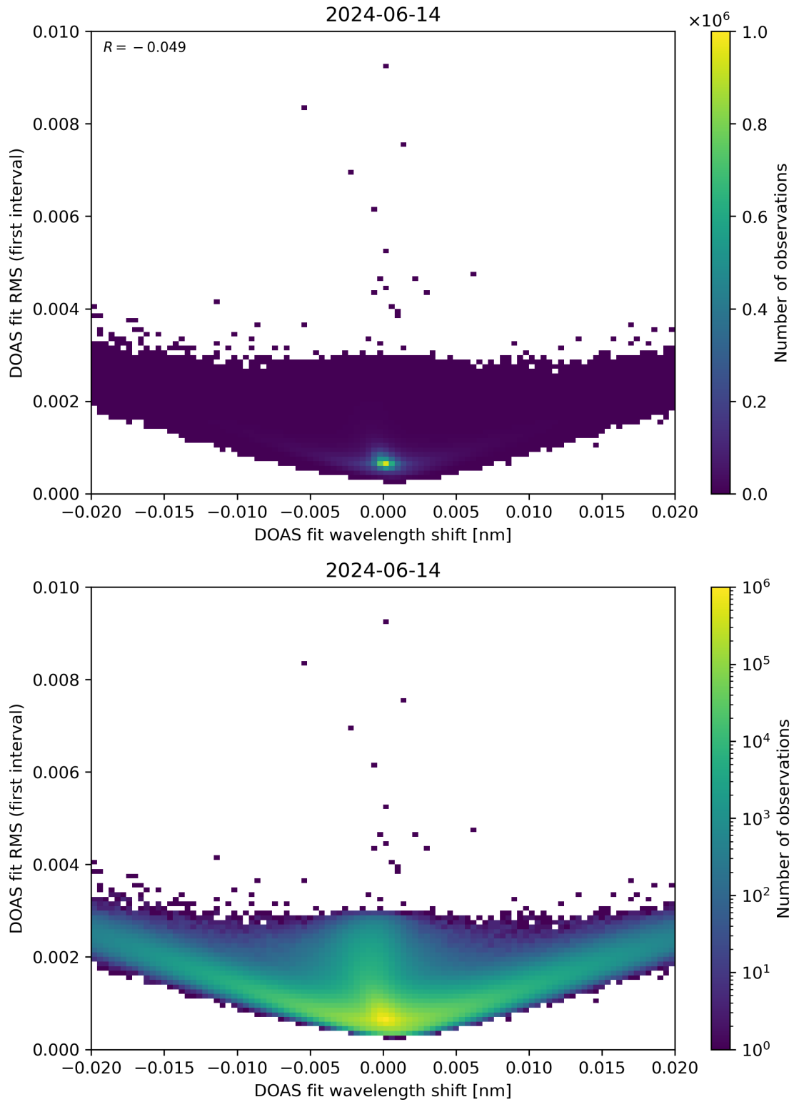
Figure 64: Scatter density plot of “DOAS fit wavelength shift” against “DOAS fit RMS (first interval)” for 2024-06-13 to 2024-06-15.
