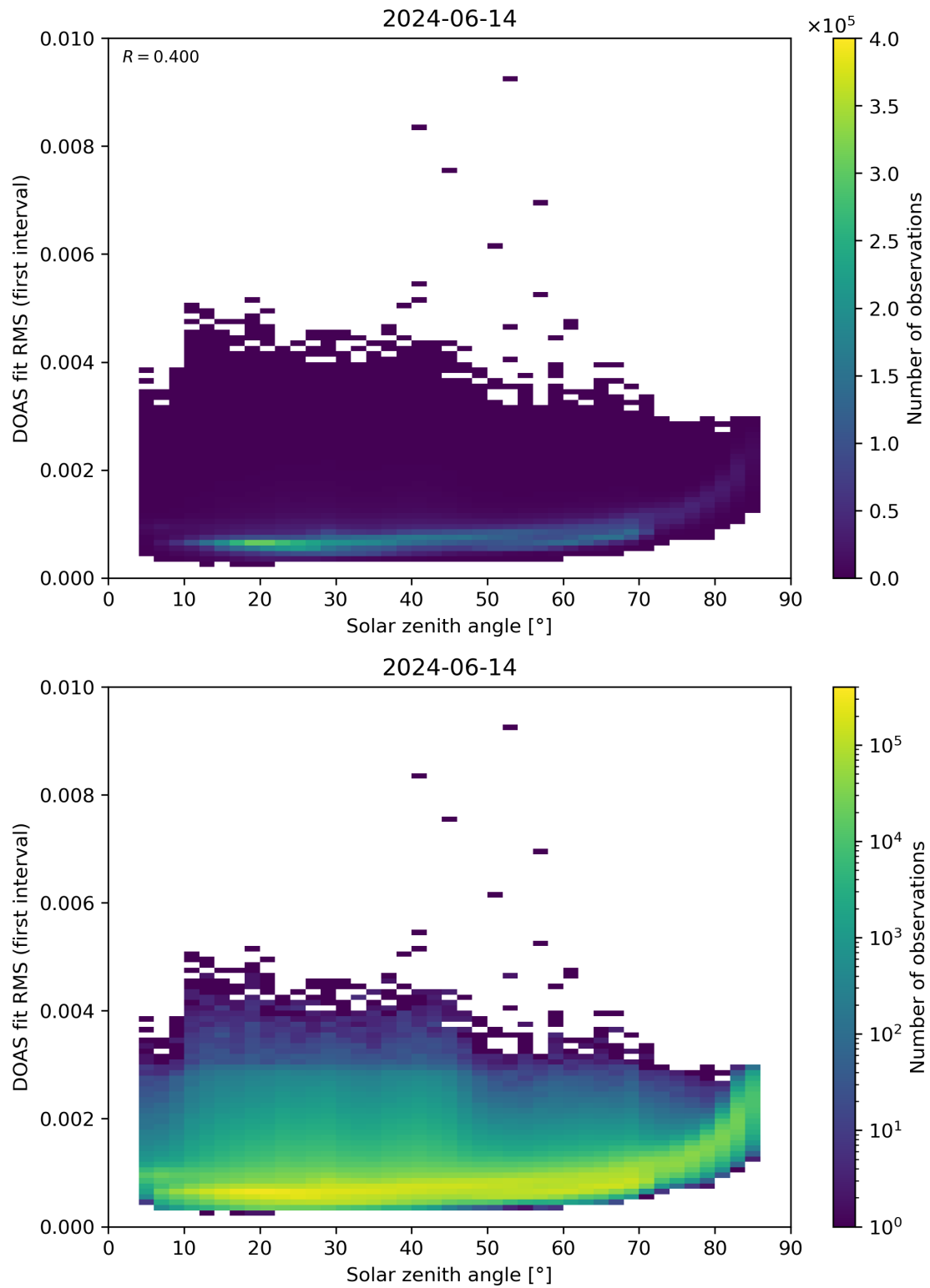
Figure 167: Scatter density plot of “Solar zenith angle” against “DOAS fit RMS (first interval)” for 2024-06-13 to 2024-06-15.
