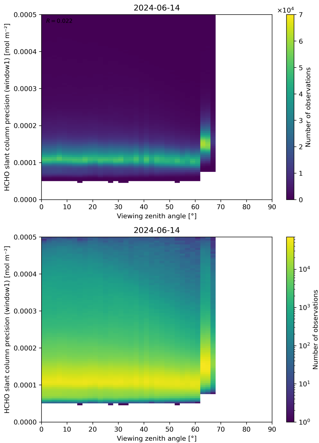
Figure 189: Scatter density plot of “Viewing zenith angle” against “HCHO slant column precision (window1)” for 2024-06-13 to 2024-06-15.
