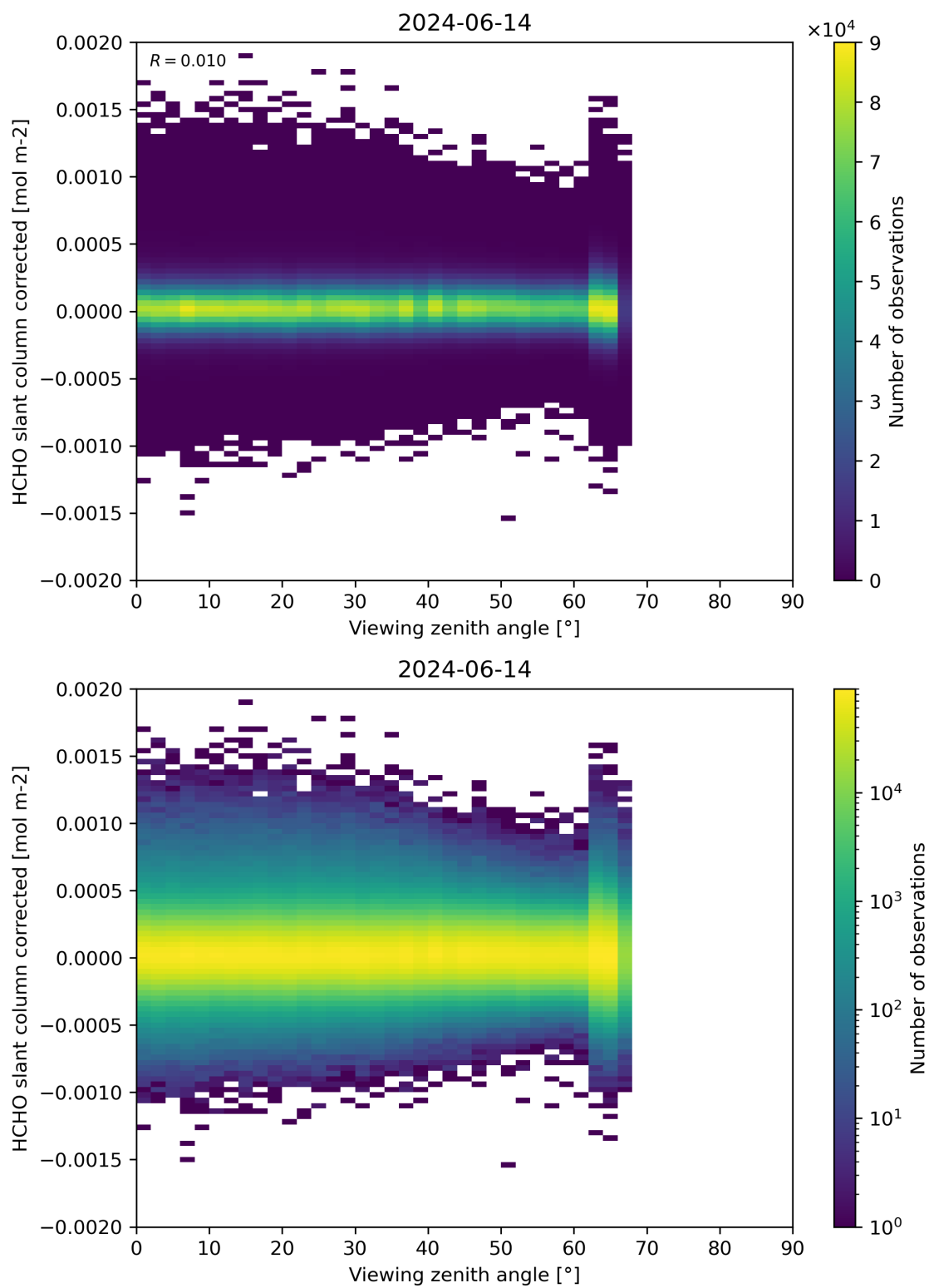
Figure 186: Scatter density plot of “Viewing zenith angle” against “HCHO slant column corrected” for 2024-06-13 to 2024-06-15.
