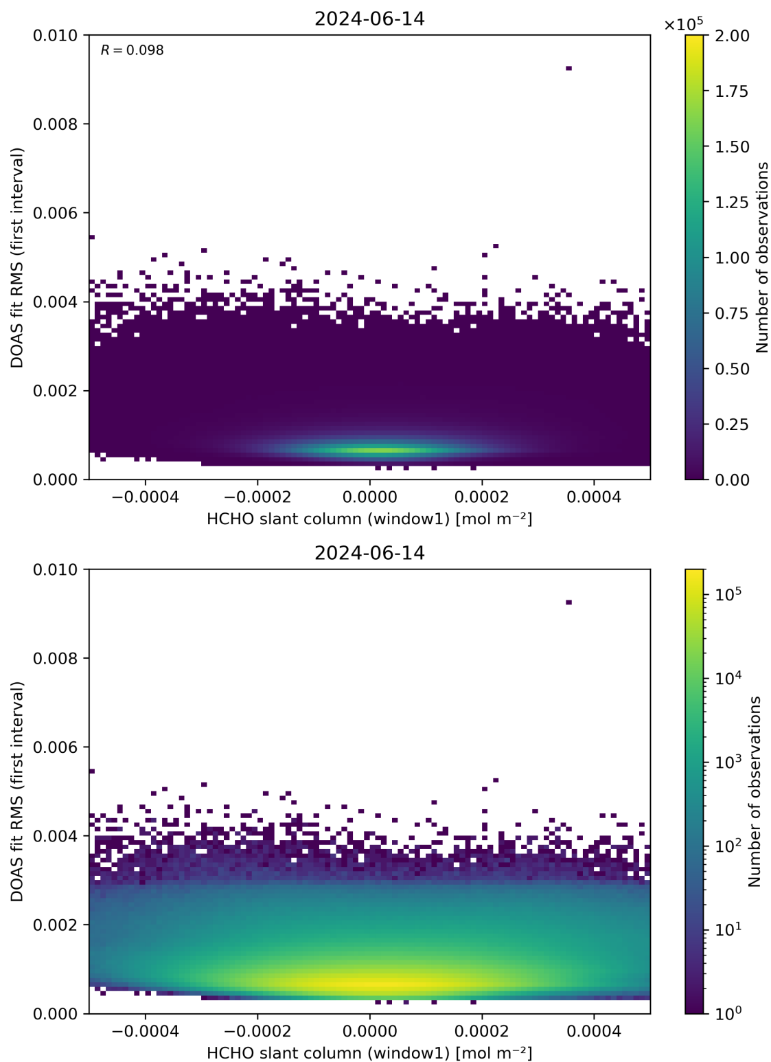
Figure 78: Scatter density plot of “HCHO slant column (window1)” against “DOAS fit RMS (first interval)” for 2024-06-13 to 2024-06-15.
