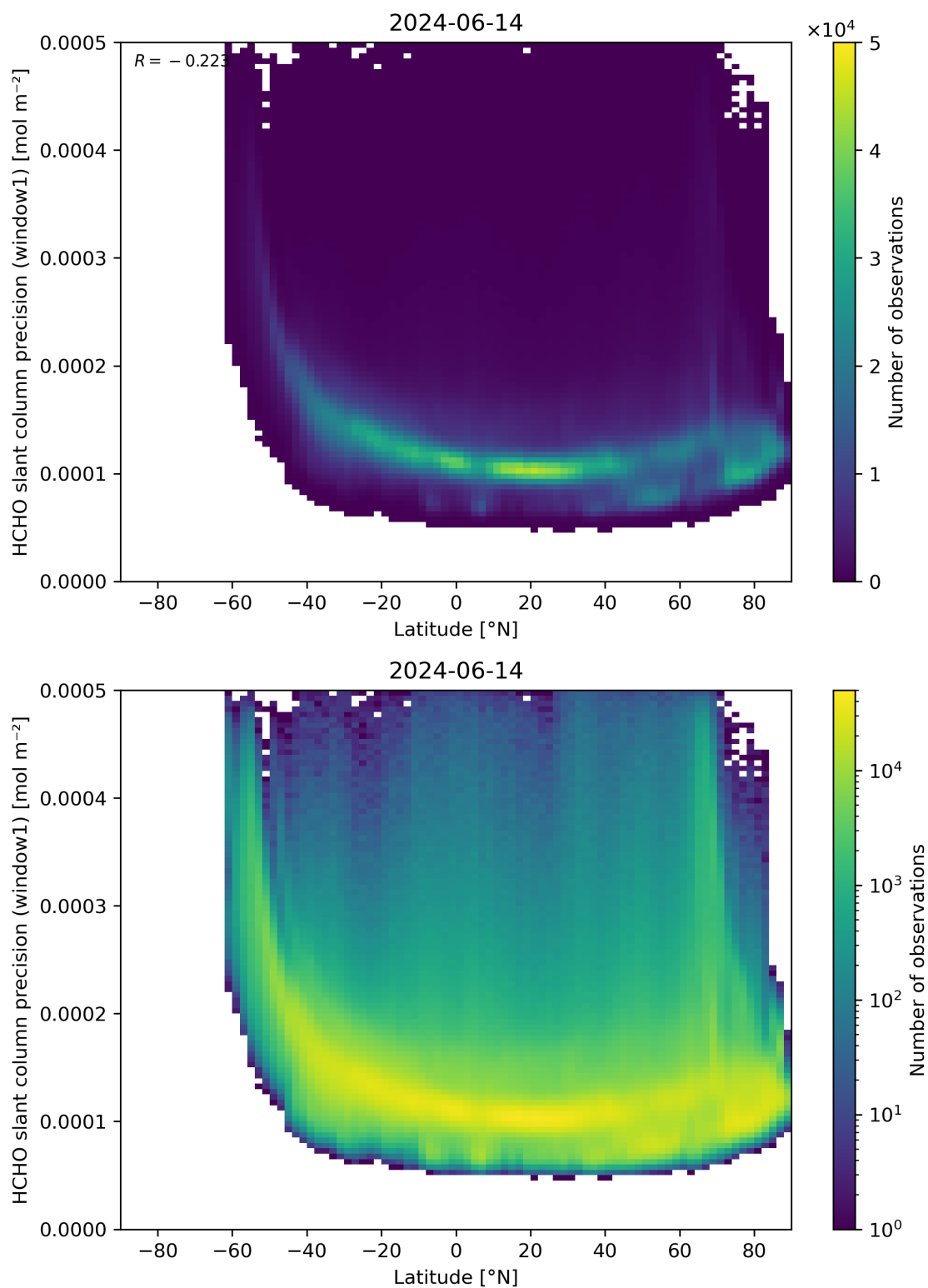
Figure 160: Scatter density plot of “Latitude” against “HCHO slant column precision (window1)” for 2024-06-13 to 2024-06-15.
