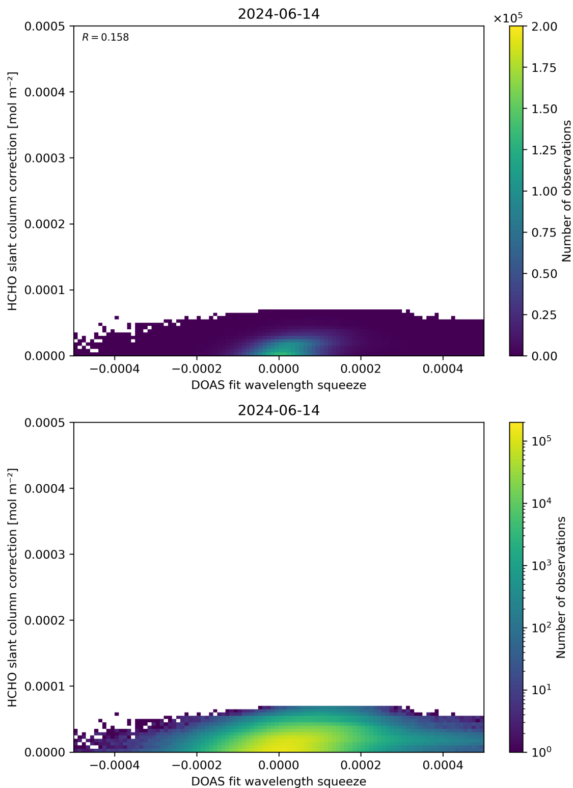
Figure 70: Scatter density plot of “DOAS fit wavelength squeeze” against “HCHO slant column correction” for 2024-06-13 to 2024-06-15.
