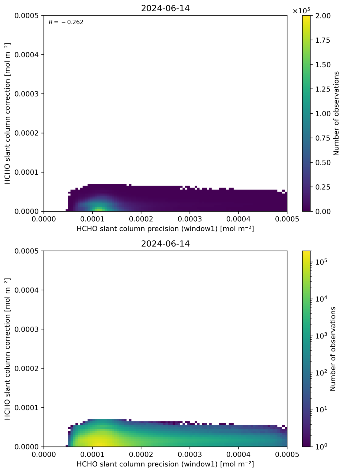
Figure 93: Scatter density plot of “HCHO slant column precision (window1)” against “HCHO slant column correction” for 2024-06-13 to 2024-06-15.
