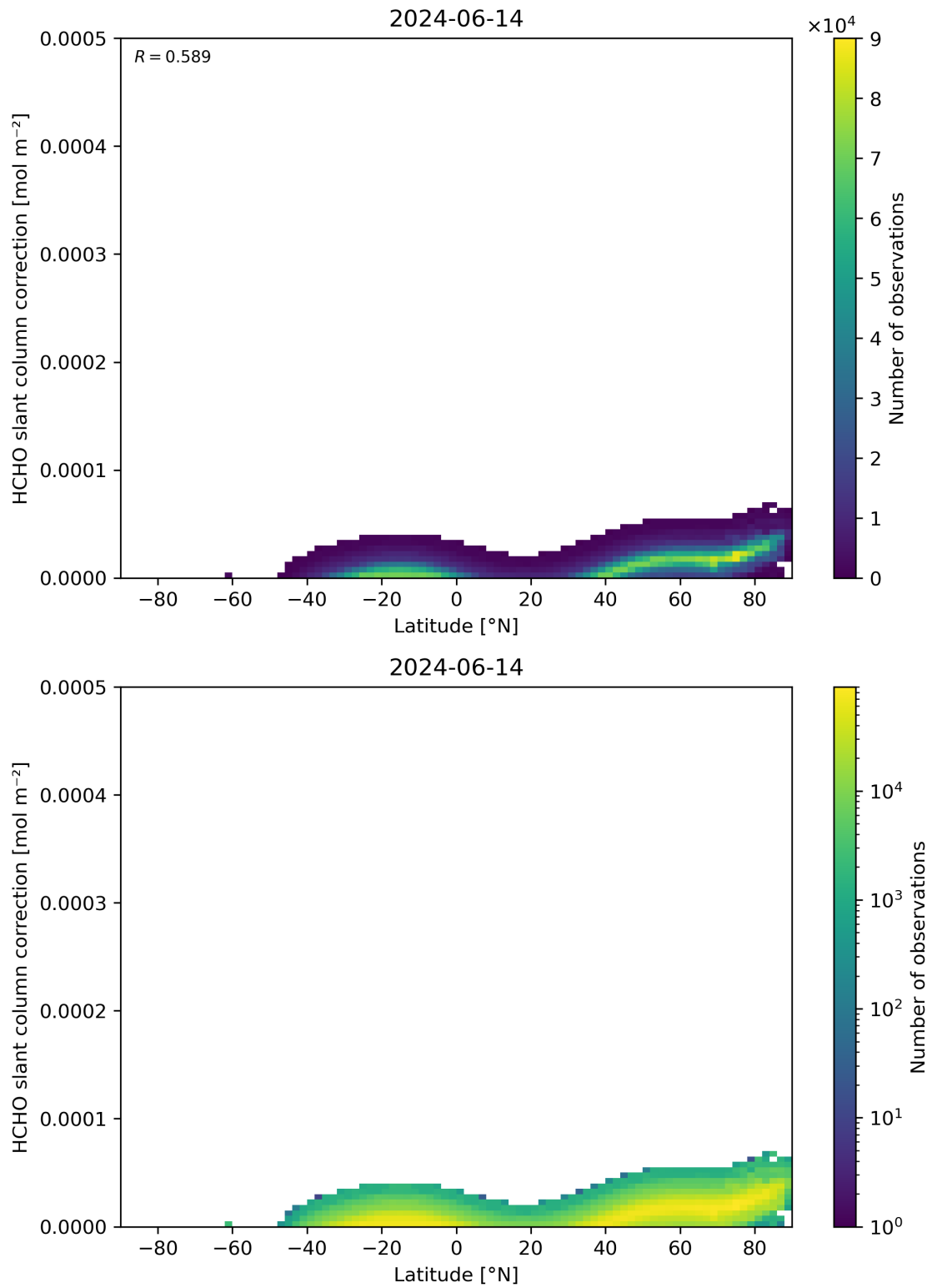
Figure 158: Scatter density plot of “Latitude” against “HCHO slant column correction” for 2024-06-13 to 2024-06-15.
