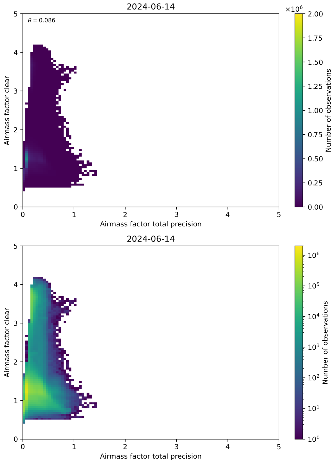
Figure 108: Scatter density plot of “Airmass factor total precision” against “Airmass factor clear” for 2024-06-13 to 2024-06-15.
