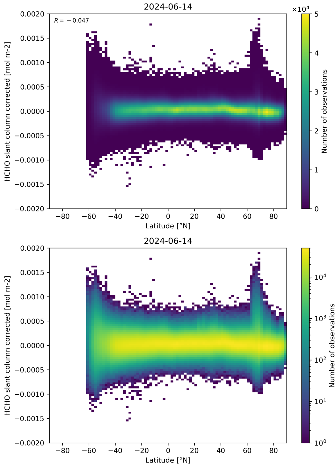
Figure 157: Scatter density plot of “Latitude” against “HCHO slant column corrected” for 2024-06-13 to 2024-06-15.
