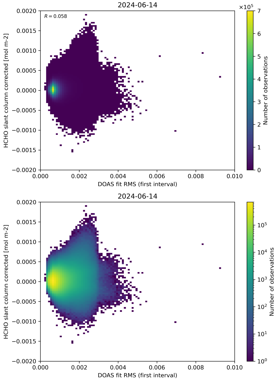
Figure 62: Scatter density plot of “DOAS fit RMS (first interval)” against “HCHO slant column corrected” for 2024-06-13 to 2024-06-15.
