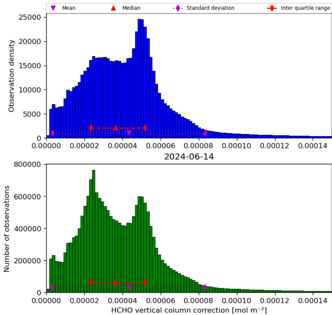
Figure 37: Histogram of “HCHO vertical column correction” for 2024-06-13 to 2024-06-15
