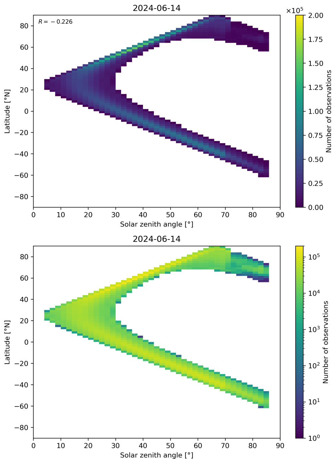
Figure 181: Scatter density plot of “Solar zenith angle” against “Latitude” for 2024-06-13 to 2024-06-15.
