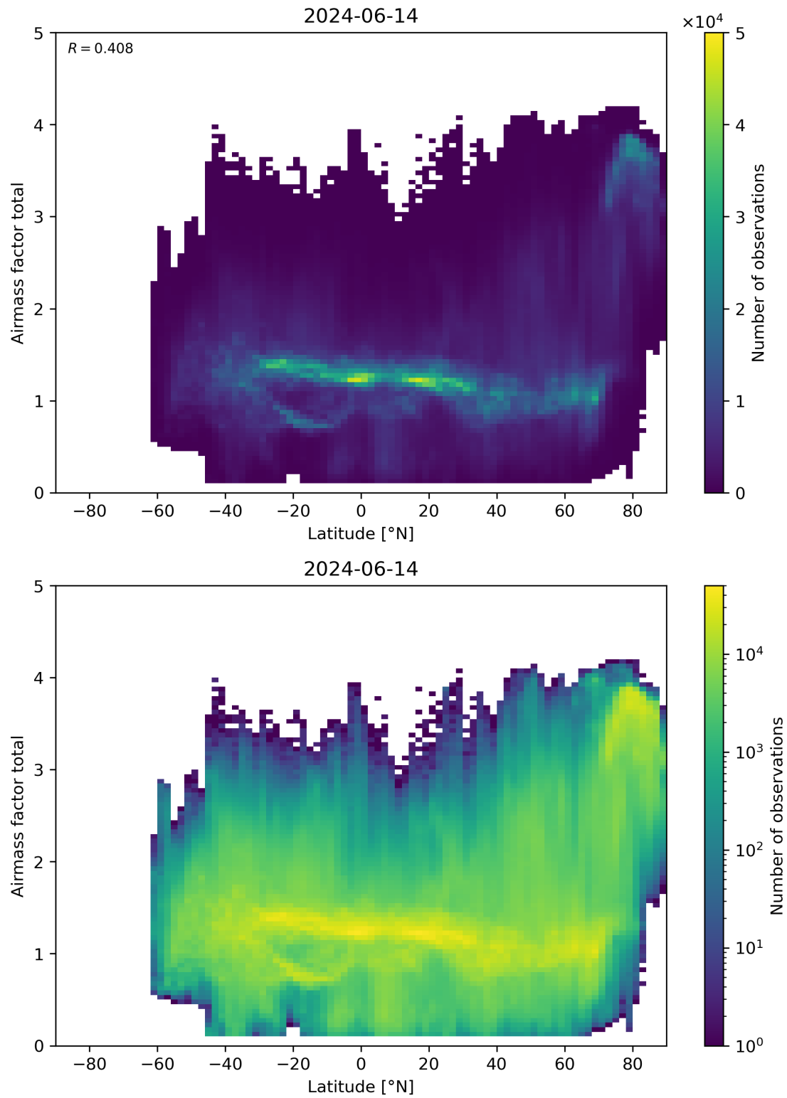
Figure 161: Scatter density plot of “Latitude” against “Airmass factor total” for 2024-06-13 to 2024-06-15.
