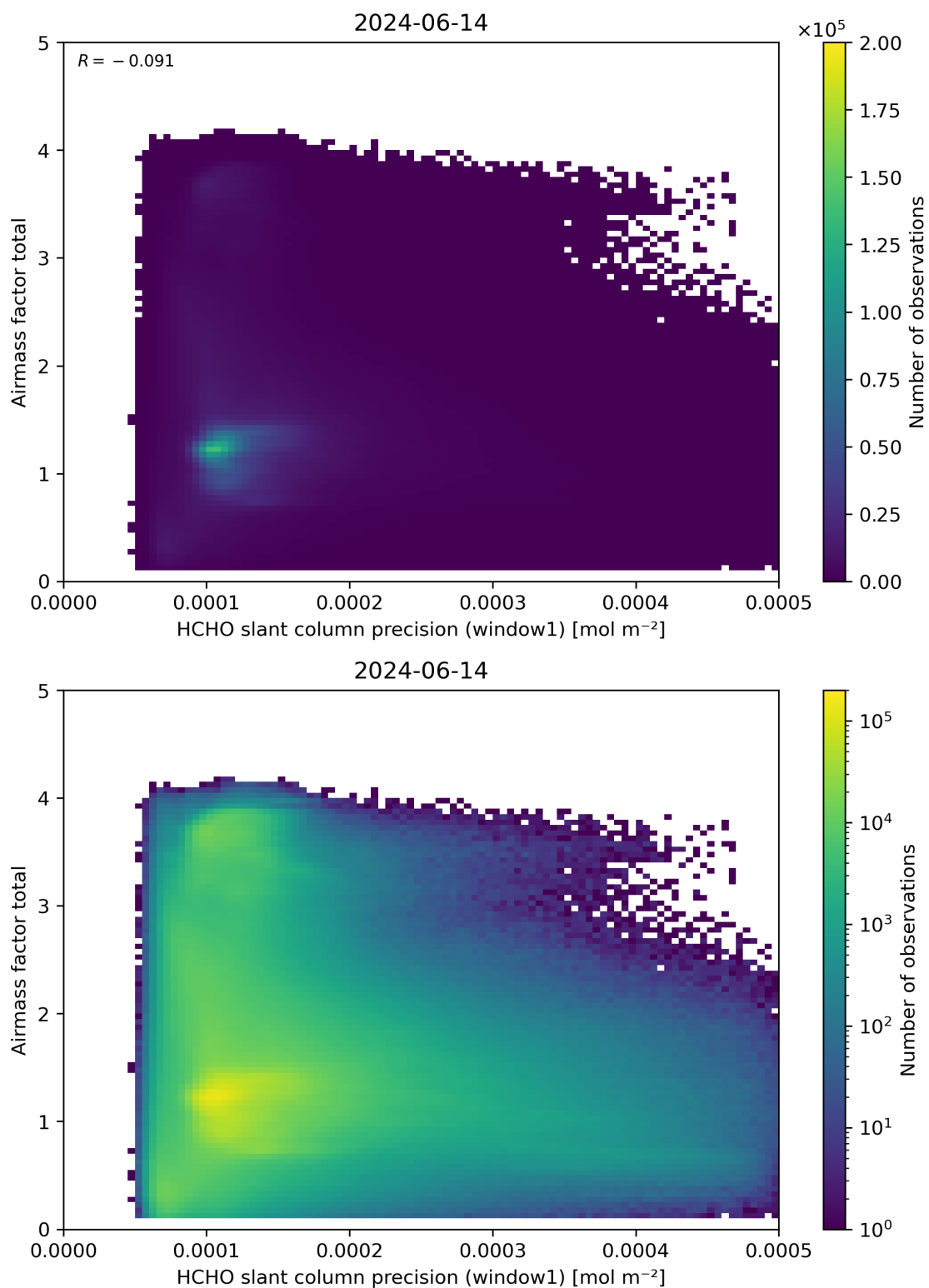
Figure 94: Scatter density plot of “HCHO slant column precision (window1)” against “Airmass factor total” for 2024-06-13 to 2024-06-15.
