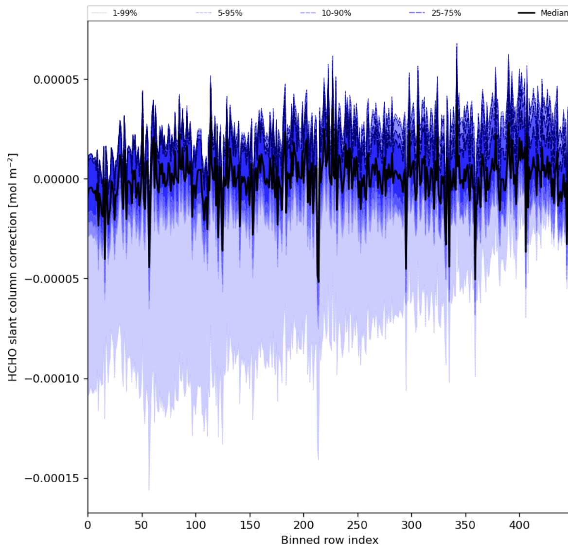
Figure 61: Along track statistics of “HCHO slant column correction” for 2024-06-13 to 2024-06-15
