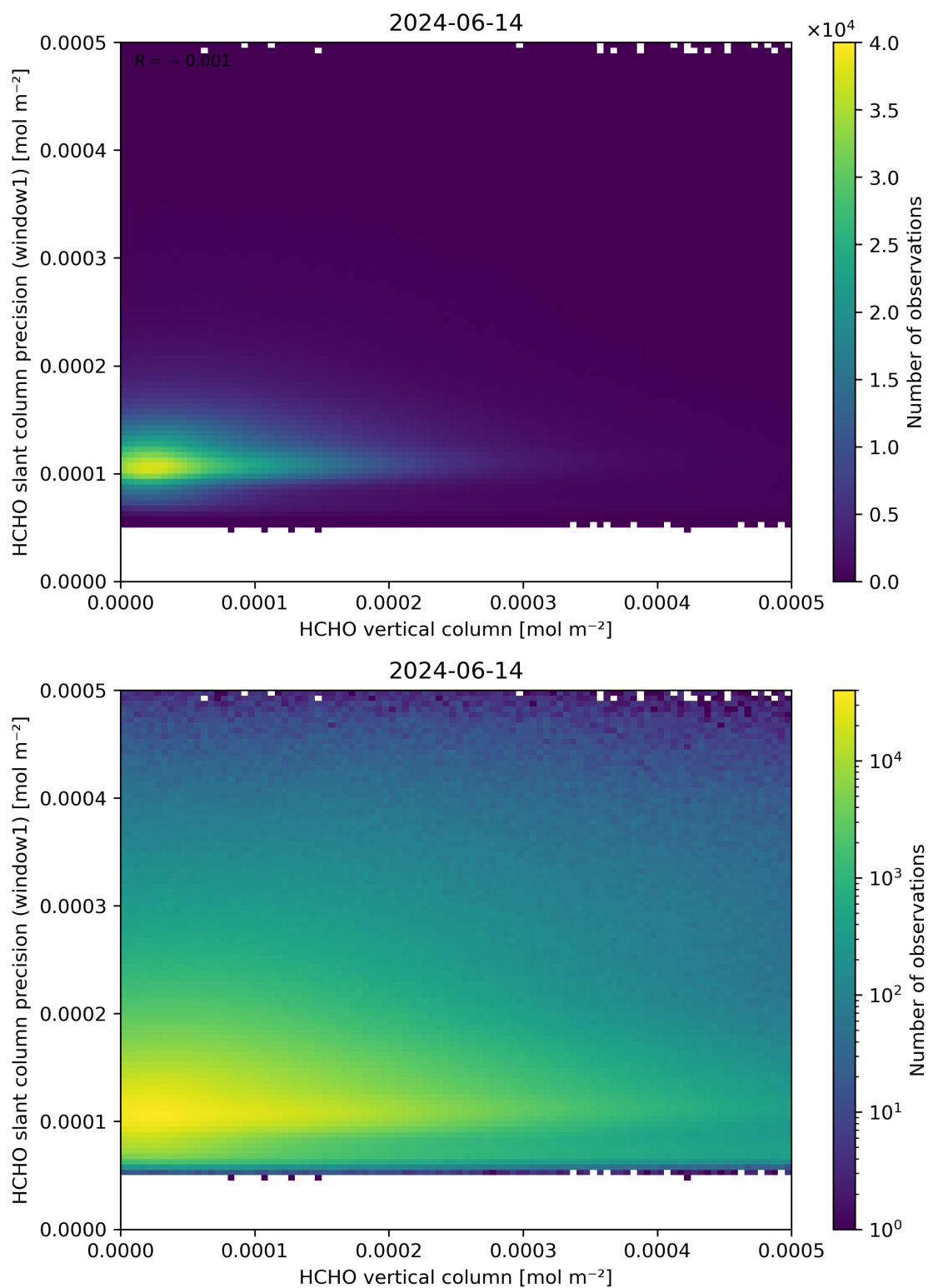
Figure 130: Scatter density plot of “HCHO vertical column” against “HCHO slant column precision (window1)” for 2024-06-13 to 2024-06-15.
