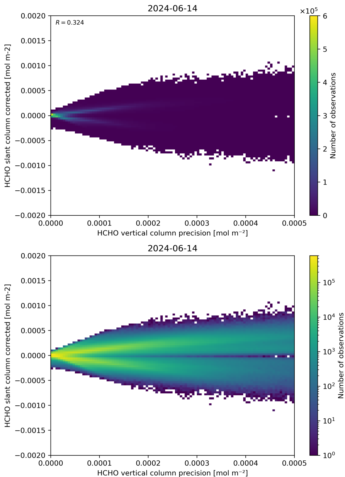
Figure 140: Scatter density plot of “HCHO vertical column precision” against “HCHO slant column corrected” for 2024-06-13 to 2024-06-15.
