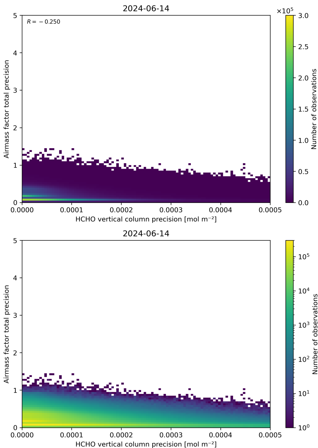
Figure 145: Scatter density plot of “HCHO vertical column precision” against “Airmass factor total precision” for 2024-06-13 to 2024-06-15.
