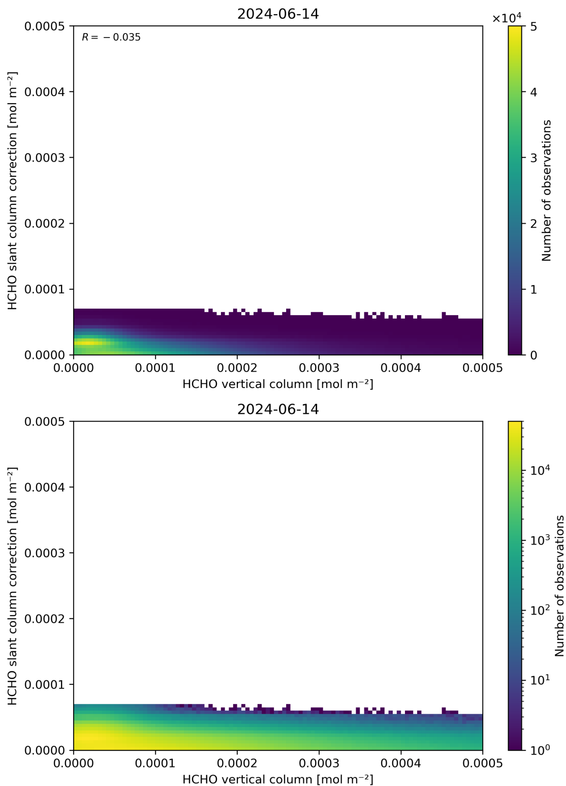
Figure 128: Scatter density plot of “HCHO vertical column” against “HCHO slant column correction” for 2024-06-13 to 2024-06-15.
