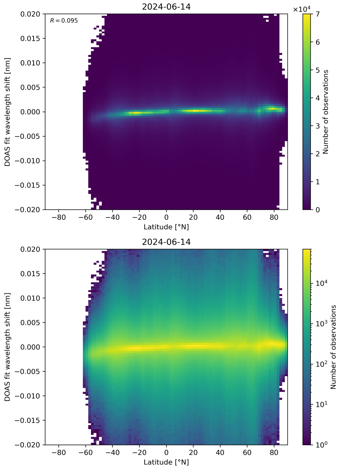
Figure 154: Scatter density plot of “Latitude” against “DOAS fit wavelength shift” for 2024-06-13 to 2024-06-15.
