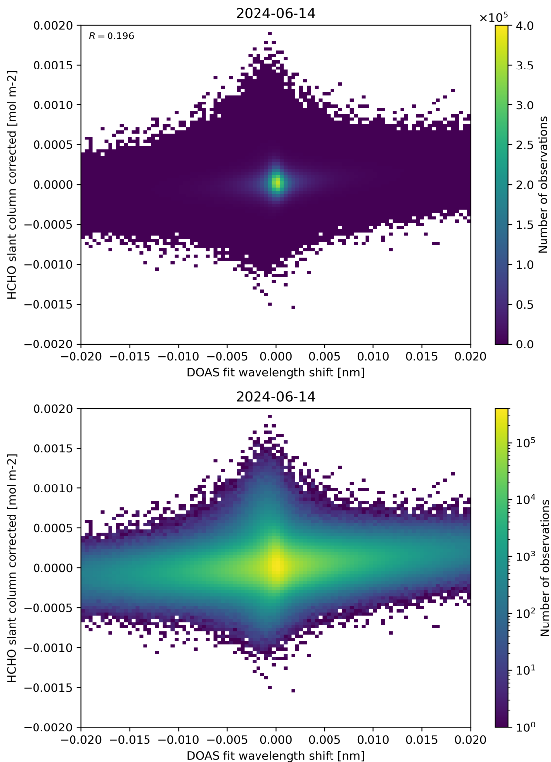
Figure 66: Scatter density plot of “DOAS fit wavelength shift” against “HCHO slant column corrected” for 2024-06-13 to 2024-06-15.
