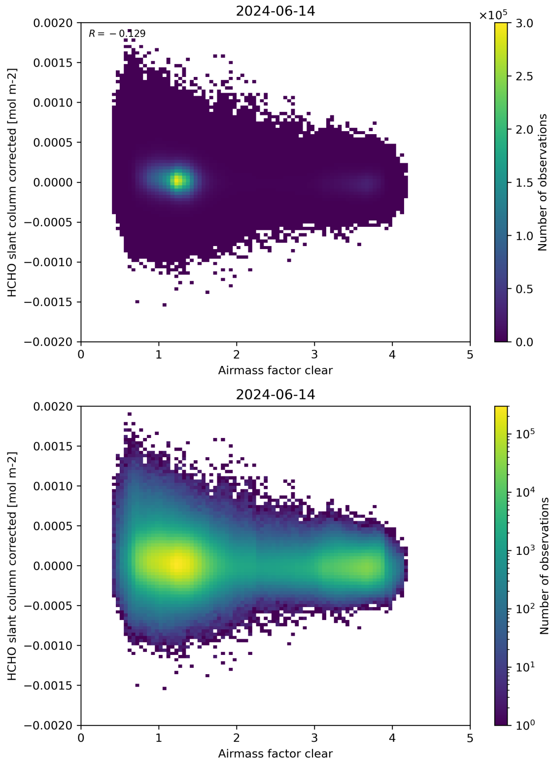
Figure 74: Scatter density plot of “Airmass factor clear” against “HCHO slant column corrected” for 2024-06-13 to 2024-06-15.
