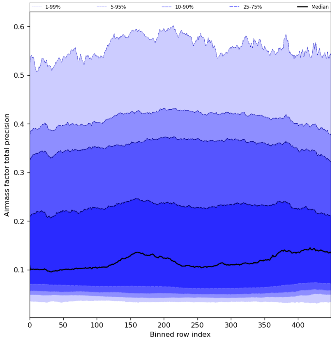
Figure 55: Along track statistics of “Airmass factor total precision” for 2024-06-13 to 2024-06-15
