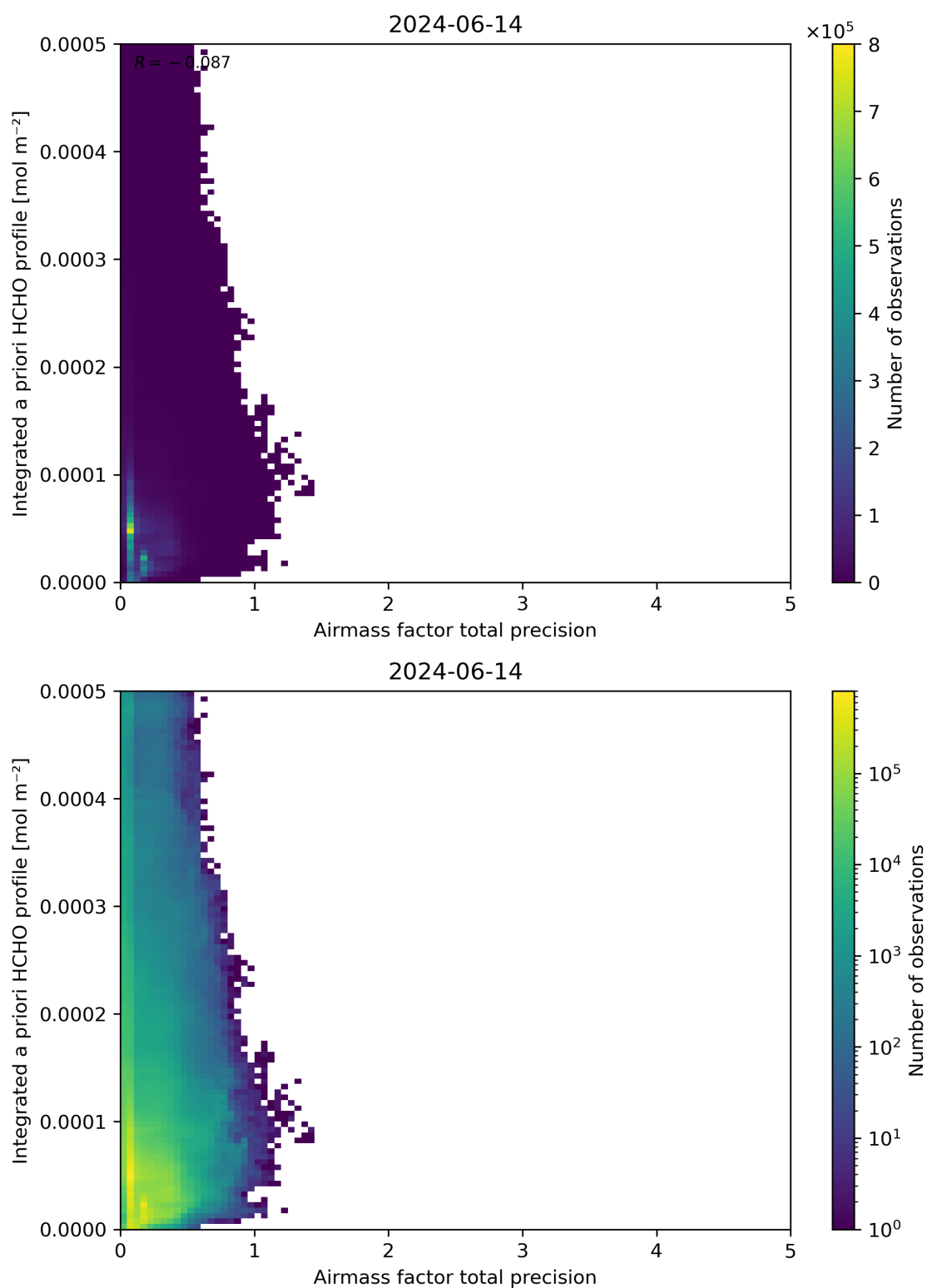
Figure 111: Scatter density plot of “Airmass factor total precision” against “Integrated a priori HCHO profile” for 2024-06-13 to 2024-06-15.
