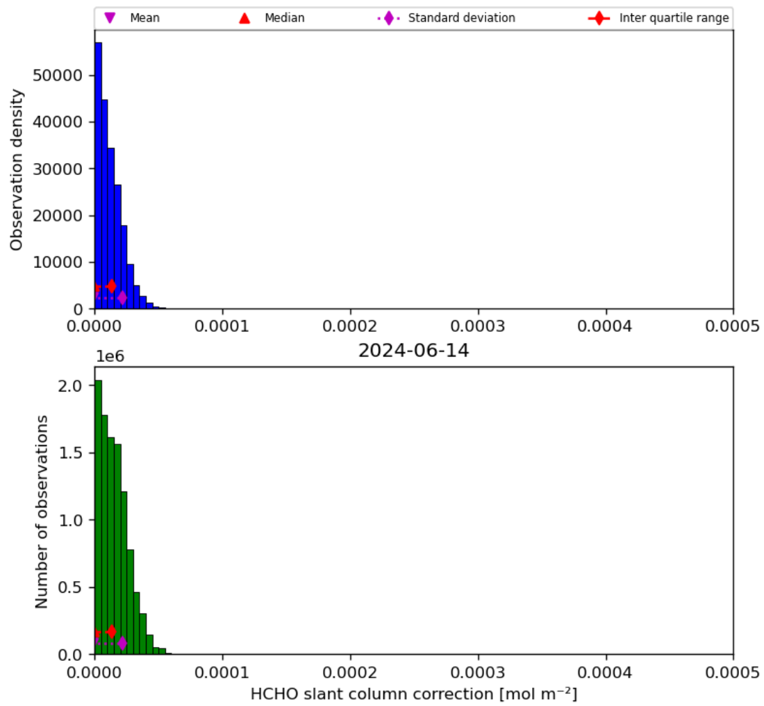
Figure 47: Histogram of “HCHO slant column correction” for 2024-06-13 to 2024-06-15
