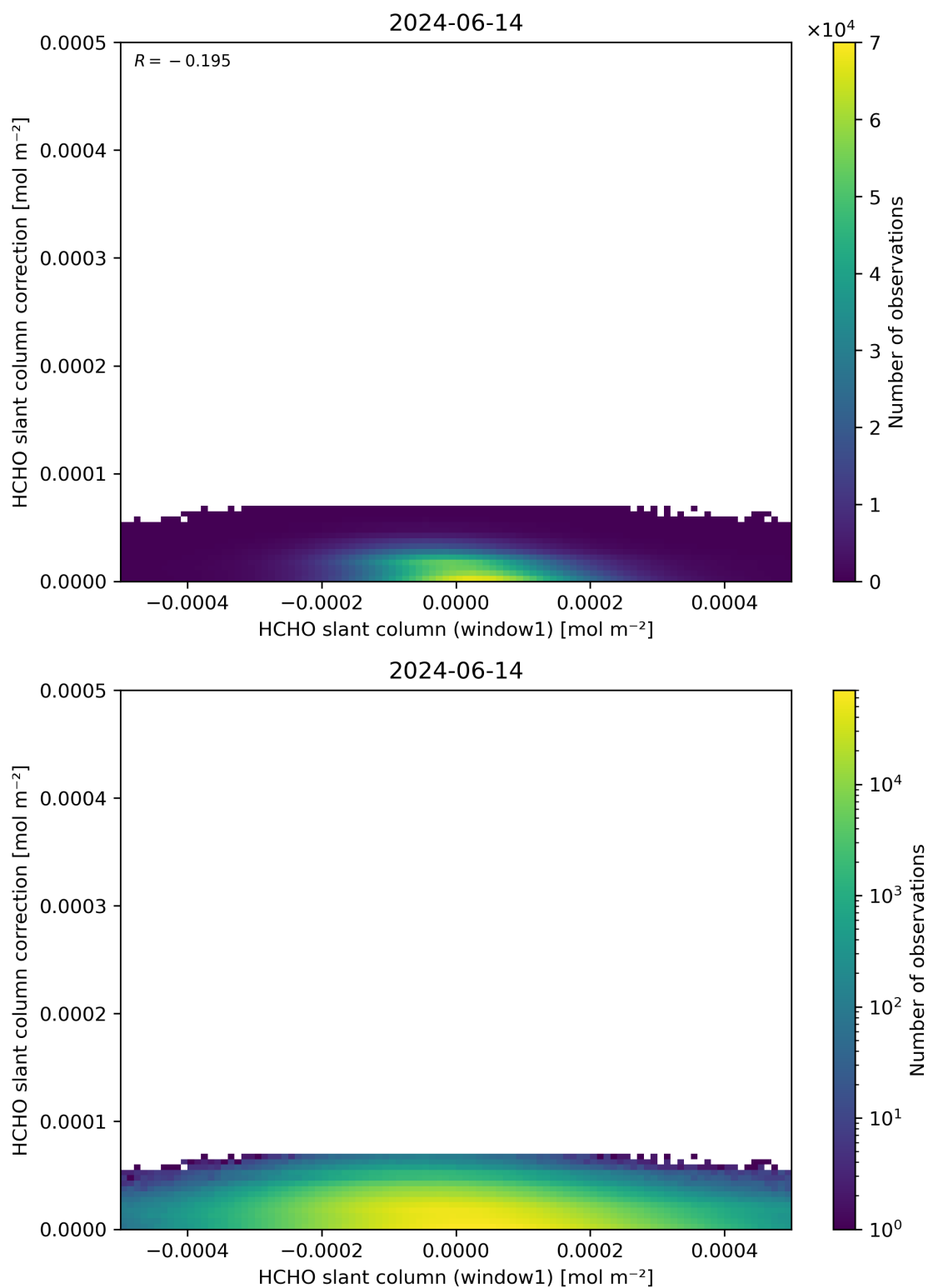
Figure 83: Scatter density plot of “HCHO slant column (window1)” against “HCHO slant column correction” for 2024-06-13 to 2024-06-15.
