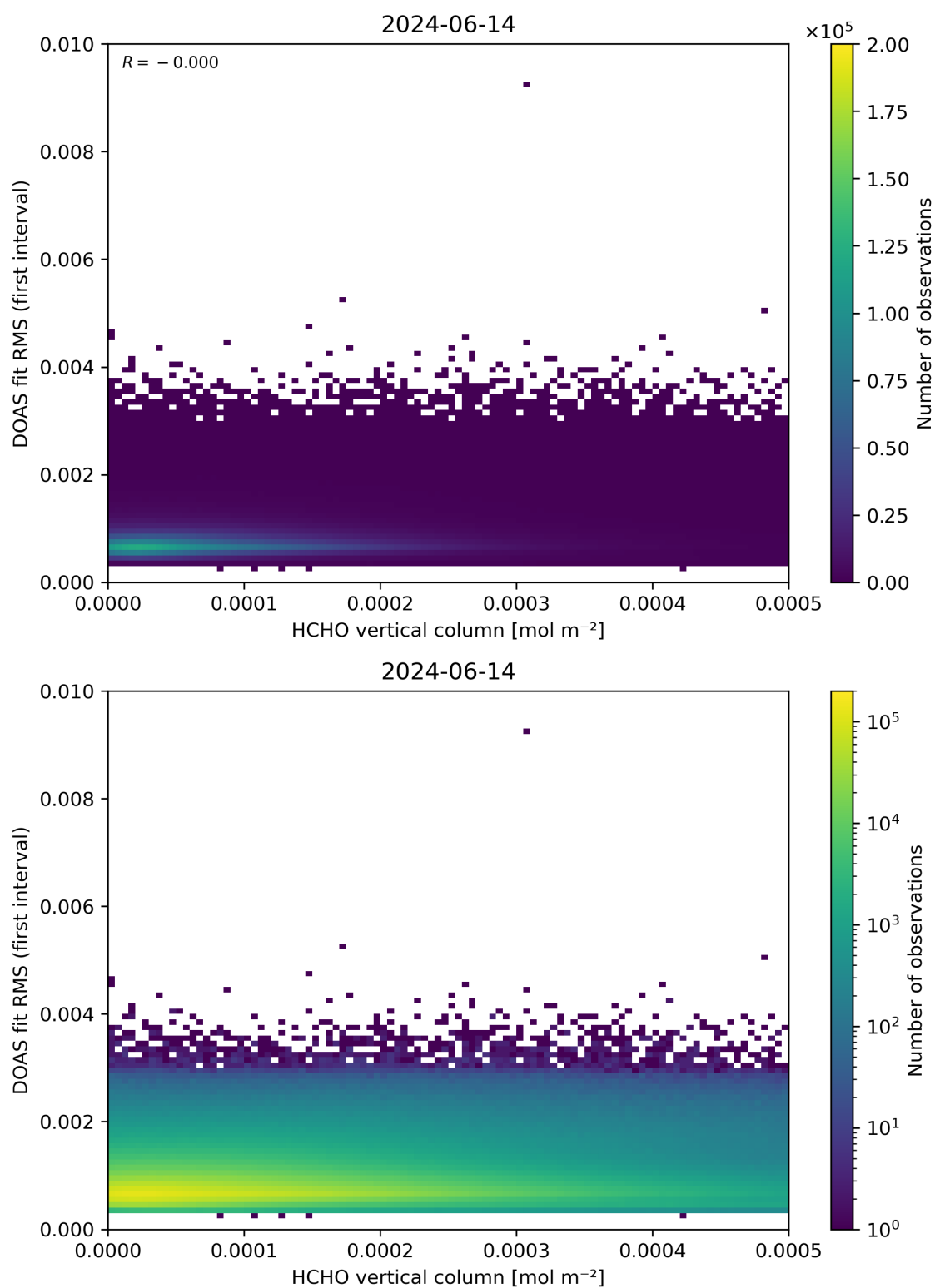
Figure 123: Scatter density plot of “HCHO vertical column” against “DOAS fit RMS (first interval)” for 2024-06-13 to 2024-06-15.
