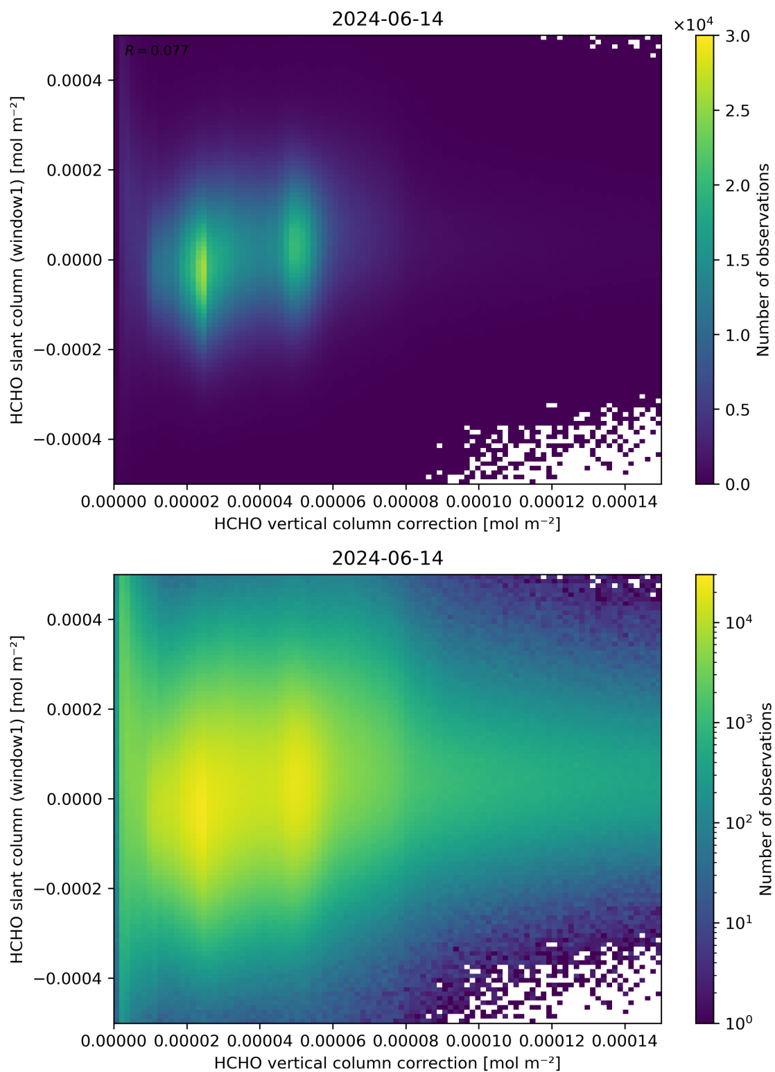
Figure 118: Scatter density plot of “HCHO vertical column correction” against “HCHO slant column (window1)” for 2024-06-13 to 2024-06-15.
