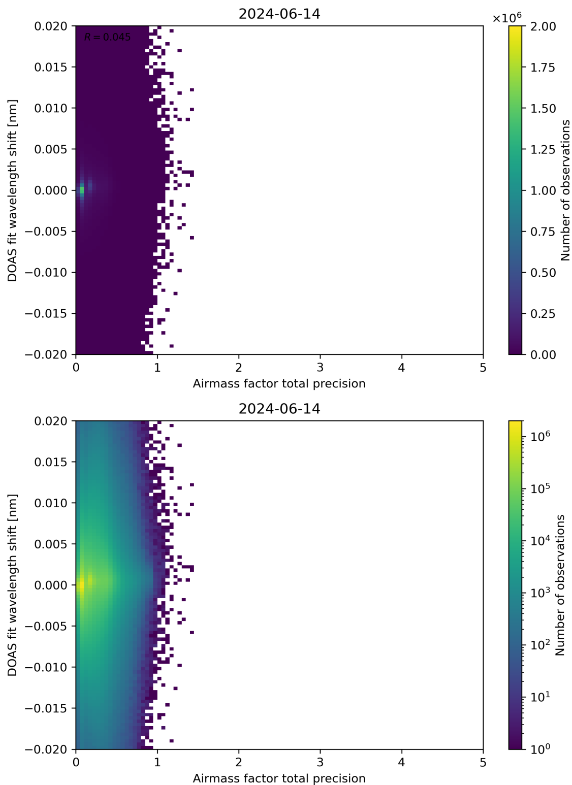
Figure 106: Scatter density plot of “Airmass factor total precision” against “DOAS fit wavelength shift” for 2024-06-13 to 2024-06-15.
