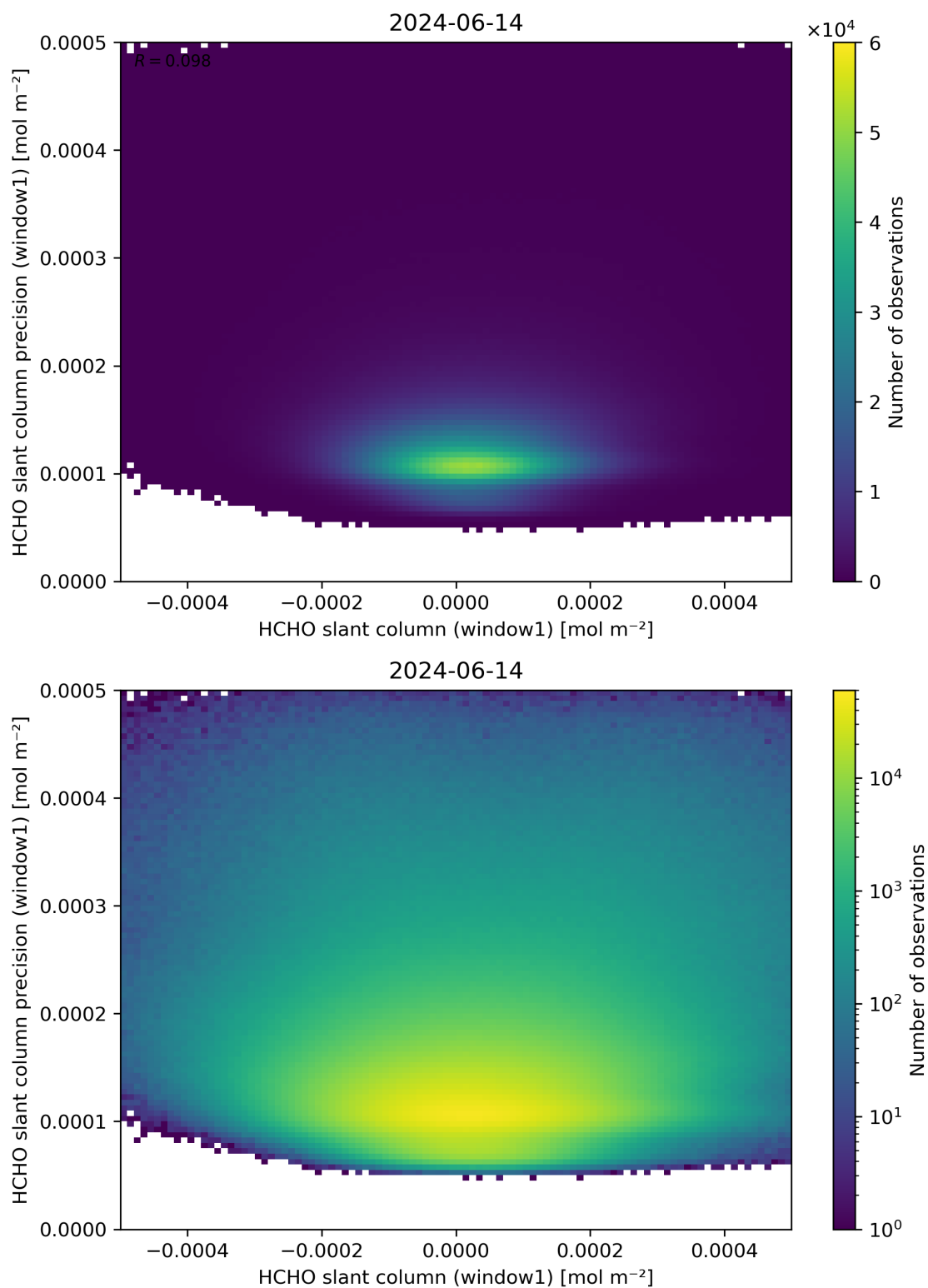
Figure 84: Scatter density plot of “HCHO slant column (window1)” against “HCHO slant column precision (window1)” for 2024-06-13 to 2024-06-15.
