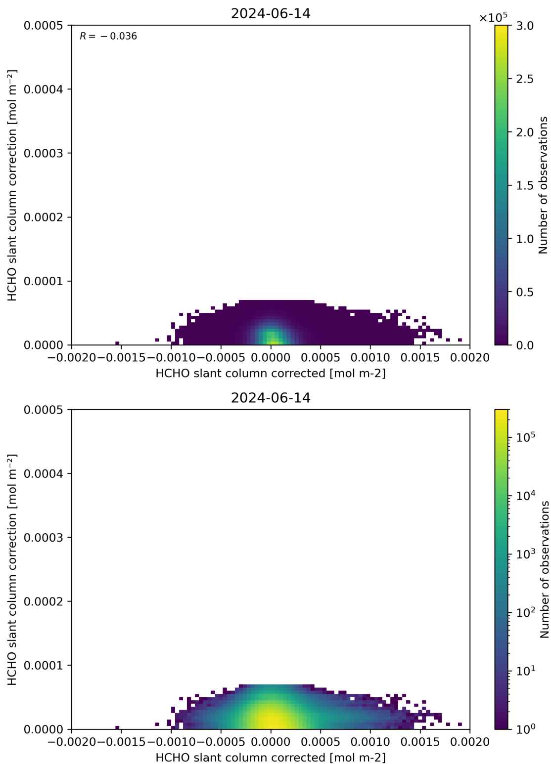
Figure 77: Scatter density plot of “HCHO slant column corrected” against “HCHO slant column correction” for 2024-06-13 to 2024-06-15.
