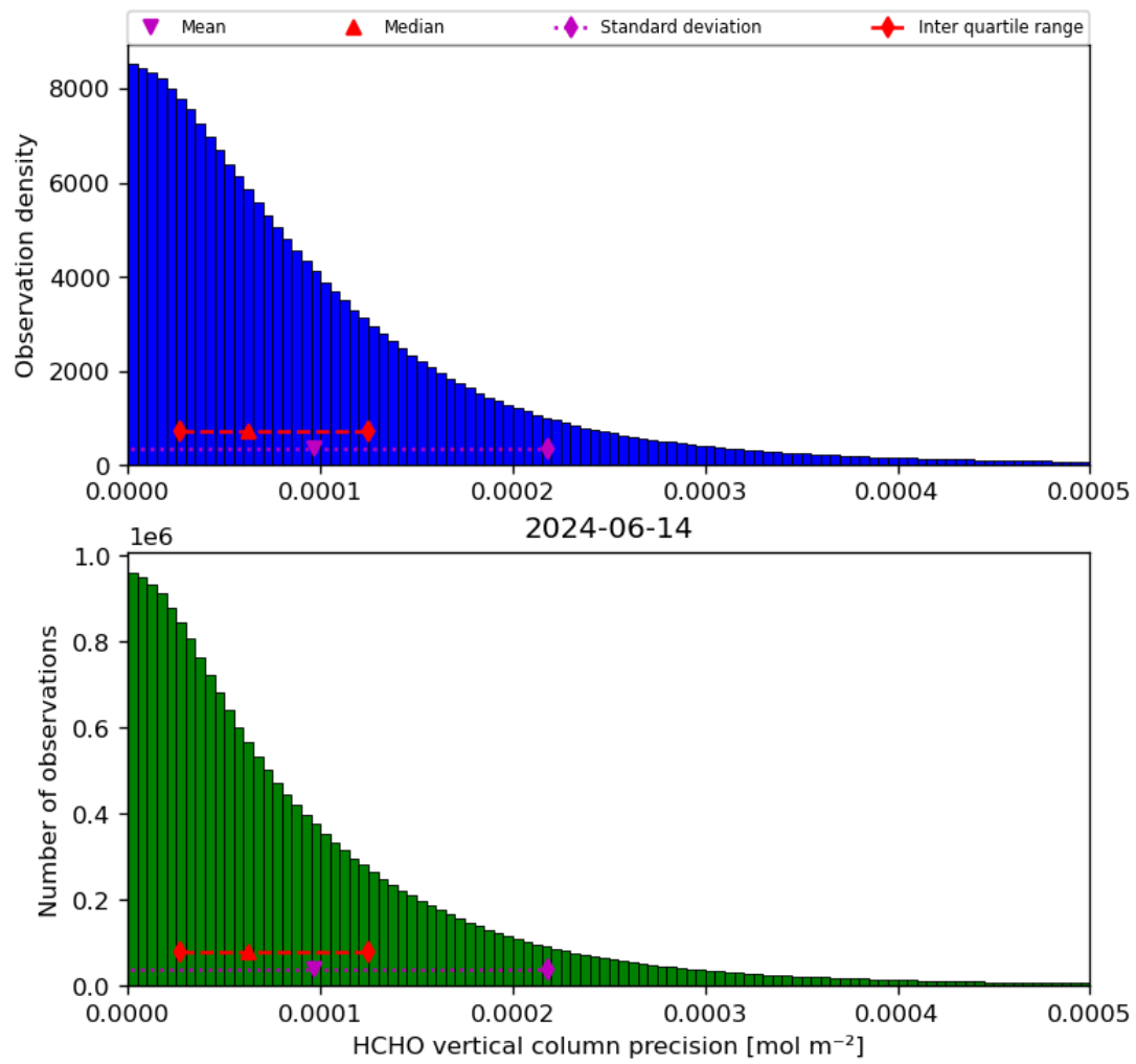
Figure 36: Histogram of “HCHO vertical column precision” for 2024-06-13 to 2024-06-15
