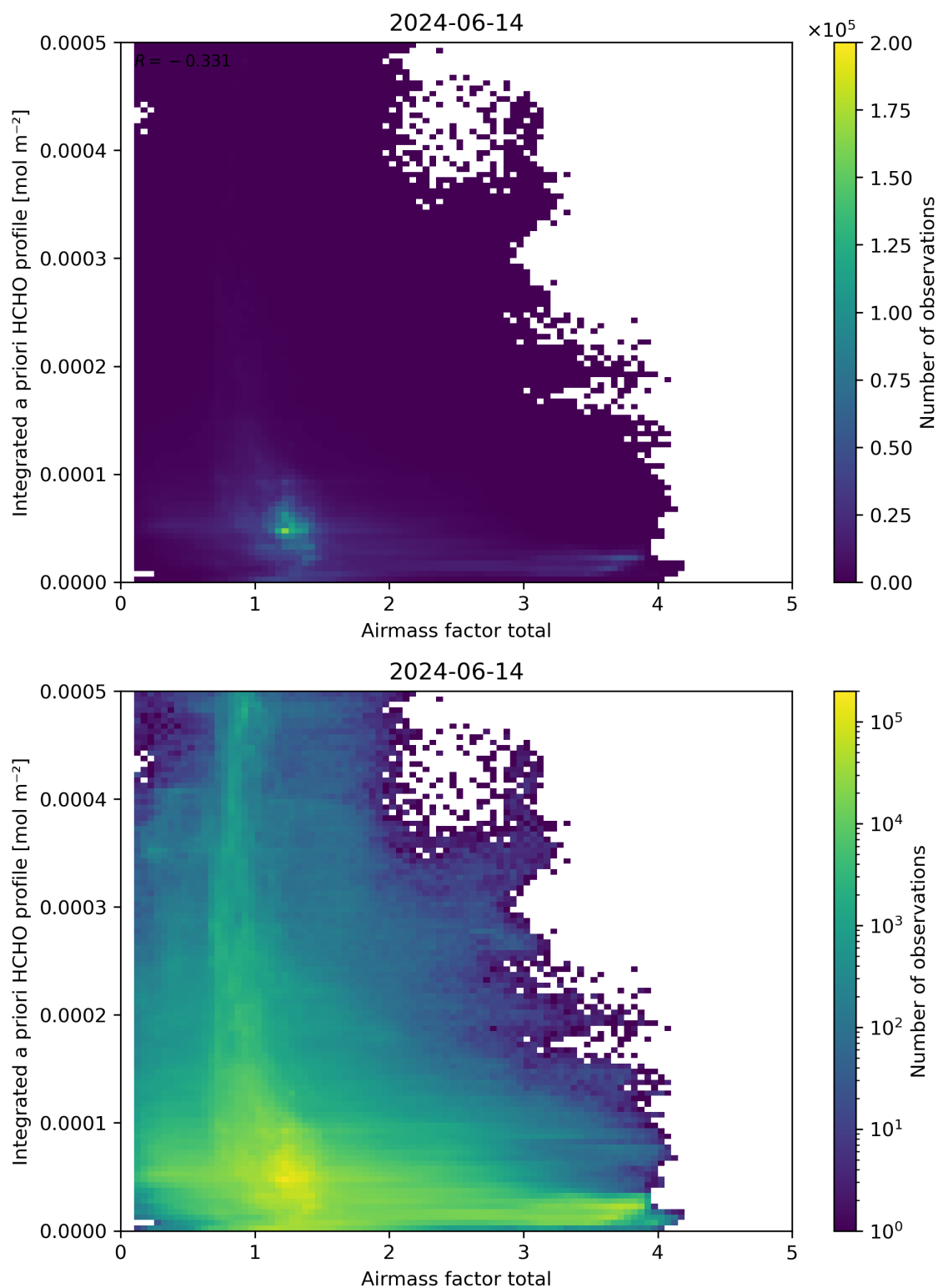
Figure 104: Scatter density plot of “Airmass factor total” against “Integrated a priori HCHO profile” for 2024-06-13 to 2024-06-15.
