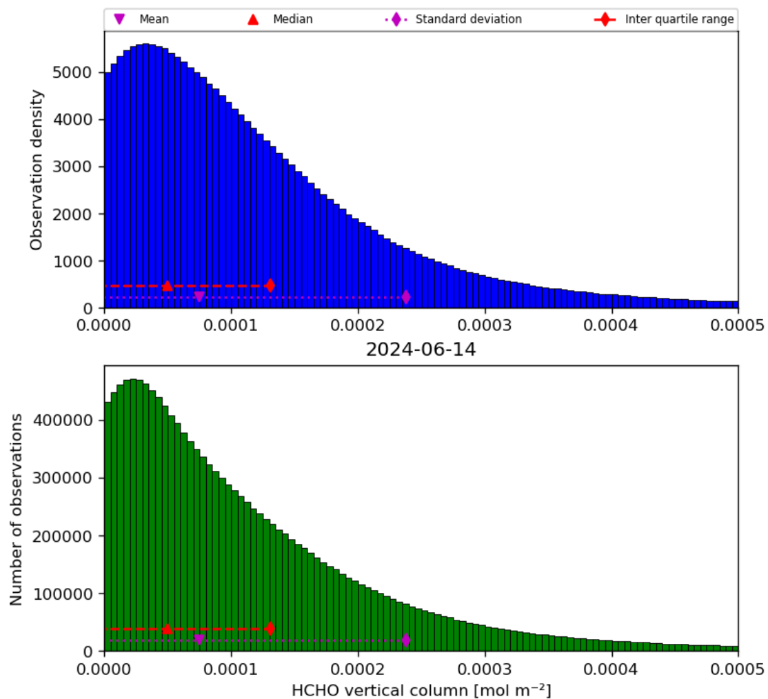
Figure 35: Histogram of “HCHO vertical column” for 2024-06-13 to 2024-06-15
