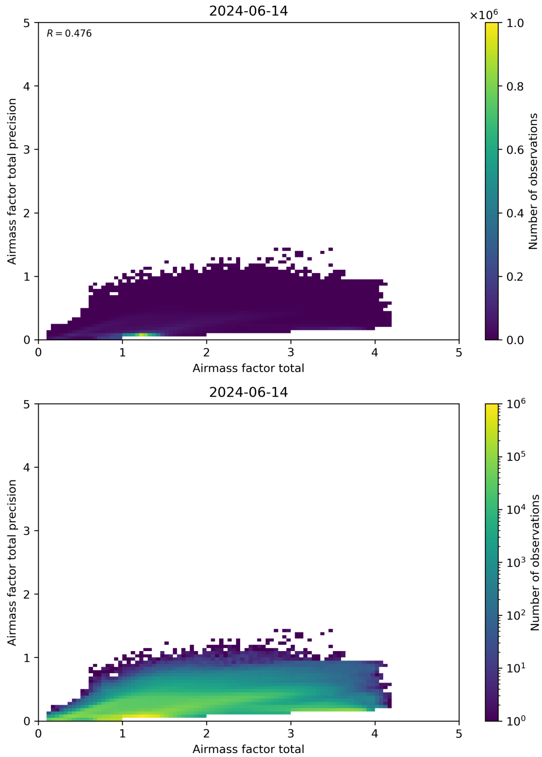
Figure 103: Scatter density plot of “Airmass factor total” against “Airmass factor total precision” for 2024-06-13 to 2024-06-15.
