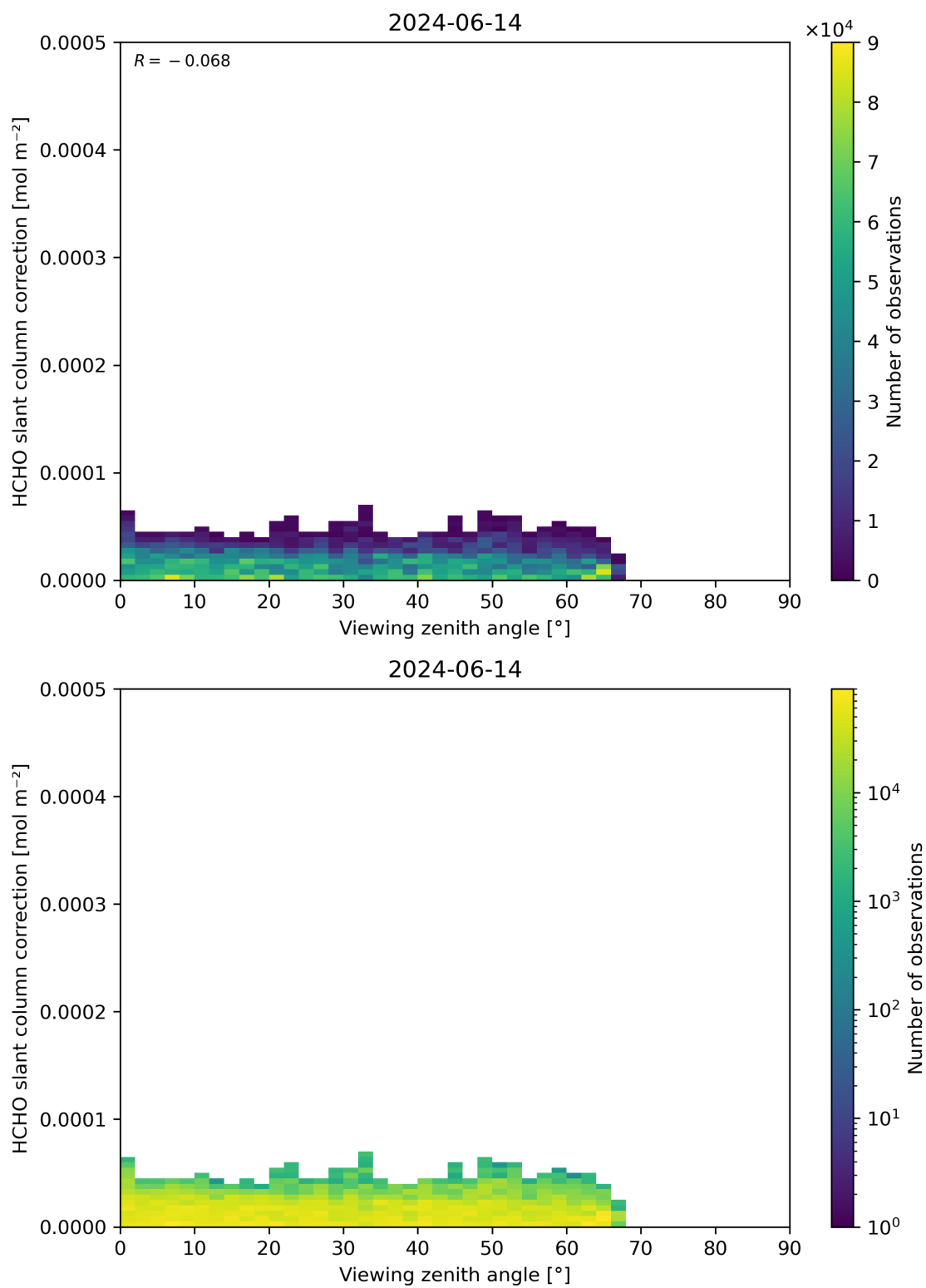
Figure 187: Scatter density plot of “Viewing zenith angle” against “HCHO slant column correction” for 2024-06-13 to 2024-06-15.
