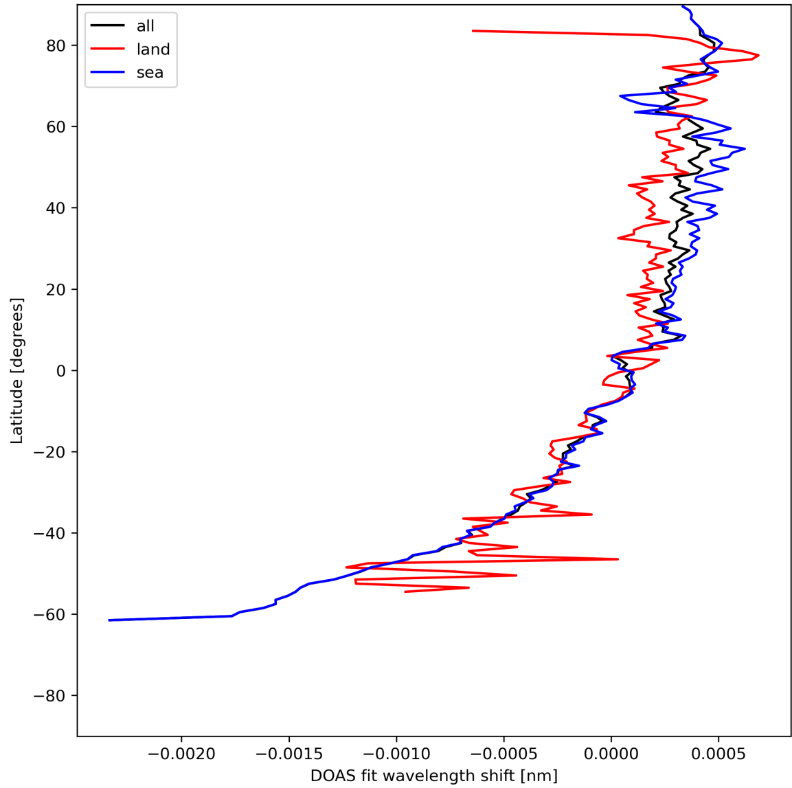
Figure 30: Zonal average of “DOAS fit wavelength shift” for 2024-06-13 to 2024-06-15.
