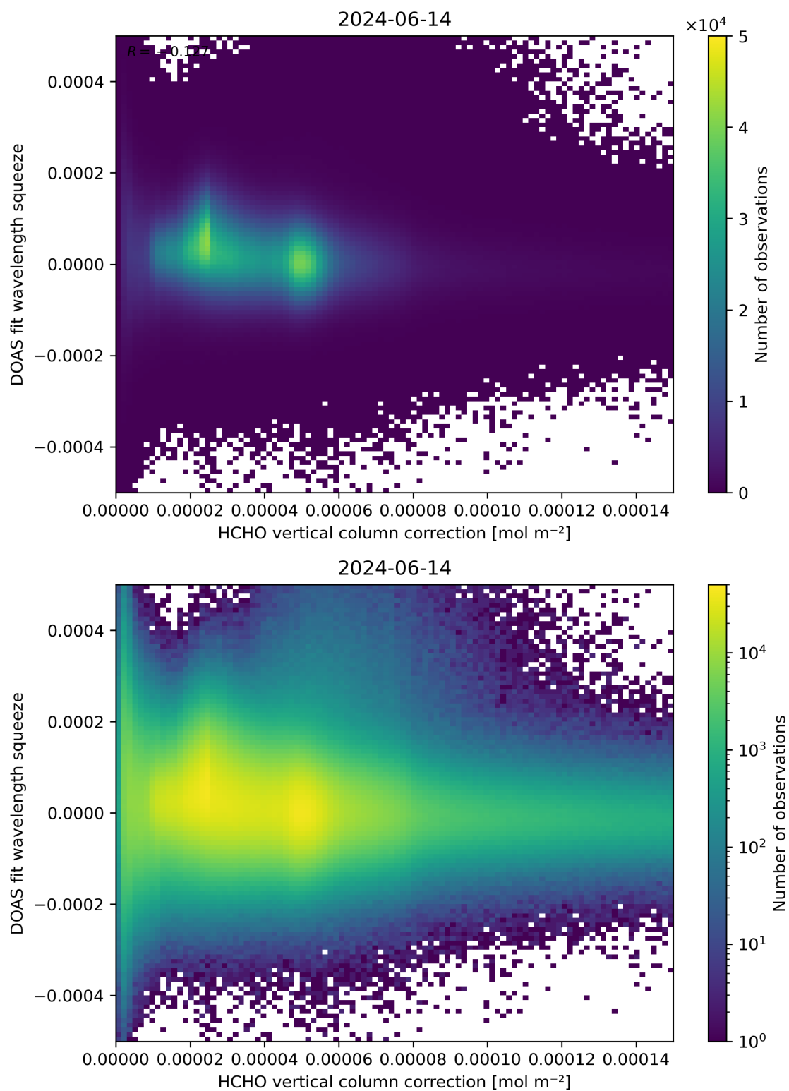
Figure 114: Scatter density plot of “HCHO vertical column correction” against “DOAS fit wavelength squeeze” for 2024-06-13 to 2024-06-15.
