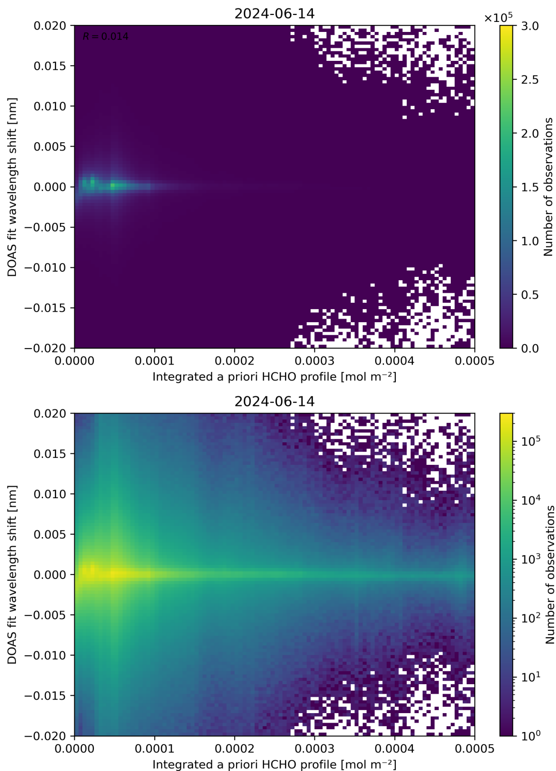
Figure 149: Scatter density plot of “Integrated a priori HCHO profile” against “DOAS fit wavelength shift” for 2024-06-13 to 2024-06-15.
