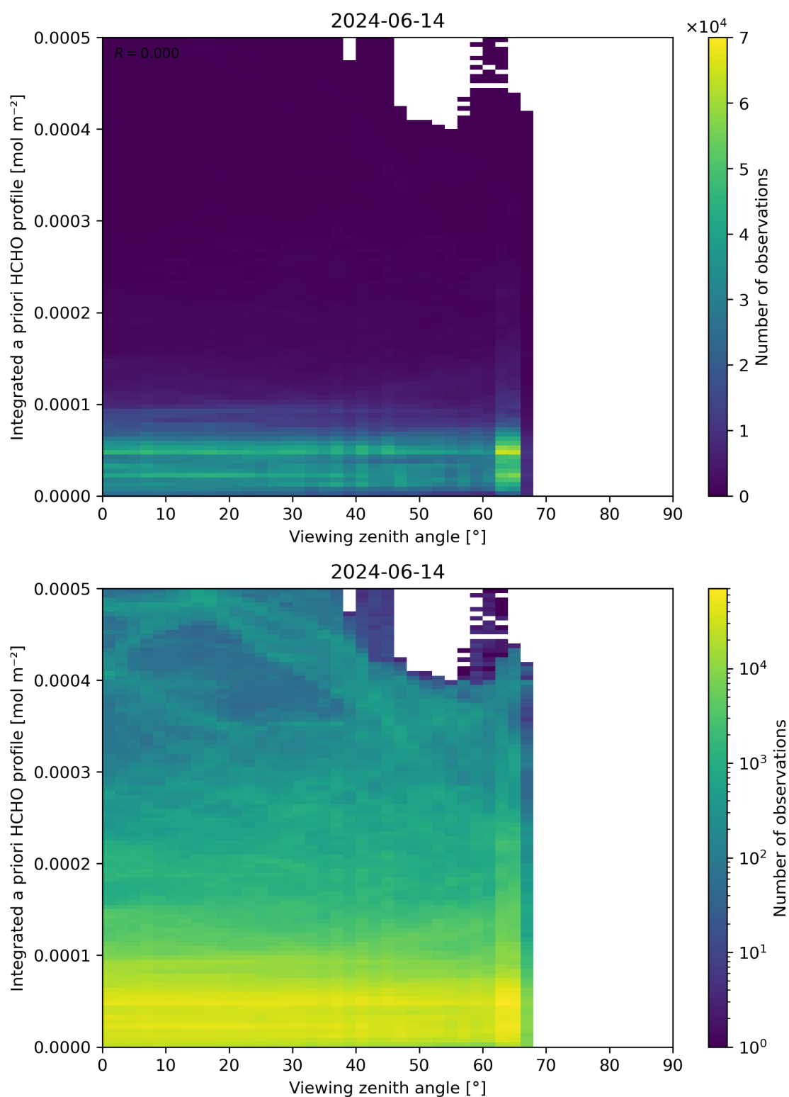
Figure 195: Scatter density plot of “Viewing zenith angle” against “Integrated a priori HCHO profile” for 2024-06-13 to 2024-06-15.
