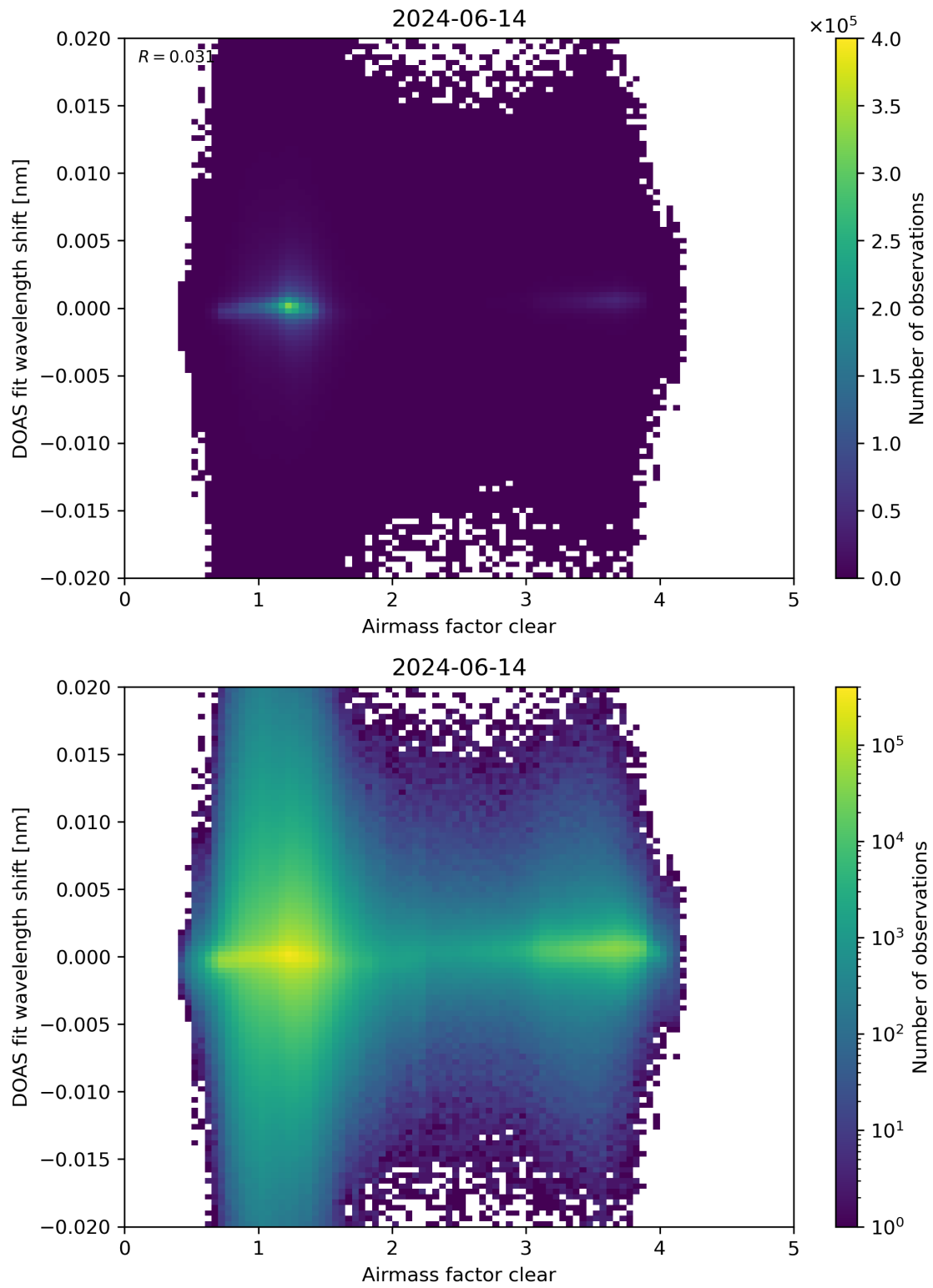
Figure 72: Scatter density plot of “Airmass factor clear” against “DOAS fit wavelength shift” for 2024-06-13 to 2024-06-15.
