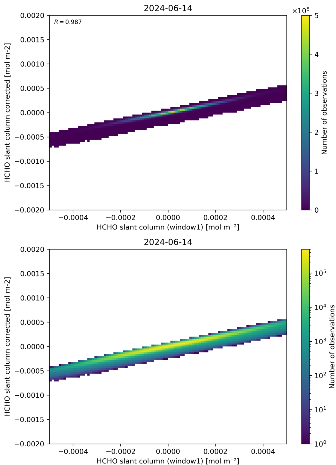
Figure 82: Scatter density plot of “HCHO slant column (window1)” against “HCHO slant column corrected” for 2024-06-13 to 2024-06-15.
