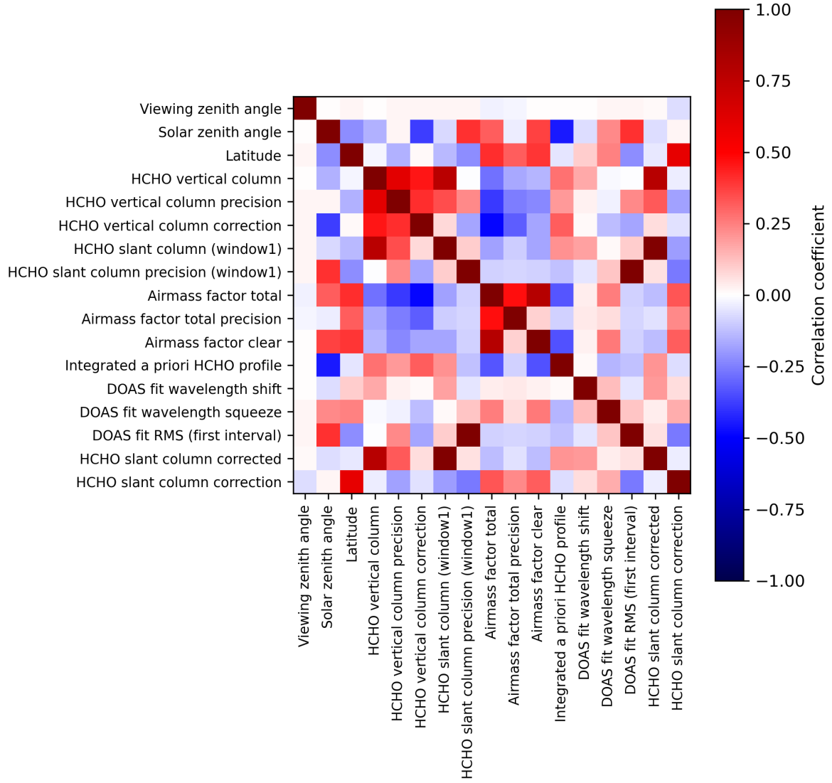
Figure 2: Map of correlation matrix for 2024-06-13 to 2024-06-15.
