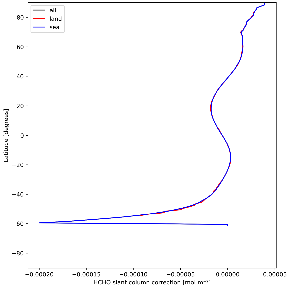
Figure 33: Zonal average of “HCHO slant column correction” for 2024-06-13 to 2024-06-15.
