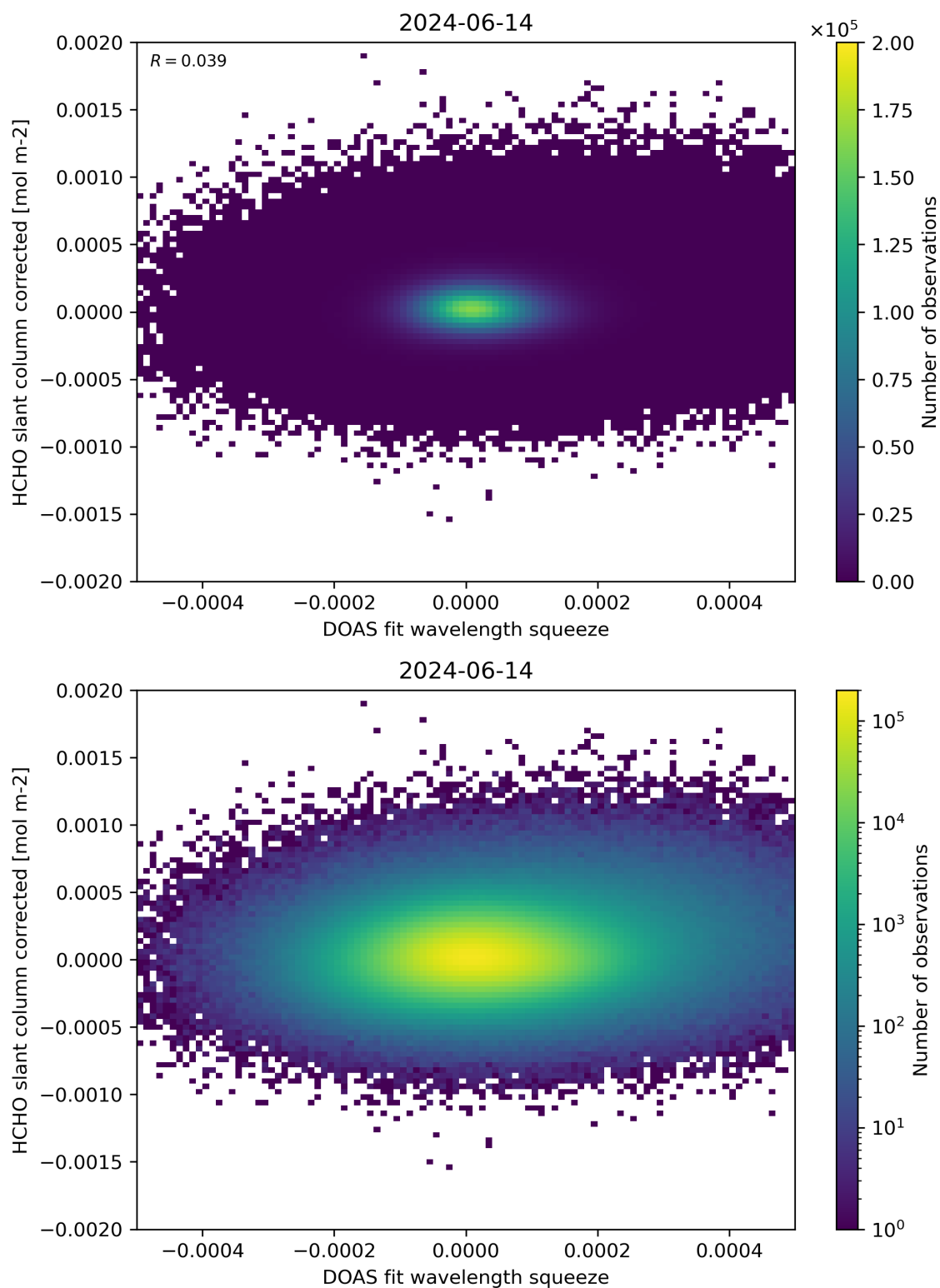
Figure 69: Scatter density plot of “DOAS fit wavelength squeeze” against “HCHO slant column corrected” for 2024-06-13 to 2024-06-15.
