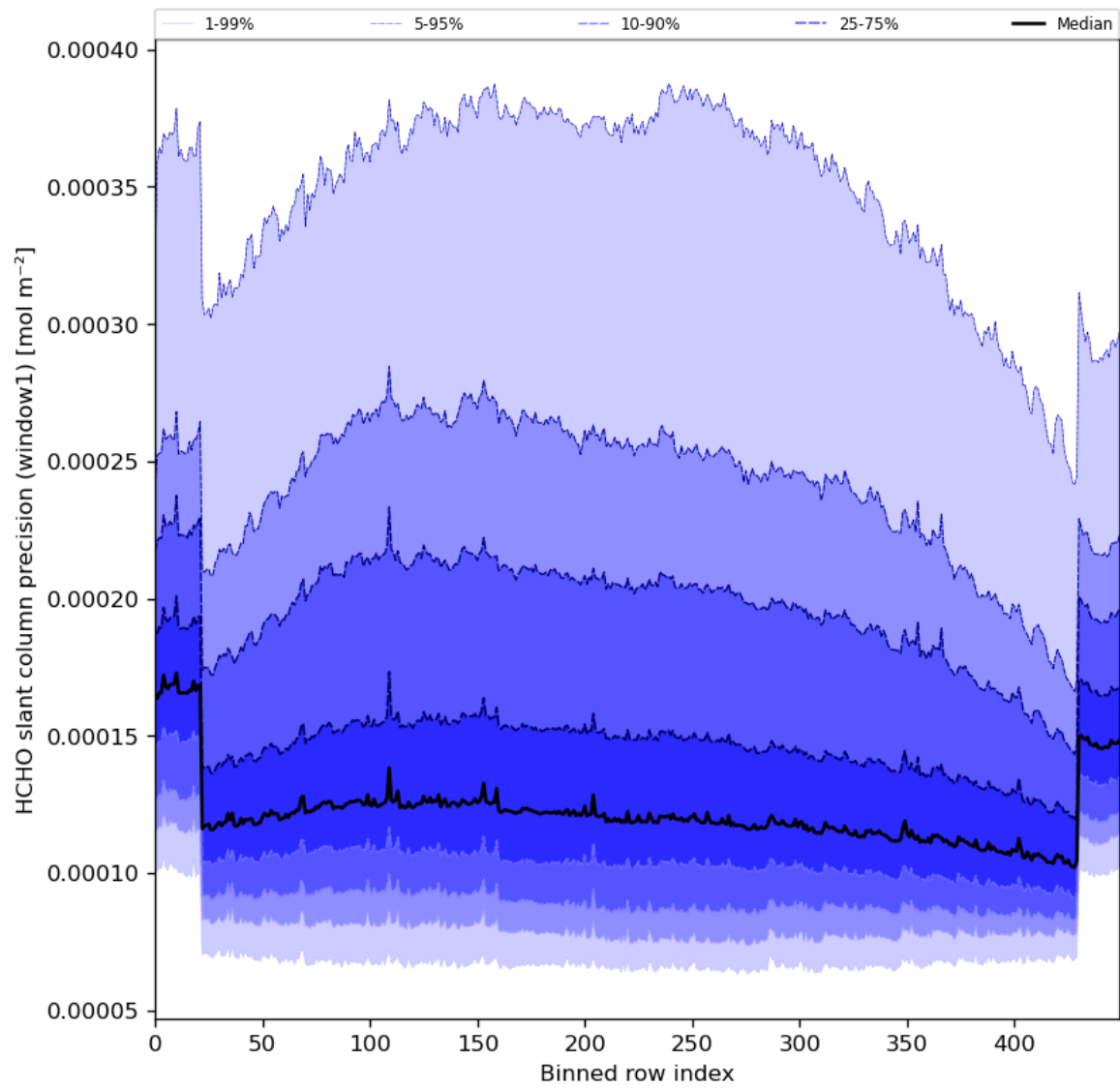
Figure 53: Along track statistics of “HCHO slant column precision (window1)” for 2024-06-13 to 2024-06-15
