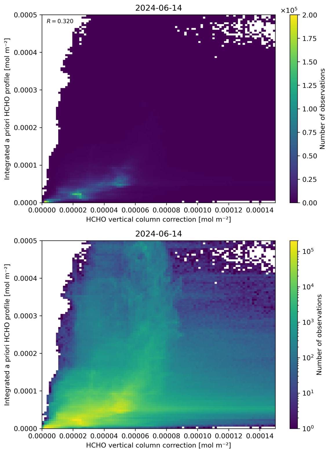
Figure 122: Scatter density plot of “HCHO vertical column correction” against “Integrated a priori HCHO profile” for 2024-06-13 to 2024-06-15.
