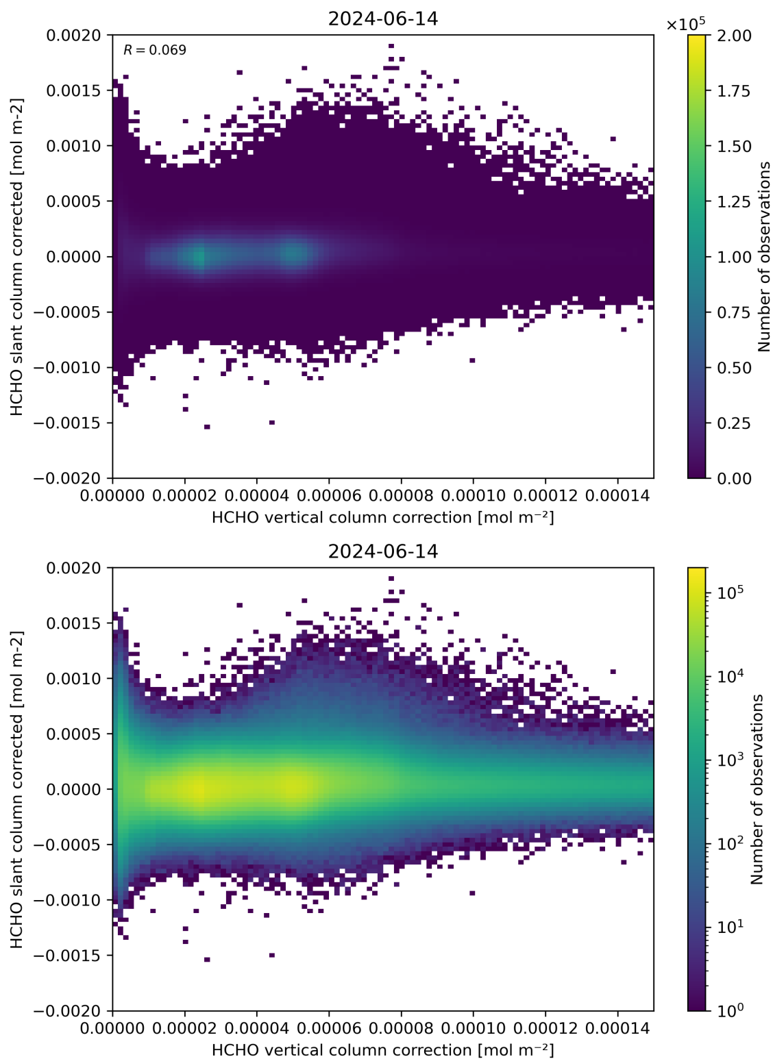
Figure 116: Scatter density plot of “HCHO vertical column correction” against “HCHO slant column corrected” for 2024-06-13 to 2024-06-15.
