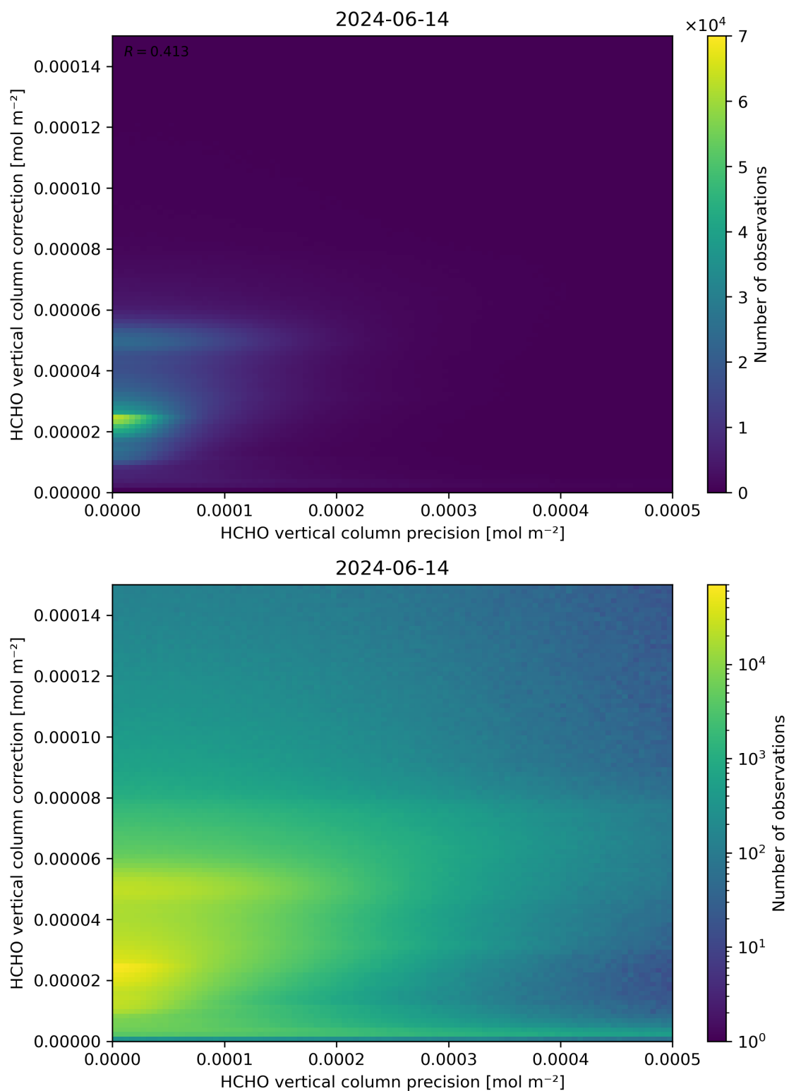
Figure 146: Scatter density plot of “HCHO vertical column precision” against “HCHO vertical column correction” for 2024-06-13 to 2024-06-15.
