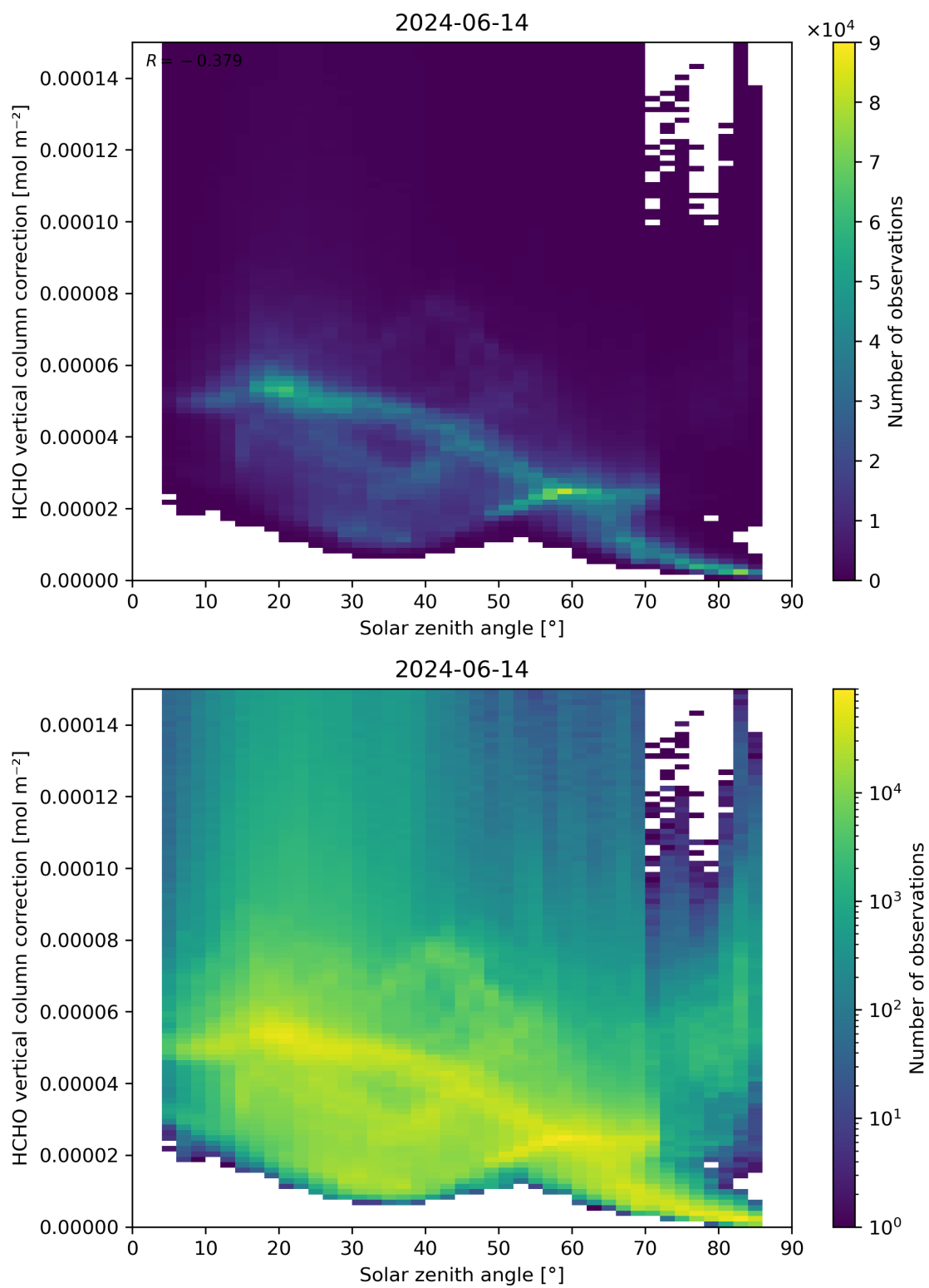
Figure 178: Scatter density plot of “Solar zenith angle” against “HCHO vertical column correction” for 2024-06-13 to 2024-06-15.
