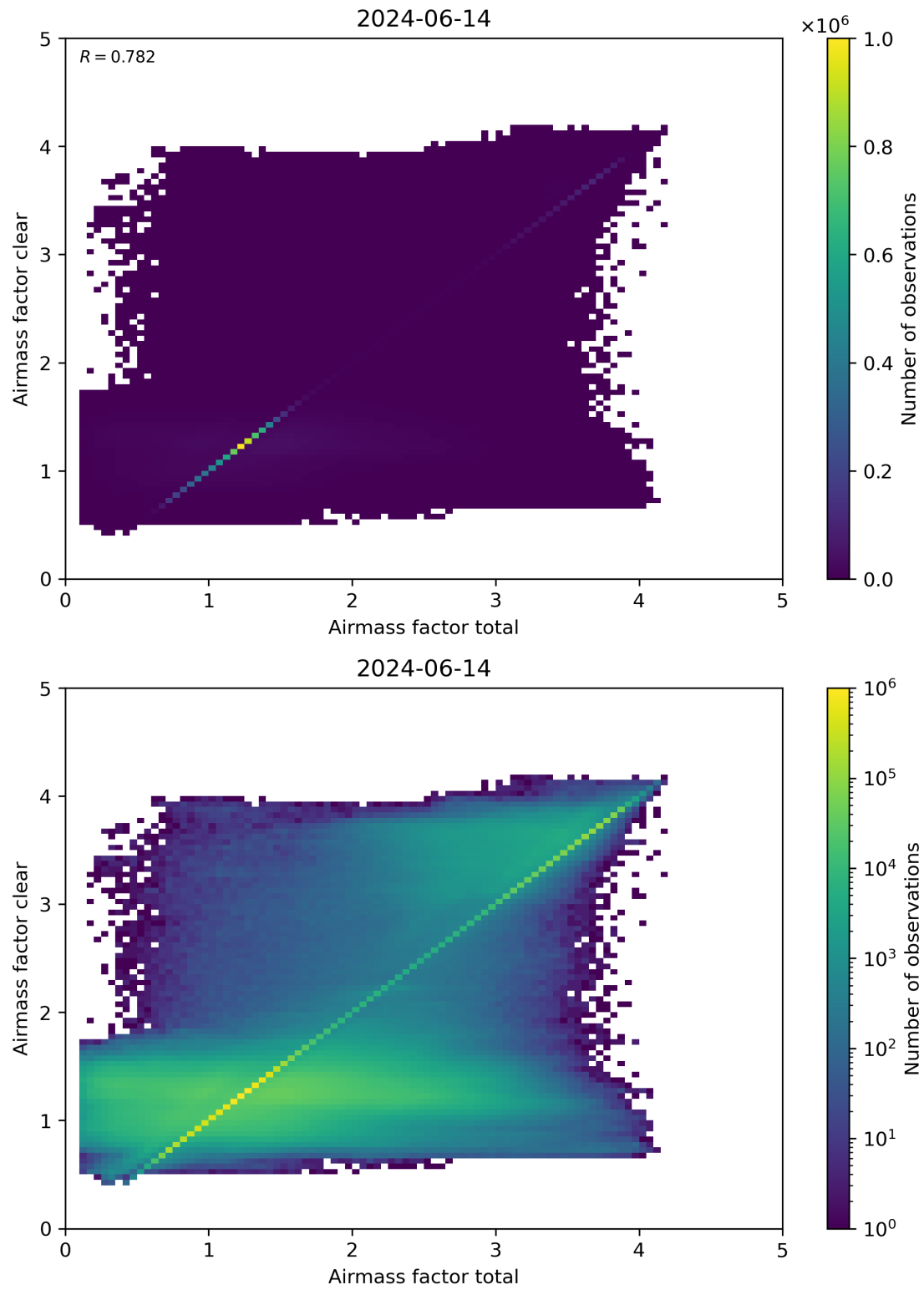
Figure 100: Scatter density plot of “Airmass factor total” against “Airmass factor clear” for 2024-06-13 to 2024-06-15.
