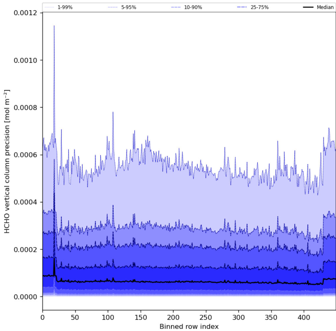
Figure 50: Along track statistics of “HCHO vertical column precision” for 2024-06-13 to 2024-06-15
