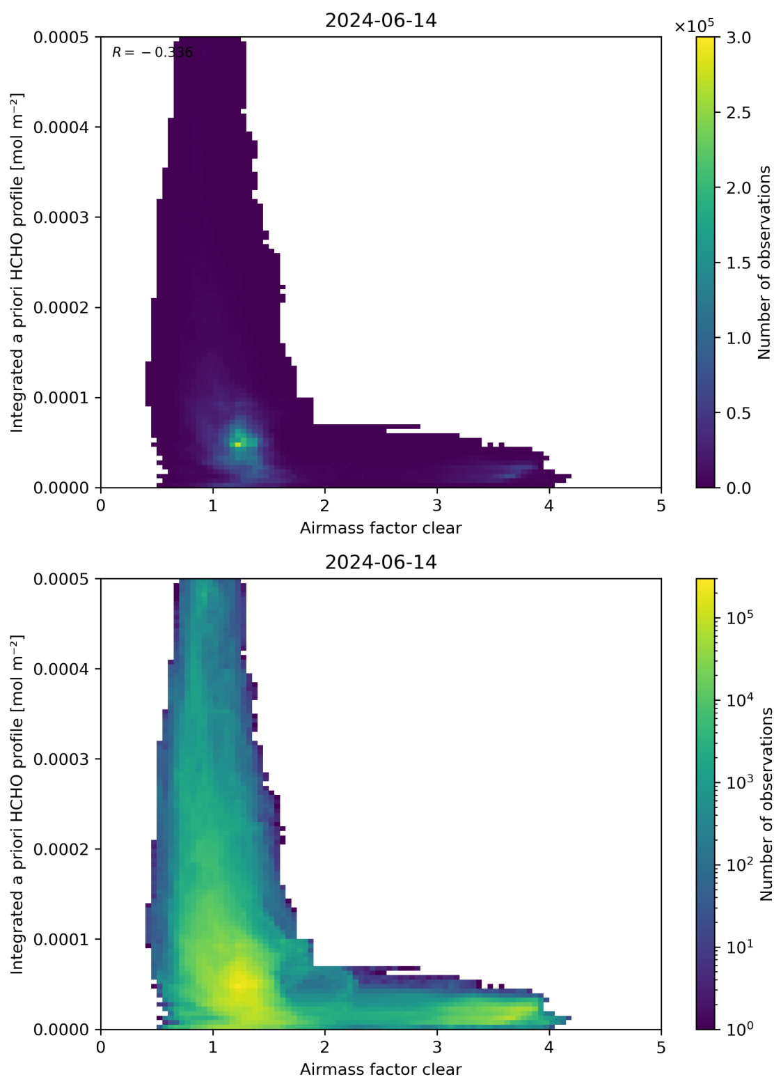
Figure 76: Scatter density plot of “Airmass factor clear” against “Integrated a priori HCHO profile” for 2024-06-13 to 2024-06-15.
