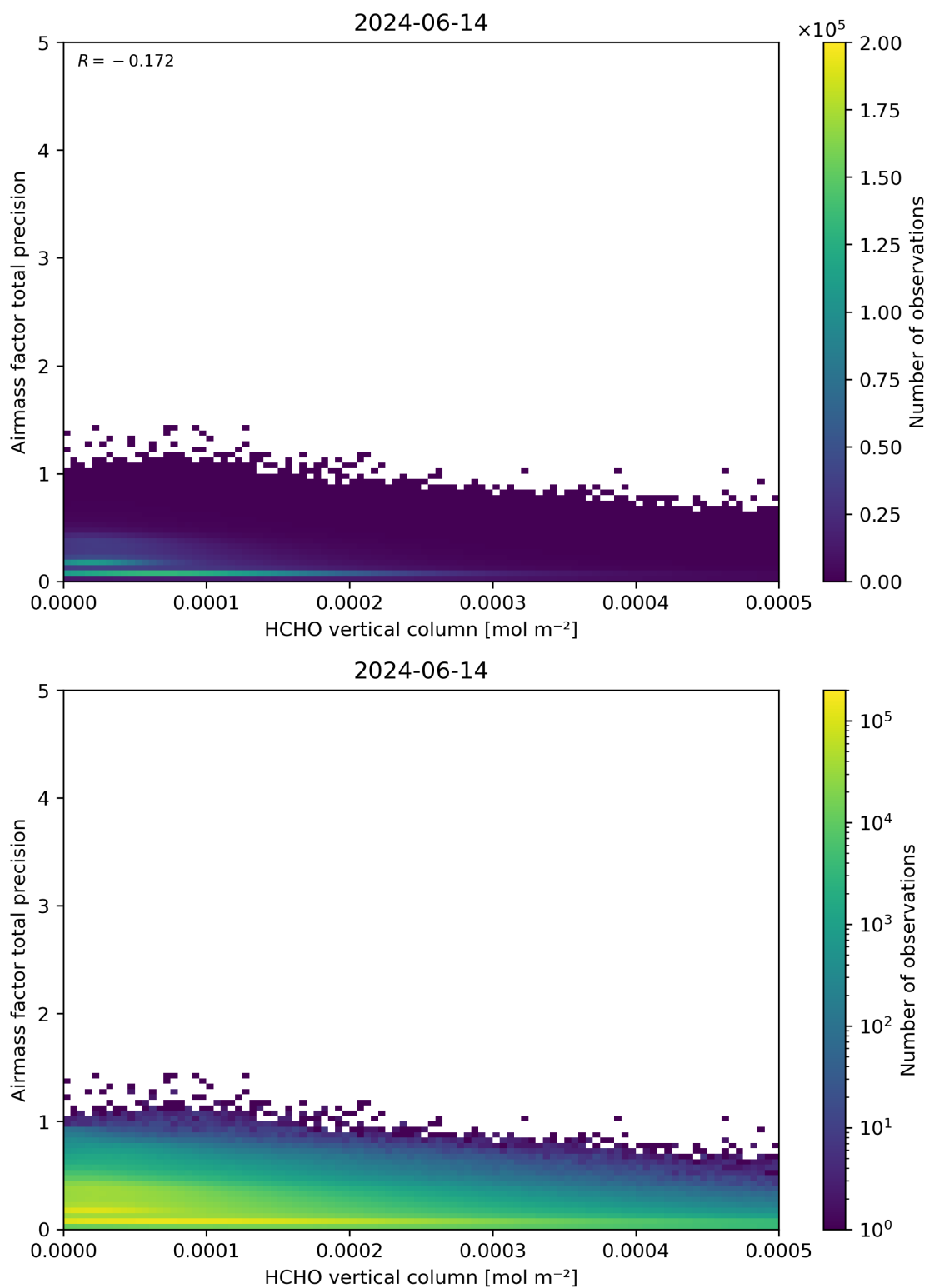
Figure 132: Scatter density plot of “HCHO vertical column” against “Airmass factor total precision” for 2024-06-13 to 2024-06-15.
