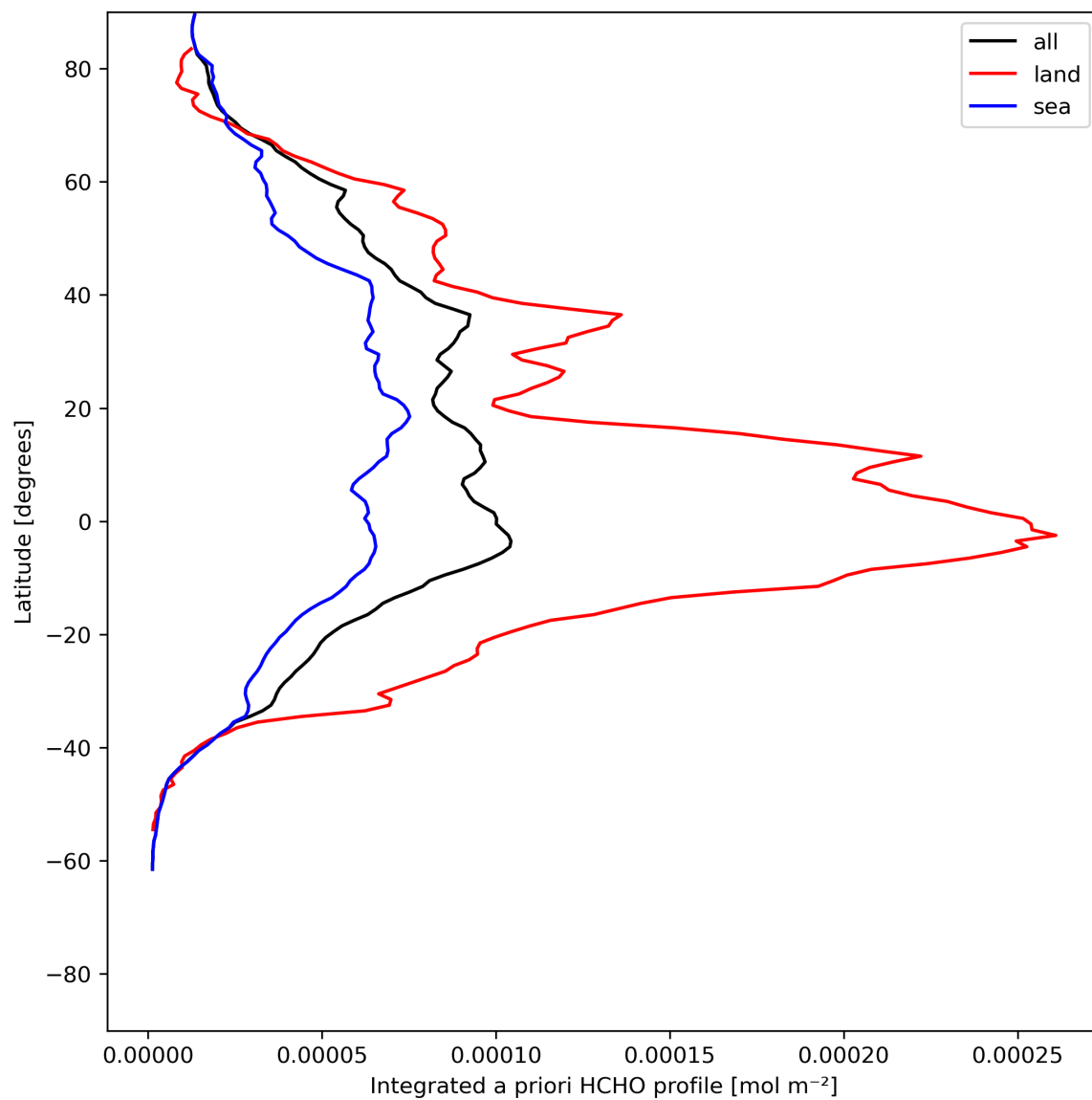
Figure 29: Zonal average of “Integrated a priori HCHO profile” for 2024-06-13 to 2024-06-15.
