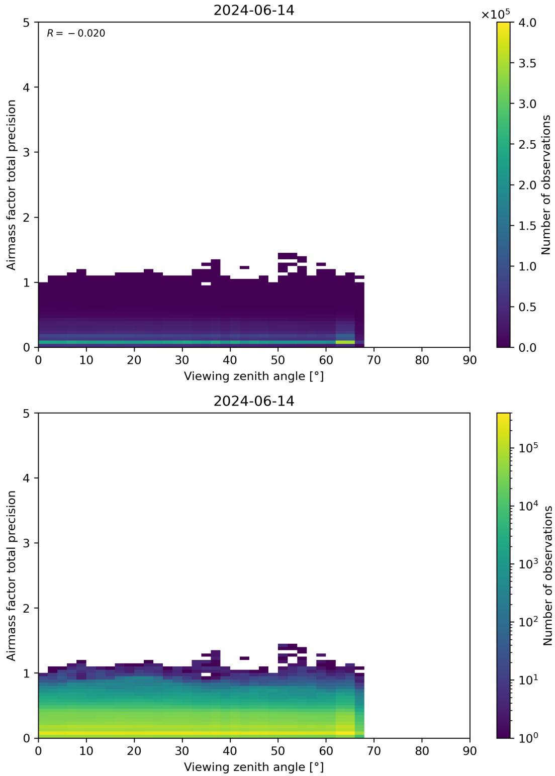
Figure 191: Scatter density plot of “Viewing zenith angle” against “Airmass factor total precision” for 2024-06-13 to 2024-06-15.
