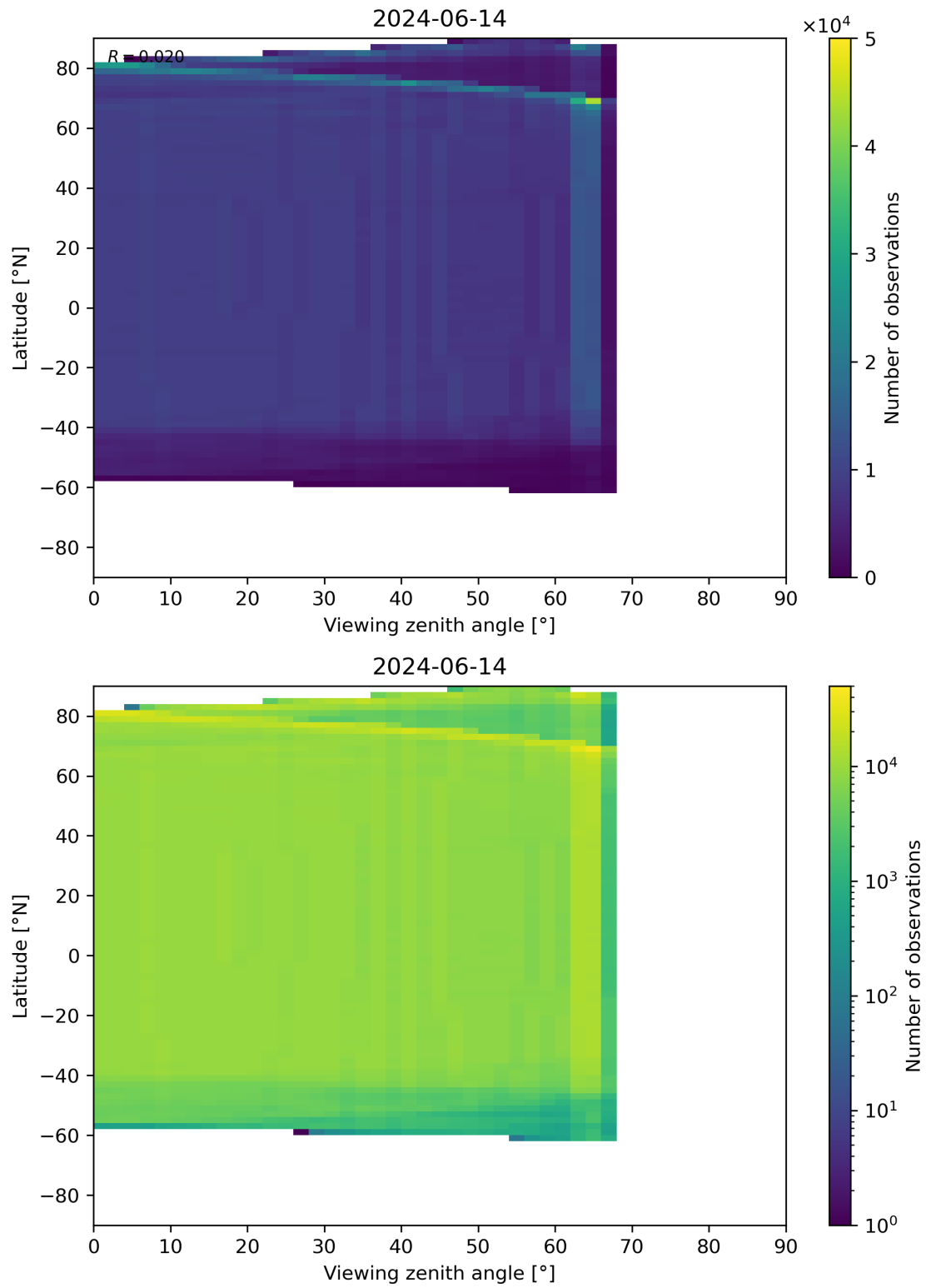
Figure 196: Scatter density plot of “Viewing zenith angle” against “Latitude” for 2024-06-13 to 2024-06-15.
