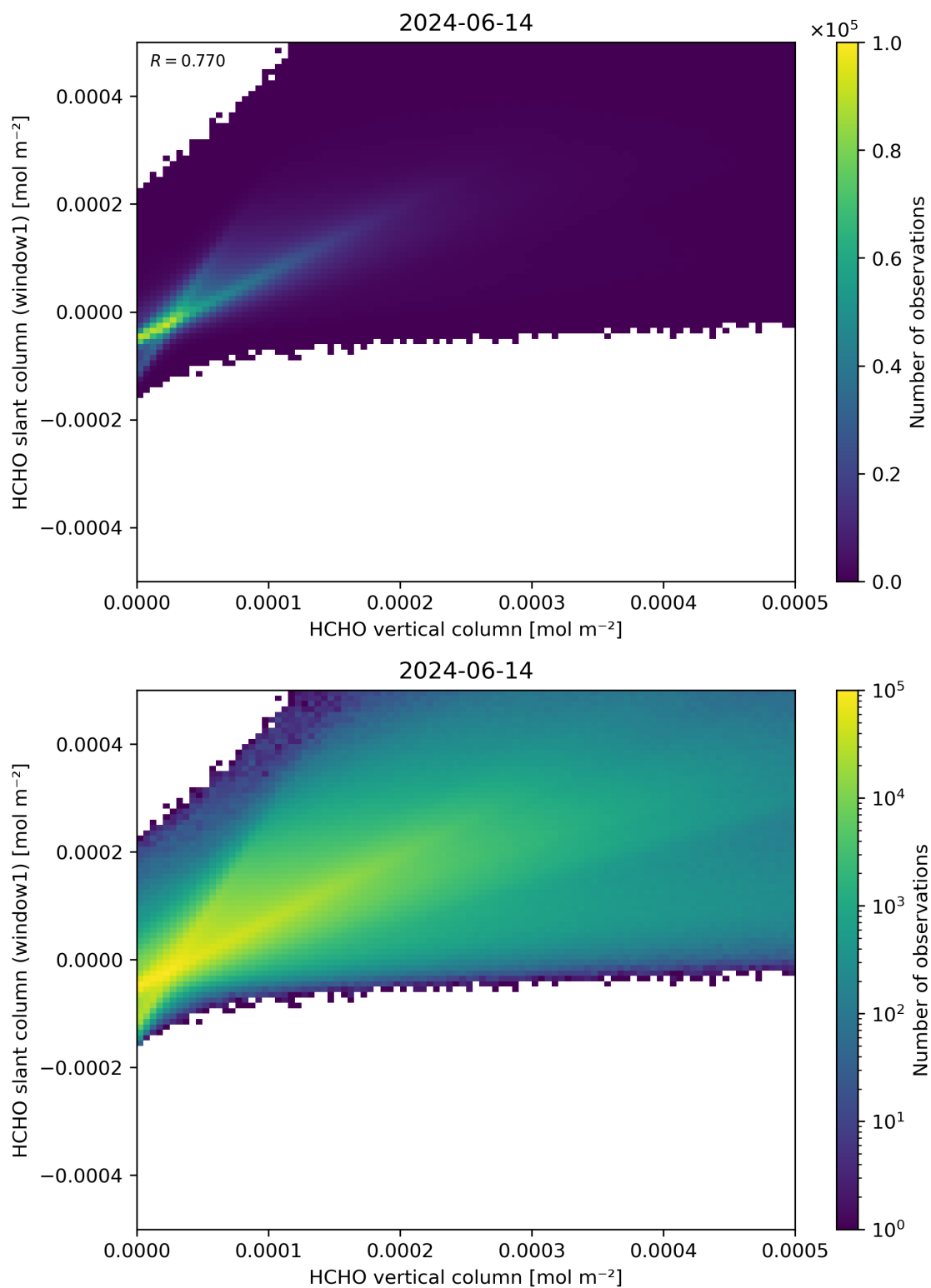
Figure 129: Scatter density plot of “HCHO vertical column” against “HCHO slant column (window1)” for 2024-06-13 to 2024-06-15.
