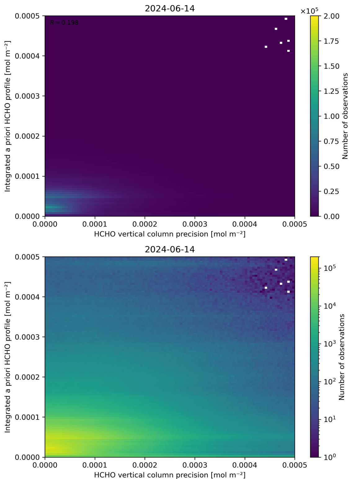
Figure 147: Scatter density plot of “HCHO vertical column precision” against “Integrated a priori HCHO profile” for 2024-06-13 to 2024-06-15.
