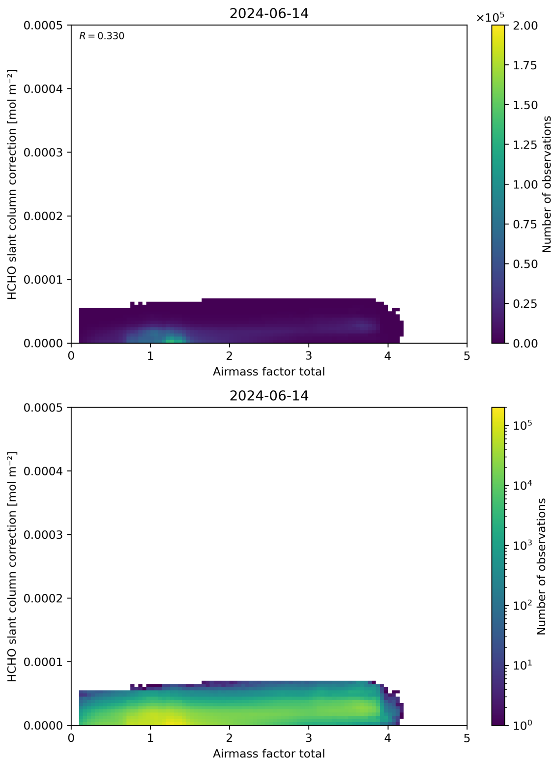
Figure 102: Scatter density plot of “Airmass factor total” against “HCHO slant column correction” for 2024-06-13 to 2024-06-15.
