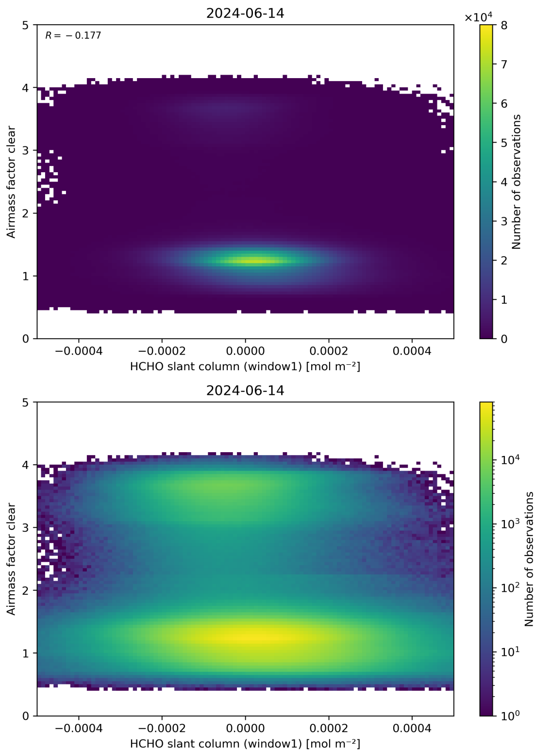
Figure 81: Scatter density plot of “HCHO slant column (window1)” against “Airmass factor clear” for 2024-06-13 to 2024-06-15.
