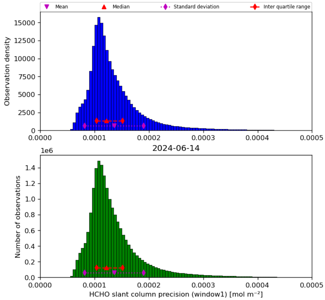
Figure 39: Histogram of “HCHO slant column precision (window1)” for 2024-06-13 to 2024-06-15
