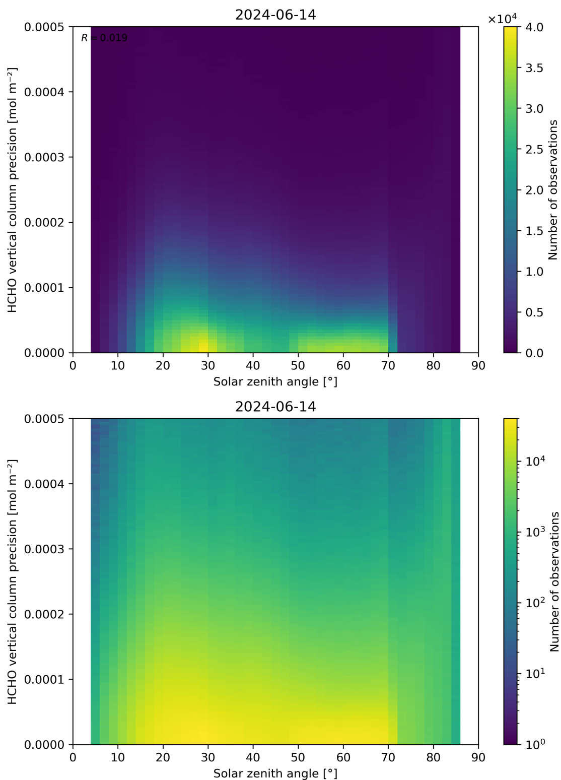
Figure 179: Scatter density plot of “Solar zenith angle” against “HCHO vertical column precision” for 2024-06-13 to 2024-06-15.
