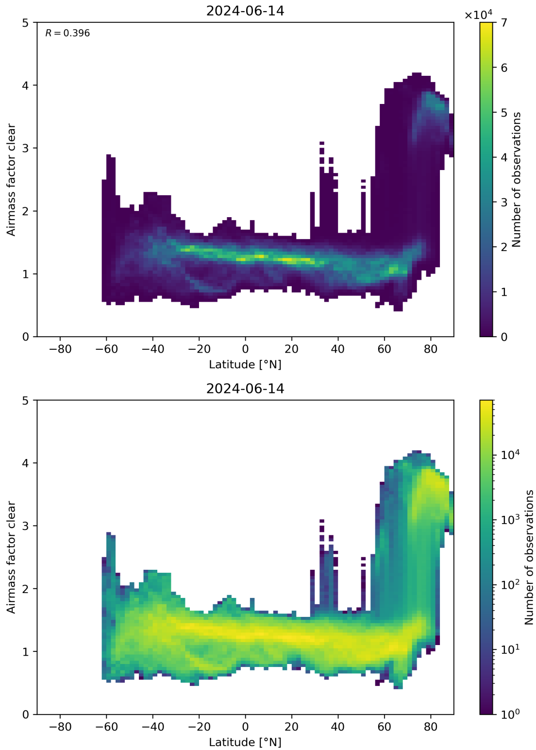
Figure 156: Scatter density plot of “Latitude” against “Airmass factor clear” for 2024-06-13 to 2024-06-15.
