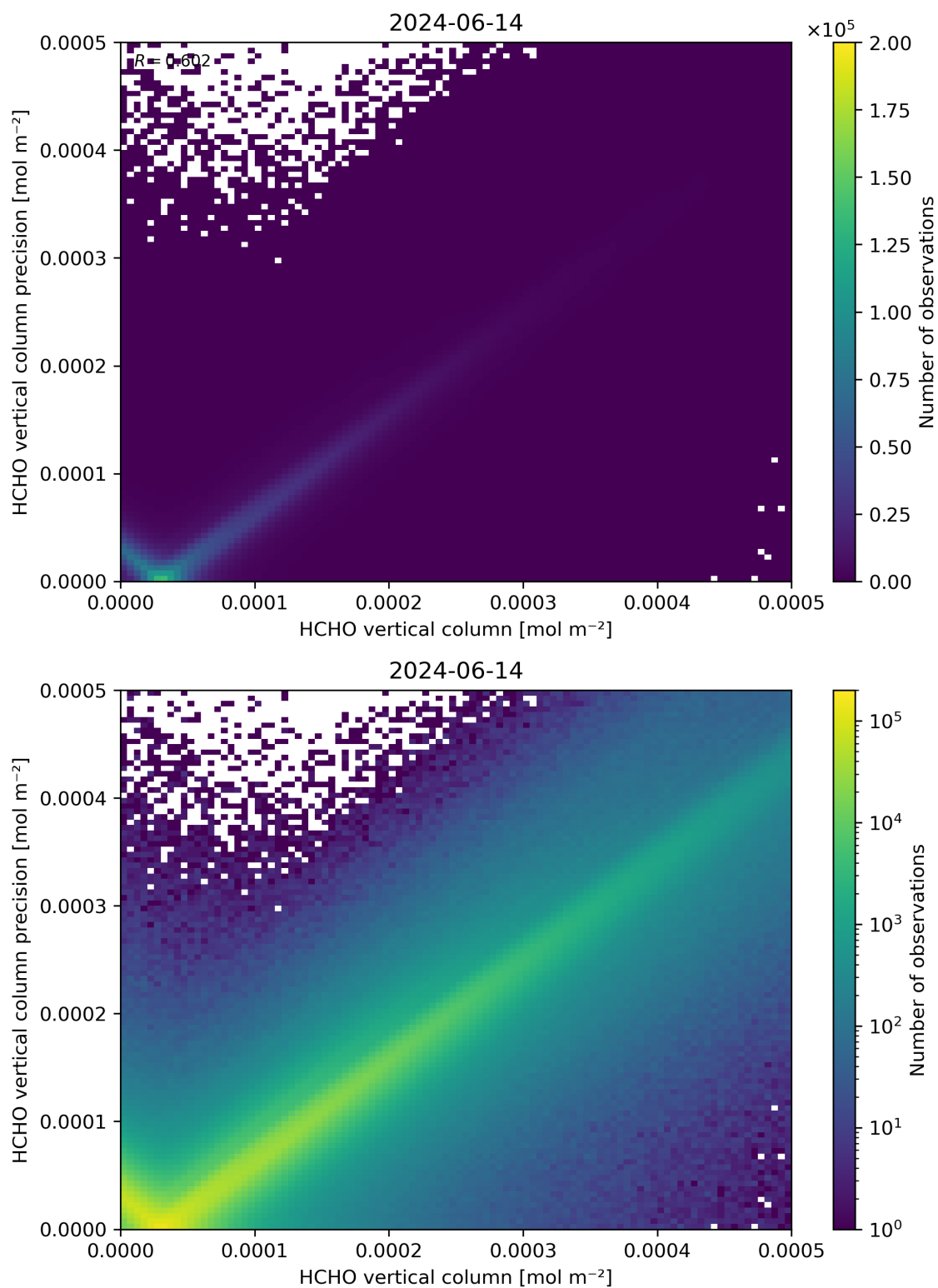
Figure 134: Scatter density plot of “HCHO vertical column” against “HCHO vertical column precision” for 2024-06-13 to 2024-06-15.
