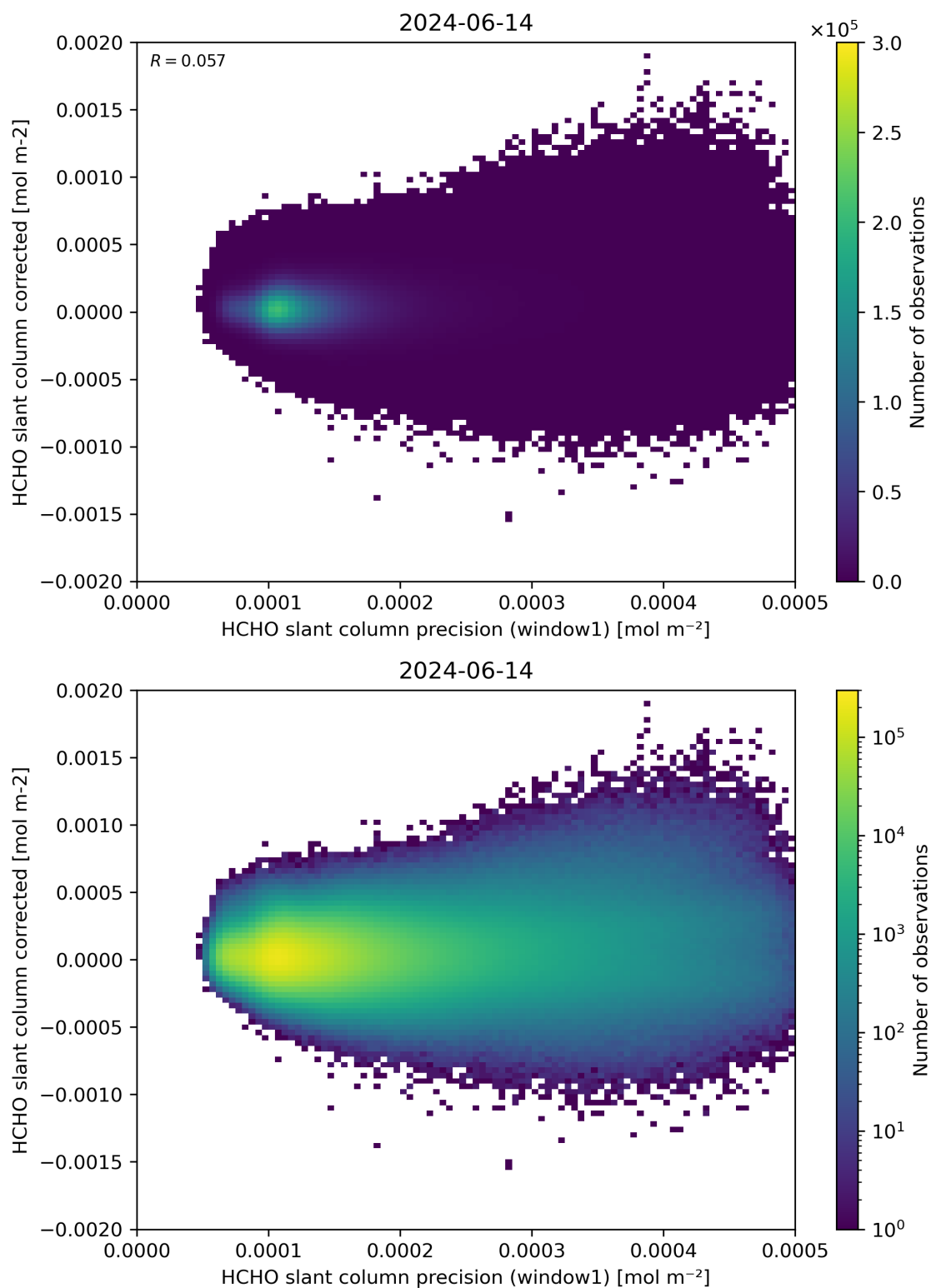
Figure 92: Scatter density plot of “HCHO slant column precision (window1)” against “HCHO slant column corrected” for 2024-06-13 to 2024-06-15.
