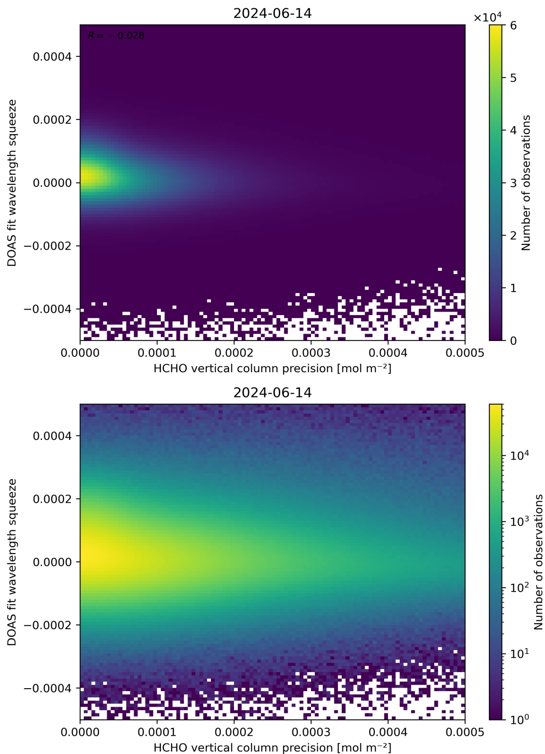
Figure 138: Scatter density plot of “HCHO vertical column precision” against “DOAS fit wavelength squeeze” for 2024-06-13 to 2024-06-15.
