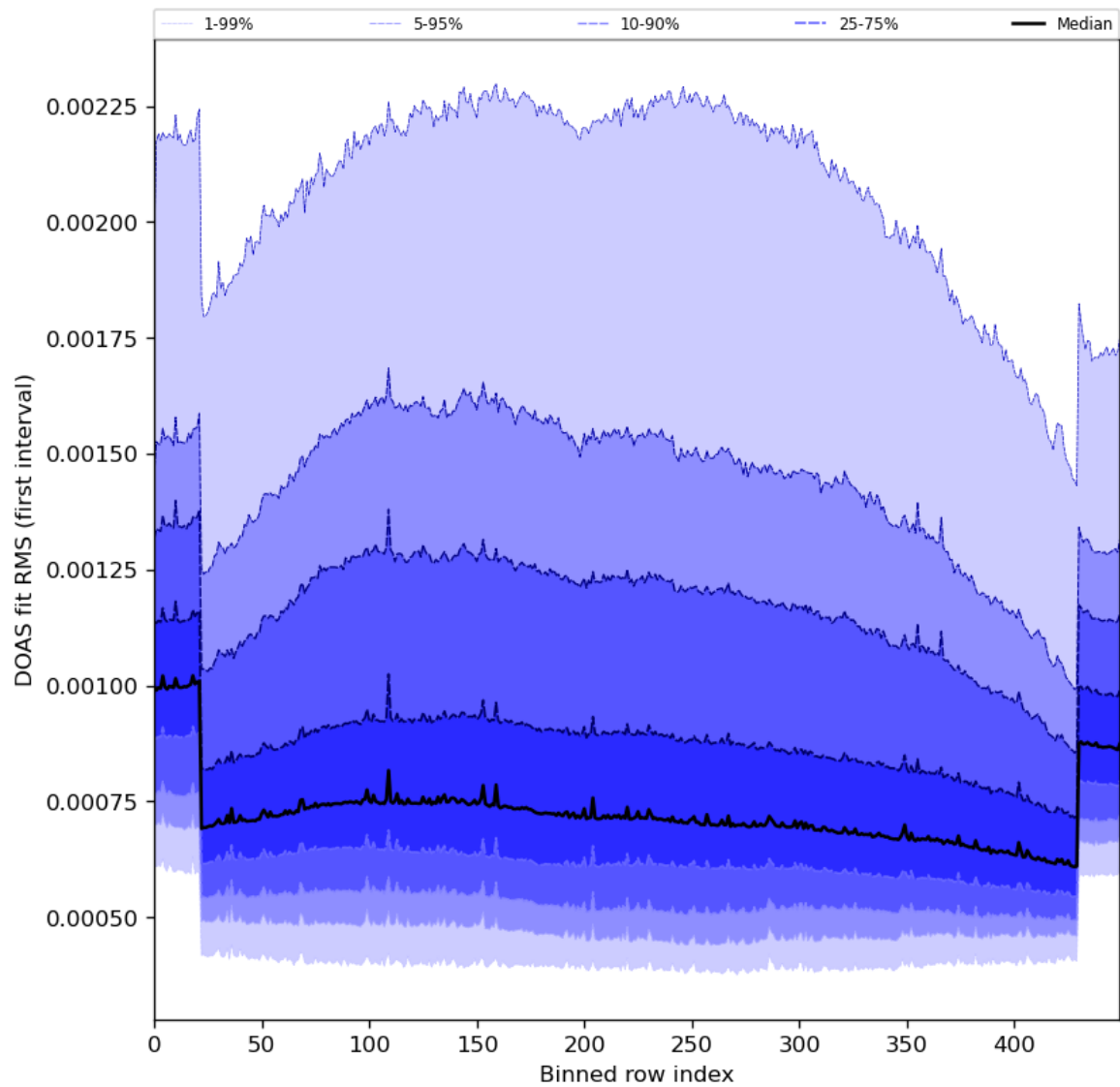
Figure 60: Along track statistics of “DOAS fit RMS (first interval)” for 2024-06-13 to 2024-06-15
