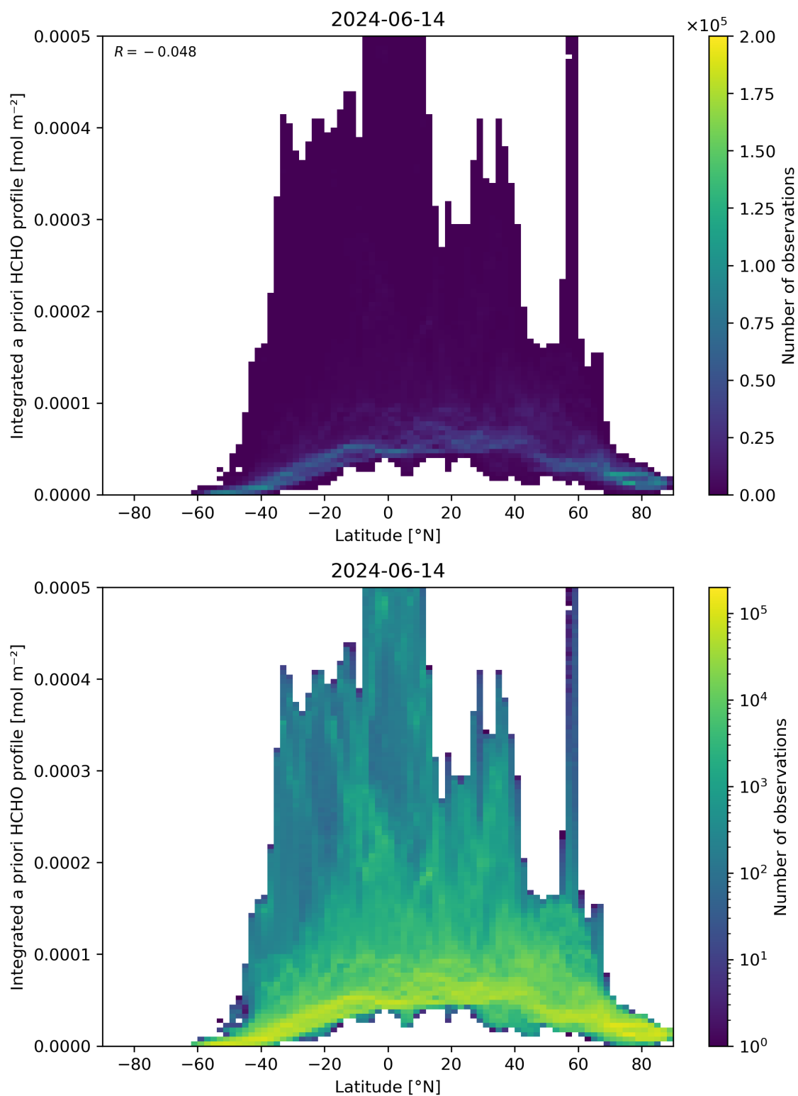
Figure 166: Scatter density plot of “Latitude” against “Integrated a priori HCHO profile” for 2024-06-13 to 2024-06-15.
