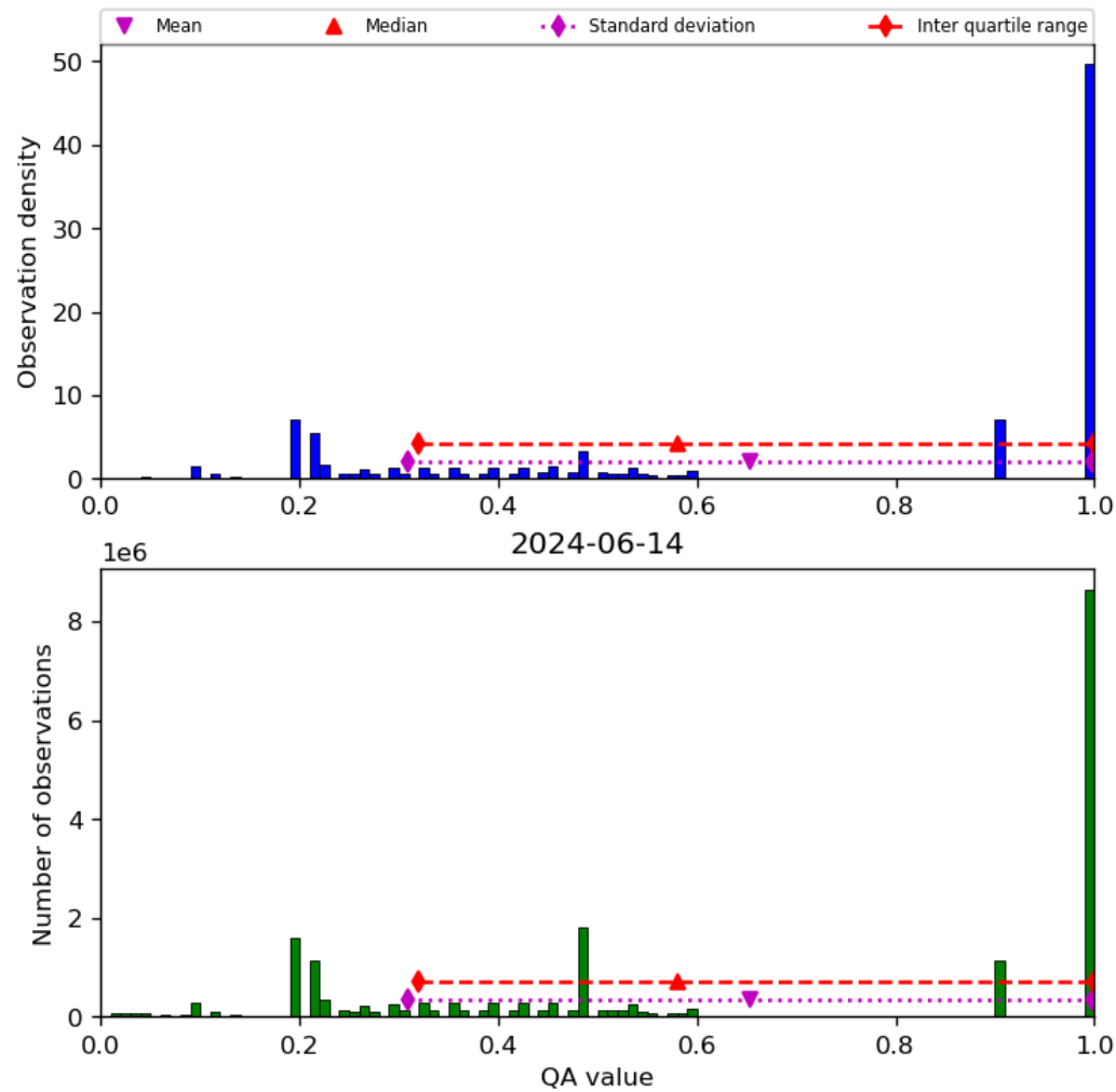
Figure 34: Histogram of “QA value” for 2024-06-13 to 2024-06-15
