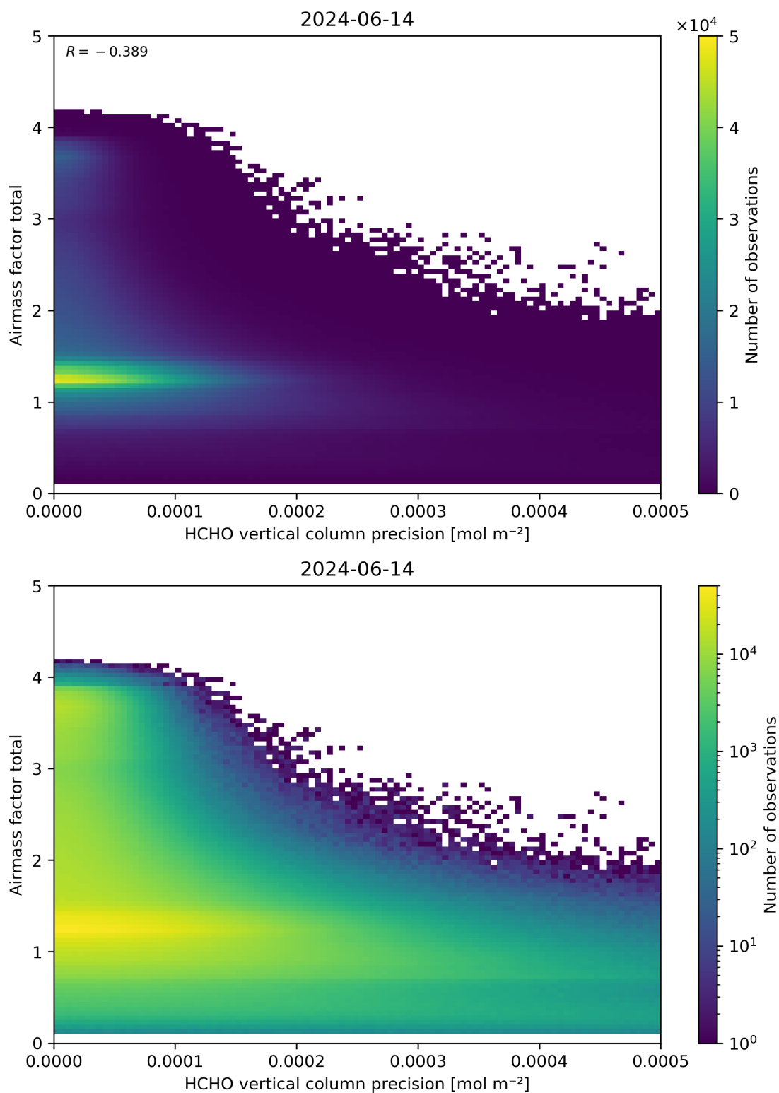
Figure 144: Scatter density plot of “HCHO vertical column precision” against “Airmass factor total” for 2024-06-13 to 2024-06-15.
