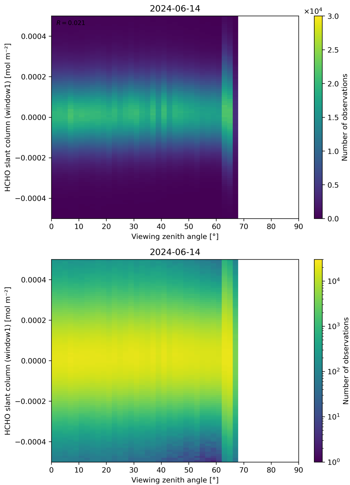
Figure 188: Scatter density plot of “Viewing zenith angle” against “HCHO slant column (window1)” for 2024-06-13 to 2024-06-15.
