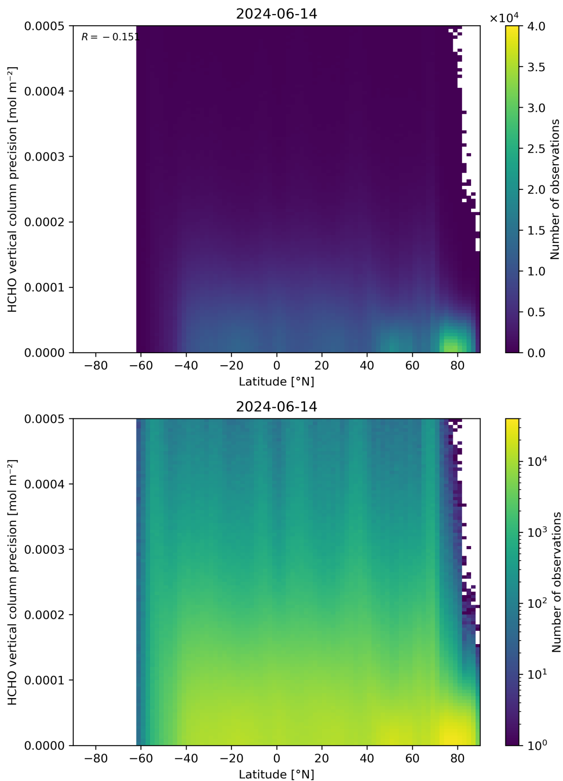
Figure 165: Scatter density plot of “Latitude” against “HCHO vertical column precision” for 2024-06-13 to 2024-06-15.
