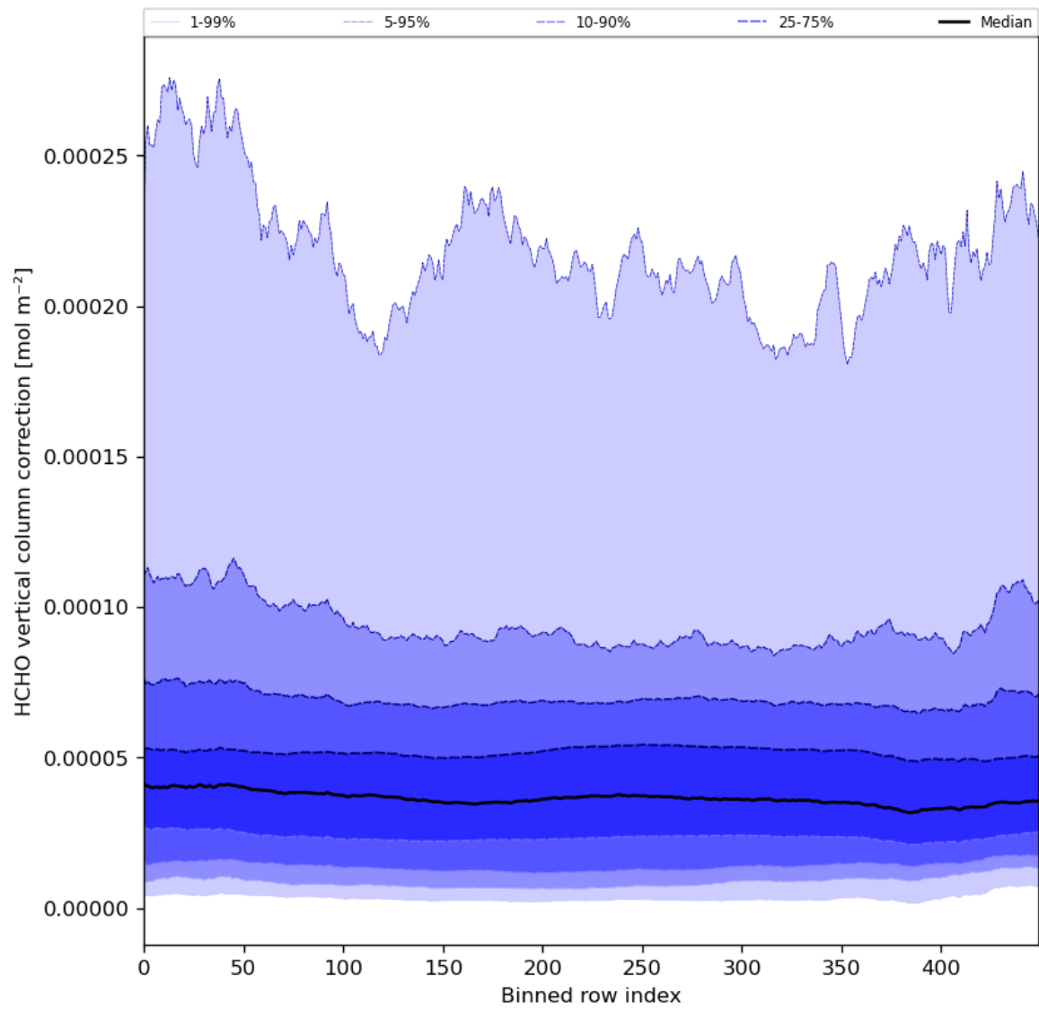
Figure 51: Along track statistics of “HCHO vertical column correction” for 2024-06-13 to 2024-06-15
