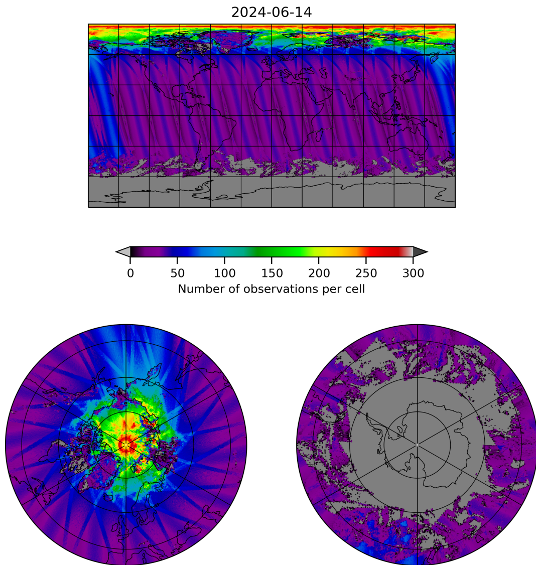
Figure 19: Map of the number of observations for 2024-06-13 to 2024-06-15
