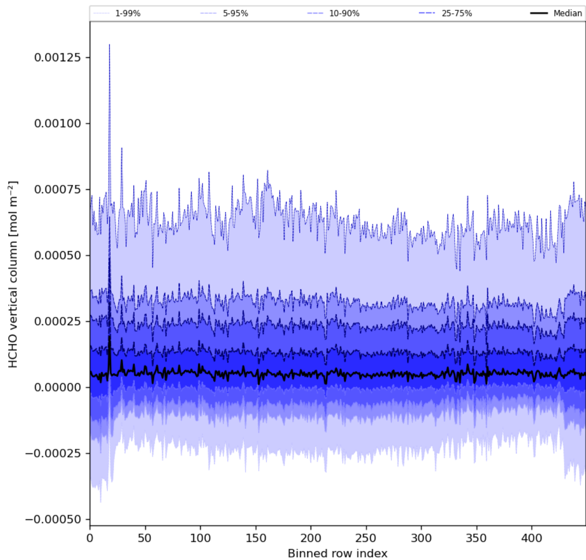
Figure 49: Along track statistics of “HCHO vertical column” for 2024-06-13 to 2024-06-15
