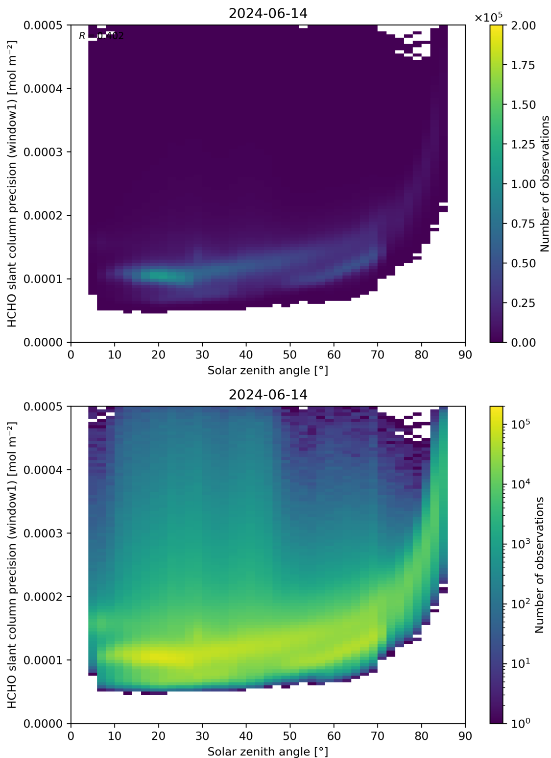
Figure 174: Scatter density plot of “Solar zenith angle” against “HCHO slant column precision (window1)” for 2024-06-13 to 2024-06-15.
