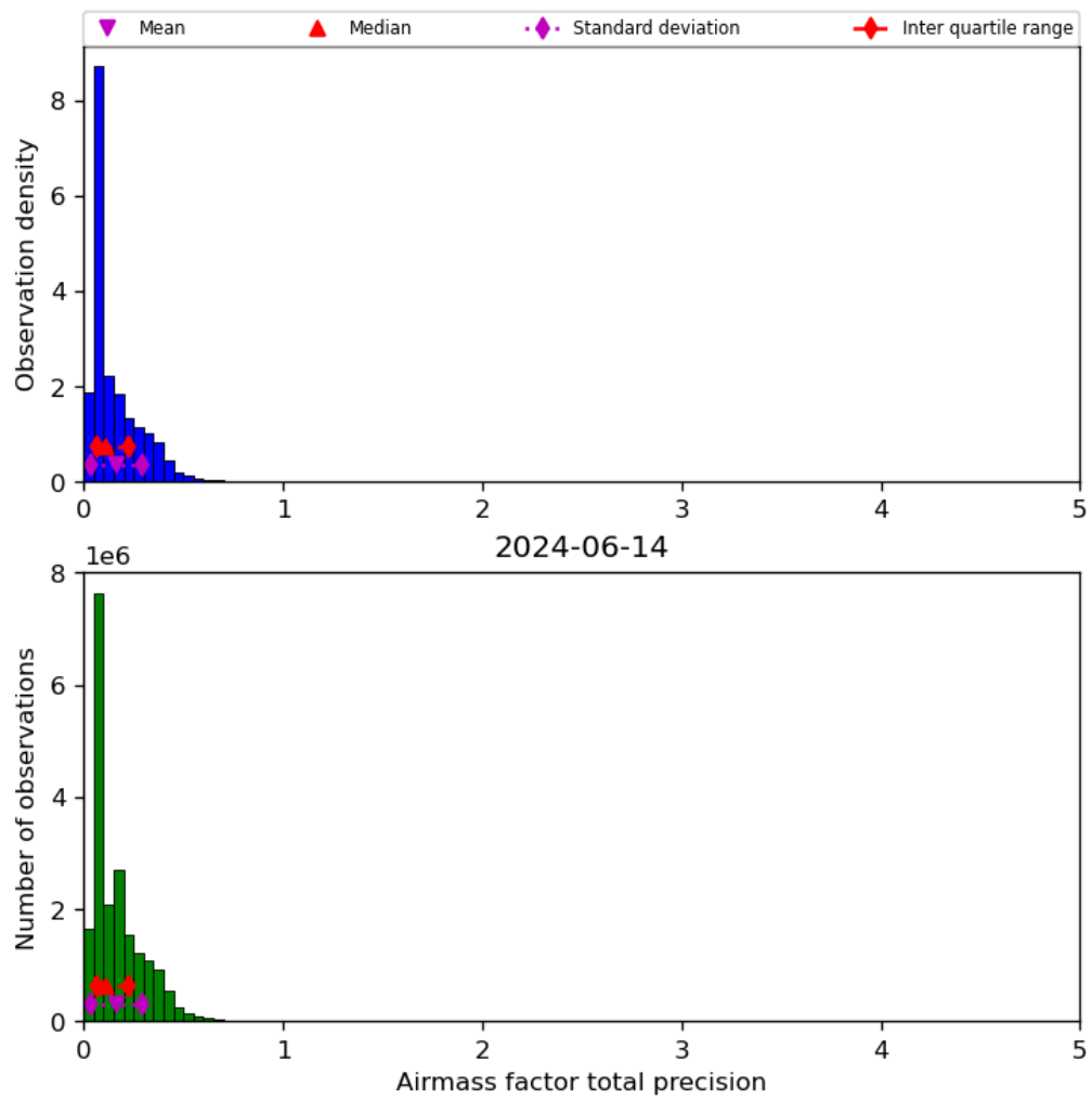
Figure 41: Histogram of “Airmass factor total precision” for 2024-06-13 to 2024-06-15
