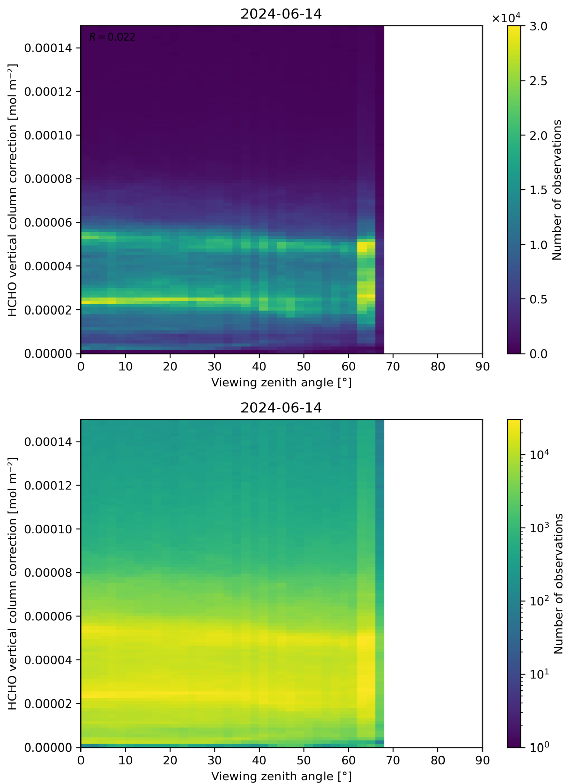
Figure 193: Scatter density plot of “Viewing zenith angle” against “HCHO vertical column correction” for 2024-06-13 to 2024-06-15.
