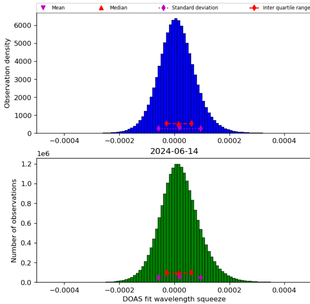
Figure 45: Histogram of “DOAS fit wavelength squeeze” for 2024-06-13 to 2024-06-15
