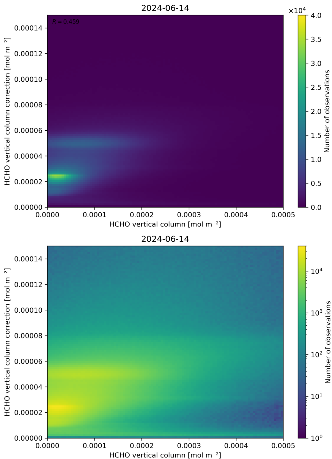
Figure 133: Scatter density plot of “HCHO vertical column” against “HCHO vertical column correction” for 2024-06-13 to 2024-06-15.
