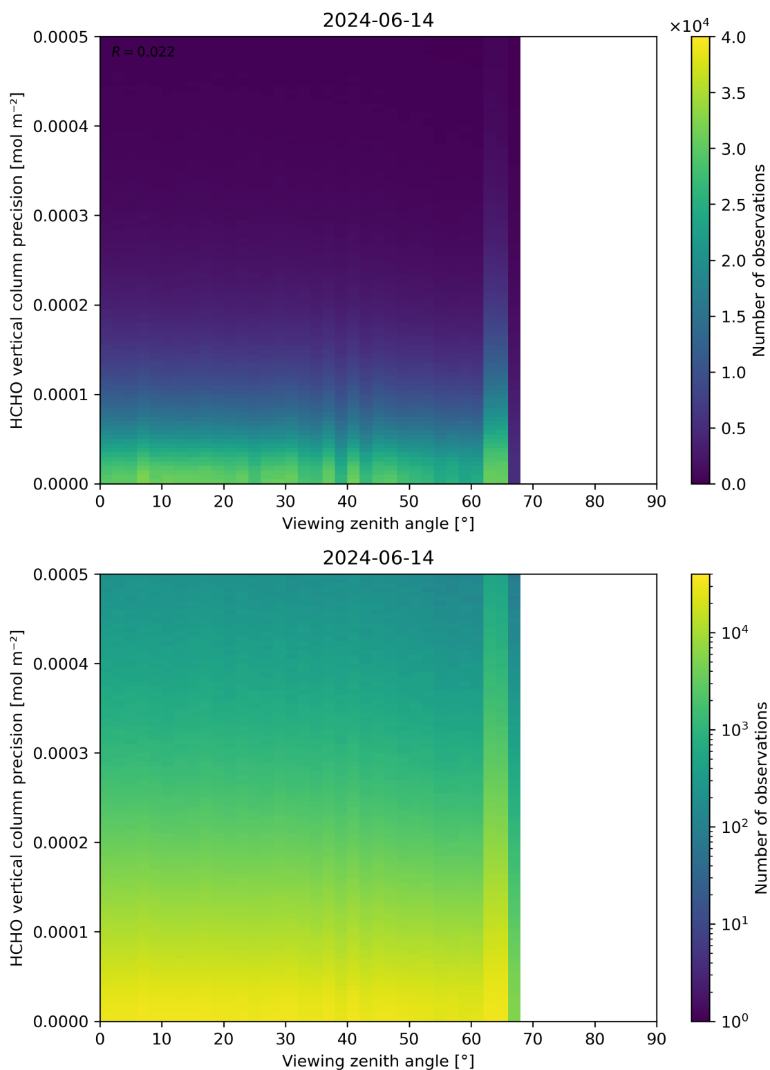
Figure 194: Scatter density plot of “Viewing zenith angle” against “HCHO vertical column precision” for 2024-06-13 to 2024-06-15.
