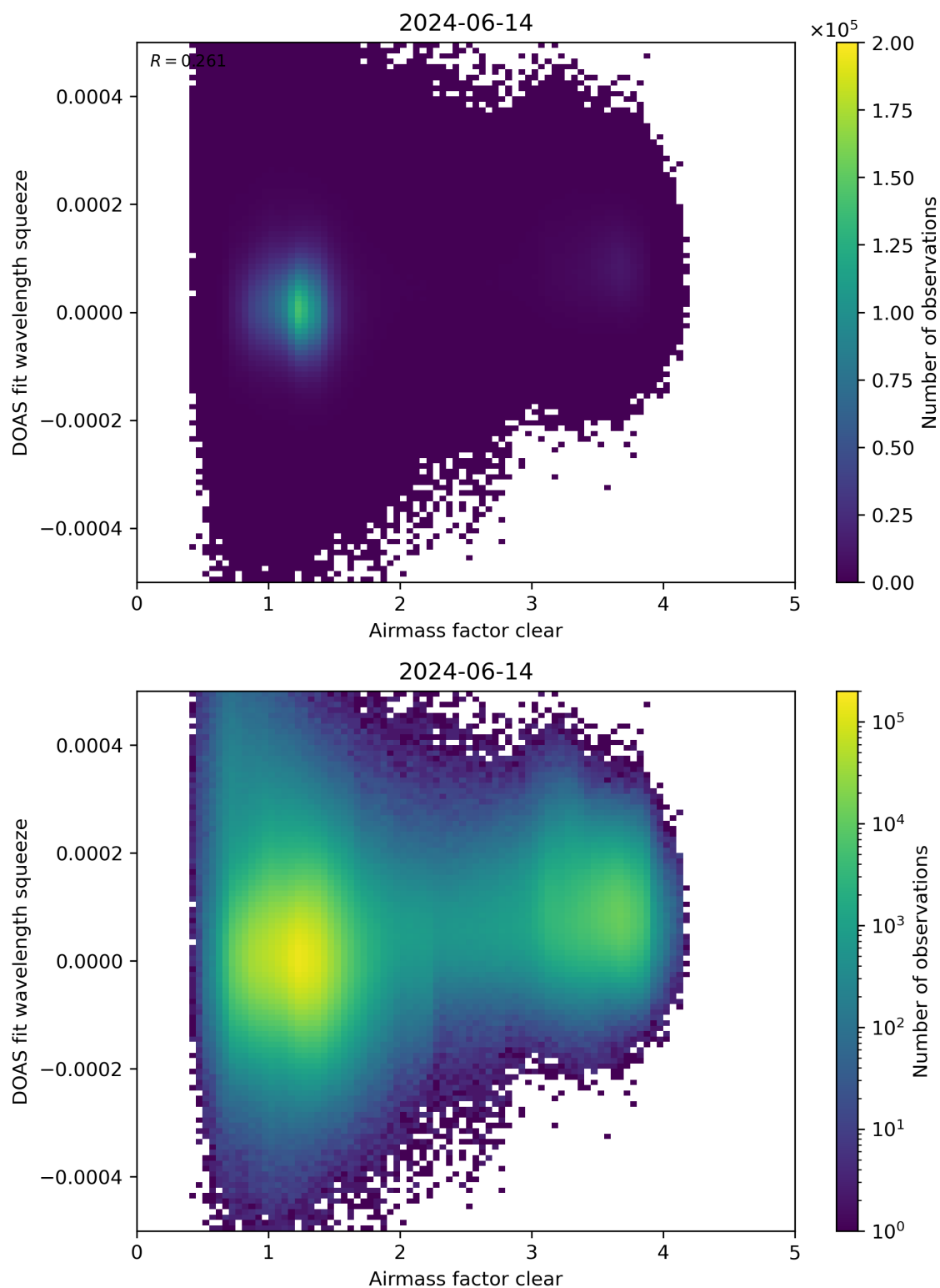
Figure 73: Scatter density plot of “Airmass factor clear” against “DOAS fit wavelength squeeze” for 2024-06-13 to 2024-06-15.
