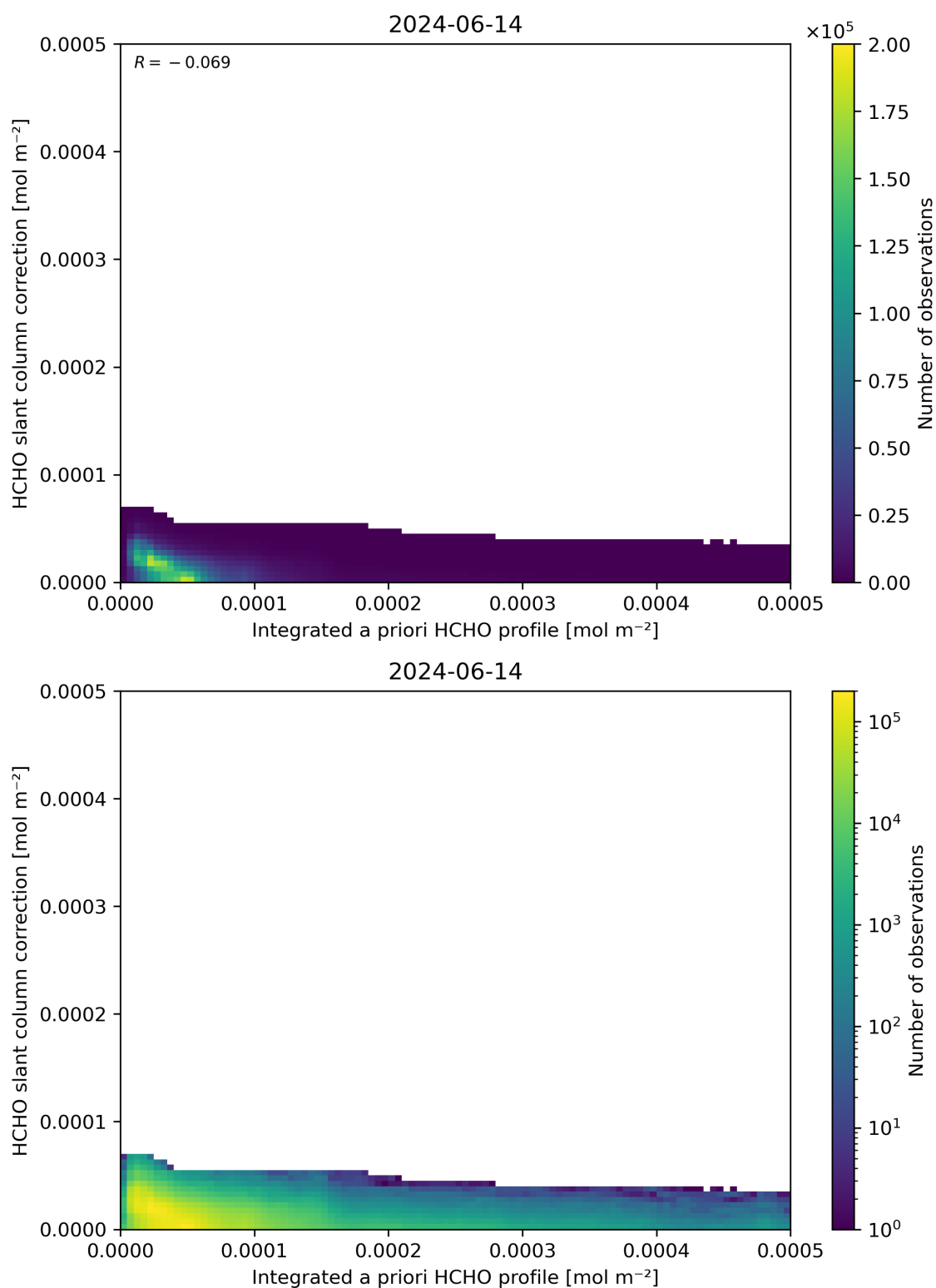
Figure 152: Scatter density plot of “Integrated a priori HCHO profile” against “HCHO slant column correction” for 2024-06-13 to 2024-06-15.
