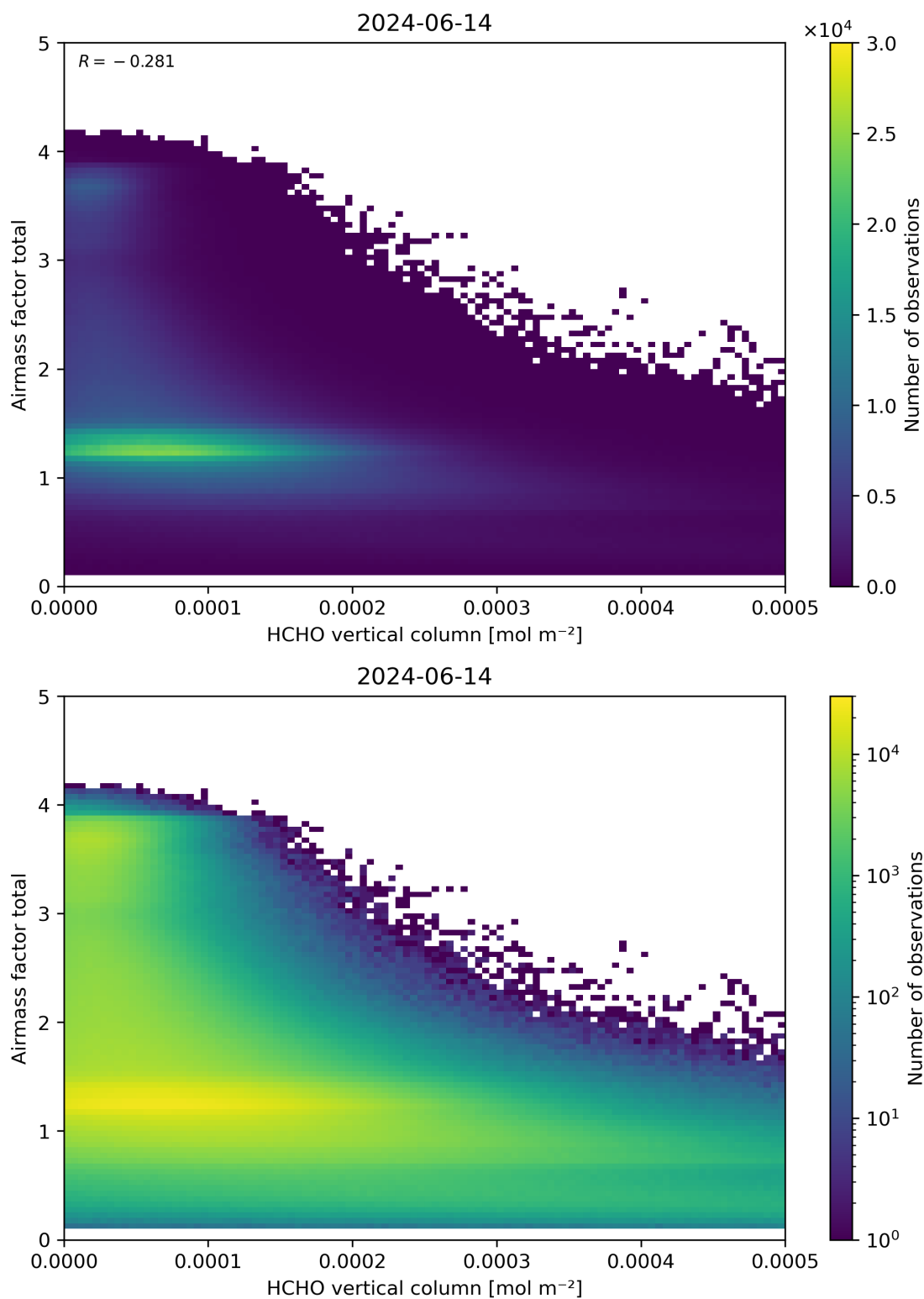
Figure 131: Scatter density plot of “HCHO vertical column” against “Airmass factor total” for 2024-06-13 to 2024-06-15.
