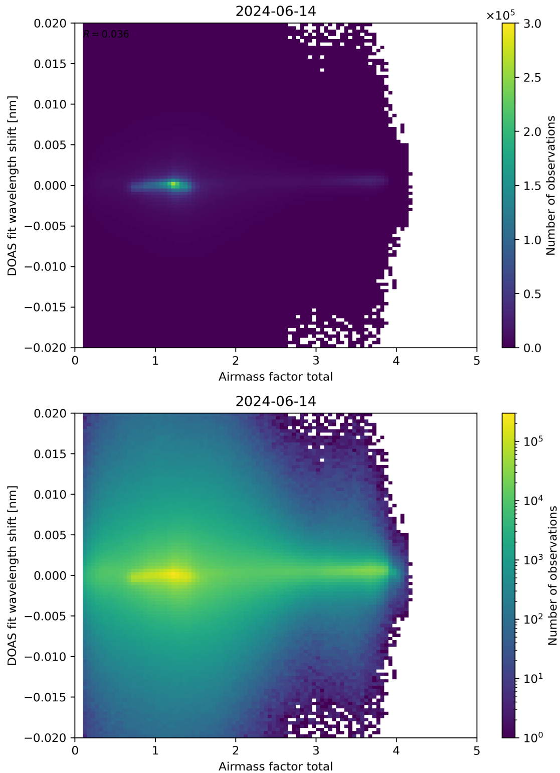
Figure 98: Scatter density plot of “Airmass factor total” against “DOAS fit wavelength shift” for 2024-06-13 to 2024-06-15.
