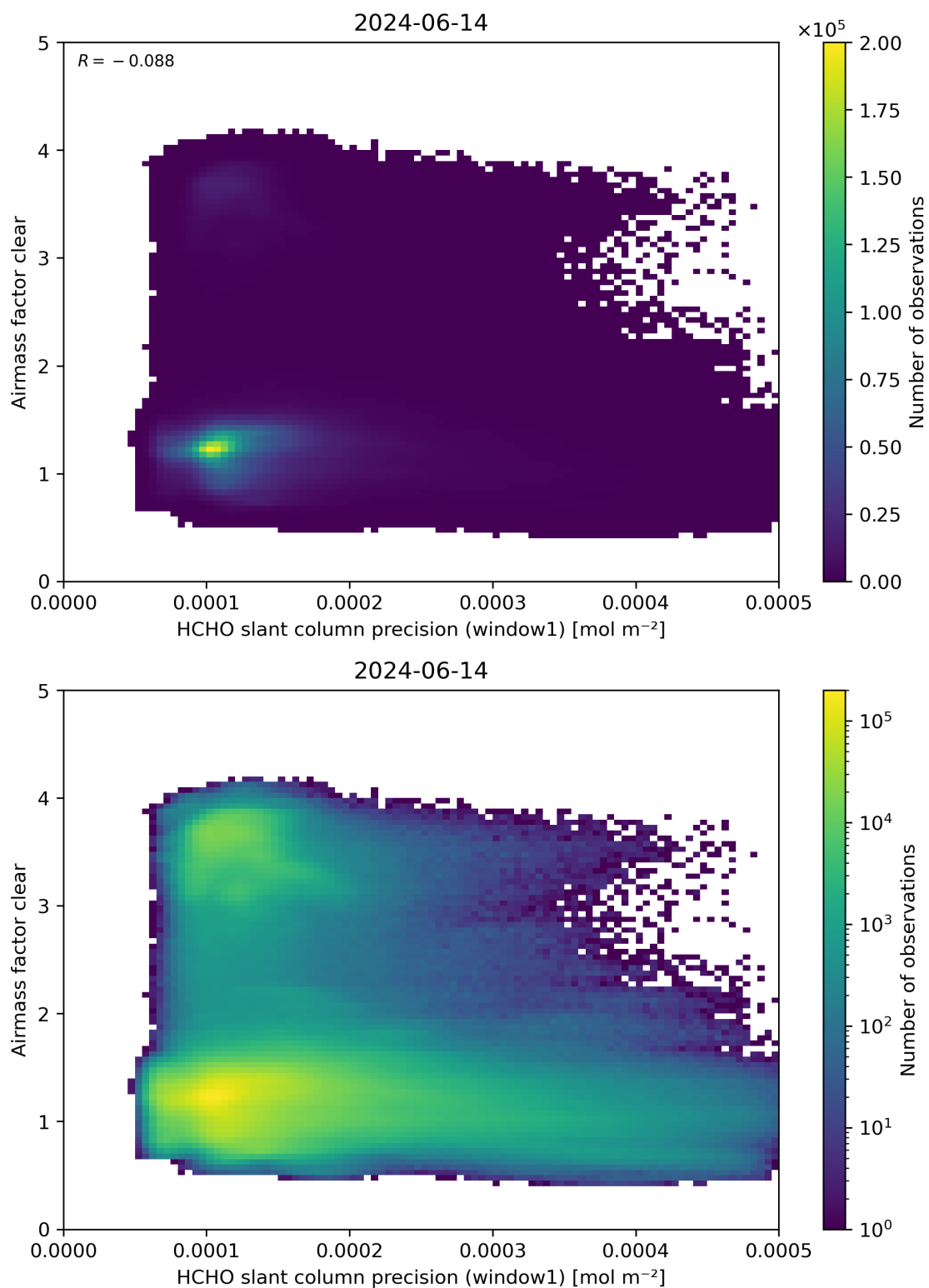
Figure 91: Scatter density plot of “HCHO slant column precision (window1)” against “Airmass factor clear” for 2024-06-13 to 2024-06-15.
