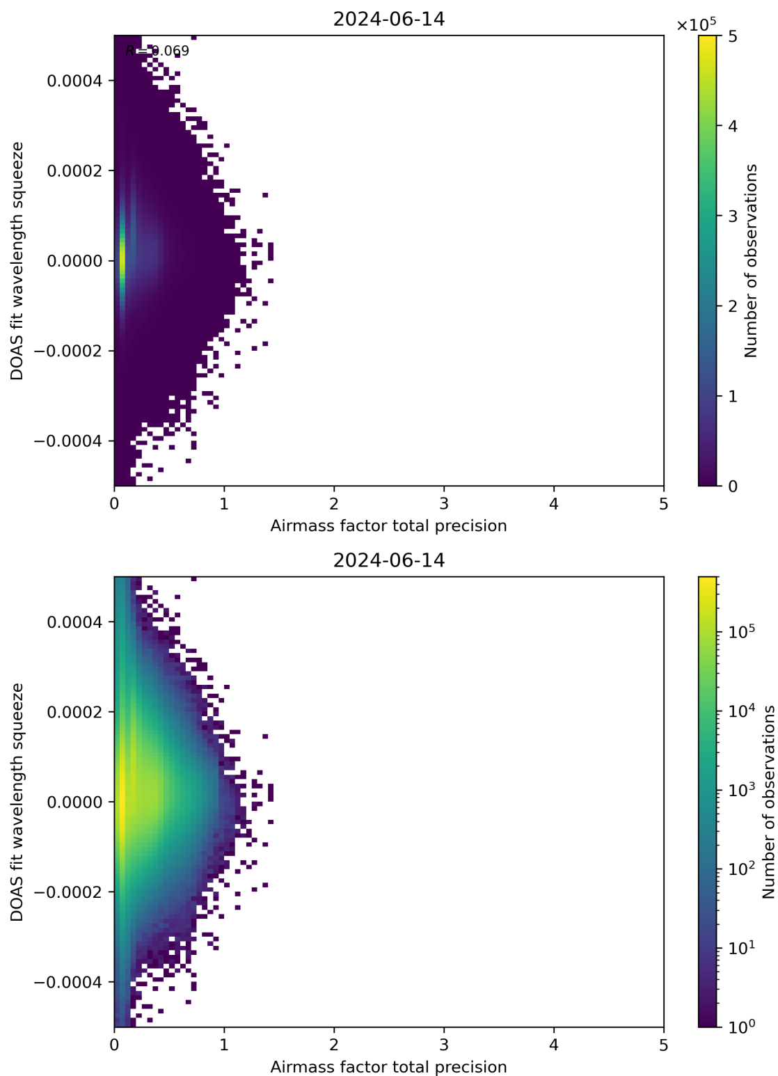
Figure 107: Scatter density plot of “Airmass factor total precision” against “DOAS fit wavelength squeeze” for 2024-06-13 to 2024-06-15.
