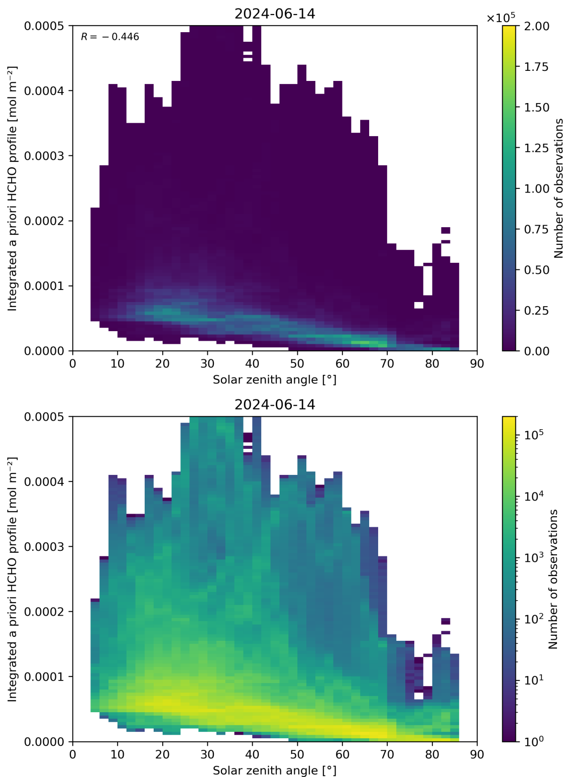
Figure 180: Scatter density plot of “Solar zenith angle” against “Integrated a priori HCHO profile” for 2024-06-13 to 2024-06-15.
