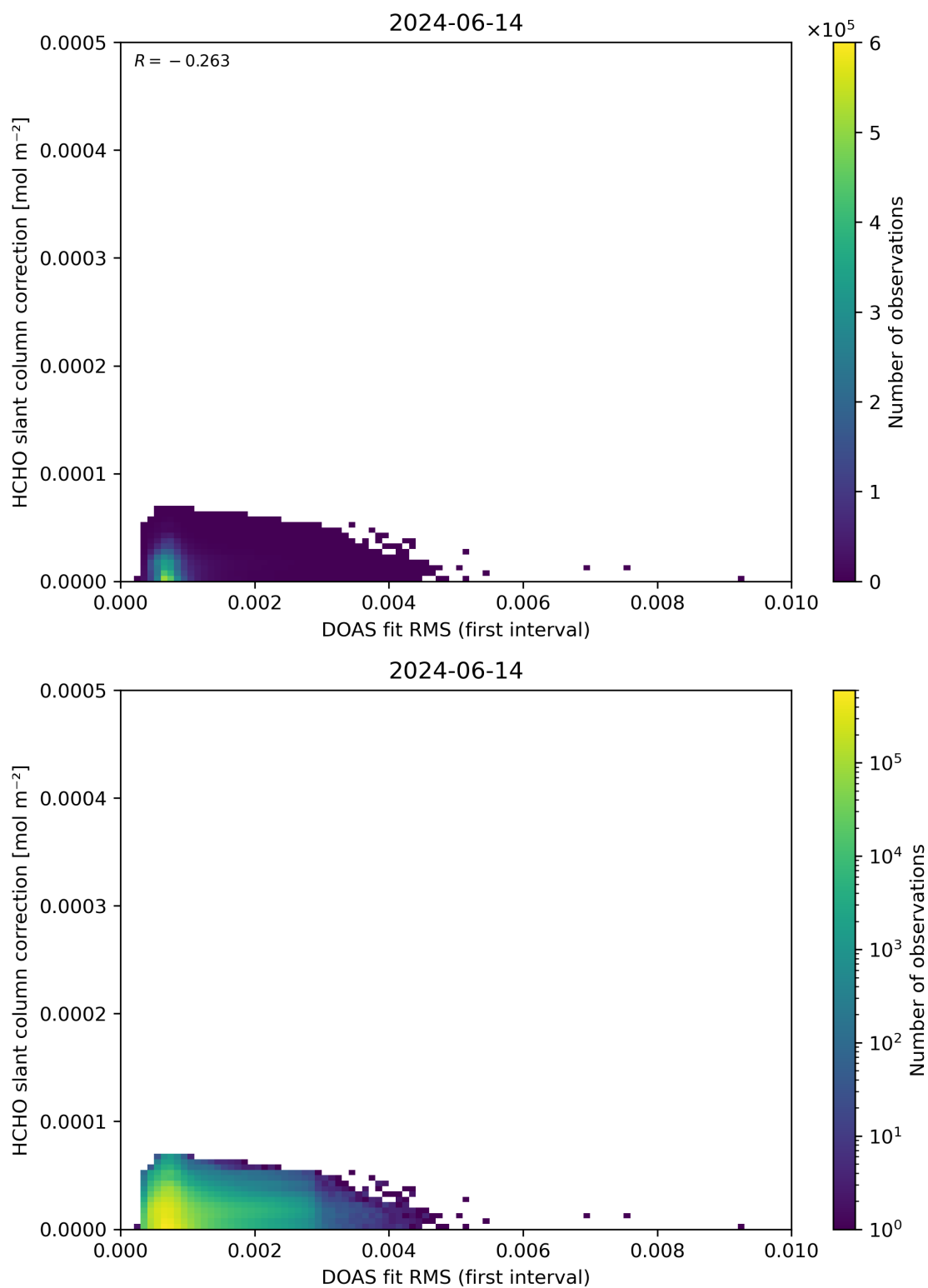
Figure 63: Scatter density plot of “DOAS fit RMS (first interval)” against “HCHO slant column correction” for 2024-06-13 to 2024-06-15.
