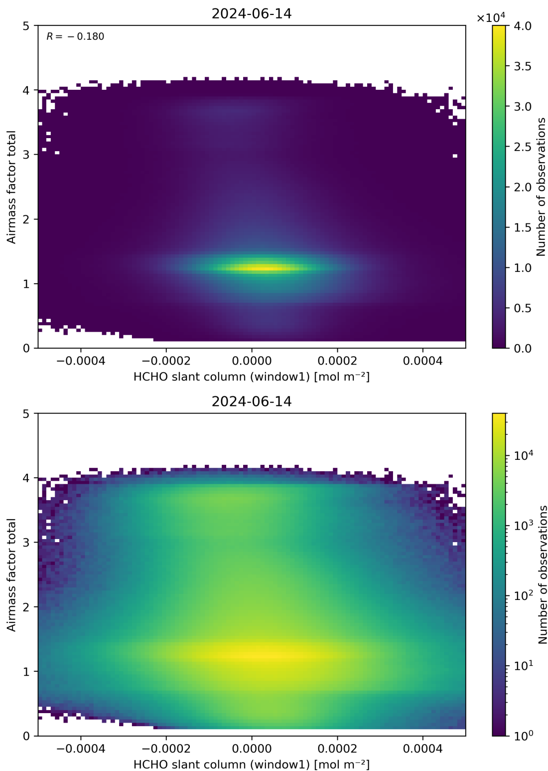
Figure 85: Scatter density plot of “HCHO slant column (window1)” against “Airmass factor total” for 2024-06-13 to 2024-06-15.
