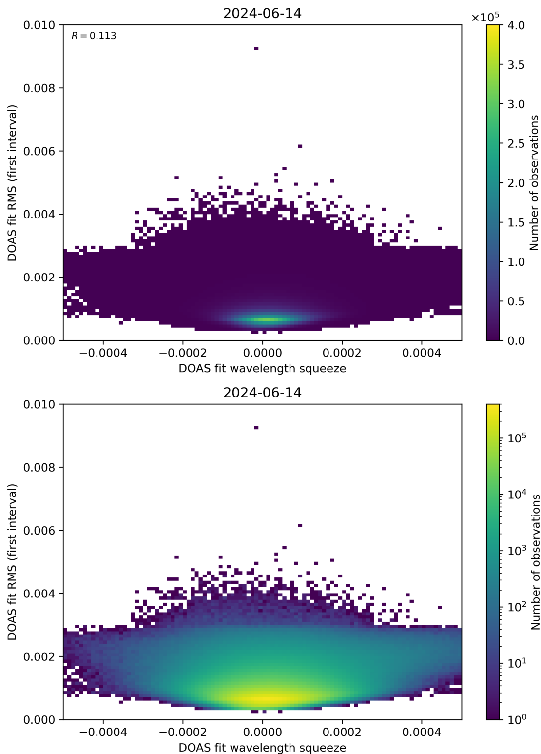
Figure 68: Scatter density plot of “DOAS fit wavelength squeeze” against “DOAS fit RMS (first interval)” for 2024-06-13 to 2024-06-15.
