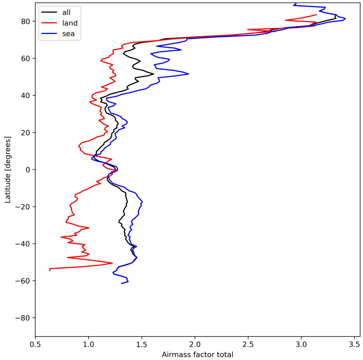
Figure 26: Zonal average of “Airmass factor total” for 2024-06-13 to 2024-06-15.
