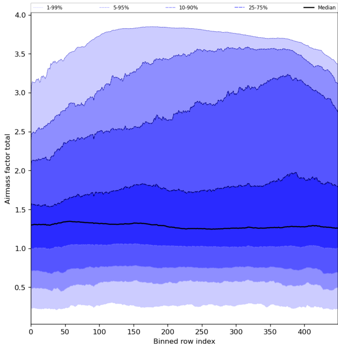
Figure 54: Along track statistics of “Airmass factor total” for 2024-06-13 to 2024-06-15
