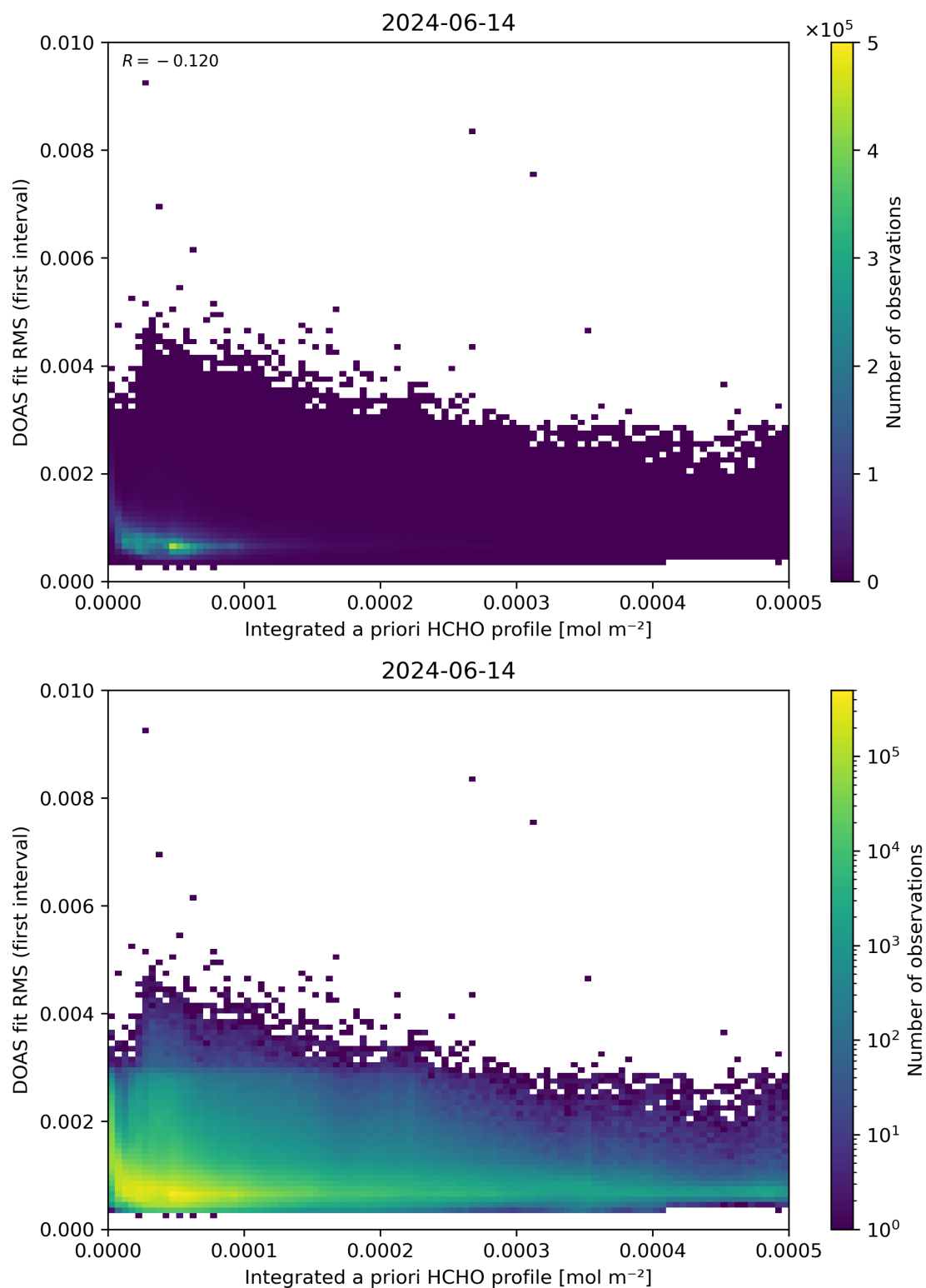
Figure 148: Scatter density plot of “Integrated a priori HCHO profile” against “DOAS fit RMS (first interval)” for 2024-06-13 to 2024-06-15.
