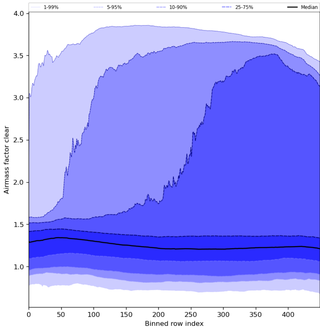
Figure 56: Along track statistics of “Airmass factor clear” for 2024-06-13 to 2024-06-15
