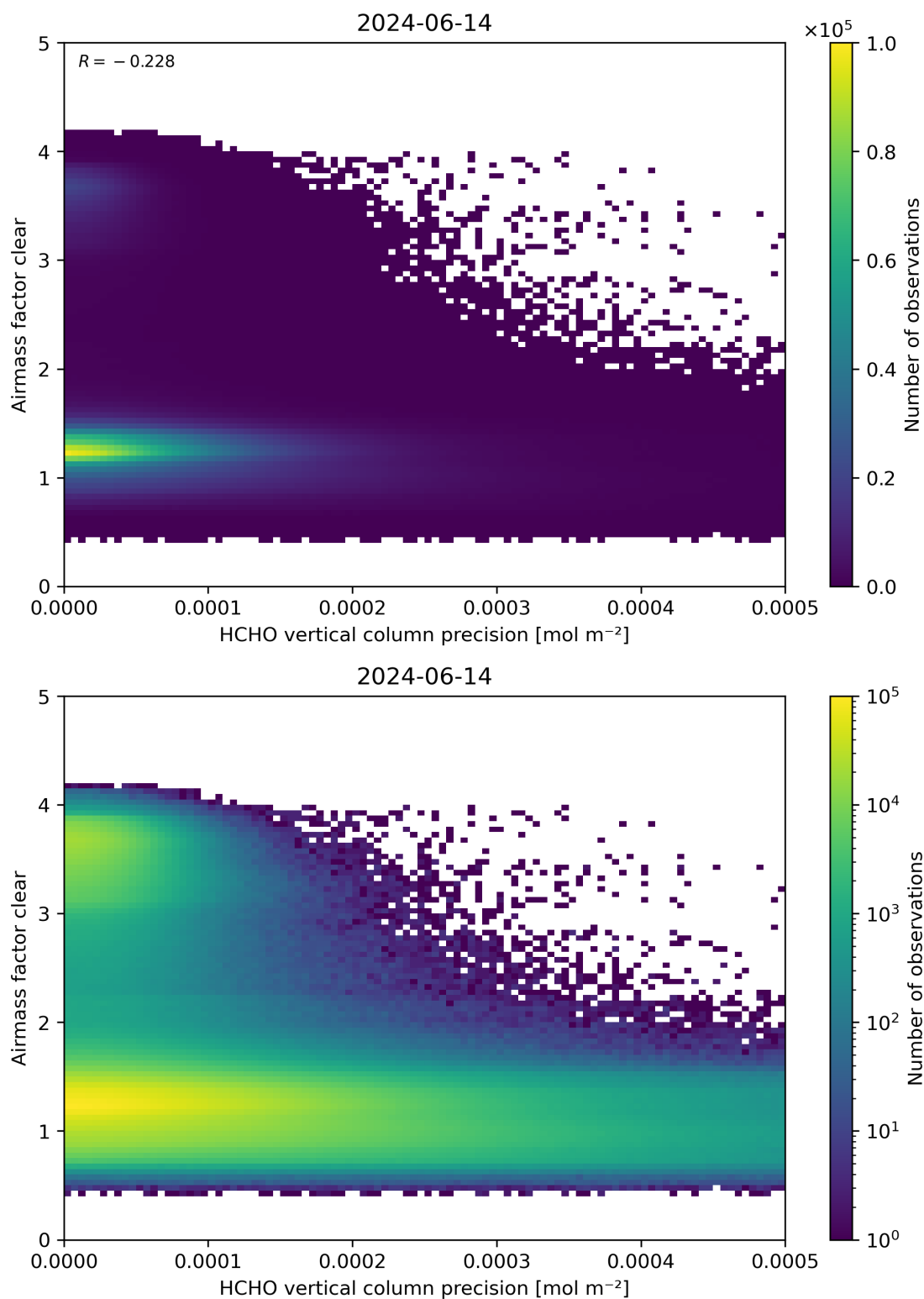
Figure 139: Scatter density plot of “HCHO vertical column precision” against “Airmass factor clear” for 2024-06-13 to 2024-06-15.
