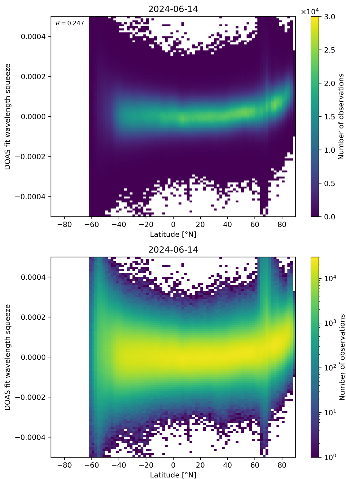
Figure 155: Scatter density plot of “Latitude” against “DOAS fit wavelength squeeze” for 2024-06-13 to 2024-06-15.
