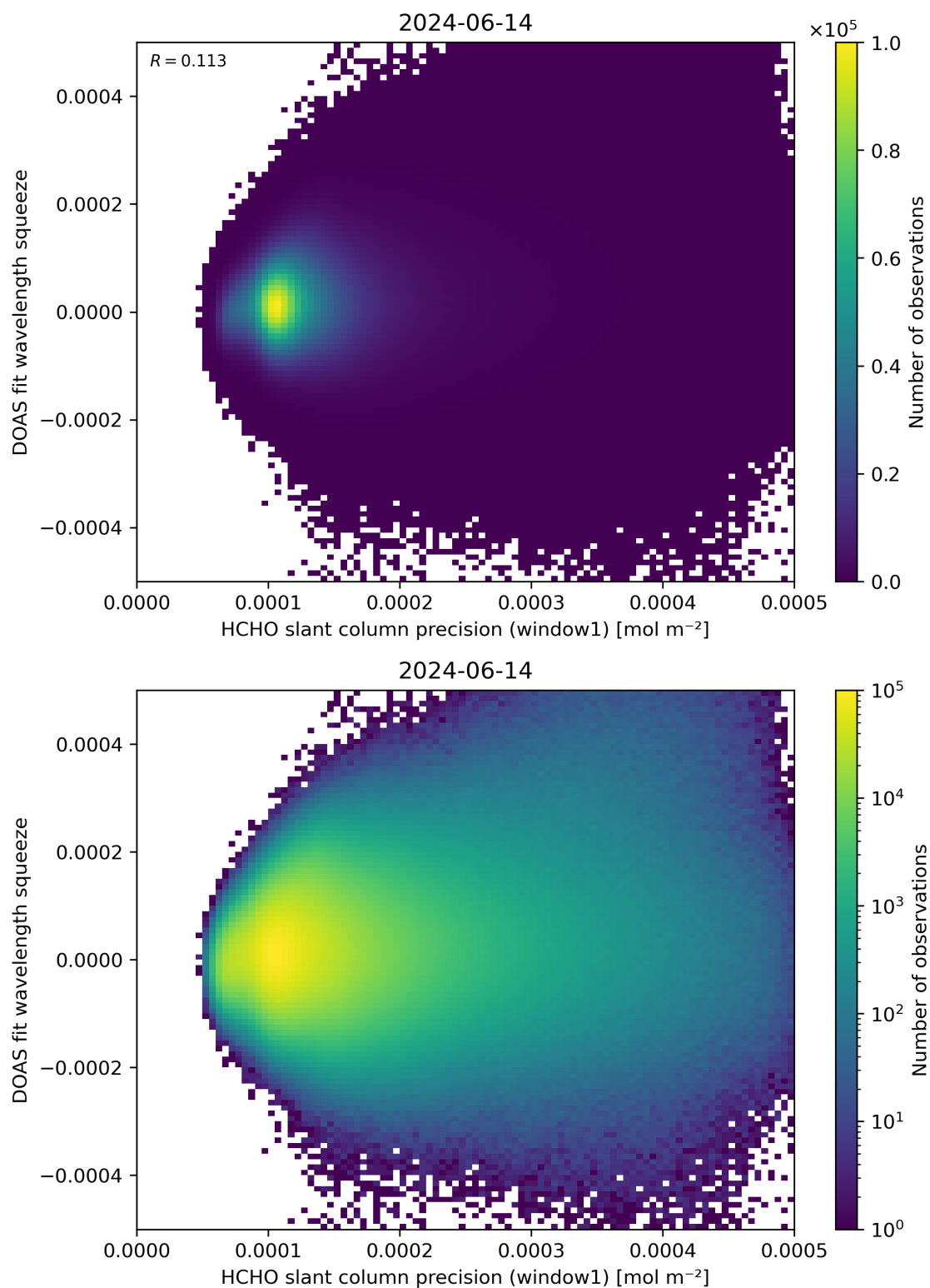
Figure 90: Scatter density plot of “HCHO slant column precision (window1)” against “DOAS fit wavelength squeeze” for 2024-06-13 to 2024-06-15.
