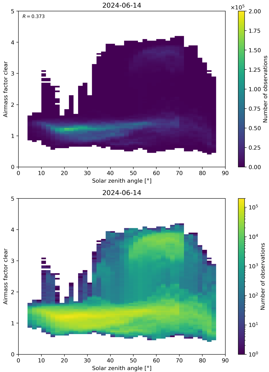
Figure 170: Scatter density plot of “Solar zenith angle” against “Airmass factor clear” for 2024-06-13 to 2024-06-15.
