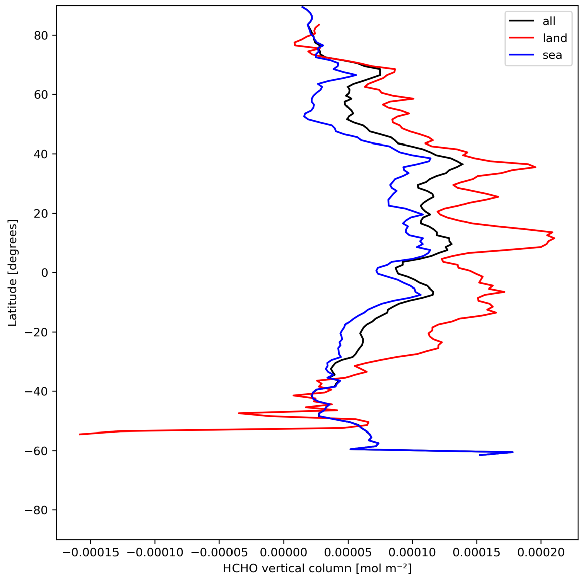
Figure 21: Zonal average of “HCHO vertical column” for 2024-06-13 to 2024-06-15.
