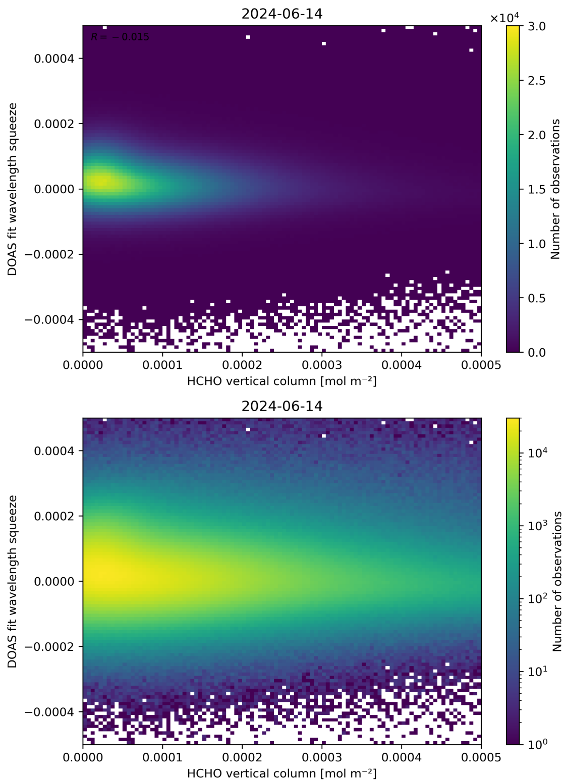
Figure 125: Scatter density plot of “HCHO vertical column” against “DOAS fit wavelength squeeze” for 2024-06-13 to 2024-06-15.
