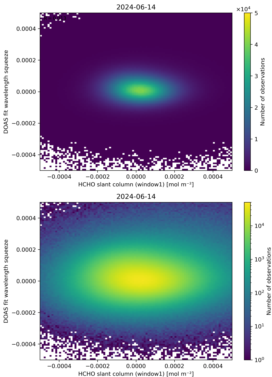
Figure 80: Scatter density plot of “HCHO slant column (window1)” against “DOAS fit wavelength squeeze” for 2024-06-13 to 2024-06-15.
