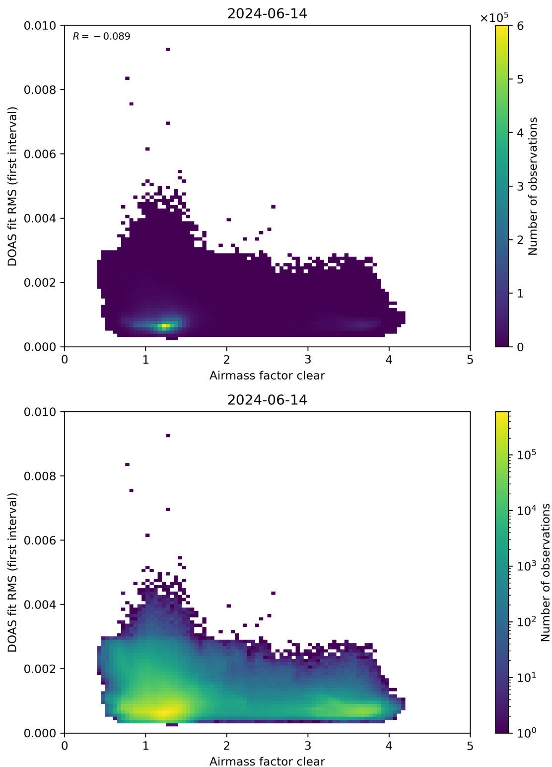
Figure 71: Scatter density plot of “Airmass factor clear” against “DOAS fit RMS (first interval)” for 2024-06-13 to 2024-06-15.
