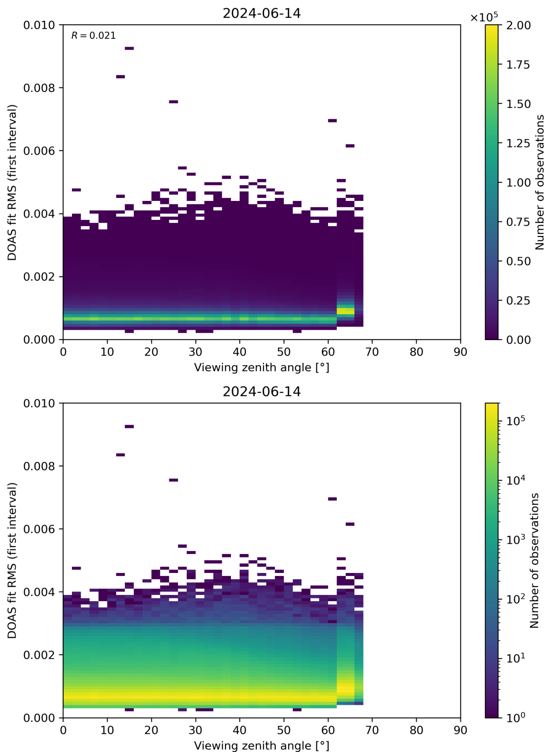
Figure 182: Scatter density plot of “Viewing zenith angle” against “DOAS fit RMS (first interval)” for 2024-06-13 to 2024-06-15.
