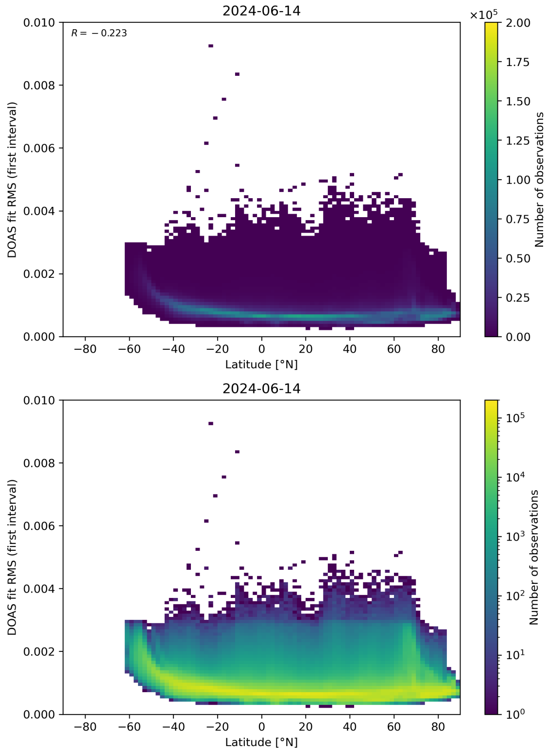
Figure 153: Scatter density plot of “Latitude” against “DOAS fit RMS (first interval)” for 2024-06-13 to 2024-06-15.
