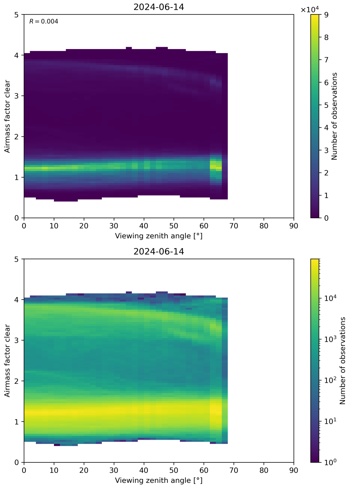
Figure 185: Scatter density plot of “Viewing zenith angle” against “Airmass factor clear” for 2024-06-13 to 2024-06-15.
