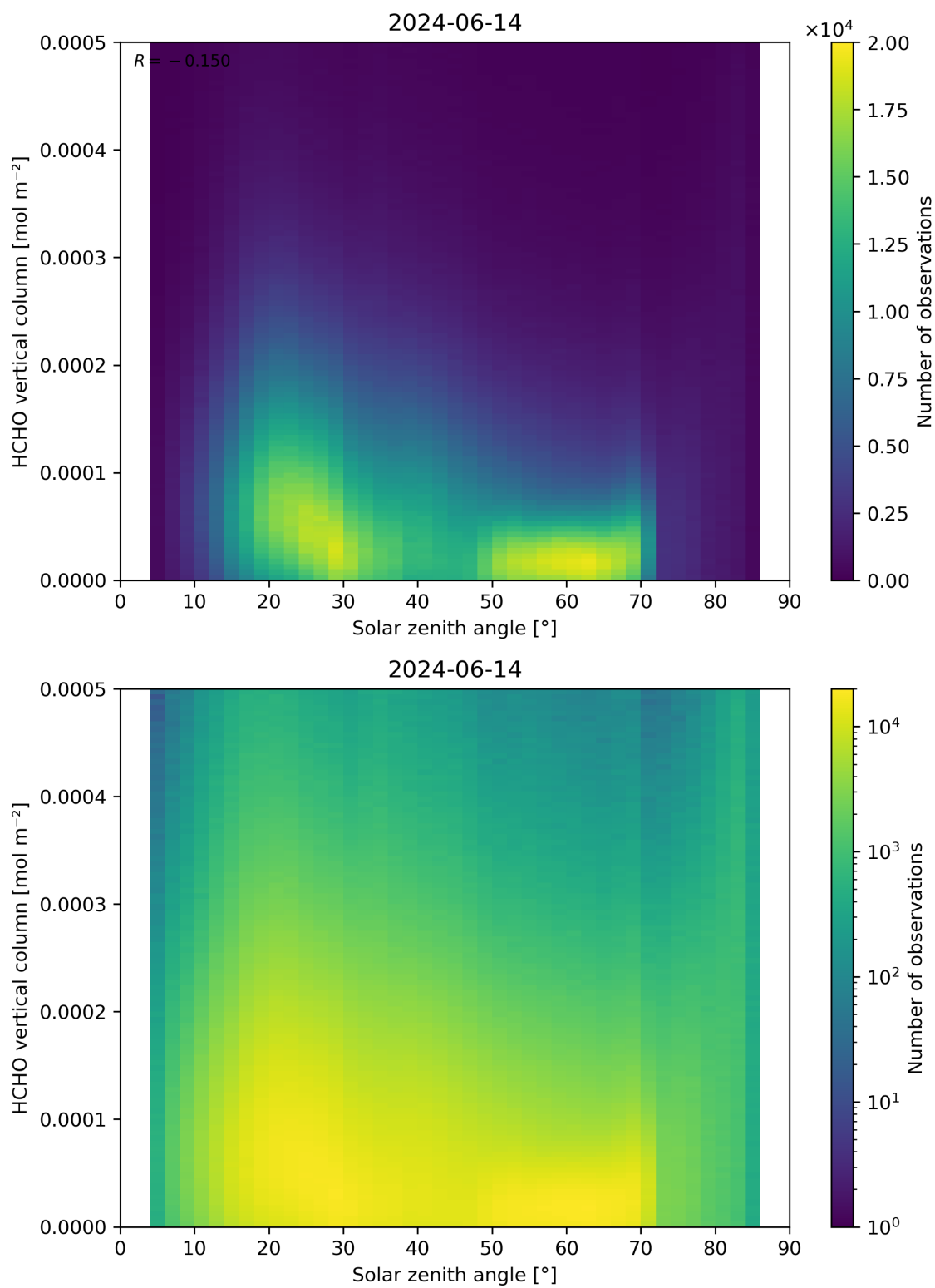
Figure 177: Scatter density plot of “Solar zenith angle” against “HCHO vertical column” for 2024-06-13 to 2024-06-15.
