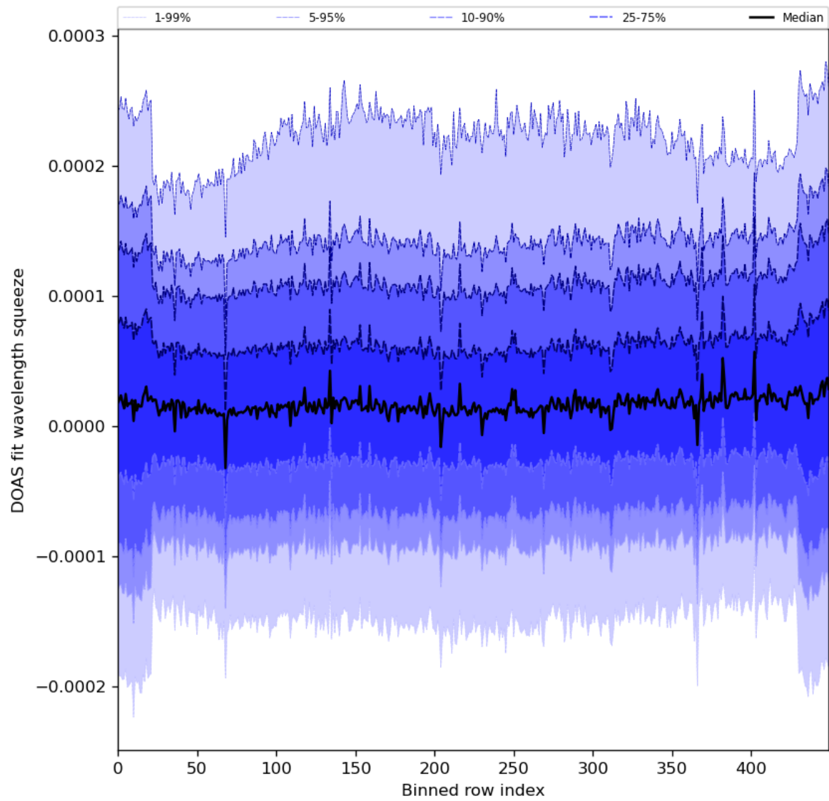
Figure 59: Along track statistics of “DOAS fit wavelength squeeze” for 2024-06-13 to 2024-06-15
