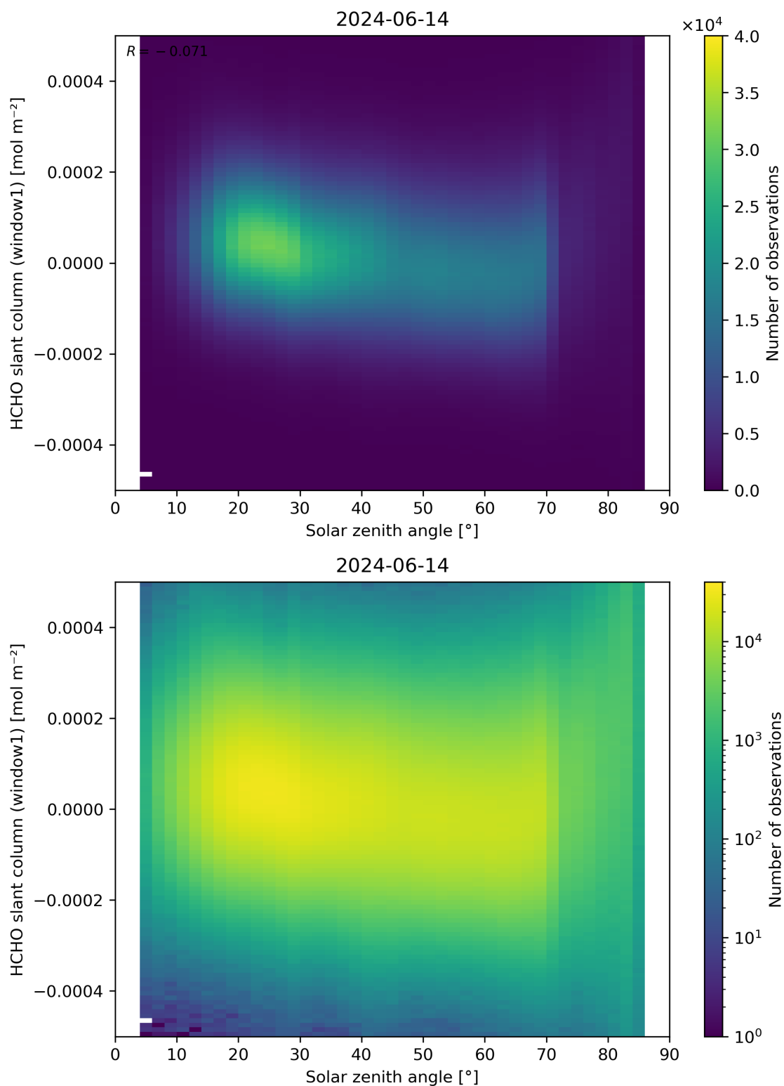
Figure 173: Scatter density plot of “Solar zenith angle” against “HCHO slant column (window1)” for 2024-06-13 to 2024-06-15.
