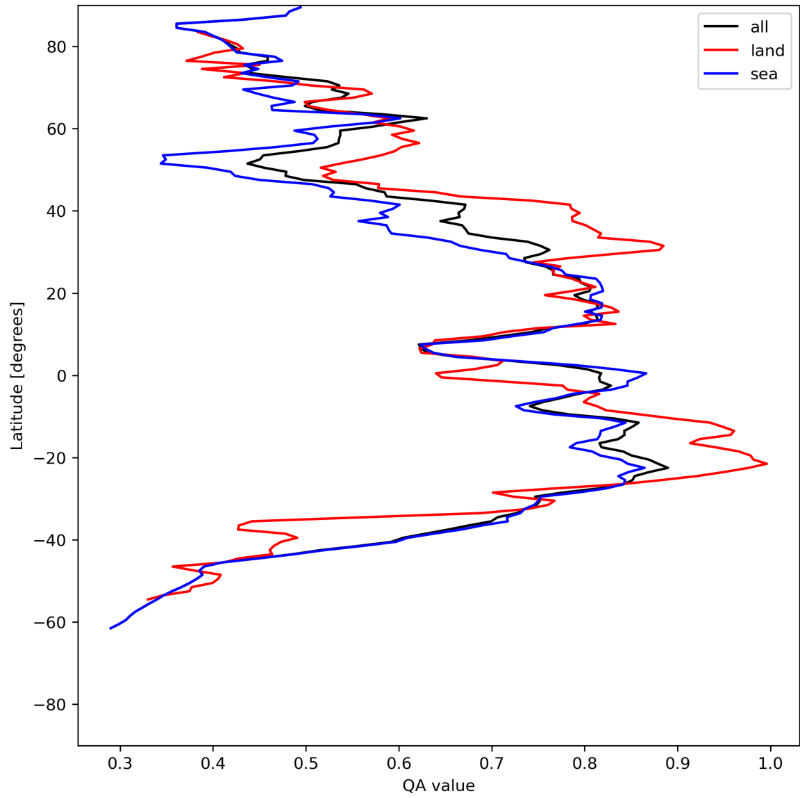
Figure 20: Zonal average of “QA value” for 2024-06-13 to 2024-06-15.
