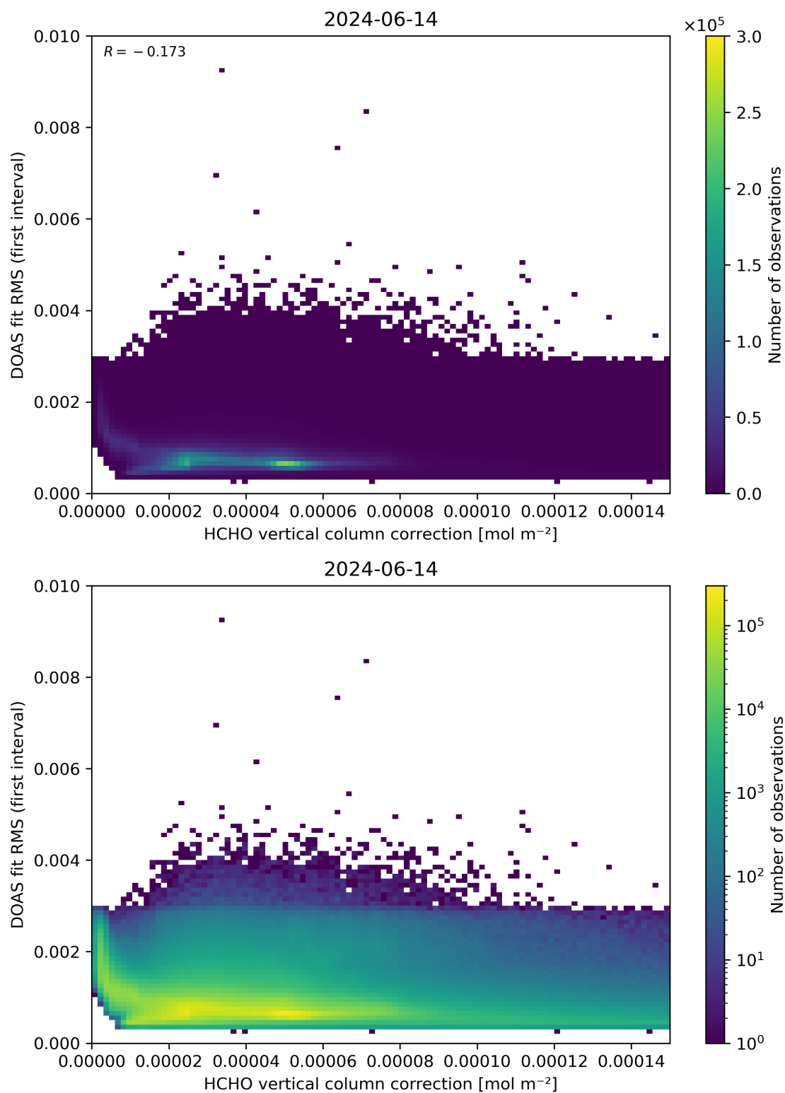
Figure 112: Scatter density plot of “HCHO vertical column correction” against “DOAS fit RMS (first interval)” for 2024-06-13 to 2024-06-15.
