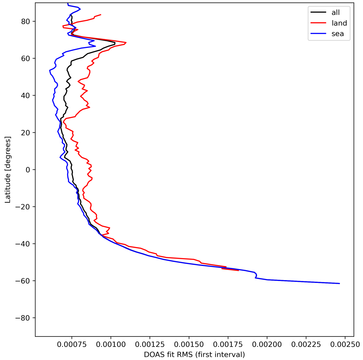
Figure 32: Zonal average of “DOAS fit RMS (first interval)” for 2024-06-13 to 2024-06-15.
