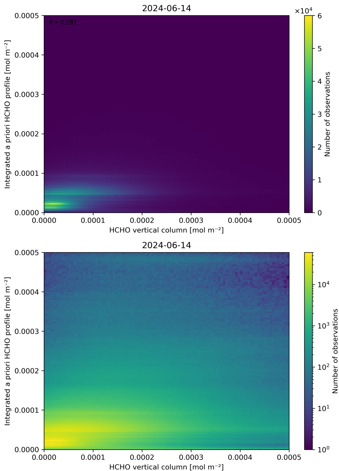
Figure 135: Scatter density plot of “HCHO vertical column” against “Integrated a priori HCHO profile” for 2024-06-13 to 2024-06-15.
