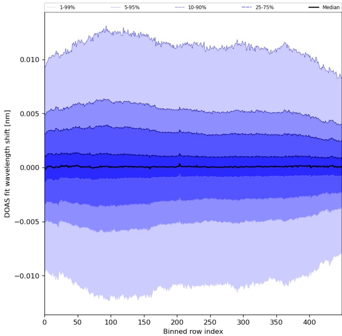
Figure 58: Along track statistics of “DOAS fit wavelength shift” for 2024-06-13 to 2024-06-15
