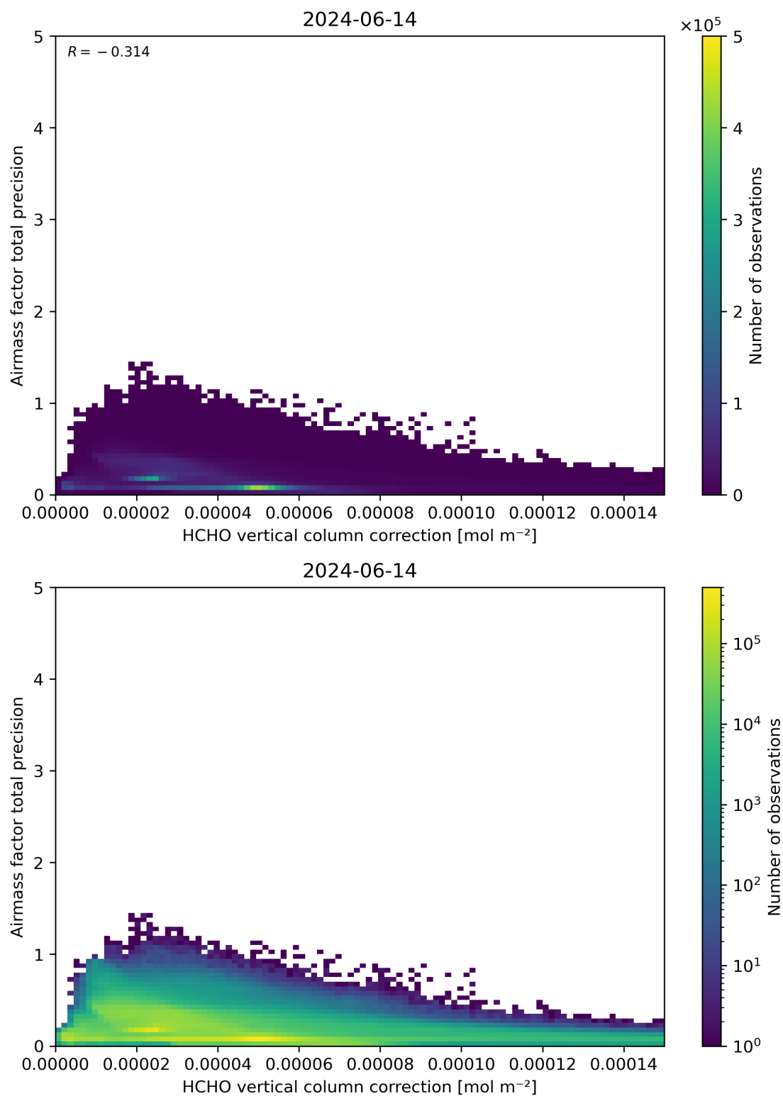
Figure 121: Scatter density plot of “HCHO vertical column correction” against “Airmass factor total precision” for 2024-06-13 to 2024-06-15.
