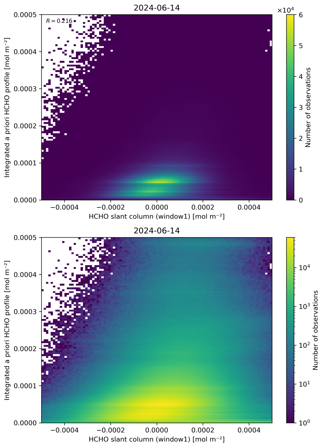
Figure 87: Scatter density plot of “HCHO slant column (window1)” against “Integrated a priori HCHO profile” for 2024-06-13 to 2024-06-15.
