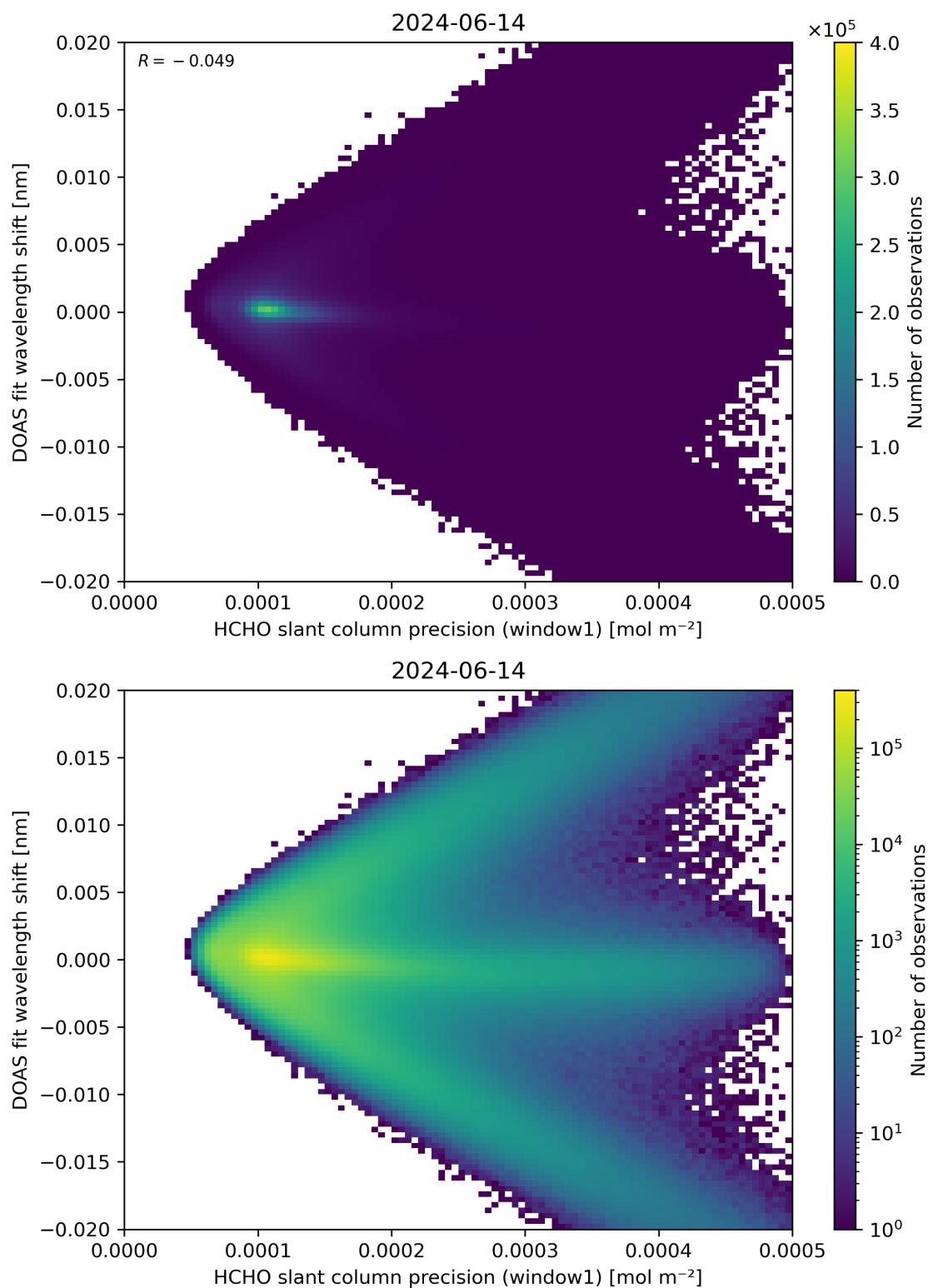
Figure 89: Scatter density plot of “HCHO slant column precision (window1)” against “DOAS fit wavelength shift” for 2024-06-13 to 2024-06-15.
