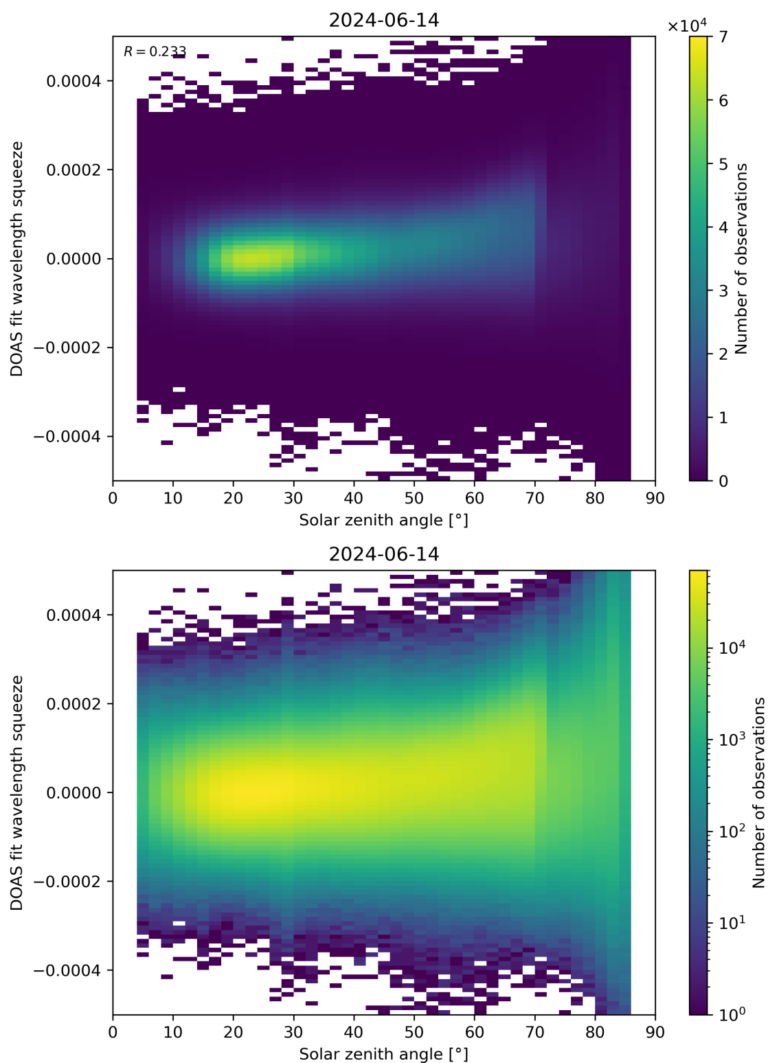
Figure 169: Scatter density plot of “Solar zenith angle” against “DOAS fit wavelength squeeze” for 2024-06-13 to 2024-06-15.
