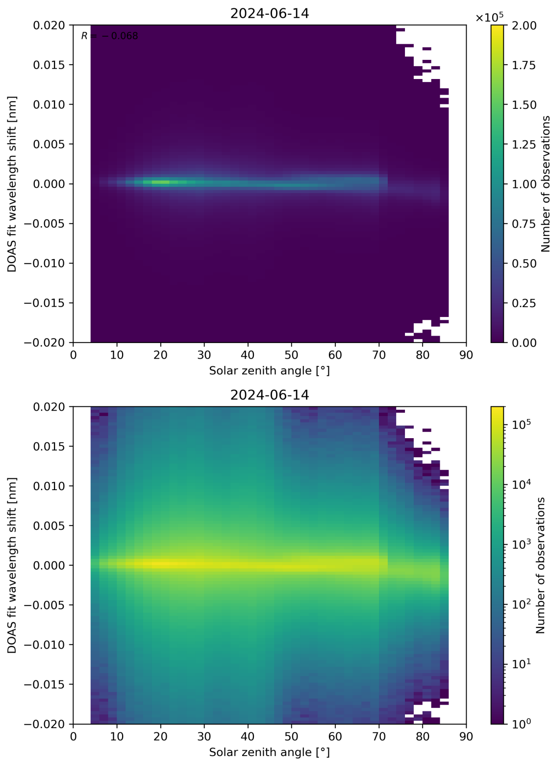
Figure 168: Scatter density plot of “Solar zenith angle” against “DOAS fit wavelength shift” for 2024-06-13 to 2024-06-15.
