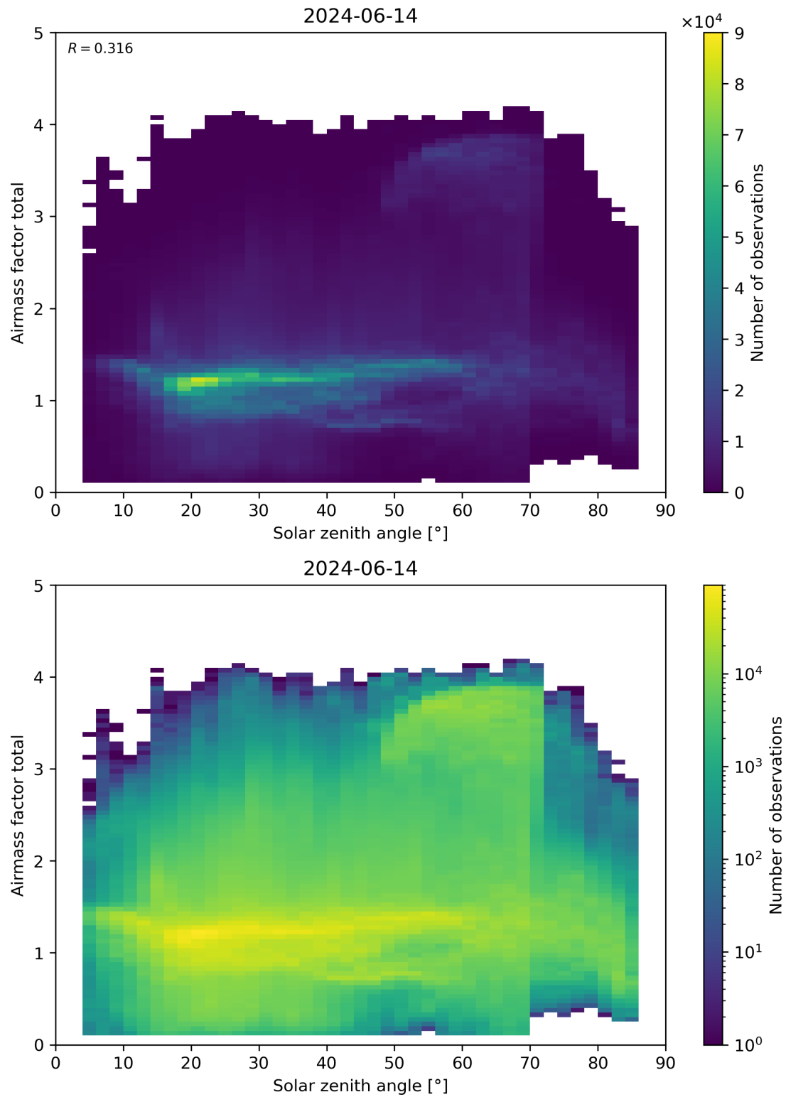
Figure 175: Scatter density plot of “Solar zenith angle” against “Airmass factor total” for 2024-06-13 to 2024-06-15.
