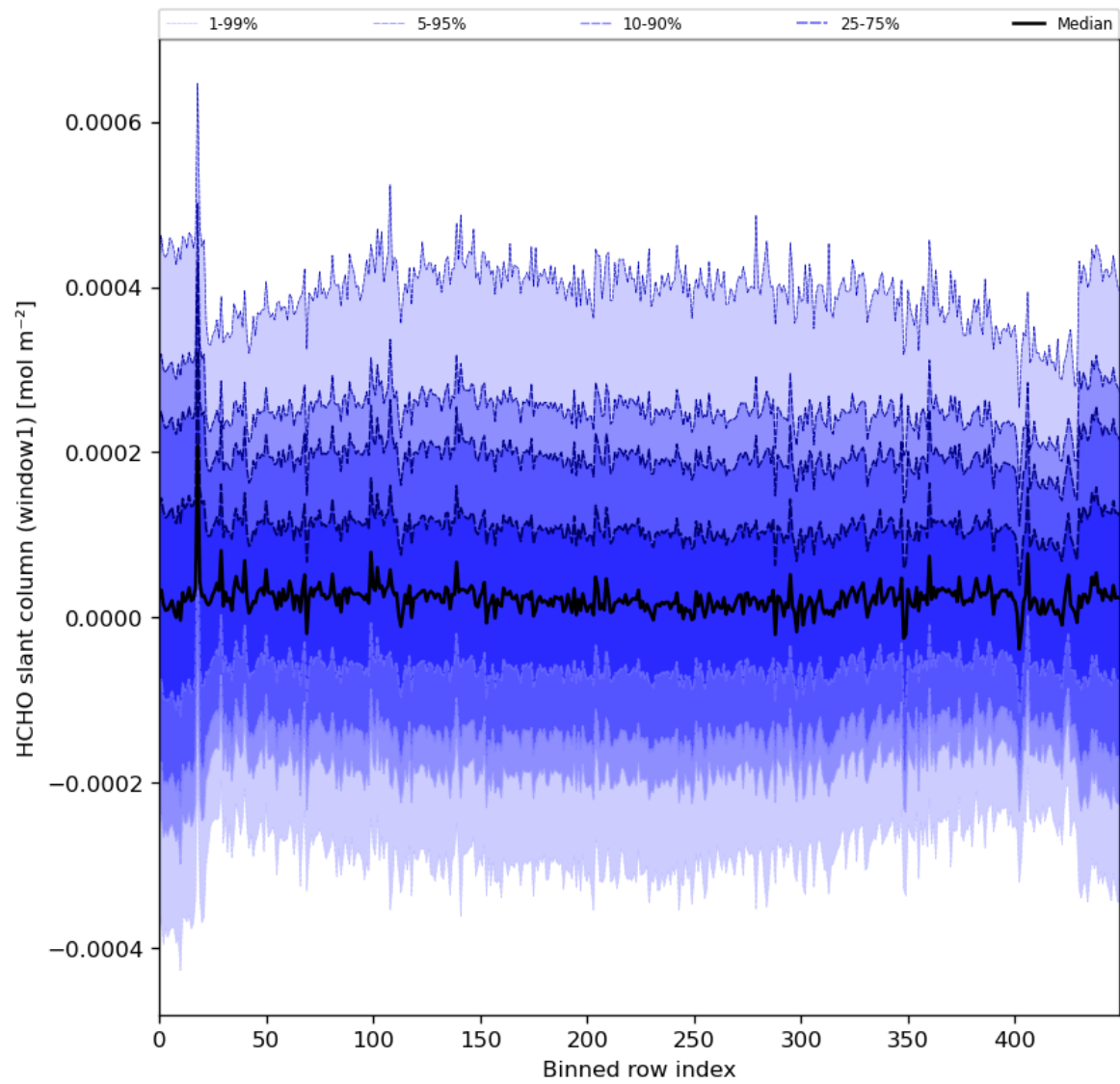
Figure 52: Along track statistics of "HCHO slant column (window1)" for 2024-06-13 to 2024-06-15
