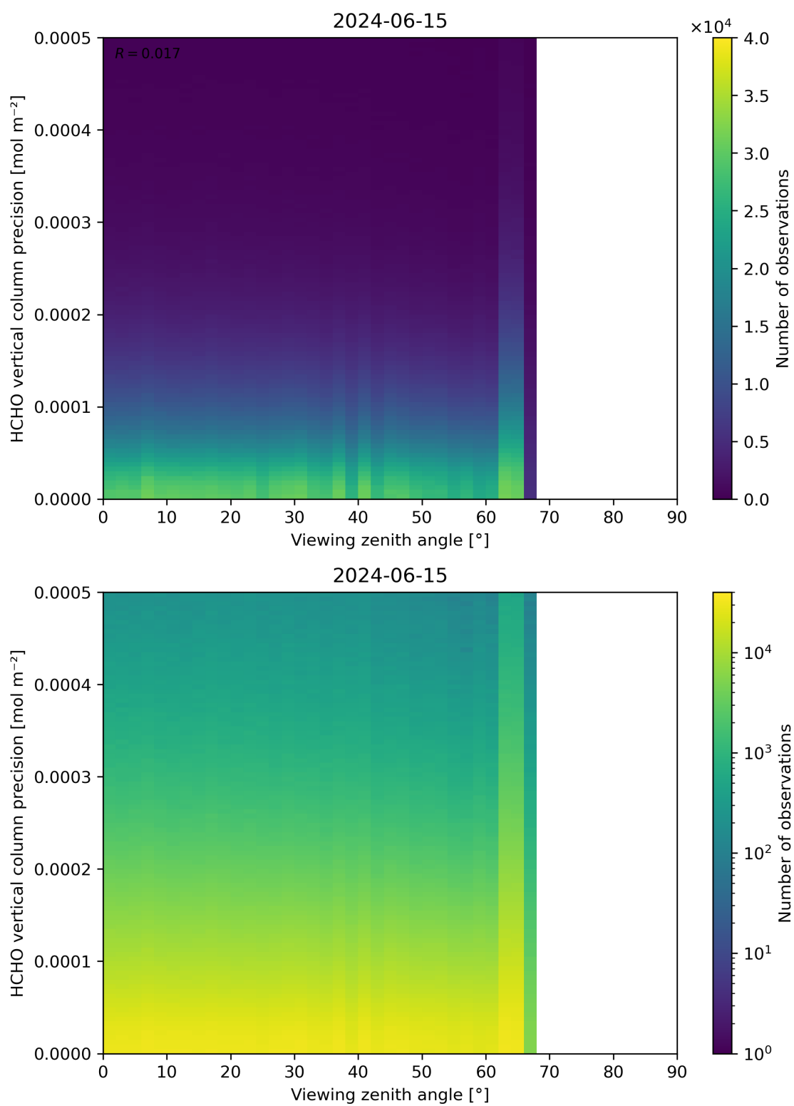
Figure 194: Scatter density plot of “Viewing zenith angle” against “HCHO vertical column precision” for 2024-06-14 to 2024-06-16.
