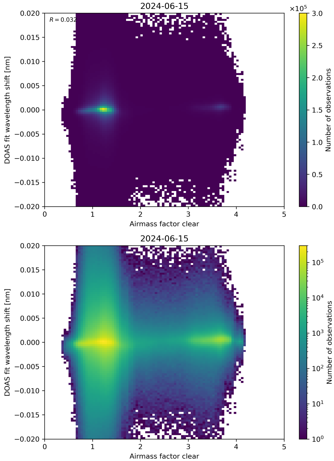
Figure 72: Scatter density plot of “Airmass factor clear” against “DOAS fit wavelength shift” for 2024-06-14 to 2024-06-16.
