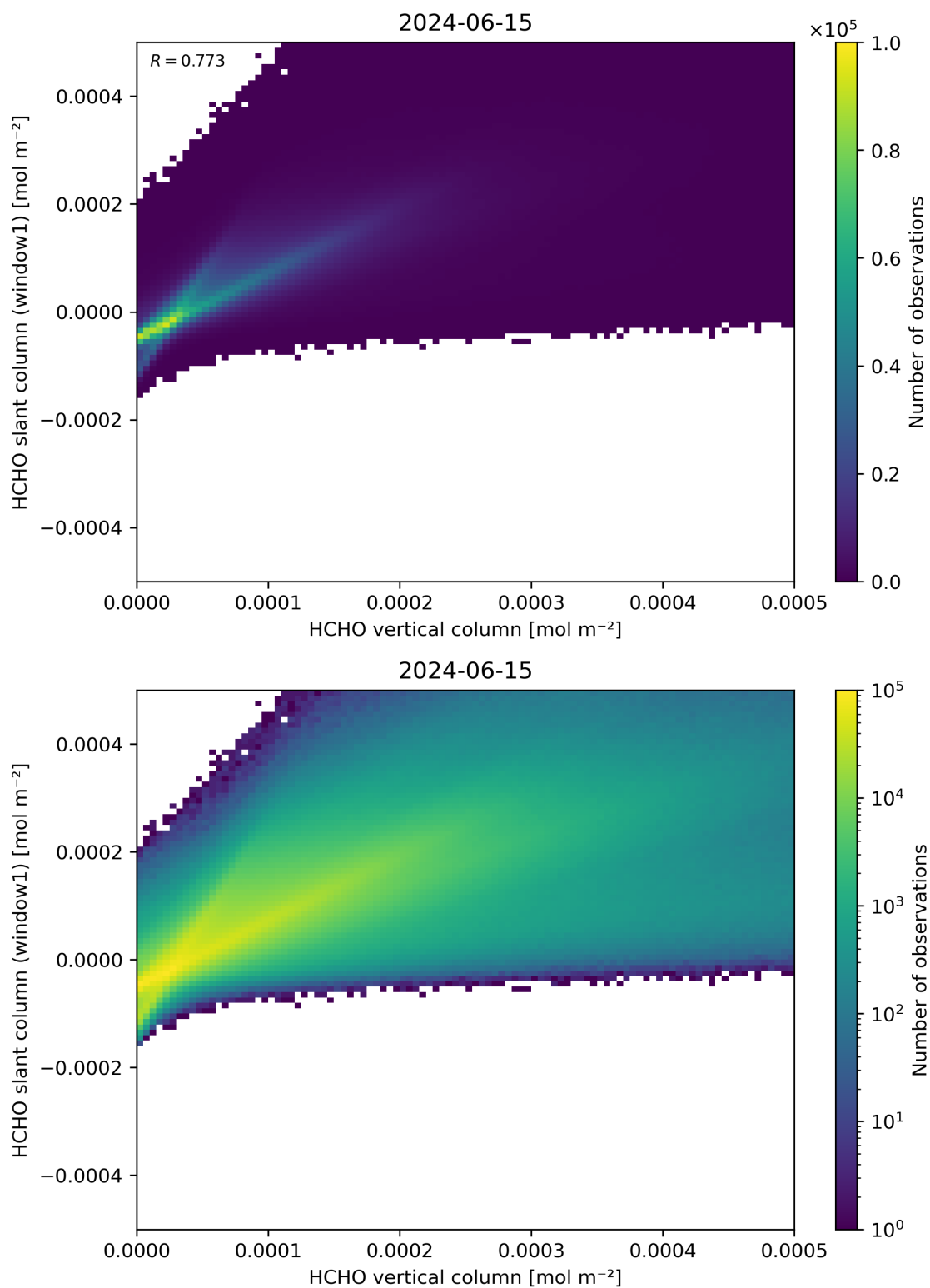
Figure 129: Scatter density plot of “HCHO vertical column” against “HCHO slant column (window1)” for 2024-06-14 to 2024-06-16.
