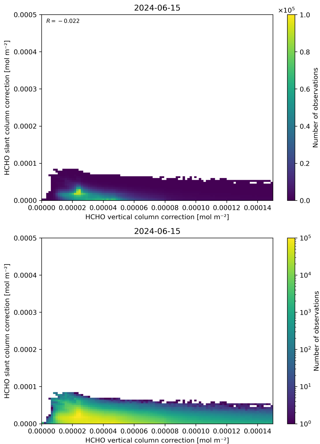
Figure 117: Scatter density plot of “HCHO vertical column correction” against “HCHO slant column correction” for 2024-06-14 to 2024-06-16.
