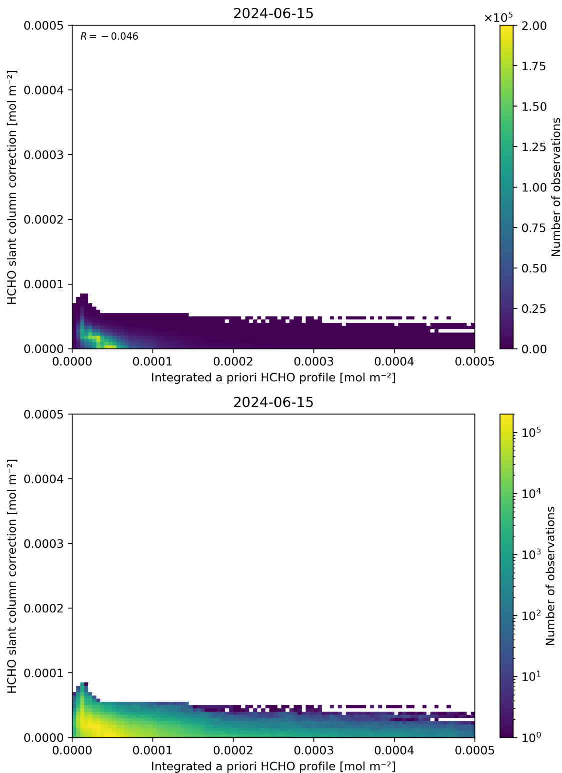
Figure 152: Scatter density plot of “Integrated a priori HCHO profile” against “HCHO slant column correction” for 2024-06-14 to 2024-06-16.
