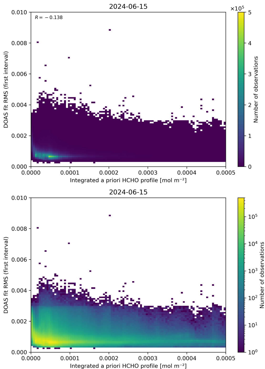
Figure 148: Scatter density plot of “Integrated a priori HCHO profile” against “DOAS fit RMS (first interval)” for 2024-06-14 to 2024-06-16.
