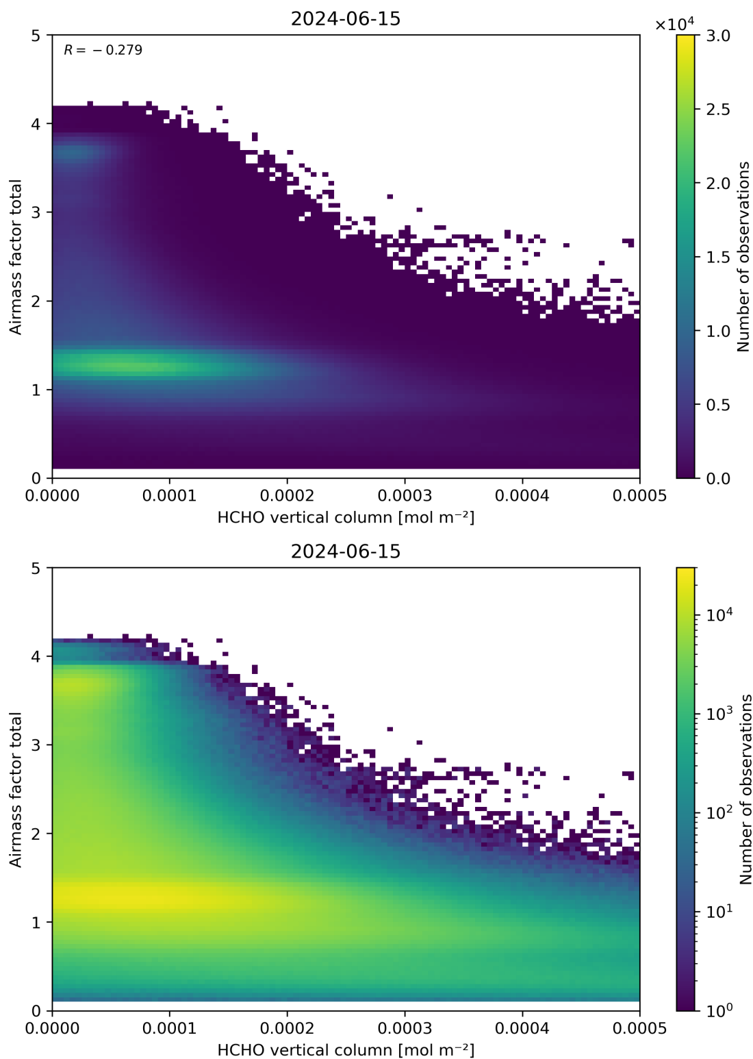
Figure 131: Scatter density plot of “HCHO vertical column” against “Airmass factor total” for 2024-06-14 to 2024-06-16.
