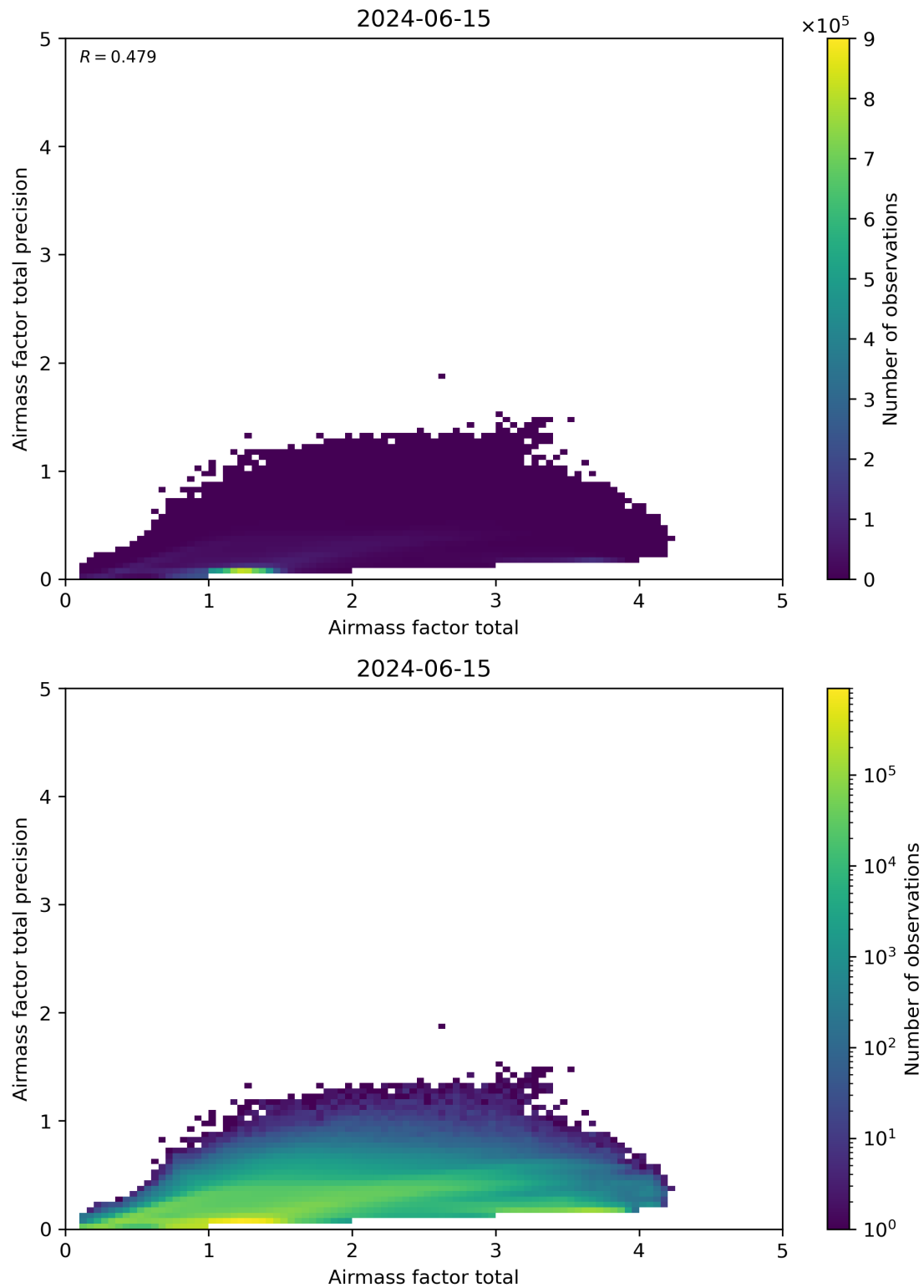
Figure 103: Scatter density plot of “Airmass factor total” against “Airmass factor total precision” for 2024-06-14 to 2024-06-16.
