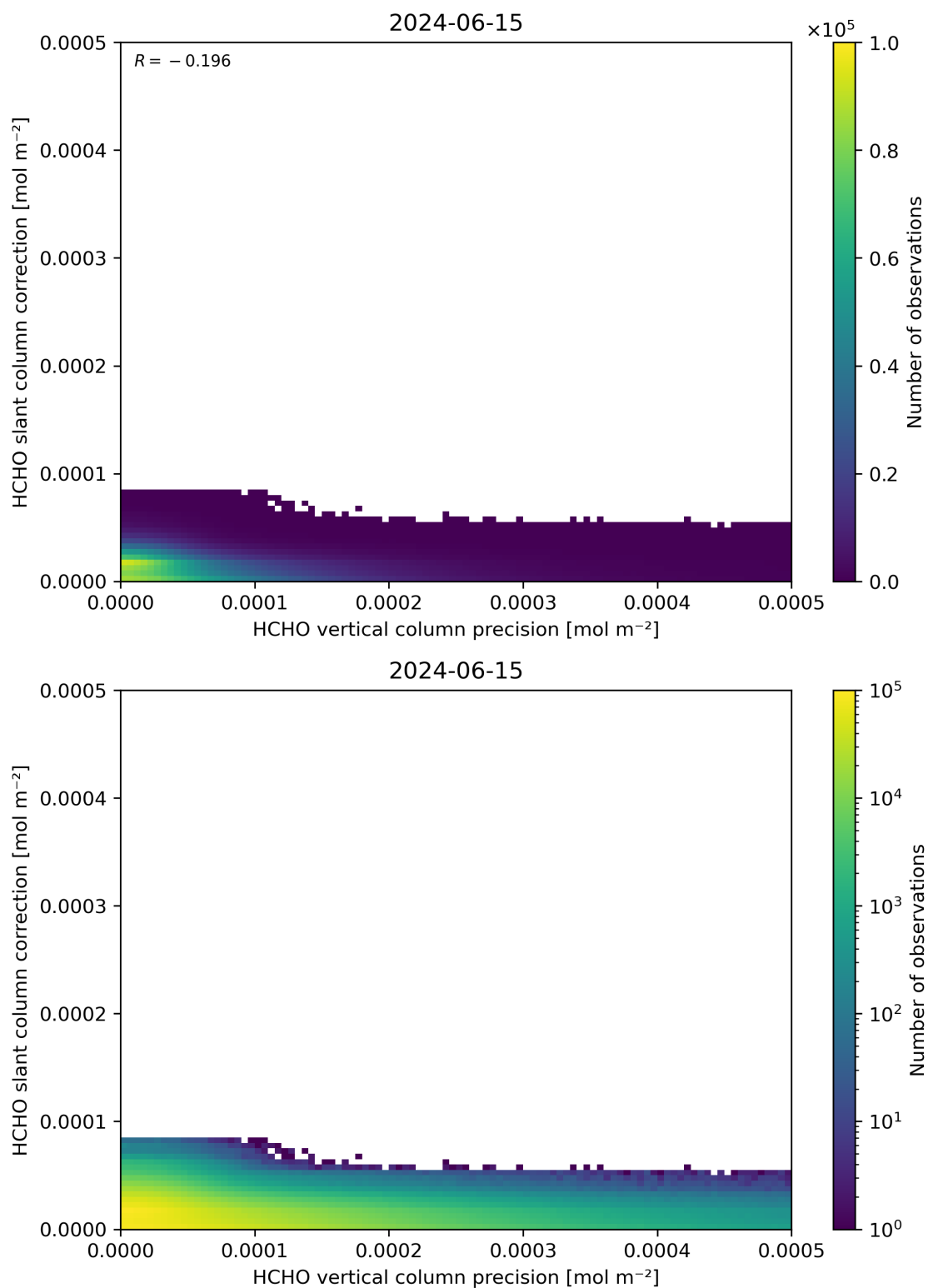
Figure 141: Scatter density plot of “HCHO vertical column precision” against “HCHO slant column correction” for 2024-06-14 to 2024-06-16.
