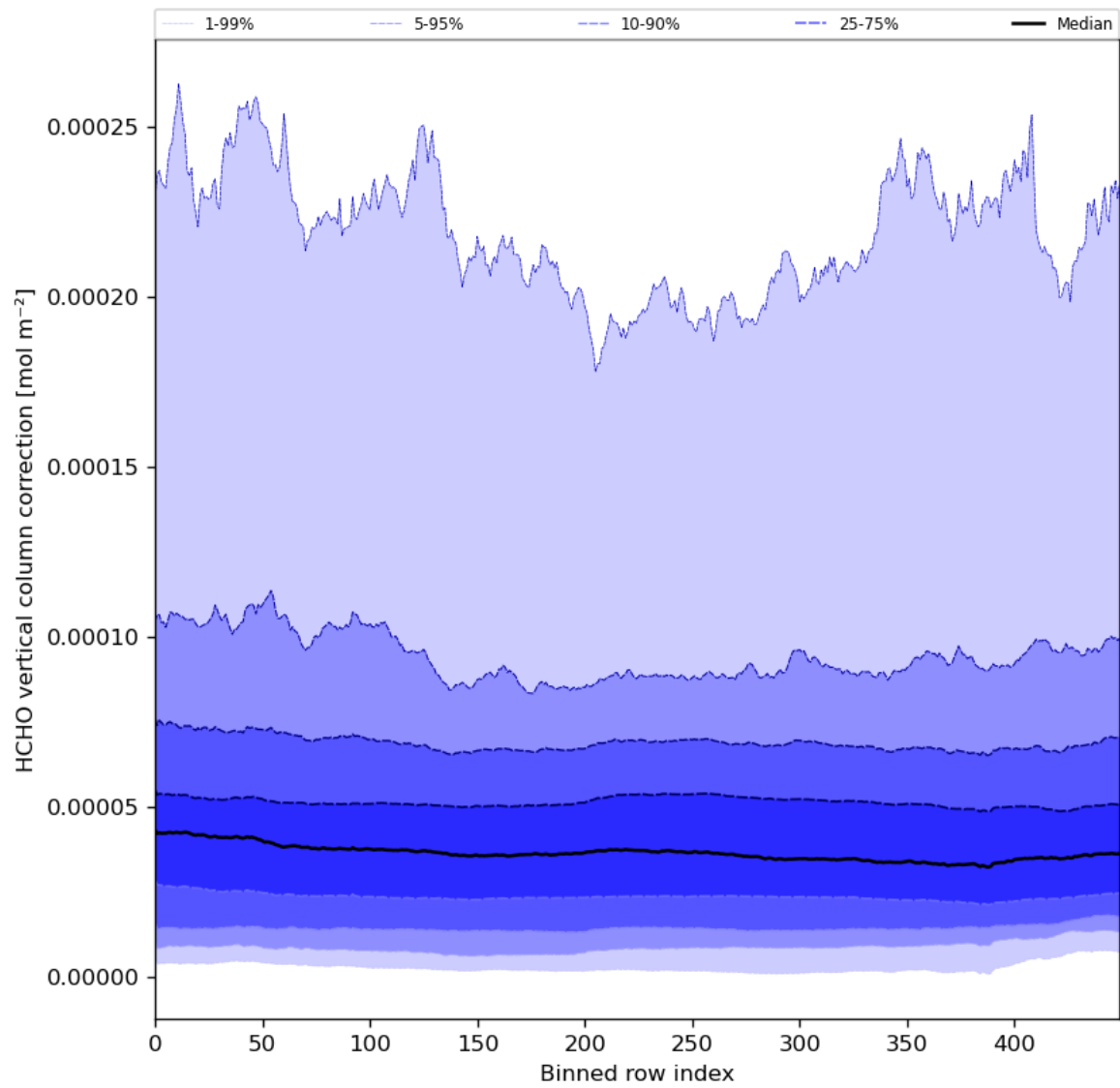
Figure 51: Along track statistics of “HCHO vertical column correction” for 2024-06-14 to 2024-06-16
