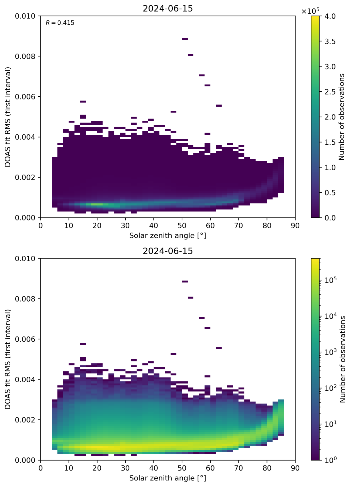
Figure 167: Scatter density plot of “Solar zenith angle” against “DOAS fit RMS (first interval)” for 2024-06-14 to 2024-06-16.
