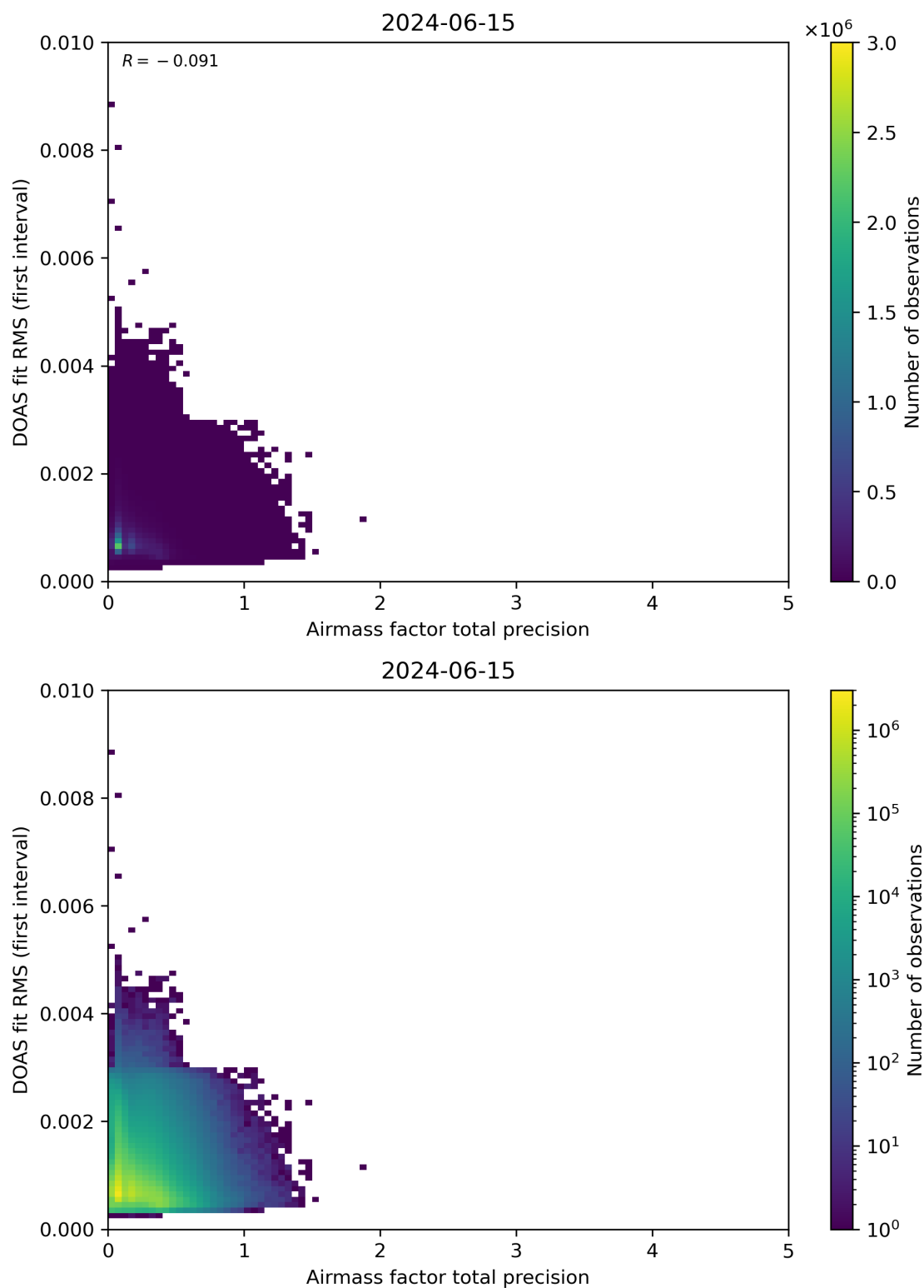
Figure 105: Scatter density plot of “Airmass factor total precision” against “DOAS fit RMS (first interval)” for 2024-06-14 to 2024-06-16.
