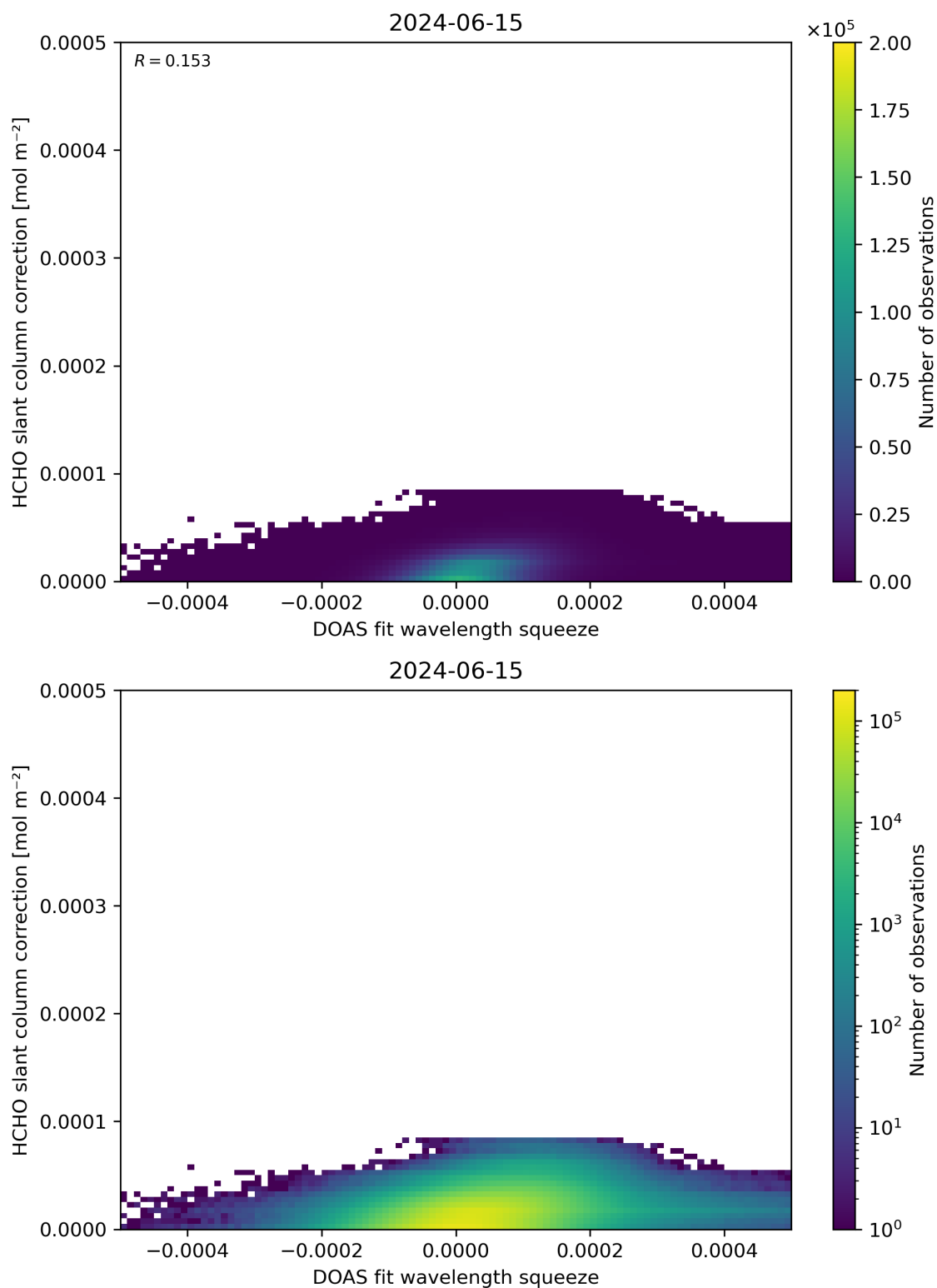
Figure 70: Scatter density plot of “DOAS fit wavelength squeeze” against “HCHO slant column correction” for 2024-06-14 to 2024-06-16.
