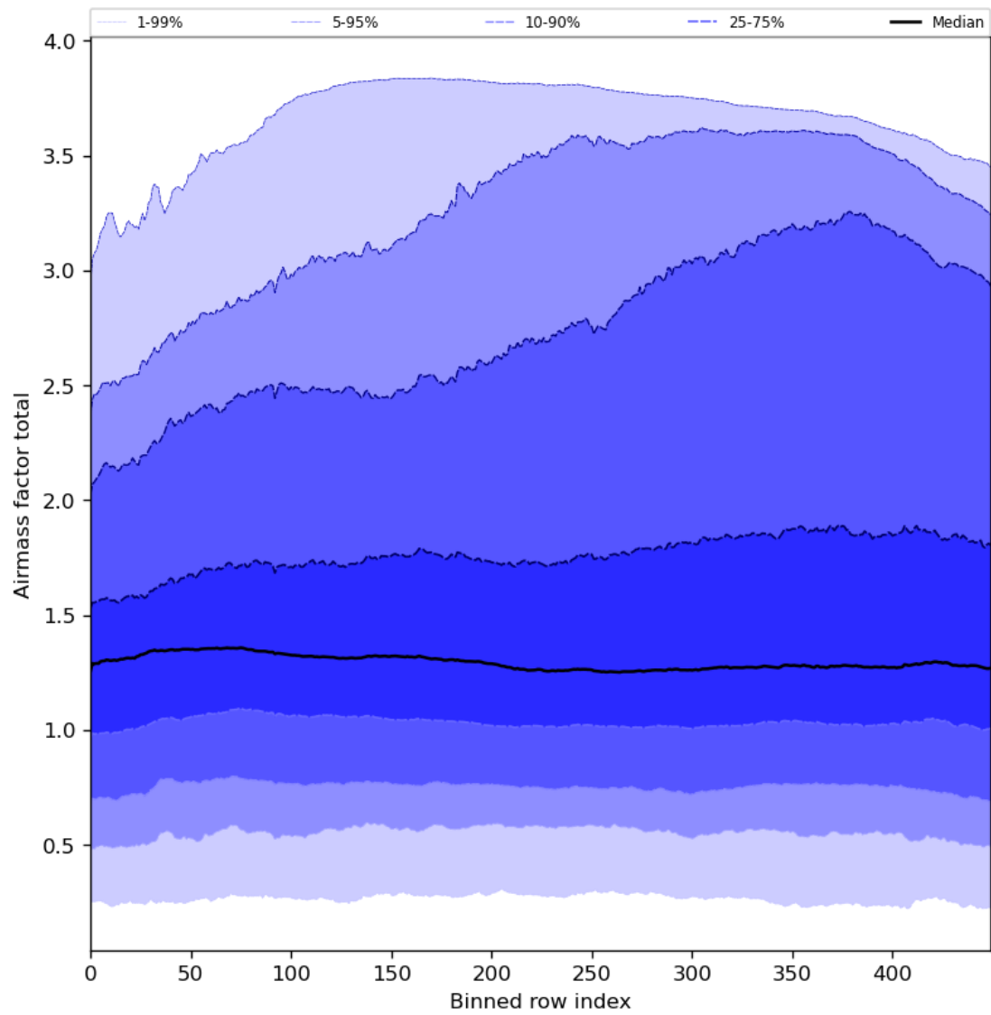
Figure 54: Along track statistics of “Airmass factor total” for 2024-06-14 to 2024-06-16
