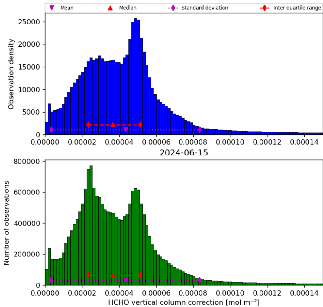
Figure 37: Histogram of “HCHO vertical column correction” for 2024-06-14 to 2024-06-16
