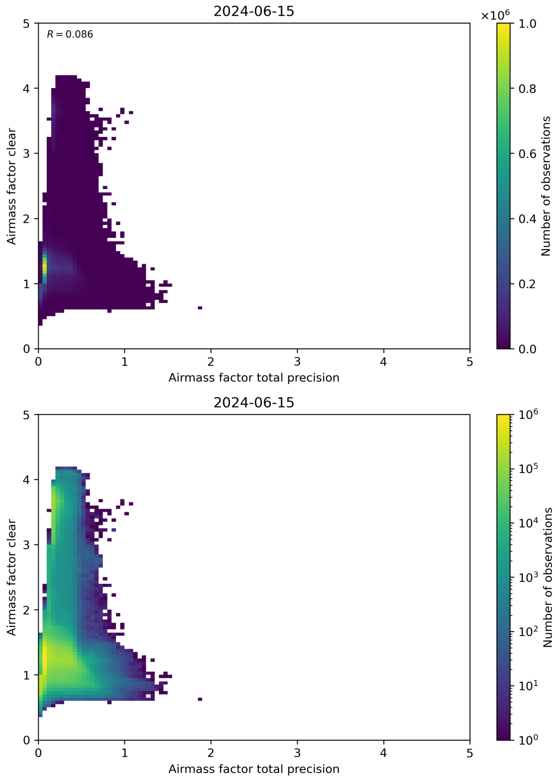
Figure 108: Scatter density plot of “Airmass factor total precision” against “Airmass factor clear” for 2024-06-14 to 2024-06-16.
