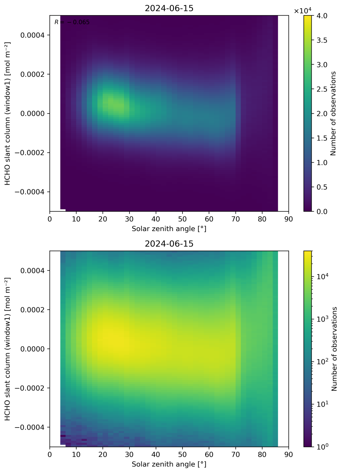
Figure 173: Scatter density plot of “Solar zenith angle” against “HCHO slant column (window1)” for 2024-06-14 to 2024-06-16.
