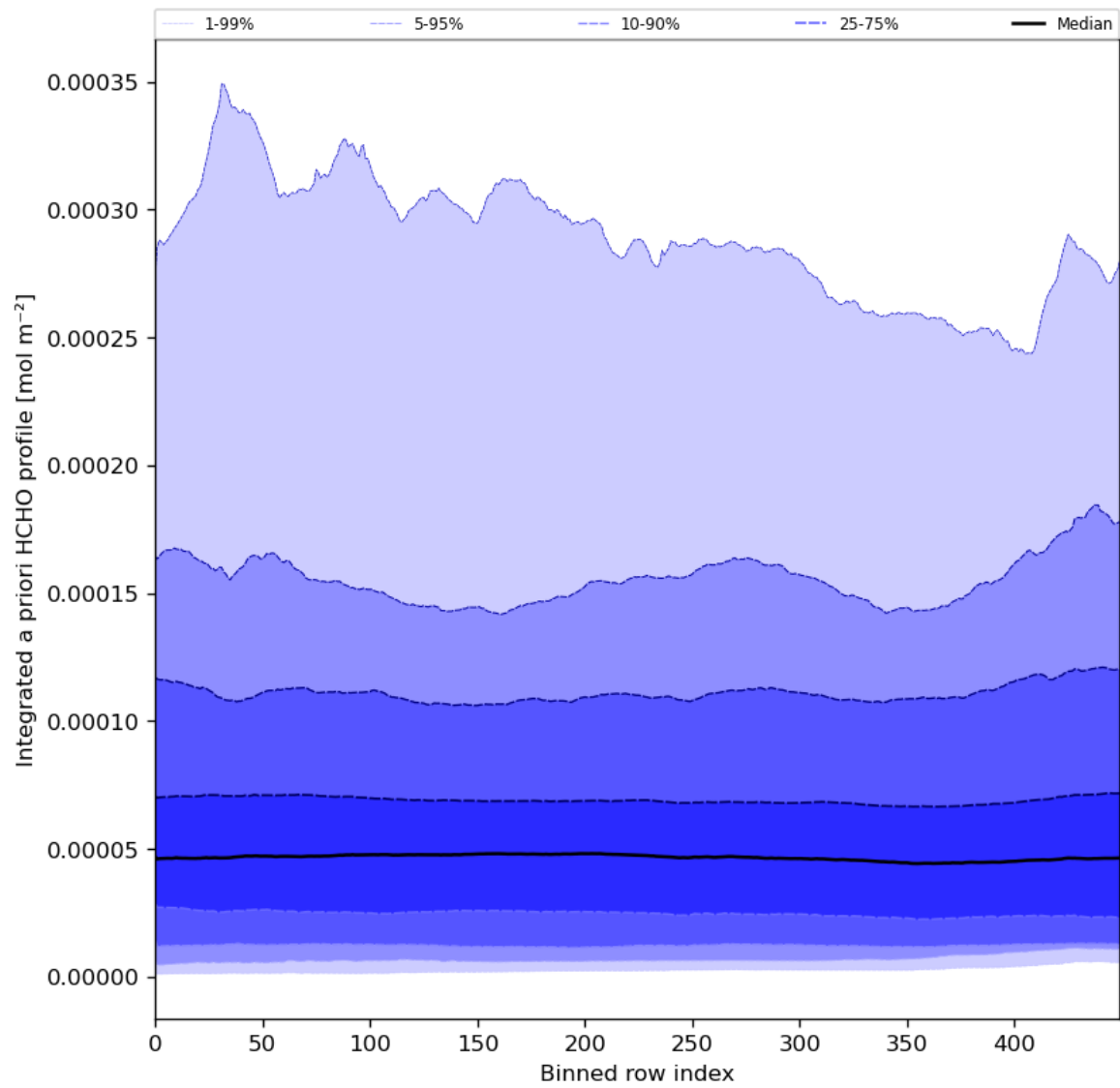
Figure 57: Along track statistics of "Integrated a priori HCHO profile" for 2024-06-14 to 2024-06-16
