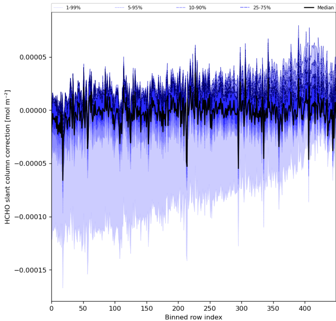
Figure 61: Along track statistics of “HCHO slant column correction” for 2024-06-14 to 2024-06-16
