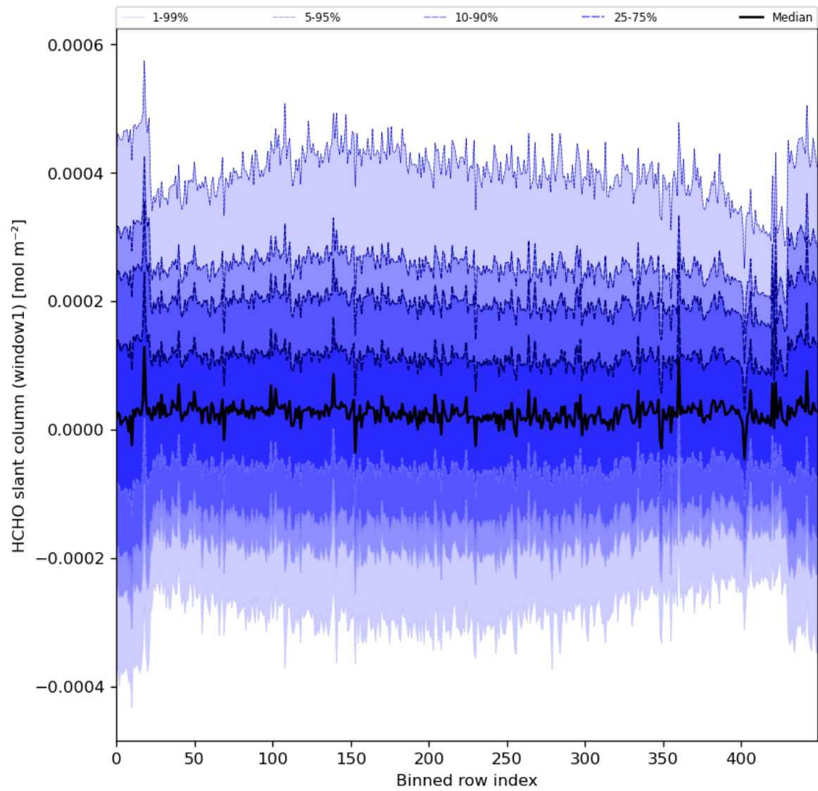
Figure 52: Along track statistics of “HCHO slant column (window1)” for 2024-06-14 to 2024-06-16
