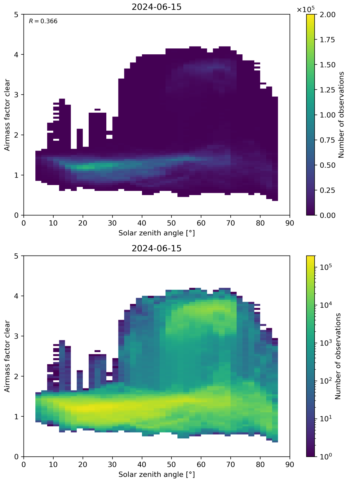
Figure 170: Scatter density plot of “Solar zenith angle” against “Airmass factor clear” for 2024-06-14 to 2024-06-16.
