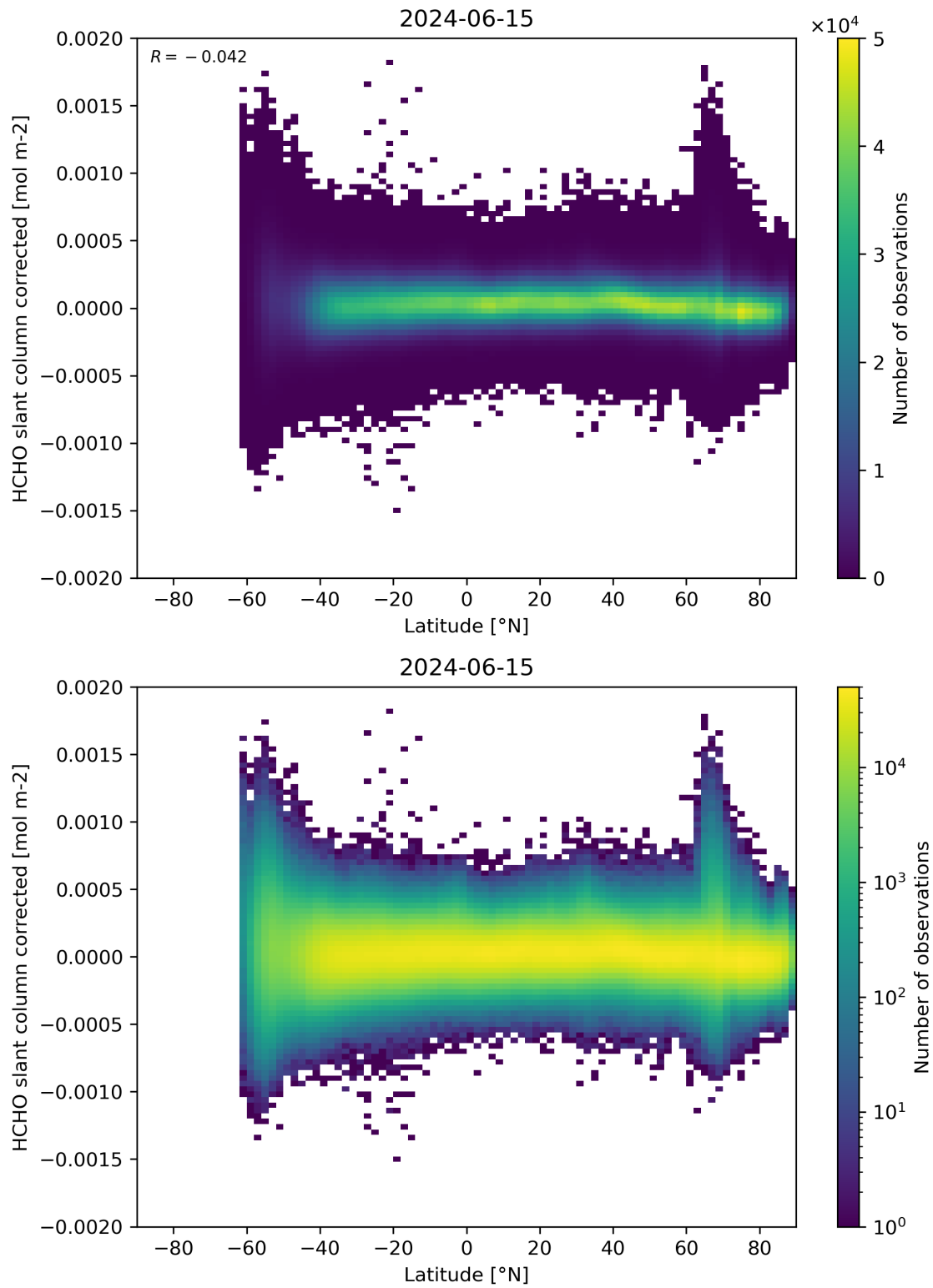
Figure 157: Scatter density plot of “Latitude” against “HCHO slant column corrected” for 2024-06-14 to 2024-06-16.
