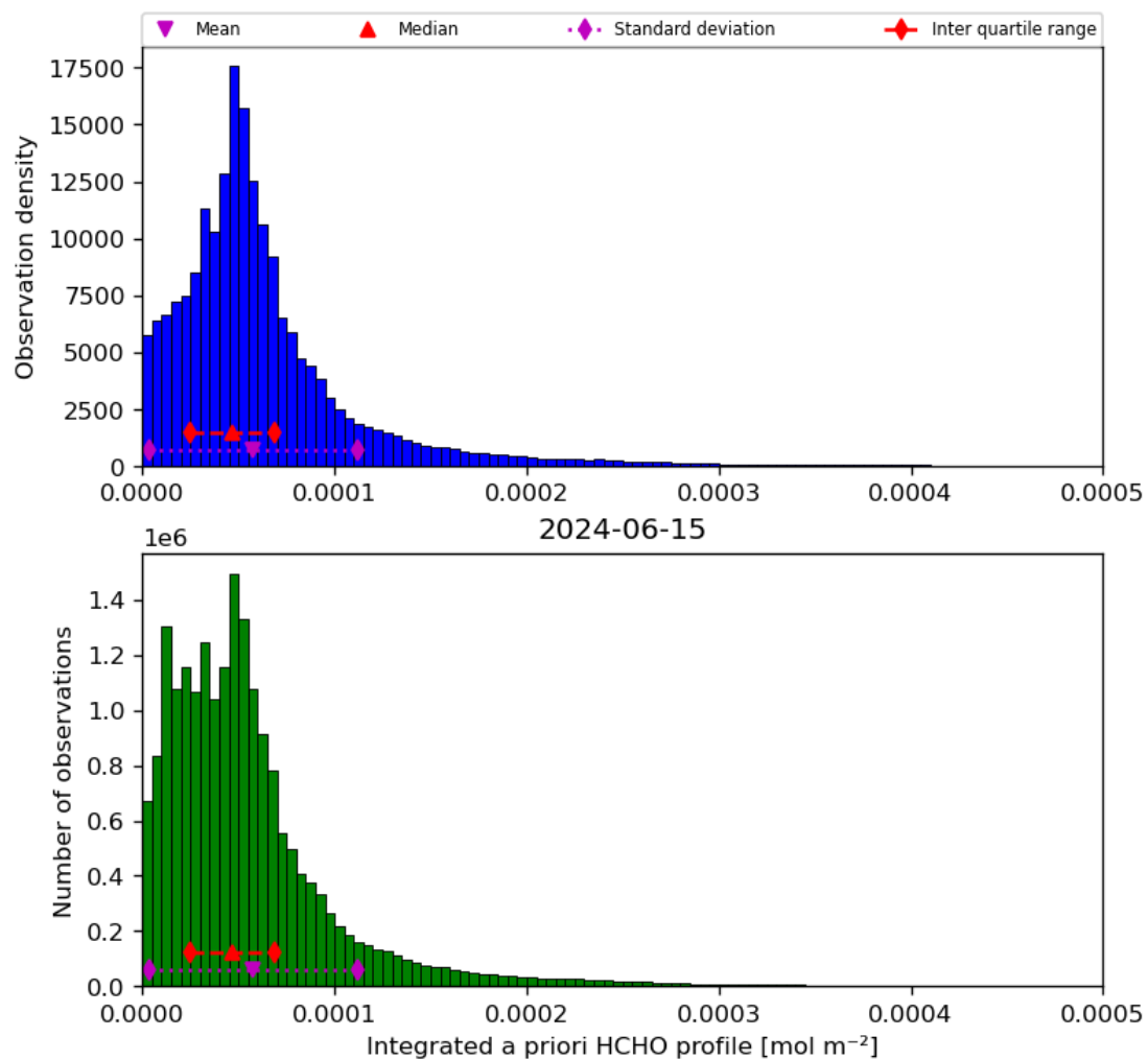
Figure 43: Histogram of “Integrated a priori HCHO profile” for 2024-06-14 to 2024-06-16
