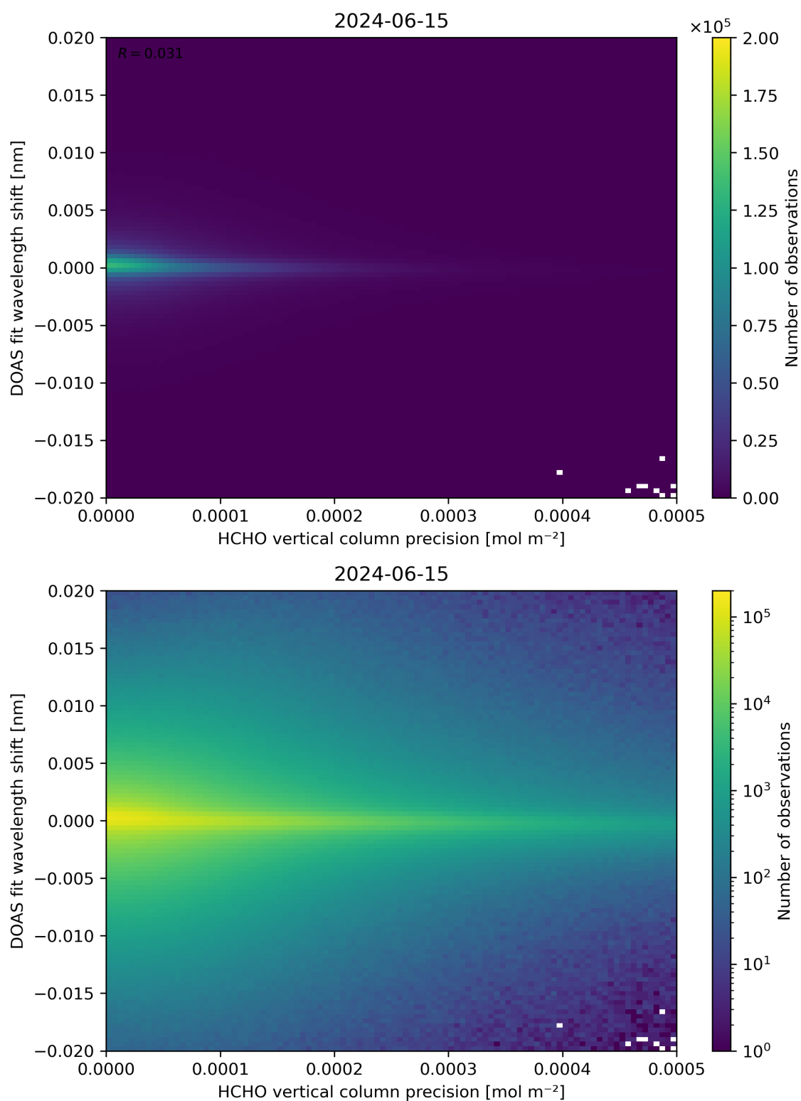
Figure 137: Scatter density plot of “HCHO vertical column precision” against “DOAS fit wavelength shift” for 2024-06-14 to 2024-06-16.
