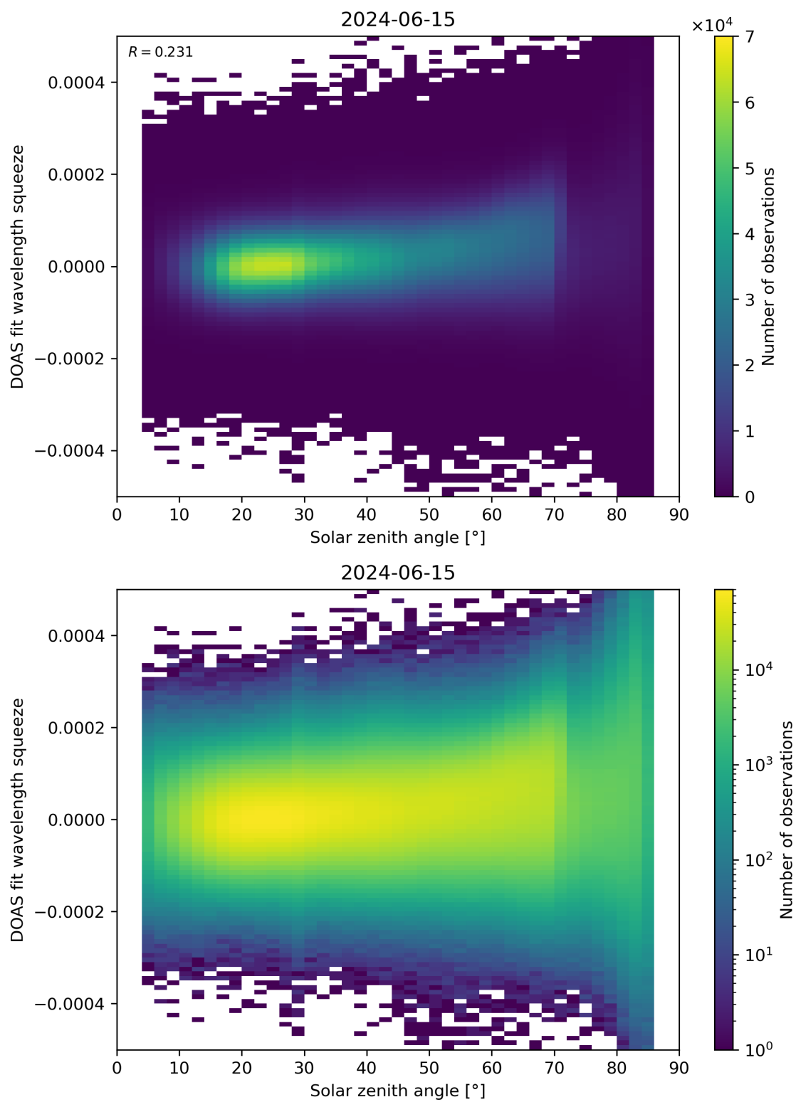
Figure 169: Scatter density plot of “Solar zenith angle” against “DOAS fit wavelength squeeze” for 2024-06-14 to 2024-06-16.
