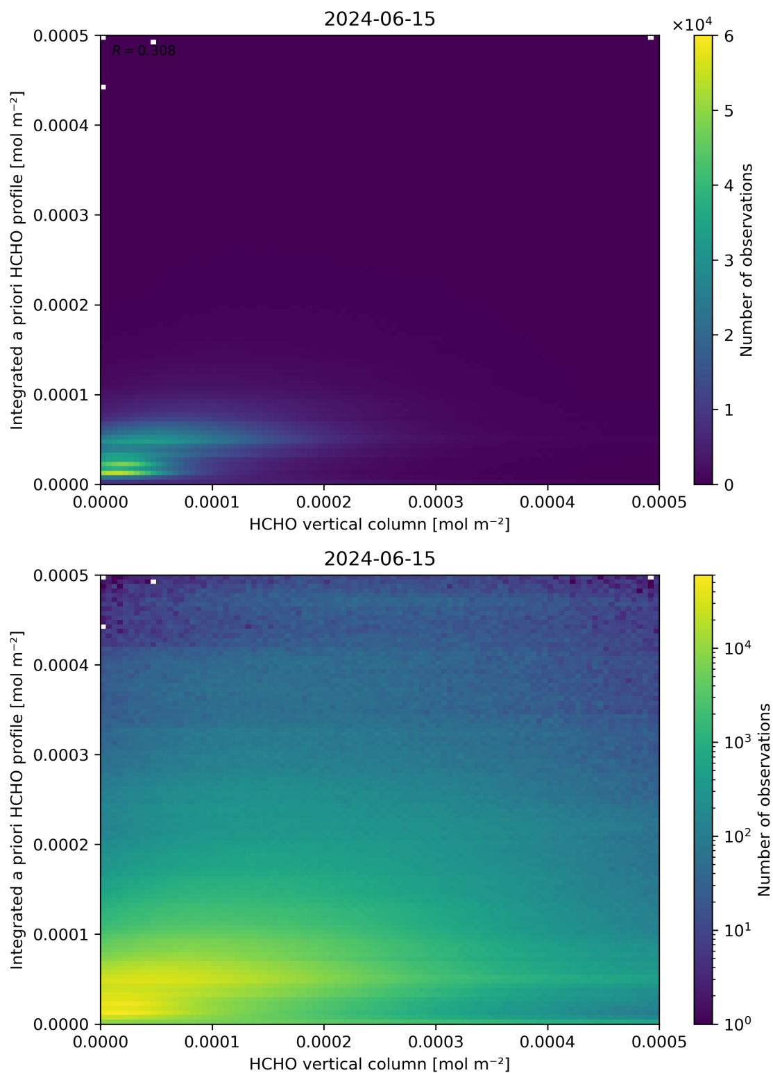
Figure 135: Scatter density plot of “HCHO vertical column” against “Integrated a priori HCHO profile” for 2024-06-14 to 2024-06-16.
