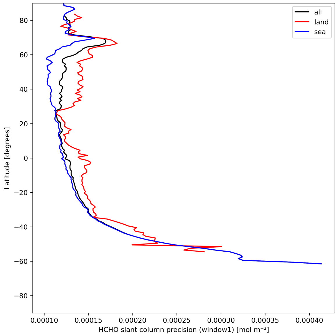
Figure 25: Zonal average of "HCHO slant column precision (window1)" for 2024-06-14 to 2024-06-16.
