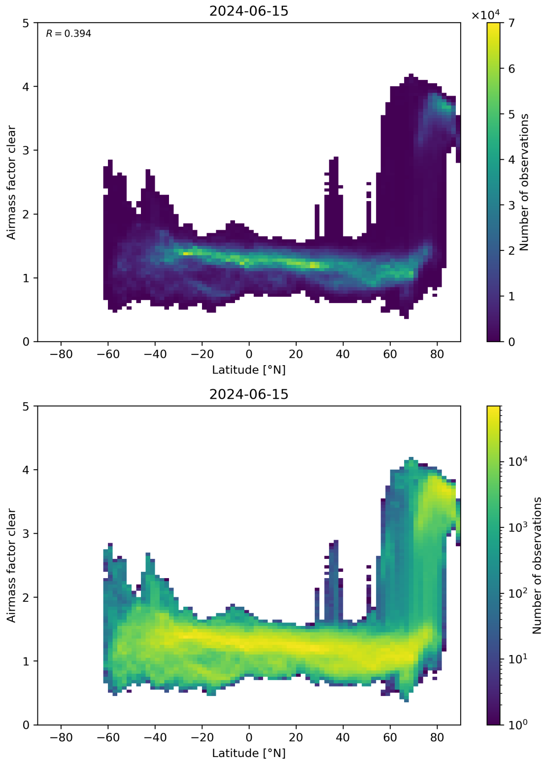
Figure 156: Scatter density plot of “Latitude” against “Airmass factor clear” for 2024-06-14 to 2024-06-16.
