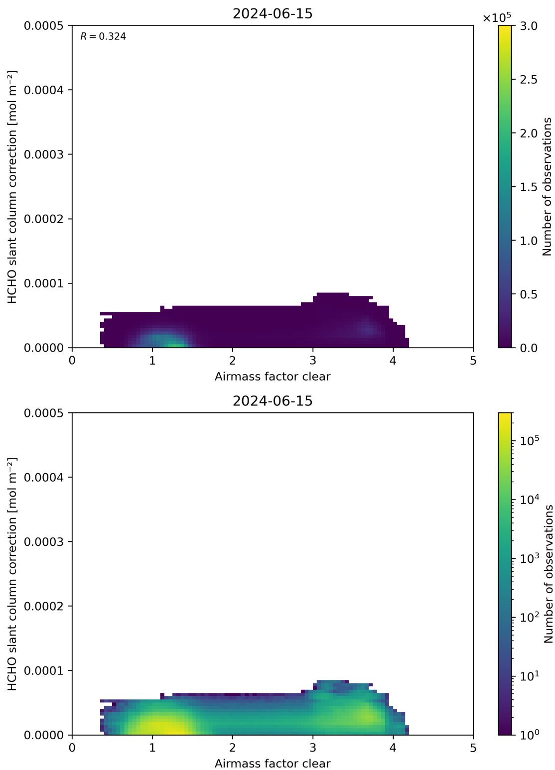
Figure 75: Scatter density plot of “Airmass factor clear” against “HCHO slant column correction” for 2024-06-14 to 2024-06-16.
