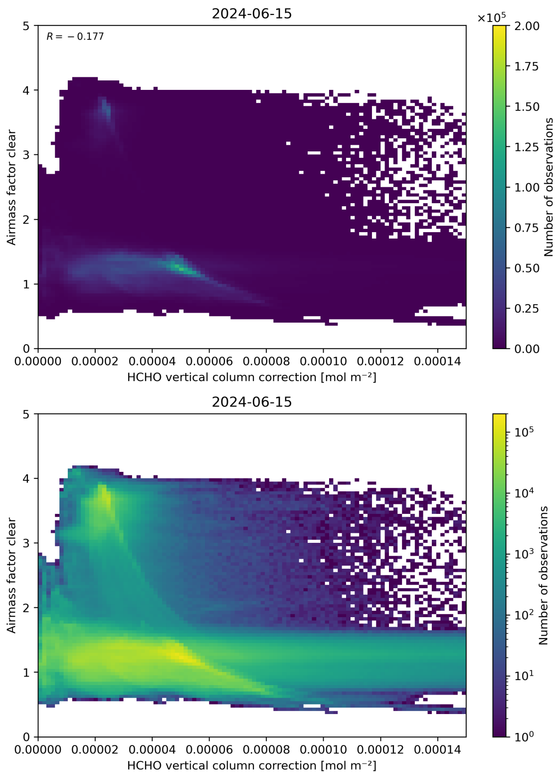
Figure 115: Scatter density plot of “HCHO vertical column correction” against “Airmass factor clear” for 2024-06-14 to 2024-06-16.
