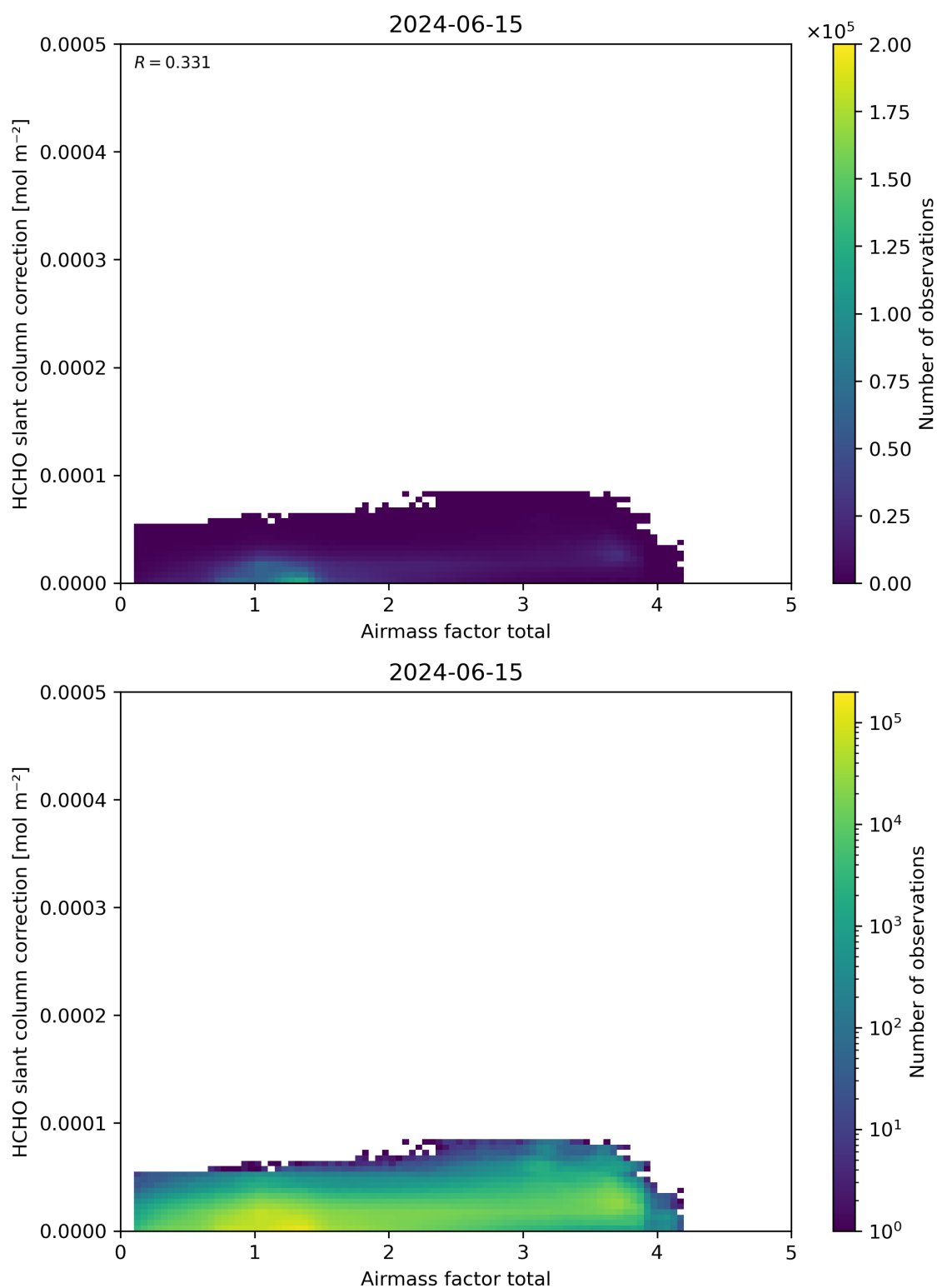
Figure 102: Scatter density plot of “Airmass factor total” against “HCHO slant column correction” for 2024-06-14 to 2024-06-16.
