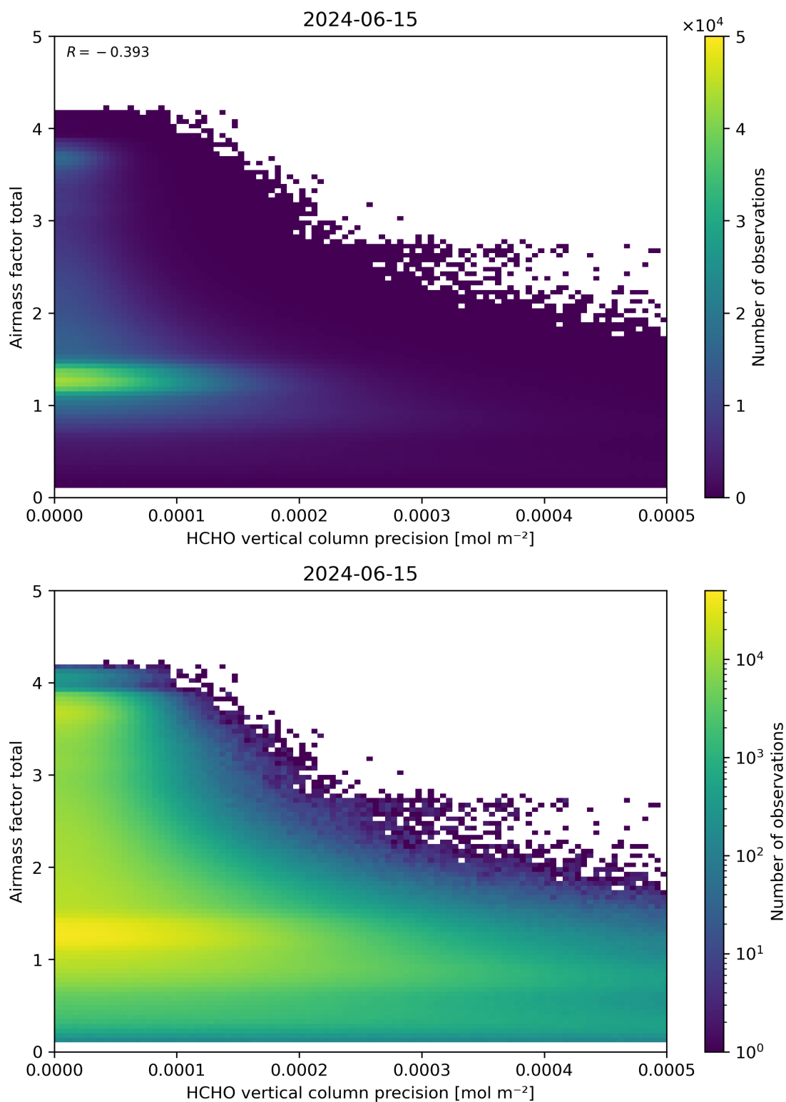
Figure 144: Scatter density plot of “HCHO vertical column precision” against “Airmass factor total” for 2024-06-14 to 2024-06-16.
