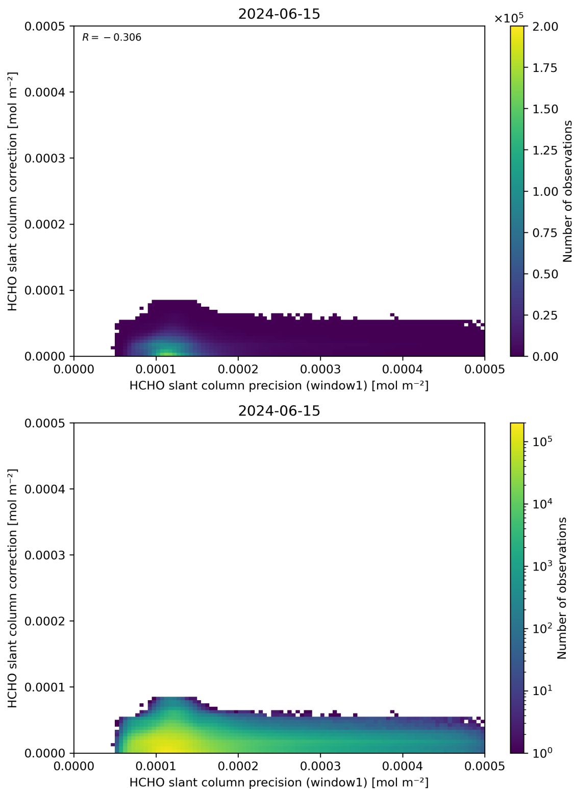
Figure 93: Scatter density plot of “HCHO slant column precision (window1)” against “HCHO slant column correction” for 2024-06-14 to 2024-06-16.
