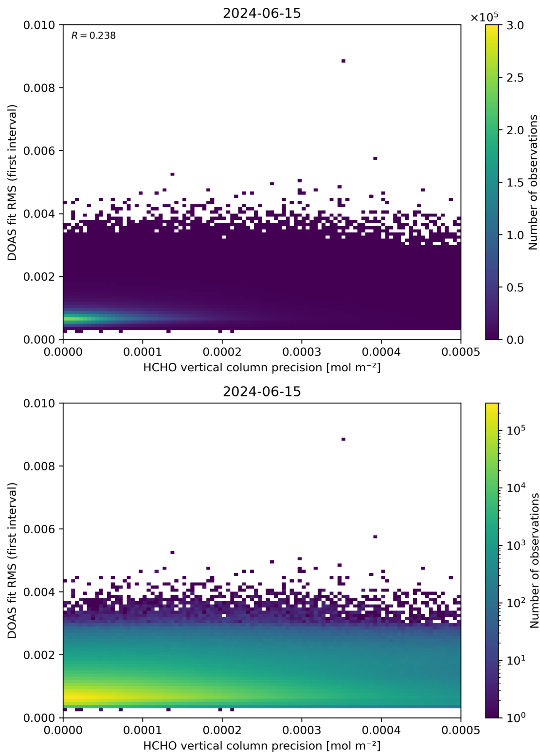
Figure 136: Scatter density plot of “HCHO vertical column precision” against “DOAS fit RMS (first interval)” for 2024-06-14 to 2024-06-16.
