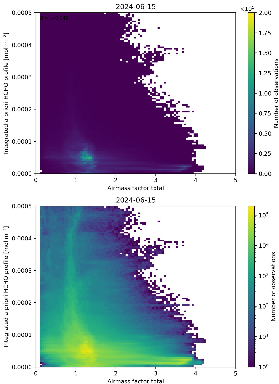
Figure 104: Scatter density plot of “Airmass factor total” against “Integrated a priori HCHO profile” for 2024-06-14 to 2024-06-16.
