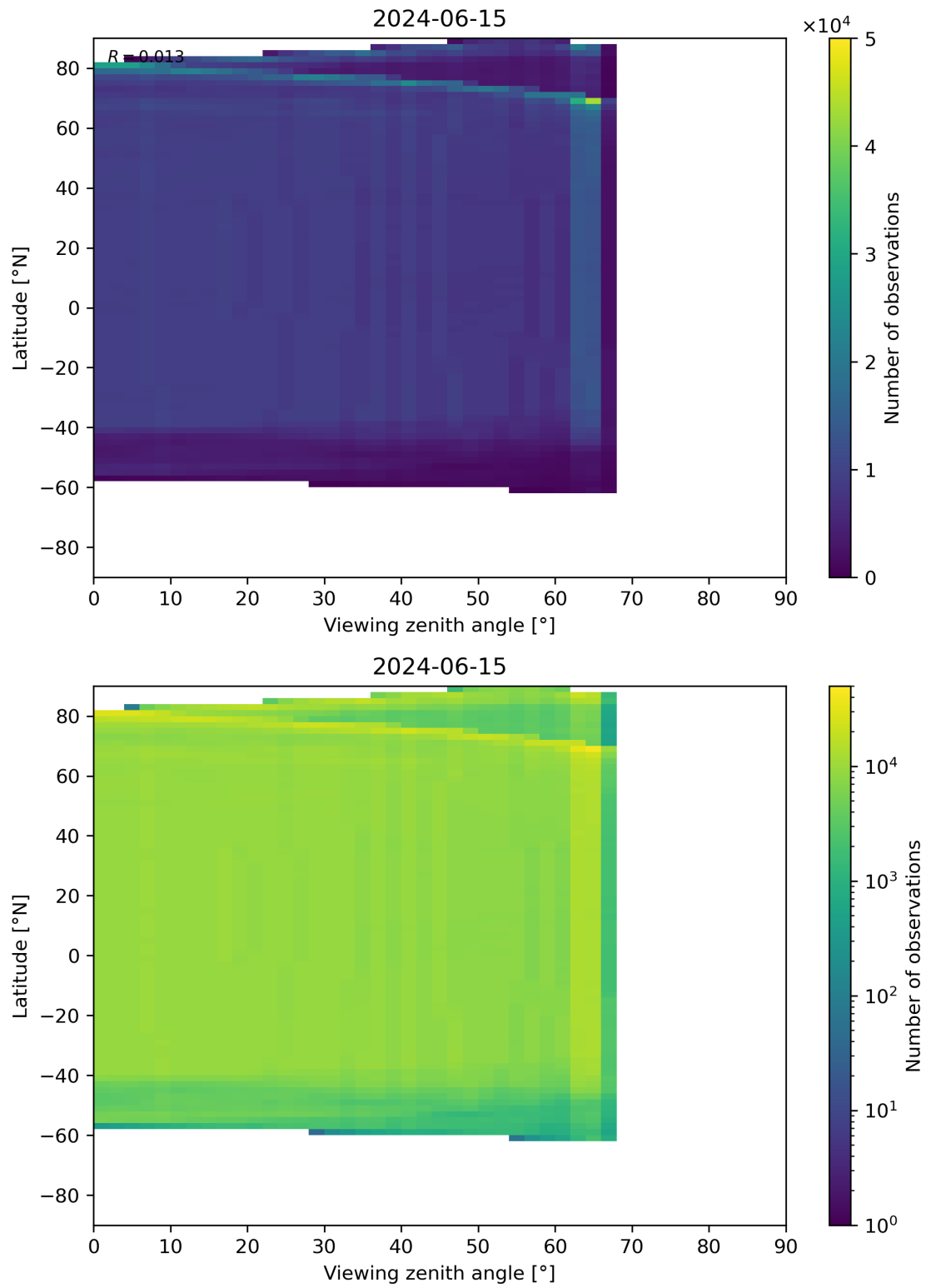
Figure 196: Scatter density plot of “Viewing zenith angle” against “Latitude” for 2024-06-14 to 2024-06-16.
