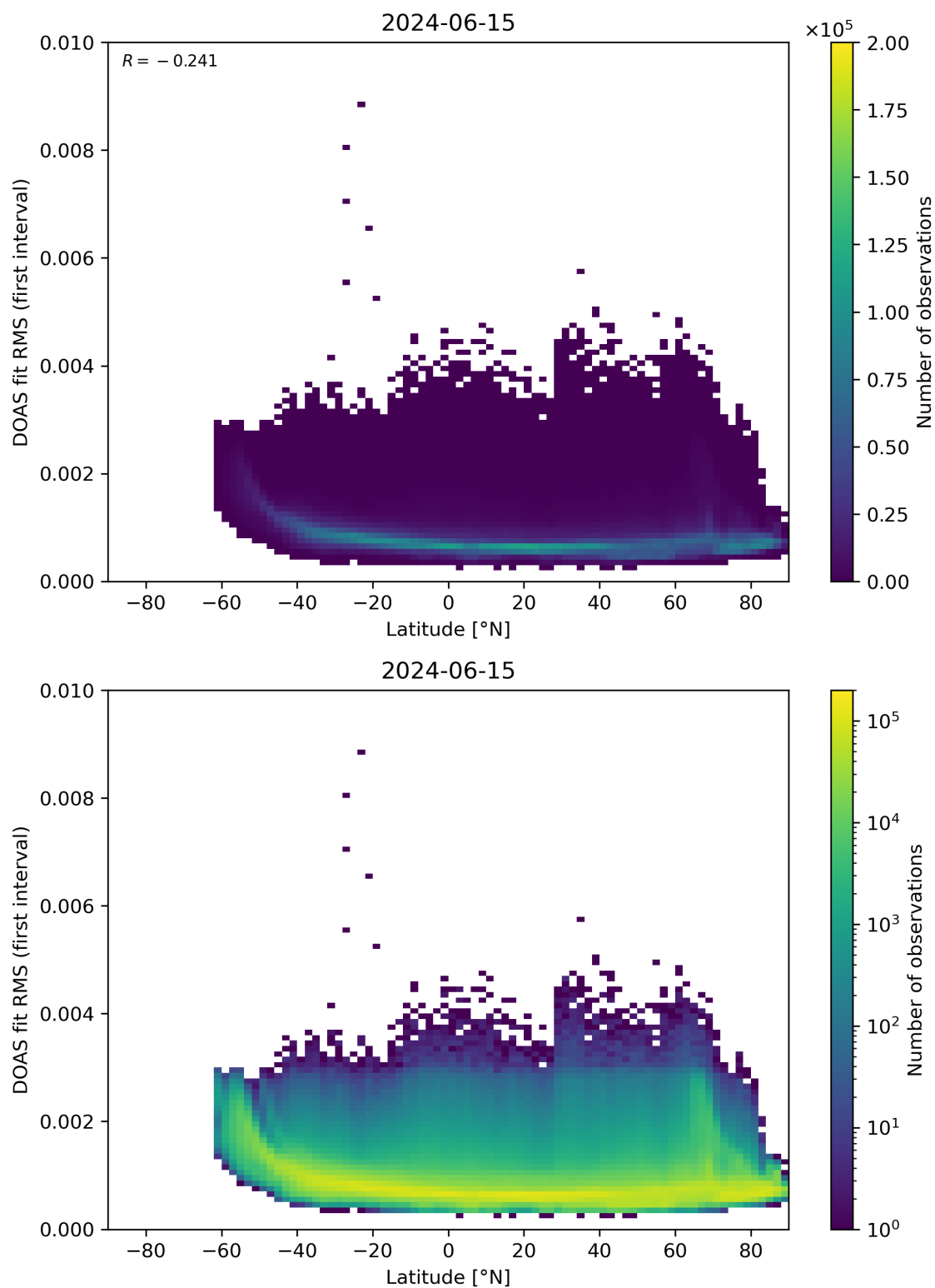
Figure 153: Scatter density plot of “Latitude” against “DOAS fit RMS (first interval)” for 2024-06-14 to 2024-06-16.
