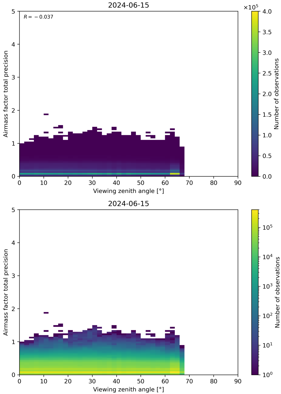
Figure 191: Scatter density plot of “Viewing zenith angle” against “Airmass factor total precision” for 2024-06-14 to 2024-06-16.
