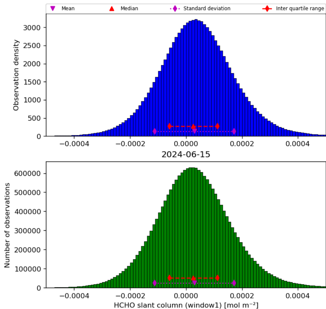
Figure 38: Histogram of “HCHO slant column (window1)” for 2024-06-14 to 2024-06-16
