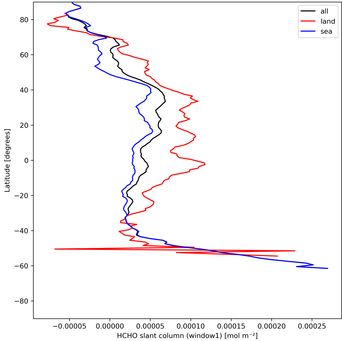
Figure 24: Zonal average of “HCHO slant column (window1)” for 2024-06-14 to 2024-06-16.
