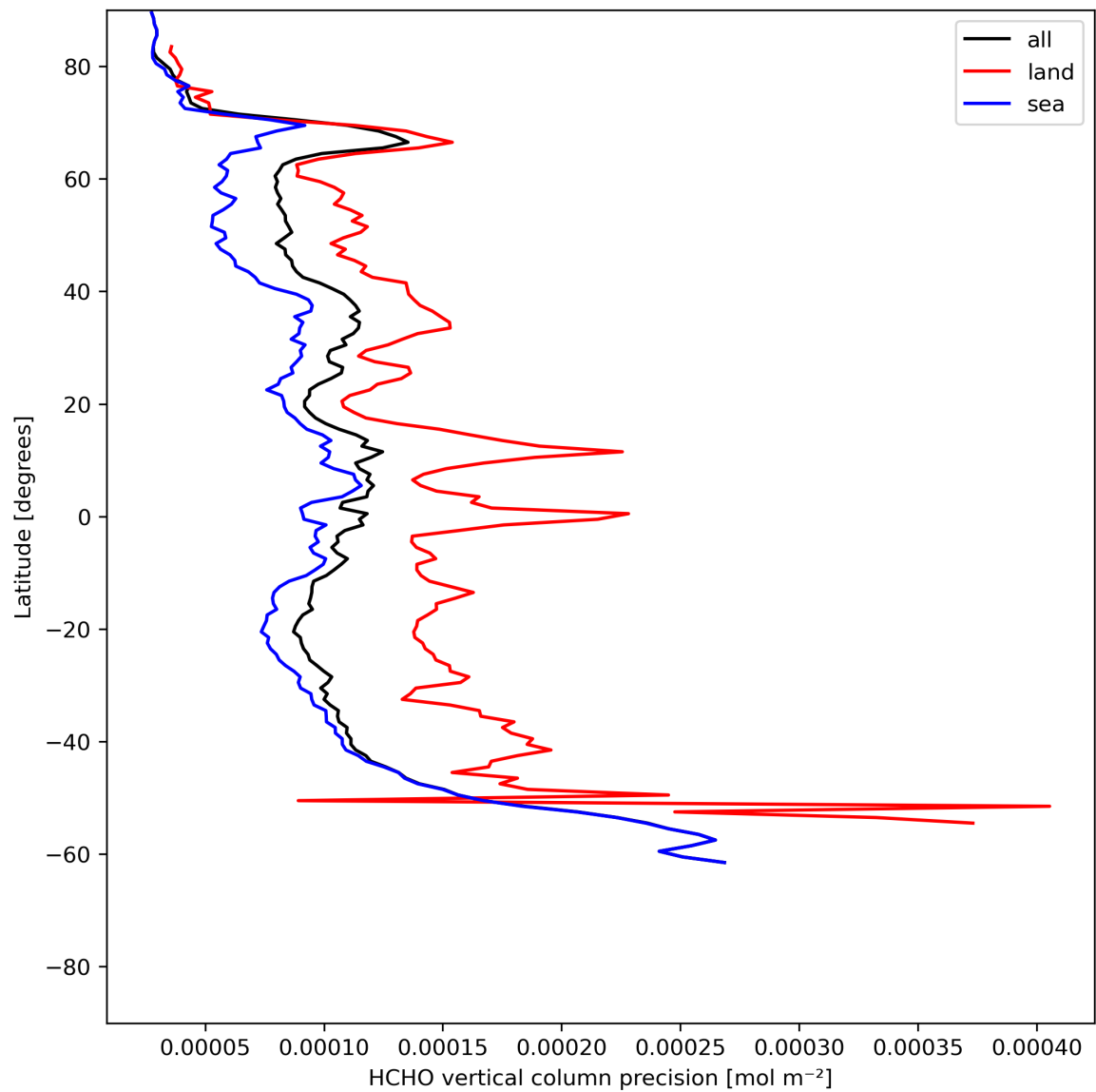
Figure 22: Zonal average of “HCHO vertical column precision” for 2024-06-14 to 2024-06-16.
