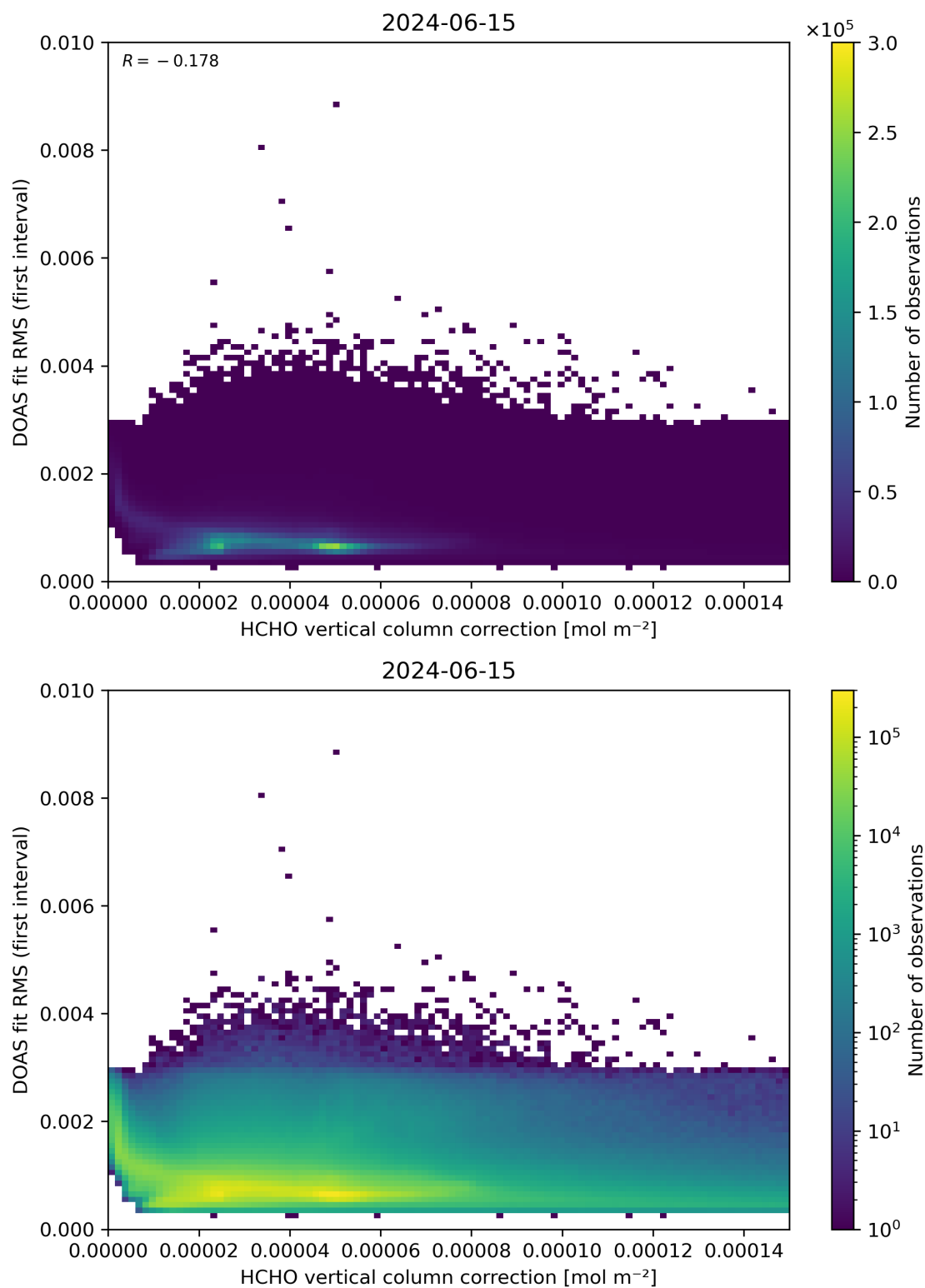
Figure 112: Scatter density plot of “HCHO vertical column correction” against “DOAS fit RMS (first interval)” for 2024-06-14 to 2024-06-16.
