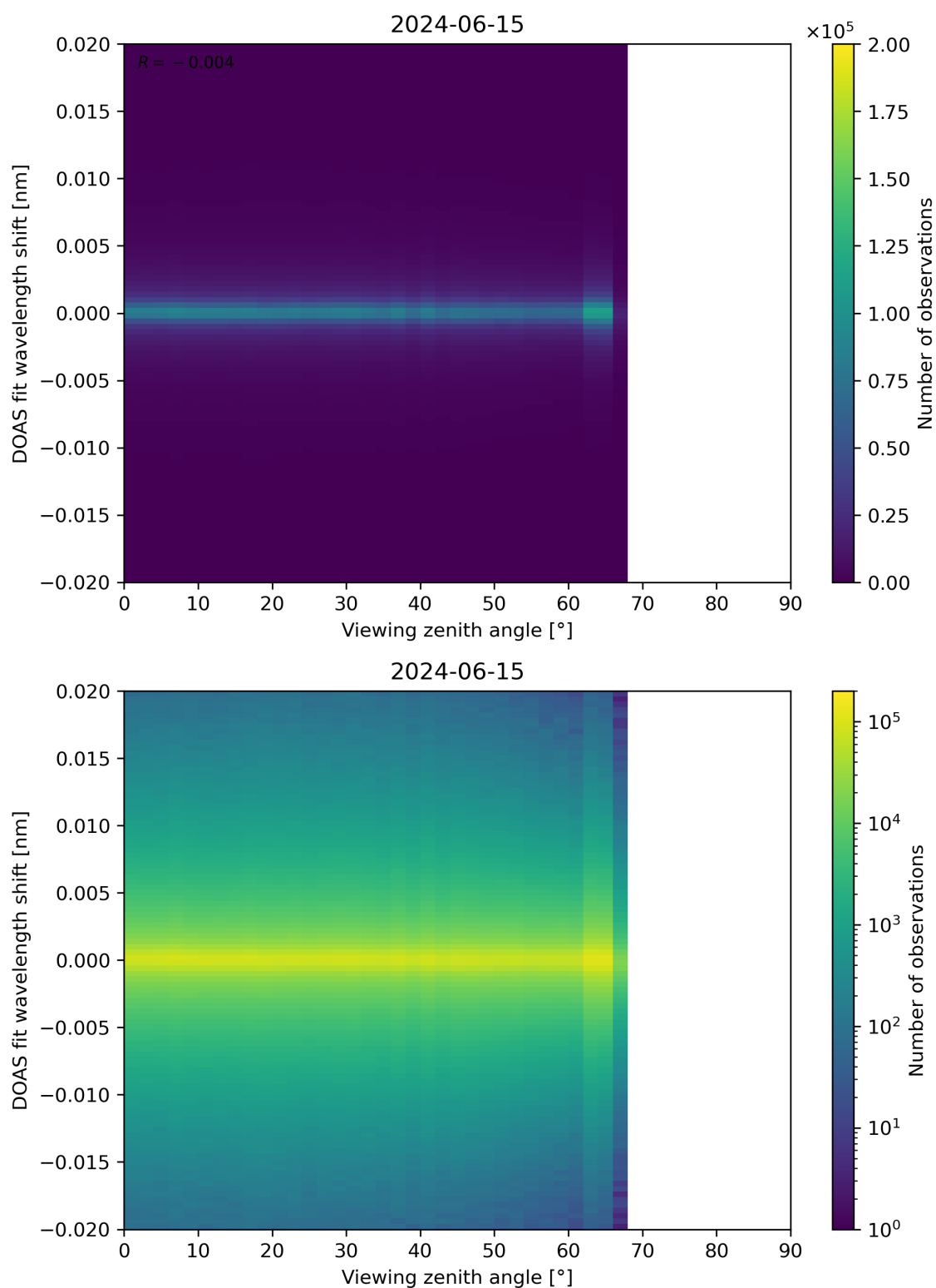
Figure 183: Scatter density plot of “Viewing zenith angle” against “DOAS fit wavelength shift” for 2024-06-14 to 2024-06-16.
