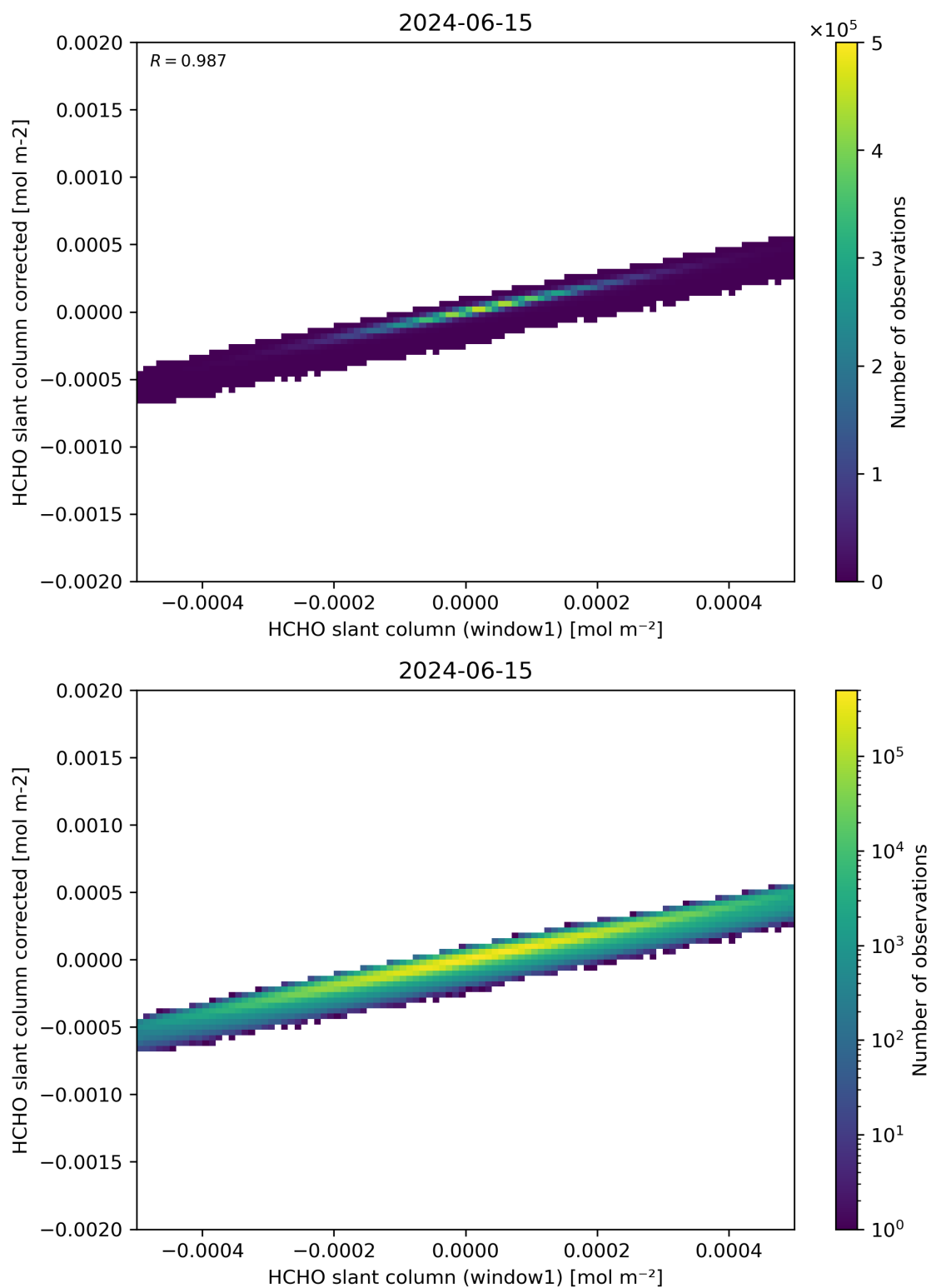
Figure 82: Scatter density plot of “HCHO slant column (window1)” against “HCHO slant column corrected” for 2024-06-14 to 2024-06-16.
