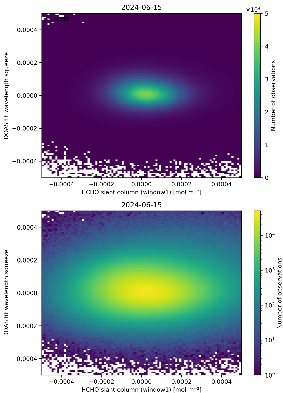
Figure 80: Scatter density plot of “HCHO slant column (window1)” against “DOAS fit wavelength squeeze” for 2024-06-14 to 2024-06-16.
