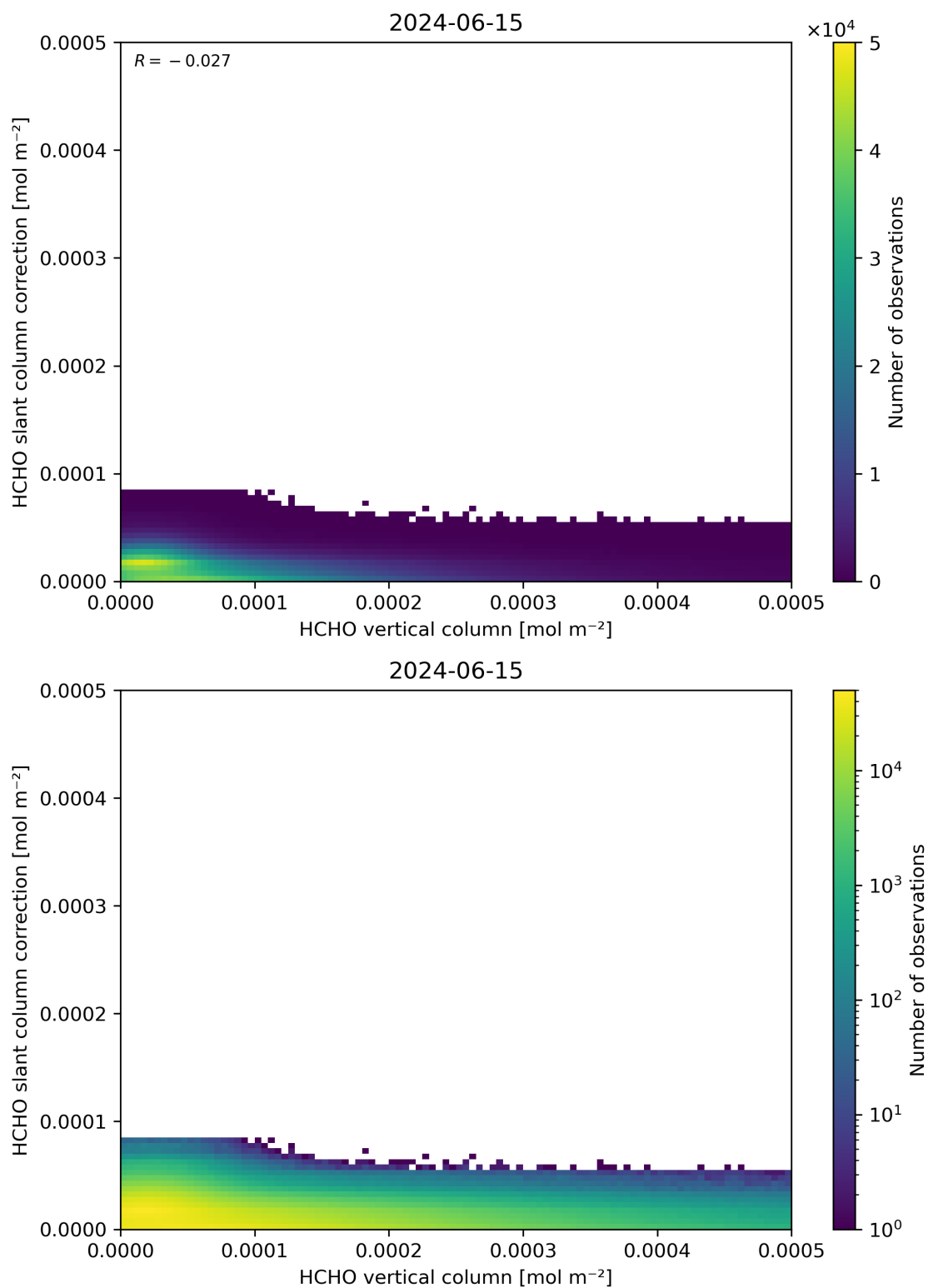
Figure 128: Scatter density plot of “HCHO vertical column” against “HCHO slant column correction” for 2024-06-14 to 2024-06-16.
