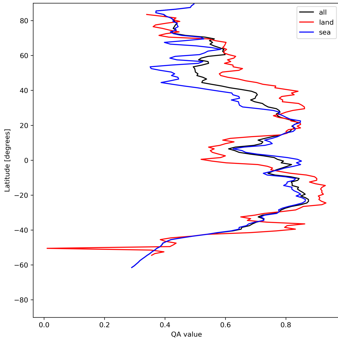
Figure 20: Zonal average of “QA value” for 2024-06-14 to 2024-06-16.
