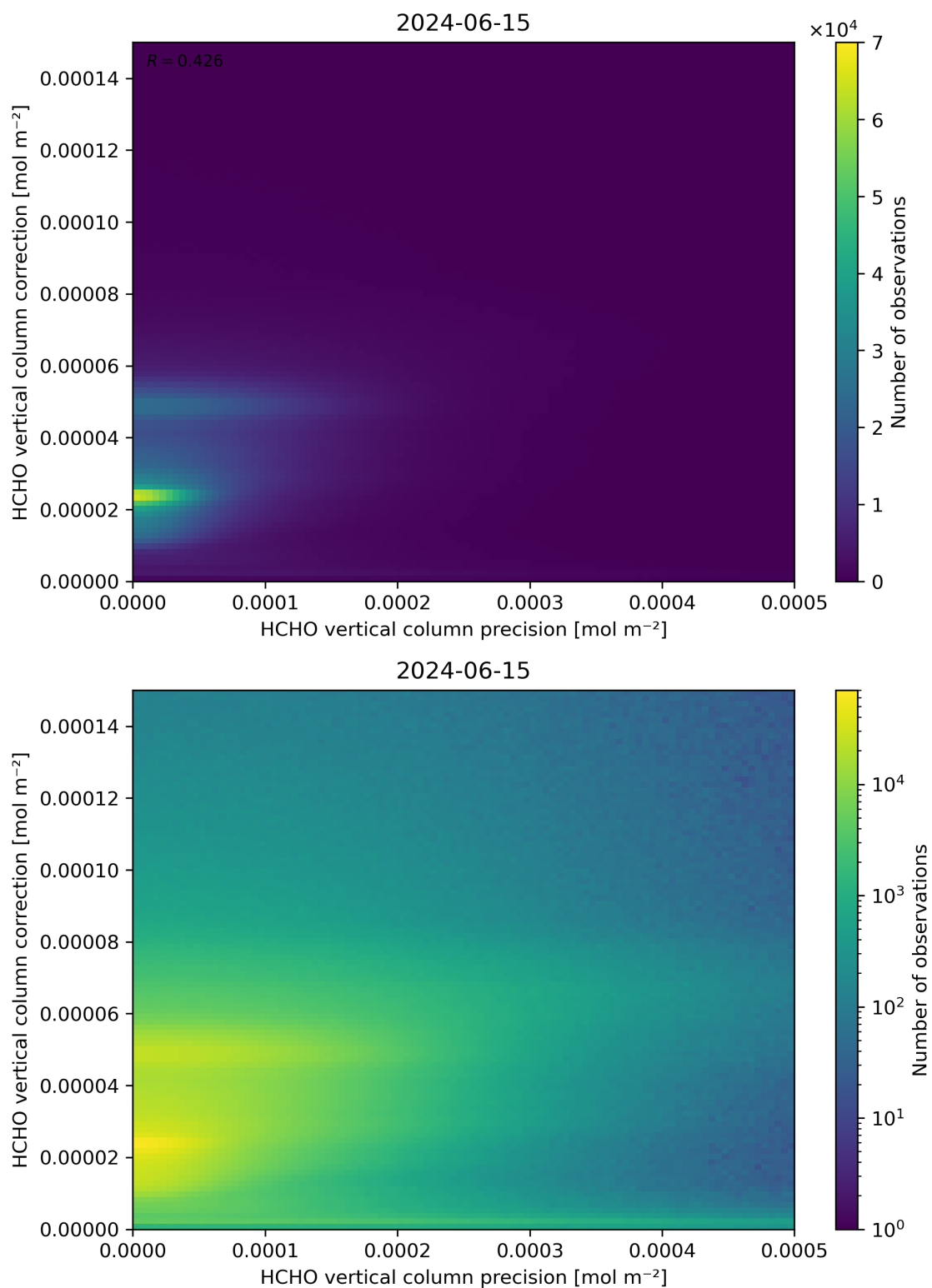
Figure 146: Scatter density plot of “HCHO vertical column precision” against “HCHO vertical column correction” for 2024-06-14 to 2024-06-16.
