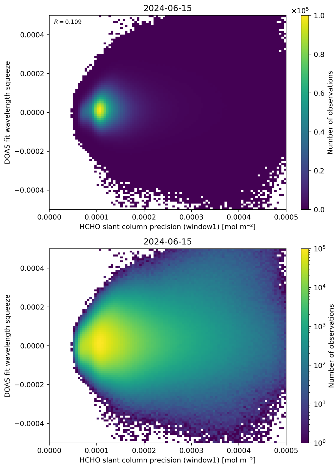
Figure 90: Scatter density plot of “HCHO slant column precision (window1)” against “DOAS fit wavelength squeeze” for 2024-06-14 to 2024-06-16.
