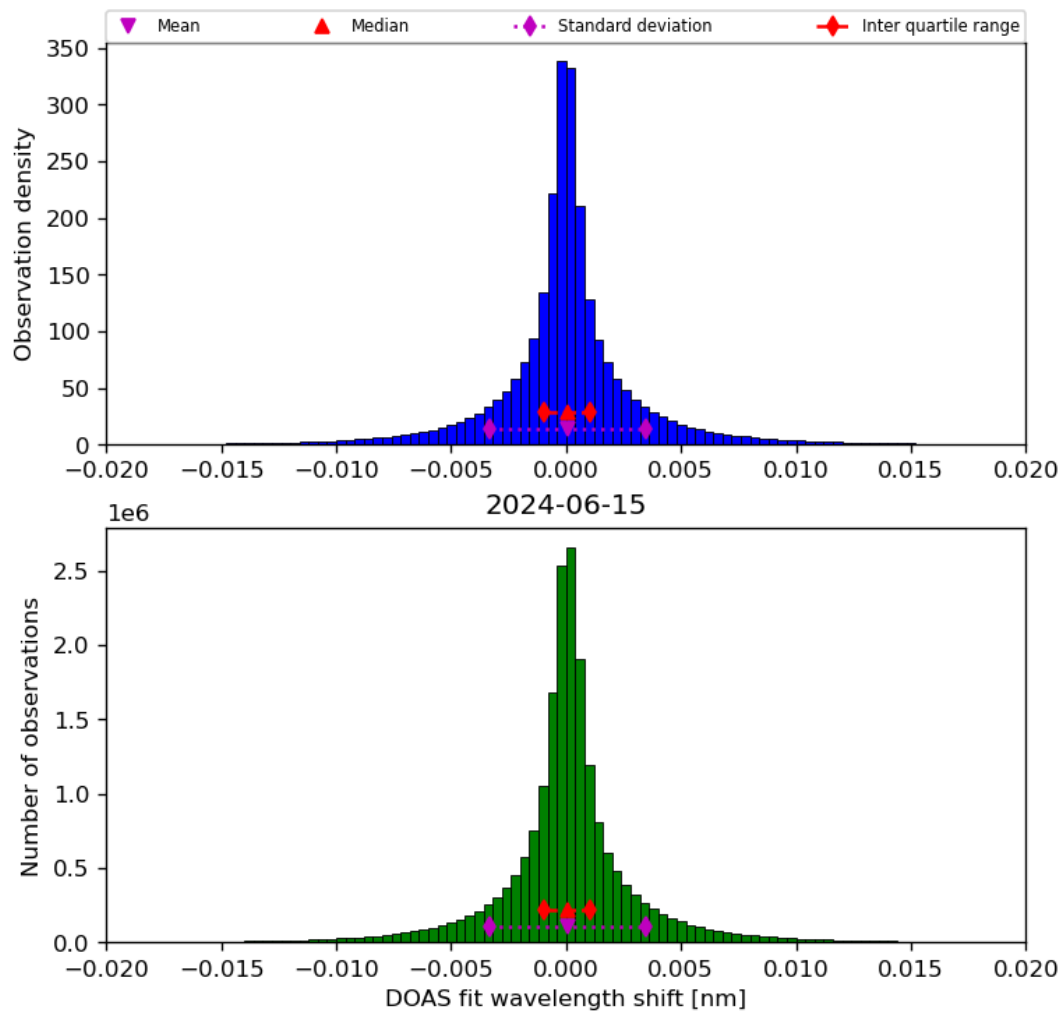
Figure 44: Histogram of “DOAS fit wavelength shift” for 2024-06-14 to 2024-06-16
