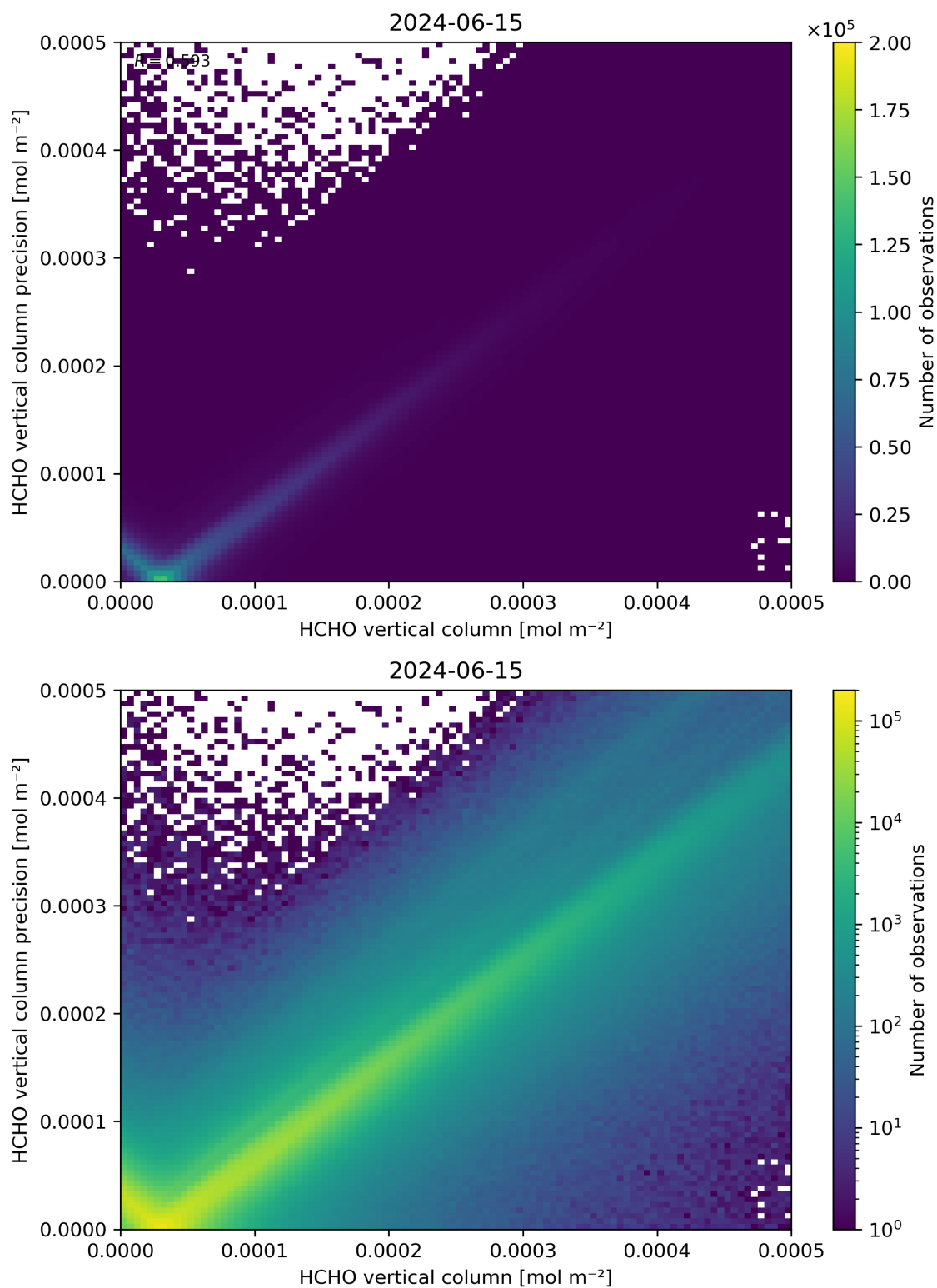
Figure 134: Scatter density plot of “HCHO vertical column” against “HCHO vertical column precision” for 2024-06-14 to 2024-06-16.
