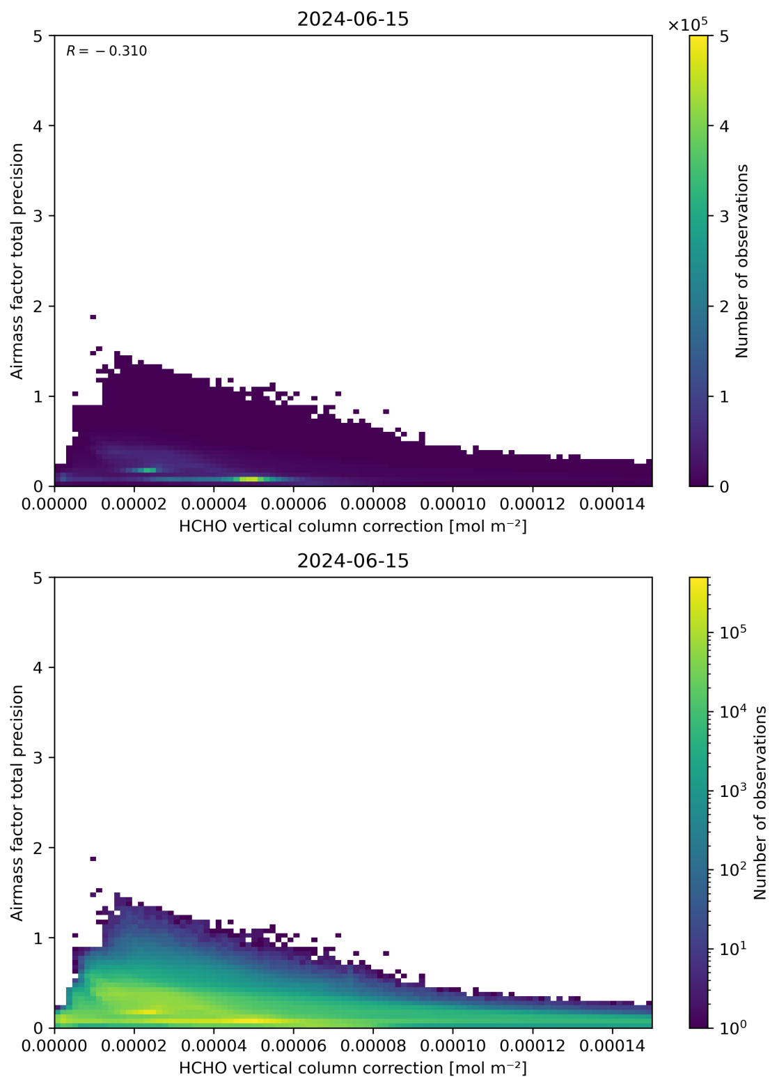
Figure 121: Scatter density plot of “HCHO vertical column correction” against “Airmass factor total precision” for 2024-06-14 to 2024-06-16.
