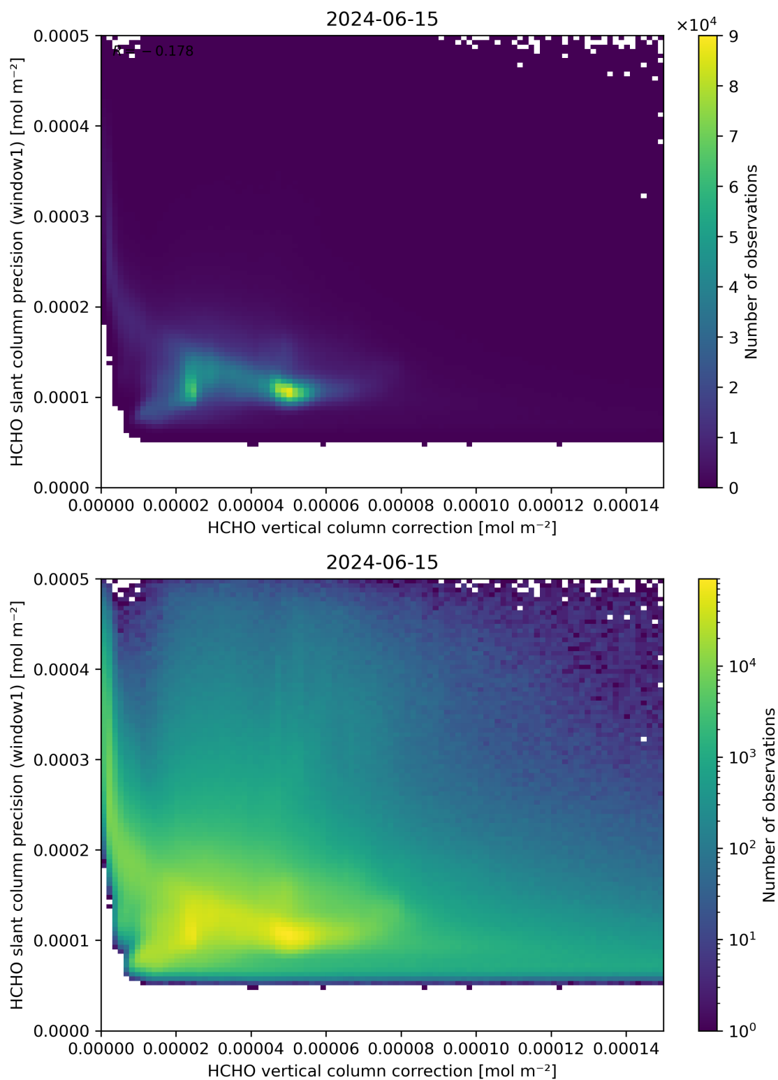
Figure 119: Scatter density plot of “HCHO vertical column correction” against “HCHO slant column precision (window1)” for 2024-06-14 to 2024-06-16.
