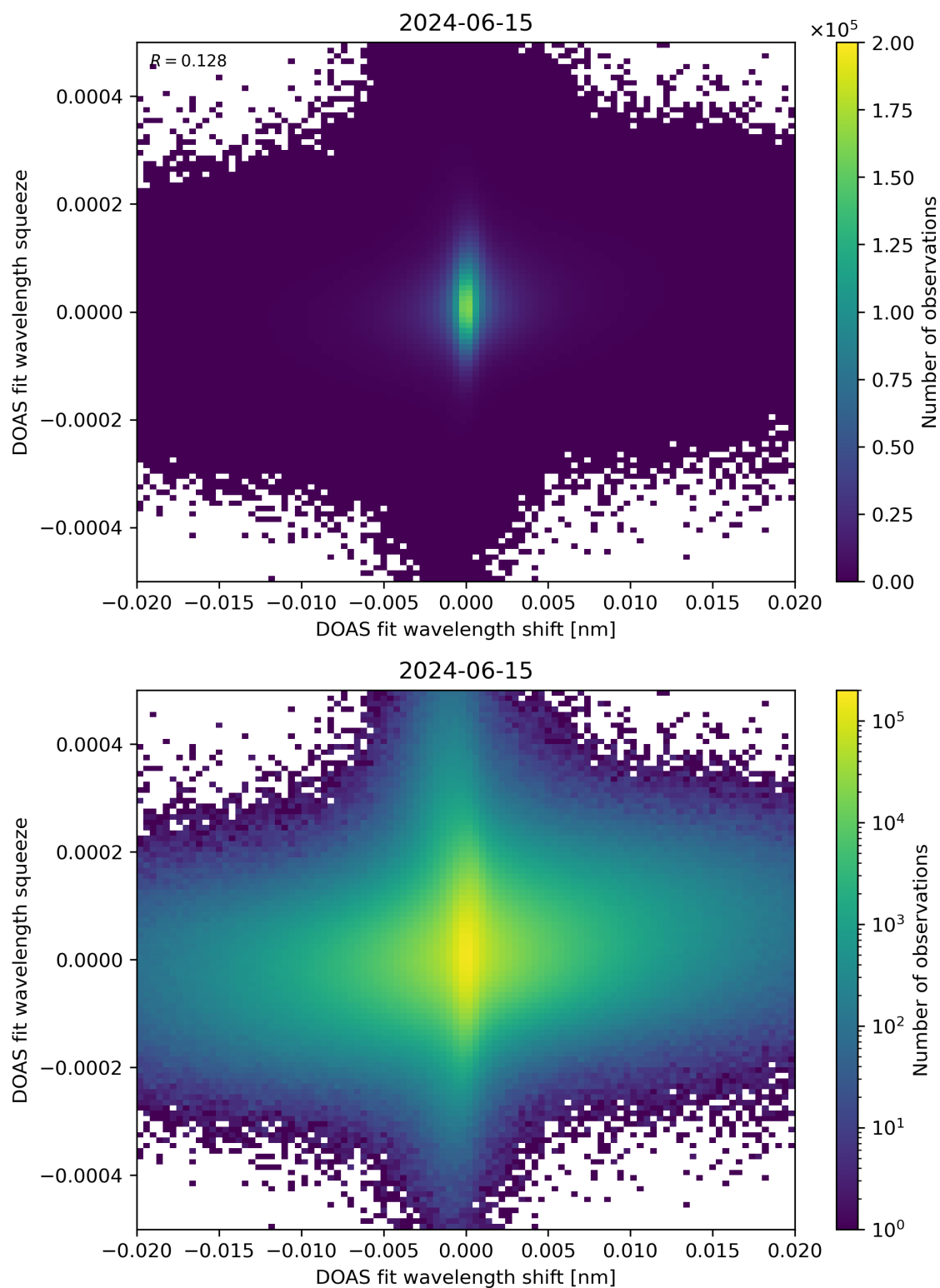
Figure 65: Scatter density plot of “DOAS fit wavelength shift” against “DOAS fit wavelength squeeze” for 2024-06-14 to 2024-06-16.
