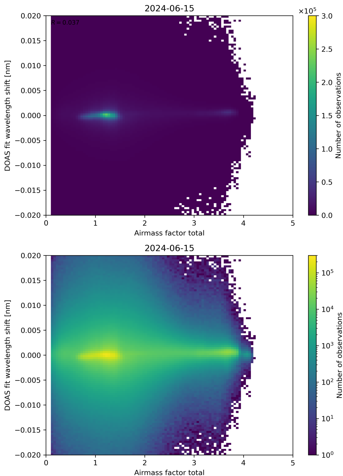
Figure 98: Scatter density plot of “Airmass factor total” against “DOAS fit wavelength shift” for 2024-06-14 to 2024-06-16.
