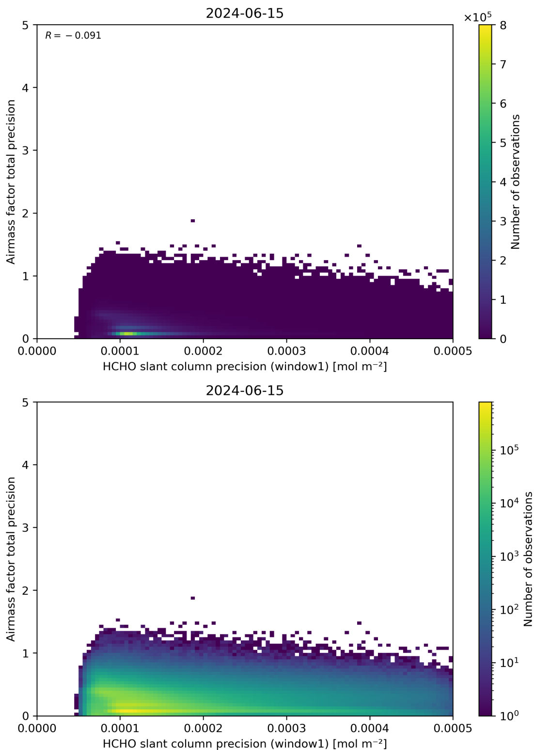
Figure 95: Scatter density plot of “HCHO slant column precision (window1)” against “Airmass factor total precision” for 2024-06-14 to 2024-06-16.
