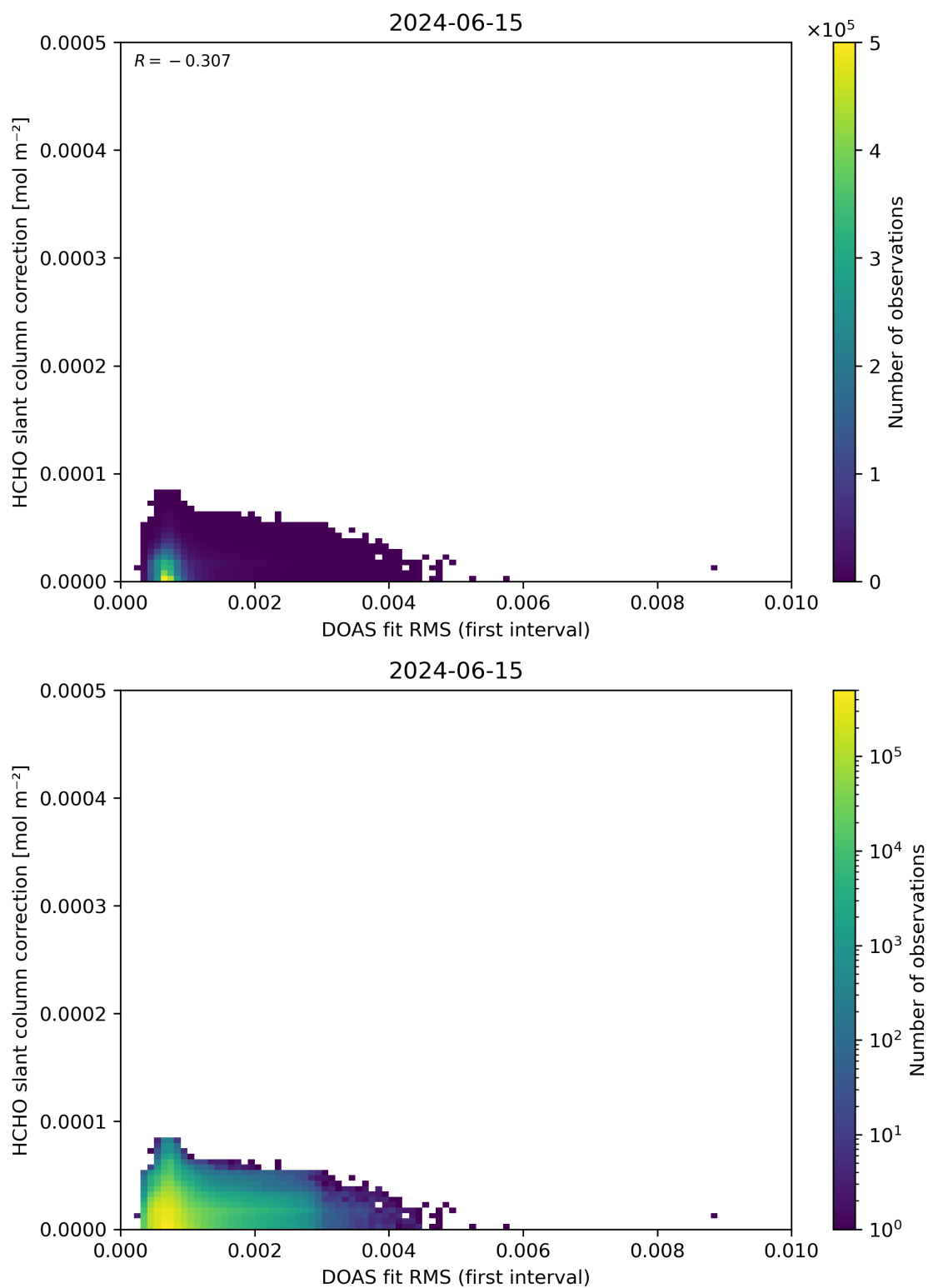
Figure 63: Scatter density plot of “DOAS fit RMS (first interval)” against “HCHO slant column correction” for 2024-06-14 to 2024-06-16.
