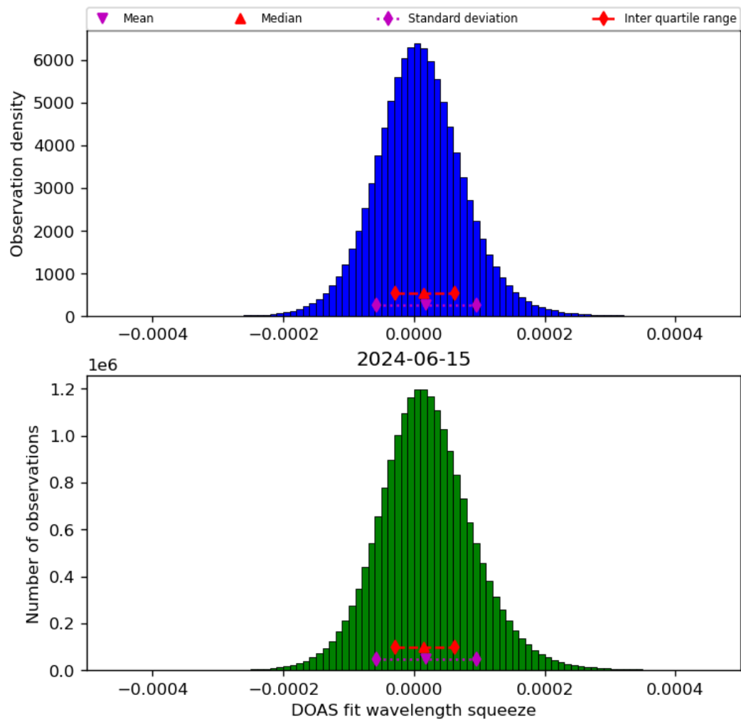
Figure 45: Histogram of “DOAS fit wavelength squeeze” for 2024-06-14 to 2024-06-16
