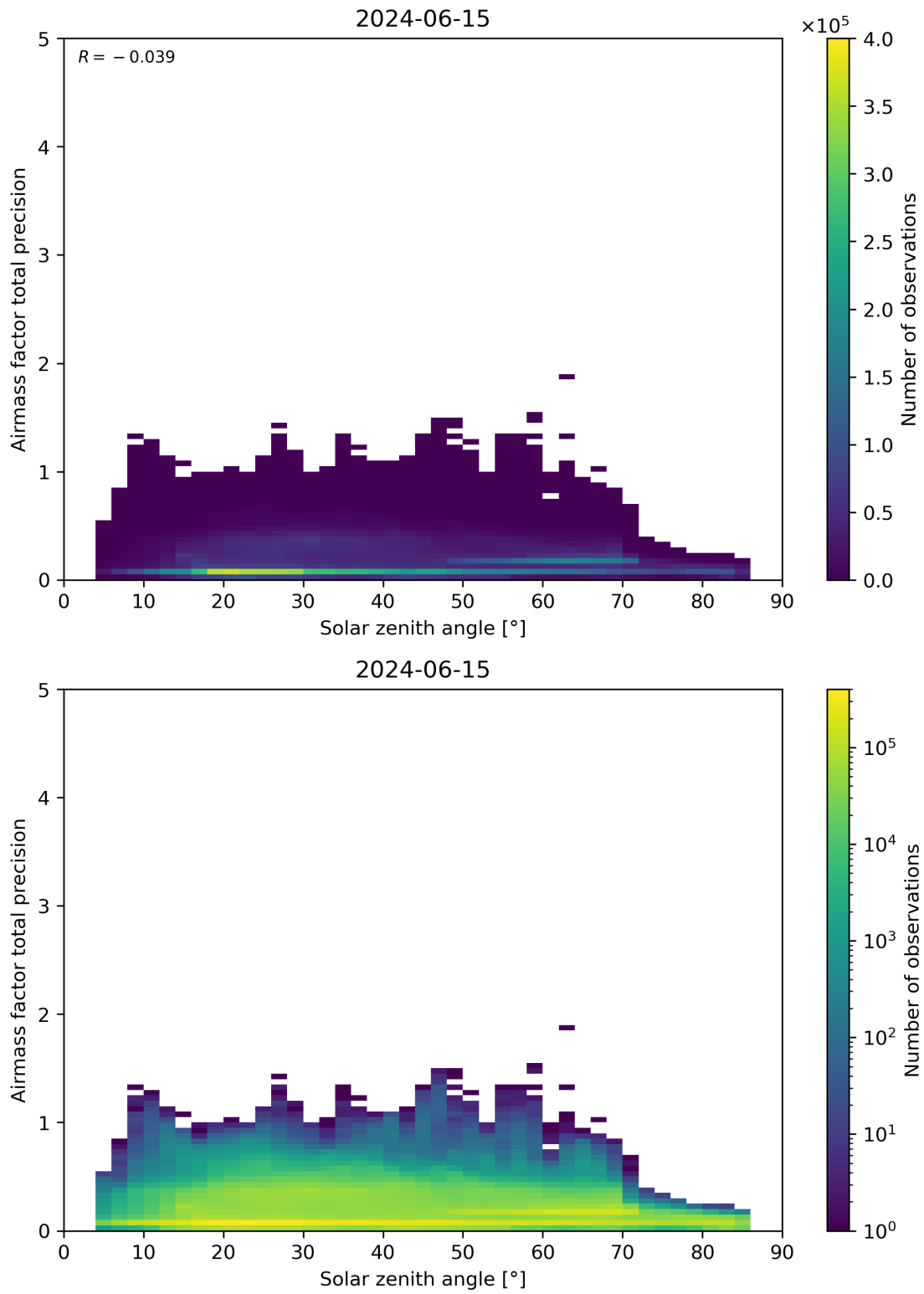
Figure 176: Scatter density plot of “Solar zenith angle” against “Airmass factor total precision” for 2024-06-14 to 2024-06-16.
