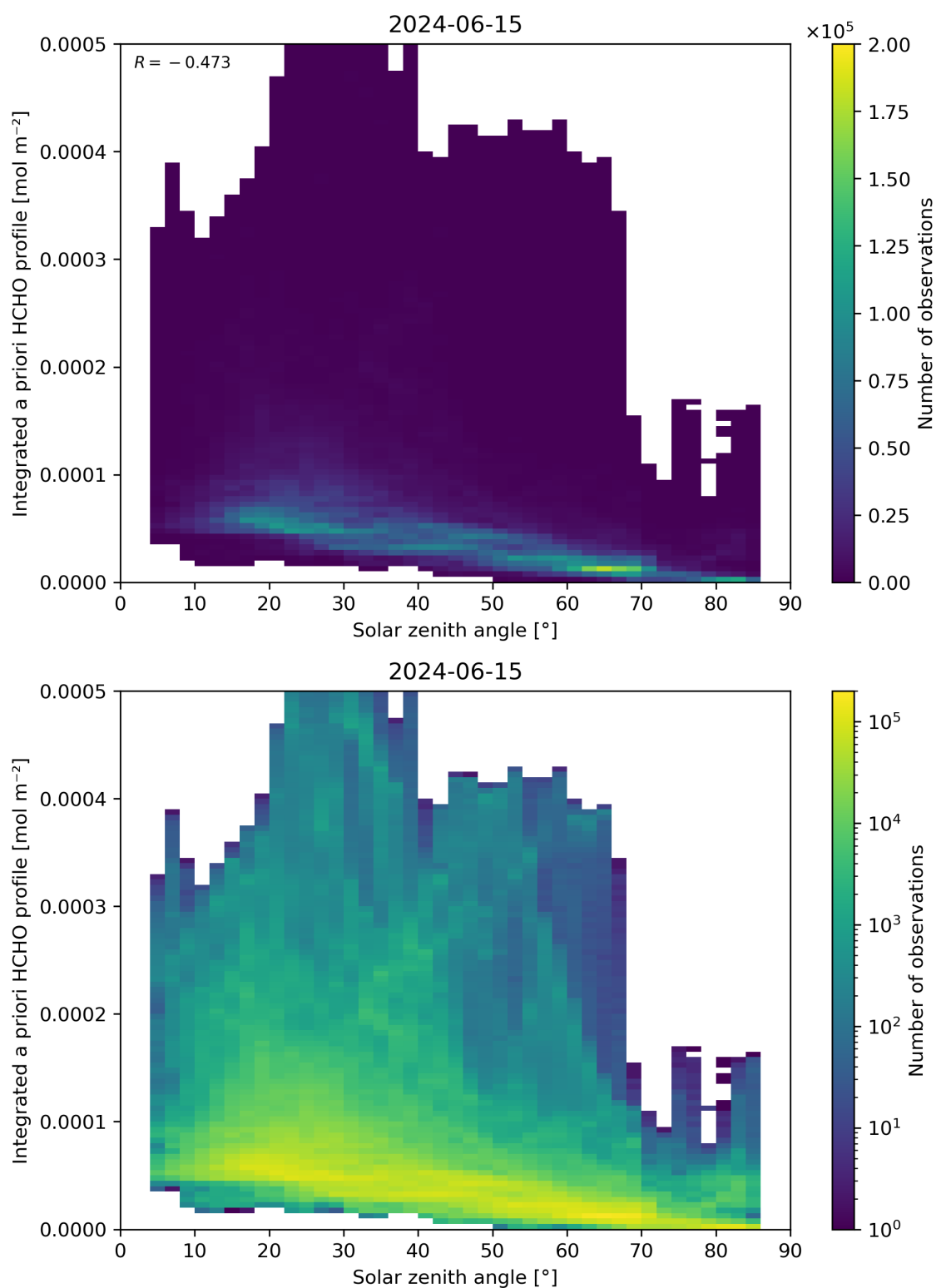
Figure 180: Scatter density plot of “Solar zenith angle” against “Integrated a priori HCHO profile” for 2024-06-14 to 2024-06-16.
