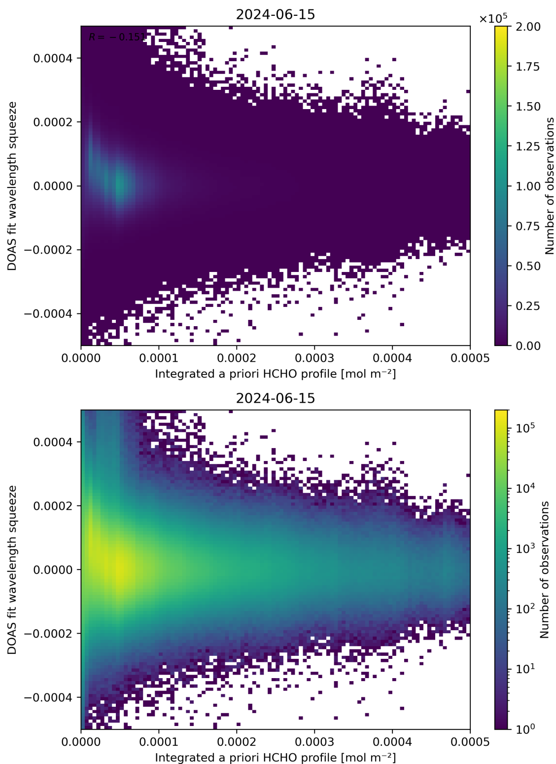
Figure 150: Scatter density plot of “Integrated a priori HCHO profile” against “DOAS fit wavelength squeeze” for 2024-06-14 to 2024-06-16.
