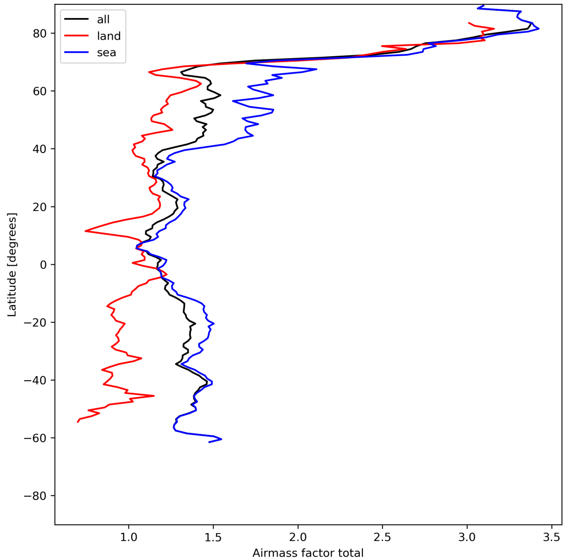
Figure 26: Zonal average of “Airmass factor total” for 2024-06-14 to 2024-06-16.
