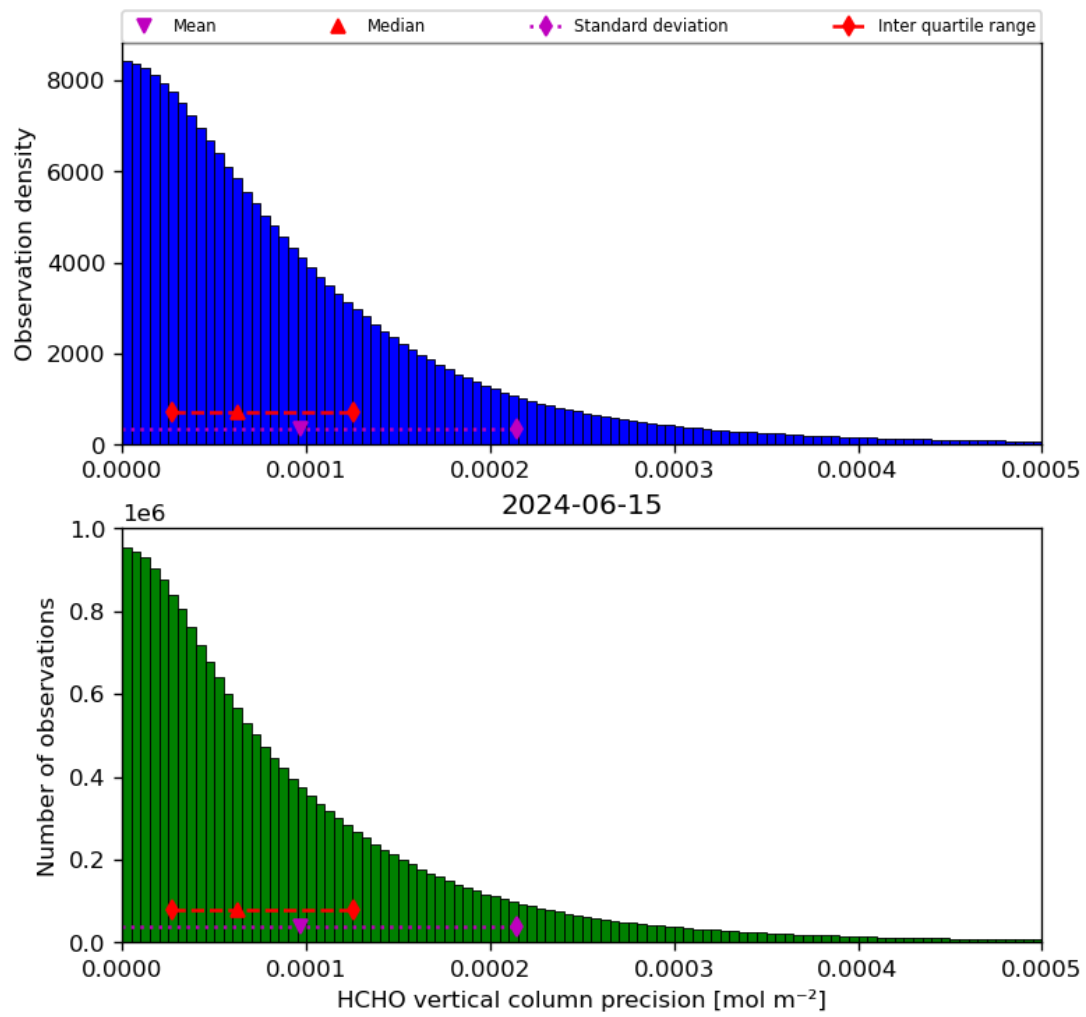
Figure 36: Histogram of “HCHO vertical column precision” for 2024-06-14 to 2024-06-16
