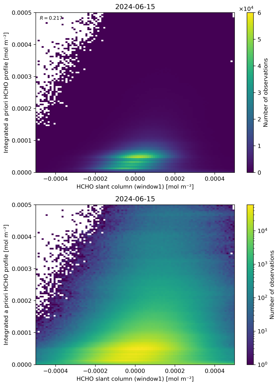
Figure 87: Scatter density plot of “HCHO slant column (window1)” against “Integrated a priori HCHO profile” for 2024-06-14 to 2024-06-16.
