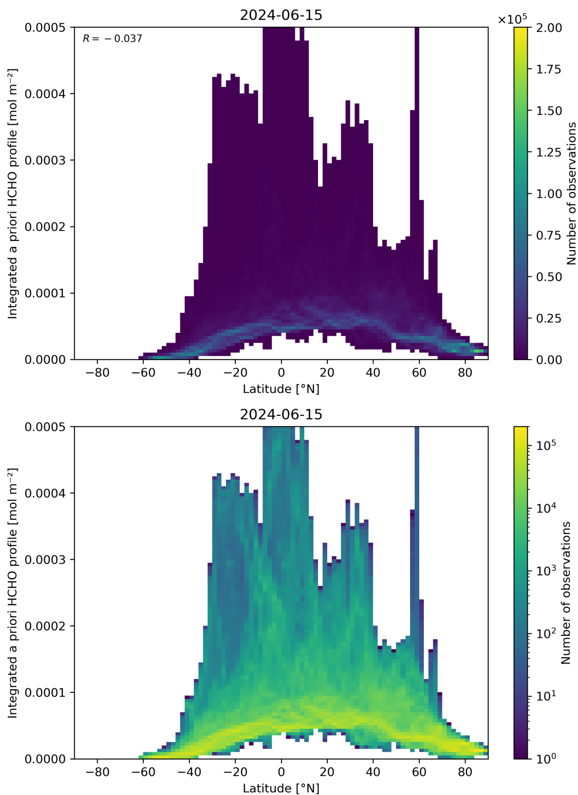
Figure 166: Scatter density plot of “Latitude” against “Integrated a priori HCHO profile” for 2024-06-14 to 2024-06-16.
