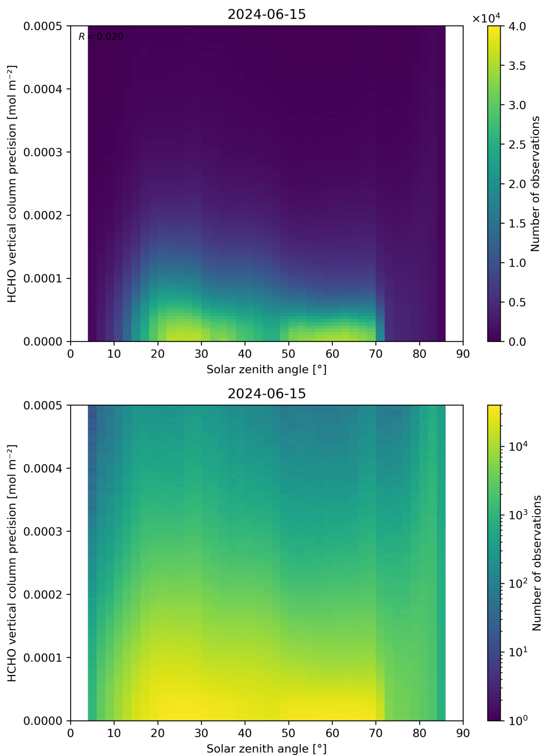
Figure 179: Scatter density plot of “Solar zenith angle” against “HCHO vertical column precision” for 2024-06-14 to 2024-06-16.
