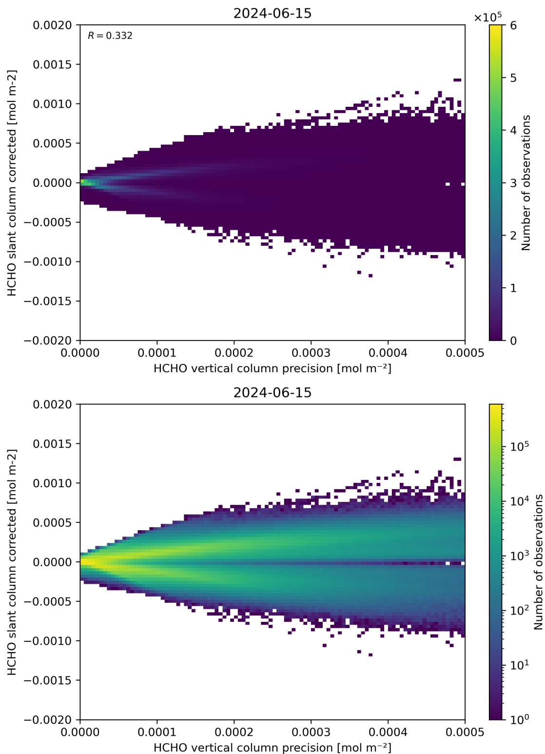
Figure 140: Scatter density plot of “HCHO vertical column precision” against “HCHO slant column corrected” for 2024-06-14 to 2024-06-16.
