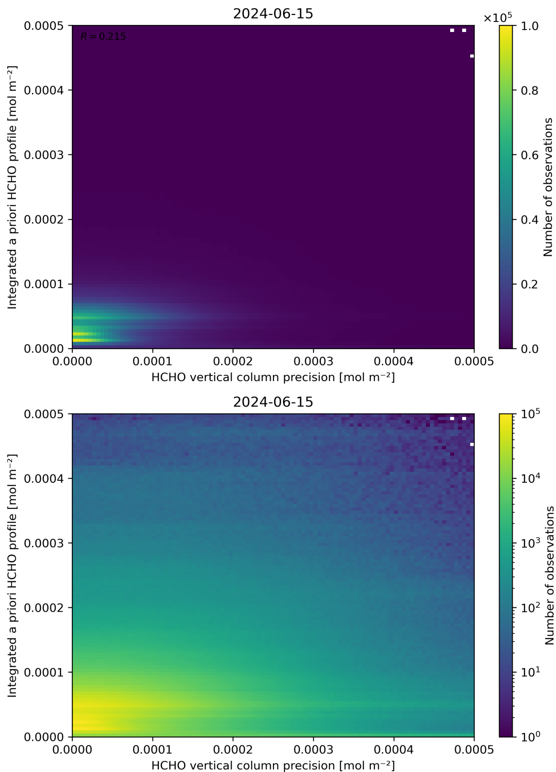
Figure 147: Scatter density plot of “HCHO vertical column precision” against “Integrated a priori HCHO profile” for 2024-06-14 to 2024-06-16.
