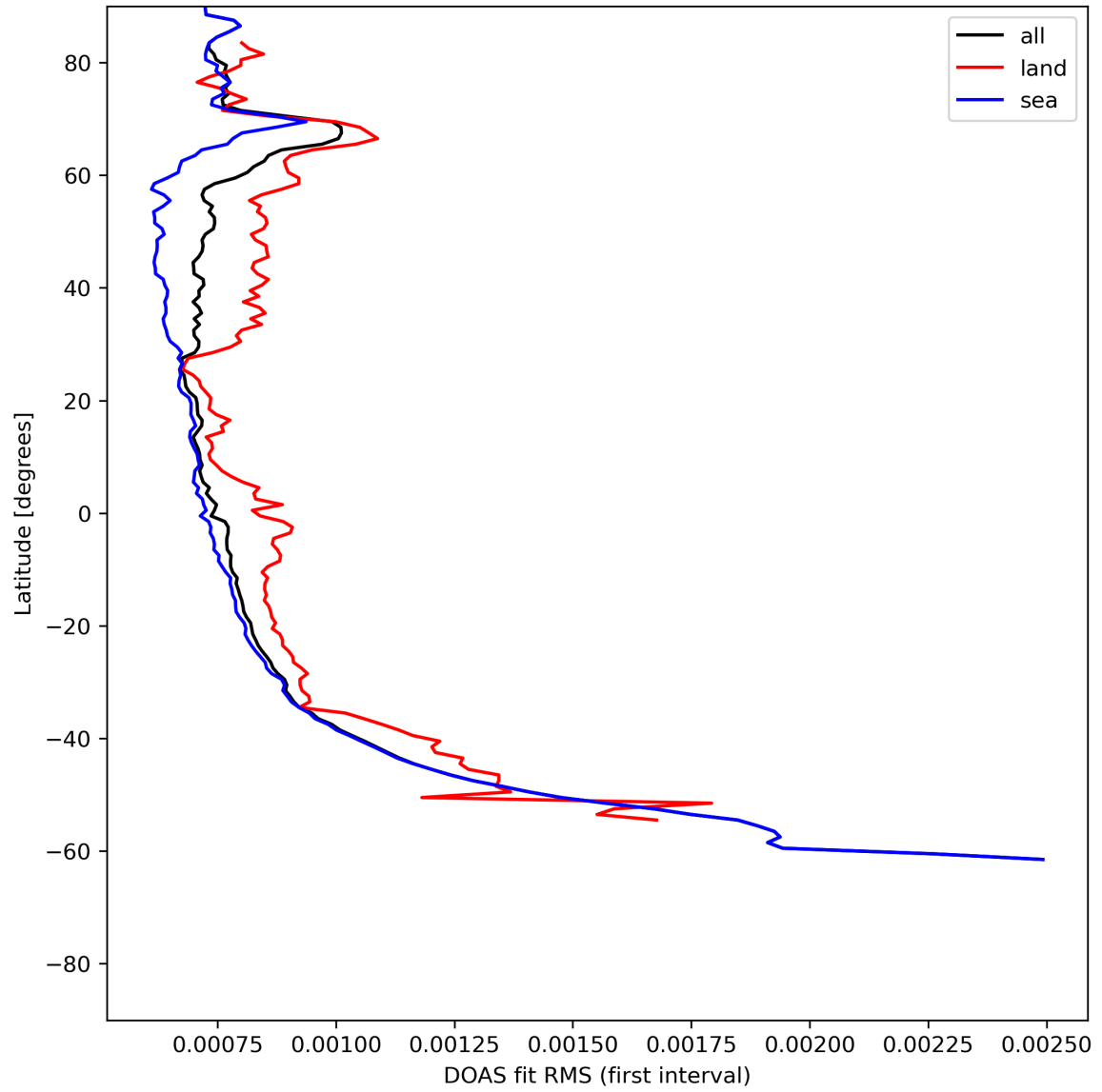
Figure 32: Zonal average of “DOAS fit RMS (first interval)” for 2024-06-14 to 2024-06-16.
