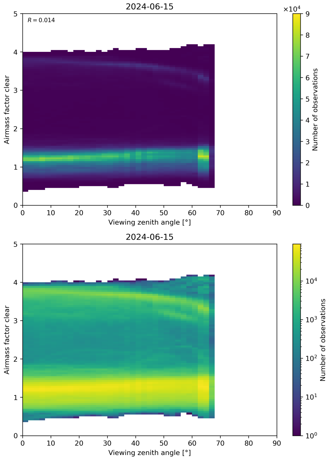
Figure 185: Scatter density plot of “Viewing zenith angle” against “Airmass factor clear” for 2024-06-14 to 2024-06-16.
