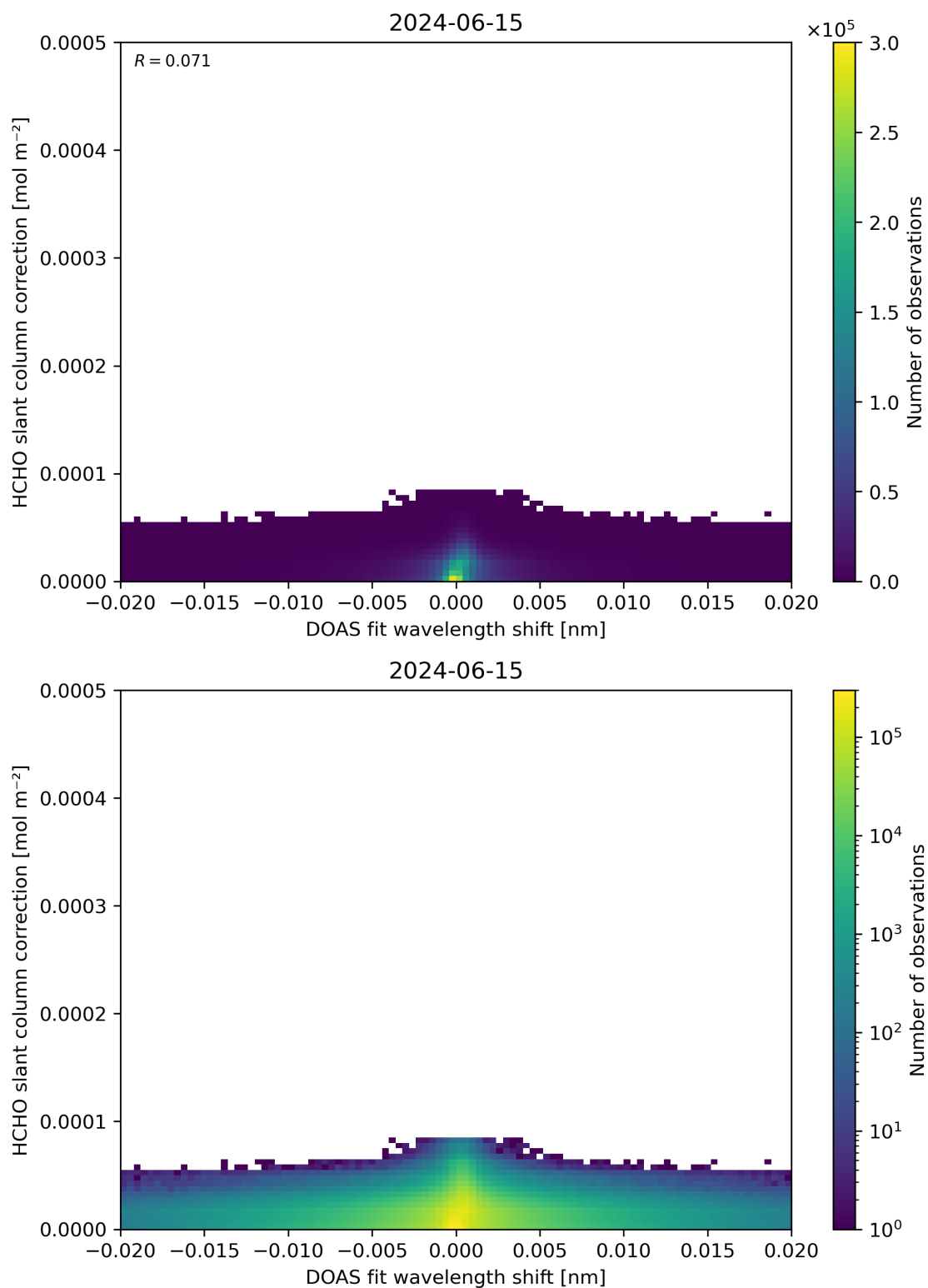
Figure 67: Scatter density plot of “DOAS fit wavelength shift” against “HCHO slant column correction” for 2024-06-14 to 2024-06-16.
