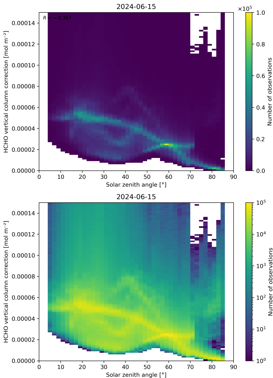
Figure 178: Scatter density plot of “Solar zenith angle” against “HCHO vertical column correction” for 2024-06-14 to 2024-06-16.
