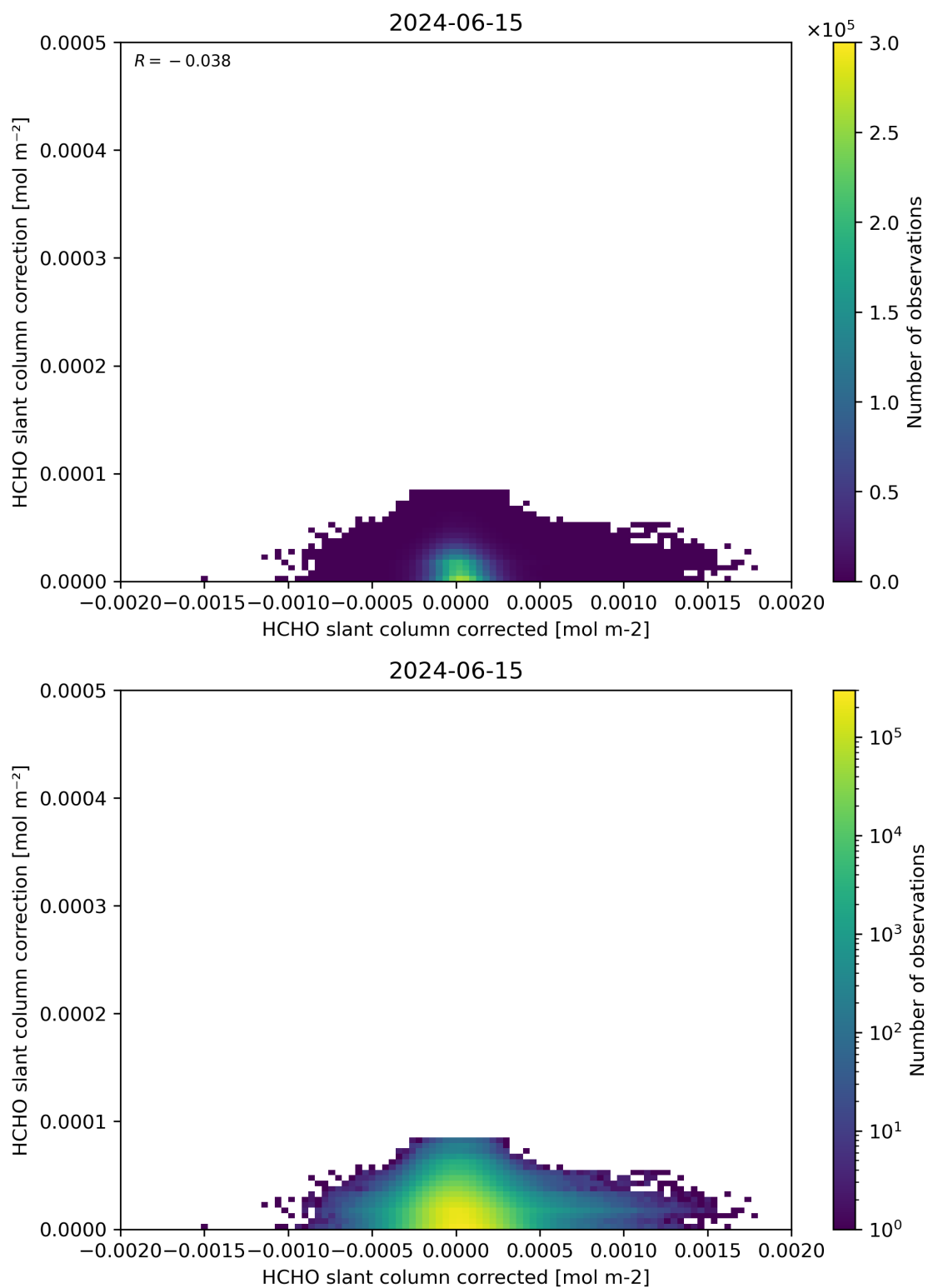
Figure 77: Scatter density plot of “HCHO slant column corrected” against “HCHO slant column correction” for 2024-06-14 to 2024-06-16.
