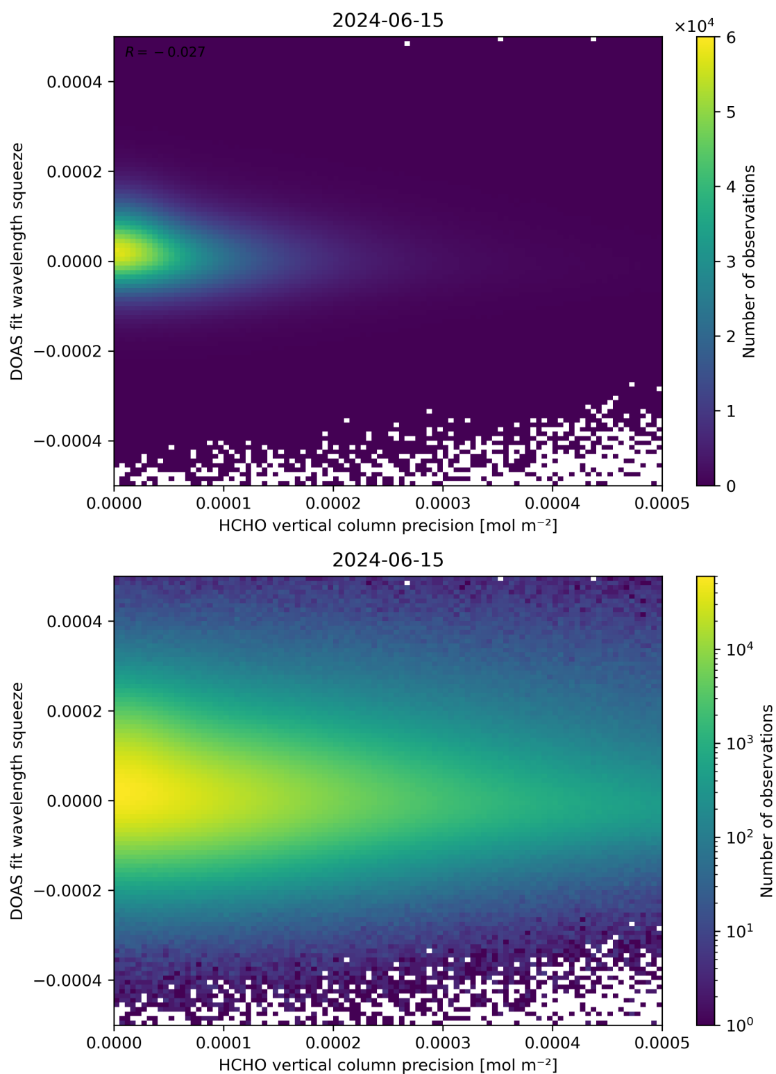
Figure 138: Scatter density plot of “HCHO vertical column precision” against “DOAS fit wavelength squeeze” for 2024-06-14 to 2024-06-16.
