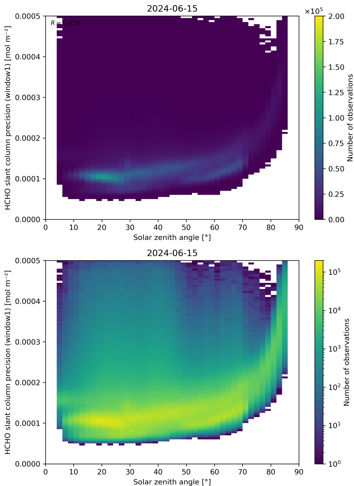
Figure 174: Scatter density plot of “Solar zenith angle” against “HCHO slant column precision (window1)” for 2024-06-14 to 2024-06-16.
