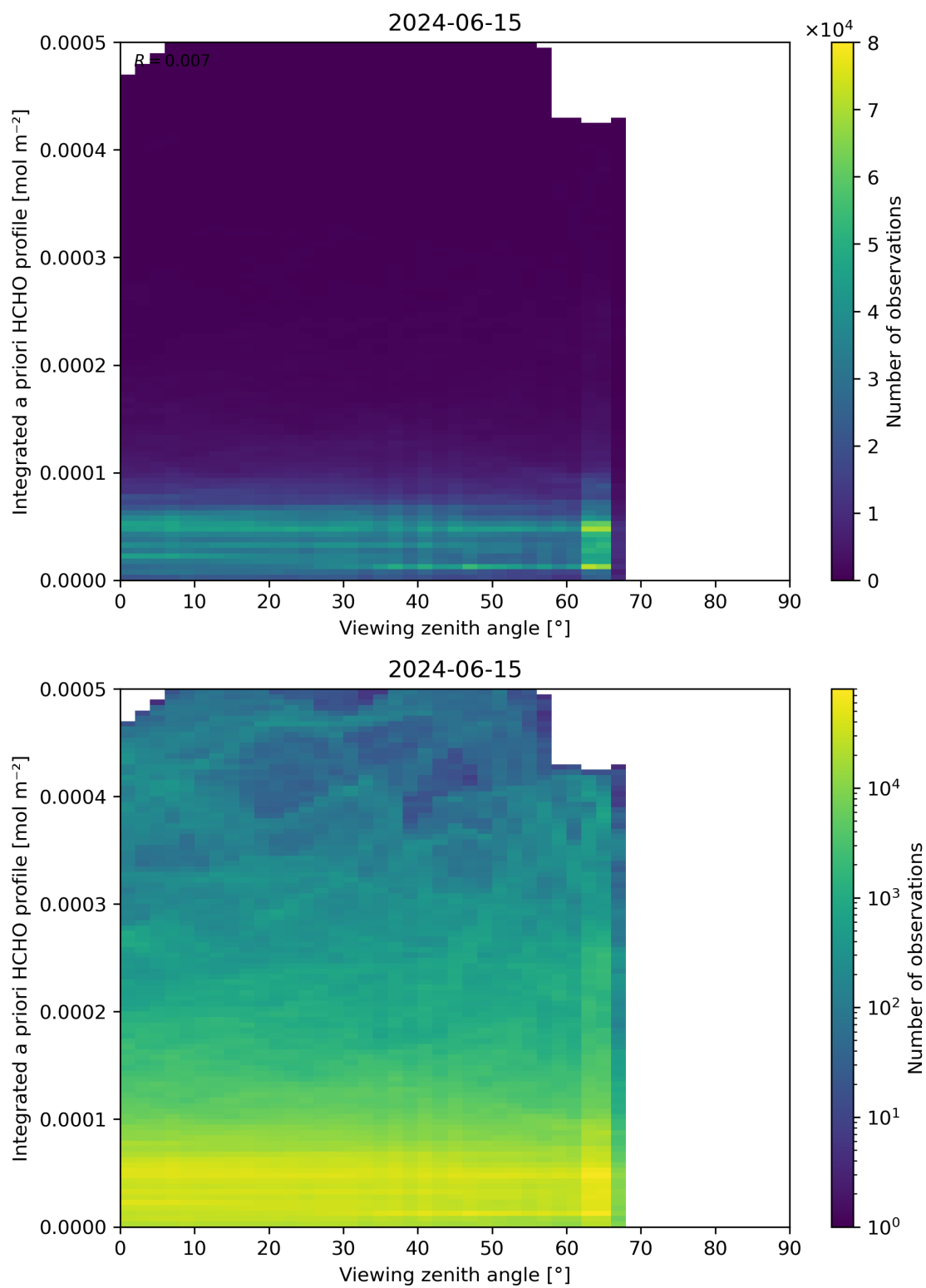
Figure 195: Scatter density plot of “Viewing zenith angle” against “Integrated a priori HCHO profile” for 2024-06-14 to 2024-06-16.
