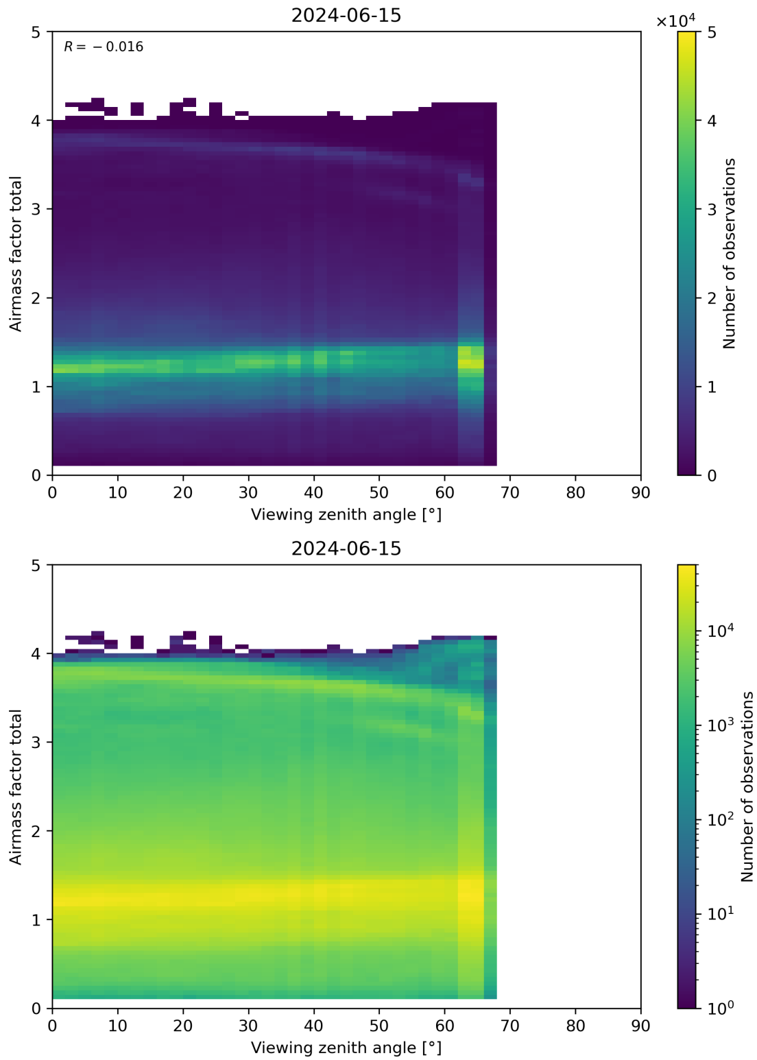
Figure 190: Scatter density plot of “Viewing zenith angle” against “Airmass factor total” for 2024-06-14 to 2024-06-16.
