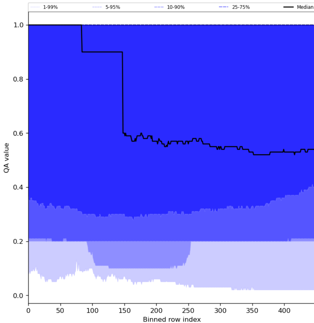
Figure 48: Along track statistics of “QA value” for 2024-06-14 to 2024-06-16
