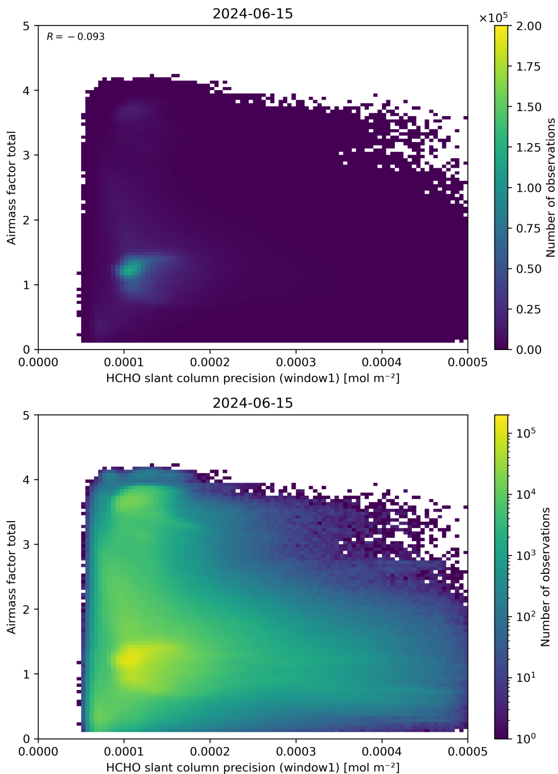
Figure 94: Scatter density plot of “HCHO slant column precision (window1)” against “Airmass factor total” for 2024-06-14 to 2024-06-16.
