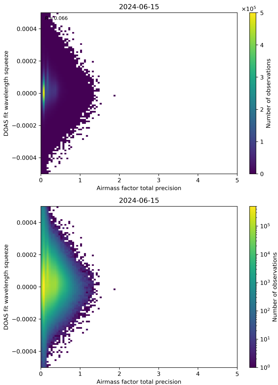
Figure 107: Scatter density plot of “Airmass factor total precision” against “DOAS fit wavelength squeeze” for 2024-06-14 to 2024-06-16.
