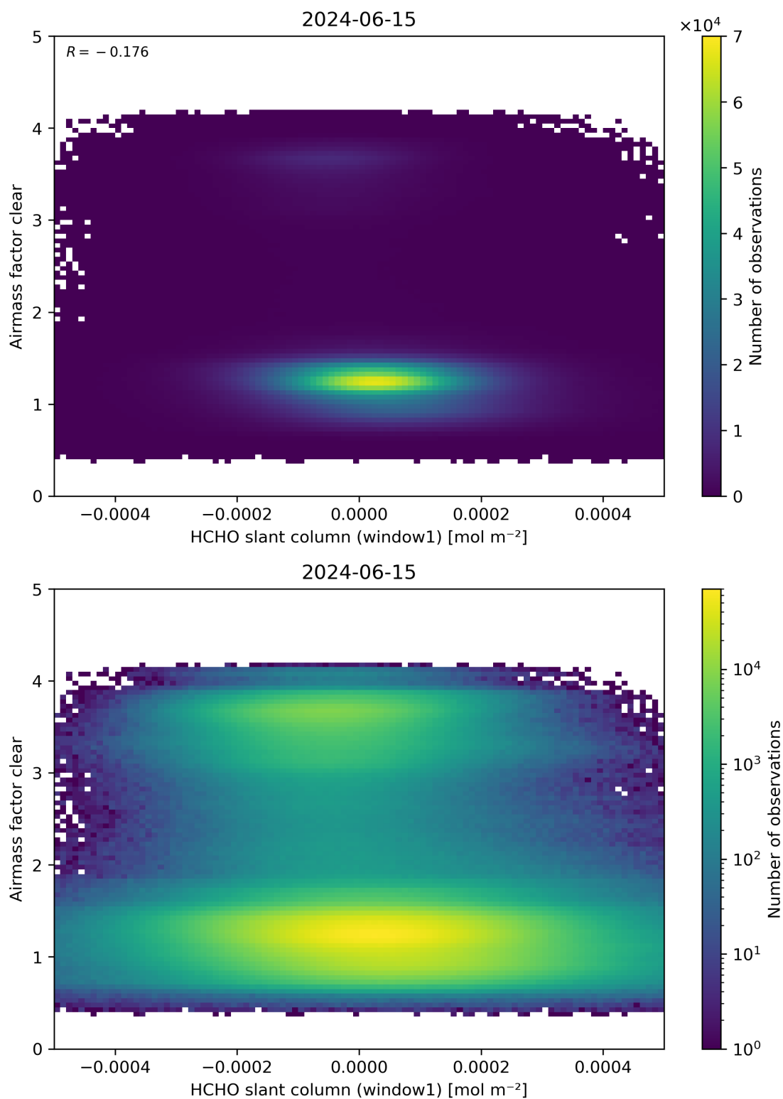
Figure 81: Scatter density plot of “HCHO slant column (window1)” against “Airmass factor clear” for 2024-06-14 to 2024-06-16.
