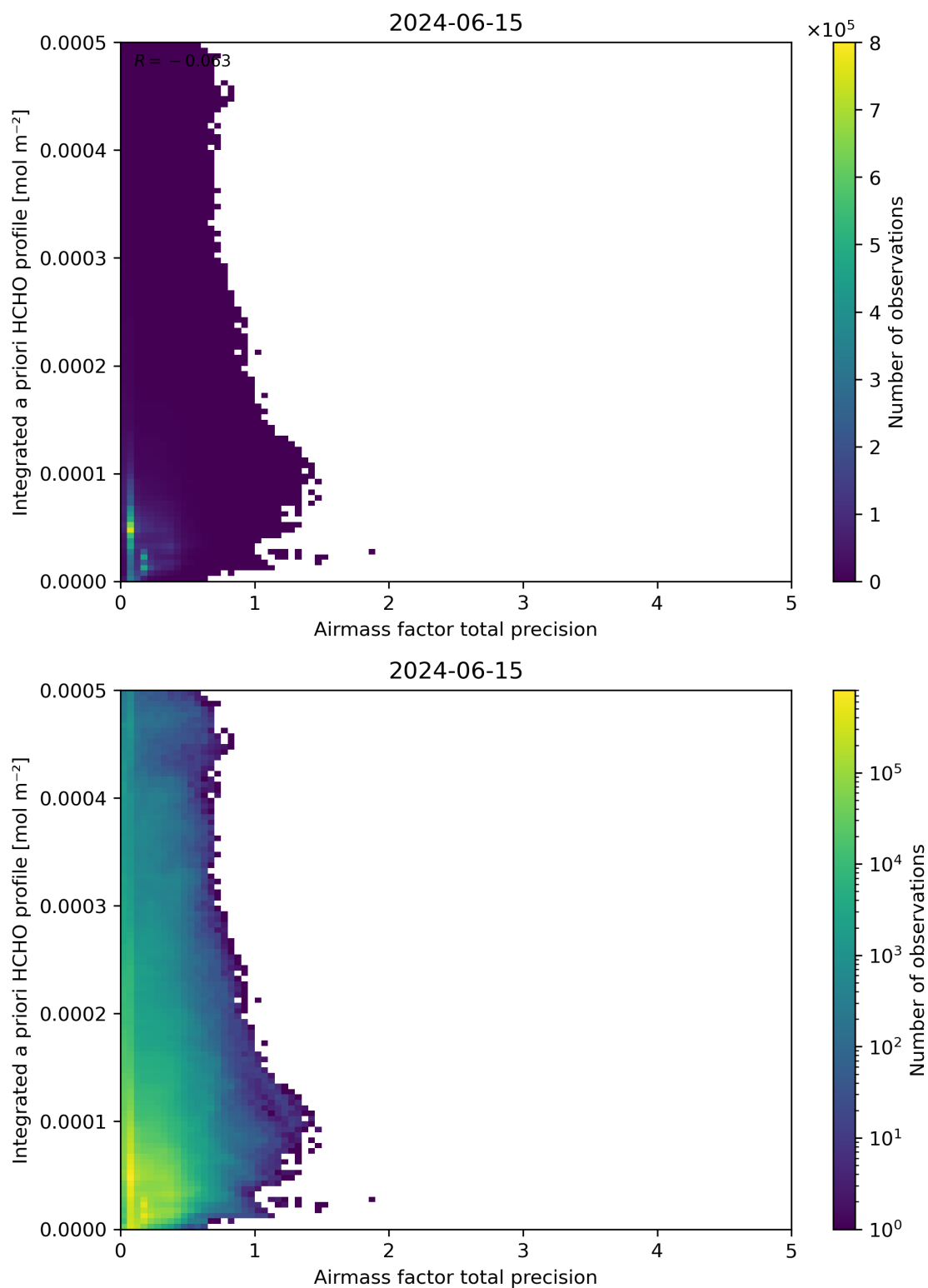
Figure 111: Scatter density plot of “Airmass factor total precision” against “Integrated a priori HCHO profile” for 2024-06-14 to 2024-06-16.
