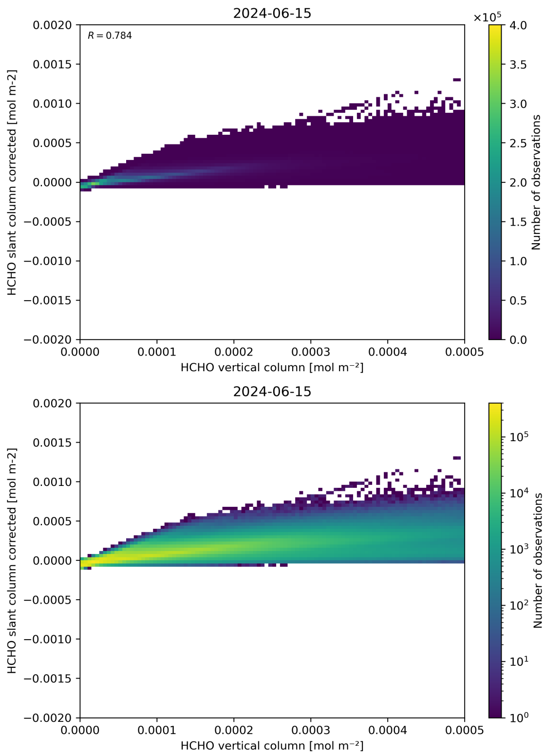
Figure 127: Scatter density plot of “HCHO vertical column” against “HCHO slant column corrected” for 2024-06-14 to 2024-06-16.
