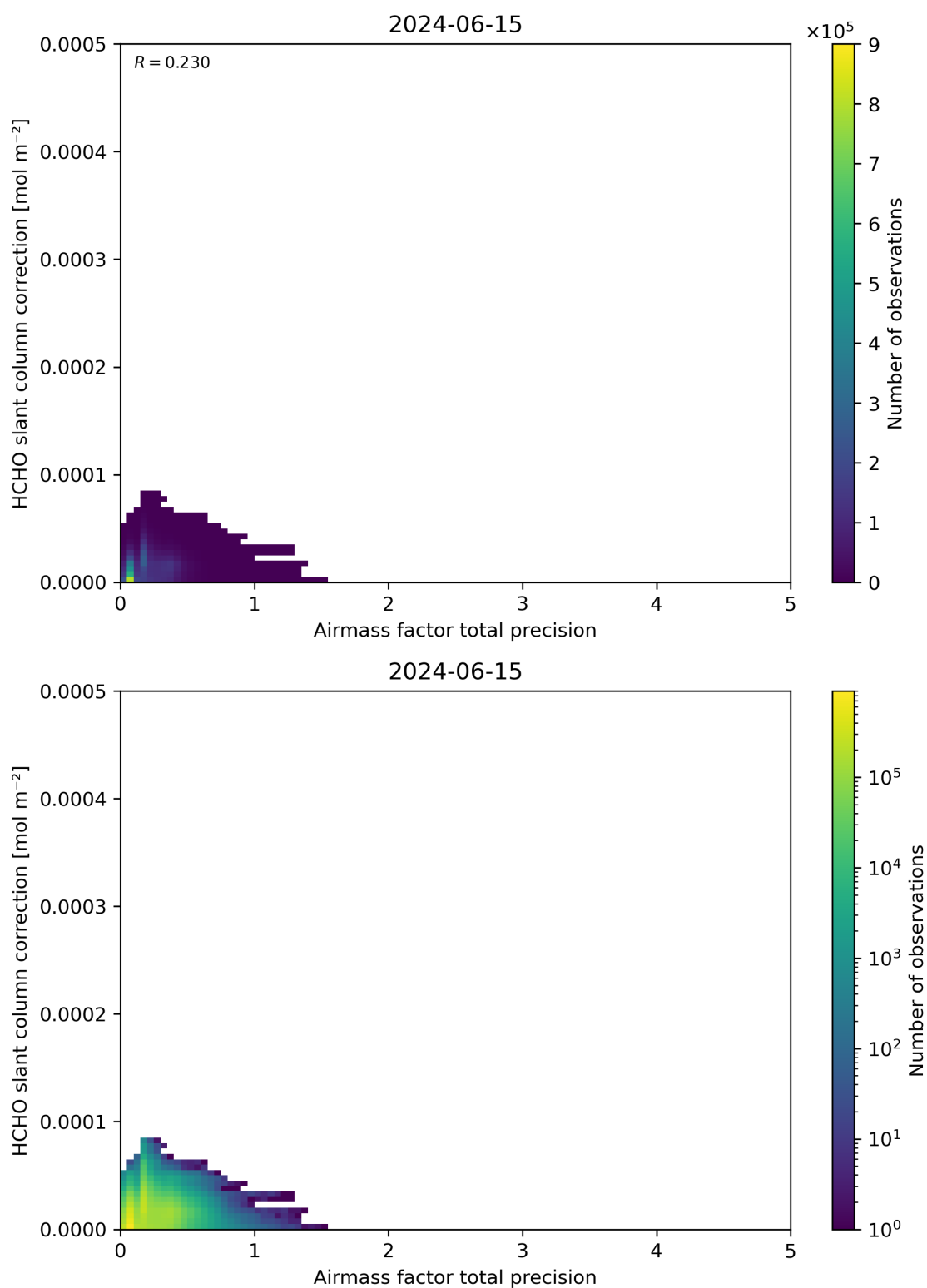
Figure 110: Scatter density plot of “Airmass factor total precision” against “HCHO slant column correction” for 2024-06-14 to 2024-06-16.
