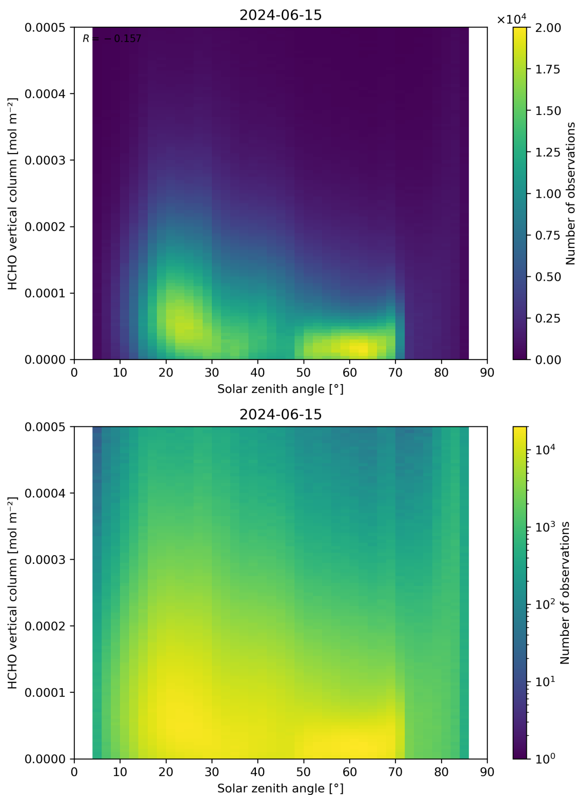
Figure 177: Scatter density plot of “Solar zenith angle” against “HCHO vertical column” for 2024-06-14 to 2024-06-16.
