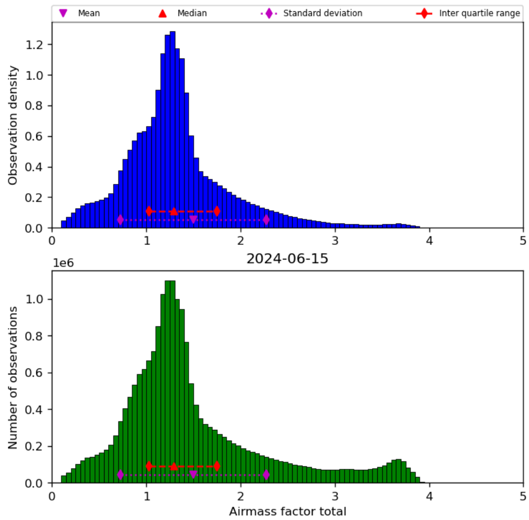
Figure 40: Histogram of “Airmass factor total” for 2024-06-14 to 2024-06-16
