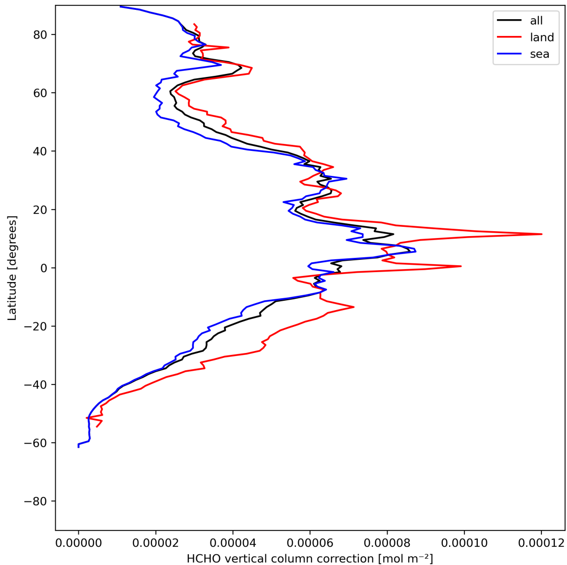
Figure 23: Zonal average of “HCHO vertical column correction” for 2024-06-14 to 2024-06-16.
