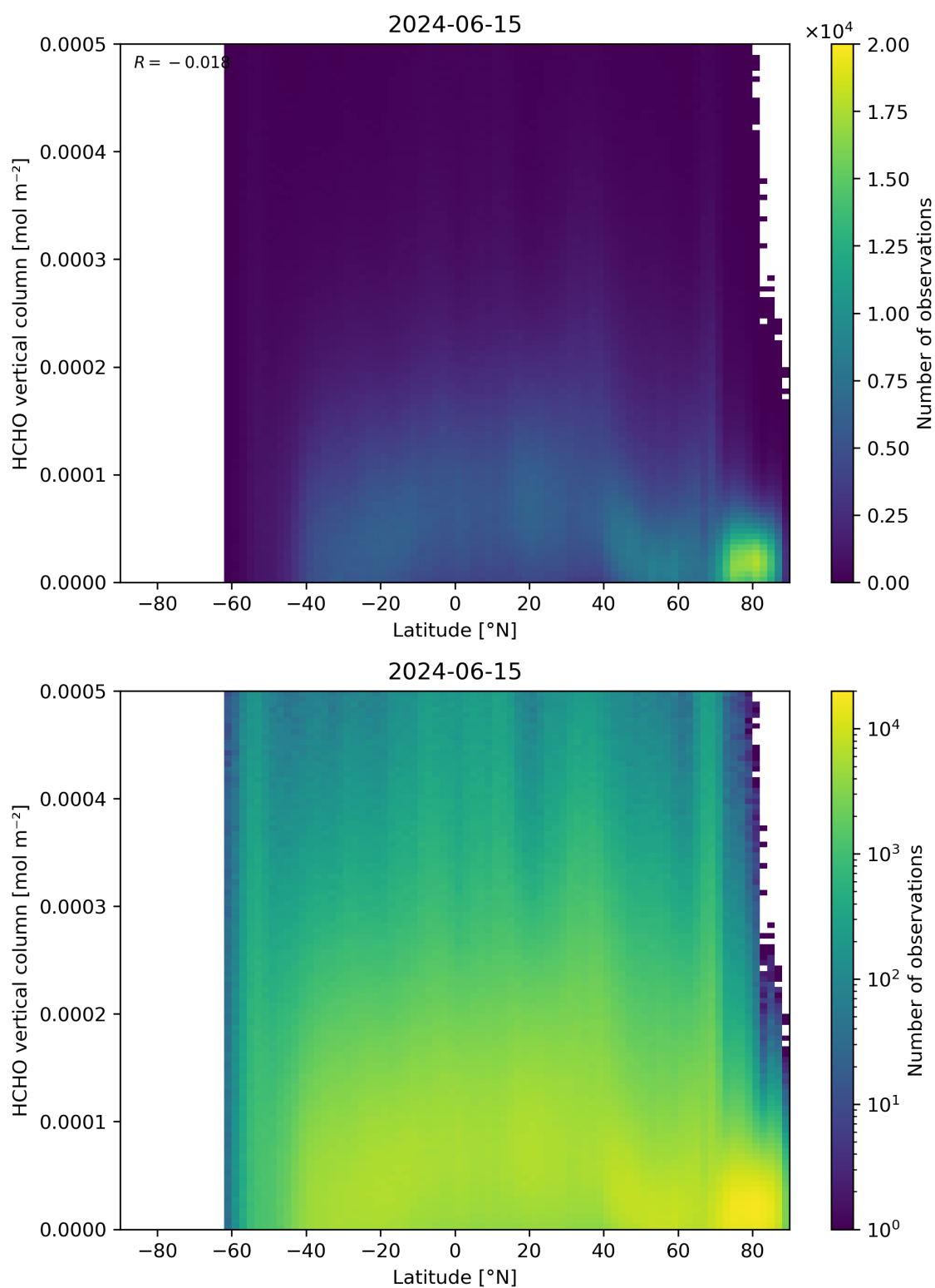
Figure 163: Scatter density plot of “Latitude” against “HCHO vertical column” for 2024-06-14 to 2024-06-16.
