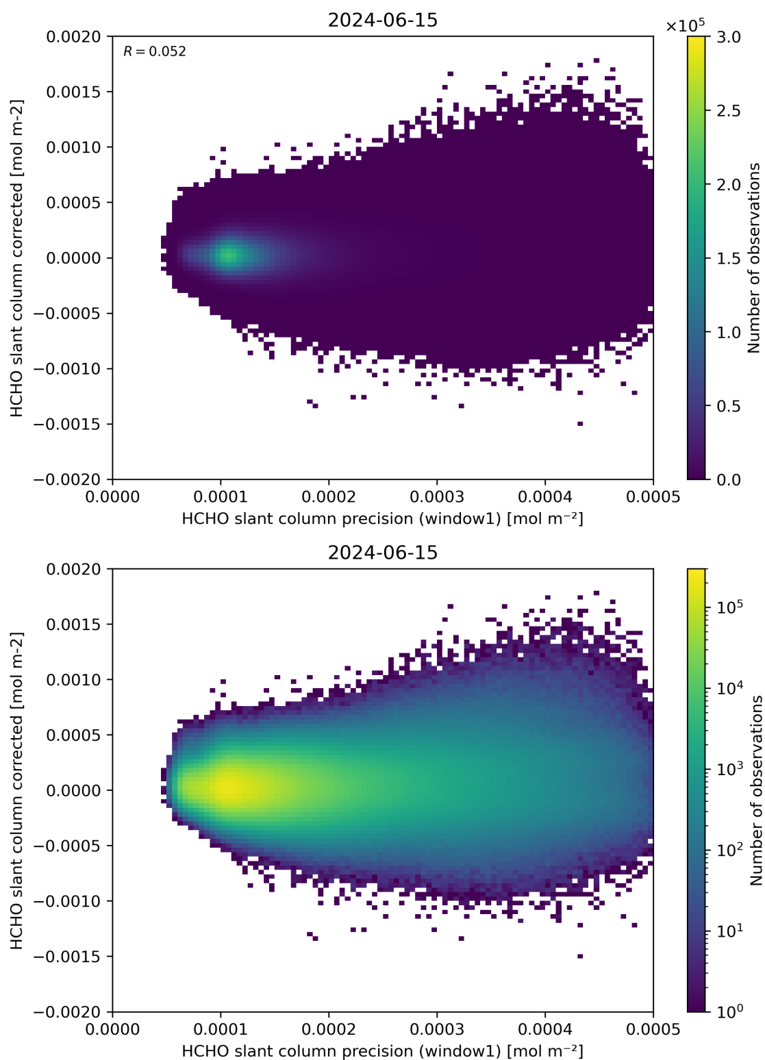
Figure 92: Scatter density plot of “HCHO slant column precision (window1)” against “HCHO slant column corrected” for 2024-06-14 to 2024-06-16.
