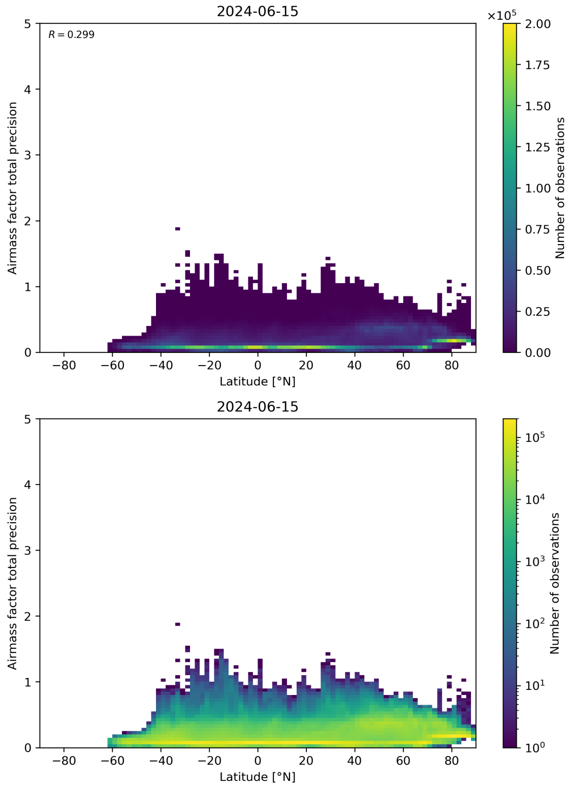
Figure 162: Scatter density plot of “Latitude” against “Airmass factor total precision” for 2024-06-14 to 2024-06-16.
