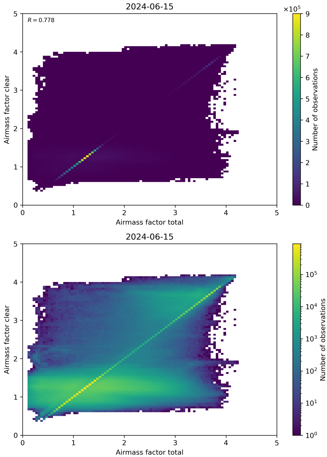
Figure 100: Scatter density plot of “Airmass factor total” against “Airmass factor clear” for 2024-06-14 to 2024-06-16.
