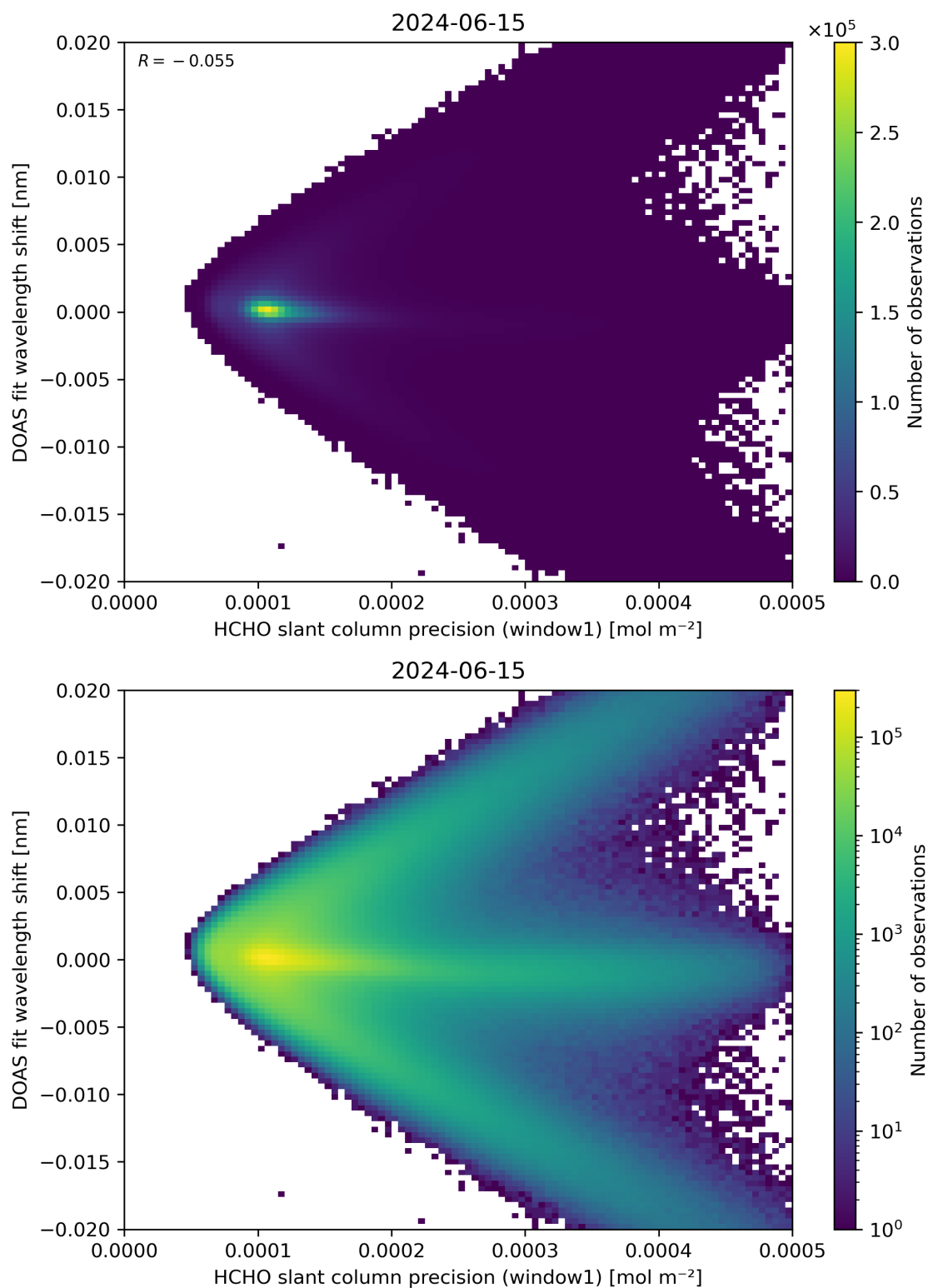
Figure 89: Scatter density plot of “HCHO slant column precision (window1)” against “DOAS fit wavelength shift” for 2024-06-14 to 2024-06-16.
