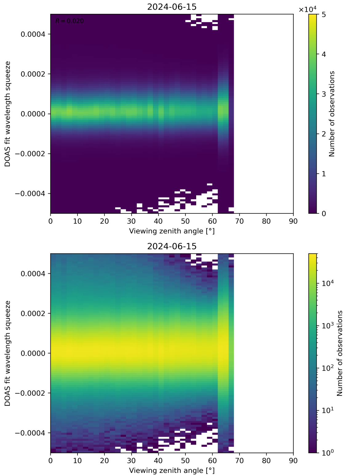
Figure 184: Scatter density plot of “Viewing zenith angle” against “DOAS fit wavelength squeeze” for 2024-06-14 to 2024-06-16.
