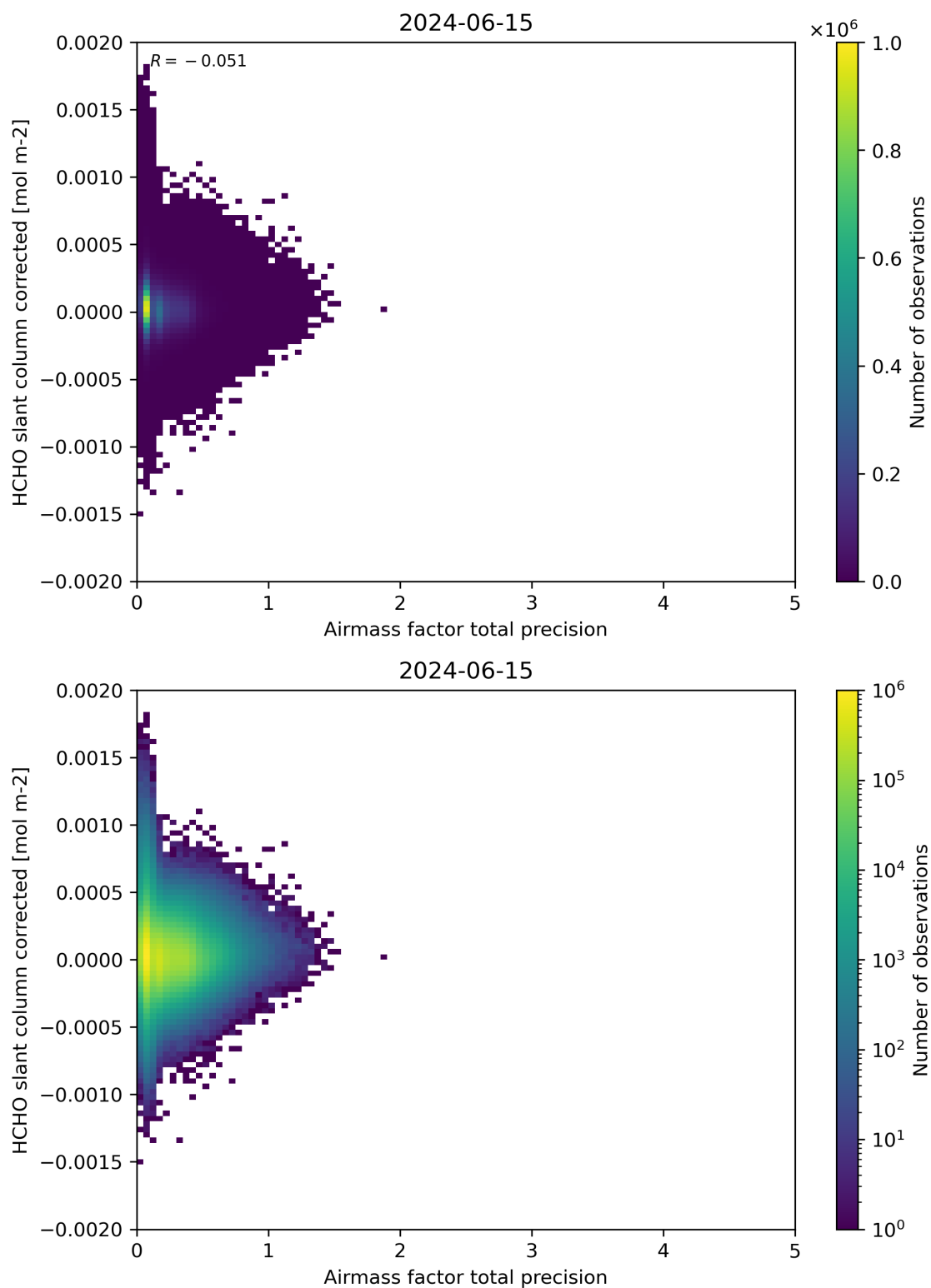
Figure 109: Scatter density plot of “Airmass factor total precision” against “HCHO slant column corrected” for 2024-06-14 to 2024-06-16.
