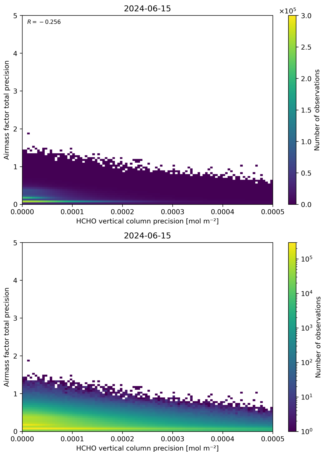
Figure 145: Scatter density plot of “HCHO vertical column precision” against “Airmass factor total precision” for 2024-06-14 to 2024-06-16.
