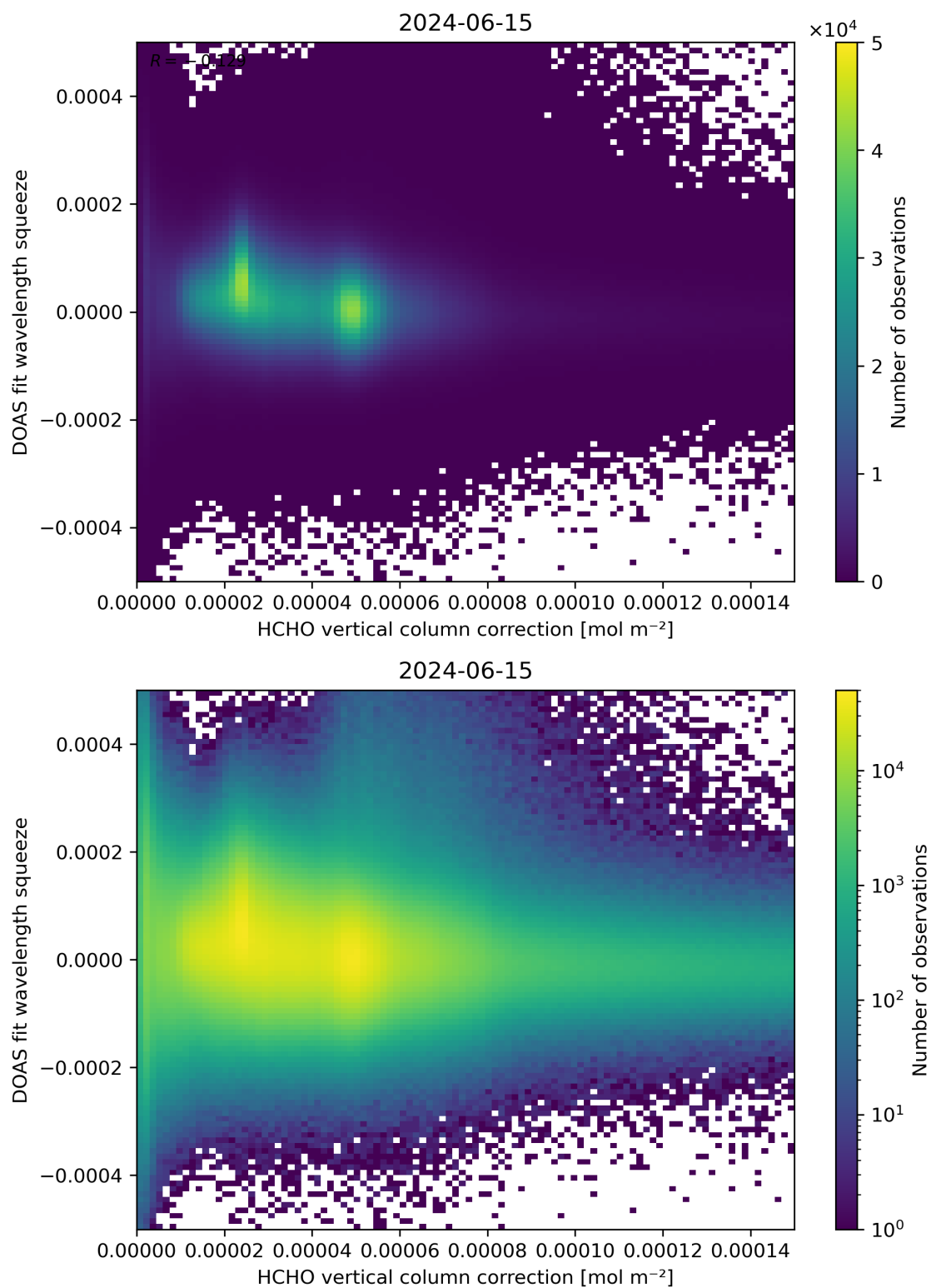
Figure 114: Scatter density plot of “HCHO vertical column correction” against “DOAS fit wavelength squeeze” for 2024-06-14 to 2024-06-16.
