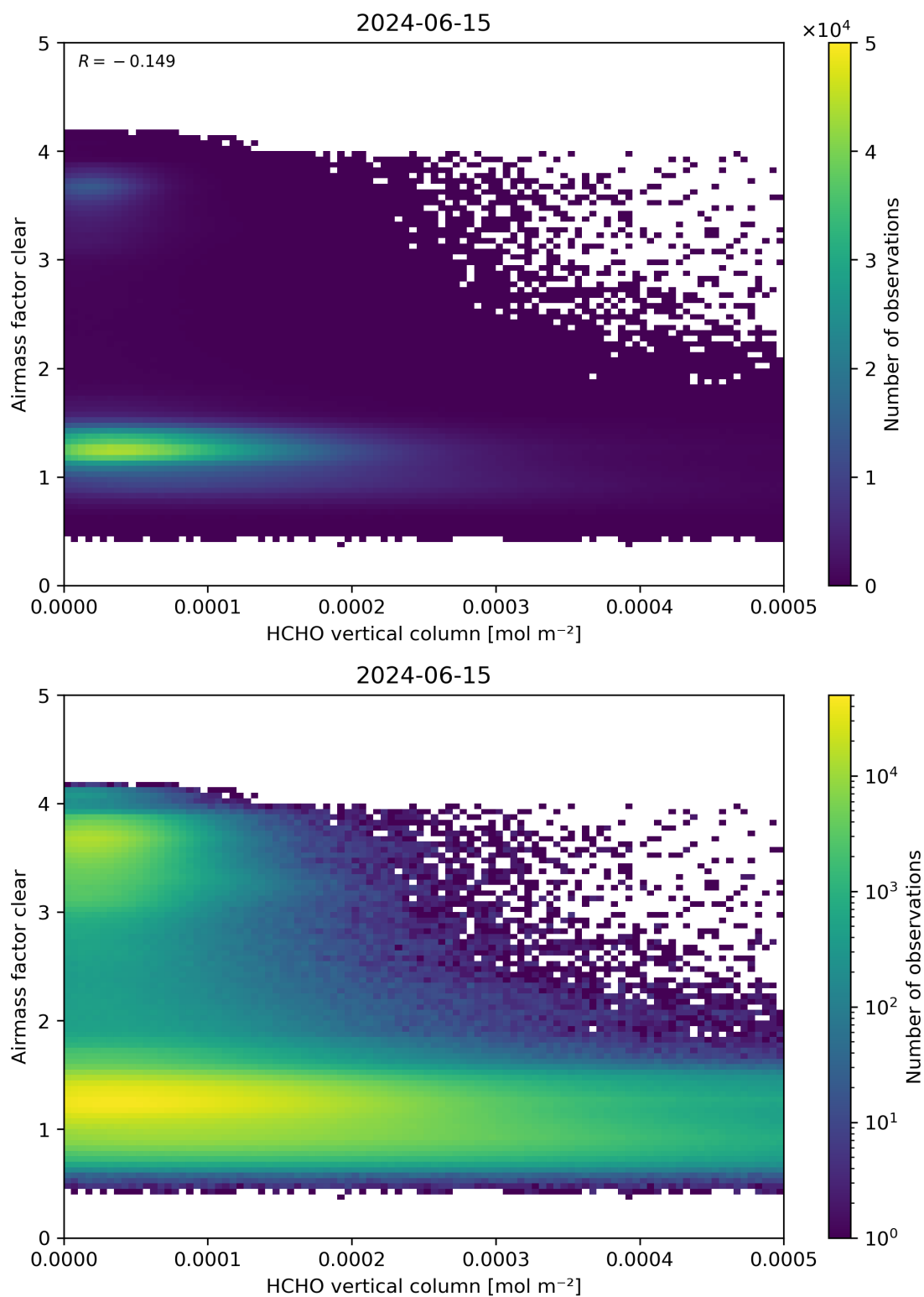
Figure 126: Scatter density plot of “HCHO vertical column” against “Airmass factor clear” for 2024-06-14 to 2024-06-16.
