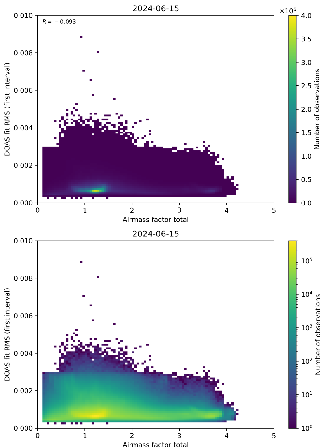
Figure 97: Scatter density plot of “Airmass factor total” against “DOAS fit RMS (first interval)” for 2024-06-14 to 2024-06-16.
