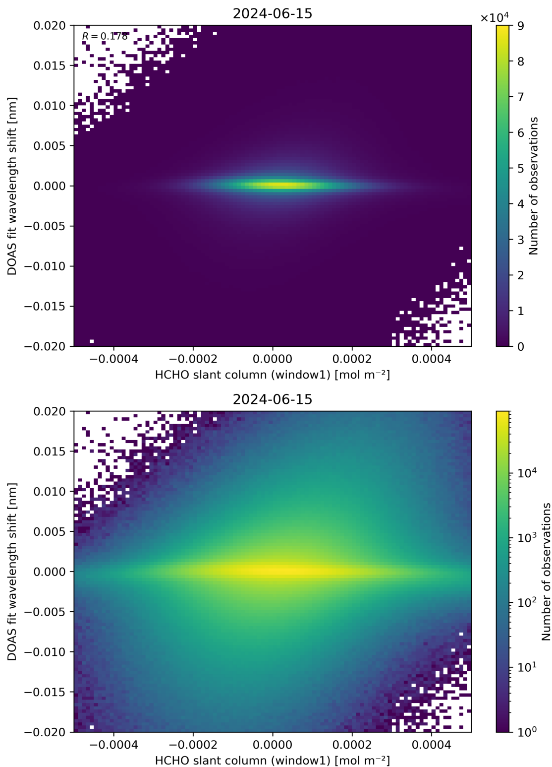
Figure 79: Scatter density plot of “HCHO slant column (window1)” against “DOAS fit wavelength shift” for 2024-06-14 to 2024-06-16.
