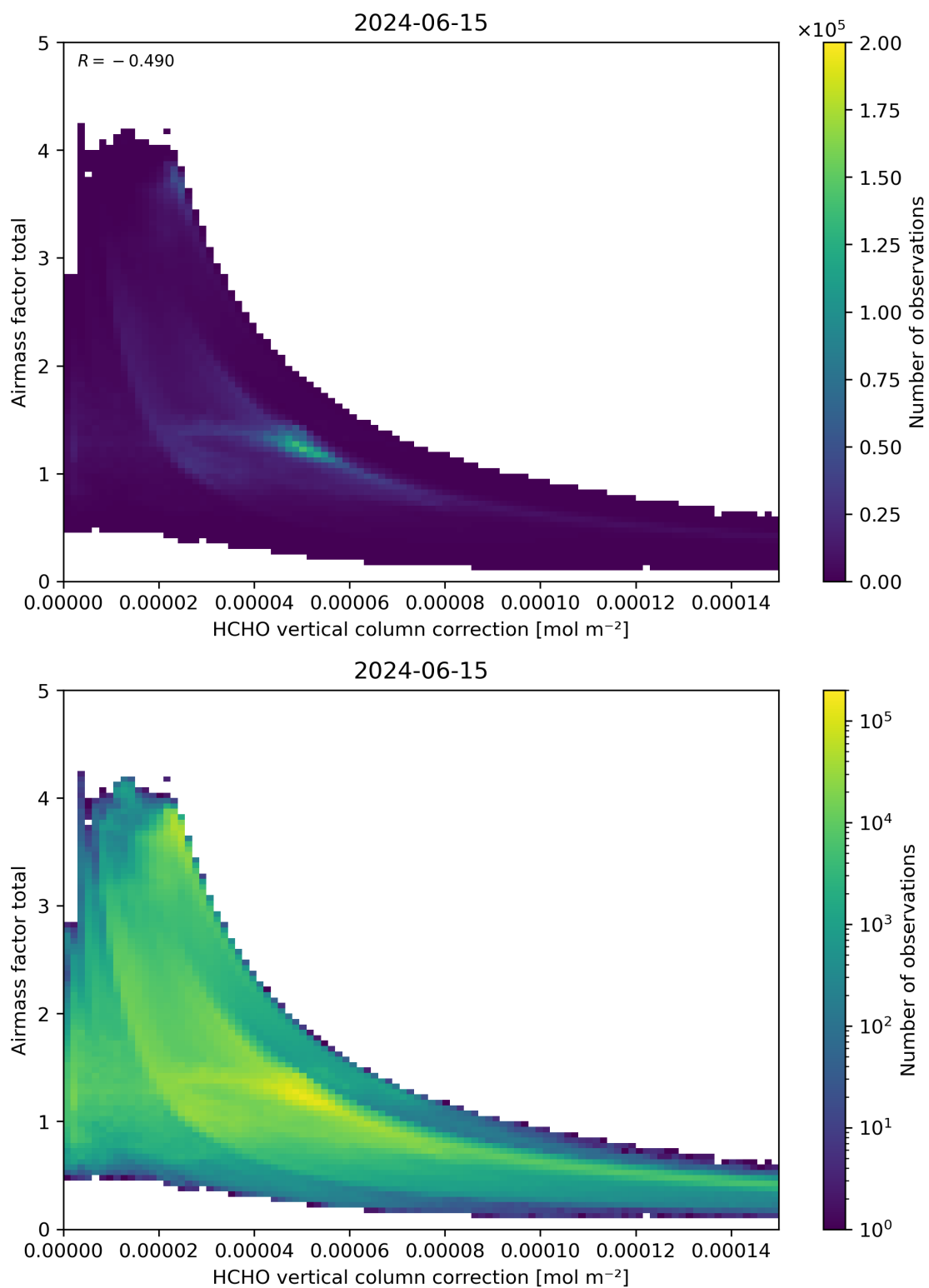
Figure 120: Scatter density plot of “HCHO vertical column correction” against “Airmass factor total” for 2024-06-14 to 2024-06-16.
