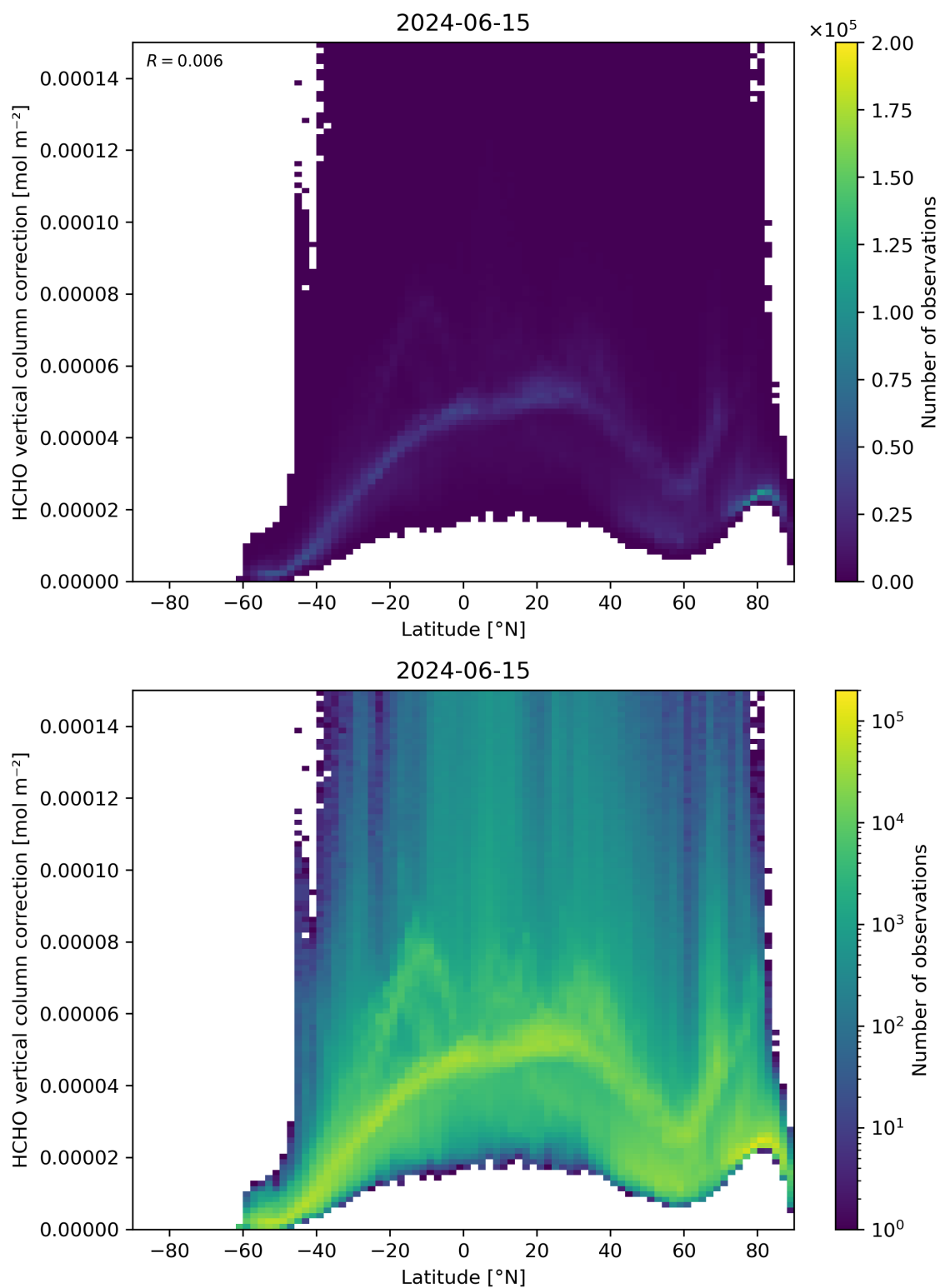
Figure 164: Scatter density plot of “Latitude” against “HCHO vertical column correction” for 2024-06-14 to 2024-06-16.
