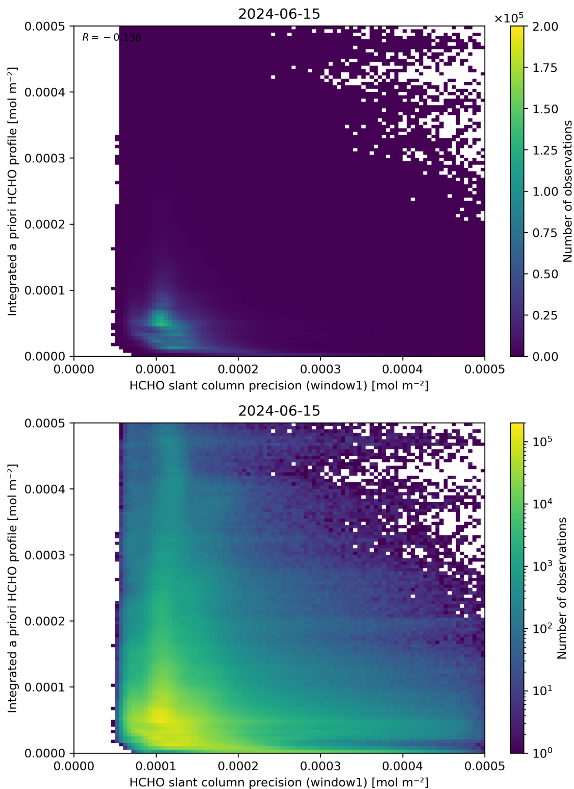
Figure 96: Scatter density plot of “HCHO slant column precision (window1)” against “Integrated a priori HCHO profile” for 2024-06-14 to 2024-06-16.
