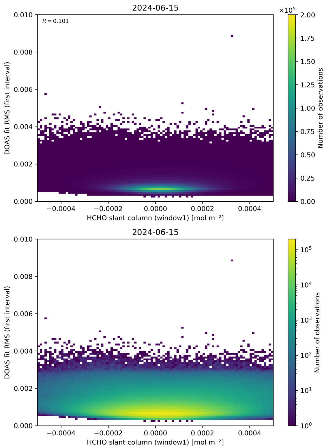
Figure 78: Scatter density plot of “HCHO slant column (window1)” against “DOAS fit RMS (first interval)” for 2024-06-14 to 2024-06-16.
