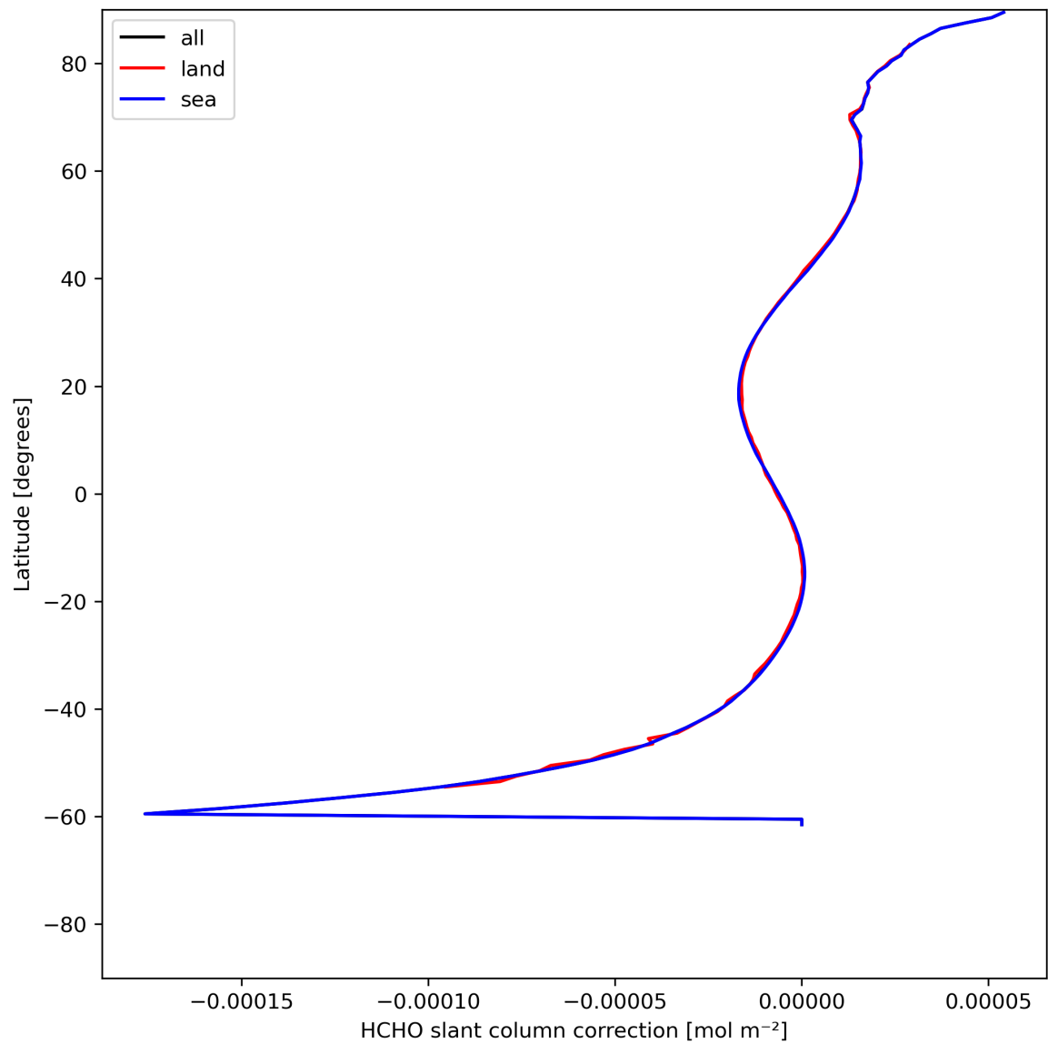
Figure 33: Zonal average of “HCHO slant column correction” for 2024-06-14 to 2024-06-16.
