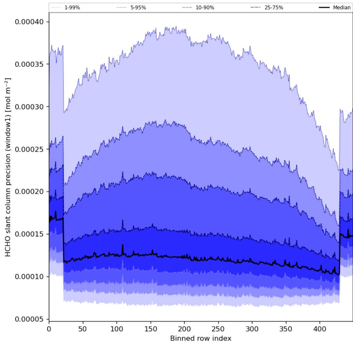
Figure 53: Along track statistics of “HCHO slant column precision (window1)” for 2024-06-14 to 2024-06-16
