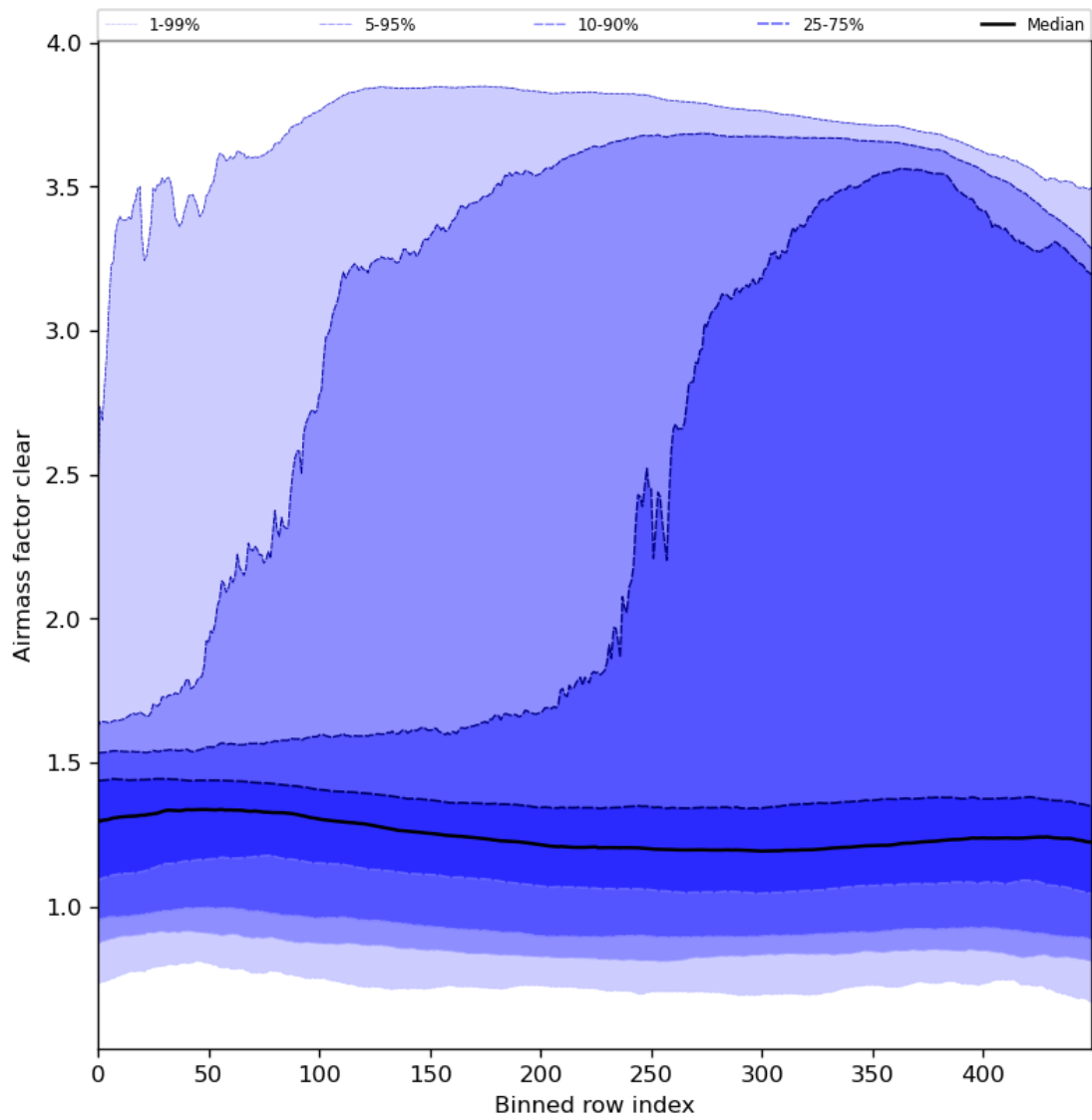
Figure 56: Along track statistics of “Airmass factor clear” for 2024-06-14 to 2024-06-16
