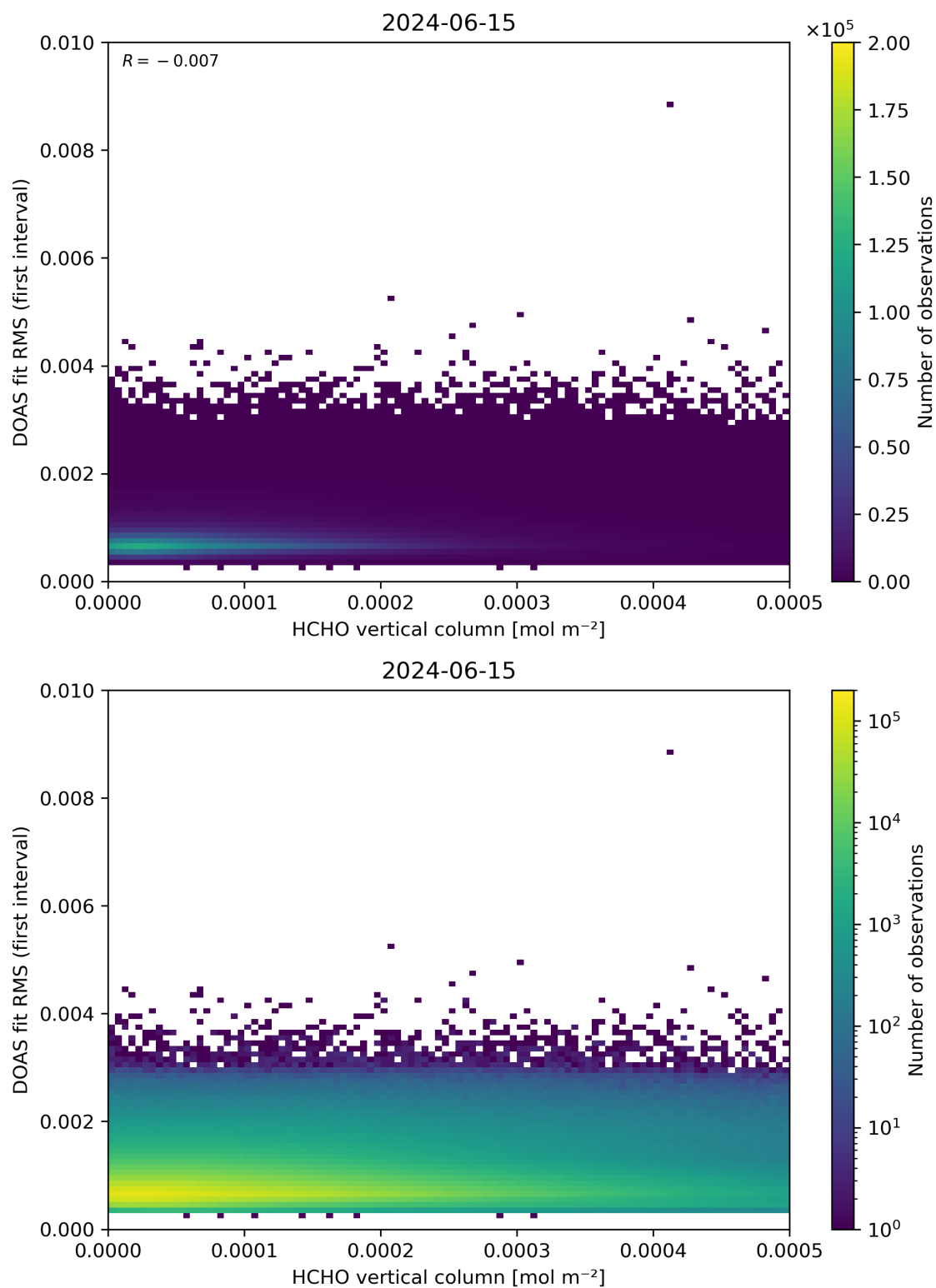
Figure 123: Scatter density plot of “HCHO vertical column” against “DOAS fit RMS (first interval)” for 2024-06-14 to 2024-06-16.
