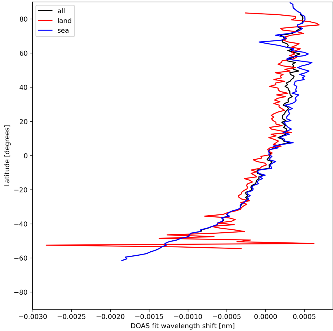
Figure 30: Zonal average of "DOAS fit wavelength shift" for 2024-06-14 to 2024-06-16.
