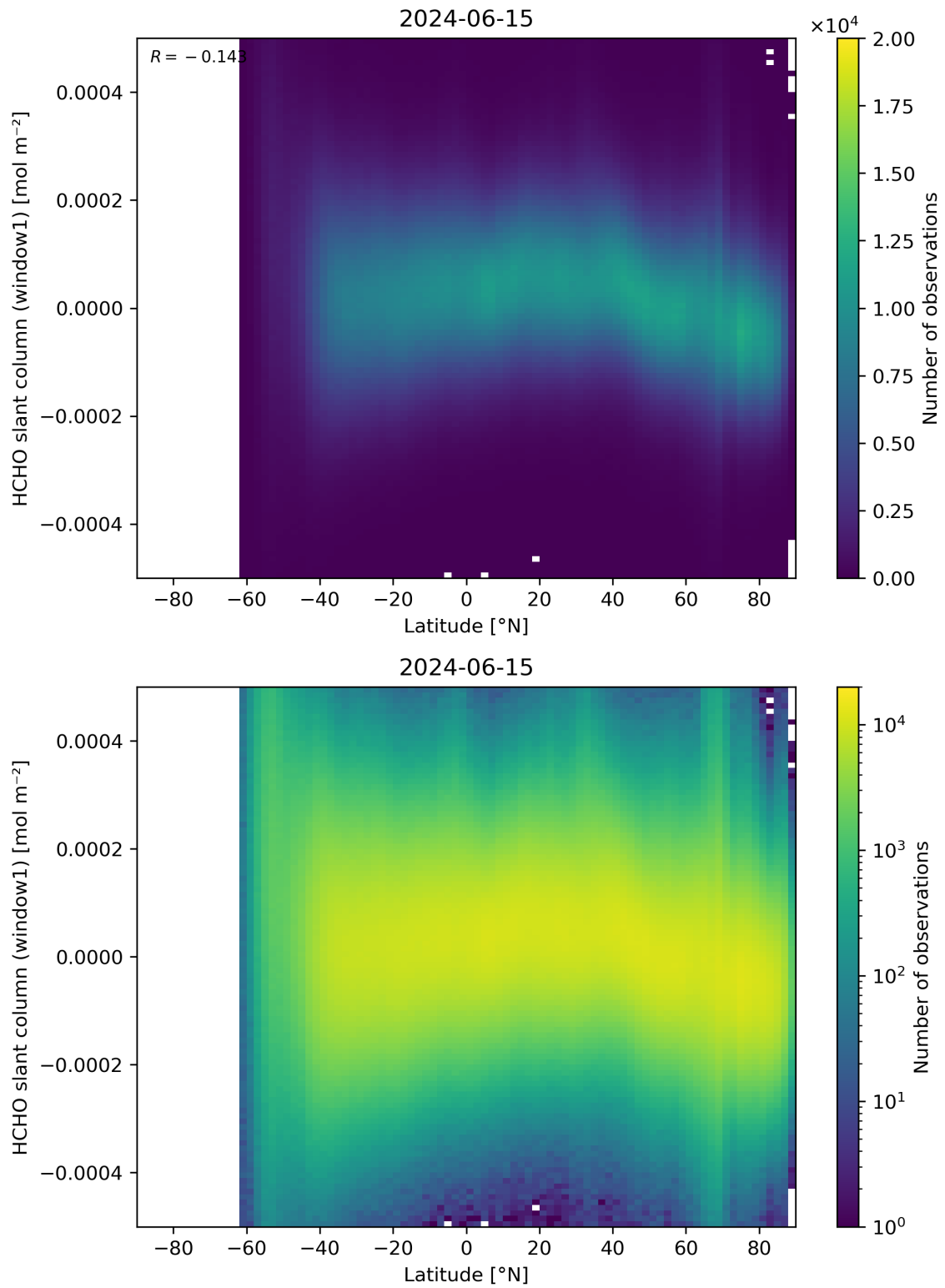
Figure 159: Scatter density plot of “Latitude” against “HCHO slant column (window1)” for 2024-06-14 to 2024-06-16.
