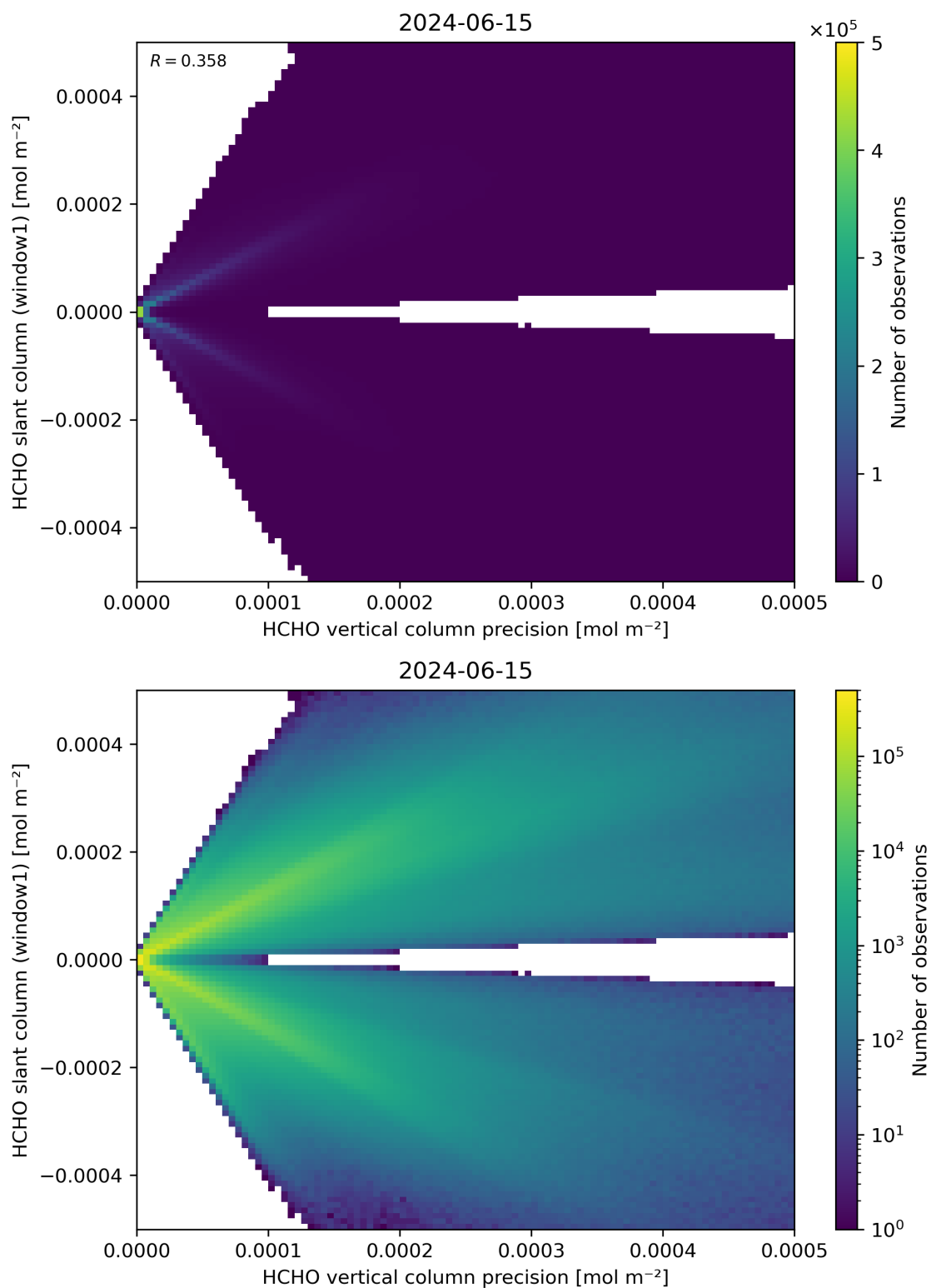
Figure 142: Scatter density plot of “HCHO vertical column precision” against “HCHO slant column (window1)” for 2024-06-14 to 2024-06-16.
