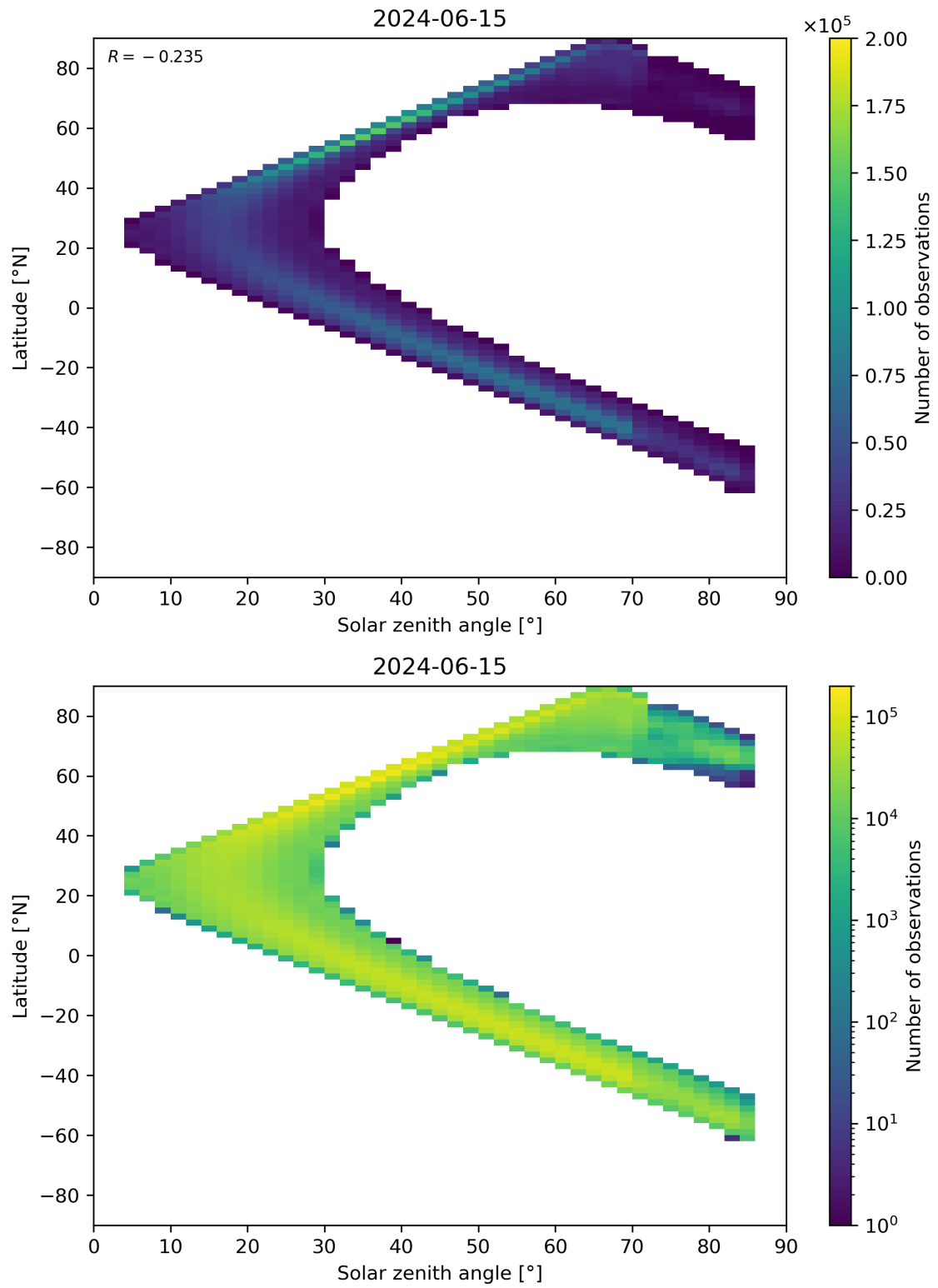
Figure 181: Scatter density plot of “Solar zenith angle” against “Latitude” for 2024-06-14 to 2024-06-16.
