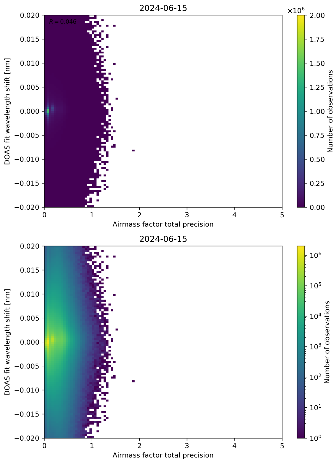
Figure 106: Scatter density plot of “Airmass factor total precision” against “DOAS fit wavelength shift” for 2024-06-14 to 2024-06-16.
