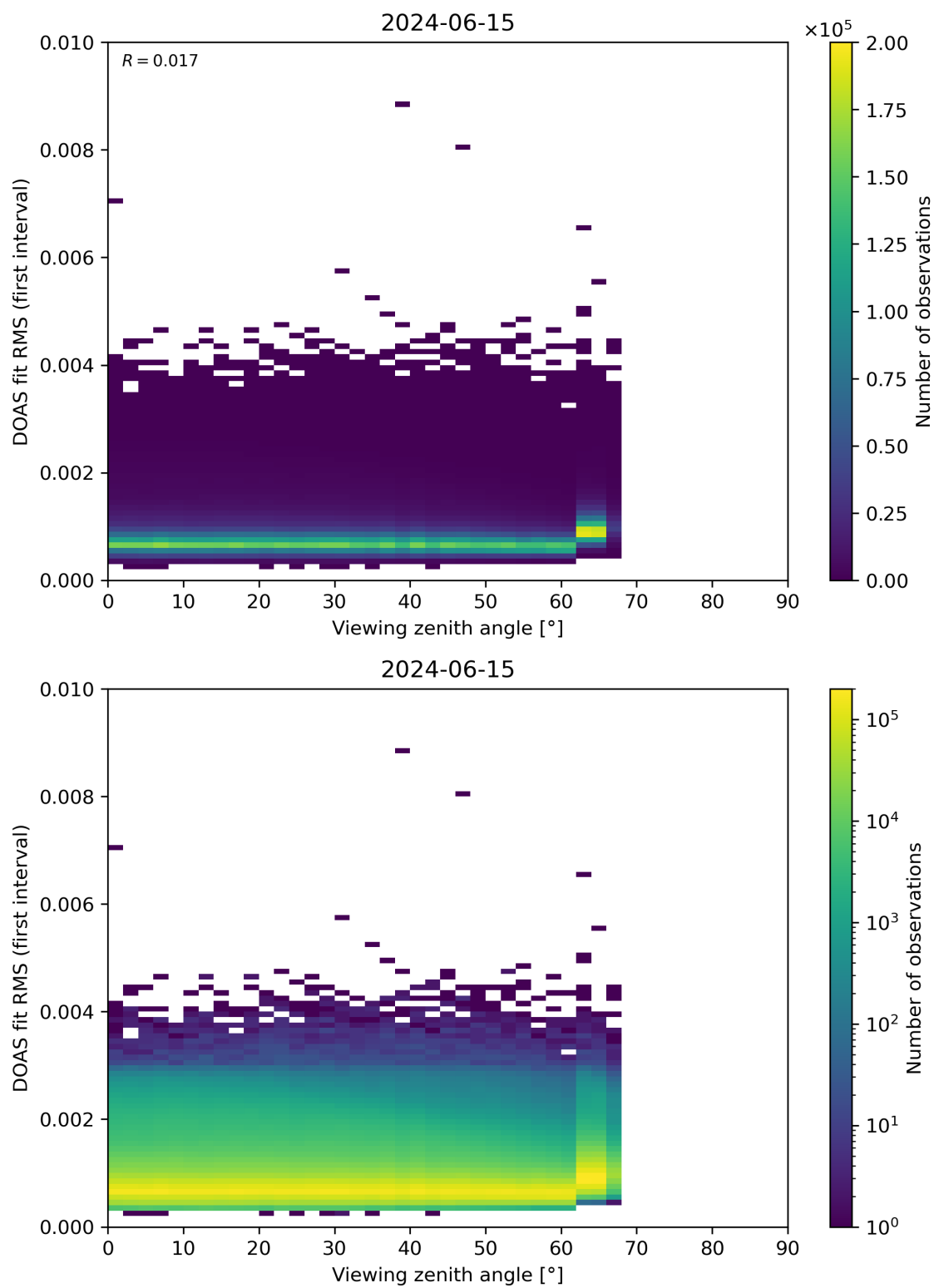
Figure 182: Scatter density plot of “Viewing zenith angle” against “DOAS fit RMS (first interval)” for 2024-06-14 to 2024-06-16.
