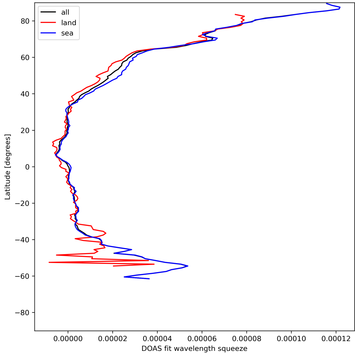
Figure 31: Zonal average of “DOAS fit wavelength squeeze” for 2024-06-14 to 2024-06-16.
