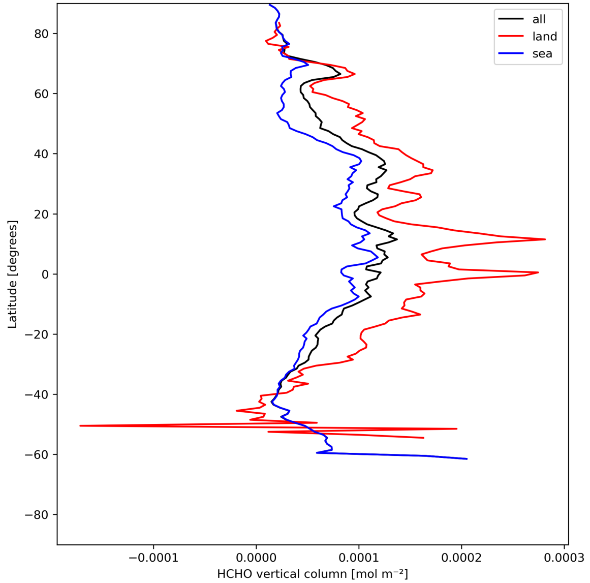
Figure 21: Zonal average of “HCHO vertical column” for 2024-06-14 to 2024-06-16.
