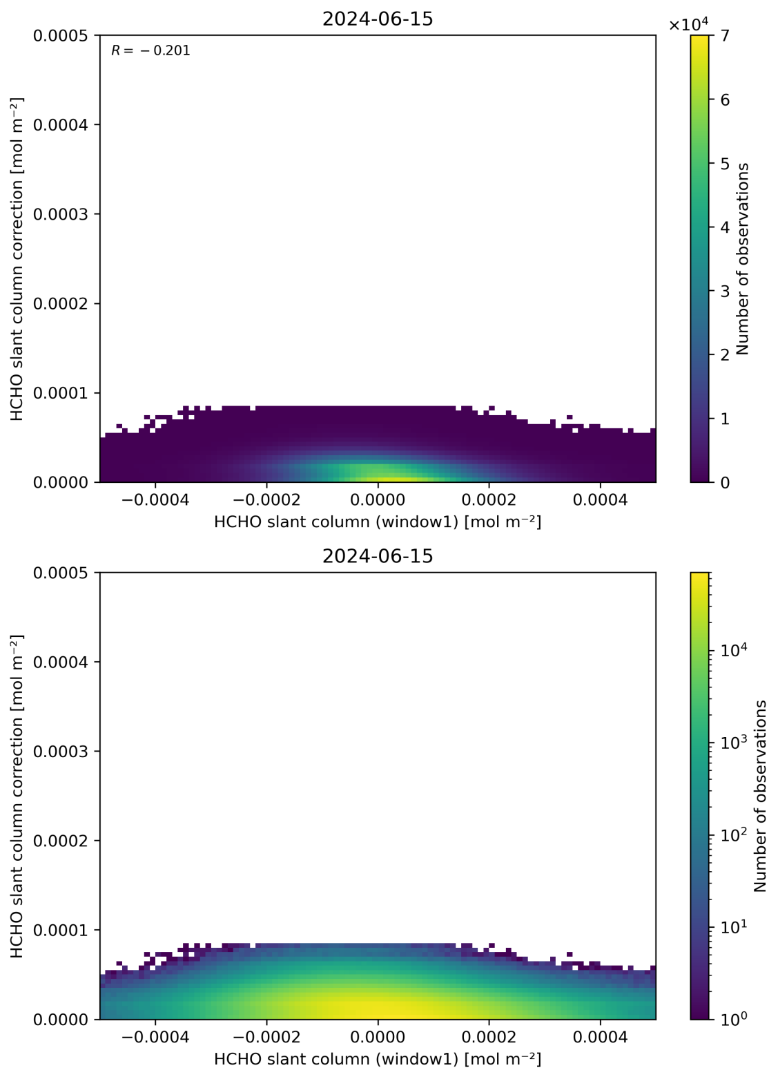
Figure 83: Scatter density plot of “HCHO slant column (window1)” against “HCHO slant column correction” for 2024-06-14 to 2024-06-16.
