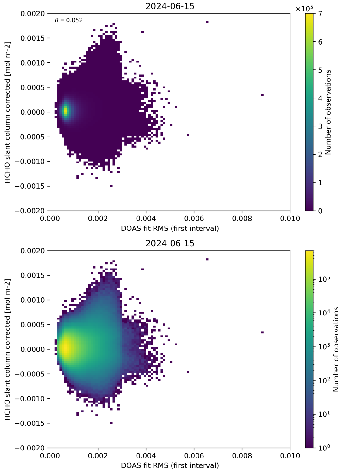
Figure 62: Scatter density plot of “DOAS fit RMS (first interval)” against “HCHO slant column corrected” for 2024-06-14 to 2024-06-16.
