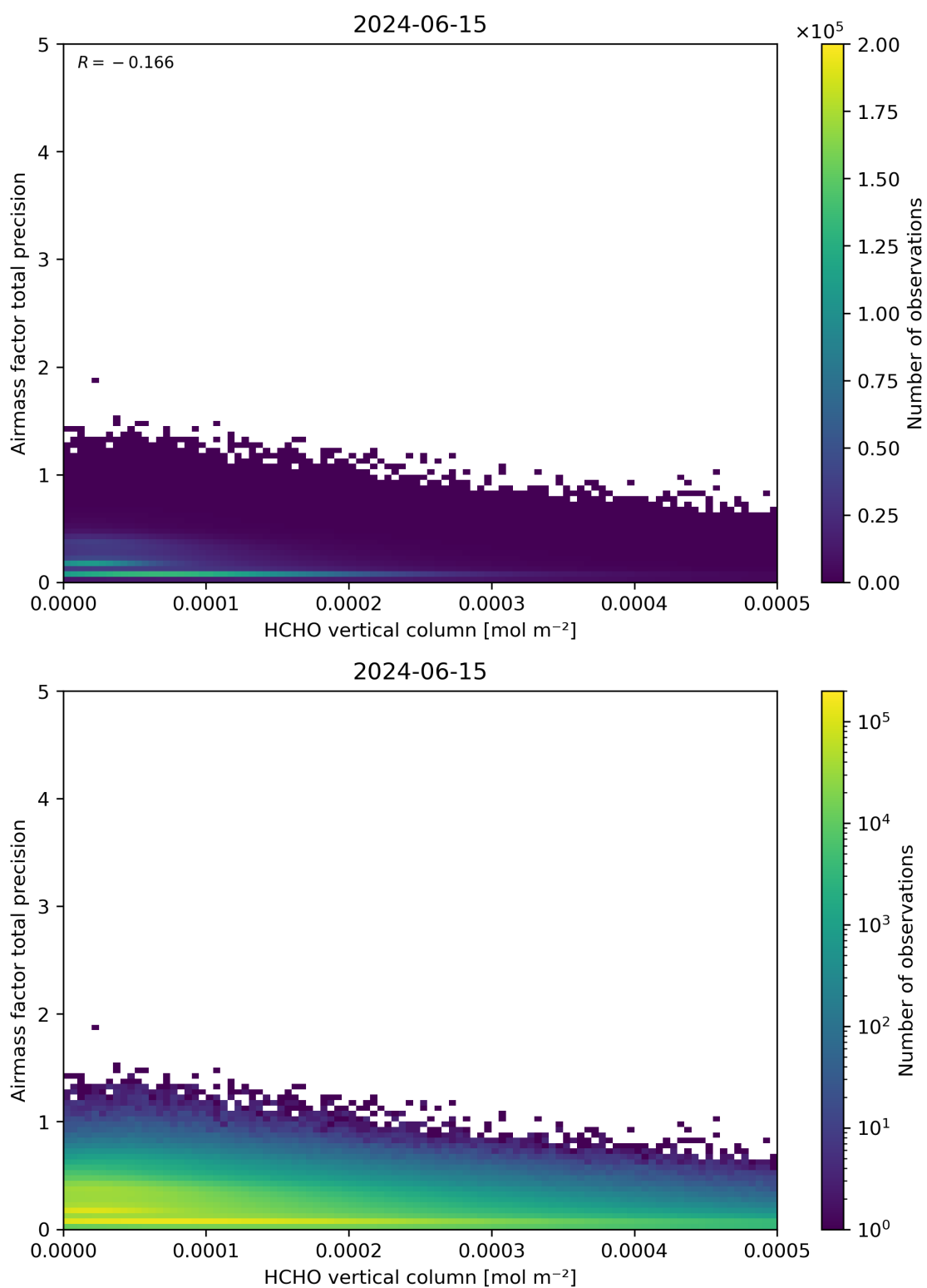
Figure 132: Scatter density plot of “HCHO vertical column” against “Airmass factor total precision” for 2024-06-14 to 2024-06-16.
