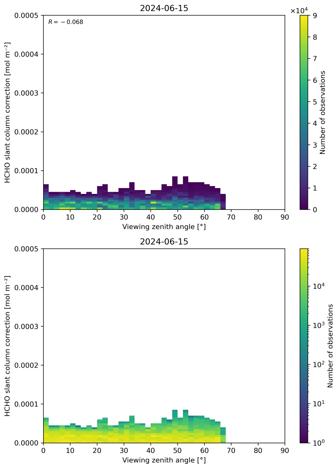
Figure 187: Scatter density plot of “Viewing zenith angle” against “HCHO slant column correction” for 2024-06-14 to 2024-06-16.
