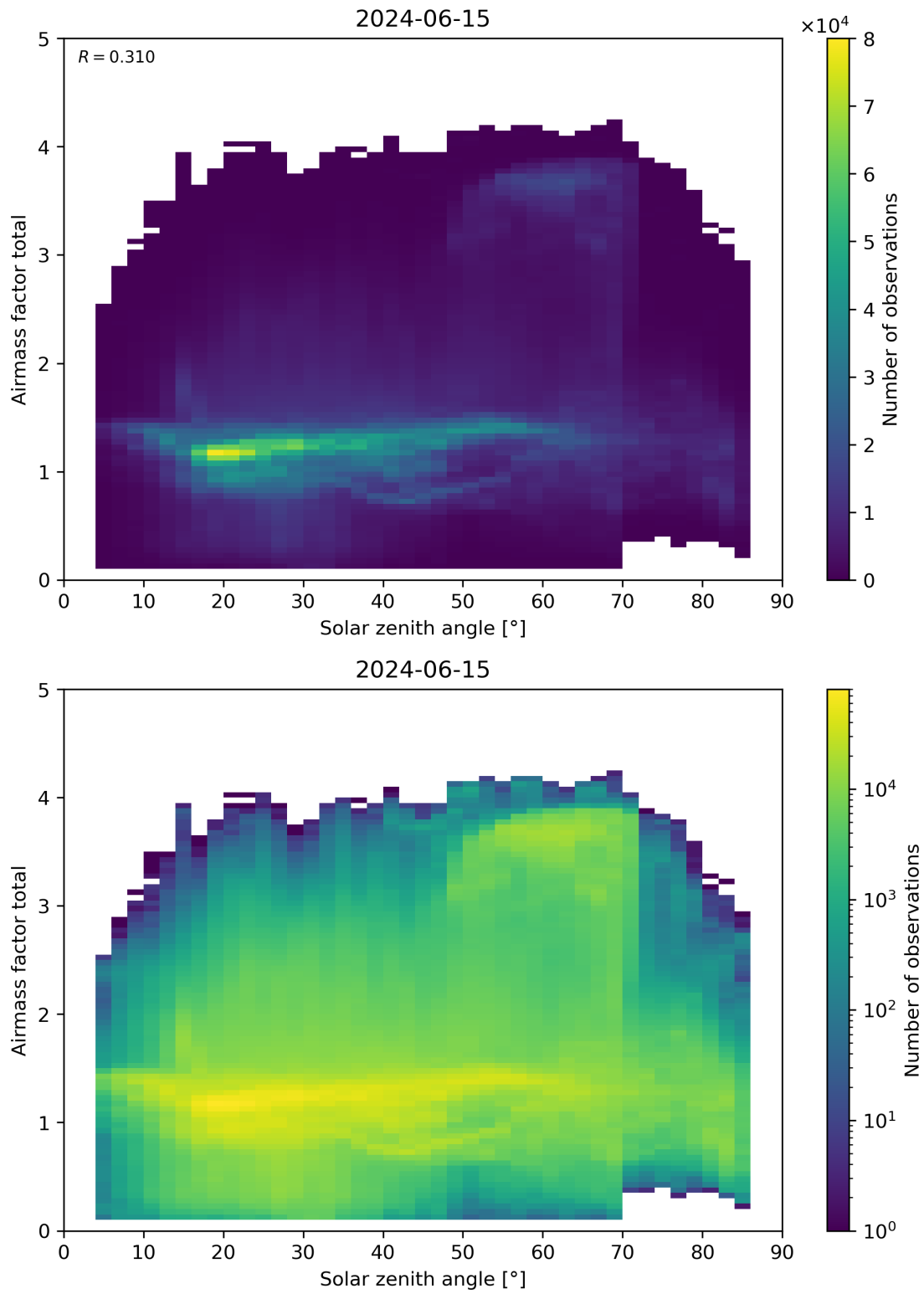
Figure 175: Scatter density plot of “Solar zenith angle” against “Airmass factor total” for 2024-06-14 to 2024-06-16.
