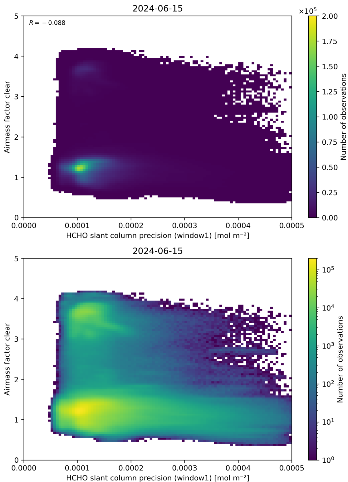
Figure 91: Scatter density plot of “HCHO slant column precision (window1)” against “Airmass factor clear” for 2024-06-14 to 2024-06-16.
