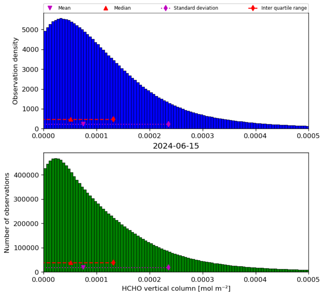
Figure 35: Histogram of “HCHO vertical column” for 2024-06-14 to 2024-06-16
