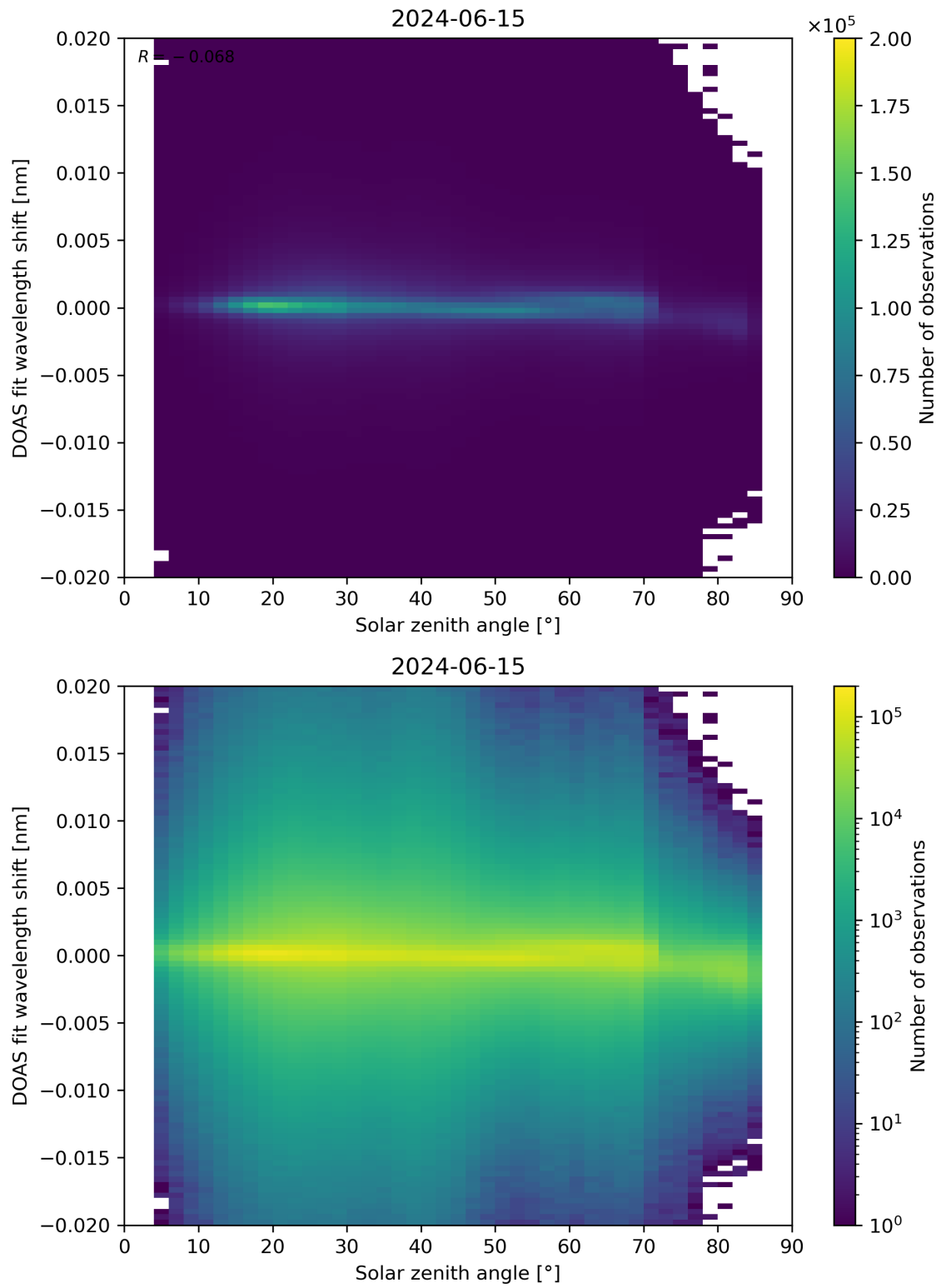
Figure 168: Scatter density plot of “Solar zenith angle” against “DOAS fit wavelength shift” for 2024-06-14 to 2024-06-16.
