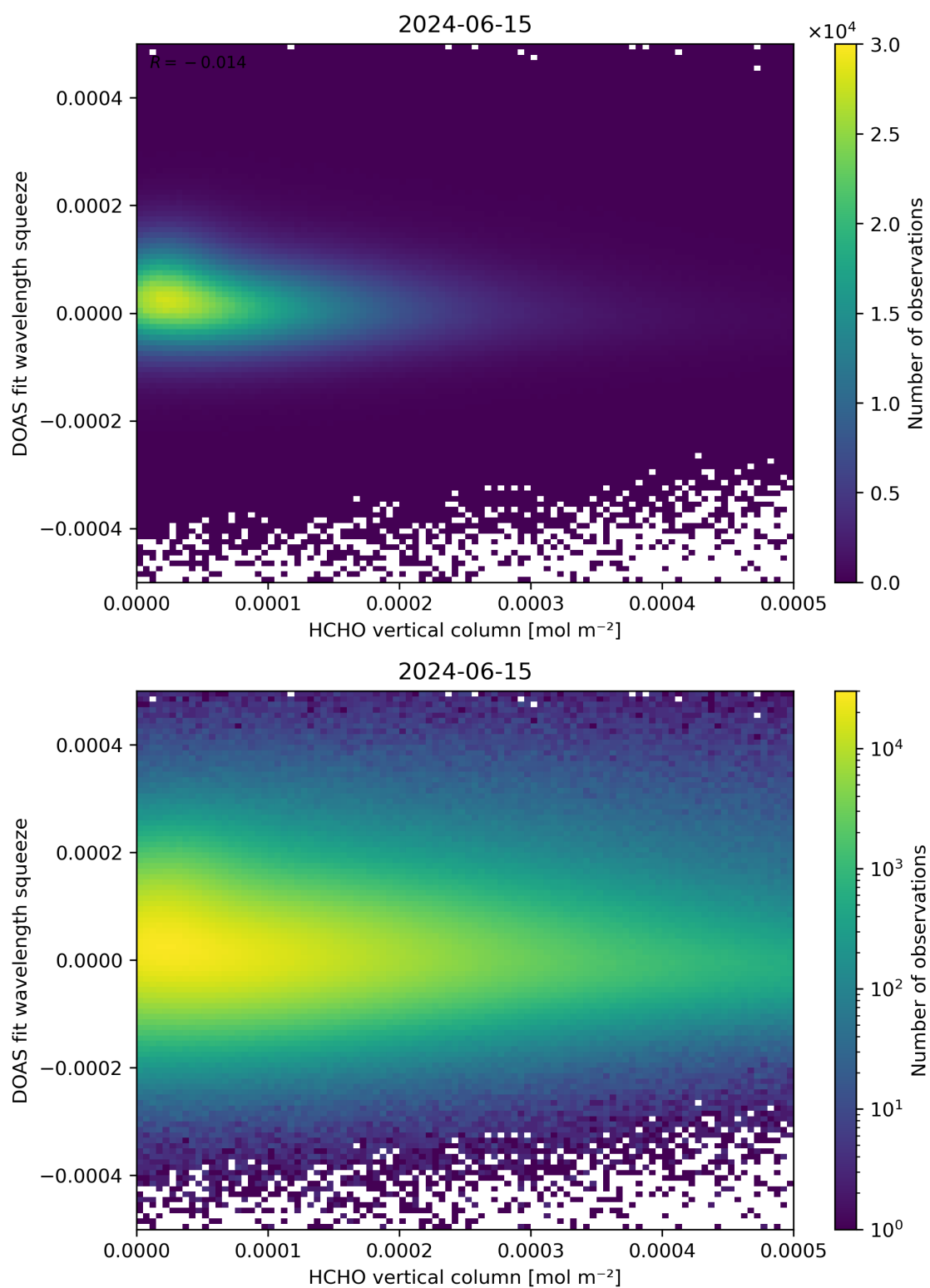
Figure 125: Scatter density plot of “HCHO vertical column” against “DOAS fit wavelength squeeze” for 2024-06-14 to 2024-06-16.
