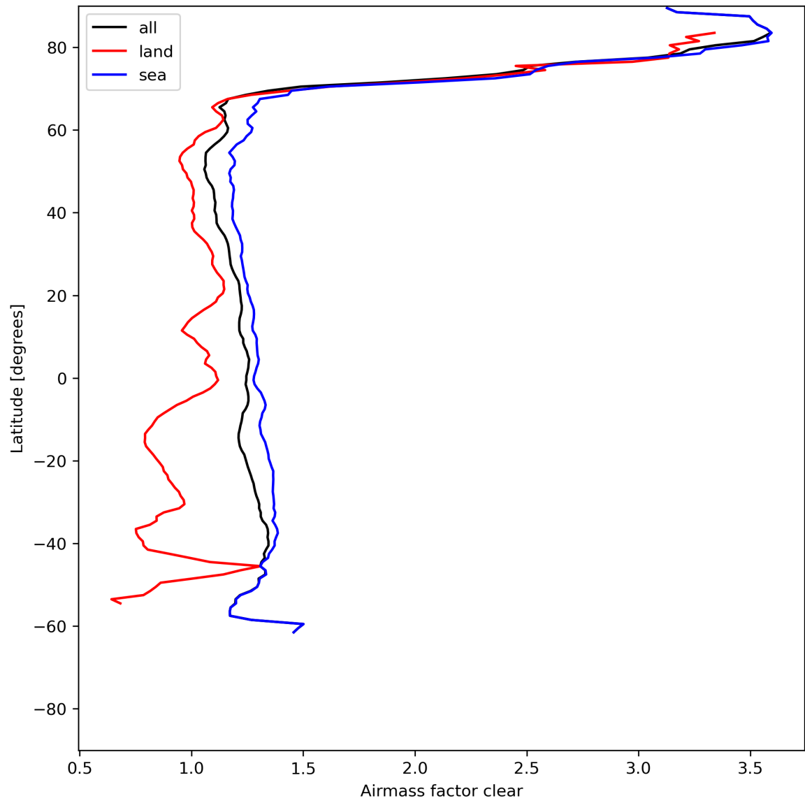
Figure 28: Zonal average of “Airmass factor clear” for 2024-06-14 to 2024-06-16.
