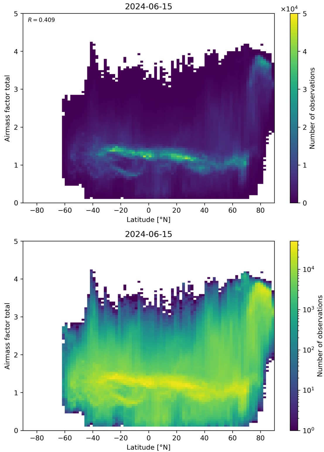
Figure 161: Scatter density plot of “Latitude” against “Airmass factor total” for 2024-06-14 to 2024-06-16.
