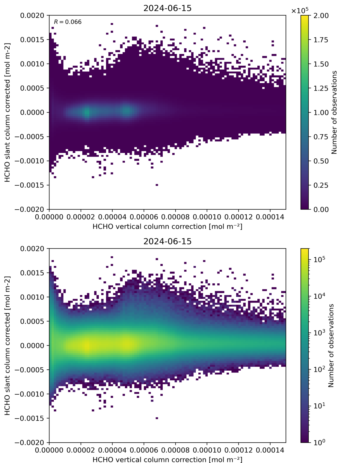
Figure 116: Scatter density plot of “HCHO vertical column correction” against “HCHO slant column corrected” for 2024-06-14 to 2024-06-16.
