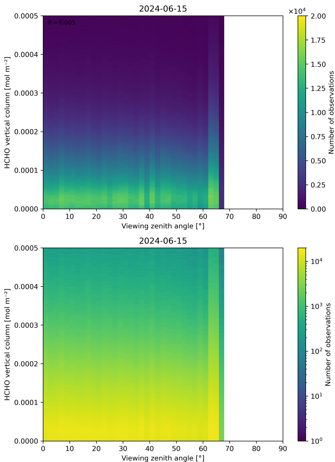
Figure 192: Scatter density plot of “Viewing zenith angle” against “HCHO vertical column” for 2024-06-14 to 2024-06-16.
