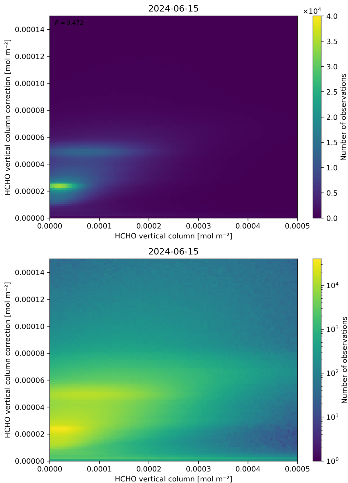
Figure 133: Scatter density plot of “HCHO vertical column” against “HCHO vertical column correction” for 2024-06-14 to 2024-06-16.
