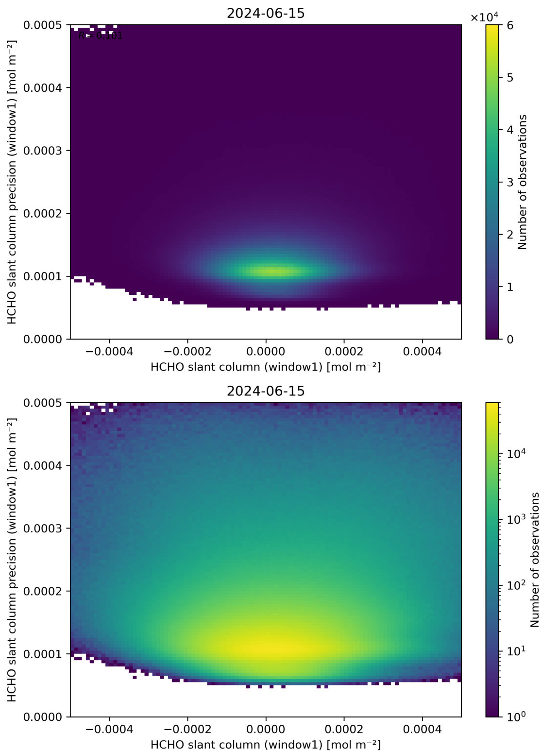
Figure 84: Scatter density plot of “HCHO slant column (window1)” against “HCHO slant column precision (window1)” for 2024-06-14 to 2024-06-16.
