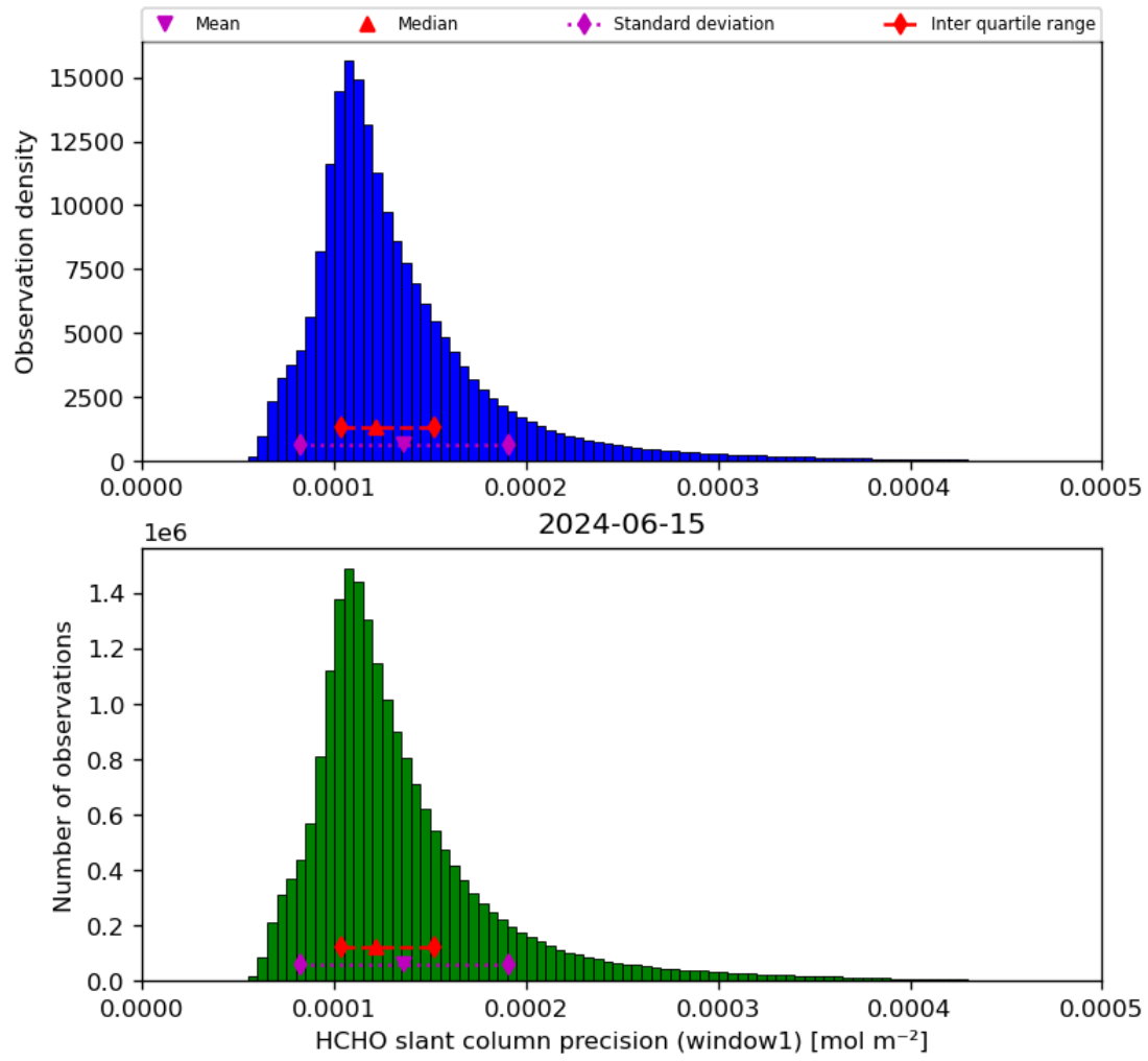
Figure 39: Histogram of “HCHO slant column precision (window1)” for 2024-06-14 to 2024-06-16
