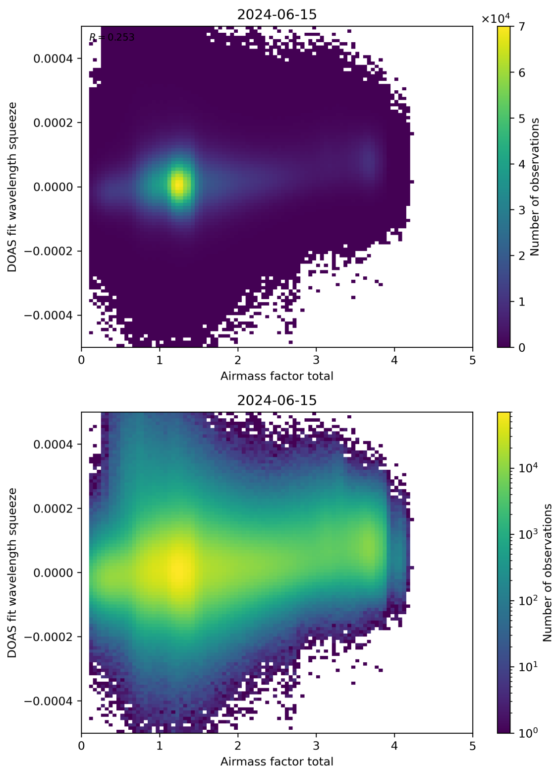
Figure 99: Scatter density plot of “Airmass factor total” against “DOAS fit wavelength squeeze” for 2024-06-14 to 2024-06-16.
