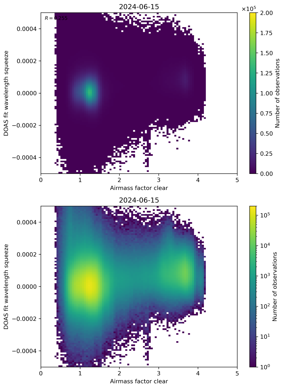
Figure 73: Scatter density plot of “Airmass factor clear” against “DOAS fit wavelength squeeze” for 2024-06-14 to 2024-06-16.
