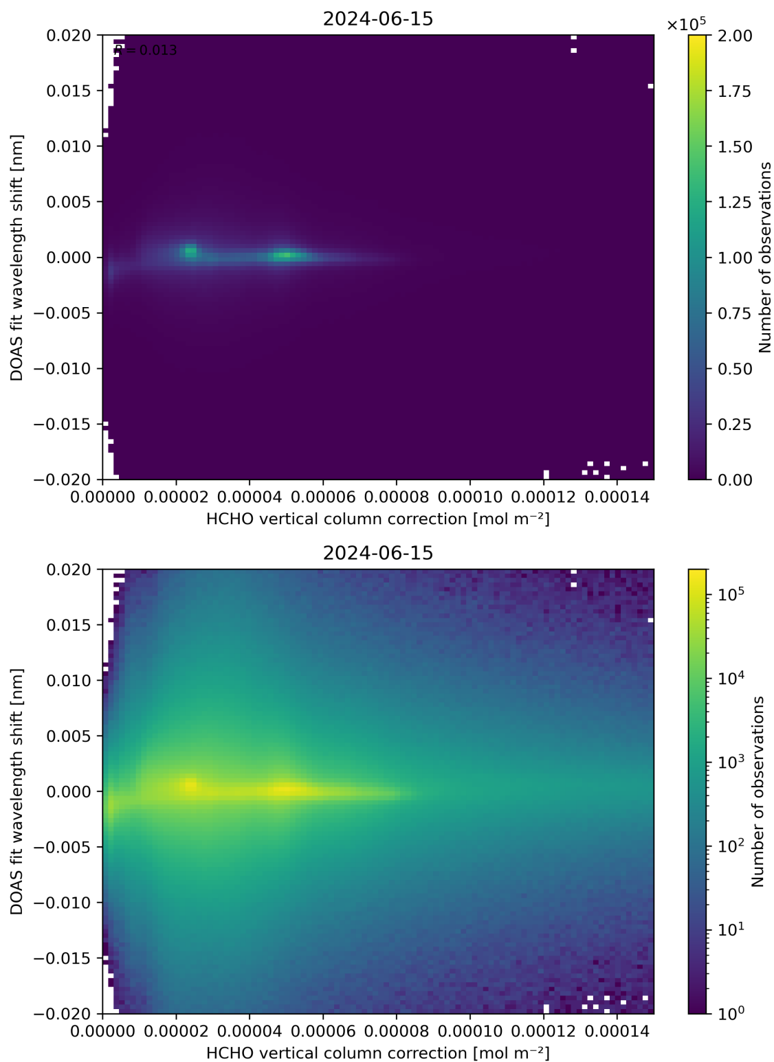
Figure 113: Scatter density plot of “HCHO vertical column correction” against “DOAS fit wavelength shift” for 2024-06-14 to 2024-06-16.
