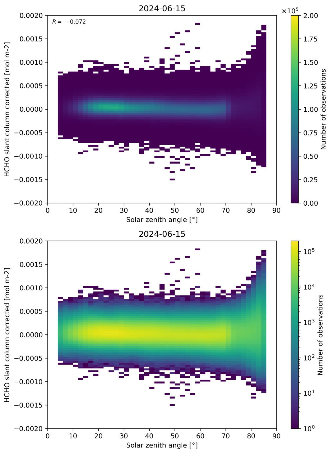
Figure 171: Scatter density plot of “Solar zenith angle” against “HCHO slant column corrected” for 2024-06-14 to 2024-06-16.
