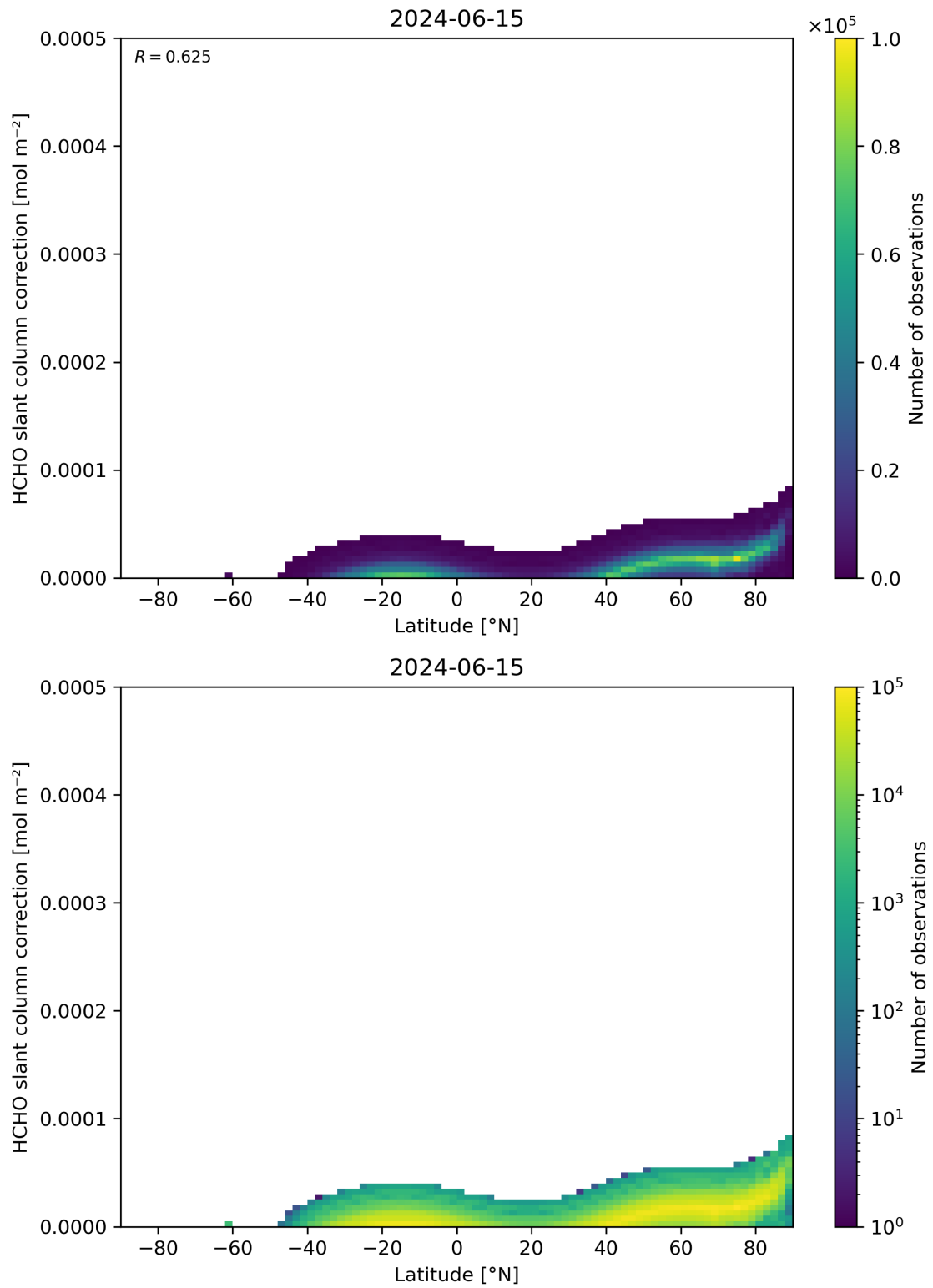
Figure 158: Scatter density plot of “Latitude” against “HCHO slant column correction” for 2024-06-14 to 2024-06-16.
