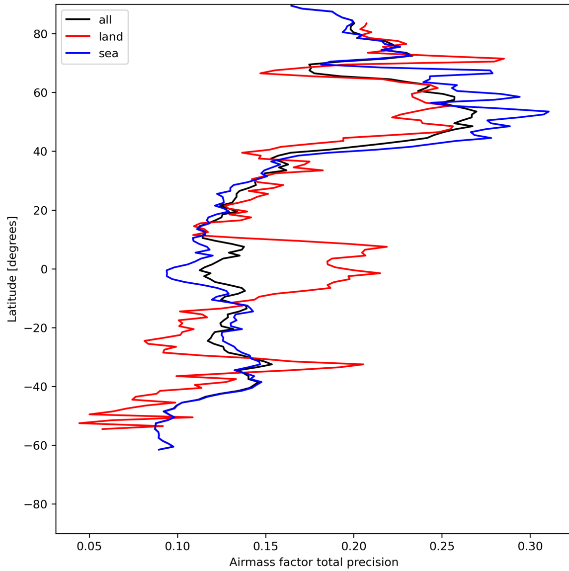
Figure 27: Zonal average of “Airmass factor total precision” for 2024-06-14 to 2024-06-16.
