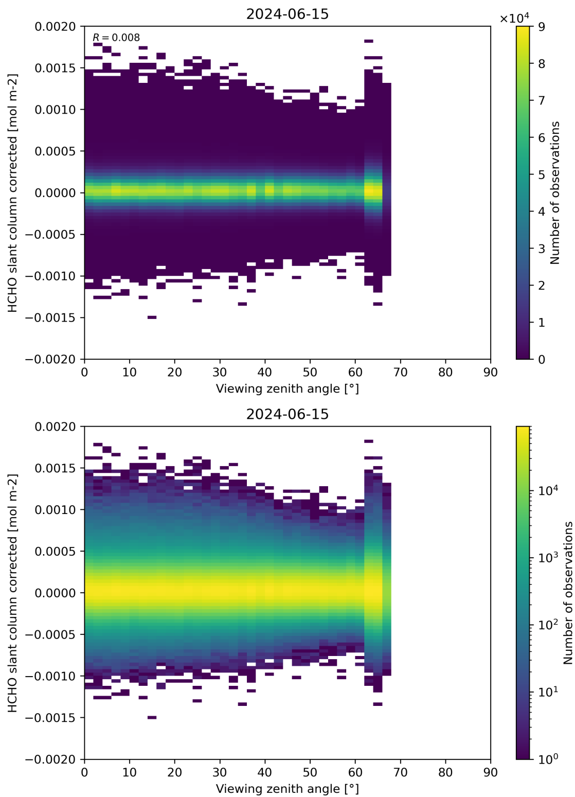
Figure 186: Scatter density plot of “Viewing zenith angle” against “HCHO slant column corrected” for 2024-06-14 to 2024-06-16.
