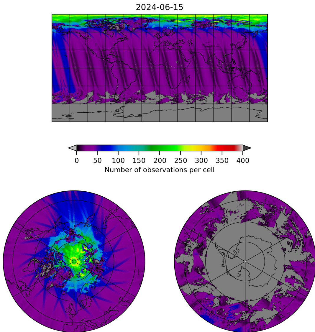
Figure 19: Map of the number of observations for 2024-06-14 to 2024-06-16
