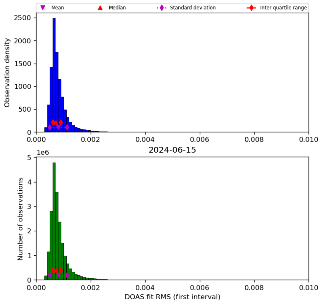
Figure 46: Histogram of “DOAS fit RMS (first interval)” for 2024-06-14 to 2024-06-16
