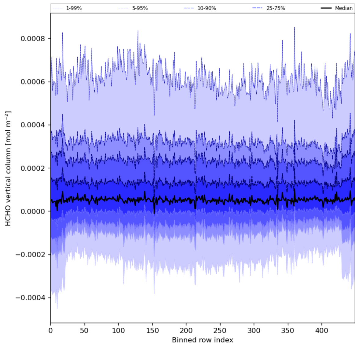
Figure 49: Along track statistics of “HCHO vertical column” for 2024-06-14 to 2024-06-16
