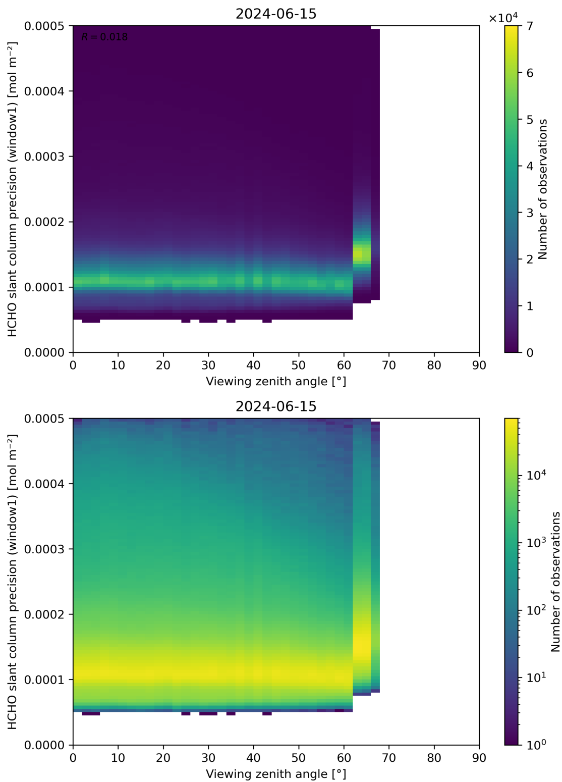
Figure 189: Scatter density plot of “Viewing zenith angle” against “HCHO slant column precision (window1)” for 2024-06-14 to 2024-06-16.
