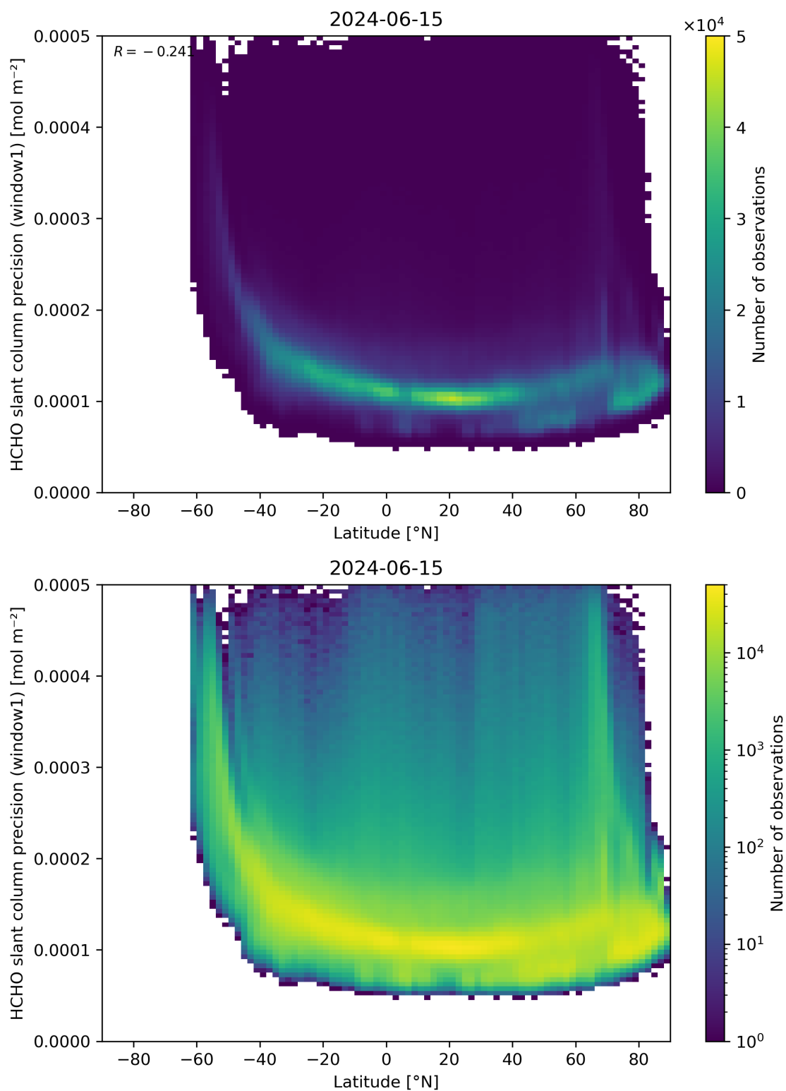
Figure 160: Scatter density plot of “Latitude” against “HCHO slant column precision (window1)” for 2024-06-14 to 2024-06-16.
