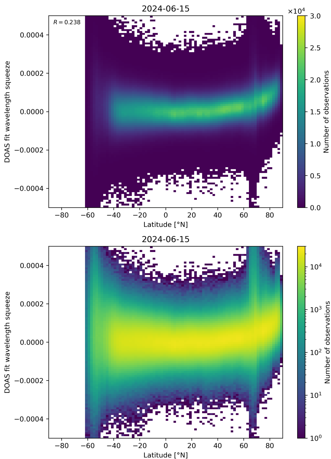
Figure 155: Scatter density plot of “Latitude” against “DOAS fit wavelength squeeze” for 2024-06-14 to 2024-06-16.
