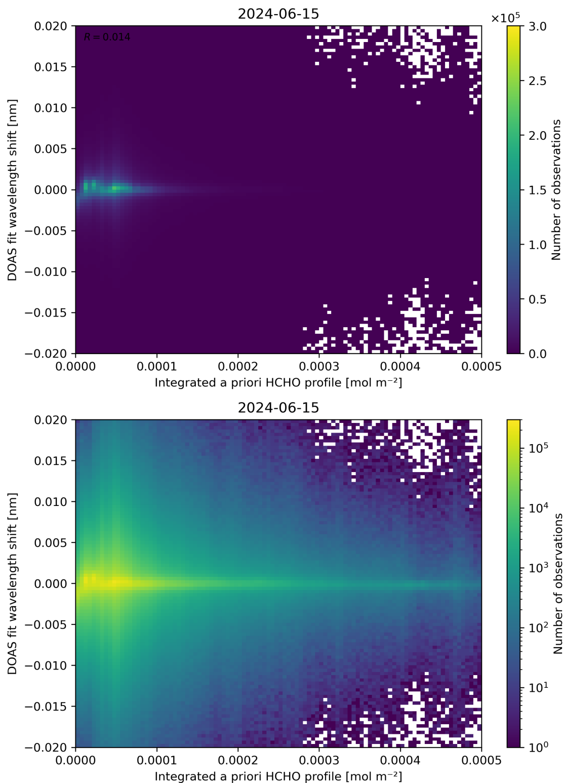
Figure 149: Scatter density plot of “Integrated a priori HCHO profile” against “DOAS fit wavelength shift” for 2024-06-14 to 2024-06-16.
