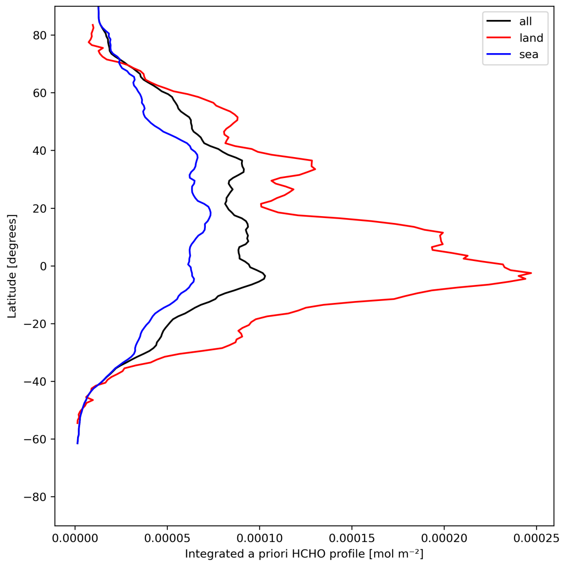
Figure 29: Zonal average of “Integrated a priori HCHO profile” for 2024-06-14 to 2024-06-16.
