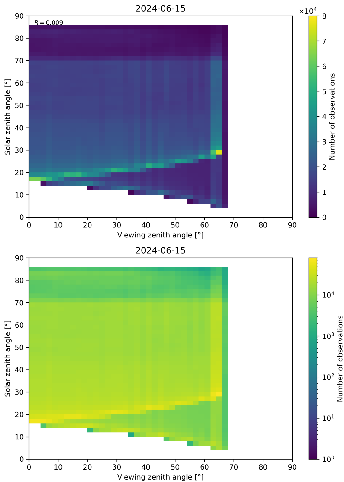
Figure 197: Scatter density plot of “Viewing zenith angle” against “Solar zenith angle” for 2024-06-14 to 2024-06-16.
