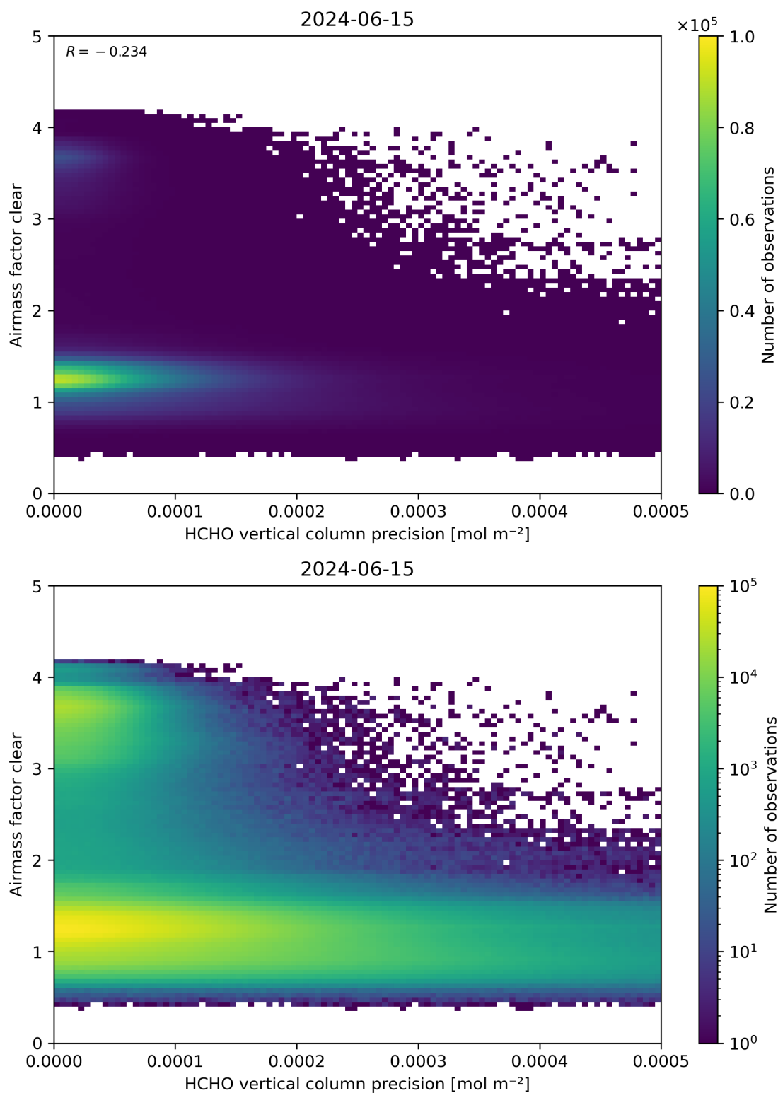
Figure 139: Scatter density plot of “HCHO vertical column precision” against “Airmass factor clear” for 2024-06-14 to 2024-06-16.
