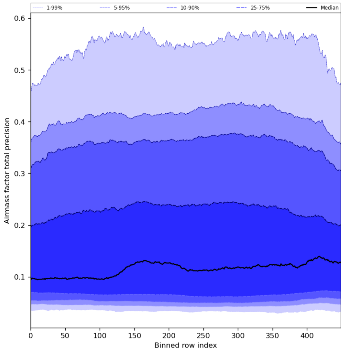
Figure 55: Along track statistics of “Airmass factor total precision” for 2024-06-14 to 2024-06-16
