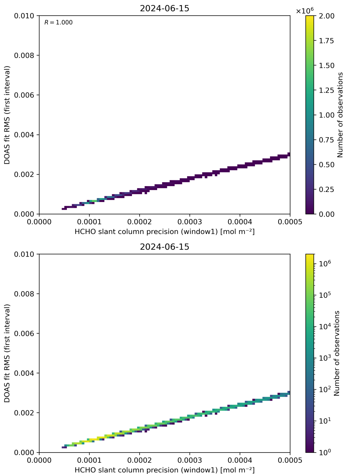
Figure 88: Scatter density plot of “HCHO slant column precision (window1)” against “DOAS fit RMS (first interval)” for 2024-06-14 to 2024-06-16.
