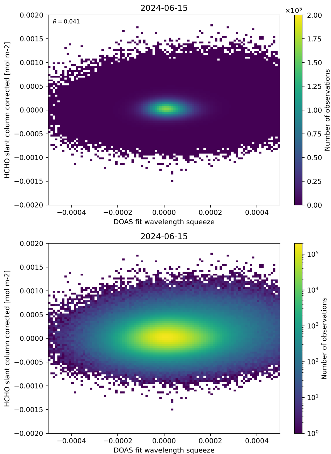
Figure 69: Scatter density plot of “DOAS fit wavelength squeeze” against “HCHO slant column corrected” for 2024-06-14 to 2024-06-16.
