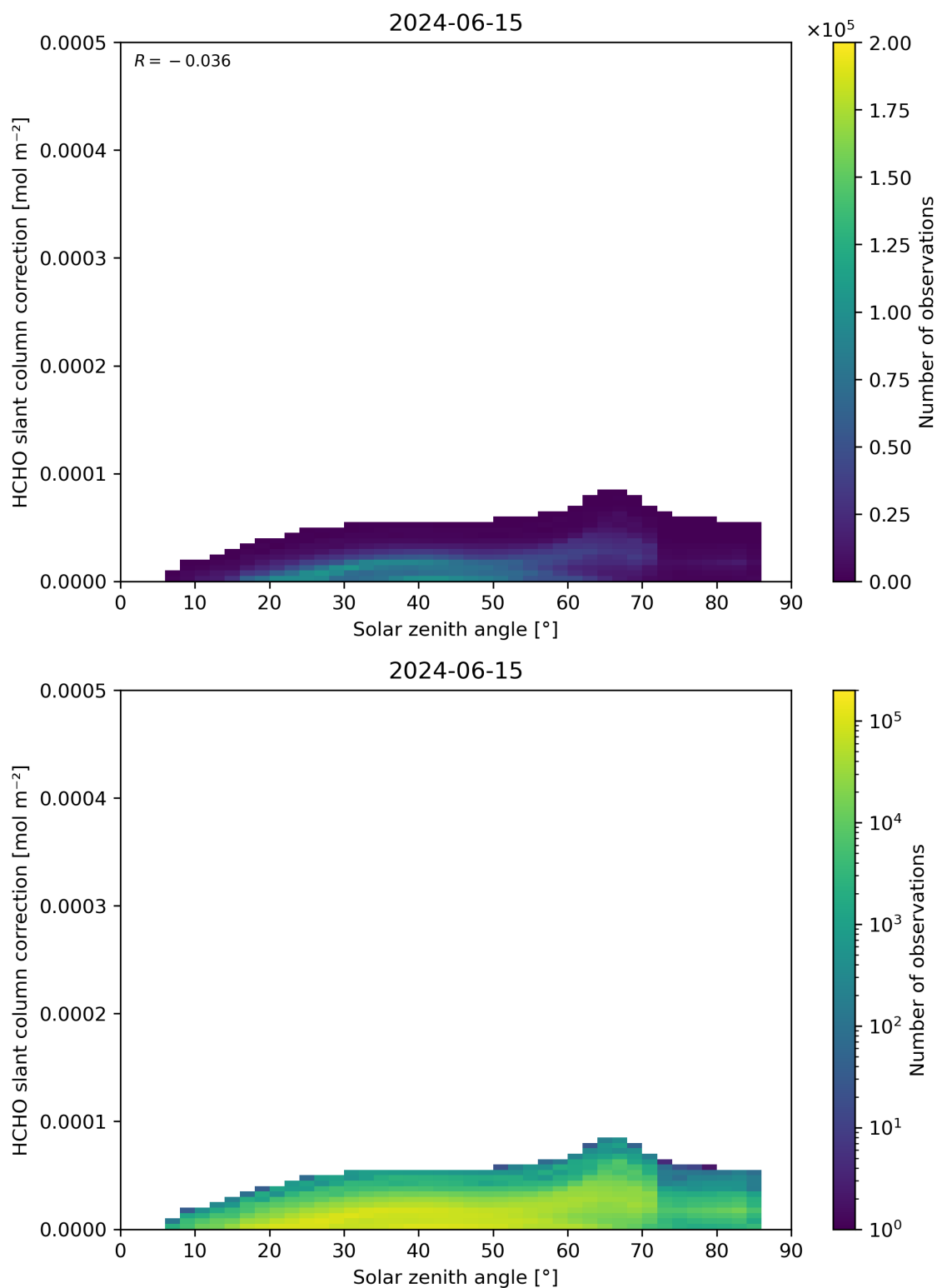
Figure 172: Scatter density plot of “Solar zenith angle” against “HCHO slant column correction” for 2024-06-14 to 2024-06-16.
