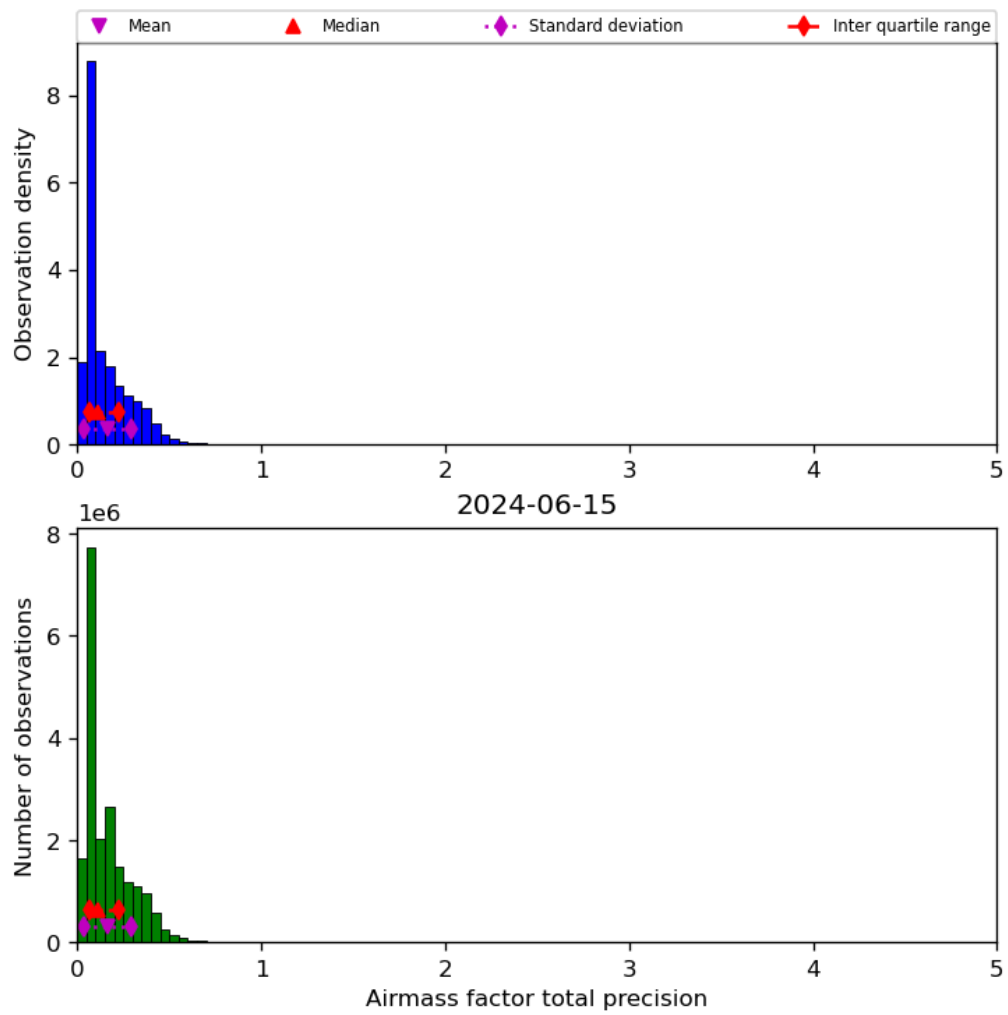
Figure 41: Histogram of “Airmass factor total precision” for 2024-06-14 to 2024-06-16
