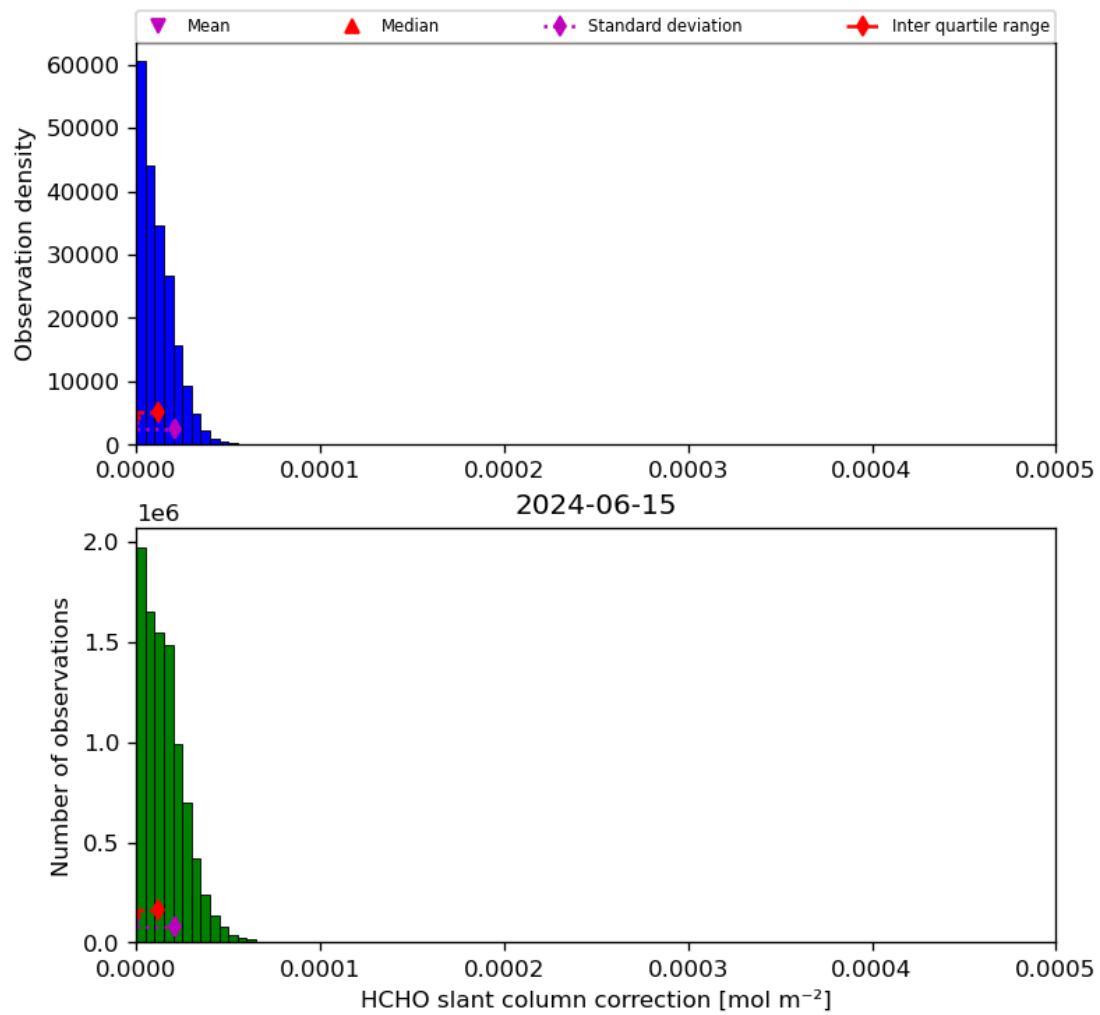
Figure 47: Histogram of “HCHO slant column correction” for 2024-06-14 to 2024-06-16
