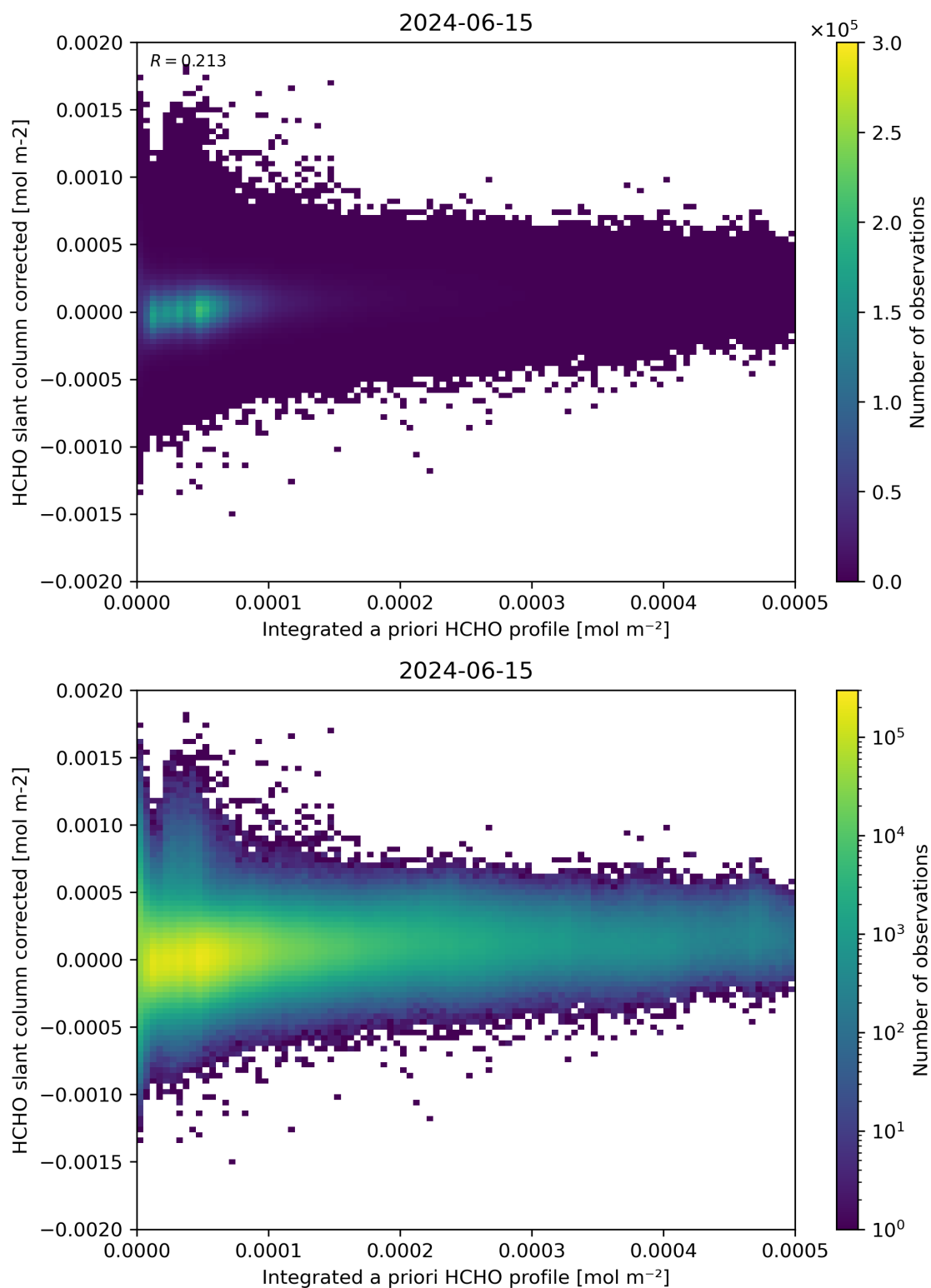
Figure 151: Scatter density plot of “Integrated a priori HCHO profile” against “HCHO slant column corrected” for 2024-06-14 to 2024-06-16.
