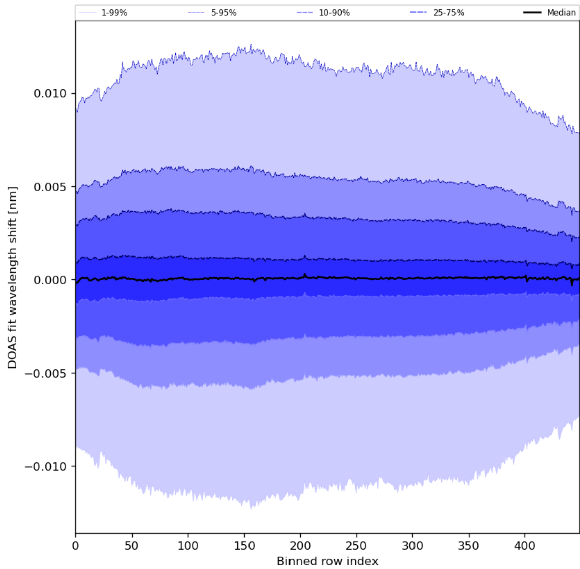
Figure 58: Along track statistics of “DOAS fit wavelength shift” for 2024-06-14 to 2024-06-16
