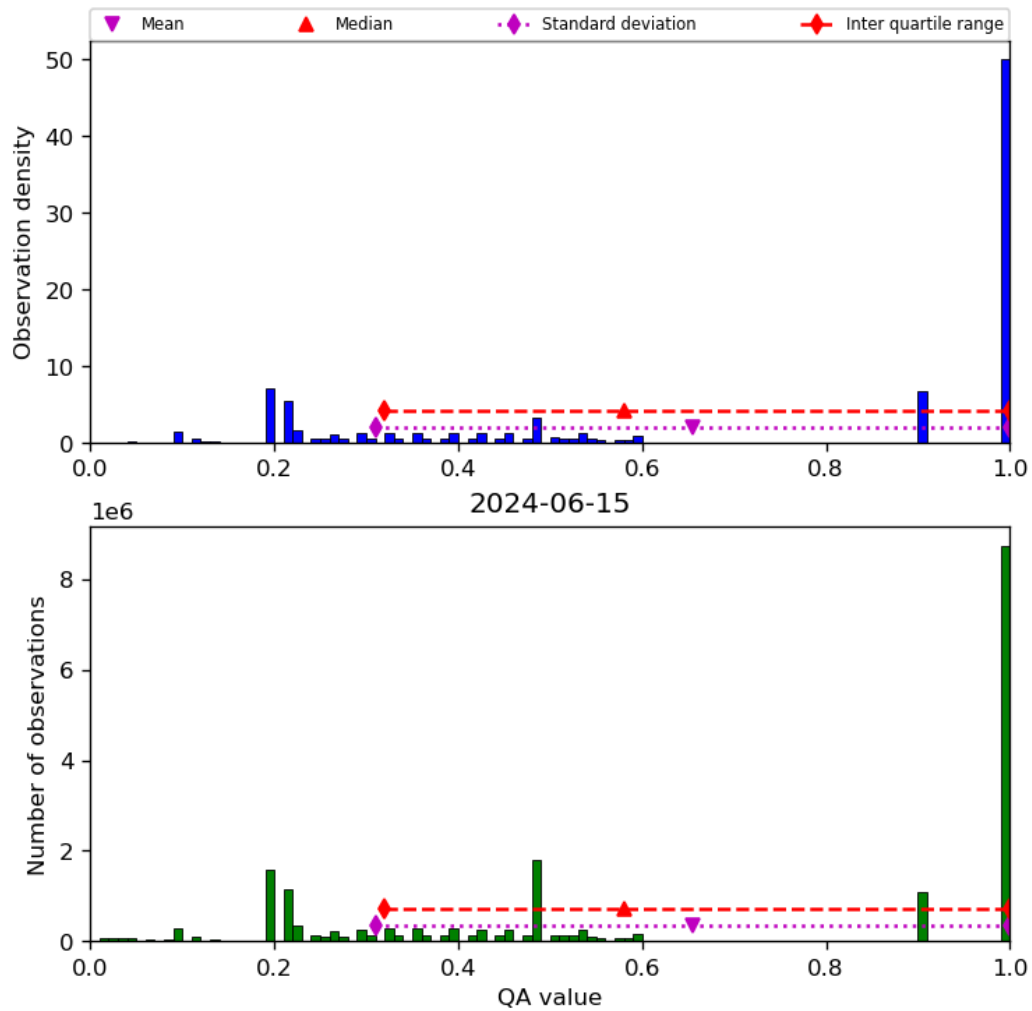
Figure 34: Histogram of “QA value” for 2024-06-14 to 2024-06-16
