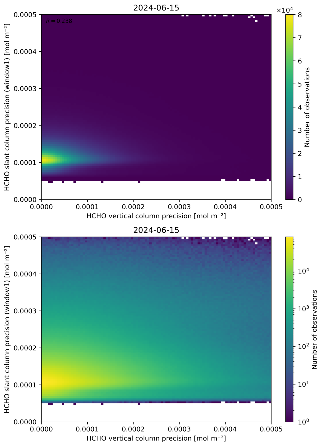
Figure 143: Scatter density plot of “HCHO vertical column precision” against “HCHO slant column precision (window1)” for 2024-06-14 to 2024-06-16.
