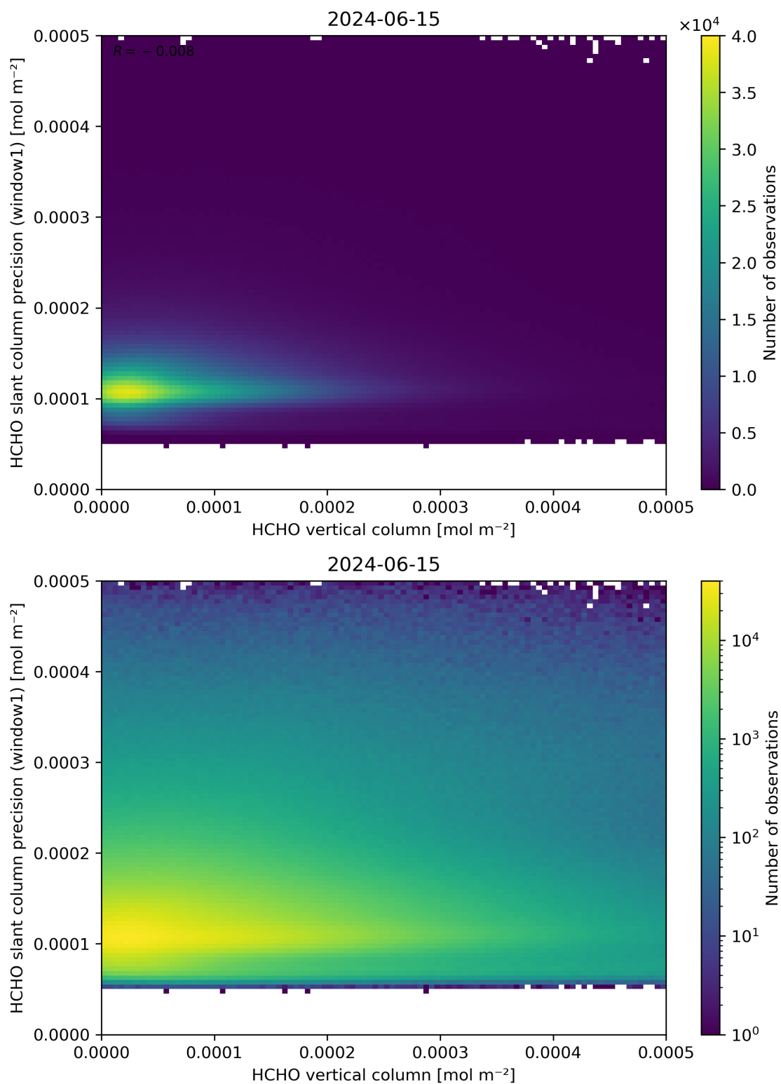
Figure 130: Scatter density plot of “HCHO vertical column” against “HCHO slant column precision (window1)” for 2024-06-14 to 2024-06-16.
