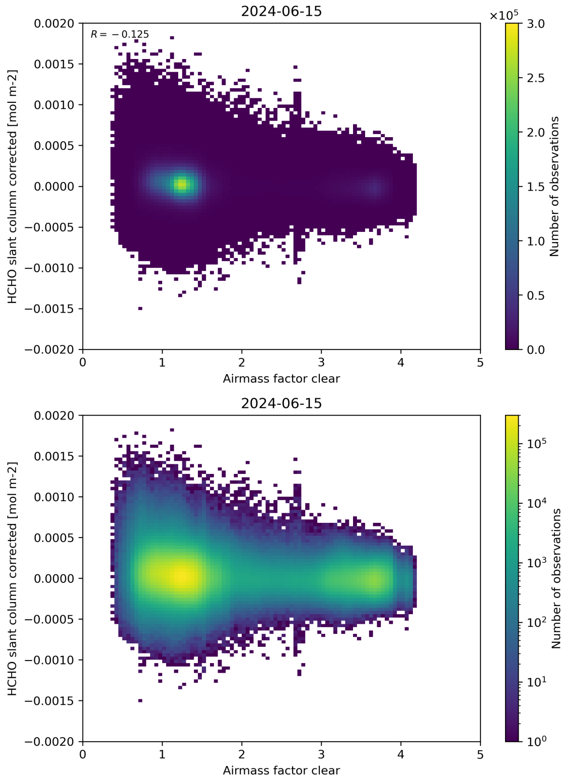
Figure 74: Scatter density plot of “Airmass factor clear” against “HCHO slant column corrected” for 2024-06-14 to 2024-06-16.
