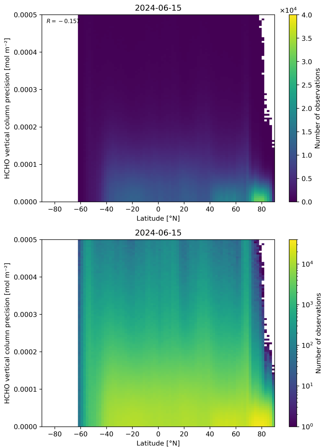
Figure 165: Scatter density plot of “Latitude” against “HCHO vertical column precision” for 2024-06-14 to 2024-06-16.
