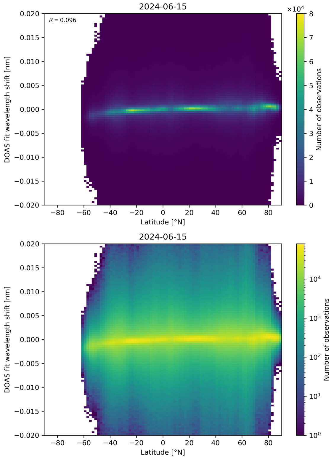
Figure 154: Scatter density plot of “Latitude” against “DOAS fit wavelength shift” for 2024-06-14 to 2024-06-16.
