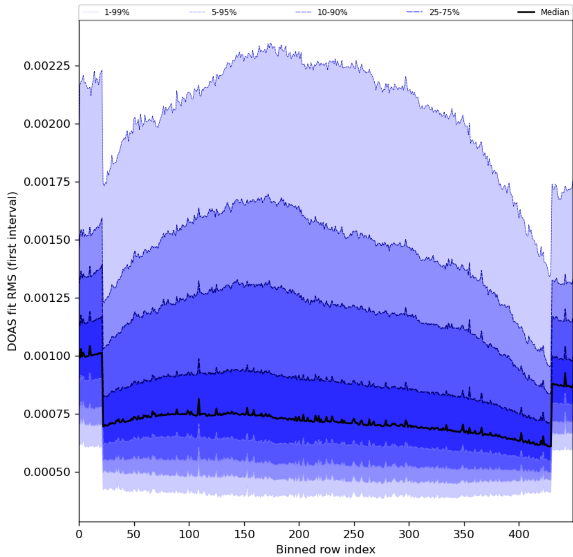
Figure 60: Along track statistics of “DOAS fit RMS (first interval)” for 2024-06-14 to 2024-06-16
