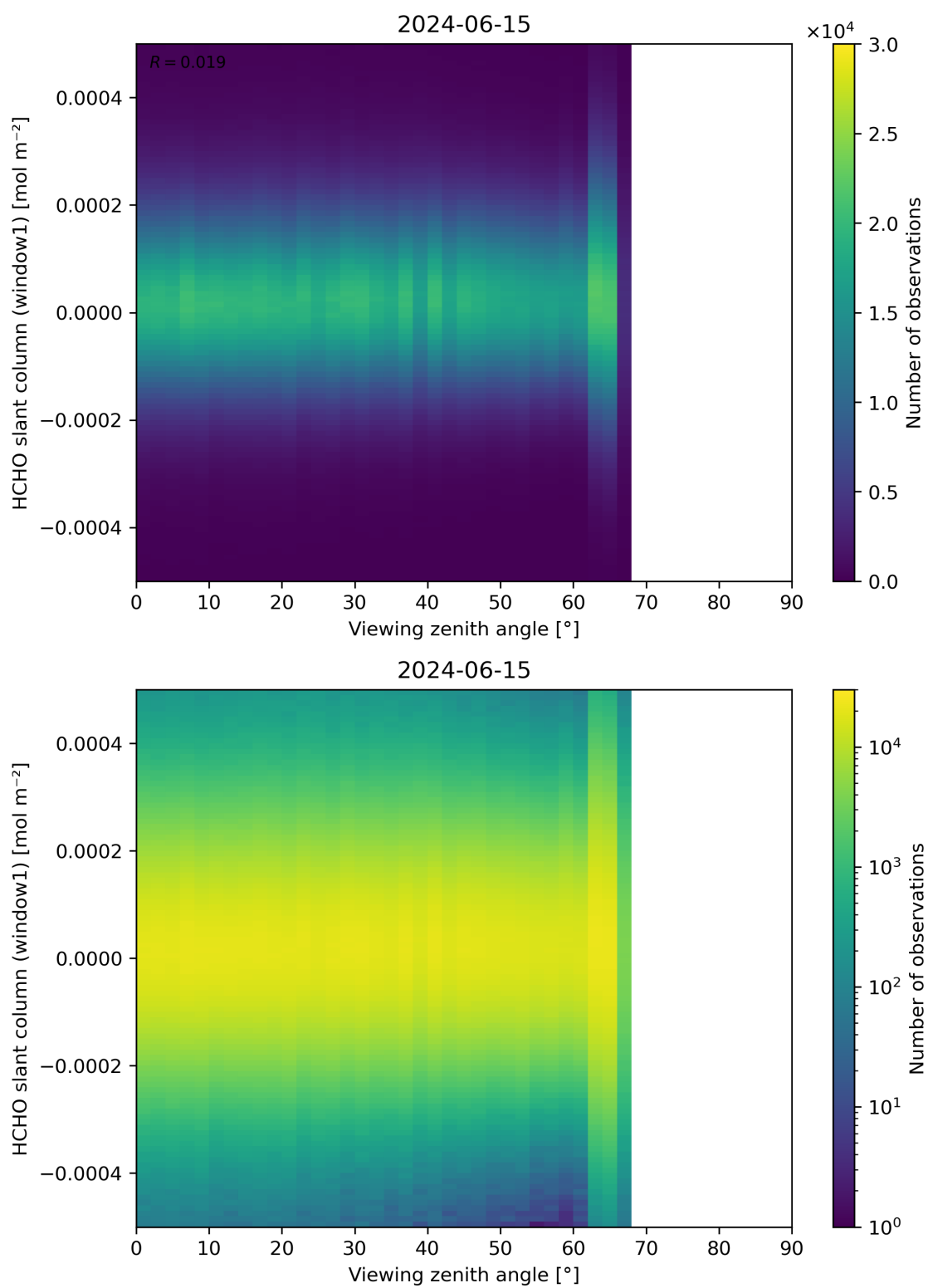
Figure 188: Scatter density plot of “Viewing zenith angle” against “HCHO slant column (window1)” for 2024-06-14 to 2024-06-16.
