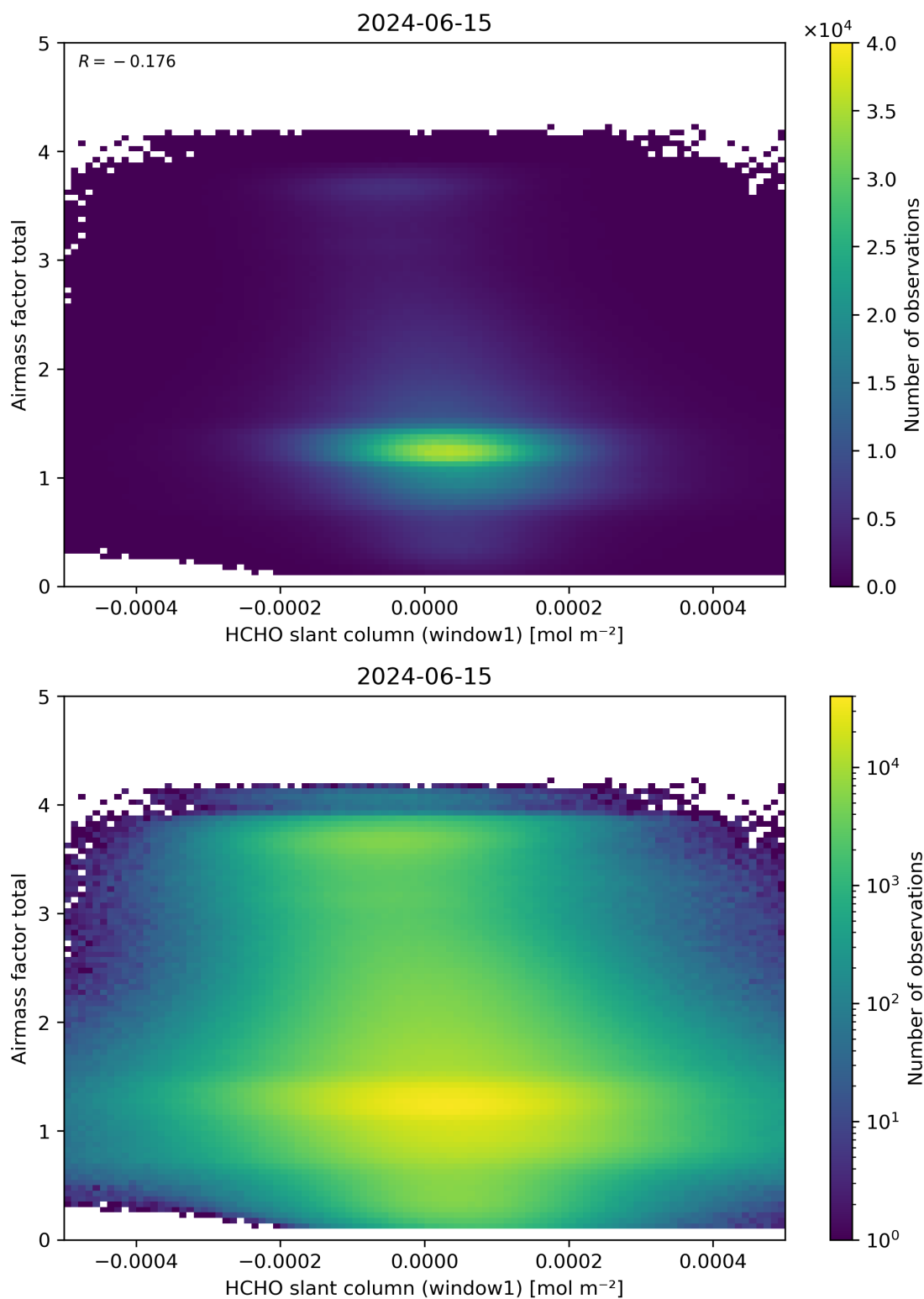
Figure 85: Scatter density plot of “HCHO slant column (window1)” against “Airmass factor total” for 2024-06-14 to 2024-06-16.
