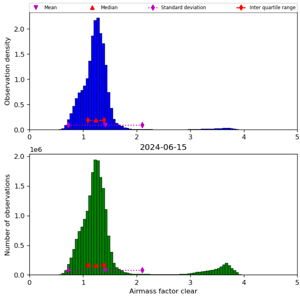
Figure 42: Histogram of “Airmass factor clear” for 2024-06-14 to 2024-06-16
