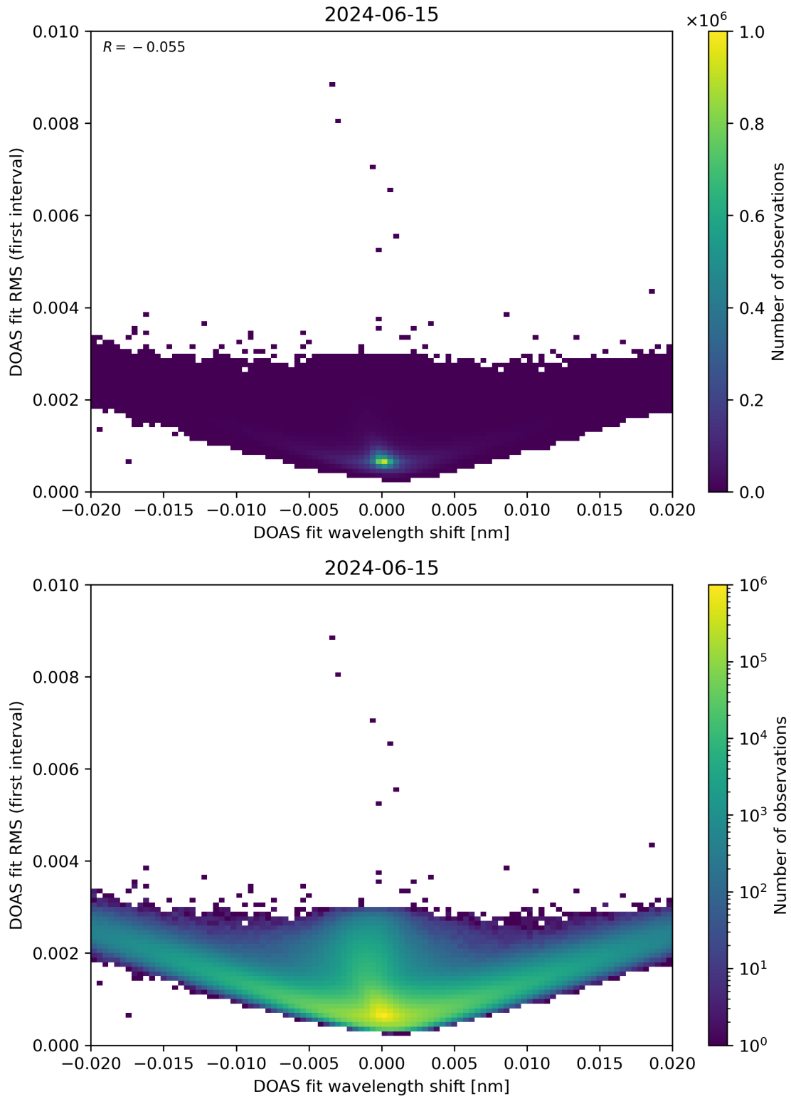
Figure 64: Scatter density plot of “DOAS fit wavelength shift” against “DOAS fit RMS (first interval)” for 2024-06-14 to 2024-06-16.
