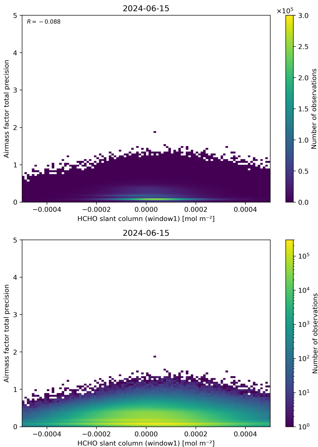
Figure 86: Scatter density plot of “HCHO slant column (window1)” against “Airmass factor total precision” for 2024-06-14 to 2024-06-16.
