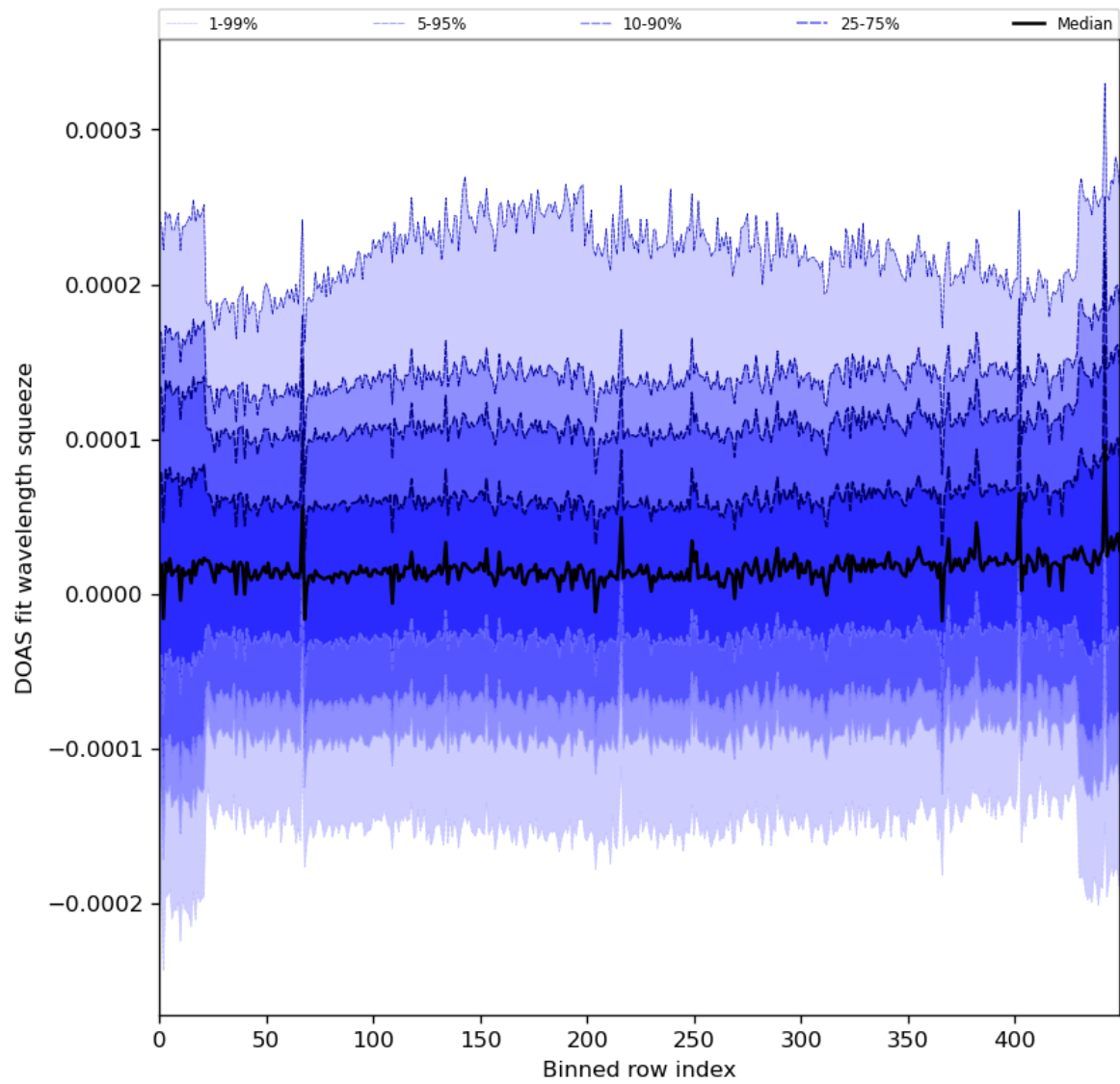
Figure 59: Along track statistics of “DOAS fit wavelength squeeze” for 2024-06-14 to 2024-06-16
