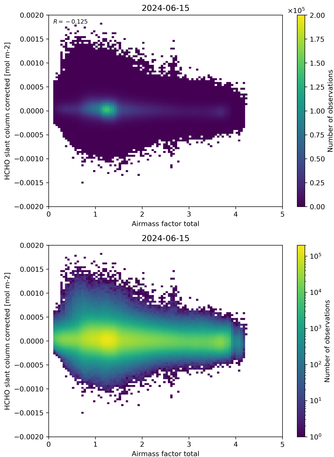
Figure 101: Scatter density plot of “Airmass factor total” against “HCHO slant column corrected” for 2024-06-14 to 2024-06-16.
