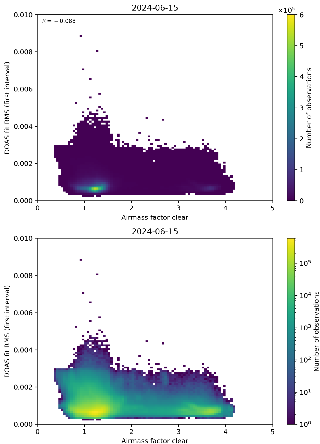
Figure 71: Scatter density plot of “Airmass factor clear” against “DOAS fit RMS (first interval)” for 2024-06-14 to 2024-06-16.
