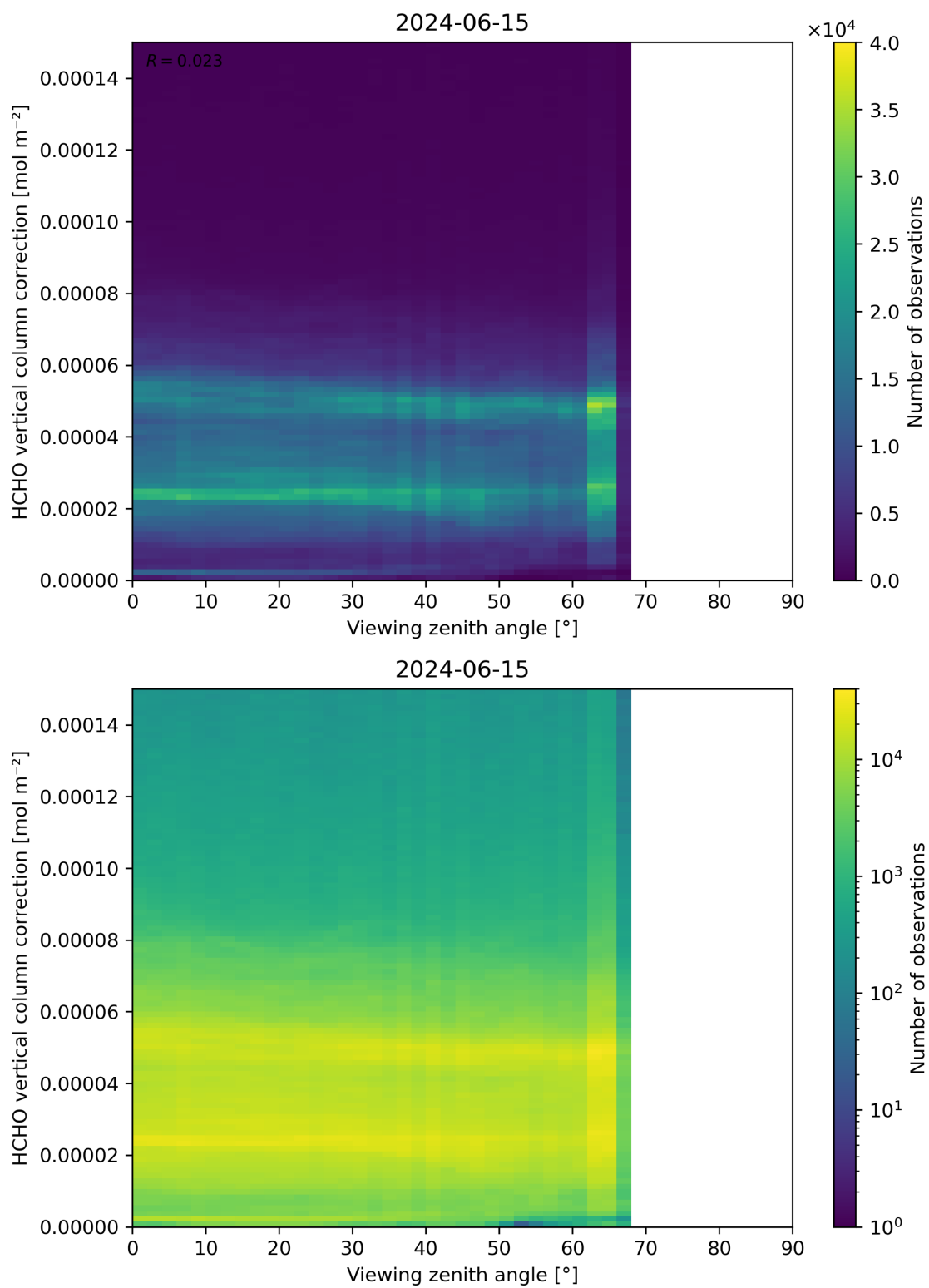
Figure 193: Scatter density plot of “Viewing zenith angle” against “HCHO vertical column correction” for 2024-06-14 to 2024-06-16.
