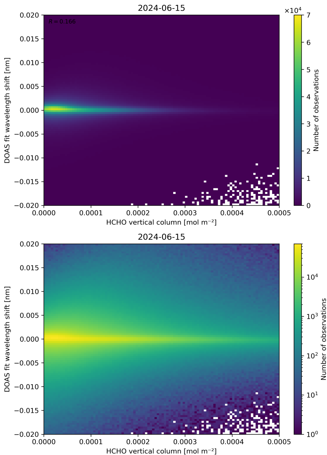
Figure 124: Scatter density plot of “HCHO vertical column” against “DOAS fit wavelength shift” for 2024-06-14 to 2024-06-16.
