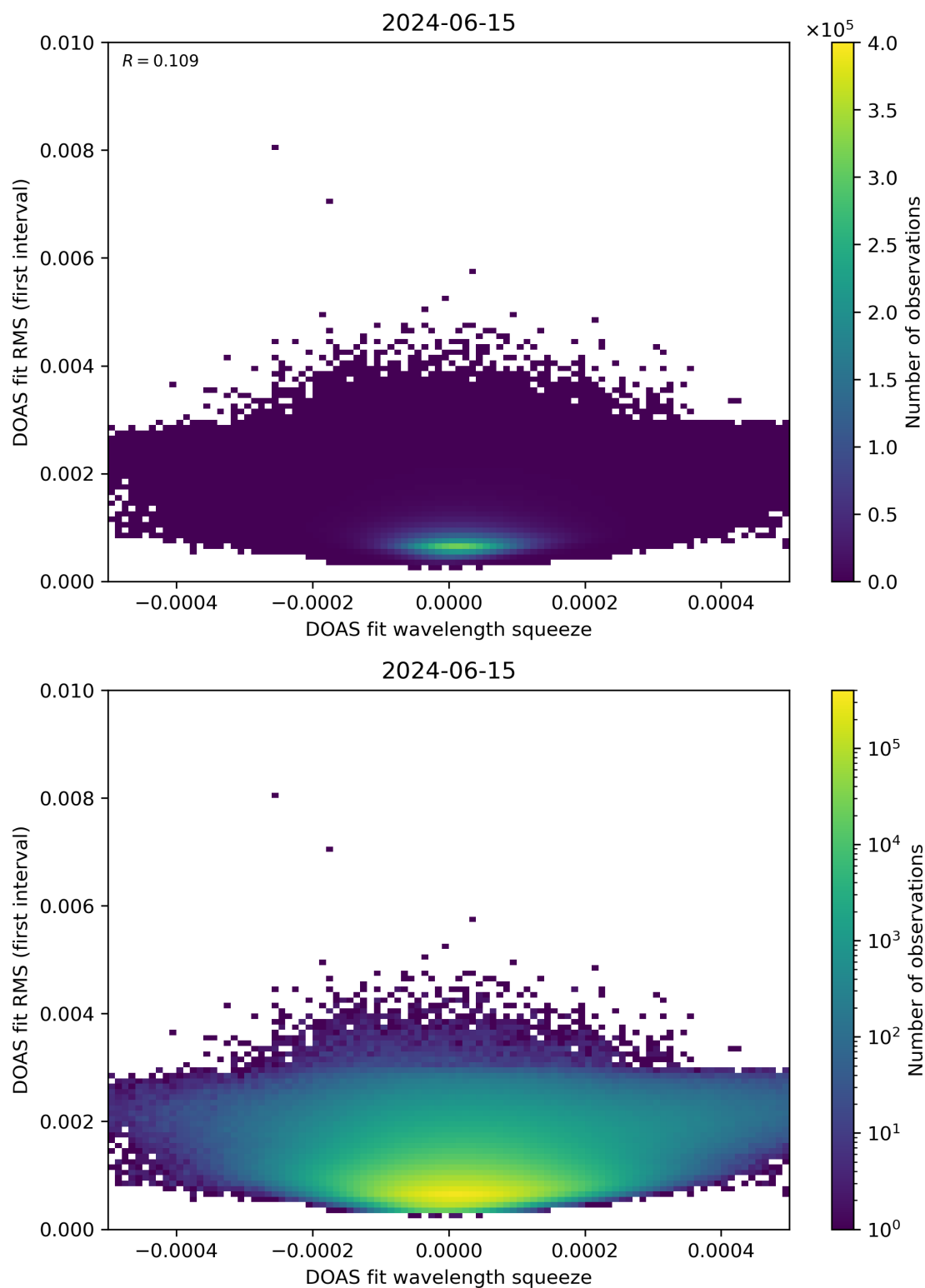
Figure 68: Scatter density plot of “DOAS fit wavelength squeeze” against “DOAS fit RMS (first interval)” for 2024-06-14 to 2024-06-16.
