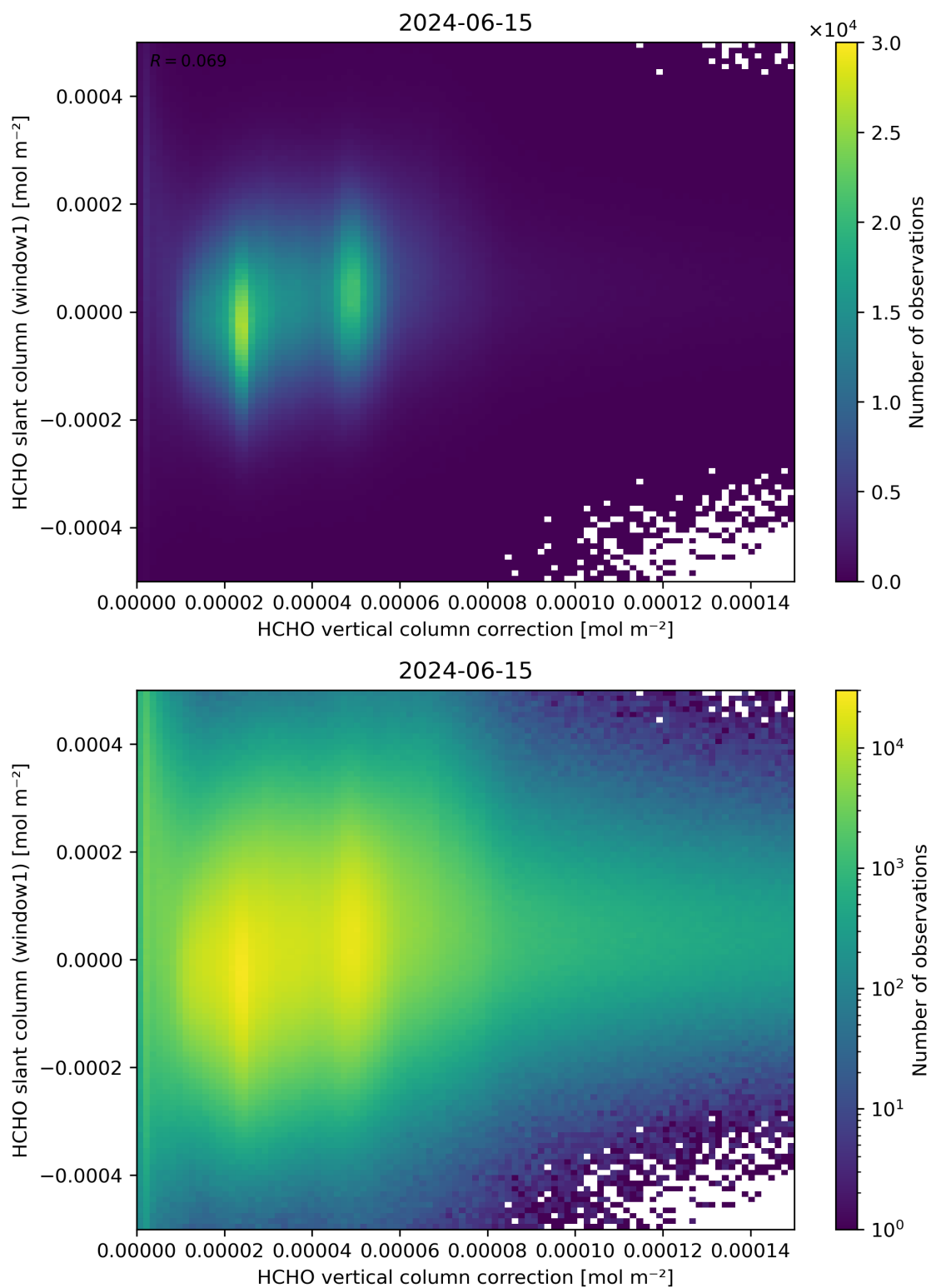
Figure 118: Scatter density plot of “HCHO vertical column correction” against “HCHO slant column (window1)” for 2024-06-14 to 2024-06-16.
