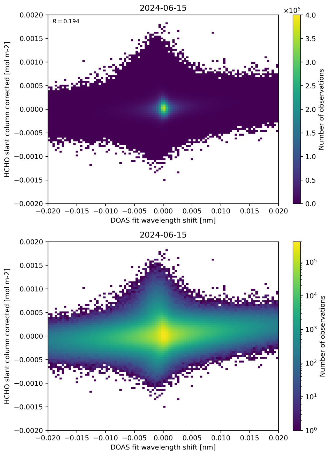
Figure 66: Scatter density plot of “DOAS fit wavelength shift” against “HCHO slant column corrected” for 2024-06-14 to 2024-06-16.
