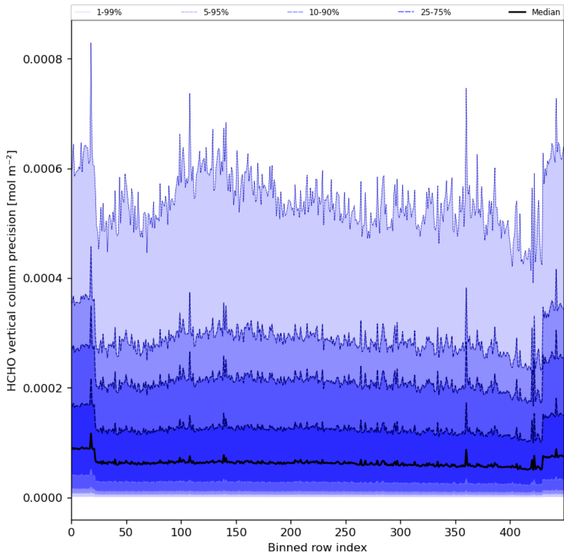
Figure 50: Along track statistics of “HCHO vertical column precision” for 2024-06-14 to 2024-06-16
