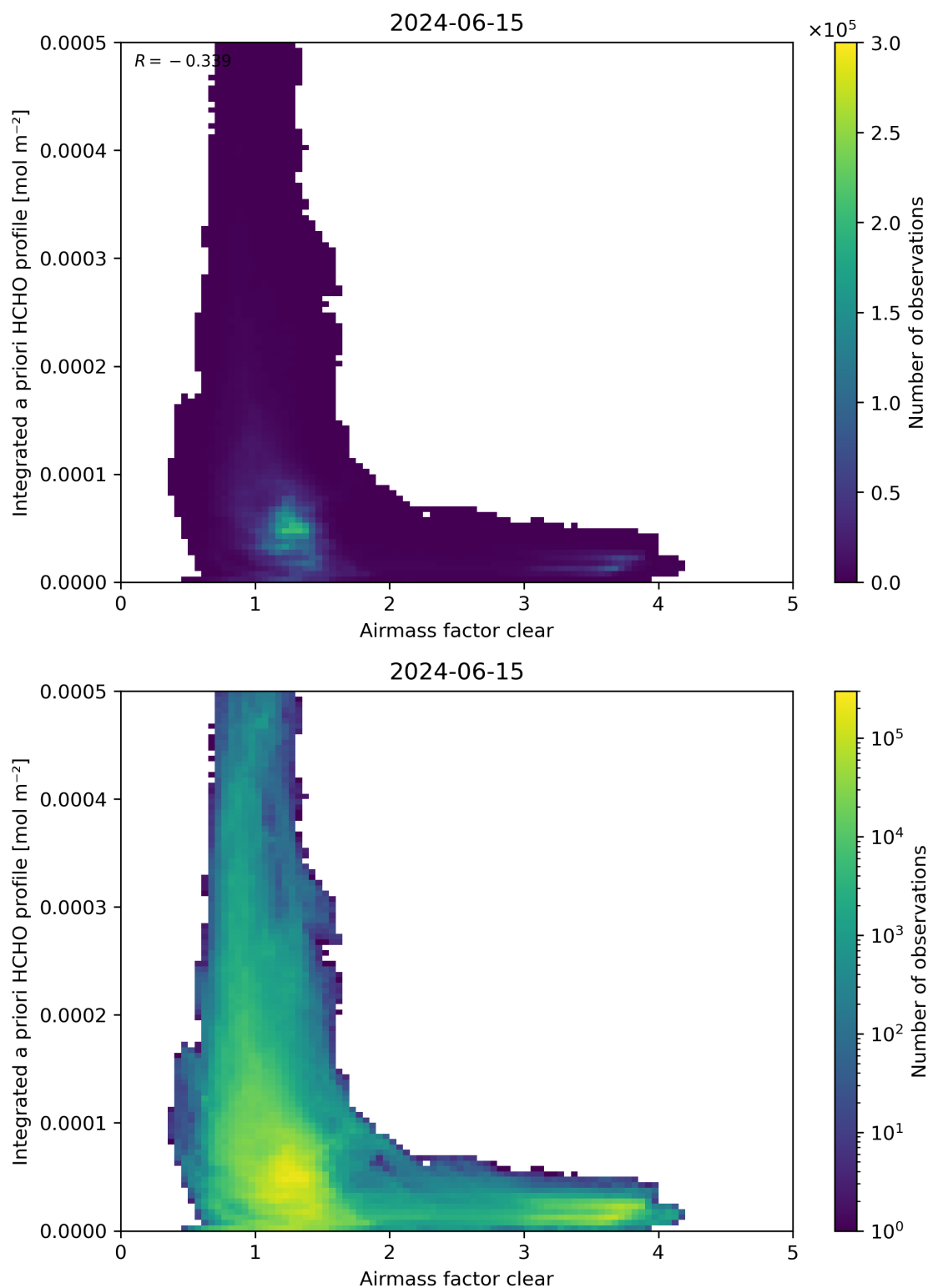
Figure 76: Scatter density plot of “Airmass factor clear” against “Integrated a priori HCHO profile” for 2024-06-14 to 2024-06-16.
