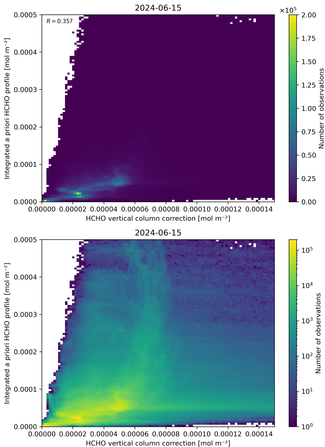
Figure 122: Scatter density plot of “HCHO vertical column correction” against “Integrated a priori HCHO profile” for 2024-06-14 to 2024-06-16.
