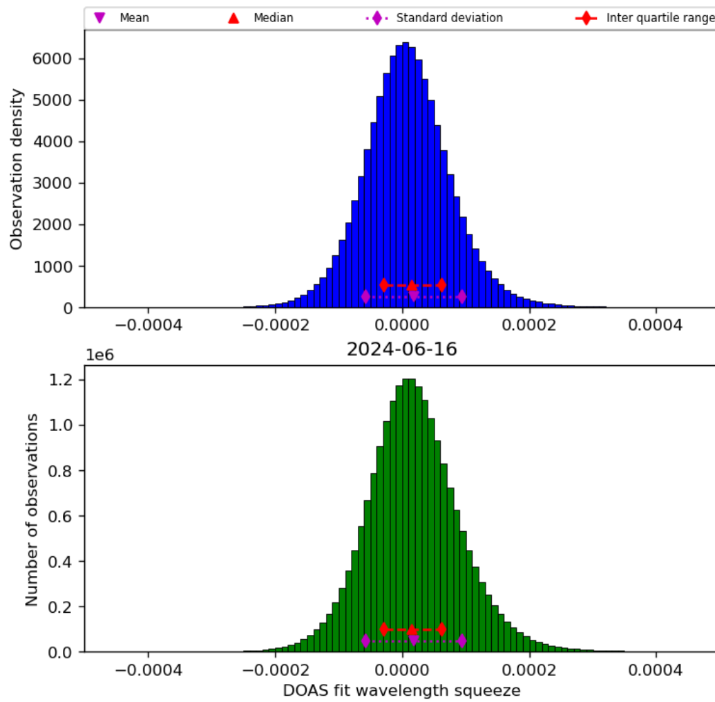
Figure 45: Histogram of “DOAS fit wavelength squeeze” for 2024-06-15 to 2024-06-17
