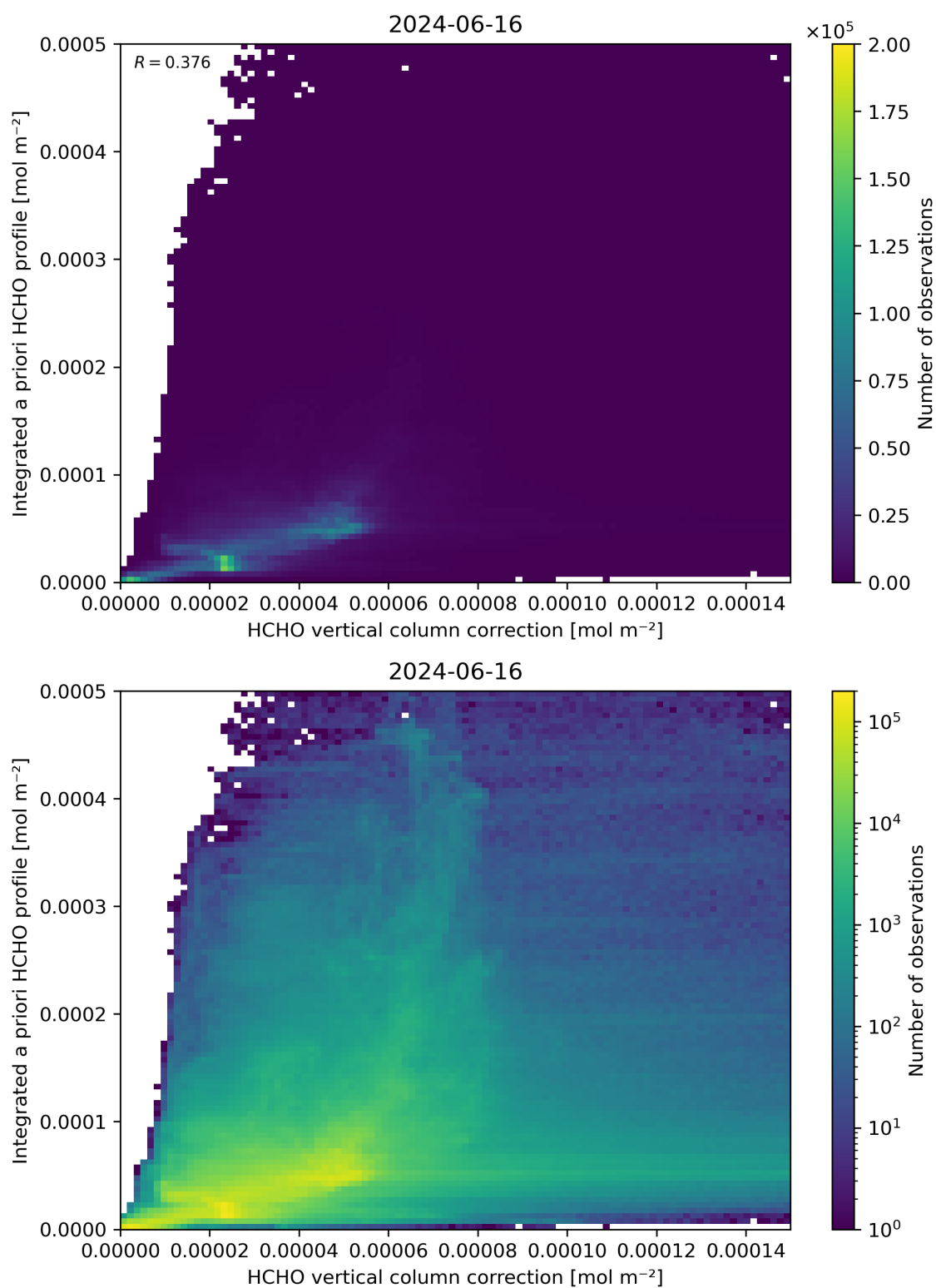
Figure 122: Scatter density plot of “HCHO vertical column correction” against “Integrated a priori HCHO profile” for 2024-06-15 to 2024-06-17.
