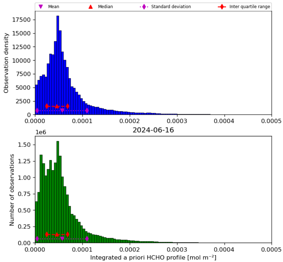
Figure 43: Histogram of “Integrated a priori HCHO profile” for 2024-06-15 to 2024-06-17
