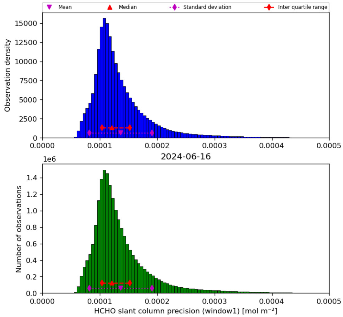
Figure 39: Histogram of “HCHO slant column precision (window1)” for 2024-06-15 to 2024-06-17
