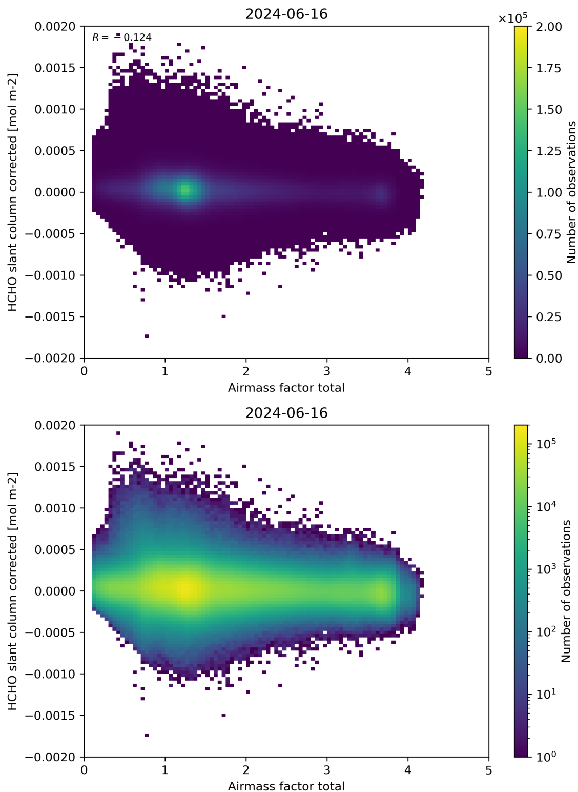
Figure 101: Scatter density plot of “Airmass factor total” against “HCHO slant column corrected” for 2024-06-15 to 2024-06-17.
