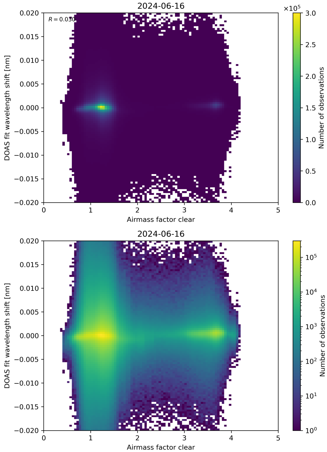
Figure 72: Scatter density plot of “Airmass factor clear” against “DOAS fit wavelength shift” for 2024-06-15 to 2024-06-17.
