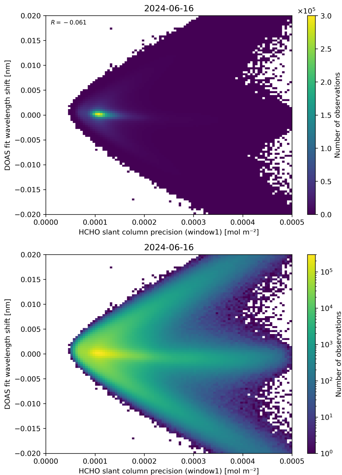
Figure 89: Scatter density plot of “HCHO slant column precision (window1)” against “DOAS fit wavelength shift” for 2024-06-15 to 2024-06-17.
