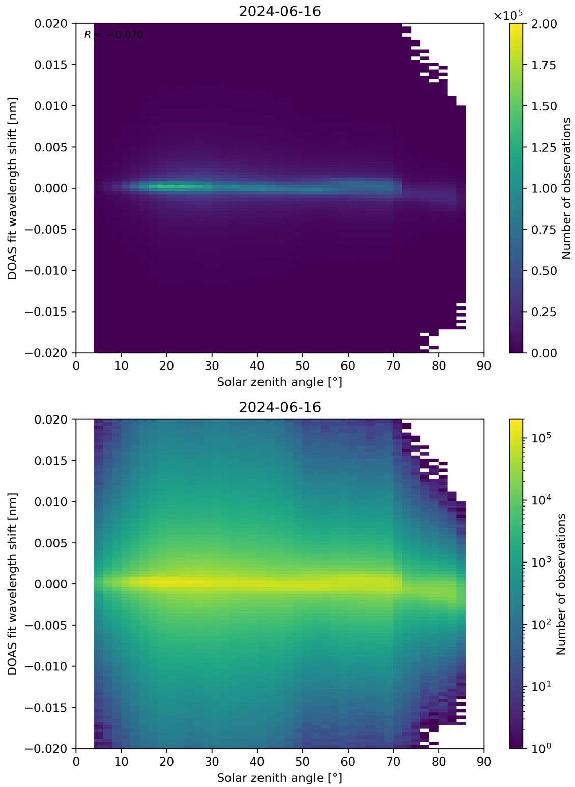
Figure 168: Scatter density plot of “Solar zenith angle” against “DOAS fit wavelength shift” for 2024-06-15 to 2024-06-17.
