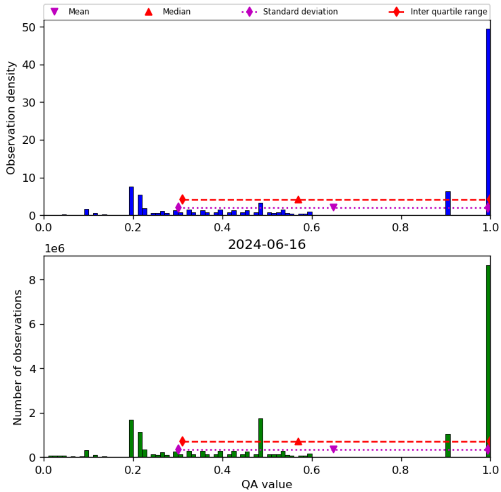
Figure 34: Histogram of “QA value” for 2024-06-15 to 2024-06-17
