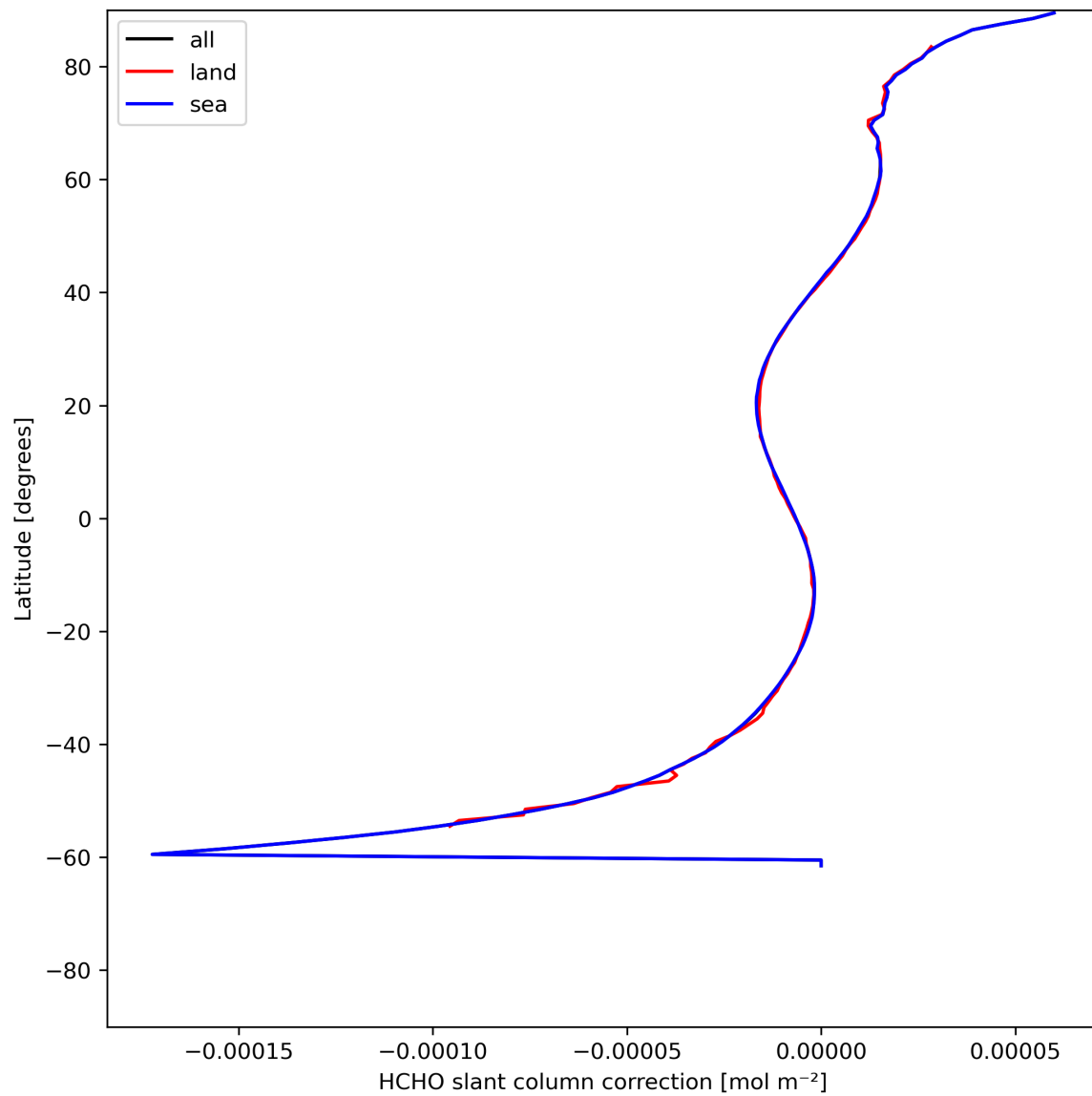
Figure 33: Zonal average of “HCHO slant column correction” for 2024-06-15 to 2024-06-17.
