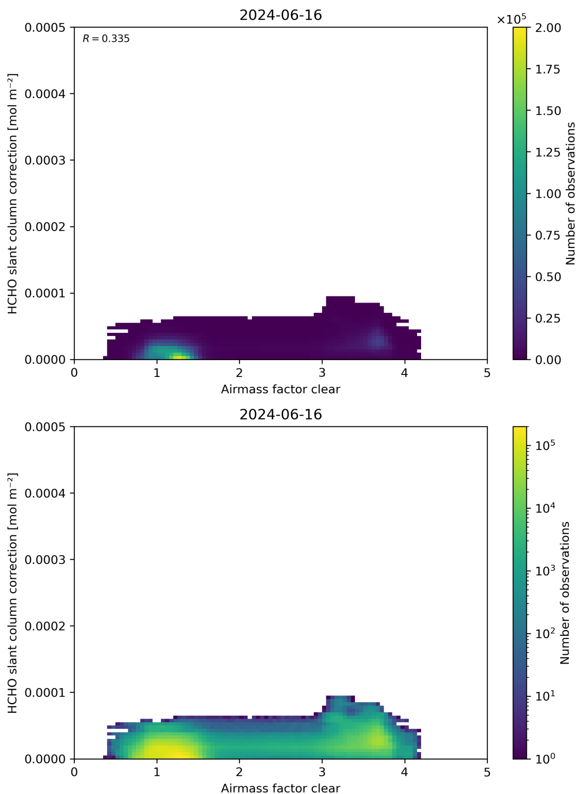
Figure 75: Scatter density plot of “Airmass factor clear” against “HCHO slant column correction” for 2024-06-15 to 2024-06-17.
