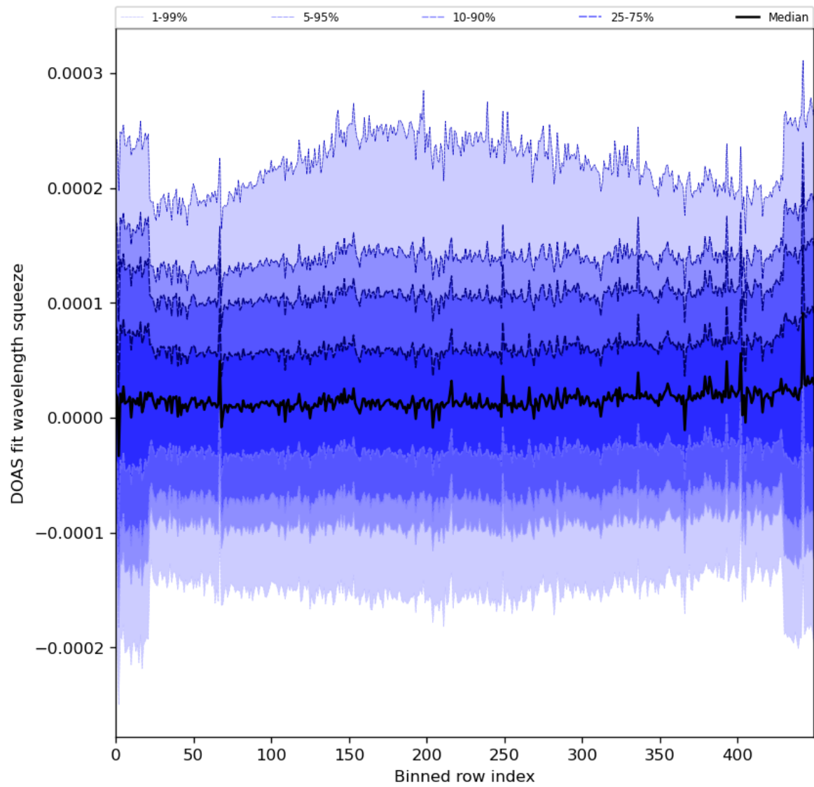
Figure 59: Along track statistics of “DOAS fit wavelength squeeze” for 2024-06-15 to 2024-06-17
