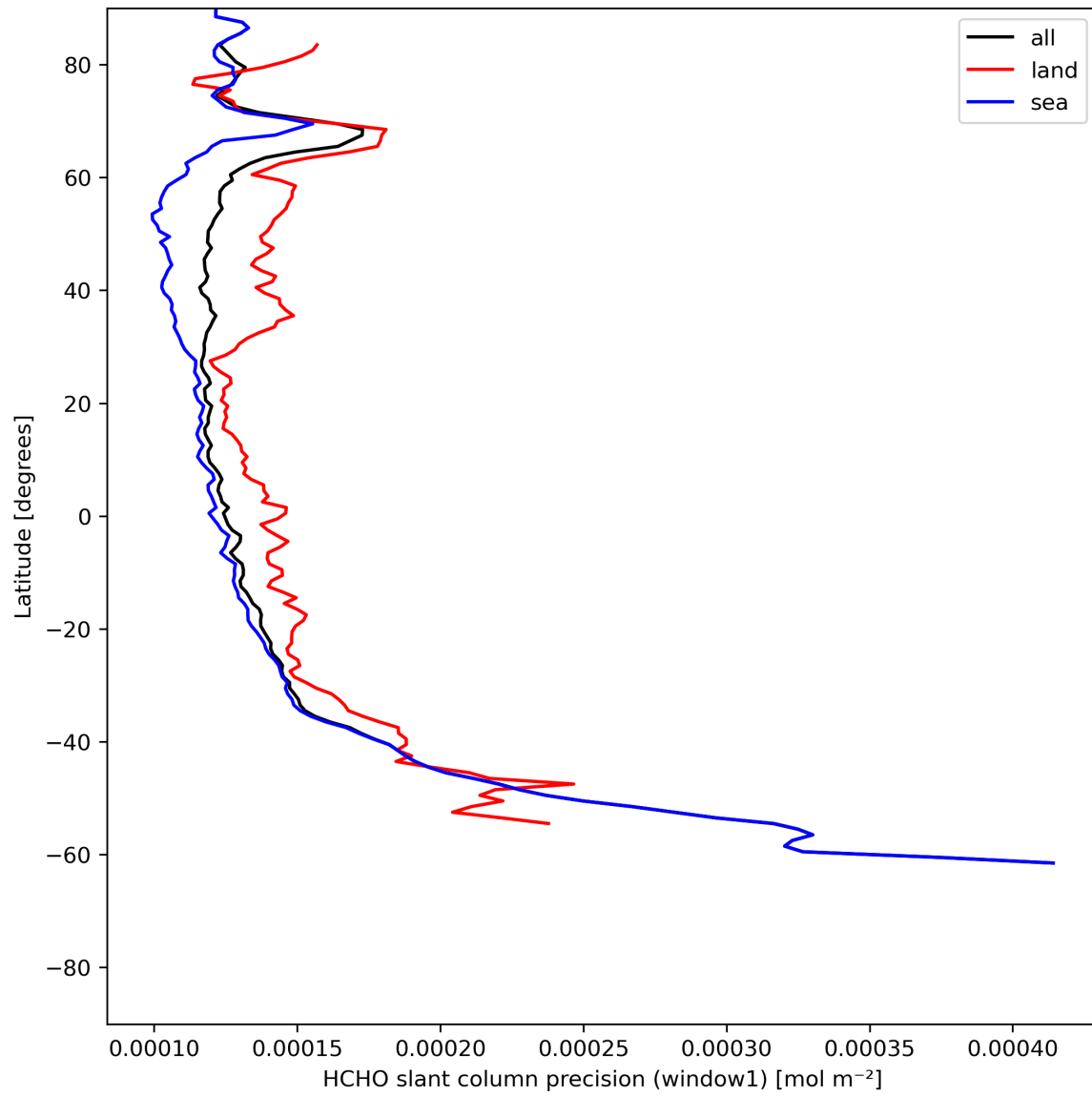
Figure 25: Zonal average of "HCHO slant column precision (window1)" for 2024-06-15 to 2024-06-17.
