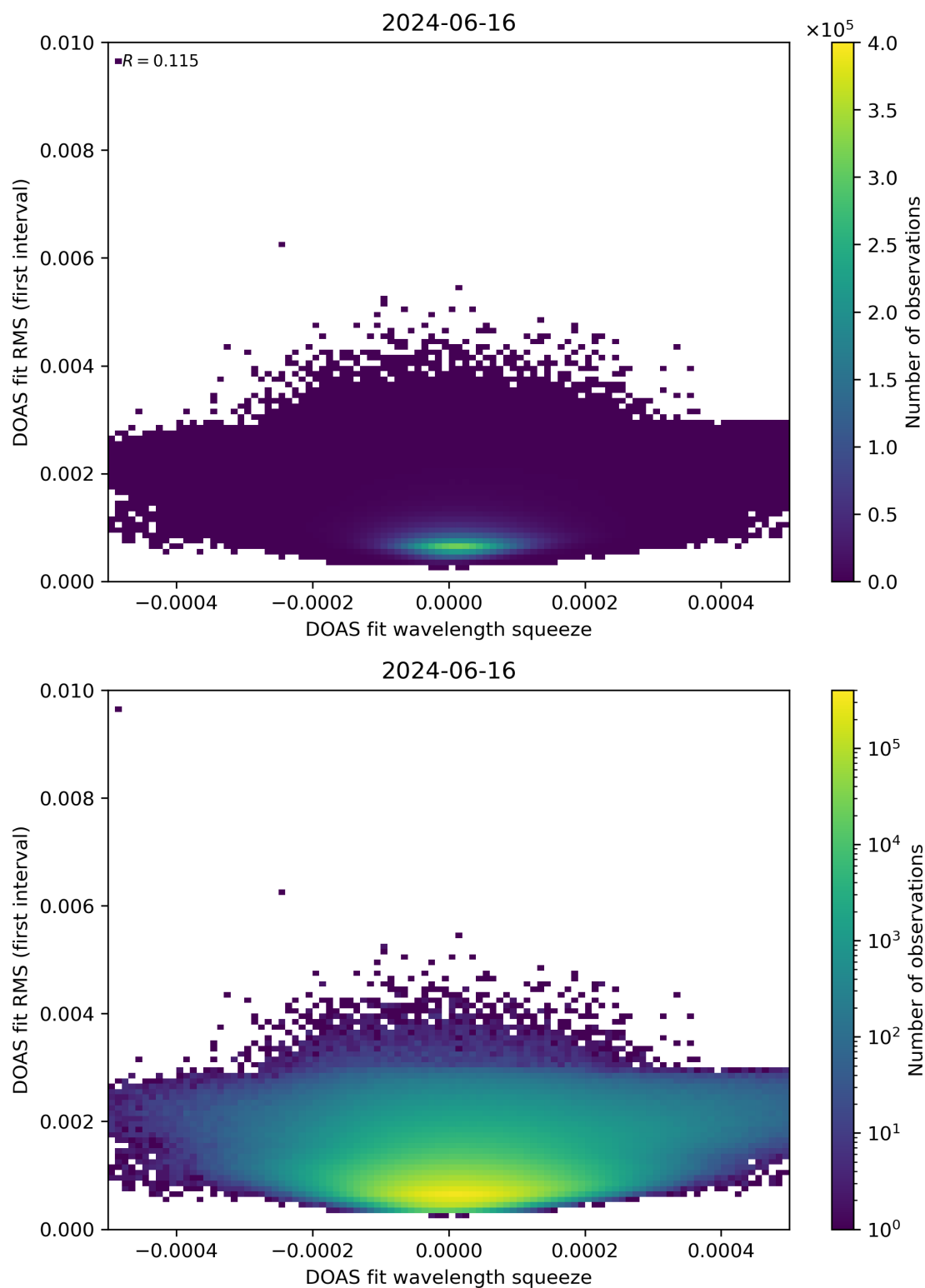
Figure 68: Scatter density plot of “DOAS fit wavelength squeeze” against “DOAS fit RMS (first interval)” for 2024-06-15 to 2024-06-17.
