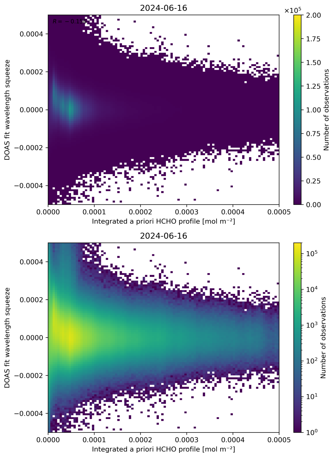
Figure 150: Scatter density plot of “Integrated a priori HCHO profile” against “DOAS fit wavelength squeeze” for 2024-06-15 to 2024-06-17.
