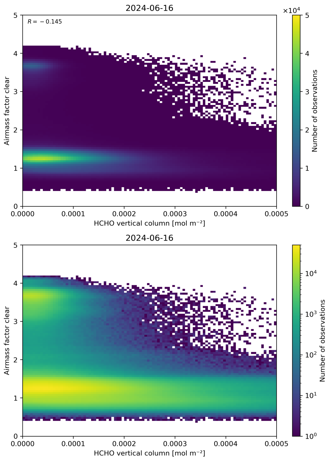
Figure 126: Scatter density plot of “HCHO vertical column” against “Airmass factor clear” for 2024-06-15 to 2024-06-17.
