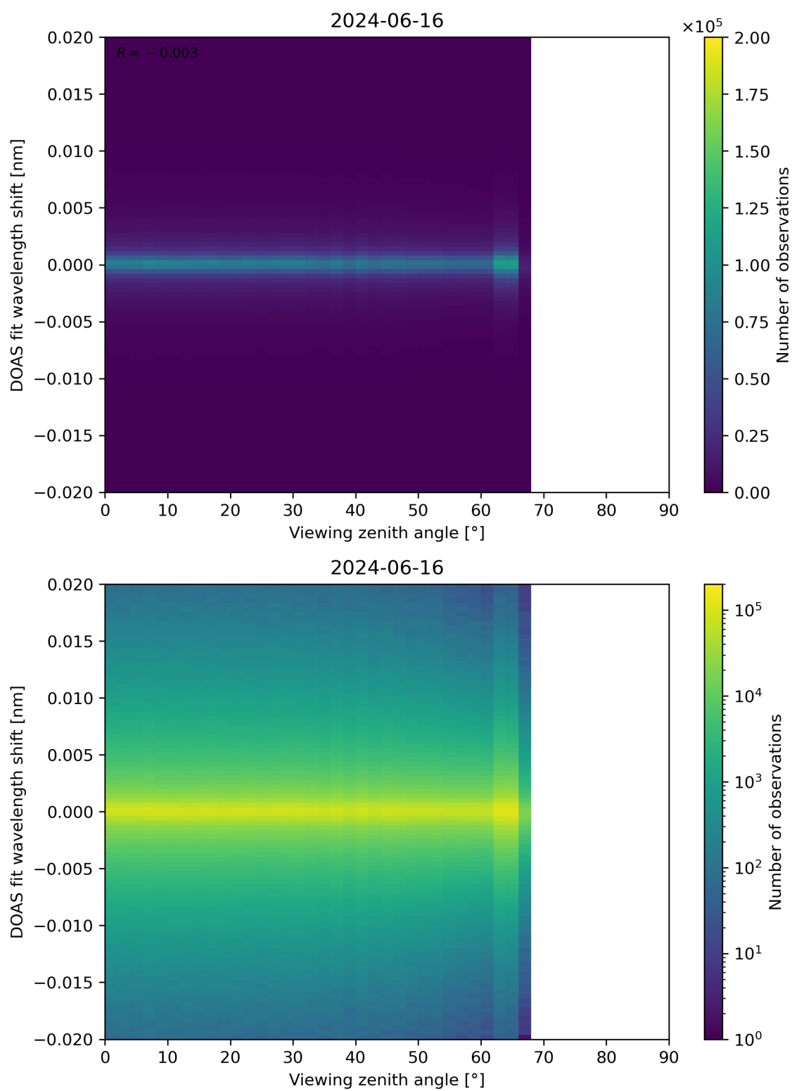
Figure 183: Scatter density plot of “Viewing zenith angle” against “DOAS fit wavelength shift” for 2024-06-15 to 2024-06-17.
