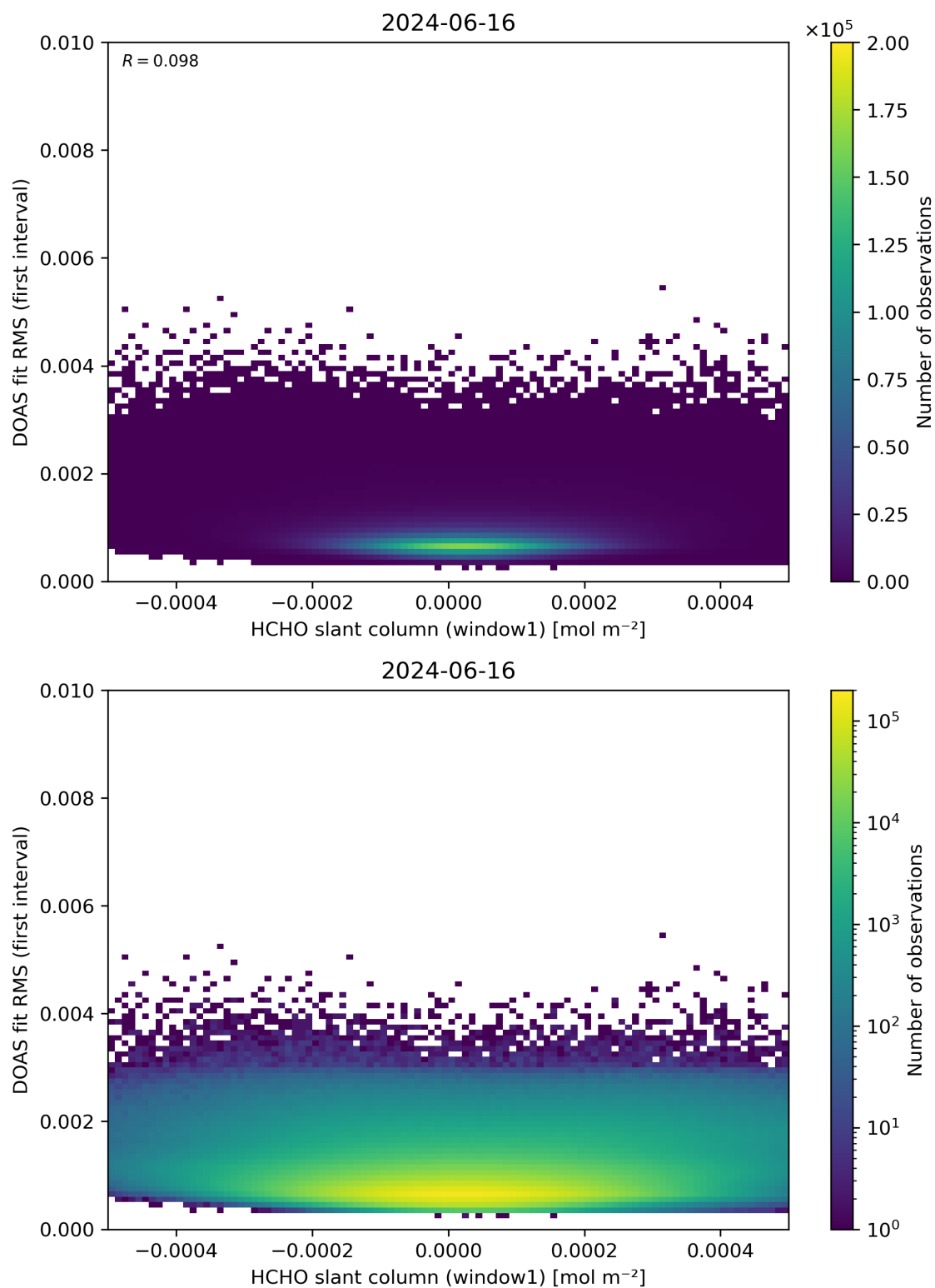
Figure 78: Scatter density plot of “HCHO slant column (window1)” against “DOAS fit RMS (first interval)” for 2024-06-15 to 2024-06-17.
