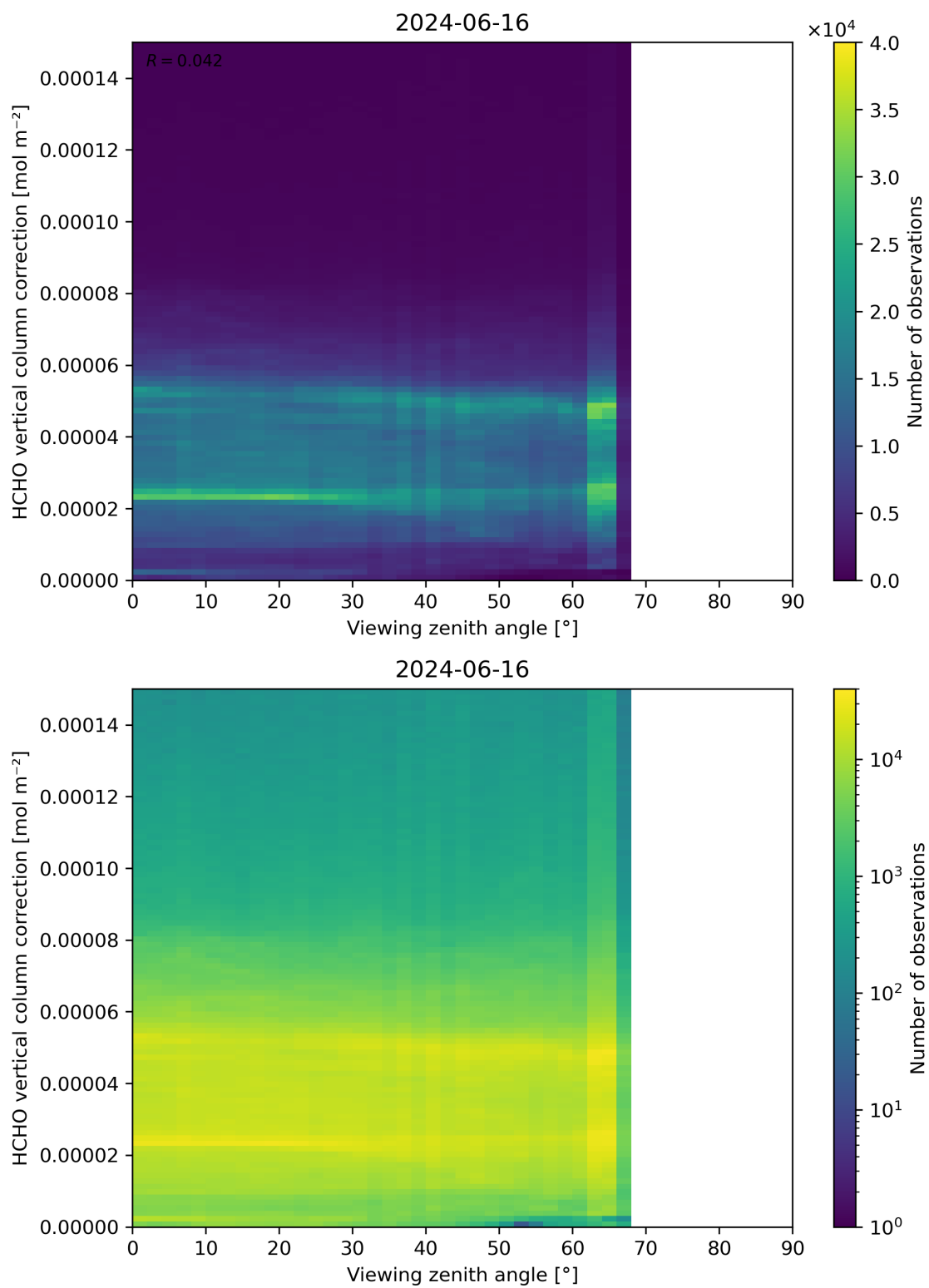
Figure 193: Scatter density plot of “Viewing zenith angle” against “HCHO vertical column correction” for 2024-06-15 to 2024-06-17.
