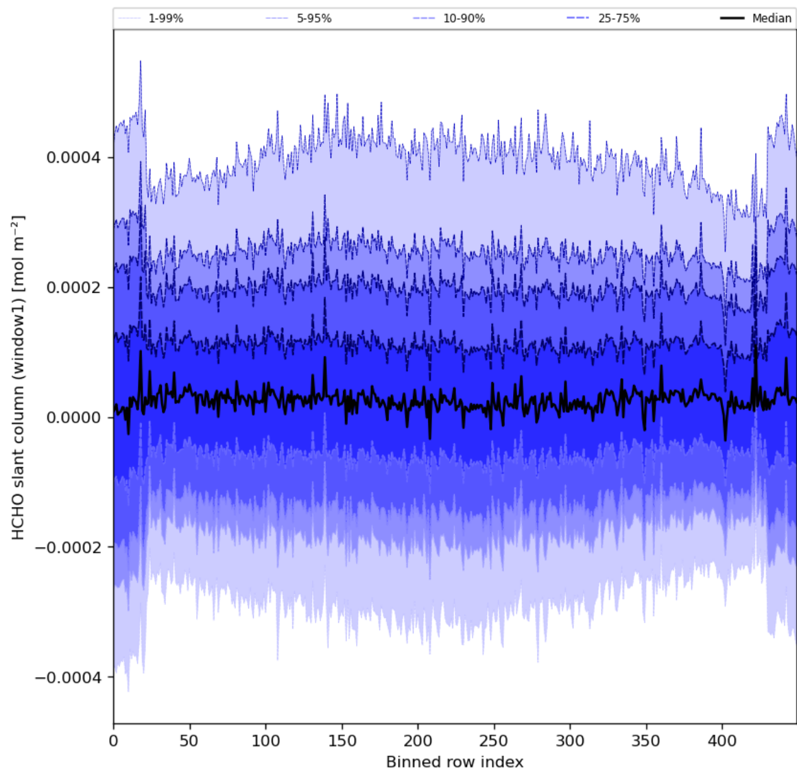
Figure 52: Along track statistics of “HCHO slant column (window1)” for 2024-06-15 to 2024-06-17
