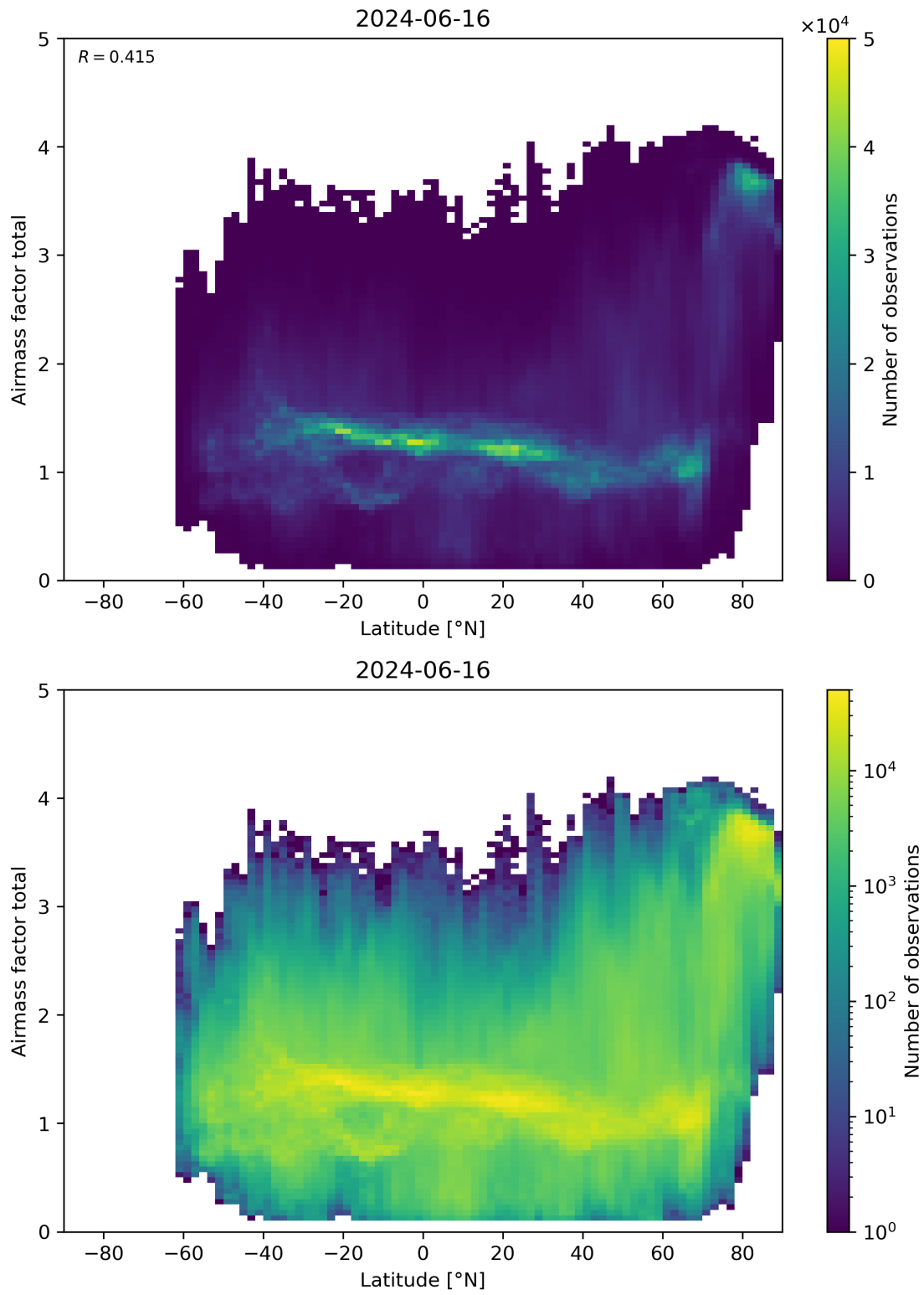
Figure 161: Scatter density plot of “Latitude” against “Airmass factor total” for 2024-06-15 to 2024-06-17.
