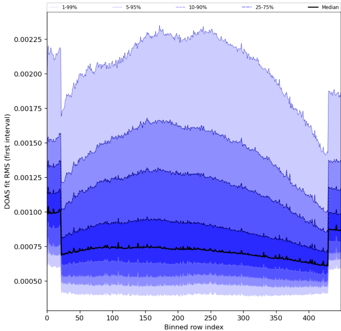
Figure 60: Along track statistics of “DOAS fit RMS (first interval)” for 2024-06-15 to 2024-06-17
