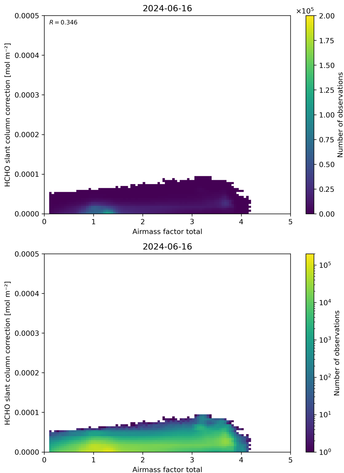
Figure 102: Scatter density plot of “Airmass factor total” against “HCHO slant column correction” for 2024-06-15 to 2024-06-17.
