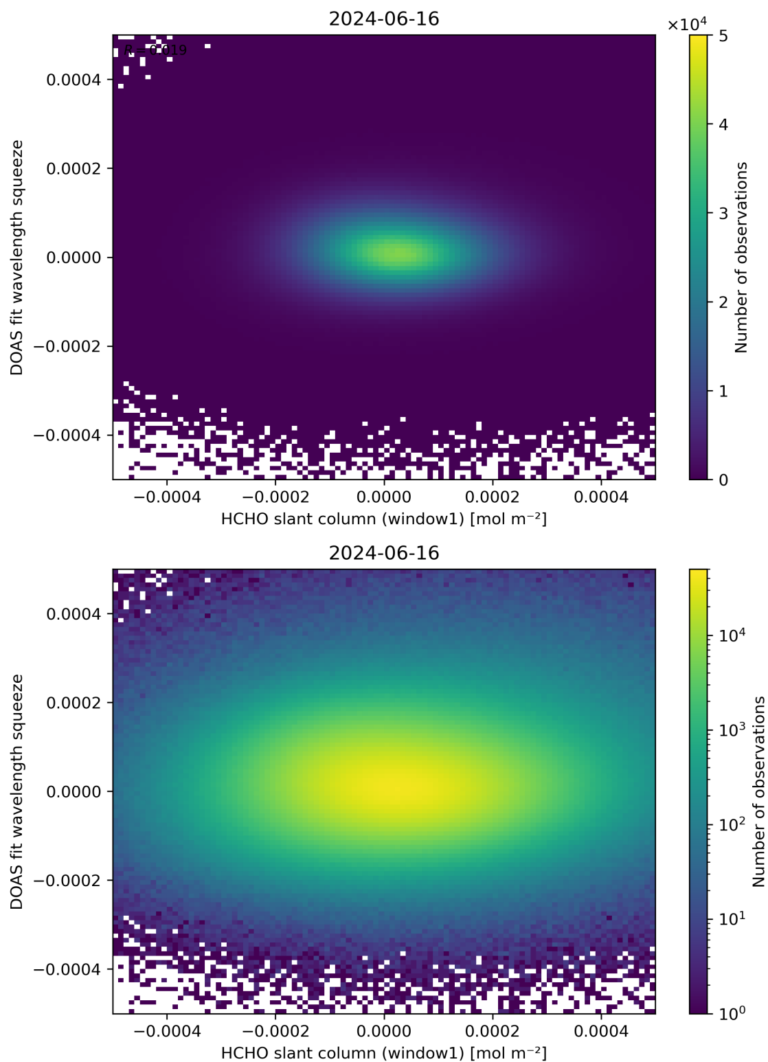
Figure 80: Scatter density plot of “HCHO slant column (window1)” against “DOAS fit wavelength squeeze” for 2024-06-15 to 2024-06-17.
