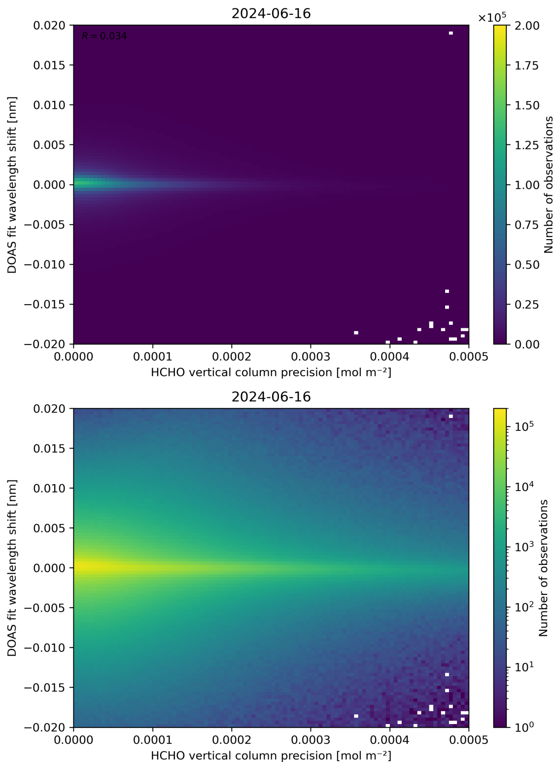
Figure 137: Scatter density plot of “HCHO vertical column precision” against “DOAS fit wavelength shift” for 2024-06-15 to 2024-06-17.
