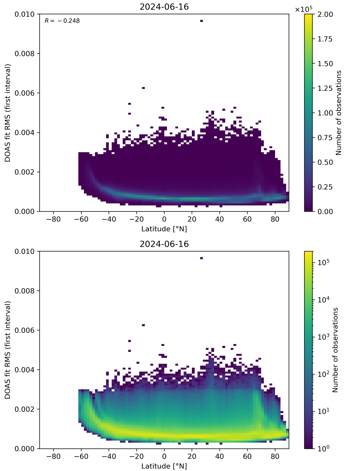
Figure 153: Scatter density plot of “Latitude” against “DOAS fit RMS (first interval)” for 2024-06-15 to 2024-06-17.
