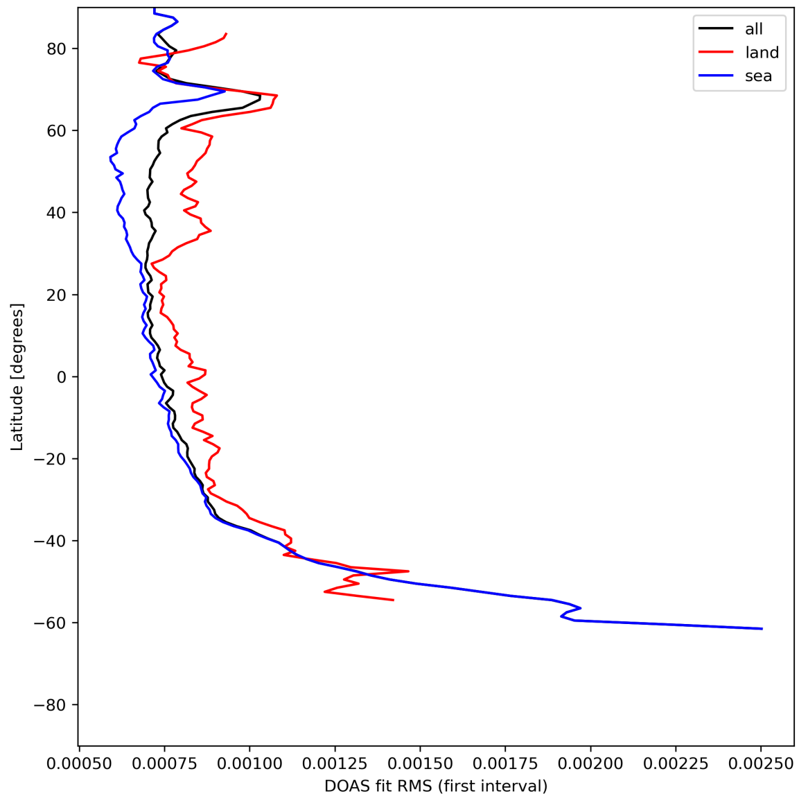
Figure 32: Zonal average of "DOAS fit RMS (first interval)" for 2024-06-15 to 2024-06-17.
