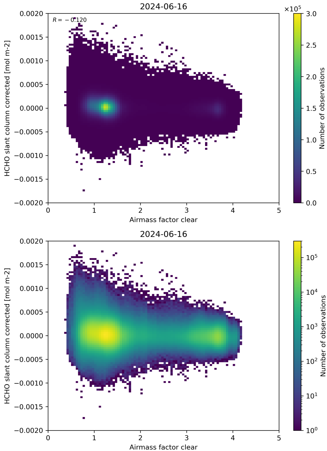
Figure 74: Scatter density plot of “Airmass factor clear” against “HCHO slant column corrected” for 2024-06-15 to 2024-06-17.
