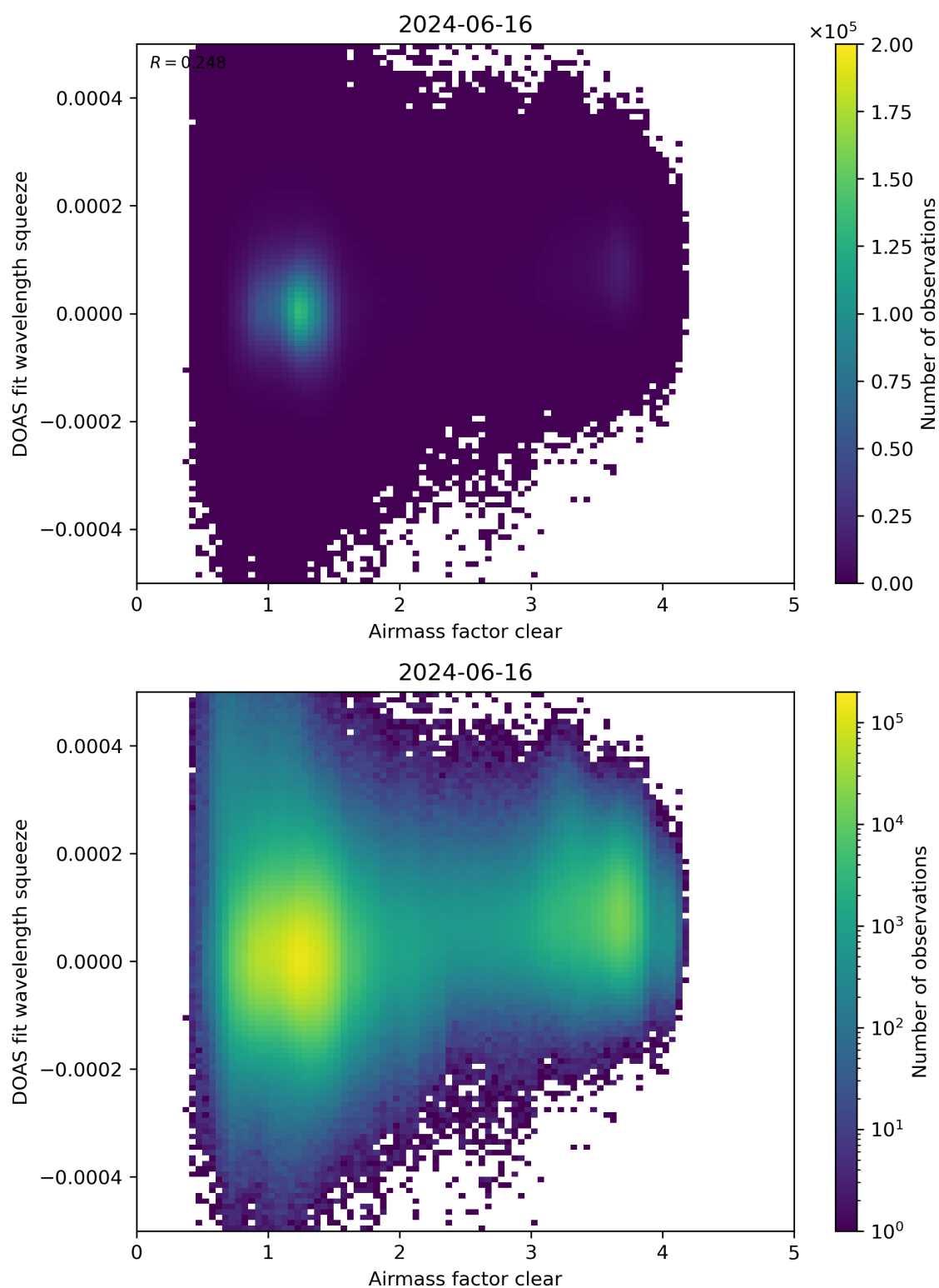
Figure 73: Scatter density plot of “Airmass factor clear” against “DOAS fit wavelength squeeze” for 2024-06-15 to 2024-06-17.
