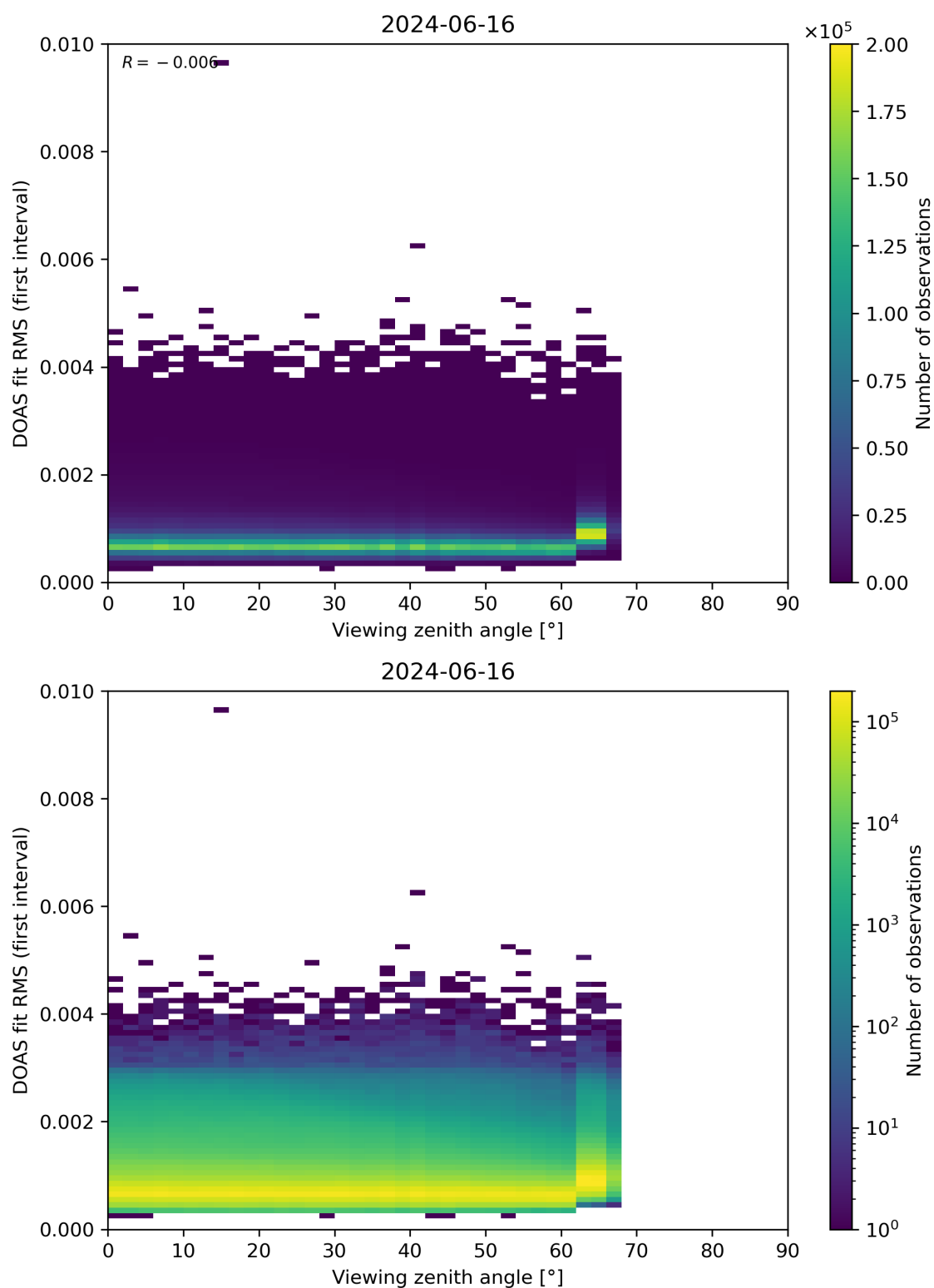
Figure 182: Scatter density plot of “Viewing zenith angle” against “DOAS fit RMS (first interval)” for 2024-06-15 to 2024-06-17.
