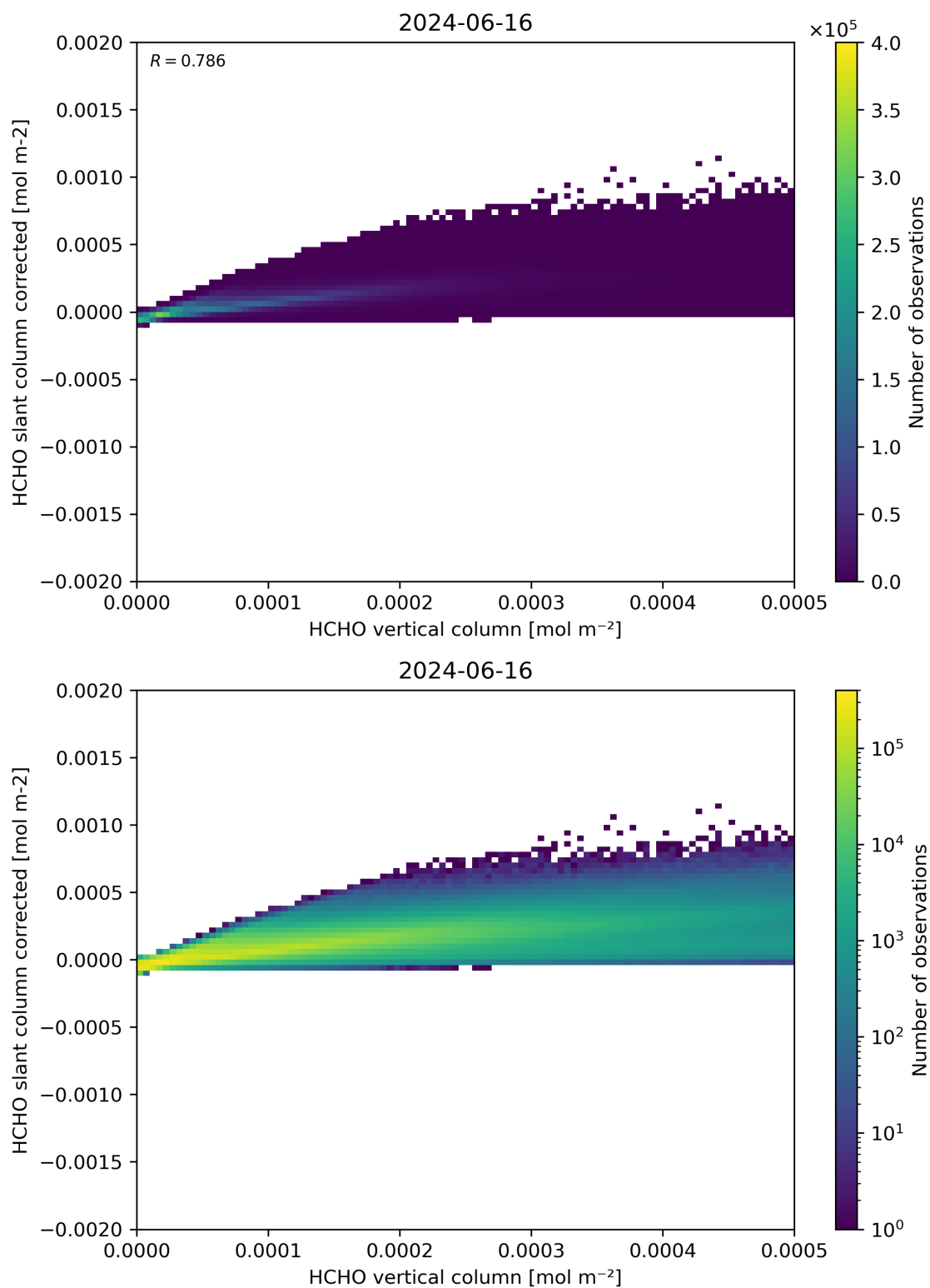
Figure 127: Scatter density plot of “HCHO vertical column” against “HCHO slant column corrected” for 2024-06-15 to 2024-06-17.
