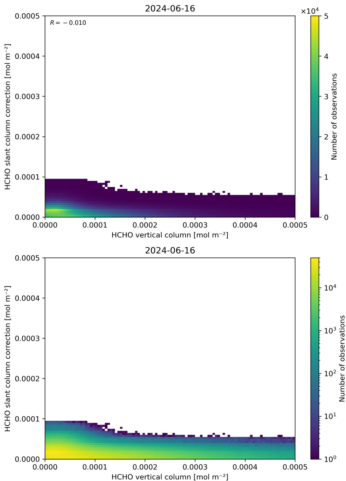
Figure 128: Scatter density plot of “HCHO vertical column” against “HCHO slant column correction” for 2024-06-15 to 2024-06-17.
