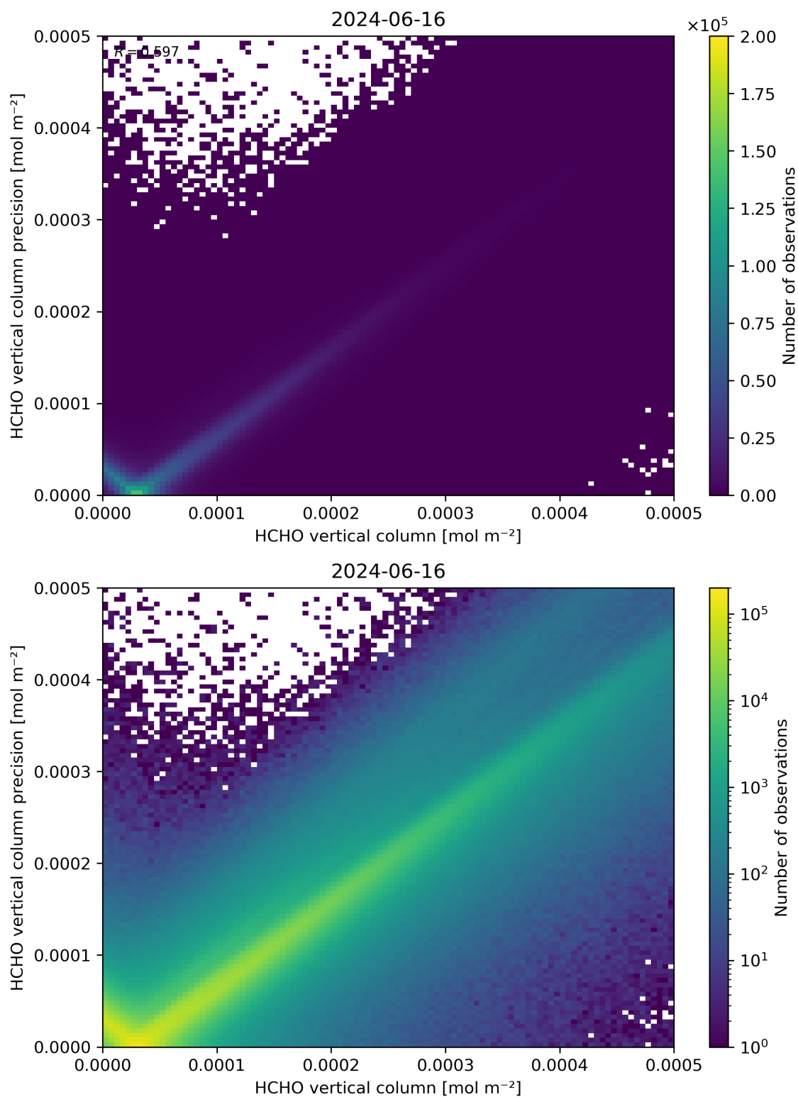
Figure 134: Scatter density plot of “HCHO vertical column” against “HCHO vertical column precision” for 2024-06-15 to 2024-06-17.
