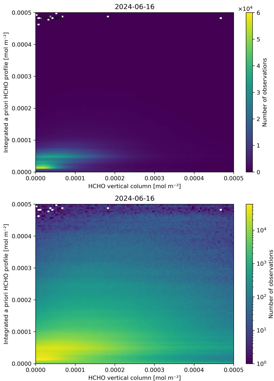
Figure 135: Scatter density plot of “HCHO vertical column” against “Integrated a priori HCHO profile” for 2024-06-15 to 2024-06-17.
