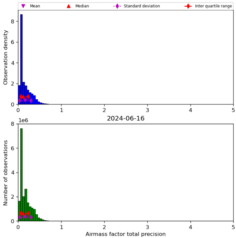
Figure 41: Histogram of “Airmass factor total precision” for 2024-06-15 to 2024-06-17
