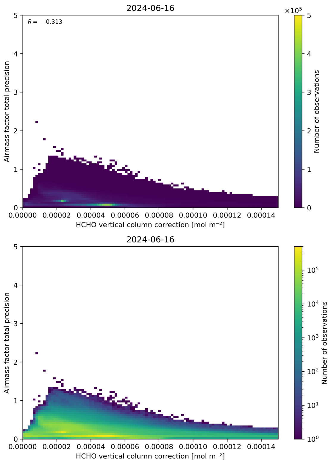
Figure 121: Scatter density plot of “HCHO vertical column correction” against “Airmass factor total precision” for 2024-06-15 to 2024-06-17.
