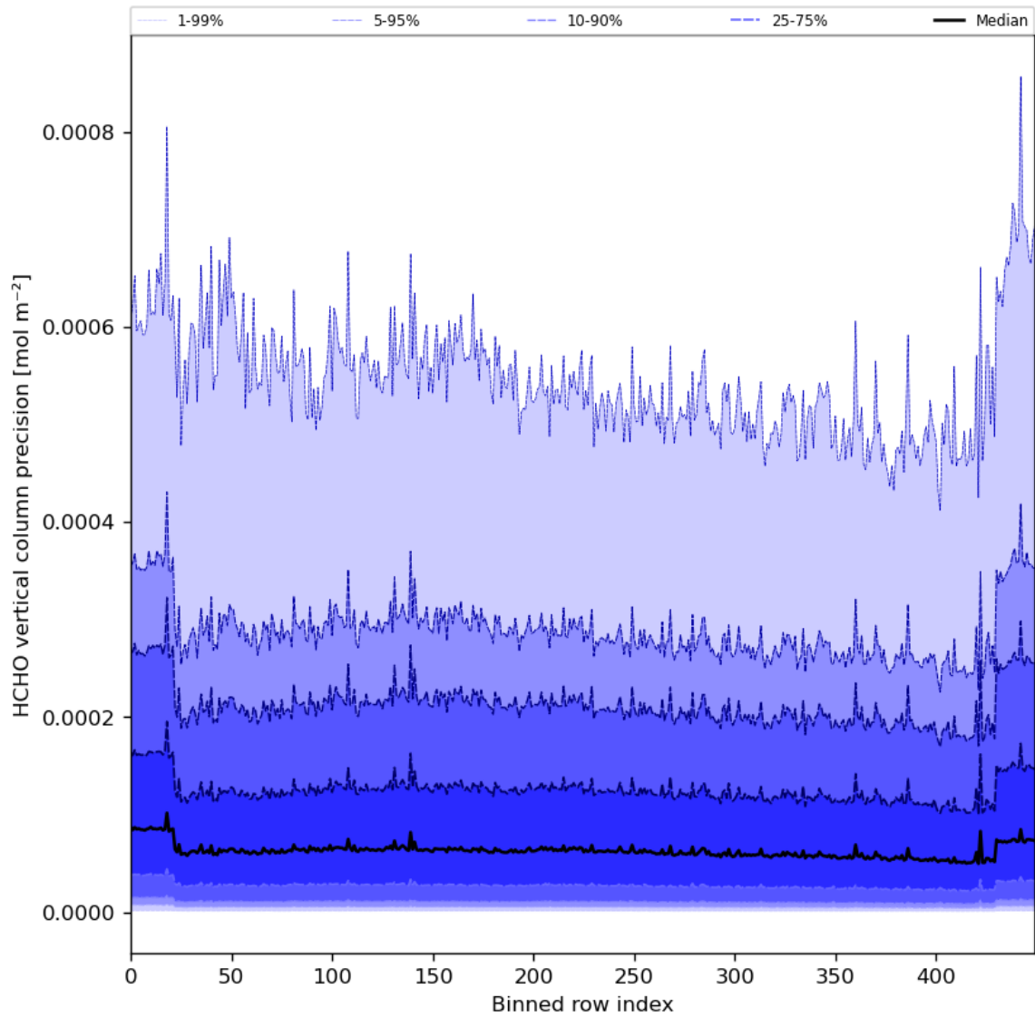
Figure 50: Along track statistics of “HCHO vertical column precision” for 2024-06-15 to 2024-06-17
