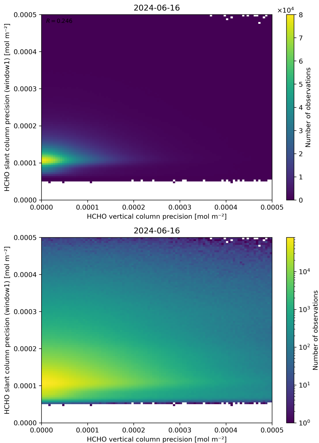
Figure 143: Scatter density plot of “HCHO vertical column precision” against “HCHO slant column precision (window1)” for 2024-06-15 to 2024-06-17.
