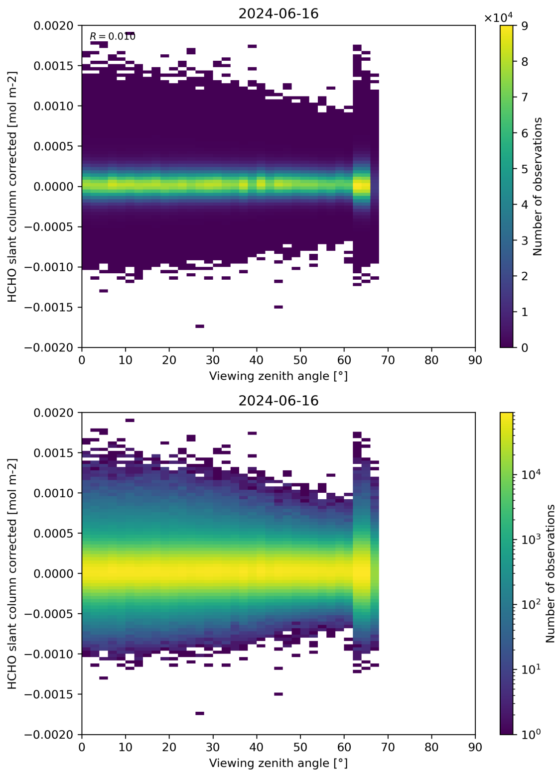
Figure 186: Scatter density plot of “Viewing zenith angle” against “HCHO slant column corrected” for 2024-06-15 to 2024-06-17.
