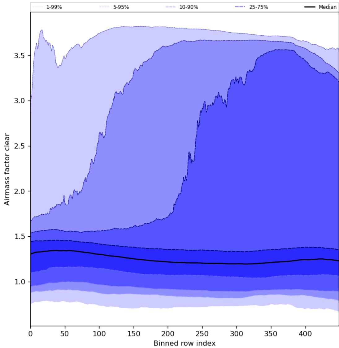
Figure 56: Along track statistics of “Airmass factor clear” for 2024-06-15 to 2024-06-17
