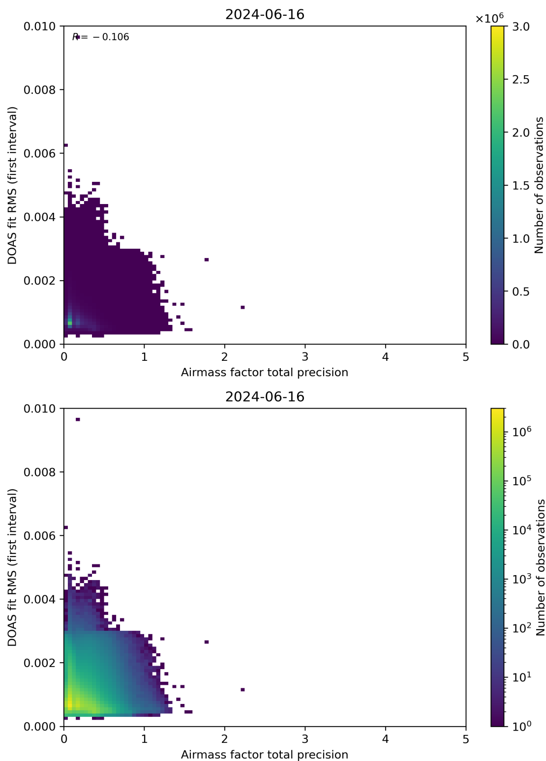
Figure 105: Scatter density plot of “Airmass factor total precision” against “DOAS fit RMS (first interval)” for 2024-06-15 to 2024-06-17.
