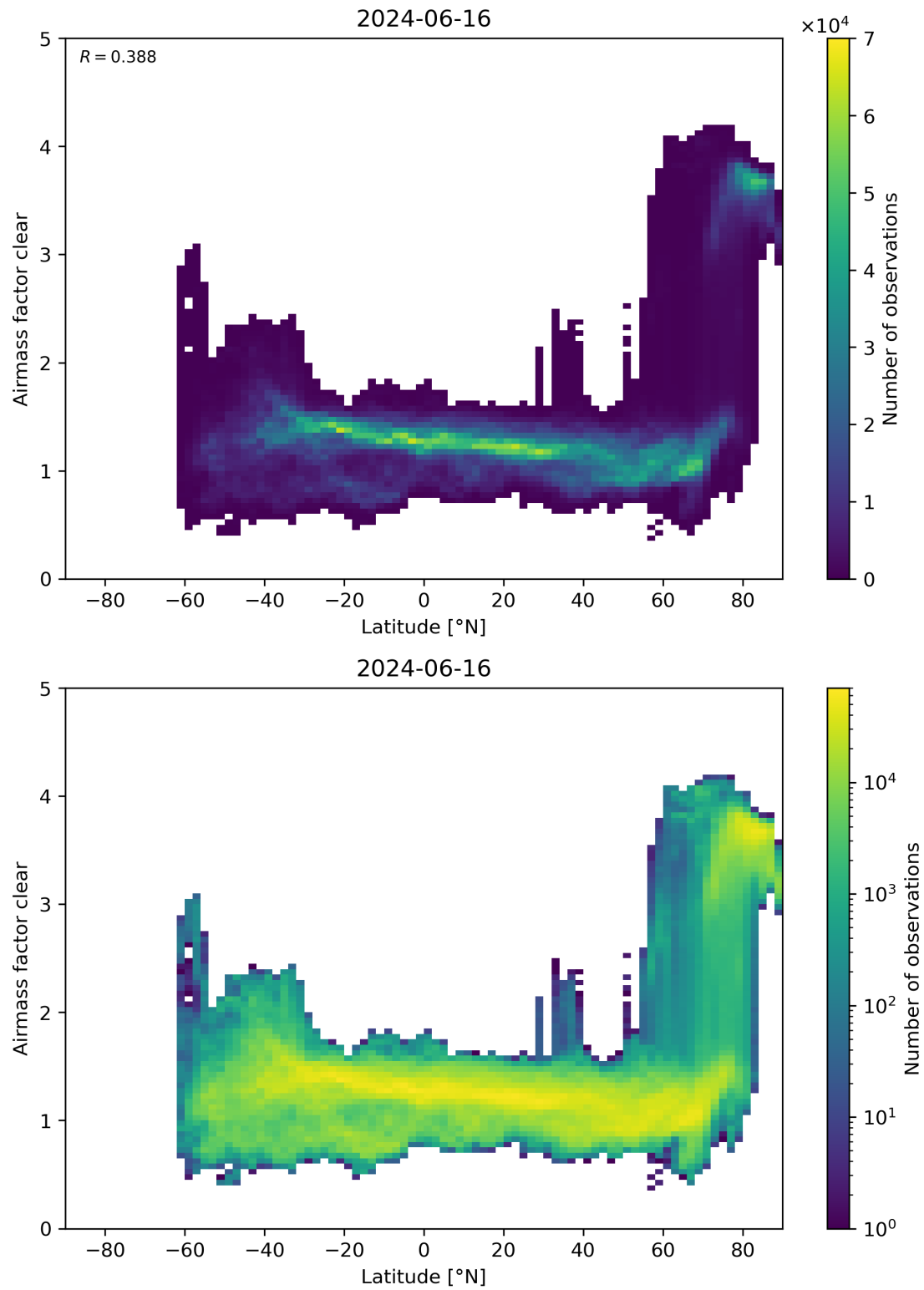
Figure 156: Scatter density plot of “Latitude” against “Airmass factor clear” for 2024-06-15 to 2024-06-17.
