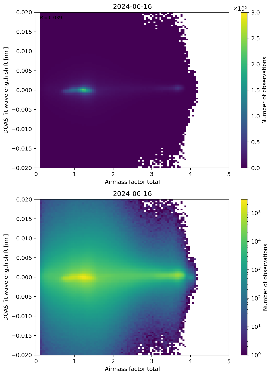
Figure 98: Scatter density plot of “Airmass factor total” against “DOAS fit wavelength shift” for 2024-06-15 to 2024-06-17.
