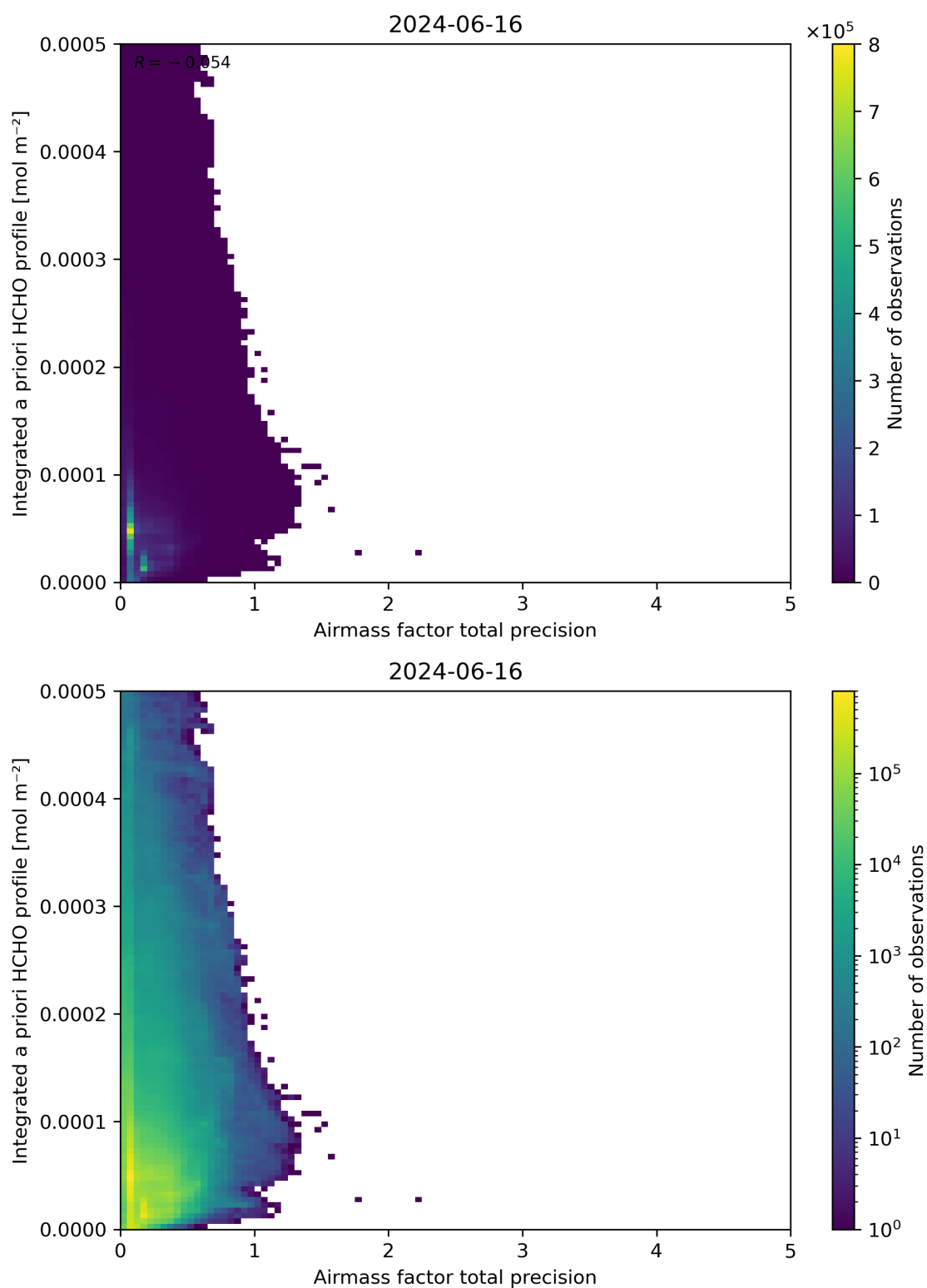
Figure 111: Scatter density plot of “Airmass factor total precision” against “Integrated a priori HCHO profile” for 2024-06-15 to 2024-06-17.
