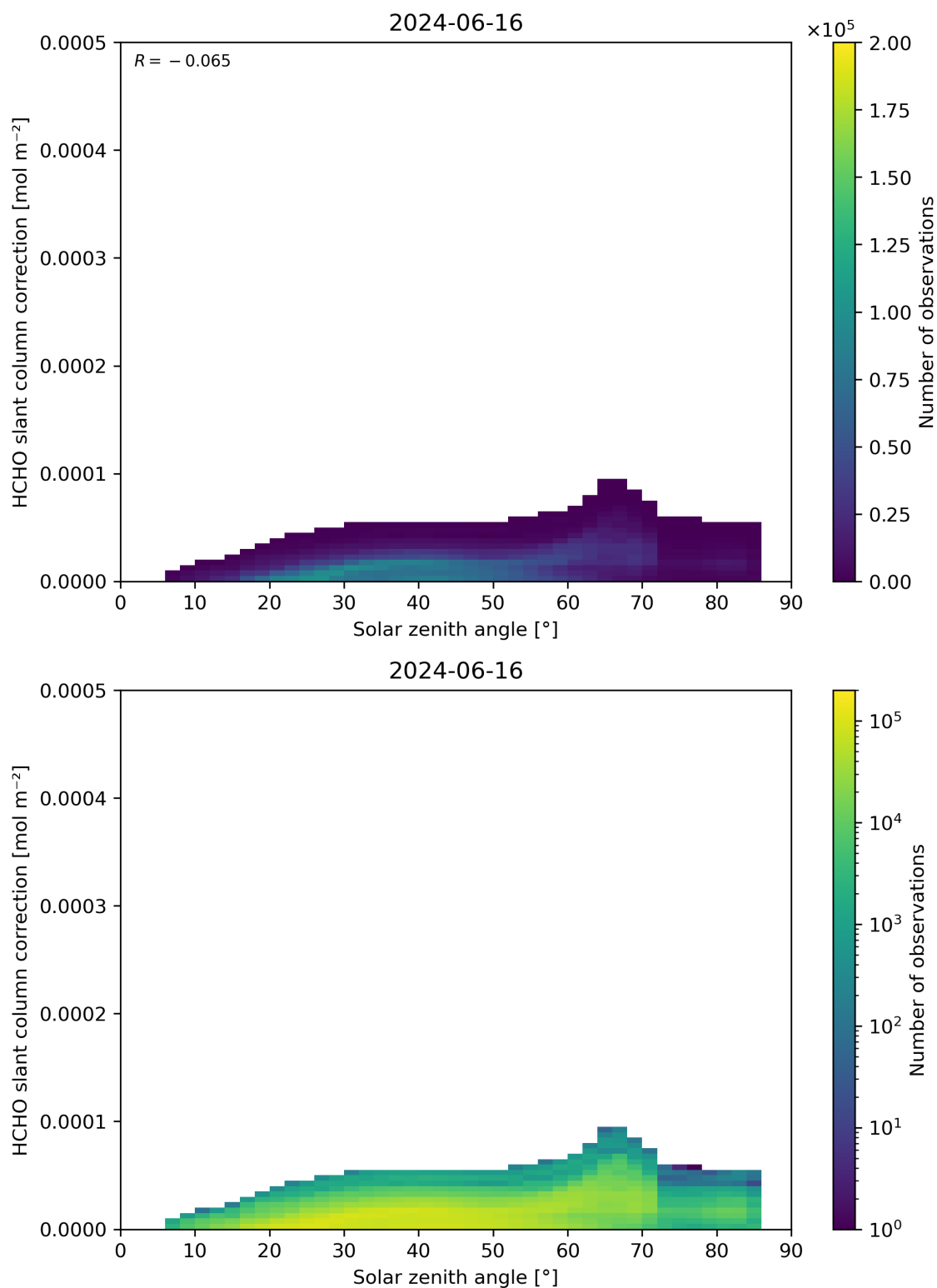
Figure 172: Scatter density plot of “Solar zenith angle” against “HCHO slant column correction” for 2024-06-15 to 2024-06-17.
