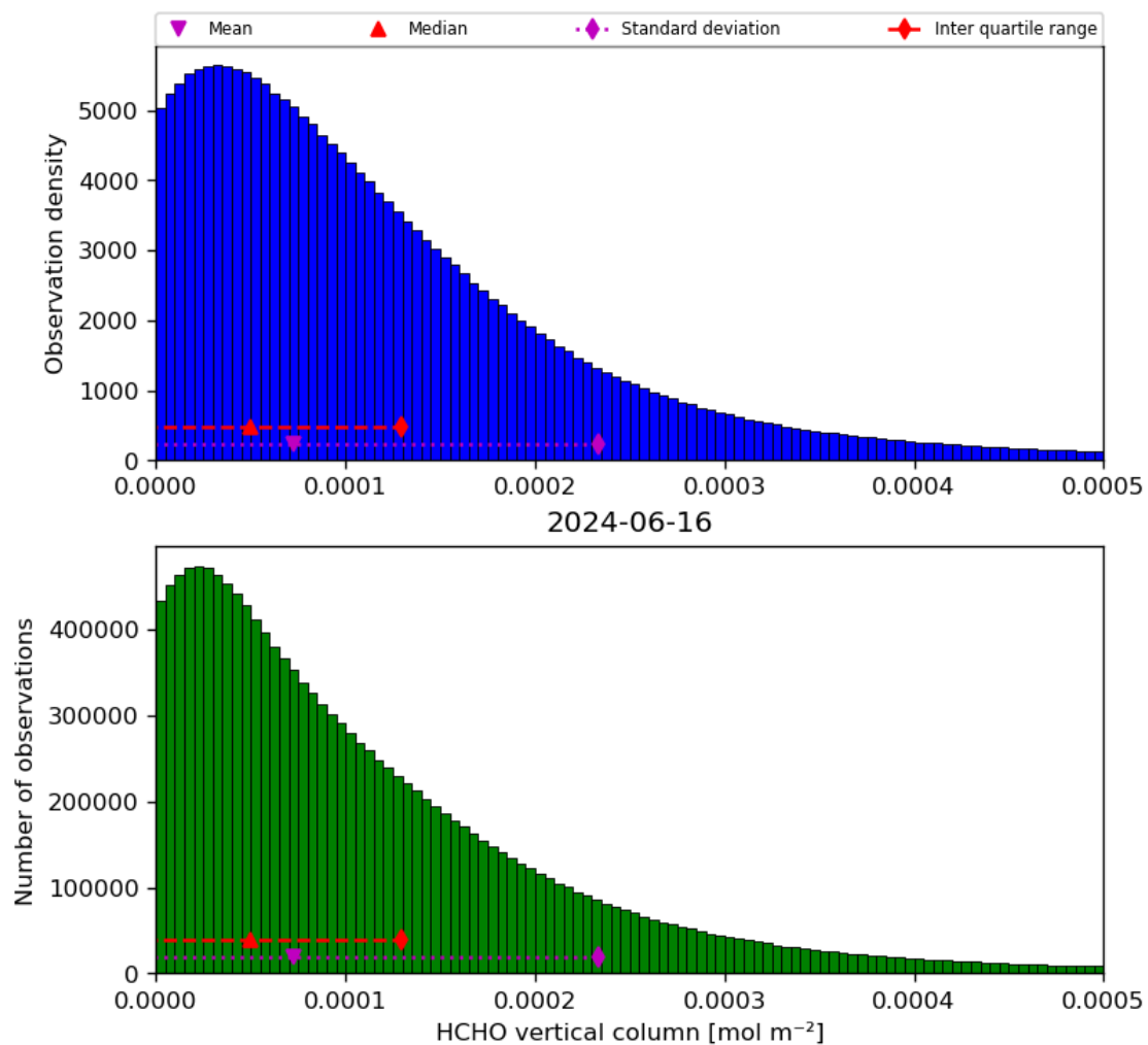
Figure 35: Histogram of “HCHO vertical column” for 2024-06-15 to 2024-06-17
