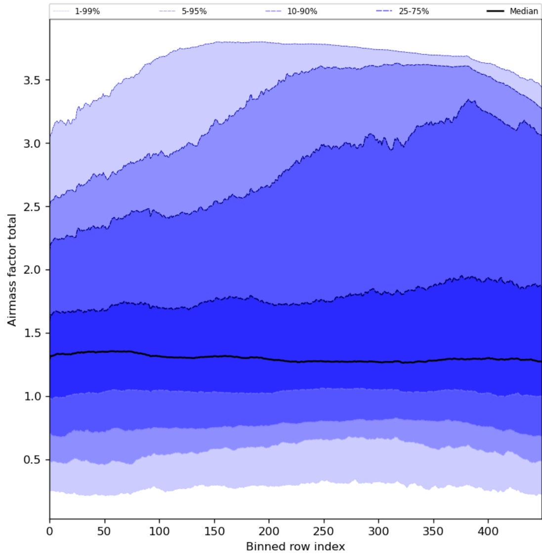
Figure 54: Along track statistics of “Airmass factor total” for 2024-06-15 to 2024-06-17
