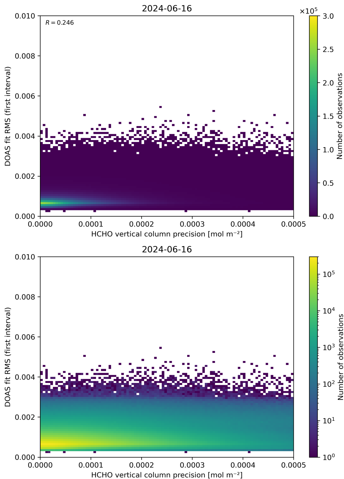
Figure 136: Scatter density plot of “HCHO vertical column precision” against “DOAS fit RMS (first interval)” for 2024-06-15 to 2024-06-17.
