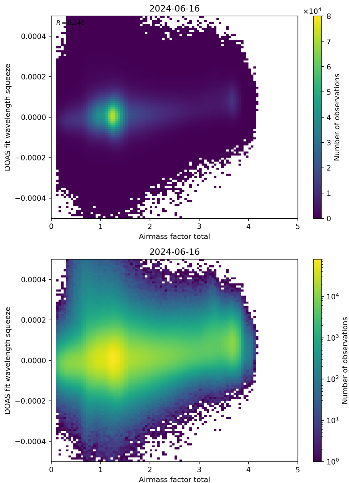
Figure 99: Scatter density plot of “Airmass factor total” against “DOAS fit wavelength squeeze” for 2024-06-15 to 2024-06-17.
