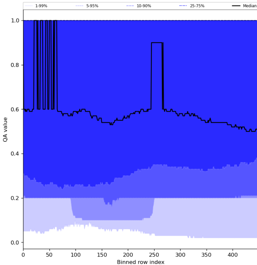
Figure 48: Along track statistics of “QA value” for 2024-06-15 to 2024-06-17
