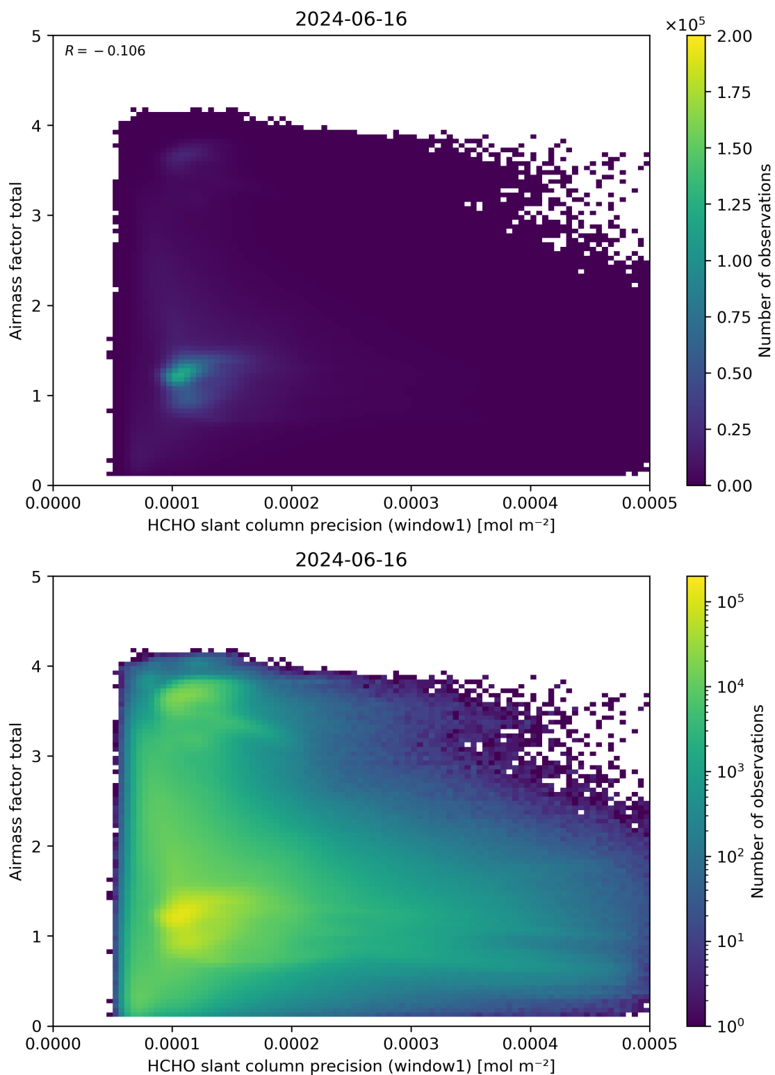
Figure 94: Scatter density plot of “HCHO slant column precision (window1)” against “Airmass factor total” for 2024-06-15 to 2024-06-17.
