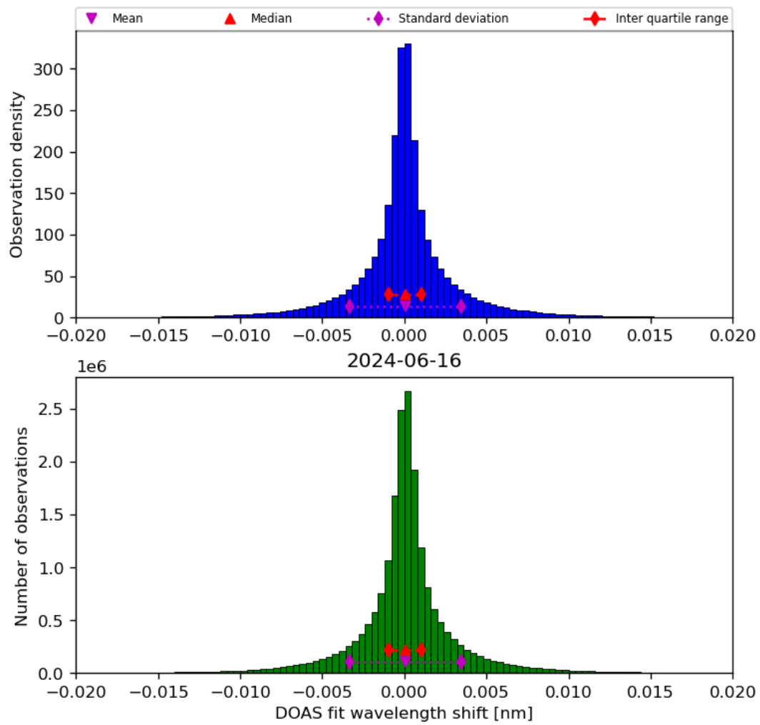
Figure 44: Histogram of “DOAS fit wavelength shift” for 2024-06-15 to 2024-06-17
