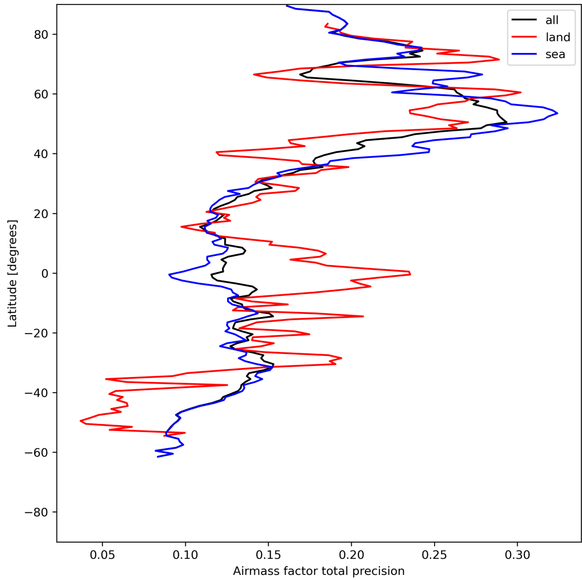
Figure 27: Zonal average of “Airmass factor total precision” for 2024-06-15 to 2024-06-17.
