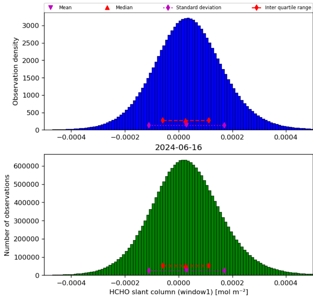
Figure 38: Histogram of “HCHO slant column (window1)” for 2024-06-15 to 2024-06-17
