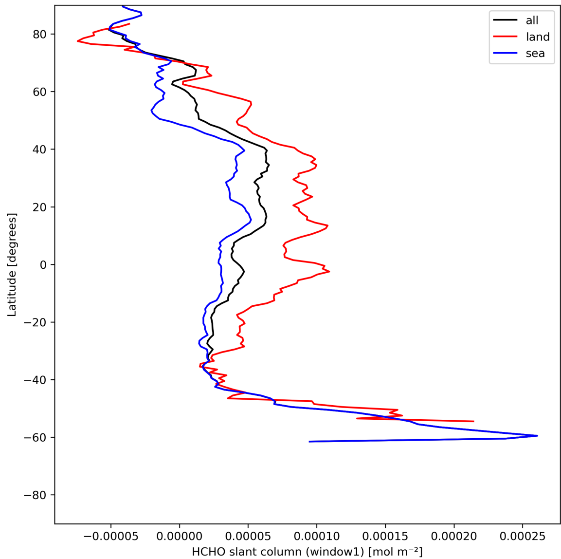
Figure 24: Zonal average of “HCHO slant column (window1)” for 2024-06-15 to 2024-06-17.
