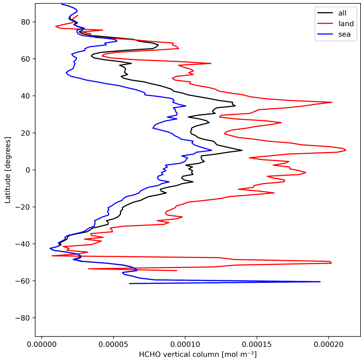
Figure 21: Zonal average of “HCHO vertical column” for 2024-06-15 to 2024-06-17.
