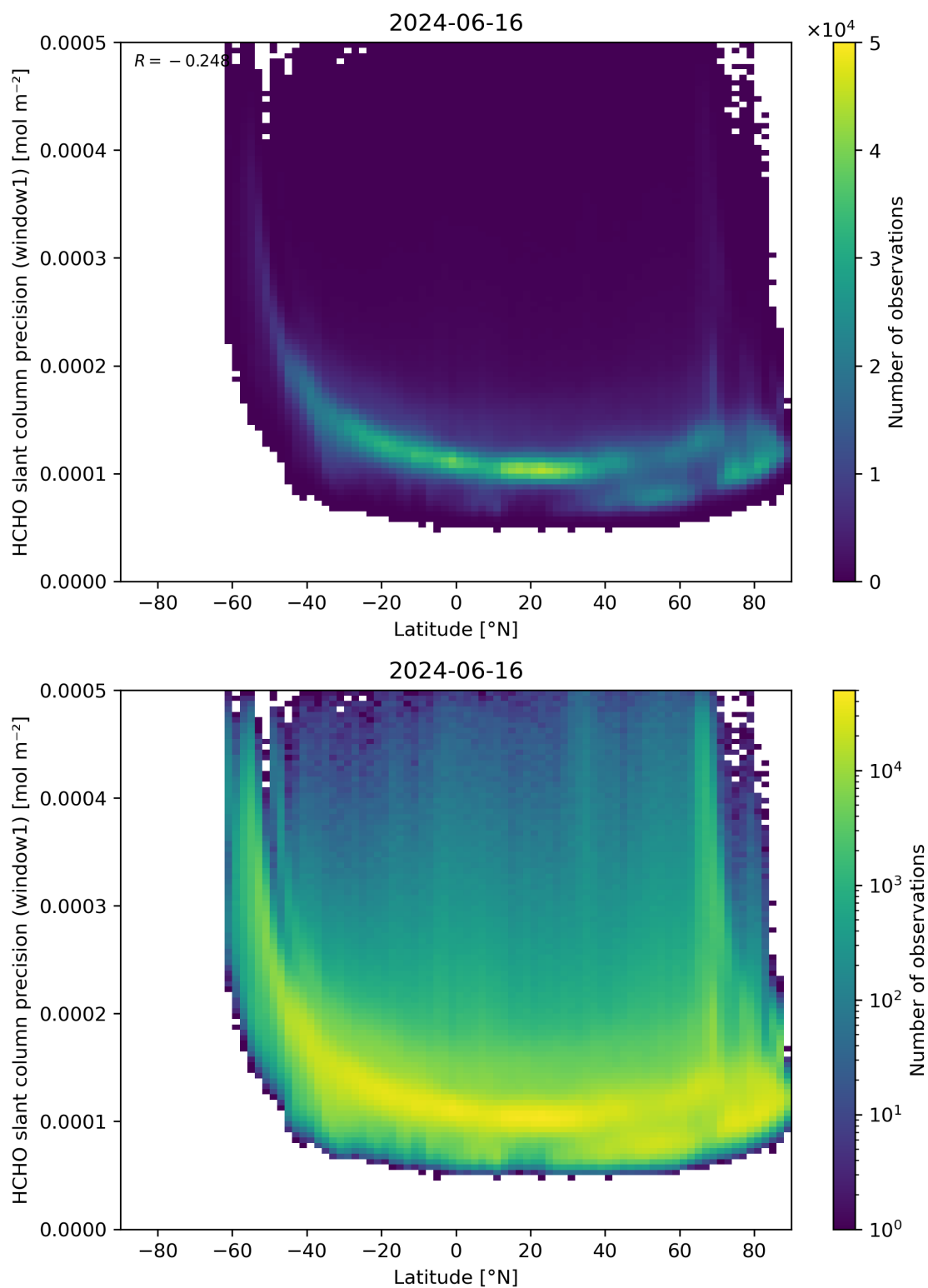
Figure 160: Scatter density plot of “Latitude” against “HCHO slant column precision (window1)” for 2024-06-15 to 2024-06-17.
