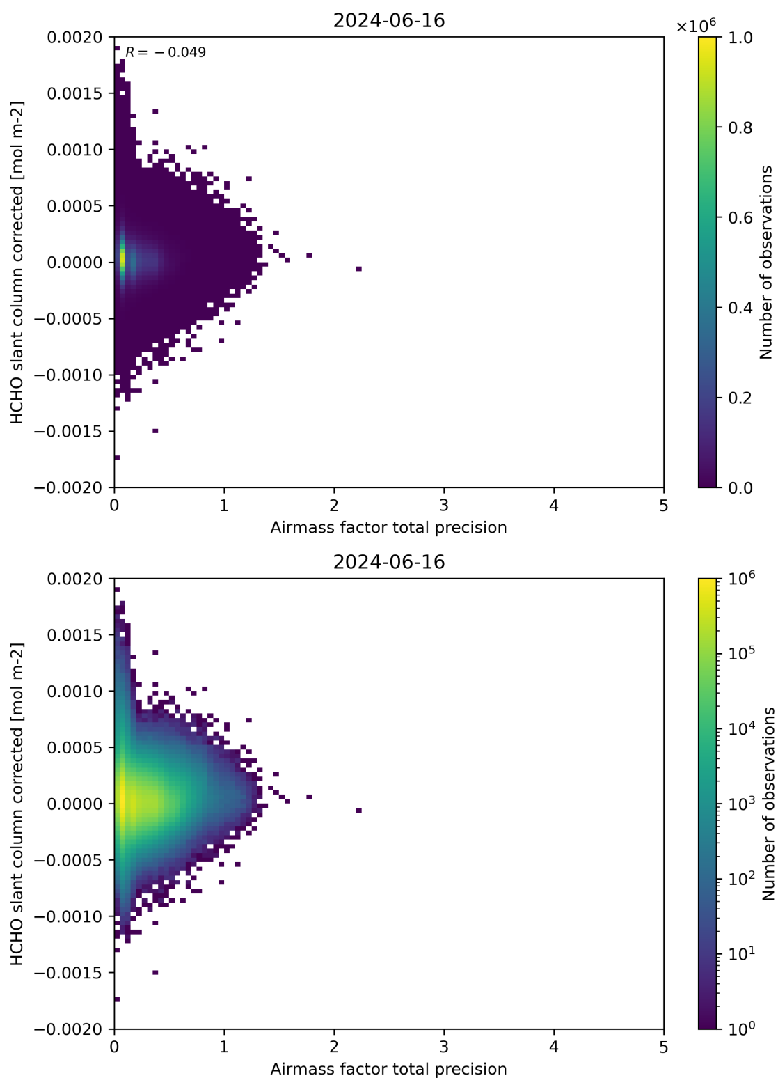
Figure 109: Scatter density plot of “Airmass factor total precision” against “HCHO slant column corrected” for 2024-06-15 to 2024-06-17.
