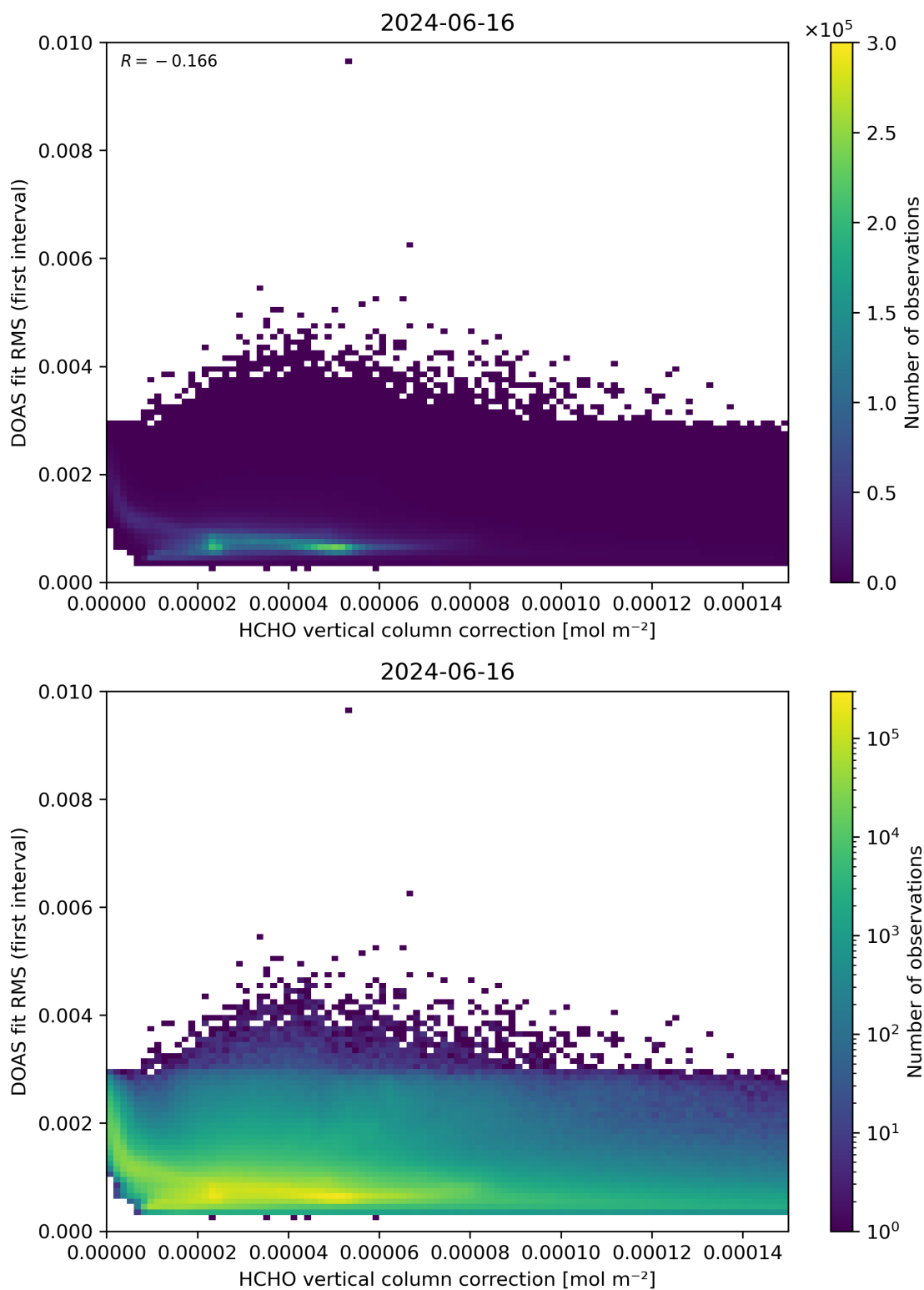
Figure 112: Scatter density plot of “HCHO vertical column correction” against “DOAS fit RMS (first interval)” for 2024-06-15 to 2024-06-17.
