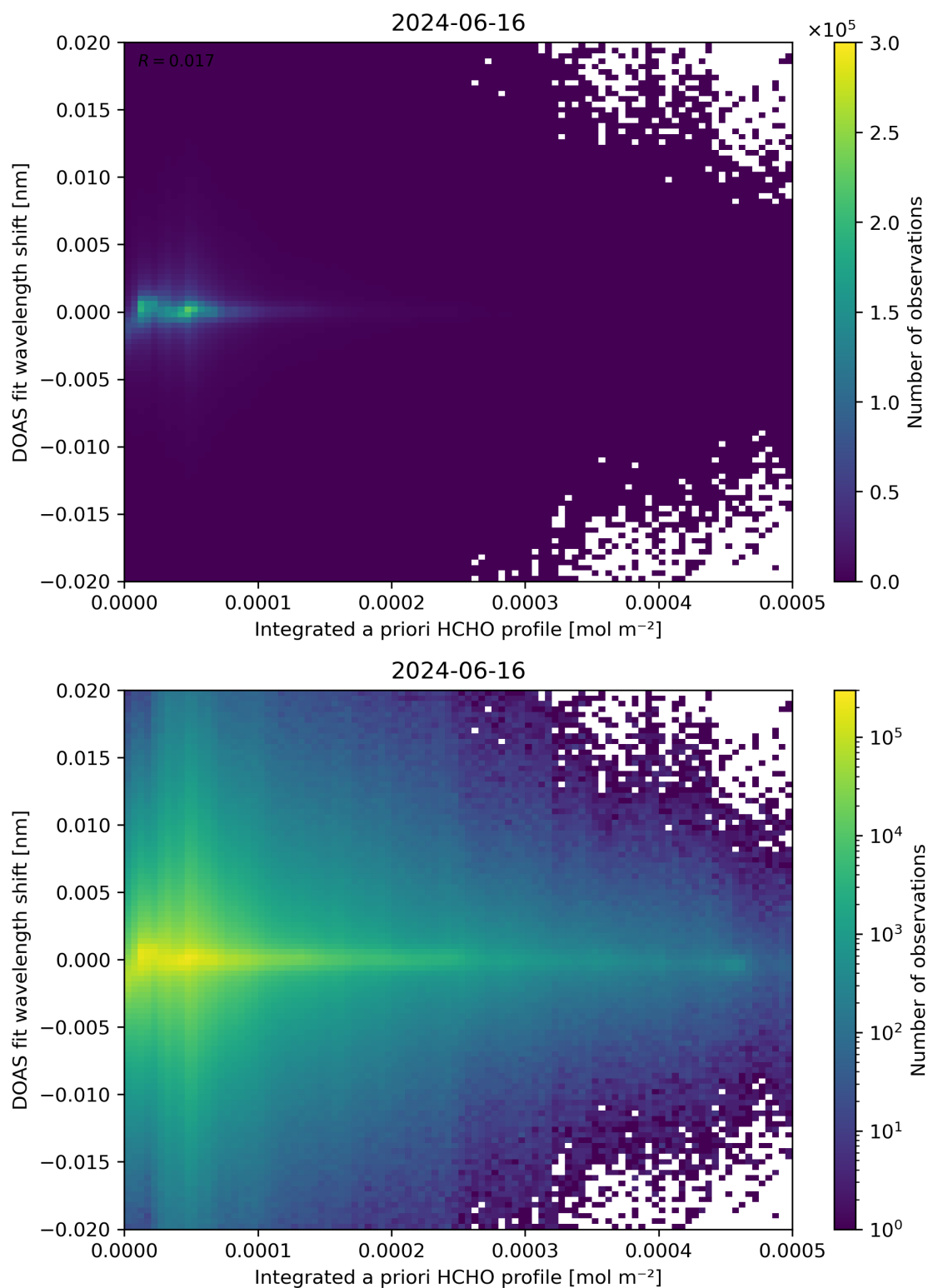
Figure 149: Scatter density plot of “Integrated a priori HCHO profile” against “DOAS fit wavelength shift” for 2024-06-15 to 2024-06-17.
