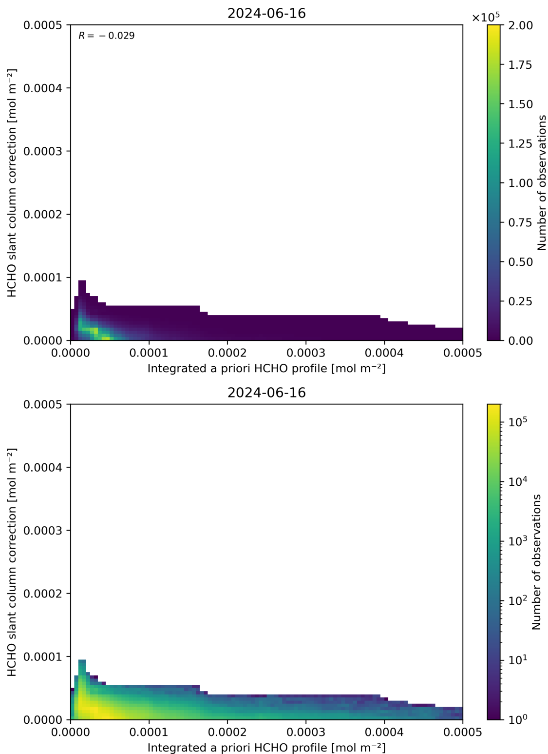
Figure 152: Scatter density plot of “Integrated a priori HCHO profile” against “HCHO slant column correction” for 2024-06-15 to 2024-06-17.
