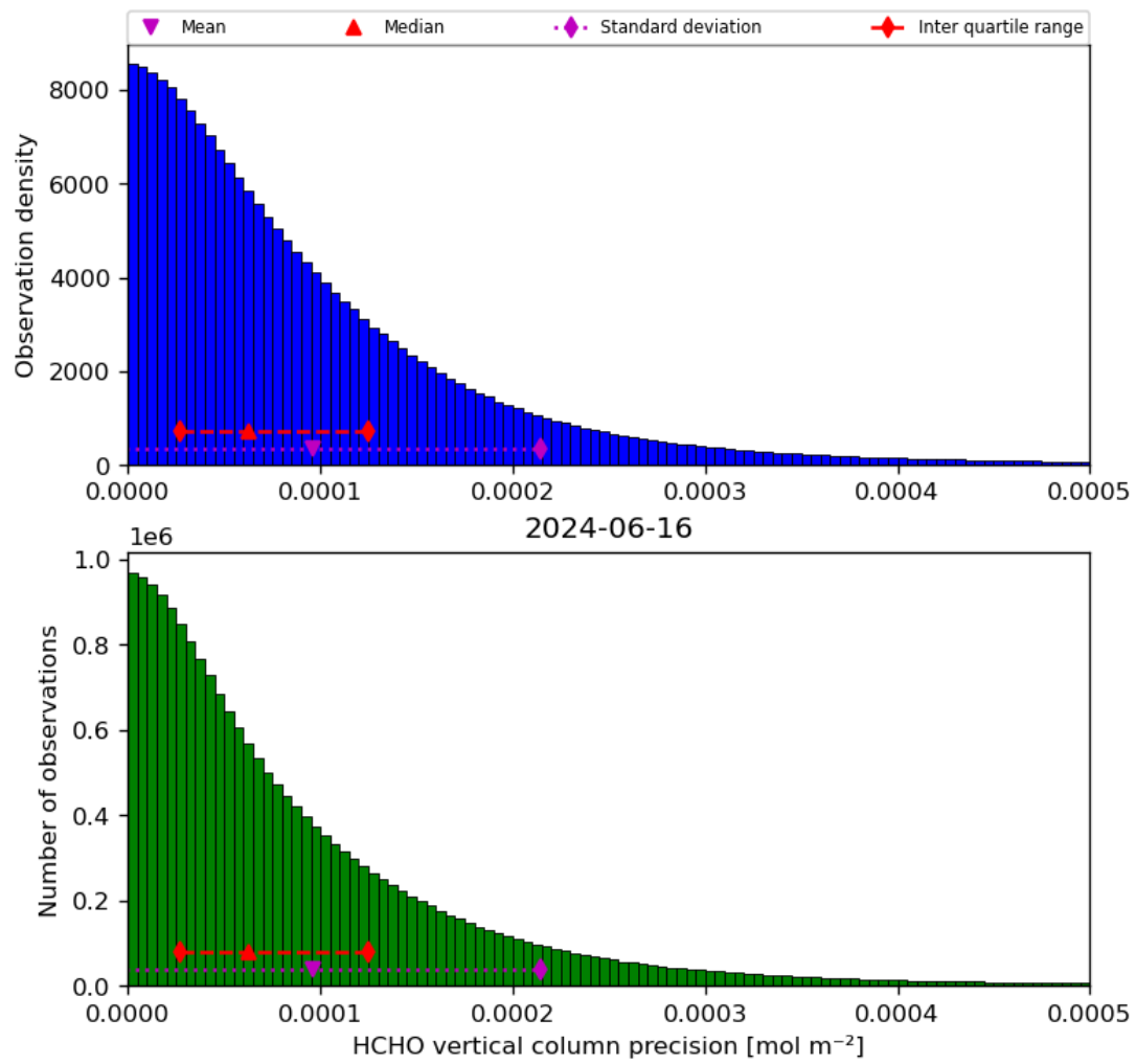
Figure 36: Histogram of “HCHO vertical column precision” for 2024-06-15 to 2024-06-17
