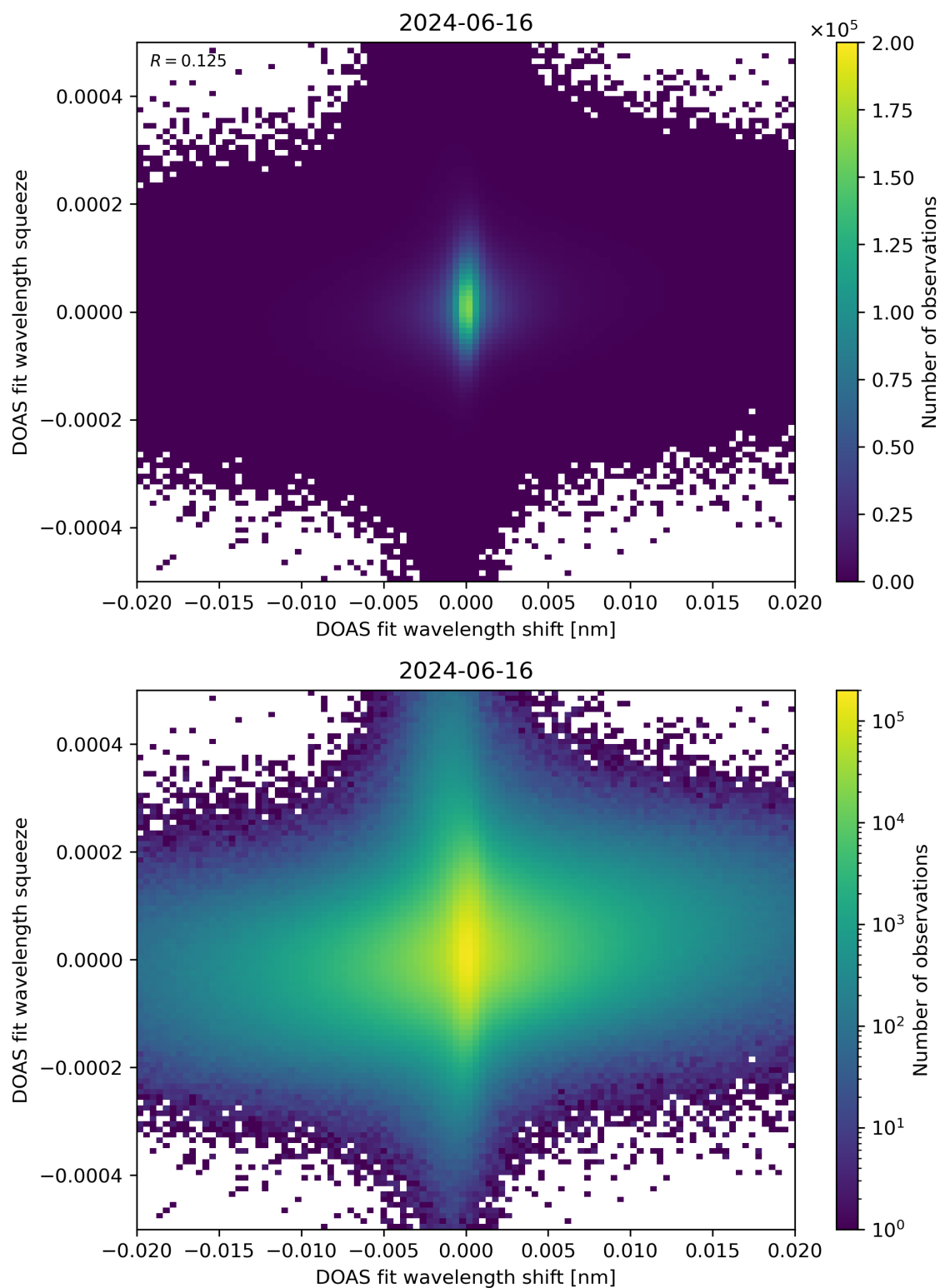
Figure 65: Scatter density plot of “DOAS fit wavelength shift” against “DOAS fit wavelength squeeze” for 2024-06-15 to 2024-06-17.
