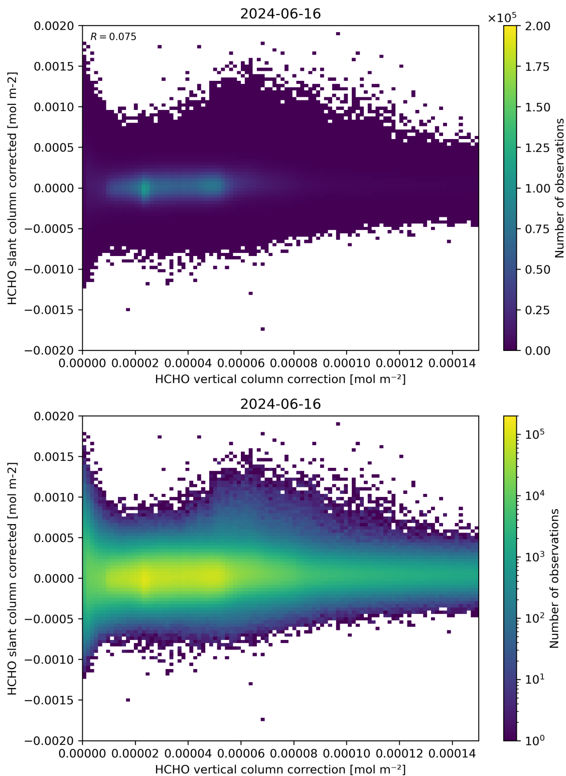
Figure 116: Scatter density plot of “HCHO vertical column correction” against “HCHO slant column corrected” for 2024-06-15 to 2024-06-17.
