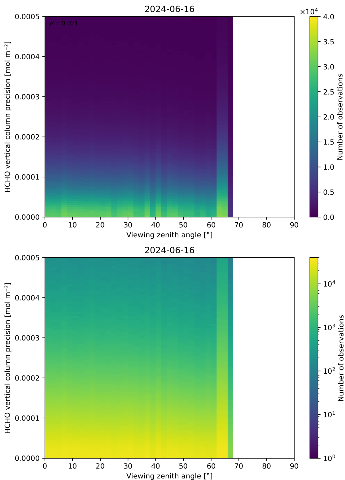
Figure 194: Scatter density plot of “Viewing zenith angle” against “HCHO vertical column precision” for 2024-06-15 to 2024-06-17.
