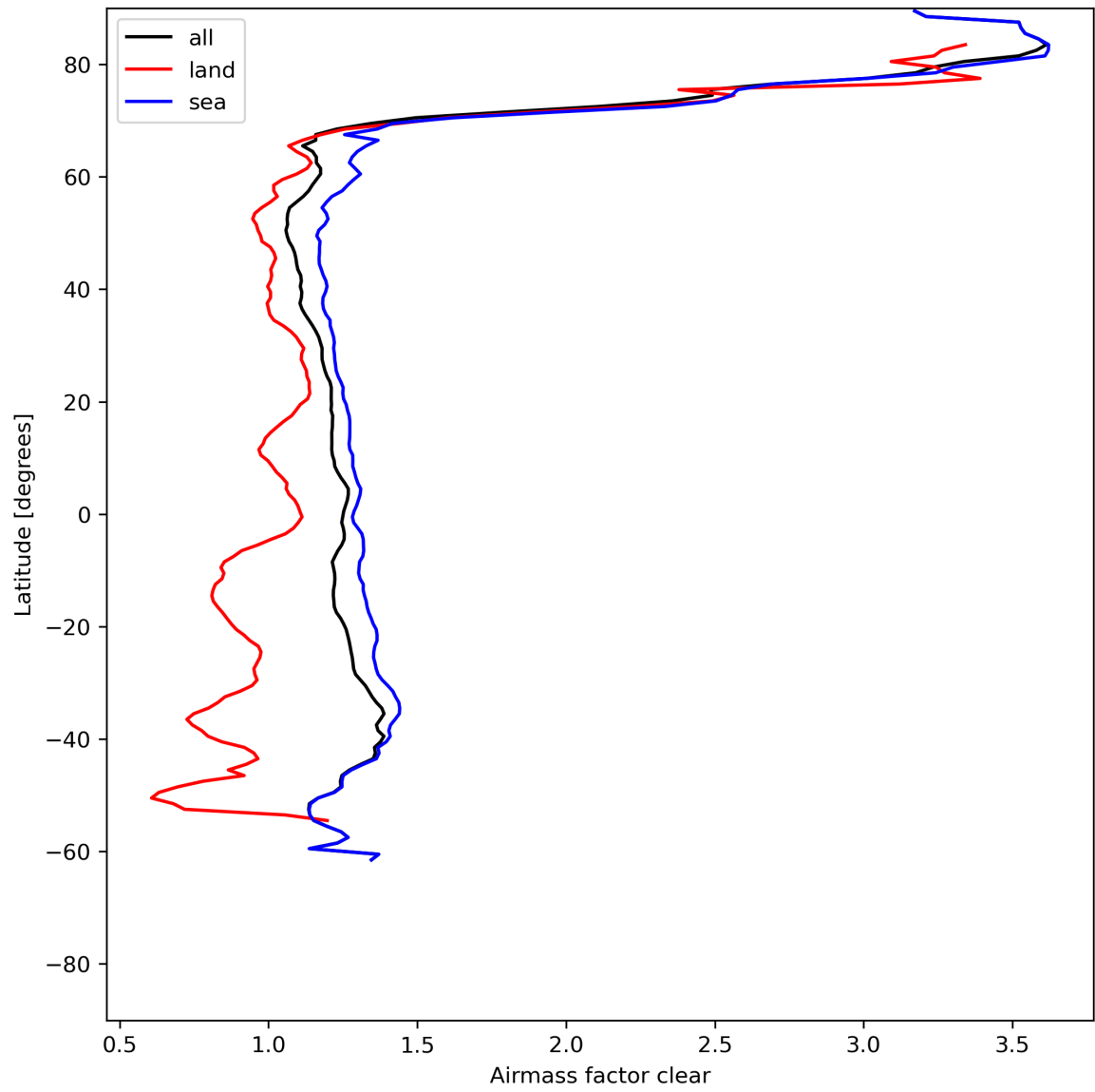
Figure 28: Zonal average of “Airmass factor clear” for 2024-06-15 to 2024-06-17.
