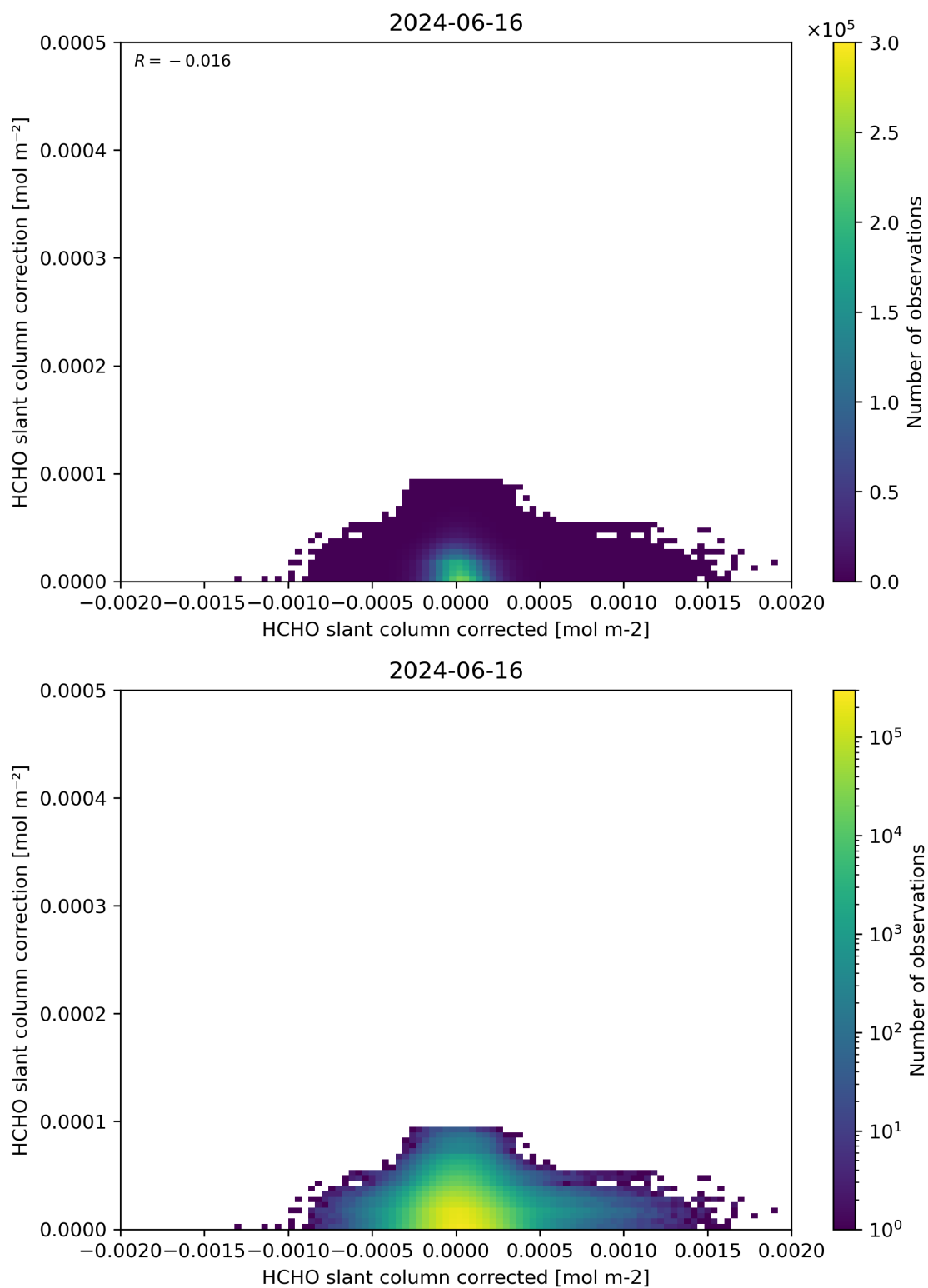
Figure 77: Scatter density plot of “HCHO slant column corrected” against “HCHO slant column correction” for 2024-06-15 to 2024-06-17.
