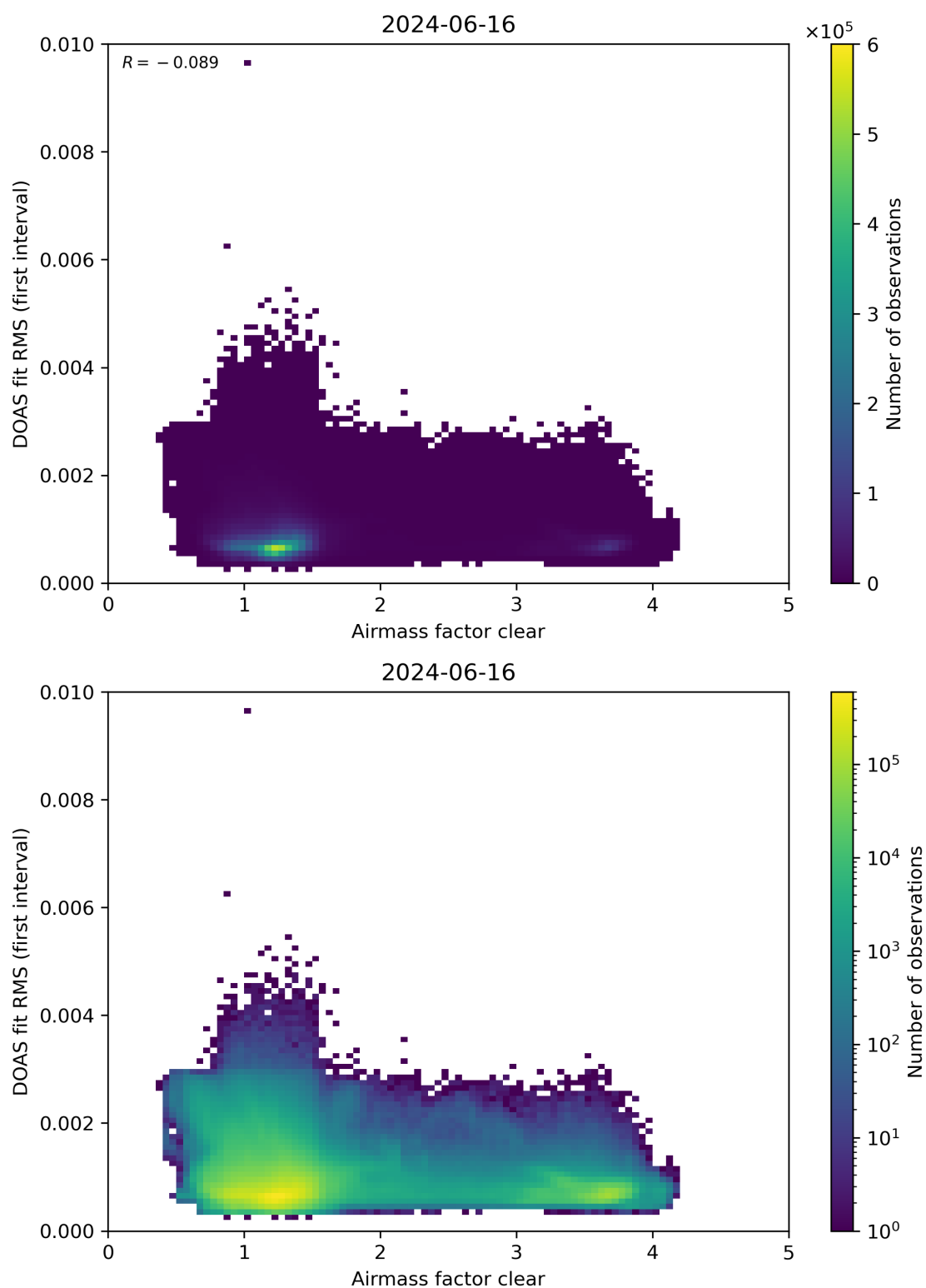
Figure 71: Scatter density plot of “Airmass factor clear” against “DOAS fit RMS (first interval)” for 2024-06-15 to 2024-06-17.
