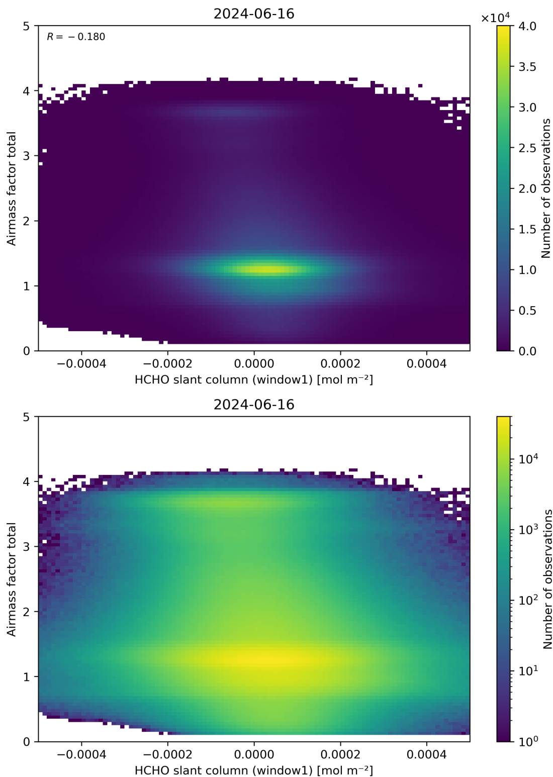
Figure 85: Scatter density plot of “HCHO slant column (window1)” against “Airmass factor total” for 2024-06-15 to 2024-06-17.
