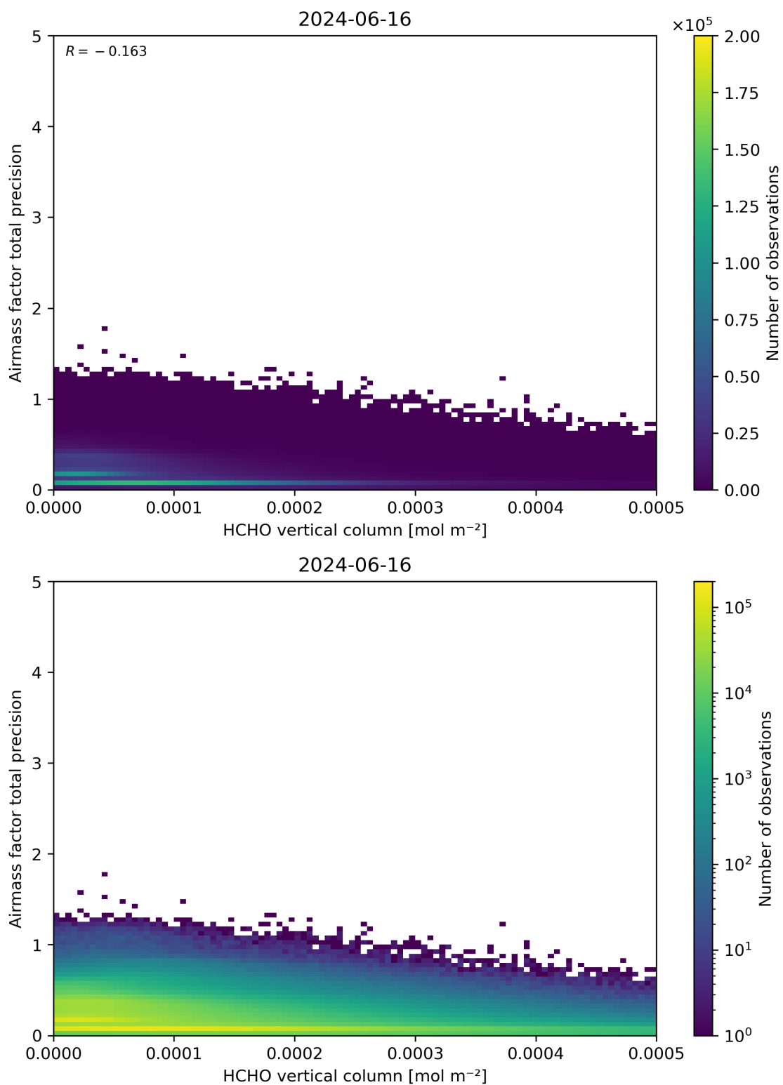
Figure 132: Scatter density plot of “HCHO vertical column” against “Airmass factor total precision” for 2024-06-15 to 2024-06-17.
