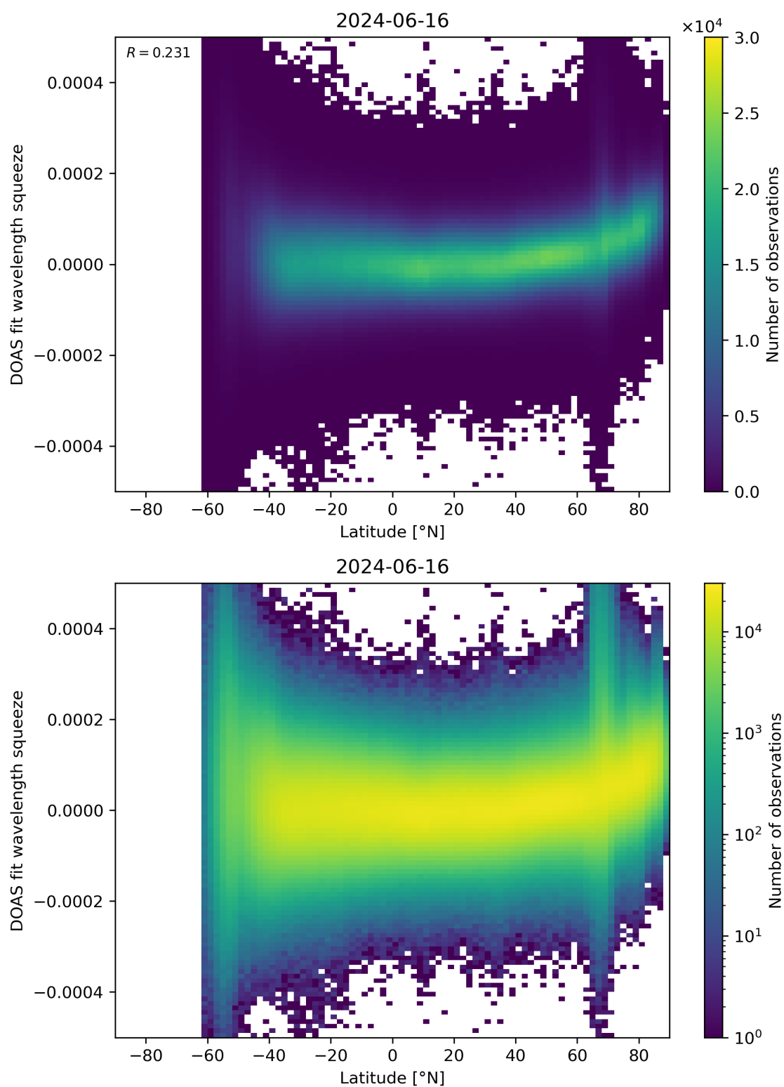
Figure 155: Scatter density plot of “Latitude” against “DOAS fit wavelength squeeze” for 2024-06-15 to 2024-06-17.
