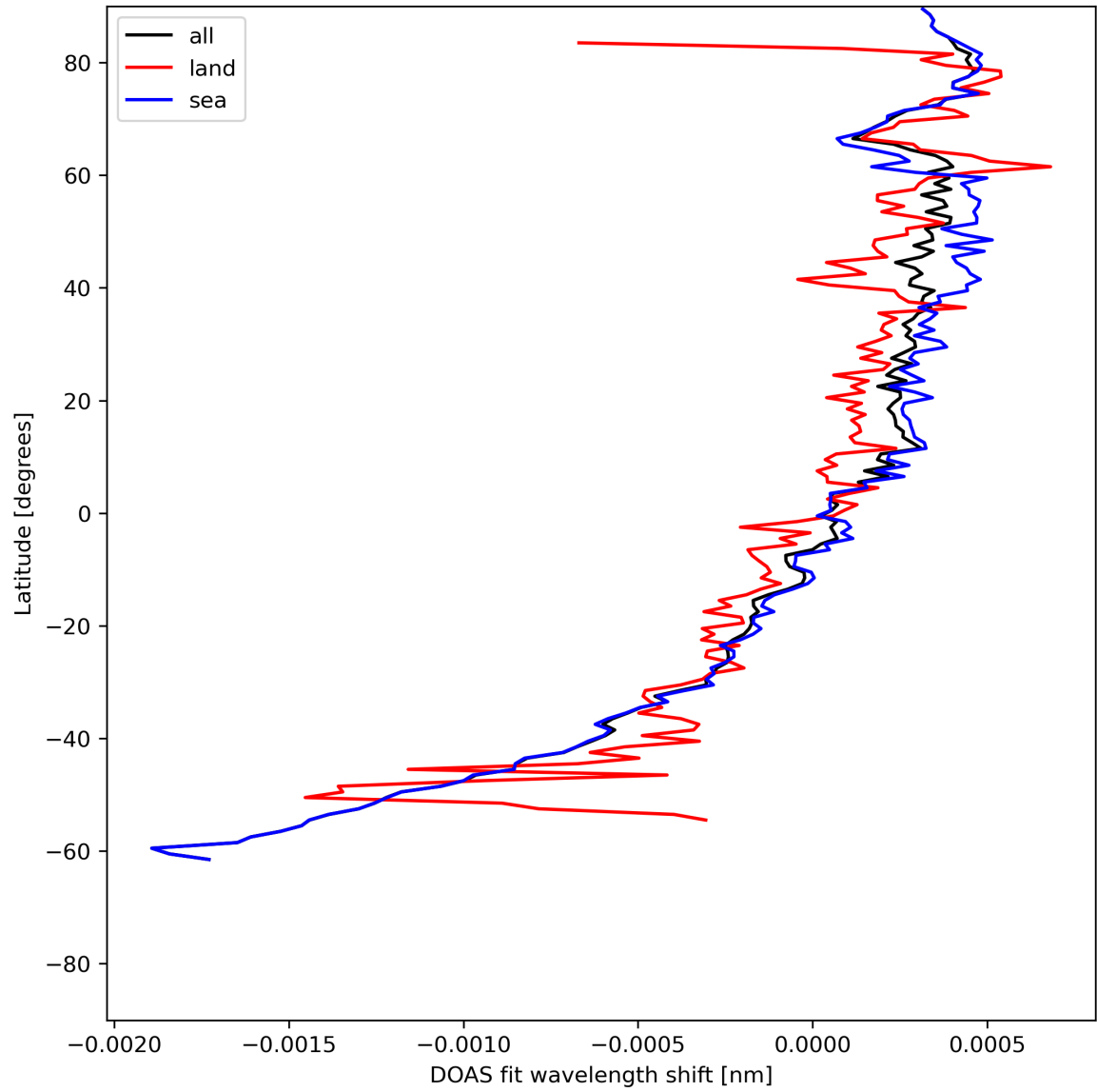
Figure 30: Zonal average of “DOAS fit wavelength shift” for 2024-06-15 to 2024-06-17.
