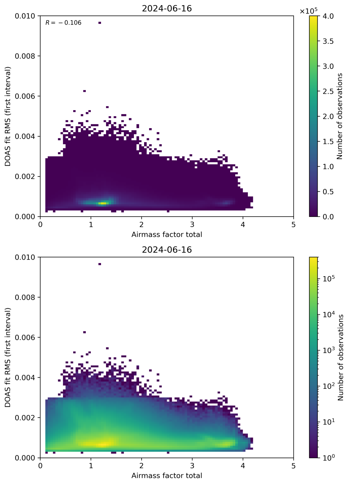
Figure 97: Scatter density plot of “Airmass factor total” against “DOAS fit RMS (first interval)” for 2024-06-15 to 2024-06-17.
