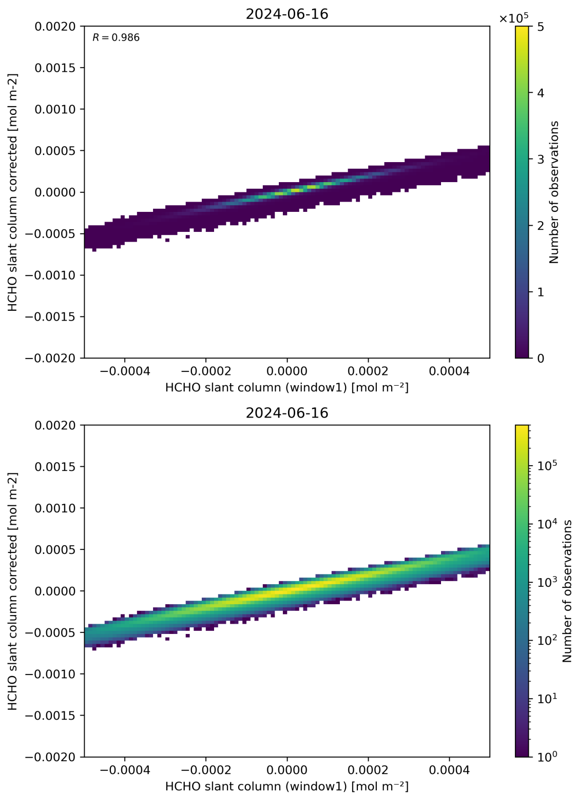
Figure 82: Scatter density plot of “HCHO slant column (window1)” against “HCHO slant column corrected” for 2024-06-15 to 2024-06-17.
