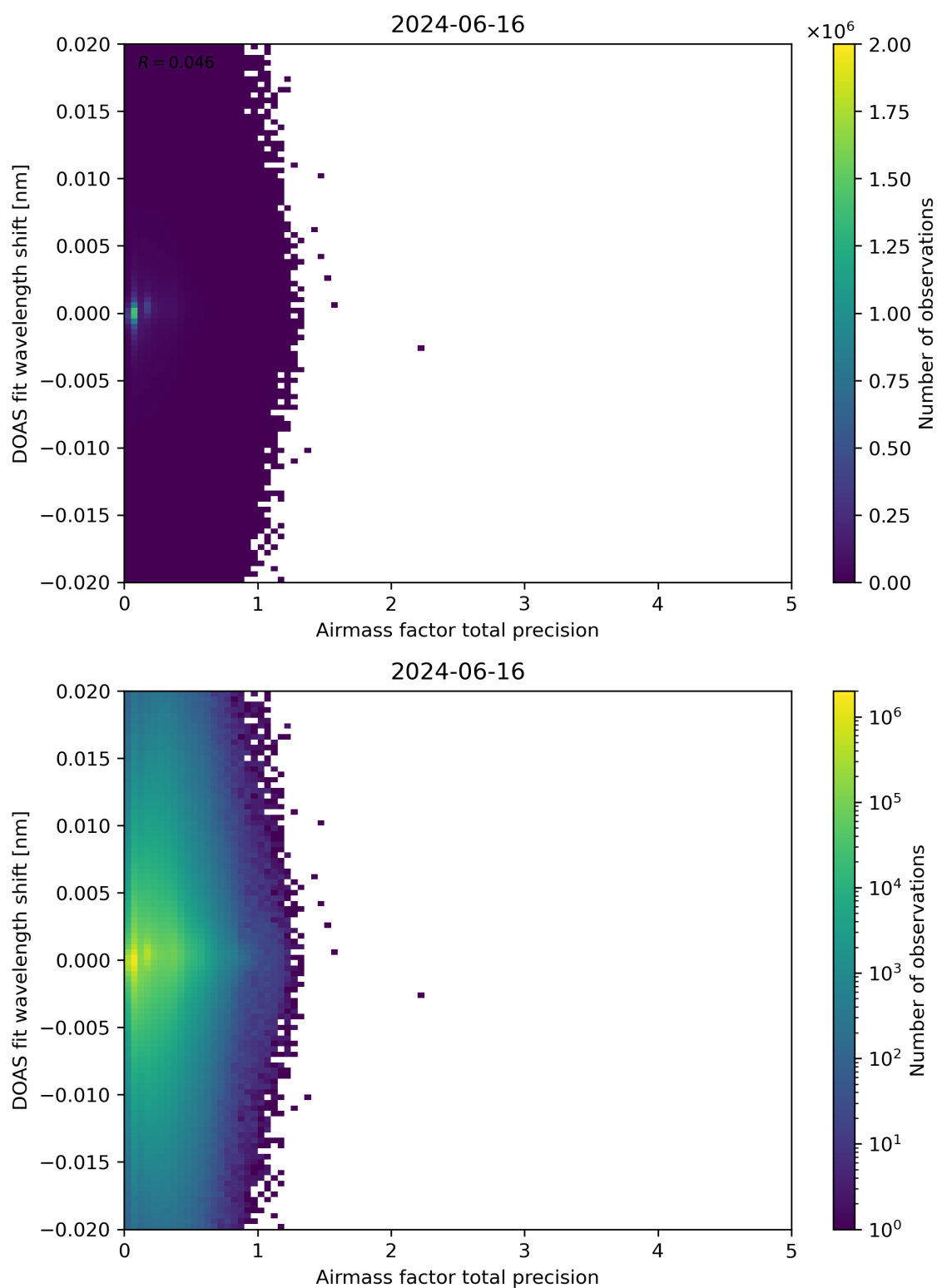
Figure 106: Scatter density plot of “Airmass factor total precision” against “DOAS fit wavelength shift” for 2024-06-15 to 2024-06-17.
