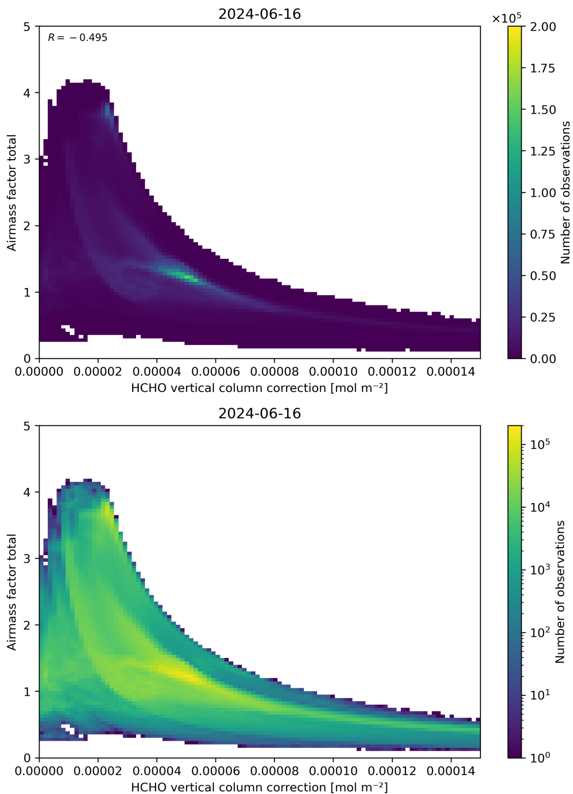
Figure 120: Scatter density plot of “HCHO vertical column correction” against “Airmass factor total” for 2024-06-15 to 2024-06-17.
