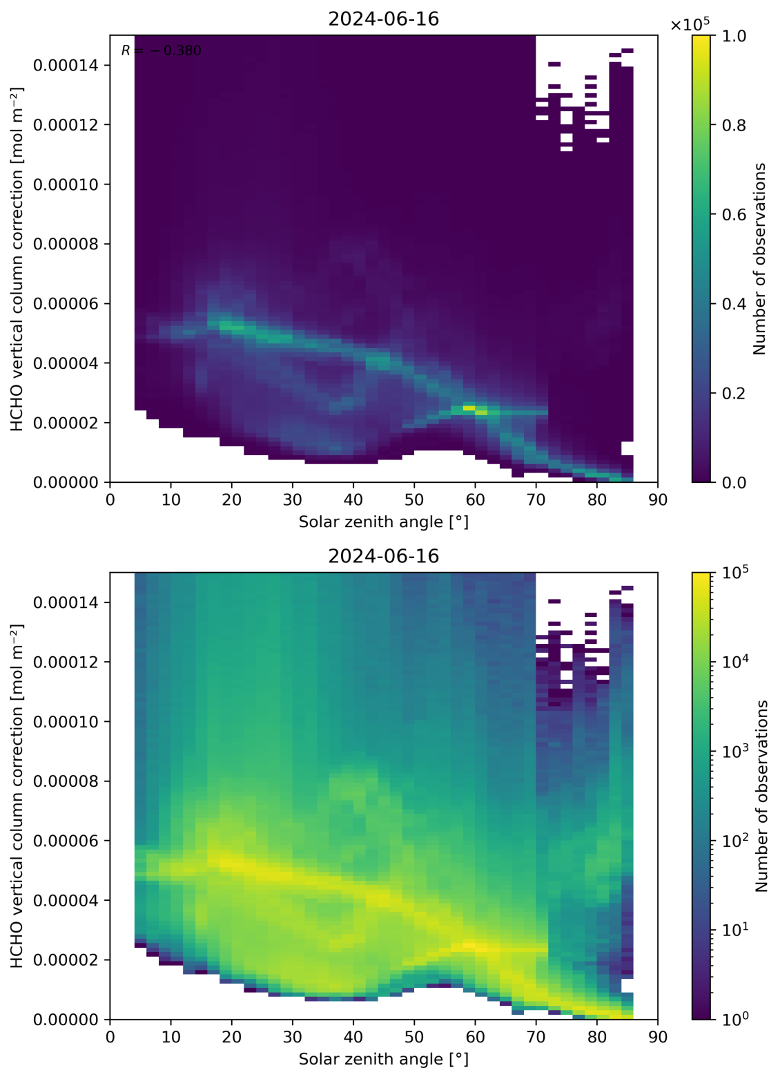
Figure 178: Scatter density plot of “Solar zenith angle” against “HCHO vertical column correction” for 2024-06-15 to 2024-06-17.
