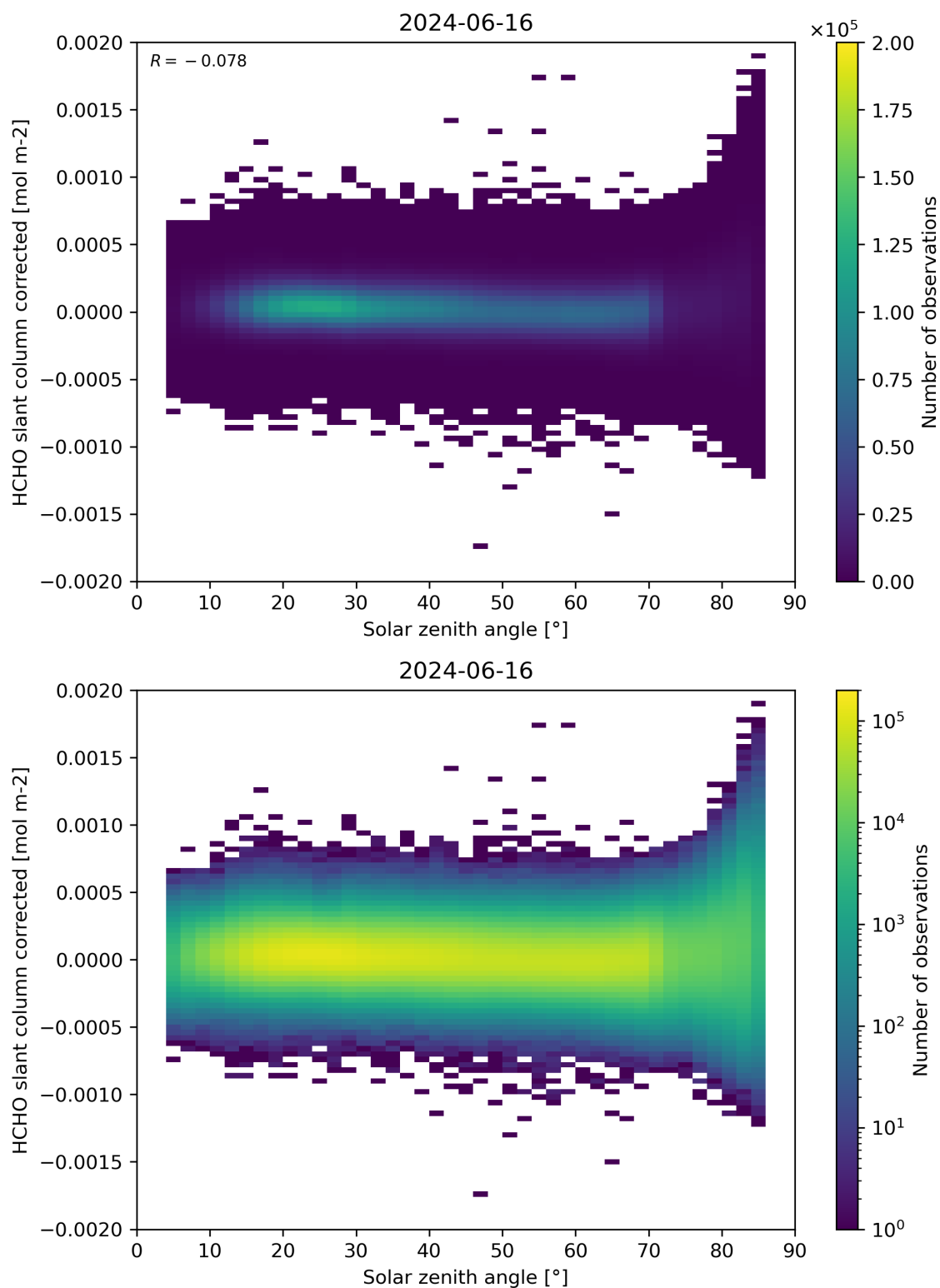
Figure 171: Scatter density plot of “Solar zenith angle” against “HCHO slant column corrected” for 2024-06-15 to 2024-06-17.
