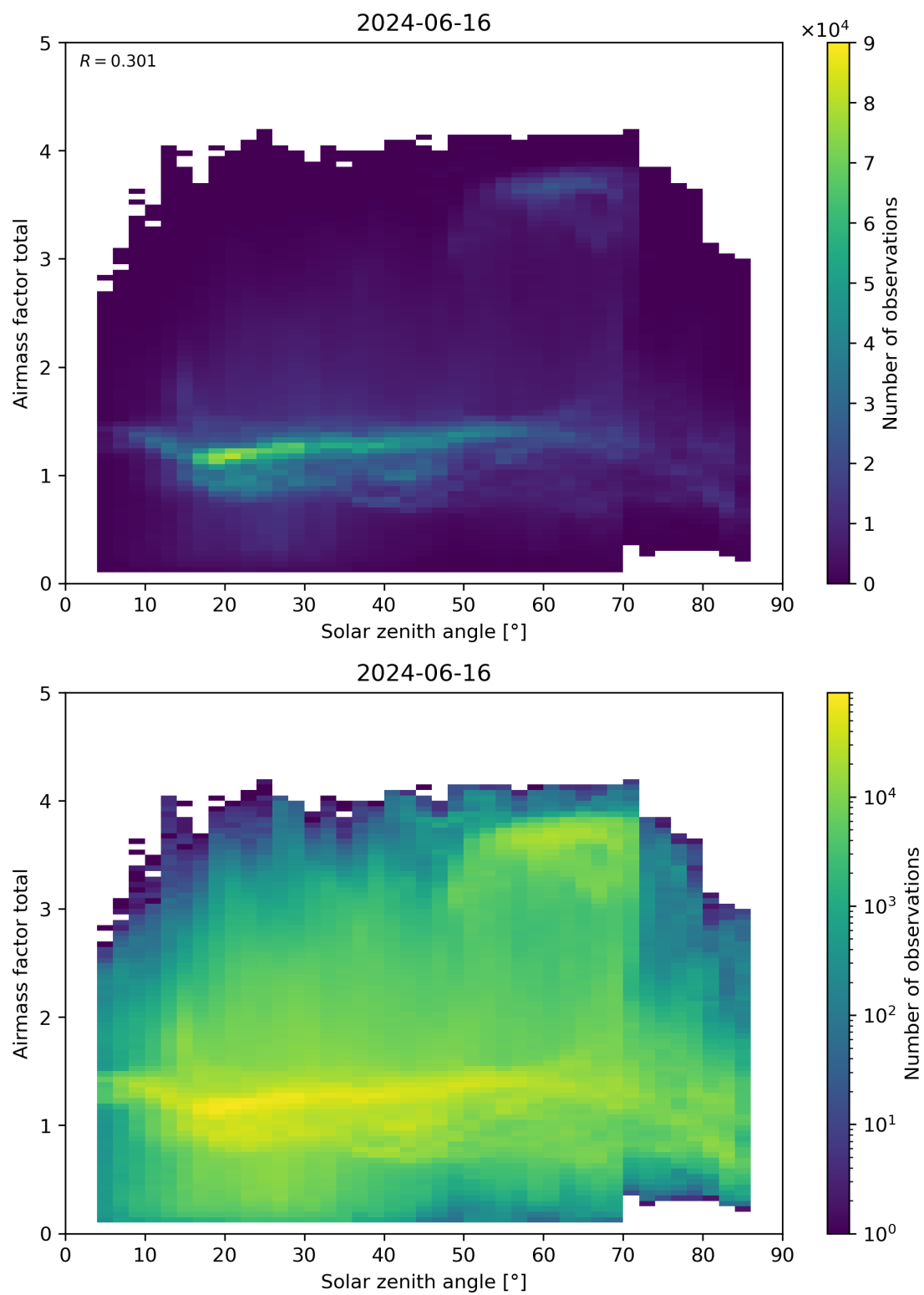
Figure 175: Scatter density plot of “Solar zenith angle” against “Airmass factor total” for 2024-06-15 to 2024-06-17.
