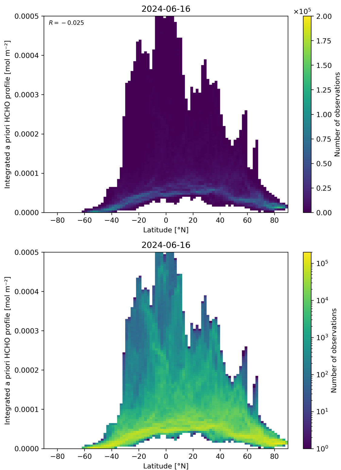
Figure 166: Scatter density plot of “Latitude” against “Integrated a priori HCHO profile” for 2024-06-15 to 2024-06-17.
