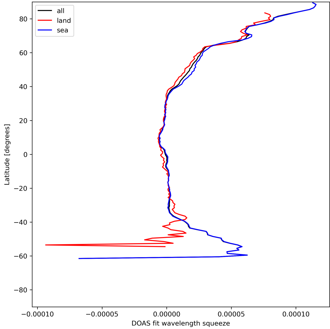
Figure 31: Zonal average of “DOAS fit wavelength squeeze” for 2024-06-15 to 2024-06-17.
