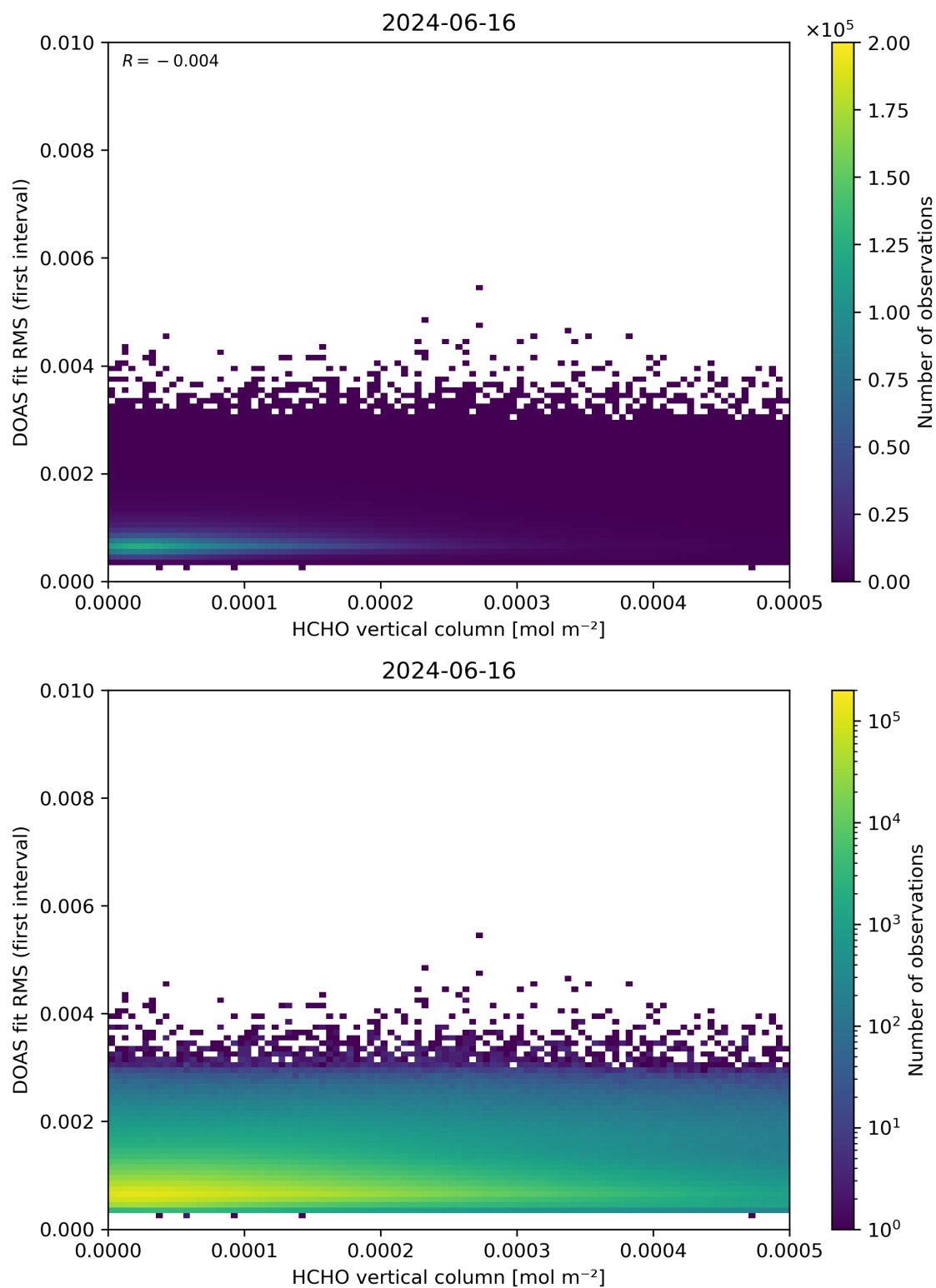
Figure 123: Scatter density plot of “HCHO vertical column” against “DOAS fit RMS (first interval)” for 2024-06-15 to 2024-06-17.
