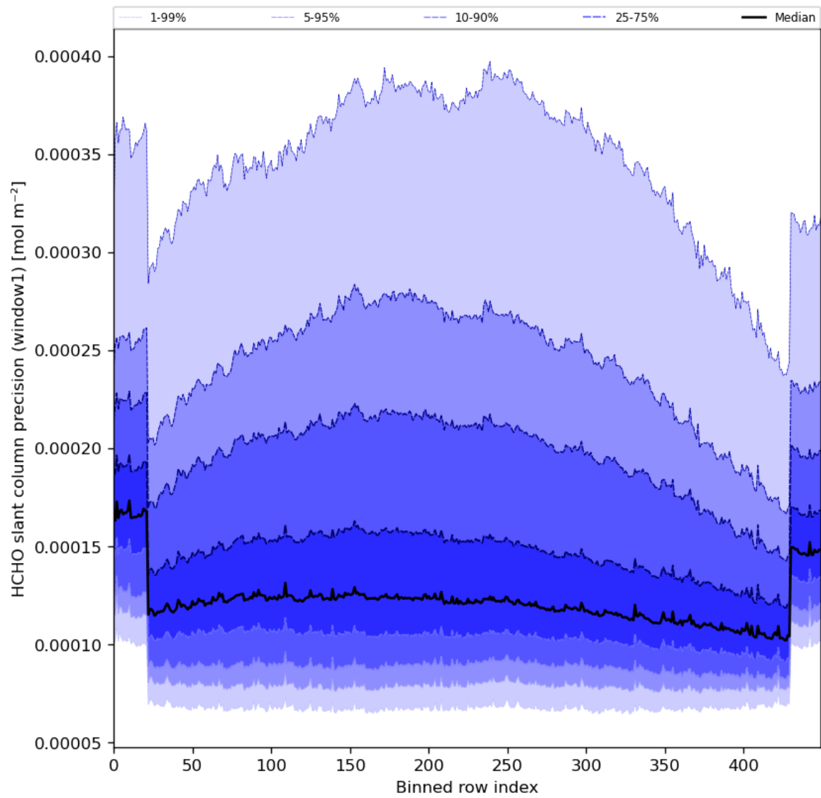
Figure 53: Along track statistics of “HCHO slant column precision (window1)” for 2024-06-15 to 2024-06-17
