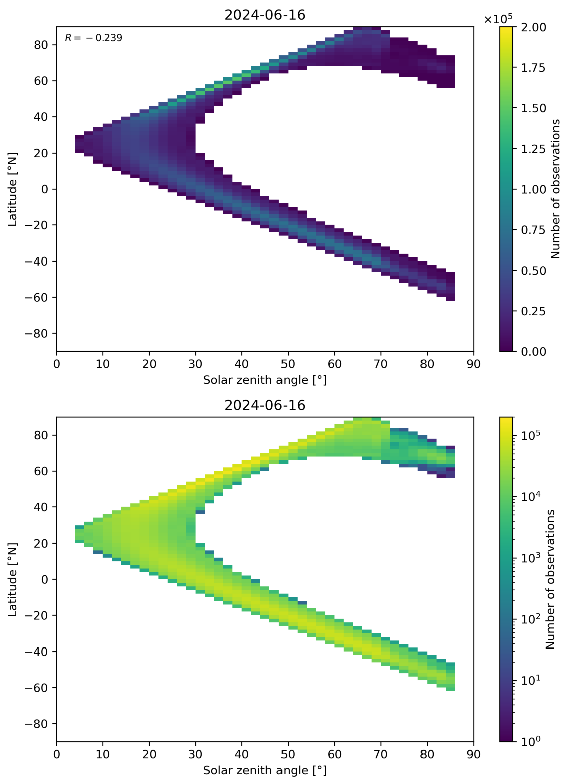
Figure 181: Scatter density plot of “Solar zenith angle” against “Latitude” for 2024-06-15 to 2024-06-17.
