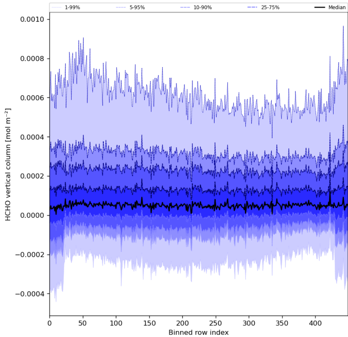
Figure 49: Along track statistics of “HCHO vertical column” for 2024-06-15 to 2024-06-17
