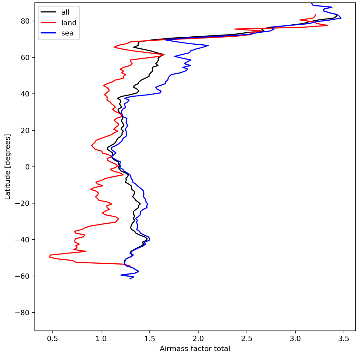
Figure 26: Zonal average of “Airmass factor total” for 2024-06-15 to 2024-06-17.
