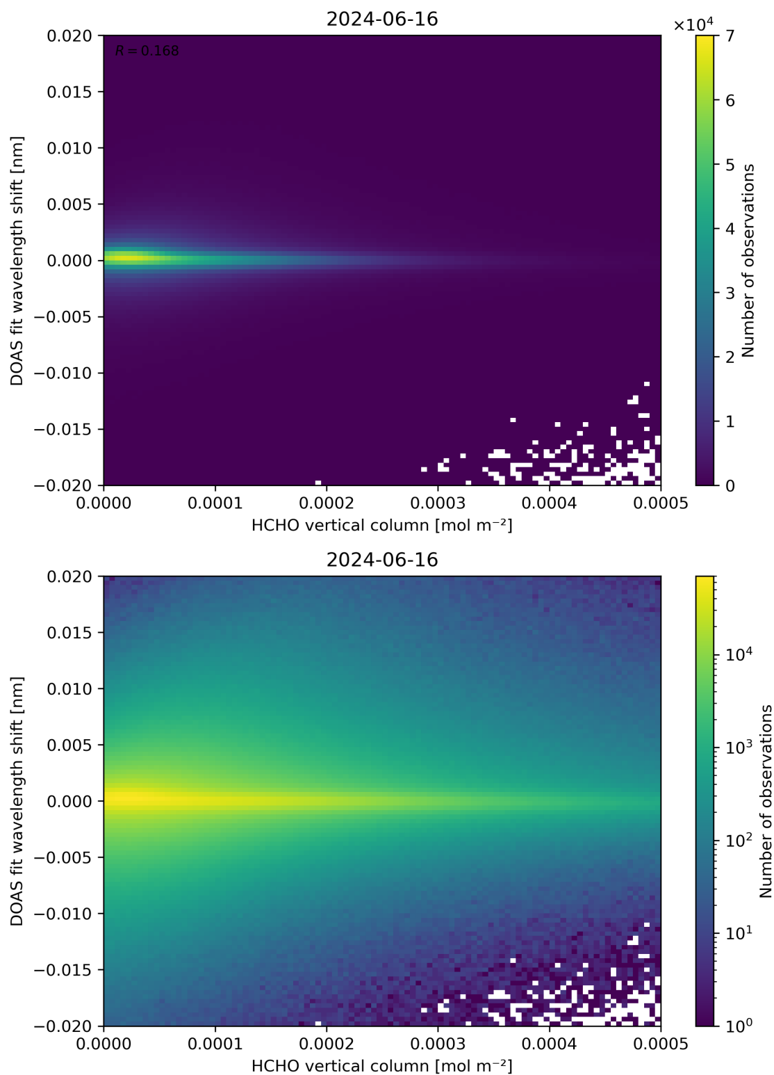
Figure 124: Scatter density plot of “HCHO vertical column” against “DOAS fit wavelength shift” for 2024-06-15 to 2024-06-17.
