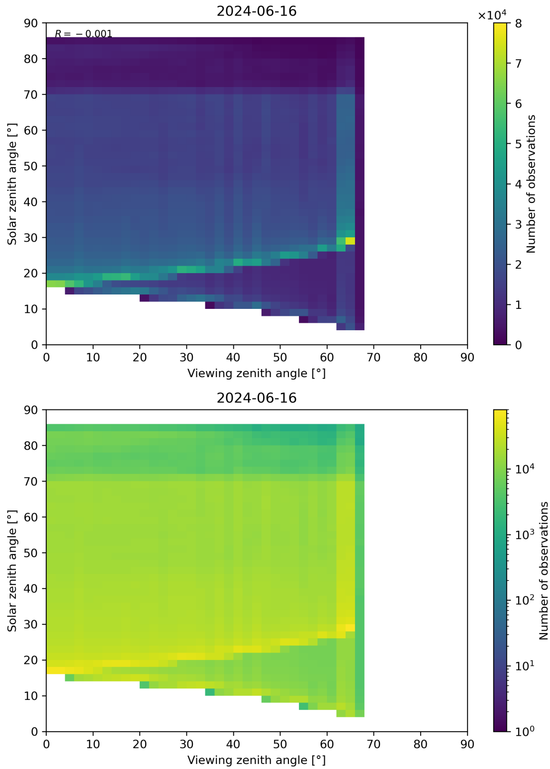
Figure 197: Scatter density plot of “Viewing zenith angle” against “Solar zenith angle” for 2024-06-15 to 2024-06-17.
