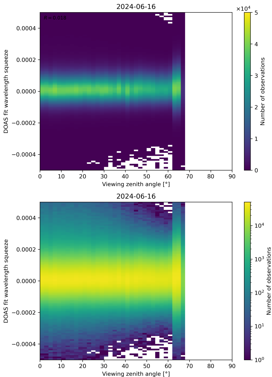
Figure 184: Scatter density plot of “Viewing zenith angle” against “DOAS fit wavelength squeeze” for 2024-06-15 to 2024-06-17.
