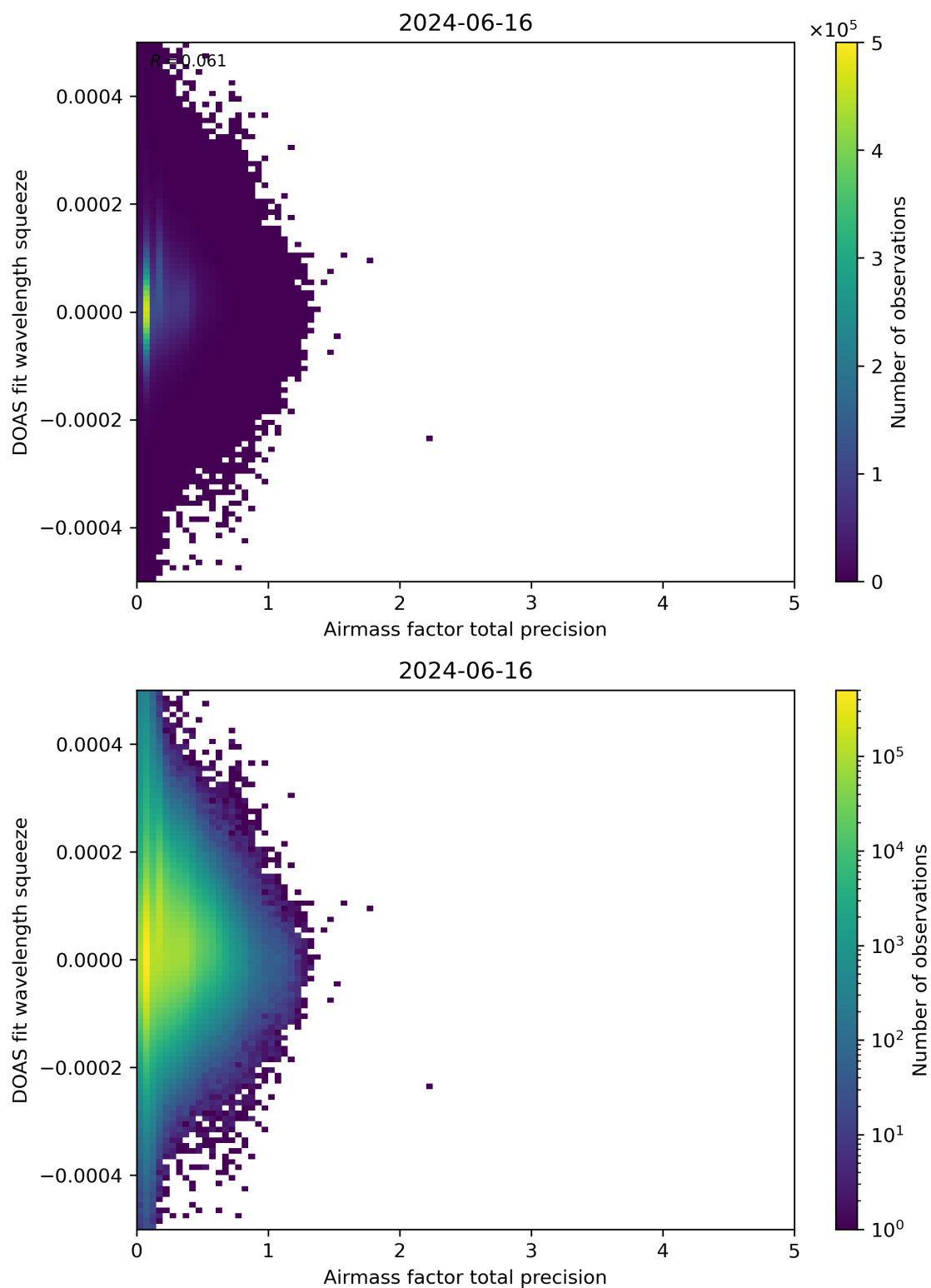
Figure 107: Scatter density plot of “Airmass factor total precision” against “DOAS fit wavelength squeeze” for 2024-06-15 to 2024-06-17.
