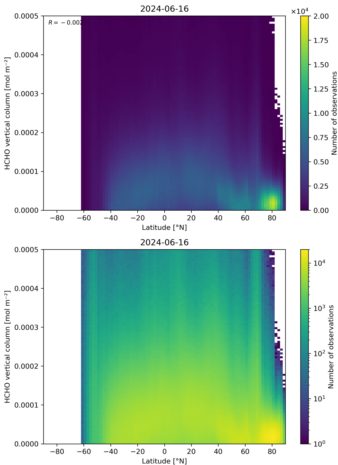
Figure 163: Scatter density plot of “Latitude” against “HCHO vertical column” for 2024-06-15 to 2024-06-17.
