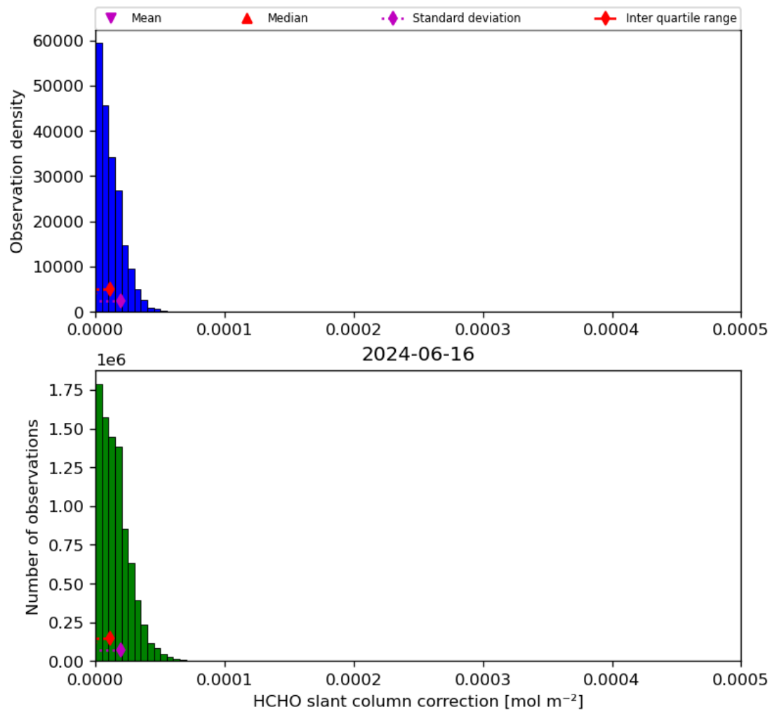
Figure 47: Histogram of “HCHO slant column correction” for 2024-06-15 to 2024-06-17
