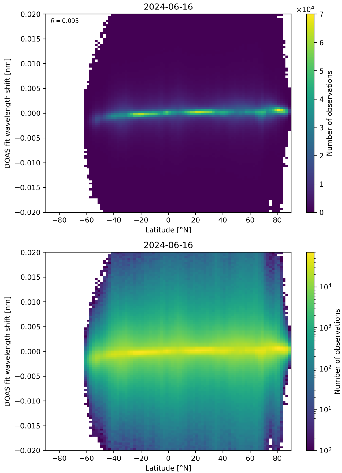
Figure 154: Scatter density plot of “Latitude” against “DOAS fit wavelength shift” for 2024-06-15 to 2024-06-17.
