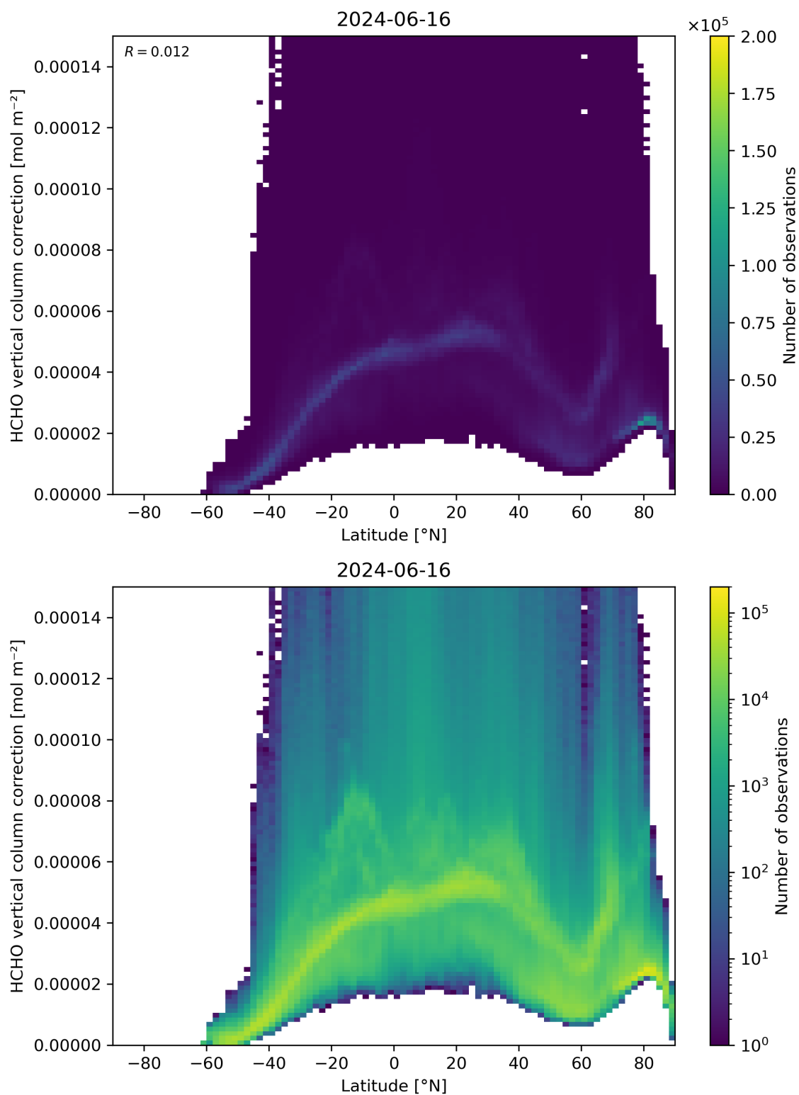
Figure 164: Scatter density plot of “Latitude” against “HCHO vertical column correction” for 2024-06-15 to 2024-06-17.
