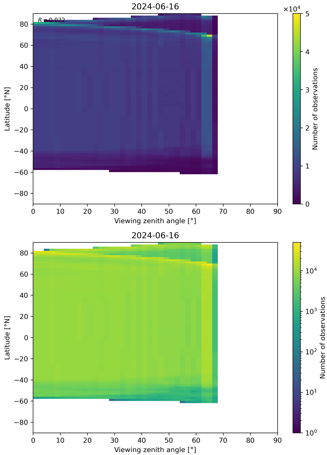
Figure 196: Scatter density plot of “Viewing zenith angle” against “Latitude” for 2024-06-15 to 2024-06-17.
