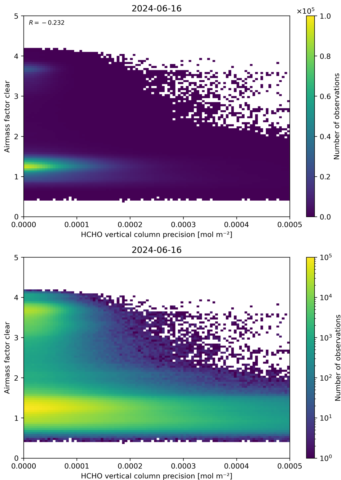
Figure 139: Scatter density plot of “HCHO vertical column precision” against “Airmass factor clear” for 2024-06-15 to 2024-06-17.
