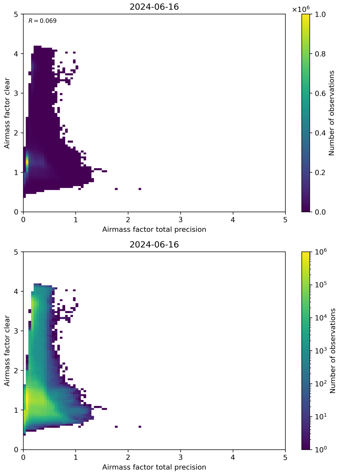
Figure 108: Scatter density plot of “Airmass factor total precision” against “Airmass factor clear” for 2024-06-15 to 2024-06-17.
