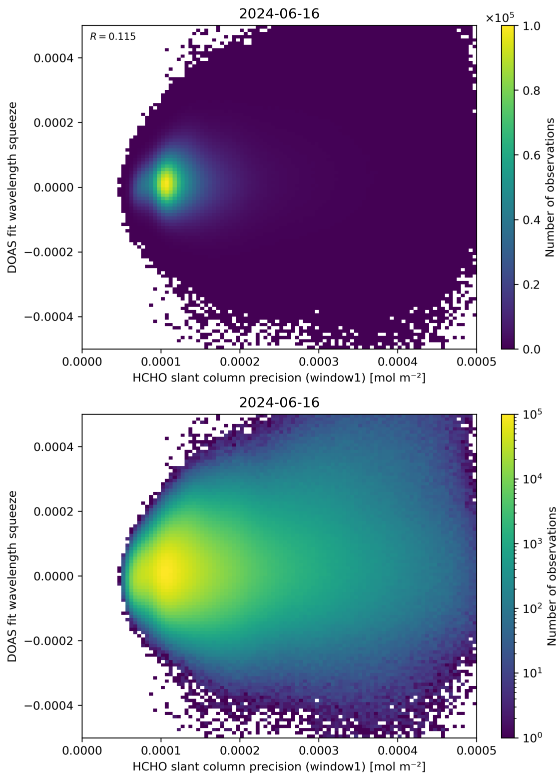
Figure 90: Scatter density plot of “HCHO slant column precision (window1)” against “DOAS fit wavelength squeeze” for 2024-06-15 to 2024-06-17.
