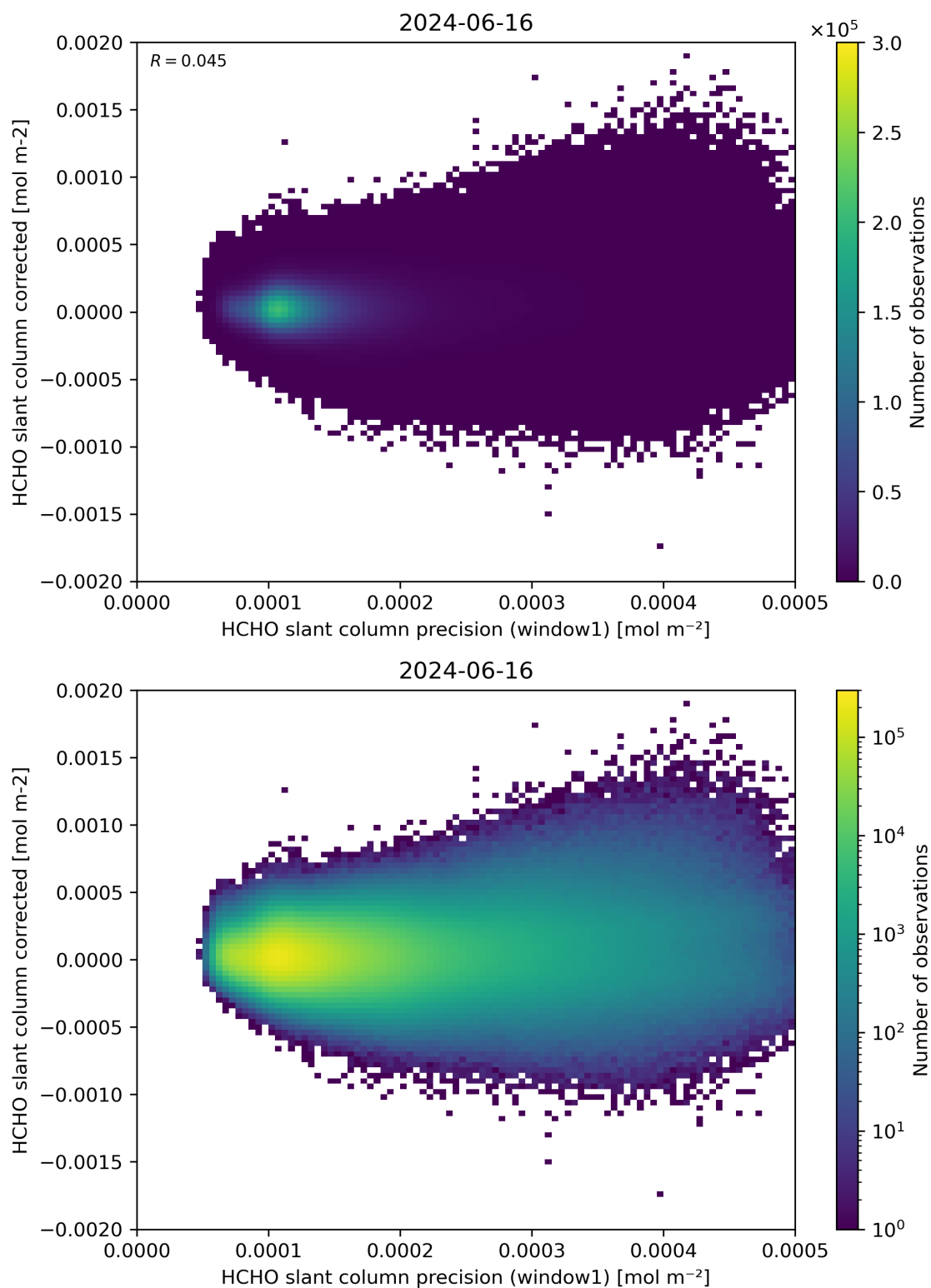
Figure 92: Scatter density plot of “HCHO slant column precision (window1)” against “HCHO slant column corrected” for 2024-06-15 to 2024-06-17.
