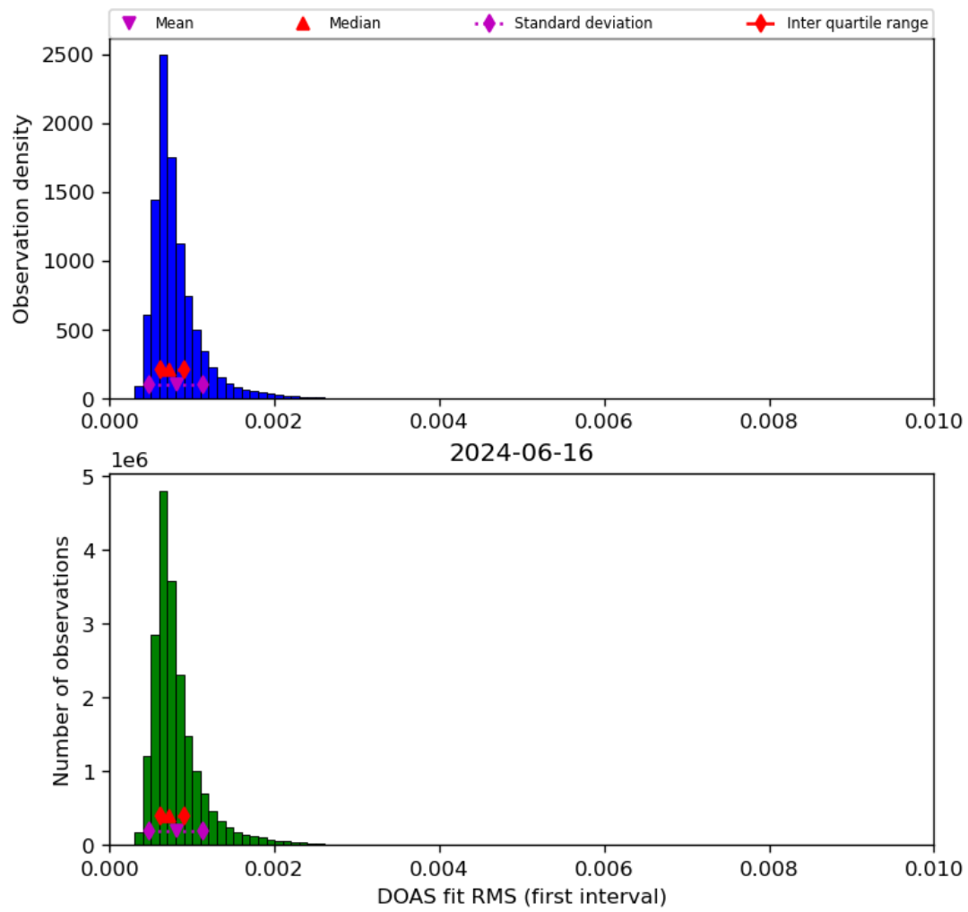
Figure 46: Histogram of “DOAS fit RMS (first interval)” for 2024-06-15 to 2024-06-17
