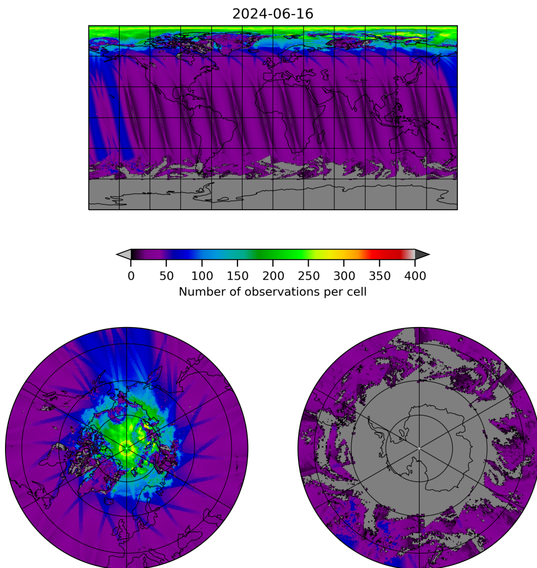
Figure 19: Map of the number of observations for 2024-06-15 to 2024-06-17
