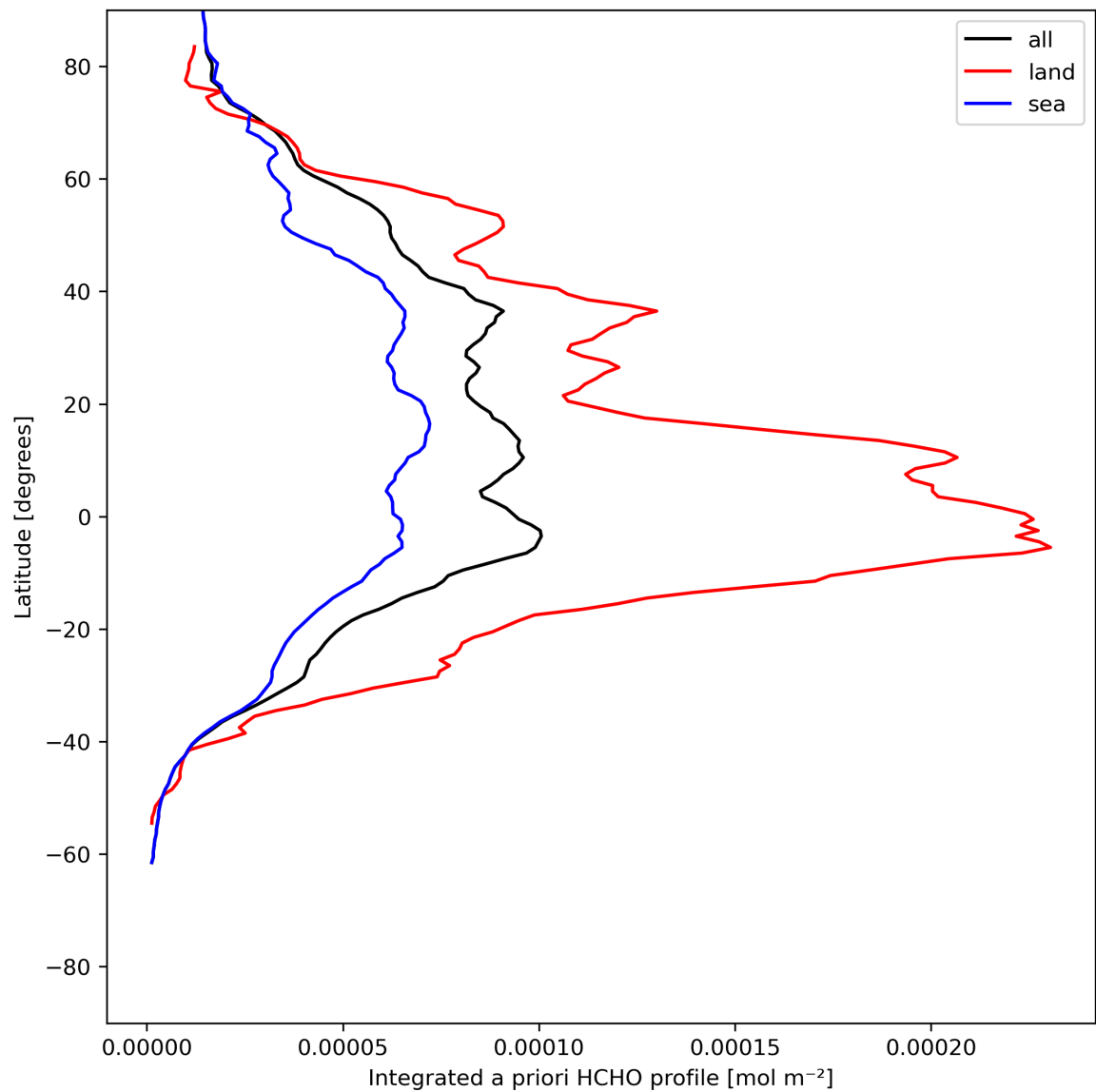
Figure 29: Zonal average of “Integrated a priori HCHO profile” for 2024-06-15 to 2024-06-17.
