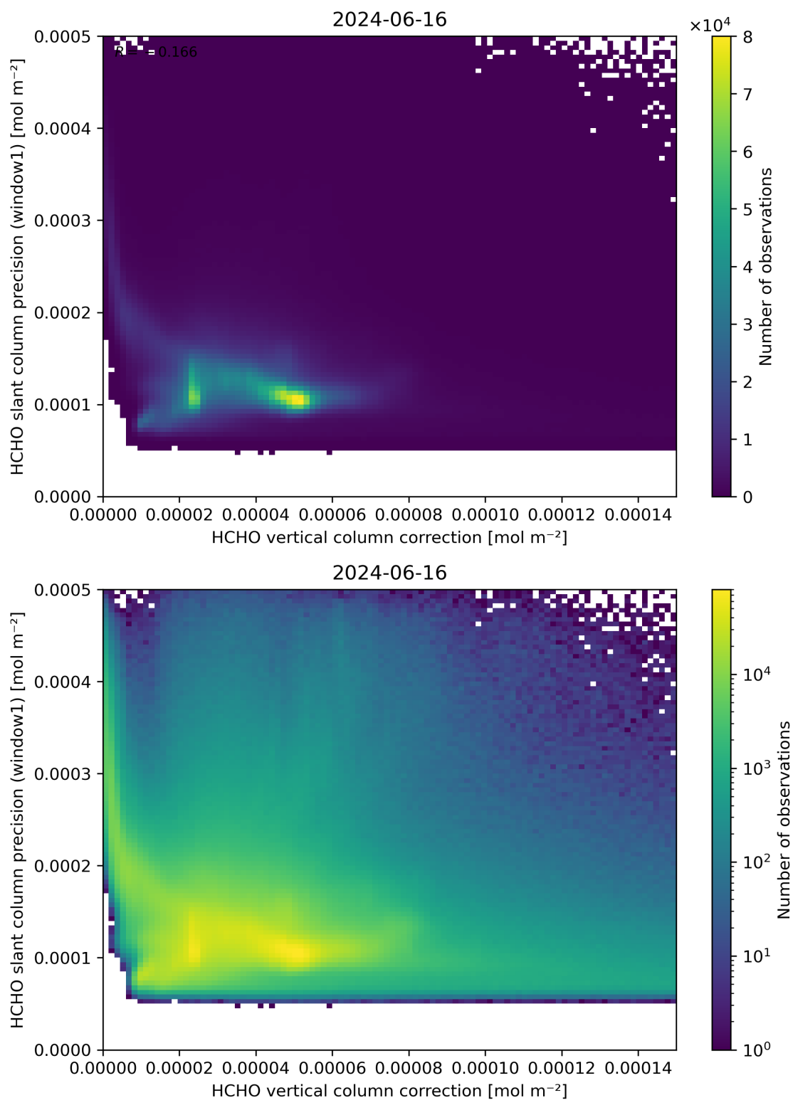
Figure 119: Scatter density plot of “HCHO vertical column correction” against “HCHO slant column precision (window1)” for 2024-06-15 to 2024-06-17.
