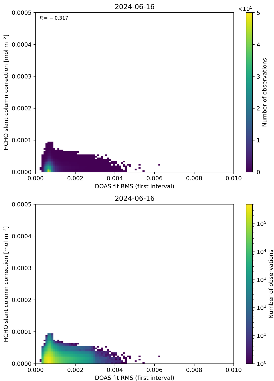
Figure 63: Scatter density plot of “DOAS fit RMS (first interval)” against “HCHO slant column correction” for 2024-06-15 to 2024-06-17.
