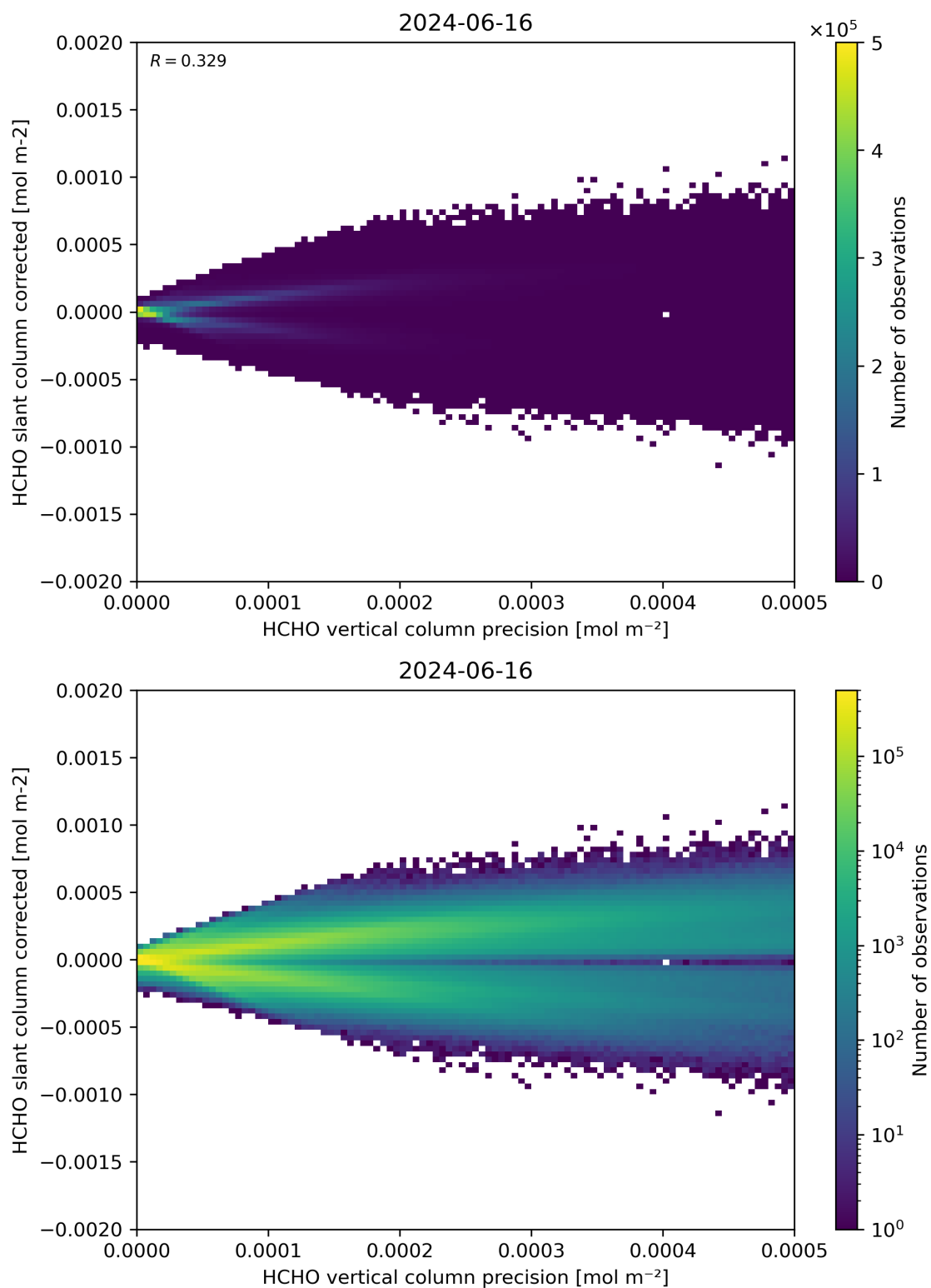
Figure 140: Scatter density plot of “HCHO vertical column precision” against “HCHO slant column corrected” for 2024-06-15 to 2024-06-17.
