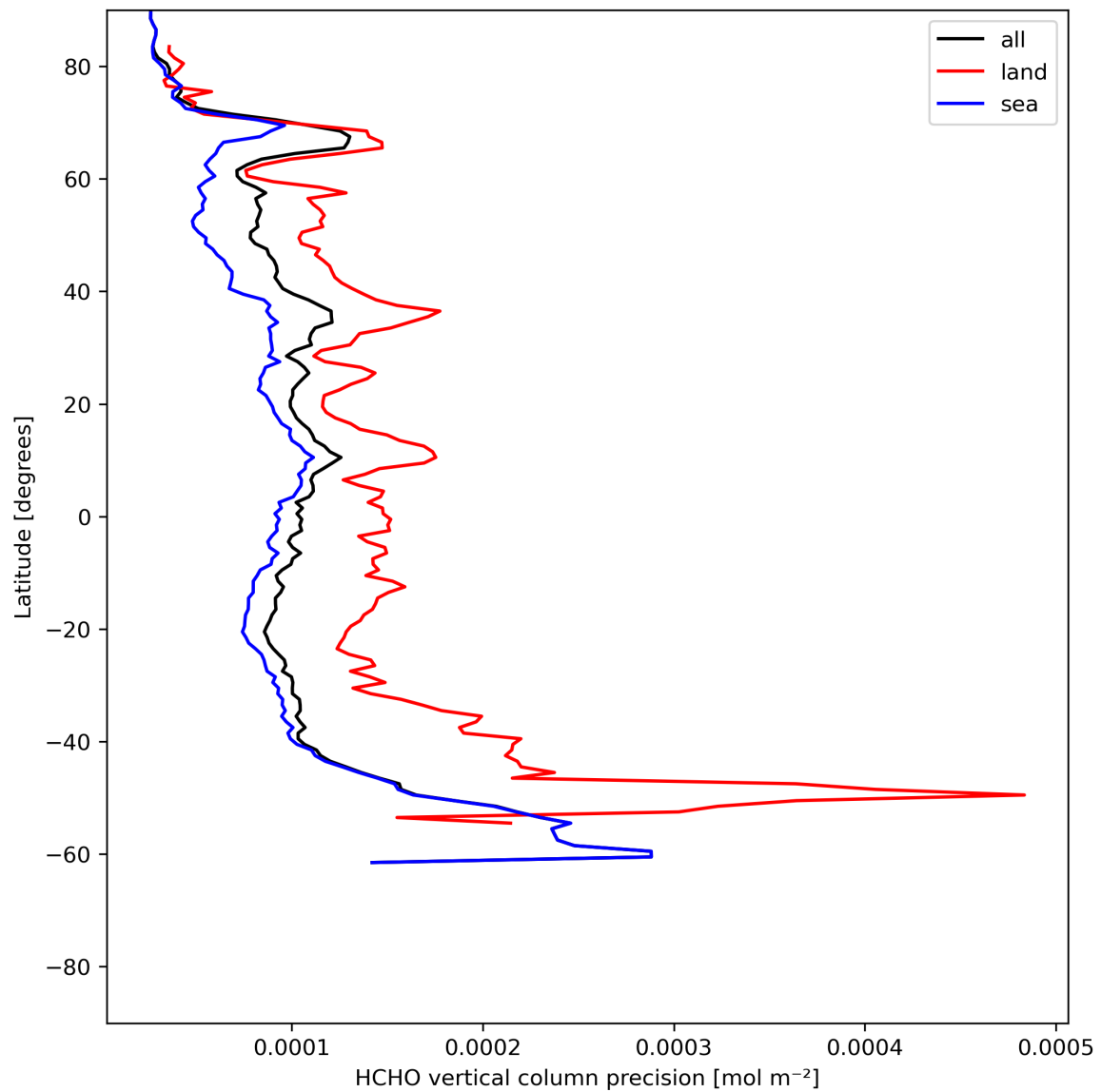
Figure 22: Zonal average of “HCHO vertical column precision” for 2024-06-15 to 2024-06-17.
