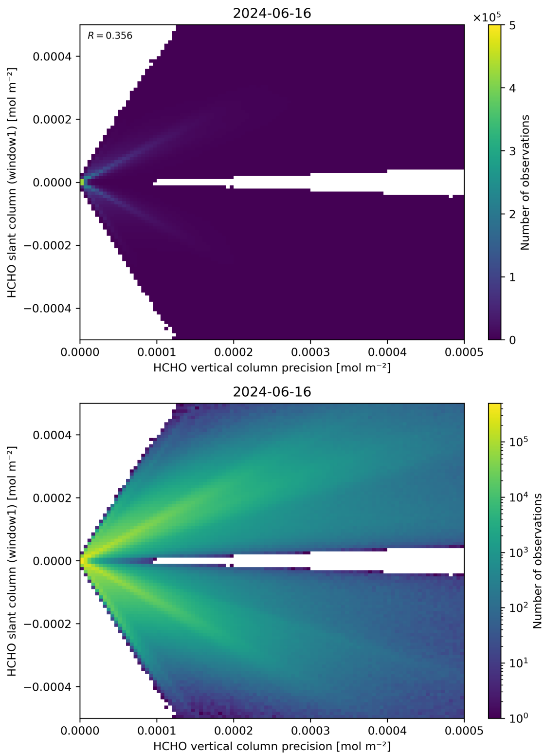
Figure 142: Scatter density plot of “HCHO vertical column precision” against “HCHO slant column (window1)” for 2024-06-15 to 2024-06-17.
