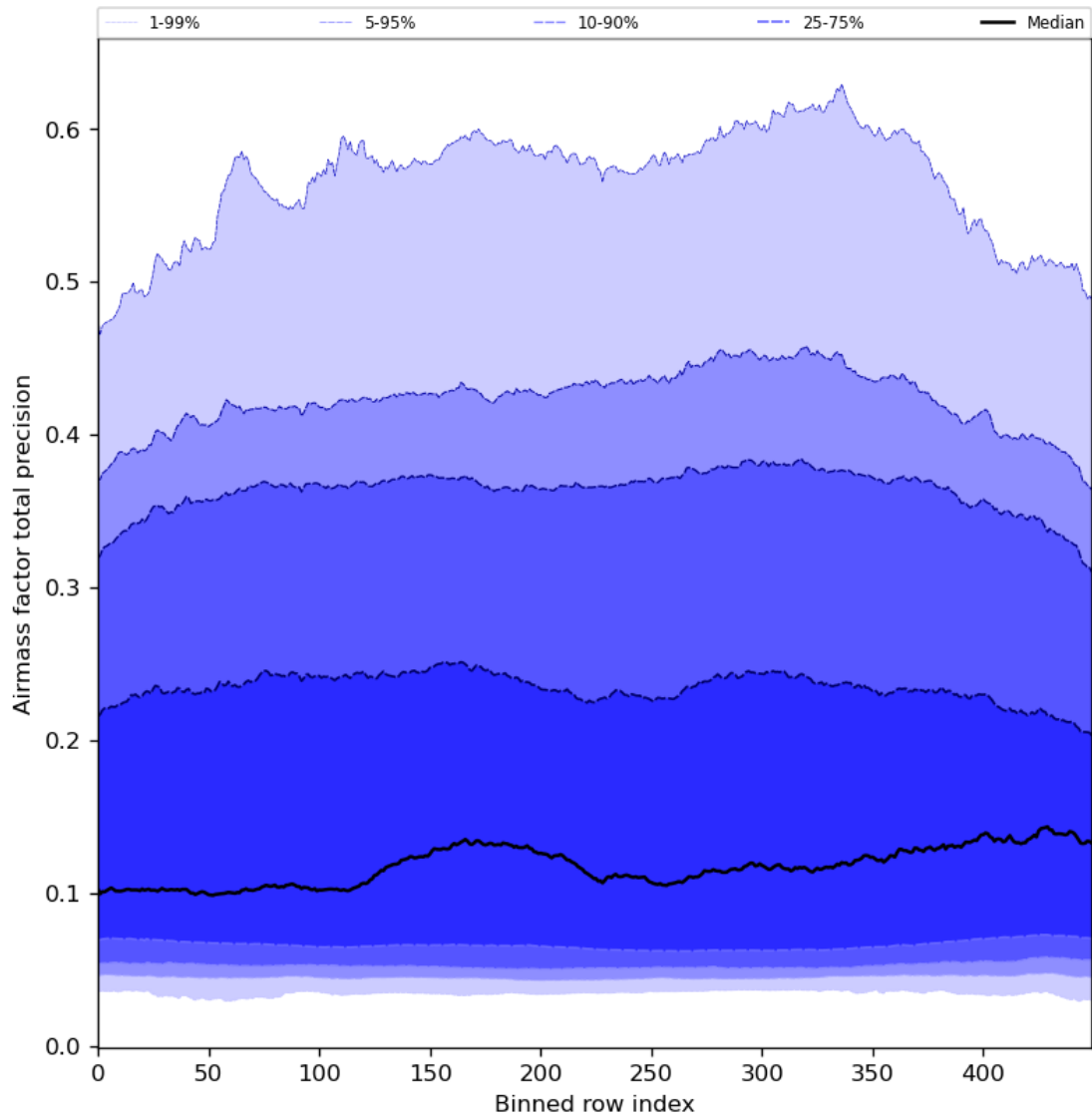
Figure 55: Along track statistics of “Airmass factor total precision” for 2024-06-15 to 2024-06-17
