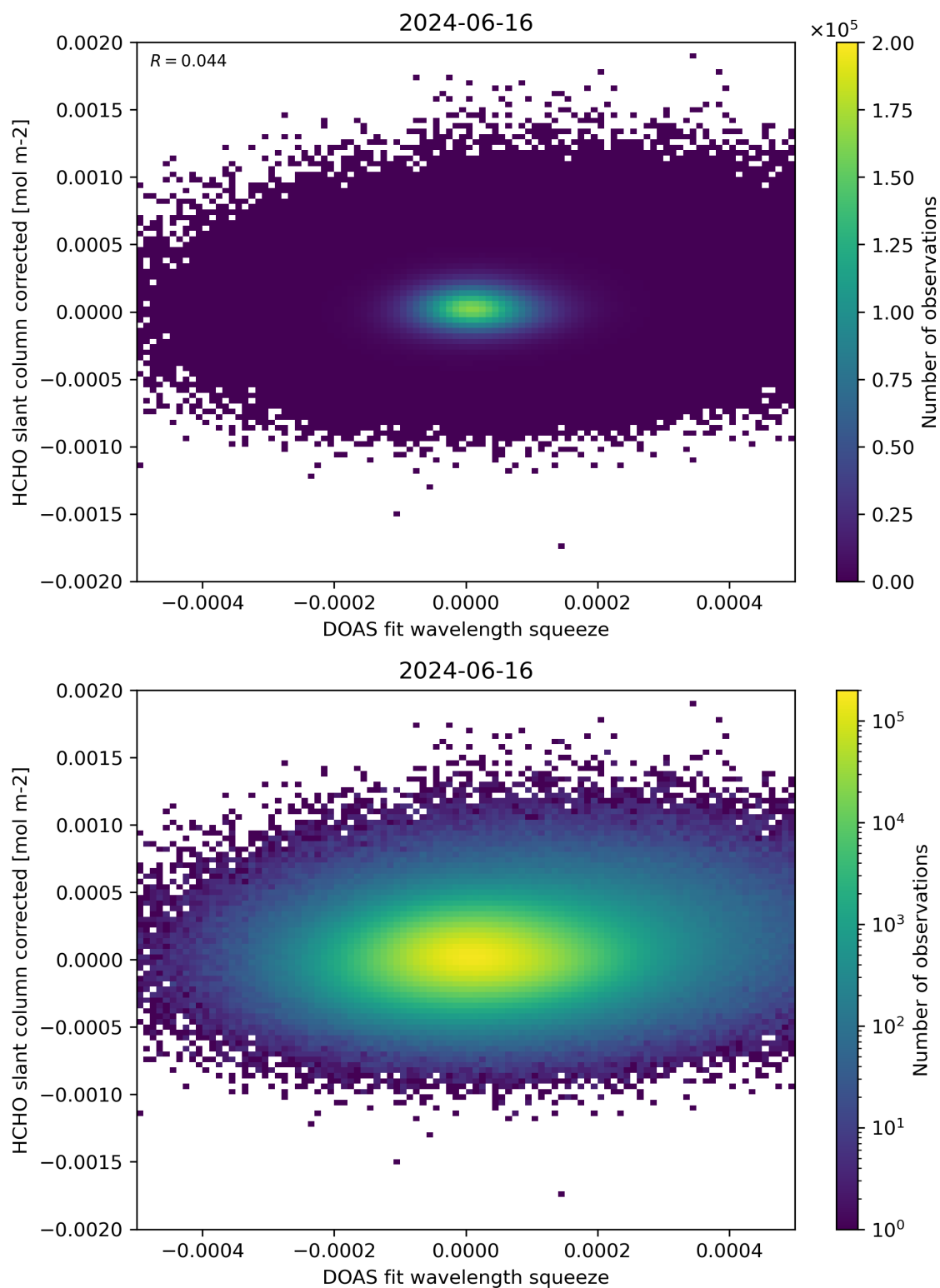
Figure 69: Scatter density plot of “DOAS fit wavelength squeeze” against “HCHO slant column corrected” for 2024-06-15 to 2024-06-17.
