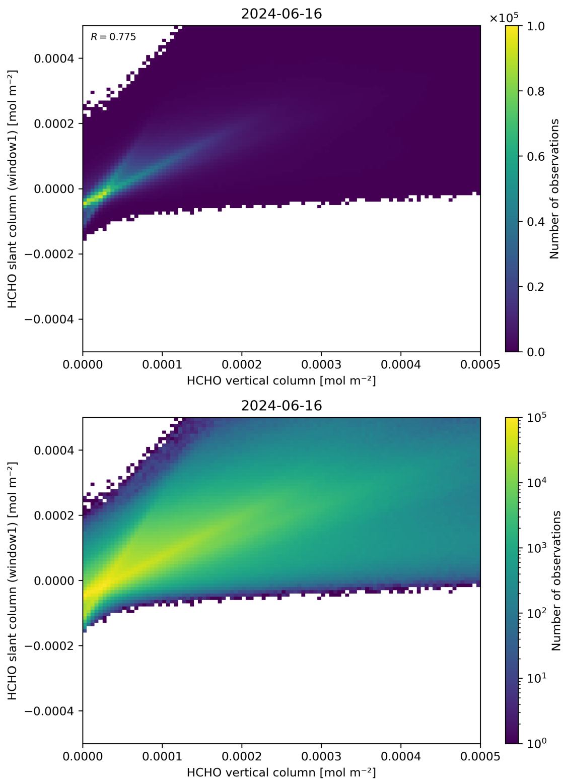
Figure 129: Scatter density plot of “HCHO vertical column” against “HCHO slant column (window1)” for 2024-06-15 to 2024-06-17.
