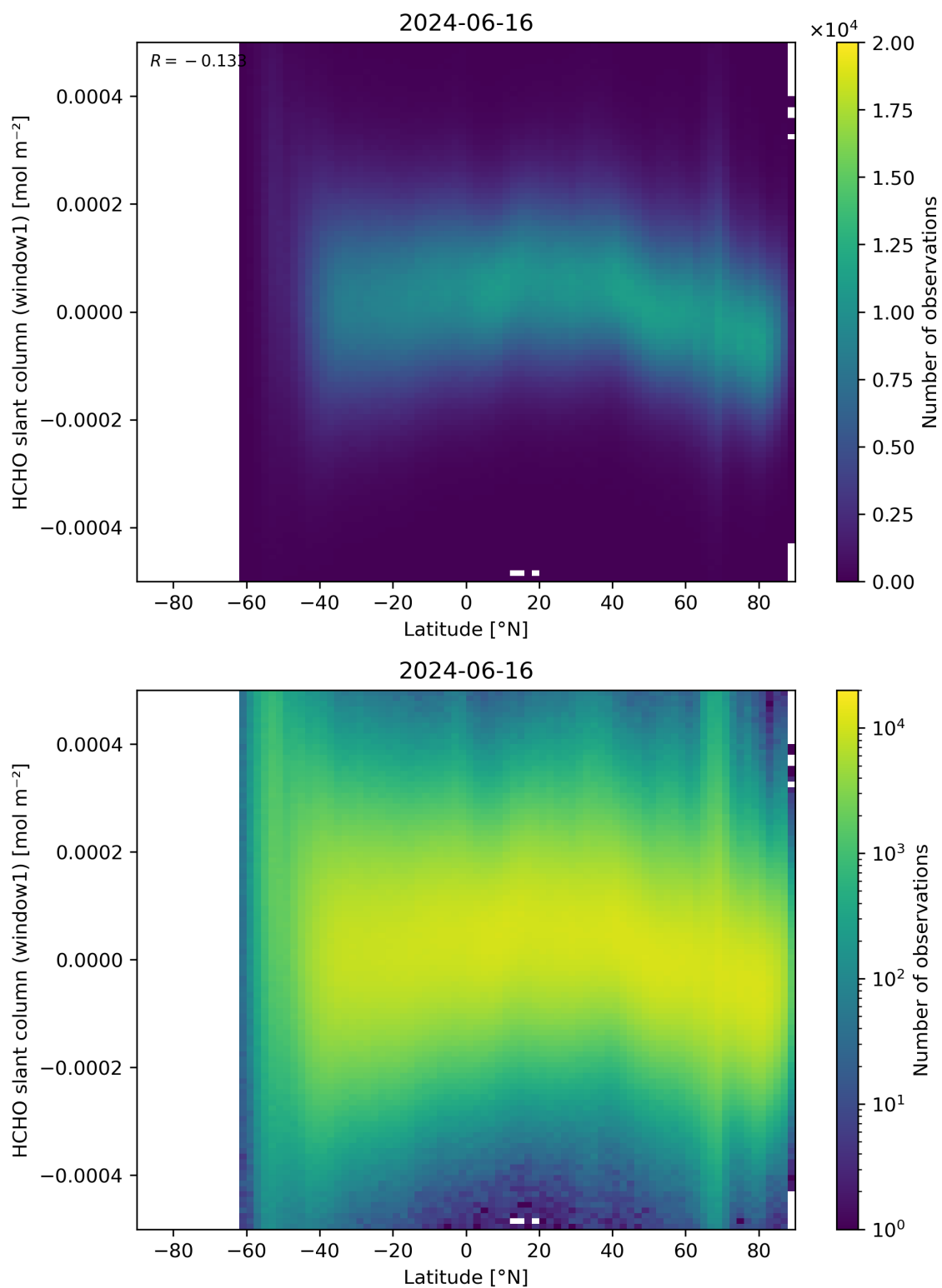
Figure 159: Scatter density plot of “Latitude” against “HCHO slant column (window1)” for 2024-06-15 to 2024-06-17.
