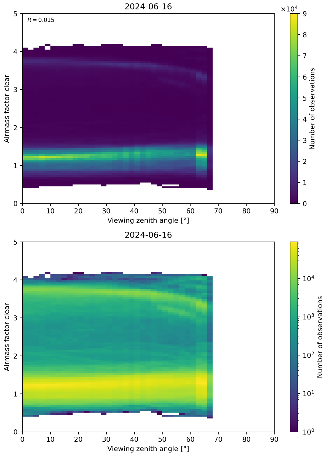
Figure 185: Scatter density plot of “Viewing zenith angle” against “Airmass factor clear” for 2024-06-15 to 2024-06-17.
