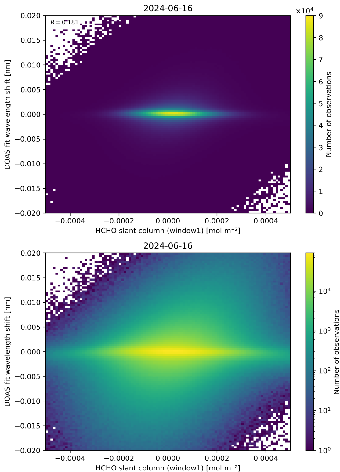
Figure 79: Scatter density plot of “HCHO slant column (window1)” against “DOAS fit wavelength shift” for 2024-06-15 to 2024-06-17.
