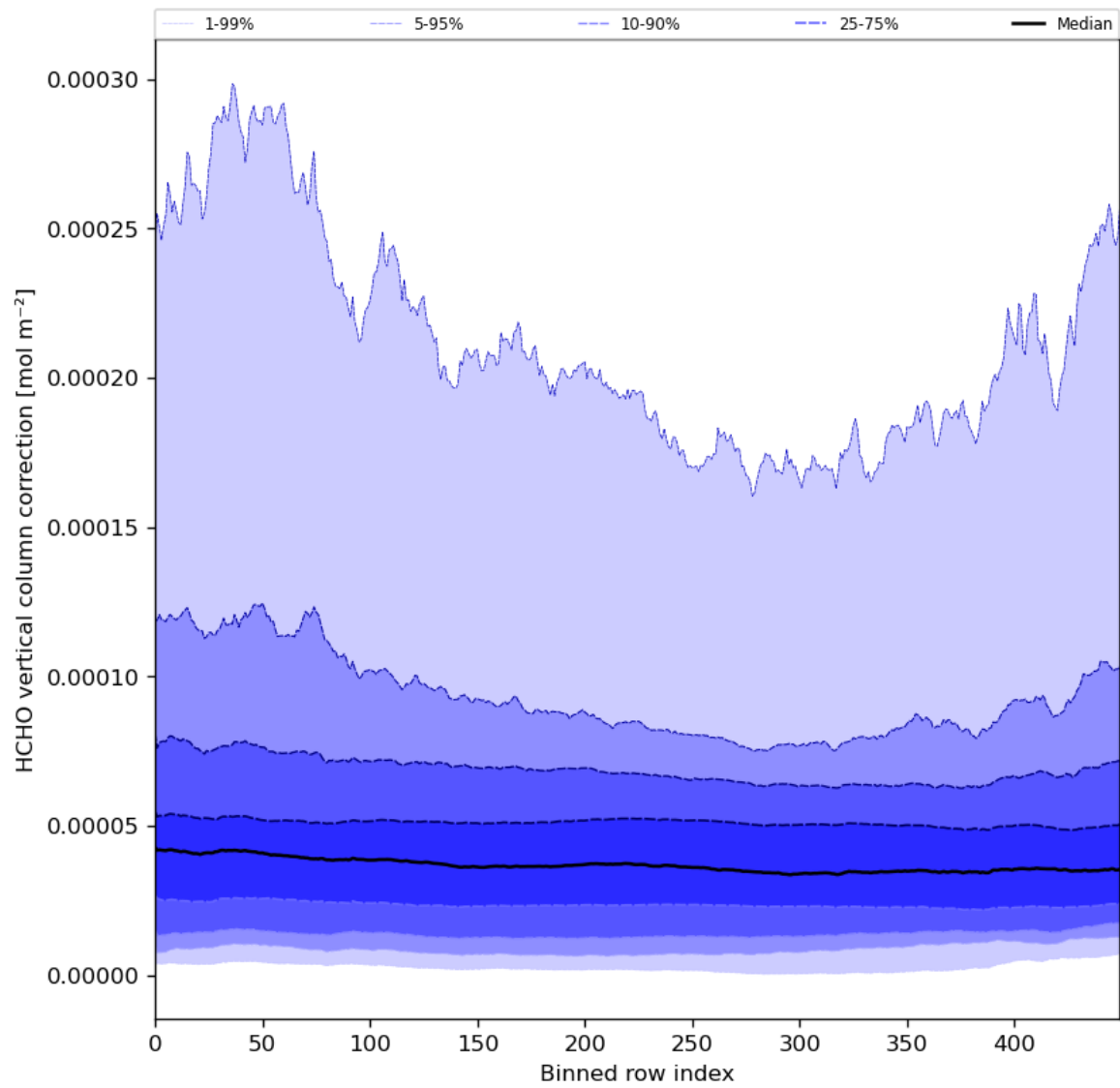
Figure 51: Along track statistics of “HCHO vertical column correction” for 2024-06-15 to 2024-06-17
