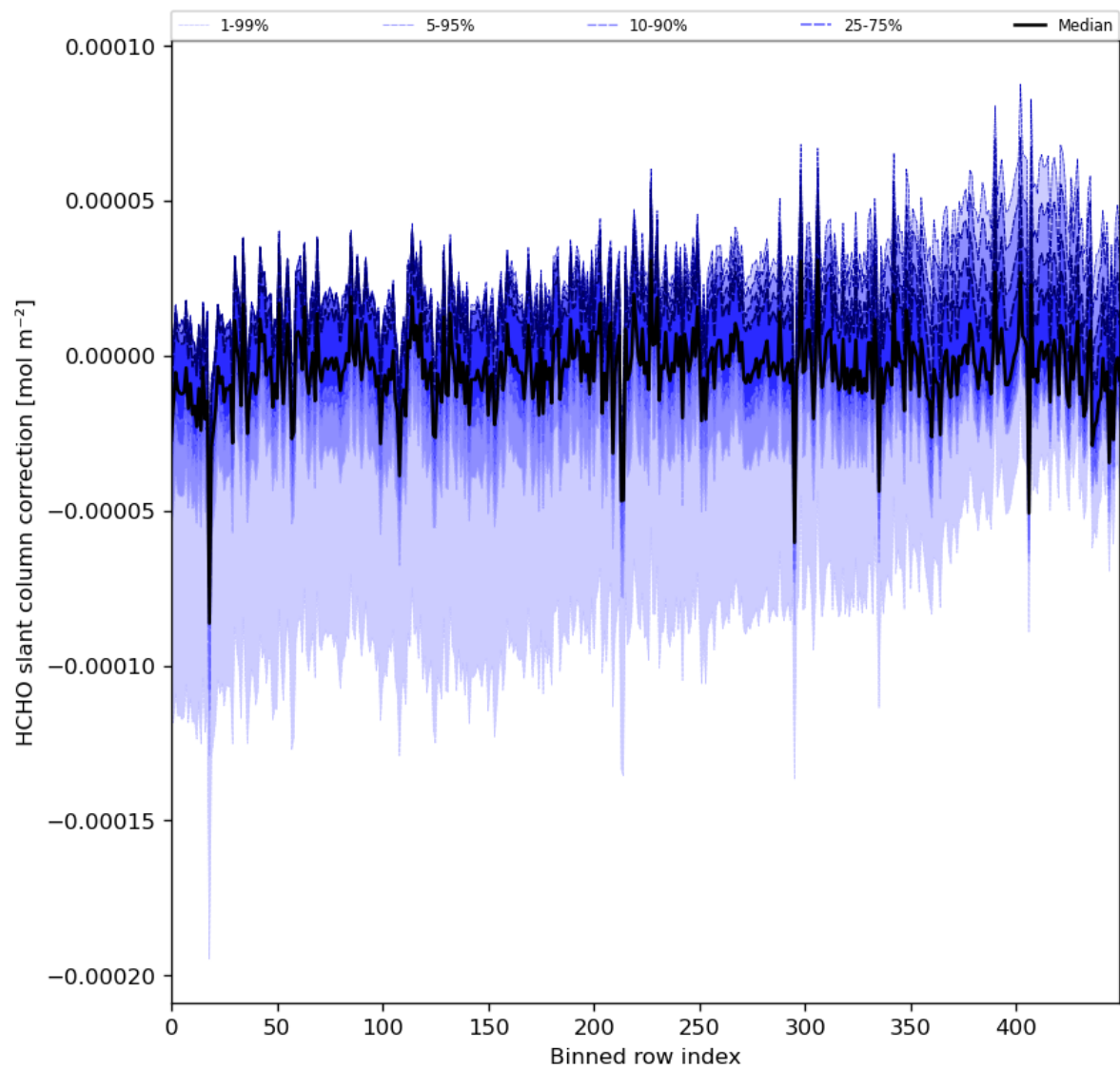
Figure 61: Along track statistics of “HCHO slant column correction” for 2024-06-15 to 2024-06-17
