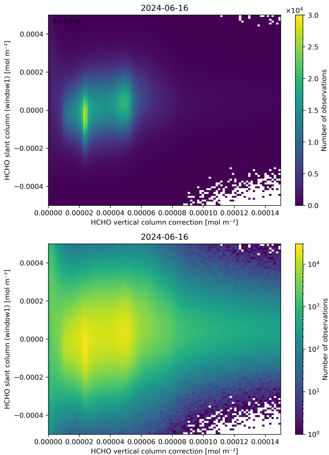
Figure 118: Scatter density plot of “HCHO vertical column correction” against “HCHO slant column (window1)” for 2024-06-15 to 2024-06-17.
