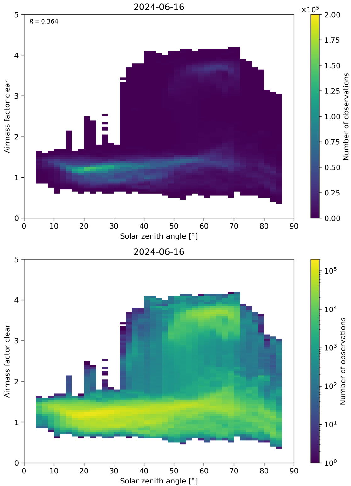
Figure 170: Scatter density plot of “Solar zenith angle” against “Airmass factor clear” for 2024-06-15 to 2024-06-17.
