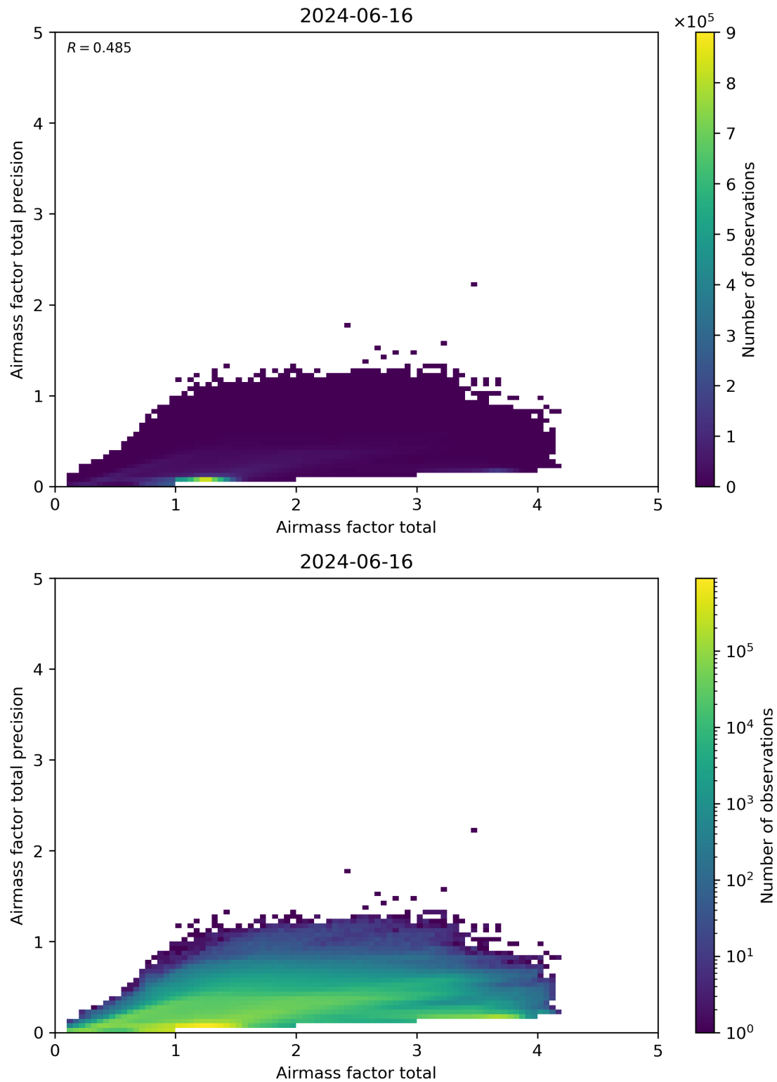
Figure 103: Scatter density plot of “Airmass factor total” against “Airmass factor total precision” for 2024-06-15 to 2024-06-17.
