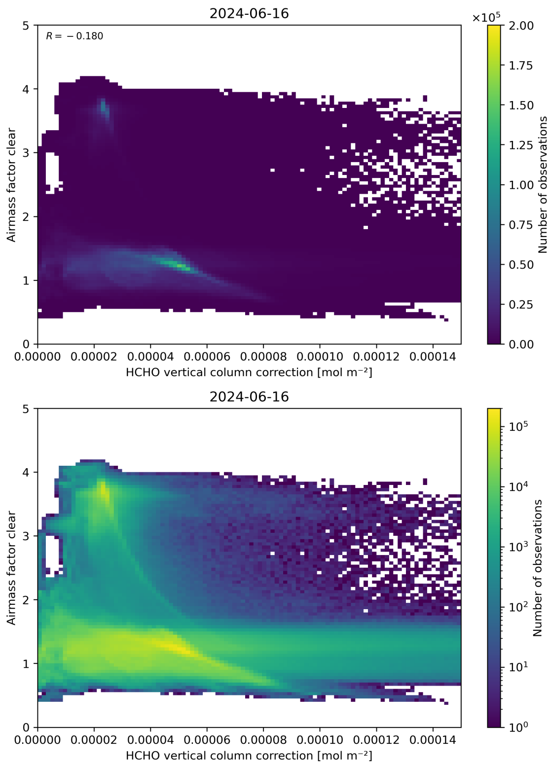
Figure 115: Scatter density plot of “HCHO vertical column correction” against “Airmass factor clear” for 2024-06-15 to 2024-06-17.
