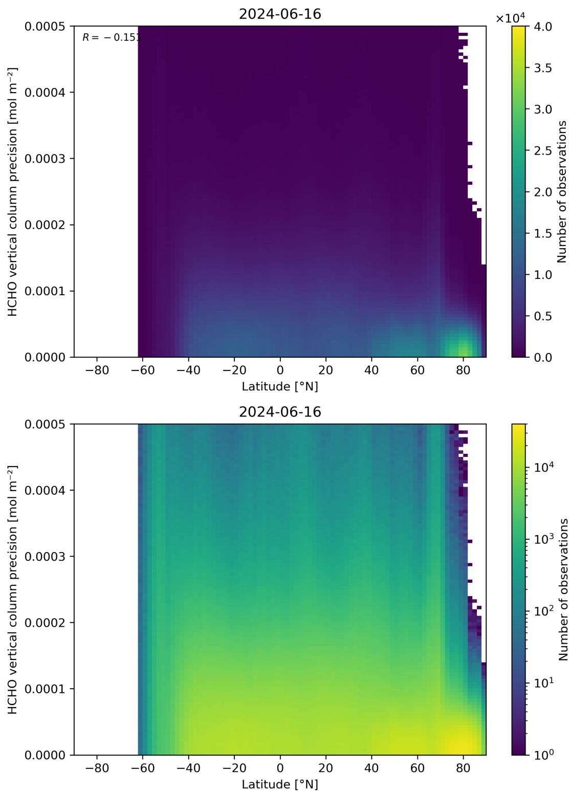
Figure 165: Scatter density plot of “Latitude” against “HCHO vertical column precision” for 2024-06-15 to 2024-06-17.
