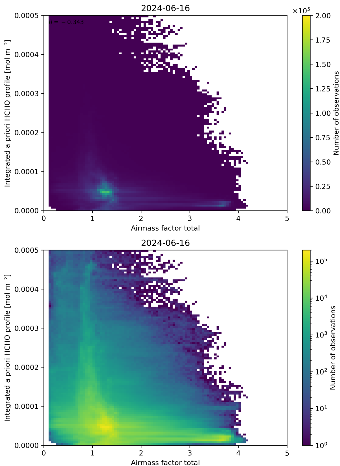
Figure 104: Scatter density plot of “Airmass factor total” against “Integrated a priori HCHO profile” for 2024-06-15 to 2024-06-17.
