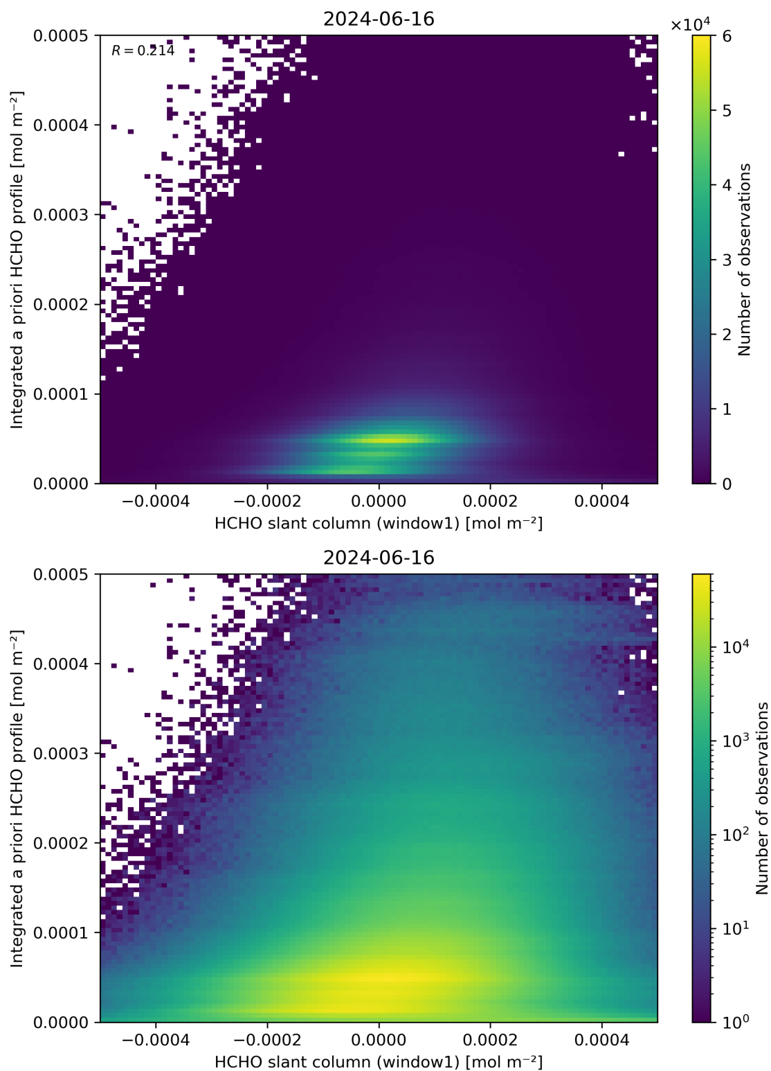
Figure 87: Scatter density plot of “HCHO slant column (window1)” against “Integrated a priori HCHO profile” for 2024-06-15 to 2024-06-17.
