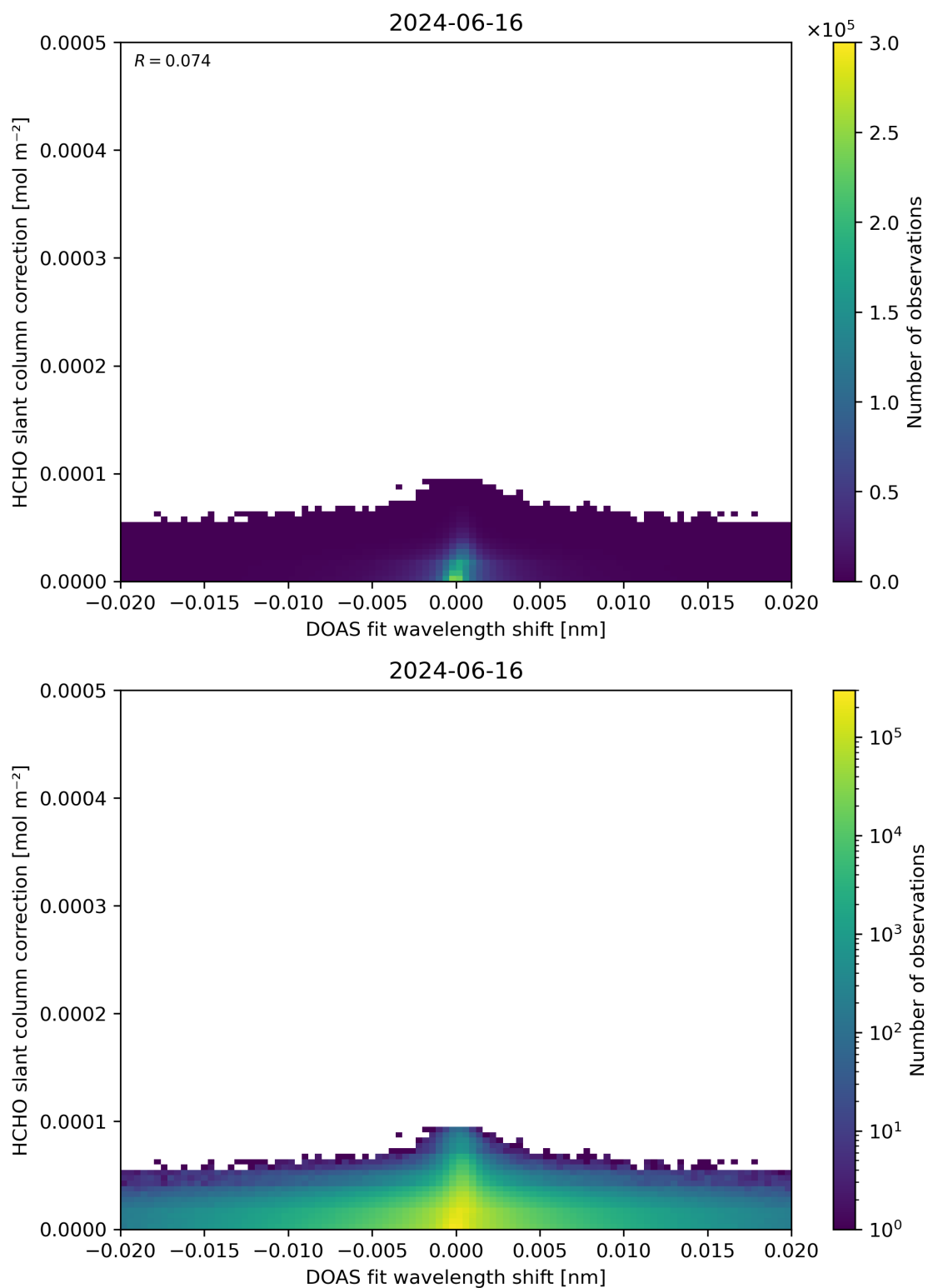
Figure 67: Scatter density plot of “DOAS fit wavelength shift” against “HCHO slant column correction” for 2024-06-15 to 2024-06-17.
