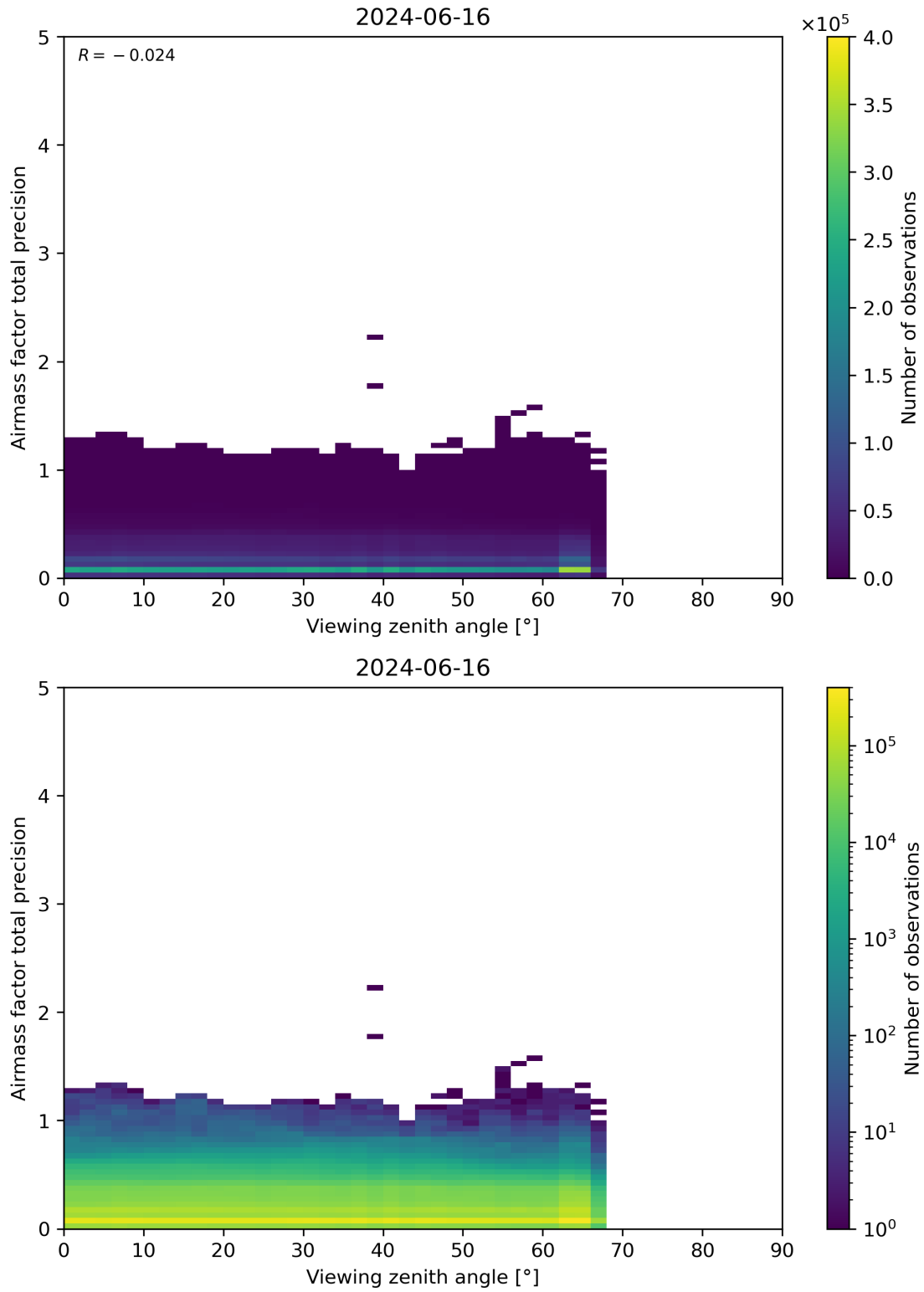
Figure 191: Scatter density plot of “Viewing zenith angle” against “Airmass factor total precision” for 2024-06-15 to 2024-06-17.
