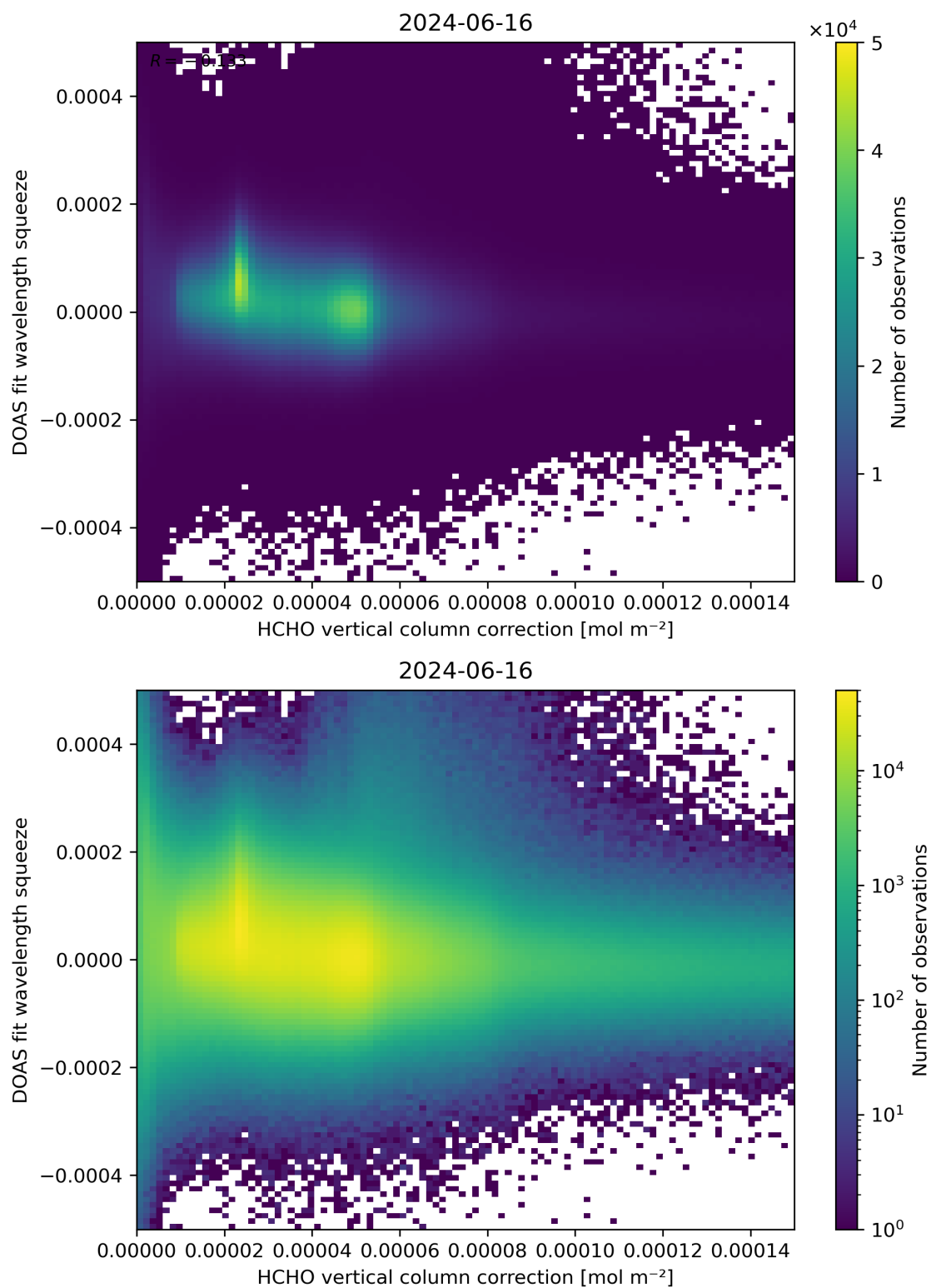
Figure 114: Scatter density plot of “HCHO vertical column correction” against “DOAS fit wavelength squeeze” for 2024-06-15 to 2024-06-17.
