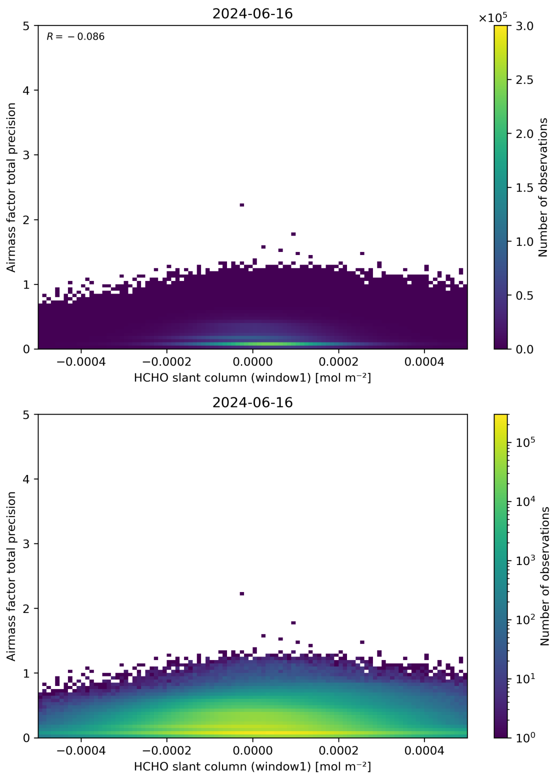
Figure 86: Scatter density plot of “HCHO slant column (window1)” against “Airmass factor total precision” for 2024-06-15 to 2024-06-17.
