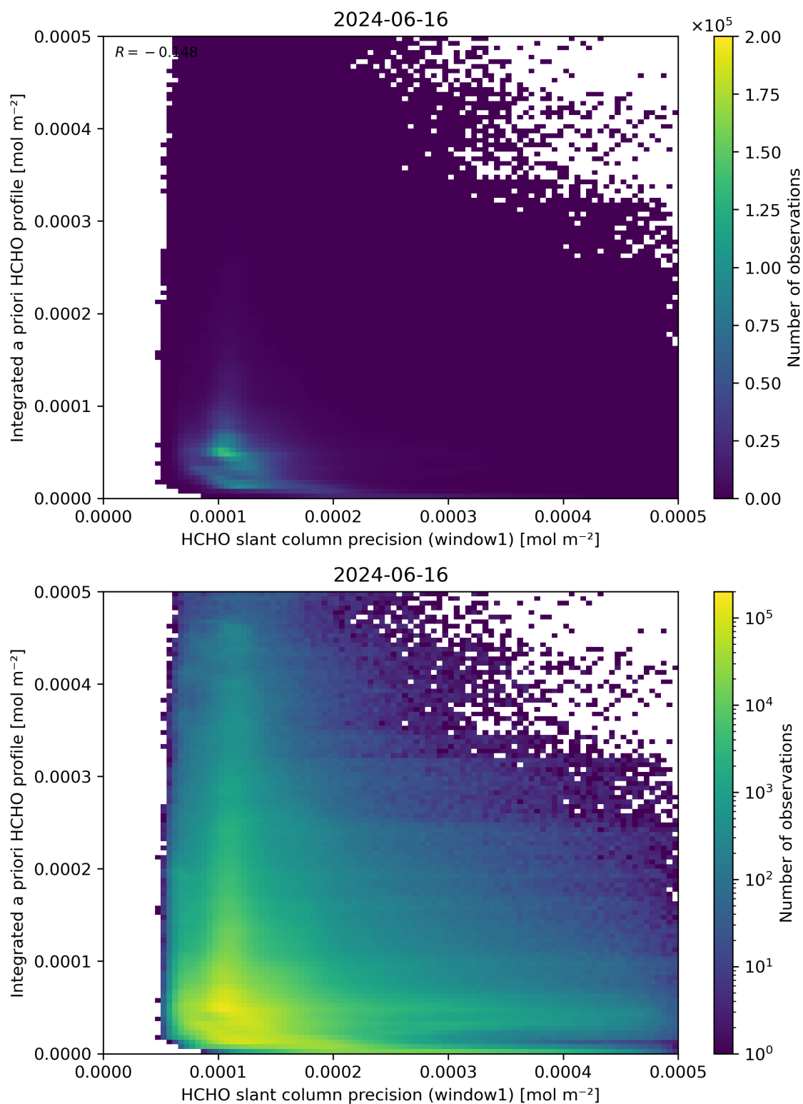
Figure 96: Scatter density plot of “HCHO slant column precision (window1)” against “Integrated a priori HCHO profile” for 2024-06-15 to 2024-06-17.
