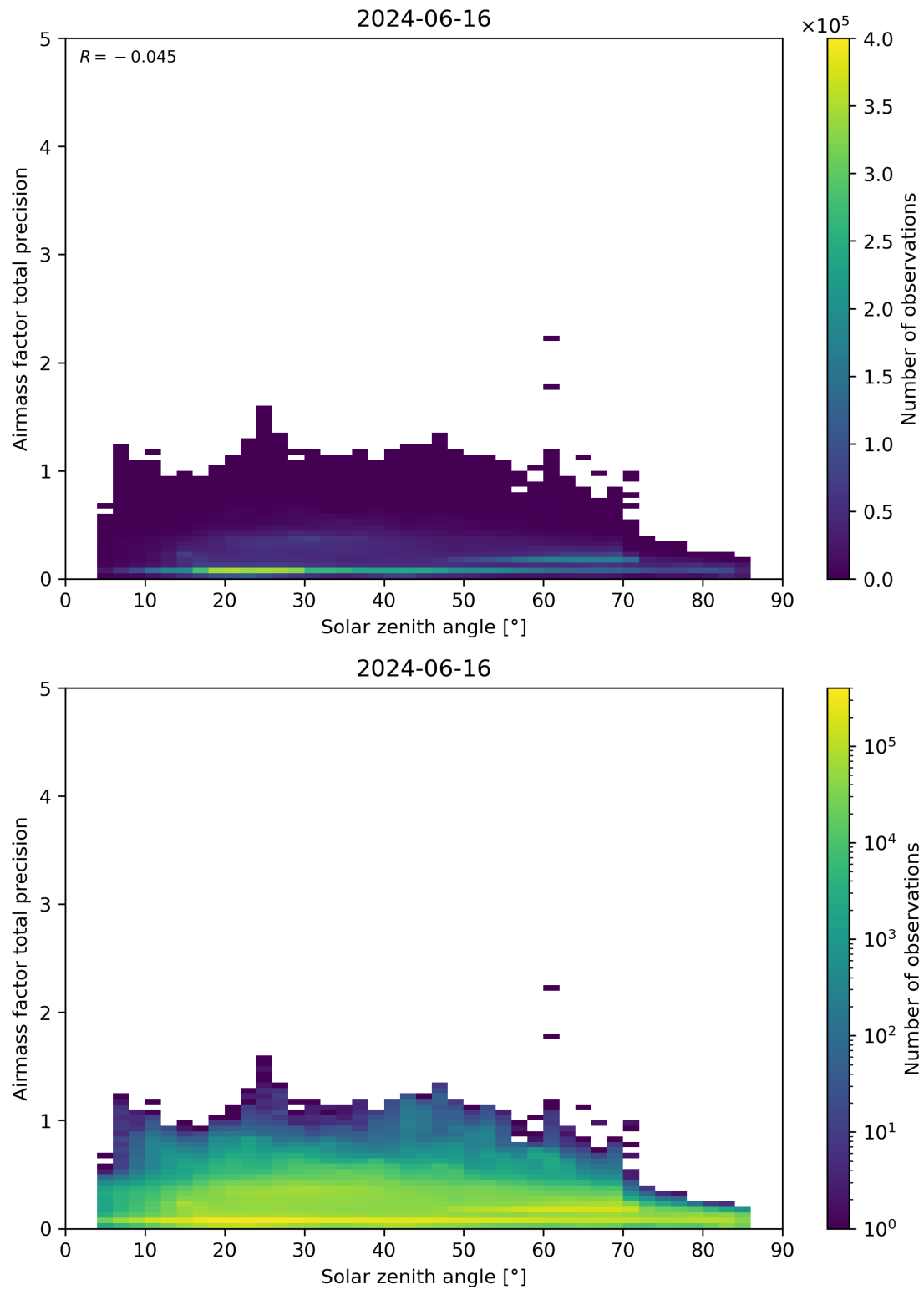
Figure 176: Scatter density plot of “Solar zenith angle” against “Airmass factor total precision” for 2024-06-15 to 2024-06-17.
