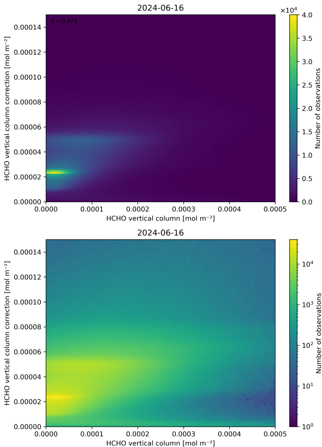
Figure 133: Scatter density plot of “HCHO vertical column” against “HCHO vertical column correction” for 2024-06-15 to 2024-06-17.
