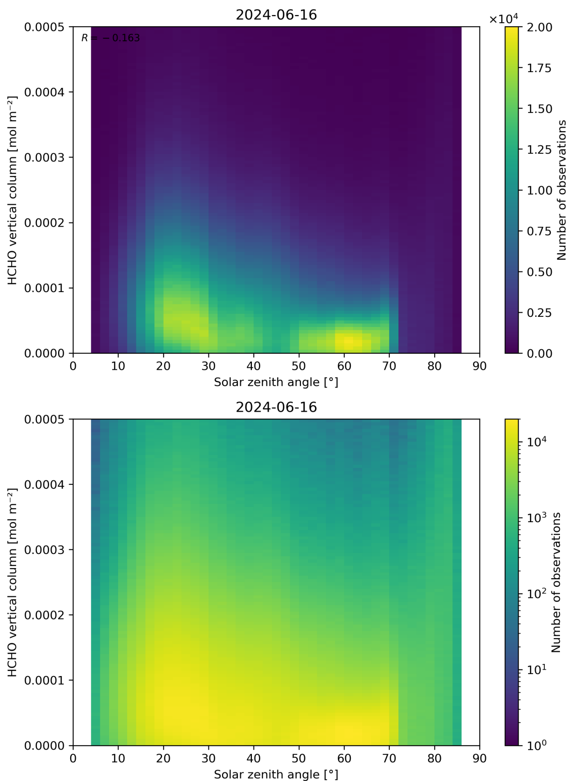
Figure 177: Scatter density plot of “Solar zenith angle” against “HCHO vertical column” for 2024-06-15 to 2024-06-17.
