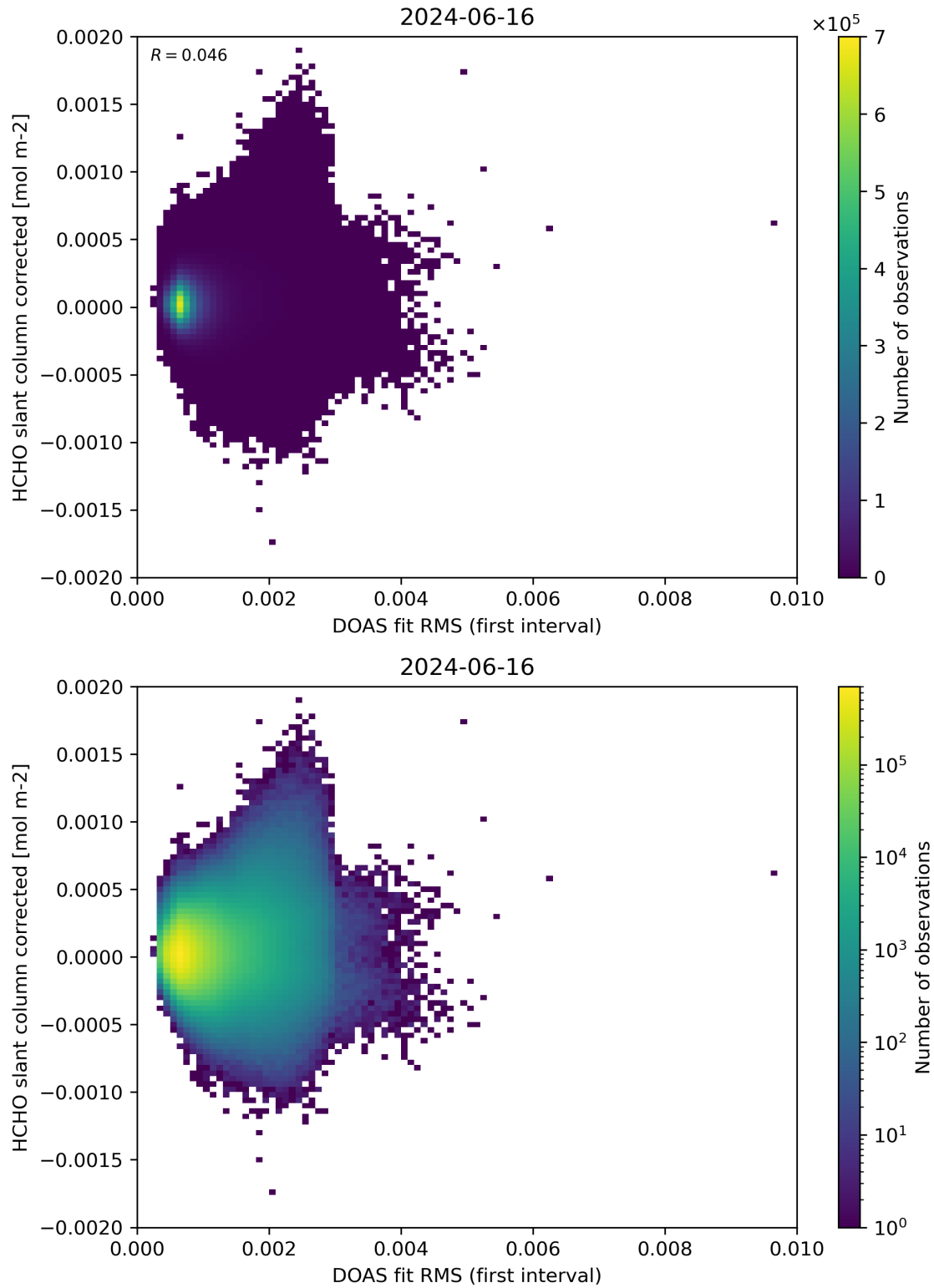
Figure 62: Scatter density plot of “DOAS fit RMS (first interval)” against “HCHO slant column corrected” for 2024-06-15 to 2024-06-17.
