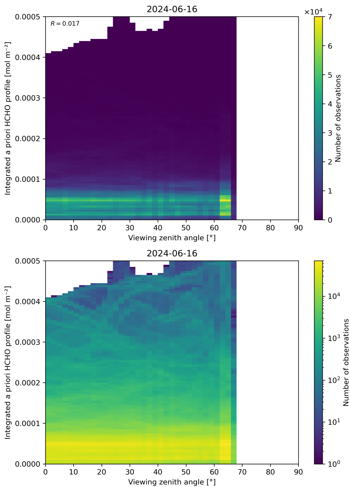
Figure 195: Scatter density plot of “Viewing zenith angle” against “Integrated a priori HCHO profile” for 2024-06-15 to 2024-06-17.
