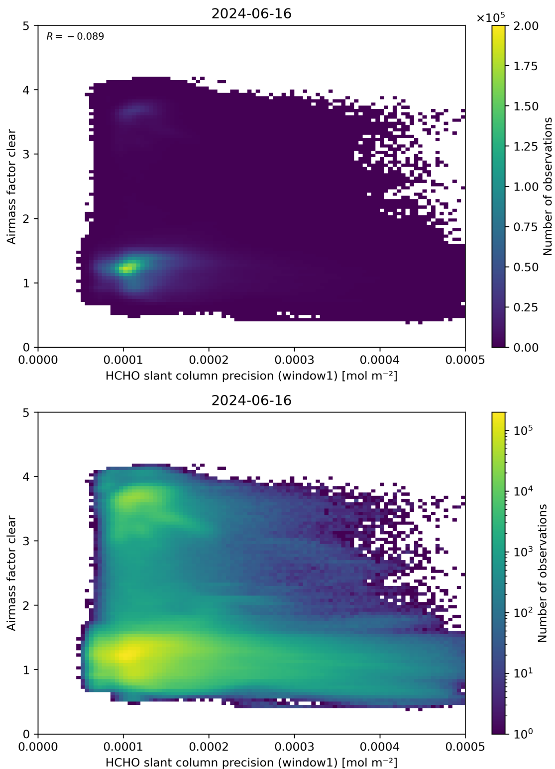
Figure 91: Scatter density plot of “HCHO slant column precision (window1)” against “Airmass factor clear” for 2024-06-15 to 2024-06-17.
