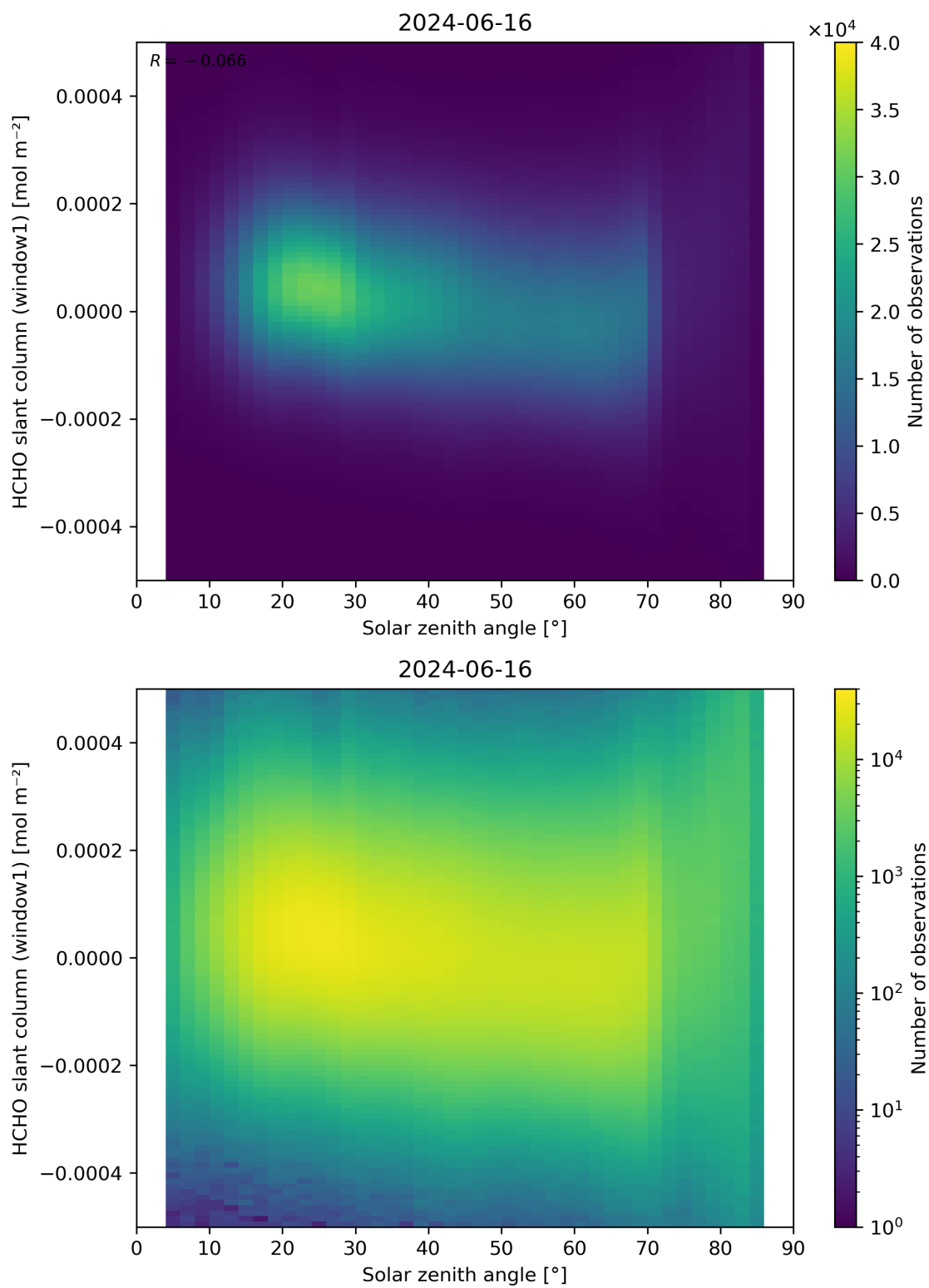
Figure 173: Scatter density plot of “Solar zenith angle” against “HCHO slant column (window1)” for 2024-06-15 to 2024-06-17.
