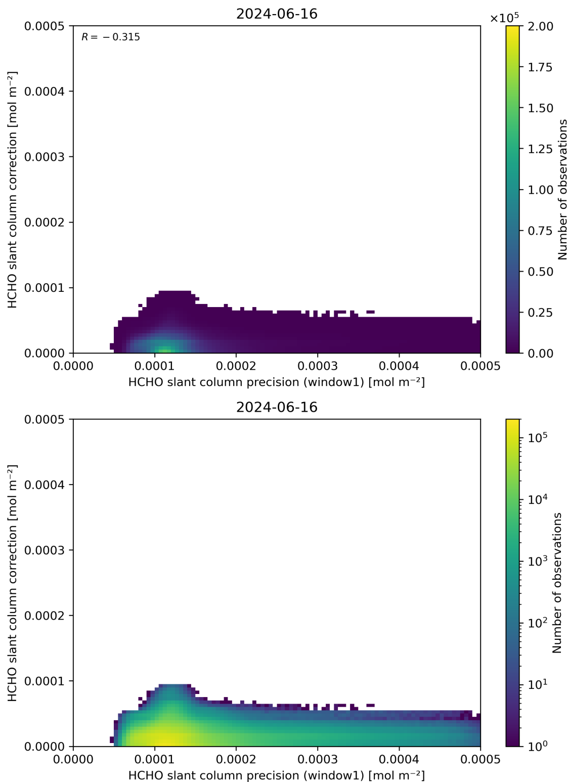
Figure 93: Scatter density plot of “HCHO slant column precision (window1)” against “HCHO slant column correction” for 2024-06-15 to 2024-06-17.
