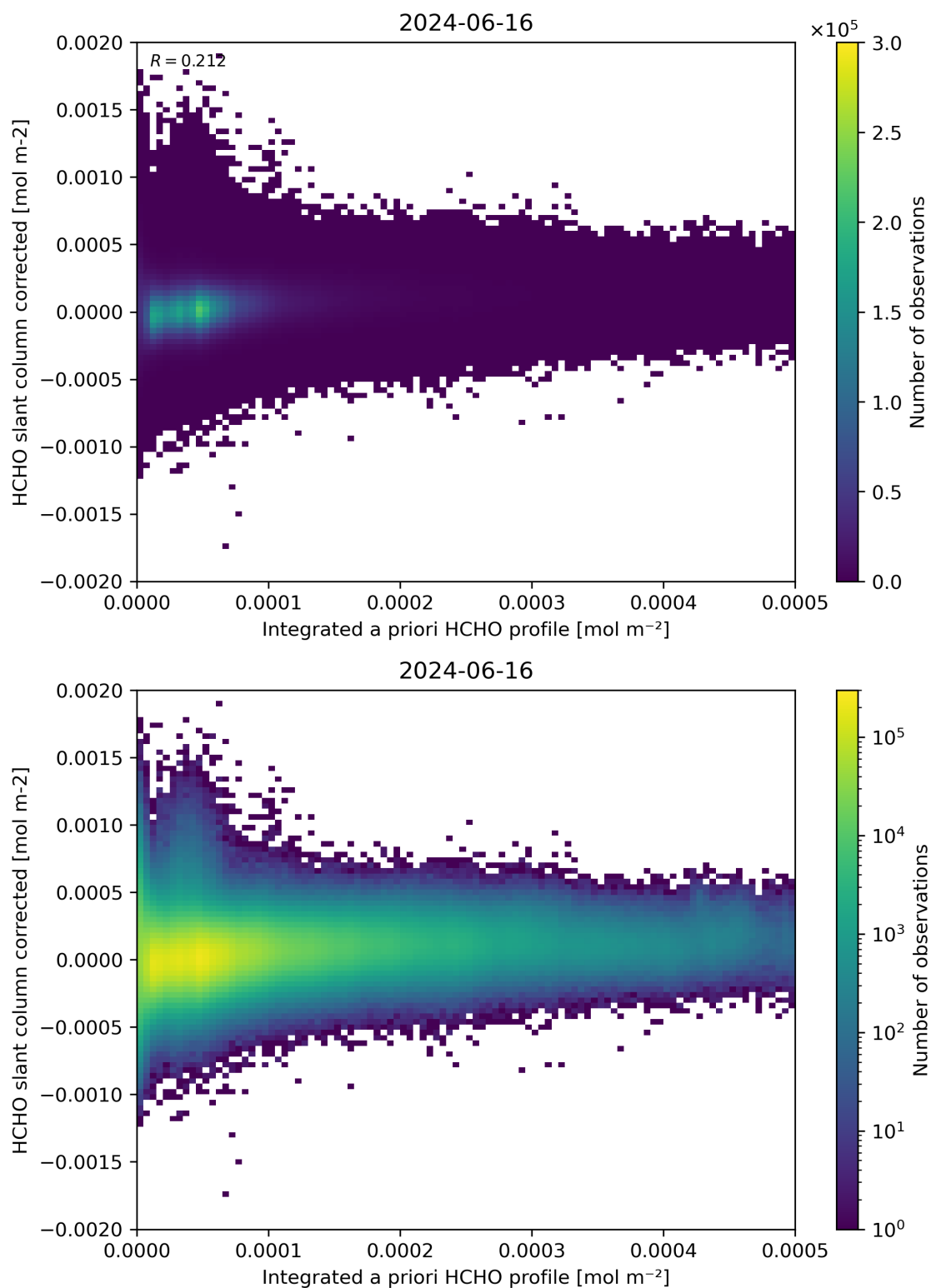
Figure 151: Scatter density plot of “Integrated a priori HCHO profile” against “HCHO slant column corrected” for 2024-06-15 to 2024-06-17.
