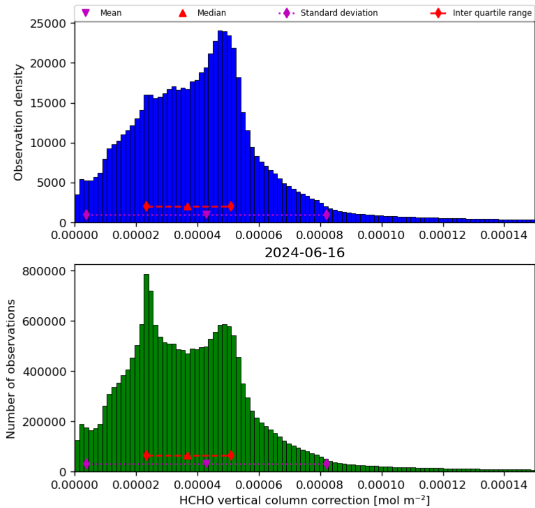
Figure 37: Histogram of “HCHO vertical column correction” for 2024-06-15 to 2024-06-17
