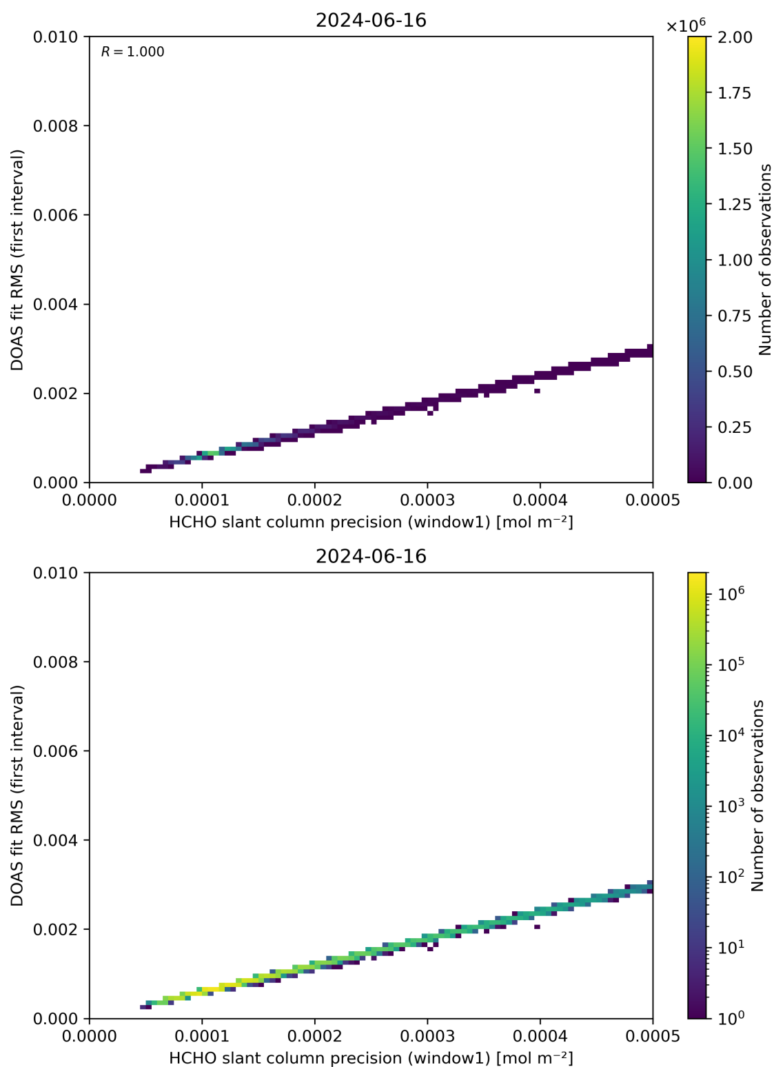
Figure 88: Scatter density plot of “HCHO slant column precision (window1)” against “DOAS fit RMS (first interval)” for 2024-06-15 to 2024-06-17.
