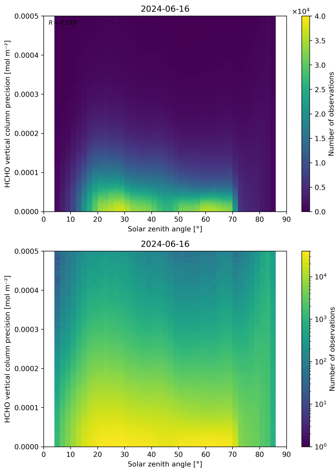
Figure 179: Scatter density plot of “Solar zenith angle” against “HCHO vertical column precision” for 2024-06-15 to 2024-06-17.
