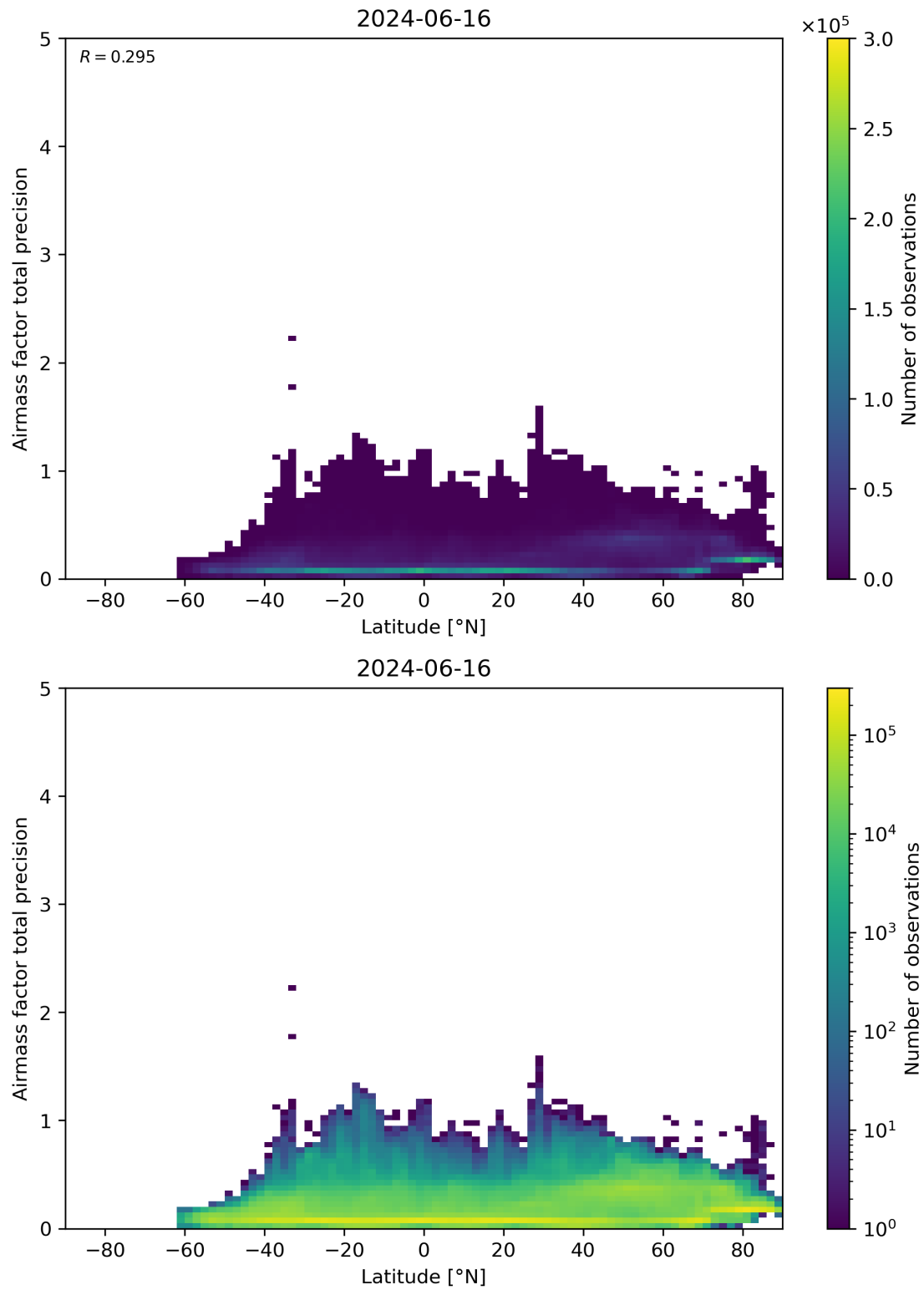
Figure 162: Scatter density plot of “Latitude” against “Airmass factor total precision” for 2024-06-15 to 2024-06-17.
