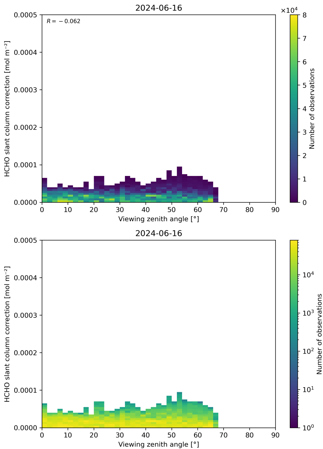
Figure 187: Scatter density plot of “Viewing zenith angle” against “HCHO slant column correction” for 2024-06-15 to 2024-06-17.
