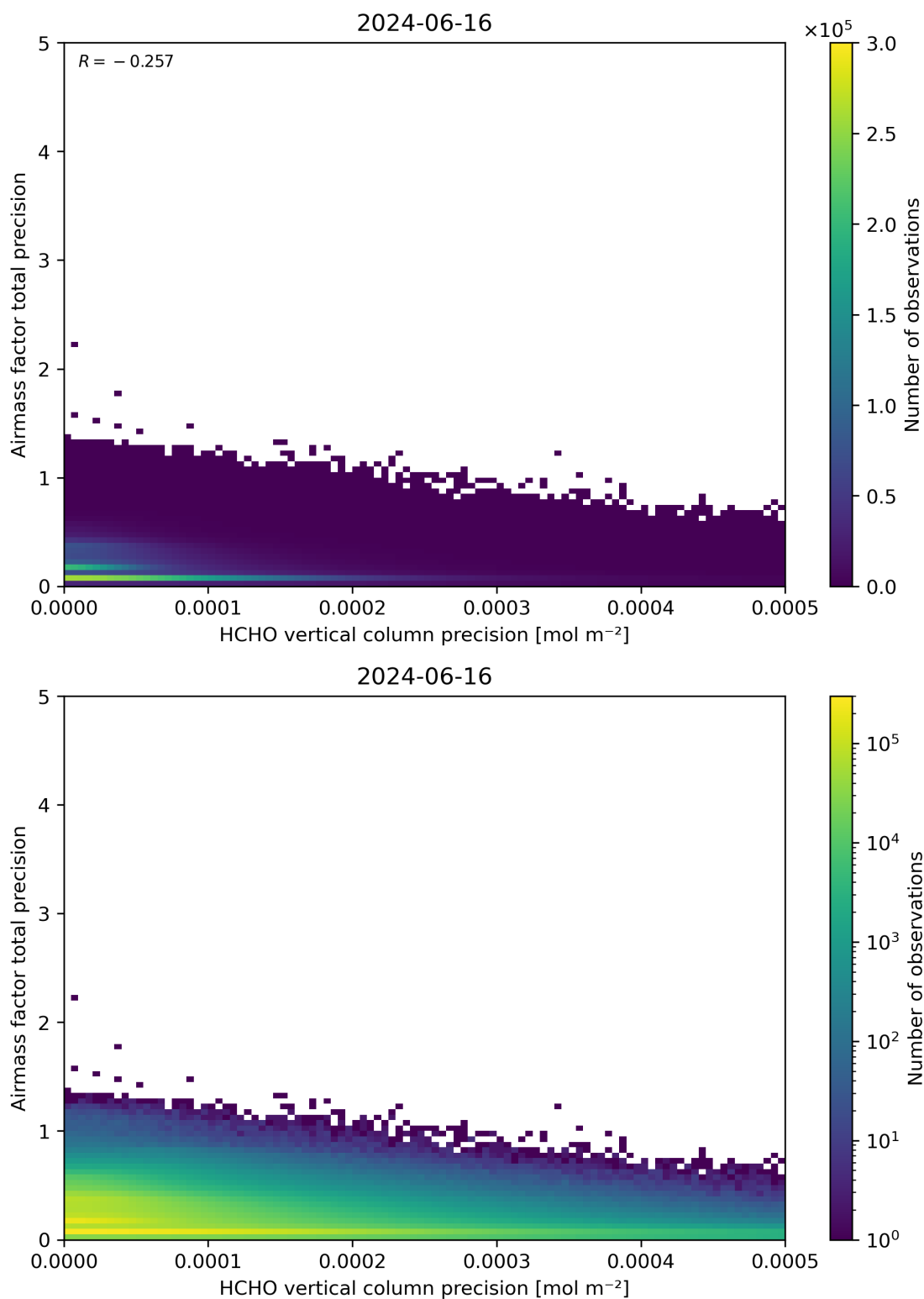
Figure 145: Scatter density plot of “HCHO vertical column precision” against “Airmass factor total precision” for 2024-06-15 to 2024-06-17.
