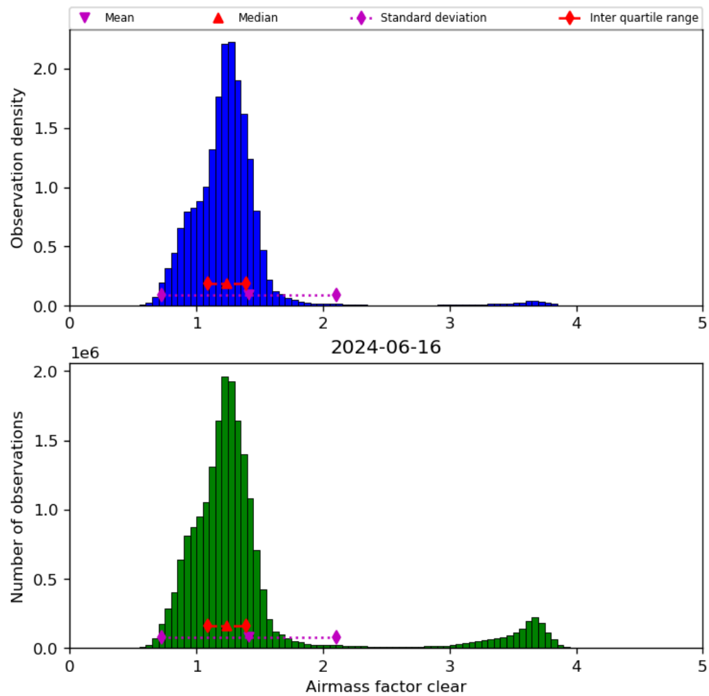
Figure 42: Histogram of “Airmass factor clear” for 2024-06-15 to 2024-06-17
