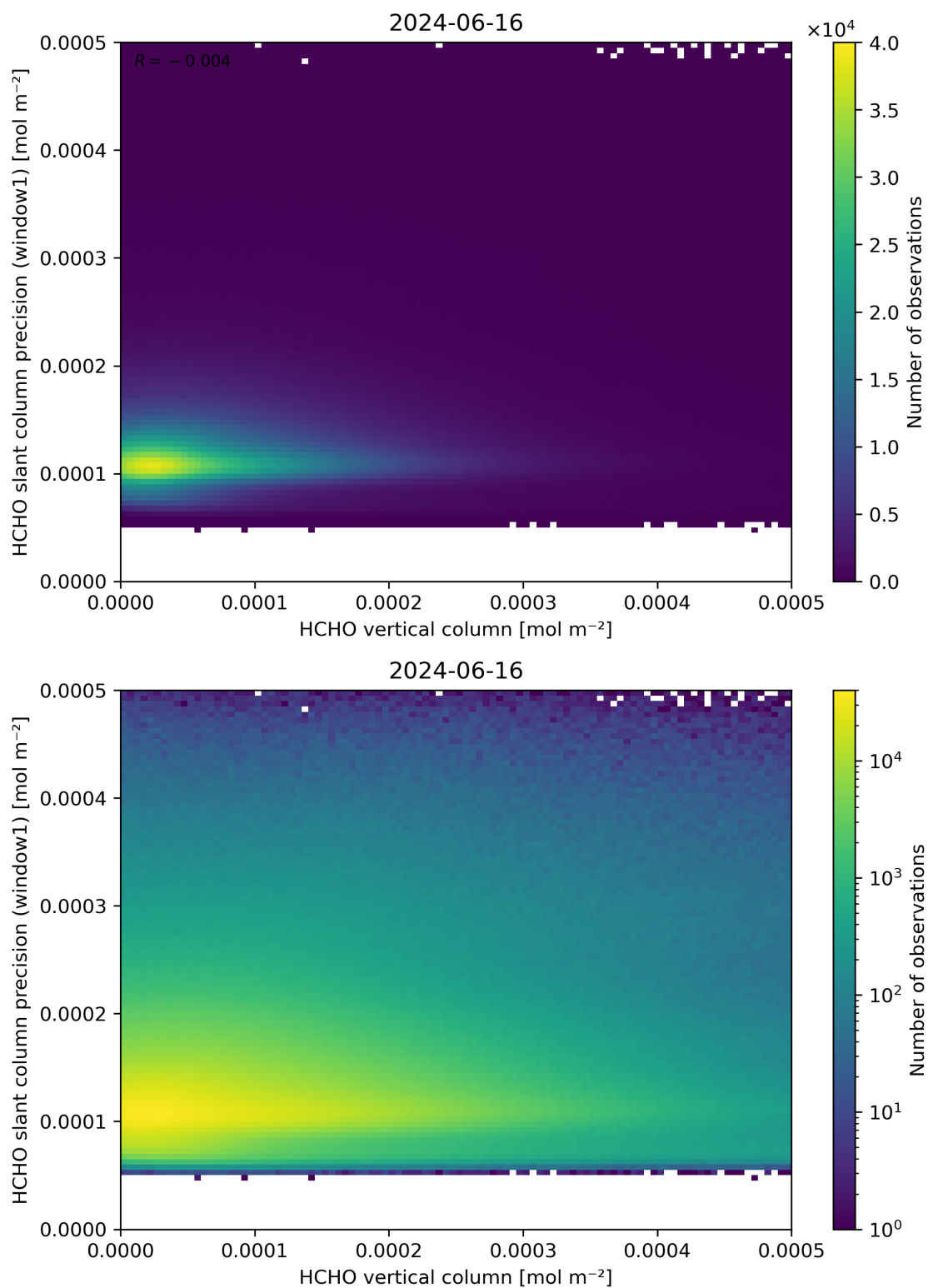
Figure 130: Scatter density plot of “HCHO vertical column” against “HCHO slant column precision (window1)” for 2024-06-15 to 2024-06-17.
