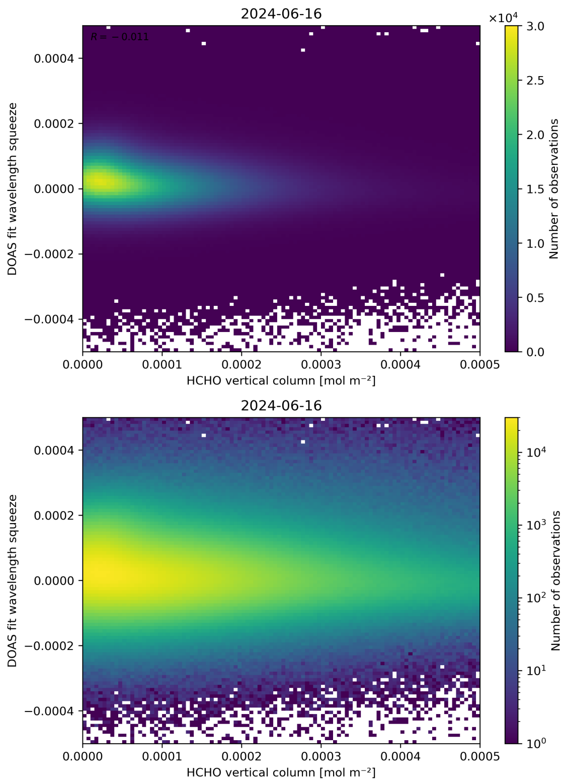
Figure 125: Scatter density plot of “HCHO vertical column” against “DOAS fit wavelength squeeze” for 2024-06-15 to 2024-06-17.
