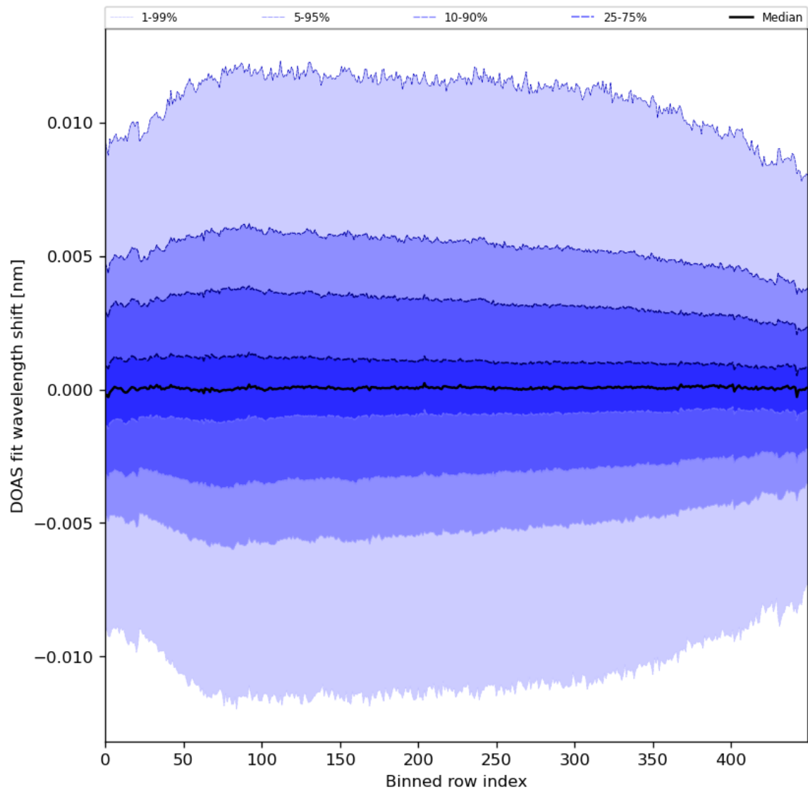
Figure 58: Along track statistics of “DOAS fit wavelength shift” for 2024-06-15 to 2024-06-17
