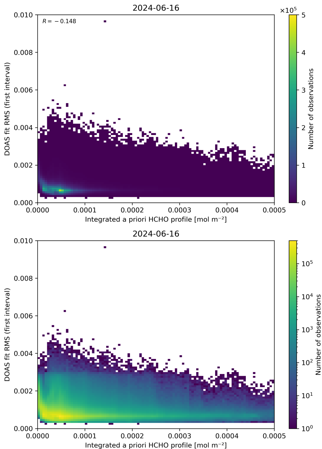
Figure 148: Scatter density plot of “Integrated a priori HCHO profile” against “DOAS fit RMS (first interval)” for 2024-06-15 to 2024-06-17.
