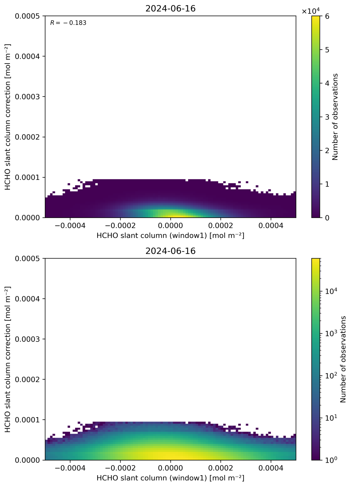
Figure 83: Scatter density plot of “HCHO slant column (window1)” against “HCHO slant column correction” for 2024-06-15 to 2024-06-17.
