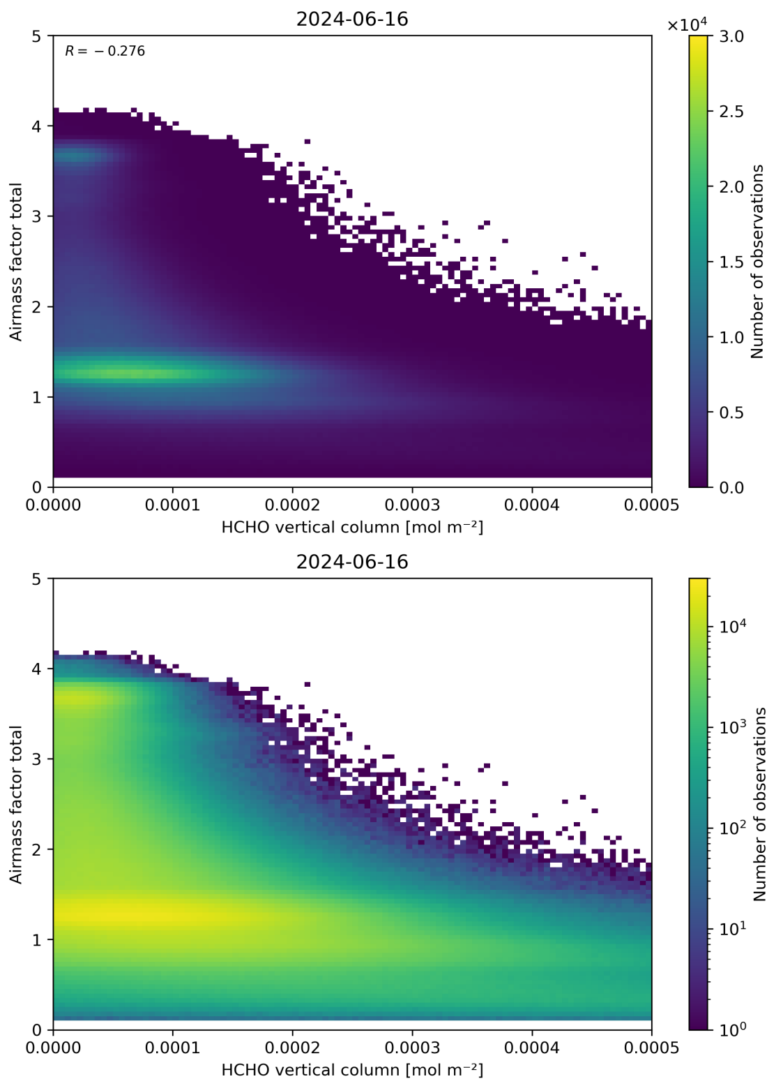
Figure 131: Scatter density plot of “HCHO vertical column” against “Airmass factor total” for 2024-06-15 to 2024-06-17.
