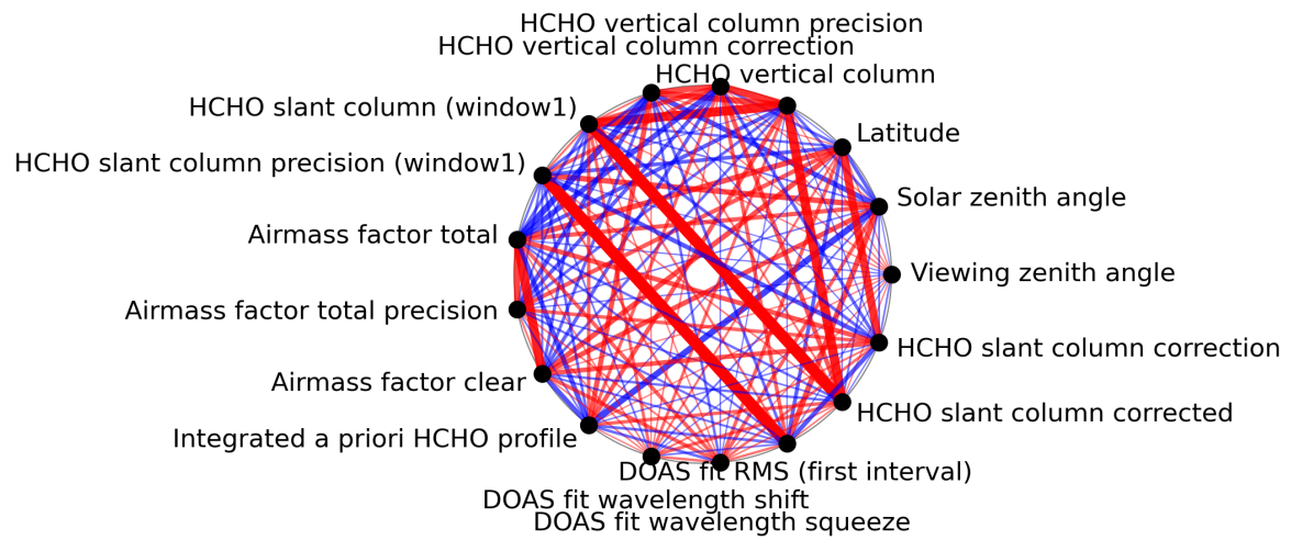
Figure 1: Map of correlation graph for 2024-06-15 to 2024-06-17.
