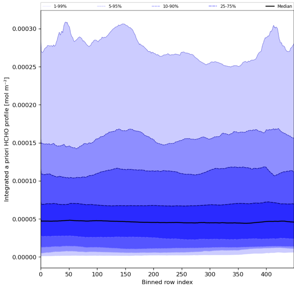
Figure 57: Along track statistics of "Integrated a priori HCHO profile" for 2024-06-15 to 2024-06-17
