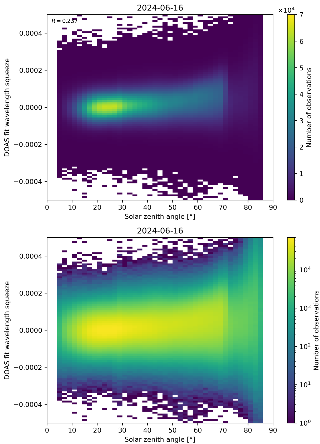
Figure 169: Scatter density plot of “Solar zenith angle” against “DOAS fit wavelength squeeze” for 2024-06-15 to 2024-06-17.
