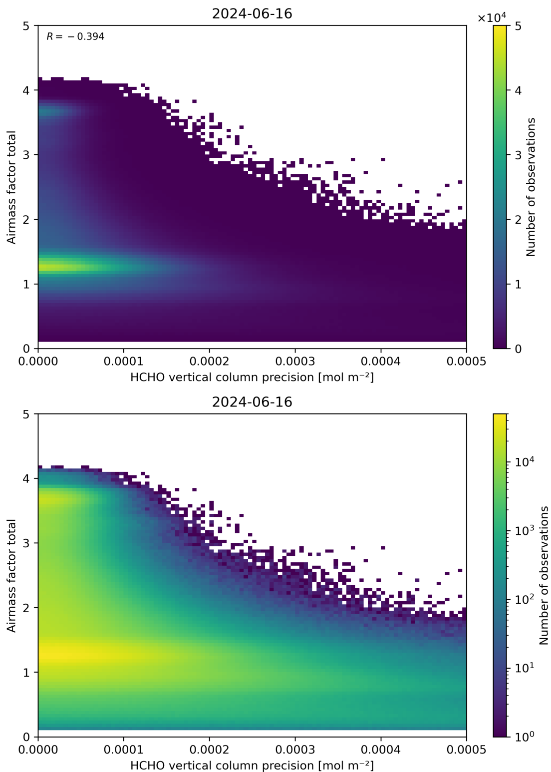
Figure 144: Scatter density plot of “HCHO vertical column precision” against “Airmass factor total” for 2024-06-15 to 2024-06-17.
