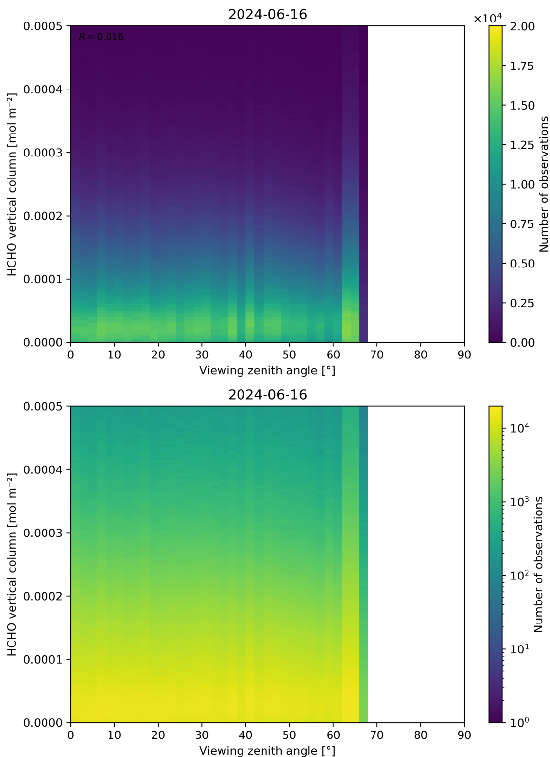
Figure 192: Scatter density plot of “Viewing zenith angle” against “HCHO vertical column” for 2024-06-15 to 2024-06-17.
