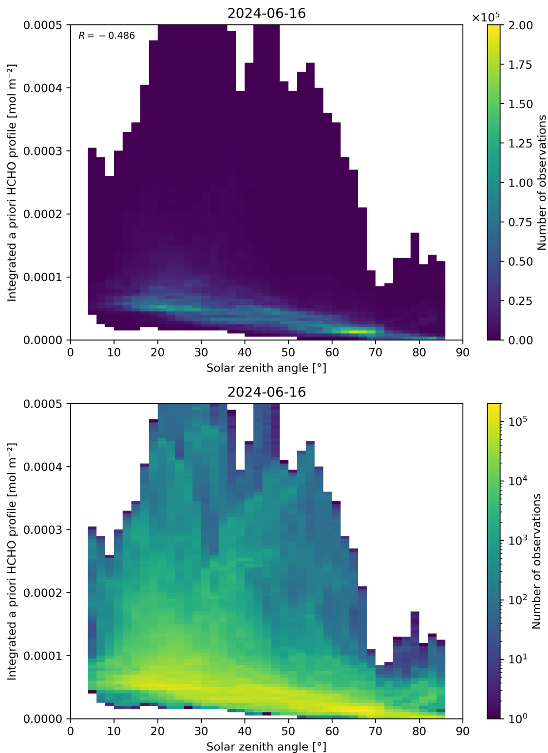
Figure 180: Scatter density plot of “Solar zenith angle” against “Integrated a priori HCHO profile” for 2024-06-15 to 2024-06-17.
