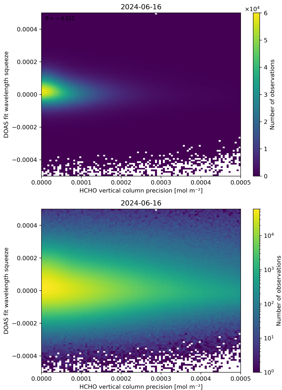
Figure 138: Scatter density plot of “HCHO vertical column precision” against “DOAS fit wavelength squeeze” for 2024-06-15 to 2024-06-17.
