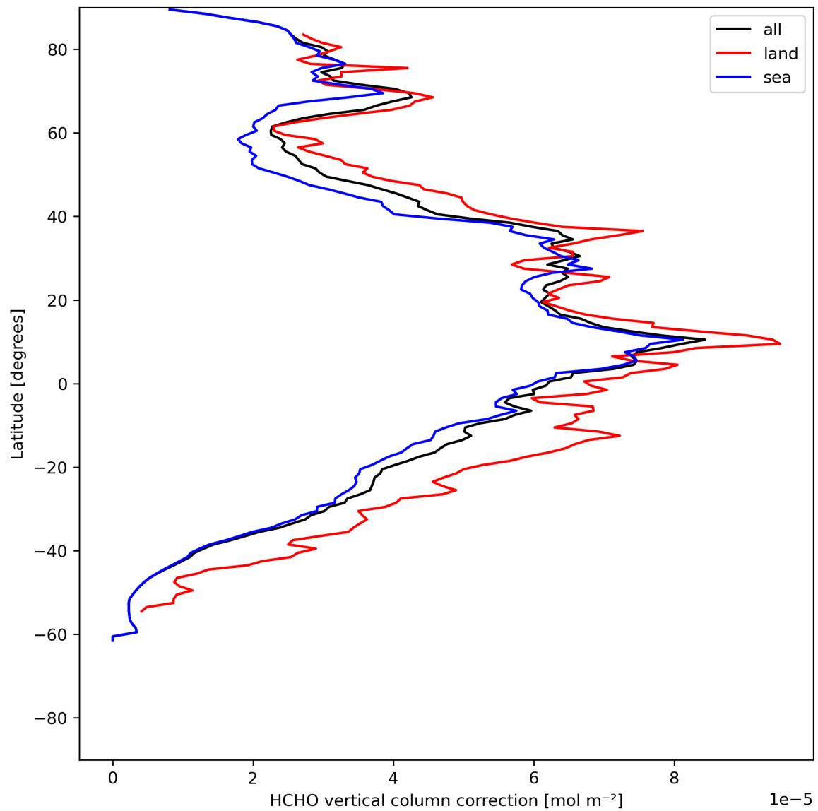
Figure 23: Zonal average of “HCHO vertical column correction” for 2024-06-15 to 2024-06-17.
