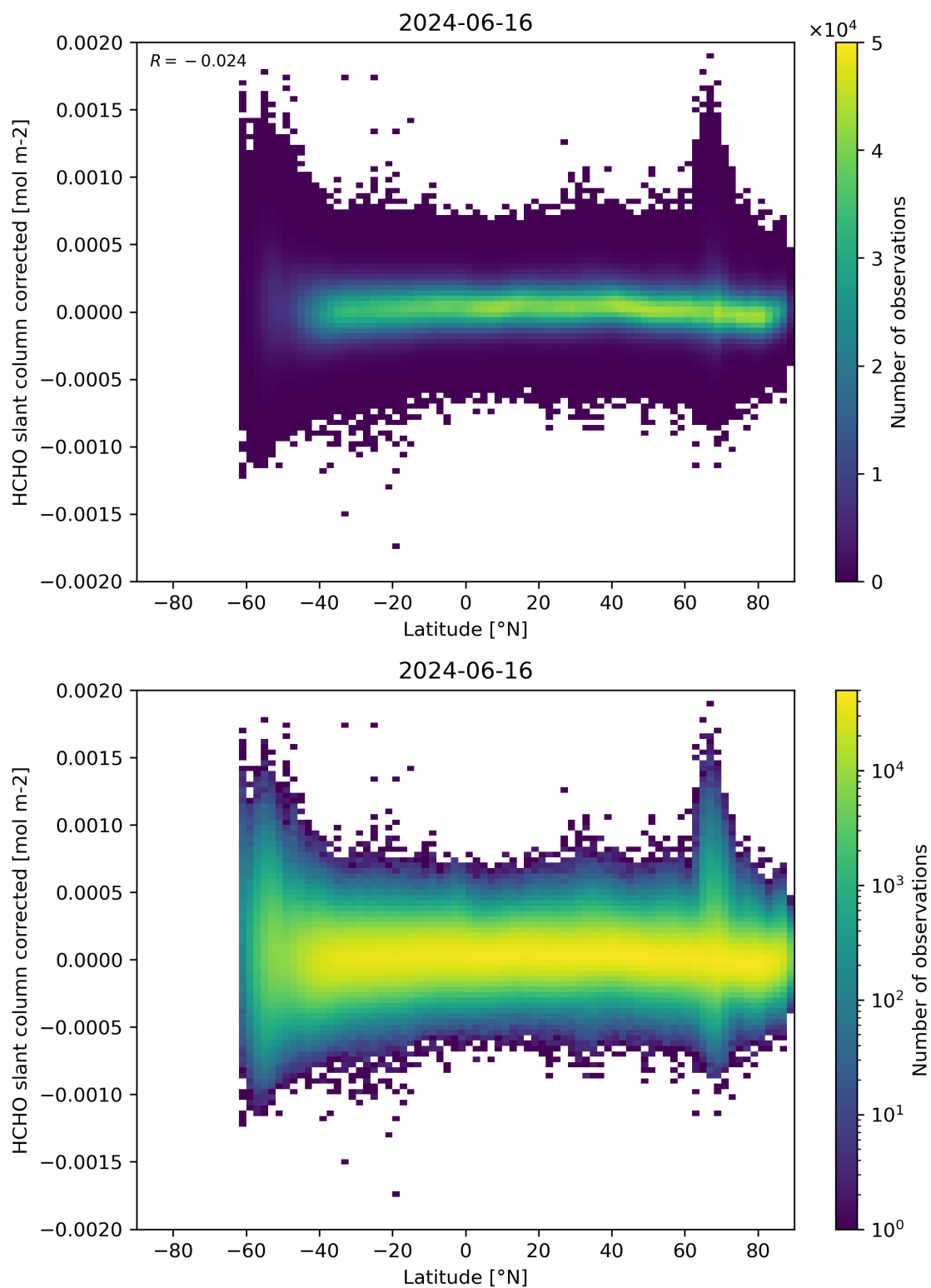
Figure 157: Scatter density plot of “Latitude” against “HCHO slant column corrected” for 2024-06-15 to 2024-06-17.
