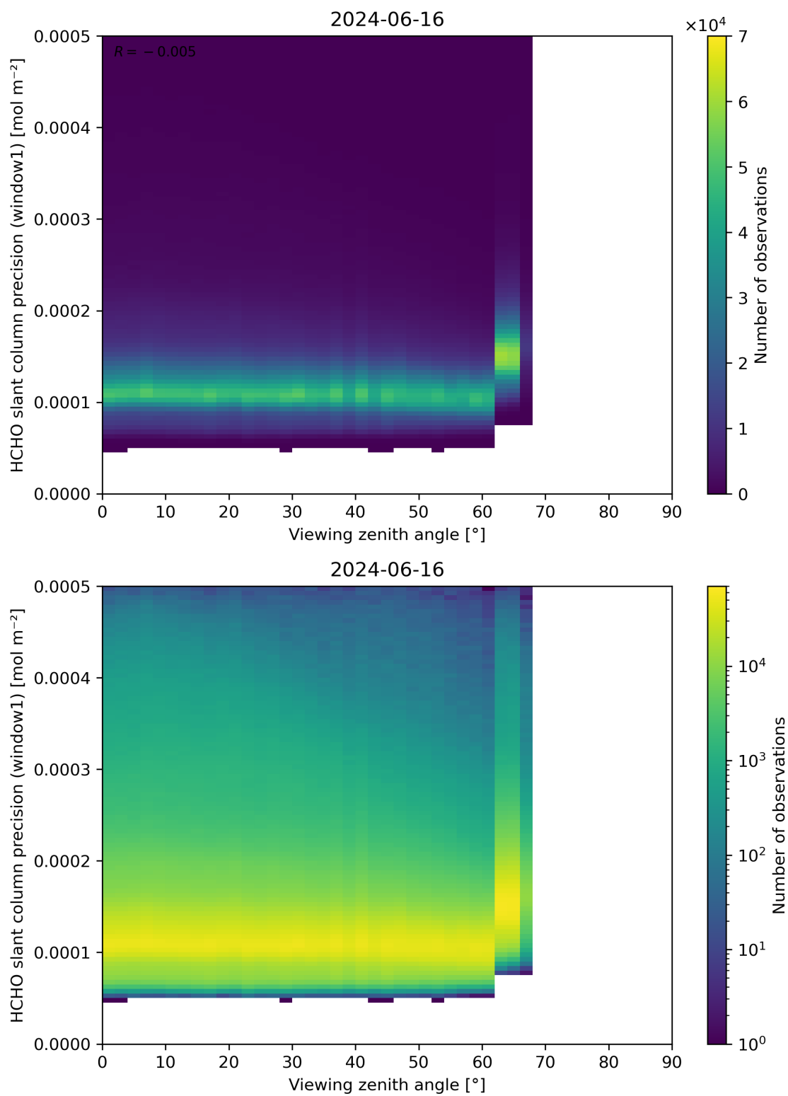
Figure 189: Scatter density plot of “Viewing zenith angle” against “HCHO slant column precision (window1)” for 2024-06-15 to 2024-06-17.
