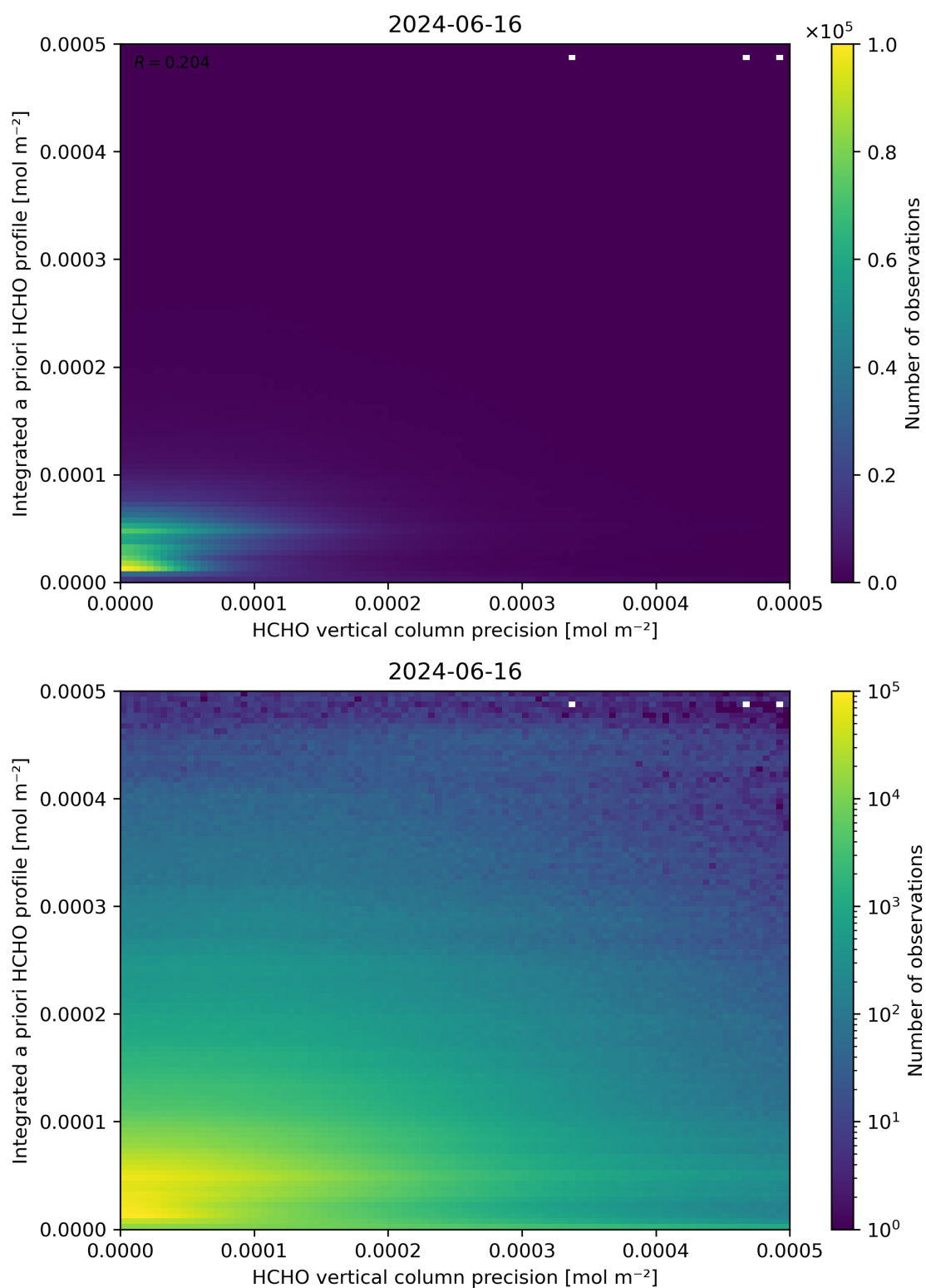
Figure 147: Scatter density plot of “HCHO vertical column precision” against “Integrated a priori HCHO profile” for 2024-06-15 to 2024-06-17.
