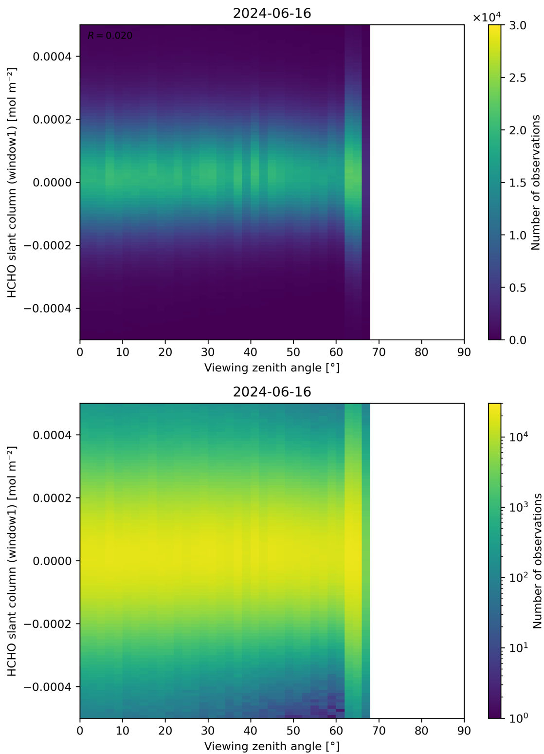
Figure 188: Scatter density plot of “Viewing zenith angle” against “HCHO slant column (window1)” for 2024-06-15 to 2024-06-17.
