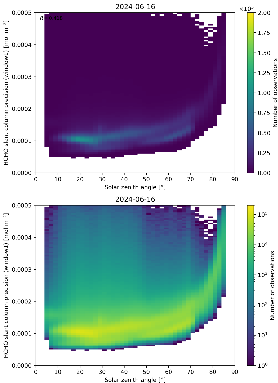
Figure 174: Scatter density plot of “Solar zenith angle” against “HCHO slant column precision (window1)” for 2024-06-15 to 2024-06-17.
