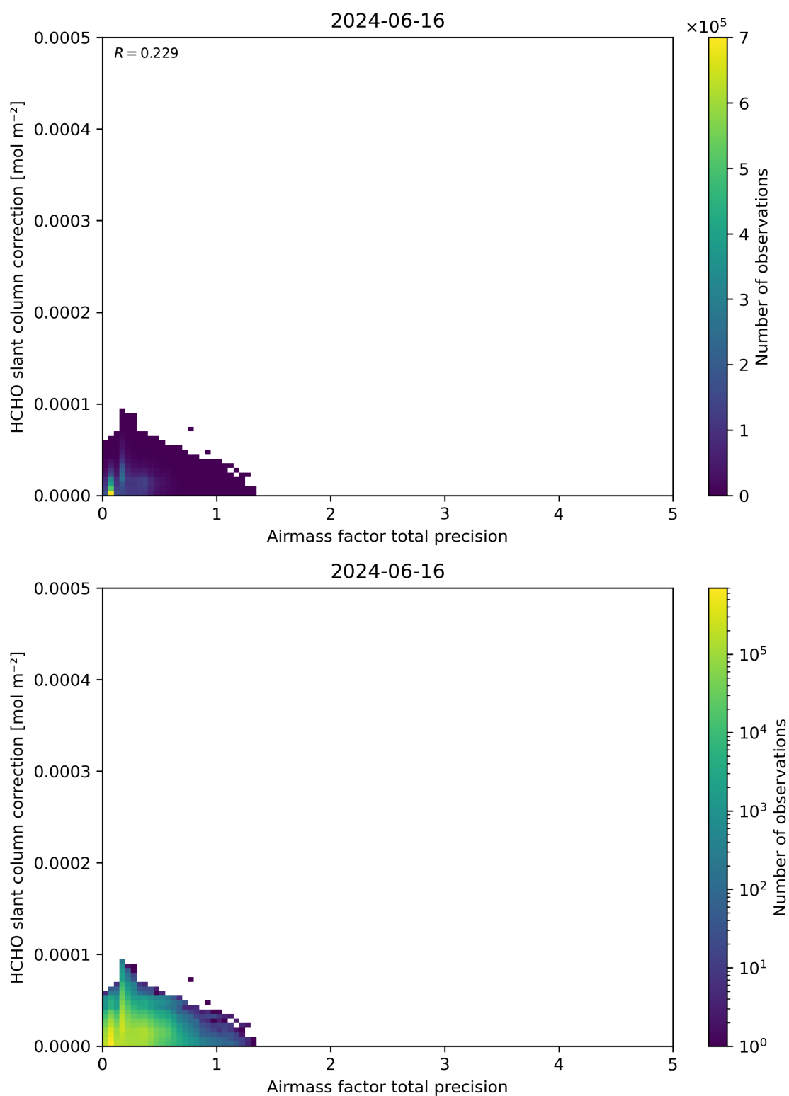
Figure 110: Scatter density plot of “Airmass factor total precision” against “HCHO slant column correction” for 2024-06-15 to 2024-06-17.
