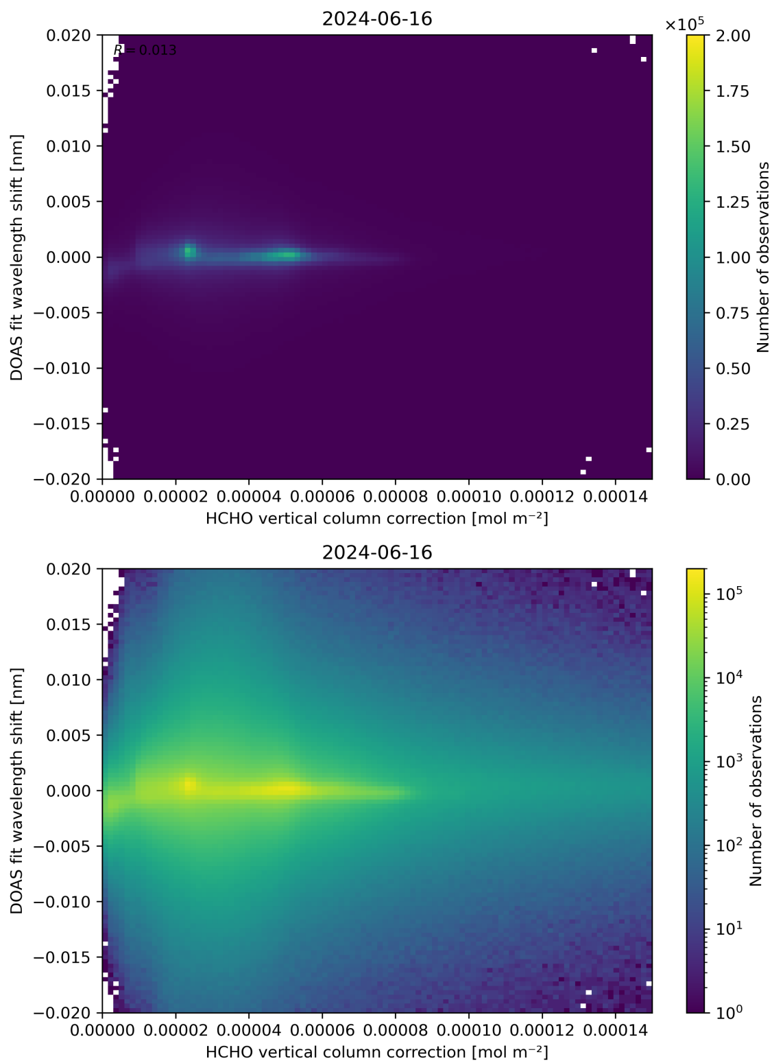
Figure 113: Scatter density plot of “HCHO vertical column correction” against “DOAS fit wavelength shift” for 2024-06-15 to 2024-06-17.
