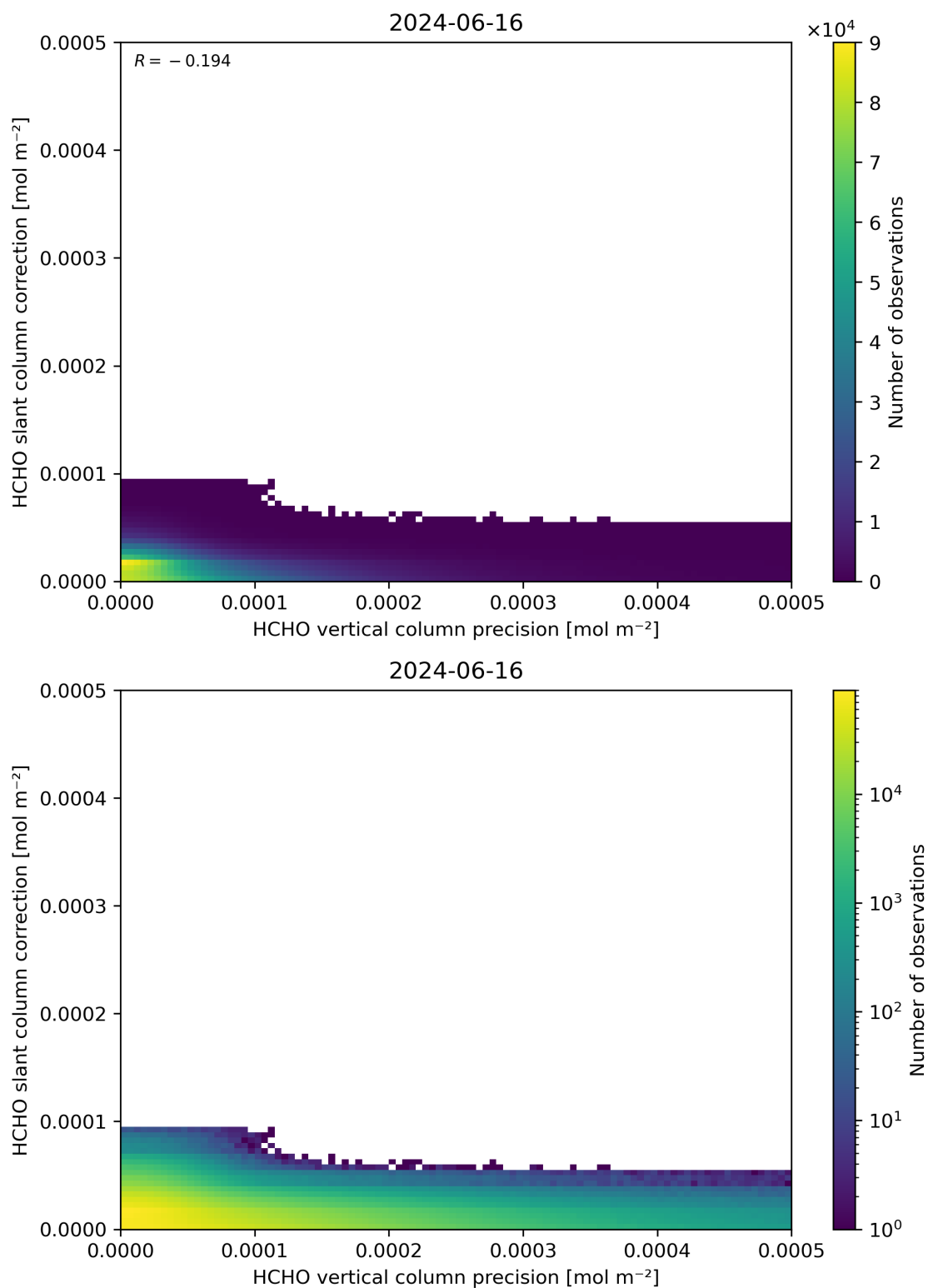
Figure 141: Scatter density plot of “HCHO vertical column precision” against “HCHO slant column correction” for 2024-06-15 to 2024-06-17.
