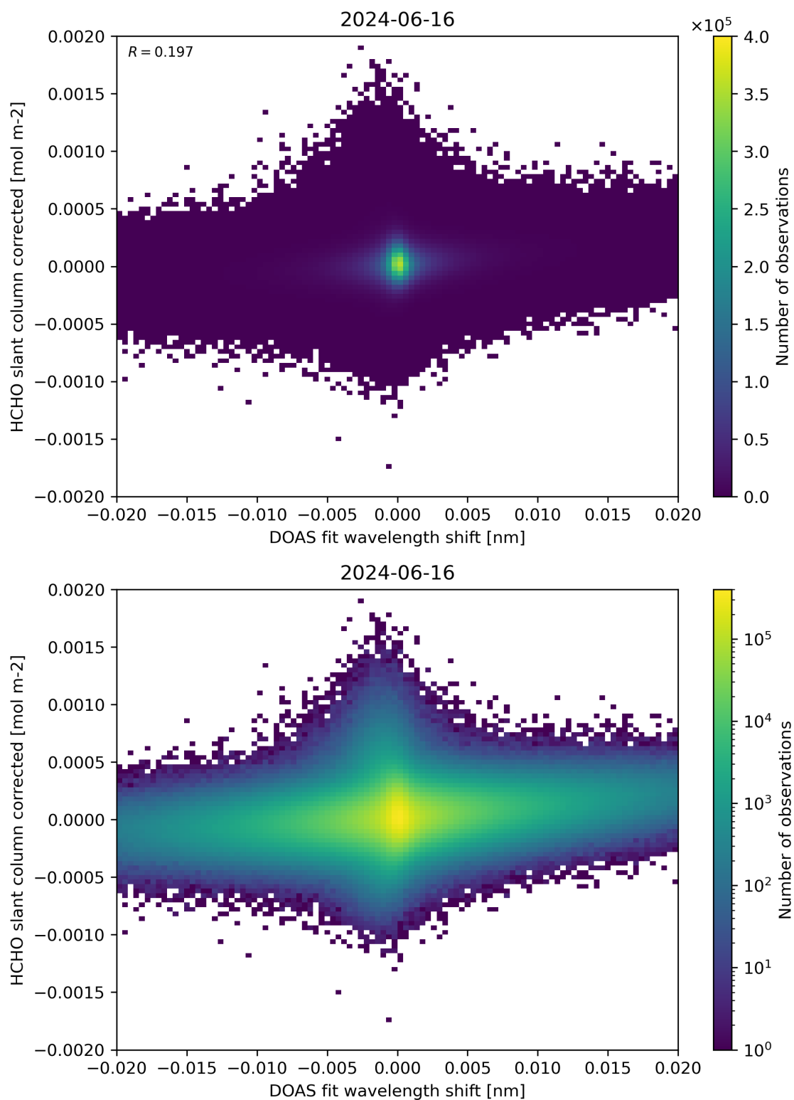
Figure 66: Scatter density plot of “DOAS fit wavelength shift” against “HCHO slant column corrected” for 2024-06-15 to 2024-06-17.
