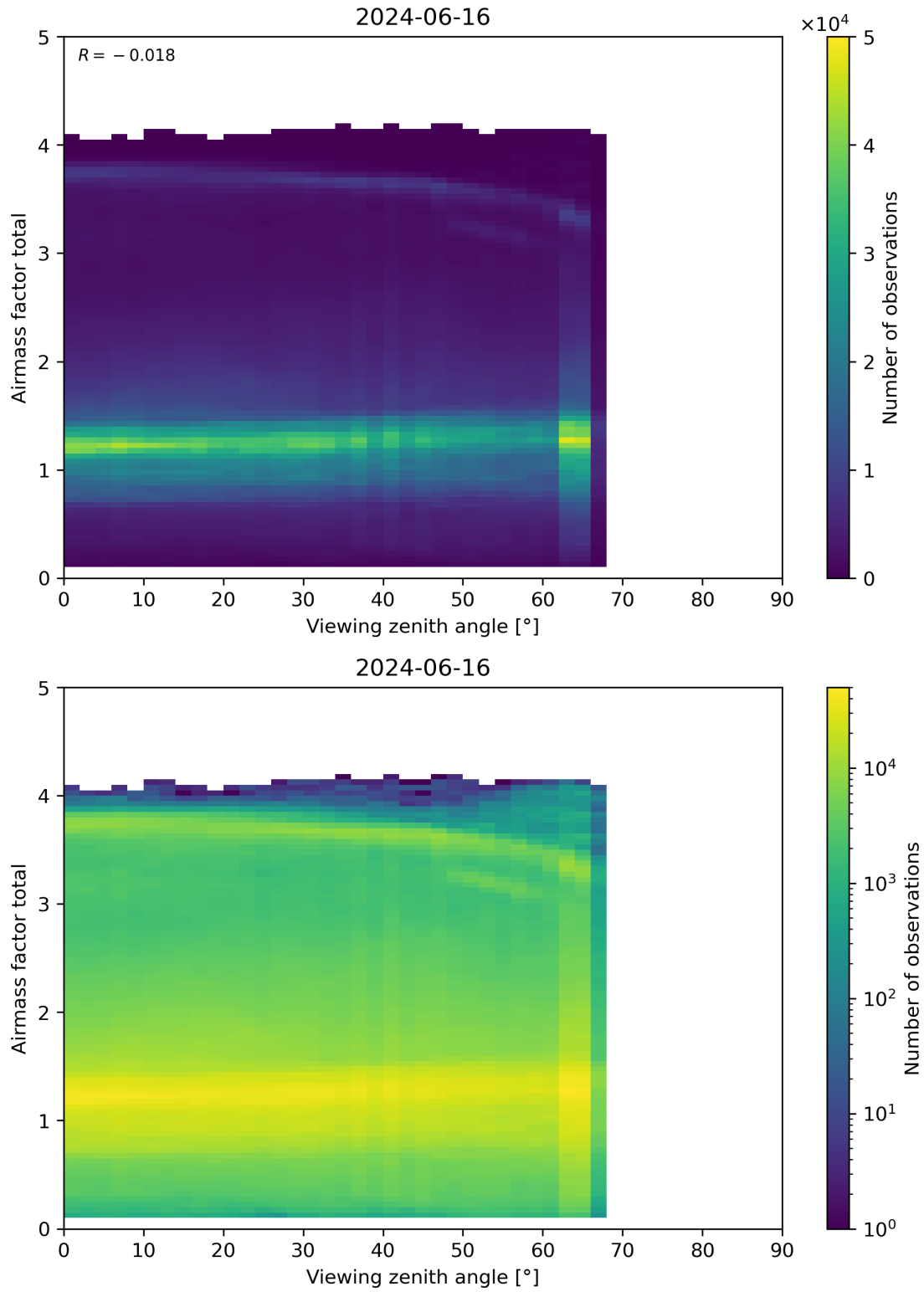
Figure 190: Scatter density plot of “Viewing zenith angle” against “Airmass factor total” for 2024-06-15 to 2024-06-17.
