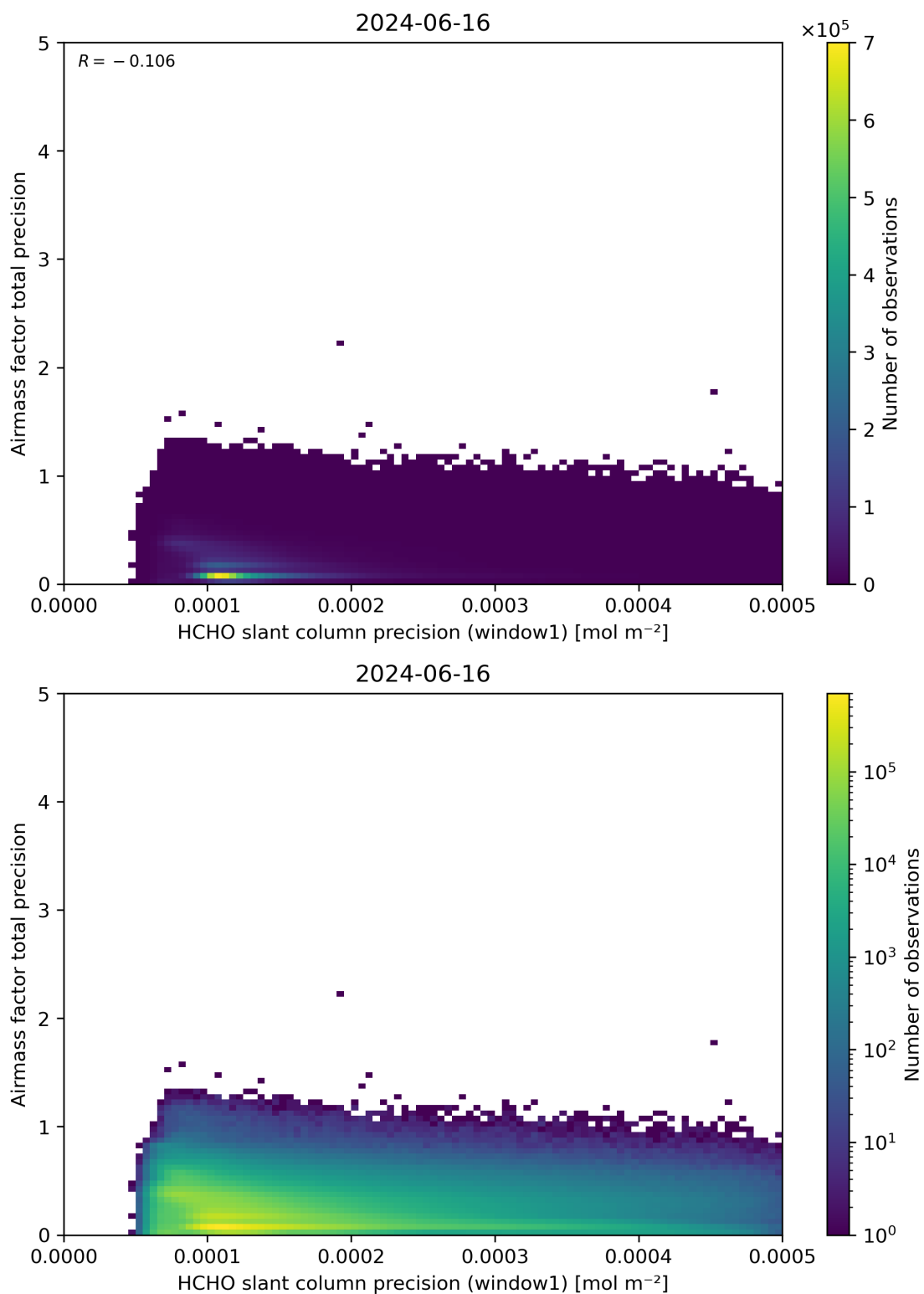
Figure 95: Scatter density plot of “HCHO slant column precision (window1)” against “Airmass factor total precision” for 2024-06-15 to 2024-06-17.
