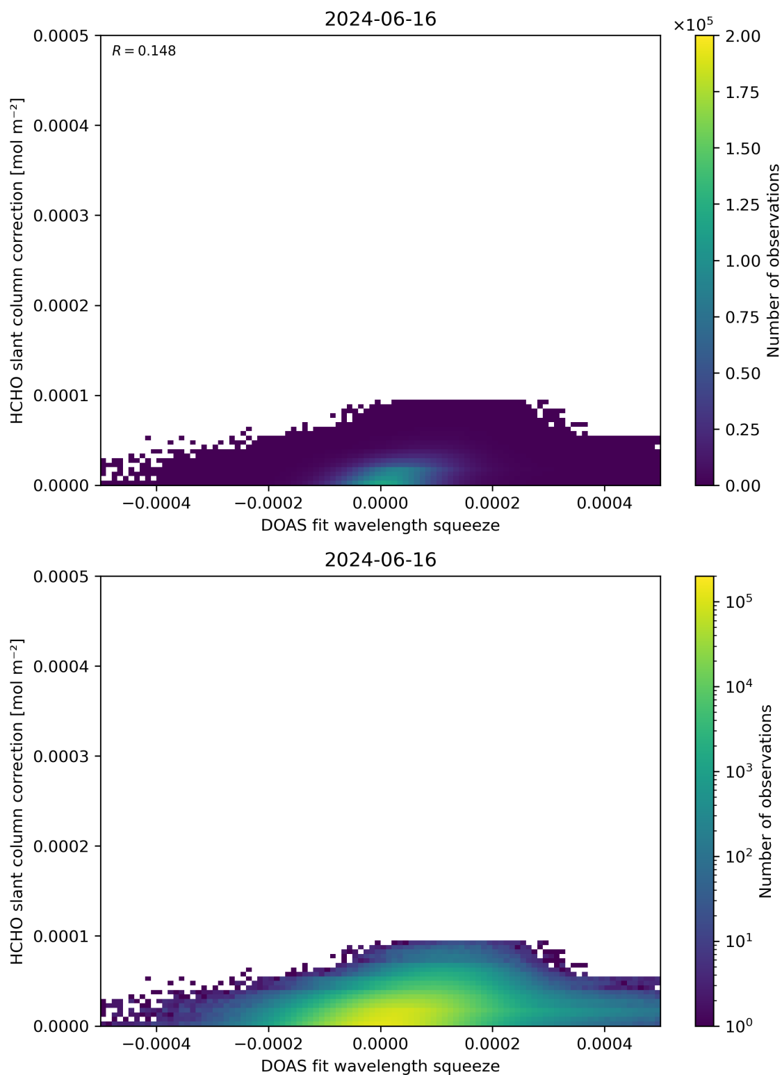
Figure 70: Scatter density plot of “DOAS fit wavelength squeeze” against “HCHO slant column correction” for 2024-06-15 to 2024-06-17.
