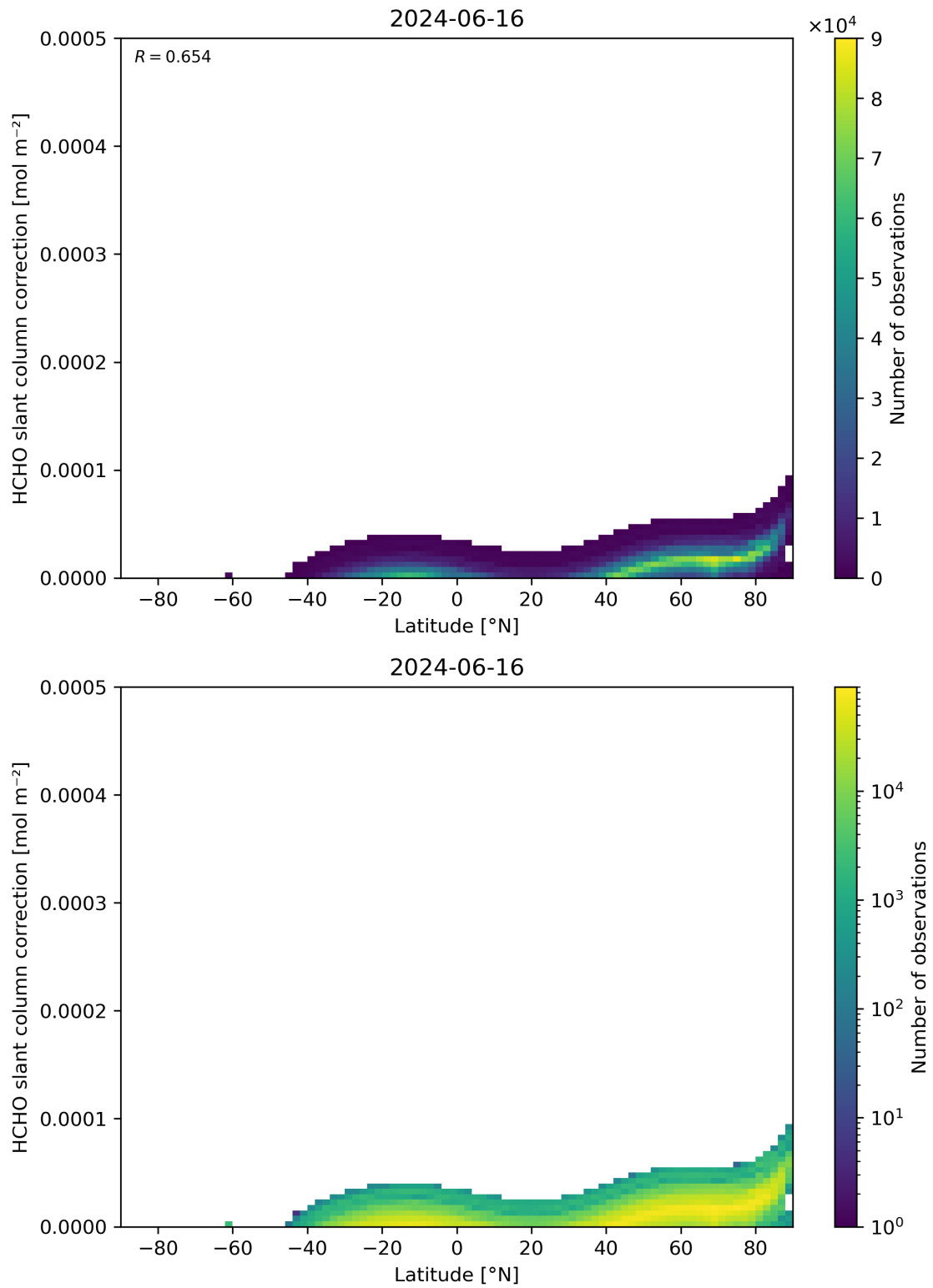
Figure 158: Scatter density plot of “Latitude” against “HCHO slant column correction” for 2024-06-15 to 2024-06-17.
