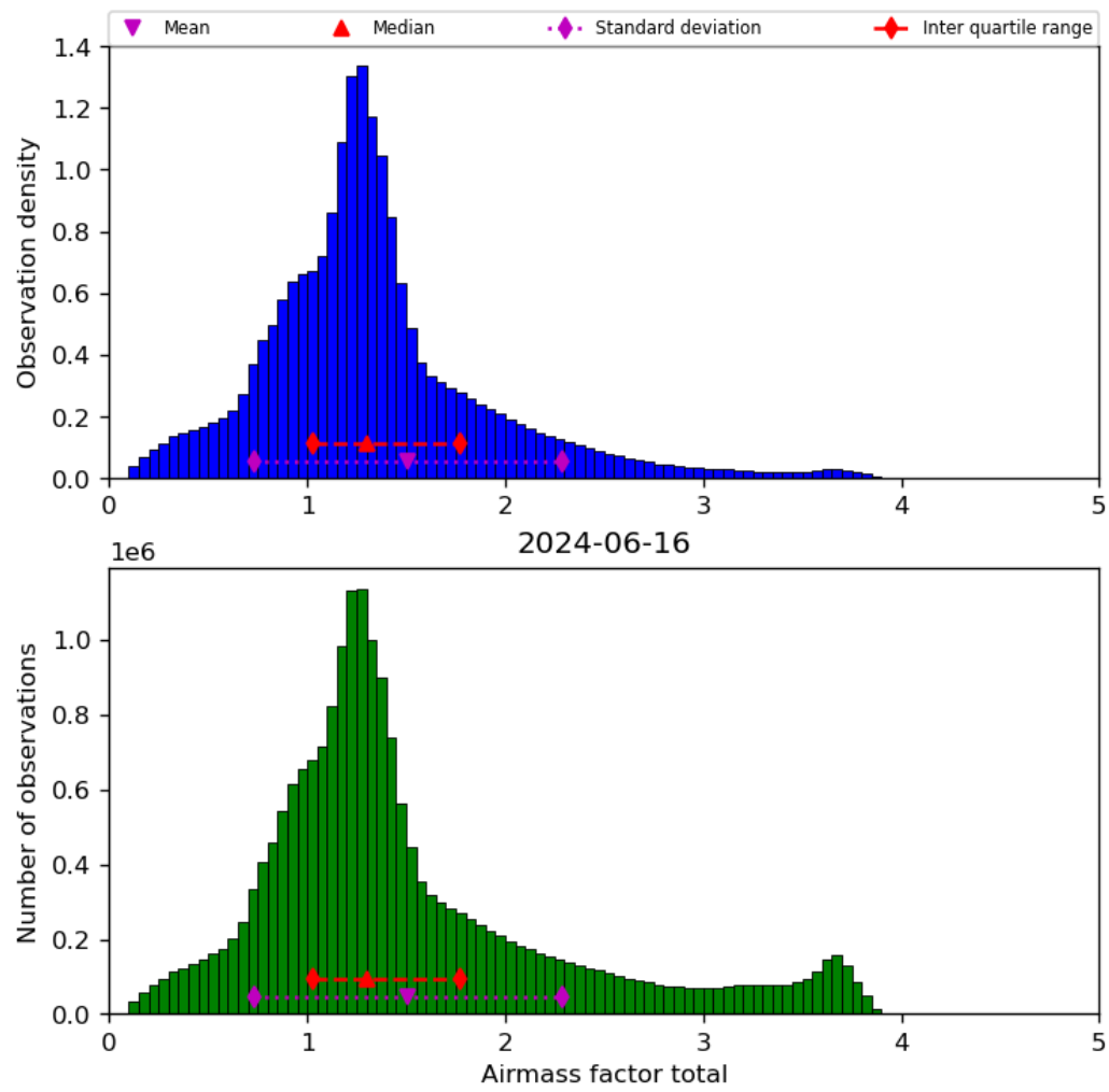
Figure 40: Histogram of “Airmass factor total” for 2024-06-15 to 2024-06-17
