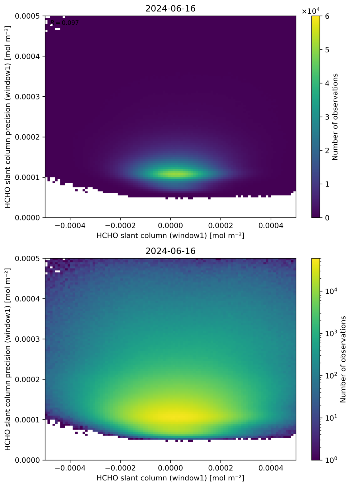
Figure 84: Scatter density plot of “HCHO slant column (window1)” against “HCHO slant column precision (window1)” for 2024-06-15 to 2024-06-17.
