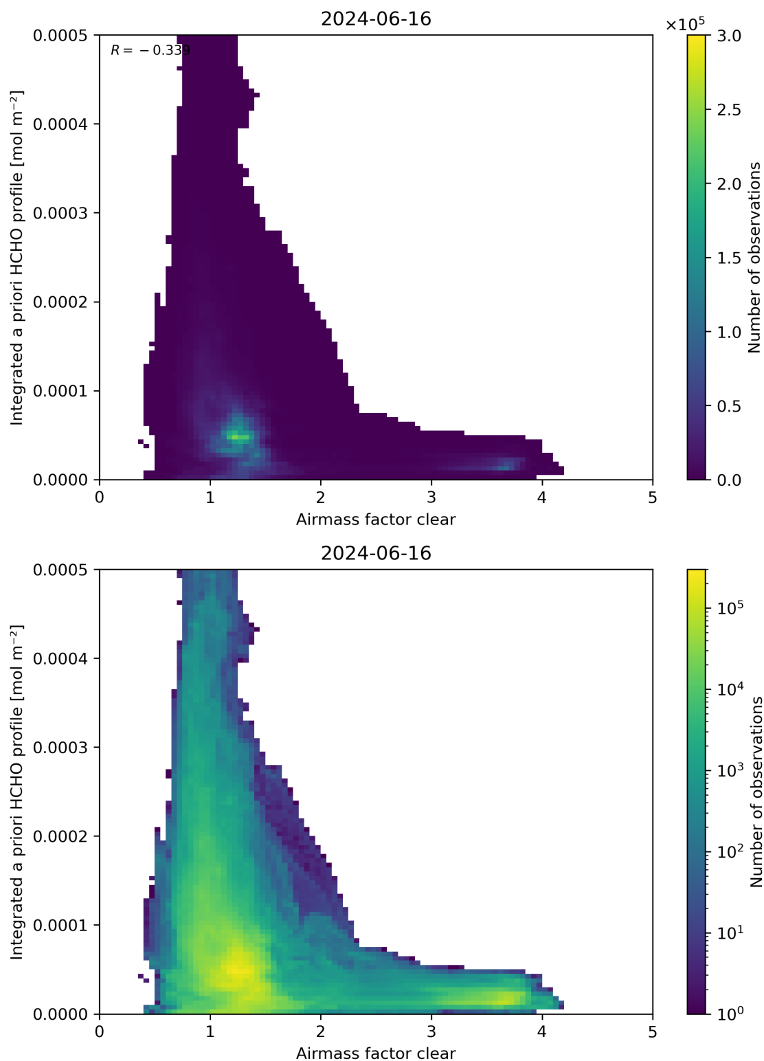
Figure 76: Scatter density plot of “Airmass factor clear” against “Integrated a priori HCHO profile” for 2024-06-15 to 2024-06-17.
