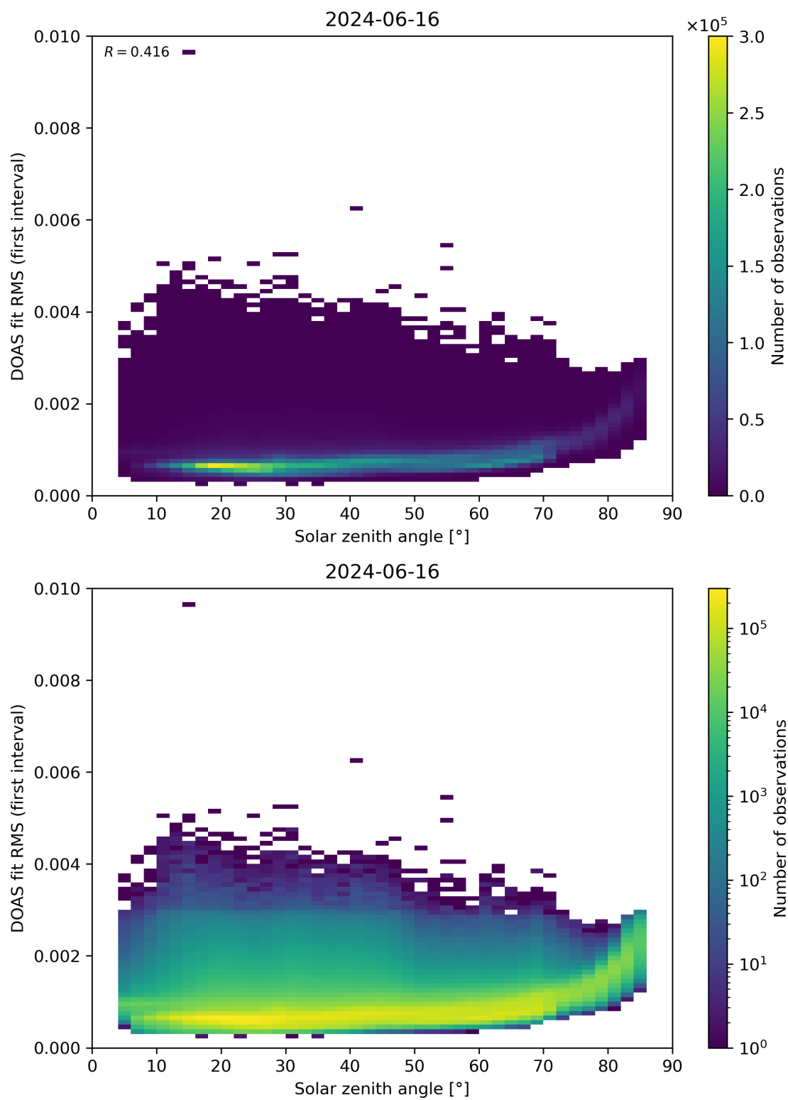
Figure 167: Scatter density plot of “Solar zenith angle” against “DOAS fit RMS (first interval)” for 2024-06-15 to 2024-06-17.
