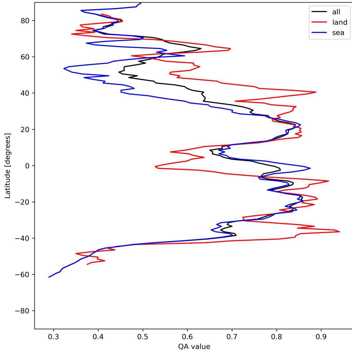
Figure 20: Zonal average of “QA value” for 2024-06-15 to 2024-06-17.
