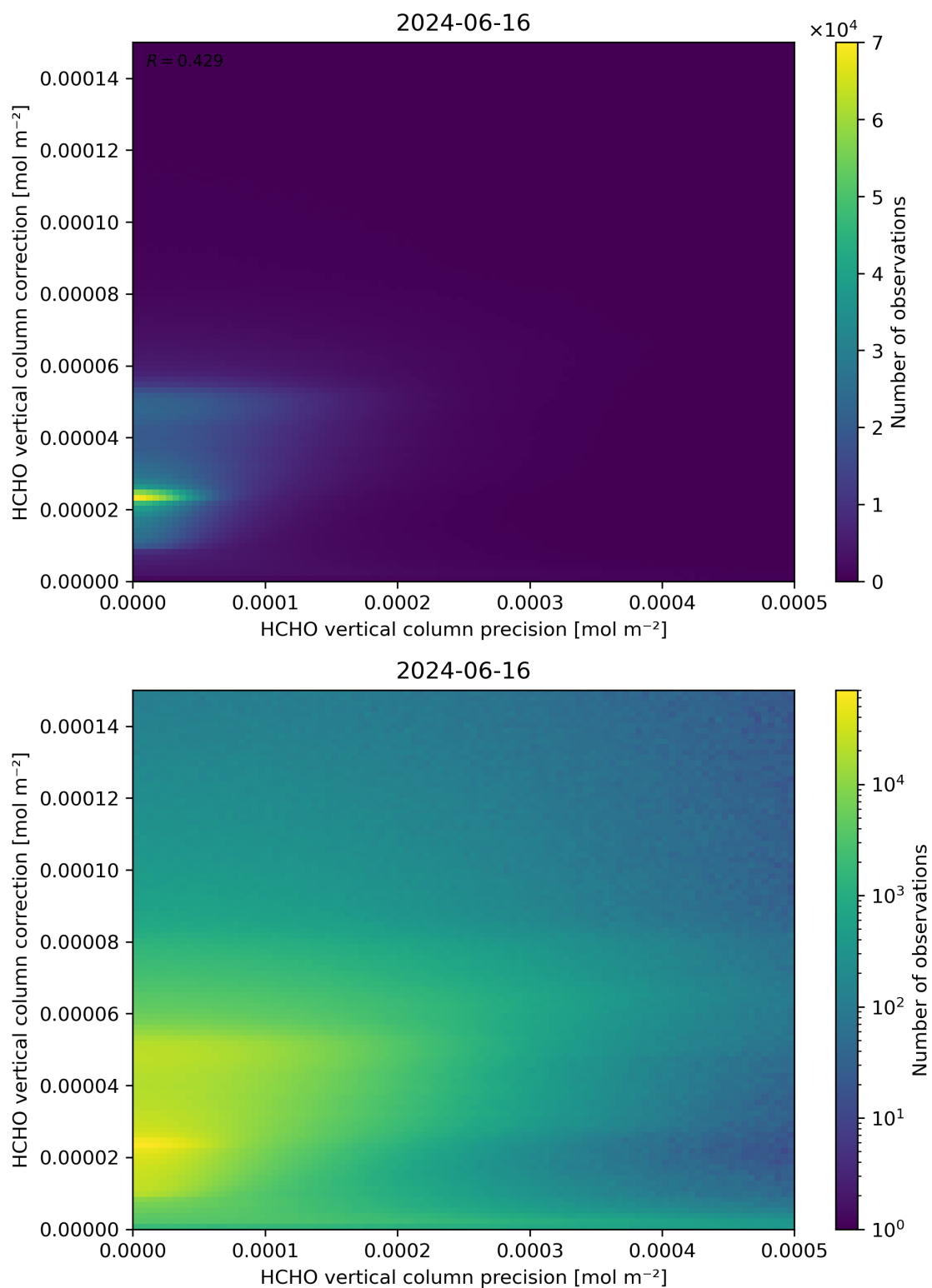
Figure 146: Scatter density plot of “HCHO vertical column precision” against “HCHO vertical column correction” for 2024-06-15 to 2024-06-17.
