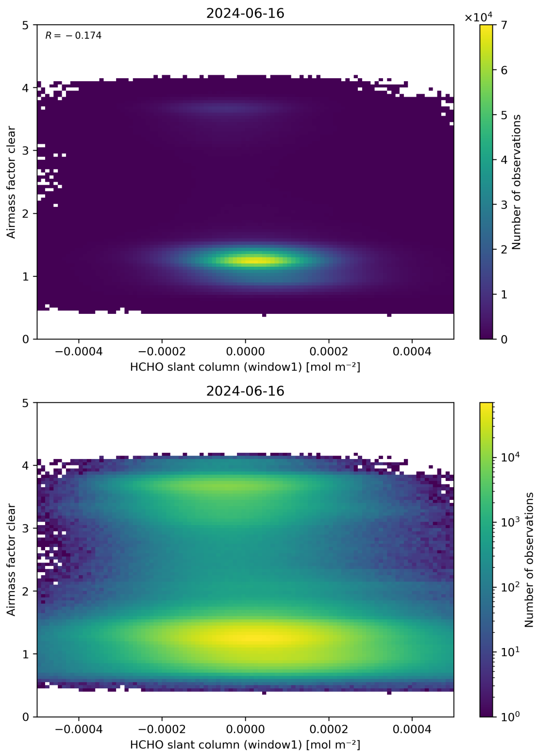
Figure 81: Scatter density plot of “HCHO slant column (window1)” against “Airmass factor clear” for 2024-06-15 to 2024-06-17.
