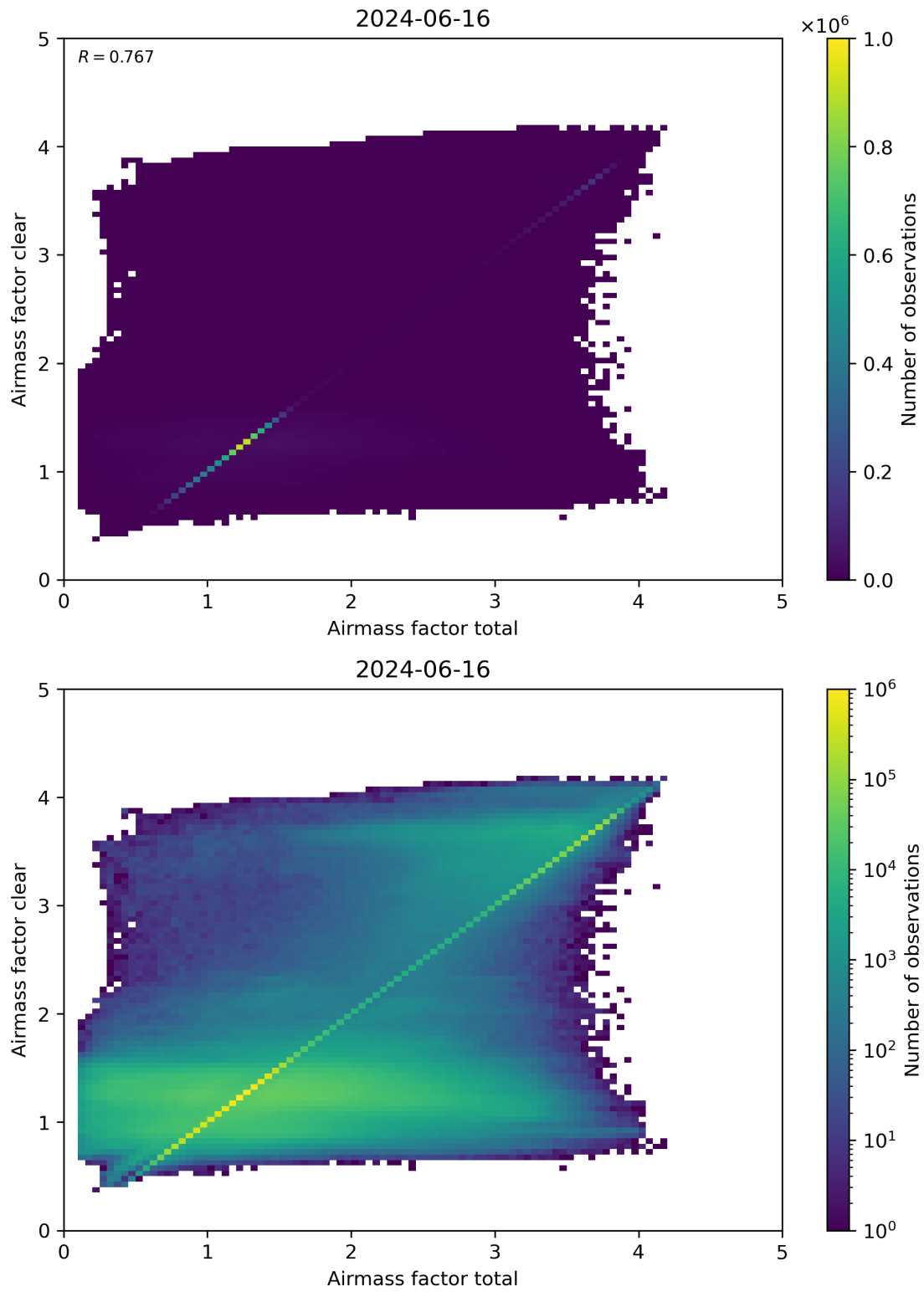
Figure 100: Scatter density plot of “Airmass factor total” against “Airmass factor clear” for 2024-06-15 to 2024-06-17.
