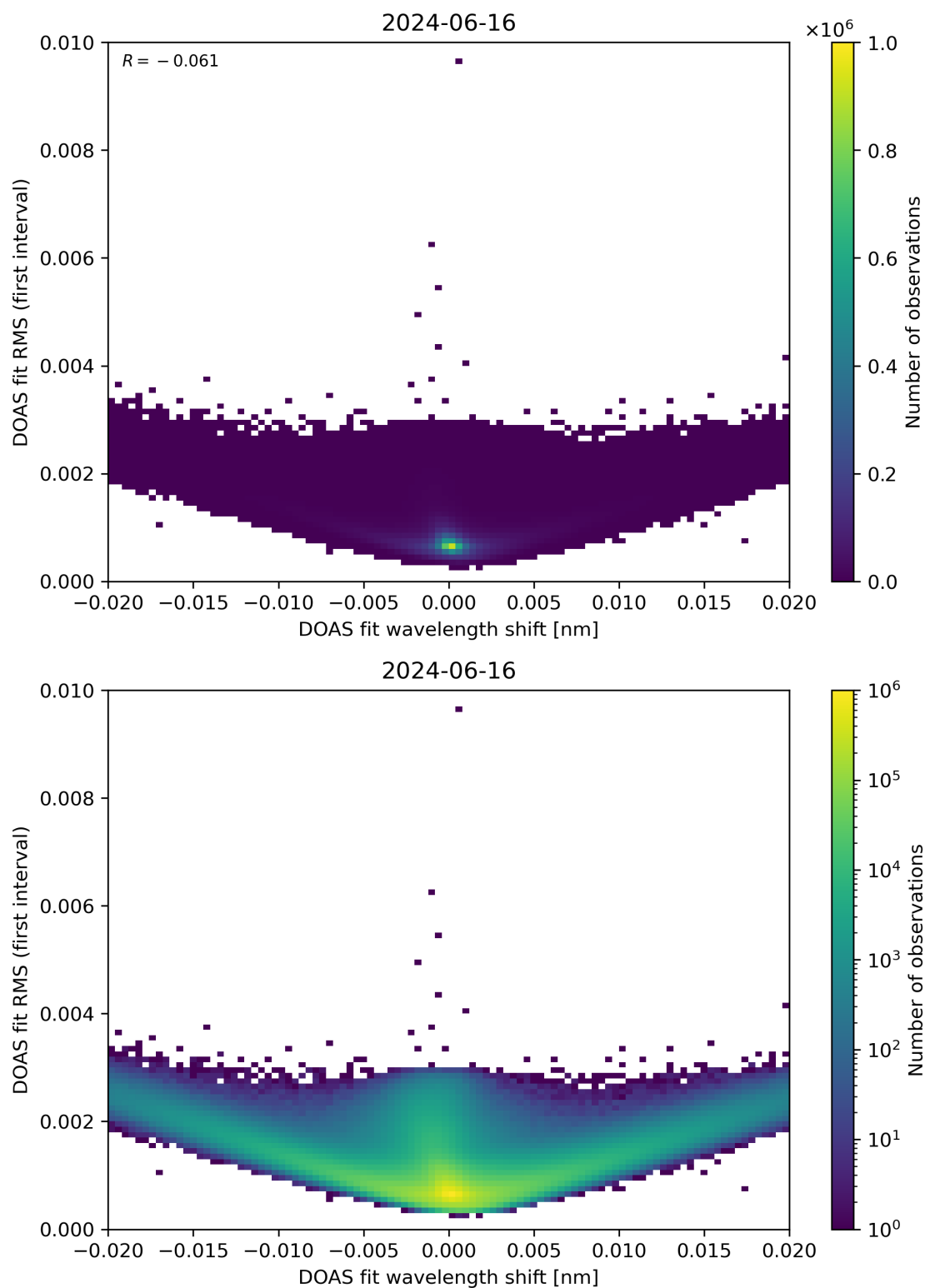
Figure 64: Scatter density plot of “DOAS fit wavelength shift” against “DOAS fit RMS (first interval)” for 2024-06-15 to 2024-06-17.
