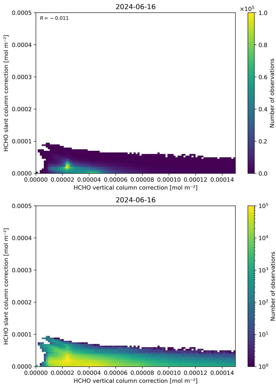
Figure 117: Scatter density plot of “HCHO vertical column correction” against “HCHO slant column correction” for 2024-06-15 to 2024-06-17.
