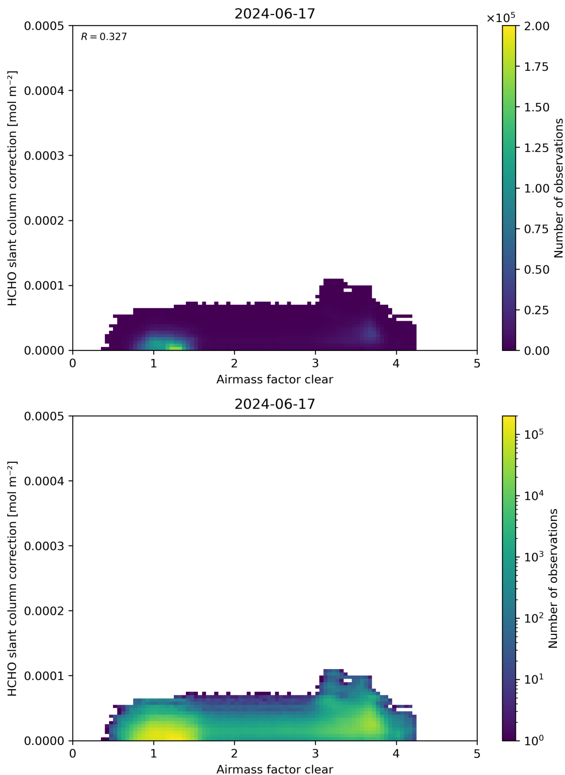
Figure 75: Scatter density plot of “Airmass factor clear” against “HCHO slant column correction” for 2024-06-16 to 2024-06-18.
