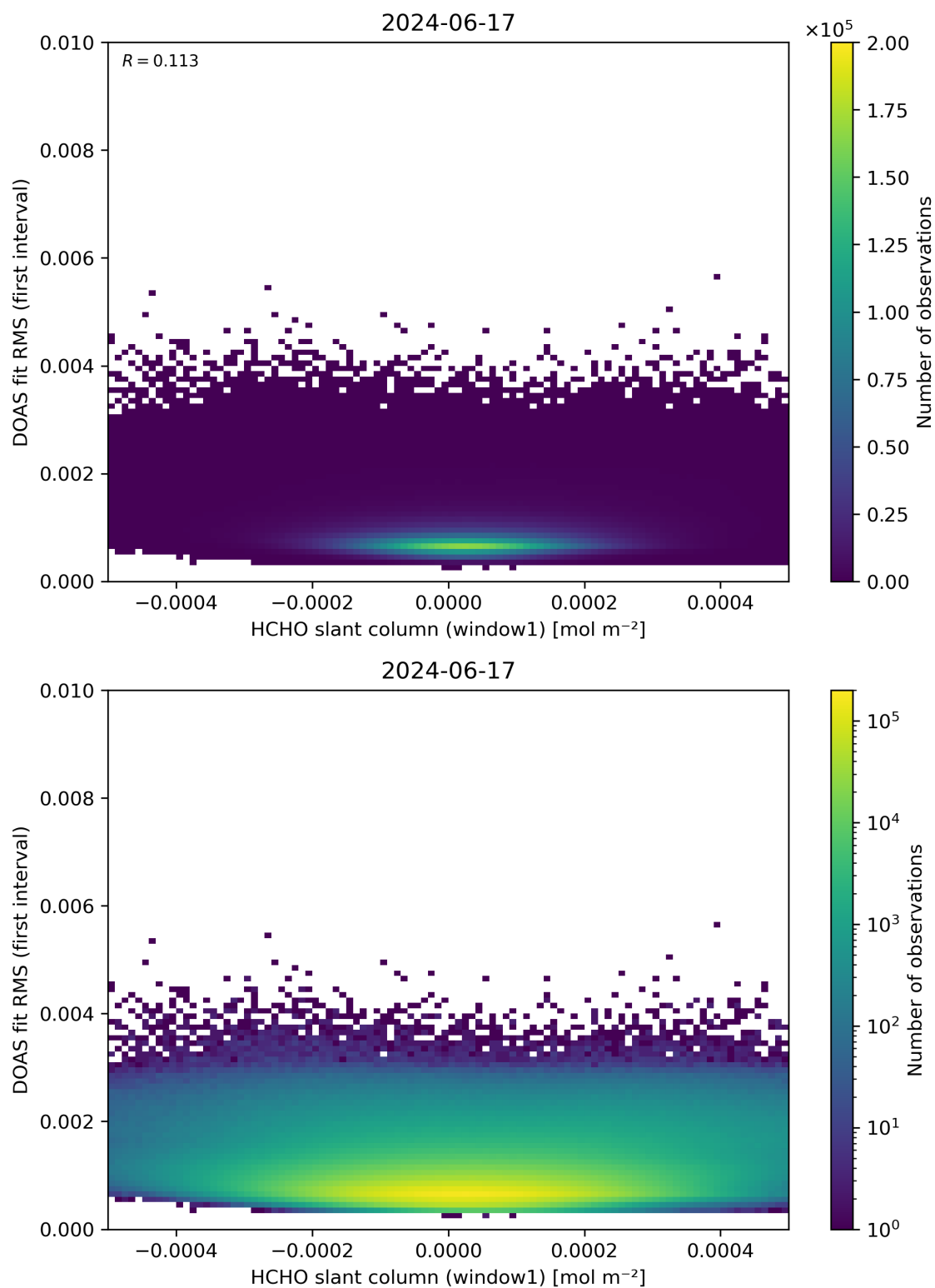
Figure 78: Scatter density plot of “HCHO slant column (window1)” against “DOAS fit RMS (first interval)” for 2024-06-16 to 2024-06-18.
