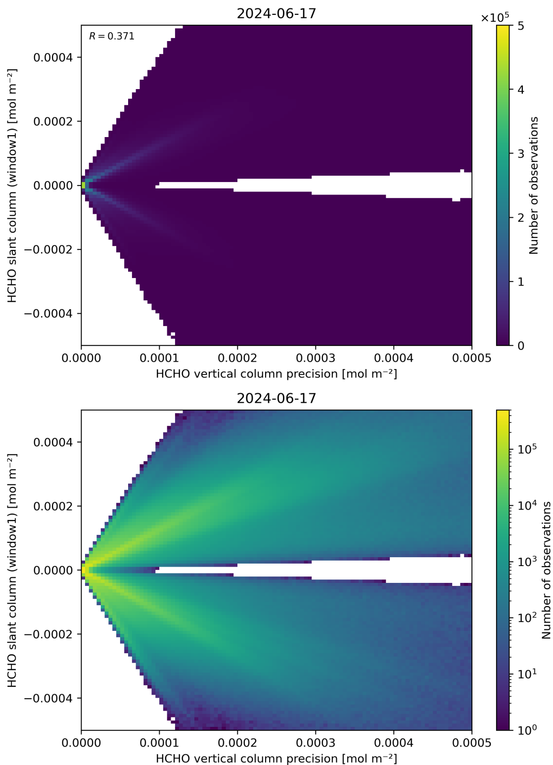
Figure 142: Scatter density plot of “HCHO vertical column precision” against “HCHO slant column (window1)” for 2024-06-16 to 2024-06-18.
