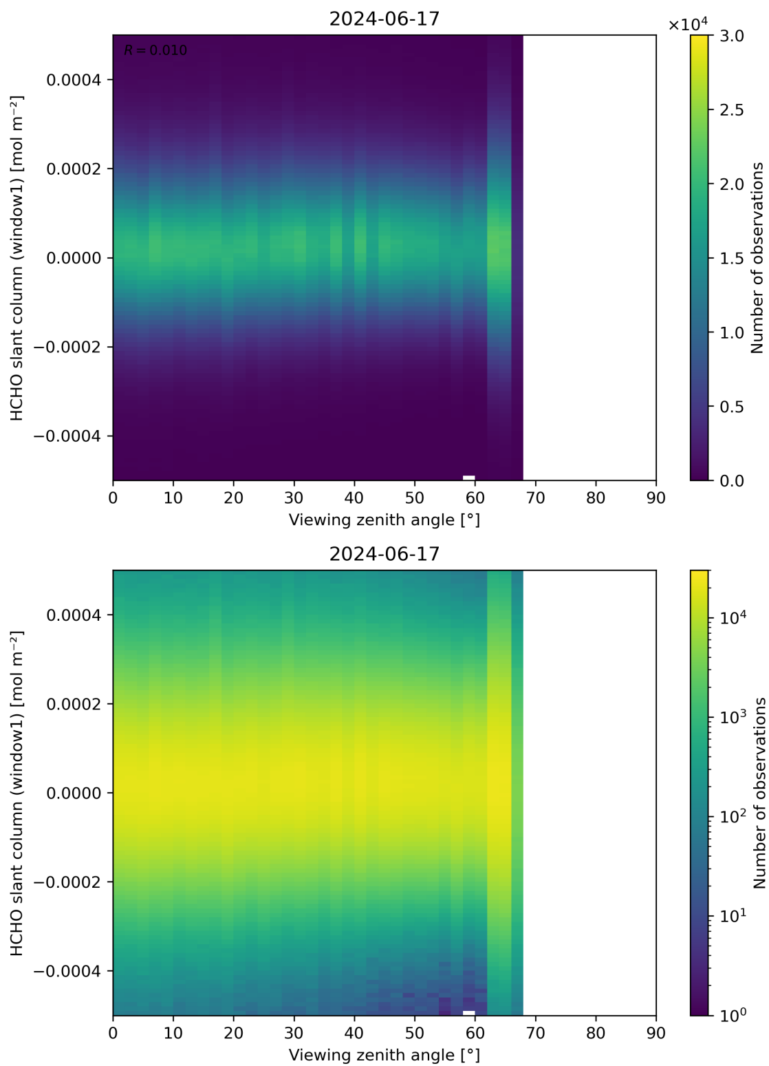
Figure 188: Scatter density plot of “Viewing zenith angle” against “HCHO slant column (window1)” for 2024-06-16 to 2024-06-18.
