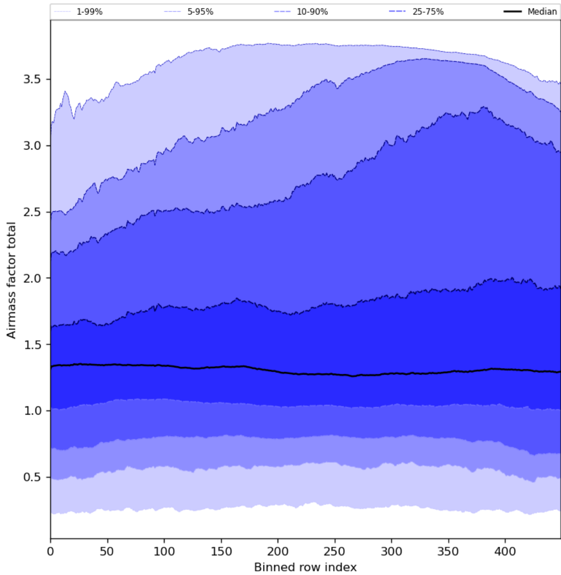
Figure 54: Along track statistics of “Airmass factor total” for 2024-06-16 to 2024-06-18
