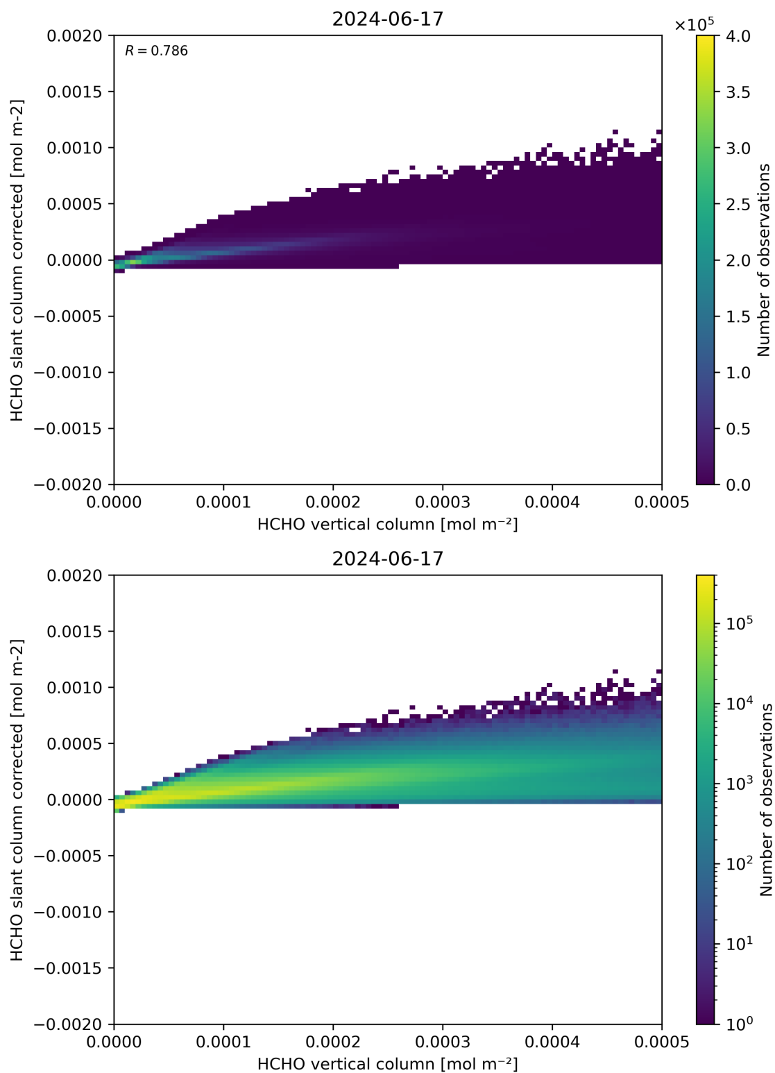
Figure 127: Scatter density plot of “HCHO vertical column” against “HCHO slant column corrected” for 2024-06-16 to 2024-06-18.
