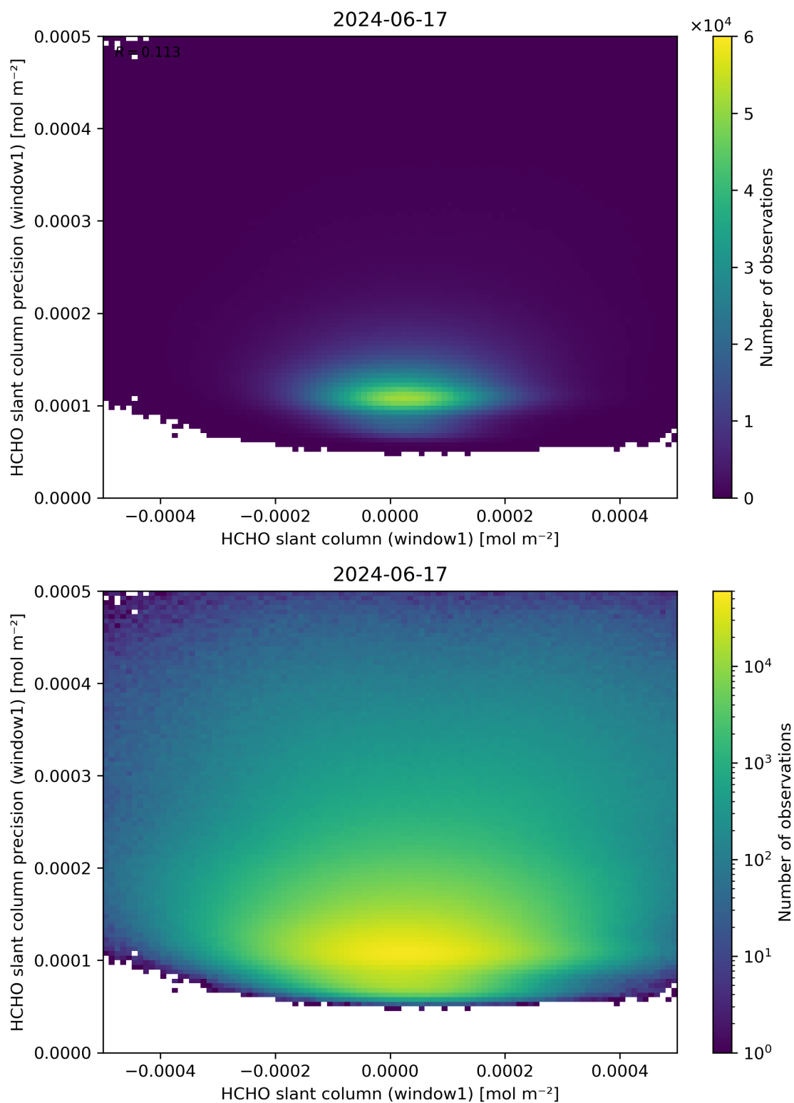
Figure 84: Scatter density plot of “HCHO slant column (window1)” against “HCHO slant column precision (window1)” for 2024-06-16 to 2024-06-18.
