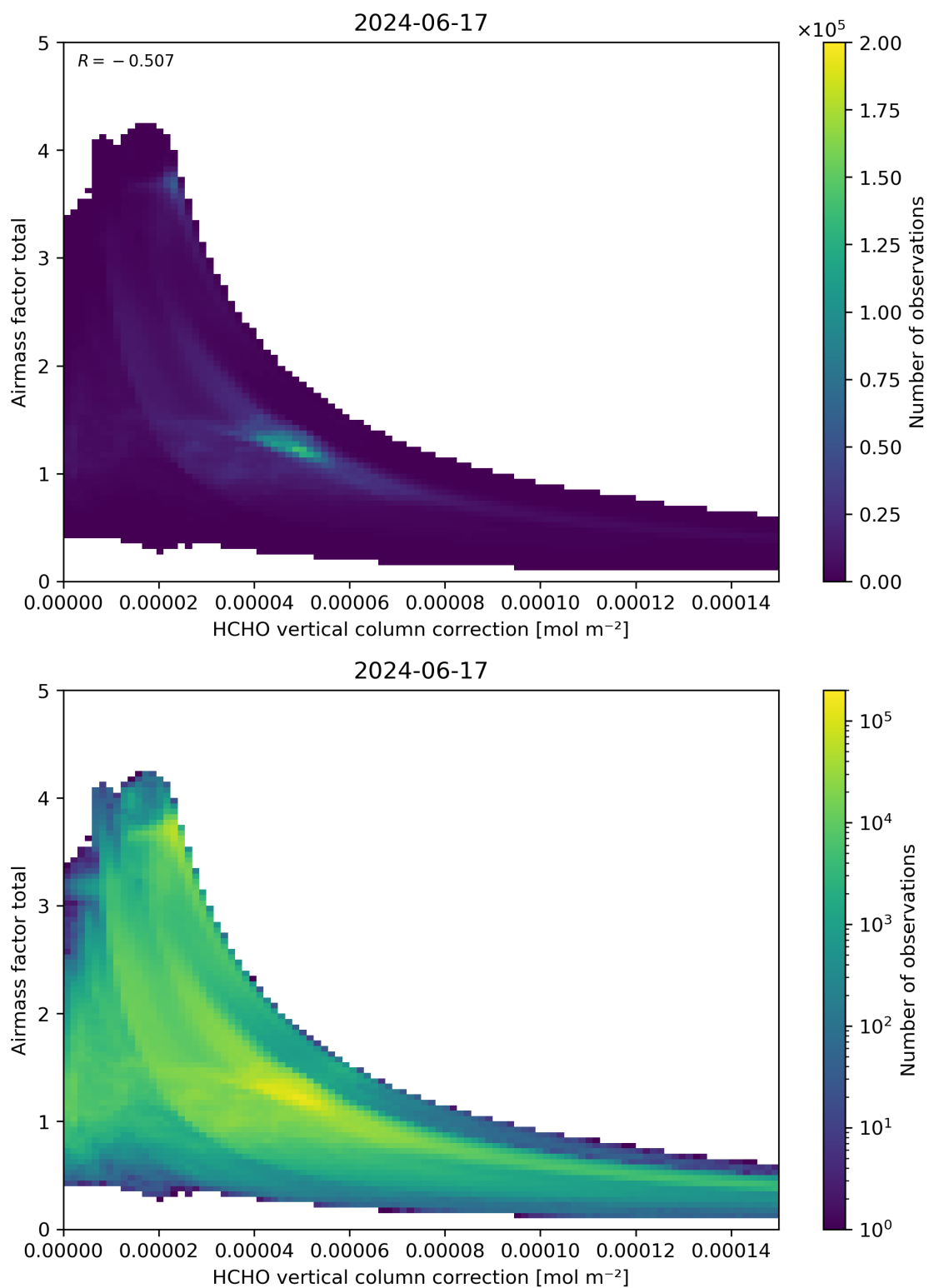
Figure 120: Scatter density plot of “HCHO vertical column correction” against “Airmass factor total” for 2024-06-16 to 2024-06-18.
