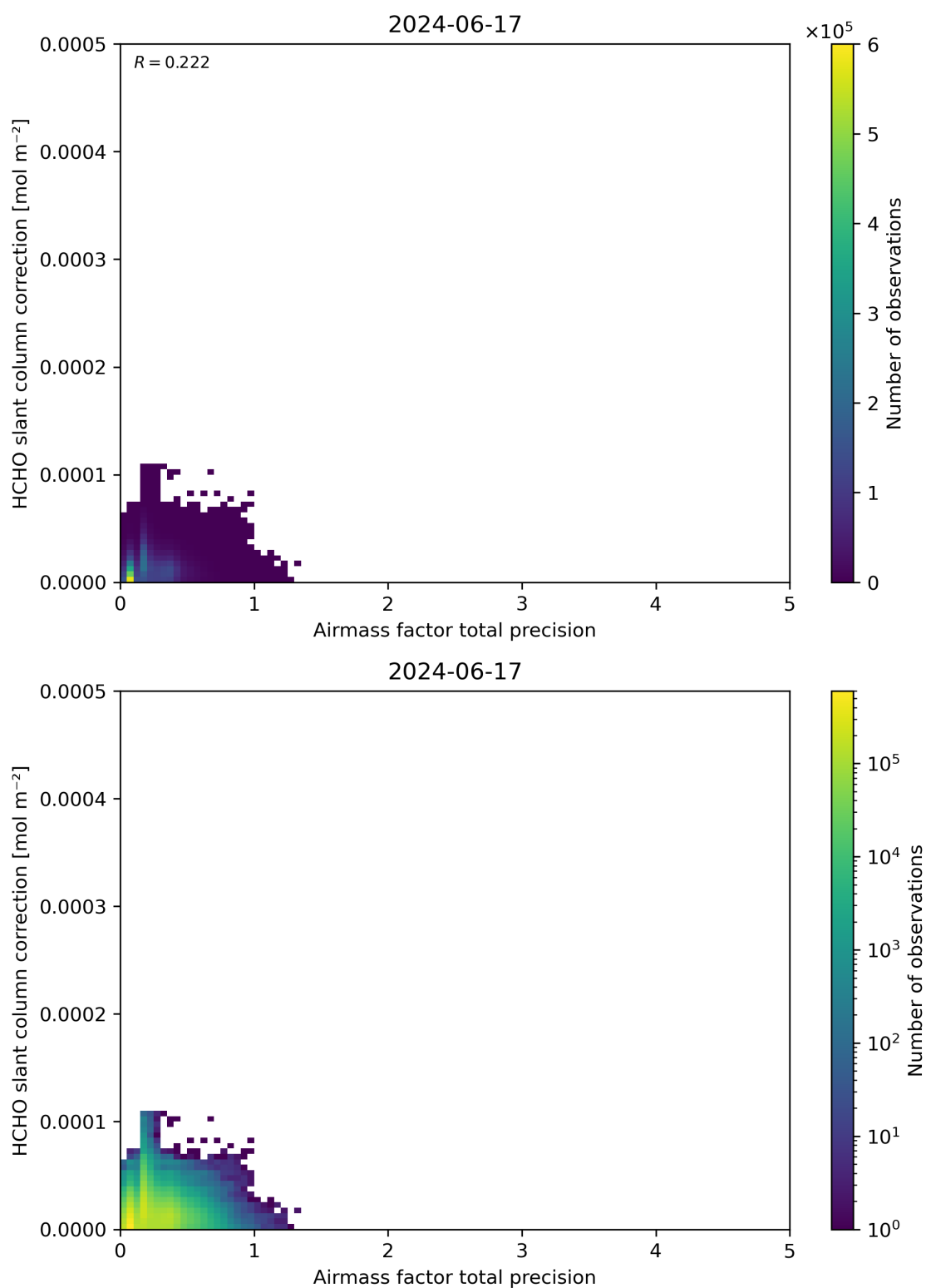
Figure 110: Scatter density plot of “Airmass factor total precision” against “HCHO slant column correction” for 2024-06-16 to 2024-06-18.
