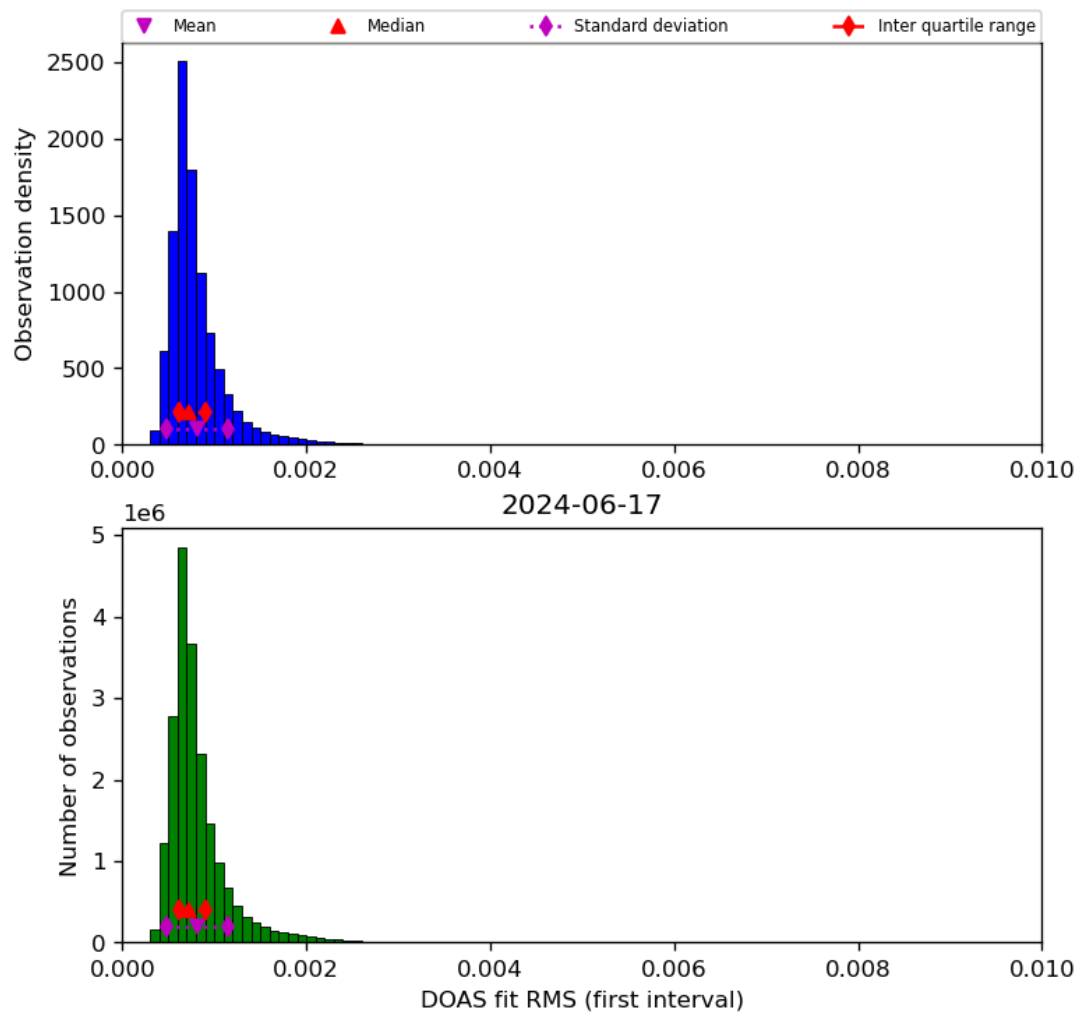
Figure 46: Histogram of “DOAS fit RMS (first interval)” for 2024-06-16 to 2024-06-18
