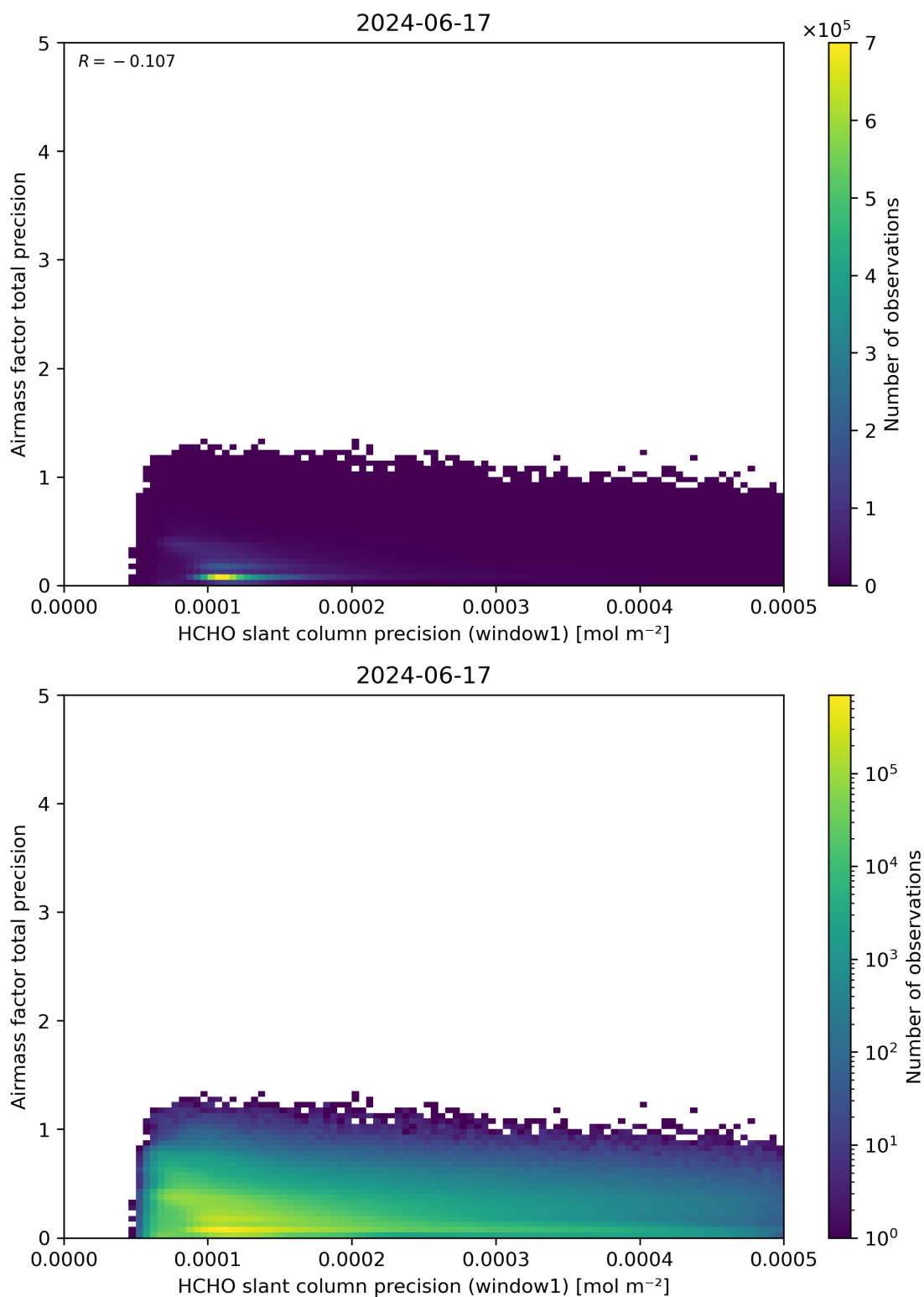
Figure 95: Scatter density plot of “HCHO slant column precision (window1)” against “Airmass factor total precision” for 2024-06-16 to 2024-06-18.
