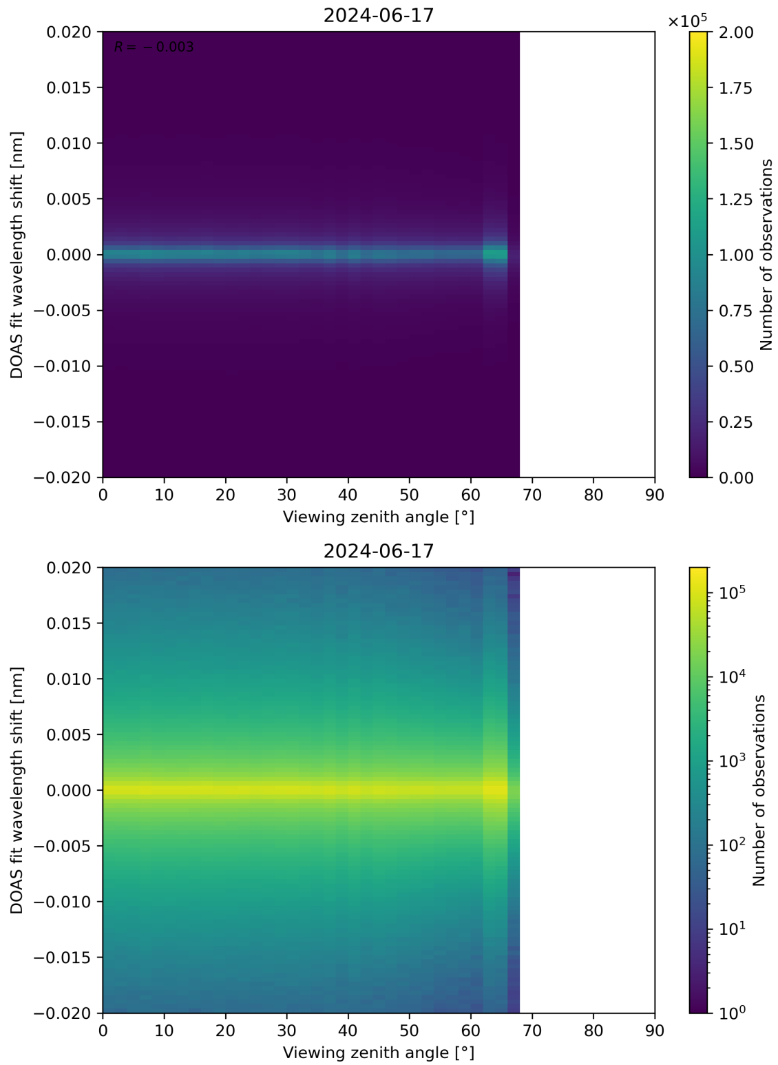
Figure 183: Scatter density plot of “Viewing zenith angle” against “DOAS fit wavelength shift” for 2024-06-16 to 2024-06-18.
