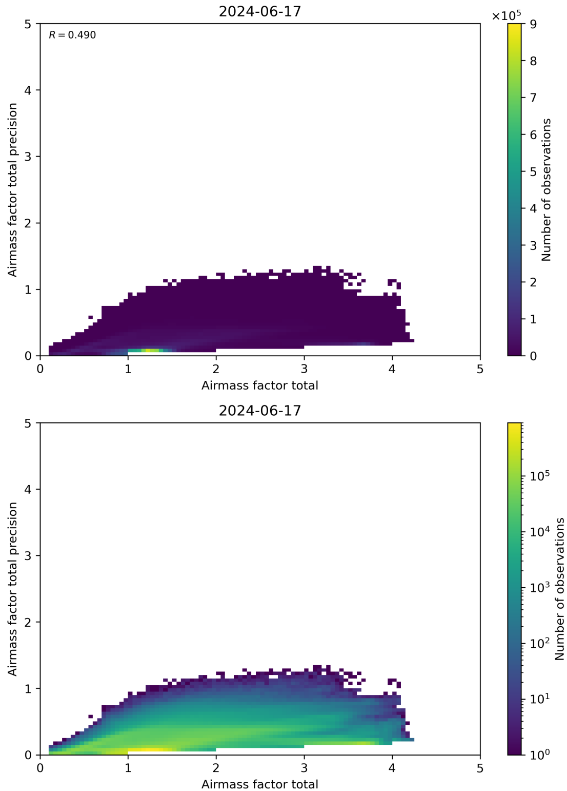
Figure 103: Scatter density plot of “Airmass factor total” against “Airmass factor total precision” for 2024-06-16 to 2024-06-18.
