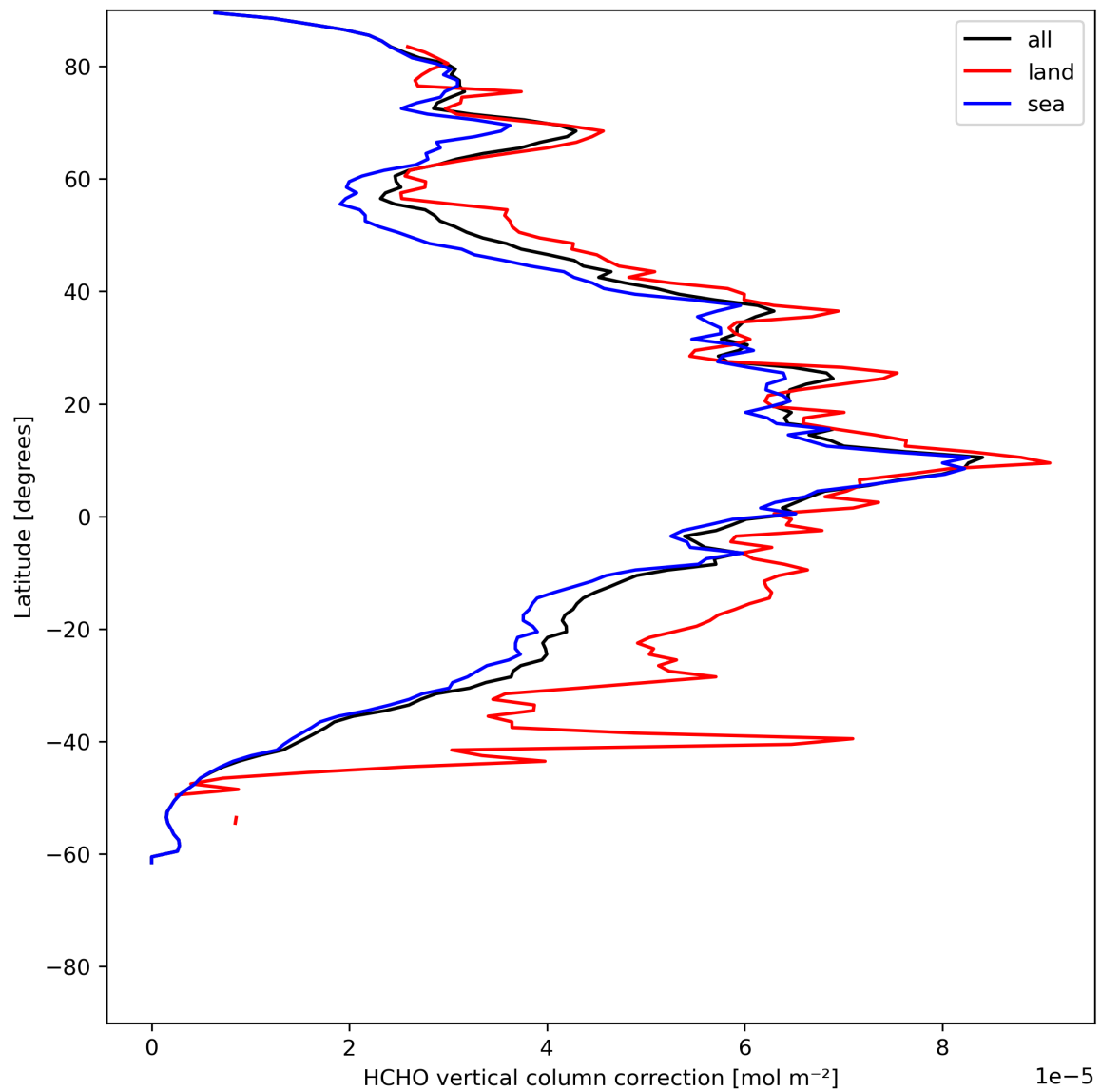
Figure 23: Zonal average of “HCHO vertical column correction” for 2024-06-16 to 2024-06-18.
