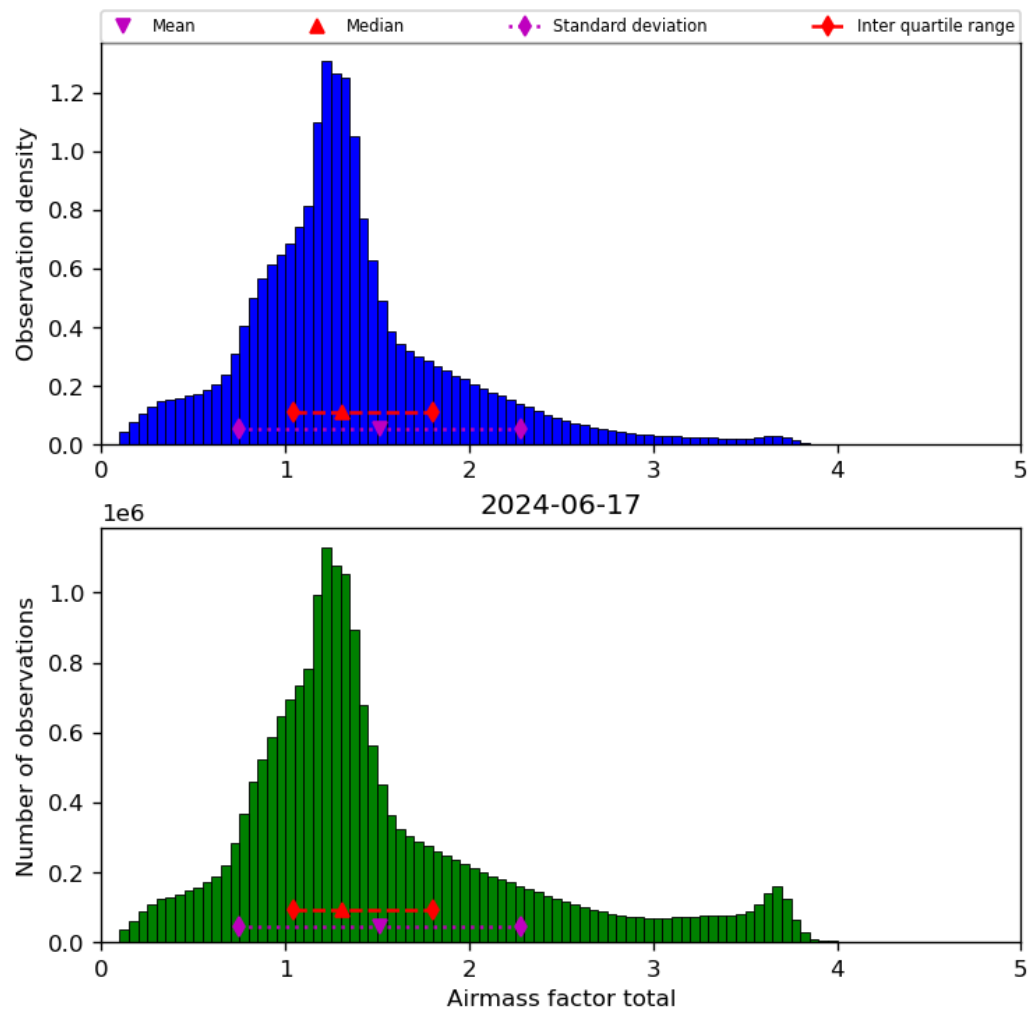
Figure 40: Histogram of “Airmass factor total” for 2024-06-16 to 2024-06-18
