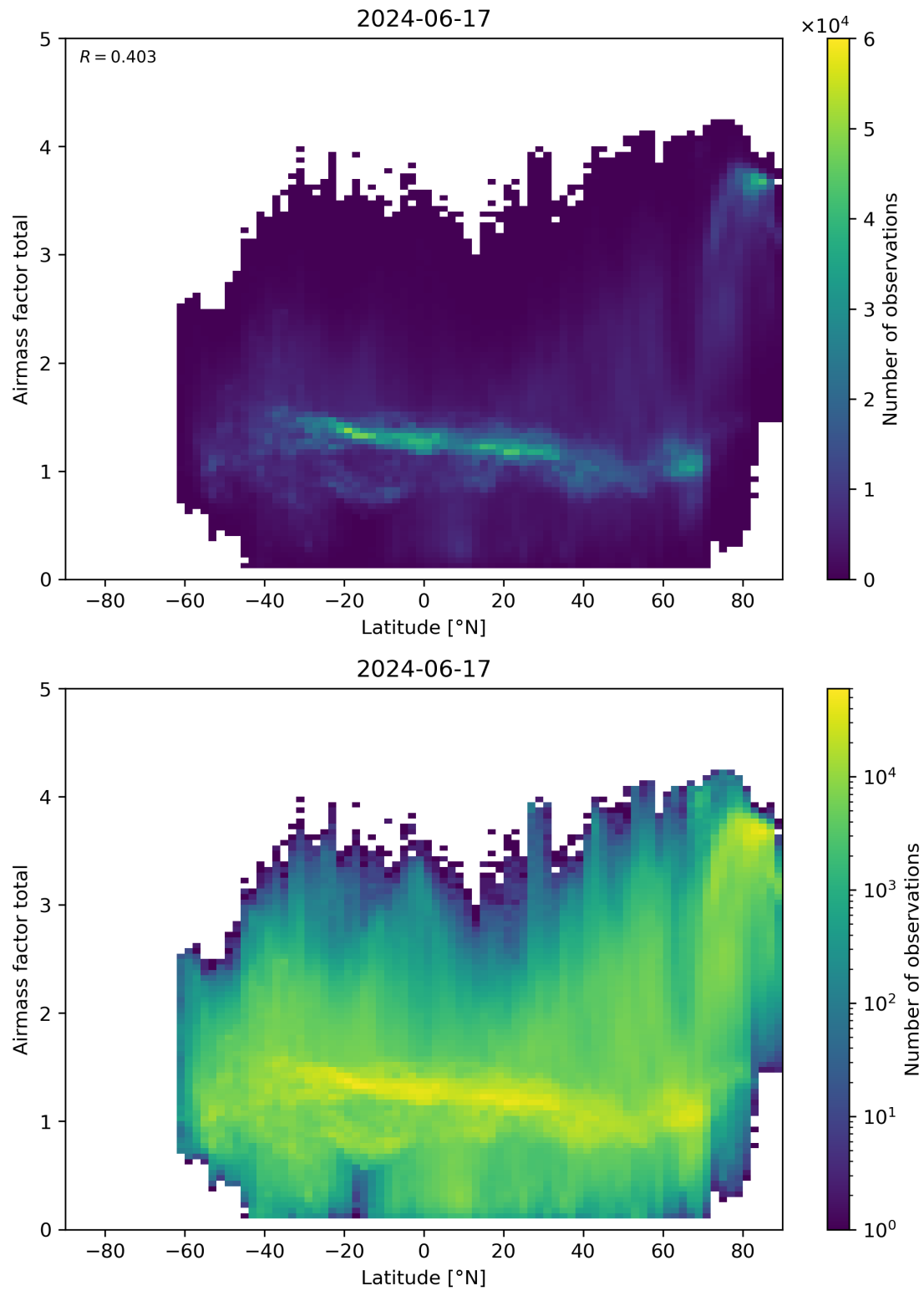
Figure 161: Scatter density plot of “Latitude” against “Airmass factor total” for 2024-06-16 to 2024-06-18.
