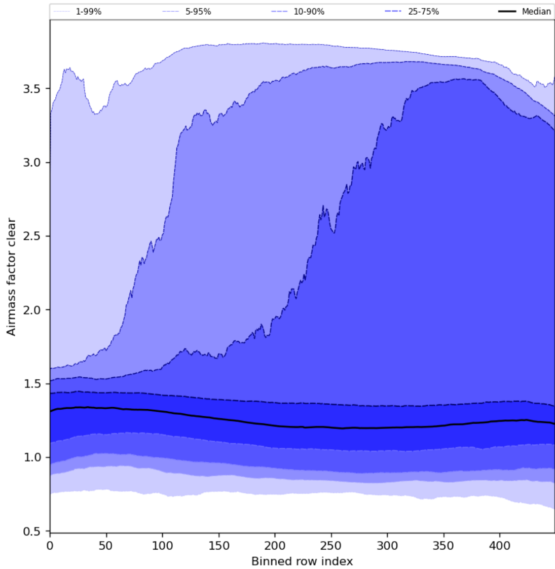
Figure 56: Along track statistics of “Airmass factor clear” for 2024-06-16 to 2024-06-18
