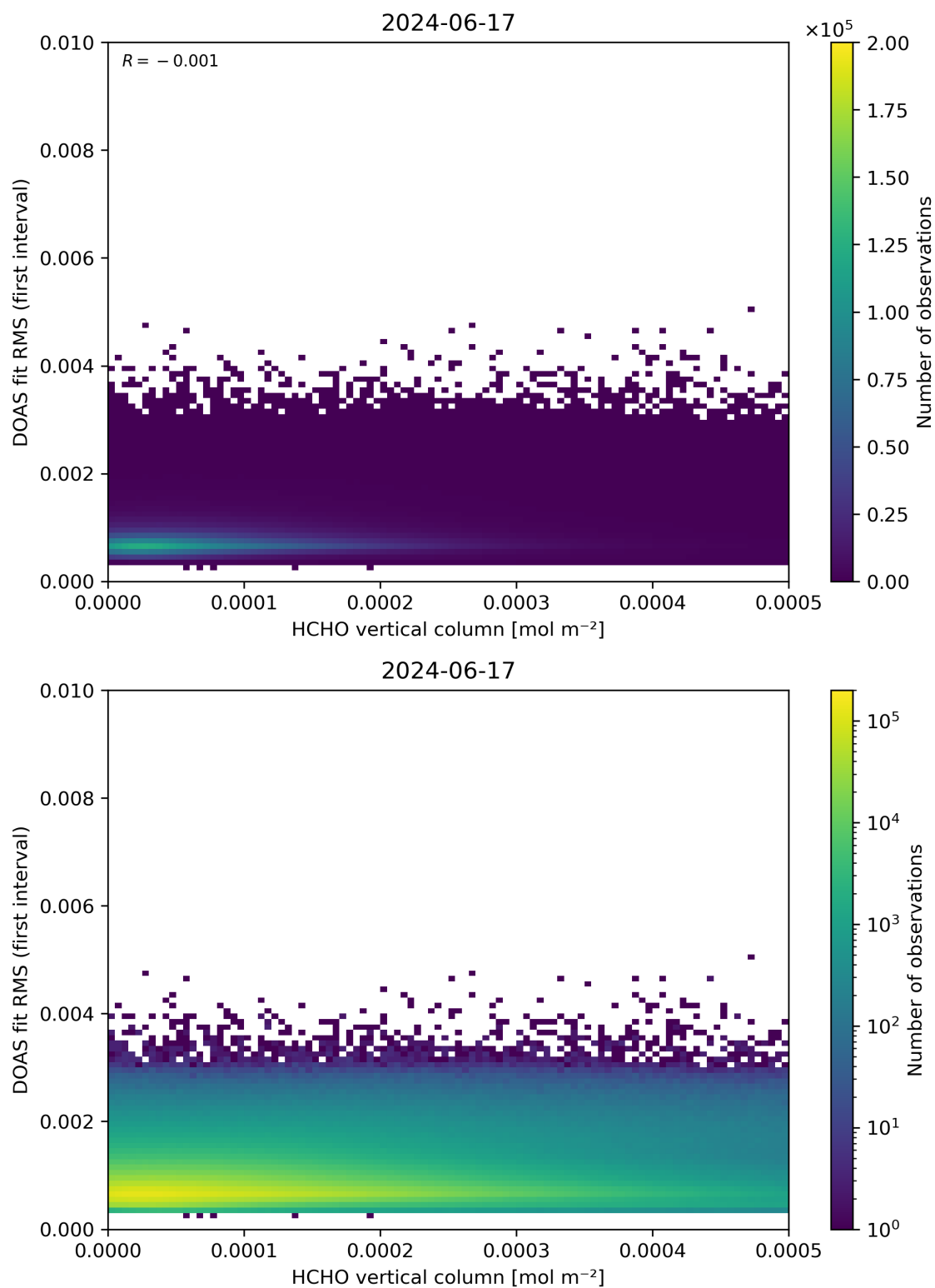
Figure 123: Scatter density plot of “HCHO vertical column” against “DOAS fit RMS (first interval)” for 2024-06-16 to 2024-06-18.
