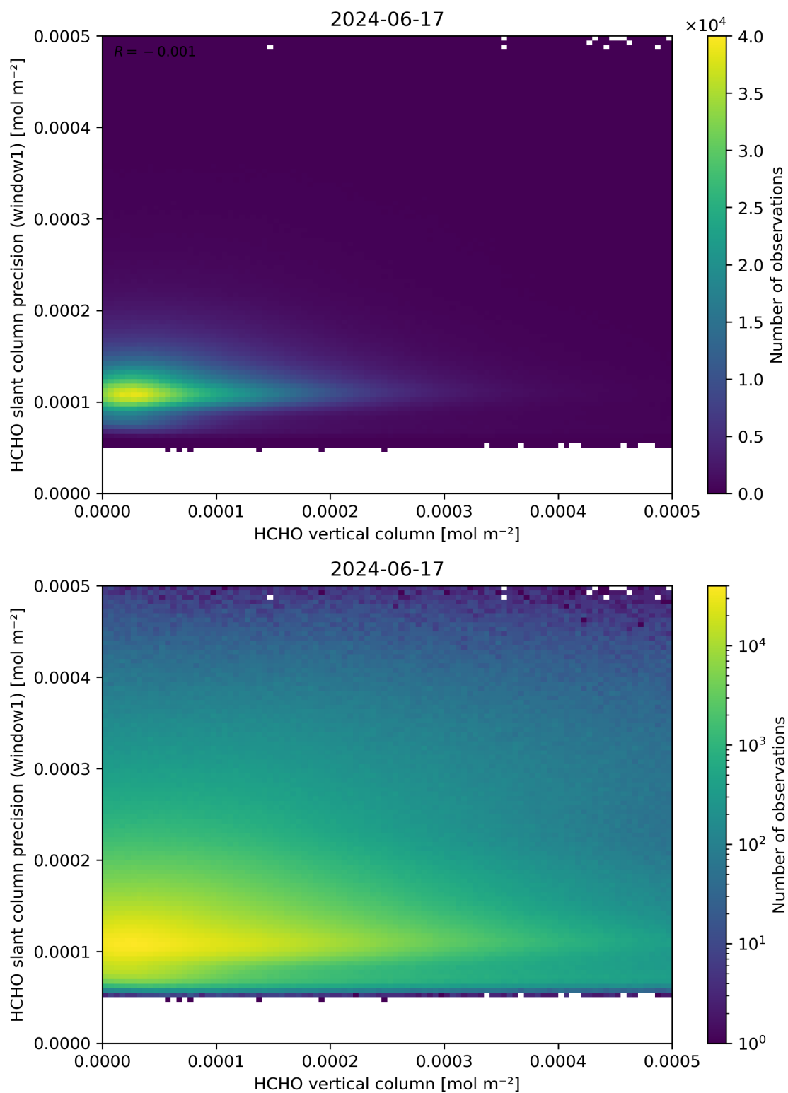
Figure 130: Scatter density plot of “HCHO vertical column” against “HCHO slant column precision (window1)” for 2024-06-16 to 2024-06-18.
