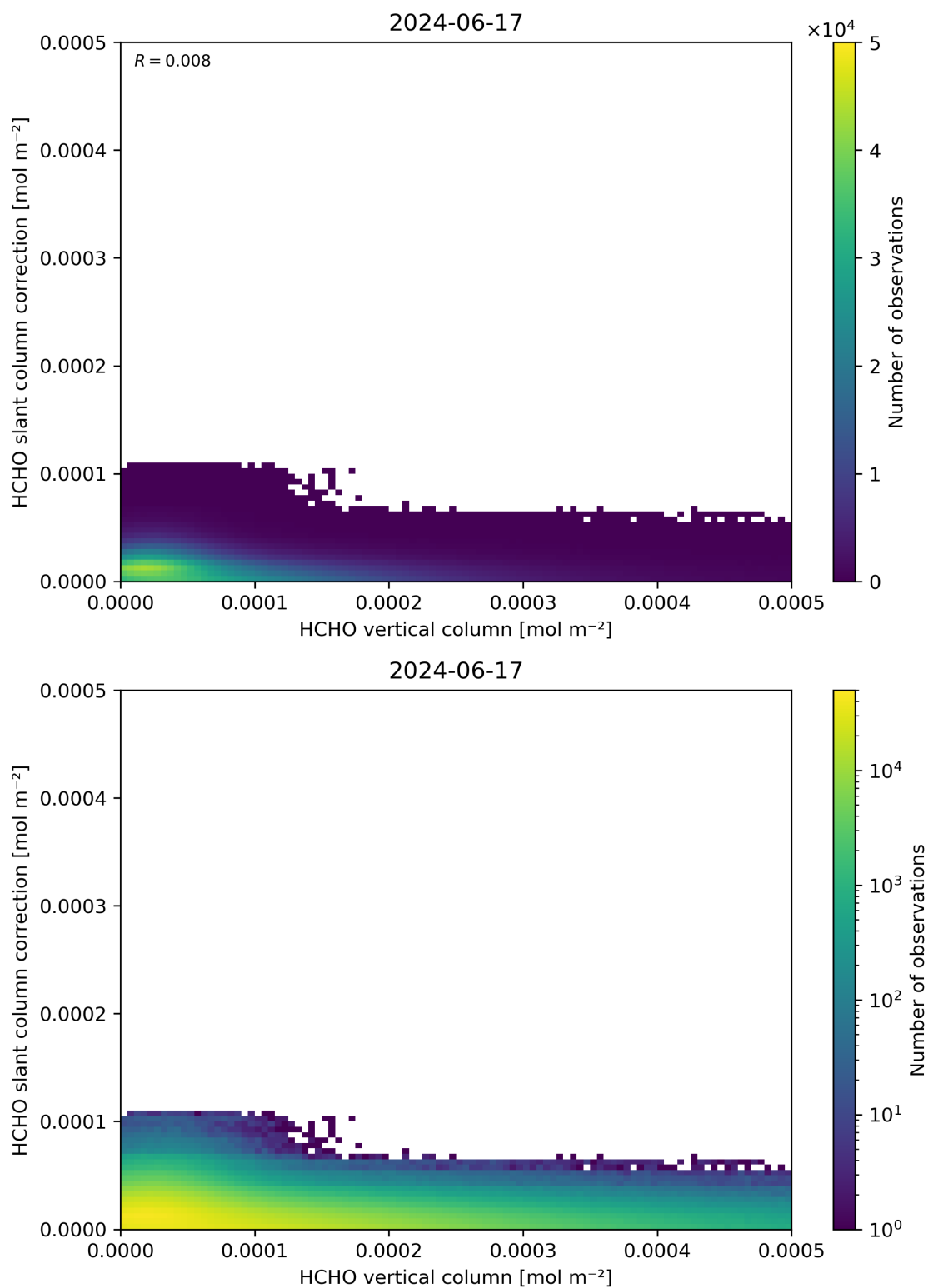
Figure 128: Scatter density plot of “HCHO vertical column” against “HCHO slant column correction” for 2024-06-16 to 2024-06-18.
