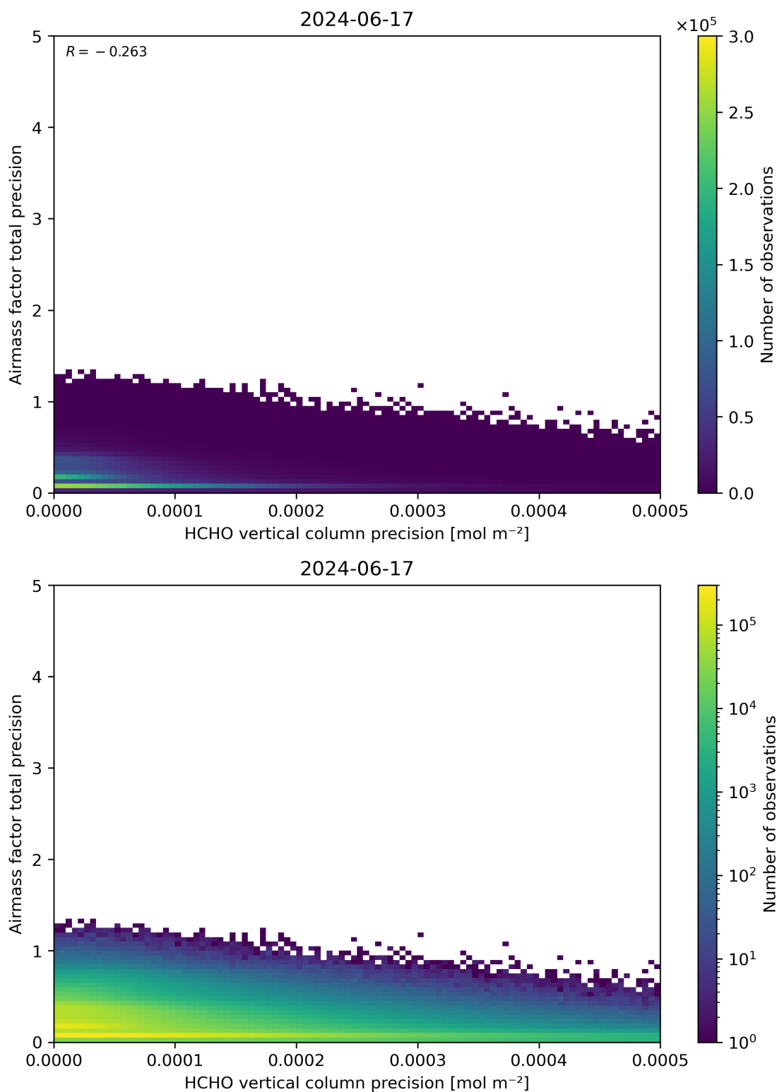
Figure 145: Scatter density plot of “HCHO vertical column precision” against “Airmass factor total precision” for 2024-06-16 to 2024-06-18.
