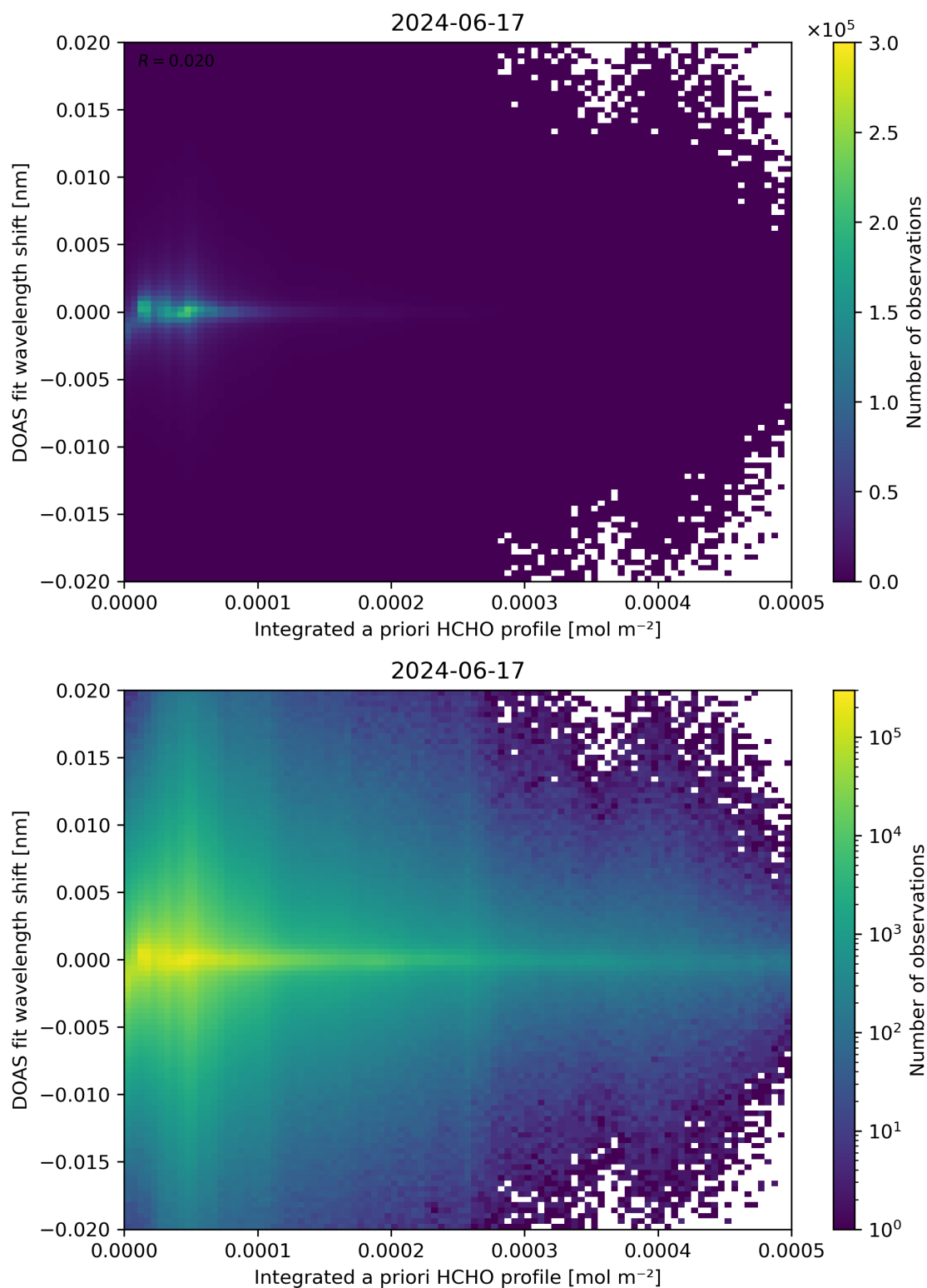
Figure 149: Scatter density plot of “Integrated a priori HCHO profile” against “DOAS fit wavelength shift” for 2024-06-16 to 2024-06-18.
