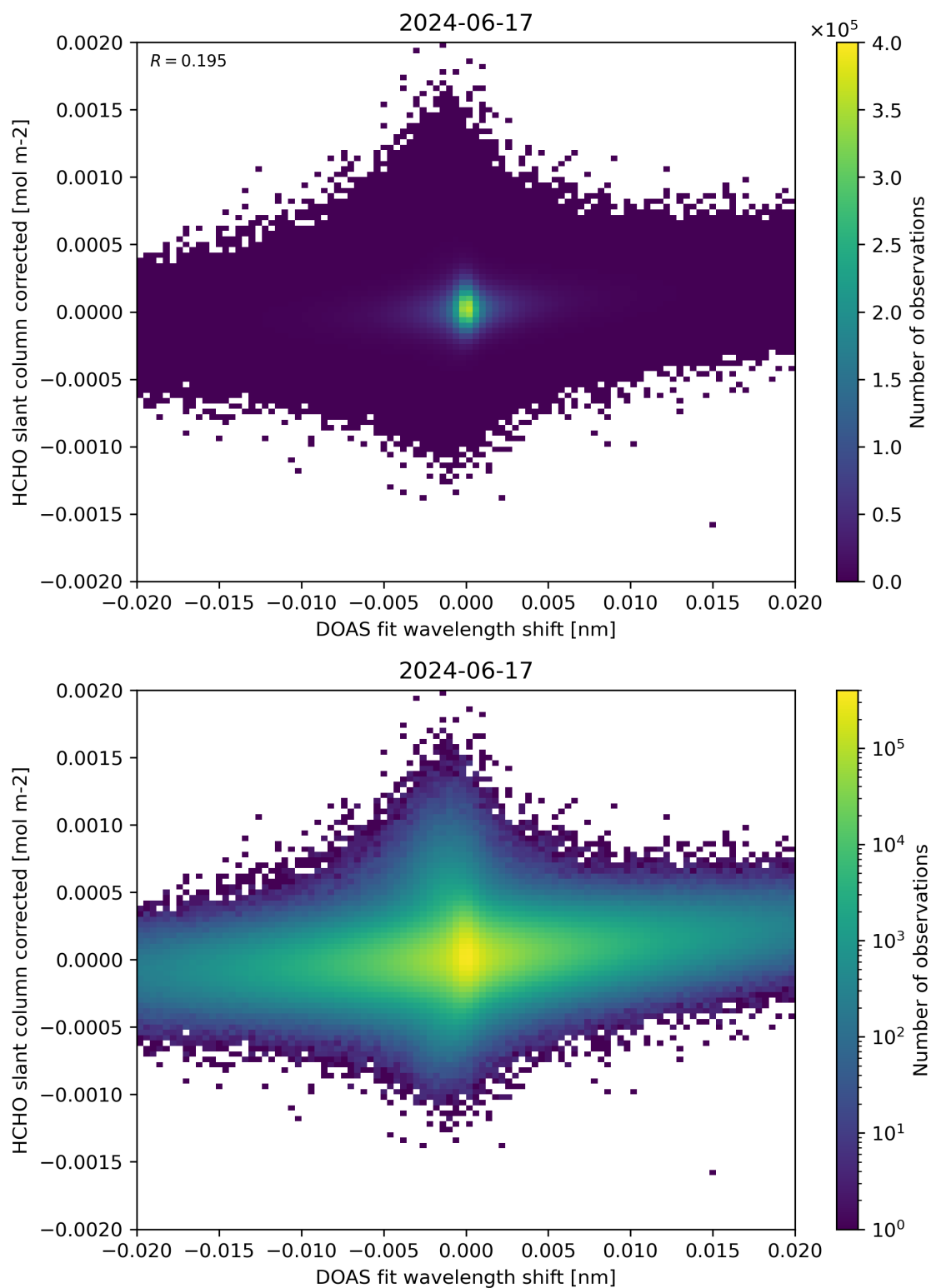
Figure 66: Scatter density plot of “DOAS fit wavelength shift” against “HCHO slant column corrected” for 2024-06-16 to 2024-06-18.
