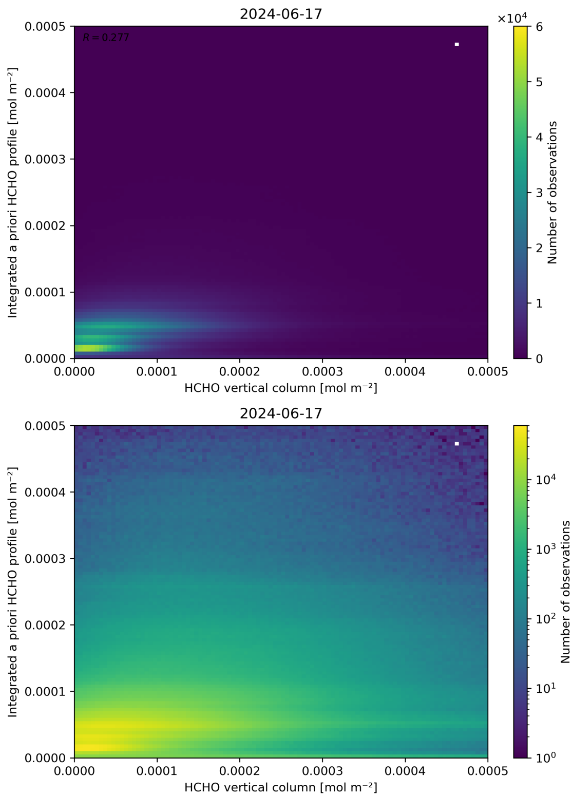
Figure 135: Scatter density plot of “HCHO vertical column” against “Integrated a priori HCHO profile” for 2024-06-16 to 2024-06-18.
