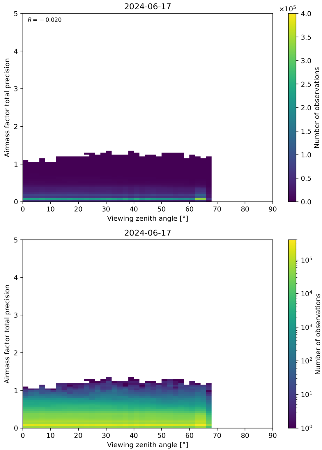
Figure 191: Scatter density plot of “Viewing zenith angle” against “Airmass factor total precision” for 2024-06-16 to 2024-06-18.
