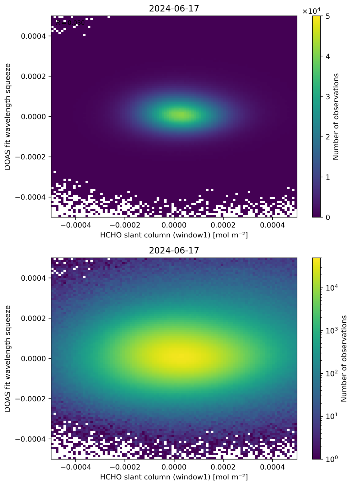
Figure 80: Scatter density plot of “HCHO slant column (window1)” against “DOAS fit wavelength squeeze” for 2024-06-16 to 2024-06-18.
