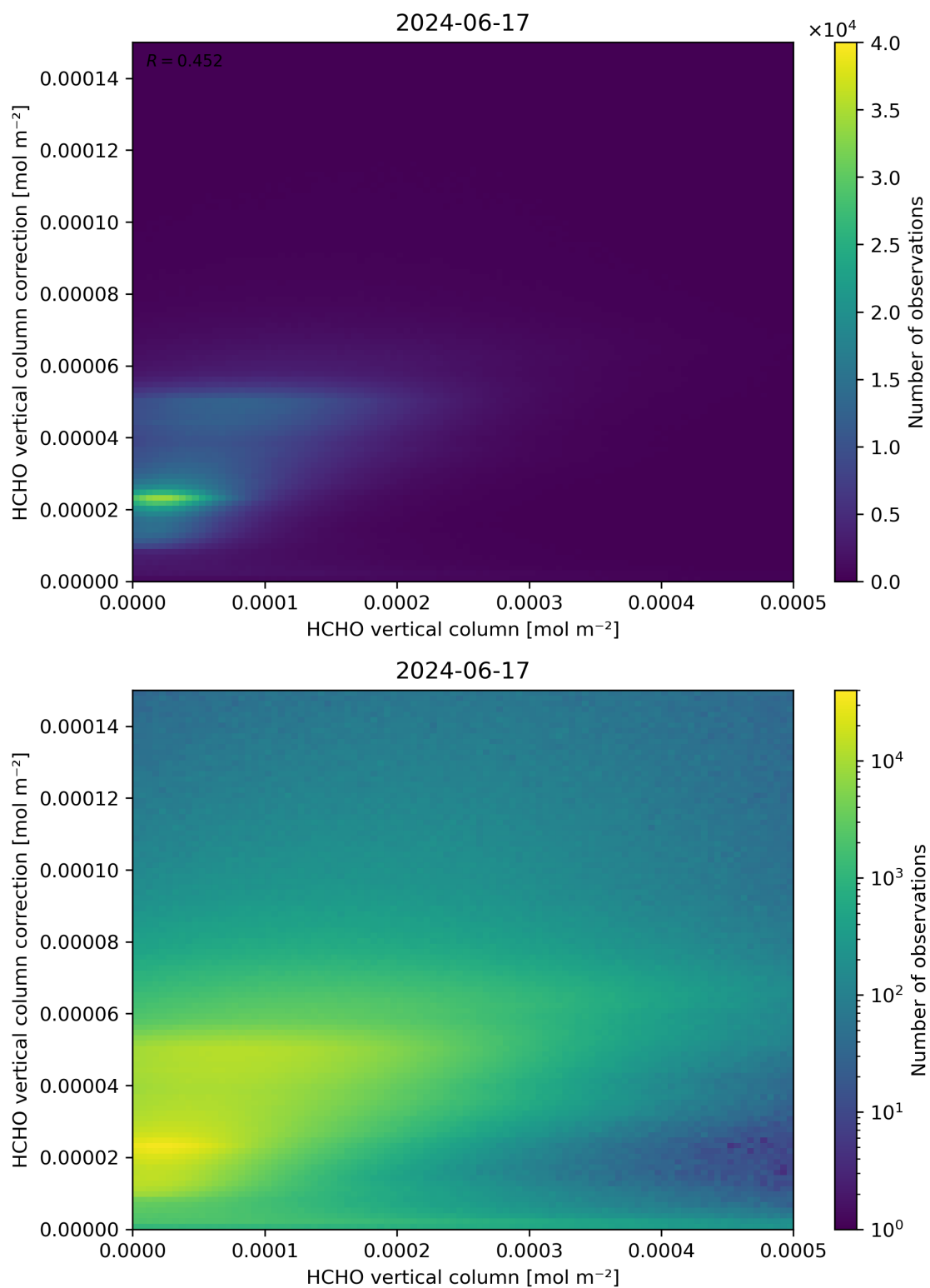
Figure 133: Scatter density plot of “HCHO vertical column” against “HCHO vertical column correction” for 2024-06-16 to 2024-06-18.
