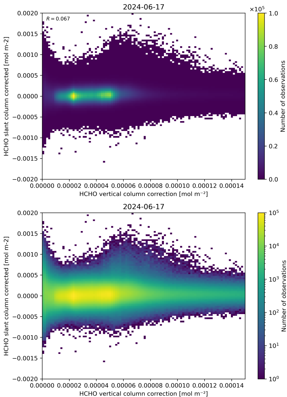
Figure 116: Scatter density plot of “HCHO vertical column correction” against “HCHO slant column corrected” for 2024-06-16 to 2024-06-18.
