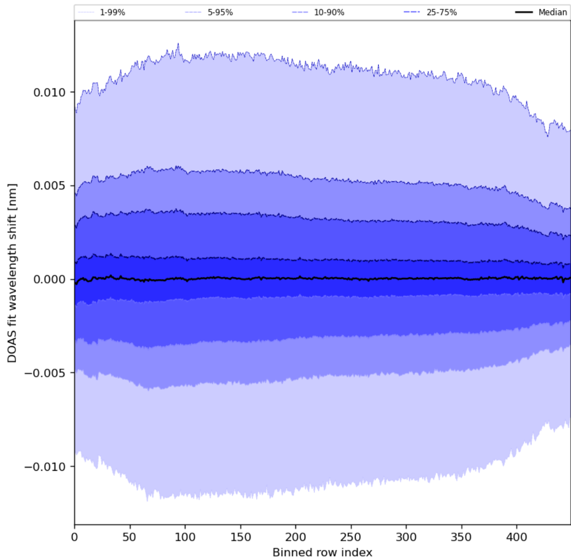
Figure 58: Along track statistics of “DOAS fit wavelength shift” for 2024-06-16 to 2024-06-18
