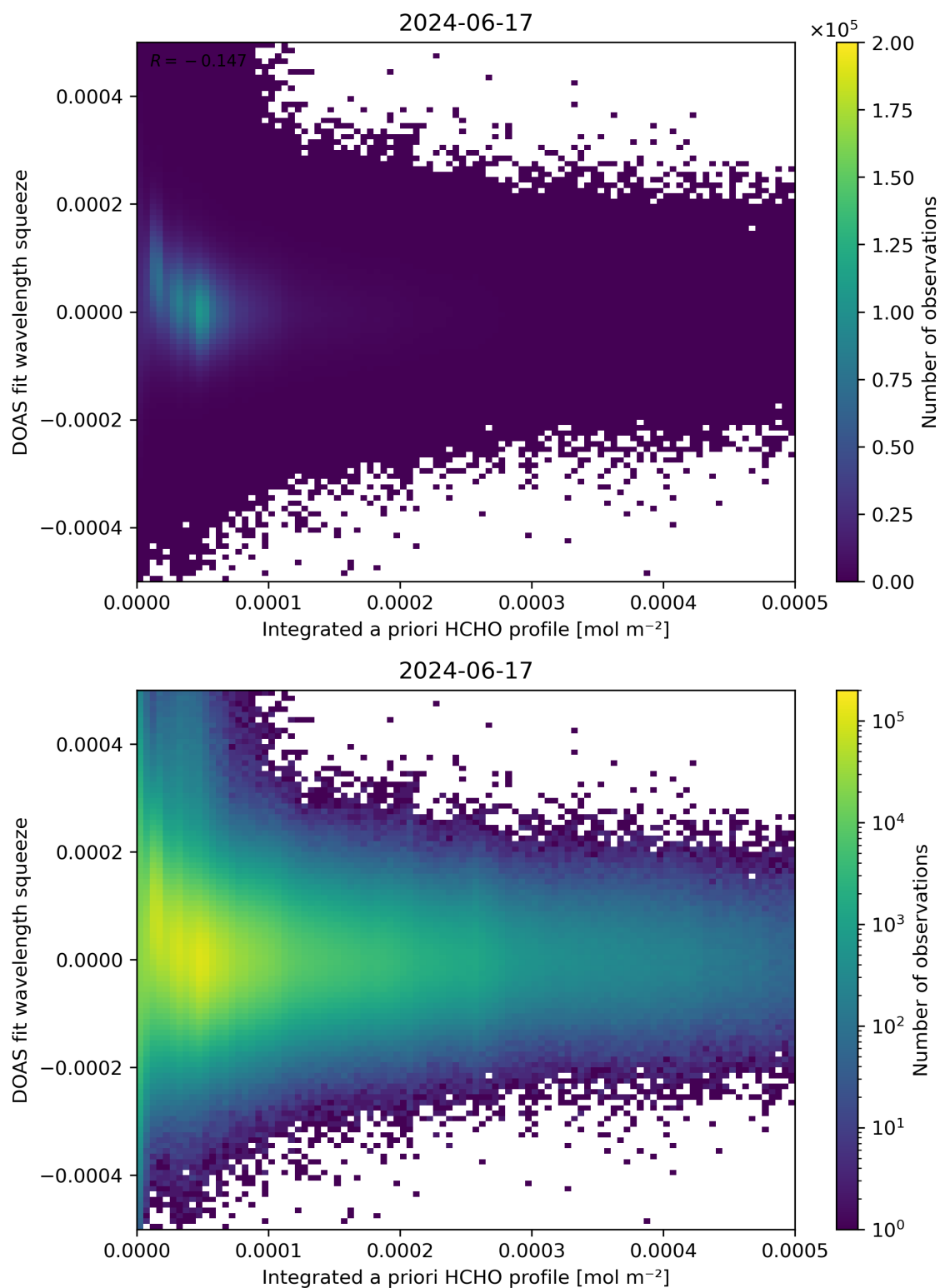
Figure 150: Scatter density plot of “Integrated a priori HCHO profile” against “DOAS fit wavelength squeeze” for 2024-06-16 to 2024-06-18.
