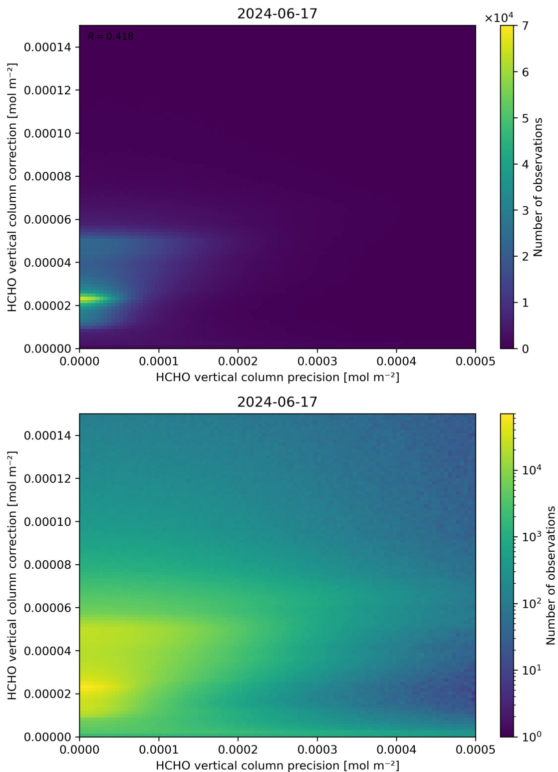
Figure 146: Scatter density plot of “HCHO vertical column precision” against “HCHO vertical column correction” for 2024-06-16 to 2024-06-18.
