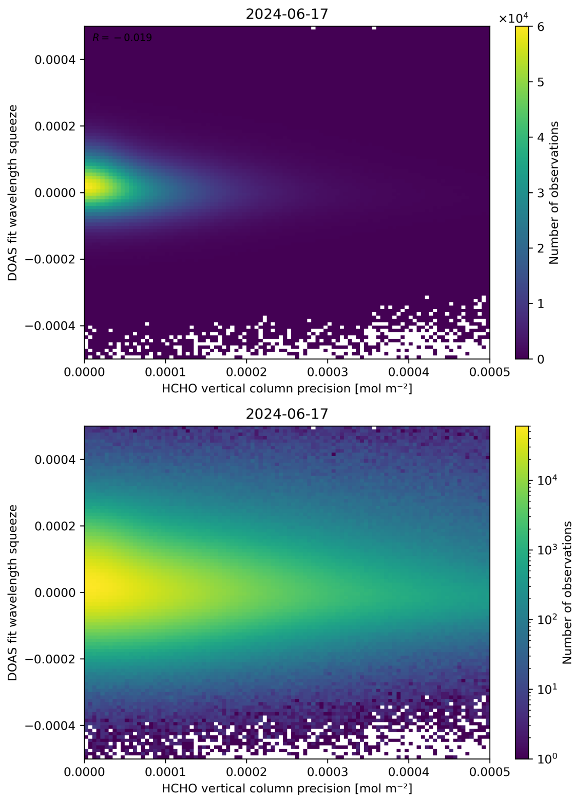
Figure 138: Scatter density plot of “HCHO vertical column precision” against “DOAS fit wavelength squeeze” for 2024-06-16 to 2024-06-18.
