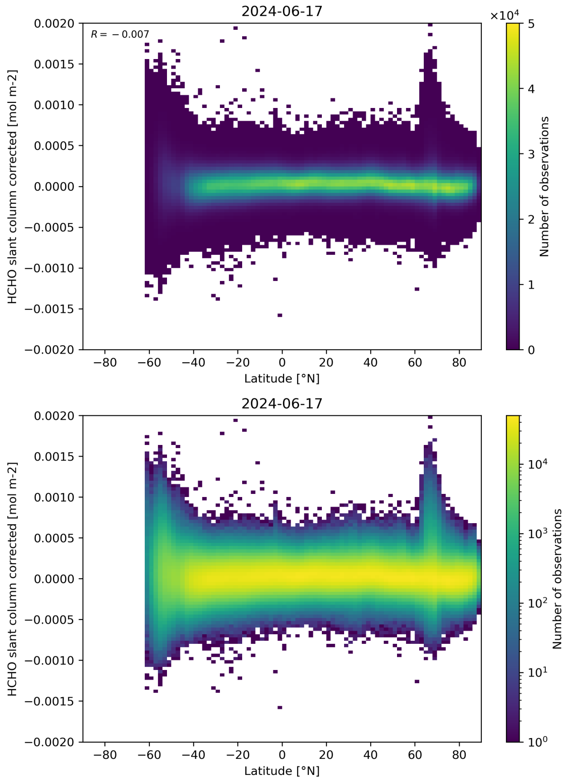
Figure 157: Scatter density plot of “Latitude” against “HCHO slant column corrected” for 2024-06-16 to 2024-06-18.
