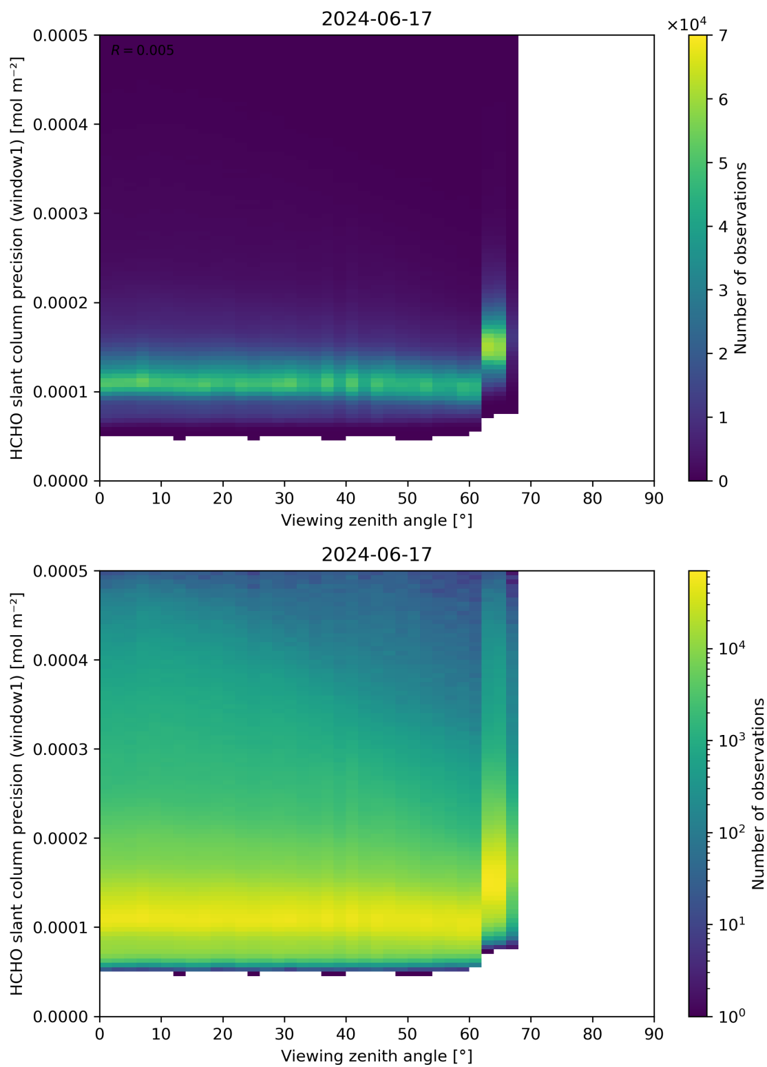
Figure 189: Scatter density plot of “Viewing zenith angle” against “HCHO slant column precision (window1)” for 2024-06-16 to 2024-06-18.
