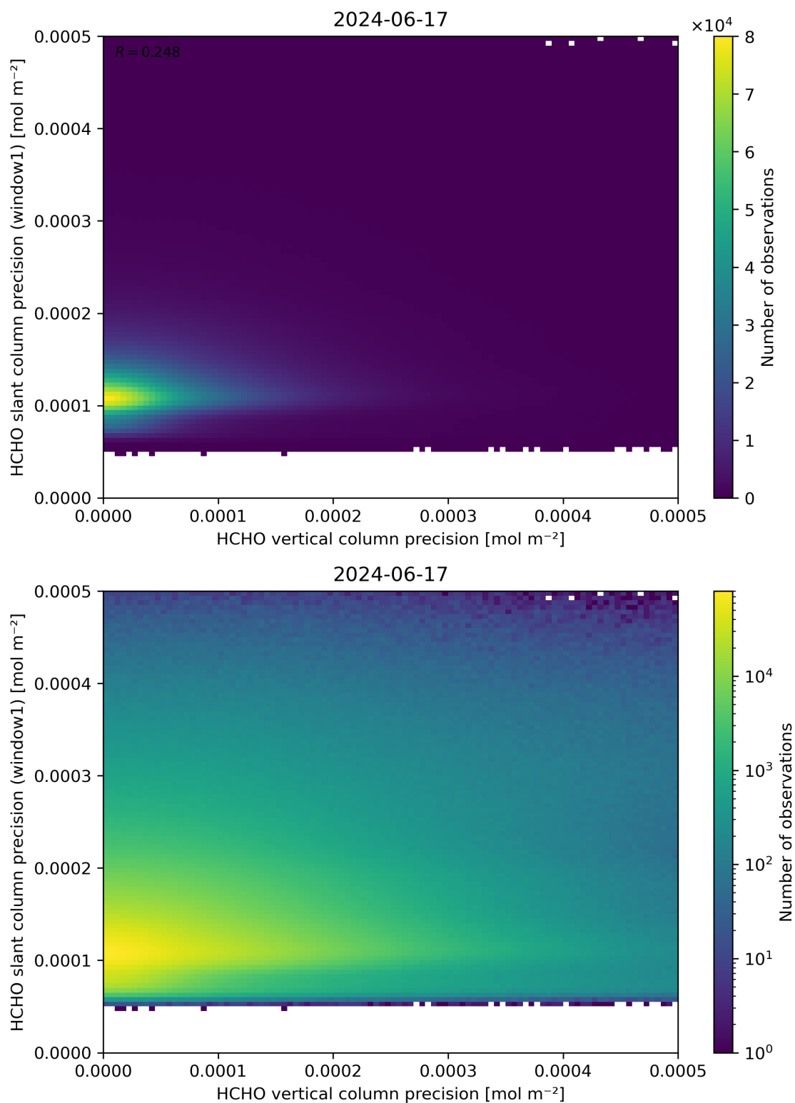
Figure 143: Scatter density plot of “HCHO vertical column precision” against “HCHO slant column precision (window1)” for 2024-06-16 to 2024-06-18.
