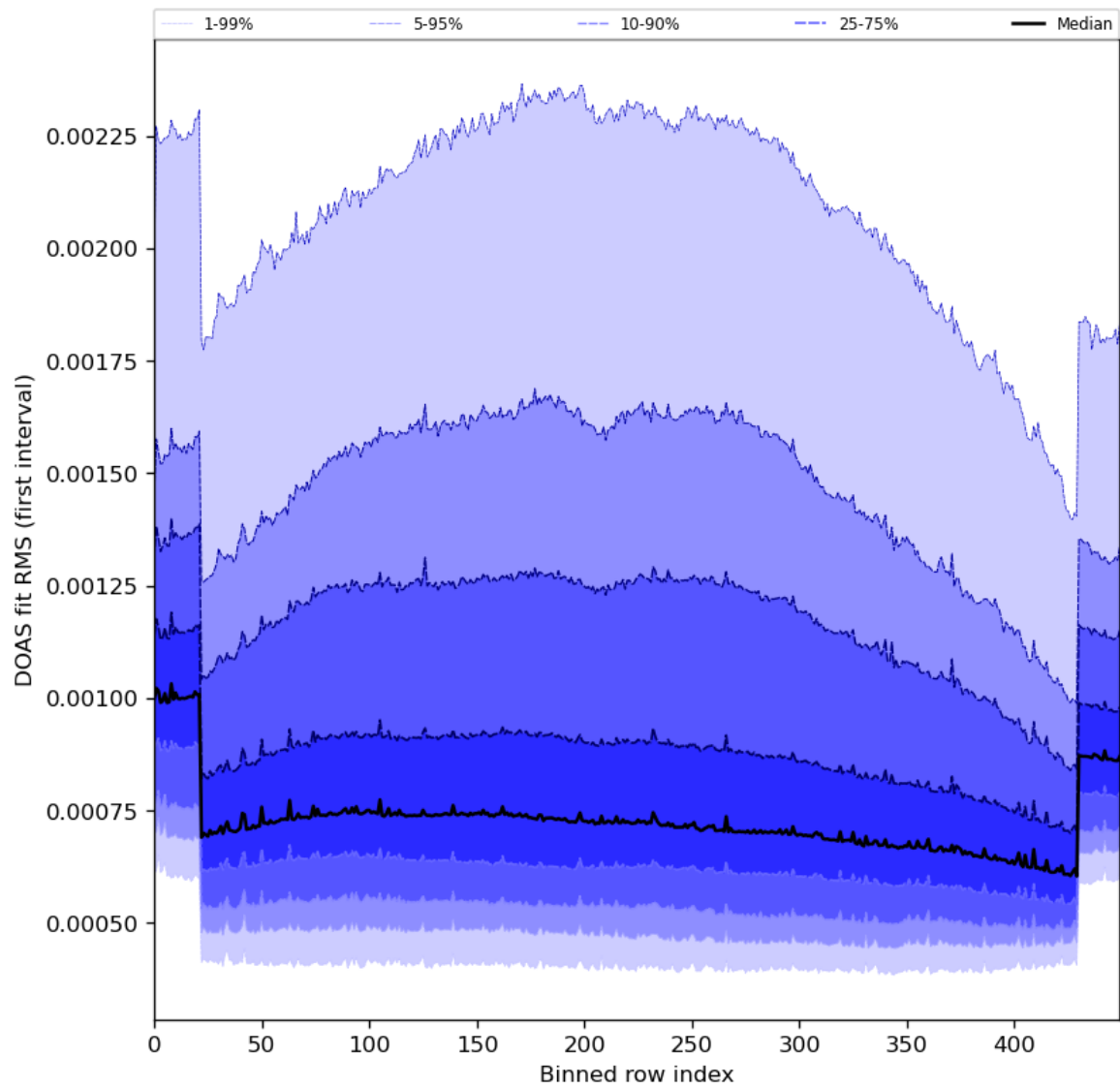
Figure 60: Along track statistics of “DOAS fit RMS (first interval)” for 2024-06-16 to 2024-06-18
