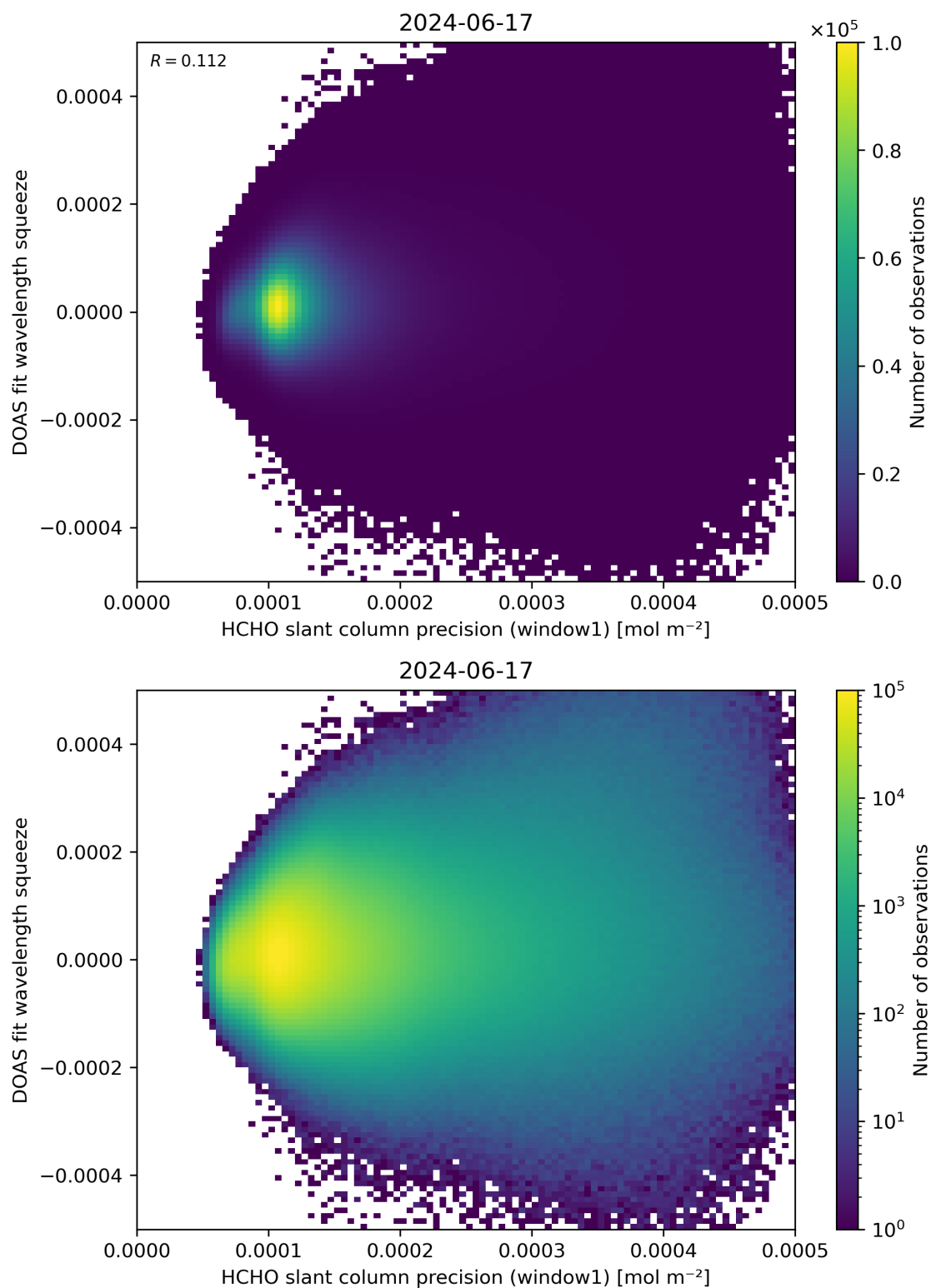
Figure 90: Scatter density plot of “HCHO slant column precision (window1)” against “DOAS fit wavelength squeeze” for 2024-06-16 to 2024-06-18.
