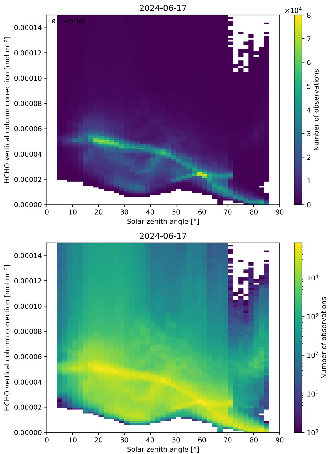
Figure 178: Scatter density plot of “Solar zenith angle” against “HCHO vertical column correction” for 2024-06-16 to 2024-06-18.
