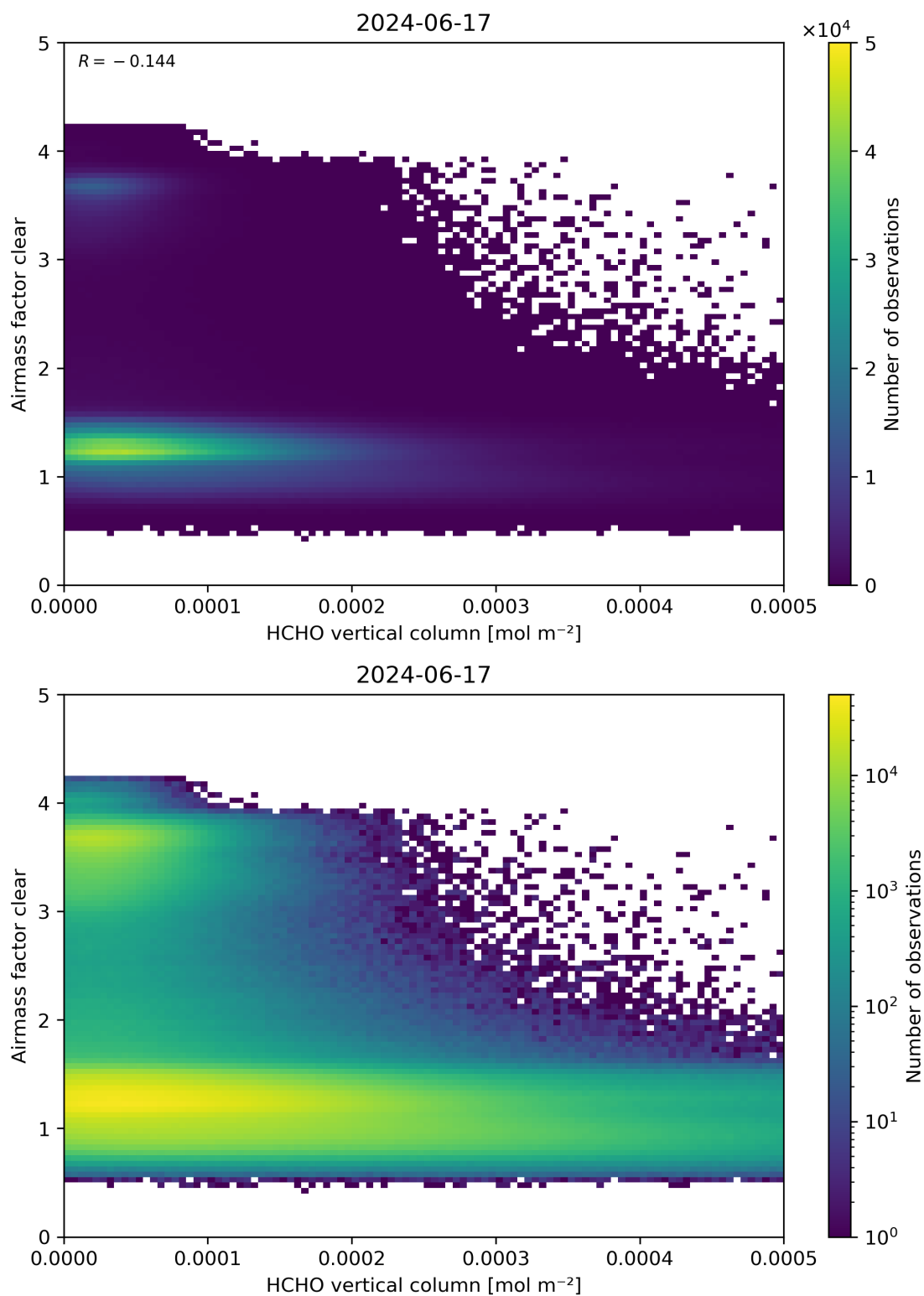
Figure 126: Scatter density plot of “HCHO vertical column” against “Airmass factor clear” for 2024-06-16 to 2024-06-18.
