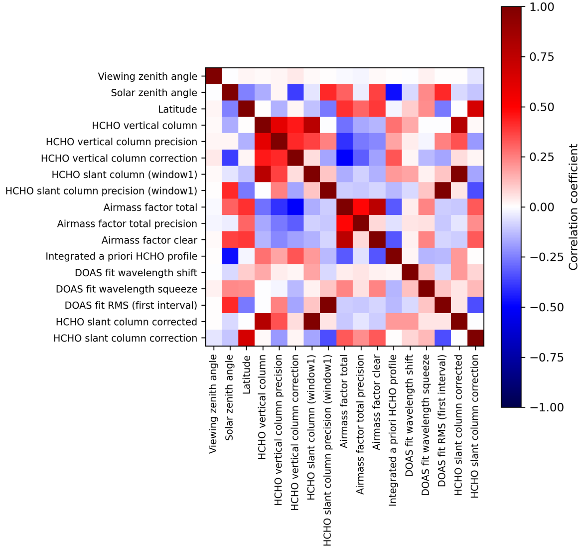
Figure 2: Map of correlation matrix for 2024-06-16 to 2024-06-18.
