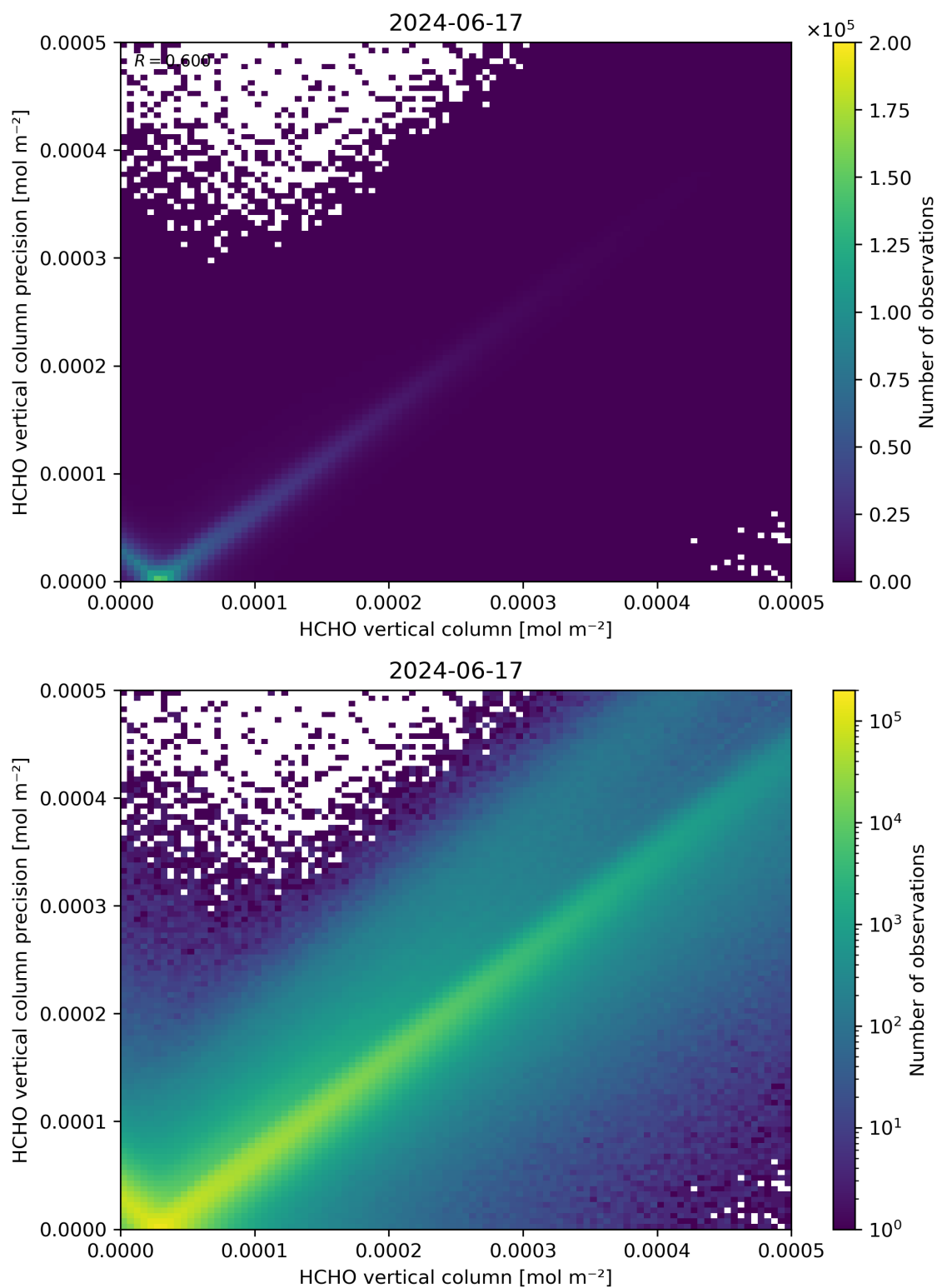
Figure 134: Scatter density plot of “HCHO vertical column” against “HCHO vertical column precision” for 2024-06-16 to 2024-06-18.
