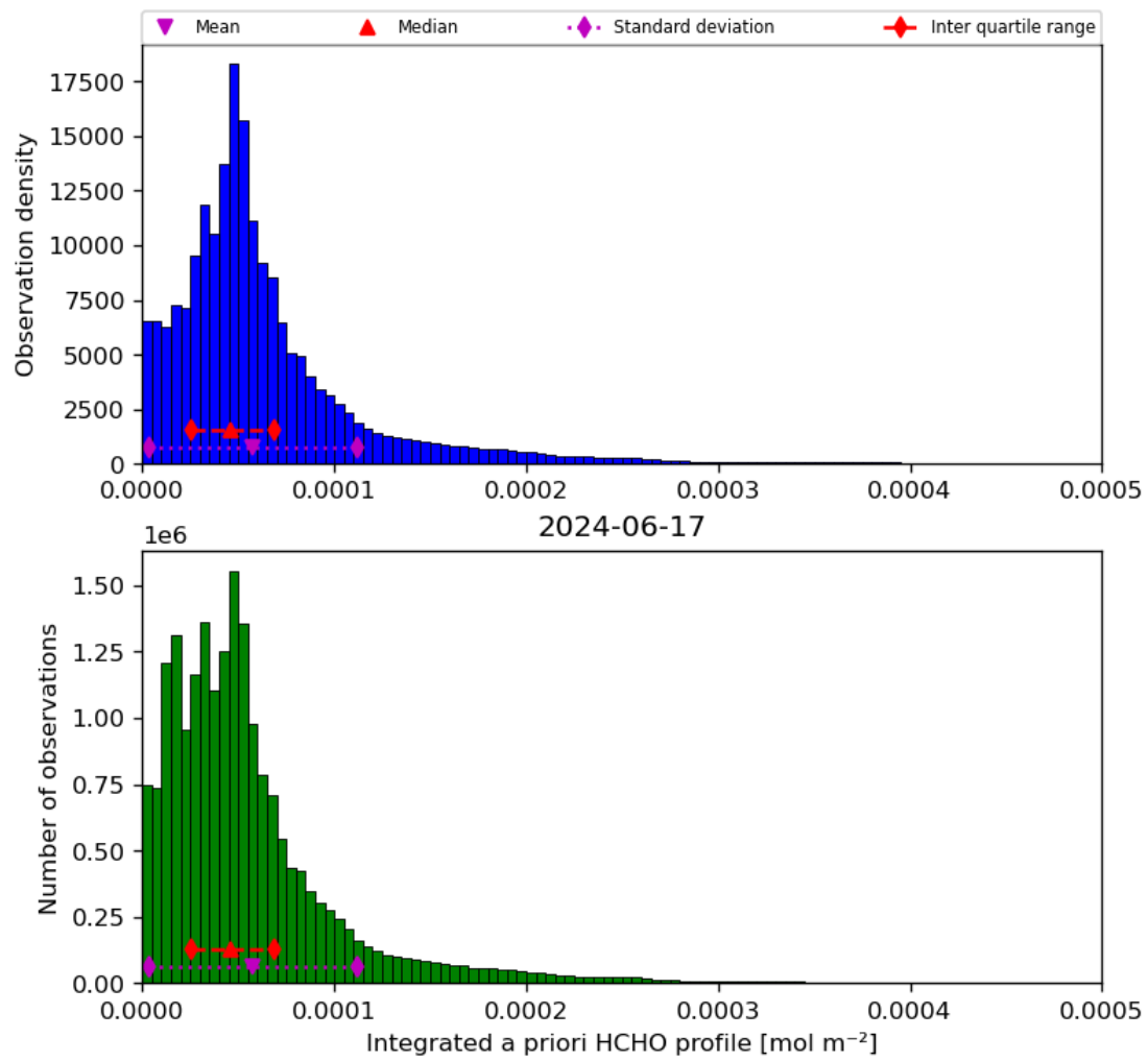
Figure 43: Histogram of “Integrated a priori HCHO profile” for 2024-06-16 to 2024-06-18
