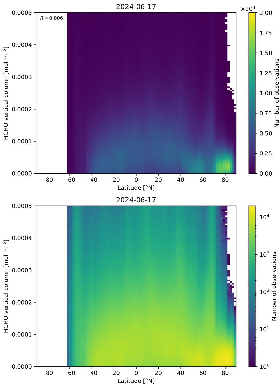
Figure 163: Scatter density plot of “Latitude” against “HCHO vertical column” for 2024-06-16 to 2024-06-18.
