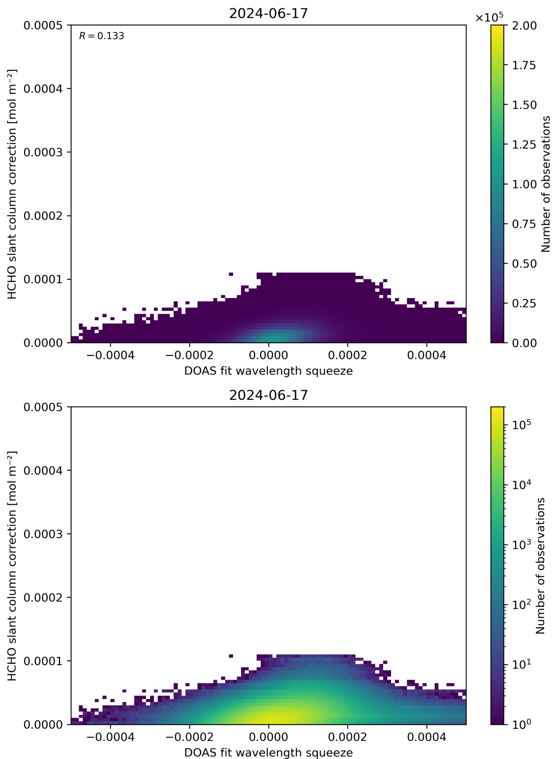
Figure 70: Scatter density plot of “DOAS fit wavelength squeeze” against “HCHO slant column correction” for 2024-06-16 to 2024-06-18.
