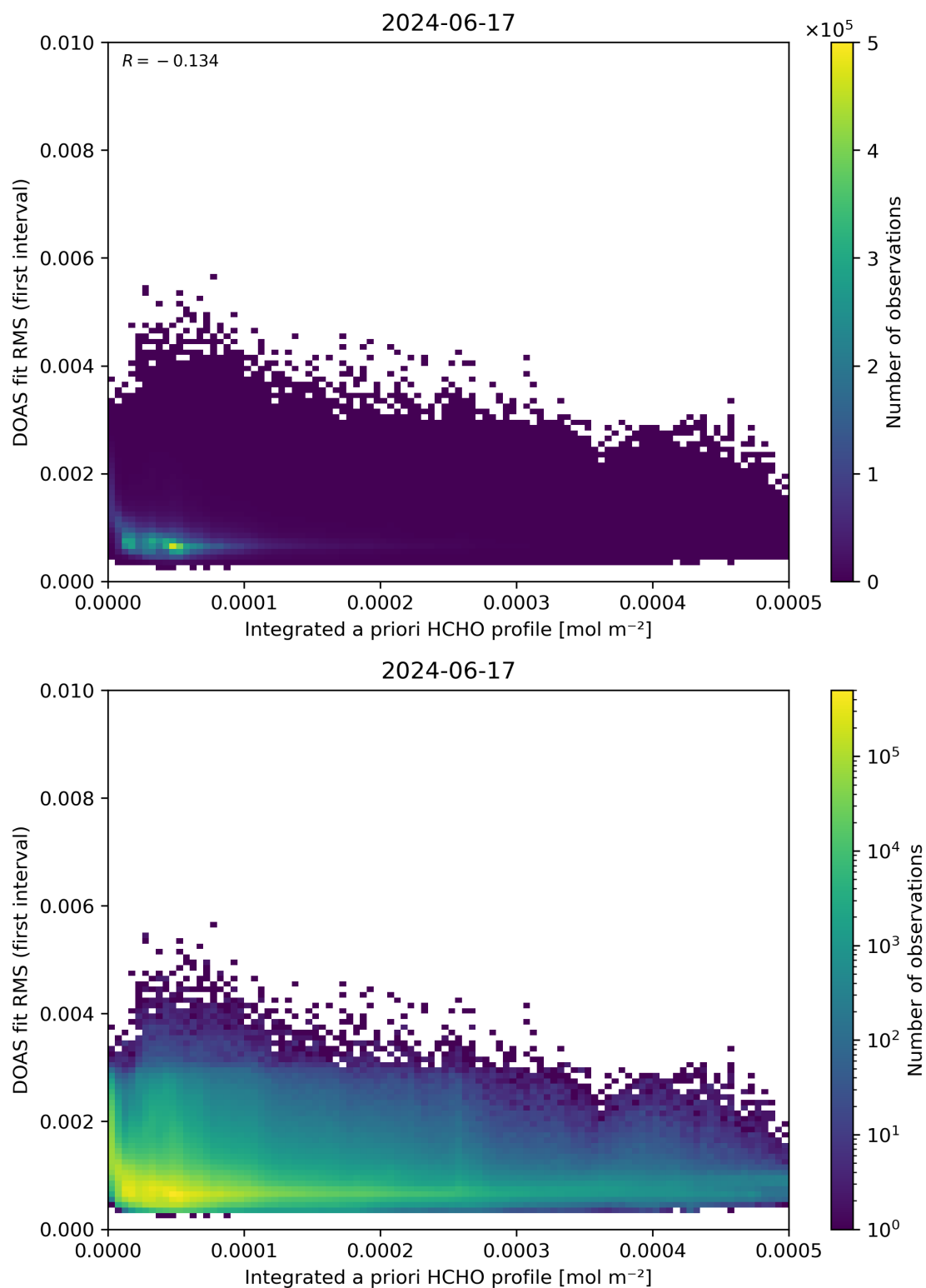
Figure 148: Scatter density plot of “Integrated a priori HCHO profile” against “DOAS fit RMS (first interval)” for 2024-06-16 to 2024-06-18.
