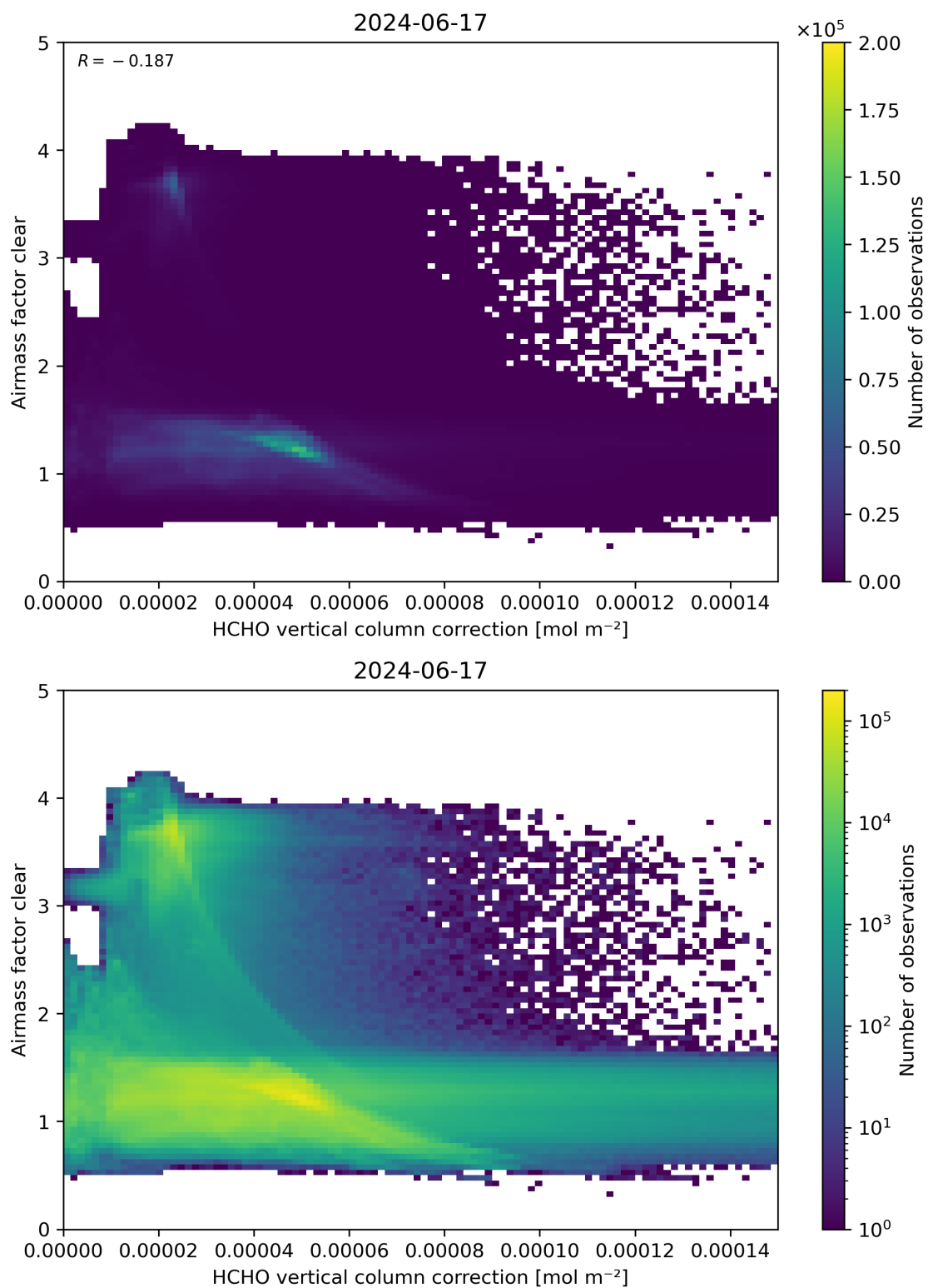
Figure 115: Scatter density plot of “HCHO vertical column correction” against “Airmass factor clear” for 2024-06-16 to 2024-06-18.
