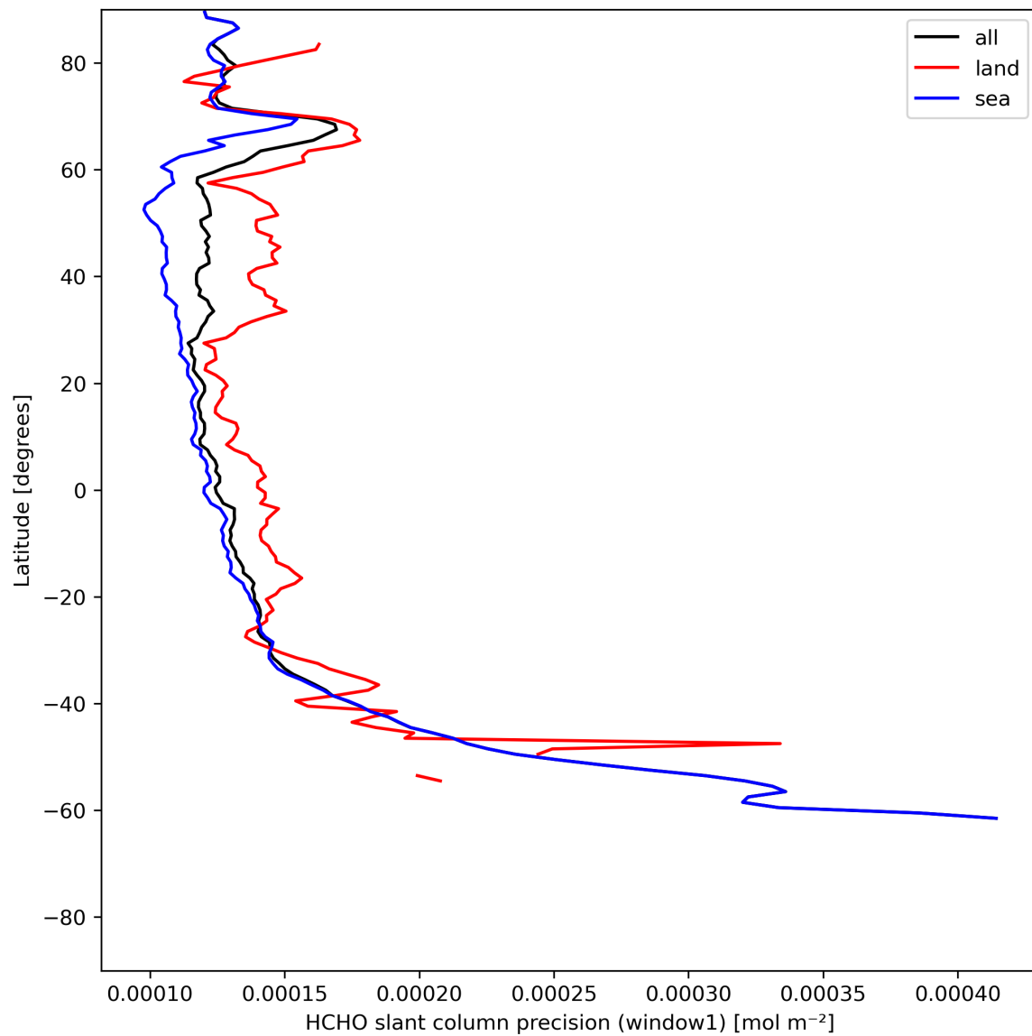
Figure 25: Zonal average of “HCHO slant column precision (window1)” for 2024-06-16 to 2024-06-18.
