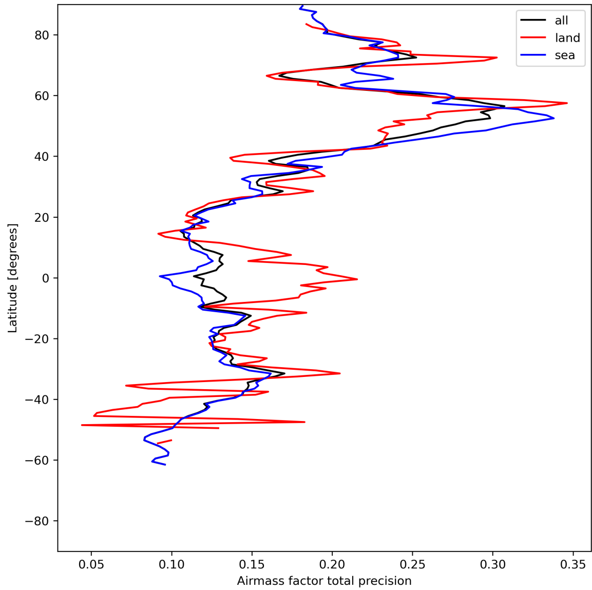
Figure 27: Zonal average of “Airmass factor total precision” for 2024-06-16 to 2024-06-18.
