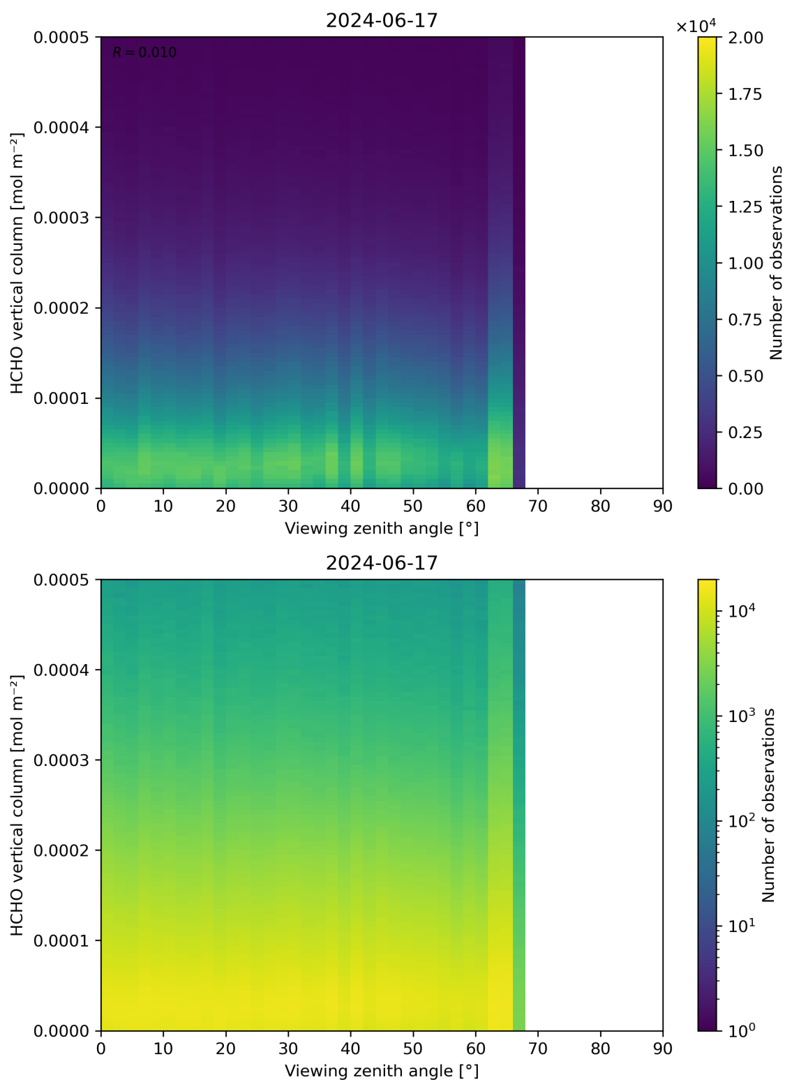
Figure 192: Scatter density plot of “Viewing zenith angle” against “HCHO vertical column” for 2024-06-16 to 2024-06-18.
