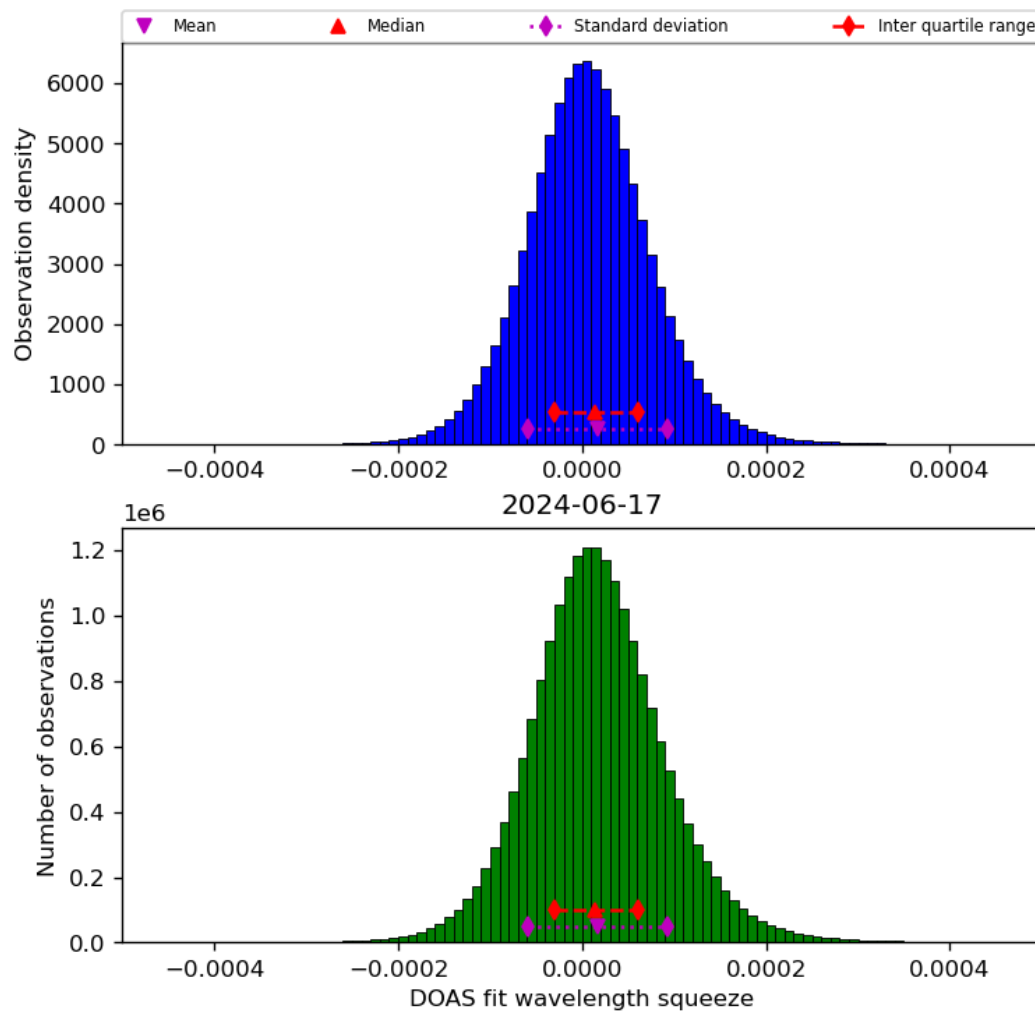
Figure 45: Histogram of “DOAS fit wavelength squeeze” for 2024-06-16 to 2024-06-18
