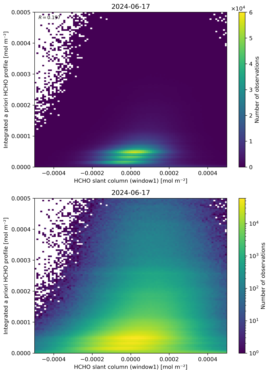
Figure 87: Scatter density plot of “HCHO slant column (window1)” against “Integrated a priori HCHO profile” for 2024-06-16 to 2024-06-18.
