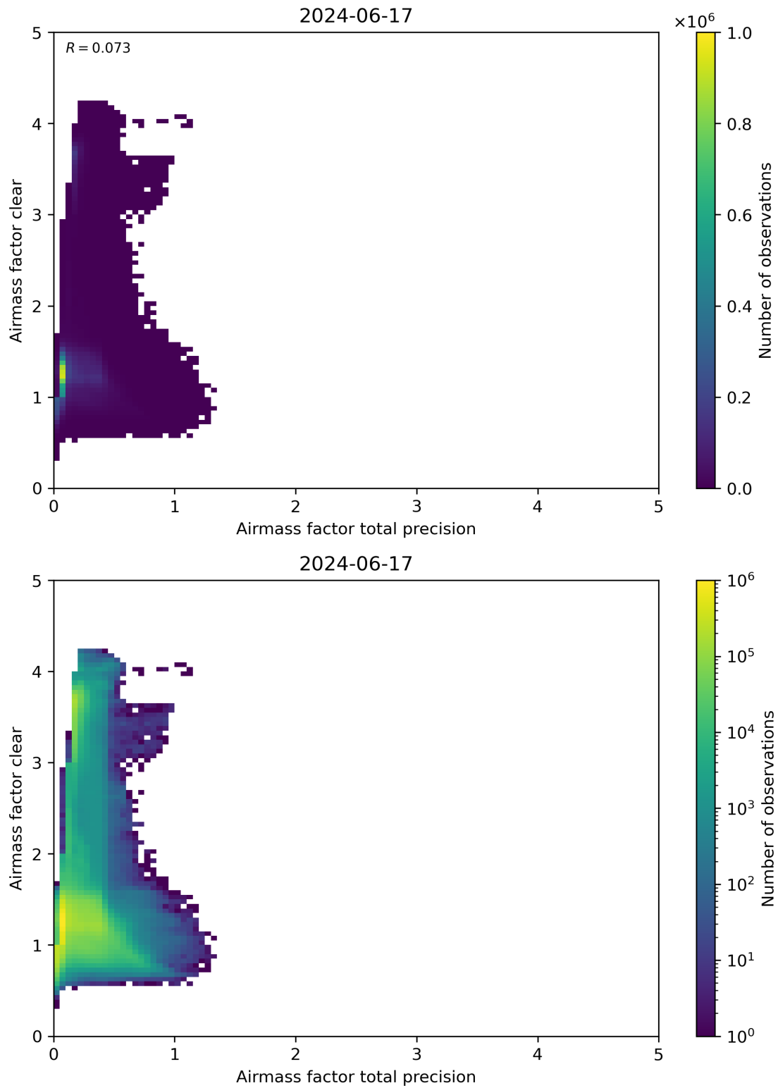
Figure 108: Scatter density plot of “Airmass factor total precision” against “Airmass factor clear” for 2024-06-16 to 2024-06-18.
