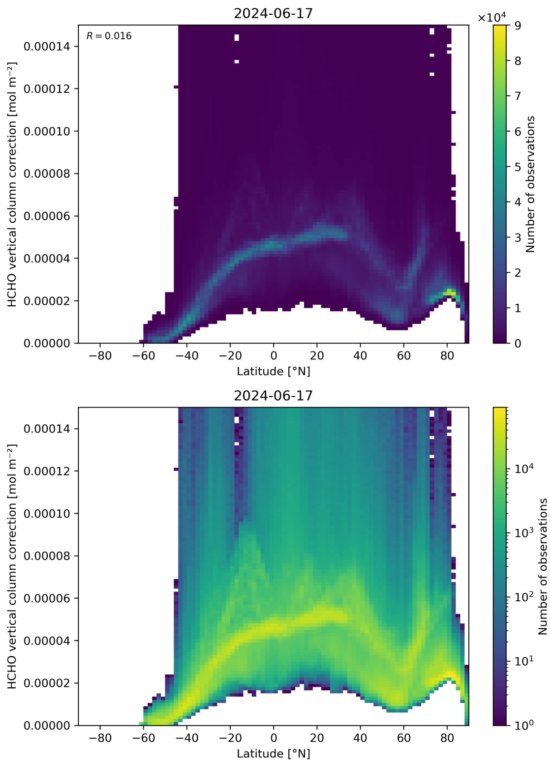
Figure 164: Scatter density plot of “Latitude” against “HCHO vertical column correction” for 2024-06-16 to 2024-06-18.
