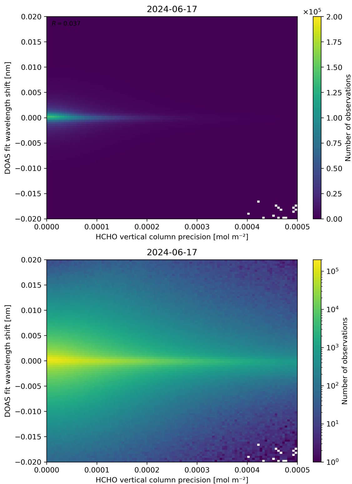
Figure 137: Scatter density plot of “HCHO vertical column precision” against “DOAS fit wavelength shift” for 2024-06-16 to 2024-06-18.
