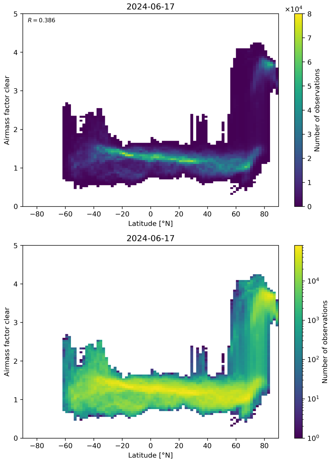
Figure 156: Scatter density plot of “Latitude” against “Airmass factor clear” for 2024-06-16 to 2024-06-18.
