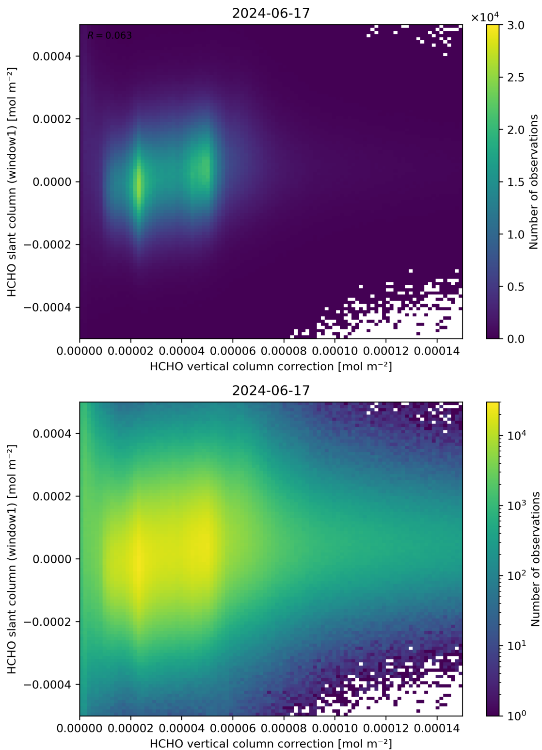
Figure 118: Scatter density plot of “HCHO vertical column correction” against “HCHO slant column (window1)” for 2024-06-16 to 2024-06-18.
