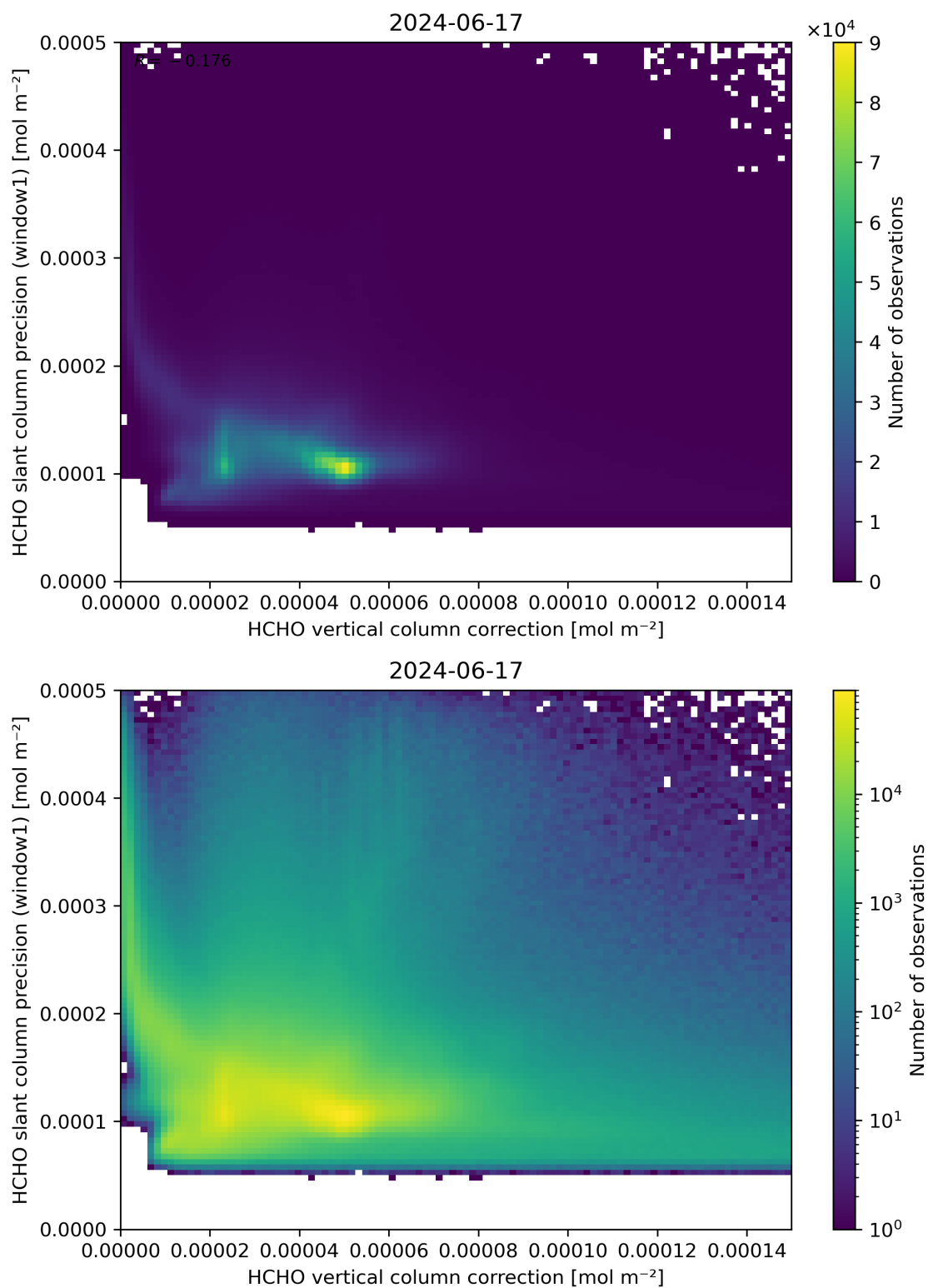
Figure 119: Scatter density plot of “HCHO vertical column correction” against “HCHO slant column precision (window1)” for 2024-06-16 to 2024-06-18.
