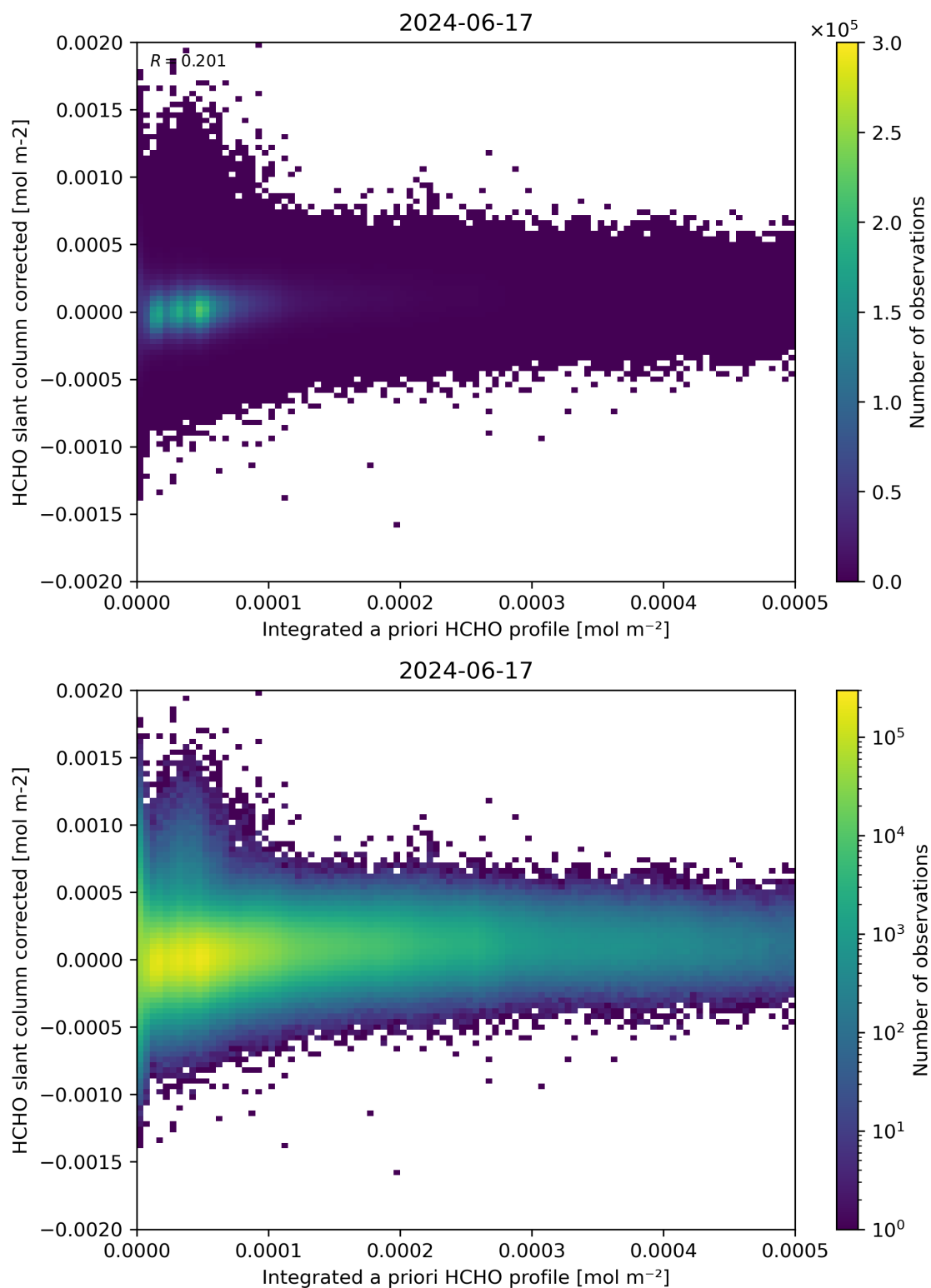
Figure 151: Scatter density plot of “Integrated a priori HCHO profile” against “HCHO slant column corrected” for 2024-06-16 to 2024-06-18.
