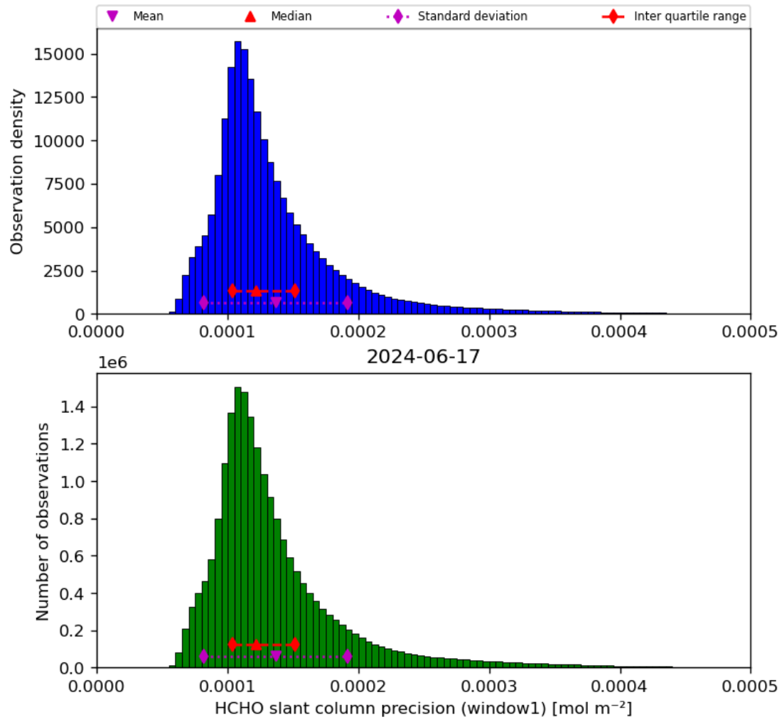
Figure 39: Histogram of “HCHO slant column precision (window1)” for 2024-06-16 to 2024-06-18
