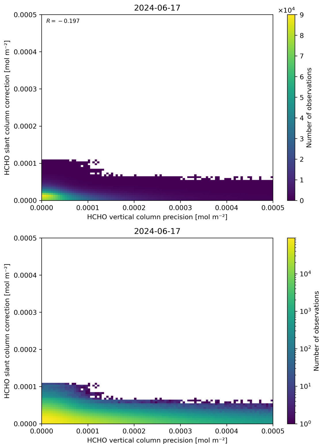
Figure 141: Scatter density plot of “HCHO vertical column precision” against “HCHO slant column correction” for 2024-06-16 to 2024-06-18.
