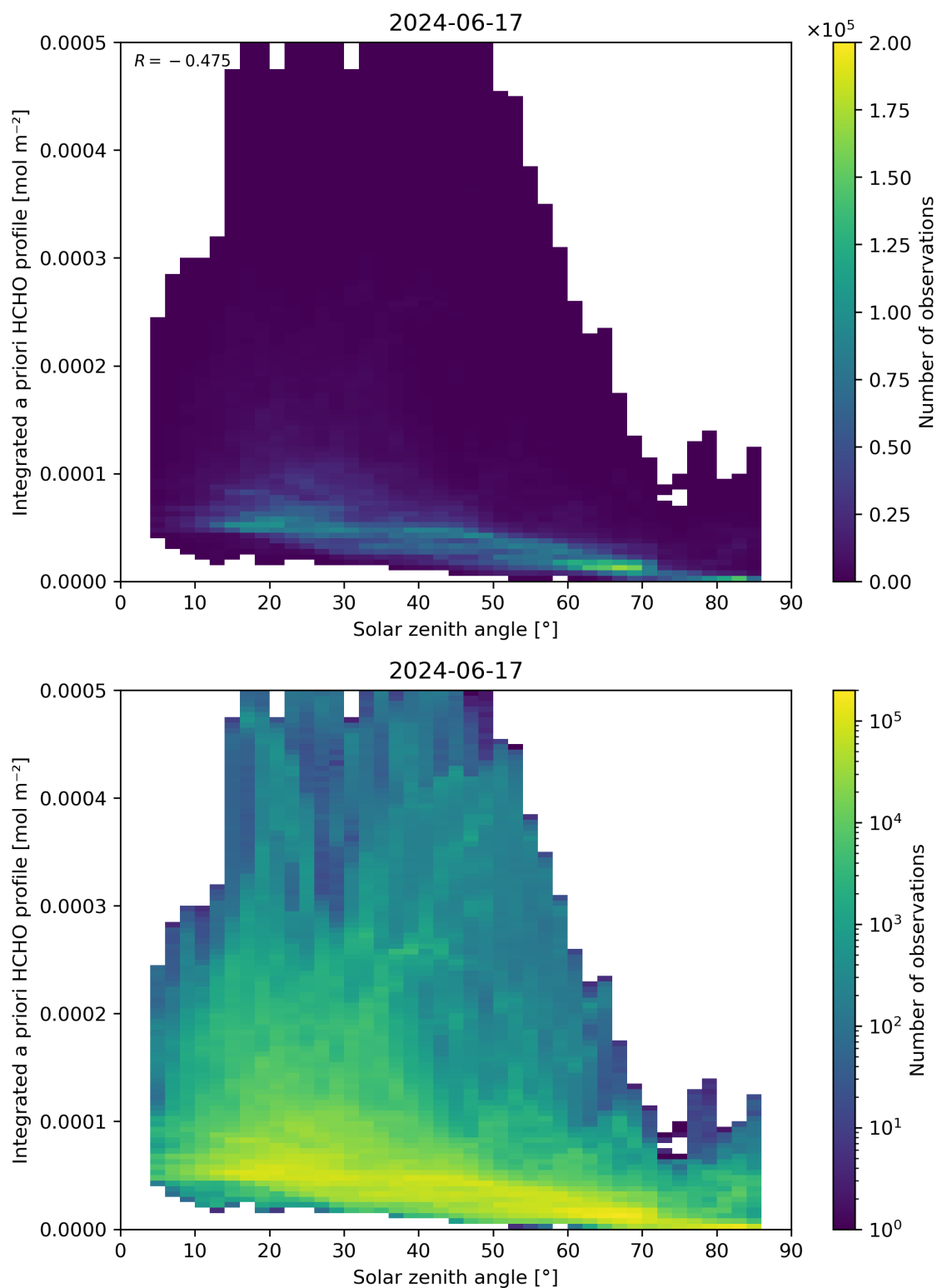
Figure 180: Scatter density plot of “Solar zenith angle” against “Integrated a priori HCHO profile” for 2024-06-16 to 2024-06-18.
