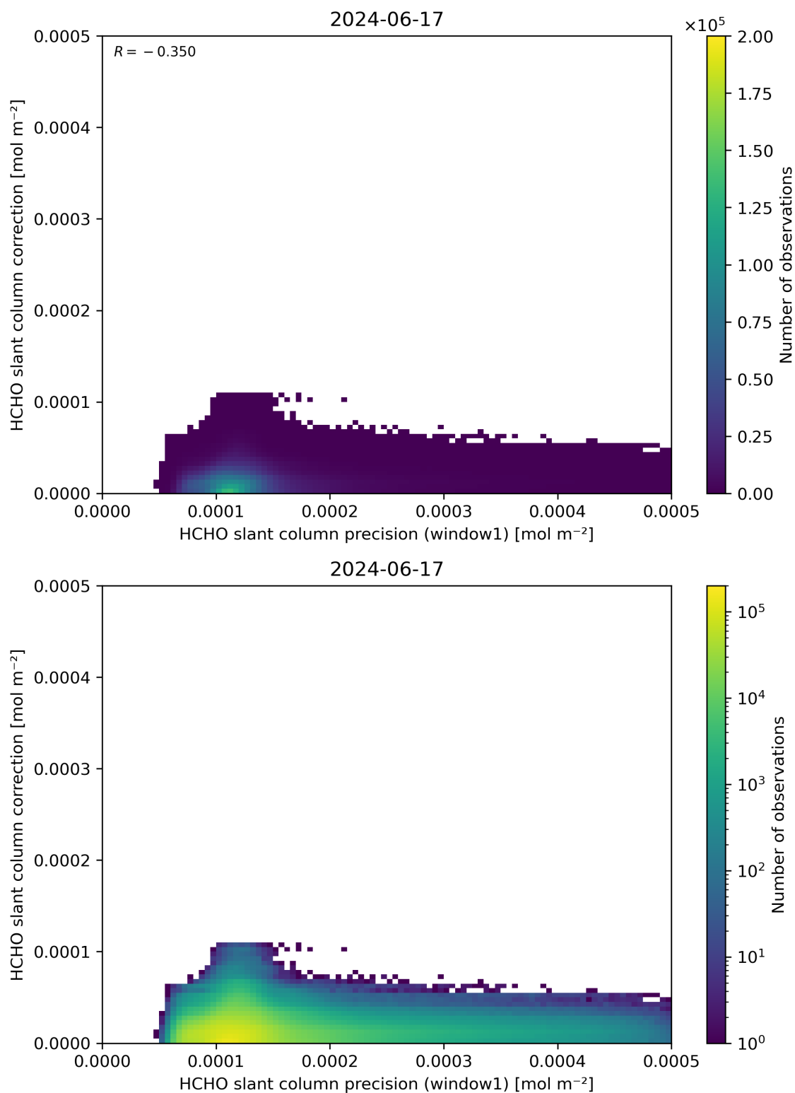
Figure 93: Scatter density plot of “HCHO slant column precision (window1)” against “HCHO slant column correction” for 2024-06-16 to 2024-06-18.
