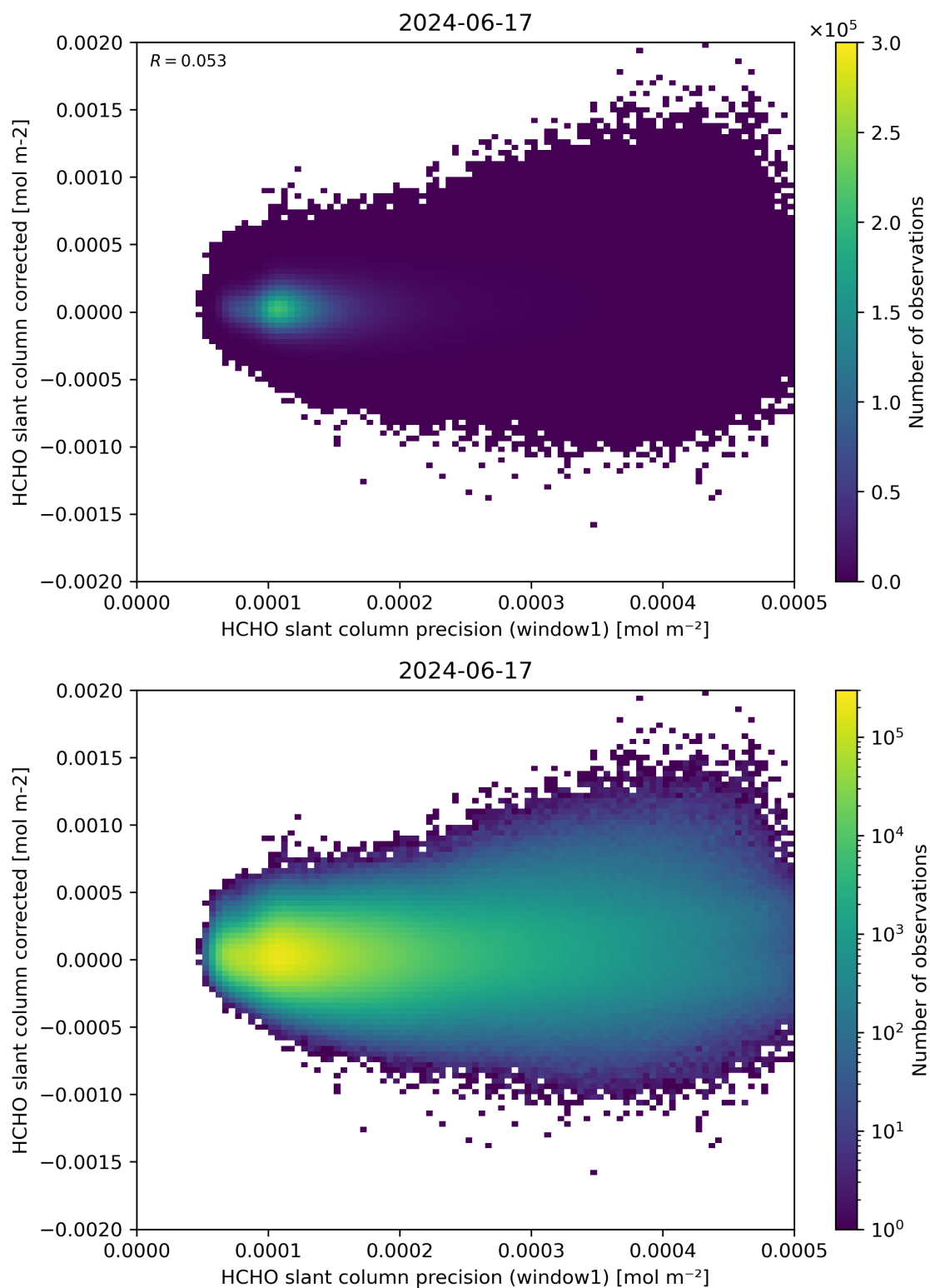
Figure 92: Scatter density plot of “HCHO slant column precision (window1)” against “HCHO slant column corrected” for 2024-06-16 to 2024-06-18.
