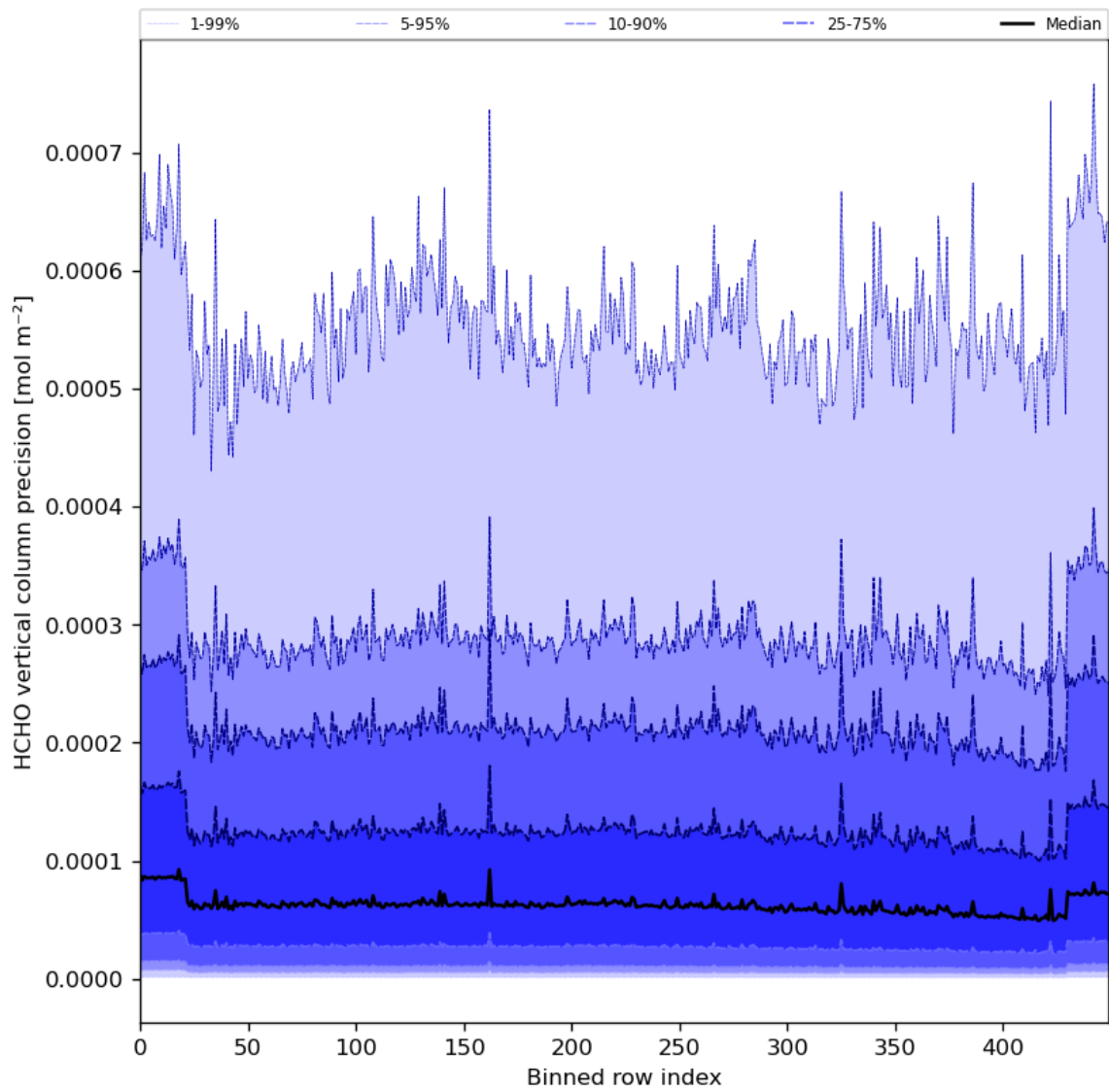
Figure 50: Along track statistics of “HCHO vertical column precision” for 2024-06-16 to 2024-06-18
