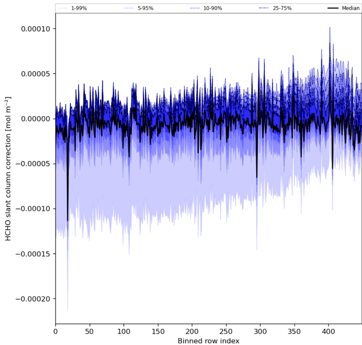
Figure 61: Along track statistics of “HCHO slant column correction” for 2024-06-16 to 2024-06-18
