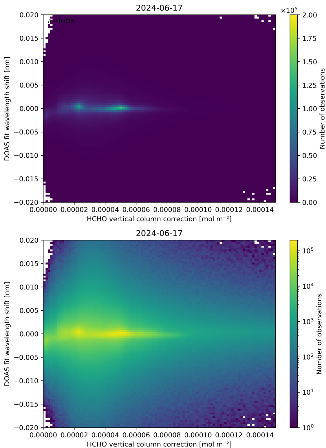
Figure 113: Scatter density plot of “HCHO vertical column correction” against “DOAS fit wavelength shift” for 2024-06-16 to 2024-06-18.
