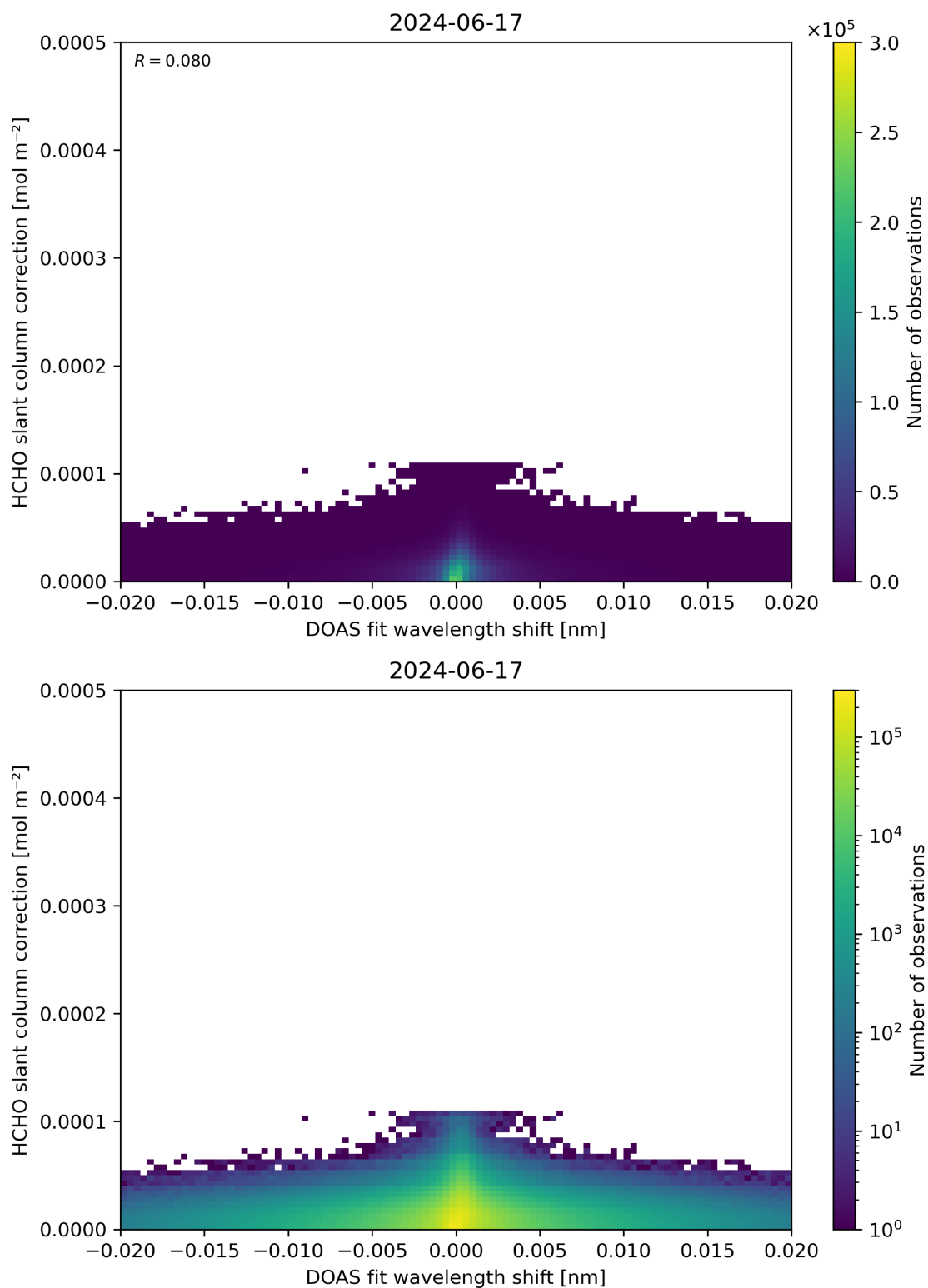
Figure 67: Scatter density plot of “DOAS fit wavelength shift” against “HCHO slant column correction” for 2024-06-16 to 2024-06-18.
