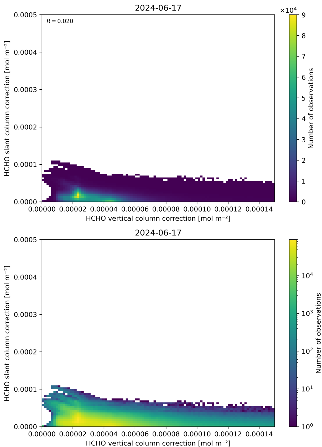
Figure 117: Scatter density plot of “HCHO vertical column correction” against “HCHO slant column correction” for 2024-06-16 to 2024-06-18.
