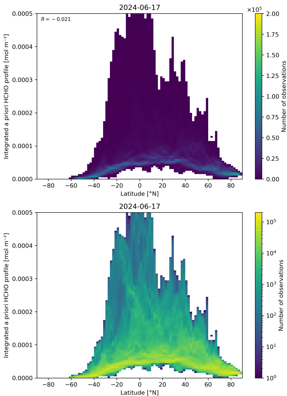
Figure 166: Scatter density plot of “Latitude” against “Integrated a priori HCHO profile” for 2024-06-16 to 2024-06-18.
