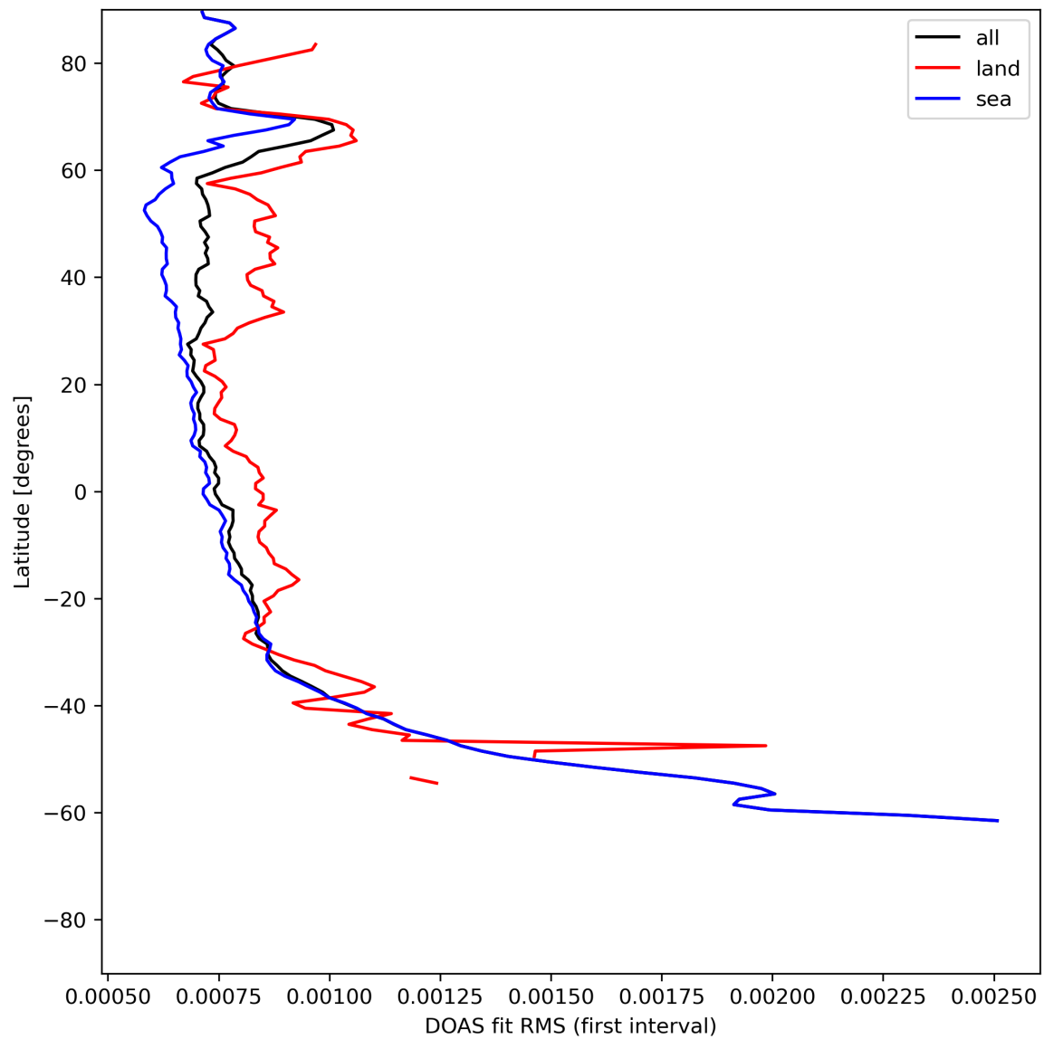
Figure 32: Zonal average of “DOAS fit RMS (first interval)” for 2024-06-16 to 2024-06-18.
