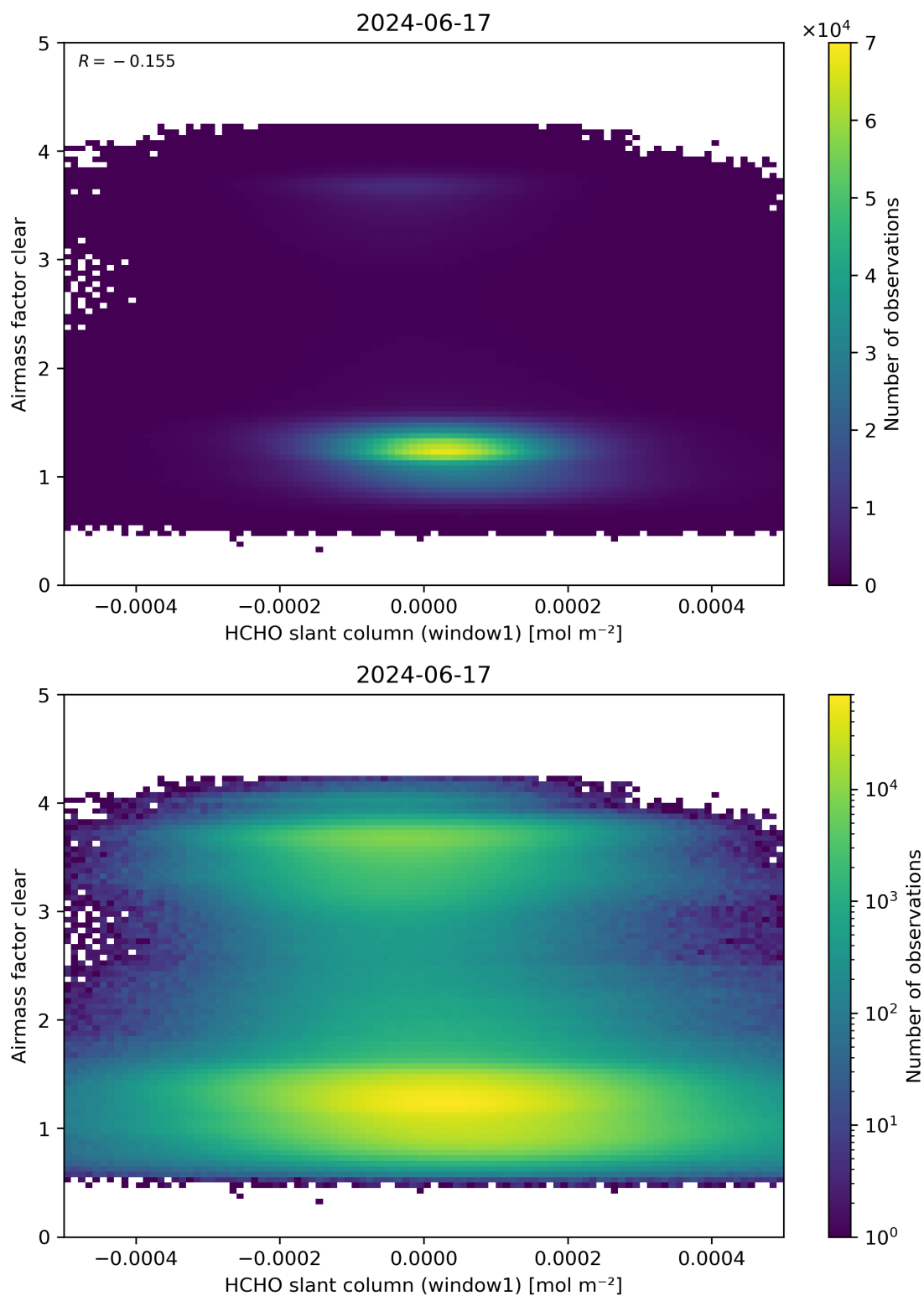
Figure 81: Scatter density plot of “HCHO slant column (window1)” against “Airmass factor clear” for 2024-06-16 to 2024-06-18.
