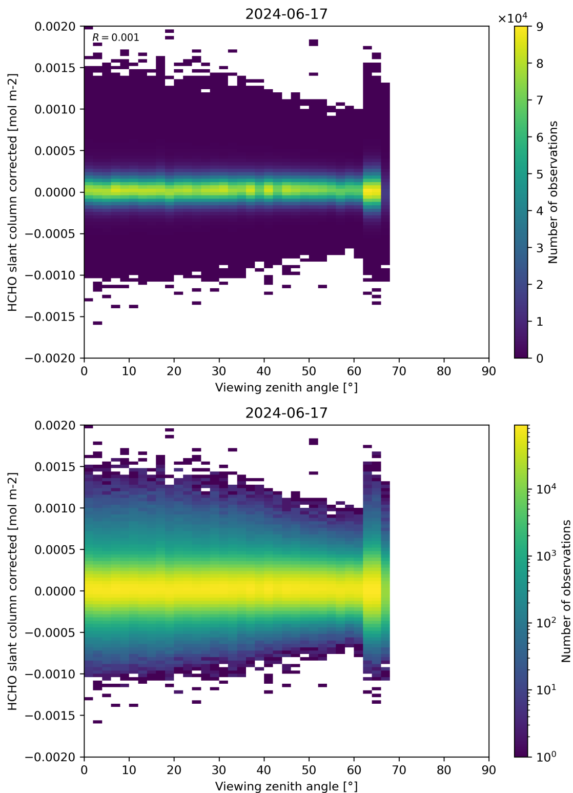
Figure 186: Scatter density plot of “Viewing zenith angle” against “HCHO slant column corrected” for 2024-06-16 to 2024-06-18.
