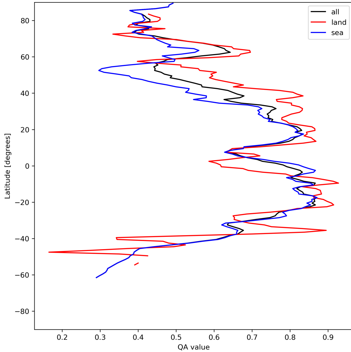
Figure 20: Zonal average of “QA value” for 2024-06-16 to 2024-06-18.
