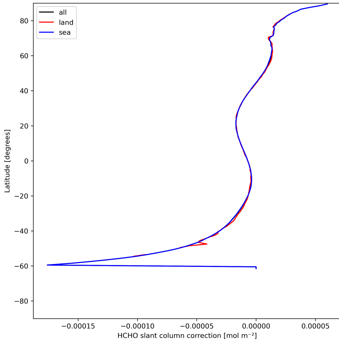
Figure 33: Zonal average of “HCHO slant column correction” for 2024-06-16 to 2024-06-18.
