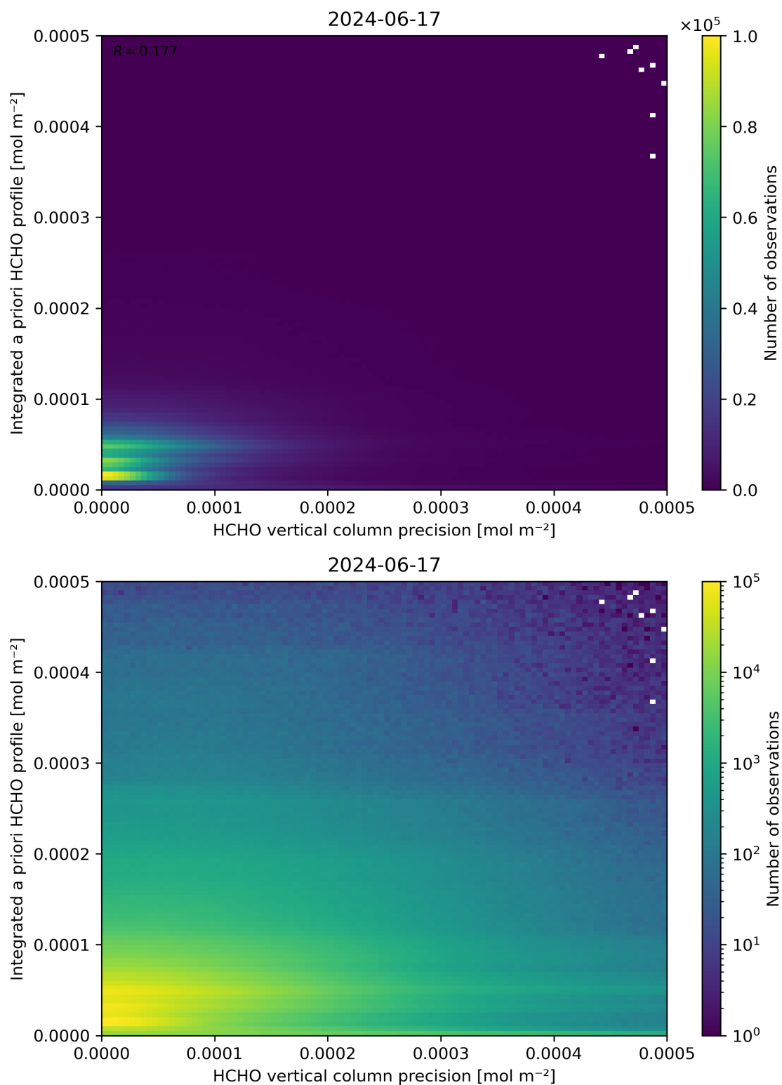
Figure 147: Scatter density plot of “HCHO vertical column precision” against “Integrated a priori HCHO profile” for 2024-06-16 to 2024-06-18.
