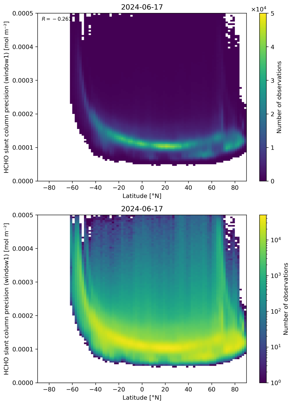
Figure 160: Scatter density plot of “Latitude” against “HCHO slant column precision (window1)” for 2024-06-16 to 2024-06-18.
