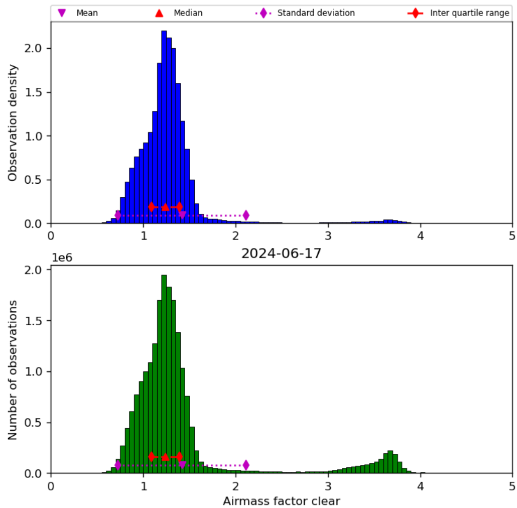
Figure 42: Histogram of “Airmass factor clear” for 2024-06-16 to 2024-06-18
