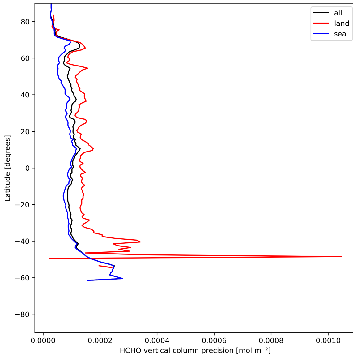
Figure 22: Zonal average of “HCHO vertical column precision” for 2024-06-16 to 2024-06-18.
