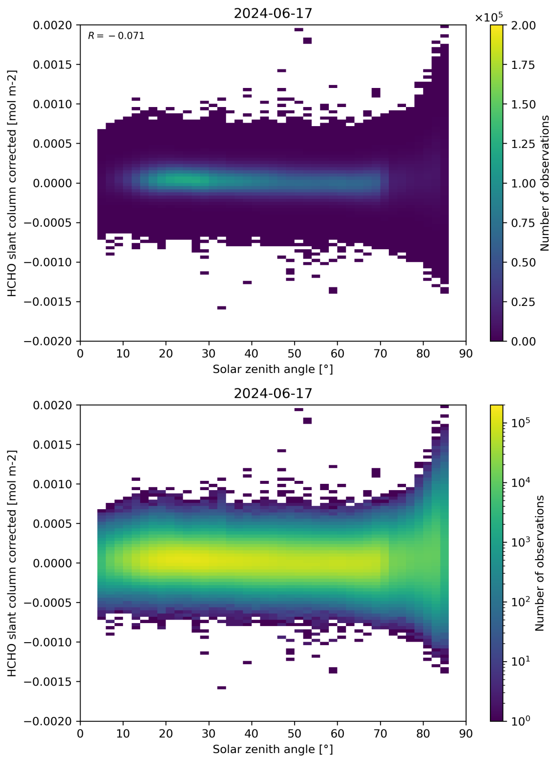
Figure 171: Scatter density plot of “Solar zenith angle” against “HCHO slant column corrected” for 2024-06-16 to 2024-06-18.
