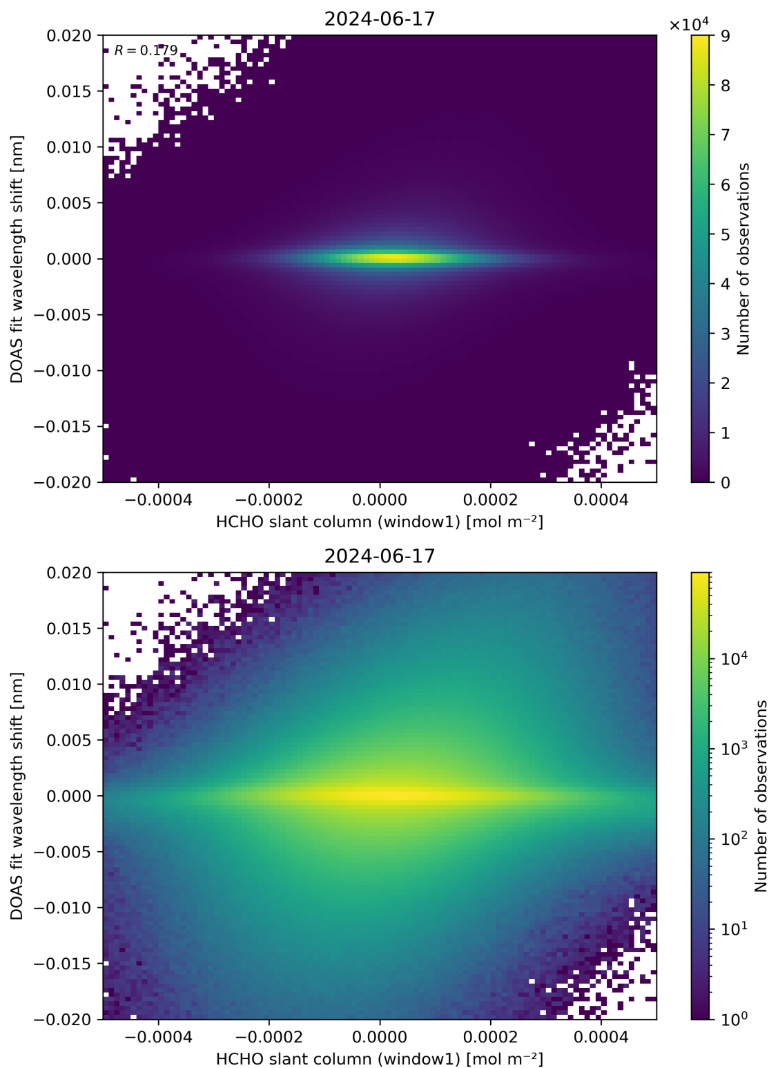
Figure 79: Scatter density plot of “HCHO slant column (window1)” against “DOAS fit wavelength shift” for 2024-06-16 to 2024-06-18.
