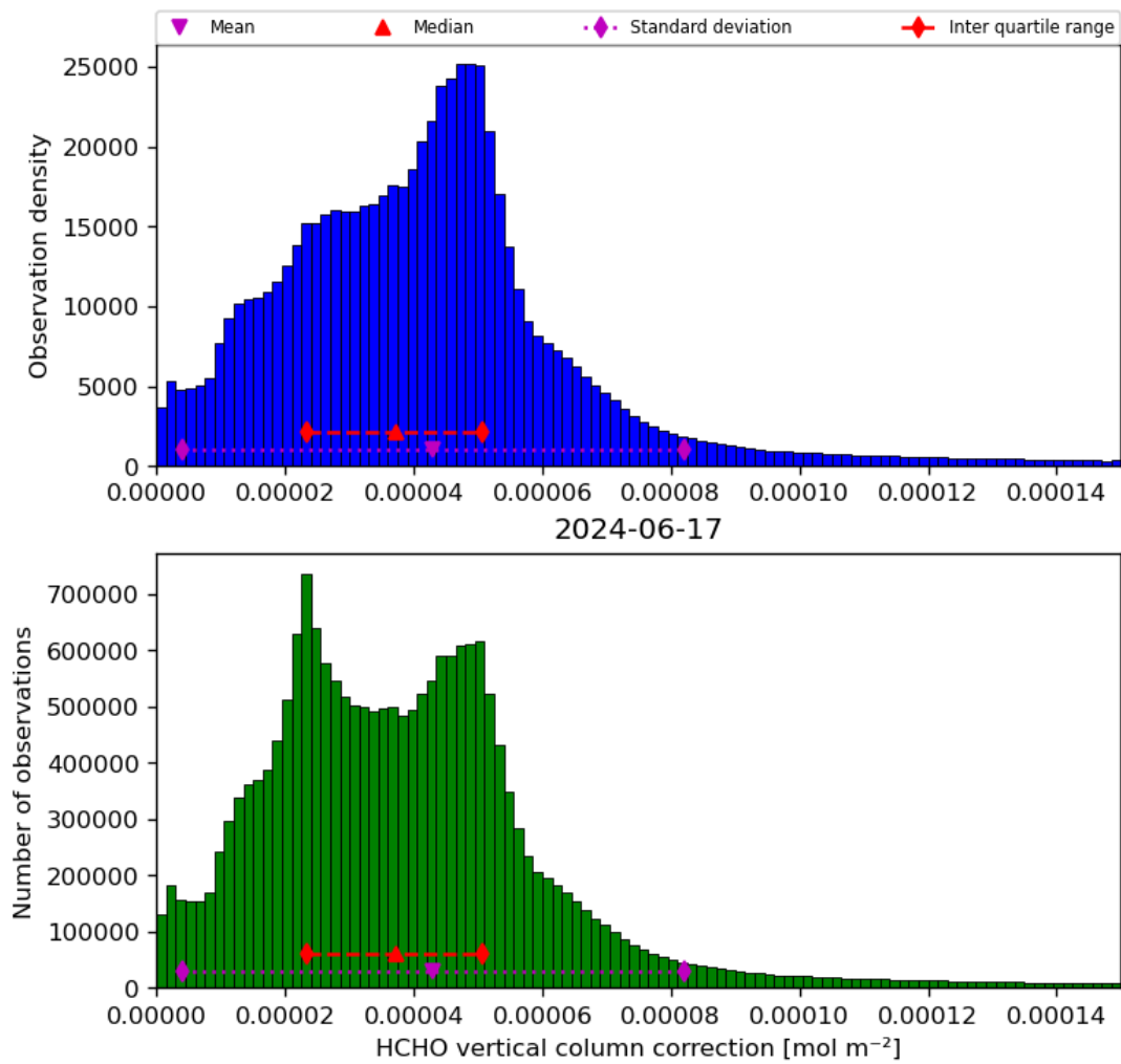
Figure 37: Histogram of “HCHO vertical column correction” for 2024-06-16 to 2024-06-18
