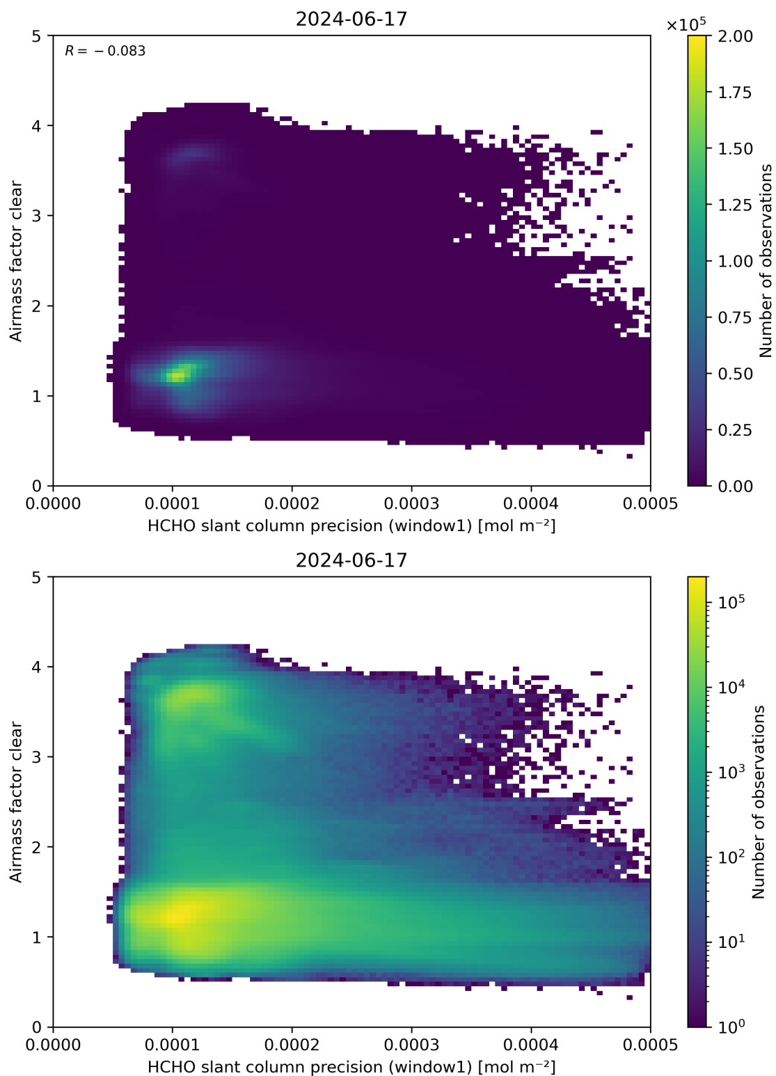
Figure 91: Scatter density plot of “HCHO slant column precision (window1)” against “Airmass factor clear” for 2024-06-16 to 2024-06-18.
