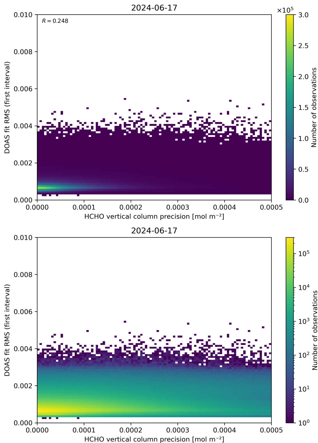
Figure 136: Scatter density plot of “HCHO vertical column precision” against “DOAS fit RMS (first interval)” for 2024-06-16 to 2024-06-18.
