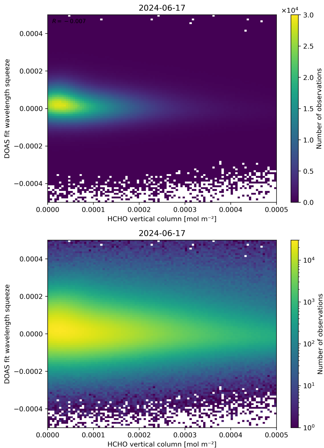
Figure 125: Scatter density plot of “HCHO vertical column” against “DOAS fit wavelength squeeze” for 2024-06-16 to 2024-06-18.
