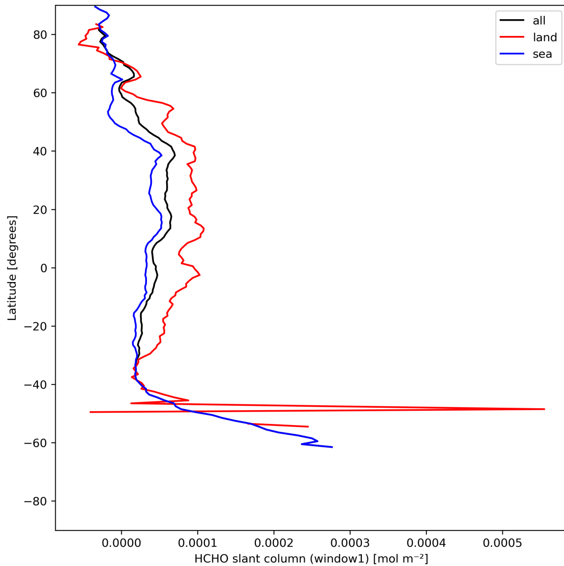
Figure 24: Zonal average of “HCHO slant column (window1)” for 2024-06-16 to 2024-06-18.
