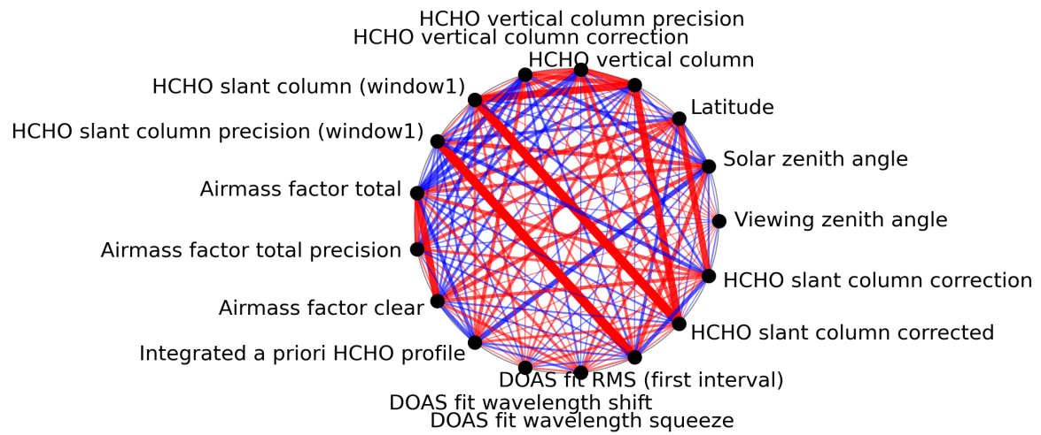
Figure 1: Map of correlation graph for 2024-06-16 to 2024-06-18.
