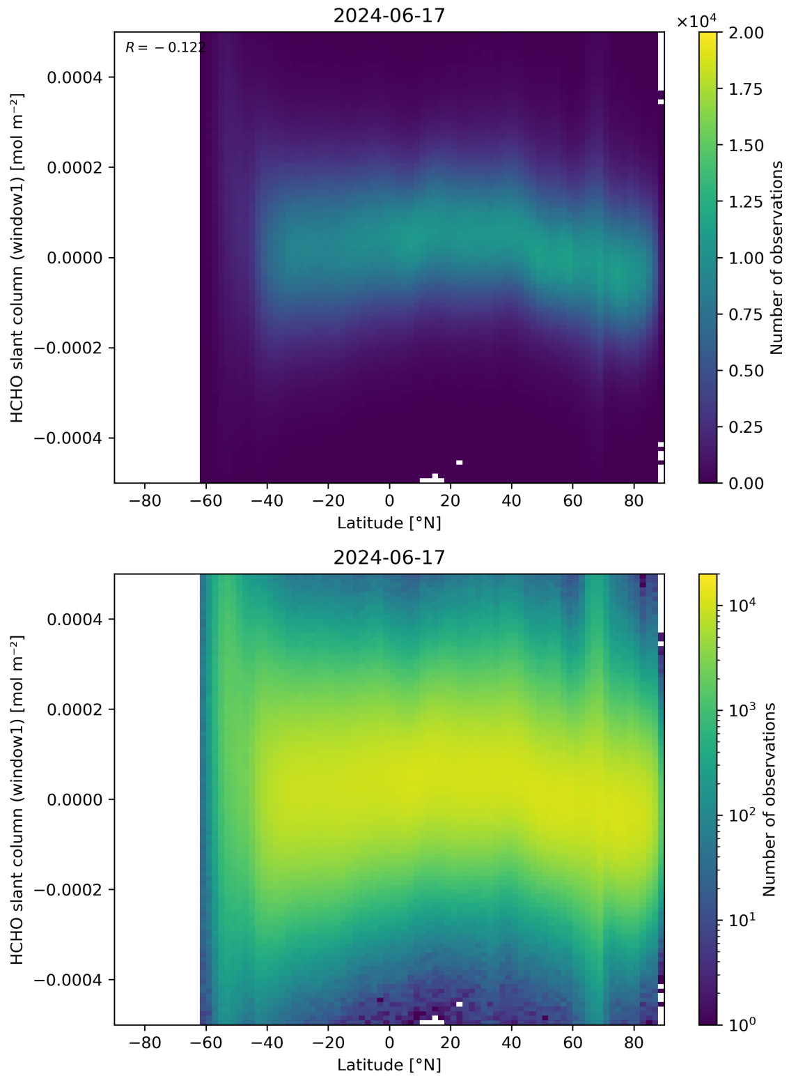
Figure 159: Scatter density plot of “Latitude” against “HCHO slant column (window1)” for 2024-06-16 to 2024-06-18.
