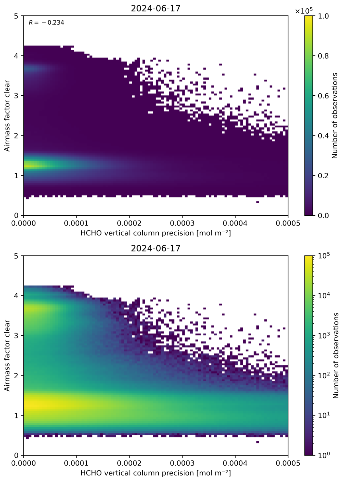
Figure 139: Scatter density plot of “HCHO vertical column precision” against “Airmass factor clear” for 2024-06-16 to 2024-06-18.
