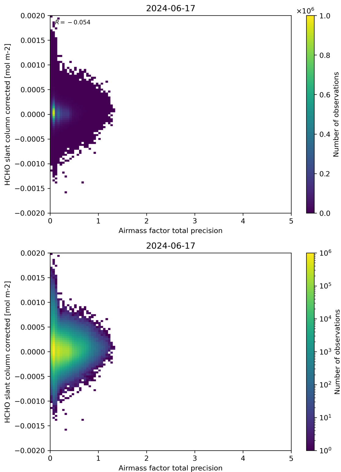
Figure 109: Scatter density plot of “Airmass factor total precision” against “HCHO slant column corrected” for 2024-06-16 to 2024-06-18.
