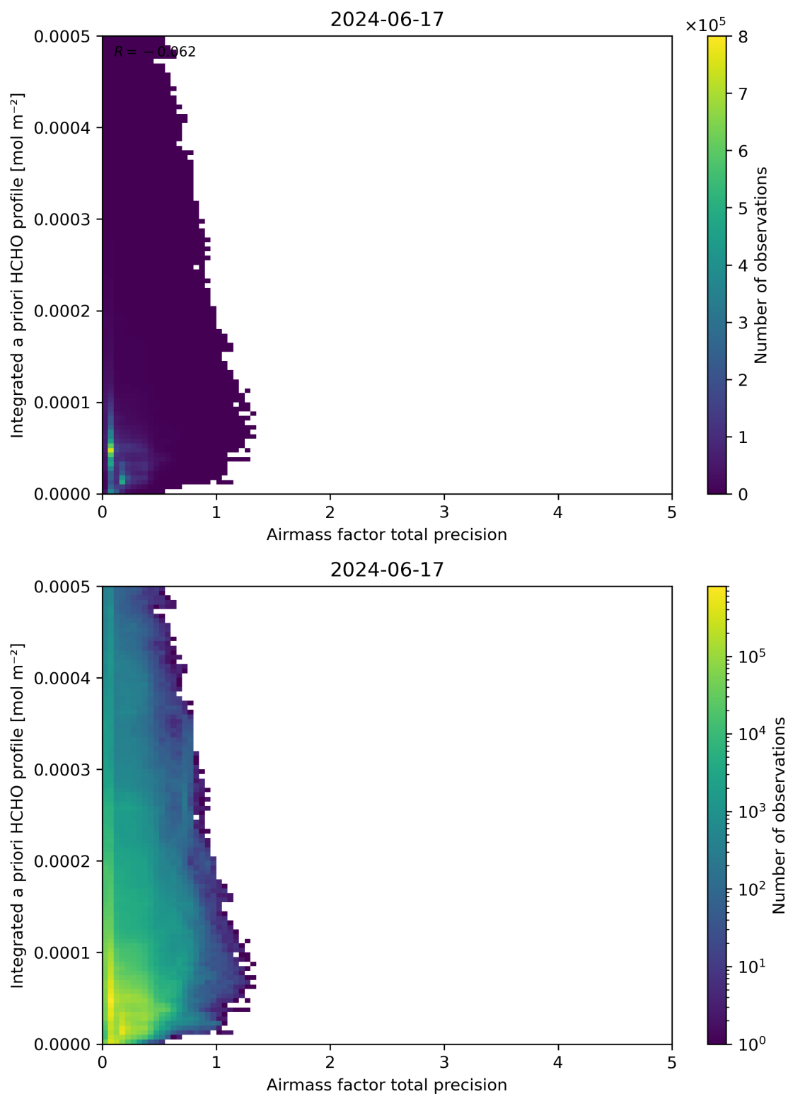
Figure 111: Scatter density plot of “Airmass factor total precision” against “Integrated a priori HCHO profile” for 2024-06-16 to 2024-06-18.
