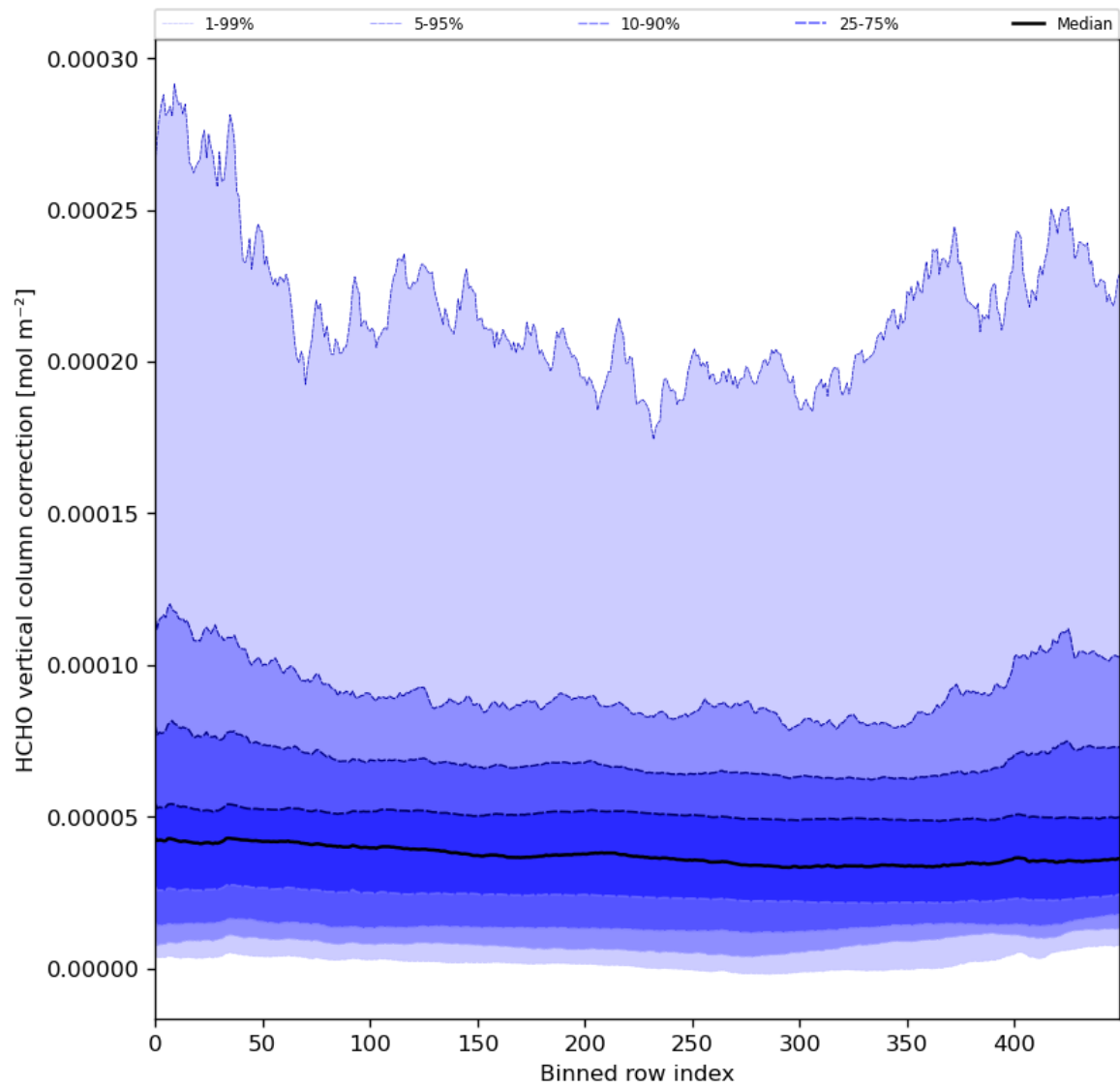
Figure 51: Along track statistics of “HCHO vertical column correction” for 2024-06-16 to 2024-06-18
