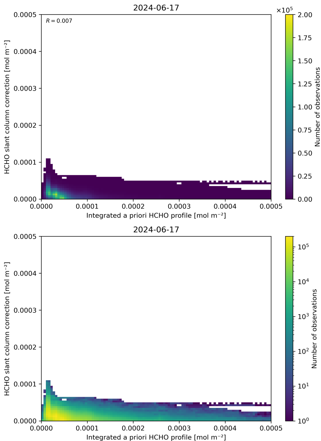
Figure 152: Scatter density plot of “Integrated a priori HCHO profile” against “HCHO slant column correction” for 2024-06-16 to 2024-06-18.
