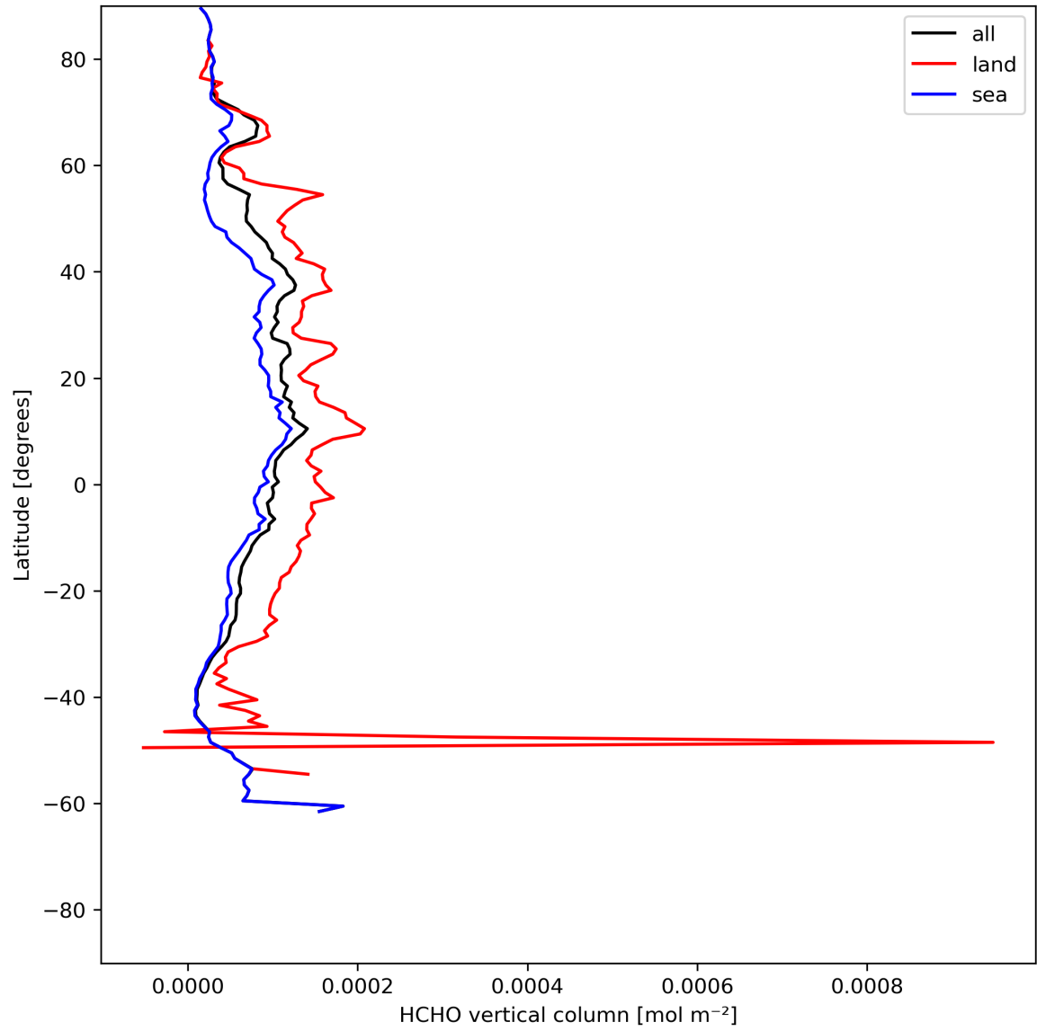
Figure 21: Zonal average of “HCHO vertical column” for 2024-06-16 to 2024-06-18.
