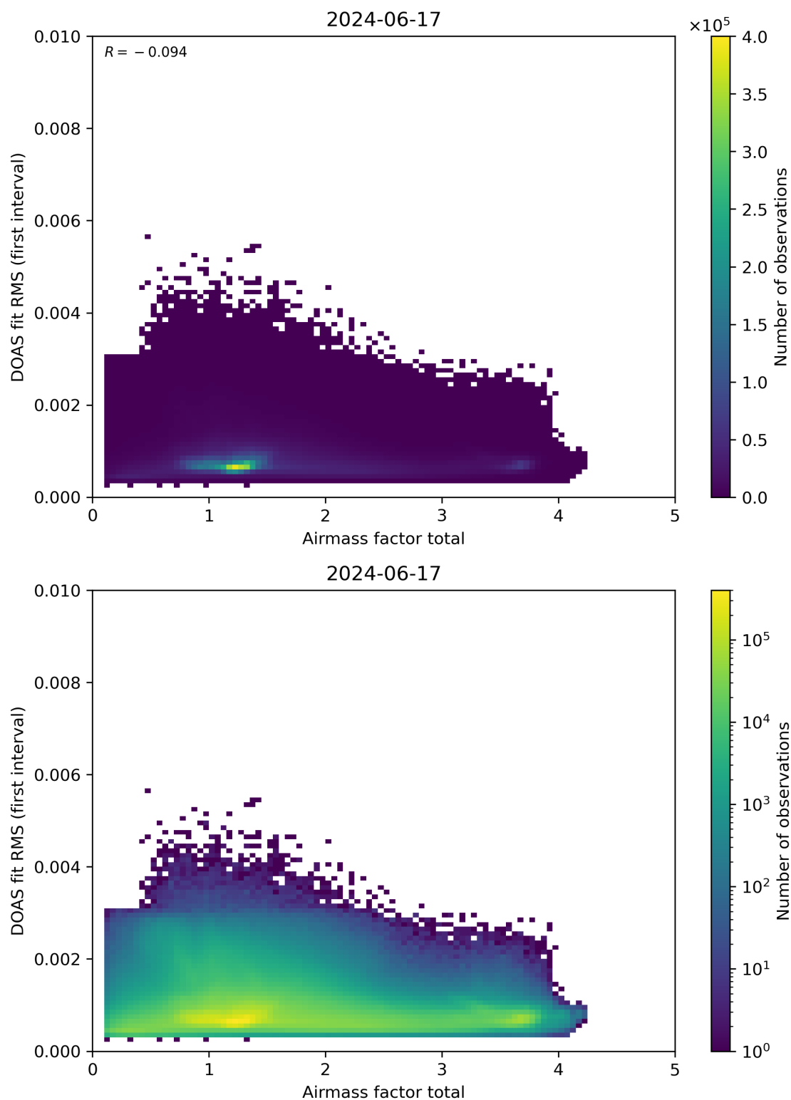
Figure 97: Scatter density plot of “Airmass factor total” against “DOAS fit RMS (first interval)” for 2024-06-16 to 2024-06-18.
