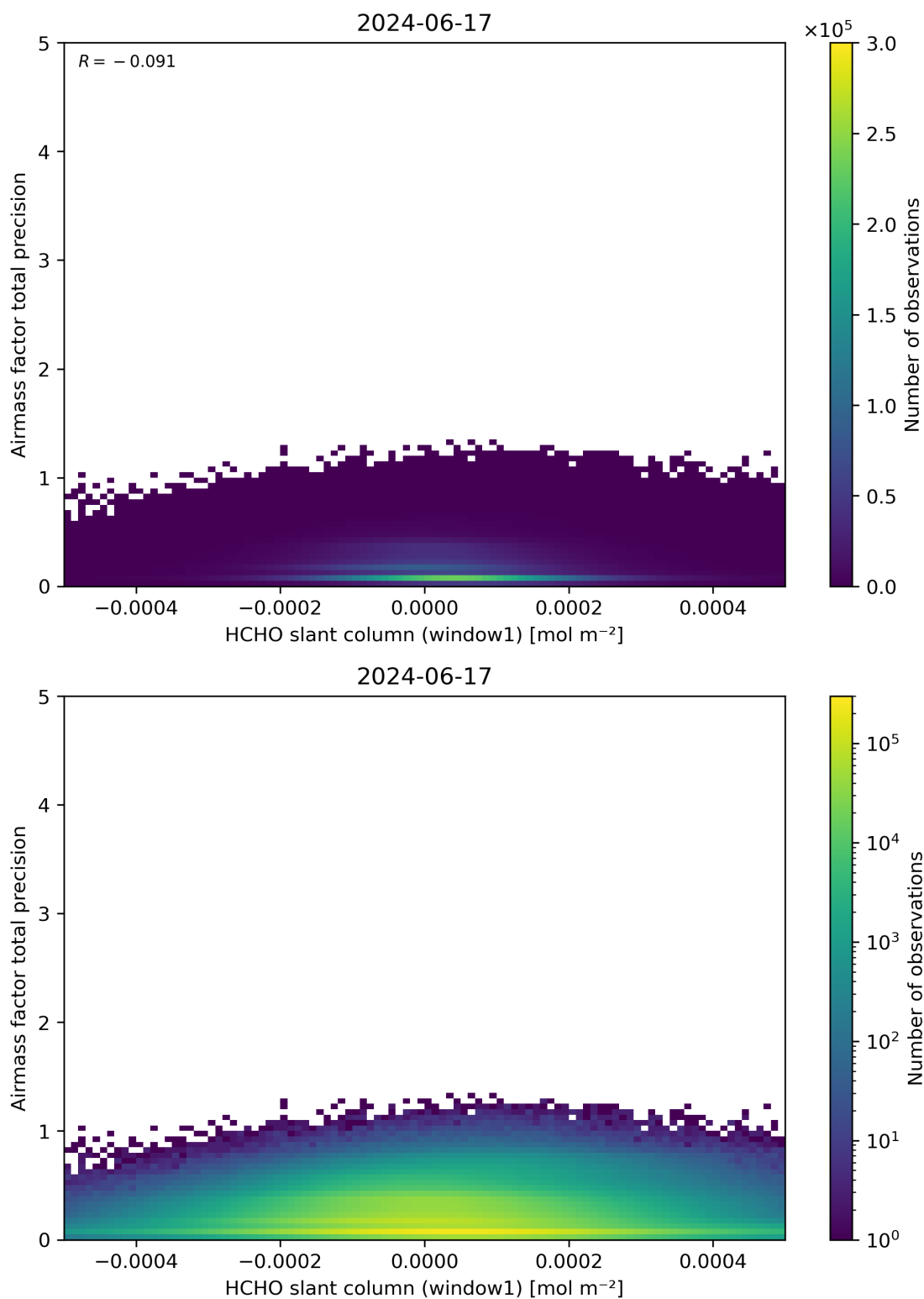
Figure 86: Scatter density plot of “HCHO slant column (window1)” against “Airmass factor total precision” for 2024-06-16 to 2024-06-18.
