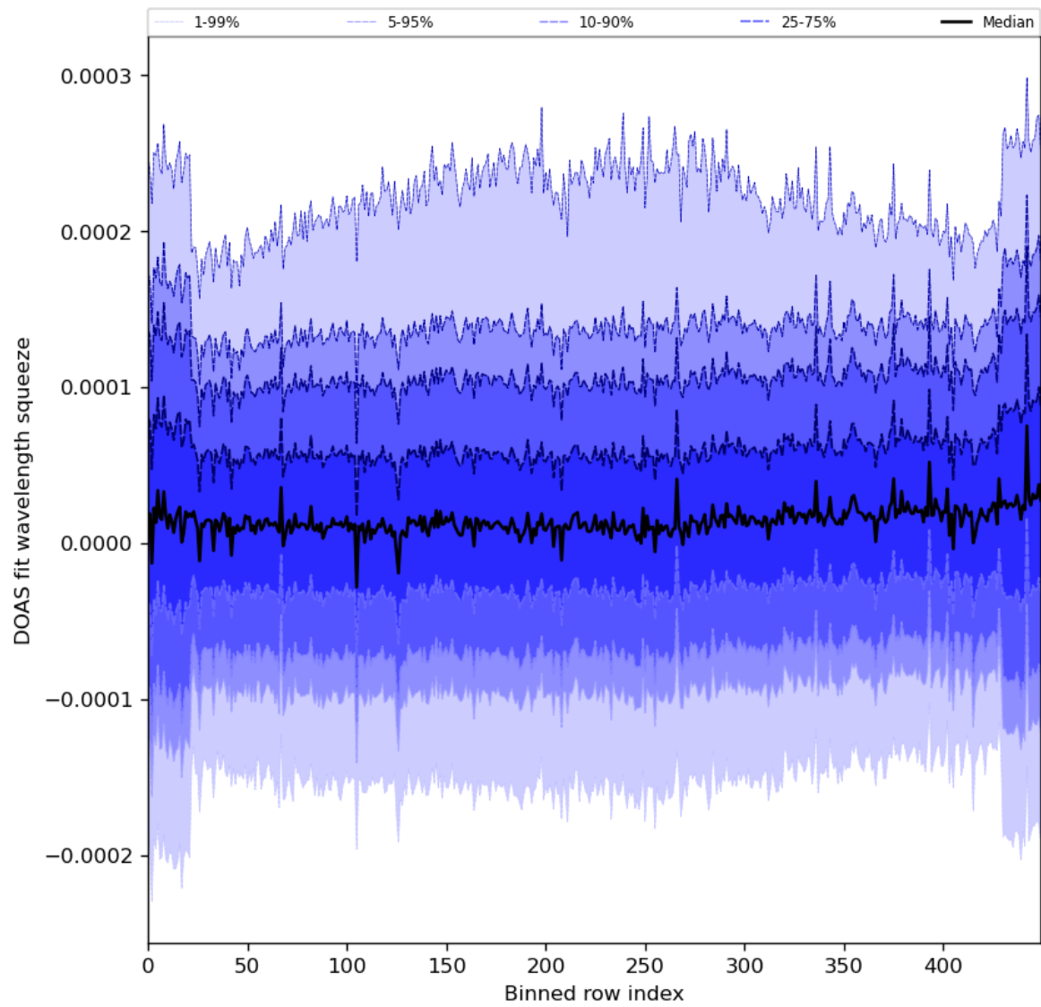
Figure 59: Along track statistics of “DOAS fit wavelength squeeze” for 2024-06-16 to 2024-06-18
