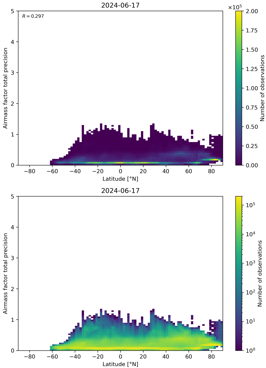
Figure 162: Scatter density plot of “Latitude” against “Airmass factor total precision” for 2024-06-16 to 2024-06-18.
