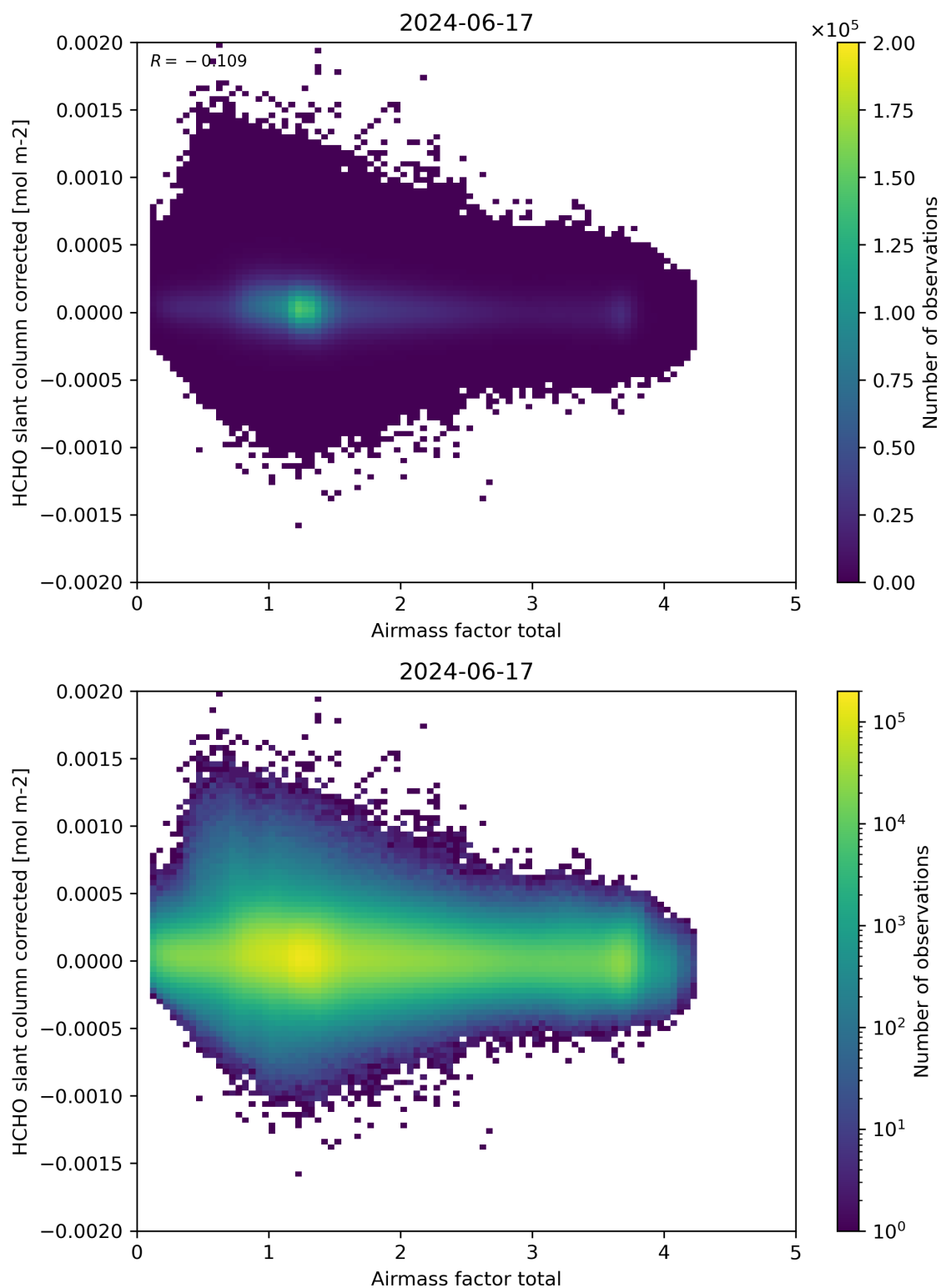
Figure 101: Scatter density plot of “Airmass factor total” against “HCHO slant column corrected” for 2024-06-16 to 2024-06-18.
