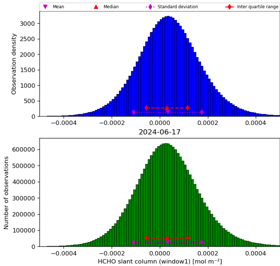
Figure 38: Histogram of “HCHO slant column (window1)” for 2024-06-16 to 2024-06-18
