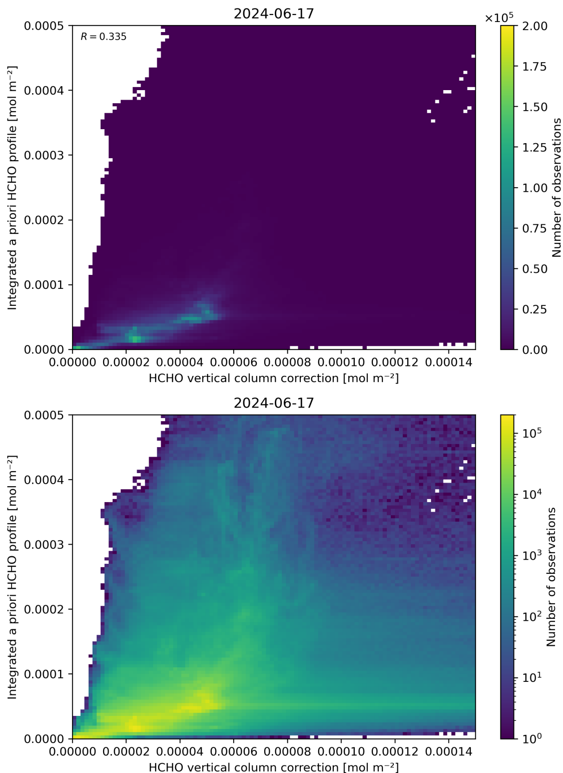
Figure 122: Scatter density plot of “HCHO vertical column correction” against “Integrated a priori HCHO profile” for 2024-06-16 to 2024-06-18.
