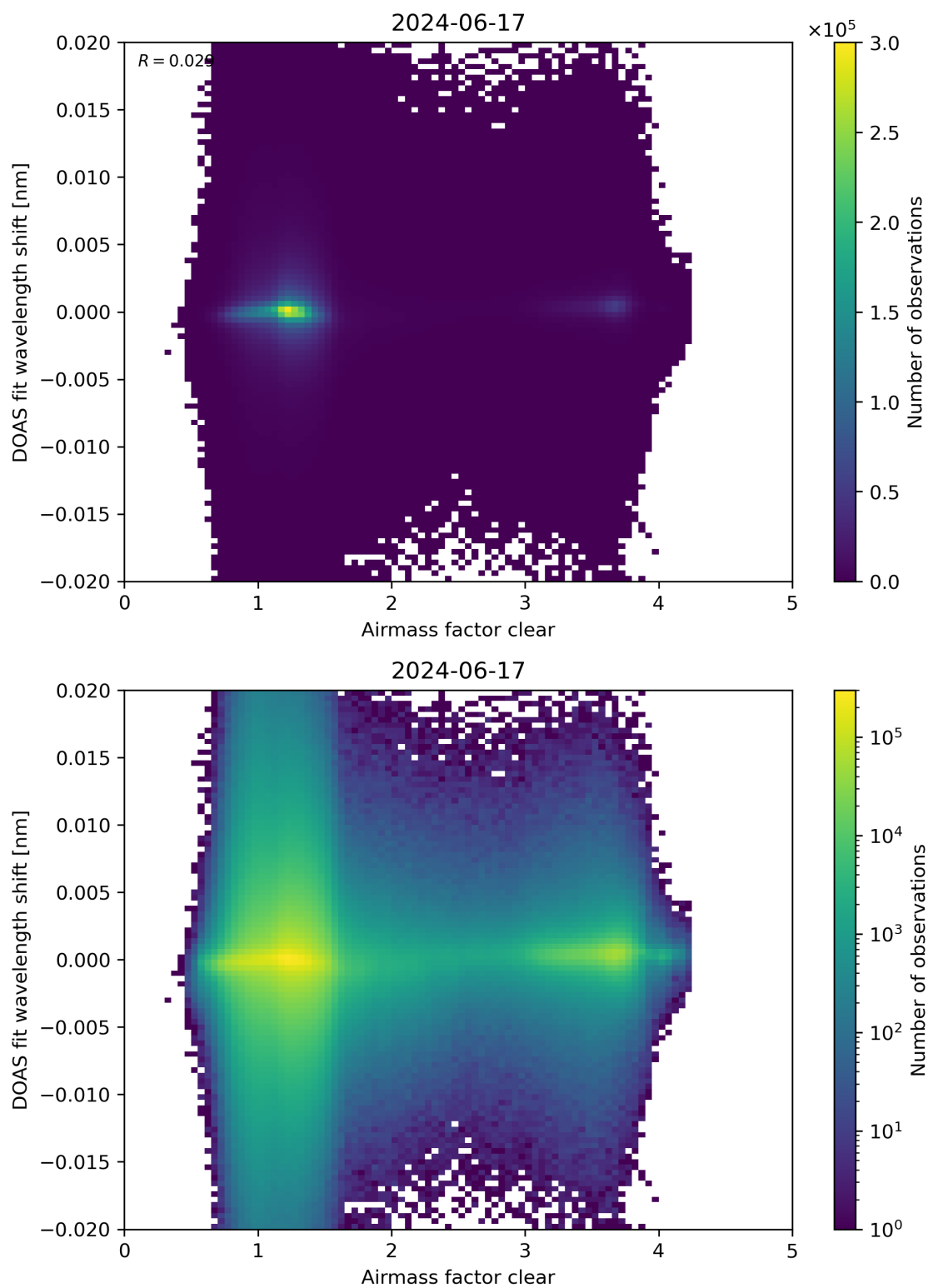
Figure 72: Scatter density plot of “Airmass factor clear” against “DOAS fit wavelength shift” for 2024-06-16 to 2024-06-18.
