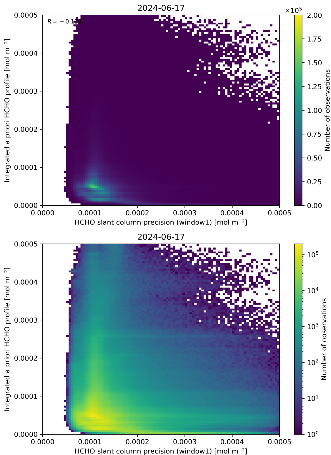
Figure 96: Scatter density plot of “HCHO slant column precision (window1)” against “Integrated a priori HCHO profile” for 2024-06-16 to 2024-06-18.
