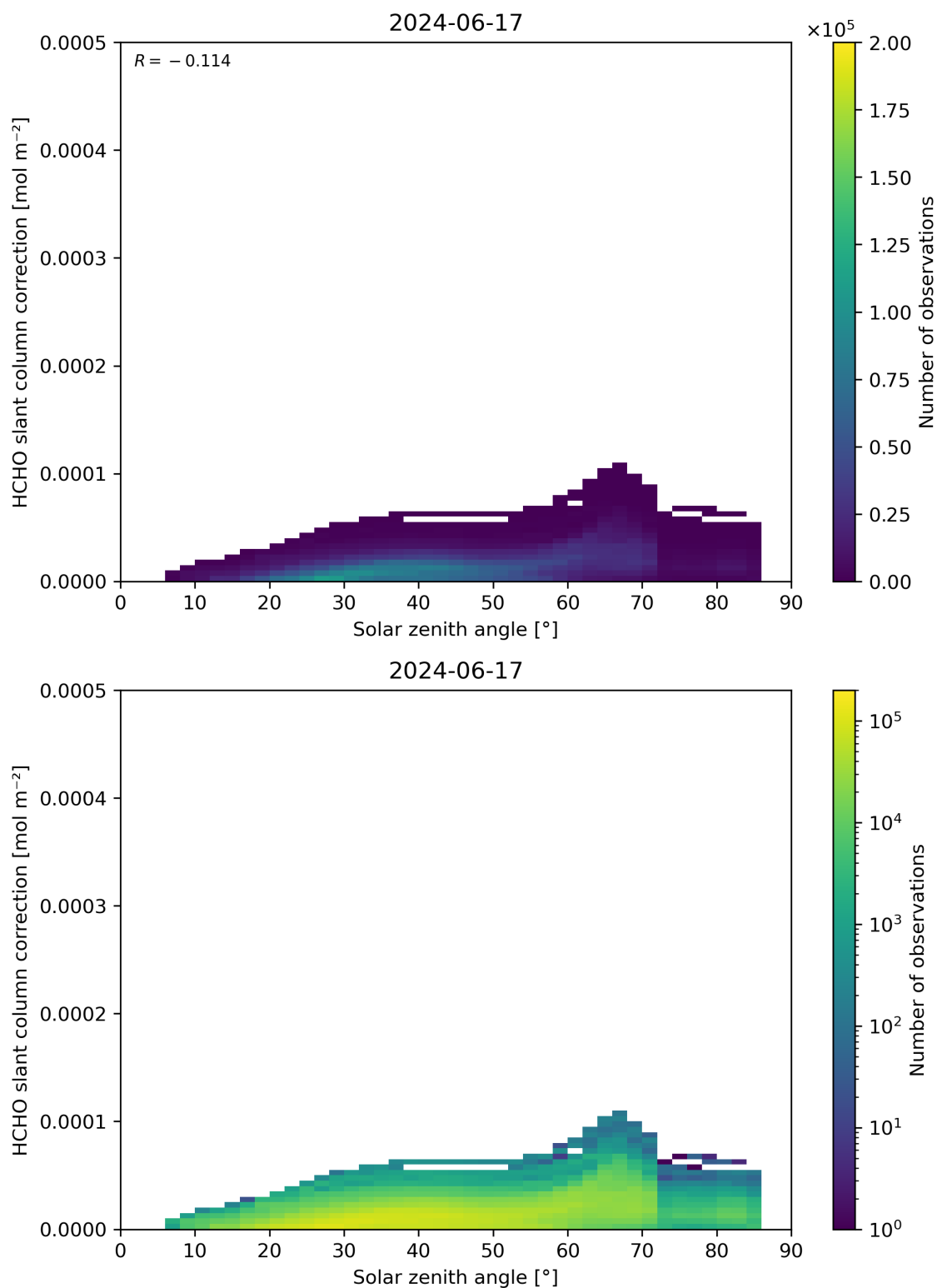
Figure 172: Scatter density plot of “Solar zenith angle” against “HCHO slant column correction” for 2024-06-16 to 2024-06-18.
