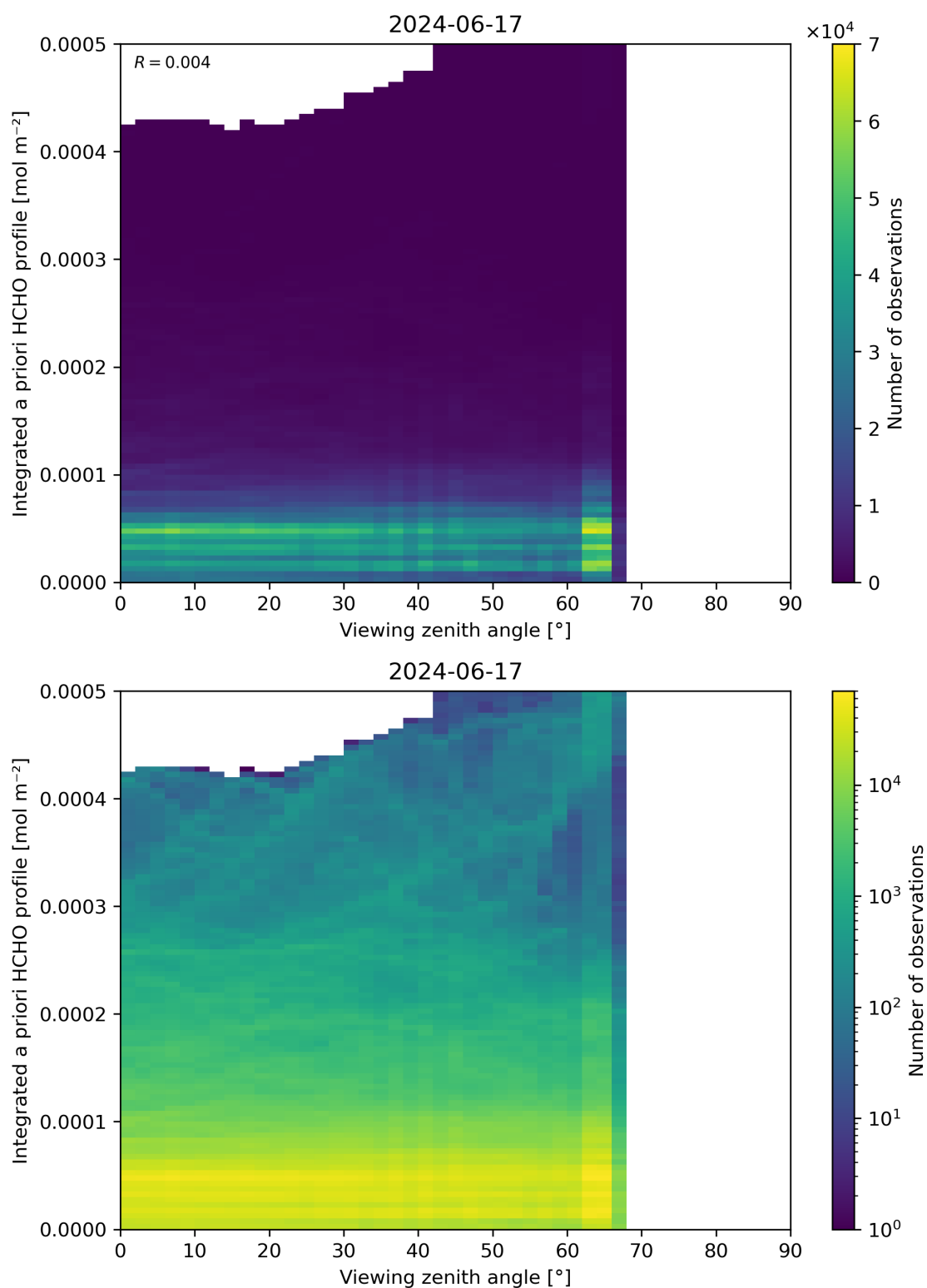
Figure 195: Scatter density plot of “Viewing zenith angle” against “Integrated a priori HCHO profile” for 2024-06-16 to 2024-06-18.
