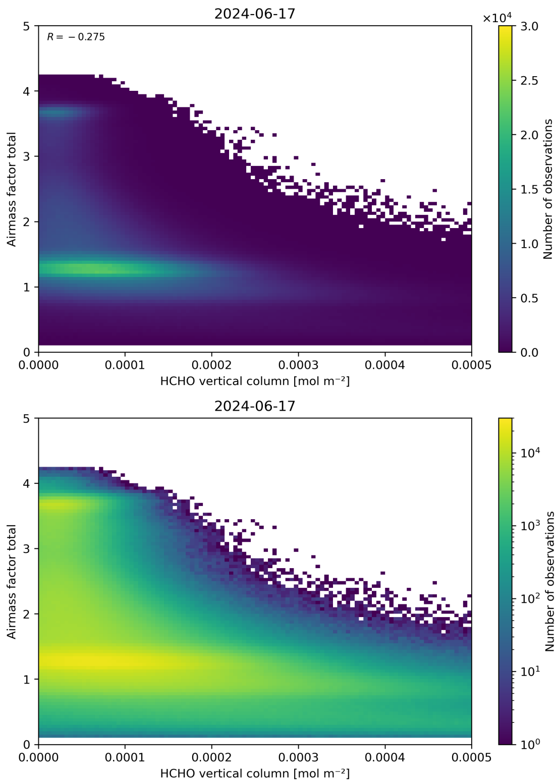
Figure 131: Scatter density plot of “HCHO vertical column” against “Airmass factor total” for 2024-06-16 to 2024-06-18.
