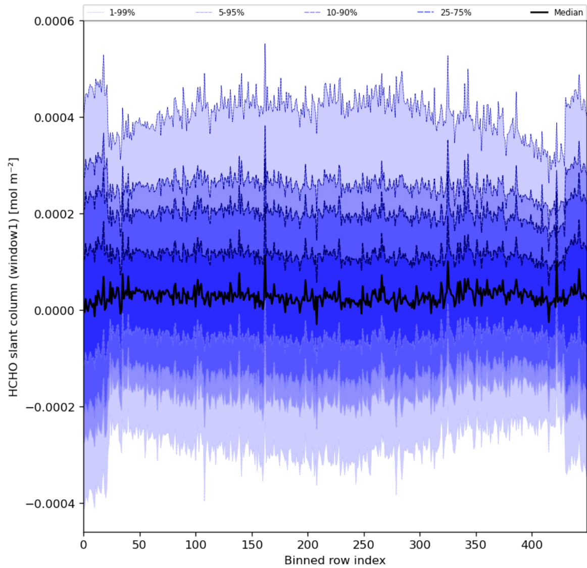
Figure 52: Along track statistics of “HCHO slant column (window1)” for 2024-06-16 to 2024-06-18
