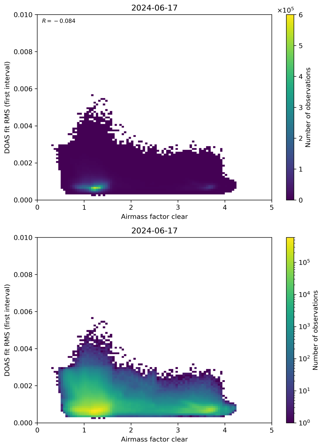
Figure 71: Scatter density plot of “Airmass factor clear” against “DOAS fit RMS (first interval)” for 2024-06-16 to 2024-06-18.
