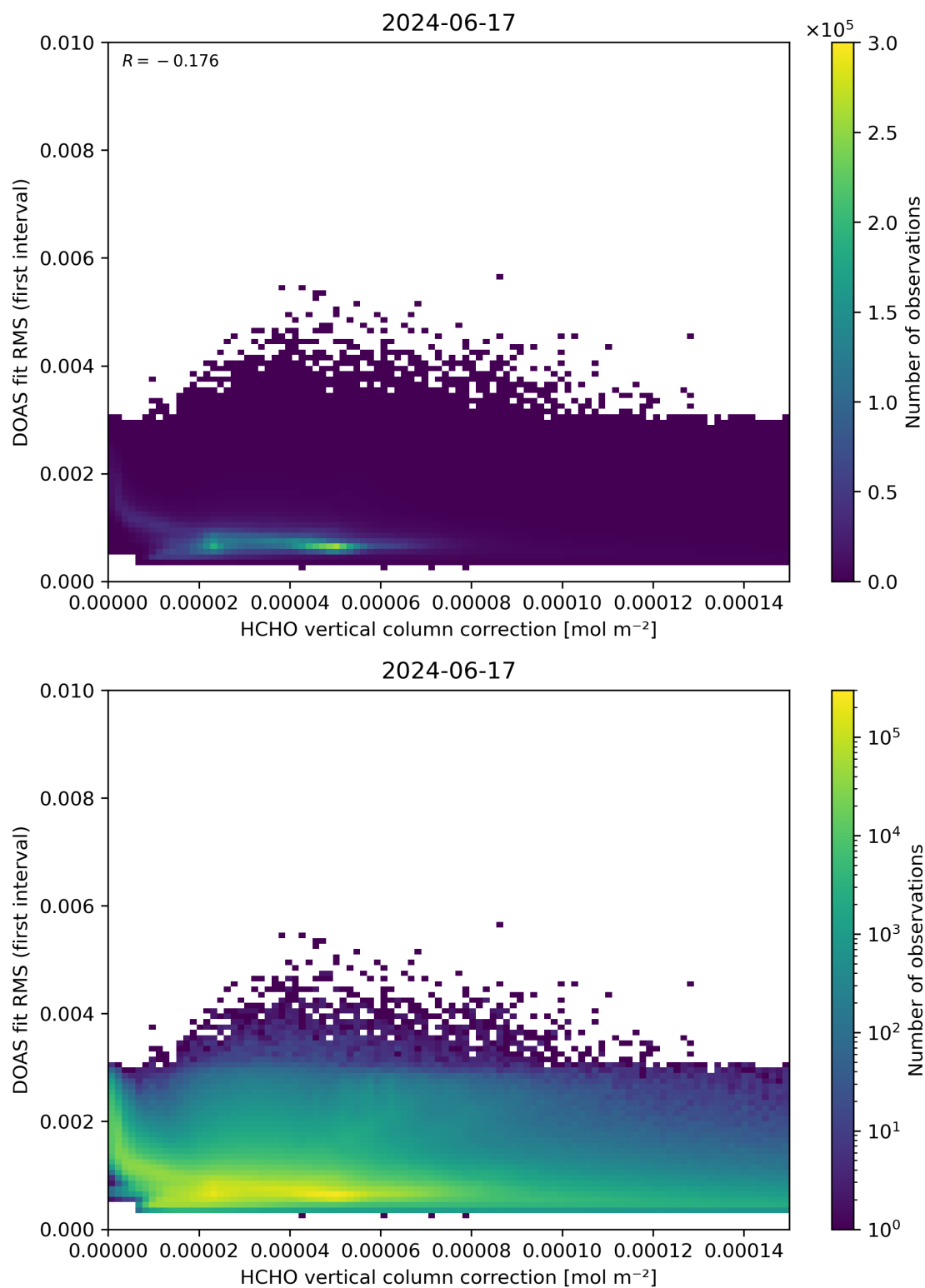
Figure 112: Scatter density plot of “HCHO vertical column correction” against “DOAS fit RMS (first interval)” for 2024-06-16 to 2024-06-18.
