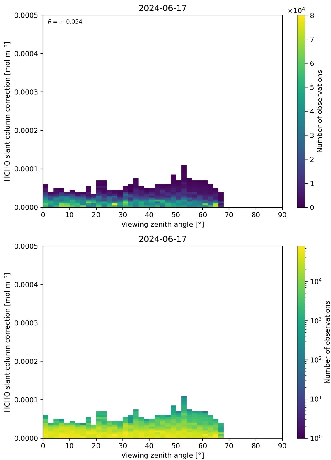
Figure 187: Scatter density plot of “Viewing zenith angle” against “HCHO slant column correction” for 2024-06-16 to 2024-06-18.
