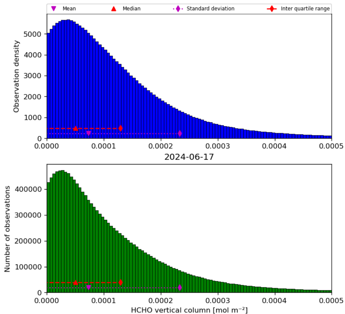
Figure 35: Histogram of “HCHO vertical column” for 2024-06-16 to 2024-06-18
