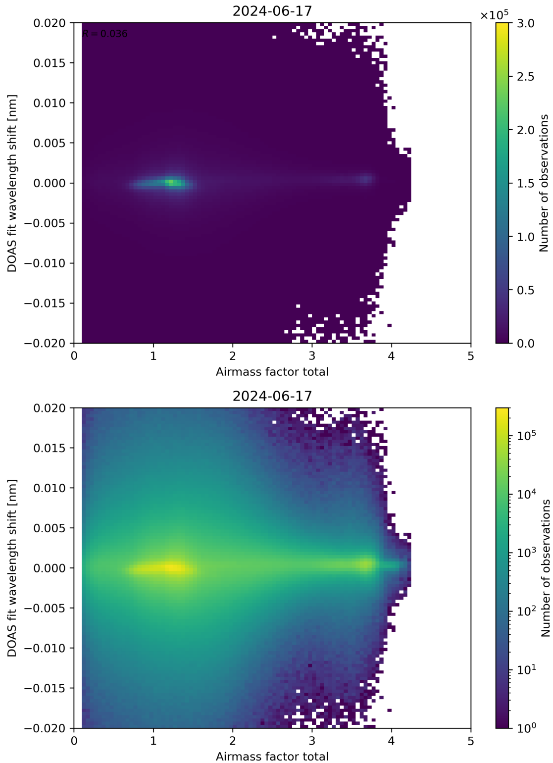
Figure 98: Scatter density plot of “Airmass factor total” against “DOAS fit wavelength shift” for 2024-06-16 to 2024-06-18.
