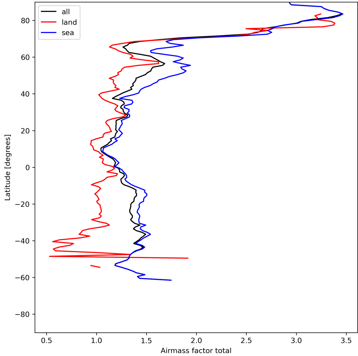
Figure 26: Zonal average of “Airmass factor total” for 2024-06-16 to 2024-06-18.
