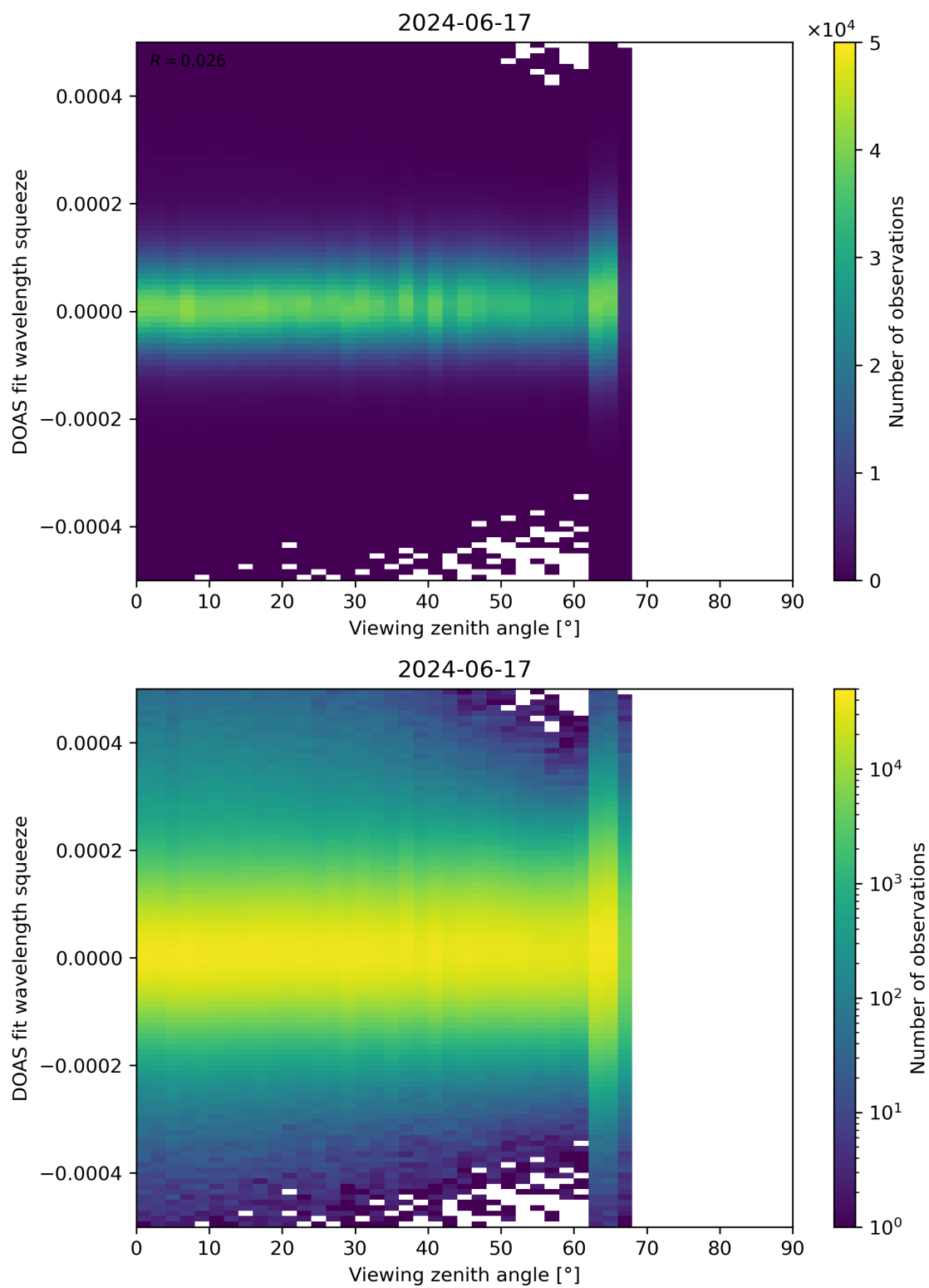
Figure 184: Scatter density plot of “Viewing zenith angle” against “DOAS fit wavelength squeeze” for 2024-06-16 to 2024-06-18.
