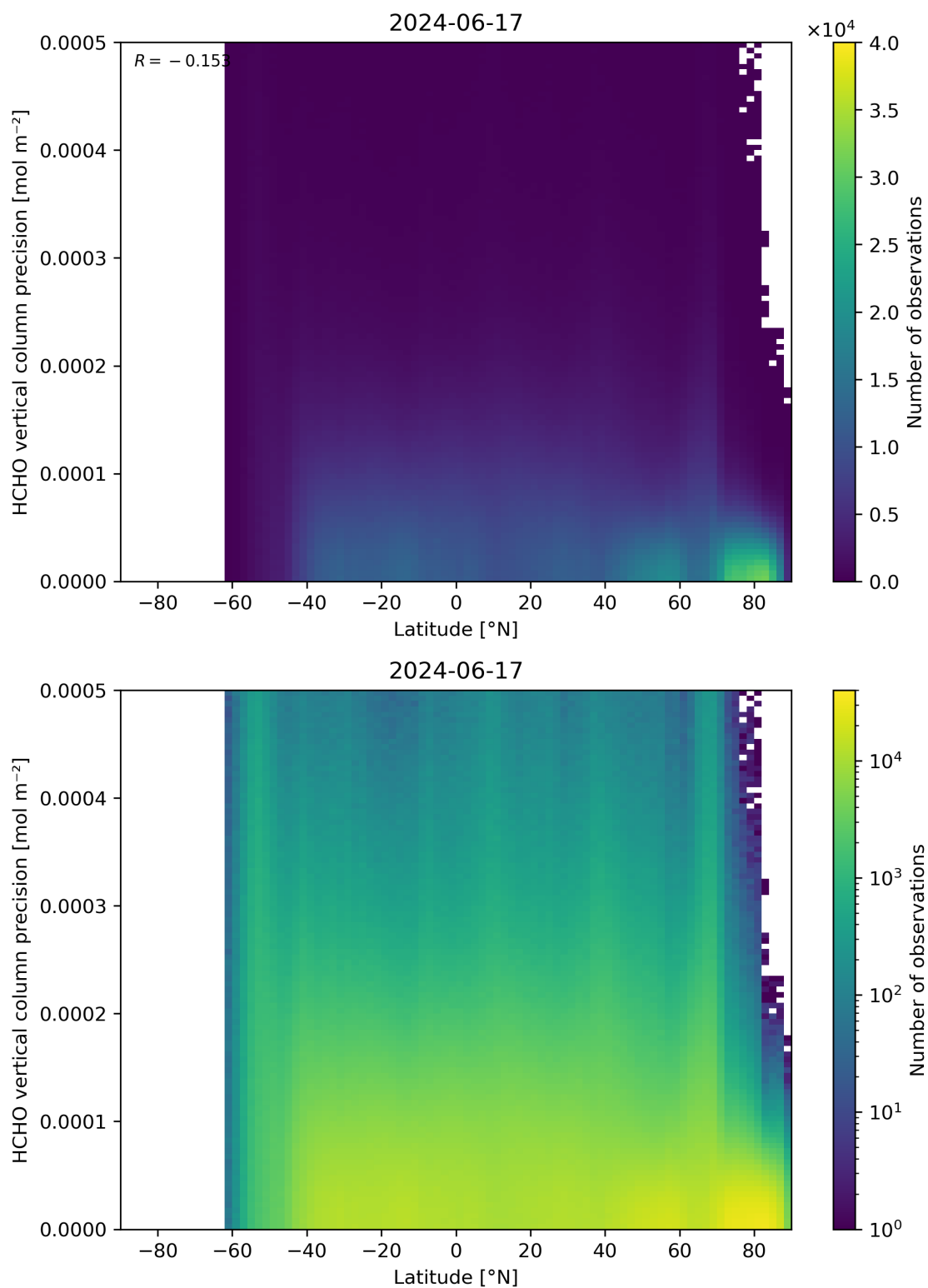
Figure 165: Scatter density plot of “Latitude” against “HCHO vertical column precision” for 2024-06-16 to 2024-06-18.
