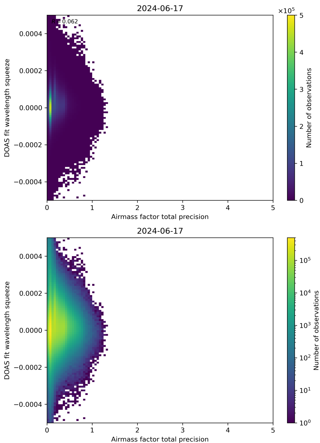
Figure 107: Scatter density plot of “Airmass factor total precision” against “DOAS fit wavelength squeeze” for 2024-06-16 to 2024-06-18.
