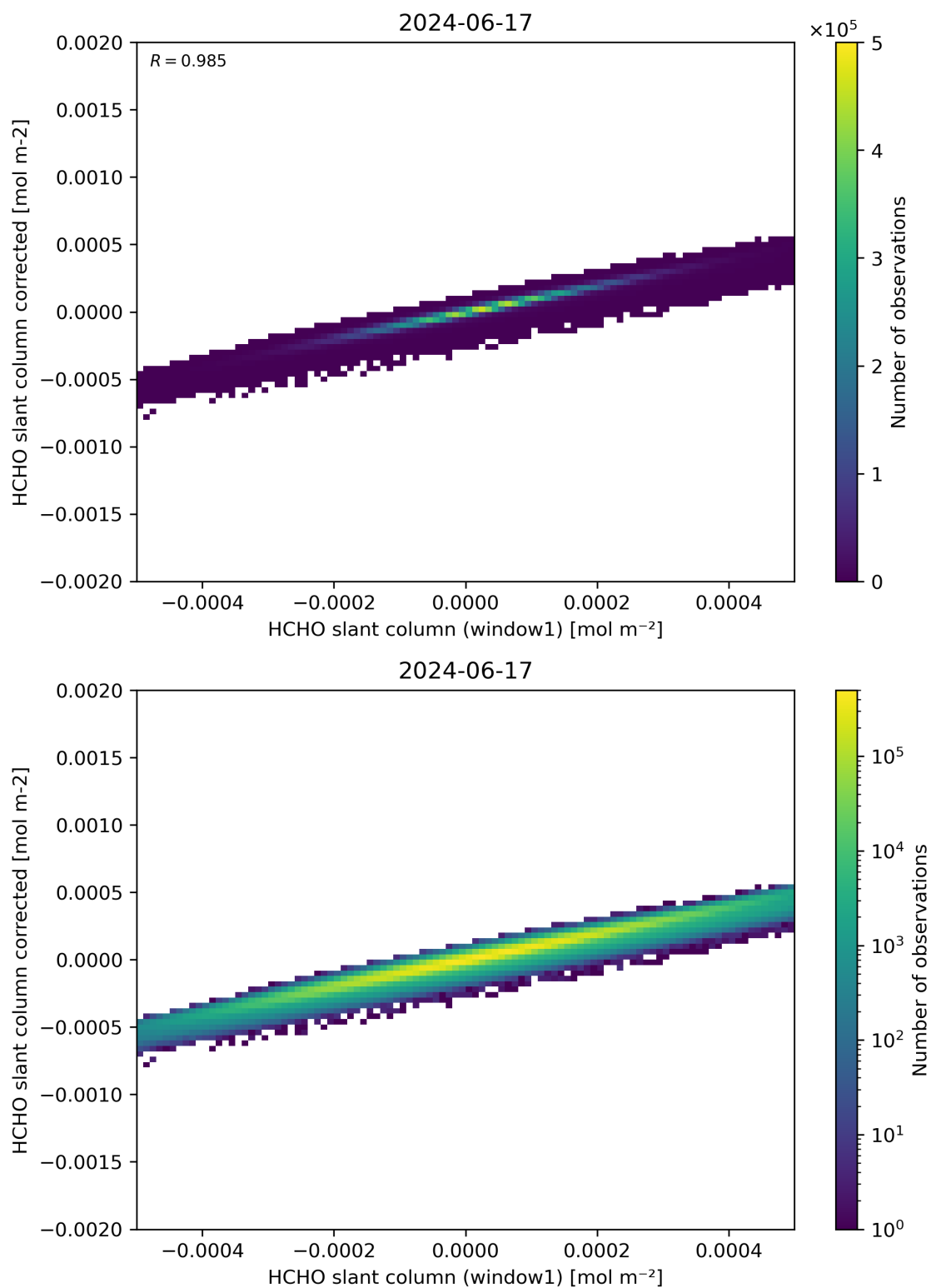
Figure 82: Scatter density plot of “HCHO slant column (window1)” against “HCHO slant column corrected” for 2024-06-16 to 2024-06-18.
