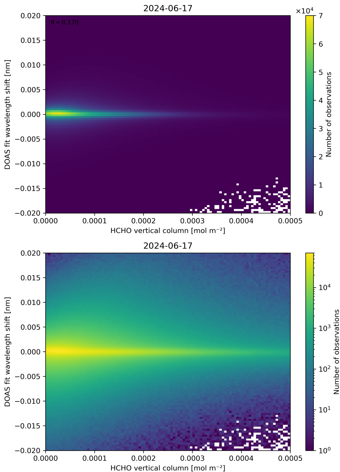
Figure 124: Scatter density plot of “HCHO vertical column” against “DOAS fit wavelength shift” for 2024-06-16 to 2024-06-18.
