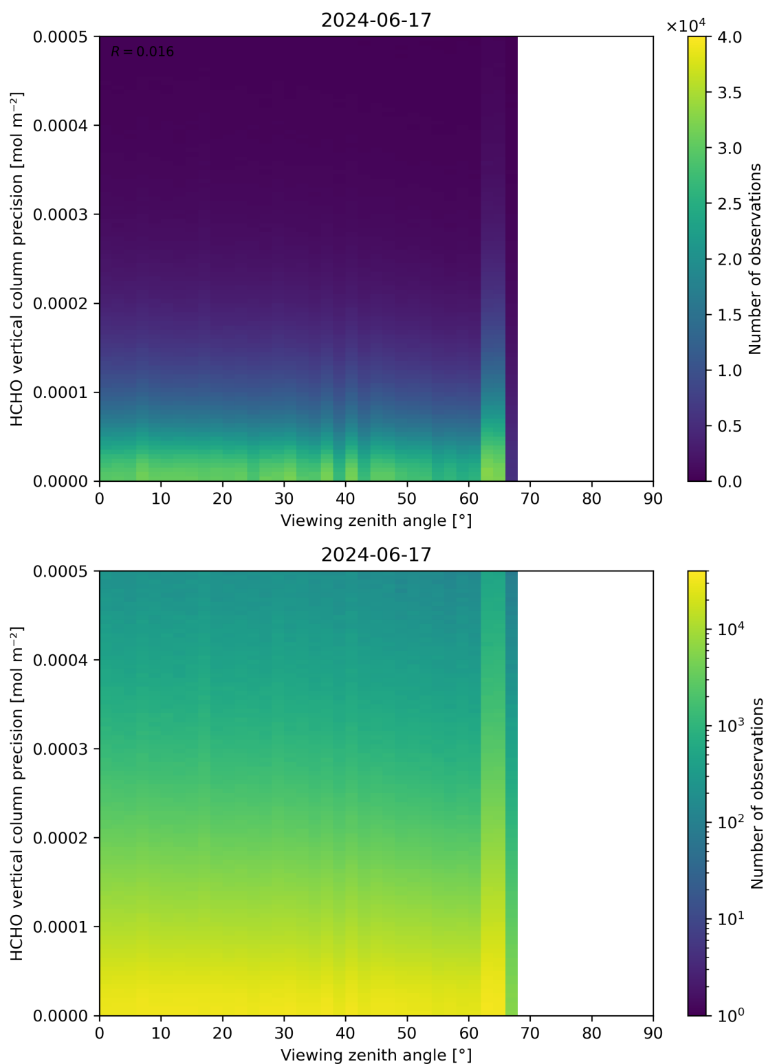
Figure 194: Scatter density plot of “Viewing zenith angle” against “HCHO vertical column precision” for 2024-06-16 to 2024-06-18.
