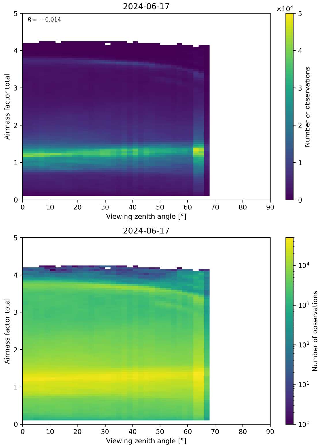
Figure 190: Scatter density plot of “Viewing zenith angle” against “Airmass factor total” for 2024-06-16 to 2024-06-18.
