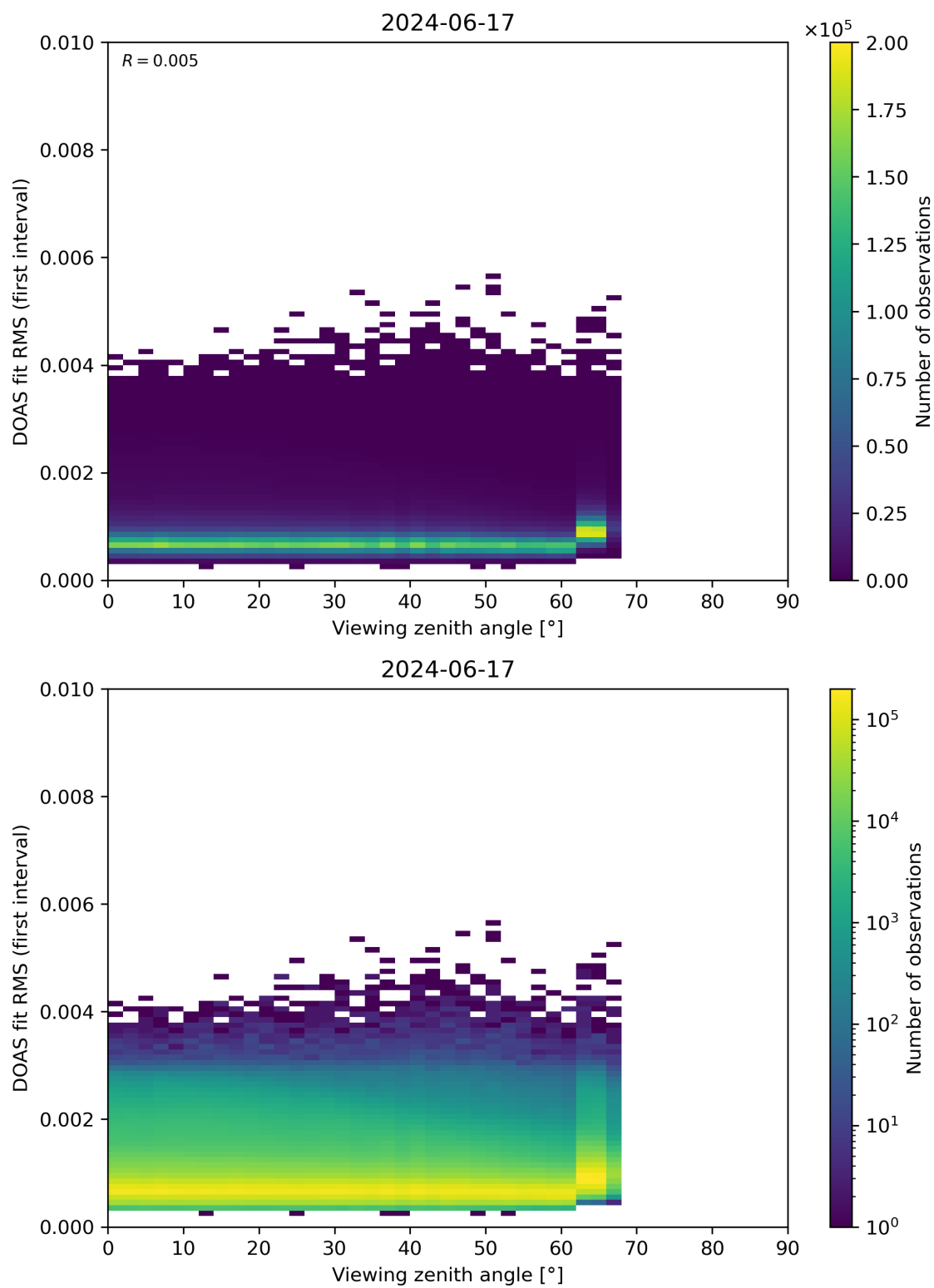
Figure 182: Scatter density plot of “Viewing zenith angle” against “DOAS fit RMS (first interval)” for 2024-06-16 to 2024-06-18.
