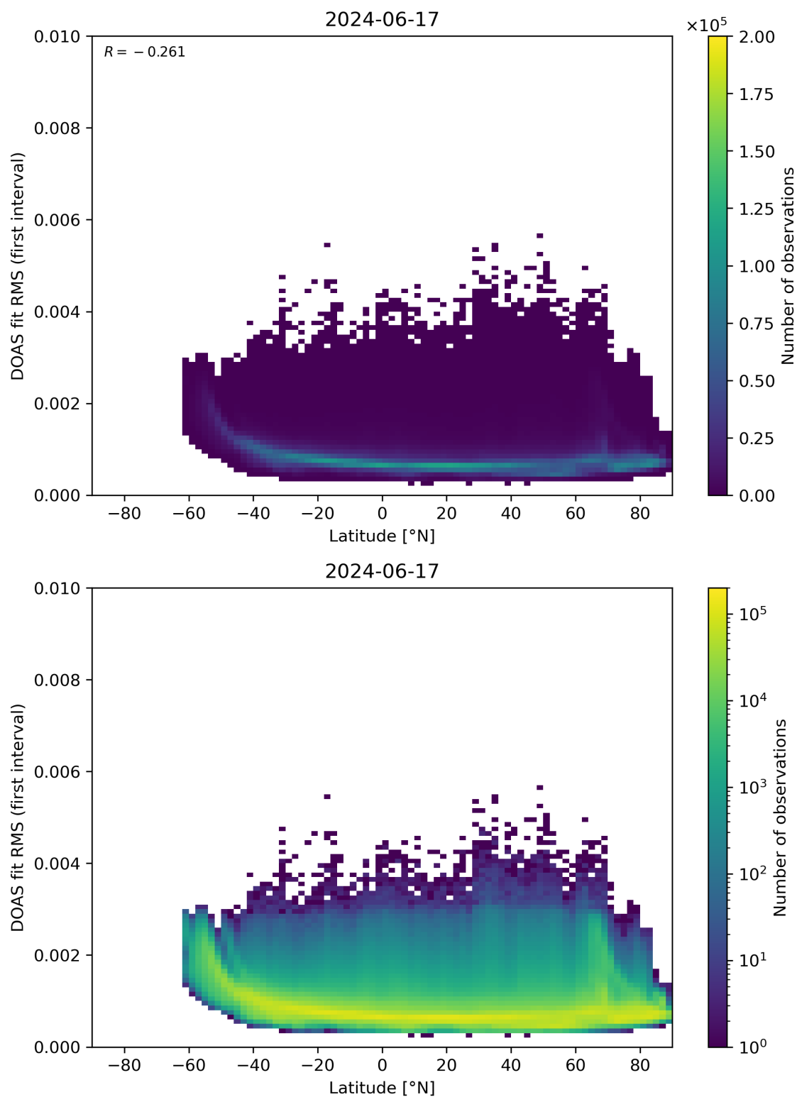
Figure 153: Scatter density plot of “Latitude” against “DOAS fit RMS (first interval)” for 2024-06-16 to 2024-06-18.
