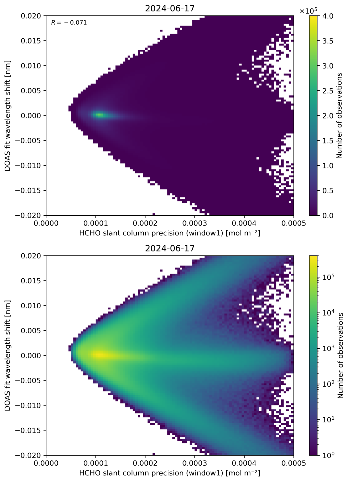
Figure 89: Scatter density plot of “HCHO slant column precision (window1)” against “DOAS fit wavelength shift” for 2024-06-16 to 2024-06-18.
