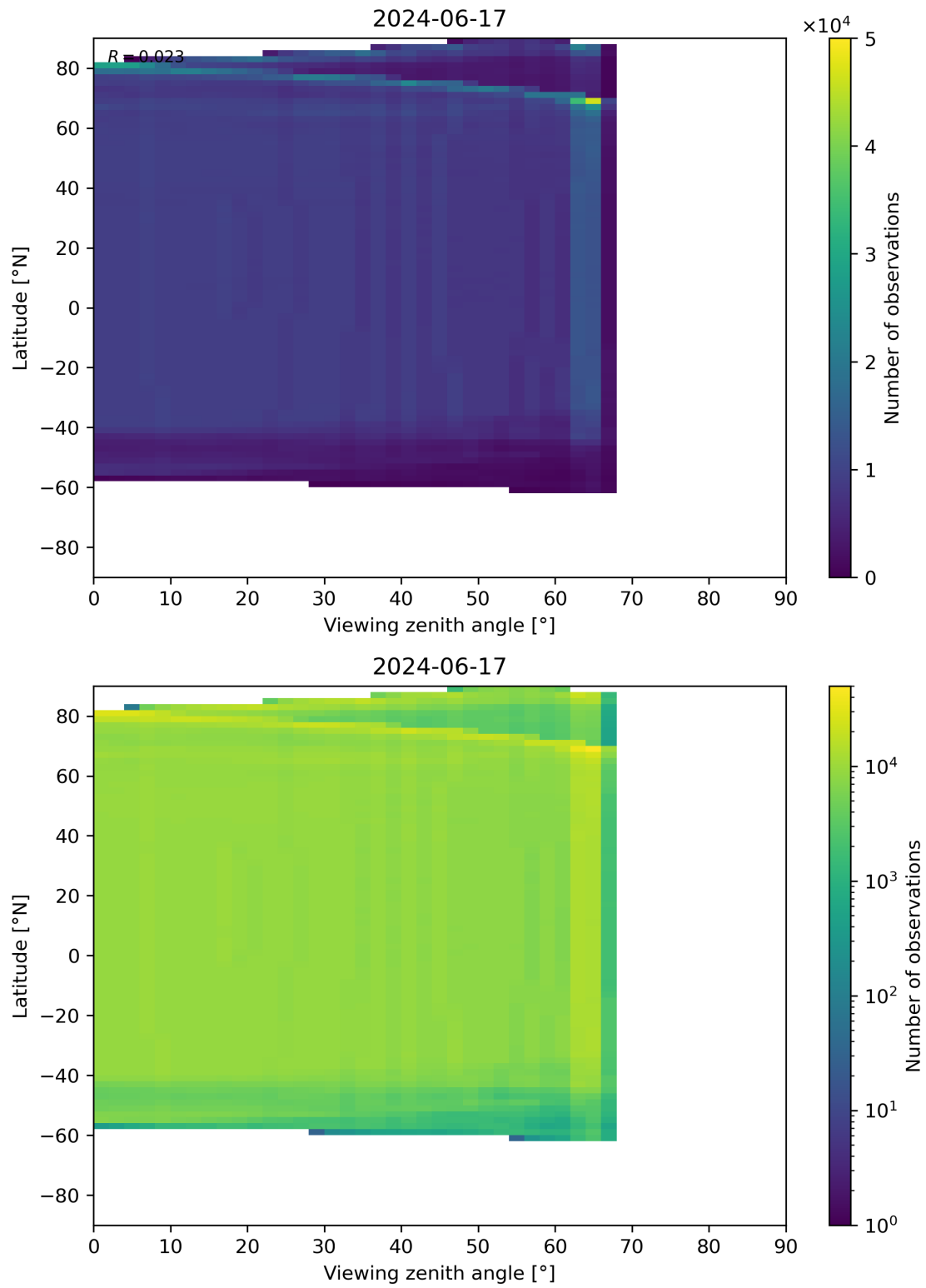
Figure 196: Scatter density plot of “Viewing zenith angle” against “Latitude” for 2024-06-16 to 2024-06-18.
