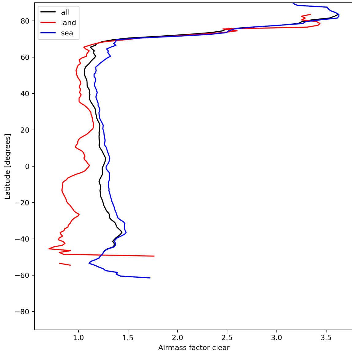
Figure 28: Zonal average of “Airmass factor clear” for 2024-06-16 to 2024-06-18.
