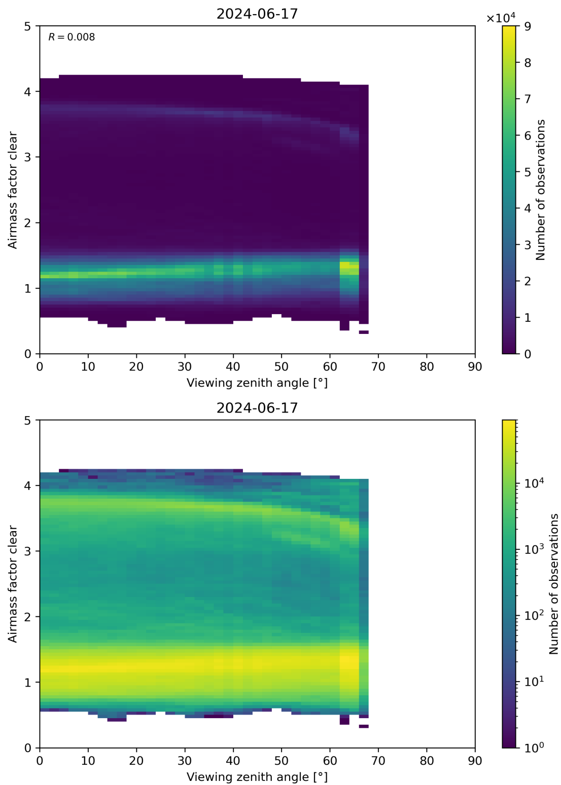
Figure 185: Scatter density plot of “Viewing zenith angle” against “Airmass factor clear” for 2024-06-16 to 2024-06-18.
