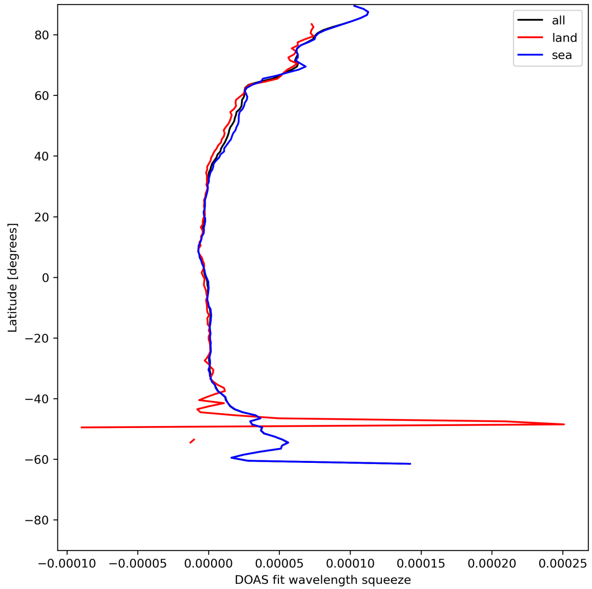
Figure 31: Zonal average of “DOAS fit wavelength squeeze” for 2024-06-16 to 2024-06-18.
