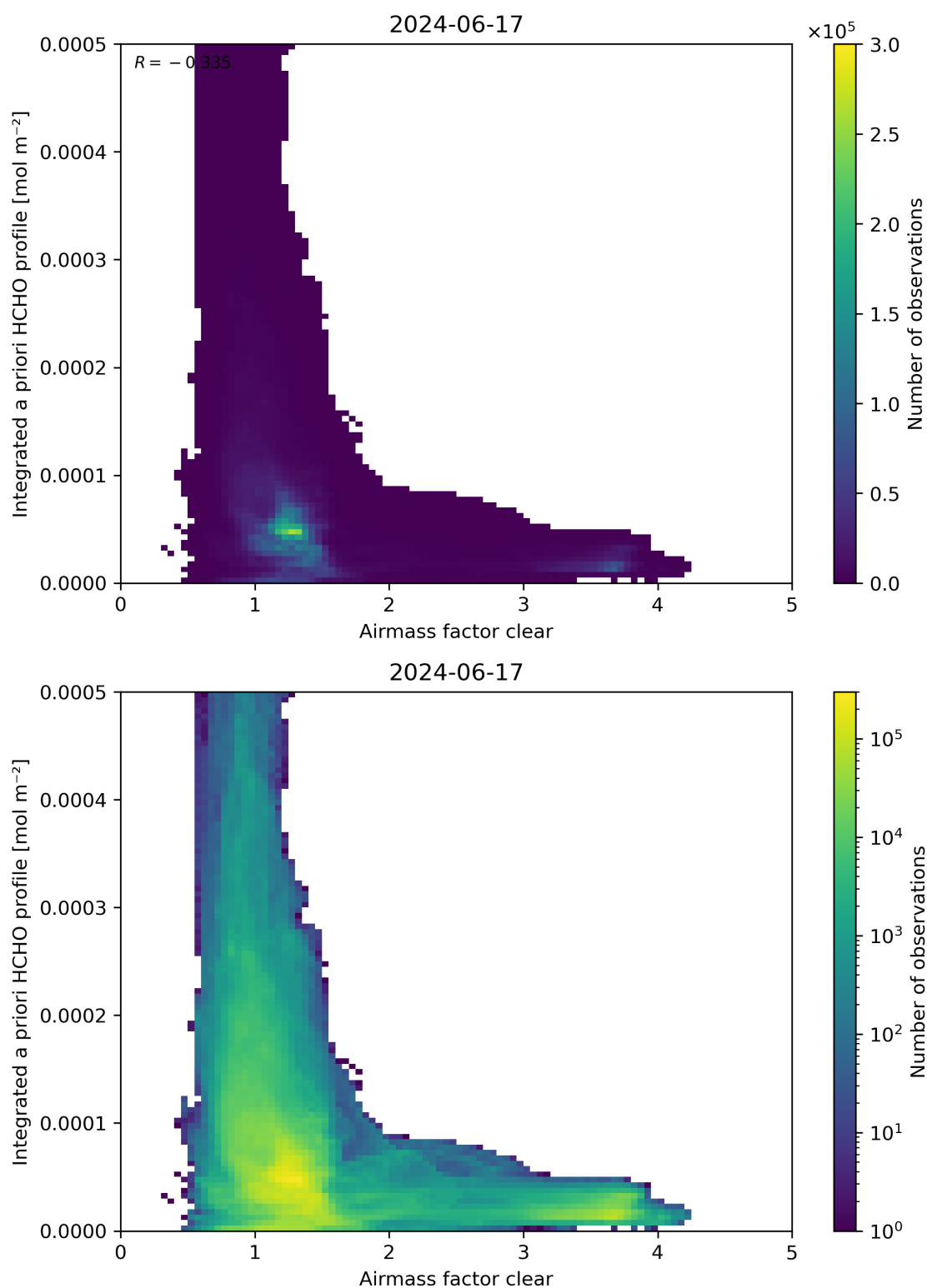
Figure 76: Scatter density plot of “Airmass factor clear” against “Integrated a priori HCHO profile” for 2024-06-16 to 2024-06-18.
