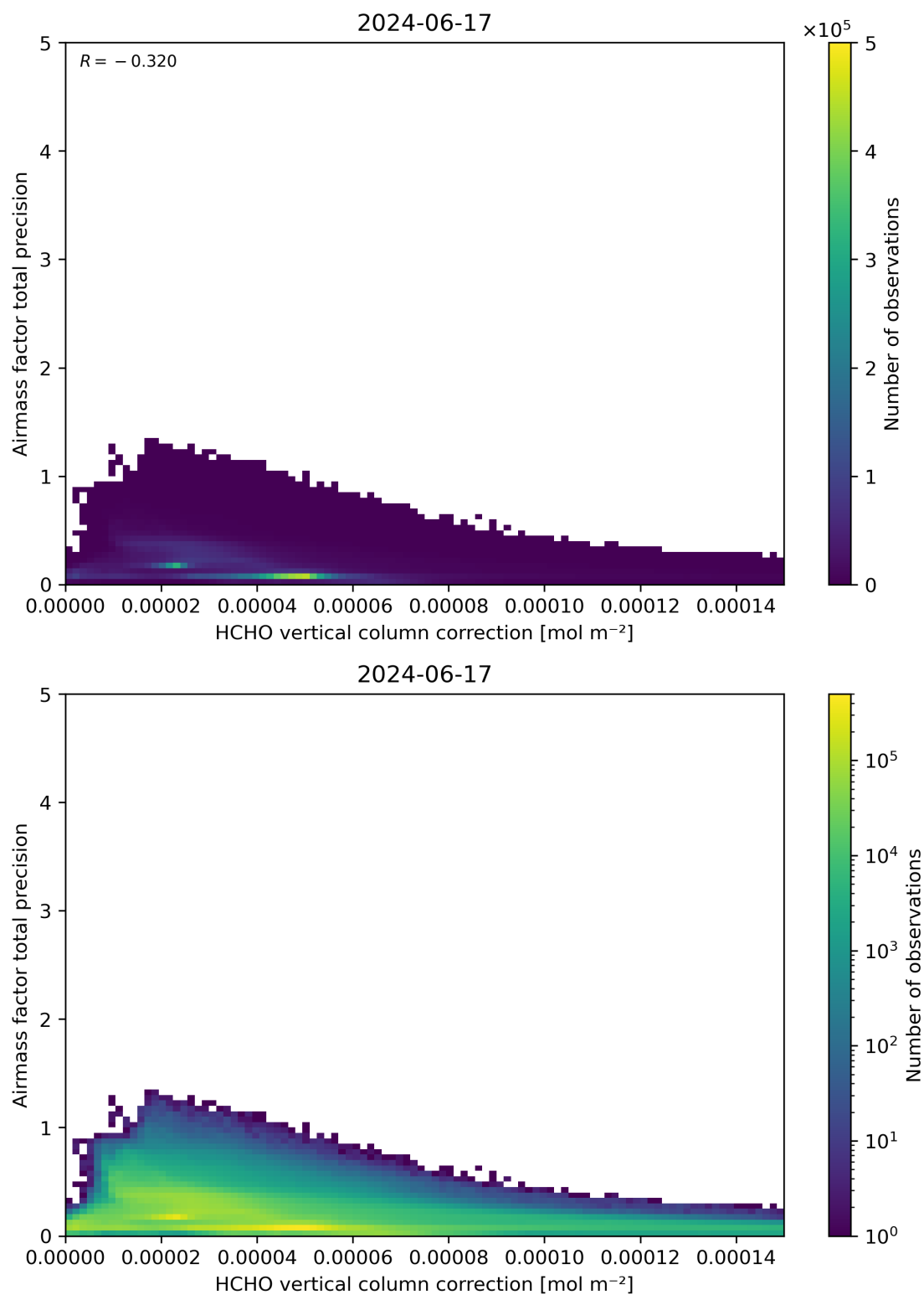
Figure 121: Scatter density plot of “HCHO vertical column correction” against “Airmass factor total precision” for 2024-06-16 to 2024-06-18.
