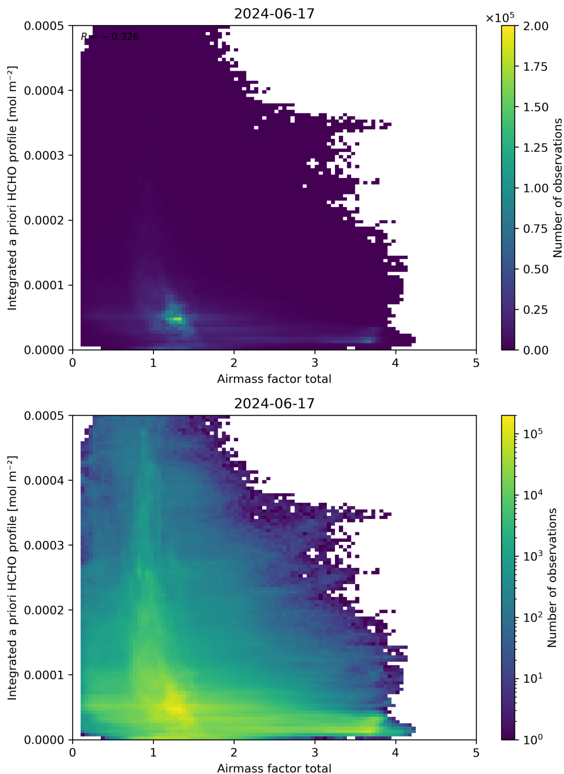
Figure 104: Scatter density plot of “Airmass factor total” against “Integrated a priori HCHO profile” for 2024-06-16 to 2024-06-18.
