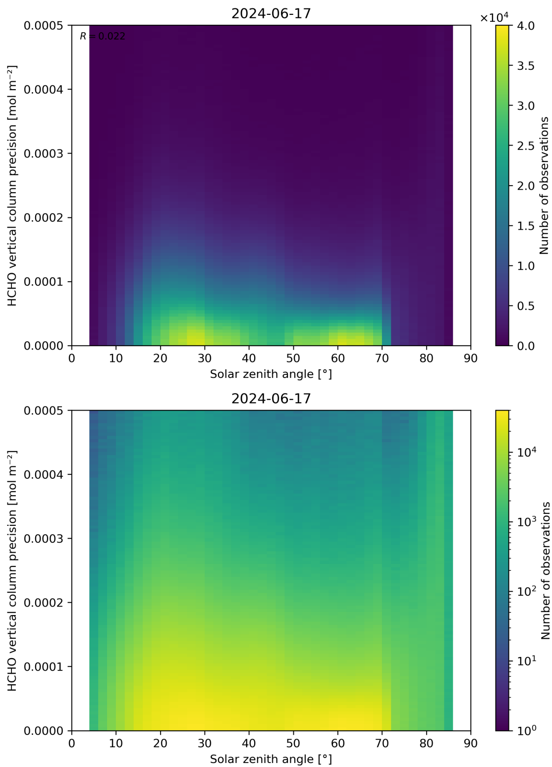
Figure 179: Scatter density plot of “Solar zenith angle” against “HCHO vertical column precision” for 2024-06-16 to 2024-06-18.
