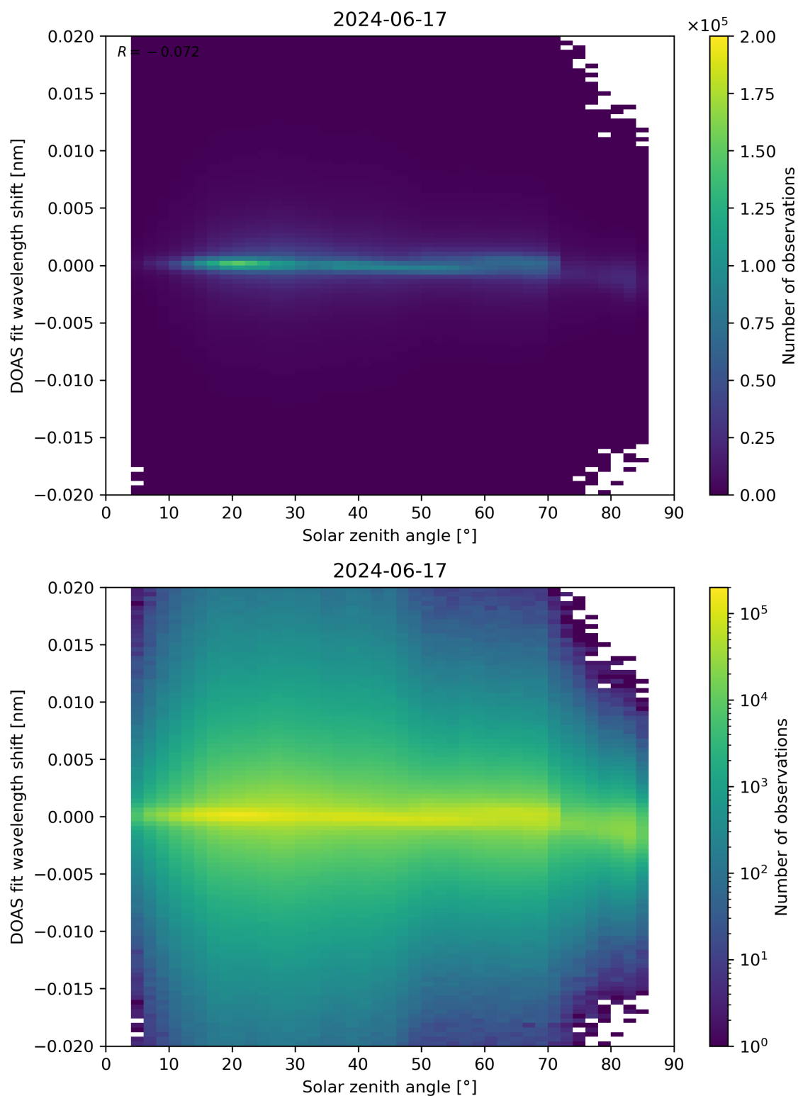
Figure 168: Scatter density plot of “Solar zenith angle” against “DOAS fit wavelength shift” for 2024-06-16 to 2024-06-18.
