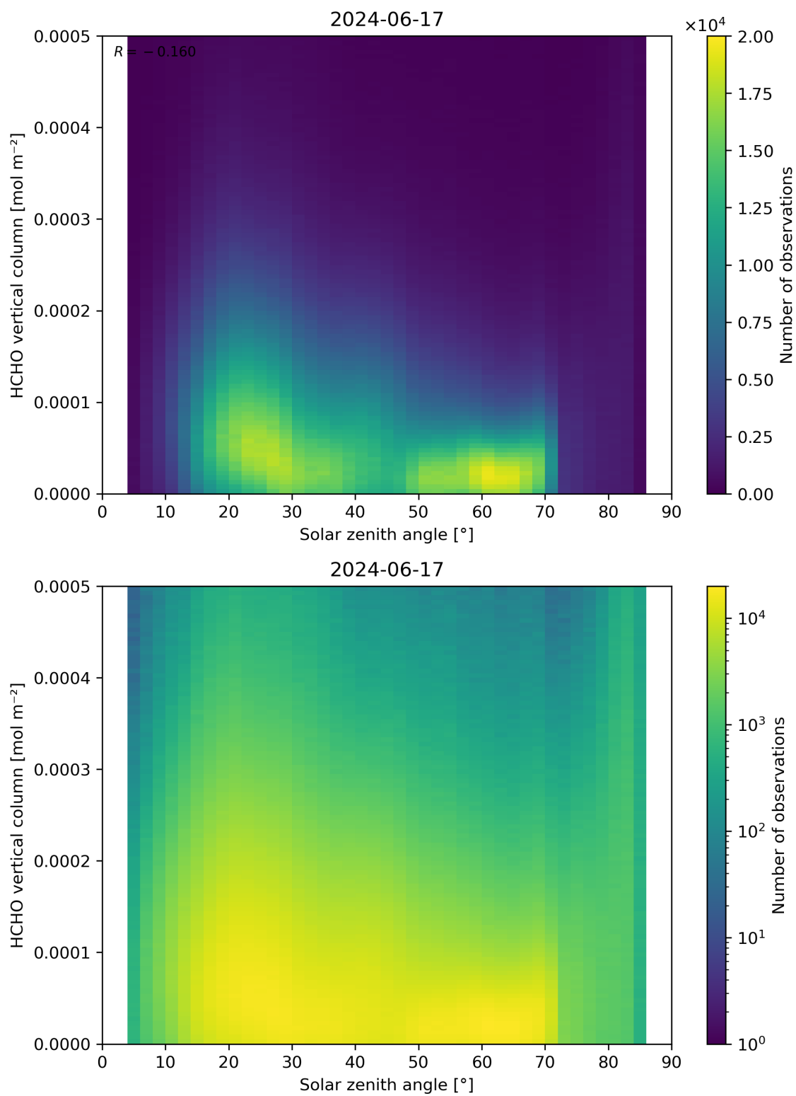
Figure 177: Scatter density plot of “Solar zenith angle” against “HCHO vertical column” for 2024-06-16 to 2024-06-18.
