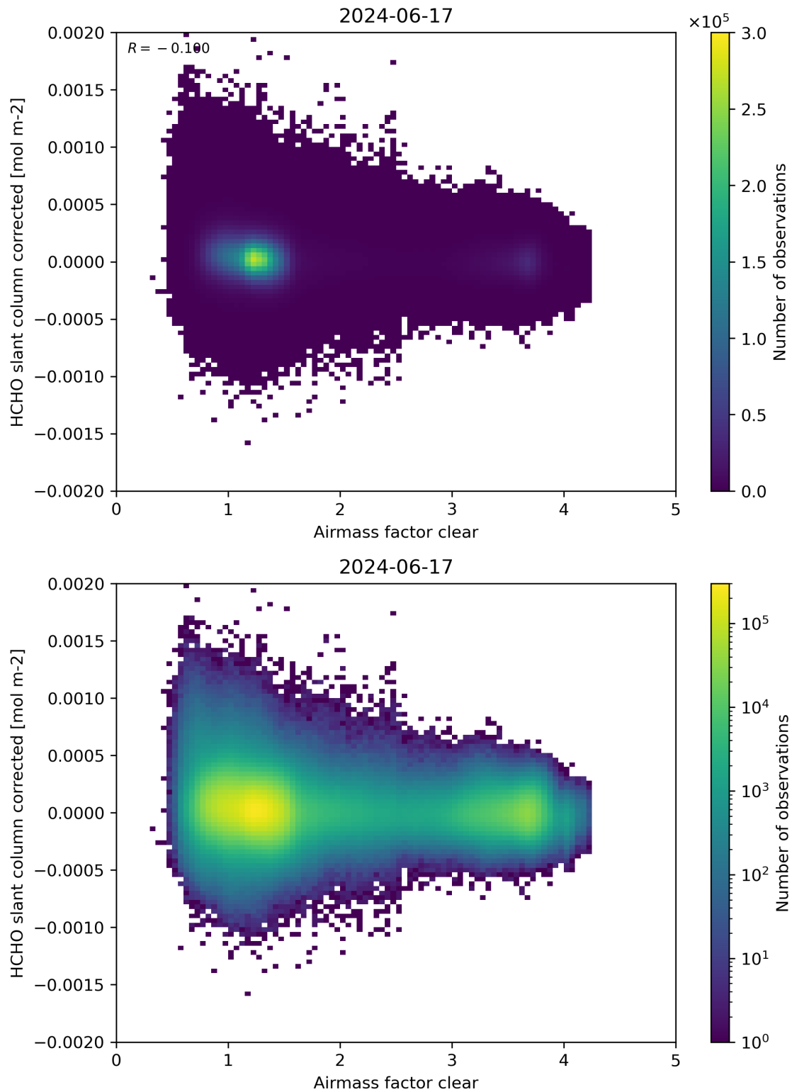
Figure 74: Scatter density plot of “Airmass factor clear” against “HCHO slant column corrected” for 2024-06-16 to 2024-06-18.
