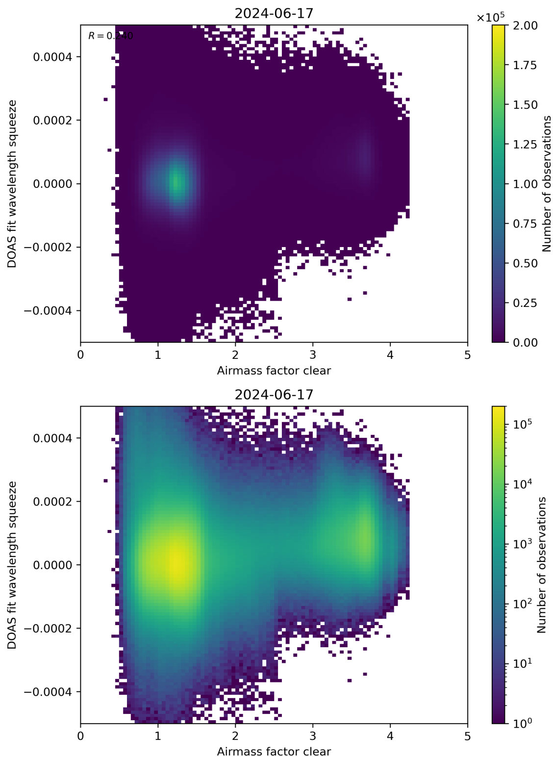
Figure 73: Scatter density plot of “Airmass factor clear” against “DOAS fit wavelength squeeze” for 2024-06-16 to 2024-06-18.
