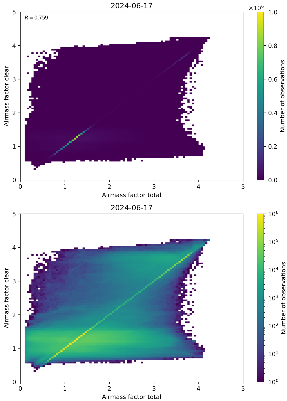
Figure 100: Scatter density plot of “Airmass factor total” against “Airmass factor clear” for 2024-06-16 to 2024-06-18.
