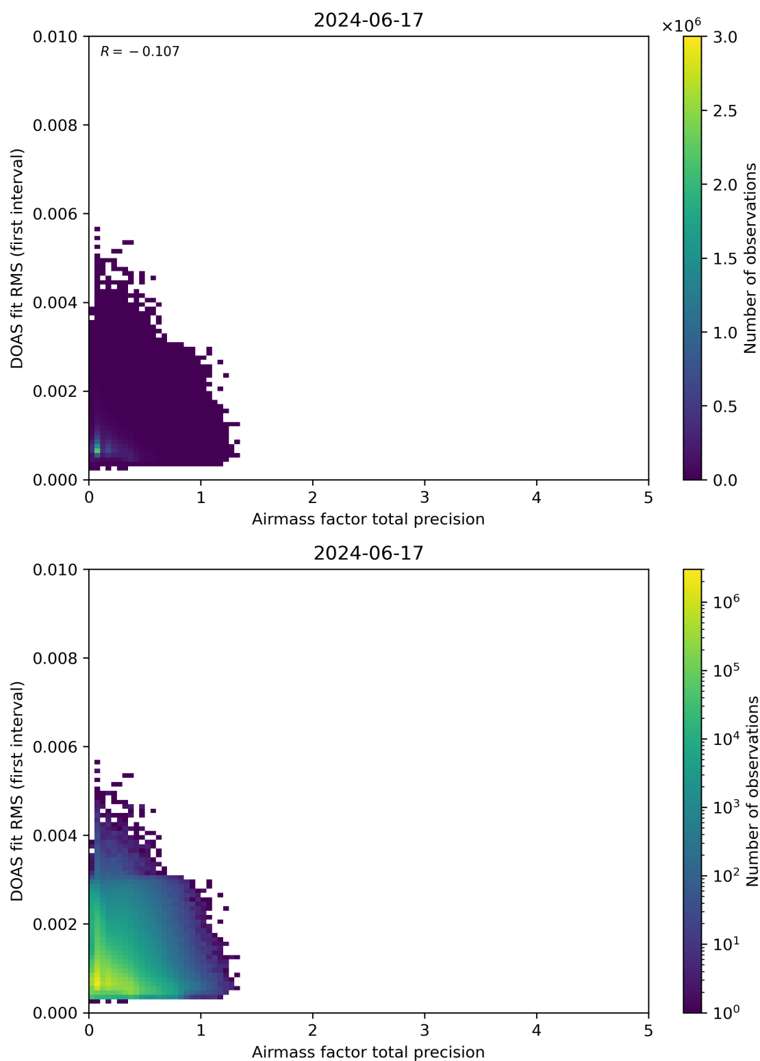
Figure 105: Scatter density plot of “Airmass factor total precision” against “DOAS fit RMS (first interval)” for 2024-06-16 to 2024-06-18.
