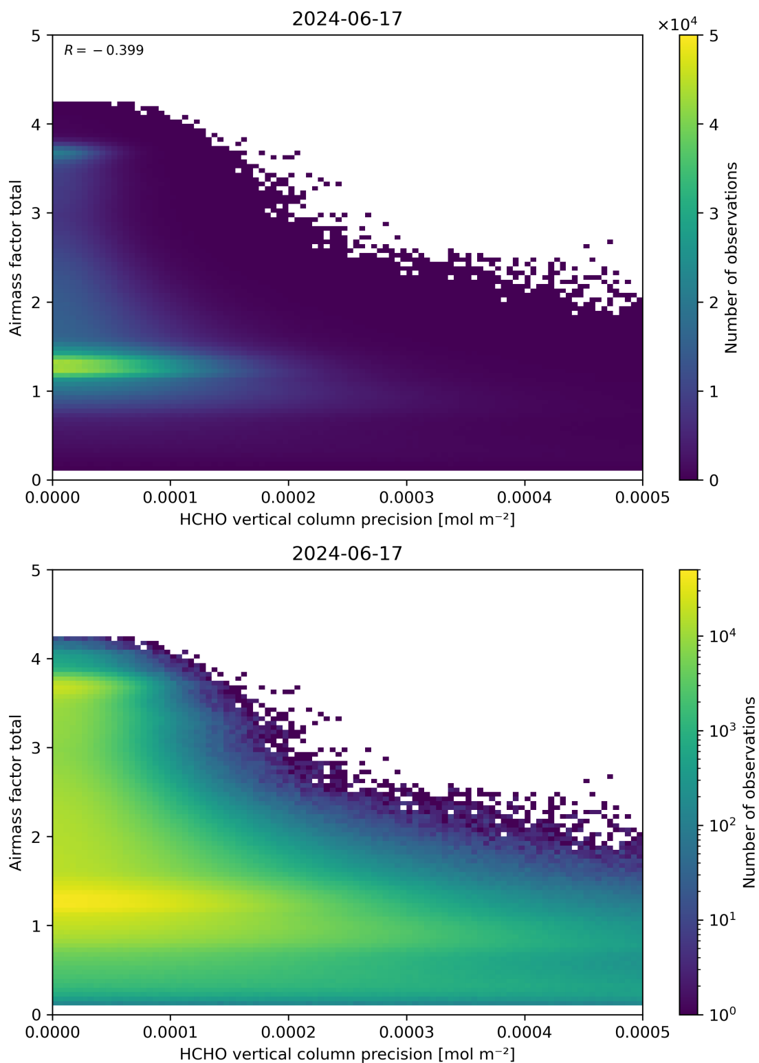
Figure 144: Scatter density plot of “HCHO vertical column precision” against “Airmass factor total” for 2024-06-16 to 2024-06-18.
