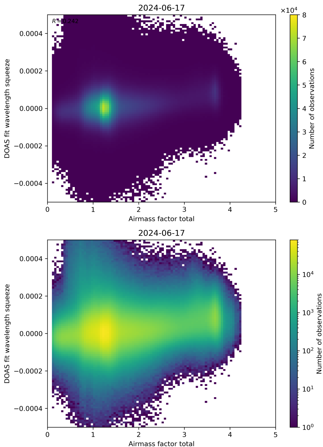
Figure 99: Scatter density plot of “Airmass factor total” against “DOAS fit wavelength squeeze” for 2024-06-16 to 2024-06-18.
