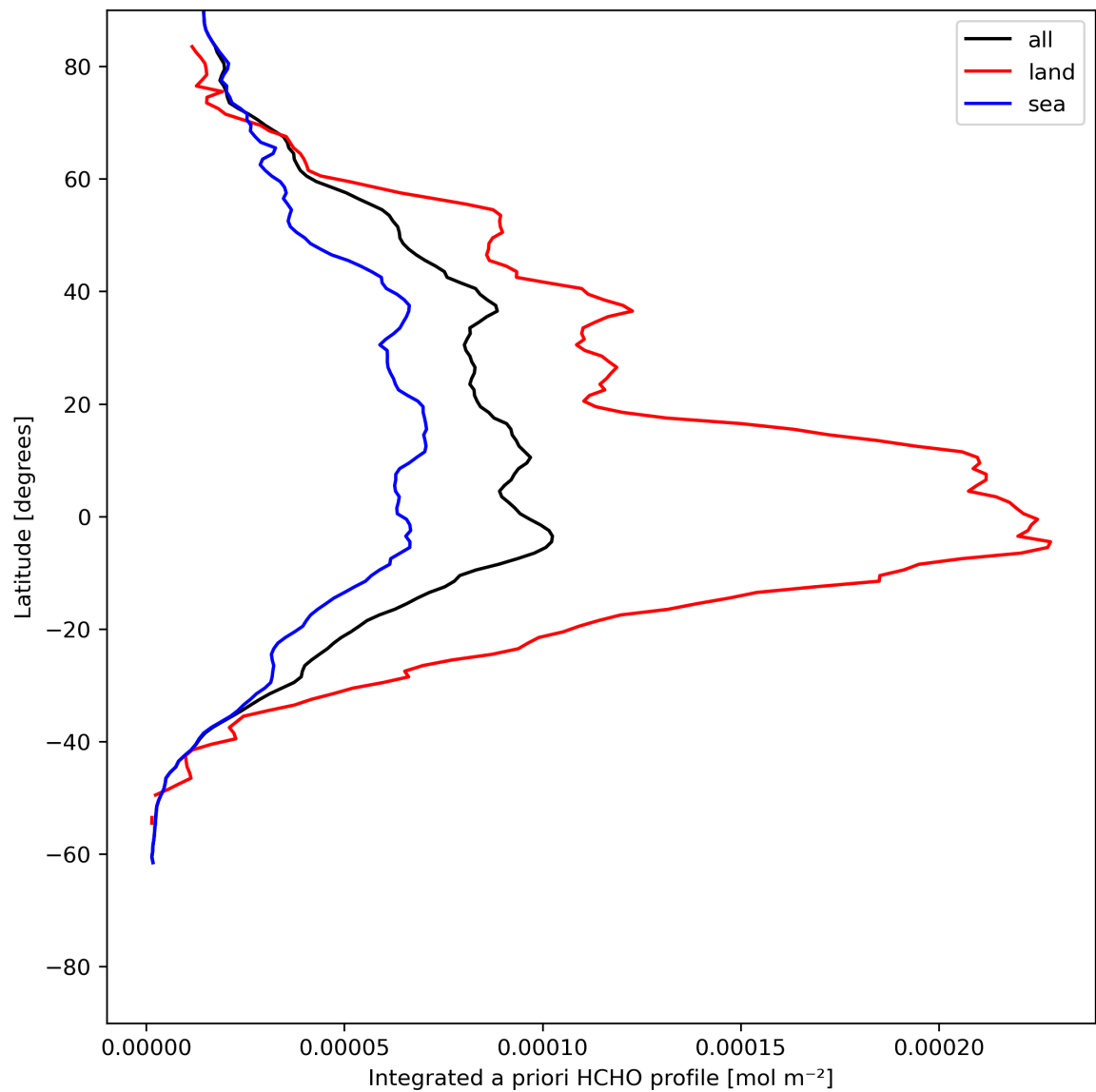
Figure 29: Zonal average of “Integrated a priori HCHO profile” for 2024-06-16 to 2024-06-18.
