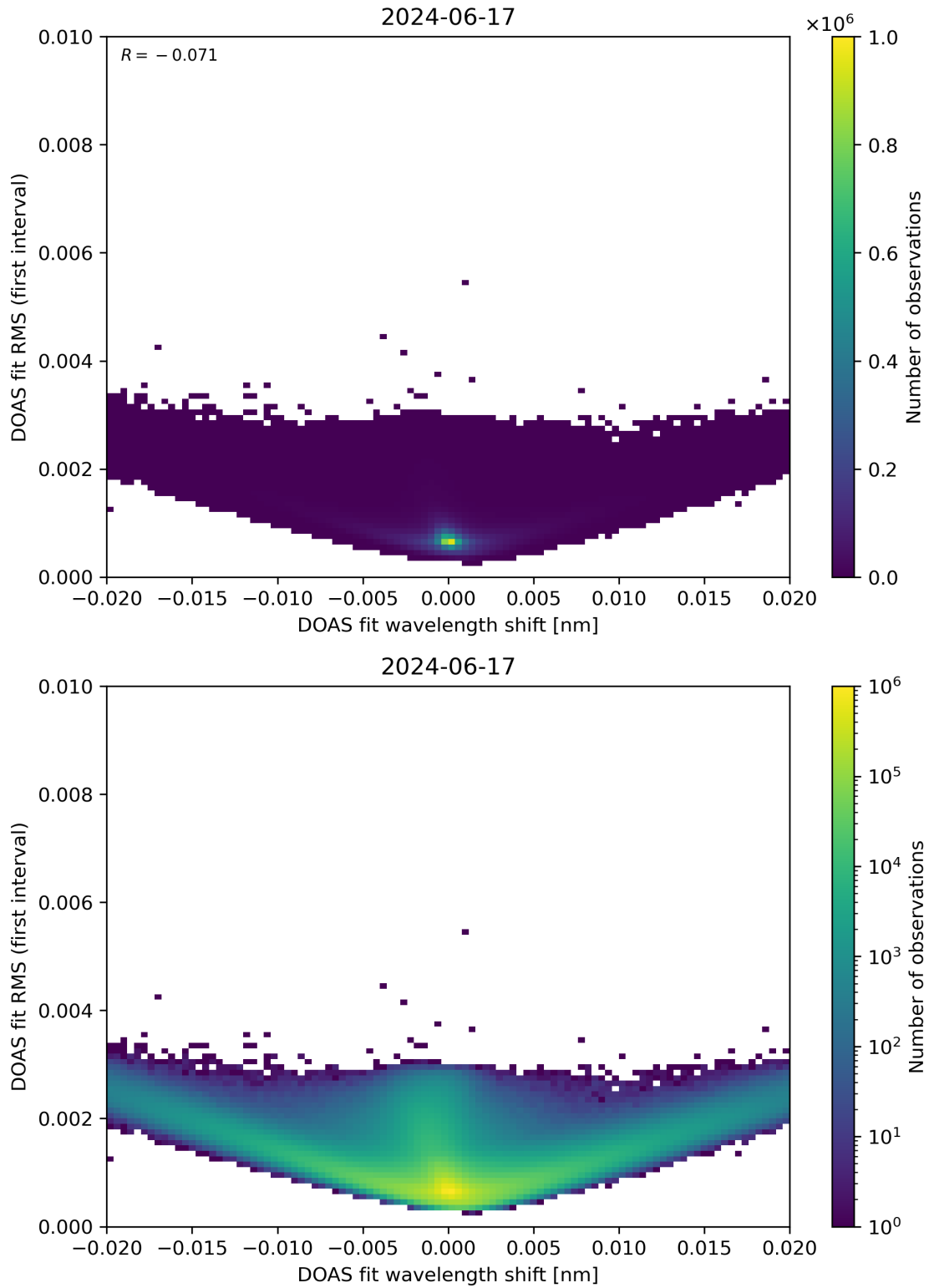
Figure 64: Scatter density plot of “DOAS fit wavelength shift” against “DOAS fit RMS (first interval)” for 2024-06-16 to 2024-06-18.
