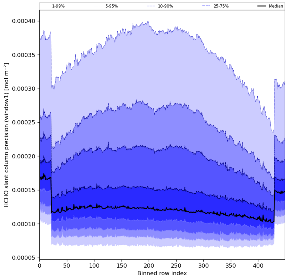
Figure 53: Along track statistics of “HCHO slant column precision (window1)” for 2024-06-16 to 2024-06-18
