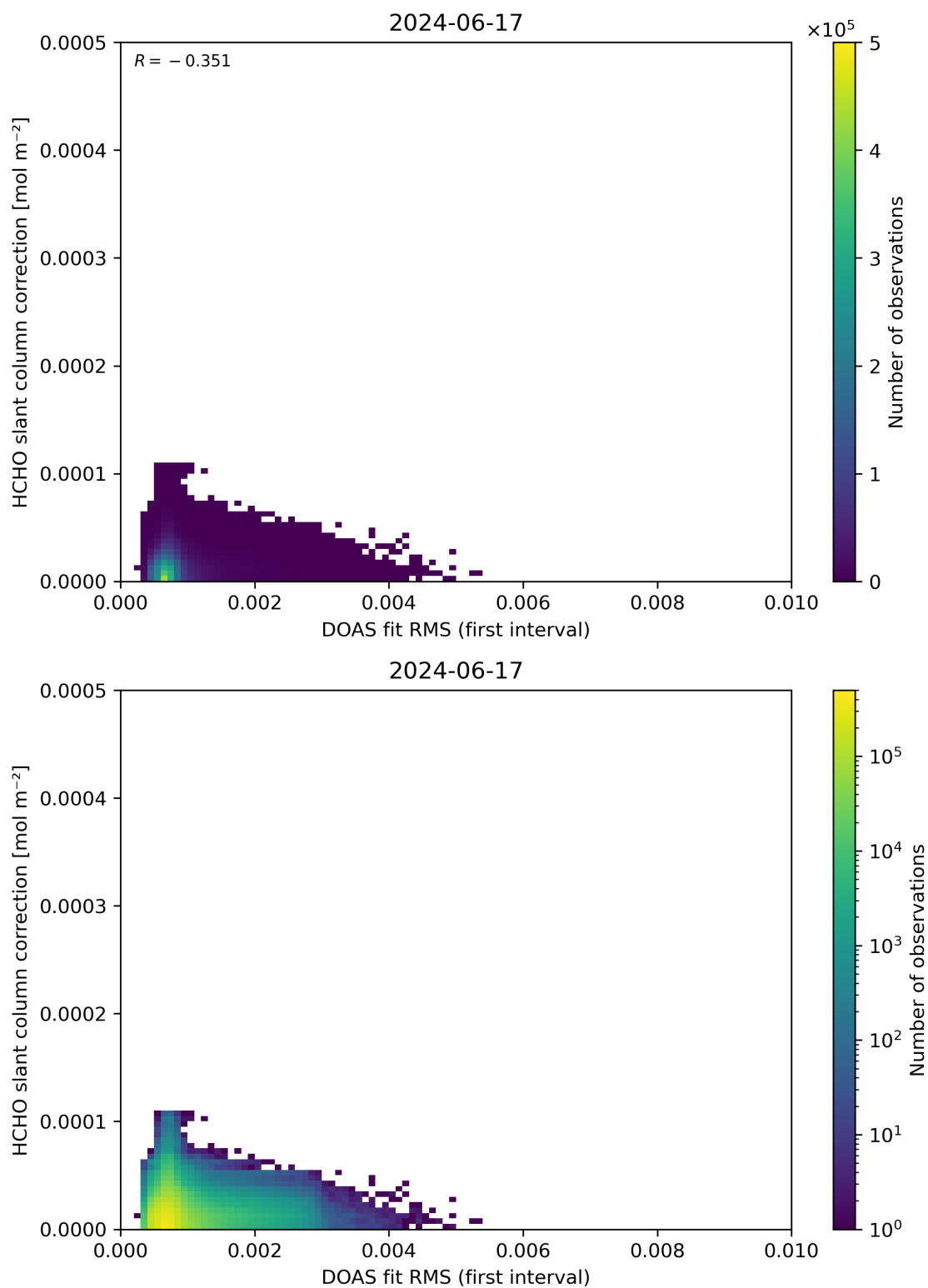
Figure 63: Scatter density plot of “DOAS fit RMS (first interval)” against “HCHO slant column correction” for 2024-06-16 to 2024-06-18.
