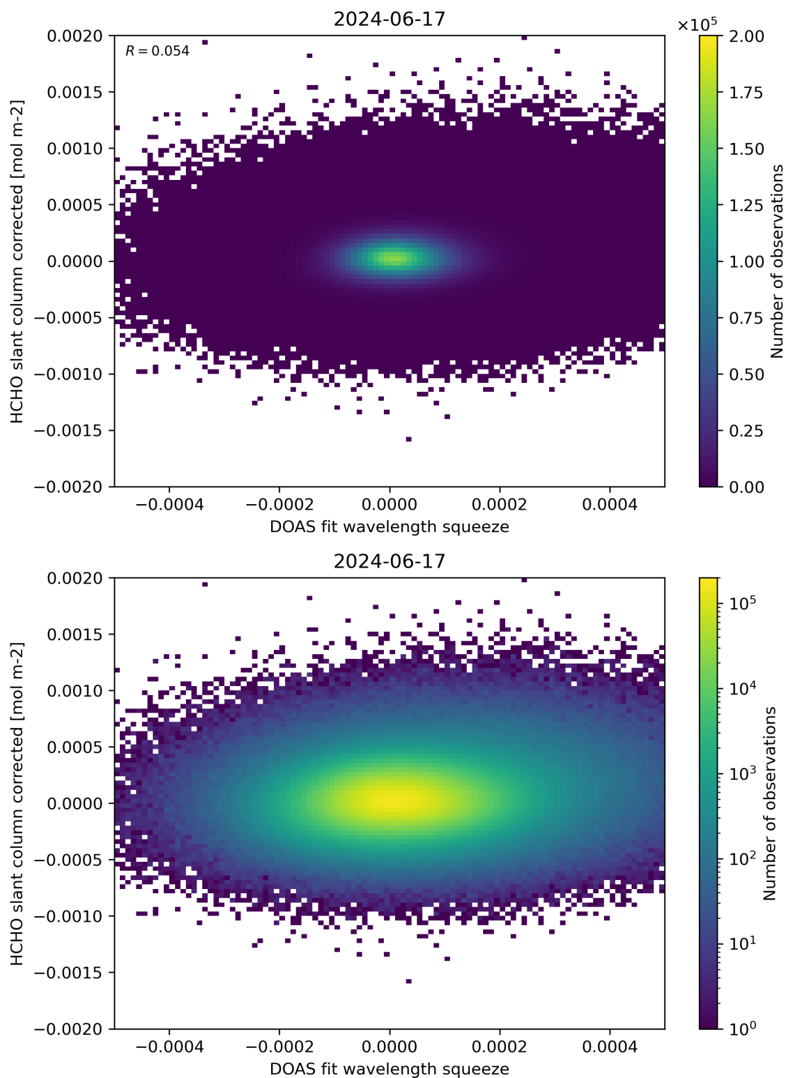
Figure 69: Scatter density plot of “DOAS fit wavelength squeeze” against “HCHO slant column corrected” for 2024-06-16 to 2024-06-18.
