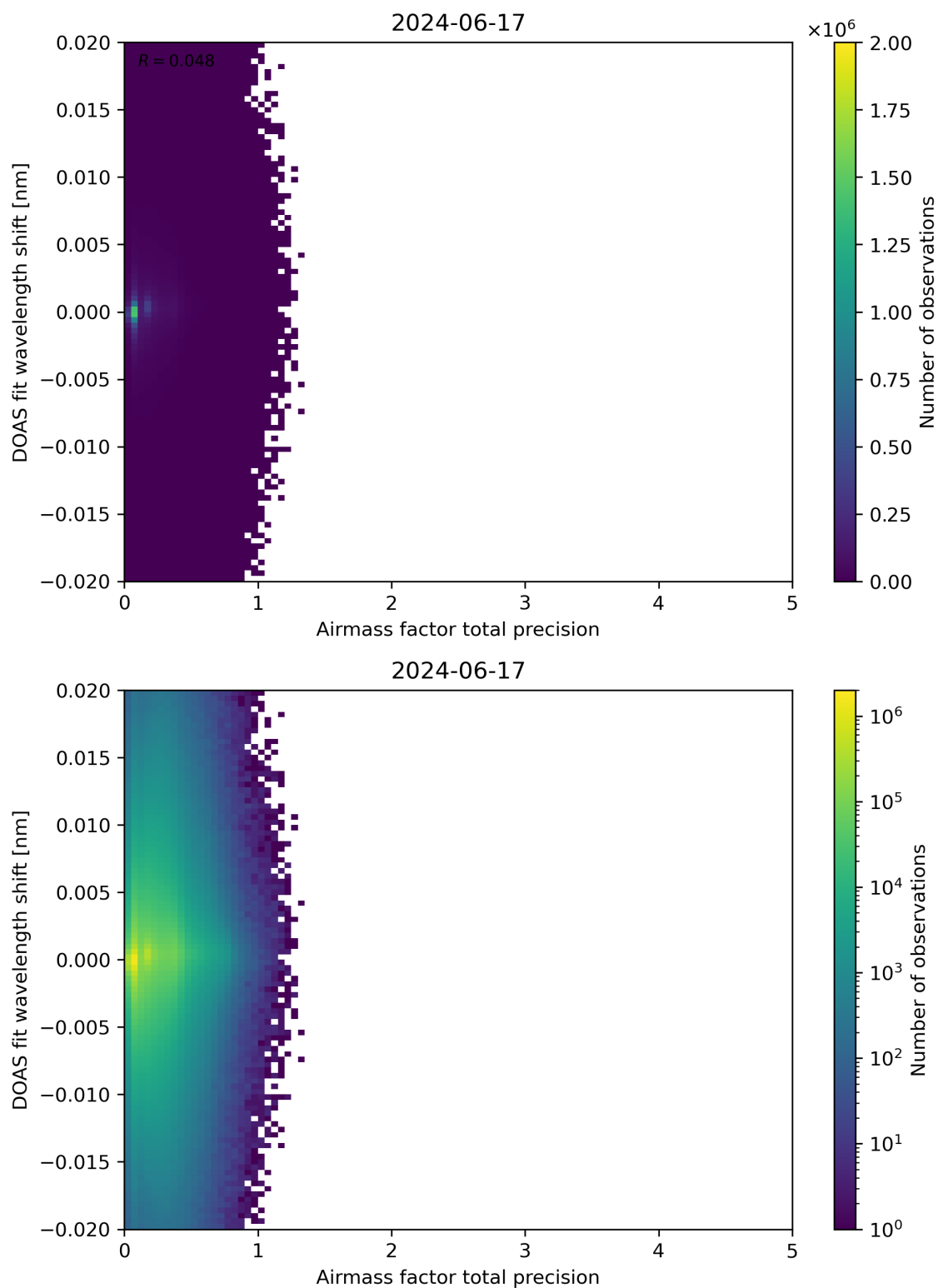
Figure 106: Scatter density plot of “Airmass factor total precision” against “DOAS fit wavelength shift” for 2024-06-16 to 2024-06-18.
