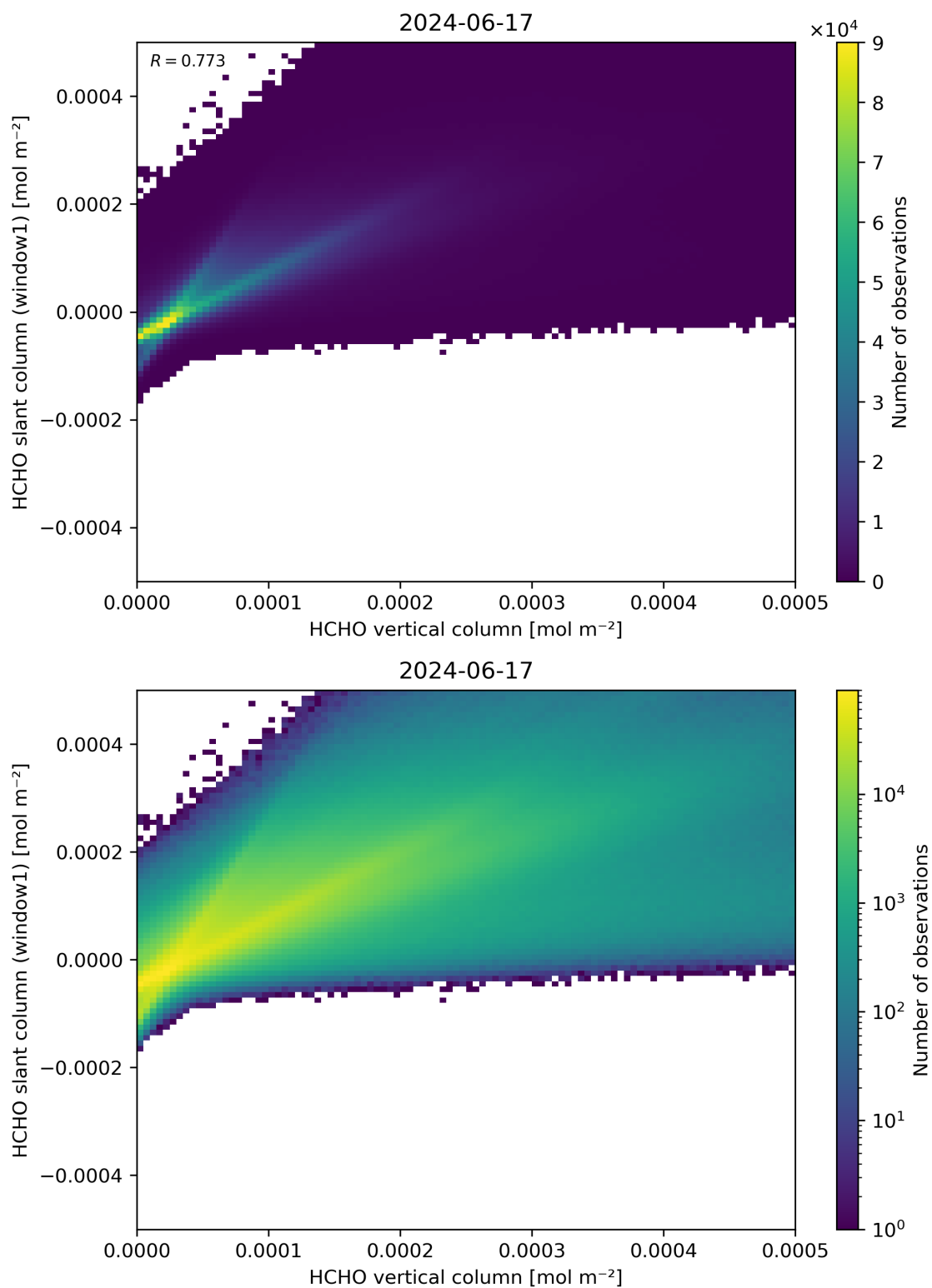
Figure 129: Scatter density plot of “HCHO vertical column” against “HCHO slant column (window1)” for 2024-06-16 to 2024-06-18.
