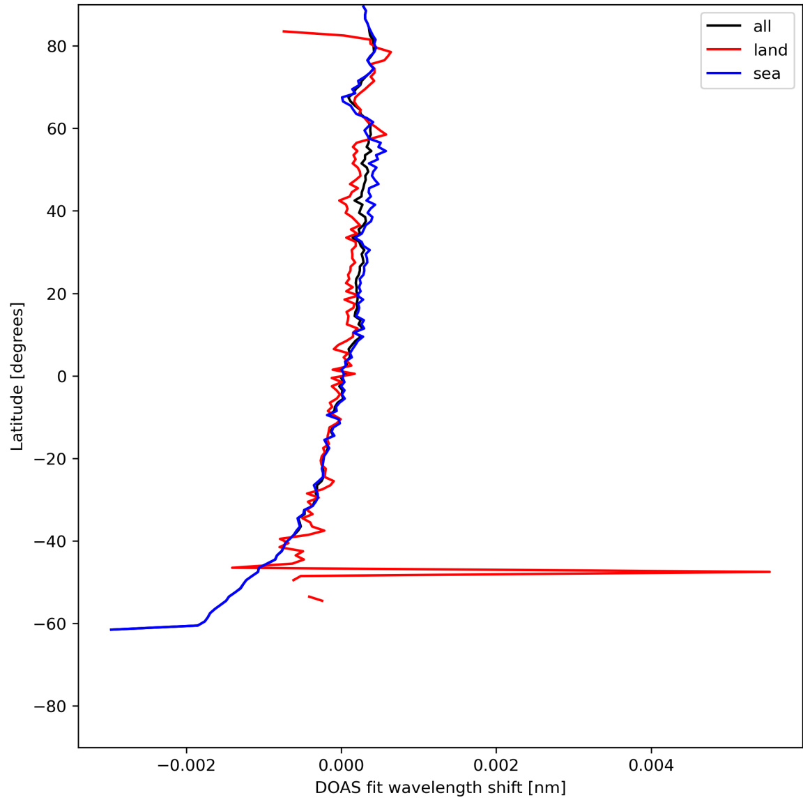
Figure 30: Zonal average of “DOAS fit wavelength shift” for 2024-06-16 to 2024-06-18.
