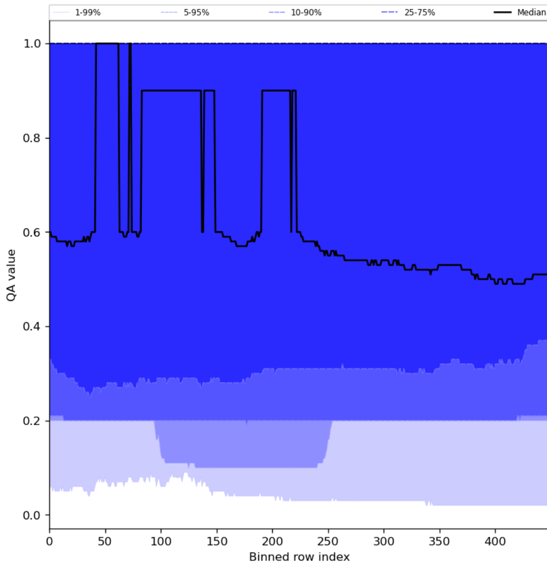
Figure 48: Along track statistics of “QA value” for 2024-06-16 to 2024-06-18
