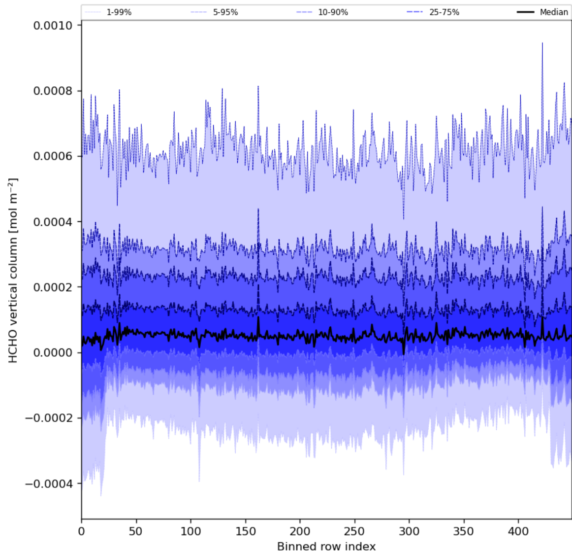
Figure 49: Along track statistics of “HCHO vertical column” for 2024-06-16 to 2024-06-18
