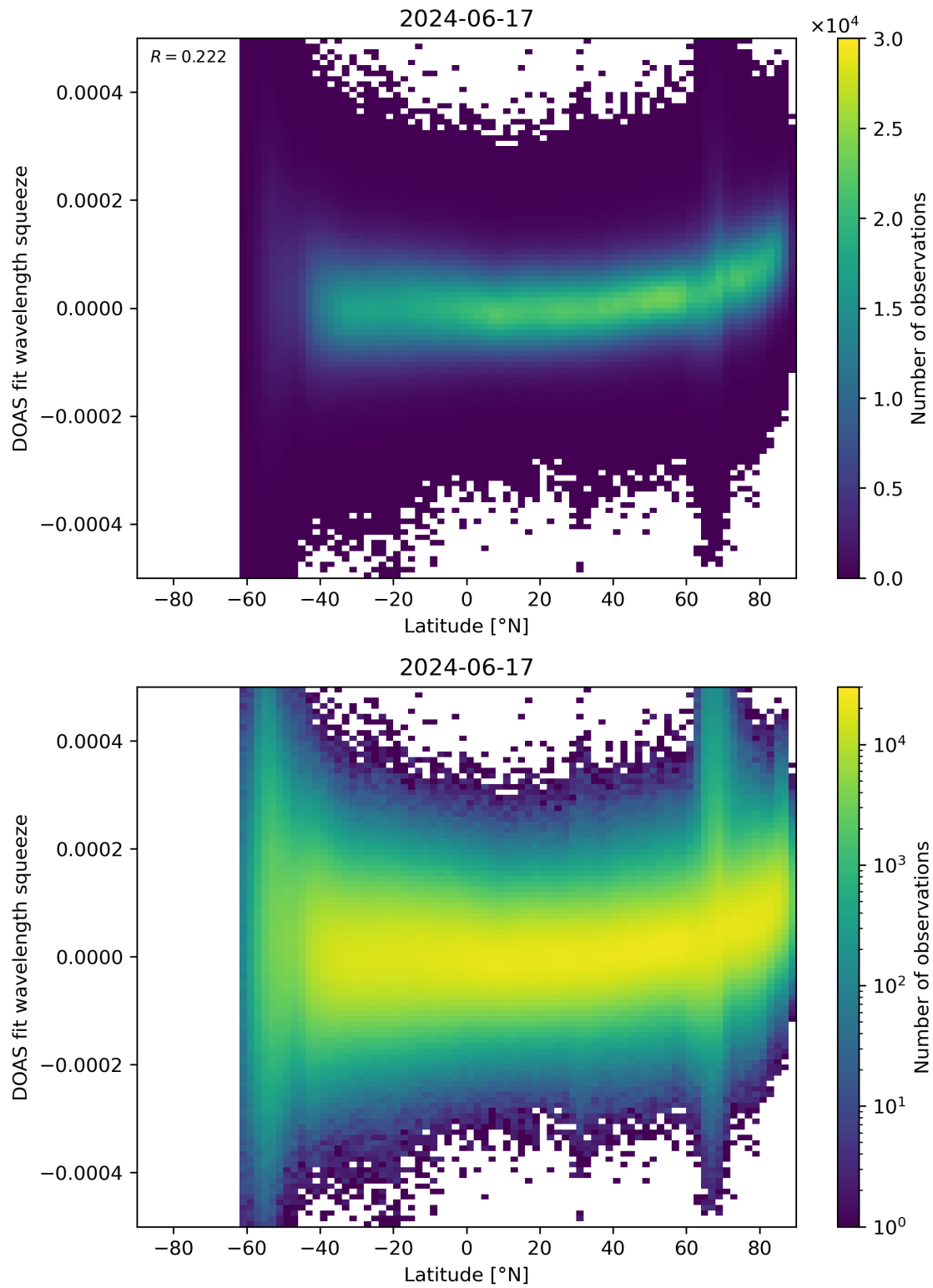
Figure 155: Scatter density plot of “Latitude” against “DOAS fit wavelength squeeze” for 2024-06-16 to 2024-06-18.
