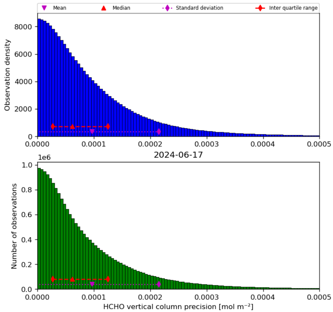
Figure 36: Histogram of “HCHO vertical column precision” for 2024-06-16 to 2024-06-18
