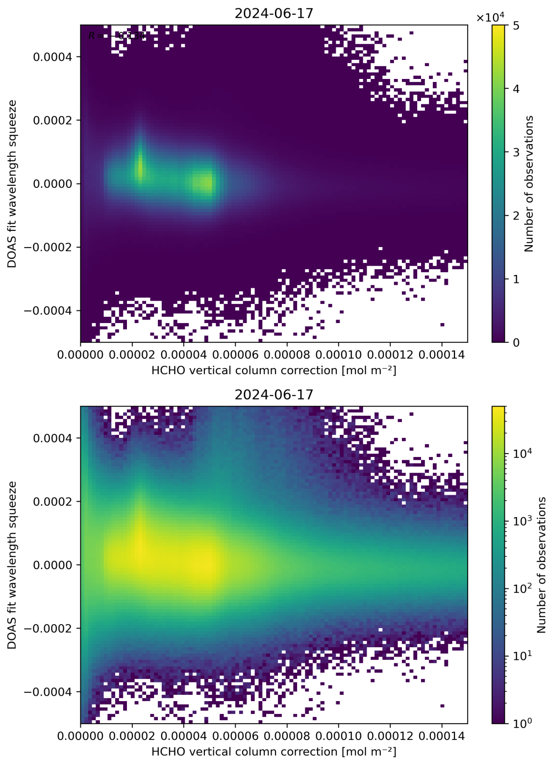
Figure 114: Scatter density plot of “HCHO vertical column correction” against “DOAS fit wavelength squeeze” for 2024-06-16 to 2024-06-18.
