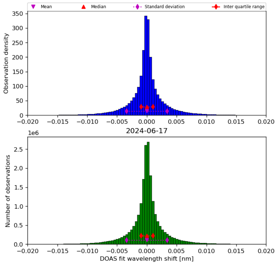
Figure 44: Histogram of “DOAS fit wavelength shift” for 2024-06-16 to 2024-06-18
