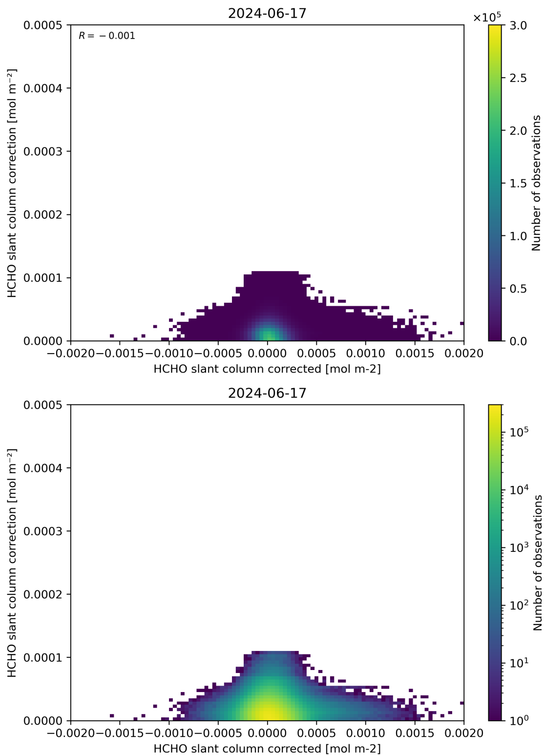
Figure 77: Scatter density plot of “HCHO slant column corrected” against “HCHO slant column correction” for 2024-06-16 to 2024-06-18.
