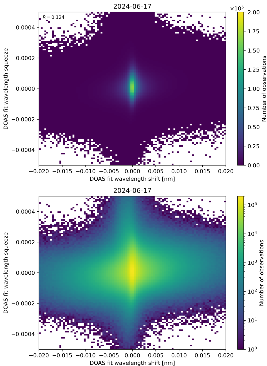
Figure 65: Scatter density plot of “DOAS fit wavelength shift” against “DOAS fit wavelength squeeze” for 2024-06-16 to 2024-06-18.
