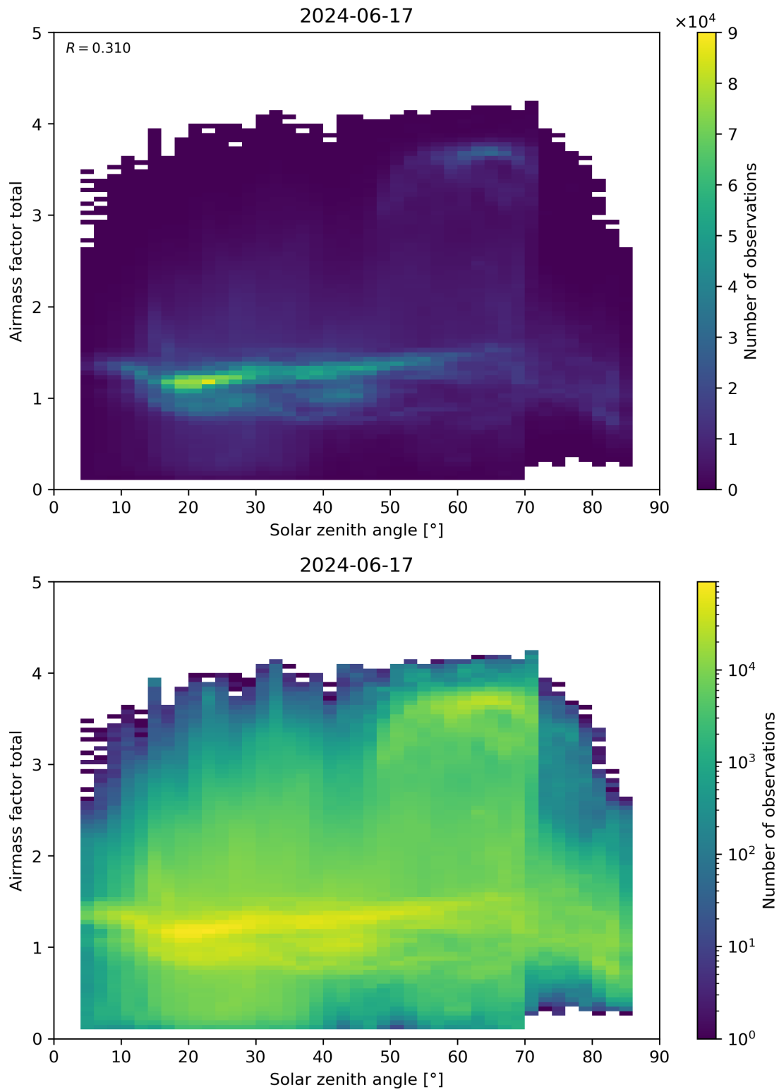
Figure 175: Scatter density plot of “Solar zenith angle” against “Airmass factor total” for 2024-06-16 to 2024-06-18.
