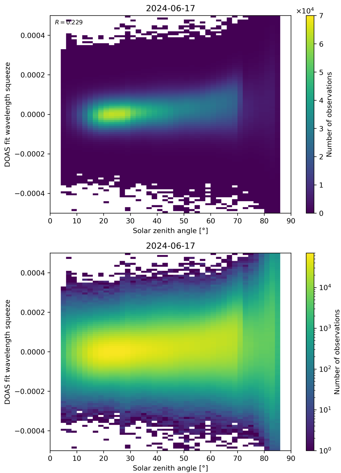
Figure 169: Scatter density plot of “Solar zenith angle” against “DOAS fit wavelength squeeze” for 2024-06-16 to 2024-06-18.
