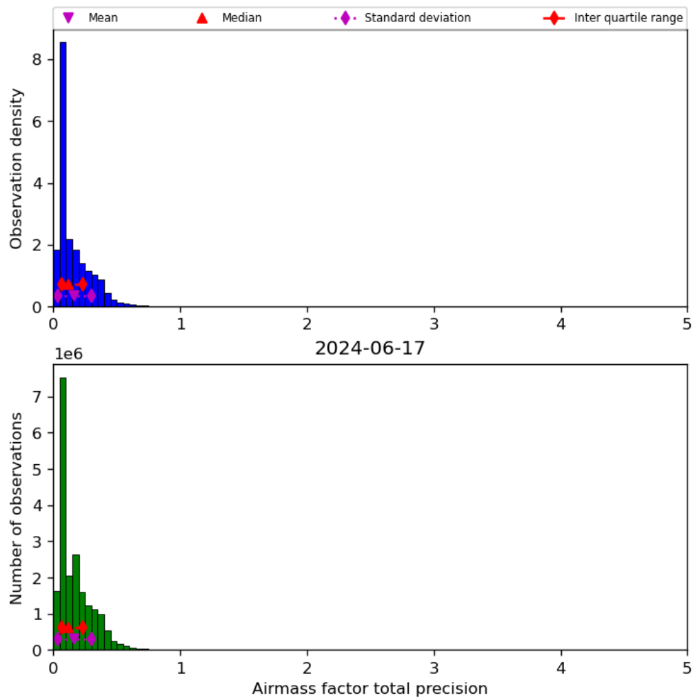
Figure 41: Histogram of "Airmass factor total precision" for 2024-06-16 to 2024-06-18
