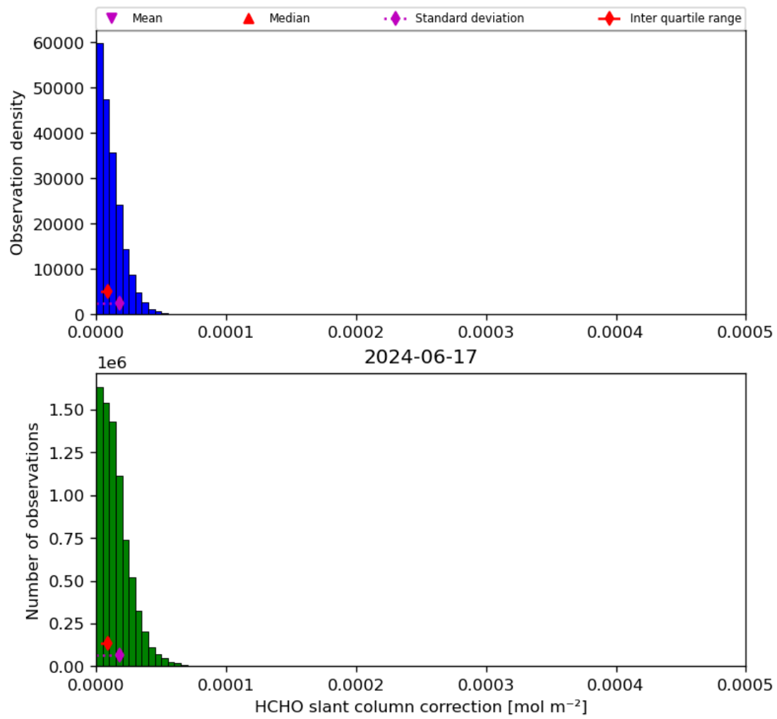
Figure 47: Histogram of “HCHO slant column correction” for 2024-06-16 to 2024-06-18
