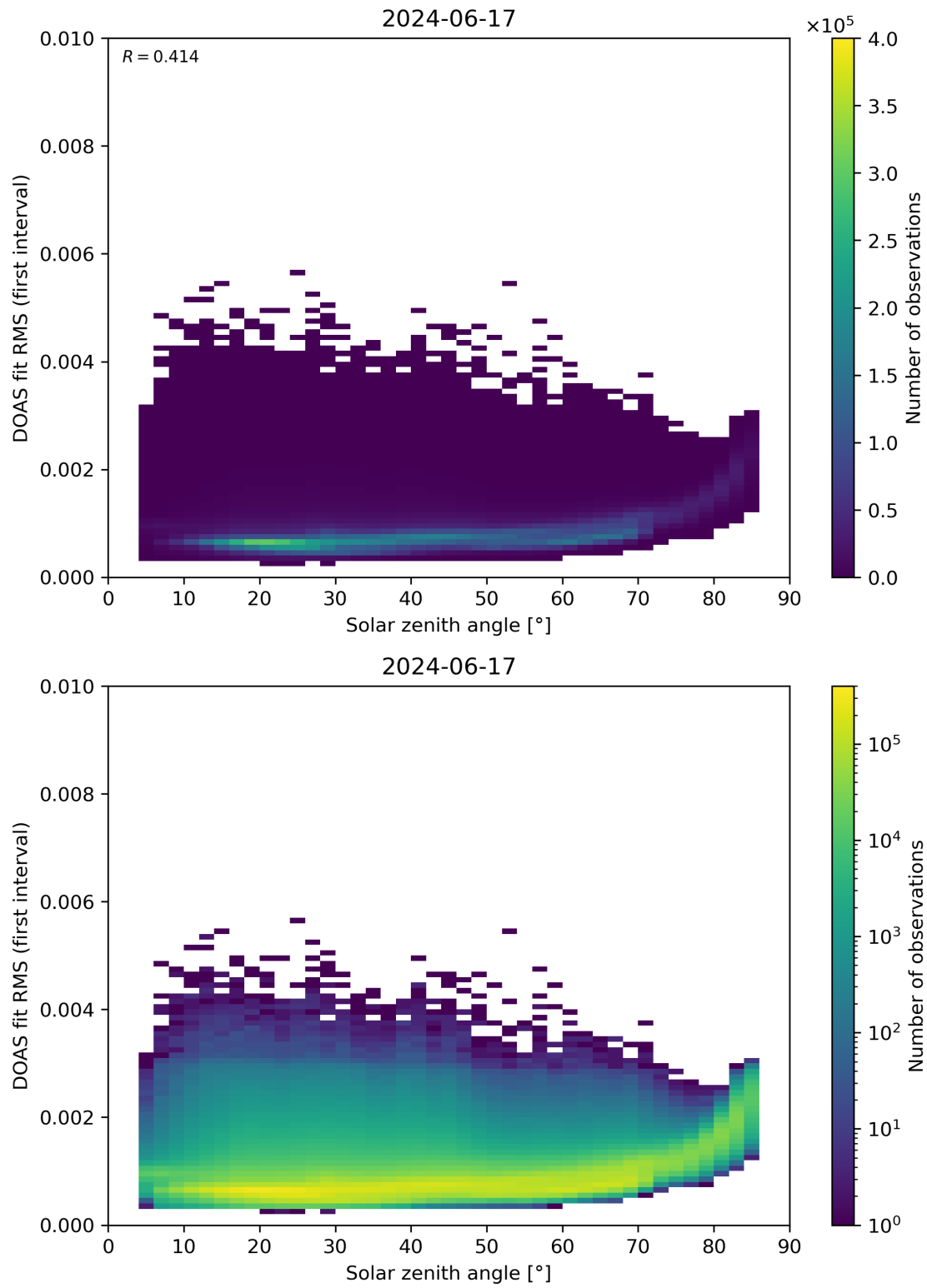
Figure 167: Scatter density plot of “Solar zenith angle” against “DOAS fit RMS (first interval)” for 2024-06-16 to 2024-06-18.
