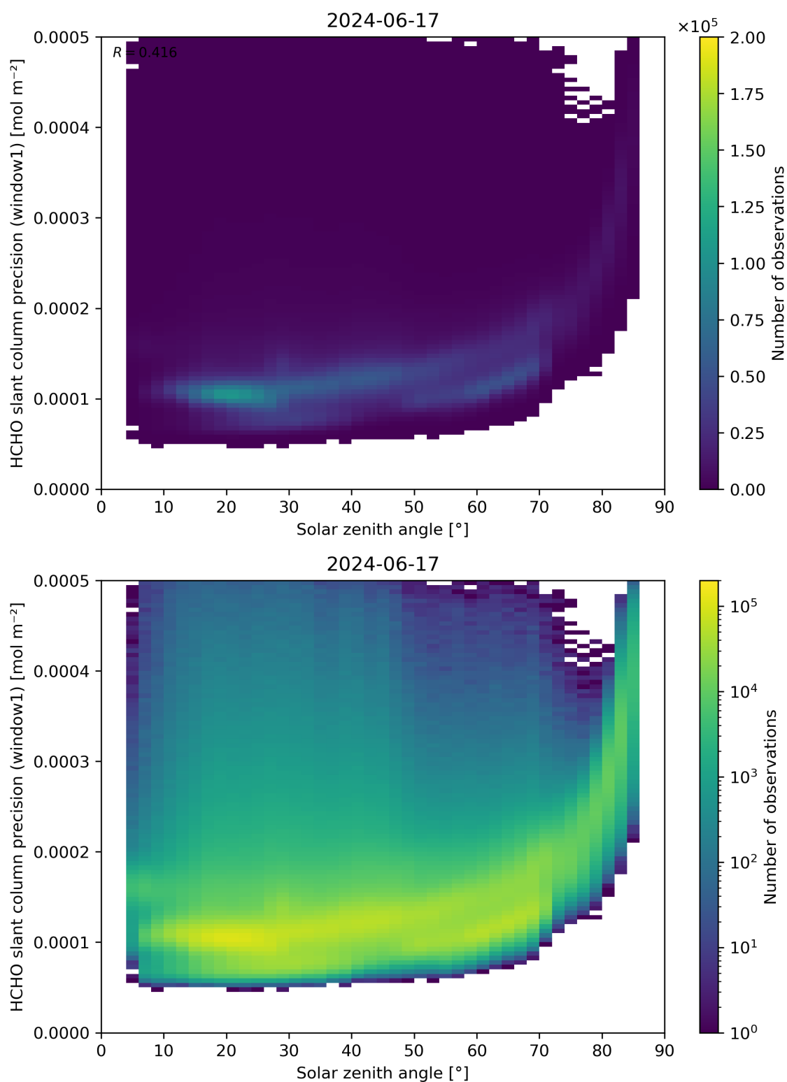
Figure 174: Scatter density plot of “Solar zenith angle” against “HCHO slant column precision (window1)” for 2024-06-16 to 2024-06-18.
