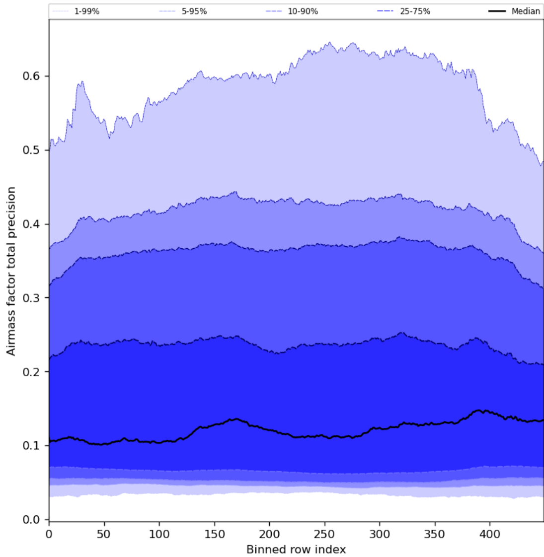
Figure 55: Along track statistics of “Airmass factor total precision” for 2024-06-16 to 2024-06-18
