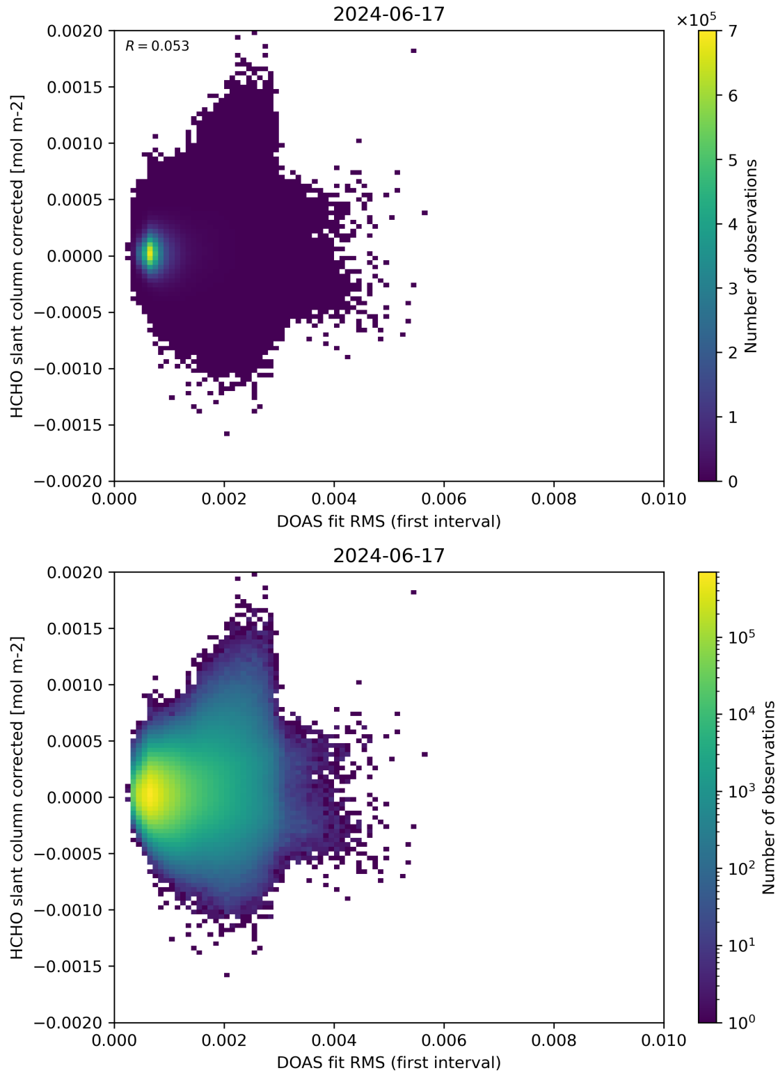
Figure 62: Scatter density plot of “DOAS fit RMS (first interval)” against “HCHO slant column corrected” for 2024-06-16 to 2024-06-18.
