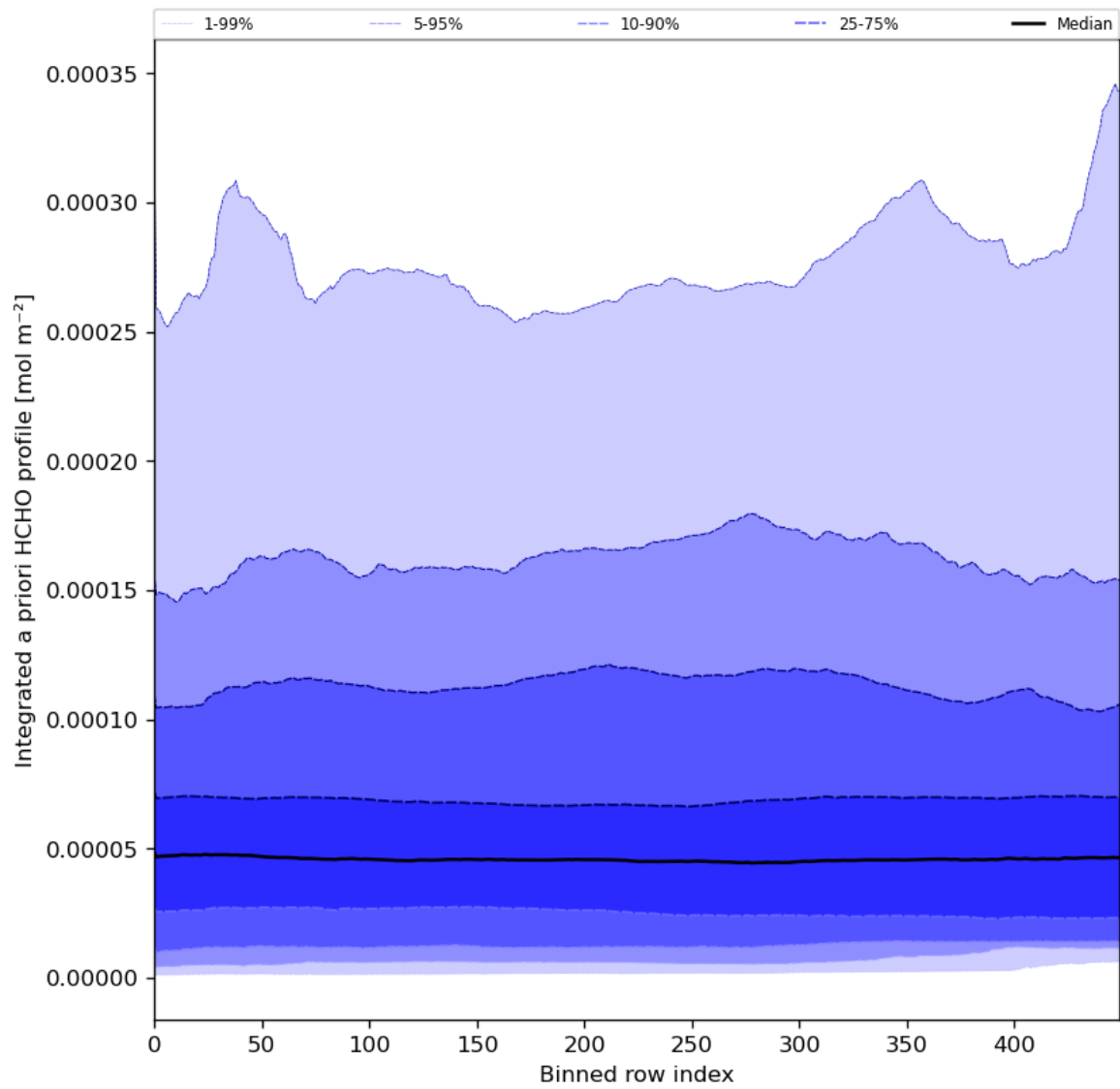
Figure 57: Along track statistics of “Integrated a priori HCHO profile” for 2024-06-16 to 2024-06-18
