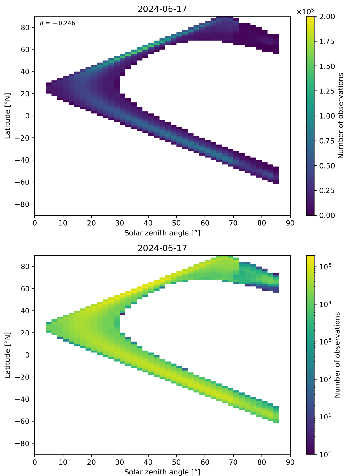
Figure 181: Scatter density plot of “Solar zenith angle” against “Latitude” for 2024-06-16 to 2024-06-18.
