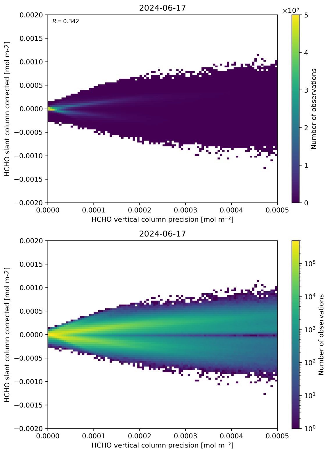
Figure 140: Scatter density plot of “HCHO vertical column precision” against “HCHO slant column corrected” for 2024-06-16 to 2024-06-18.
