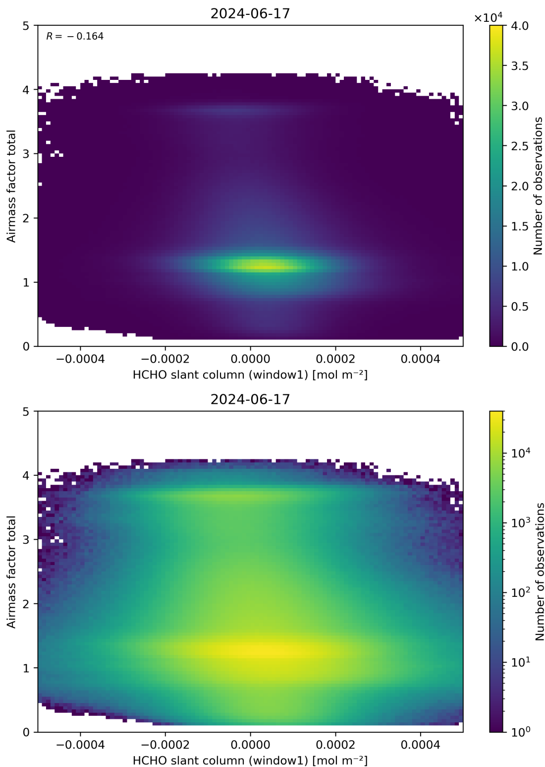
Figure 85: Scatter density plot of “HCHO slant column (window1)” against “Airmass factor total” for 2024-06-16 to 2024-06-18.
