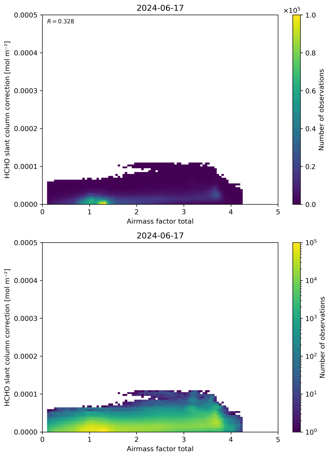
Figure 102: Scatter density plot of “Airmass factor total” against “HCHO slant column correction” for 2024-06-16 to 2024-06-18.
