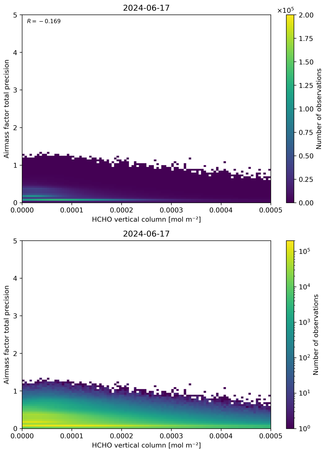
Figure 132: Scatter density plot of “HCHO vertical column” against “Airmass factor total precision” for 2024-06-16 to 2024-06-18.
