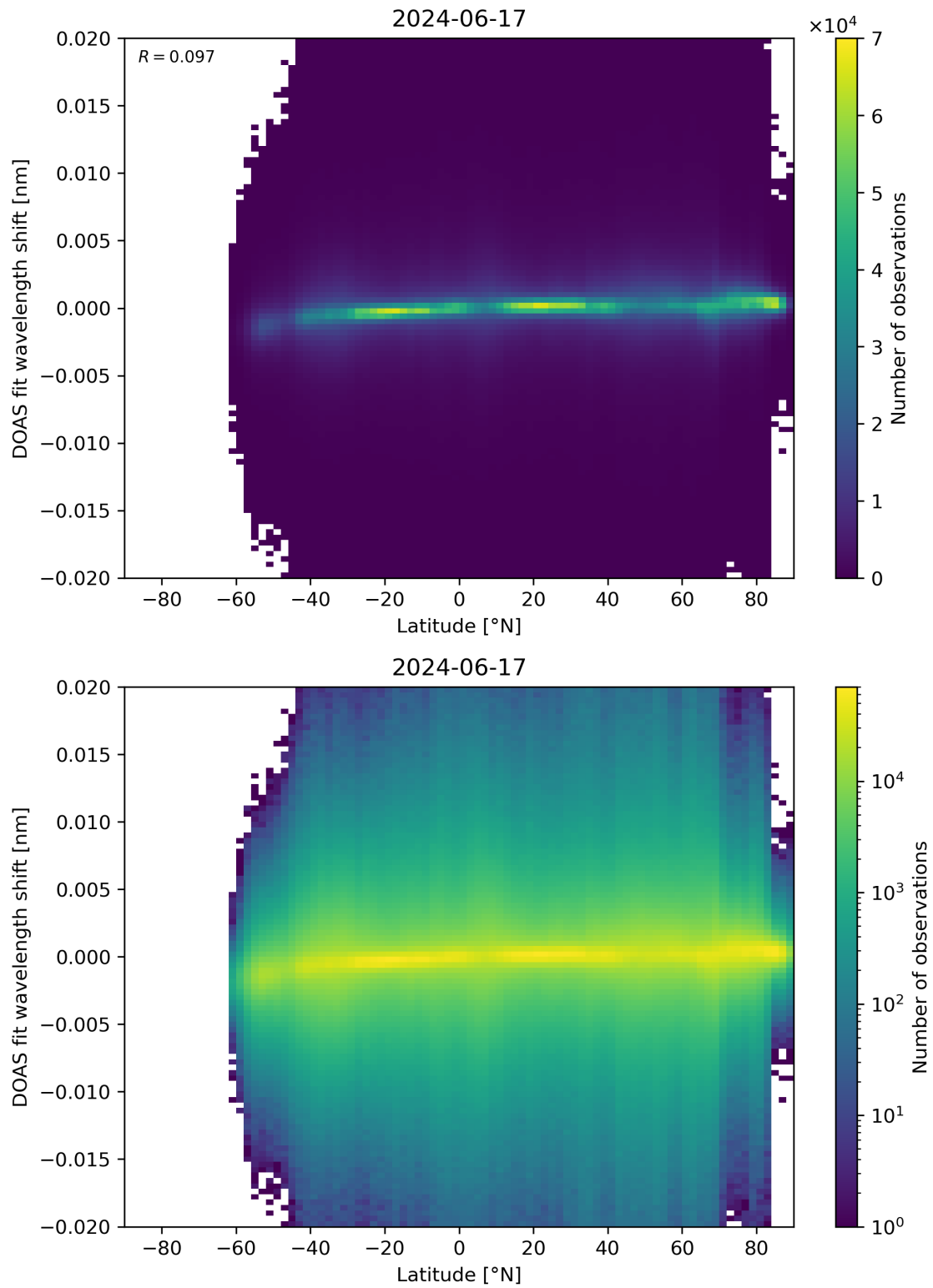
Figure 154: Scatter density plot of “Latitude” against “DOAS fit wavelength shift” for 2024-06-16 to 2024-06-18.
