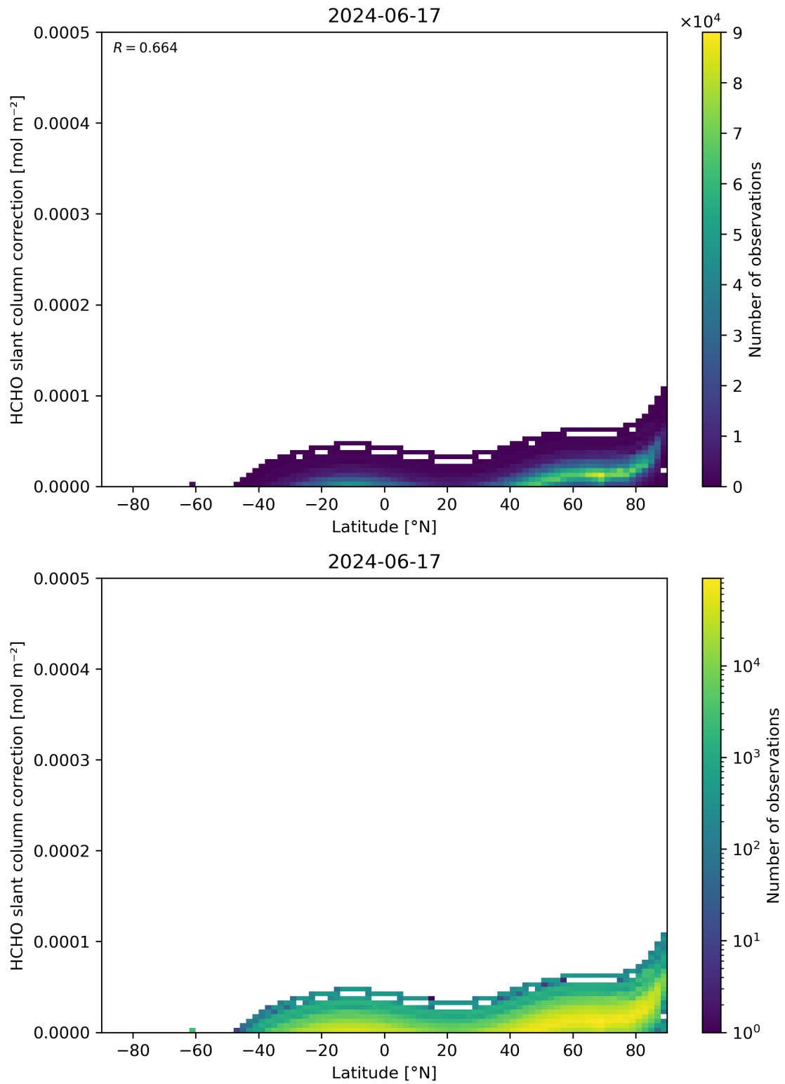
Figure 158: Scatter density plot of “Latitude” against “HCHO slant column correction” for 2024-06-16 to 2024-06-18.
