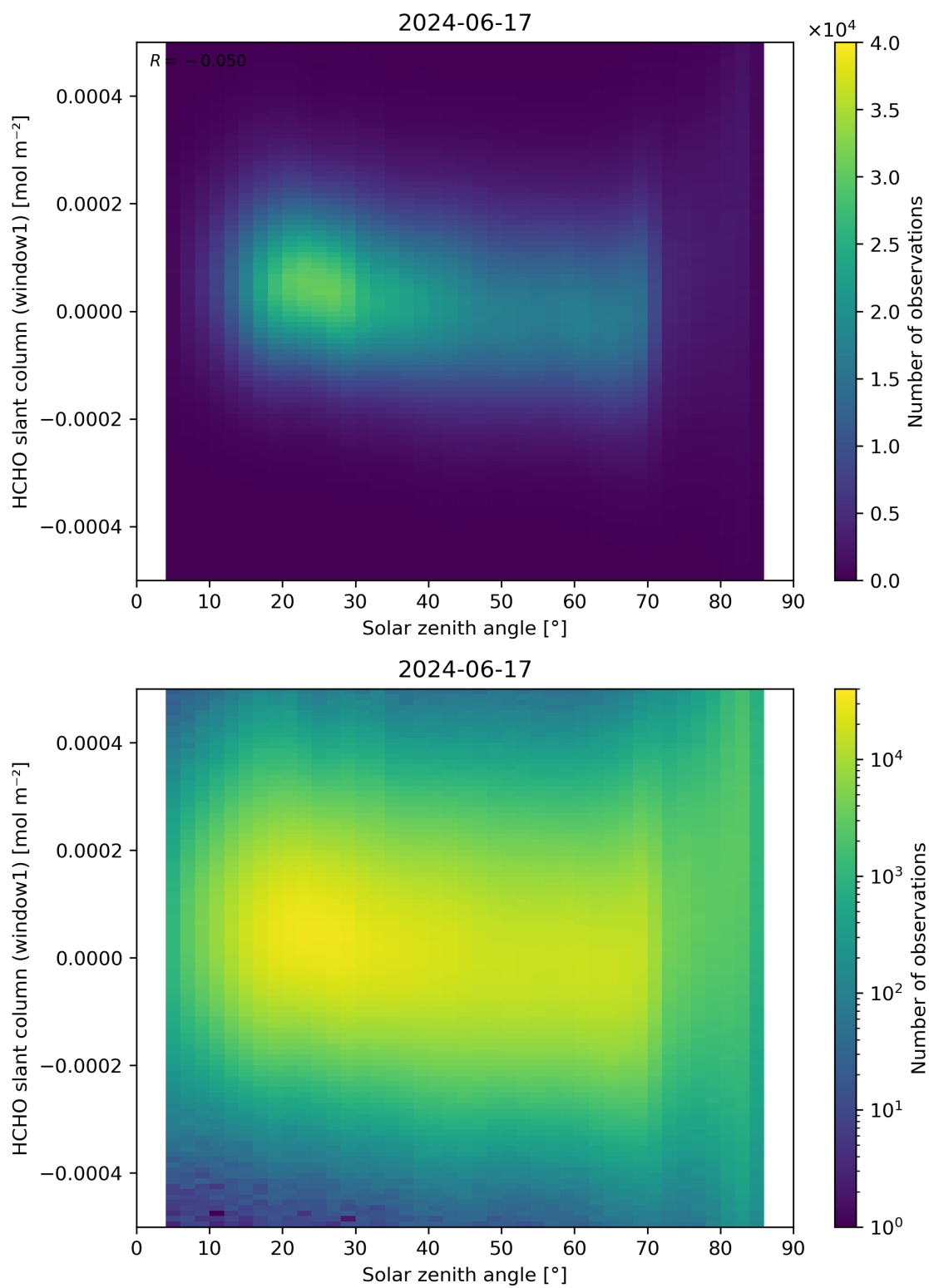
Figure 173: Scatter density plot of “Solar zenith angle” against “HCHO slant column (window1)” for 2024-06-16 to 2024-06-18.
