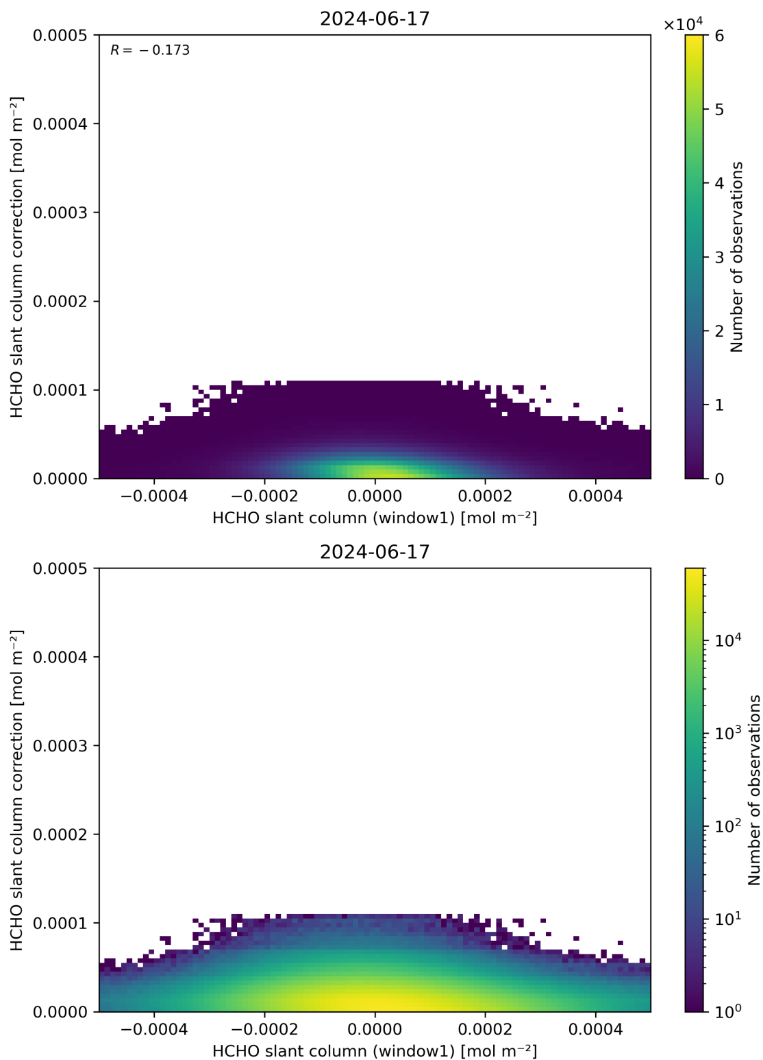
Figure 83: Scatter density plot of “HCHO slant column (window1)” against “HCHO slant column correction” for 2024-06-16 to 2024-06-18.
