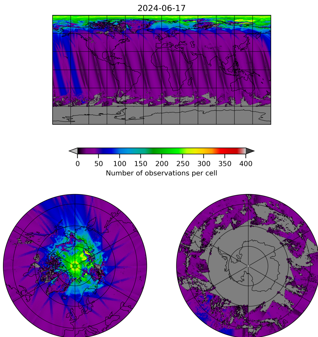
Figure 19: Map of the number of observations for 2024-06-16 to 2024-06-18
