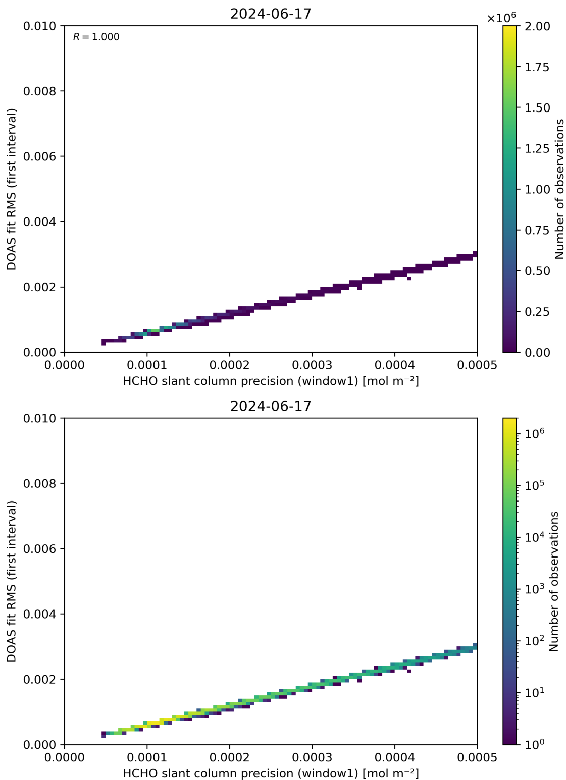
Figure 88: Scatter density plot of “HCHO slant column precision (window1)” against “DOAS fit RMS (first interval)” for 2024-06-16 to 2024-06-18.
