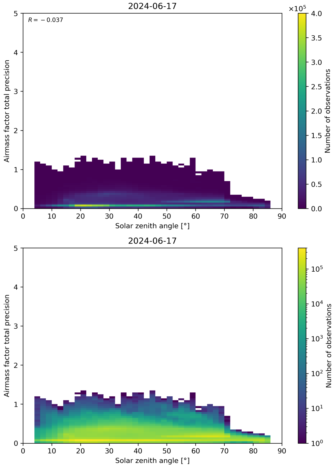
Figure 176: Scatter density plot of “Solar zenith angle” against “Airmass factor total precision” for 2024-06-16 to 2024-06-18.
