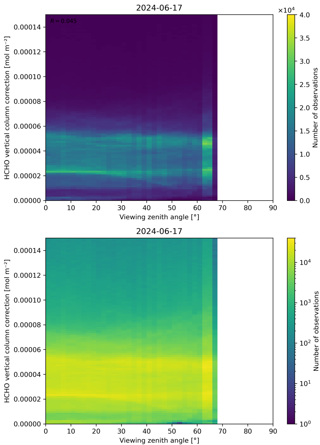
Figure 193: Scatter density plot of “Viewing zenith angle” against “HCHO vertical column correction” for 2024-06-16 to 2024-06-18.
