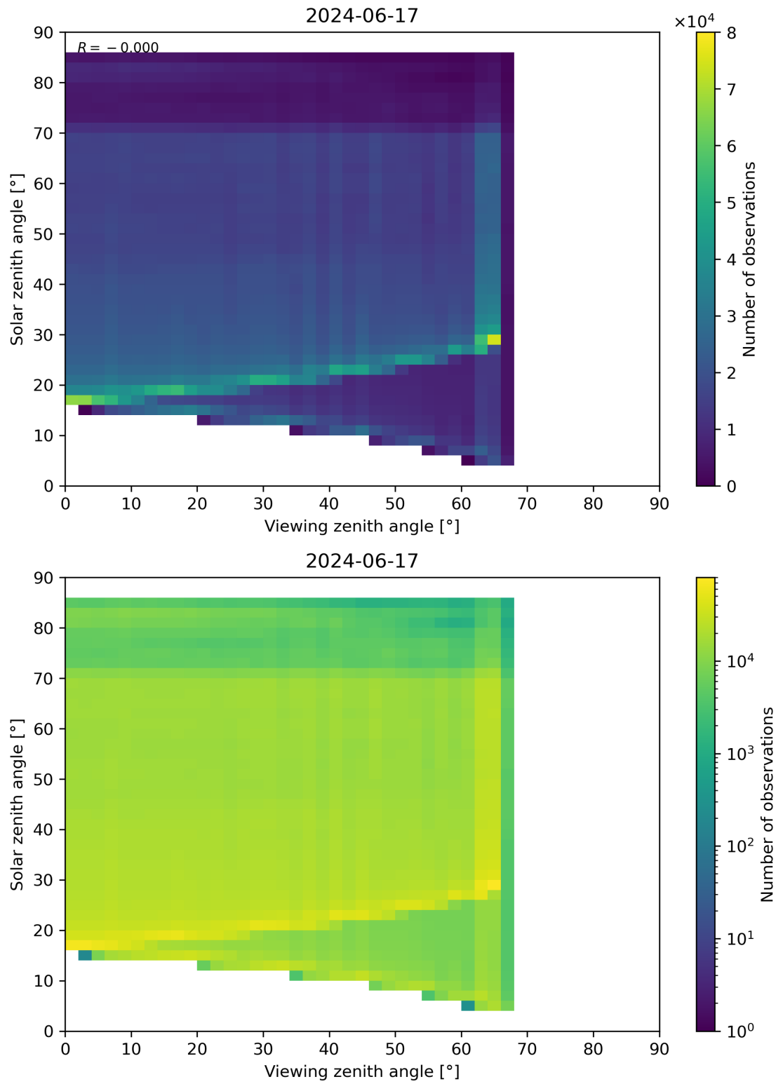
Figure 197: Scatter density plot of “Viewing zenith angle” against “Solar zenith angle” for 2024-06-16 to 2024-06-18.
