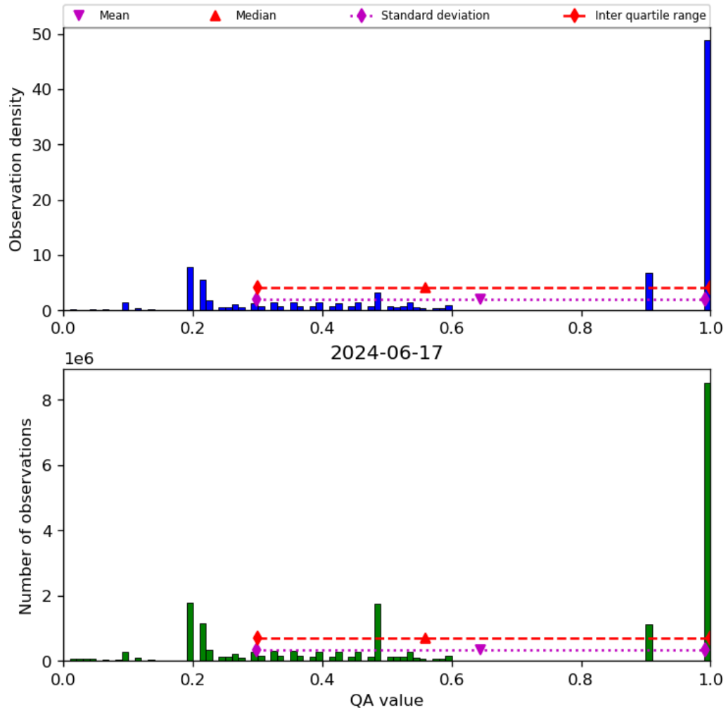
Figure 34: Histogram of “QA value” for 2024-06-16 to 2024-06-18
