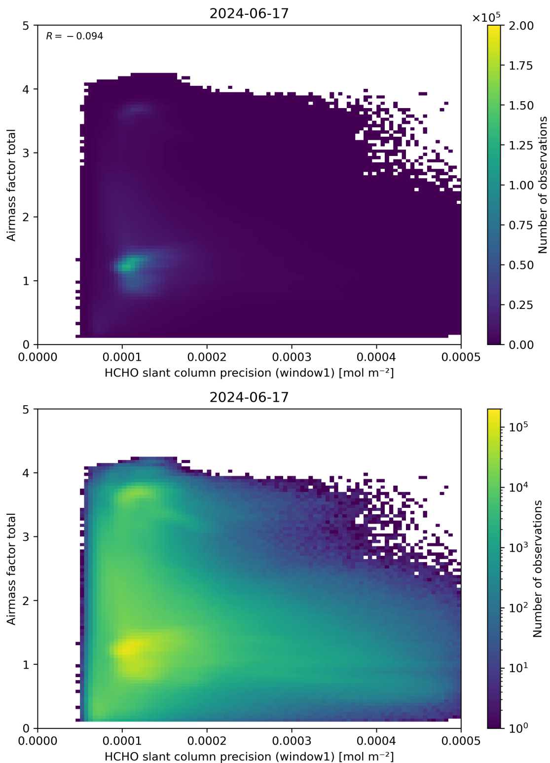
Figure 94: Scatter density plot of “HCHO slant column precision (window1)” against “Airmass factor total” for 2024-06-16 to 2024-06-18.
