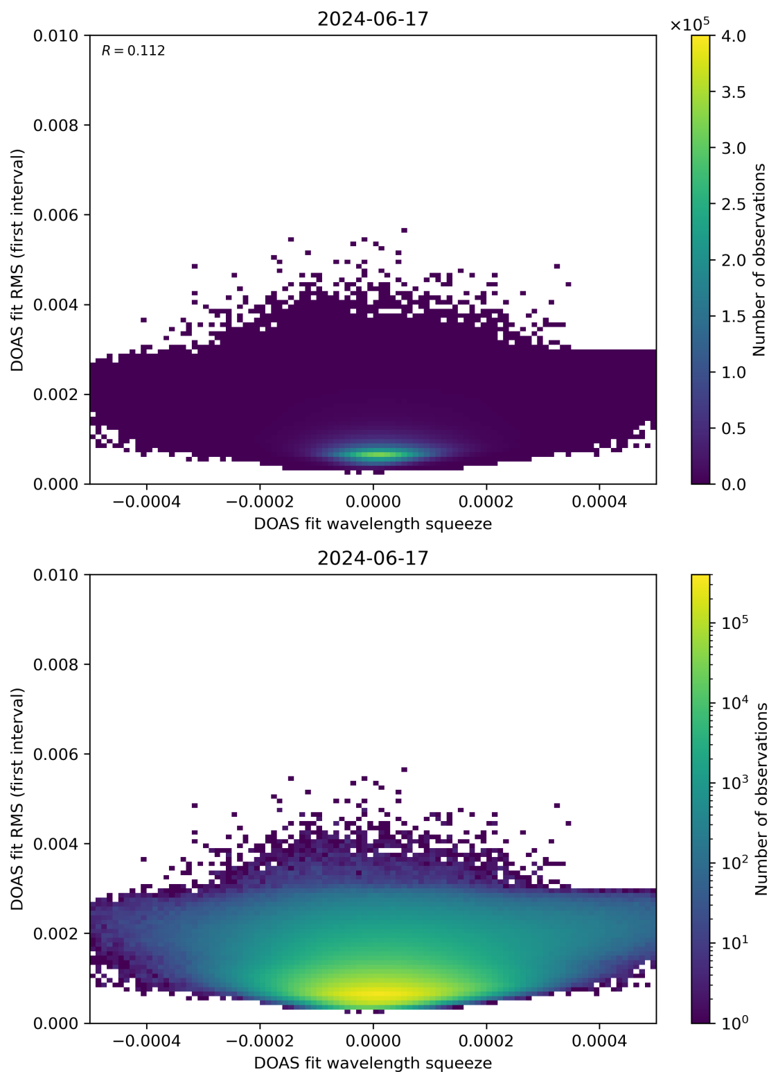
Figure 68: Scatter density plot of “DOAS fit wavelength squeeze” against “DOAS fit RMS (first interval)” for 2024-06-16 to 2024-06-18.
