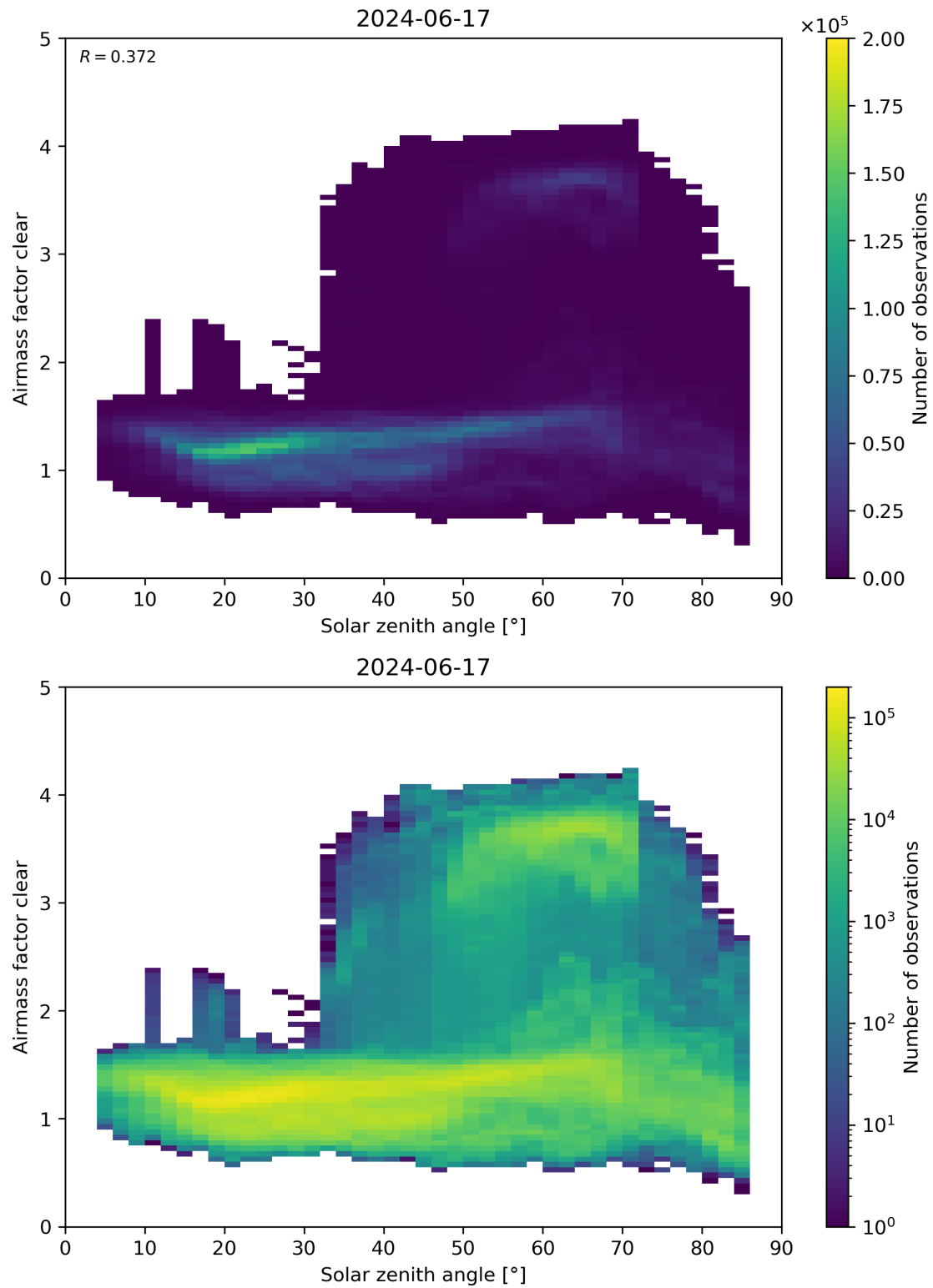
Figure 170: Scatter density plot of “Solar zenith angle” against “Airmass factor clear” for 2024-06-16 to 2024-06-18.
