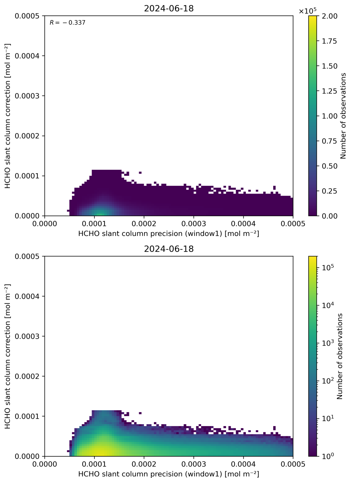
Figure 93: Scatter density plot of “HCHO slant column precision (window1)” against “HCHO slant column correction” for 2024-06-17 to 2024-06-19.
