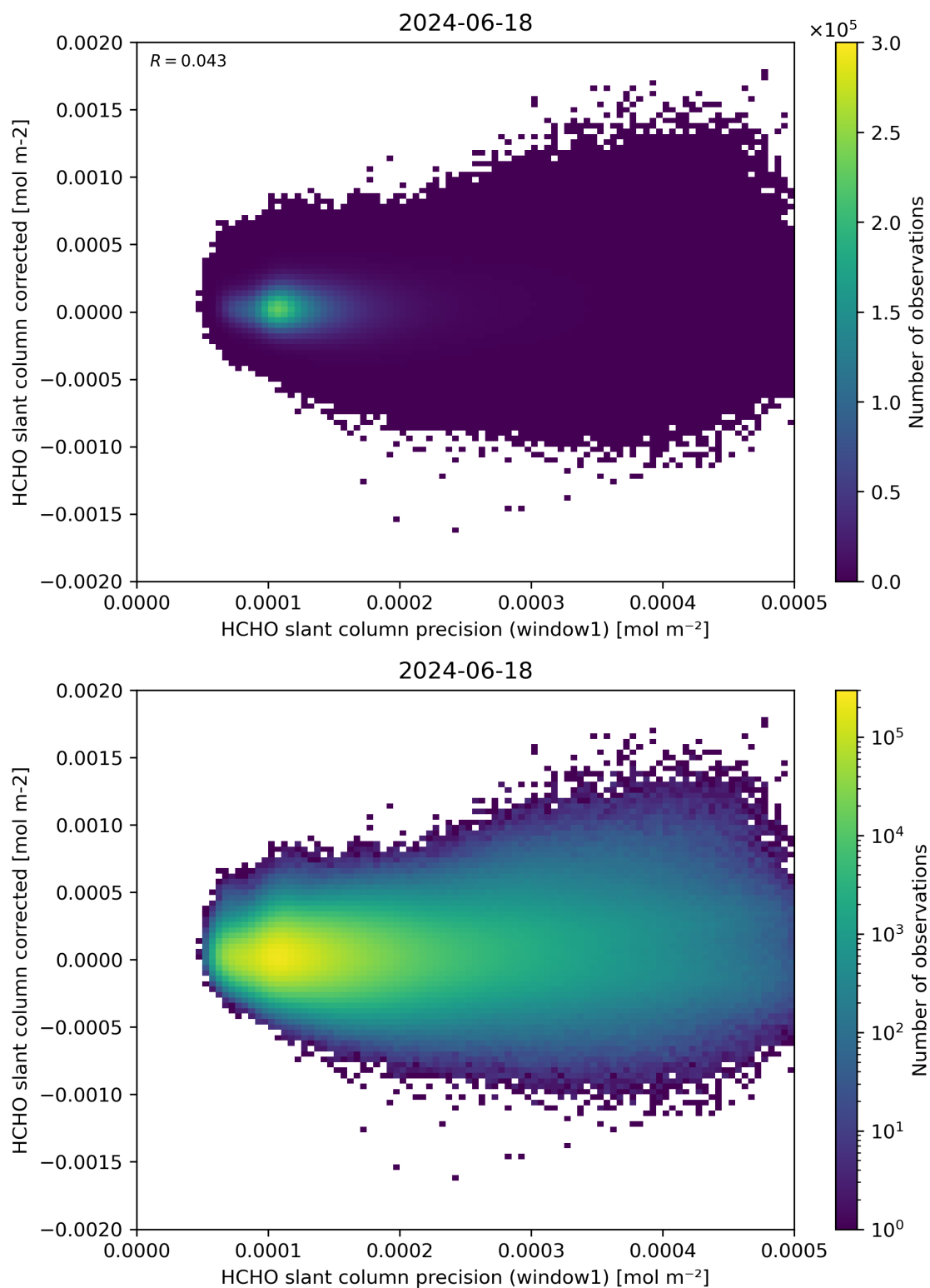
Figure 92: Scatter density plot of “HCHO slant column precision (window1)” against “HCHO slant column corrected” for 2024-06-17 to 2024-06-19.
