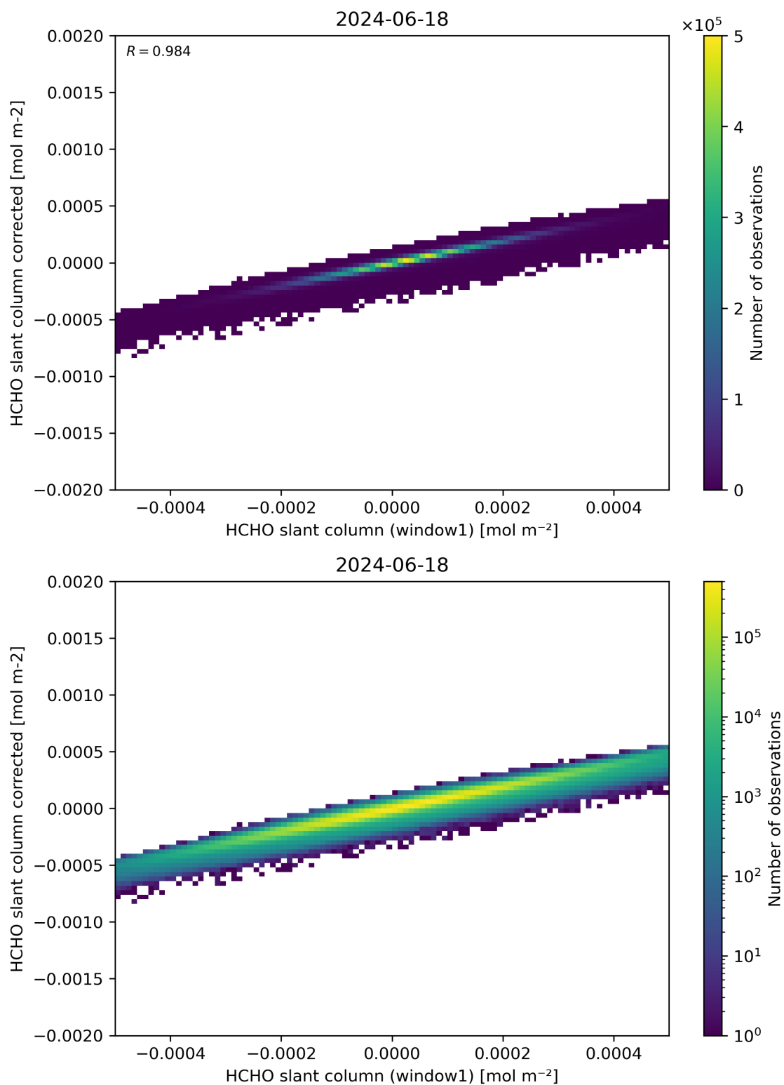
Figure 82: Scatter density plot of “HCHO slant column (window1)” against “HCHO slant column corrected” for 2024-06-17 to 2024-06-19.
