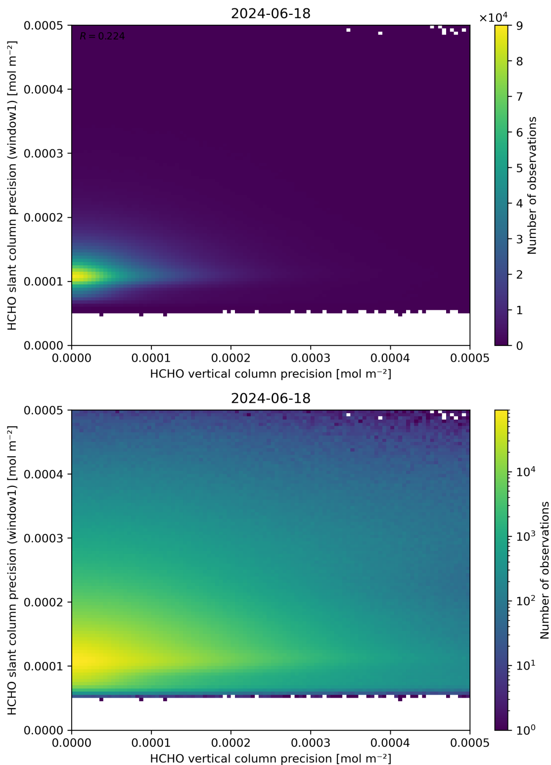
Figure 143: Scatter density plot of “HCHO vertical column precision” against “HCHO slant column precision (window1)” for 2024-06-17 to 2024-06-19.
