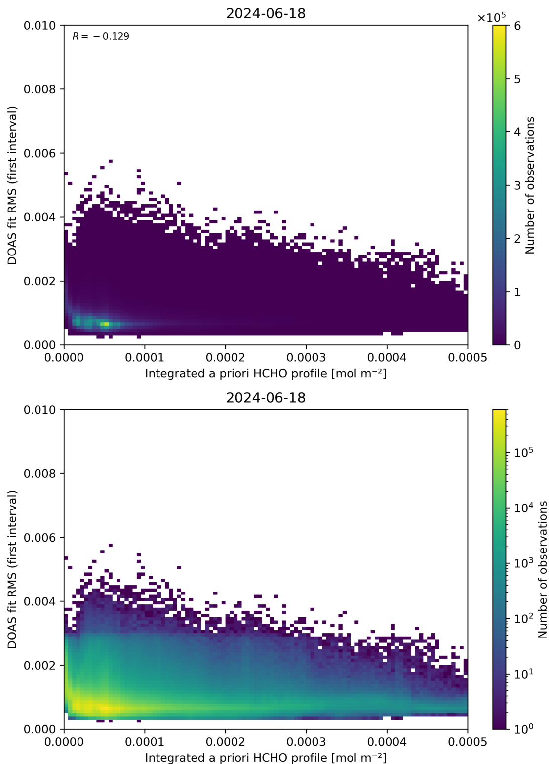
Figure 148: Scatter density plot of “Integrated a priori HCHO profile” against “DOAS fit RMS (first interval)” for 2024-06-17 to 2024-06-19.
