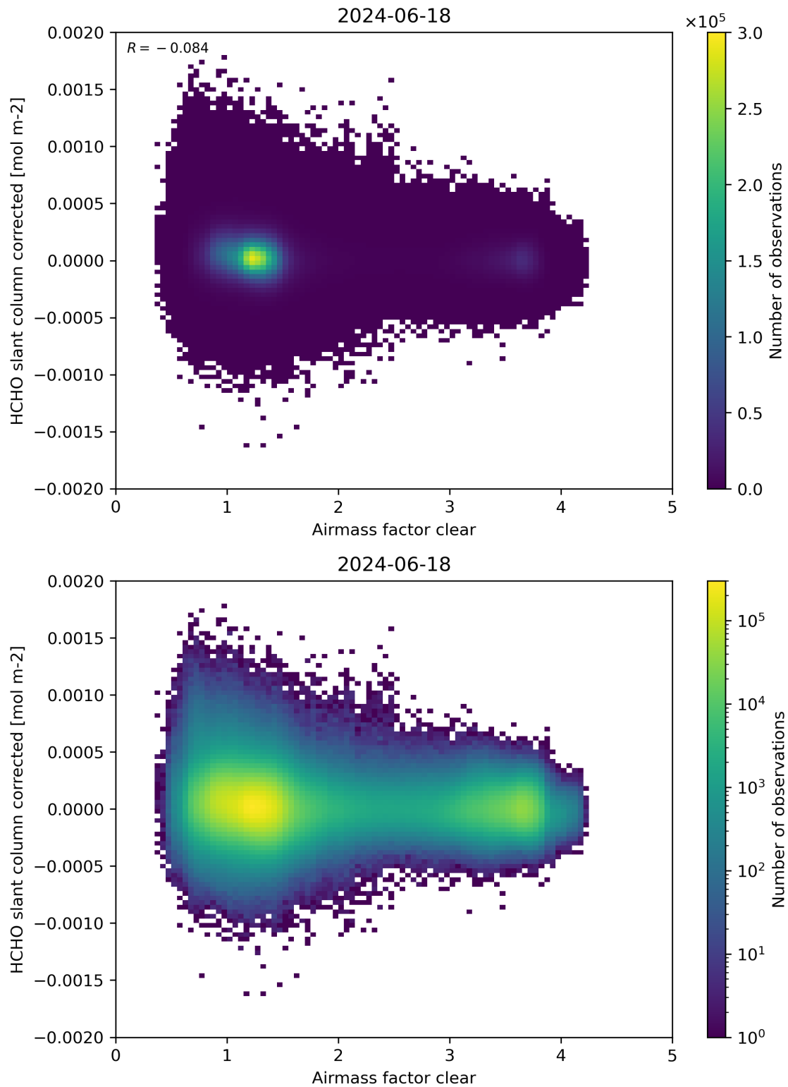
Figure 74: Scatter density plot of “Airmass factor clear” against “HCHO slant column corrected” for 2024-06-17 to 2024-06-19.
