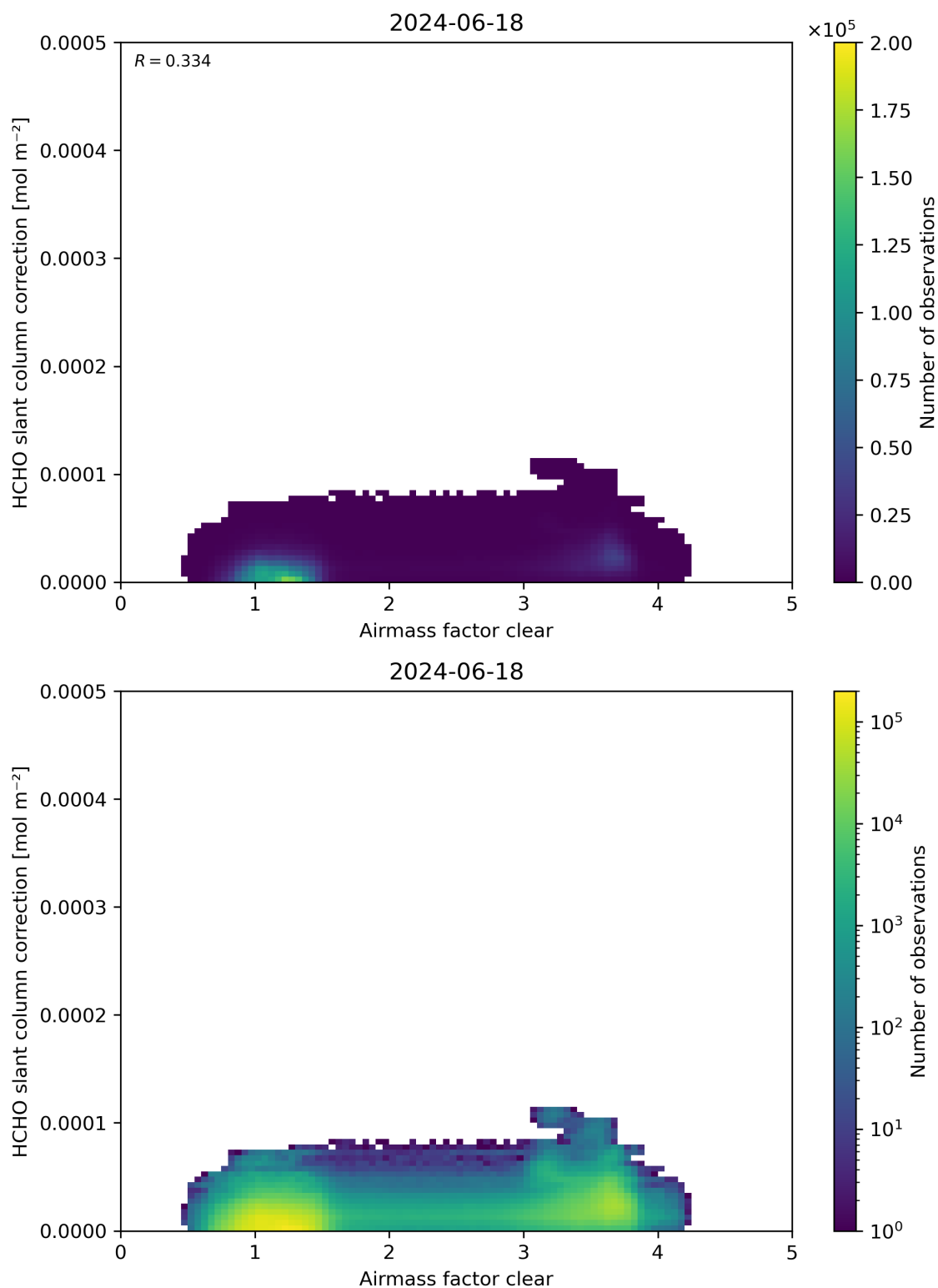
Figure 75: Scatter density plot of “Airmass factor clear” against “HCHO slant column correction” for 2024-06-17 to 2024-06-19.
