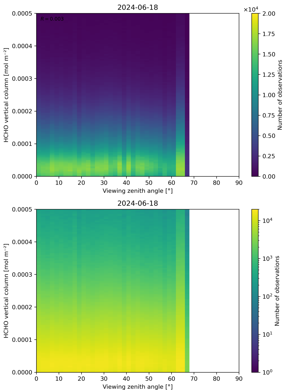
Figure 192: Scatter density plot of “Viewing zenith angle” against “HCHO vertical column” for 2024-06-17 to 2024-06-19.
