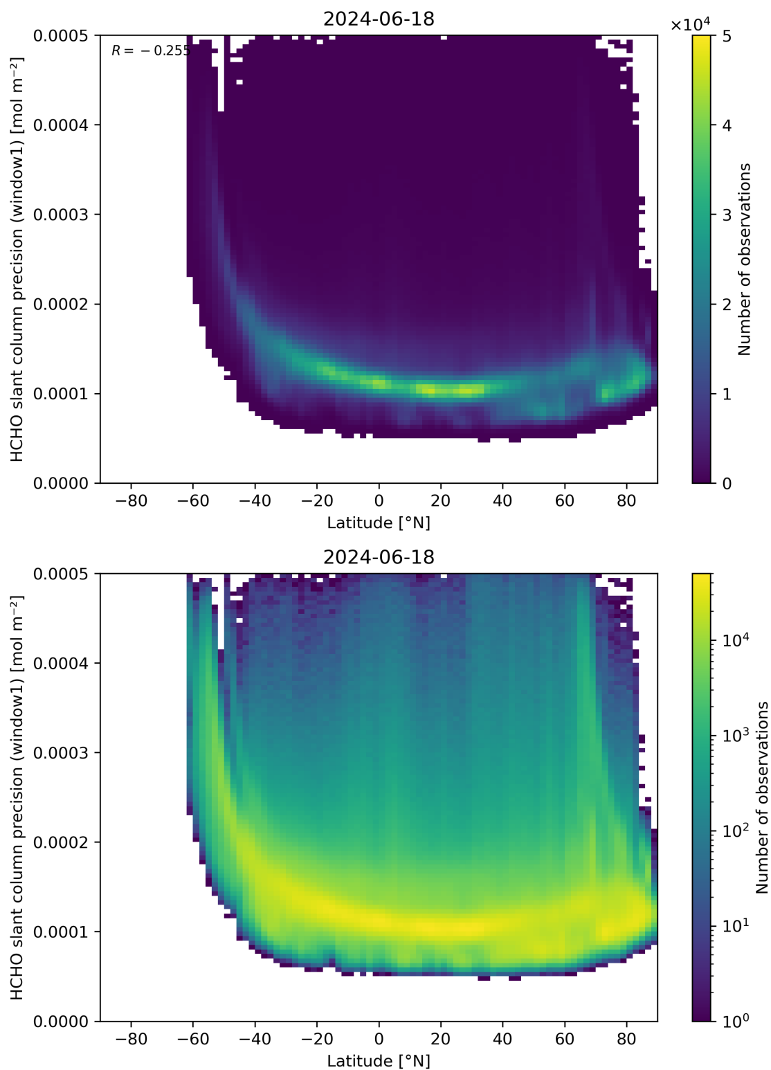
Figure 160: Scatter density plot of “Latitude” against “HCHO slant column precision (window1)” for 2024-06-17 to 2024-06-19.
