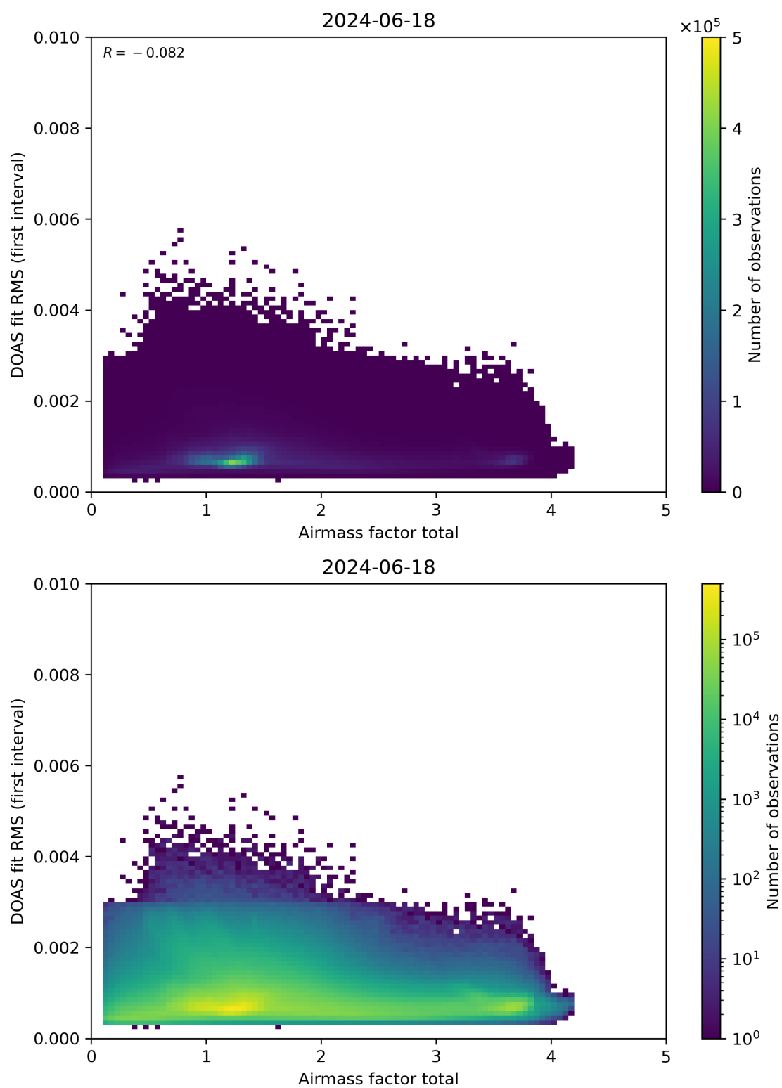
Figure 97: Scatter density plot of “Airmass factor total” against “DOAS fit RMS (first interval)” for 2024-06-17 to 2024-06-19.
