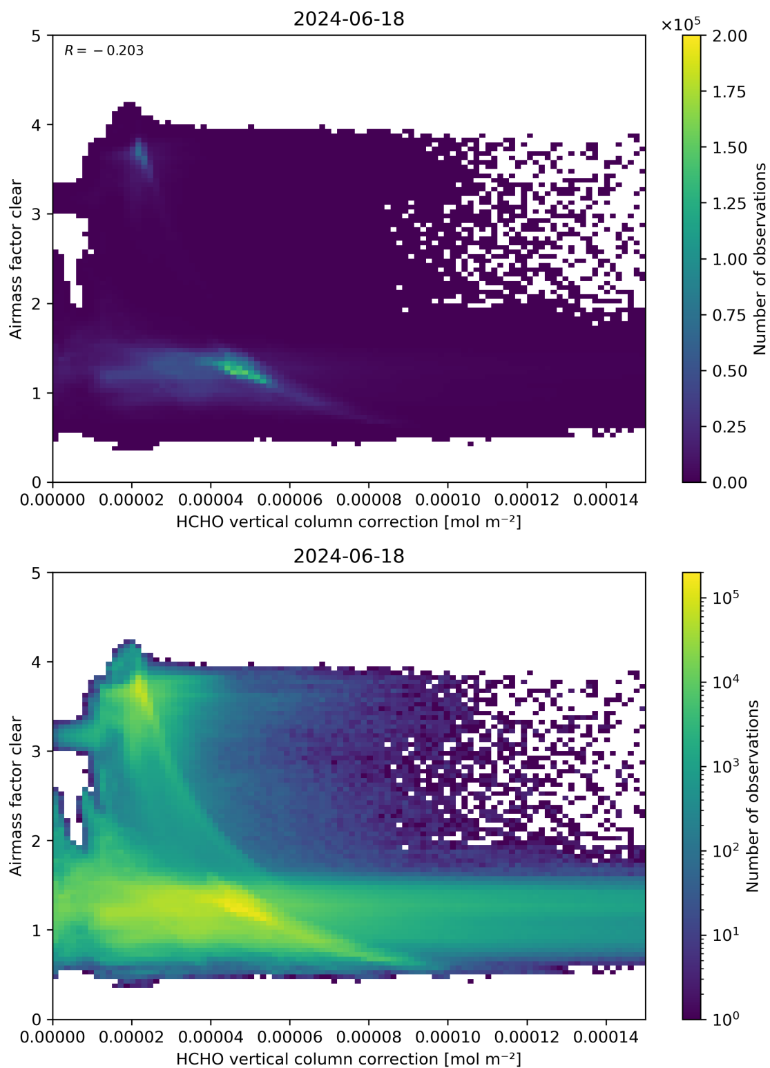
Figure 115: Scatter density plot of “HCHO vertical column correction” against “Airmass factor clear” for 2024-06-17 to 2024-06-19.
