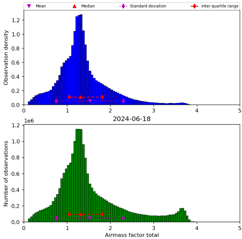
Figure 40: Histogram of “Airmass factor total” for 2024-06-17 to 2024-06-19
