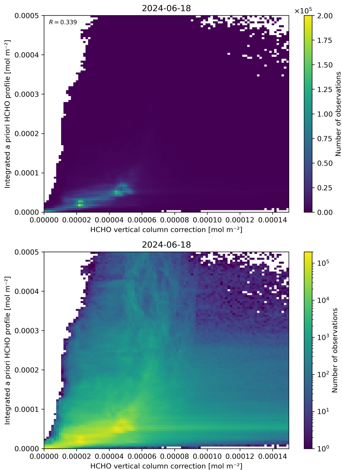
Figure 122: Scatter density plot of “HCHO vertical column correction” against “Integrated a priori HCHO profile” for 2024-06-17 to 2024-06-19.
