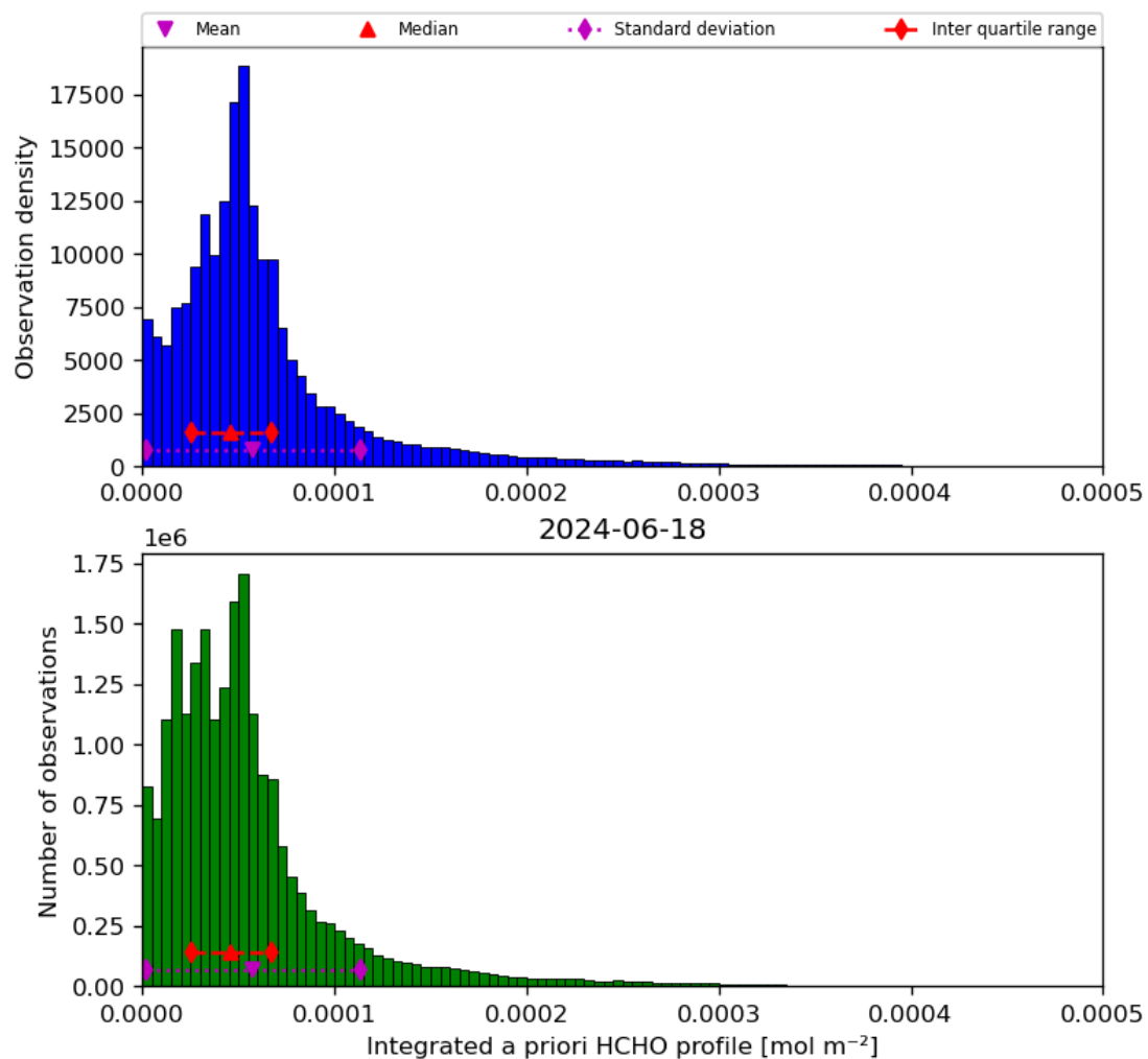
Figure 43: Histogram of “Integrated a priori HCHO profile” for 2024-06-17 to 2024-06-19
