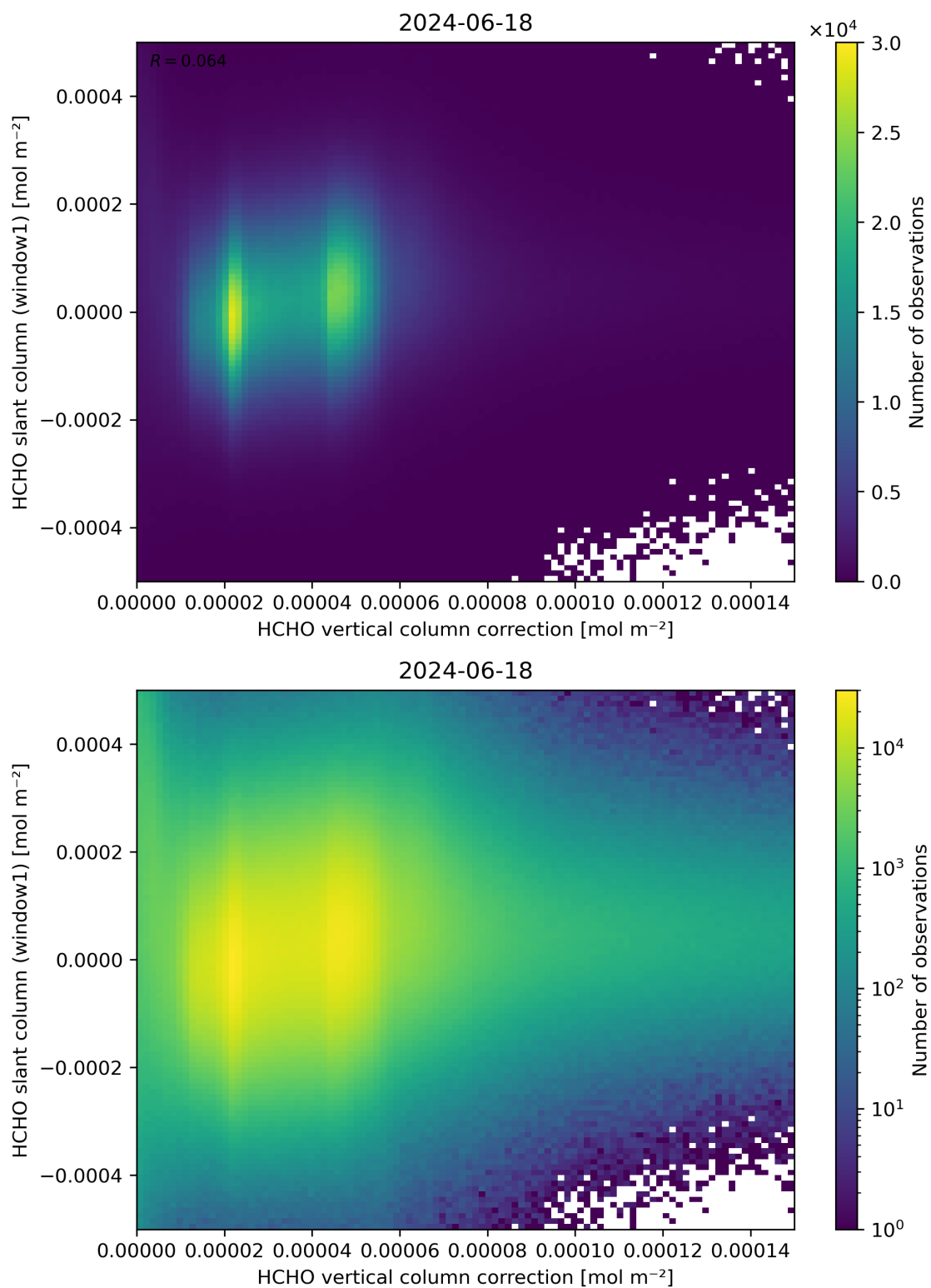
Figure 118: Scatter density plot of “HCHO vertical column correction” against “HCHO slant column (window1)” for 2024-06-17 to 2024-06-19.
