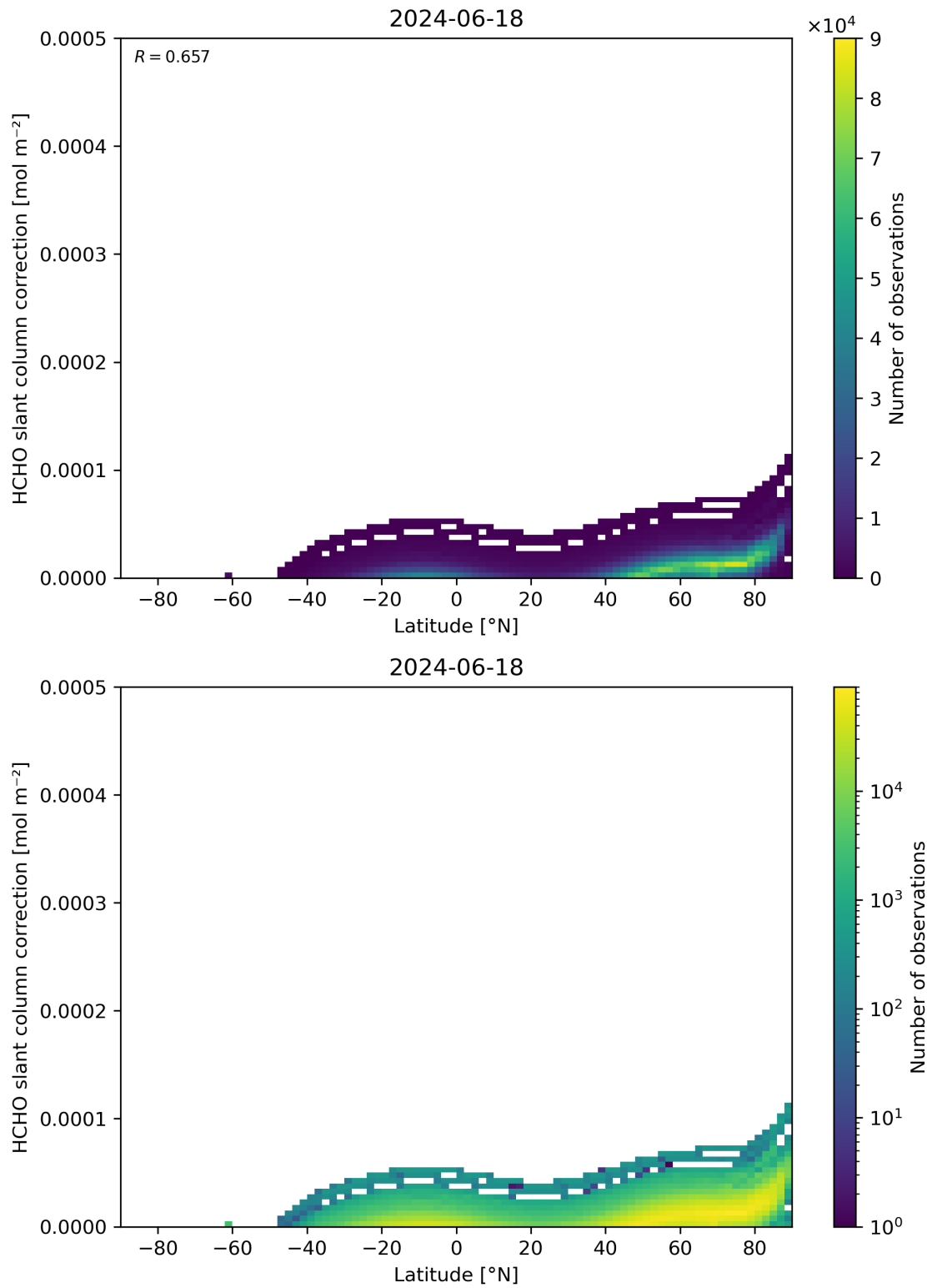
Figure 158: Scatter density plot of “Latitude” against “HCHO slant column correction” for 2024-06-17 to 2024-06-19.
