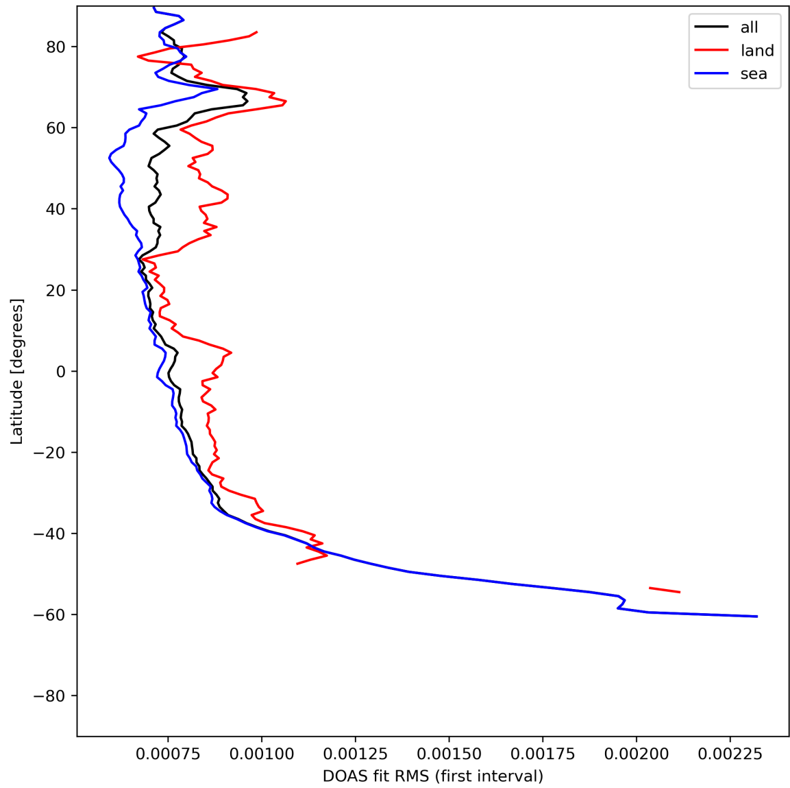
Figure 32: Zonal average of “DOAS fit RMS (first interval)” for 2024-06-17 to 2024-06-19.
