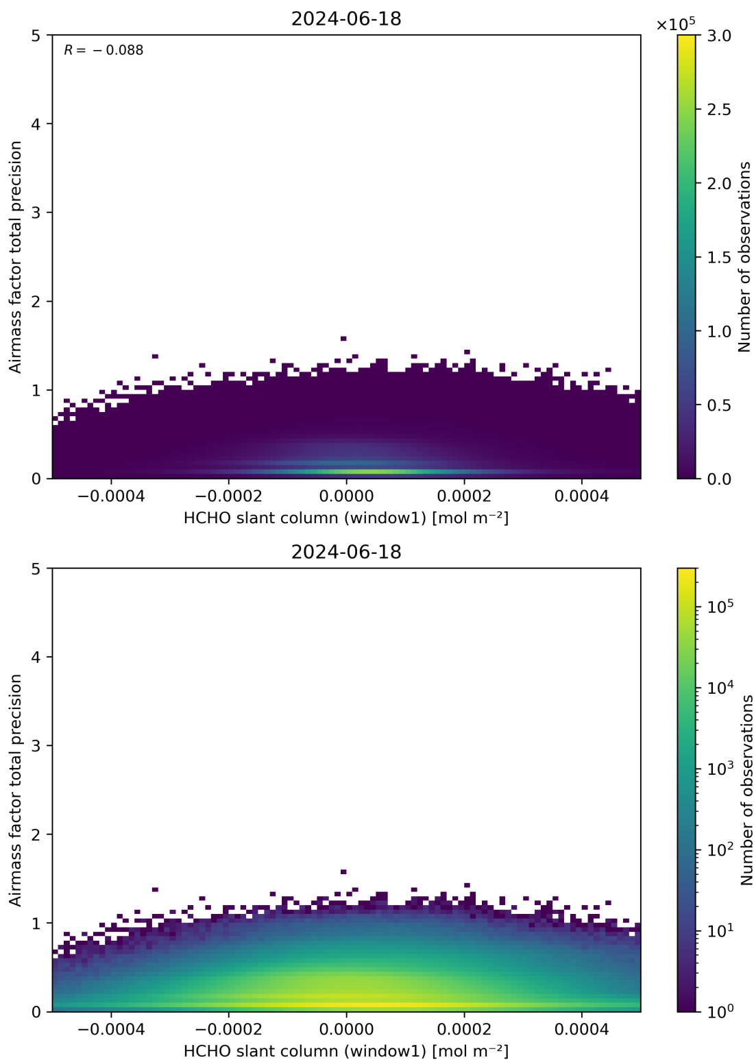
Figure 86: Scatter density plot of “HCHO slant column (window1)” against “Airmass factor total precision” for 2024-06-17 to 2024-06-19.
