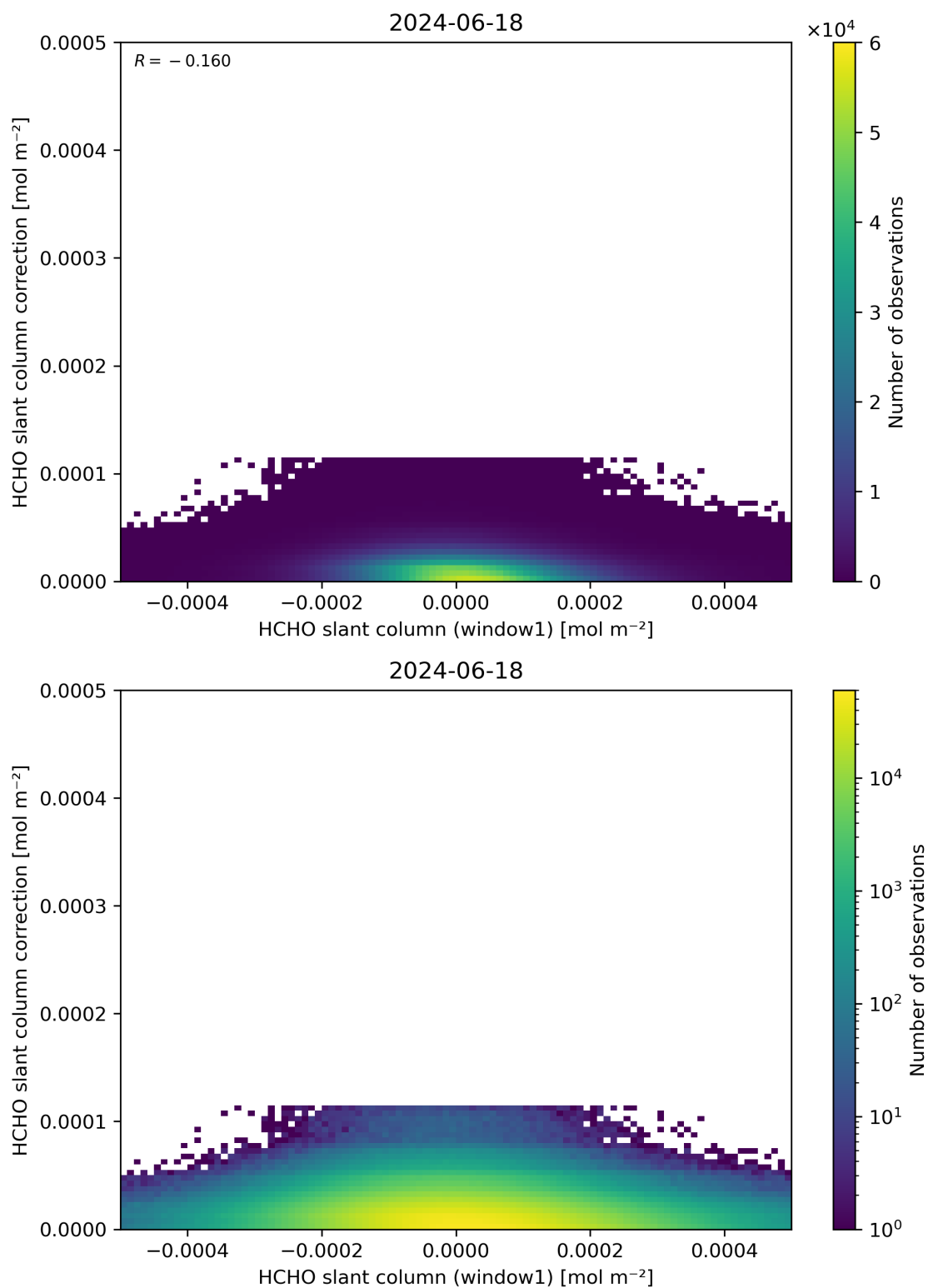
Figure 83: Scatter density plot of “HCHO slant column (window1)” against “HCHO slant column correction” for 2024-06-17 to 2024-06-19.
