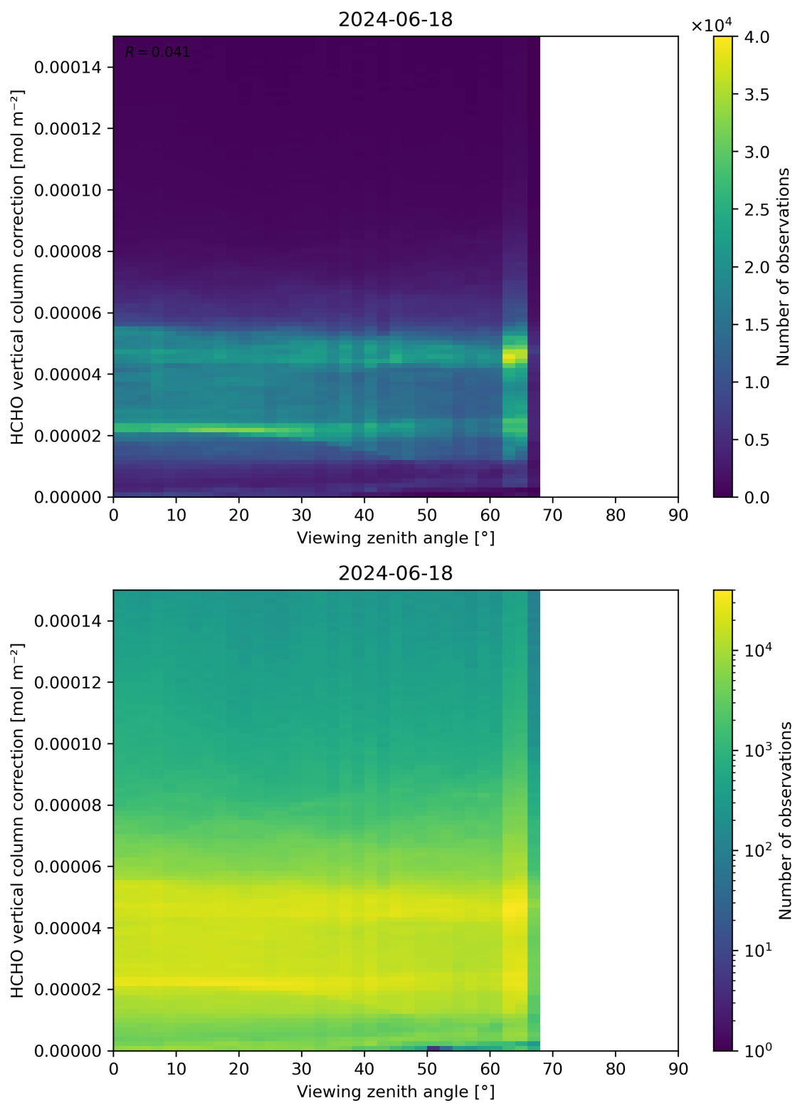
Figure 193: Scatter density plot of “Viewing zenith angle” against “HCHO vertical column correction” for 2024-06-17 to 2024-06-19.
