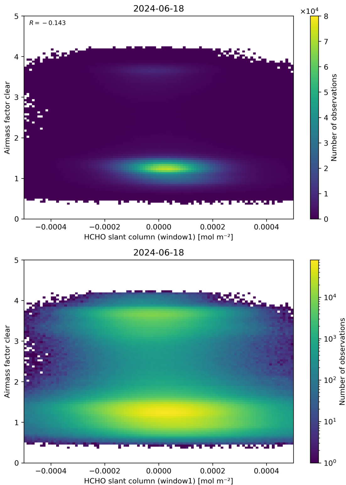
Figure 81: Scatter density plot of “HCHO slant column (window1)” against “Airmass factor clear” for 2024-06-17 to 2024-06-19.
