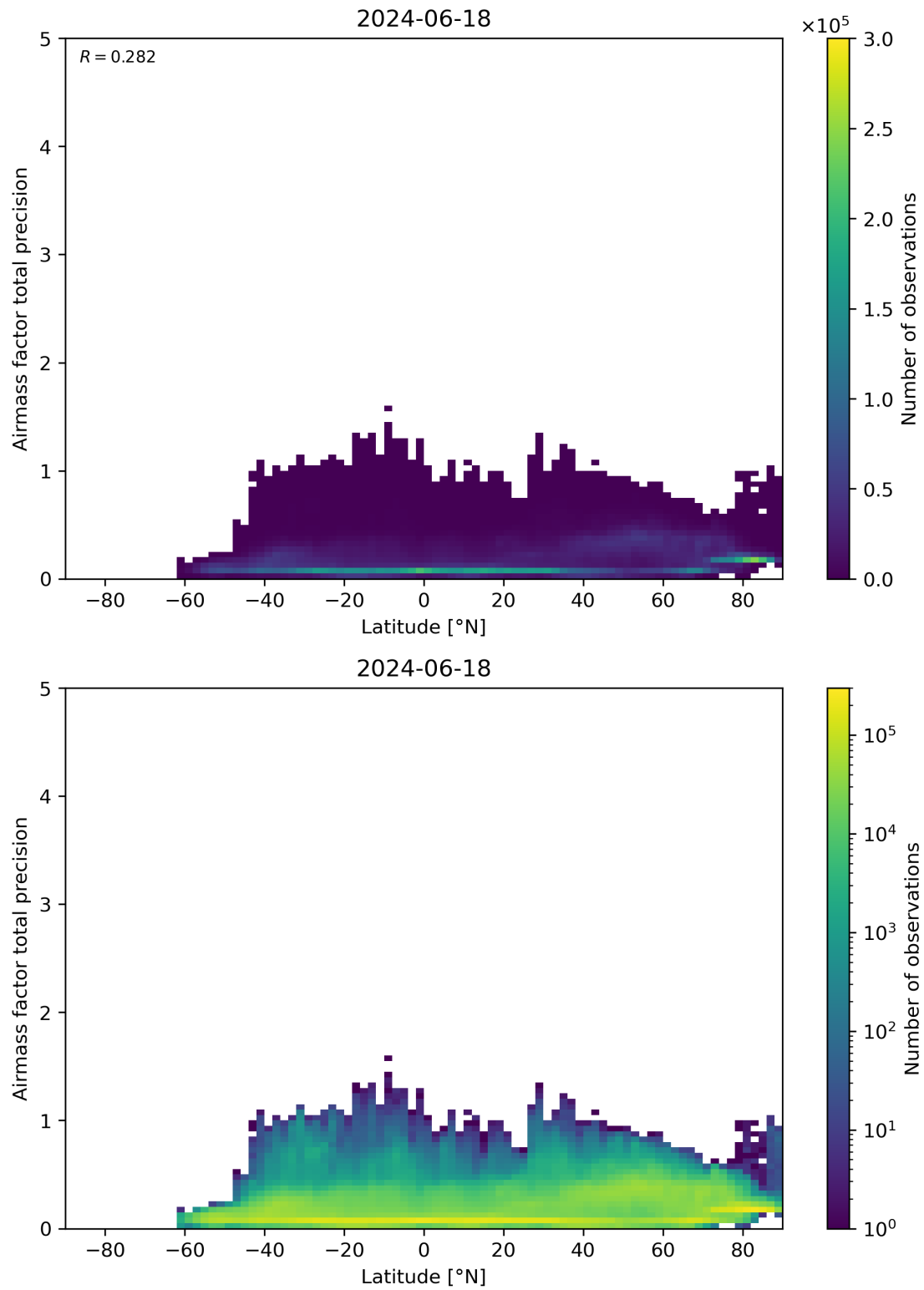
Figure 162: Scatter density plot of “Latitude” against “Airmass factor total precision” for 2024-06-17 to 2024-06-19.
