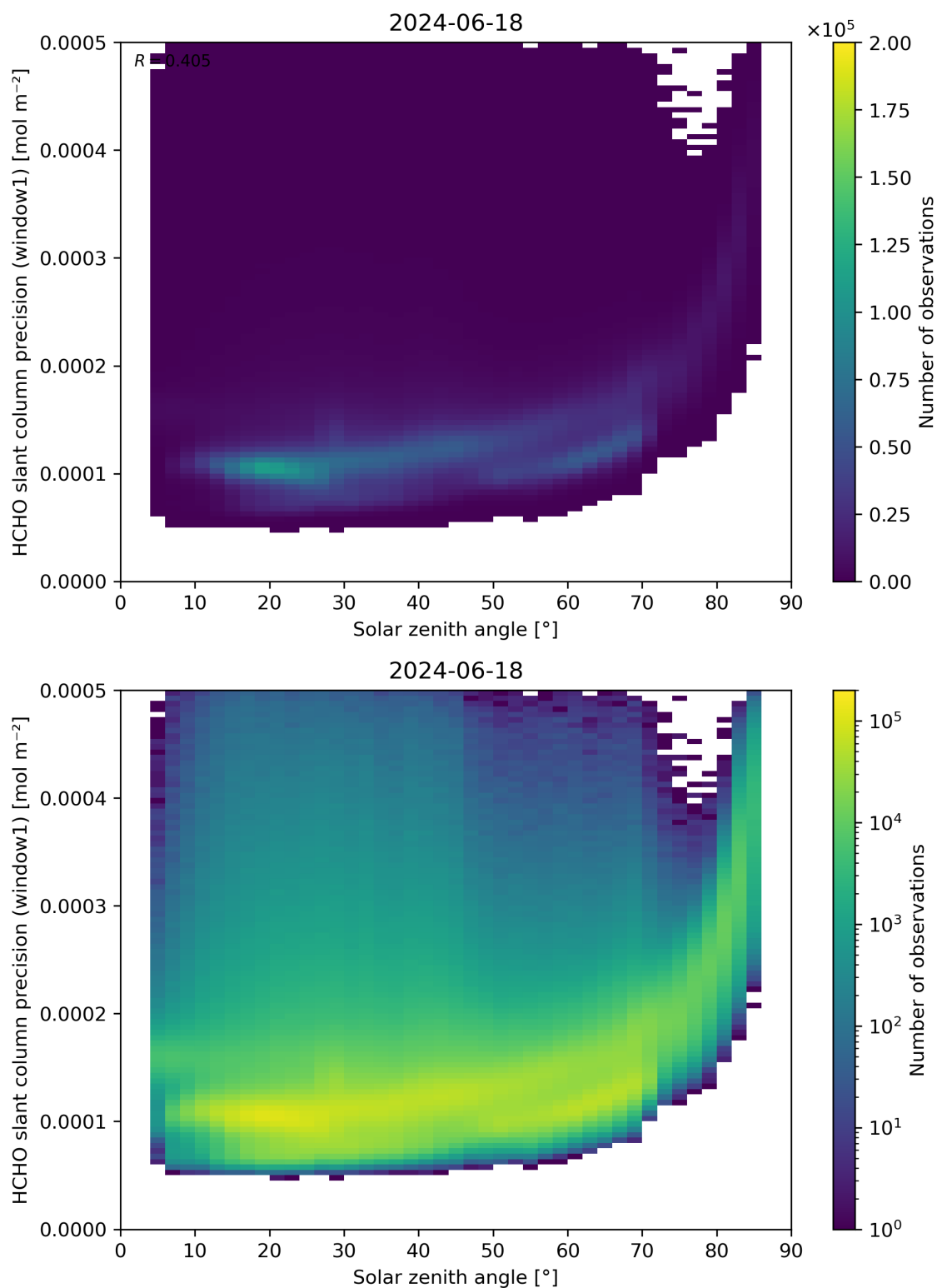
Figure 174: Scatter density plot of “Solar zenith angle” against “HCHO slant column precision (window1)” for 2024-06-17 to 2024-06-19.
