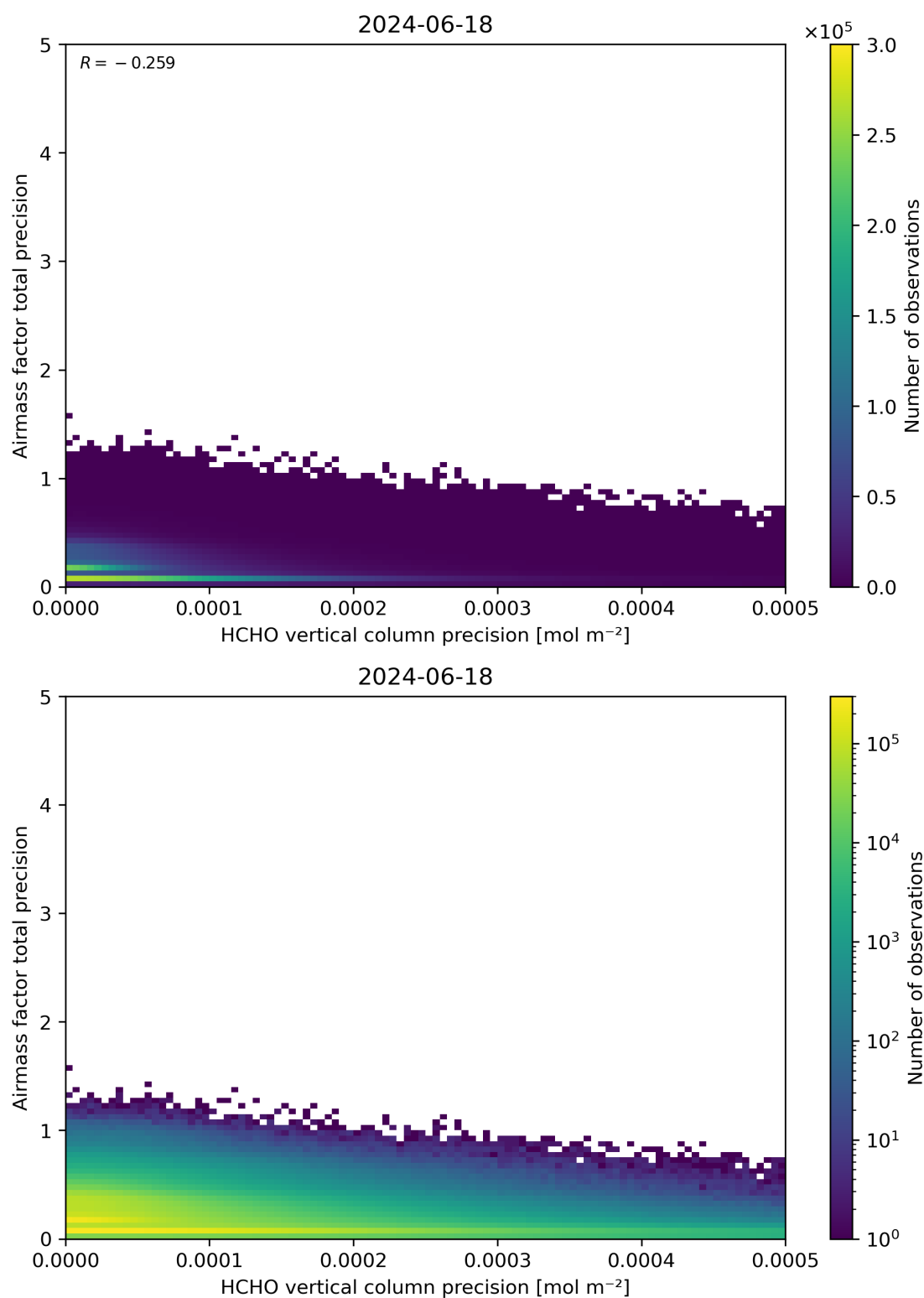
Figure 145: Scatter density plot of “HCHO vertical column precision” against “Airmass factor total precision” for 2024-06-17 to 2024-06-19.
