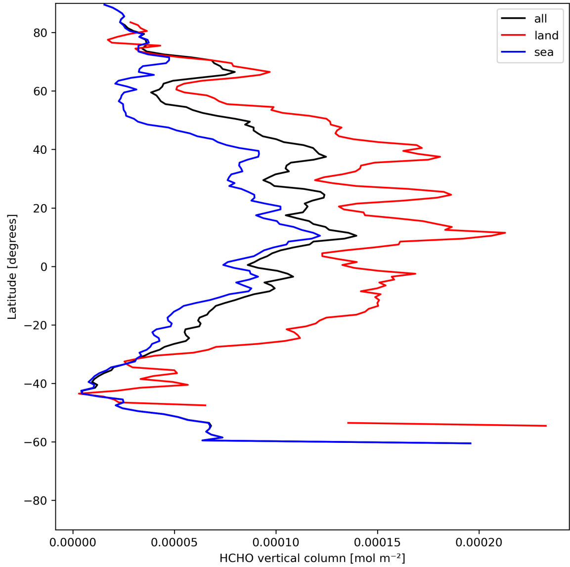
Figure 21: Zonal average of “HCHO vertical column” for 2024-06-17 to 2024-06-19.
