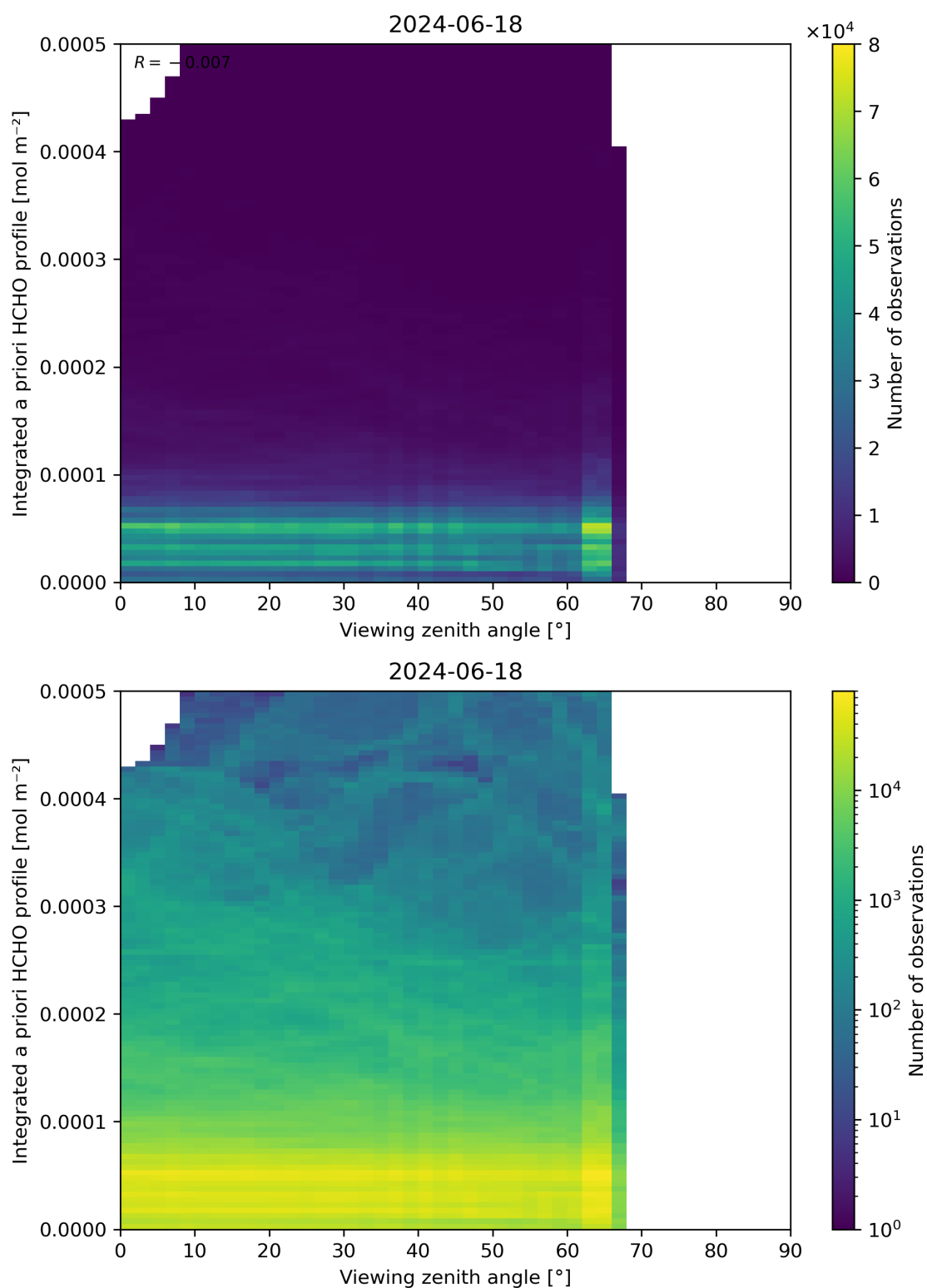
Figure 195: Scatter density plot of “Viewing zenith angle” against “Integrated a priori HCHO profile” for 2024-06-17 to 2024-06-19.
