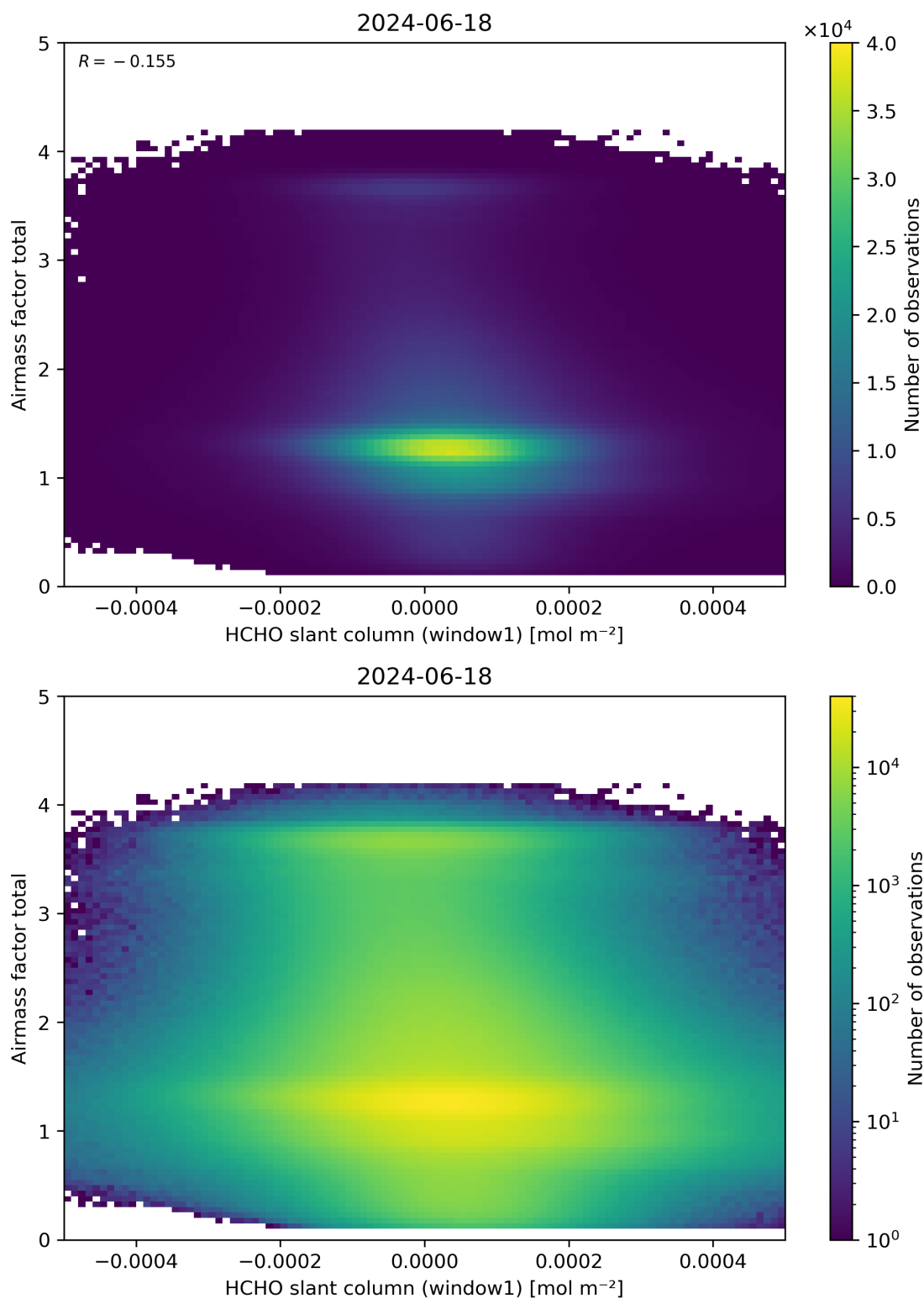
Figure 85: Scatter density plot of “HCHO slant column (window1)” against “Airmass factor total” for 2024-06-17 to 2024-06-19.
