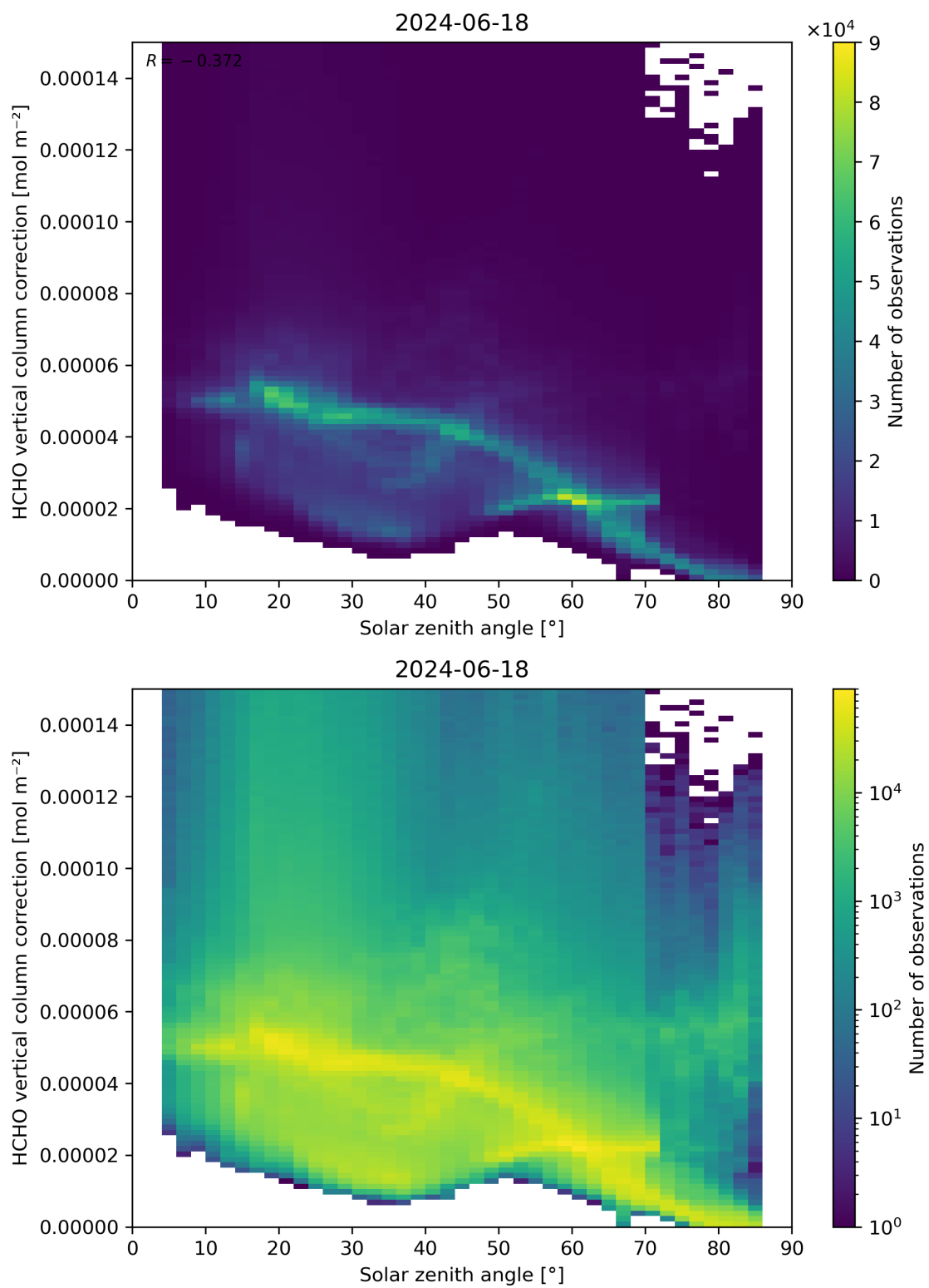
Figure 178: Scatter density plot of “Solar zenith angle” against “HCHO vertical column correction” for 2024-06-17 to 2024-06-19.
