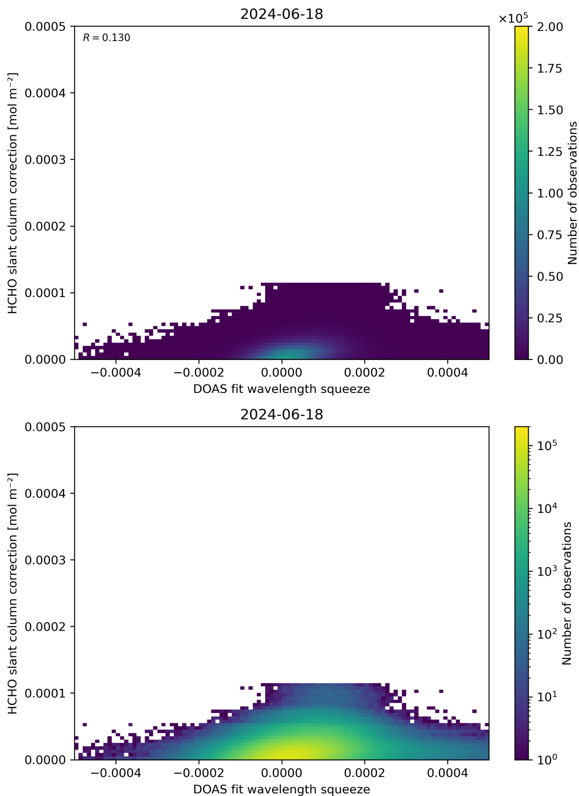
Figure 70: Scatter density plot of “DOAS fit wavelength squeeze” against “HCHO slant column correction” for 2024-06-17 to 2024-06-19.
