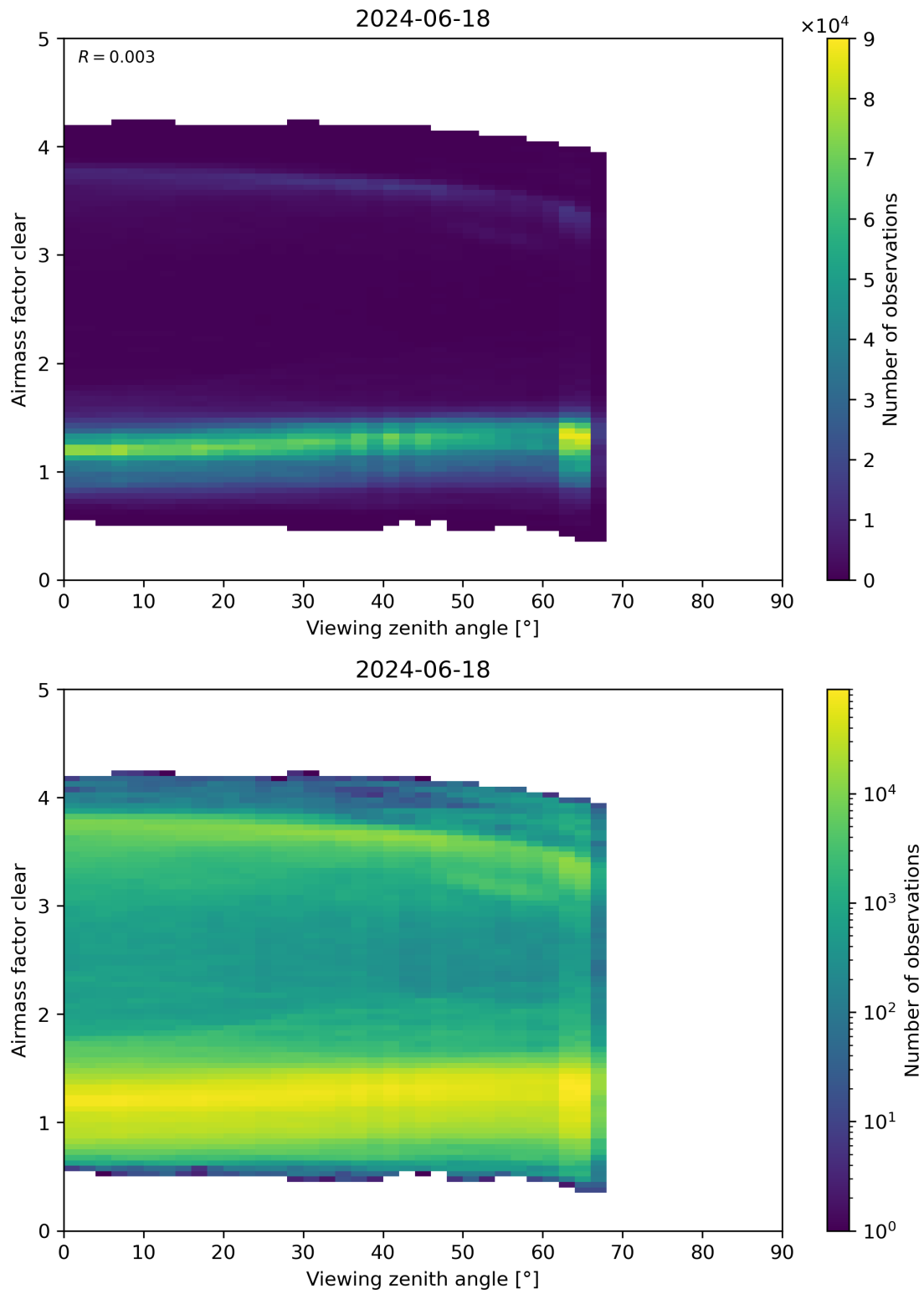
Figure 185: Scatter density plot of “Viewing zenith angle” against “Airmass factor clear” for 2024-06-17 to 2024-06-19.
