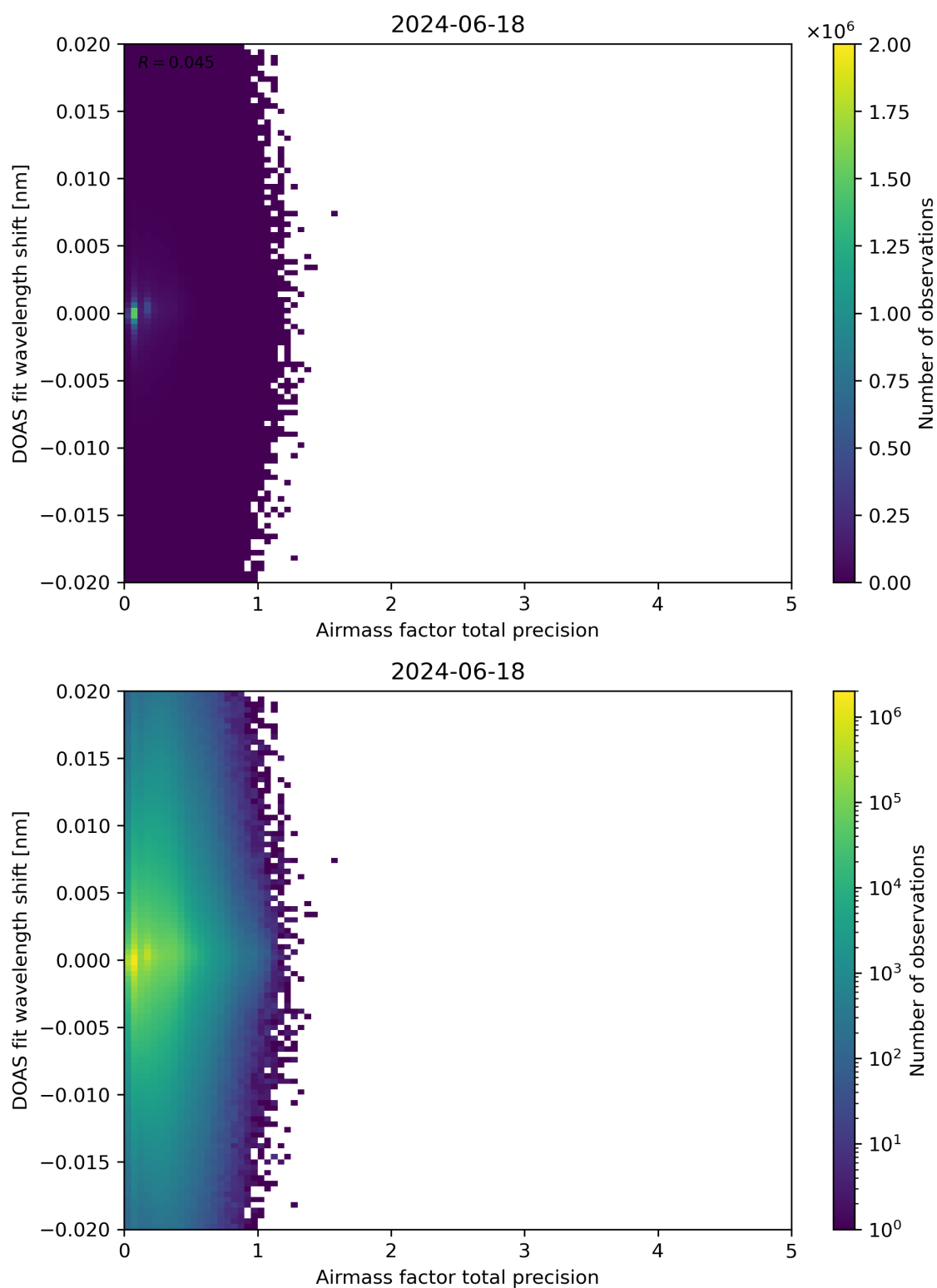
Figure 106: Scatter density plot of “Airmass factor total precision” against “DOAS fit wavelength shift” for 2024-06-17 to 2024-06-19.
