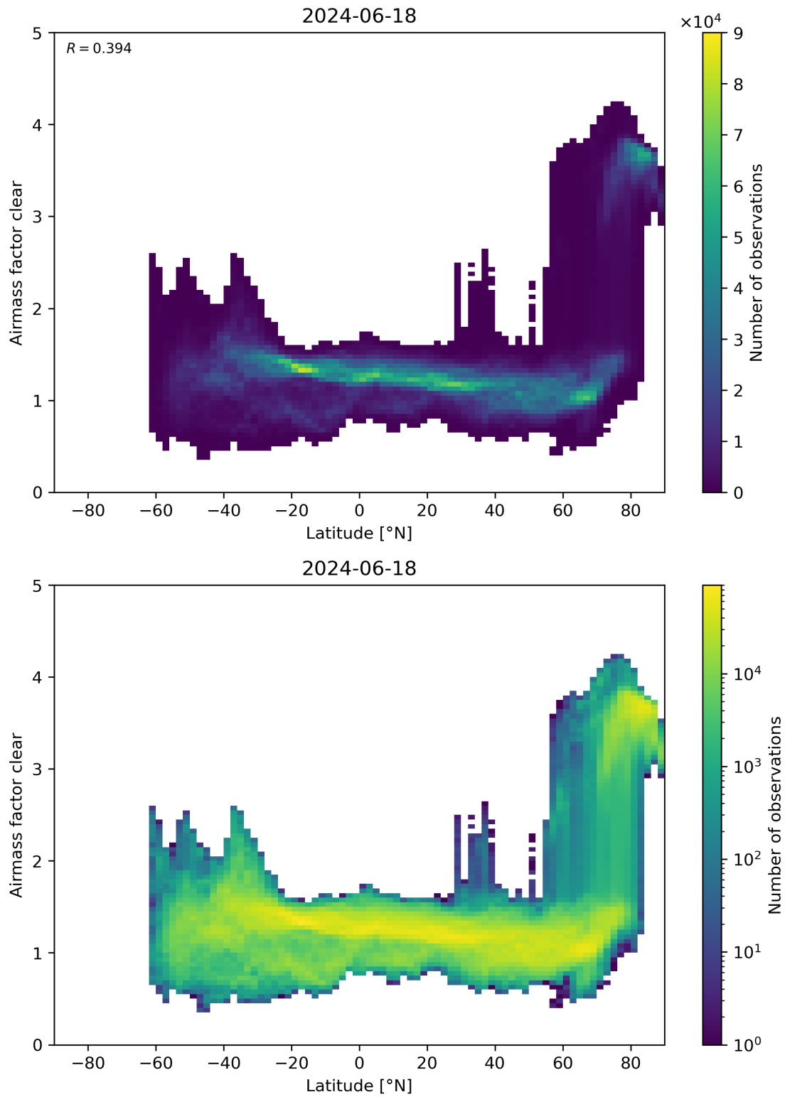
Figure 156: Scatter density plot of “Latitude” against “Airmass factor clear” for 2024-06-17 to 2024-06-19.
