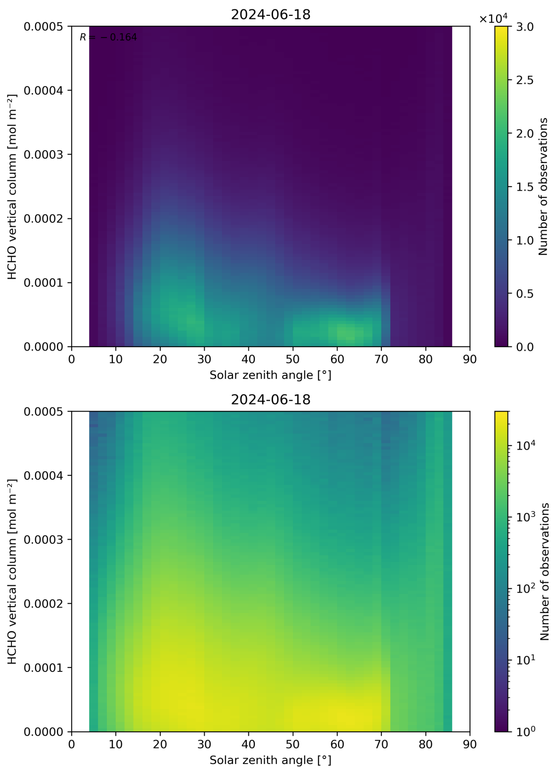
Figure 177: Scatter density plot of “Solar zenith angle” against “HCHO vertical column” for 2024-06-17 to 2024-06-19.
