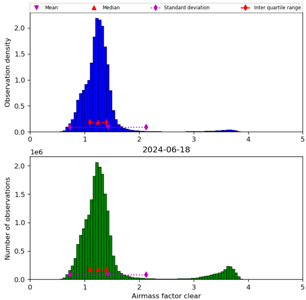
Figure 42: Histogram of “Airmass factor clear” for 2024-06-17 to 2024-06-19
