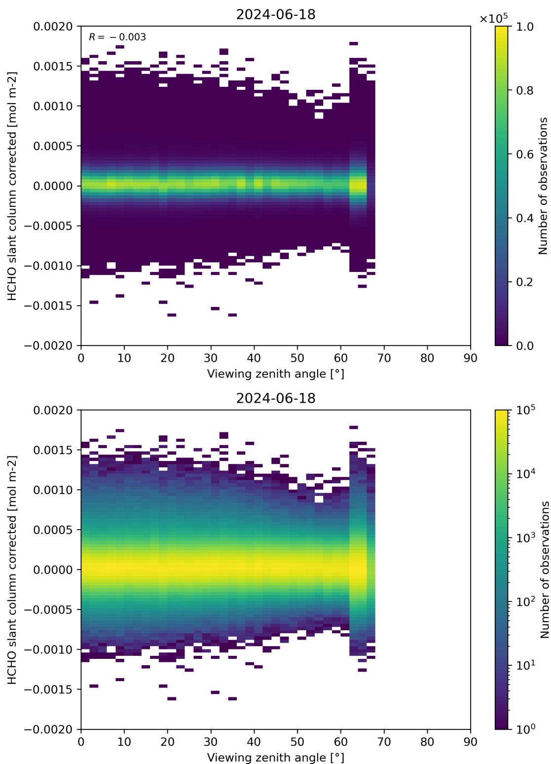
Figure 186: Scatter density plot of “Viewing zenith angle” against “HCHO slant column corrected” for 2024-06-17 to 2024-06-19.
