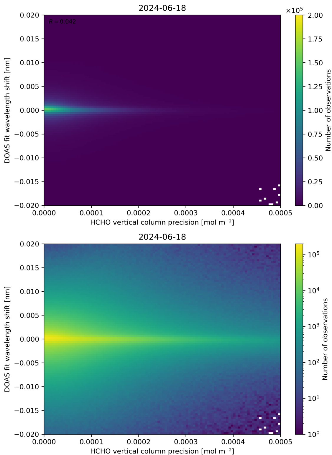
Figure 137: Scatter density plot of “HCHO vertical column precision” against “DOAS fit wavelength shift” for 2024-06-17 to 2024-06-19.
