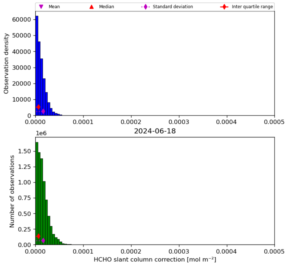
Figure 47: Histogram of “HCHO slant column correction” for 2024-06-17 to 2024-06-19
