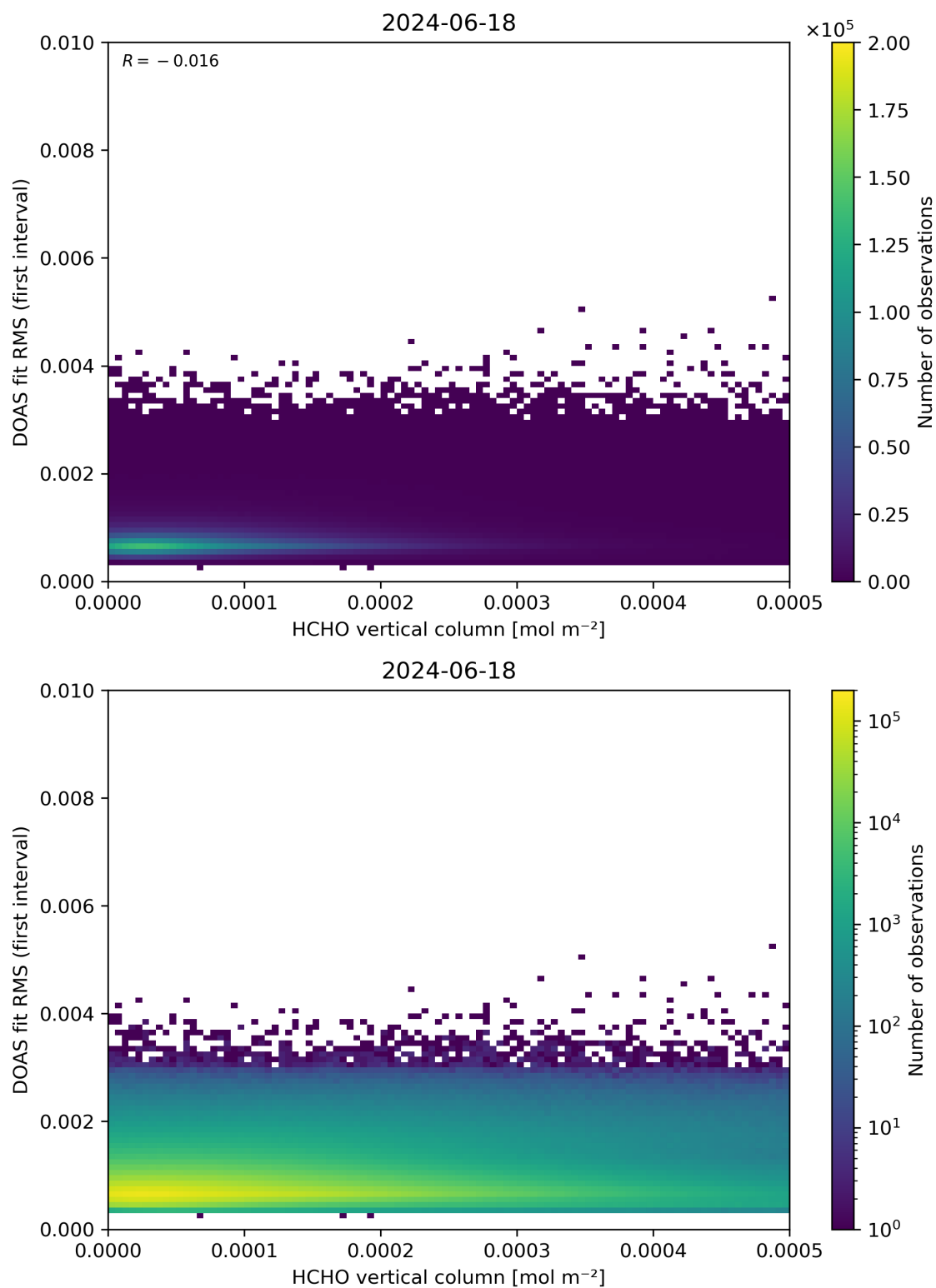
Figure 123: Scatter density plot of “HCHO vertical column” against “DOAS fit RMS (first interval)” for 2024-06-17 to 2024-06-19.
