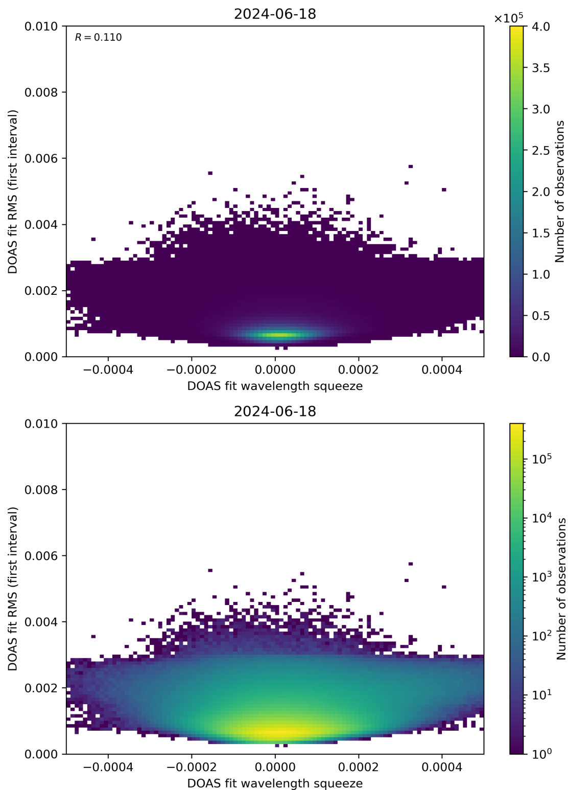
Figure 68: Scatter density plot of “DOAS fit wavelength squeeze” against “DOAS fit RMS (first interval)” for 2024-06-17 to 2024-06-19.
