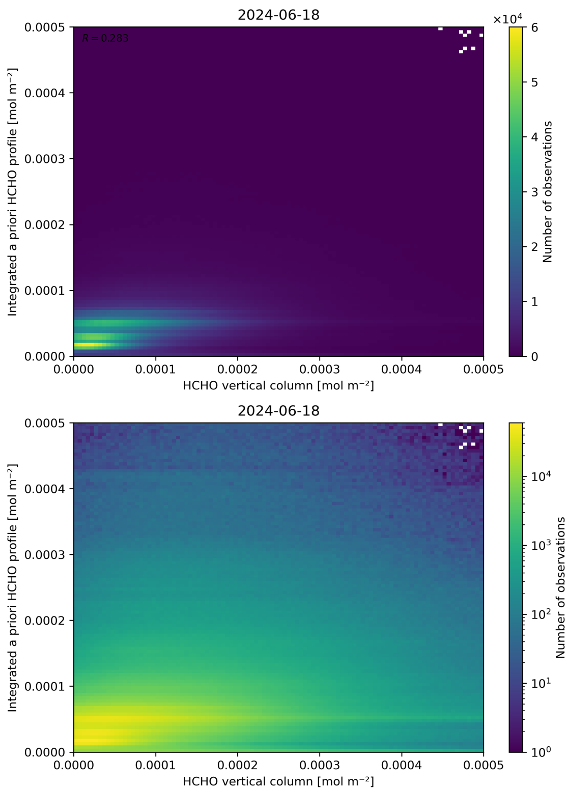
Figure 135: Scatter density plot of “HCHO vertical column” against “Integrated a priori HCHO profile” for 2024-06-17 to 2024-06-19.
