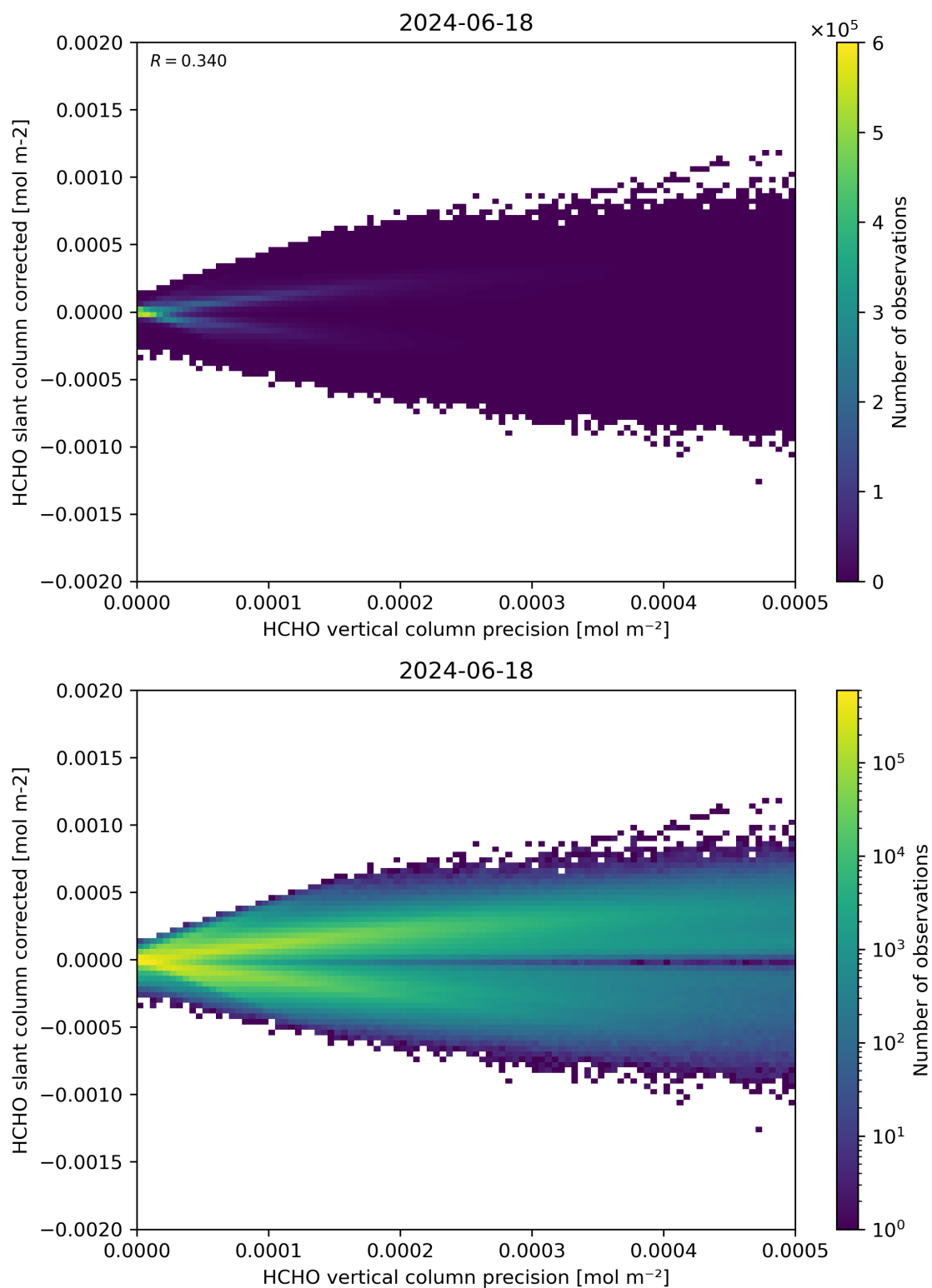
Figure 140: Scatter density plot of “HCHO vertical column precision” against “HCHO slant column corrected” for 2024-06-17 to 2024-06-19.
