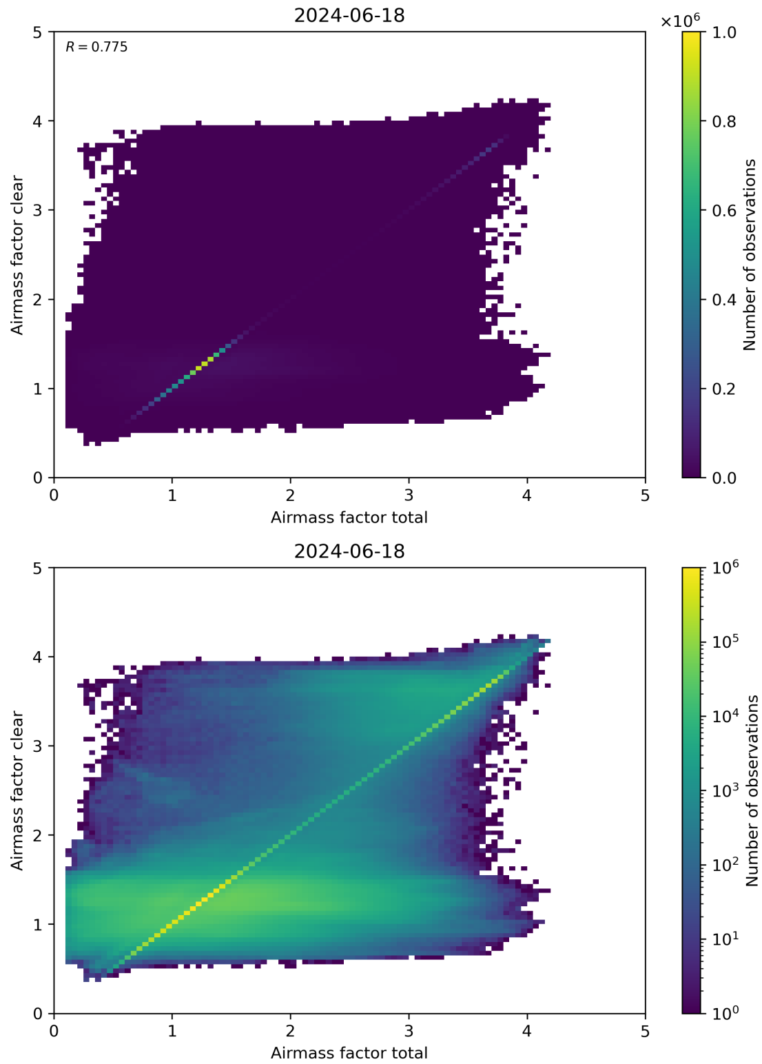
Figure 100: Scatter density plot of “Airmass factor total” against “Airmass factor clear” for 2024-06-17 to 2024-06-19.
