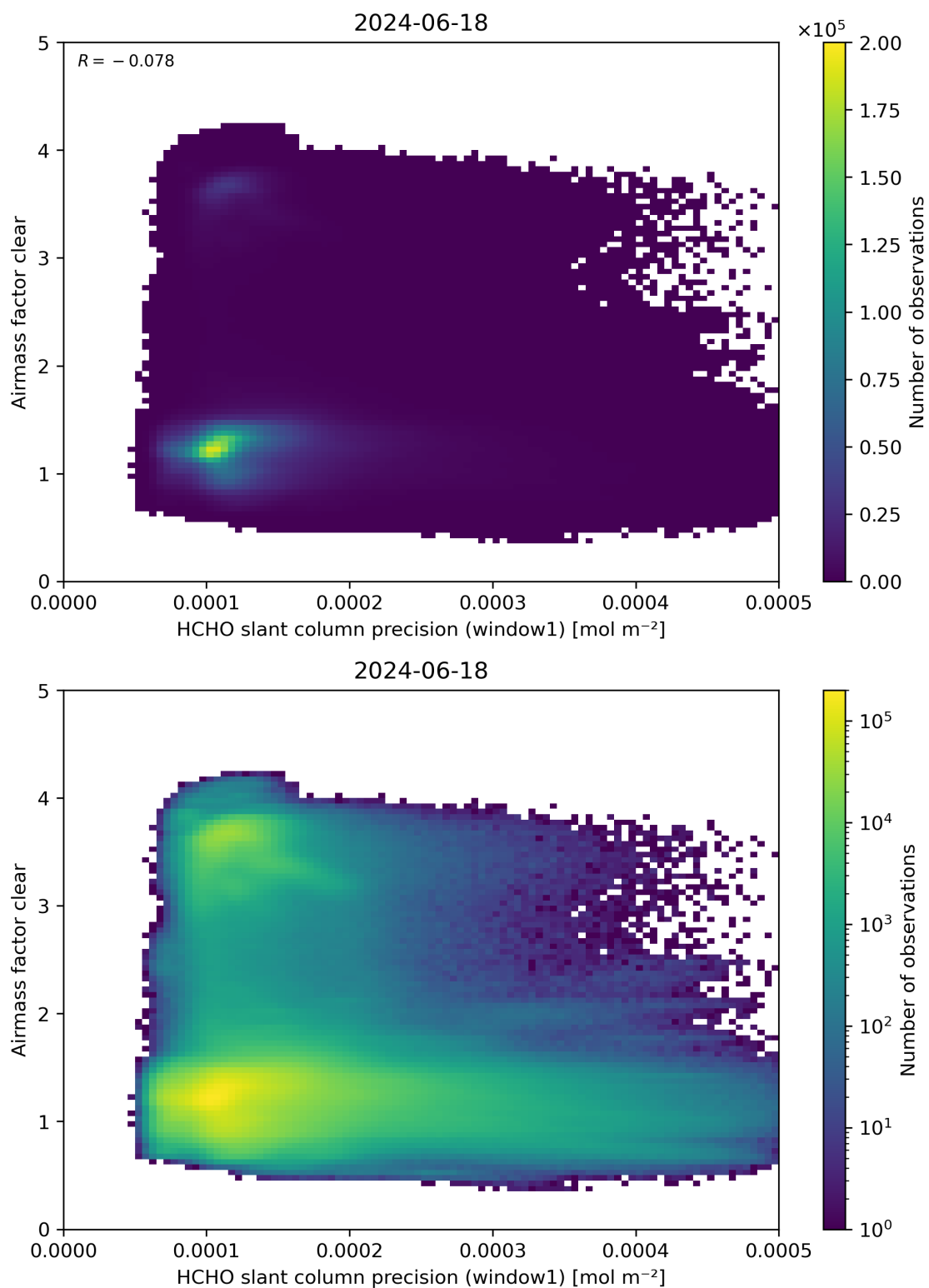
Figure 91: Scatter density plot of “HCHO slant column precision (window1)” against “Airmass factor clear” for 2024-06-17 to 2024-06-19.
