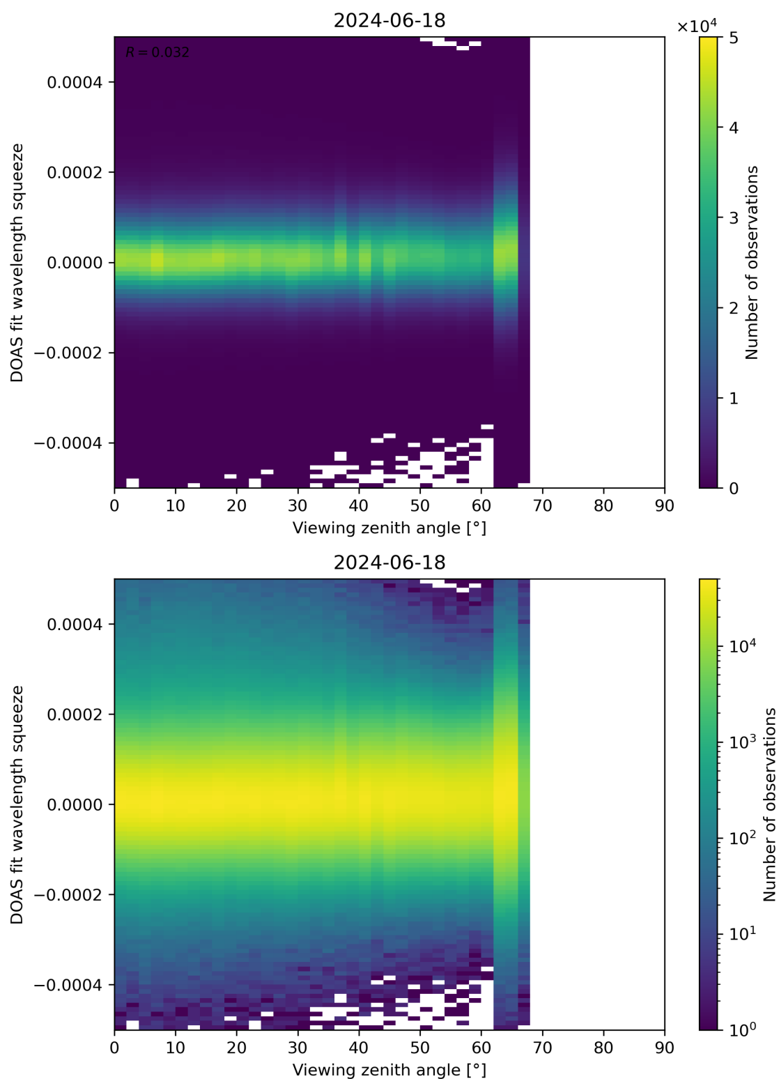
Figure 184: Scatter density plot of “Viewing zenith angle” against “DOAS fit wavelength squeeze” for 2024-06-17 to 2024-06-19.
