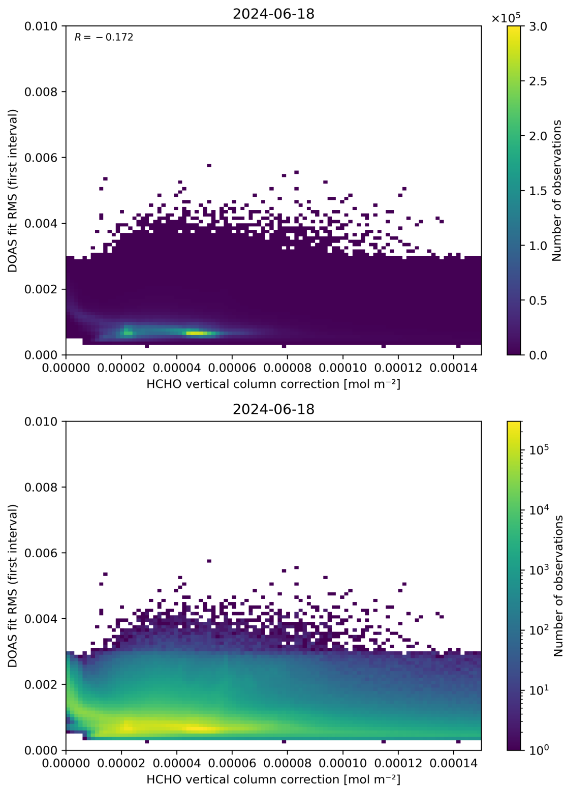
Figure 112: Scatter density plot of “HCHO vertical column correction” against “DOAS fit RMS (first interval)” for 2024-06-17 to 2024-06-19.
