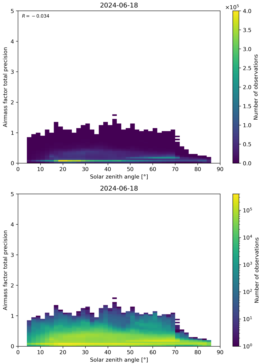
Figure 176: Scatter density plot of “Solar zenith angle” against “Airmass factor total precision” for 2024-06-17 to 2024-06-19.
