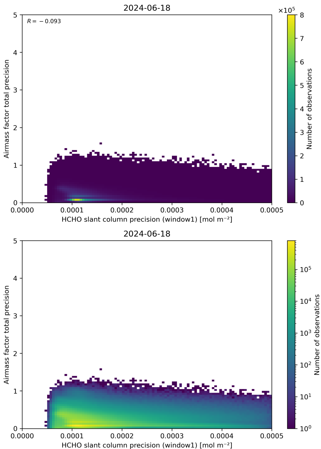
Figure 95: Scatter density plot of “HCHO slant column precision (window1)” against “Airmass factor total precision” for 2024-06-17 to 2024-06-19.
