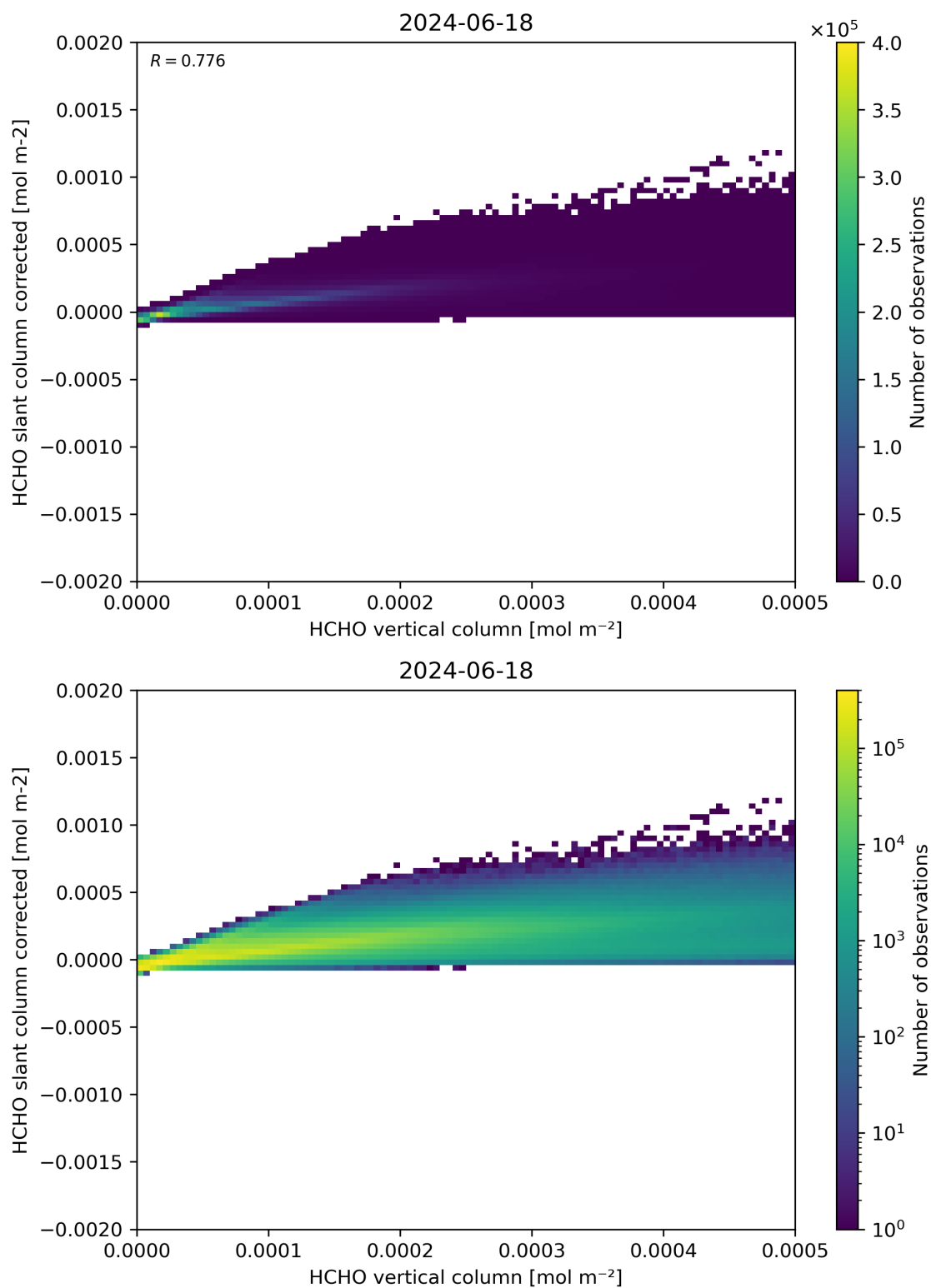
Figure 127: Scatter density plot of “HCHO vertical column” against “HCHO slant column corrected” for 2024-06-17 to 2024-06-19.
