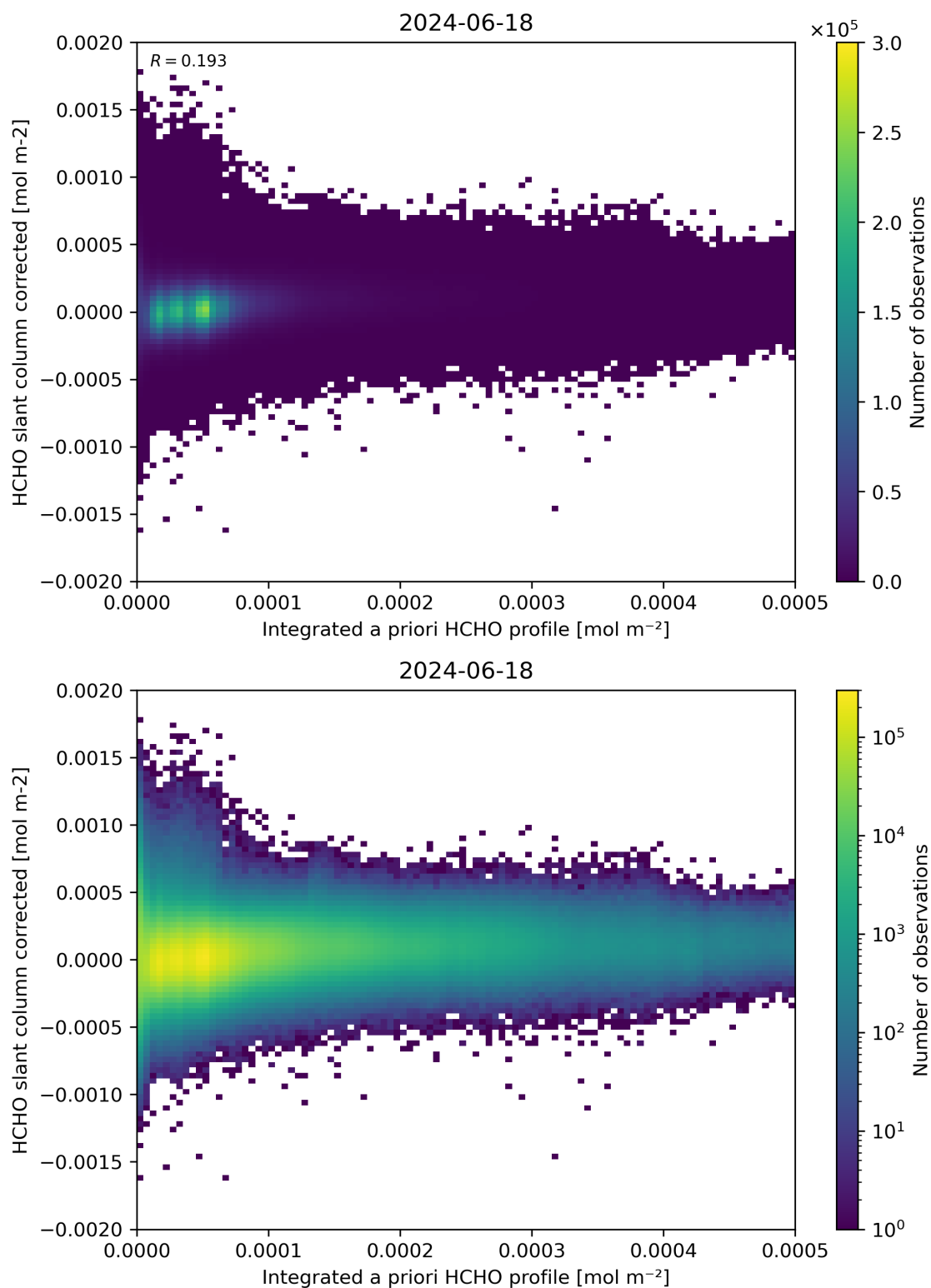
Figure 151: Scatter density plot of “Integrated a priori HCHO profile” against “HCHO slant column corrected” for 2024-06-17 to 2024-06-19.
