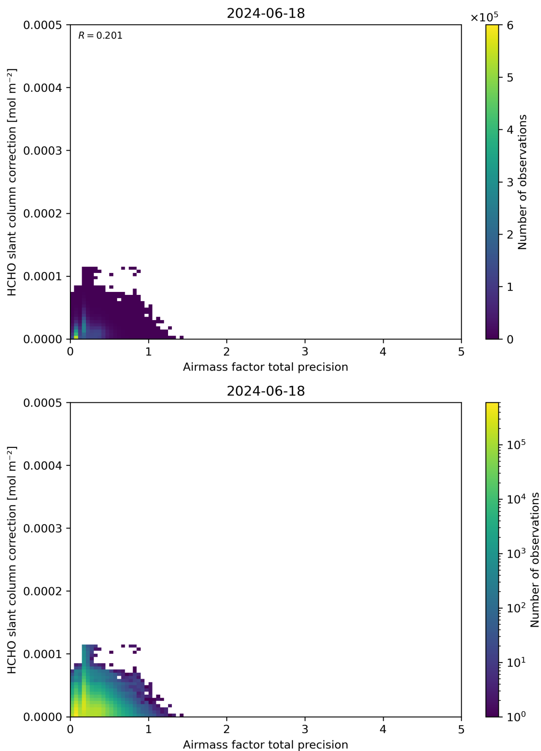
Figure 110: Scatter density plot of “Airmass factor total precision” against “HCHO slant column correction” for 2024-06-17 to 2024-06-19.
