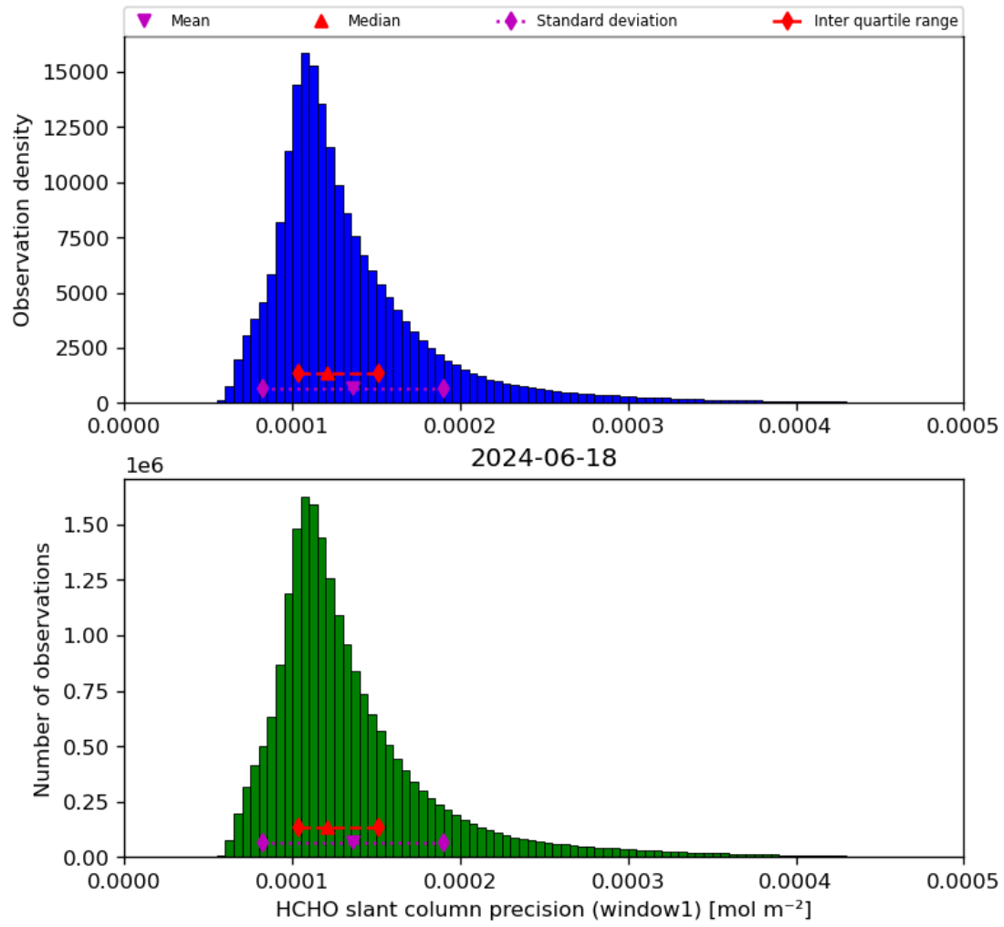
Figure 39: Histogram of “HCHO slant column precision (window1)” for 2024-06-17 to 2024-06-19
