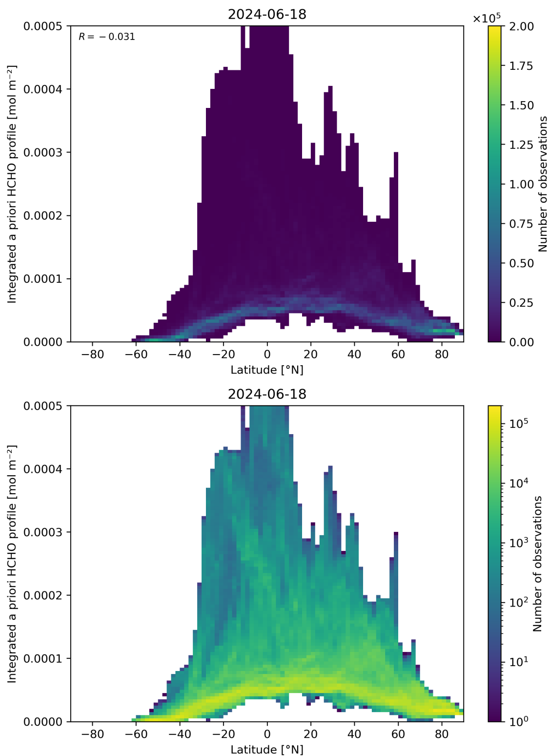
Figure 166: Scatter density plot of “Latitude” against “Integrated a priori HCHO profile” for 2024-06-17 to 2024-06-19.
