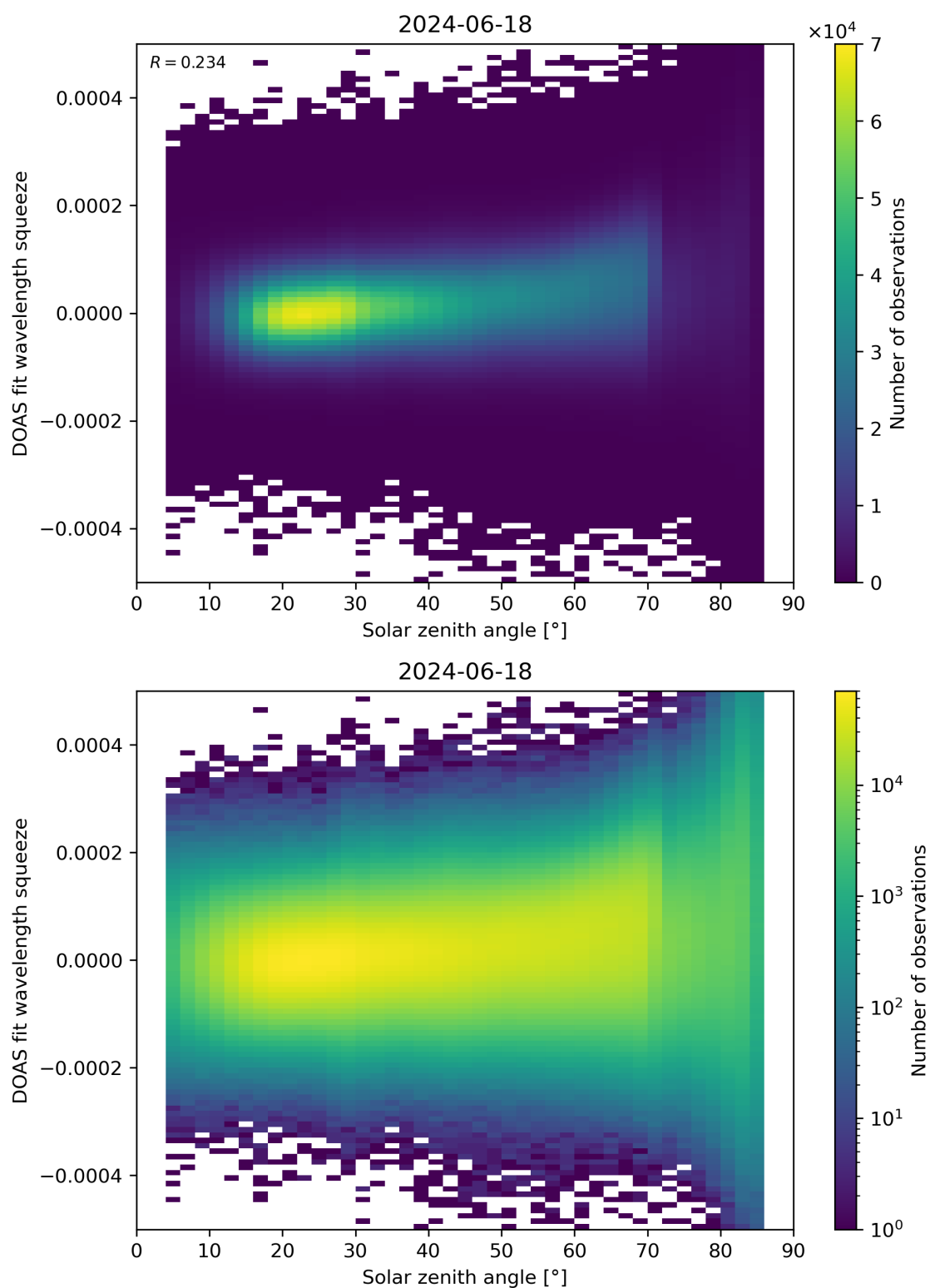
Figure 169: Scatter density plot of “Solar zenith angle” against “DOAS fit wavelength squeeze” for 2024-06-17 to 2024-06-19.
