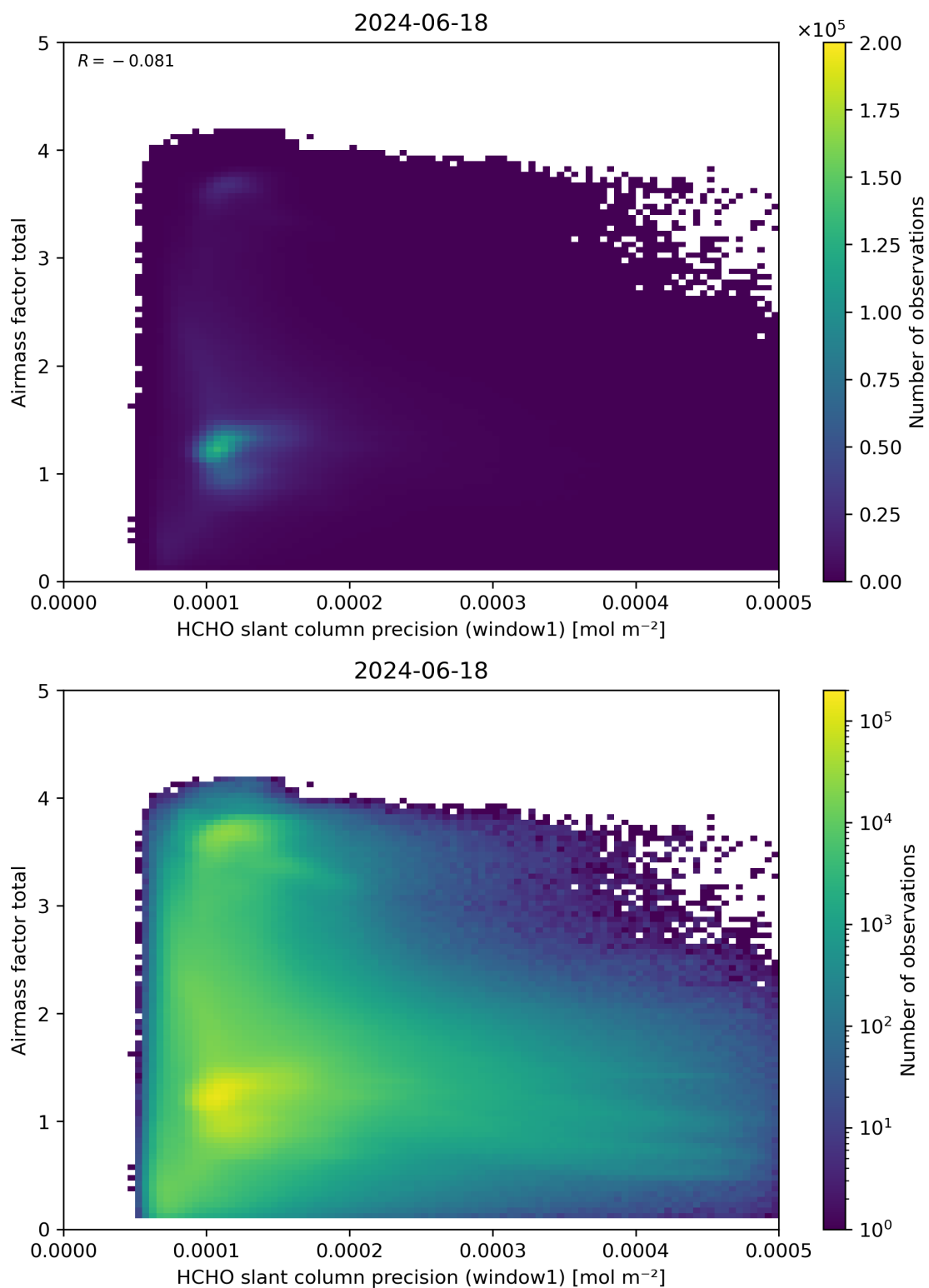
Figure 94: Scatter density plot of “HCHO slant column precision (window1)” against “Airmass factor total” for 2024-06-17 to 2024-06-19.
