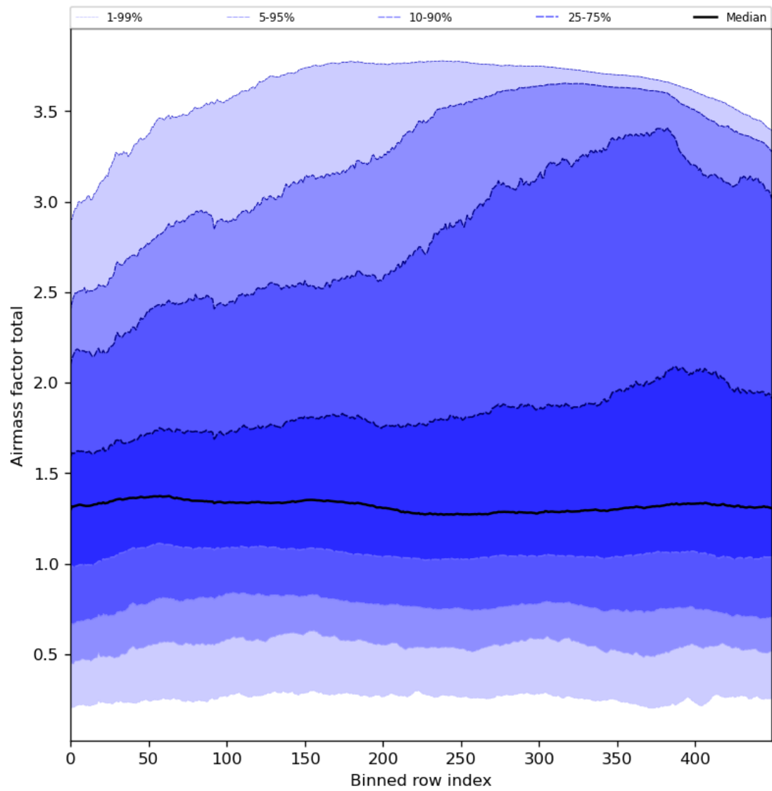
Figure 54: Along track statistics of “Airmass factor total” for 2024-06-17 to 2024-06-19
