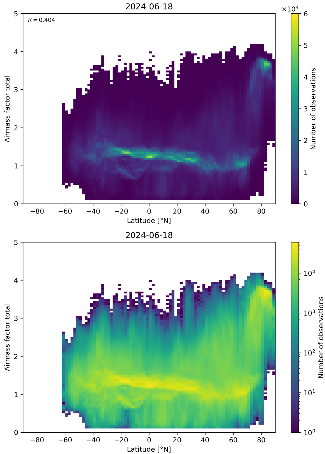
Figure 161: Scatter density plot of “Latitude” against “Airmass factor total” for 2024-06-17 to 2024-06-19.
