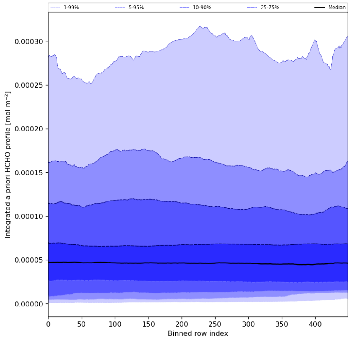
Figure 57: Along track statistics of "Integrated a priori HCHO profile" for 2024-06-17 to 2024-06-19
