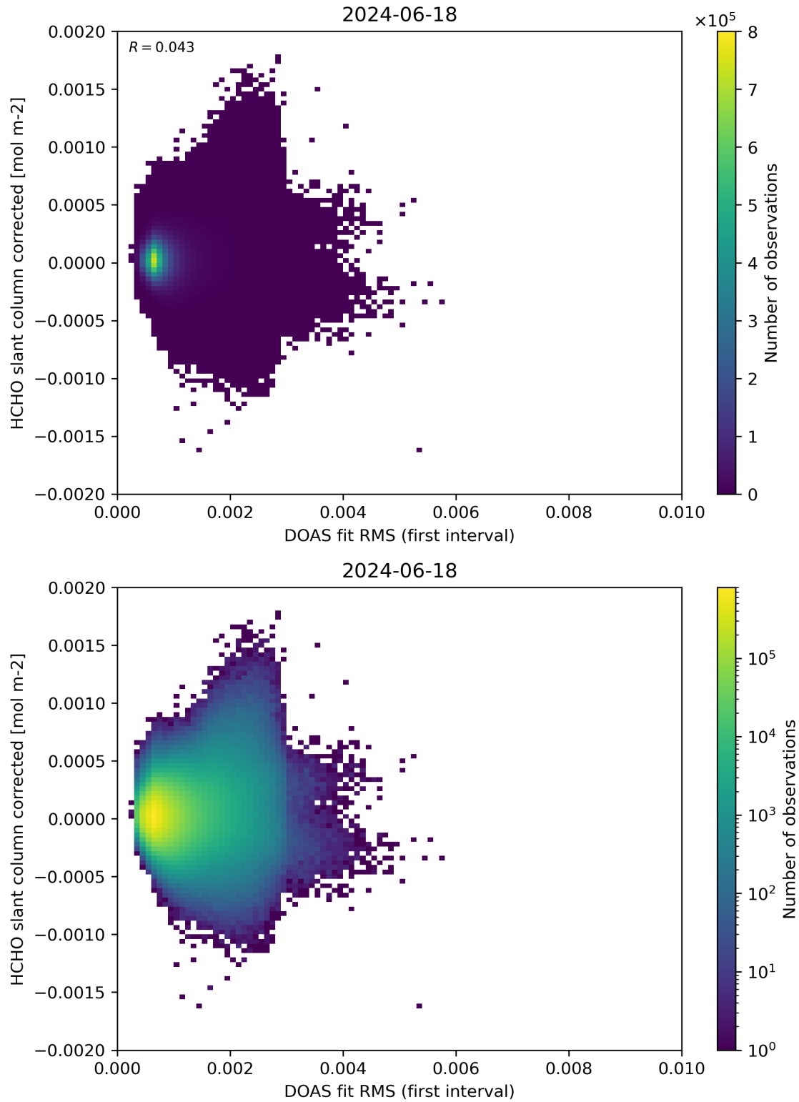
Figure 62: Scatter density plot of “DOAS fit RMS (first interval)” against “HCHO slant column corrected” for 2024-06-17 to 2024-06-19.
