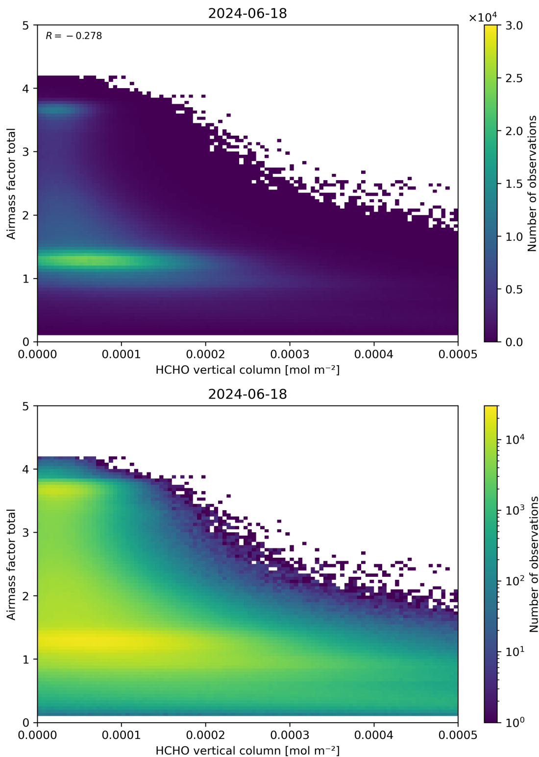
Figure 131: Scatter density plot of “HCHO vertical column” against “Airmass factor total” for 2024-06-17 to 2024-06-19.
