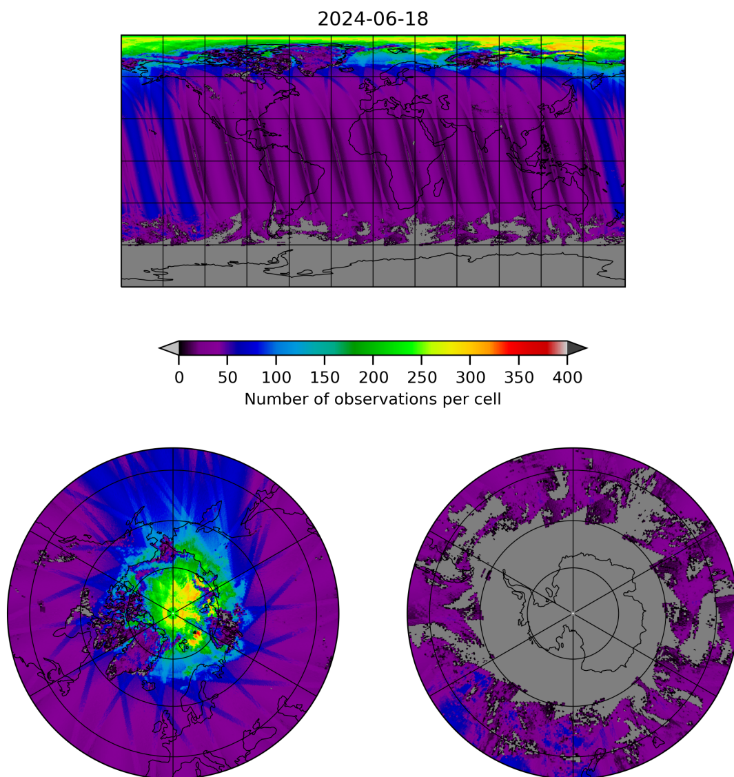
Figure 19: Map of the number of observations for 2024-06-17 to 2024-06-19
