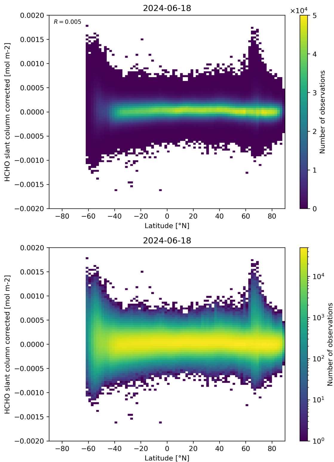
Figure 157: Scatter density plot of “Latitude” against “HCHO slant column corrected” for 2024-06-17 to 2024-06-19.
