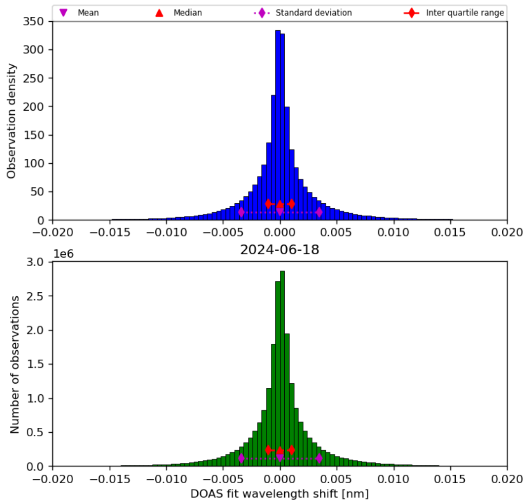
Figure 44: Histogram of “DOAS fit wavelength shift” for 2024-06-17 to 2024-06-19
