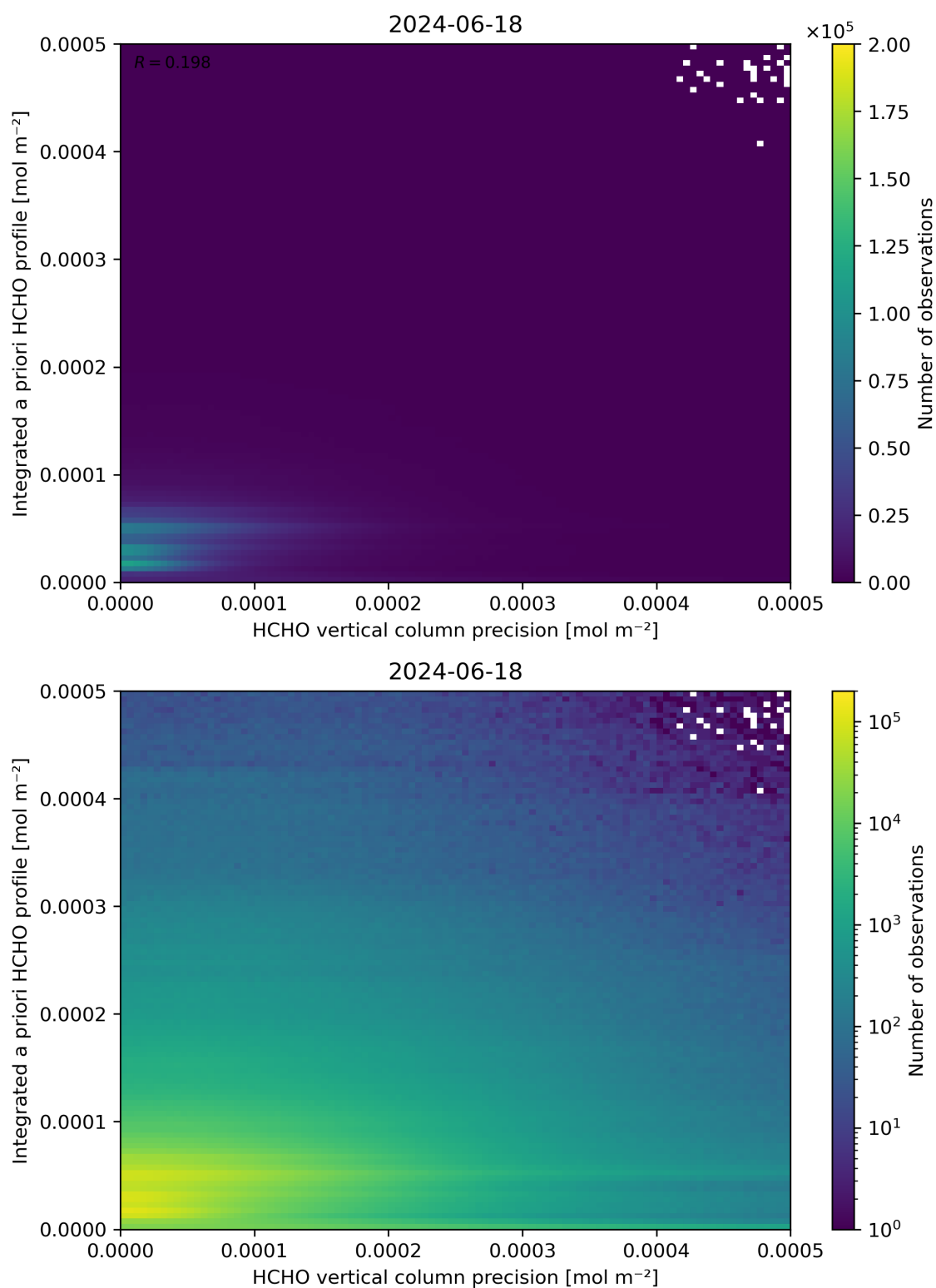
Figure 147: Scatter density plot of “HCHO vertical column precision” against “Integrated a priori HCHO profile” for 2024-06-17 to 2024-06-19.
