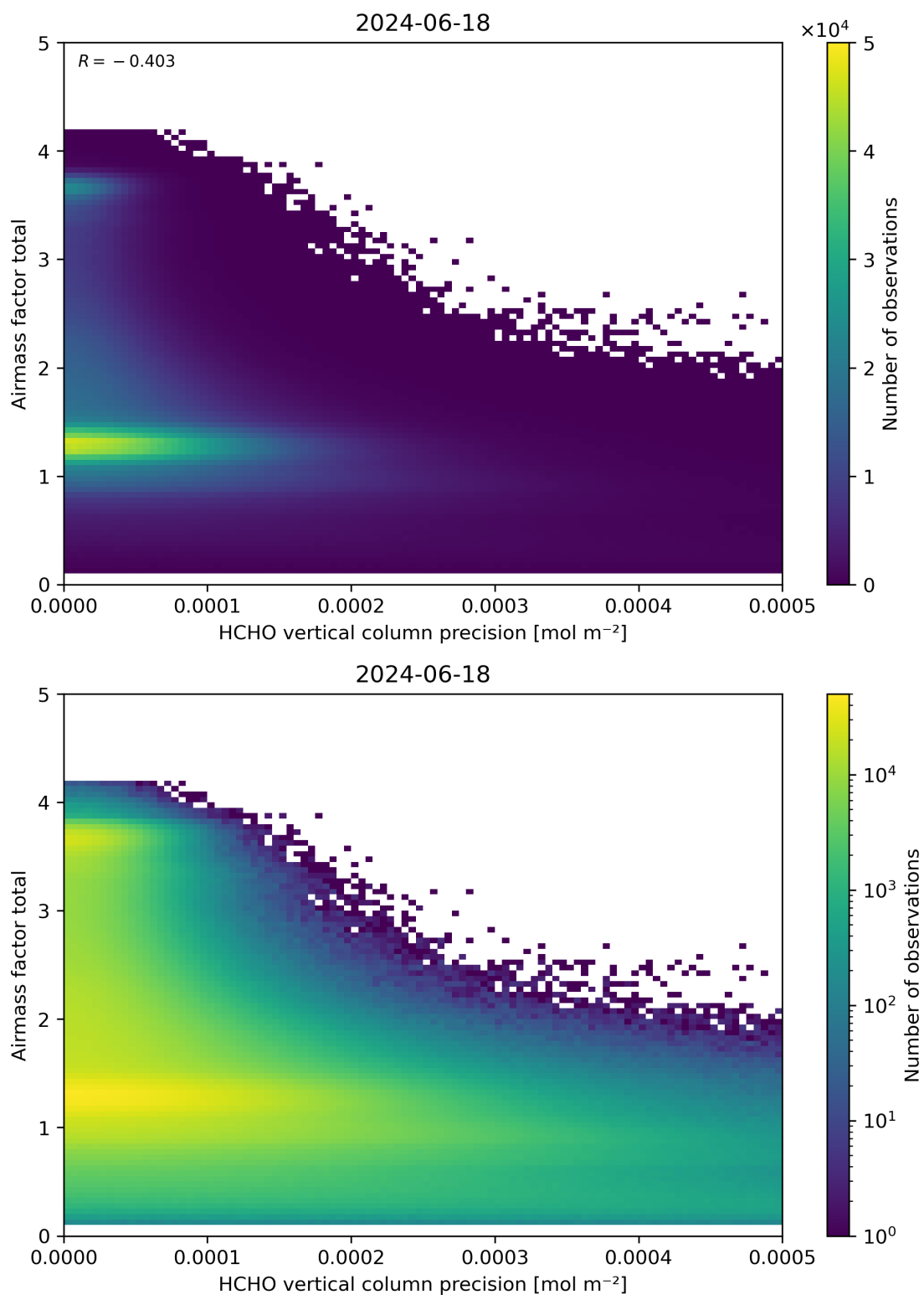
Figure 144: Scatter density plot of “HCHO vertical column precision” against “Airmass factor total” for 2024-06-17 to 2024-06-19.
