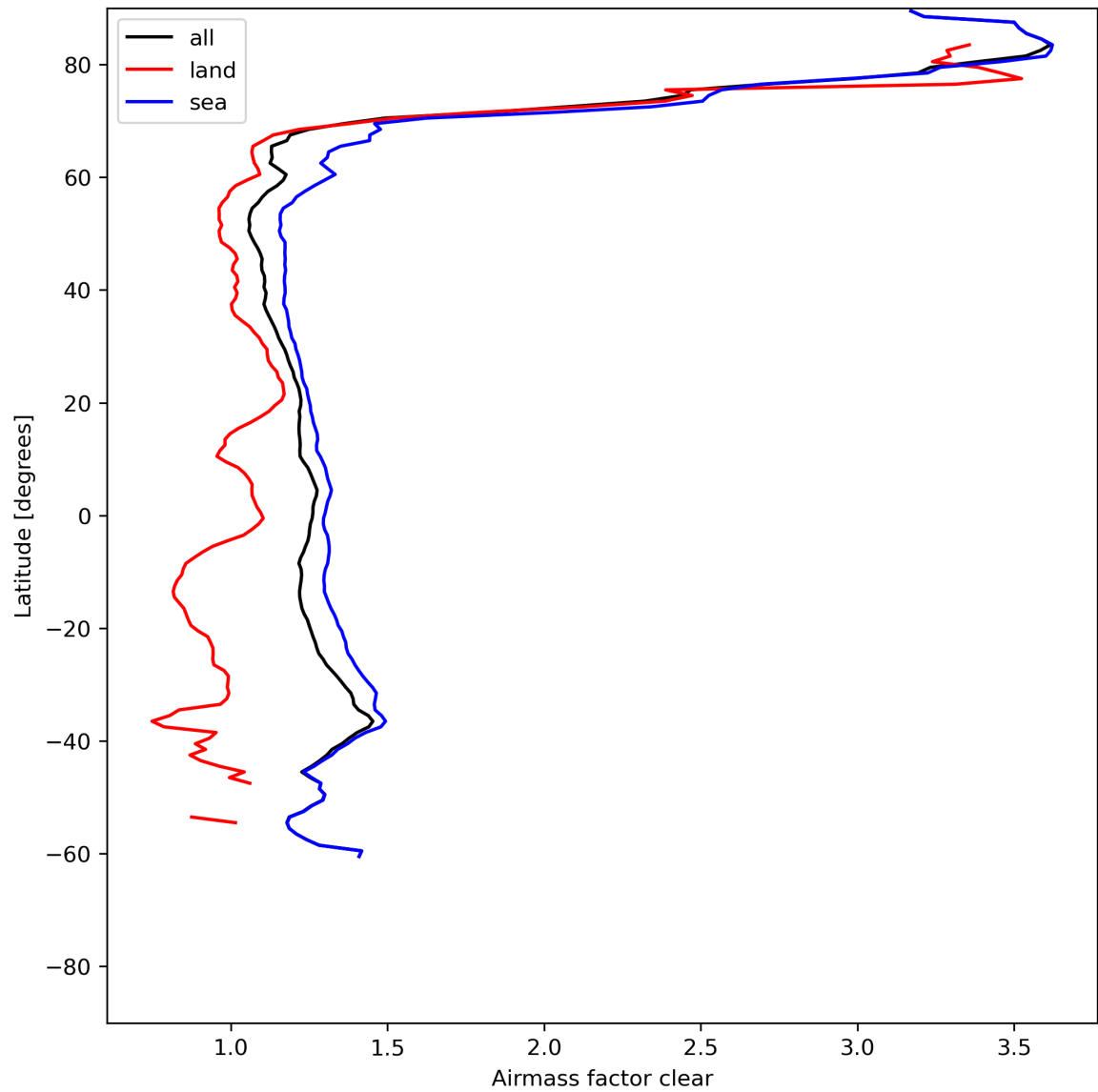
Figure 28: Zonal average of “Airmass factor clear” for 2024-06-17 to 2024-06-19.
