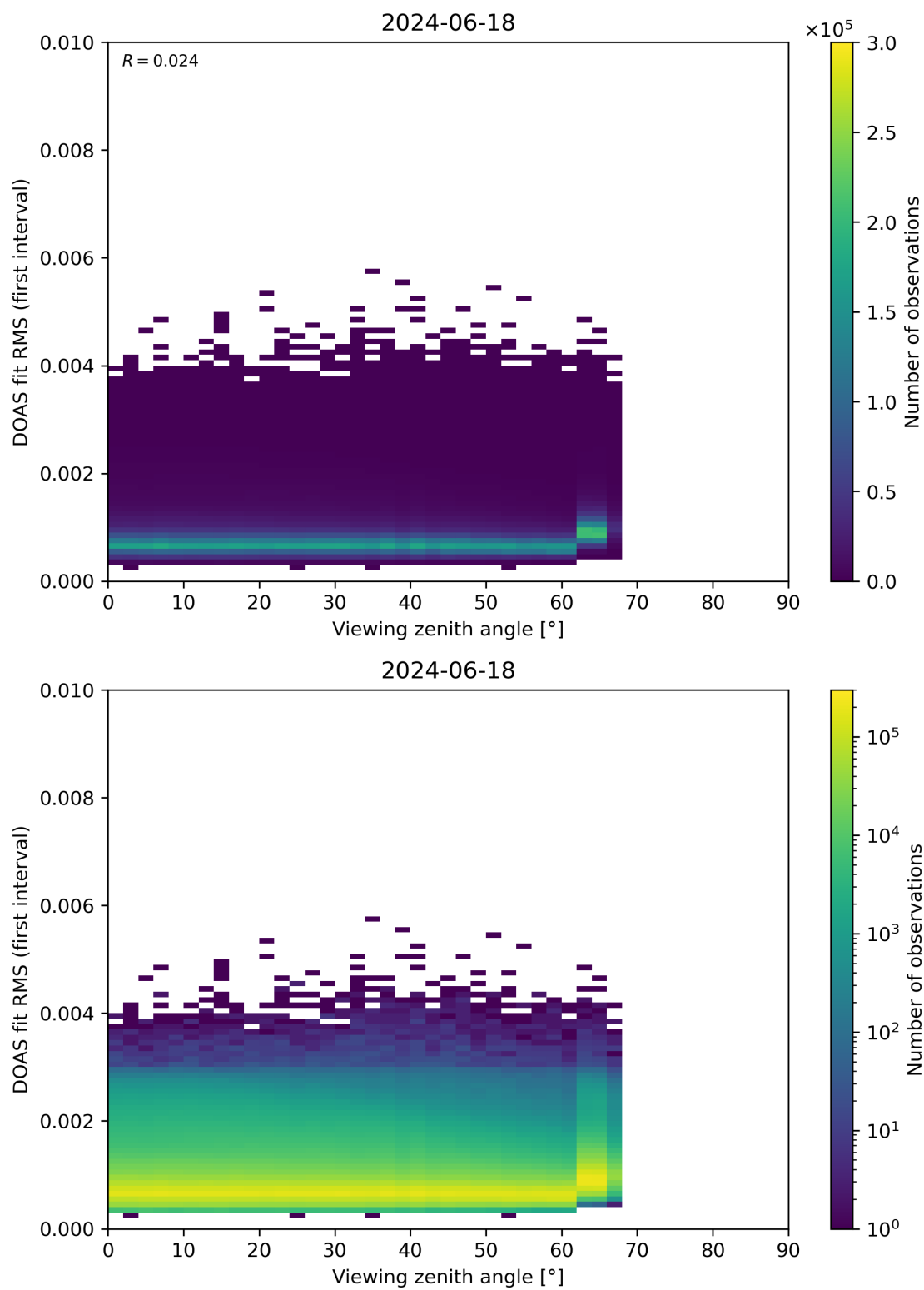
Figure 182: Scatter density plot of “Viewing zenith angle” against “DOAS fit RMS (first interval)” for 2024-06-17 to 2024-06-19.
