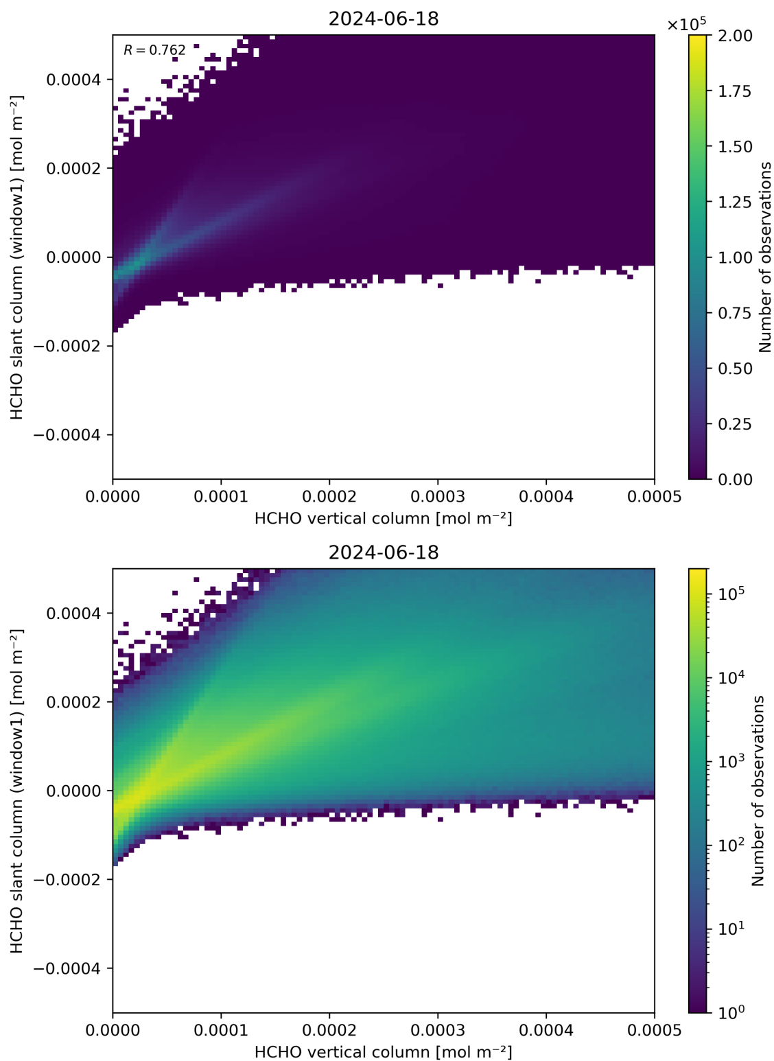
Figure 129: Scatter density plot of “HCHO vertical column” against “HCHO slant column (window1)” for 2024-06-17 to 2024-06-19.
