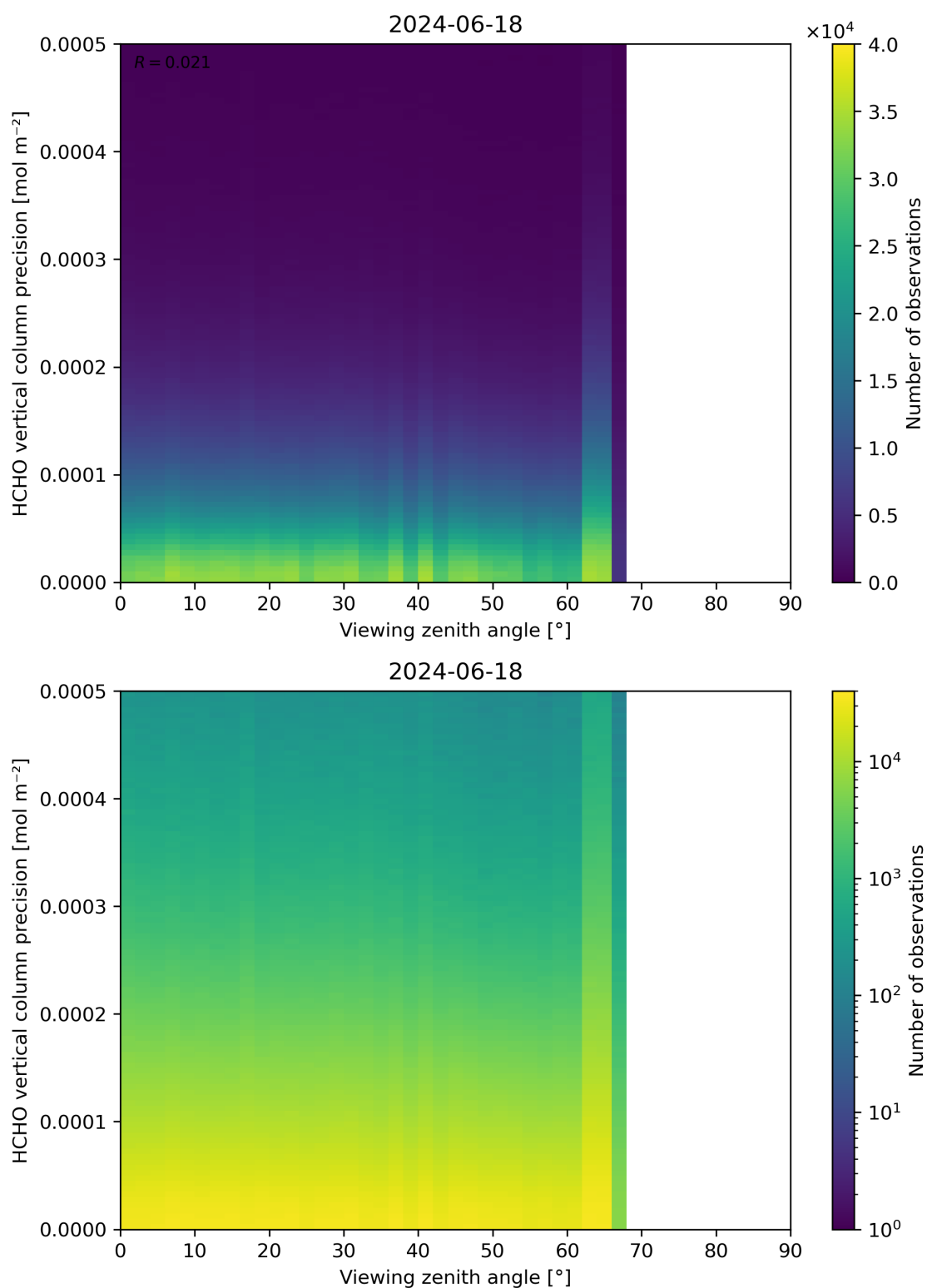
Figure 194: Scatter density plot of “Viewing zenith angle” against “HCHO vertical column precision” for 2024-06-17 to 2024-06-19.
