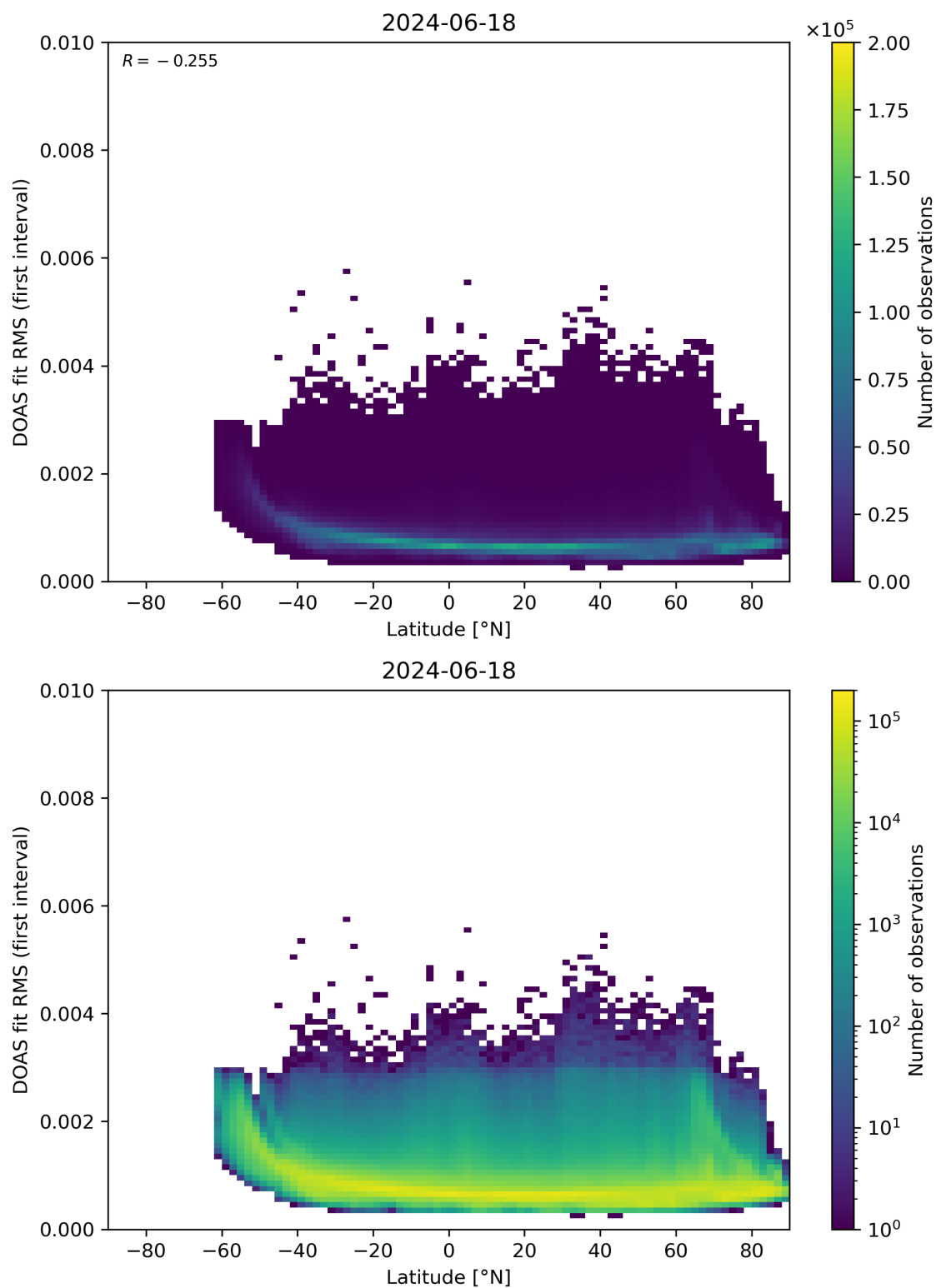
Figure 153: Scatter density plot of “Latitude” against “DOAS fit RMS (first interval)” for 2024-06-17 to 2024-06-19.
