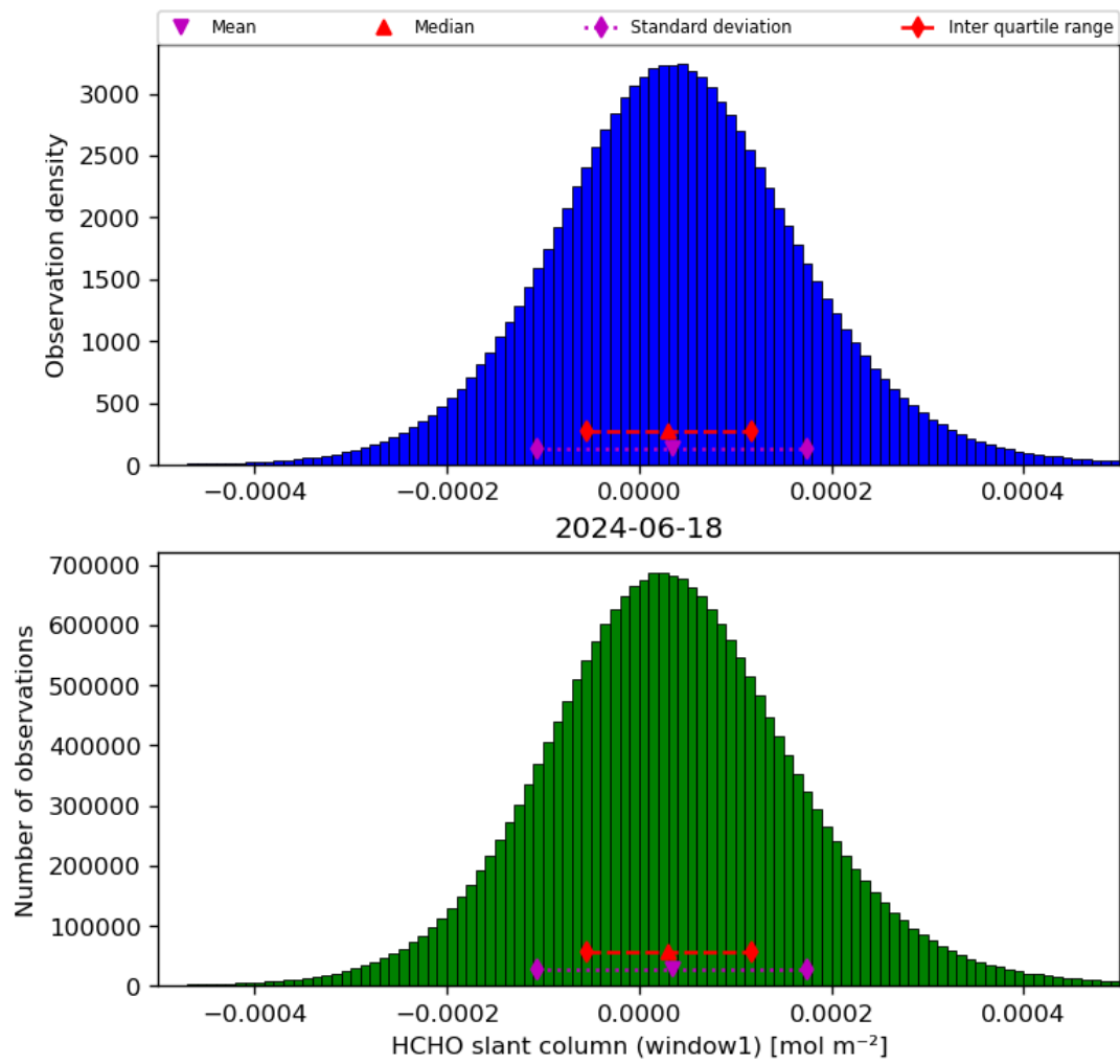
Figure 38: Histogram of “HCHO slant column (window1)” for 2024-06-17 to 2024-06-19
