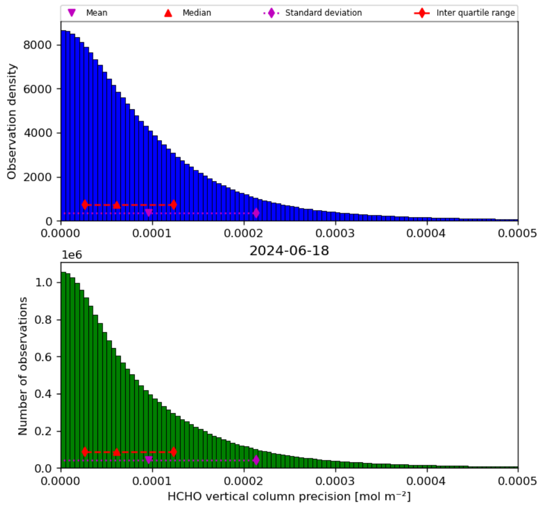
Figure 36: Histogram of “HCHO vertical column precision” for 2024-06-17 to 2024-06-19
