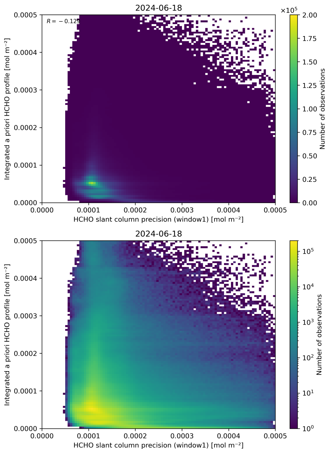
Figure 96: Scatter density plot of “HCHO slant column precision (window1)” against “Integrated a priori HCHO profile” for 2024-06-17 to 2024-06-19.
