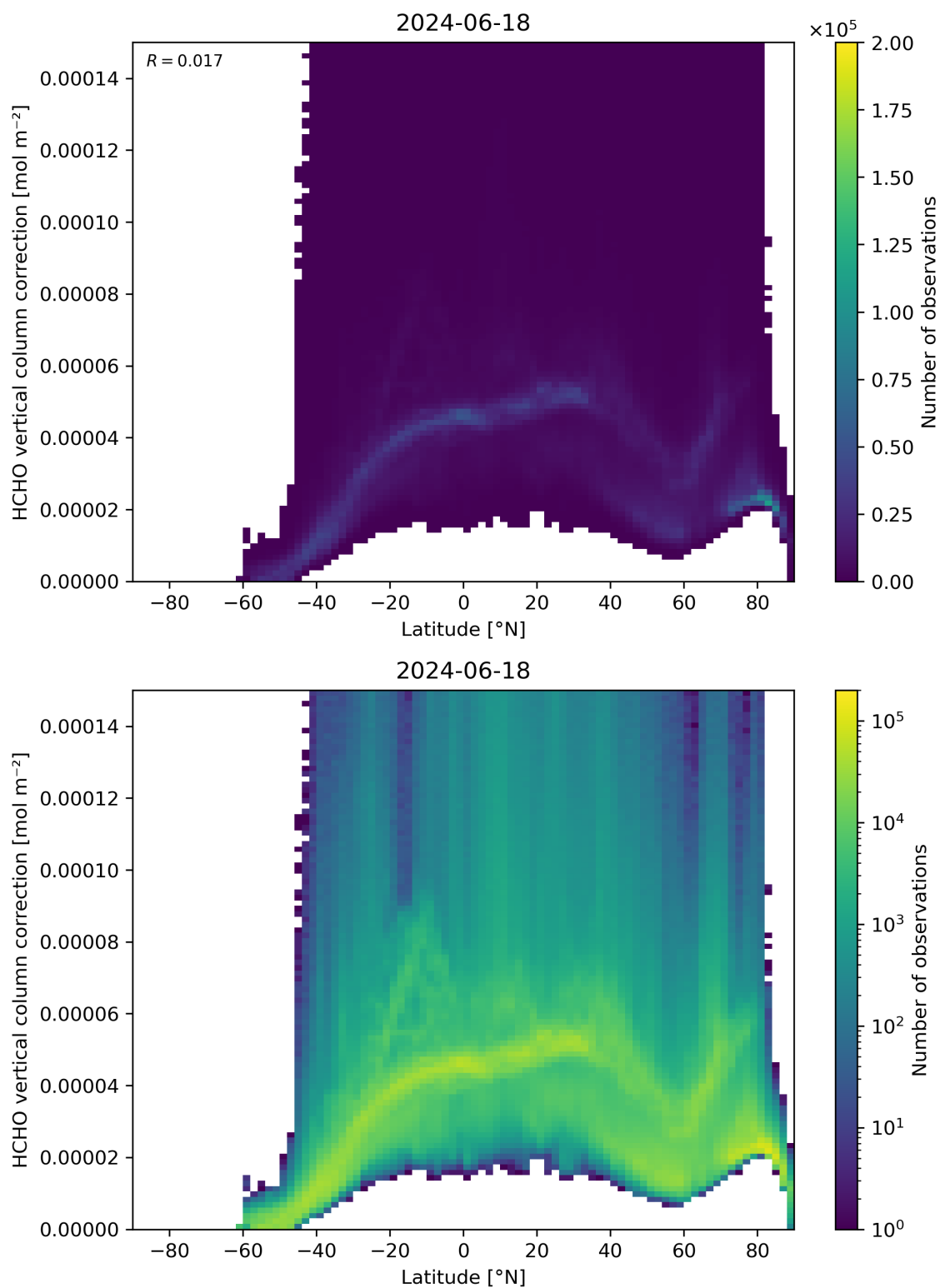
Figure 164: Scatter density plot of “Latitude” against “HCHO vertical column correction” for 2024-06-17 to 2024-06-19.
