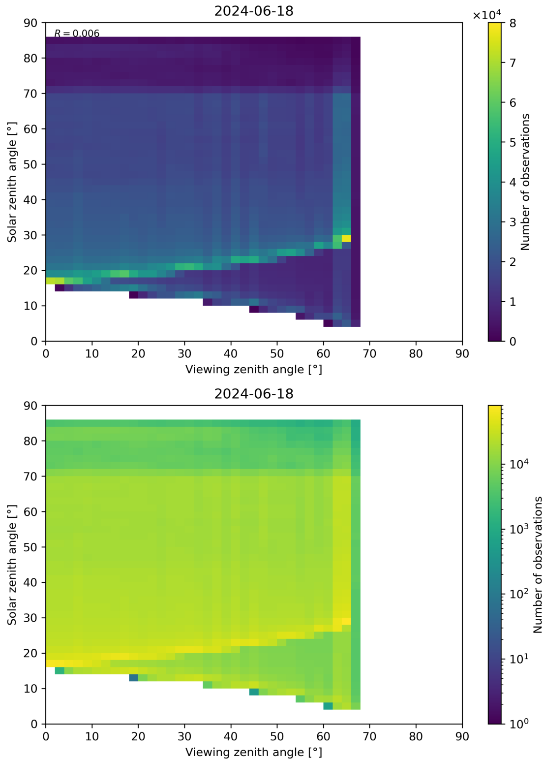
Figure 197: Scatter density plot of “Viewing zenith angle” against “Solar zenith angle” for 2024-06-17 to 2024-06-19.
