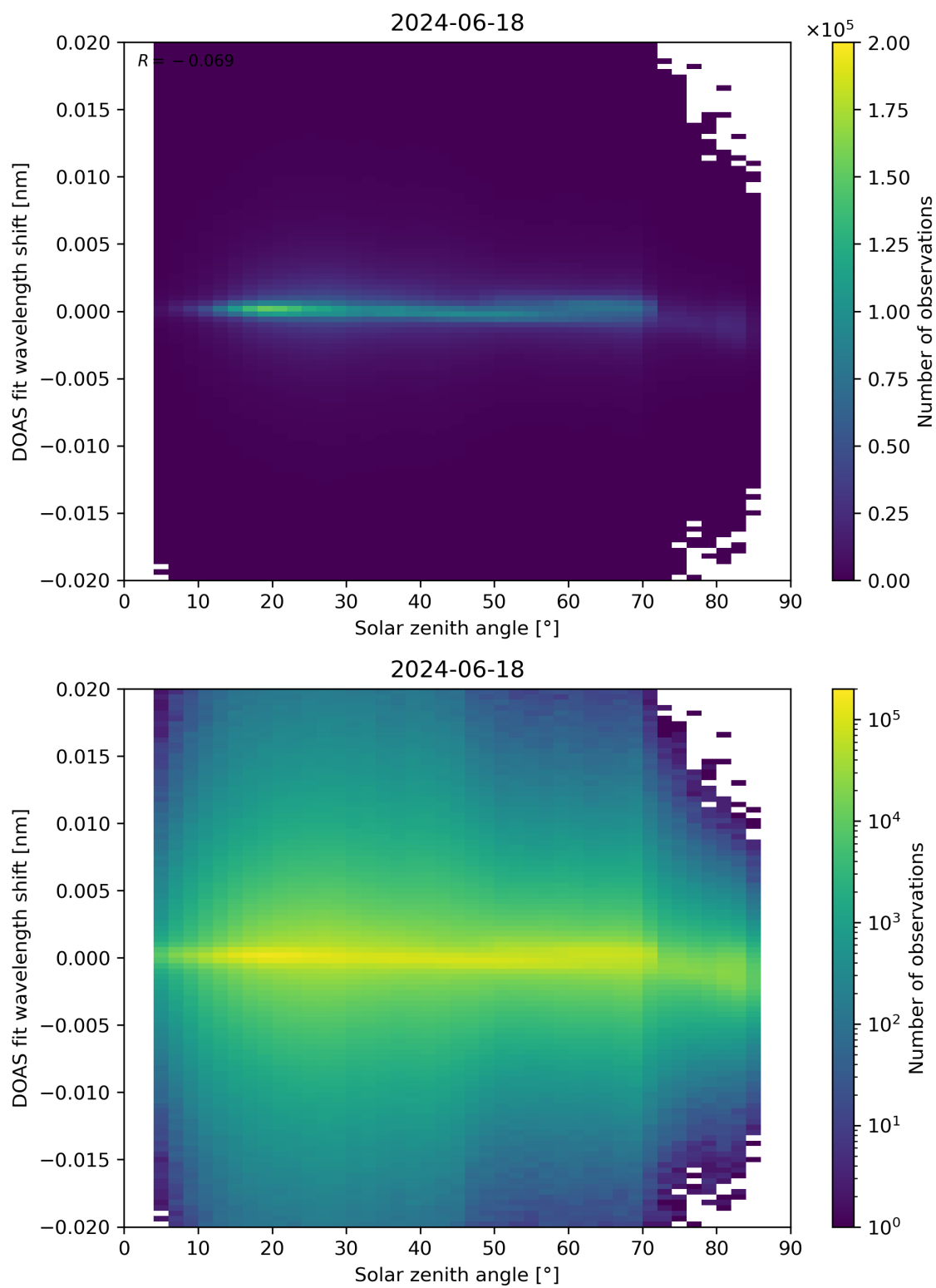
Figure 168: Scatter density plot of “Solar zenith angle” against “DOAS fit wavelength shift” for 2024-06-17 to 2024-06-19.
