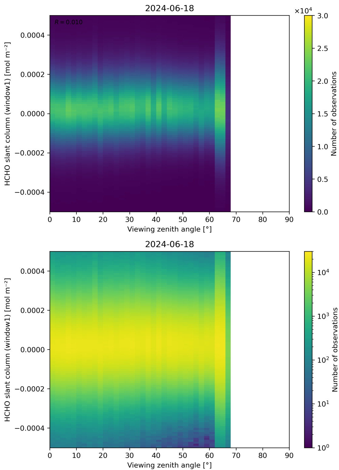
Figure 188: Scatter density plot of “Viewing zenith angle” against “HCHO slant column (window1)” for 2024-06-17 to 2024-06-19.
