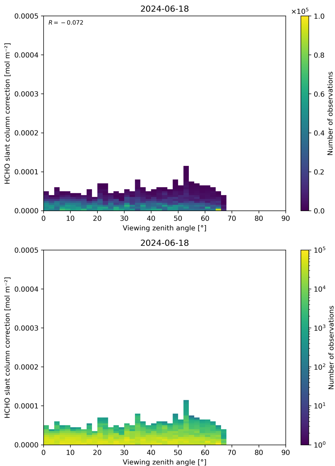
Figure 187: Scatter density plot of “Viewing zenith angle” against “HCHO slant column correction” for 2024-06-17 to 2024-06-19.
