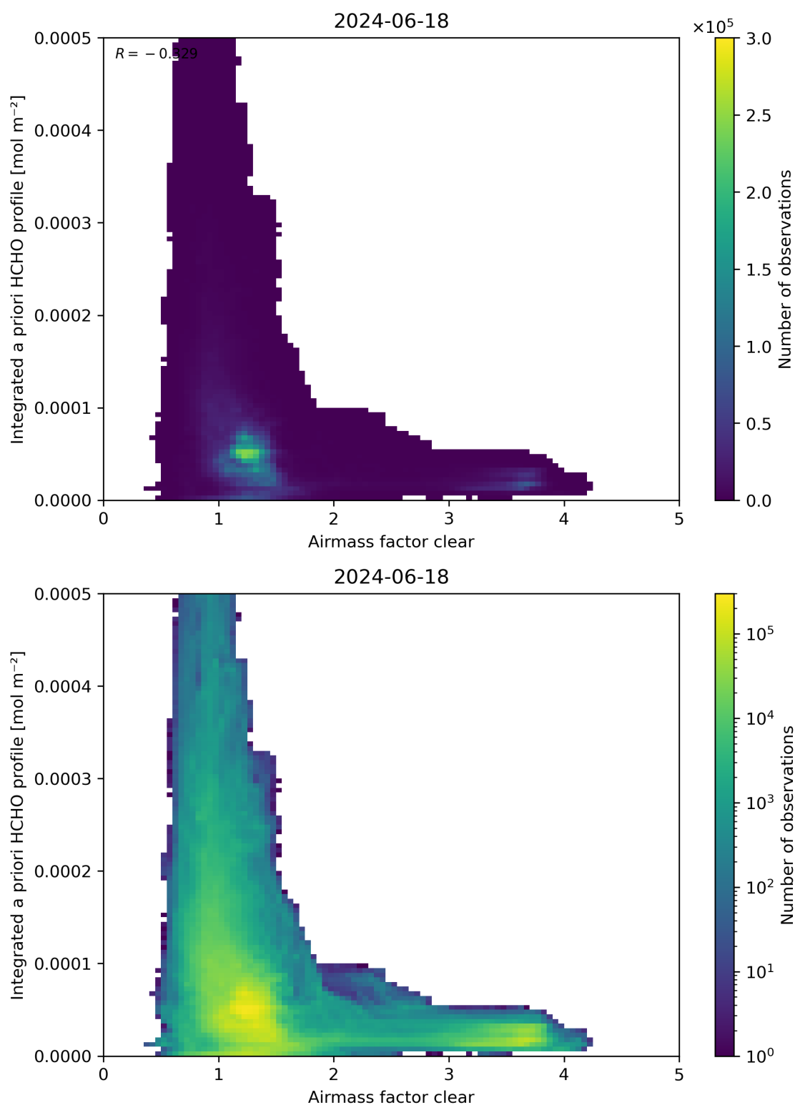
Figure 76: Scatter density plot of “Airmass factor clear” against “Integrated a priori HCHO profile” for 2024-06-17 to 2024-06-19.
