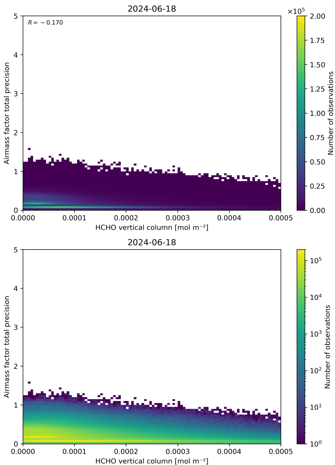
Figure 132: Scatter density plot of “HCHO vertical column” against “Airmass factor total precision” for 2024-06-17 to 2024-06-19.
