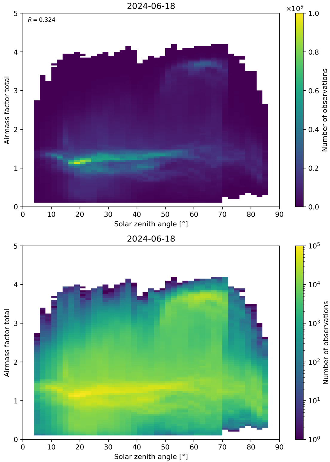
Figure 175: Scatter density plot of “Solar zenith angle” against “Airmass factor total” for 2024-06-17 to 2024-06-19.
