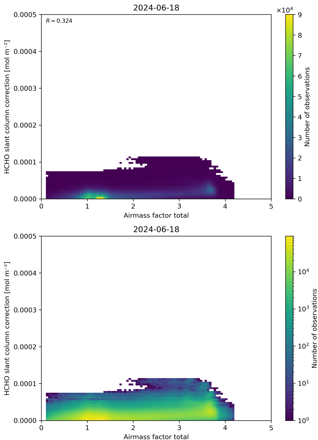
Figure 102: Scatter density plot of “Airmass factor total” against “HCHO slant column correction” for 2024-06-17 to 2024-06-19.
