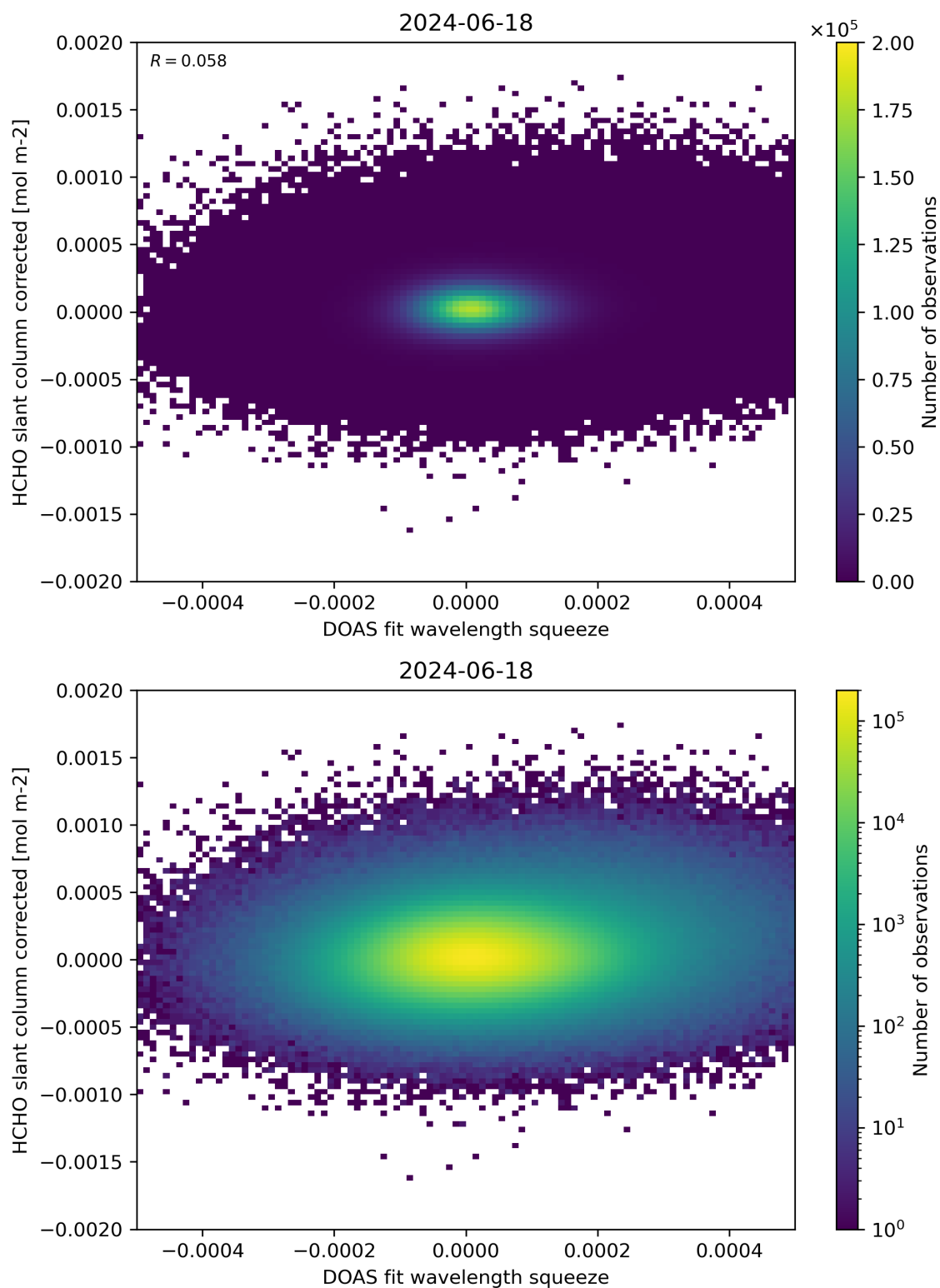
Figure 69: Scatter density plot of “DOAS fit wavelength squeeze” against “HCHO slant column corrected” for 2024-06-17 to 2024-06-19.
