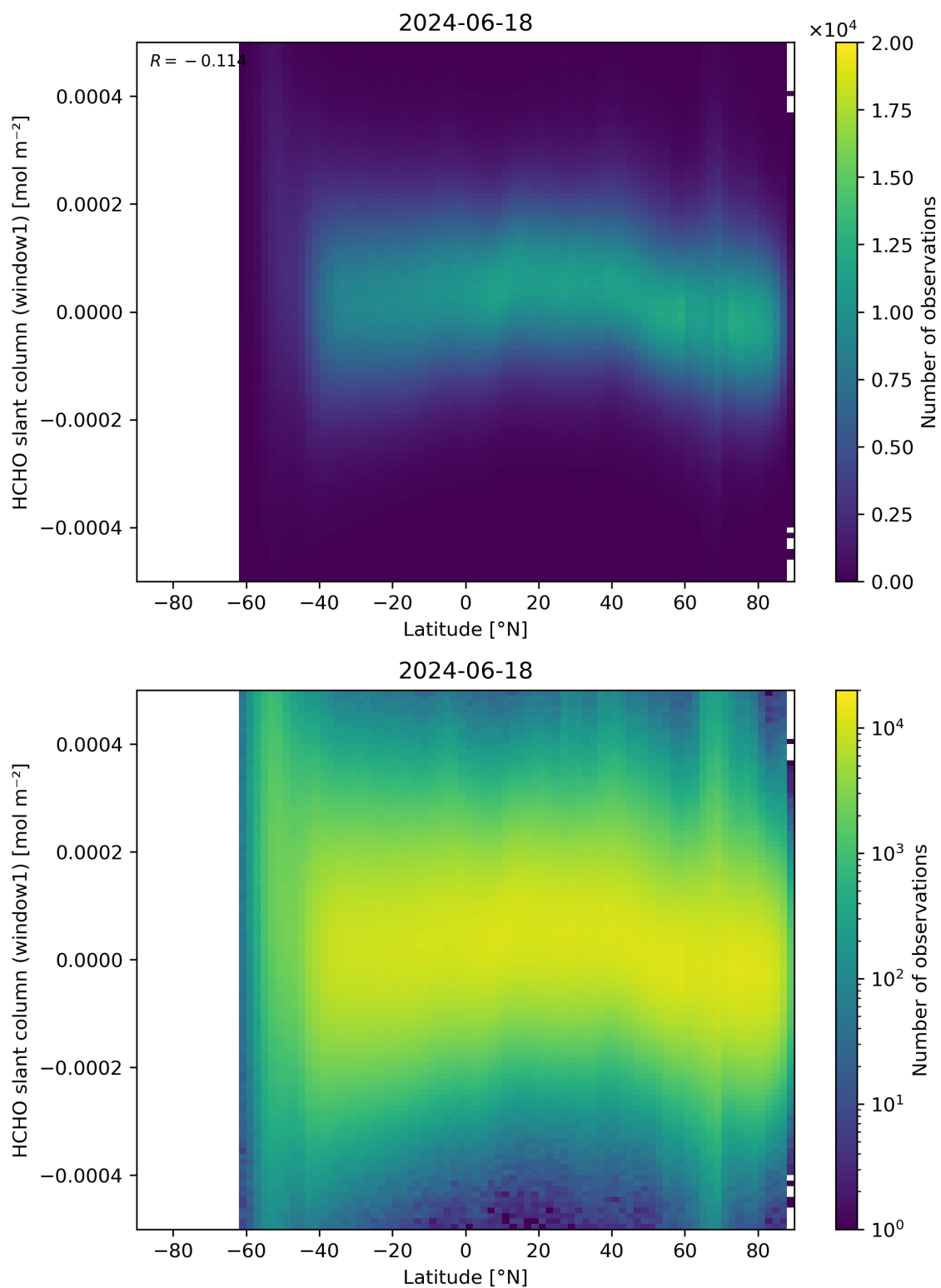
Figure 159: Scatter density plot of “Latitude” against “HCHO slant column (window1)” for 2024-06-17 to 2024-06-19.
