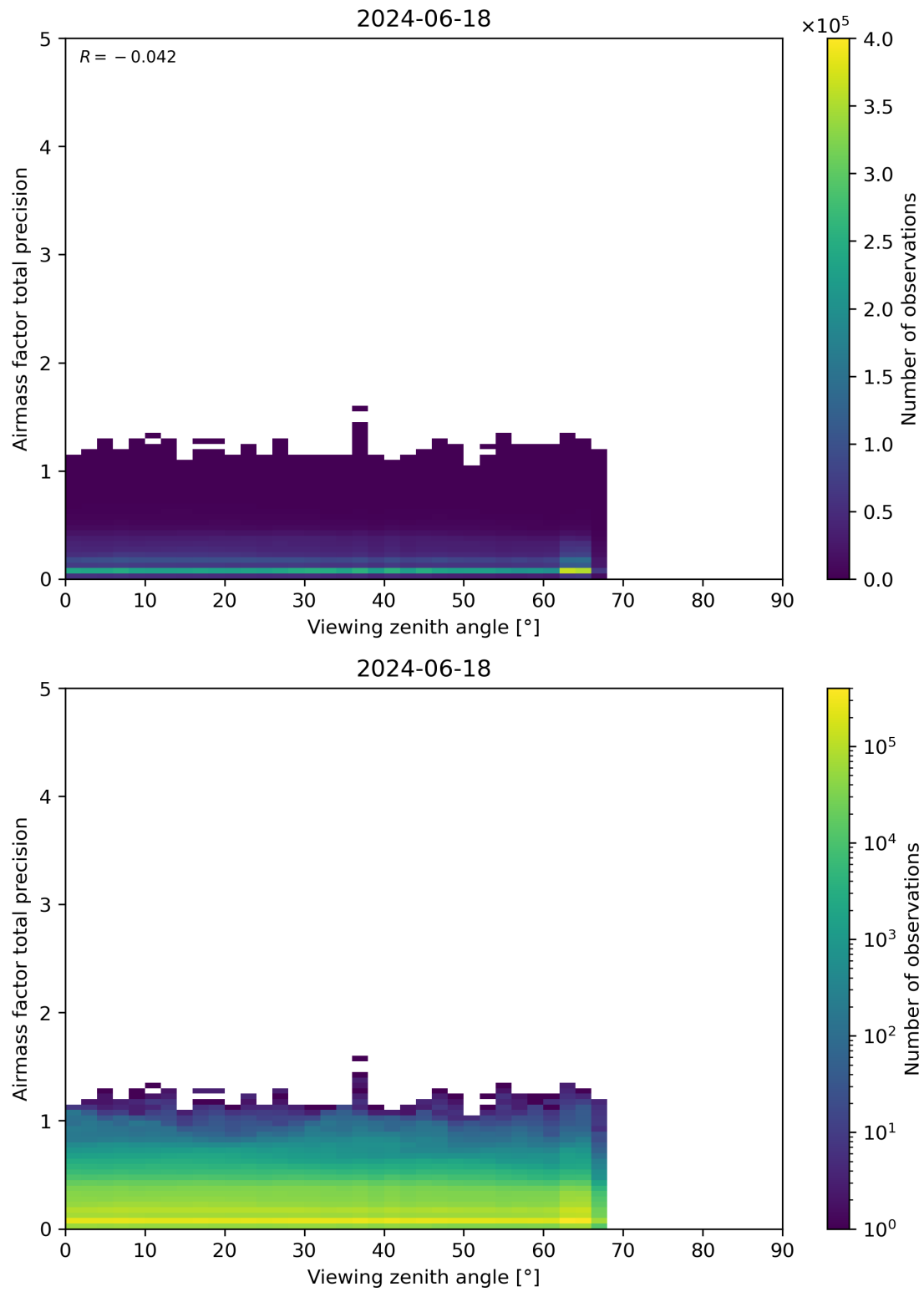
Figure 191: Scatter density plot of “Viewing zenith angle” against “Airmass factor total precision” for 2024-06-17 to 2024-06-19.
