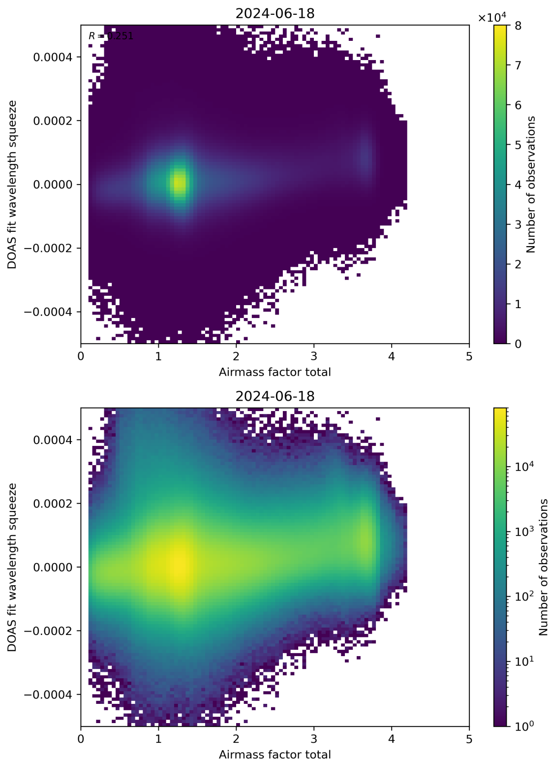
Figure 99: Scatter density plot of “Airmass factor total” against “DOAS fit wavelength squeeze” for 2024-06-17 to 2024-06-19.
