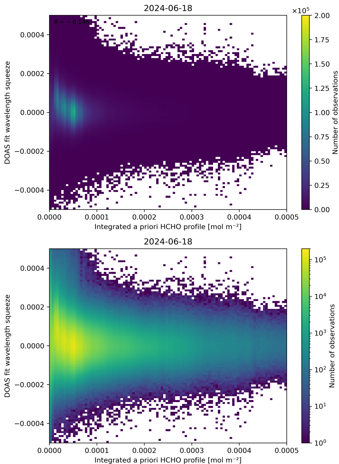
Figure 150: Scatter density plot of “Integrated a priori HCHO profile” against “DOAS fit wavelength squeeze” for 2024-06-17 to 2024-06-19.
