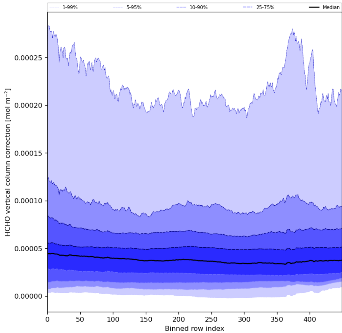
Figure 51: Along track statistics of “HCHO vertical column correction” for 2024-06-17 to 2024-06-19
