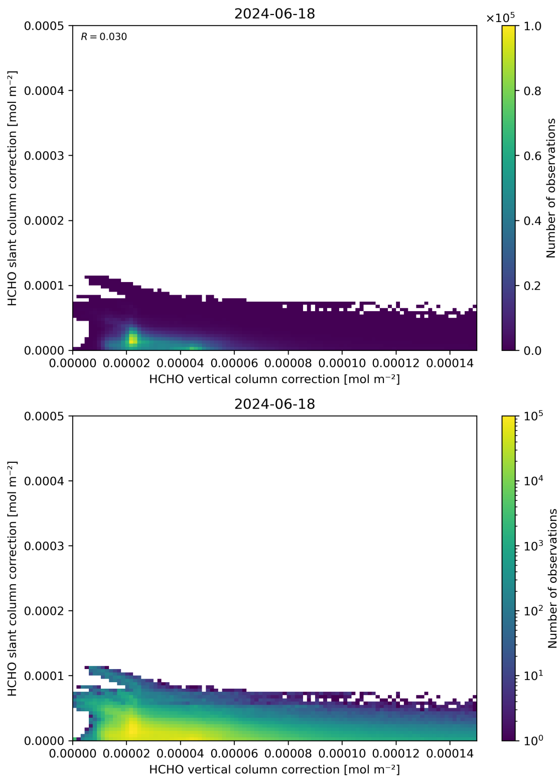
Figure 117: Scatter density plot of “HCHO vertical column correction” against “HCHO slant column correction” for 2024-06-17 to 2024-06-19.
