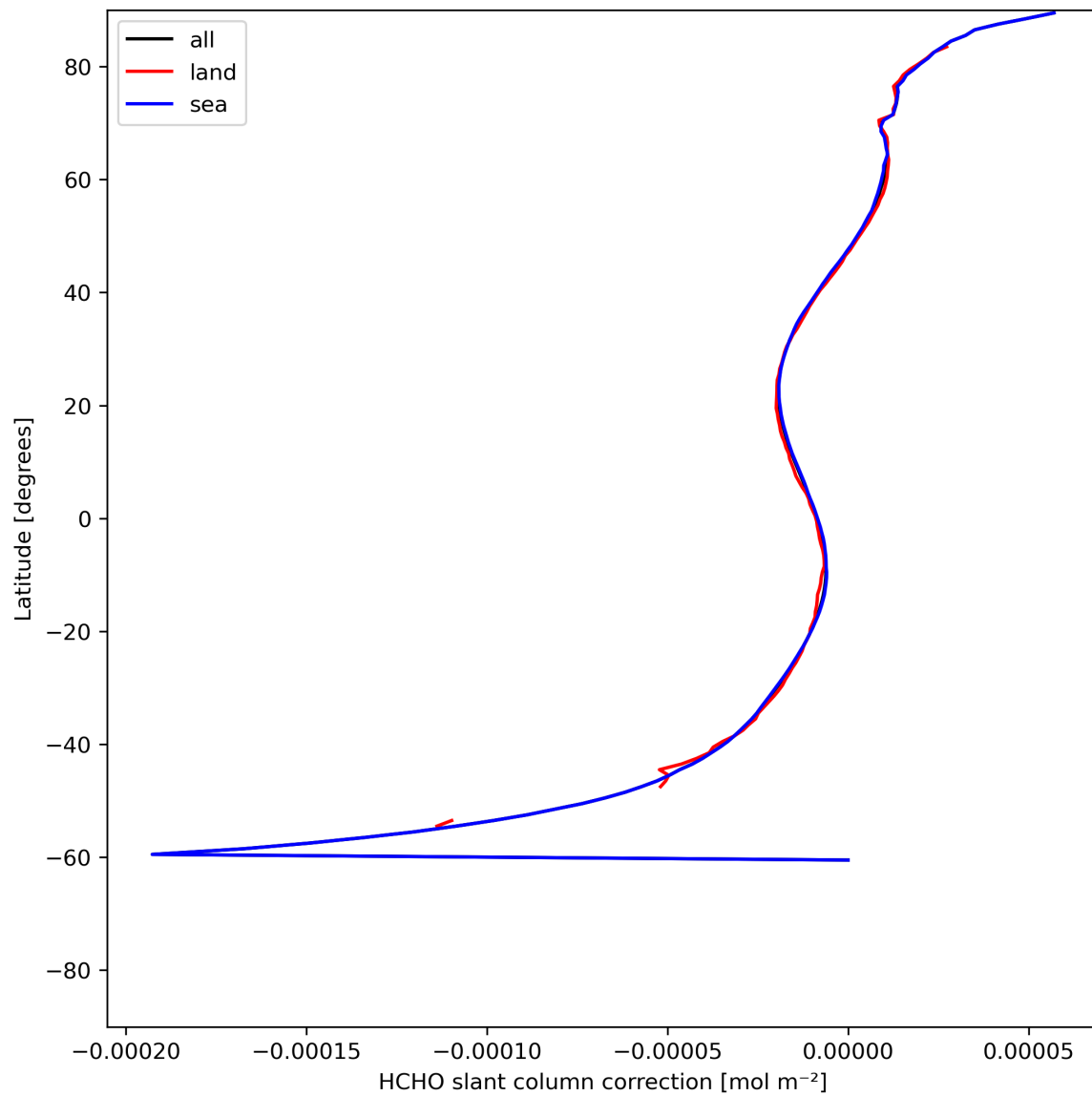
Figure 33: Zonal average of “HCHO slant column correction” for 2024-06-17 to 2024-06-19.
