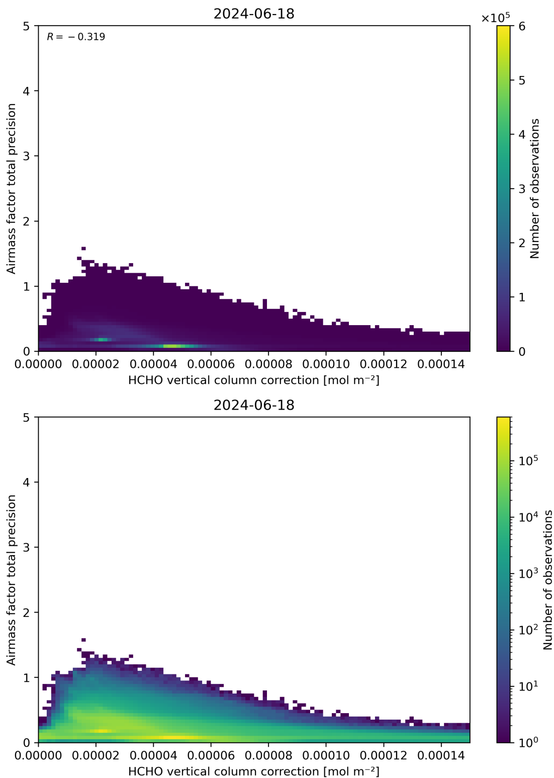
Figure 121: Scatter density plot of “HCHO vertical column correction” against “Airmass factor total precision” for 2024-06-17 to 2024-06-19.
