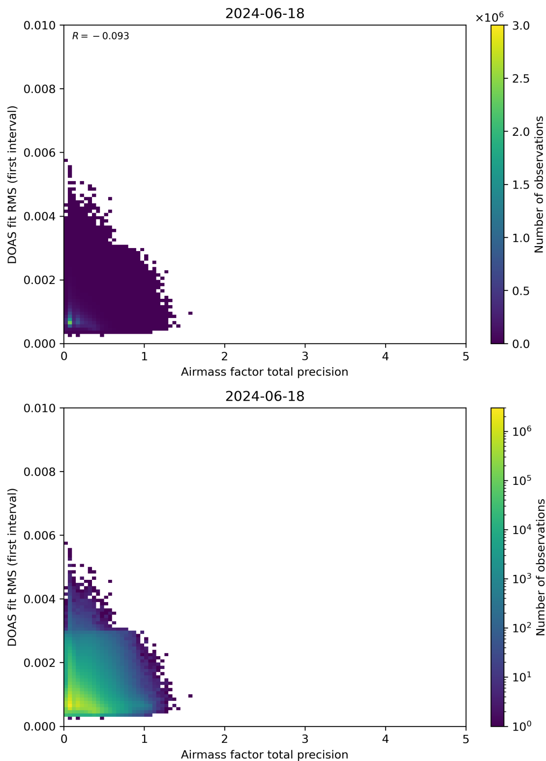
Figure 105: Scatter density plot of “Airmass factor total precision” against “DOAS fit RMS (first interval)” for 2024-06-17 to 2024-06-19.
