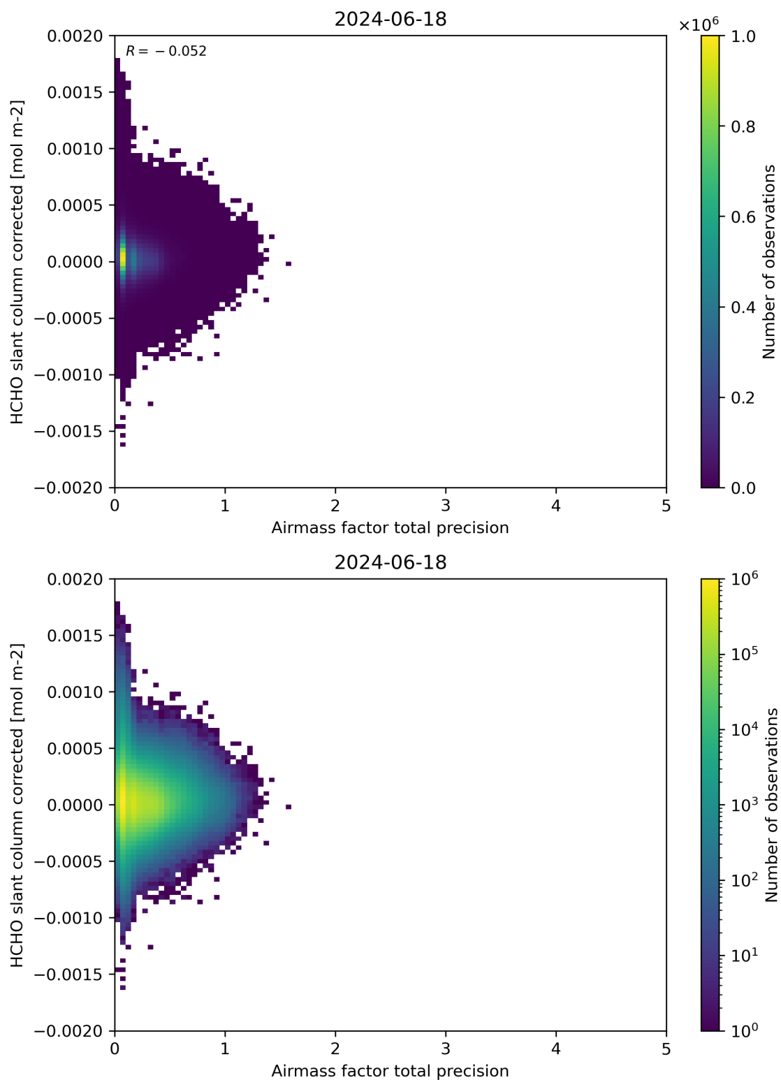
Figure 109: Scatter density plot of “Airmass factor total precision” against “HCHO slant column corrected” for 2024-06-17 to 2024-06-19.
