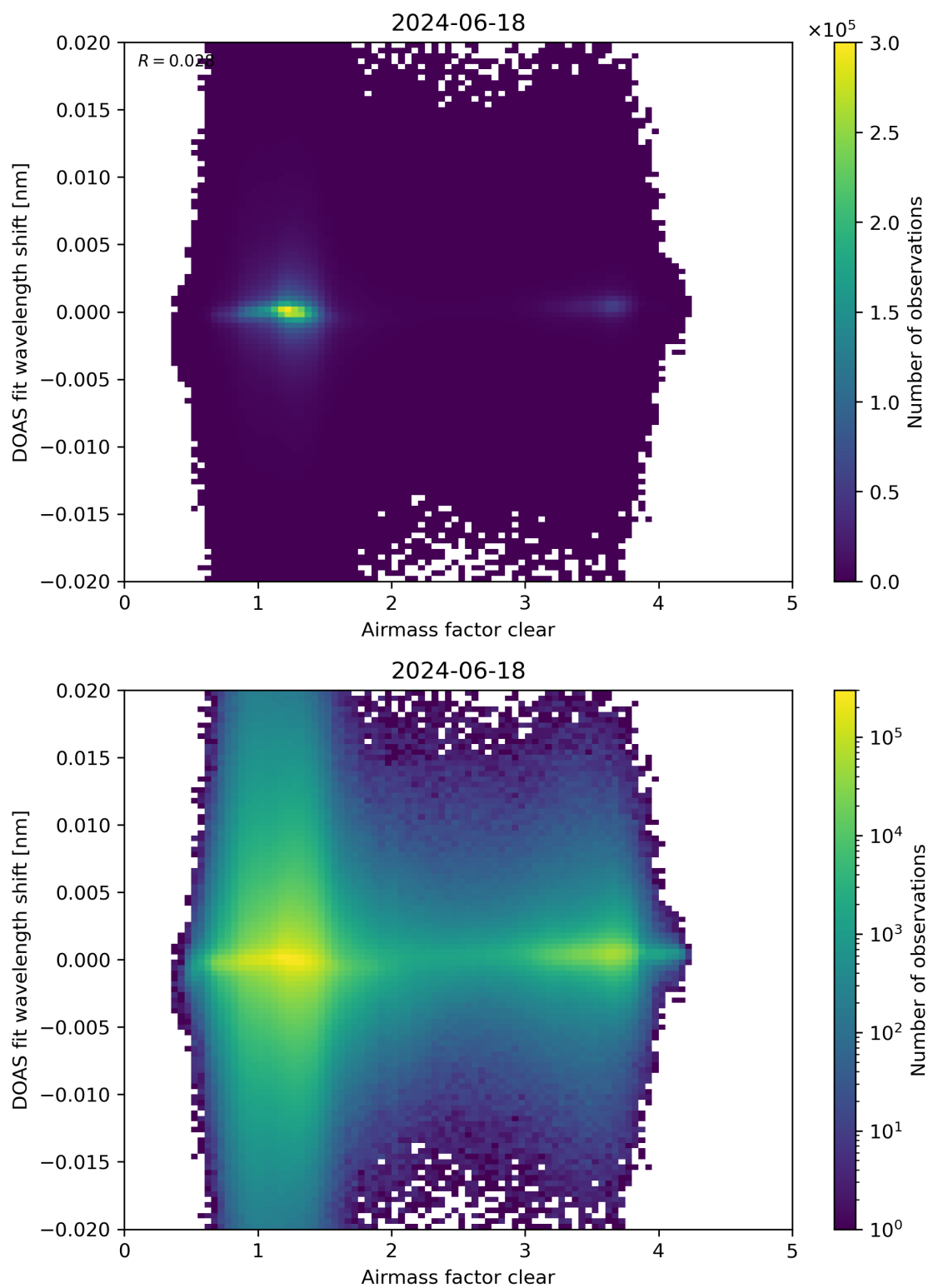
Figure 72: Scatter density plot of “Airmass factor clear” against “DOAS fit wavelength shift” for 2024-06-17 to 2024-06-19.
