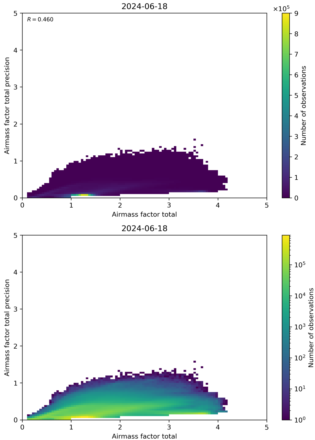
Figure 103: Scatter density plot of “Airmass factor total” against “Airmass factor total precision” for 2024-06-17 to 2024-06-19.
