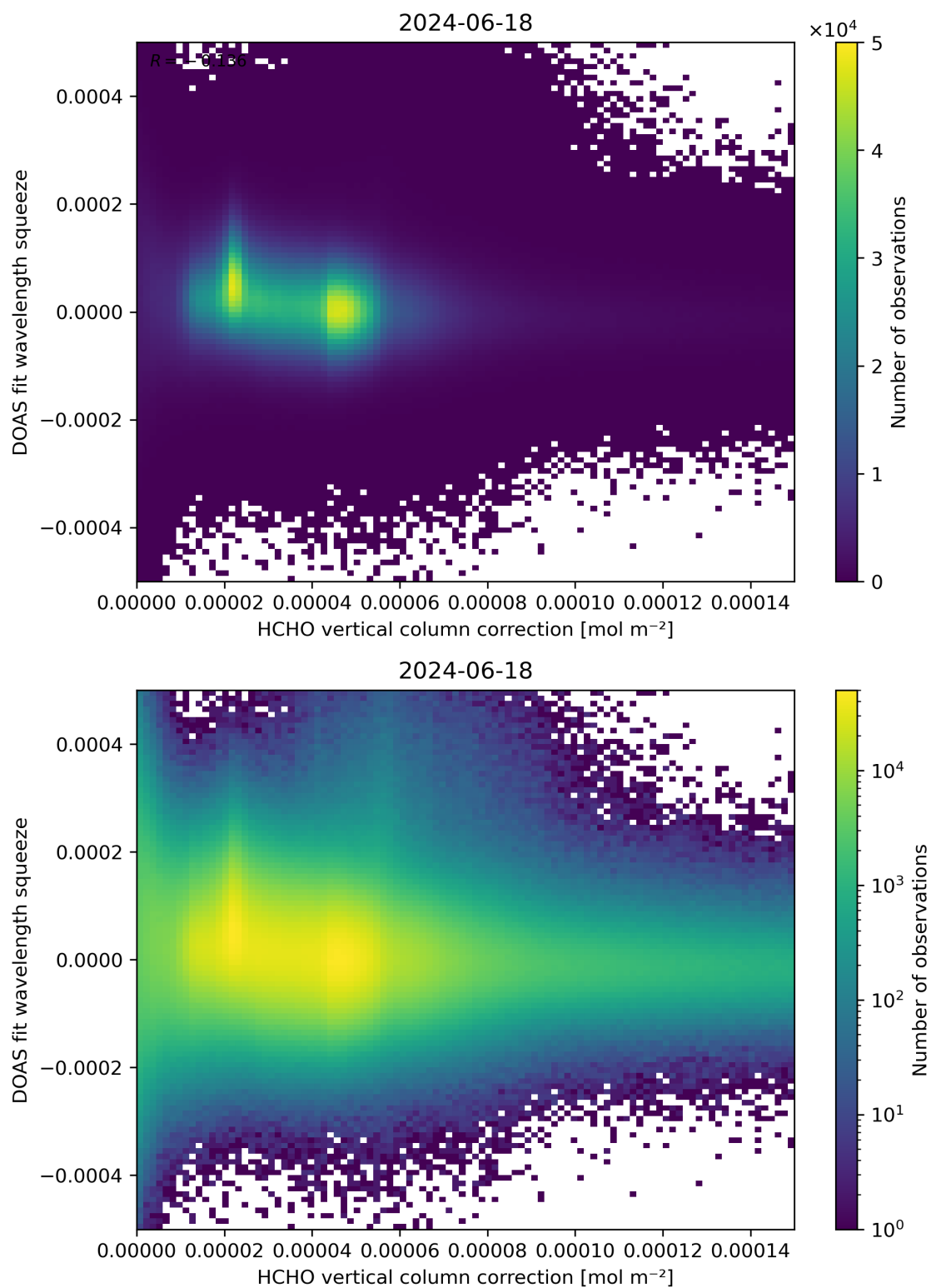
Figure 114: Scatter density plot of “HCHO vertical column correction” against “DOAS fit wavelength squeeze” for 2024-06-17 to 2024-06-19.
