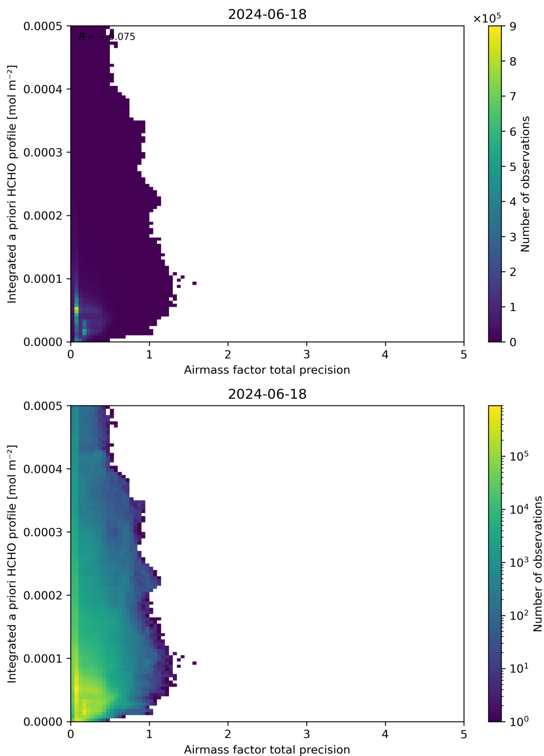
Figure 111: Scatter density plot of “Airmass factor total precision” against “Integrated a priori HCHO profile” for 2024-06-17 to 2024-06-19.
