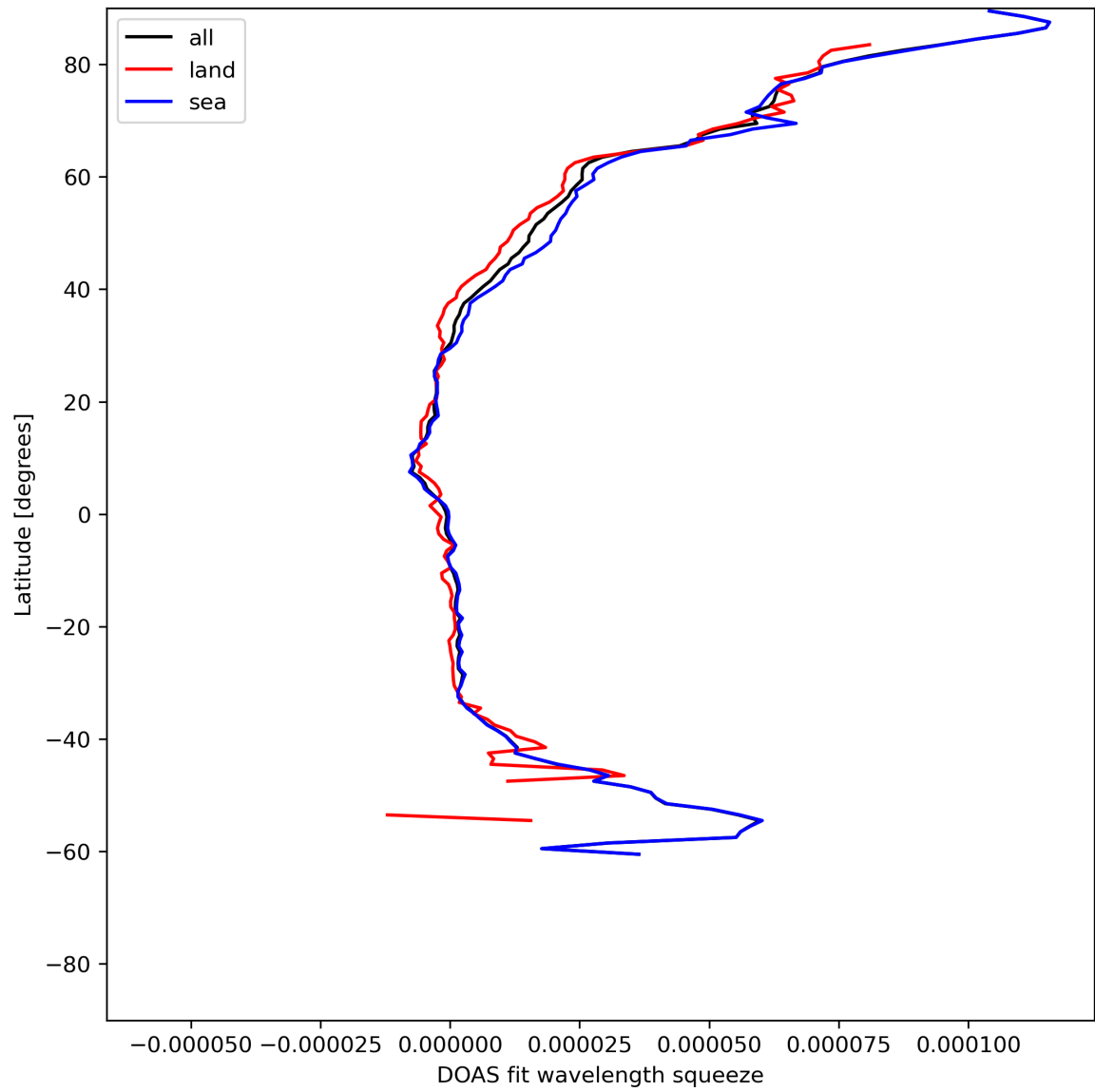
Figure 31: Zonal average of “DOAS fit wavelength squeeze” for 2024-06-17 to 2024-06-19.
