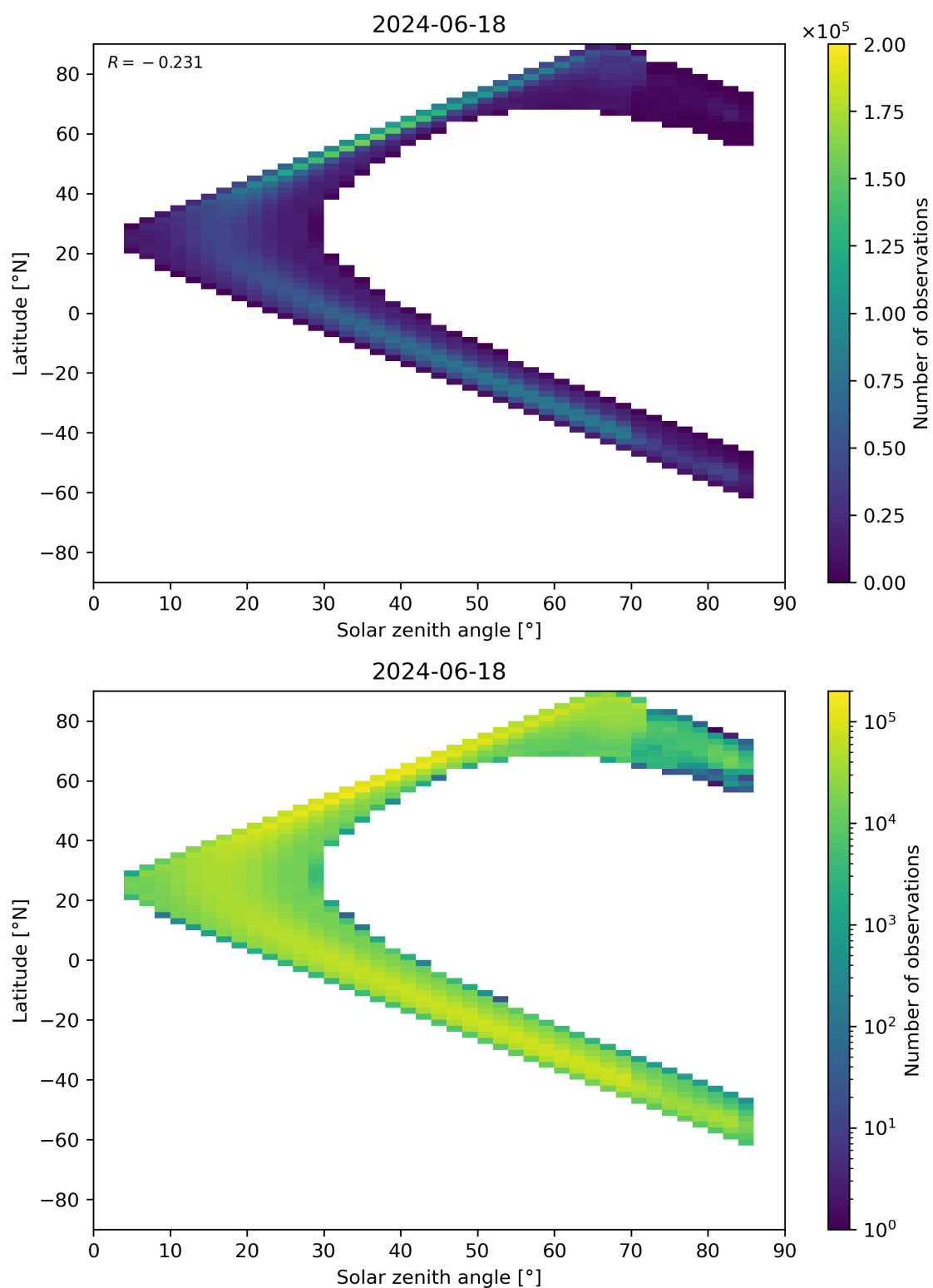
Figure 181: Scatter density plot of “Solar zenith angle” against “Latitude” for 2024-06-17 to 2024-06-19.
