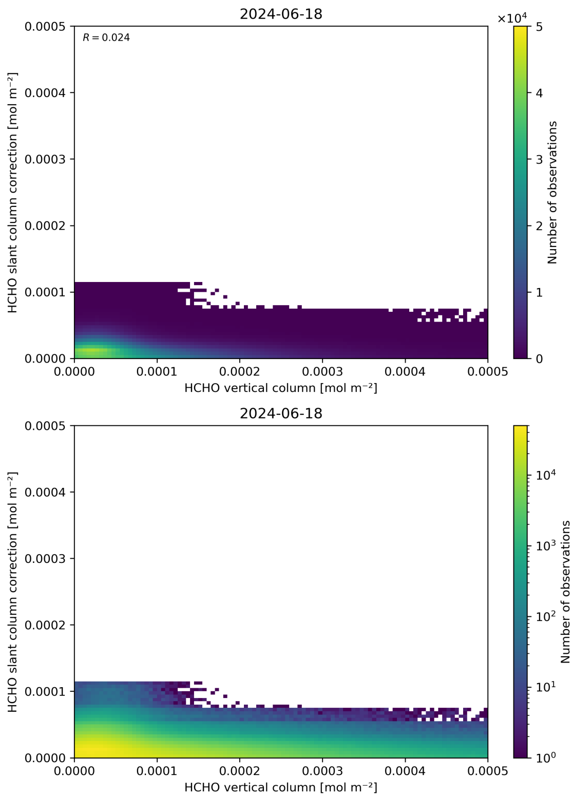
Figure 128: Scatter density plot of “HCHO vertical column” against “HCHO slant column correction” for 2024-06-17 to 2024-06-19.
