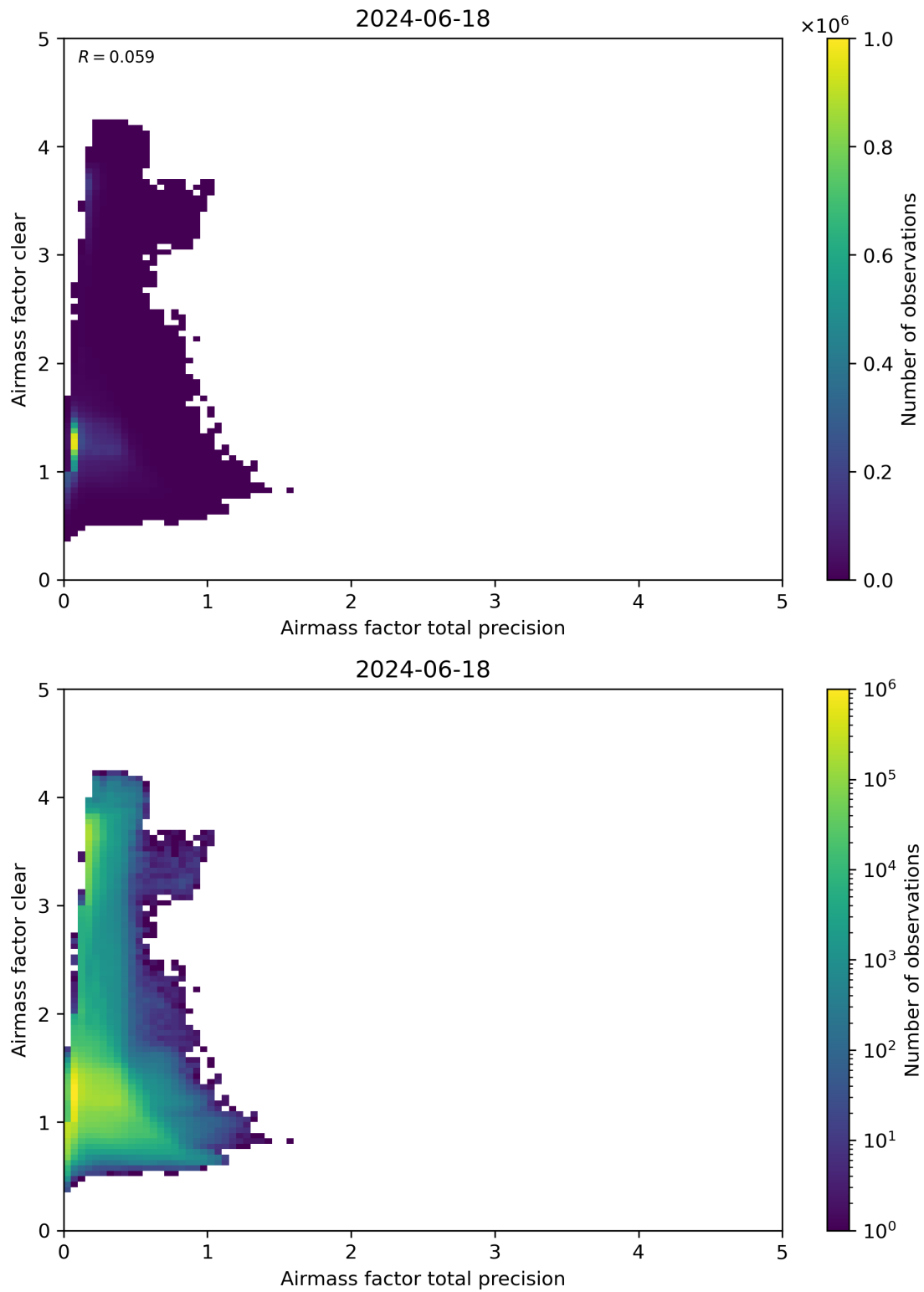
Figure 108: Scatter density plot of “Airmass factor total precision” against “Airmass factor clear” for 2024-06-17 to 2024-06-19.
