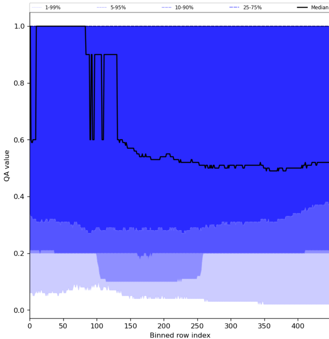
Figure 48: Along track statistics of “QA value” for 2024-06-17 to 2024-06-19
