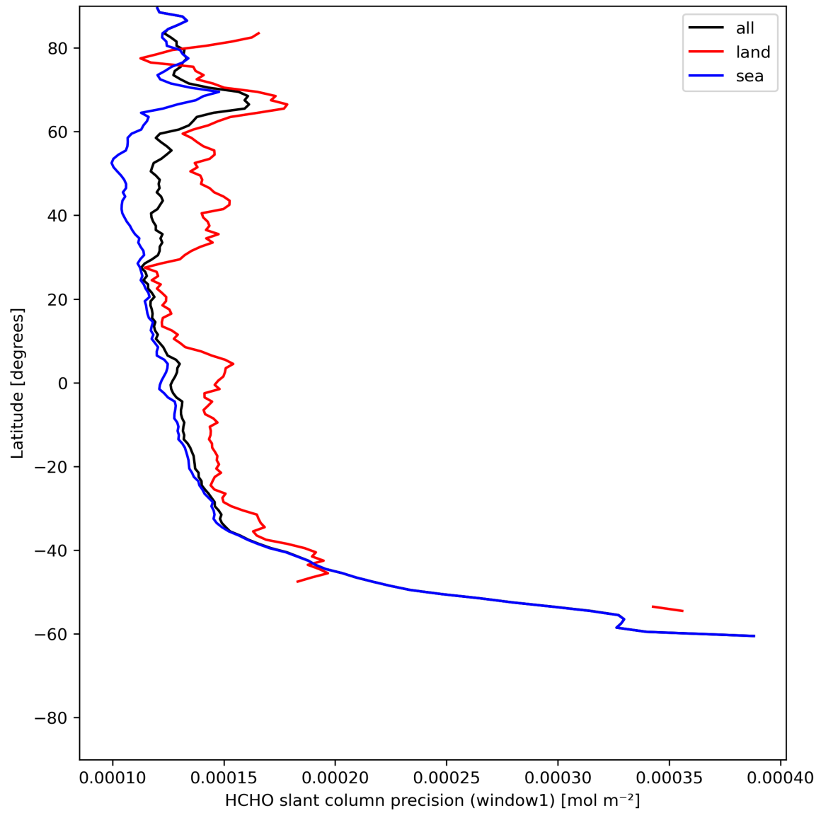
Figure 25: Zonal average of “HCHO slant column precision (window1)” for 2024-06-17 to 2024-06-19.
