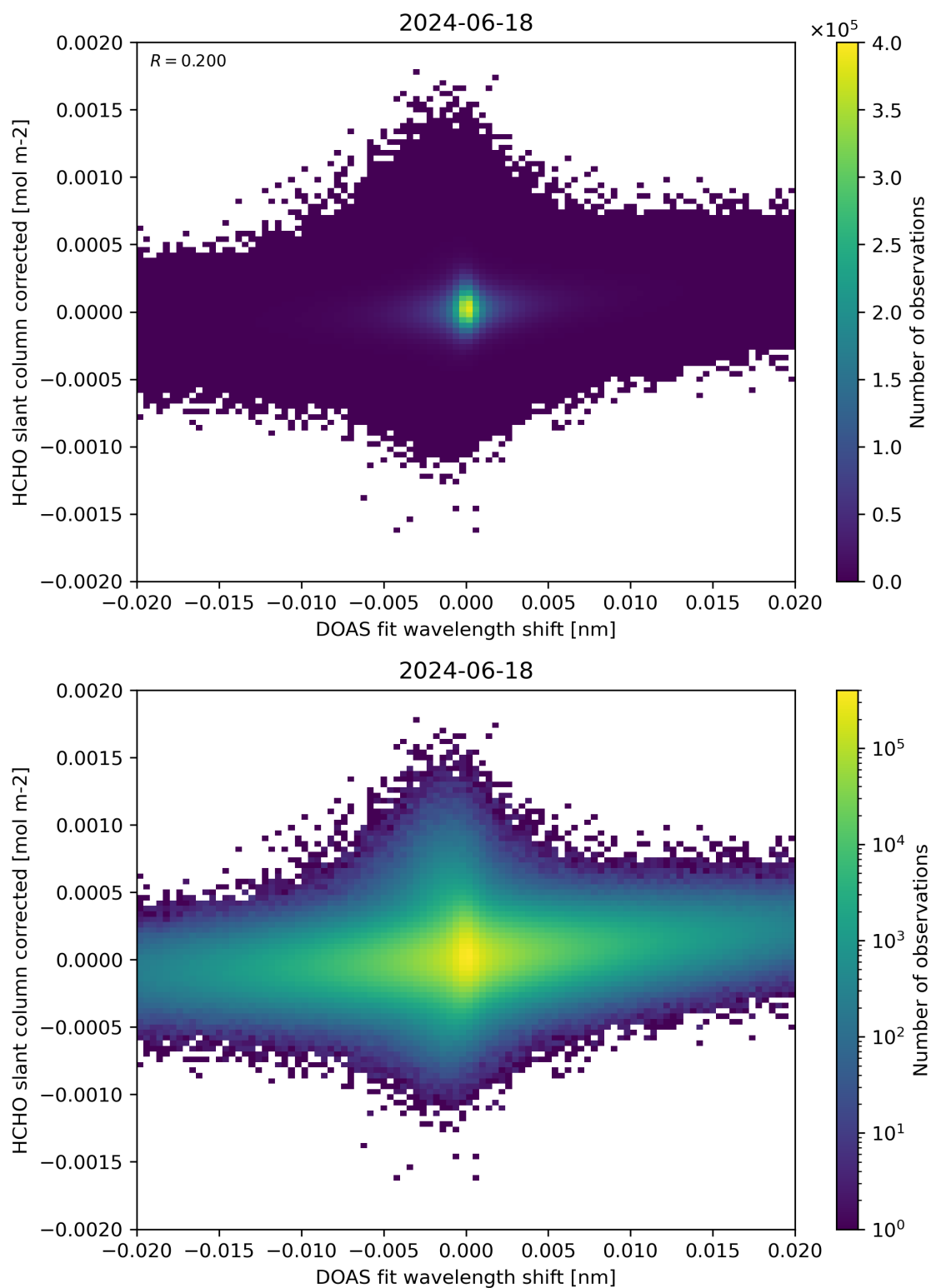
Figure 66: Scatter density plot of “DOAS fit wavelength shift” against “HCHO slant column corrected” for 2024-06-17 to 2024-06-19.
