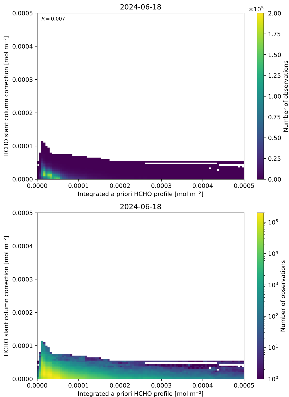
Figure 152: Scatter density plot of “Integrated a priori HCHO profile” against “HCHO slant column correction” for 2024-06-17 to 2024-06-19.
