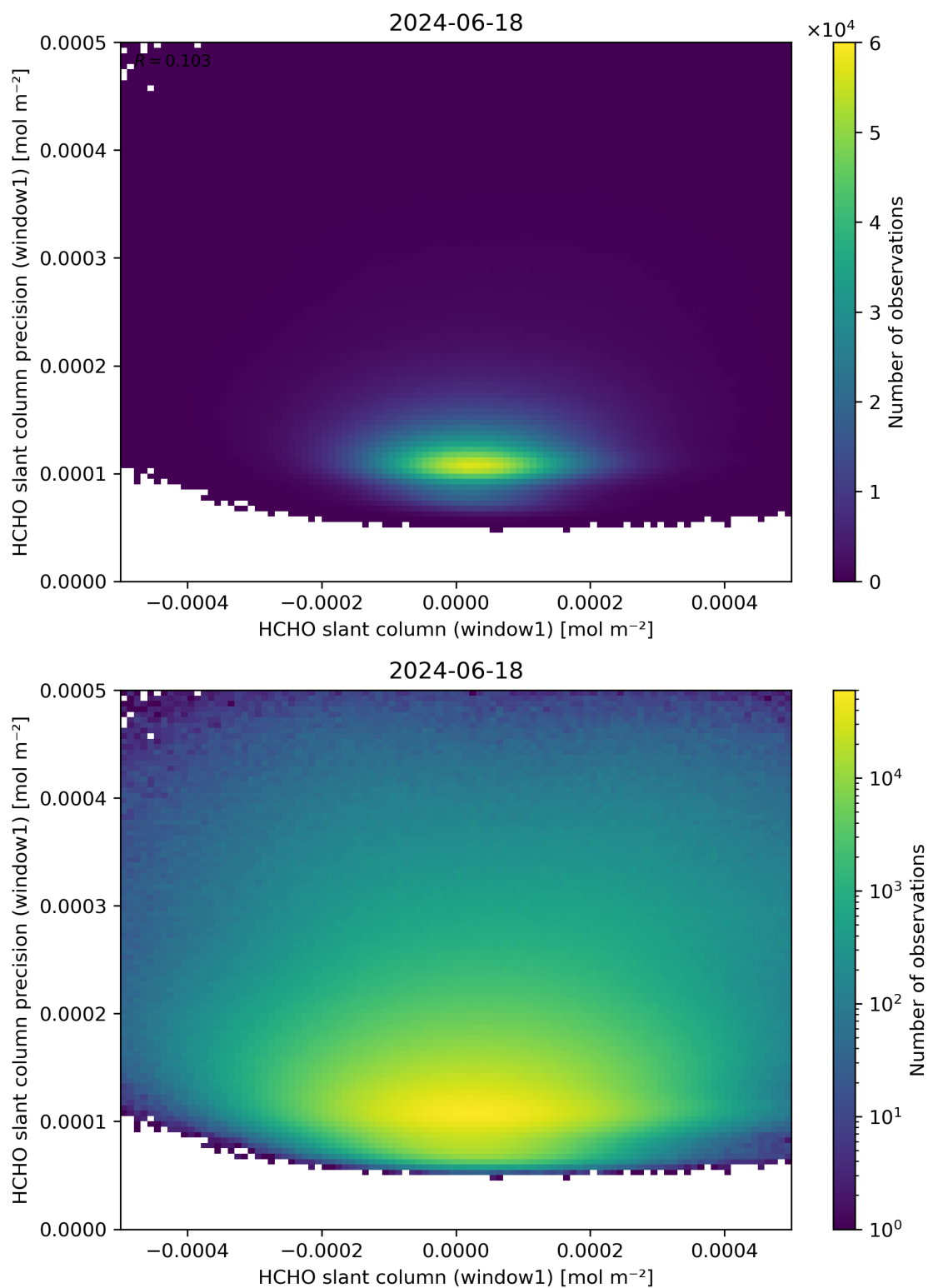
Figure 84: Scatter density plot of “HCHO slant column (window1)” against “HCHO slant column precision (window1)” for 2024-06-17 to 2024-06-19.
