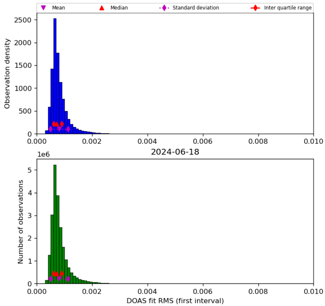
Figure 46: Histogram of “DOAS fit RMS (first interval)” for 2024-06-17 to 2024-06-19
