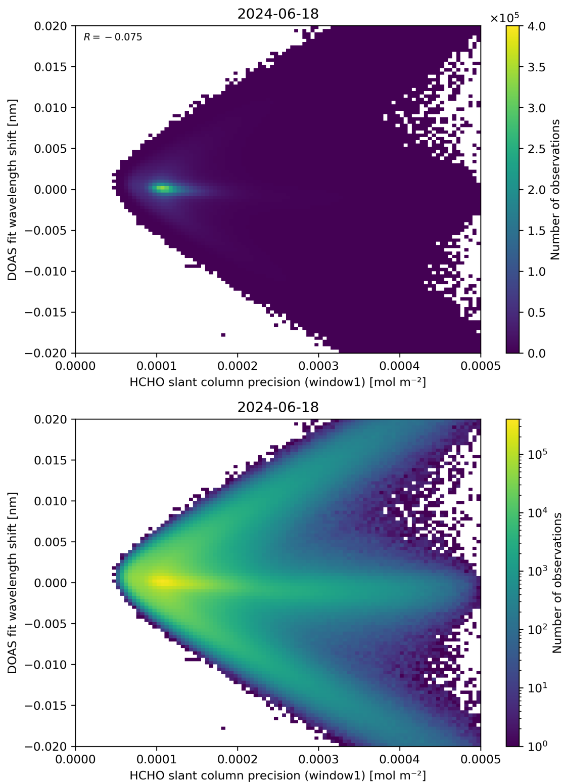
Figure 89: Scatter density plot of “HCHO slant column precision (window1)” against “DOAS fit wavelength shift” for 2024-06-17 to 2024-06-19.
