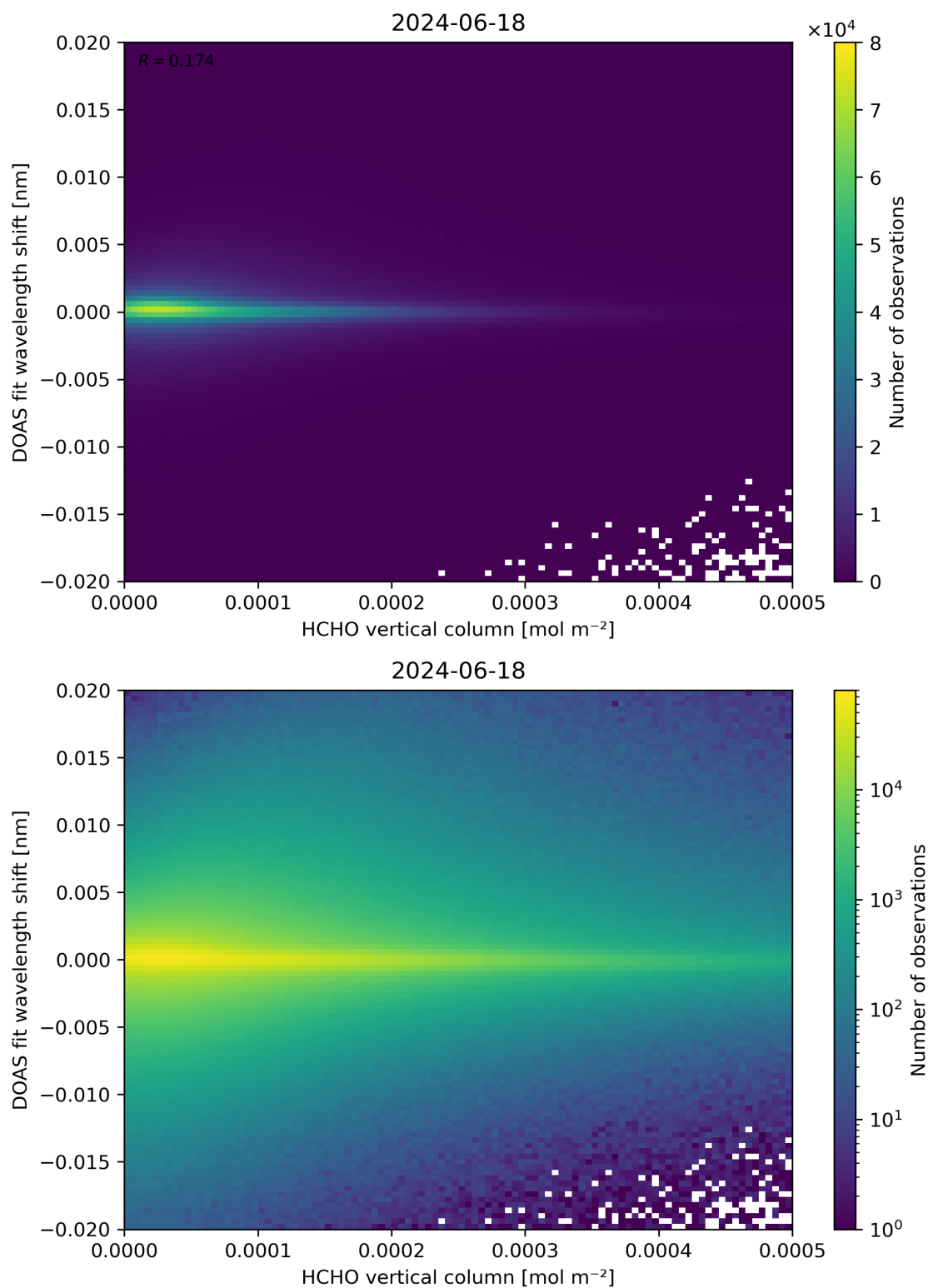
Figure 124: Scatter density plot of “HCHO vertical column” against “DOAS fit wavelength shift” for 2024-06-17 to 2024-06-19.
