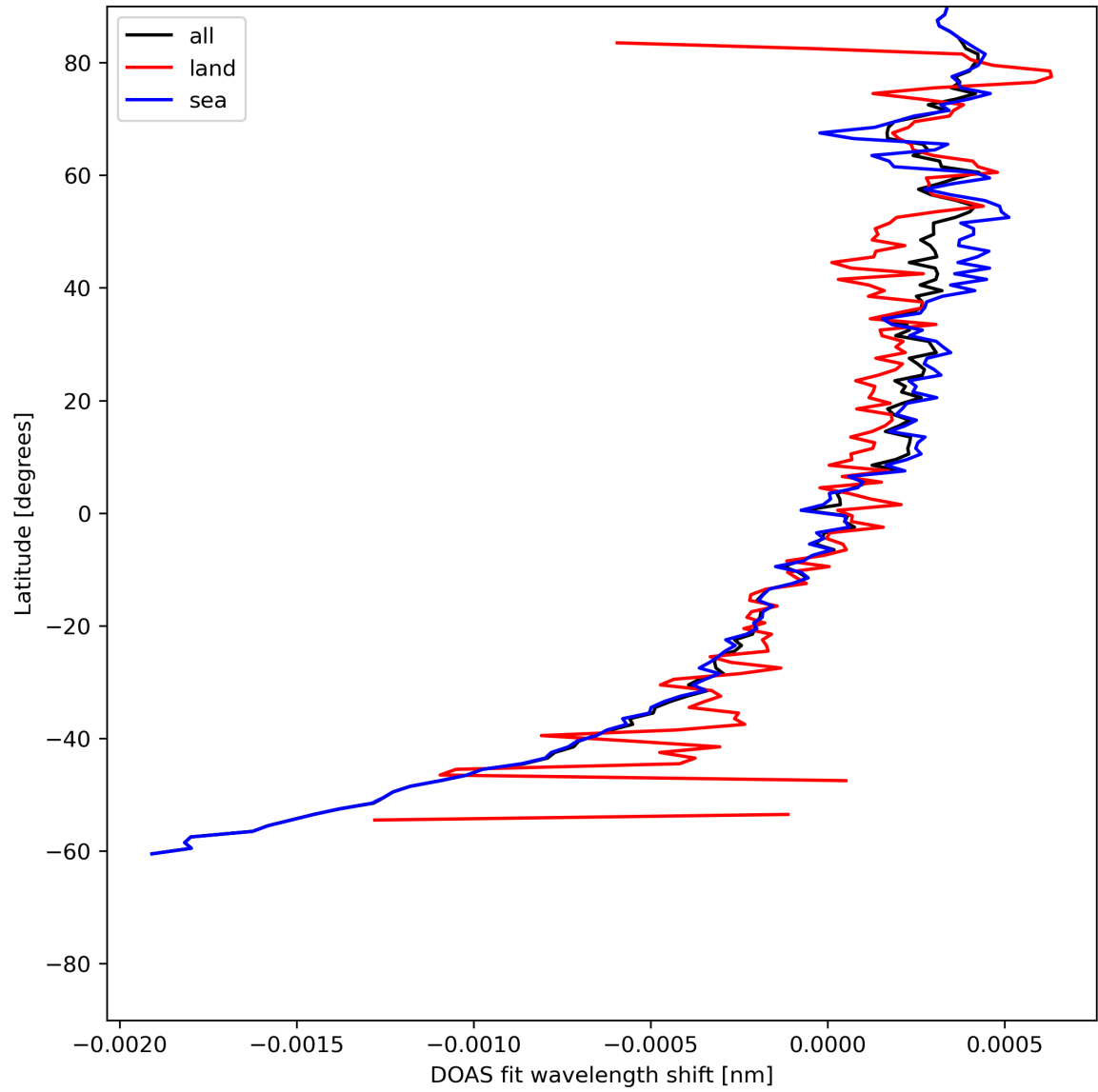
Figure 30: Zonal average of “DOAS fit wavelength shift” for 2024-06-17 to 2024-06-19.
