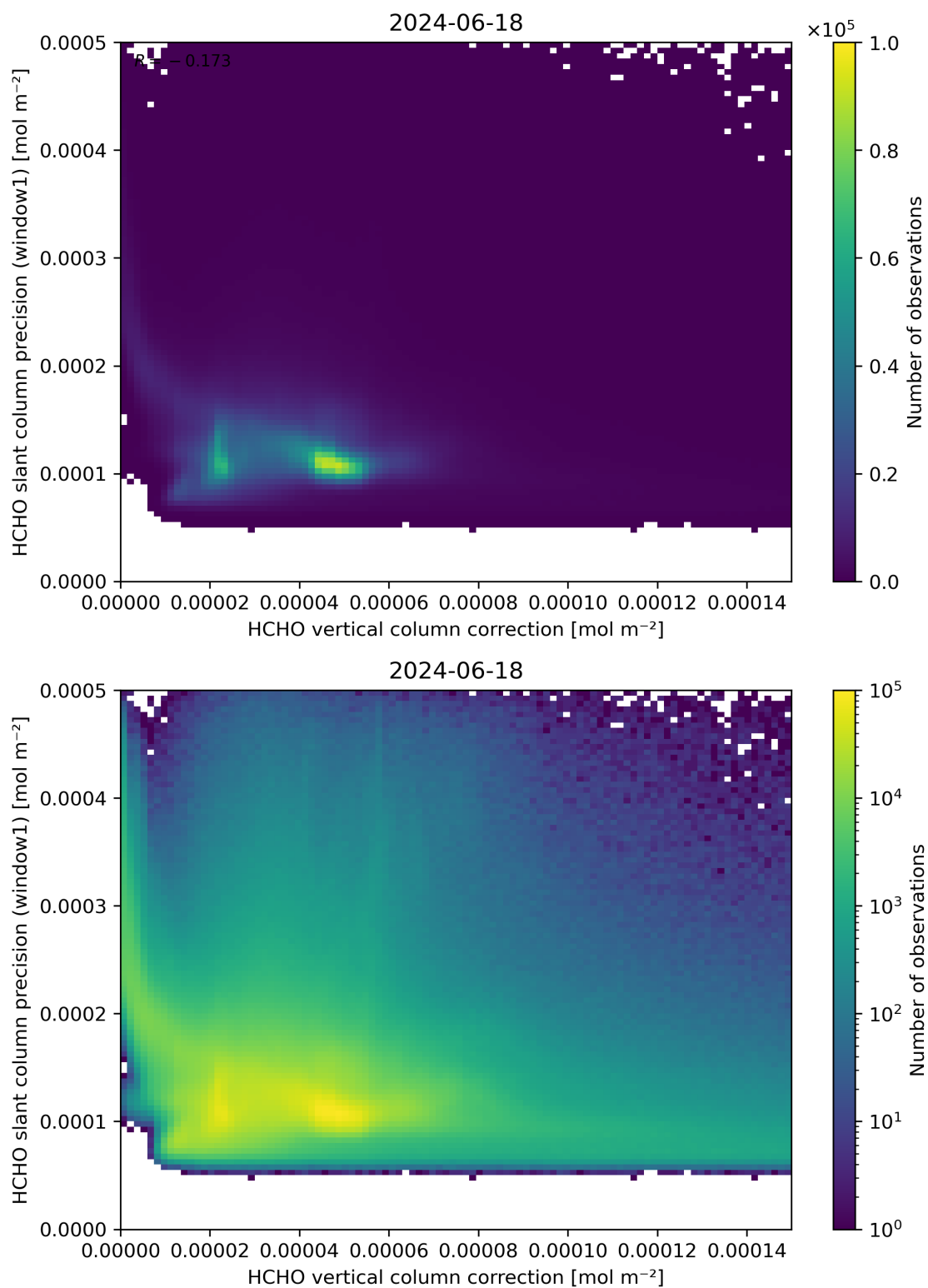
Figure 119: Scatter density plot of “HCHO vertical column correction” against “HCHO slant column precision (window1)” for 2024-06-17 to 2024-06-19.
