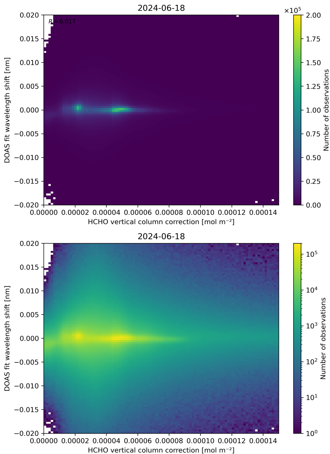
Figure 113: Scatter density plot of “HCHO vertical column correction” against “DOAS fit wavelength shift” for 2024-06-17 to 2024-06-19.
