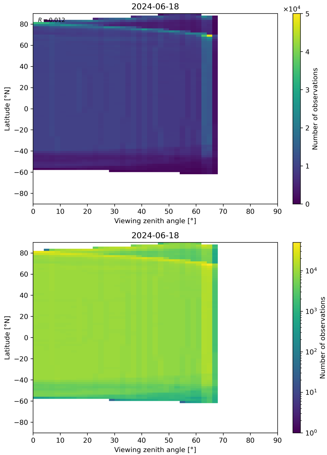
Figure 196: Scatter density plot of “Viewing zenith angle” against “Latitude” for 2024-06-17 to 2024-06-19.
