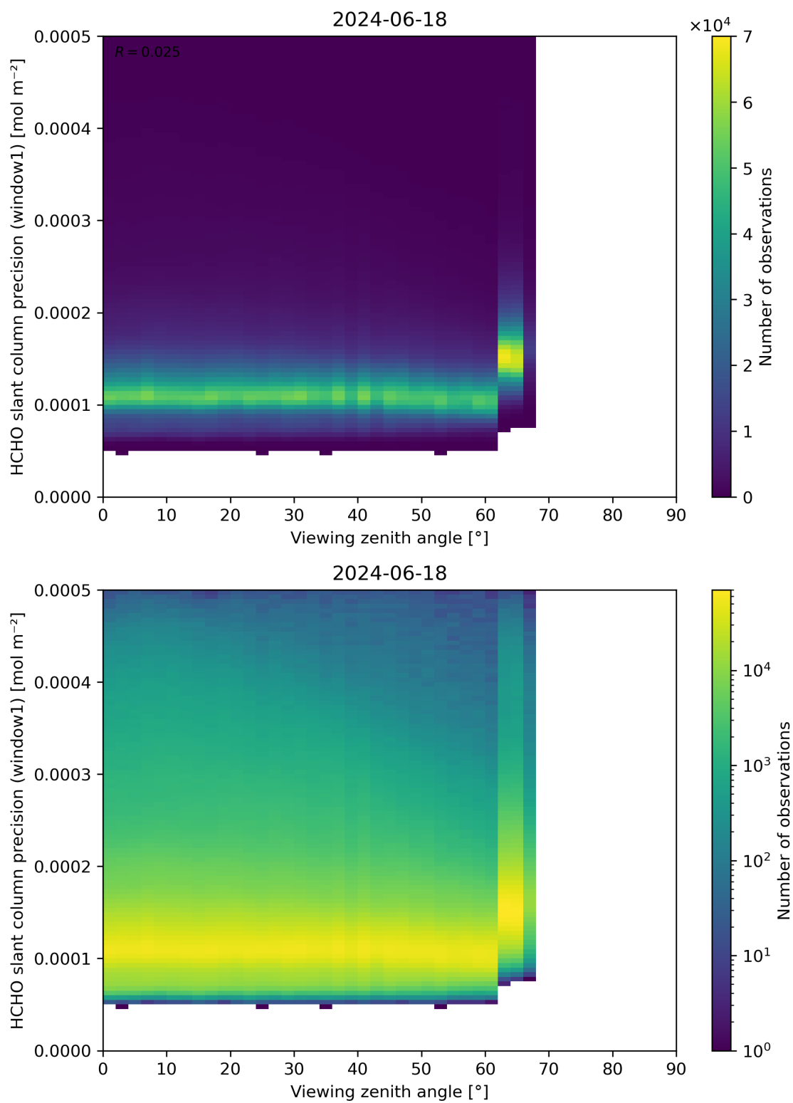
Figure 189: Scatter density plot of “Viewing zenith angle” against “HCHO slant column precision (window1)” for 2024-06-17 to 2024-06-19.
