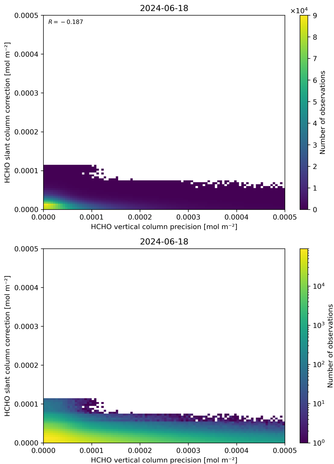
Figure 141: Scatter density plot of “HCHO vertical column precision” against “HCHO slant column correction” for 2024-06-17 to 2024-06-19.
