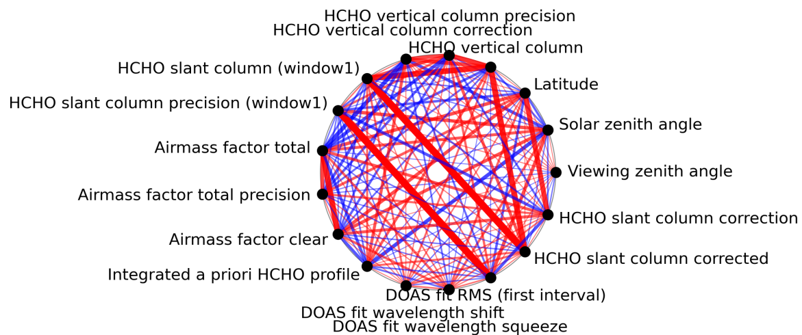
Figure 1: Map of correlation graph for 2024-06-17 to 2024-06-19.
