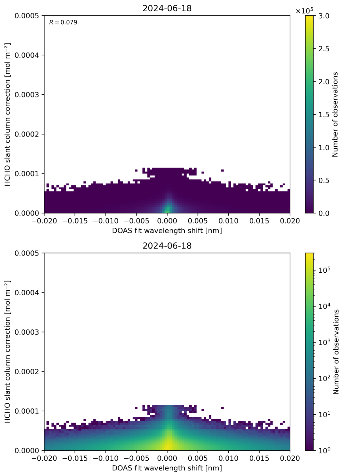
Figure 67: Scatter density plot of “DOAS fit wavelength shift” against “HCHO slant column correction” for 2024-06-17 to 2024-06-19.
