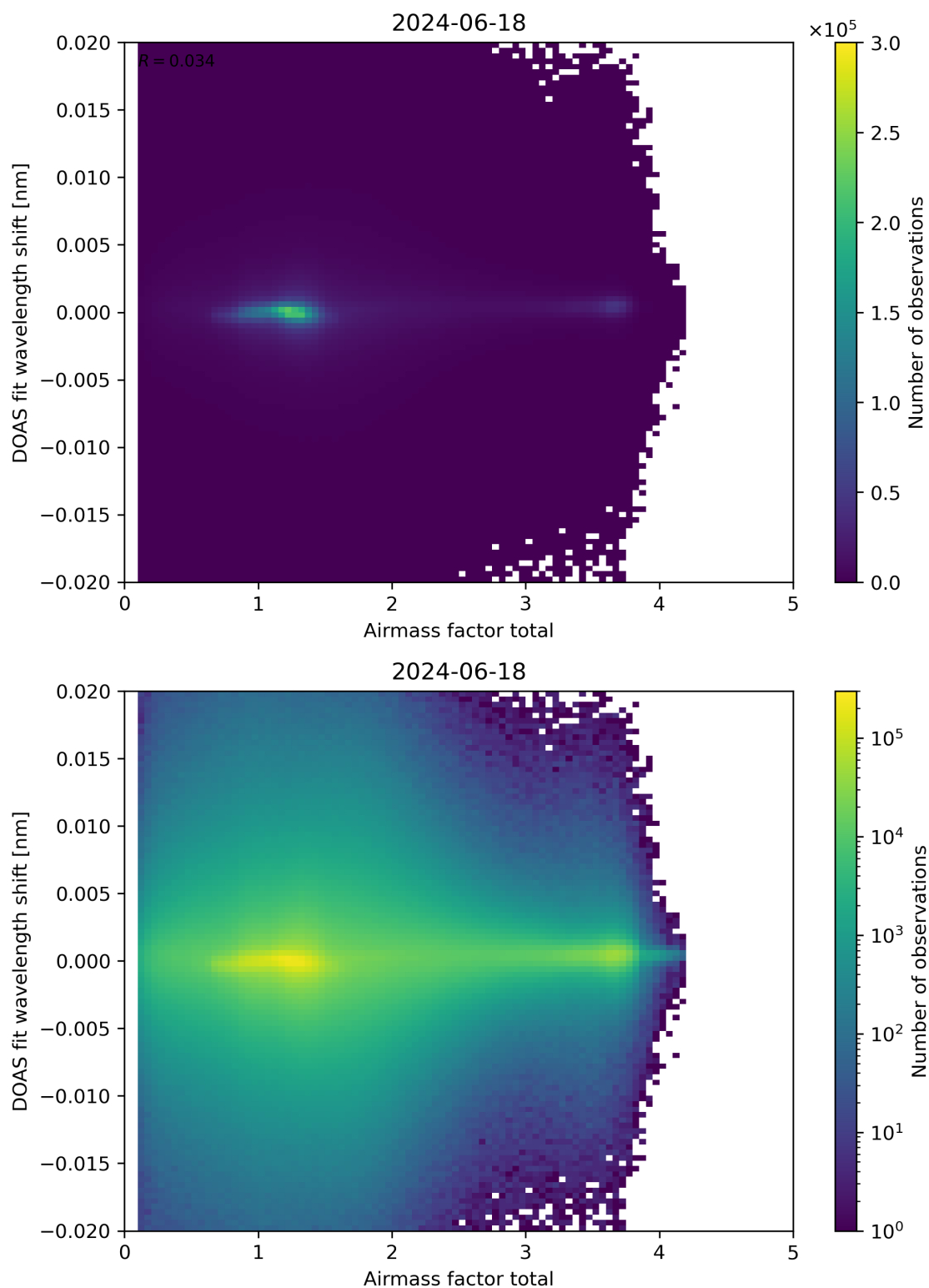
Figure 98: Scatter density plot of “Airmass factor total” against “DOAS fit wavelength shift” for 2024-06-17 to 2024-06-19.
