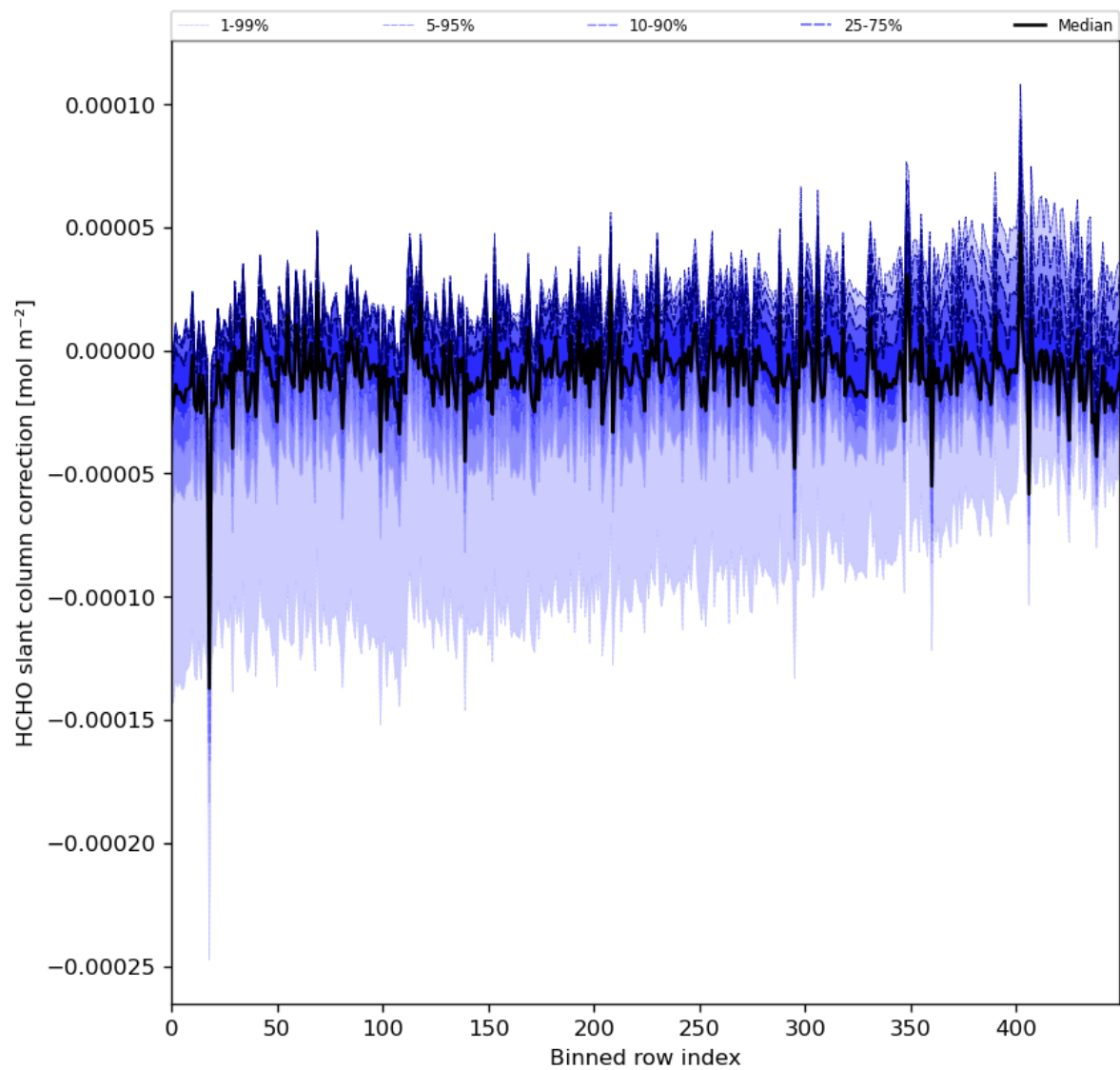
Figure 61: Along track statistics of “HCHO slant column correction” for 2024-06-17 to 2024-06-19
