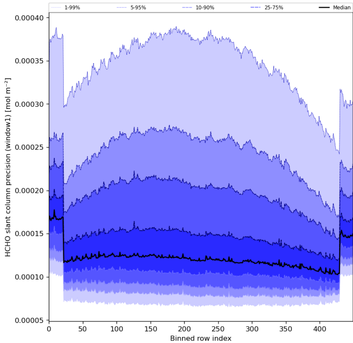
Figure 53: Along track statistics of “HCHO slant column precision (window1)” for 2024-06-17 to 2024-06-19
