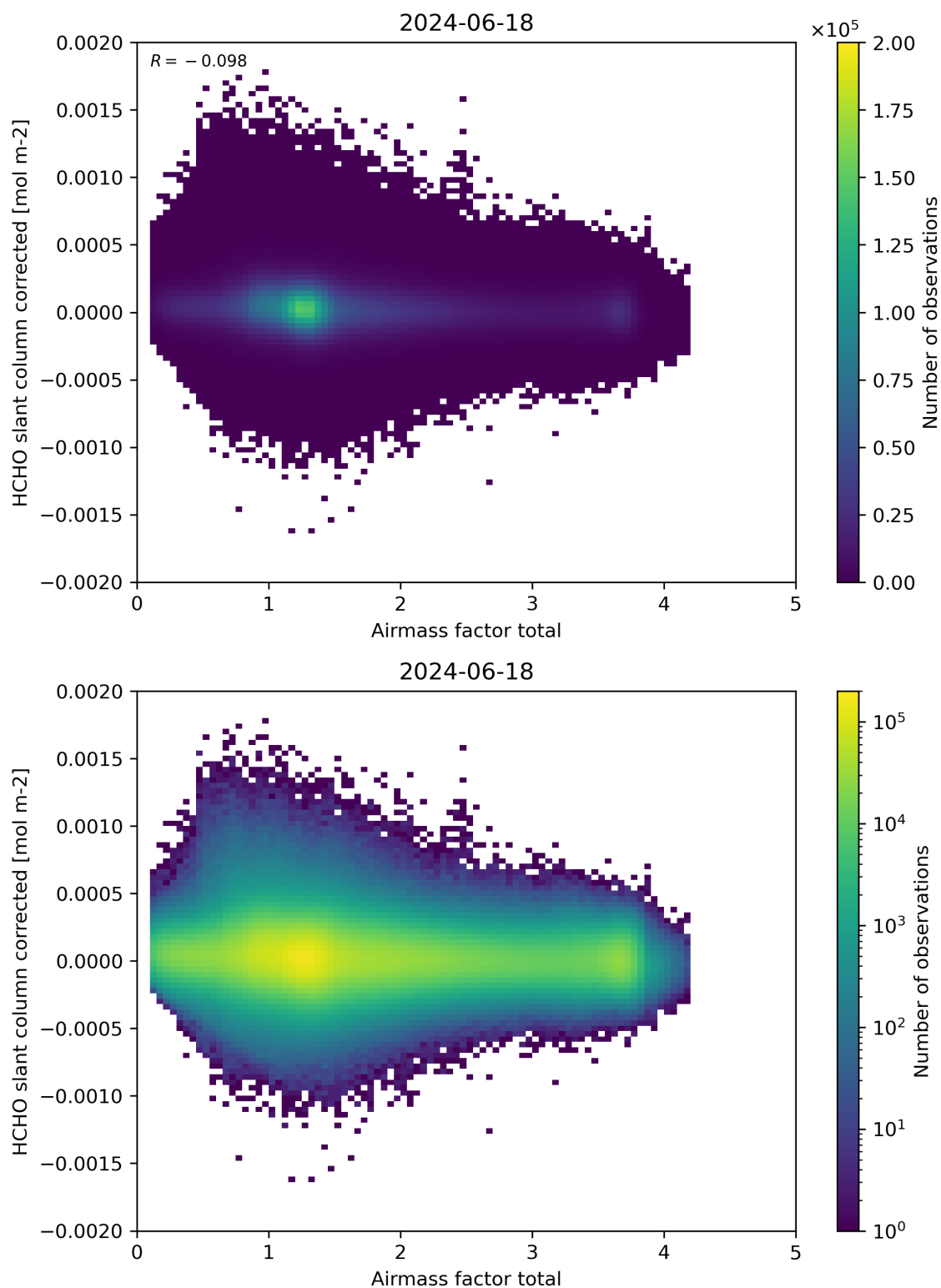
Figure 101: Scatter density plot of “Airmass factor total” against “HCHO slant column corrected” for 2024-06-17 to 2024-06-19.
