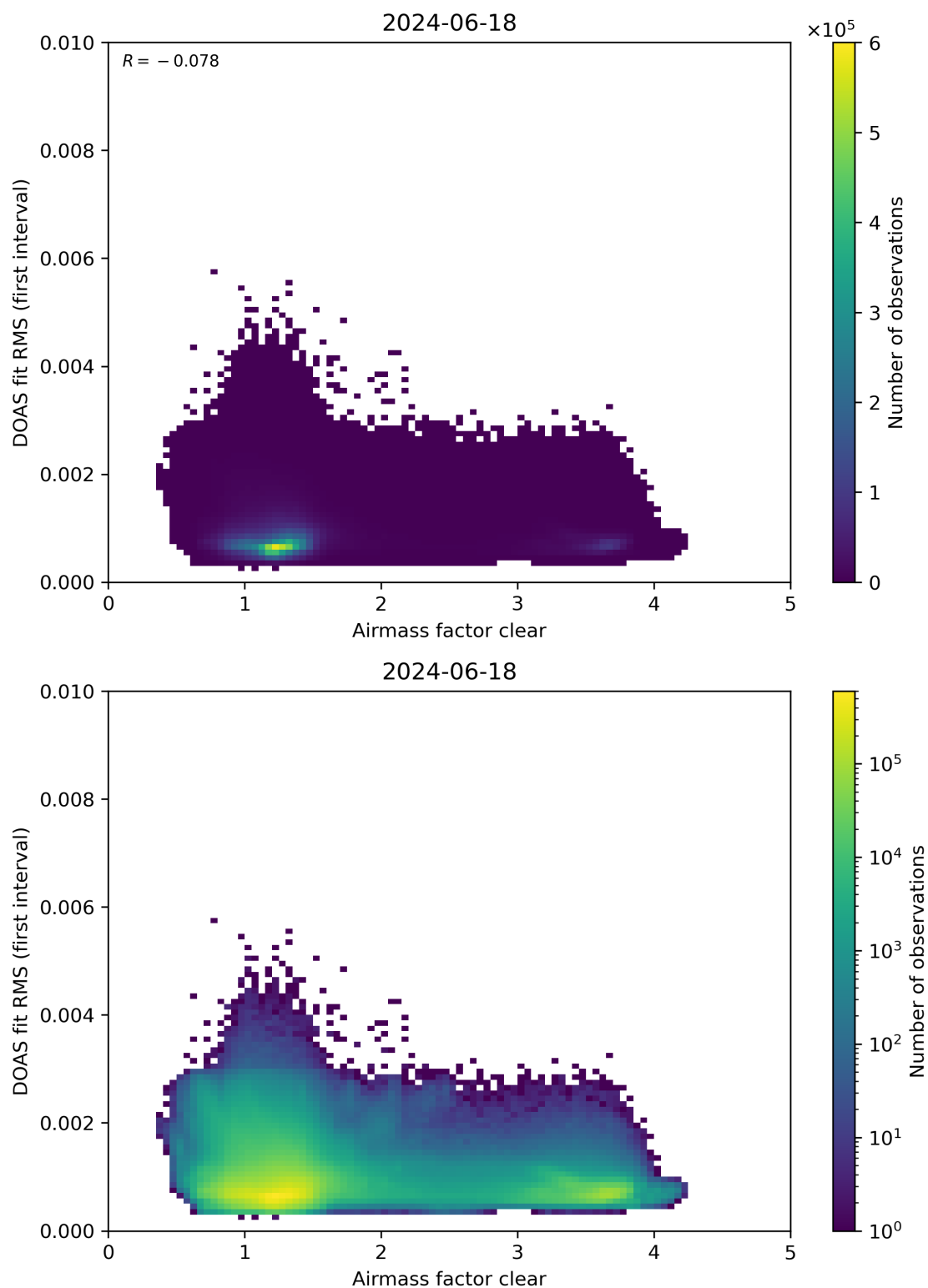
Figure 71: Scatter density plot of “Airmass factor clear” against “DOAS fit RMS (first interval)” for 2024-06-17 to 2024-06-19.
