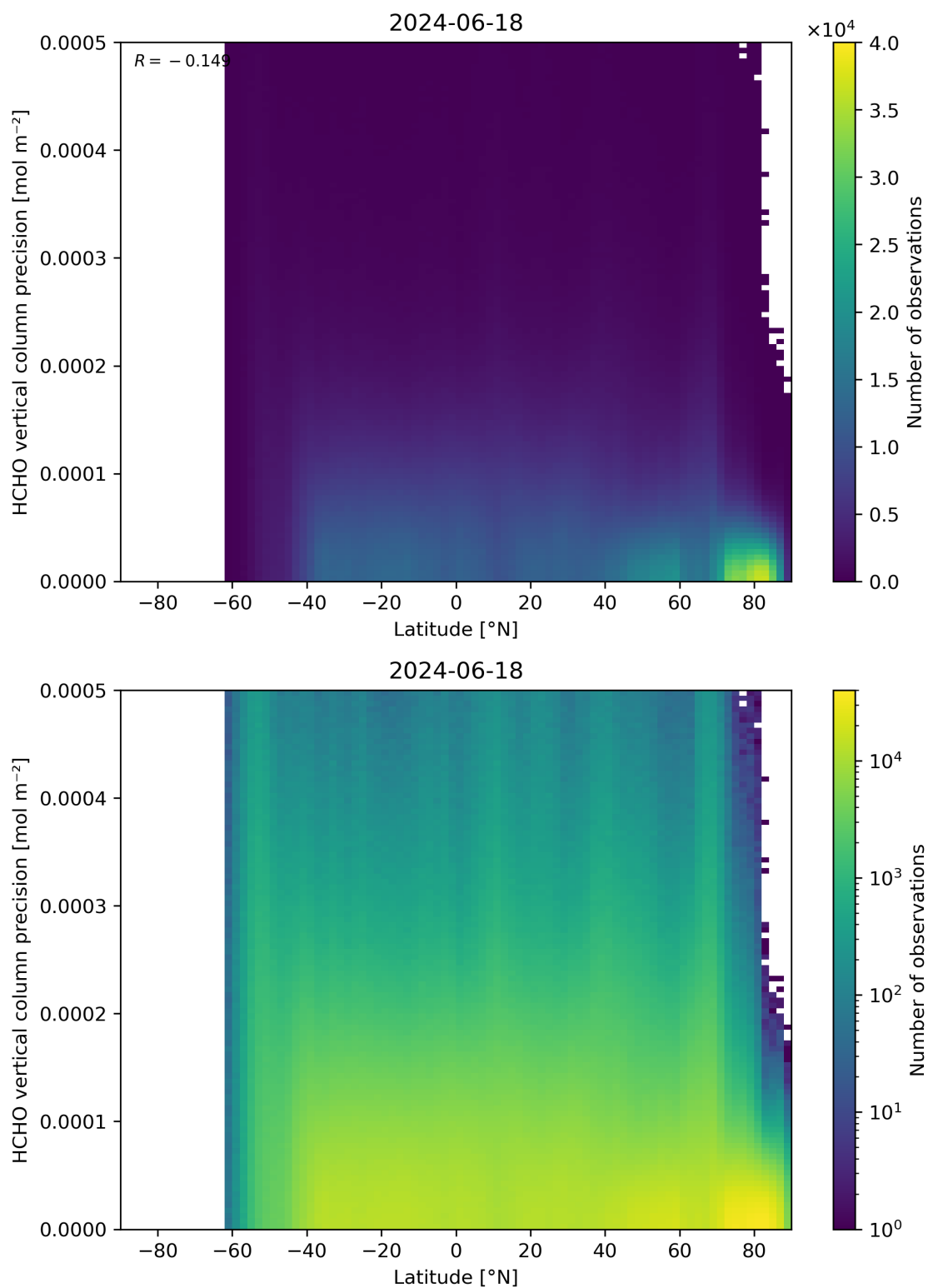
Figure 165: Scatter density plot of “Latitude” against “HCHO vertical column precision” for 2024-06-17 to 2024-06-19.
