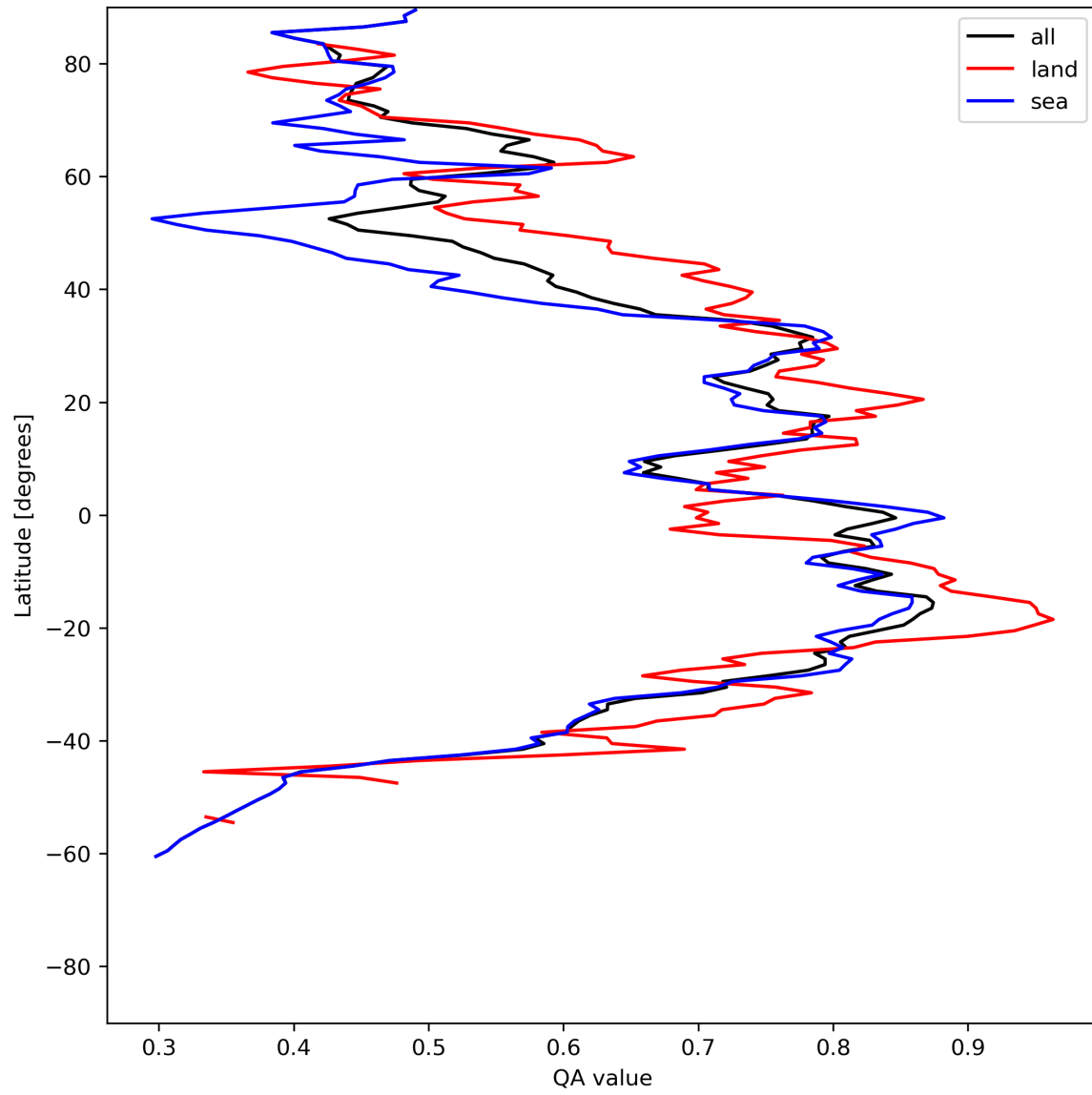
Figure 20: Zonal average of “QA value” for 2024-06-17 to 2024-06-19.
