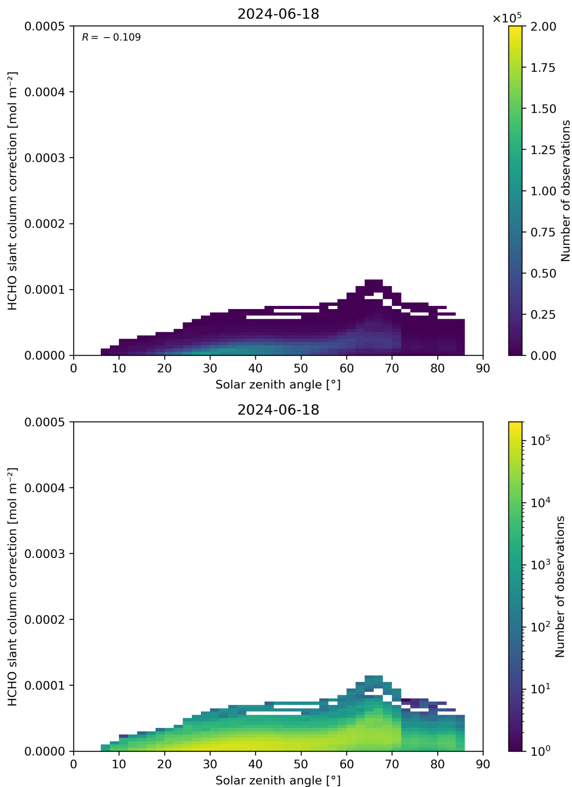
Figure 172: Scatter density plot of “Solar zenith angle” against “HCHO slant column correction” for 2024-06-17 to 2024-06-19.
