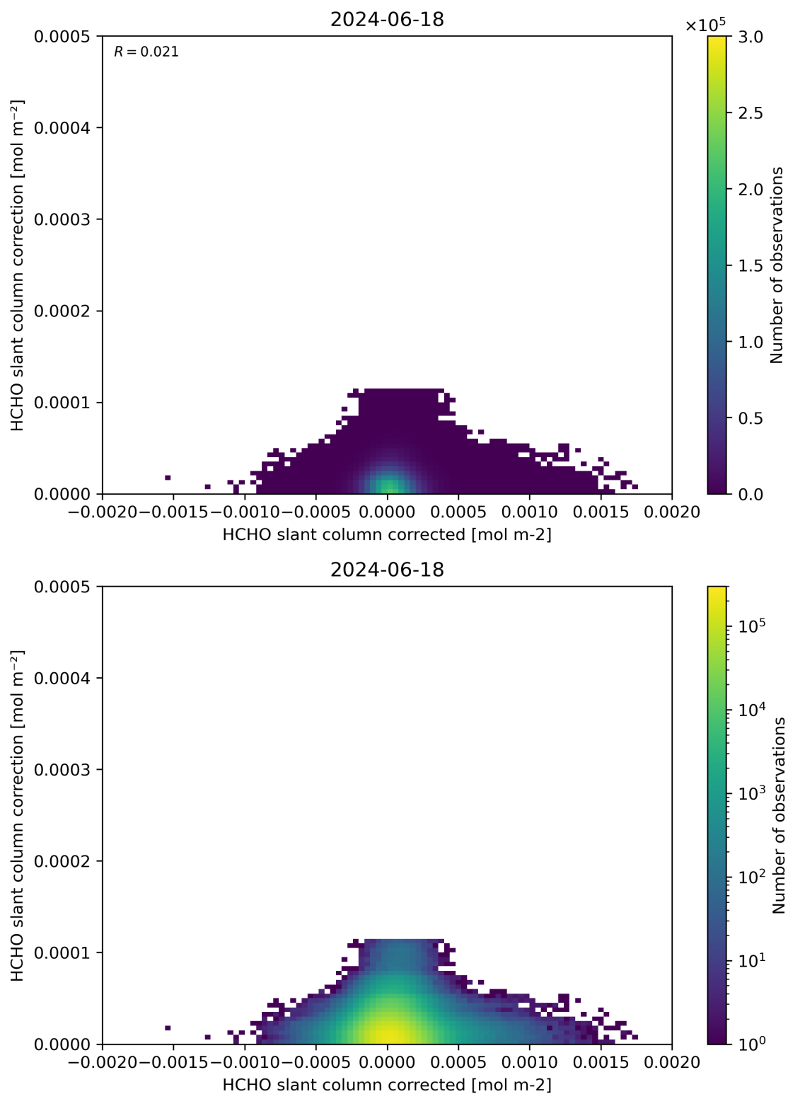
Figure 77: Scatter density plot of “HCHO slant column corrected” against “HCHO slant column correction” for 2024-06-17 to 2024-06-19.
