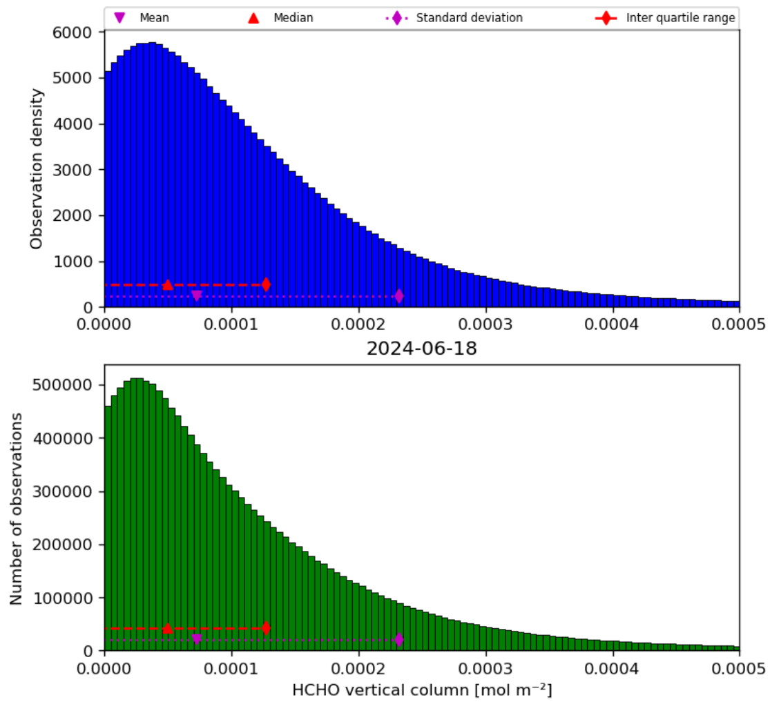
Figure 35: Histogram of “HCHO vertical column” for 2024-06-17 to 2024-06-19
