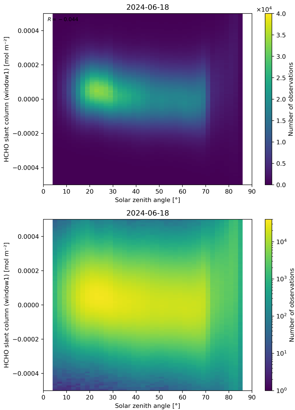
Figure 173: Scatter density plot of “Solar zenith angle” against “HCHO slant column (window1)” for 2024-06-17 to 2024-06-19.
