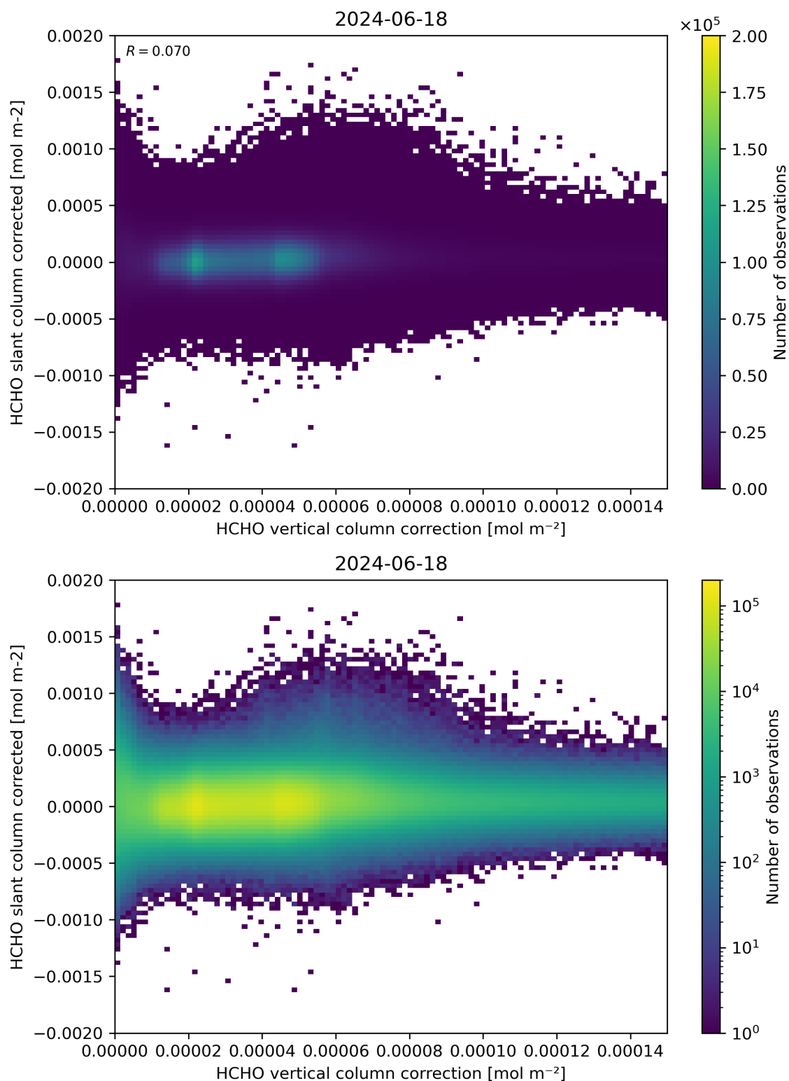
Figure 116: Scatter density plot of “HCHO vertical column correction” against “HCHO slant column corrected” for 2024-06-17 to 2024-06-19.
