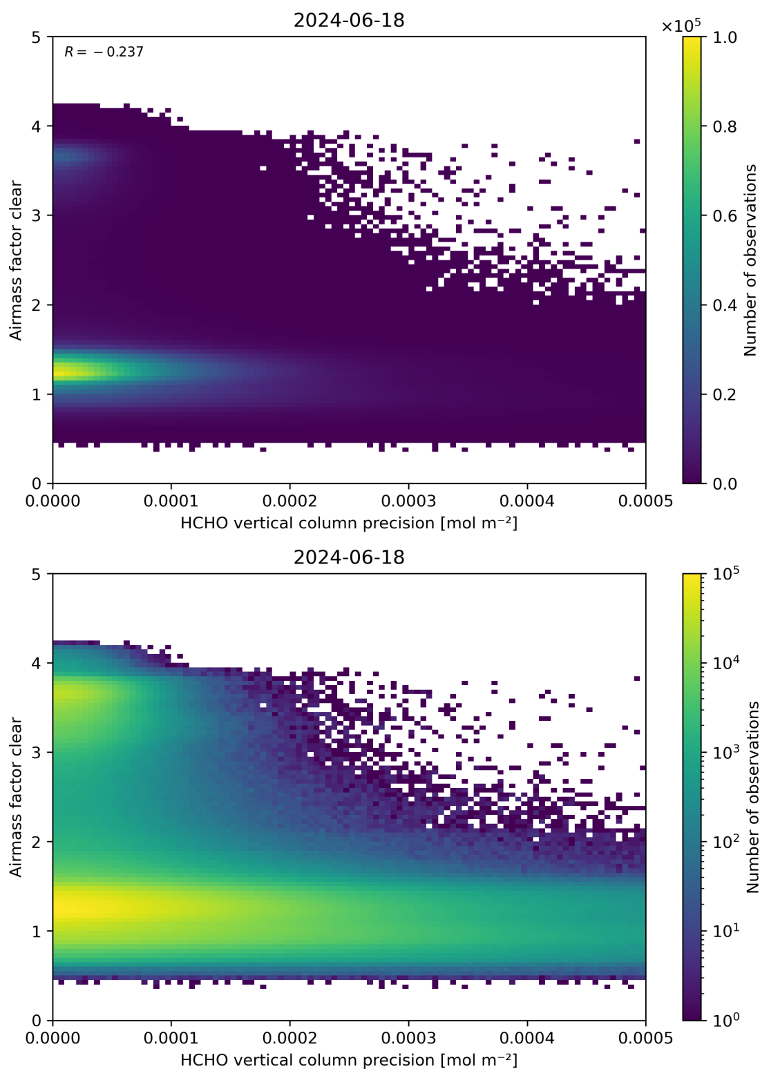
Figure 139: Scatter density plot of “HCHO vertical column precision” against “Airmass factor clear” for 2024-06-17 to 2024-06-19.
