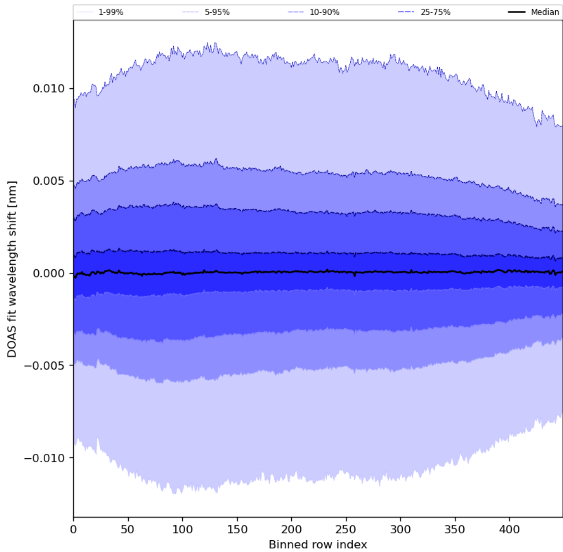
Figure 58: Along track statistics of “DOAS fit wavelength shift” for 2024-06-17 to 2024-06-19
