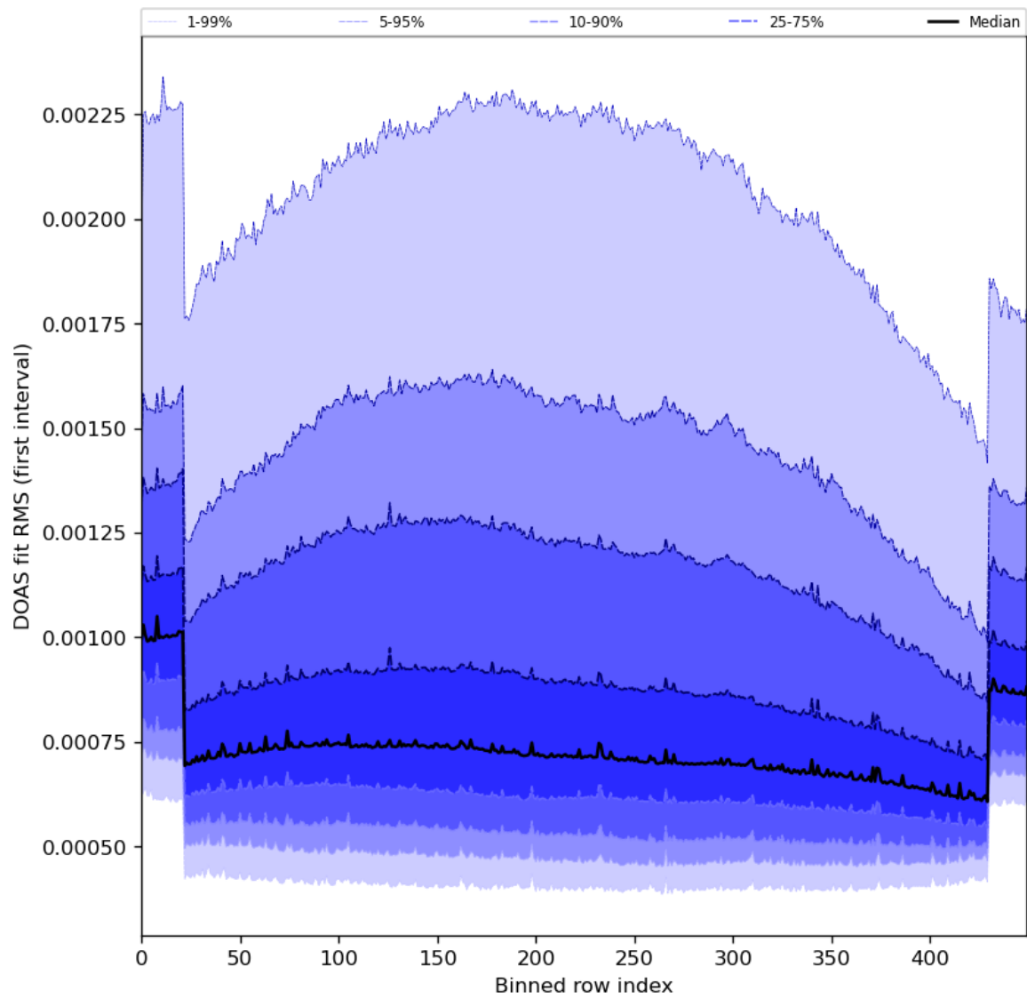
Figure 60: Along track statistics of “DOAS fit RMS (first interval)” for 2024-06-17 to 2024-06-19
