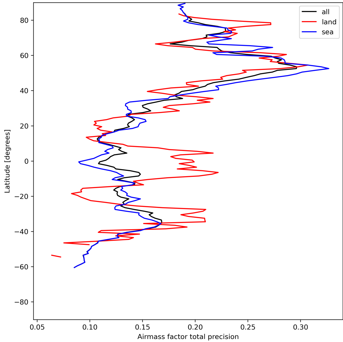
Figure 27: Zonal average of “Airmass factor total precision” for 2024-06-17 to 2024-06-19.
