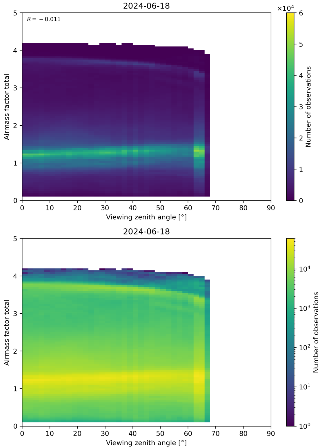
Figure 190: Scatter density plot of “Viewing zenith angle” against “Airmass factor total” for 2024-06-17 to 2024-06-19.
