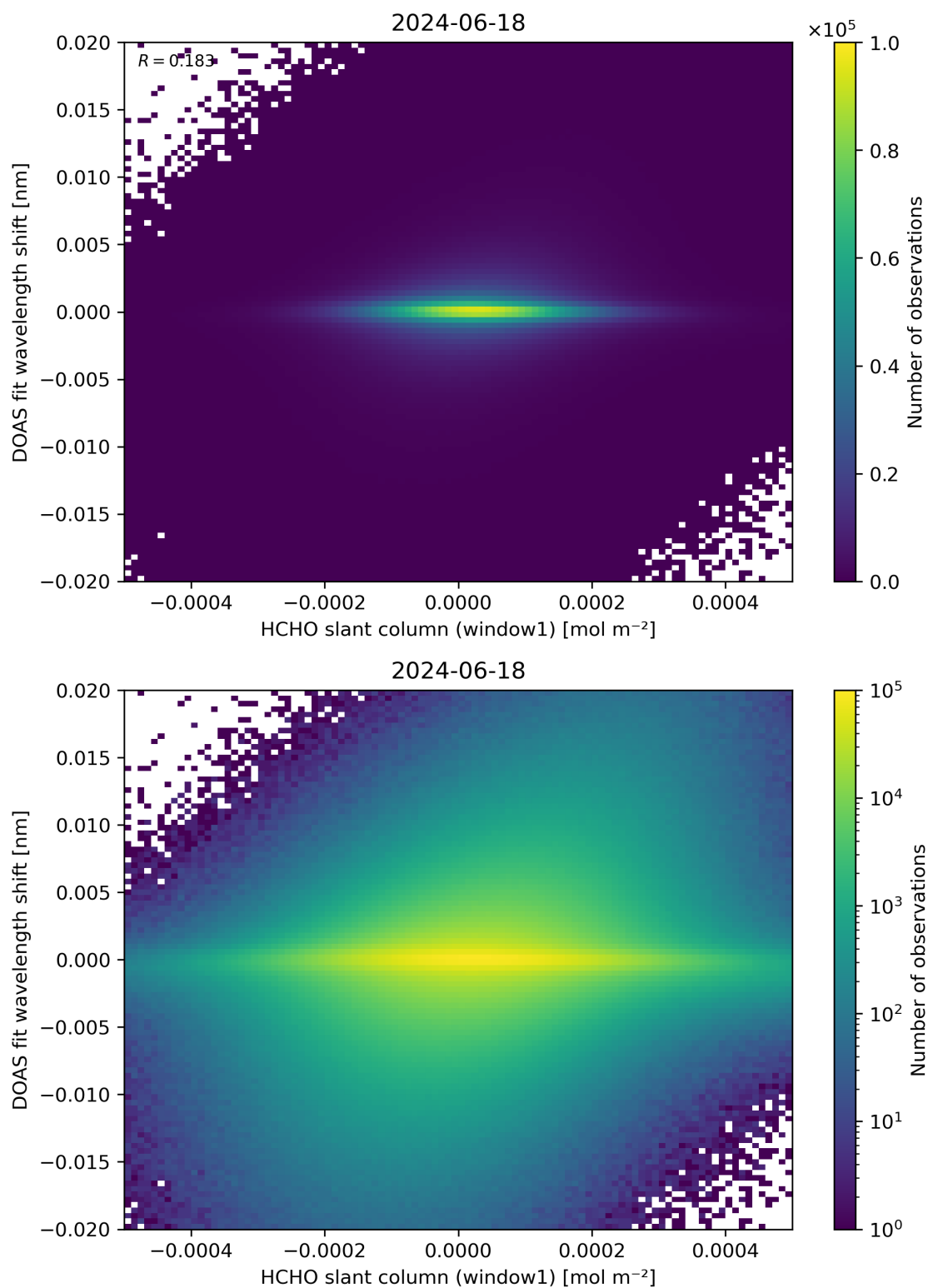
Figure 79: Scatter density plot of “HCHO slant column (window1)” against “DOAS fit wavelength shift” for 2024-06-17 to 2024-06-19.
