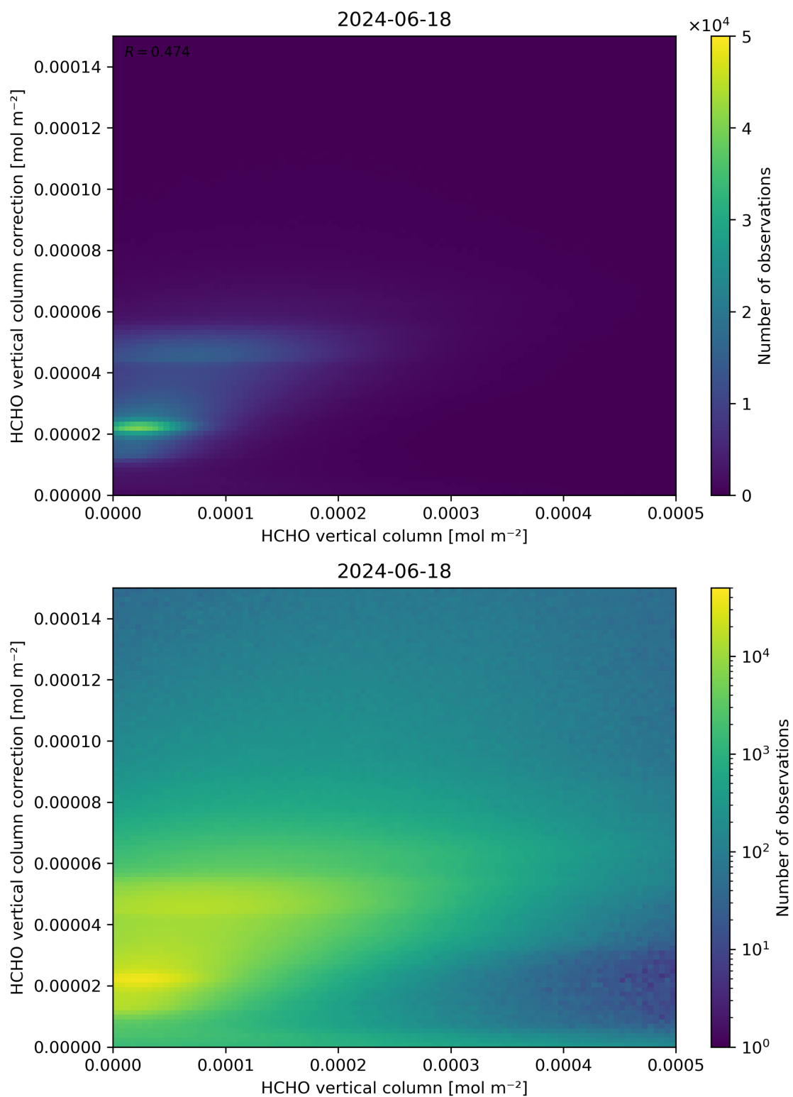
Figure 133: Scatter density plot of “HCHO vertical column” against “HCHO vertical column correction” for 2024-06-17 to 2024-06-19.
