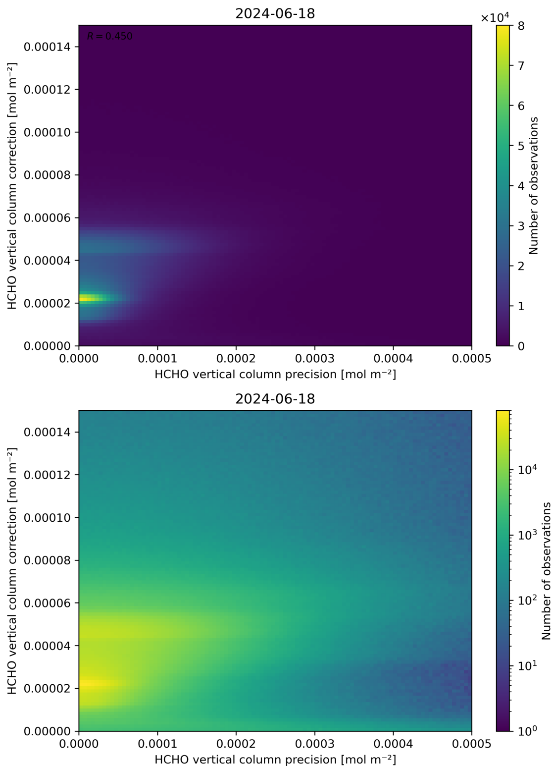
Figure 146: Scatter density plot of “HCHO vertical column precision” against “HCHO vertical column correction” for 2024-06-17 to 2024-06-19.
