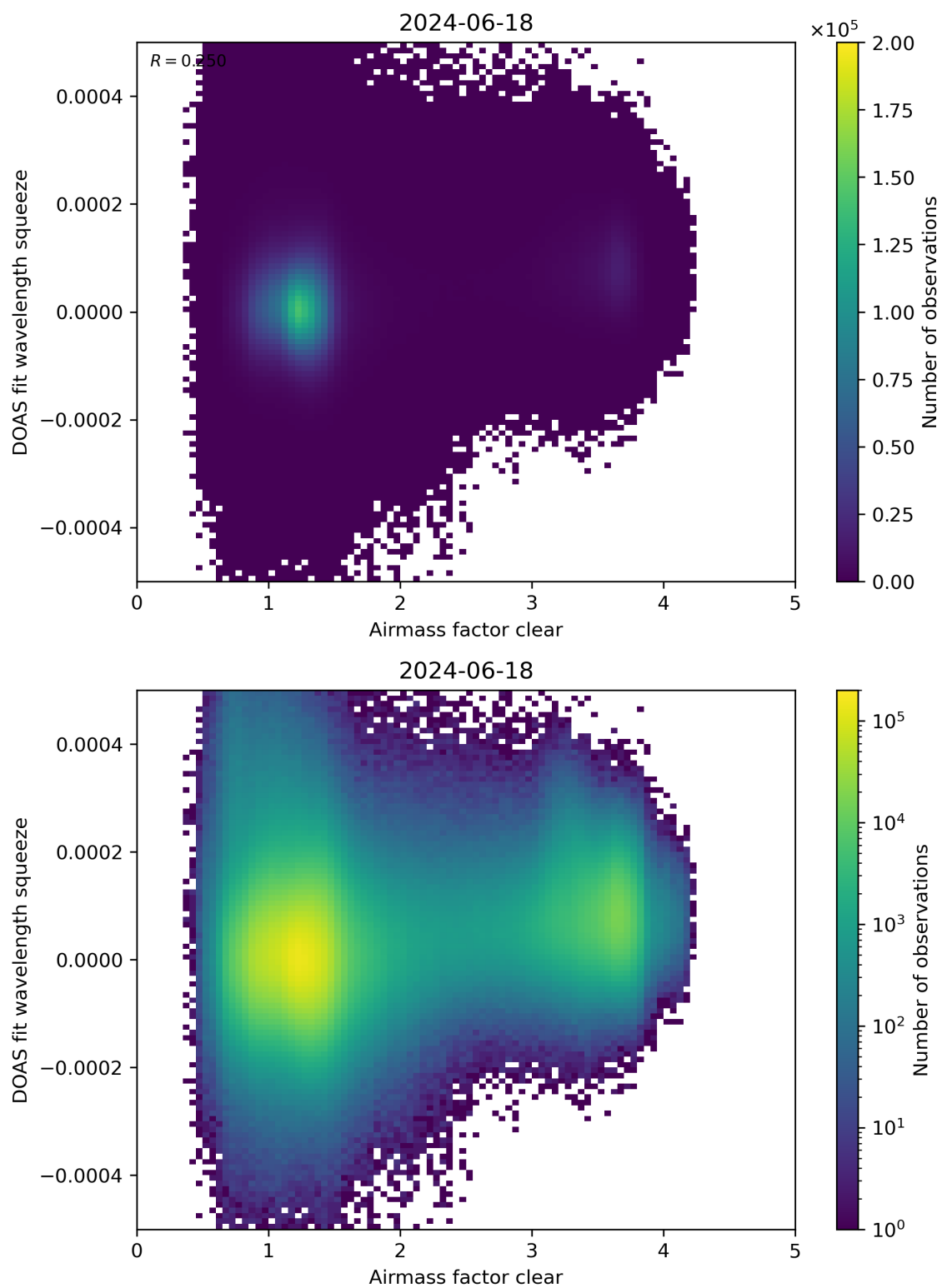
Figure 73: Scatter density plot of “Airmass factor clear” against “DOAS fit wavelength squeeze” for 2024-06-17 to 2024-06-19.
