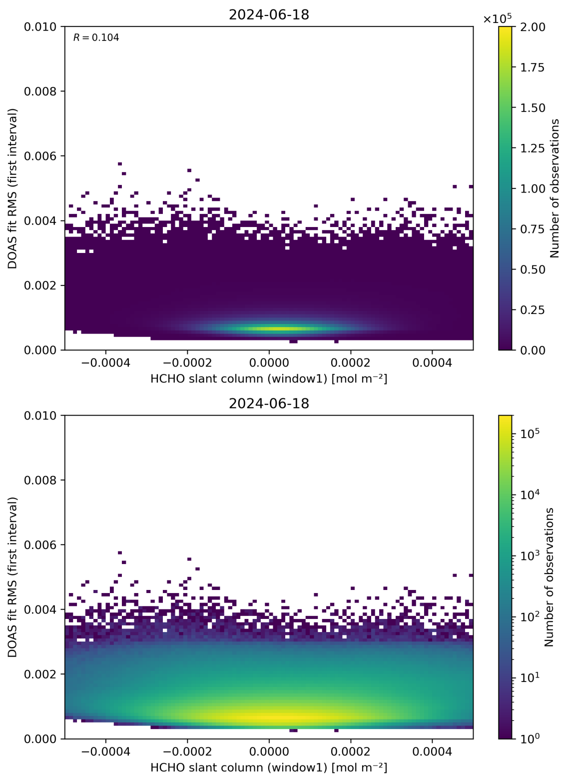
Figure 78: Scatter density plot of “HCHO slant column (window1)” against “DOAS fit RMS (first interval)” for 2024-06-17 to 2024-06-19.
