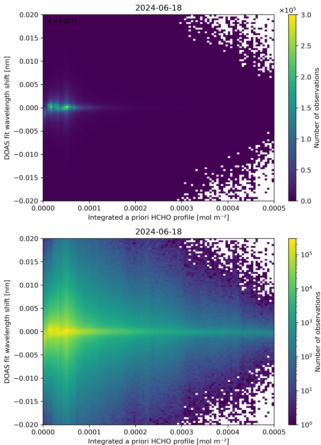
Figure 149: Scatter density plot of “Integrated a priori HCHO profile” against “DOAS fit wavelength shift” for 2024-06-17 to 2024-06-19.
