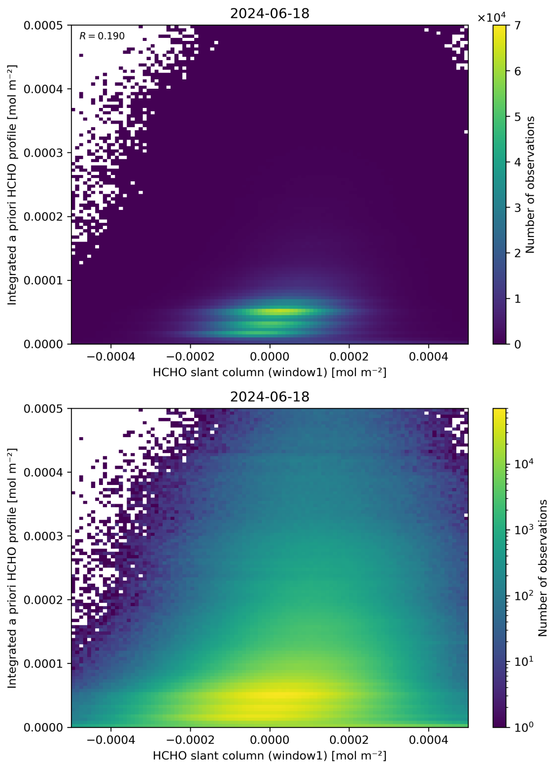
Figure 87: Scatter density plot of “HCHO slant column (window1)” against “Integrated a priori HCHO profile” for 2024-06-17 to 2024-06-19.
