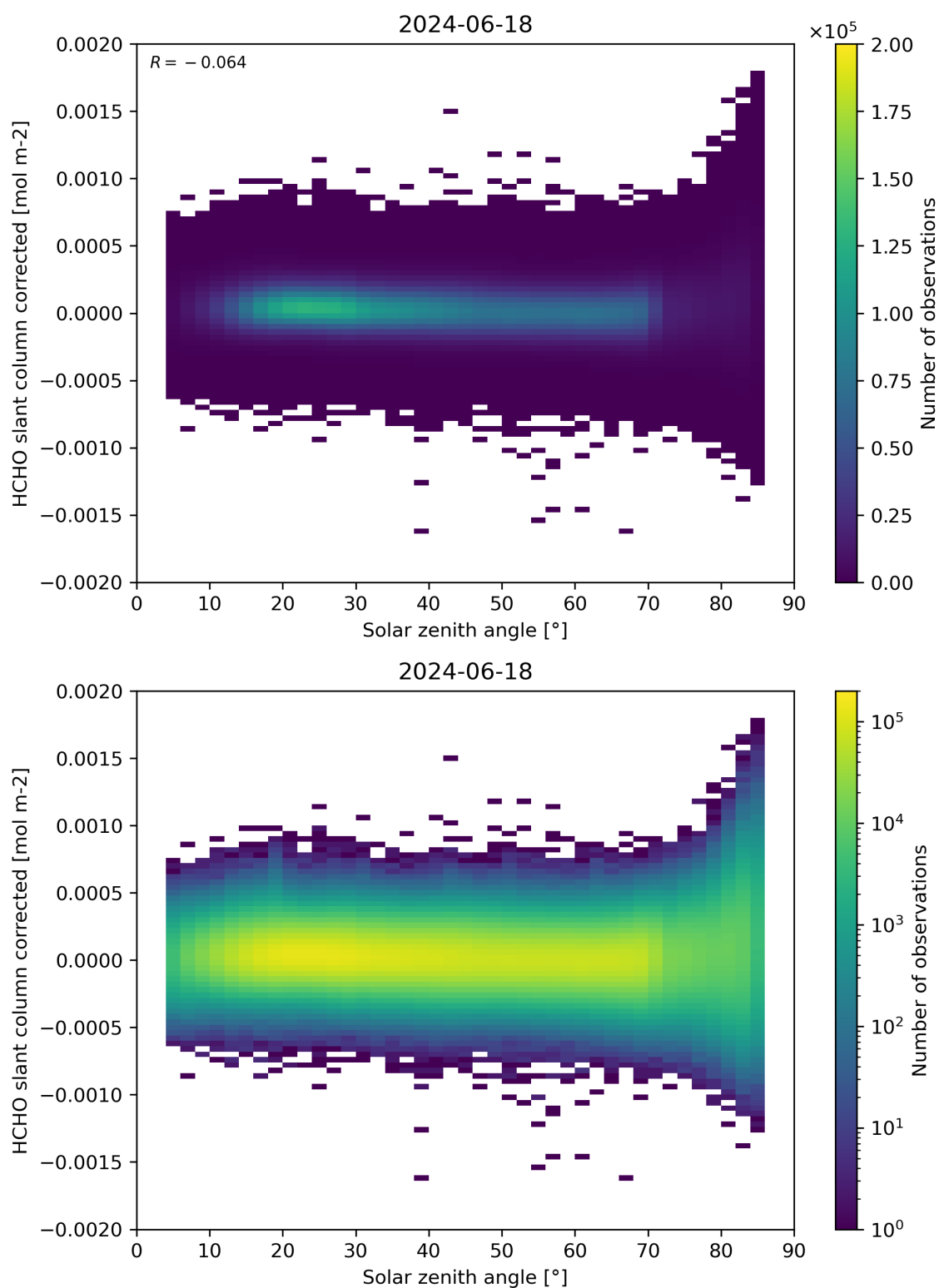
Figure 171: Scatter density plot of “Solar zenith angle” against “HCHO slant column corrected” for 2024-06-17 to 2024-06-19.
