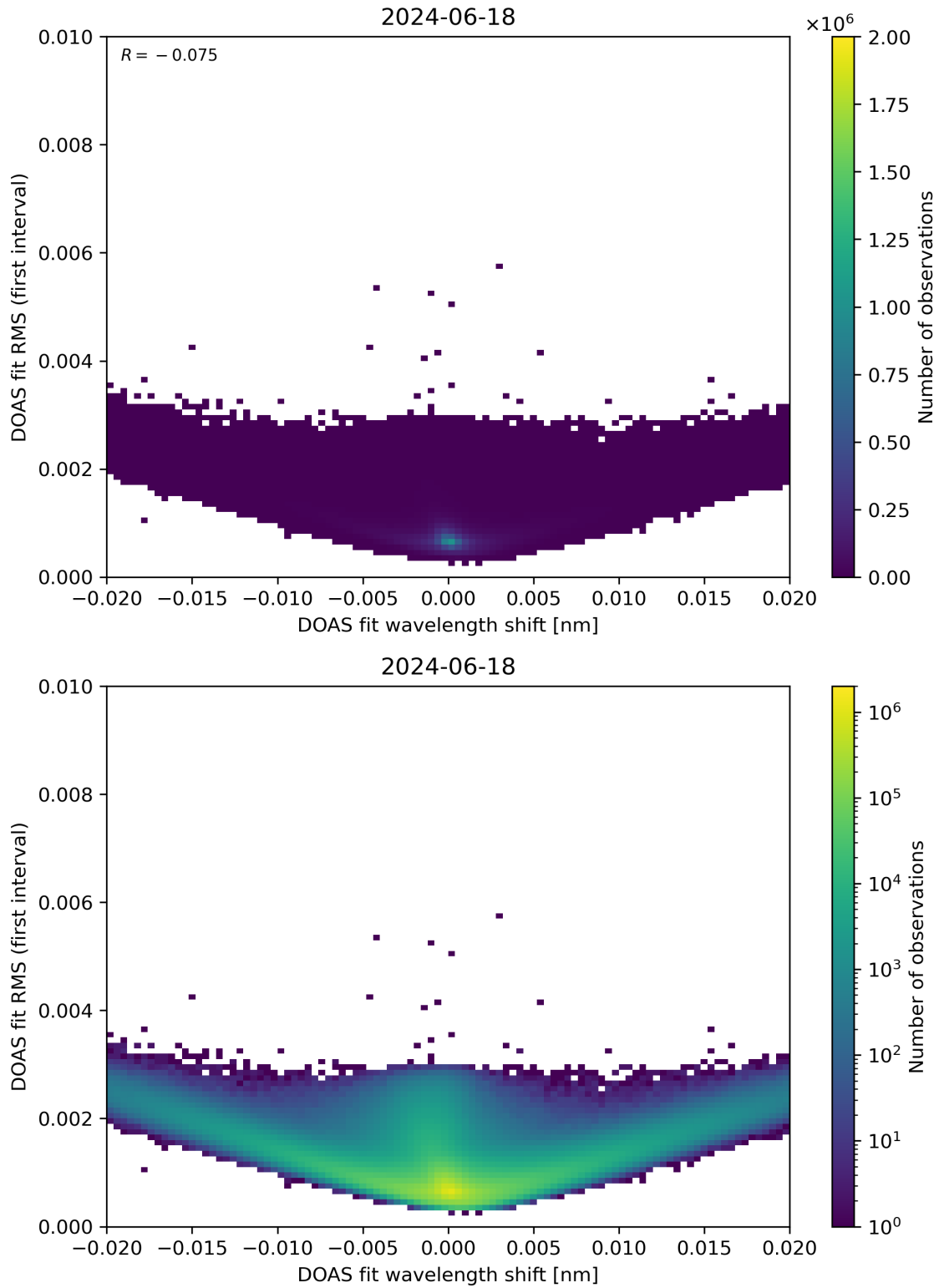
Figure 64: Scatter density plot of “DOAS fit wavelength shift” against “DOAS fit RMS (first interval)” for 2024-06-17 to 2024-06-19.
