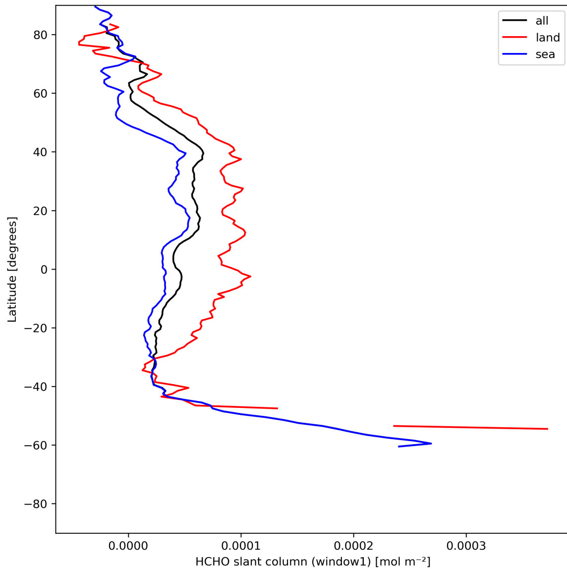
Figure 24: Zonal average of “HCHO slant column (window1)” for 2024-06-17 to 2024-06-19.
