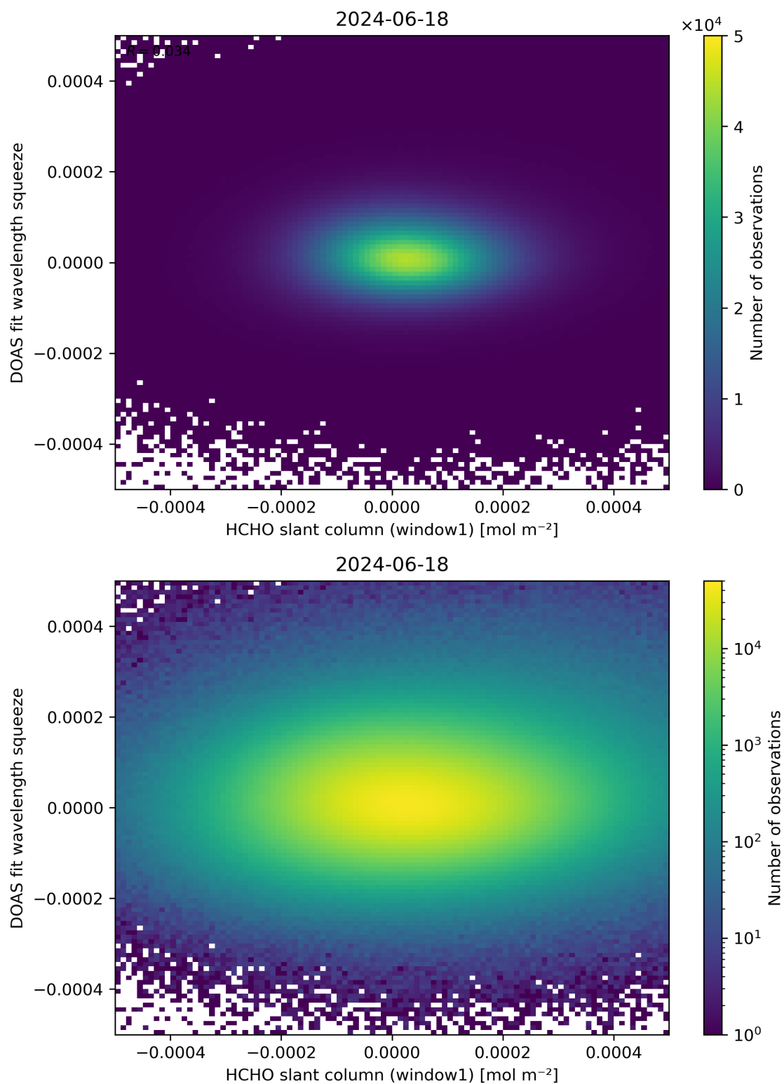
Figure 80: Scatter density plot of “HCHO slant column (window1)” against “DOAS fit wavelength squeeze” for 2024-06-17 to 2024-06-19.
