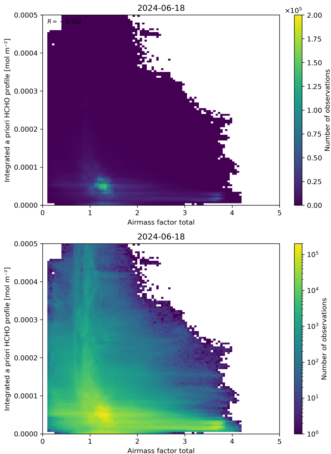
Figure 104: Scatter density plot of “Airmass factor total” against “Integrated a priori HCHO profile” for 2024-06-17 to 2024-06-19.
