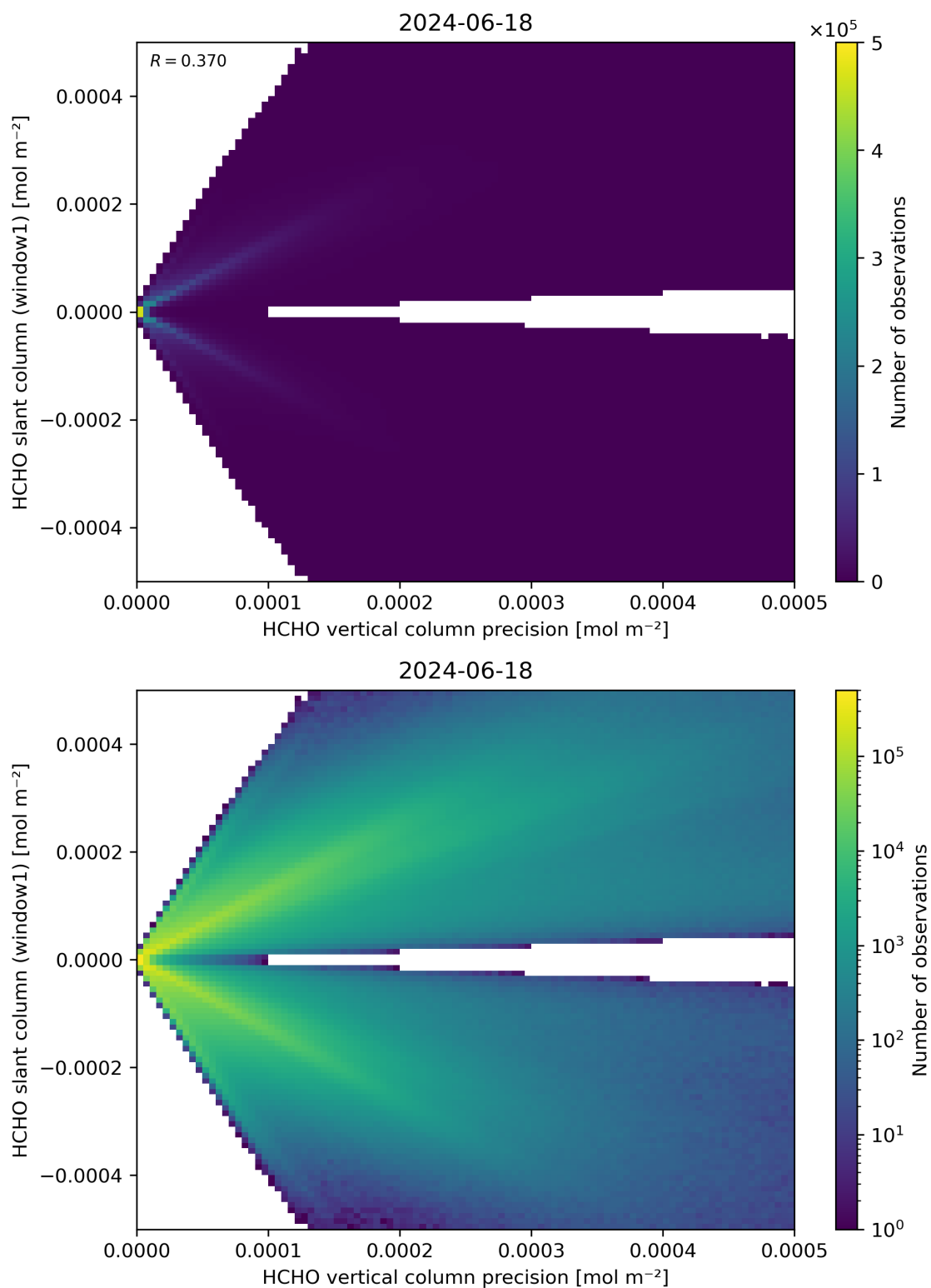
Figure 142: Scatter density plot of “HCHO vertical column precision” against “HCHO slant column (window1)” for 2024-06-17 to 2024-06-19.
