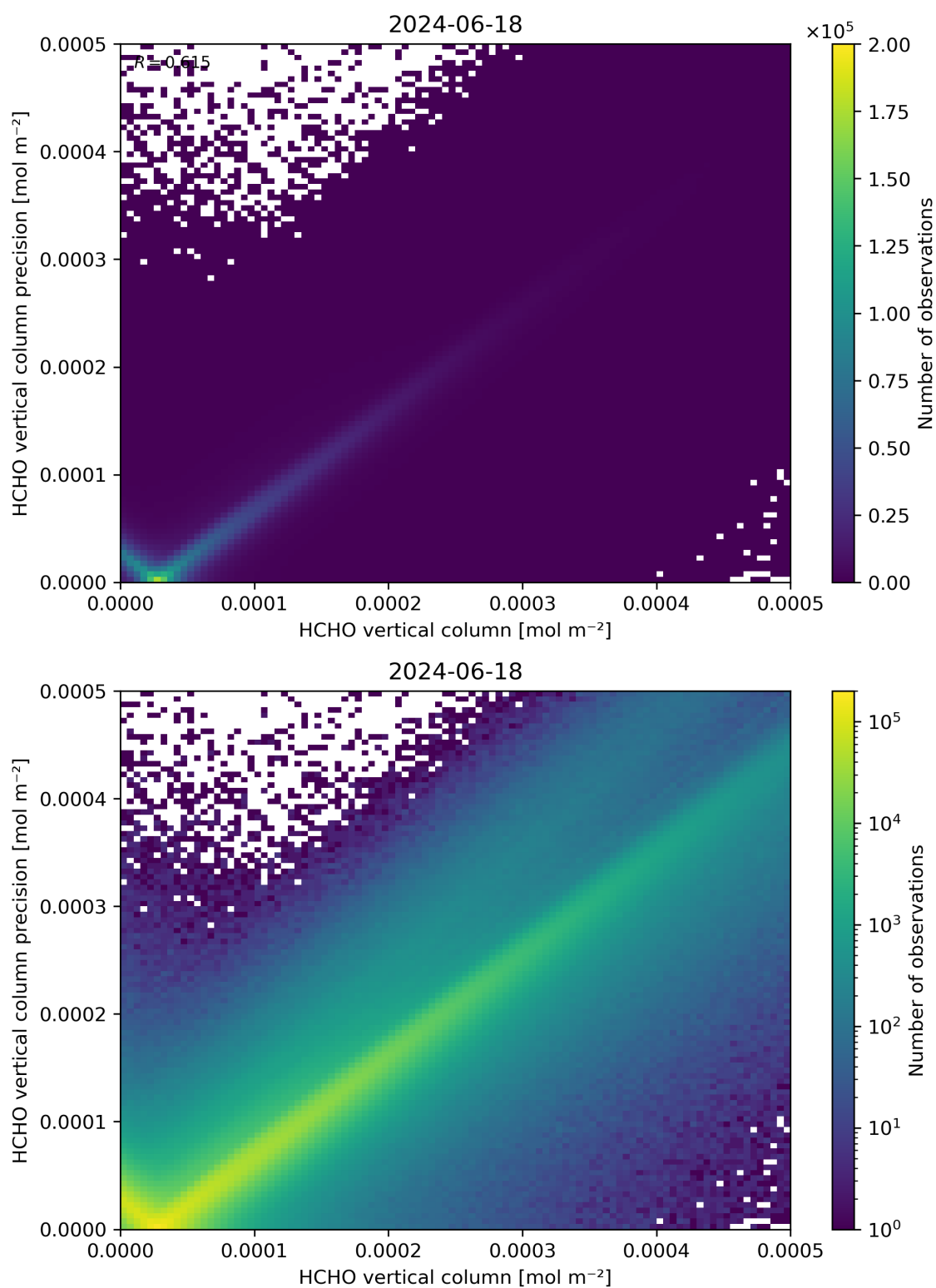
Figure 134: Scatter density plot of “HCHO vertical column” against “HCHO vertical column precision” for 2024-06-17 to 2024-06-19.
