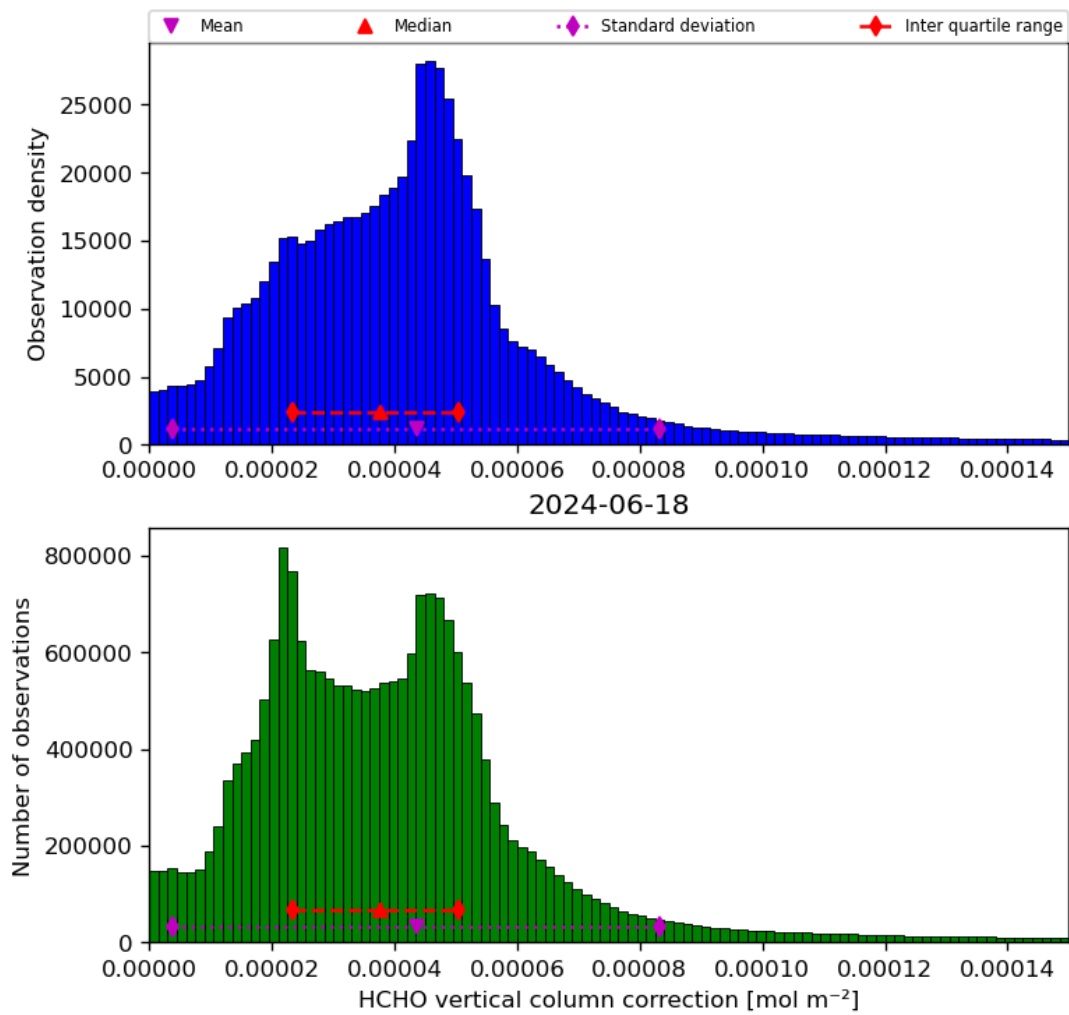
Figure 37: Histogram of “HCHO vertical column correction” for 2024-06-17 to 2024-06-19
