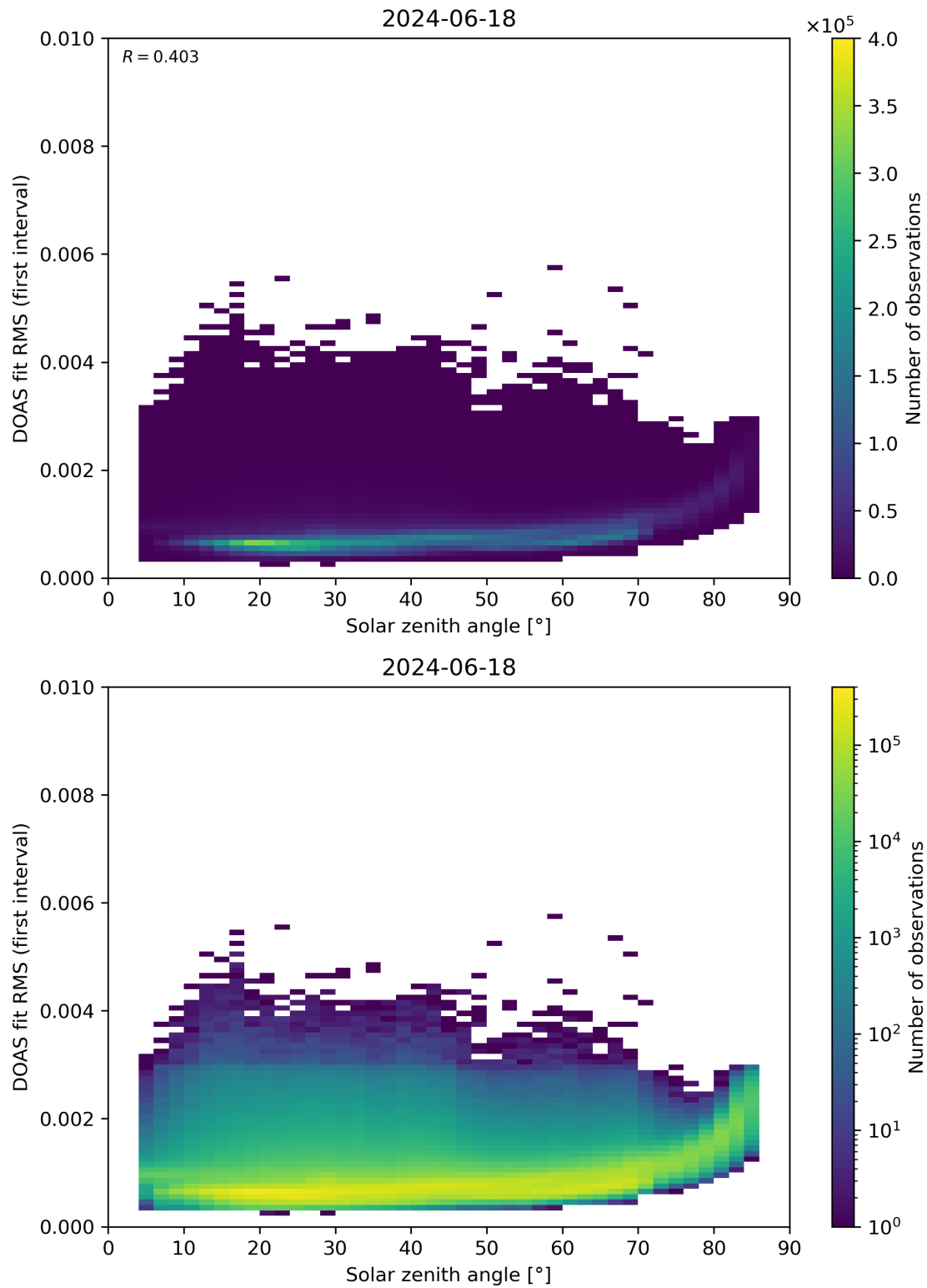
Figure 167: Scatter density plot of “Solar zenith angle” against “DOAS fit RMS (first interval)” for 2024-06-17 to 2024-06-19.
