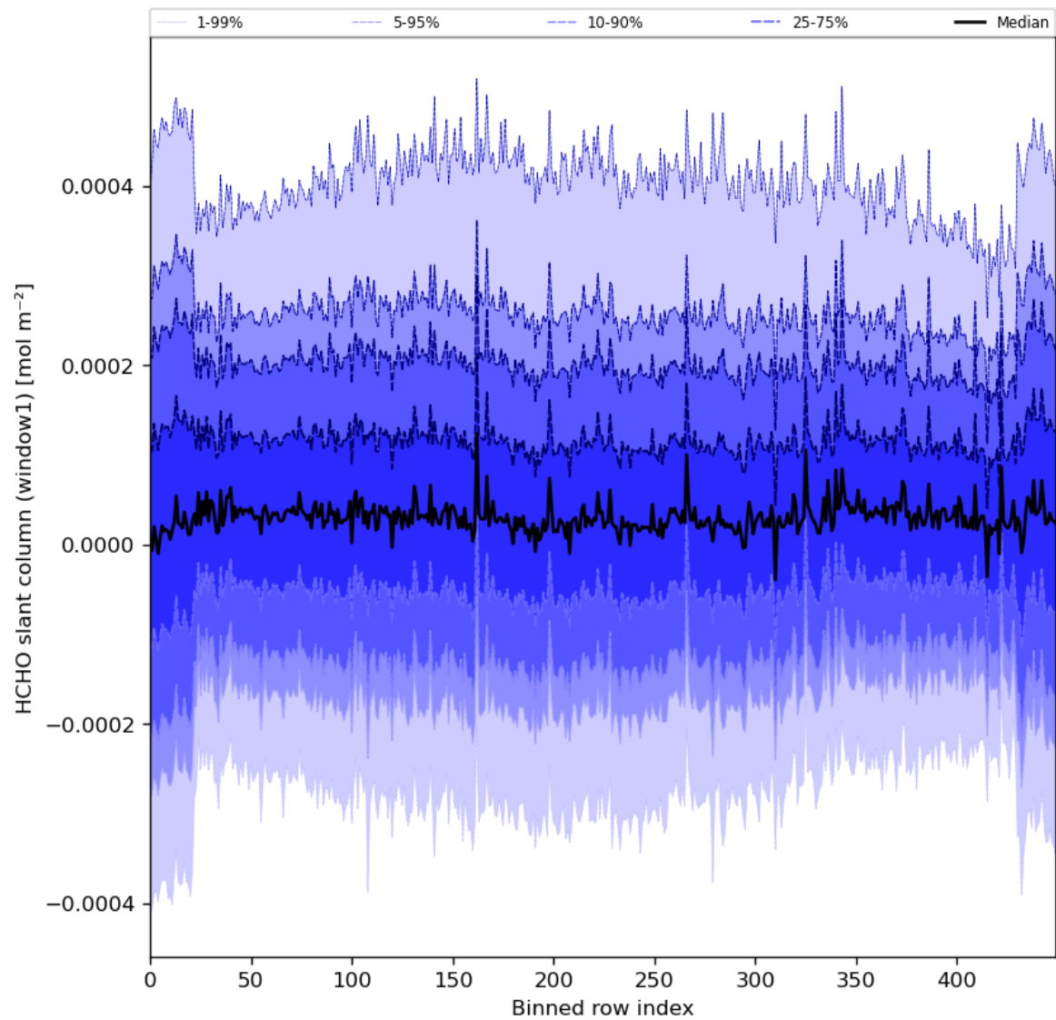
Figure 52: Along track statistics of “HCHO slant column (window1)” for 2024-06-17 to 2024-06-19
