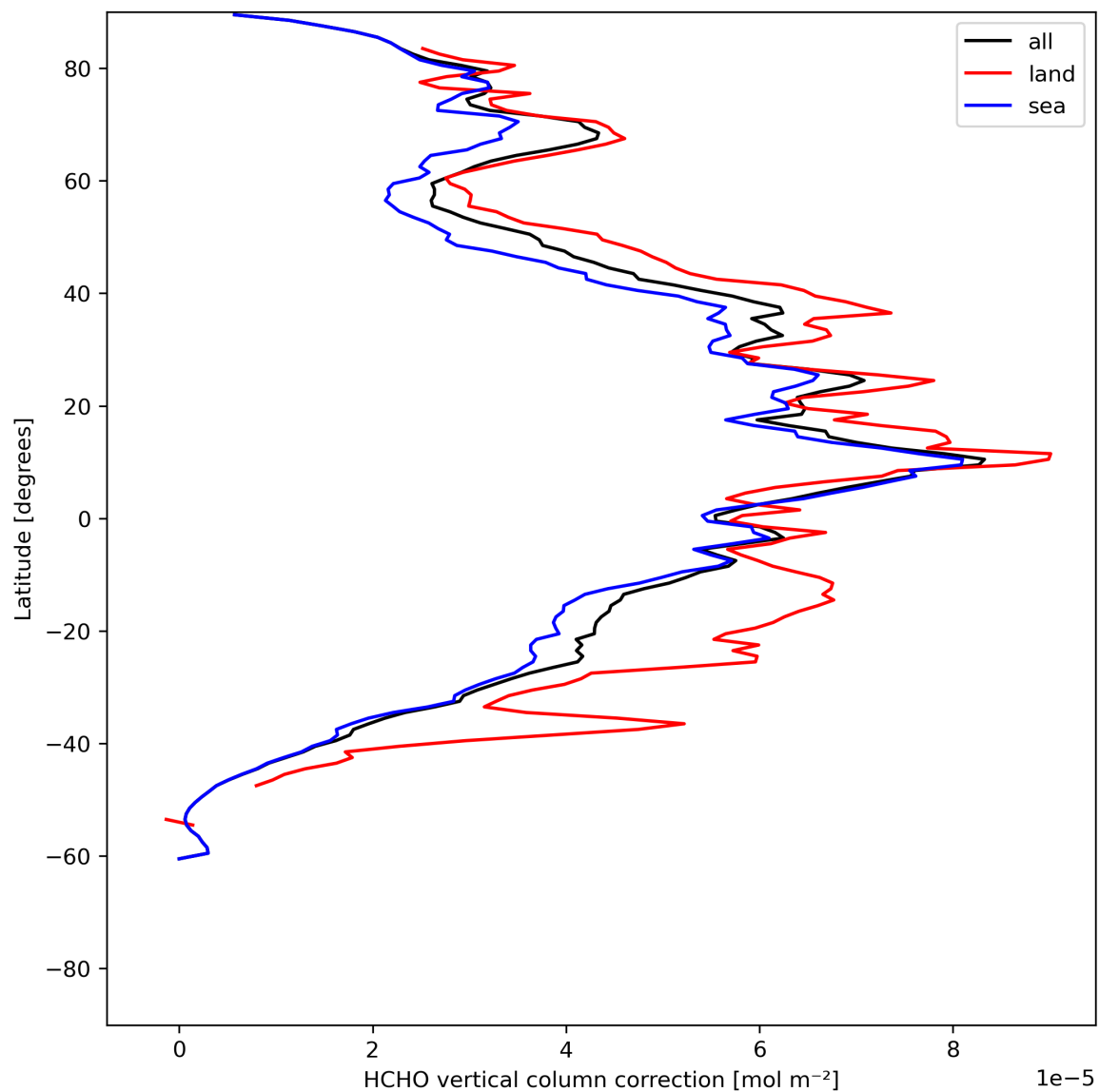
Figure 23: Zonal average of “HCHO vertical column correction” for 2024-06-17 to 2024-06-19.
