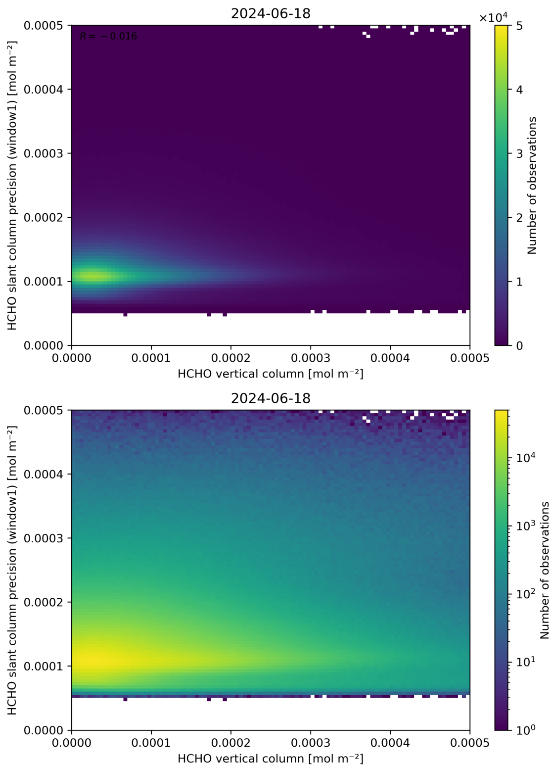
Figure 130: Scatter density plot of “HCHO vertical column” against “HCHO slant column precision (window1)” for 2024-06-17 to 2024-06-19.
