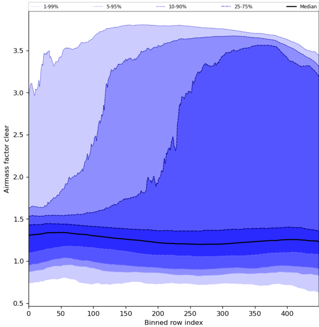
Figure 56: Along track statistics of “Airmass factor clear” for 2024-06-17 to 2024-06-19
