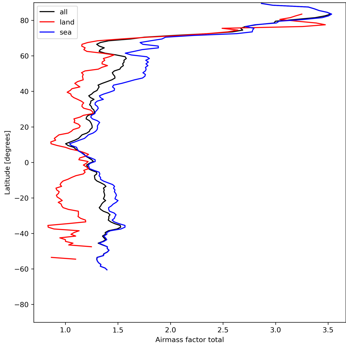
Figure 26: Zonal average of “Airmass factor total” for 2024-06-17 to 2024-06-19.
