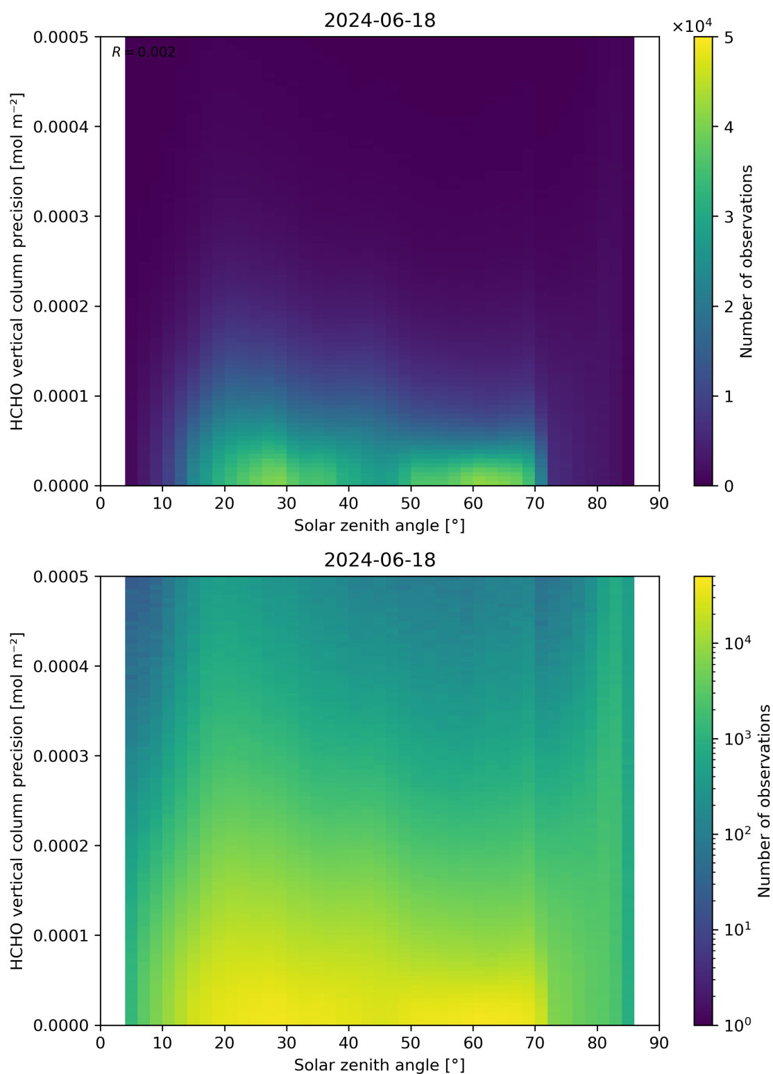
Figure 179: Scatter density plot of “Solar zenith angle” against “HCHO vertical column precision” for 2024-06-17 to 2024-06-19.
