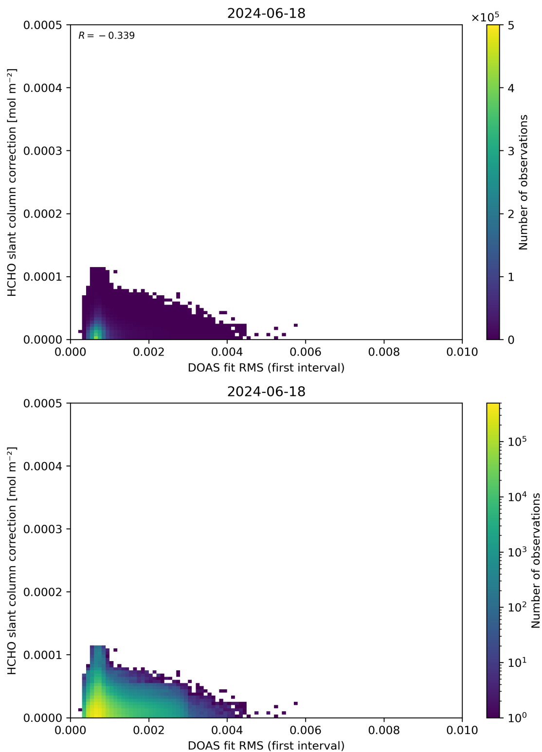
Figure 63: Scatter density plot of “DOAS fit RMS (first interval)” against “HCHO slant column correction” for 2024-06-17 to 2024-06-19.
