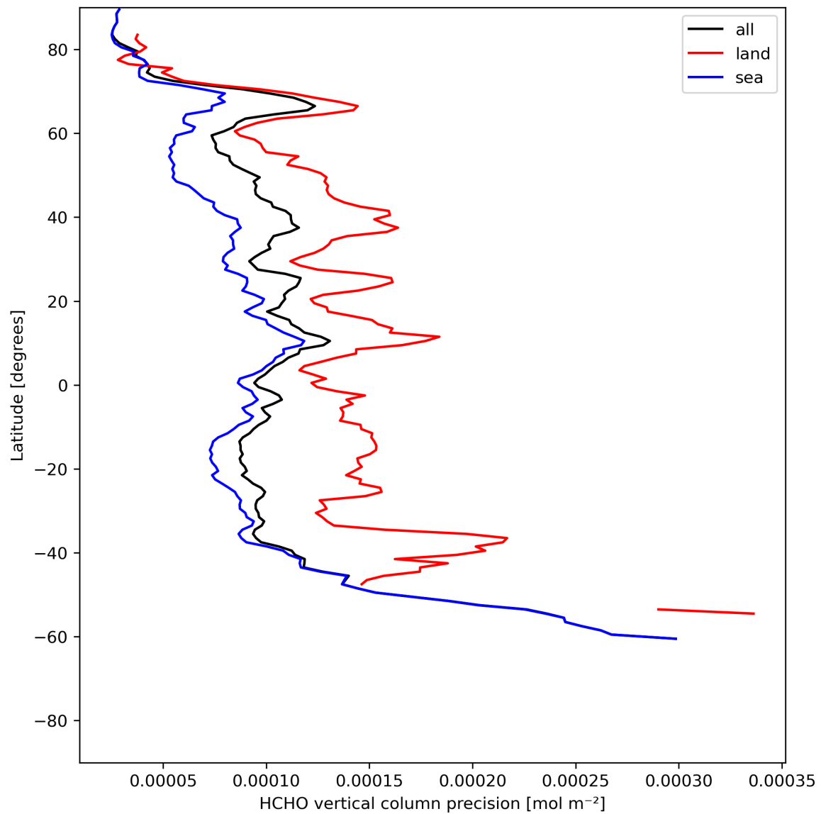
Figure 22: Zonal average of “HCHO vertical column precision” for 2024-06-17 to 2024-06-19.
