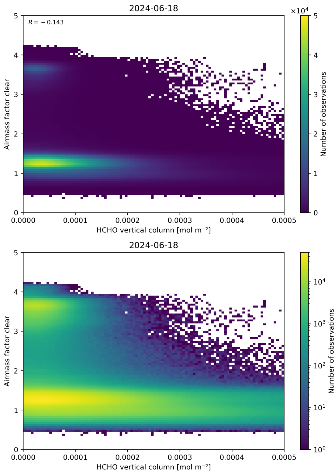
Figure 126: Scatter density plot of “HCHO vertical column” against “Airmass factor clear” for 2024-06-17 to 2024-06-19.
