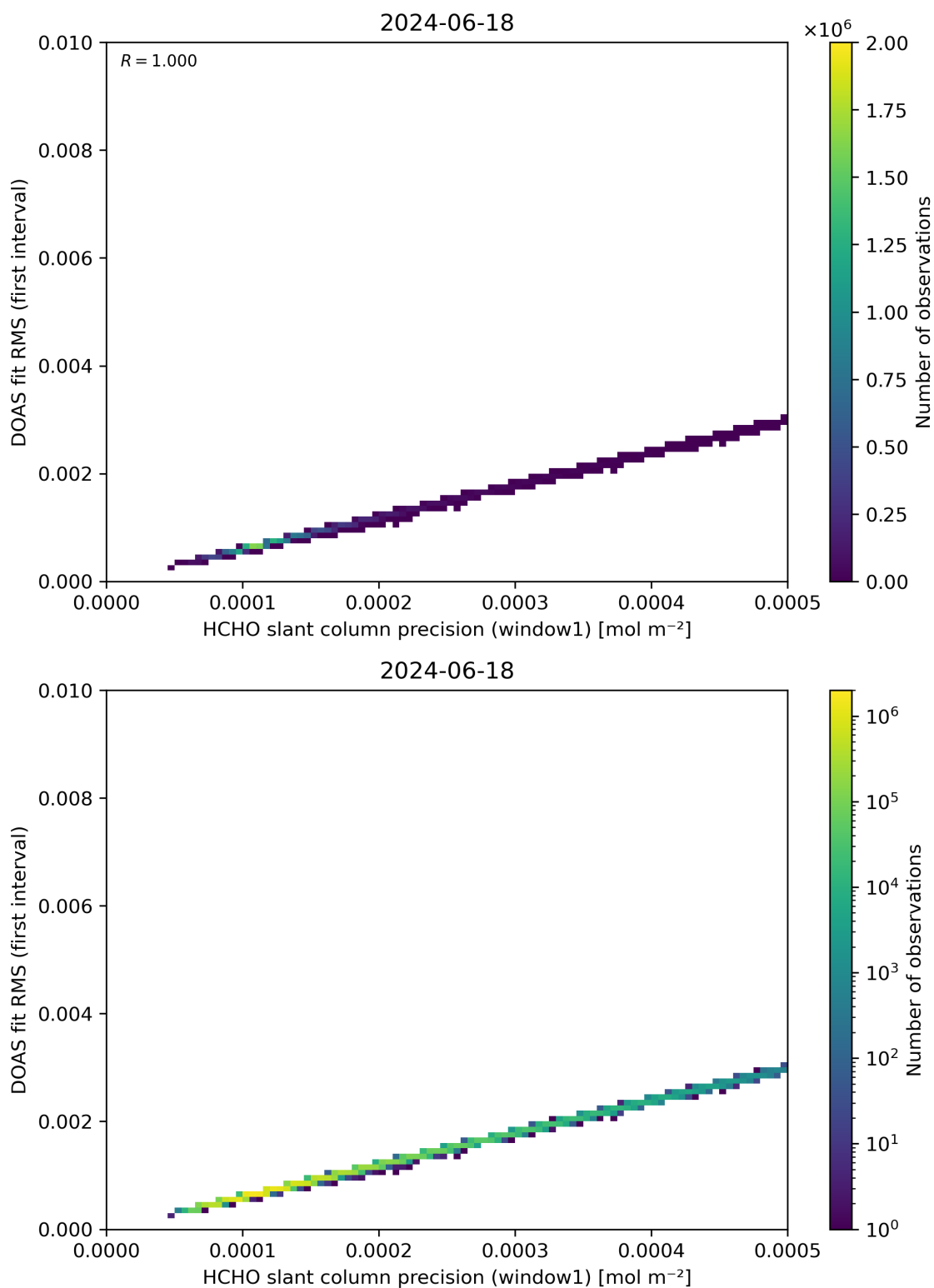
Figure 88: Scatter density plot of “HCHO slant column precision (window1)” against “DOAS fit RMS (first interval)” for 2024-06-17 to 2024-06-19.
