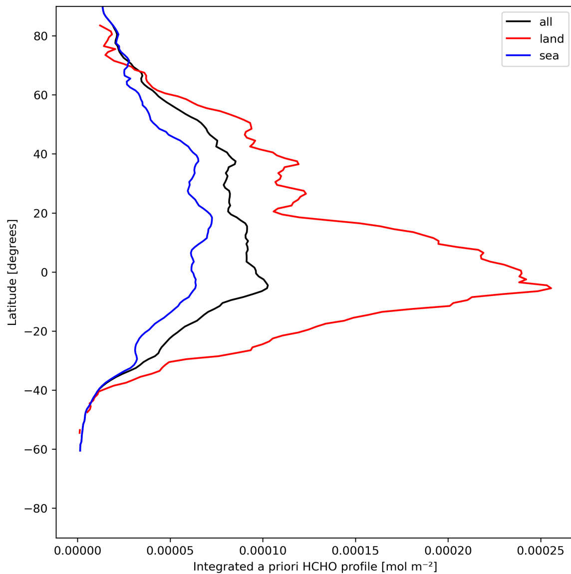
Figure 29: Zonal average of “Integrated a priori HCHO profile” for 2024-06-17 to 2024-06-19.
