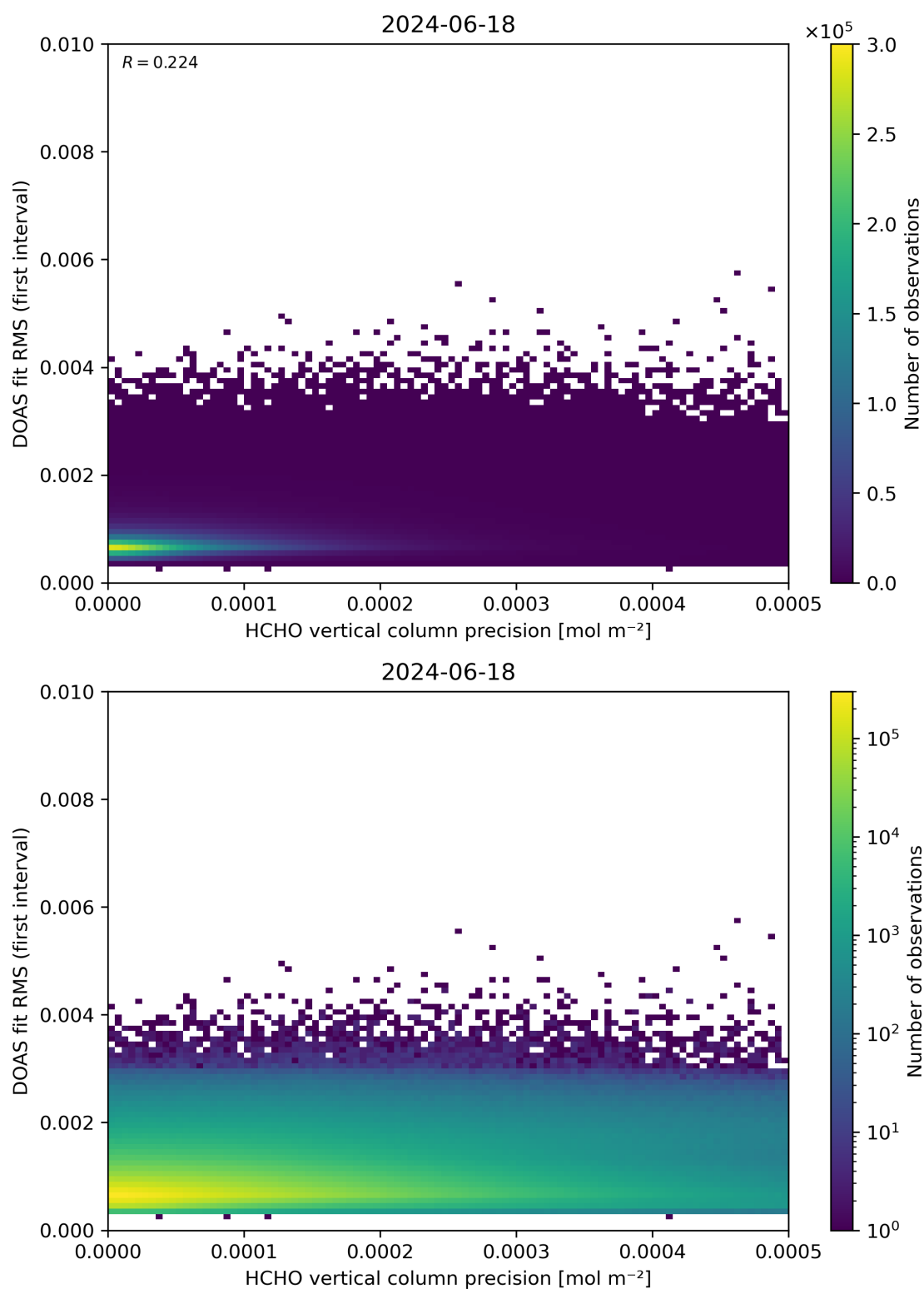
Figure 136: Scatter density plot of “HCHO vertical column precision” against “DOAS fit RMS (first interval)” for 2024-06-17 to 2024-06-19.
