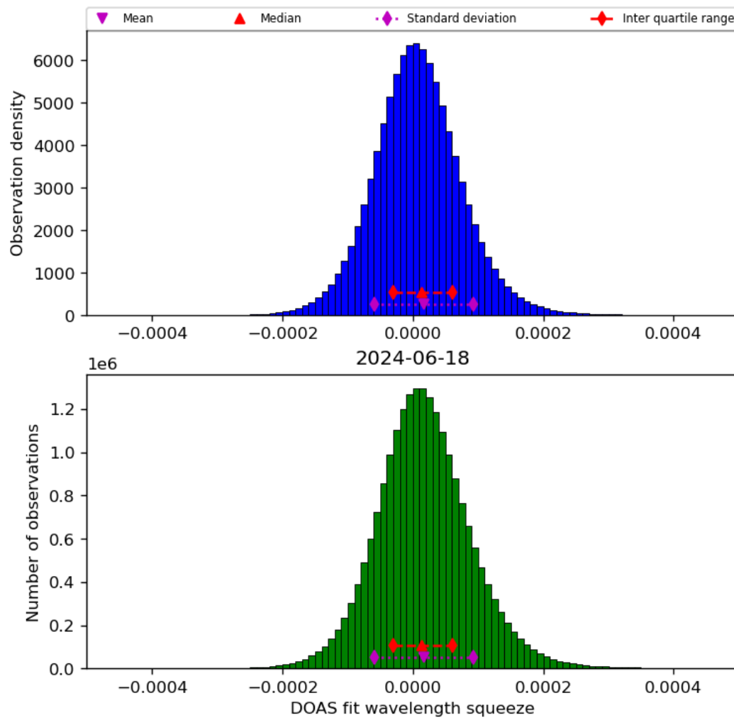
Figure 45: Histogram of “DOAS fit wavelength squeeze” for 2024-06-17 to 2024-06-19
