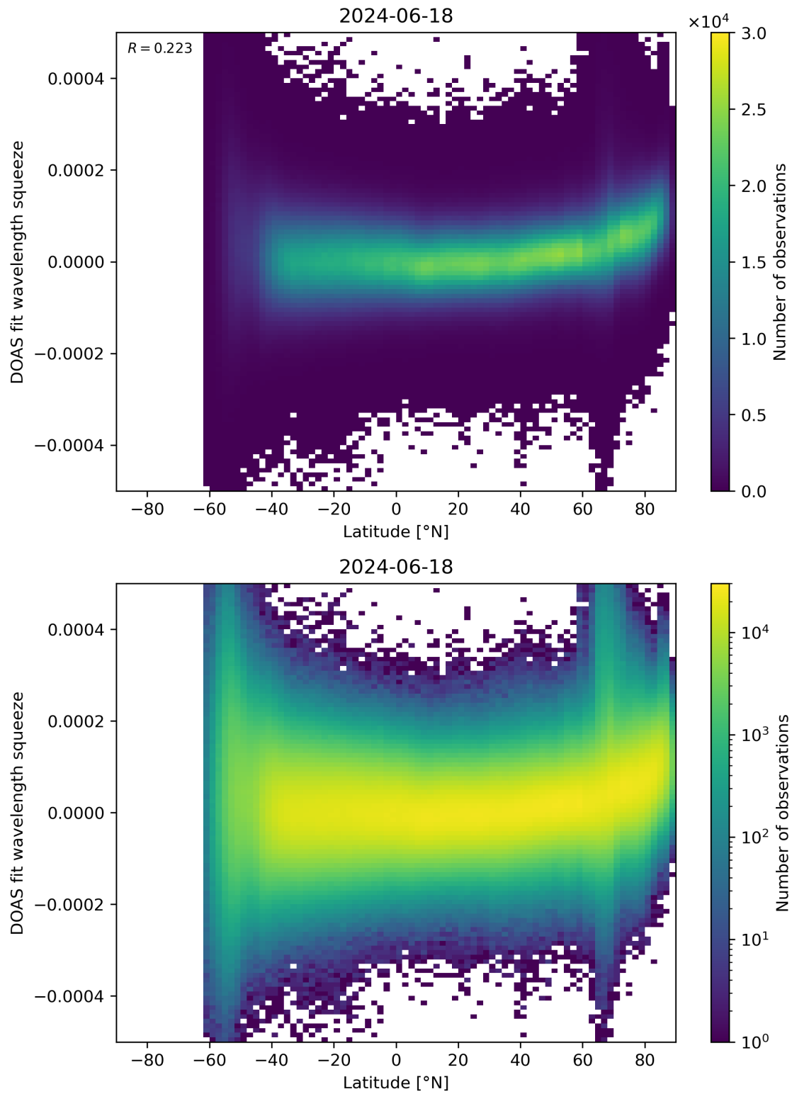
Figure 155: Scatter density plot of “Latitude” against “DOAS fit wavelength squeeze” for 2024-06-17 to 2024-06-19.
