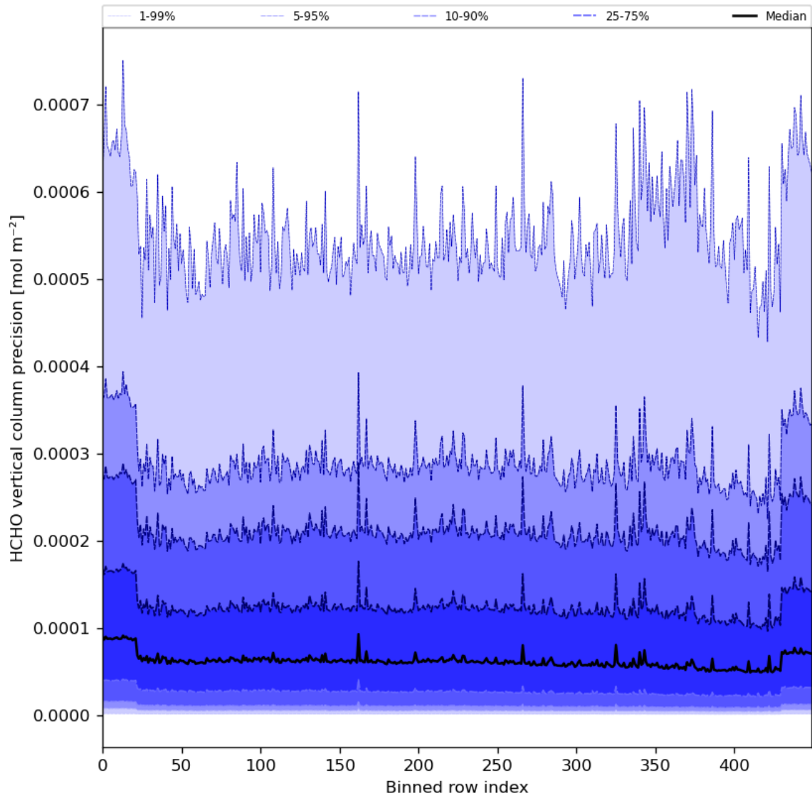
Figure 50: Along track statistics of “HCHO vertical column precision” for 2024-06-17 to 2024-06-19
