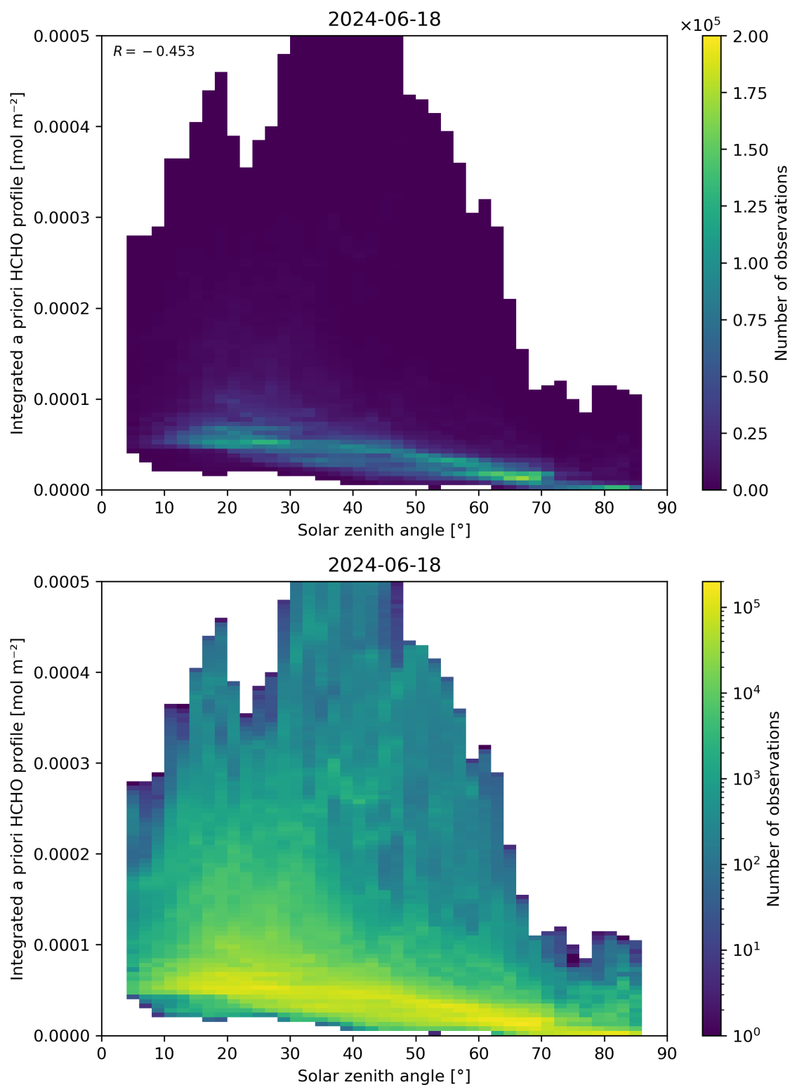
Figure 180: Scatter density plot of “Solar zenith angle” against “Integrated a priori HCHO profile” for 2024-06-17 to 2024-06-19.
