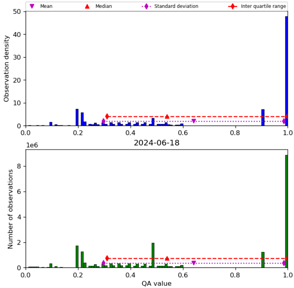
Figure 34: Histogram of “QA value” for 2024-06-17 to 2024-06-19
