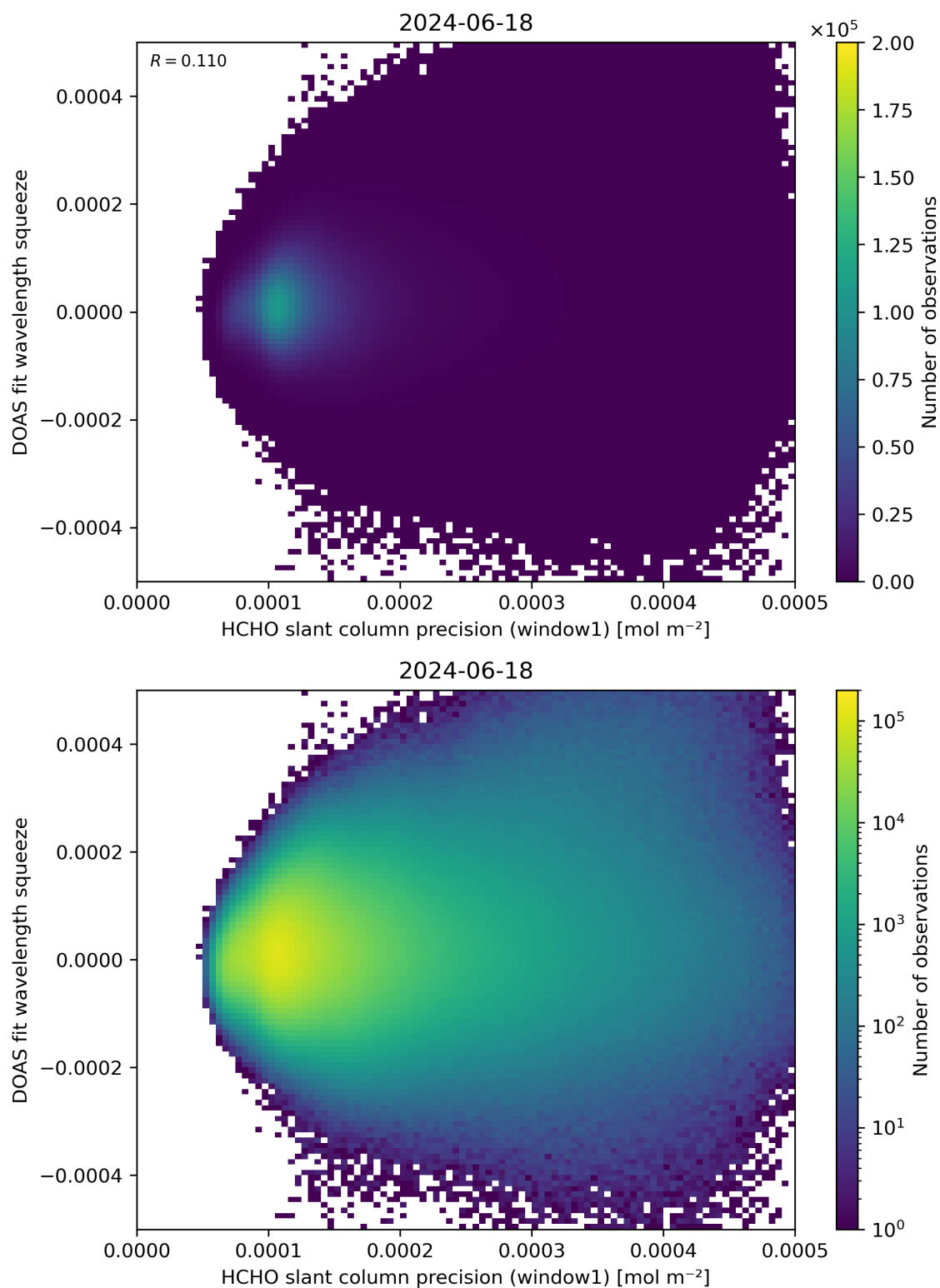
Figure 90: Scatter density plot of “HCHO slant column precision (window1)” against “DOAS fit wavelength squeeze” for 2024-06-17 to 2024-06-19.
