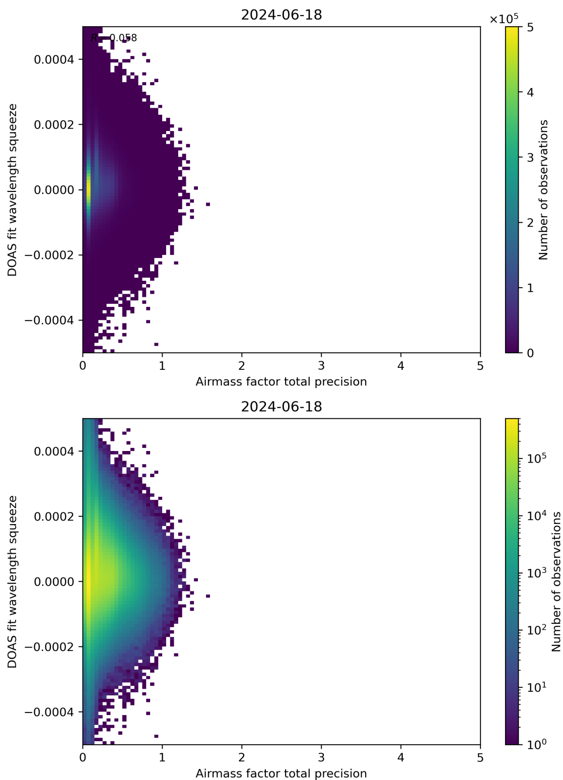
Figure 107: Scatter density plot of “Airmass factor total precision” against “DOAS fit wavelength squeeze” for 2024-06-17 to 2024-06-19.
