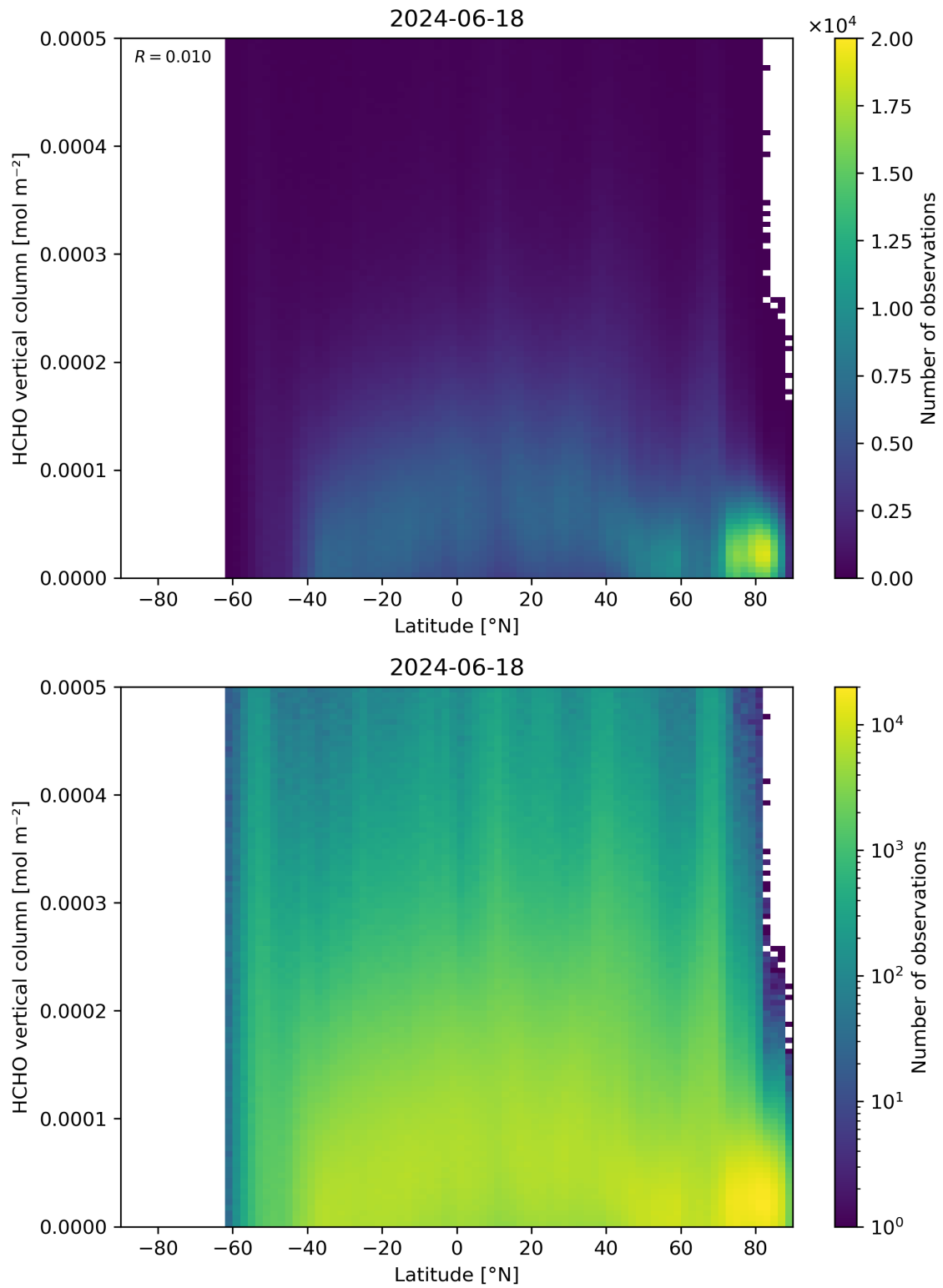
Figure 163: Scatter density plot of “Latitude” against “HCHO vertical column” for 2024-06-17 to 2024-06-19.
