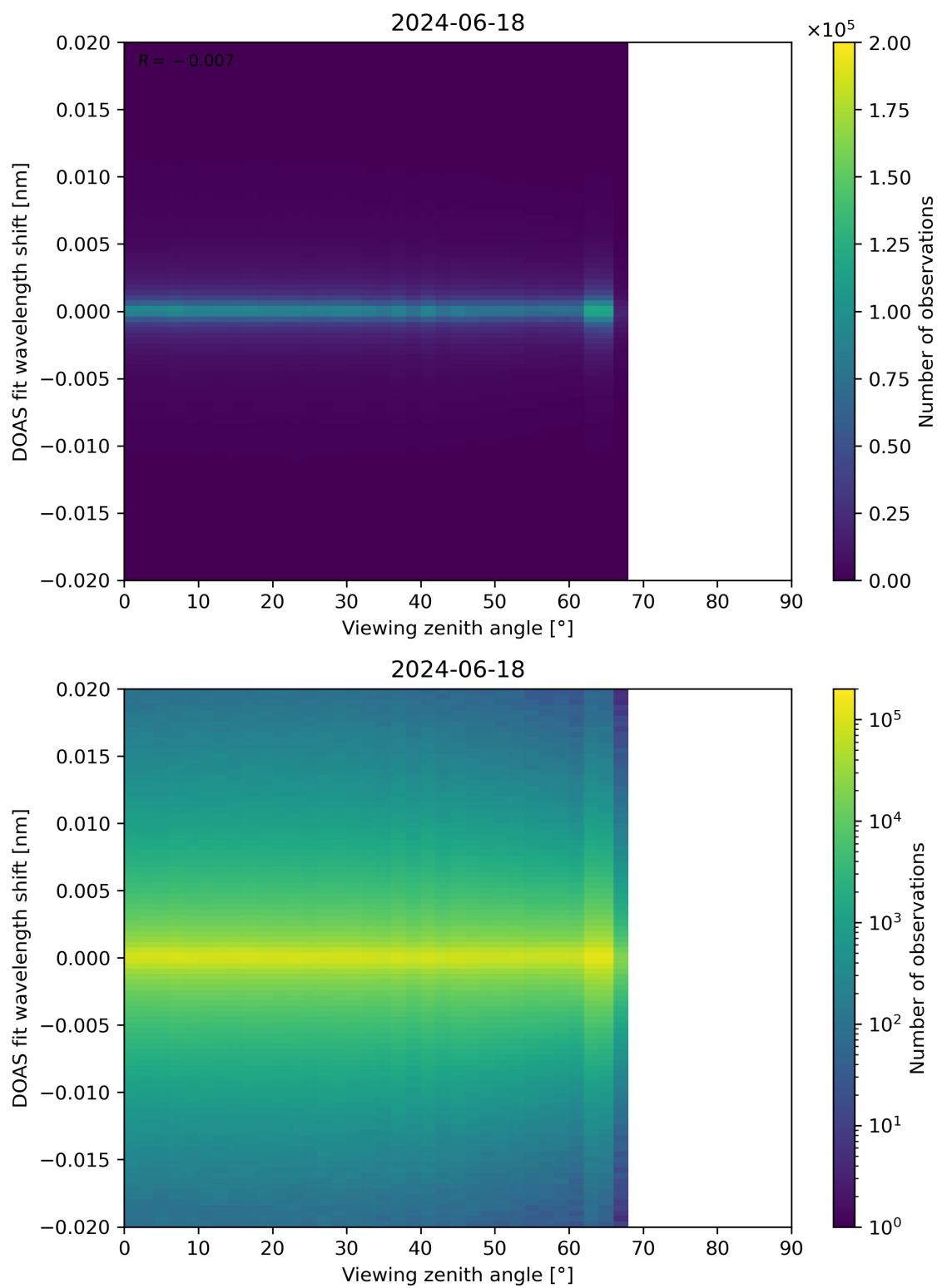
Figure 183: Scatter density plot of “Viewing zenith angle” against “DOAS fit wavelength shift” for 2024-06-17 to 2024-06-19.
