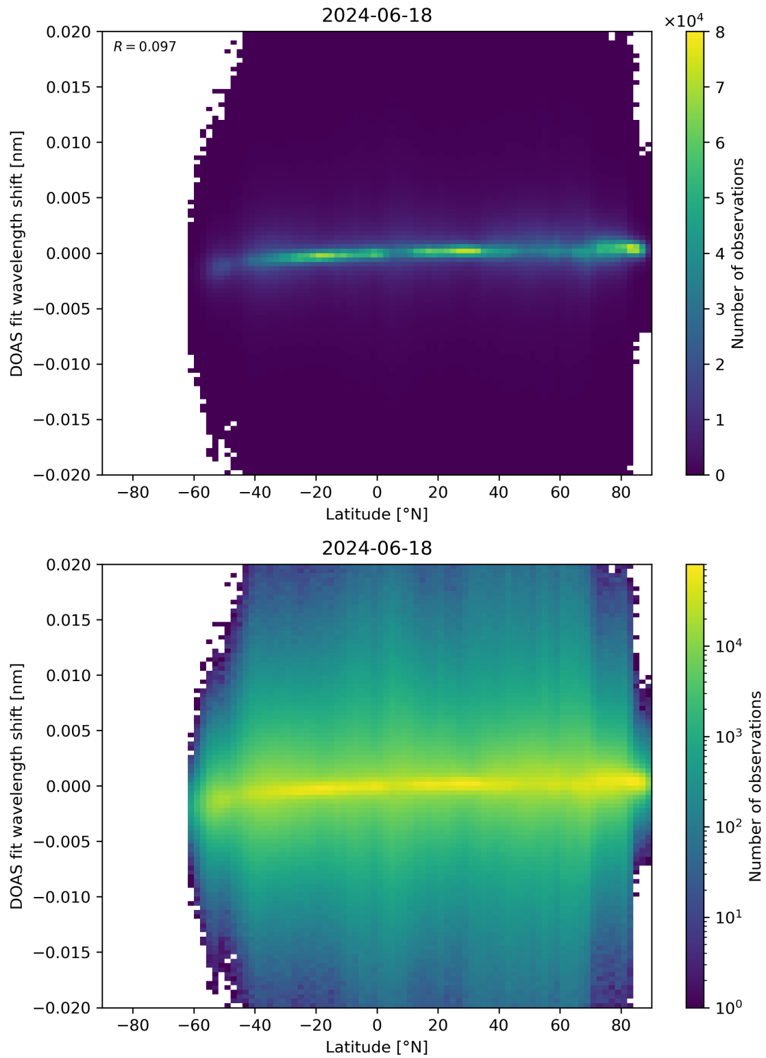
Figure 154: Scatter density plot of “Latitude” against “DOAS fit wavelength shift” for 2024-06-17 to 2024-06-19.
