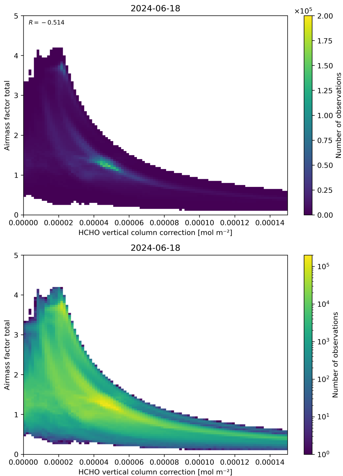
Figure 120: Scatter density plot of “HCHO vertical column correction” against “Airmass factor total” for 2024-06-17 to 2024-06-19.
