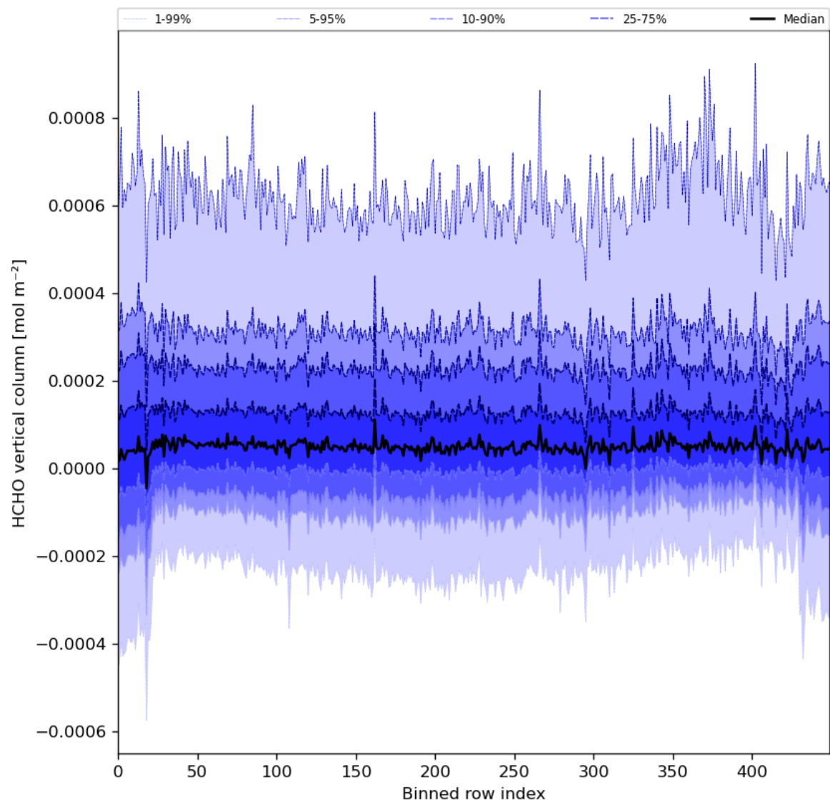
Figure 49: Along track statistics of “HCHO vertical column” for 2024-06-17 to 2024-06-19
