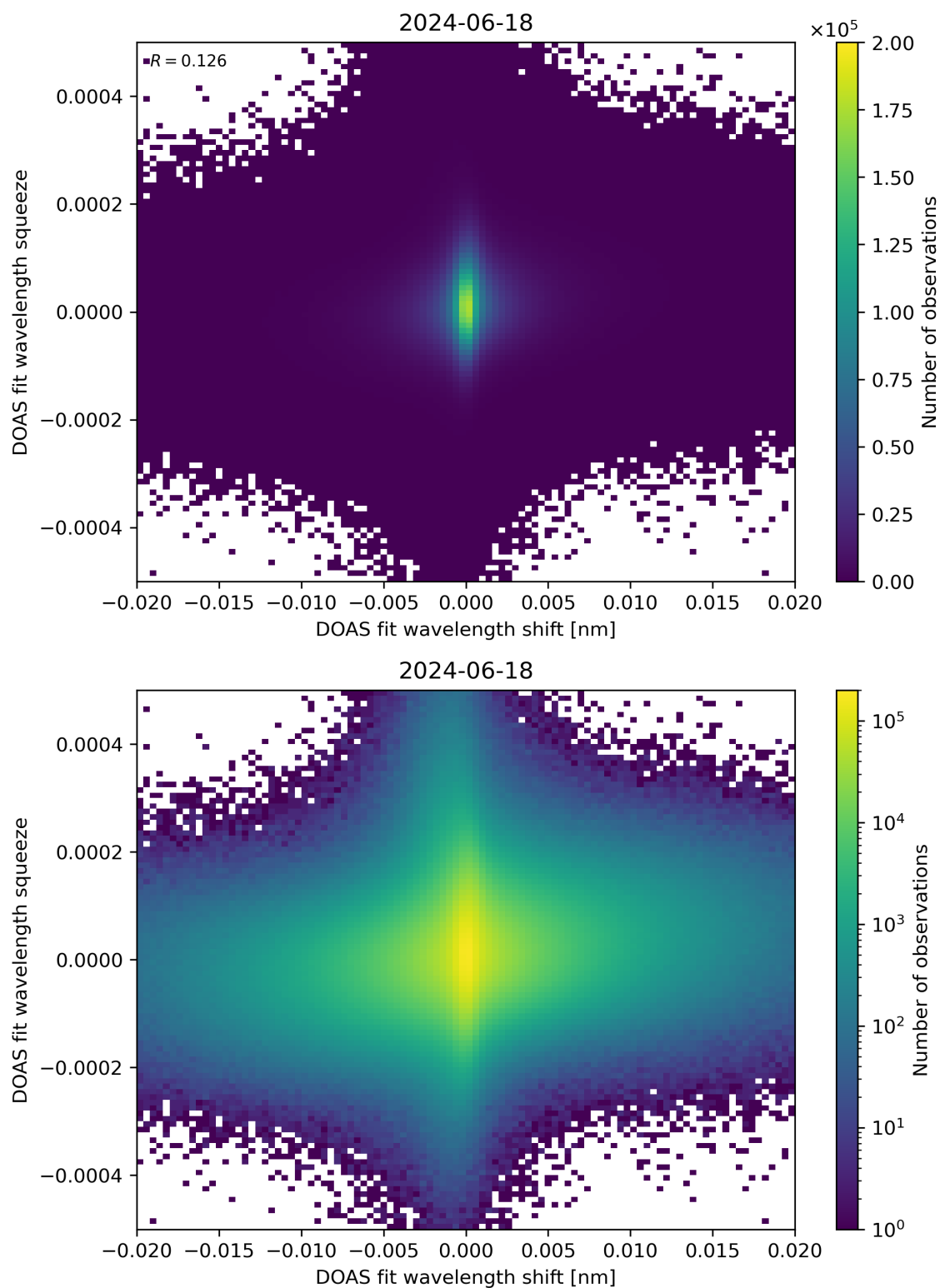
Figure 65: Scatter density plot of “DOAS fit wavelength shift” against “DOAS fit wavelength squeeze” for 2024-06-17 to 2024-06-19.
