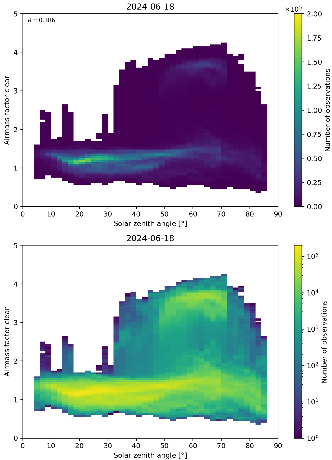
Figure 170: Scatter density plot of “Solar zenith angle” against “Airmass factor clear” for 2024-06-17 to 2024-06-19.
