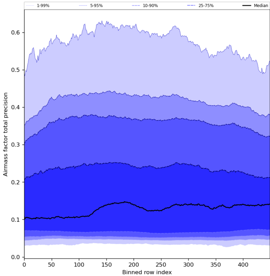
Figure 55: Along track statistics of “Airmass factor total precision” for 2024-06-17 to 2024-06-19
