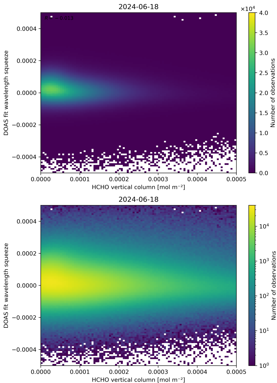
Figure 125: Scatter density plot of “HCHO vertical column” against “DOAS fit wavelength squeeze” for 2024-06-17 to 2024-06-19.
