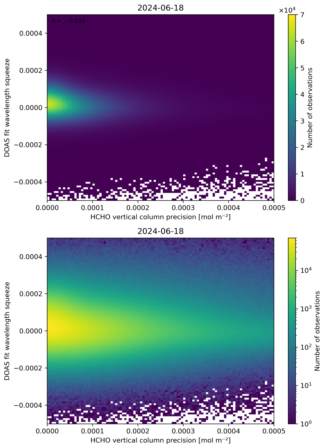
Figure 138: Scatter density plot of “HCHO vertical column precision” against “DOAS fit wavelength squeeze” for 2024-06-17 to 2024-06-19.
