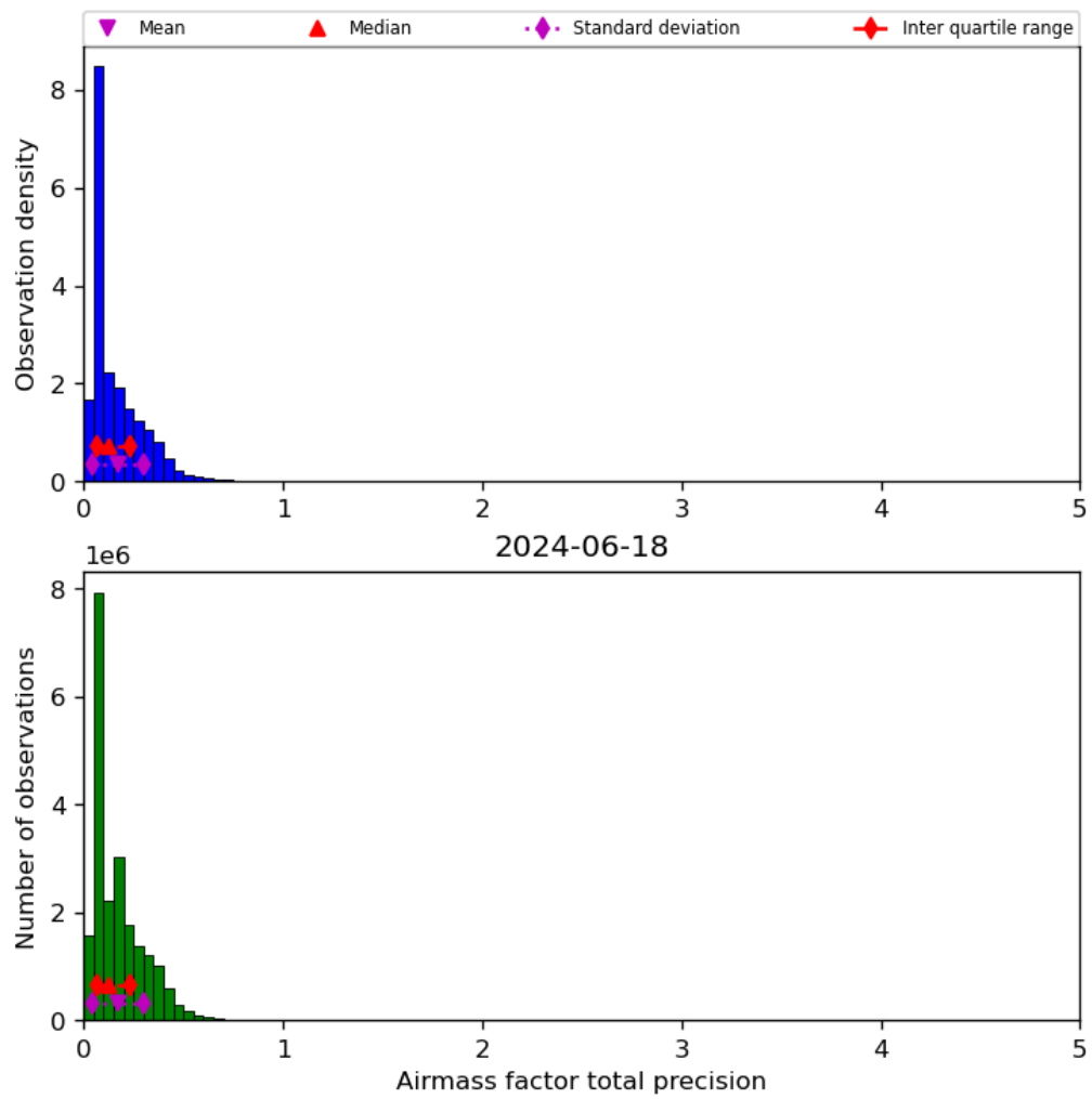
Figure 41: Histogram of “Airmass factor total precision” for 2024-06-17 to 2024-06-19
