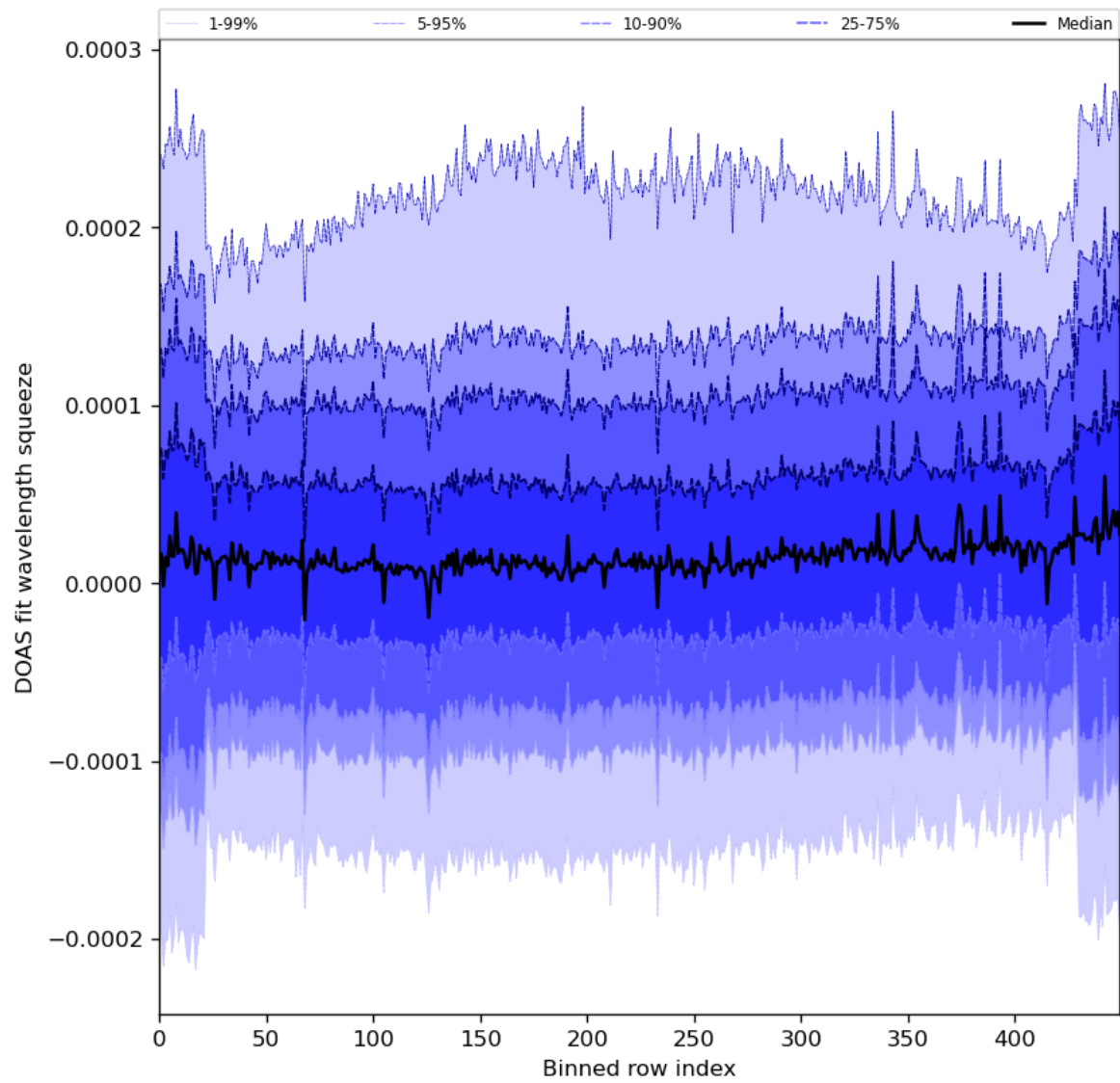
Figure 59: Along track statistics of “DOAS fit wavelength squeeze” for 2024-06-17 to 2024-06-19
