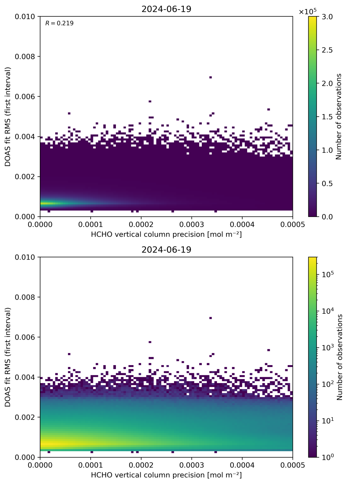
Figure 136: Scatter density plot of “HCHO vertical column precision” against “DOAS fit RMS (first interval)” for 2024-06-19 to 2024-06-20.
