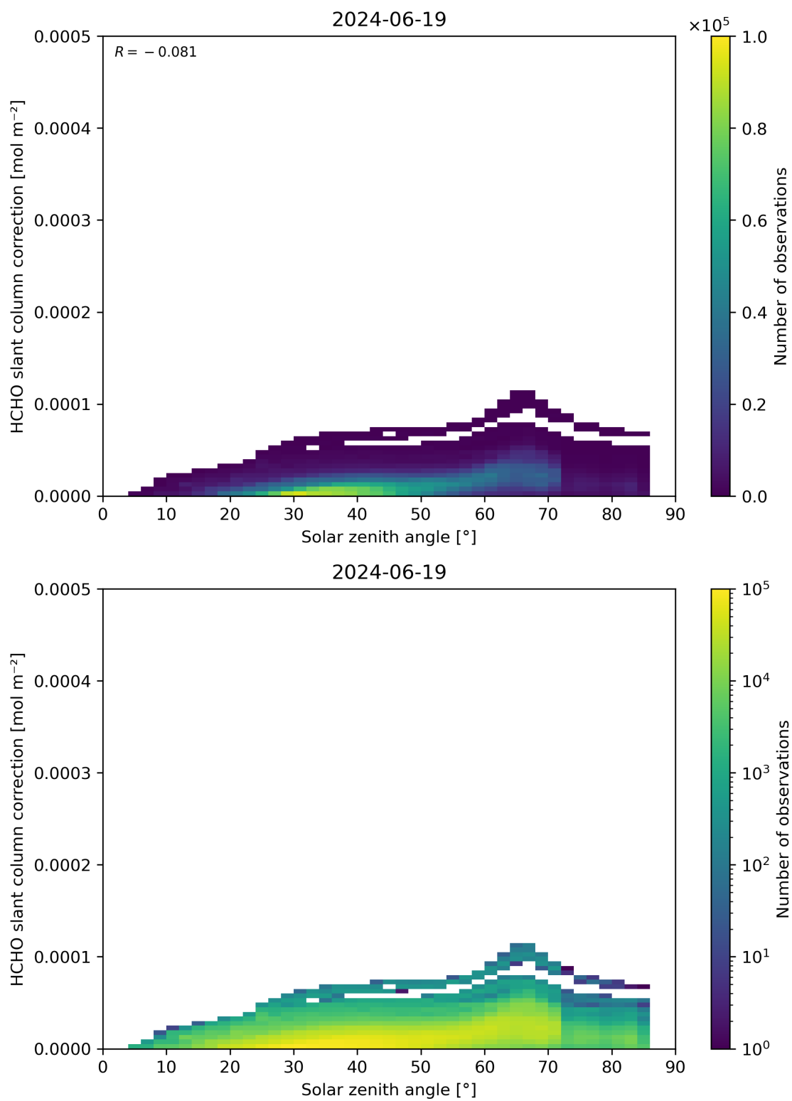
Figure 172: Scatter density plot of “Solar zenith angle” against “HCHO slant column correction” for 2024-06-19 to 2024-06-20.
