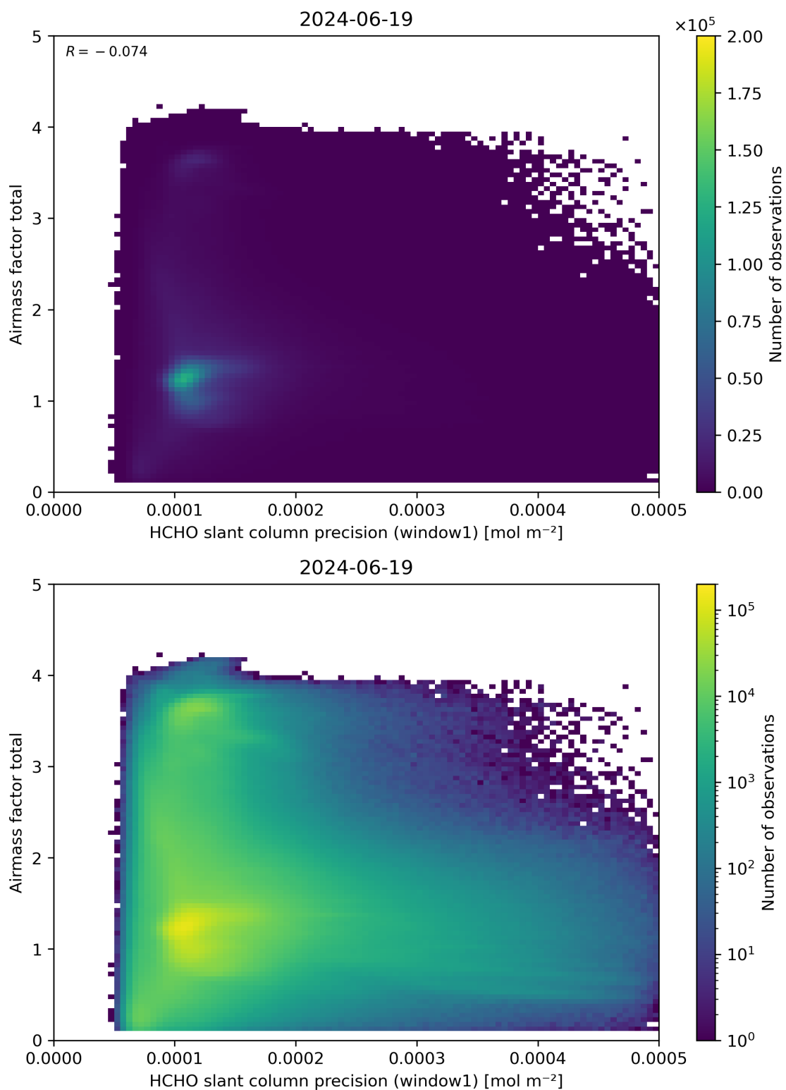
Figure 94: Scatter density plot of “HCHO slant column precision (window1)” against “Airmass factor total” for 2024-06-19 to 2024-06-20.
