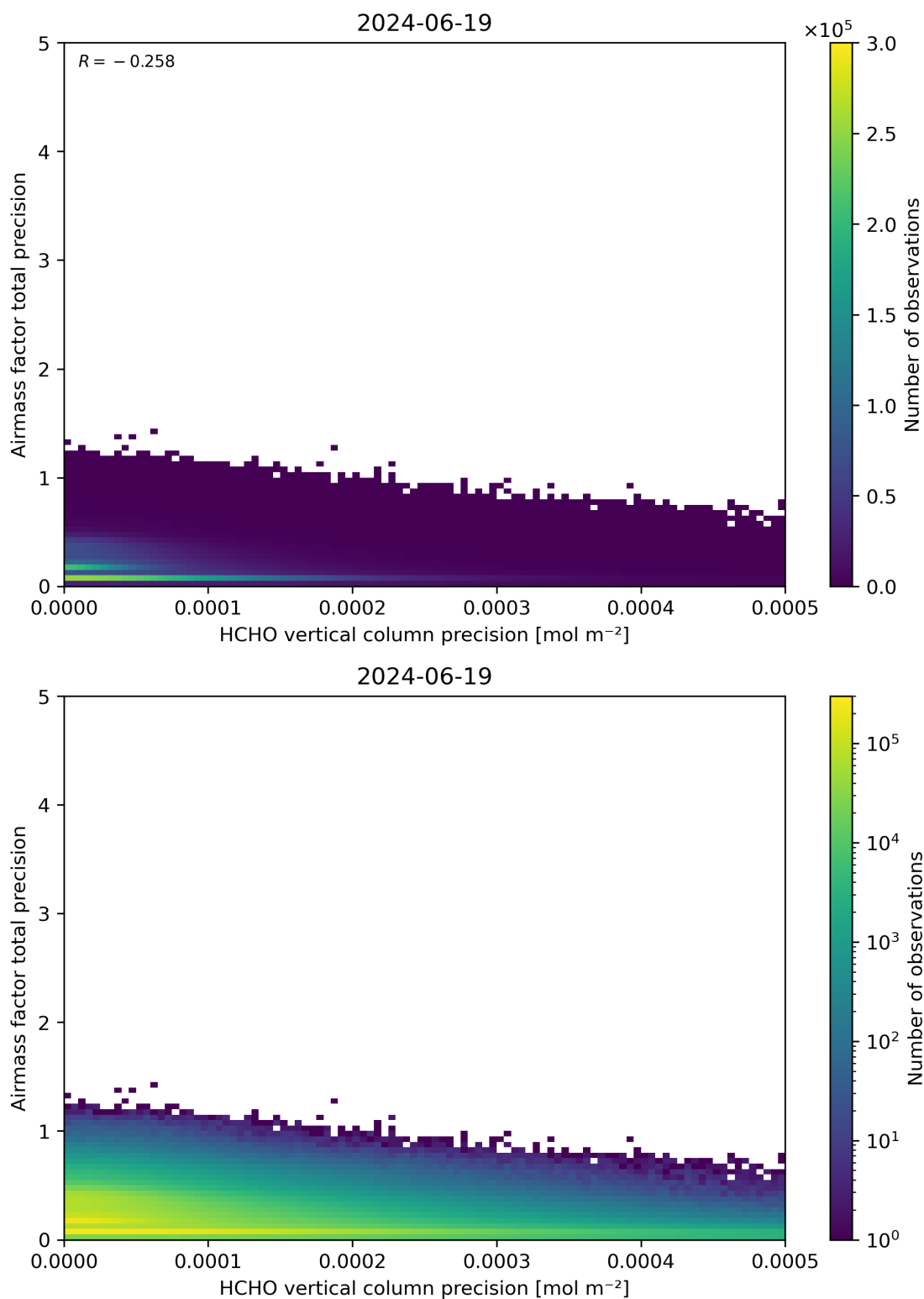
Figure 145: Scatter density plot of “HCHO vertical column precision” against “Airmass factor total precision” for 2024-06-19 to 2024-06-20.
