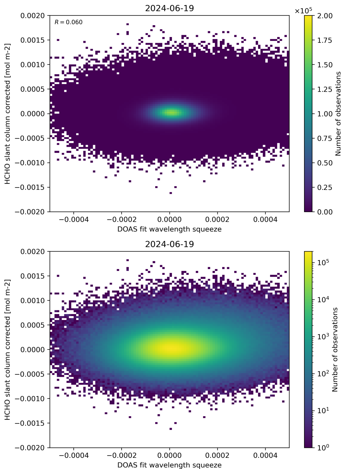
Figure 69: Scatter density plot of “DOAS fit wavelength squeeze” against “HCHO slant column corrected” for 2024-06-19 to 2024-06-20.
