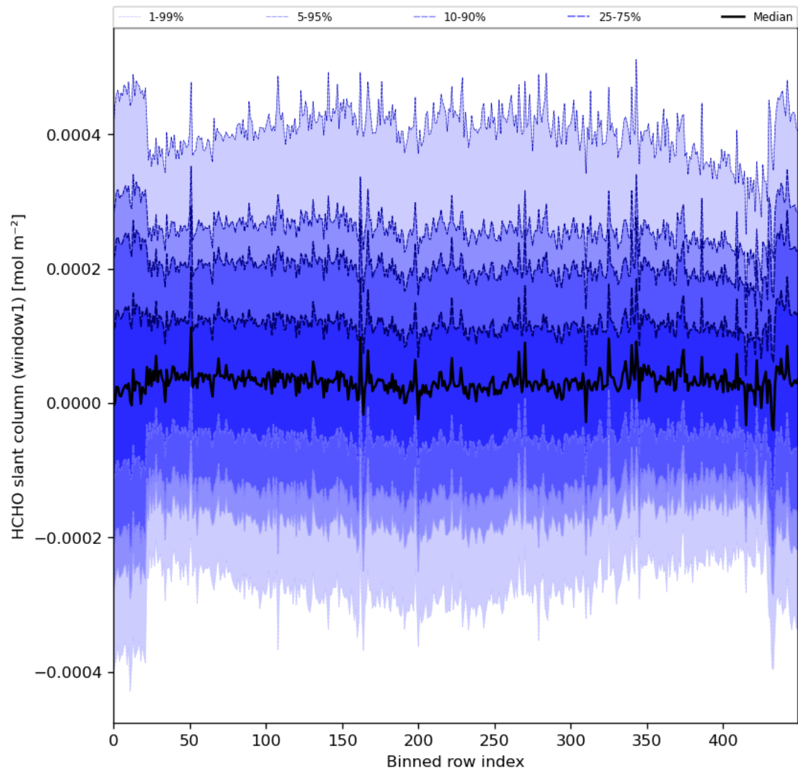
Figure 52: Along track statistics of “HCHO slant column (window1)” for 2024-06-19 to 2024-06-20
