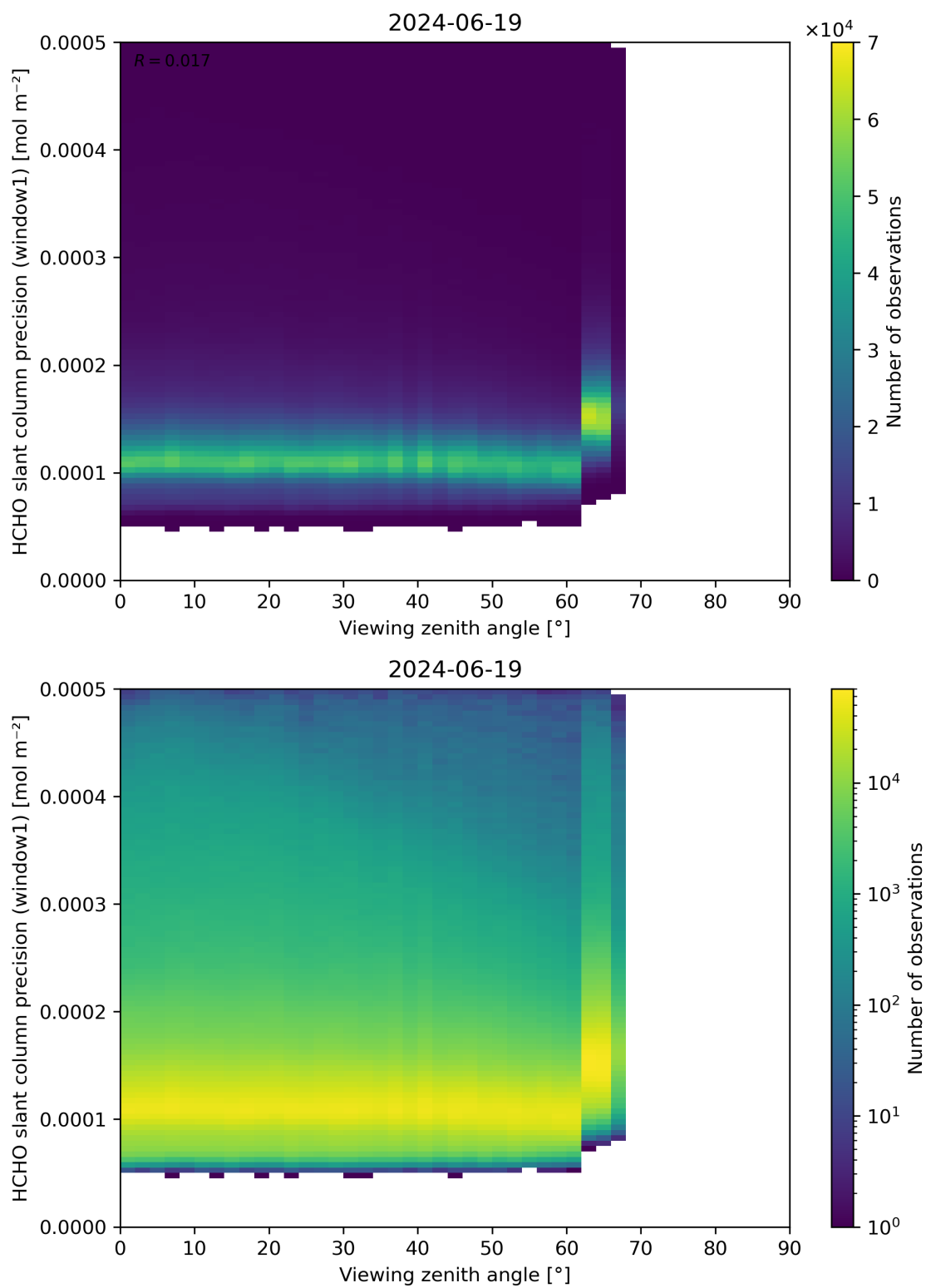
Figure 189: Scatter density plot of “Viewing zenith angle” against “HCHO slant column precision (window1)” for 2024-06-19 to 2024-06-20.
