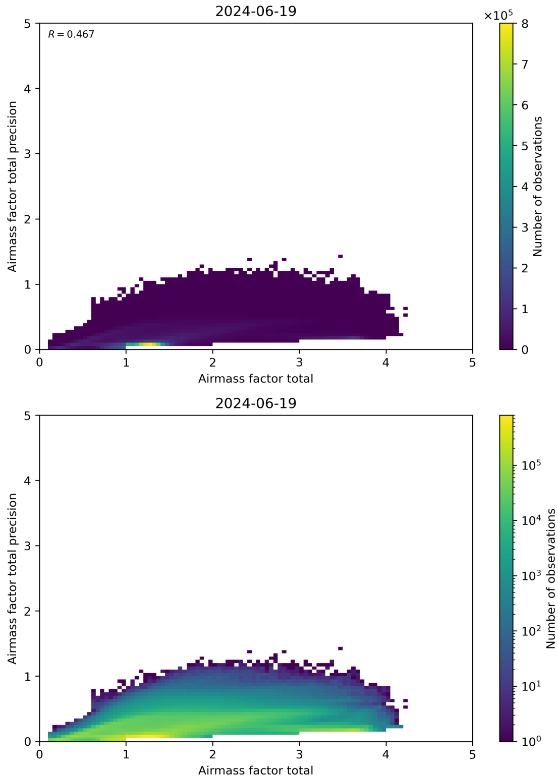
Figure 103: Scatter density plot of “Airmass factor total” against “Airmass factor total precision” for 2024-06-19 to 2024-06-20.
