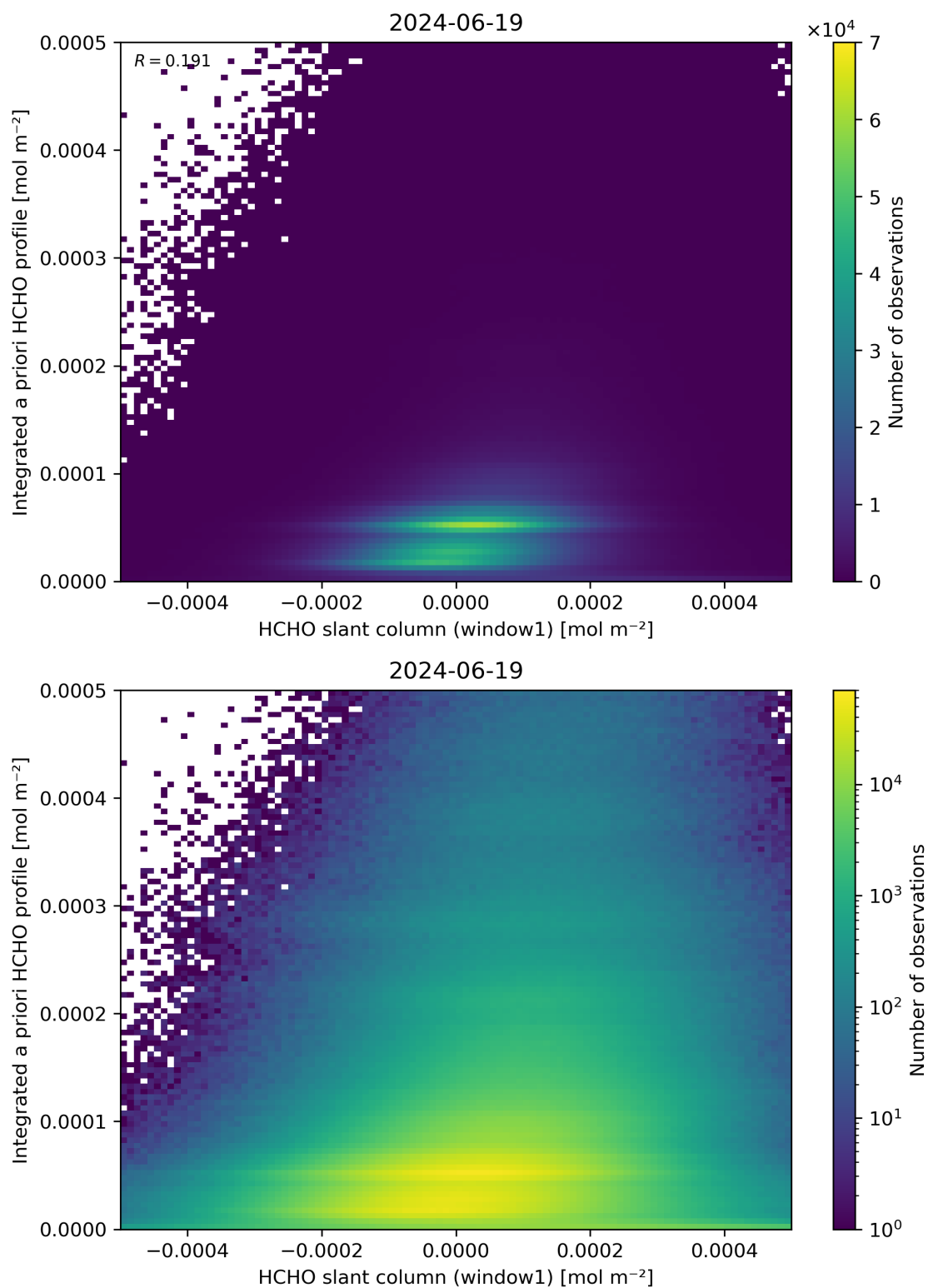
Figure 87: Scatter density plot of “HCHO slant column (window1)” against “Integrated a priori HCHO profile” for 2024-06-19 to 2024-06-20.
