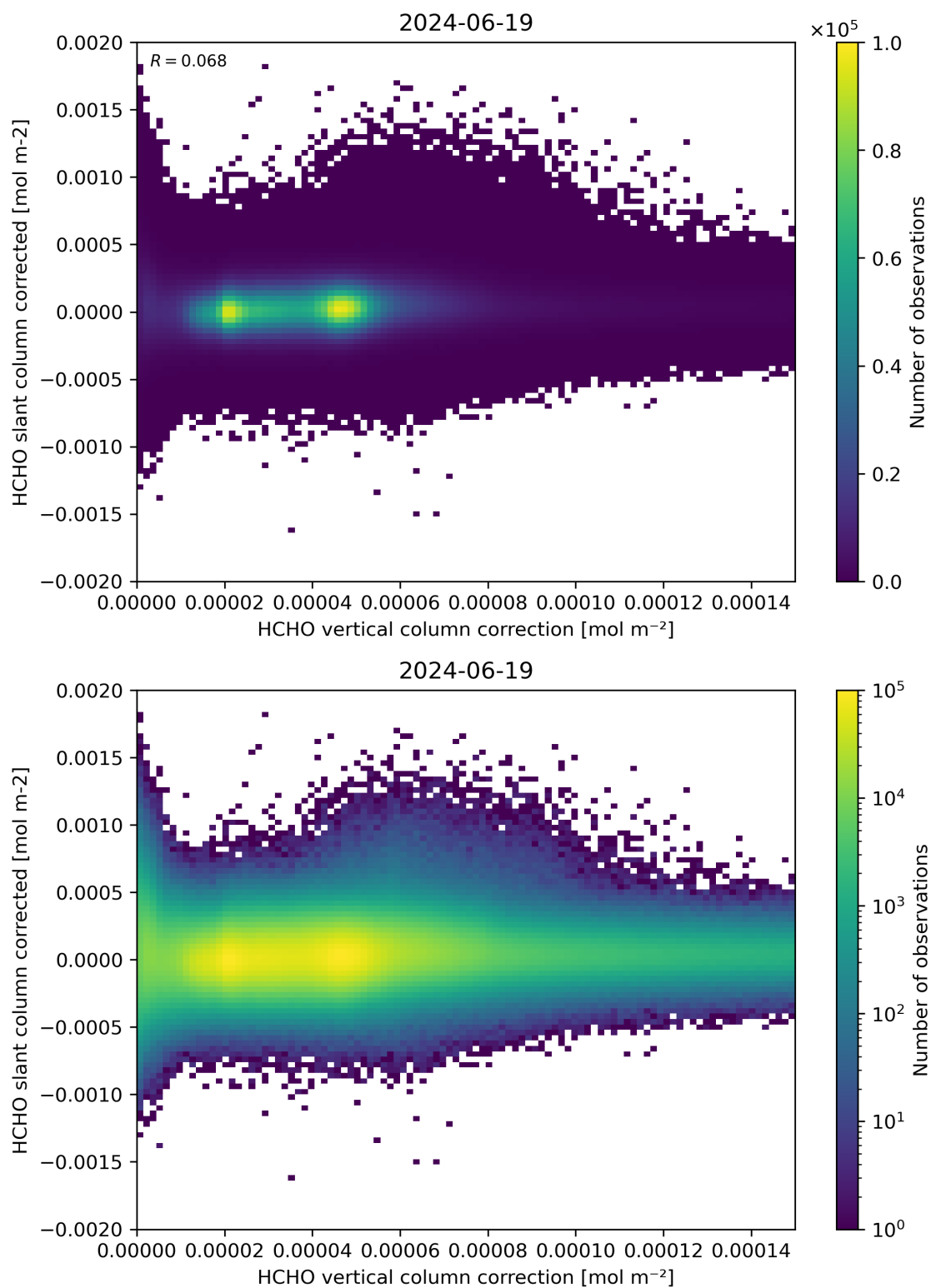
Figure 116: Scatter density plot of “HCHO vertical column correction” against “HCHO slant column corrected” for 2024-06-19 to 2024-06-20.
