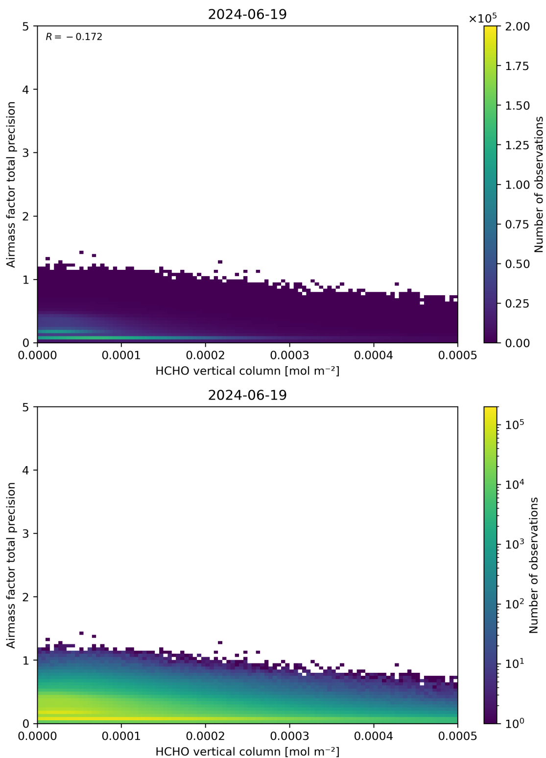
Figure 132: Scatter density plot of “HCHO vertical column” against “Airmass factor total precision” for 2024-06-19 to 2024-06-20.
