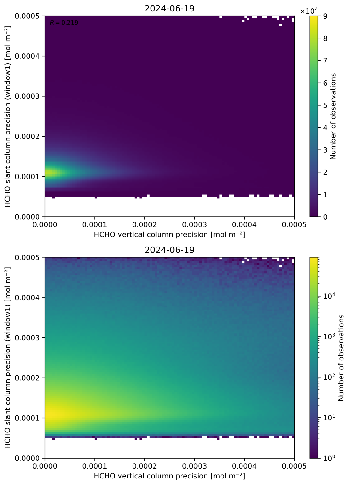
Figure 143: Scatter density plot of “HCHO vertical column precision” against “HCHO slant column precision (window1)” for 2024-06-19 to 2024-06-20.
