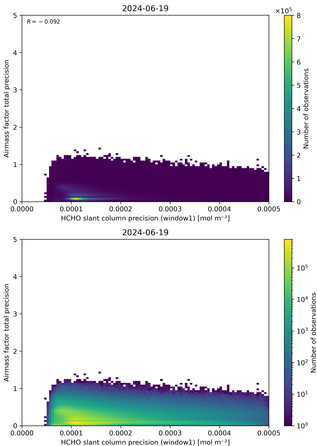
Figure 95: Scatter density plot of “HCHO slant column precision (window1)” against “Airmass factor total precision” for 2024-06-19 to 2024-06-20.
