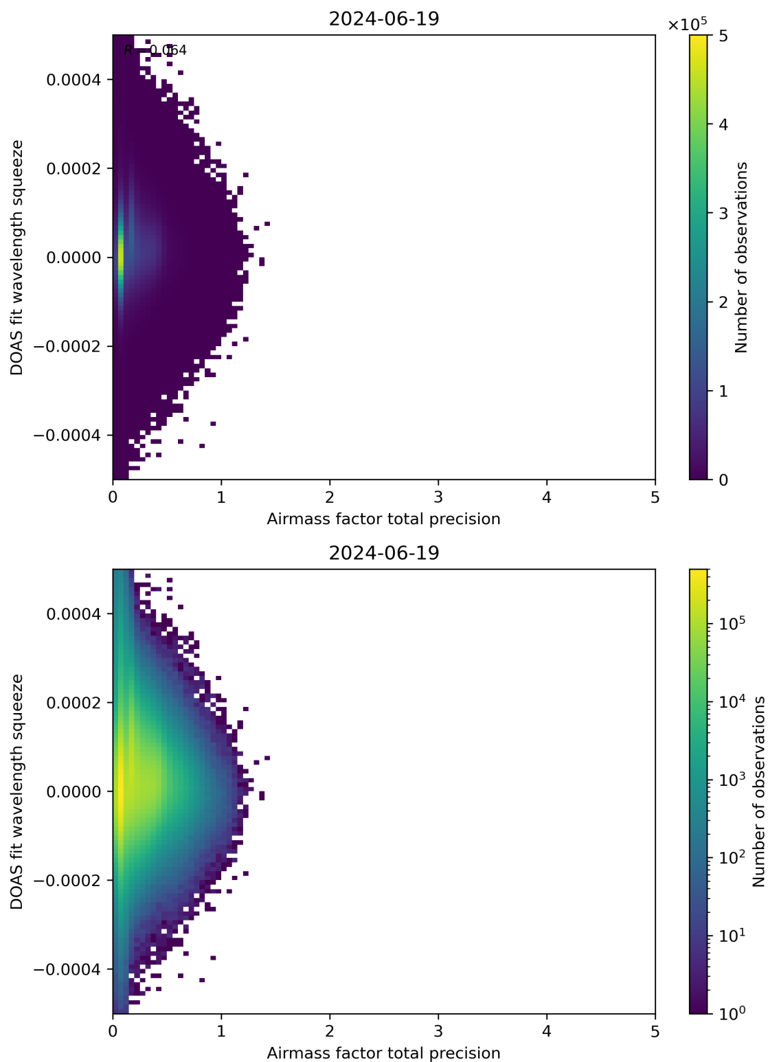
Figure 107: Scatter density plot of “Airmass factor total precision” against “DOAS fit wavelength squeeze” for 2024-06-19 to 2024-06-20.
