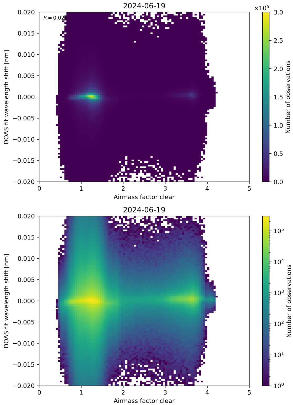
Figure 72: Scatter density plot of “Airmass factor clear” against “DOAS fit wavelength shift” for 2024-06-19 to 2024-06-20.
