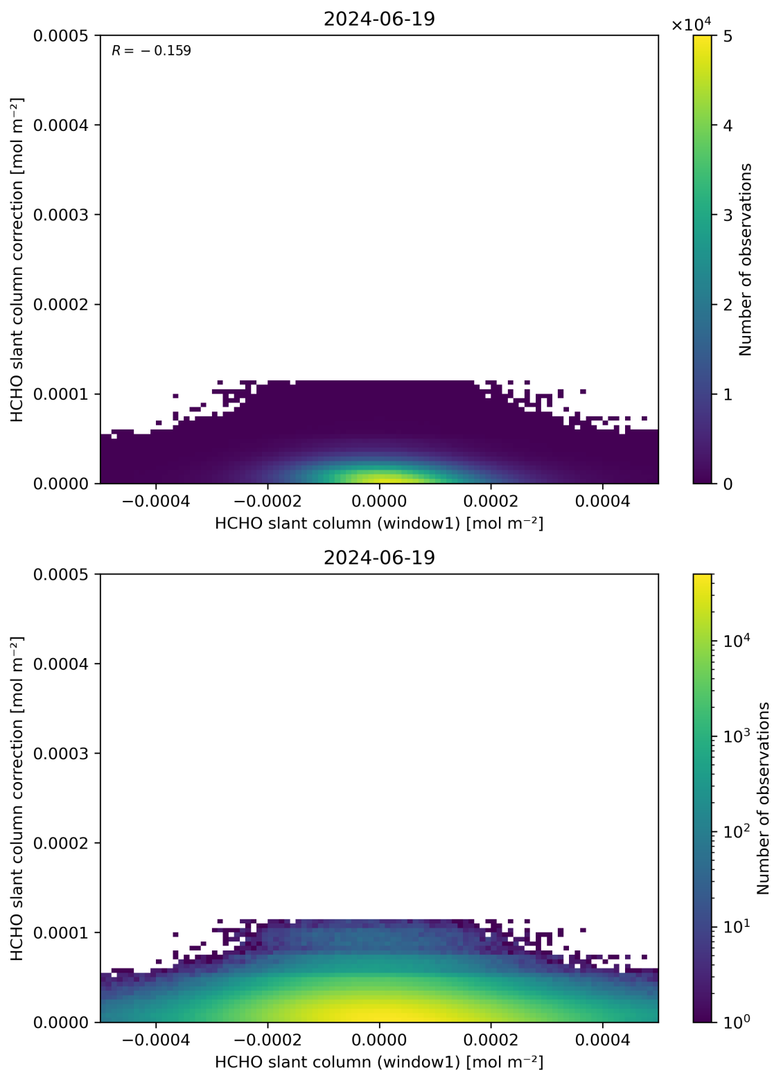
Figure 83: Scatter density plot of “HCHO slant column (window1)” against “HCHO slant column correction” for 2024-06-19 to 2024-06-20.
