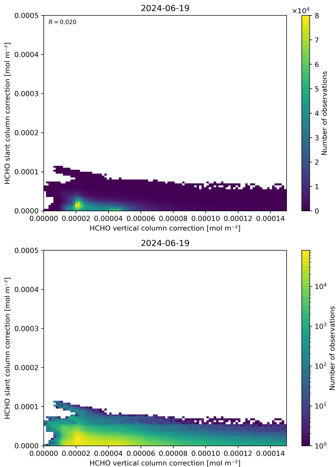
Figure 117: Scatter density plot of “HCHO vertical column correction” against “HCHO slant column correction” for 2024-06-19 to 2024-06-20.
