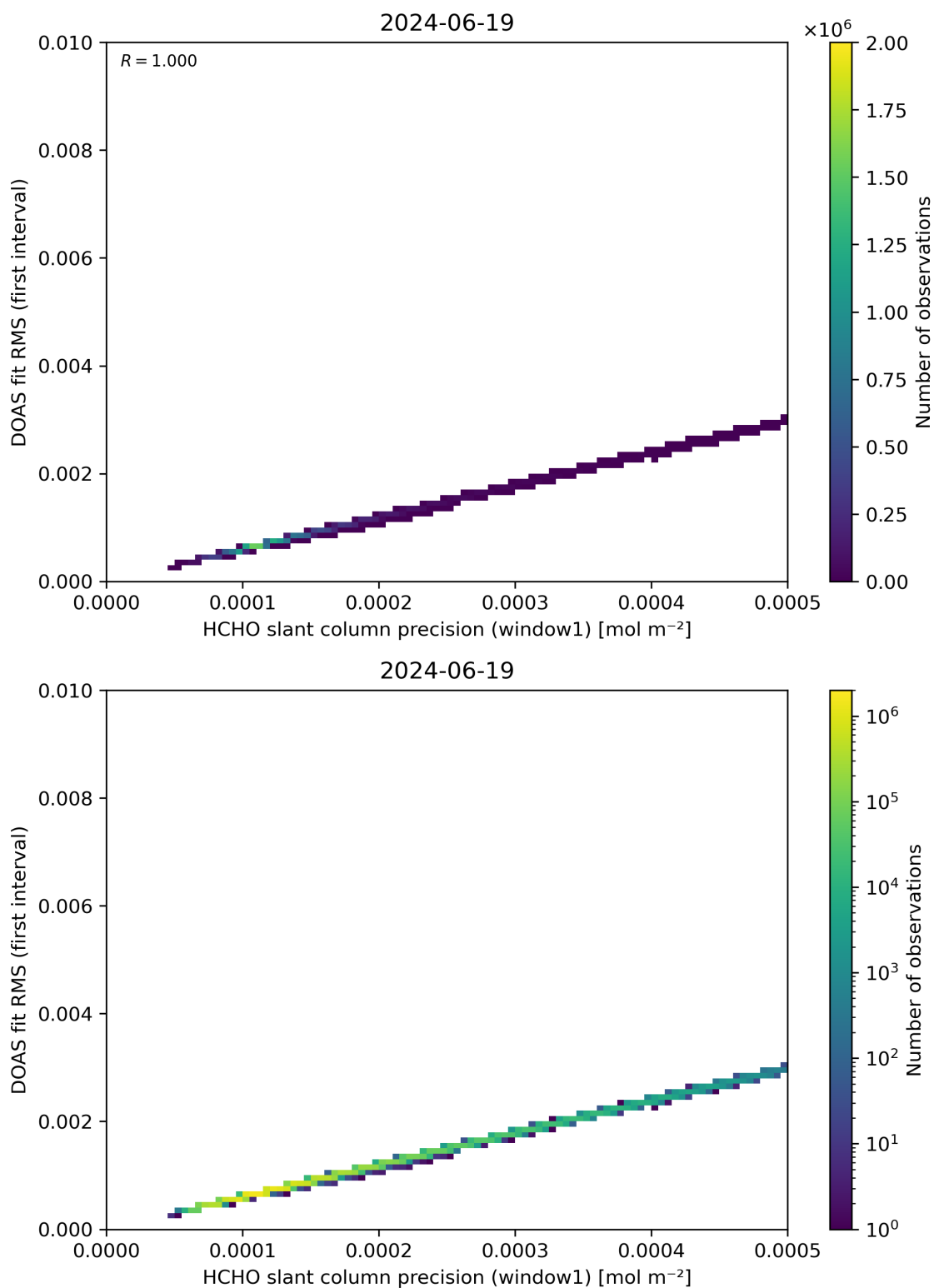
Figure 88: Scatter density plot of “HCHO slant column precision (window1)” against “DOAS fit RMS (first interval)” for 2024-06-19 to 2024-06-20.
