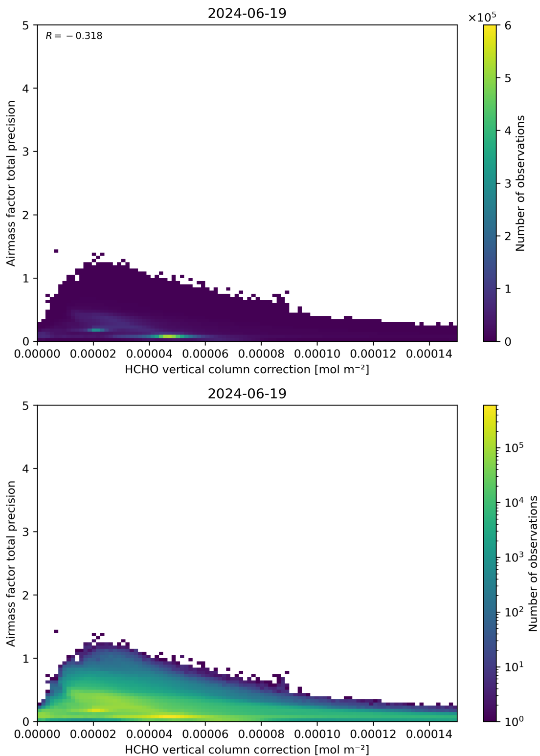
Figure 121: Scatter density plot of “HCHO vertical column correction” against “Airmass factor total precision” for 2024-06-19 to 2024-06-20.
