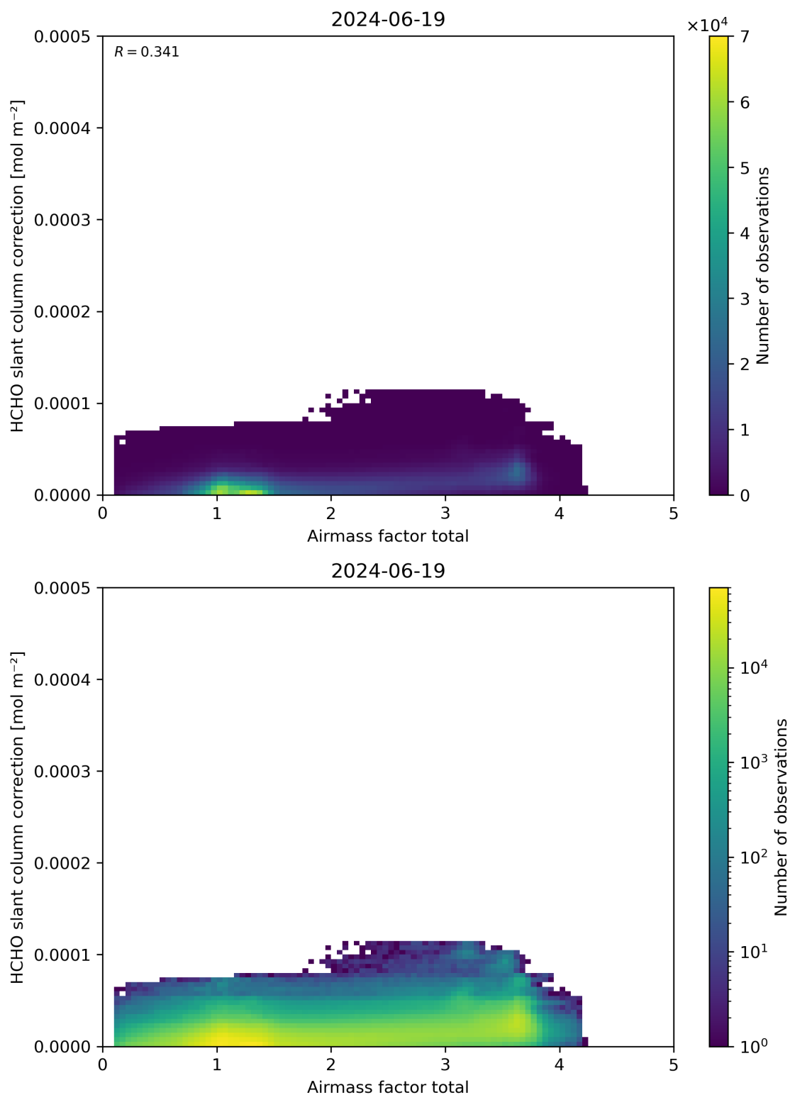
Figure 102: Scatter density plot of “Airmass factor total” against “HCHO slant column correction” for 2024-06-19 to 2024-06-20.
