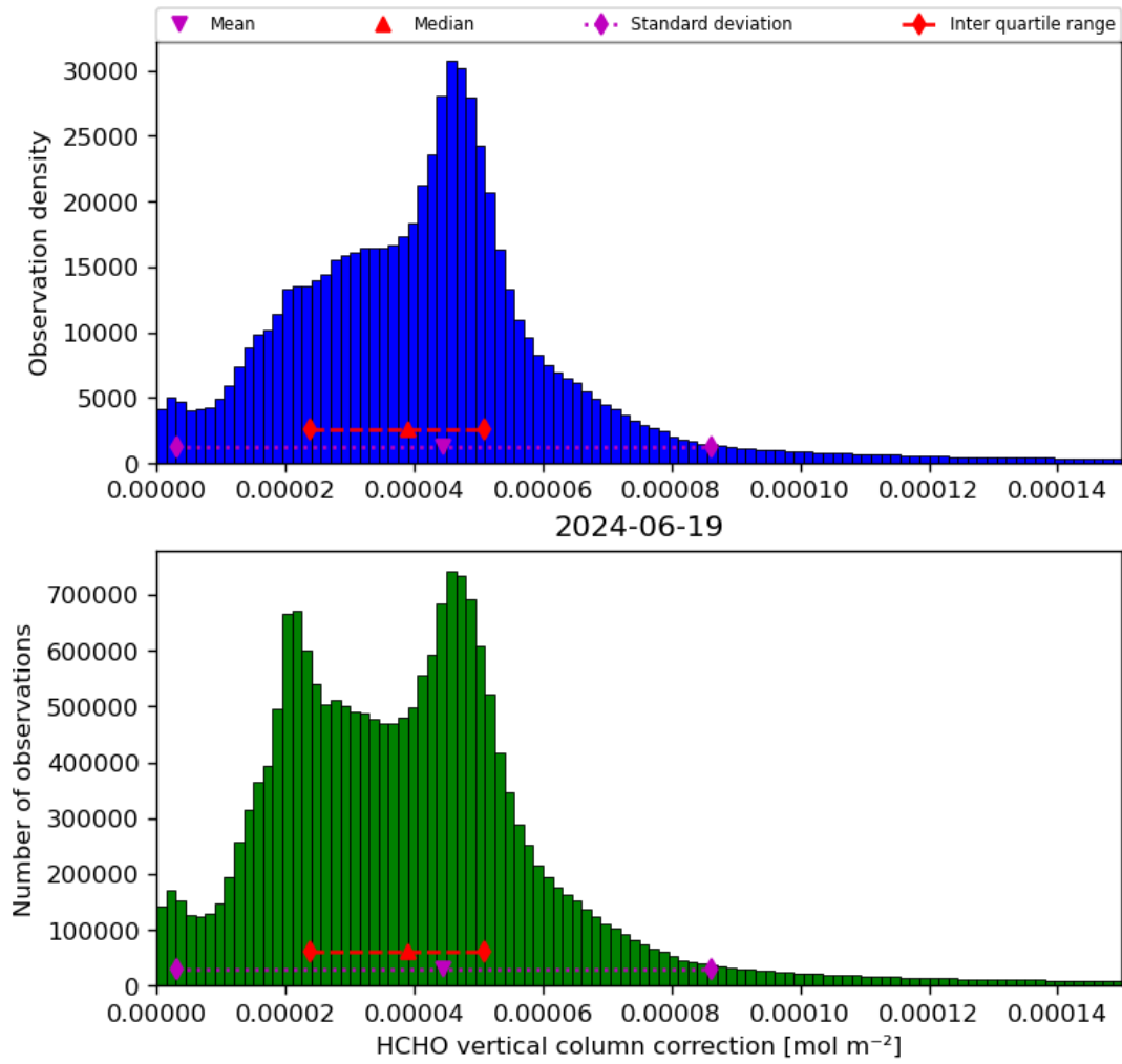
Figure 37: Histogram of “HCHO vertical column correction” for 2024-06-19 to 2024-06-20
