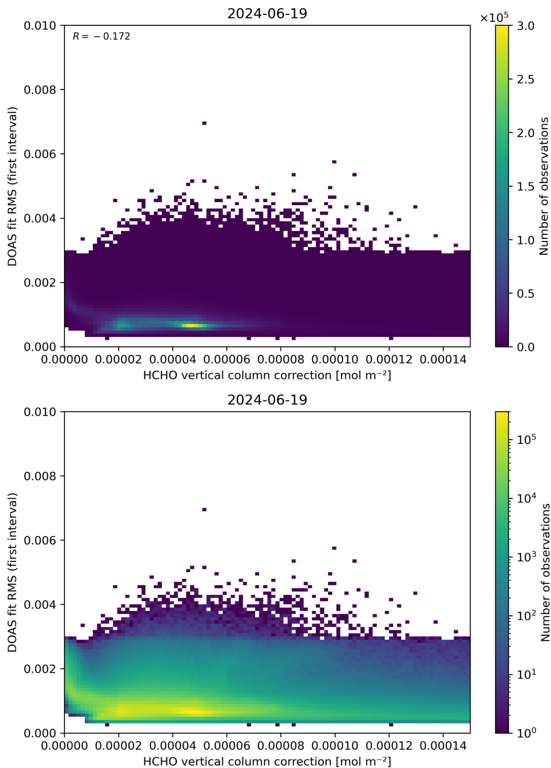
Figure 112: Scatter density plot of “HCHO vertical column correction” against “DOAS fit RMS (first interval)” for 2024-06-19 to 2024-06-20.
