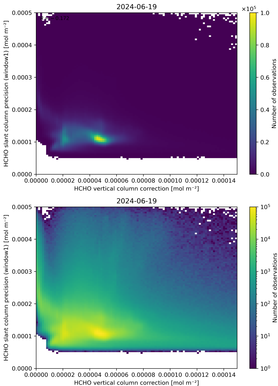
Figure 119: Scatter density plot of “HCHO vertical column correction” against “HCHO slant column precision (window1)” for 2024-06-19 to 2024-06-20.
