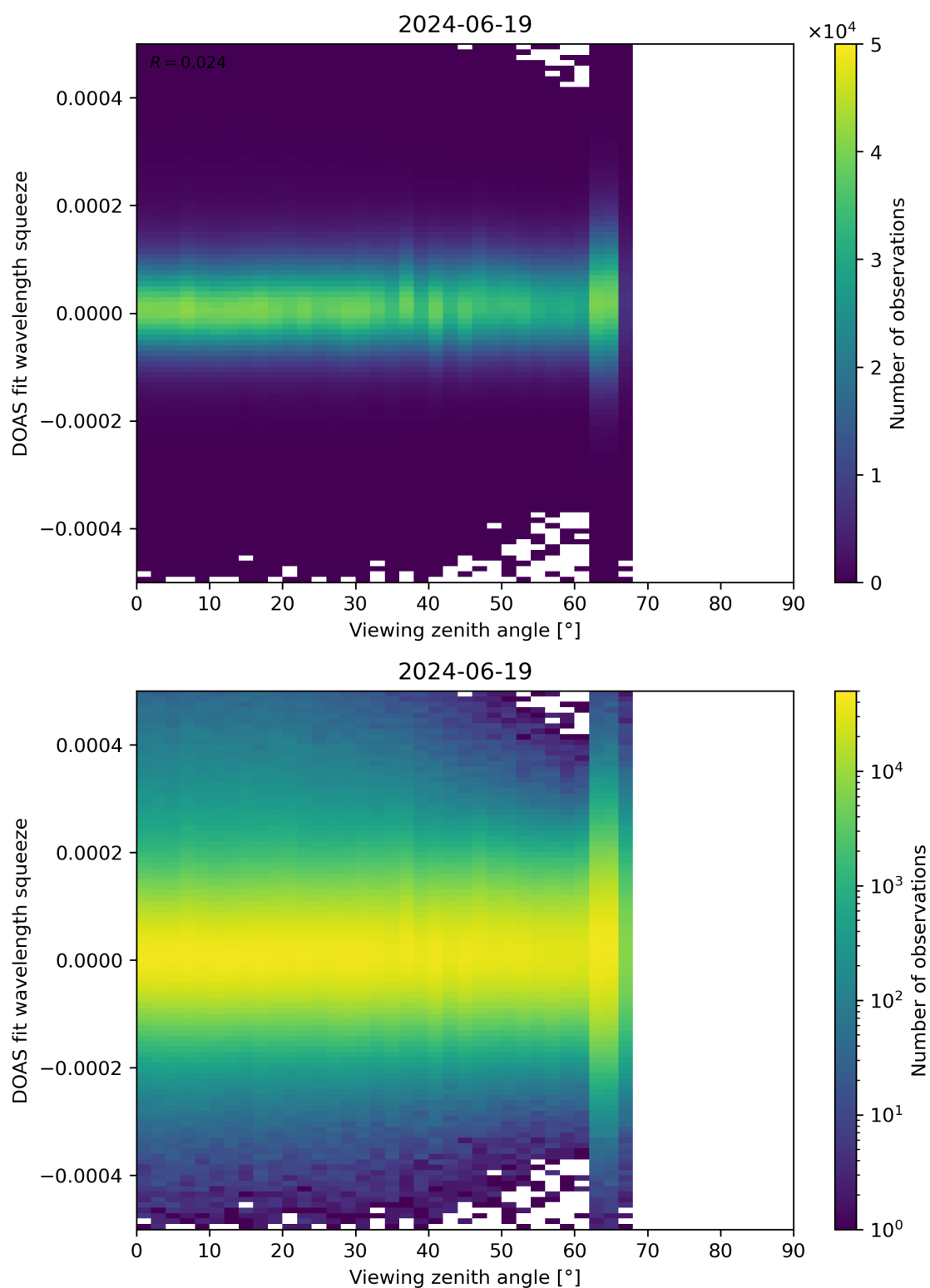
Figure 184: Scatter density plot of “Viewing zenith angle” against “DOAS fit wavelength squeeze” for 2024-06-19 to 2024-06-20.
