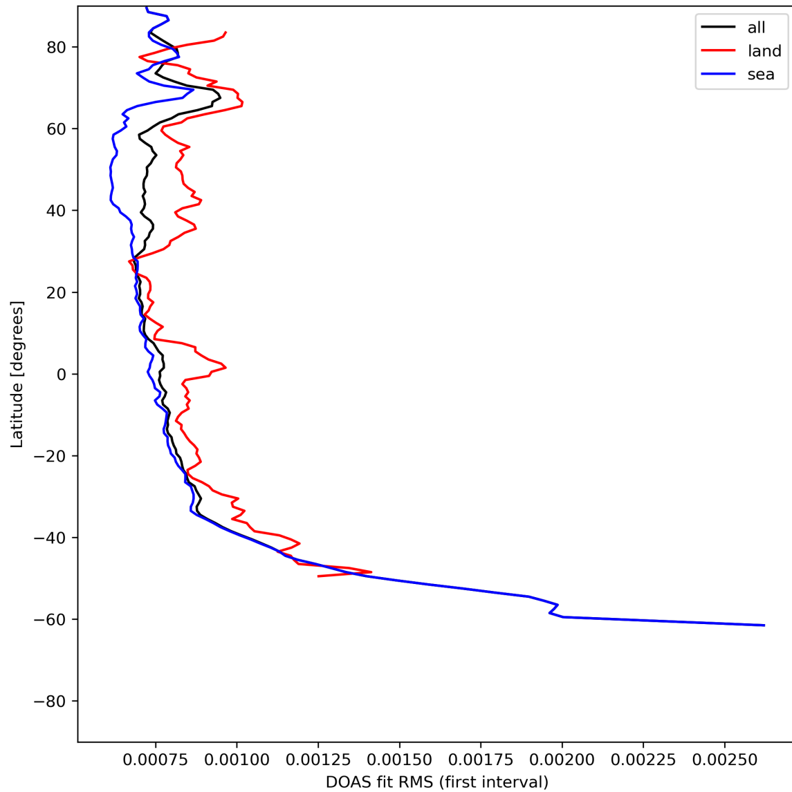
Figure 32: Zonal average of “DOAS fit RMS (first interval)” for 2024-06-19 to 2024-06-20.
