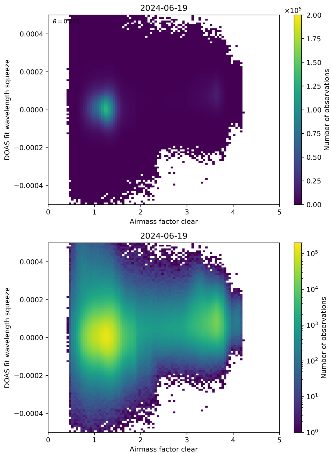
Figure 73: Scatter density plot of “Airmass factor clear” against “DOAS fit wavelength squeeze” for 2024-06-19 to 2024-06-20.
