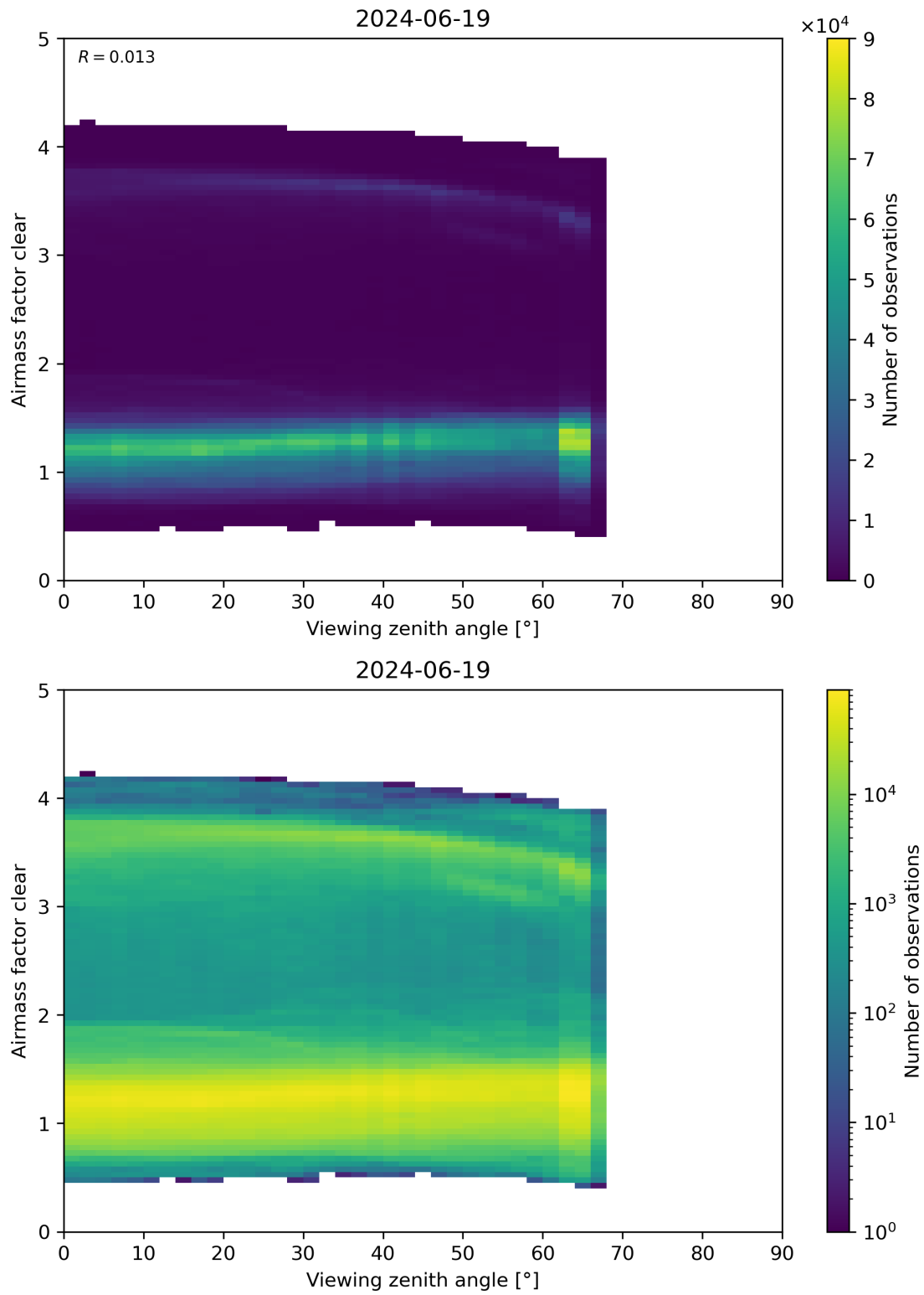
Figure 185: Scatter density plot of “Viewing zenith angle” against “Airmass factor clear” for 2024-06-19 to 2024-06-20.
