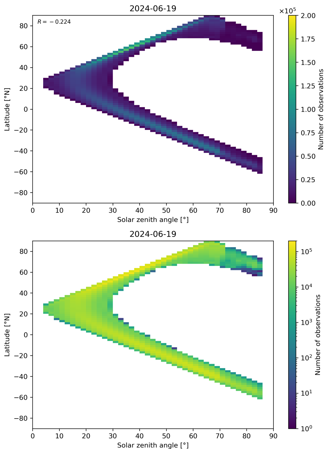
Figure 181: Scatter density plot of “Solar zenith angle” against “Latitude” for 2024-06-19 to 2024-06-20.
