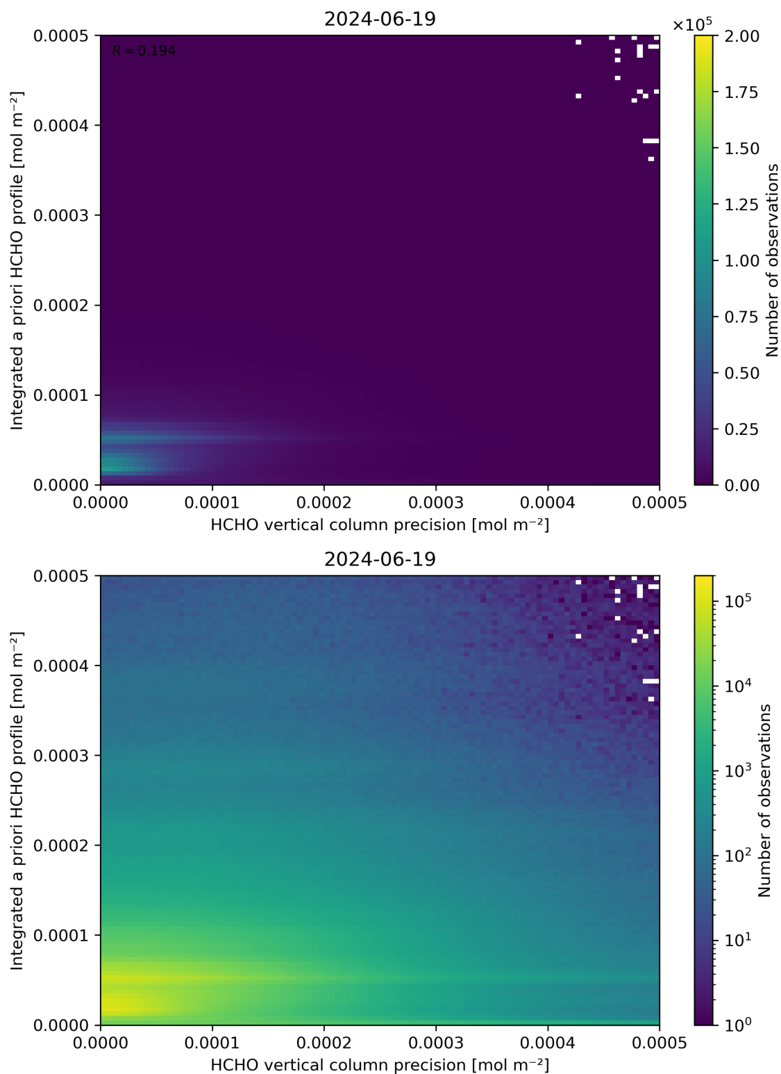
Figure 147: Scatter density plot of “HCHO vertical column precision” against “Integrated a priori HCHO profile” for 2024-06-19 to 2024-06-20.
