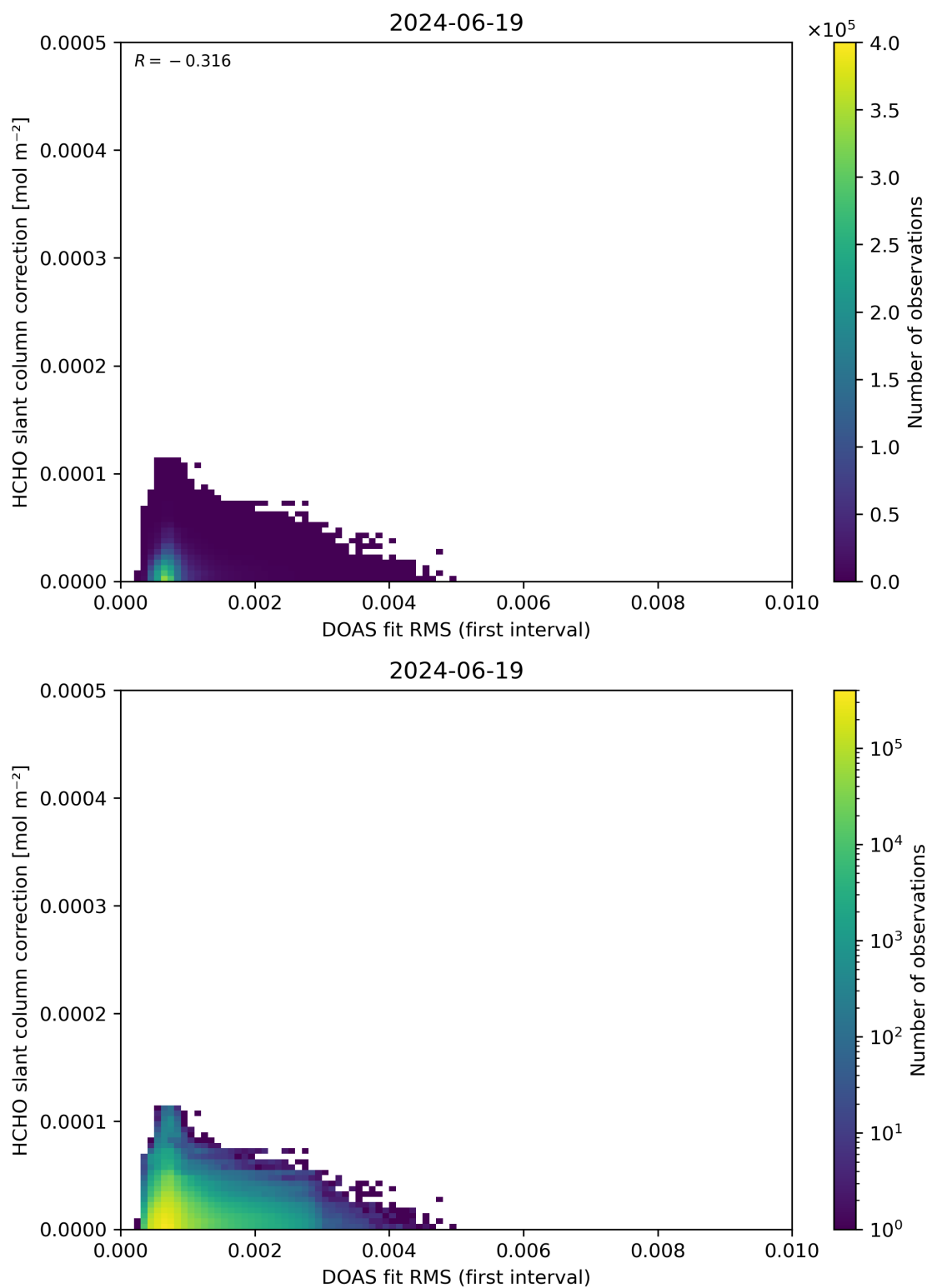
Figure 63: Scatter density plot of “DOAS fit RMS (first interval)” against “HCHO slant column correction” for 2024-06-19 to 2024-06-20.
