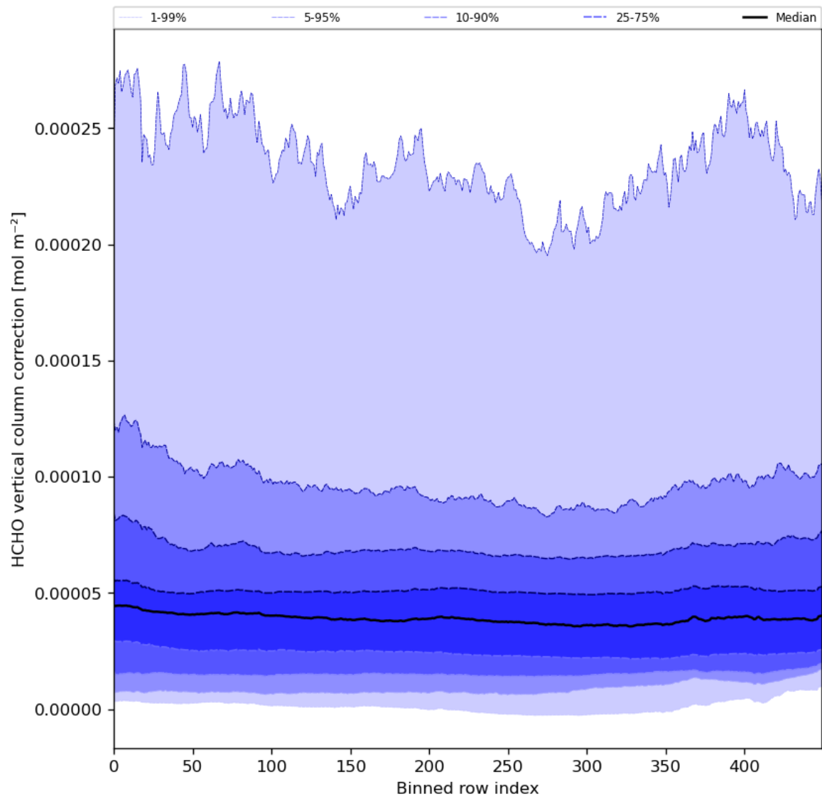
Figure 51: Along track statistics of “HCHO vertical column correction” for 2024-06-19 to 2024-06-20
