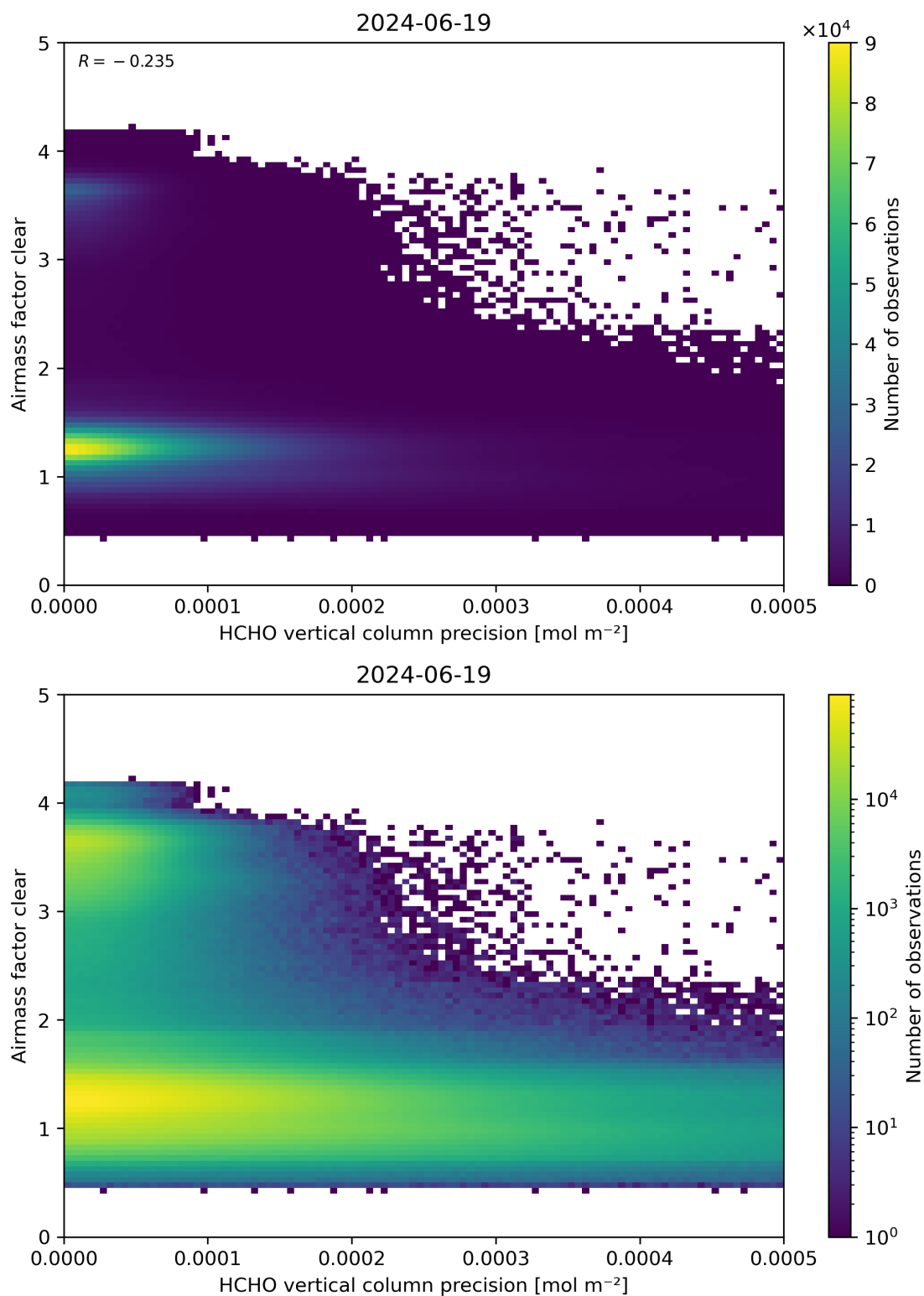
Figure 139: Scatter density plot of “HCHO vertical column precision” against “Airmass factor clear” for 2024-06-19 to 2024-06-20.
