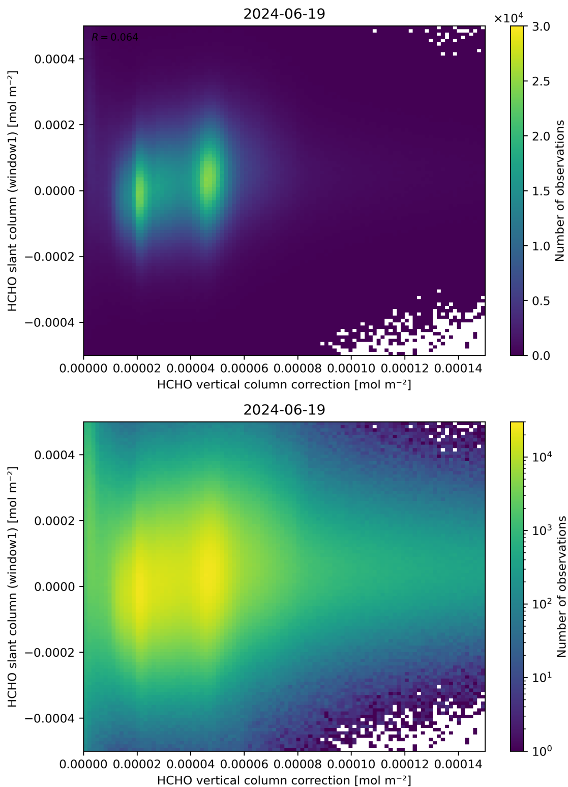
Figure 118: Scatter density plot of “HCHO vertical column correction” against “HCHO slant column (window1)” for 2024-06-19 to 2024-06-20.
