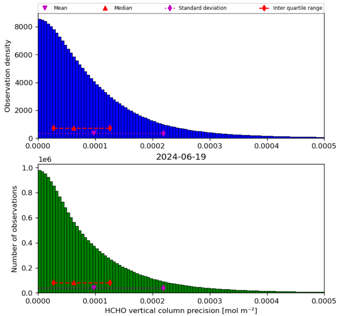
Figure 36: Histogram of “HCHO vertical column precision” for 2024-06-19 to 2024-06-20
