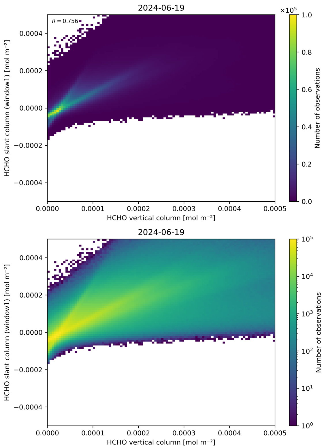
Figure 129: Scatter density plot of “HCHO vertical column” against “HCHO slant column (window1)” for 2024-06-19 to 2024-06-20.
