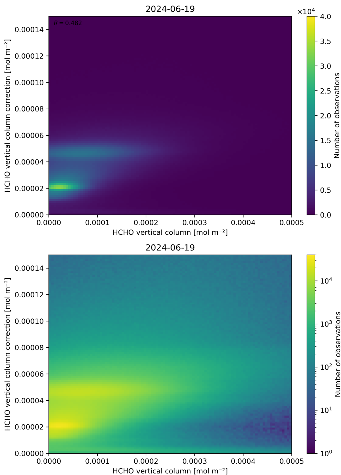
Figure 133: Scatter density plot of “HCHO vertical column” against “HCHO vertical column correction” for 2024-06-19 to 2024-06-20.
