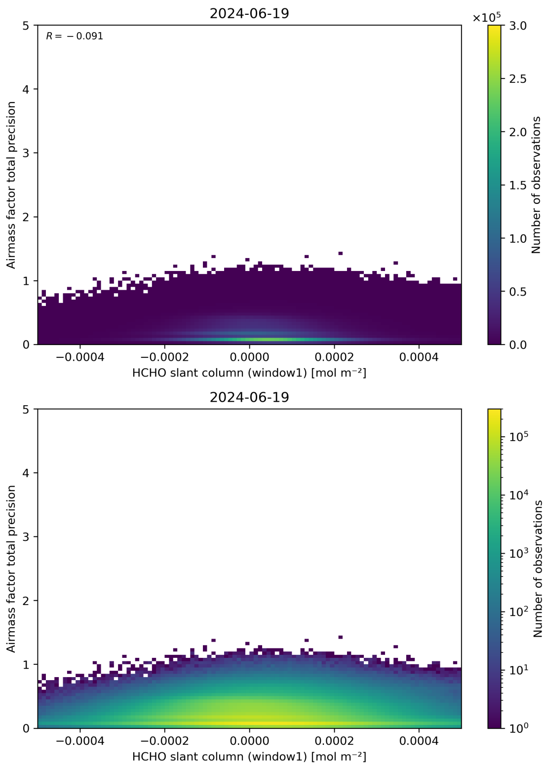
Figure 86: Scatter density plot of “HCHO slant column (window1)” against “Airmass factor total precision” for 2024-06-19 to 2024-06-20.
