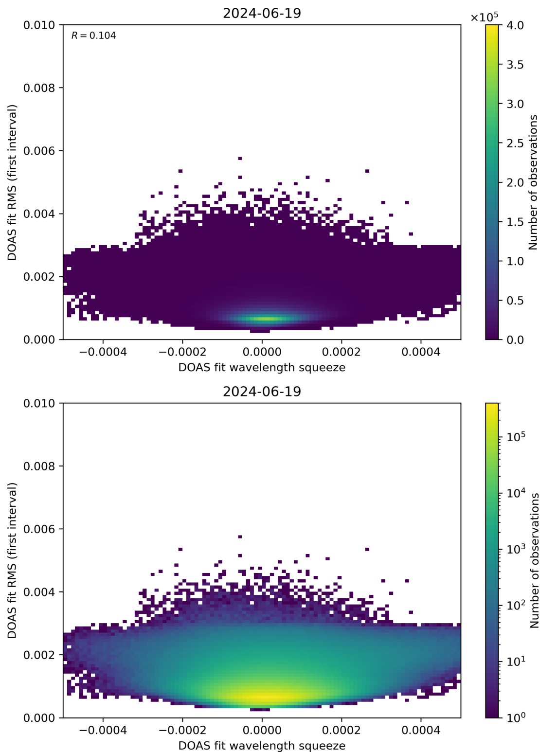
Figure 68: Scatter density plot of “DOAS fit wavelength squeeze” against “DOAS fit RMS (first interval)” for 2024-06-19 to 2024-06-20.
