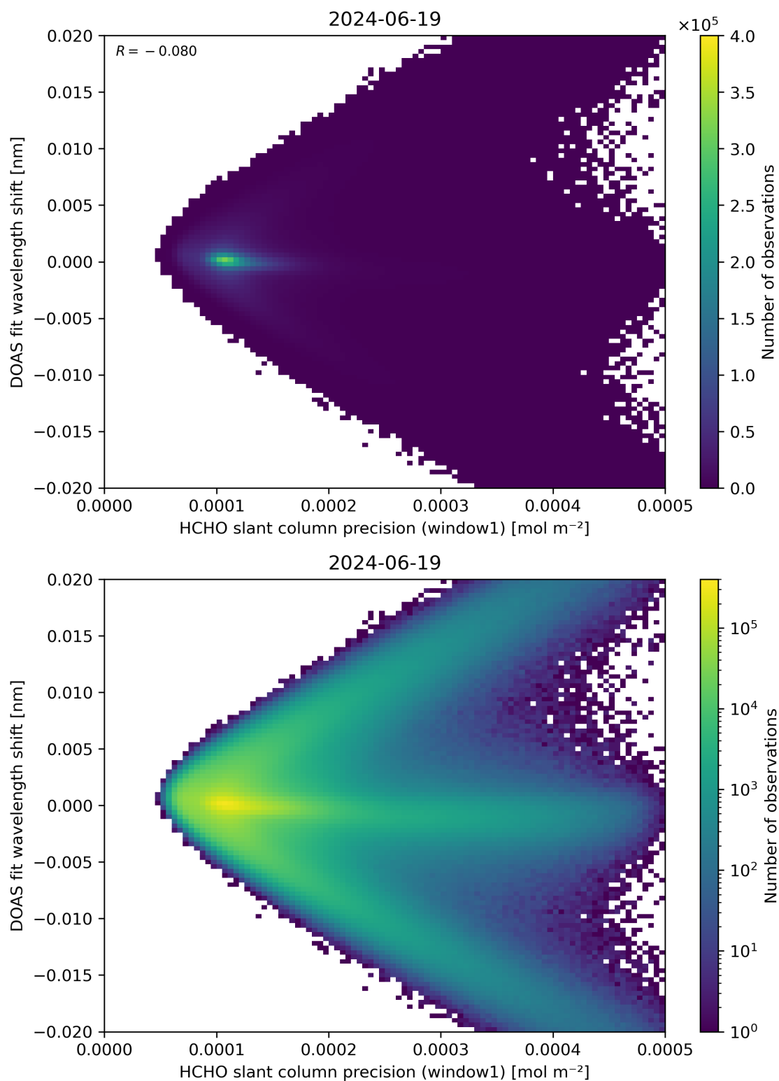
Figure 89: Scatter density plot of “HCHO slant column precision (window1)” against “DOAS fit wavelength shift” for 2024-06-19 to 2024-06-20.
