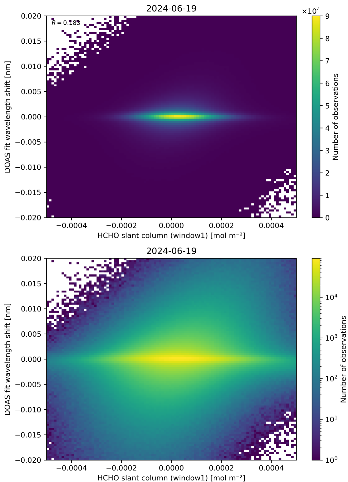
Figure 79: Scatter density plot of “HCHO slant column (window1)” against “DOAS fit wavelength shift” for 2024-06-19 to 2024-06-20.
