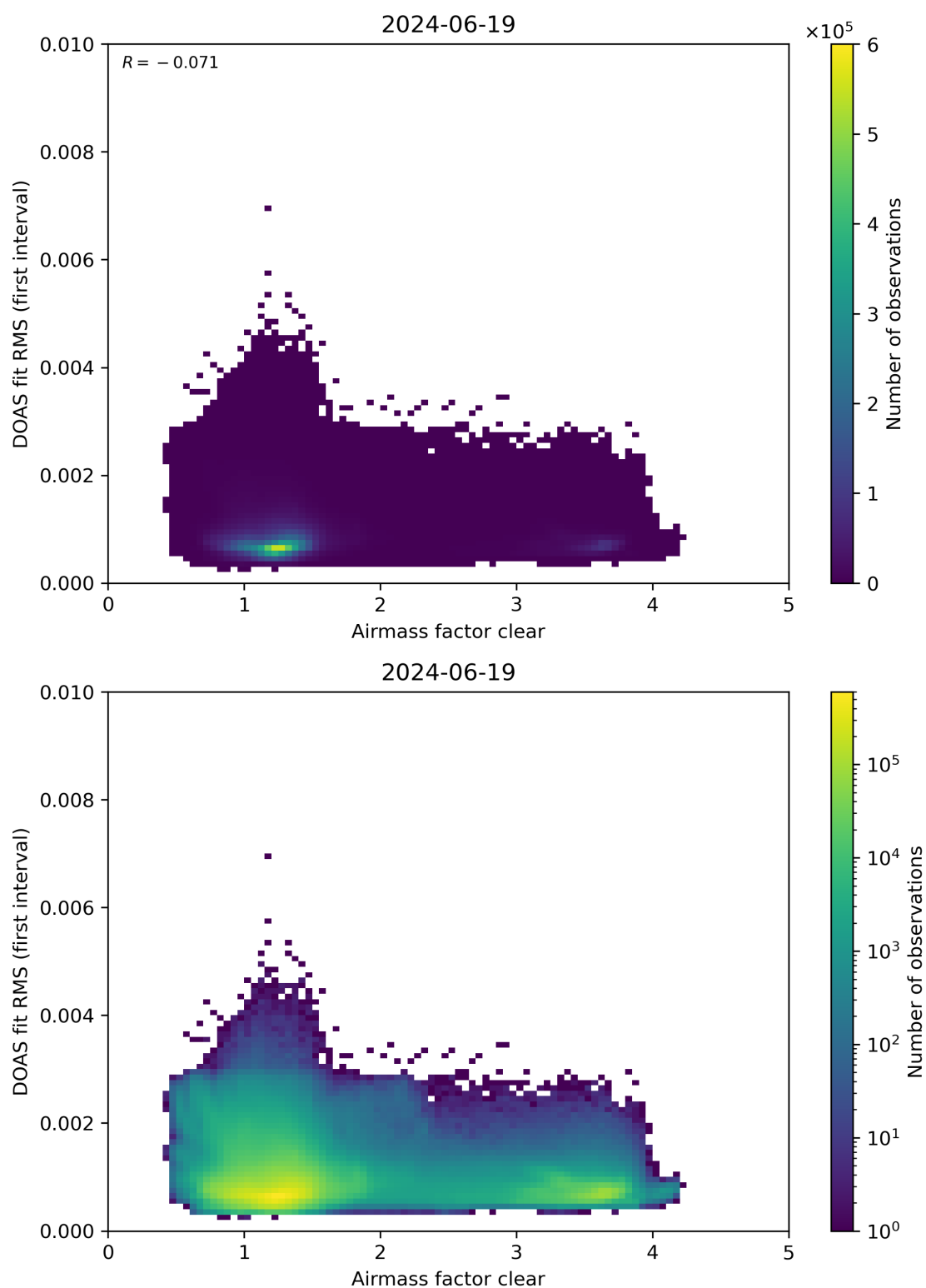
Figure 71: Scatter density plot of “Airmass factor clear” against “DOAS fit RMS (first interval)” for 2024-06-19 to 2024-06-20.
