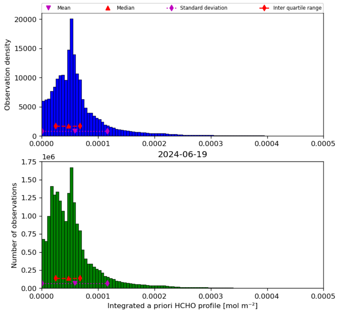
Figure 43: Histogram of “Integrated a priori HCHO profile” for 2024-06-19 to 2024-06-20
