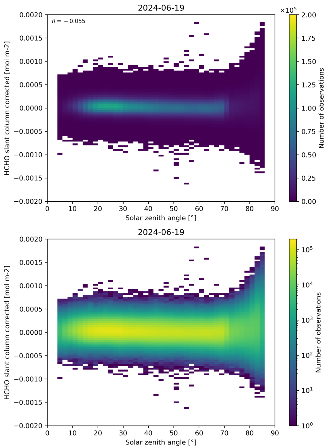
Figure 171: Scatter density plot of “Solar zenith angle” against “HCHO slant column corrected” for 2024-06-19 to 2024-06-20.
