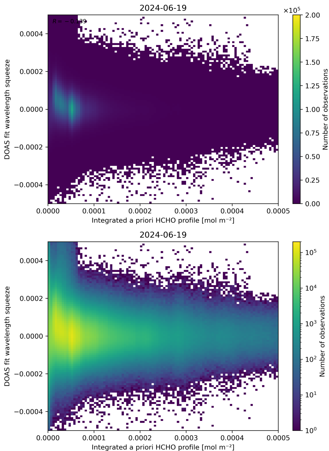
Figure 150: Scatter density plot of “Integrated a priori HCHO profile” against “DOAS fit wavelength squeeze” for 2024-06-19 to 2024-06-20.
