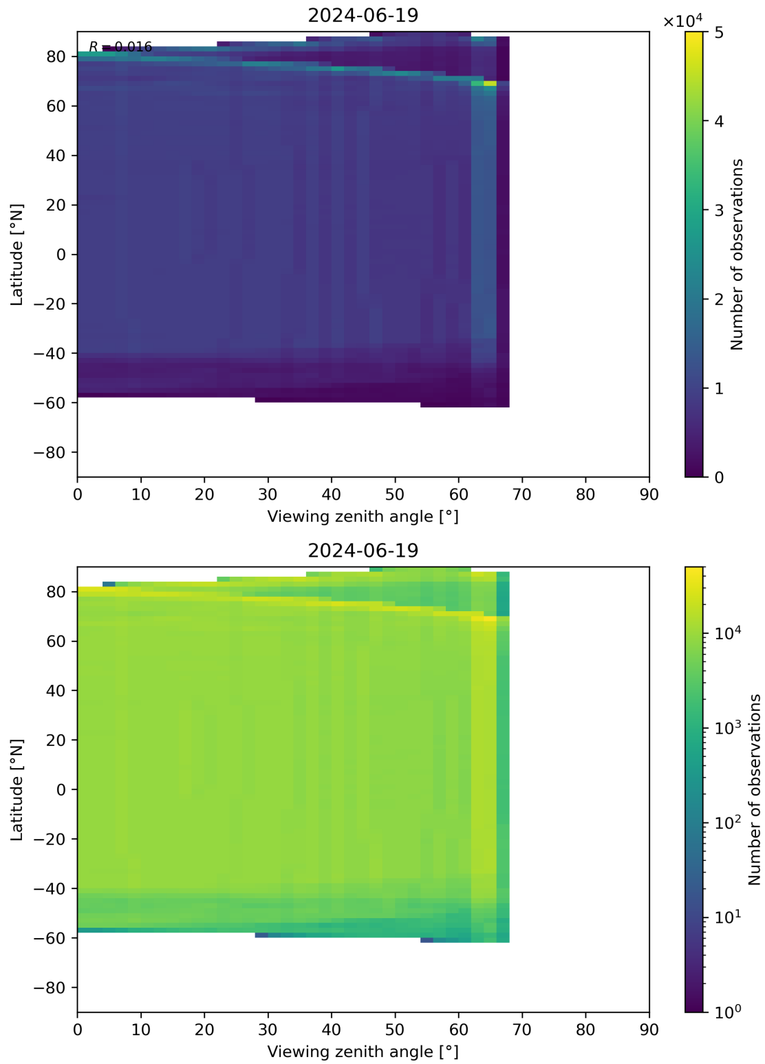
Figure 196: Scatter density plot of “Viewing zenith angle” against “Latitude” for 2024-06-19 to 2024-06-20.
