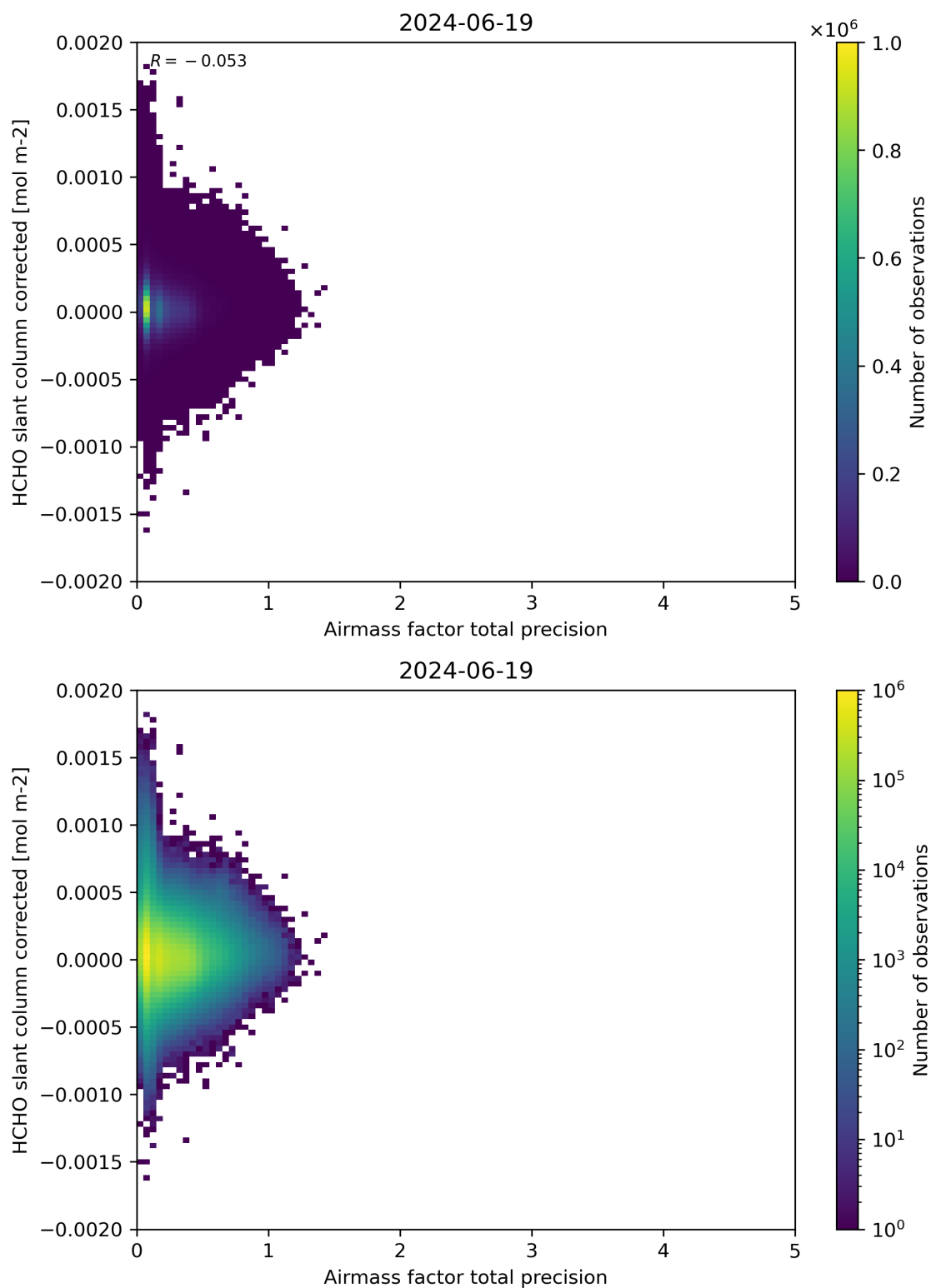
Figure 109: Scatter density plot of “Airmass factor total precision” against “HCHO slant column corrected” for 2024-06-19 to 2024-06-20.
