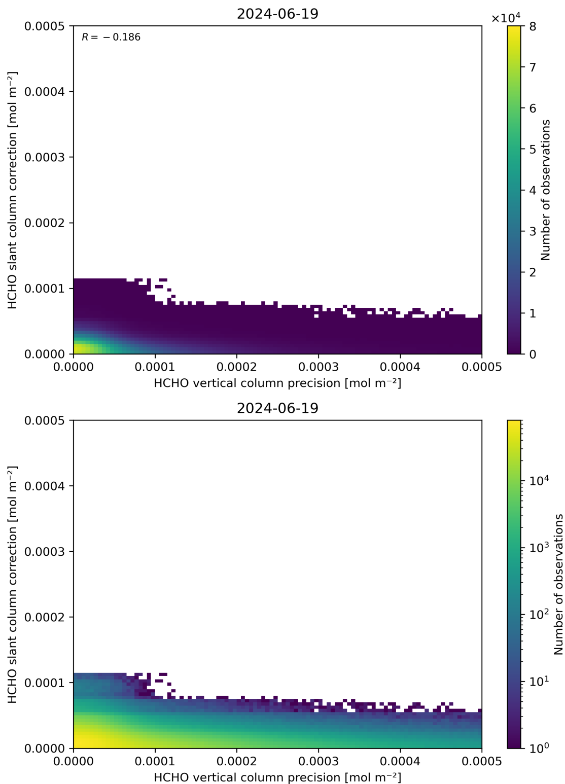
Figure 141: Scatter density plot of “HCHO vertical column precision” against “HCHO slant column correction” for 2024-06-19 to 2024-06-20.
