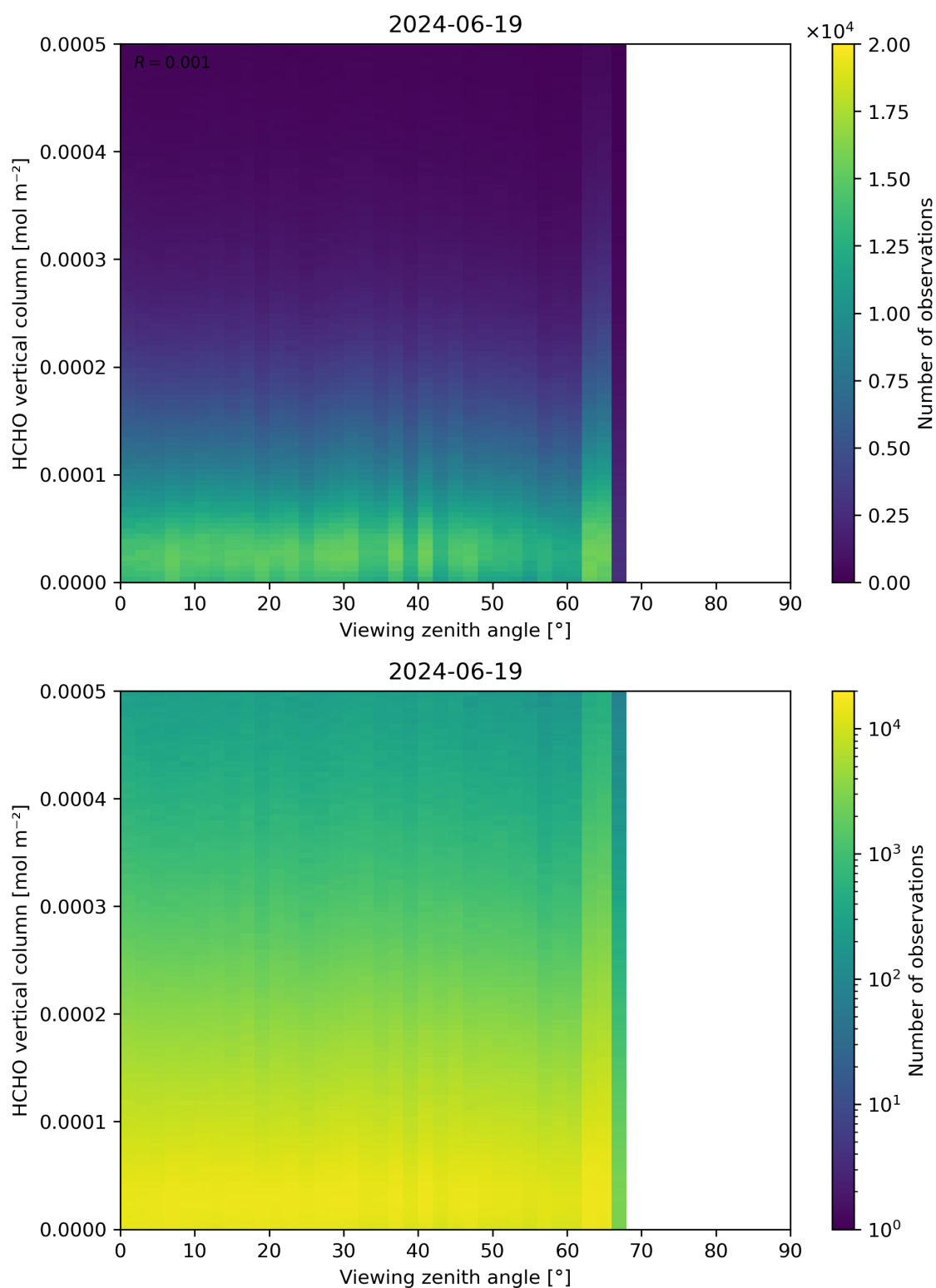
Figure 192: Scatter density plot of “Viewing zenith angle” against “HCHO vertical column” for 2024-06-19 to 2024-06-20.
