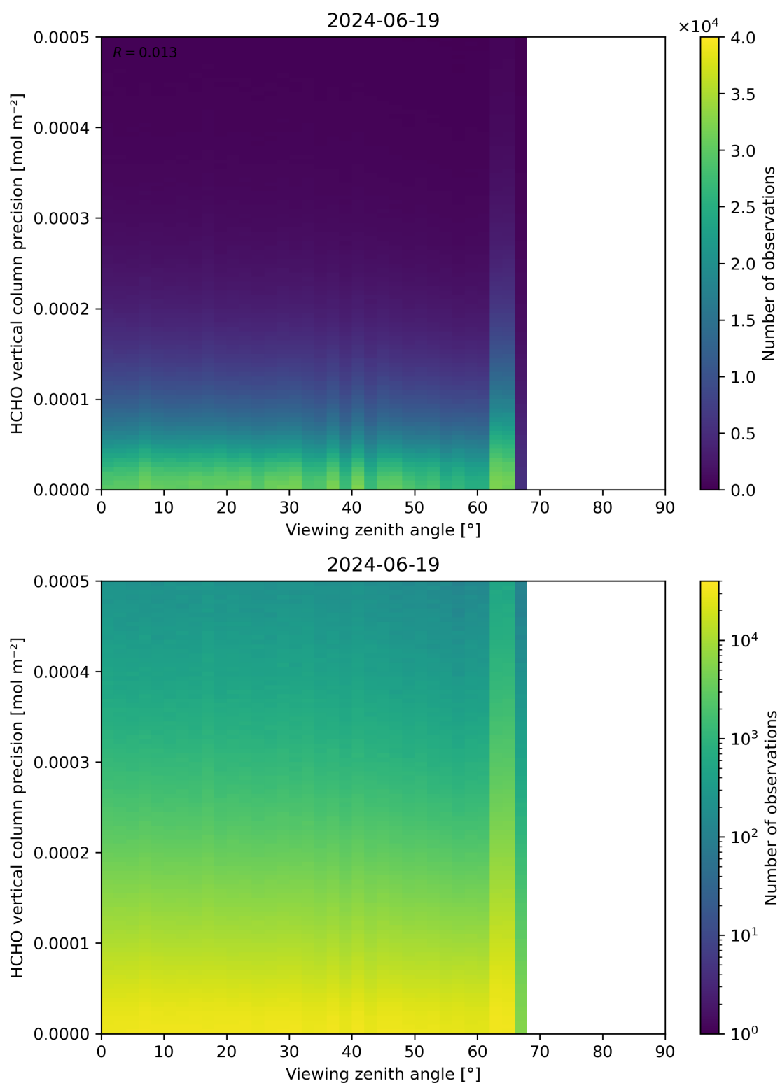
Figure 194: Scatter density plot of “Viewing zenith angle” against “HCHO vertical column precision” for 2024-06-19 to 2024-06-20.
