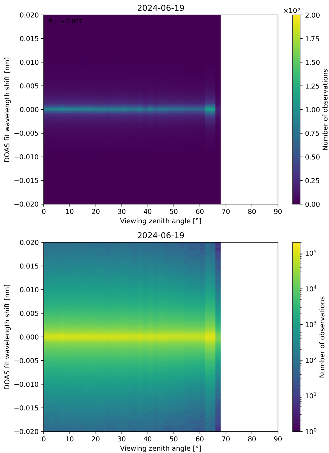
Figure 183: Scatter density plot of “Viewing zenith angle” against “DOAS fit wavelength shift” for 2024-06-19 to 2024-06-20.
