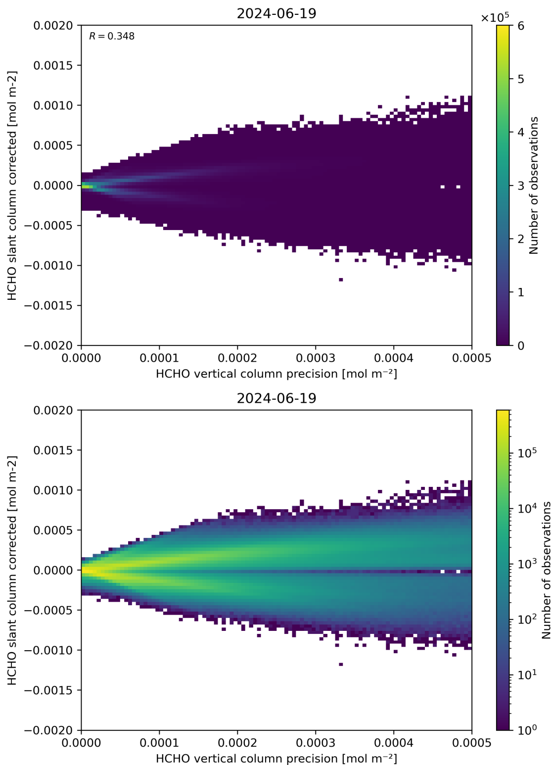
Figure 140: Scatter density plot of “HCHO vertical column precision” against “HCHO slant column corrected” for 2024-06-19 to 2024-06-20.
