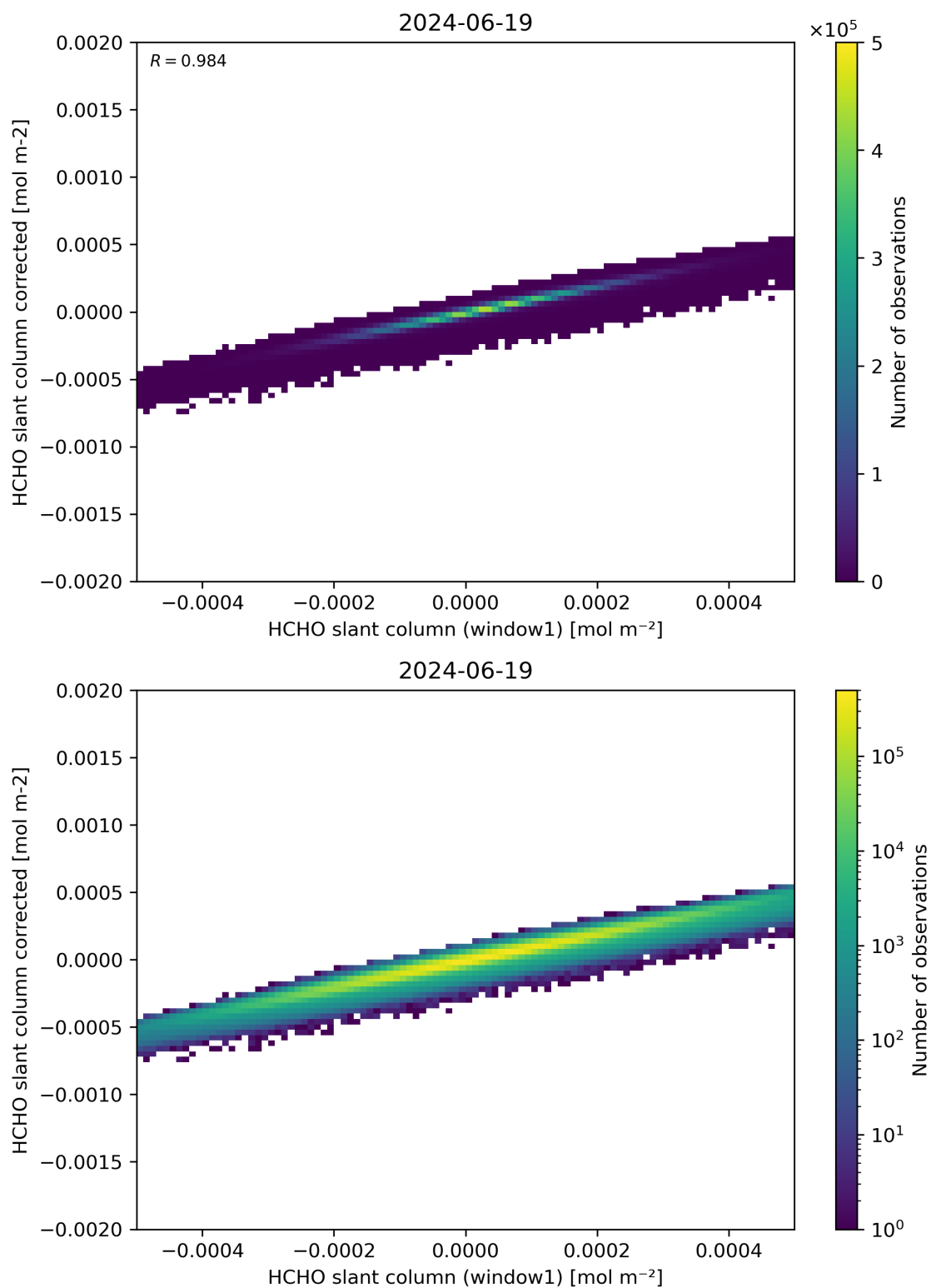
Figure 82: Scatter density plot of “HCHO slant column (window1)” against “HCHO slant column corrected” for 2024-06-19 to 2024-06-20.
