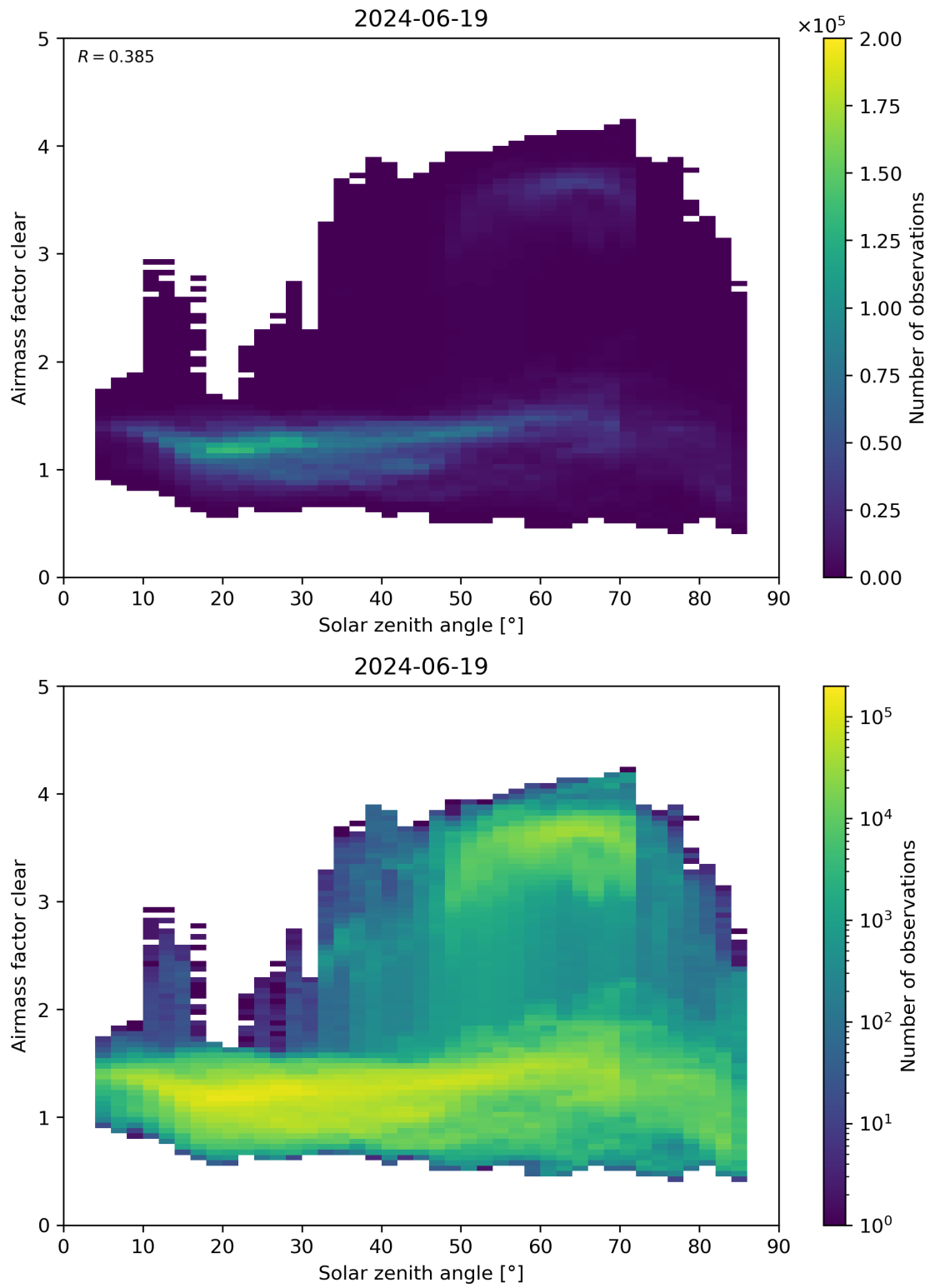
Figure 170: Scatter density plot of “Solar zenith angle” against “Airmass factor clear” for 2024-06-19 to 2024-06-20.
