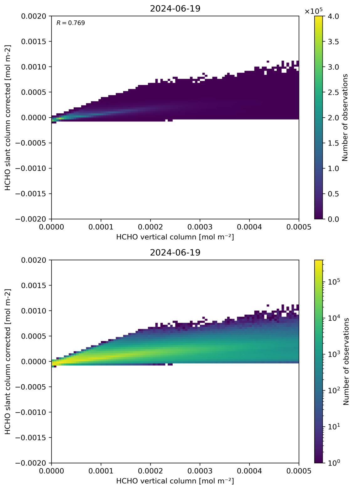
Figure 127: Scatter density plot of “HCHO vertical column” against “HCHO slant column corrected” for 2024-06-19 to 2024-06-20.
