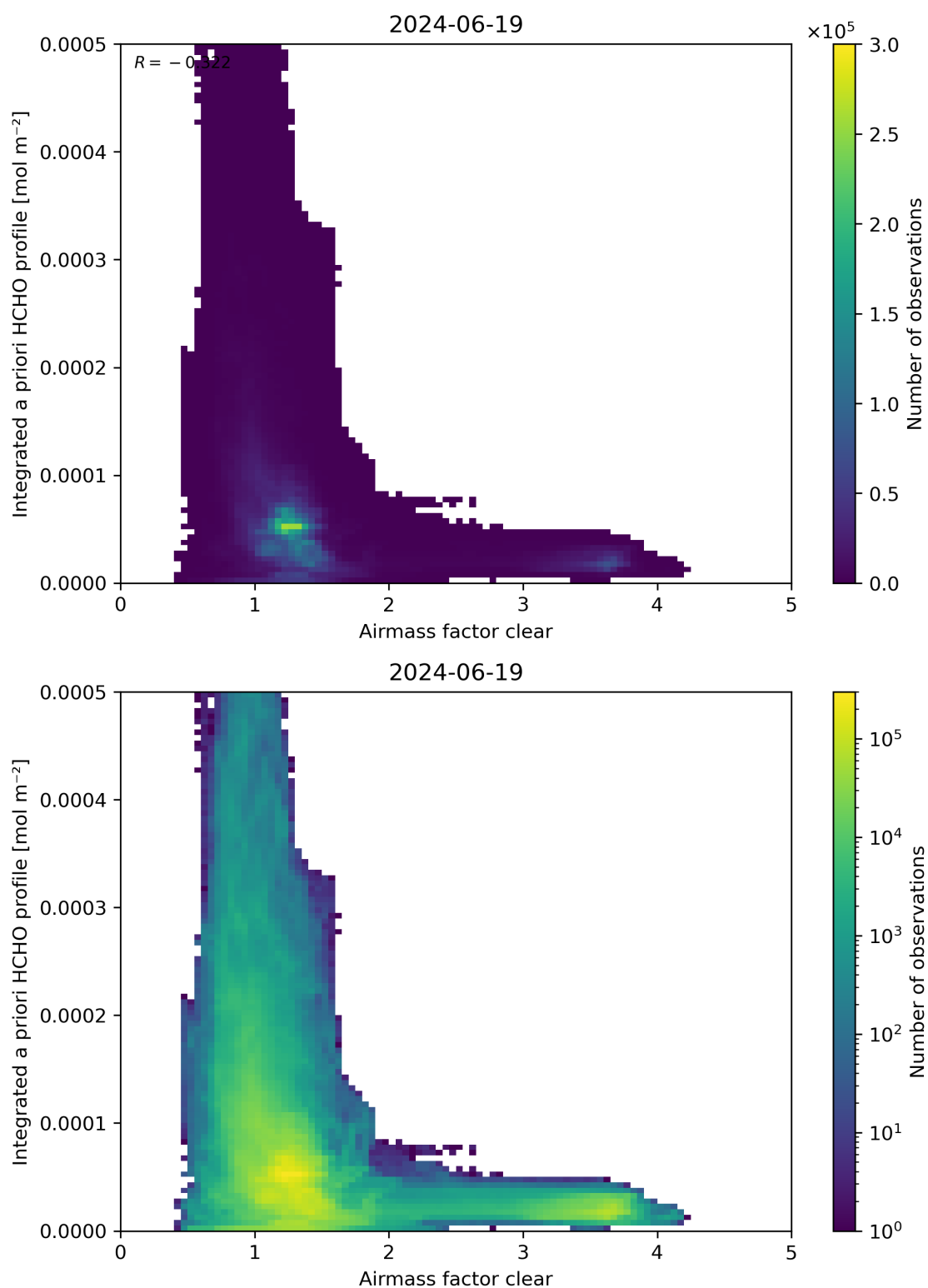
Figure 76: Scatter density plot of “Airmass factor clear” against “Integrated a priori HCHO profile” for 2024-06-19 to 2024-06-20.
