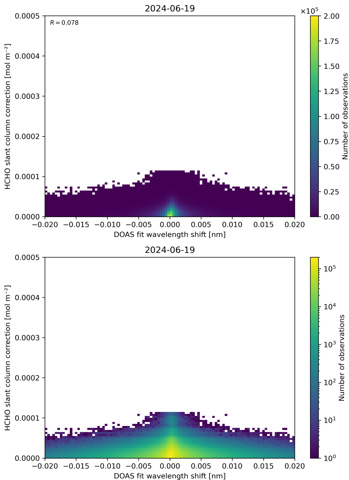
Figure 67: Scatter density plot of “DOAS fit wavelength shift” against “HCHO slant column correction” for 2024-06-19 to 2024-06-20.
