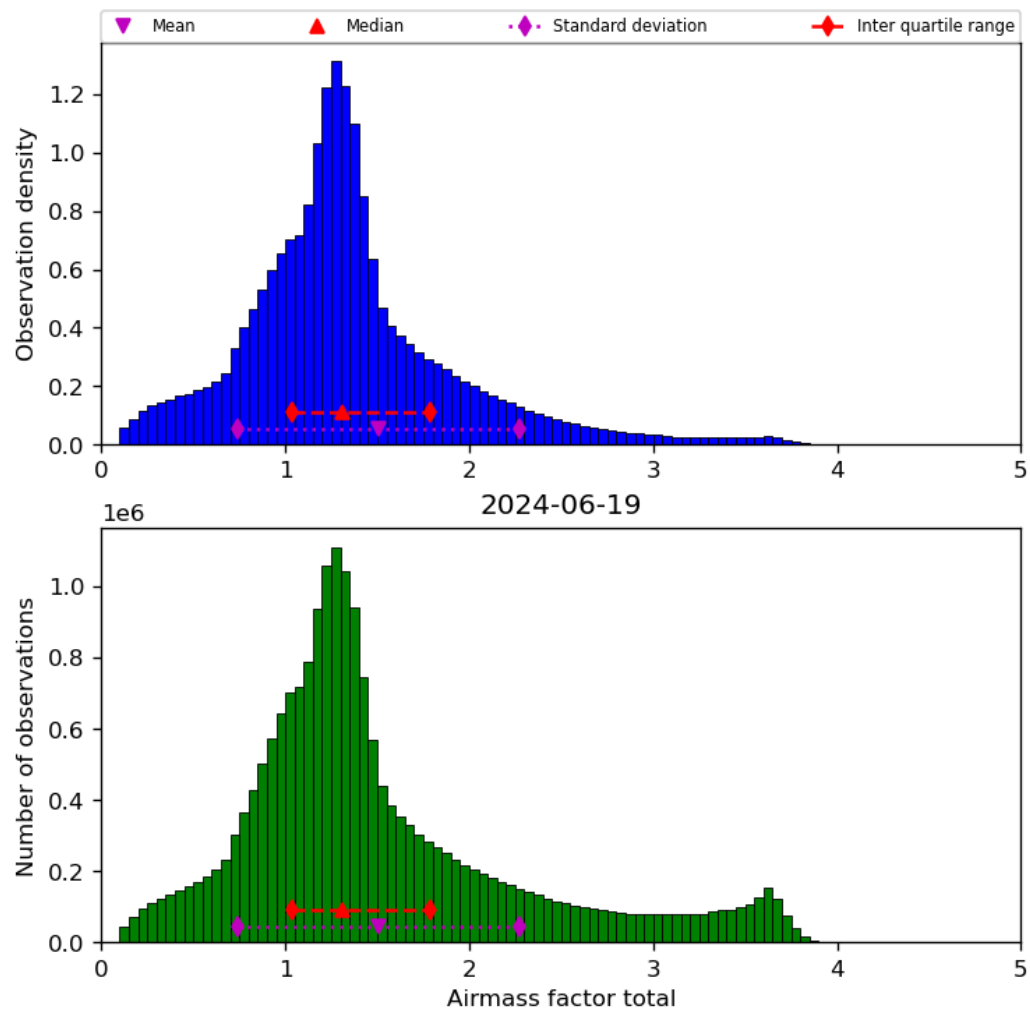
Figure 40: Histogram of “Airmass factor total” for 2024-06-19 to 2024-06-20
