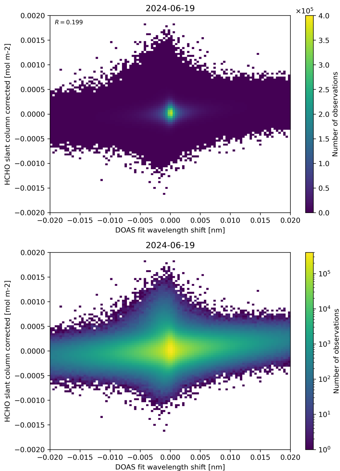
Figure 66: Scatter density plot of “DOAS fit wavelength shift” against “HCHO slant column corrected” for 2024-06-19 to 2024-06-20.
