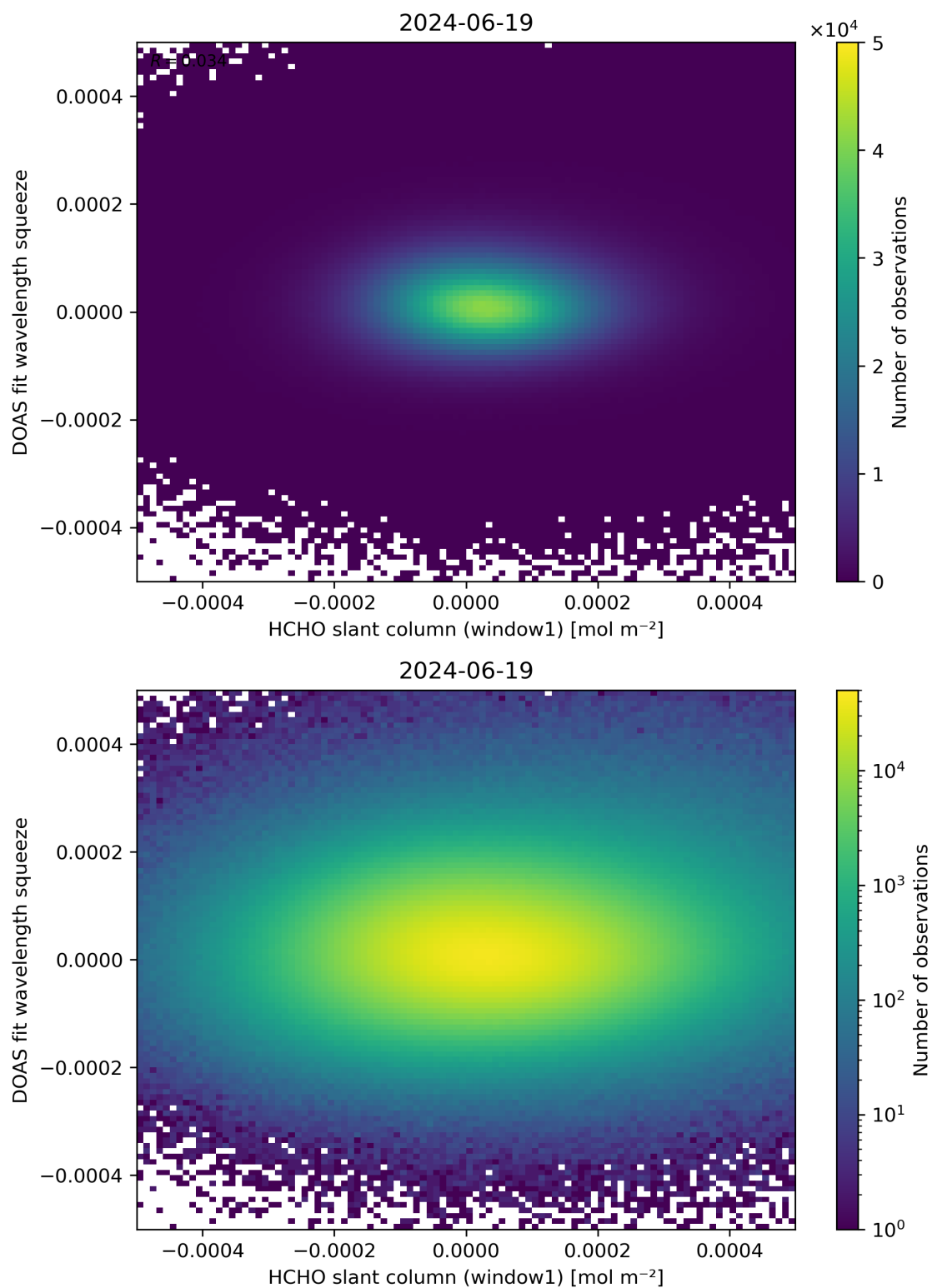
Figure 80: Scatter density plot of “HCHO slant column (window1)” against “DOAS fit wavelength squeeze” for 2024-06-19 to 2024-06-20.
