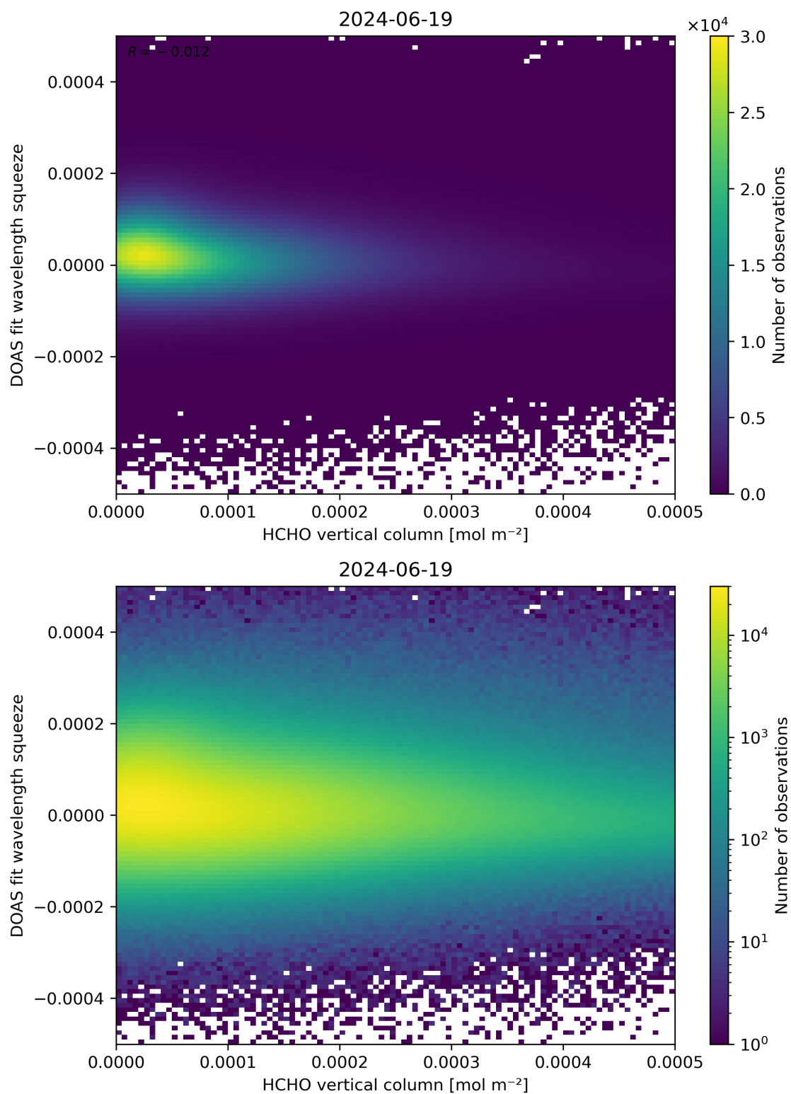
Figure 125: Scatter density plot of “HCHO vertical column” against “DOAS fit wavelength squeeze” for 2024-06-19 to 2024-06-20.
