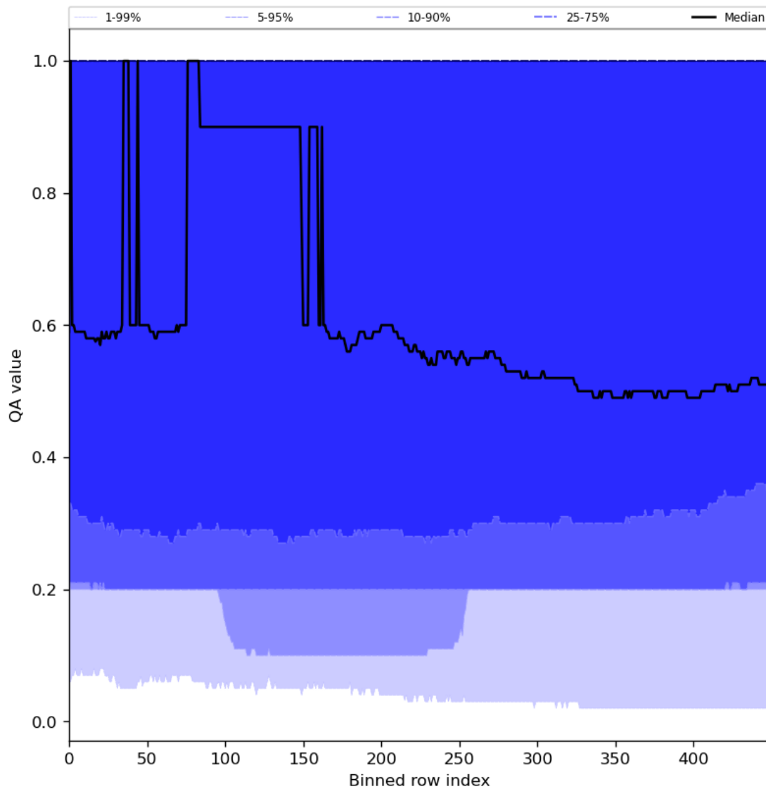
Figure 48: Along track statistics of “QA value” for 2024-06-19 to 2024-06-20
