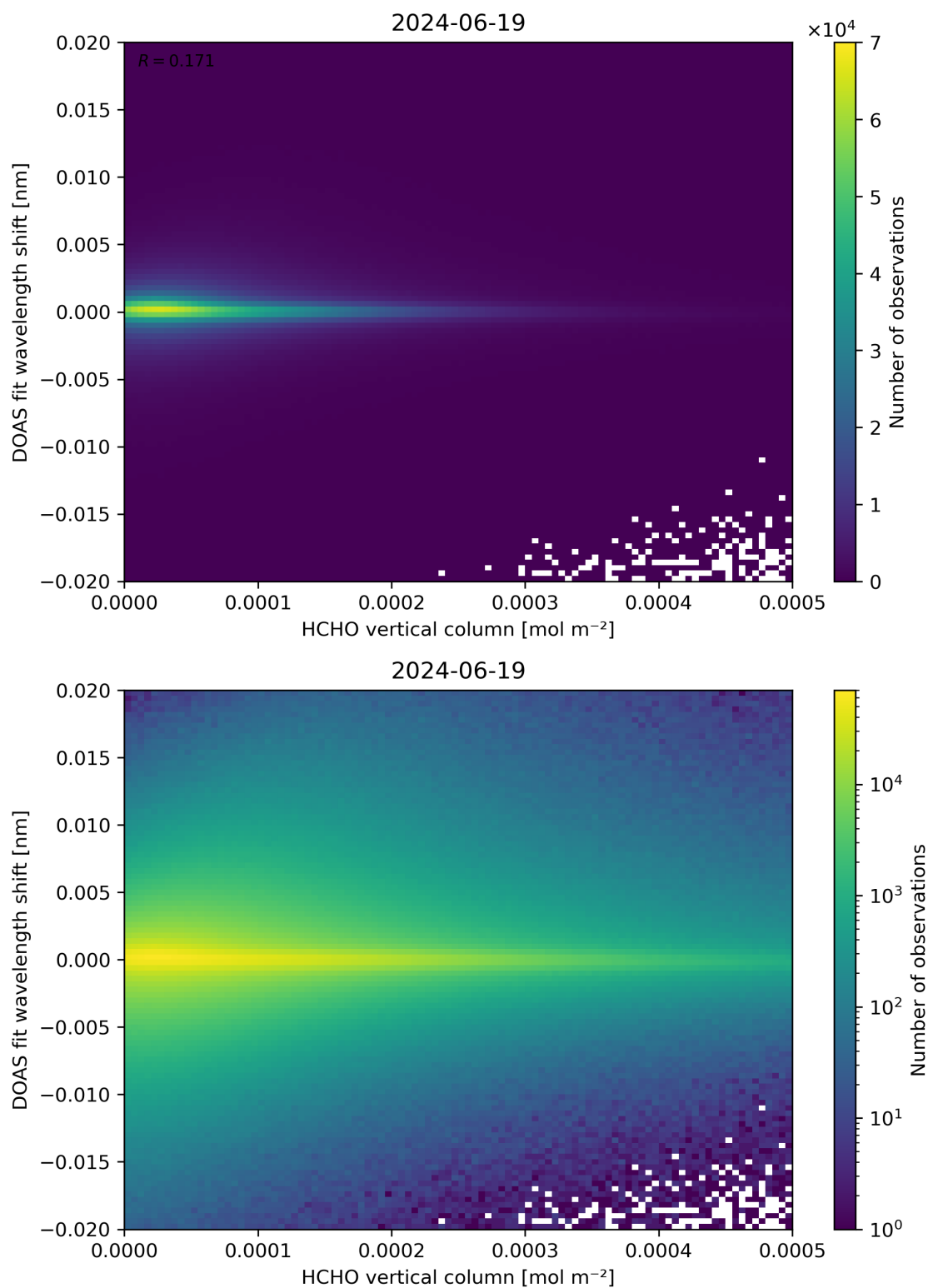
Figure 124: Scatter density plot of “HCHO vertical column” against “DOAS fit wavelength shift” for 2024-06-19 to 2024-06-20.
