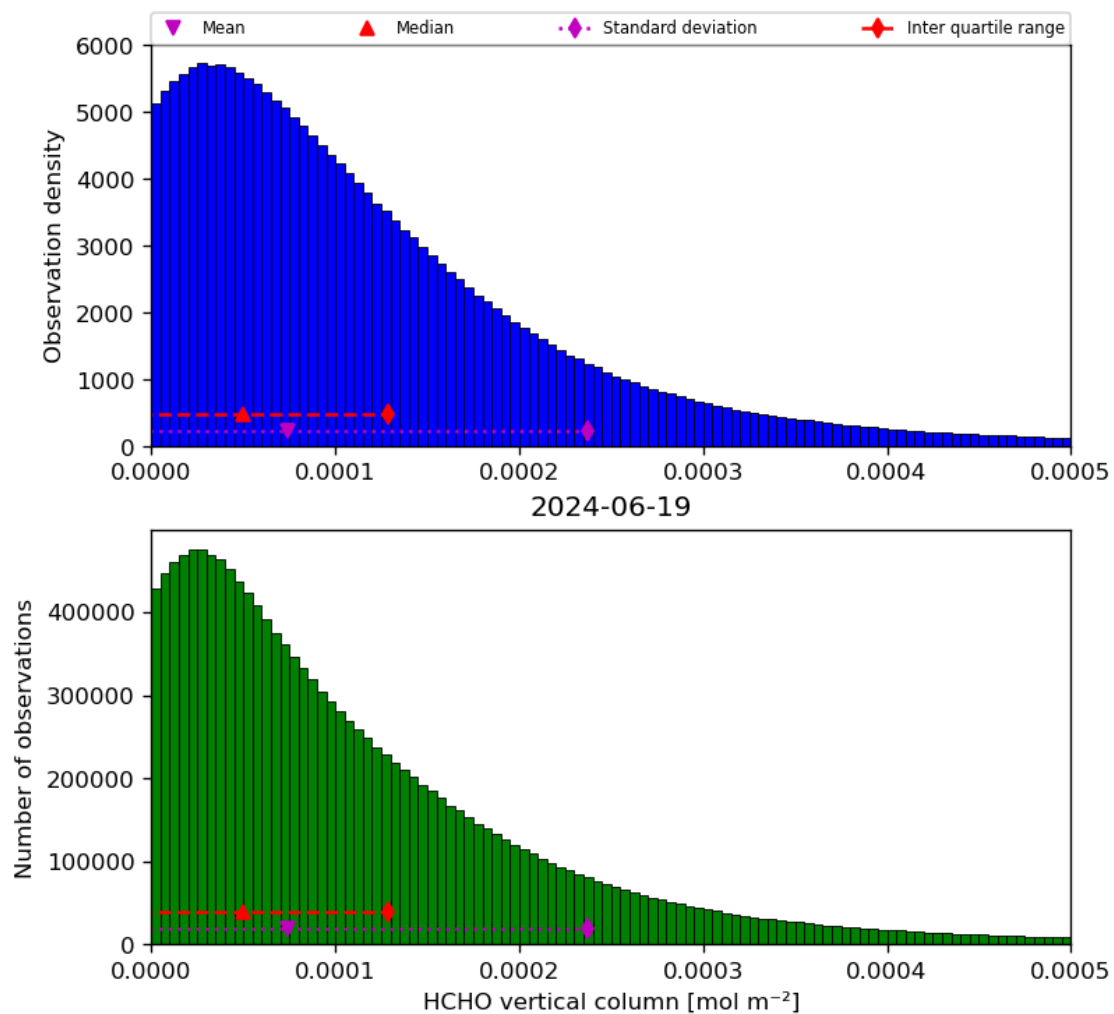
Figure 35: Histogram of “HCHO vertical column” for 2024-06-19 to 2024-06-20
