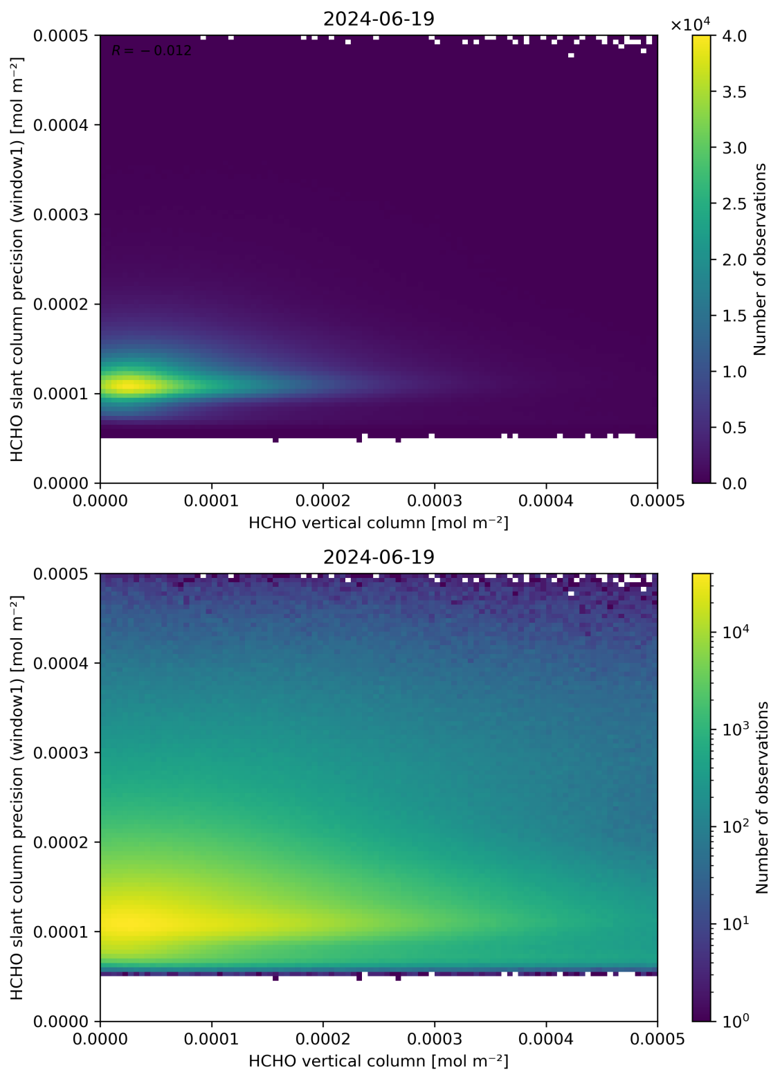
Figure 130: Scatter density plot of “HCHO vertical column” against “HCHO slant column precision (window1)” for 2024-06-19 to 2024-06-20.
