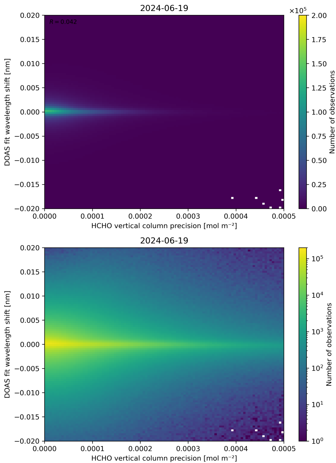
Figure 137: Scatter density plot of “HCHO vertical column precision” against “DOAS fit wavelength shift” for 2024-06-19 to 2024-06-20.
