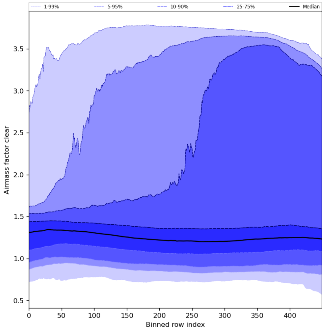
Figure 56: Along track statistics of “Airmass factor clear” for 2024-06-19 to 2024-06-20
