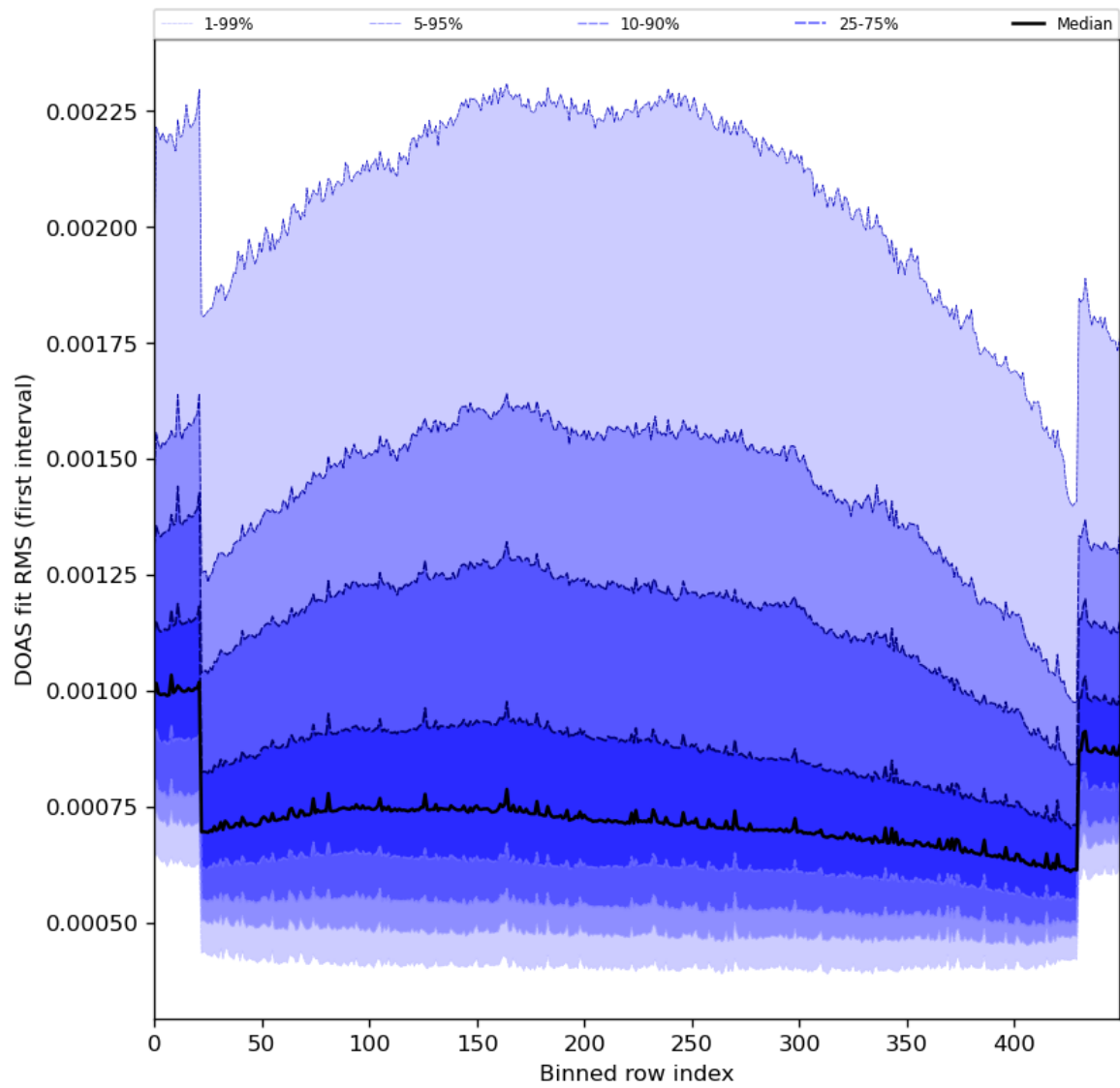
Figure 60: Along track statistics of “DOAS fit RMS (first interval)” for 2024-06-19 to 2024-06-20
