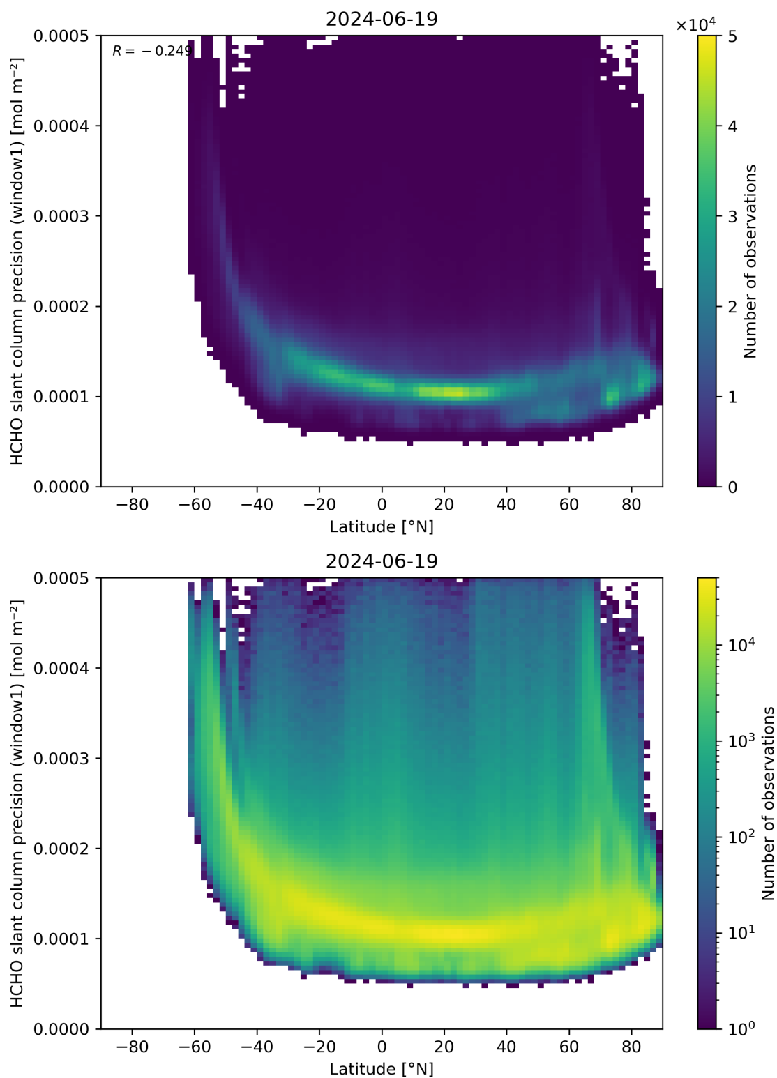
Figure 160: Scatter density plot of “Latitude” against “HCHO slant column precision (window1)” for 2024-06-19 to 2024-06-20.
