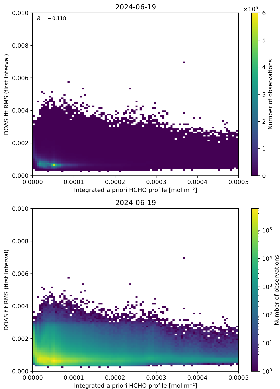
Figure 148: Scatter density plot of “Integrated a priori HCHO profile” against “DOAS fit RMS (first interval)” for 2024-06-19 to 2024-06-20.
