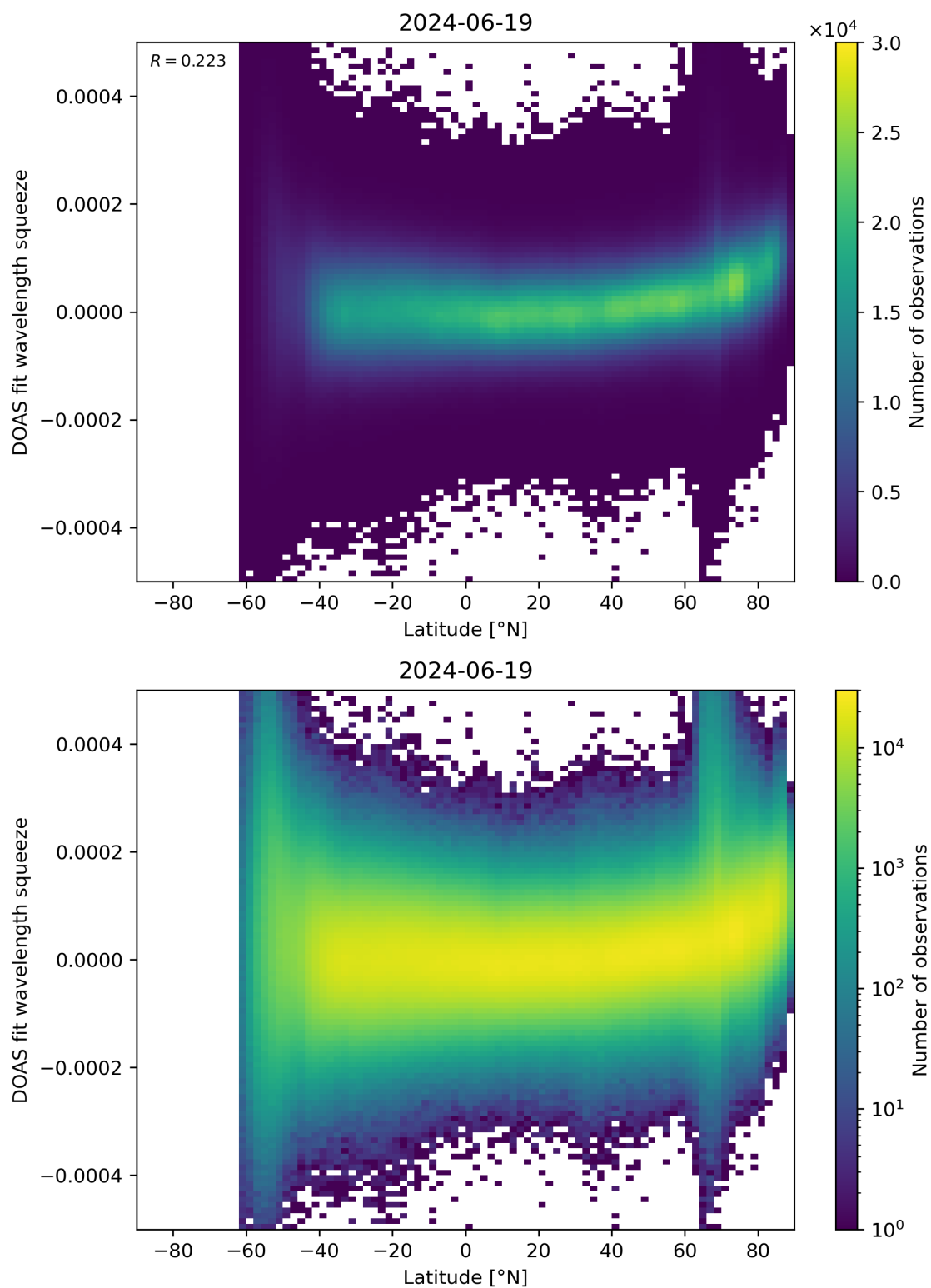
Figure 155: Scatter density plot of “Latitude” against “DOAS fit wavelength squeeze” for 2024-06-19 to 2024-06-20.
