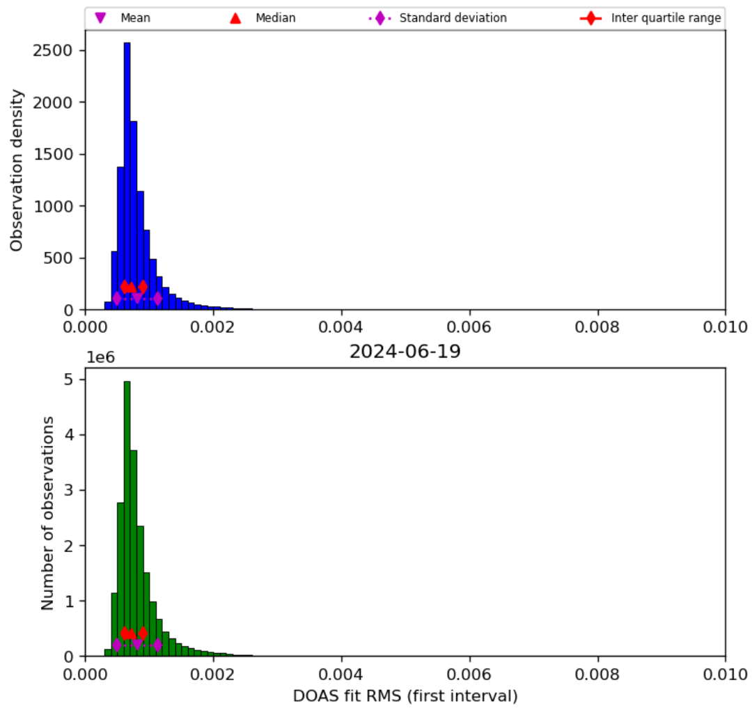
Figure 46: Histogram of “DOAS fit RMS (first interval)” for 2024-06-19 to 2024-06-20
