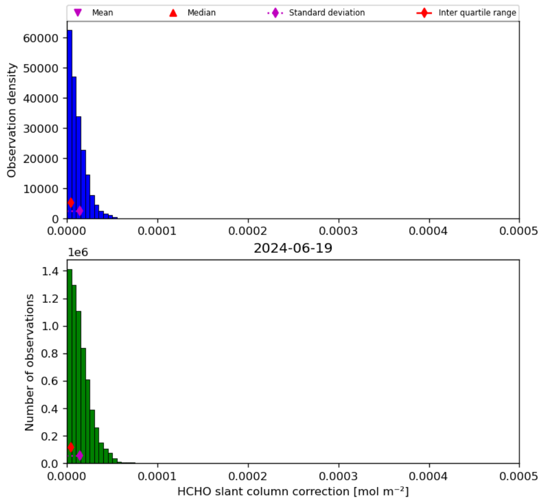
Figure 47: Histogram of “HCHO slant column correction” for 2024-06-19 to 2024-06-20
