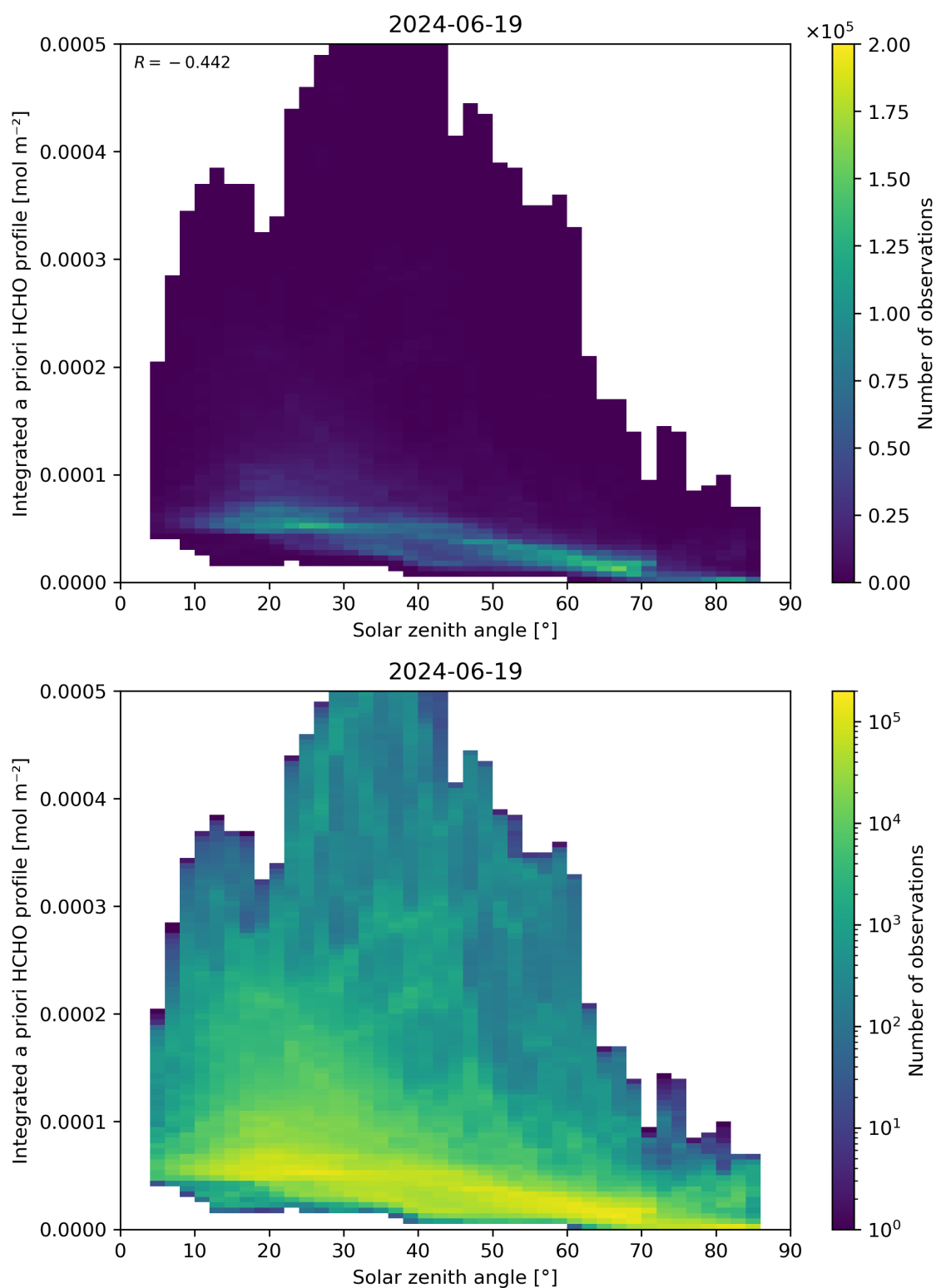
Figure 180: Scatter density plot of “Solar zenith angle” against “Integrated a priori HCHO profile” for 2024-06-19 to 2024-06-20.
