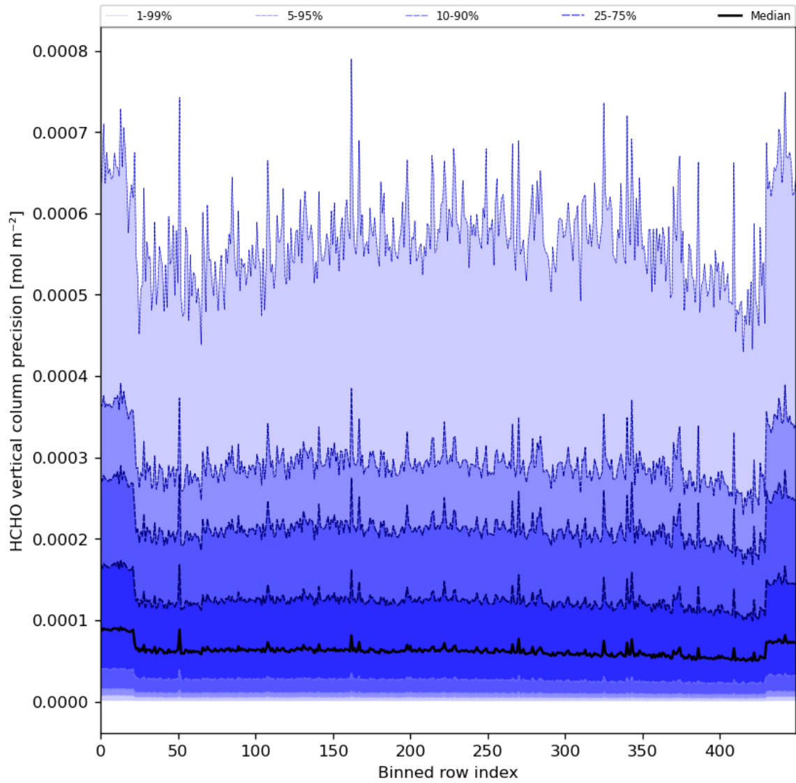
Figure 50: Along track statistics of “HCHO vertical column precision” for 2024-06-19 to 2024-06-20
