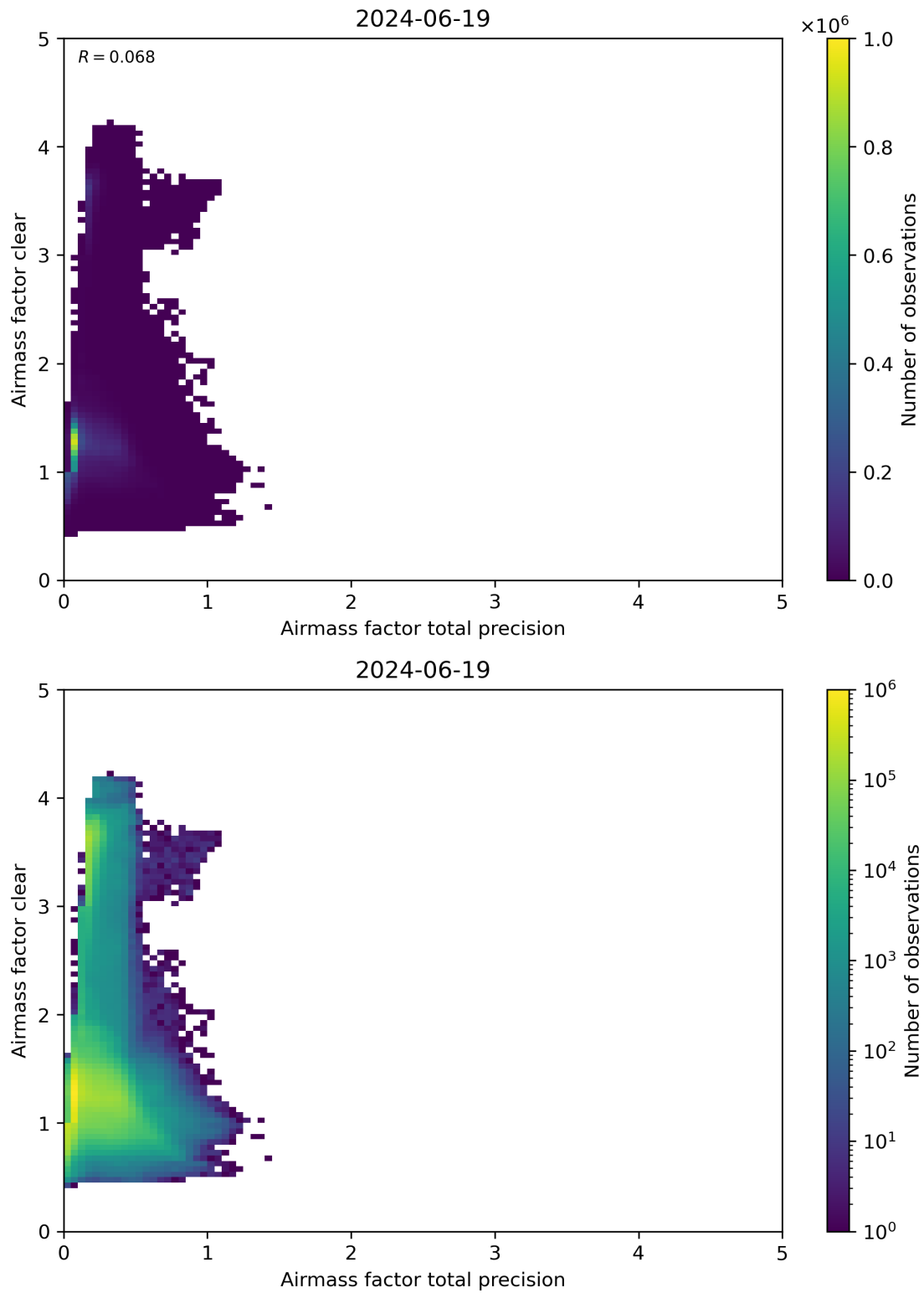
Figure 108: Scatter density plot of “Airmass factor total precision” against “Airmass factor clear” for 2024-06-19 to 2024-06-20.
