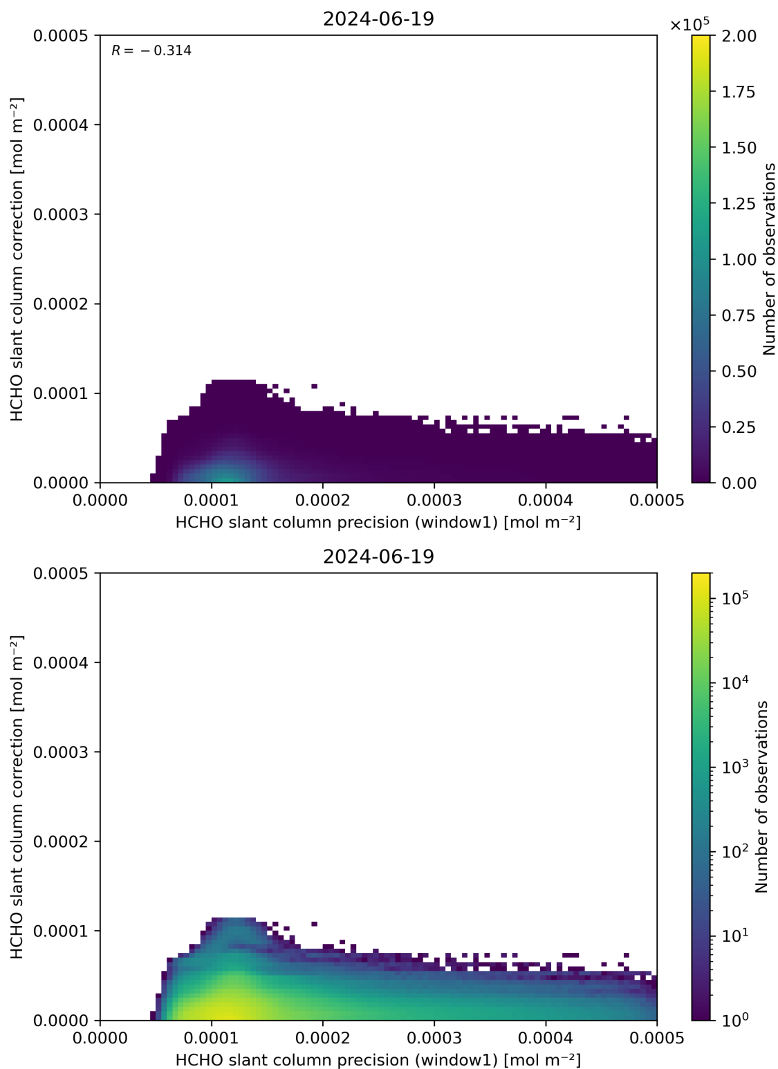
Figure 93: Scatter density plot of “HCHO slant column precision (window1)” against “HCHO slant column correction” for 2024-06-19 to 2024-06-20.
