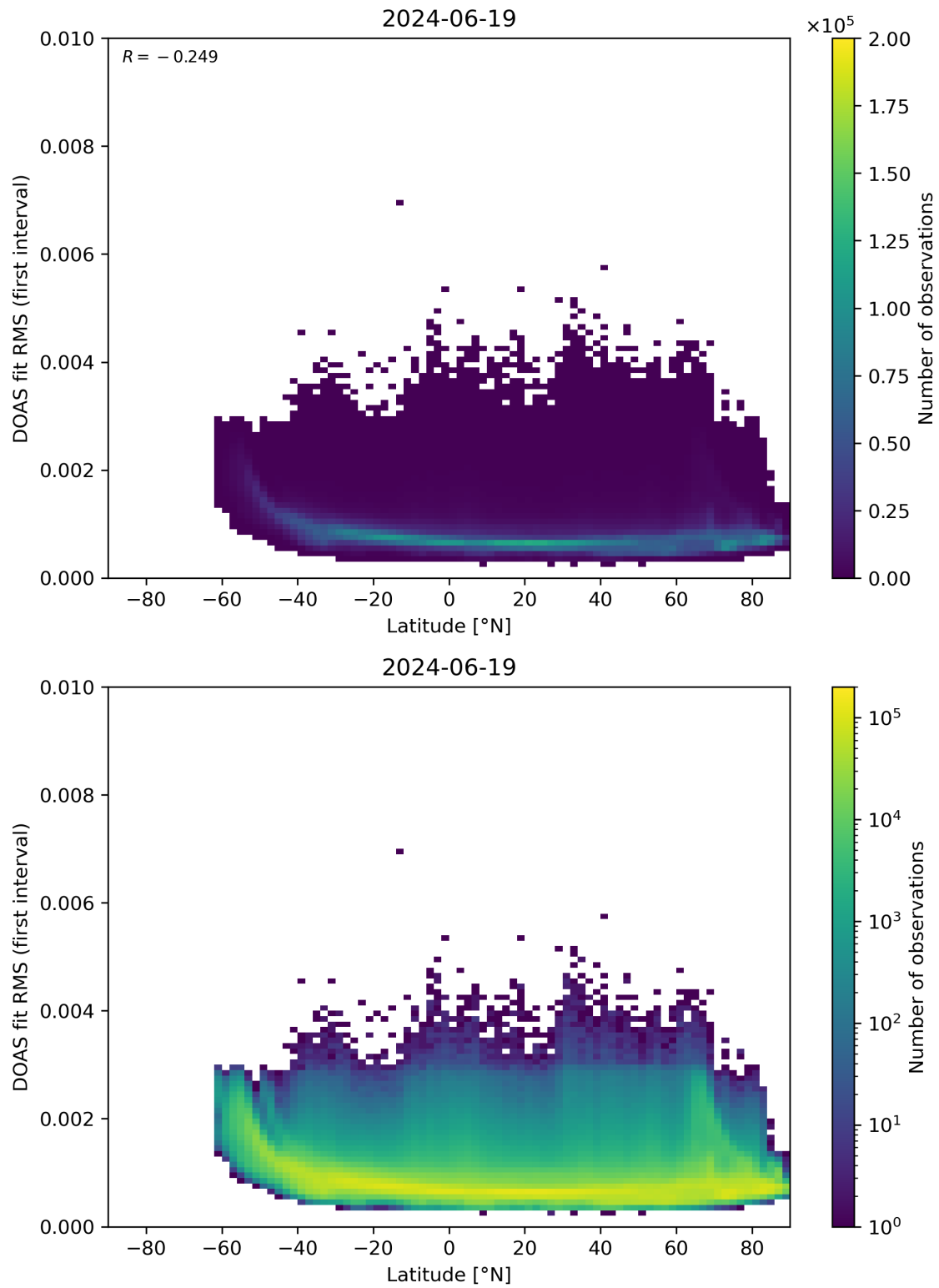
Figure 153: Scatter density plot of “Latitude” against “DOAS fit RMS (first interval)” for 2024-06-19 to 2024-06-20.
