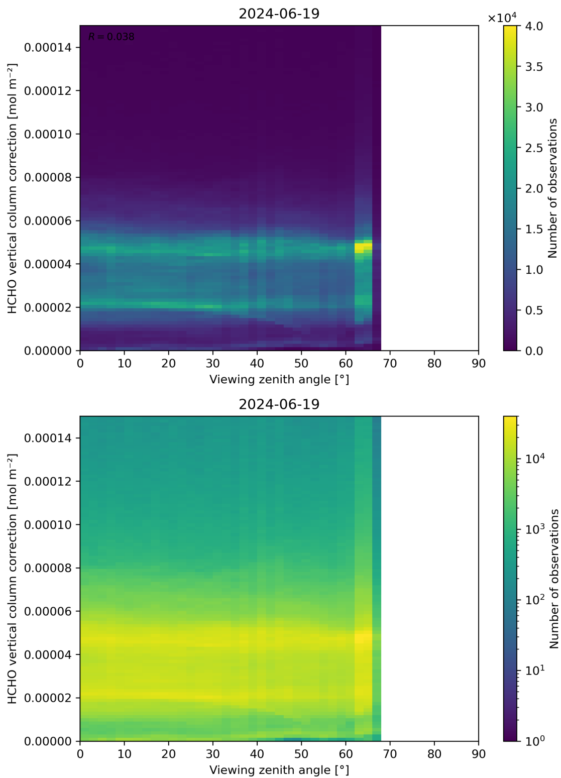
Figure 193: Scatter density plot of “Viewing zenith angle” against “HCHO vertical column correction” for 2024-06-19 to 2024-06-20.
