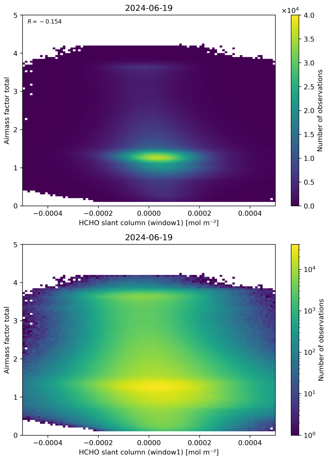
Figure 85: Scatter density plot of “HCHO slant column (window1)” against “Airmass factor total” for 2024-06-19 to 2024-06-20.
