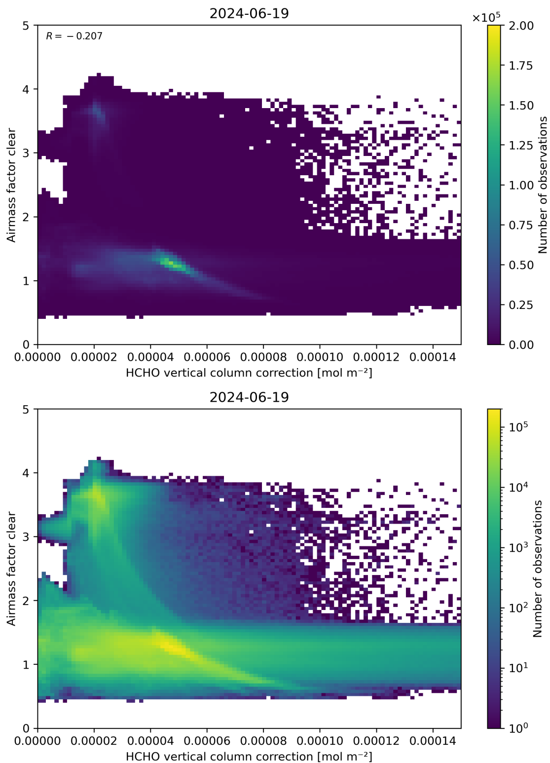
Figure 115: Scatter density plot of “HCHO vertical column correction” against “Airmass factor clear” for 2024-06-19 to 2024-06-20.
