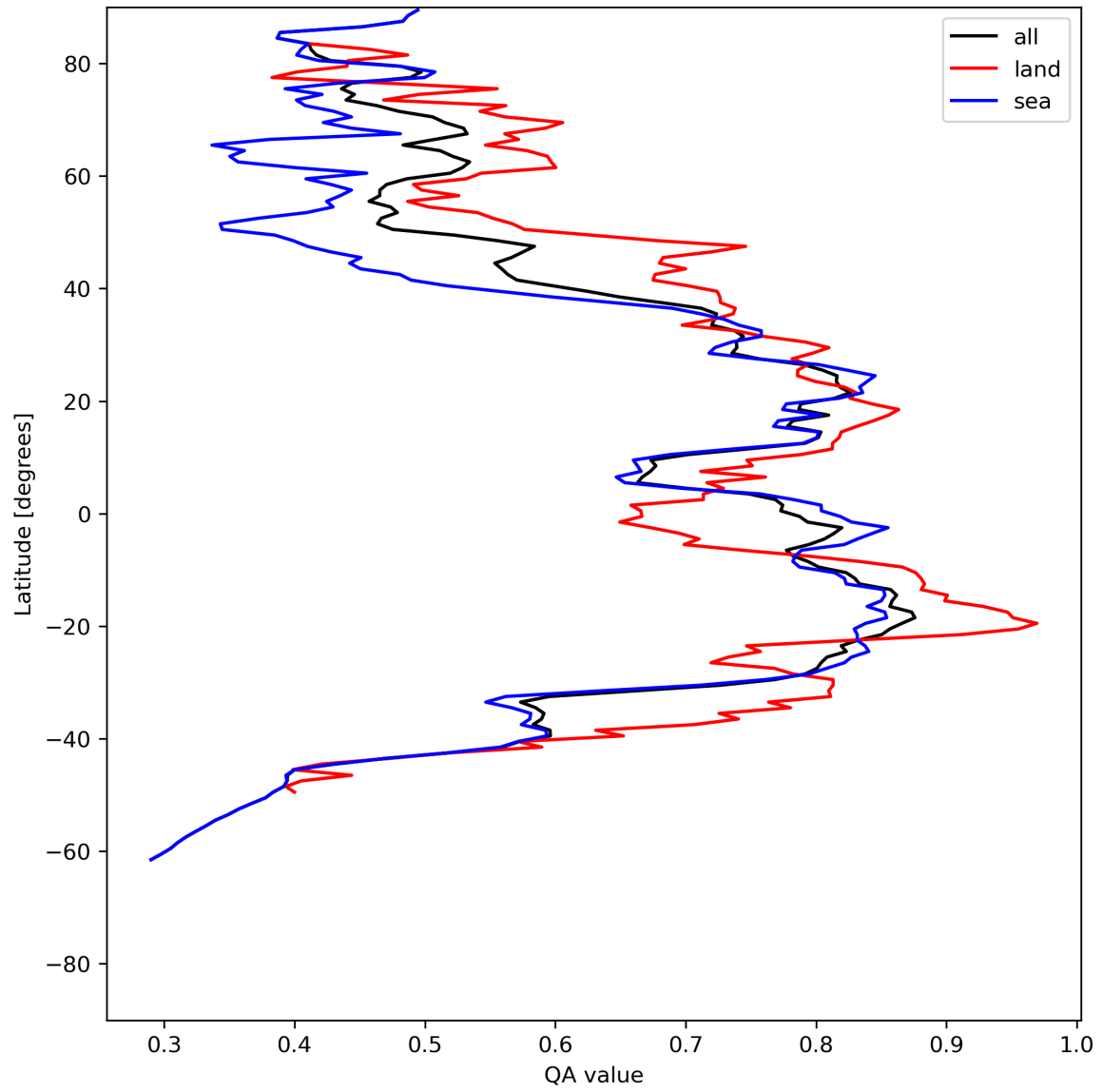
Figure 20: Zonal average of “QA value” for 2024-06-19 to 2024-06-20.
