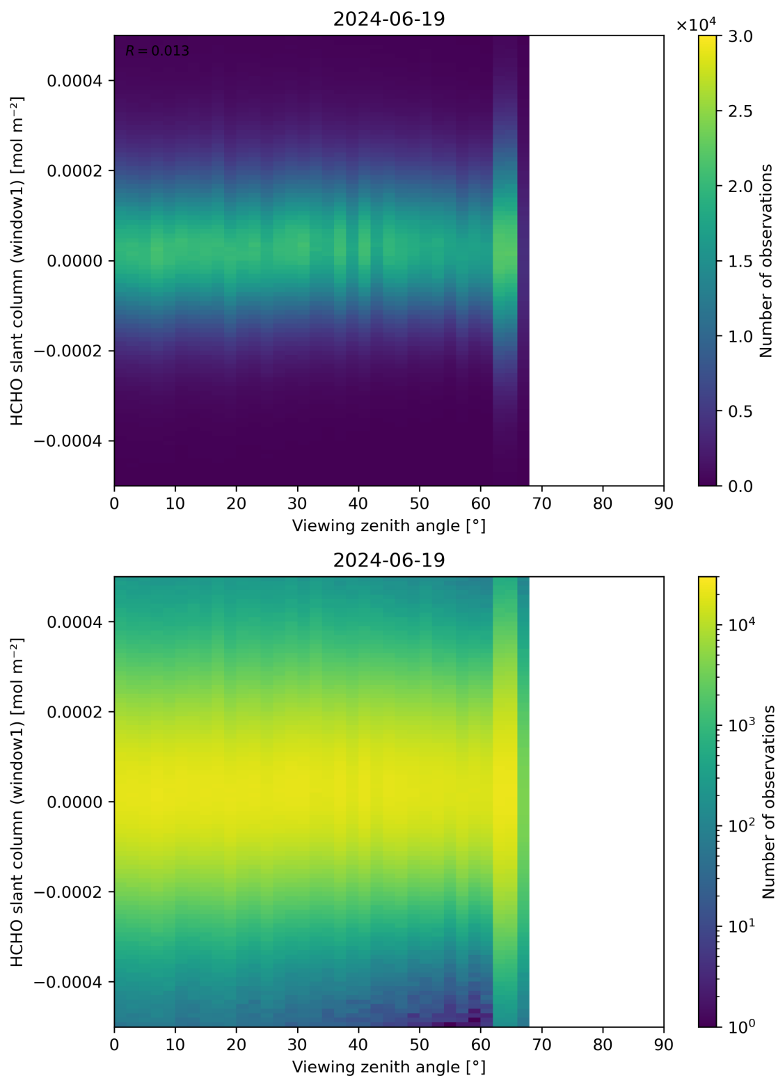
Figure 188: Scatter density plot of “Viewing zenith angle” against “HCHO slant column (window1)” for 2024-06-19 to 2024-06-20.
