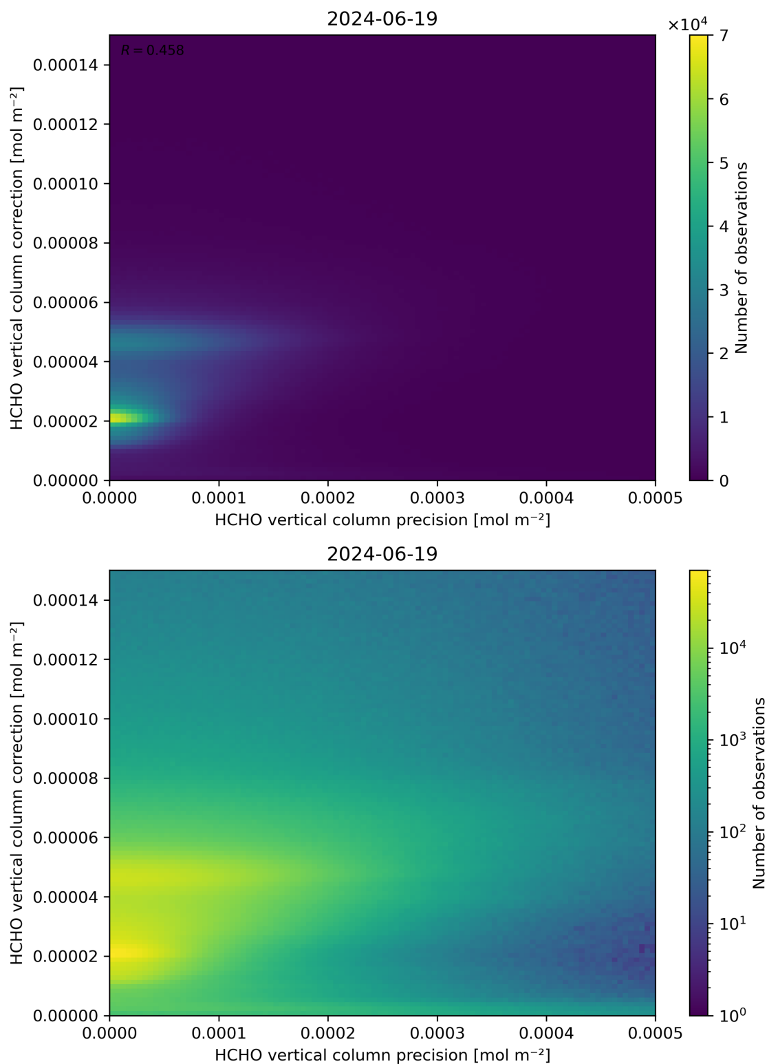
Figure 146: Scatter density plot of “HCHO vertical column precision” against “HCHO vertical column correction” for 2024-06-19 to 2024-06-20.
