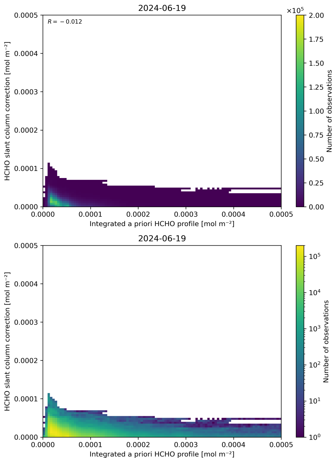
Figure 152: Scatter density plot of “Integrated a priori HCHO profile” against “HCHO slant column correction” for 2024-06-19 to 2024-06-20.
