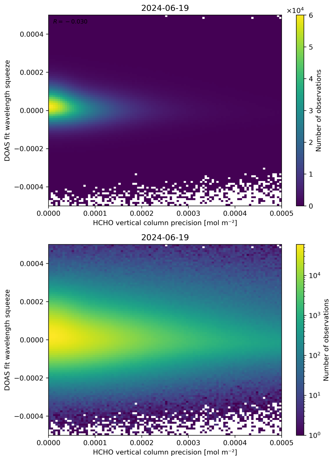
Figure 138: Scatter density plot of “HCHO vertical column precision” against “DOAS fit wavelength squeeze” for 2024-06-19 to 2024-06-20.
