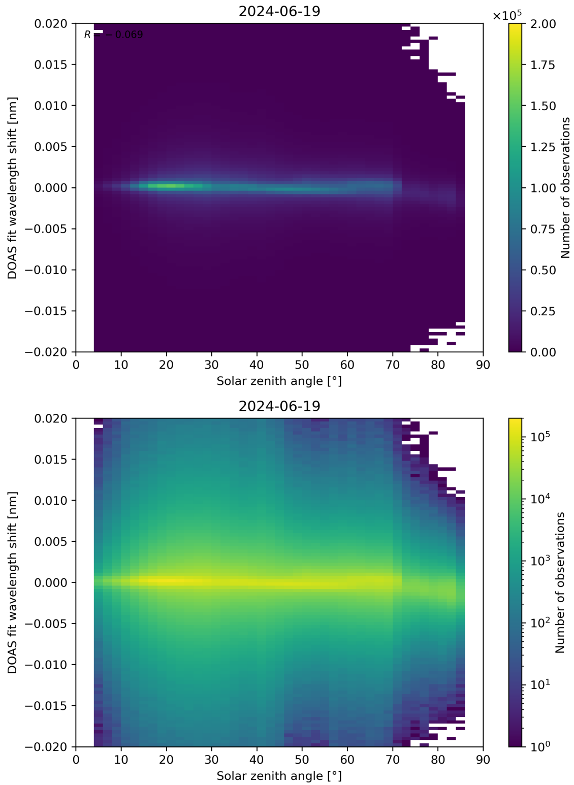
Figure 168: Scatter density plot of “Solar zenith angle” against “DOAS fit wavelength shift” for 2024-06-19 to 2024-06-20.
