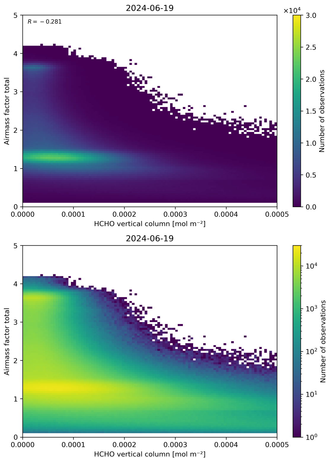
Figure 131: Scatter density plot of “HCHO vertical column” against “Airmass factor total” for 2024-06-19 to 2024-06-20.
