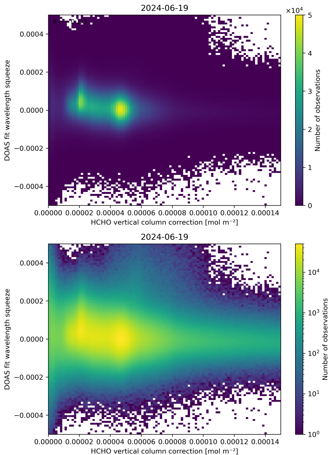
Figure 114: Scatter density plot of “HCHO vertical column correction” against “DOAS fit wavelength squeeze” for 2024-06-19 to 2024-06-20.
