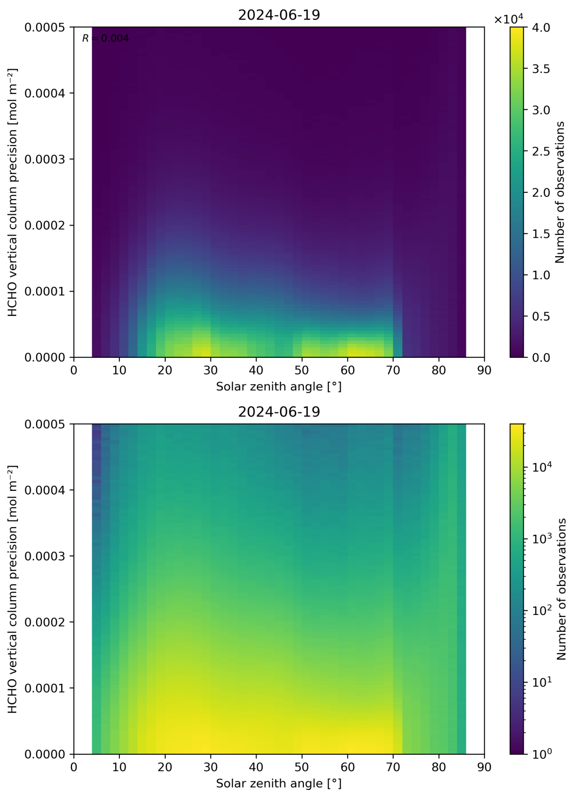
Figure 179: Scatter density plot of “Solar zenith angle” against “HCHO vertical column precision” for 2024-06-19 to 2024-06-20.
