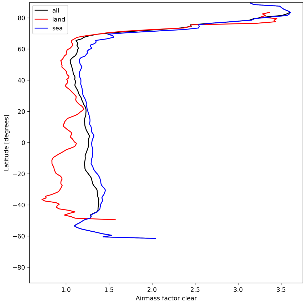
Figure 28: Zonal average of “Airmass factor clear” for 2024-06-19 to 2024-06-20.
