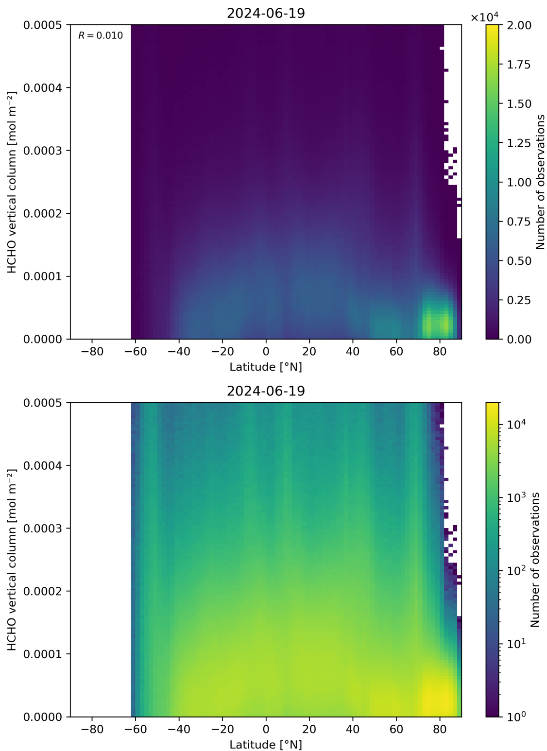
Figure 163: Scatter density plot of “Latitude” against “HCHO vertical column” for 2024-06-19 to 2024-06-20.
