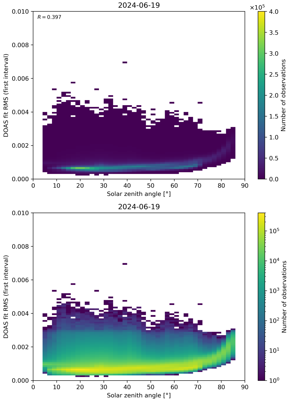
Figure 167: Scatter density plot of “Solar zenith angle” against “DOAS fit RMS (first interval)” for 2024-06-19 to 2024-06-20.
