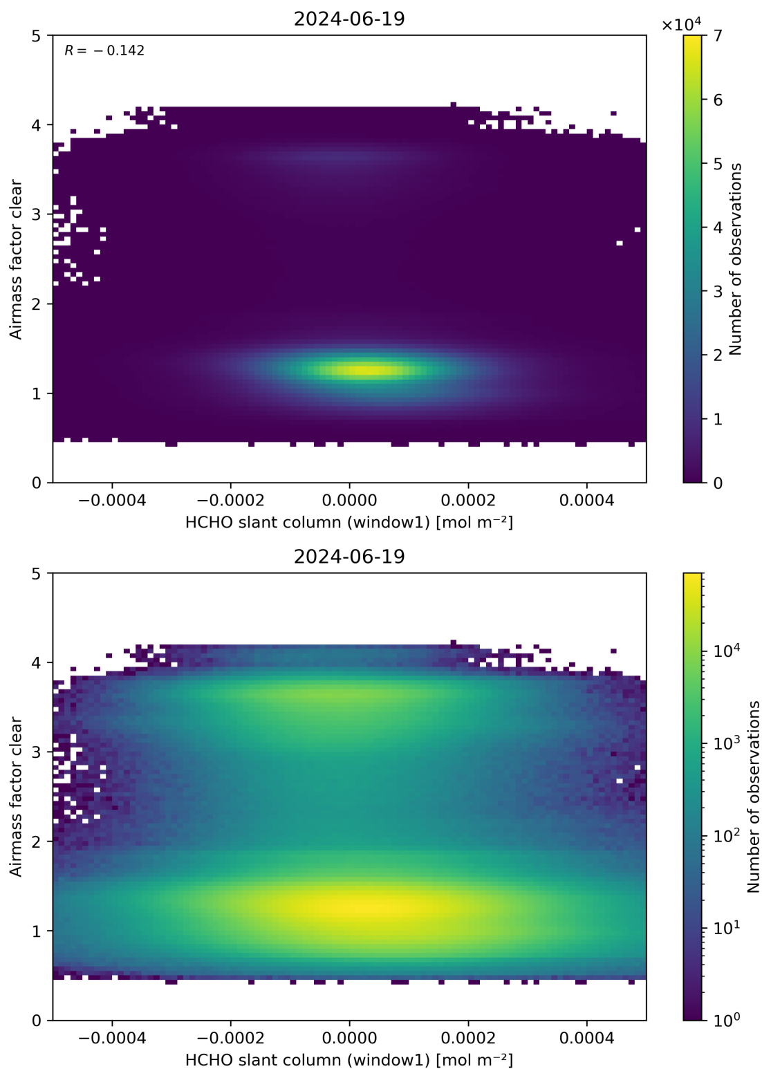
Figure 81: Scatter density plot of “HCHO slant column (window1)” against “Airmass factor clear” for 2024-06-19 to 2024-06-20.
