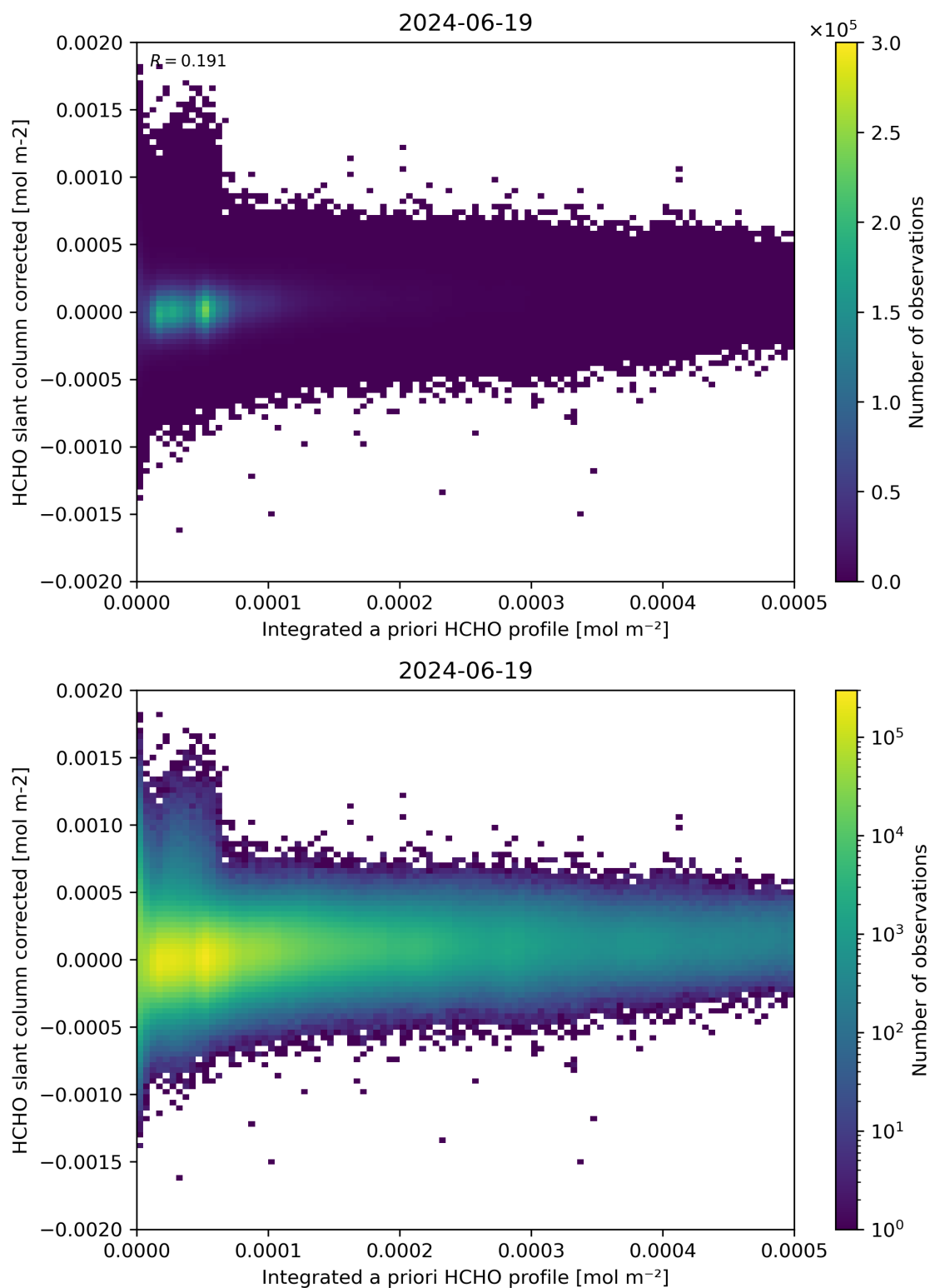
Figure 151: Scatter density plot of “Integrated a priori HCHO profile” against “HCHO slant column corrected” for 2024-06-19 to 2024-06-20.
