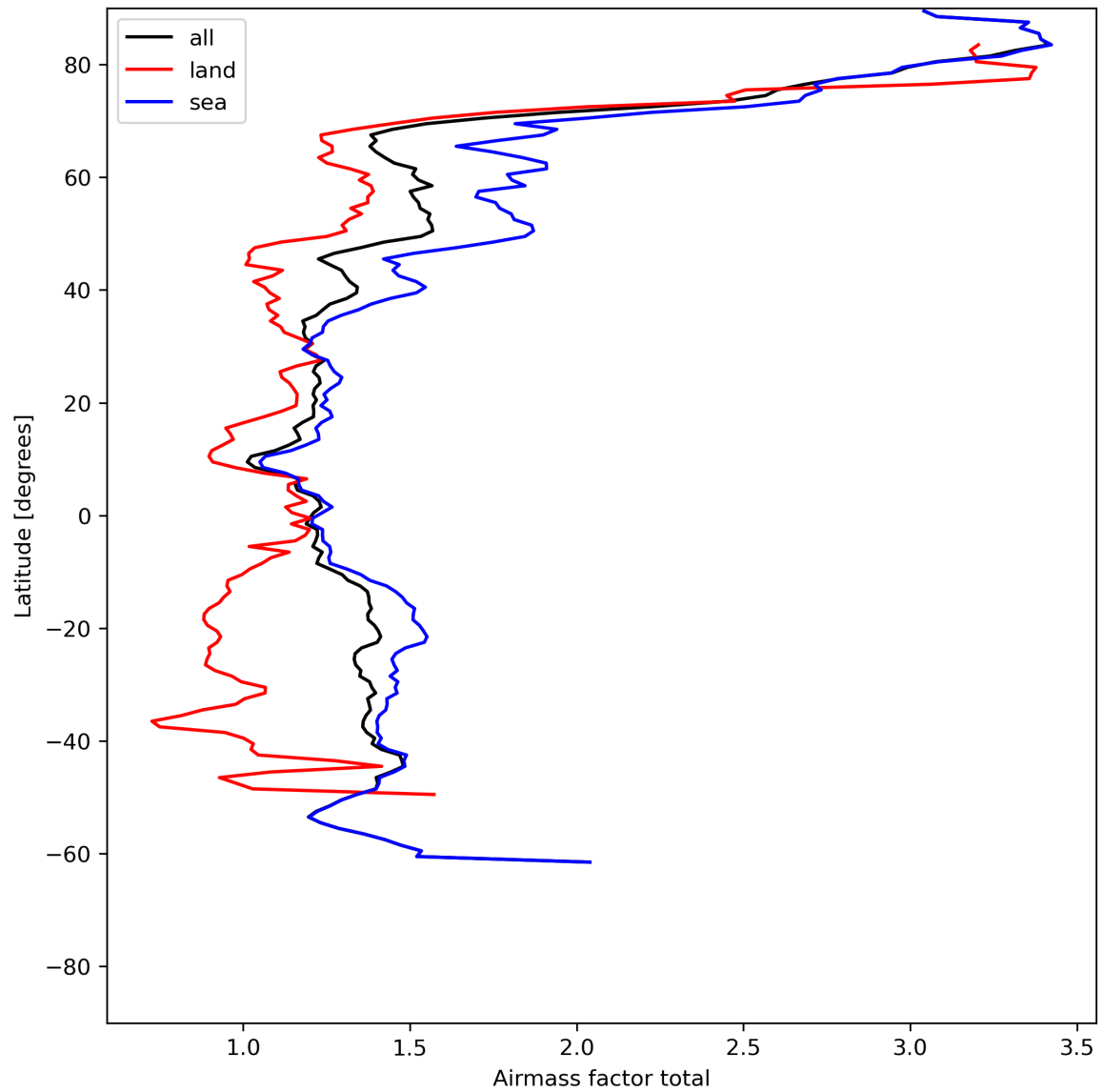
Figure 26: Zonal average of “Airmass factor total” for 2024-06-19 to 2024-06-20.
