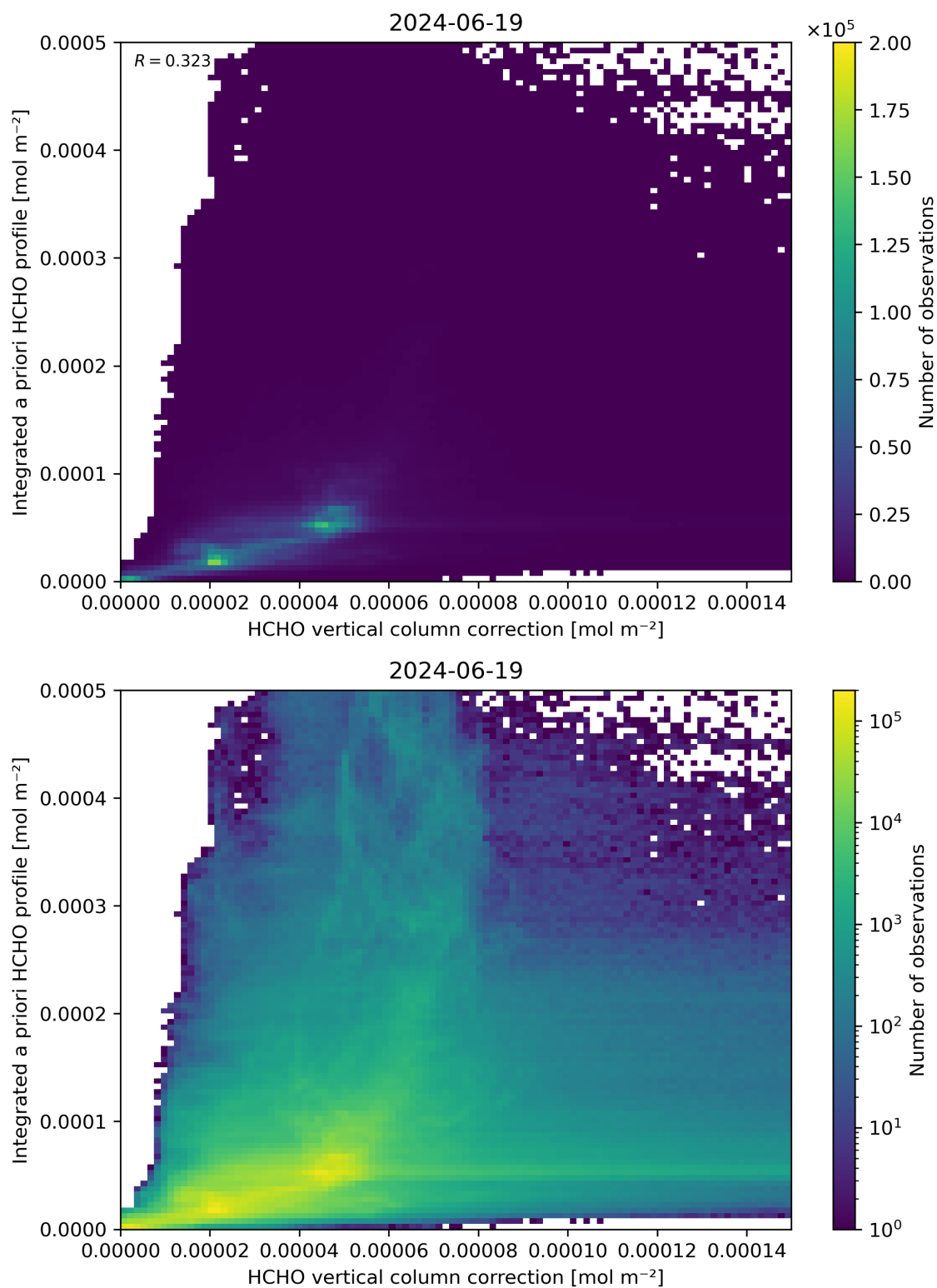
Figure 122: Scatter density plot of “HCHO vertical column correction” against “Integrated a priori HCHO profile” for 2024-06-19 to 2024-06-20.
