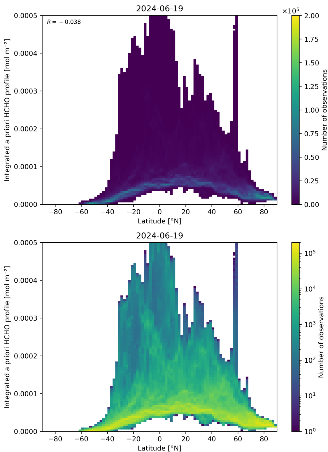
Figure 166: Scatter density plot of “Latitude” against “Integrated a priori HCHO profile” for 2024-06-19 to 2024-06-20.
