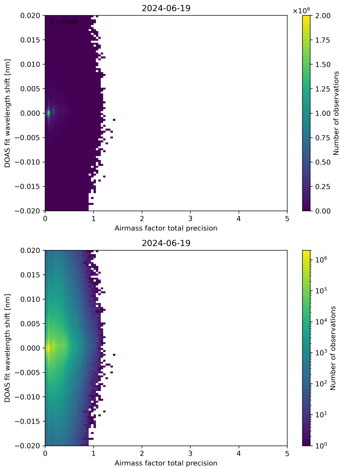
Figure 106: Scatter density plot of “Airmass factor total precision” against “DOAS fit wavelength shift” for 2024-06-19 to 2024-06-20.
