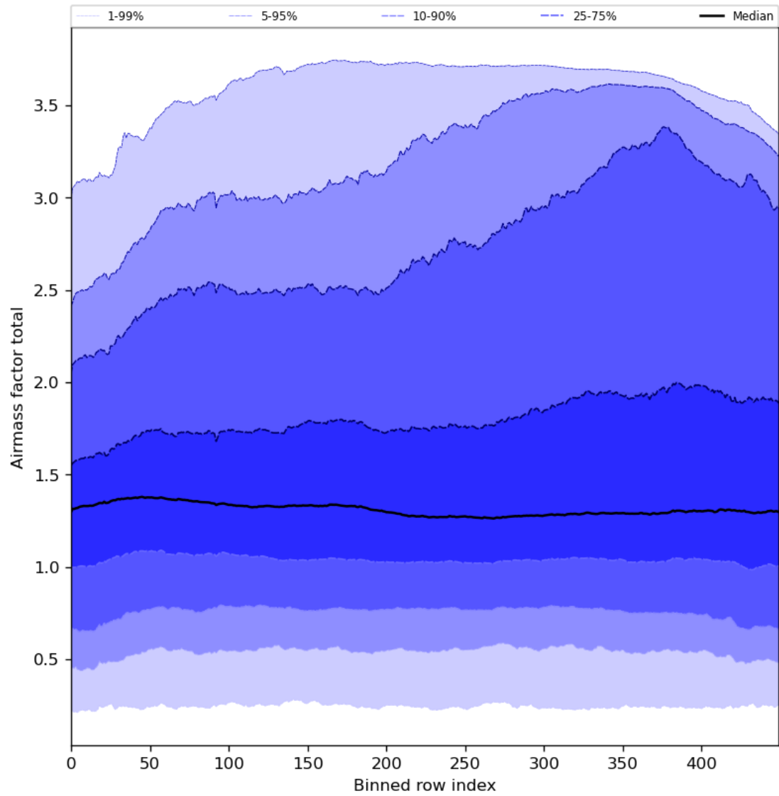
Figure 54: Along track statistics of “Airmass factor total” for 2024-06-19 to 2024-06-20
