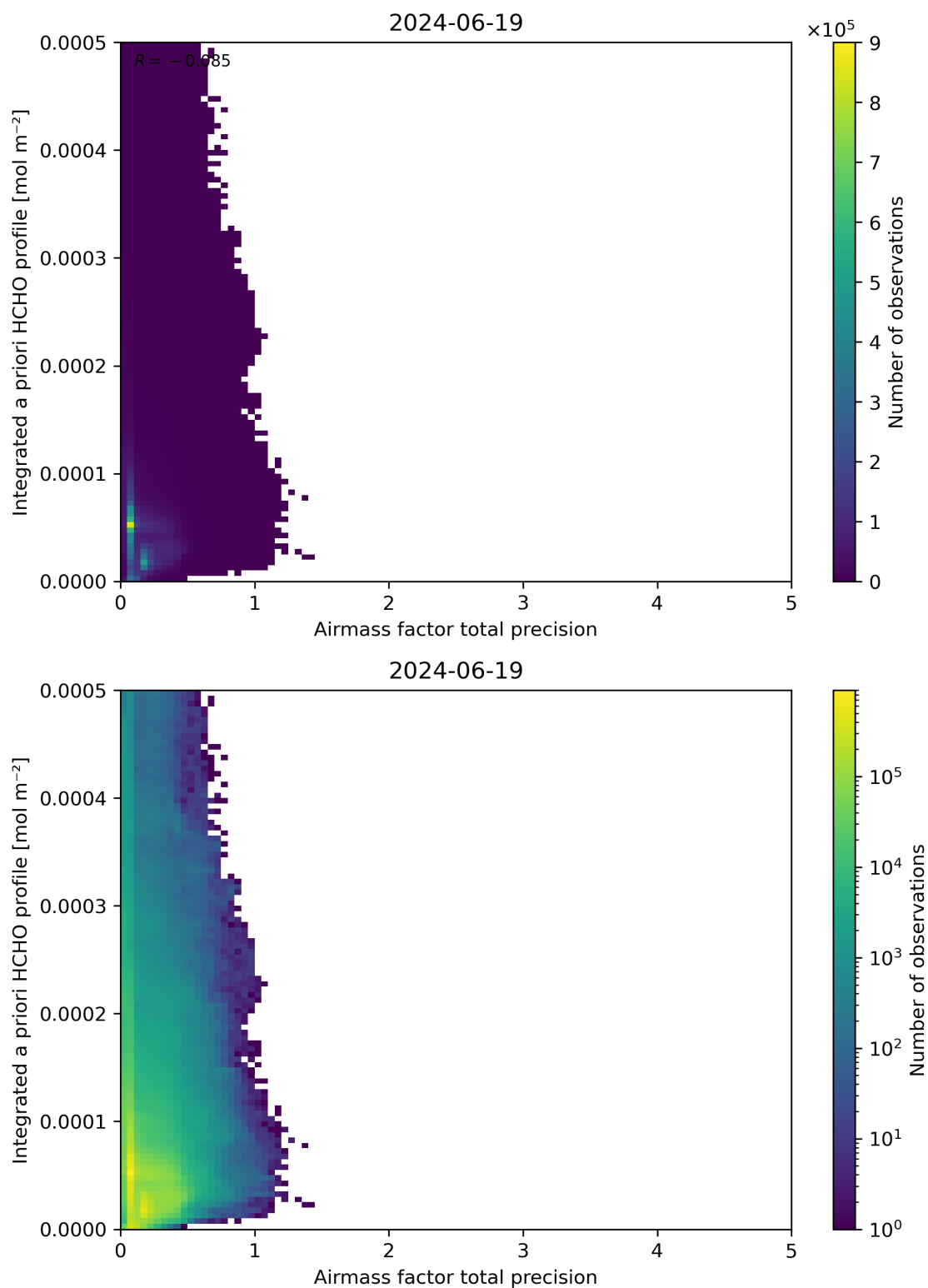
Figure 111: Scatter density plot of “Airmass factor total precision” against “Integrated a priori HCHO profile” for 2024-06-19 to 2024-06-20.
