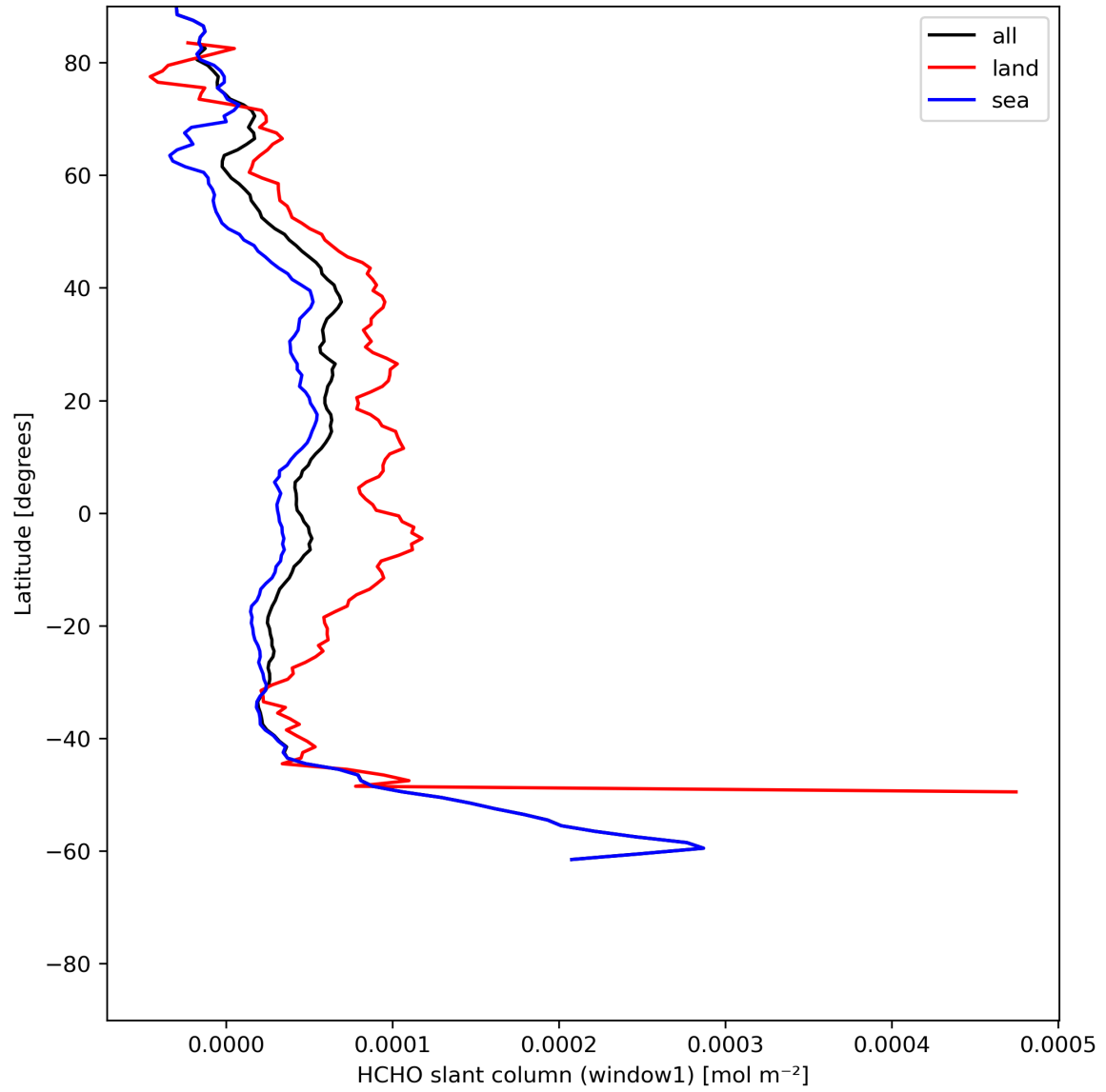
Figure 24: Zonal average of “HCHO slant column (window1)” for 2024-06-19 to 2024-06-20.
