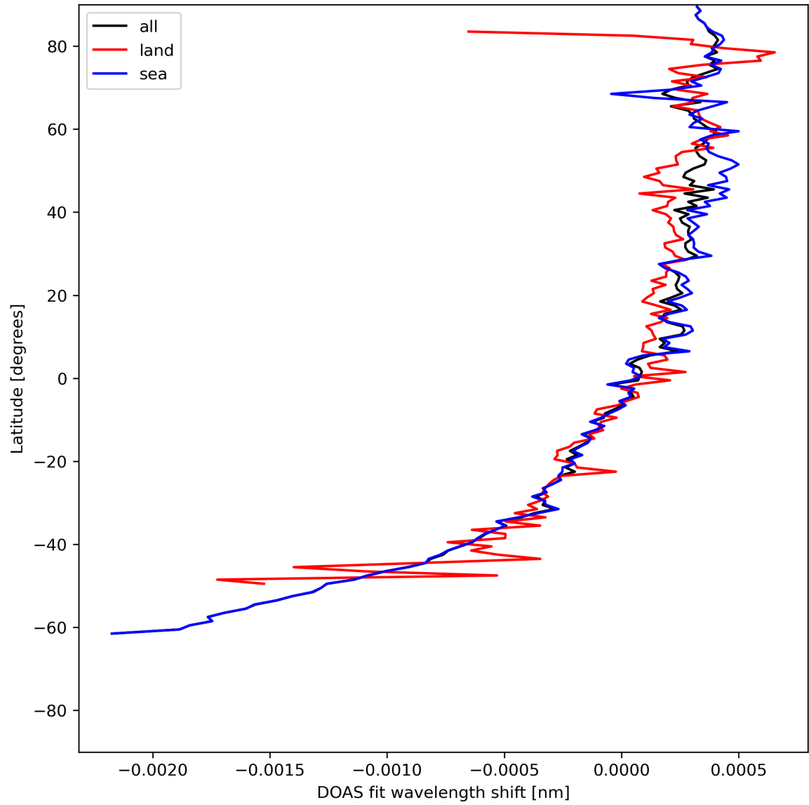
Figure 30: Zonal average of “DOAS fit wavelength shift” for 2024-06-19 to 2024-06-20.
