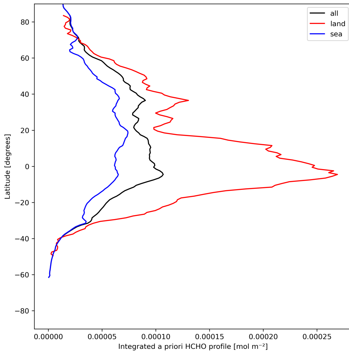
Figure 29: Zonal average of “Integrated a priori HCHO profile” for 2024-06-19 to 2024-06-20.
