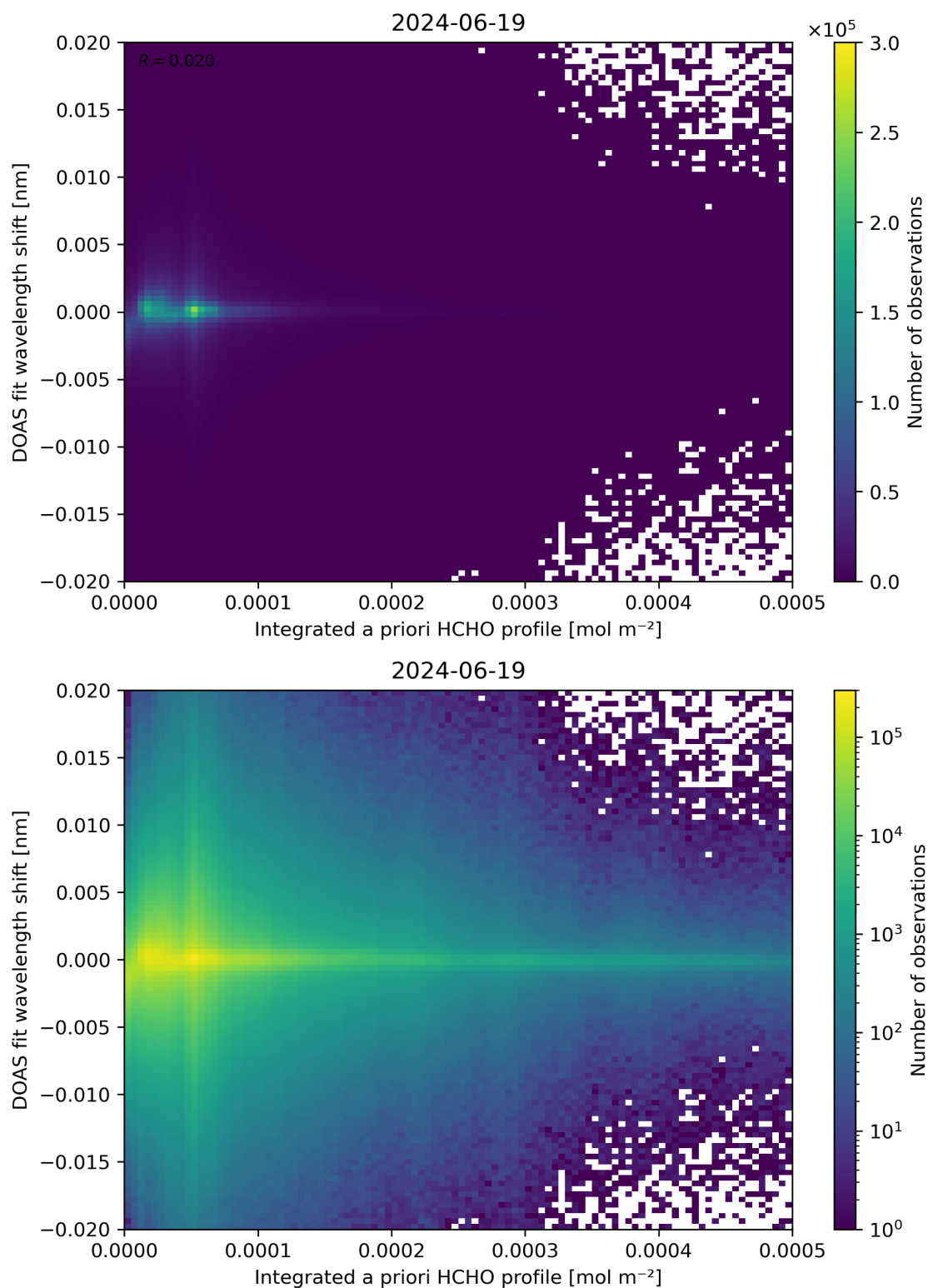
Figure 149: Scatter density plot of “Integrated a priori HCHO profile” against “DOAS fit wavelength shift” for 2024-06-19 to 2024-06-20.
