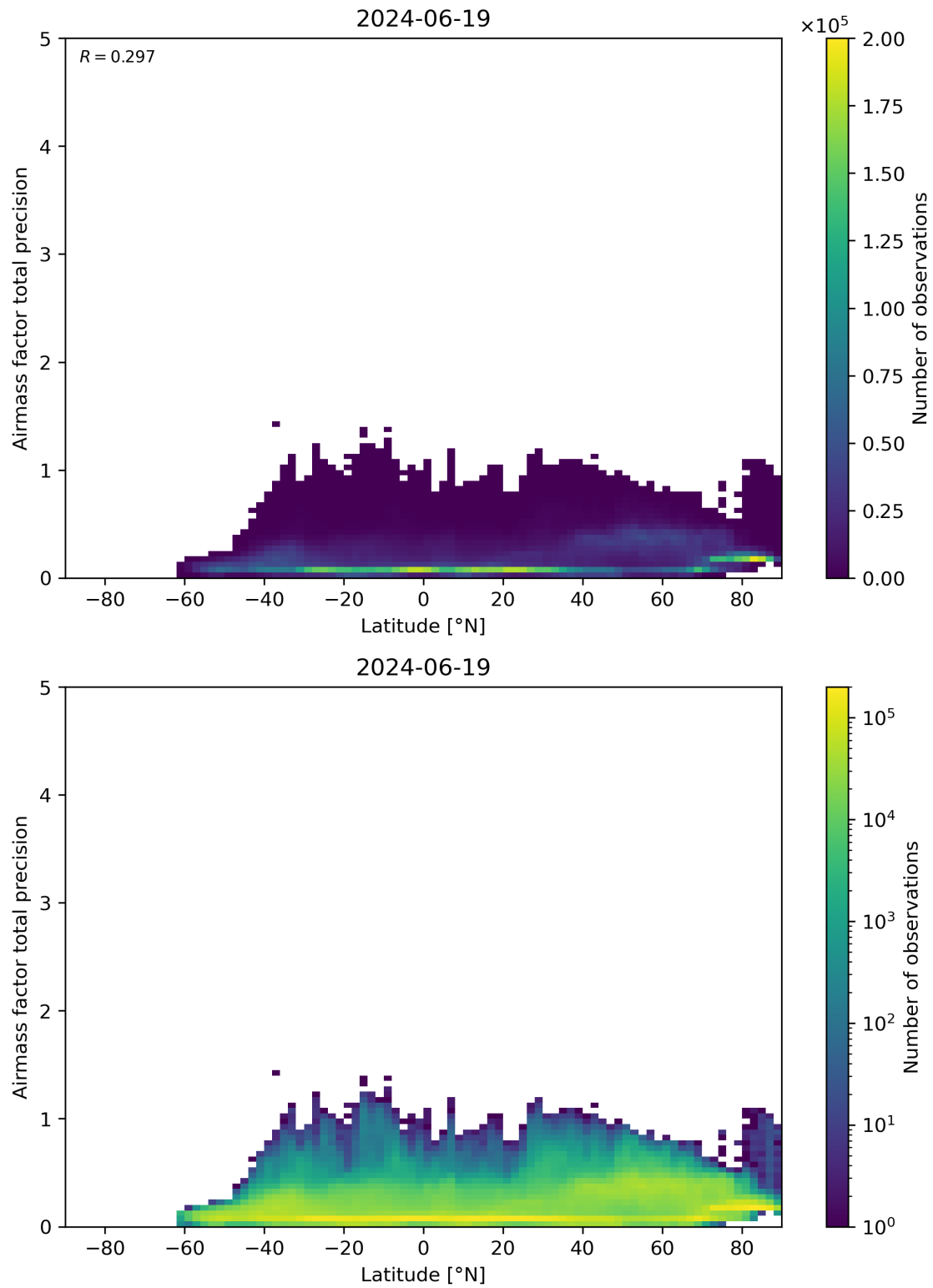
Figure 162: Scatter density plot of “Latitude” against “Airmass factor total precision” for 2024-06-19 to 2024-06-20.
