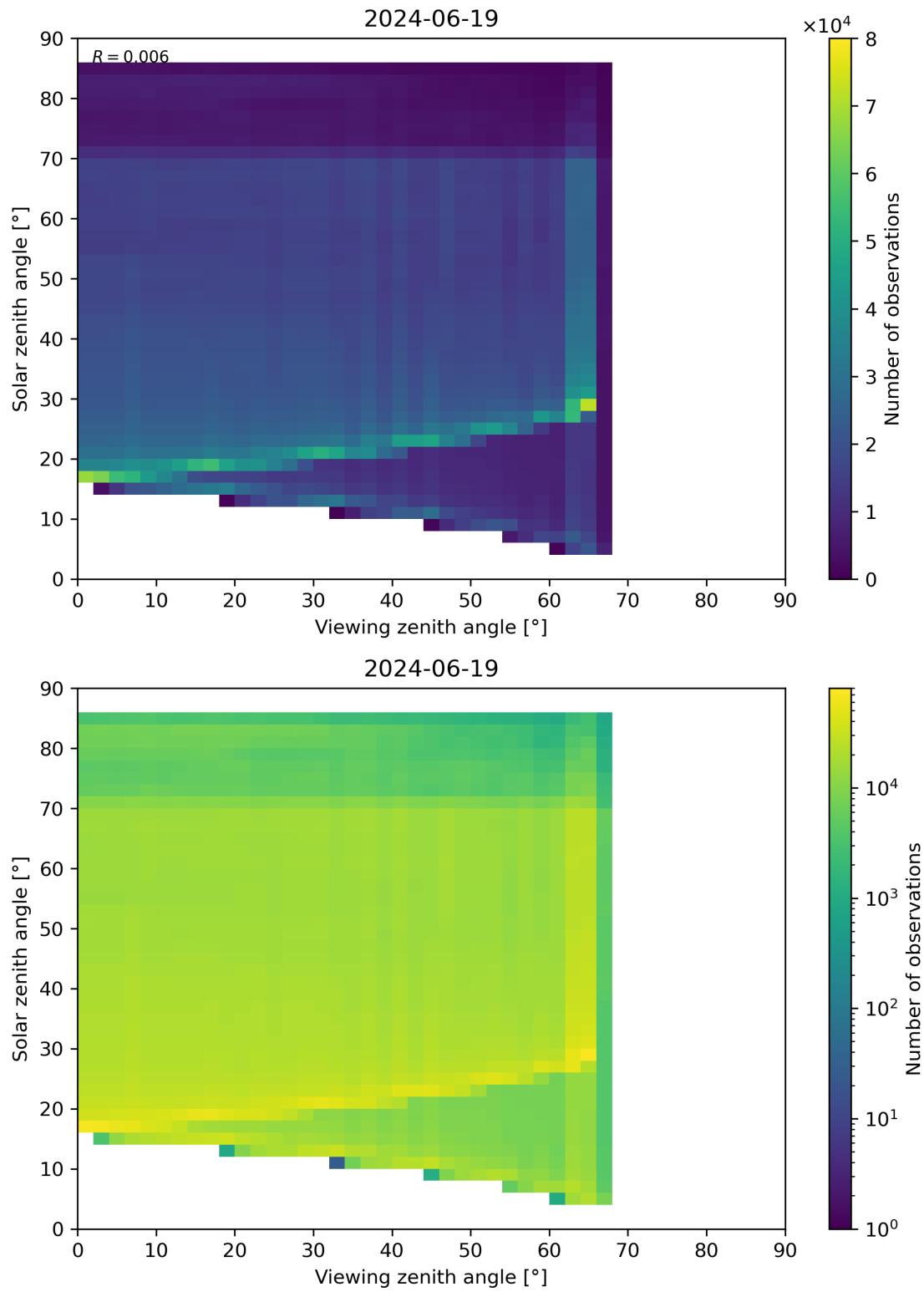
Figure 197: Scatter density plot of “Viewing zenith angle” against “Solar zenith angle” for 2024-06-19 to 2024-06-20.
