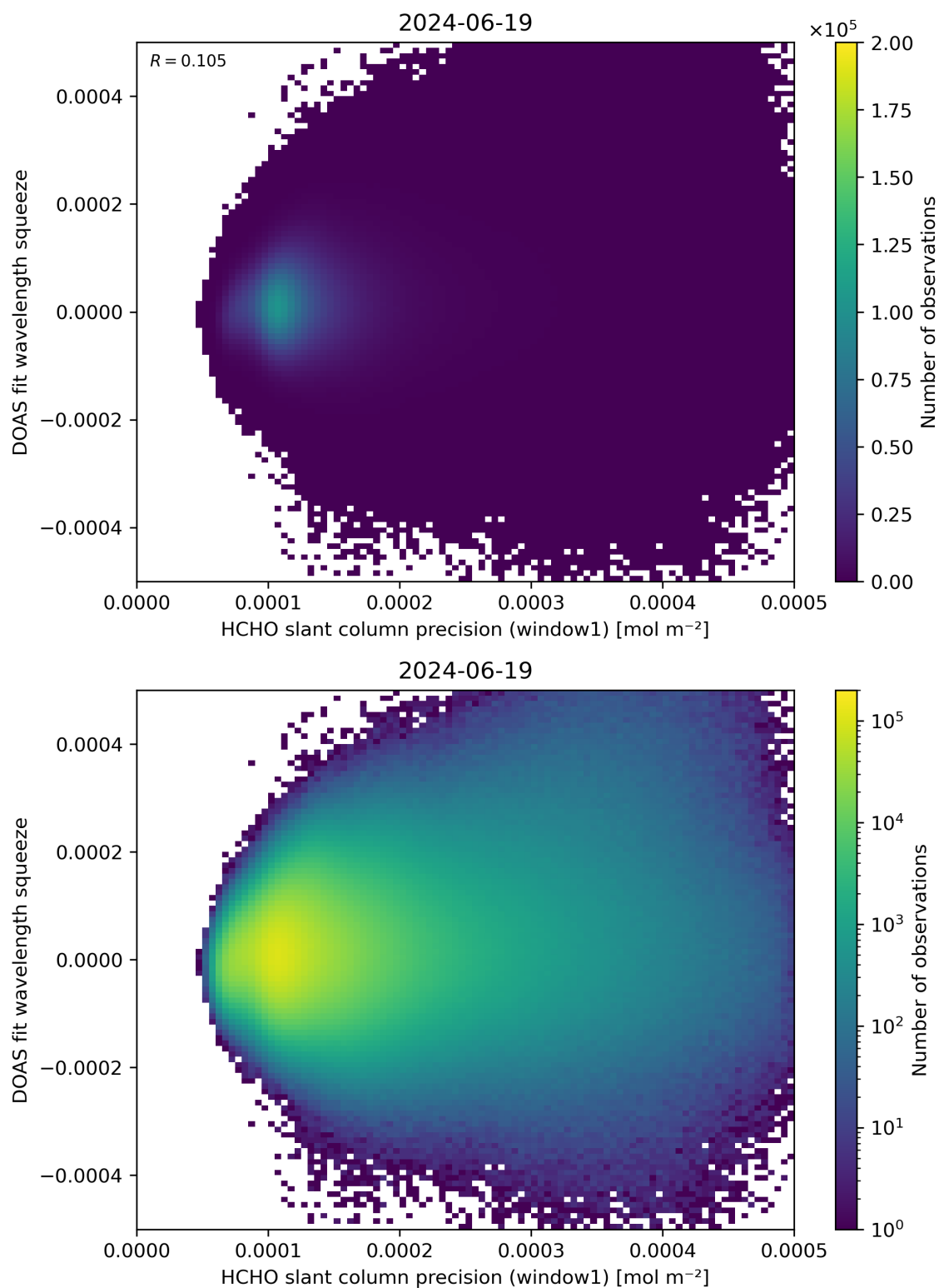
Figure 90: Scatter density plot of “HCHO slant column precision (window1)” against “DOAS fit wavelength squeeze” for 2024-06-19 to 2024-06-20.
