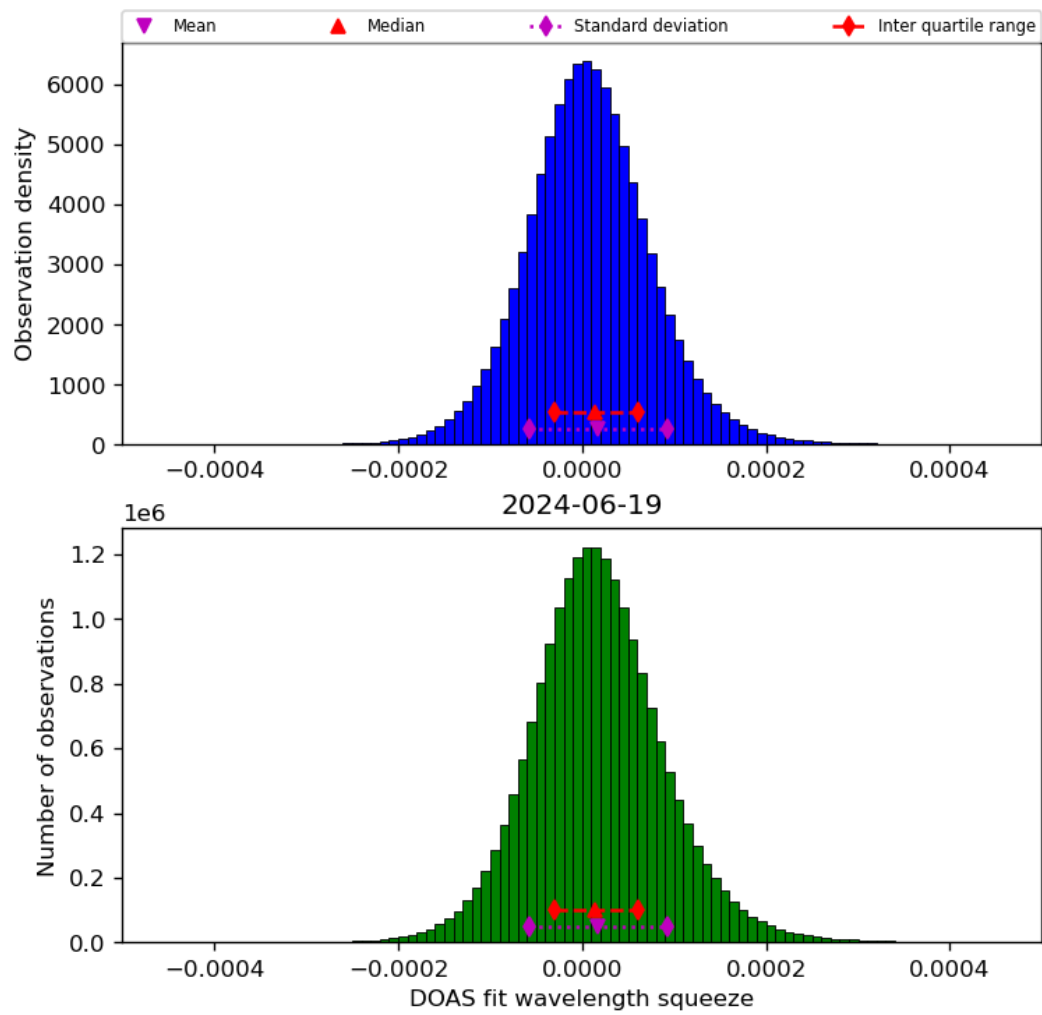
Figure 45: Histogram of “DOAS fit wavelength squeeze” for 2024-06-19 to 2024-06-20
