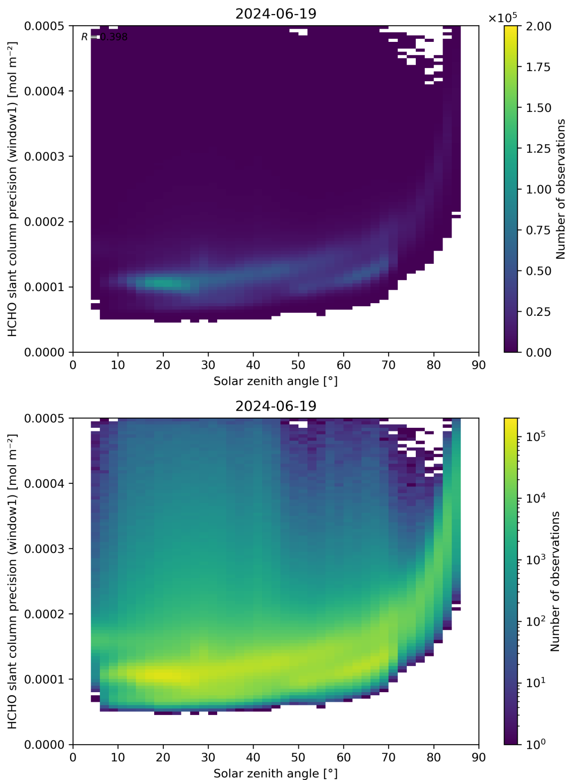
Figure 174: Scatter density plot of “Solar zenith angle” against “HCHO slant column precision (window1)” for 2024-06-19 to 2024-06-20.
