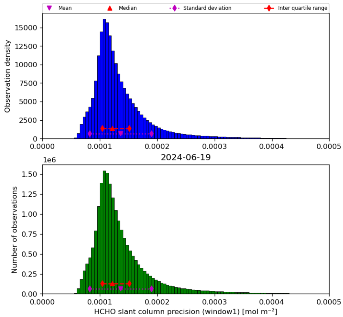
Figure 39: Histogram of “HCHO slant column precision (window1)” for 2024-06-19 to 2024-06-20
