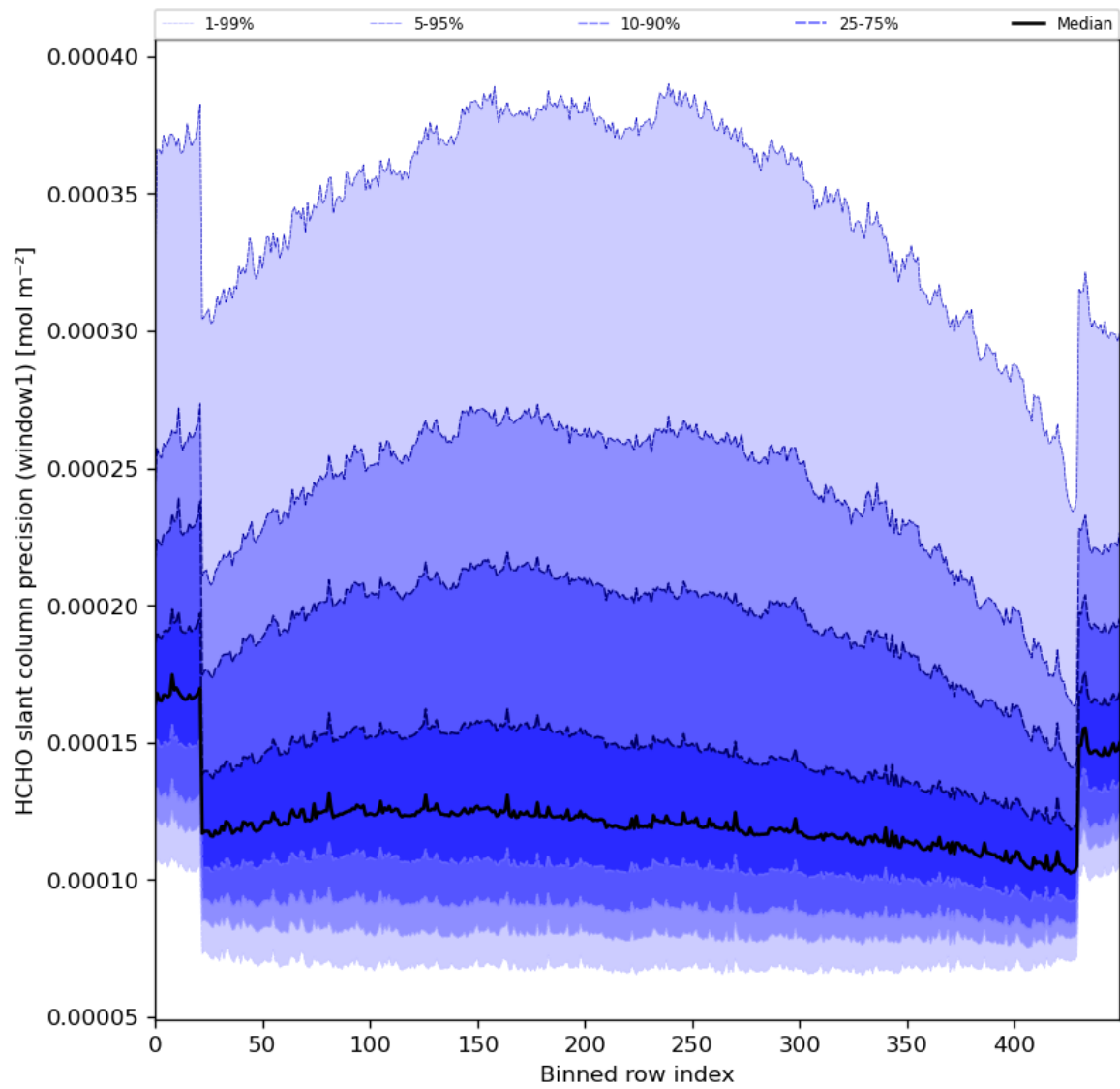
Figure 53: Along track statistics of “HCHO slant column precision (window1)” for 2024-06-19 to 2024-06-20
