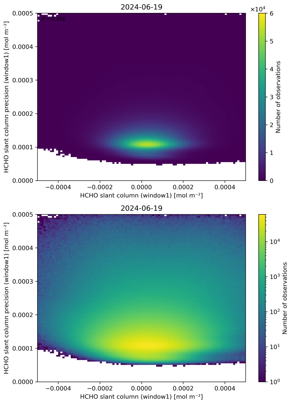
Figure 84: Scatter density plot of “HCHO slant column (window1)” against “HCHO slant column precision (window1)” for 2024-06-19 to 2024-06-20.
