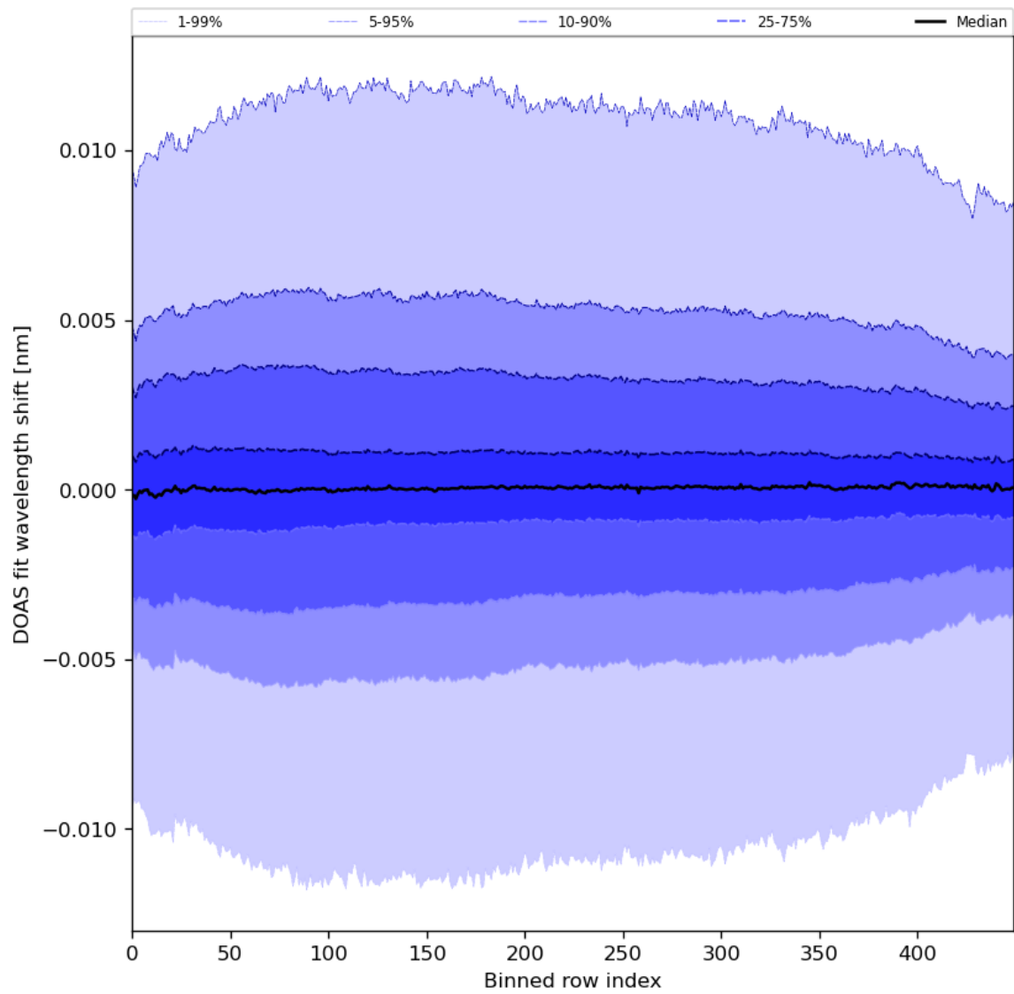
Figure 58: Along track statistics of “DOAS fit wavelength shift” for 2024-06-19 to 2024-06-20
