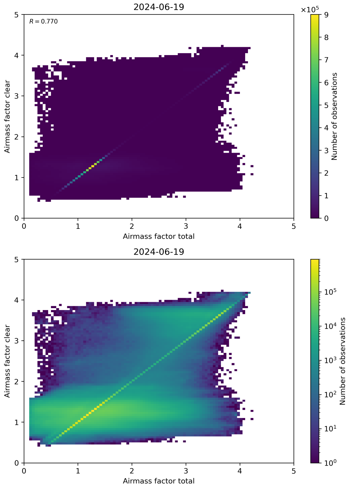
Figure 100: Scatter density plot of “Airmass factor total” against “Airmass factor clear” for 2024-06-19 to 2024-06-20.
