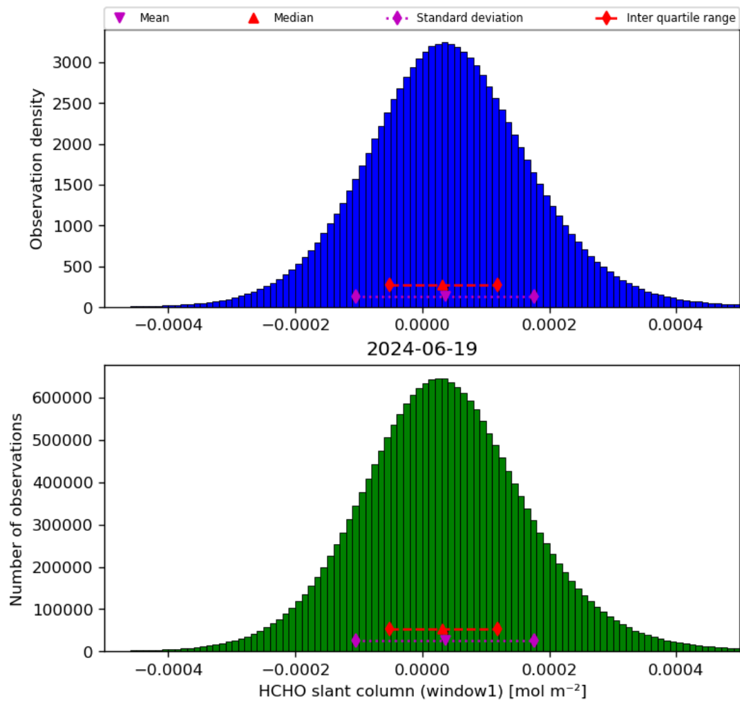
Figure 38: Histogram of “HCHO slant column (window1)” for 2024-06-19 to 2024-06-20
