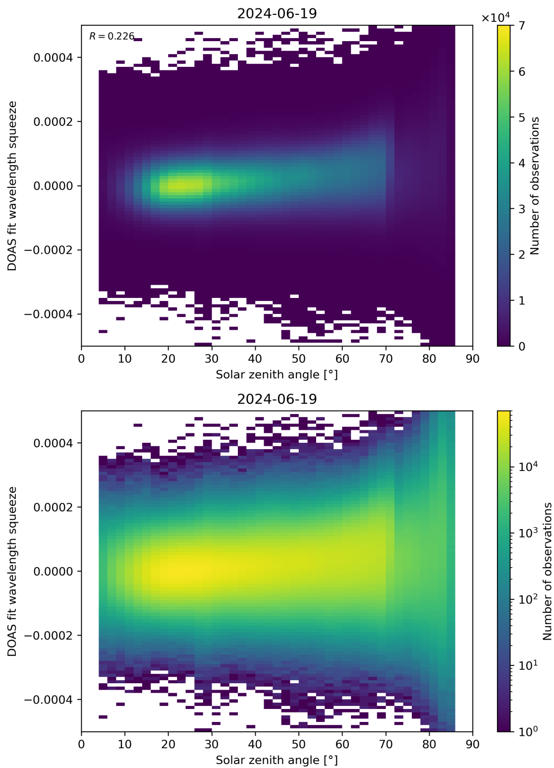
Figure 169: Scatter density plot of “Solar zenith angle” against “DOAS fit wavelength squeeze” for 2024-06-19 to 2024-06-20.
