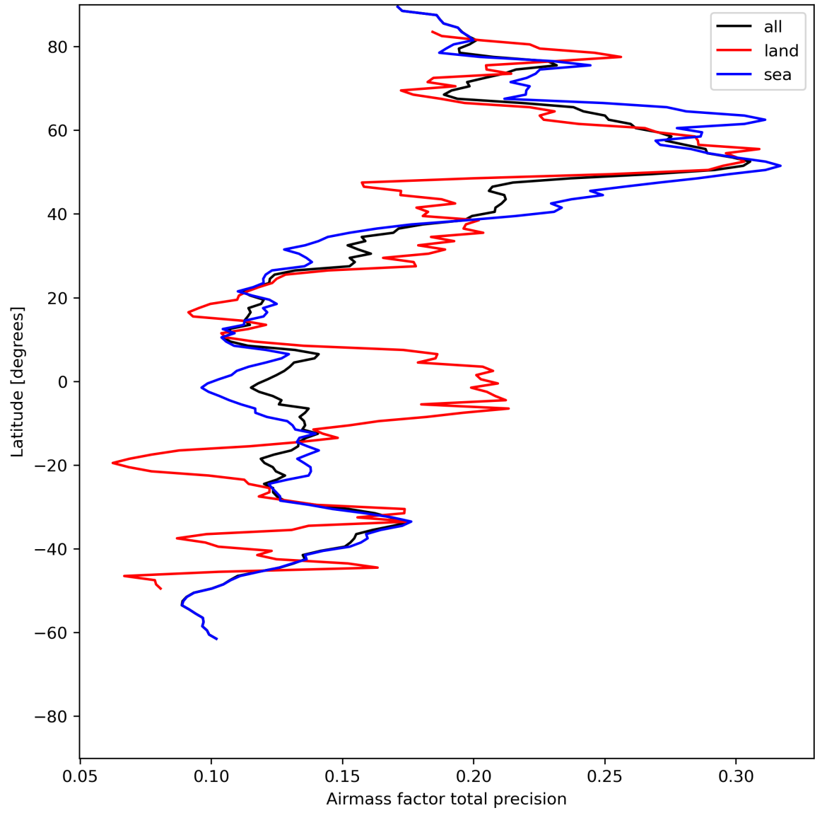
Figure 27: Zonal average of “Airmass factor total precision” for 2024-06-19 to 2024-06-20.
