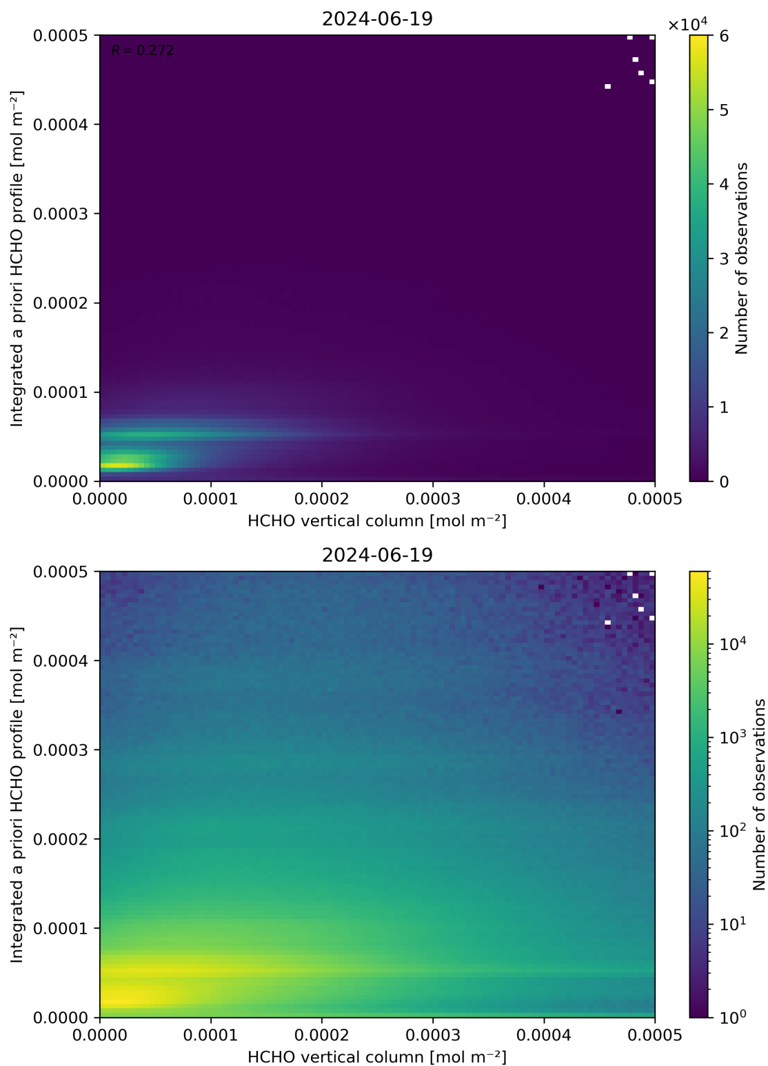
Figure 135: Scatter density plot of “HCHO vertical column” against “Integrated a priori HCHO profile” for 2024-06-19 to 2024-06-20.
