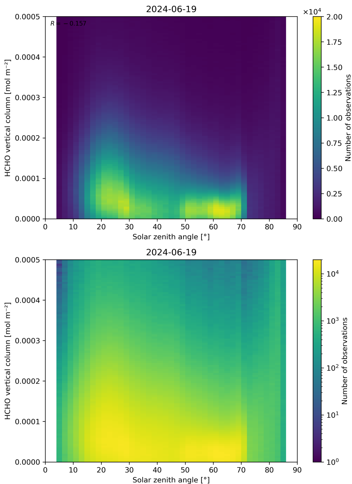
Figure 177: Scatter density plot of “Solar zenith angle” against “HCHO vertical column” for 2024-06-19 to 2024-06-20.
