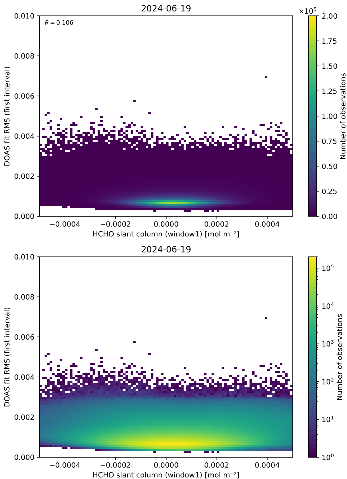
Figure 78: Scatter density plot of “HCHO slant column (window1)” against “DOAS fit RMS (first interval)” for 2024-06-19 to 2024-06-20.
