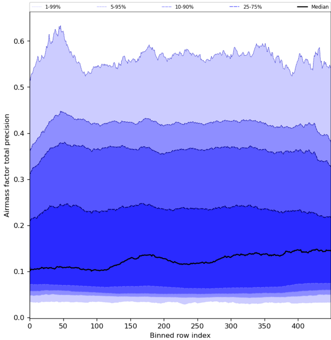
Figure 55: Along track statistics of “Airmass factor total precision” for 2024-06-19 to 2024-06-20
