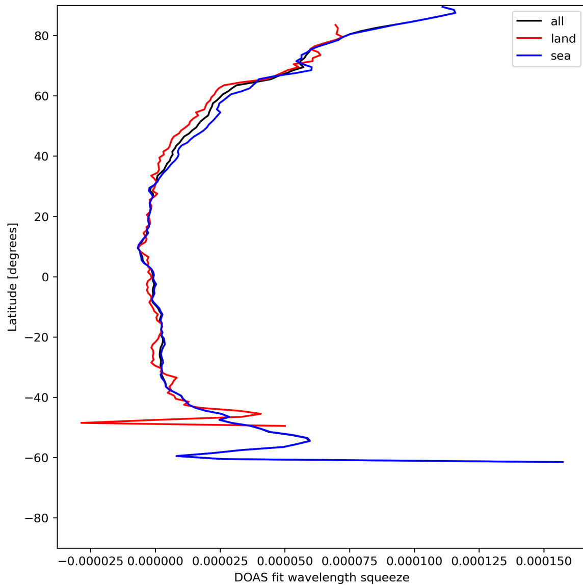
Figure 31: Zonal average of “DOAS fit wavelength squeeze” for 2024-06-19 to 2024-06-20.
