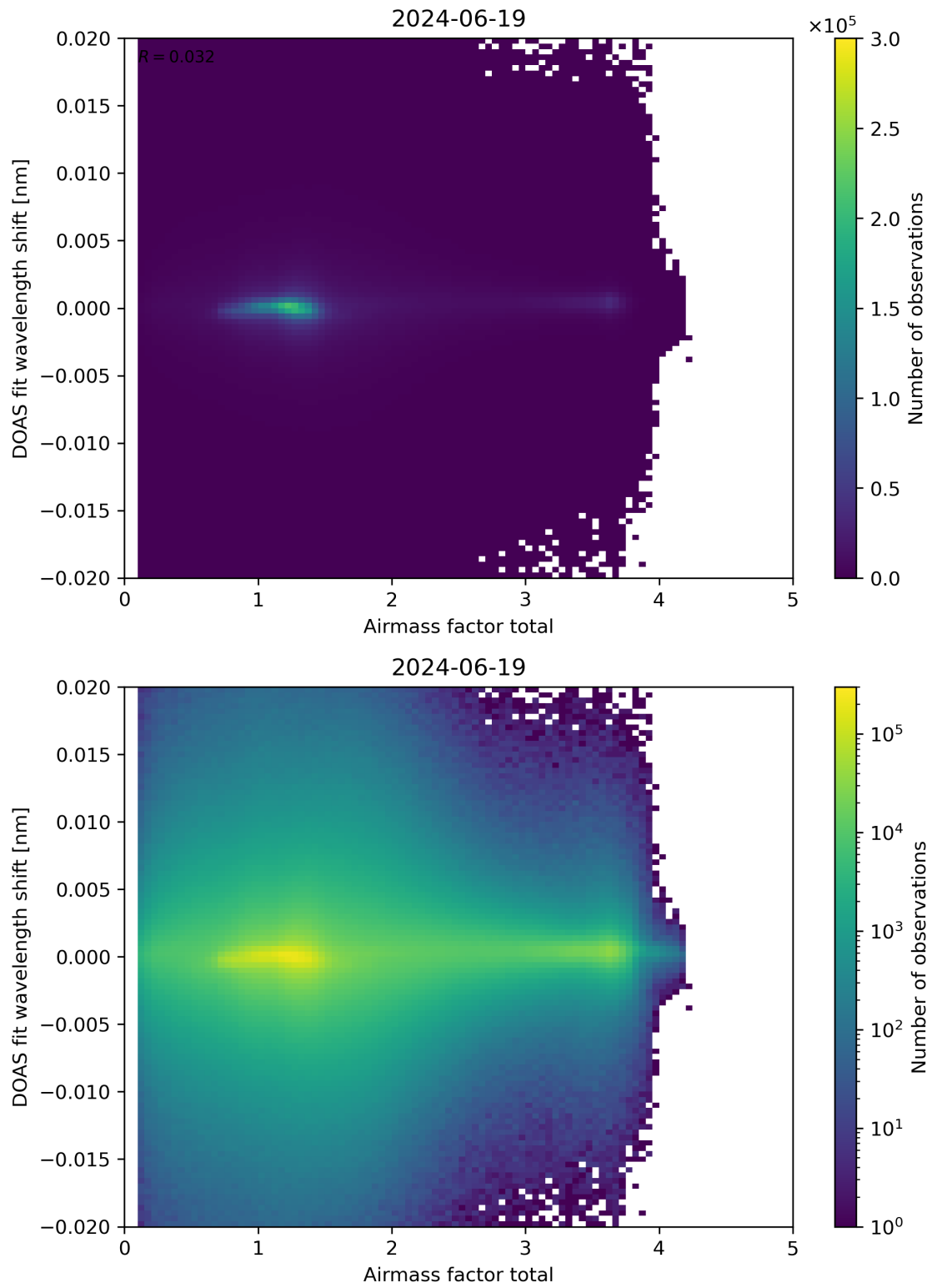
Figure 98: Scatter density plot of “Airmass factor total” against “DOAS fit wavelength shift” for 2024-06-19 to 2024-06-20.
