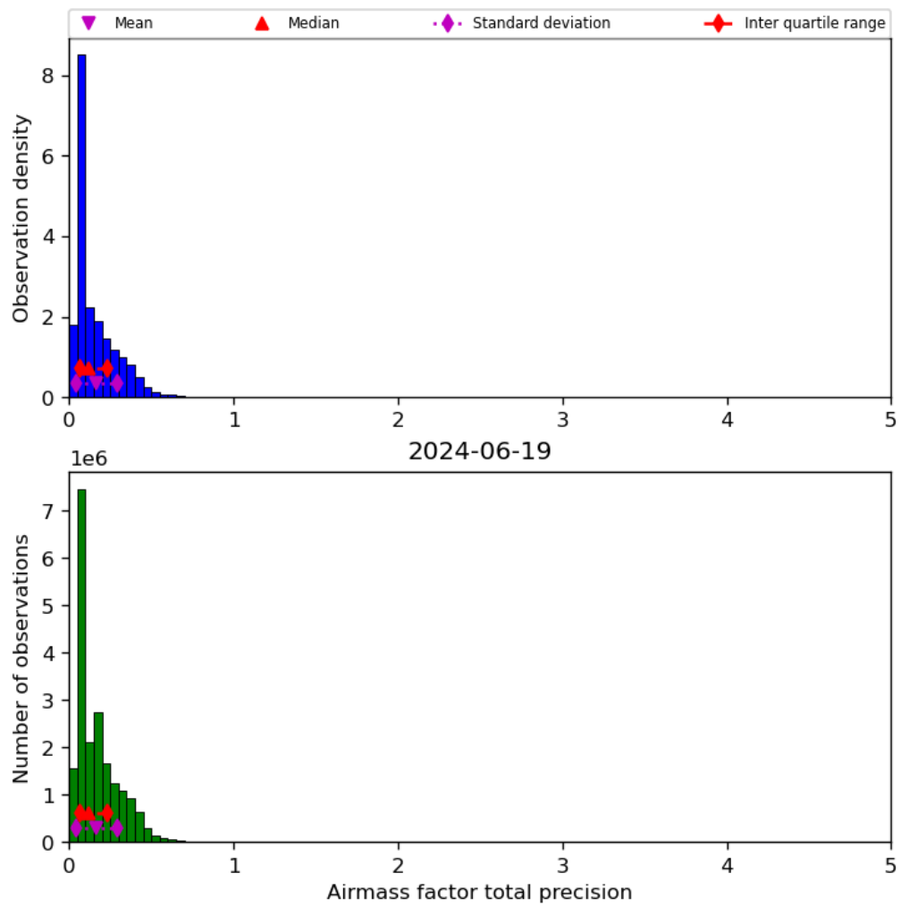
Figure 41: Histogram of “Airmass factor total precision” for 2024-06-19 to 2024-06-20
