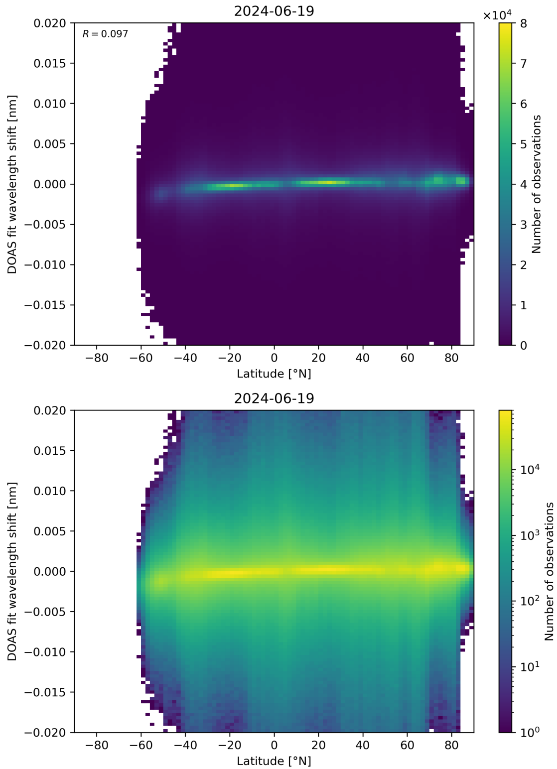
Figure 154: Scatter density plot of “Latitude” against “DOAS fit wavelength shift” for 2024-06-19 to 2024-06-20.
