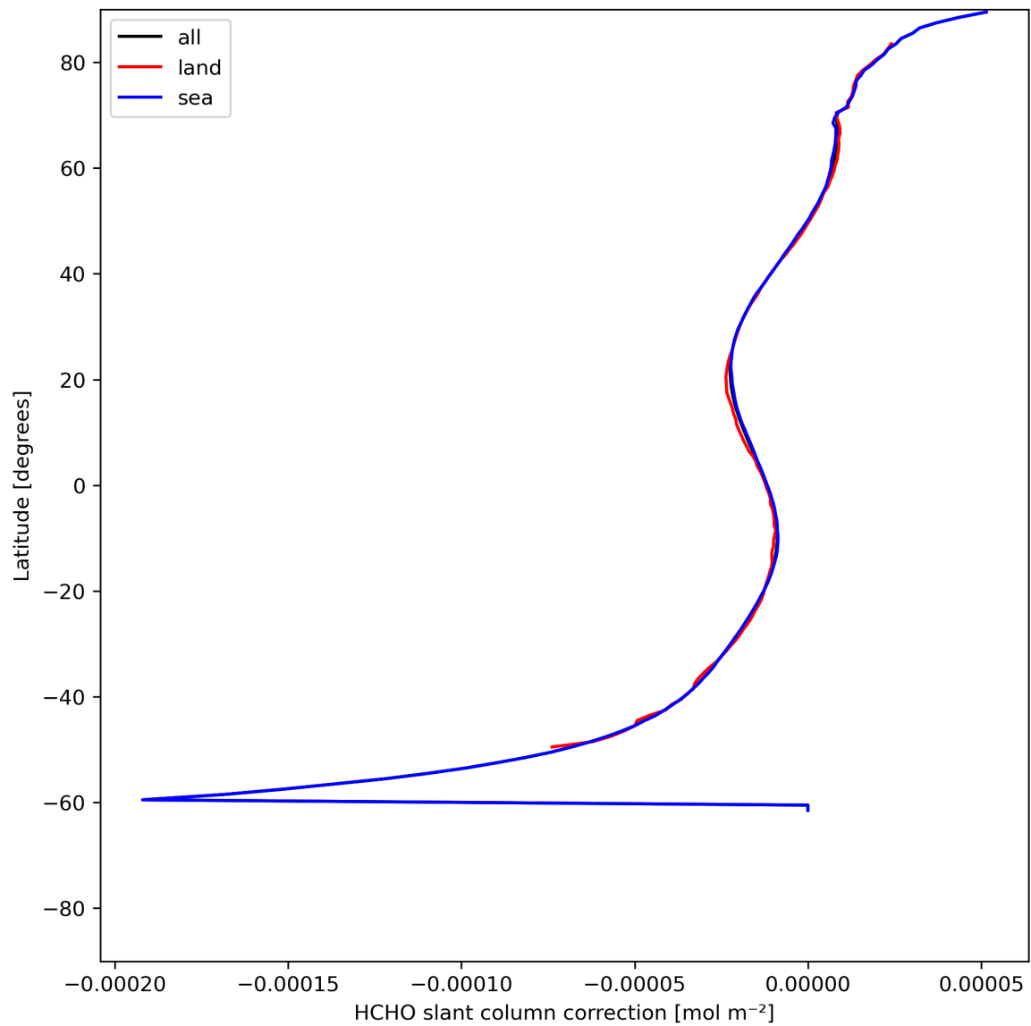
Figure 33: Zonal average of “HCHO slant column correction” for 2024-06-19 to 2024-06-20.
