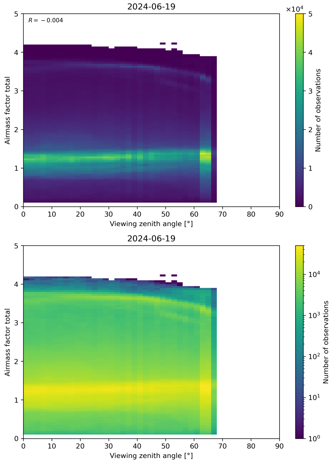
Figure 190: Scatter density plot of “Viewing zenith angle” against “Airmass factor total” for 2024-06-19 to 2024-06-20.
