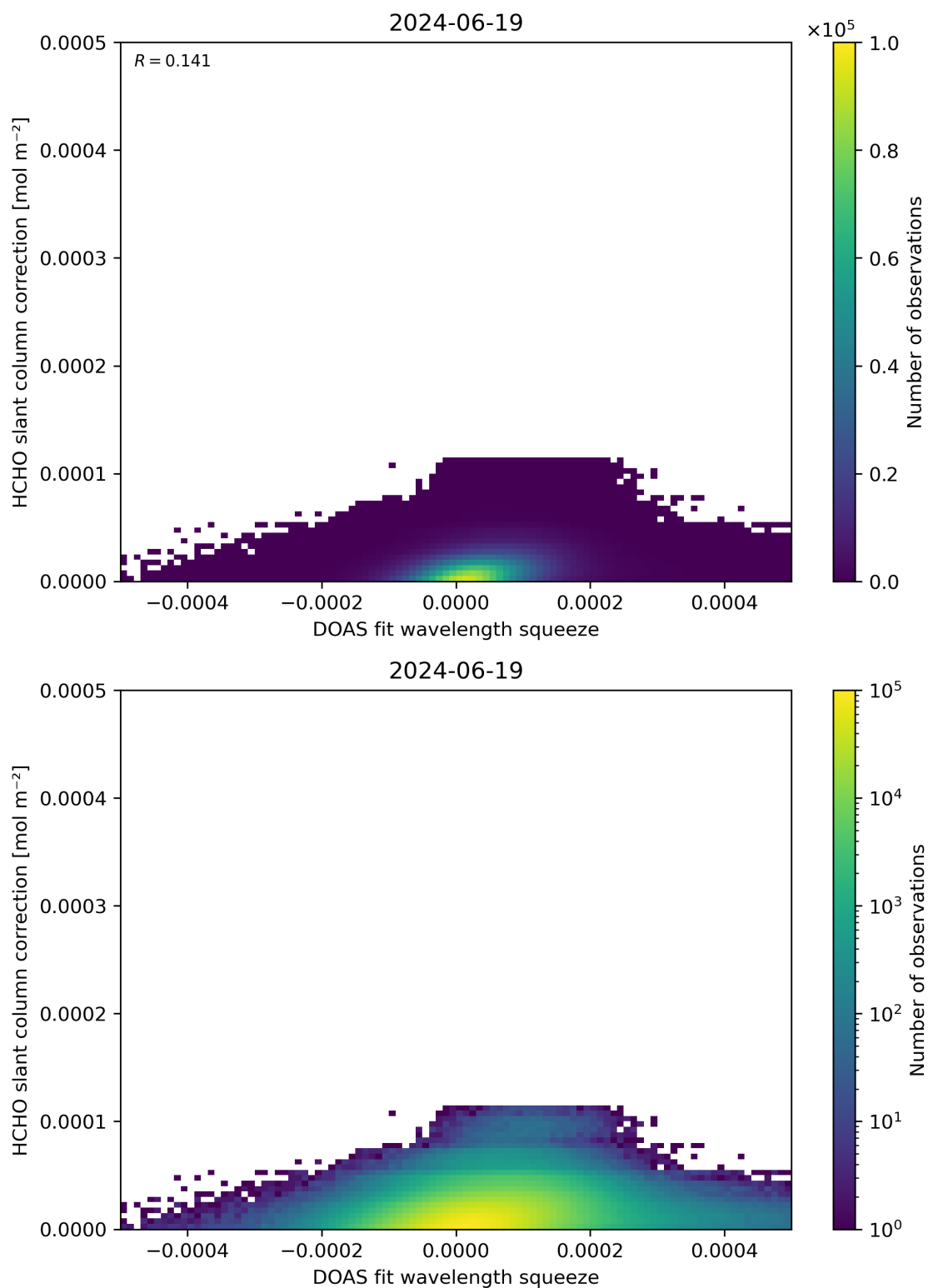
Figure 70: Scatter density plot of “DOAS fit wavelength squeeze” against “HCHO slant column correction” for 2024-06-19 to 2024-06-20.
