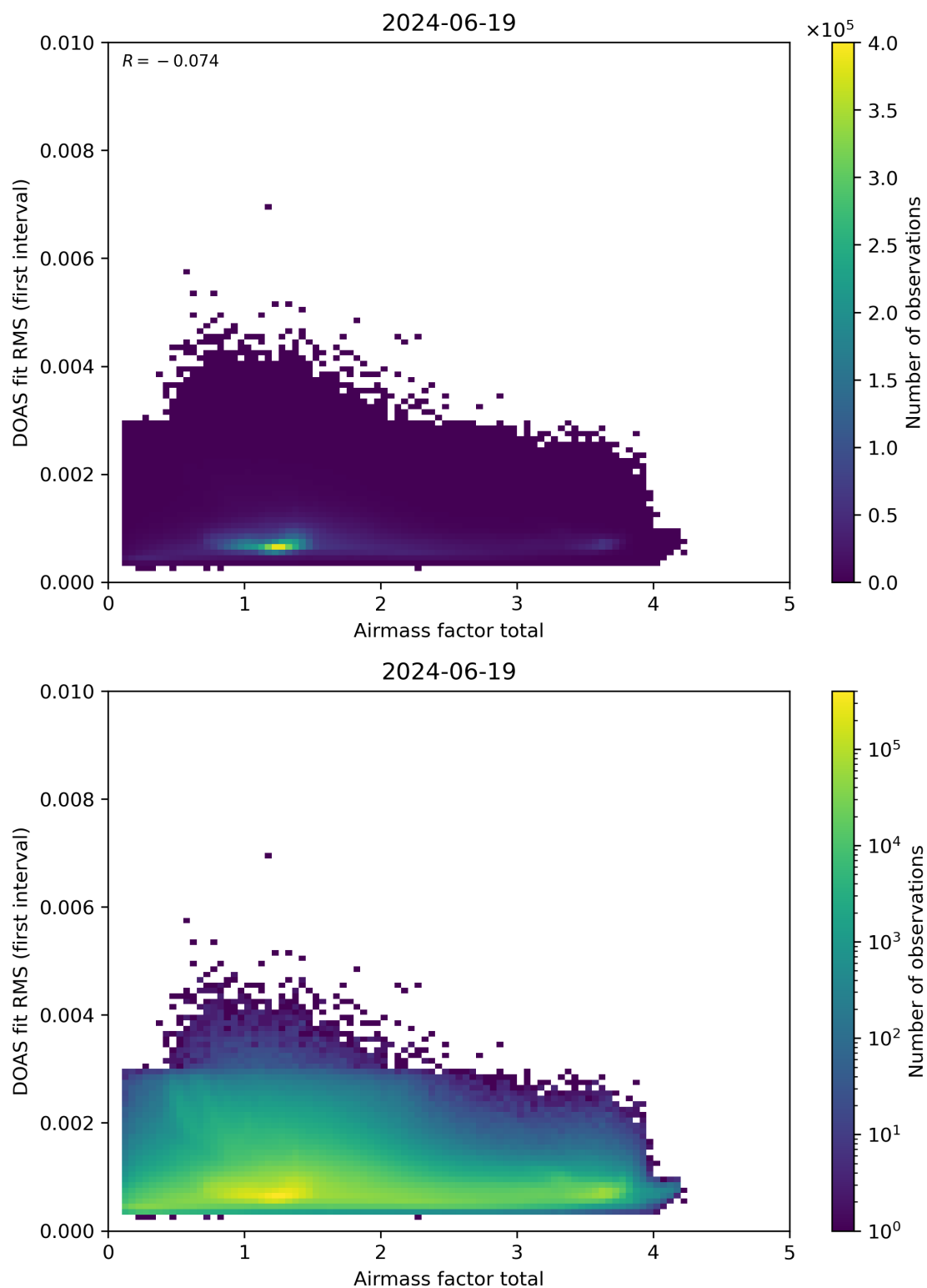
Figure 97: Scatter density plot of “Airmass factor total” against “DOAS fit RMS (first interval)” for 2024-06-19 to 2024-06-20.
