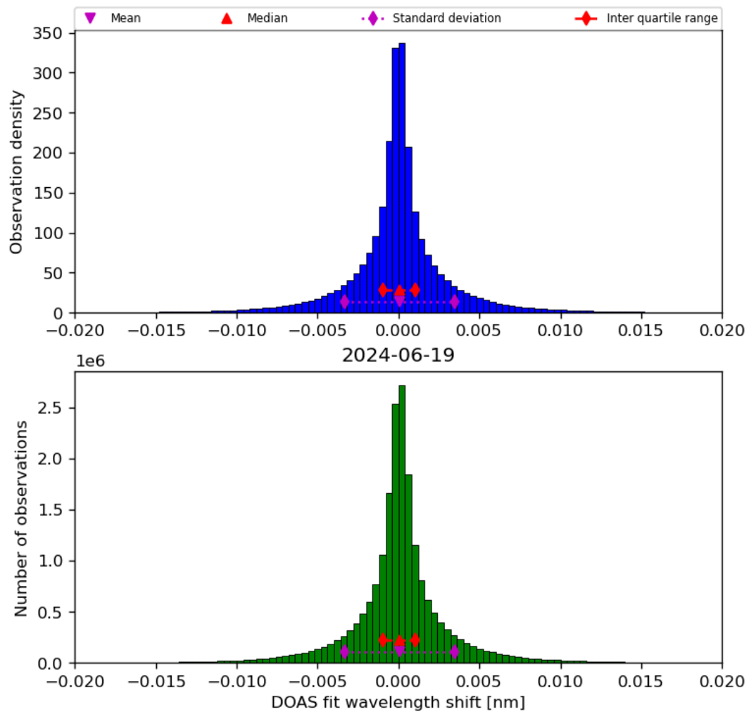
Figure 44: Histogram of “DOAS fit wavelength shift” for 2024-06-19 to 2024-06-20
