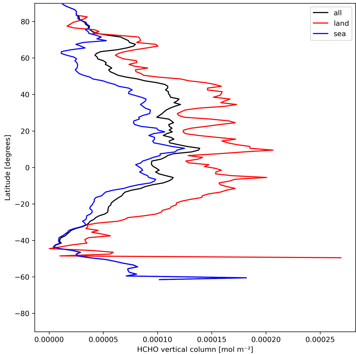
Figure 21: Zonal average of “HCHO vertical column” for 2024-06-19 to 2024-06-20.
