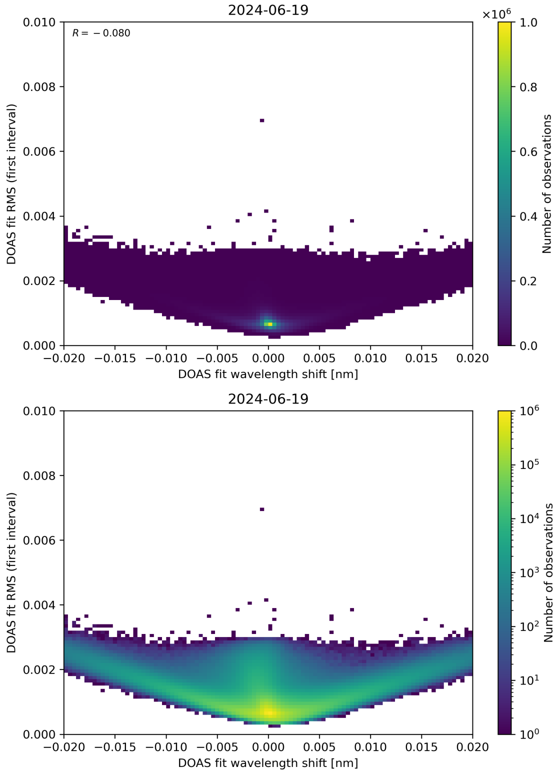
Figure 64: Scatter density plot of “DOAS fit wavelength shift” against “DOAS fit RMS (first interval)” for 2024-06-19 to 2024-06-20.
