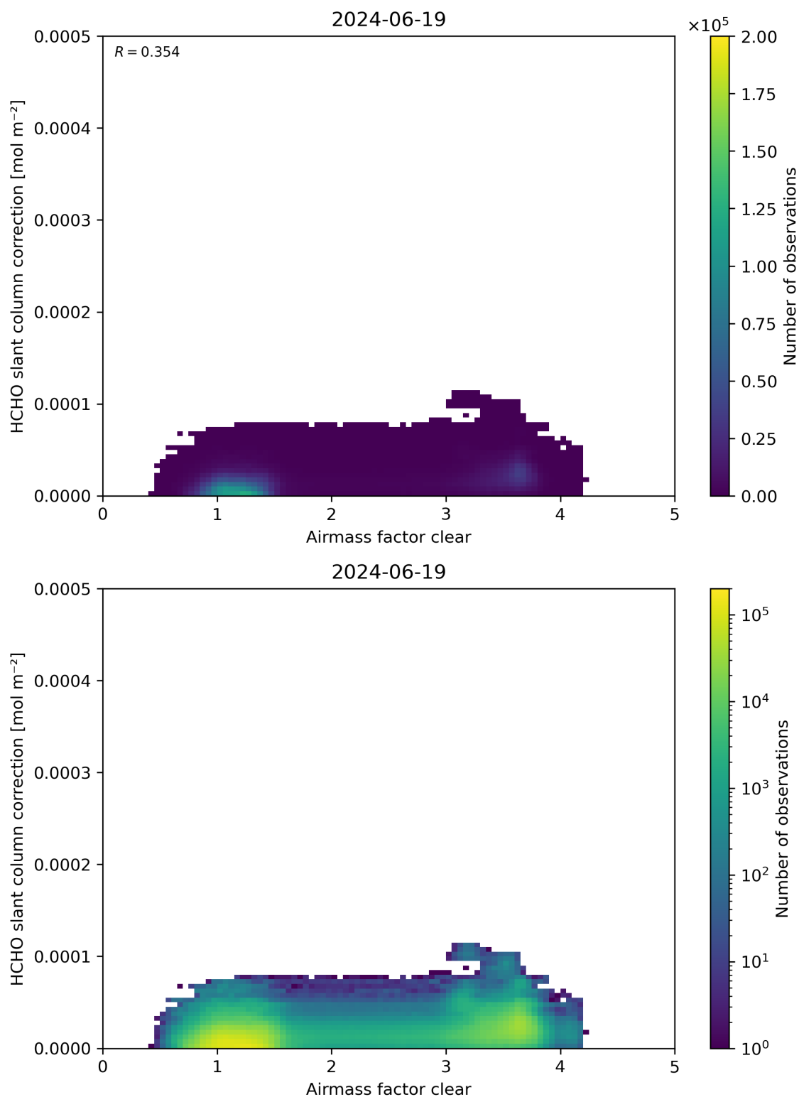
Figure 75: Scatter density plot of “Airmass factor clear” against “HCHO slant column correction” for 2024-06-19 to 2024-06-20.
