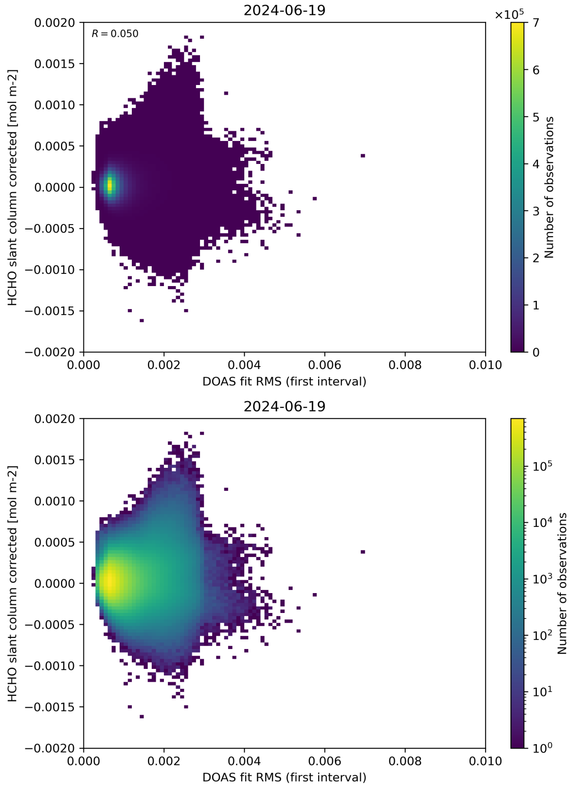
Figure 62: Scatter density plot of “DOAS fit RMS (first interval)” against “HCHO slant column corrected” for 2024-06-19 to 2024-06-20.
