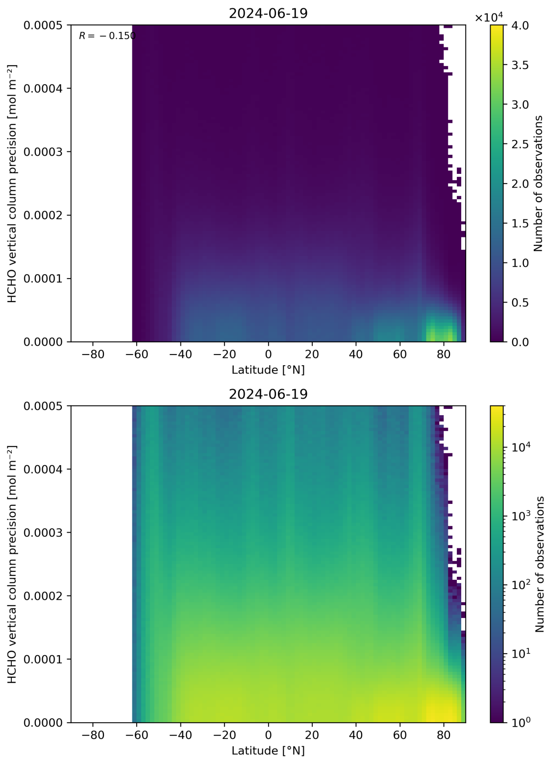
Figure 165: Scatter density plot of “Latitude” against “HCHO vertical column precision” for 2024-06-19 to 2024-06-20.
