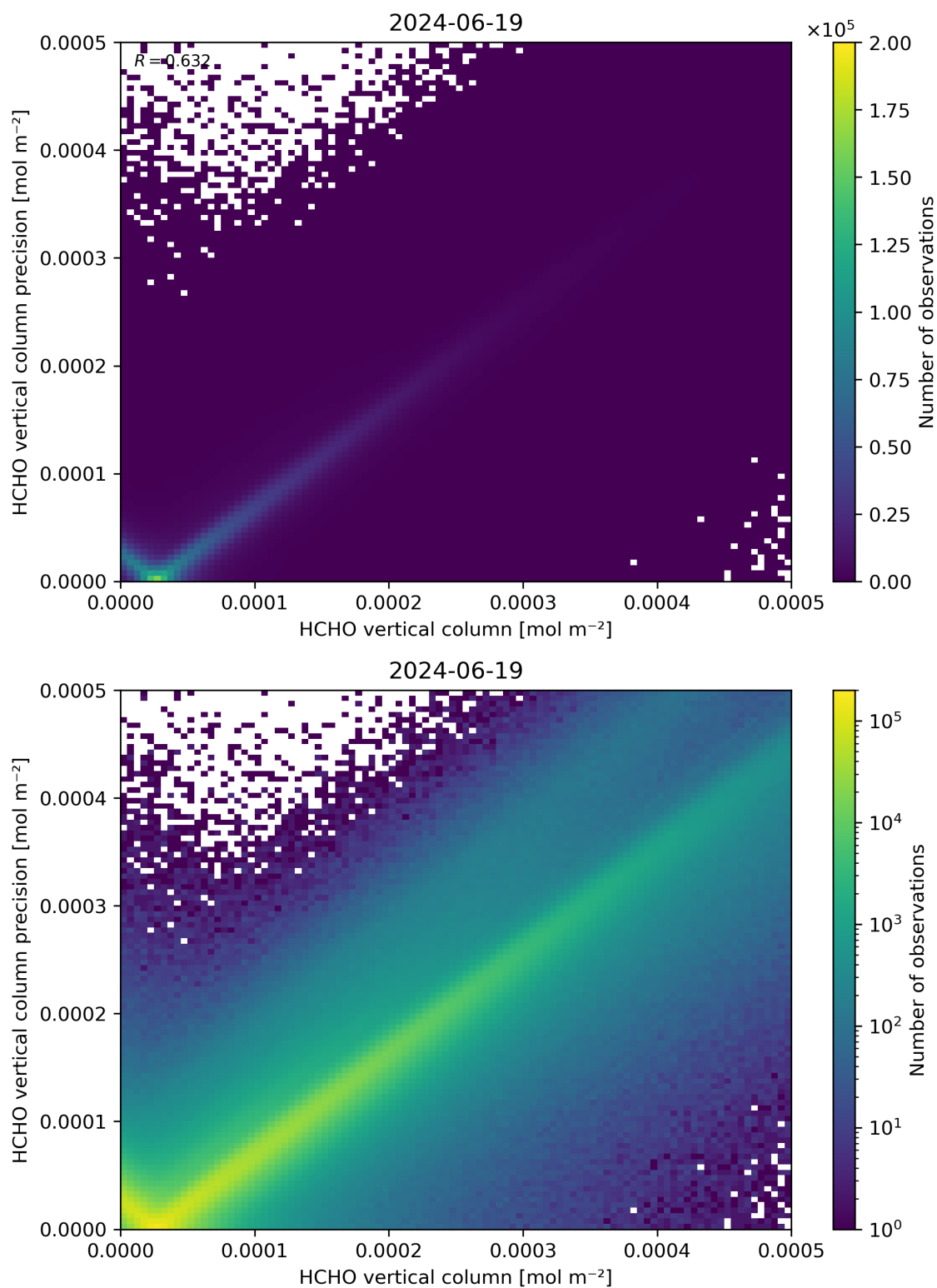
Figure 134: Scatter density plot of “HCHO vertical column” against “HCHO vertical column precision” for 2024-06-19 to 2024-06-20.
