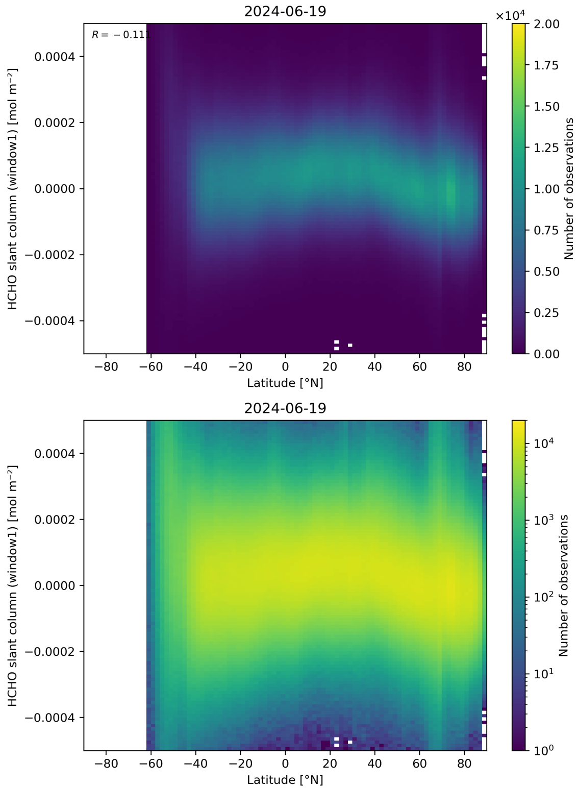
Figure 159: Scatter density plot of “Latitude” against “HCHO slant column (window1)” for 2024-06-19 to 2024-06-20.
