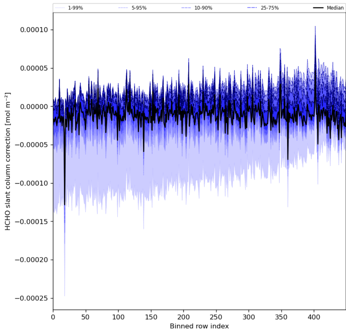
Figure 61: Along track statistics of “HCHO slant column correction” for 2024-06-19 to 2024-06-20
