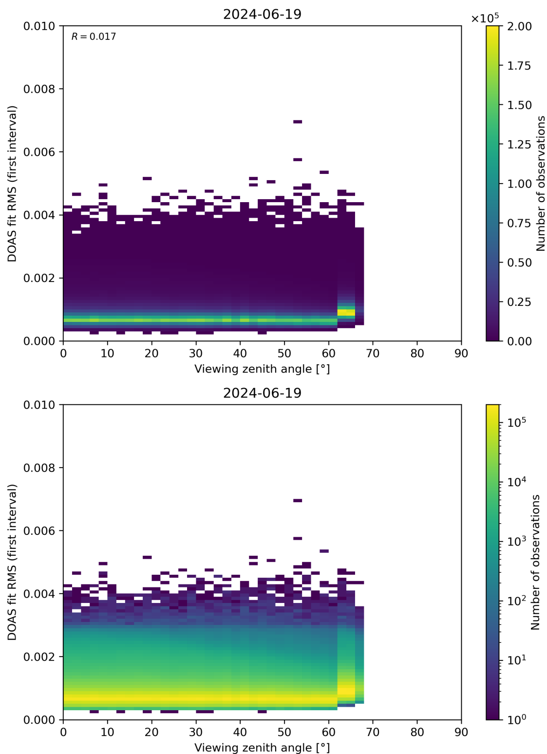
Figure 182: Scatter density plot of “Viewing zenith angle” against “DOAS fit RMS (first interval)” for 2024-06-19 to 2024-06-20.
