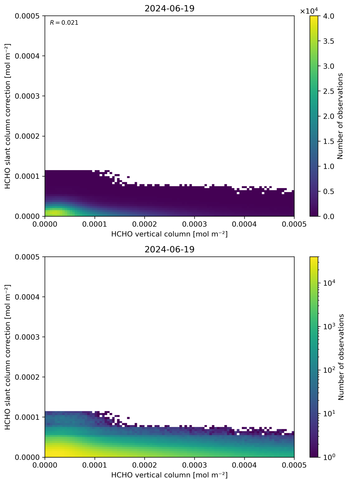
Figure 128: Scatter density plot of “HCHO vertical column” against “HCHO slant column correction” for 2024-06-19 to 2024-06-20.
