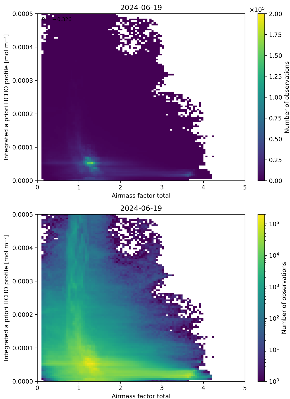
Figure 104: Scatter density plot of “Airmass factor total” against “Integrated a priori HCHO profile” for 2024-06-19 to 2024-06-20.
