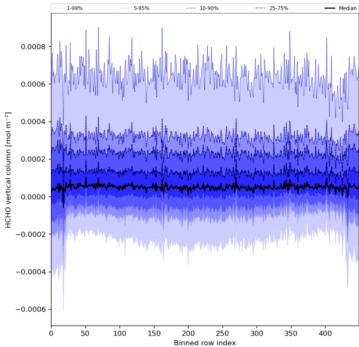
Figure 49: Along track statistics of “HCHO vertical column” for 2024-06-19 to 2024-06-20
