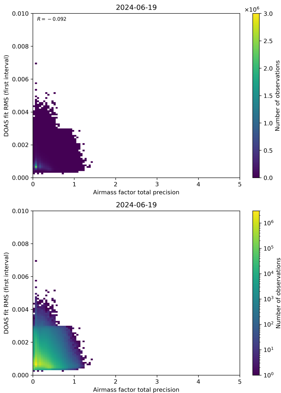
Figure 105: Scatter density plot of “Airmass factor total precision” against “DOAS fit RMS (first interval)” for 2024-06-19 to 2024-06-20.
