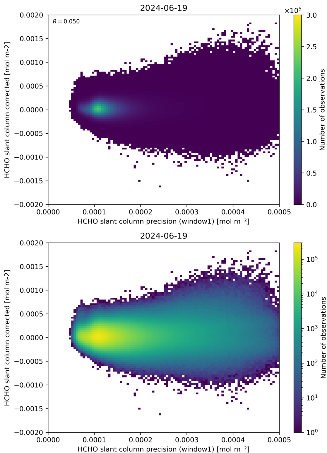
Figure 92: Scatter density plot of “HCHO slant column precision (window1)” against “HCHO slant column corrected” for 2024-06-19 to 2024-06-20.
