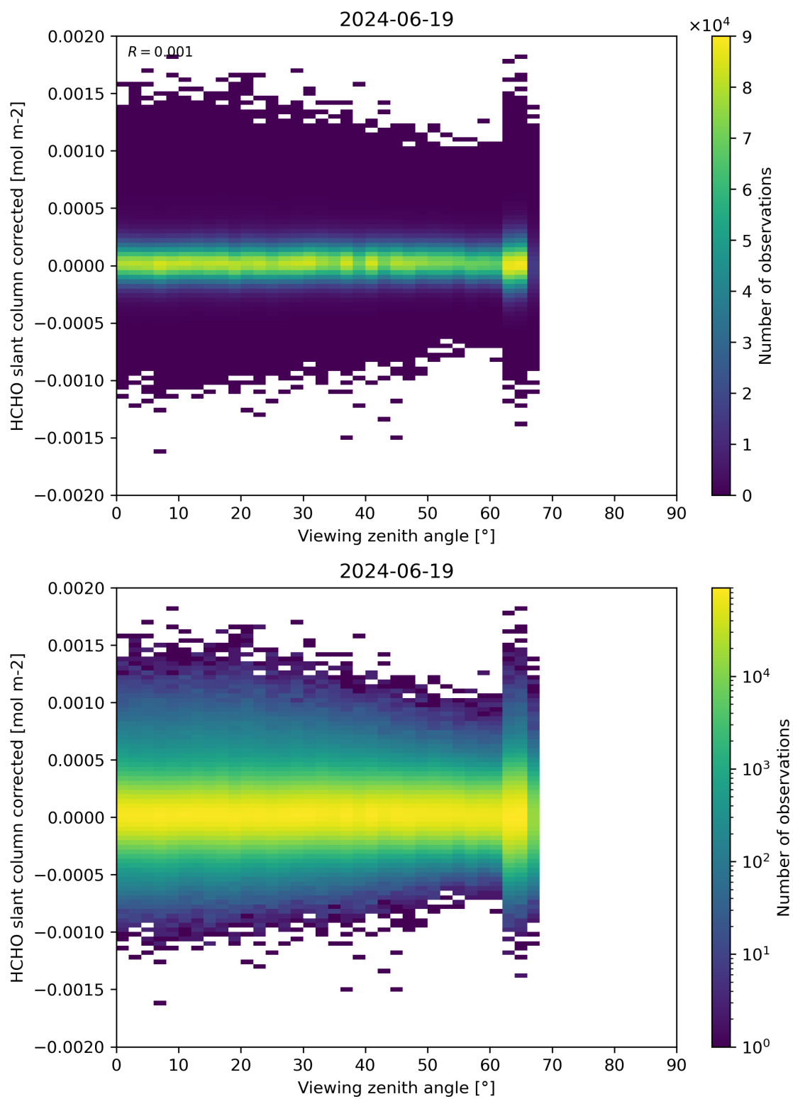
Figure 186: Scatter density plot of “Viewing zenith angle” against “HCHO slant column corrected” for 2024-06-19 to 2024-06-20.
