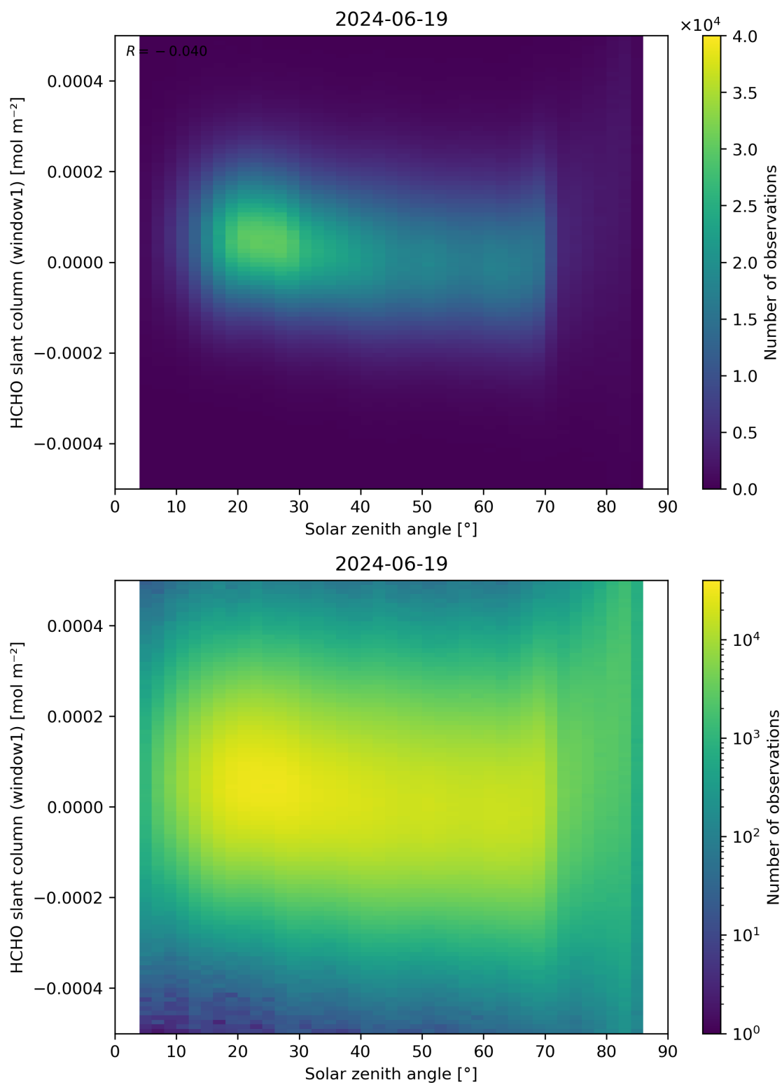
Figure 173: Scatter density plot of “Solar zenith angle” against “HCHO slant column (window1)” for 2024-06-19 to 2024-06-20.
