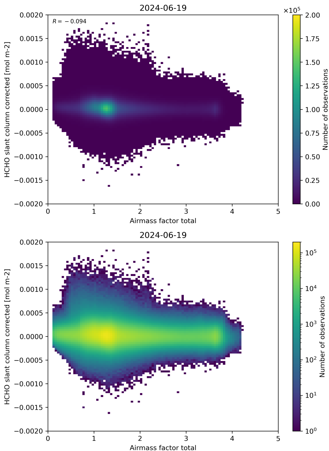
Figure 101: Scatter density plot of “Airmass factor total” against “HCHO slant column corrected” for 2024-06-19 to 2024-06-20.
