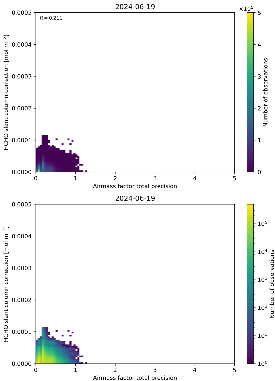
Figure 110: Scatter density plot of “Airmass factor total precision” against “HCHO slant column correction” for 2024-06-19 to 2024-06-20.
