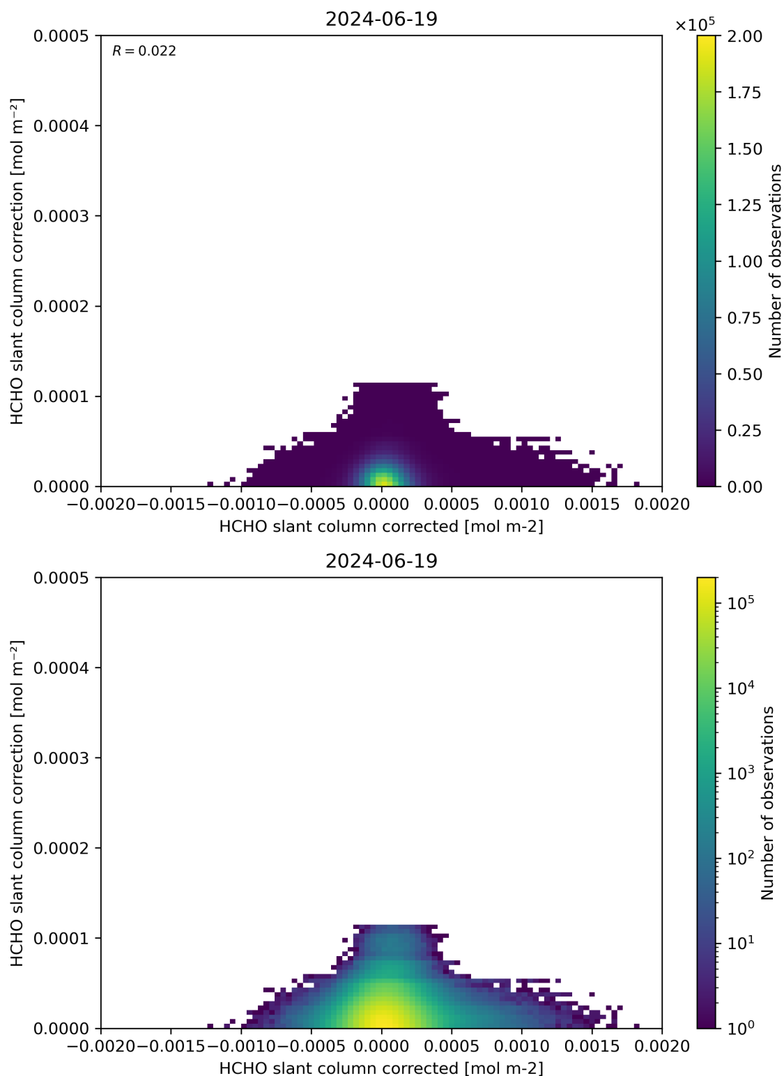
Figure 77: Scatter density plot of “HCHO slant column corrected” against “HCHO slant column correction” for 2024-06-19 to 2024-06-20.
