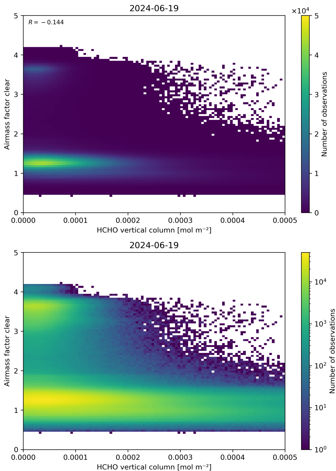
Figure 126: Scatter density plot of “HCHO vertical column” against “Airmass factor clear” for 2024-06-19 to 2024-06-20.
