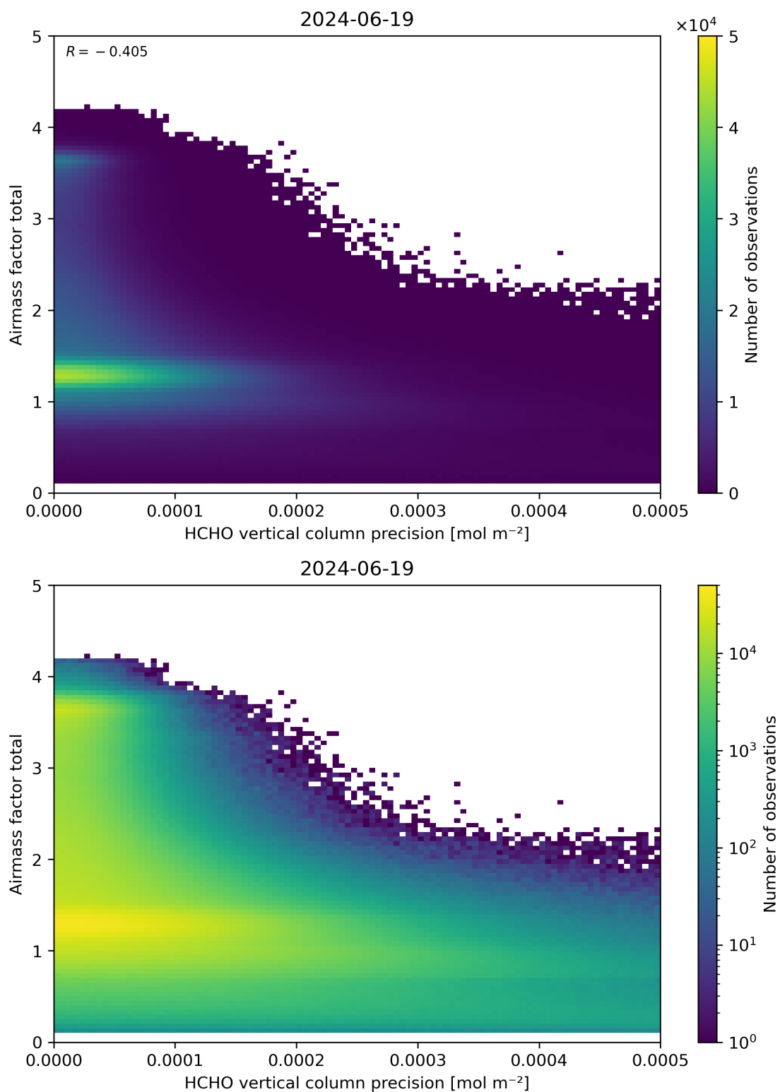
Figure 144: Scatter density plot of “HCHO vertical column precision” against “Airmass factor total” for 2024-06-19 to 2024-06-20.
