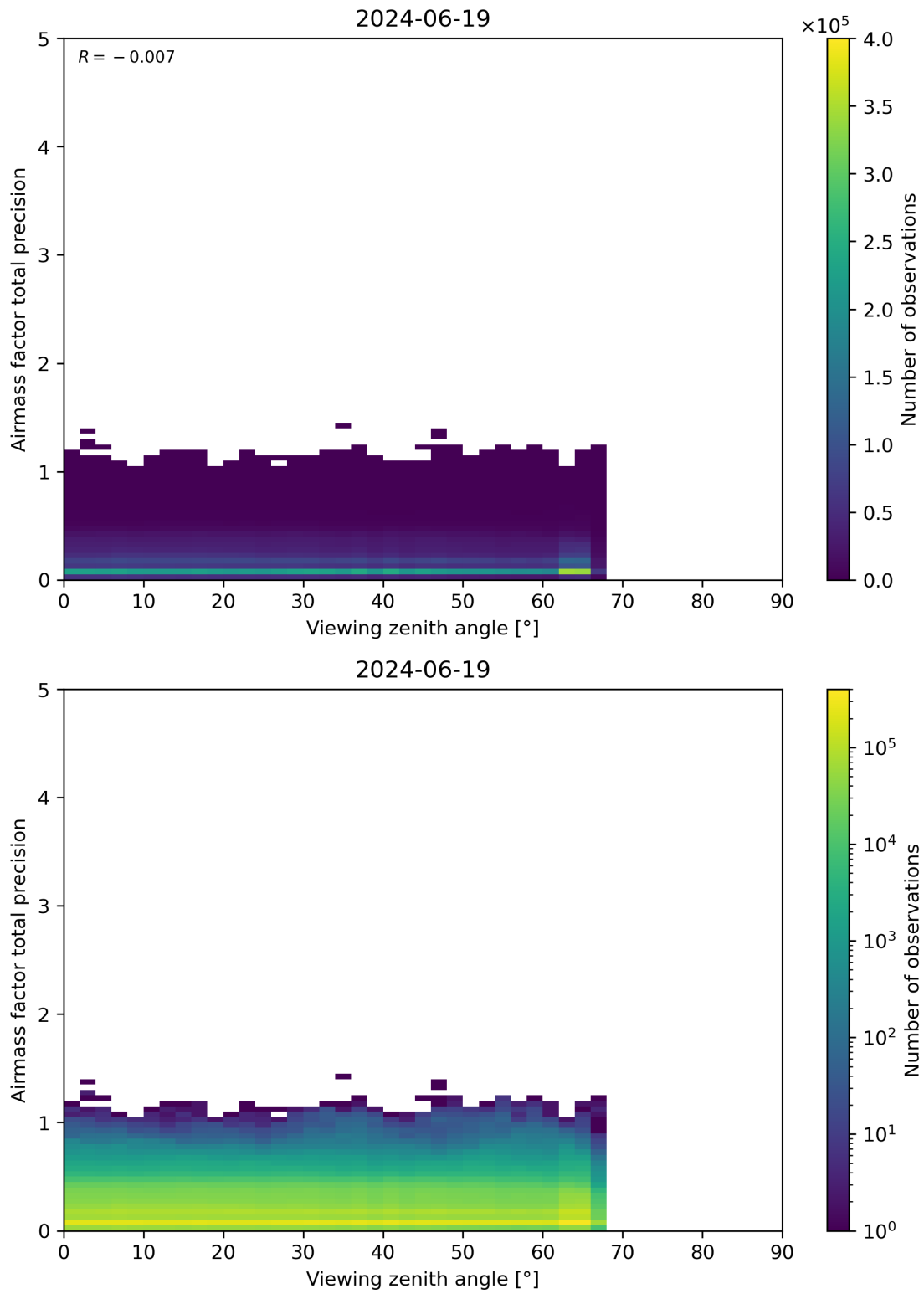
Figure 191: Scatter density plot of “Viewing zenith angle” against “Airmass factor total precision” for 2024-06-19 to 2024-06-20.
