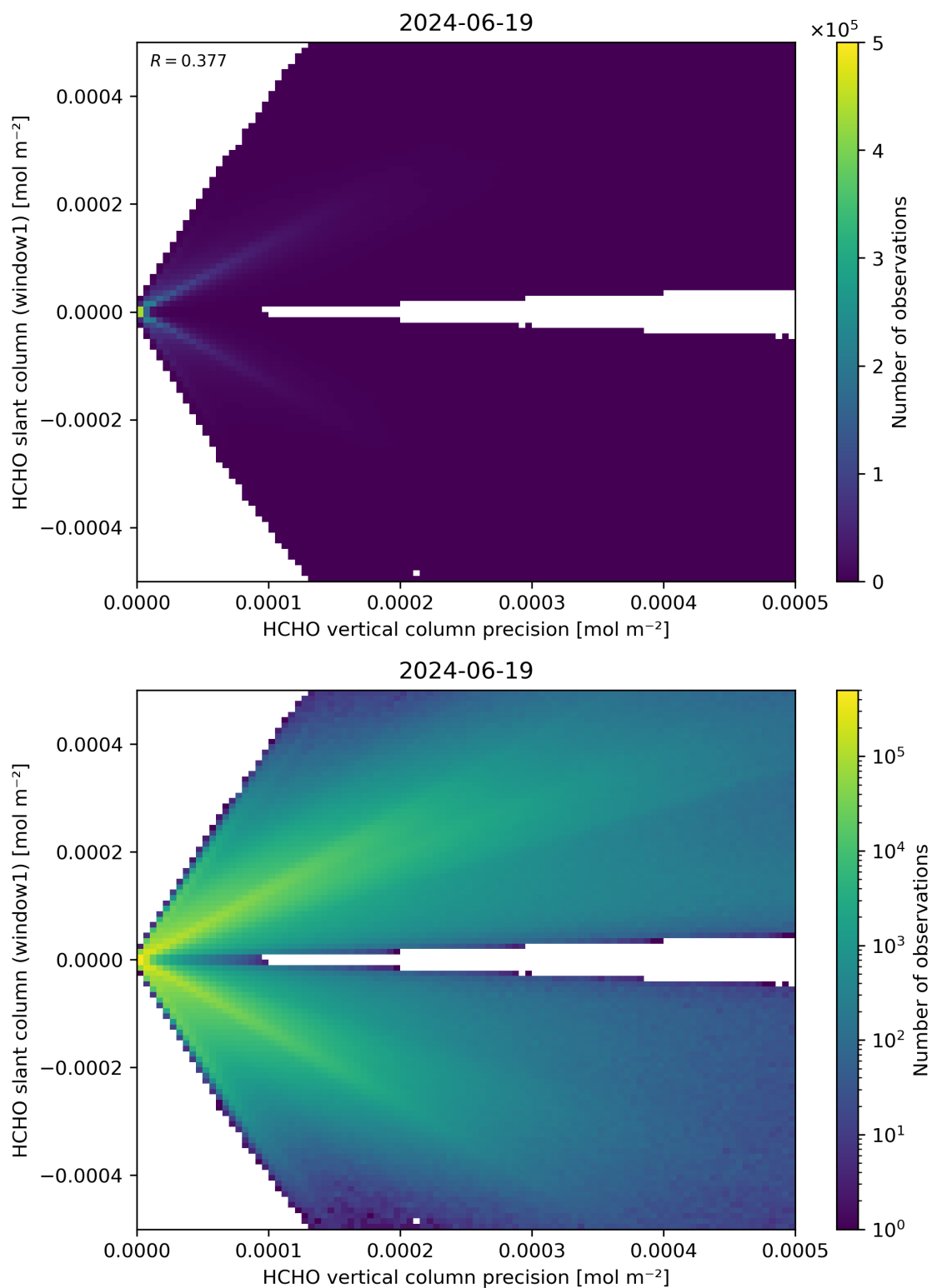
Figure 142: Scatter density plot of “HCHO vertical column precision” against “HCHO slant column (window1)” for 2024-06-19 to 2024-06-20.
