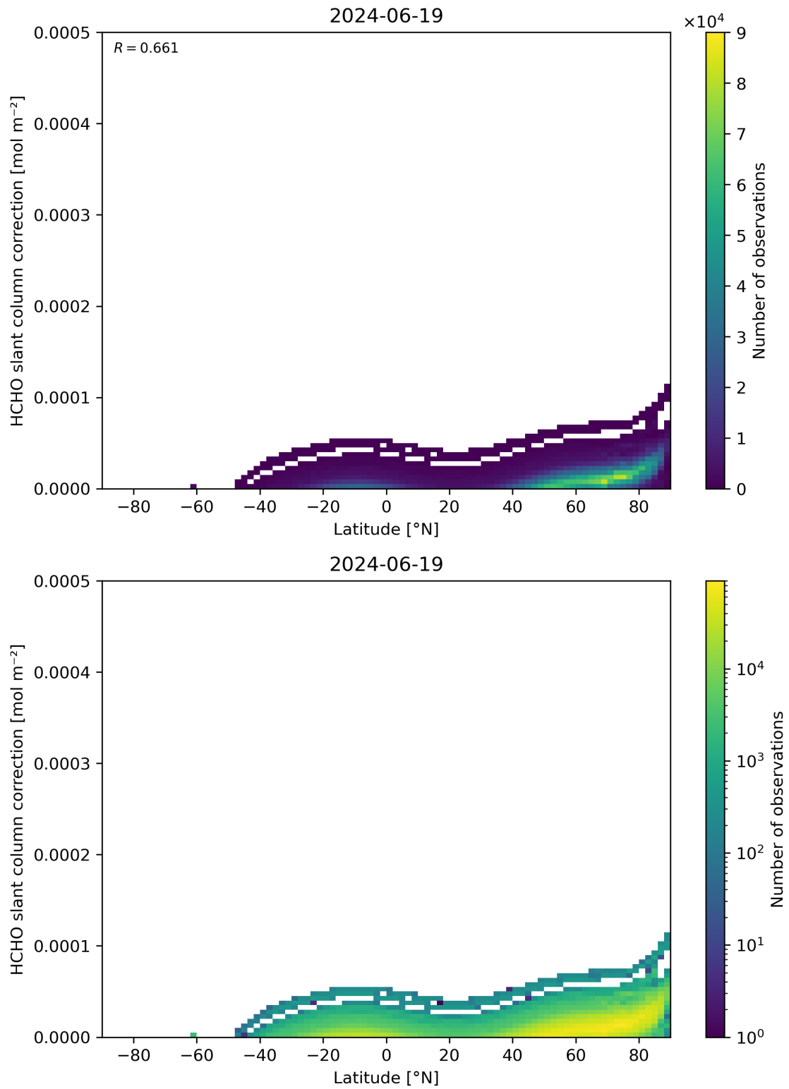
Figure 158: Scatter density plot of “Latitude” against “HCHO slant column correction” for 2024-06-19 to 2024-06-20.
