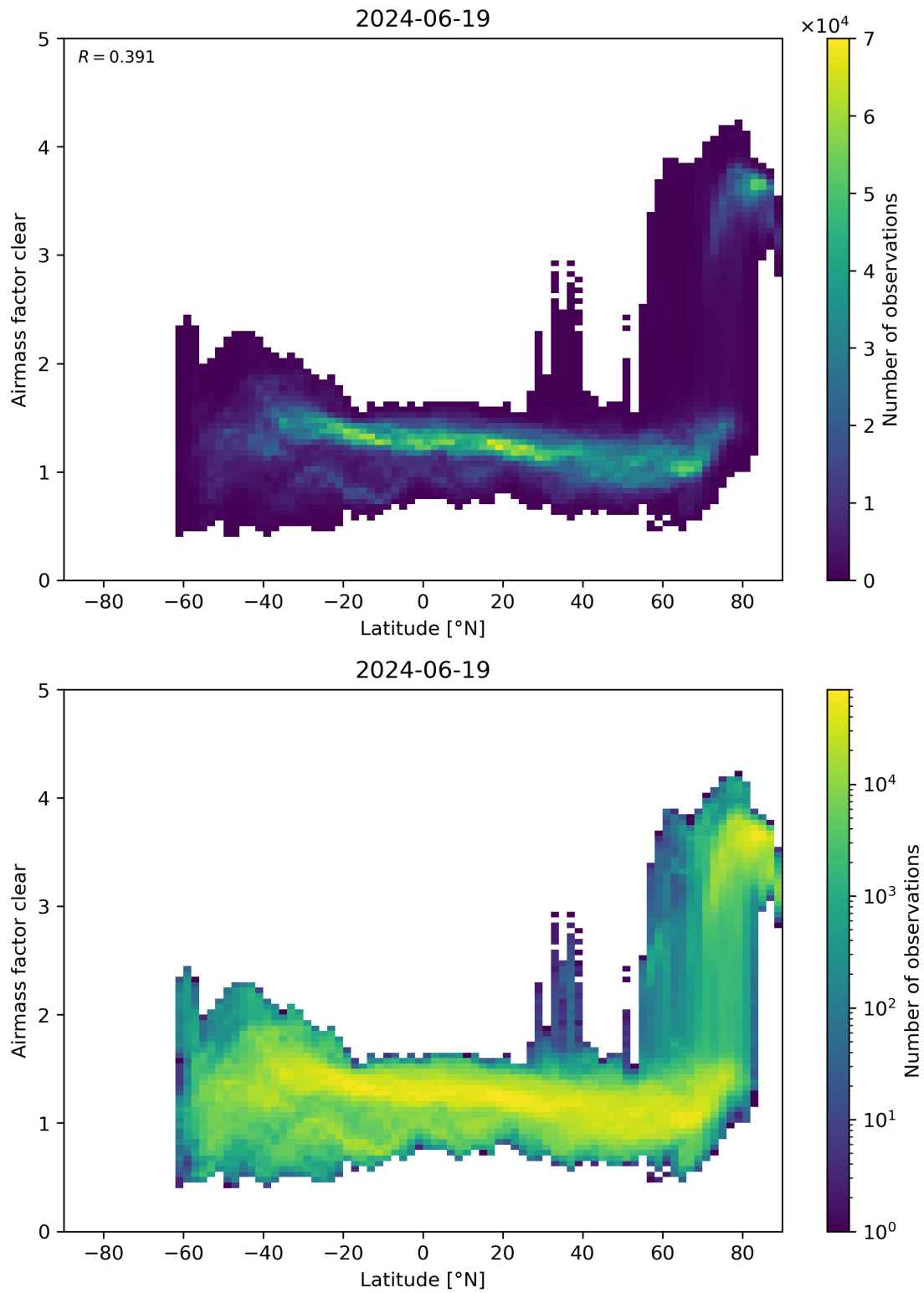
Figure 156: Scatter density plot of “Latitude” against “Airmass factor clear” for 2024-06-19 to 2024-06-20.
