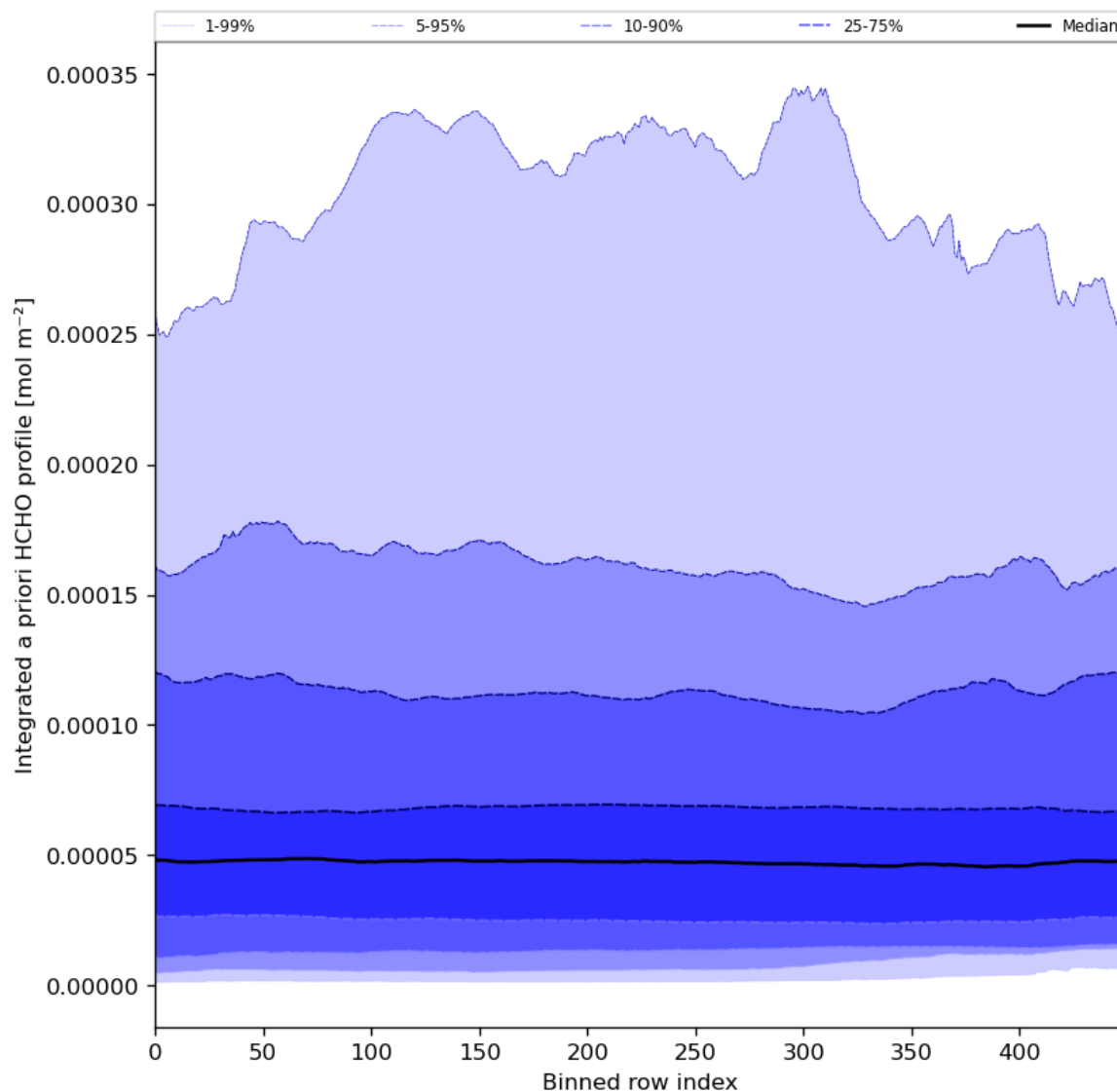
Figure 57: Along track statistics of "Integrated a priori HCHO profile" for 2024-06-19 to 2024-06-20
