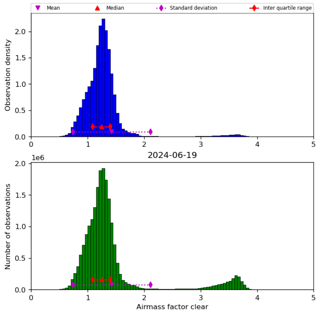
Figure 42: Histogram of “Airmass factor clear” for 2024-06-19 to 2024-06-20
