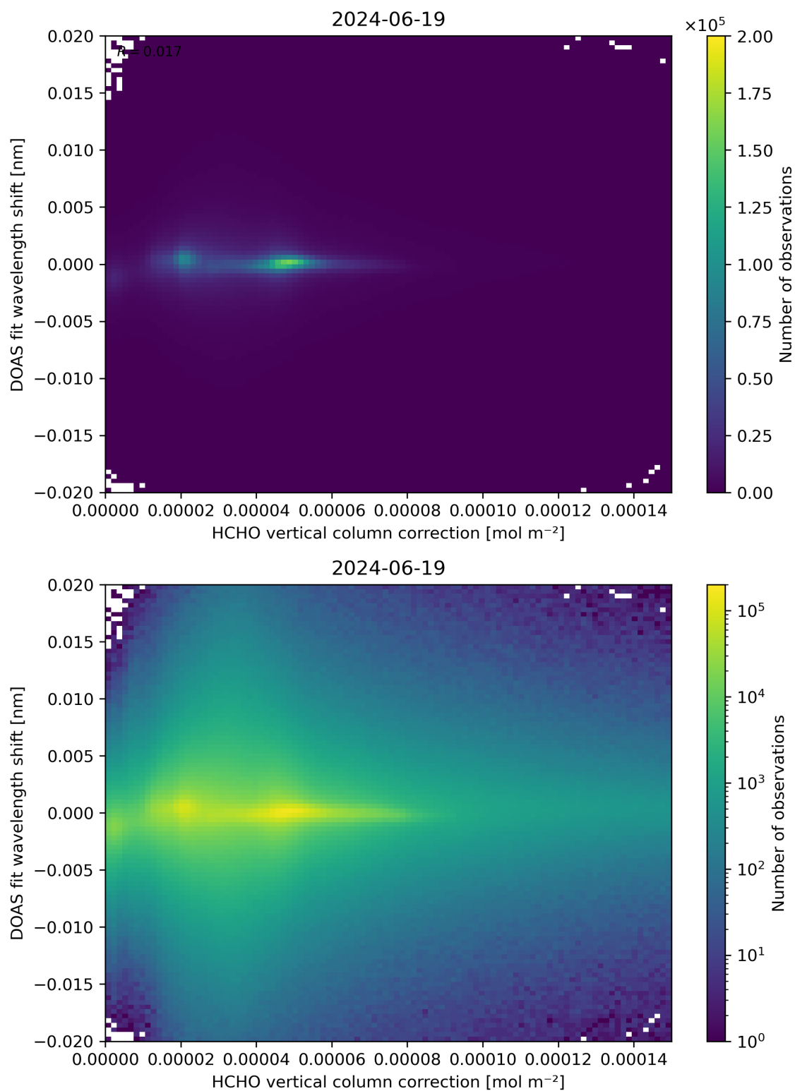
Figure 113: Scatter density plot of “HCHO vertical column correction” against “DOAS fit wavelength shift” for 2024-06-19 to 2024-06-20.
