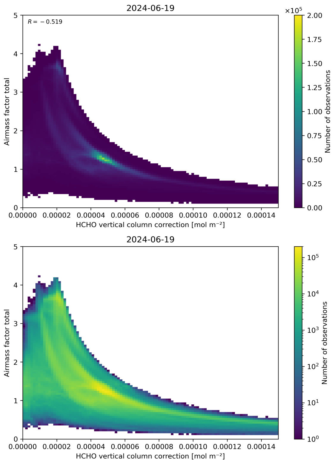
Figure 120: Scatter density plot of “HCHO vertical column correction” against “Airmass factor total” for 2024-06-19 to 2024-06-20.
