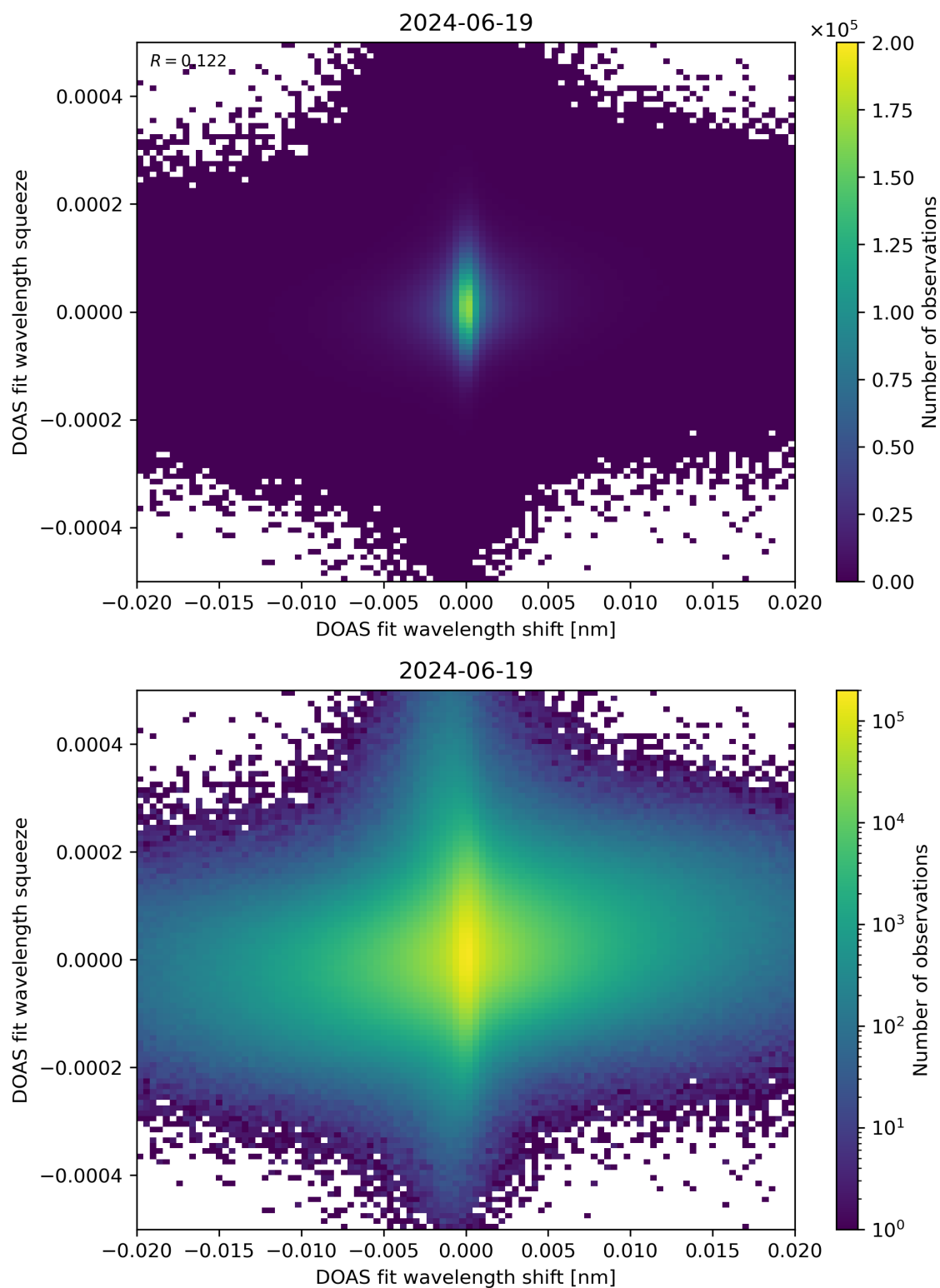
Figure 65: Scatter density plot of “DOAS fit wavelength shift” against “DOAS fit wavelength squeeze” for 2024-06-19 to 2024-06-20.
