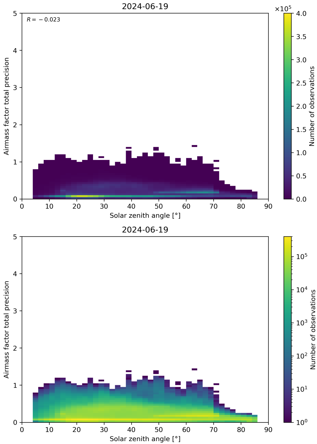
Figure 176: Scatter density plot of “Solar zenith angle” against “Airmass factor total precision” for 2024-06-19 to 2024-06-20.
