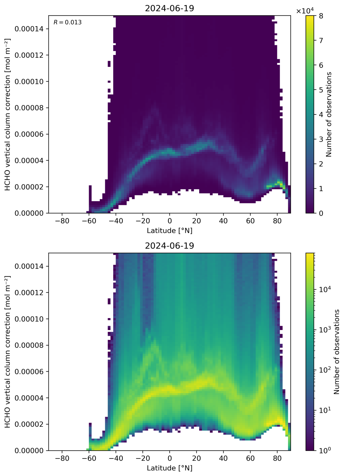
Figure 164: Scatter density plot of “Latitude” against “HCHO vertical column correction” for 2024-06-19 to 2024-06-20.
