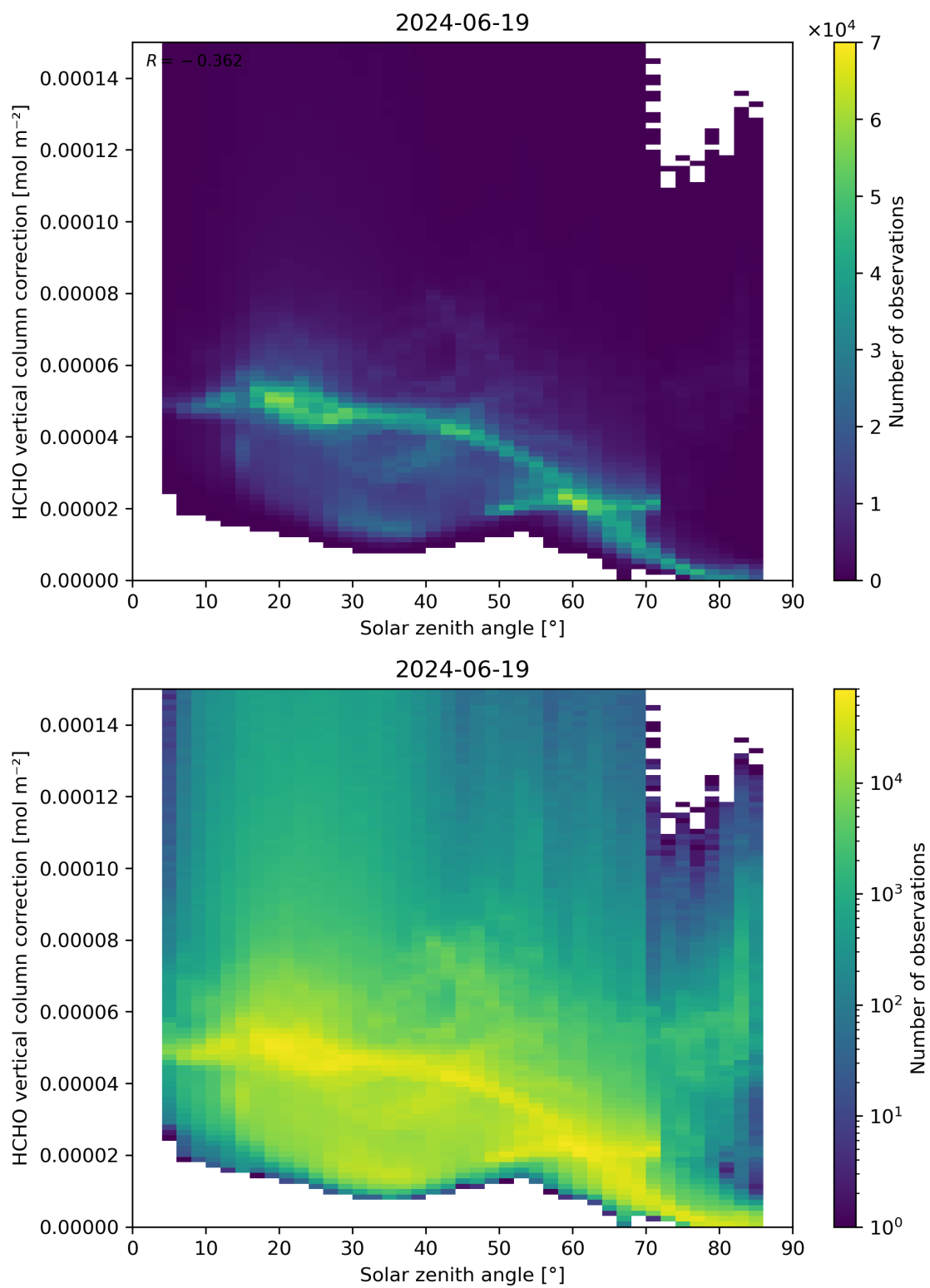
Figure 178: Scatter density plot of “Solar zenith angle” against “HCHO vertical column correction” for 2024-06-19 to 2024-06-20.
