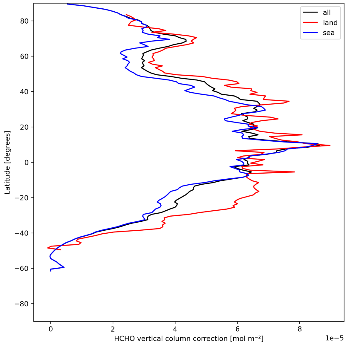
Figure 23: Zonal average of “HCHO vertical column correction” for 2024-06-19 to 2024-06-20.
