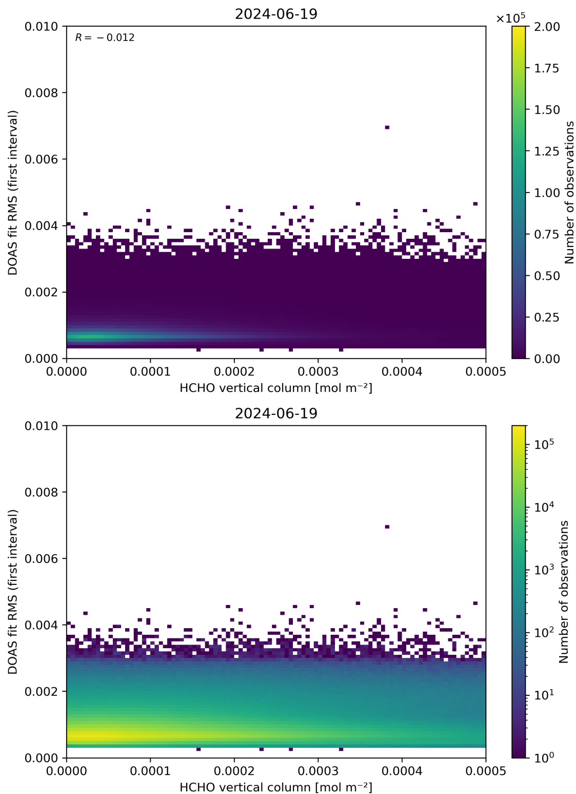
Figure 123: Scatter density plot of “HCHO vertical column” against “DOAS fit RMS (first interval)” for 2024-06-19 to 2024-06-20.
