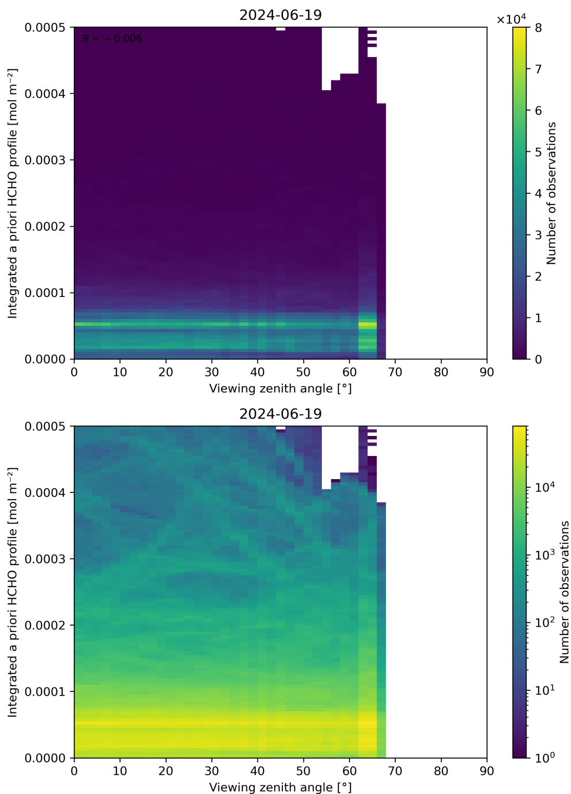
Figure 195: Scatter density plot of “Viewing zenith angle” against “Integrated a priori HCHO profile” for 2024-06-19 to 2024-06-20.
