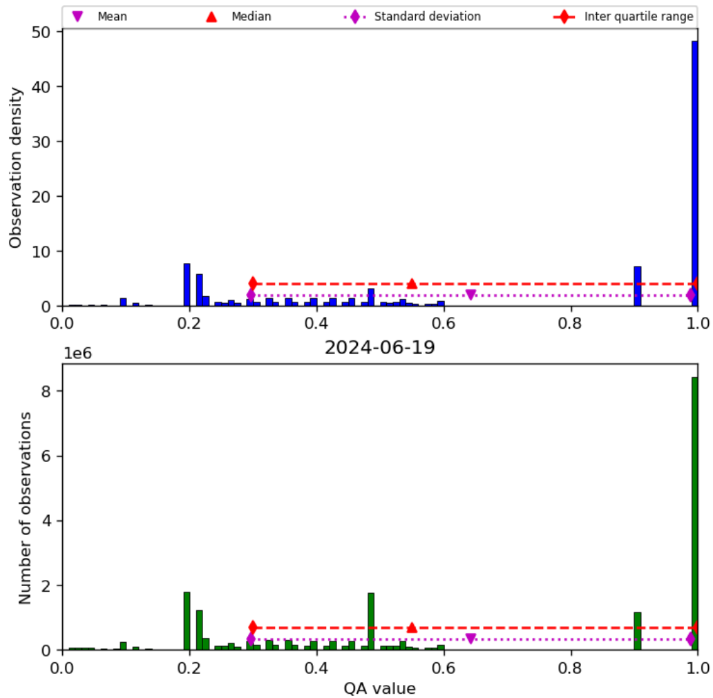
Figure 34: Histogram of “QA value” for 2024-06-19 to 2024-06-20
