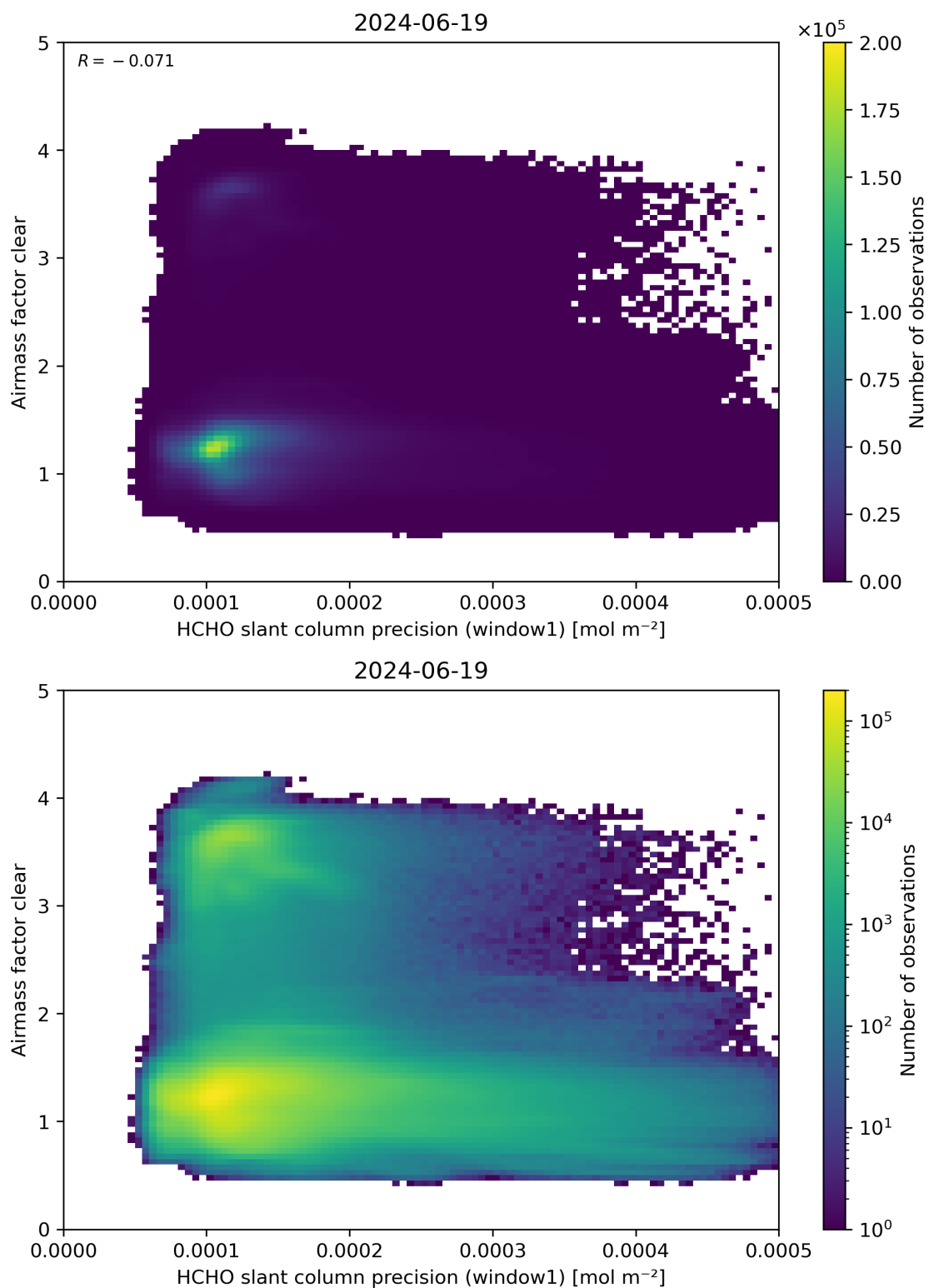
Figure 91: Scatter density plot of “HCHO slant column precision (window1)” against “Airmass factor clear” for 2024-06-19 to 2024-06-20.
