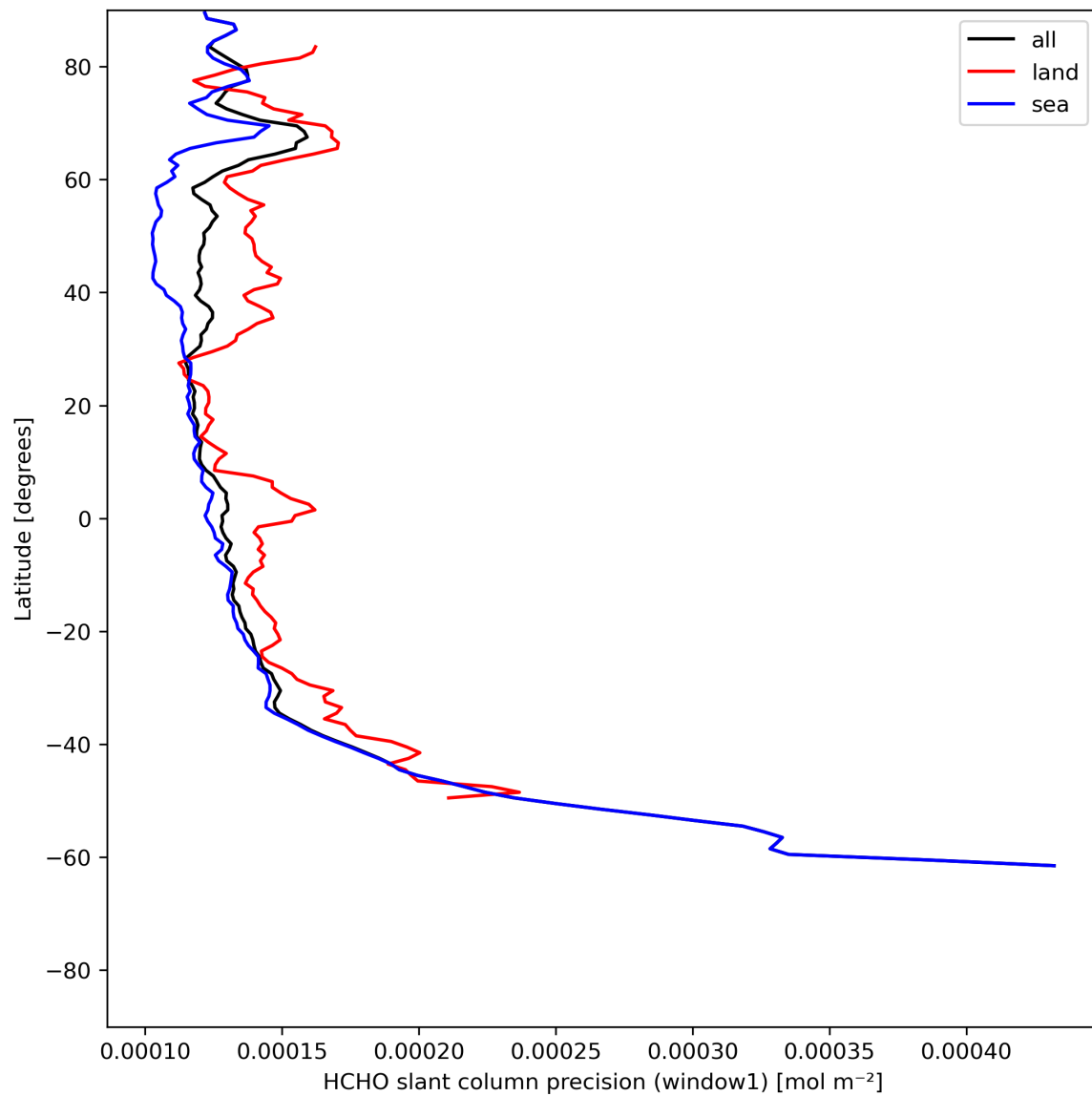
Figure 25: Zonal average of “HCHO slant column precision (window1)” for 2024-06-19 to 2024-06-20.
