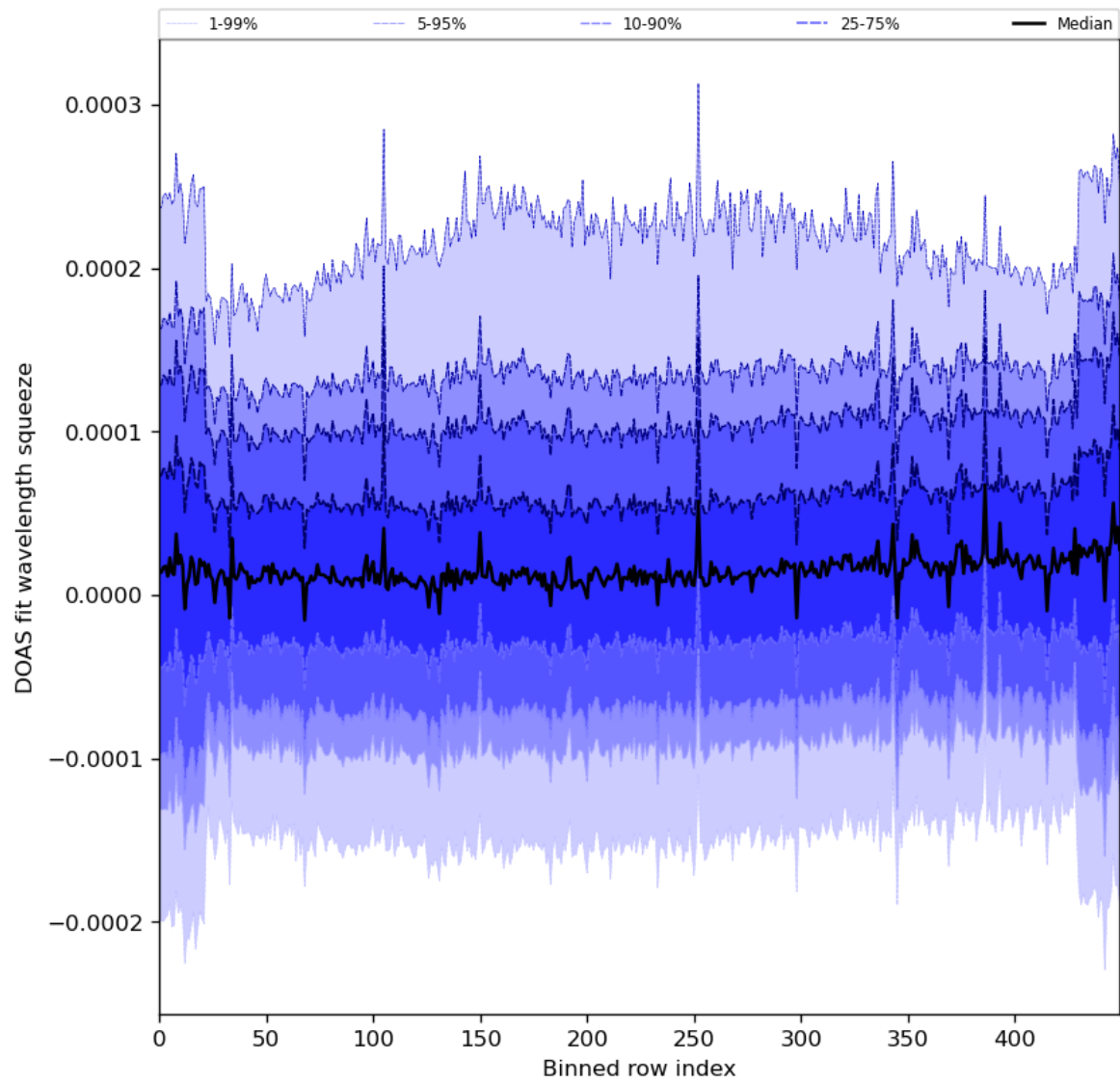
Figure 59: Along track statistics of “DOAS fit wavelength squeeze” for 2024-06-19 to 2024-06-20
