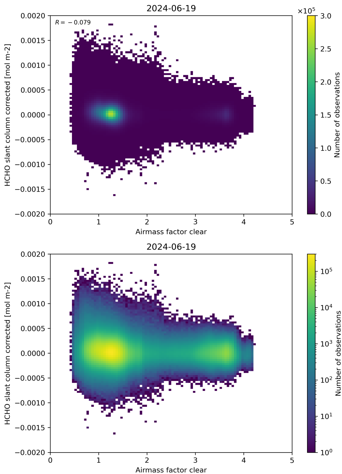
Figure 74: Scatter density plot of “Airmass factor clear” against “HCHO slant column corrected” for 2024-06-19 to 2024-06-20.
