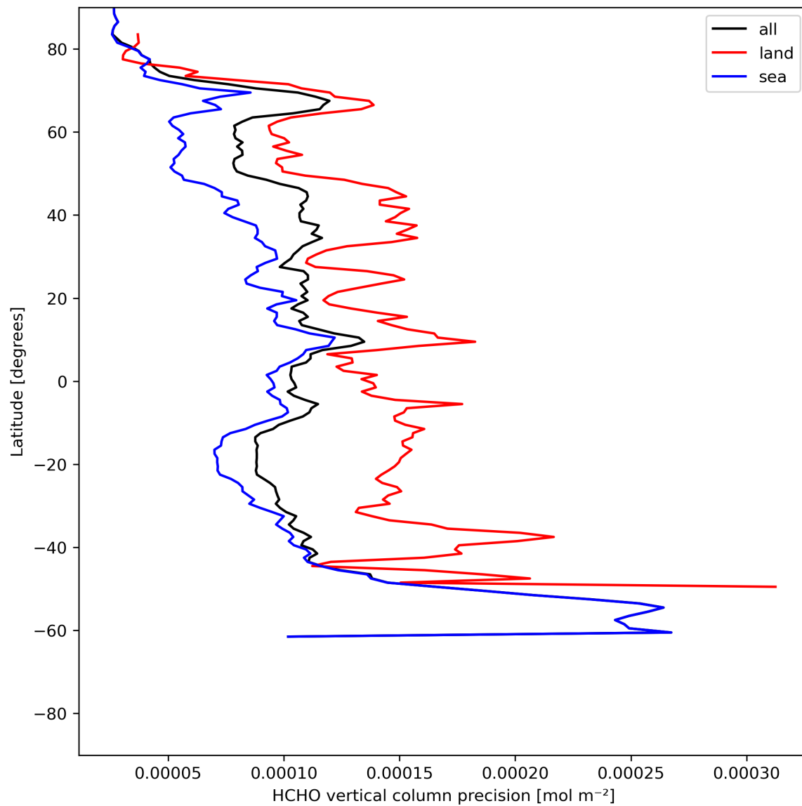
Figure 22: Zonal average of “HCHO vertical column precision” for 2024-06-19 to 2024-06-20.
