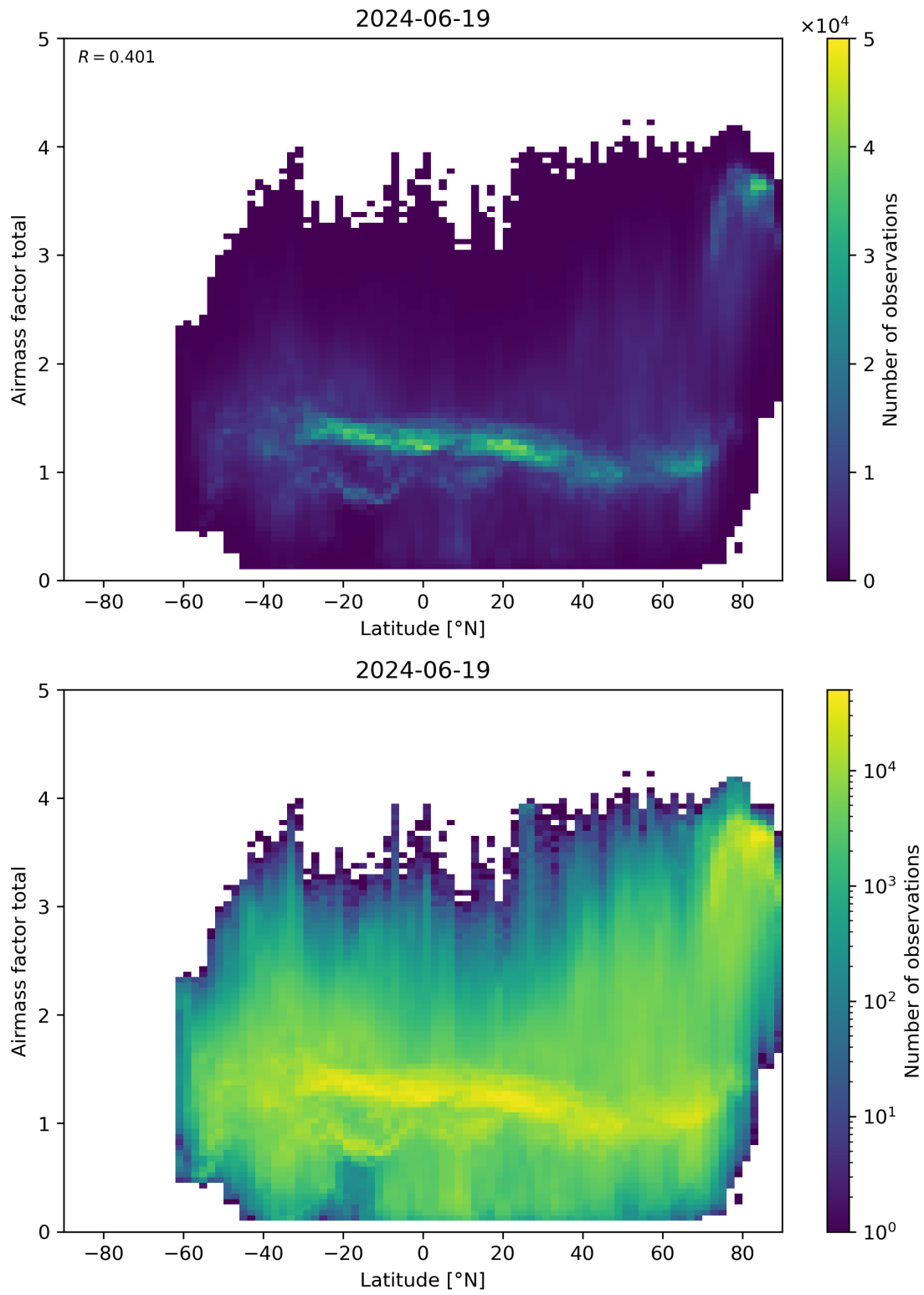
Figure 161: Scatter density plot of “Latitude” against “Airmass factor total” for 2024-06-19 to 2024-06-20.
