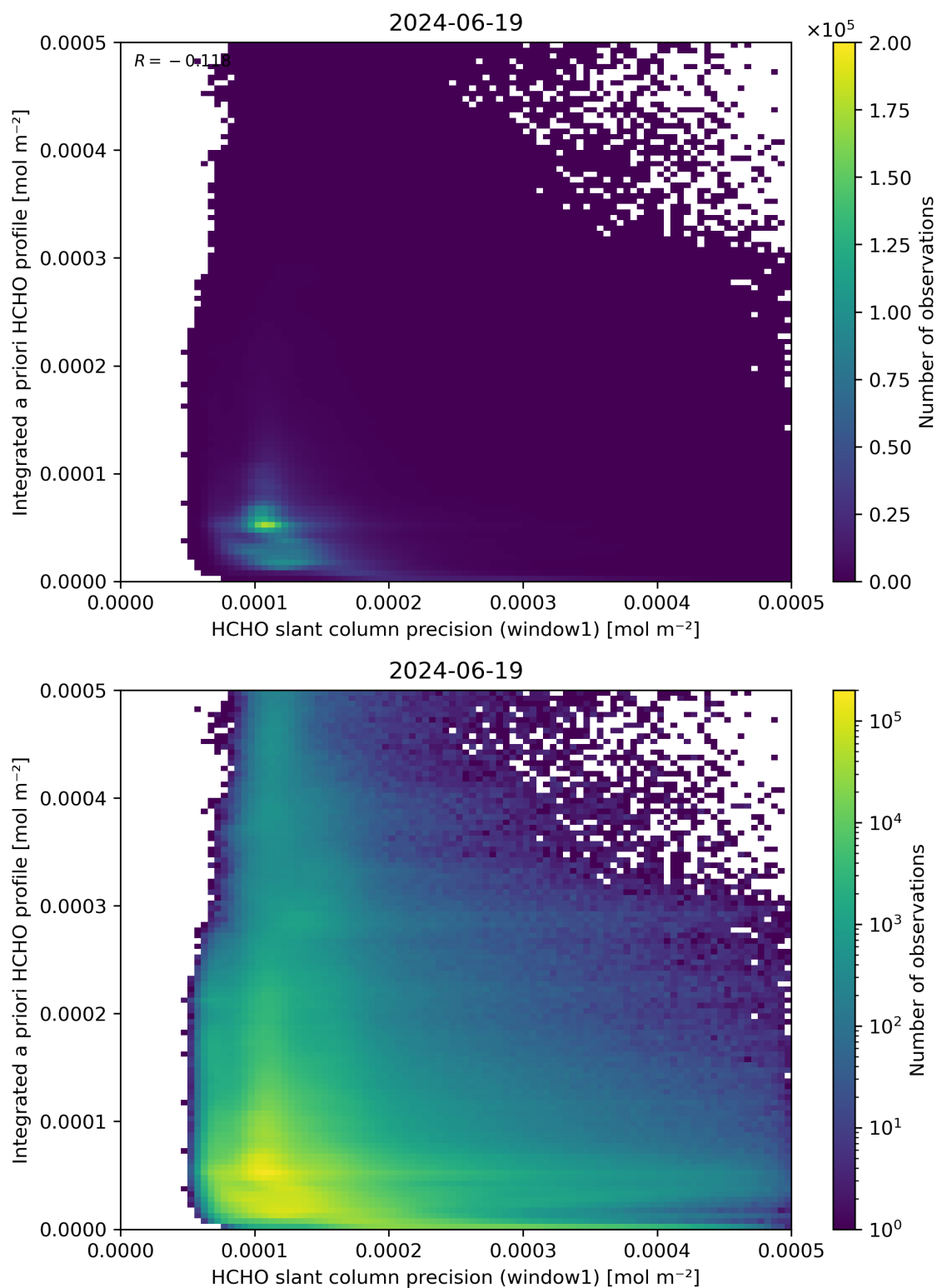
Figure 96: Scatter density plot of “HCHO slant column precision (window1)” against “Integrated a priori HCHO profile” for 2024-06-19 to 2024-06-20.
