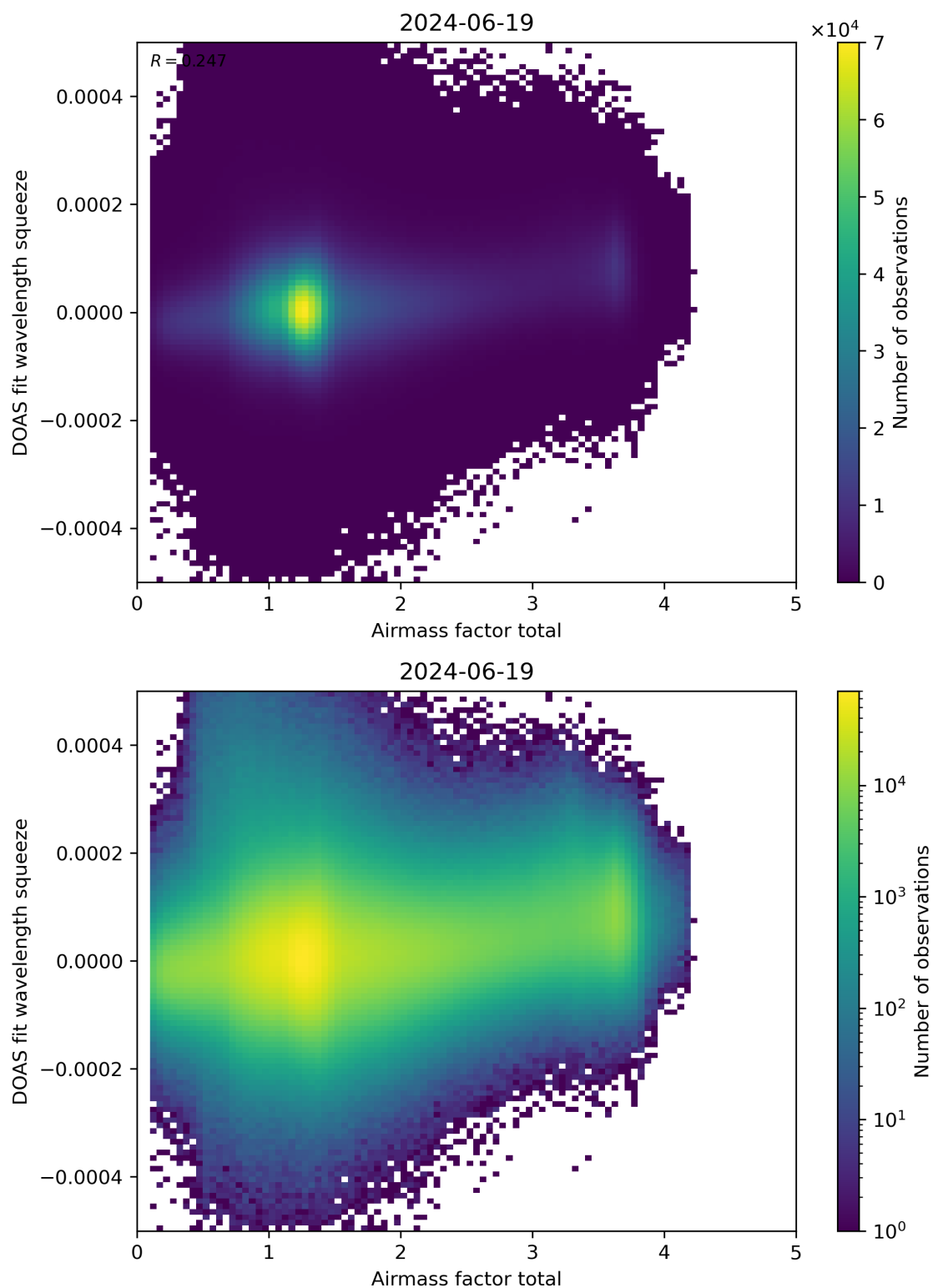
Figure 99: Scatter density plot of “Airmass factor total” against “DOAS fit wavelength squeeze” for 2024-06-19 to 2024-06-20.
