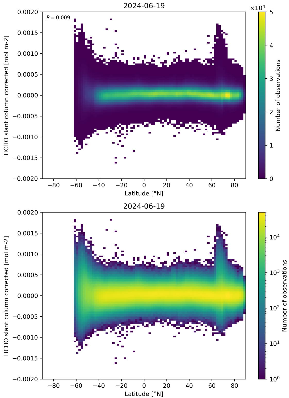
Figure 157: Scatter density plot of “Latitude” against “HCHO slant column corrected” for 2024-06-19 to 2024-06-20.
