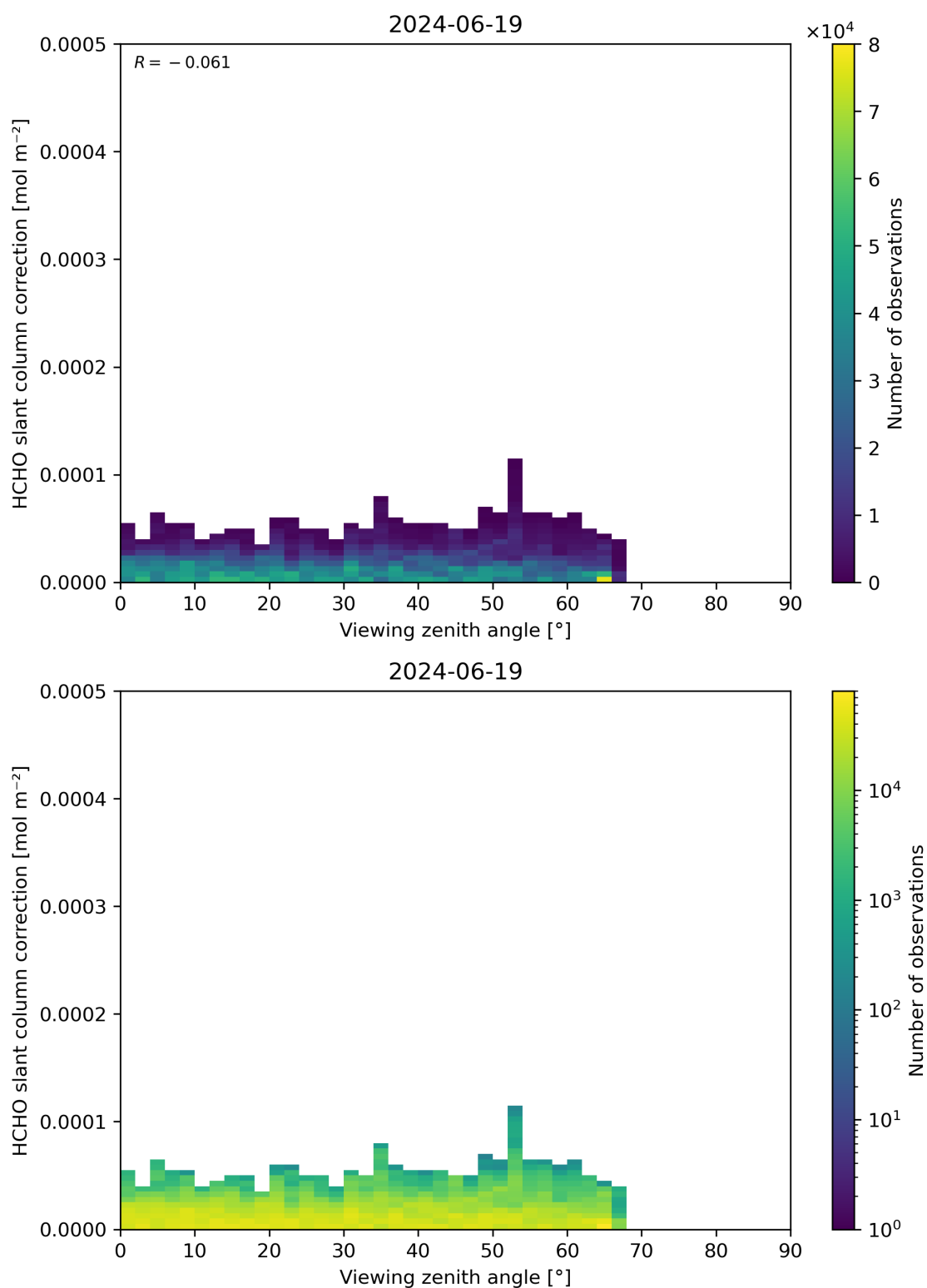
Figure 187: Scatter density plot of “Viewing zenith angle” against “HCHO slant column correction” for 2024-06-19 to 2024-06-20.
