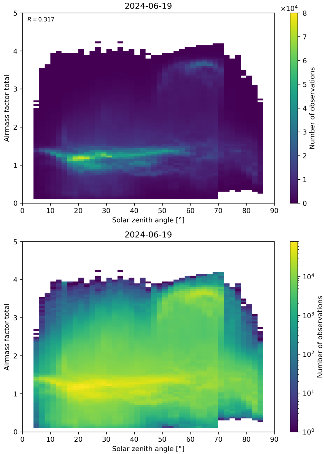
Figure 175: Scatter density plot of “Solar zenith angle” against “Airmass factor total” for 2024-06-19 to 2024-06-20.
