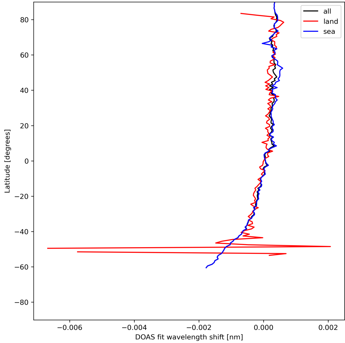
Figure 30: Zonal average of “DOAS fit wavelength shift” for 2024-06-19 to 2024-06-21.
