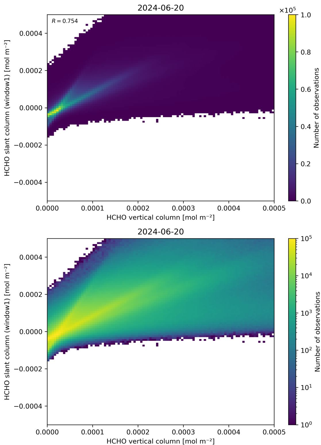
Figure 129: Scatter density plot of “HCHO vertical column” against “HCHO slant column (window1)” for 2024-06-19 to 2024-06-21.
