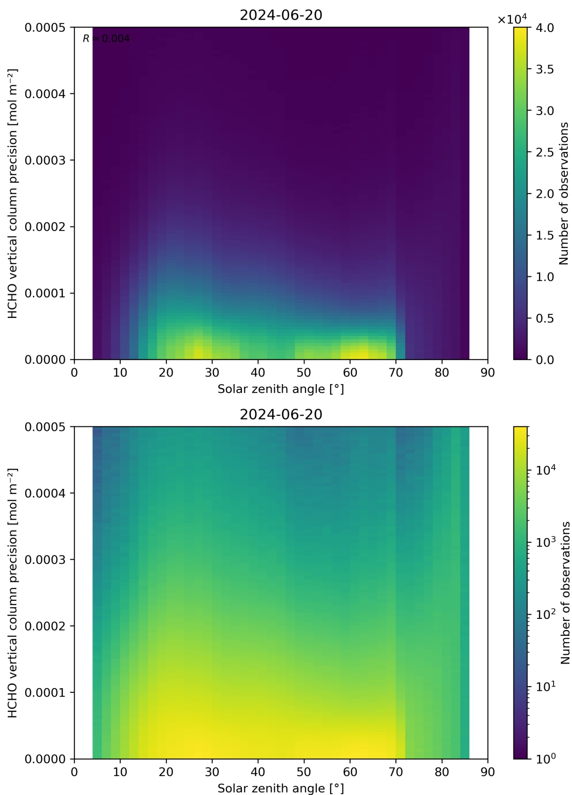
Figure 179: Scatter density plot of “Solar zenith angle” against “HCHO vertical column precision” for 2024-06-19 to 2024-06-21.
