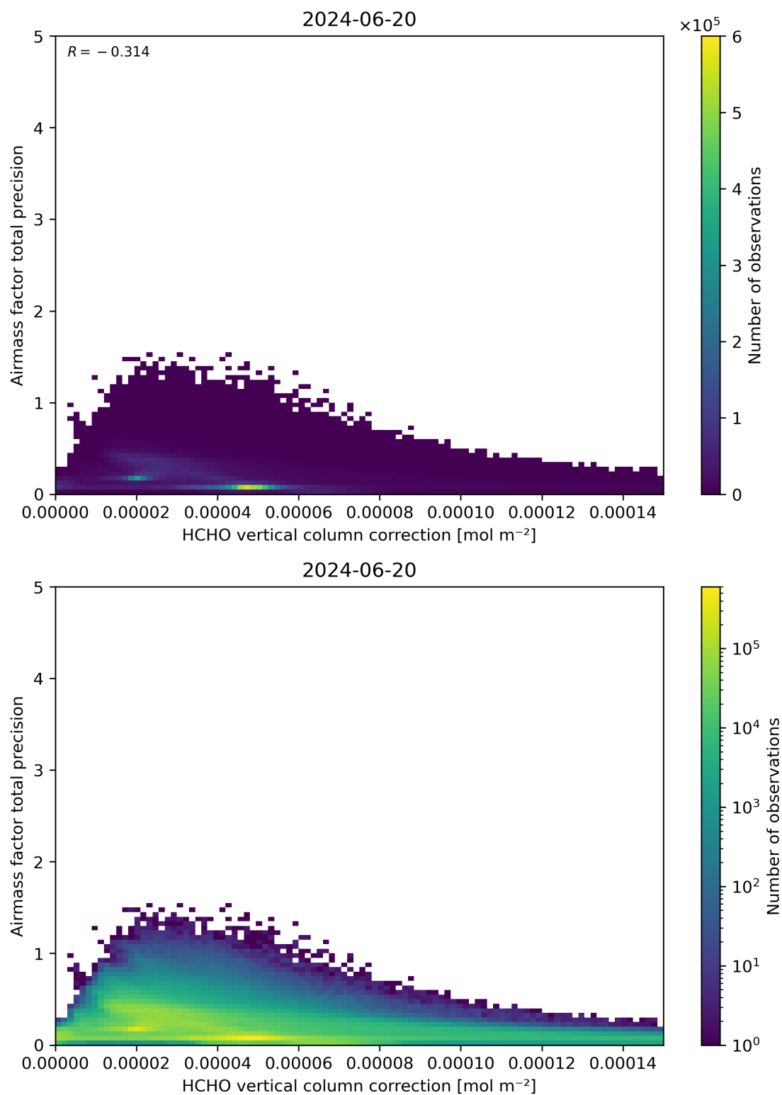
Figure 121: Scatter density plot of “HCHO vertical column correction” against “Airmass factor total precision” for 2024-06-19 to 2024-06-21.
