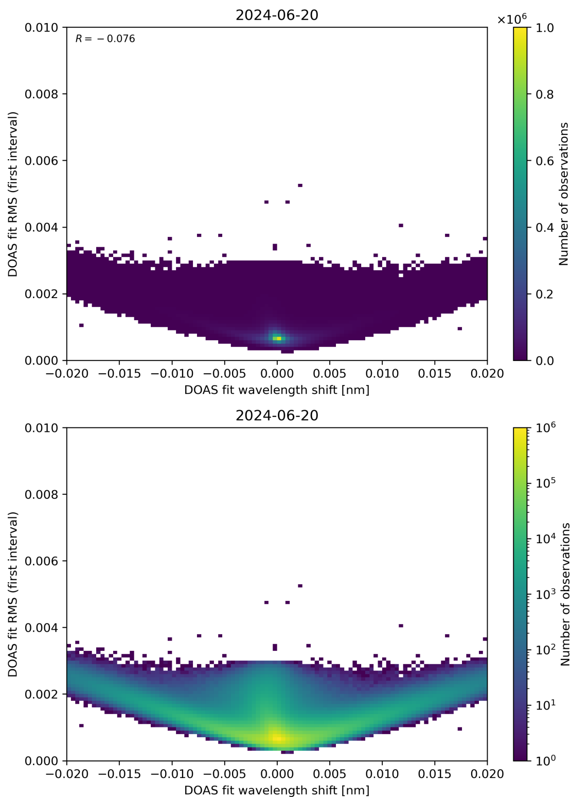
Figure 64: Scatter density plot of “DOAS fit wavelength shift” against “DOAS fit RMS (first interval)” for 2024-06-19 to 2024-06-21.
