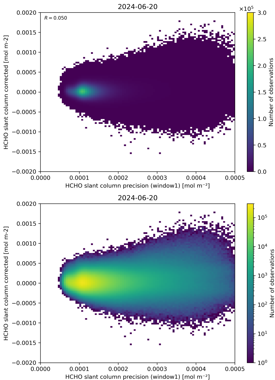
Figure 92: Scatter density plot of “HCHO slant column precision (window1)” against “HCHO slant column corrected” for 2024-06-19 to 2024-06-21.
