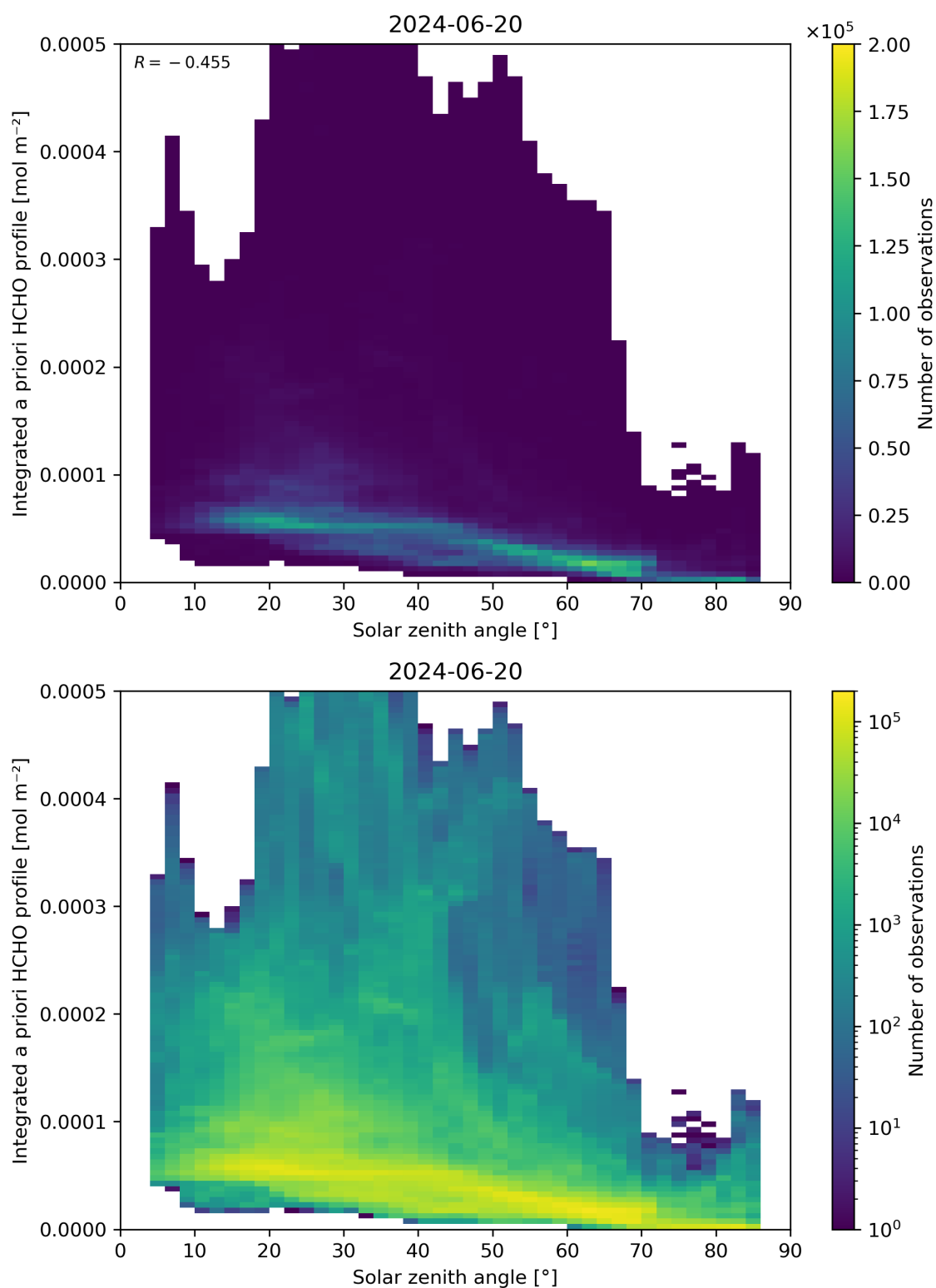
Figure 180: Scatter density plot of “Solar zenith angle” against “Integrated a priori HCHO profile” for 2024-06-19 to 2024-06-21.
