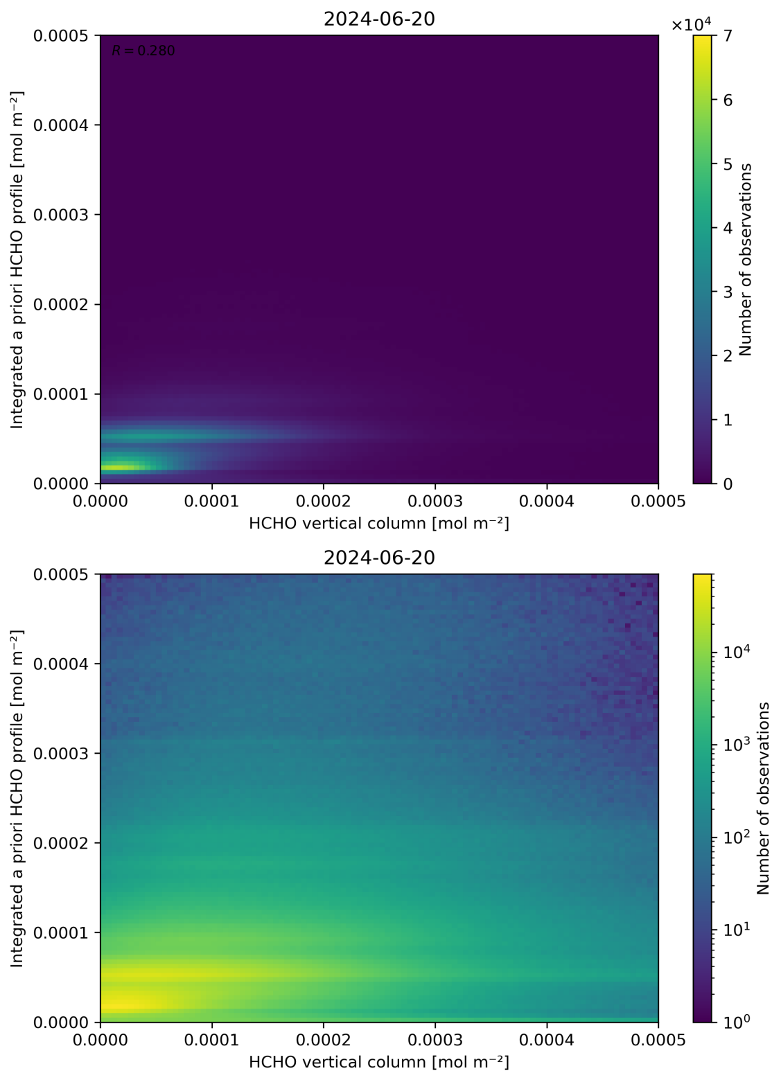
Figure 135: Scatter density plot of “HCHO vertical column” against “Integrated a priori HCHO profile” for 2024-06-19 to 2024-06-21.
