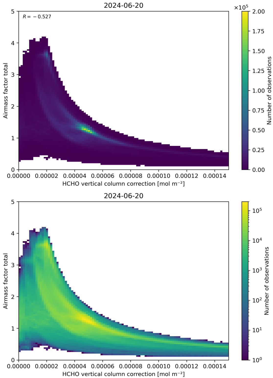
Figure 120: Scatter density plot of “HCHO vertical column correction” against “Airmass factor total” for 2024-06-19 to 2024-06-21.
