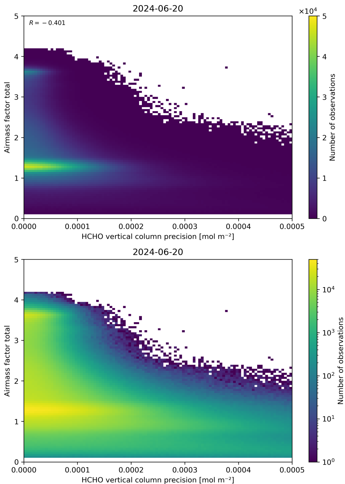
Figure 144: Scatter density plot of “HCHO vertical column precision” against “Airmass factor total” for 2024-06-19 to 2024-06-21.
