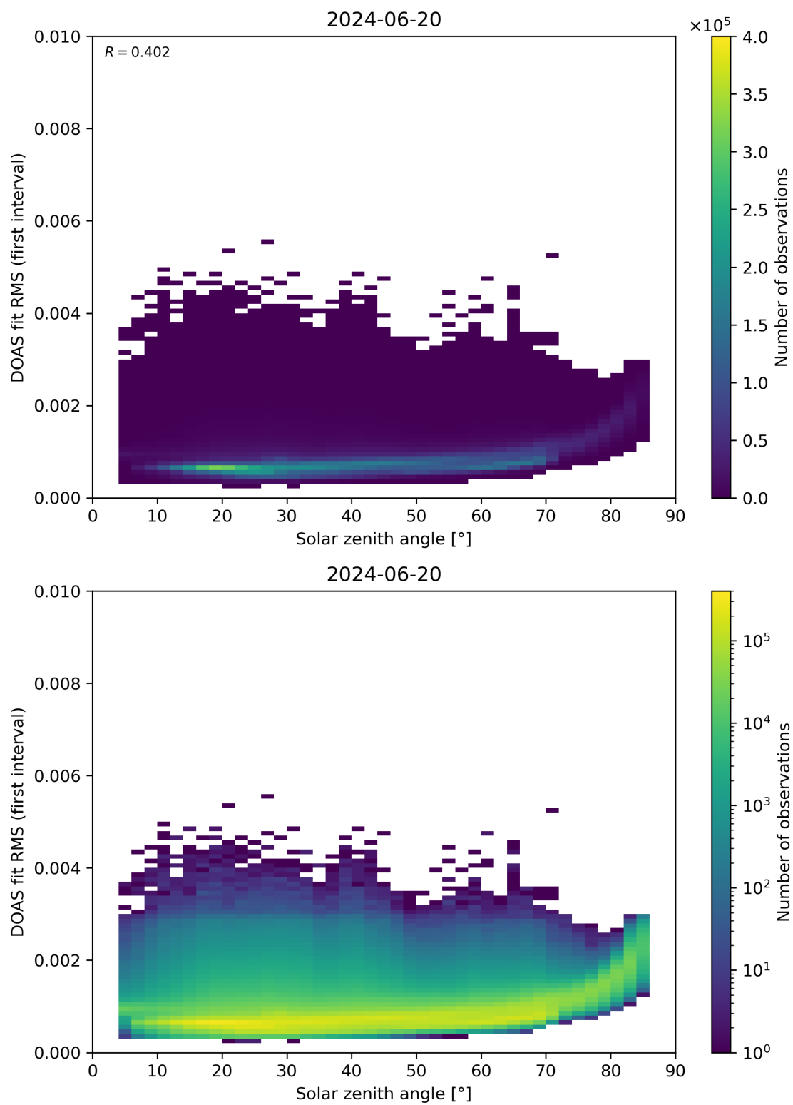
Figure 167: Scatter density plot of “Solar zenith angle” against “DOAS fit RMS (first interval)” for 2024-06-19 to 2024-06-21.
