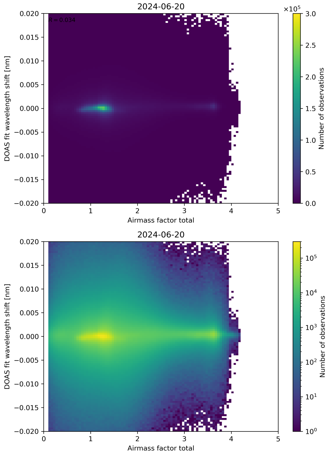
Figure 98: Scatter density plot of “Airmass factor total” against “DOAS fit wavelength shift” for 2024-06-19 to 2024-06-21.
