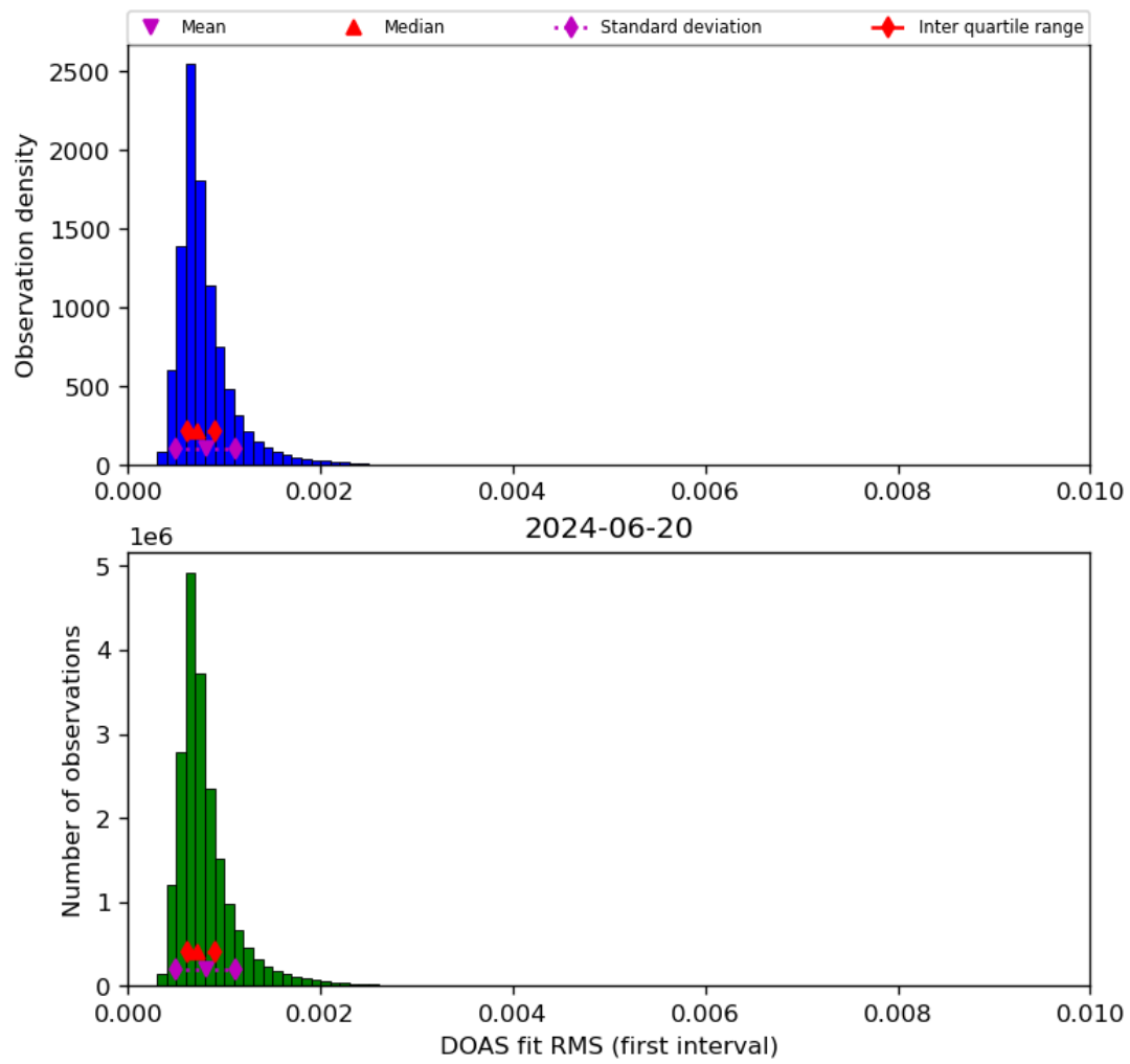
Figure 46: Histogram of “DOAS fit RMS (first interval)” for 2024-06-19 to 2024-06-21
