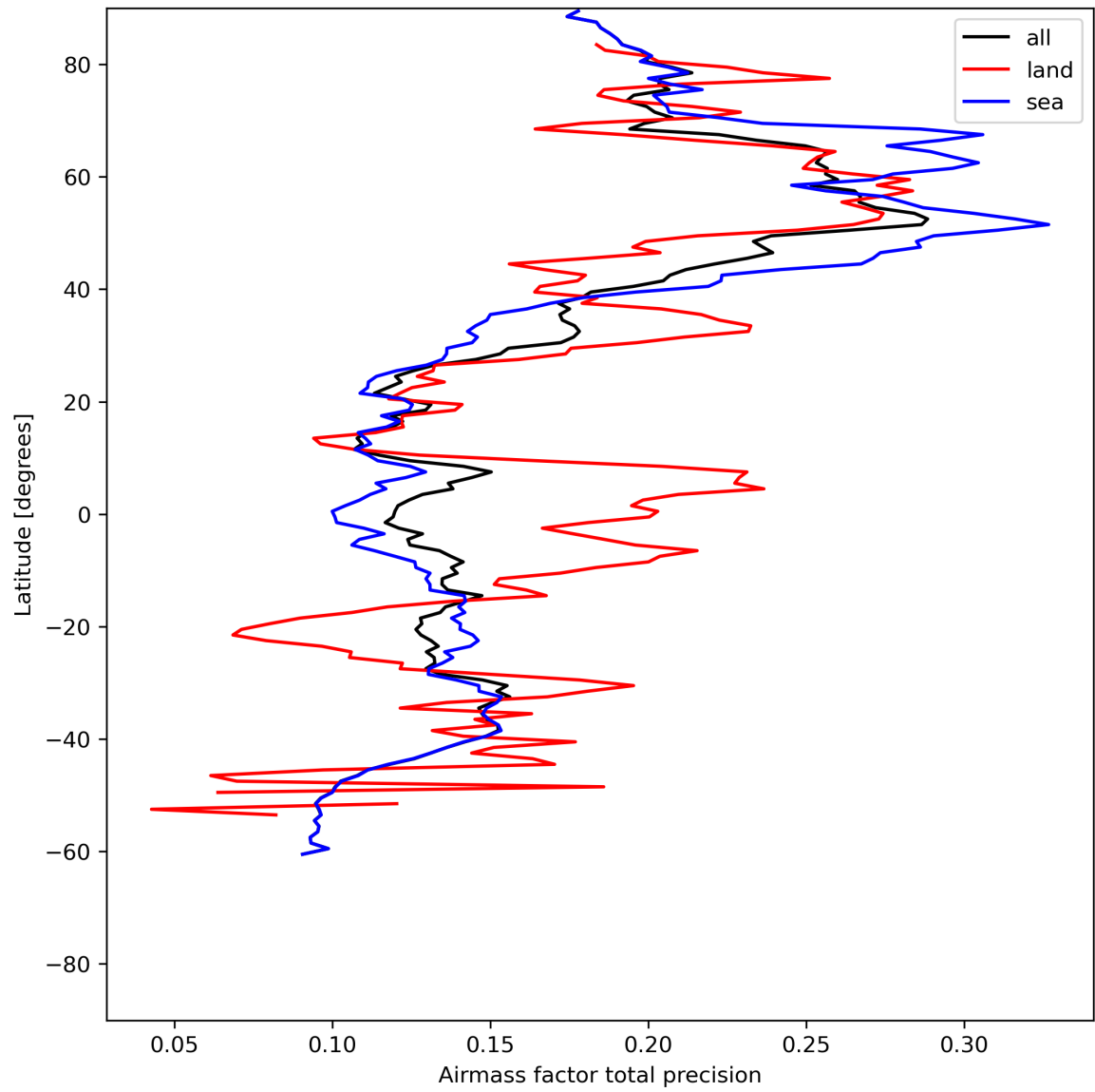
Figure 27: Zonal average of “Airmass factor total precision” for 2024-06-19 to 2024-06-21.
