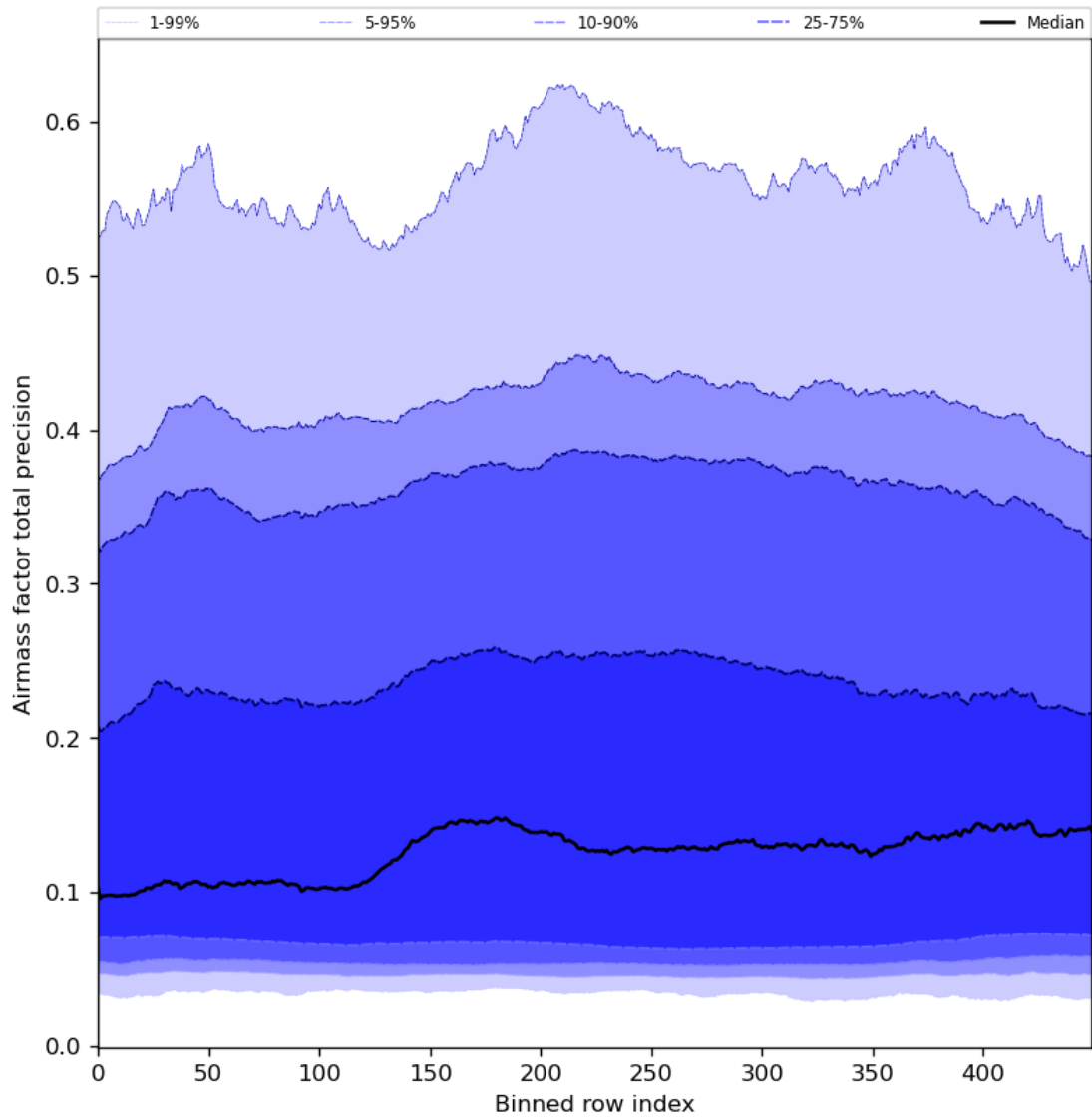
Figure 55: Along track statistics of “Airmass factor total precision” for 2024-06-19 to 2024-06-21
