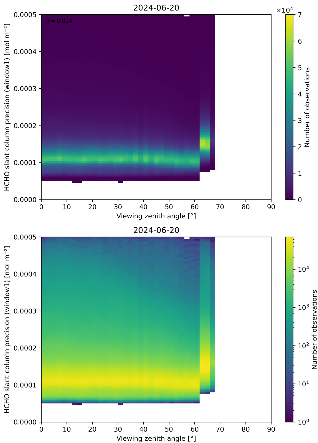
Figure 189: Scatter density plot of “Viewing zenith angle” against “HCHO slant column precision (window1)” for 2024-06-19 to 2024-06-21.
