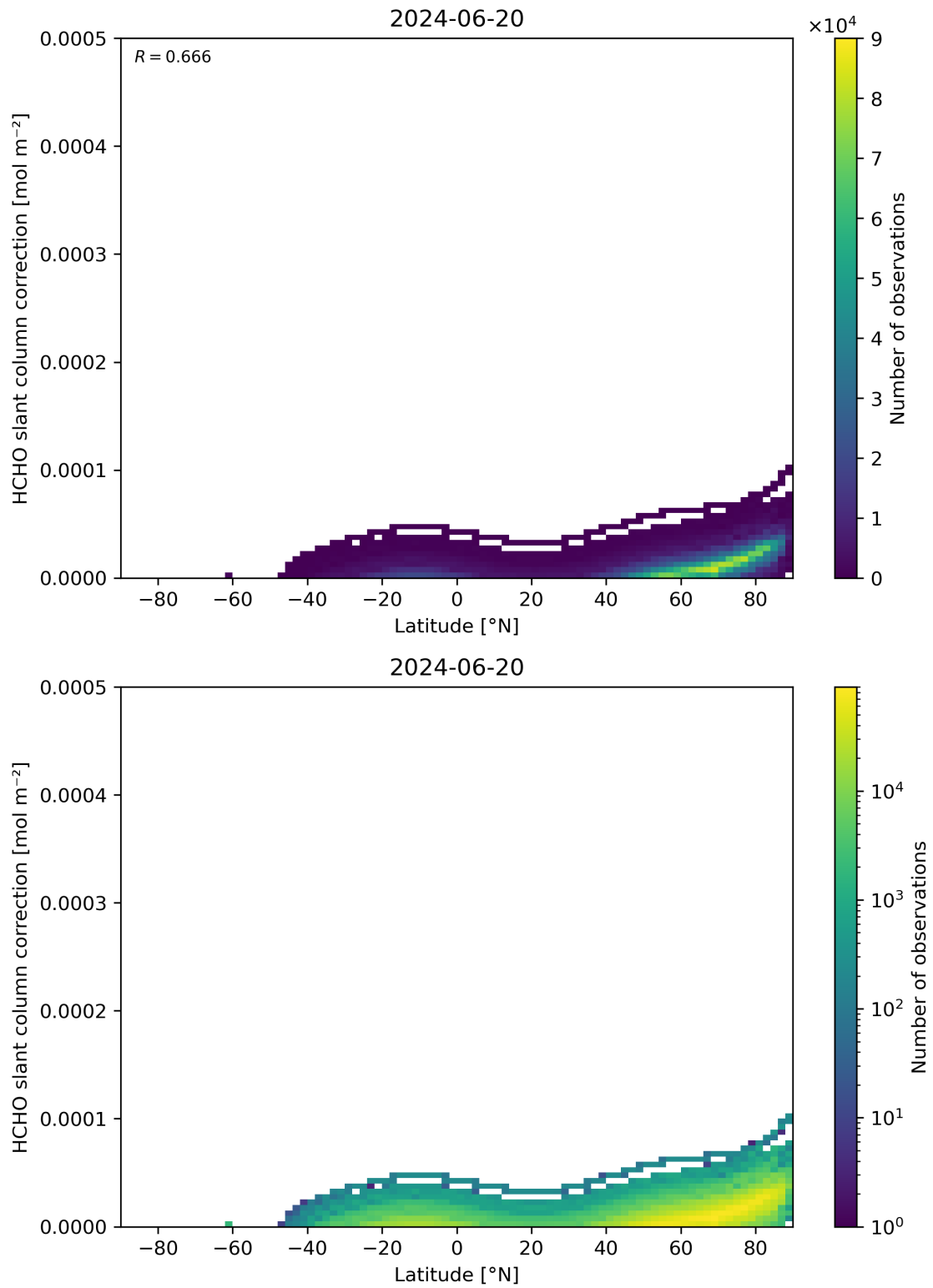
Figure 158: Scatter density plot of “Latitude” against “HCHO slant column correction” for 2024-06-19 to 2024-06-21.
