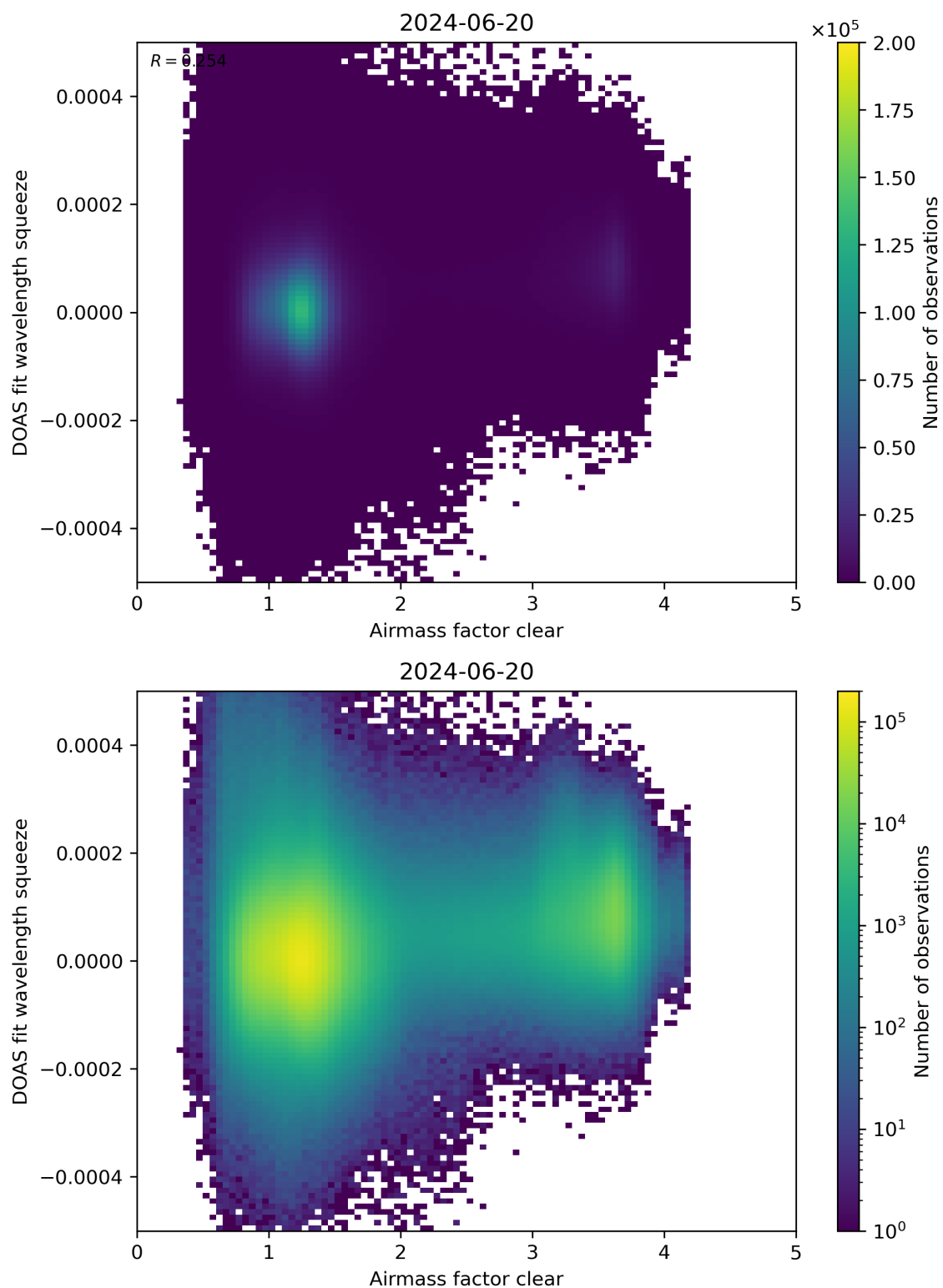
Figure 73: Scatter density plot of “Airmass factor clear” against “DOAS fit wavelength squeeze” for 2024-06-19 to 2024-06-21.
