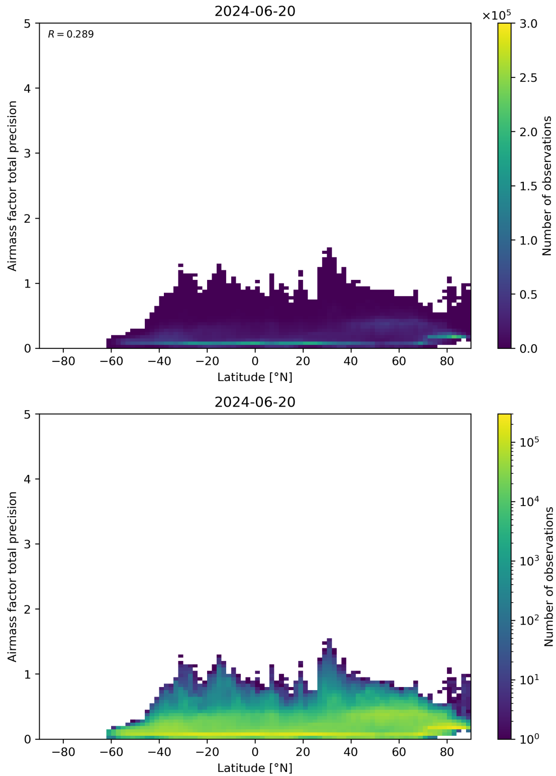
Figure 162: Scatter density plot of “Latitude” against “Airmass factor total precision” for 2024-06-19 to 2024-06-21.
