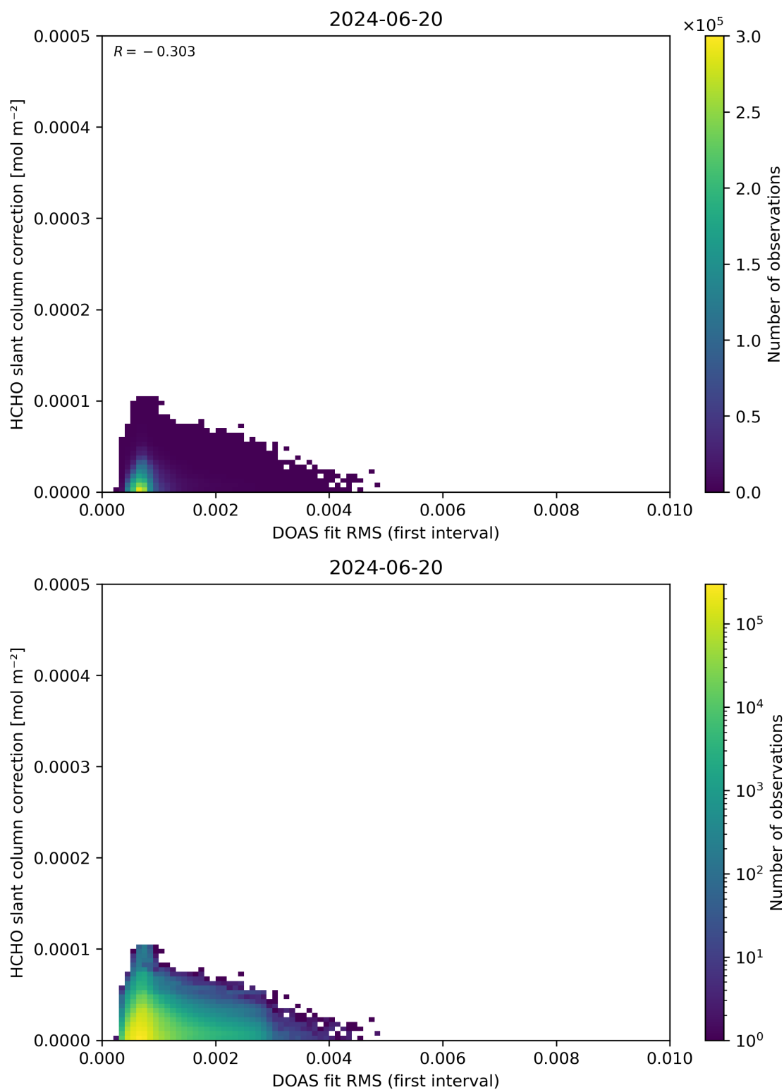
Figure 63: Scatter density plot of “DOAS fit RMS (first interval)” against “HCHO slant column correction” for 2024-06-19 to 2024-06-21.
