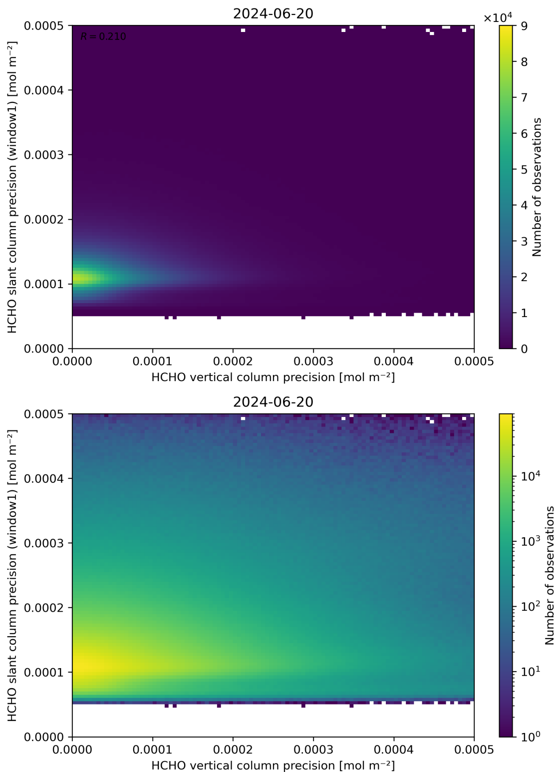
Figure 143: Scatter density plot of “HCHO vertical column precision” against “HCHO slant column precision (window1)” for 2024-06-19 to 2024-06-21.
