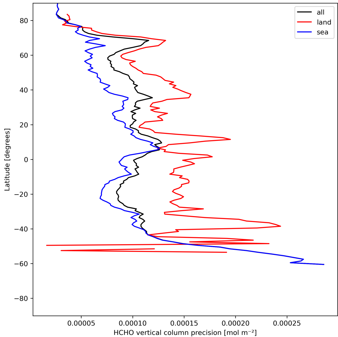
Figure 22: Zonal average of “HCHO vertical column precision” for 2024-06-19 to 2024-06-21.
