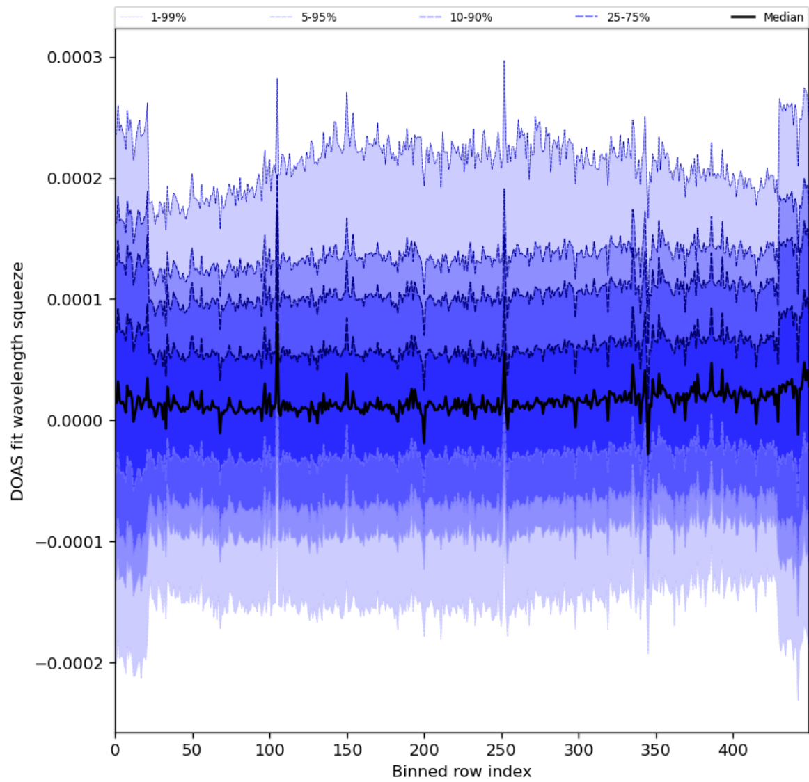
Figure 59: Along track statistics of “DOAS fit wavelength squeeze” for 2024-06-19 to 2024-06-21
