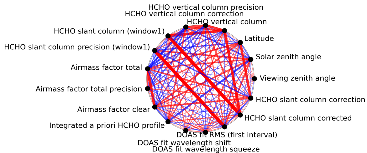
Figure 1: Map of correlation graph for 2024-06-19 to 2024-06-21.
