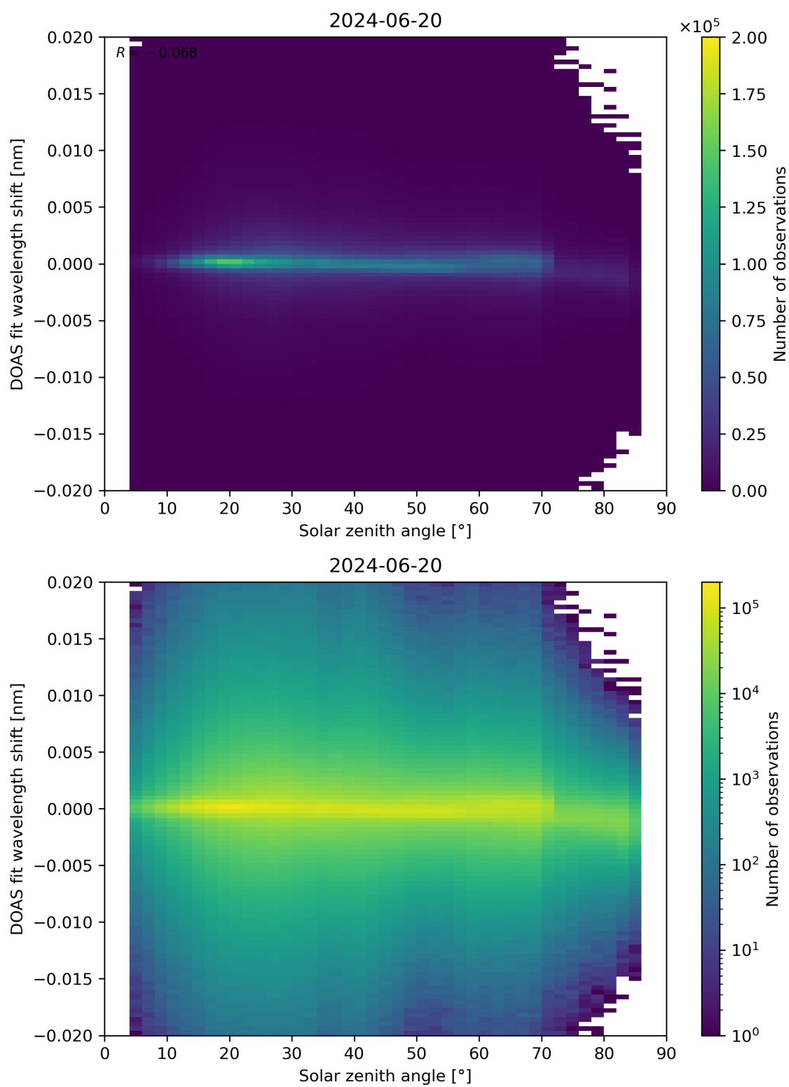
Figure 168: Scatter density plot of “Solar zenith angle” against “DOAS fit wavelength shift” for 2024-06-19 to 2024-06-21.
