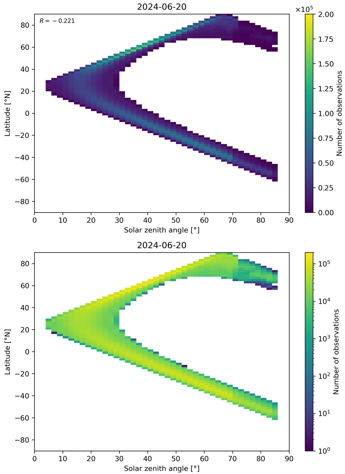
Figure 181: Scatter density plot of “Solar zenith angle” against “Latitude” for 2024-06-19 to 2024-06-21.
