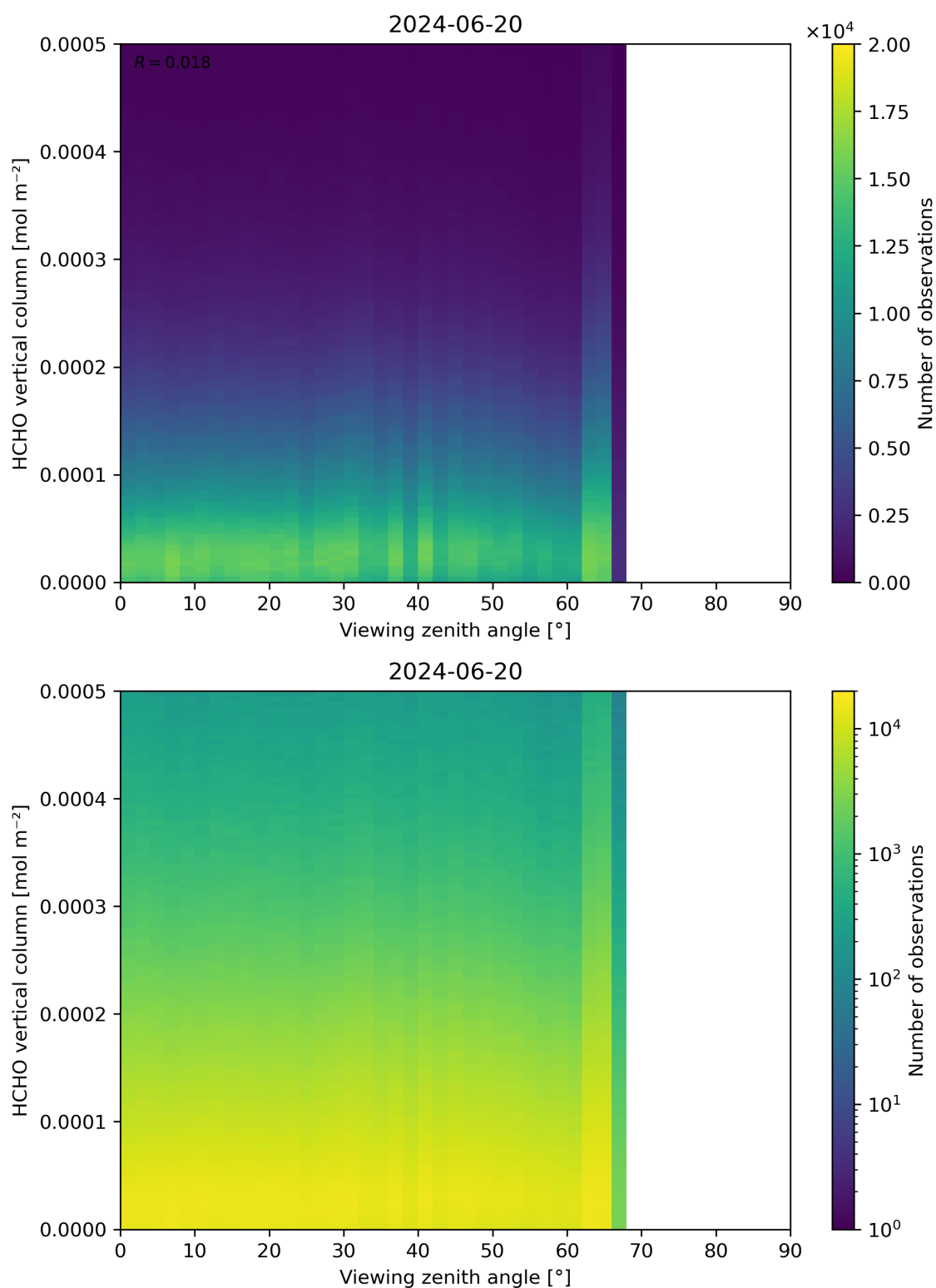
Figure 192: Scatter density plot of “Viewing zenith angle” against “HCHO vertical column” for 2024-06-19 to 2024-06-21.
