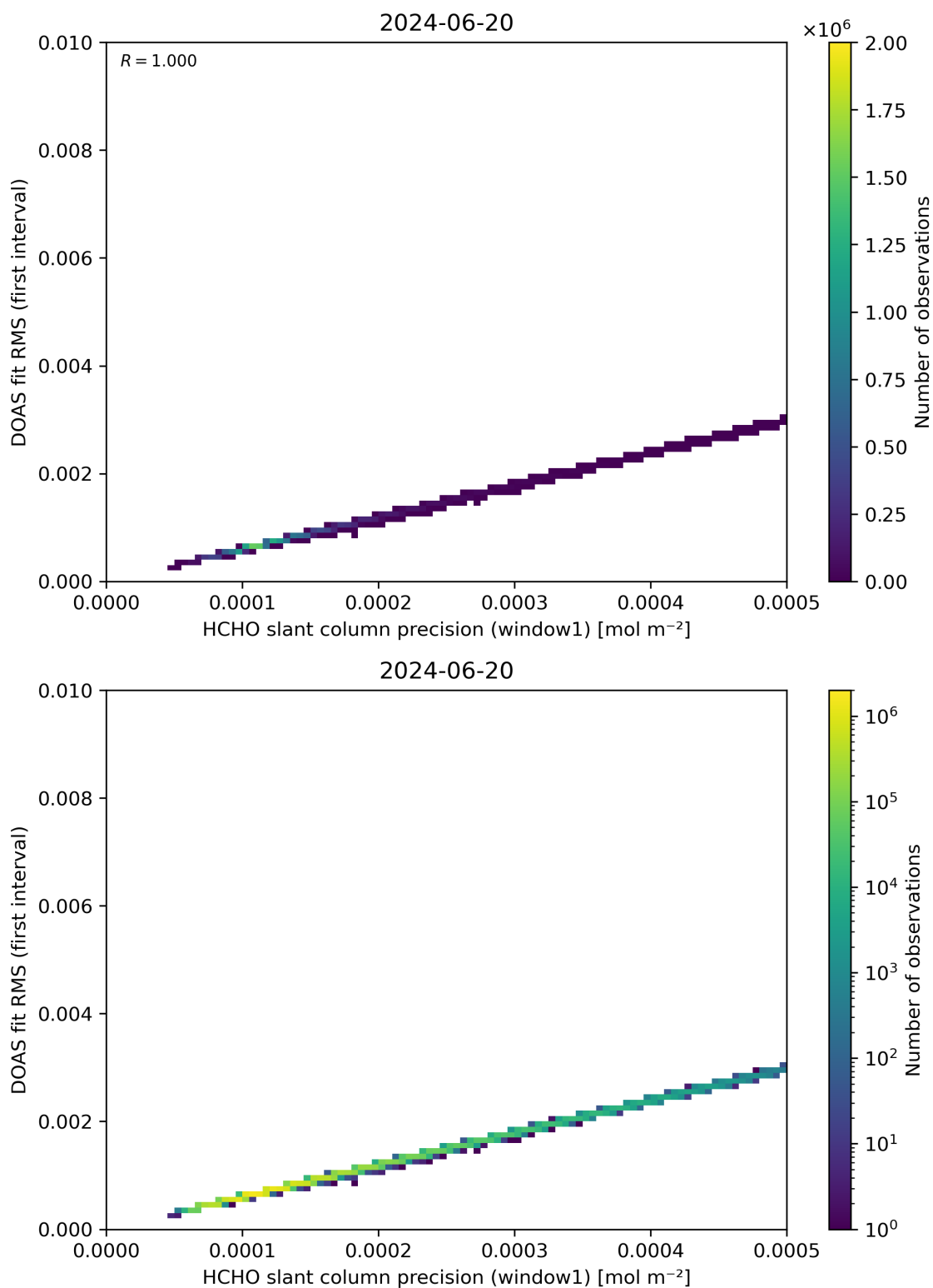
Figure 88: Scatter density plot of “HCHO slant column precision (window1)” against “DOAS fit RMS (first interval)” for 2024-06-19 to 2024-06-21.
