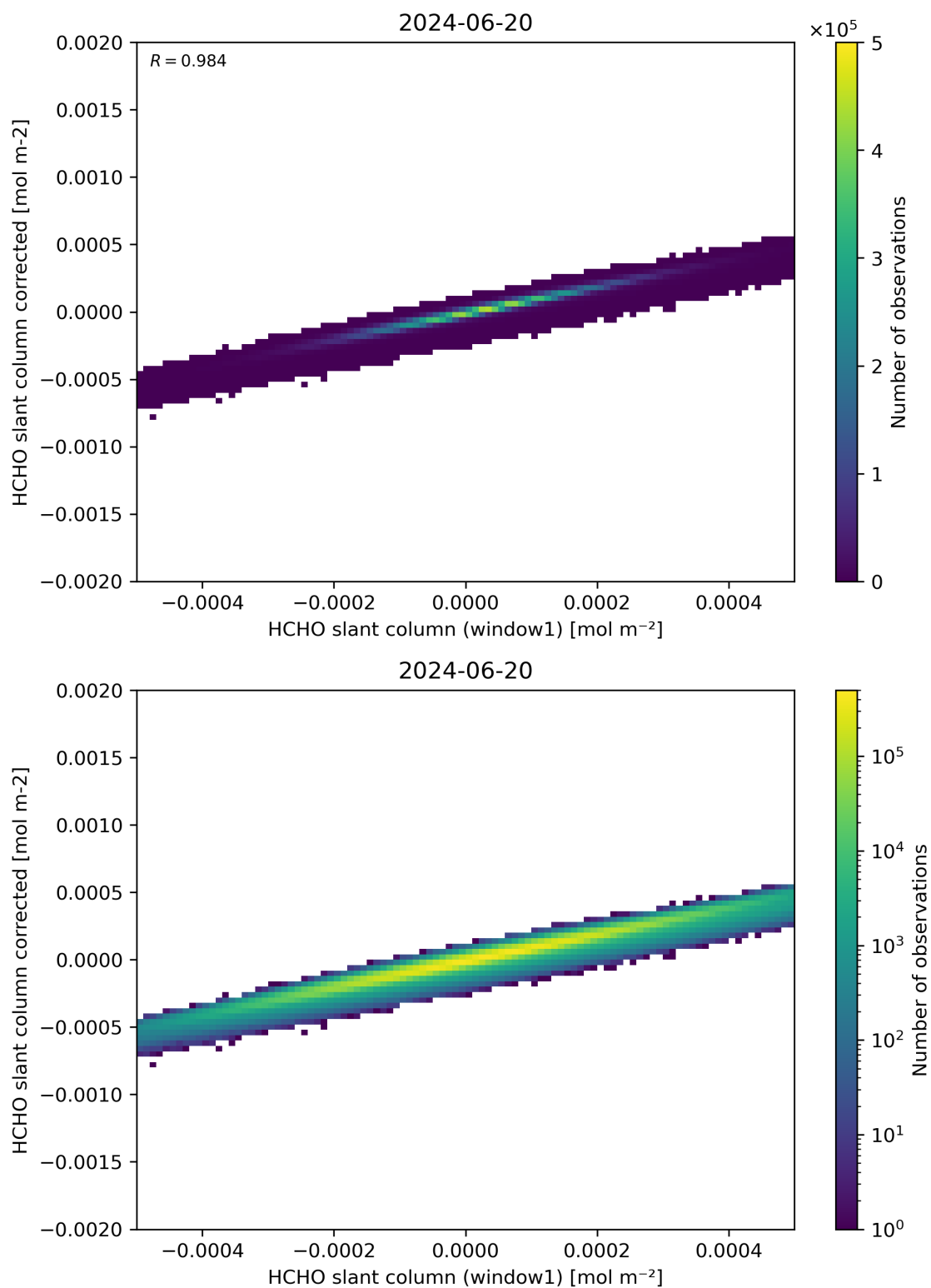
Figure 82: Scatter density plot of “HCHO slant column (window1)” against “HCHO slant column corrected” for 2024-06-19 to 2024-06-21.
