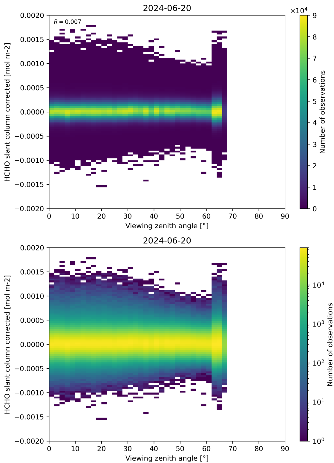
Figure 186: Scatter density plot of “Viewing zenith angle” against “HCHO slant column corrected” for 2024-06-19 to 2024-06-21.
