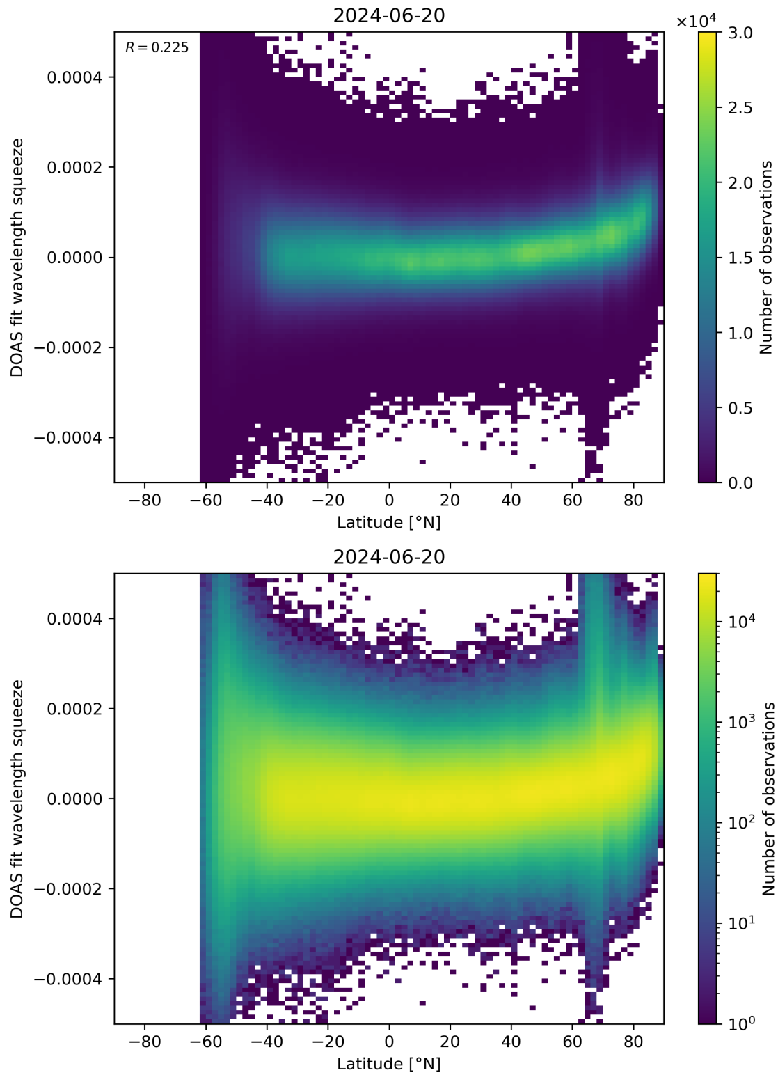
Figure 155: Scatter density plot of “Latitude” against “DOAS fit wavelength squeeze” for 2024-06-19 to 2024-06-21.
