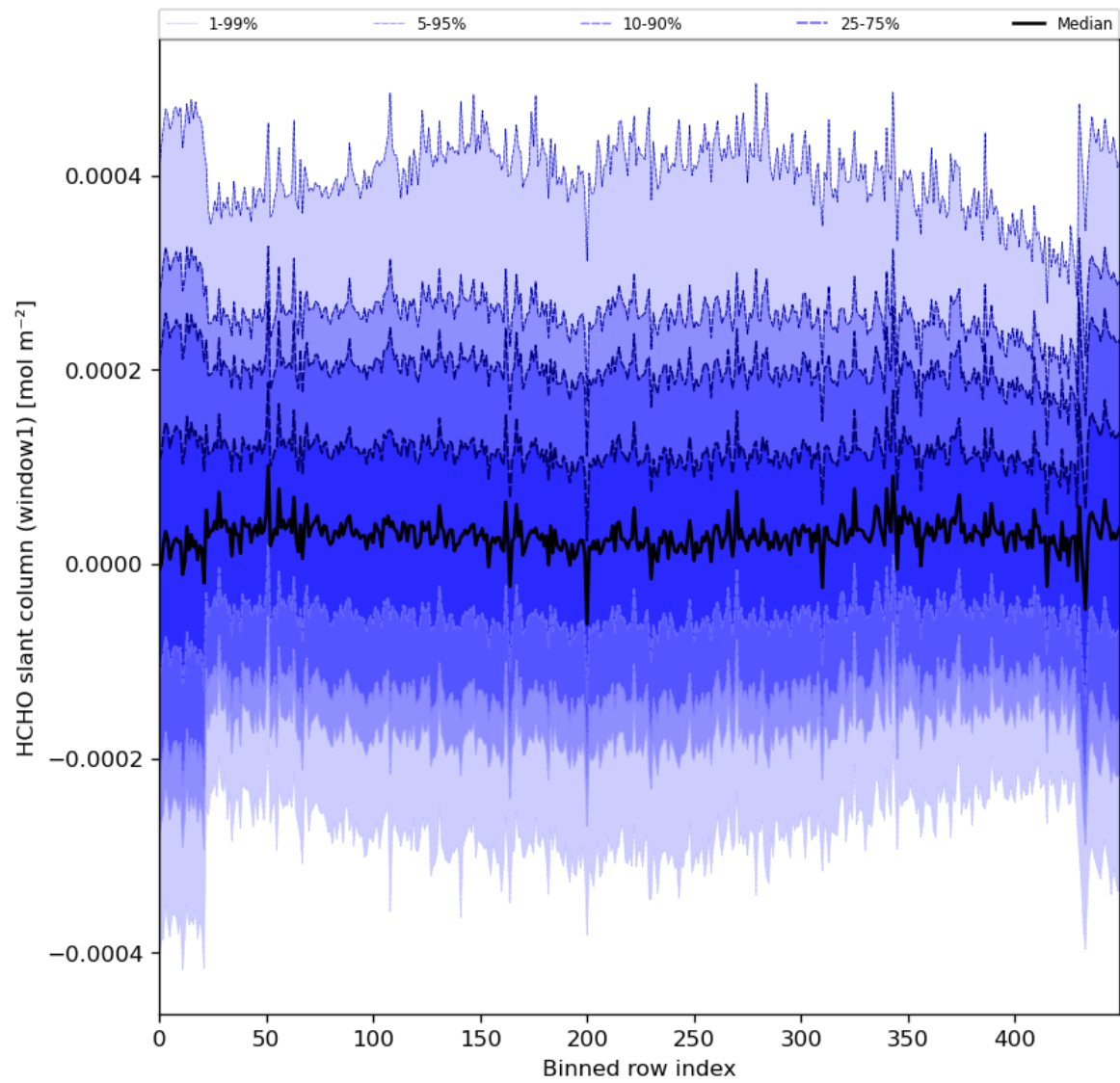
Figure 52: Along track statistics of “HCHO slant column (window1)” for 2024-06-19 to 2024-06-21
