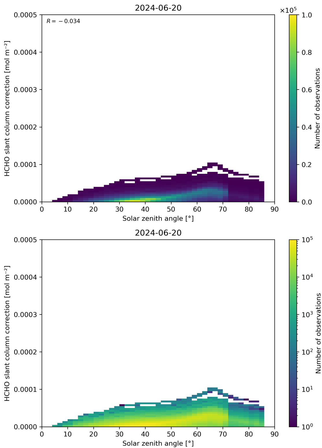
Figure 172: Scatter density plot of “Solar zenith angle” against “HCHO slant column correction” for 2024-06-19 to 2024-06-21.
