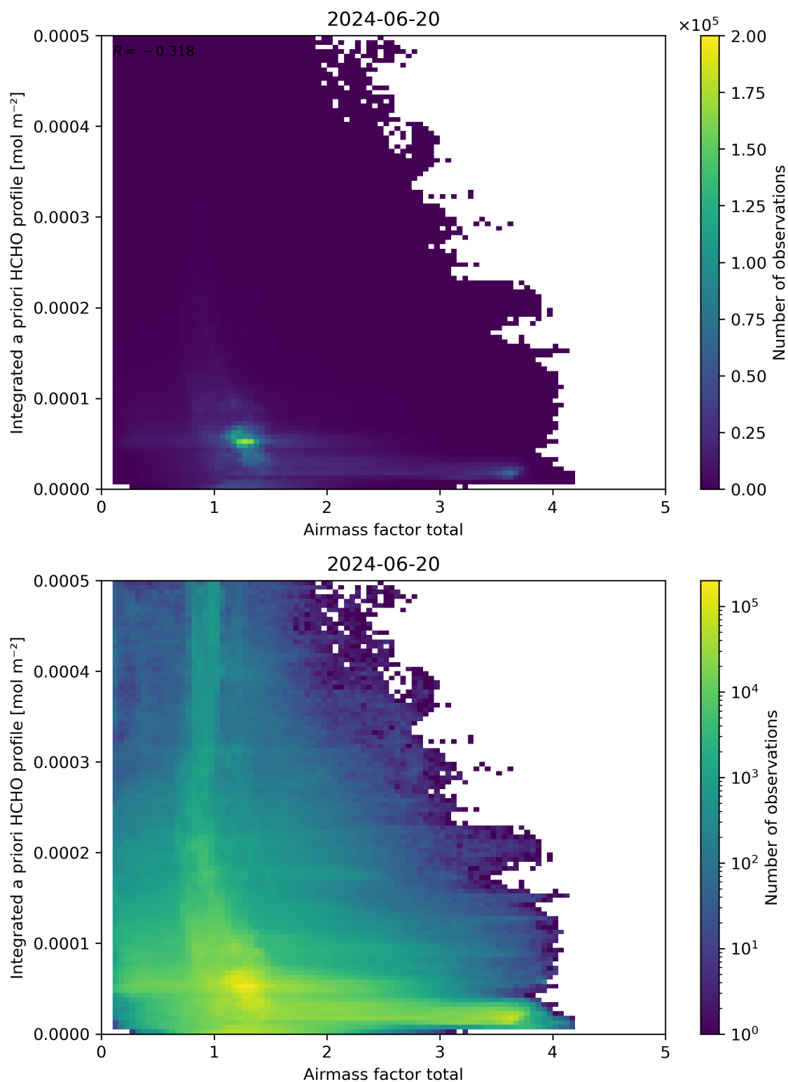
Figure 104: Scatter density plot of “Air mass factor total” against “Integrated a priori HCHO profile” for 2024-06-19 to 2024-06-21.
