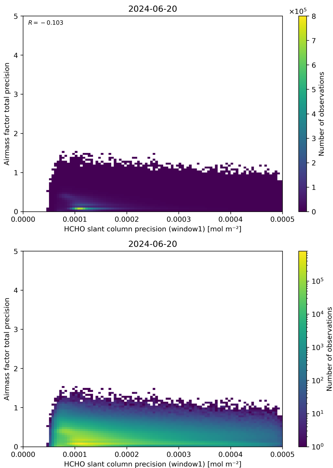
Figure 95: Scatter density plot of “HCHO slant column precision (window1)” against “Airmass factor total precision” for 2024-06-19 to 2024-06-21.
