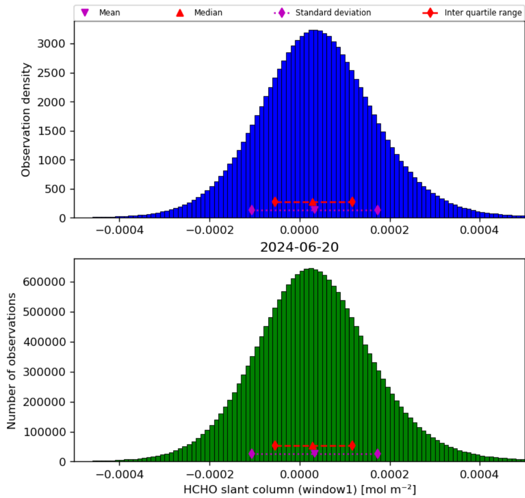
Figure 38: Histogram of “HCHO slant column (window1)” for 2024-06-19 to 2024-06-21
