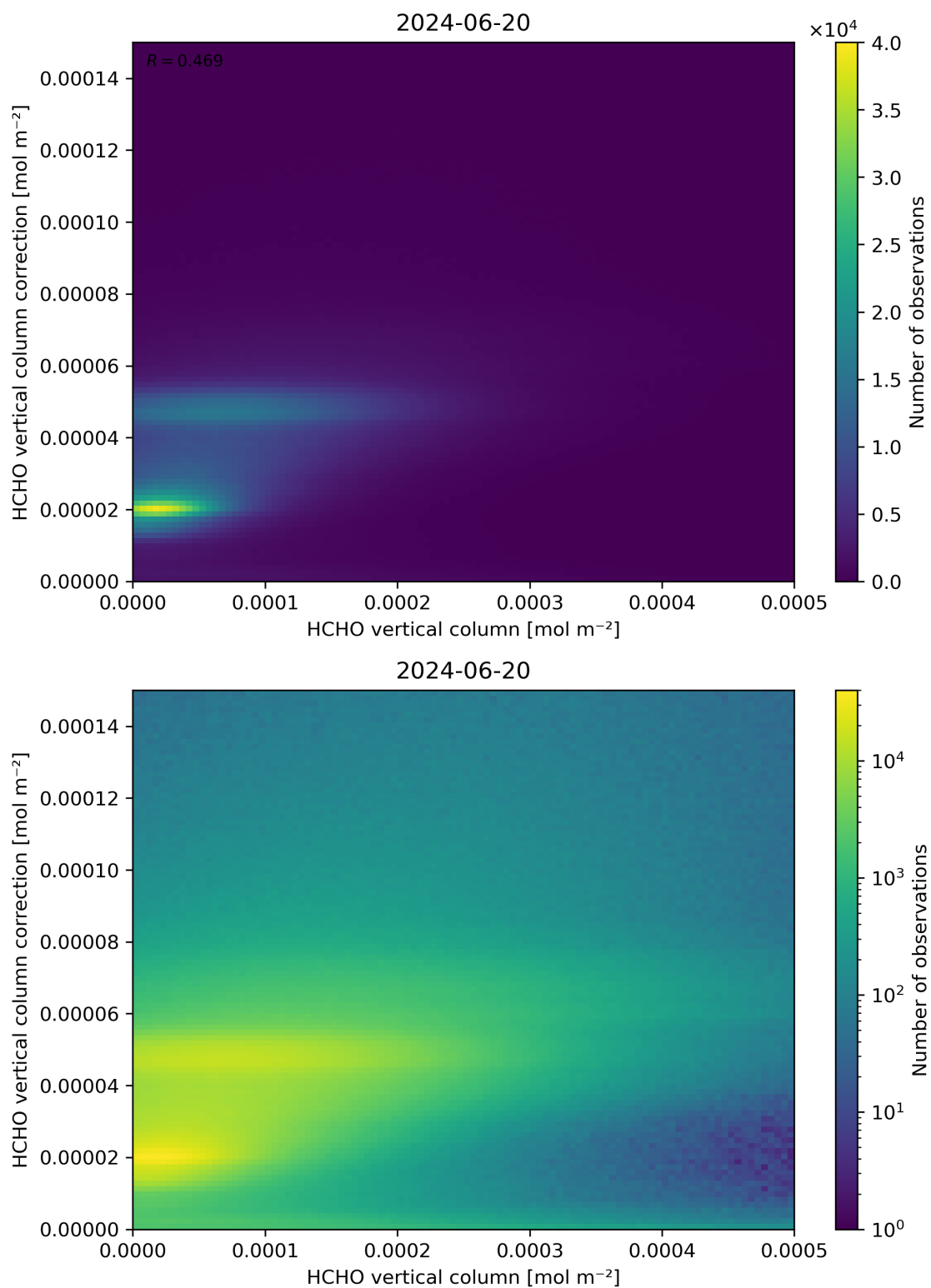
Figure 133: Scatter density plot of “HCHO vertical column” against “HCHO vertical column correction” for 2024-06-19 to 2024-06-21.
