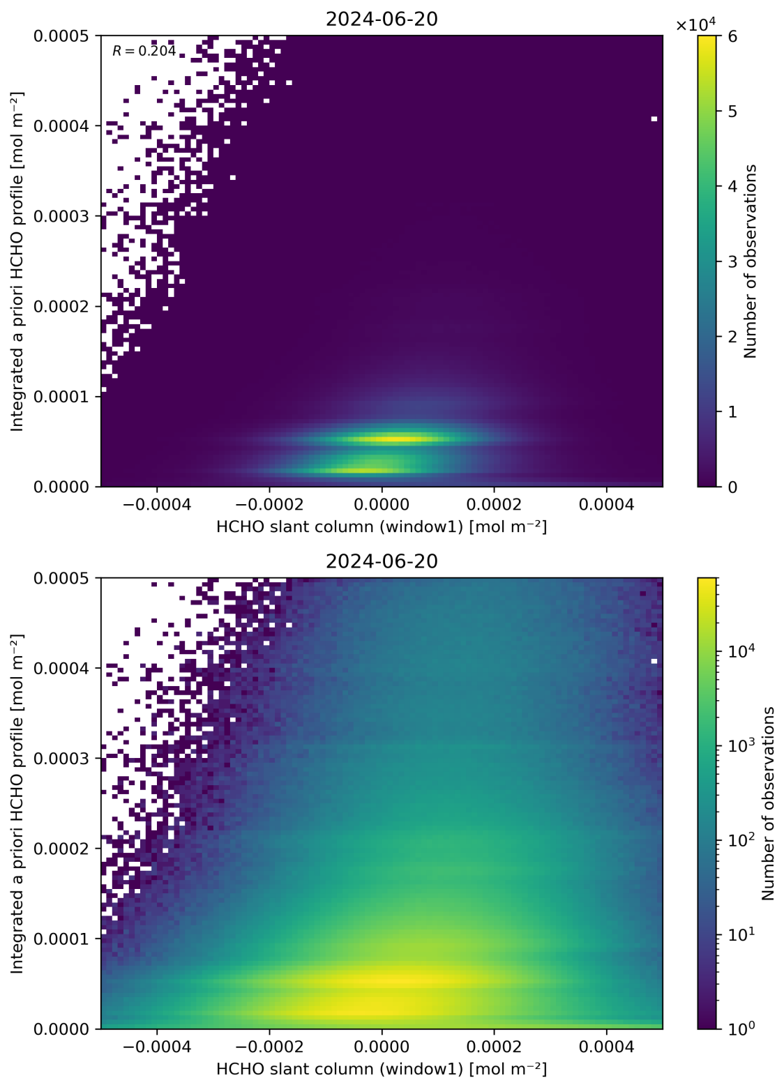
Figure 87: Scatter density plot of “HCHO slant column (window1)” against “Integrated a priori HCHO profile” for 2024-06-19 to 2024-06-21.
