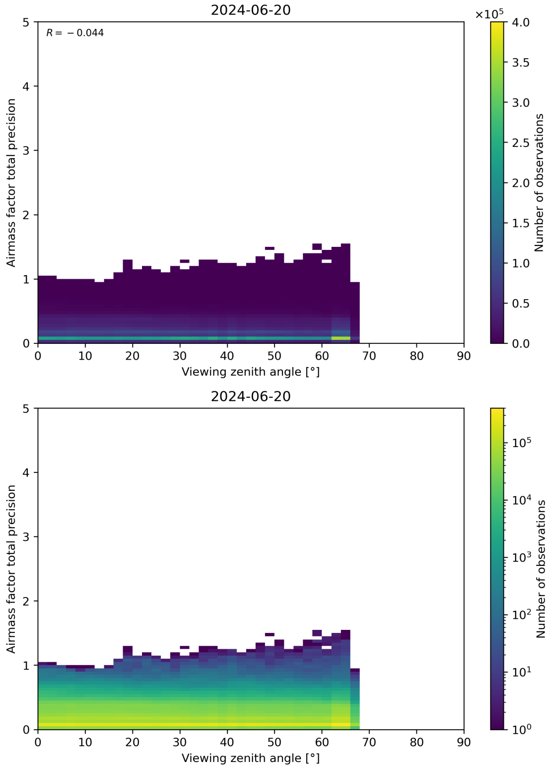
Figure 191: Scatter density plot of “Viewing zenith angle” against “Airmass factor total precision” for 2024-06-19 to 2024-06-21.
