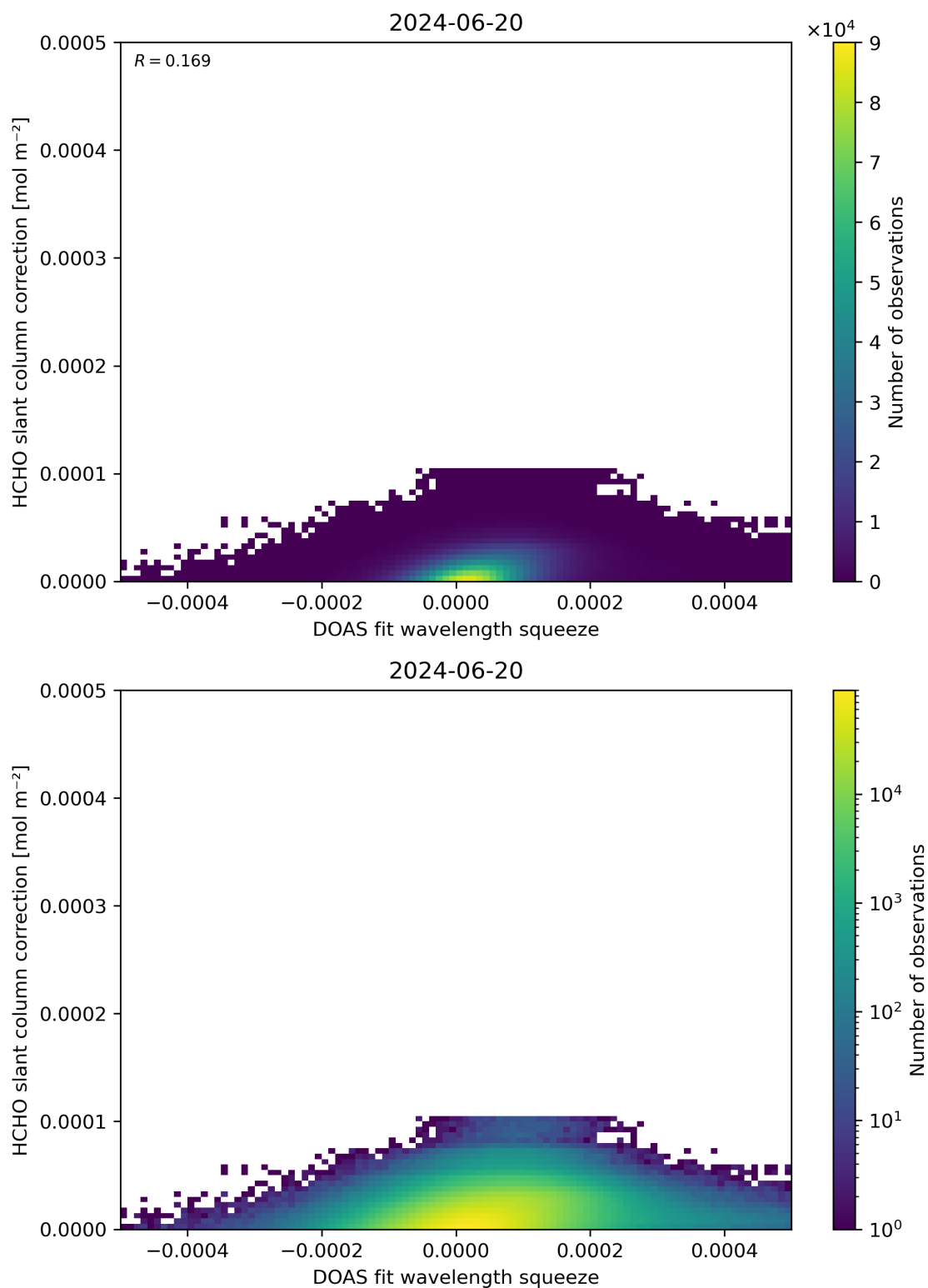
Figure 70: Scatter density plot of “DOAS fit wavelength squeeze” against “HCHO slant column correction” for 2024-06-19 to 2024-06-21.
