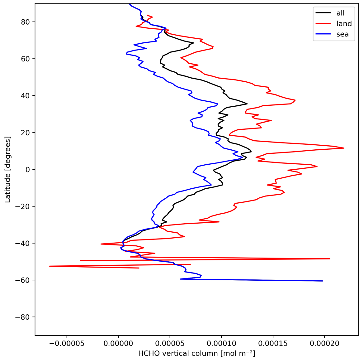
Figure 21: Zonal average of “HCHO vertical column” for 2024-06-19 to 2024-06-21.
