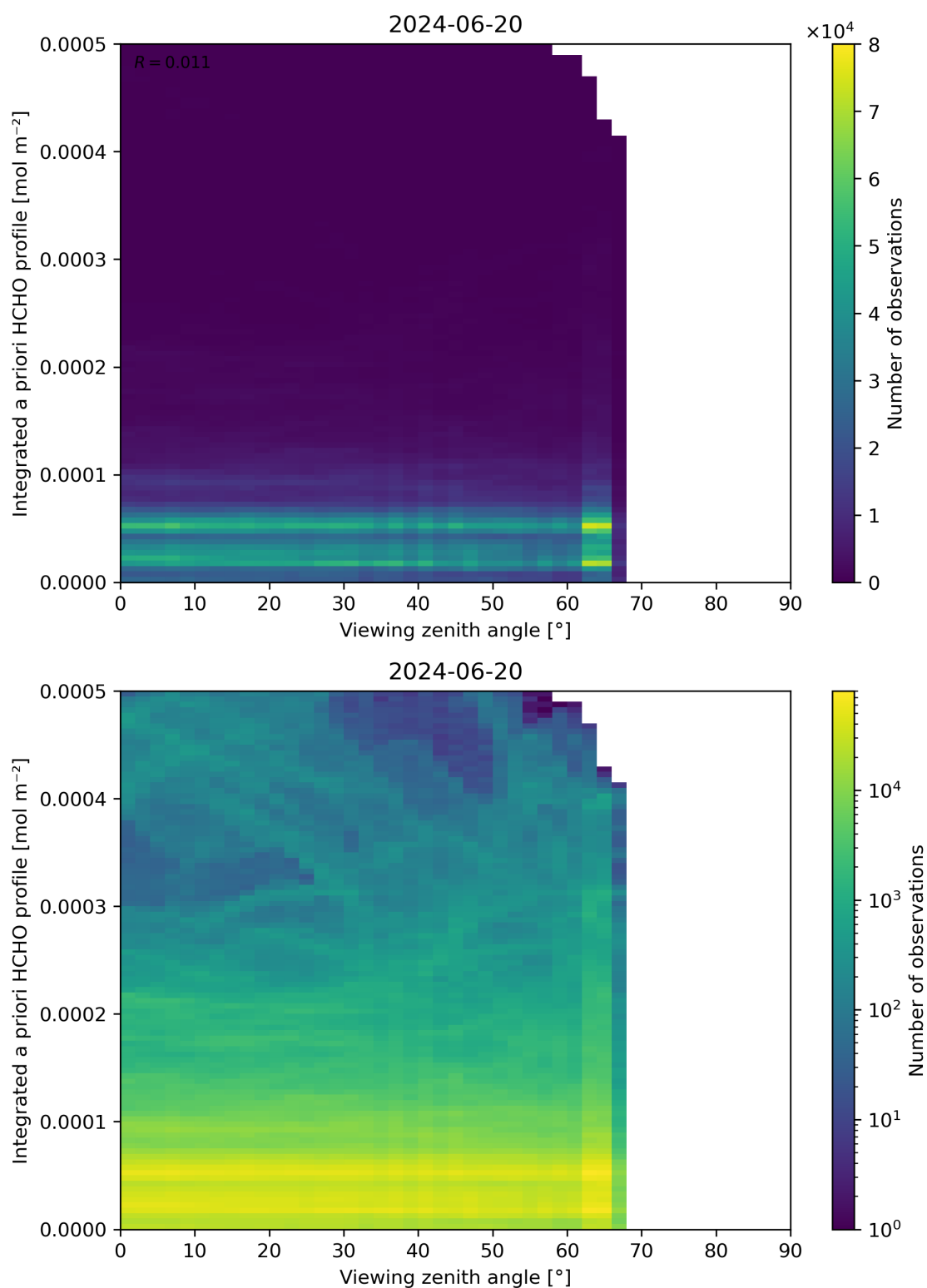
Figure 195: Scatter density plot of “Viewing zenith angle” against “Integrated a priori HCHO profile” for 2024-06-19 to 2024-06-21.
