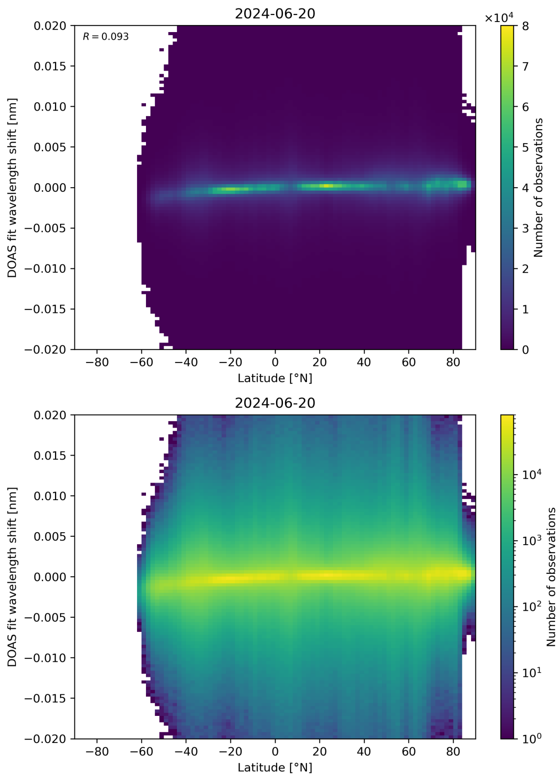
Figure 154: Scatter density plot of “Latitude” against “DOAS fit wavelength shift” for 2024-06-19 to 2024-06-21.
