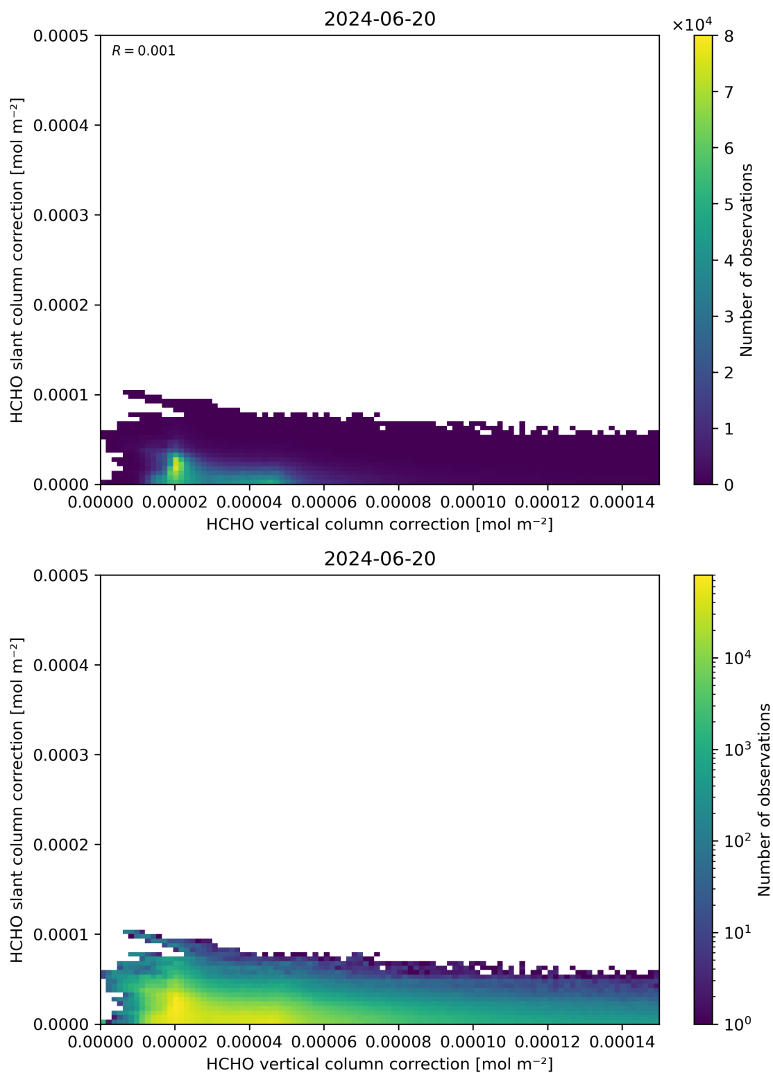
Figure 117: Scatter density plot of “HCHO vertical column correction” against “HCHO slant column correction” for 2024-06-19 to 2024-06-21.
