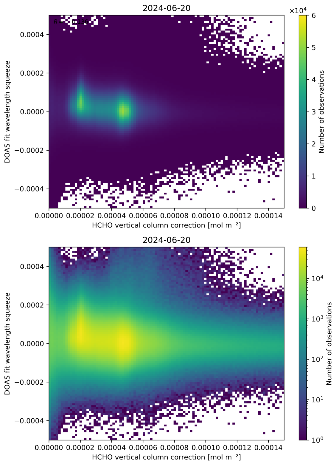
Figure 114: Scatter density plot of “HCHO vertical column correction” against “DOAS fit wavelength squeeze” for 2024-06-19 to 2024-06-21.
