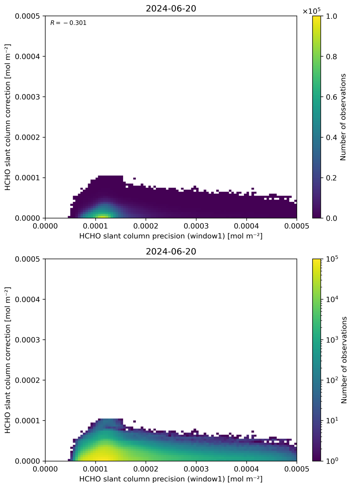
Figure 93: Scatter density plot of “HCHO slant column precision (window1)” against “HCHO slant column correction” for 2024-06-19 to 2024-06-21.
