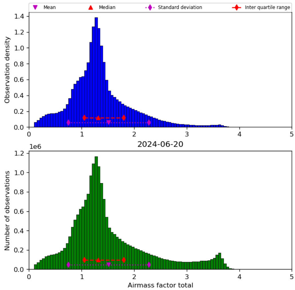
Figure 40: Histogram of “Airmass factor total” for 2024-06-19 to 2024-06-21
