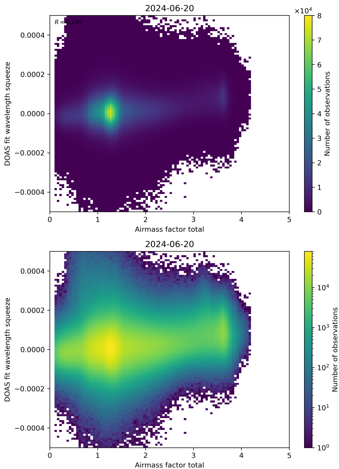
Figure 99: Scatter density plot of “Airmass factor total” against “DOAS fit wavelength squeeze” for 2024-06-19 to 2024-06-21.
