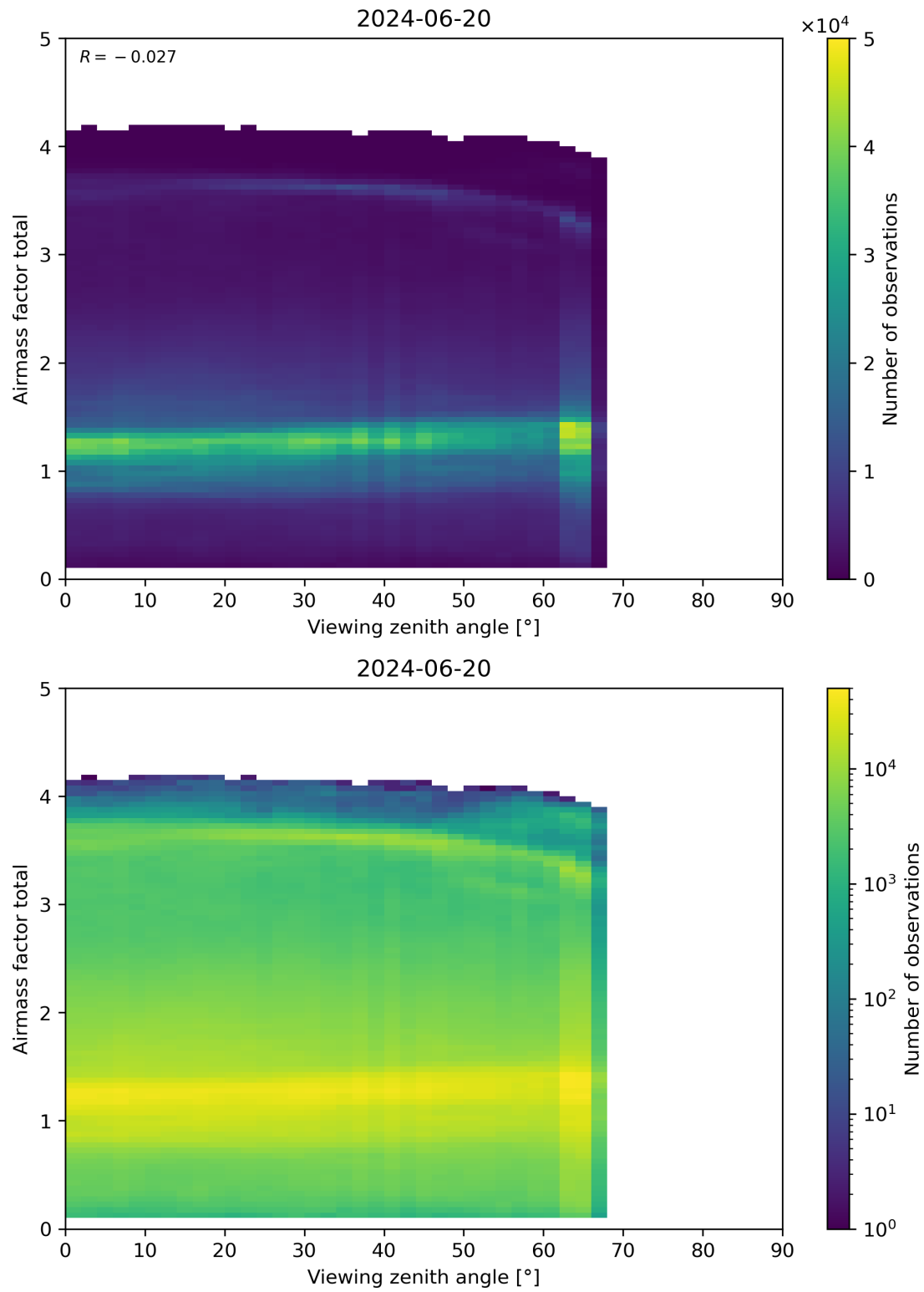
Figure 190: Scatter density plot of “Viewing zenith angle” against “Airmass factor total” for 2024-06-19 to 2024-06-21.
