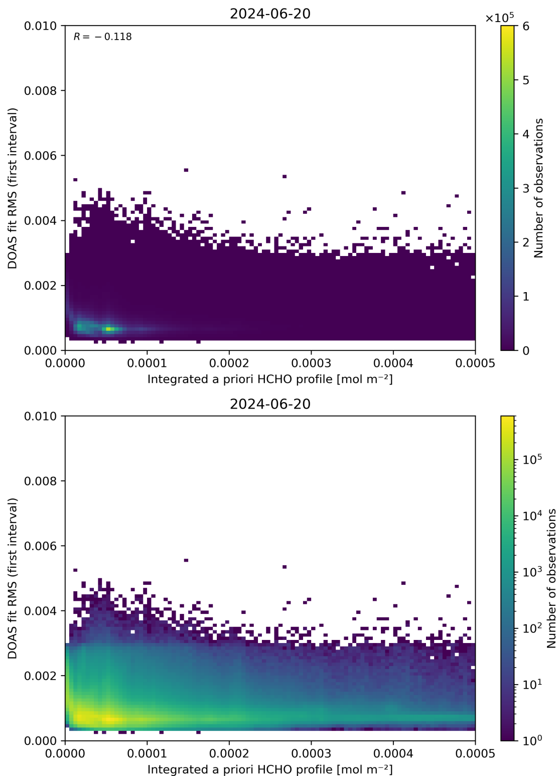
Figure 148: Scatter density plot of “Integrated a priori HCHO profile” against “DOAS fit RMS (first interval)” for 2024-06-19 to 2024-06-21.
