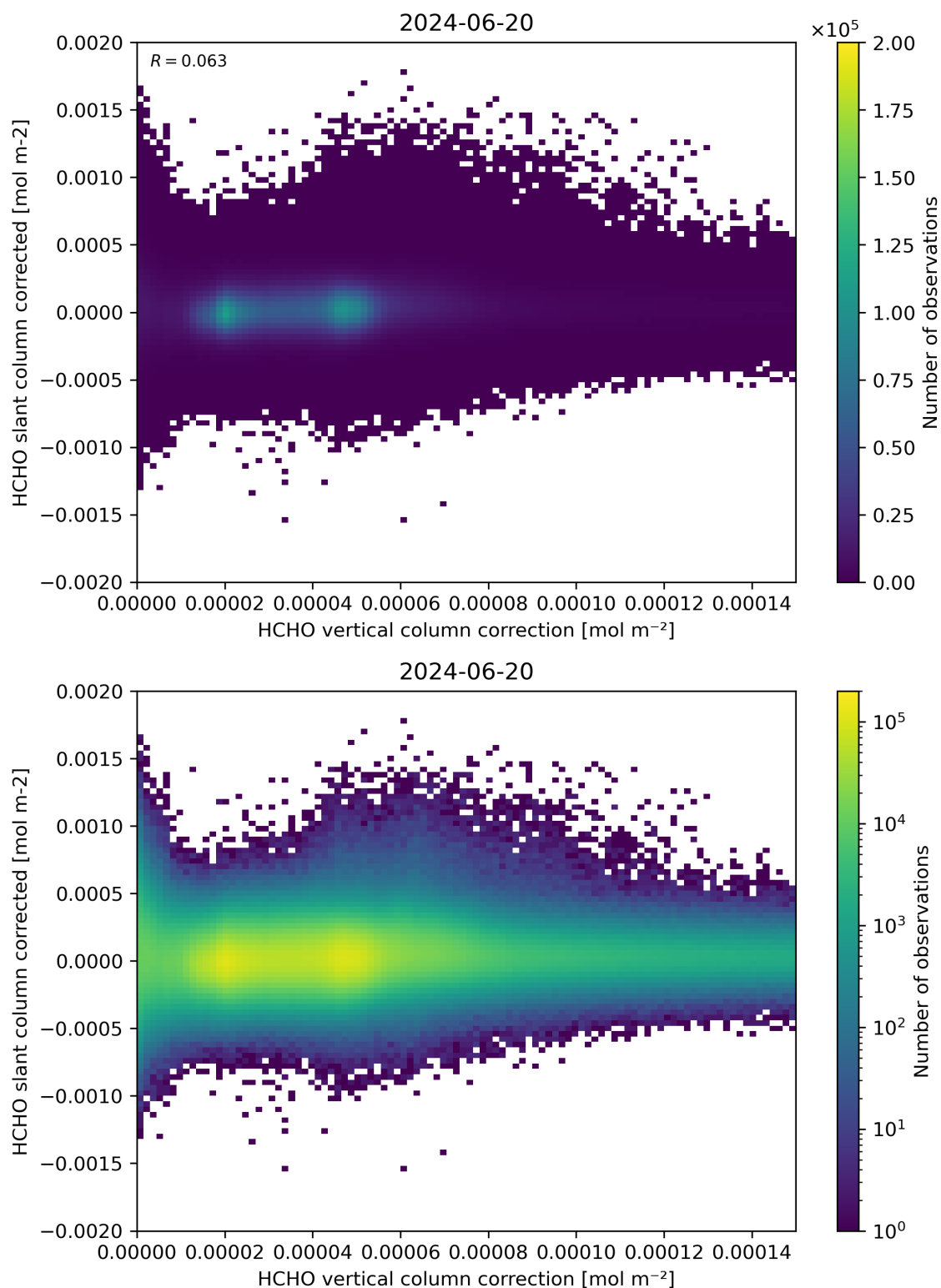
Figure 116: Scatter density plot of “HCHO vertical column correction” against “HCHO slant column corrected” for 2024-06-19 to 2024-06-21.
