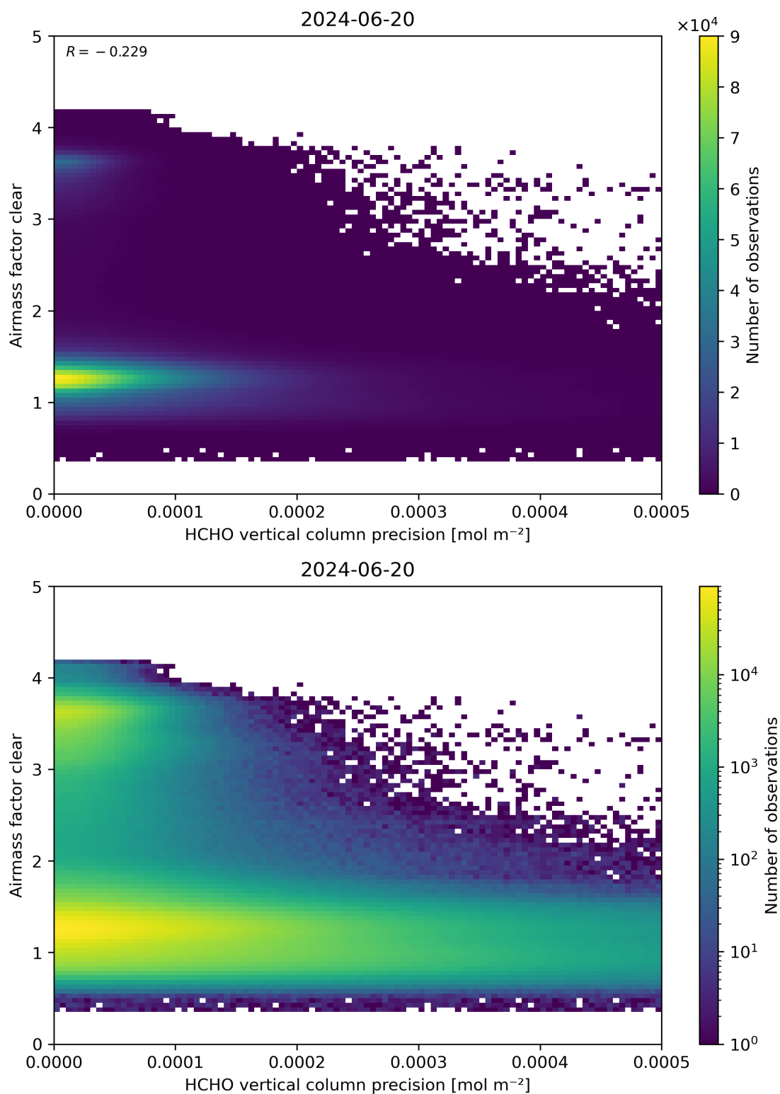
Figure 139: Scatter density plot of “HCHO vertical column precision” against “Airmass factor clear” for 2024-06-19 to 2024-06-21.
