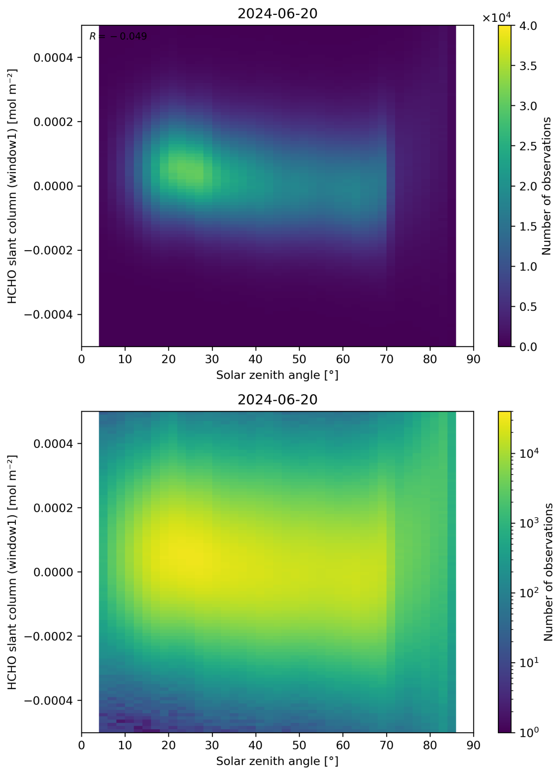
Figure 173: Scatter density plot of “Solar zenith angle” against “HCHO slant column (window1)” for 2024-06-19 to 2024-06-21.
