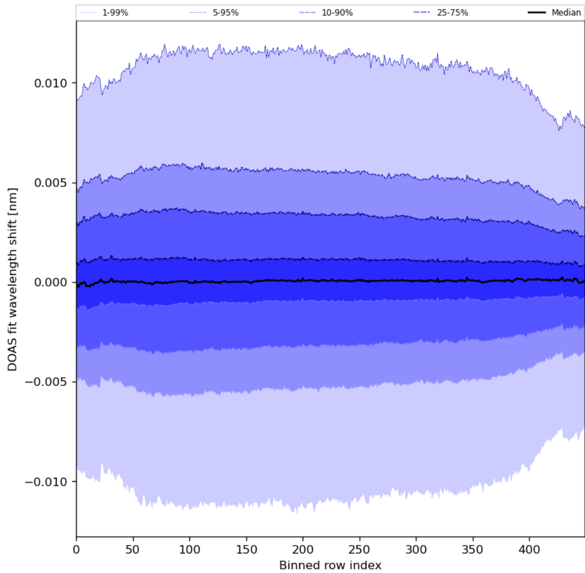
Figure 58: Along track statistics of “DOAS fit wavelength shift” for 2024-06-19 to 2024-06-21
