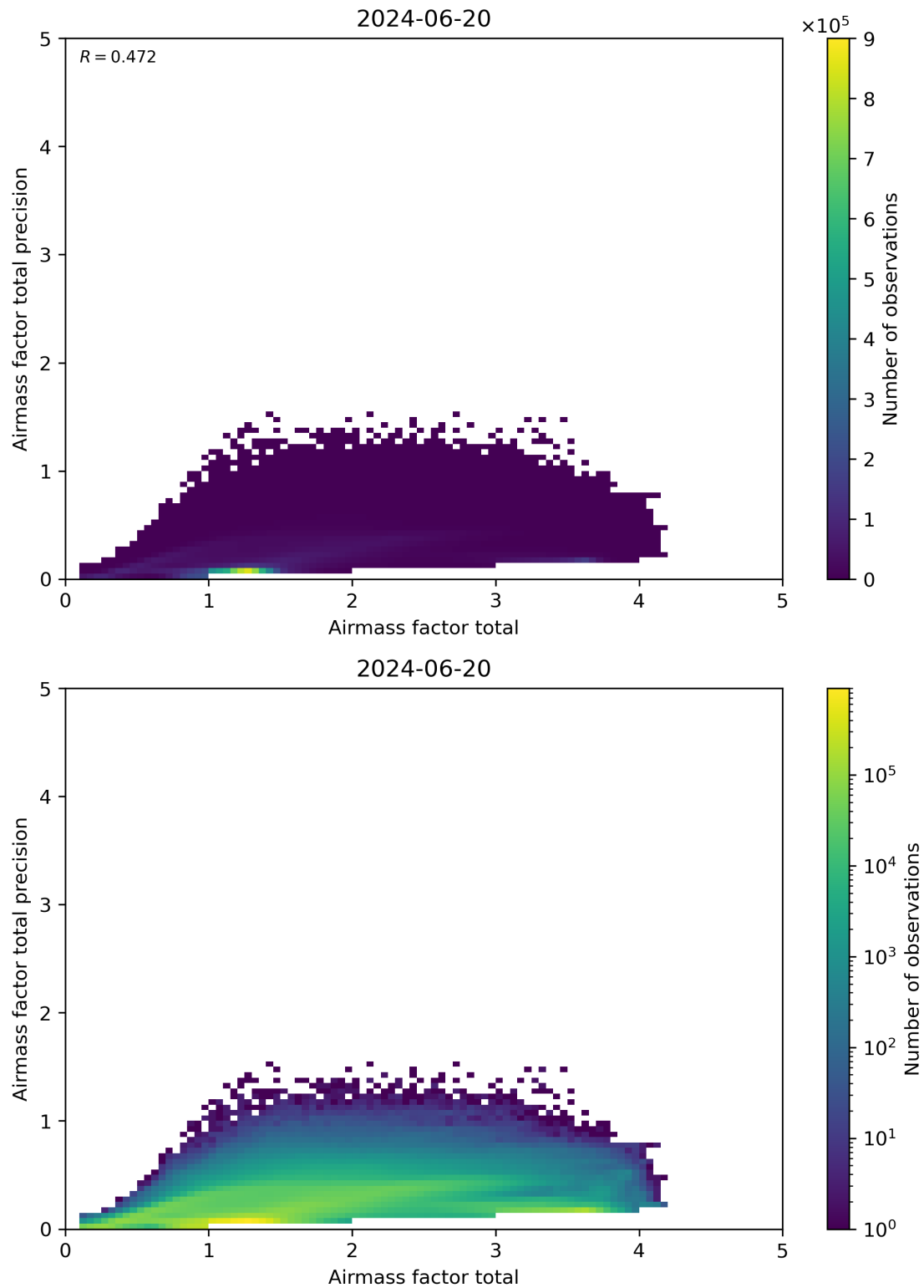
Figure 103: Scatter density plot of “Airmass factor total” against “Airmass factor total precision” for 2024-06-19 to 2024-06-21.
