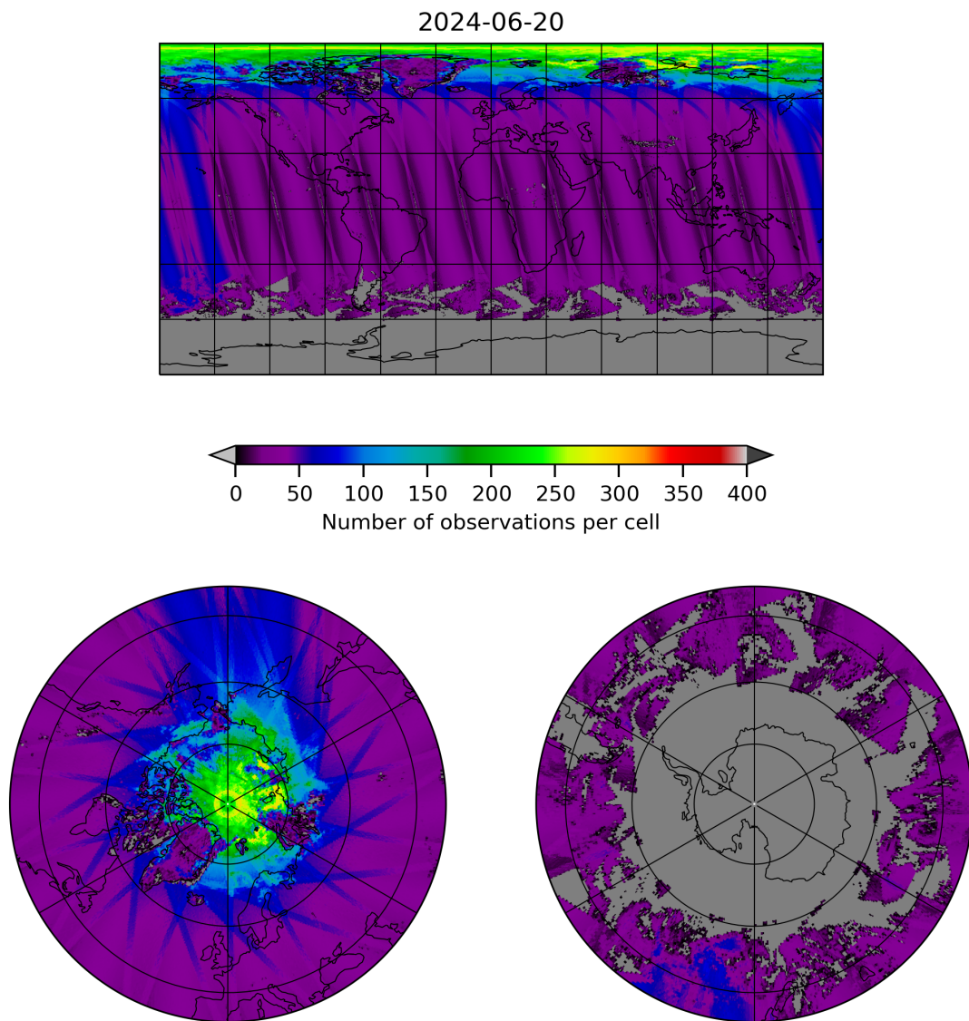
Figure 19: Map of the number of observations for 2024-06-19 to 2024-06-21
