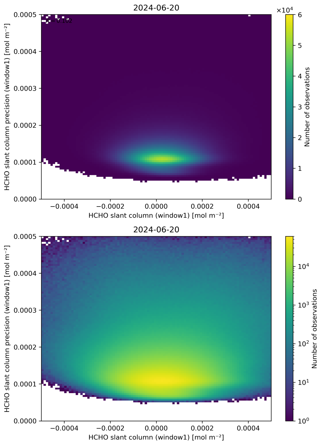
Figure 84: Scatter density plot of “HCHO slant column (window1)” against “HCHO slant column precision (window1)” for 2024-06-19 to 2024-06-21.
