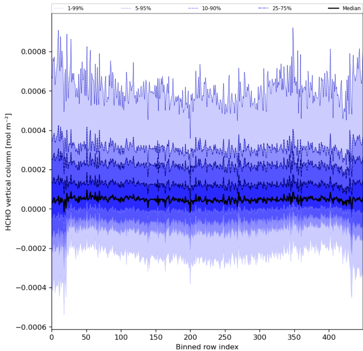
Figure 49: Along track statistics of “HCHO vertical column” for 2024-06-19 to 2024-06-21
