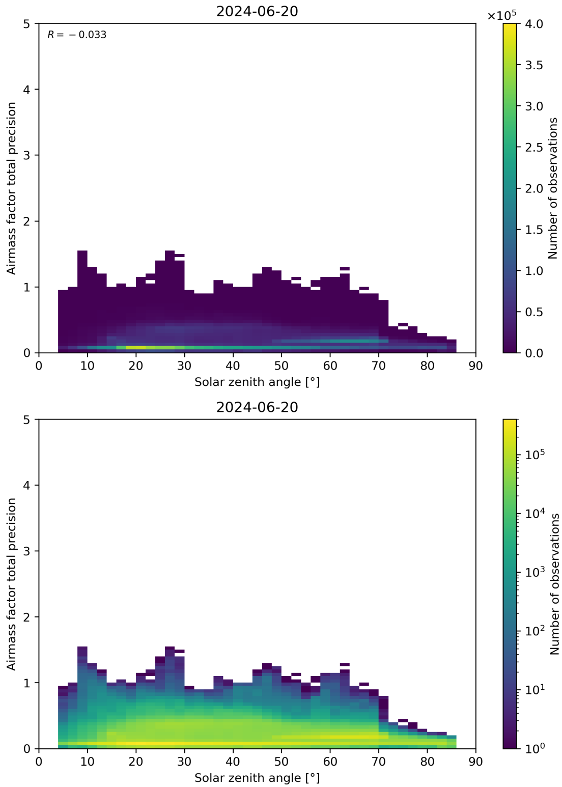
Figure 176: Scatter density plot of “Solar zenith angle” against “Airmass factor total precision” for 2024-06-19 to 2024-06-21.
