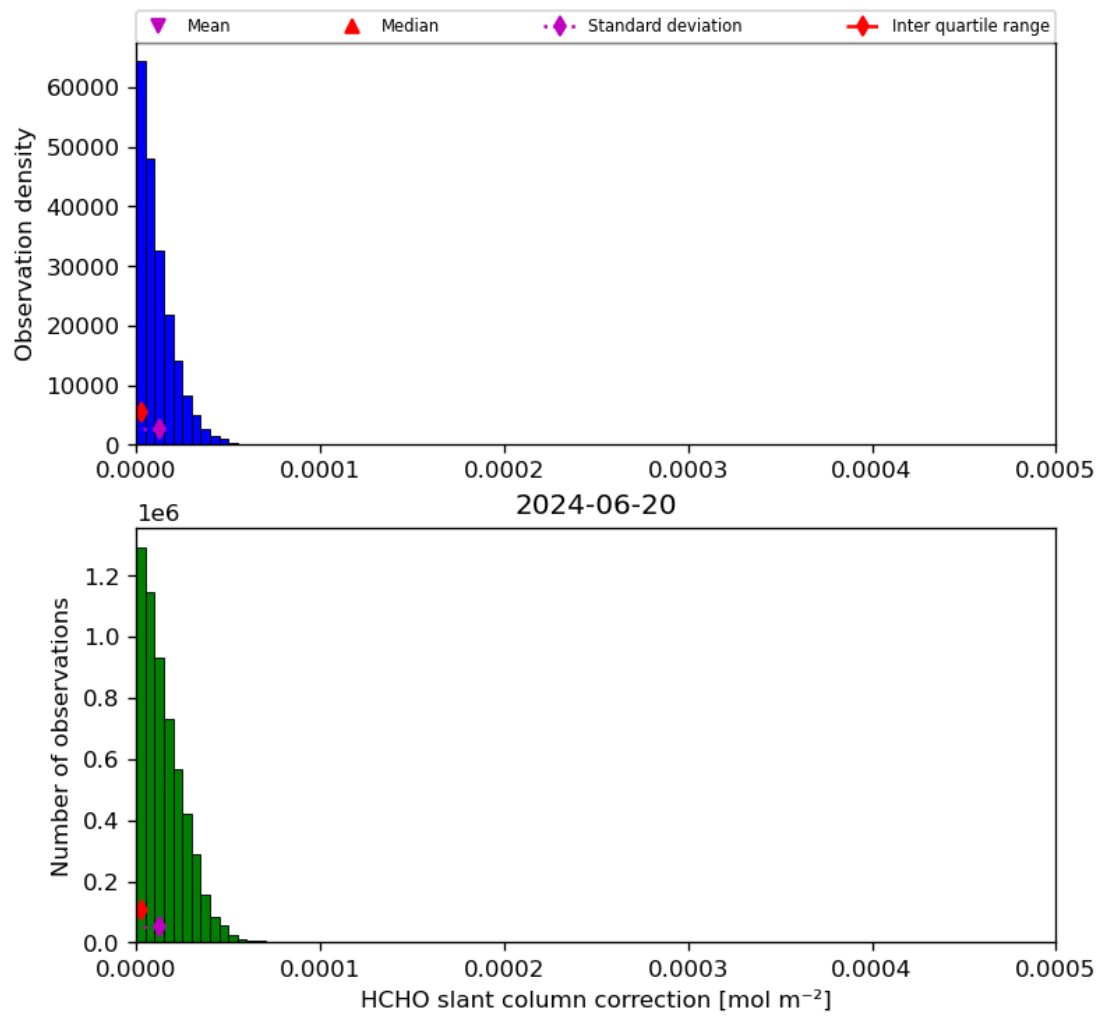
Figure 47: Histogram of “HCHO slant column correction” for 2024-06-19 to 2024-06-21
