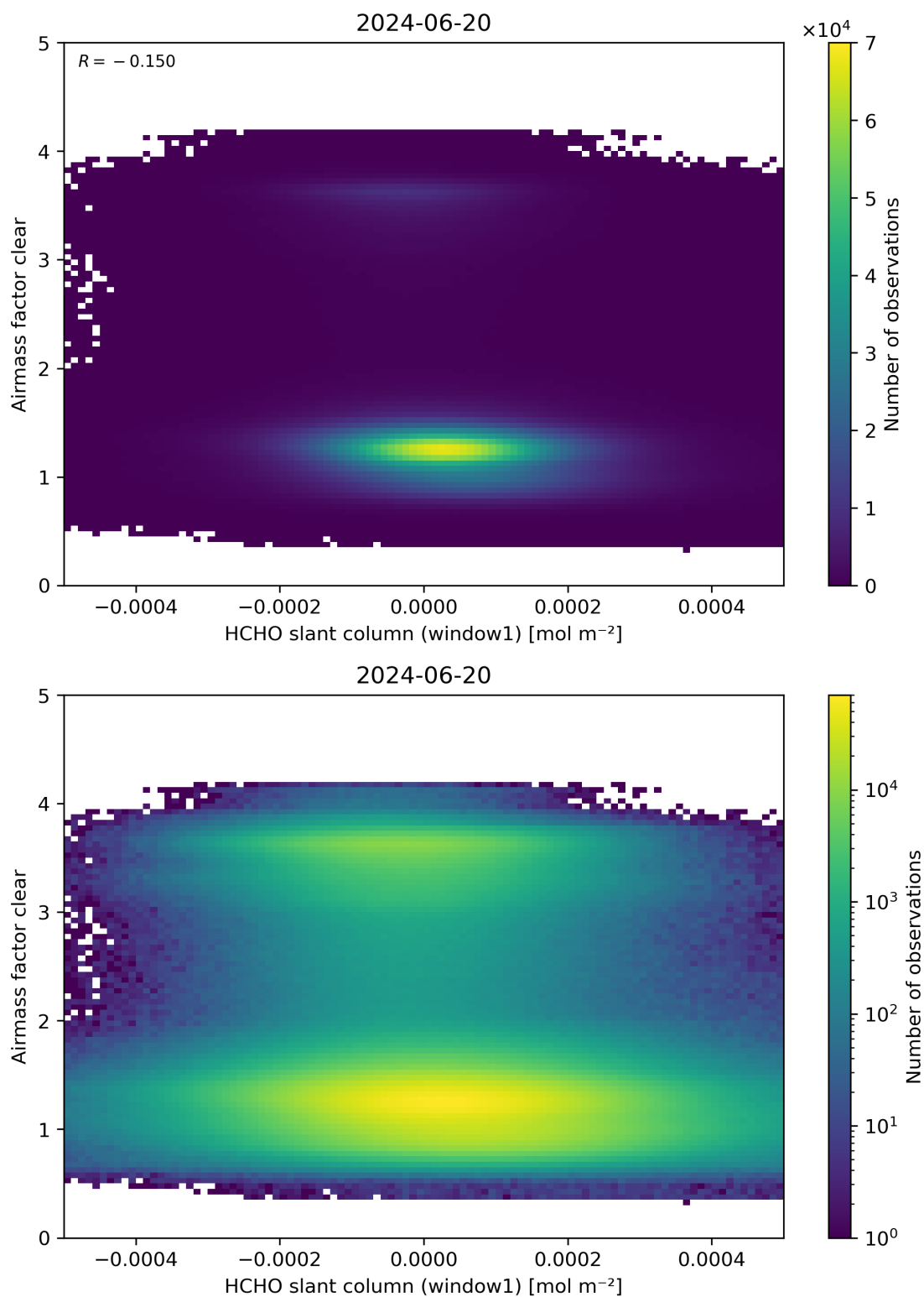
Figure 81: Scatter density plot of “HCHO slant column (window1)” against “Airmass factor clear” for 2024-06-19 to 2024-06-21.
