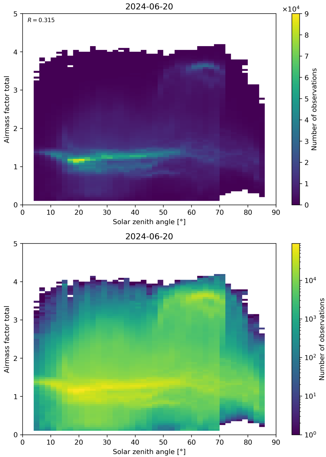
Figure 175: Scatter density plot of “Solar zenith angle” against “Airmass factor total” for 2024-06-19 to 2024-06-21.
