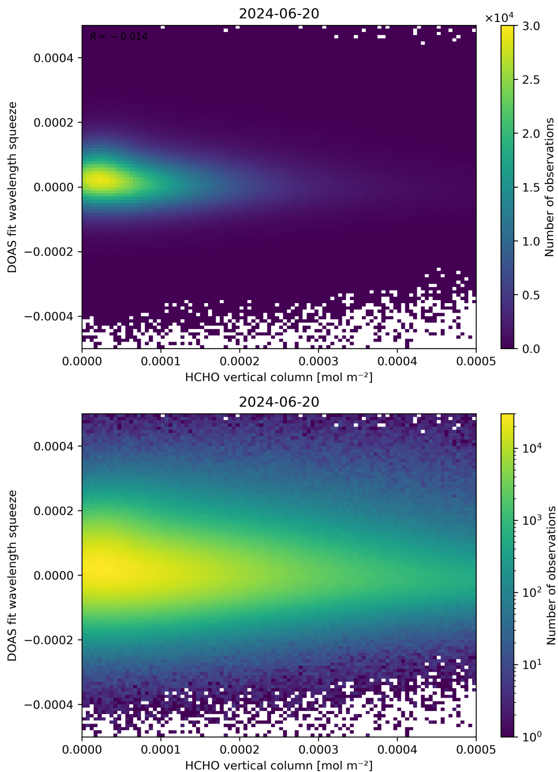
Figure 125: Scatter density plot of “HCHO vertical column” against “DOAS fit wavelength squeeze” for 2024-06-19 to 2024-06-21.
