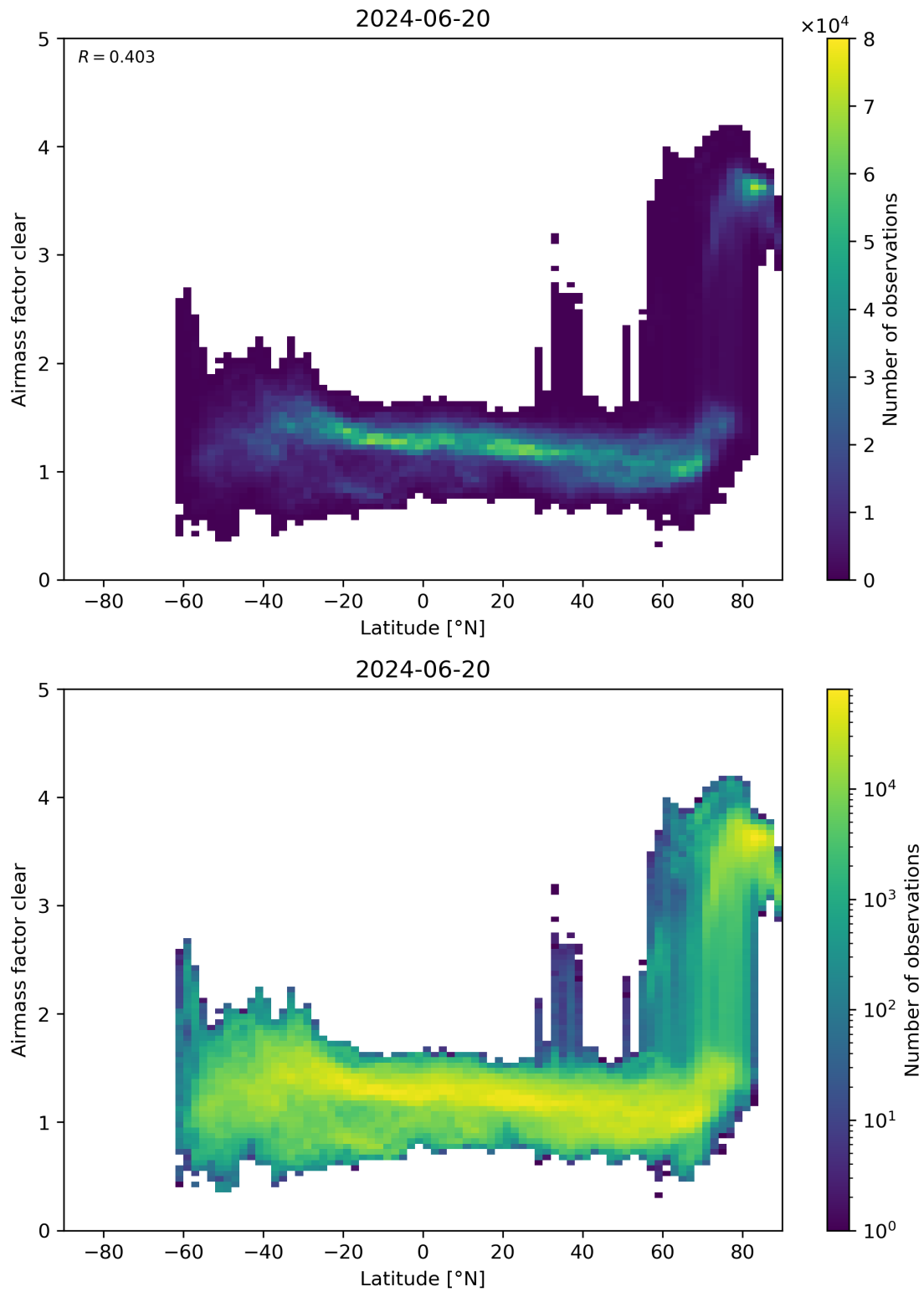
Figure 156: Scatter density plot of “Latitude” against “Airmass factor clear” for 2024-06-19 to 2024-06-21.
