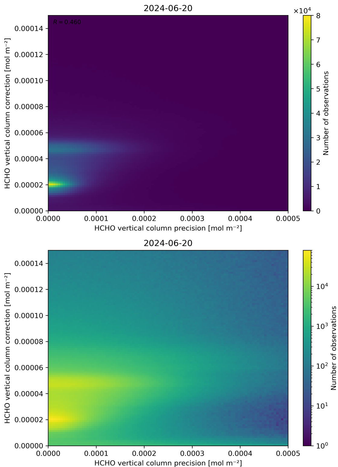
Figure 146: Scatter density plot of “HCHO vertical column precision” against “HCHO vertical column correction” for 2024-06-19 to 2024-06-21.
