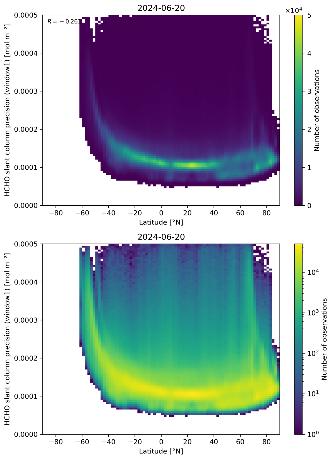
Figure 160: Scatter density plot of “Latitude” against “HCHO slant column precision (window1)” for 2024-06-19 to 2024-06-21.
