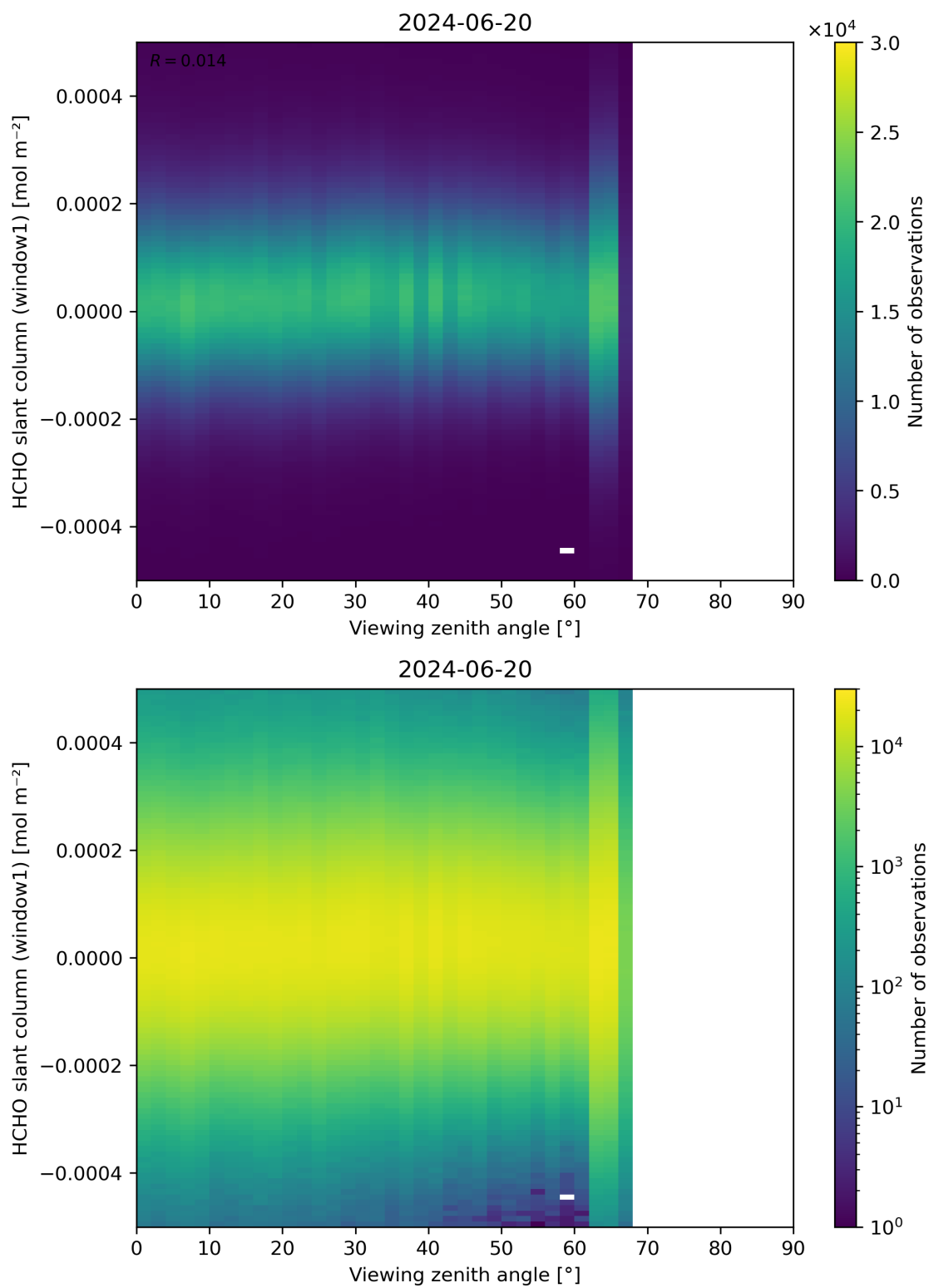
Figure 188: Scatter density plot of “Viewing zenith angle” against “HCHO slant column (window1)” for 2024-06-19 to 2024-06-21.
