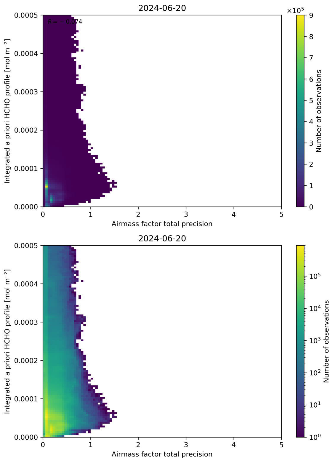
Figure 111: Scatter density plot of “Airmass factor total precision” against “Integrated a priori HCHO profile” for 2024-06-19 to 2024-06-21.
