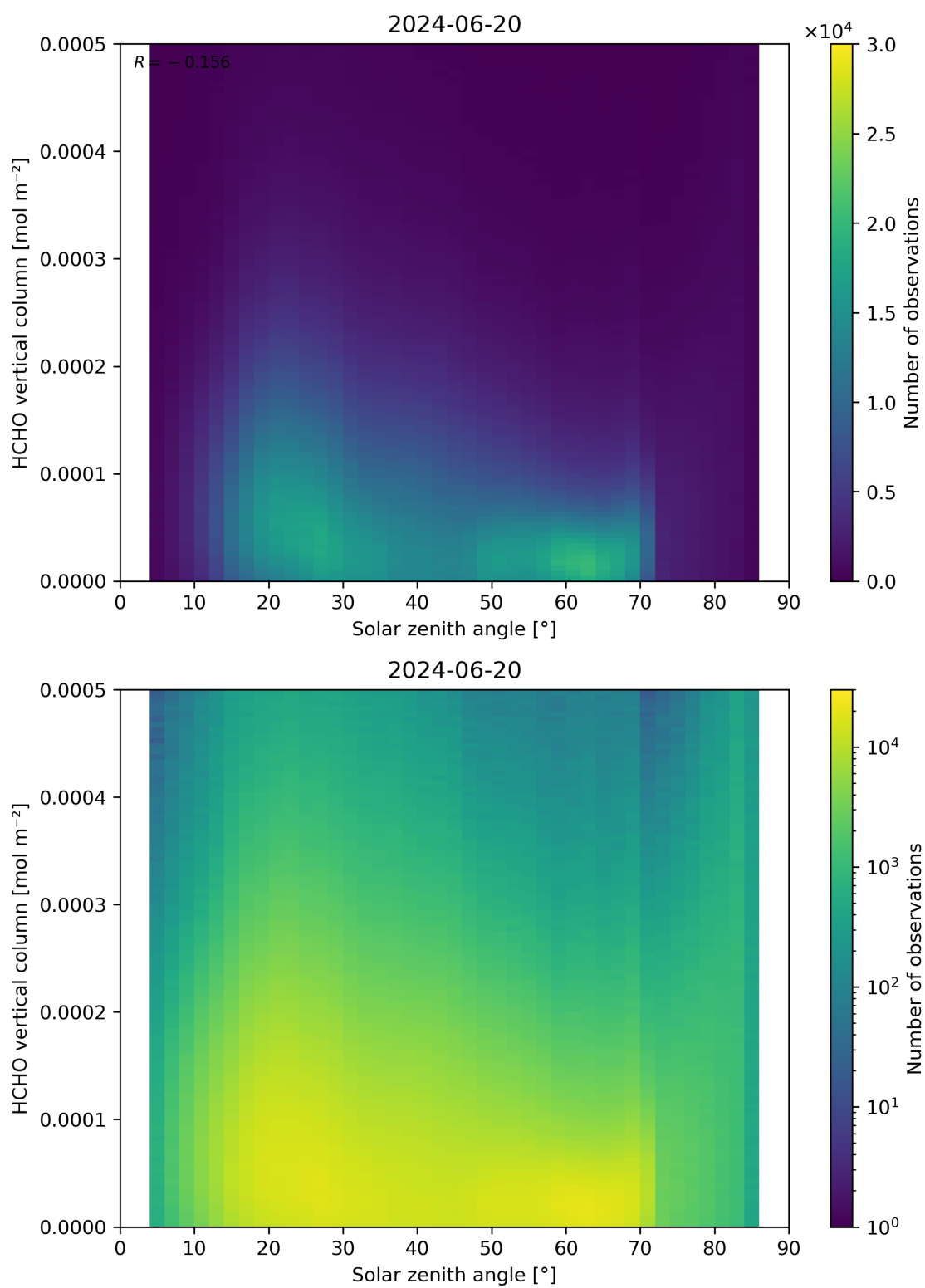
Figure 177: Scatter density plot of “Solar zenith angle” against “HCHO vertical column” for 2024-06-19 to 2024-06-21.
