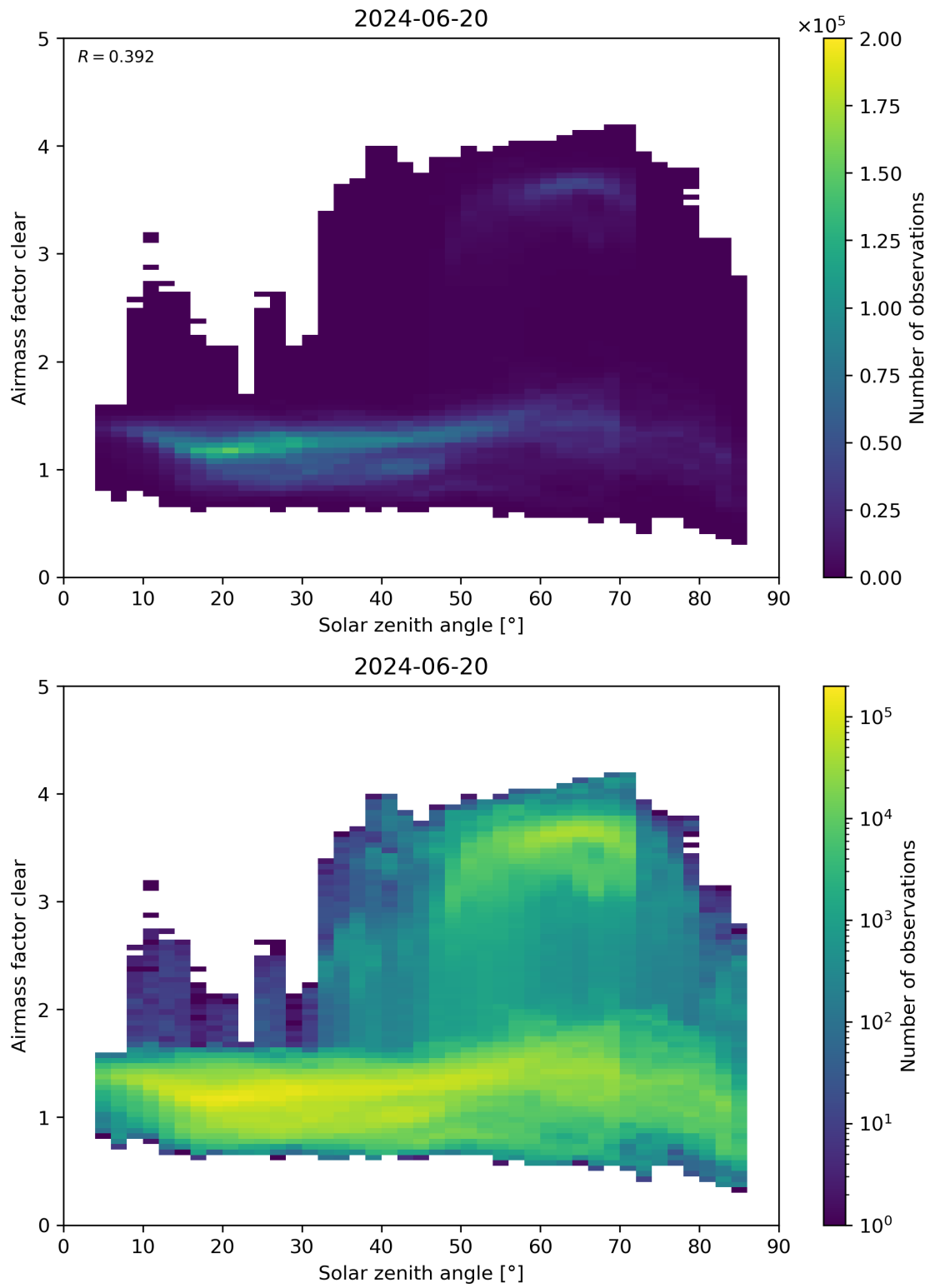
Figure 170: Scatter density plot of “Solar zenith angle” against “Airmass factor clear” for 2024-06-19 to 2024-06-21.
