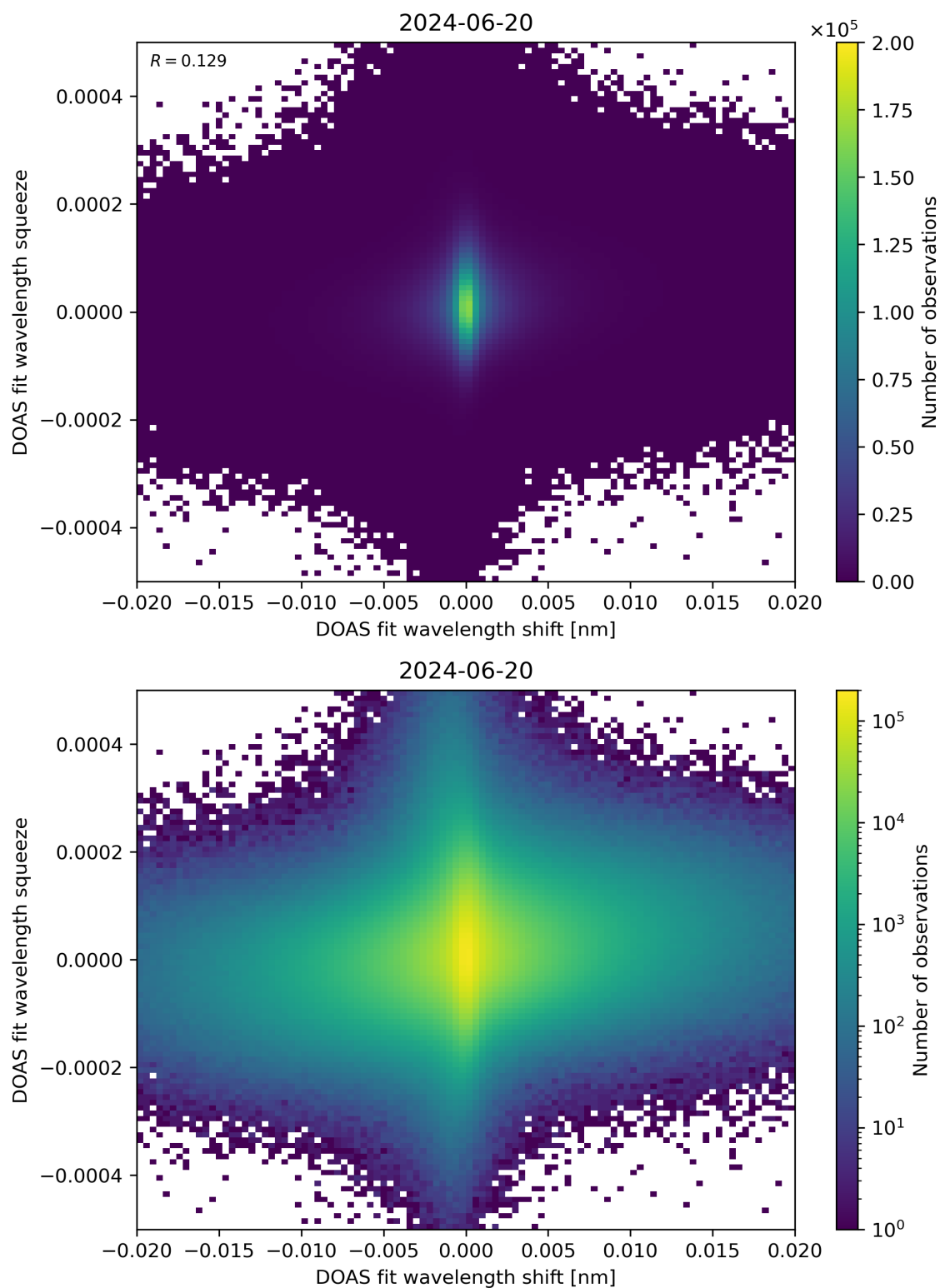
Figure 65: Scatter density plot of “DOAS fit wavelength shift” against “DOAS fit wavelength squeeze” for 2024-06-19 to 2024-06-21.
