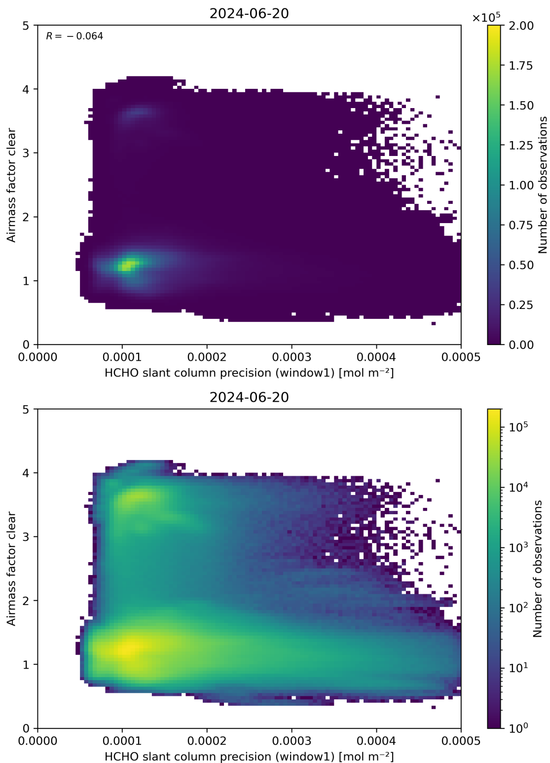
Figure 91: Scatter density plot of “HCHO slant column precision (window1)” against “Airmass factor clear” for 2024-06-19 to 2024-06-21.
