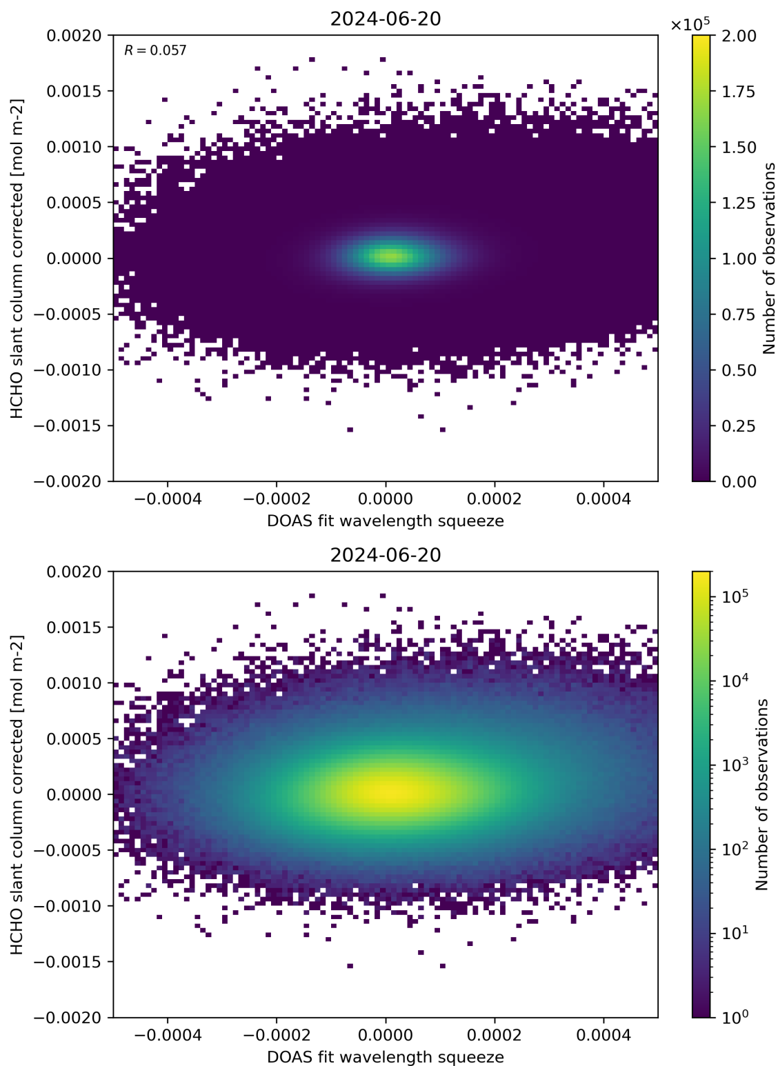
Figure 69: Scatter density plot of “DOAS fit wavelength squeeze” against “HCHO slant column corrected” for 2024-06-19 to 2024-06-21.
