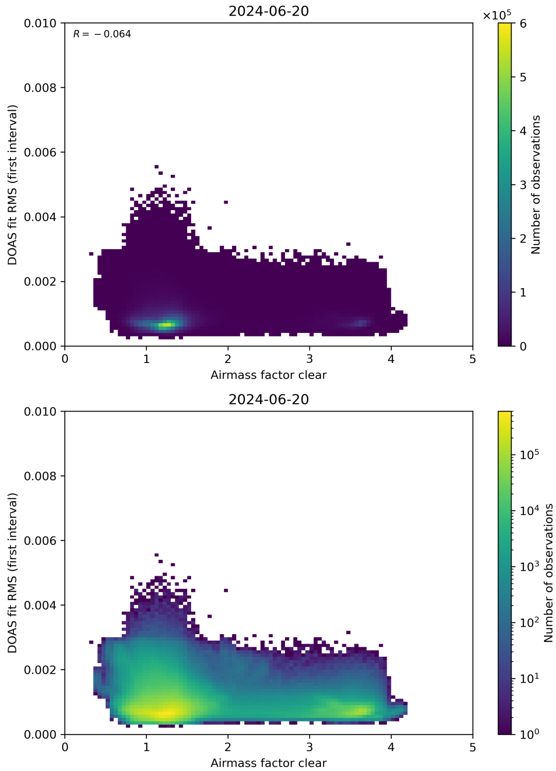
Figure 71: Scatter density plot of “Airmass factor clear” against “DOAS fit RMS (first interval)” for 2024-06-19 to 2024-06-21.
