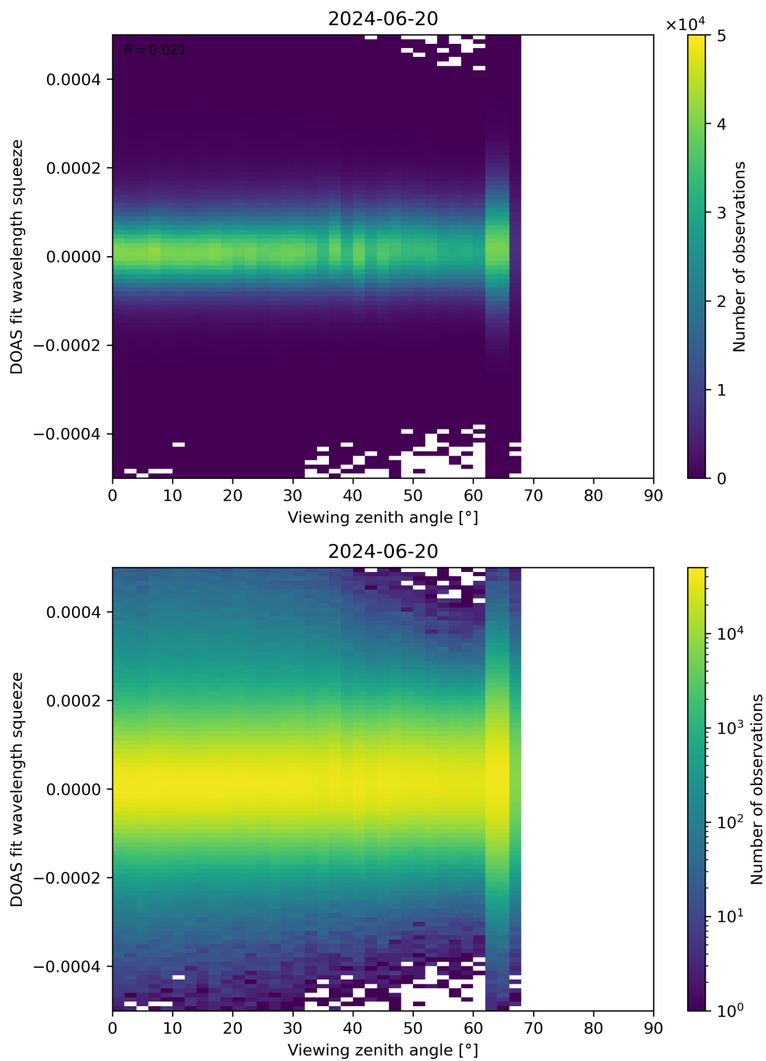
Figure 184: Scatter density plot of “Viewing zenith angle” against “DOAS fit wavelength squeeze” for 2024-06-19 to 2024-06-21.
