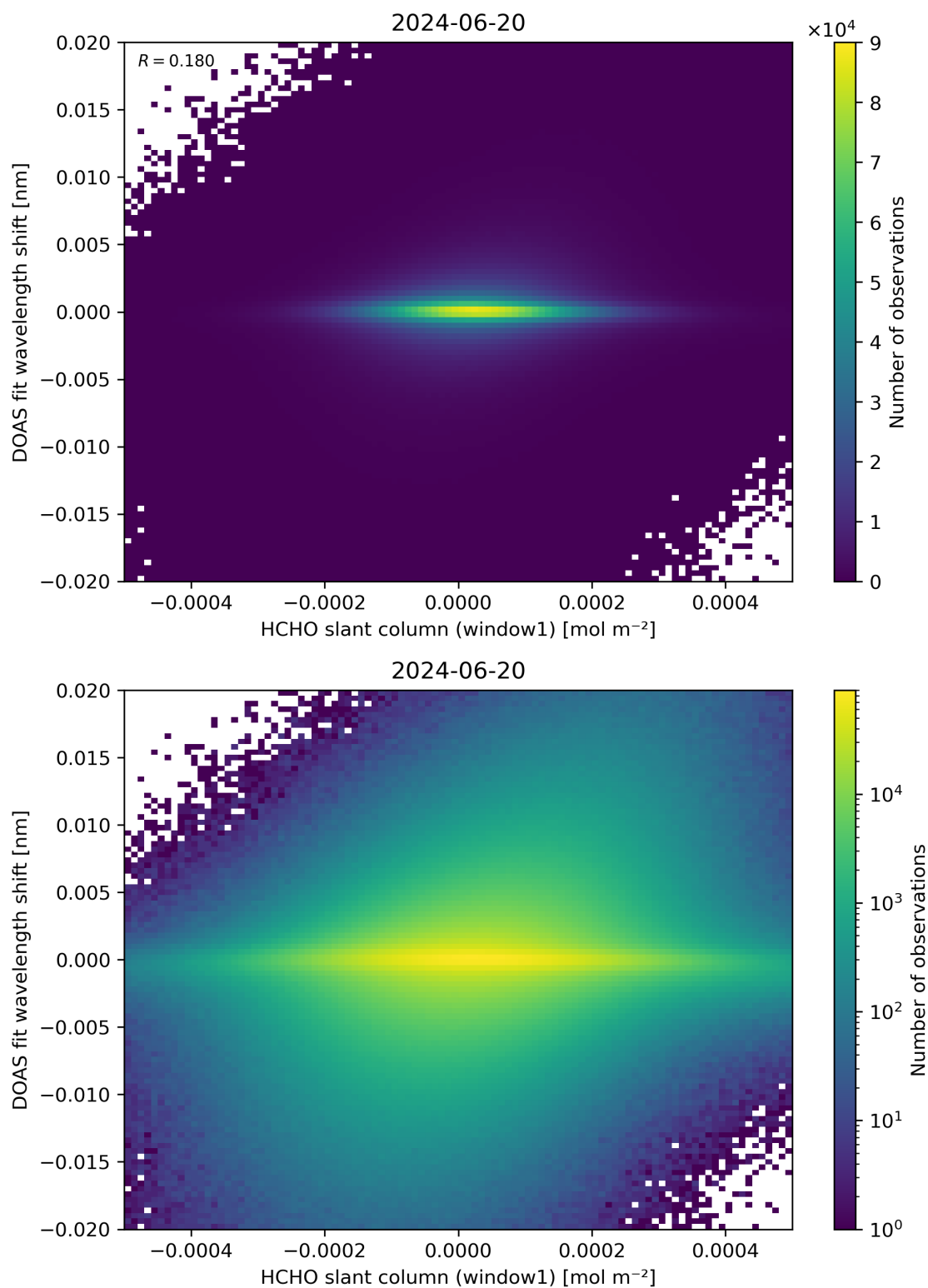
Figure 79: Scatter density plot of “HCHO slant column (window1)” against “DOAS fit wavelength shift” for 2024-06-19 to 2024-06-21.
