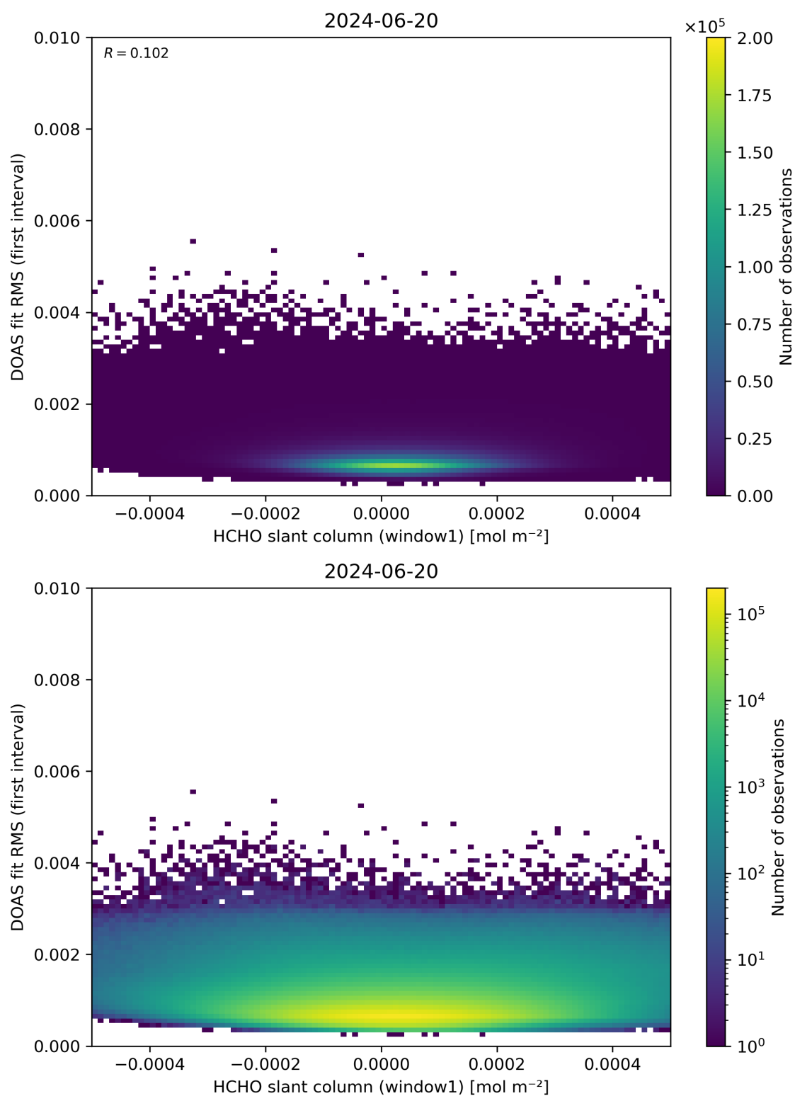
Figure 78: Scatter density plot of “HCHO slant column (window1)” against “DOAS fit RMS (first interval)” for 2024-06-19 to 2024-06-21.
