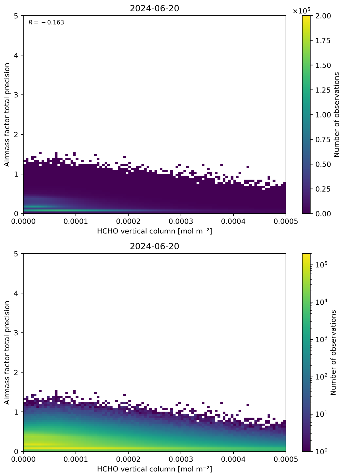
Figure 132: Scatter density plot of “HCHO vertical column” against “Airmass factor total precision” for 2024-06-19 to 2024-06-21.
