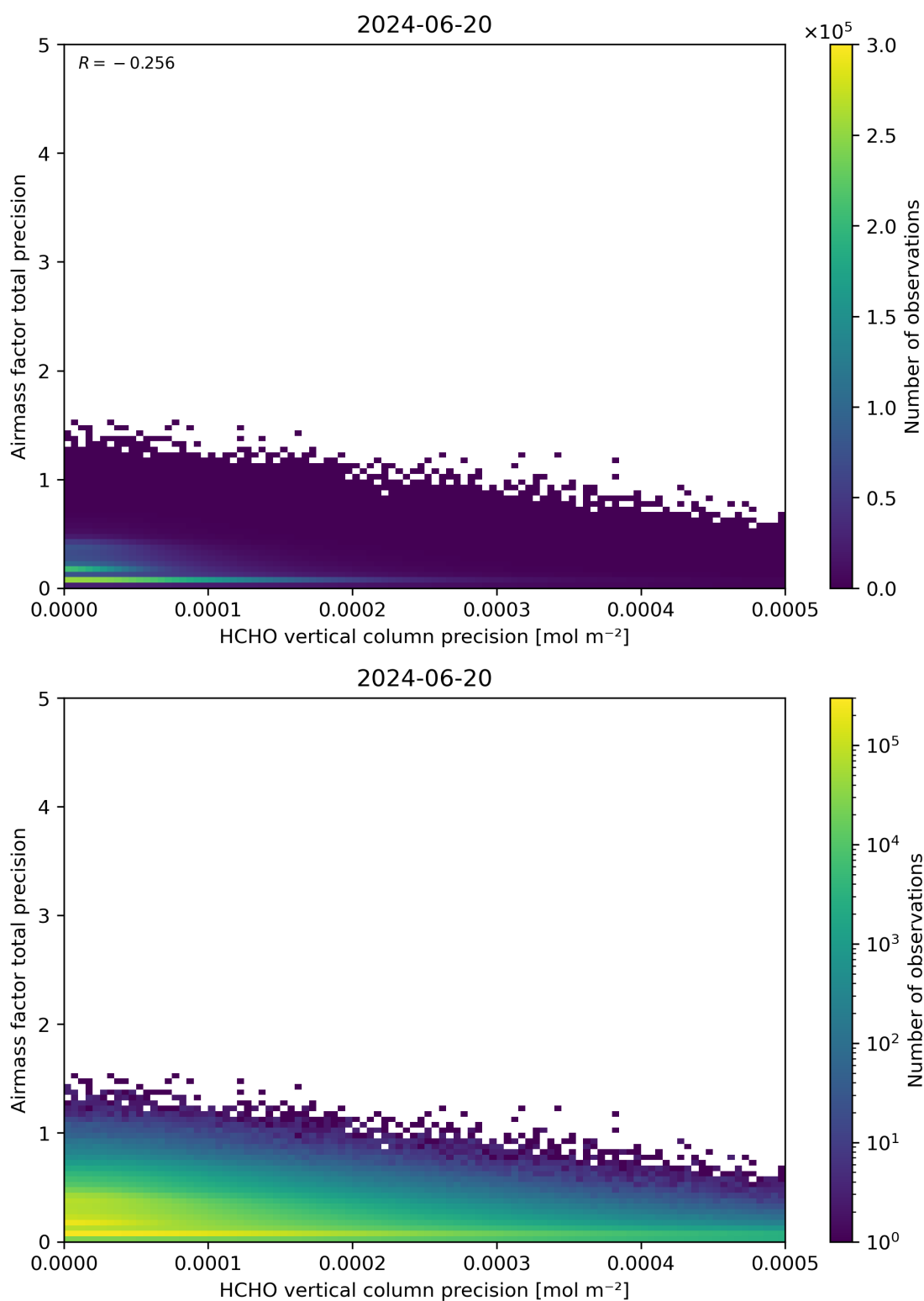
Figure 145: Scatter density plot of “HCHO vertical column precision” against “Airmass factor total precision” for 2024-06-19 to 2024-06-21.
