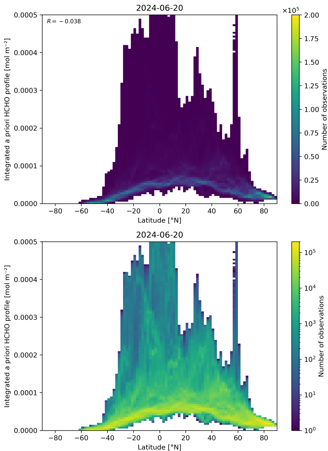
Figure 166: Scatter density plot of “Latitude” against “Integrated a priori HCHO profile” for 2024-06-19 to 2024-06-21.
