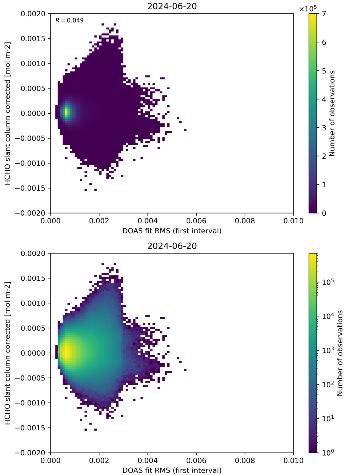
Figure 62: Scatter density plot of “DOAS fit RMS (first interval)” against “HCHO slant column corrected” for 2024-06-19 to 2024-06-21.
