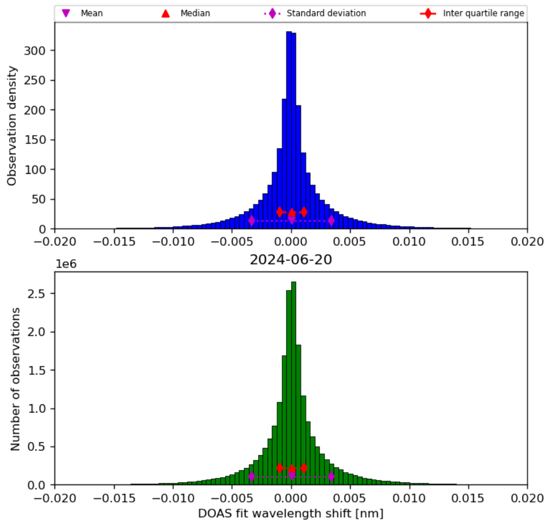
Figure 44: Histogram of “DOAS fit wavelength shift” for 2024-06-19 to 2024-06-21
