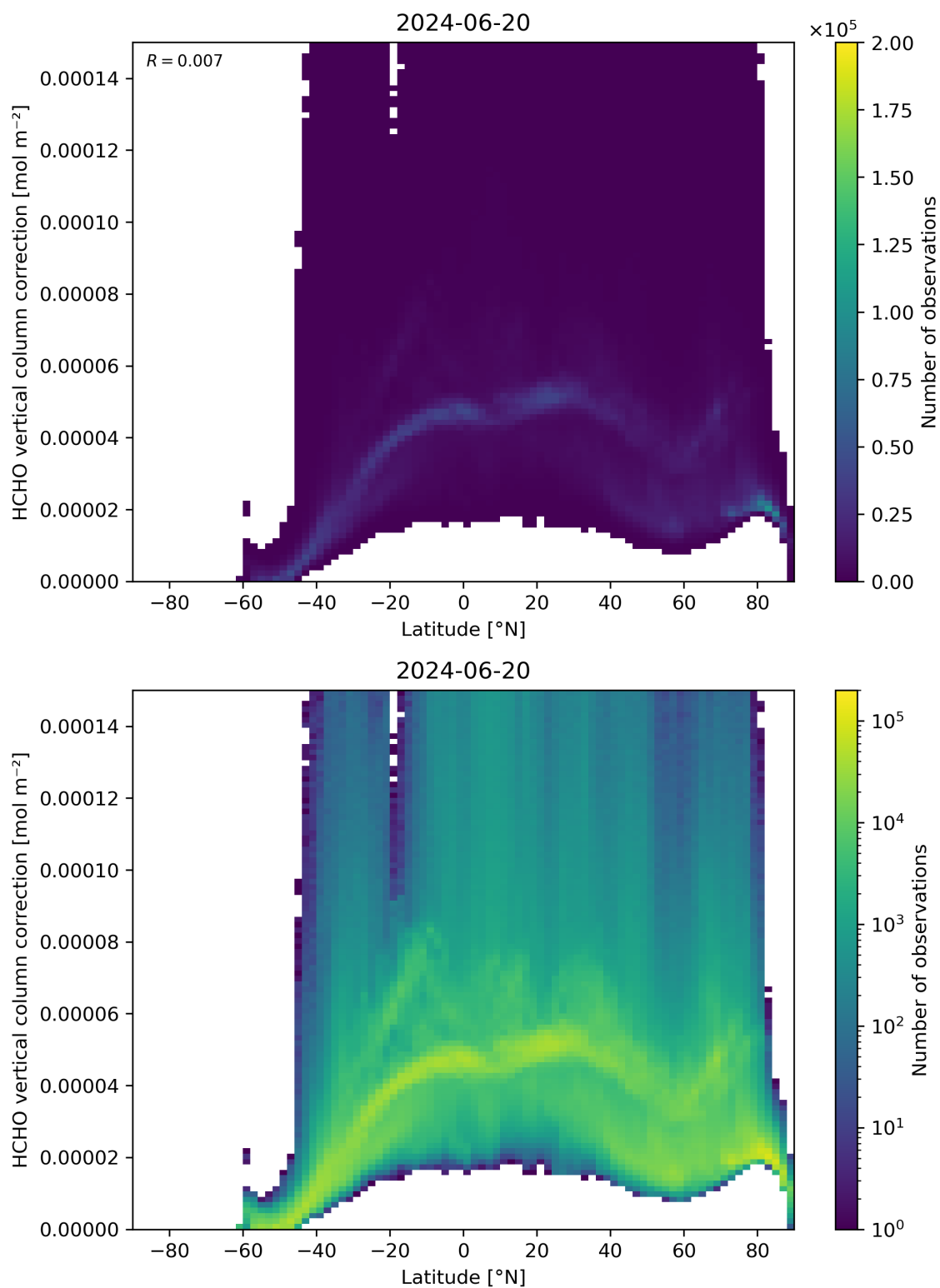
Figure 164: Scatter density plot of “Latitude” against “HCHO vertical column correction” for 2024-06-19 to 2024-06-21.
