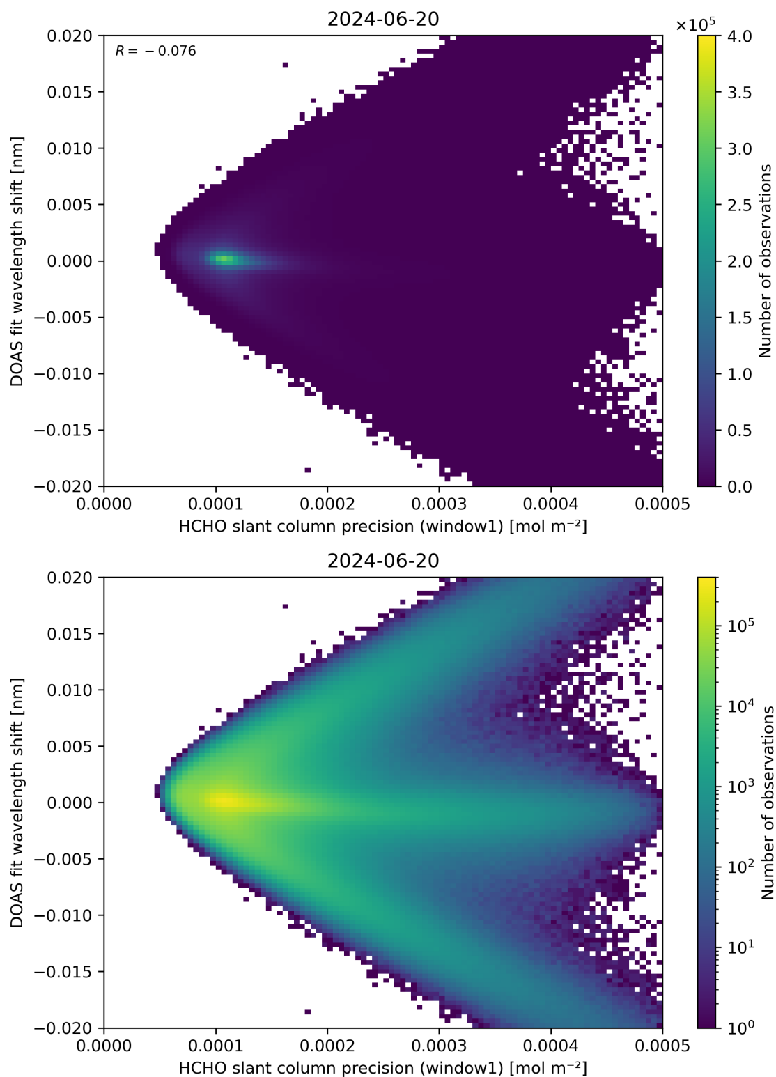
Figure 89: Scatter density plot of “HCHO slant column precision (window1)” against “DOAS fit wavelength shift” for 2024-06-19 to 2024-06-21.
