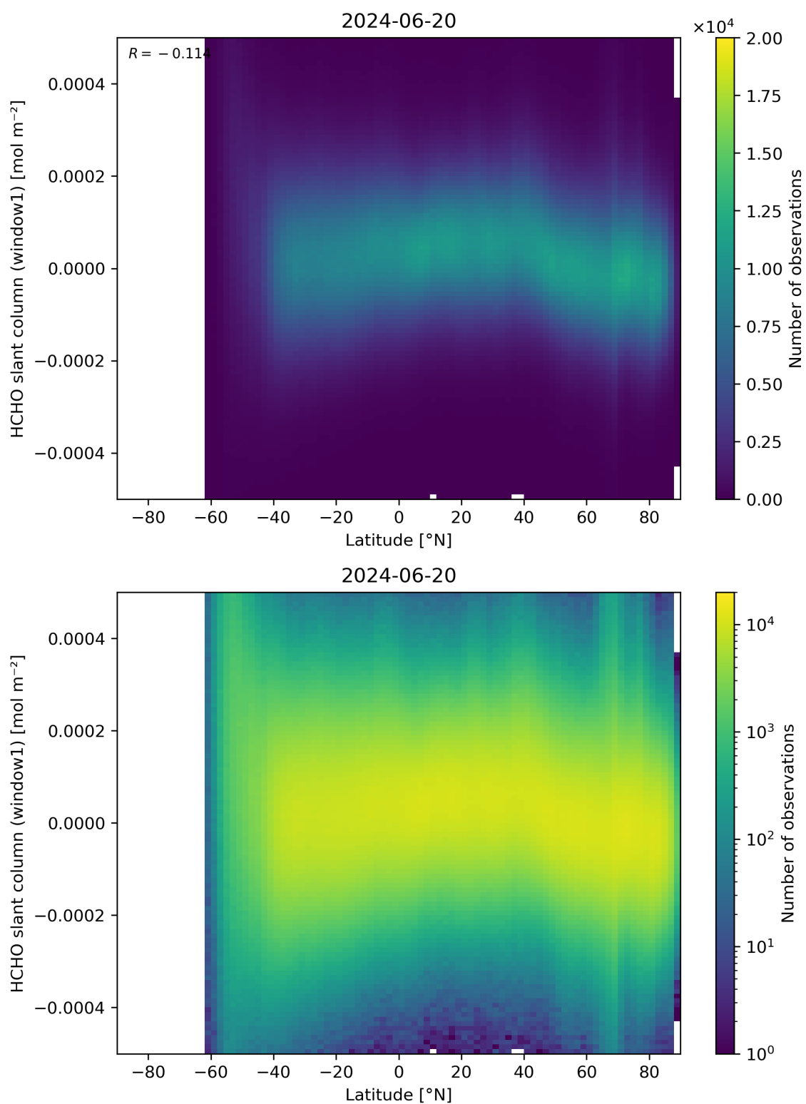
Figure 159: Scatter density plot of “Latitude” against “HCHO slant column (window1)” for 2024-06-19 to 2024-06-21.
