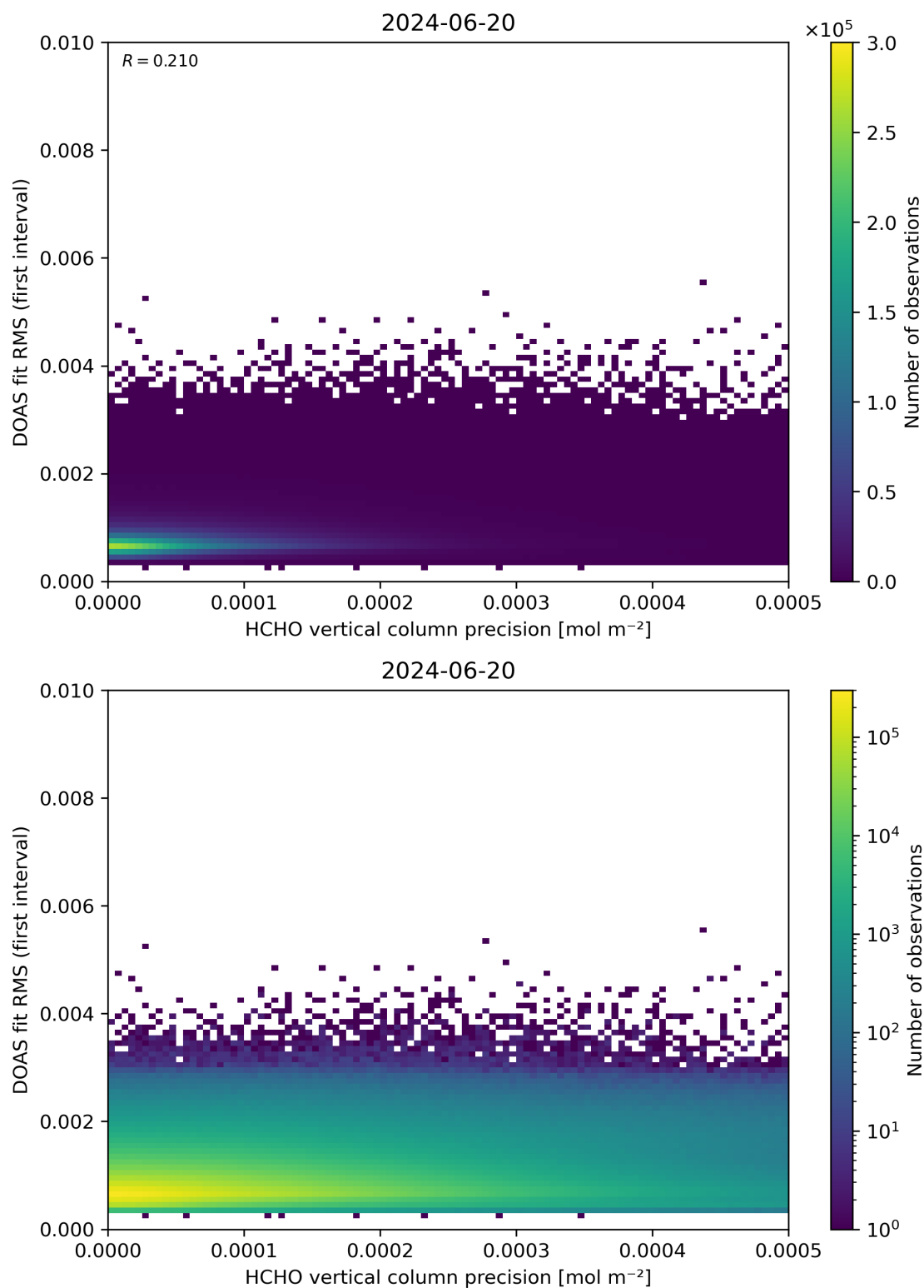
Figure 136: Scatter density plot of “HCHO vertical column precision” against “DOAS fit RMS (first interval)” for 2024-06-19 to 2024-06-21.
