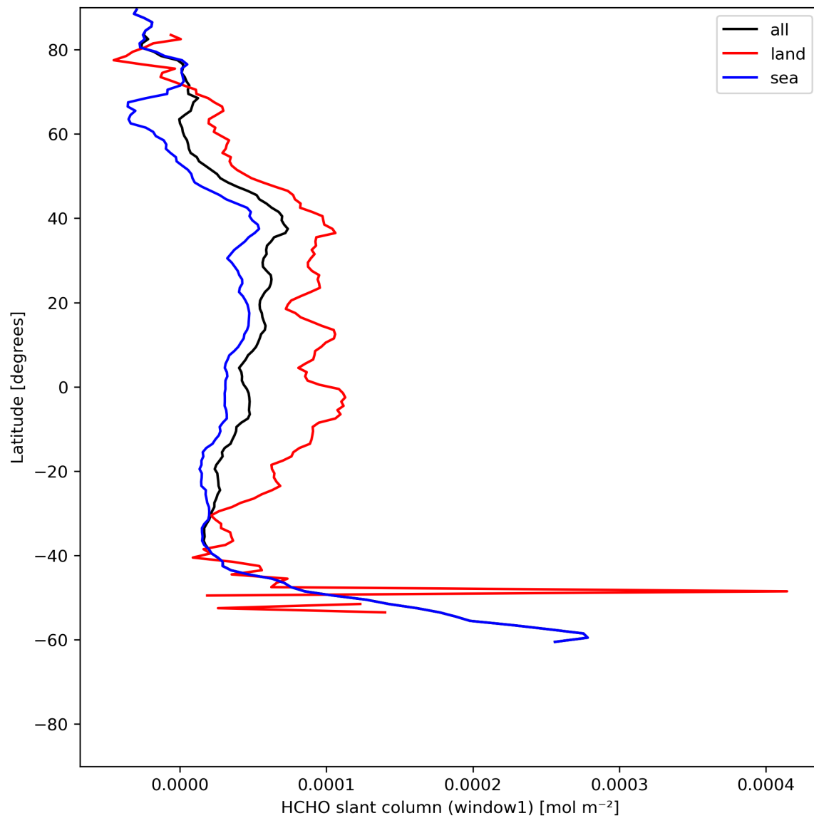
Figure 24: Zonal average of “HCHO slant column (window1)” for 2024-06-19 to 2024-06-21.
