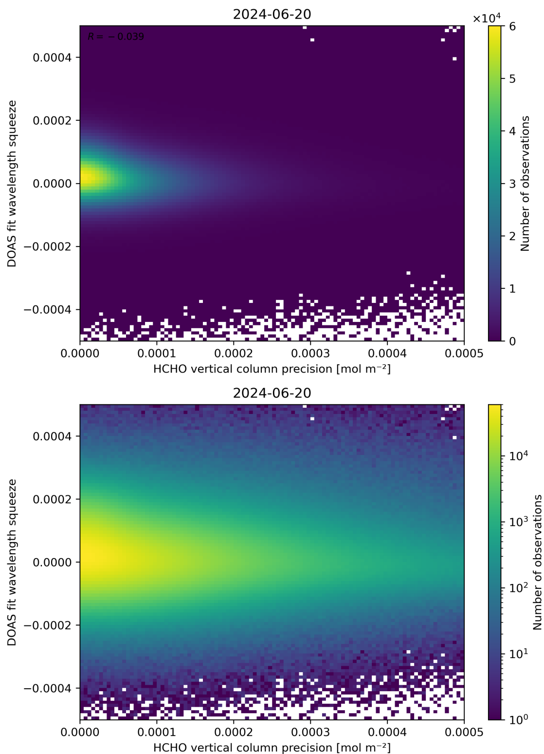
Figure 138: Scatter density plot of “HCHO vertical column precision” against “DOAS fit wavelength squeeze” for 2024-06-19 to 2024-06-21.
