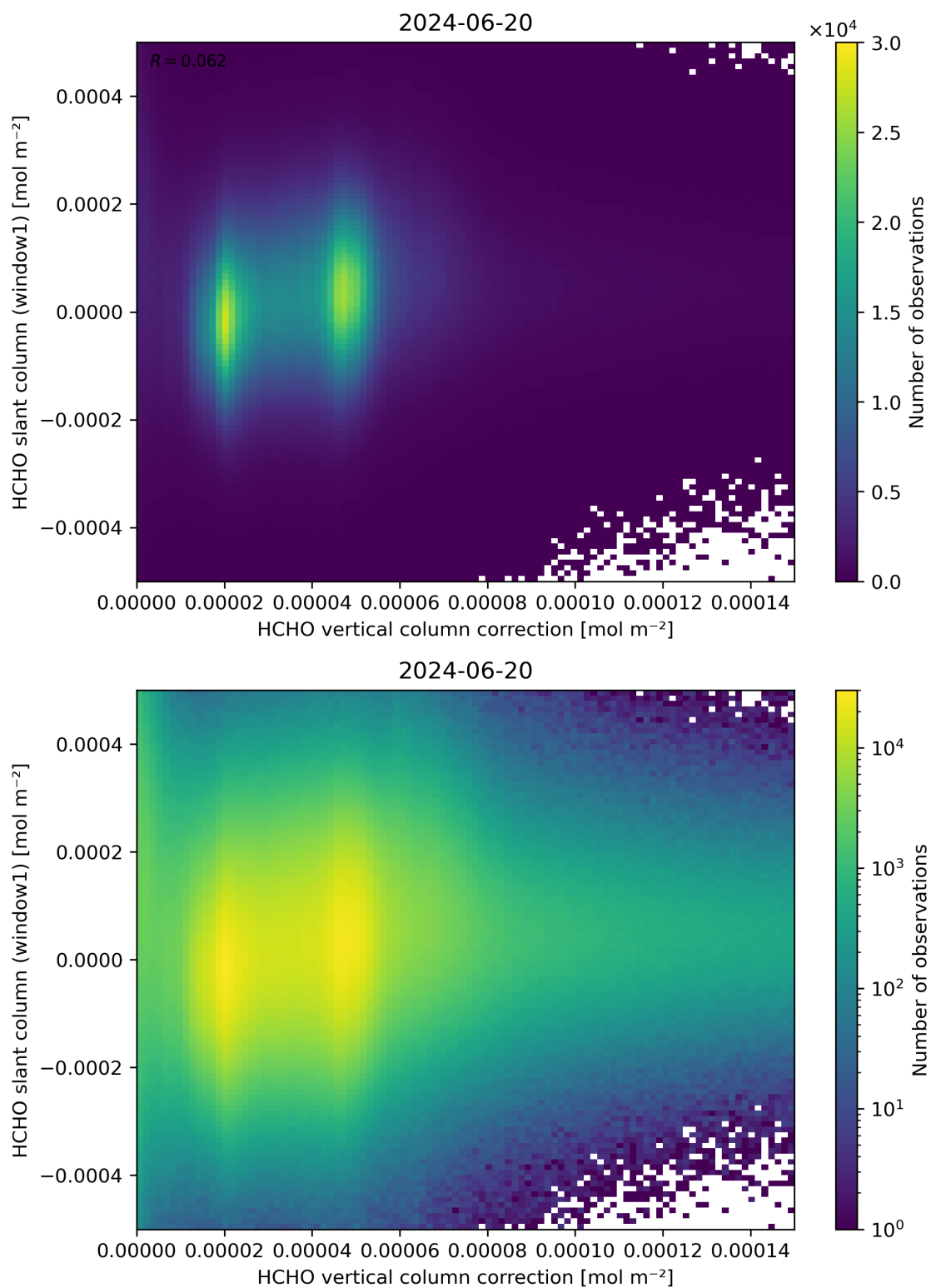
Figure 118: Scatter density plot of “HCHO vertical column correction” against “HCHO slant column (window1)” for 2024-06-19 to 2024-06-21.
