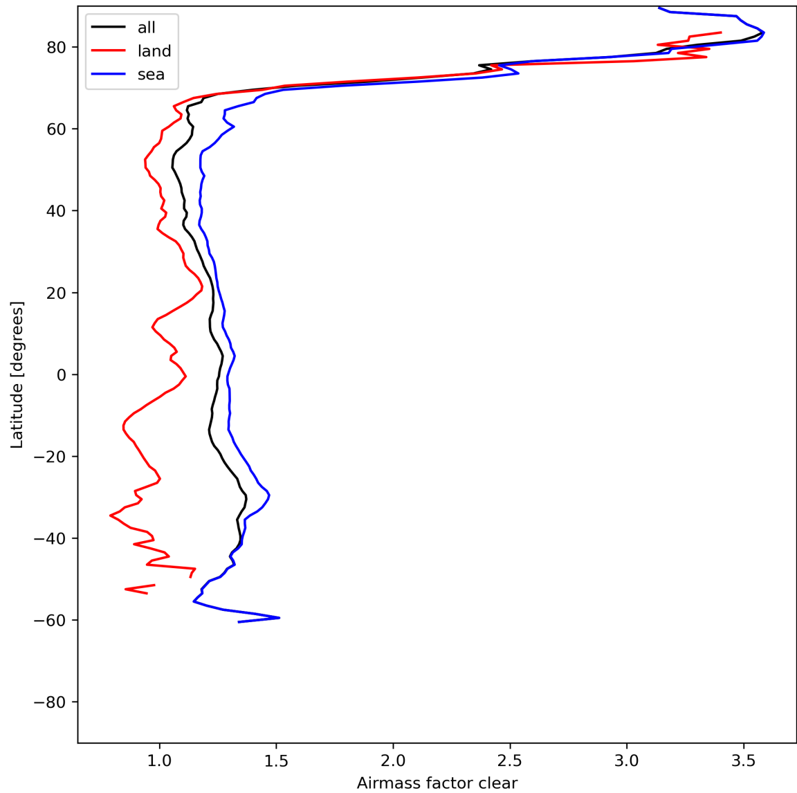
Figure 28: Zonal average of “Airmass factor clear” for 2024-06-19 to 2024-06-21.
