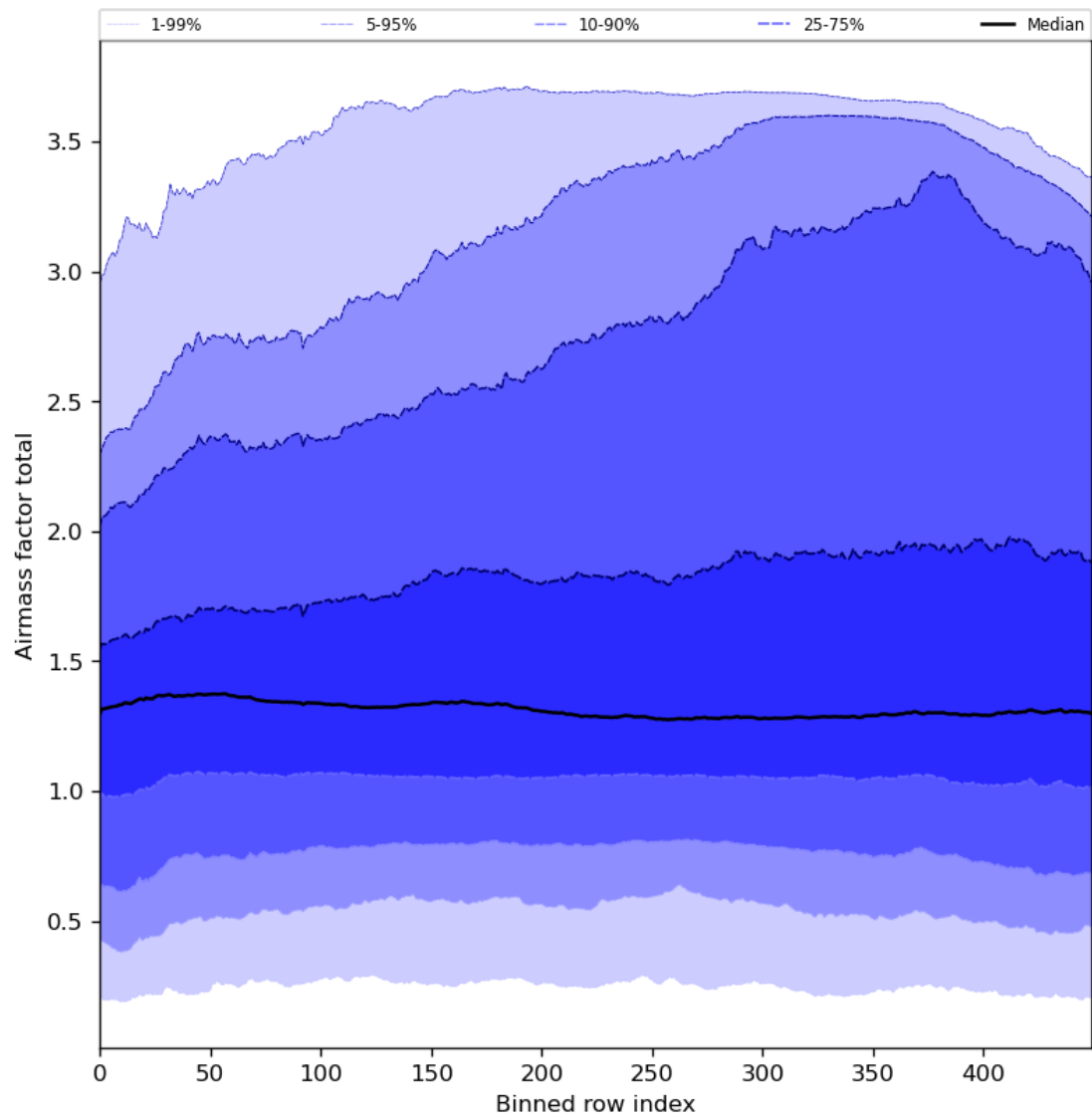
Figure 54: Along track statistics of “Airmass factor total” for 2024-06-19 to 2024-06-21
