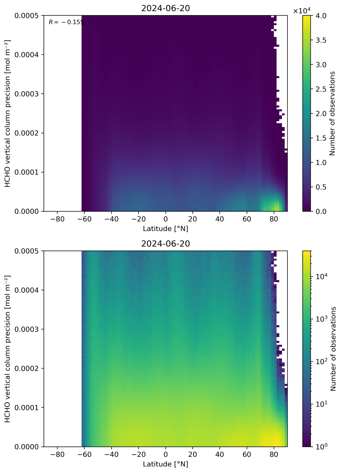
Figure 165: Scatter density plot of “Latitude” against “HCHO vertical column precision” for 2024-06-19 to 2024-06-21.
