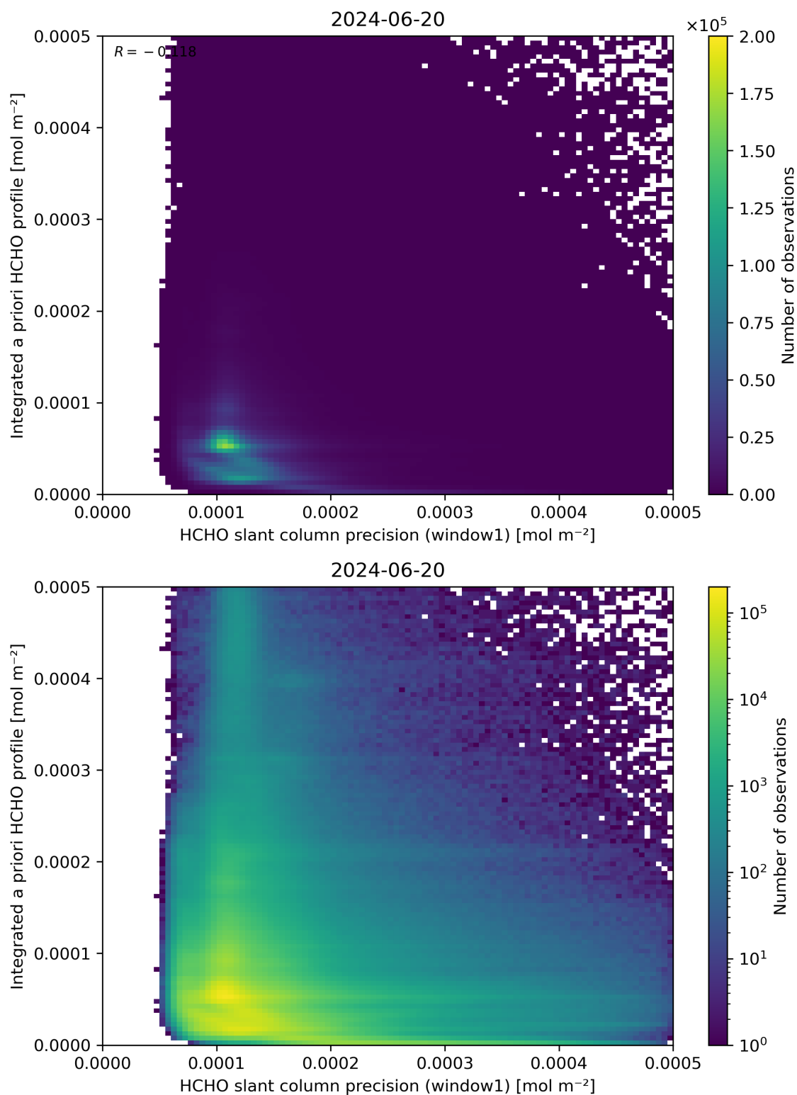
Figure 96: Scatter density plot of “HCHO slant column precision (window1)” against “Integrated a priori HCHO profile” for 2024-06-19 to 2024-06-21.
