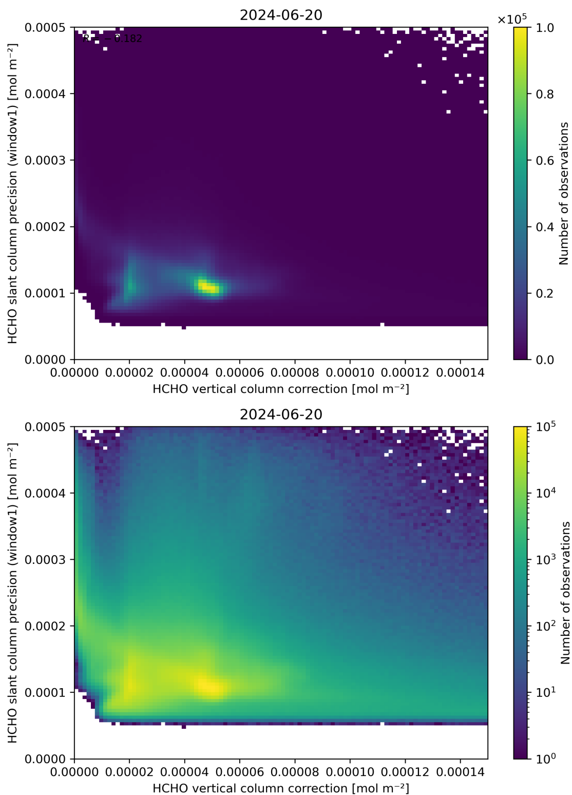
Figure 119: Scatter density plot of “HCHO vertical column correction” against “HCHO slant column precision (window1)” for 2024-06-19 to 2024-06-21.
