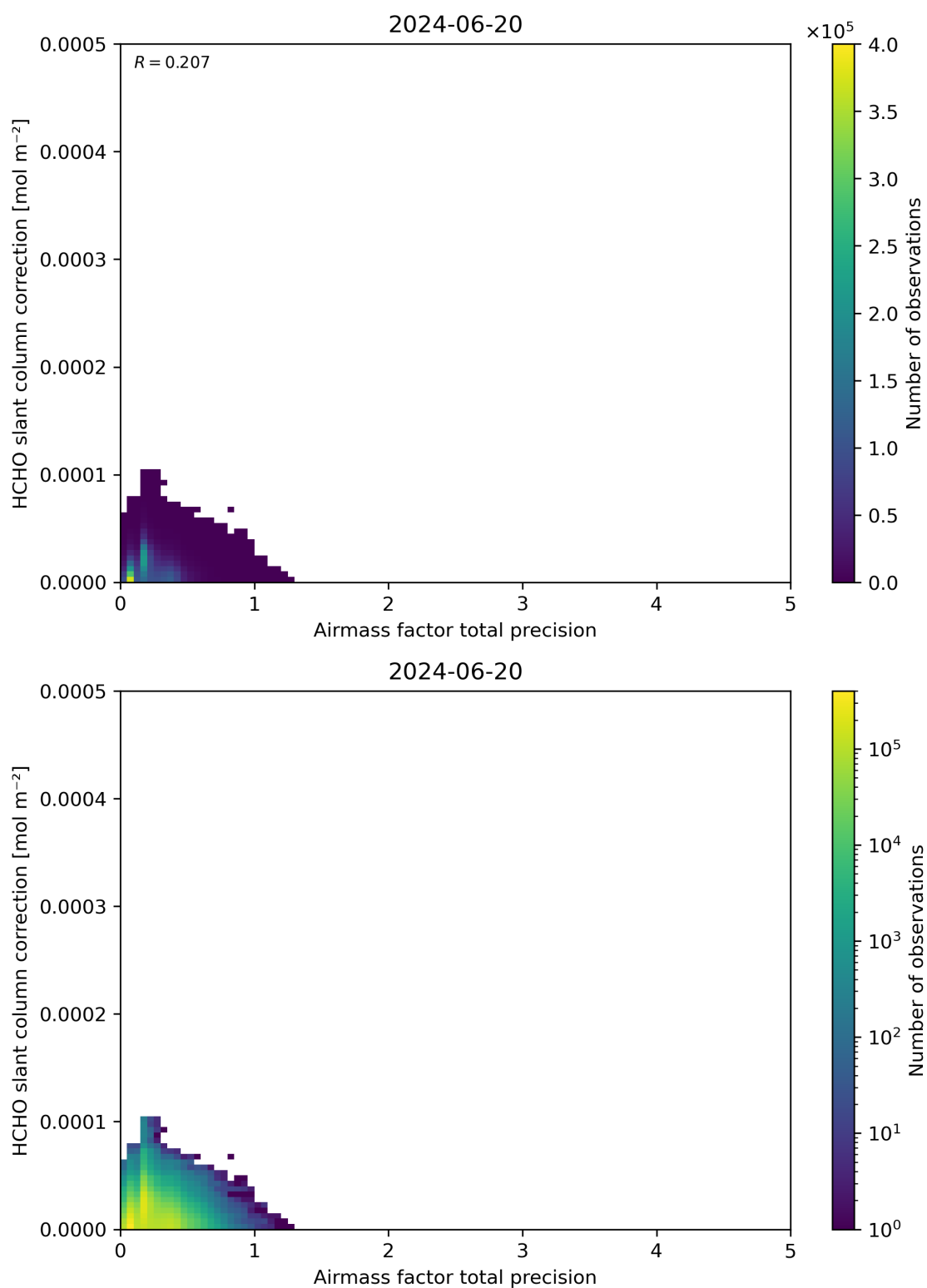
Figure 110: Scatter density plot of “Airmass factor total precision” against “HCHO slant column correction” for 2024-06-19 to 2024-06-21.
