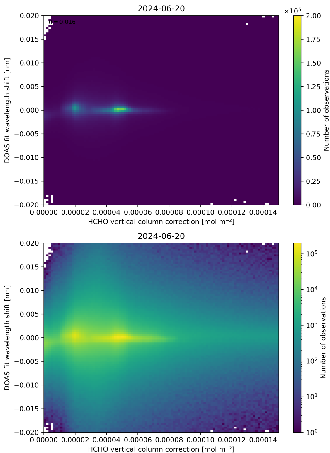
Figure 113: Scatter density plot of “HCHO vertical column correction” against “DOAS fit wavelength shift” for 2024-06-19 to 2024-06-21.
