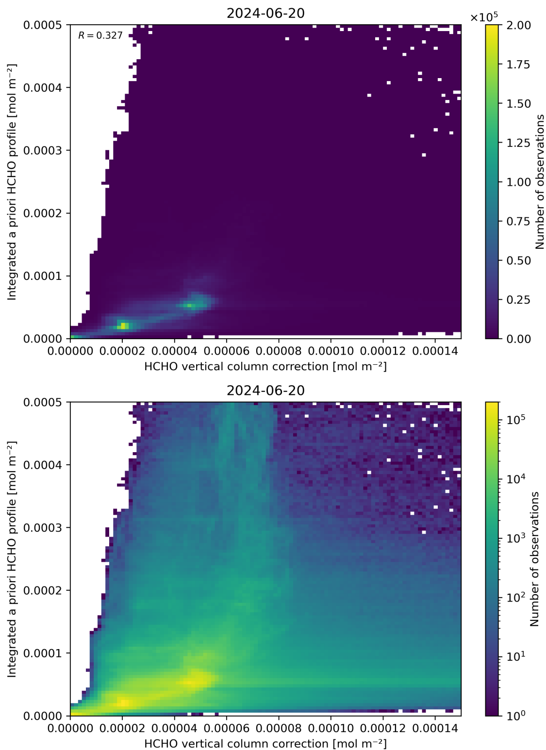
Figure 122: Scatter density plot of “HCHO vertical column correction” against “Integrated a priori HCHO profile” for 2024-06-19 to 2024-06-21.
