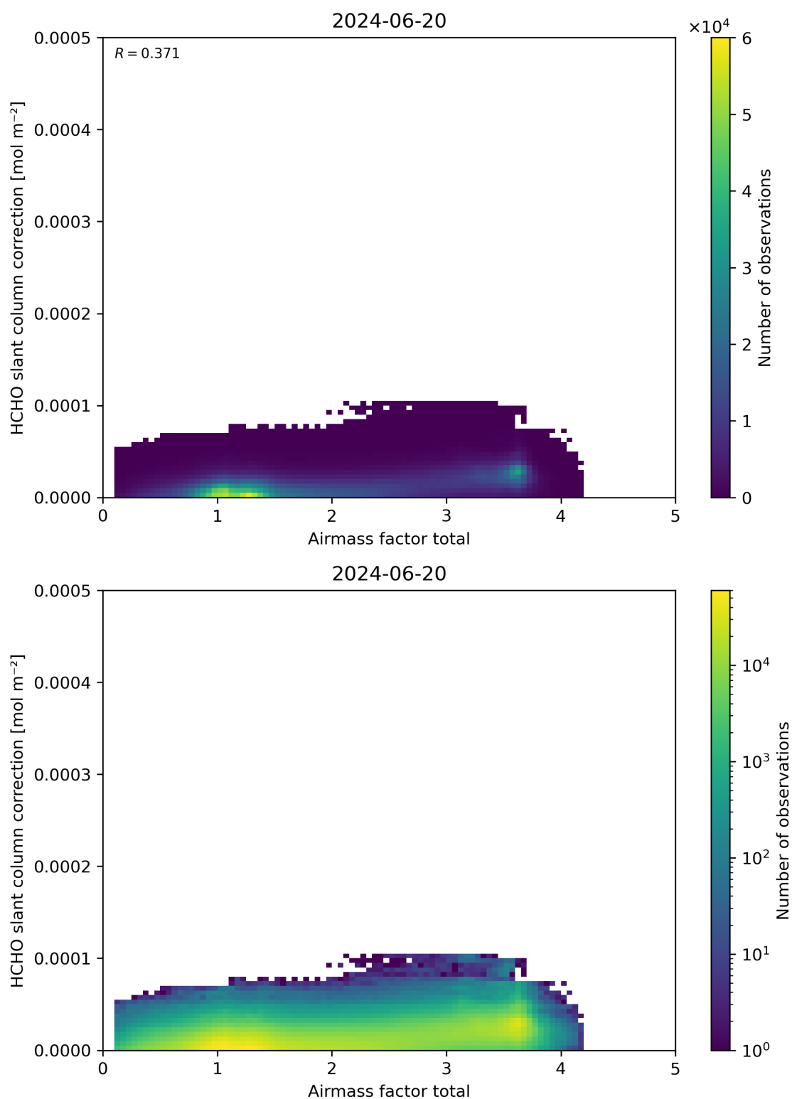
Figure 102: Scatter density plot of “Airmass factor total” against “HCHO slant column correction” for 2024-06-19 to 2024-06-21.
