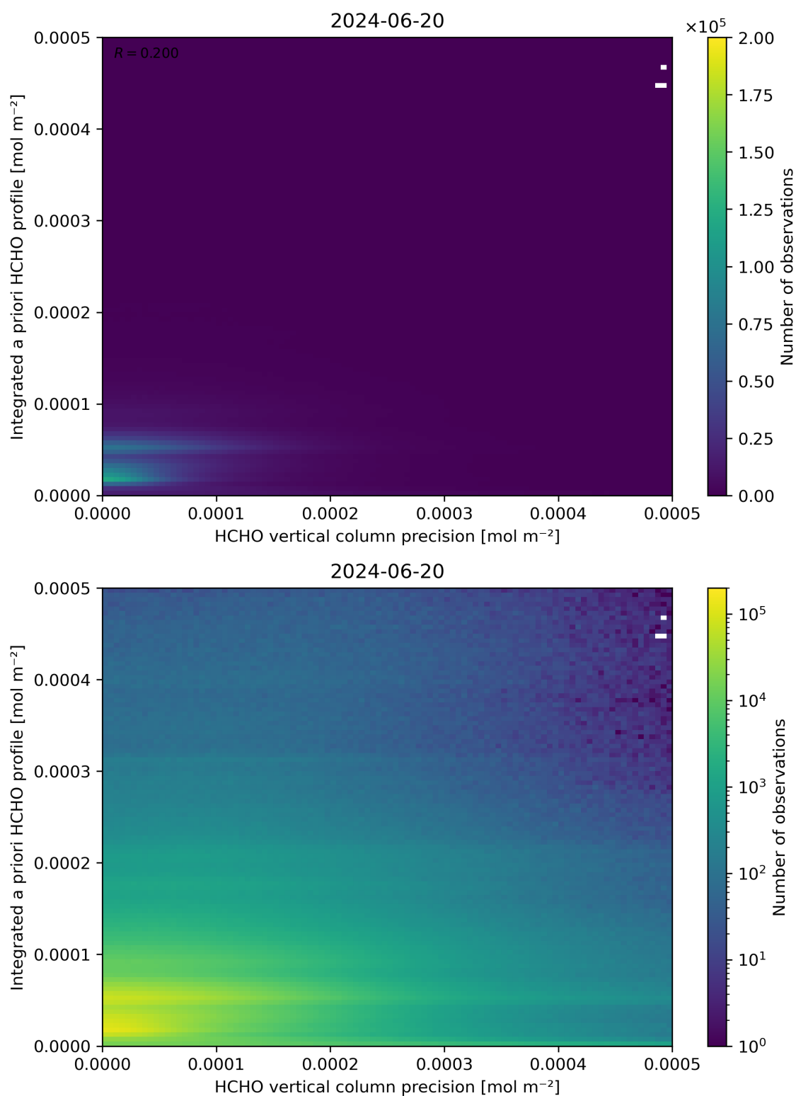
Figure 147: Scatter density plot of “HCHO vertical column precision” against “Integrated a priori HCHO profile” for 2024-06-19 to 2024-06-21.
