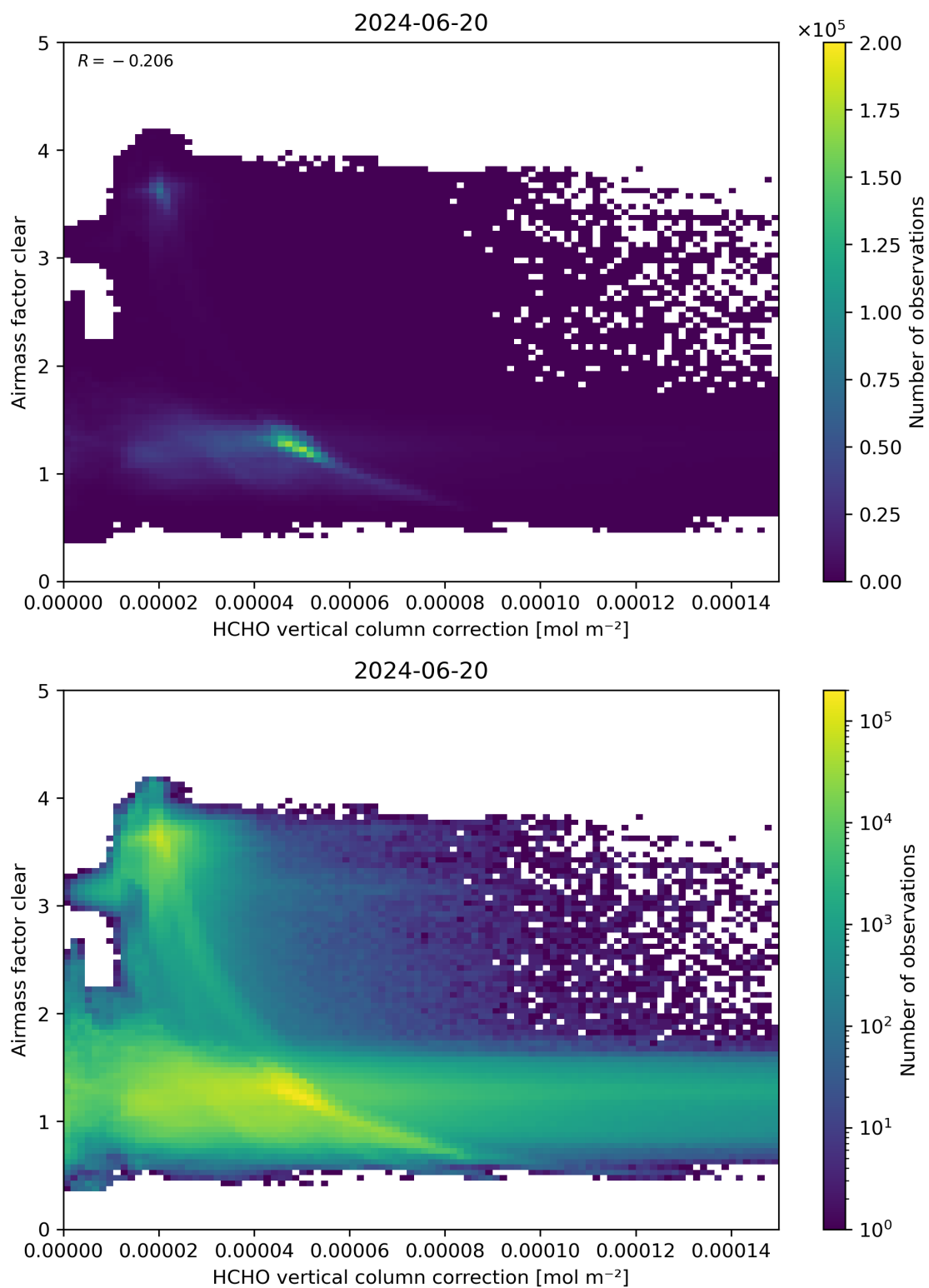
Figure 115: Scatter density plot of “HCHO vertical column correction” against “Airmass factor clear” for 2024-06-19 to 2024-06-21.
