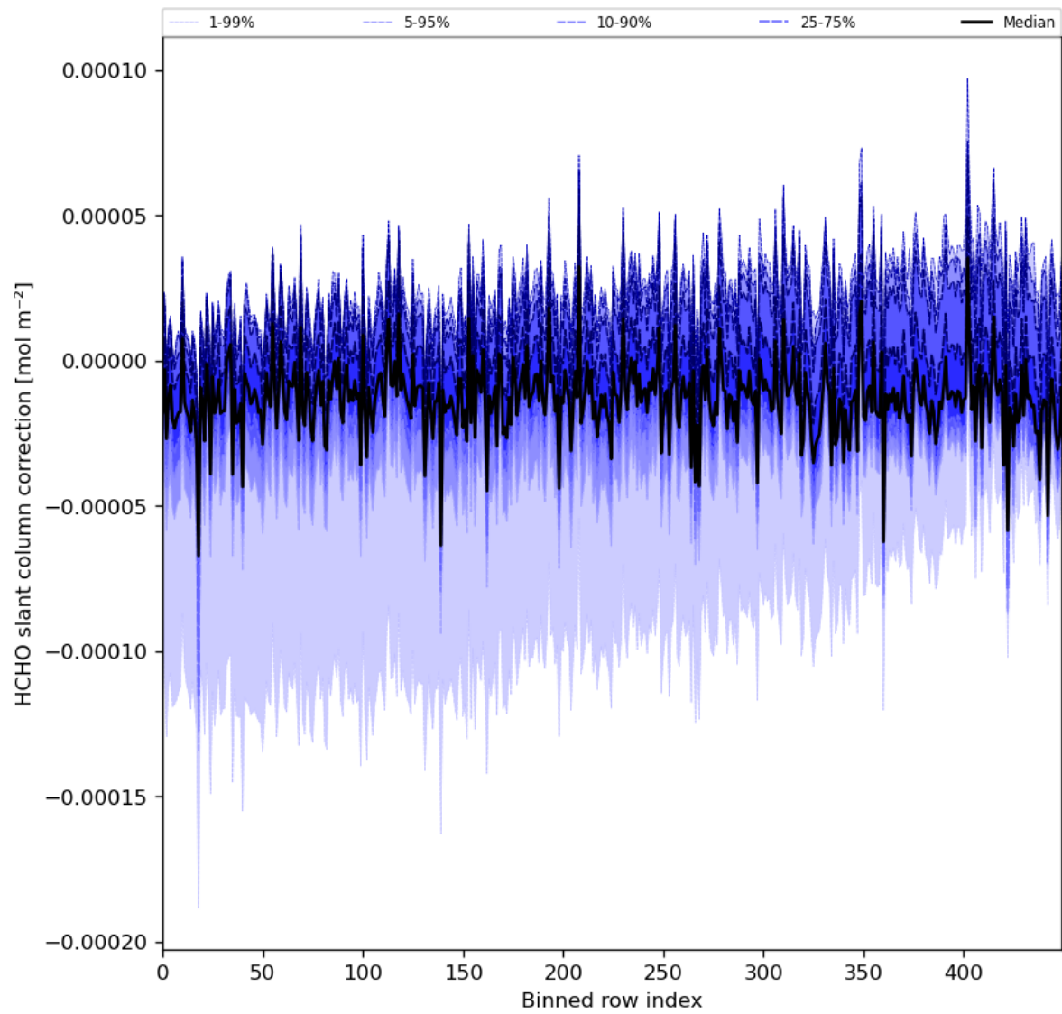
Figure 61: Along track statistics of “HCHO slant column correction” for 2024-06-19 to 2024-06-21
