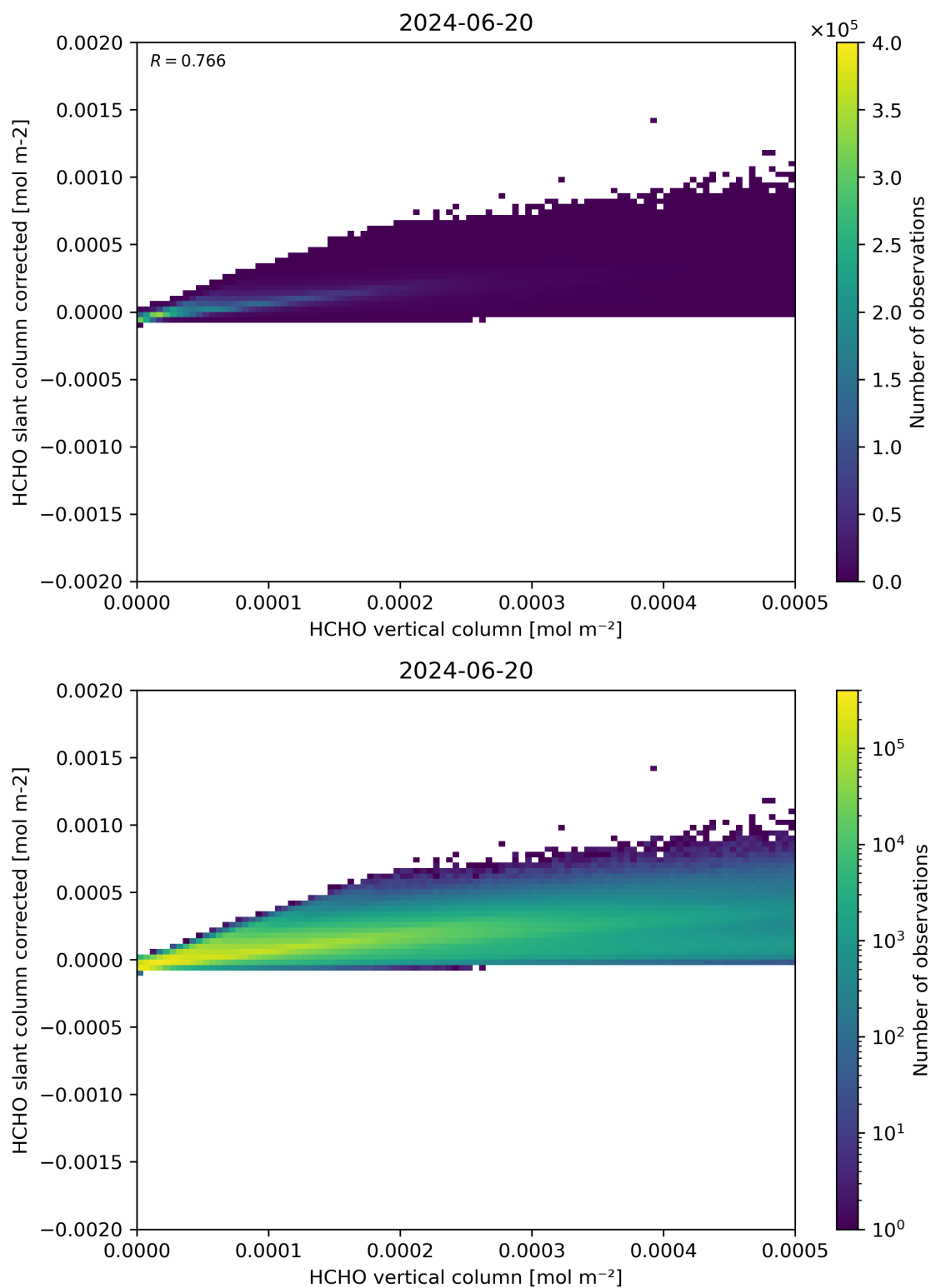
Figure 127: Scatter density plot of “HCHO vertical column” against “HCHO slant column corrected” for 2024-06-19 to 2024-06-21.
