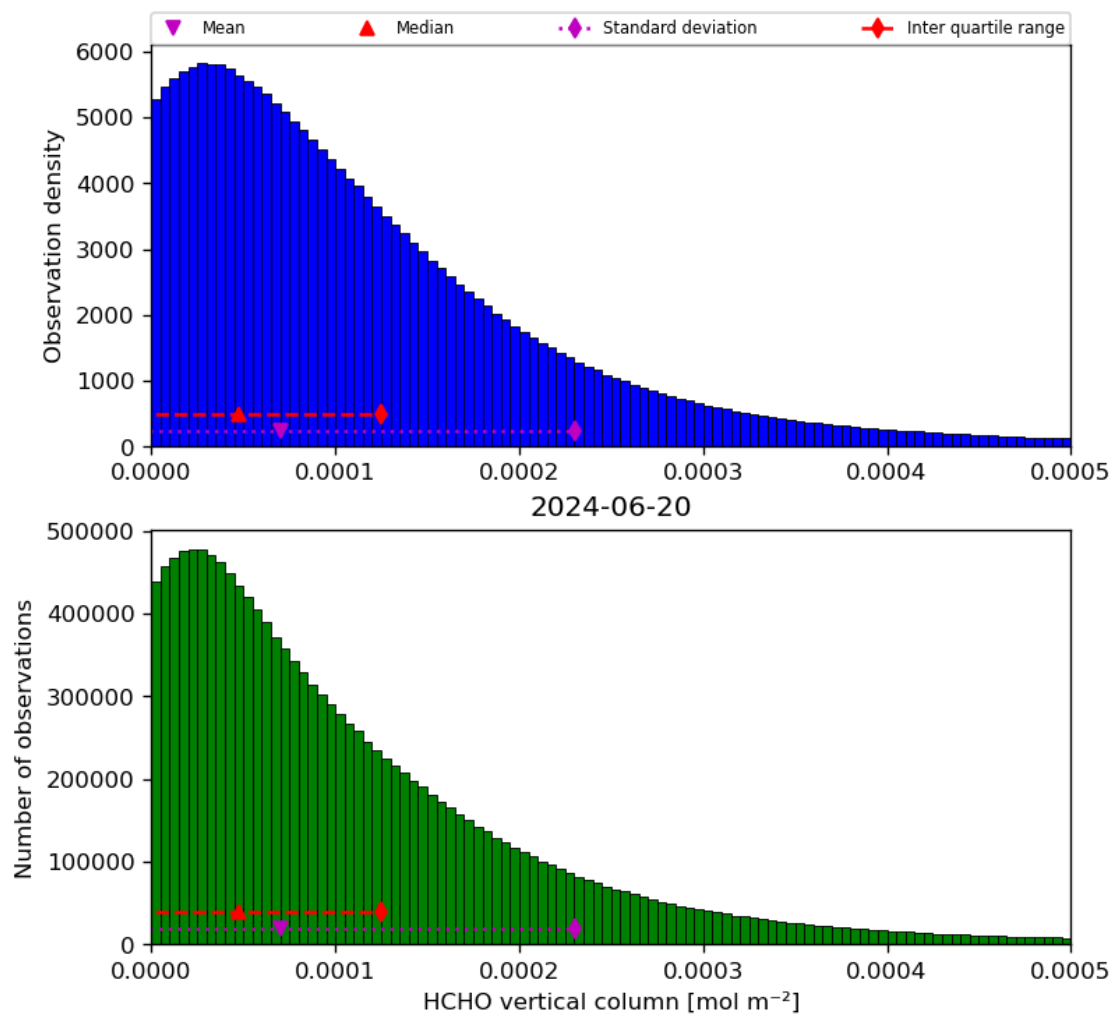
Figure 35: Histogram of “HCHO vertical column” for 2024-06-19 to 2024-06-21
