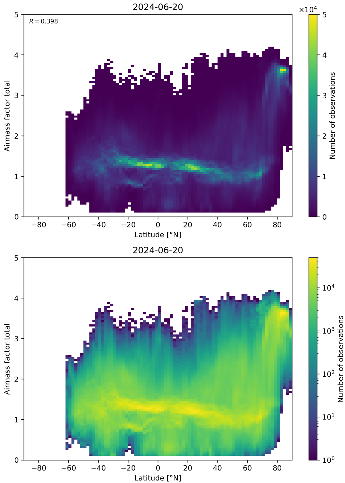
Figure 161: Scatter density plot of “Latitude” against “Airmass factor total” for 2024-06-19 to 2024-06-21.
