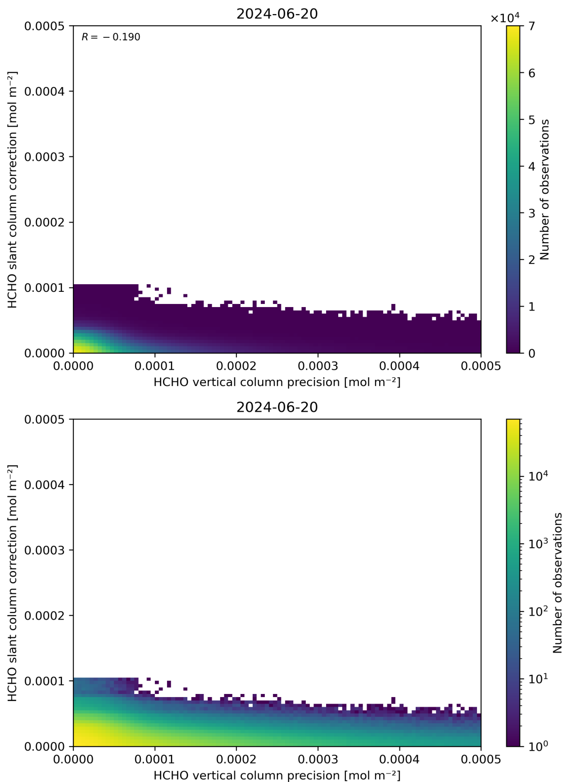
Figure 141: Scatter density plot of “HCHO vertical column precision” against “HCHO slant column correction” for 2024-06-19 to 2024-06-21.
