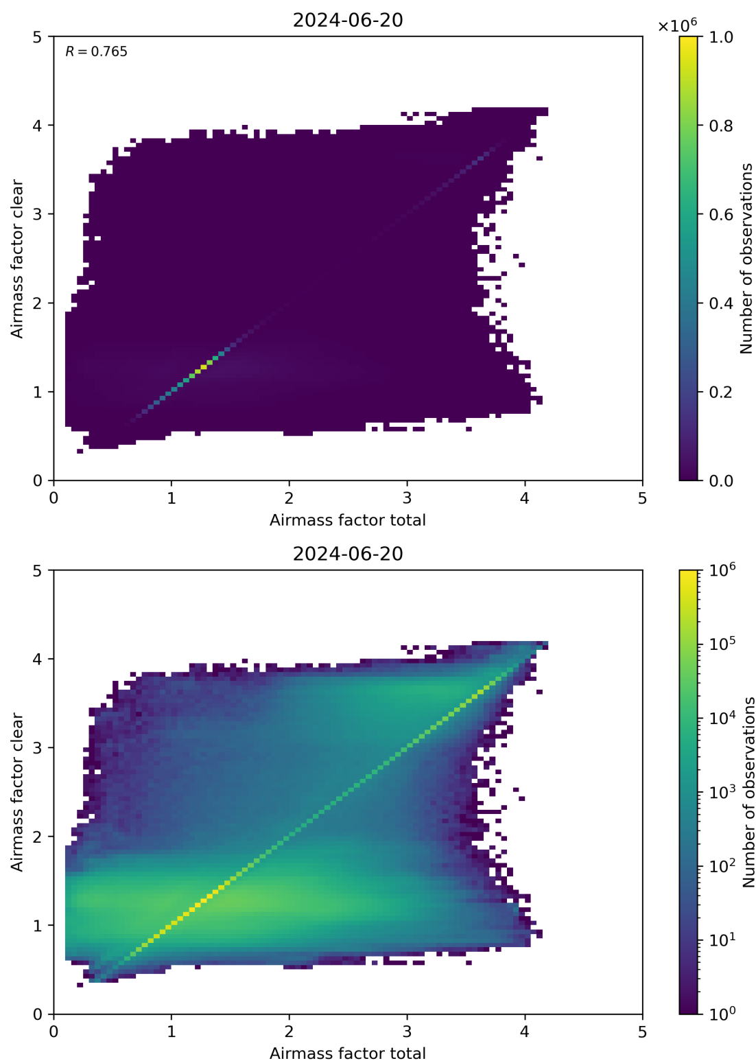
Figure 100: Scatter density plot of “Airmass factor total” against “Airmass factor clear” for 2024-06-19 to 2024-06-21.
