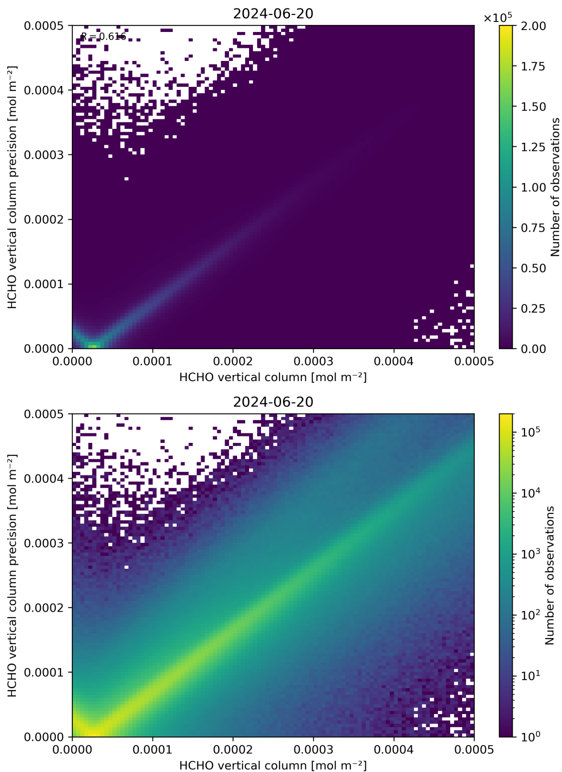
Figure 134: Scatter density plot of “HCHO vertical column” against “HCHO vertical column precision” for 2024-06-19 to 2024-06-21.
