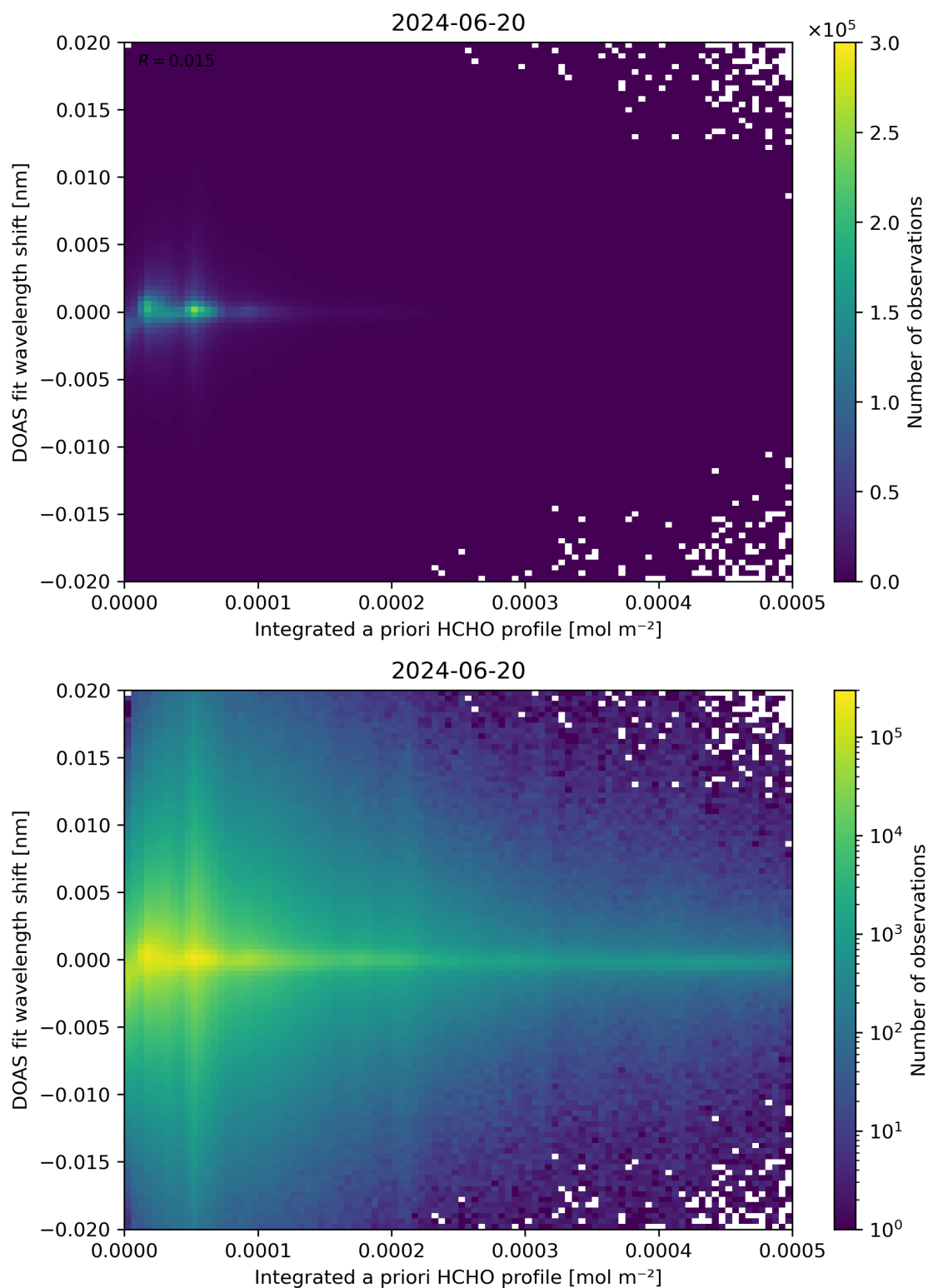
Figure 149: Scatter density plot of “Integrated a priori HCHO profile” against “DOAS fit wavelength shift” for 2024-06-19 to 2024-06-21.
