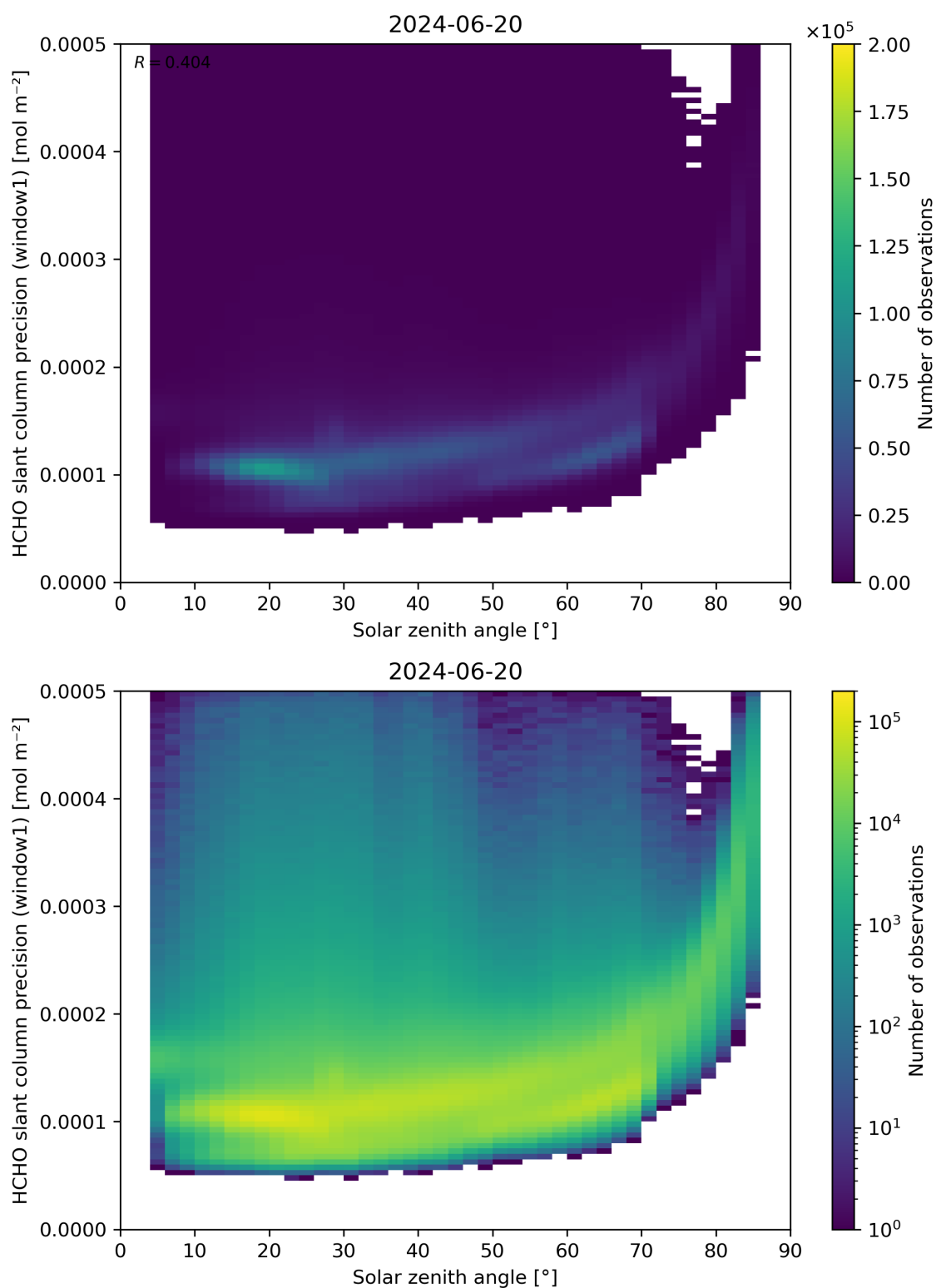
Figure 174: Scatter density plot of “Solar zenith angle” against “HCHO slant column precision (window1)” for 2024-06-19 to 2024-06-21.
