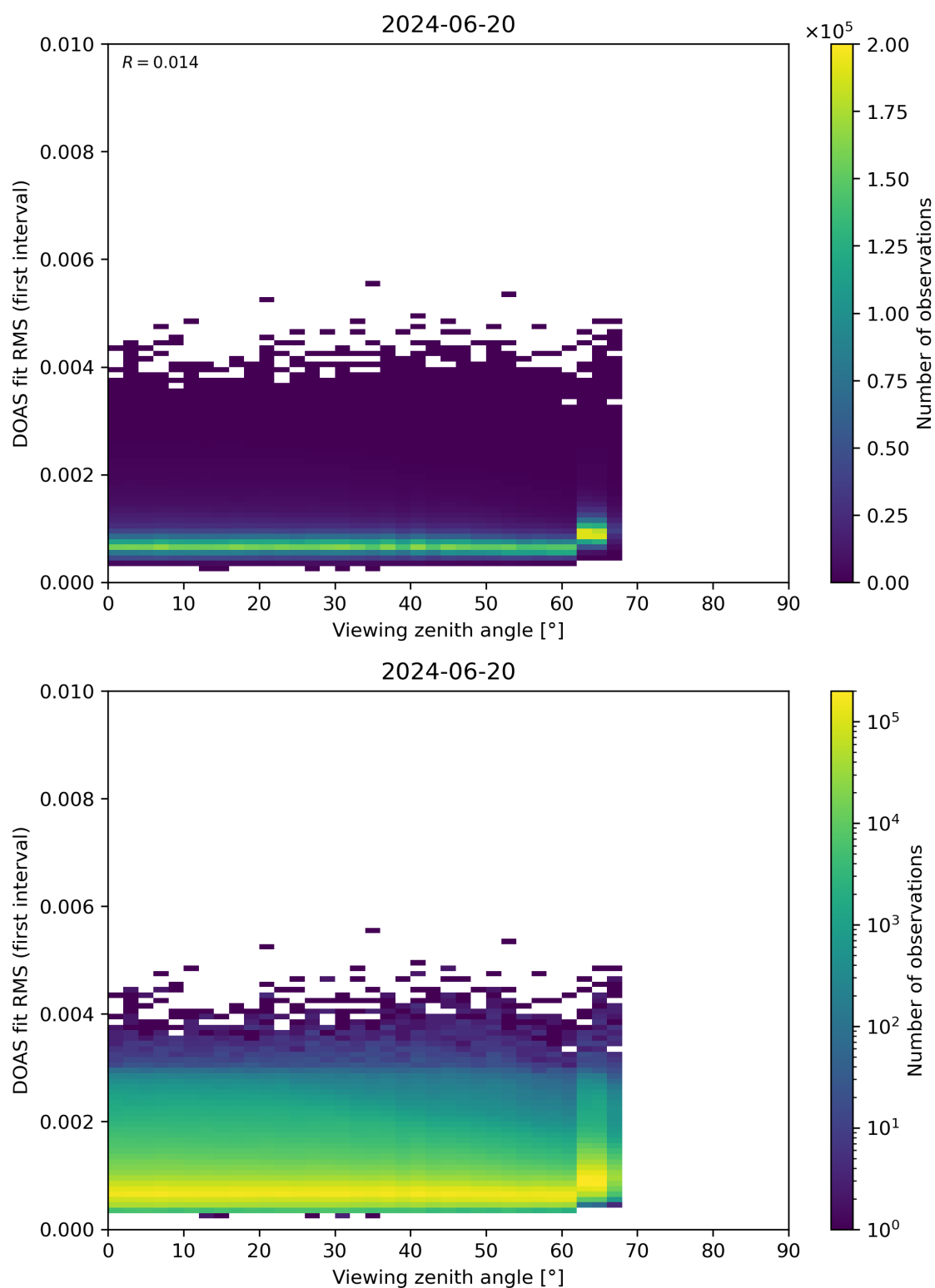
Figure 182: Scatter density plot of “Viewing zenith angle” against “DOAS fit RMS (first interval)” for 2024-06-19 to 2024-06-21.
