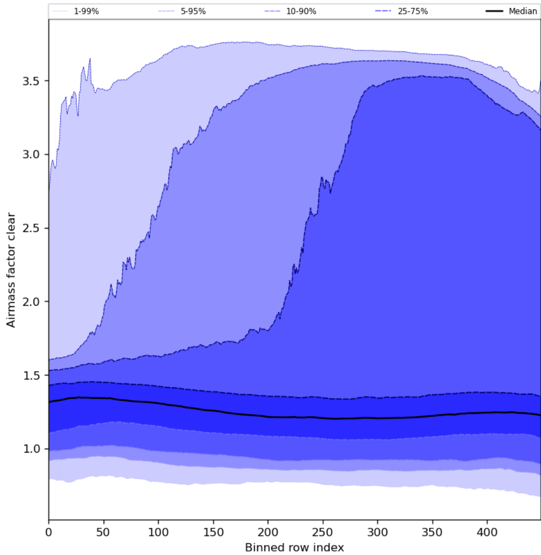
Figure 56: Along track statistics of “Airmass factor clear” for 2024-06-19 to 2024-06-21
