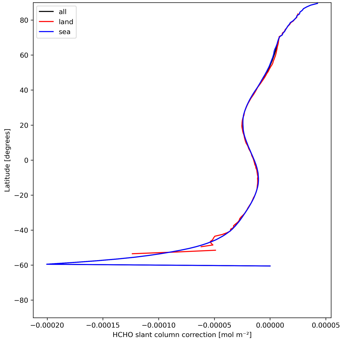
Figure 33: Zonal average of “HCHO slant column correction” for 2024-06-19 to 2024-06-21.
