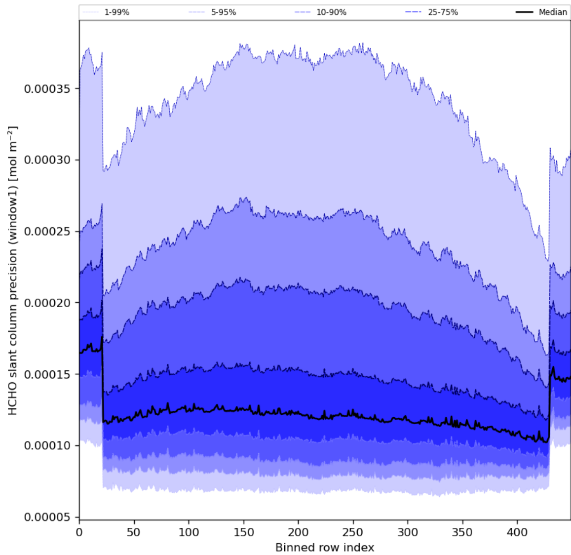
Figure 53: Along track statistics of “HCHO slant column precision (window1)” for 2024-06-19 to 2024-06-21
