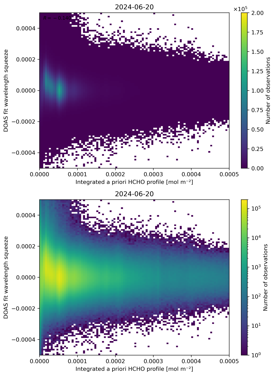
Figure 150: Scatter density plot of “Integrated a priori HCHO profile” against “DOAS fit wavelength squeeze” for 2024-06-19 to 2024-06-21.
