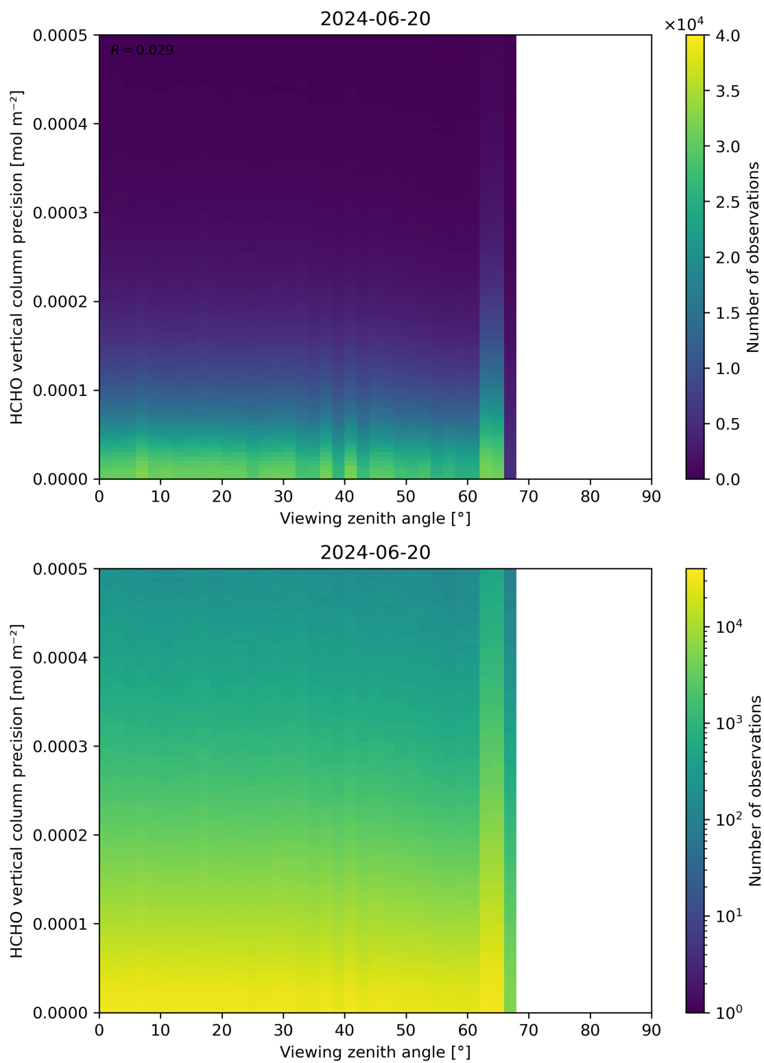
Figure 194: Scatter density plot of “Viewing zenith angle” against “HCHO vertical column precision” for 2024-06-19 to 2024-06-21.
