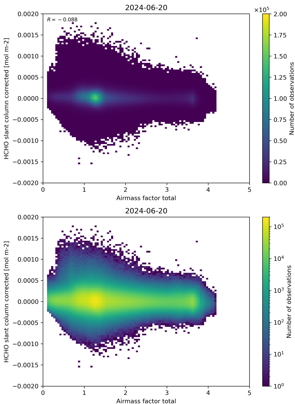
Figure 101: Scatter density plot of “Airmass factor total” against “HCHO slant column corrected” for 2024-06-19 to 2024-06-21.
