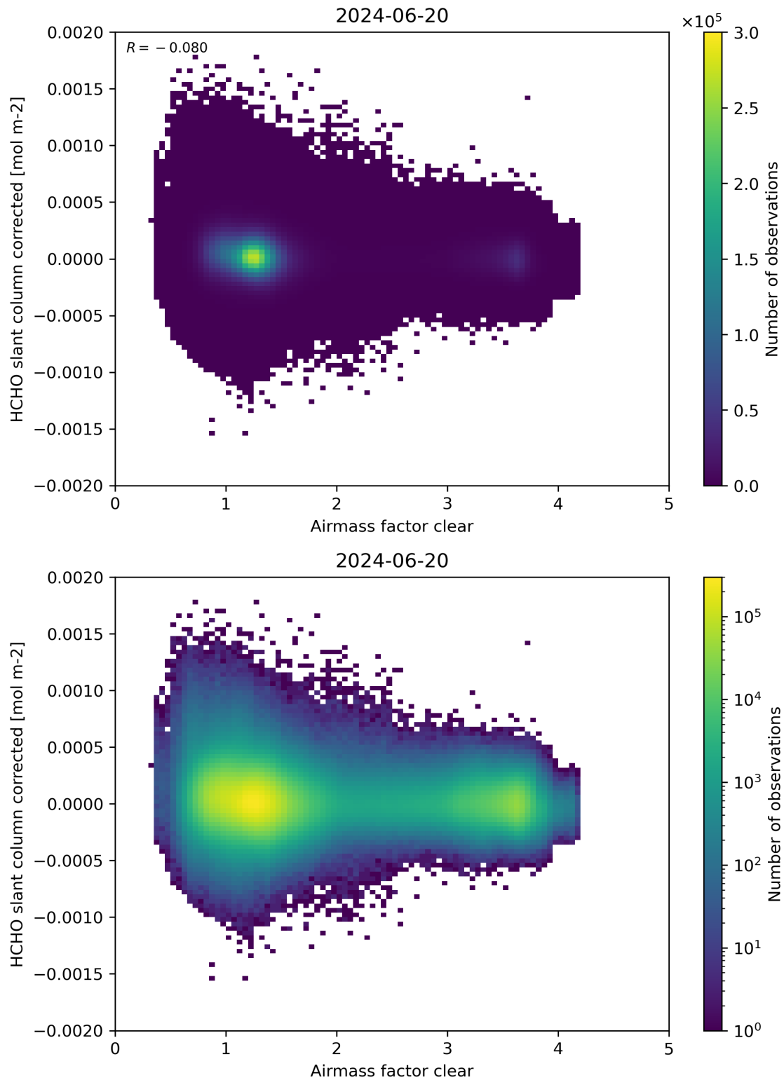
Figure 74: Scatter density plot of “Airmass factor clear” against “HCHO slant column corrected” for 2024-06-19 to 2024-06-21.
