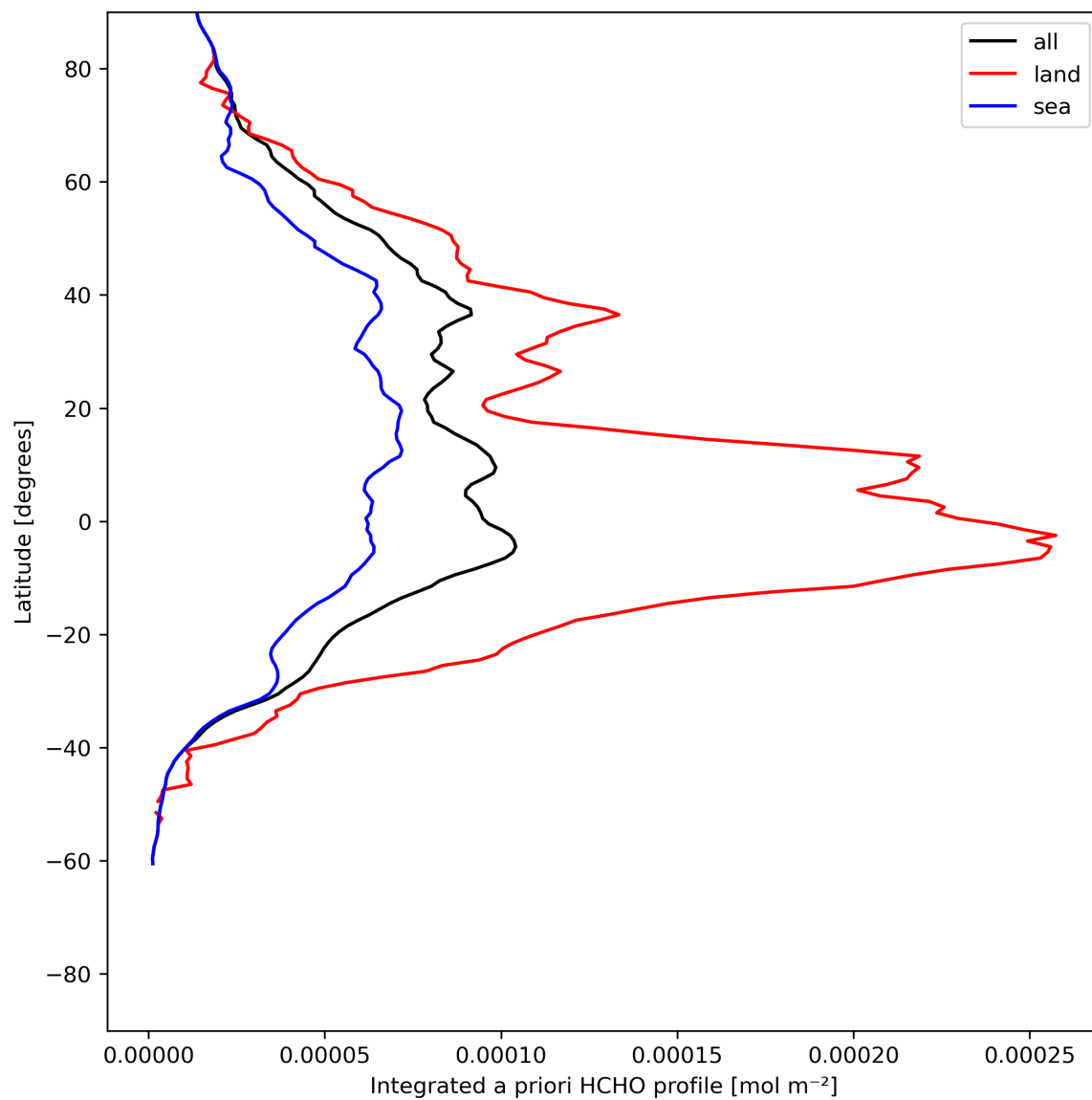
Figure 29: Zonal average of “Integrated a priori HCHO profile” for 2024-06-19 to 2024-06-21.
