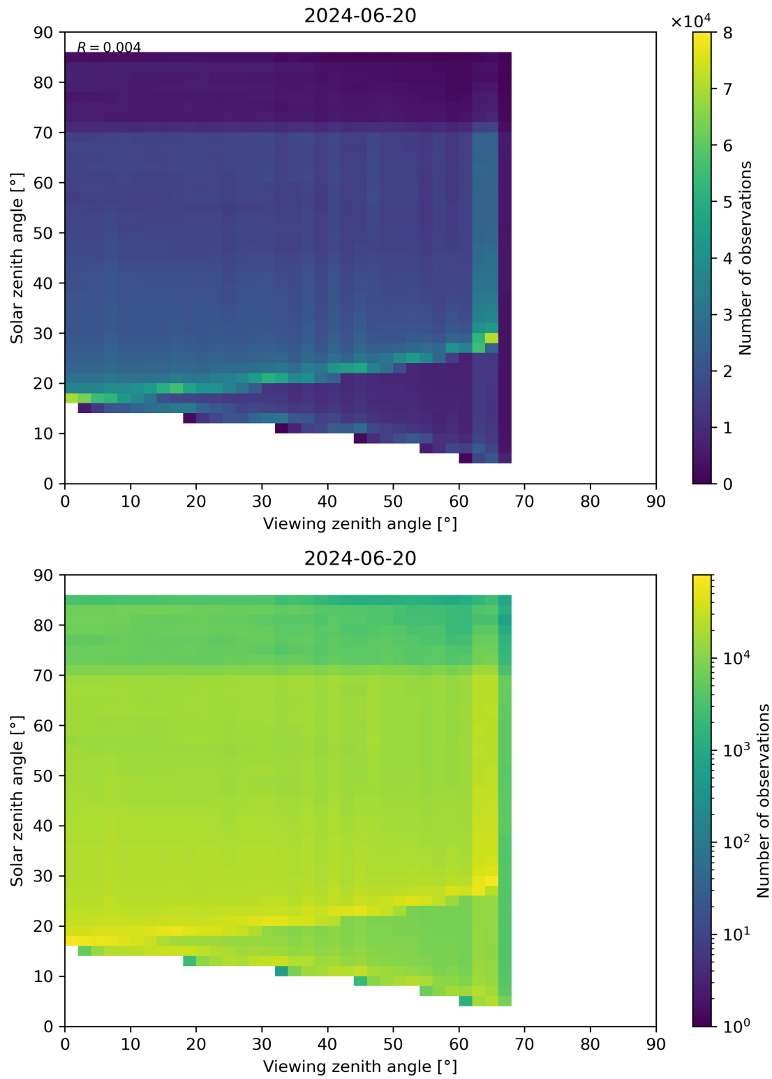
Figure 197: Scatter density plot of “Viewing zenith angle” against “Solar zenith angle” for 2024-06-19 to 2024-06-21.
