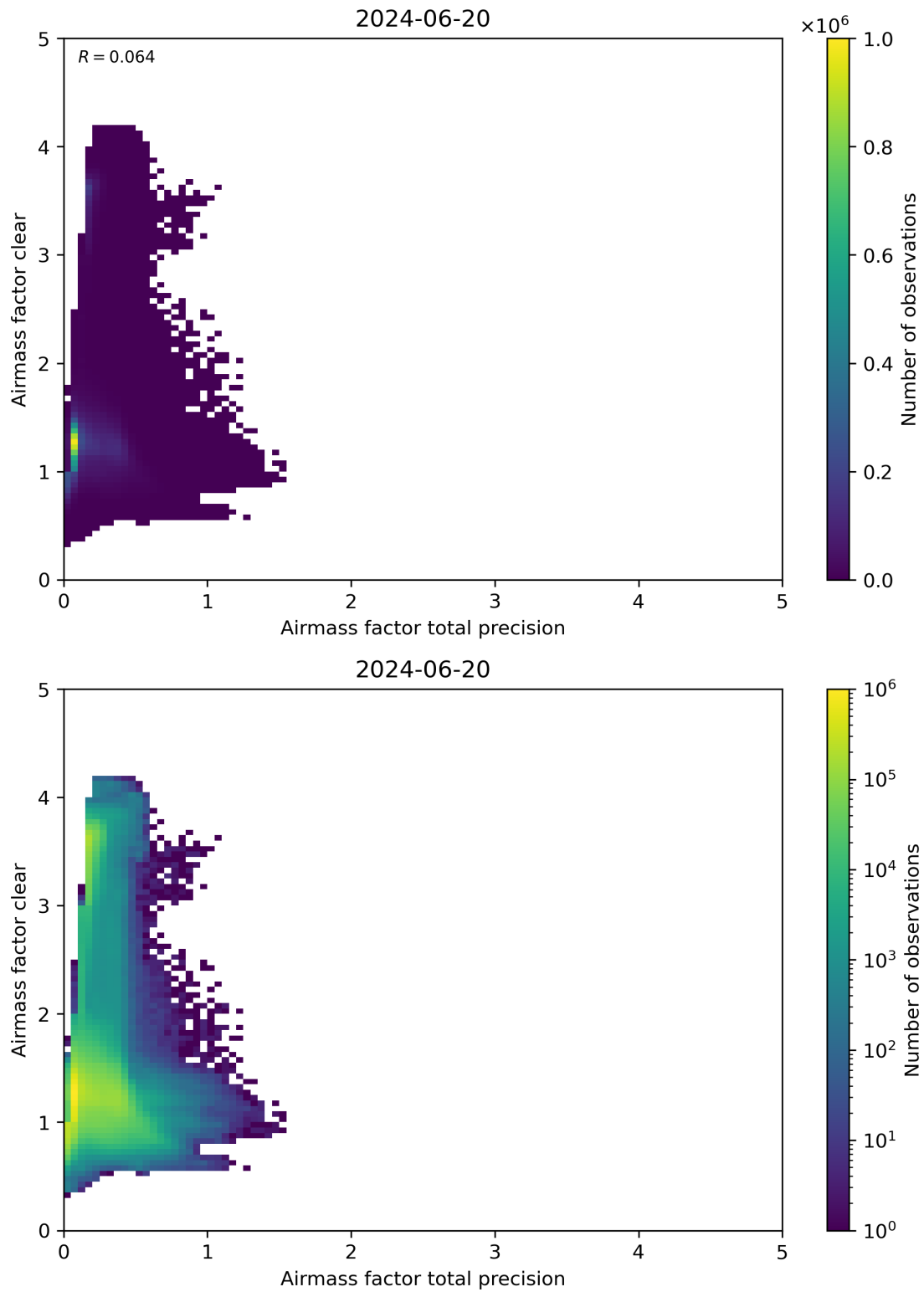
Figure 108: Scatter density plot of “Airmass factor total precision” against “Airmass factor clear” for 2024-06-19 to 2024-06-21.
