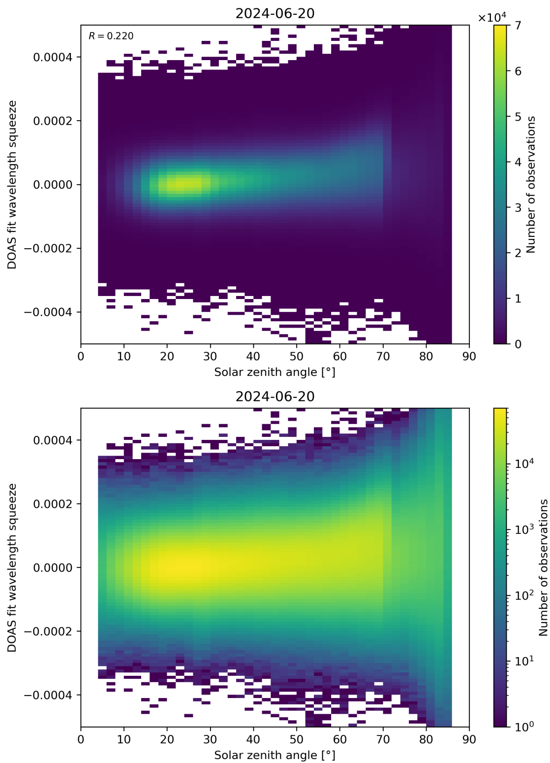
Figure 169: Scatter density plot of “Solar zenith angle” against “DOAS fit wavelength squeeze” for 2024-06-19 to 2024-06-21.
