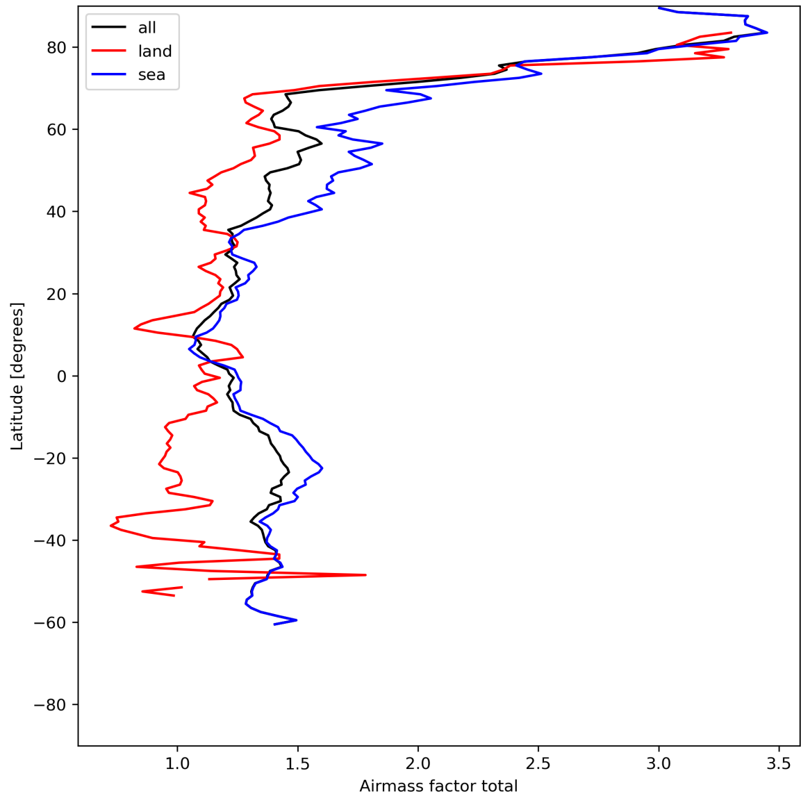
Figure 26: Zonal average of “Airmass factor total” for 2024-06-19 to 2024-06-21.
