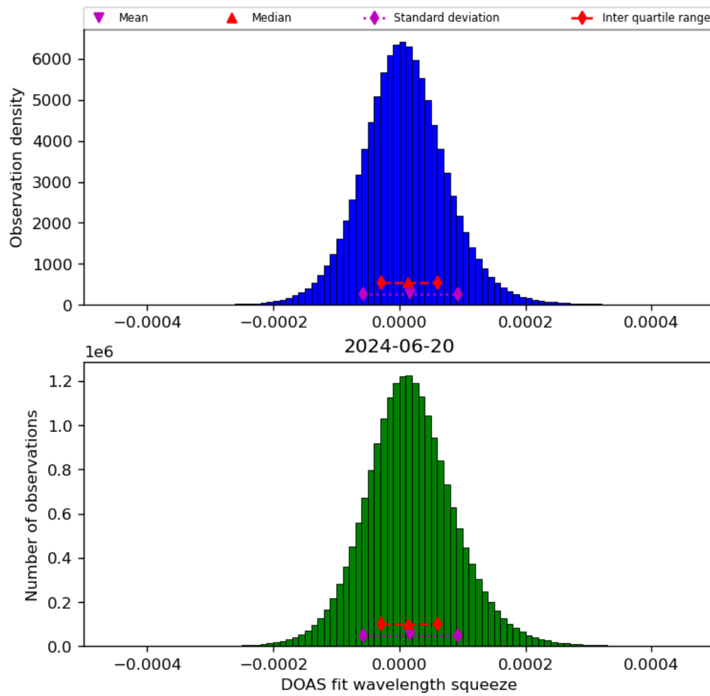
Figure 45: Histogram of “DOAS fit wavelength squeeze” for 2024-06-19 to 2024-06-21
