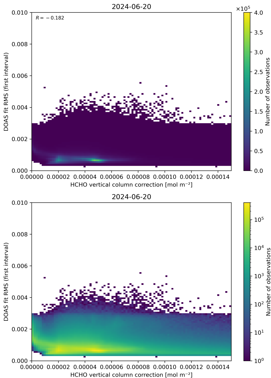
Figure 112: Scatter density plot of “HCHO vertical column correction” against “DOAS fit RMS (first interval)” for 2024-06-19 to 2024-06-21.
