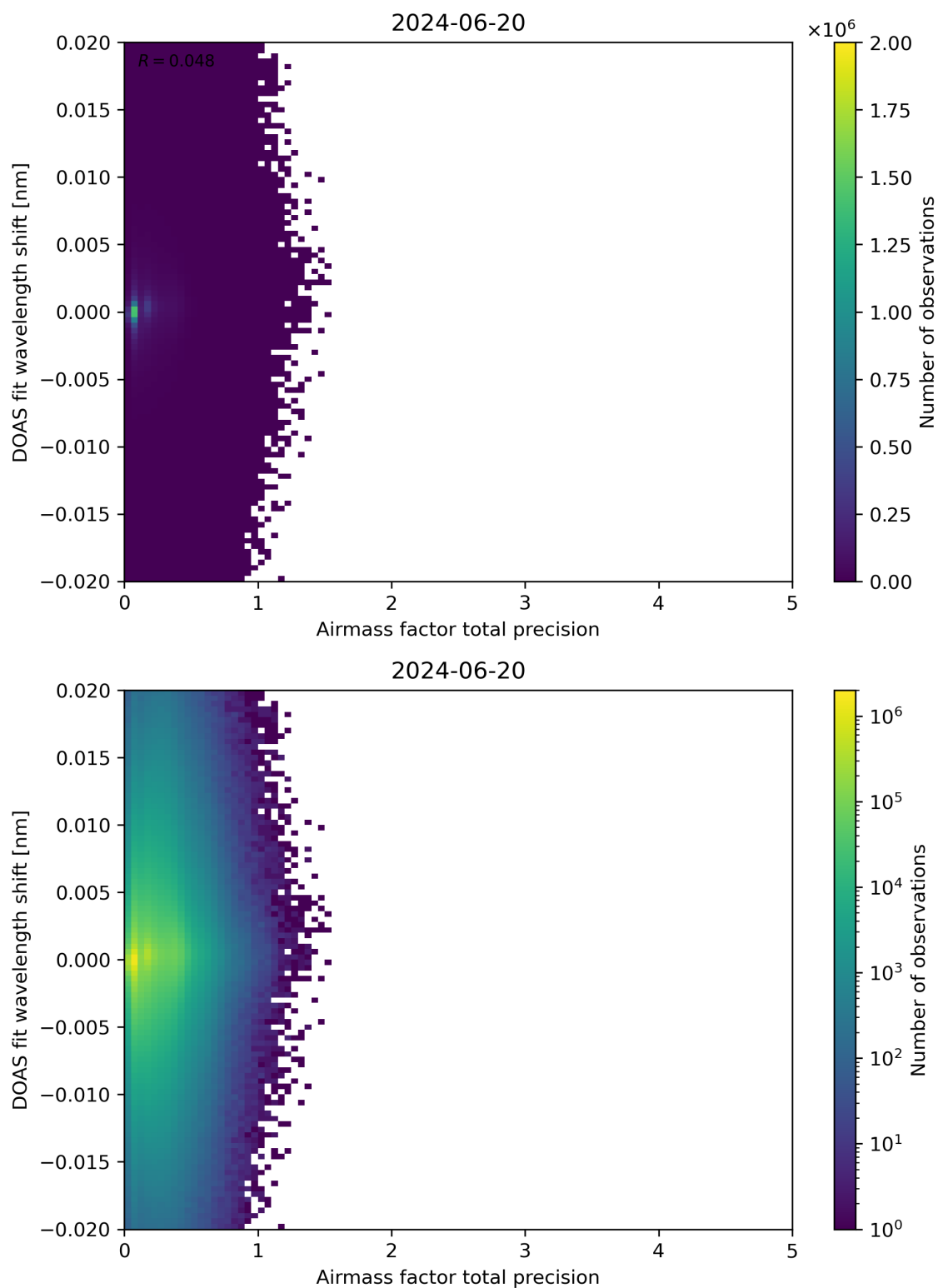
Figure 106: Scatter density plot of “Airmass factor total precision” against “DOAS fit wavelength shift” for 2024-06-19 to 2024-06-21.
