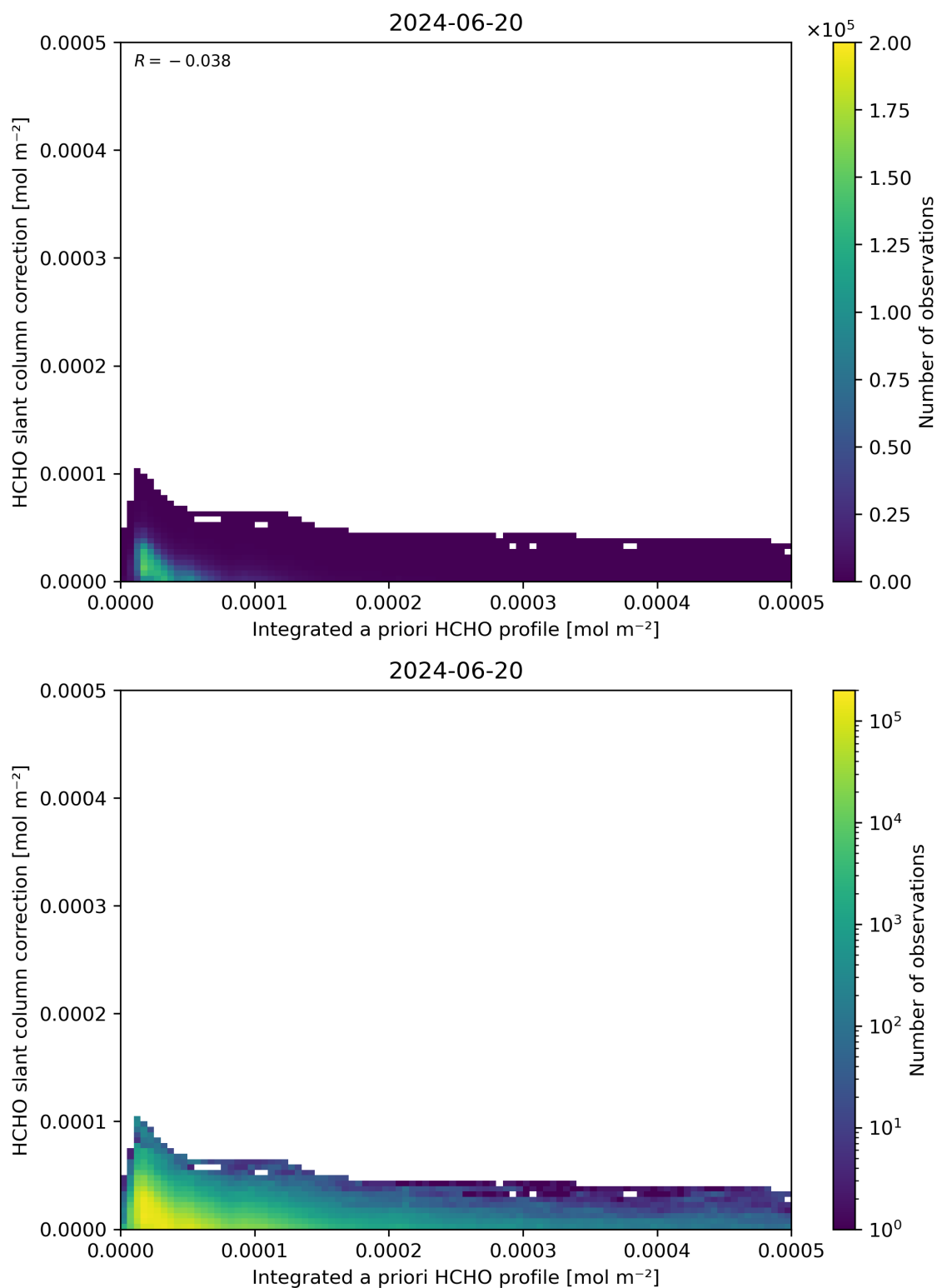
Figure 152: Scatter density plot of “Integrated a priori HCHO profile” against “HCHO slant column correction” for 2024-06-19 to 2024-06-21.
