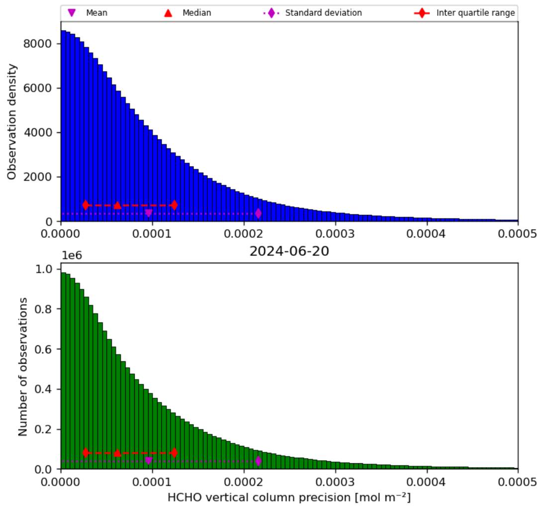
Figure 36: Histogram of “HCHO vertical column precision” for 2024-06-19 to 2024-06-21
