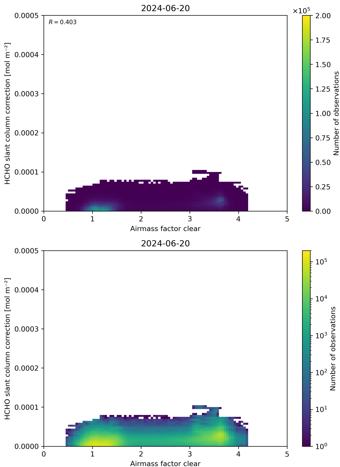
Figure 75: Scatter density plot of “Airmass factor clear” against “HCHO slant column correction” for 2024-06-19 to 2024-06-21.
