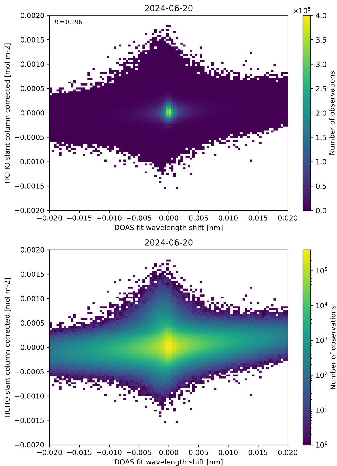
Figure 66: Scatter density plot of “DOAS fit wavelength shift” against “HCHO slant column corrected” for 2024-06-19 to 2024-06-21.
