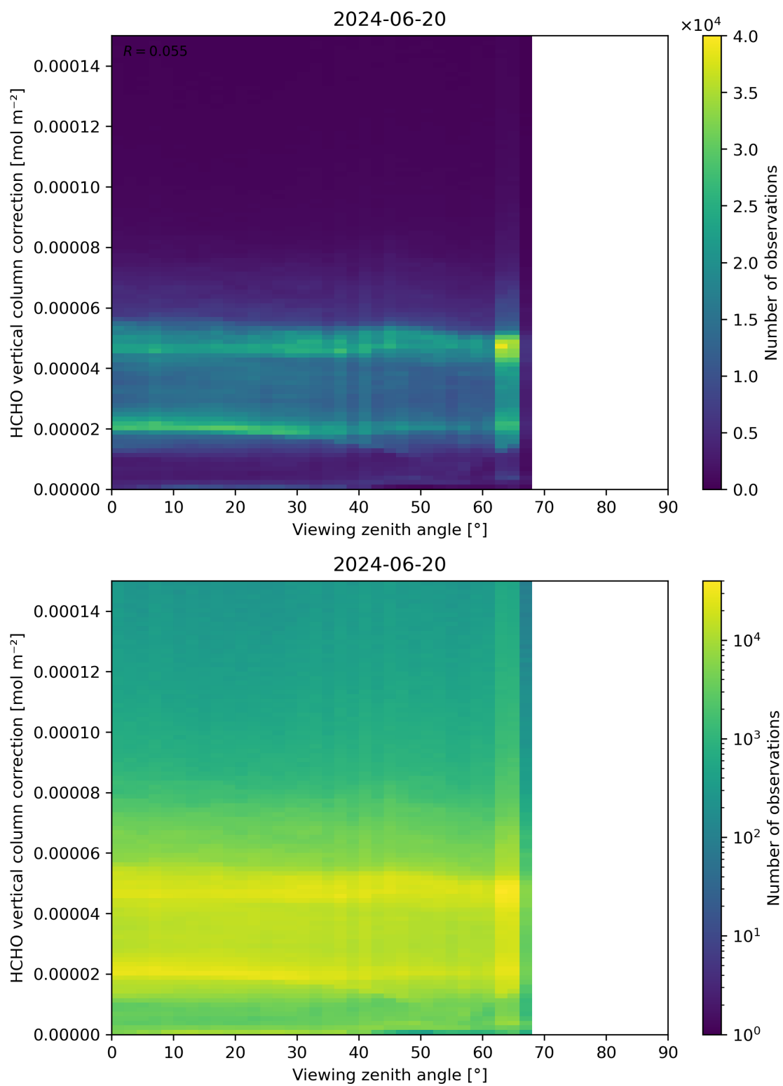
Figure 193: Scatter density plot of “Viewing zenith angle” against “HCHO vertical column correction” for 2024-06-19 to 2024-06-21.
