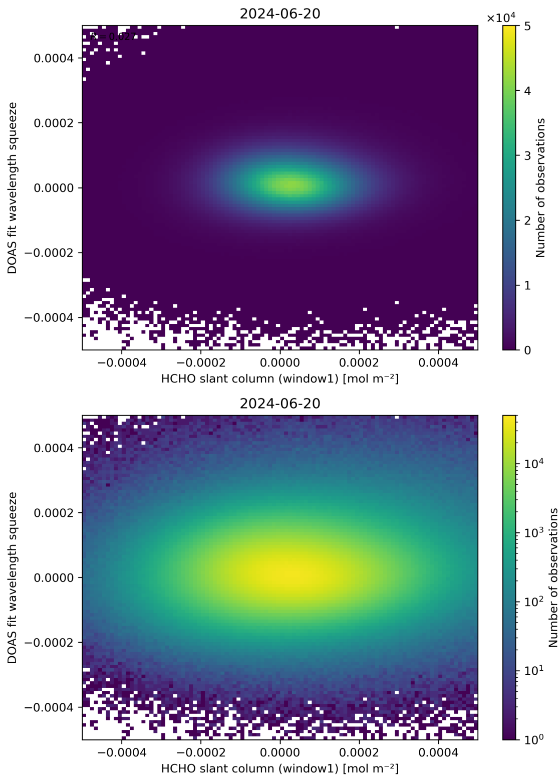
Figure 80: Scatter density plot of “HCHO slant column (window1)” against “DOAS fit wavelength squeeze” for 2024-06-19 to 2024-06-21.
