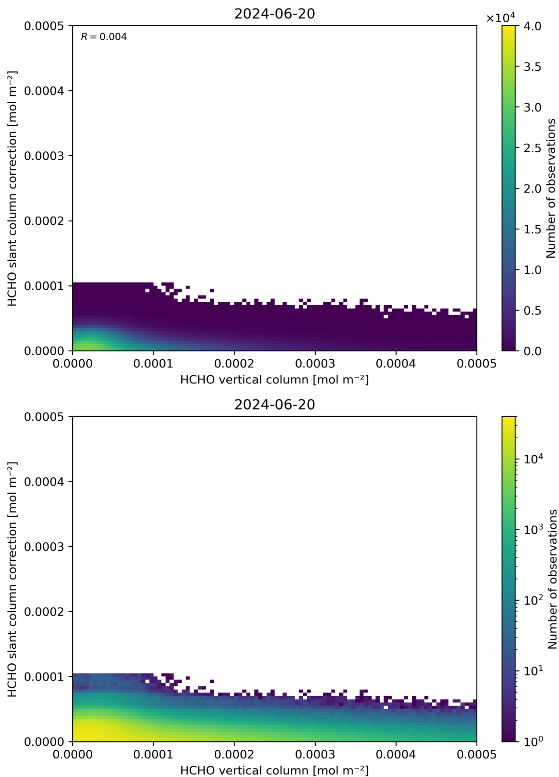
Figure 128: Scatter density plot of “HCHO vertical column” against “HCHO slant column correction” for 2024-06-19 to 2024-06-21.
