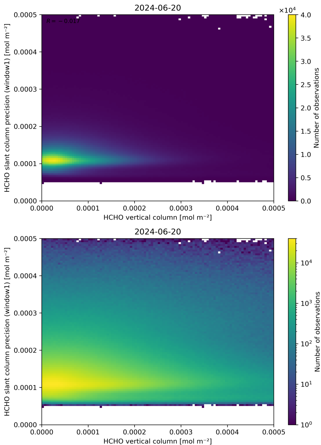
Figure 130: Scatter density plot of “HCHO vertical column” against “HCHO slant column precision (window1)” for 2024-06-19 to 2024-06-21.
