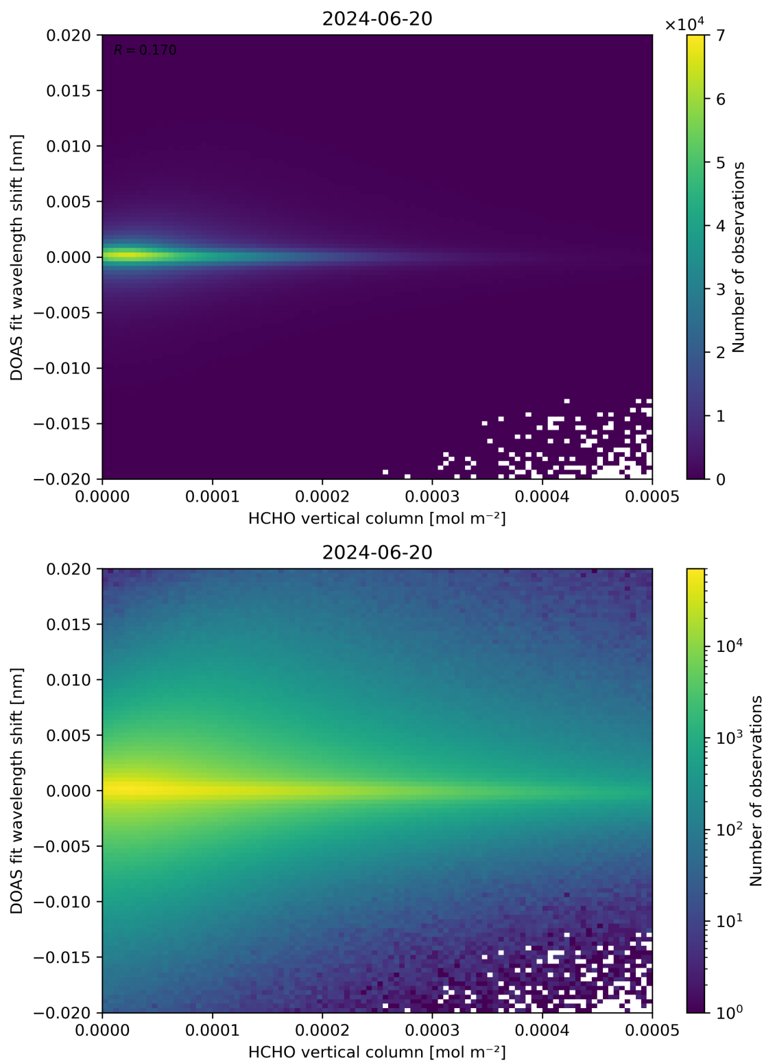
Figure 124: Scatter density plot of “HCHO vertical column” against “DOAS fit wavelength shift” for 2024-06-19 to 2024-06-21.
