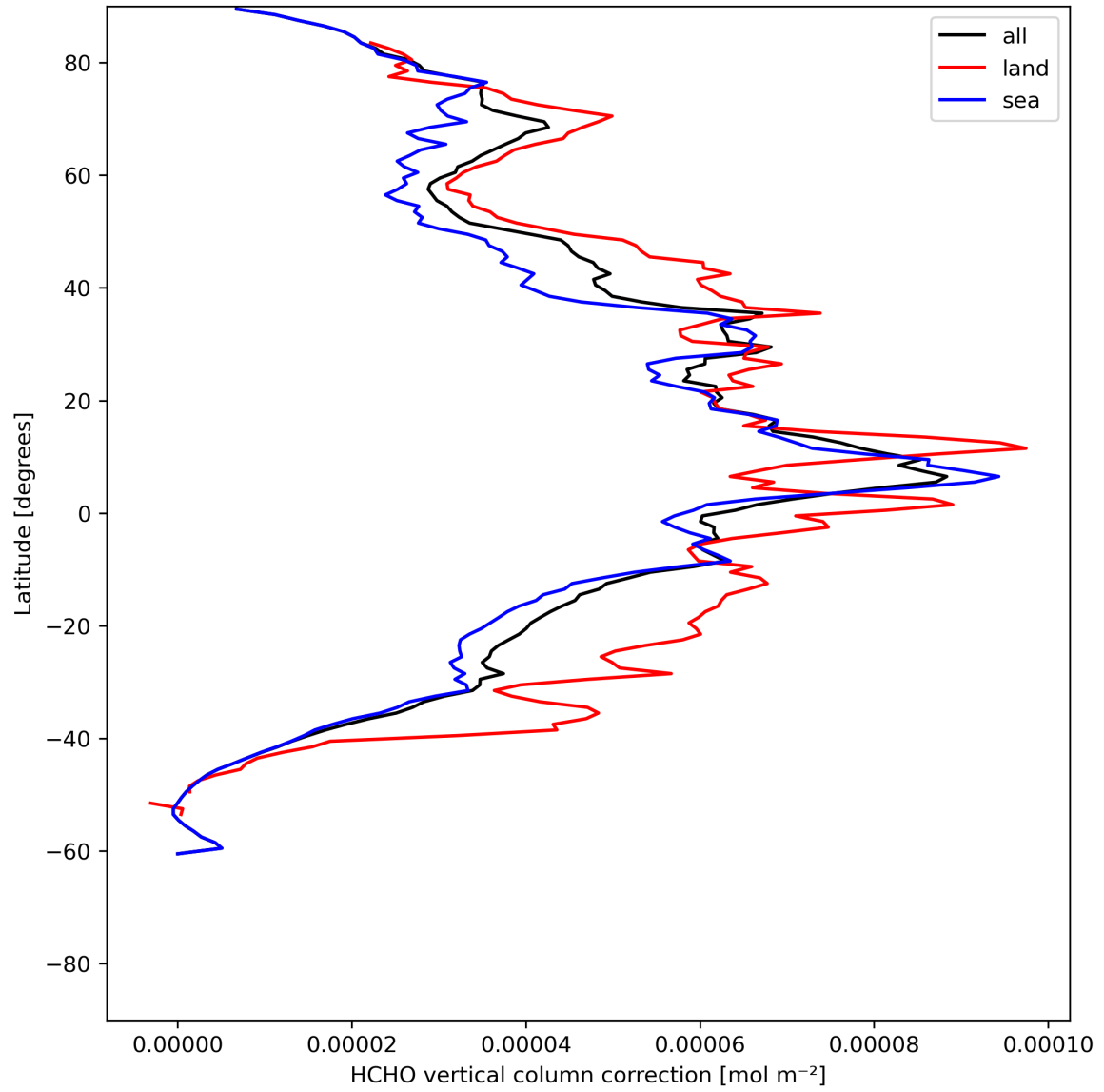
Figure 23: Zonal average of “HCHO vertical column correction” for 2024-06-19 to 2024-06-21.
