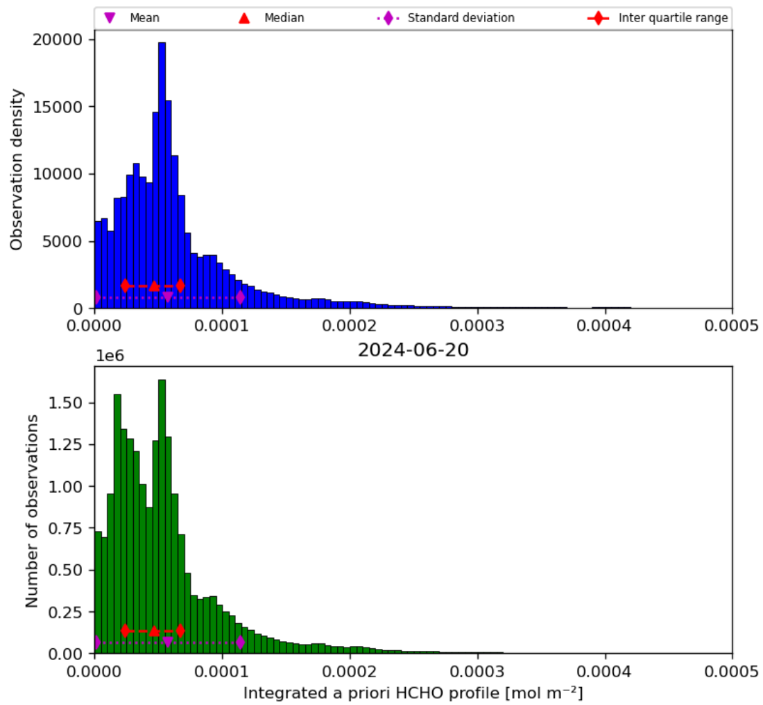
Figure 43: Histogram of “Integrated a priori HCHO profile” for 2024-06-19 to 2024-06-21
