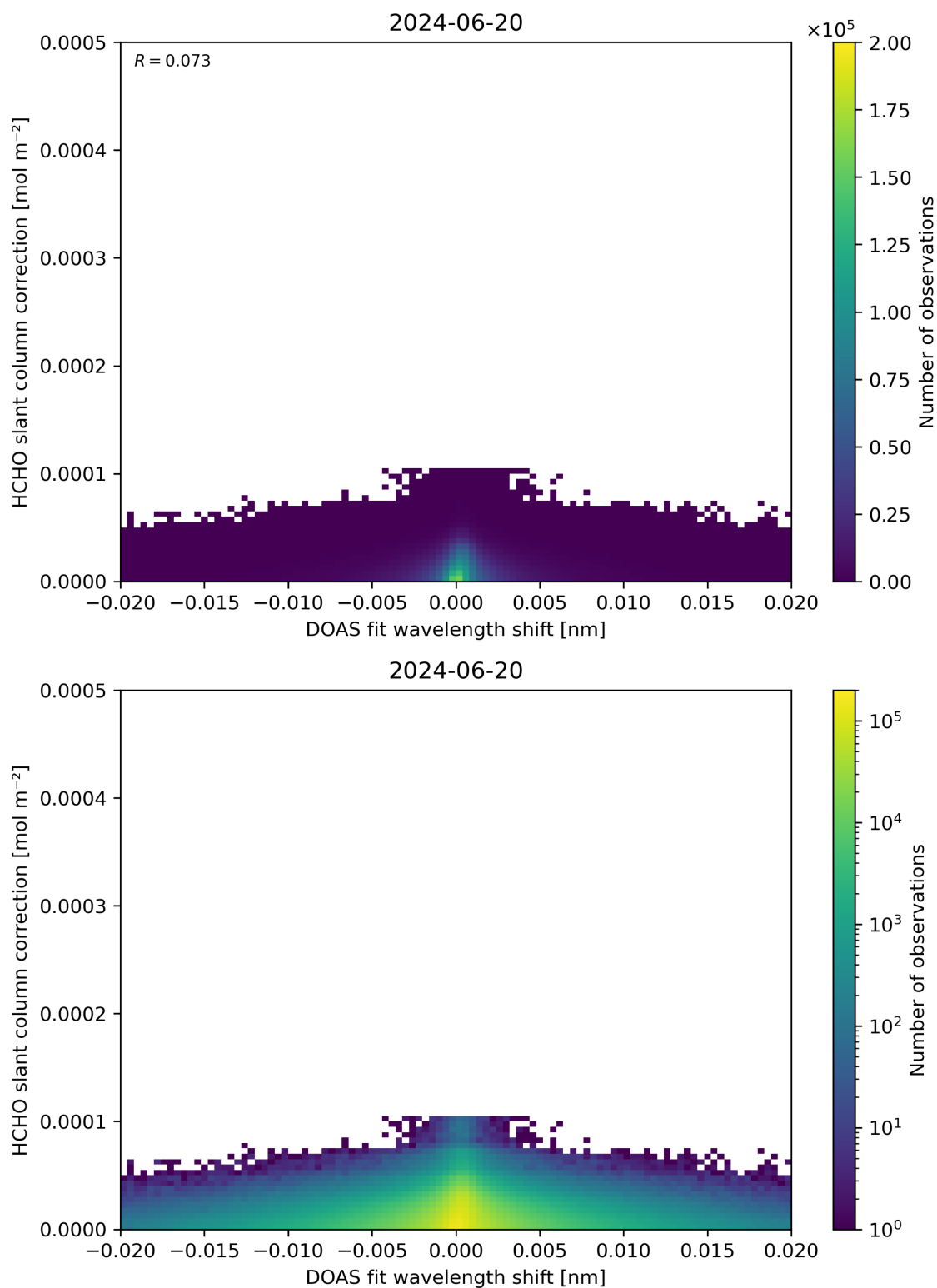
Figure 67: Scatter density plot of “DOAS fit wavelength shift” against “HCHO slant column correction” for 2024-06-19 to 2024-06-21.
