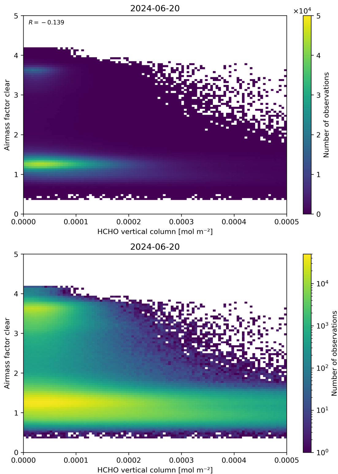
Figure 126: Scatter density plot of “HCHO vertical column” against “Airmass factor clear” for 2024-06-19 to 2024-06-21.
