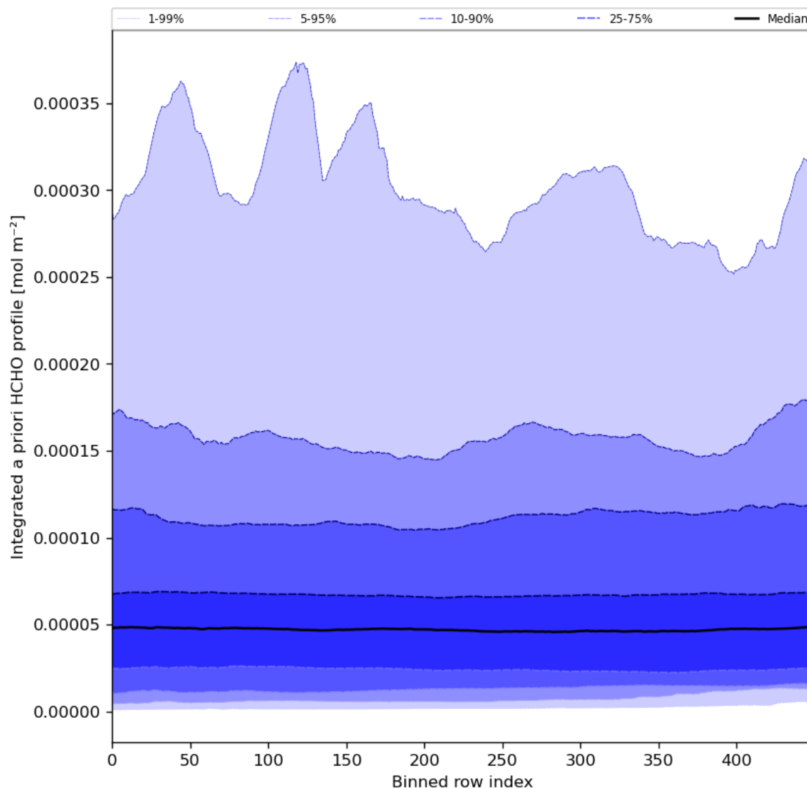
Figure 57: Along track statistics of “Integrated a priori HCHO profile” for 2024-06-19 to 2024-06-21
