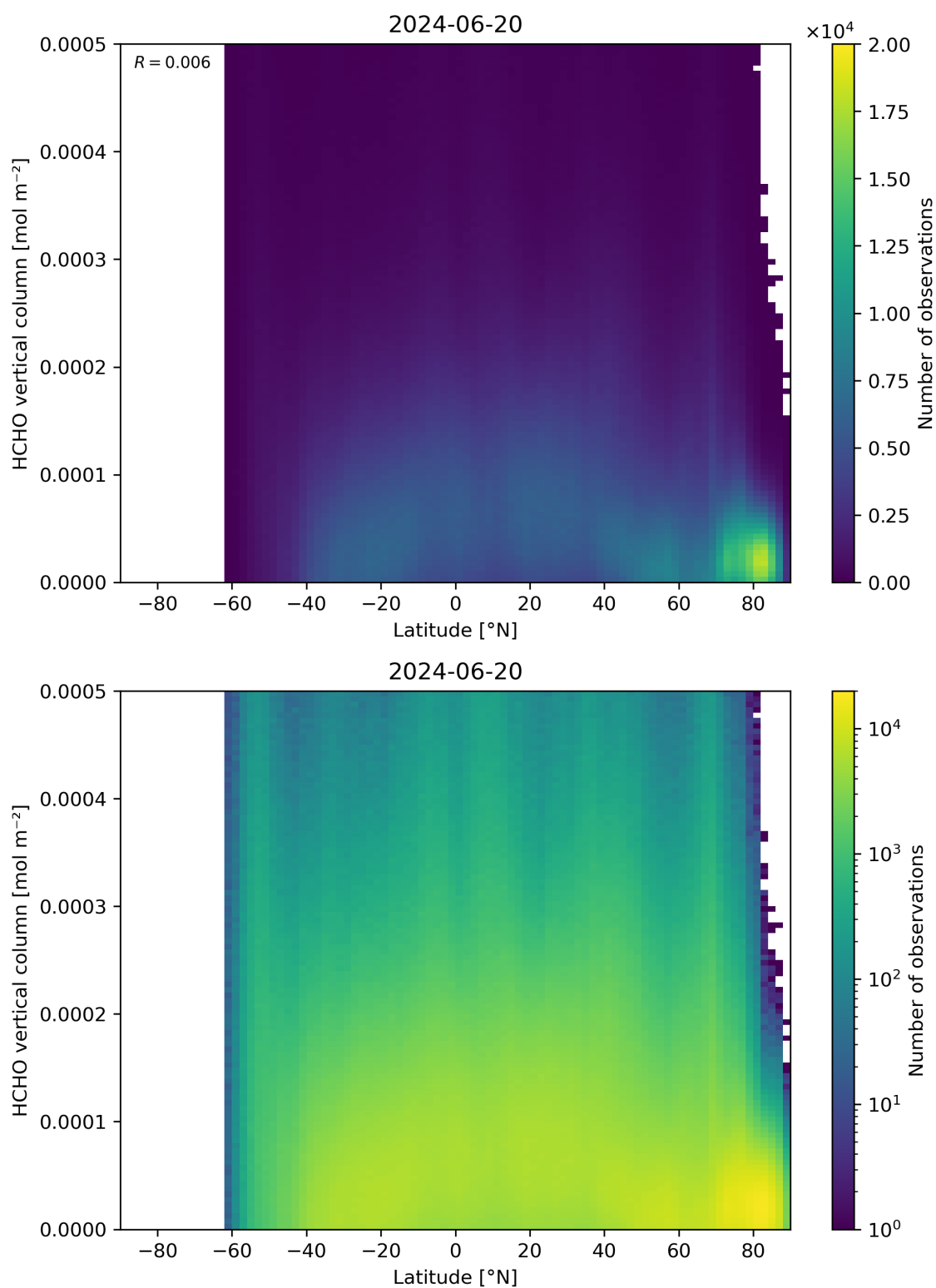
Figure 163: Scatter density plot of “Latitude” against “HCHO vertical column” for 2024-06-19 to 2024-06-21.
