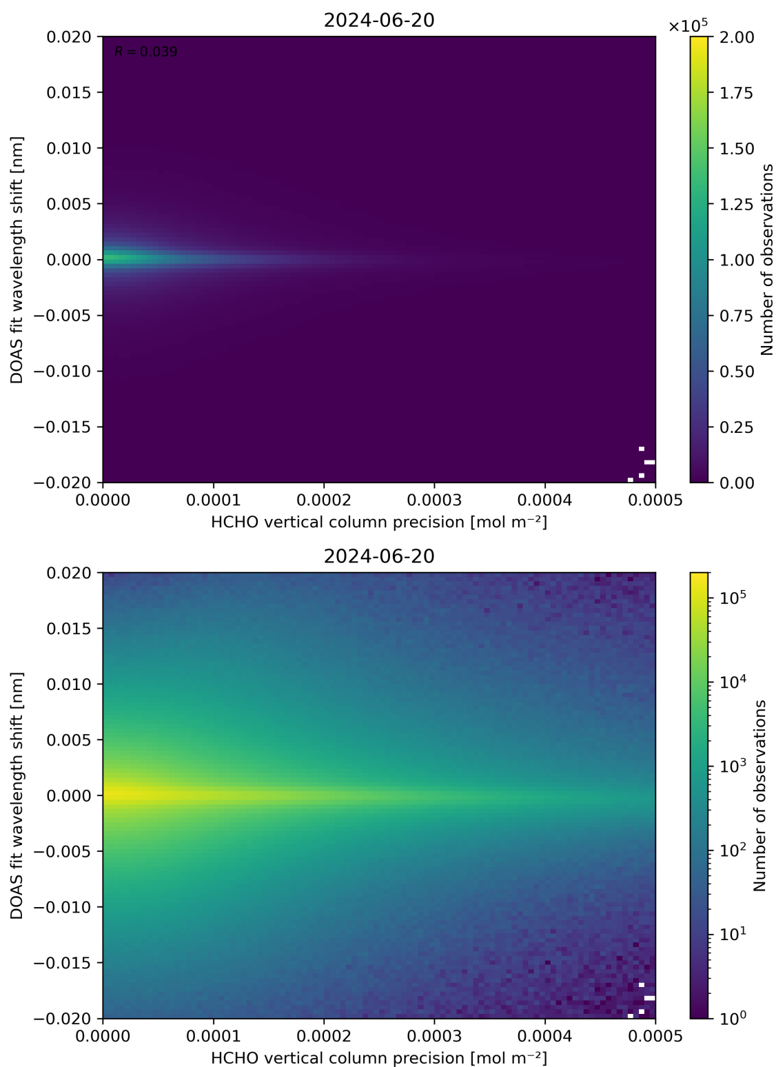
Figure 137: Scatter density plot of “HCHO vertical column precision” against “DOAS fit wavelength shift” for 2024-06-19 to 2024-06-21.
