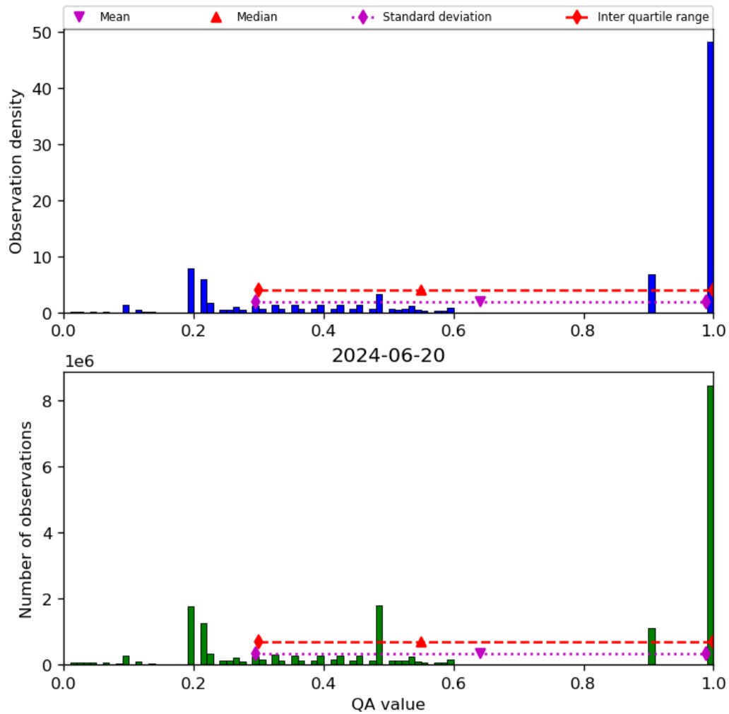
Figure 34: Histogram of “QA value” for 2024-06-19 to 2024-06-21
