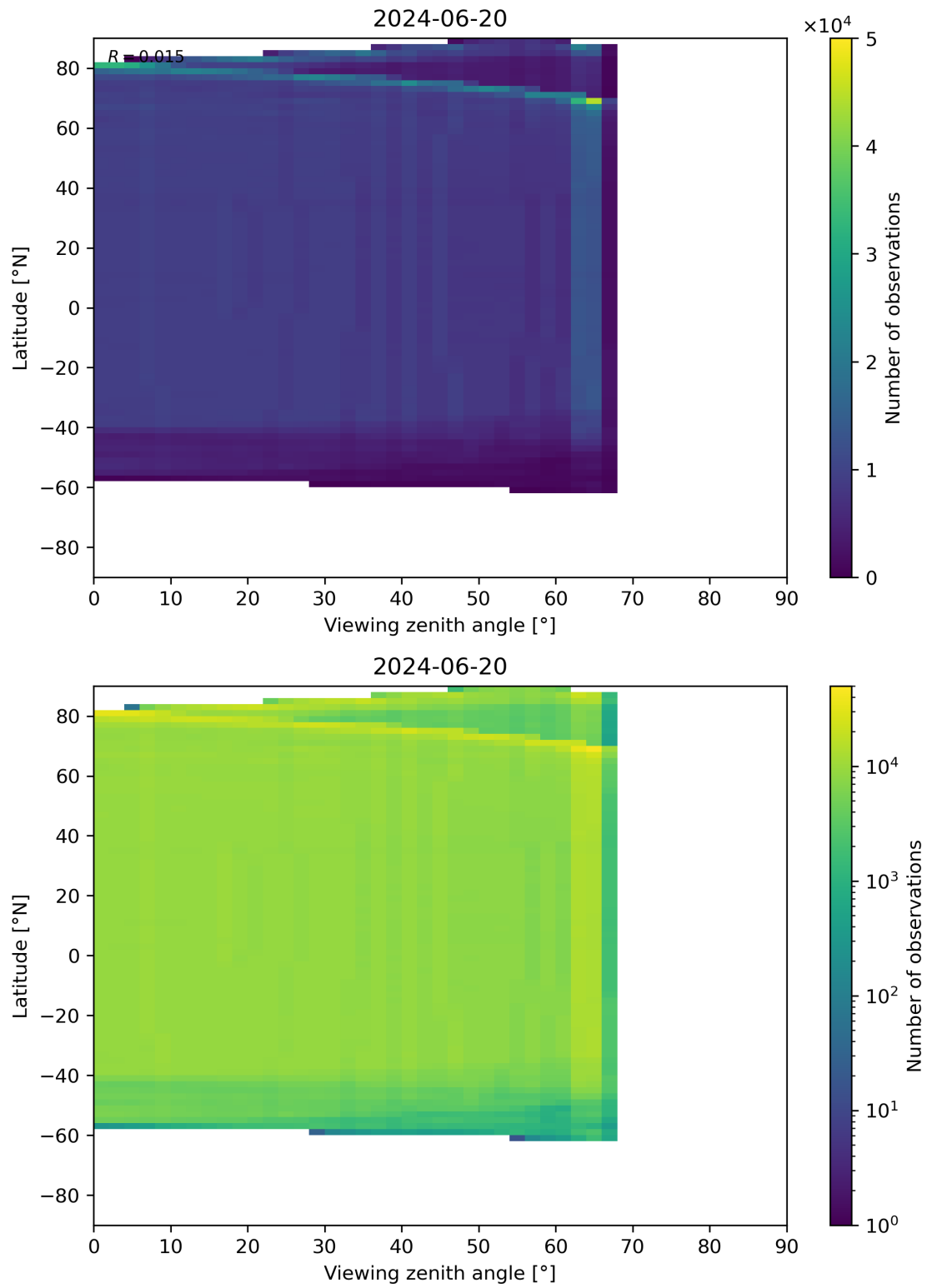
Figure 196: Scatter density plot of “Viewing zenith angle” against “Latitude” for 2024-06-19 to 2024-06-21.
