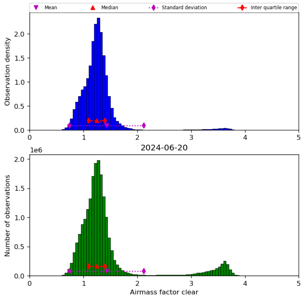
Figure 42: Histogram of “Airmass factor clear” for 2024-06-19 to 2024-06-21
