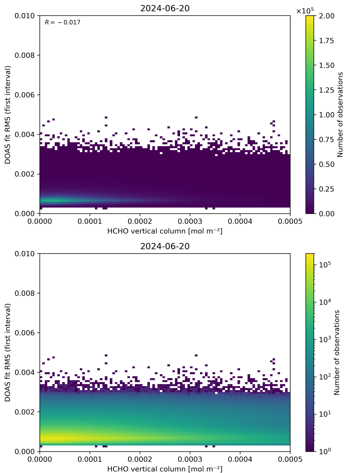
Figure 123: Scatter density plot of “HCHO vertical column” against “DOAS fit RMS (first interval)” for 2024-06-19 to 2024-06-21.
