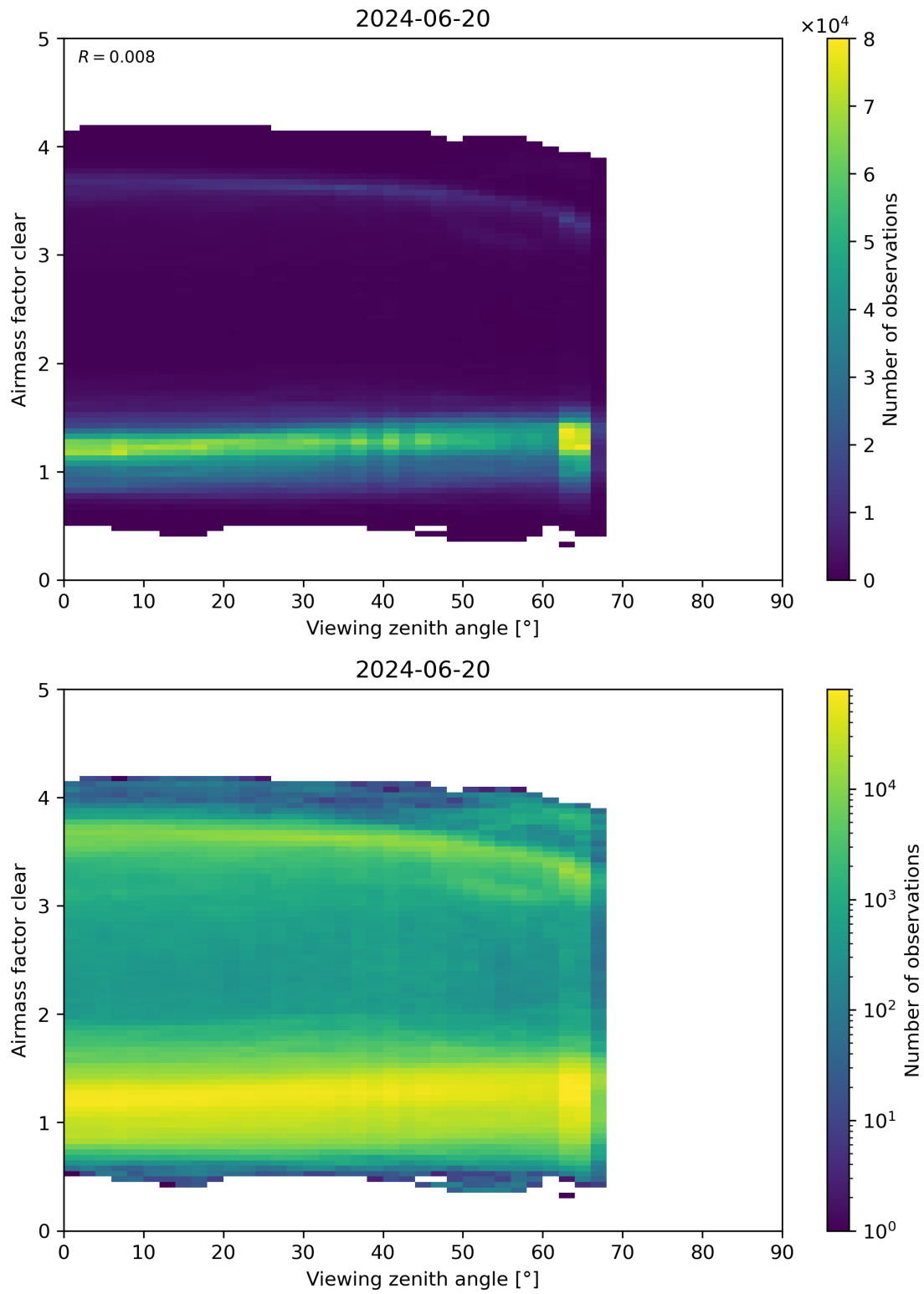
Figure 185: Scatter density plot of “Viewing zenith angle” against “Airmass factor clear” for 2024-06-19 to 2024-06-21.
