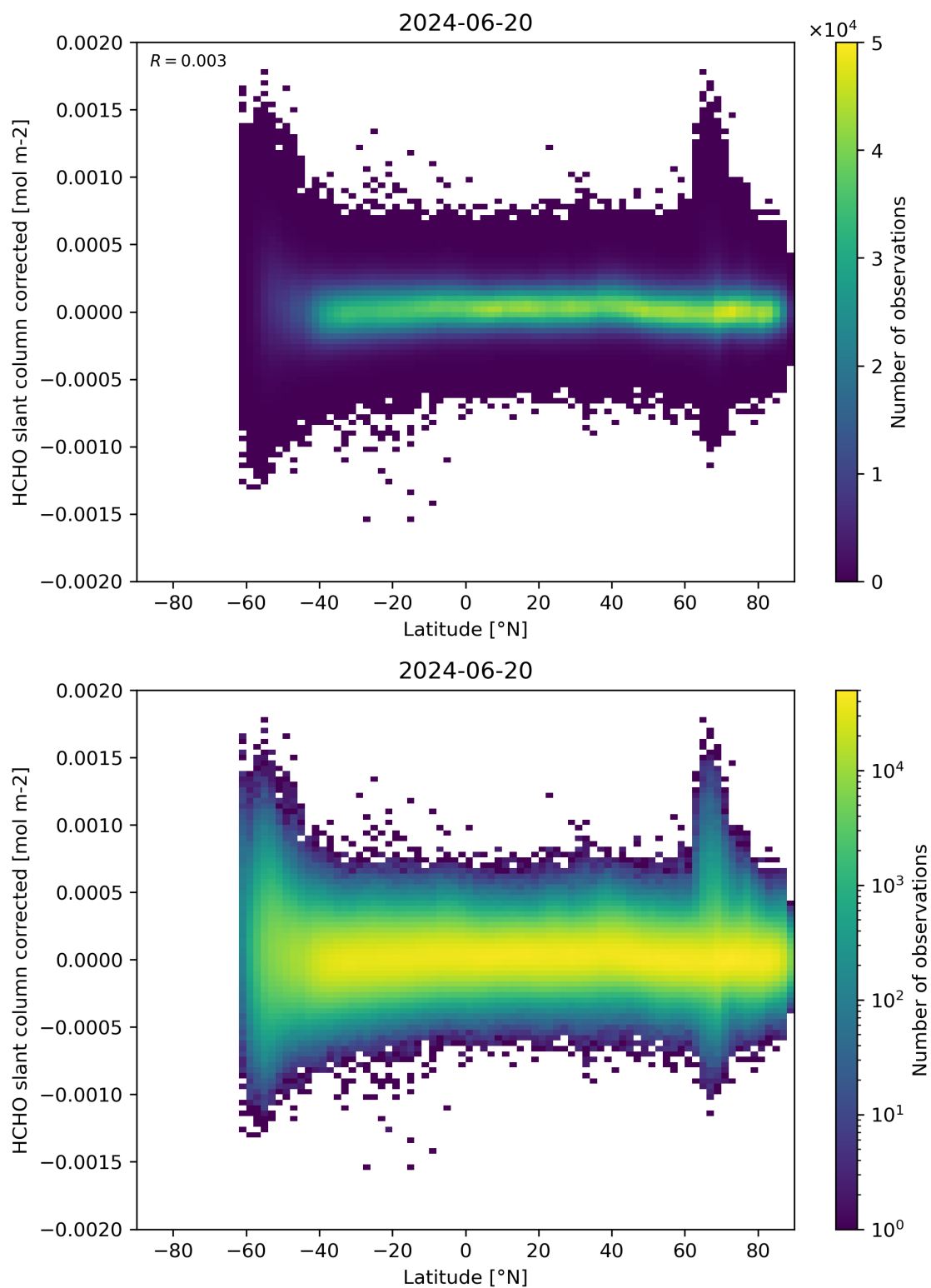
Figure 157: Scatter density plot of “Latitude” against “HCHO slant column corrected” for 2024-06-19 to 2024-06-21.
