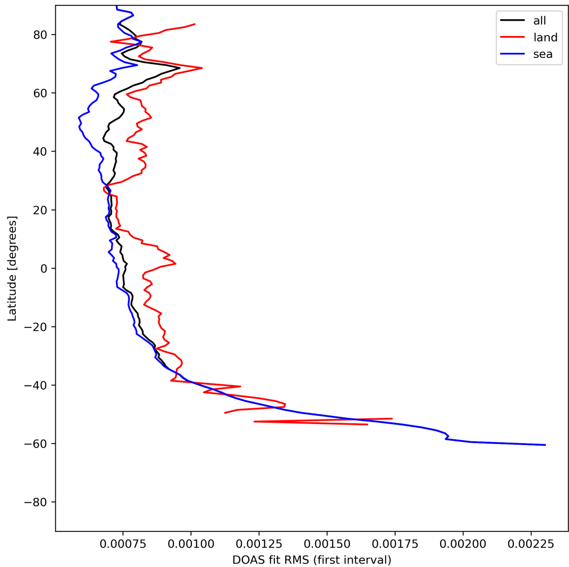
Figure 32: Zonal average of “DOAS fit RMS (first interval)” for 2024-06-19 to 2024-06-21.
