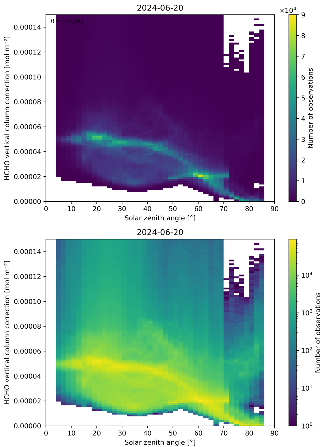
Figure 178: Scatter density plot of “Solar zenith angle” against “HCHO vertical column correction” for 2024-06-19 to 2024-06-21.
