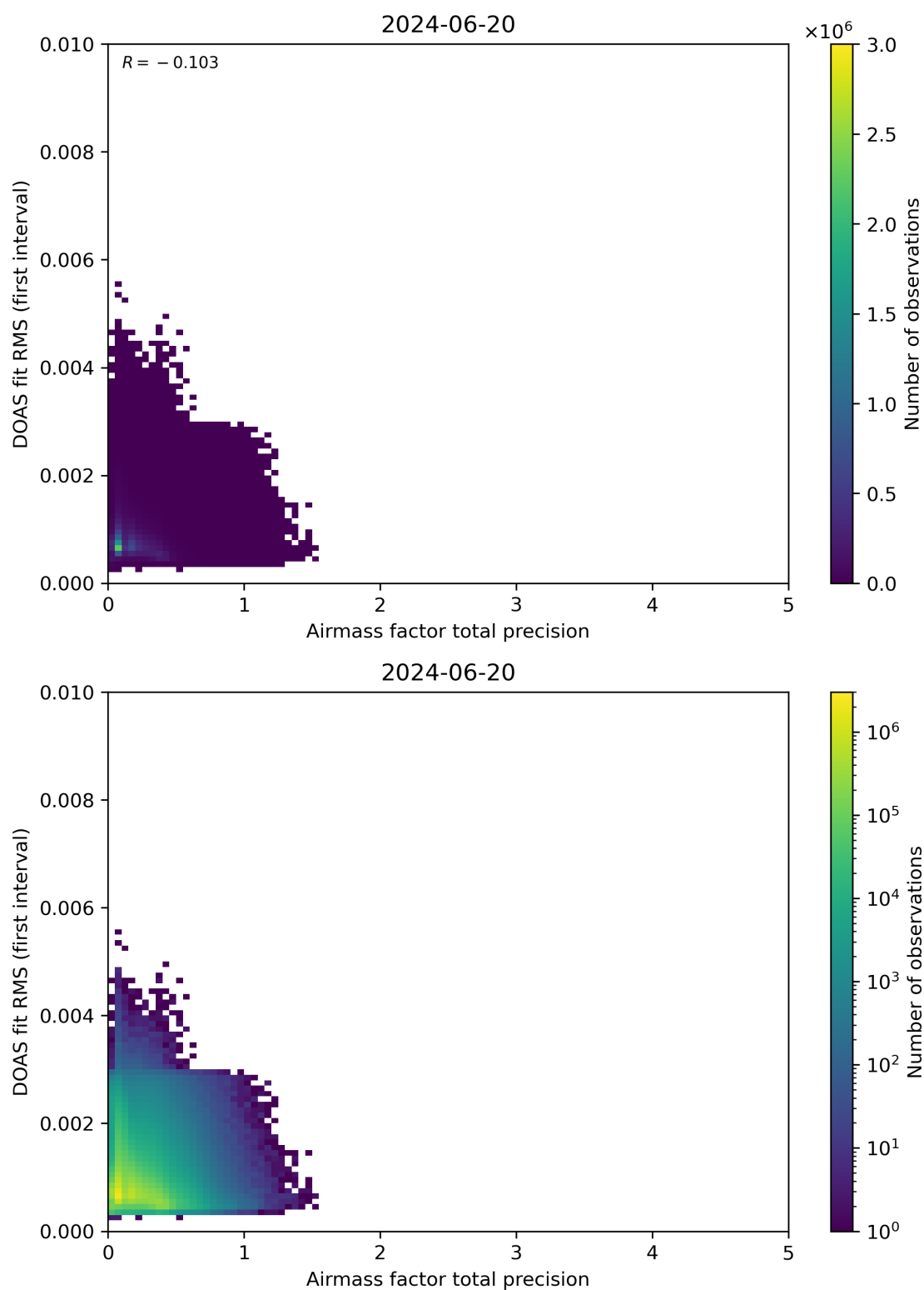
Figure 105: Scatter density plot of “Airmass factor total precision” against “DOAS fit RMS (first interval)” for 2024-06-19 to 2024-06-21.
