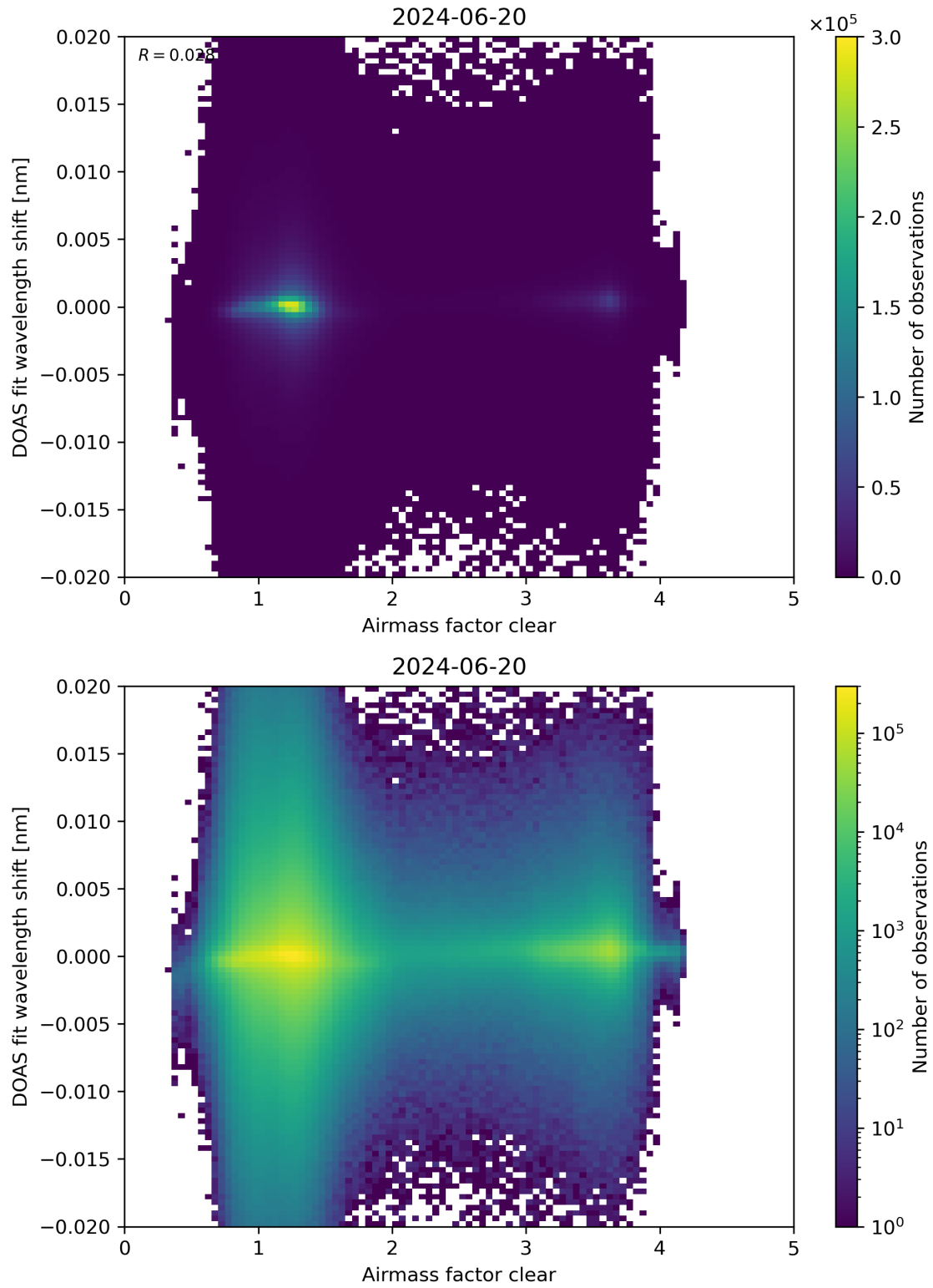
Figure 72: Scatter density plot of “Airmass factor clear” against “DOAS fit wavelength shift” for 2024-06-19 to 2024-06-21.
