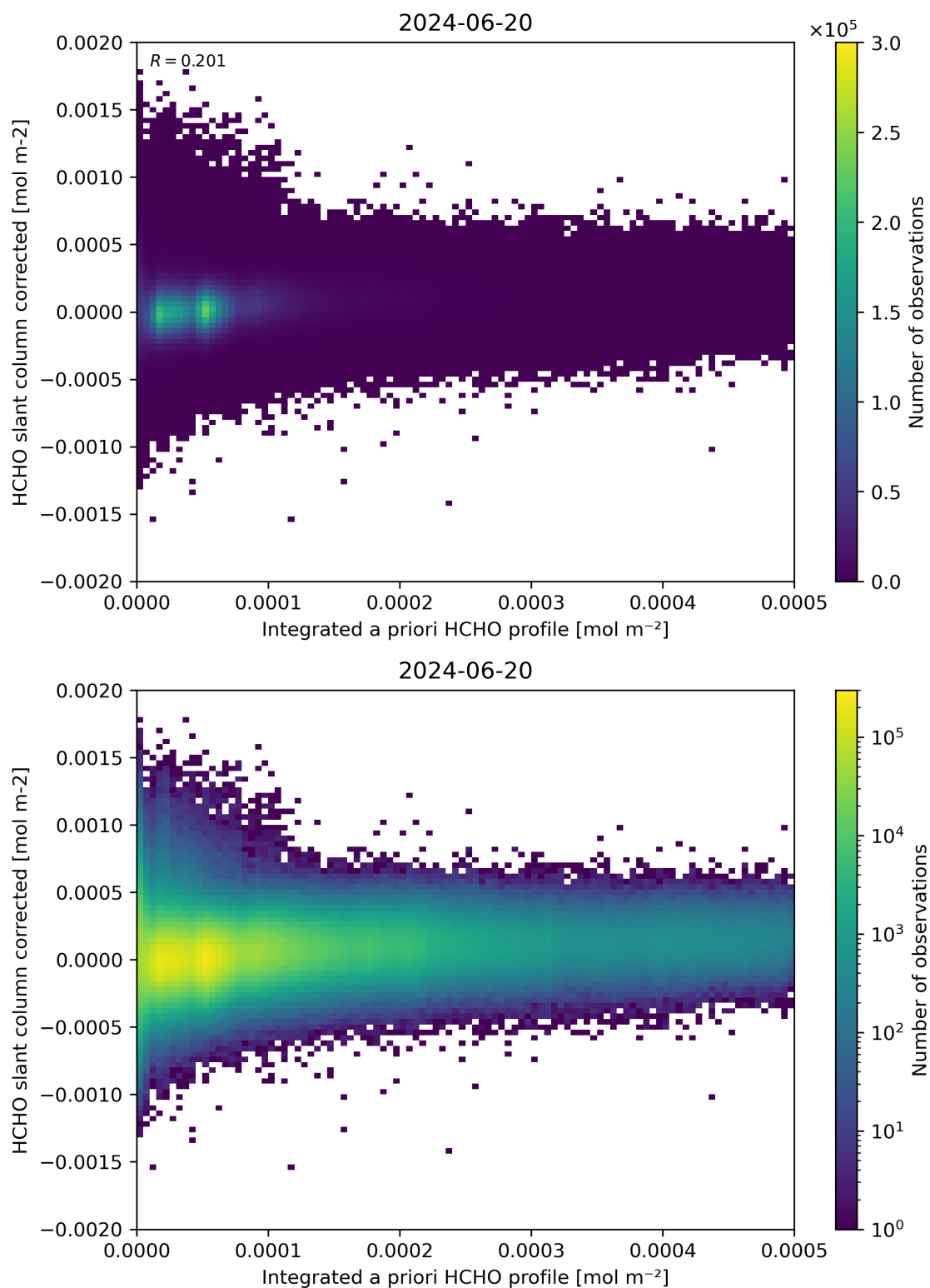
Figure 151: Scatter density plot of “Integrated a priori HCHO profile” against “HCHO slant column corrected” for 2024-06-19 to 2024-06-21.
