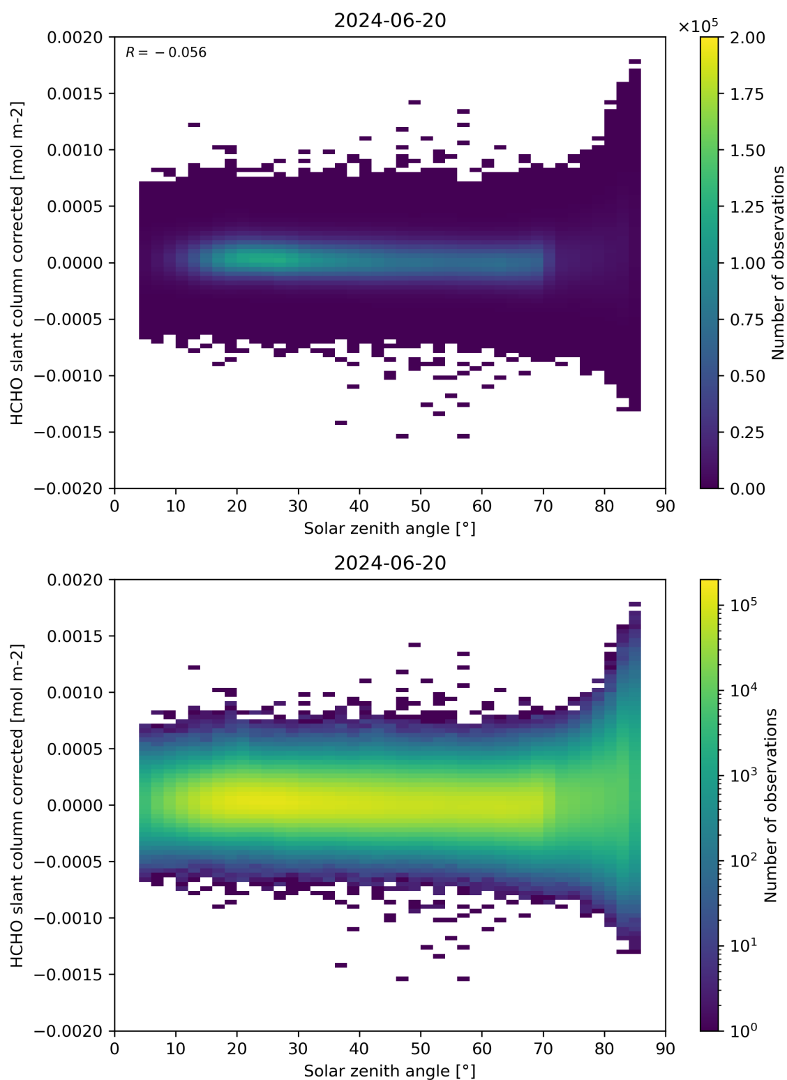
Figure 171: Scatter density plot of “Solar zenith angle” against “HCHO slant column corrected” for 2024-06-19 to 2024-06-21.
