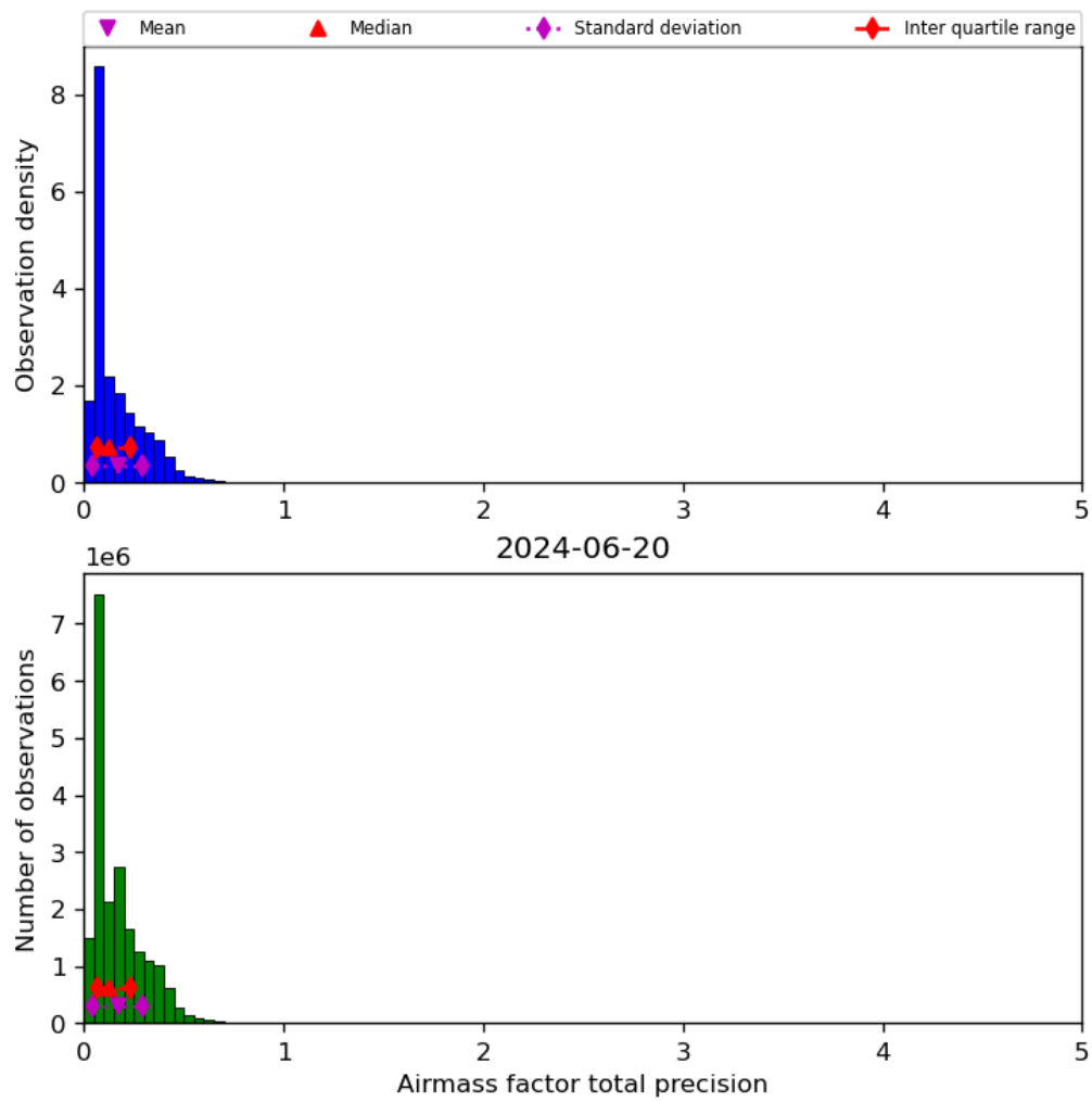
Figure 41: Histogram of “Airmass factor total precision” for 2024-06-19 to 2024-06-21
