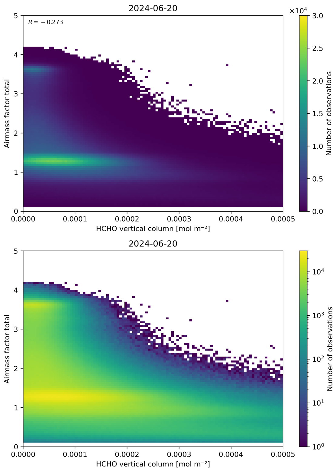
Figure 131: Scatter density plot of “HCHO vertical column” against “Airmass factor total” for 2024-06-19 to 2024-06-21.
