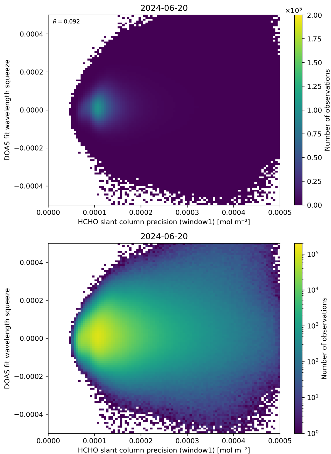
Figure 90: Scatter density plot of “HCHO slant column precision (window1)” against “DOAS fit wavelength squeeze” for 2024-06-19 to 2024-06-21.
