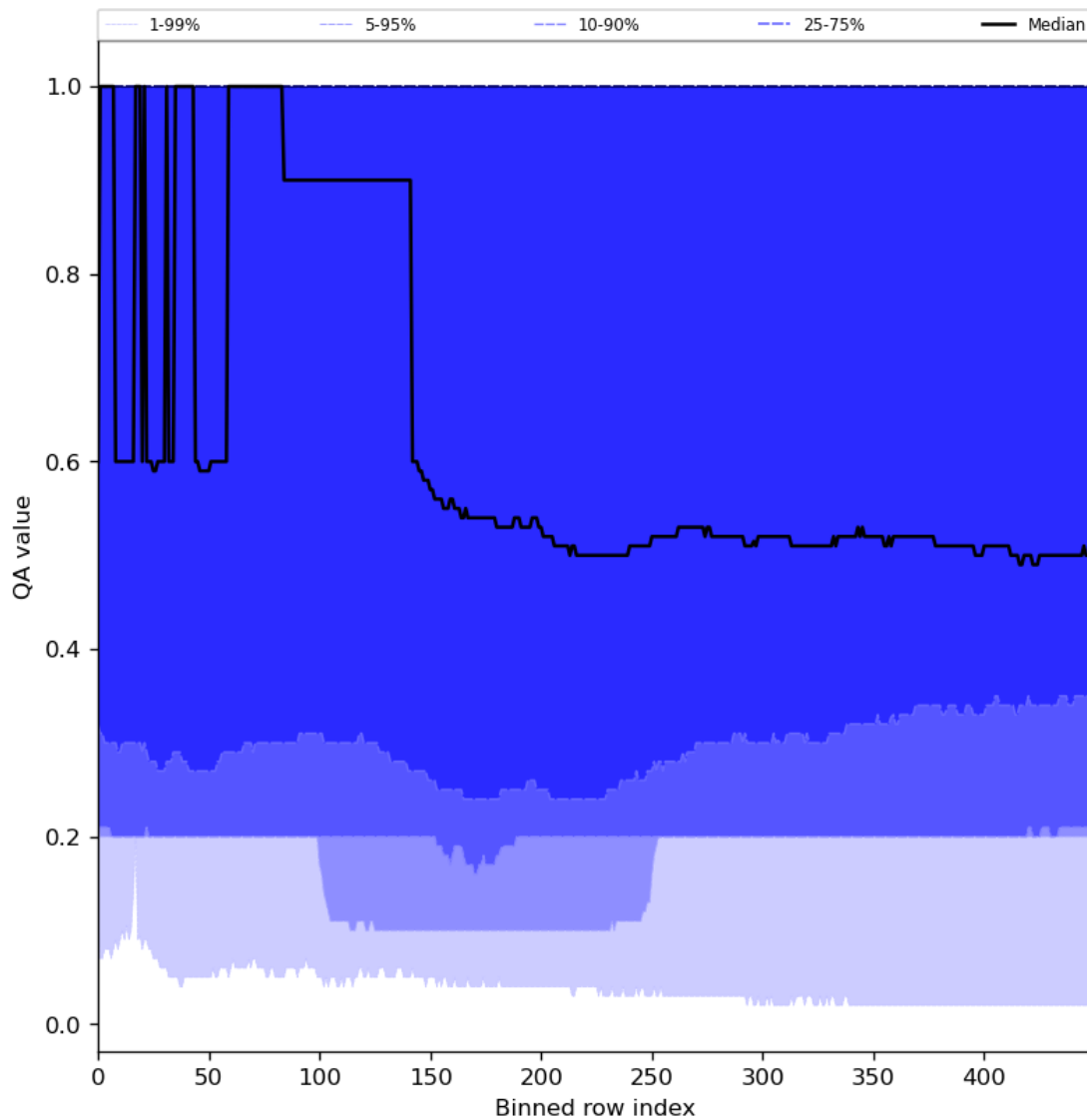
Figure 48: Along track statistics of “QA value” for 2024-06-19 to 2024-06-21
