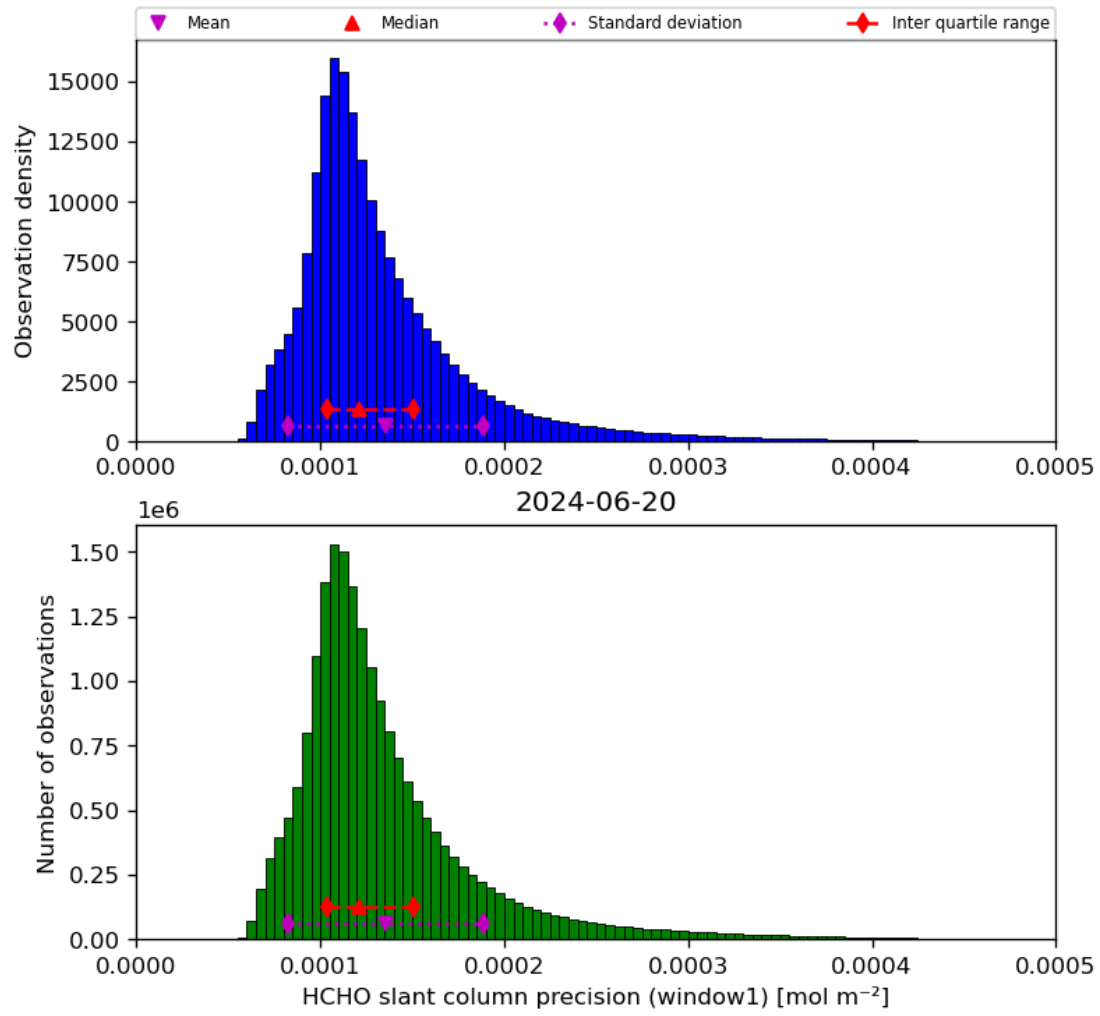
Figure 39: Histogram of “HCHO slant column precision (window1)” for 2024-06-19 to 2024-06-21
