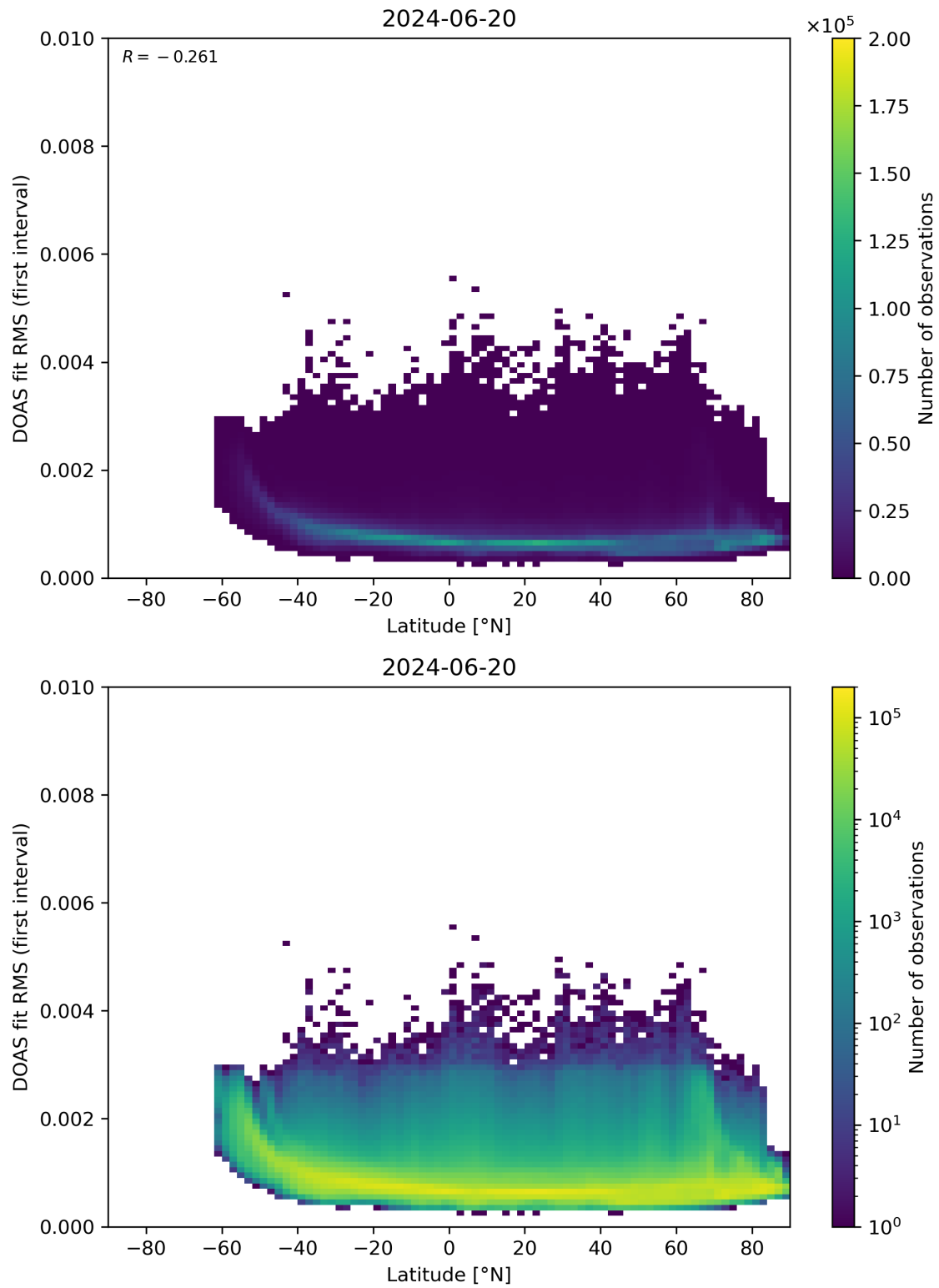
Figure 153: Scatter density plot of “Latitude” against “DOAS fit RMS (first interval)” for 2024-06-19 to 2024-06-21.
