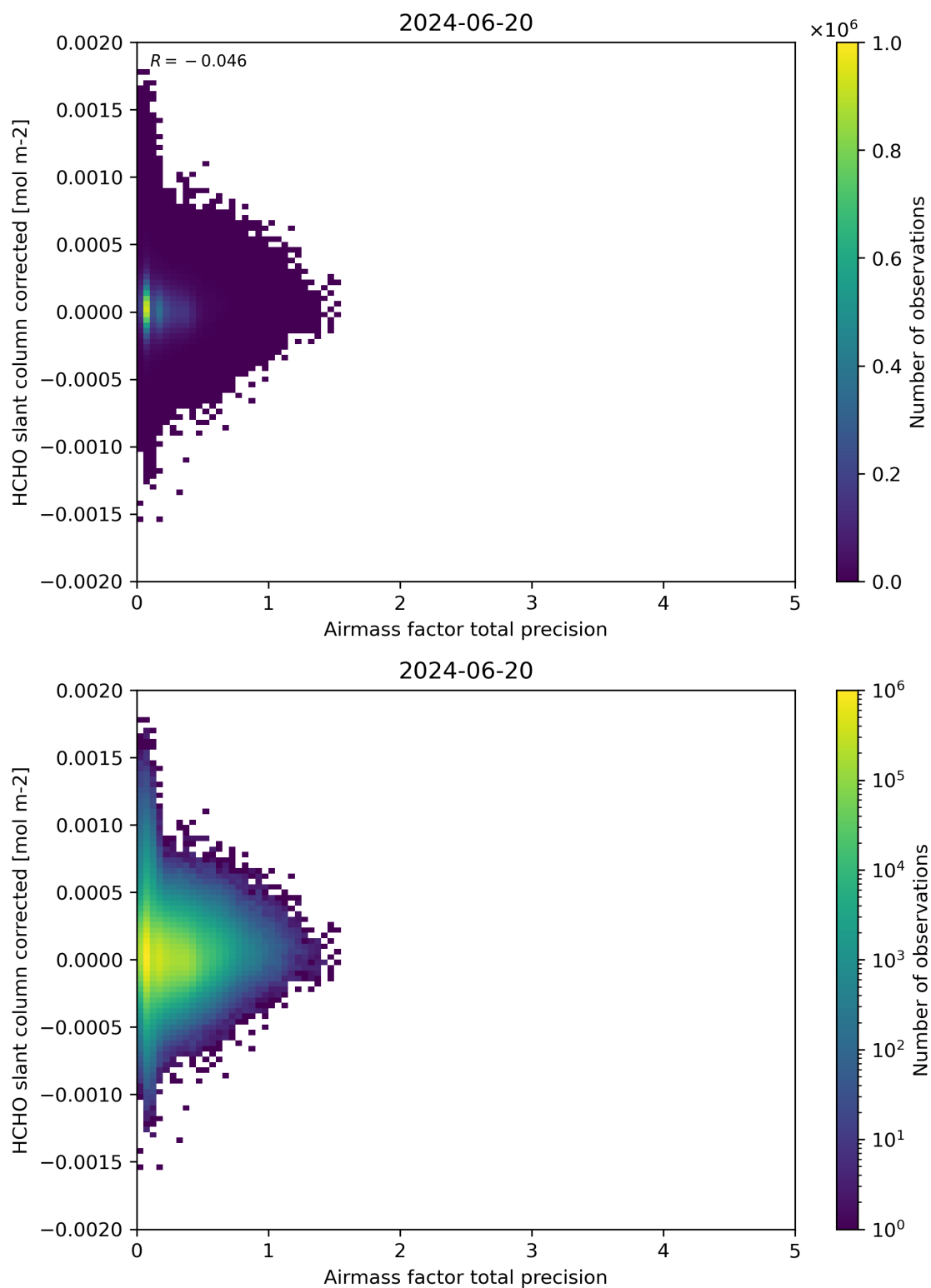
Figure 109: Scatter density plot of “Airmass factor total precision” against “HCHO slant column corrected” for 2024-06-19 to 2024-06-21.
