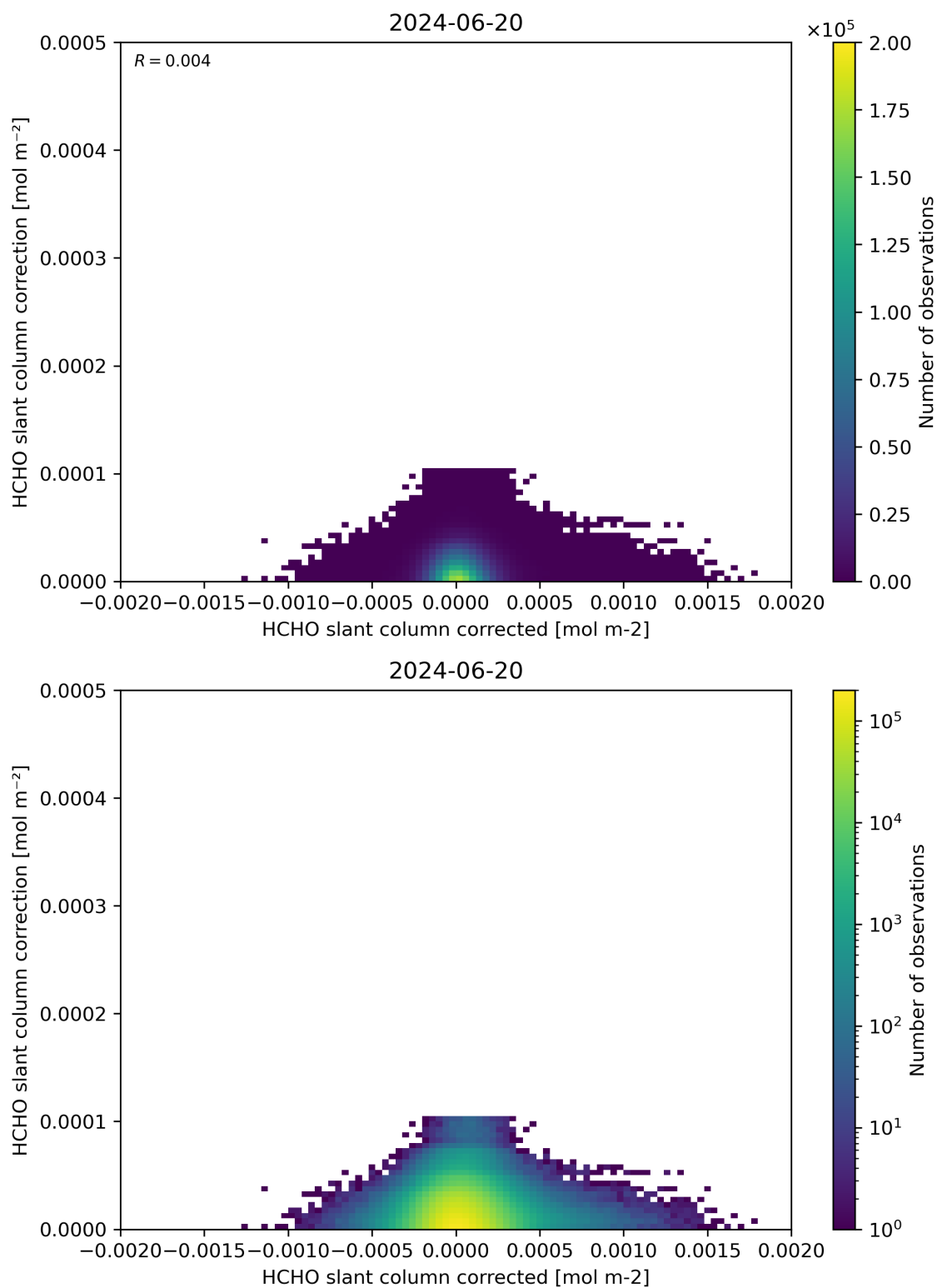
Figure 77: Scatter density plot of “HCHO slant column corrected” against “HCHO slant column correction” for 2024-06-19 to 2024-06-21.
