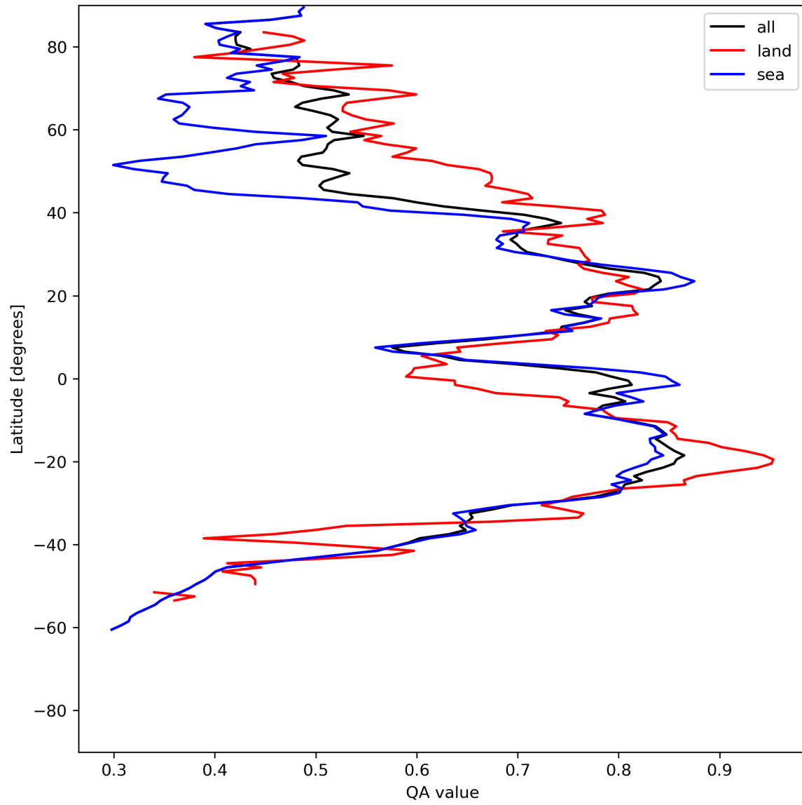
Figure 20: Zonal average of “QA value” for 2024-06-19 to 2024-06-21.
