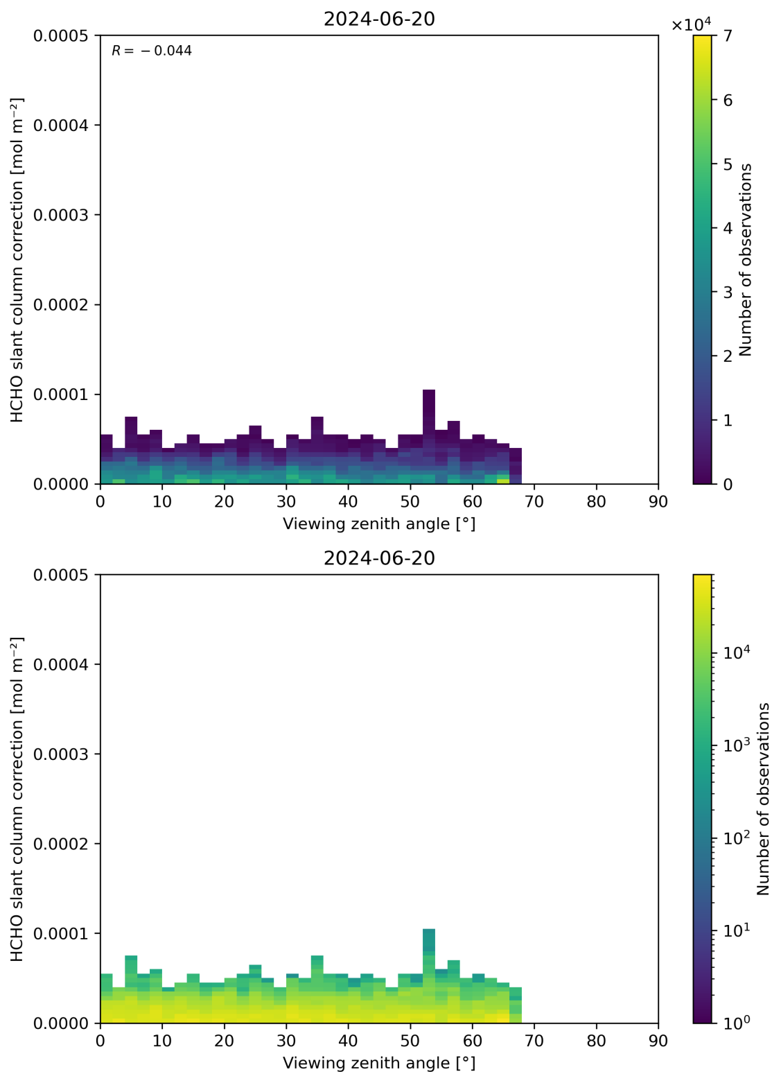
Figure 187: Scatter density plot of “Viewing zenith angle” against “HCHO slant column correction” for 2024-06-19 to 2024-06-21.
