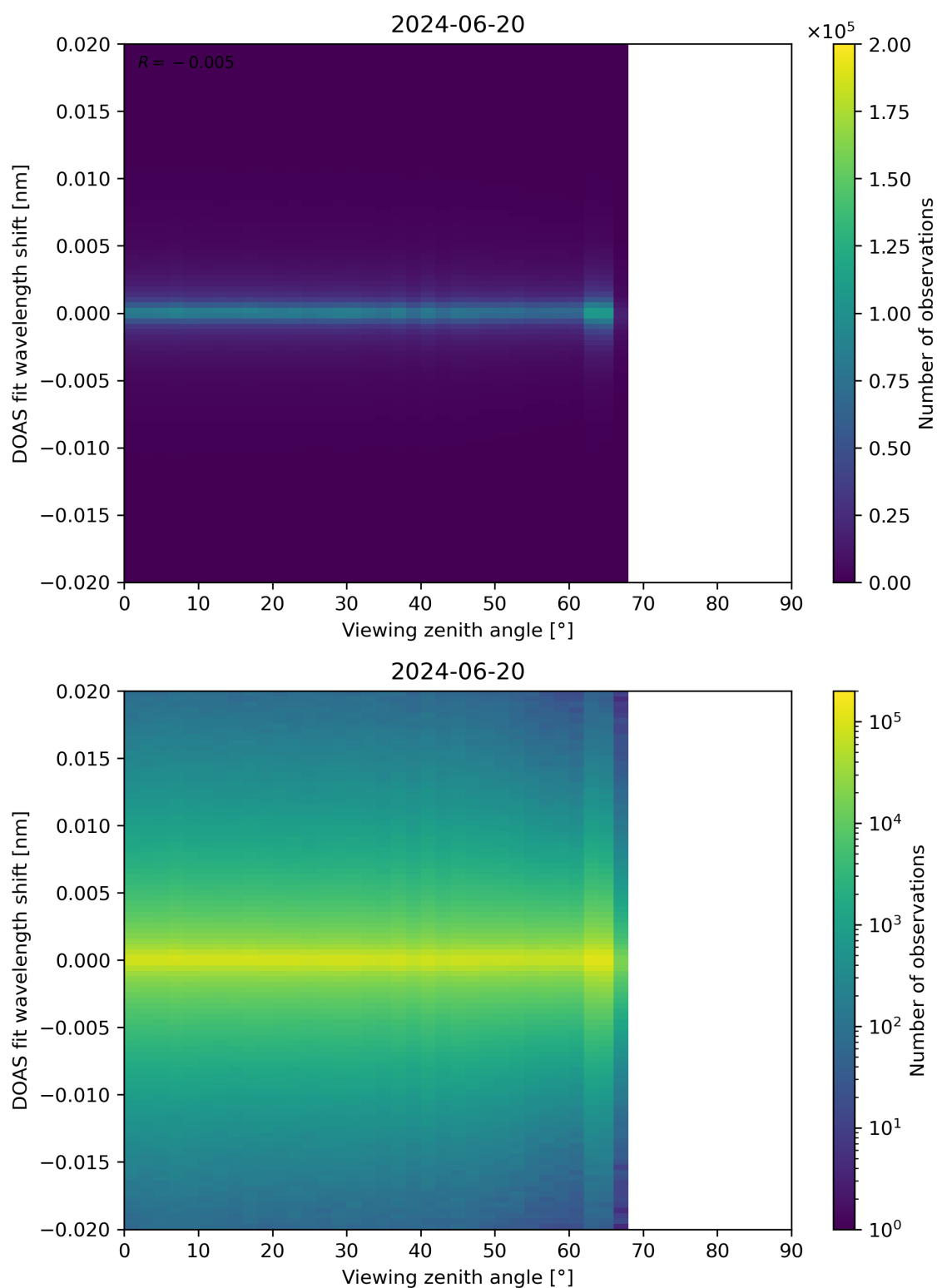
Figure 183: Scatter density plot of “Viewing zenith angle” against “DOAS fit wavelength shift” for 2024-06-19 to 2024-06-21.
