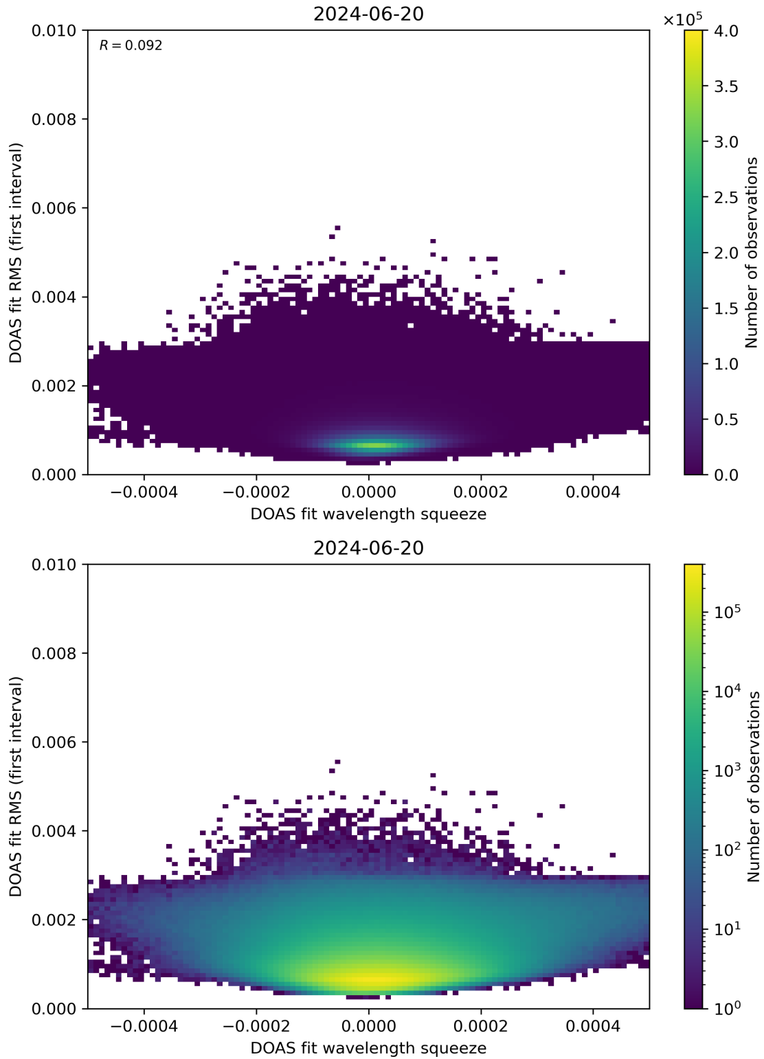
Figure 68: Scatter density plot of “DOAS fit wavelength squeeze” against “DOAS fit RMS (first interval)” for 2024-06-19 to 2024-06-21.
