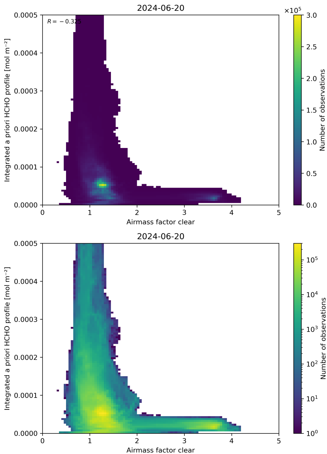
Figure 76: Scatter density plot of “Airmass factor clear” against “Integrated a priori HCHO profile” for 2024-06-19 to 2024-06-21.
