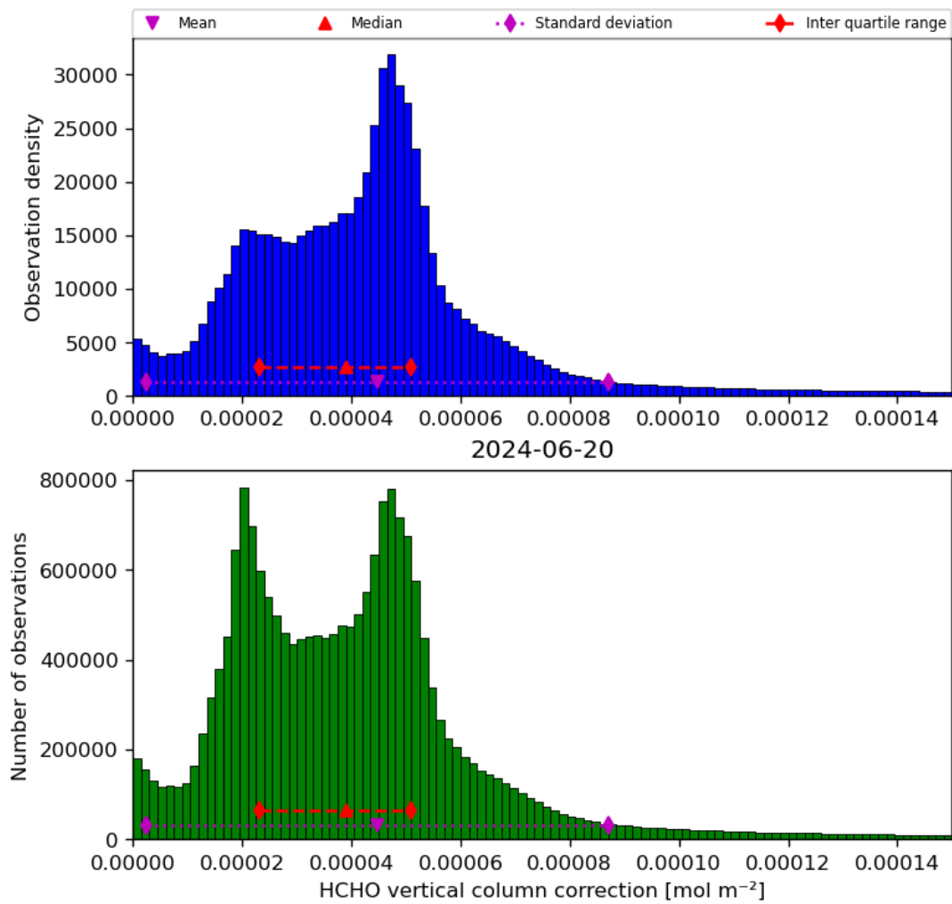
Figure 37: Histogram of “HCHO vertical column correction” for 2024-06-19 to 2024-06-21
