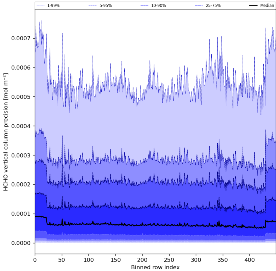
Figure 50: Along track statistics of “HCHO vertical column precision” for 2024-06-19 to 2024-06-21
