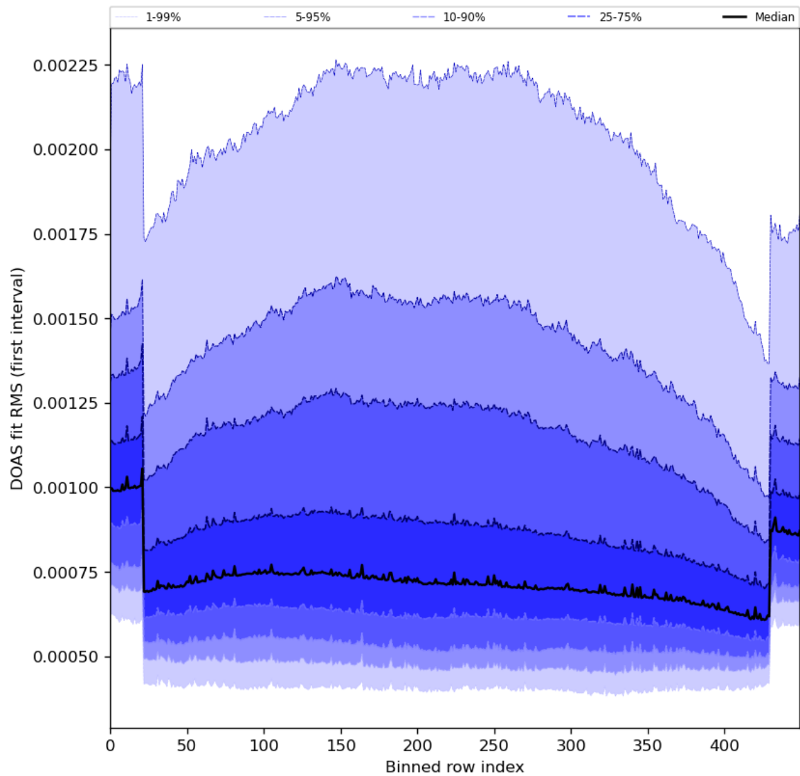
Figure 60: Along track statistics of “DOAS fit RMS (first interval)” for 2024-06-19 to 2024-06-21
