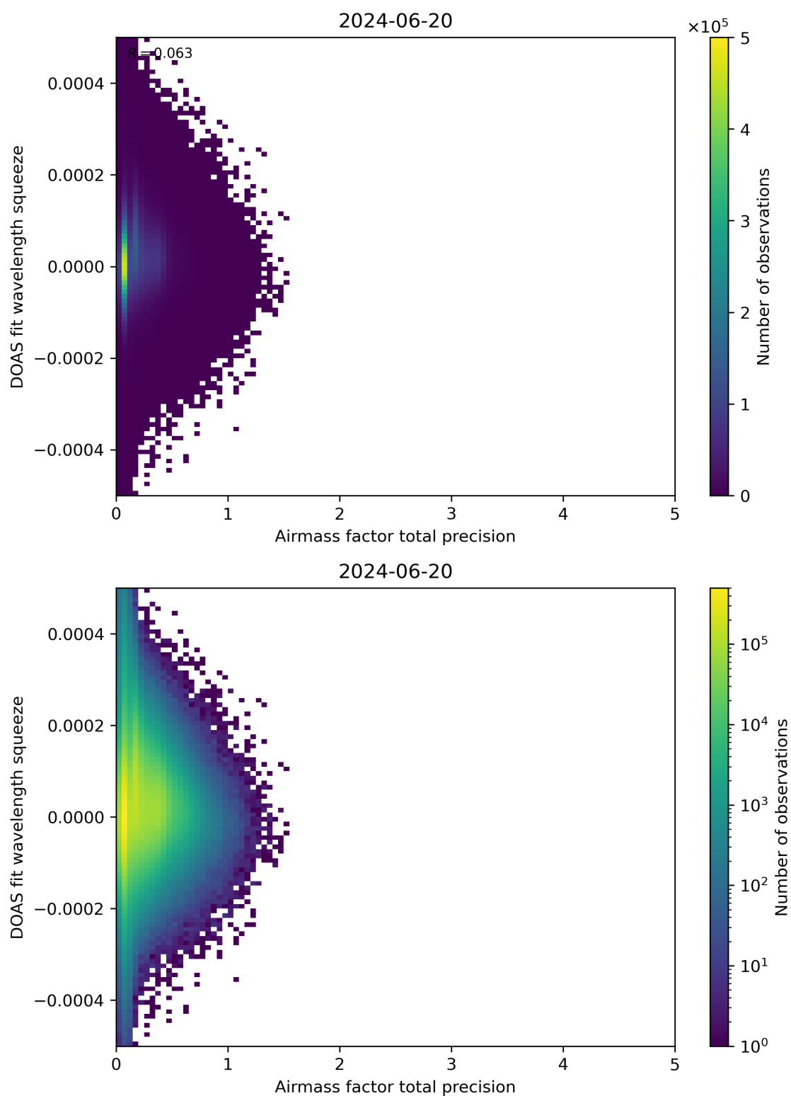
Figure 107: Scatter density plot of “Airmass factor total precision” against “DOAS fit wavelength squeeze” for 2024-06-19 to 2024-06-21.
