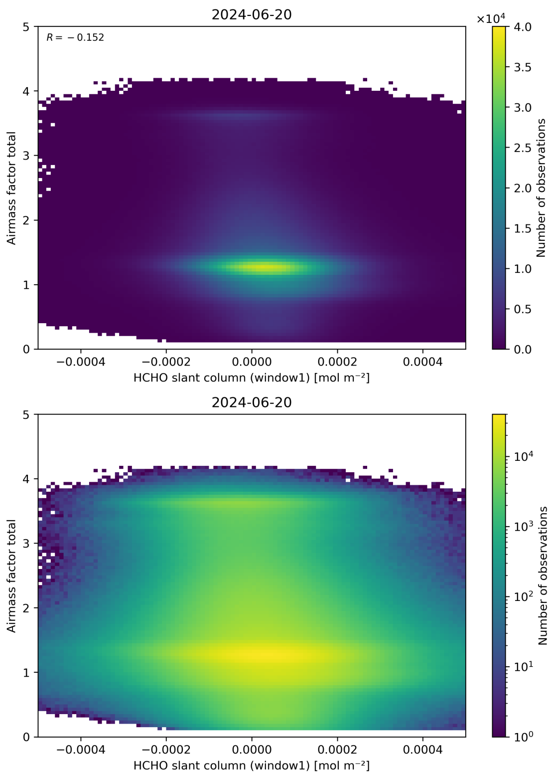
Figure 85: Scatter density plot of “HCHO slant column (window1)” against “Airmass factor total” for 2024-06-19 to 2024-06-21.
