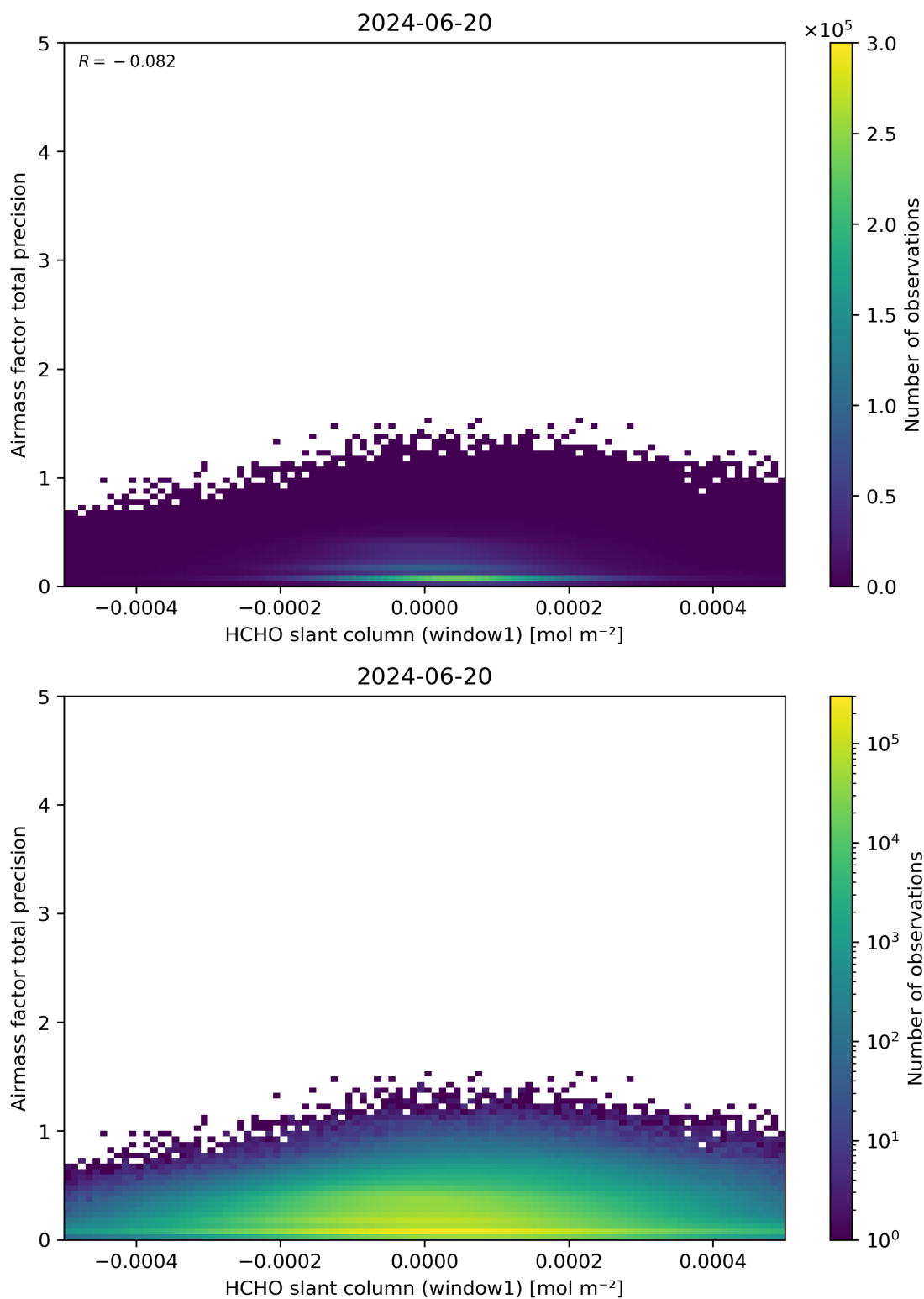
Figure 86: Scatter density plot of “HCHO slant column (window1)” against “Airmass factor total precision” for 2024-06-19 to 2024-06-21.
