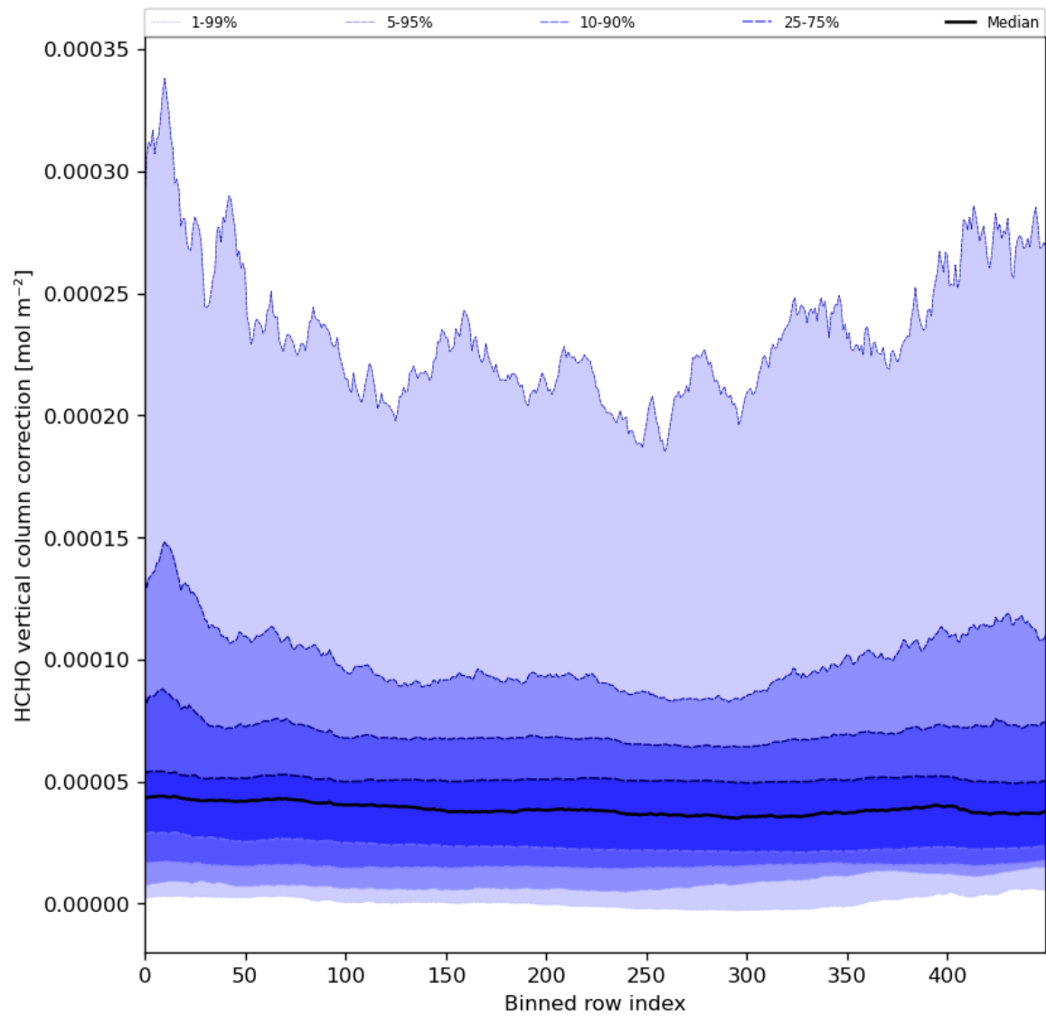
Figure 51: Along track statistics of “HCHO vertical column correction” for 2024-06-19 to 2024-06-21
