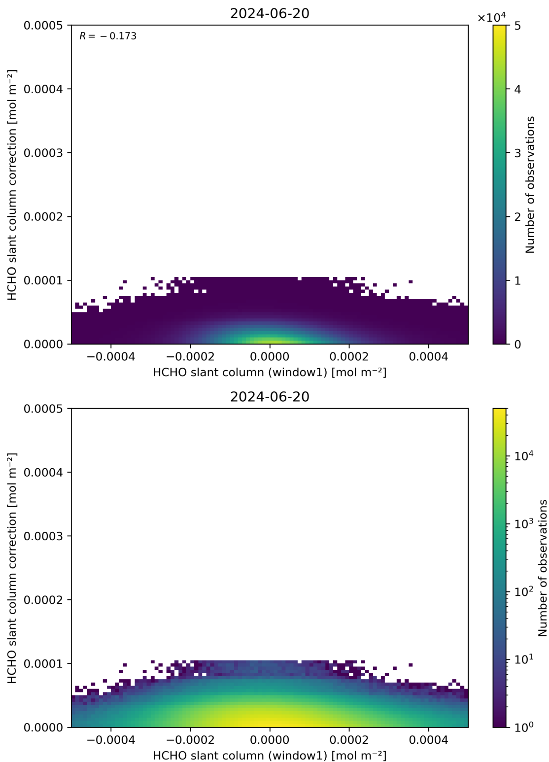
Figure 83: Scatter density plot of “HCHO slant column (window1)” against “HCHO slant column correction” for 2024-06-19 to 2024-06-21.
