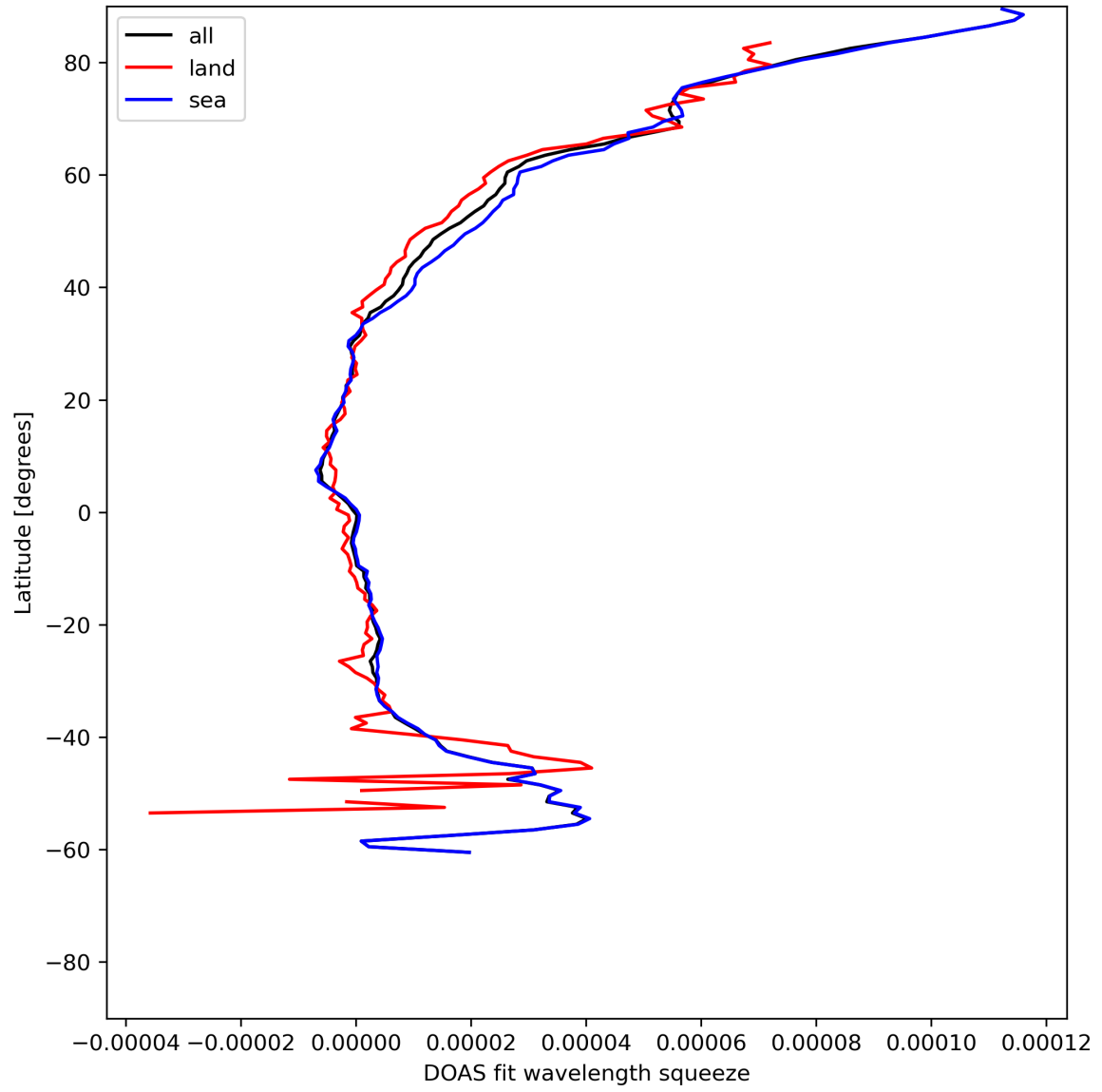
Figure 31: Zonal average of “DOAS fit wavelength squeeze” for 2024-06-19 to 2024-06-21.
