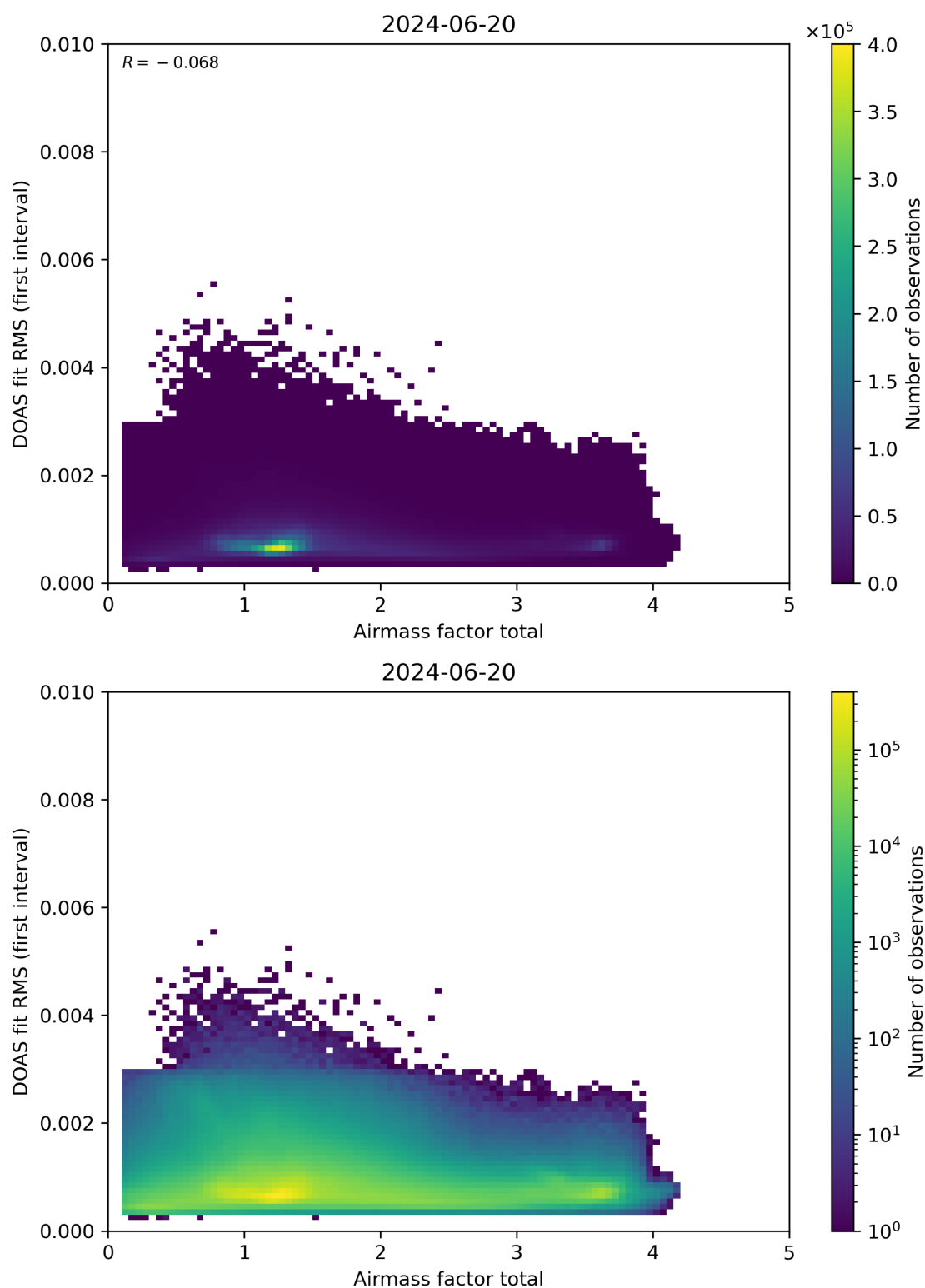
Figure 97: Scatter density plot of “Airmass factor total” against “DOAS fit RMS (first interval)” for 2024-06-19 to 2024-06-21.
