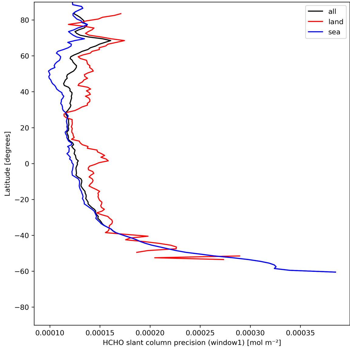
Figure 25: Zonal average of "HCHO slant column precision (window1)" for 2024-06-19 to 2024-06-21.
