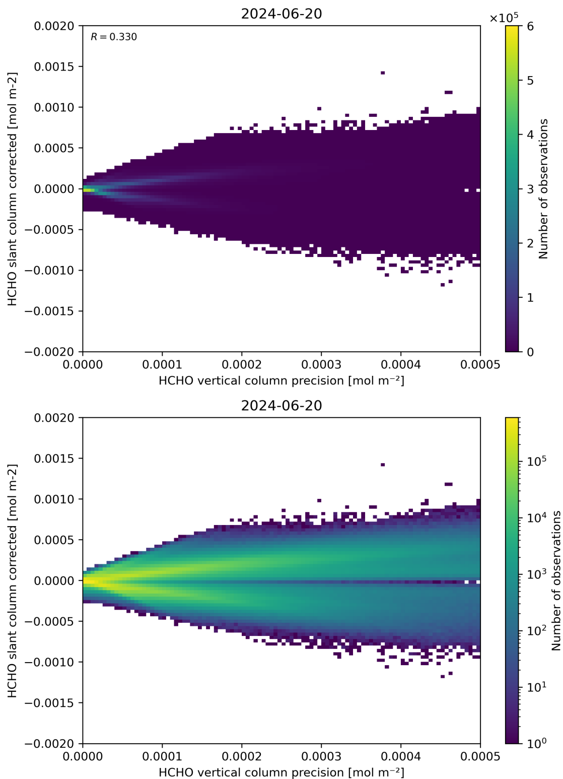
Figure 140: Scatter density plot of “HCHO vertical column precision” against “HCHO slant column corrected” for 2024-06-19 to 2024-06-21.
