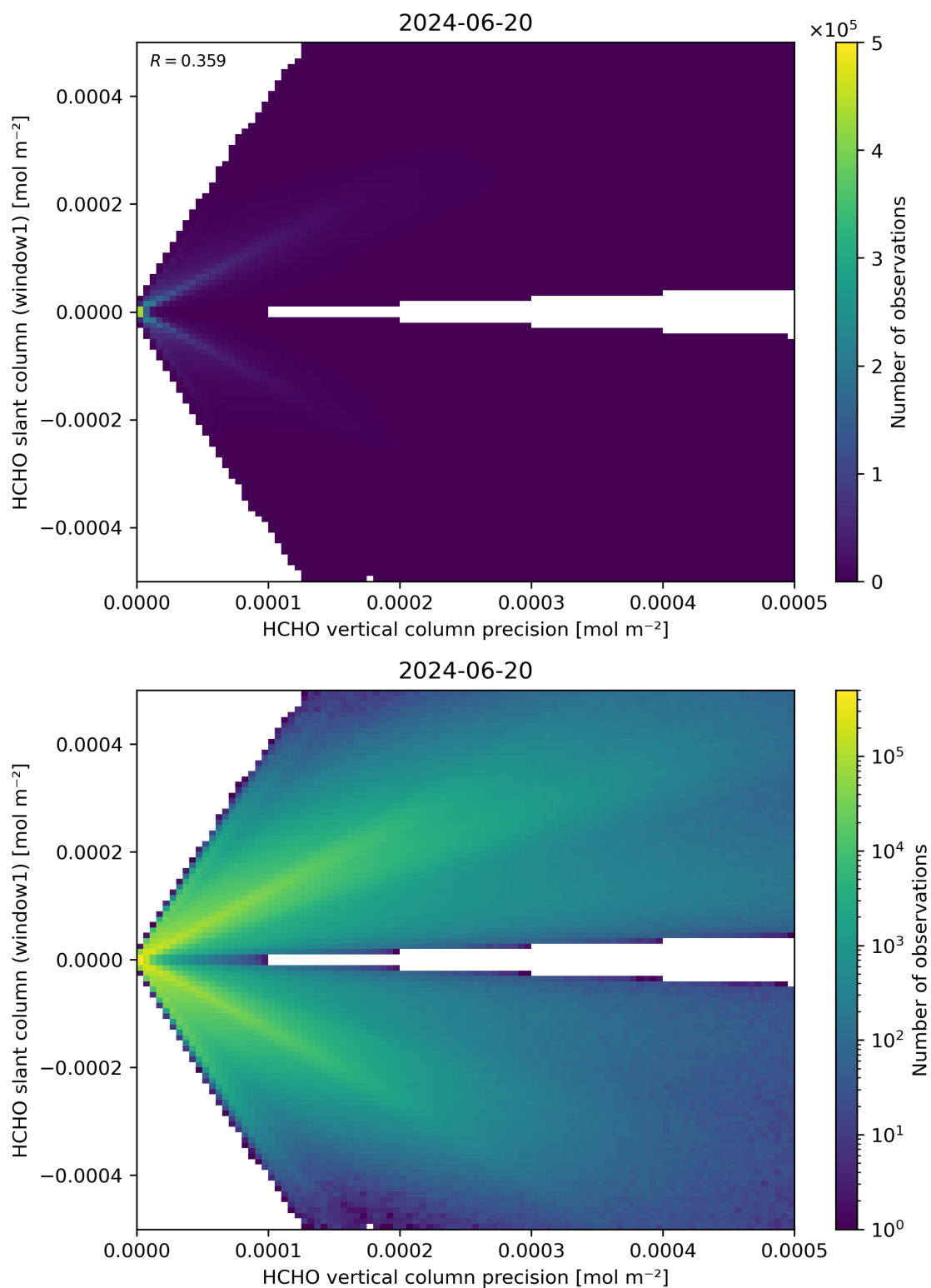
Figure 142: Scatter density plot of “HCHO vertical column precision” against “HCHO slant column (window1)” for 2024-06-19 to 2024-06-21.
