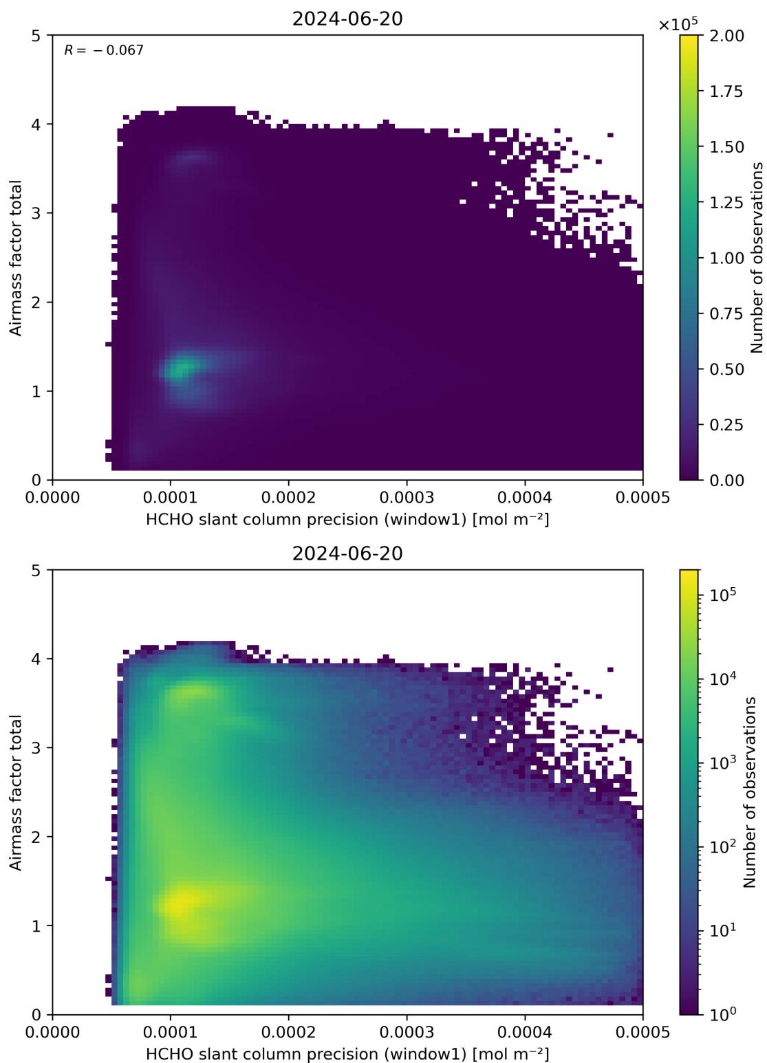
Figure 94: Scatter density plot of “HCHO slant column precision (window1)” against “Airmass factor total” for 2024-06-19 to 2024-06-21.
