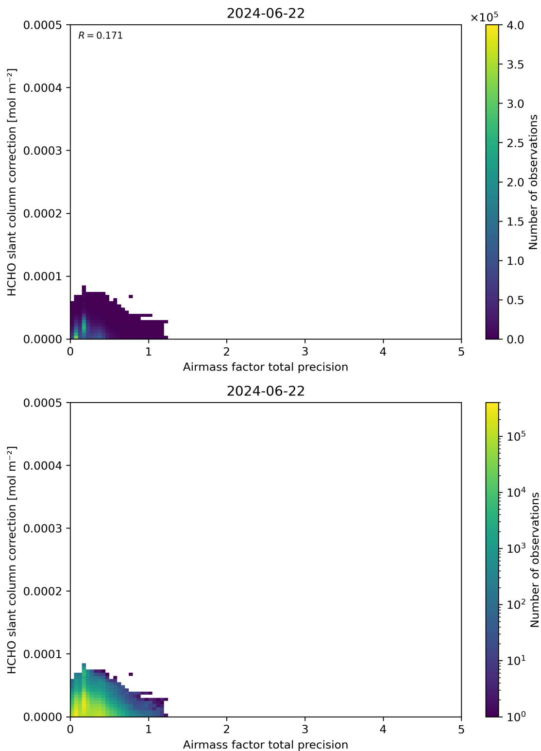
Figure 110: Scatter density plot of “Airmass factor total precision” against “HCHO slant column correction” for 2024-06-21 to 2024-06-23.
