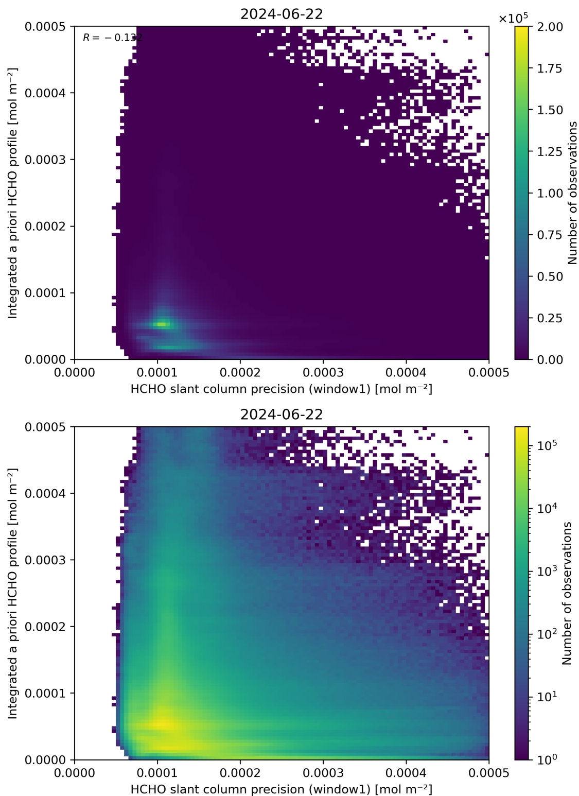
Figure 96: Scatter density plot of “HCHO slant column precision (window1)” against “Integrated a priori HCHO profile” for 2024-06-21 to 2024-06-23.
