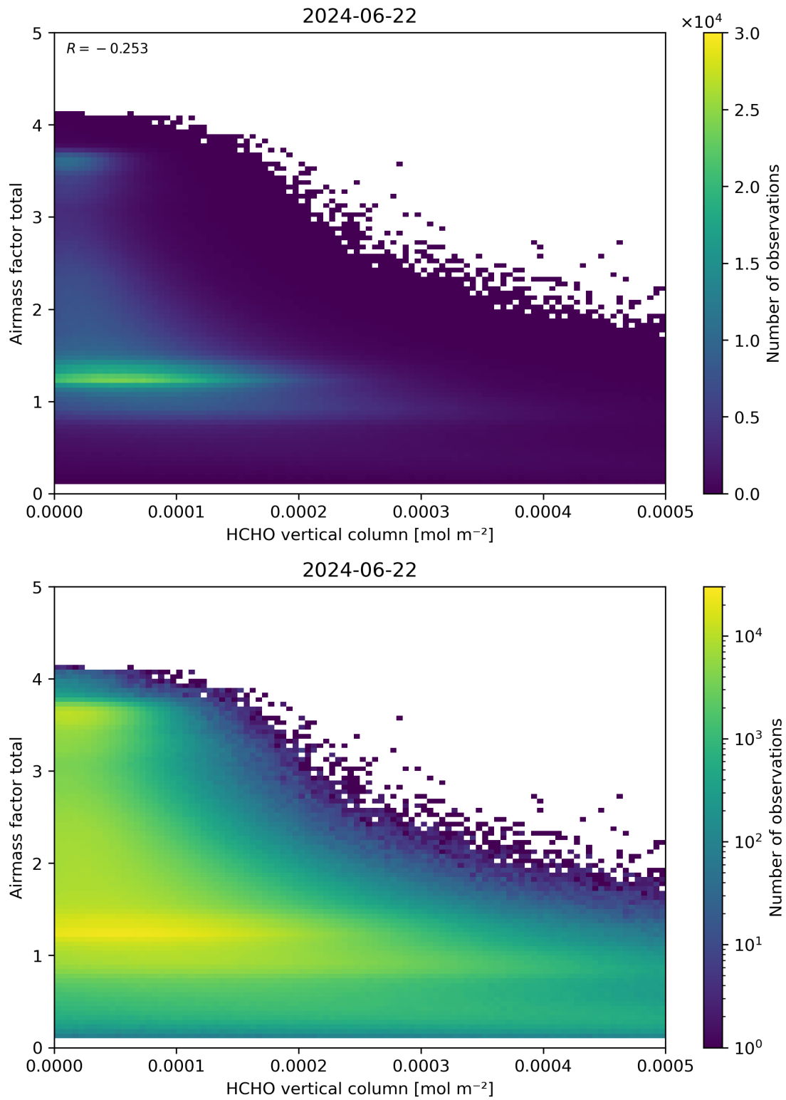
Figure 131: Scatter density plot of “HCHO vertical column” against “Airmass factor total” for 2024-06-21 to 2024-06-23.
