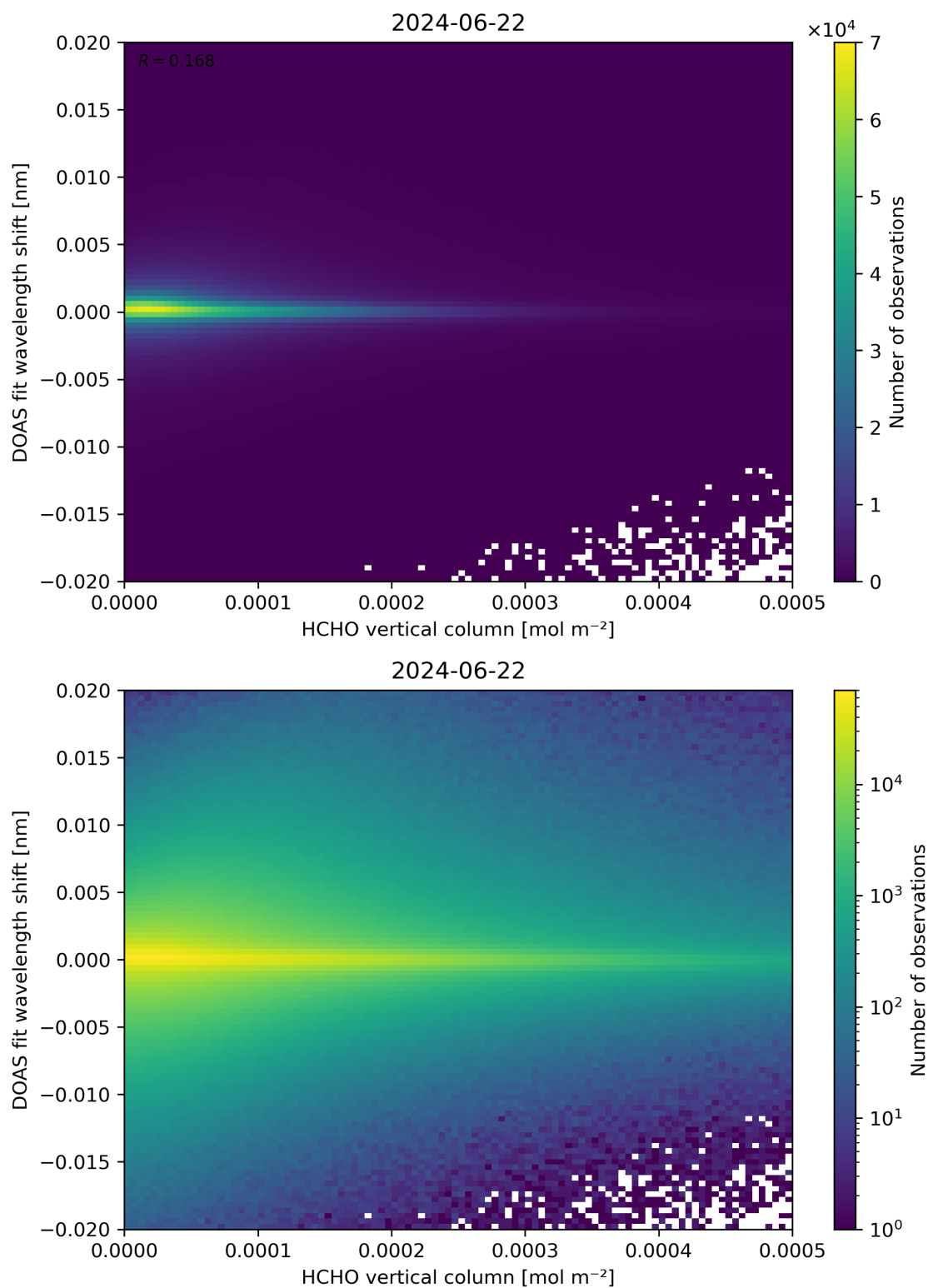
Figure 124: Scatter density plot of “HCHO vertical column” against “DOAS fit wavelength shift” for 2024-06-21 to 2024-06-23.
