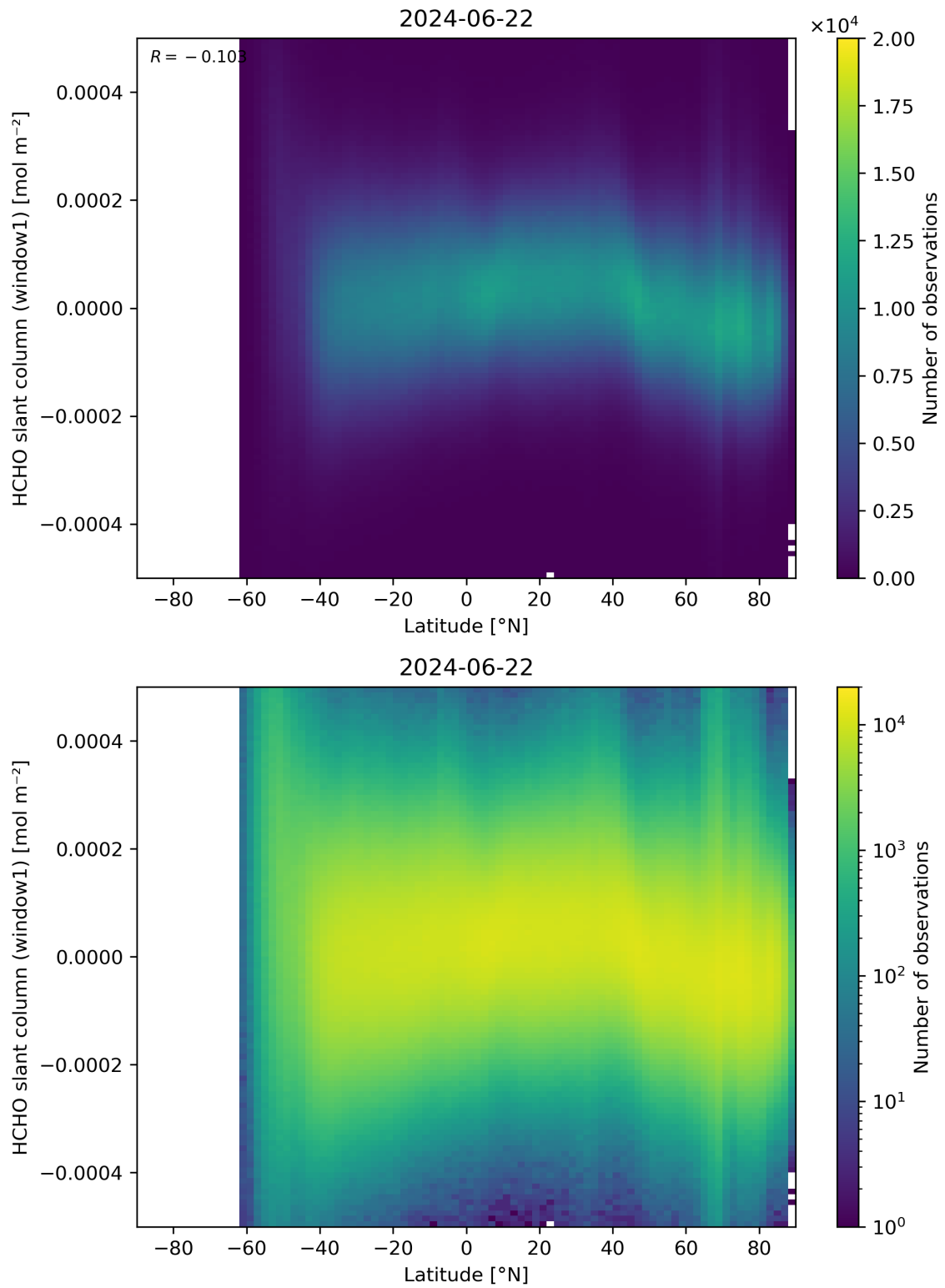
Figure 159: Scatter density plot of “Latitude” against “HCHO slant column (window1)” for 2024-06-21 to 2024-06-23.
