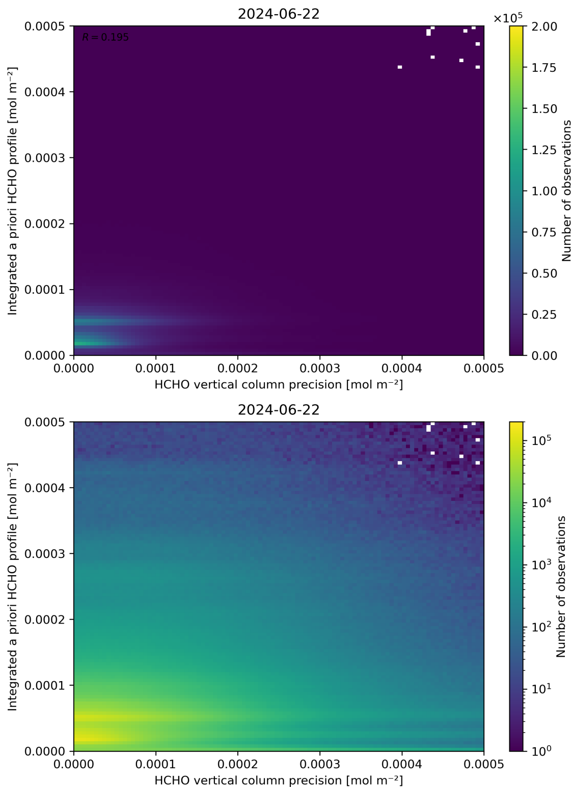
Figure 147: Scatter density plot of “HCHO vertical column precision” against “Integrated a priori HCHO profile” for 2024-06-21 to 2024-06-23.
