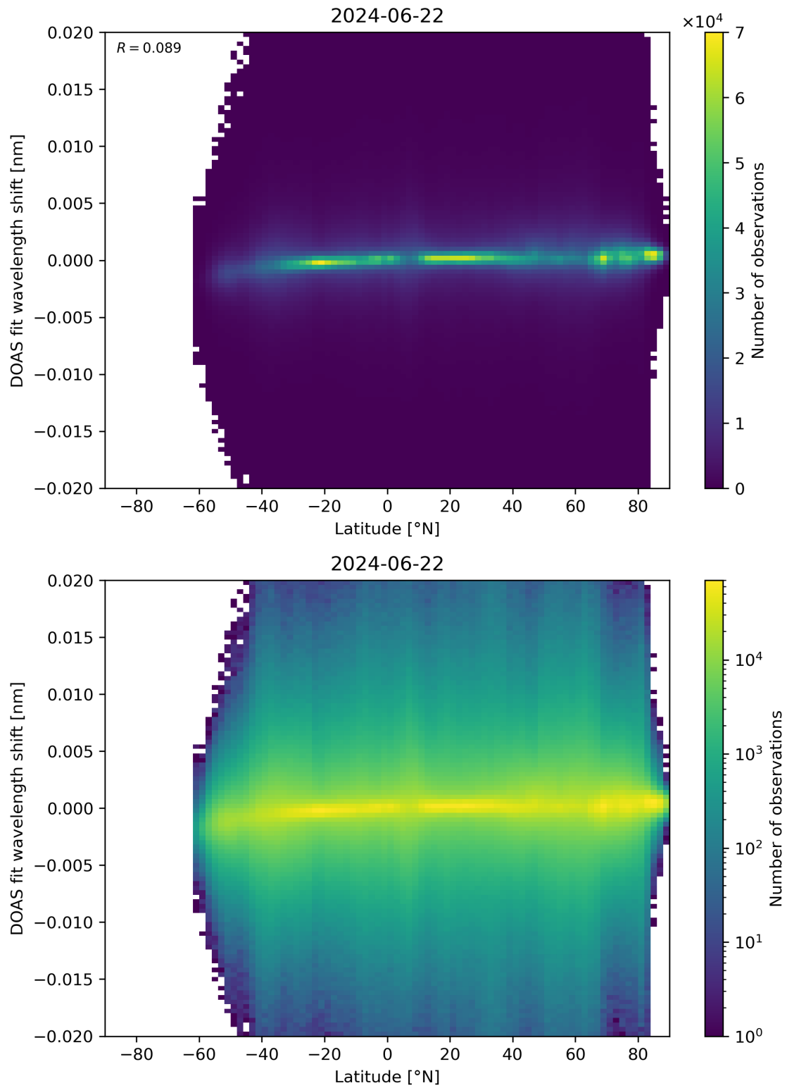
Figure 154: Scatter density plot of “Latitude” against “DOAS fit wavelength shift” for 2024-06-21 to 2024-06-23.
