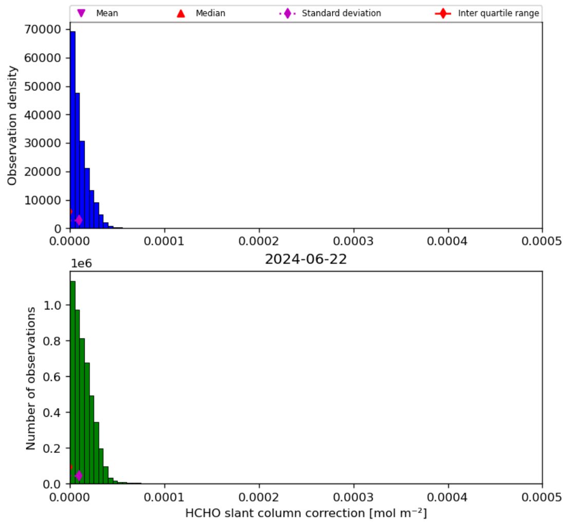
Figure 47: Histogram of “HCHO slant column correction” for 2024-06-21 to 2024-06-23
