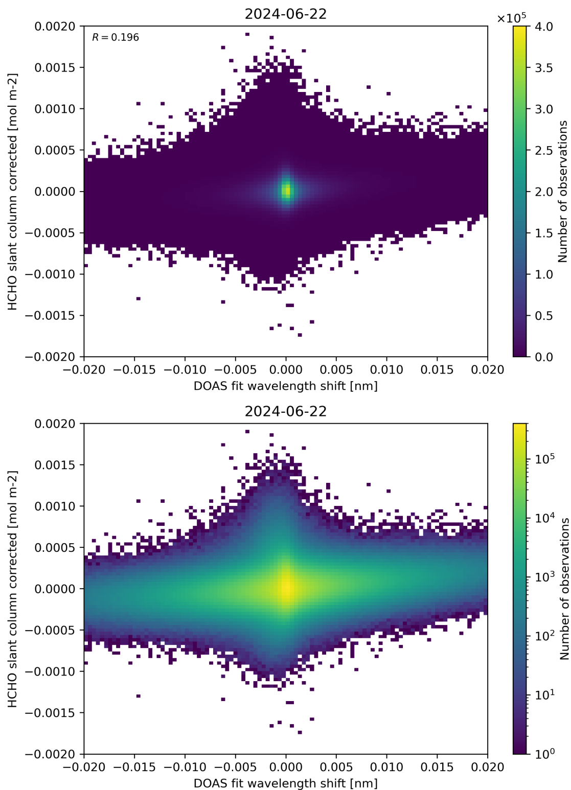
Figure 66: Scatter density plot of “DOAS fit wavelength shift” against “HCHO slant column corrected” for 2024-06-21 to 2024-06-23.
