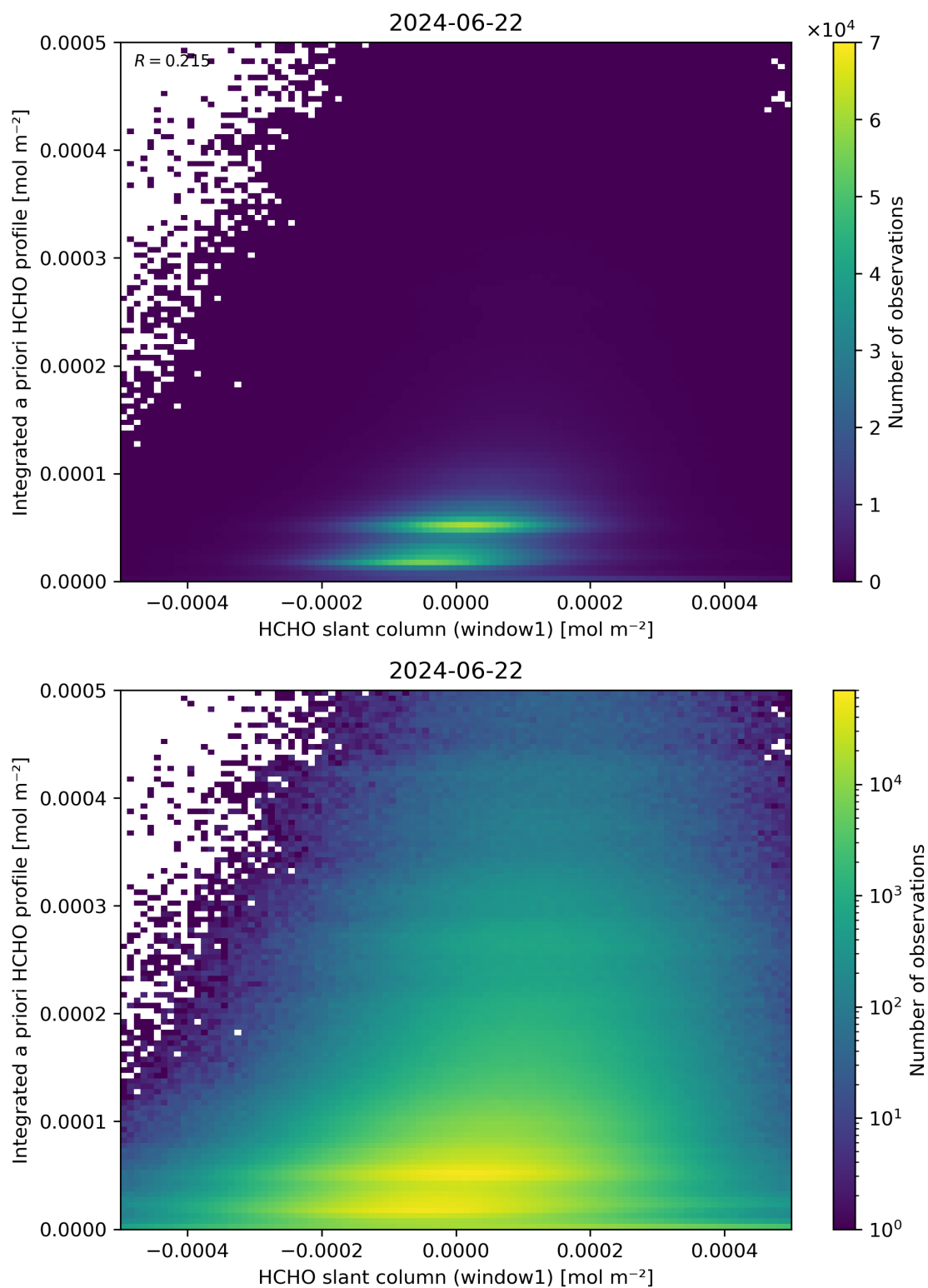
Figure 87: Scatter density plot of “HCHO slant column (window1)” against “Integrated a priori HCHO profile” for 2024-06-21 to 2024-06-23.
