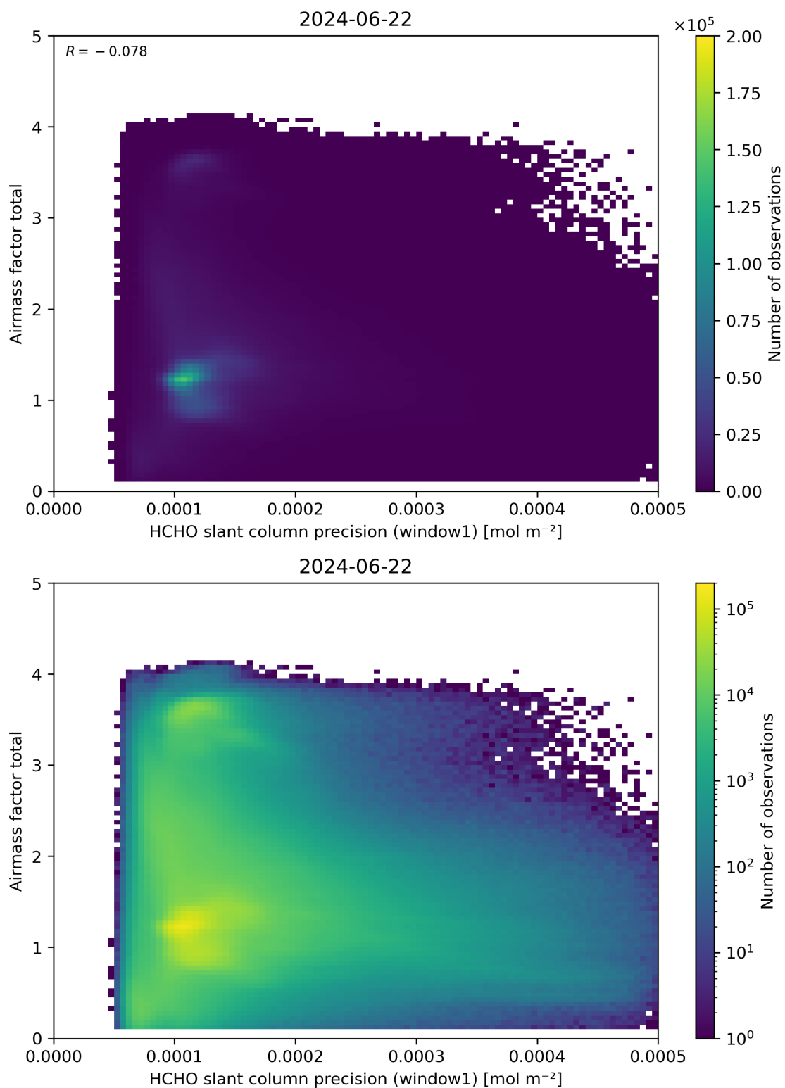
Figure 94: Scatter density plot of “HCHO slant column precision (window1)” against “Airmass factor total” for 2024-06-21 to 2024-06-23.
