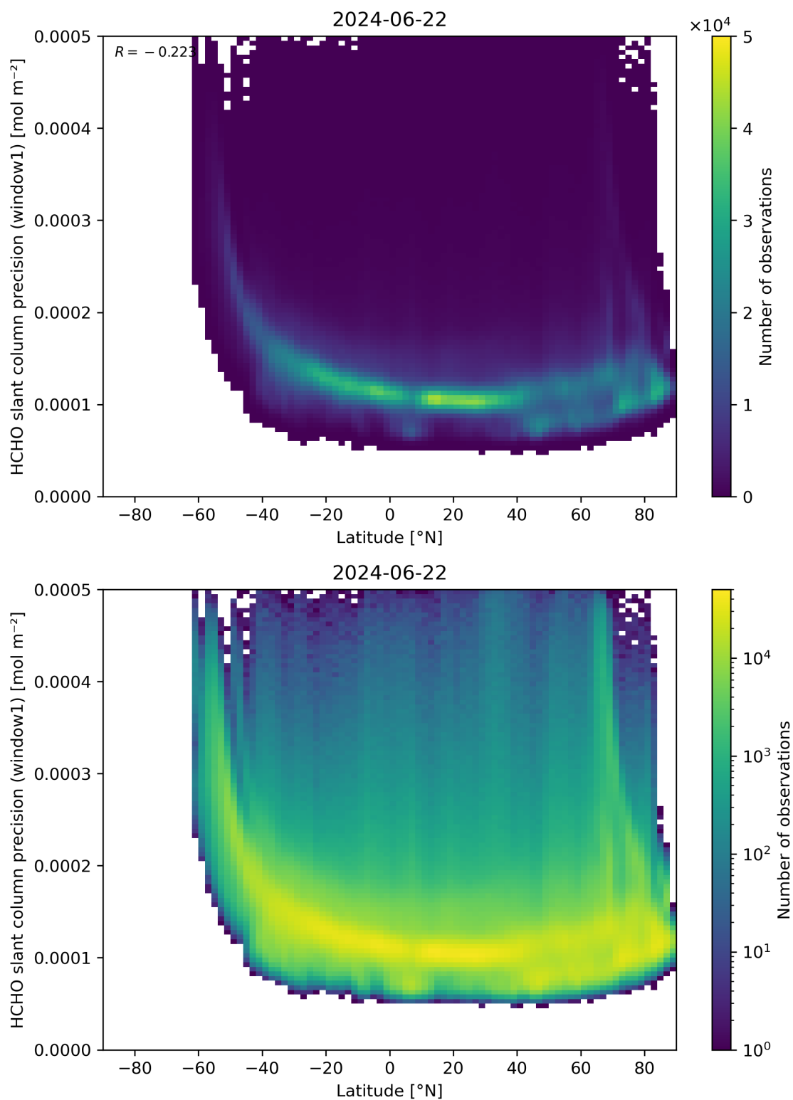
Figure 160: Scatter density plot of “Latitude” against “HCHO slant column precision (window1)” for 2024-06-21 to 2024-06-23.
