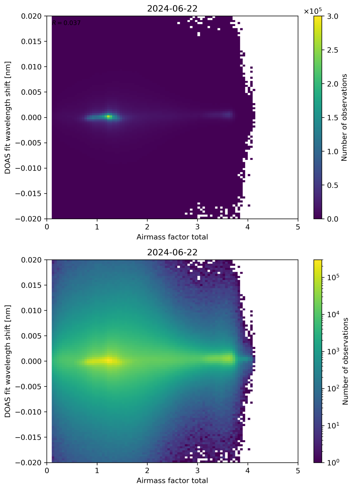
Figure 98: Scatter density plot of “Airmass factor total” against “DOAS fit wavelength shift” for 2024-06-21 to 2024-06-23.
