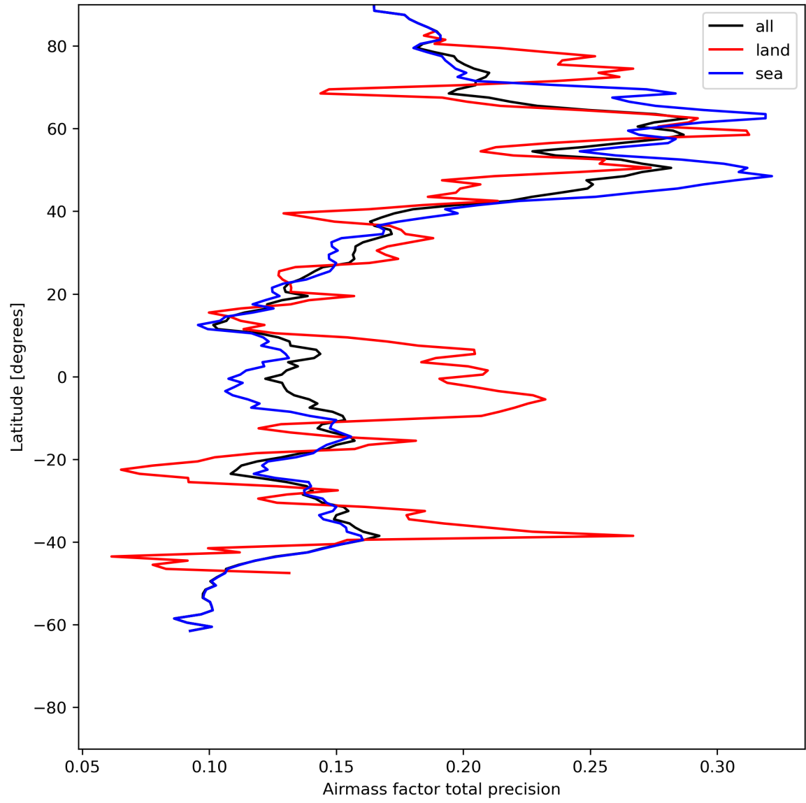
Figure 27: Zonal average of “Airmass factor total precision” for 2024-06-21 to 2024-06-23.
