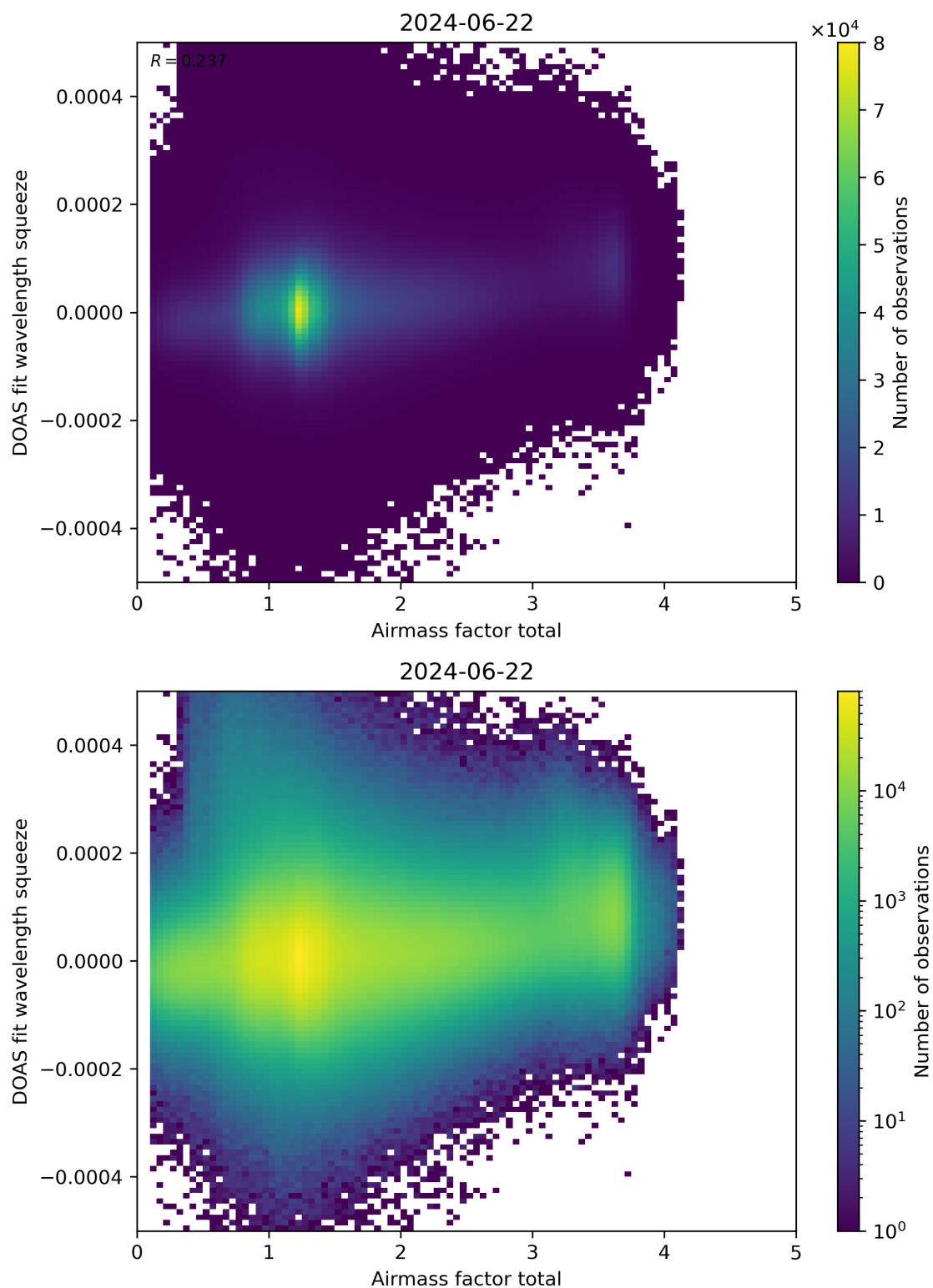
Figure 99: Scatter density plot of “Airmass factor total” against “DOAS fit wavelength squeeze” for 2024-06-21 to 2024-06-23.
