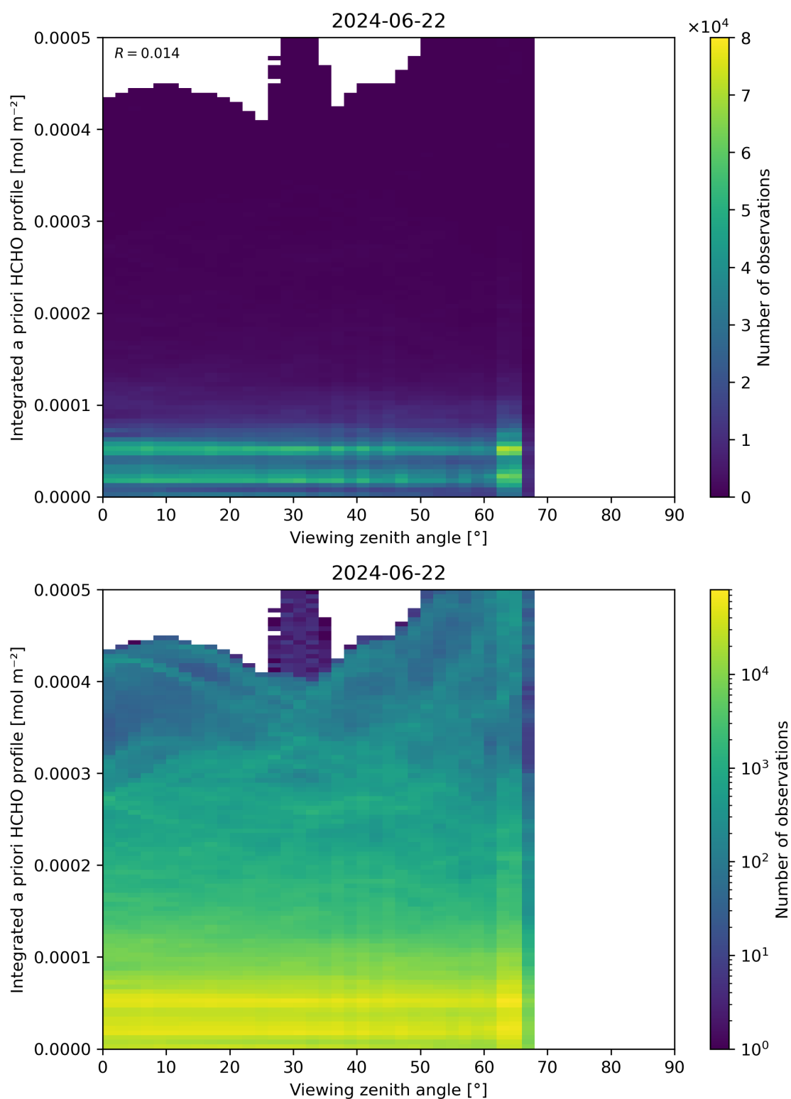
Figure 195: Scatter density plot of “Viewing zenith angle” against “Integrated a priori HCHO profile” for 2024-06-21 to 2024-06-23.
