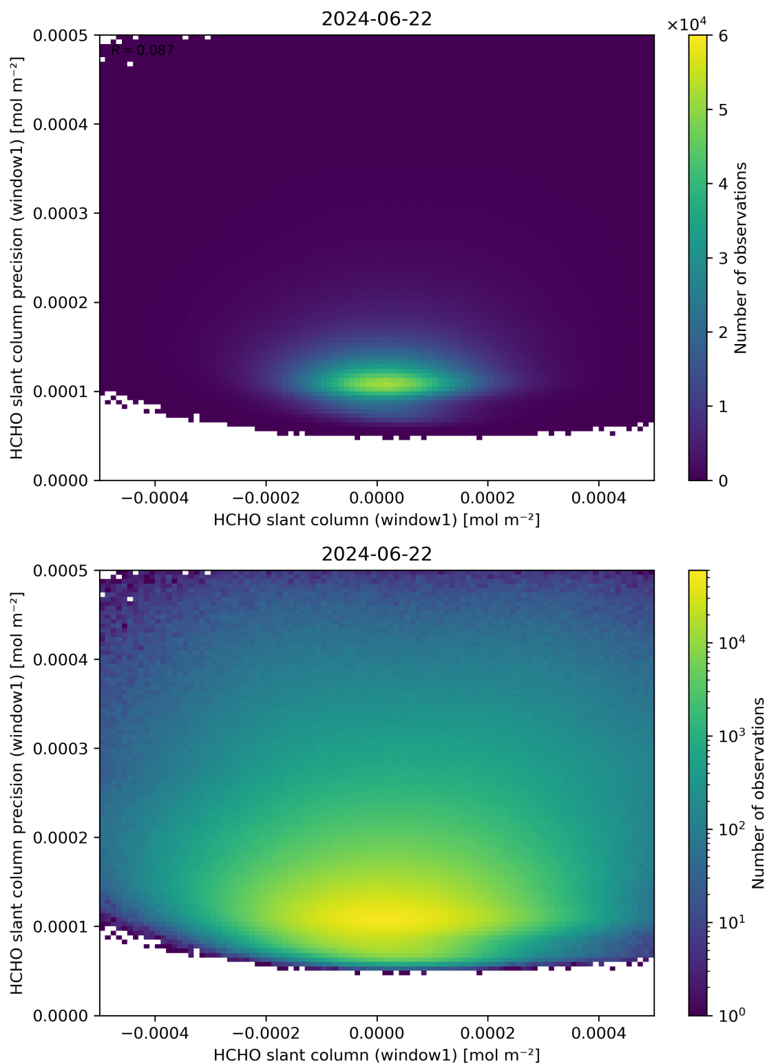
Figure 84: Scatter density plot of “HCHO slant column (window1)” against “HCHO slant column precision (window1)” for 2024-06-21 to 2024-06-23.
