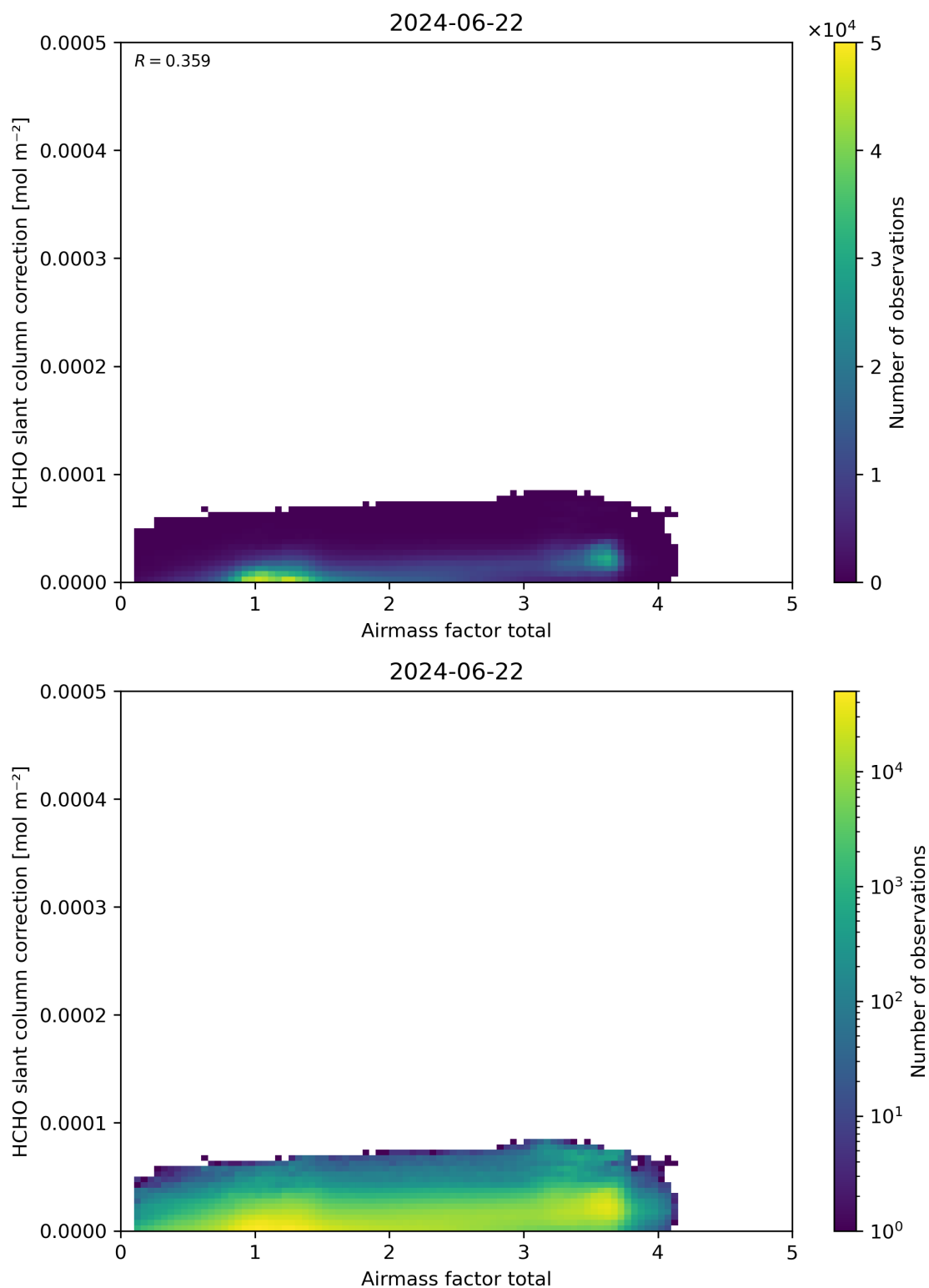
Figure 102: Scatter density plot of “Airmass factor total” against “HCHO slant column correction” for 2024-06-21 to 2024-06-23.
