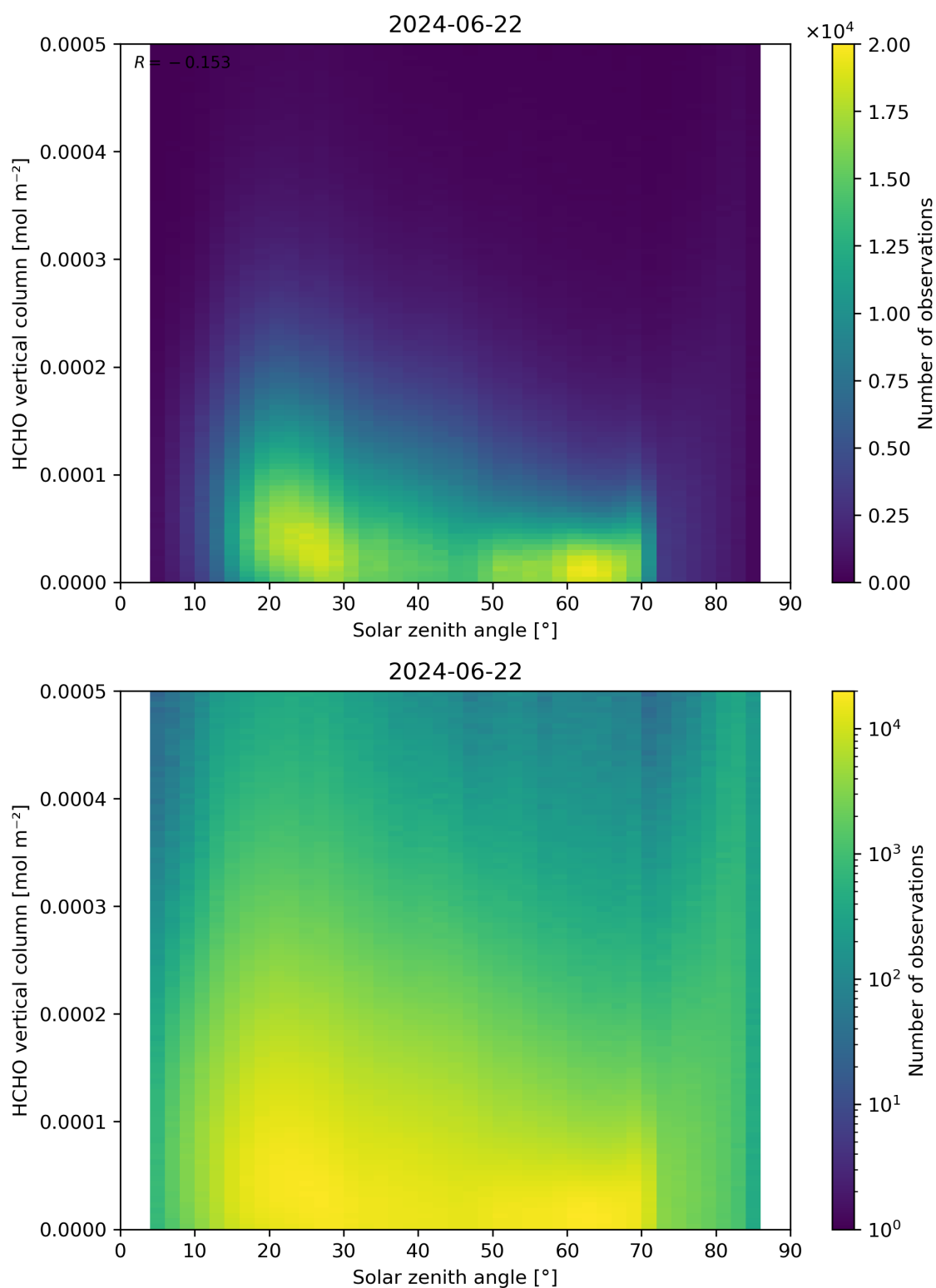
Figure 177: Scatter density plot of “Solar zenith angle” against “HCHO vertical column” for 2024-06-21 to 2024-06-23.
