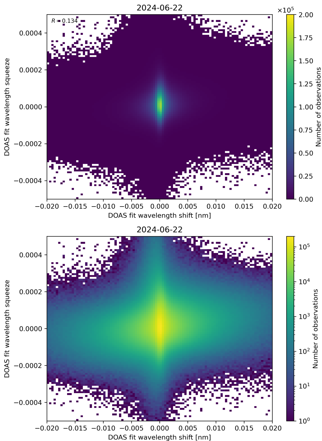
Figure 65: Scatter density plot of “DOAS fit wavelength shift” against “DOAS fit wavelength squeeze” for 2024-06-21 to 2024-06-23.
