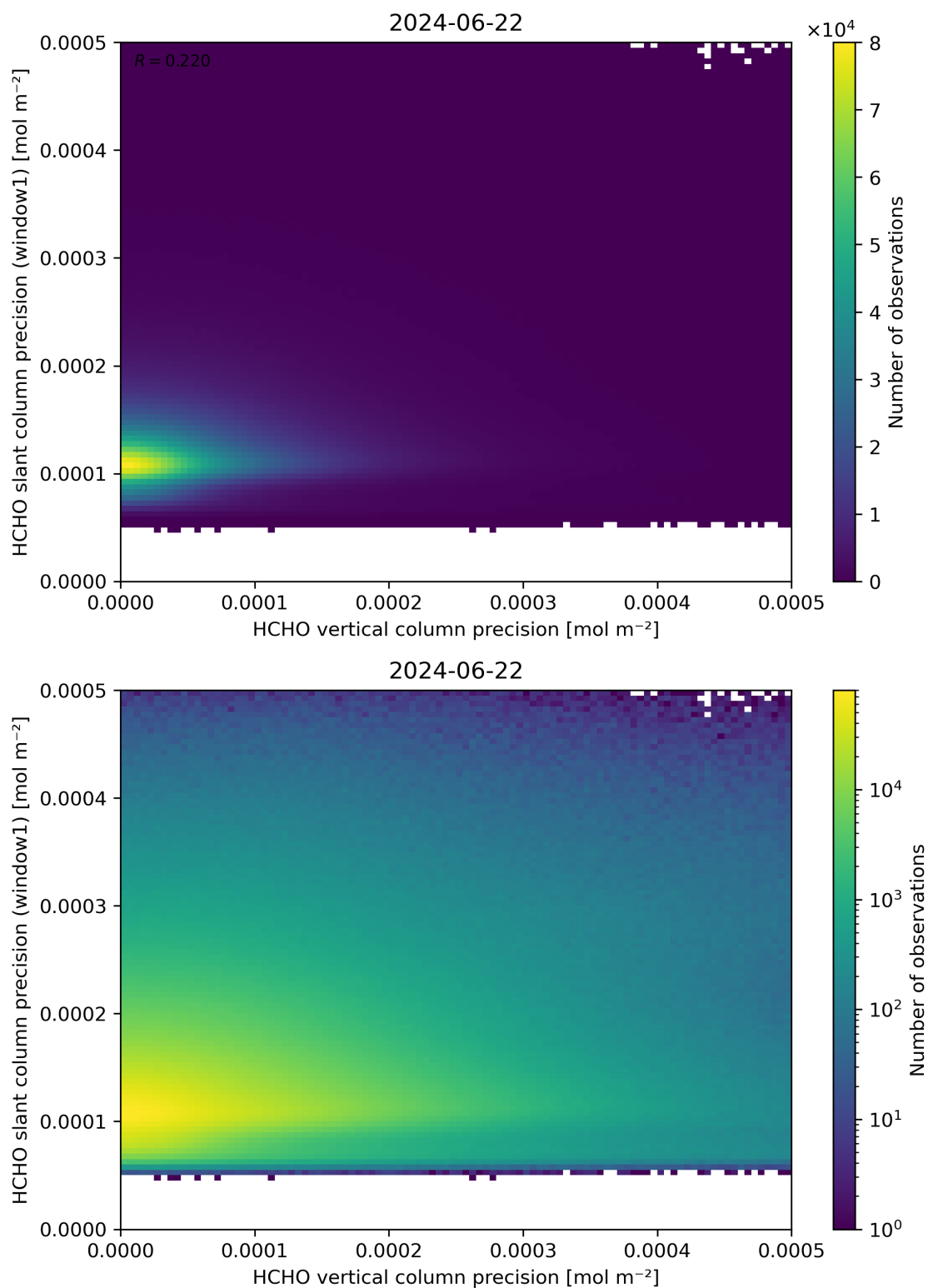
Figure 143: Scatter density plot of “HCHO vertical column precision” against “HCHO slant column precision (window1)” for 2024-06-21 to 2024-06-23.
