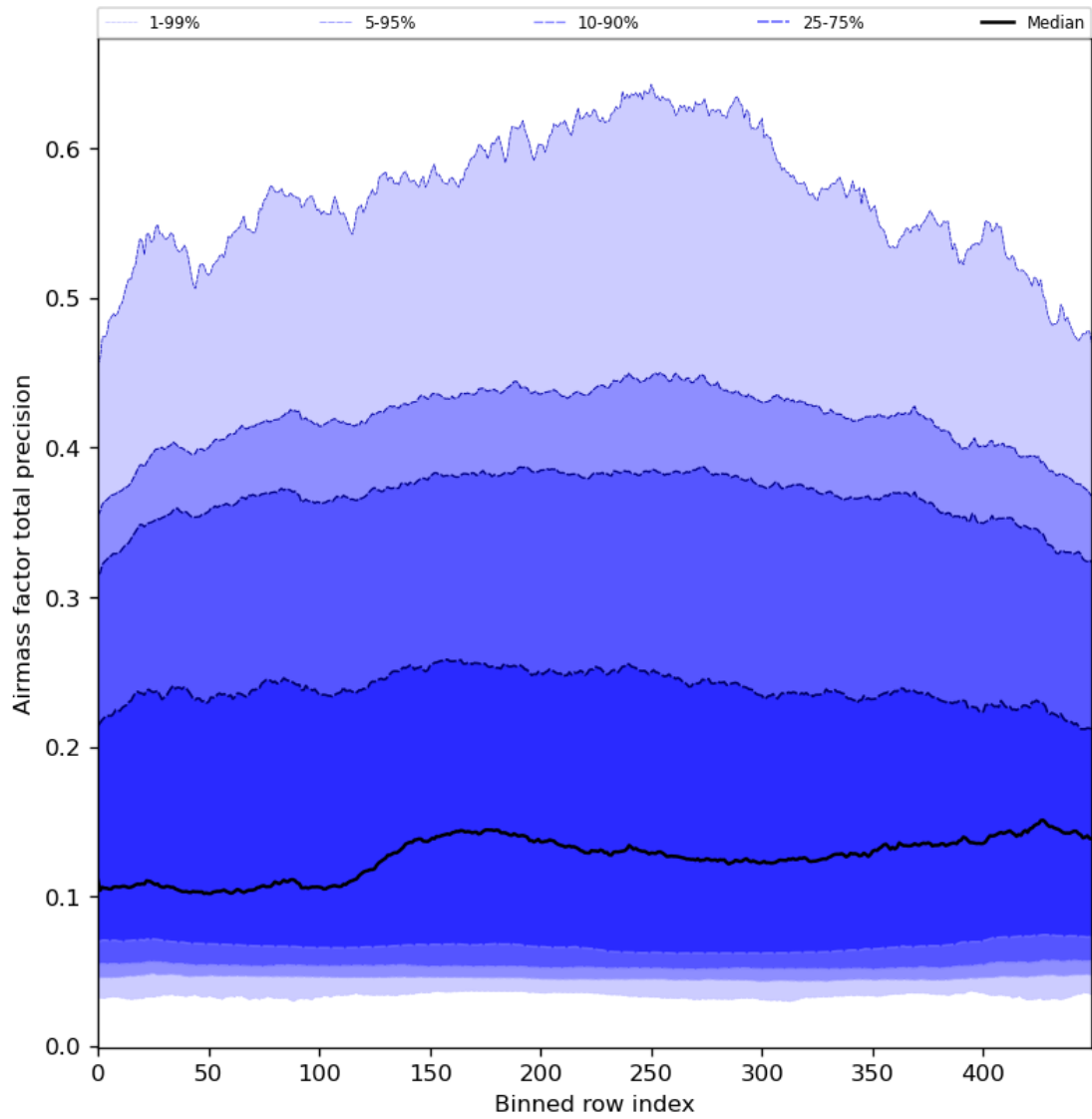
Figure 55: Along track statistics of “Airmass factor total precision” for 2024-06-21 to 2024-06-23
