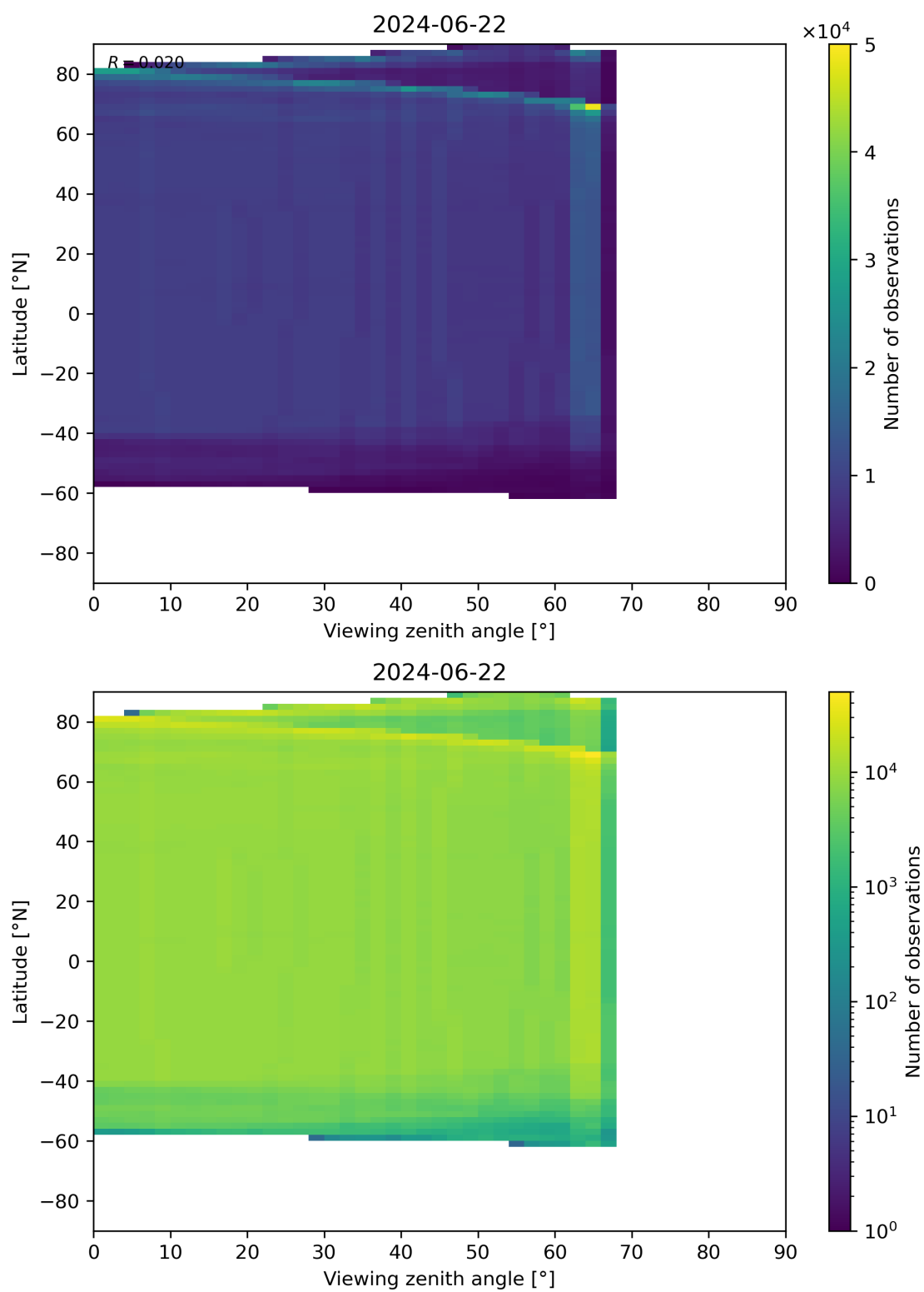
Figure 196: Scatter density plot of “Viewing zenith angle” against “Latitude” for 2024-06-21 to 2024-06-23.
