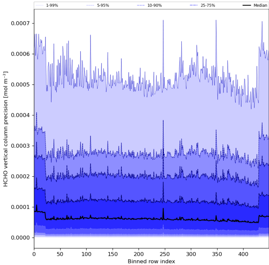
Figure 50: Along track statistics of “HCHO vertical column precision” for 2024-06-21 to 2024-06-23
