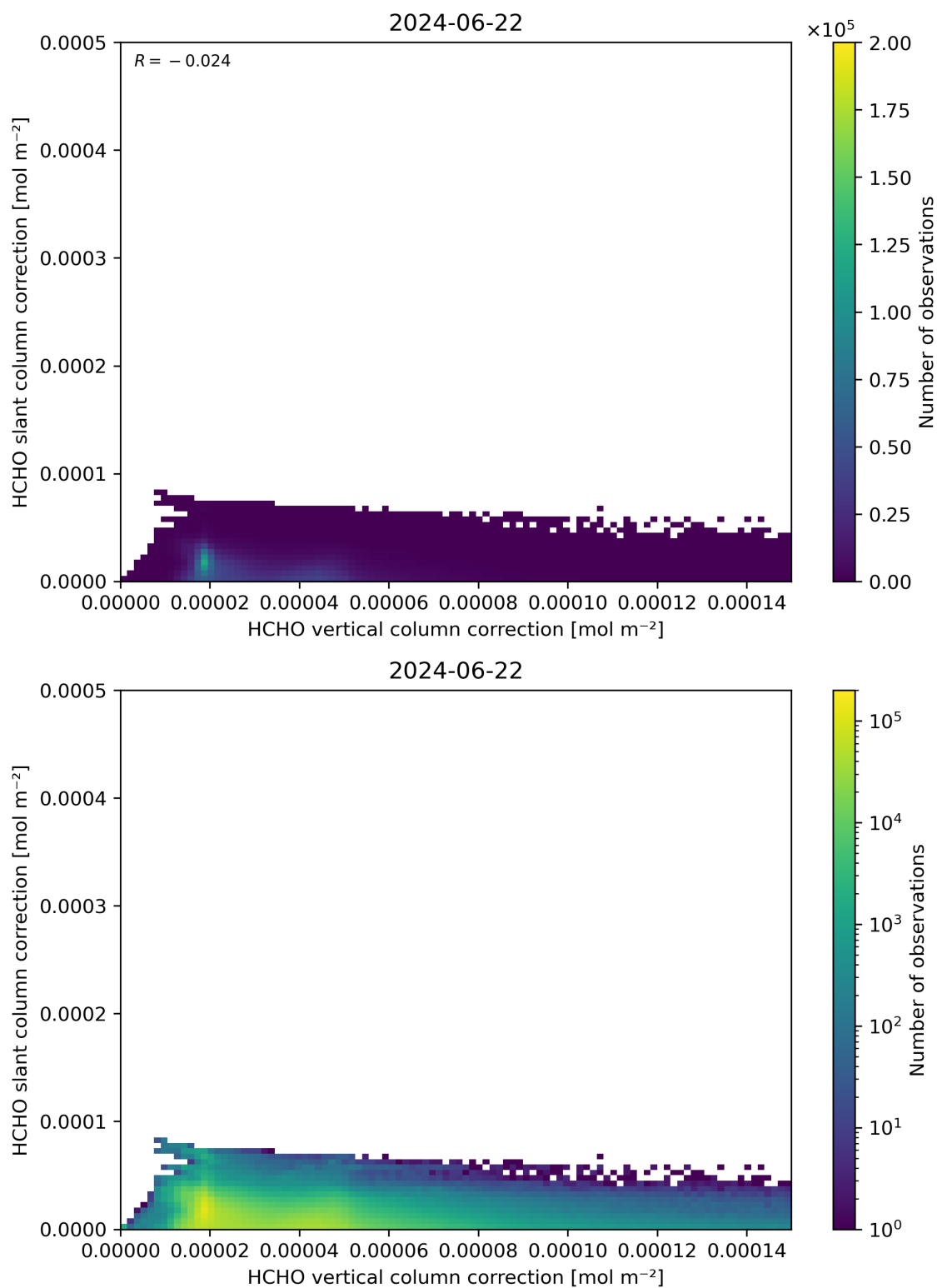
Figure 117: Scatter density plot of “HCHO vertical column correction” against “HCHO slant column correction” for 2024-06-21 to 2024-06-23.
