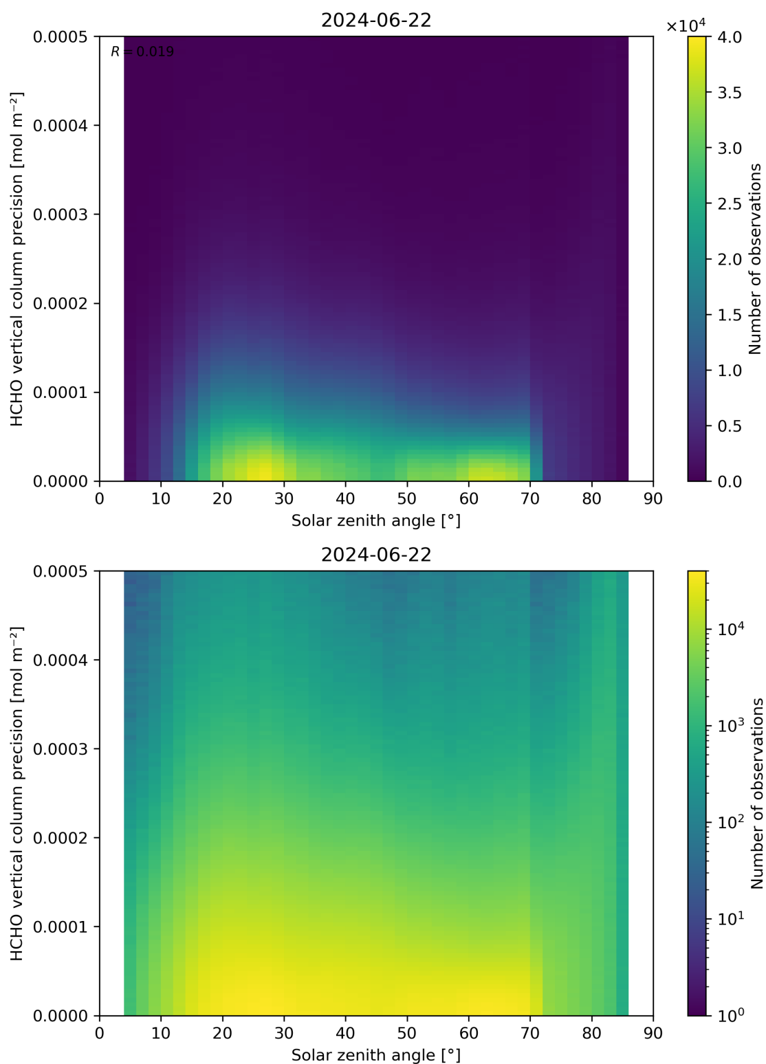
Figure 179: Scatter density plot of “Solar zenith angle” against “HCHO vertical column precision” for 2024-06-21 to 2024-06-23.
