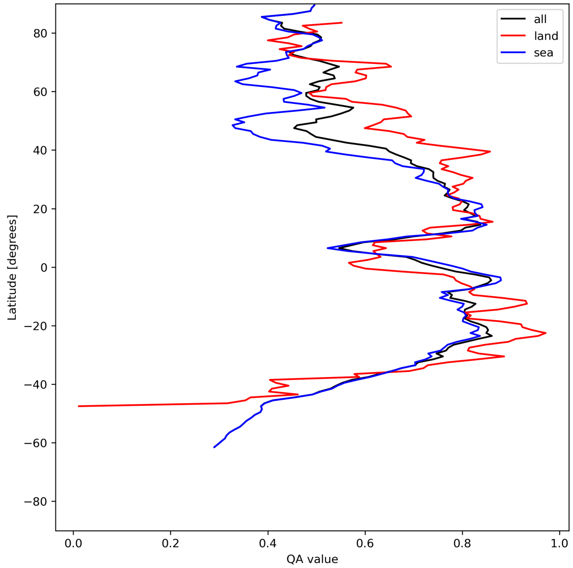
Figure 20: Zonal average of “QA value” for 2024-06-21 to 2024-06-23.
