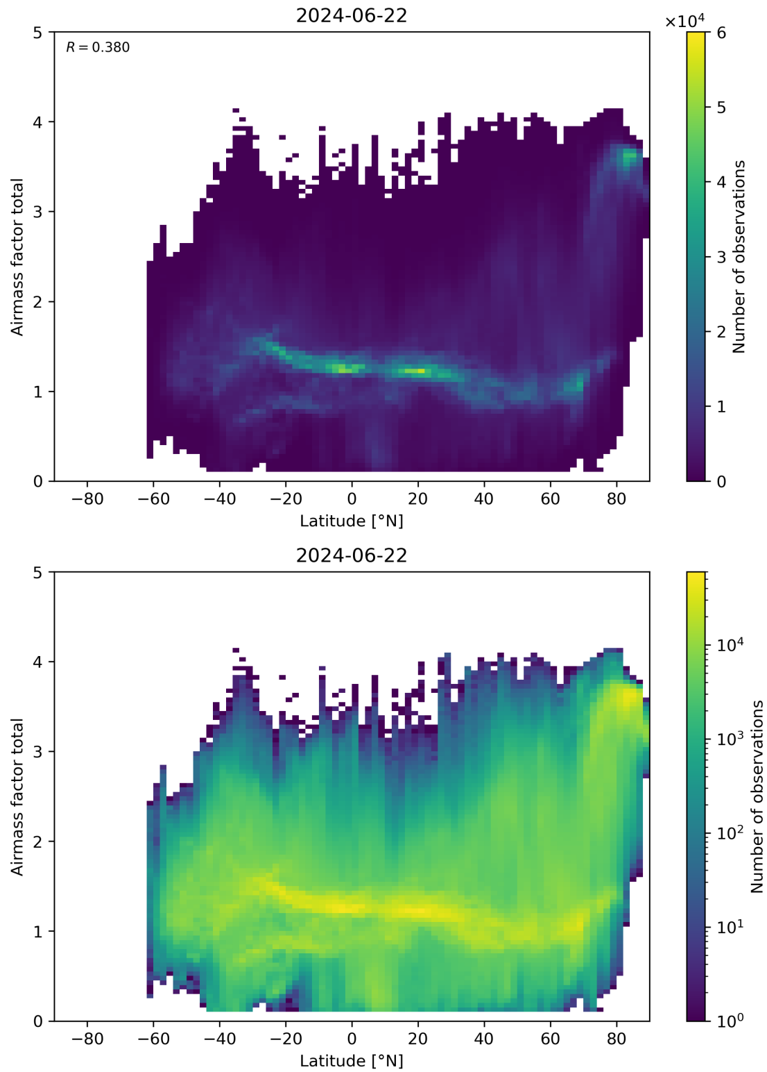
Figure 161: Scatter density plot of “Latitude” against “Airmass factor total” for 2024-06-21 to 2024-06-23.
