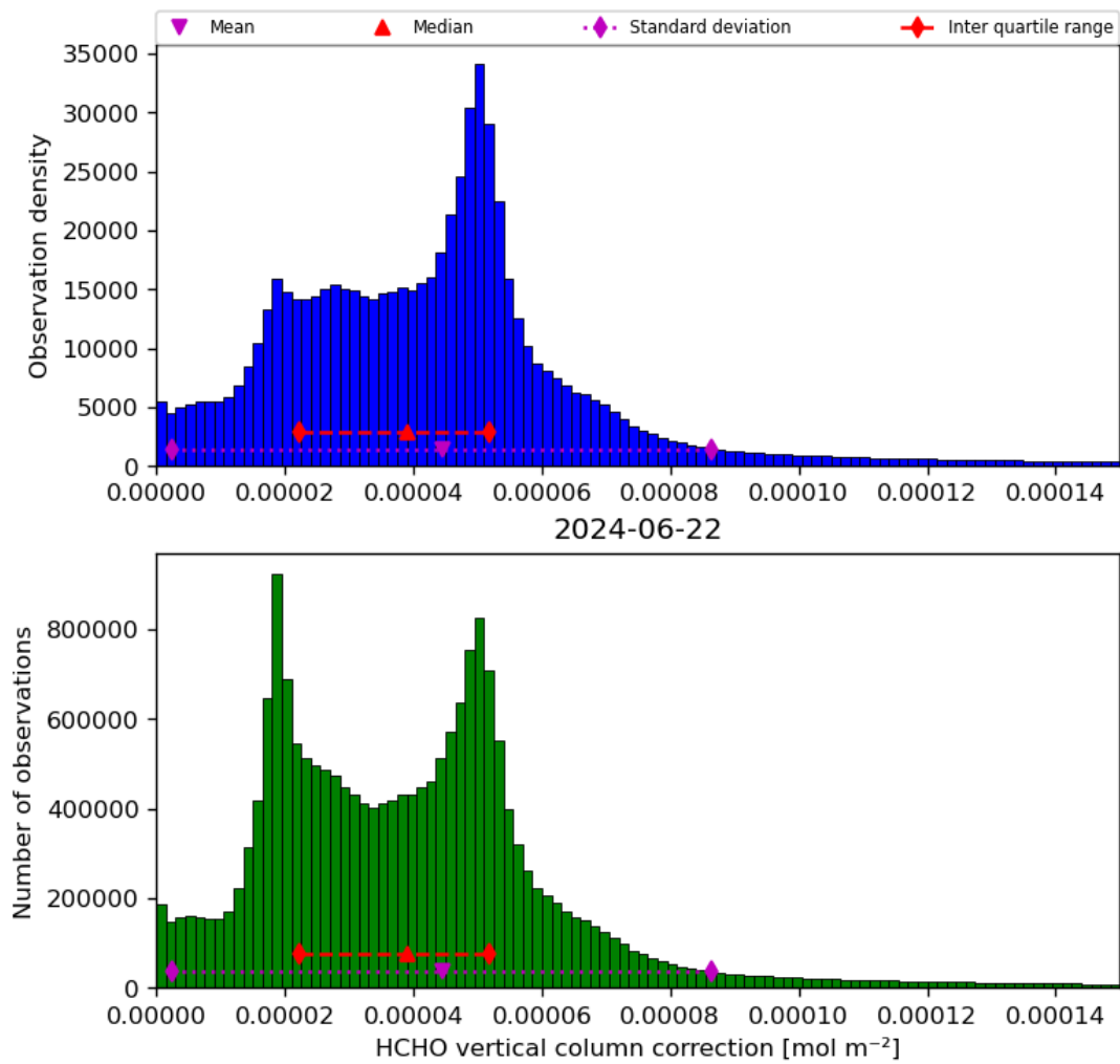
Figure 37: Histogram of “HCHO vertical column correction” for 2024-06-21 to 2024-06-23
