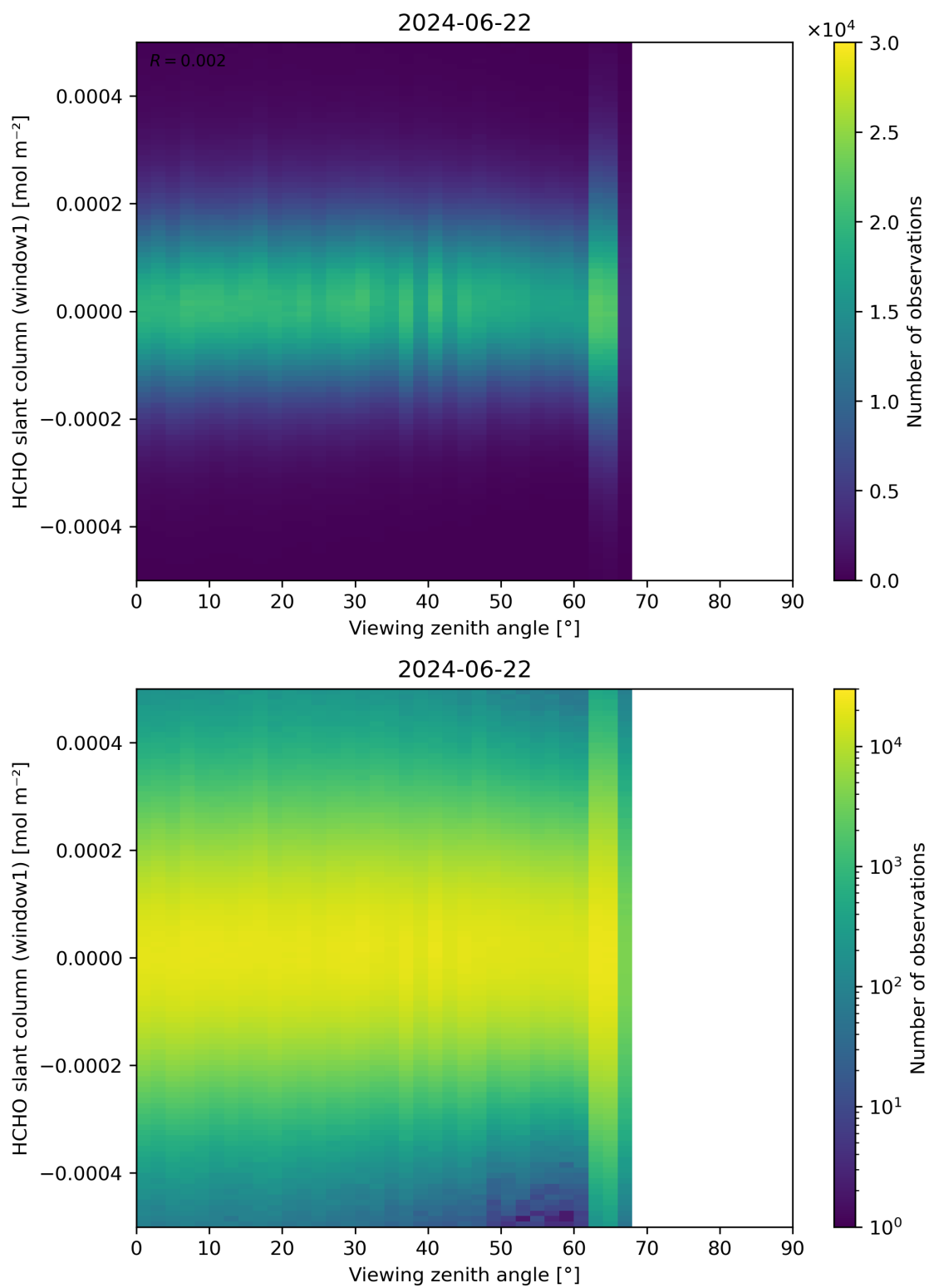
Figure 188: Scatter density plot of “Viewing zenith angle” against “HCHO slant column (window1)” for 2024-06-21 to 2024-06-23.
