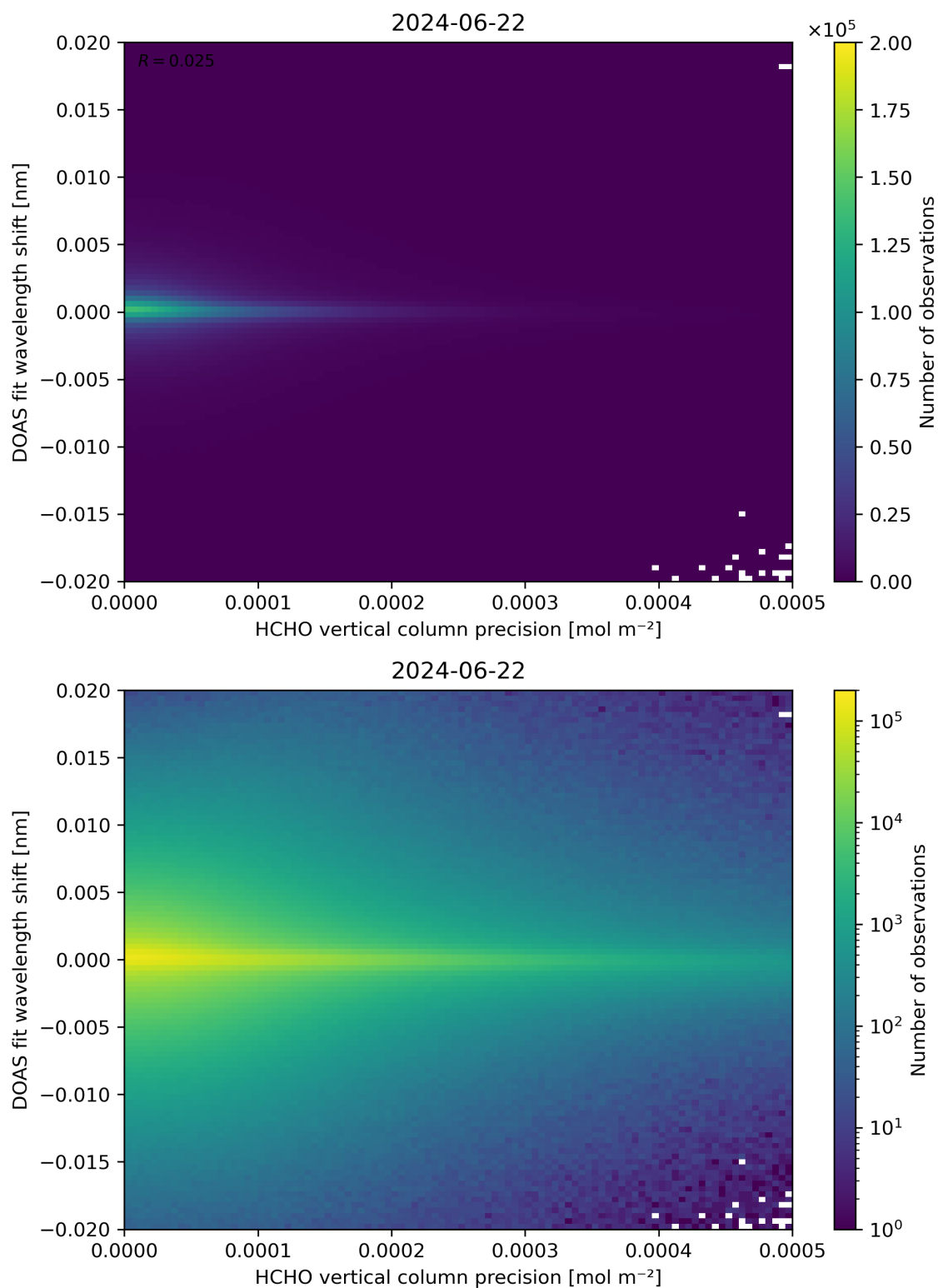
Figure 137: Scatter density plot of “HCHO vertical column precision” against “DOAS fit wavelength shift” for 2024-06-21 to 2024-06-23.
