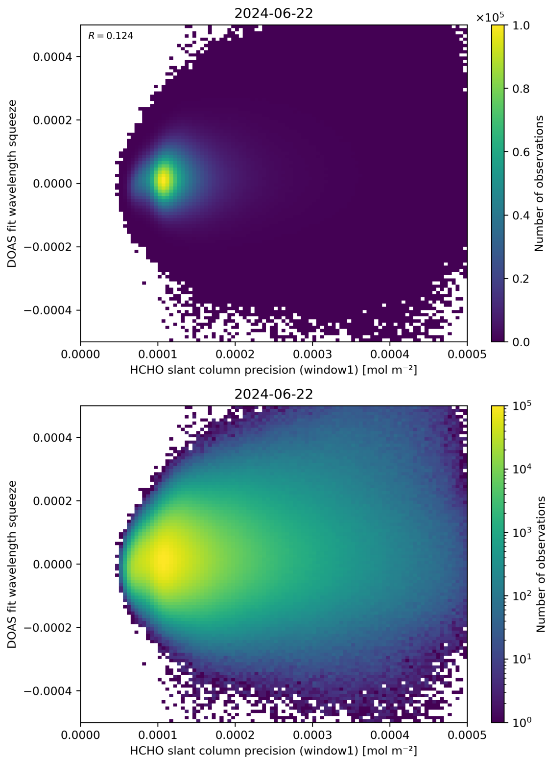
Figure 90: Scatter density plot of “HCHO slant column precision (window1)” against “DOAS fit wavelength squeeze” for 2024-06-21 to 2024-06-23.
