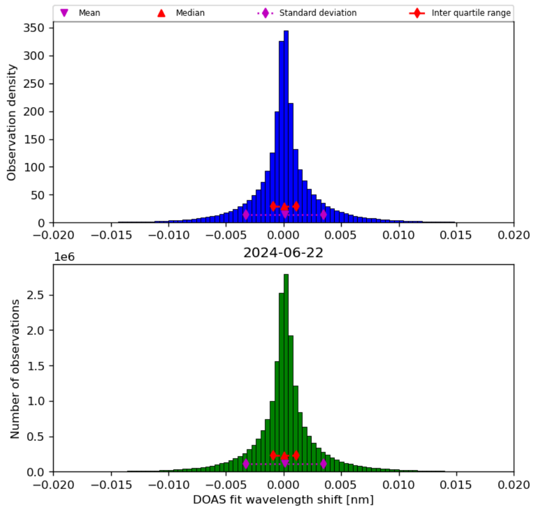
Figure 44: Histogram of “DOAS fit wavelength shift” for 2024-06-21 to 2024-06-23
