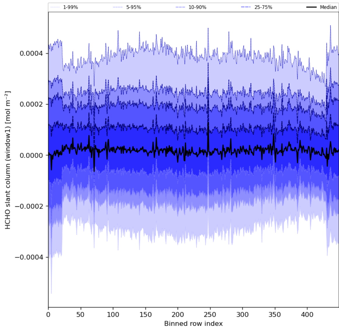
Figure 52: Along track statistics of “HCHO slant column (window1)” for 2024-06-21 to 2024-06-23
