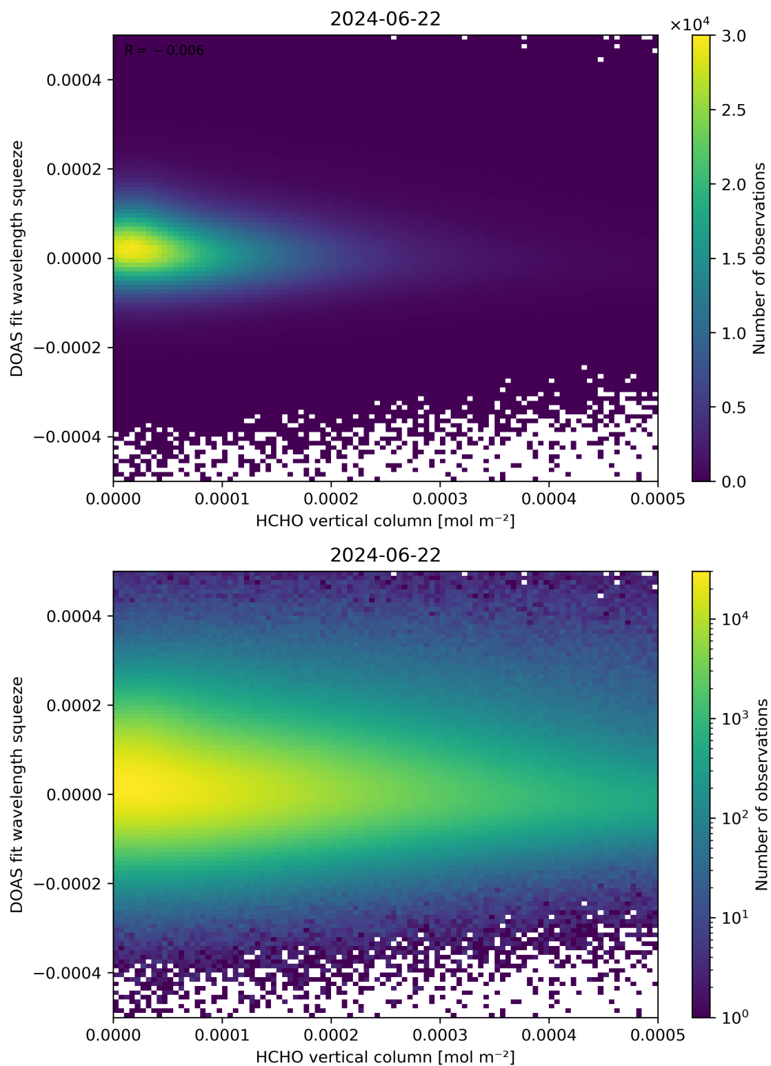
Figure 125: Scatter density plot of “HCHO vertical column” against “DOAS fit wavelength squeeze” for 2024-06-21 to 2024-06-23.
