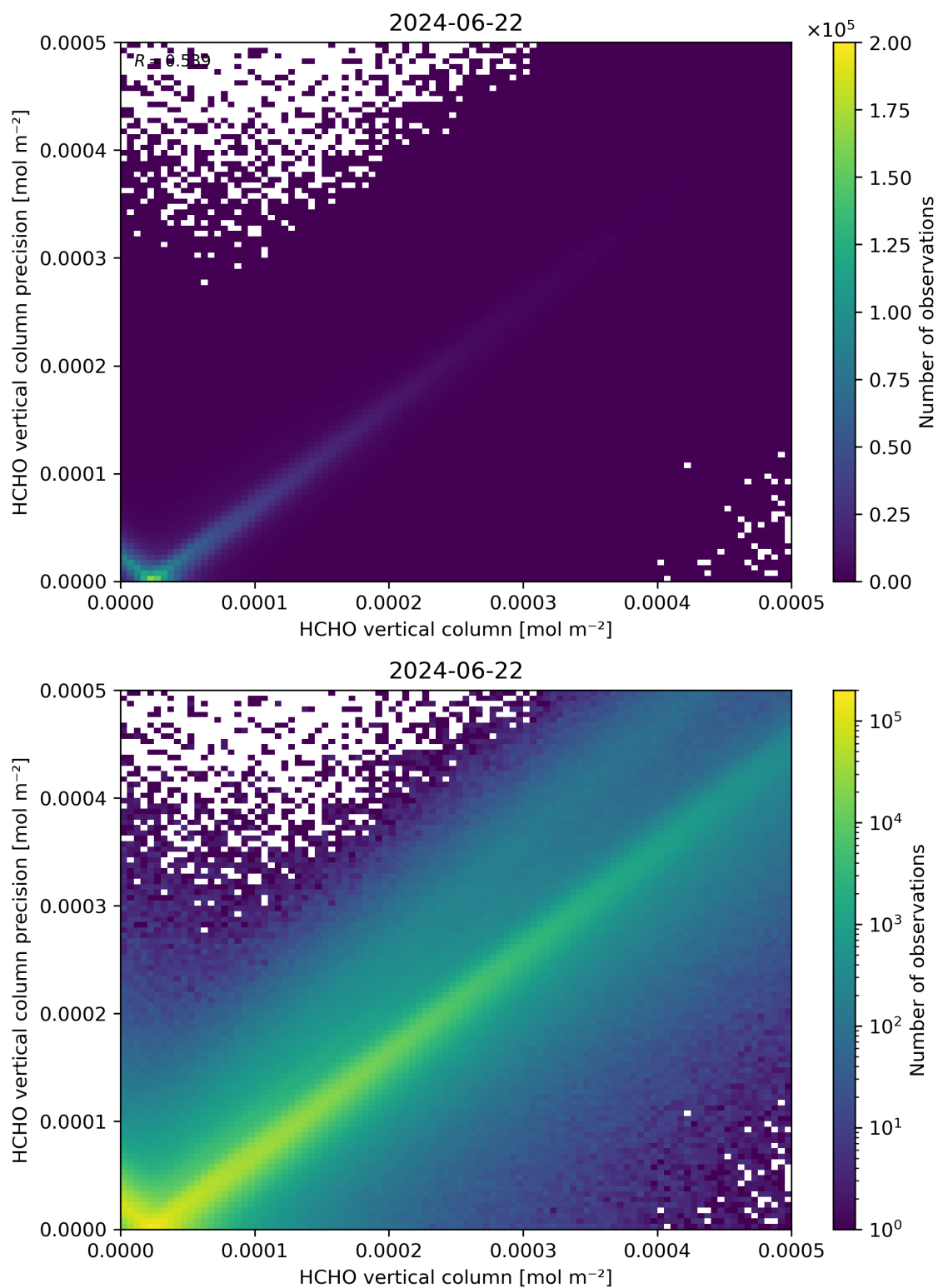
Figure 134: Scatter density plot of “HCHO vertical column” against “HCHO vertical column precision” for 2024-06-21 to 2024-06-23.
