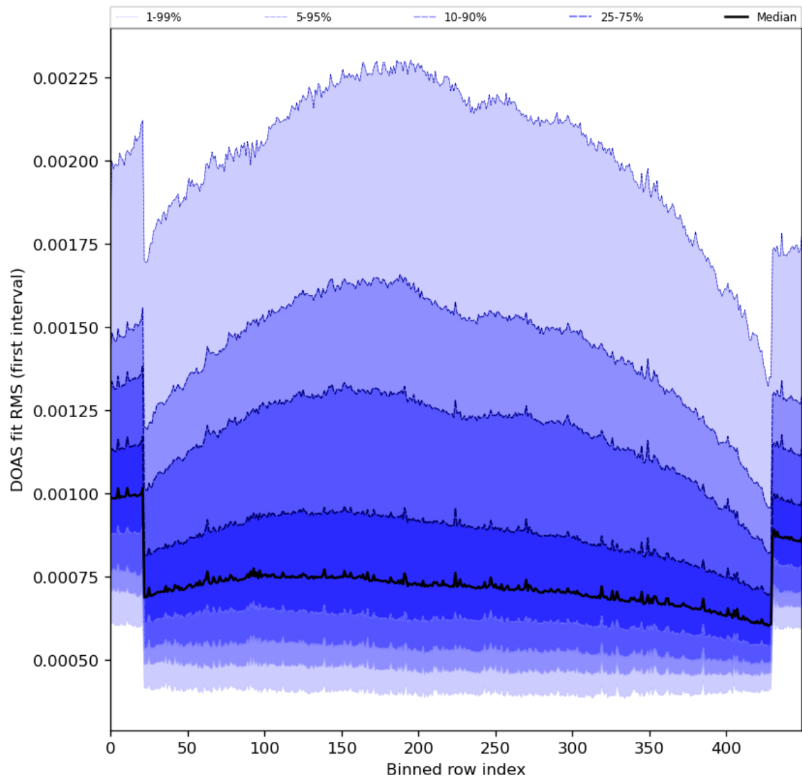
Figure 60: Along track statistics of “DOAS fit RMS (first interval)” for 2024-06-21 to 2024-06-23
