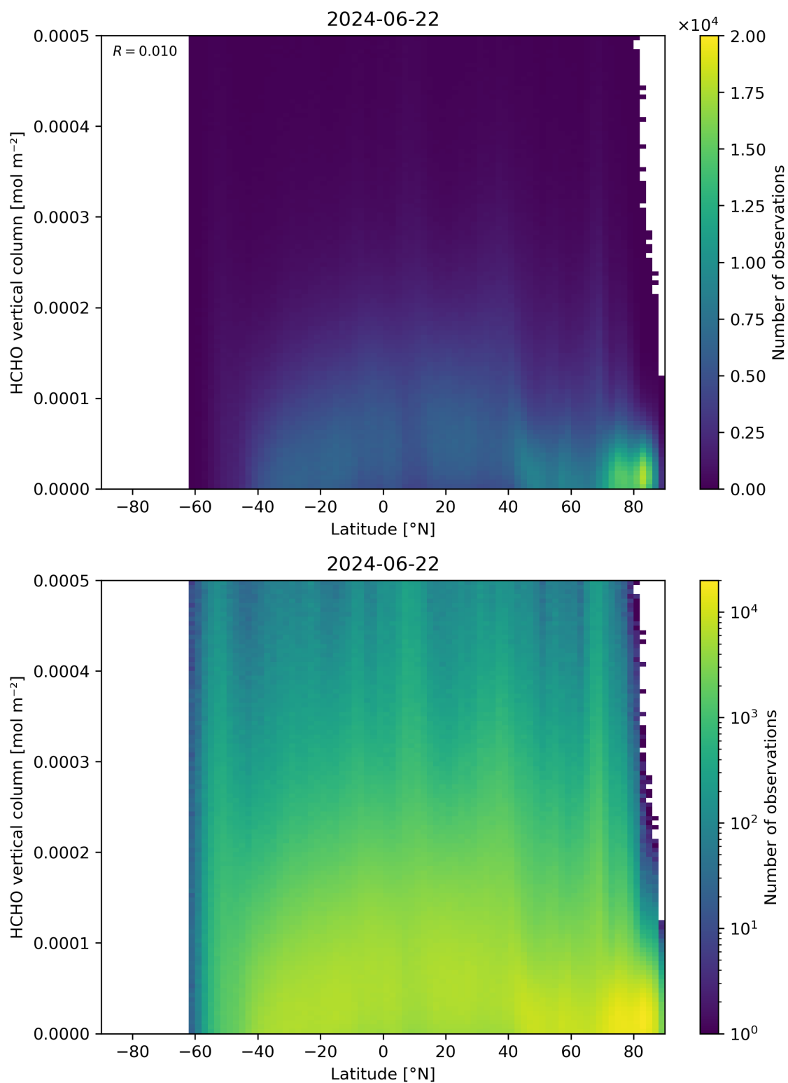
Figure 163: Scatter density plot of “Latitude” against “HCHO vertical column” for 2024-06-21 to 2024-06-23.
