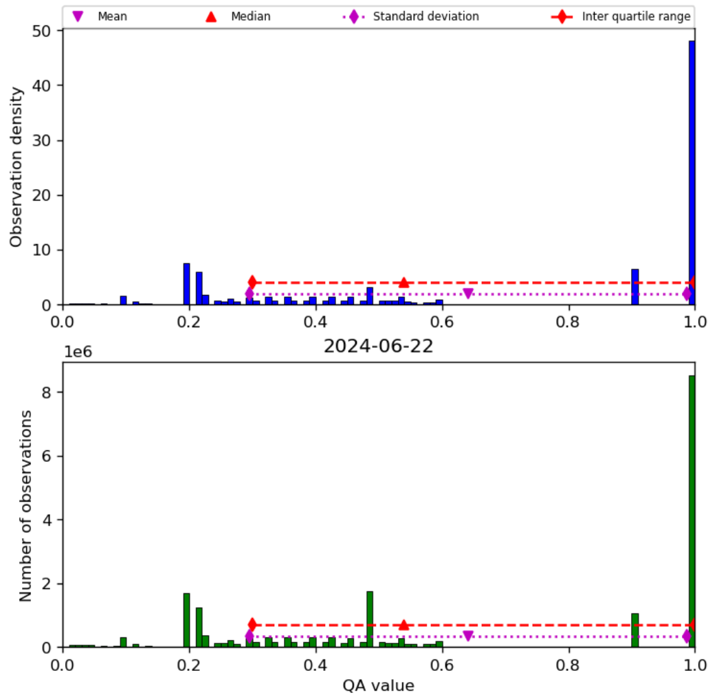
Figure 34: Histogram of “QA value” for 2024-06-21 to 2024-06-23
