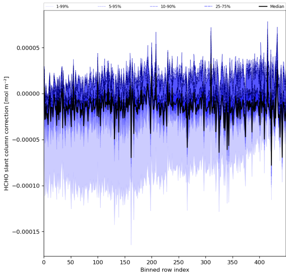
Figure 61: Along track statistics of “HCHO slant column correction” for 2024-06-21 to 2024-06-23
