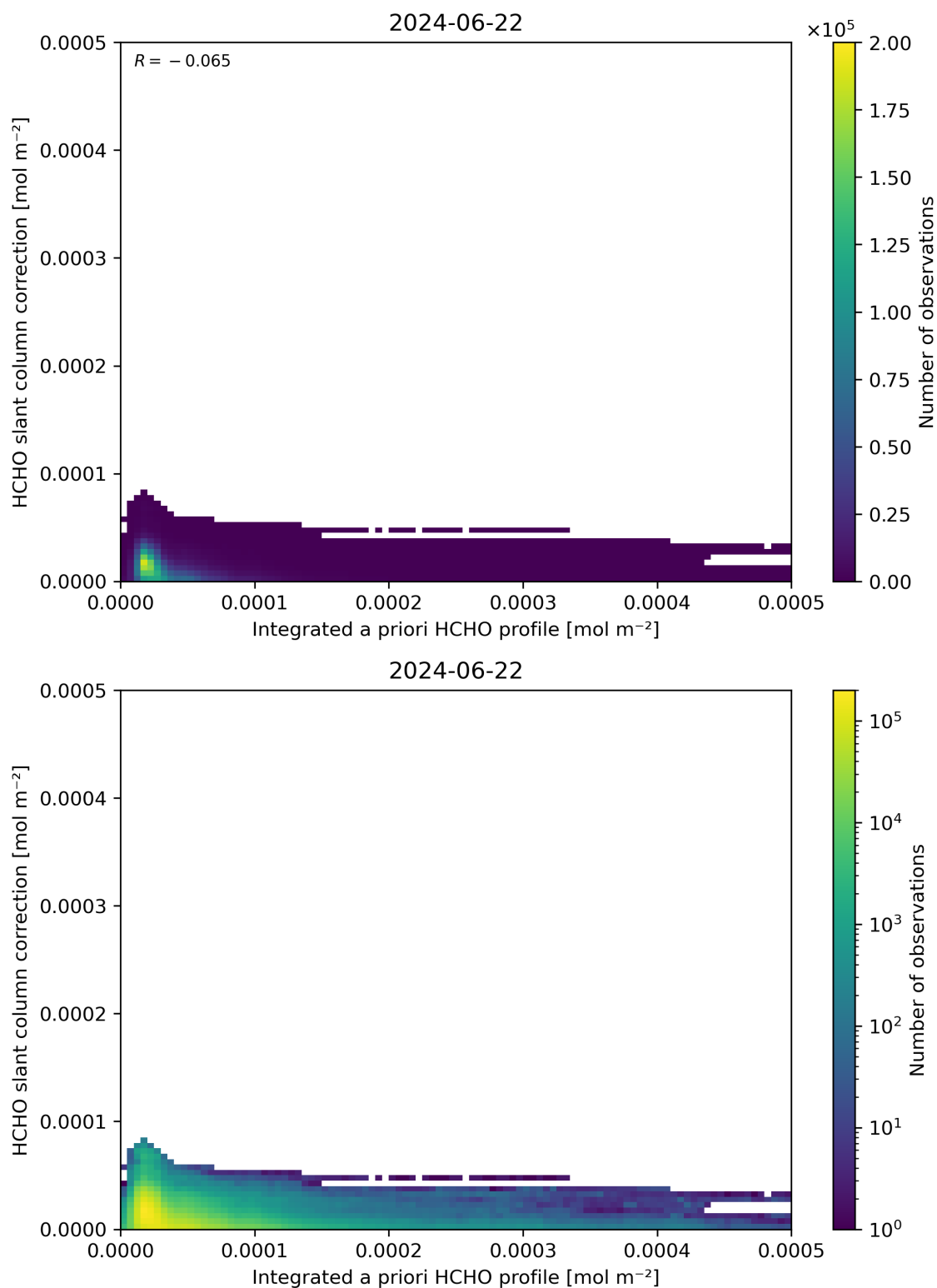
Figure 152: Scatter density plot of “Integrated a priori HCHO profile” against “HCHO slant column correction” for 2024-06-21 to 2024-06-23.
