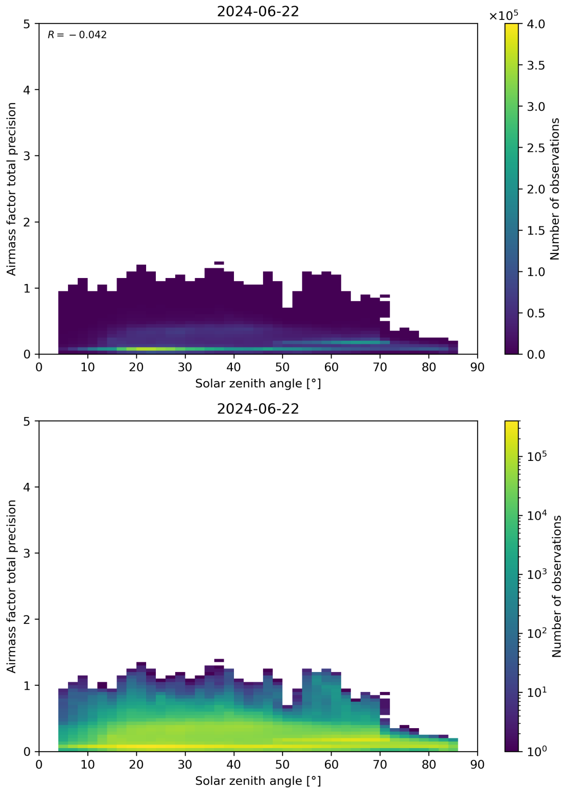
Figure 176: Scatter density plot of “Solar zenith angle” against “Airmass factor total precision” for 2024-06-21 to 2024-06-23.
