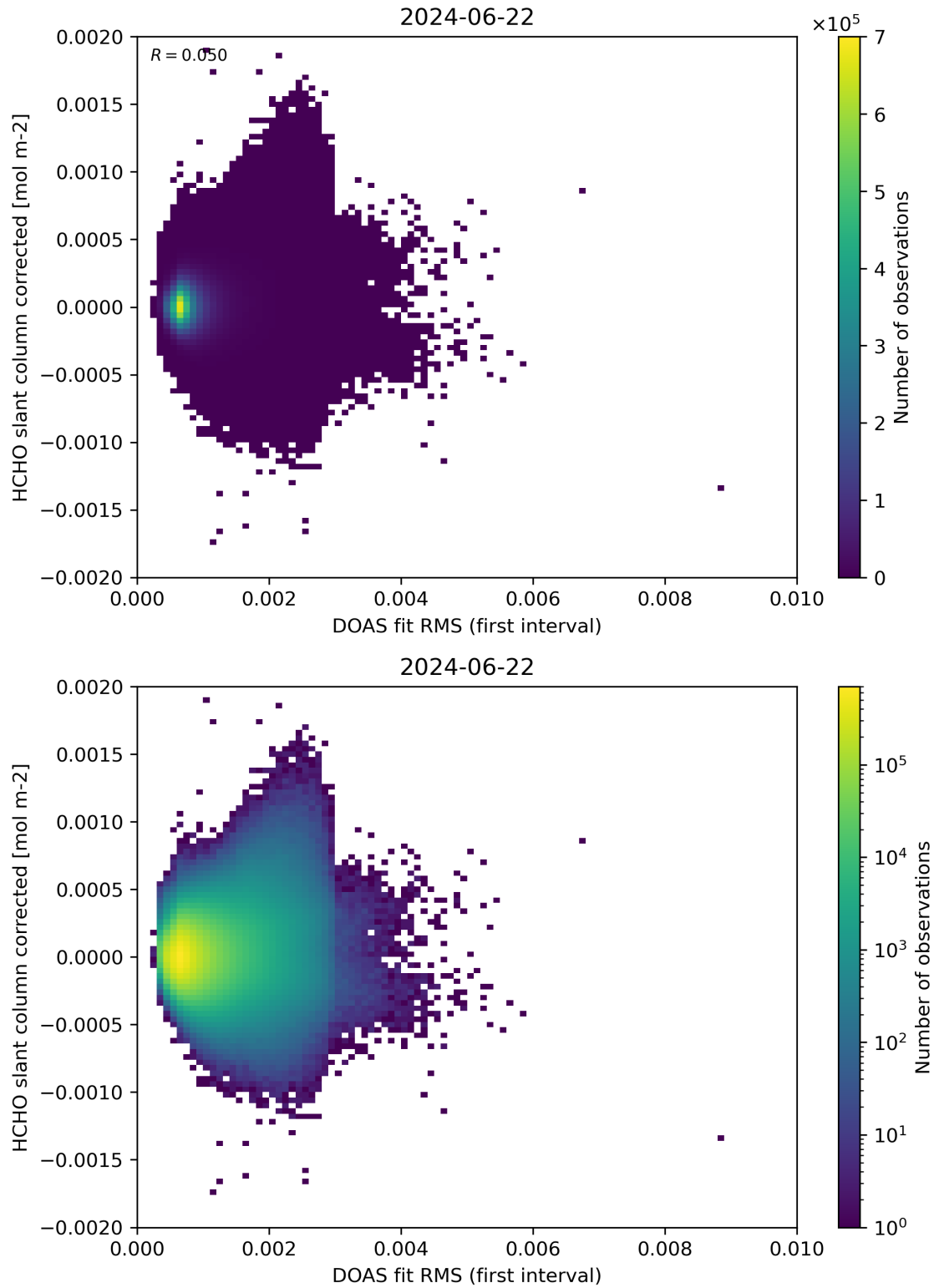
Figure 62: Scatter density plot of “DOAS fit RMS (first interval)” against “HCHO slant column corrected” for 2024-06-21 to 2024-06-23.
