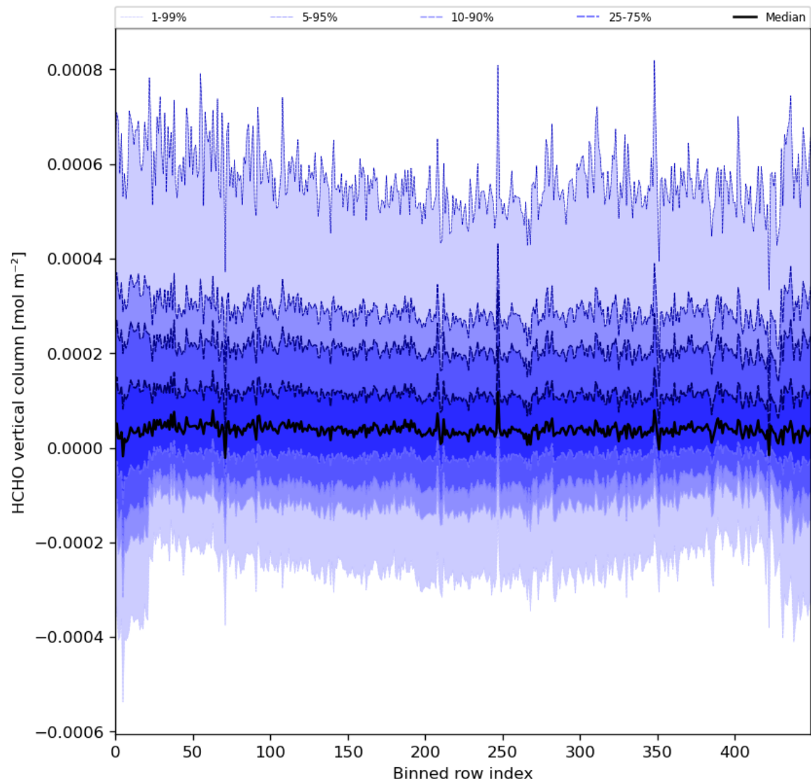
Figure 49: Along track statistics of “HCHO vertical column” for 2024-06-21 to 2024-06-23
