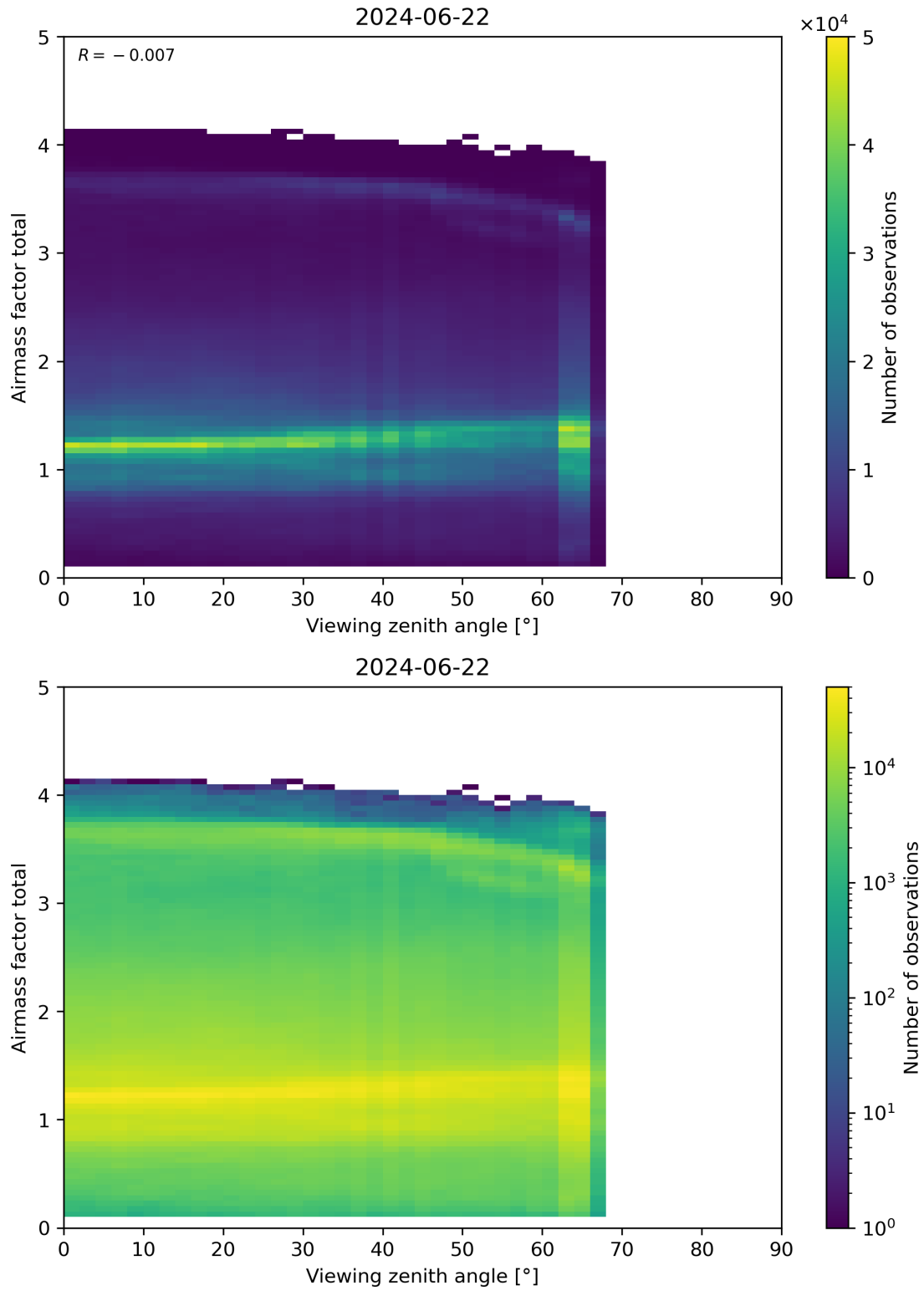
Figure 190: Scatter density plot of “Viewing zenith angle” against “Airmass factor total” for 2024-06-21 to 2024-06-23.
