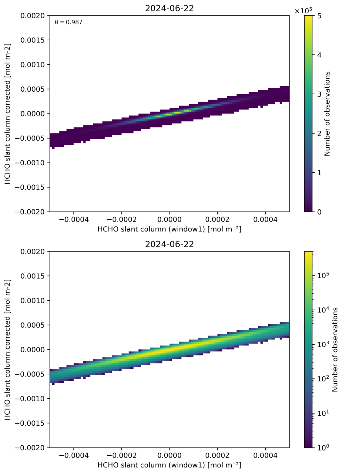
Figure 82: Scatter density plot of “HCHO slant column (window1)” against “HCHO slant column corrected” for 2024-06-21 to 2024-06-23.
