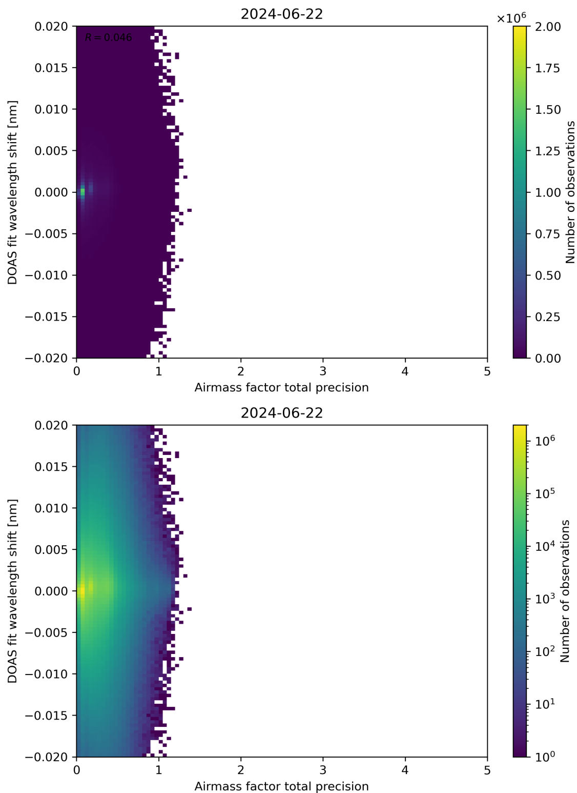
Figure 106: Scatter density plot of “Airmass factor total precision” against “DOAS fit wavelength shift” for 2024-06-21 to 2024-06-23.
