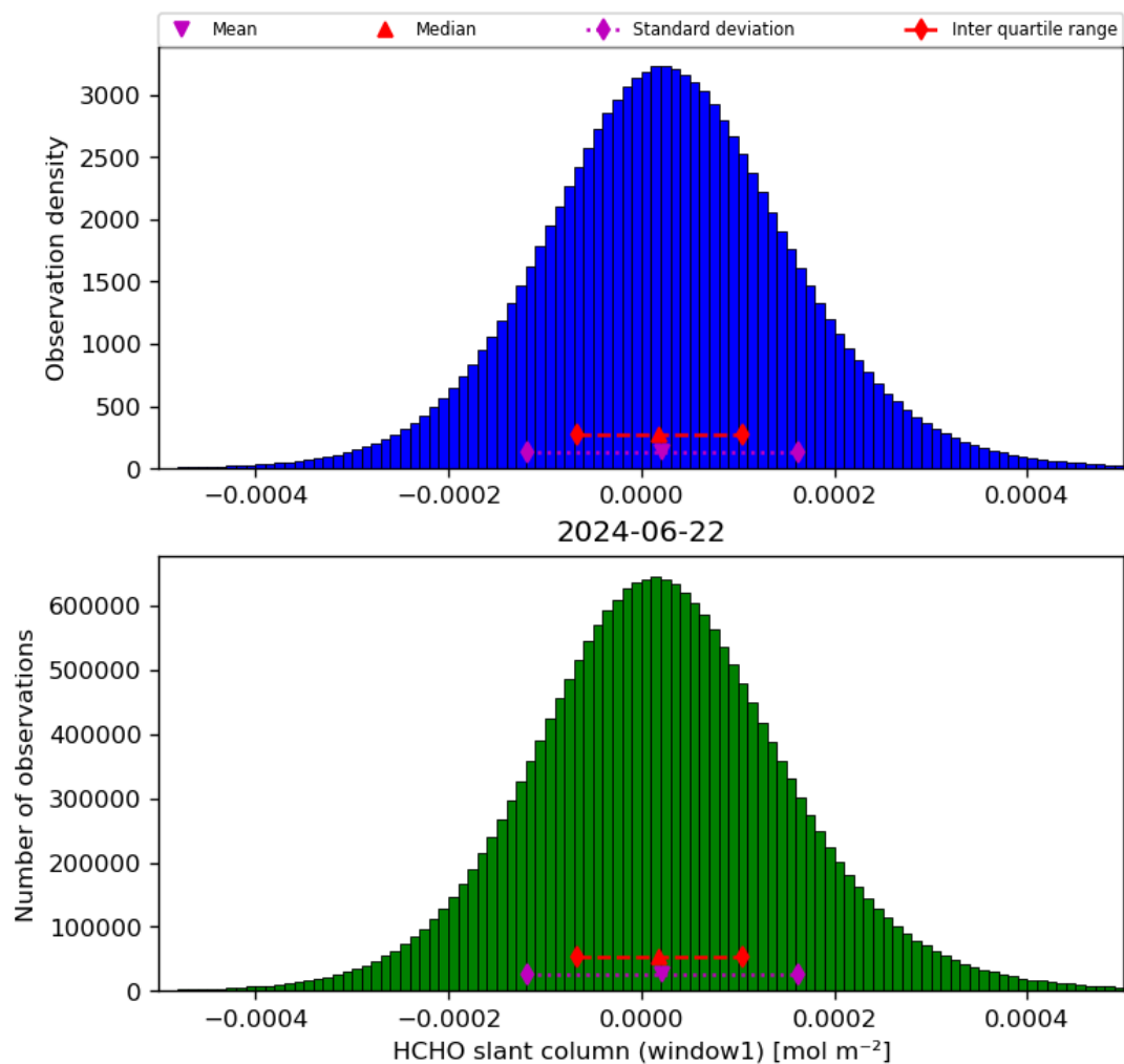
Figure 38: Histogram of “HCHO slant column (window1)” for 2024-06-21 to 2024-06-23
