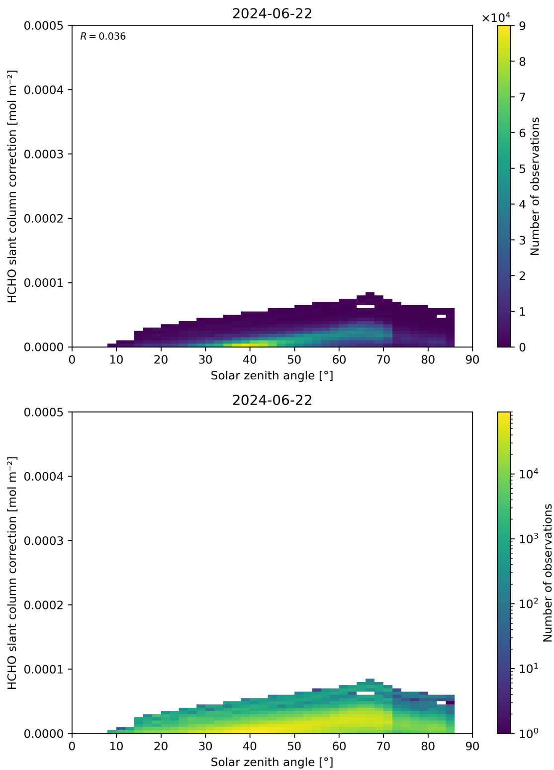
Figure 172: Scatter density plot of “Solar zenith angle” against “HCHO slant column correction” for 2024-06-21 to 2024-06-23.
