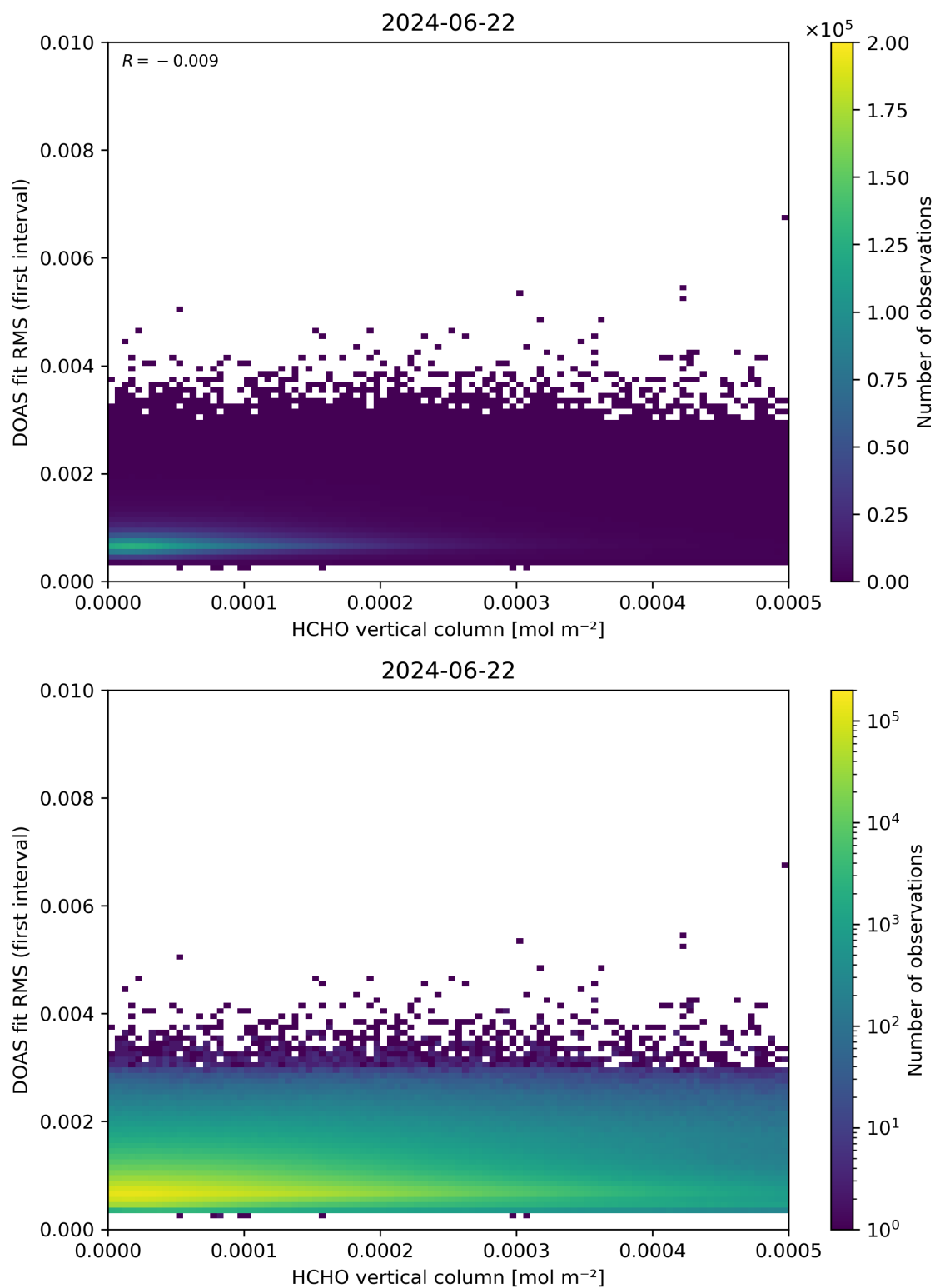
Figure 123: Scatter density plot of “HCHO vertical column” against “DOAS fit RMS (first interval)” for 2024-06-21 to 2024-06-23.
