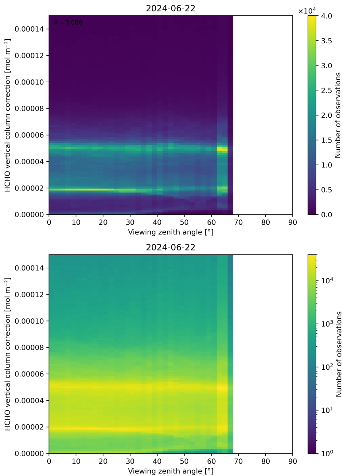
Figure 193: Scatter density plot of “Viewing zenith angle” against “HCHO vertical column correction” for 2024-06-21 to 2024-06-23.
