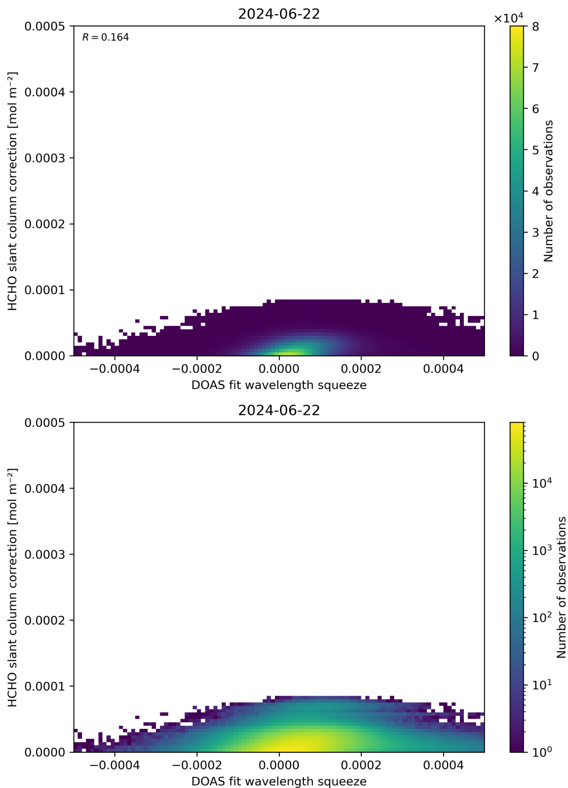
Figure 70: Scatter density plot of “DOAS fit wavelength squeeze” against “HCHO slant column correction” for 2024-06-21 to 2024-06-23.
