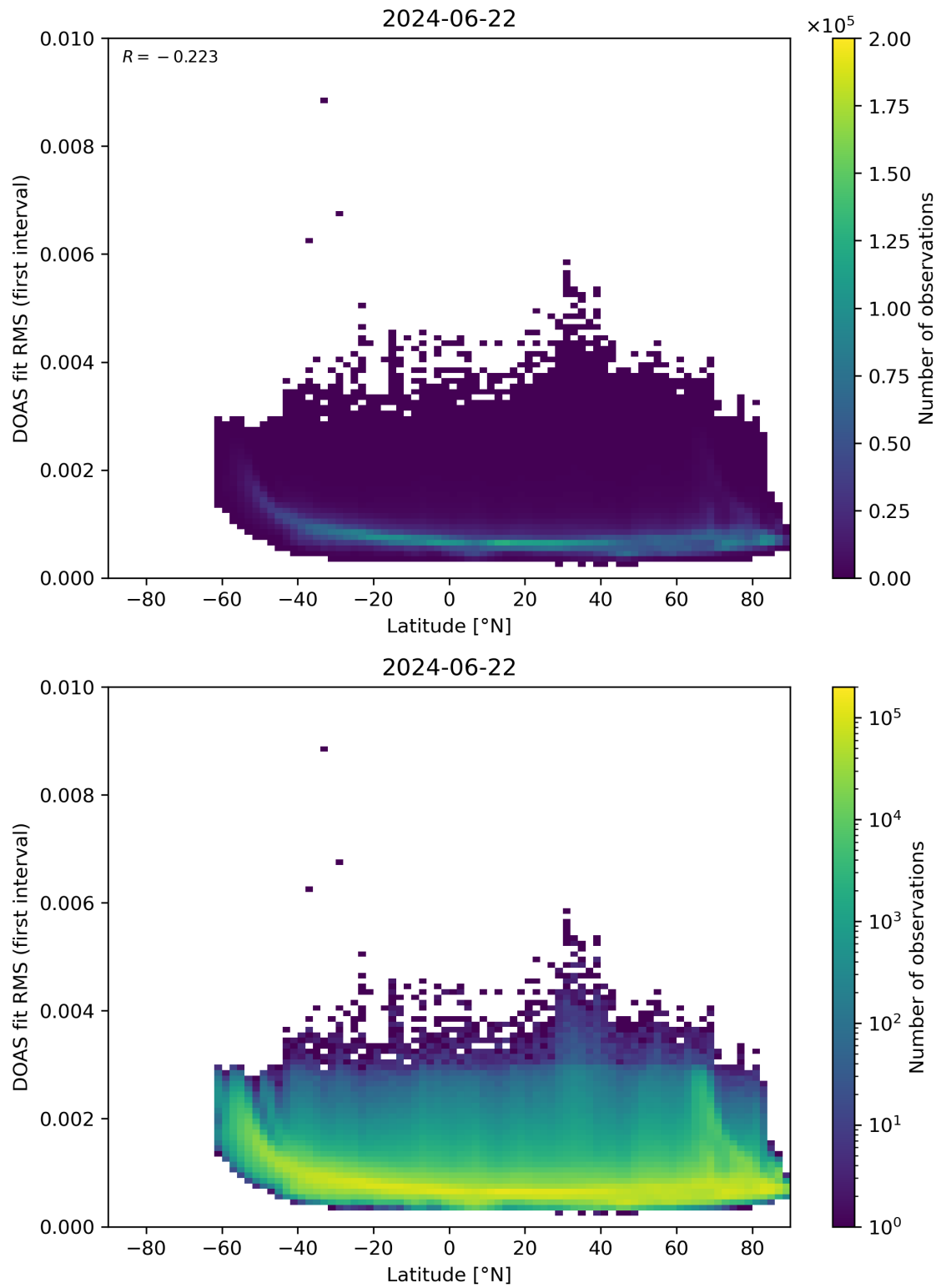
Figure 153: Scatter density plot of “Latitude” against “DOAS fit RMS (first interval)” for 2024-06-21 to 2024-06-23.
