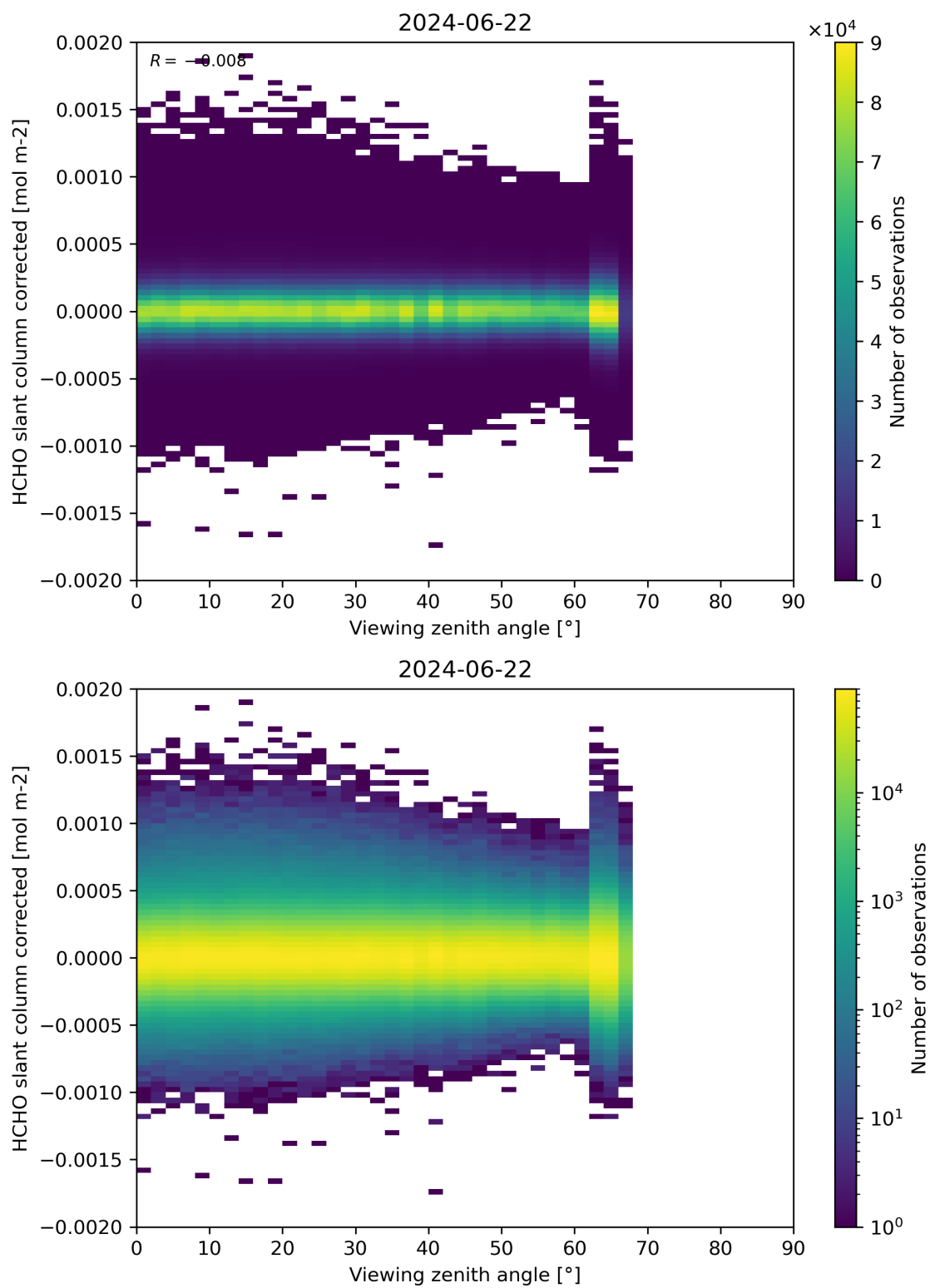
Figure 186: Scatter density plot of “Viewing zenith angle” against “HCHO slant column corrected” for 2024-06-21 to 2024-06-23.
