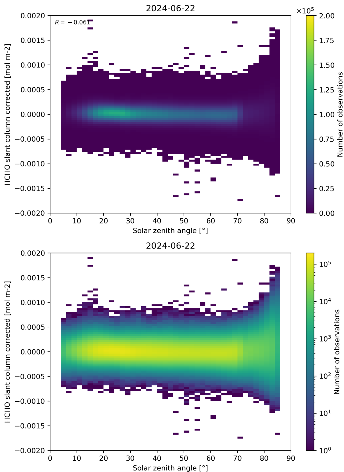
Figure 171: Scatter density plot of “Solar zenith angle” against “HCHO slant column corrected” for 2024-06-21 to 2024-06-23.
