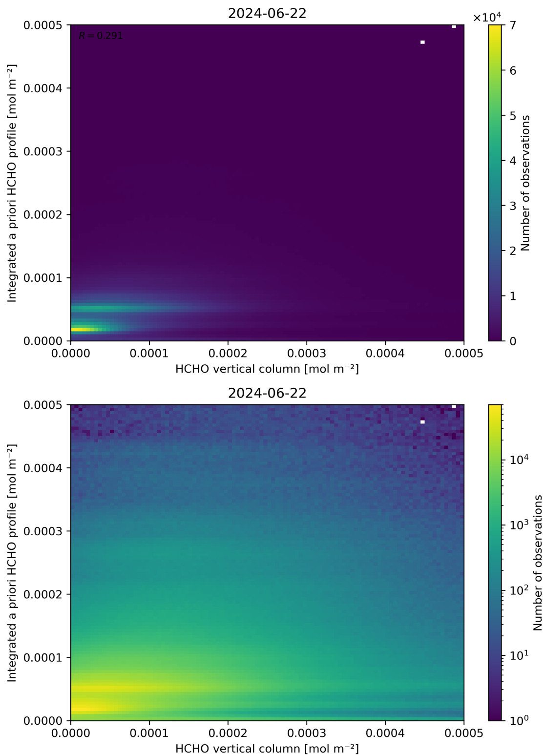
Figure 135: Scatter density plot of “HCHO vertical column” against “Integrated a priori HCHO profile” for 2024-06-21 to 2024-06-23.
