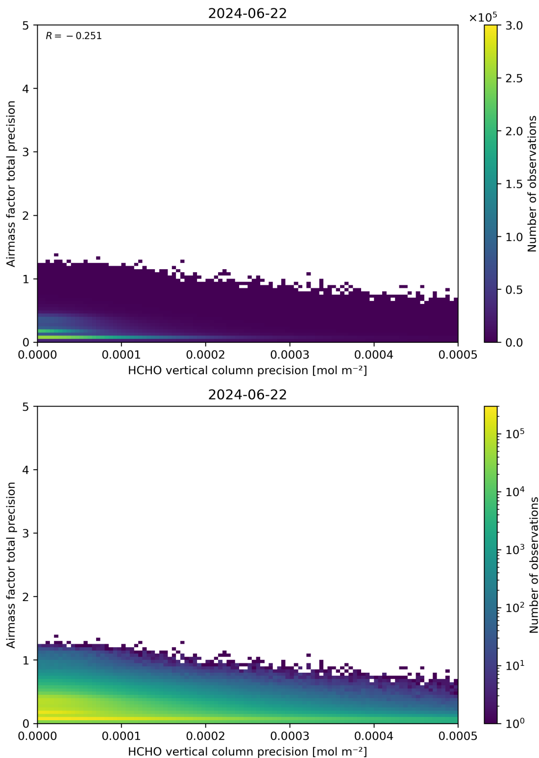
Figure 145: Scatter density plot of “HCHO vertical column precision” against “Airmass factor total precision” for 2024-06-21 to 2024-06-23.
