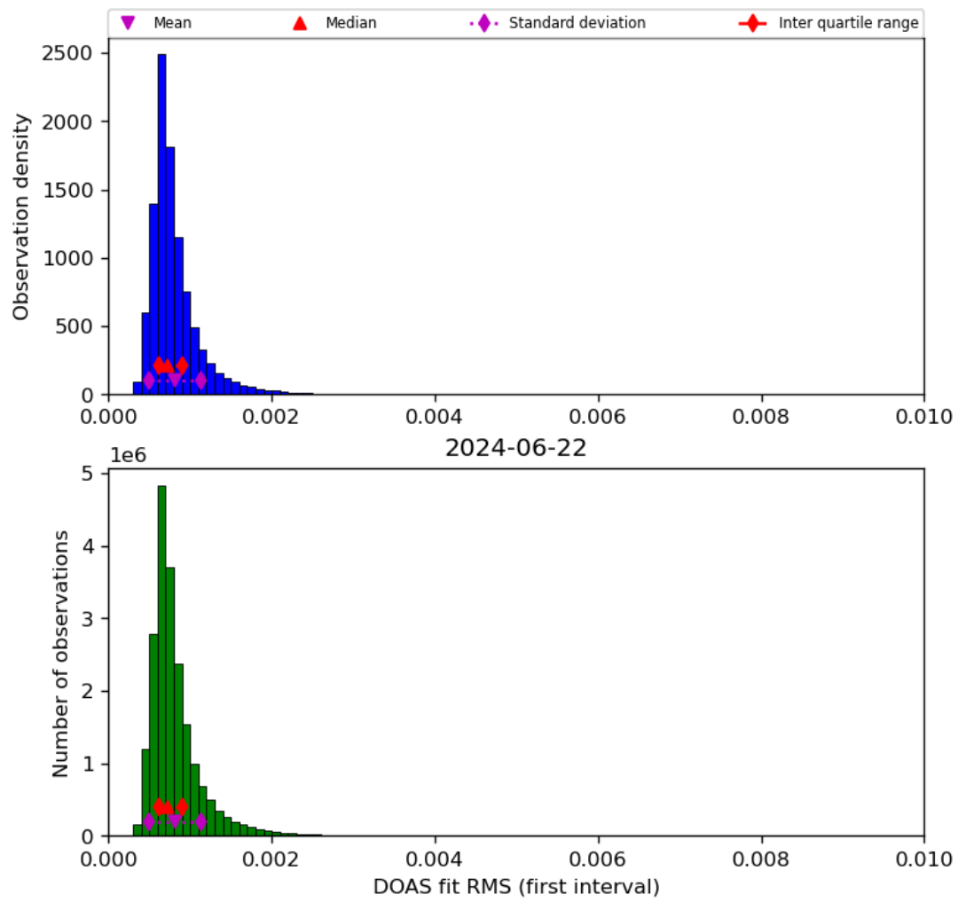
Figure 46: Histogram of “DOAS fit RMS (first interval)” for 2024-06-21 to 2024-06-23
