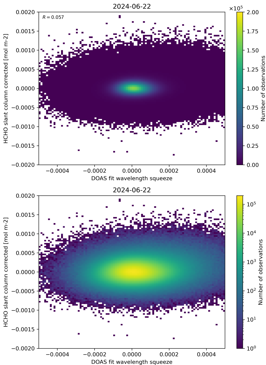
Figure 69: Scatter density plot of “DOAS fit wavelength squeeze” against “HCHO slant column corrected” for 2024-06-21 to 2024-06-23.
