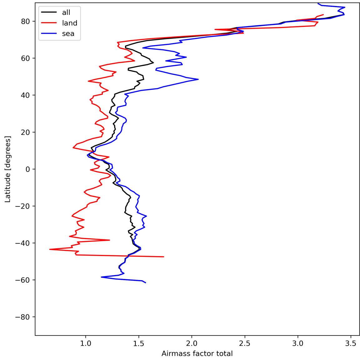
Figure 26: Zonal average of “Airmass factor total” for 2024-06-21 to 2024-06-23.
