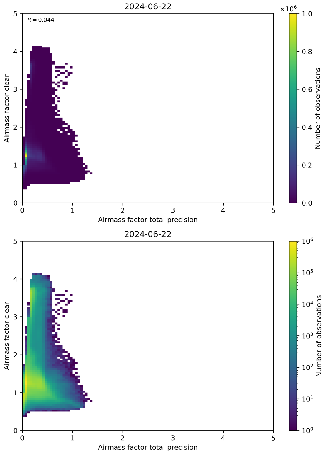
Figure 108: Scatter density plot of “Airmass factor total precision” against “Airmass factor clear” for 2024-06-21 to 2024-06-23.
