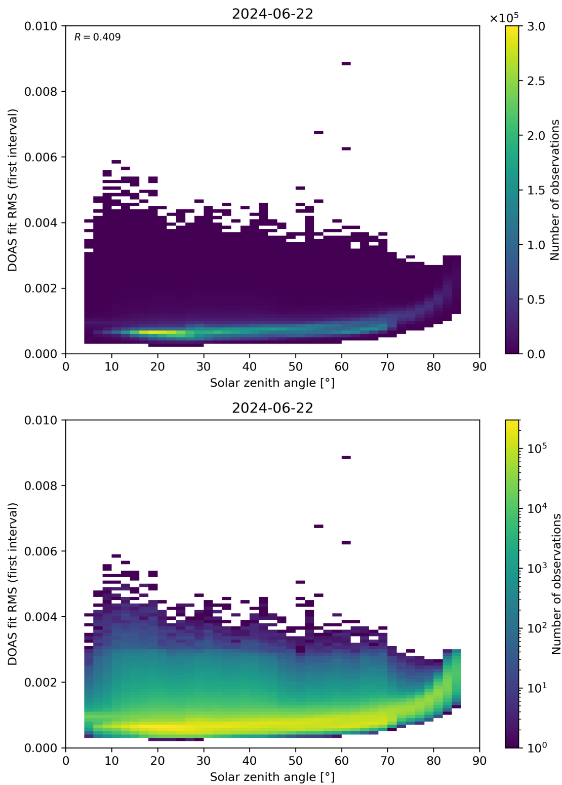
Figure 167: Scatter density plot of “Solar zenith angle” against “DOAS fit RMS (first interval)” for 2024-06-21 to 2024-06-23.
