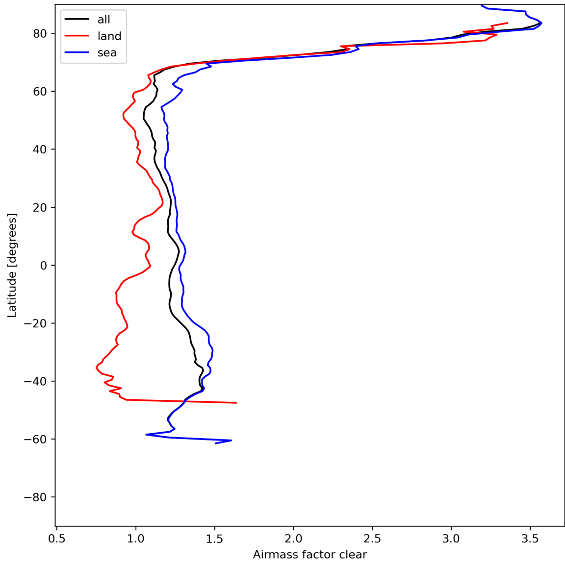
Figure 28: Zonal average of “Airmass factor clear” for 2024-06-21 to 2024-06-23.
