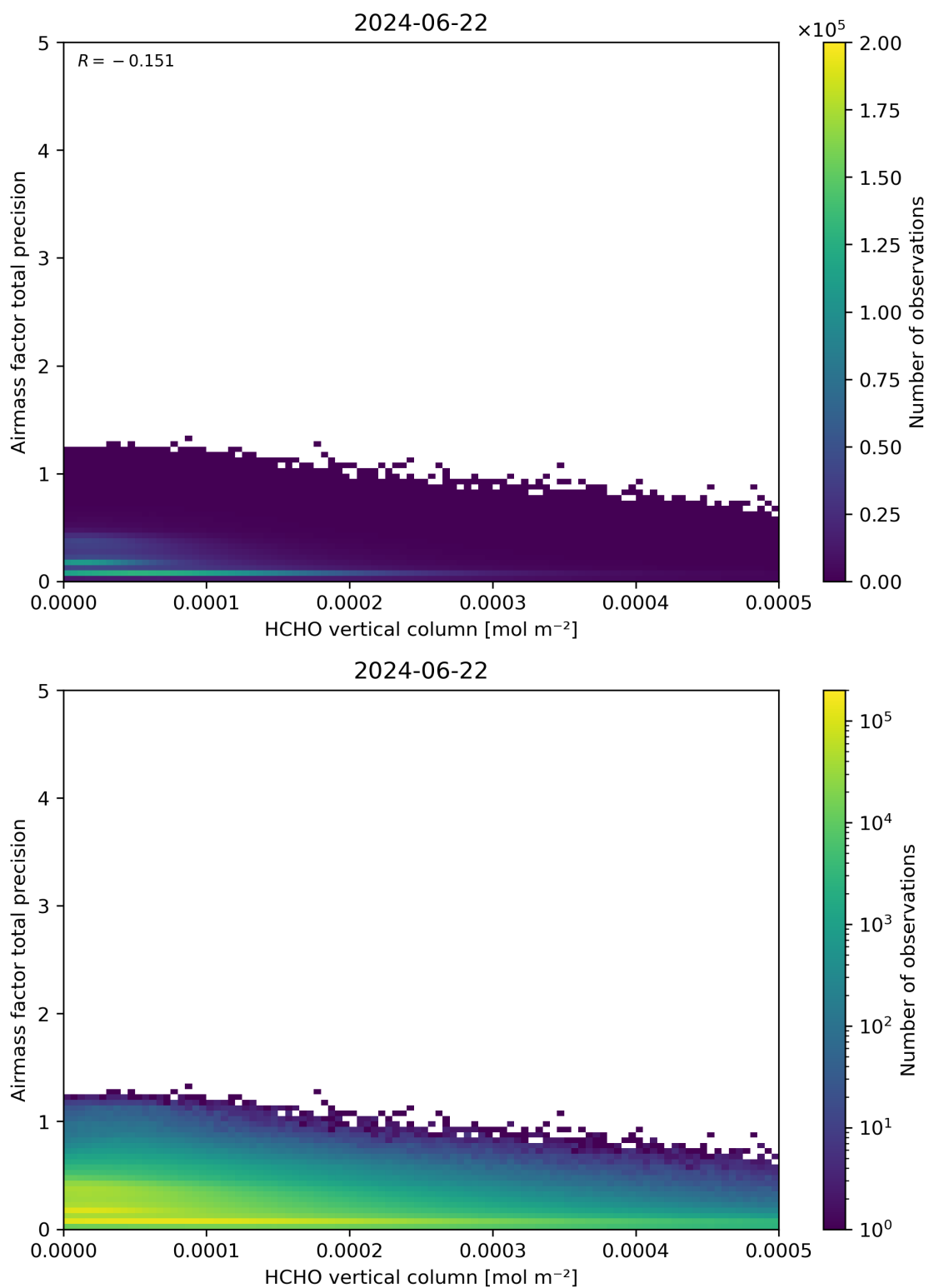
Figure 132: Scatter density plot of “HCHO vertical column” against “Airmass factor total precision” for 2024-06-21 to 2024-06-23.
