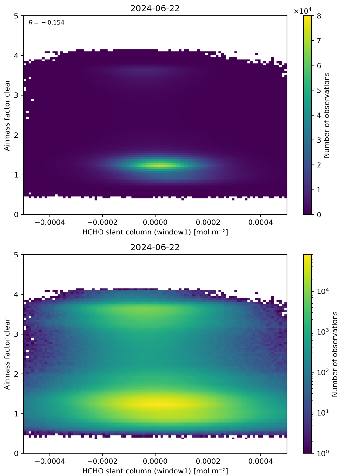
Figure 81: Scatter density plot of “HCHO slant column (window1)” against “Airmass factor clear” for 2024-06-21 to 2024-06-23.
