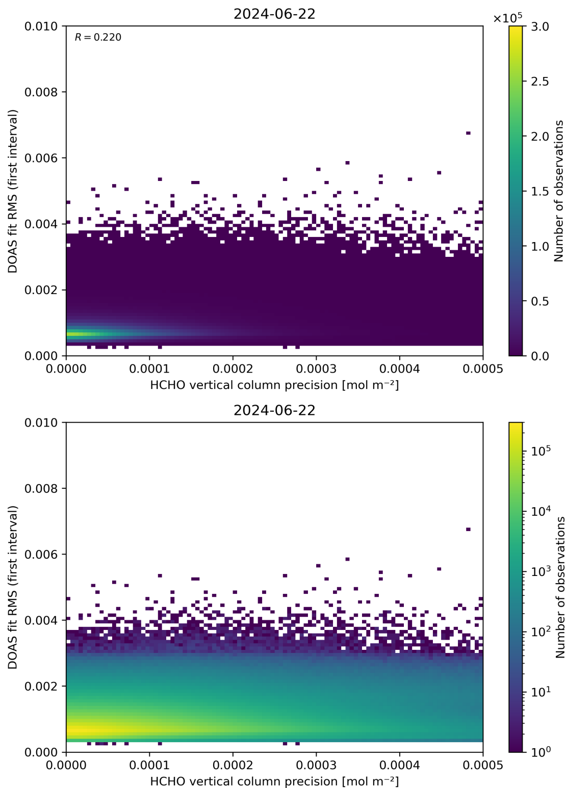
Figure 136: Scatter density plot of “HCHO vertical column precision” against “DOAS fit RMS (first interval)” for 2024-06-21 to 2024-06-23.
