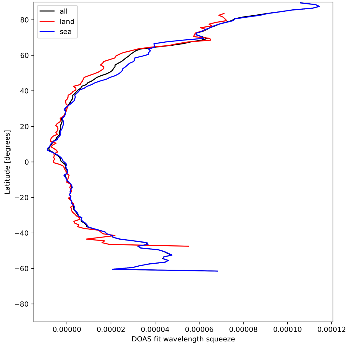
Figure 31: Zonal average of “DOAS fit wavelength squeeze” for 2024-06-21 to 2024-06-23.
