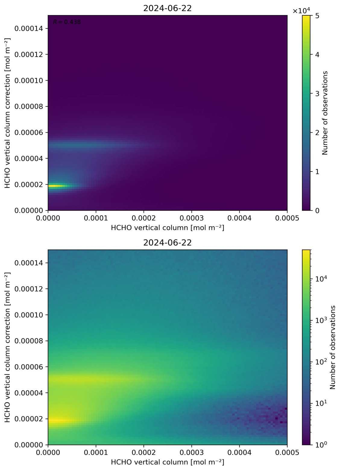
Figure 133: Scatter density plot of “HCHO vertical column” against “HCHO vertical column correction” for 2024-06-21 to 2024-06-23.
