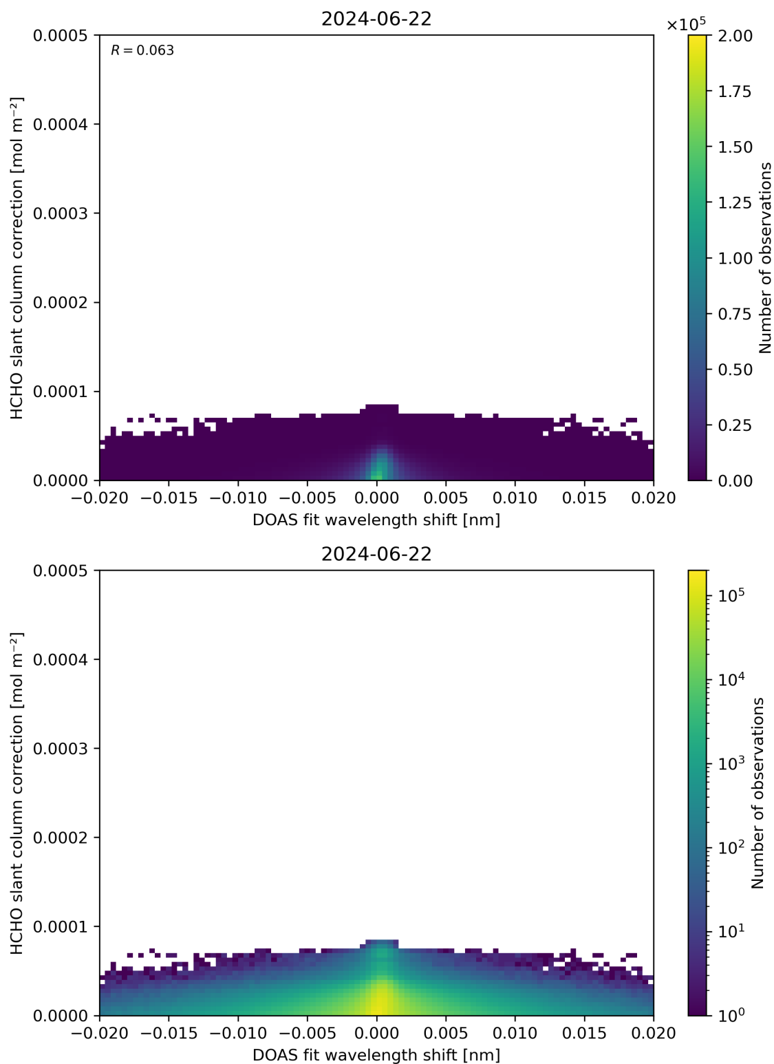
Figure 67: Scatter density plot of “DOAS fit wavelength shift” against “HCHO slant column correction” for 2024-06-21 to 2024-06-23.
