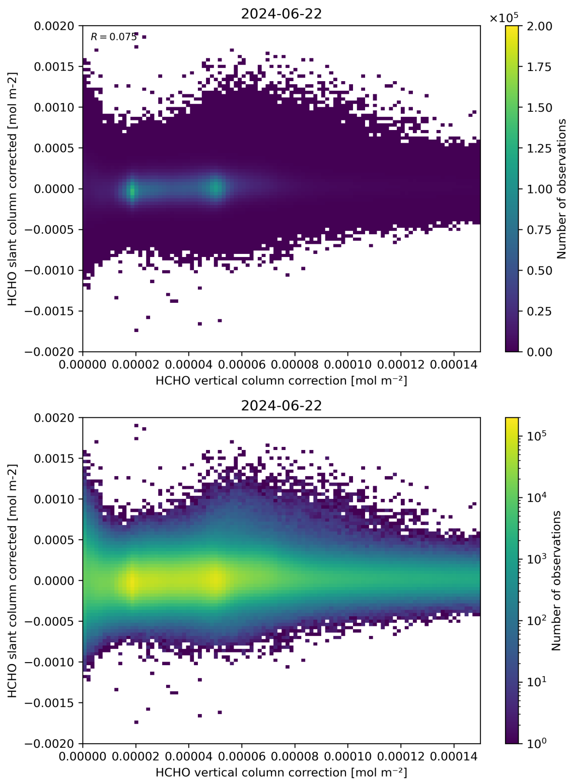
Figure 116: Scatter density plot of “HCHO vertical column correction” against “HCHO slant column corrected” for 2024-06-21 to 2024-06-23.
