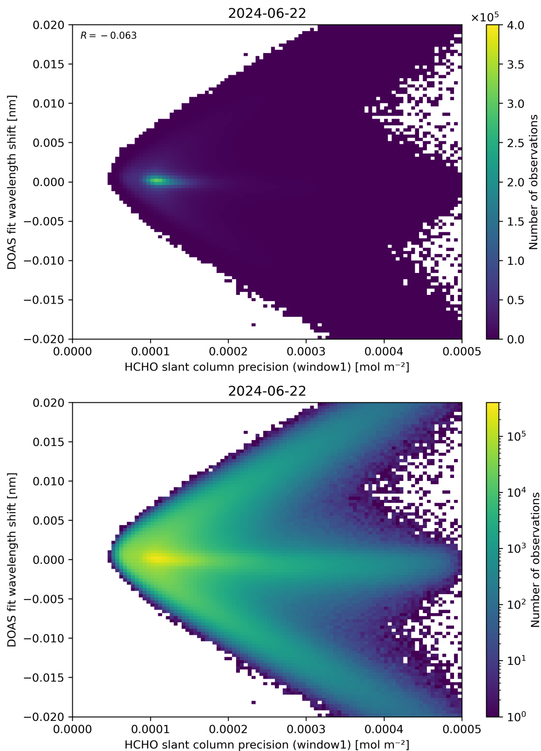
Figure 89: Scatter density plot of “HCHO slant column precision (window1)” against “DOAS fit wavelength shift” for 2024-06-21 to 2024-06-23.
