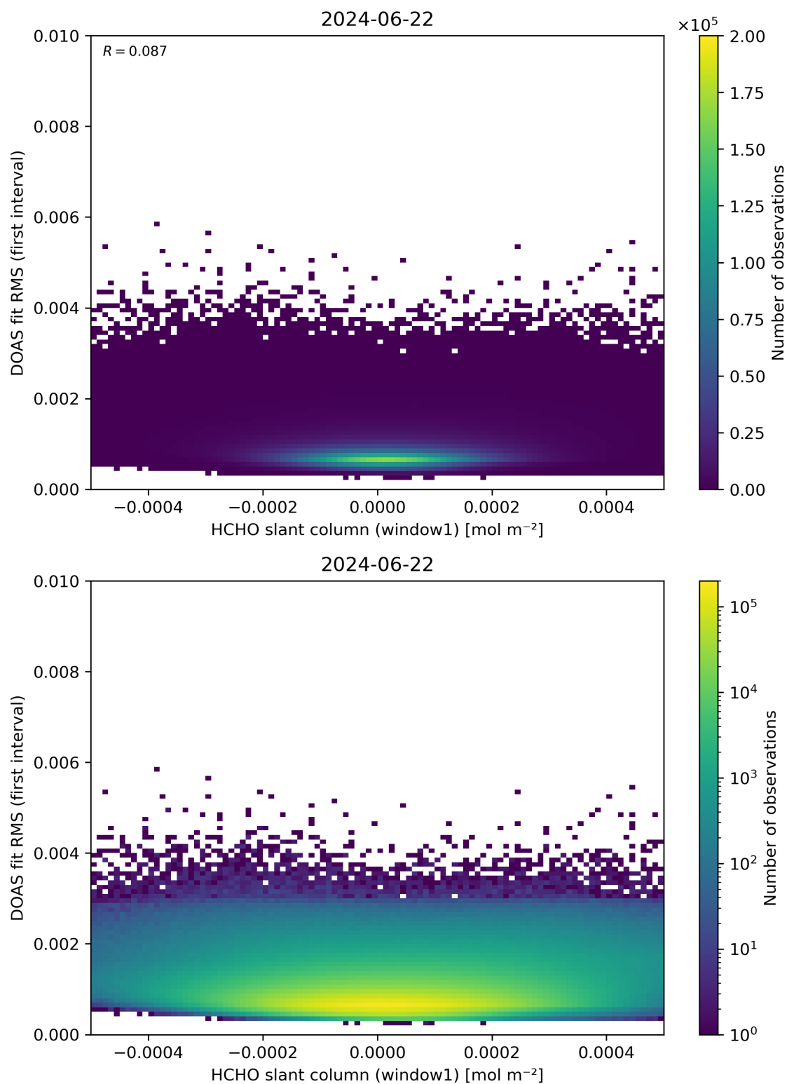
Figure 78: Scatter density plot of “HCHO slant column (window1)” against “DOAS fit RMS (first interval)” for 2024-06-21 to 2024-06-23.
