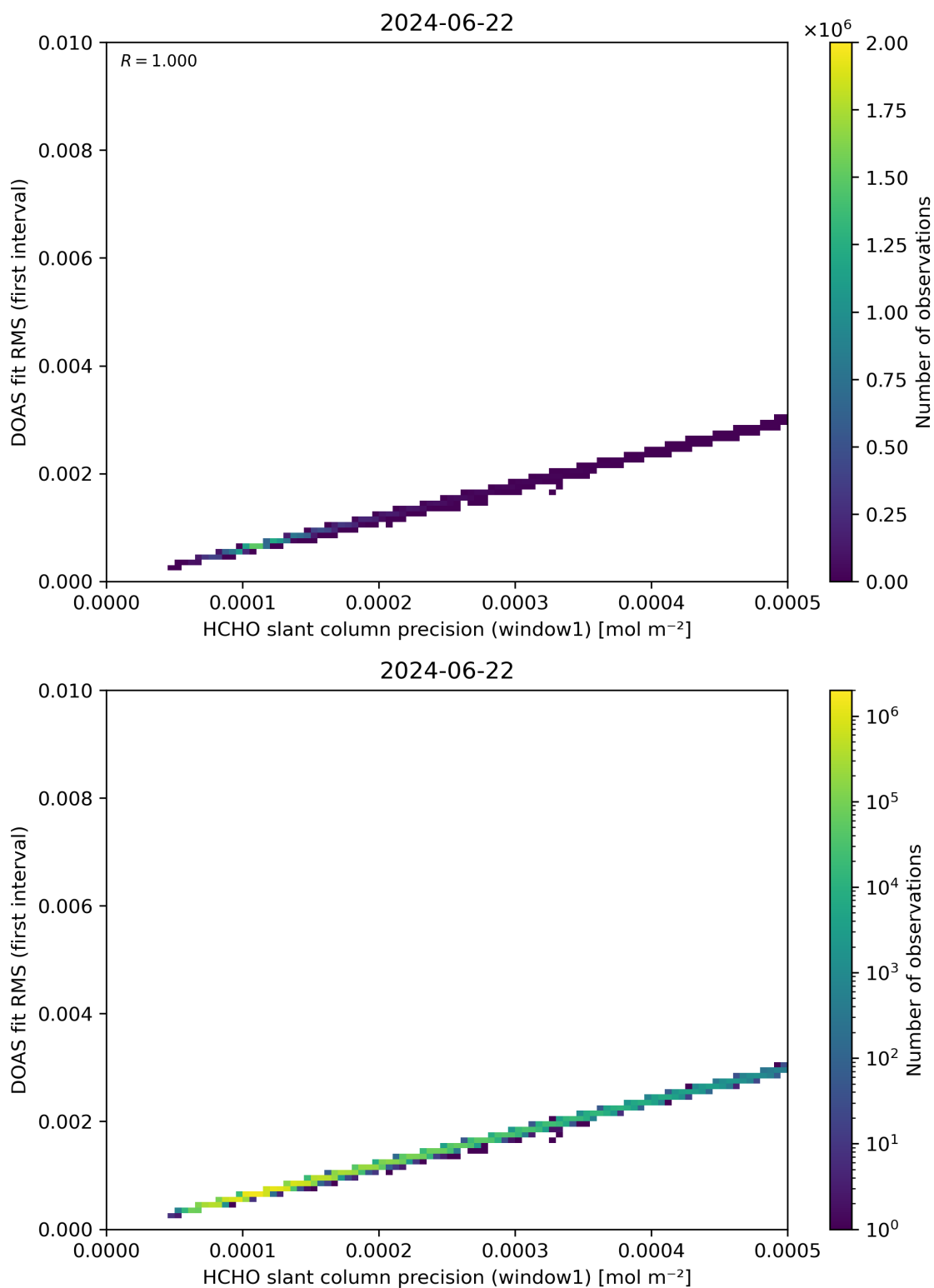
Figure 88: Scatter density plot of “HCHO slant column precision (window1)” against “DOAS fit RMS (first interval)” for 2024-06-21 to 2024-06-23.
