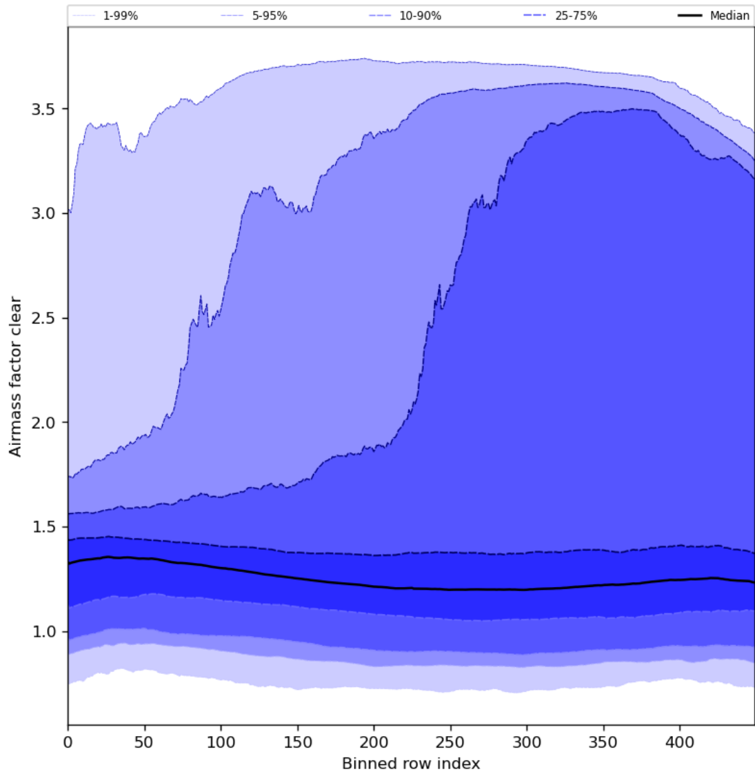
Figure 56: Along track statistics of “Airmass factor clear” for 2024-06-21 to 2024-06-23
