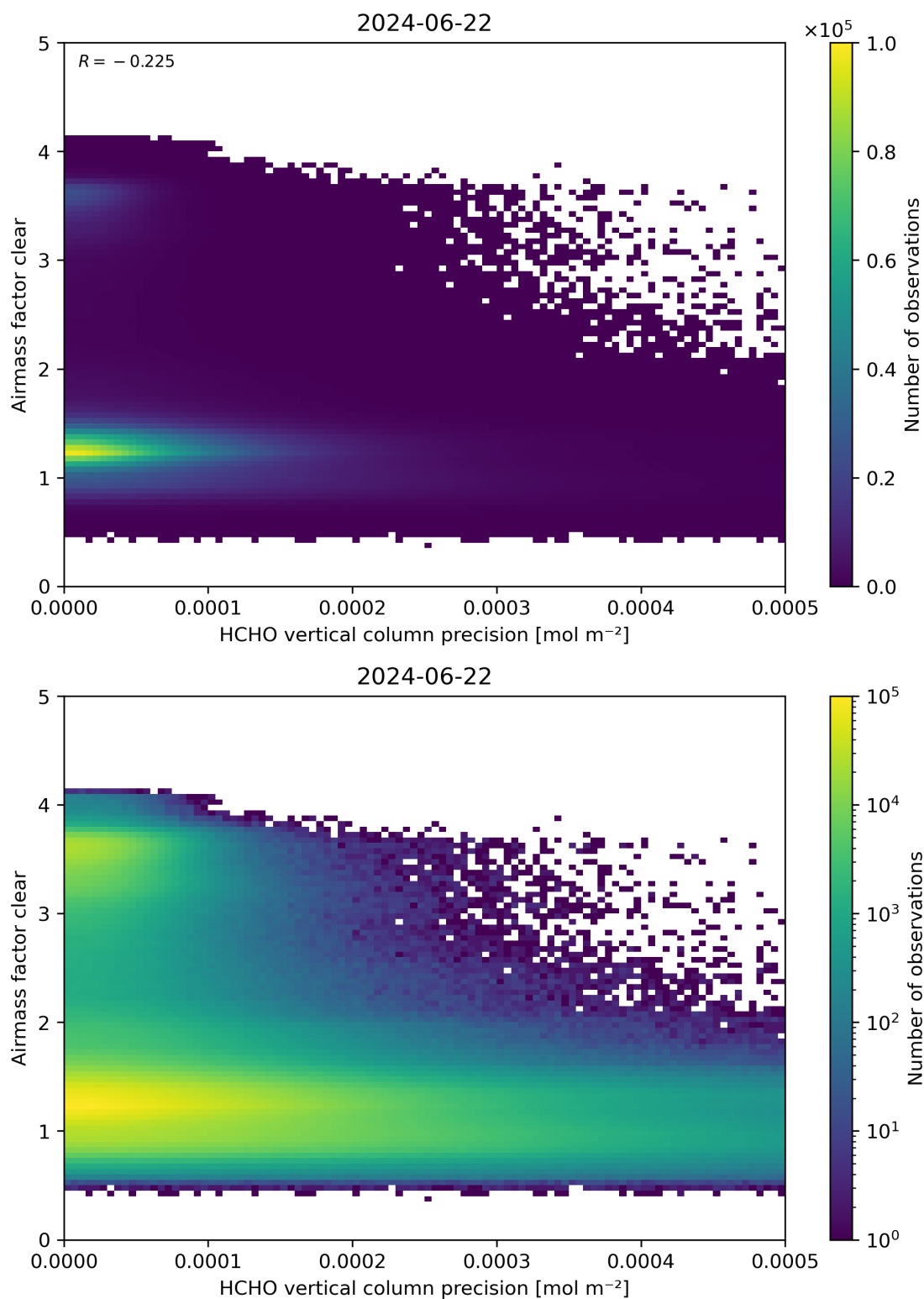
Figure 139: Scatter density plot of “HCHO vertical column precision” against “Airmass factor clear” for 2024-06-21 to 2024-06-23.
