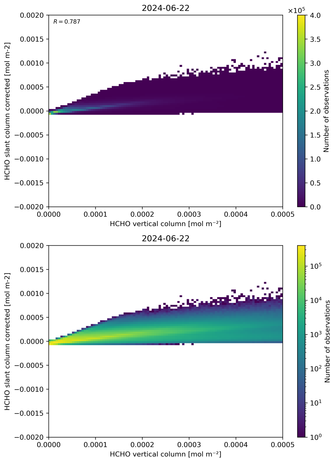
Figure 127: Scatter density plot of “HCHO vertical column” against “HCHO slant column corrected” for 2024-06-21 to 2024-06-23.
