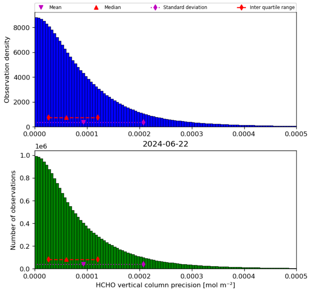
Figure 36: Histogram of “HCHO vertical column precision” for 2024-06-21 to 2024-06-23
