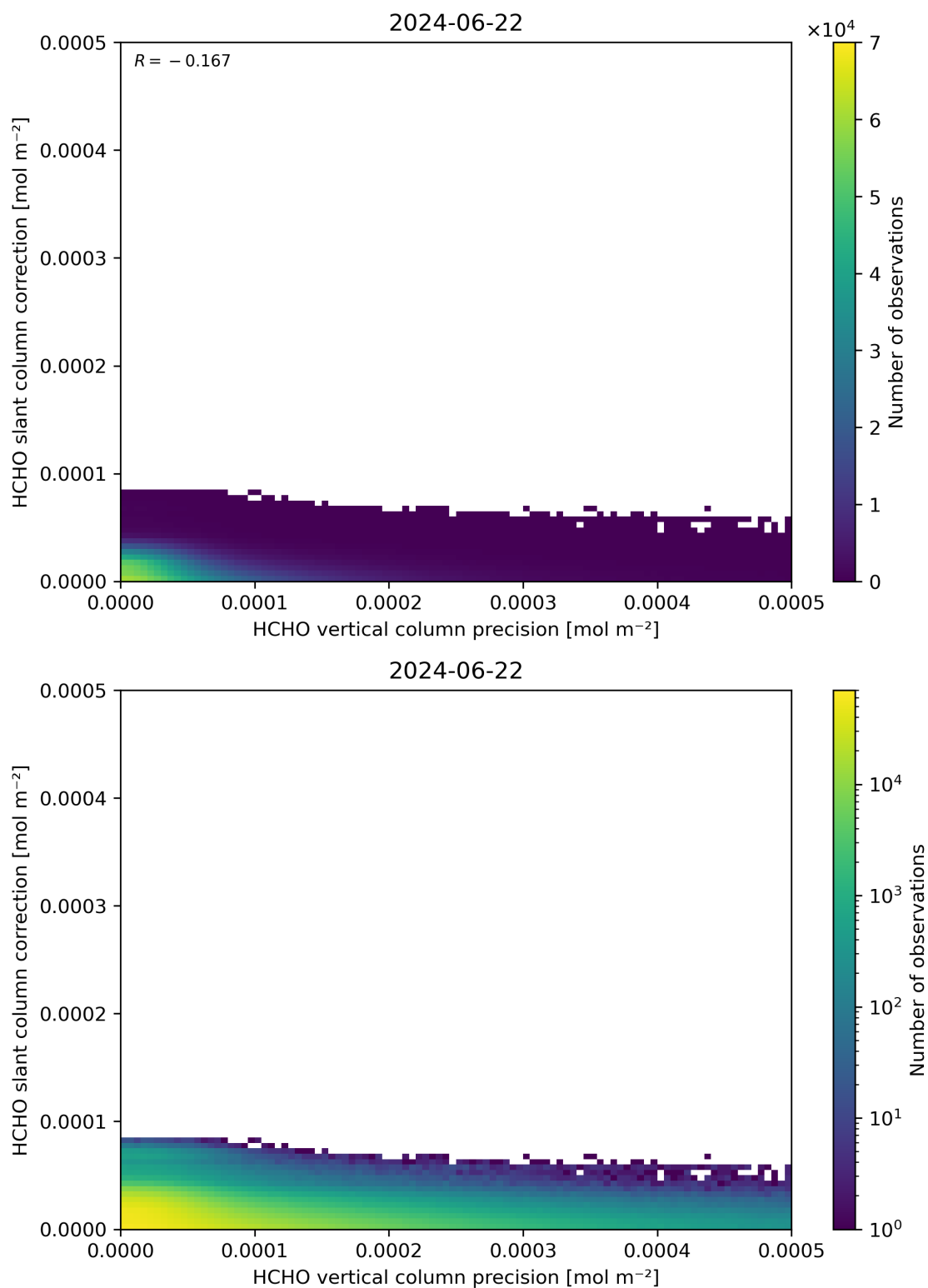
Figure 141: Scatter density plot of “HCHO vertical column precision” against “HCHO slant column correction” for 2024-06-21 to 2024-06-23.
