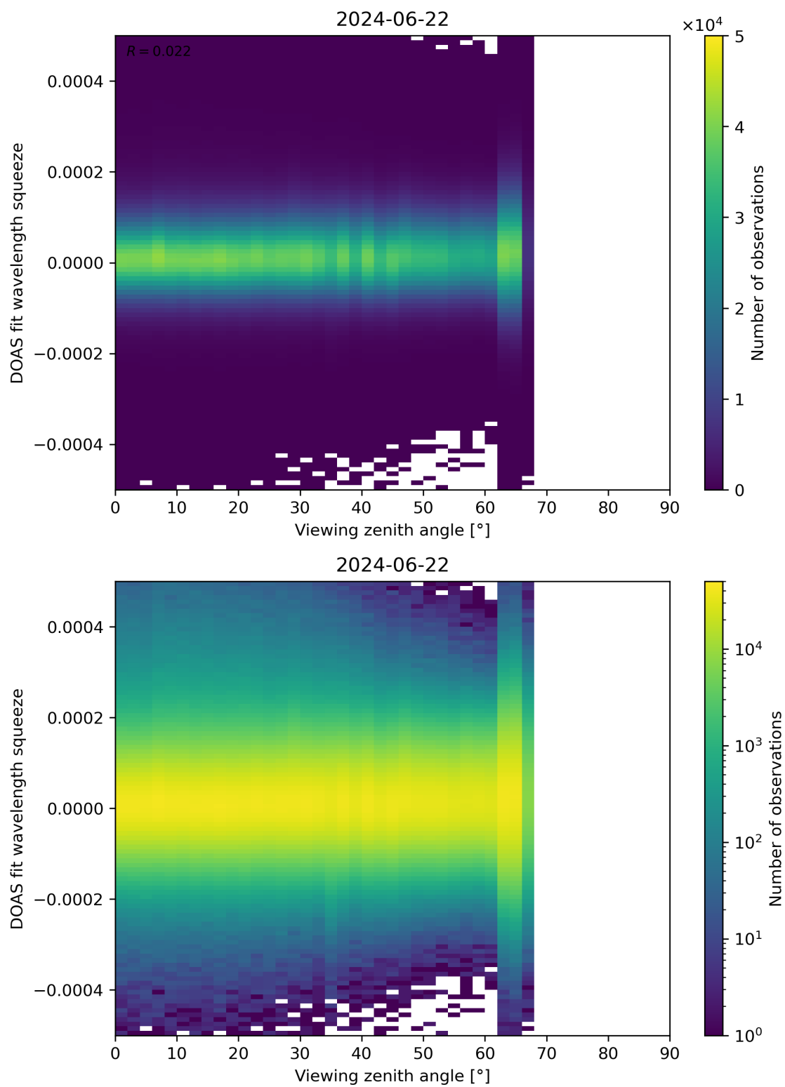
Figure 184: Scatter density plot of “Viewing zenith angle” against “DOAS fit wavelength squeeze” for 2024-06-21 to 2024-06-23.
