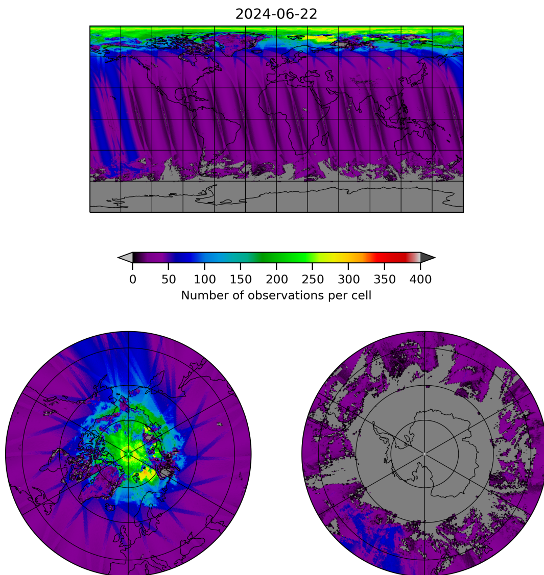
Figure 19: Map of the number of observations for 2024-06-21 to 2024-06-23
