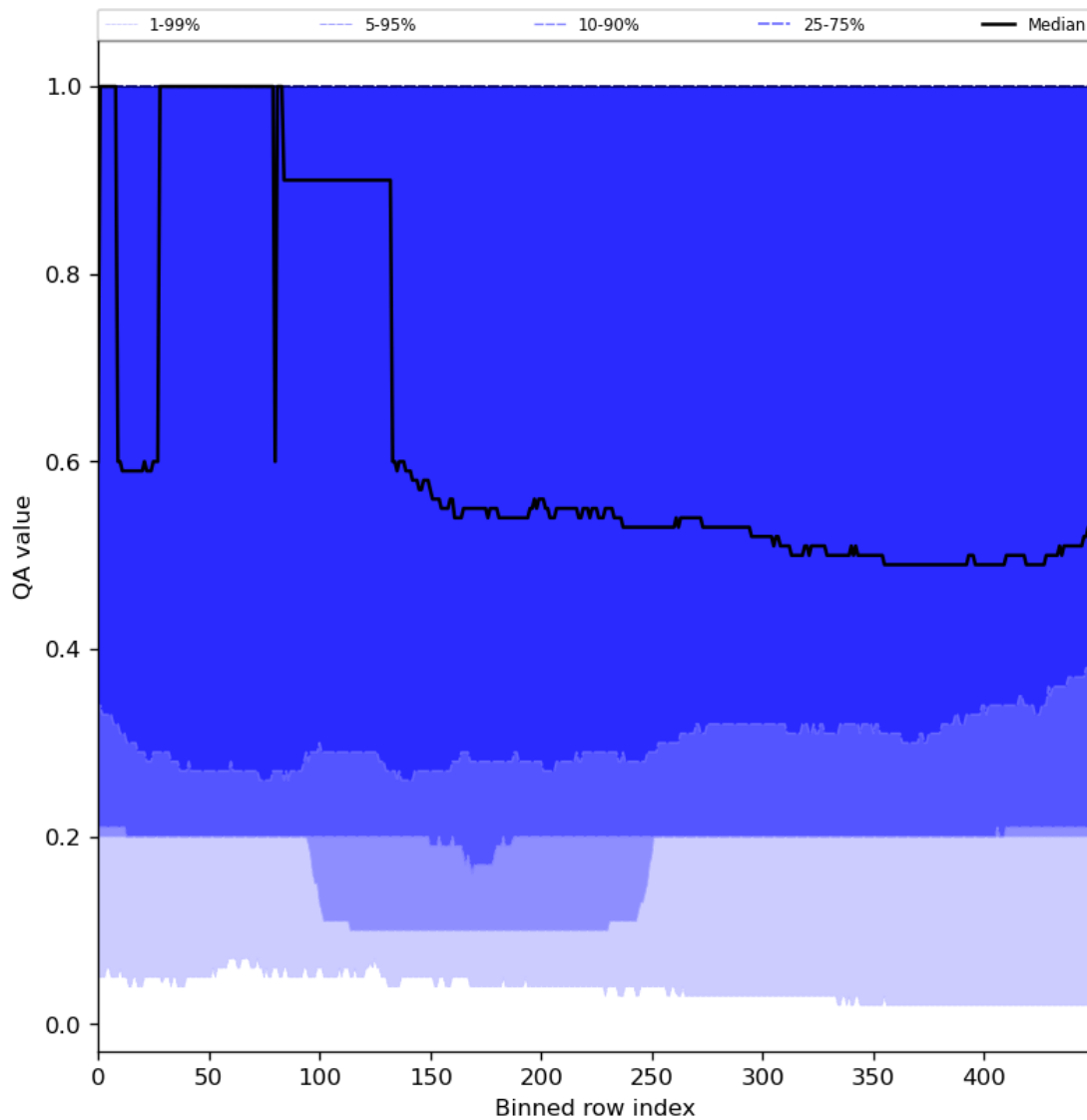
Figure 48: Along track statistics of “QA value” for 2024-06-21 to 2024-06-23
