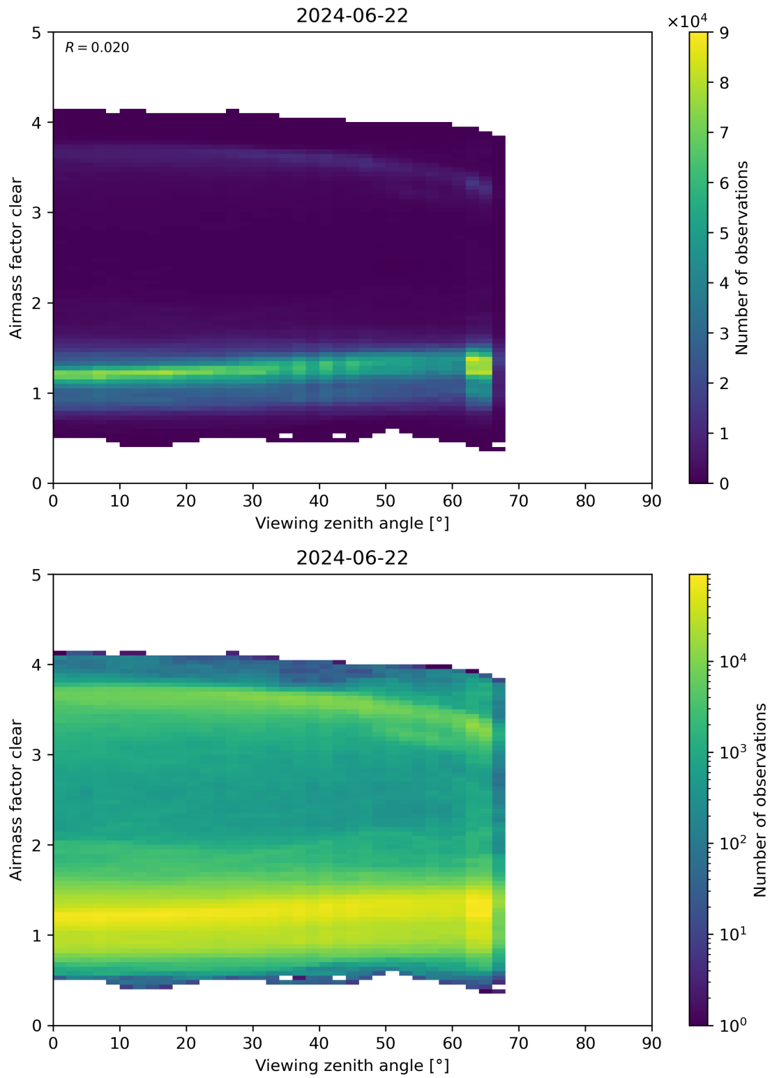
Figure 185: Scatter density plot of “Viewing zenith angle” against “Airmass factor clear” for 2024-06-21 to 2024-06-23.
