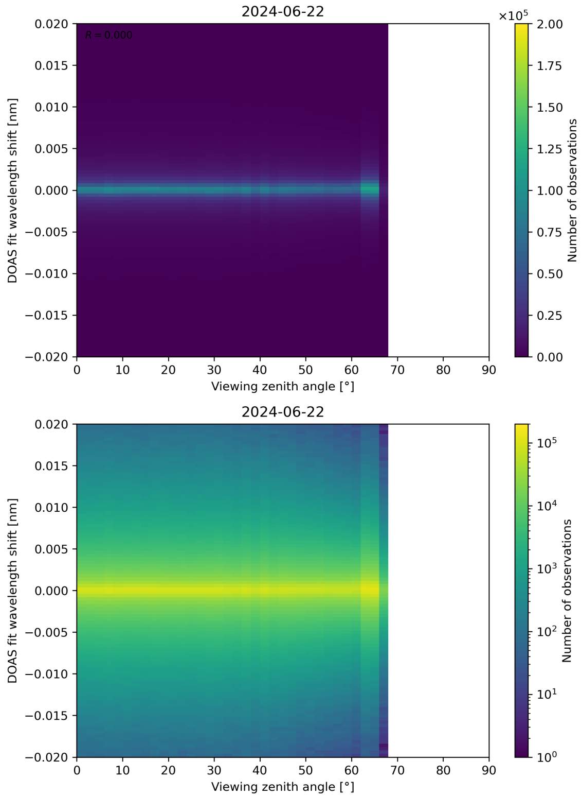
Figure 183: Scatter density plot of “Viewing zenith angle” against “DOAS fit wavelength shift” for 2024-06-21 to 2024-06-23.
