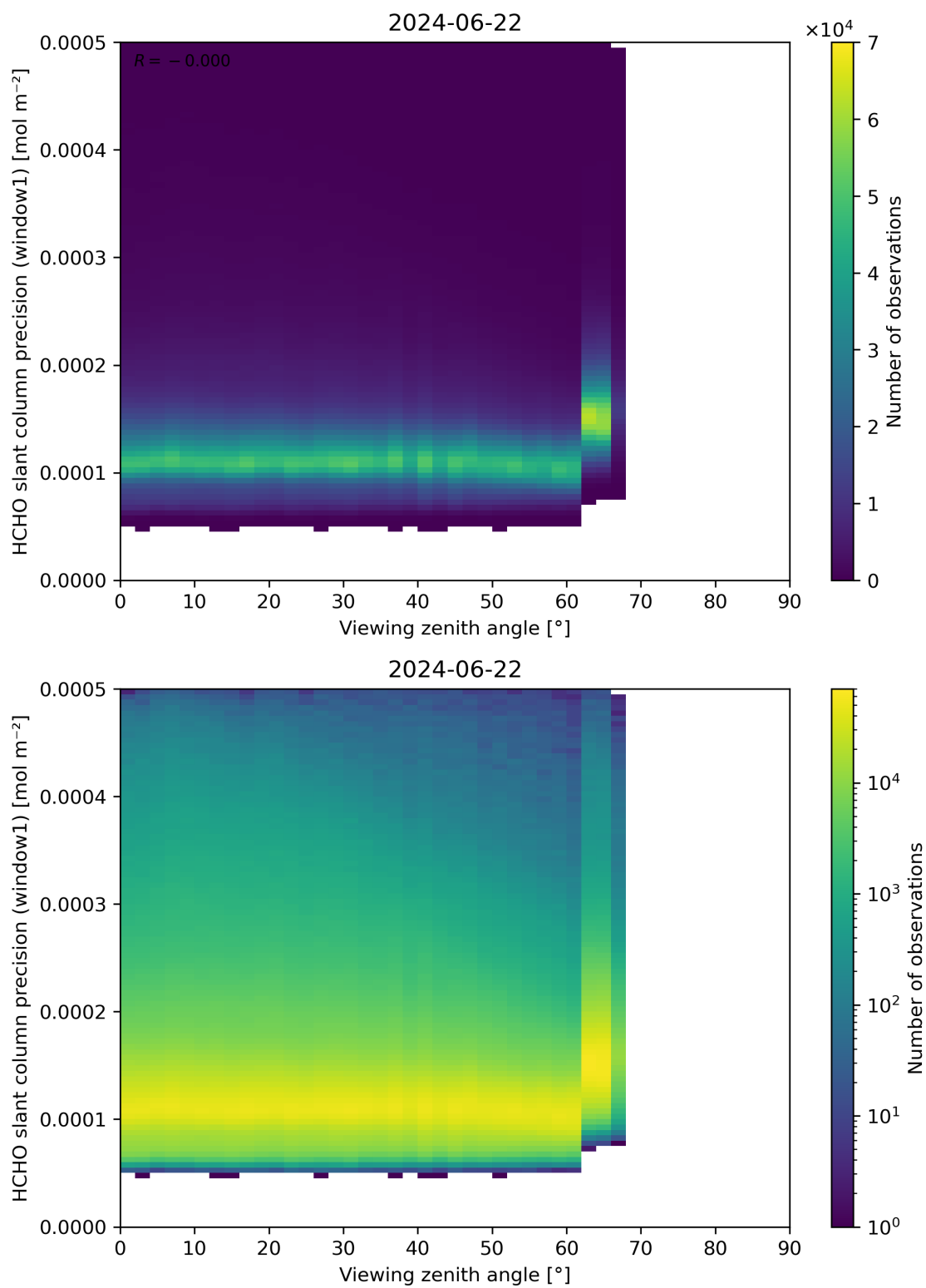
Figure 189: Scatter density plot of “Viewing zenith angle” against “HCHO slant column precision (window1)” for 2024-06-21 to 2024-06-23.
