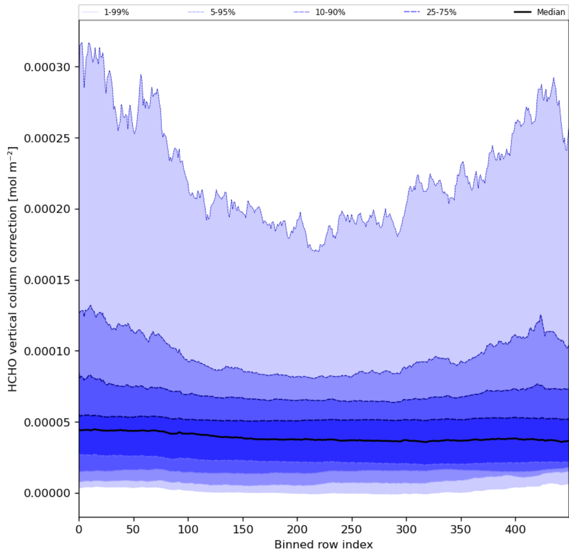
Figure 51: Along track statistics of “HCHO vertical column correction” for 2024-06-21 to 2024-06-23
