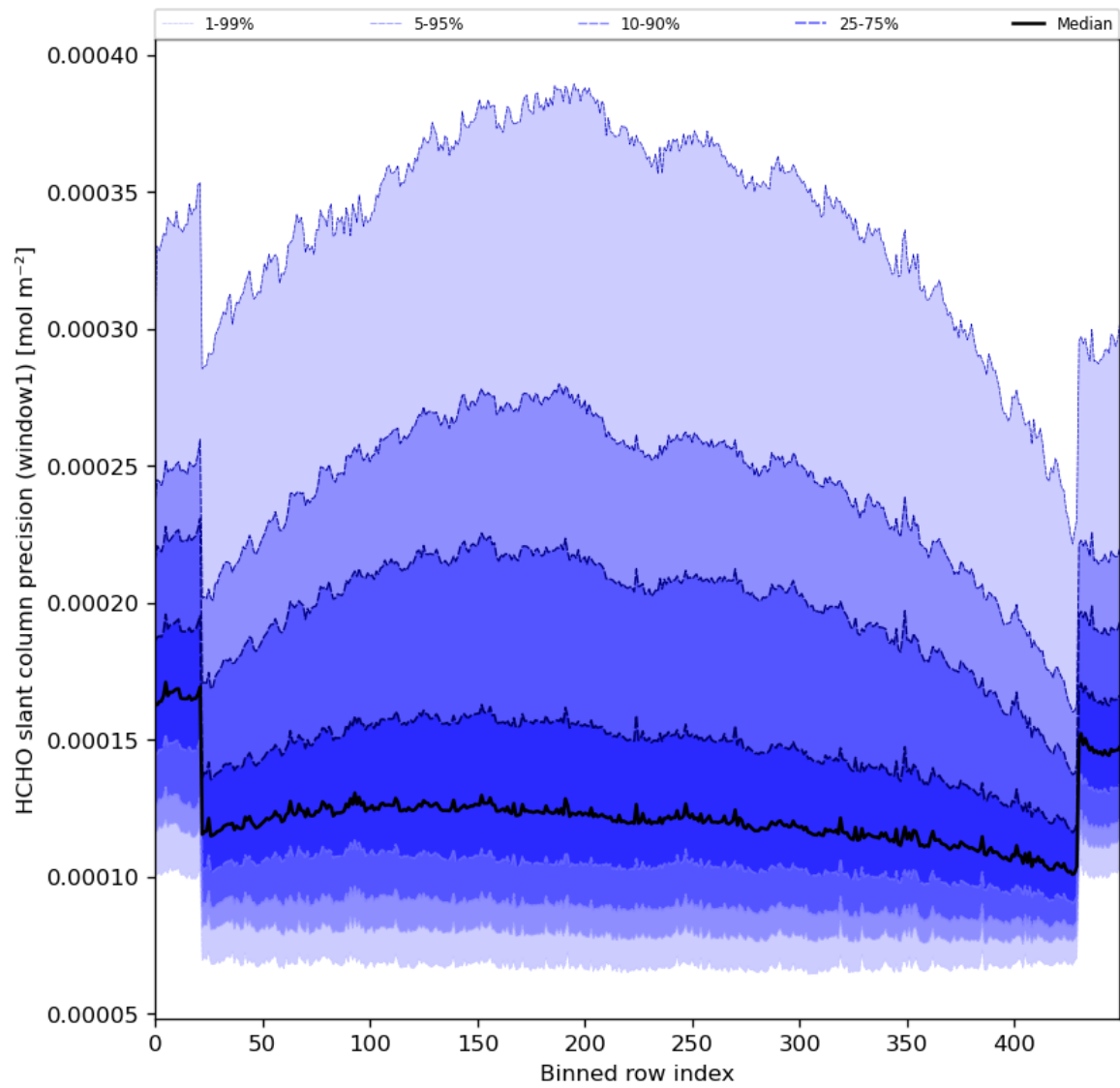
Figure 53: Along track statistics of “HCHO slant column precision (window1)” for 2024-06-21 to 2024-06-23
