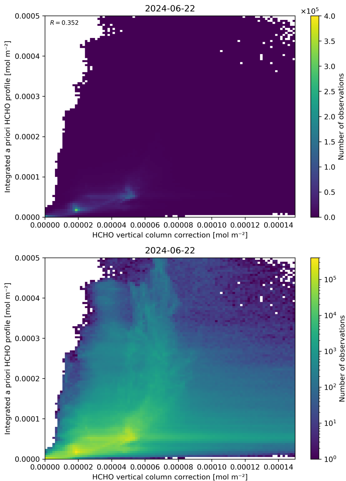
Figure 122: Scatter density plot of “HCHO vertical column correction” against “Integrated a priori HCHO profile” for 2024-06-21 to 2024-06-23.
