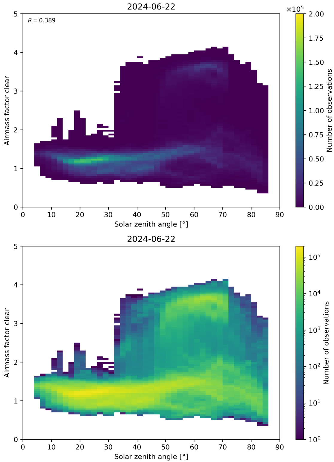
Figure 170: Scatter density plot of “Solar zenith angle” against “Airmass factor clear” for 2024-06-21 to 2024-06-23.
