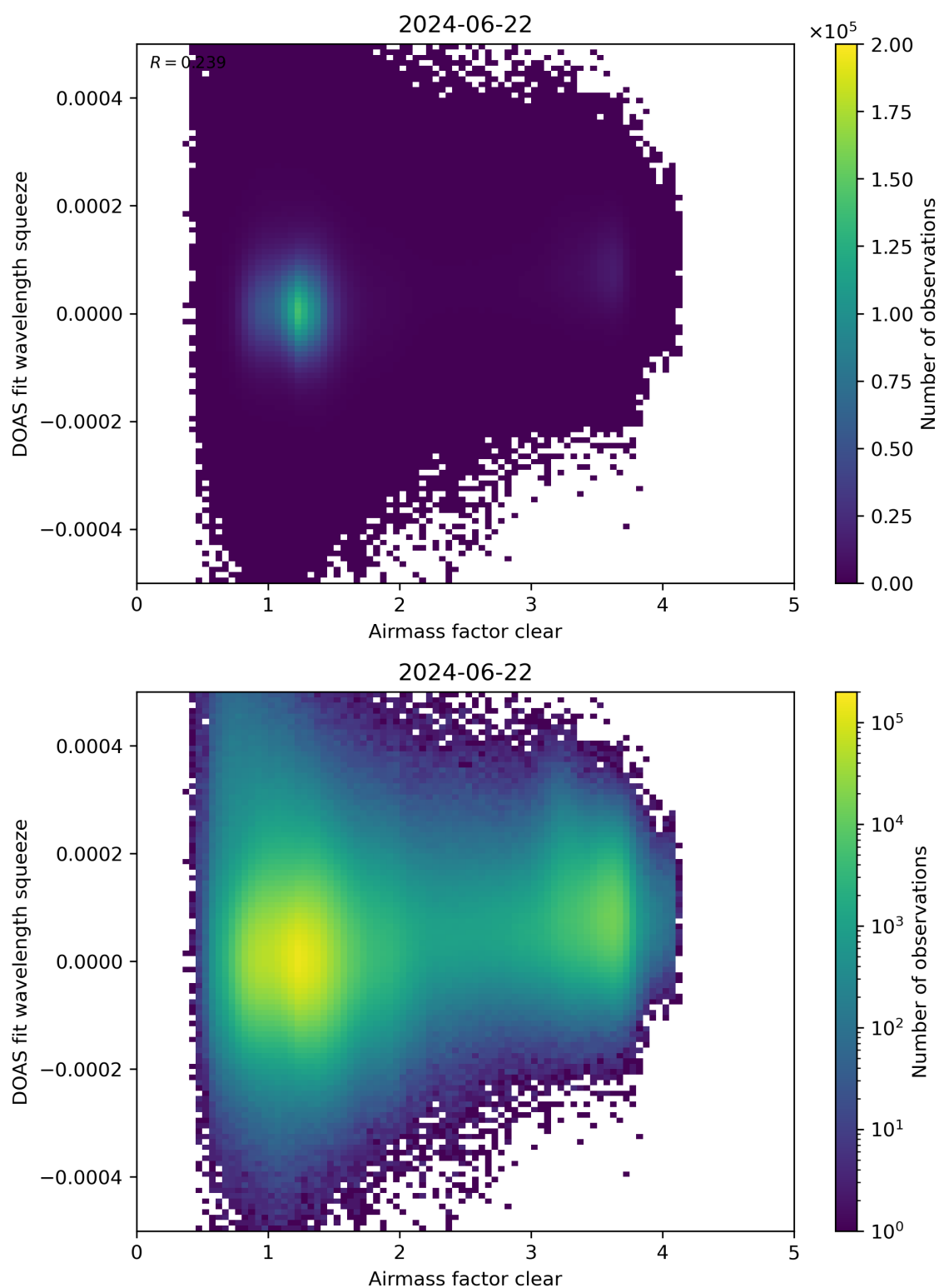
Figure 73: Scatter density plot of “Airmass factor clear” against “DOAS fit wavelength squeeze” for 2024-06-21 to 2024-06-23.
