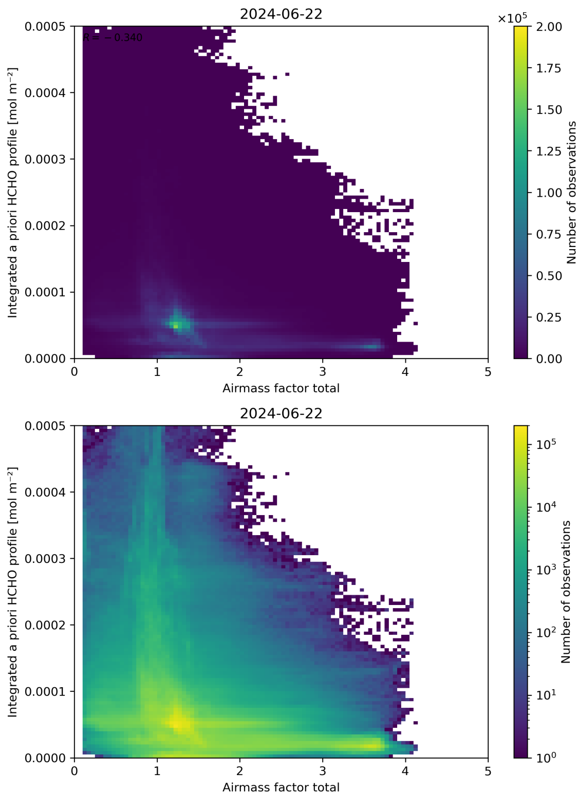
Figure 104: Scatter density plot of “Airmass factor total” against “Integrated a priori HCHO profile” for 2024-06-21 to 2024-06-23.
