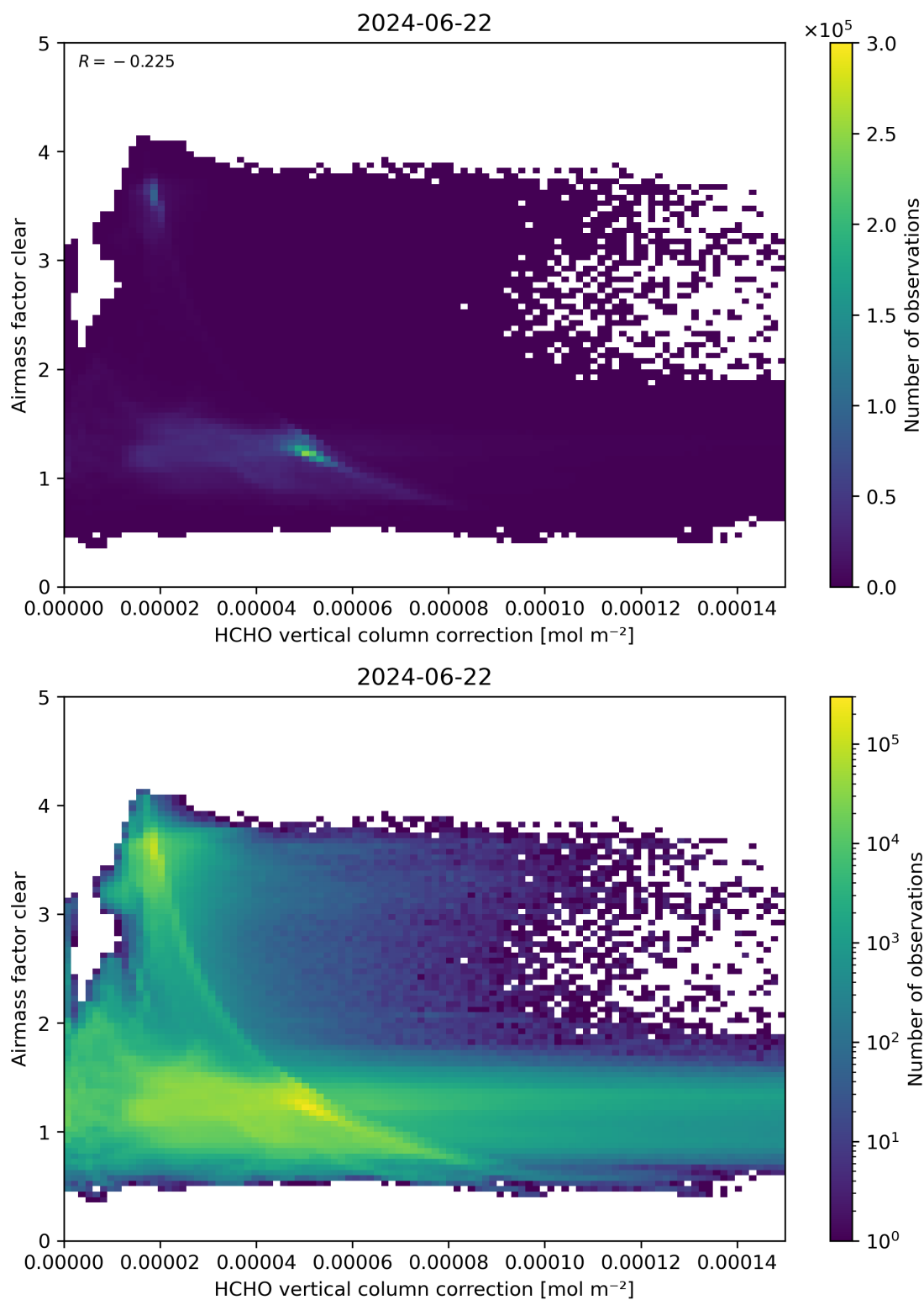
Figure 115: Scatter density plot of “HCHO vertical column correction” against “Airmass factor clear” for 2024-06-21 to 2024-06-23.
