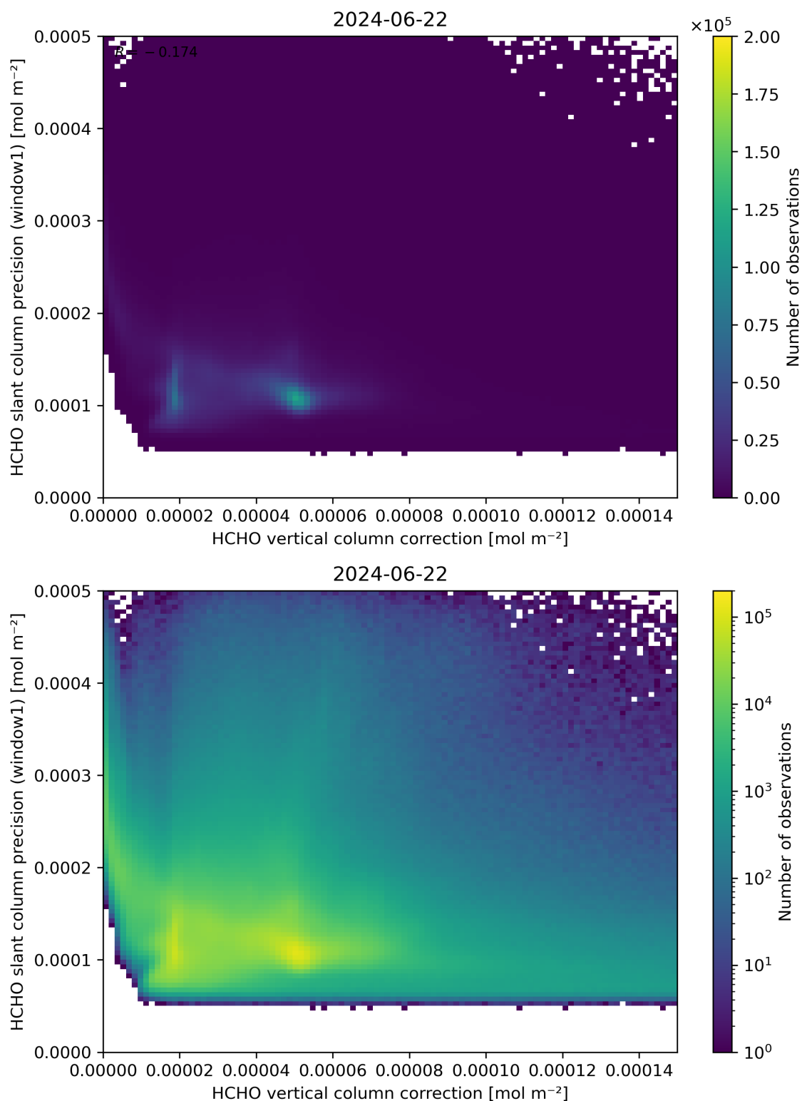
Figure 119: Scatter density plot of “HCHO vertical column correction” against “HCHO slant column precision (window1)” for 2024-06-21 to 2024-06-23.
