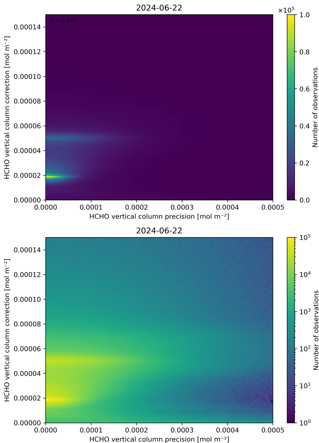
Figure 146: Scatter density plot of “HCHO vertical column precision” against “HCHO vertical column correction” for 2024-06-21 to 2024-06-23.
