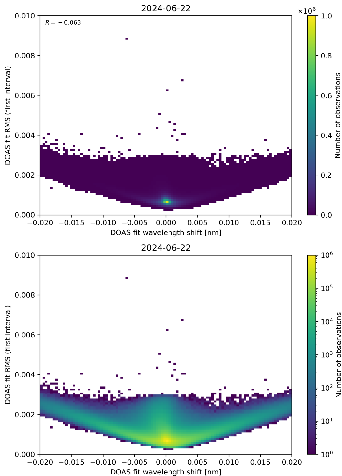
Figure 64: Scatter density plot of “DOAS fit wavelength shift” against “DOAS fit RMS (first interval)” for 2024-06-21 to 2024-06-23.
