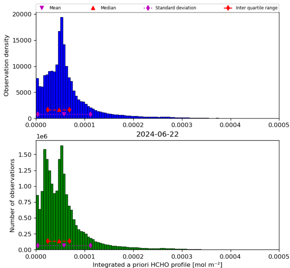
Figure 43: Histogram of “Integrated a priori HCHO profile” for 2024-06-21 to 2024-06-23
