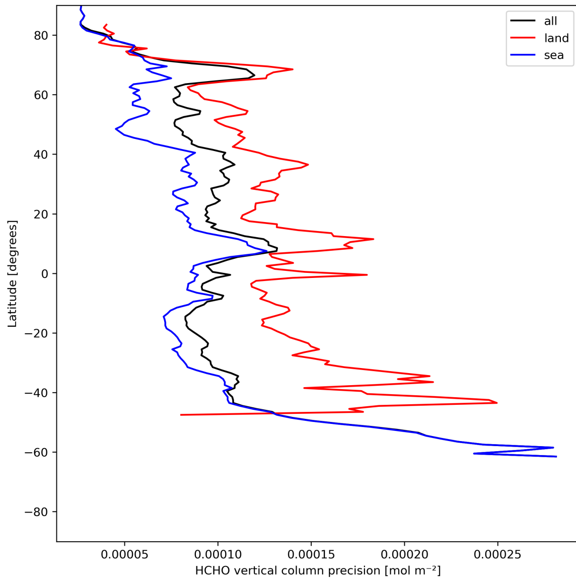
Figure 22: Zonal average of “HCHO vertical column precision” for 2024-06-21 to 2024-06-23.
