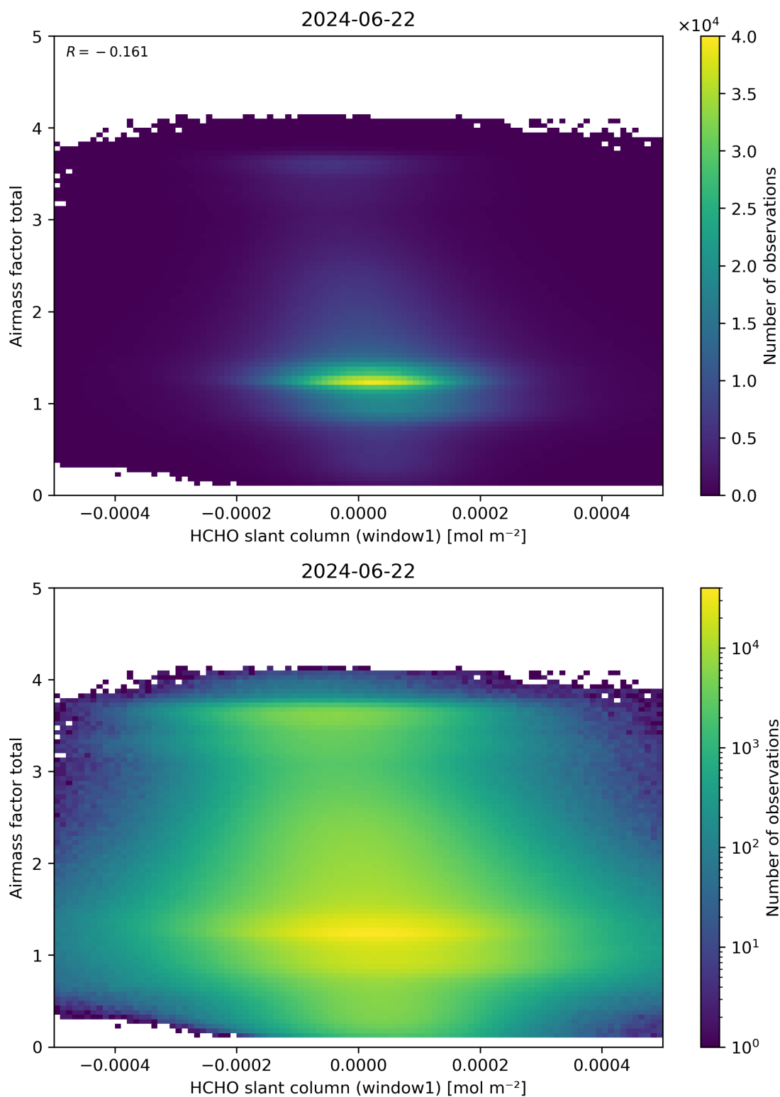
Figure 85: Scatter density plot of “HCHO slant column (window1)” against “Airmass factor total” for 2024-06-21 to 2024-06-23.
