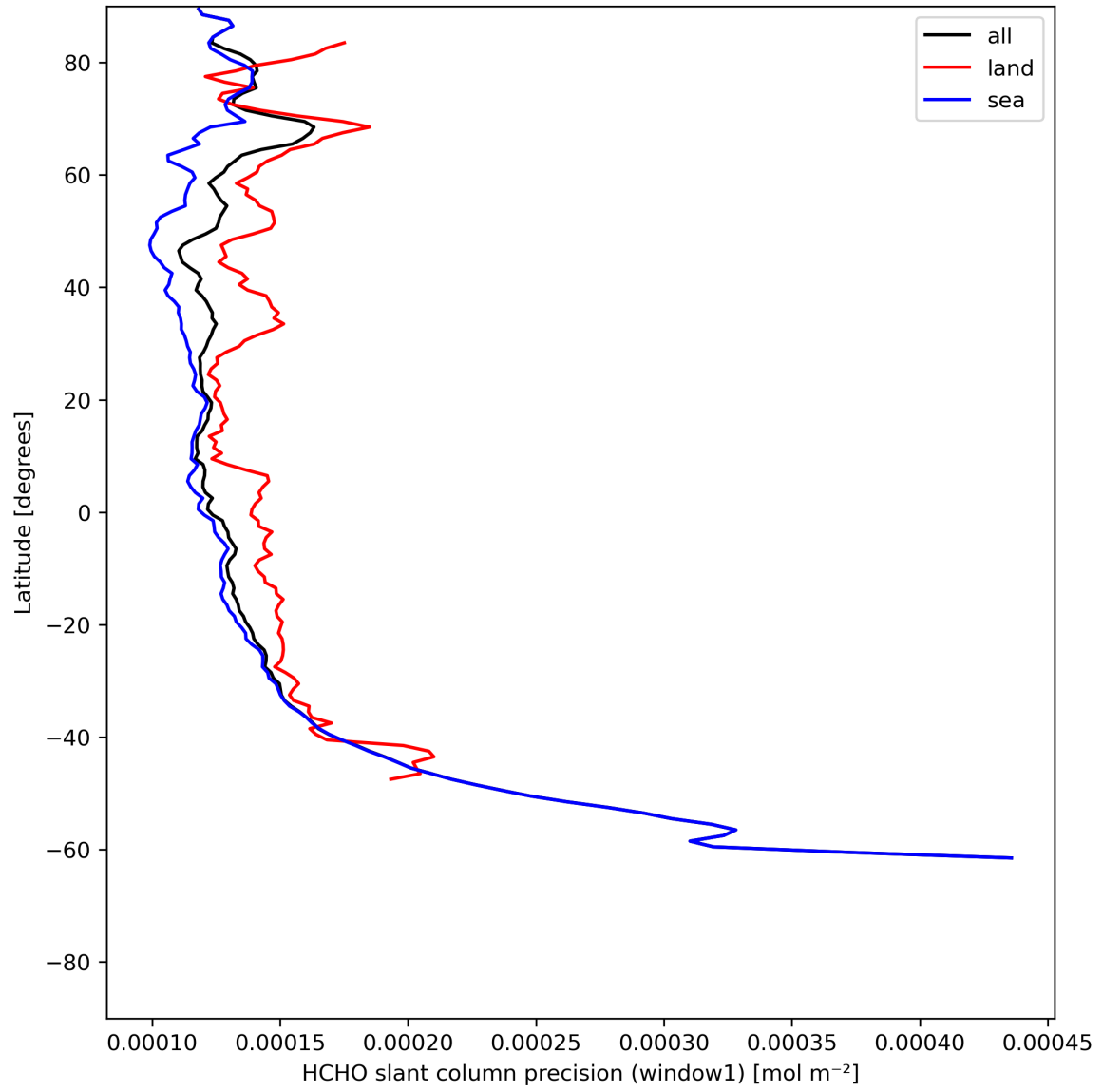
Figure 25: Zonal average of “HCHO slant column precision (window1)” for 2024-06-21 to 2024-06-23.
