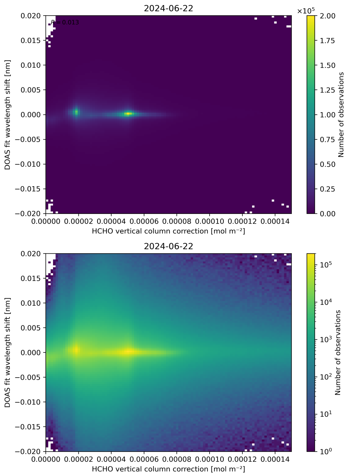
Figure 113: Scatter density plot of “HCHO vertical column correction” against “DOAS fit wavelength shift” for 2024-06-21 to 2024-06-23.
