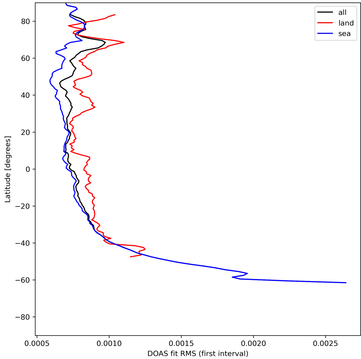
Figure 32: Zonal average of "DOAS fit RMS (first interval)" for 2024-06-21 to 2024-06-23.
