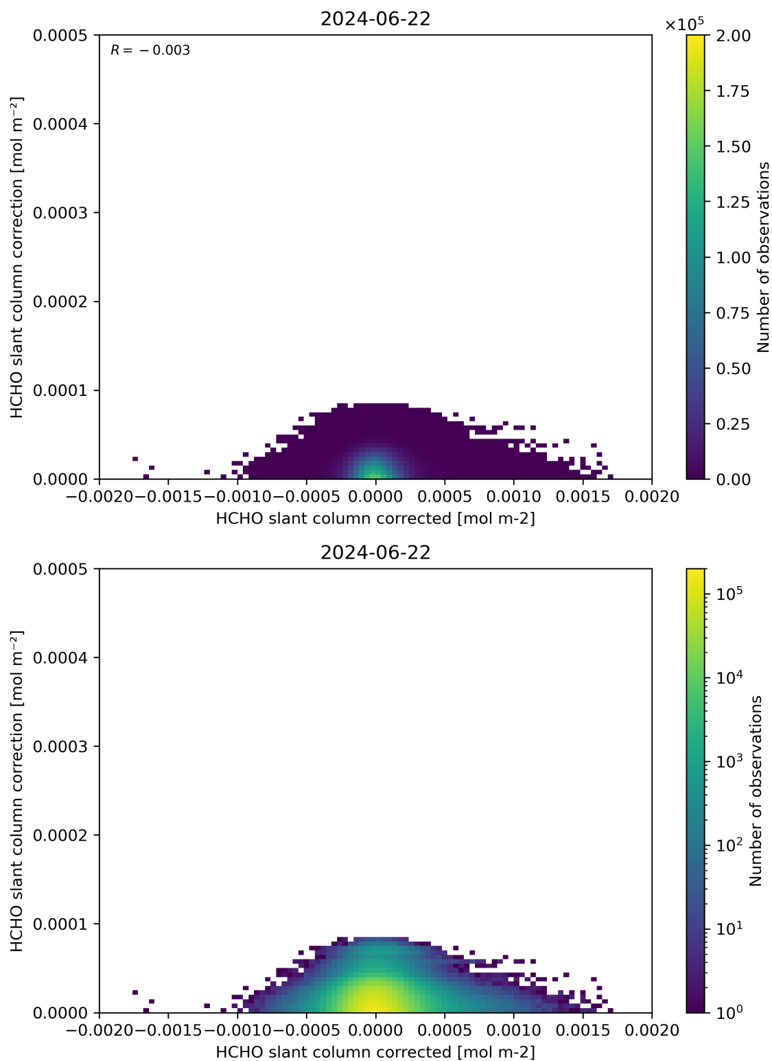
Figure 77: Scatter density plot of “HCHO slant column corrected” against “HCHO slant column correction” for 2024-06-21 to 2024-06-23.
