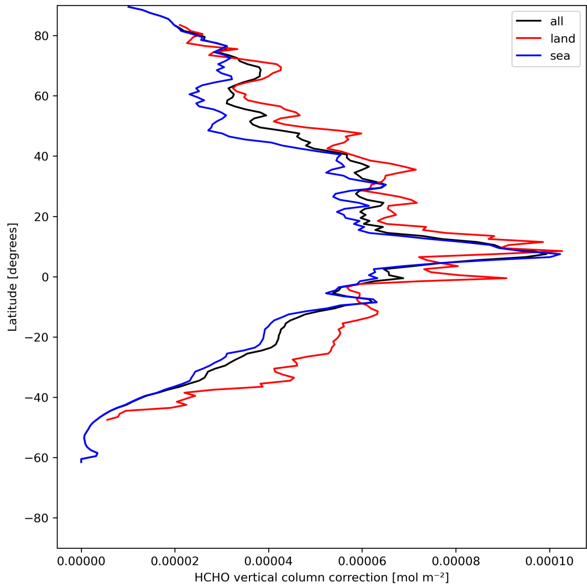
Figure 23: Zonal average of “HCHO vertical column correction” for 2024-06-21 to 2024-06-23.
