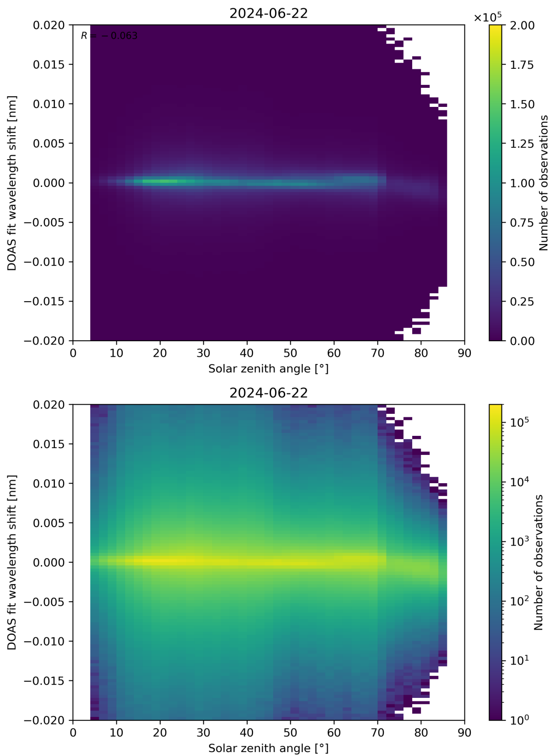
Figure 168: Scatter density plot of “Solar zenith angle” against “DOAS fit wavelength shift” for 2024-06-21 to 2024-06-23.
