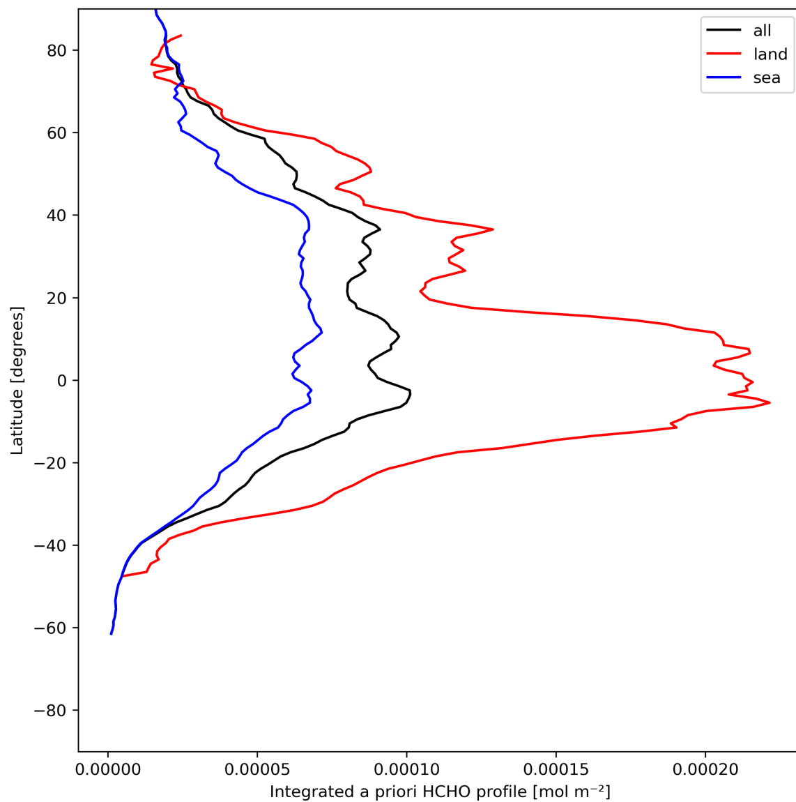
Figure 29: Zonal average of “Integrated a priori HCHO profile” for 2024-06-21 to 2024-06-23.
