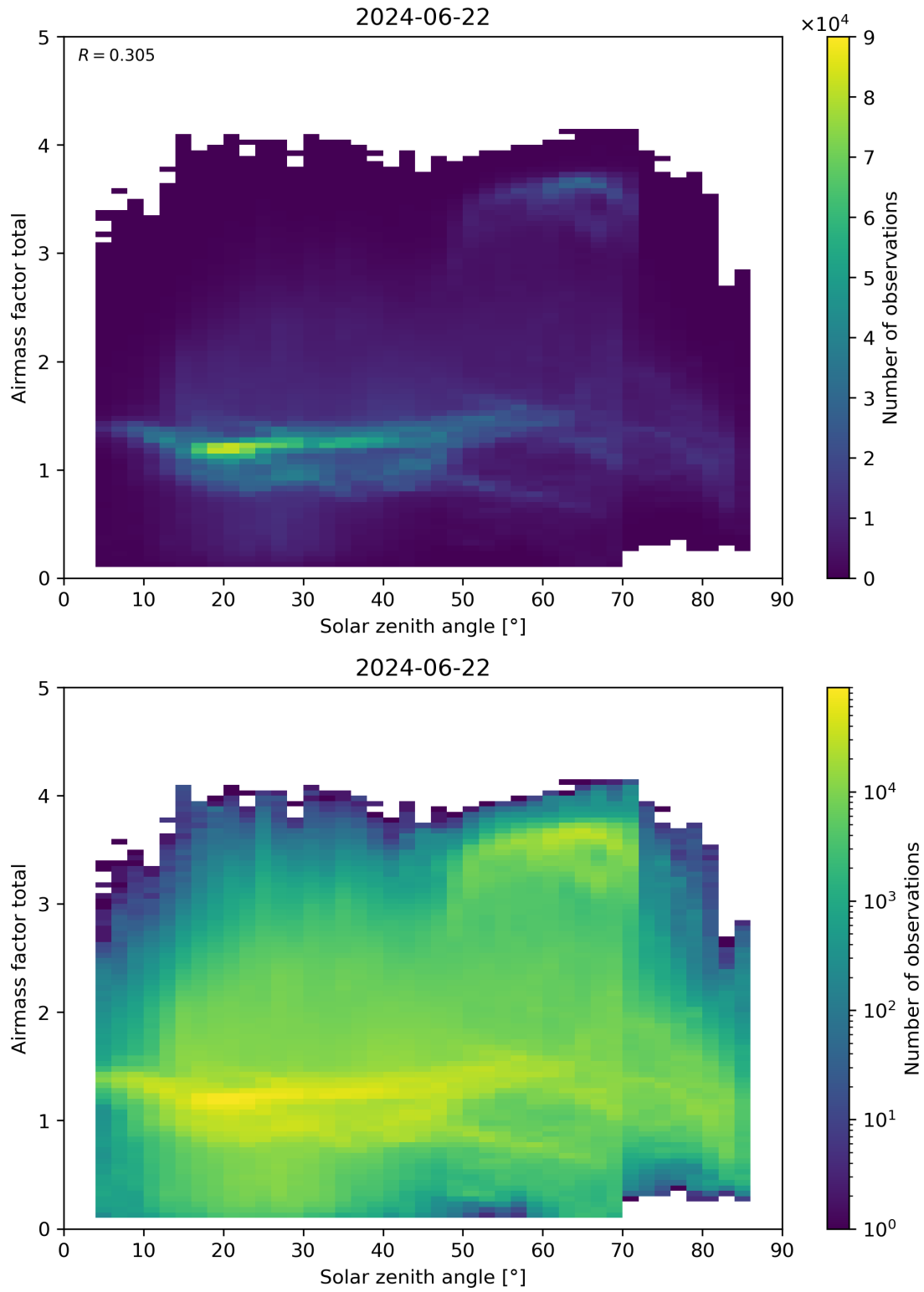
Figure 175: Scatter density plot of “Solar zenith angle” against “Airmass factor total” for 2024-06-21 to 2024-06-23.
