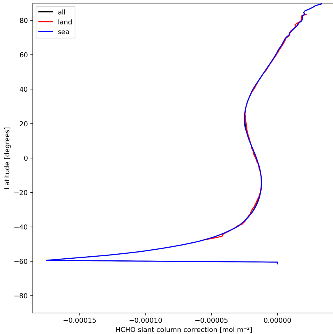
Figure 33: Zonal average of “HCHO slant column correction” for 2024-06-21 to 2024-06-23.
