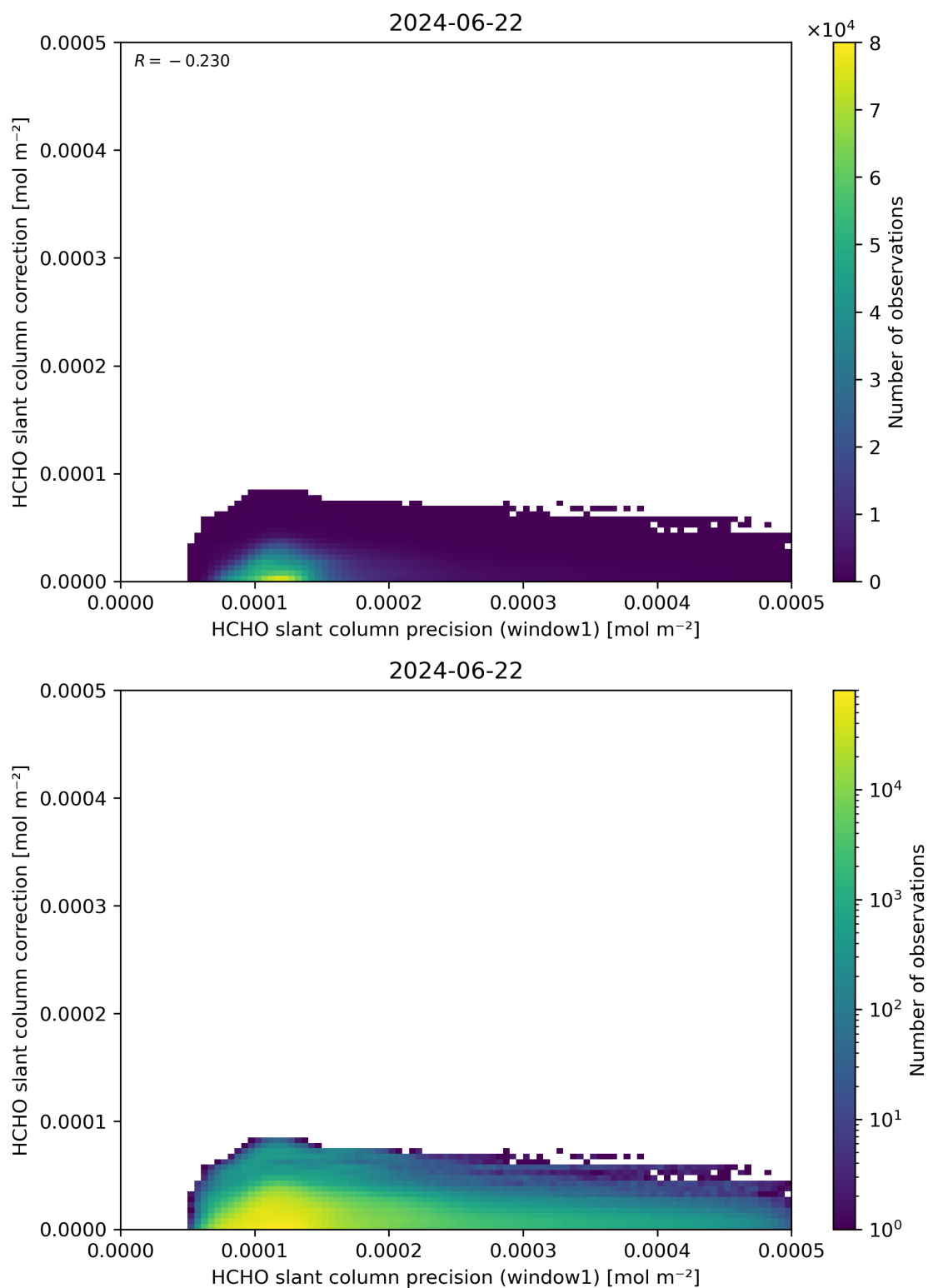
Figure 93: Scatter density plot of “HCHO slant column precision (window1)” against “HCHO slant column correction” for 2024-06-21 to 2024-06-23.
