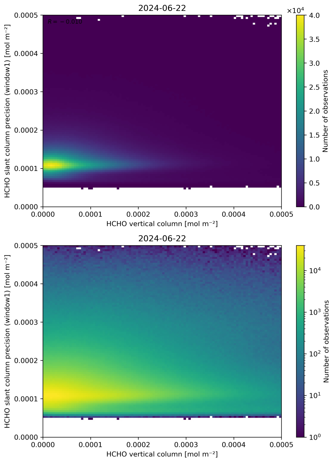
Figure 130: Scatter density plot of “HCHO vertical column” against “HCHO slant column precision (window1)” for 2024-06-21 to 2024-06-23.
