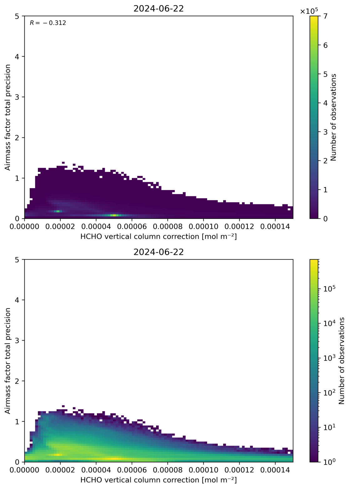
Figure 121: Scatter density plot of “HCHO vertical column correction” against “Airmass factor total precision” for 2024-06-21 to 2024-06-23.
