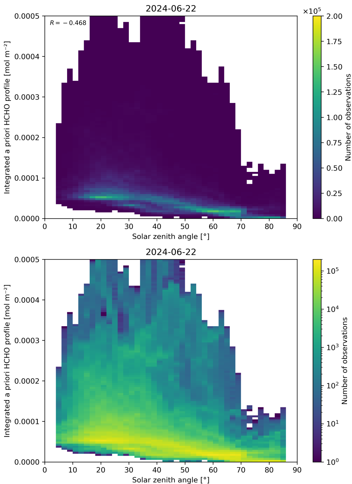
Figure 180: Scatter density plot of “Solar zenith angle” against “Integrated a priori HCHO profile” for 2024-06-21 to 2024-06-23.
