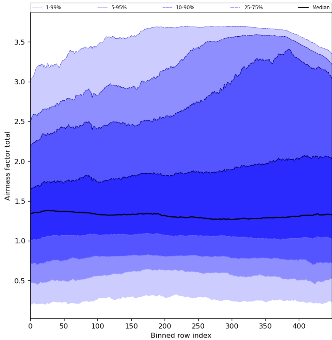
Figure 54: Along track statistics of “Airmass factor total” for 2024-06-21 to 2024-06-23
