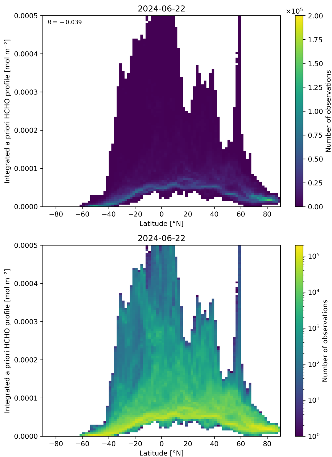
Figure 166: Scatter density plot of “Latitude” against “Integrated a priori HCHO profile” for 2024-06-21 to 2024-06-23.
