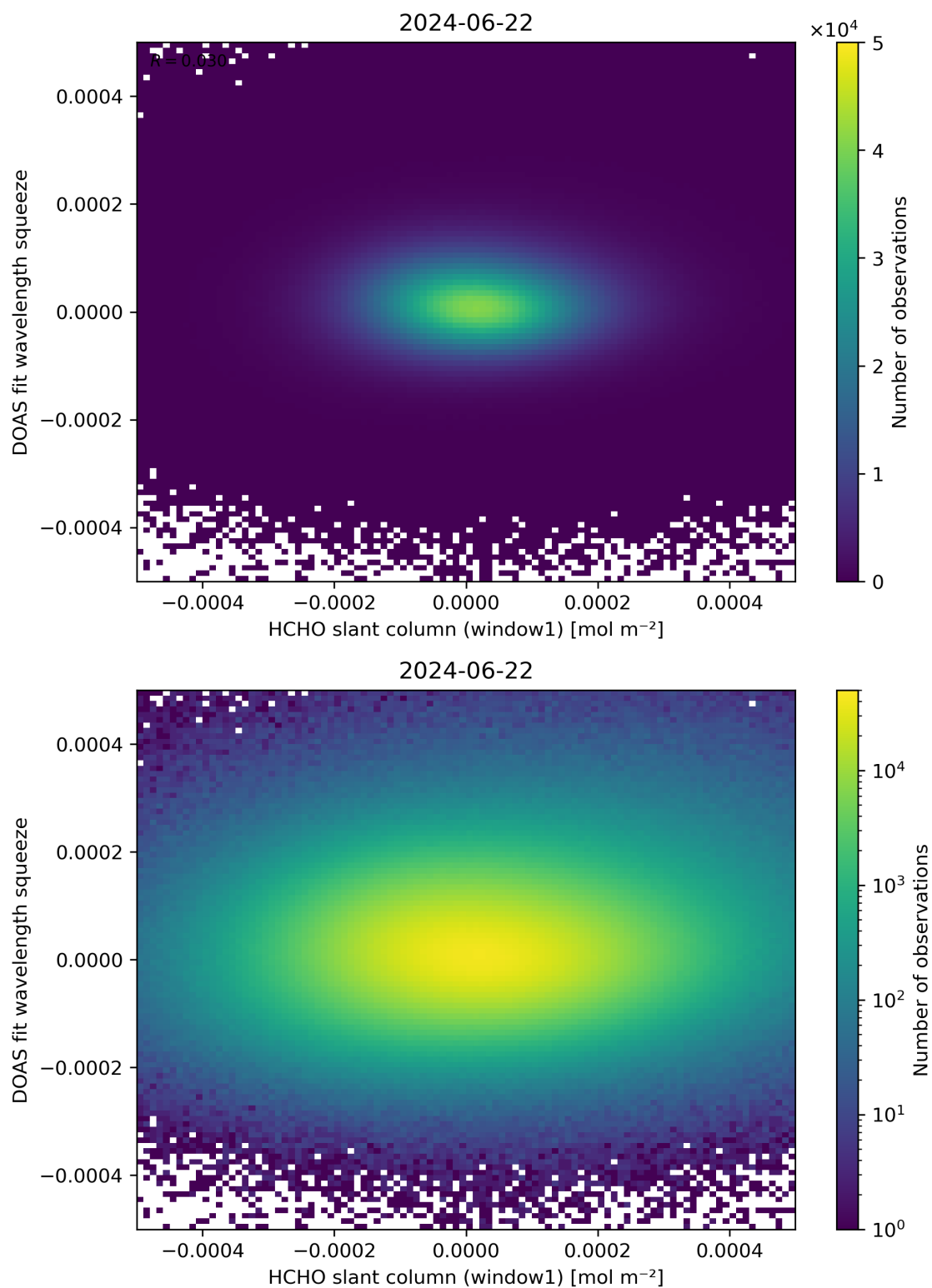
Figure 80: Scatter density plot of “HCHO slant column (window1)” against “DOAS fit wavelength squeeze” for 2024-06-21 to 2024-06-23.
