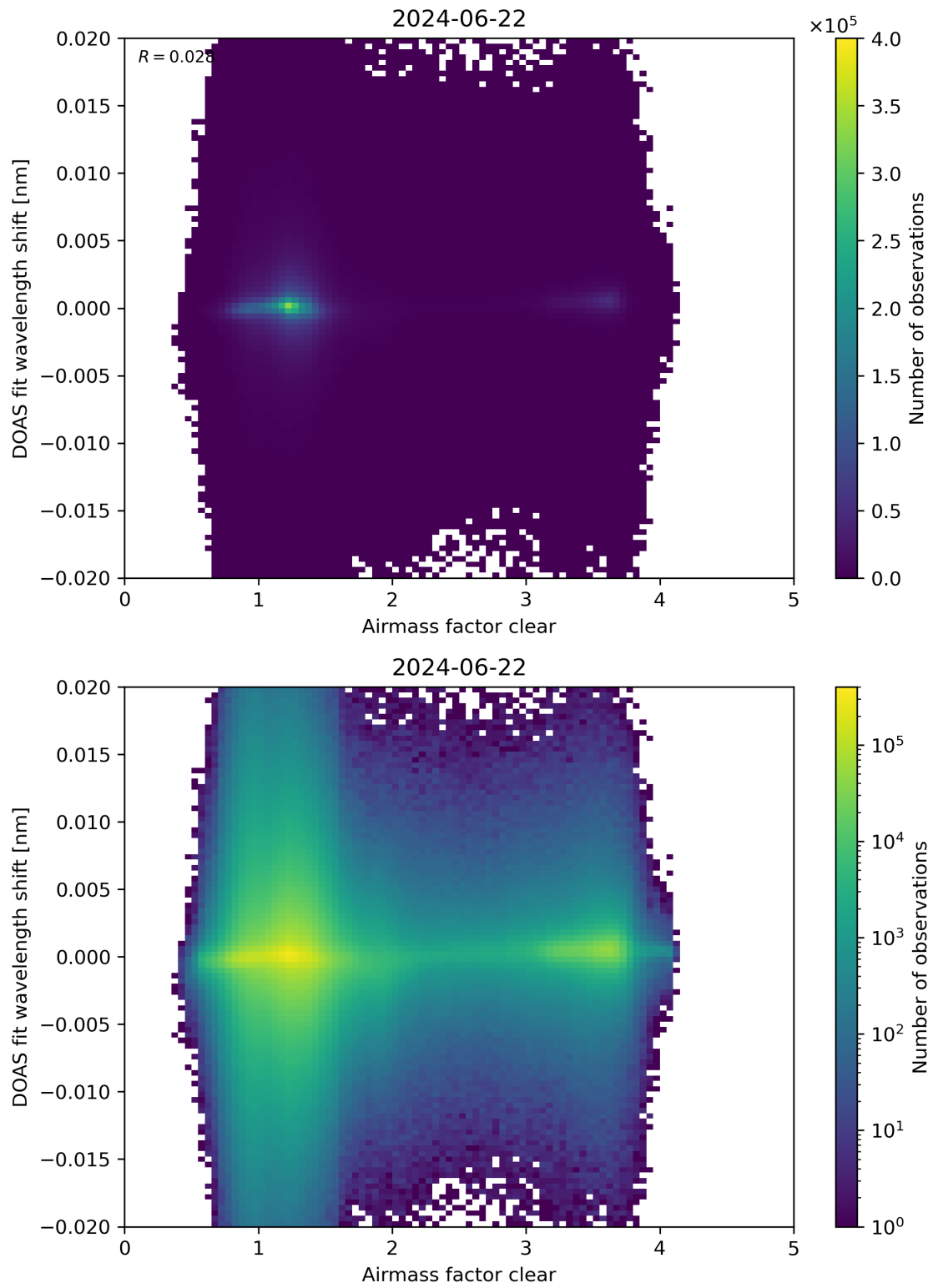
Figure 72: Scatter density plot of “Airmass factor clear” against “DOAS fit wavelength shift” for 2024-06-21 to 2024-06-23.
