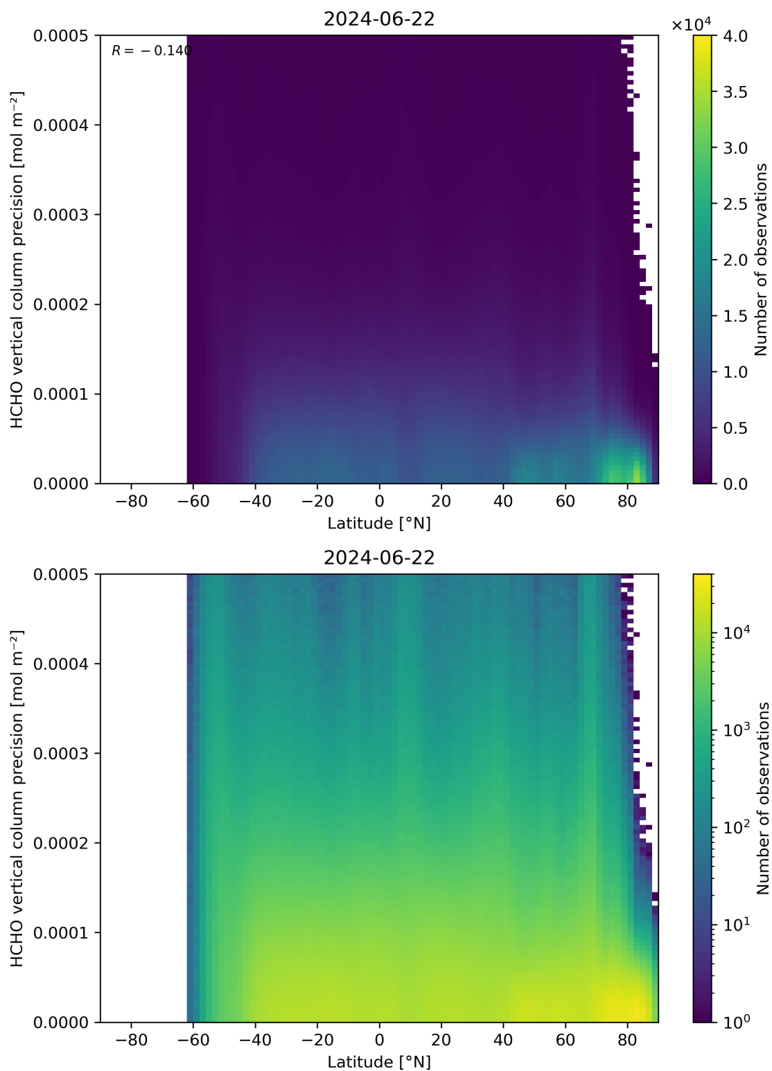
Figure 165: Scatter density plot of “Latitude” against “HCHO vertical column precision” for 2024-06-21 to 2024-06-23.
