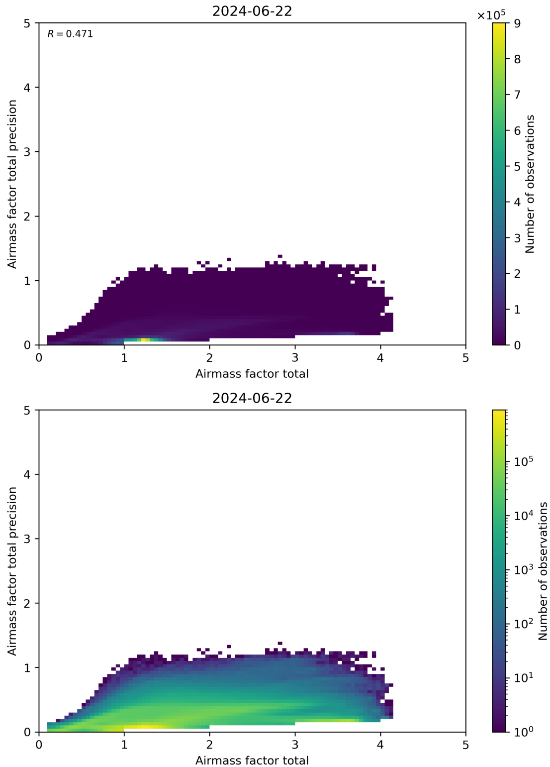
Figure 103: Scatter density plot of “Airmass factor total” against “Airmass factor total precision” for 2024-06-21 to 2024-06-23.
