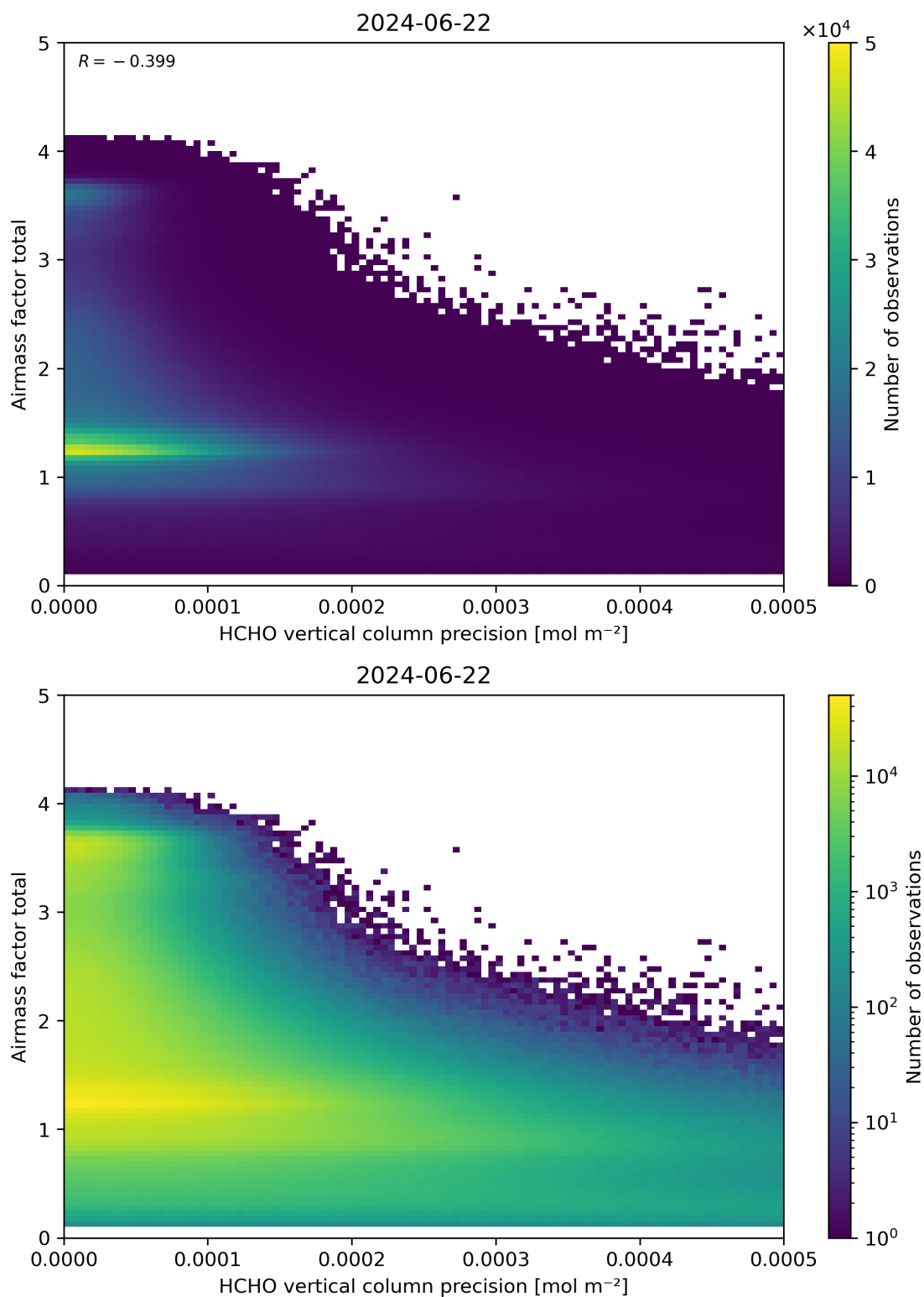
Figure 144: Scatter density plot of “HCHO vertical column precision” against “Airmass factor total” for 2024-06-21 to 2024-06-23.
