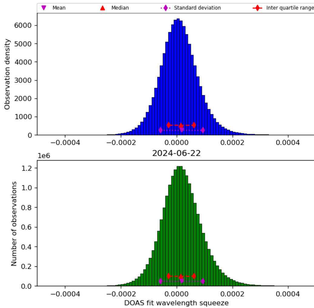
Figure 45: Histogram of “DOAS fit wavelength squeeze” for 2024-06-21 to 2024-06-23
