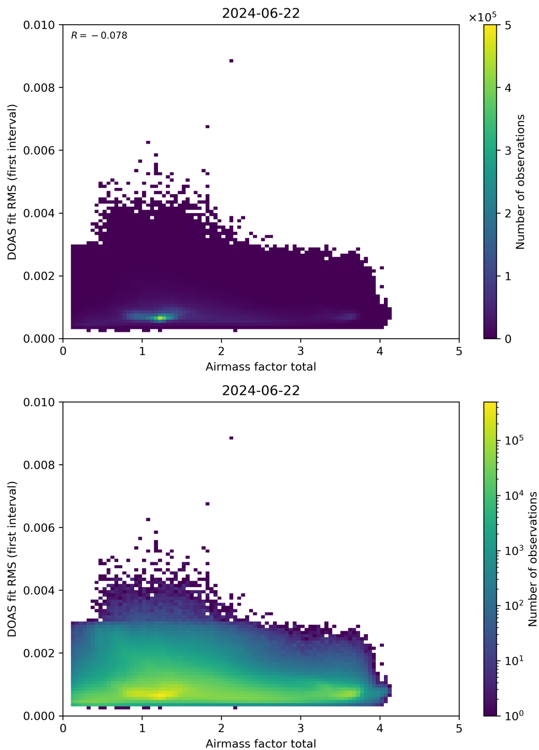
Figure 97: Scatter density plot of “Airmass factor total” against “DOAS fit RMS (first interval)” for 2024-06-21 to 2024-06-23.
