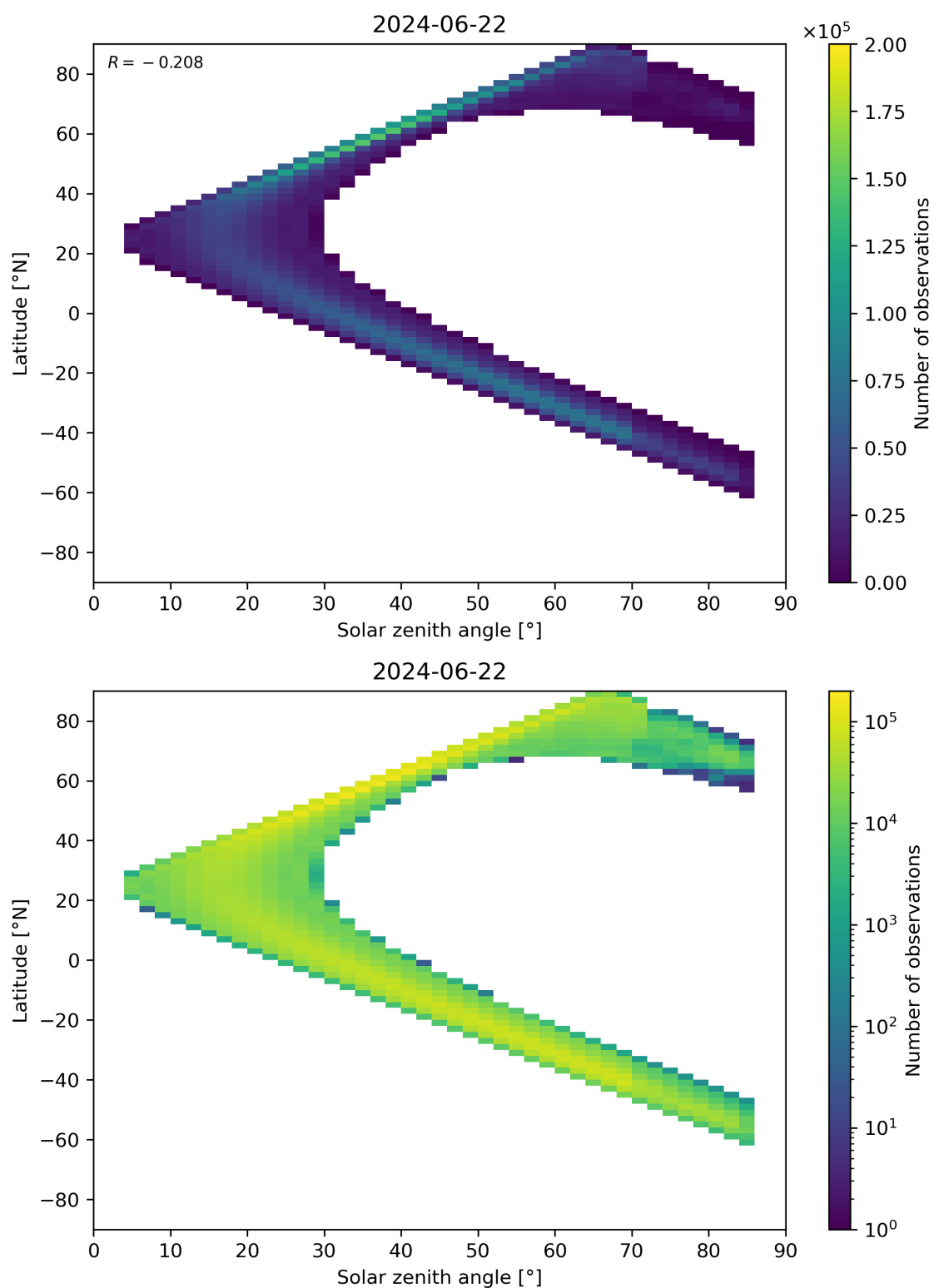
Figure 181: Scatter density plot of “Solar zenith angle” against “Latitude” for 2024-06-21 to 2024-06-23.
