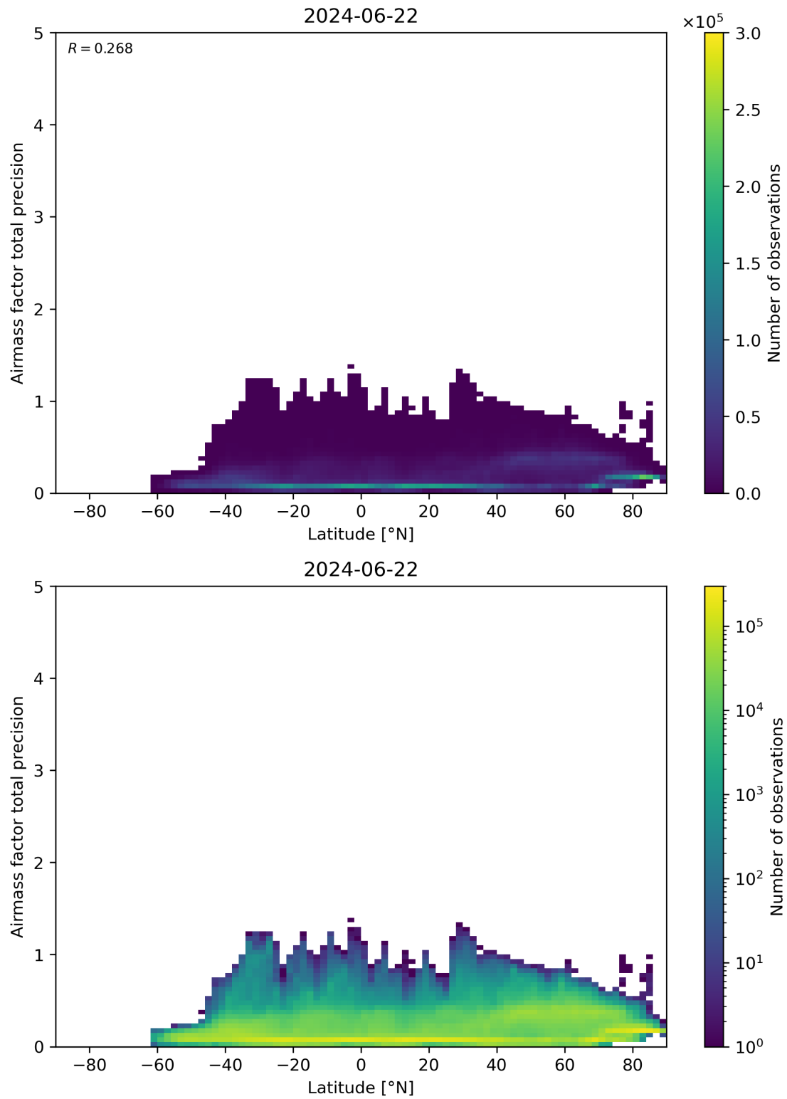
Figure 162: Scatter density plot of “Latitude” against “Airmass factor total precision” for 2024-06-21 to 2024-06-23.
