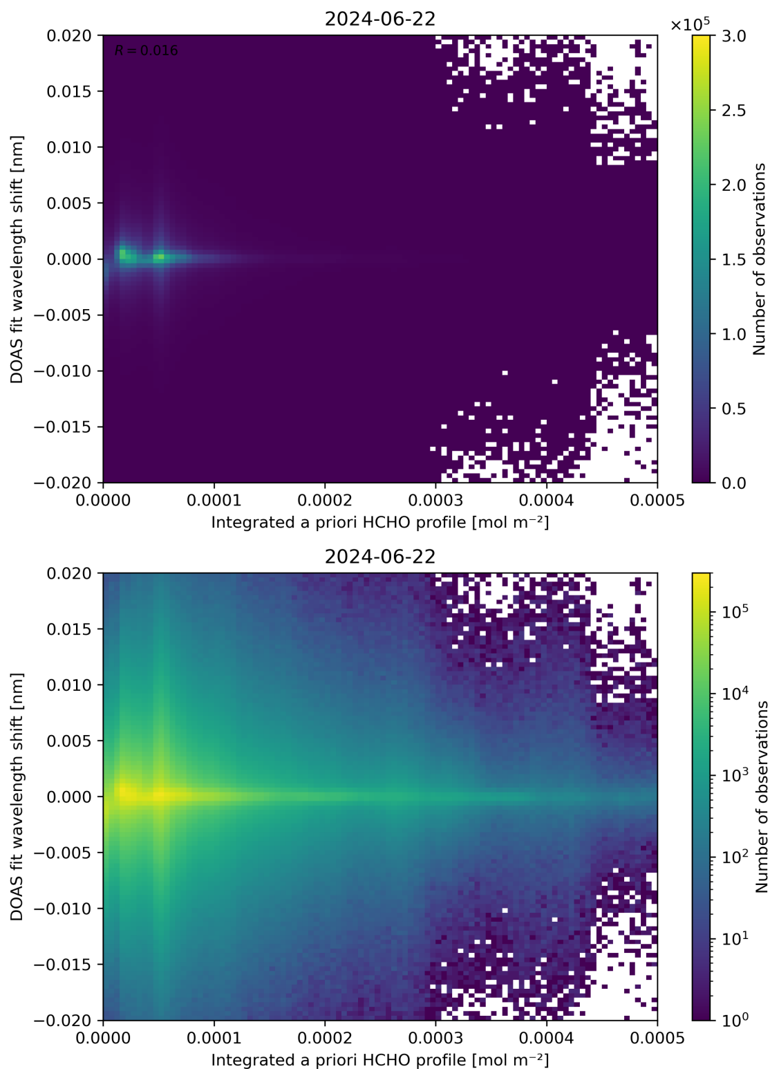
Figure 149: Scatter density plot of “Integrated a priori HCHO profile” against “DOAS fit wavelength shift” for 2024-06-21 to 2024-06-23.
