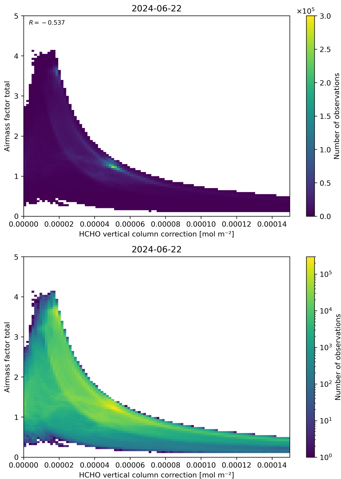
Figure 120: Scatter density plot of “HCHO vertical column correction” against “Airmass factor total” for 2024-06-21 to 2024-06-23.
