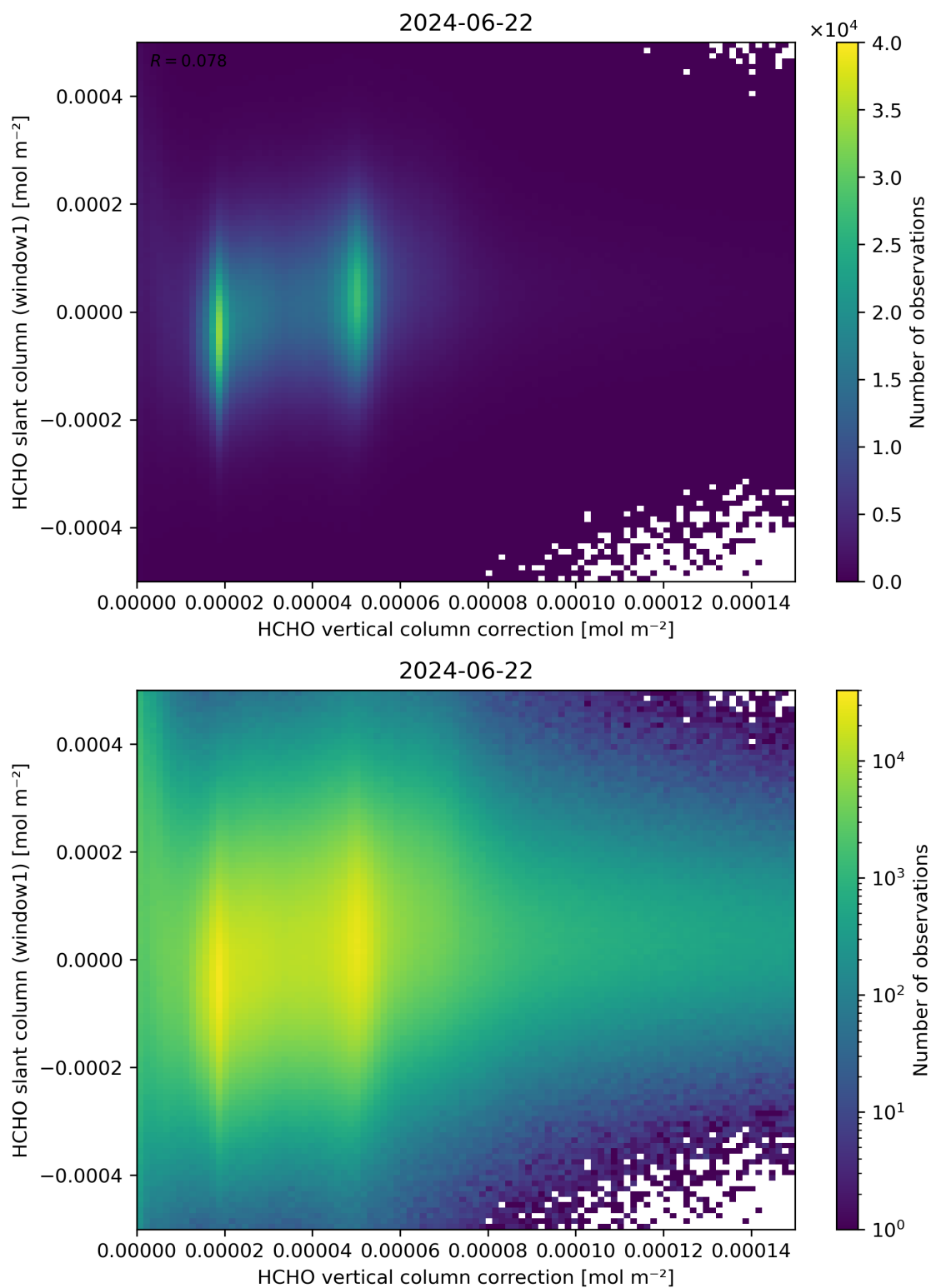
Figure 118: Scatter density plot of “HCHO vertical column correction” against “HCHO slant column (window1)” for 2024-06-21 to 2024-06-23.
