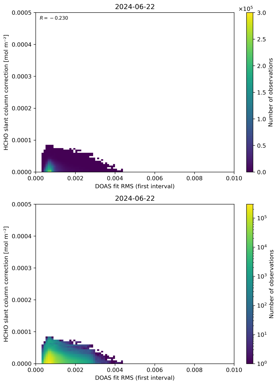
Figure 63: Scatter density plot of “DOAS fit RMS (first interval)” against “HCHO slant column correction” for 2024-06-21 to 2024-06-23.
