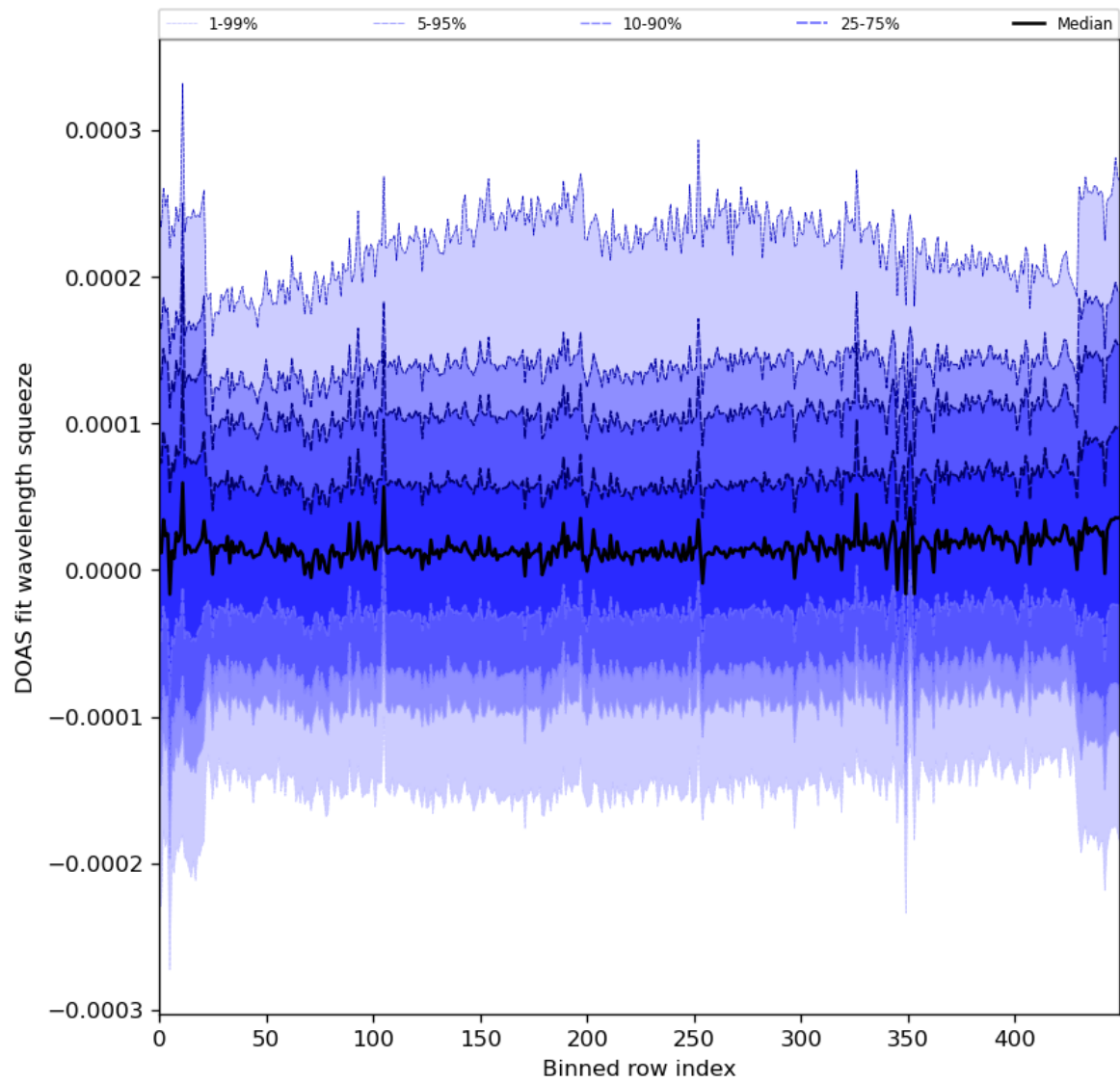
Figure 59: Along track statistics of “DOAS fit wavelength squeeze” for 2024-06-21 to 2024-06-23
