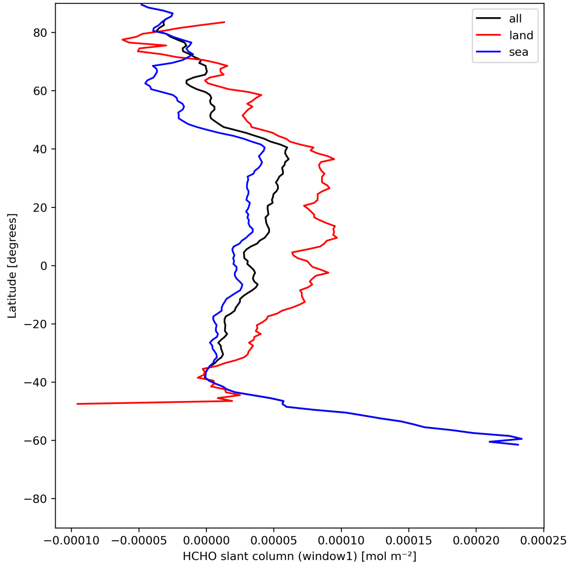
Figure 24: Zonal average of “HCHO slant column (window1)” for 2024-06-21 to 2024-06-23.
