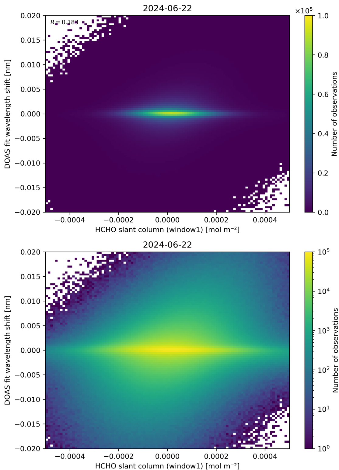
Figure 79: Scatter density plot of “HCHO slant column (window1)” against “DOAS fit wavelength shift” for 2024-06-21 to 2024-06-23.
