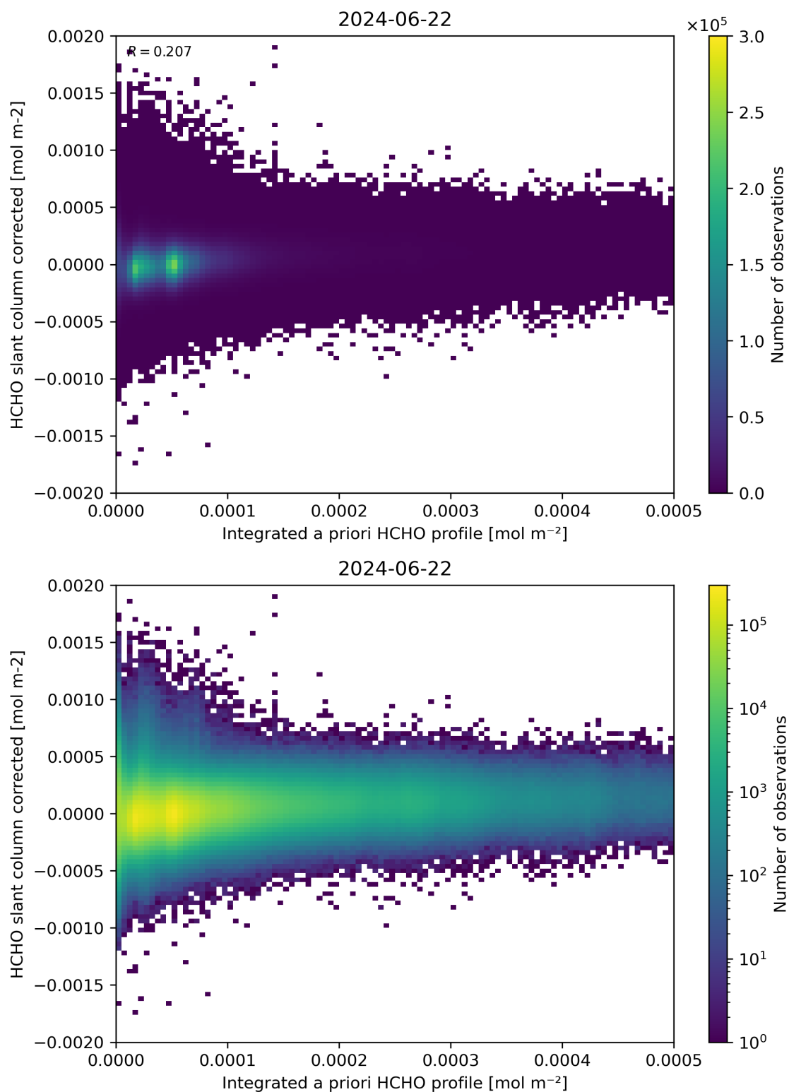
Figure 151: Scatter density plot of “Integrated a priori HCHO profile” against “HCHO slant column corrected” for 2024-06-21 to 2024-06-23.
