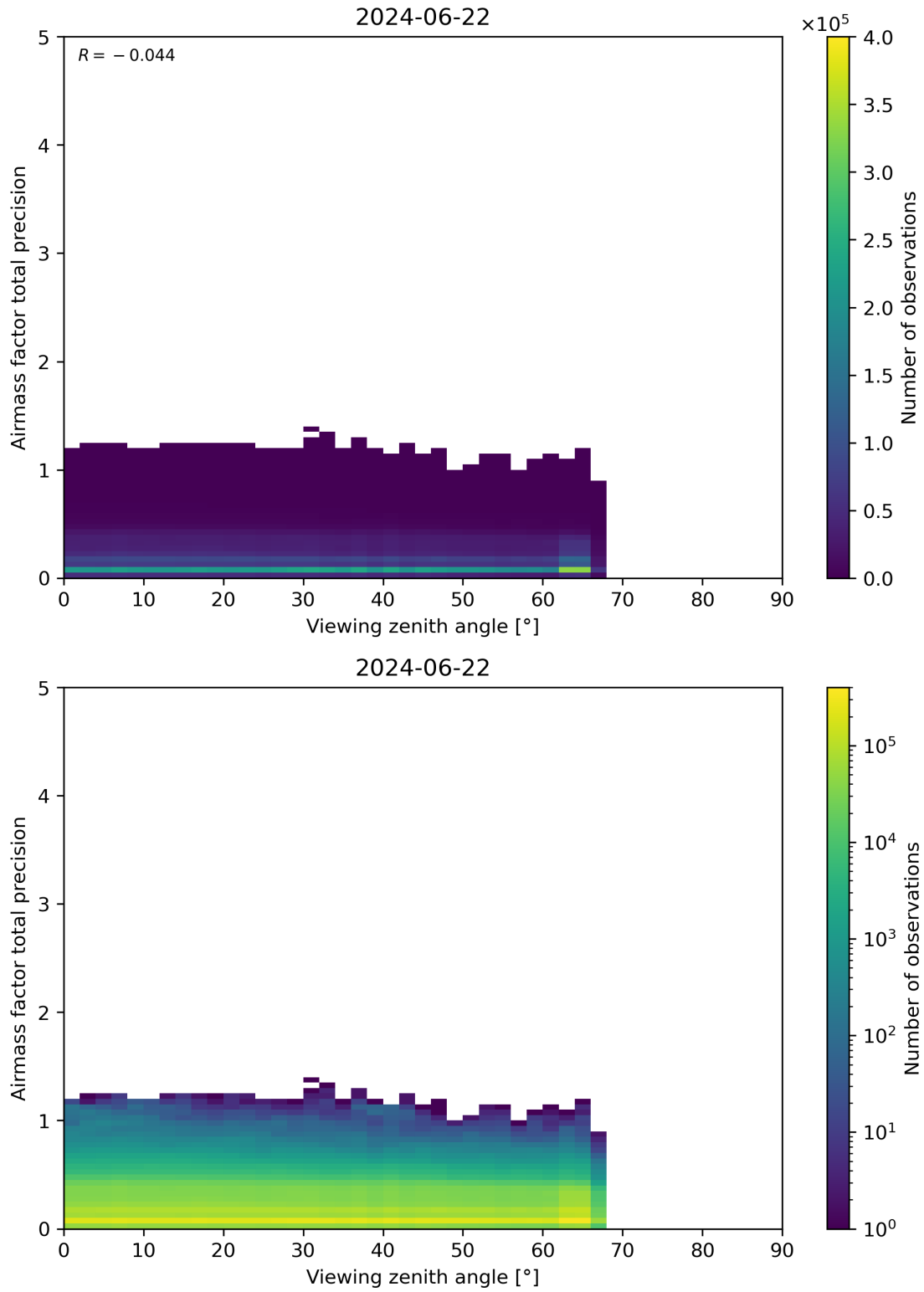
Figure 191: Scatter density plot of “Viewing zenith angle” against “Airmass factor total precision” for 2024-06-21 to 2024-06-23.
