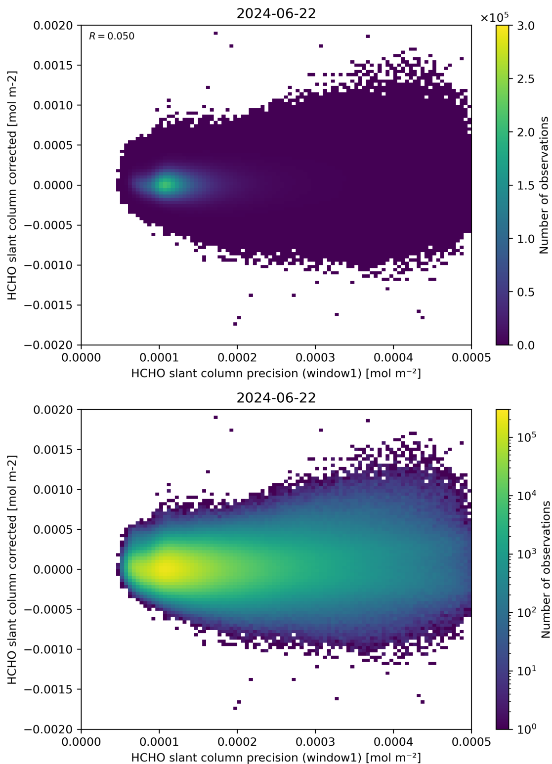
Figure 92: Scatter density plot of “HCHO slant column precision (window1)” against “HCHO slant column corrected” for 2024-06-21 to 2024-06-23.
