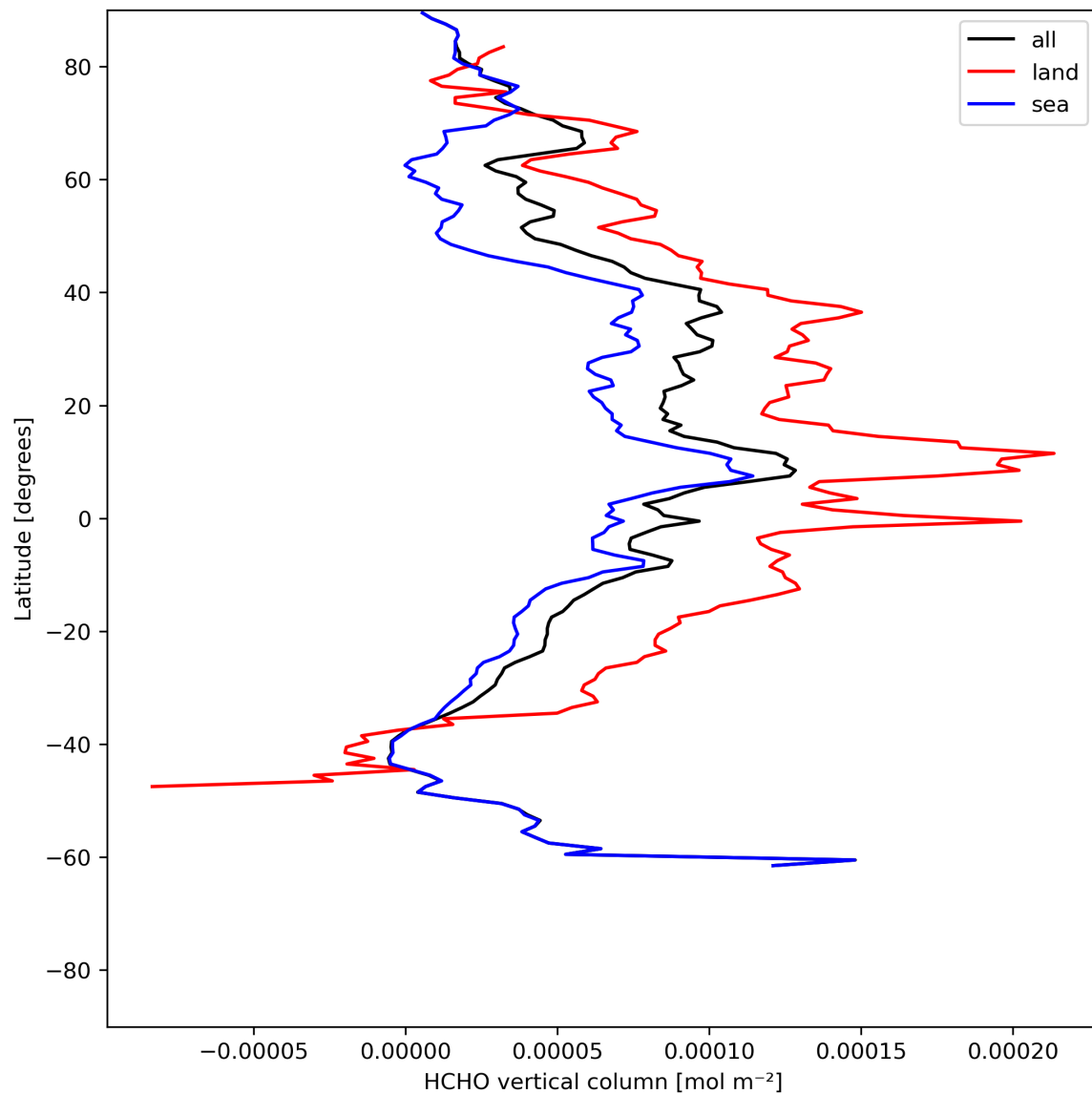
Figure 21: Zonal average of “HCHO vertical column” for 2024-06-21 to 2024-06-23.
