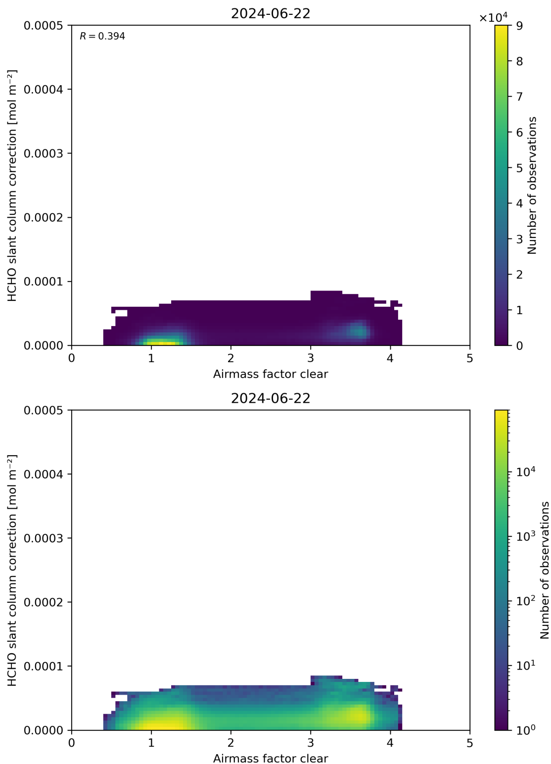
Figure 75: Scatter density plot of “Airmass factor clear” against “HCHO slant column correction” for 2024-06-21 to 2024-06-23.
