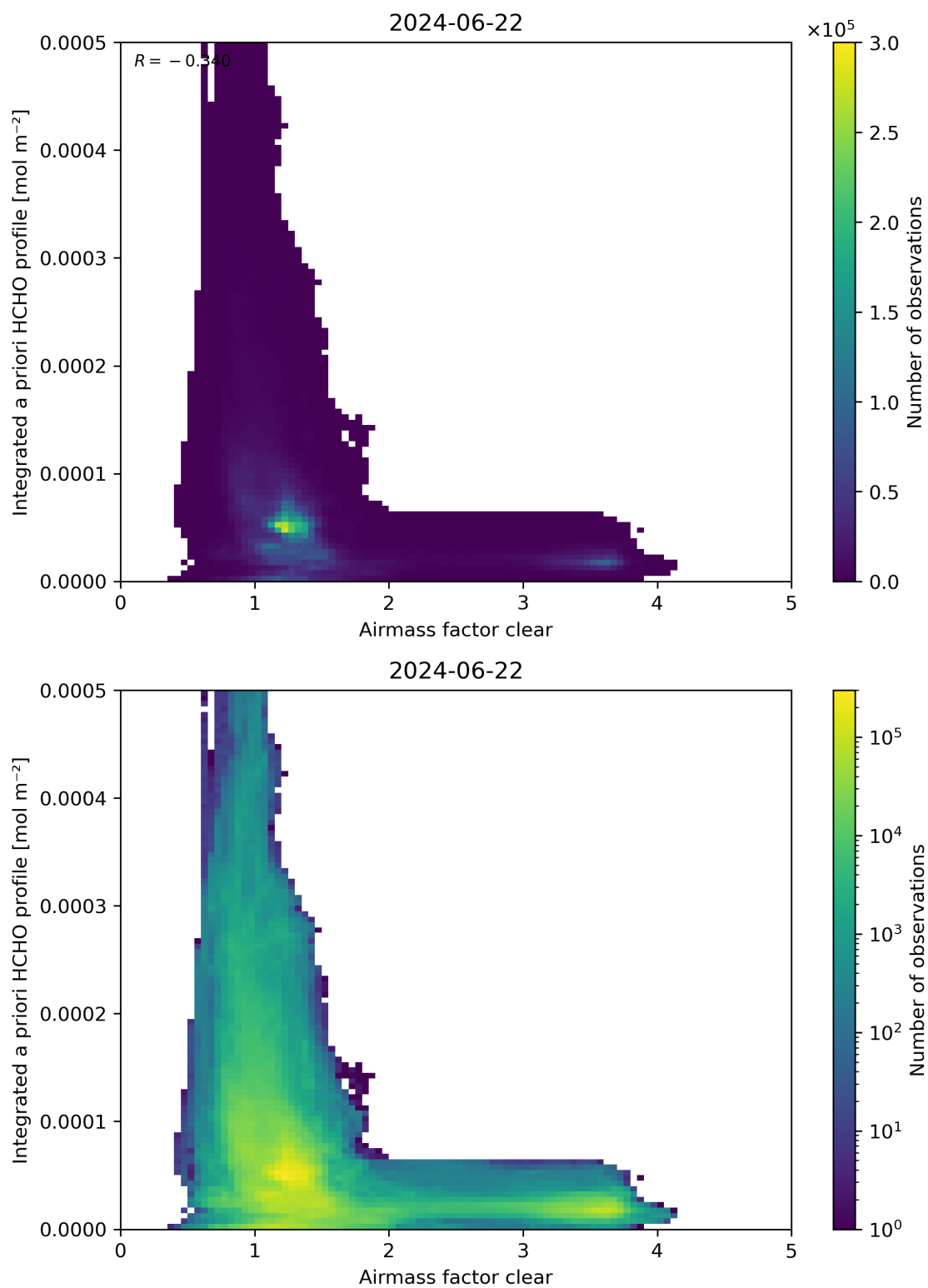
Figure 76: Scatter density plot of “Airmass factor clear” against “Integrated a priori HCHO profile” for 2024-06-21 to 2024-06-23.
