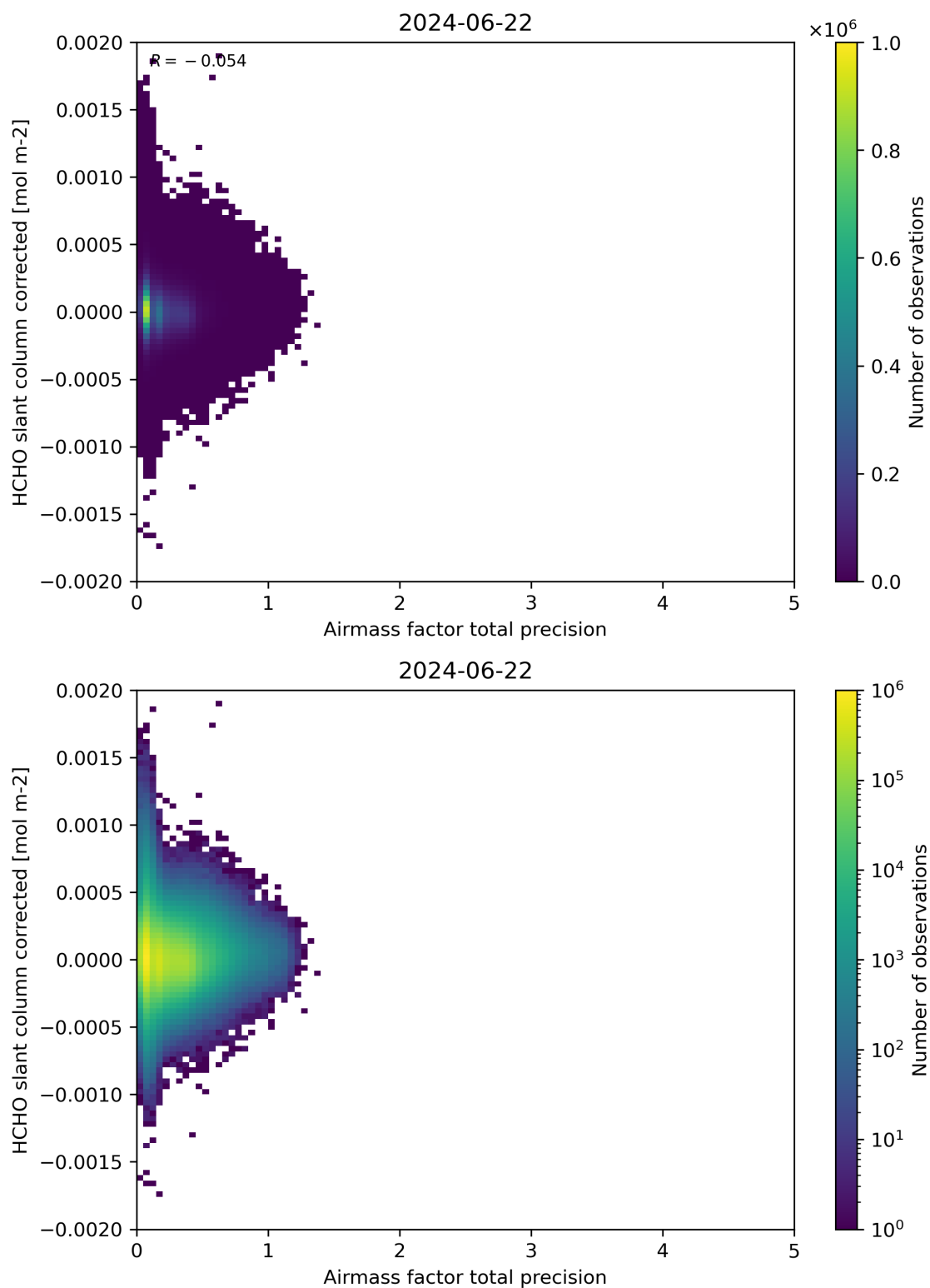
Figure 109: Scatter density plot of “Airmass factor total precision” against “HCHO slant column corrected” for 2024-06-21 to 2024-06-23.
