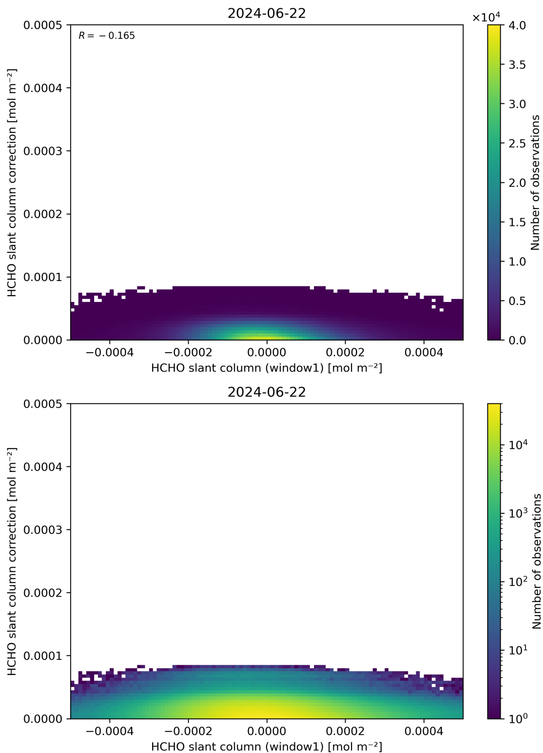
Figure 83: Scatter density plot of “HCHO slant column (window1)” against “HCHO slant column correction” for 2024-06-21 to 2024-06-23.
