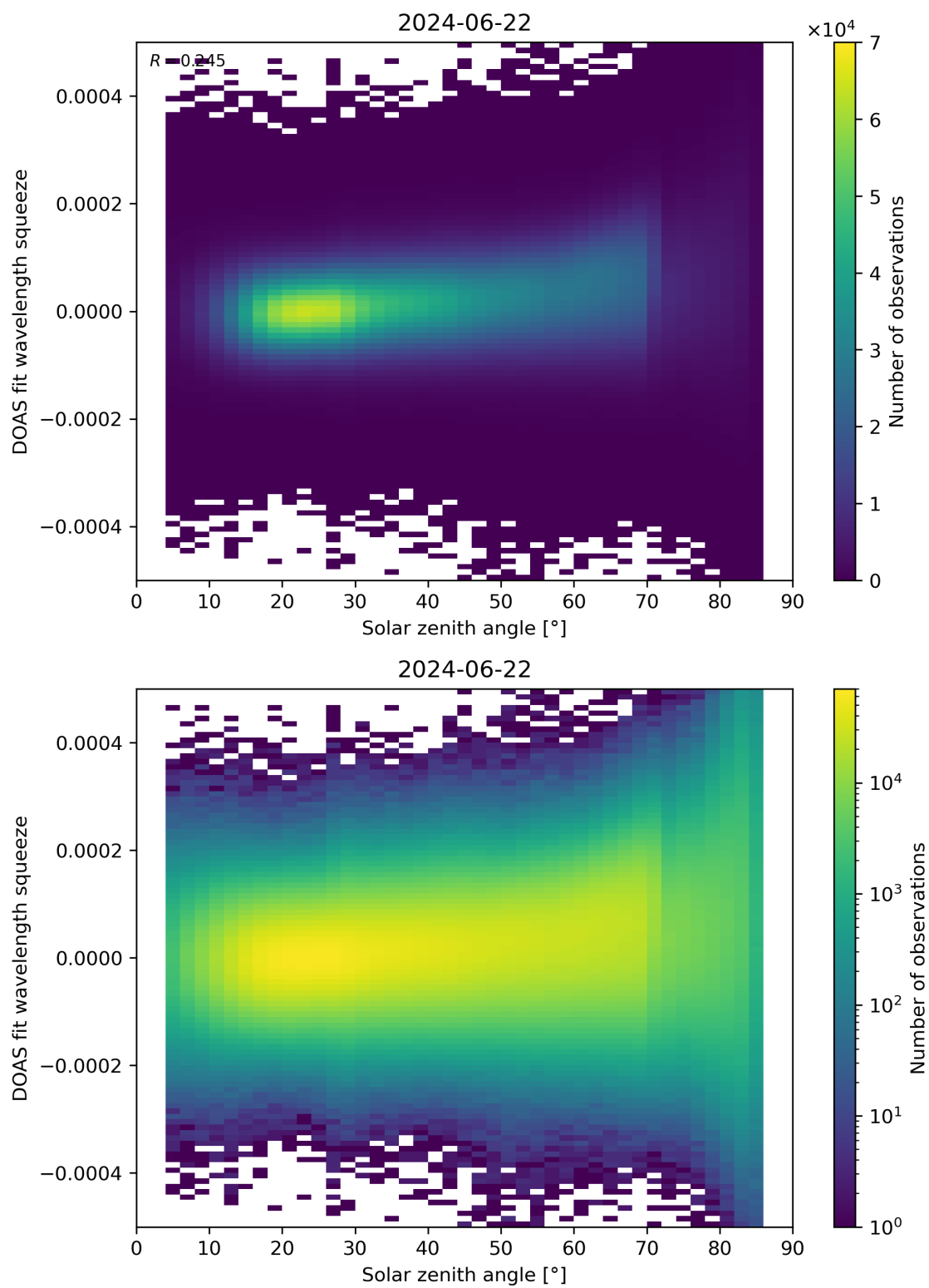
Figure 169: Scatter density plot of “Solar zenith angle” against “DOAS fit wavelength squeeze” for 2024-06-21 to 2024-06-23.
