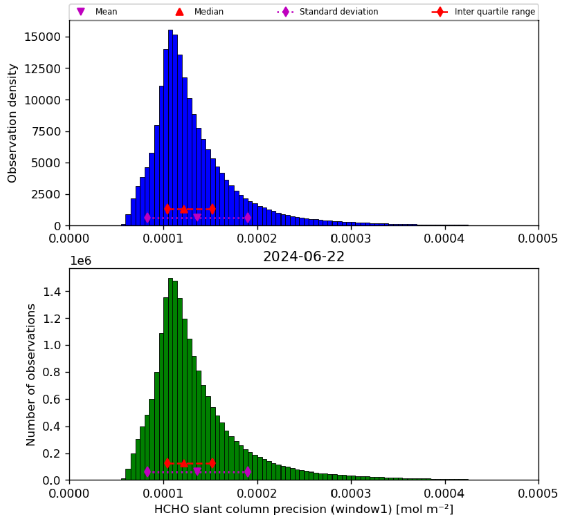
Figure 39: Histogram of “HCHO slant column precision (window1)” for 2024-06-21 to 2024-06-23
