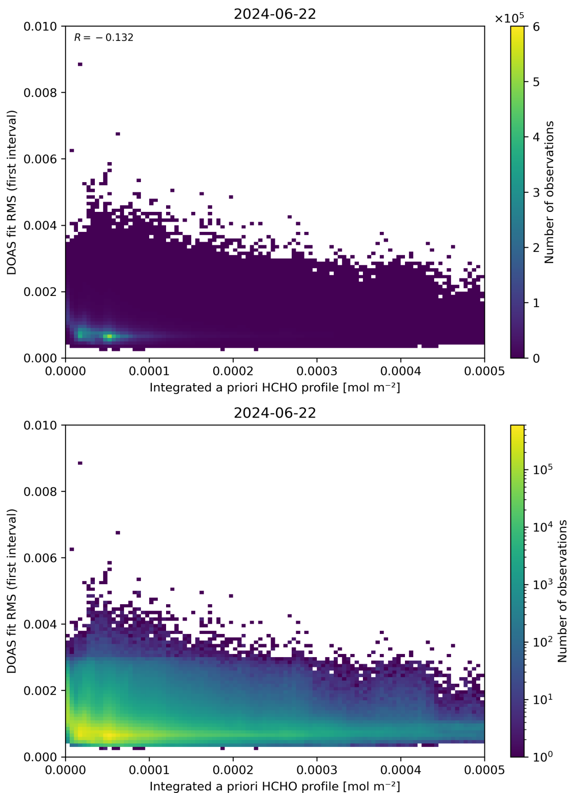
Figure 148: Scatter density plot of “Integrated a priori HCHO profile” against “DOAS fit RMS (first interval)” for 2024-06-21 to 2024-06-23.
