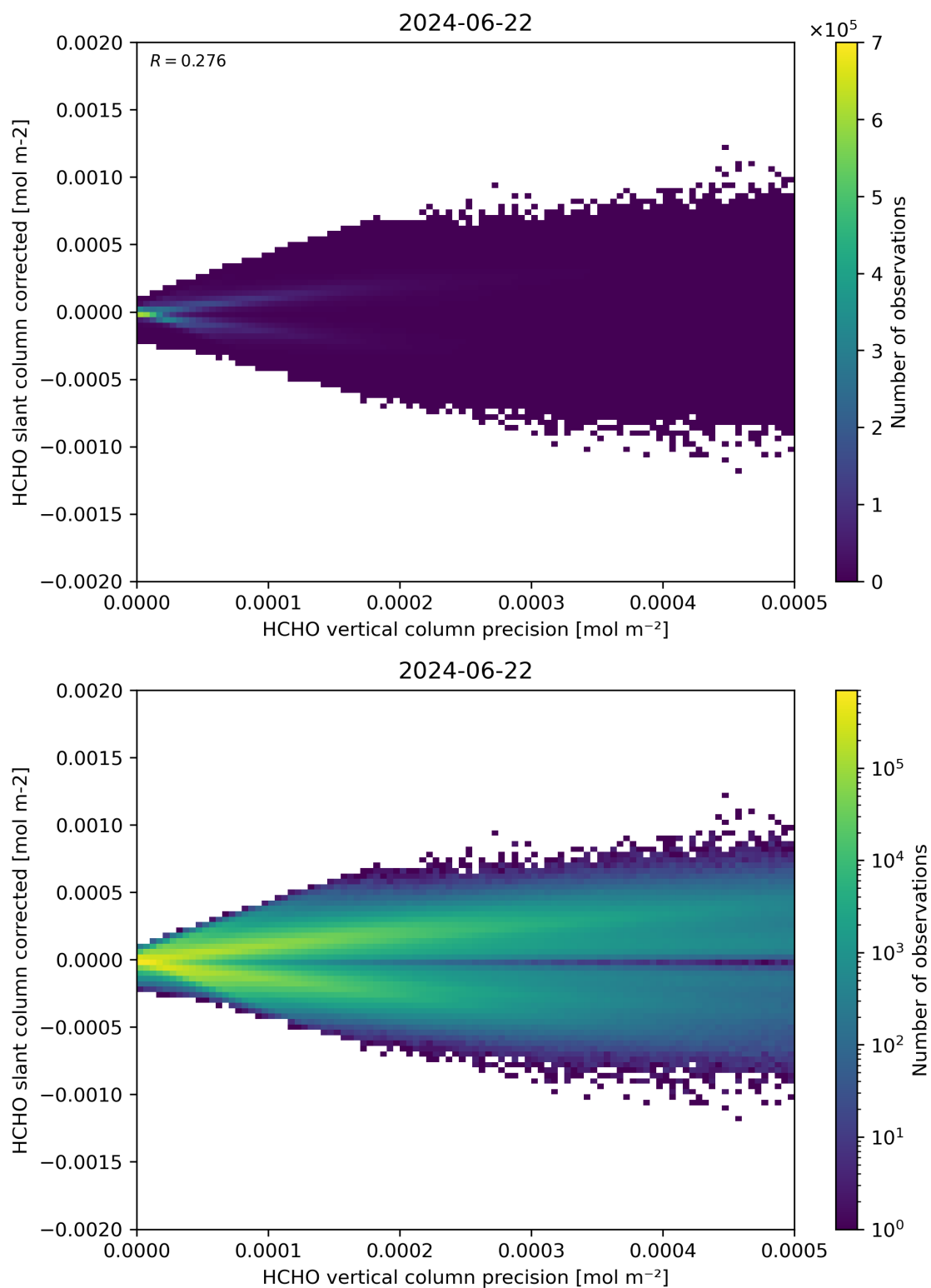
Figure 140: Scatter density plot of “HCHO vertical column precision” against “HCHO slant column corrected” for 2024-06-21 to 2024-06-23.
