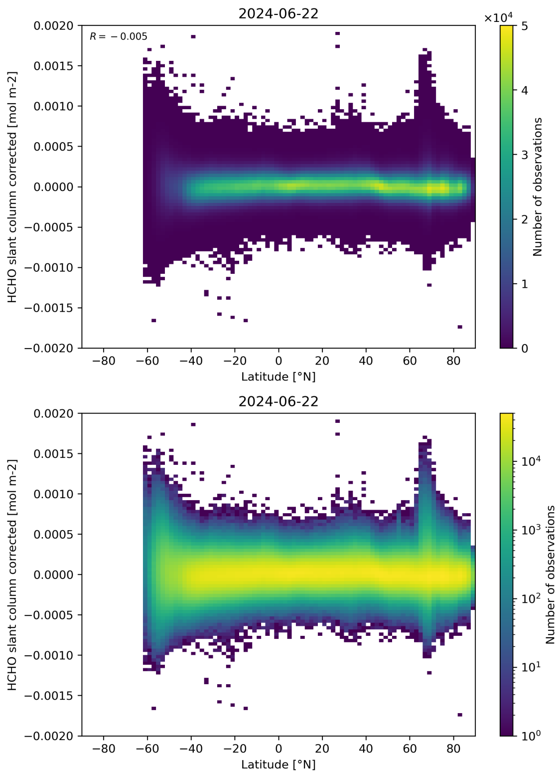
Figure 157: Scatter density plot of “Latitude” against “HCHO slant column corrected” for 2024-06-21 to 2024-06-23.
