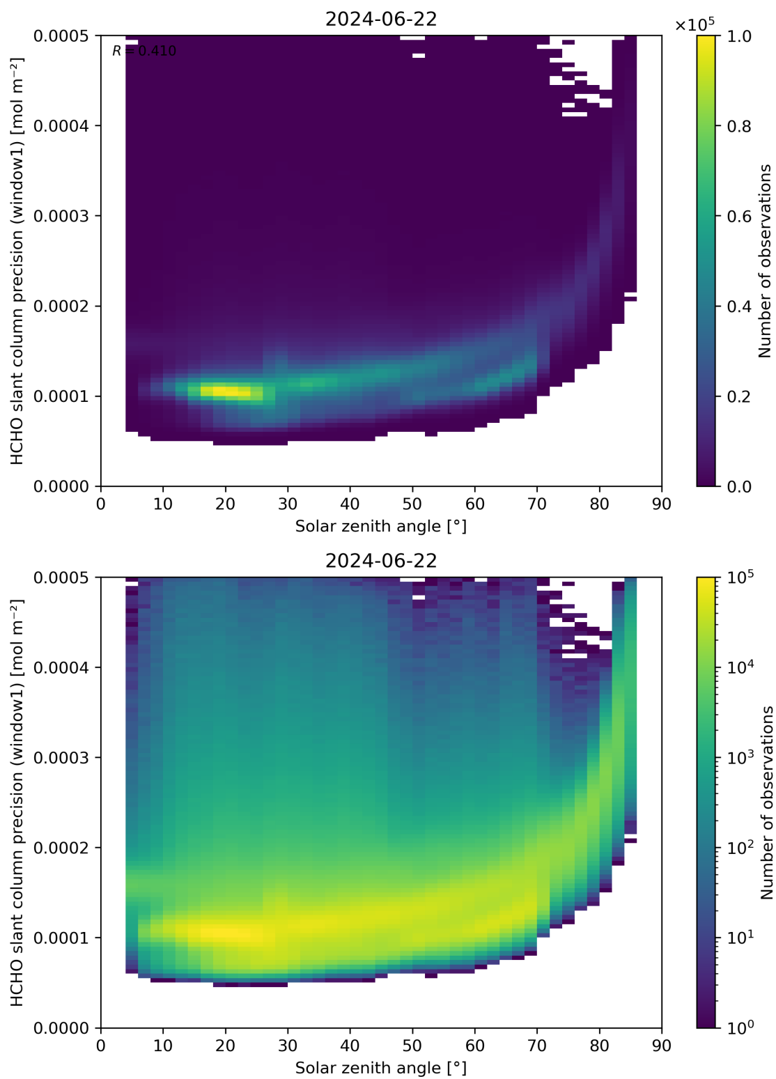
Figure 174: Scatter density plot of “Solar zenith angle” against “HCHO slant column precision (window1)” for 2024-06-21 to 2024-06-23.
