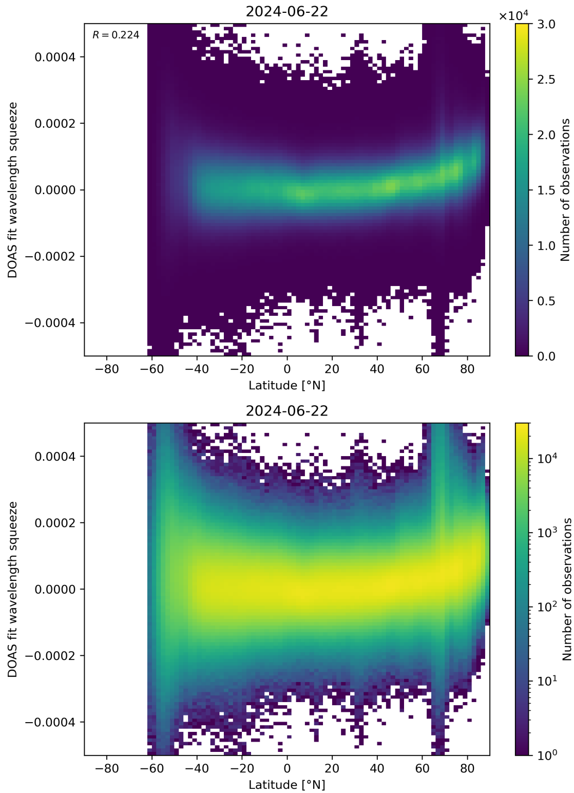
Figure 155: Scatter density plot of “Latitude” against “DOAS fit wavelength squeeze” for 2024-06-21 to 2024-06-23.
