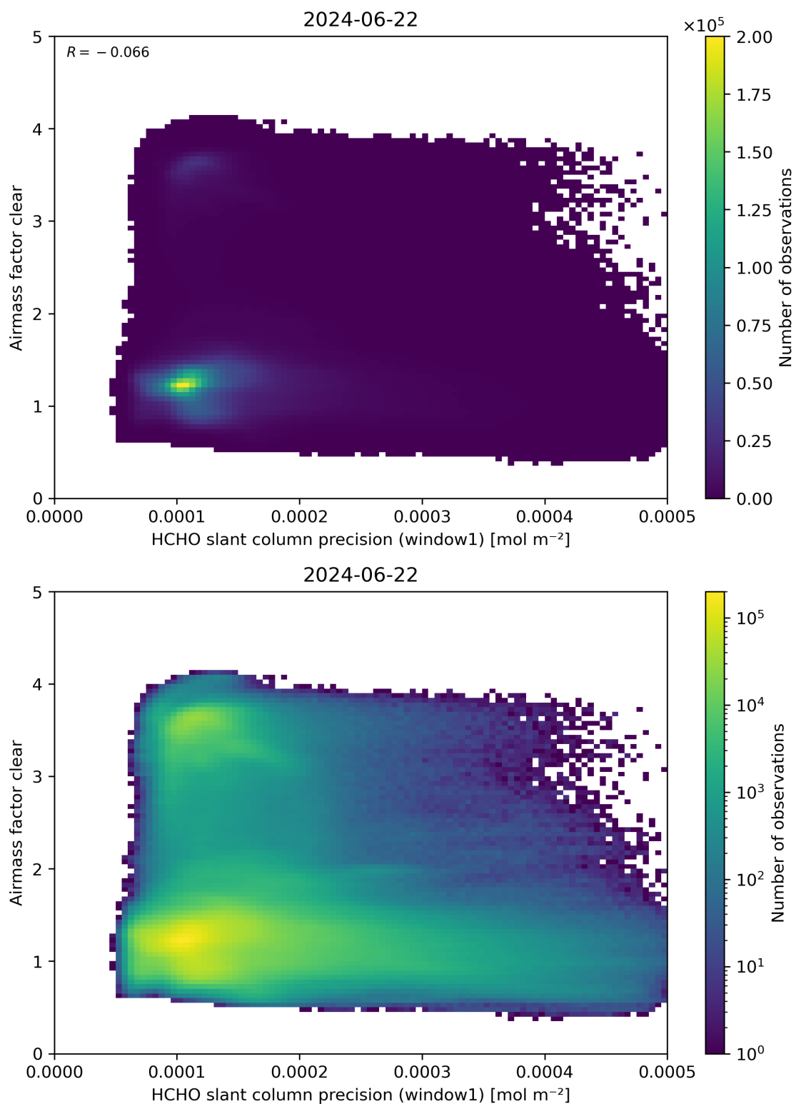
Figure 91: Scatter density plot of “HCHO slant column precision (window1)” against “Airmass factor clear” for 2024-06-21 to 2024-06-23.
