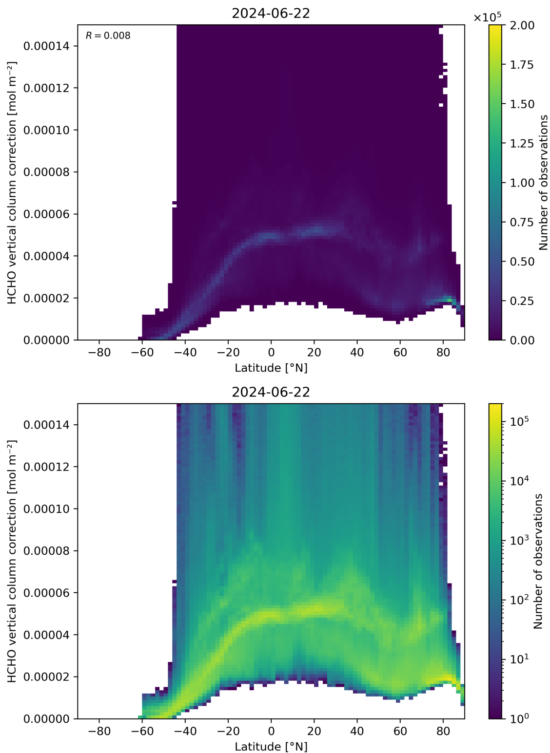
Figure 164: Scatter density plot of “Latitude” against “HCHO vertical column correction” for 2024-06-21 to 2024-06-23.
