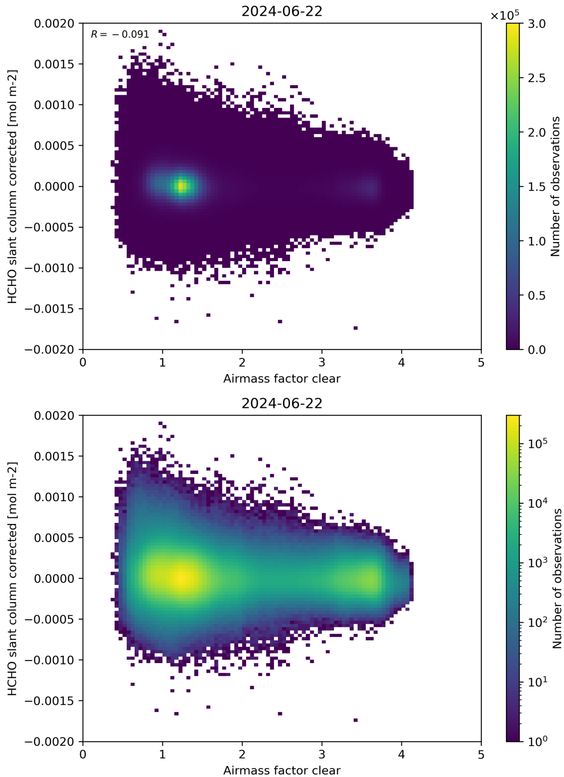
Figure 74: Scatter density plot of “Airmass factor clear” against “HCHO slant column corrected” for 2024-06-21 to 2024-06-23.
