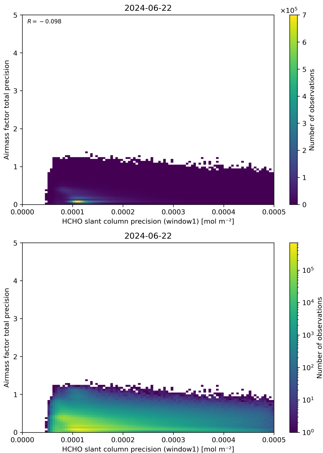
Figure 95: Scatter density plot of “HCHO slant column precision (window1)” against “Airmass factor total precision” for 2024-06-21 to 2024-06-23.
