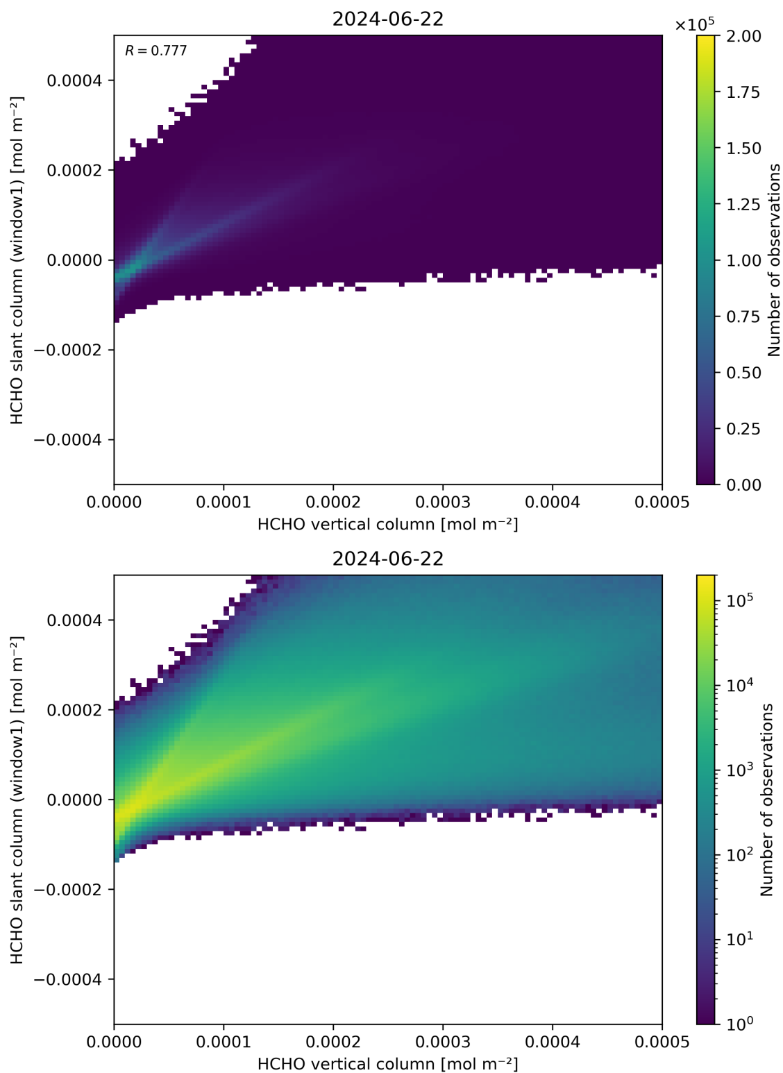
Figure 129: Scatter density plot of “HCHO vertical column” against “HCHO slant column (window1)” for 2024-06-21 to 2024-06-23.
