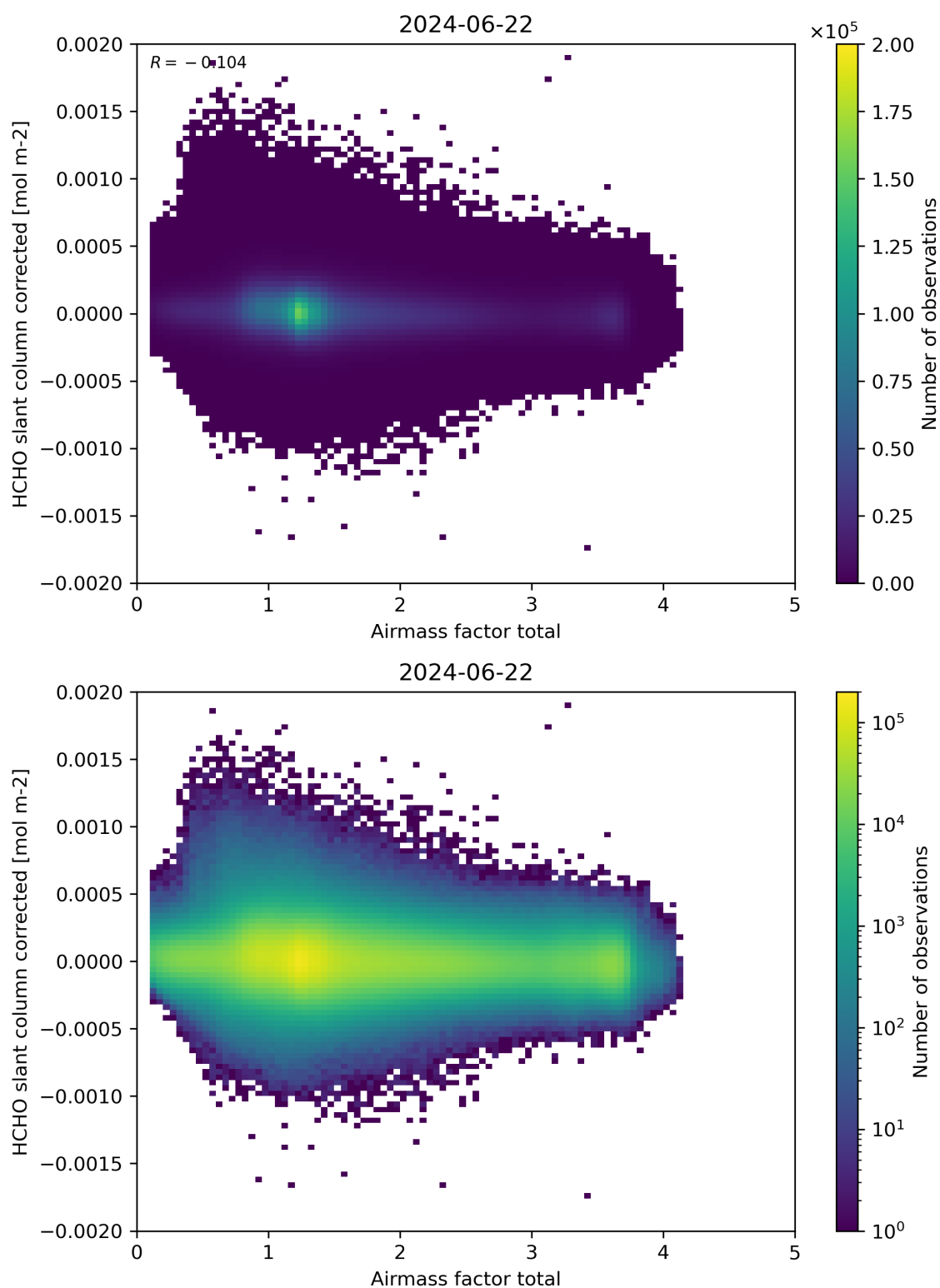
Figure 101: Scatter density plot of “Airmass factor total” against “HCHO slant column corrected” for 2024-06-21 to 2024-06-23.
