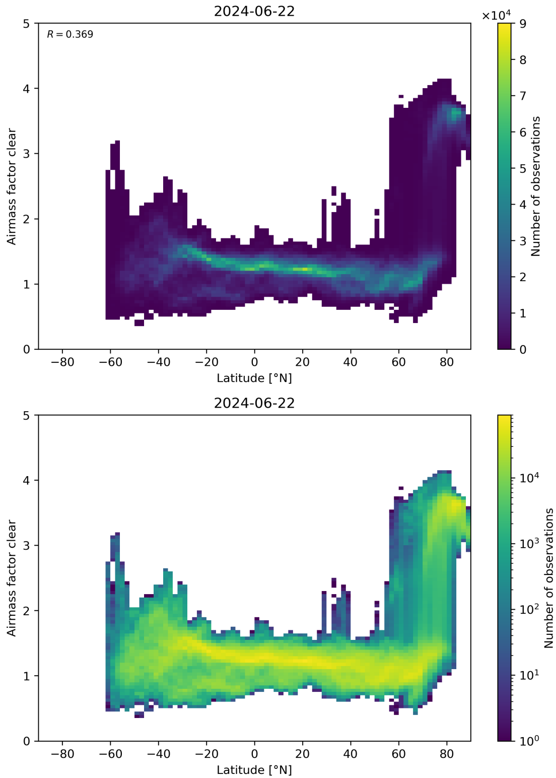
Figure 156: Scatter density plot of “Latitude” against “Airmass factor clear” for 2024-06-21 to 2024-06-23.
