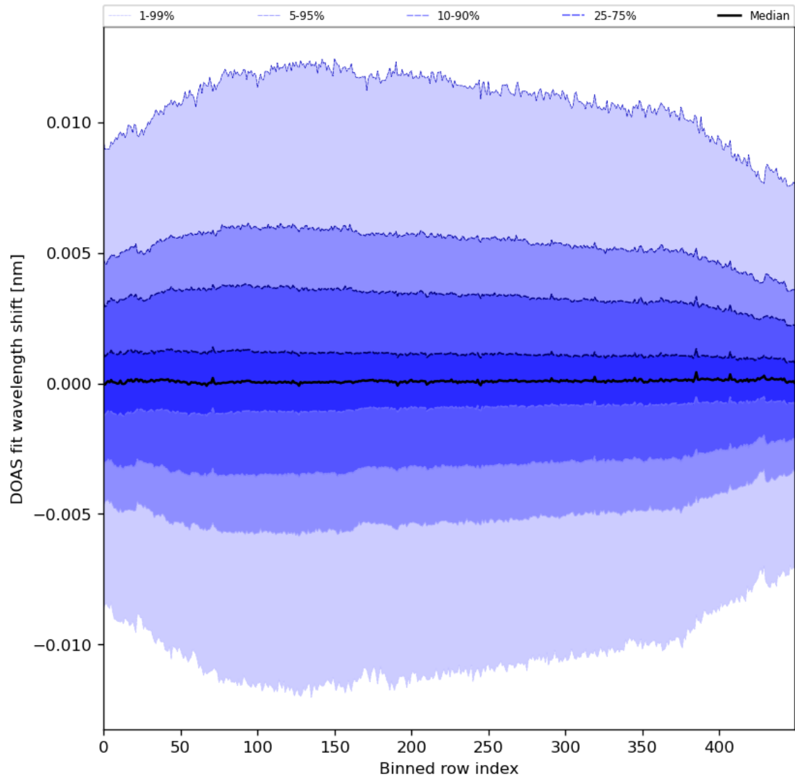
Figure 58: Along track statistics of “DOAS fit wavelength shift” for 2024-06-21 to 2024-06-23
