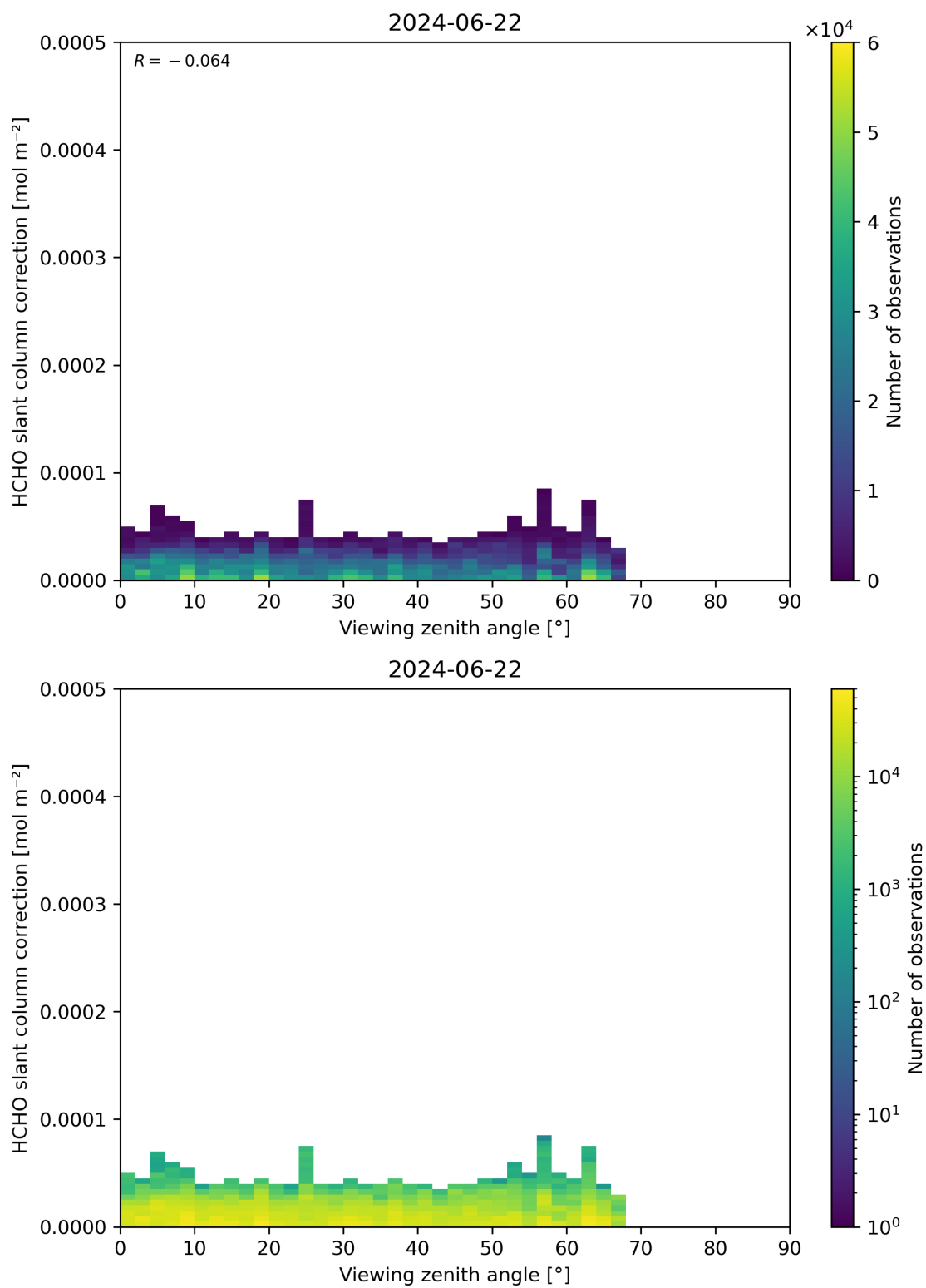
Figure 187: Scatter density plot of “Viewing zenith angle” against “HCHO slant column correction” for 2024-06-21 to 2024-06-23.
