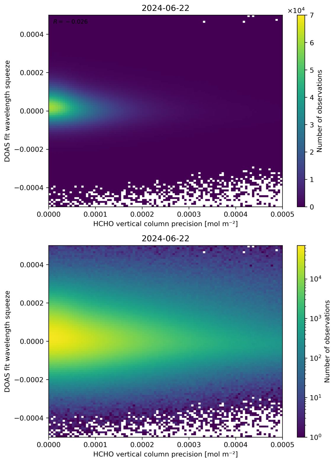
Figure 138: Scatter density plot of “HCHO vertical column precision” against “DOAS fit wavelength squeeze” for 2024-06-21 to 2024-06-23.
