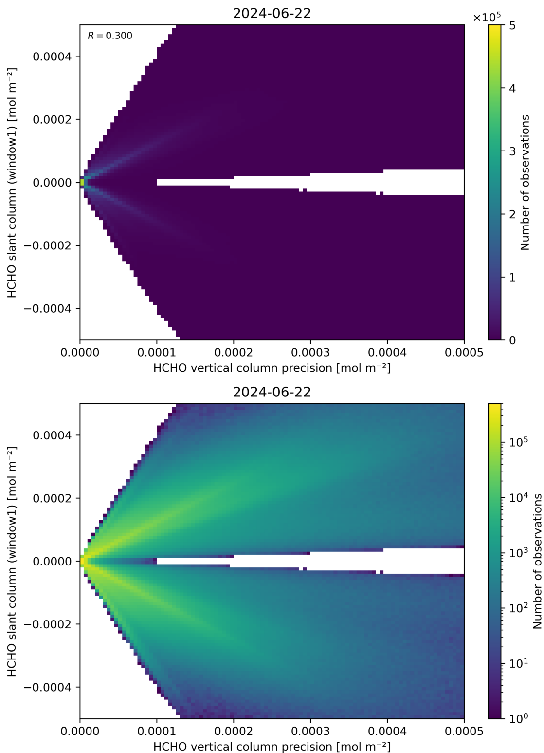
Figure 142: Scatter density plot of “HCHO vertical column precision” against “HCHO slant column (window1)” for 2024-06-21 to 2024-06-23.
