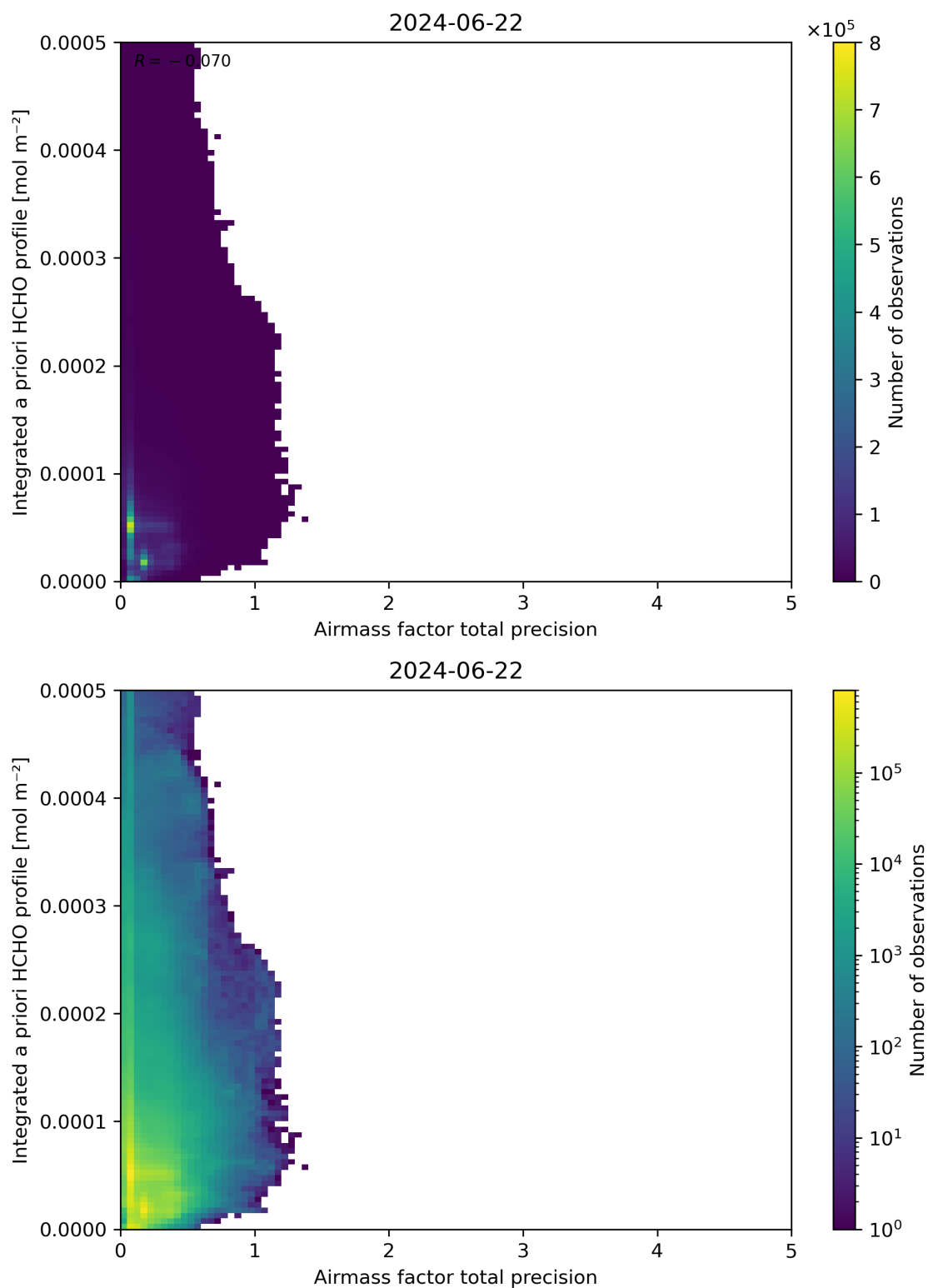
Figure 111: Scatter density plot of “Airmass factor total precision” against “Integrated a priori HCHO profile” for 2024-06-21 to 2024-06-23.
