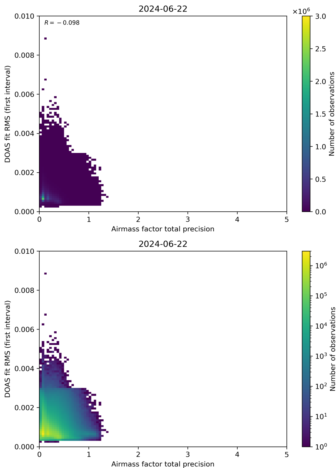
Figure 105: Scatter density plot of “Airmass factor total precision” against “DOAS fit RMS (first interval)” for 2024-06-21 to 2024-06-23.
