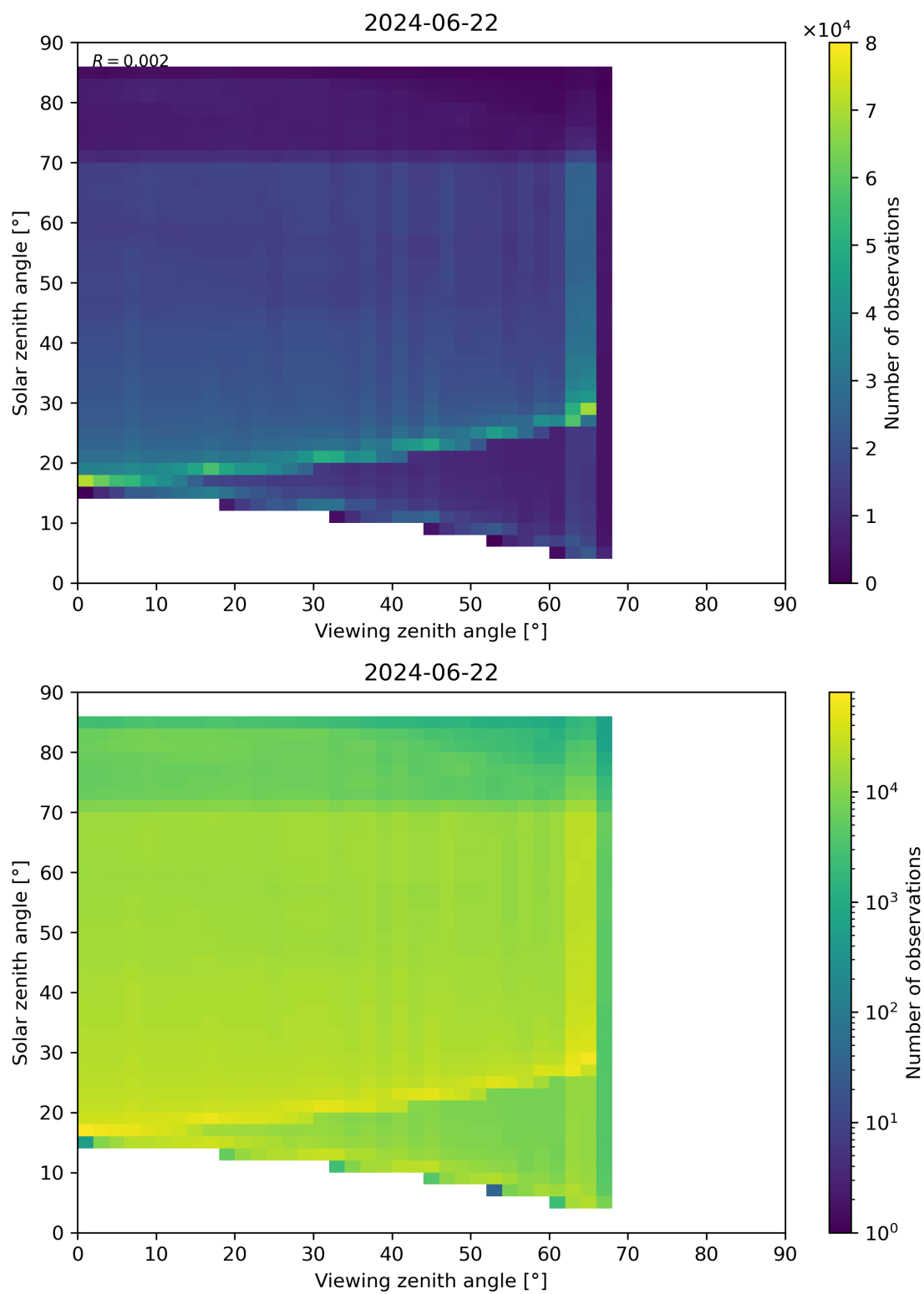
Figure 197: Scatter density plot of “Viewing zenith angle” against “Solar zenith angle” for 2024-06-21 to 2024-06-23.
