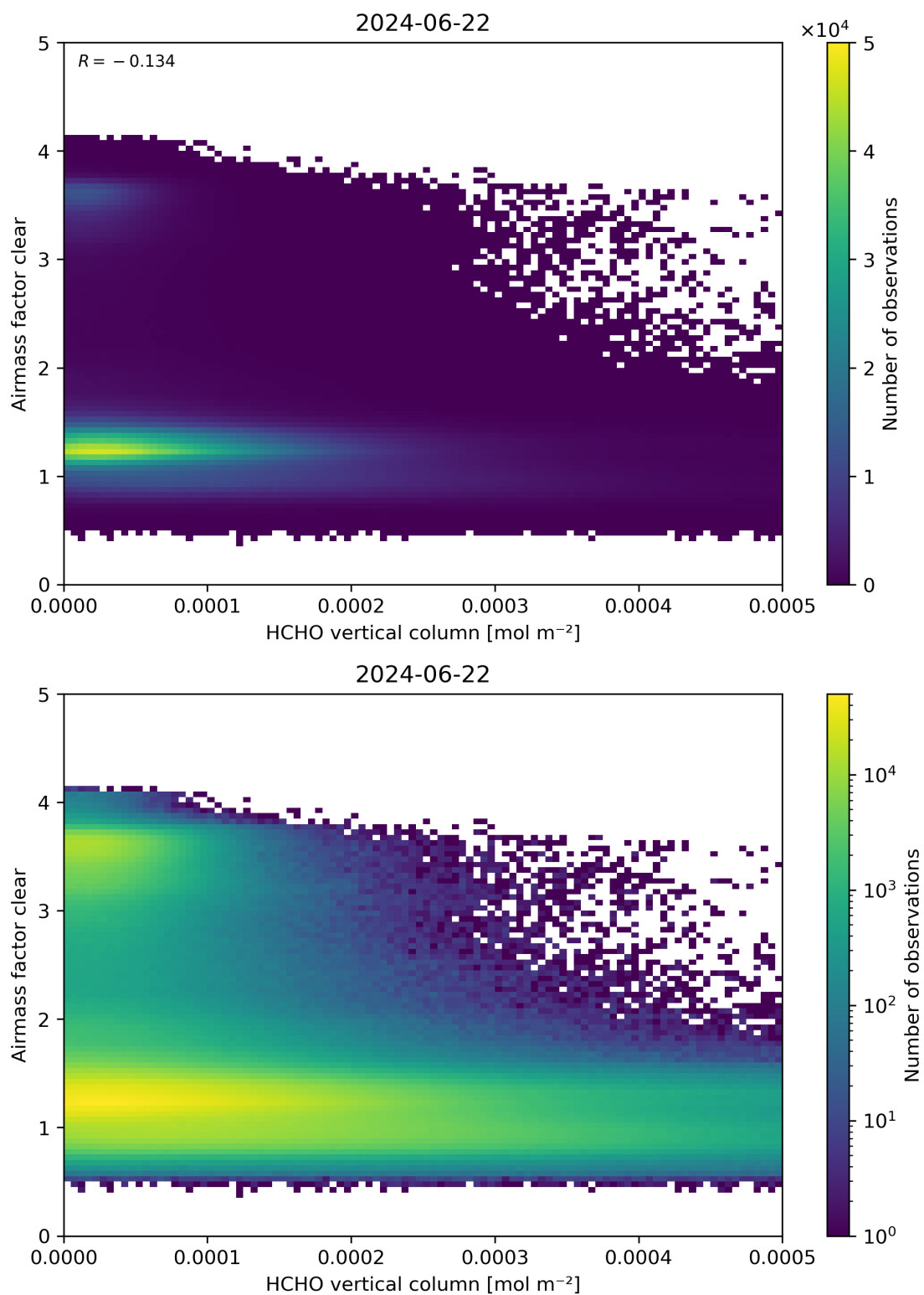
Figure 126: Scatter density plot of “HCHO vertical column” against “Airmass factor clear” for 2024-06-21 to 2024-06-23.
