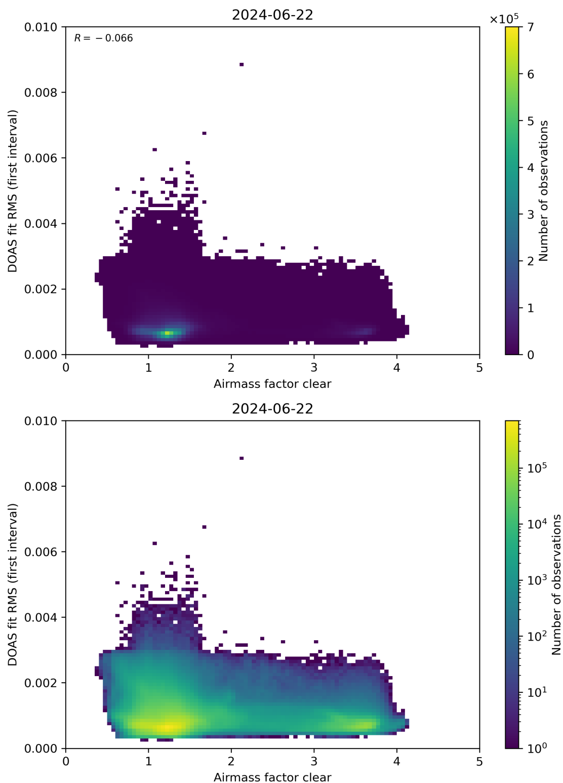
Figure 71: Scatter density plot of “Airmass factor clear” against “DOAS fit RMS (first interval)” for 2024-06-21 to 2024-06-23.
