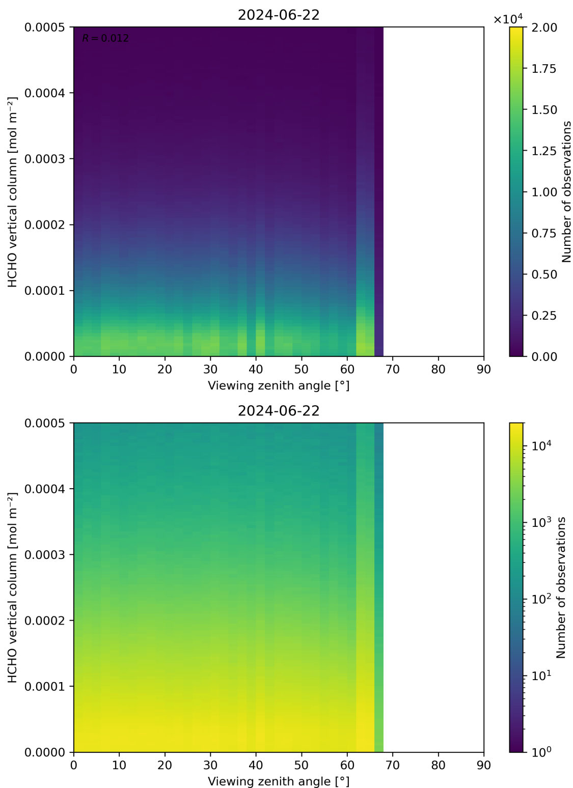
Figure 192: Scatter density plot of “Viewing zenith angle” against “HCHO vertical column” for 2024-06-21 to 2024-06-23.
