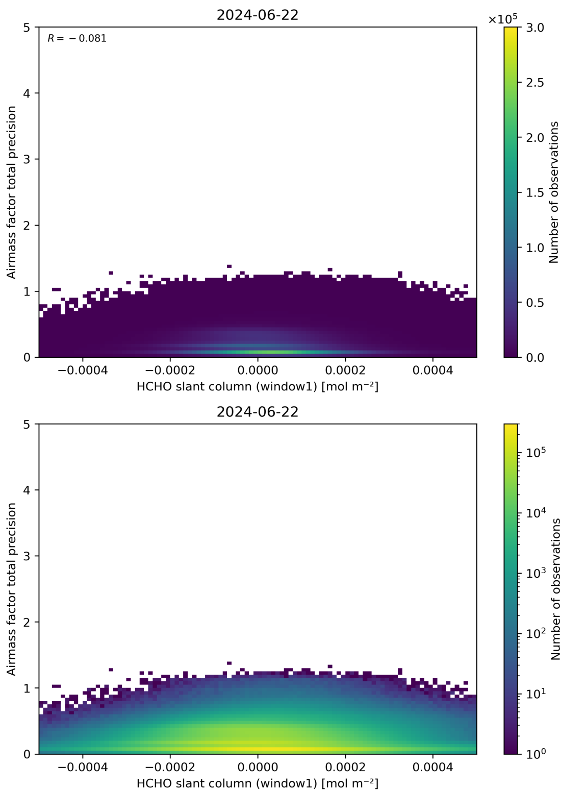
Figure 86: Scatter density plot of “HCHO slant column (window1)” against “Airmass factor total precision” for 2024-06-21 to 2024-06-23.
