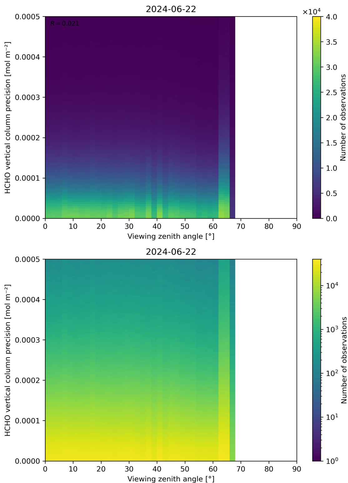
Figure 194: Scatter density plot of “Viewing zenith angle” against “HCHO vertical column precision” for 2024-06-21 to 2024-06-23.
