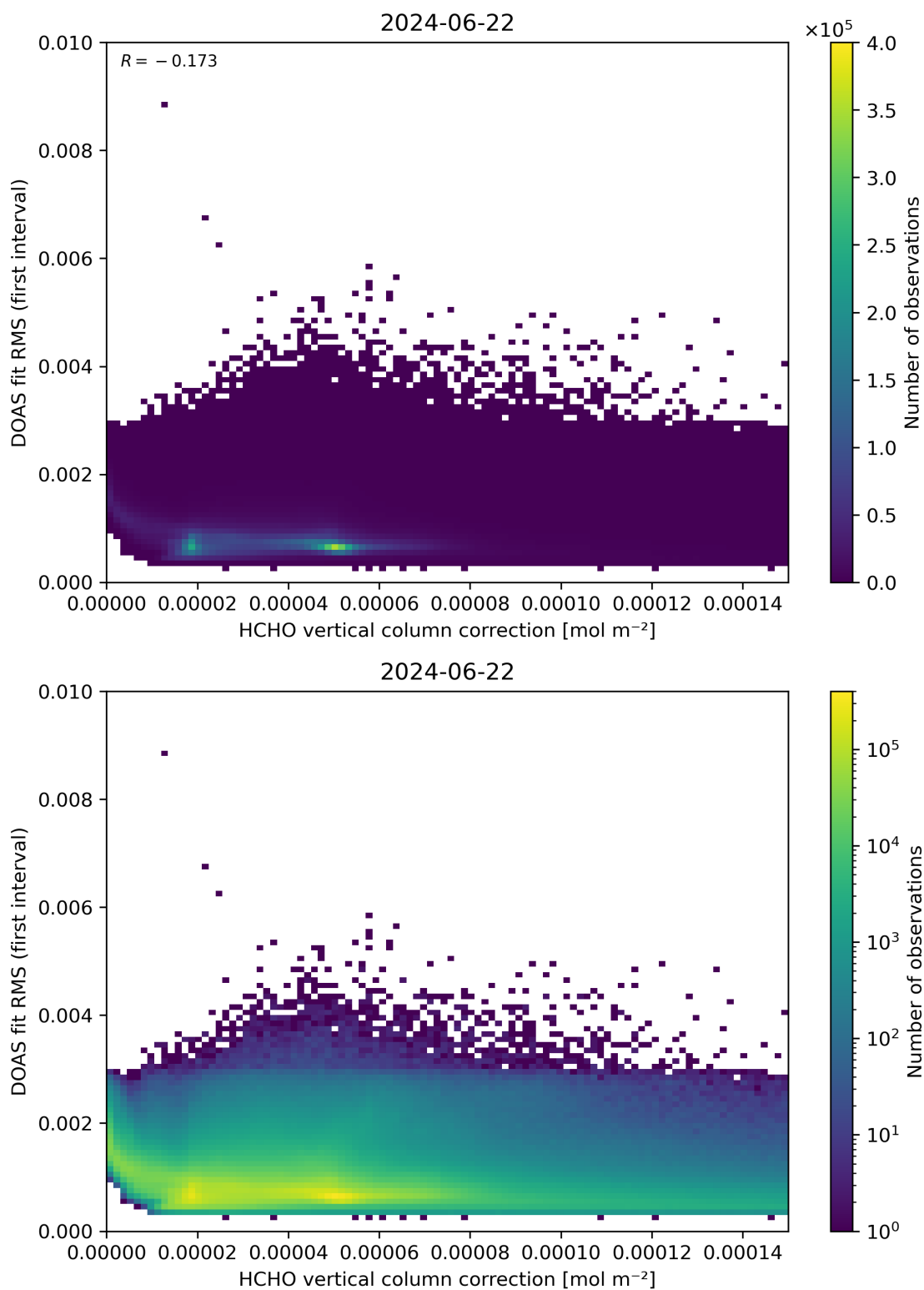
Figure 112: Scatter density plot of “HCHO vertical column correction” against “DOAS fit RMS (first interval)” for 2024-06-21 to 2024-06-23.
