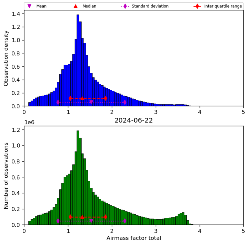
Figure 40: Histogram of “Airmass factor total” for 2024-06-21 to 2024-06-23
