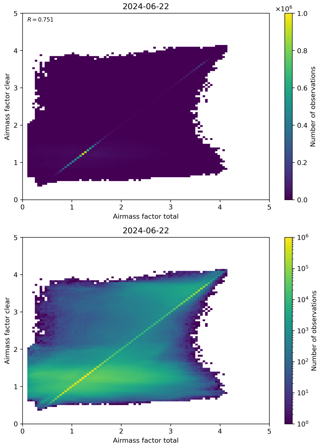
Figure 100: Scatter density plot of “Airmass factor total” against “Airmass factor clear” for 2024-06-21 to 2024-06-23.
