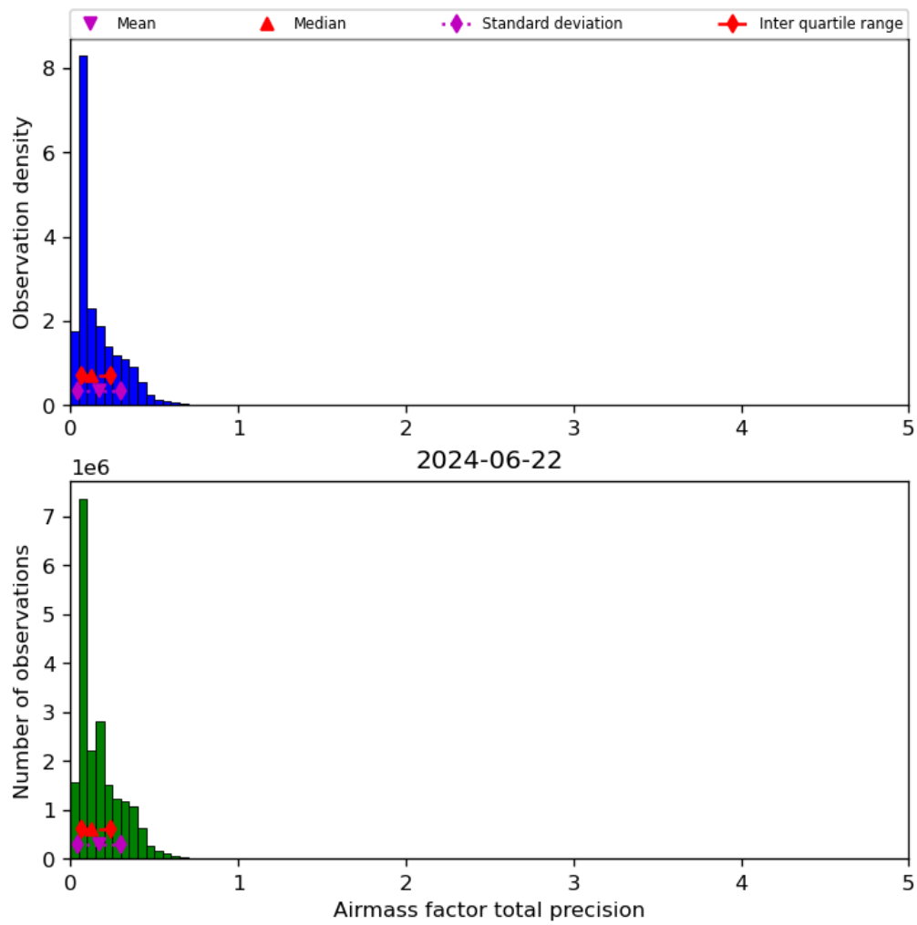
Figure 41: Histogram of "Airmass factor total precision" for 2024-06-21 to 2024-06-23
