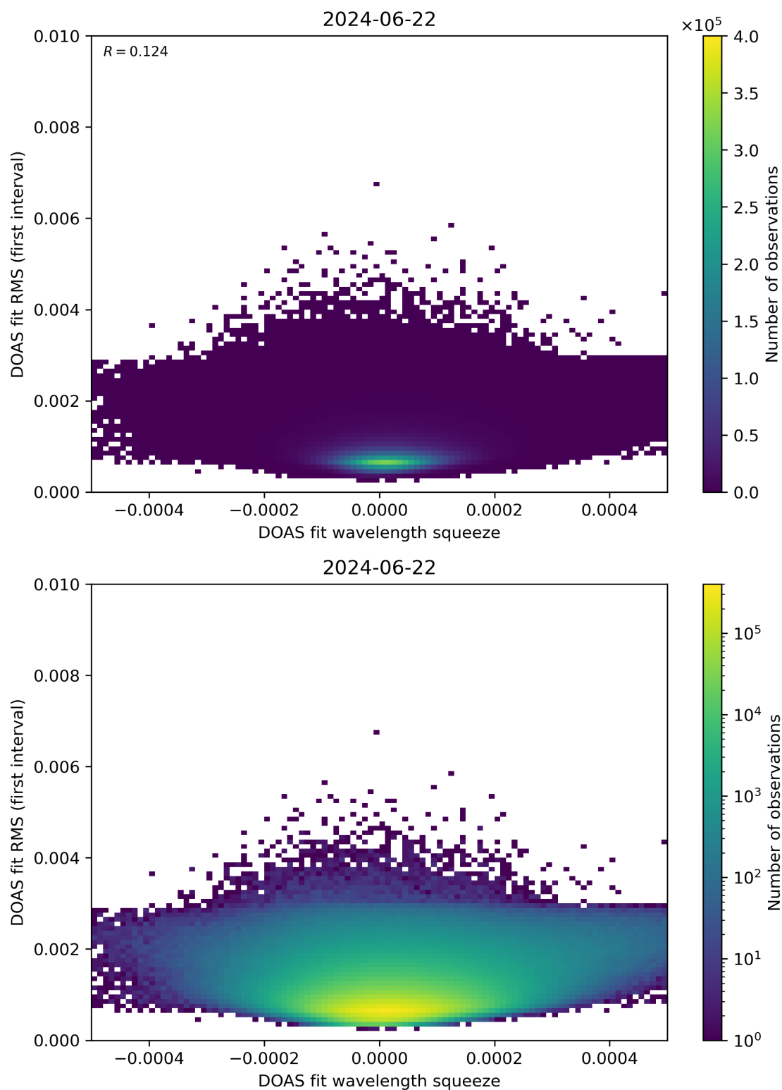
Figure 68: Scatter density plot of “DOAS fit wavelength squeeze” against “DOAS fit RMS (first interval)” for 2024-06-21 to 2024-06-23.
