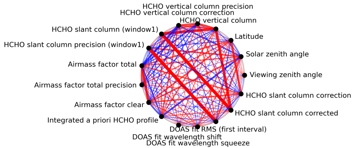
Figure 1: Map of correlation graph for 2024-06-21 to 2024-06-23.
