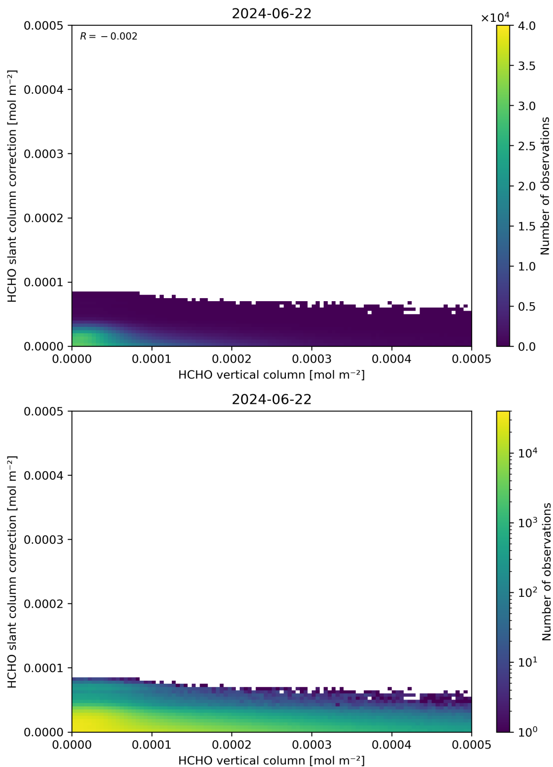
Figure 128: Scatter density plot of “HCHO vertical column” against “HCHO slant column correction” for 2024-06-21 to 2024-06-23.
