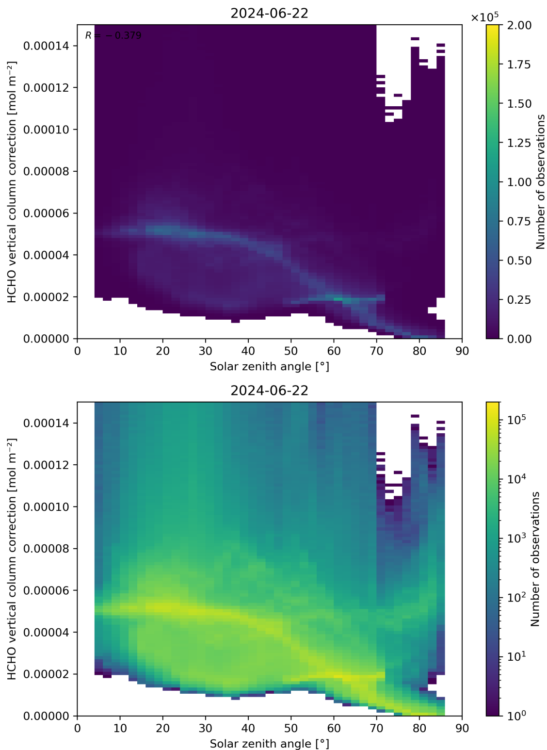
Figure 178: Scatter density plot of “Solar zenith angle” against “HCHO vertical column correction” for 2024-06-21 to 2024-06-23.
