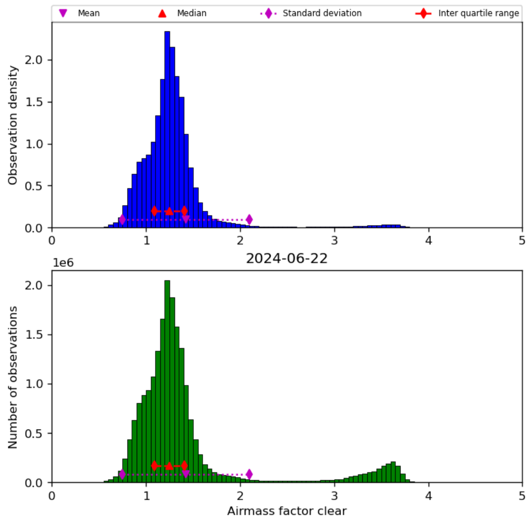
Figure 42: Histogram of “Airmass factor clear” for 2024-06-21 to 2024-06-23
