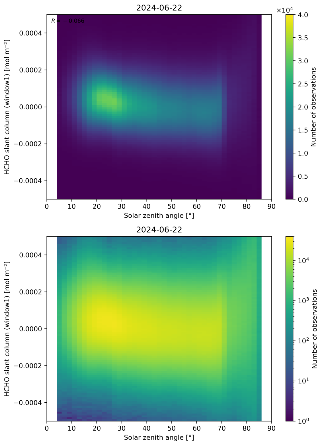
Figure 173: Scatter density plot of “Solar zenith angle” against “HCHO slant column (window1)” for 2024-06-21 to 2024-06-23.
