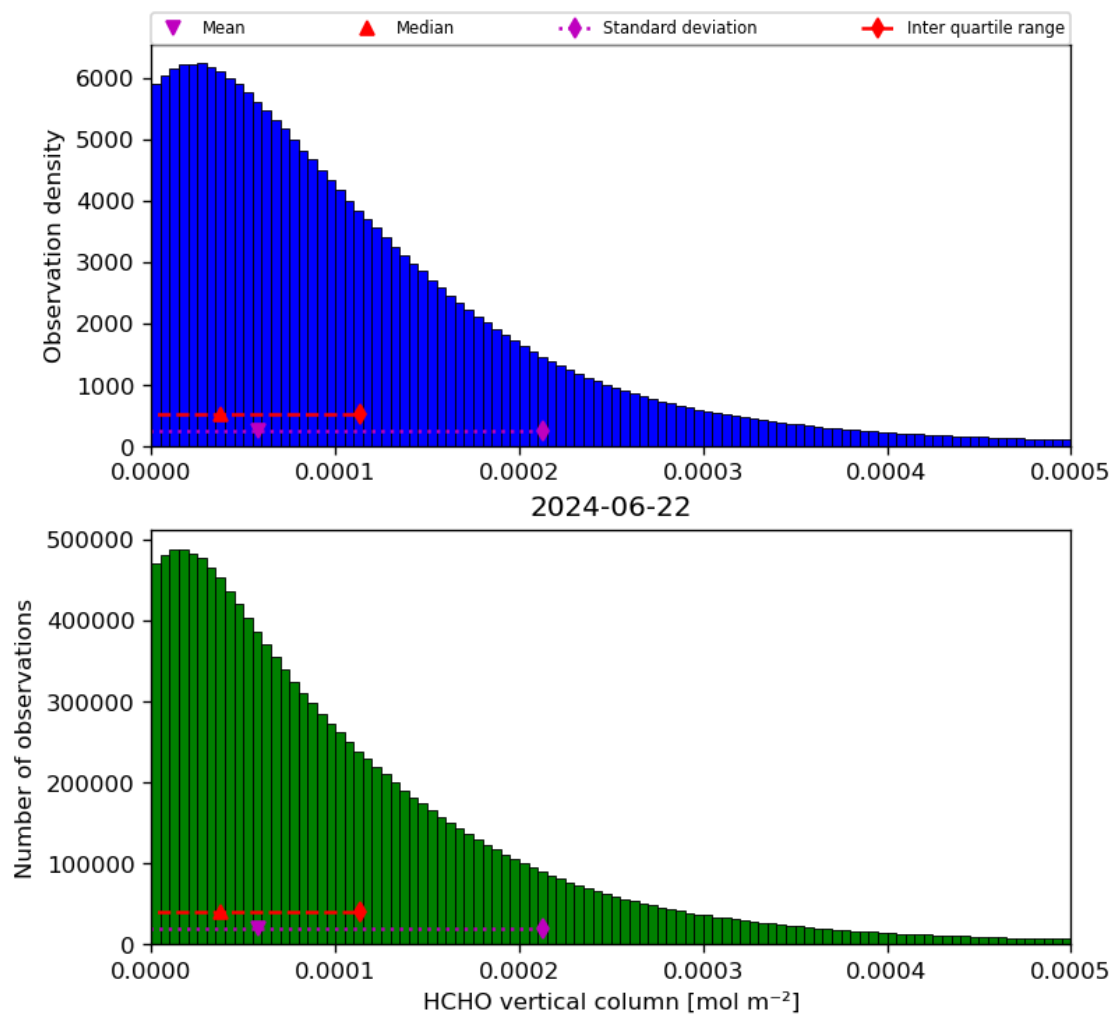
Figure 35: Histogram of “HCHO vertical column” for 2024-06-21 to 2024-06-23
