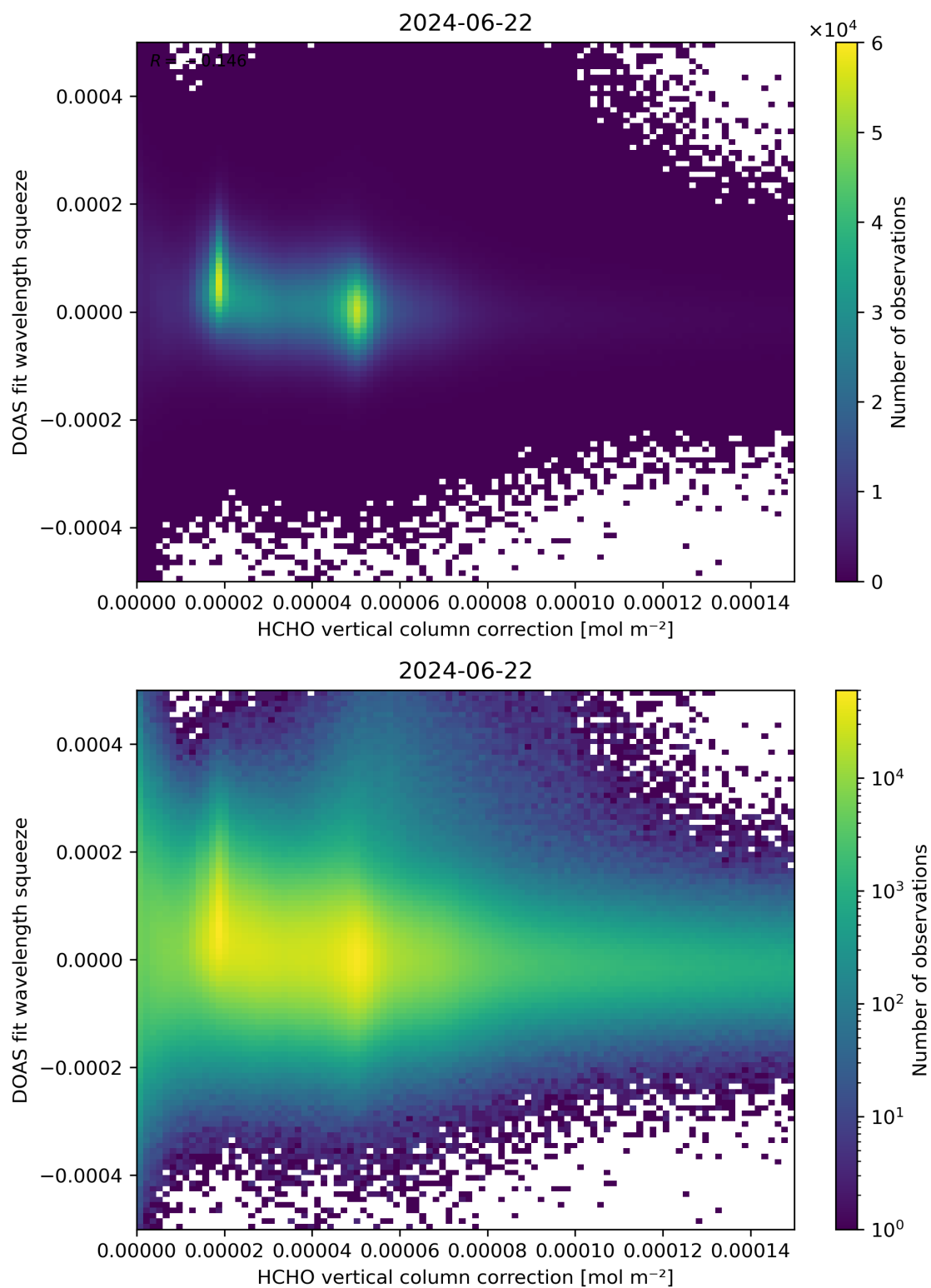
Figure 114: Scatter density plot of “HCHO vertical column correction” against “DOAS fit wavelength squeeze” for 2024-06-21 to 2024-06-23.
