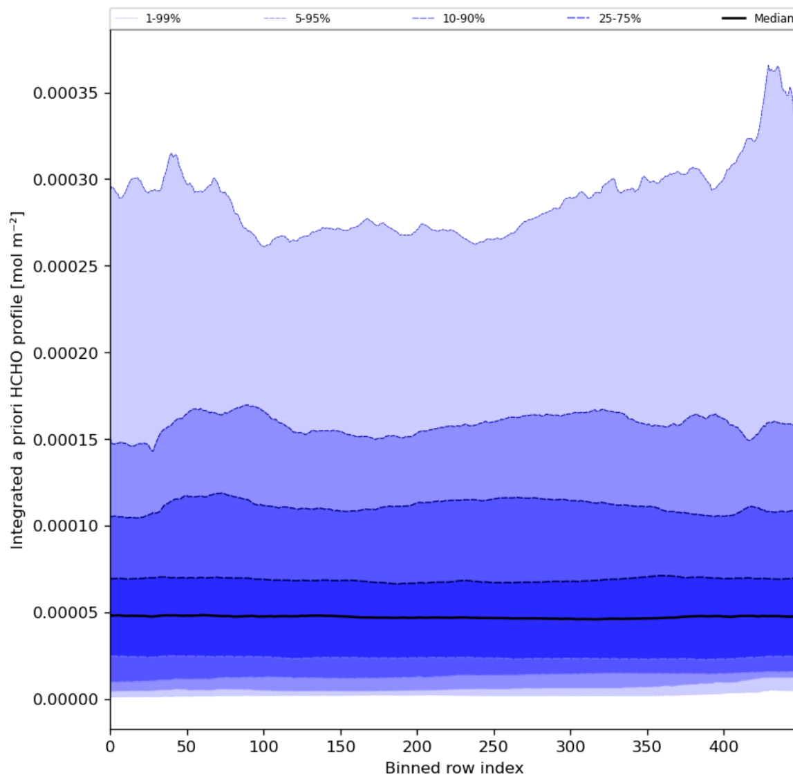
Figure 57: Along track statistics of “Integrated a priori HCHO profile” for 2024-06-21 to 2024-06-23
