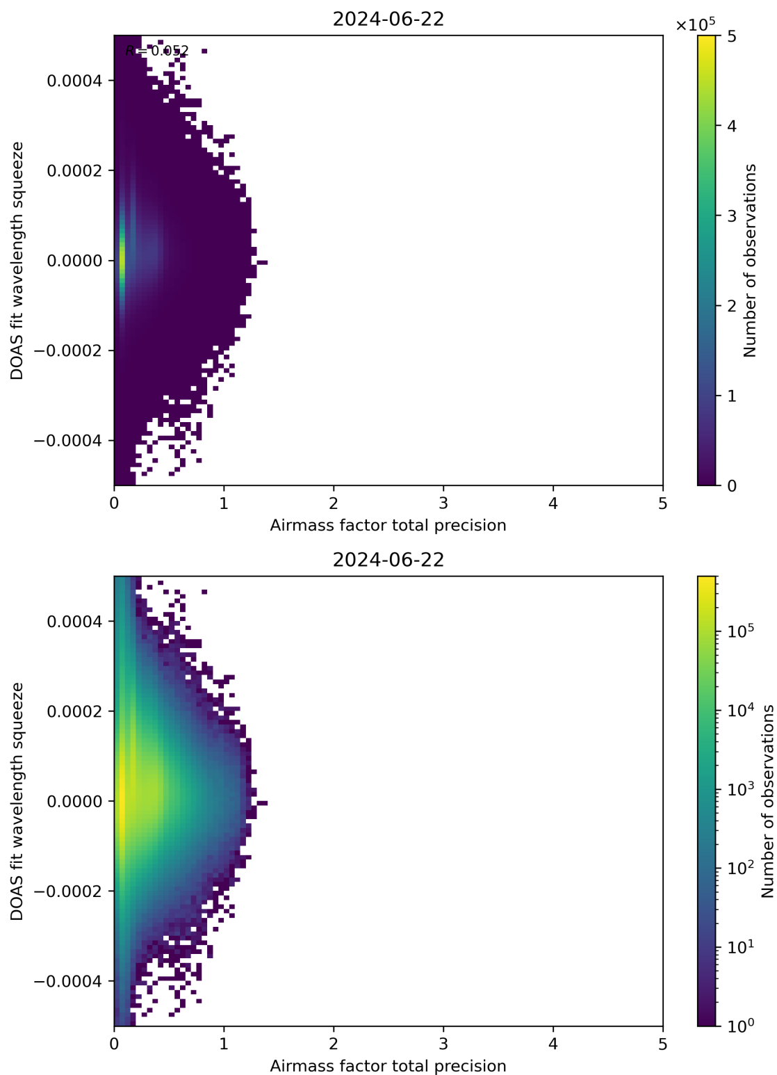
Figure 107: Scatter density plot of “Airmass factor total precision” against “DOAS fit wavelength squeeze” for 2024-06-21 to 2024-06-23.
