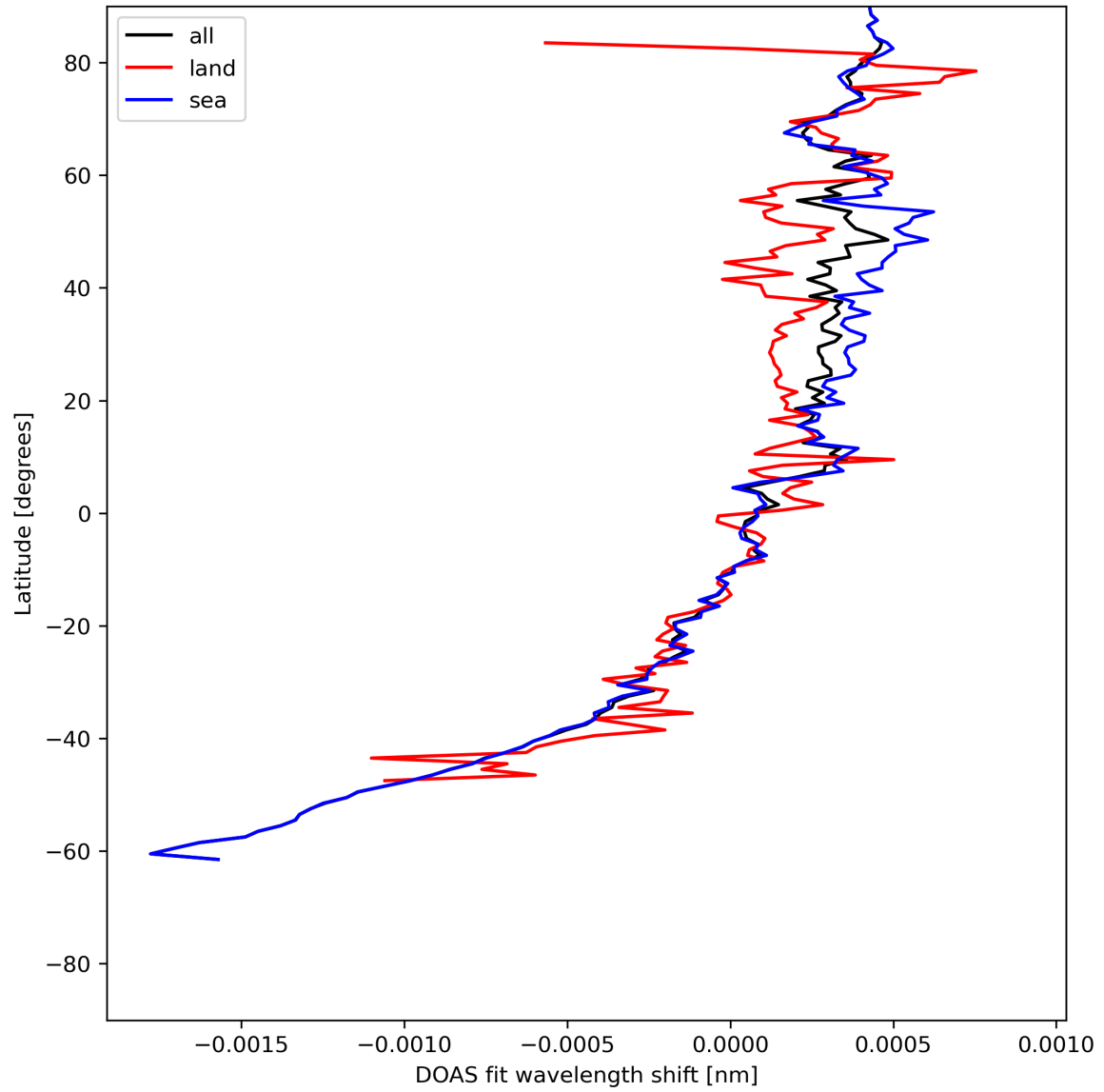
Figure 30: Zonal average of “DOAS fit wavelength shift” for 2024-06-21 to 2024-06-23.
