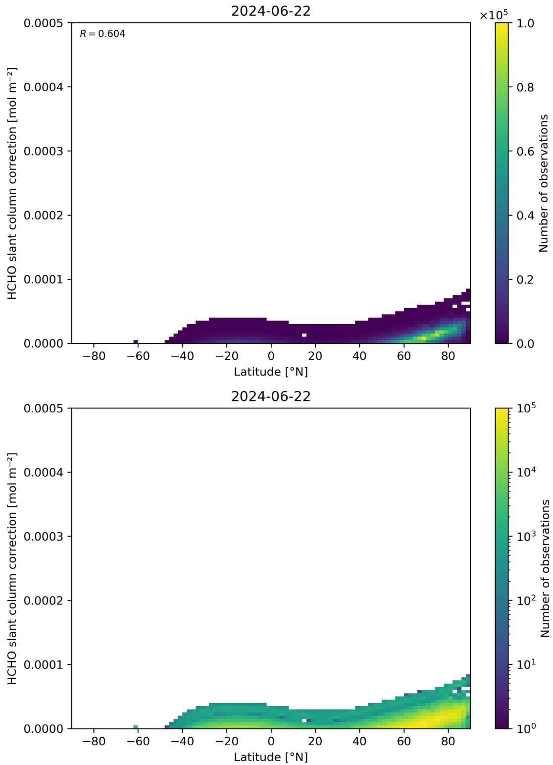
Figure 158: Scatter density plot of “Latitude” against “HCHO slant column correction” for 2024-06-21 to 2024-06-23.
