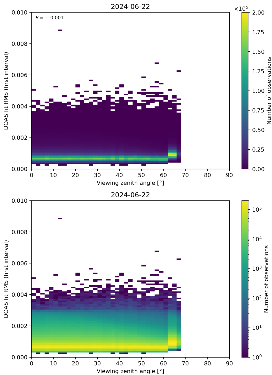
Figure 182: Scatter density plot of “Viewing zenith angle” against “DOAS fit RMS (first interval)” for 2024-06-21 to 2024-06-23.
