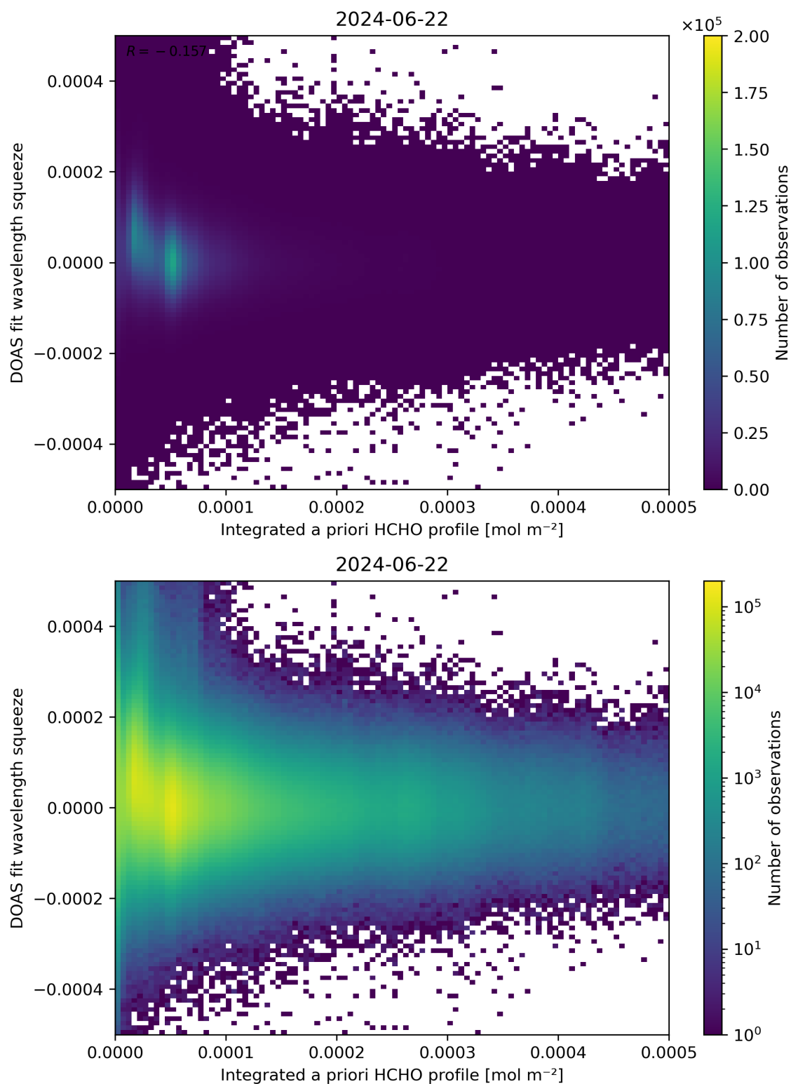
Figure 150: Scatter density plot of “Integrated a priori HCHO profile” against “DOAS fit wavelength squeeze” for 2024-06-21 to 2024-06-23.
