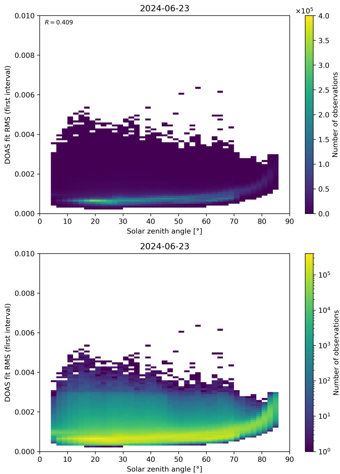
Figure 167: Scatter density plot of “Solar zenith angle” against “DOAS fit RMS (first interval)” for 2024-06-22 to 2024-06-24.
