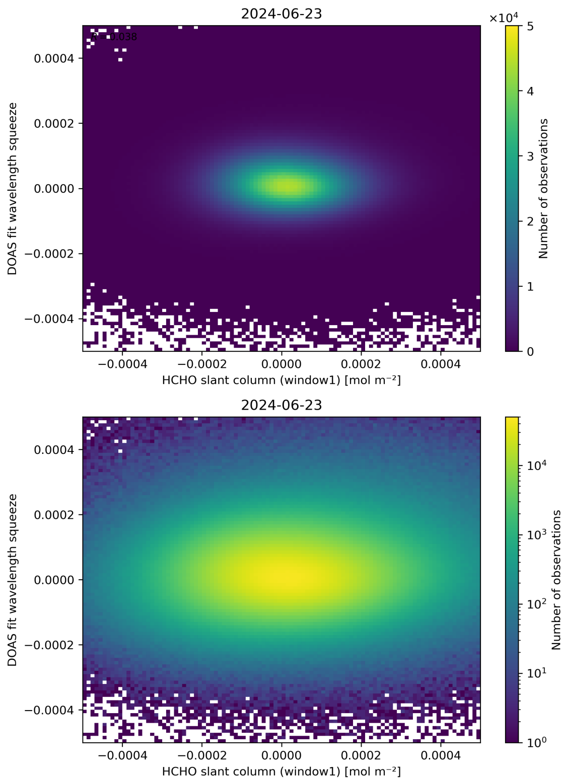
Figure 80: Scatter density plot of “HCHO slant column (window1)” against “DOAS fit wavelength squeeze” for 2024-06-22 to 2024-06-24.
