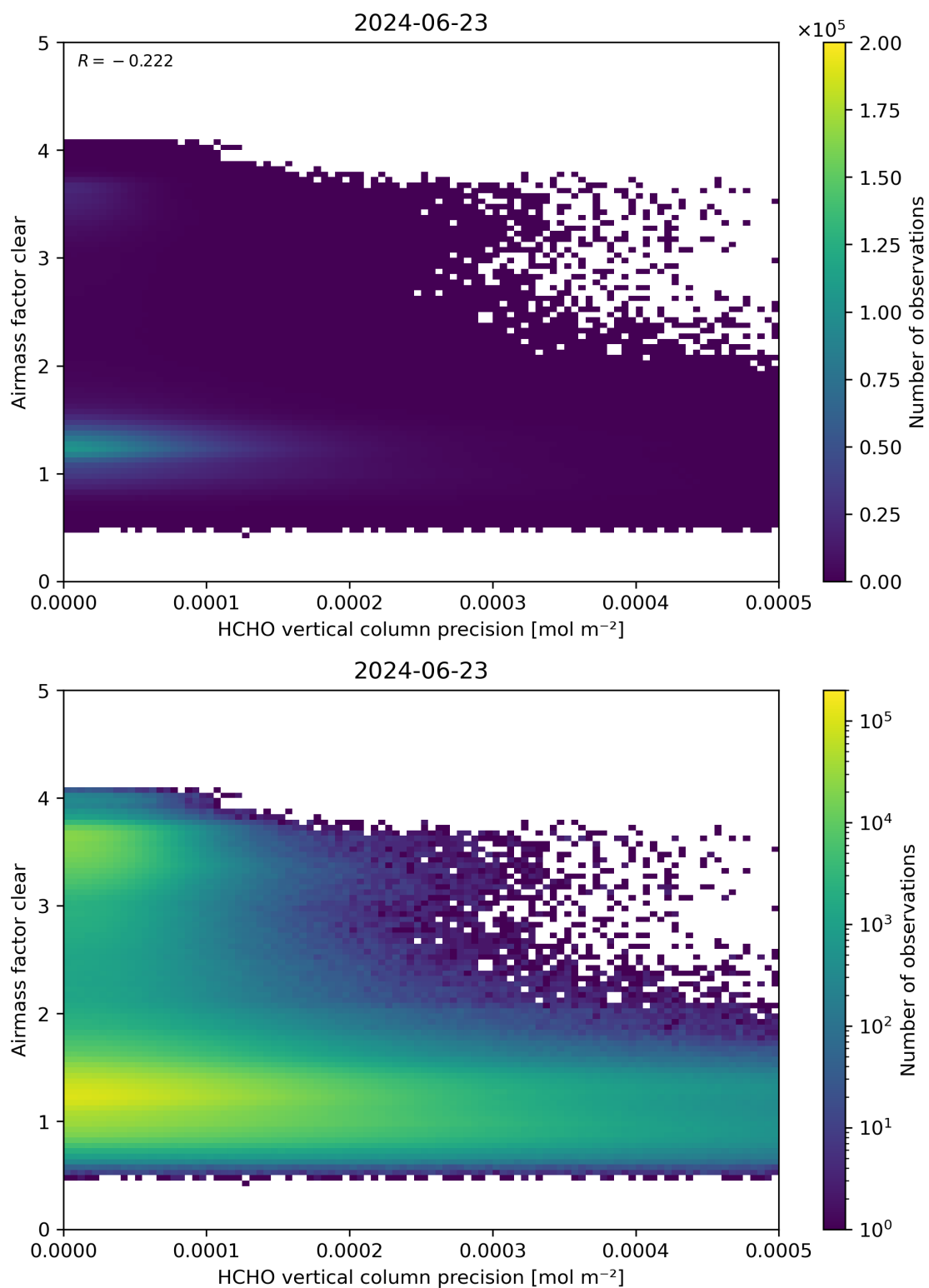
Figure 139: Scatter density plot of “HCHO vertical column precision” against “Airmass factor clear” for 2024-06-22 to 2024-06-24.
