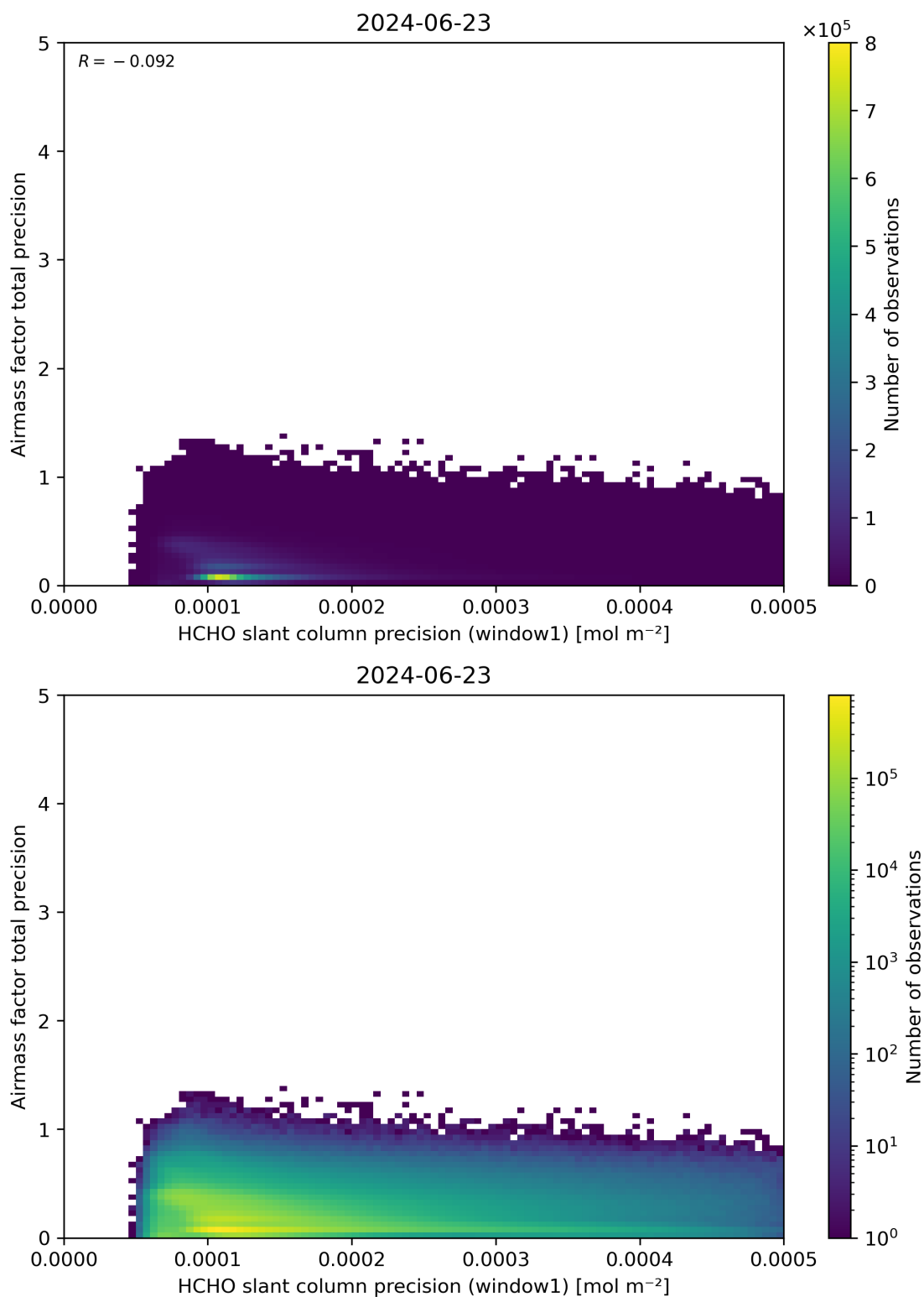
Figure 95: Scatter density plot of “HCHO slant column precision (window1)” against “Airmass factor total precision” for 2024-06-22 to 2024-06-24.
