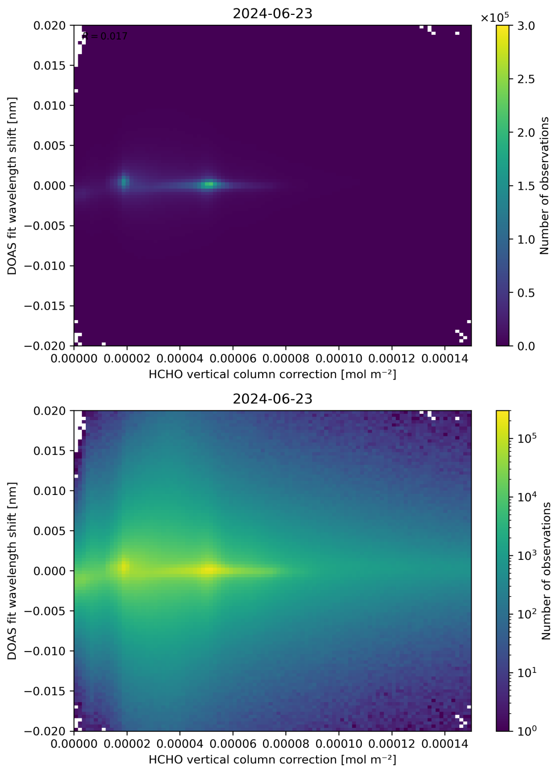
Figure 113: Scatter density plot of “HCHO vertical column correction” against “DOAS fit wavelength shift” for 2024-06-22 to 2024-06-24.
