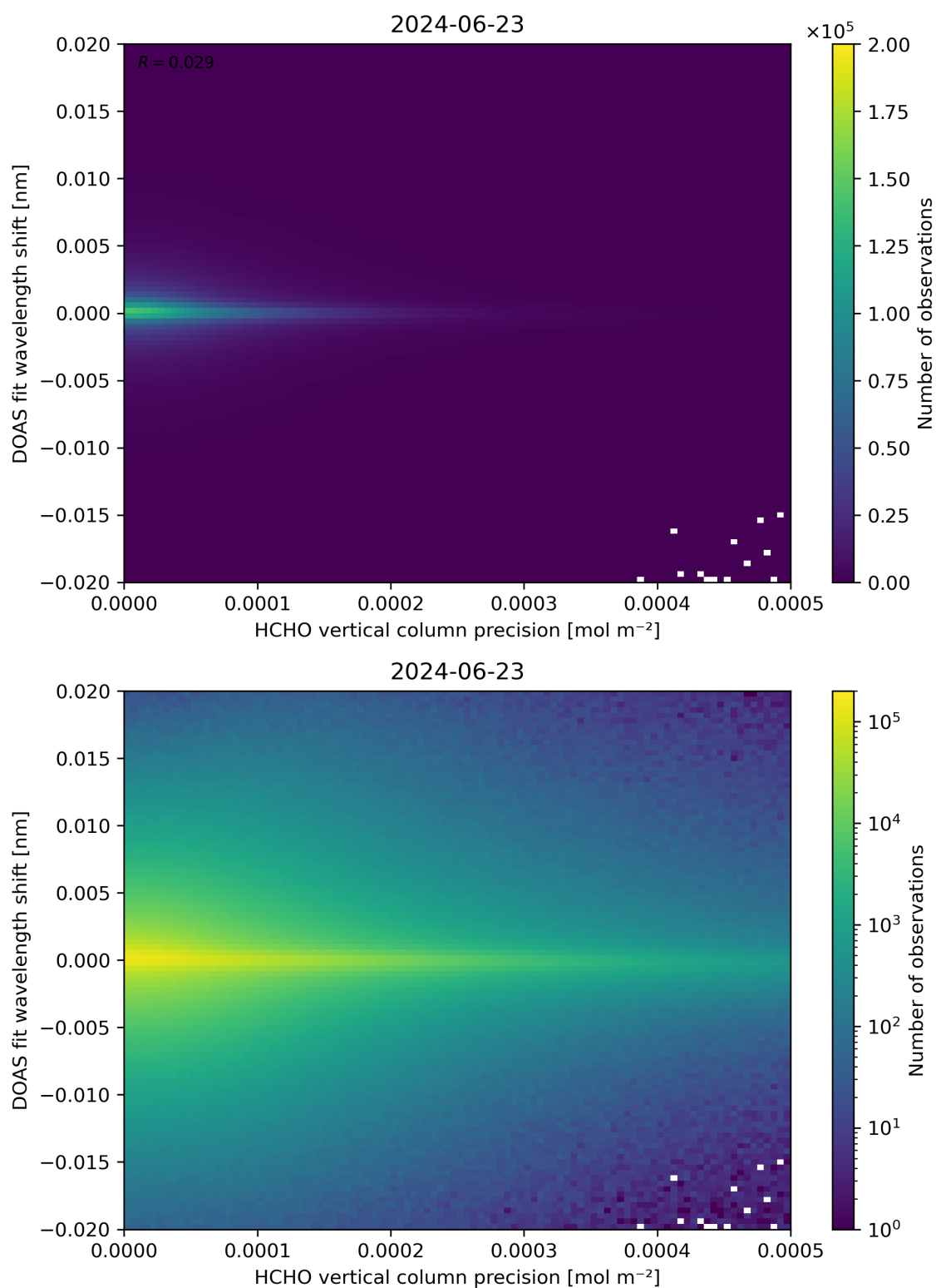
Figure 137: Scatter density plot of “HCHO vertical column precision” against “DOAS fit wavelength shift” for 2024-06-22 to 2024-06-24.
