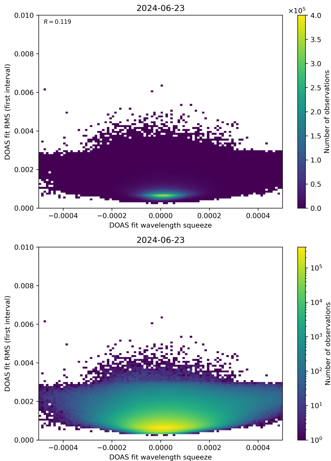
Figure 68: Scatter density plot of “DOAS fit wavelength squeeze” against “DOAS fit RMS (first interval)” for 2024-06-22 to 2024-06-24.
