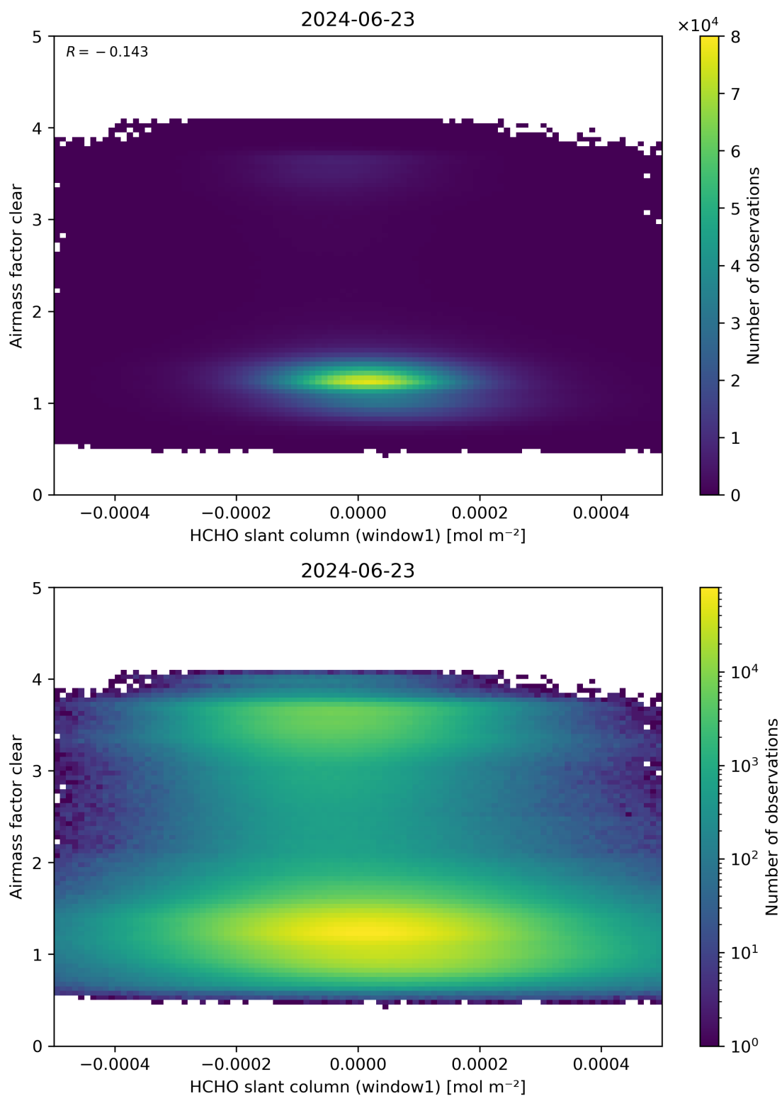
Figure 81: Scatter density plot of “HCHO slant column (window1)” against “Airmass factor clear” for 2024-06-22 to 2024-06-24.
