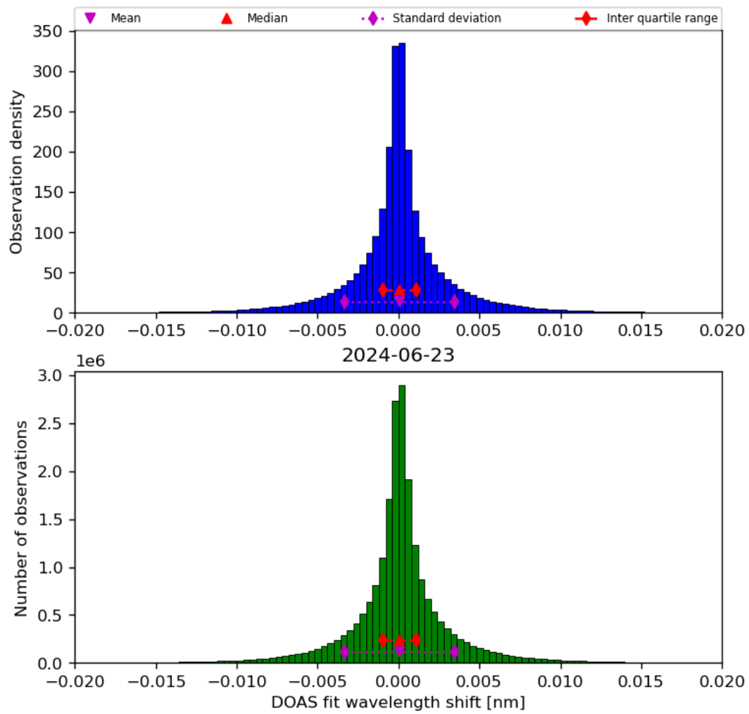
Figure 44: Histogram of “DOAS fit wavelength shift” for 2024-06-22 to 2024-06-24
