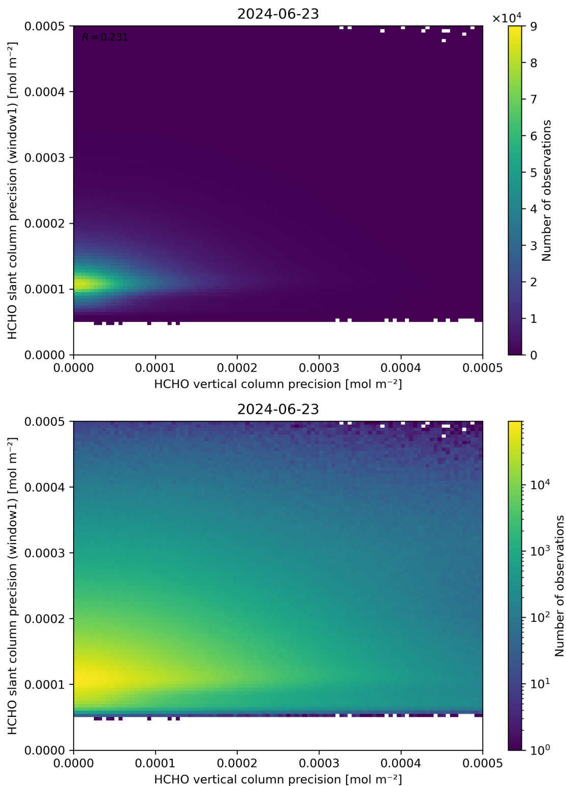
Figure 143: Scatter density plot of “HCHO vertical column precision” against “HCHO slant column precision (window1)” for 2024-06-22 to 2024-06-24.
