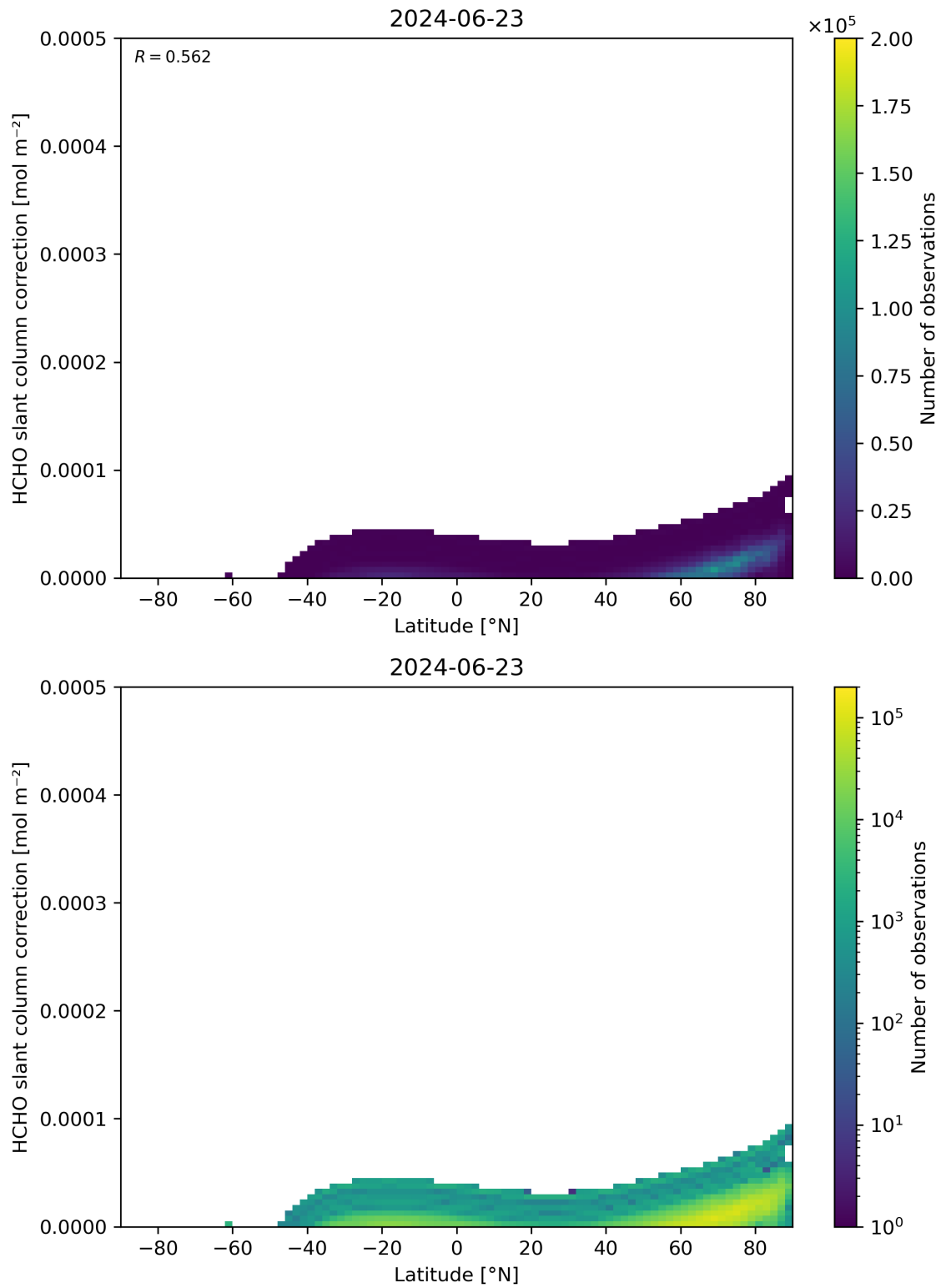
Figure 158: Scatter density plot of “Latitude” against “HCHO slant column correction” for 2024-06-22 to 2024-06-24.
