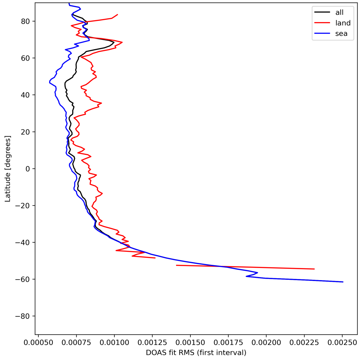
Figure 32: Zonal average of "DOAS fit RMS (first interval)" for 2024-06-22 to 2024-06-24.
