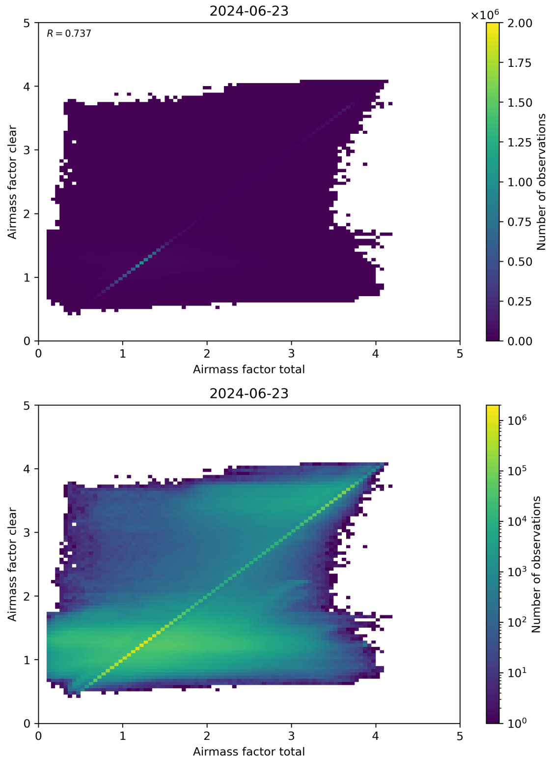
Figure 100: Scatter density plot of “Airmass factor total” against “Airmass factor clear” for 2024-06-22 to 2024-06-24.
