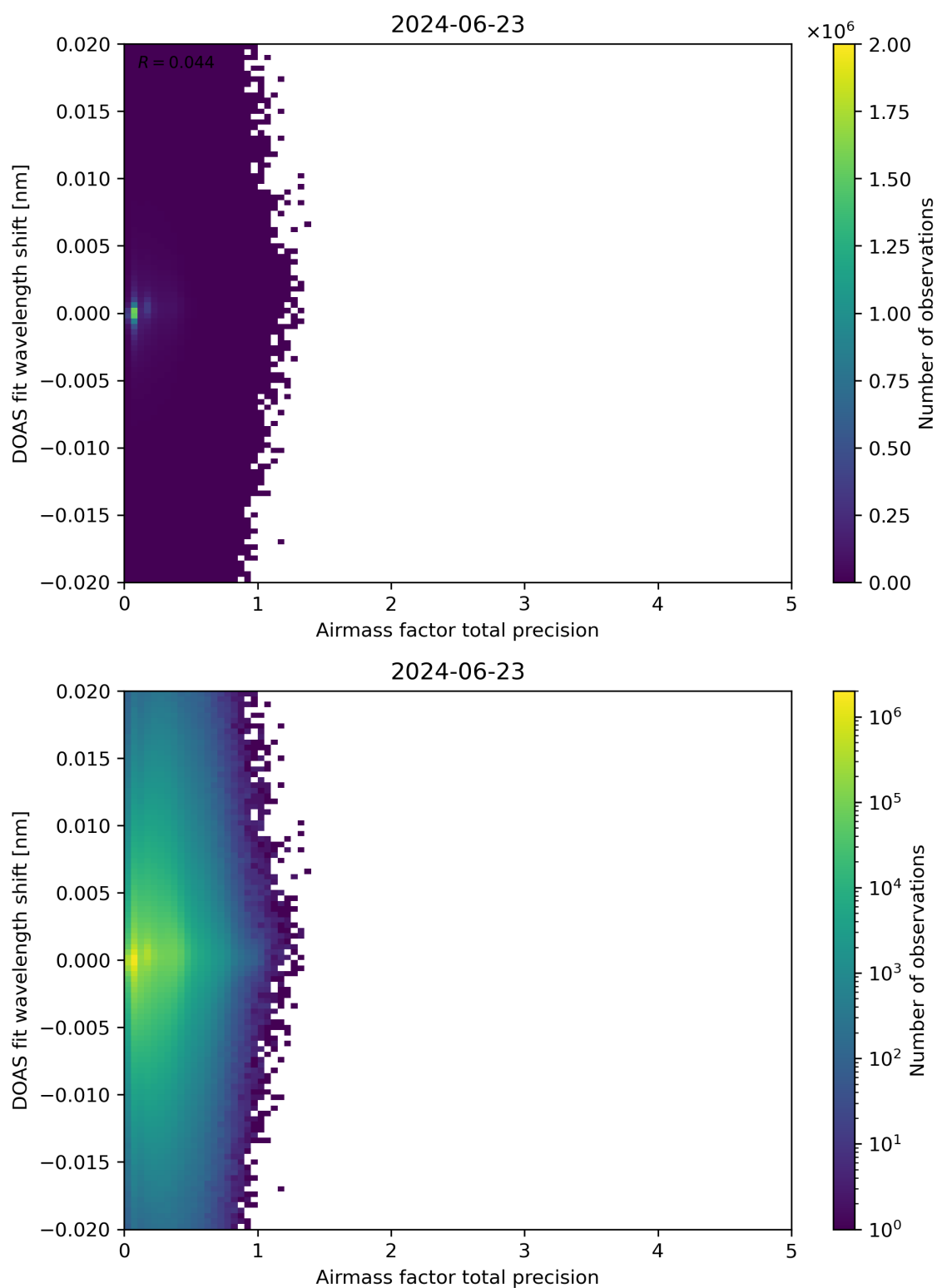
Figure 106: Scatter density plot of “Airmass factor total precision” against “DOAS fit wavelength shift” for 2024-06-22 to 2024-06-24.
