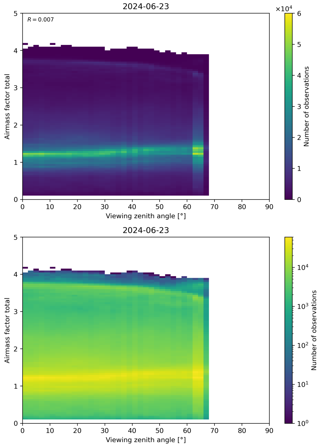
Figure 190: Scatter density plot of “Viewing zenith angle” against “Airmass factor total” for 2024-06-22 to 2024-06-24.
