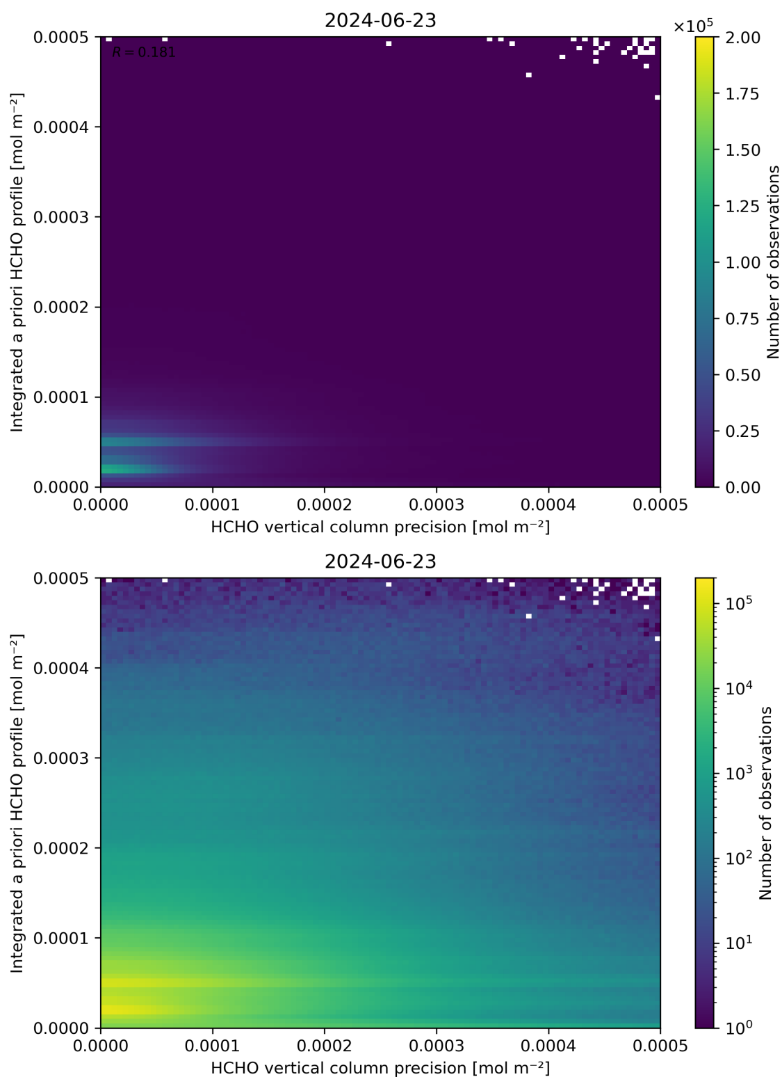
Figure 147: Scatter density plot of “HCHO vertical column precision” against “Integrated a priori HCHO profile” for 2024-06-22 to 2024-06-24.
