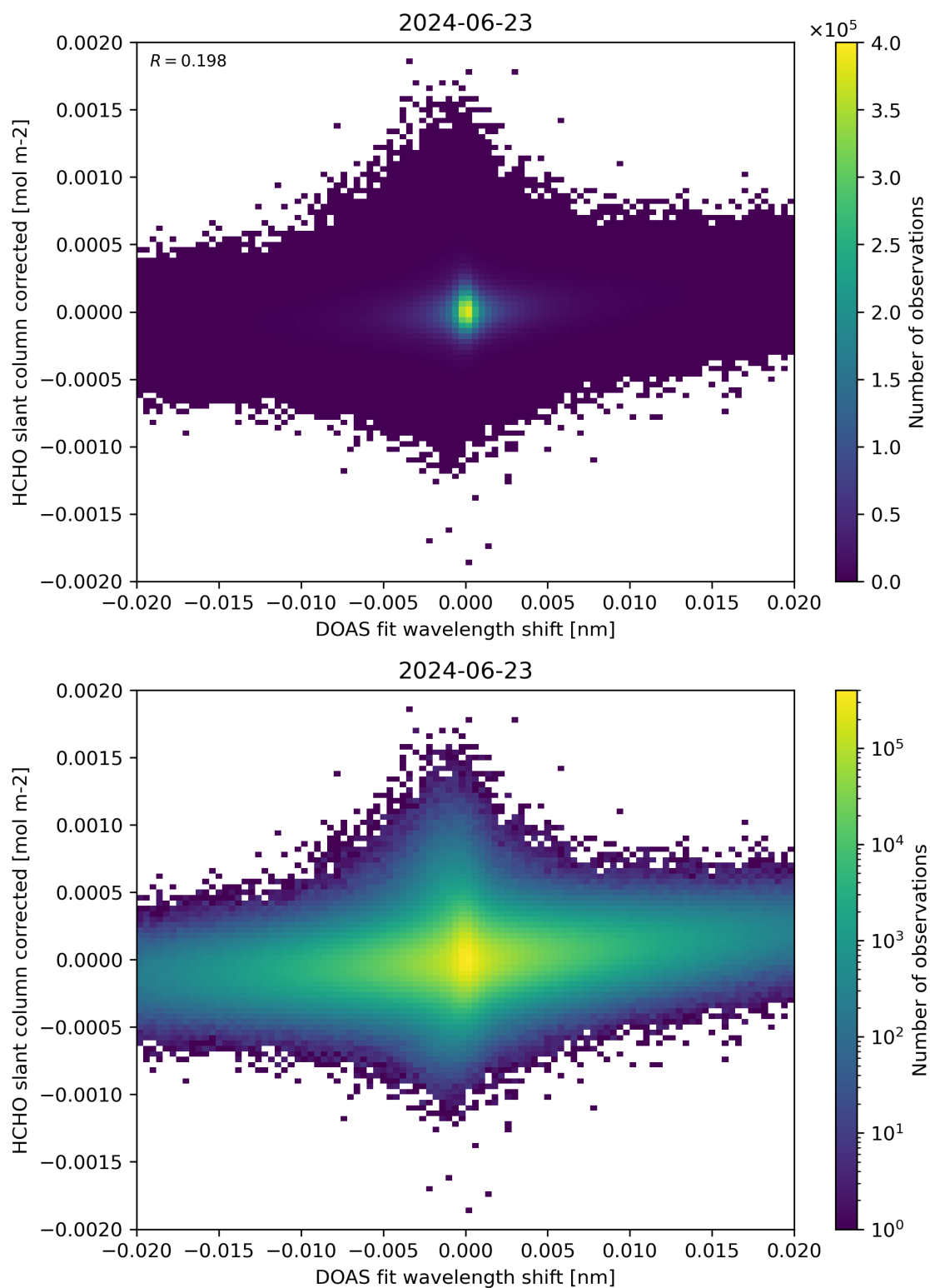
Figure 66: Scatter density plot of “DOAS fit wavelength shift” against “HCHO slant column corrected” for 2024-06-22 to 2024-06-24.
