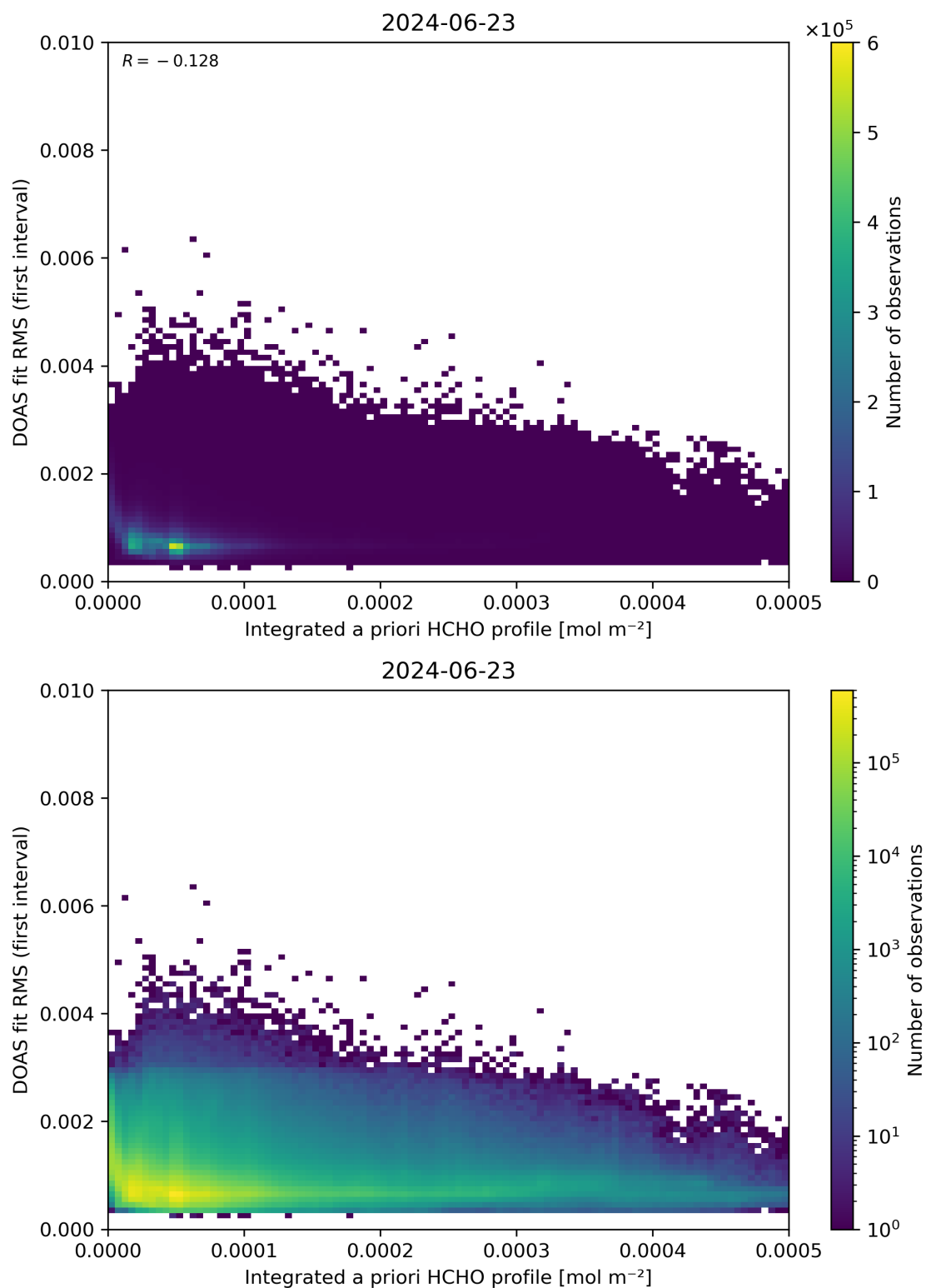
Figure 148: Scatter density plot of “Integrated a priori HCHO profile” against “DOAS fit RMS (first interval)” for 2024-06-22 to 2024-06-24.
