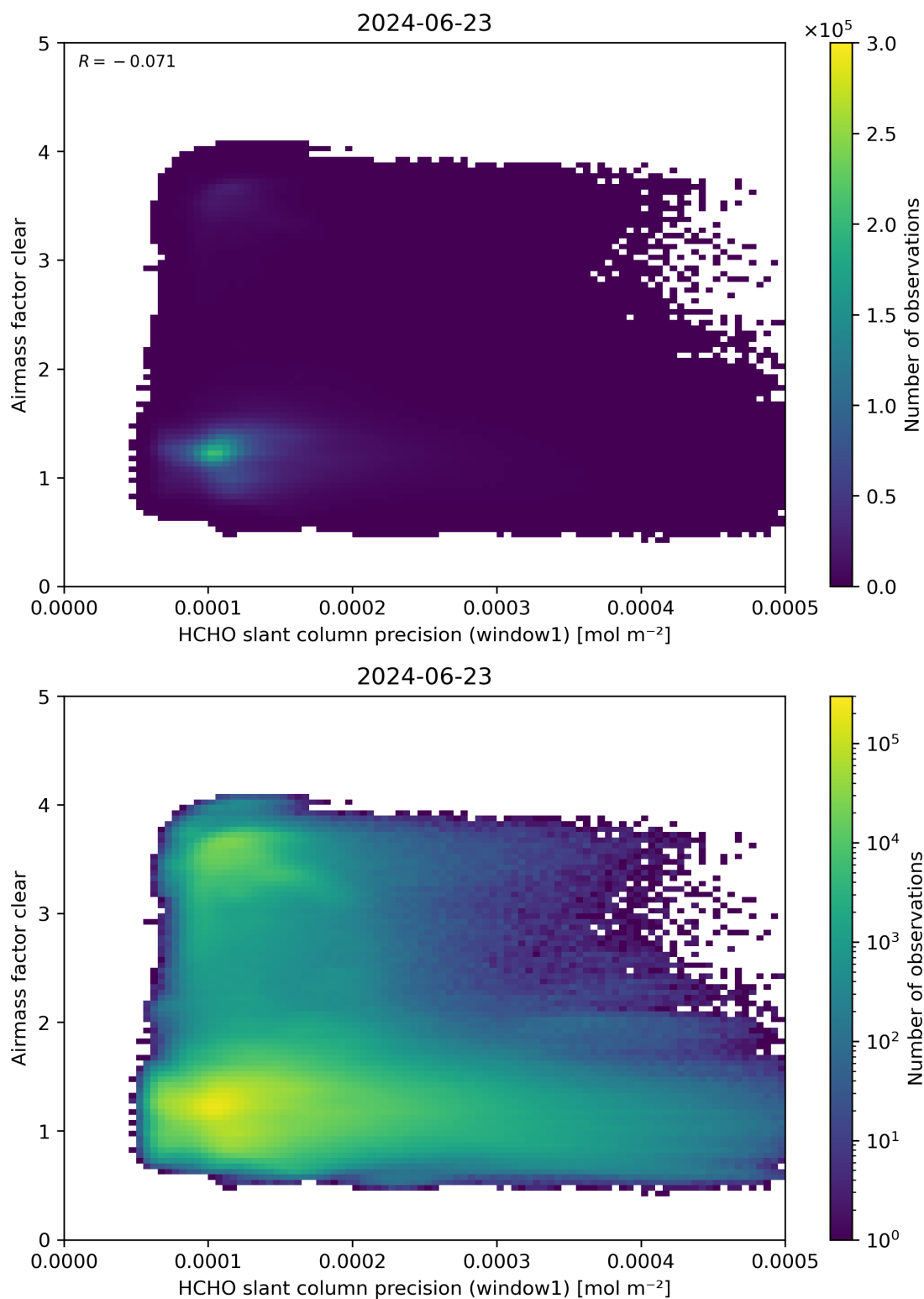
Figure 91: Scatter density plot of “HCHO slant column precision (window1)” against “Airmass factor clear” for 2024-06-22 to 2024-06-24.
