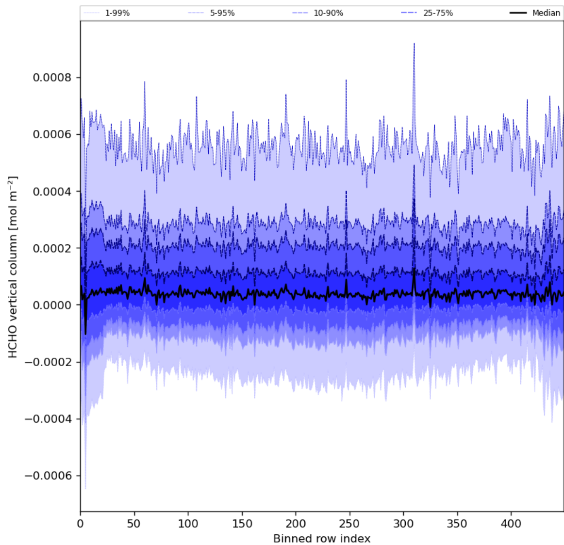
Figure 49: Along track statistics of “HCHO vertical column” for 2024-06-22 to 2024-06-24
