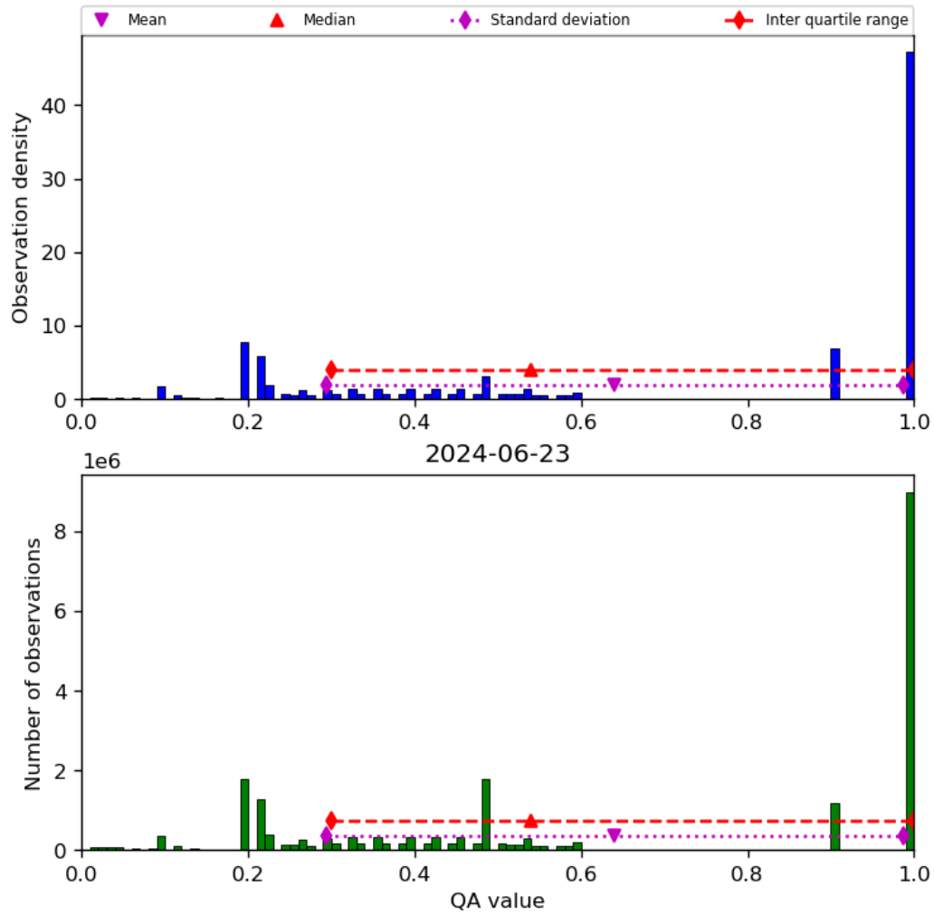
Figure 34: Histogram of “QA value” for 2024-06-22 to 2024-06-24
