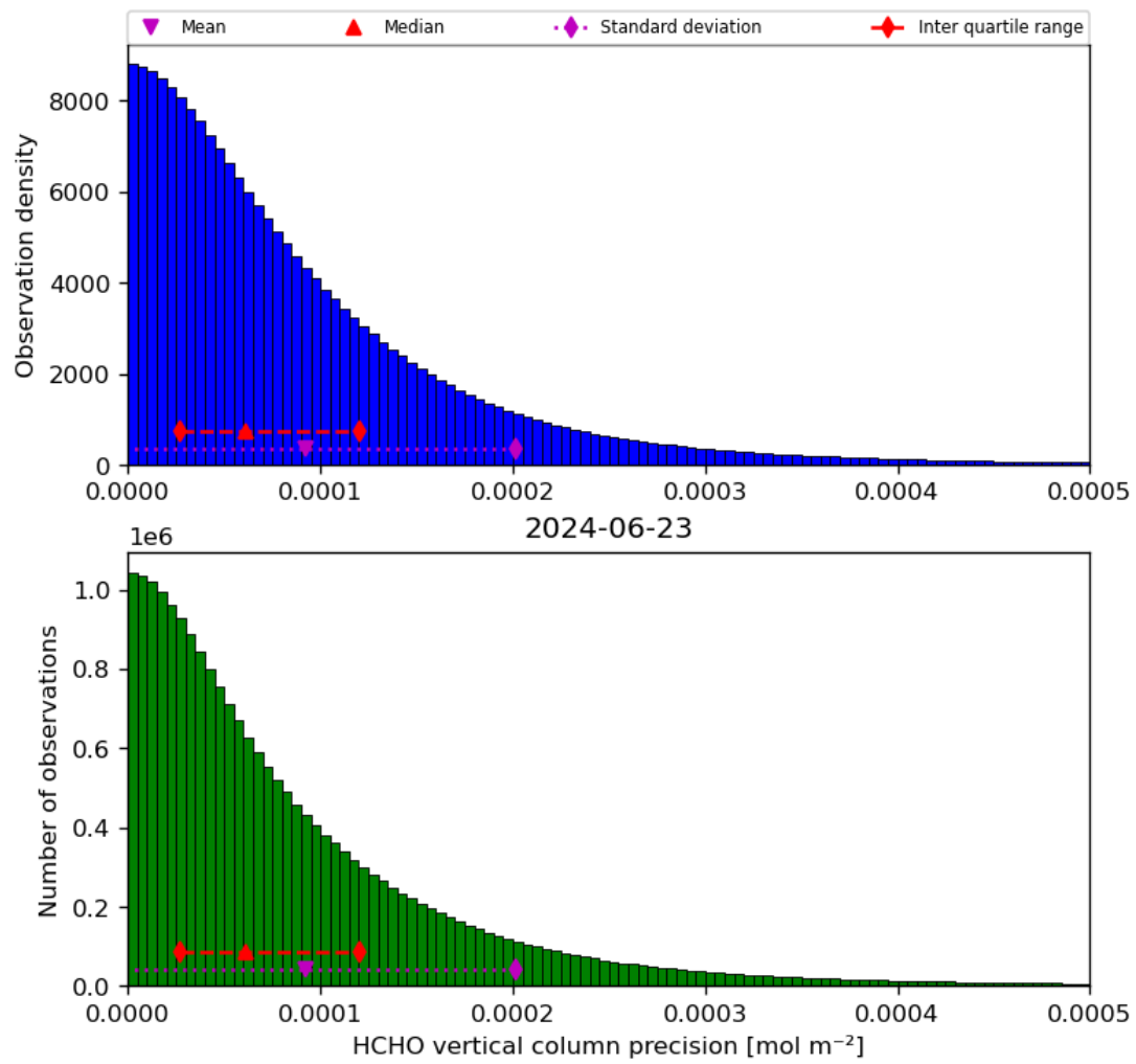
Figure 36: Histogram of “HCHO vertical column precision” for 2024-06-22 to 2024-06-24
