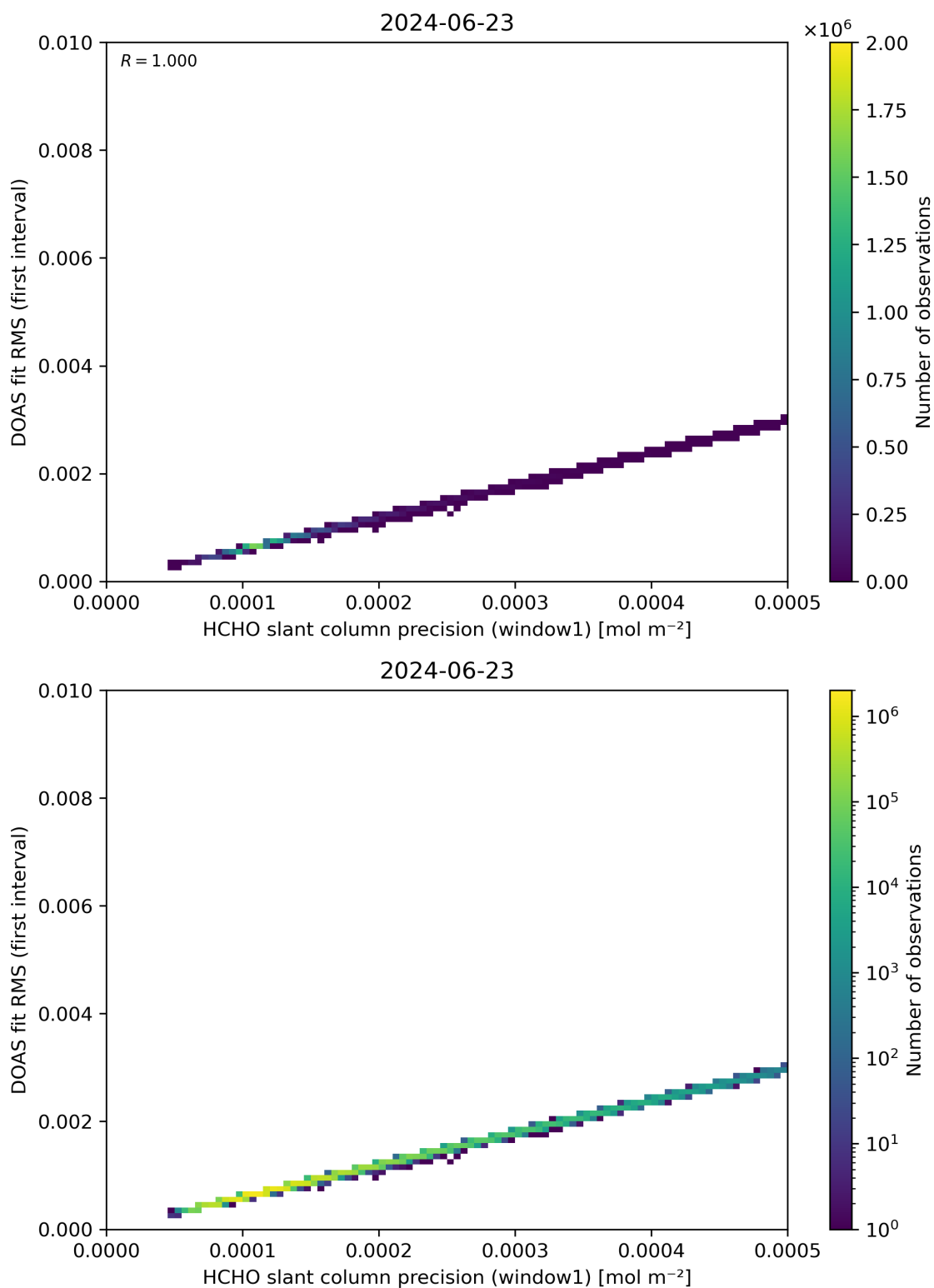
Figure 88: Scatter density plot of “HCHO slant column precision (window1)” against “DOAS fit RMS (first interval)” for 2024-06-22 to 2024-06-24.
