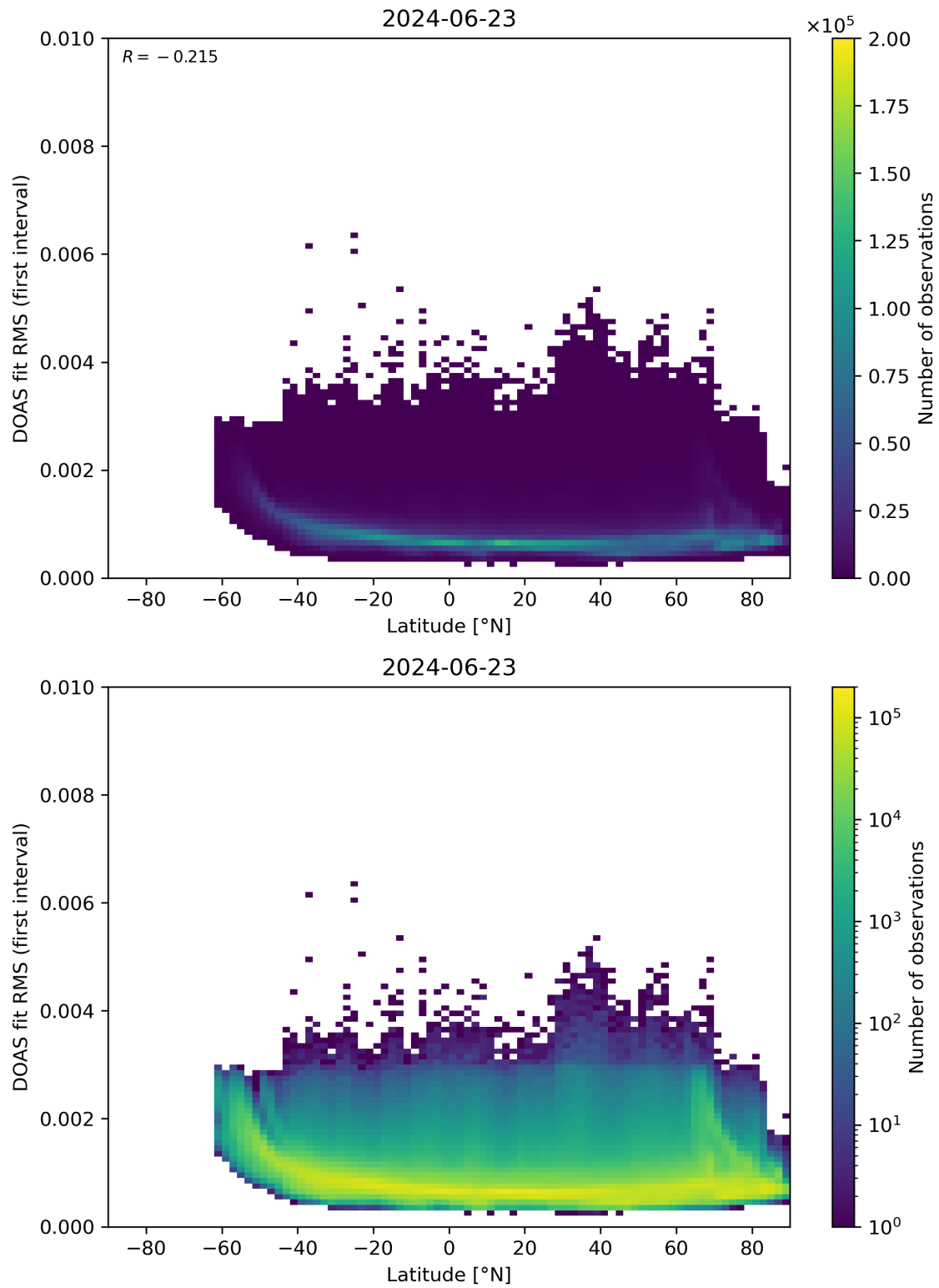
Figure 153: Scatter density plot of “Latitude” against “DOAS fit RMS (first interval)” for 2024-06-22 to 2024-06-24.
