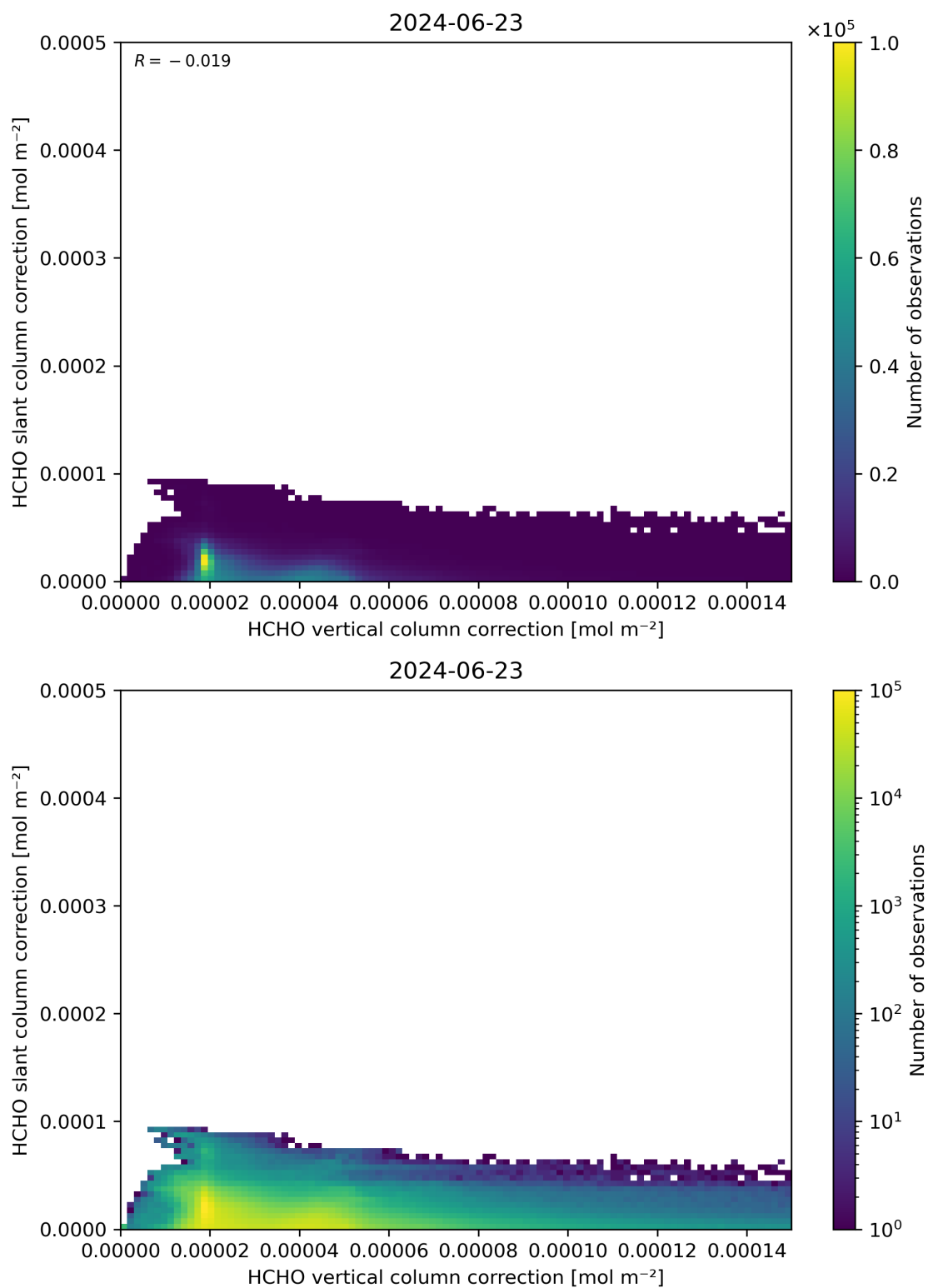
Figure 117: Scatter density plot of “HCHO vertical column correction” against “HCHO slant column correction” for 2024-06-22 to 2024-06-24.
