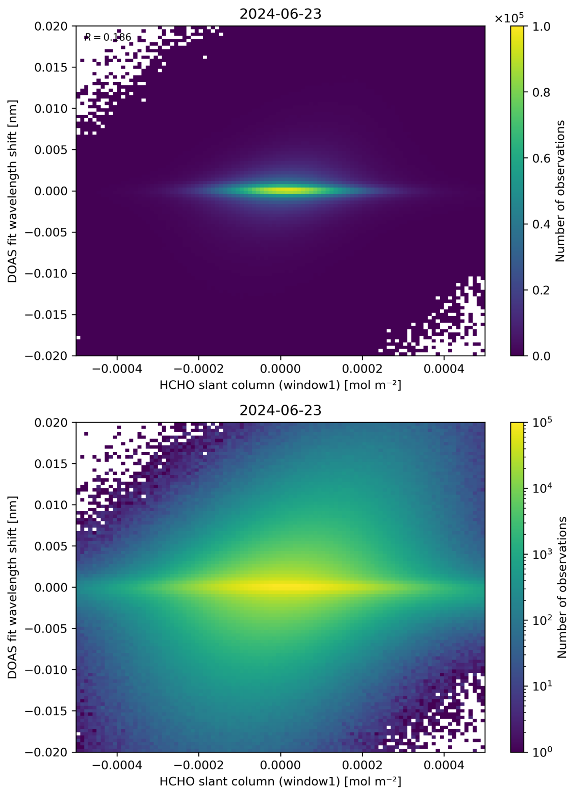
Figure 79: Scatter density plot of “HCHO slant column (window1)” against “DOAS fit wavelength shift” for 2024-06-22 to 2024-06-24.
