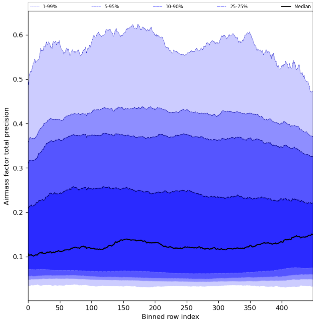
Figure 55: Along track statistics of “Airmass factor total precision” for 2024-06-22 to 2024-06-24
