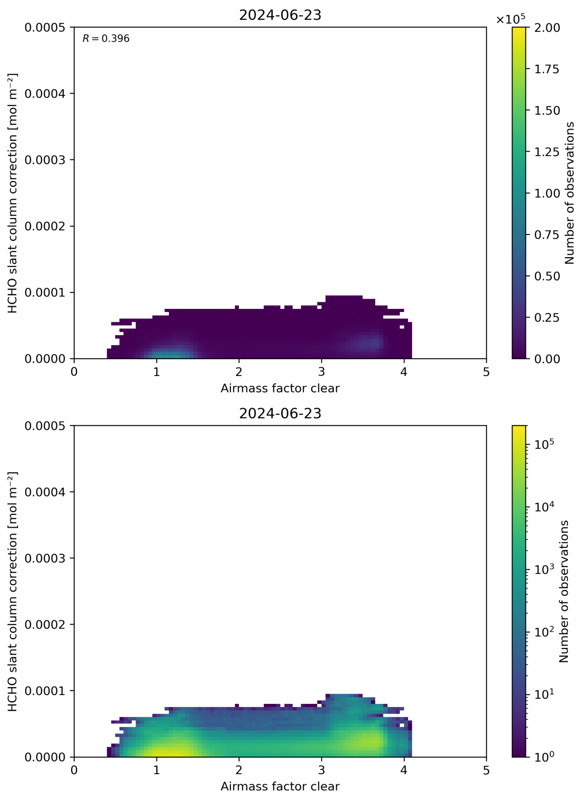
Figure 75: Scatter density plot of “Airmass factor clear” against “HCHO slant column correction” for 2024-06-22 to 2024-06-24.
