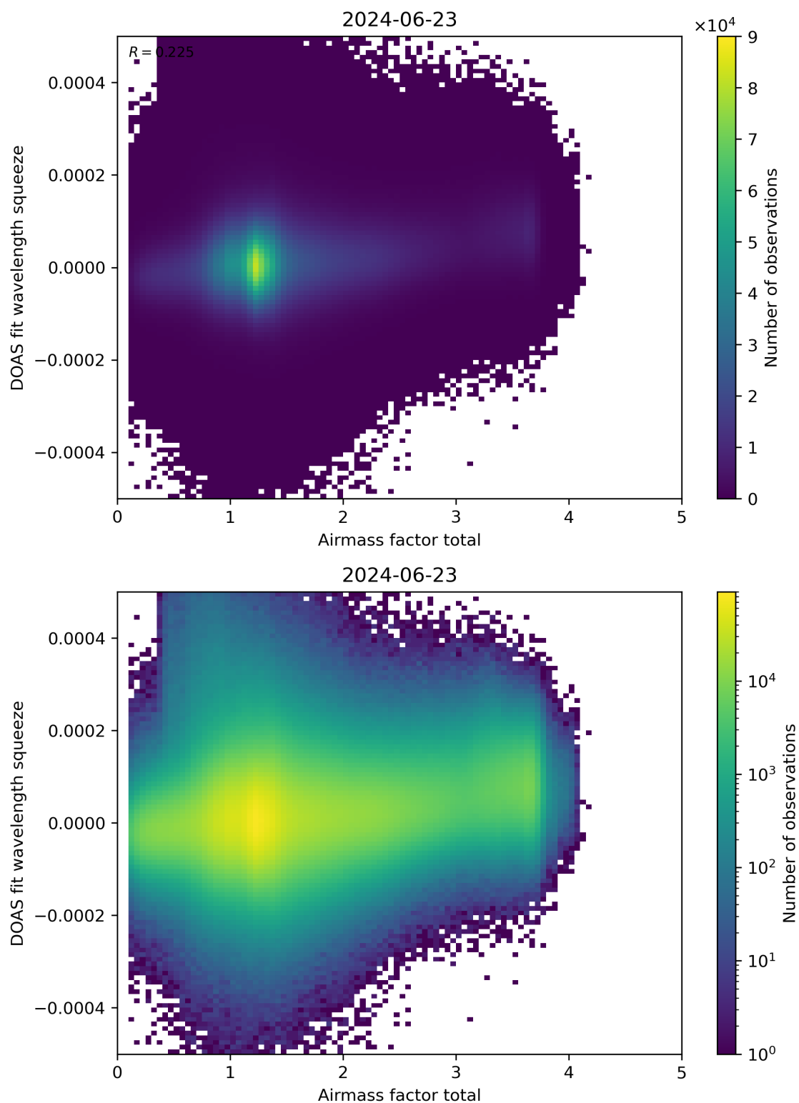
Figure 99: Scatter density plot of “Airmass factor total” against “DOAS fit wavelength squeeze” for 2024-06-22 to 2024-06-24.
