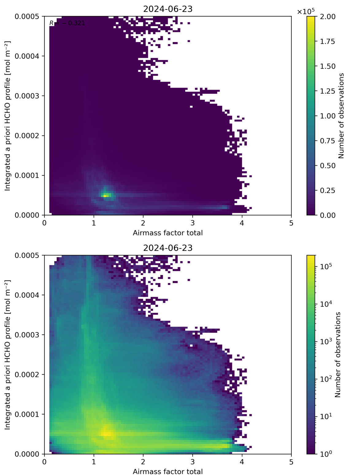
Figure 104: Scatter density plot of “Airmass factor total” against “Integrated a priori HCHO profile” for 2024-06-22 to 2024-06-24.
