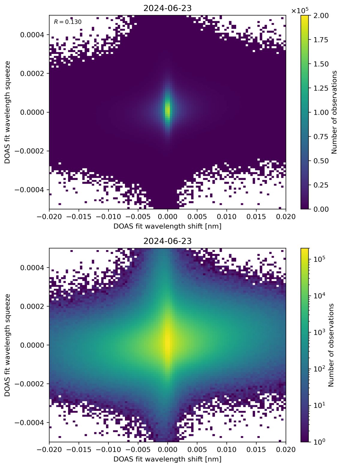
Figure 65: Scatter density plot of “DOAS fit wavelength shift” against “DOAS fit wavelength squeeze” for 2024-06-22 to 2024-06-24.
