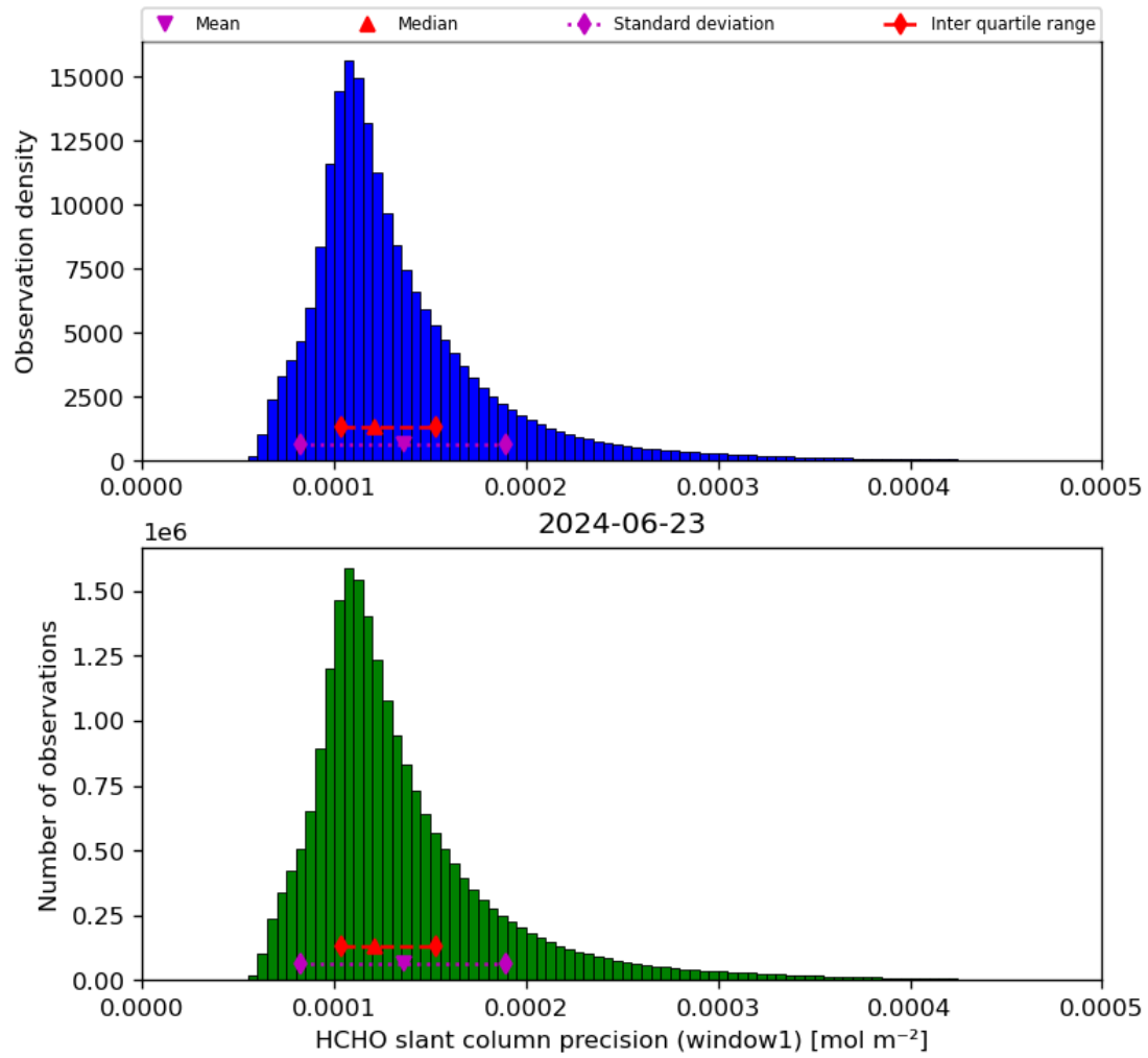
Figure 39: Histogram of “HCHO slant column precision (window1)” for 2024-06-22 to 2024-06-24
