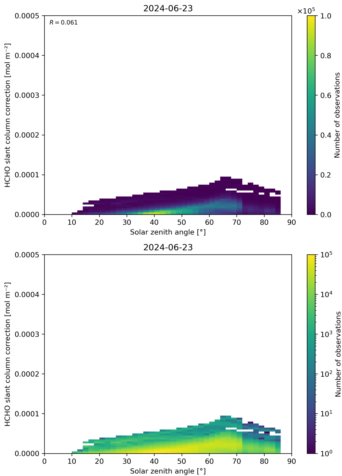
Figure 172: Scatter density plot of “Solar zenith angle” against “HCHO slant column correction” for 2024-06-22 to 2024-06-24.
