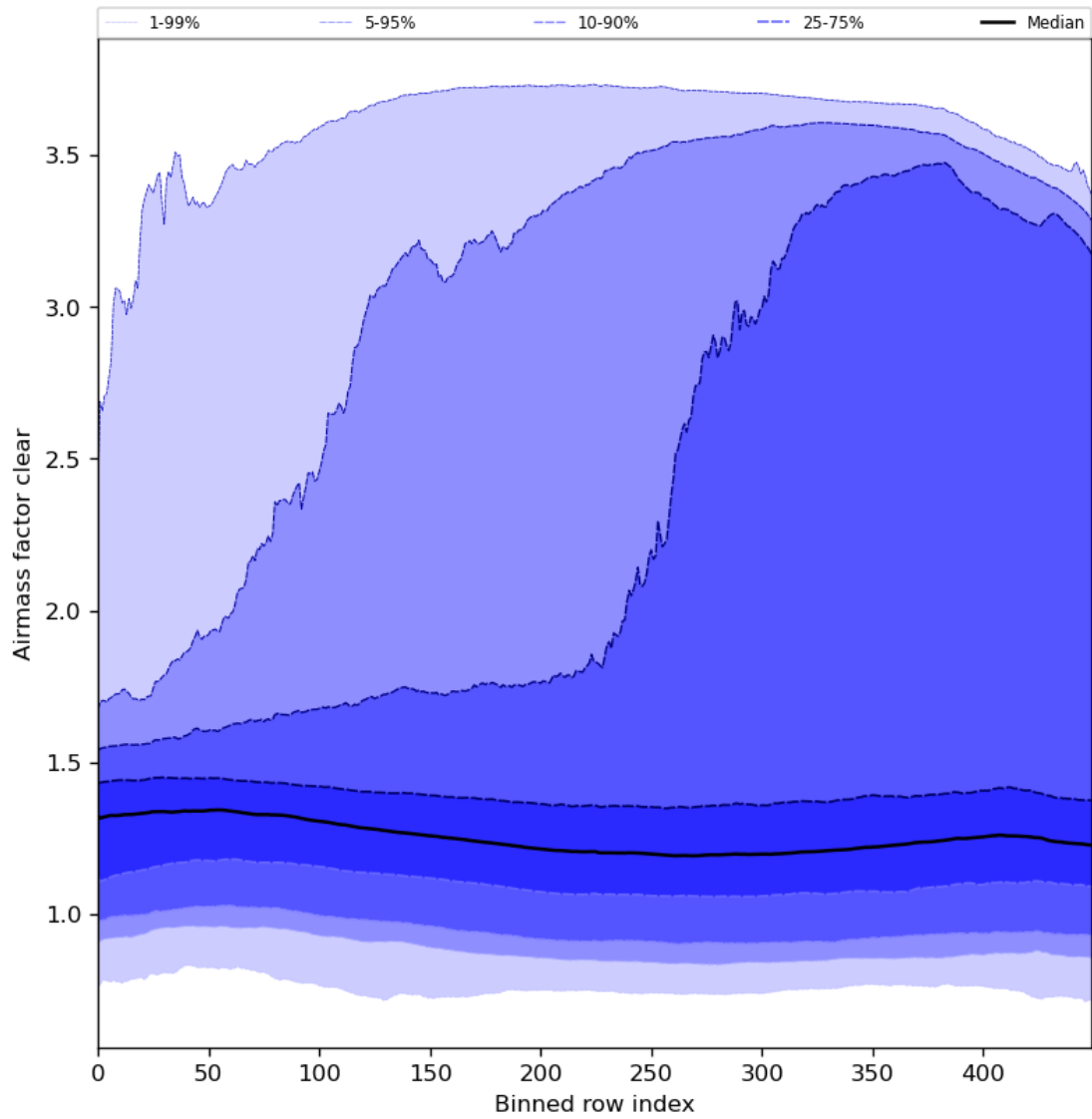
Figure 56: Along track statistics of “Airmass factor clear” for 2024-06-22 to 2024-06-24
