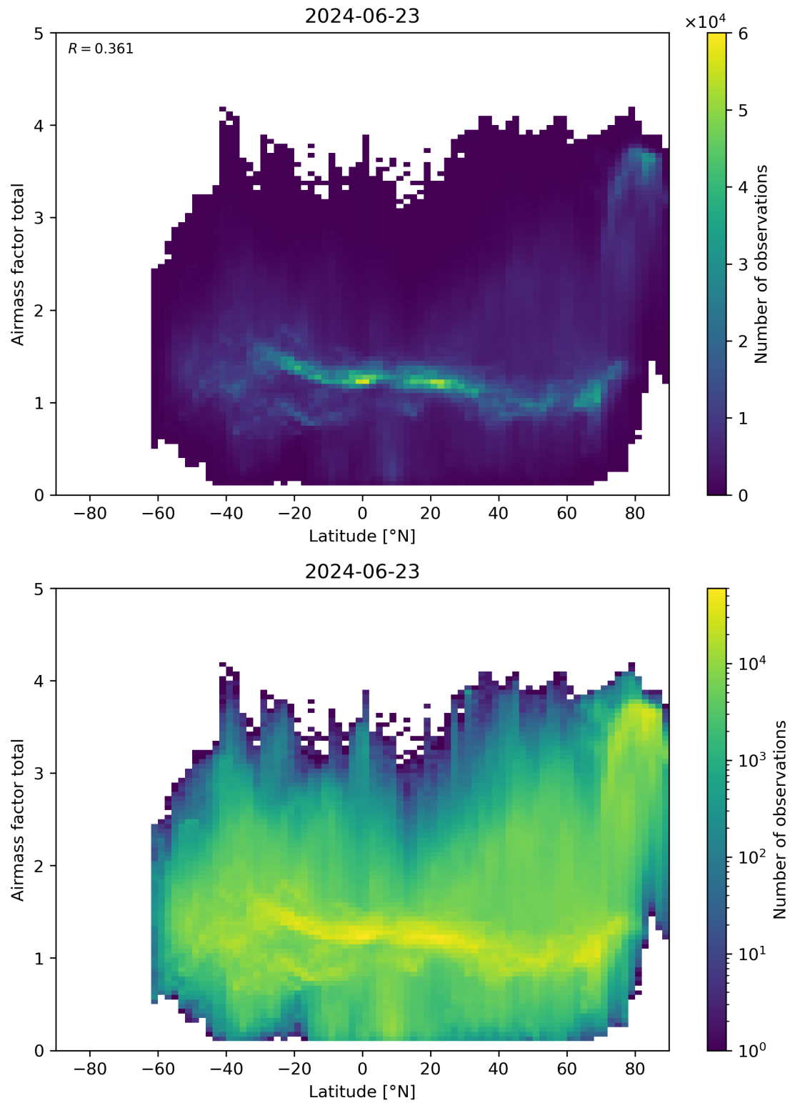
Figure 161: Scatter density plot of “Latitude” against “Airmass factor total” for 2024-06-22 to 2024-06-24.
