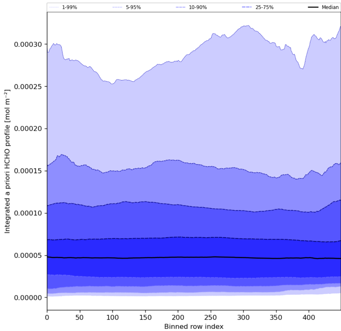
Figure 57: Along track statistics of “Integrated a priori HCHO profile” for 2024-06-22 to 2024-06-24
