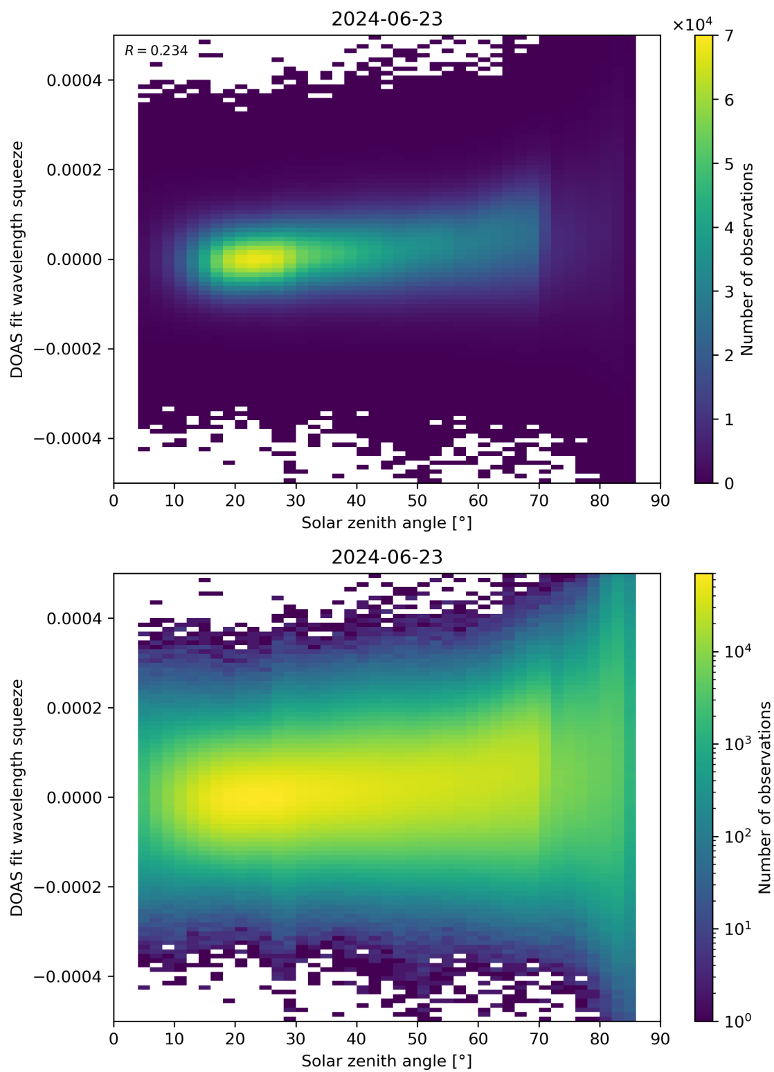
Figure 169: Scatter density plot of “Solar zenith angle” against “DOAS fit wavelength squeeze” for 2024-06-22 to 2024-06-24.
