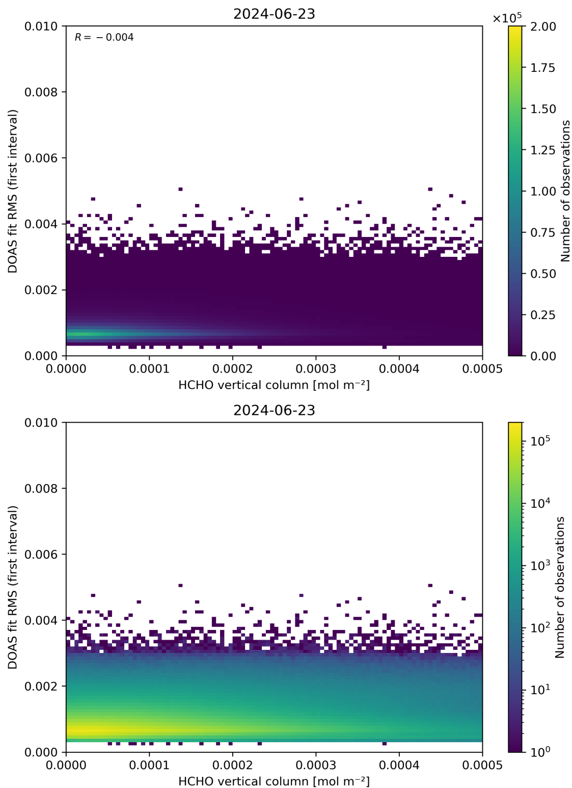
Figure 123: Scatter density plot of “HCHO vertical column” against “DOAS fit RMS (first interval)” for 2024-06-22 to 2024-06-24.
