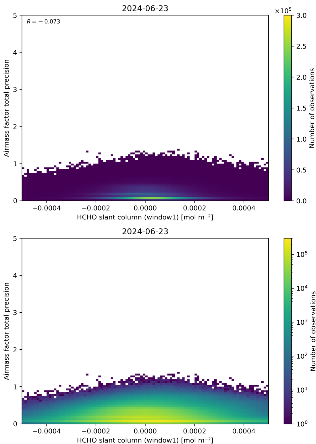
Figure 86: Scatter density plot of “HCHO slant column (window1)” against “Airmass factor total precision” for 2024-06-22 to 2024-06-24.
