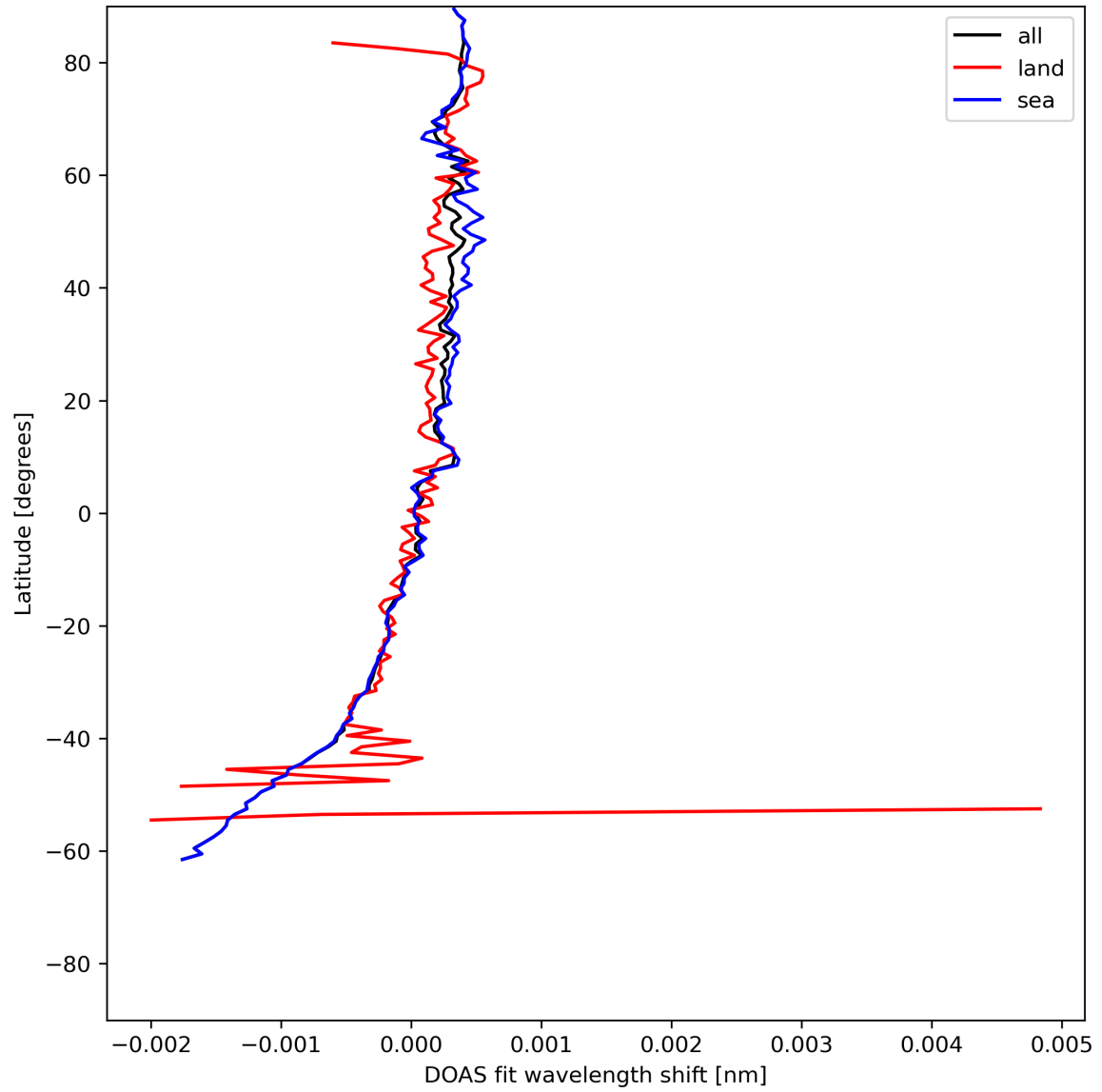
Figure 30: Zonal average of “DOAS fit wavelength shift” for 2024-06-22 to 2024-06-24.
