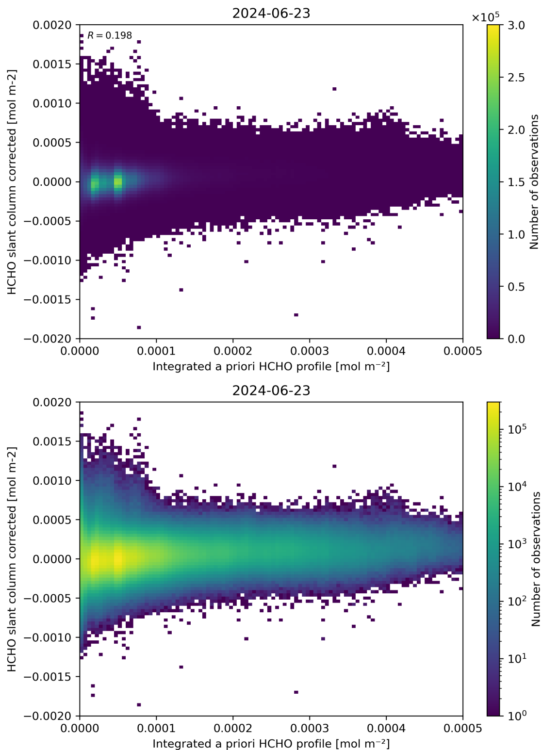
Figure 151: Scatter density plot of “Integrated a priori HCHO profile” against “HCHO slant column corrected” for 2024-06-22 to 2024-06-24.
