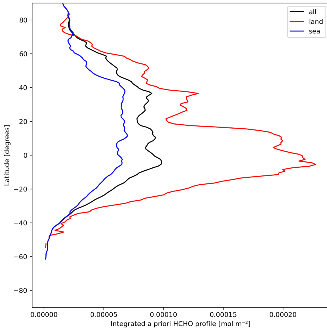
Figure 29: Zonal average of “Integrated a priori HCHO profile” for 2024-06-22 to 2024-06-24.
