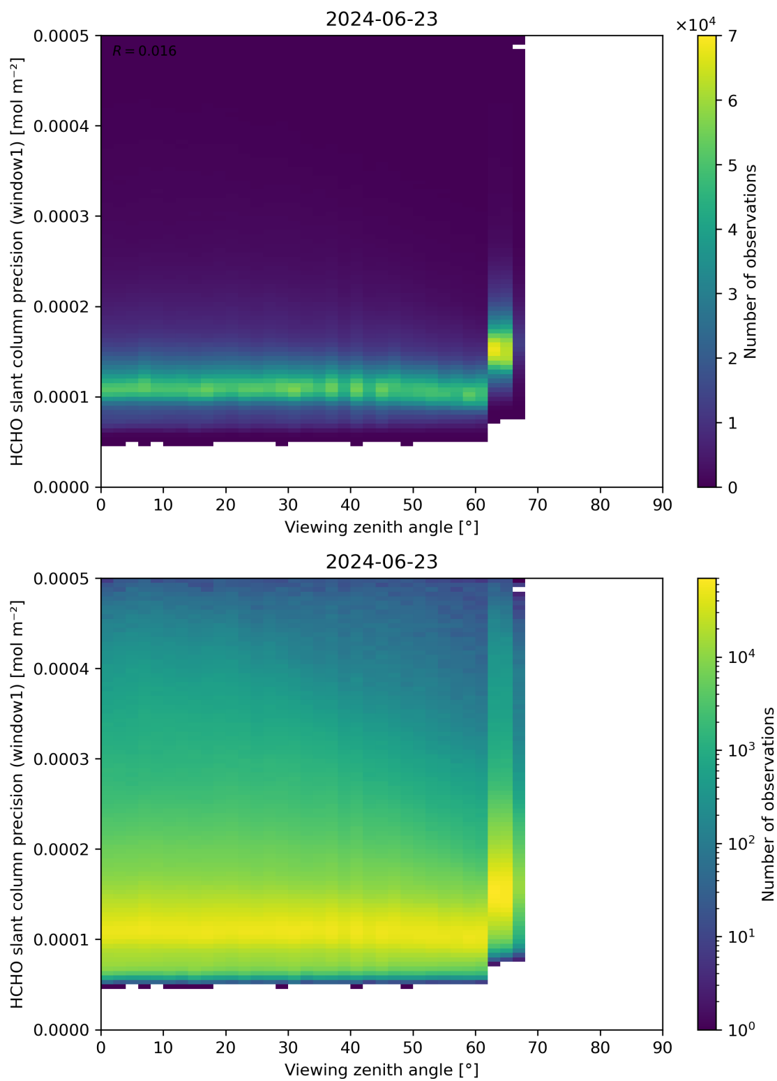
Figure 189: Scatter density plot of “Viewing zenith angle” against “HCHO slant column precision (window1)” for 2024-06-22 to 2024-06-24.
