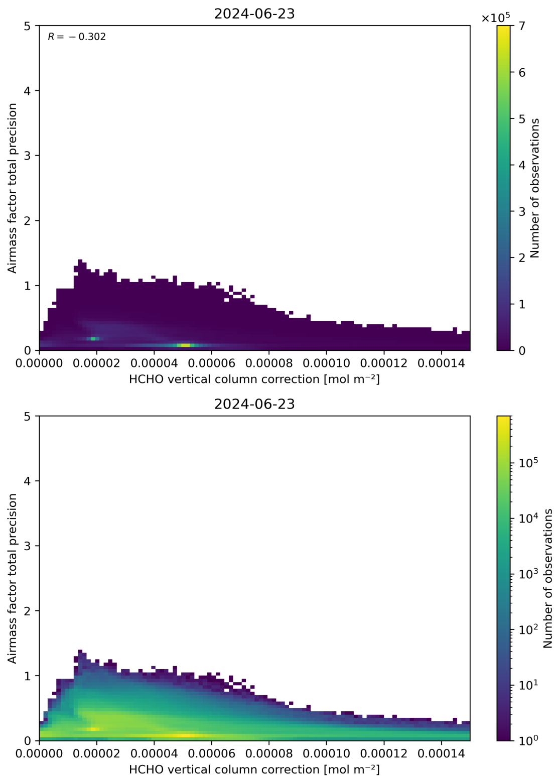
Figure 121: Scatter density plot of “HCHO vertical column correction” against “Airmass factor total precision” for 2024-06-22 to 2024-06-24.
