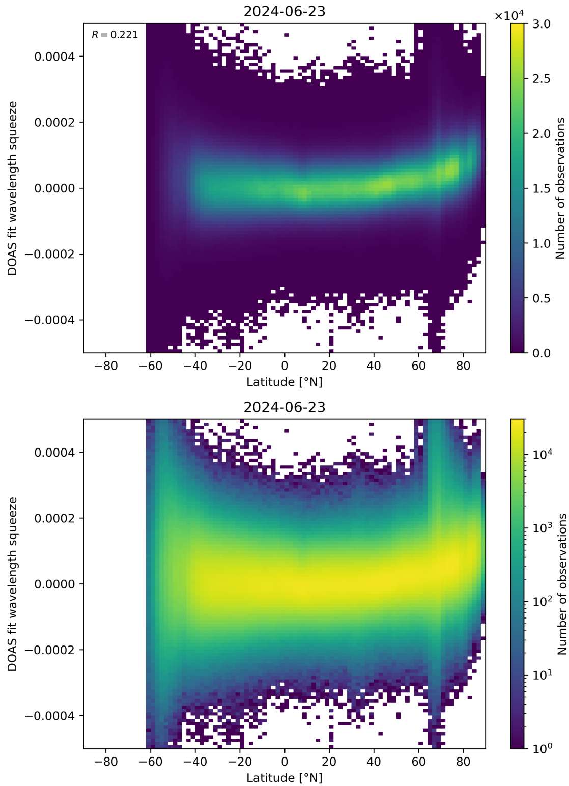
Figure 155: Scatter density plot of “Latitude” against “DOAS fit wavelength squeeze” for 2024-06-22 to 2024-06-24.
