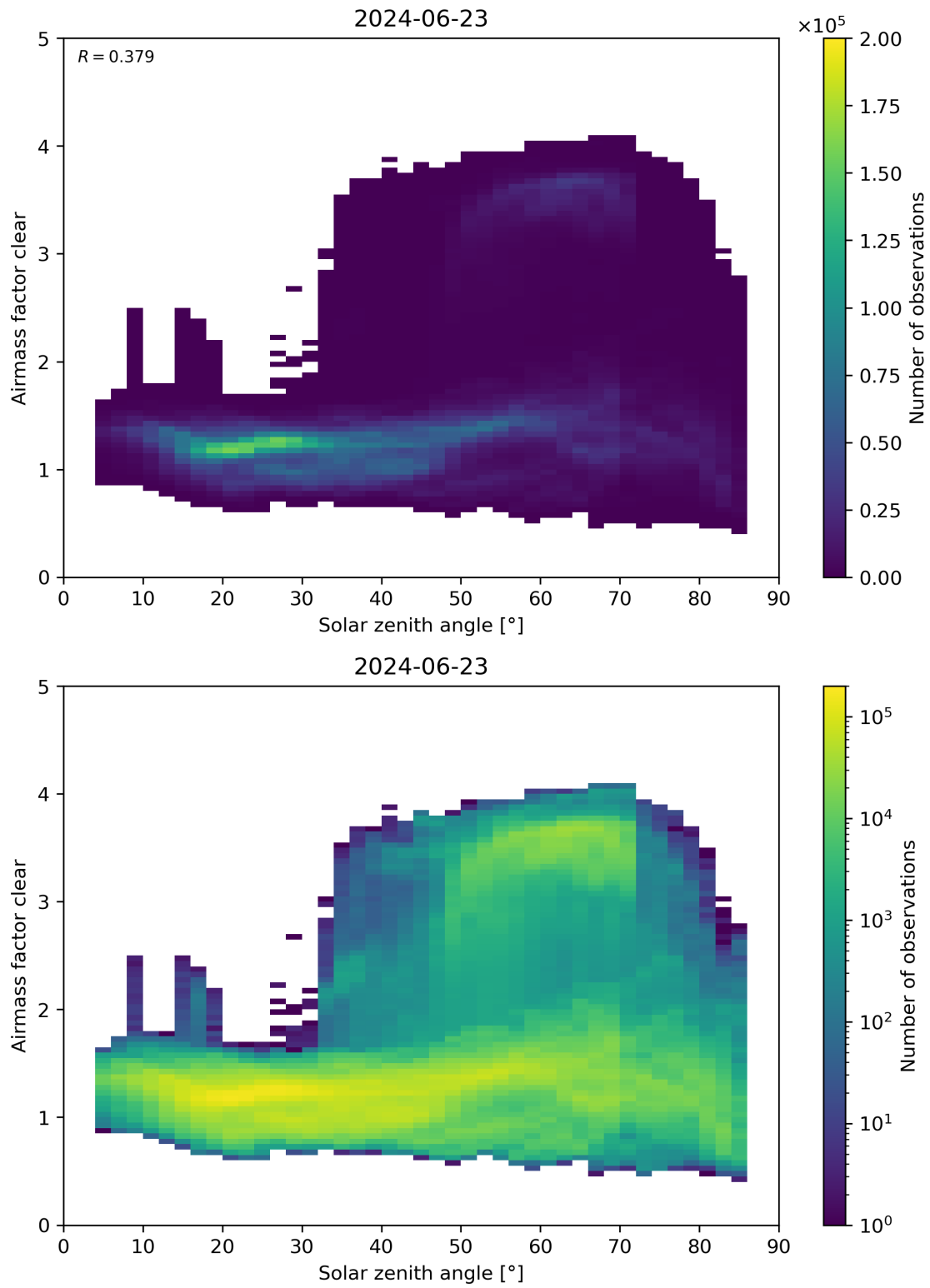
Figure 170: Scatter density plot of “Solar zenith angle” against “Airmass factor clear” for 2024-06-22 to 2024-06-24.
