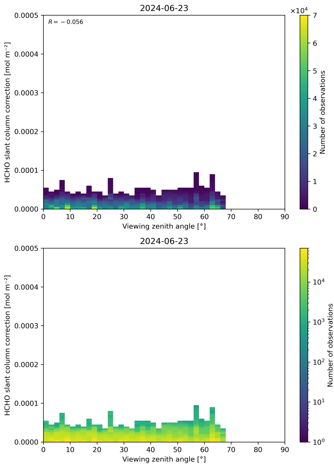
Figure 187: Scatter density plot of “Viewing zenith angle” against “HCHO slant column correction” for 2024-06-22 to 2024-06-24.
