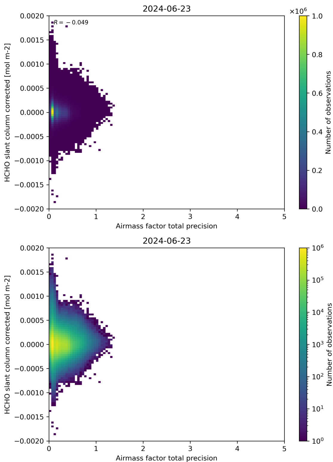
Figure 109: Scatter density plot of “Airmass factor total precision” against “HCHO slant column corrected” for 2024-06-22 to 2024-06-24.
