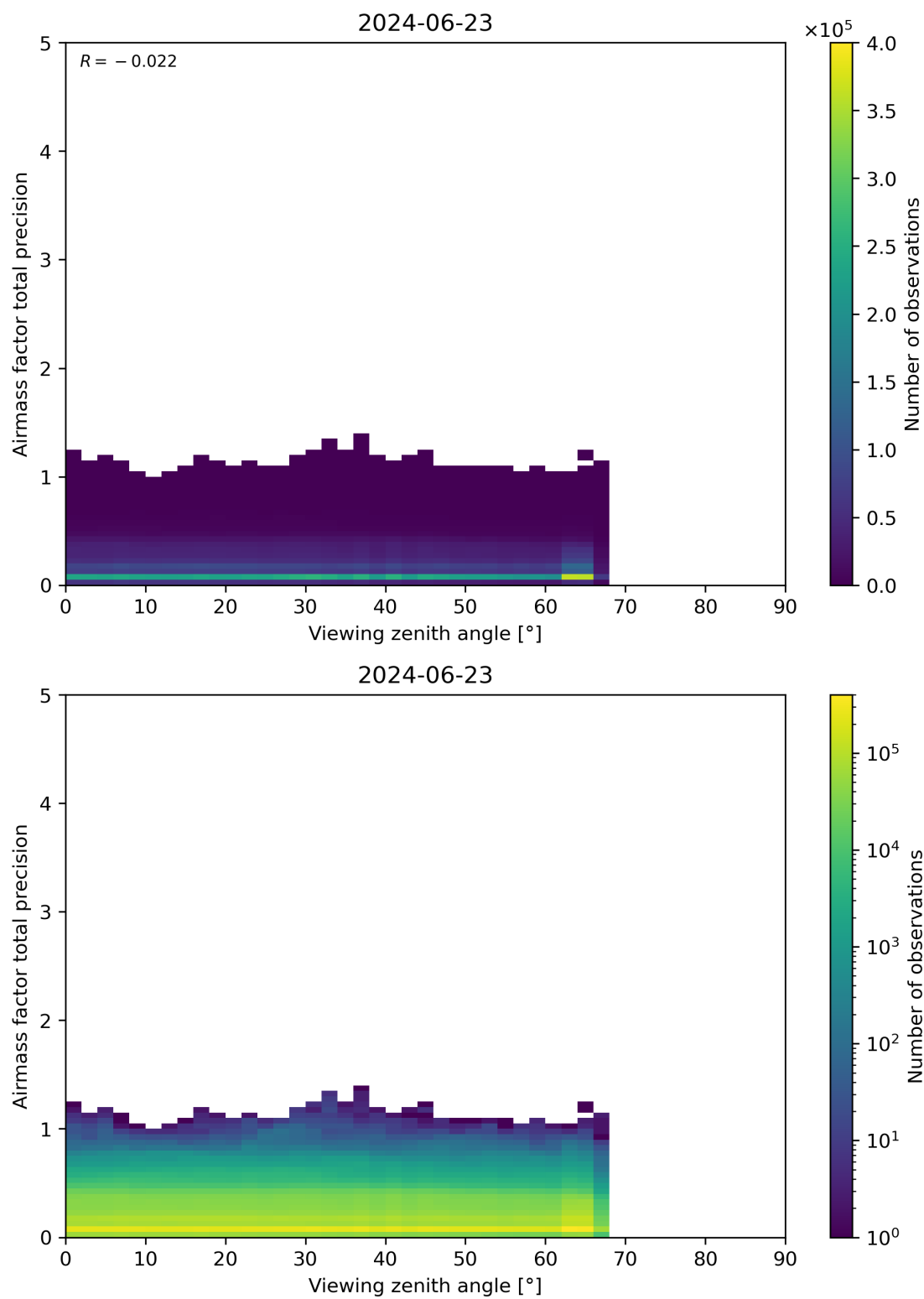
Figure 191: Scatter density plot of “Viewing zenith angle” against “Airmass factor total precision” for 2024-06-22 to 2024-06-24.
