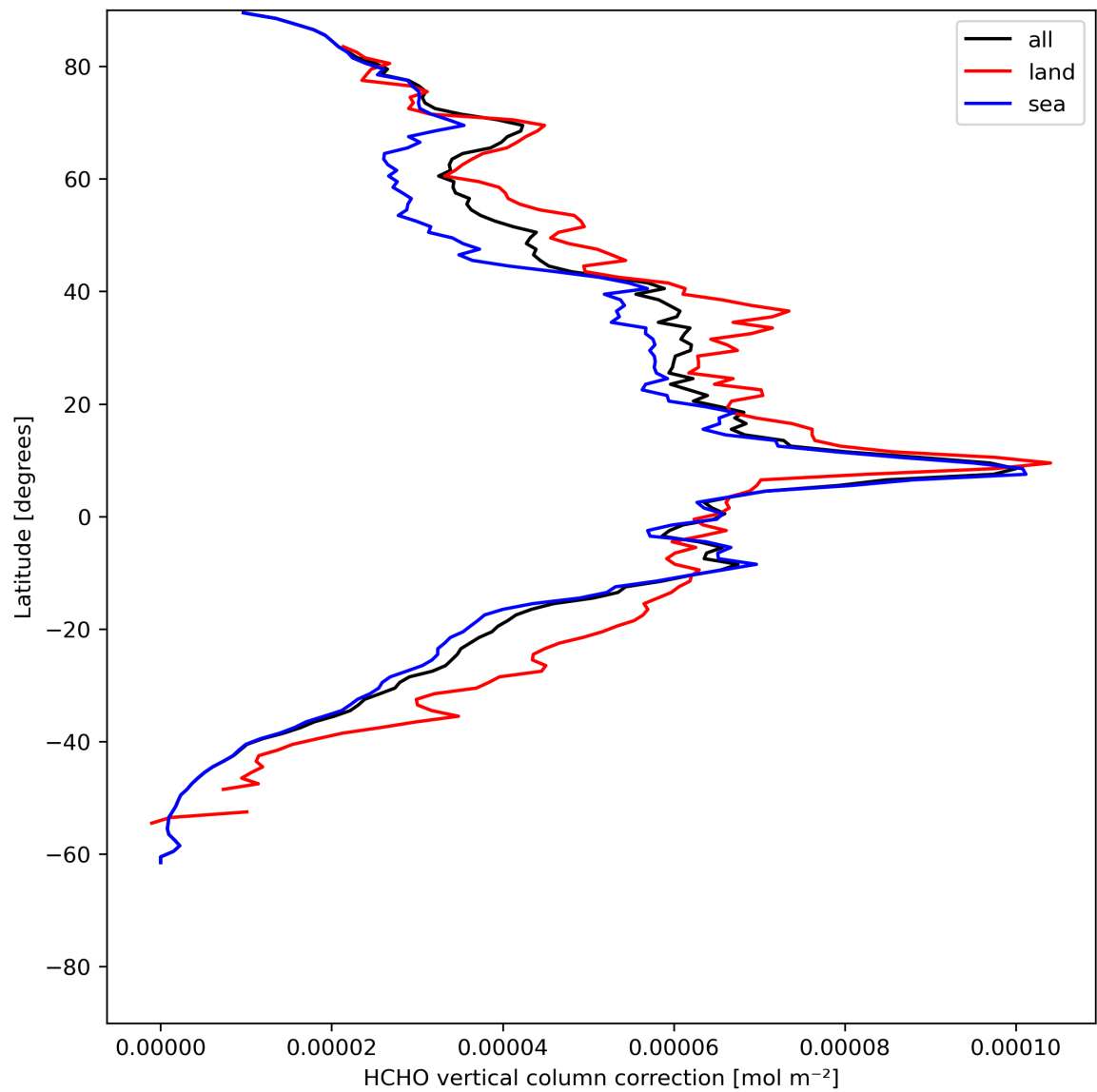
Figure 23: Zonal average of “HCHO vertical column correction” for 2024-06-22 to 2024-06-24.
