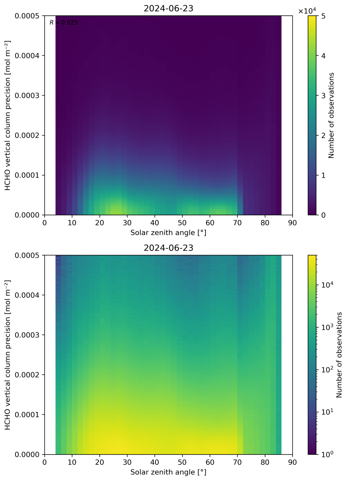
Figure 179: Scatter density plot of “Solar zenith angle” against “HCHO vertical column precision” for 2024-06-22 to 2024-06-24.
