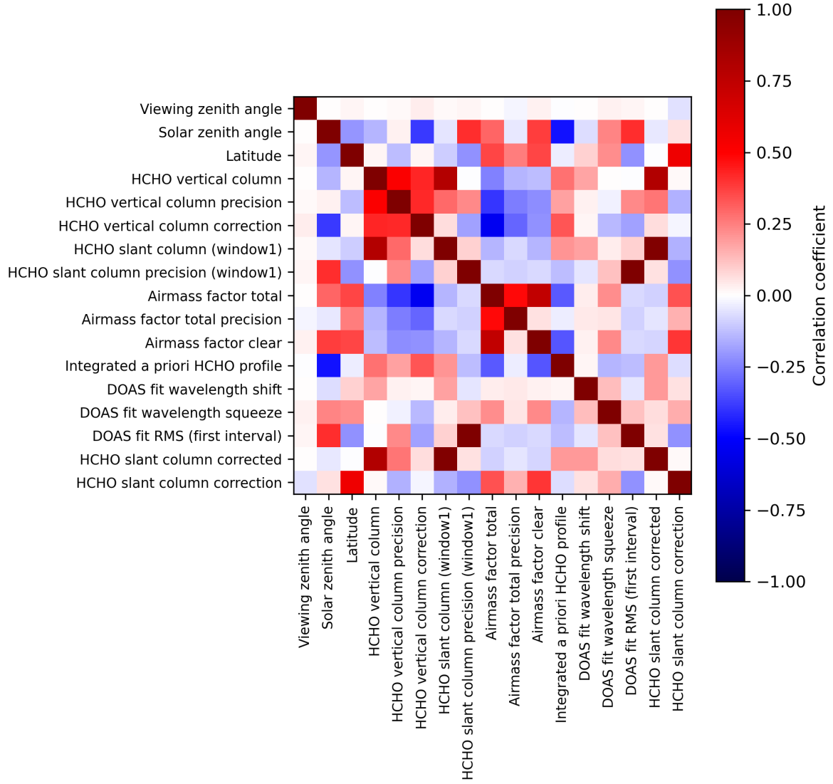
Figure 2: Map of correlation matrix for 2024-06-22 to 2024-06-24.
