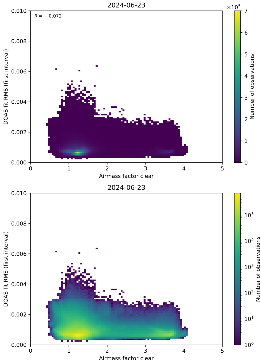
Figure 71: Scatter density plot of “Airmass factor clear” against “DOAS fit RMS (first interval)” for 2024-06-22 to 2024-06-24.
