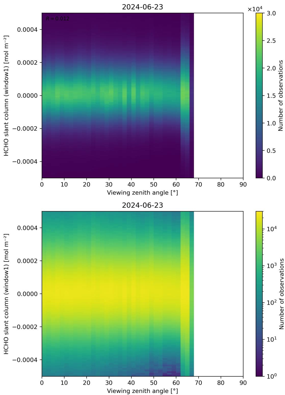
Figure 188: Scatter density plot of “Viewing zenith angle” against “HCHO slant column (window1)” for 2024-06-22 to 2024-06-24.
