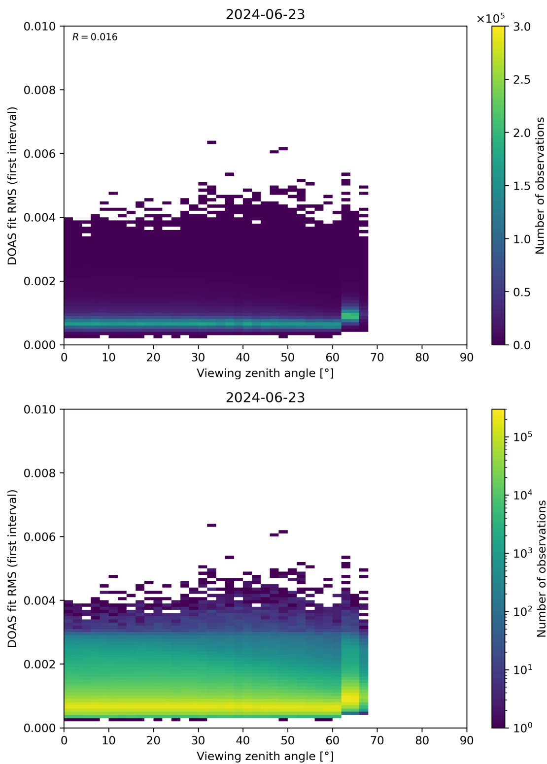
Figure 182: Scatter density plot of “Viewing zenith angle” against “DOAS fit RMS (first interval)” for 2024-06-22 to 2024-06-24.
