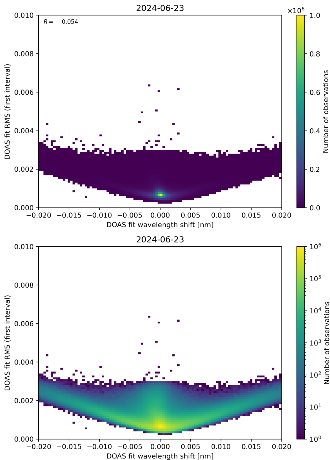
Figure 64: Scatter density plot of “DOAS fit wavelength shift” against “DOAS fit RMS (first interval)” for 2024-06-22 to 2024-06-24.
