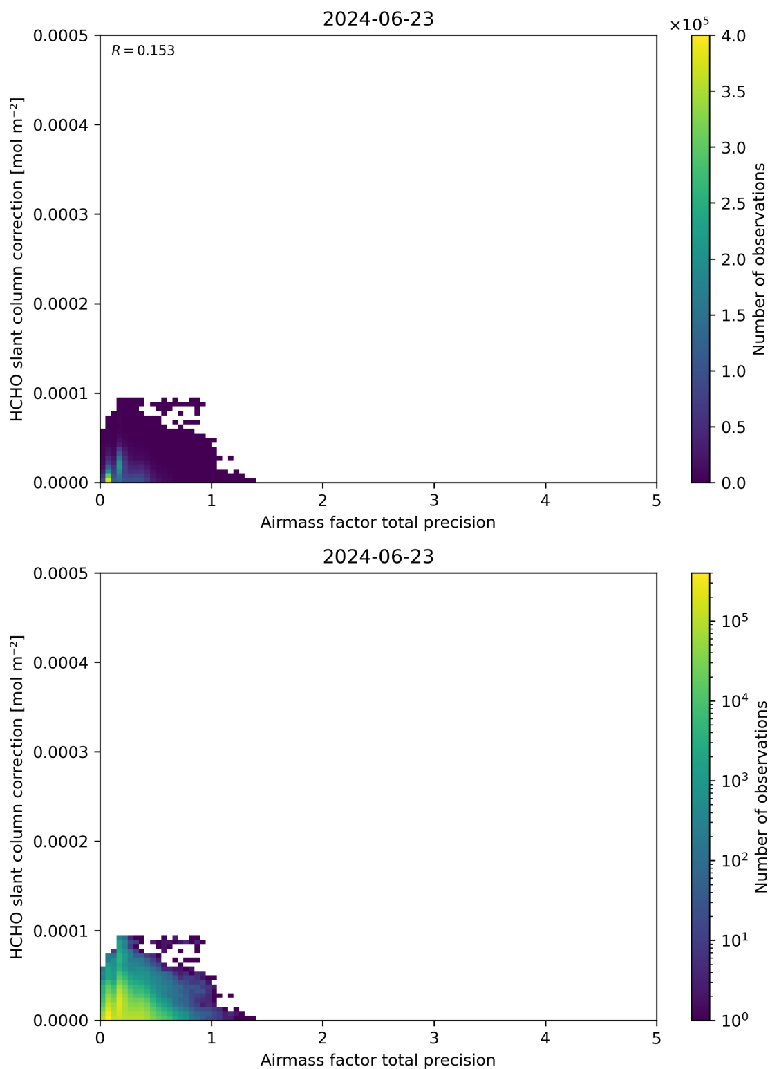
Figure 110: Scatter density plot of “Airmass factor total precision” against “HCHO slant column correction” for 2024-06-22 to 2024-06-24.
