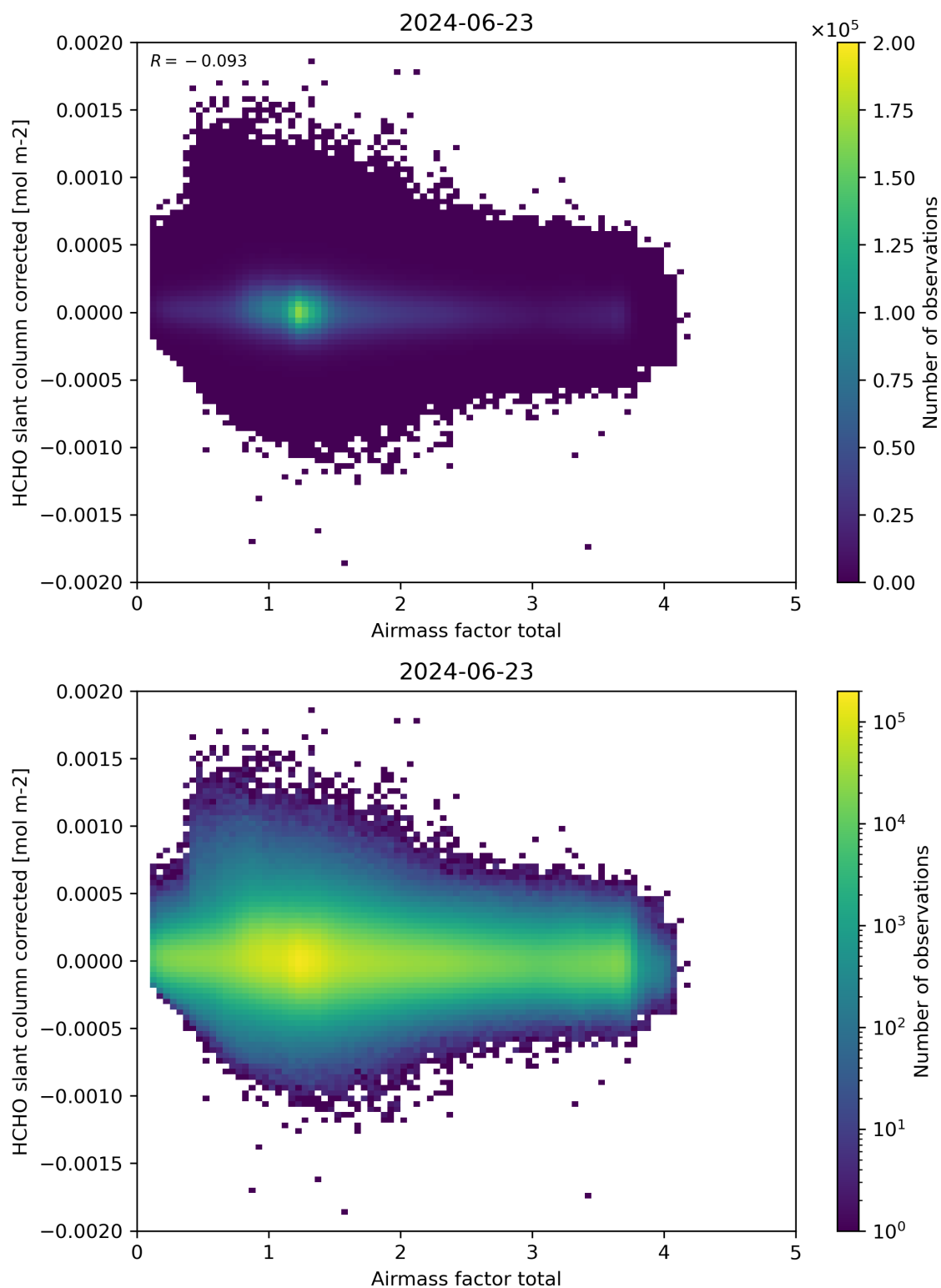
Figure 101: Scatter density plot of “Airmass factor total” against “HCHO slant column corrected” for 2024-06-22 to 2024-06-24.
