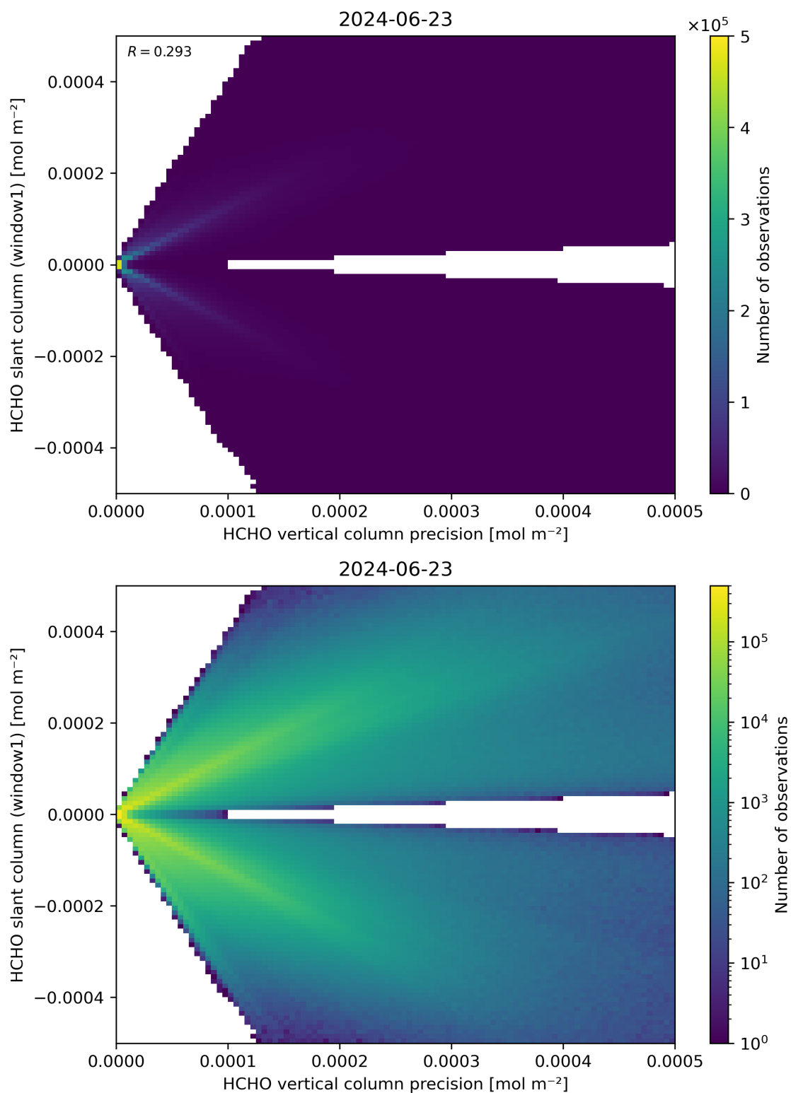
Figure 142: Scatter density plot of “HCHO vertical column precision” against “HCHO slant column (window1)” for 2024-06-22 to 2024-06-24.
