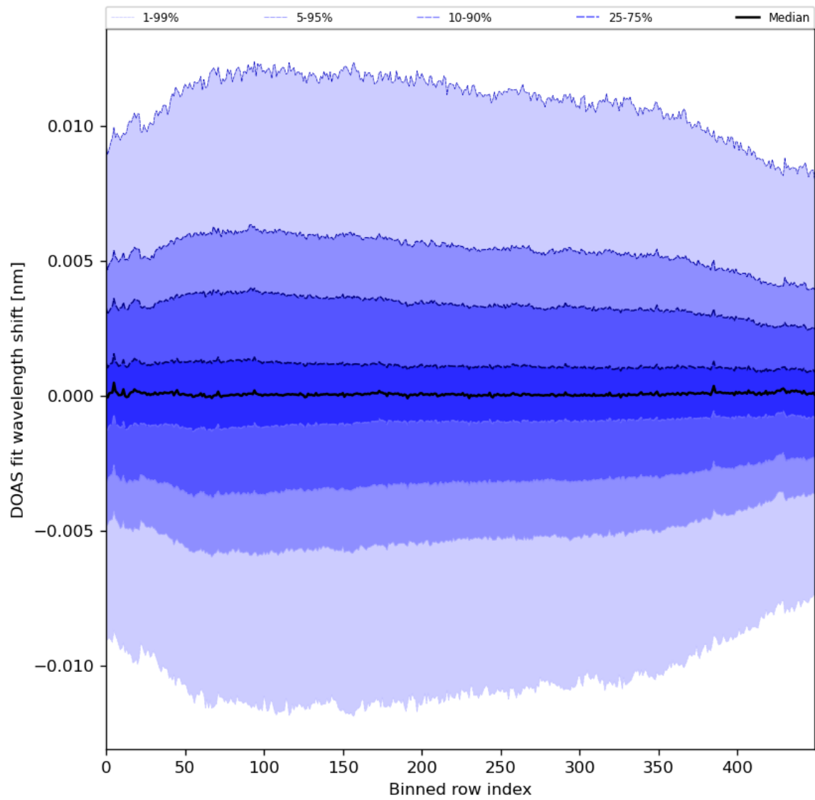
Figure 58: Along track statistics of “DOAS fit wavelength shift” for 2024-06-22 to 2024-06-24
