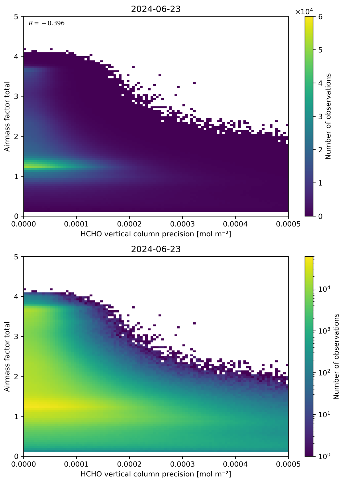
Figure 144: Scatter density plot of “HCHO vertical column precision” against “Airmass factor total” for 2024-06-22 to 2024-06-24.
