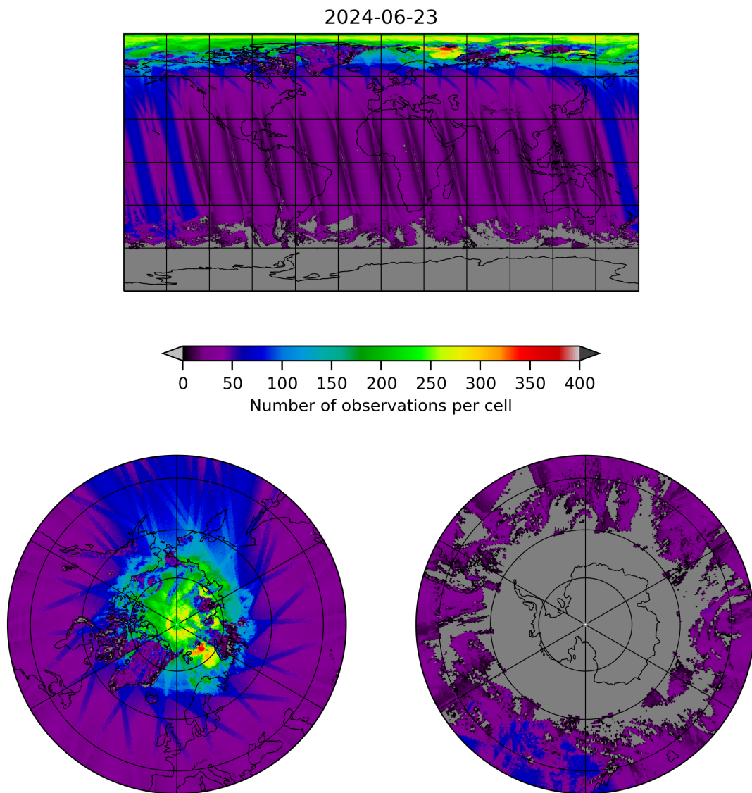
Figure 19: Map of the number of observations for 2024-06-22 to 2024-06-24
