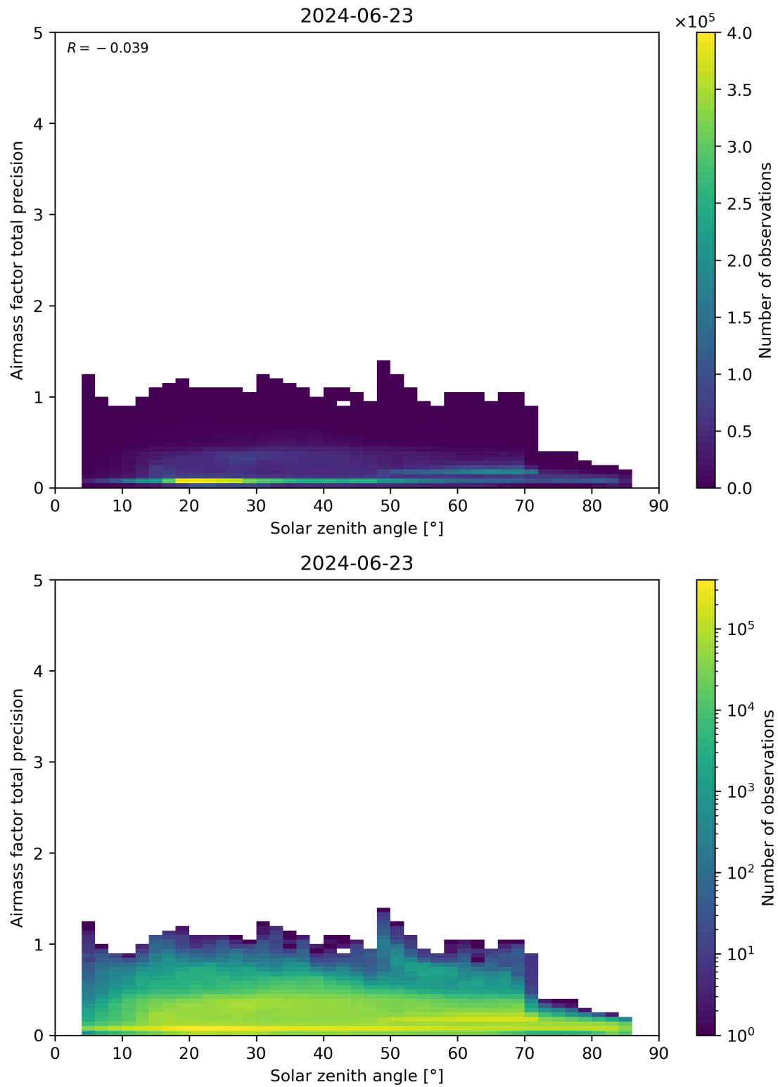
Figure 176: Scatter density plot of “Solar zenith angle” against “Airmass factor total precision” for 2024-06-22 to 2024-06-24.
