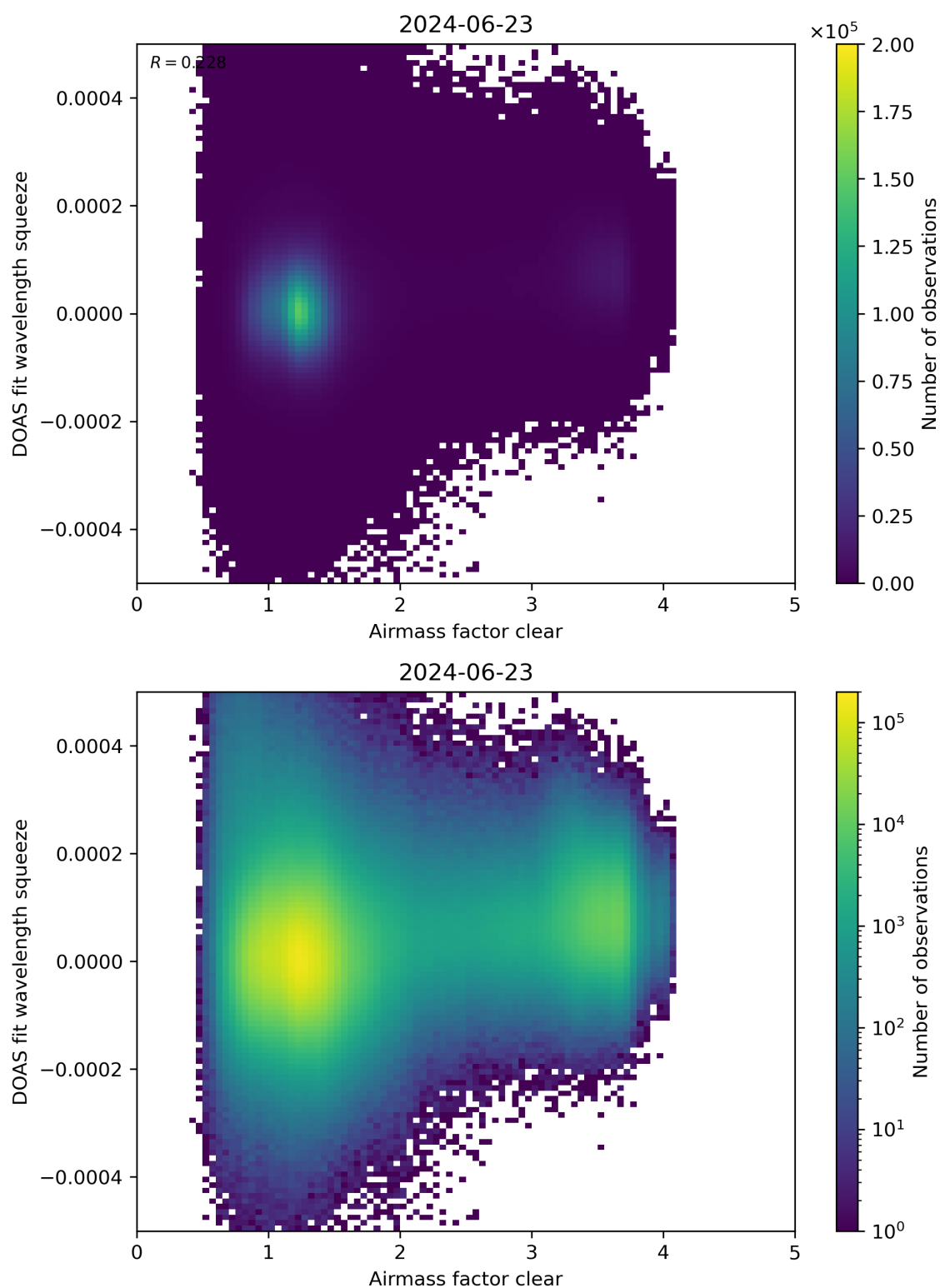
Figure 73: Scatter density plot of “Airmass factor clear” against “DOAS fit wavelength squeeze” for 2024-06-22 to 2024-06-24.
