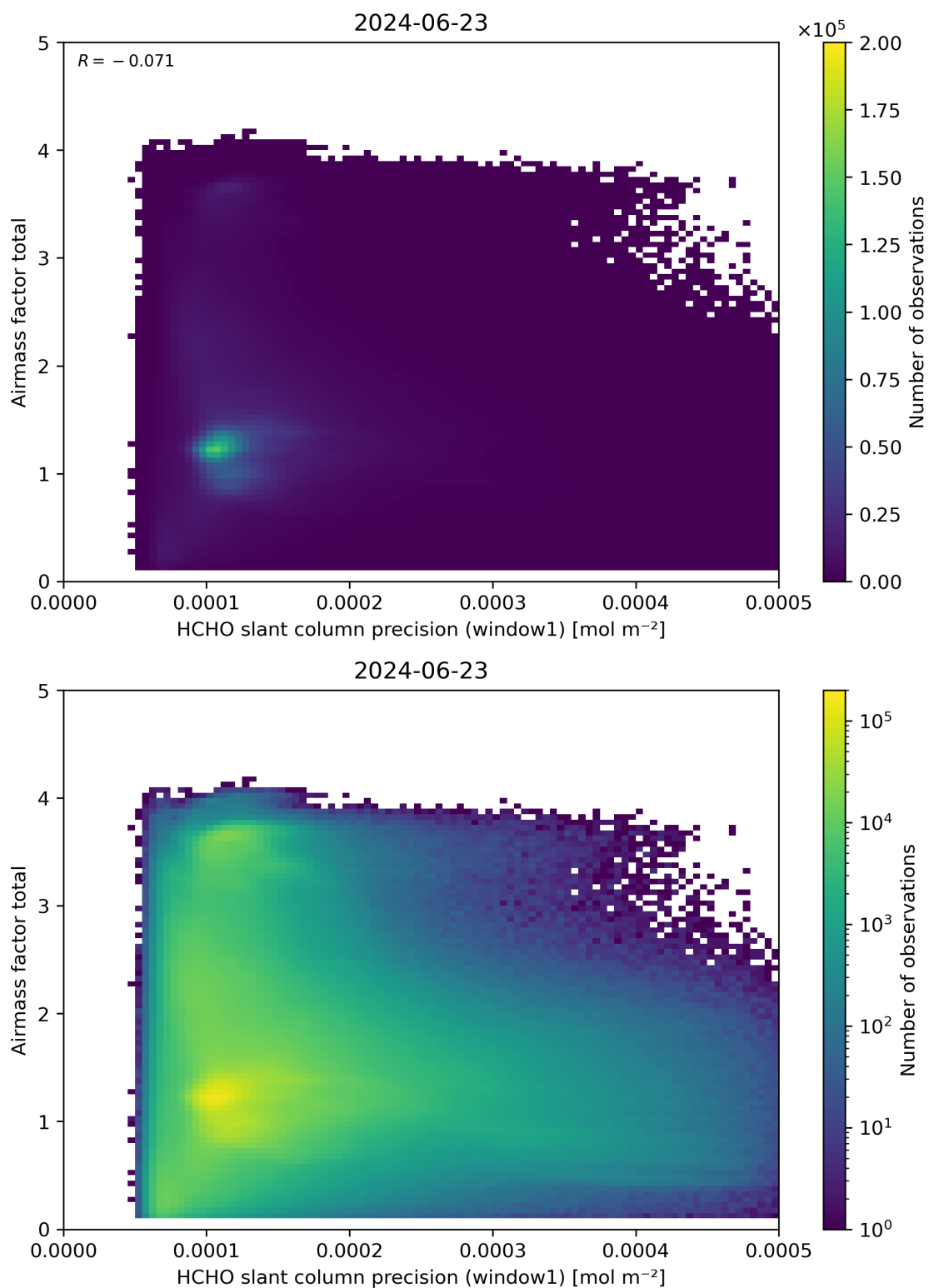
Figure 94: Scatter density plot of “HCHO slant column precision (window1)” against “Airmass factor total” for 2024-06-22 to 2024-06-24.
