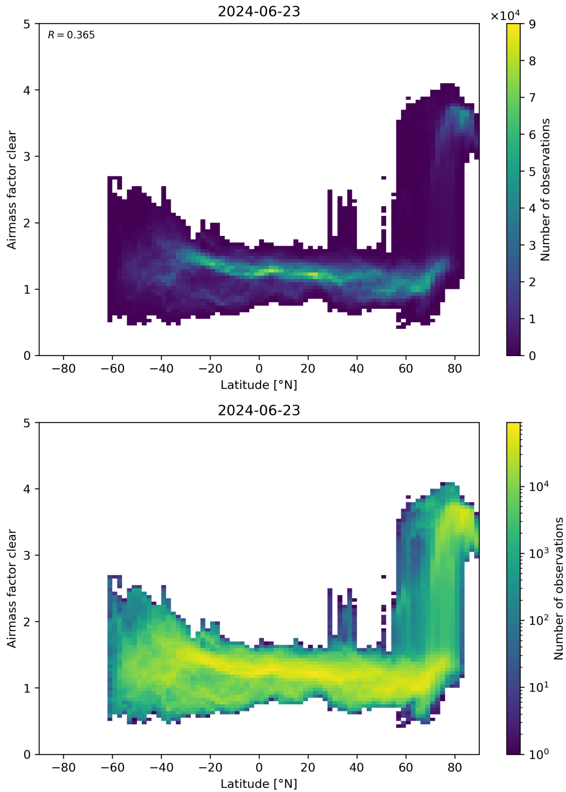
Figure 156: Scatter density plot of “Latitude” against “Airmass factor clear” for 2024-06-22 to 2024-06-24.
