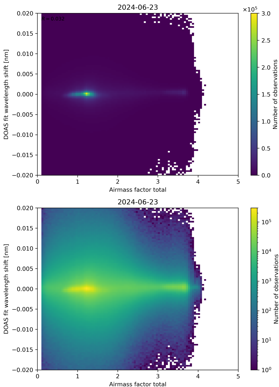
Figure 98: Scatter density plot of “Airmass factor total” against “DOAS fit wavelength shift” for 2024-06-22 to 2024-06-24.
