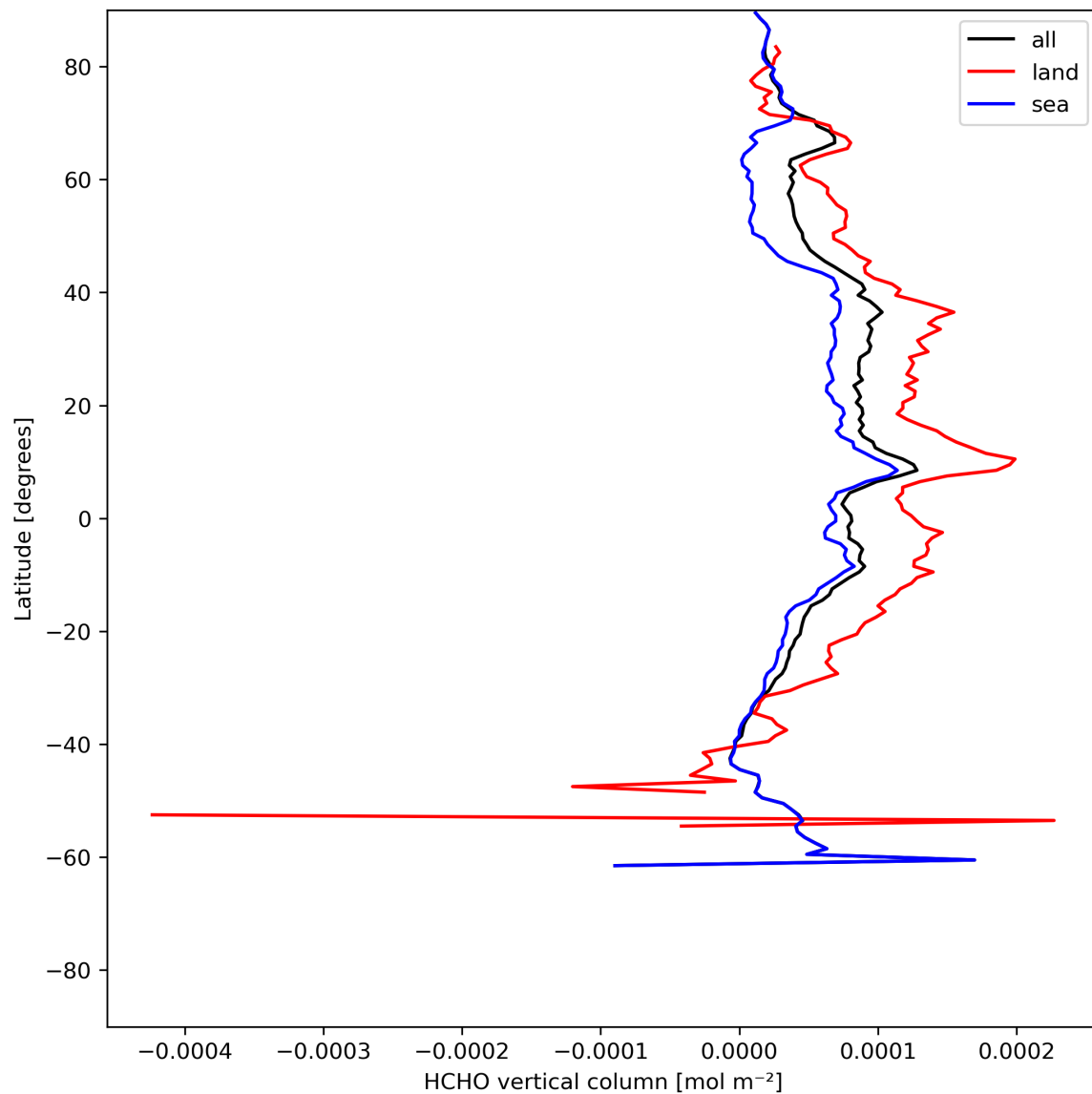
Figure 21: Zonal average of “HCHO vertical column” for 2024-06-22 to 2024-06-24.
