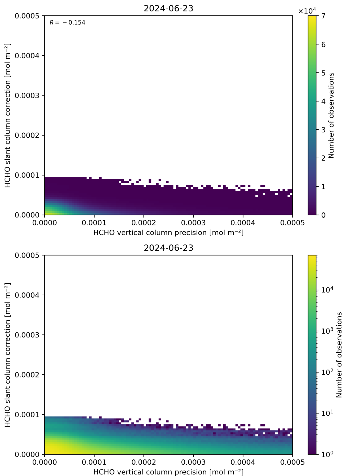
Figure 141: Scatter density plot of “HCHO vertical column precision” against “HCHO slant column correction” for 2024-06-22 to 2024-06-24.
