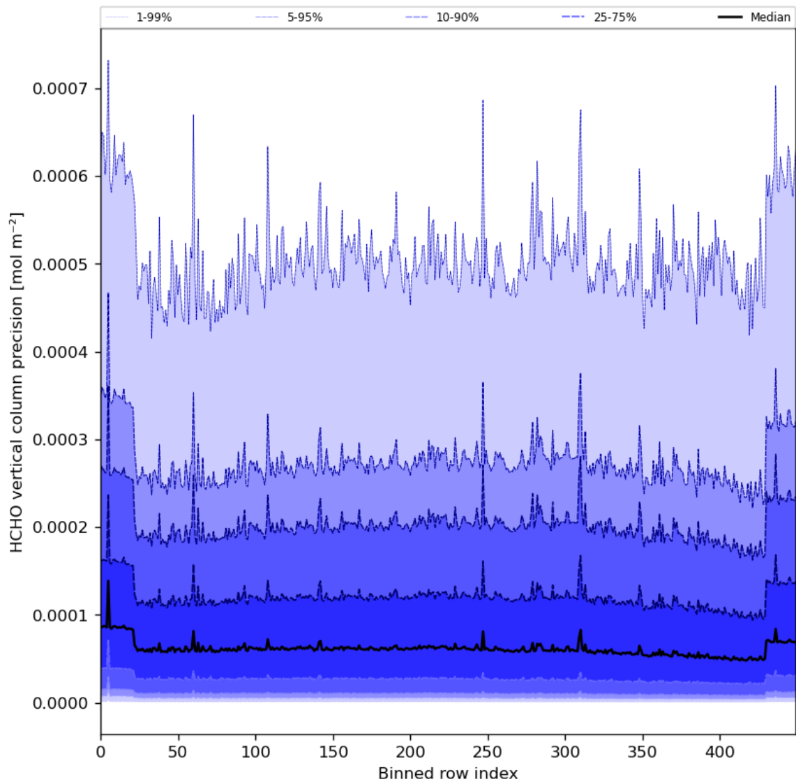
Figure 50: Along track statistics of “HCHO vertical column precision” for 2024-06-22 to 2024-06-24
