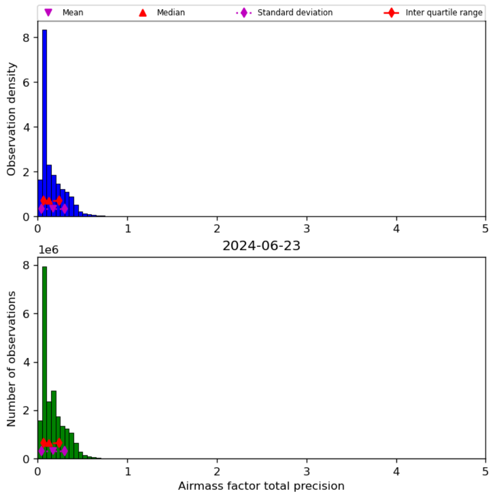
Figure 41: Histogram of “Airmass factor total precision” for 2024-06-22 to 2024-06-24
