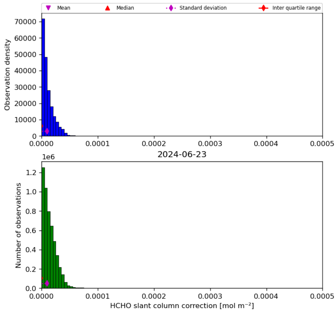
Figure 47: Histogram of “HCHO slant column correction” for 2024-06-22 to 2024-06-24
