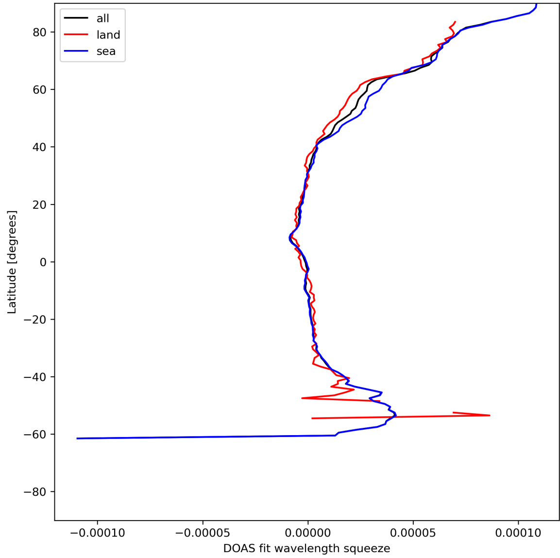
Figure 31: Zonal average of “DOAS fit wavelength squeeze” for 2024-06-22 to 2024-06-24.
