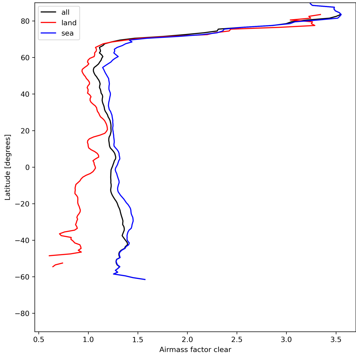
Figure 28: Zonal average of “Airmass factor clear” for 2024-06-22 to 2024-06-24.
