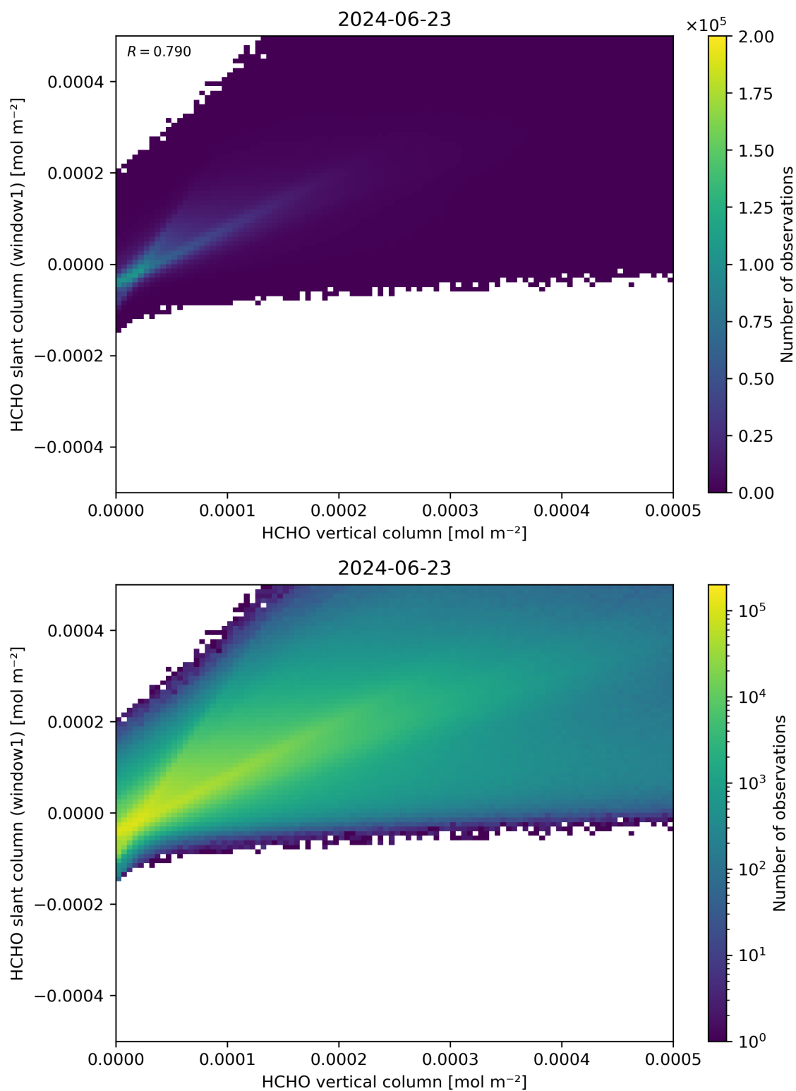
Figure 129: Scatter density plot of “HCHO vertical column” against “HCHO slant column (window1)” for 2024-06-22 to 2024-06-24.
