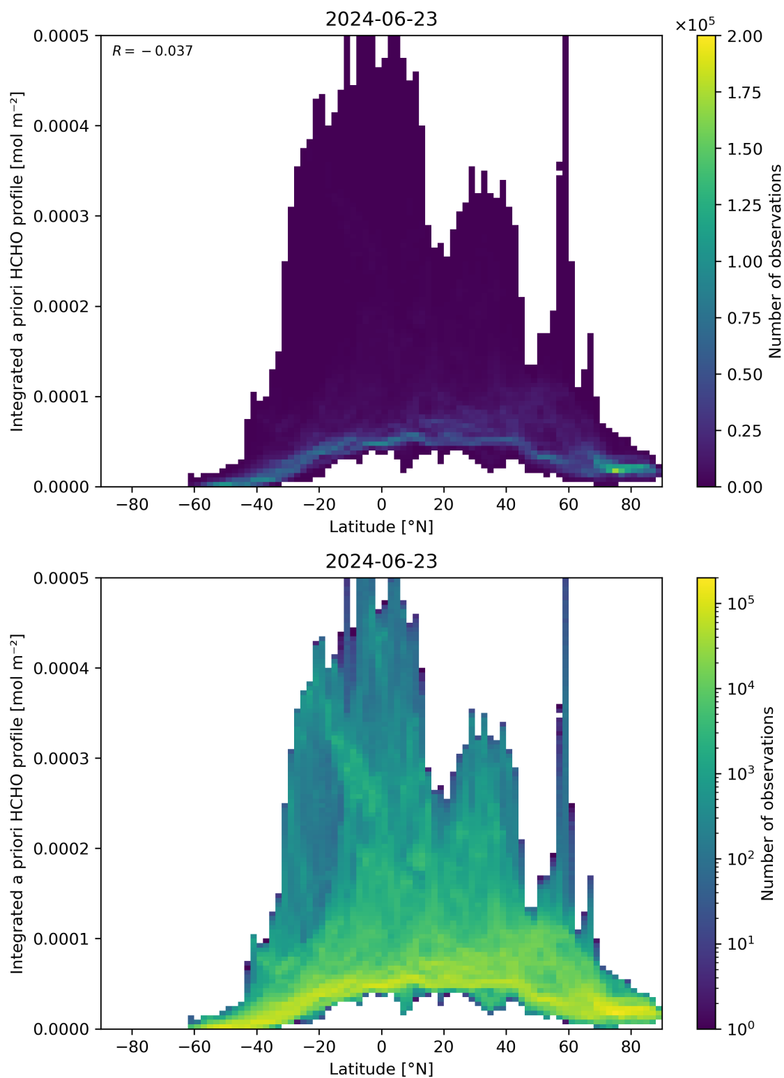
Figure 166: Scatter density plot of “Latitude” against “Integrated a priori HCHO profile” for 2024-06-22 to 2024-06-24.
