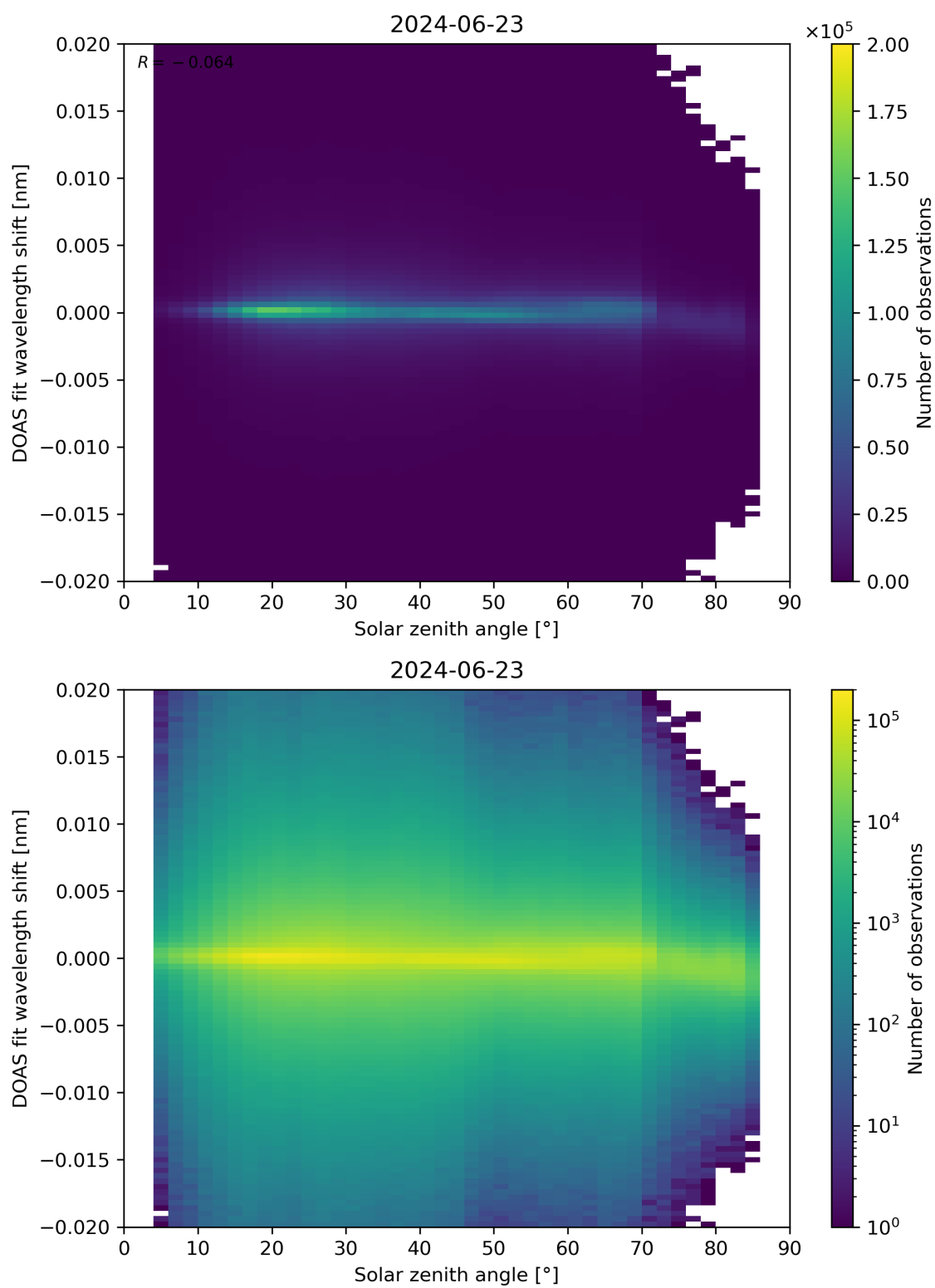
Figure 168: Scatter density plot of “Solar zenith angle” against “DOAS fit wavelength shift” for 2024-06-22 to 2024-06-24.
