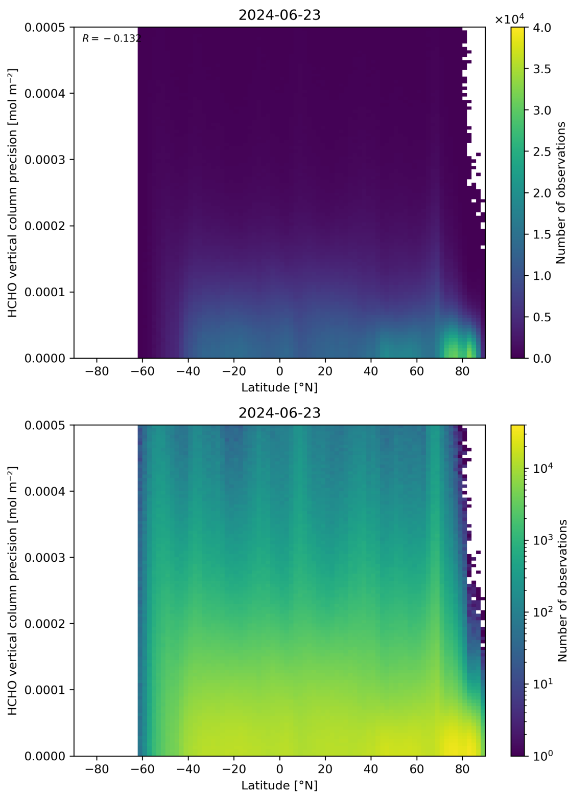
Figure 165: Scatter density plot of “Latitude” against “HCHO vertical column precision” for 2024-06-22 to 2024-06-24.
