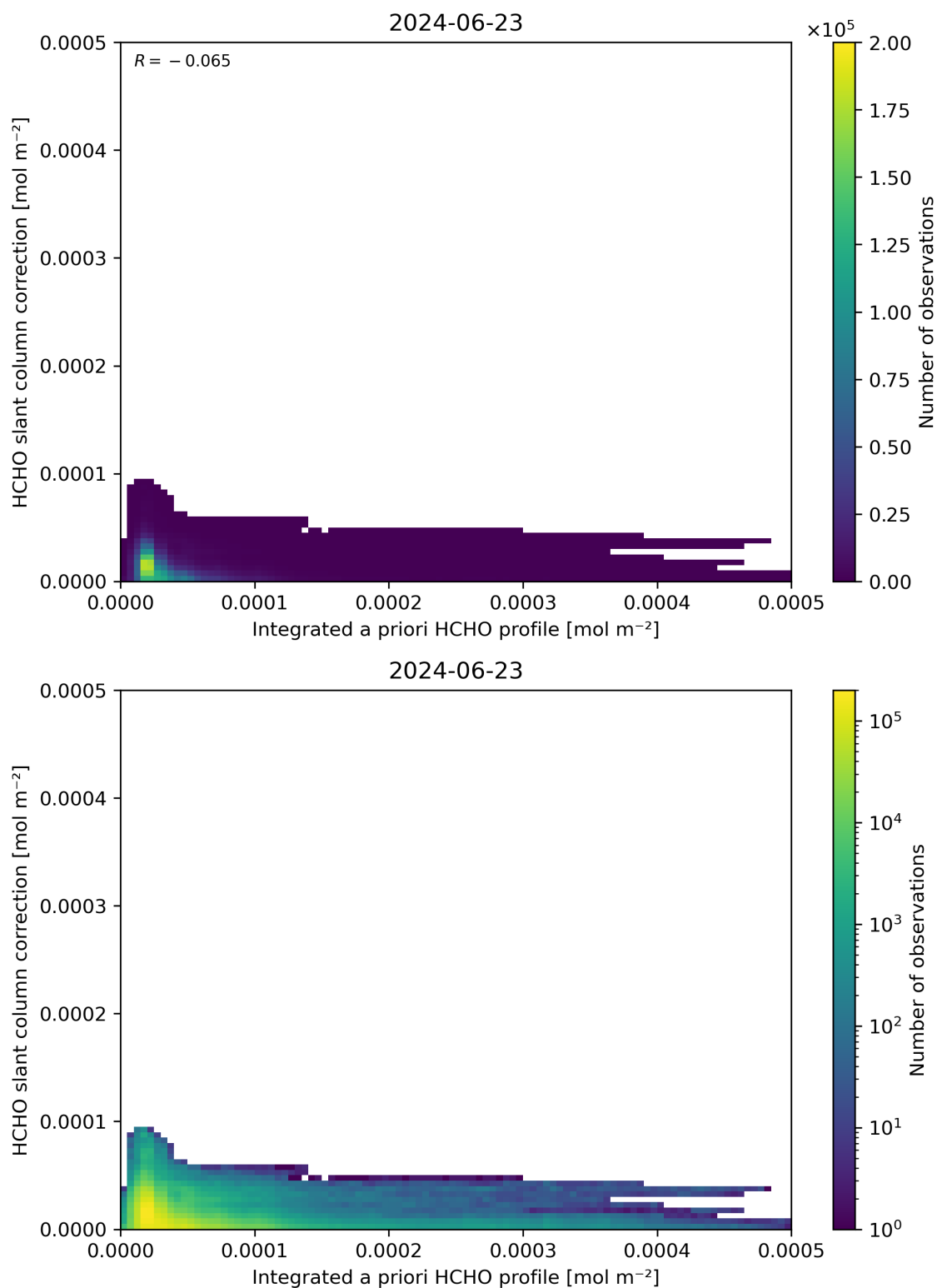
Figure 152: Scatter density plot of “Integrated a priori HCHO profile” against “HCHO slant column correction” for 2024-06-22 to 2024-06-24.
