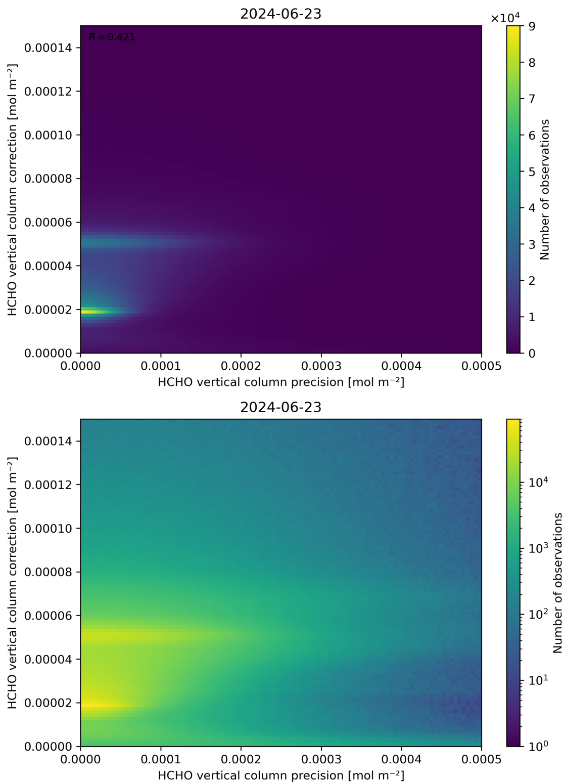
Figure 146: Scatter density plot of “HCHO vertical column precision” against “HCHO vertical column correction” for 2024-06-22 to 2024-06-24.
