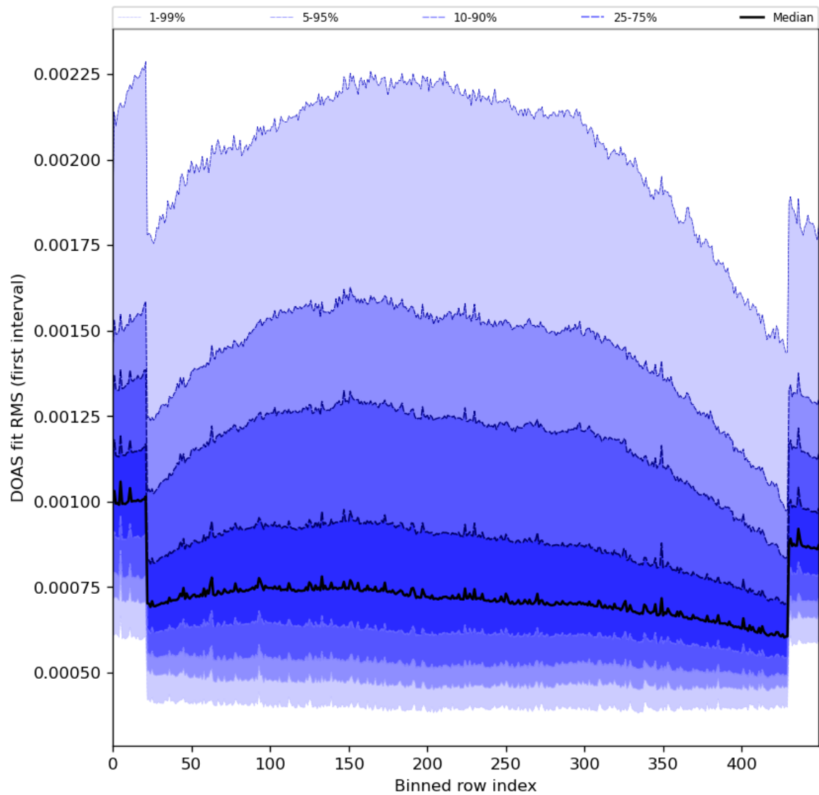
Figure 60: Along track statistics of “DOAS fit RMS (first interval)” for 2024-06-22 to 2024-06-24
