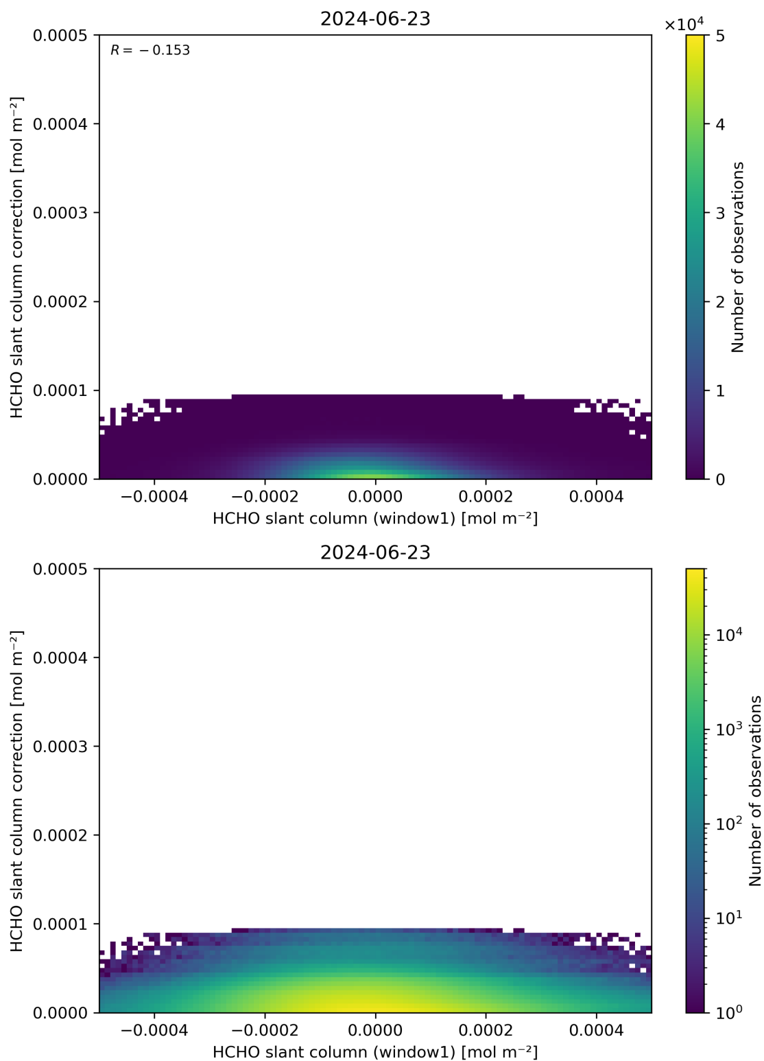
Figure 83: Scatter density plot of “HCHO slant column (window1)” against “HCHO slant column correction” for 2024-06-22 to 2024-06-24.
