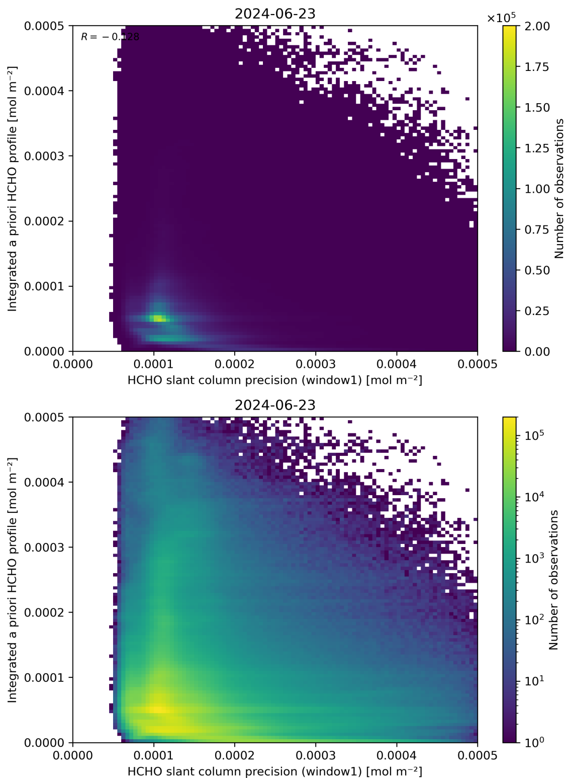
Figure 96: Scatter density plot of “HCHO slant column precision (window1)” against “Integrated a priori HCHO profile” for 2024-06-22 to 2024-06-24.
