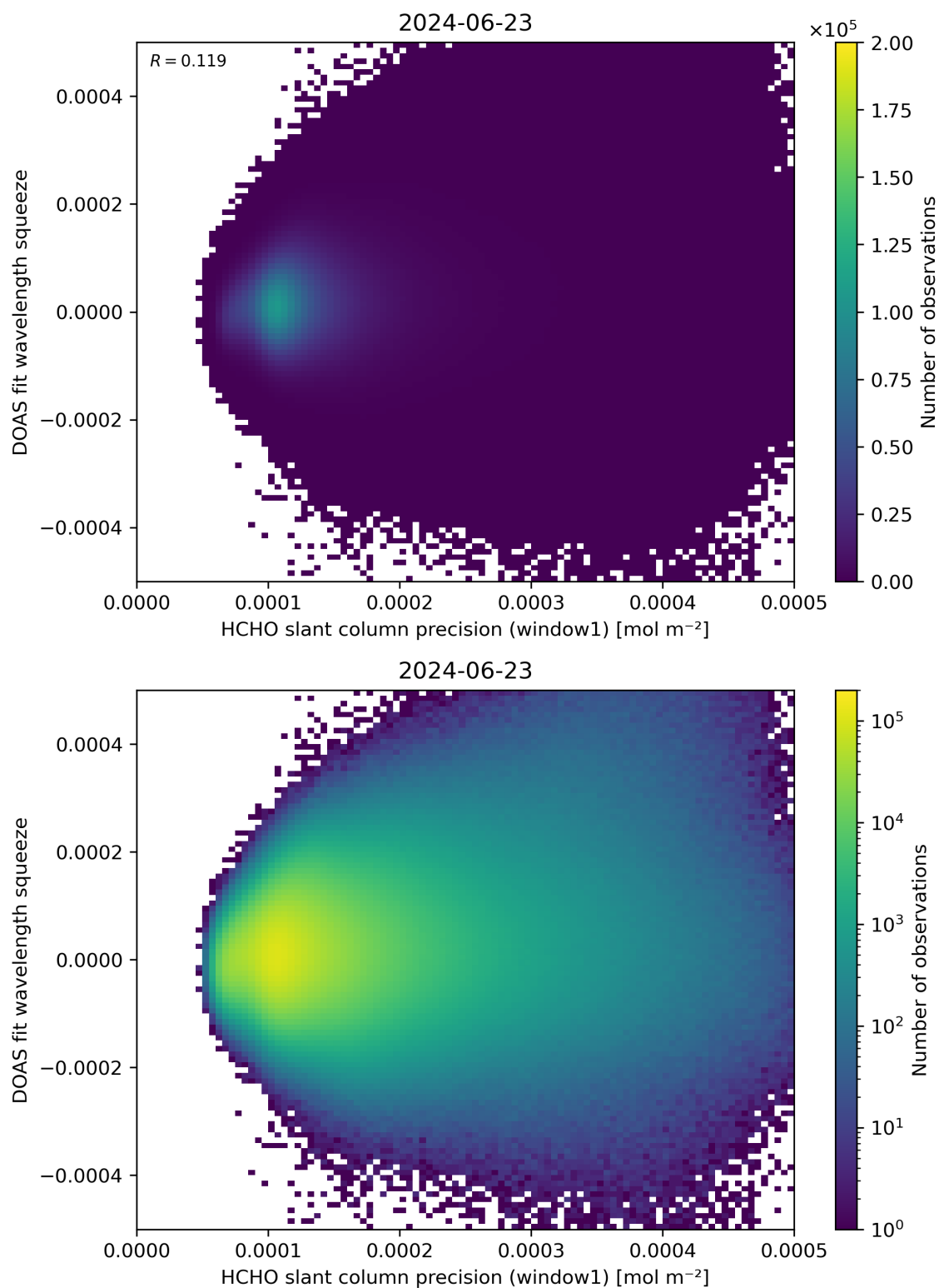
Figure 90: Scatter density plot of “HCHO slant column precision (window1)” against “DOAS fit wavelength squeeze” for 2024-06-22 to 2024-06-24.
