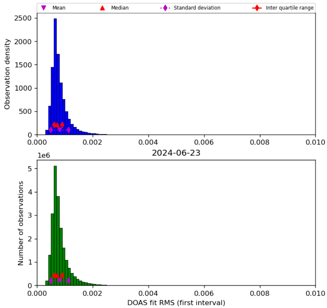
Figure 46: Histogram of “DOAS fit RMS (first interval)” for 2024-06-22 to 2024-06-24
