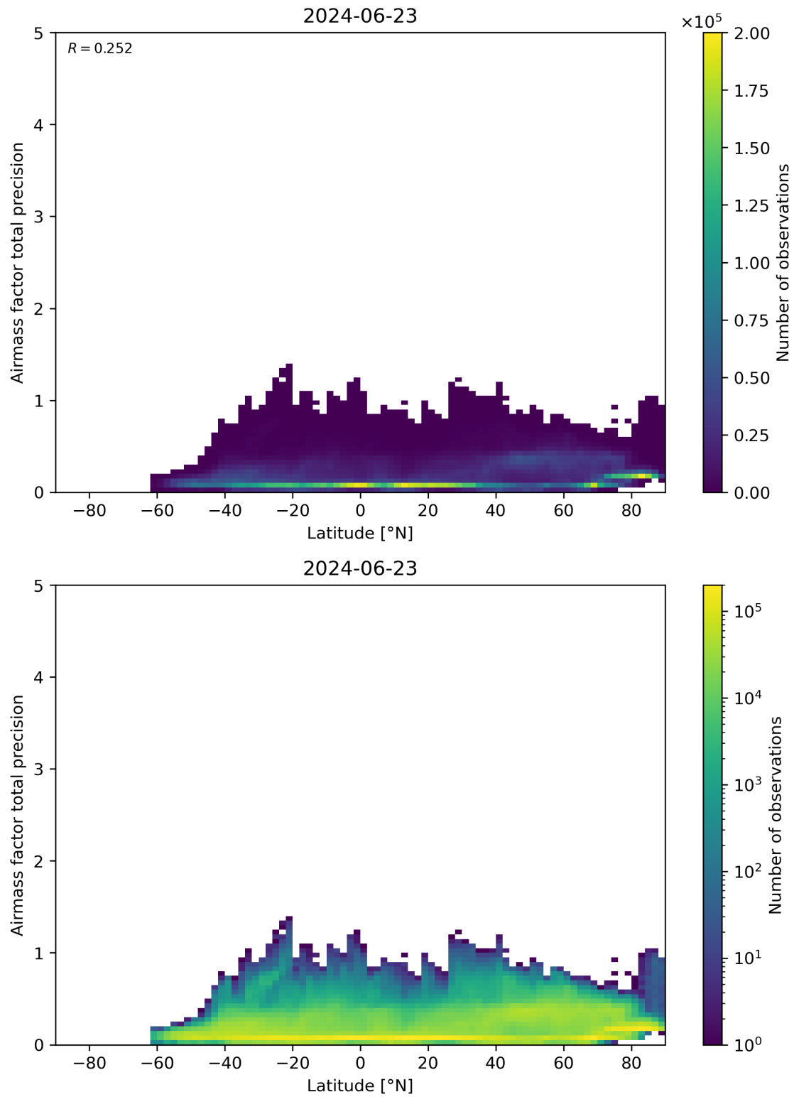
Figure 162: Scatter density plot of “Latitude” against “Airmass factor total precision” for 2024-06-22 to 2024-06-24.
