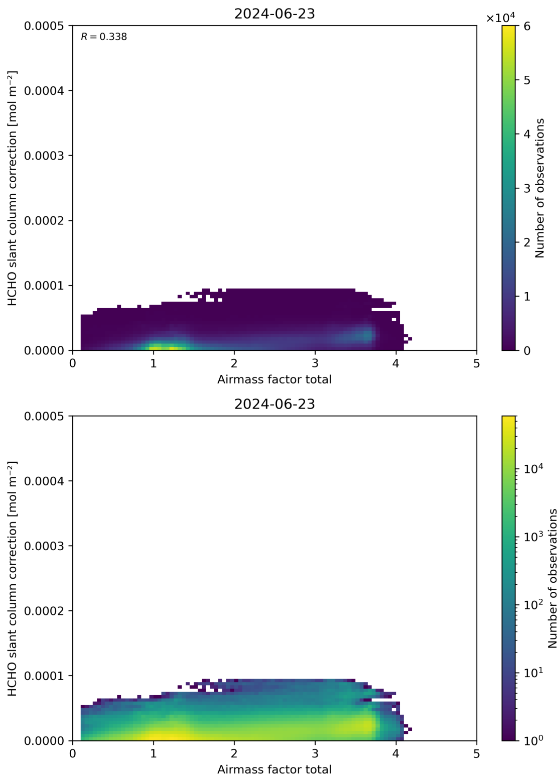
Figure 102: Scatter density plot of “Airmass factor total” against “HCHO slant column correction” for 2024-06-22 to 2024-06-24.
