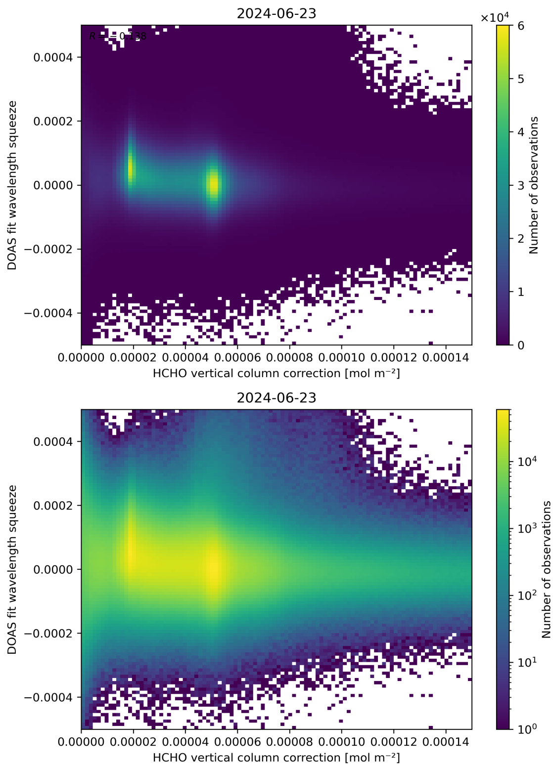
Figure 114: Scatter density plot of “HCHO vertical column correction” against “DOAS fit wavelength squeeze” for 2024-06-22 to 2024-06-24.
