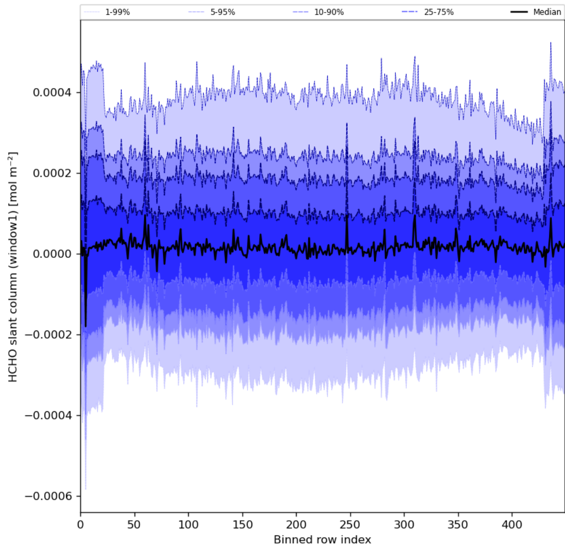
Figure 52: Along track statistics of "HCHO slant column (window1)" for 2024-06-22 to 2024-06-24
