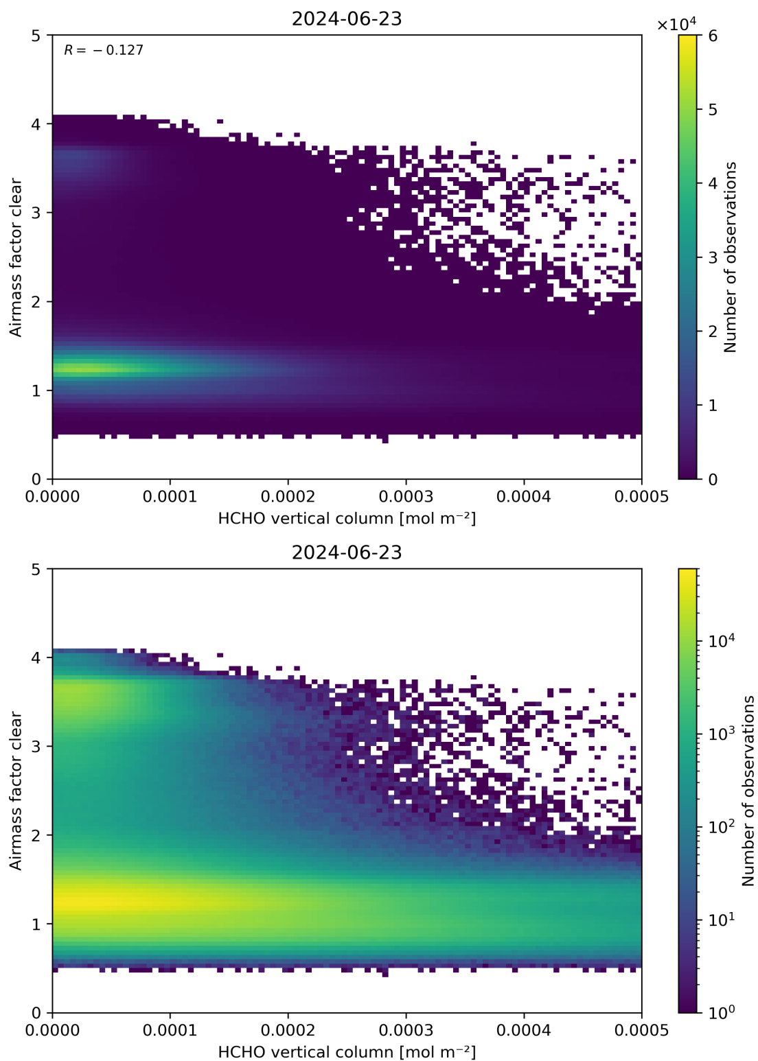
Figure 126: Scatter density plot of “HCHO vertical column” against “Airmass factor clear” for 2024-06-22 to 2024-06-24.
