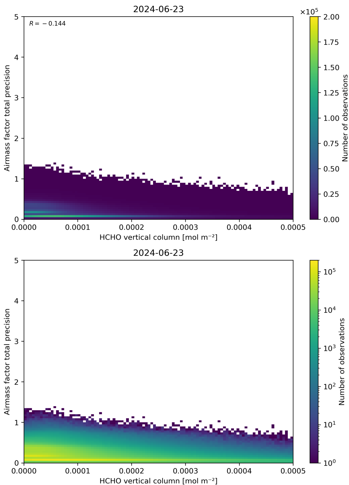
Figure 132: Scatter density plot of “HCHO vertical column” against “Airmass factor total precision” for 2024-06-22 to 2024-06-24.
