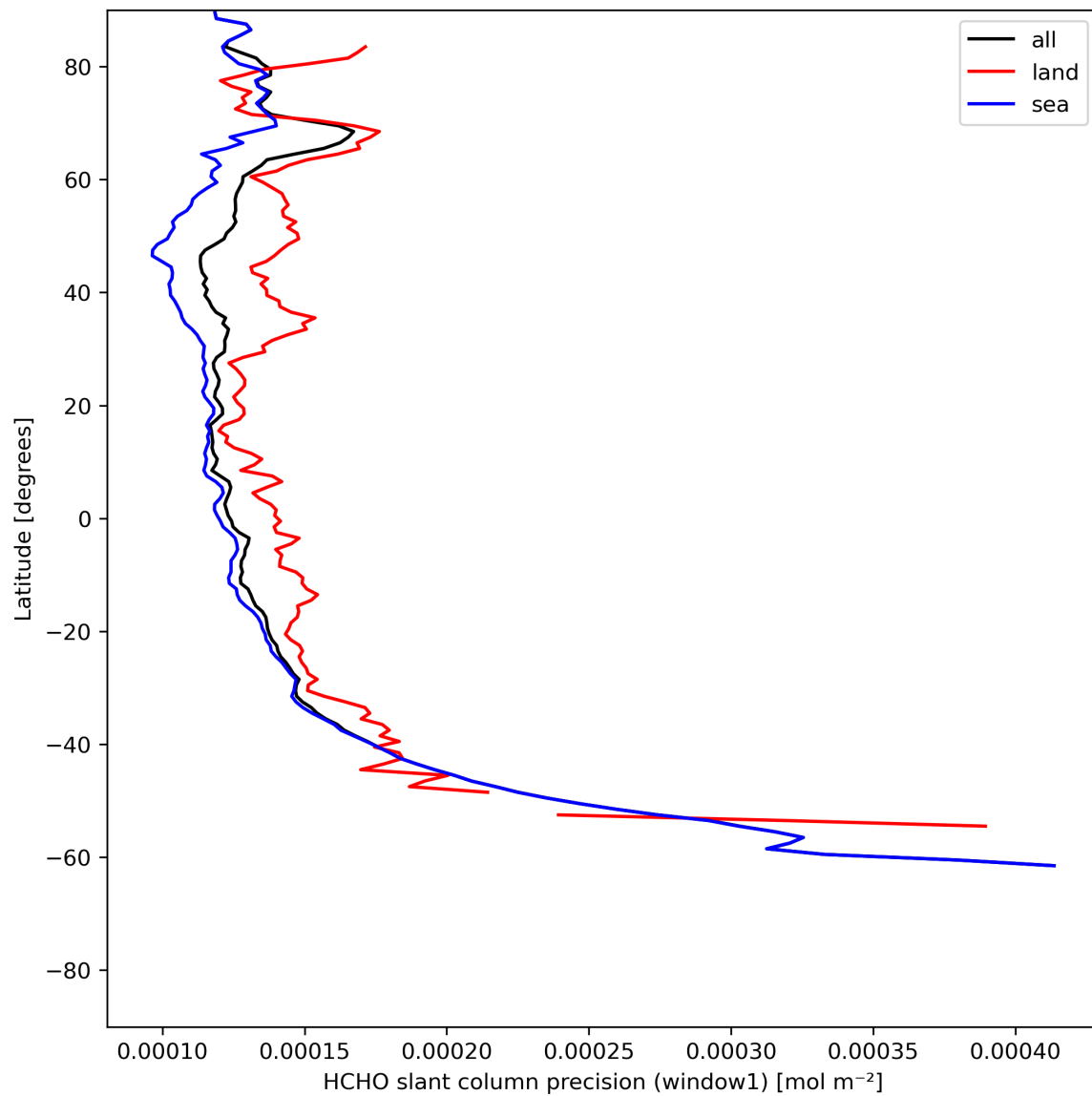
Figure 25: Zonal average of "HCHO slant column precision (window1)" for 2024-06-22 to 2024-06-24.
