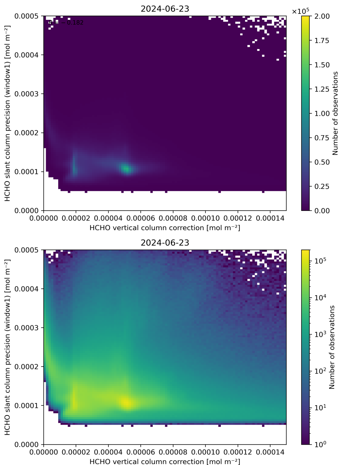
Figure 119: Scatter density plot of “HCHO vertical column correction” against “HCHO slant column precision (window1)” for 2024-06-22 to 2024-06-24.
