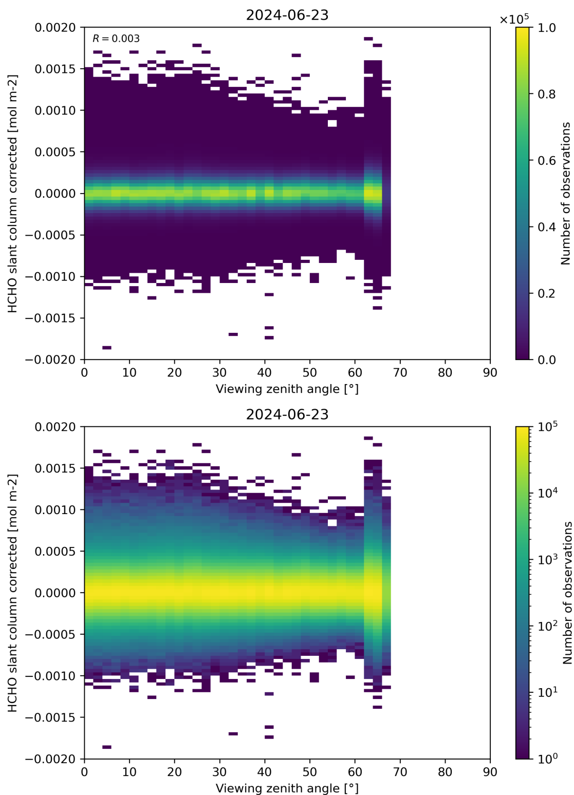
Figure 186: Scatter density plot of “Viewing zenith angle” against “HCHO slant column corrected” for 2024-06-22 to 2024-06-24.
