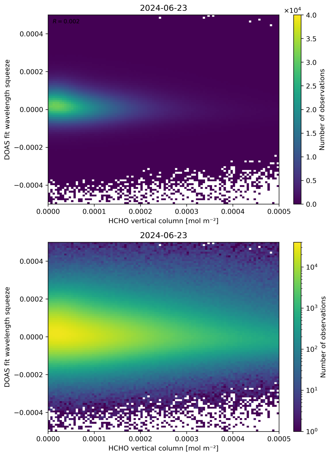
Figure 125: Scatter density plot of “HCHO vertical column” against “DOAS fit wavelength squeeze” for 2024-06-22 to 2024-06-24.
