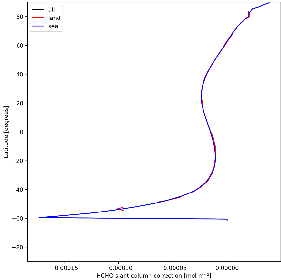
Figure 33: Zonal average of “HCHO slant column correction” for 2024-06-22 to 2024-06-24.
