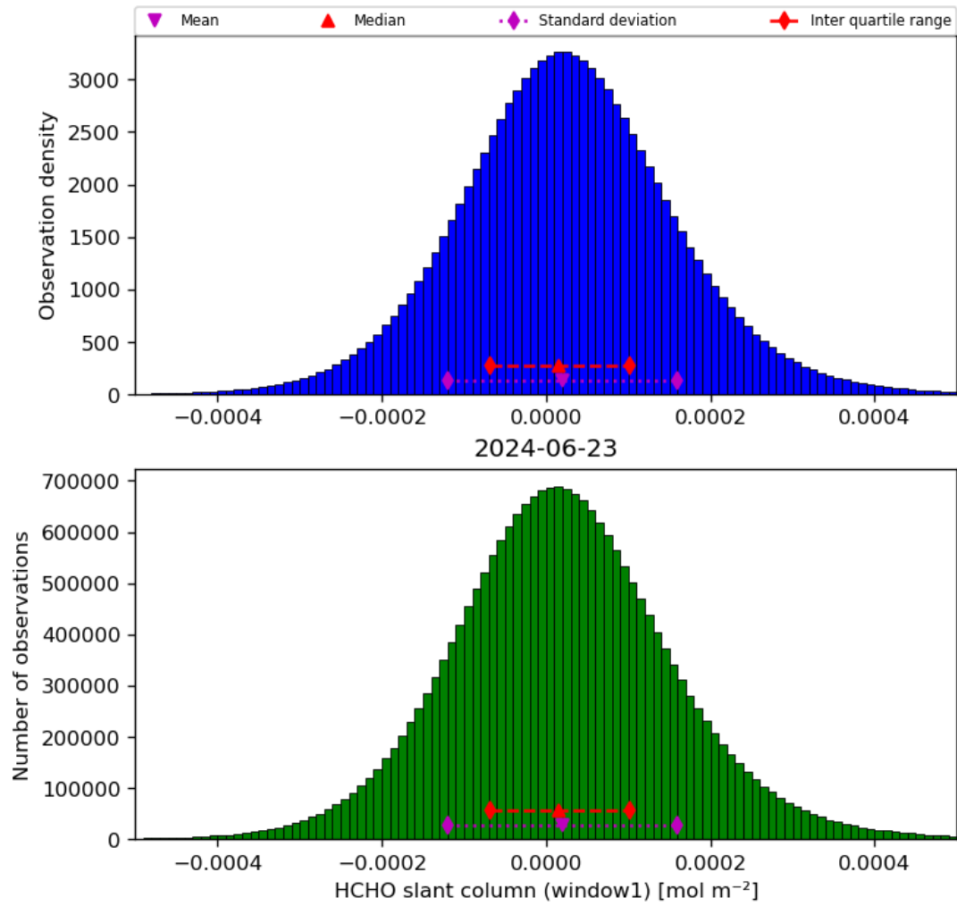
Figure 38: Histogram of “HCHO slant column (window1)” for 2024-06-22 to 2024-06-24
