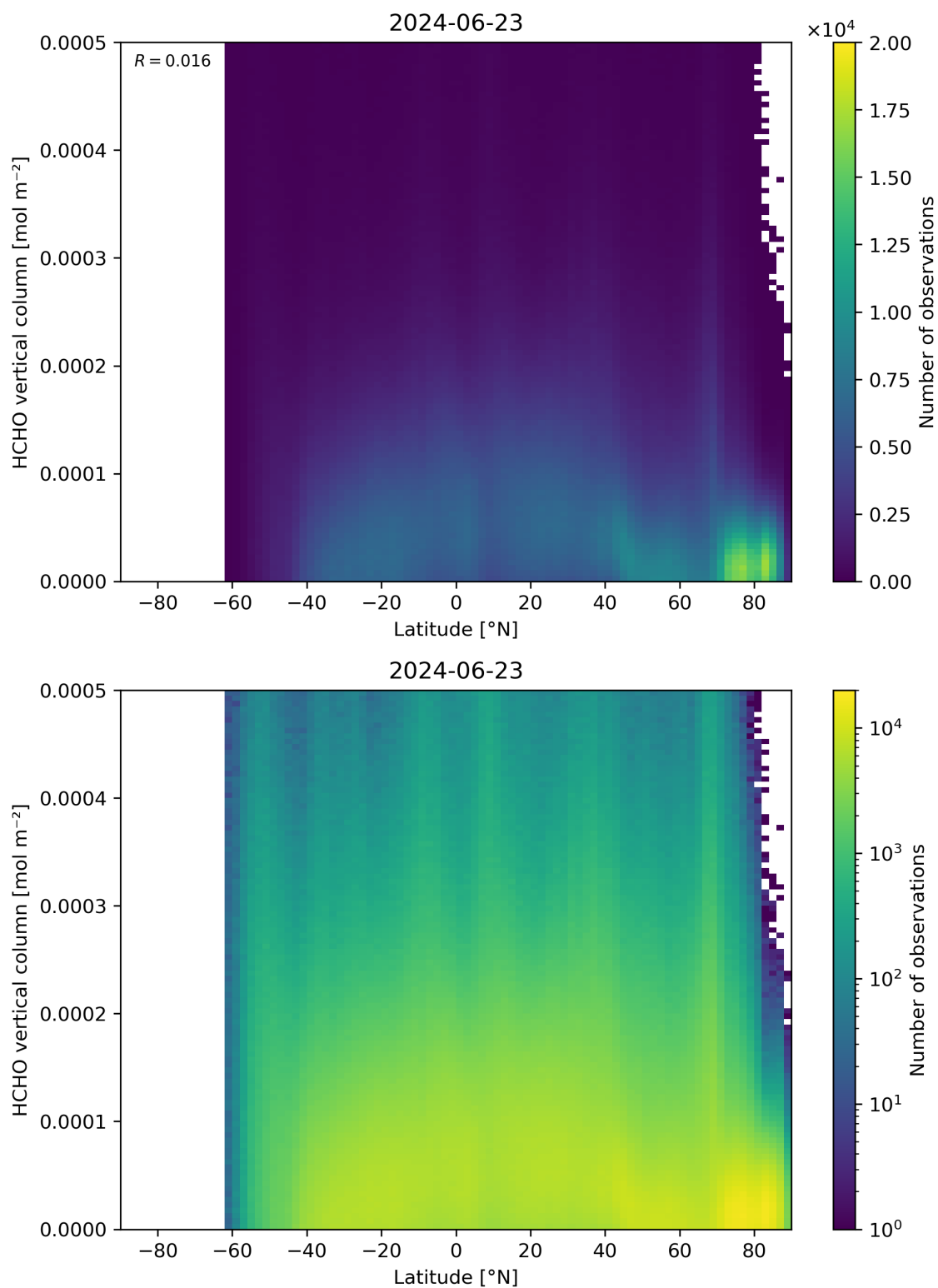
Figure 163: Scatter density plot of “Latitude” against “HCHO vertical column” for 2024-06-22 to 2024-06-24.
