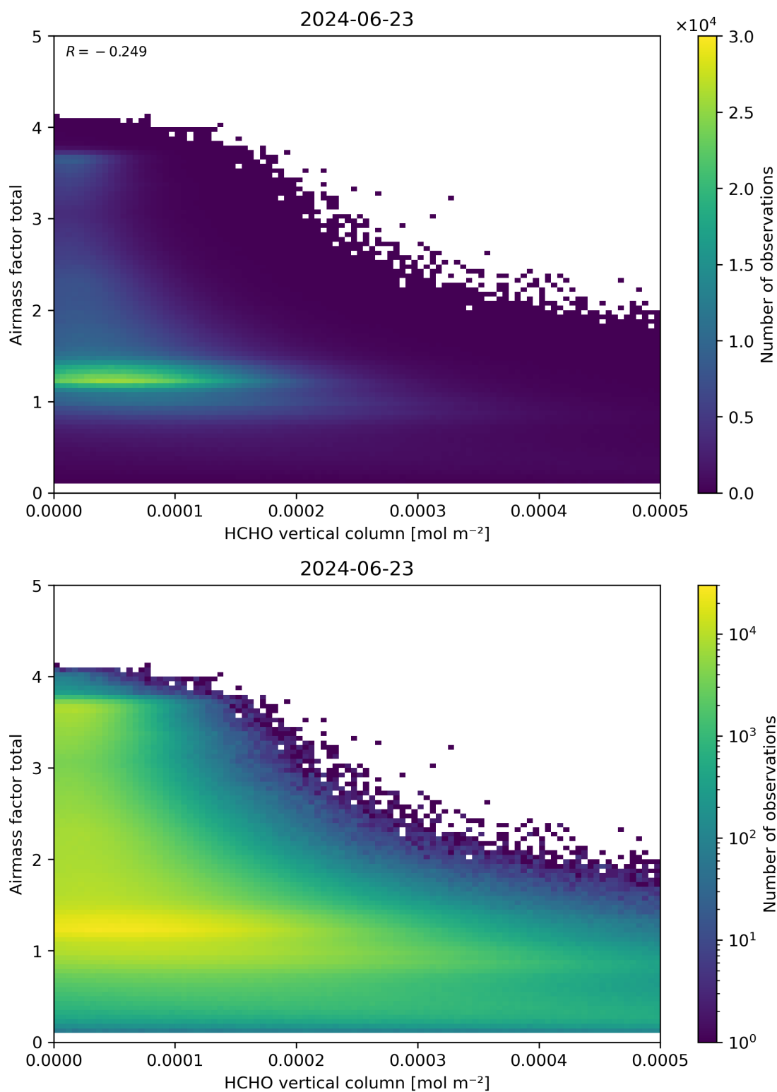
Figure 131: Scatter density plot of “HCHO vertical column” against “Airmass factor total” for 2024-06-22 to 2024-06-24.
