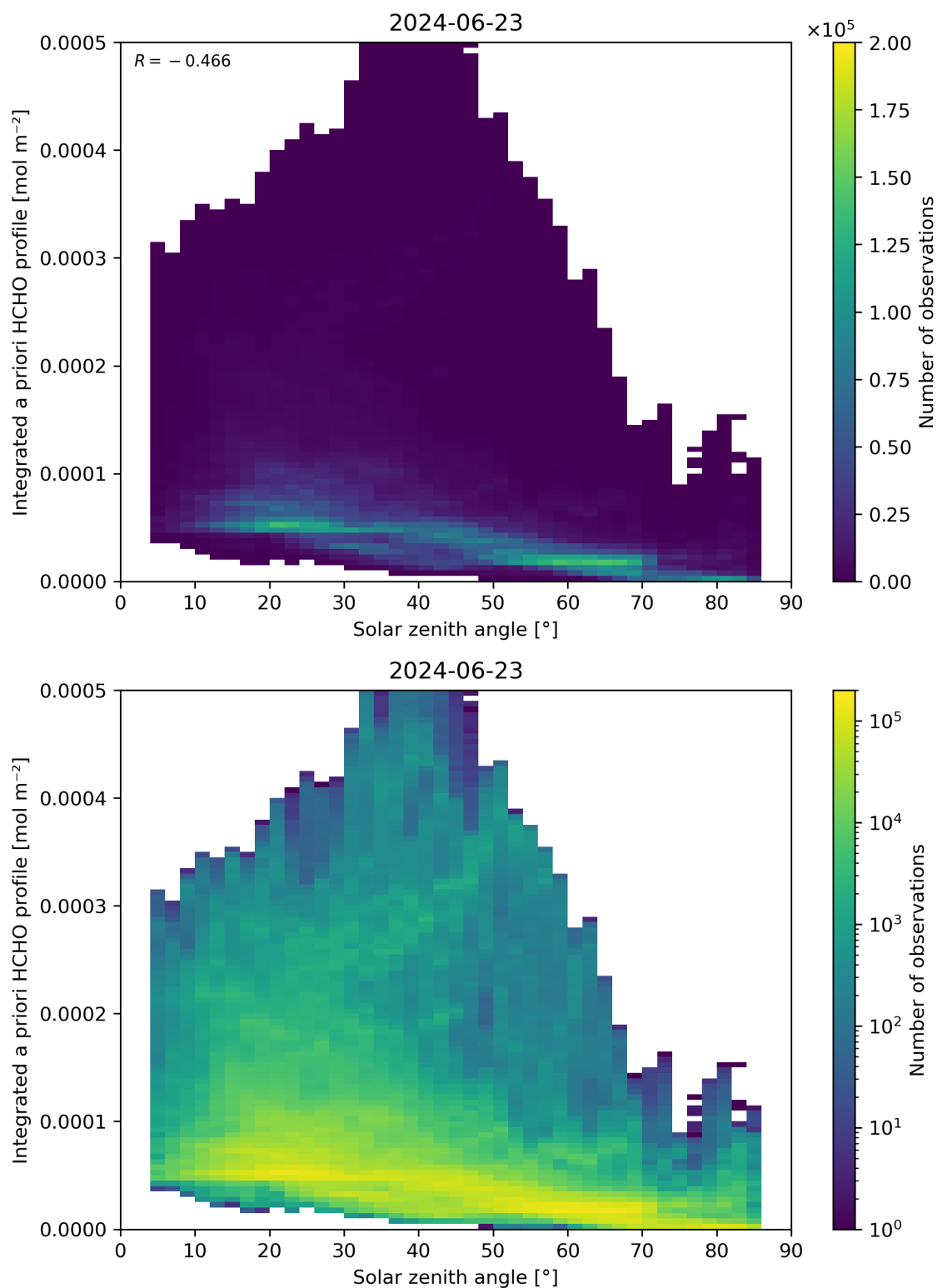
Figure 180: Scatter density plot of “Solar zenith angle” against “Integrated a priori HCHO profile” for 2024-06-22 to 2024-06-24.
