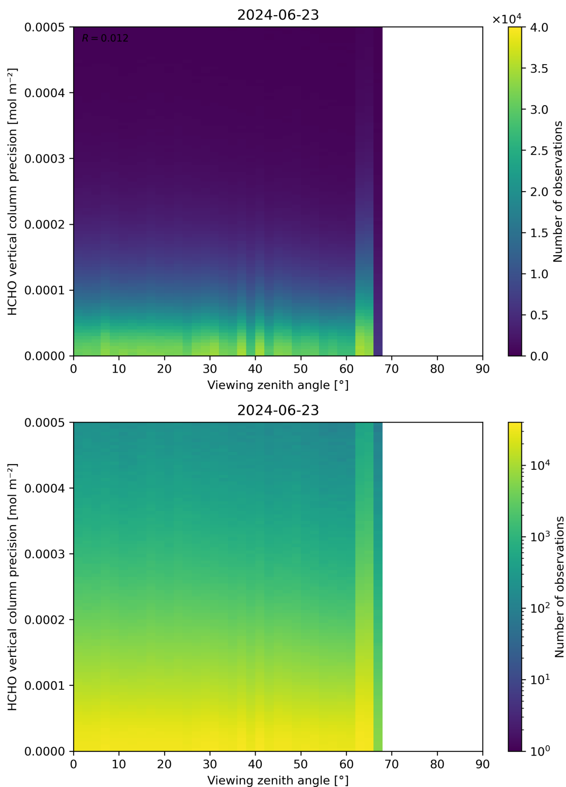
Figure 194: Scatter density plot of “Viewing zenith angle” against “HCHO vertical column precision” for 2024-06-22 to 2024-06-24.
