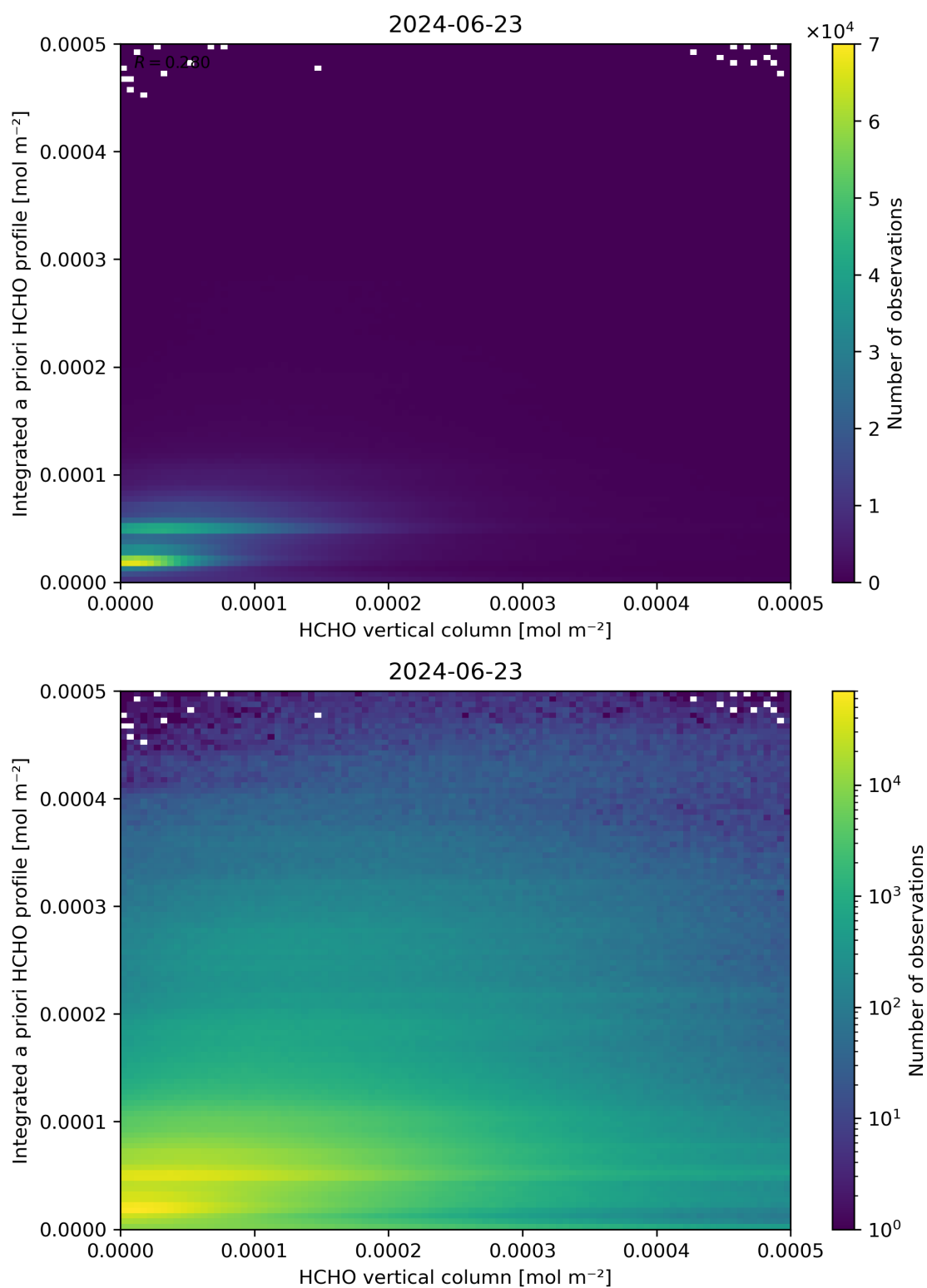
Figure 135: Scatter density plot of “HCHO vertical column” against “Integrated a priori HCHO profile” for 2024-06-22 to 2024-06-24.
