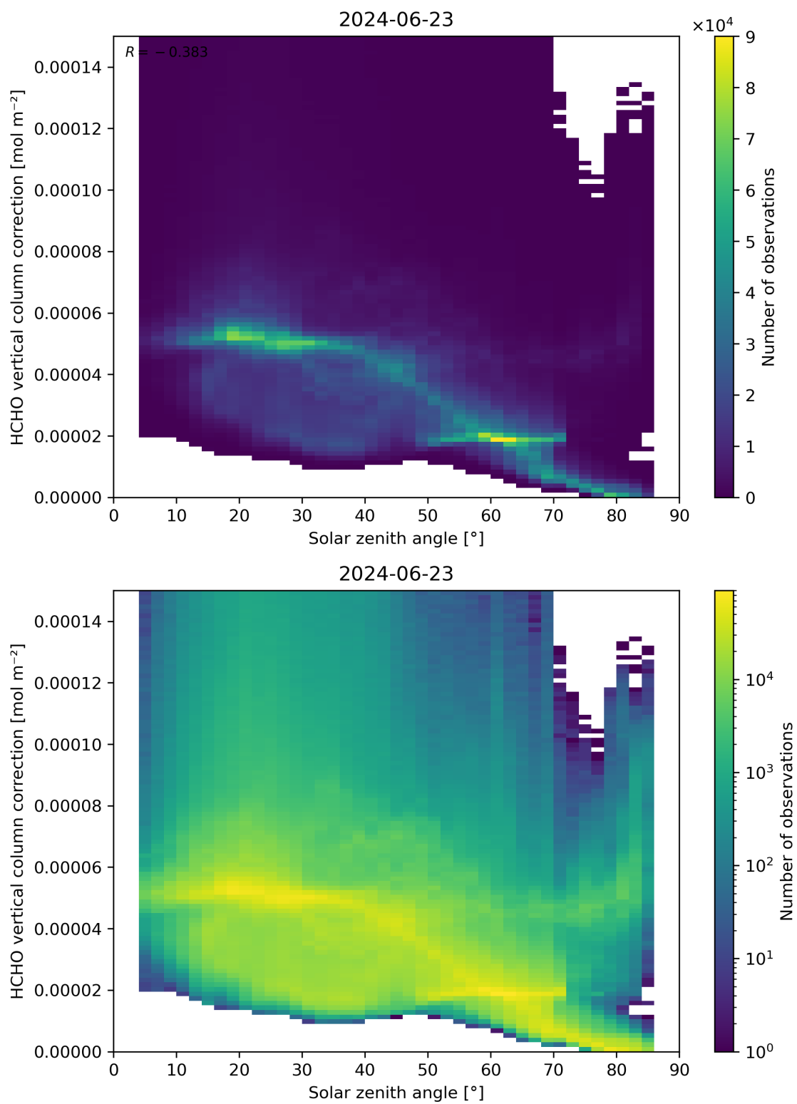
Figure 178: Scatter density plot of “Solar zenith angle” against “HCHO vertical column correction” for 2024-06-22 to 2024-06-24.
