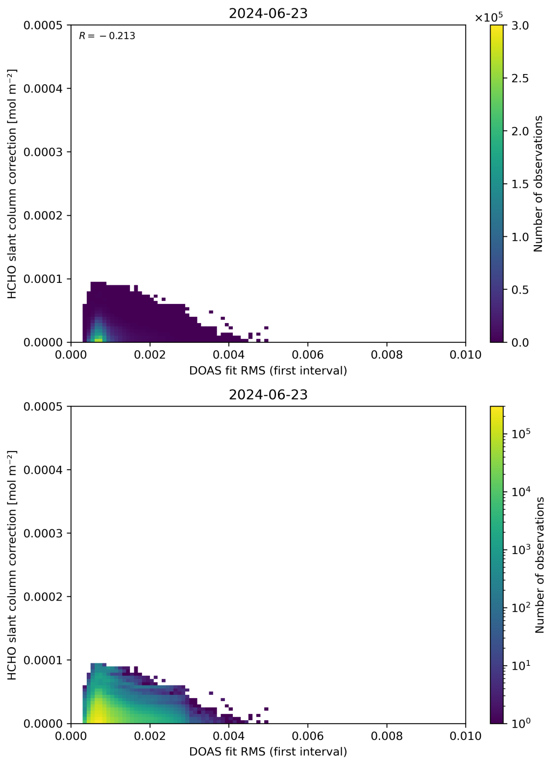
Figure 63: Scatter density plot of “DOAS fit RMS (first interval)” against “HCHO slant column correction” for 2024-06-22 to 2024-06-24.
