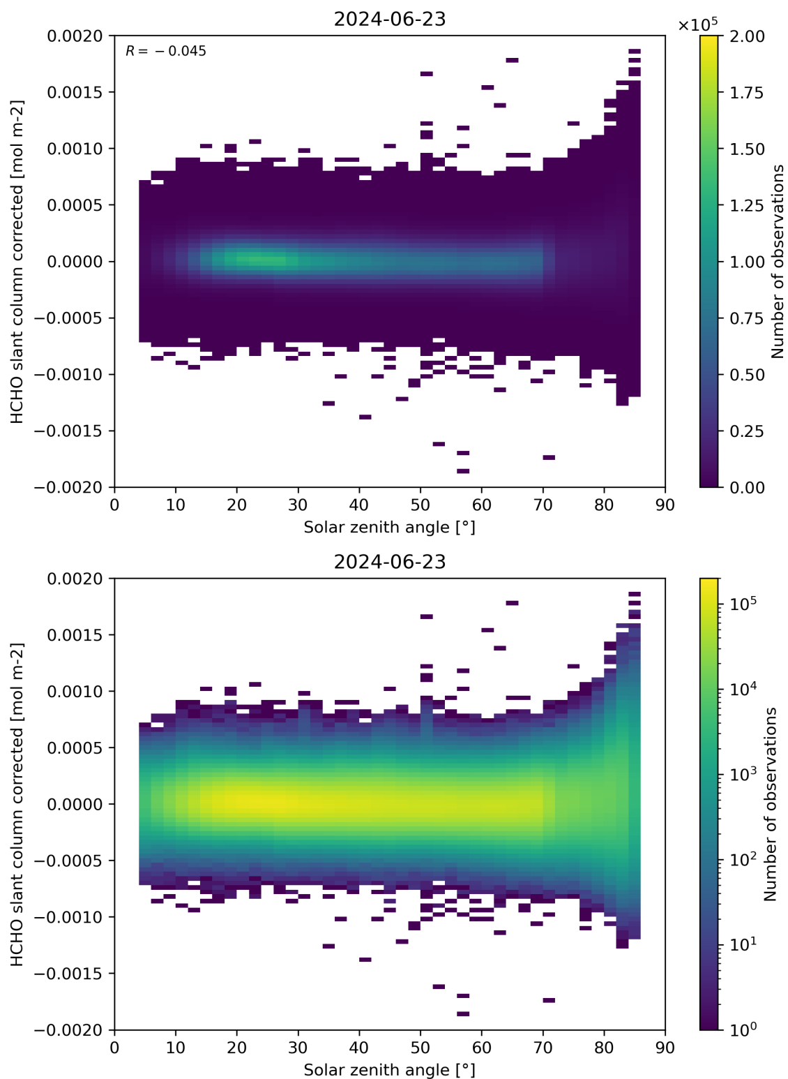
Figure 171: Scatter density plot of “Solar zenith angle” against “HCHO slant column corrected” for 2024-06-22 to 2024-06-24.
