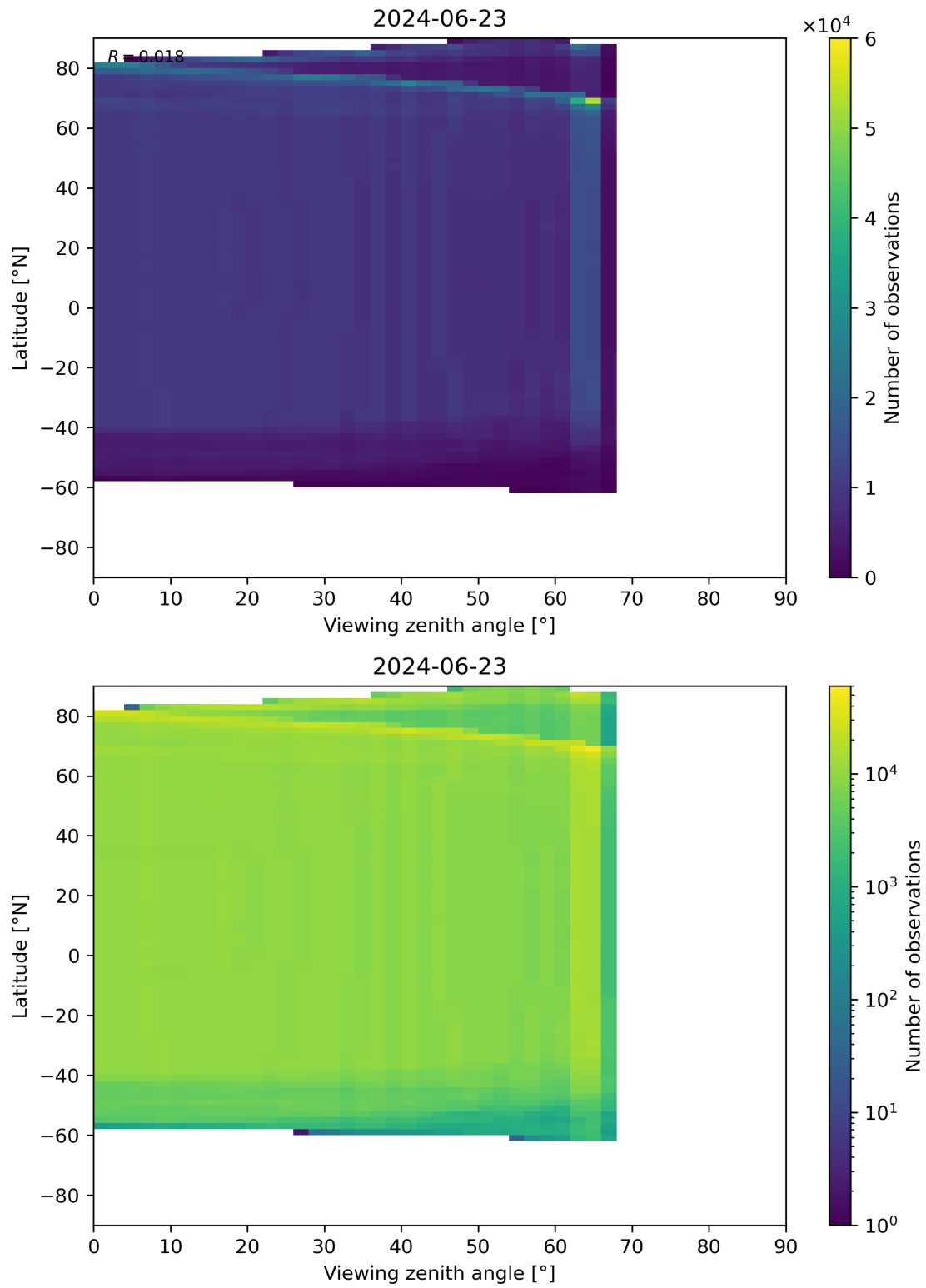
Figure 196: Scatter density plot of “Viewing zenith angle” against “Latitude” for 2024-06-22 to 2024-06-24.
