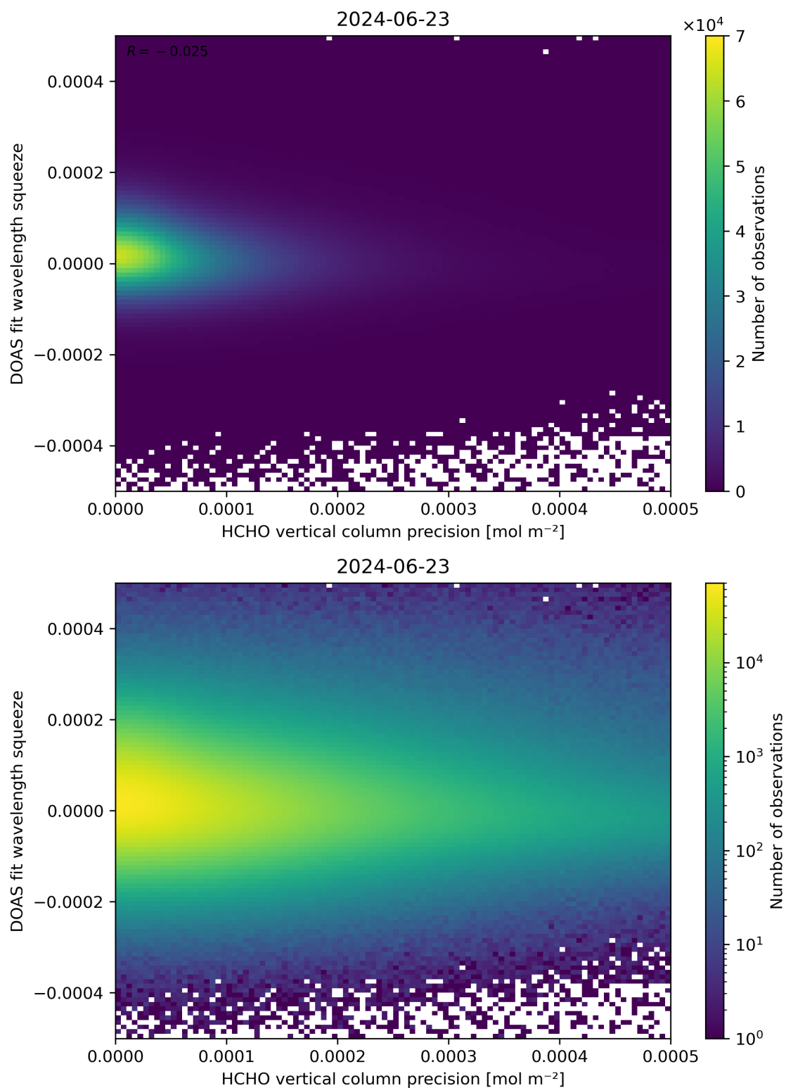
Figure 138: Scatter density plot of “HCHO vertical column precision” against “DOAS fit wavelength squeeze” for 2024-06-22 to 2024-06-24.
