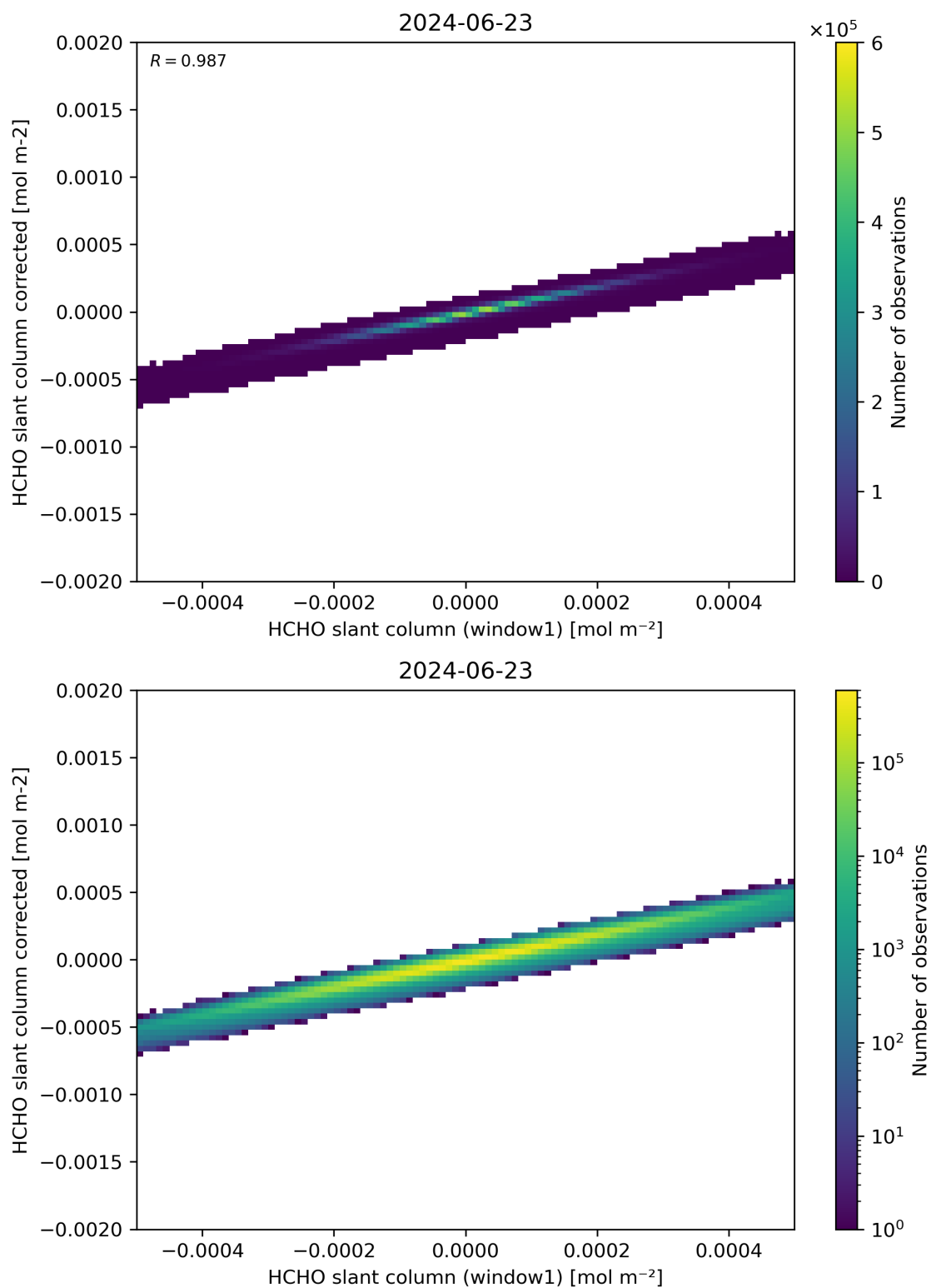
Figure 82: Scatter density plot of “HCHO slant column (window1)” against “HCHO slant column corrected” for 2024-06-22 to 2024-06-24.
