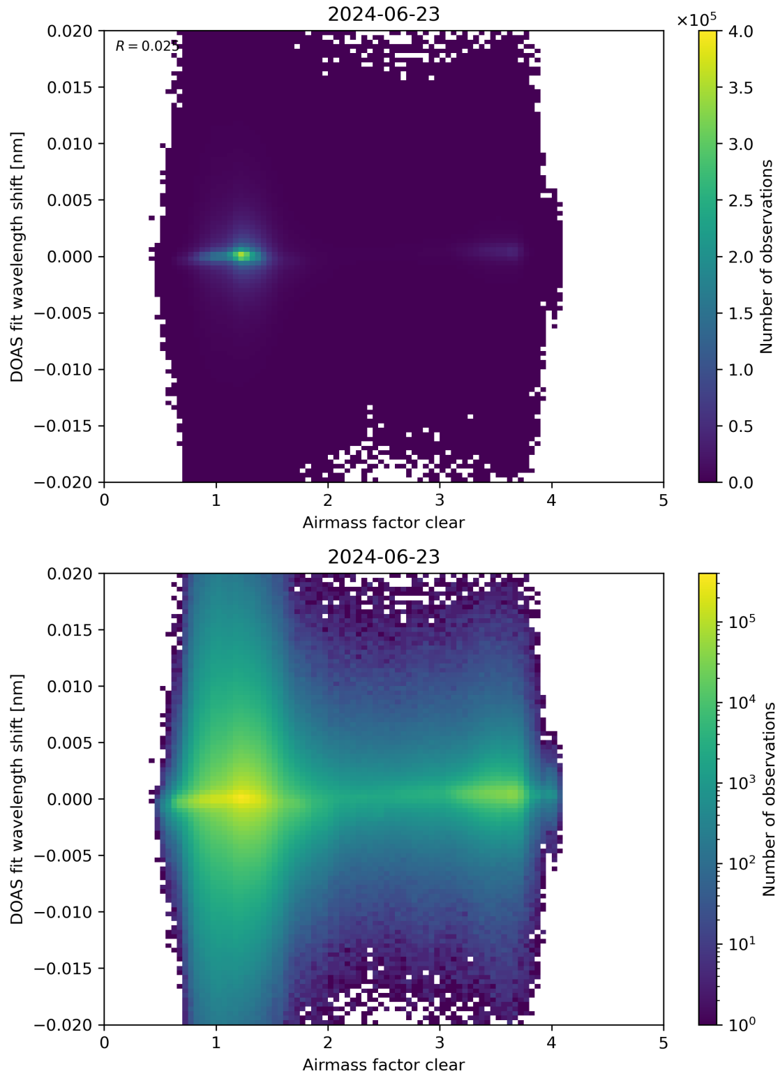
Figure 72: Scatter density plot of “Airmass factor clear” against “DOAS fit wavelength shift” for 2024-06-22 to 2024-06-24.
