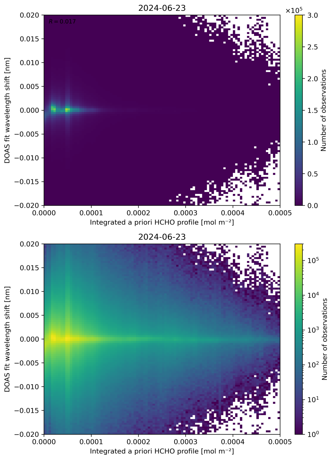
Figure 149: Scatter density plot of “Integrated a priori HCHO profile” against “DOAS fit wavelength shift” for 2024-06-22 to 2024-06-24.
