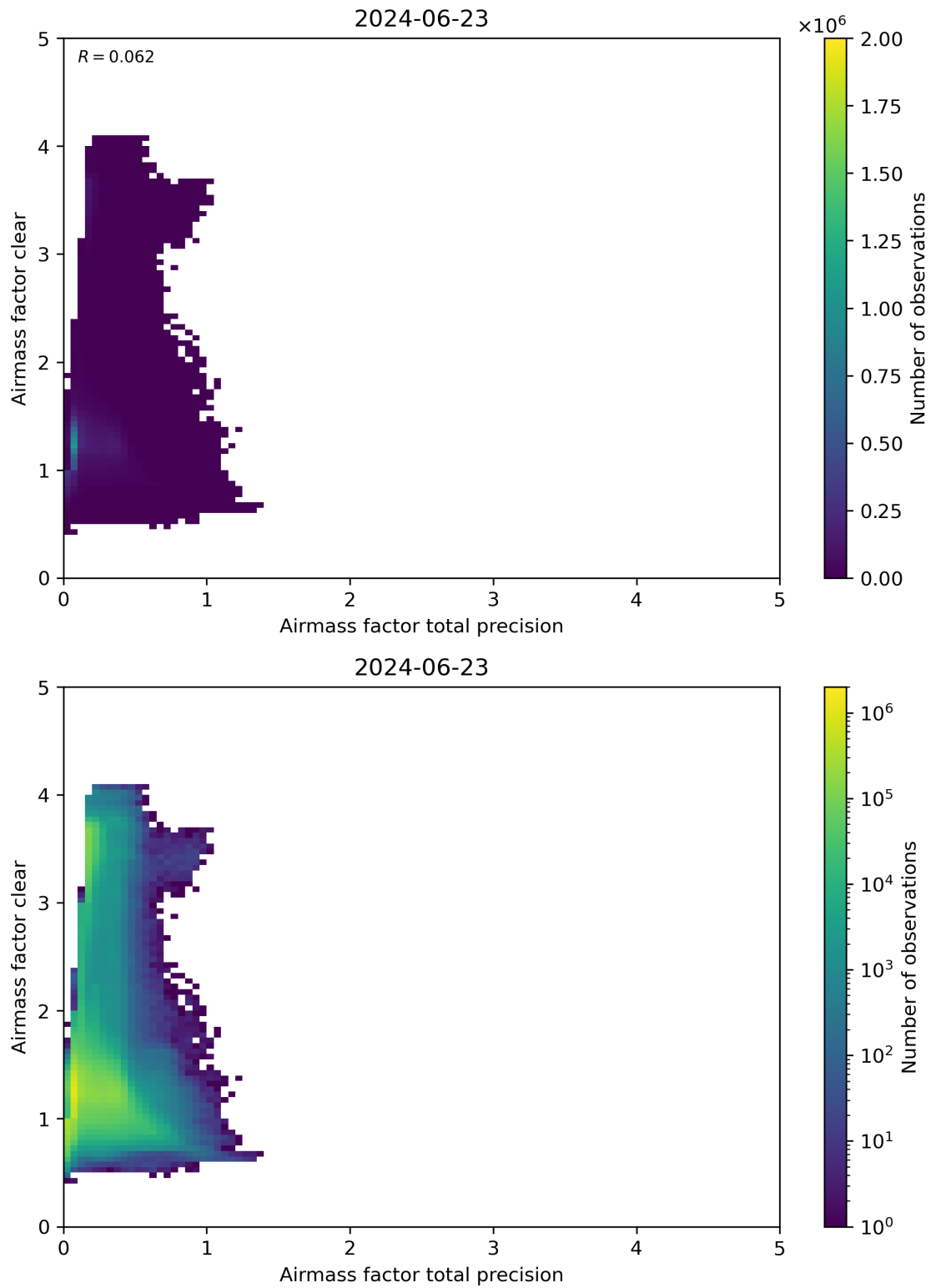
Figure 108: Scatter density plot of “Airmass factor total precision” against “Airmass factor clear” for 2024-06-22 to 2024-06-24.
