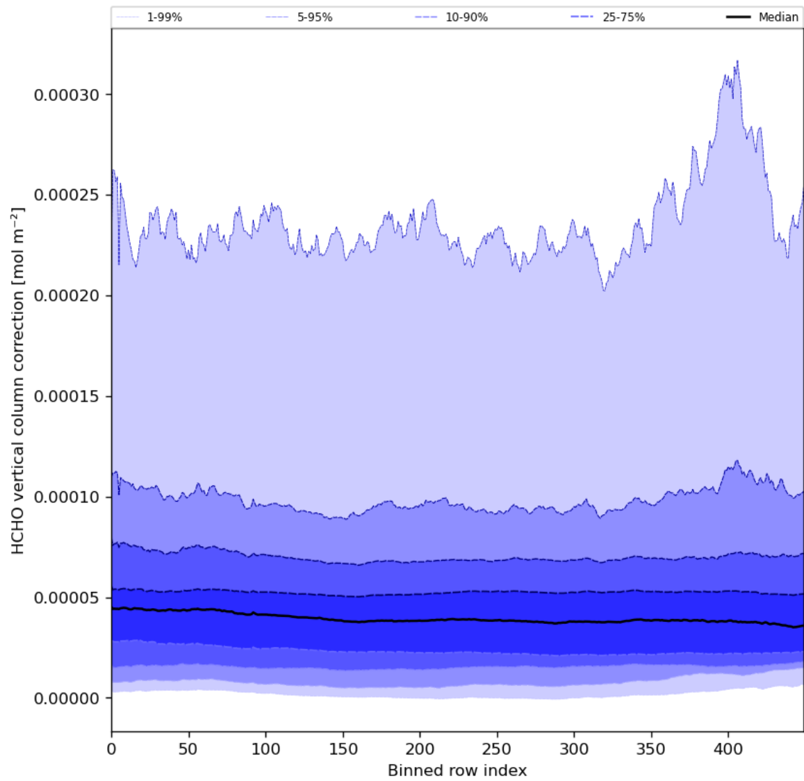
Figure 51: Along track statistics of “HCHO vertical column correction” for 2024-06-22 to 2024-06-24
