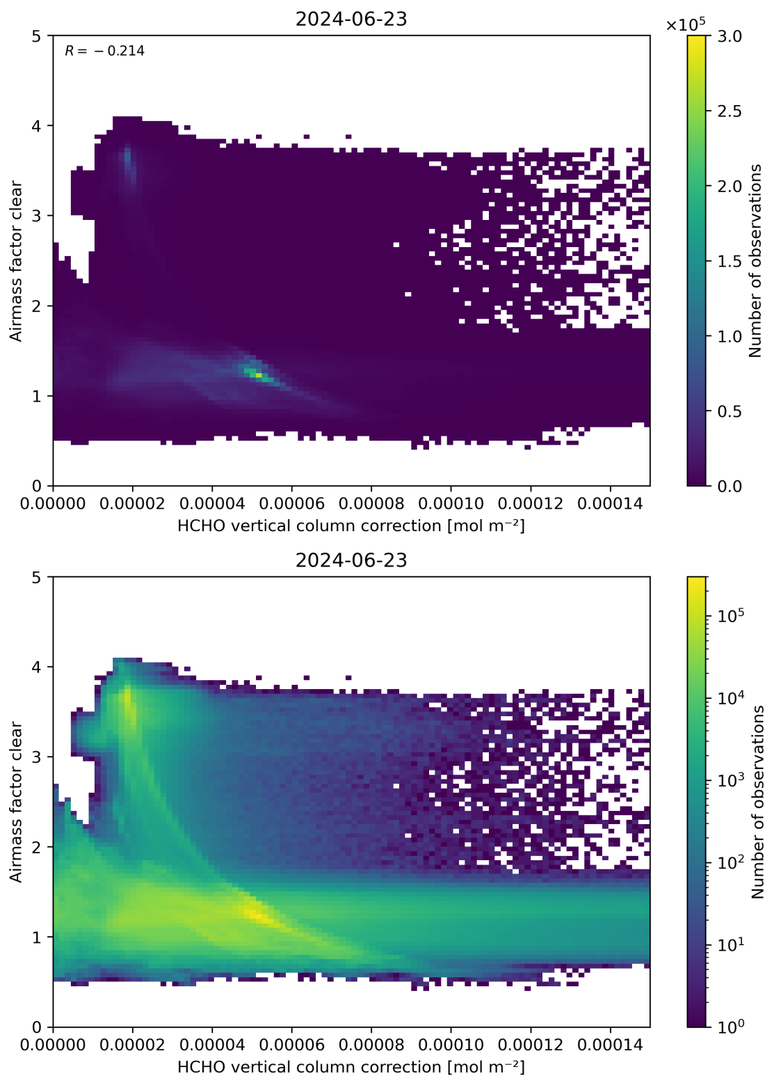
Figure 115: Scatter density plot of “HCHO vertical column correction” against “Airmass factor clear” for 2024-06-22 to 2024-06-24.
