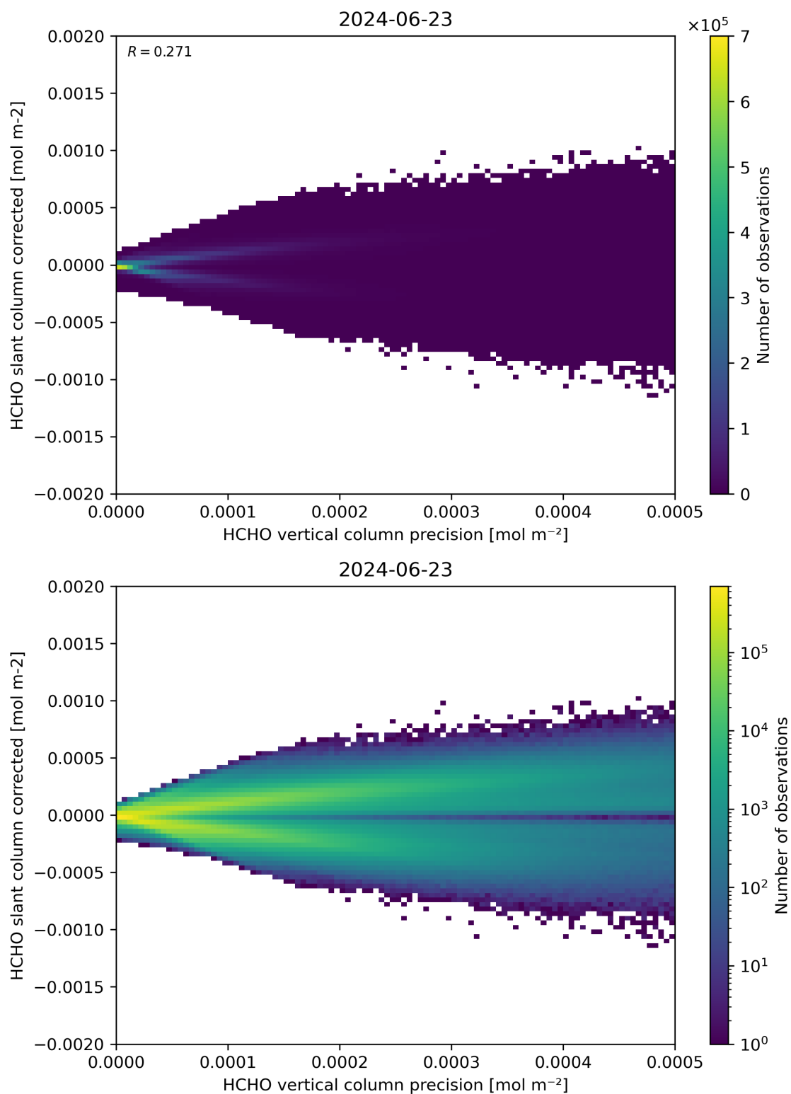
Figure 140: Scatter density plot of “HCHO vertical column precision” against “HCHO slant column corrected” for 2024-06-22 to 2024-06-24.
