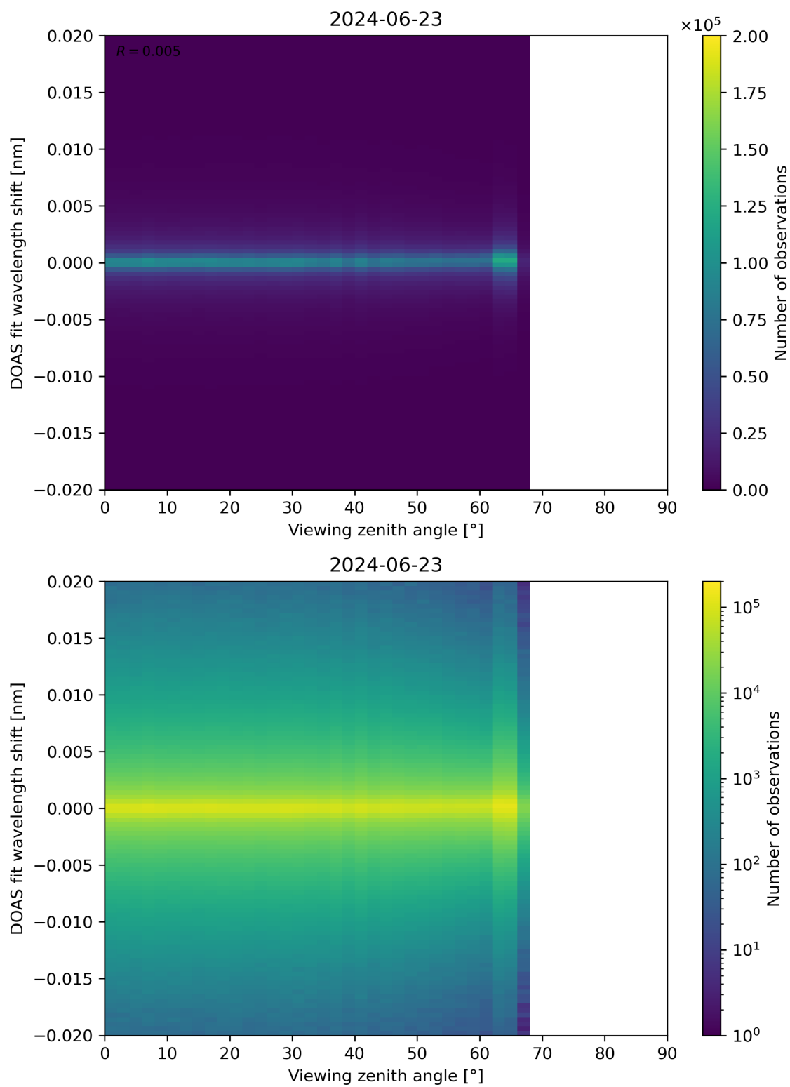
Figure 183: Scatter density plot of “Viewing zenith angle” against “DOAS fit wavelength shift” for 2024-06-22 to 2024-06-24.
