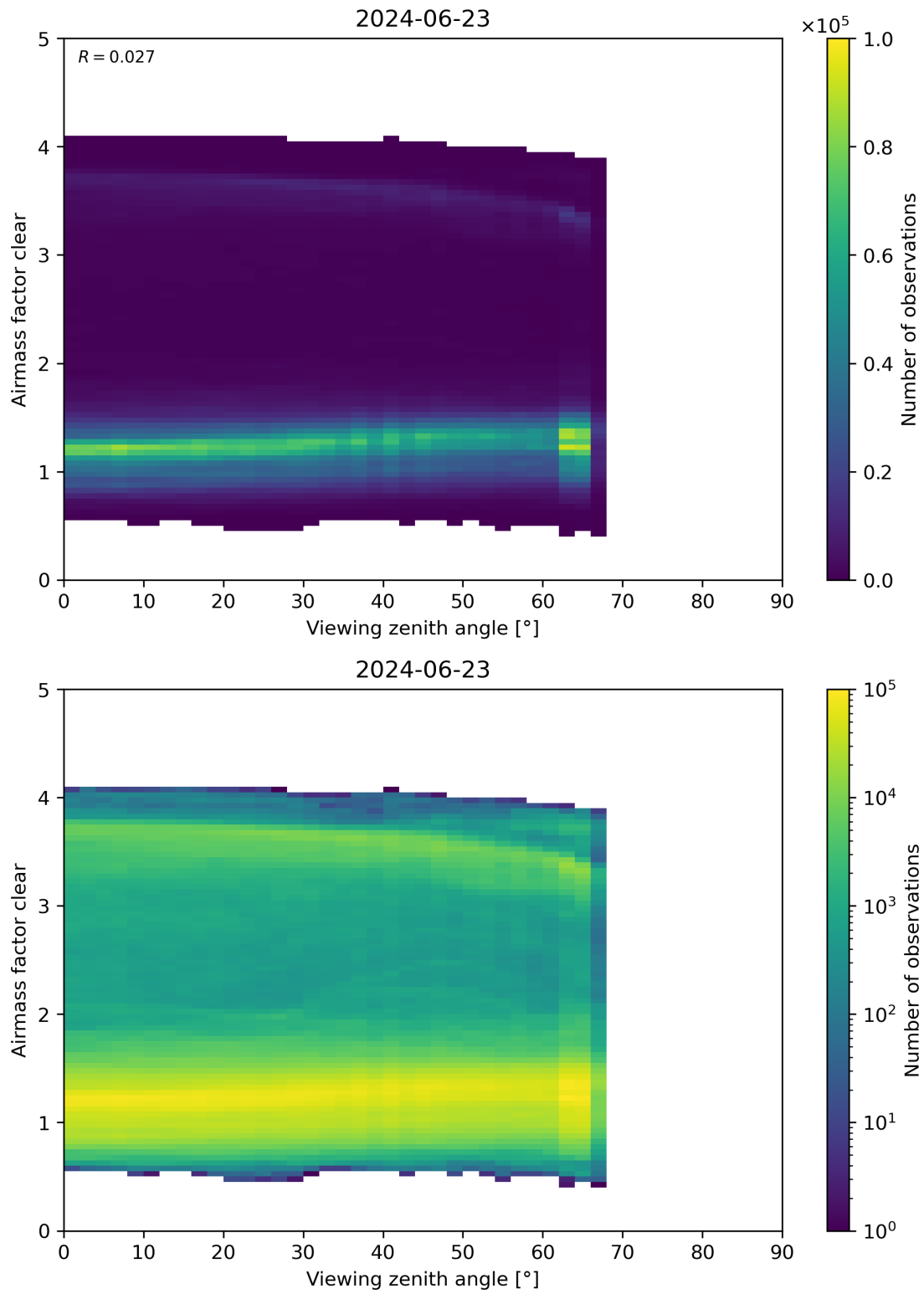
Figure 185: Scatter density plot of “Viewing zenith angle” against “Airmass factor clear” for 2024-06-22 to 2024-06-24.
