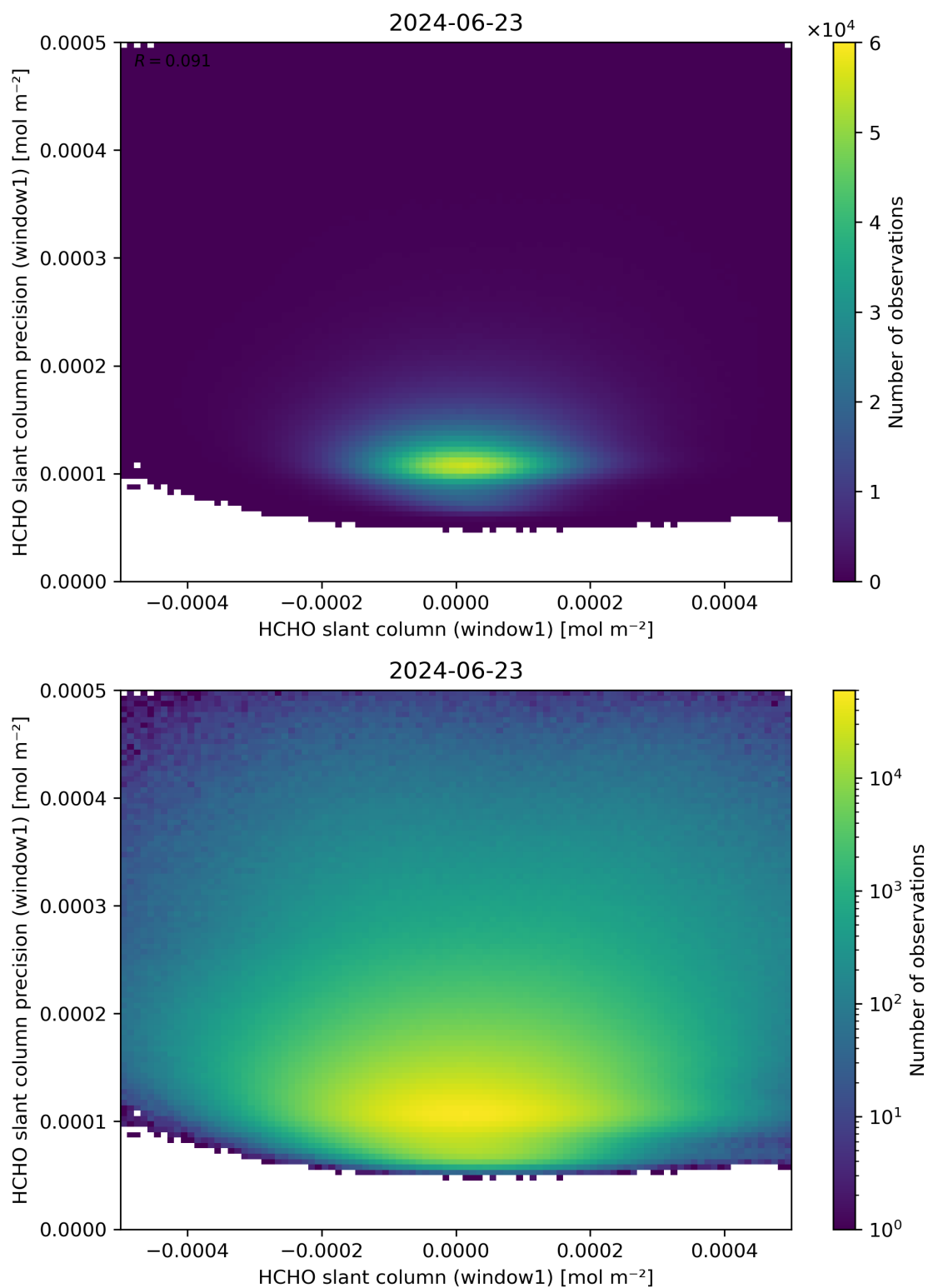
Figure 84: Scatter density plot of “HCHO slant column (window1)” against “HCHO slant column precision (window1)” for 2024-06-22 to 2024-06-24.
