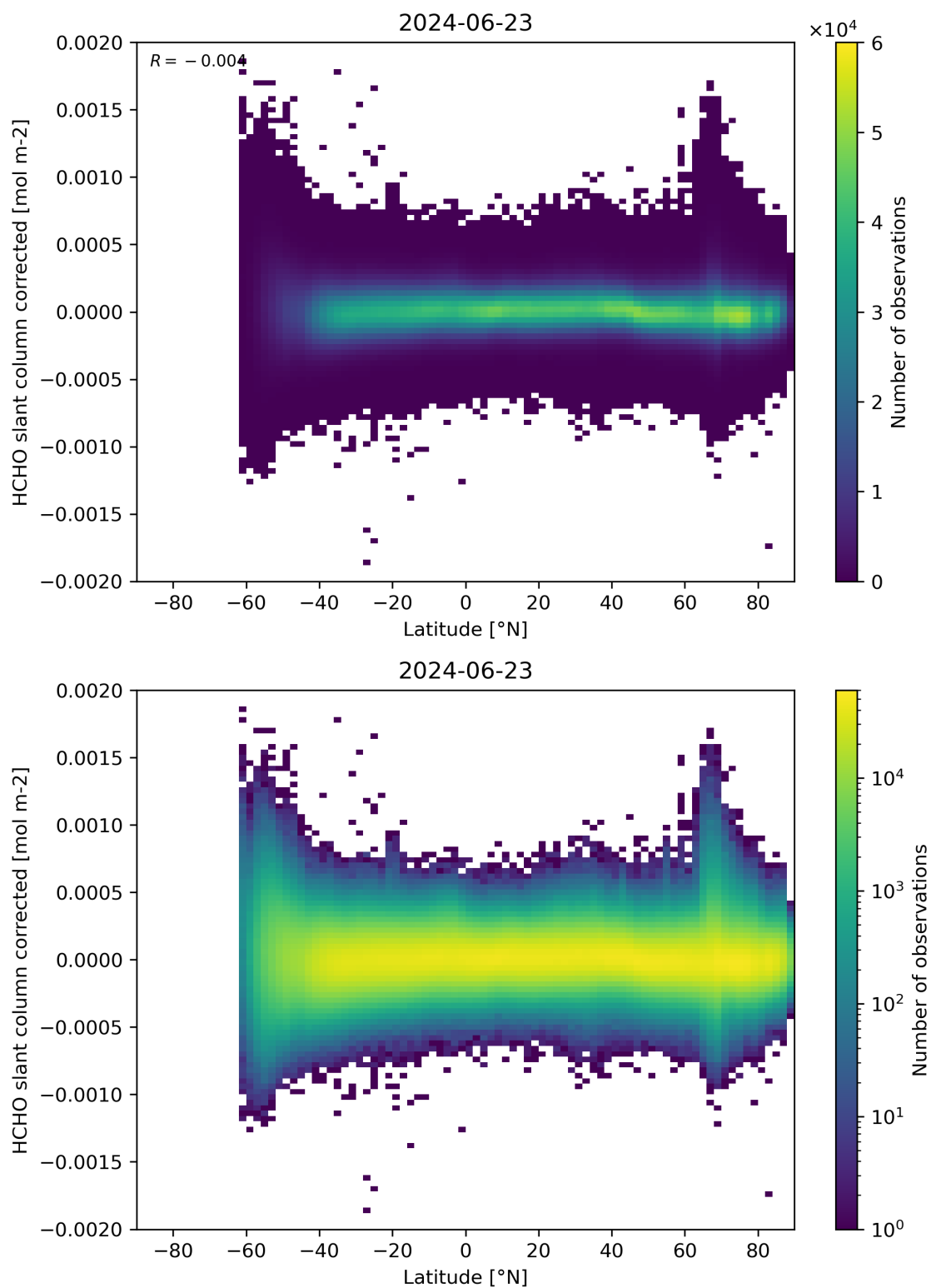
Figure 157: Scatter density plot of “Latitude” against “HCHO slant column corrected” for 2024-06-22 to 2024-06-24.
