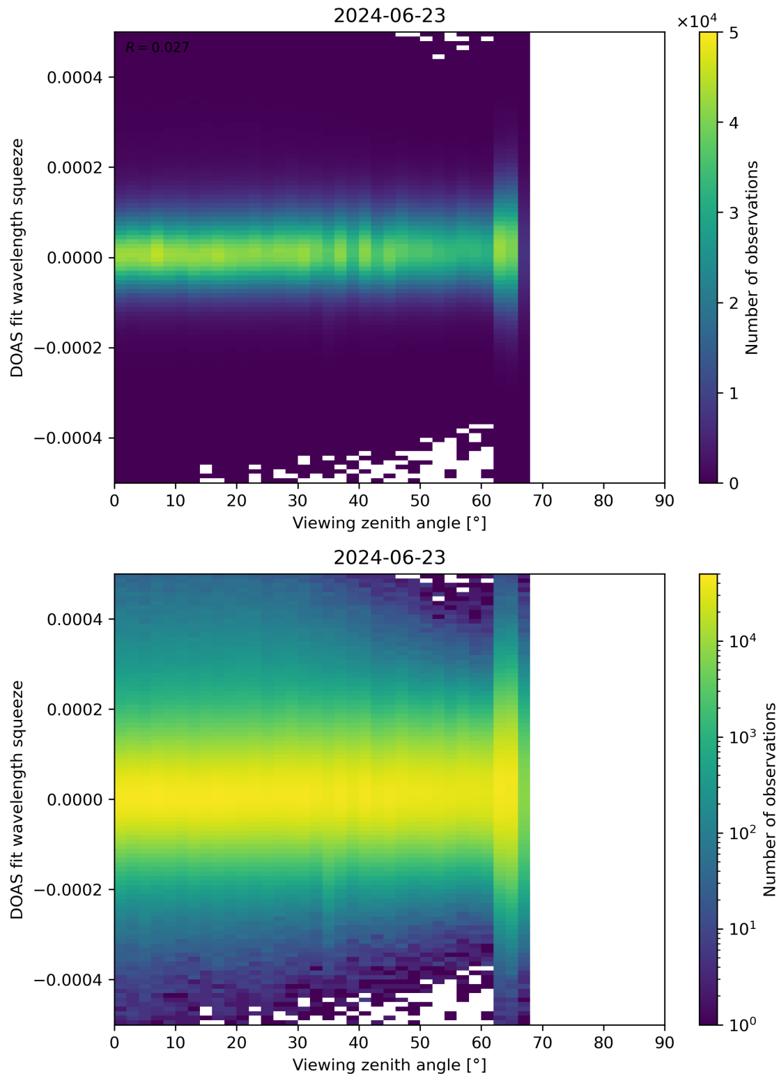
Figure 184: Scatter density plot of “Viewing zenith angle” against “DOAS fit wavelength squeeze” for 2024-06-22 to 2024-06-24.
