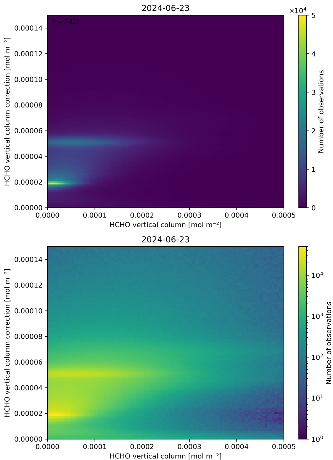
Figure 133: Scatter density plot of “HCHO vertical column” against “HCHO vertical column correction” for 2024-06-22 to 2024-06-24.
