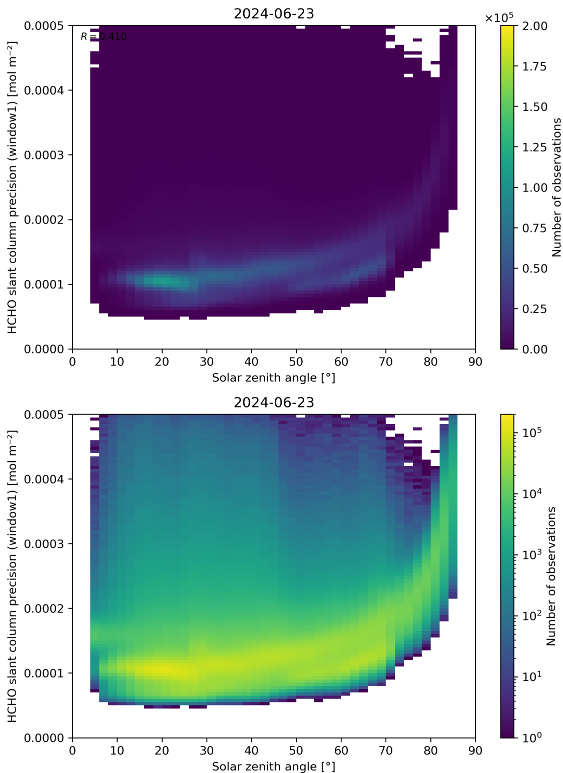
Figure 174: Scatter density plot of “Solar zenith angle” against “HCHO slant column precision (window1)” for 2024-06-22 to 2024-06-24.
