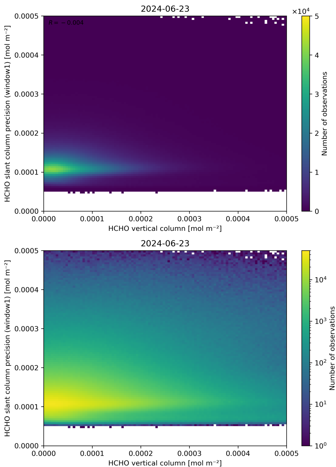
Figure 130: Scatter density plot of “HCHO vertical column” against “HCHO slant column precision (window1)” for 2024-06-22 to 2024-06-24.
