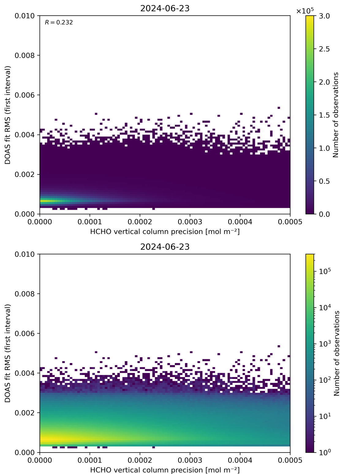
Figure 136: Scatter density plot of “HCHO vertical column precision” against “DOAS fit RMS (first interval)” for 2024-06-22 to 2024-06-24.
