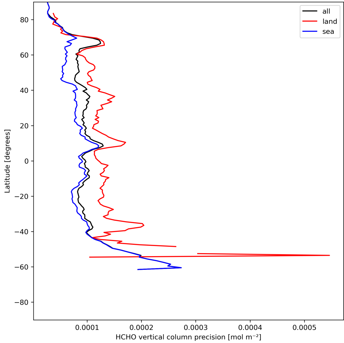
Figure 22: Zonal average of “HCHO vertical column precision” for 2024-06-22 to 2024-06-24.
