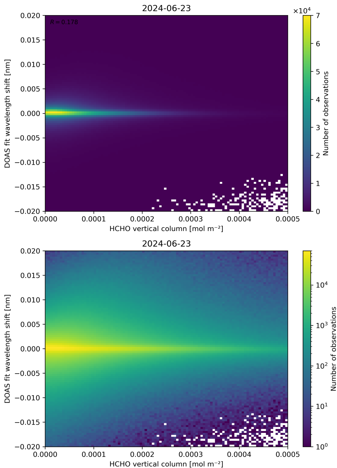
Figure 124: Scatter density plot of “HCHO vertical column” against “DOAS fit wavelength shift” for 2024-06-22 to 2024-06-24.
