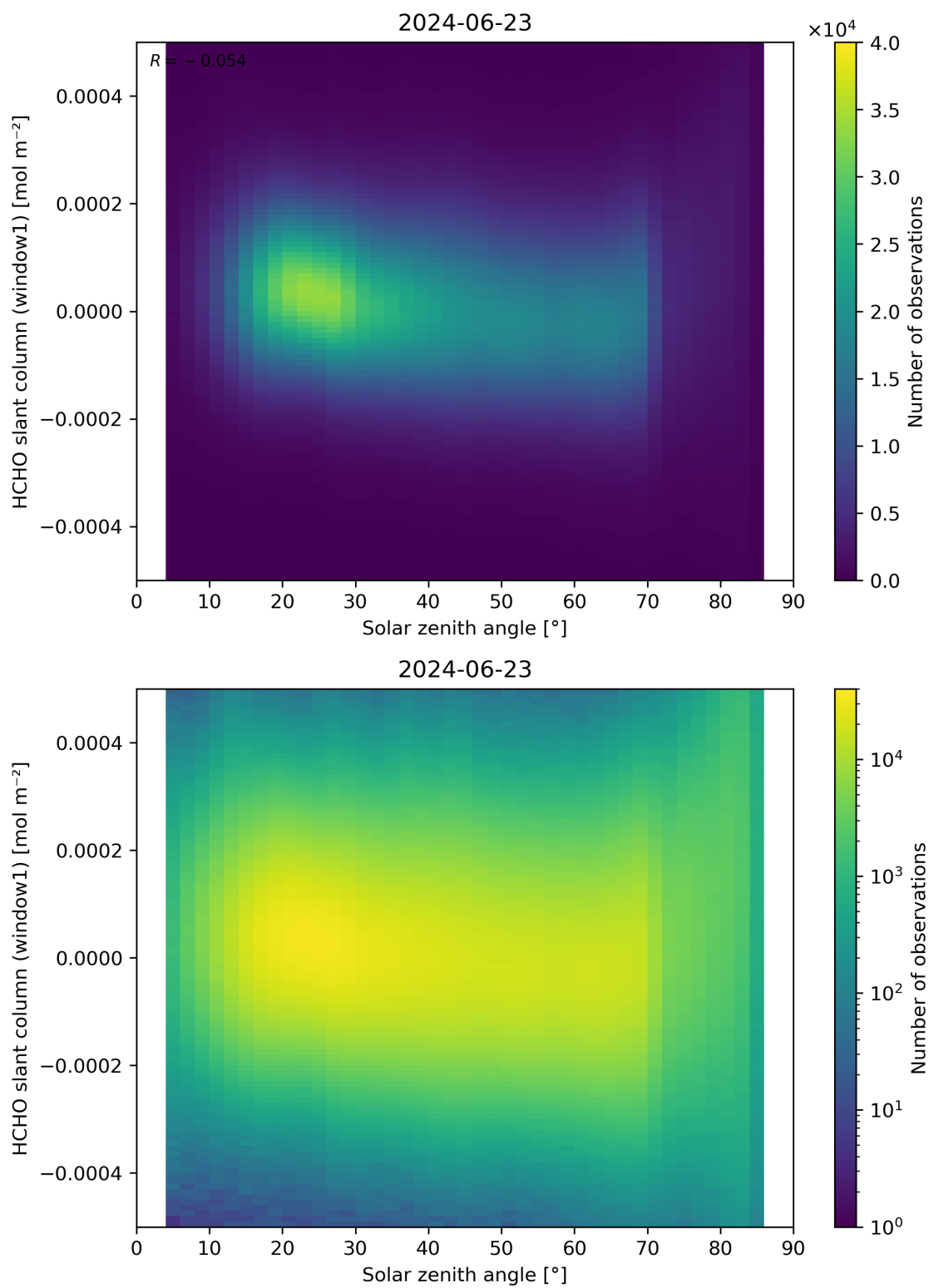
Figure 173: Scatter density plot of “Solar zenith angle” against “HCHO slant column (window1)” for 2024-06-22 to 2024-06-24.
