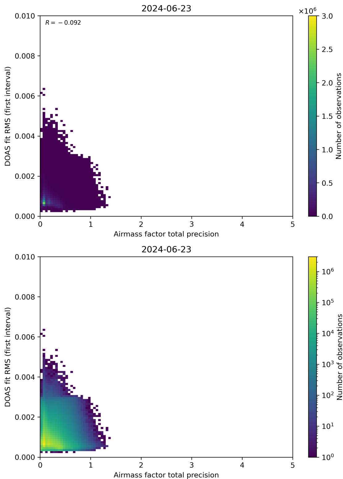
Figure 105: Scatter density plot of “Airmass factor total precision” against “DOAS fit RMS (first interval)” for 2024-06-22 to 2024-06-24.
