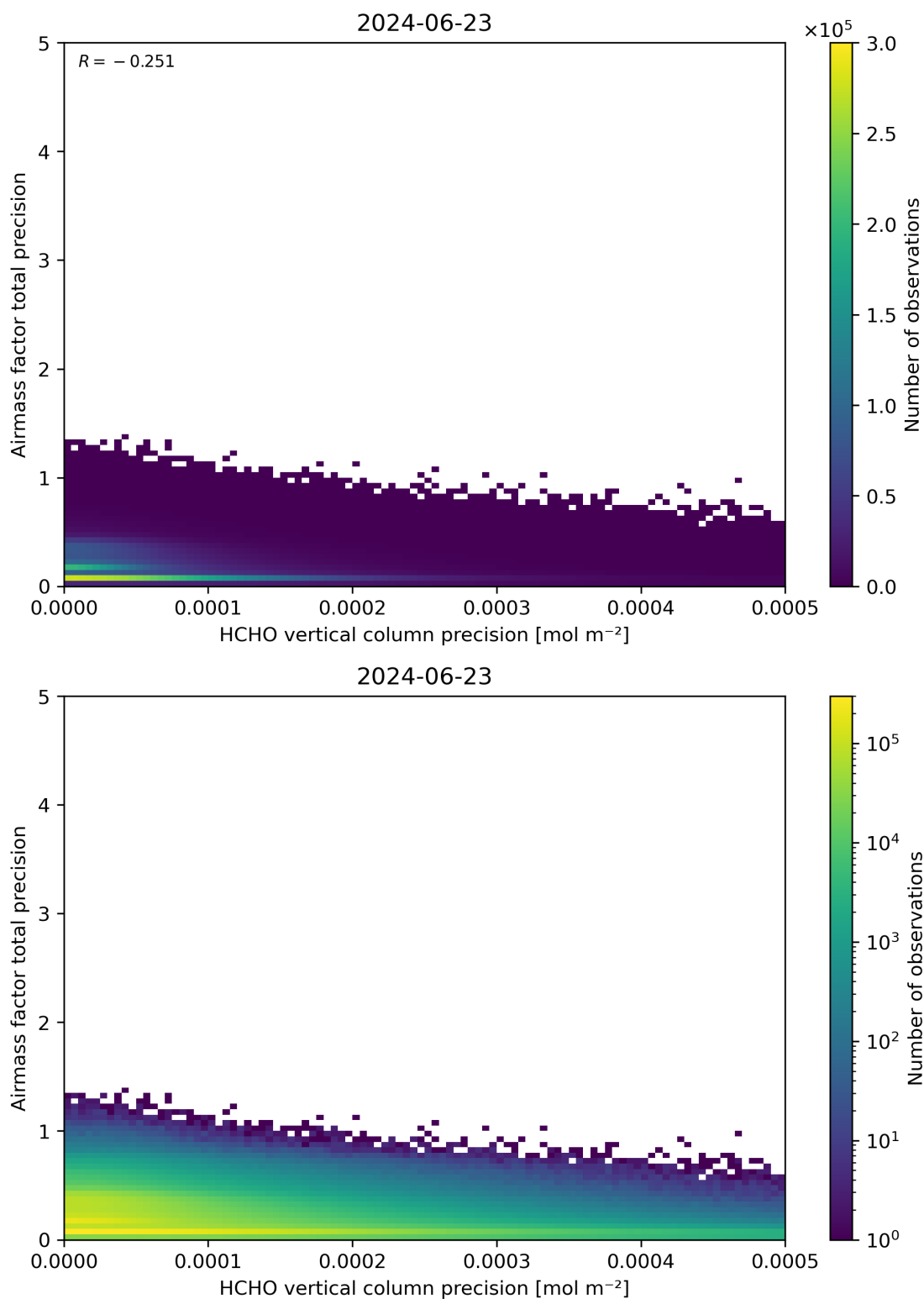
Figure 145: Scatter density plot of “HCHO vertical column precision” against “Airmass factor total precision” for 2024-06-22 to 2024-06-24.
