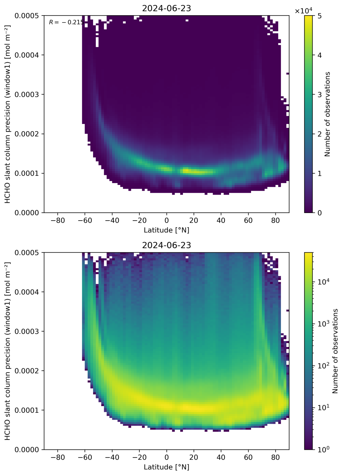
Figure 160: Scatter density plot of “Latitude” against “HCHO slant column precision (window1)” for 2024-06-22 to 2024-06-24.
