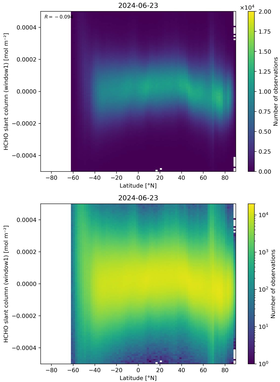
Figure 159: Scatter density plot of “Latitude” against “HCHO slant column (window1)” for 2024-06-22 to 2024-06-24.
