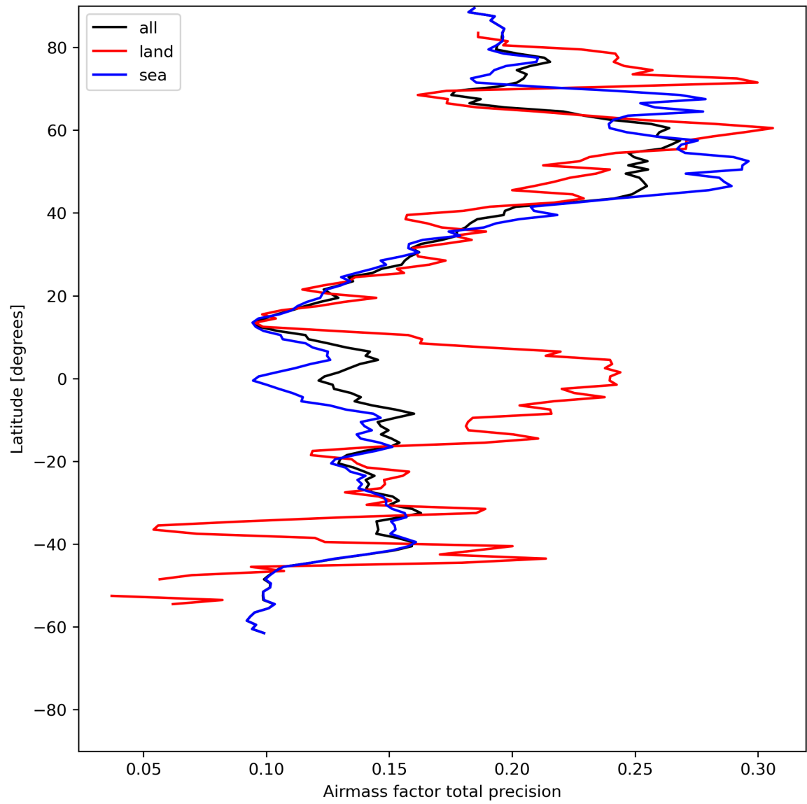
Figure 27: Zonal average of “Airmass factor total precision” for 2024-06-22 to 2024-06-24.
