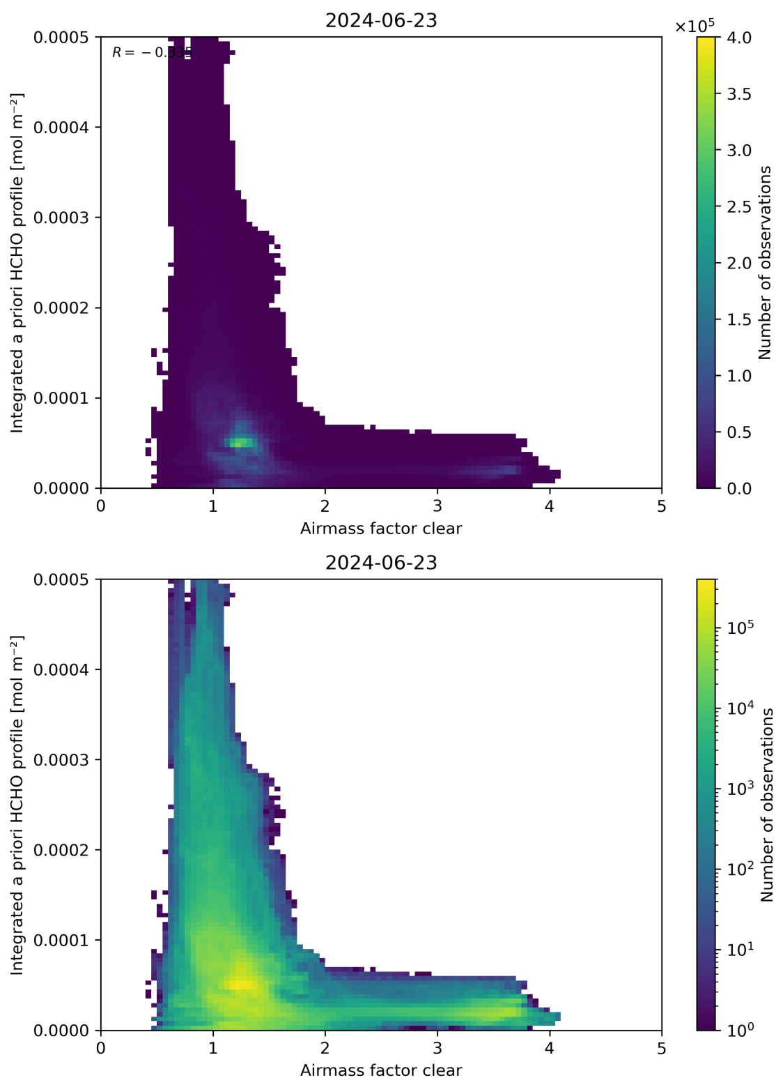
Figure 76: Scatter density plot of “Airmass factor clear” against “Integrated a priori HCHO profile” for 2024-06-22 to 2024-06-24.
