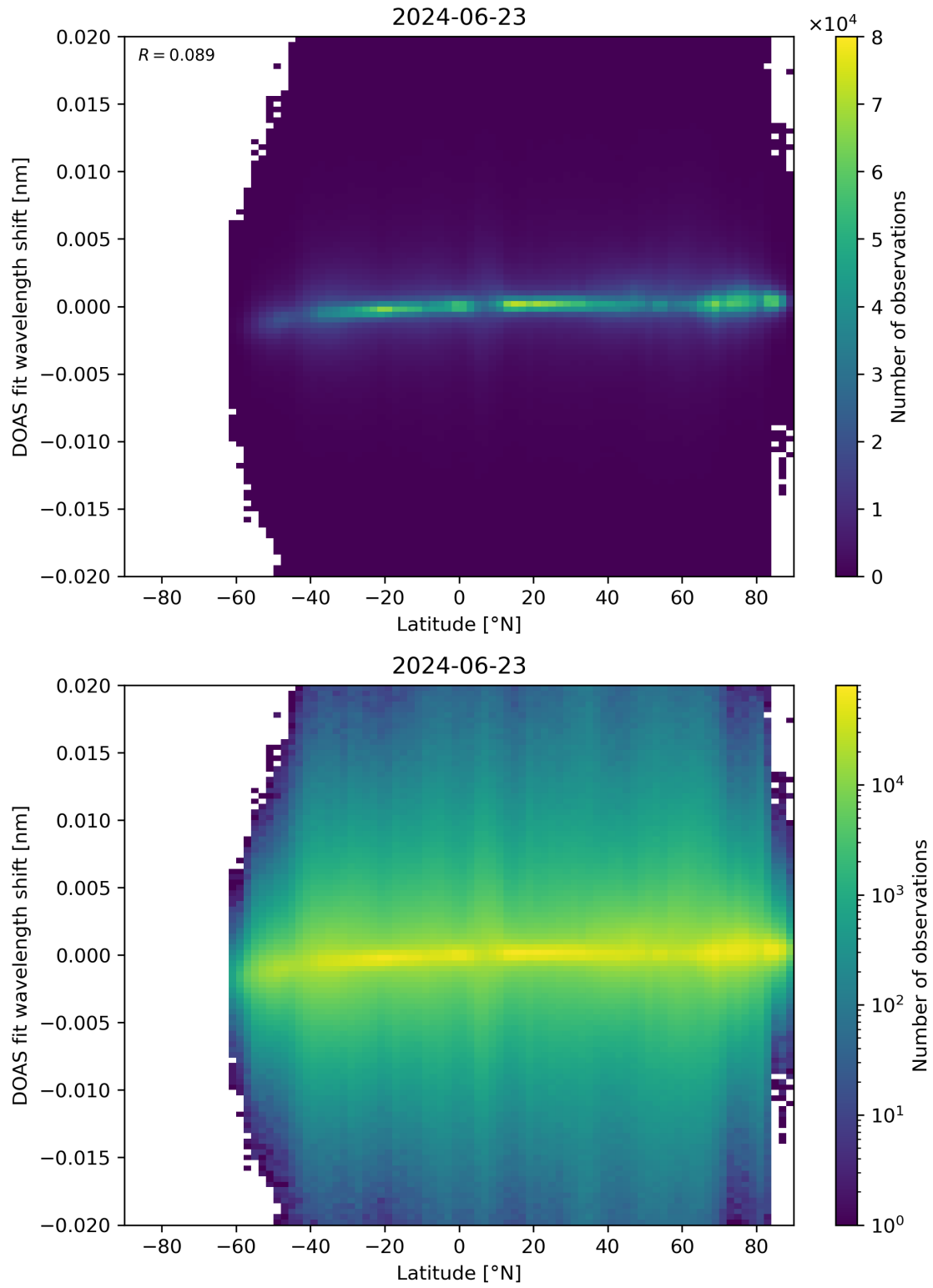
Figure 154: Scatter density plot of “Latitude” against “DOAS fit wavelength shift” for 2024-06-22 to 2024-06-24.
