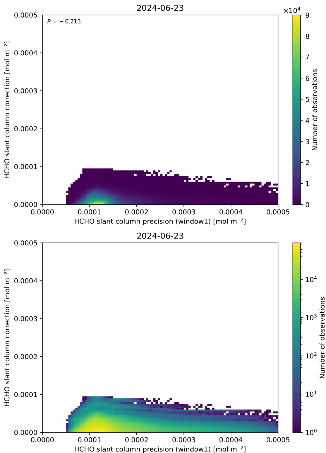
Figure 93: Scatter density plot of “HCHO slant column precision (window1)” against “HCHO slant column correction” for 2024-06-22 to 2024-06-24.
