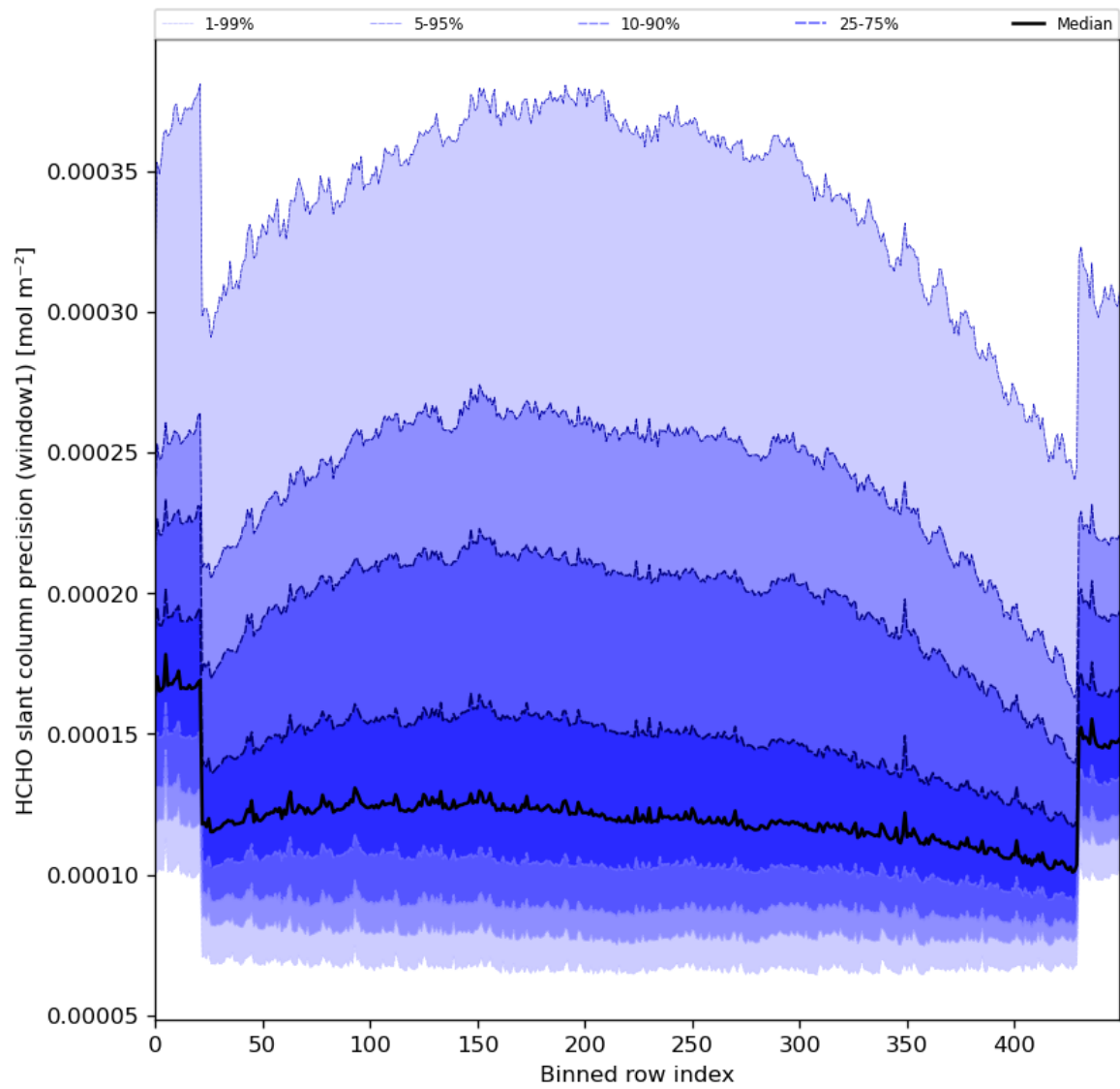
Figure 53: Along track statistics of “HCHO slant column precision (window1)” for 2024-06-22 to 2024-06-24
