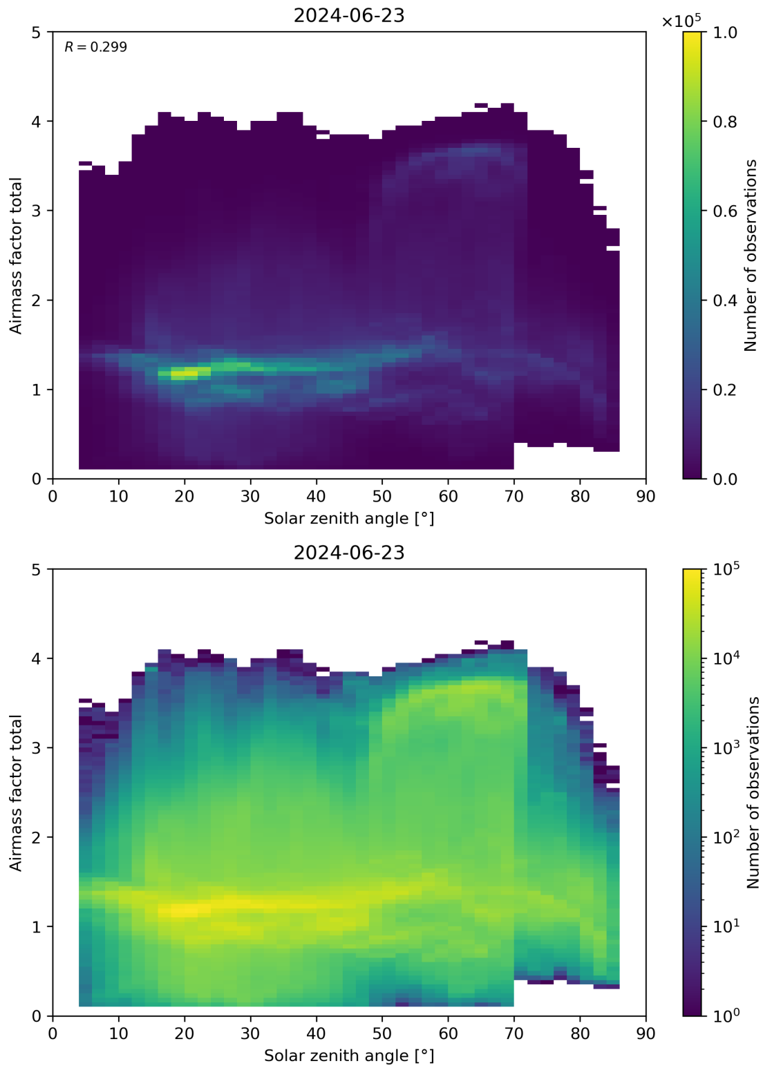
Figure 175: Scatter density plot of “Solar zenith angle” against “Airmass factor total” for 2024-06-22 to 2024-06-24.
