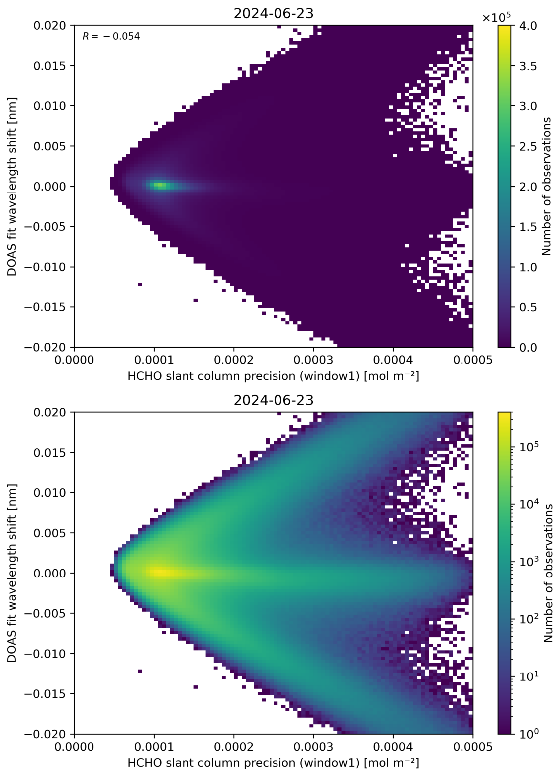
Figure 89: Scatter density plot of “HCHO slant column precision (window1)” against “DOAS fit wavelength shift” for 2024-06-22 to 2024-06-24.
