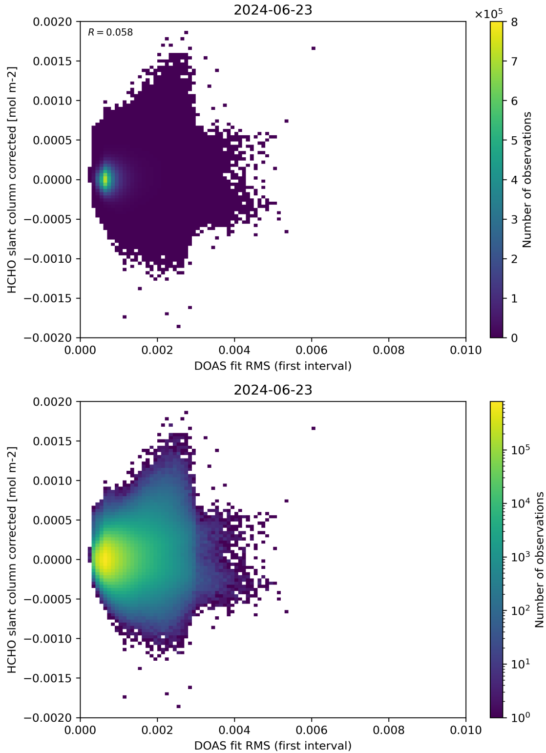
Figure 62: Scatter density plot of “DOAS fit RMS (first interval)” against “HCHO slant column corrected” for 2024-06-22 to 2024-06-24.
