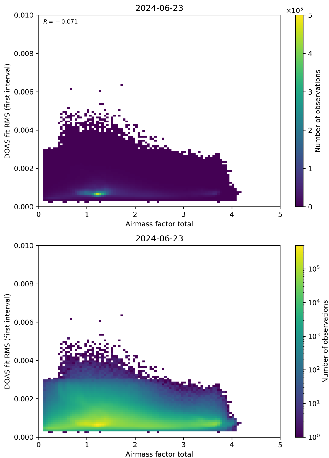
Figure 97: Scatter density plot of “Airmass factor total” against “DOAS fit RMS (first interval)” for 2024-06-22 to 2024-06-24.
