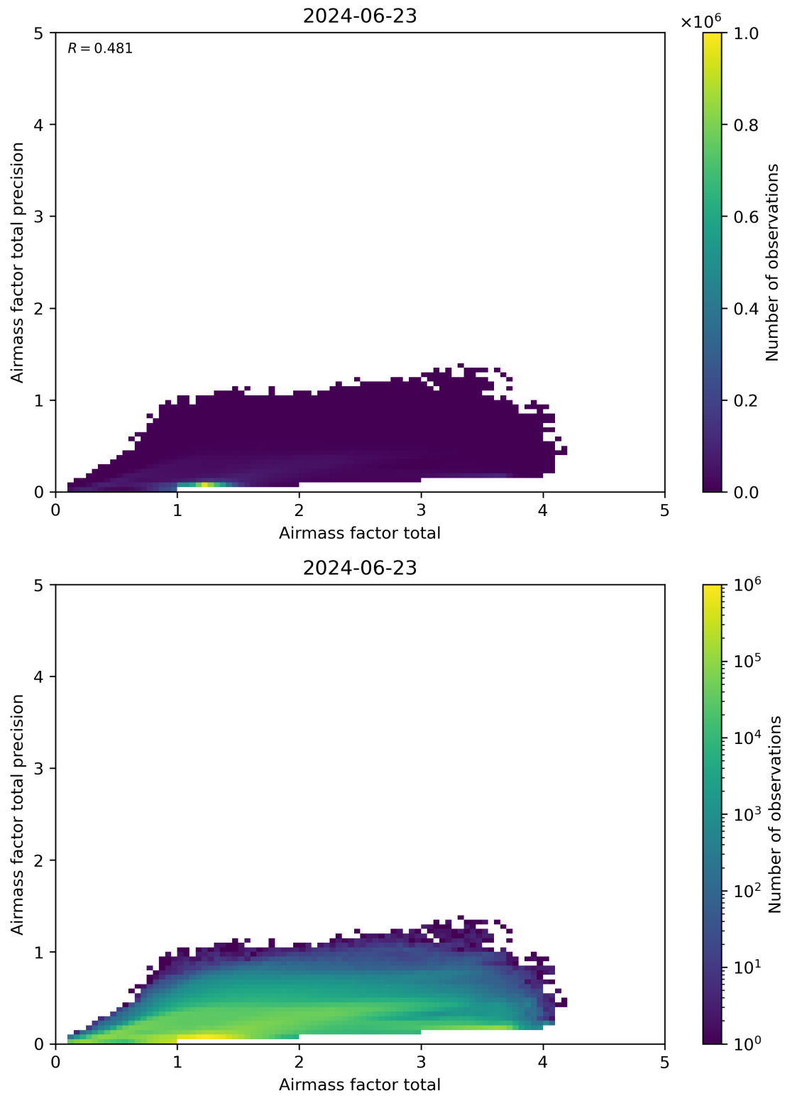
Figure 103: Scatter density plot of “Airmass factor total” against “Airmass factor total precision” for 2024-06-22 to 2024-06-24.
