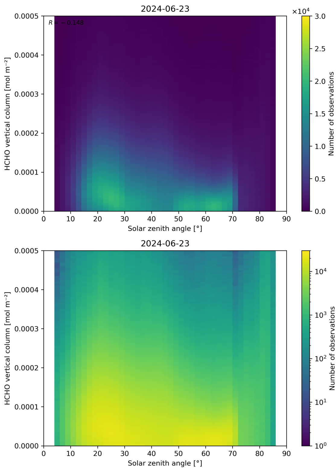
Figure 177: Scatter density plot of “Solar zenith angle” against “HCHO vertical column” for 2024-06-22 to 2024-06-24.
