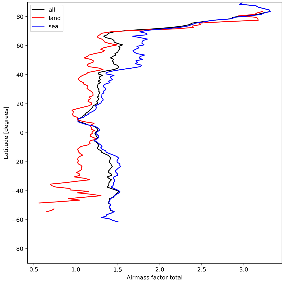
Figure 26: Zonal average of “Airmass factor total” for 2024-06-22 to 2024-06-24.
