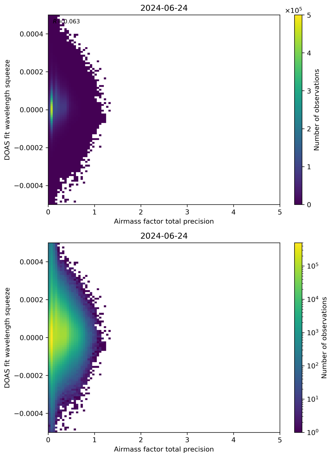
Figure 107: Scatter density plot of “Airmass factor total precision” against “DOAS fit wavelength squeeze” for 2024-06-24 to 2024-06-25.
