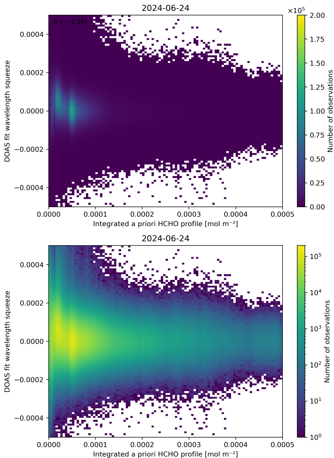
Figure 150: Scatter density plot of “Integrated a priori HCHO profile” against “DOAS fit wavelength squeeze” for 2024-06-24 to 2024-06-25.
