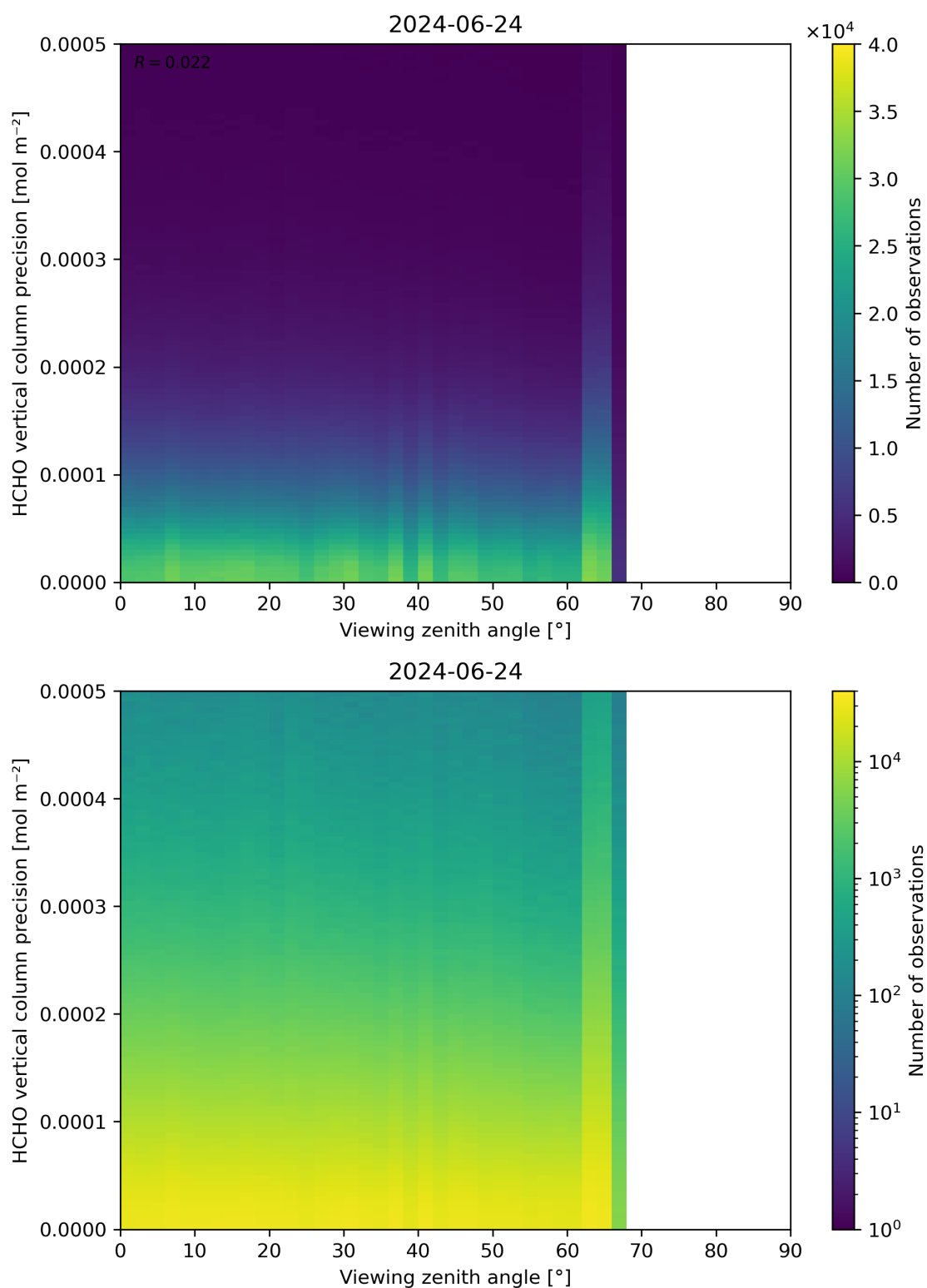
Figure 194: Scatter density plot of “Viewing zenith angle” against “HCHO vertical column precision” for 2024-06-24 to 2024-06-25.
