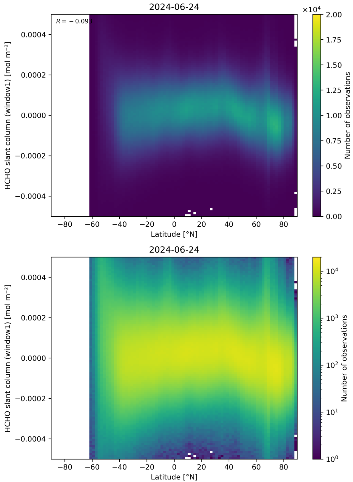
Figure 159: Scatter density plot of “Latitude” against “HCHO slant column (window1)” for 2024-06-24 to 2024-06-25.
