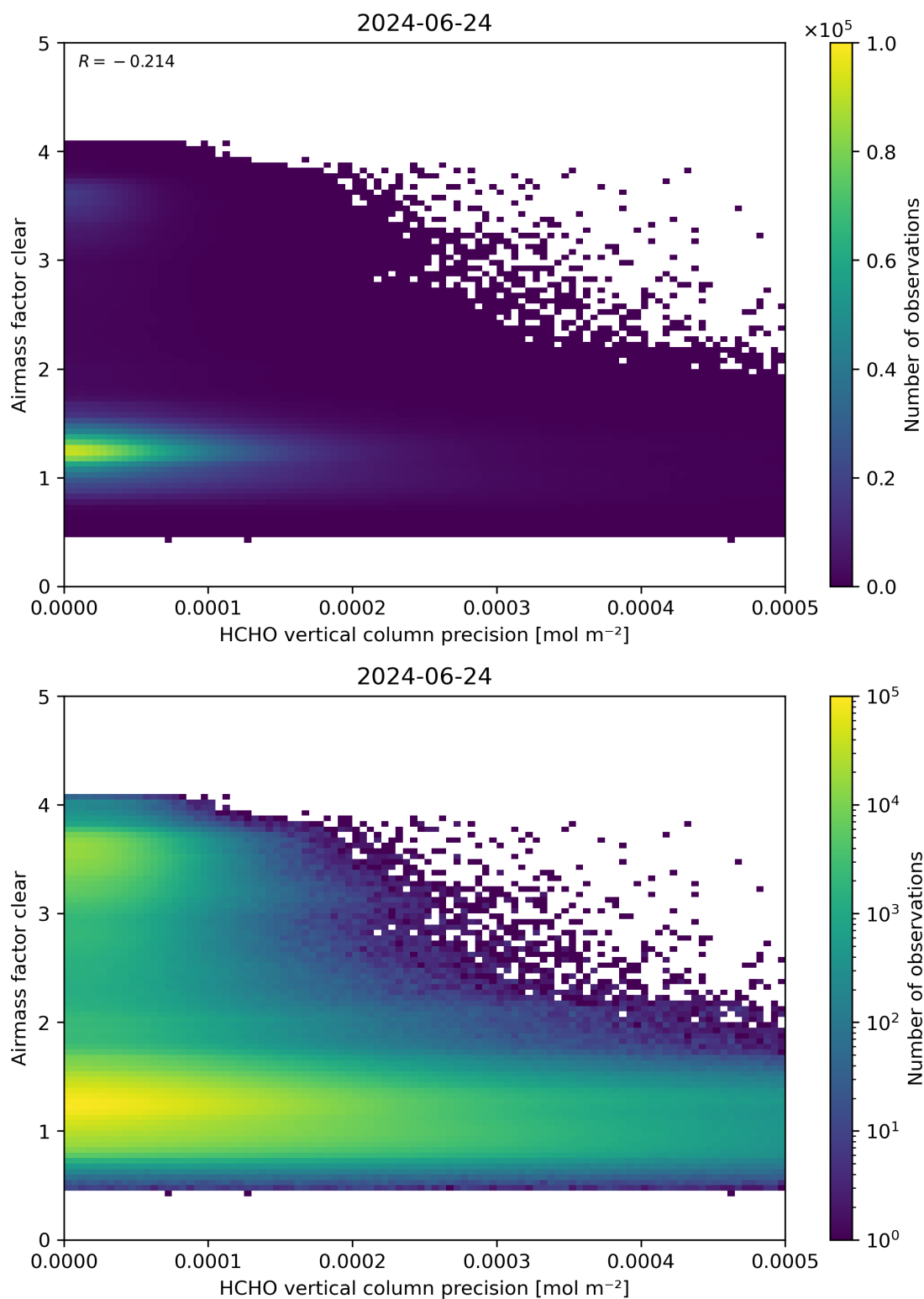
Figure 139: Scatter density plot of “HCHO vertical column precision” against “Airmass factor clear” for 2024-06-24 to 2024-06-25.
