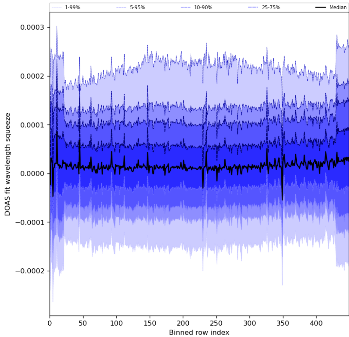
Figure 59: Along track statistics of “DOAS fit wavelength squeeze” for 2024-06-24 to 2024-06-25
