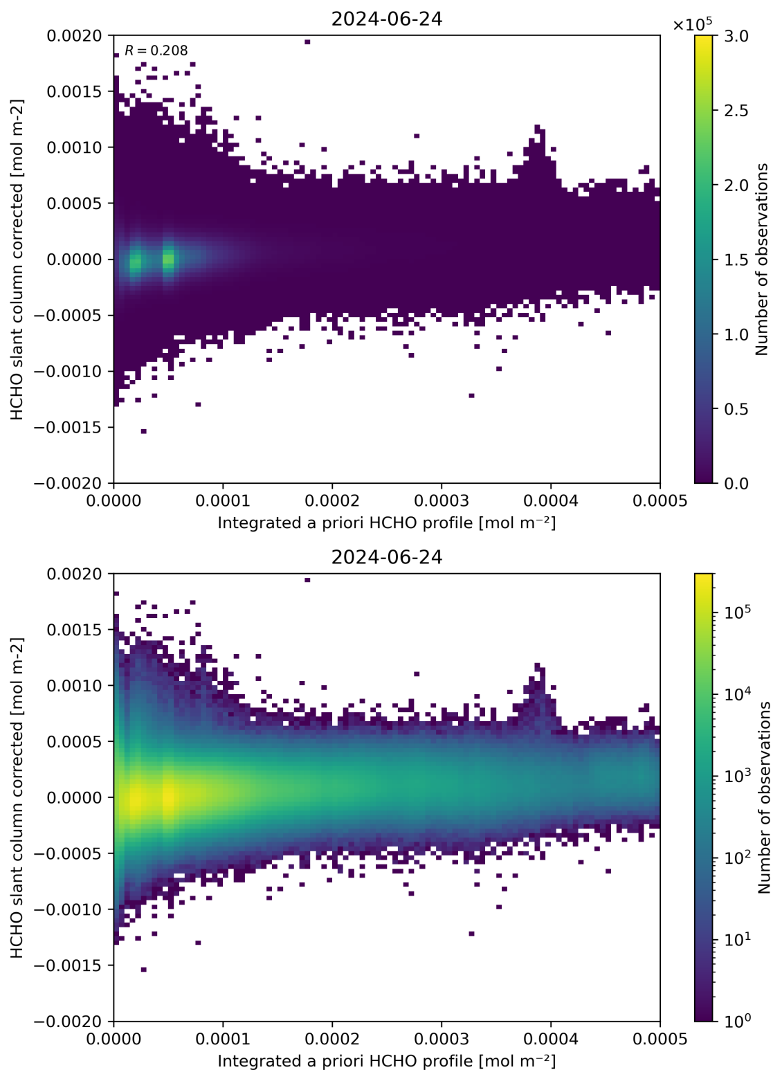
Figure 151: Scatter density plot of “Integrated a priori HCHO profile” against “HCHO slant column corrected” for 2024-06-24 to 2024-06-25.
