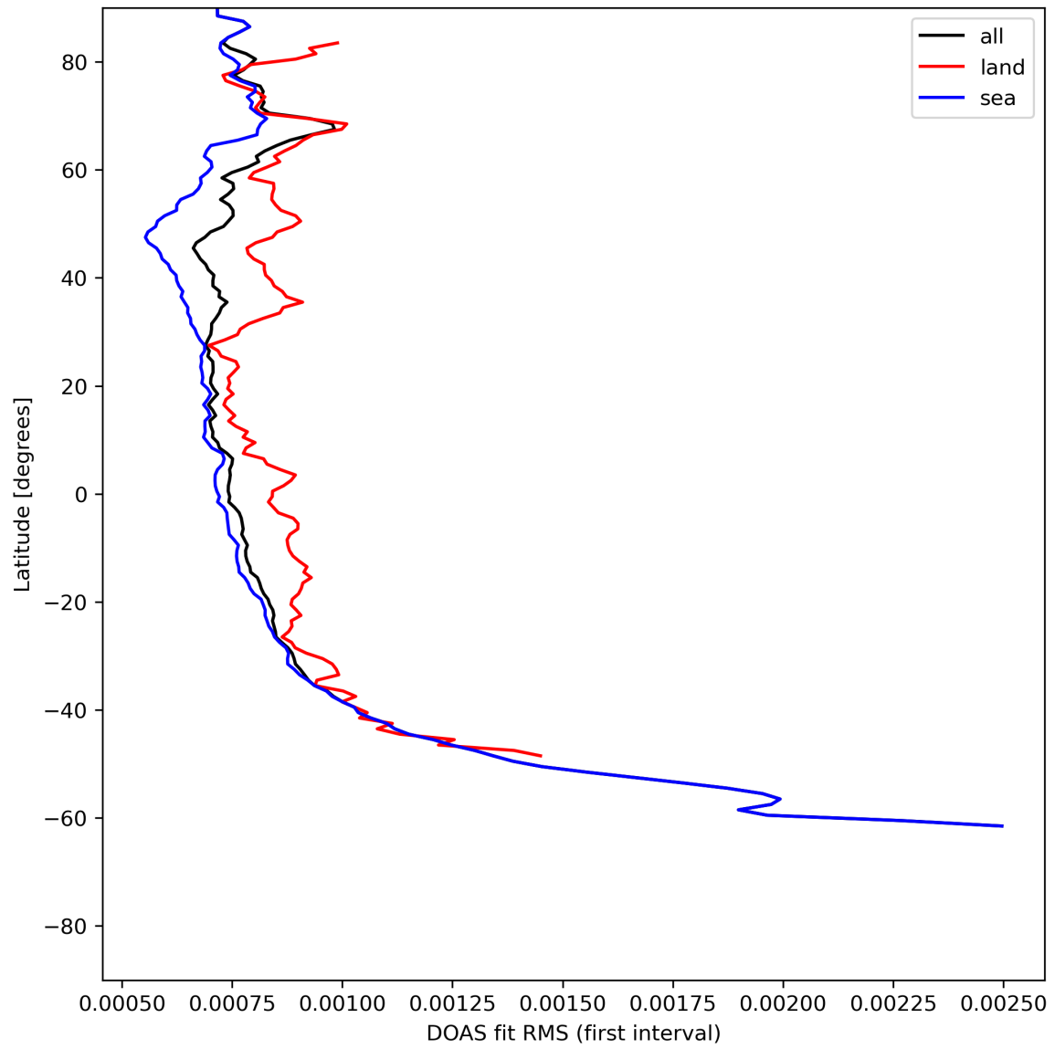
Figure 32: Zonal average of “DOAS fit RMS (first interval)” for 2024-06-24 to 2024-06-25.
