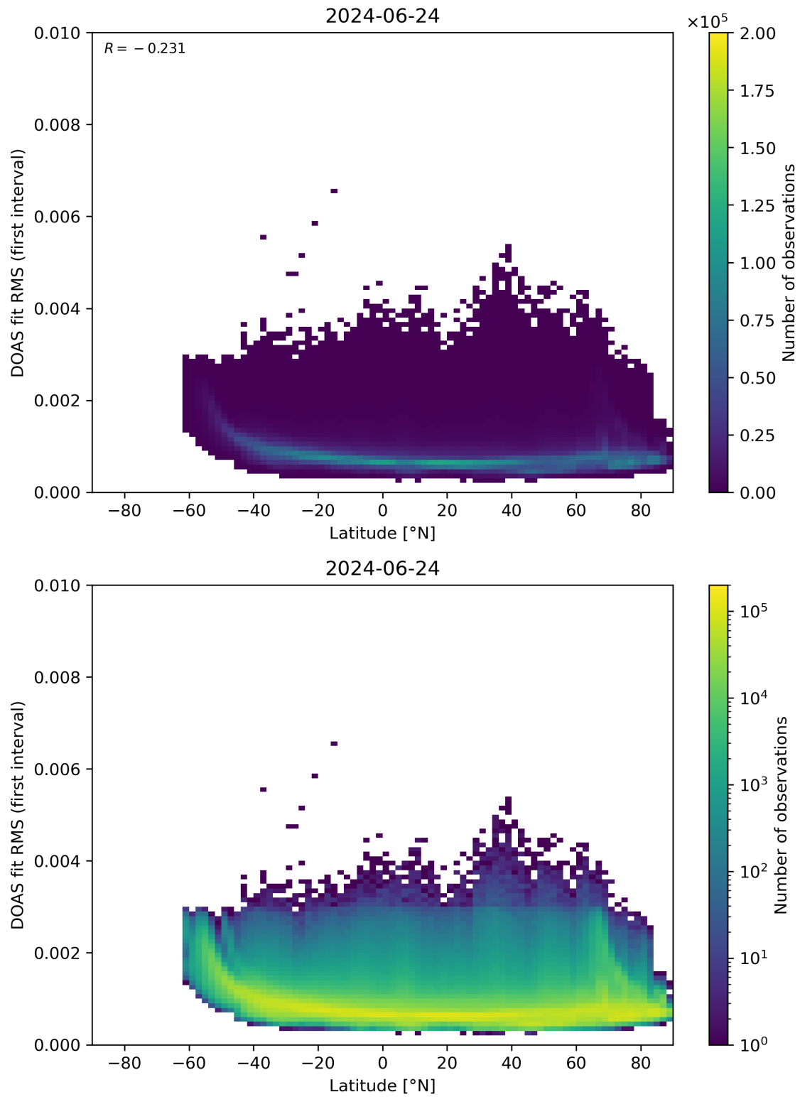
Figure 153: Scatter density plot of “Latitude” against “DOAS fit RMS (first interval)” for 2024-06-24 to 2024-06-25.
