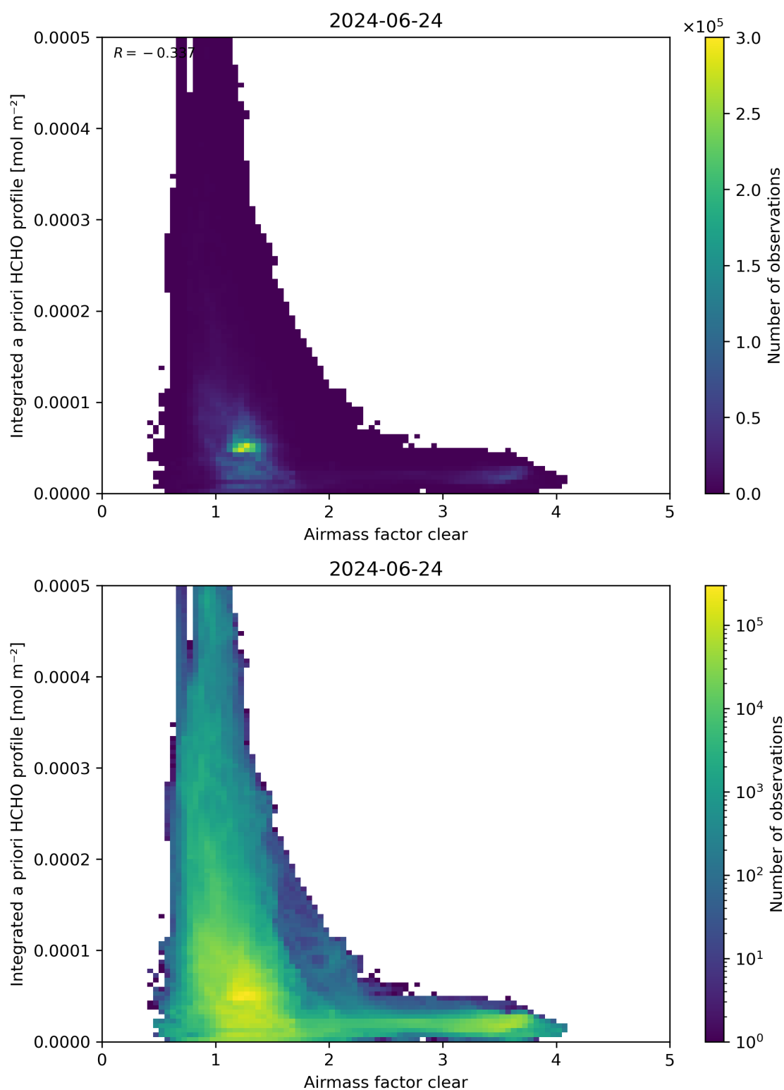
Figure 76: Scatter density plot of “Airmass factor clear” against “Integrated a priori HCHO profile” for 2024-06-24 to 2024-06-25.
