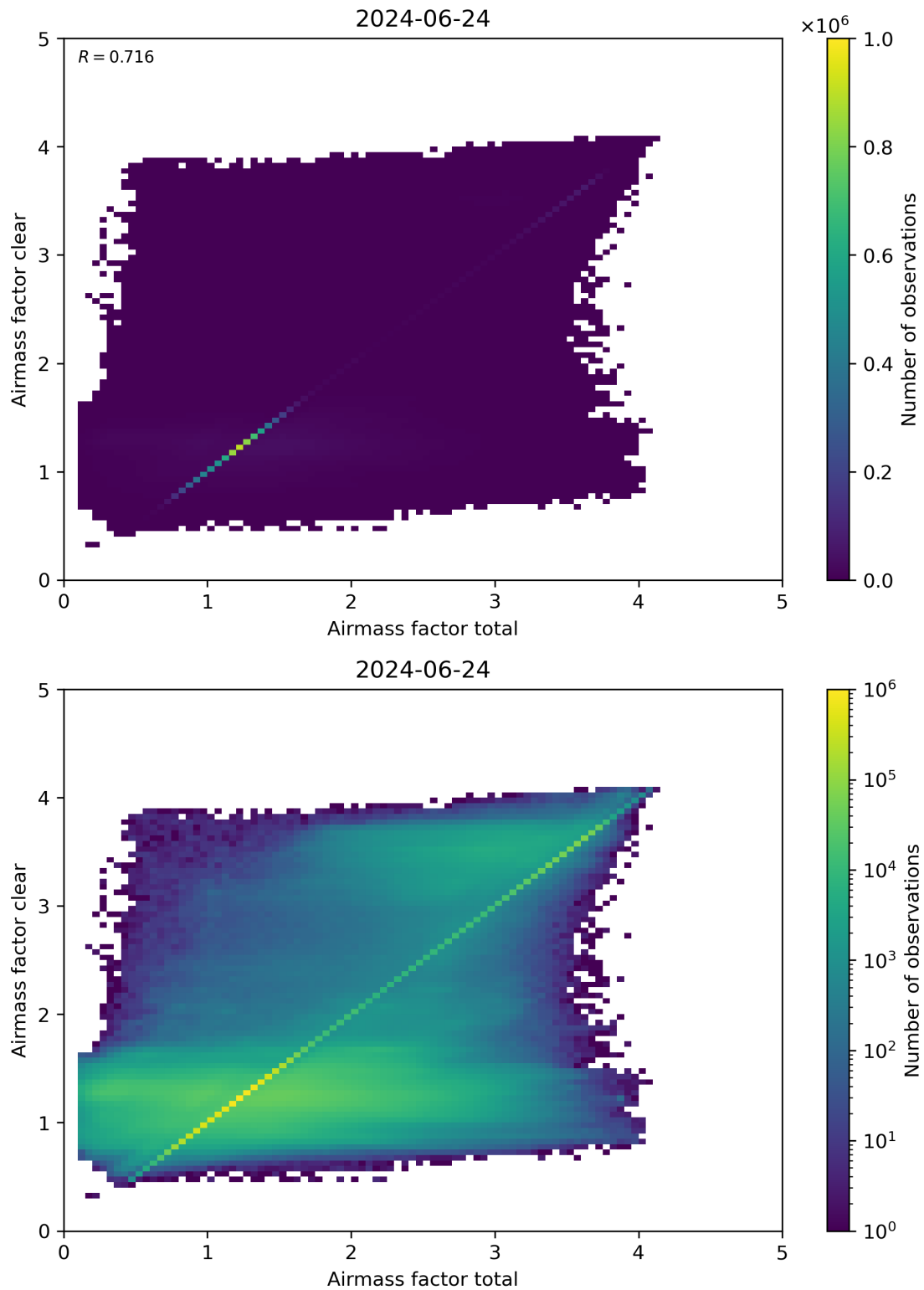
Figure 100: Scatter density plot of “Airmass factor total” against “Airmass factor clear” for 2024-06-24 to 2024-06-25.
