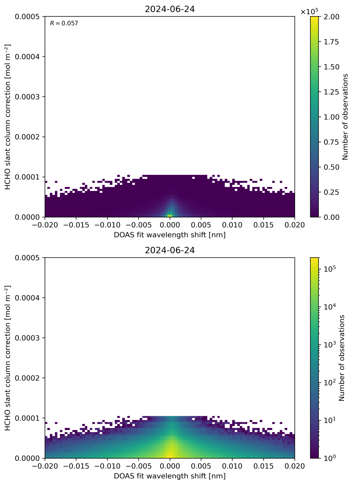
Figure 67: Scatter density plot of “DOAS fit wavelength shift” against “HCHO slant column correction” for 2024-06-24 to 2024-06-25.
