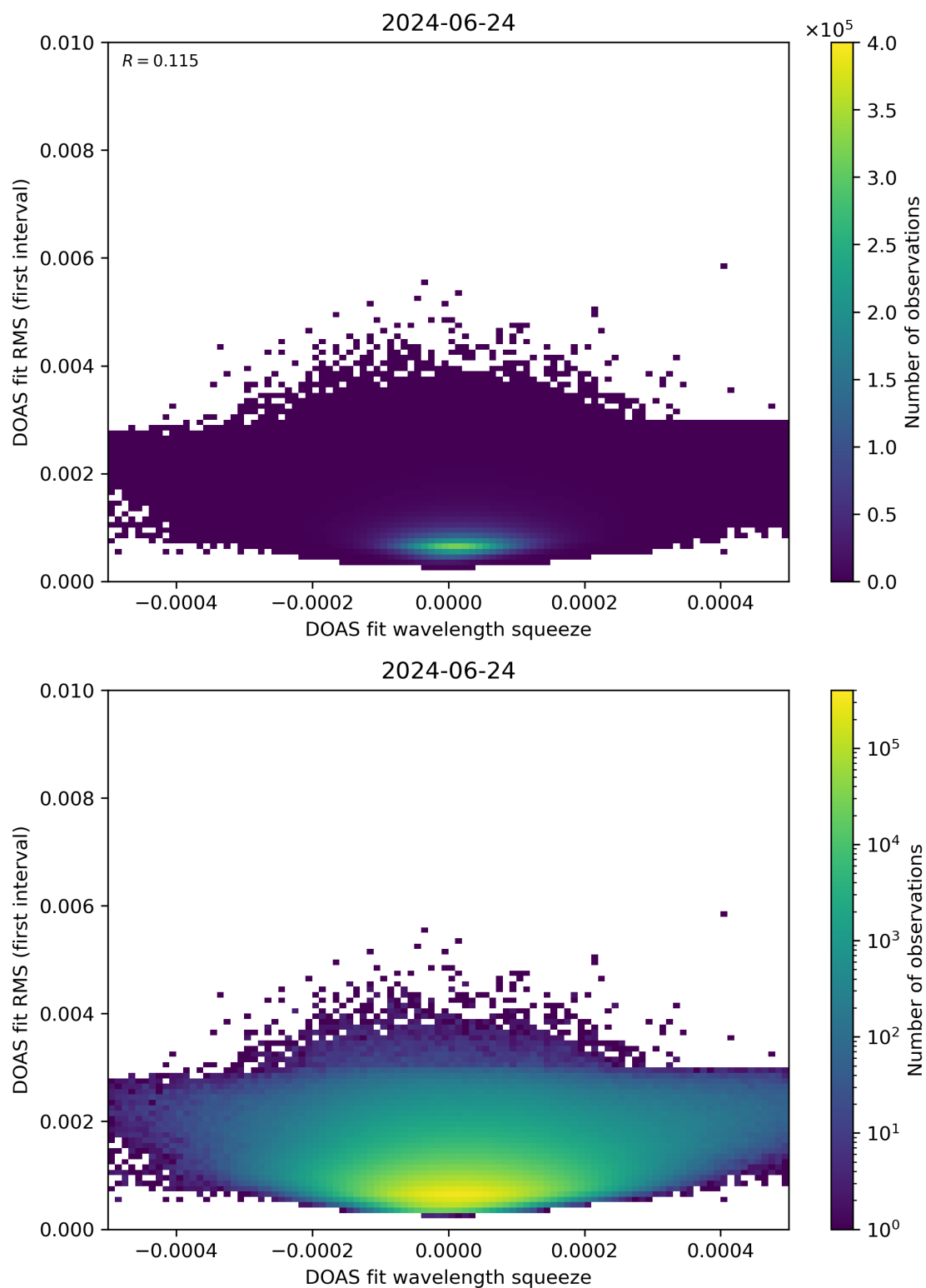
Figure 68: Scatter density plot of “DOAS fit wavelength squeeze” against “DOAS fit RMS (first interval)” for 2024-06-24 to 2024-06-25.
