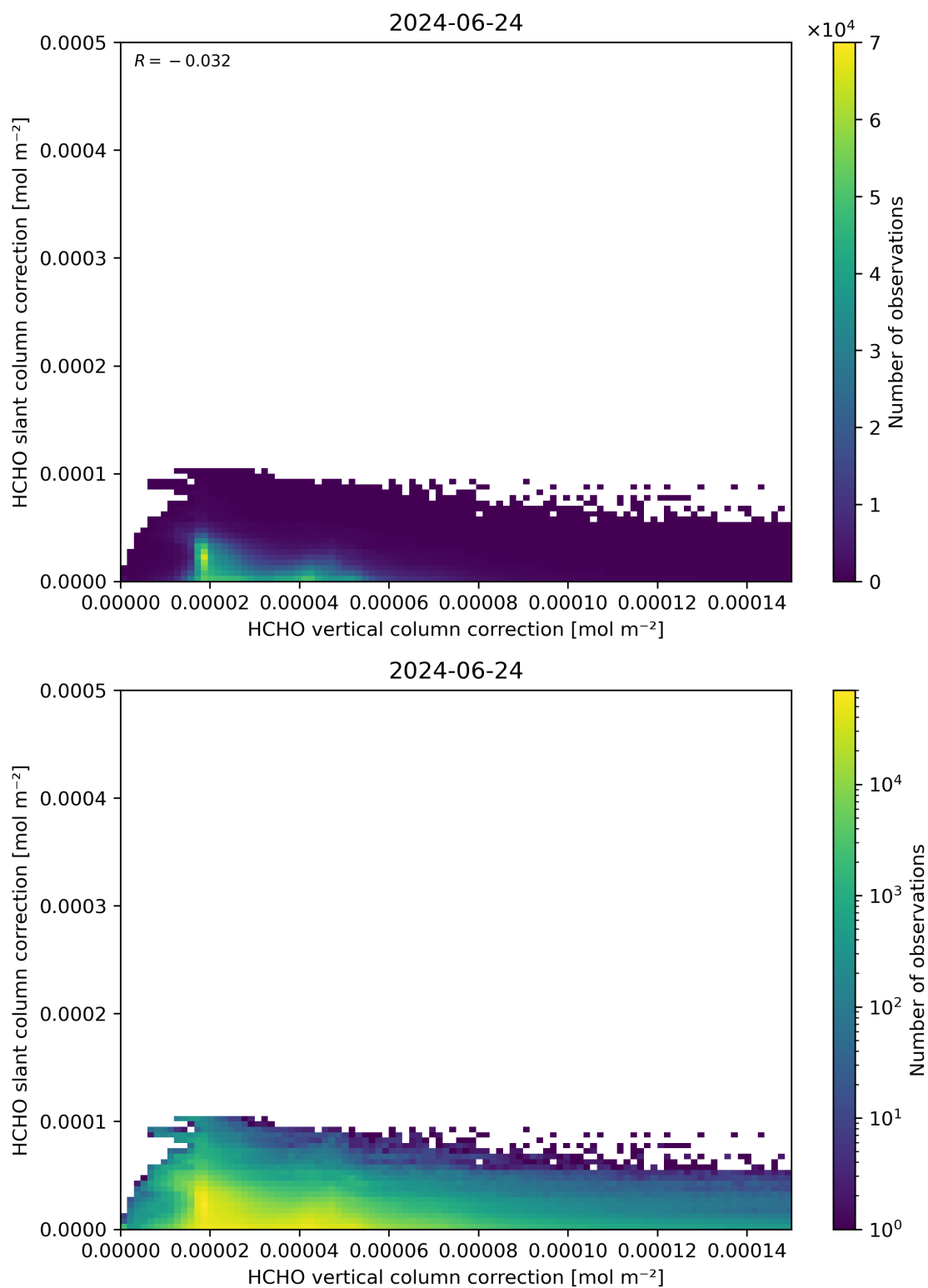
Figure 117: Scatter density plot of “HCHO vertical column correction” against “HCHO slant column correction” for 2024-06-24 to 2024-06-25.
