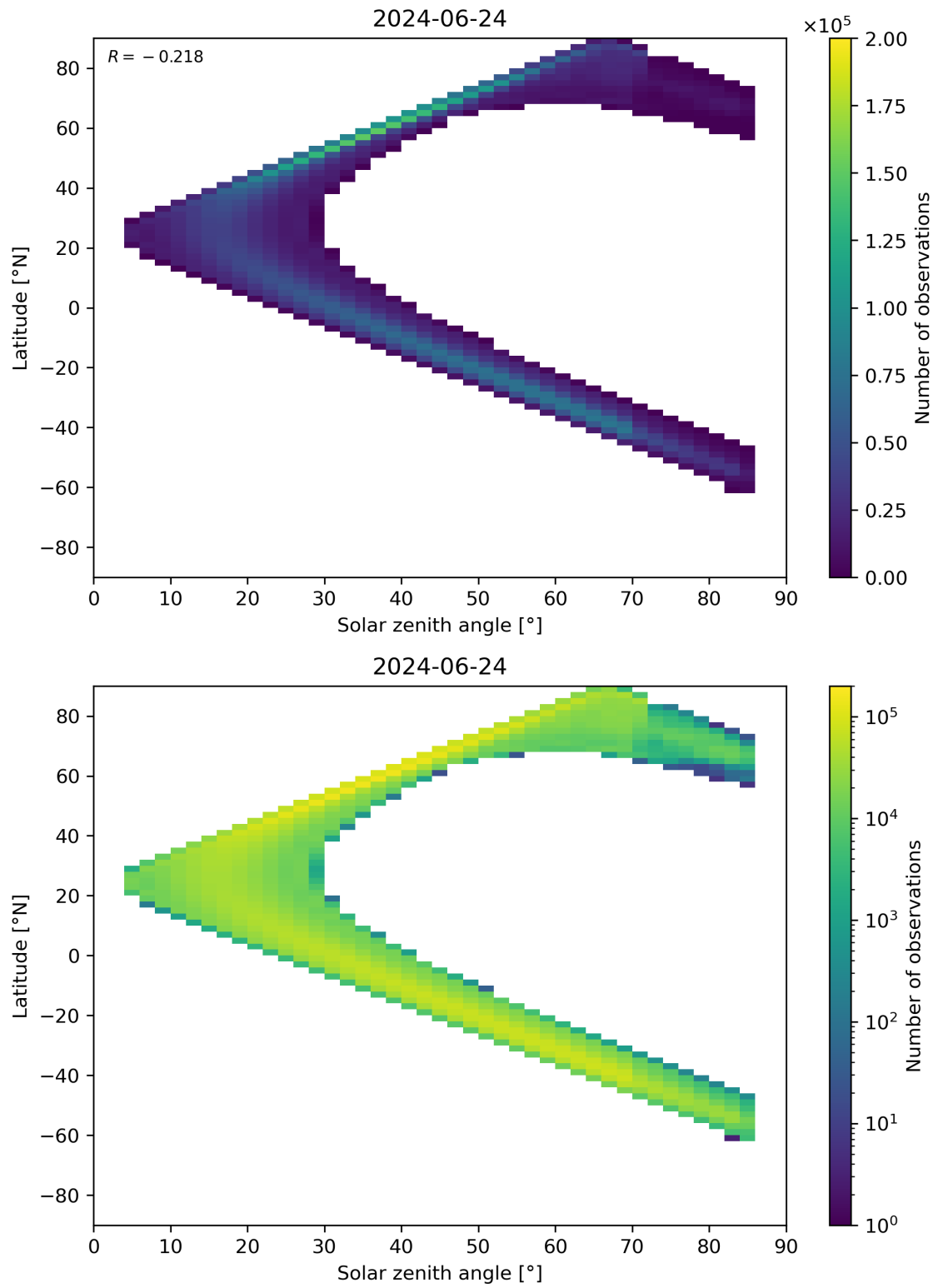
Figure 181: Scatter density plot of “Solar zenith angle” against “Latitude” for 2024-06-24 to 2024-06-25.
