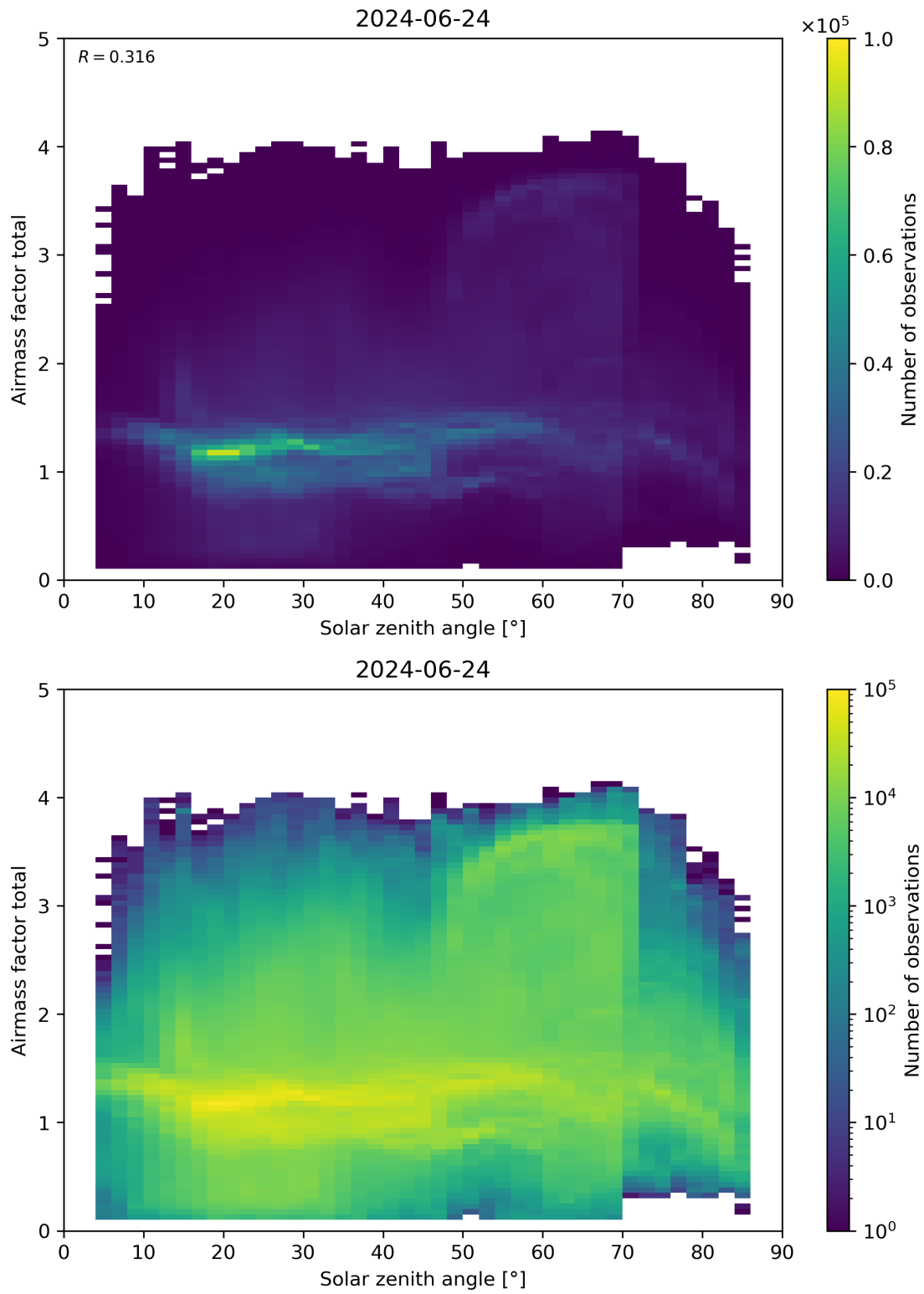
Figure 175: Scatter density plot of “Solar zenith angle” against “Airmass factor total” for 2024-06-24 to 2024-06-25.
