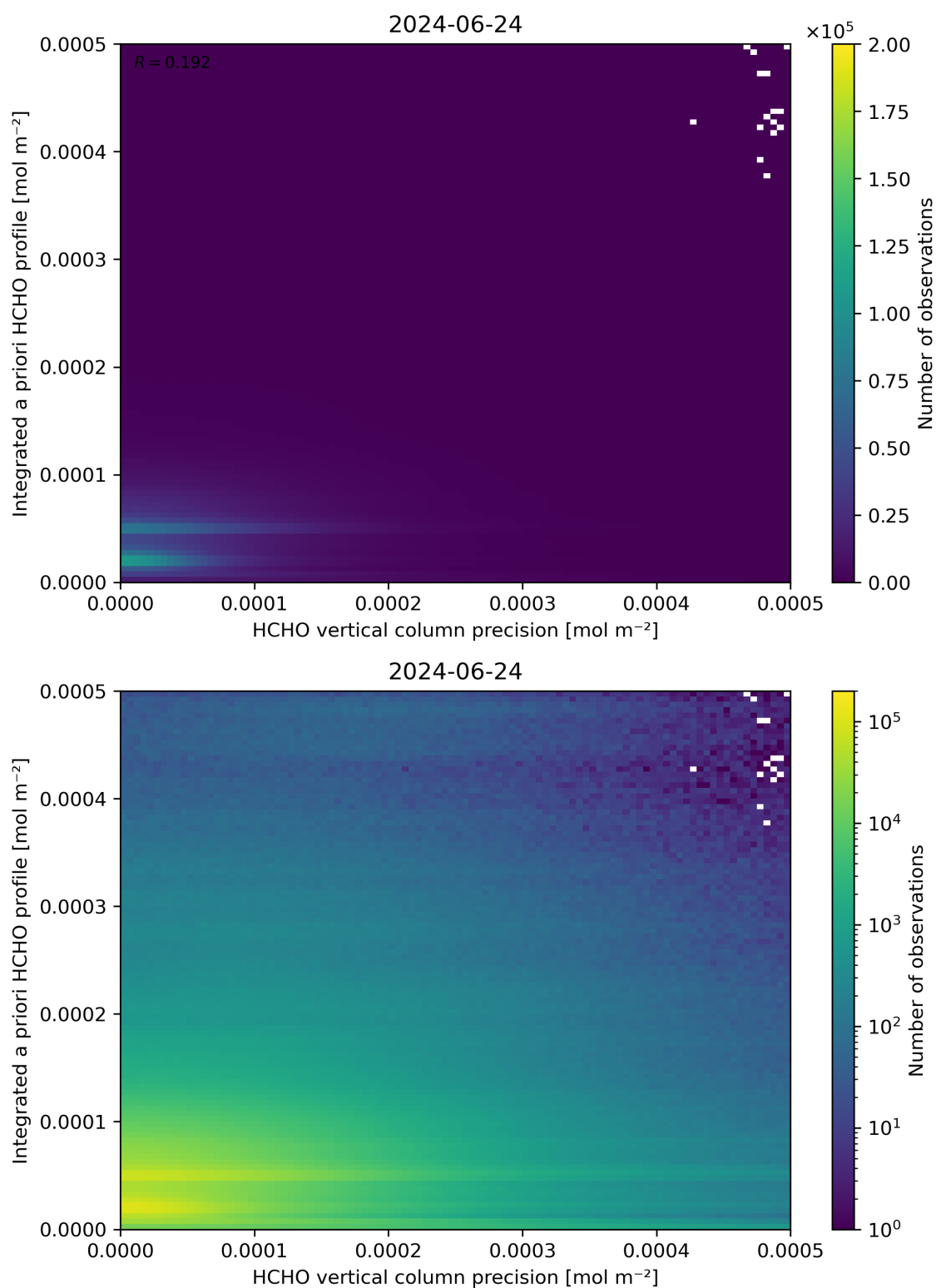
Figure 147: Scatter density plot of “HCHO vertical column precision” against “Integrated a priori HCHO profile” for 2024-06-24 to 2024-06-25.
