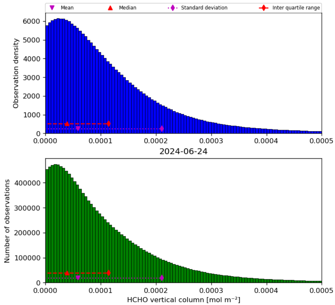
Figure 35: Histogram of “HCHO vertical column” for 2024-06-24 to 2024-06-25
