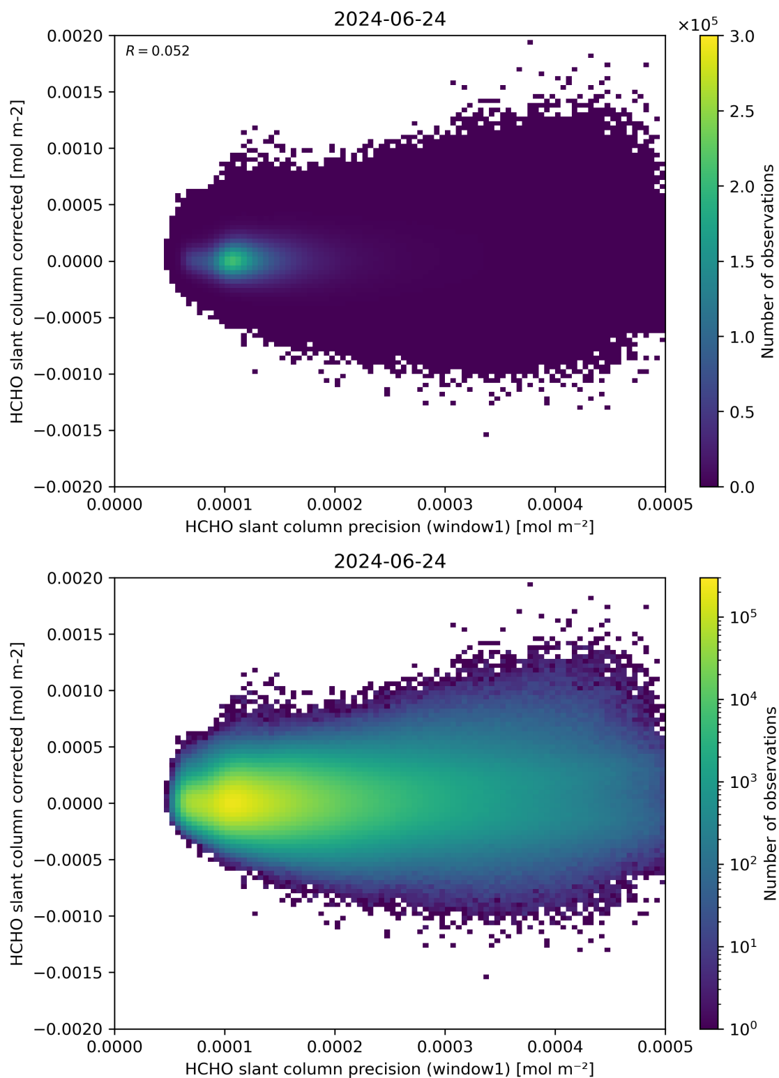
Figure 92: Scatter density plot of “HCHO slant column precision (window1)” against “HCHO slant column corrected” for 2024-06-24 to 2024-06-25.
