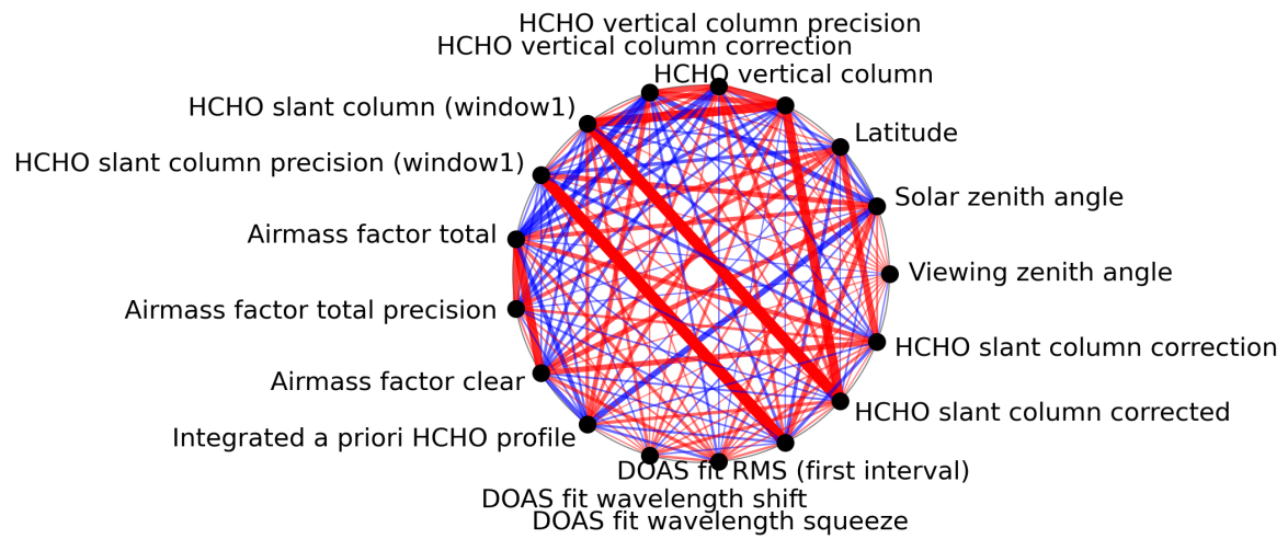
Figure 1: Map of correlation graph for 2024-06-24 to 2024-06-25.
