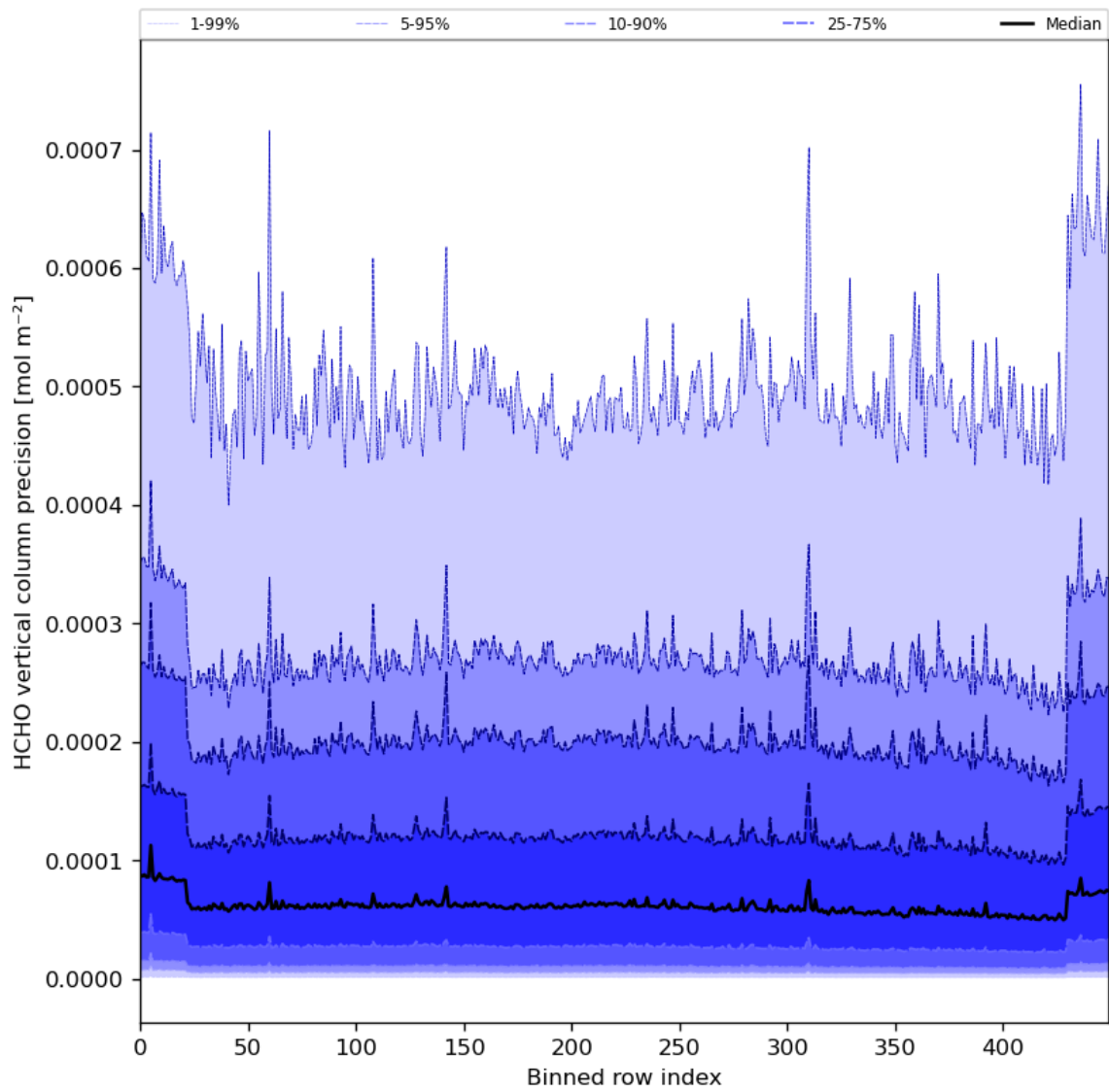
Figure 50: Along track statistics of “HCHO vertical column precision” for 2024-06-24 to 2024-06-25
