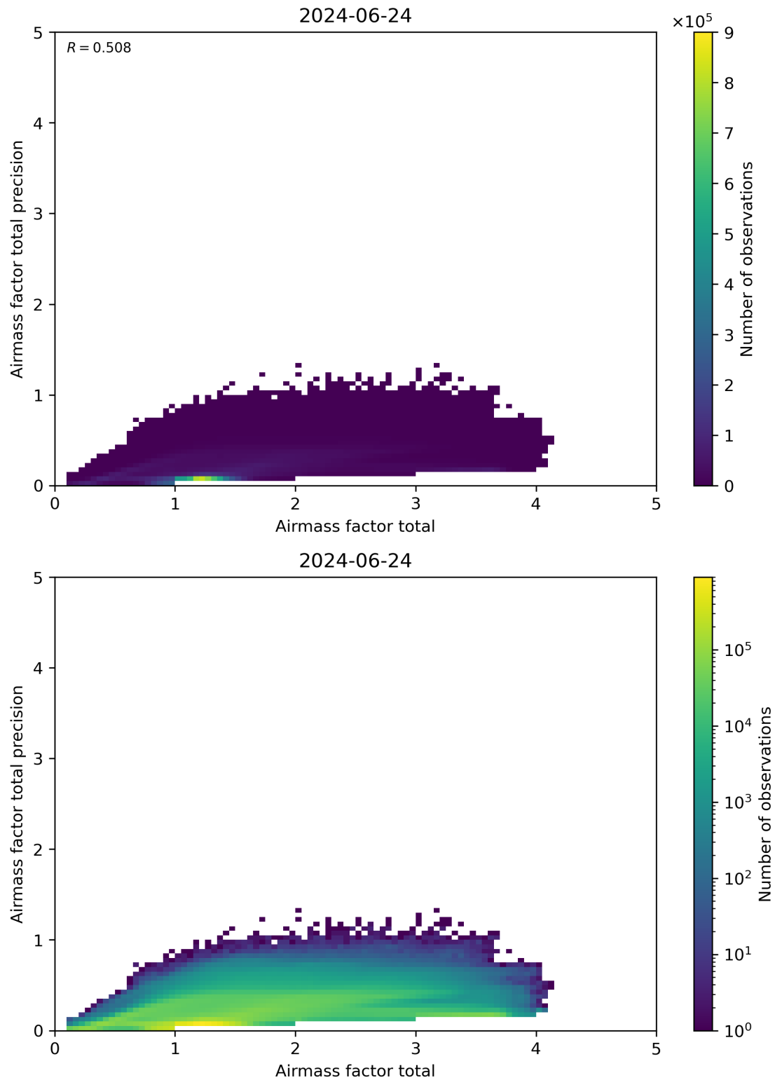
Figure 103: Scatter density plot of “Airmass factor total” against “Airmass factor total precision” for 2024-06-24 to 2024-06-25.
