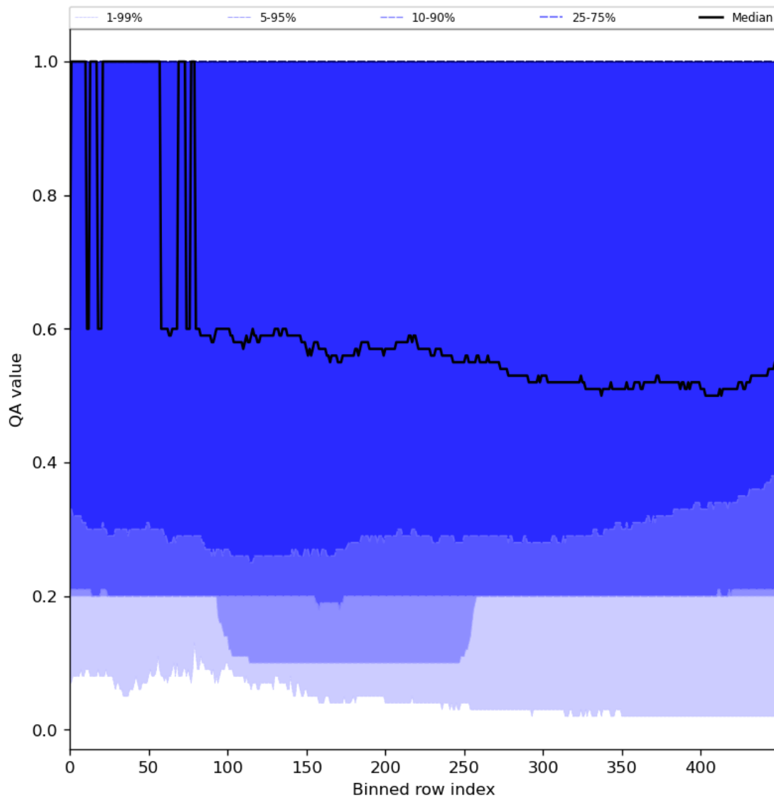
Figure 48: Along track statistics of “QA value” for 2024-06-24 to 2024-06-25
