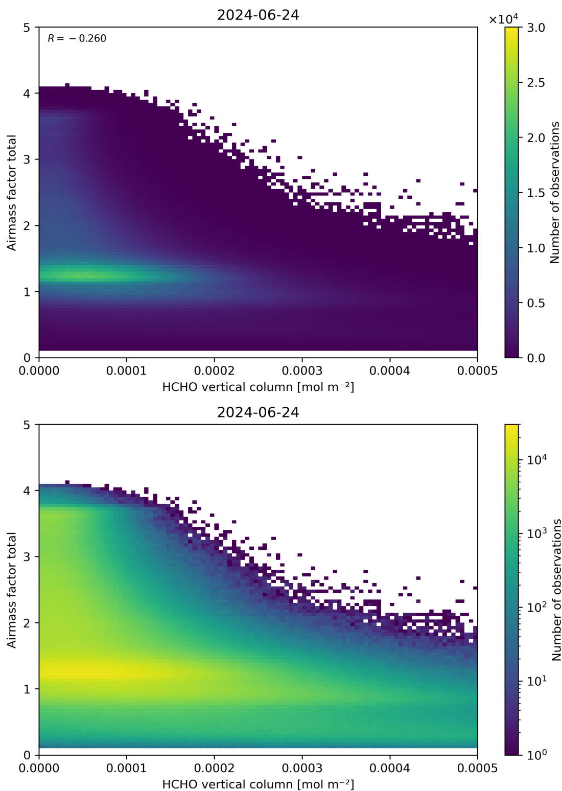
Figure 131: Scatter density plot of “HCHO vertical column” against “Airmass factor total” for 2024-06-24 to 2024-06-25.
