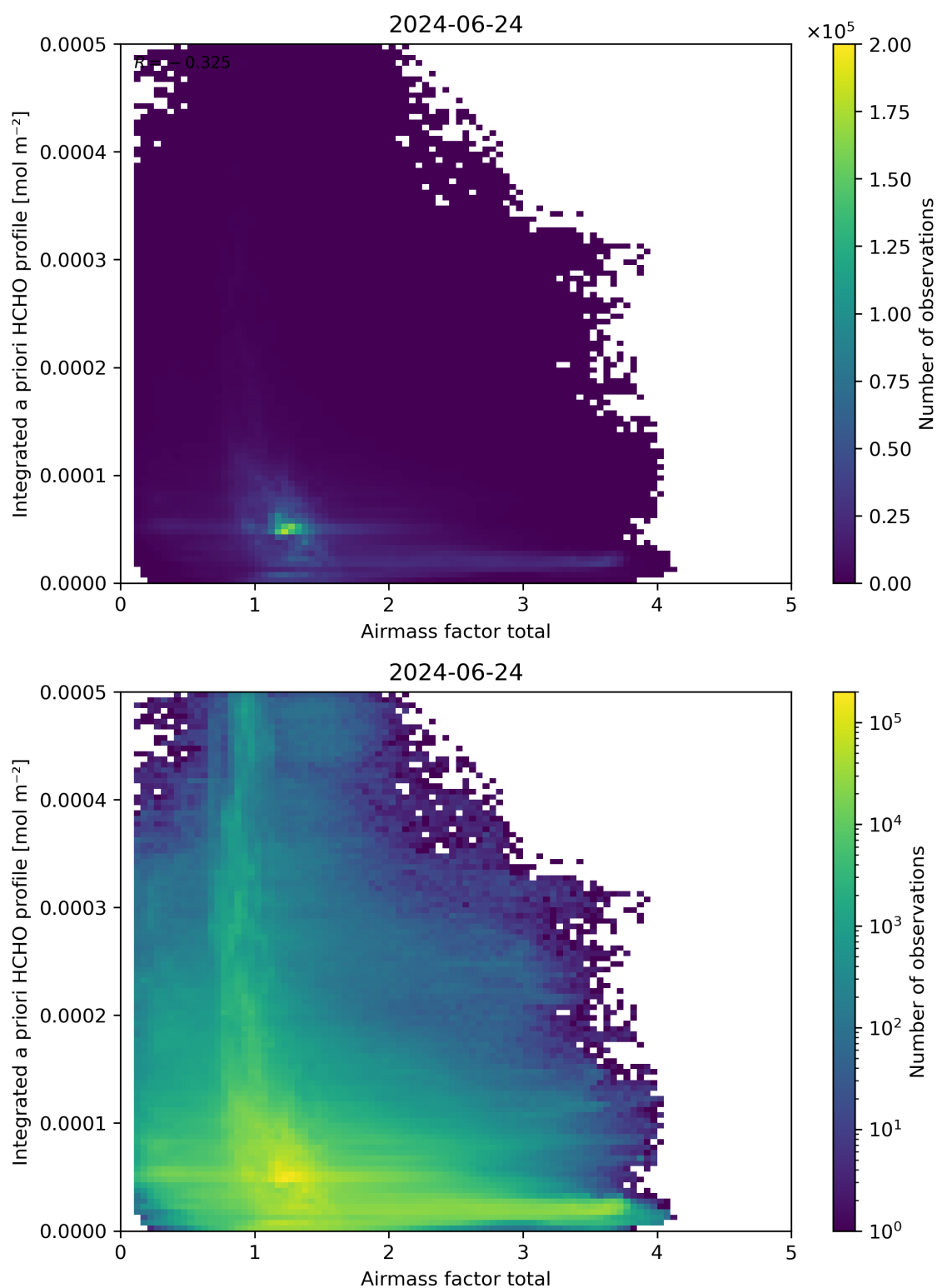
Figure 104: Scatter density plot of “Airmass factor total” against “Integrated a priori HCHO profile” for 2024-06-24 to 2024-06-25.
