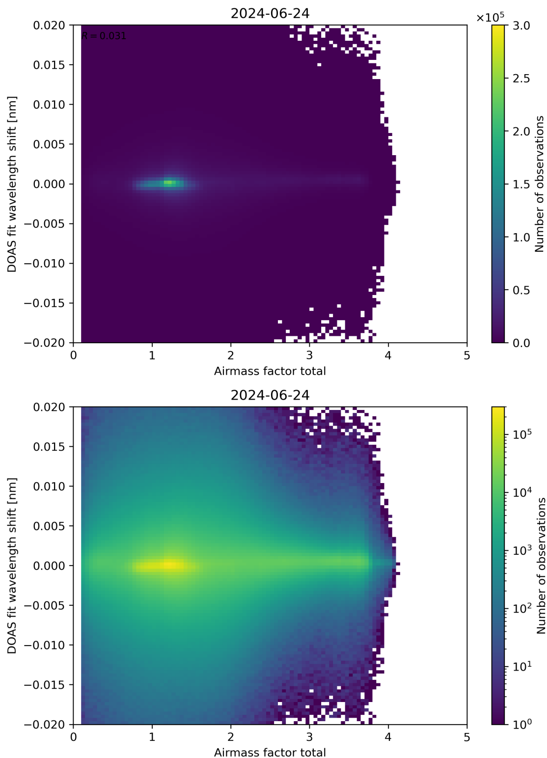
Figure 98: Scatter density plot of “Airmass factor total” against “DOAS fit wavelength shift” for 2024-06-24 to 2024-06-25.
