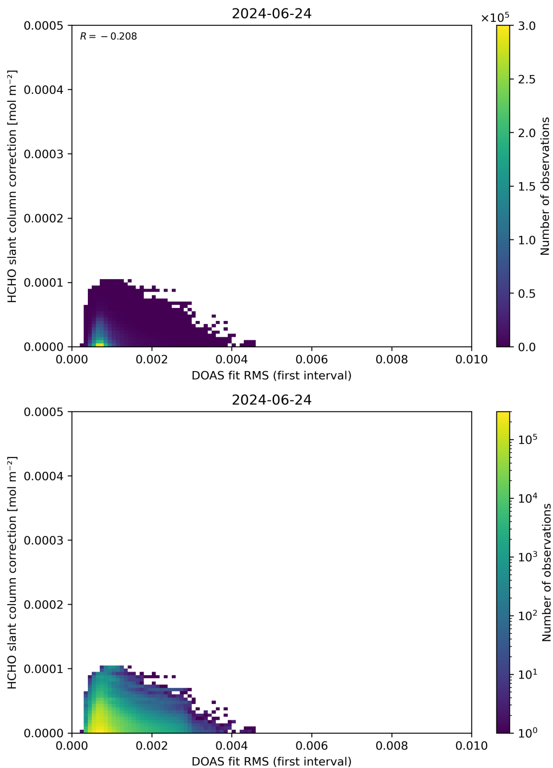
Figure 63: Scatter density plot of “DOAS fit RMS (first interval)” against “HCHO slant column correction” for 2024-06-24 to 2024-06-25.
