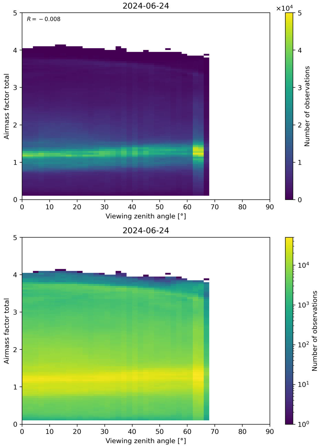
Figure 190: Scatter density plot of “Viewing zenith angle” against “Airmass factor total” for 2024-06-24 to 2024-06-25.
