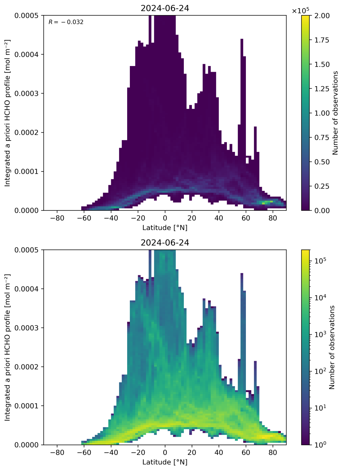
Figure 166: Scatter density plot of “Latitude” against “Integrated a priori HCHO profile” for 2024-06-24 to 2024-06-25.
