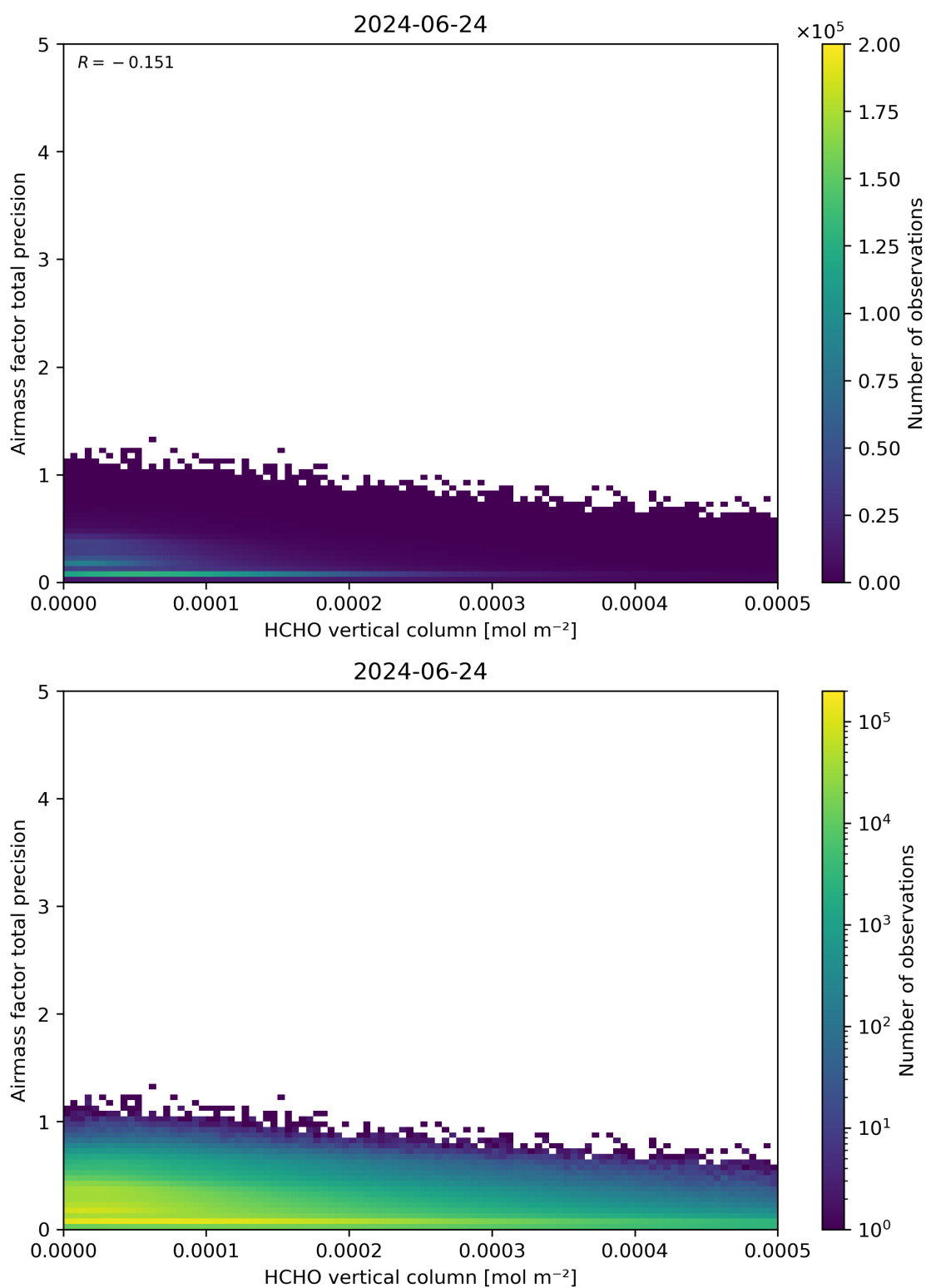
Figure 132: Scatter density plot of “HCHO vertical column” against “Airmass factor total precision” for 2024-06-24 to 2024-06-25.
