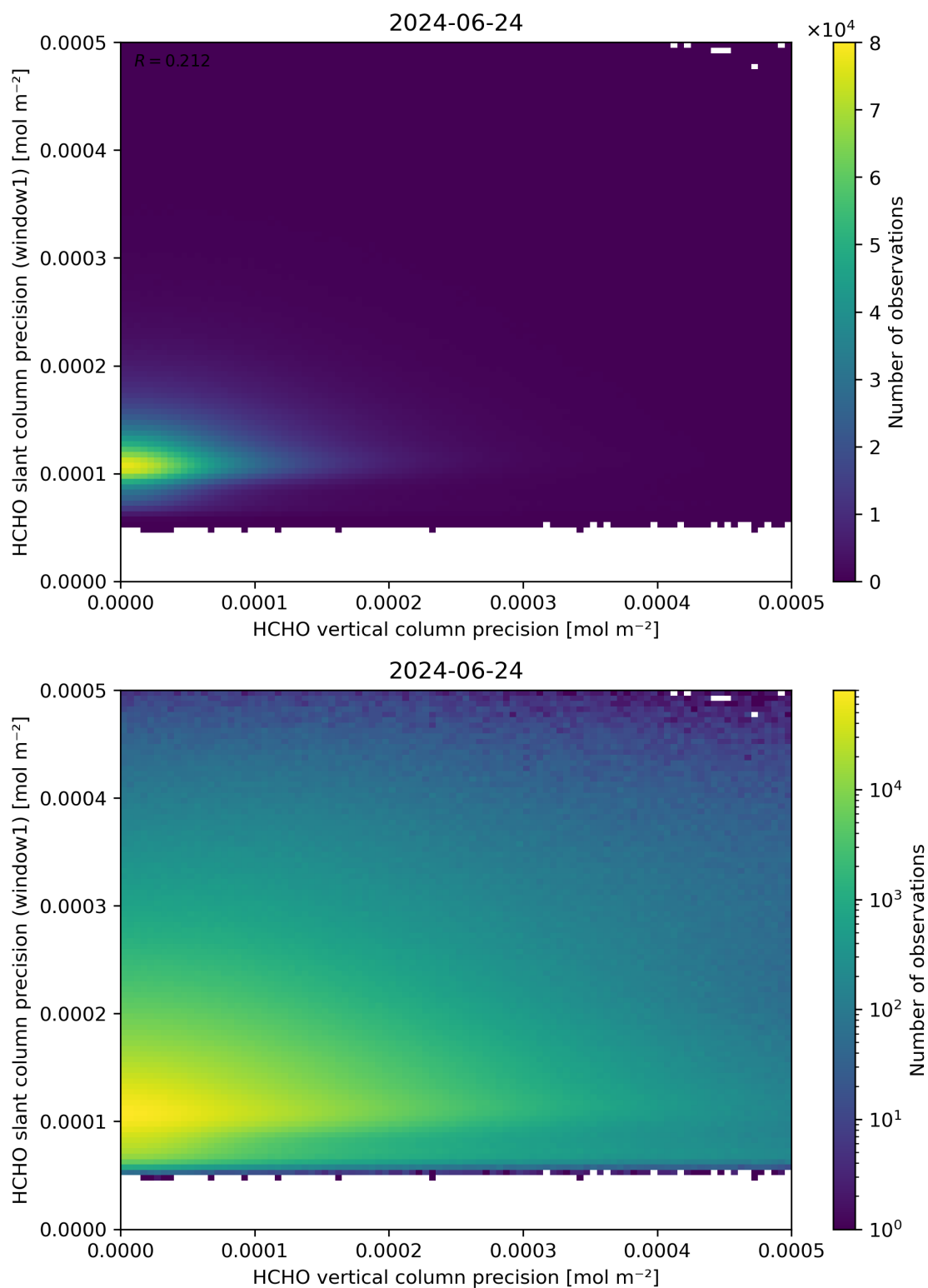
Figure 143: Scatter density plot of “HCHO vertical column precision” against “HCHO slant column precision (window1)” for 2024-06-24 to 2024-06-25.
