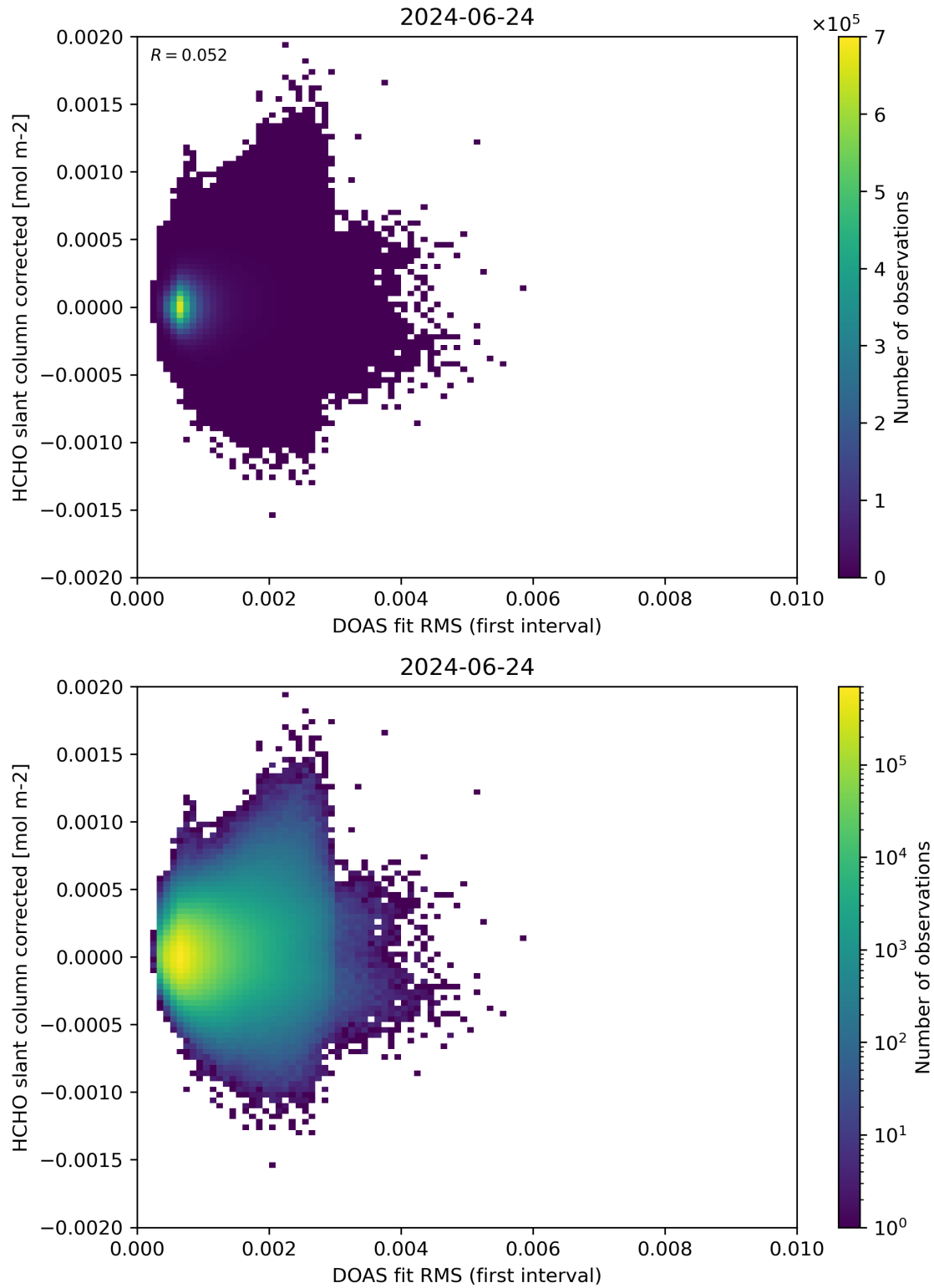
Figure 62: Scatter density plot of “DOAS fit RMS (first interval)” against “HCHO slant column corrected” for 2024-06-24 to 2024-06-25.
