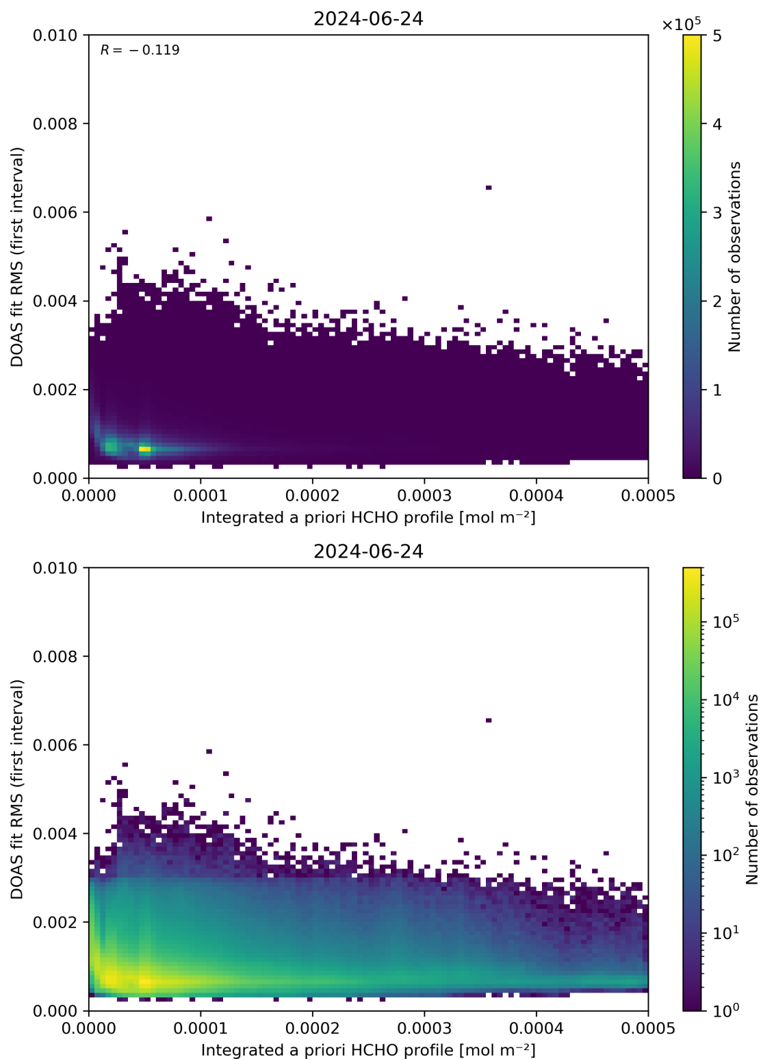
Figure 148: Scatter density plot of “Integrated a priori HCHO profile” against “DOAS fit RMS (first interval)” for 2024-06-24 to 2024-06-25.
