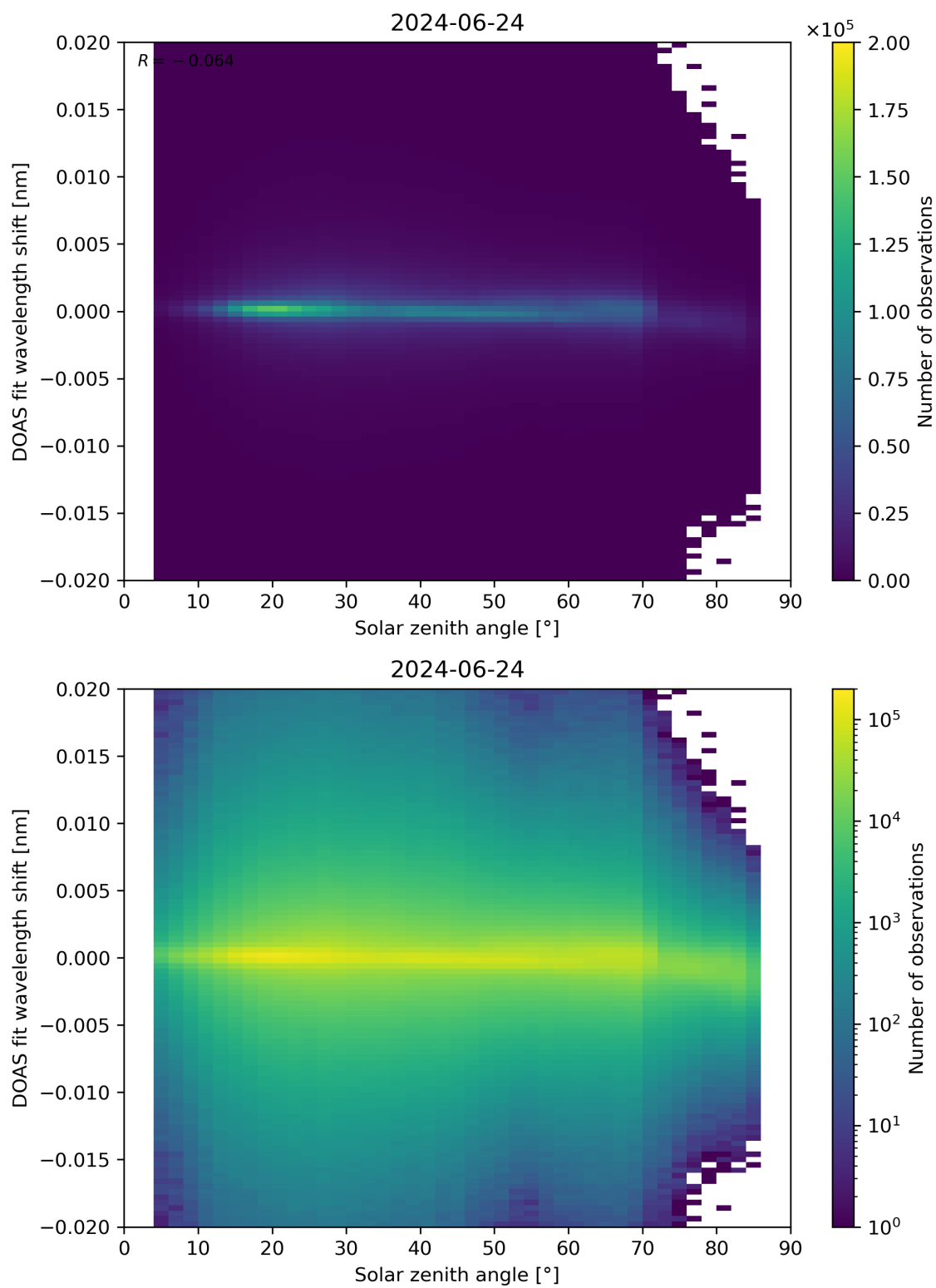
Figure 168: Scatter density plot of “Solar zenith angle” against “DOAS fit wavelength shift” for 2024-06-24 to 2024-06-25.
