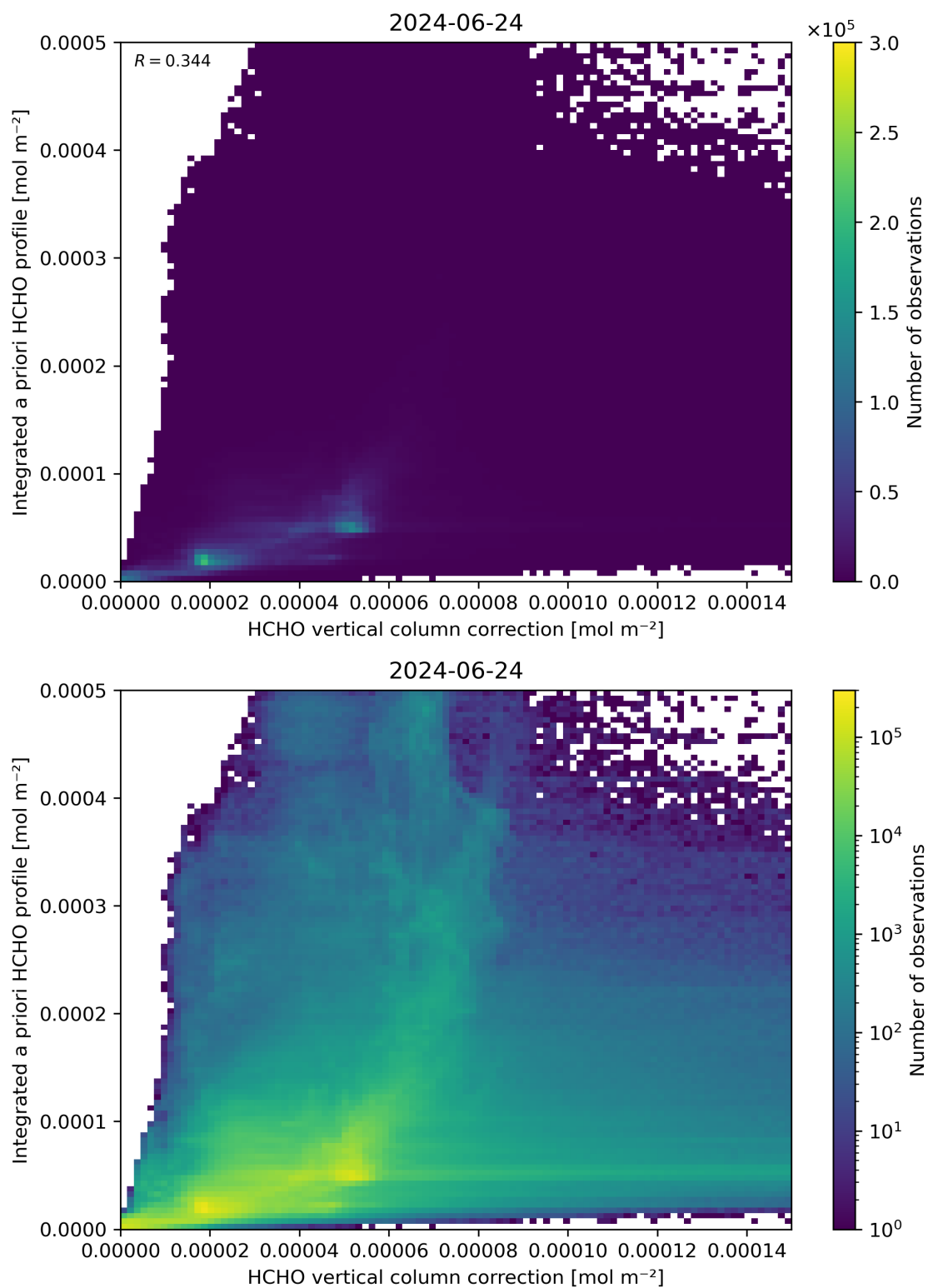
Figure 122: Scatter density plot of “HCHO vertical column correction” against “Integrated a priori HCHO profile” for 2024-06-24 to 2024-06-25.
