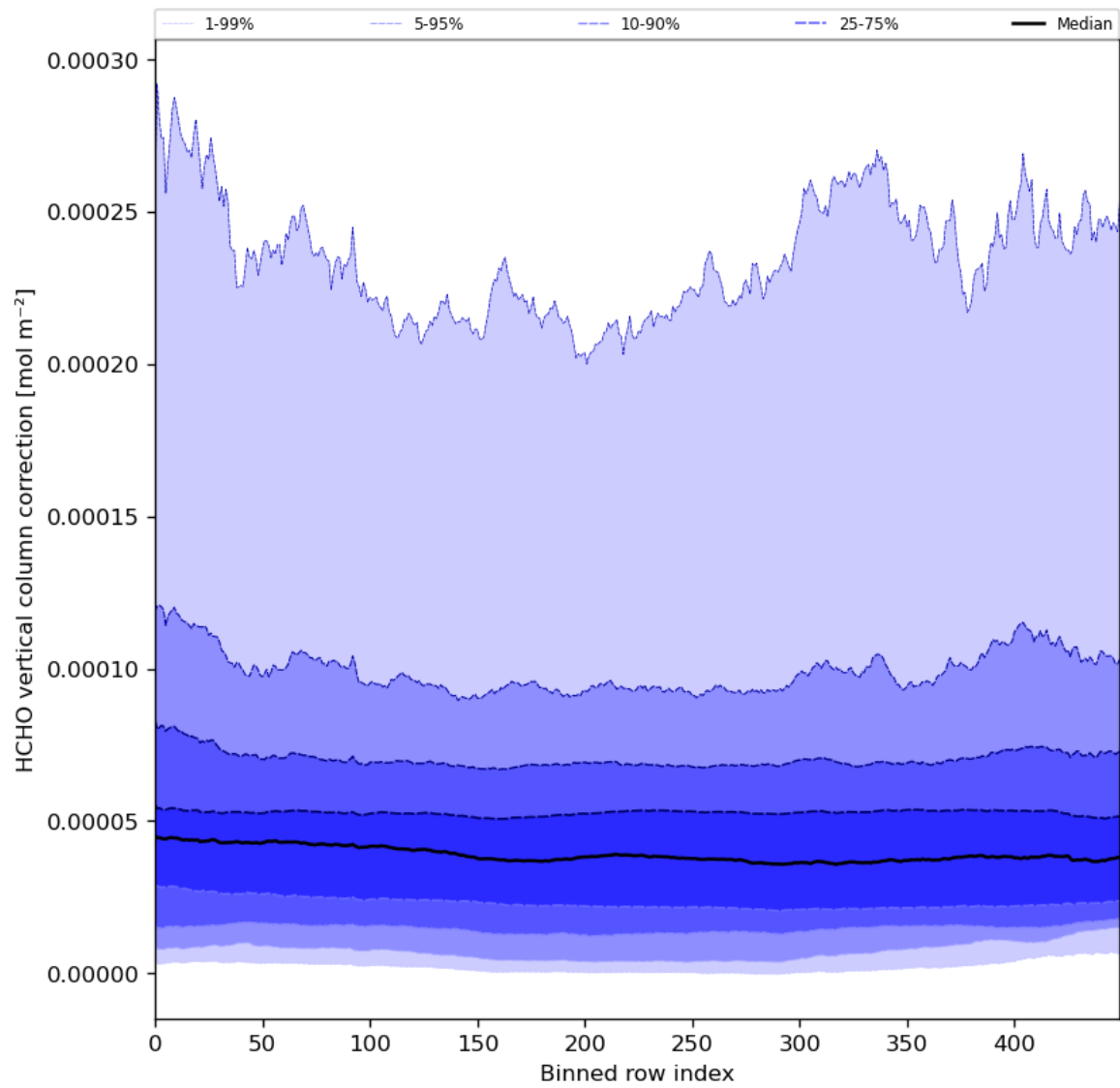
Figure 51: Along track statistics of “HCHO vertical column correction” for 2024-06-24 to 2024-06-25
