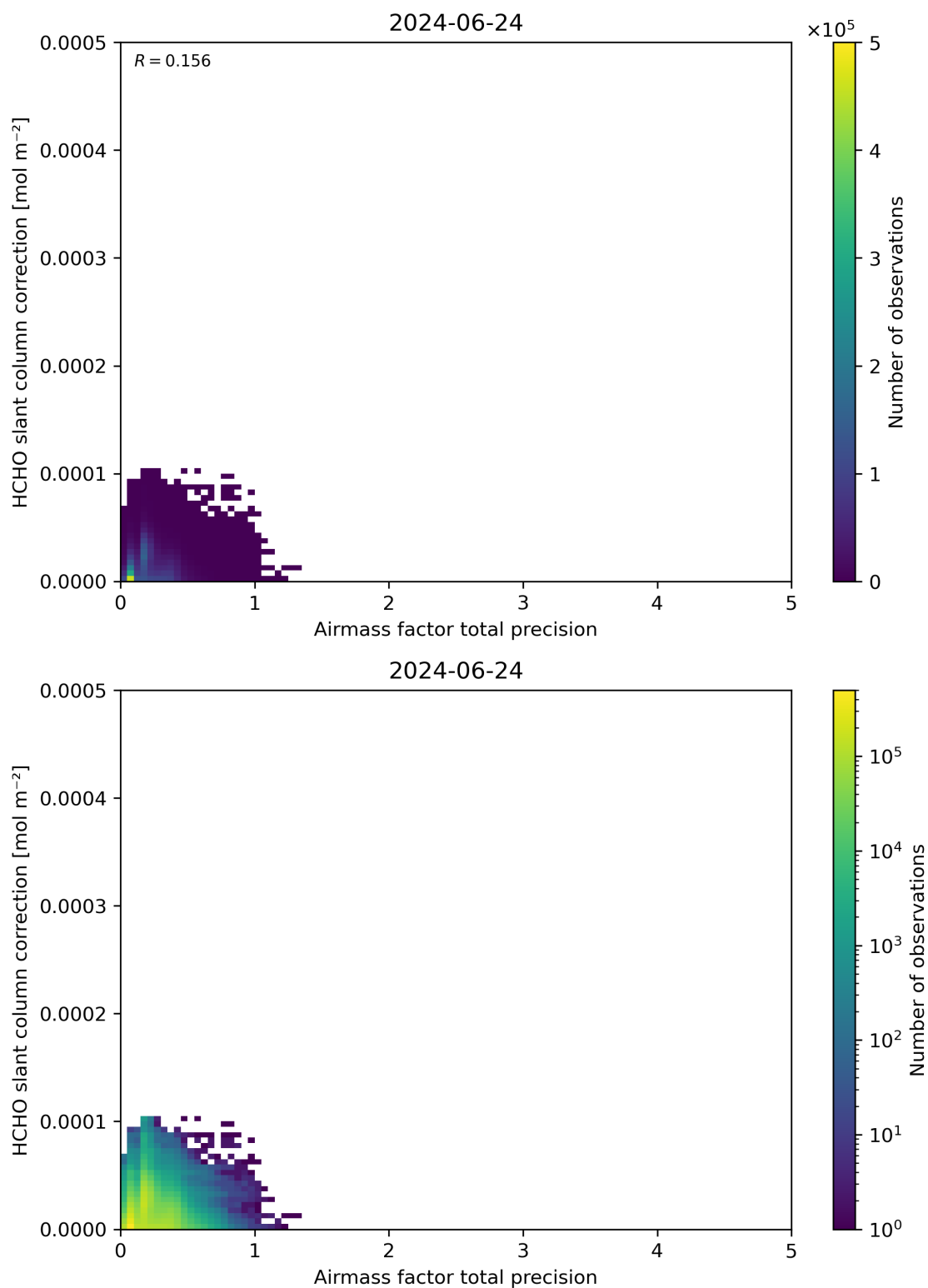
Figure 110: Scatter density plot of “Airmass factor total precision” against “HCHO slant column correction” for 2024-06-24 to 2024-06-25.
