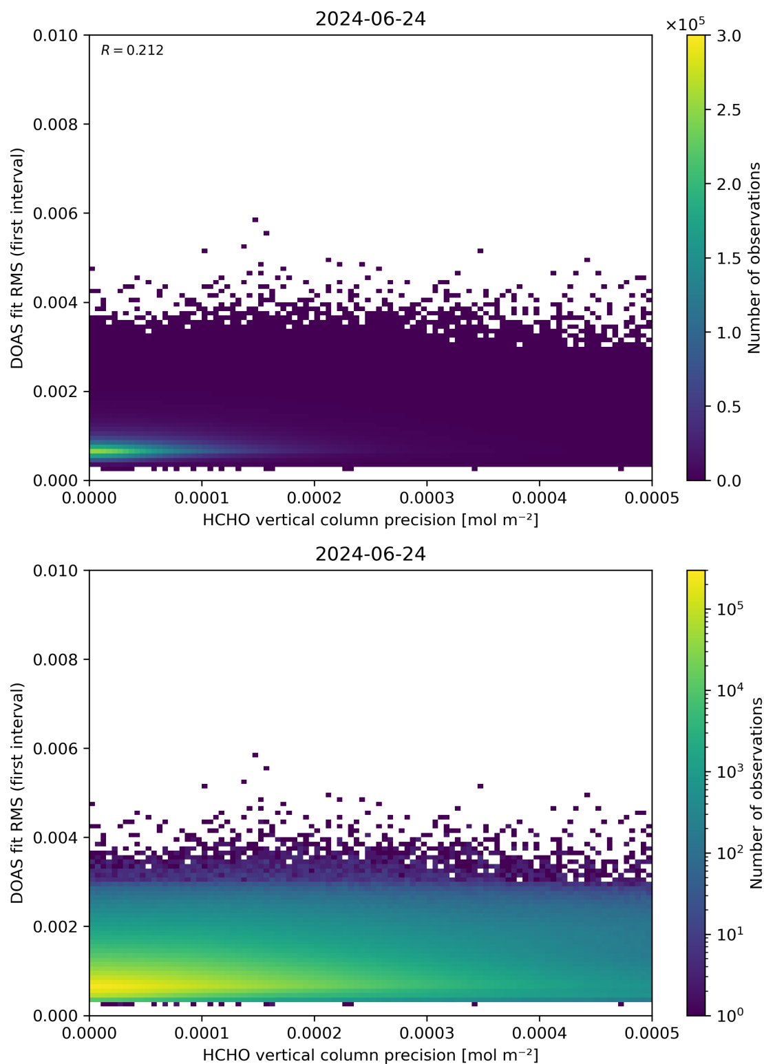
Figure 136: Scatter density plot of “HCHO vertical column precision” against “DOAS fit RMS (first interval)” for 2024-06-24 to 2024-06-25.
