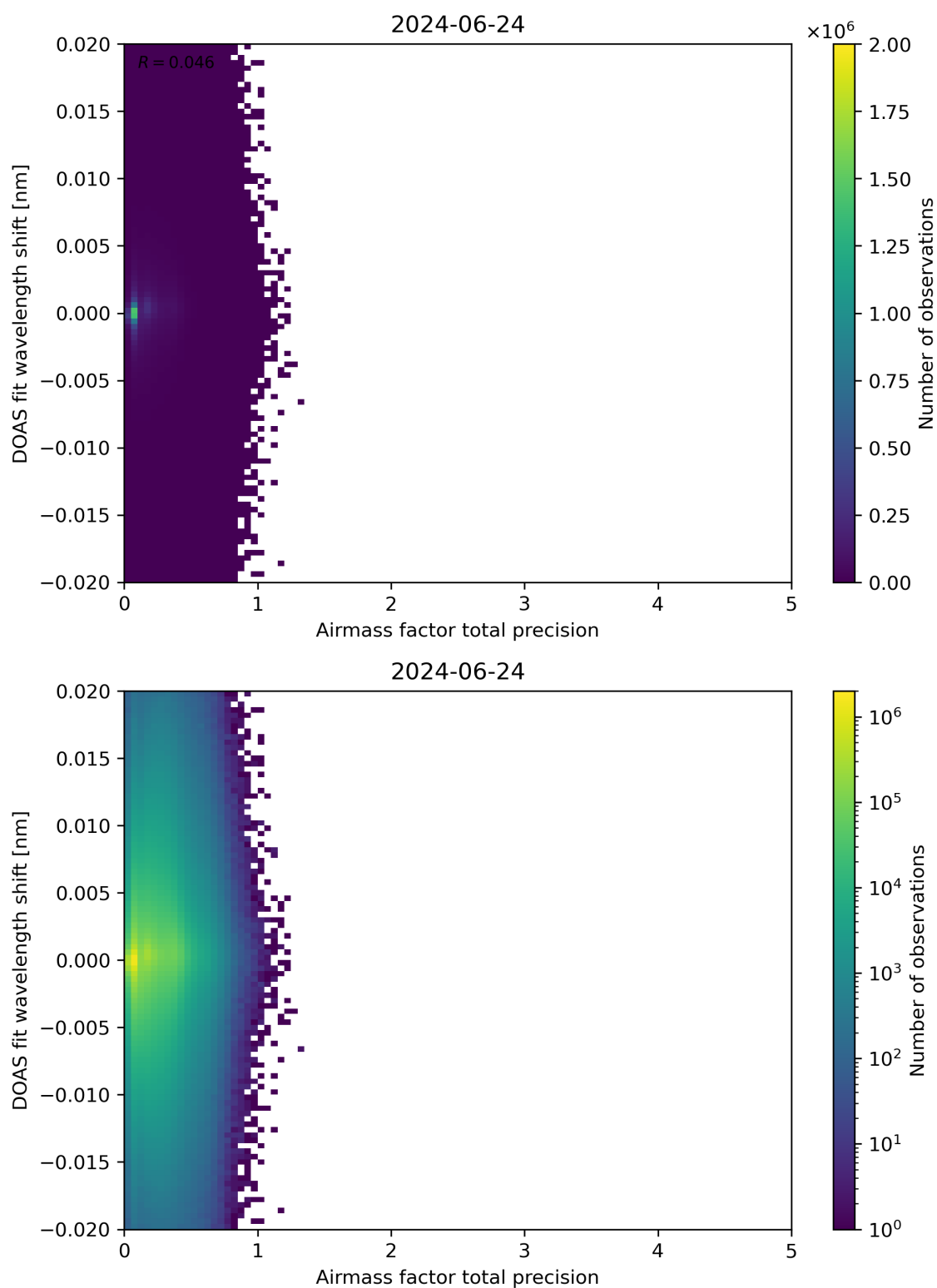
Figure 106: Scatter density plot of “Airmass factor total precision” against “DOAS fit wavelength shift” for 2024-06-24 to 2024-06-25.
