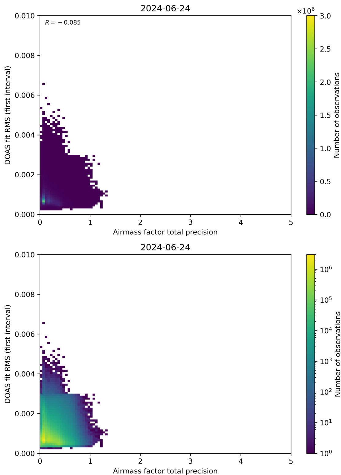
Figure 105: Scatter density plot of “Airmass factor total precision” against “DOAS fit RMS (first interval)” for 2024-06-24 to 2024-06-25.
