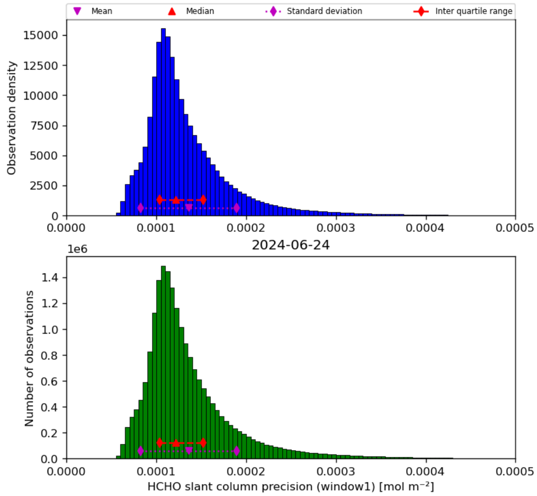
Figure 39: Histogram of “HCHO slant column precision (window1)” for 2024-06-24 to 2024-06-25
