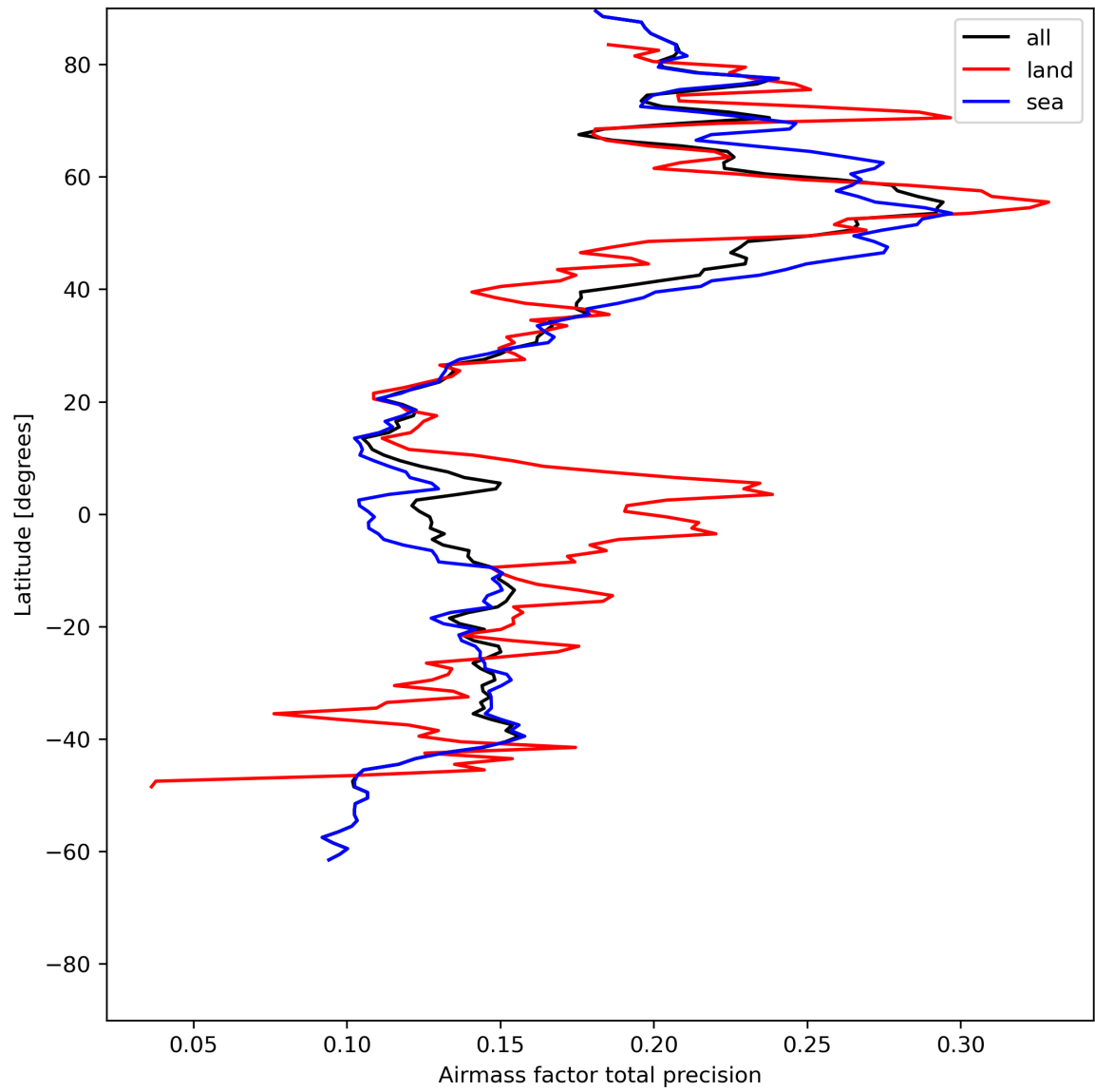
Figure 27: Zonal average of “Airmass factor total precision” for 2024-06-24 to 2024-06-25.
