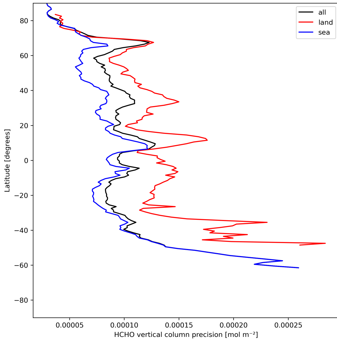
Figure 22: Zonal average of “HCHO vertical column precision” for 2024-06-24 to 2024-06-25.
