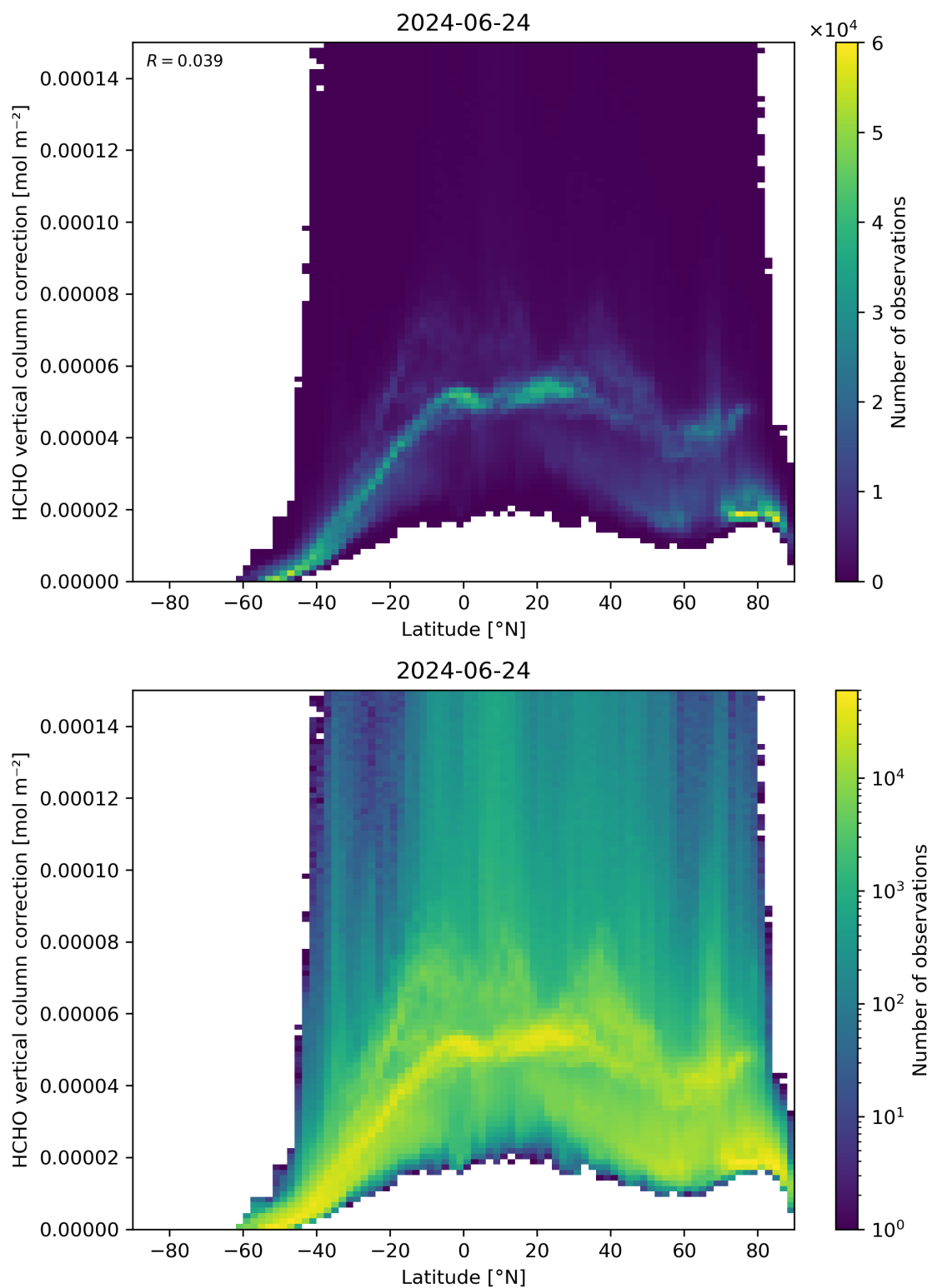
Figure 164: Scatter density plot of “Latitude” against “HCHO vertical column correction” for 2024-06-24 to 2024-06-25.
