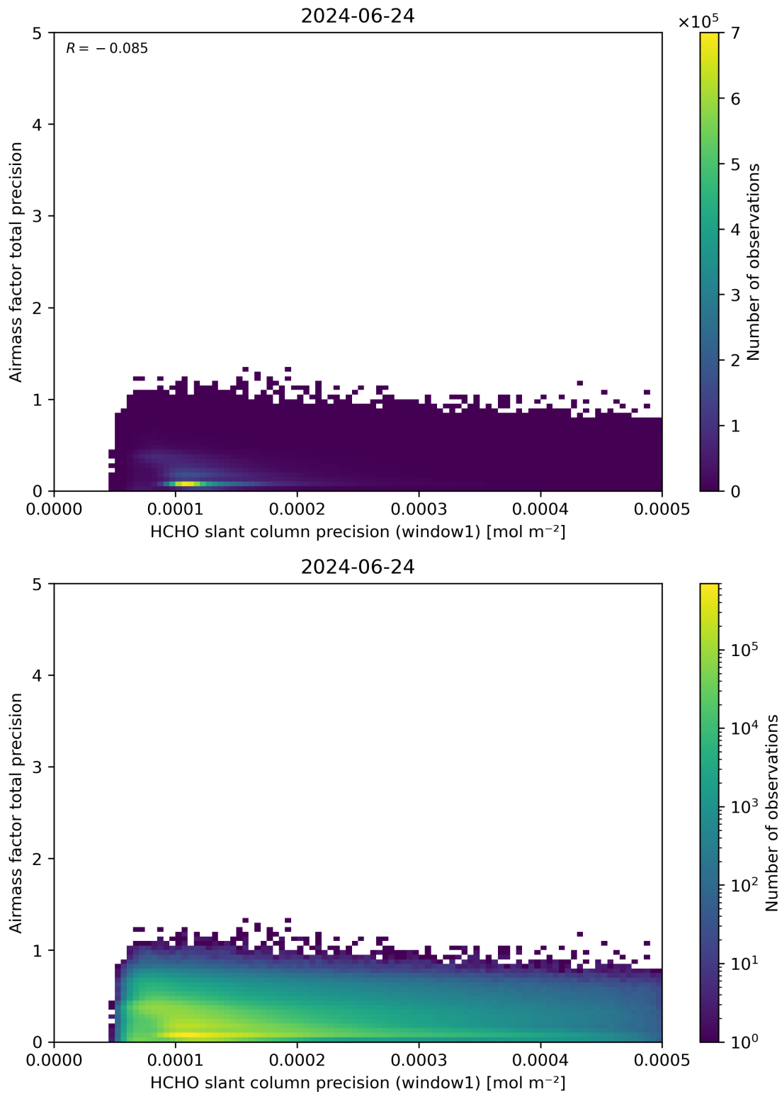
Figure 95: Scatter density plot of “HCHO slant column precision (window1)” against “Airmass factor total precision” for 2024-06-24 to 2024-06-25.
