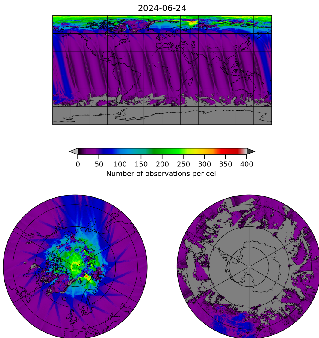
Figure 19: Map of the number of observations for 2024-06-24 to 2024-06-25
