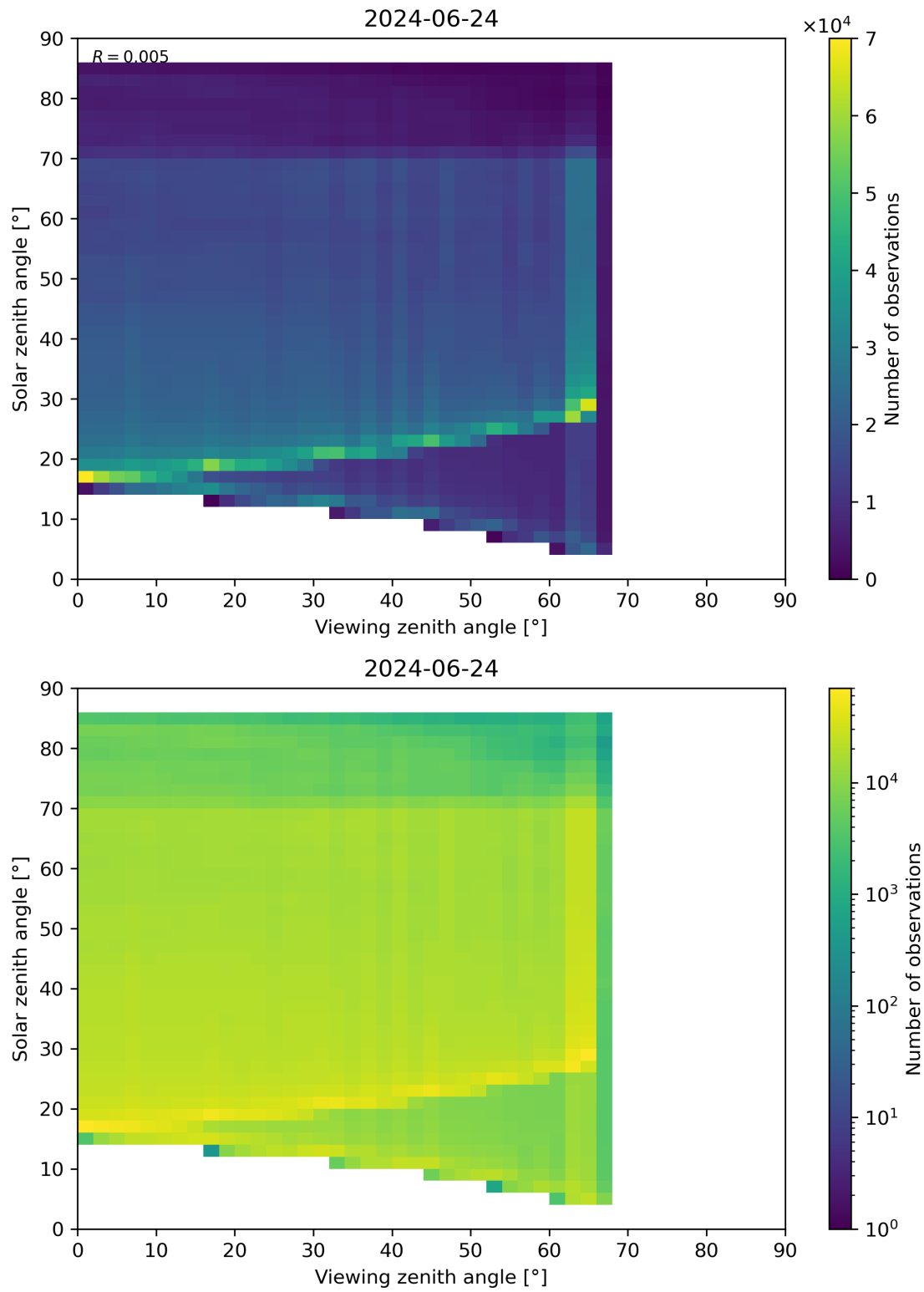
Figure 197: Scatter density plot of “Viewing zenith angle” against “Solar zenith angle” for 2024-06-24 to 2024-06-25.
