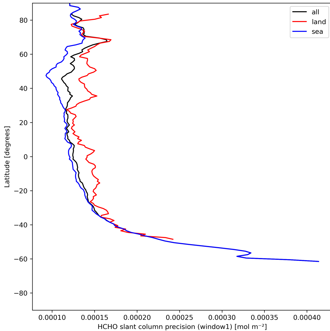
Figure 25: Zonal average of "HCHO slant column precision (window1)" for 2024-06-24 to 2024-06-25.
