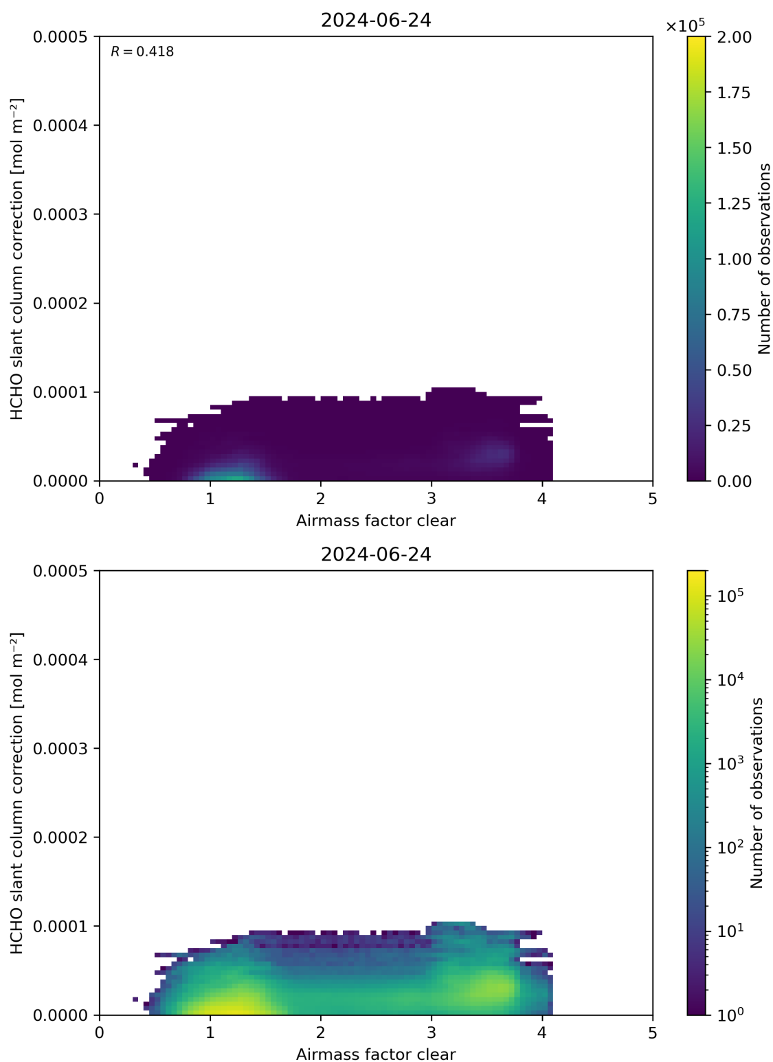
Figure 75: Scatter density plot of “Airmass factor clear” against “HCHO slant column correction” for 2024-06-24 to 2024-06-25.
