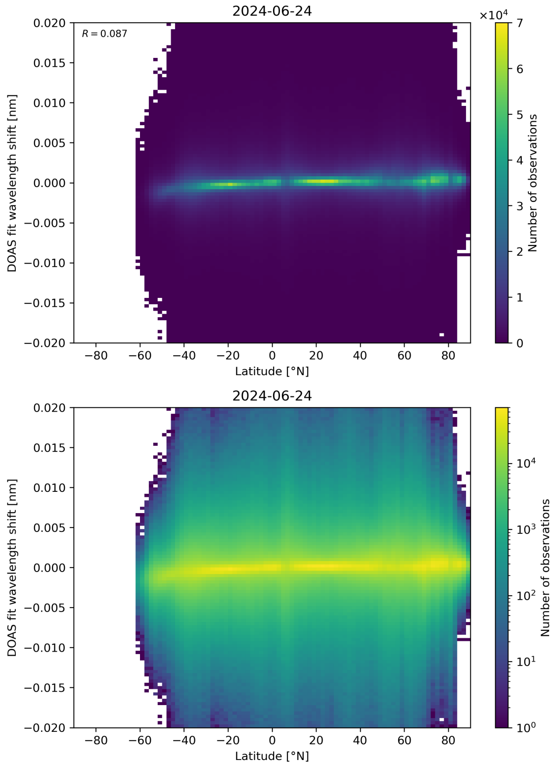
Figure 154: Scatter density plot of “Latitude” against “DOAS fit wavelength shift” for 2024-06-24 to 2024-06-25.
