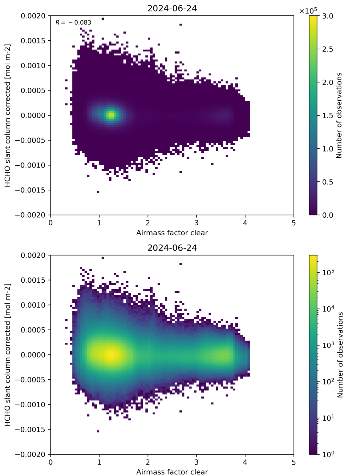
Figure 74: Scatter density plot of “Airmass factor clear” against “HCHO slant column corrected” for 2024-06-24 to 2024-06-25.
