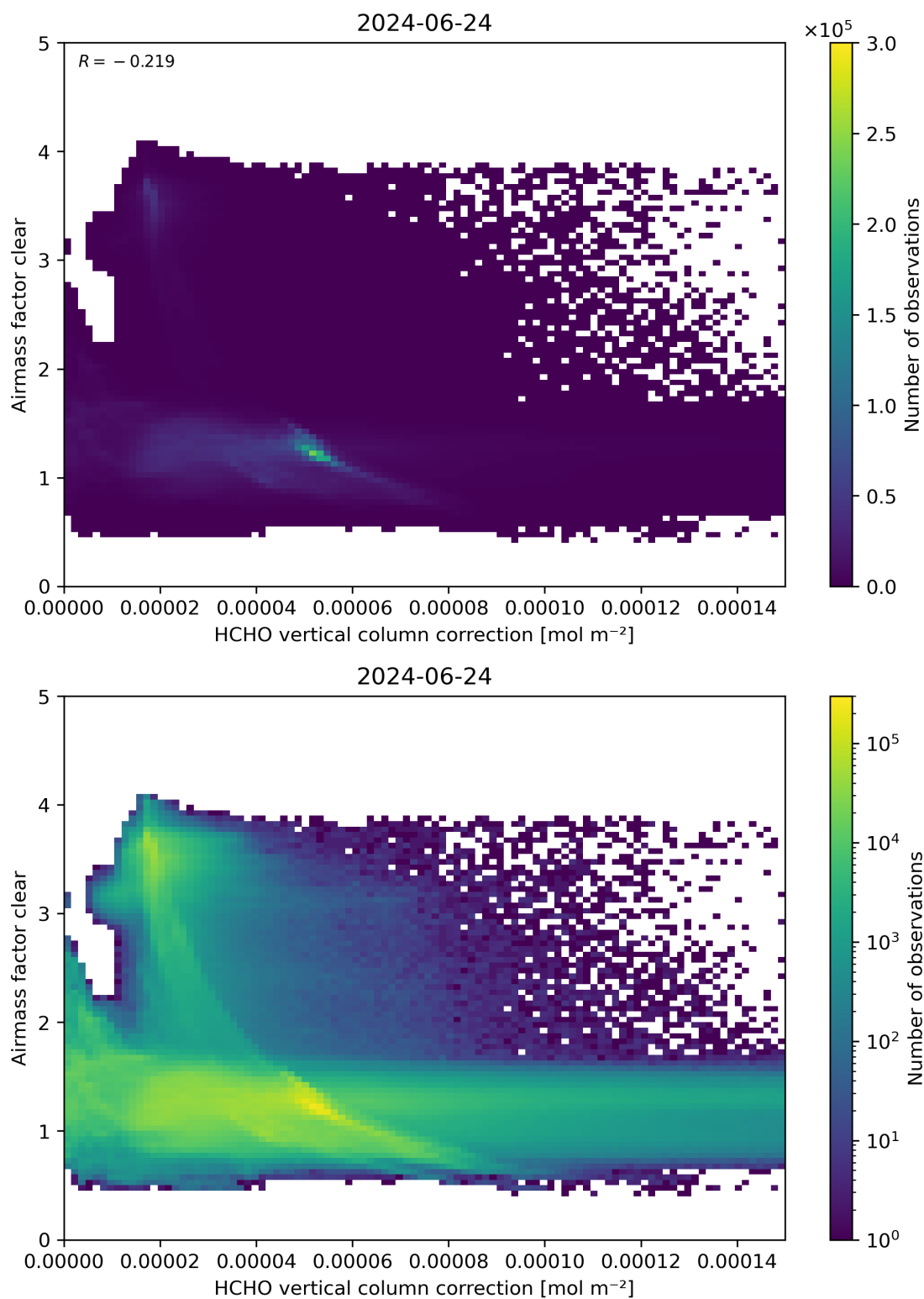
Figure 115: Scatter density plot of “HCHO vertical column correction” against “Airmass factor clear” for 2024-06-24 to 2024-06-25.
