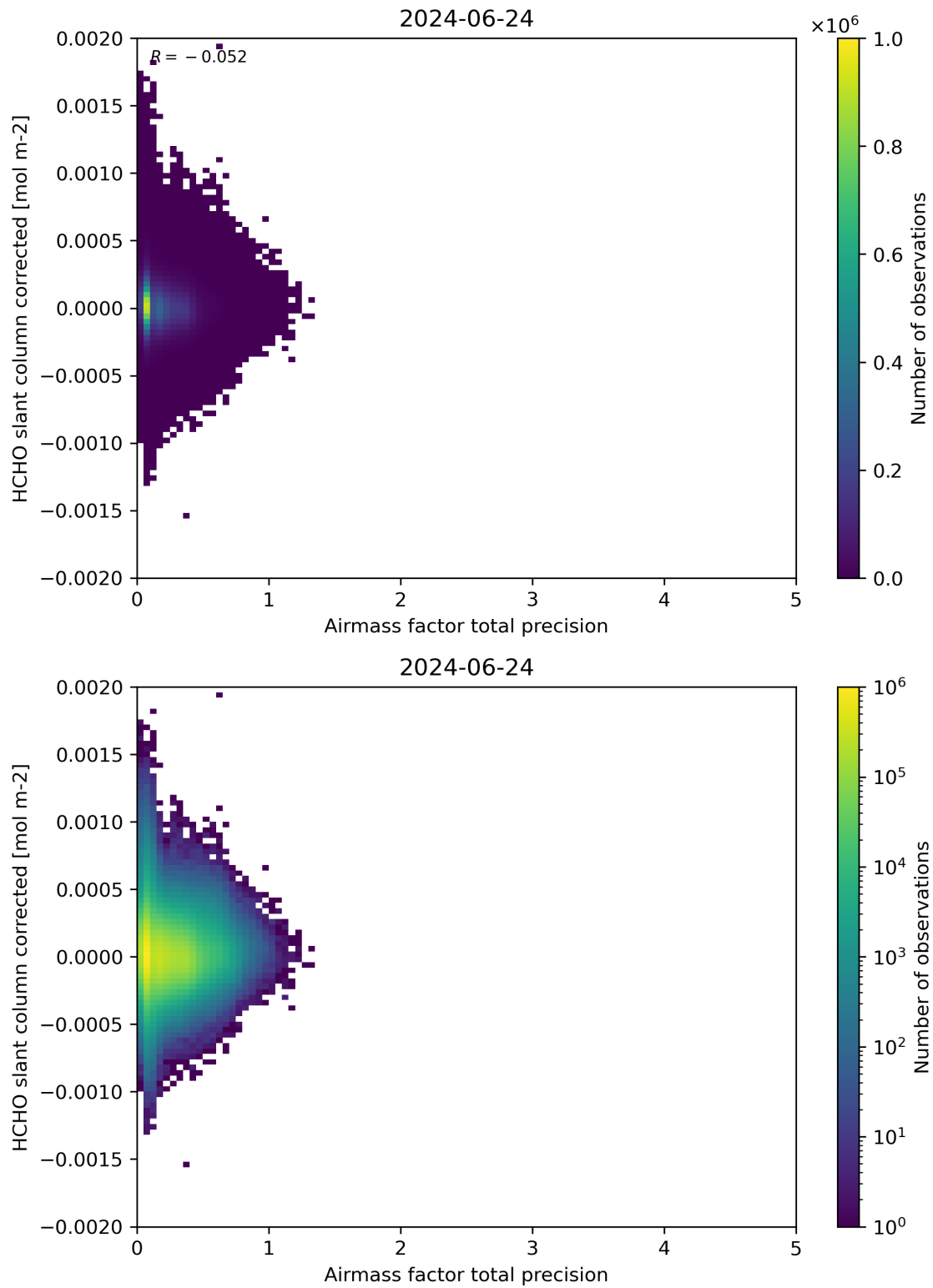
Figure 109: Scatter density plot of “Airmass factor total precision” against “HCHO slant column corrected” for 2024-06-24 to 2024-06-25.
