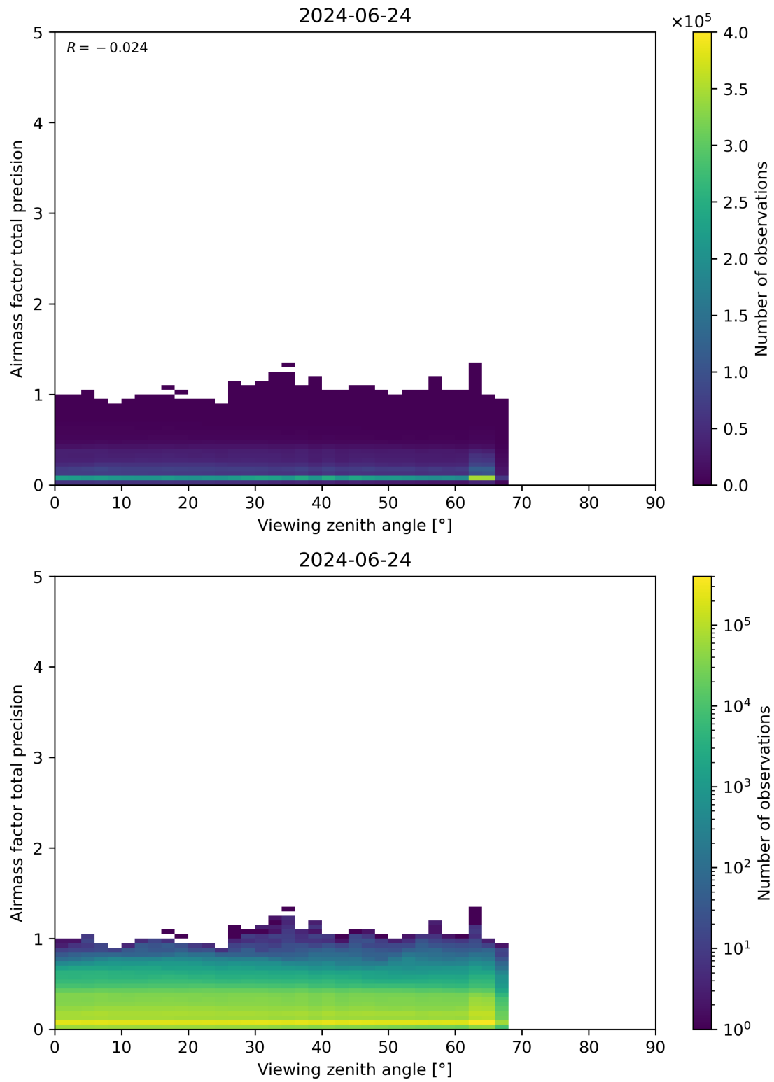
Figure 191: Scatter density plot of “Viewing zenith angle” against “Airmass factor total precision” for 2024-06-24 to 2024-06-25.
