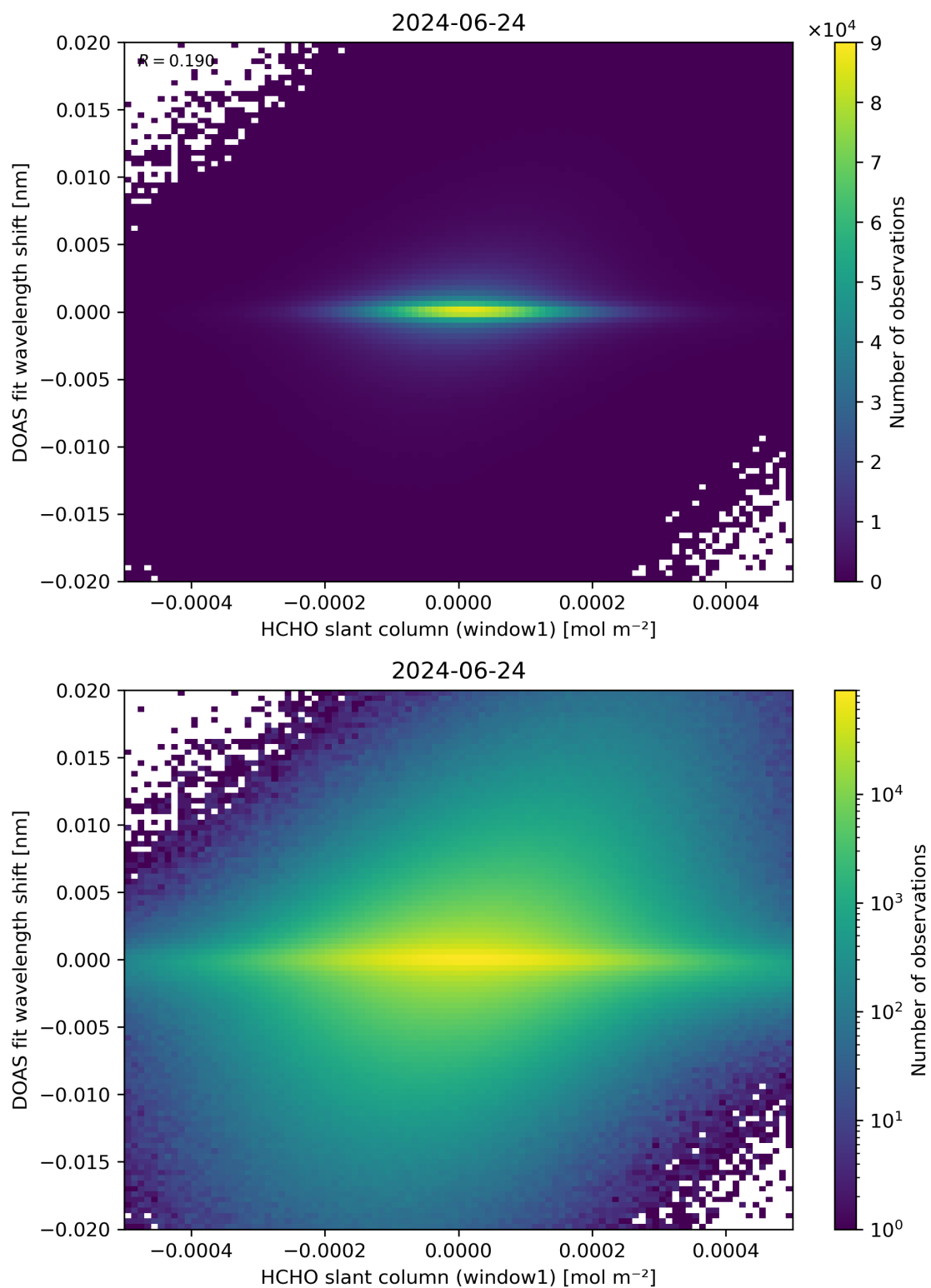
Figure 79: Scatter density plot of “HCHO slant column (window1)” against “DOAS fit wavelength shift” for 2024-06-24 to 2024-06-25.
