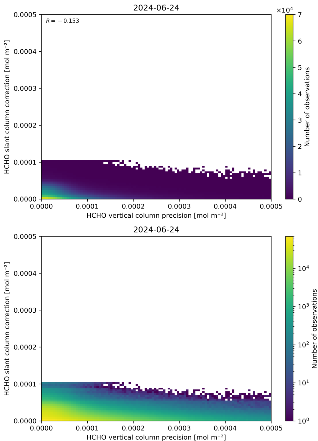
Figure 141: Scatter density plot of “HCHO vertical column precision” against “HCHO slant column correction” for 2024-06-24 to 2024-06-25.
