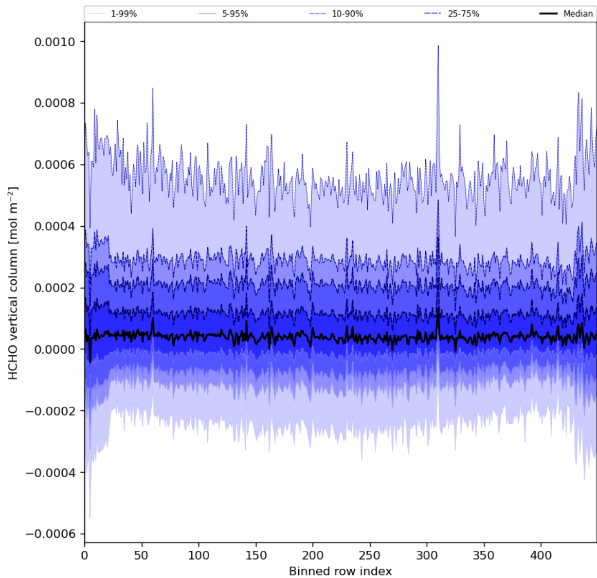
Figure 49: Along track statistics of “HCHO vertical column” for 2024-06-24 to 2024-06-25
