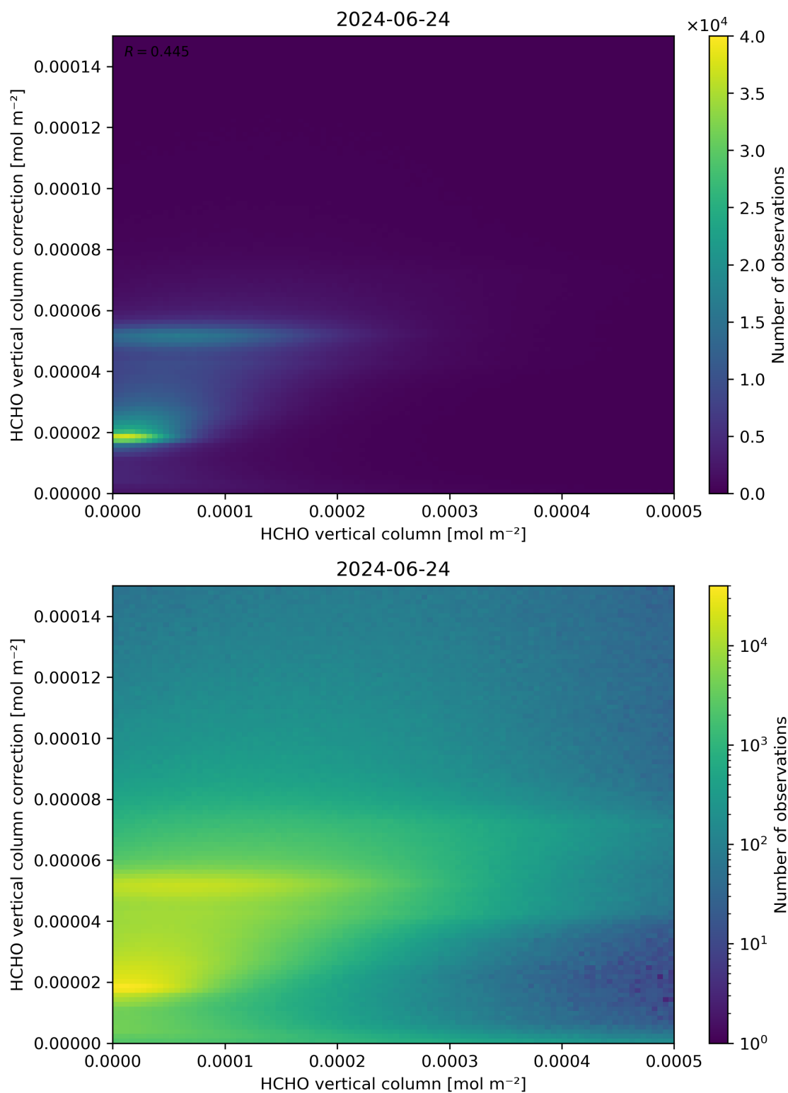
Figure 133: Scatter density plot of “HCHO vertical column” against “HCHO vertical column correction” for 2024-06-24 to 2024-06-25.
