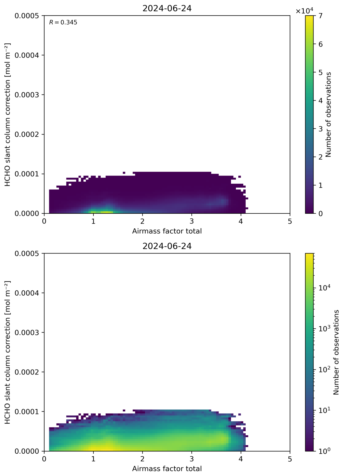
Figure 102: Scatter density plot of “Airmass factor total” against “HCHO slant column correction” for 2024-06-24 to 2024-06-25.
