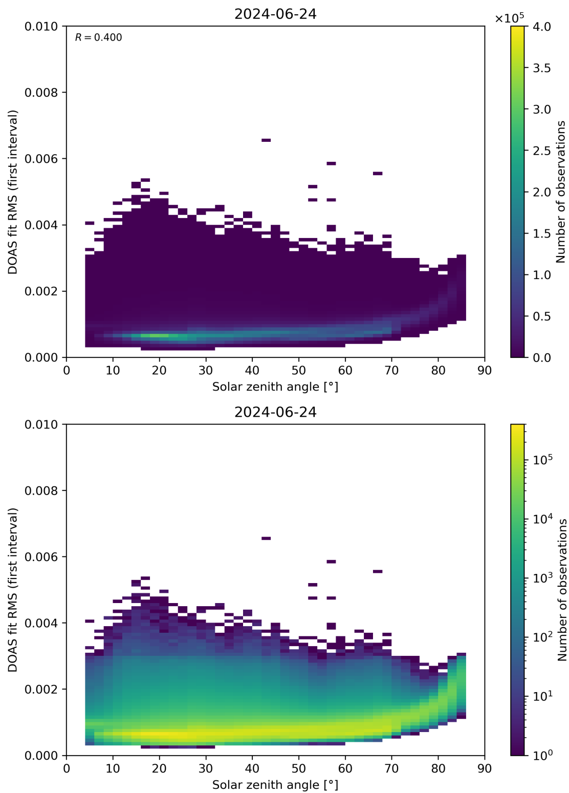
Figure 167: Scatter density plot of “Solar zenith angle” against “DOAS fit RMS (first interval)” for 2024-06-24 to 2024-06-25.
