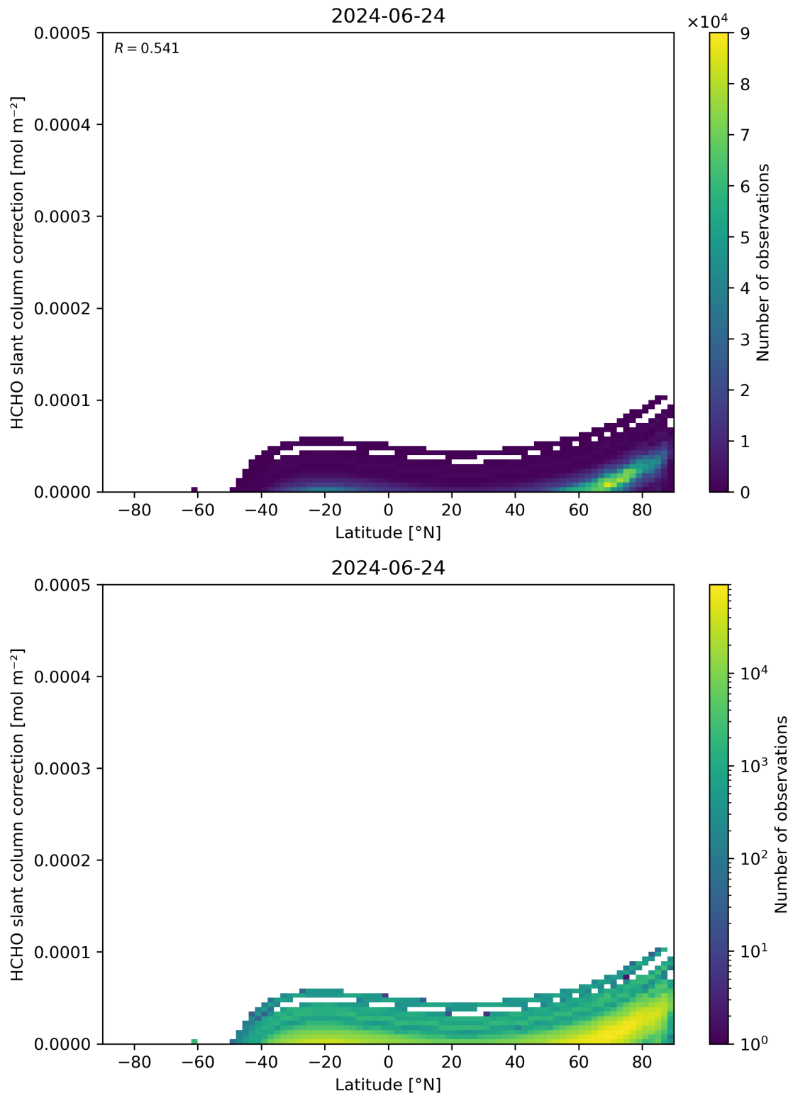
Figure 158: Scatter density plot of “Latitude” against “HCHO slant column correction” for 2024-06-24 to 2024-06-25.
