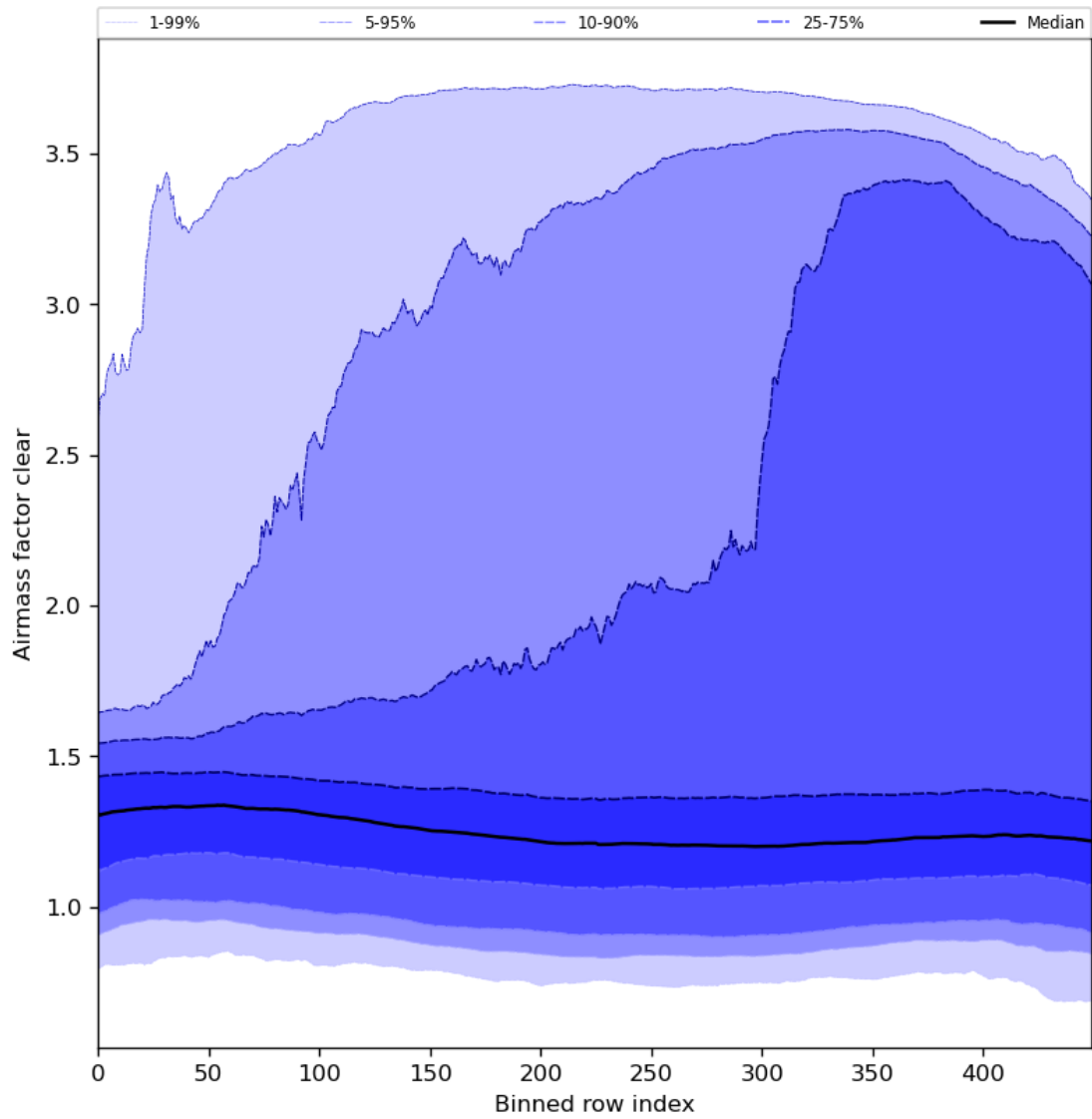
Figure 56: Along track statistics of “Airmass factor clear” for 2024-06-24 to 2024-06-25
