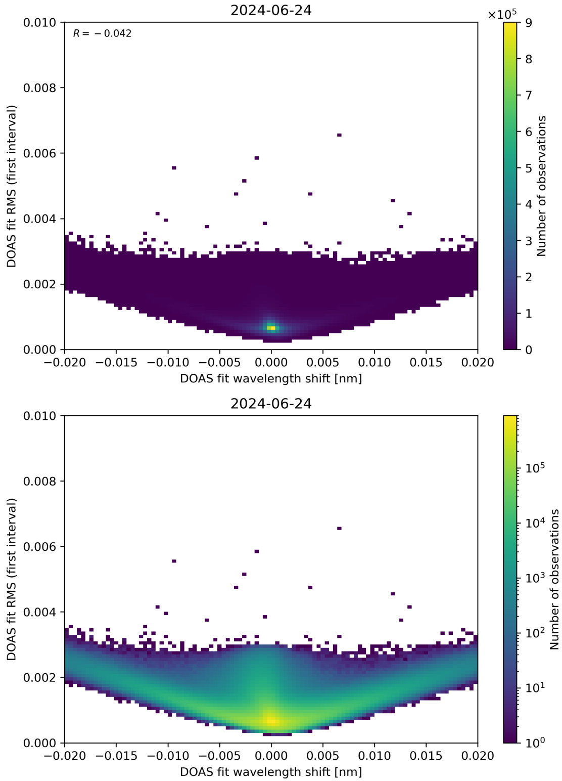
Figure 64: Scatter density plot of “DOAS fit wavelength shift” against “DOAS fit RMS (first interval)” for 2024-06-24 to 2024-06-25.
