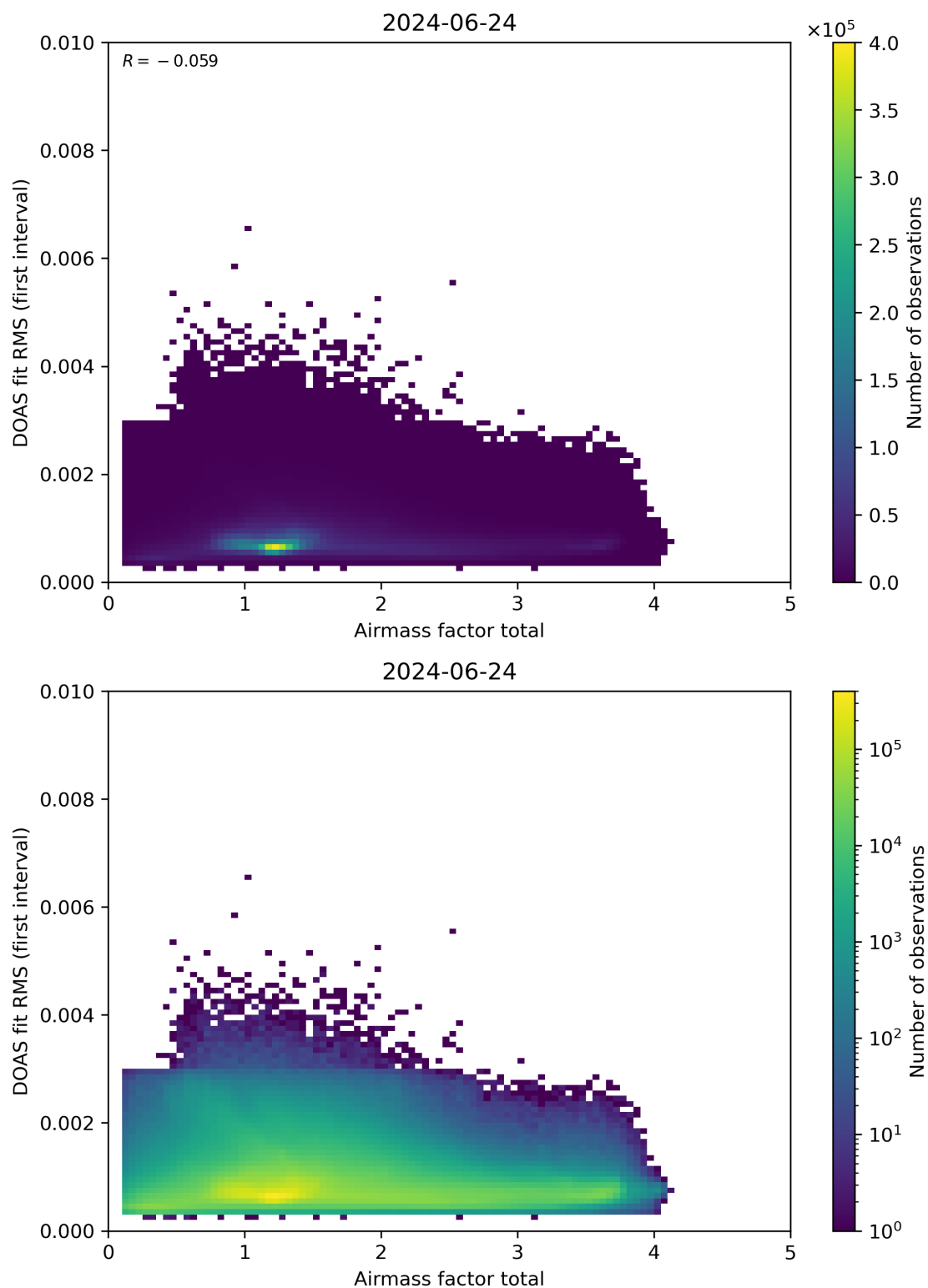
Figure 97: Scatter density plot of “Airmass factor total” against “DOAS fit RMS (first interval)” for 2024-06-24 to 2024-06-25.
