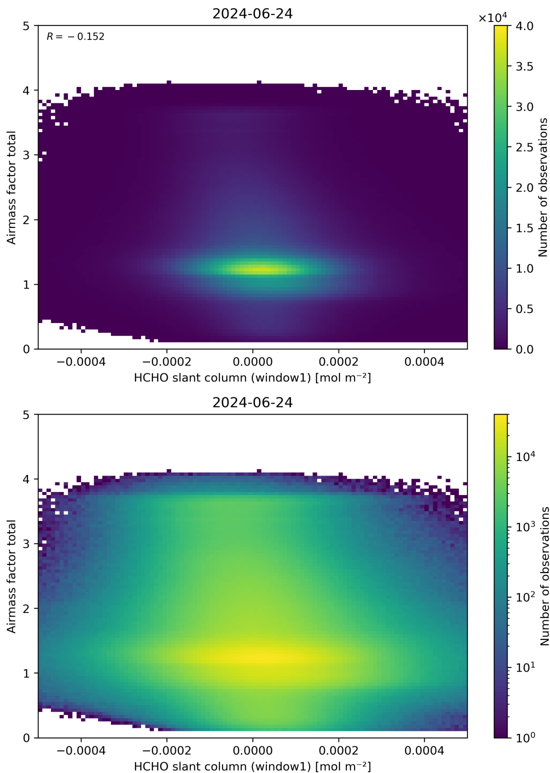
Figure 85: Scatter density plot of “HCHO slant column (window1)” against “Airmass factor total” for 2024-06-24 to 2024-06-25.
