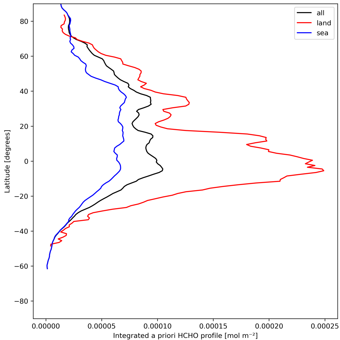
Figure 29: Zonal average of “Integrated a priori HCHO profile” for 2024-06-24 to 2024-06-25.
