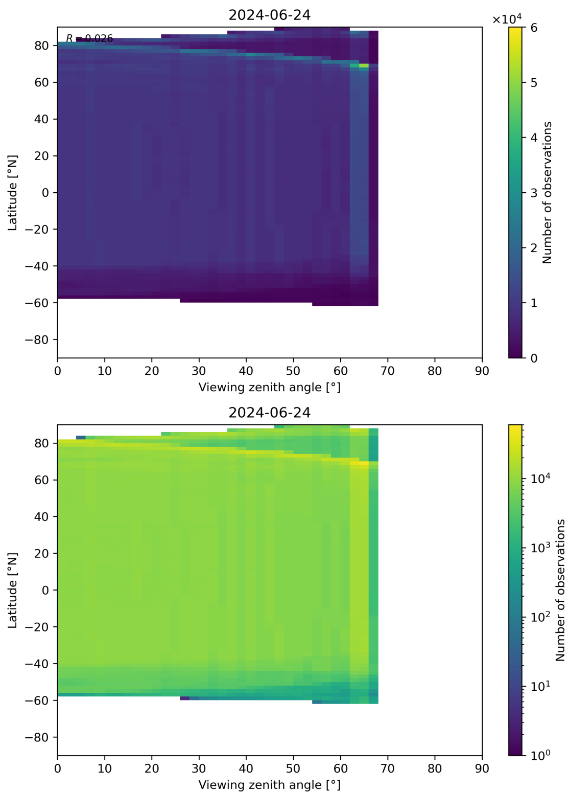
Figure 196: Scatter density plot of “Viewing zenith angle” against “Latitude” for 2024-06-24 to 2024-06-25.
