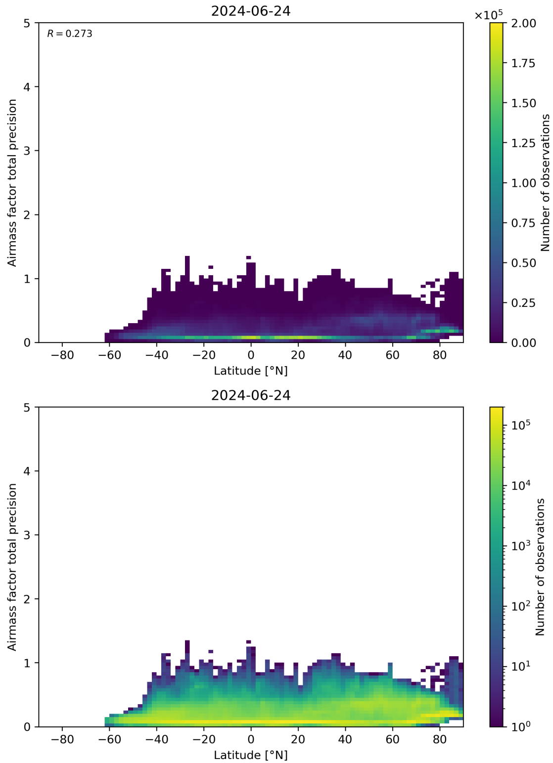
Figure 162: Scatter density plot of “Latitude” against “Airmass factor total precision” for 2024-06-24 to 2024-06-25.
