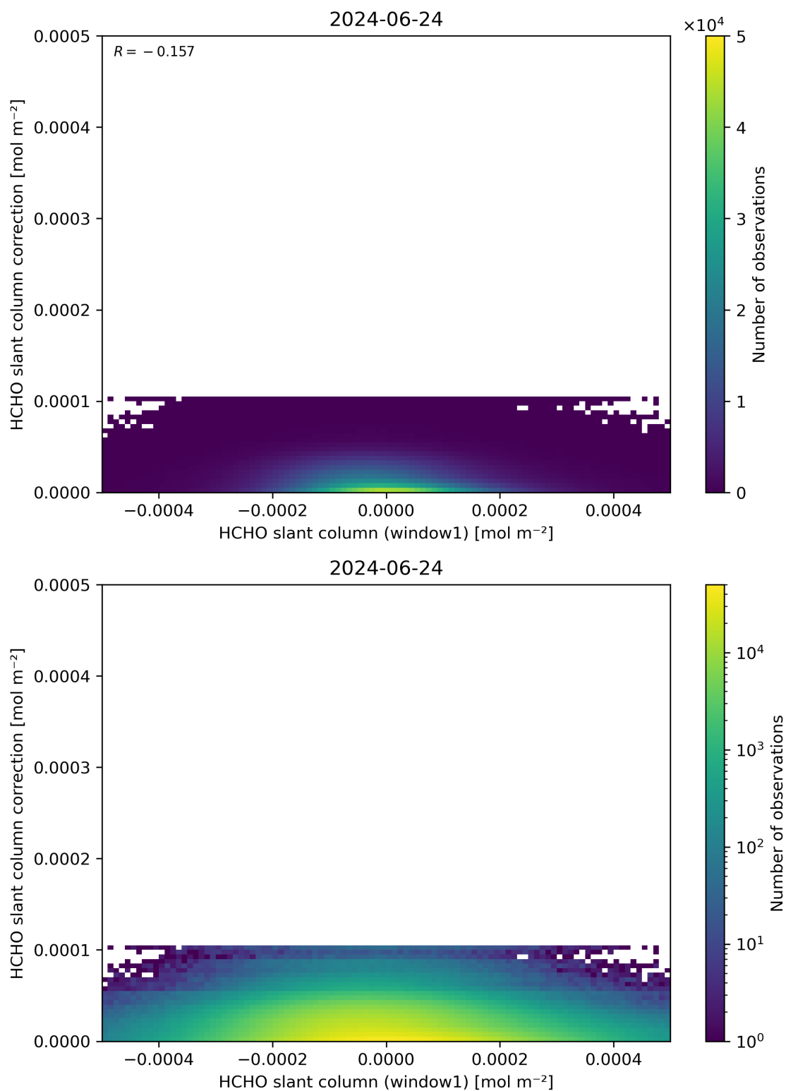
Figure 83: Scatter density plot of “HCHO slant column (window1)” against “HCHO slant column correction” for 2024-06-24 to 2024-06-25.
