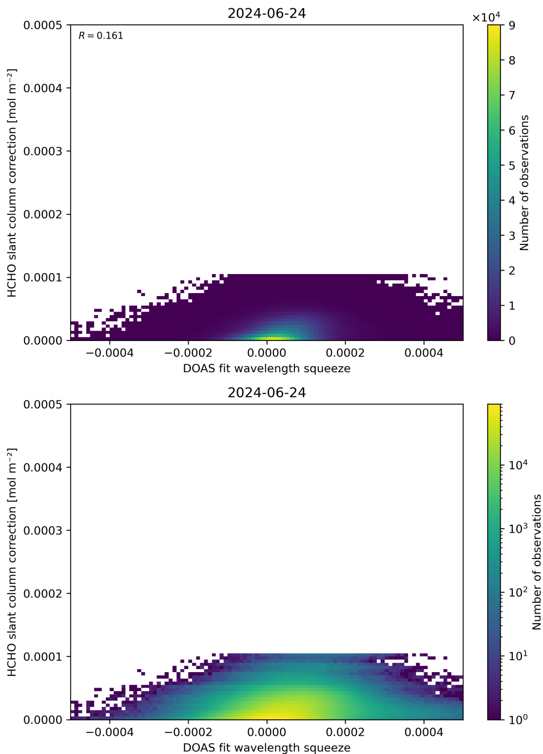
Figure 70: Scatter density plot of “DOAS fit wavelength squeeze” against “HCHO slant column correction” for 2024-06-24 to 2024-06-25.
