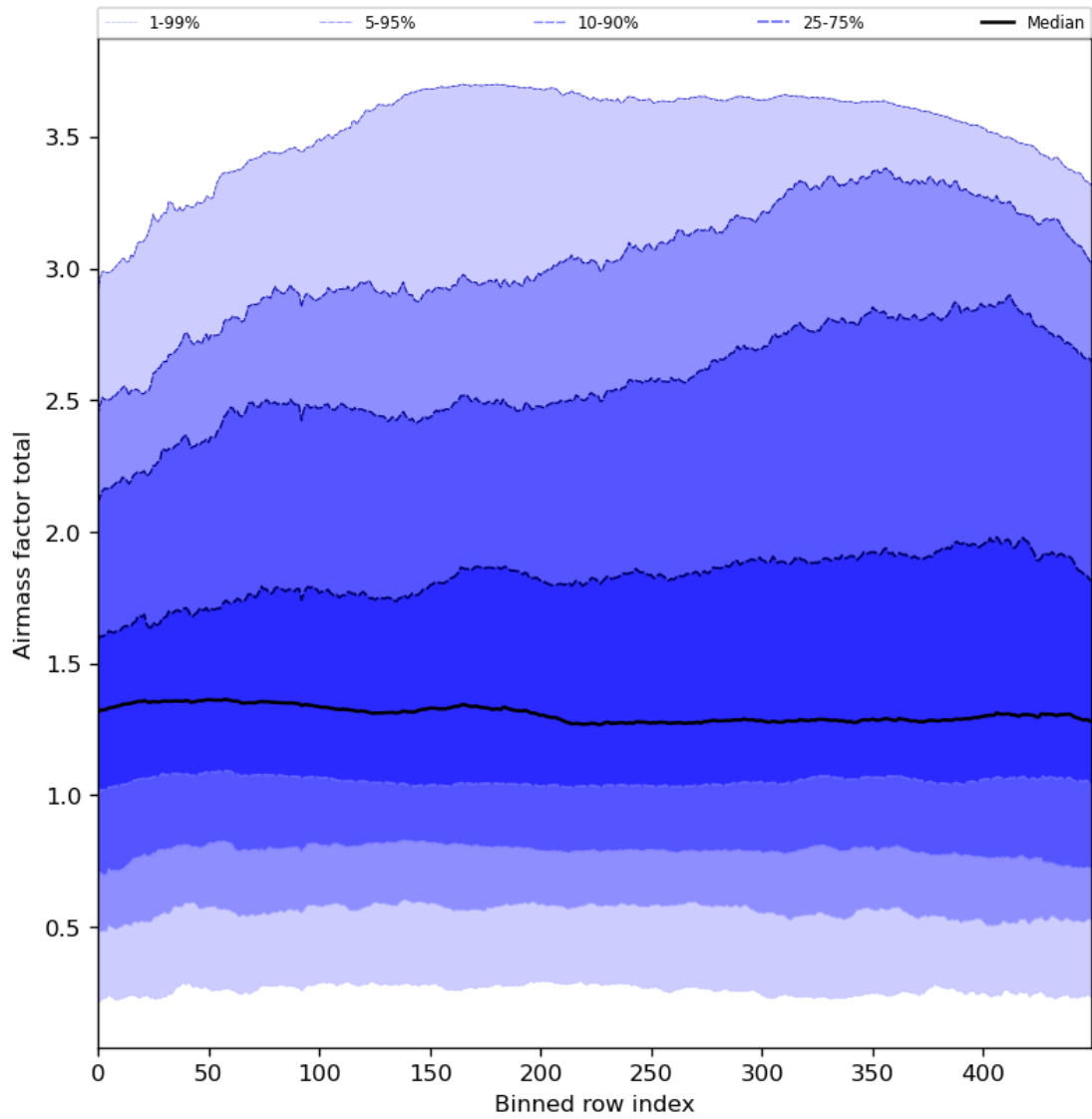
Figure 54: Along track statistics of “Airmass factor total” for 2024-06-24 to 2024-06-25
