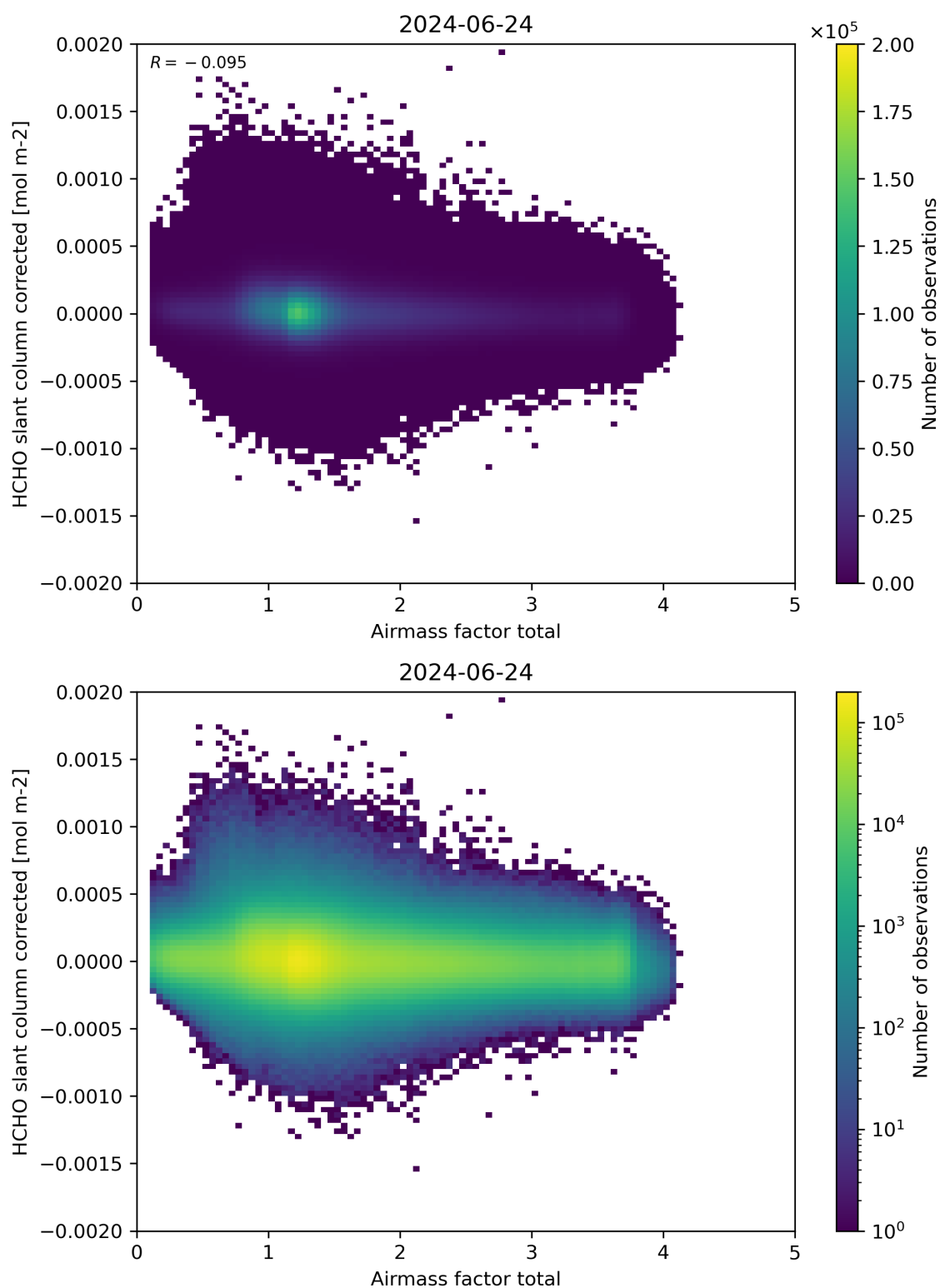
Figure 101: Scatter density plot of “Airmass factor total” against “HCHO slant column corrected” for 2024-06-24 to 2024-06-25.
