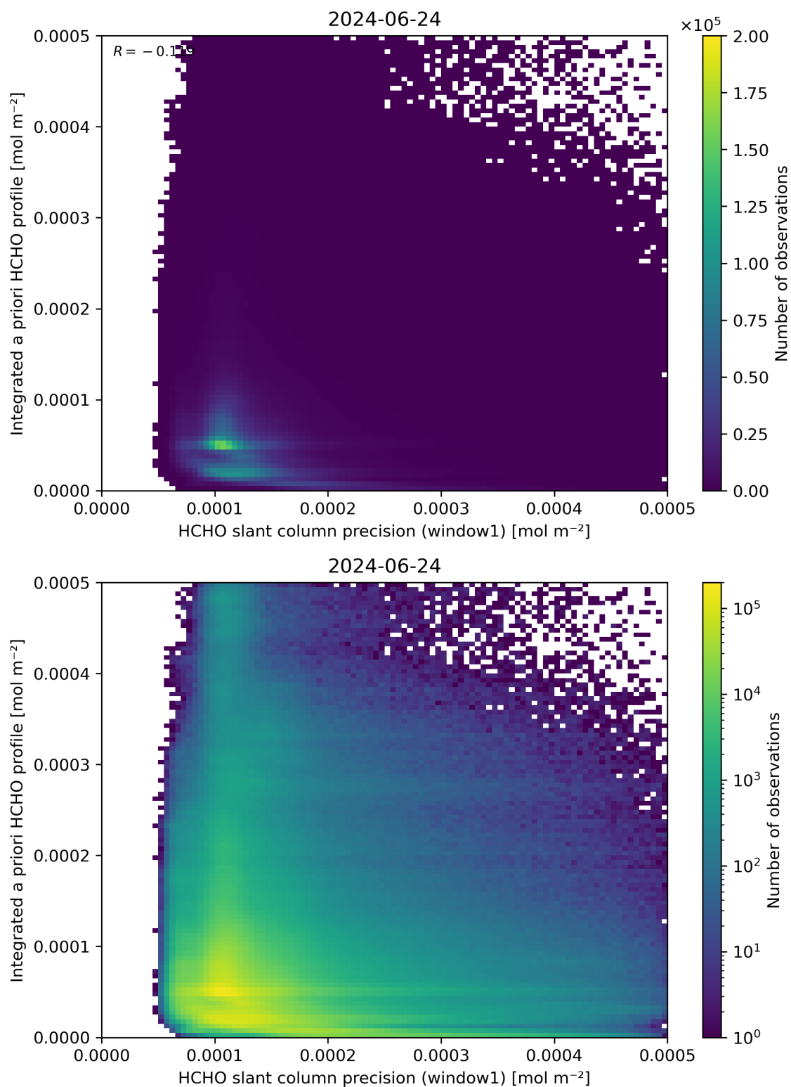
Figure 96: Scatter density plot of “HCHO slant column precision (window1)” against “Integrated a priori HCHO profile” for 2024-06-24 to 2024-06-25.
