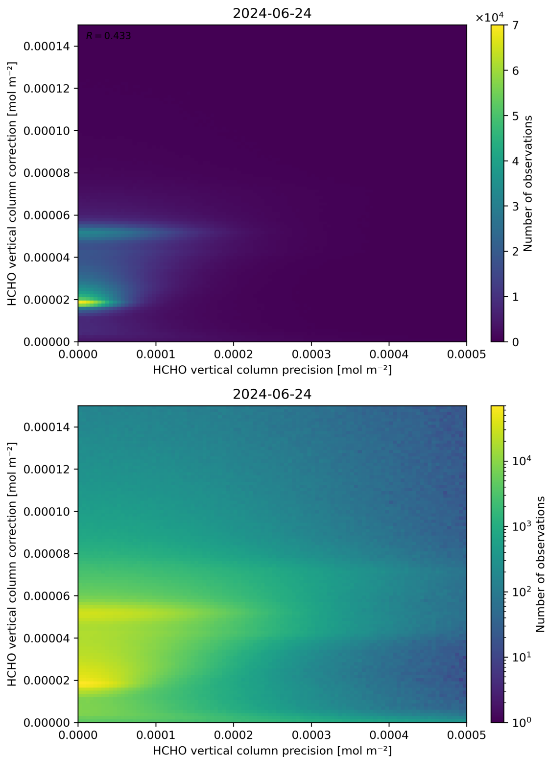
Figure 146: Scatter density plot of “HCHO vertical column precision” against “HCHO vertical column correction” for 2024-06-24 to 2024-06-25.
