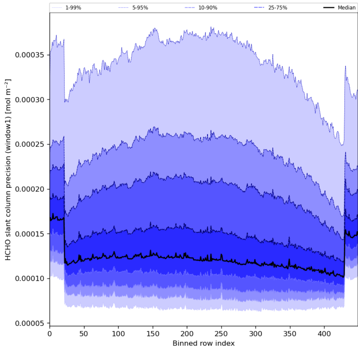
Figure 53: Along track statistics of “HCHO slant column precision (window1)” for 2024-06-24 to 2024-06-25
