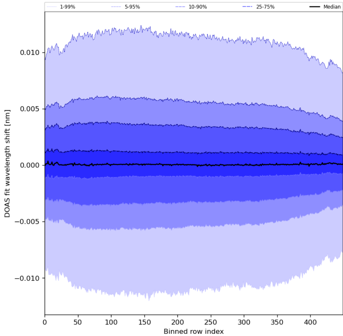
Figure 58: Along track statistics of “DOAS fit wavelength shift” for 2024-06-24 to 2024-06-25
