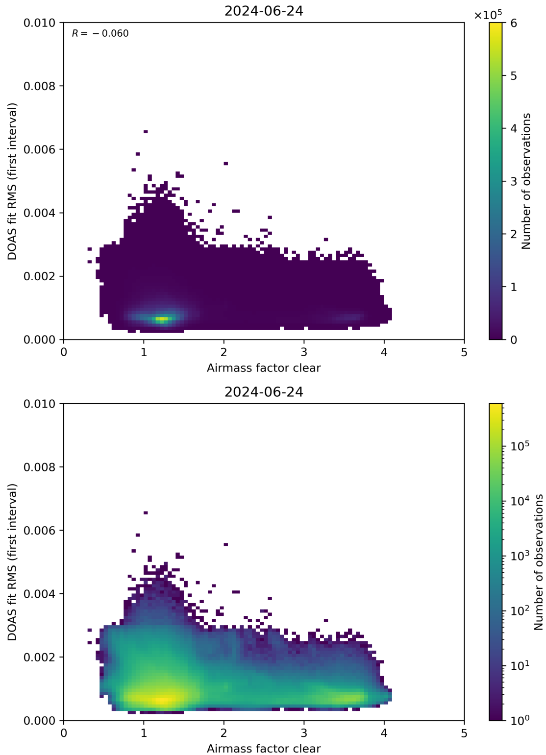
Figure 71: Scatter density plot of “Airmass factor clear” against “DOAS fit RMS (first interval)” for 2024-06-24 to 2024-06-25.
