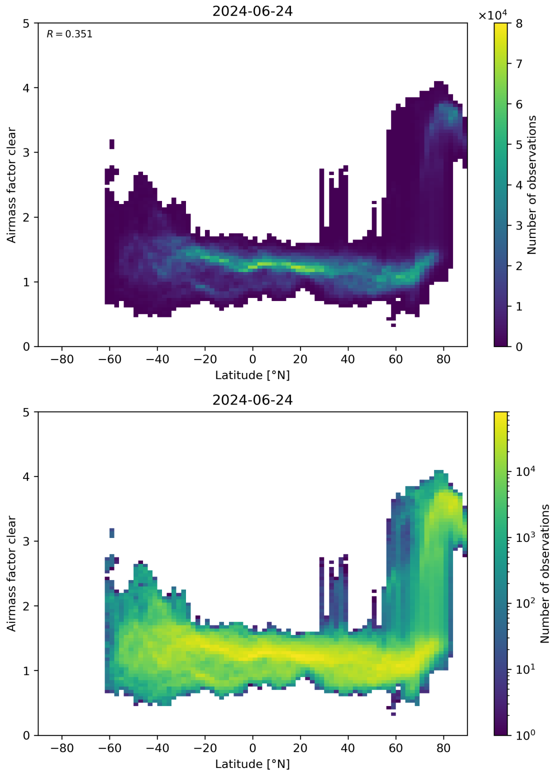
Figure 156: Scatter density plot of “Latitude” against “Airmass factor clear” for 2024-06-24 to 2024-06-25.
