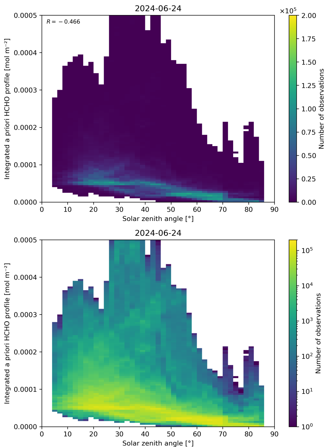
Figure 180: Scatter density plot of “Solar zenith angle” against “Integrated a priori HCHO profile” for 2024-06-24 to 2024-06-25.
