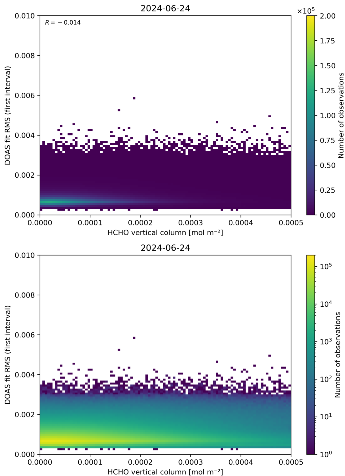
Figure 123: Scatter density plot of “HCHO vertical column” against “DOAS fit RMS (first interval)” for 2024-06-24 to 2024-06-25.
