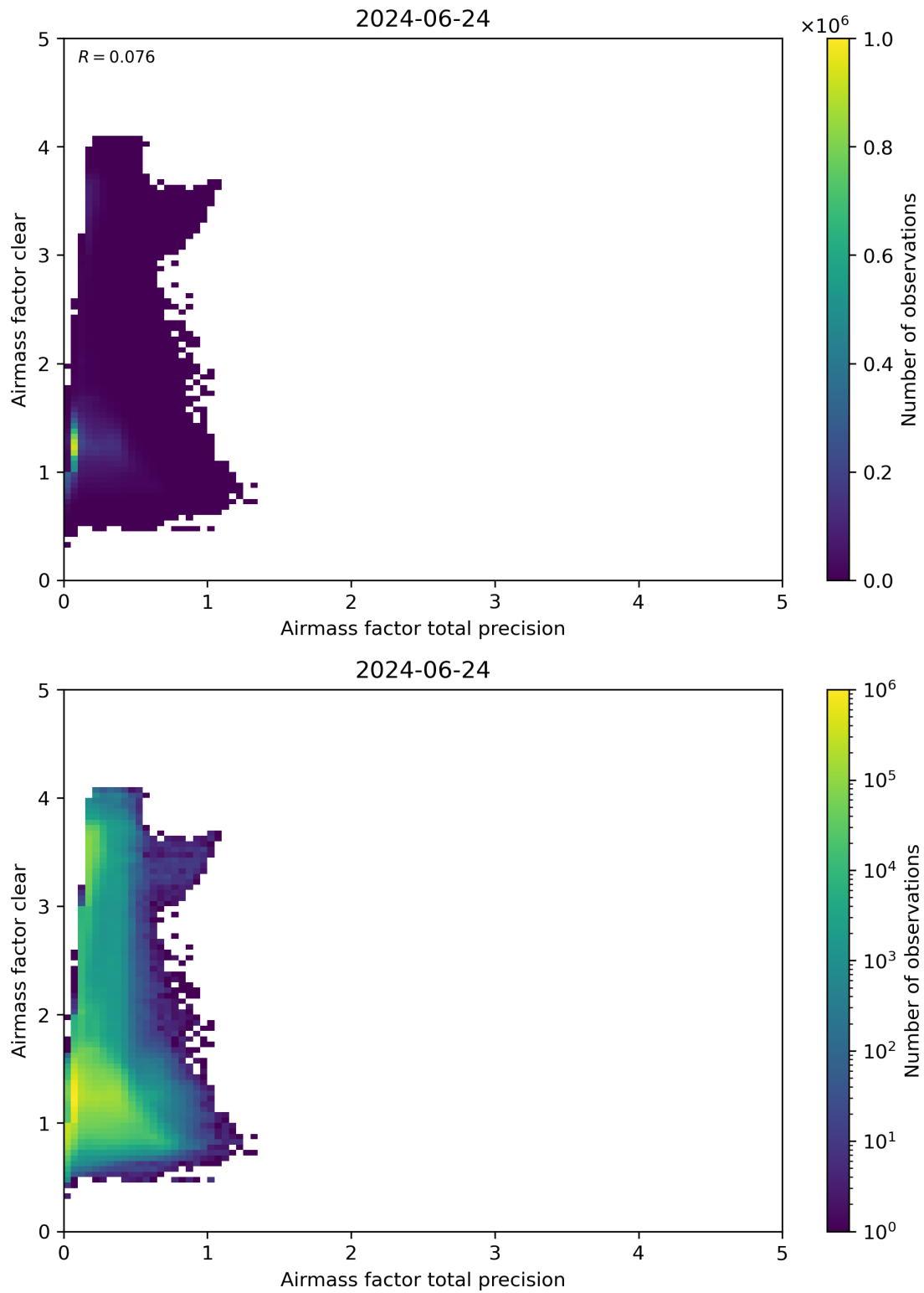
Figure 108: Scatter density plot of “Airmass factor total precision” against “Airmass factor clear” for 2024-06-24 to 2024-06-25.
