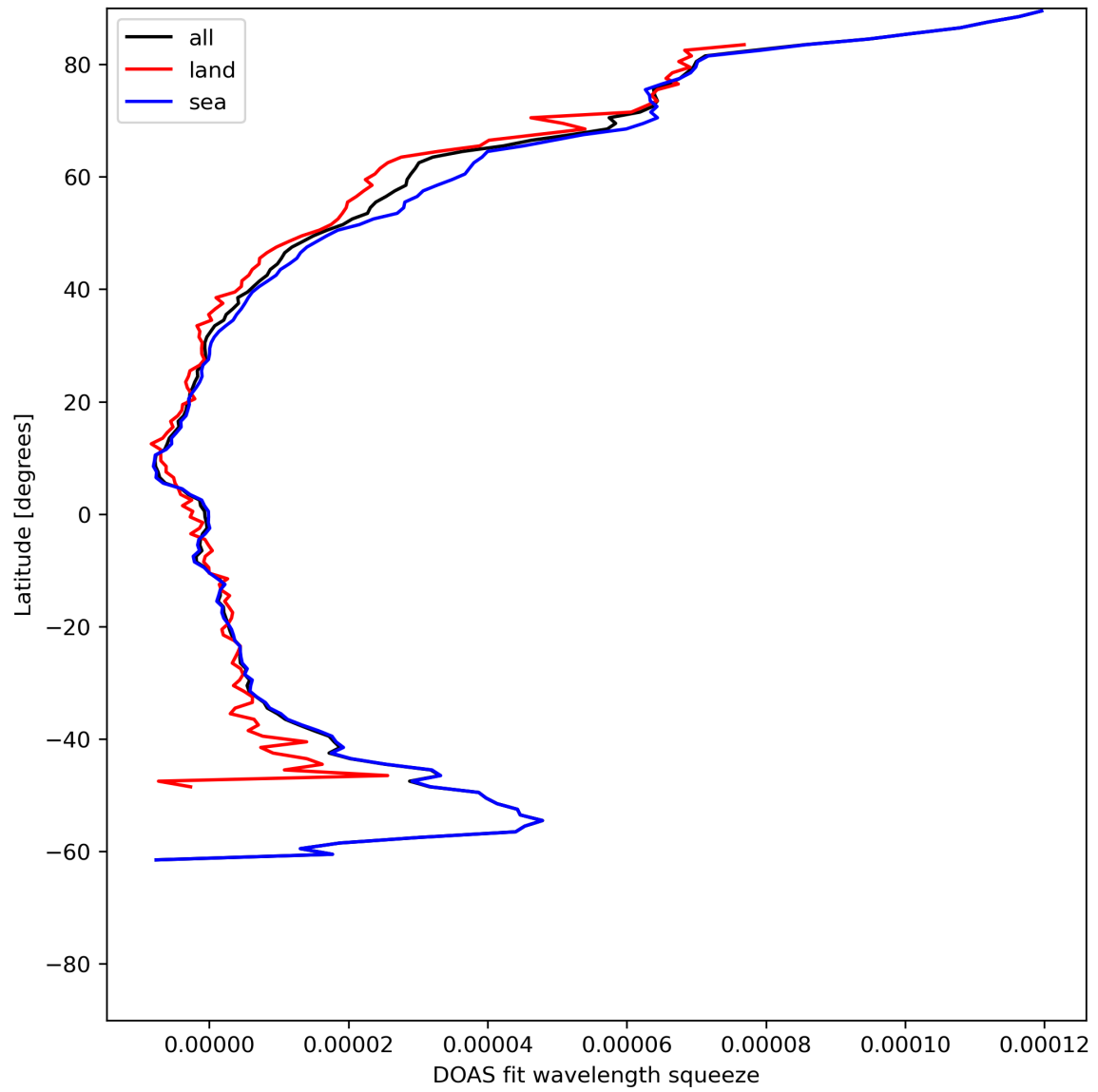
Figure 31: Zonal average of “DOAS fit wavelength squeeze” for 2024-06-24 to 2024-06-25.
