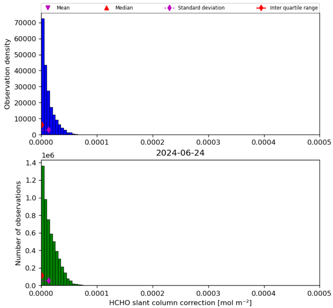
Figure 47: Histogram of “HCHO slant column correction” for 2024-06-24 to 2024-06-25
