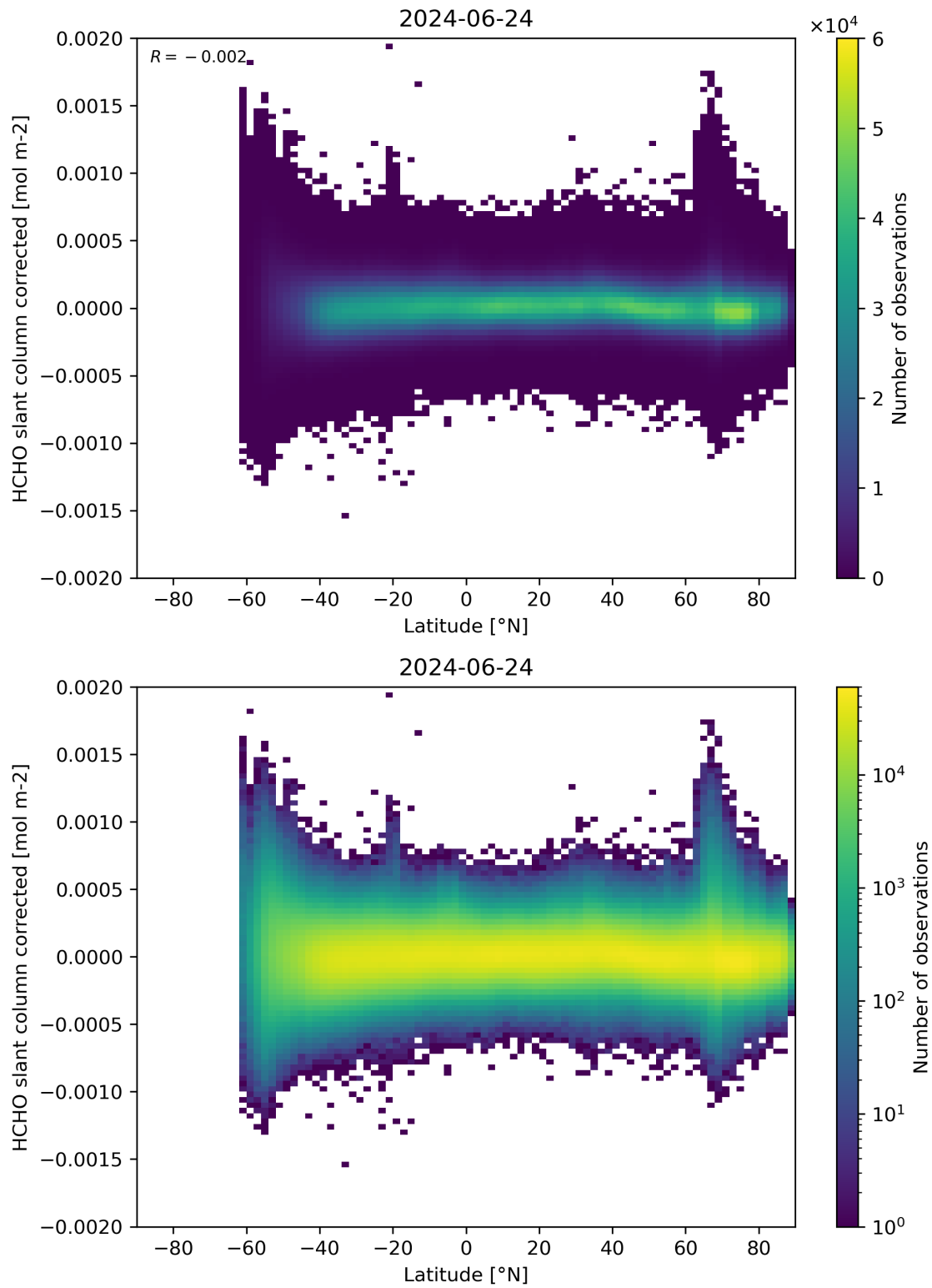
Figure 157: Scatter density plot of “Latitude” against “HCHO slant column corrected” for 2024-06-24 to 2024-06-25.
