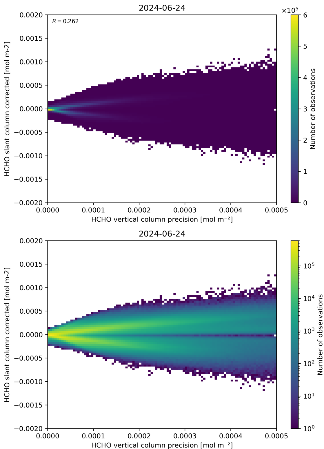
Figure 140: Scatter density plot of “HCHO vertical column precision” against “HCHO slant column corrected” for 2024-06-24 to 2024-06-25.
