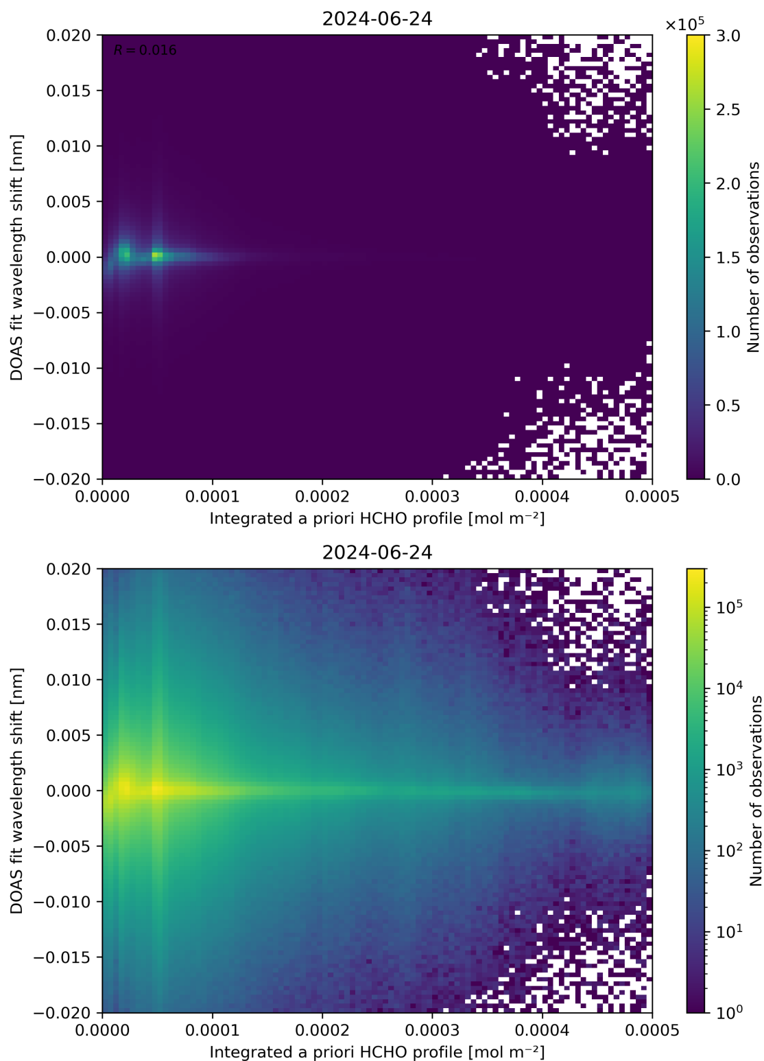
Figure 149: Scatter density plot of “Integrated a priori HCHO profile” against “DOAS fit wavelength shift” for 2024-06-24 to 2024-06-25.
