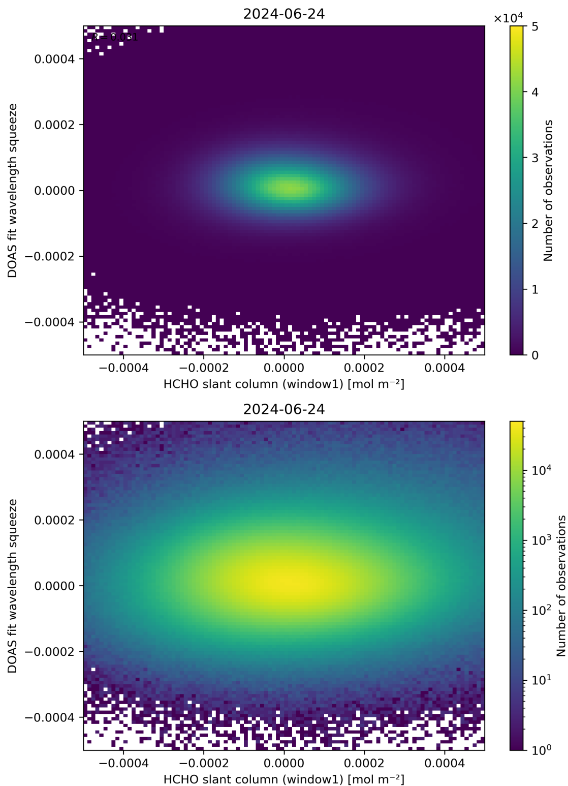
Figure 80: Scatter density plot of “HCHO slant column (window1)” against “DOAS fit wavelength squeeze” for 2024-06-24 to 2024-06-25.
