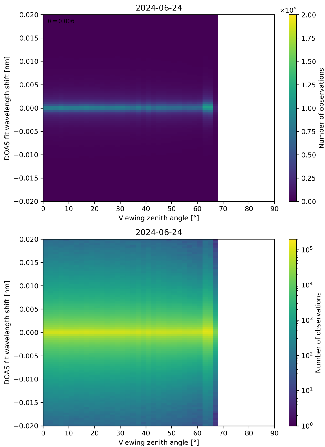
Figure 183: Scatter density plot of “Viewing zenith angle” against “DOAS fit wavelength shift” for 2024-06-24 to 2024-06-25.
