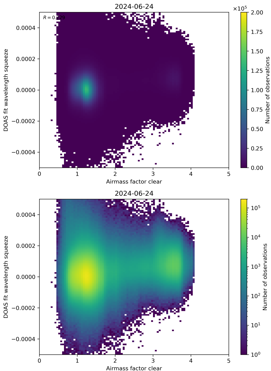
Figure 73: Scatter density plot of “Airmass factor clear” against “DOAS fit wavelength squeeze” for 2024-06-24 to 2024-06-25.
