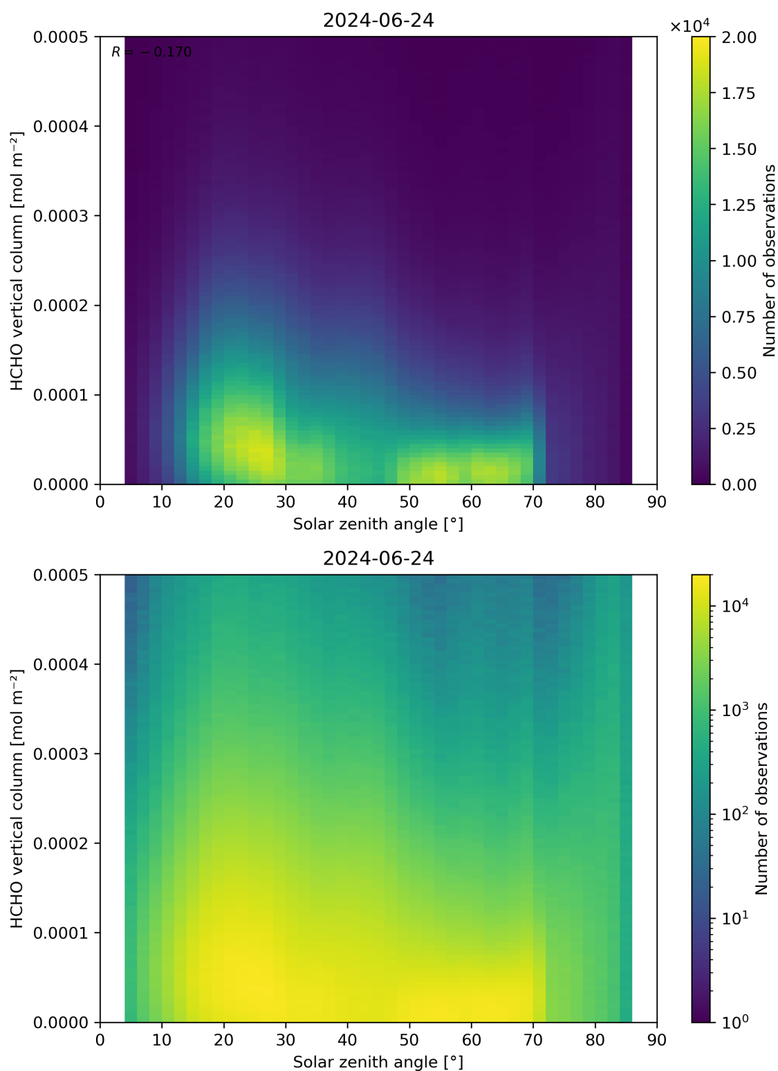
Figure 177: Scatter density plot of “Solar zenith angle” against “HCHO vertical column” for 2024-06-24 to 2024-06-25.
