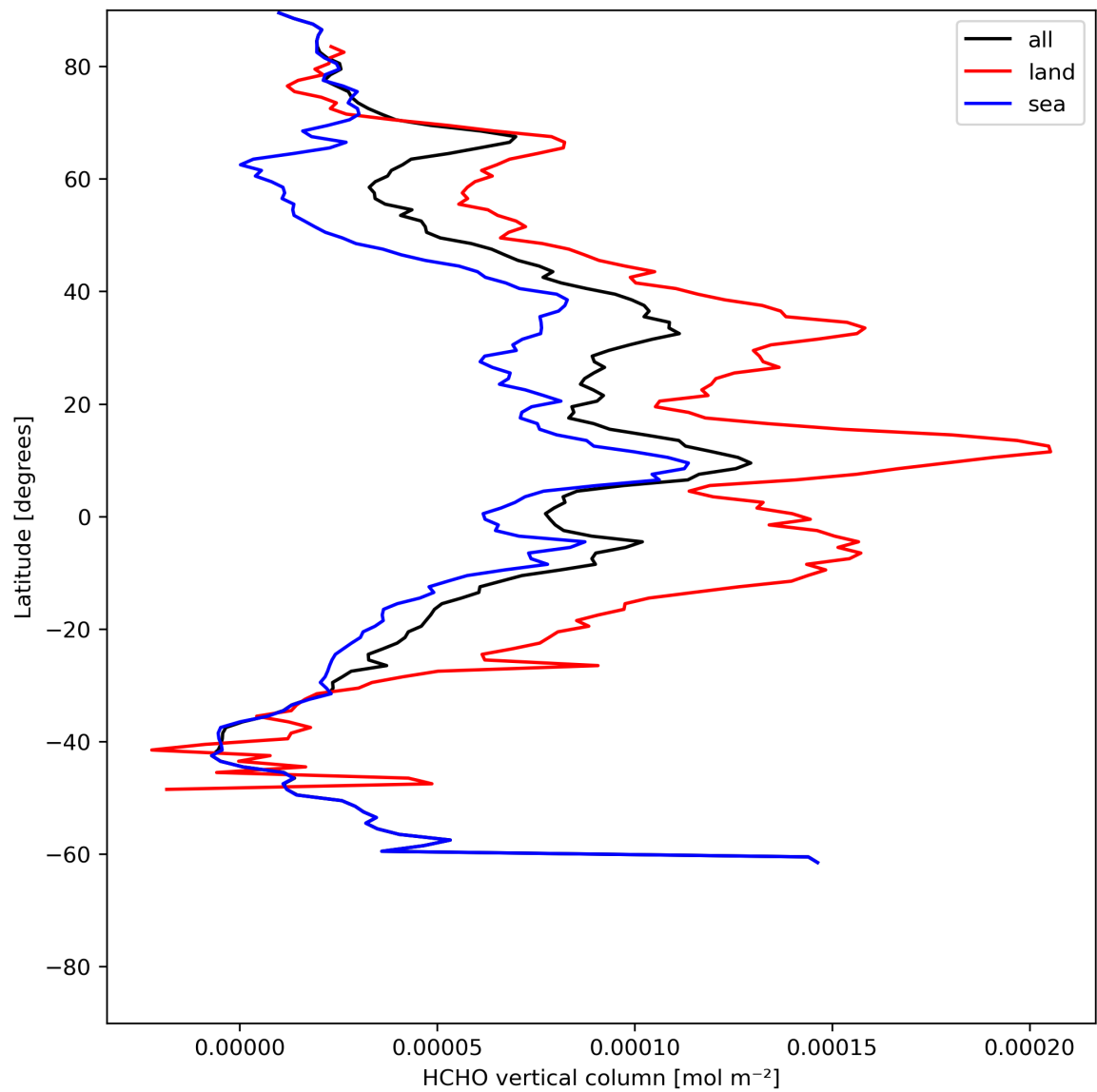
Figure 21: Zonal average of “HCHO vertical column” for 2024-06-24 to 2024-06-25.
