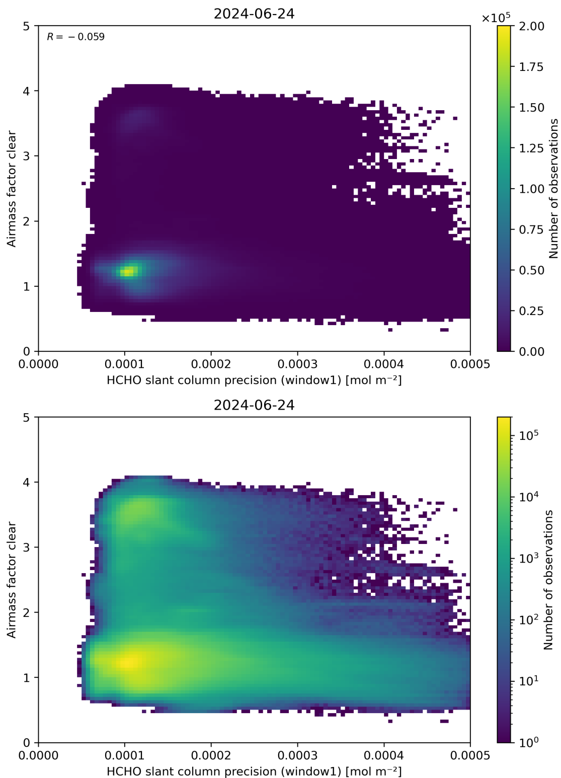
Figure 91: Scatter density plot of “HCHO slant column precision (window1)” against “Airmass factor clear” for 2024-06-24 to 2024-06-25.
