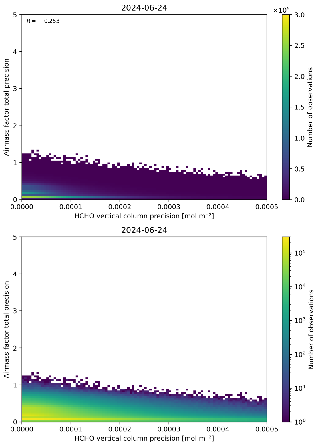
Figure 145: Scatter density plot of “HCHO vertical column precision” against “Airmass factor total precision” for 2024-06-24 to 2024-06-25.
