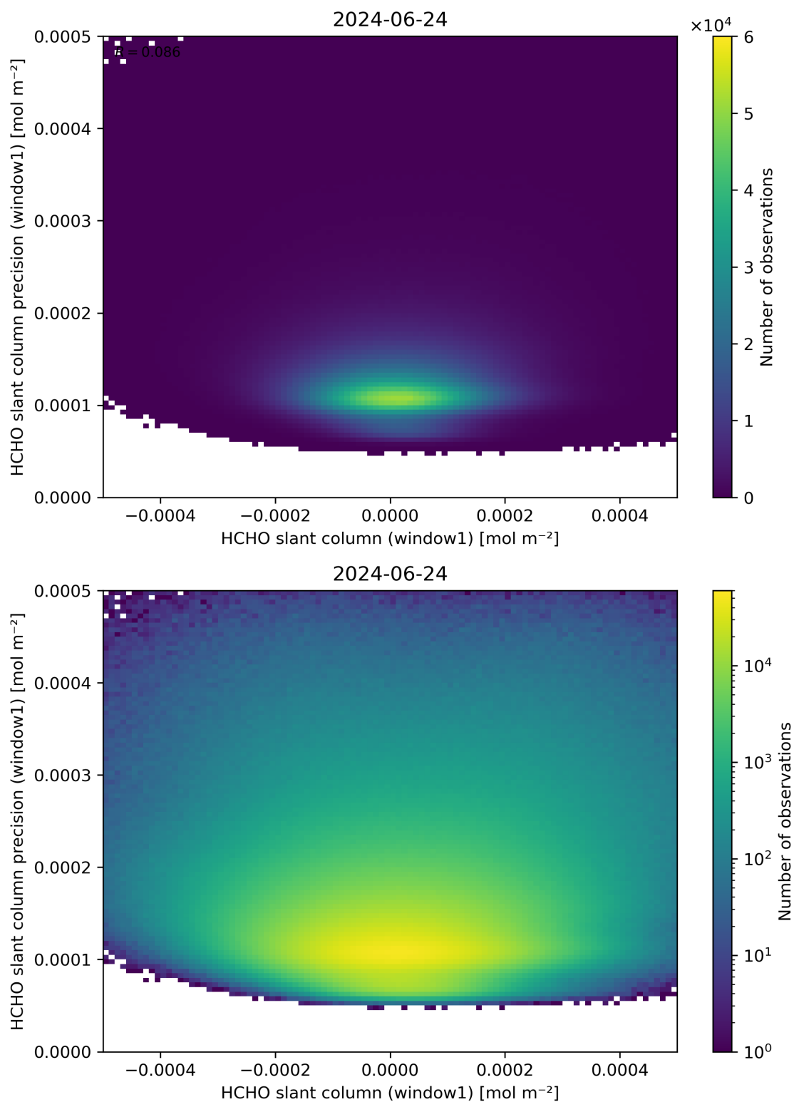
Figure 84: Scatter density plot of “HCHO slant column (window1)” against “HCHO slant column precision (window1)” for 2024-06-24 to 2024-06-25.
