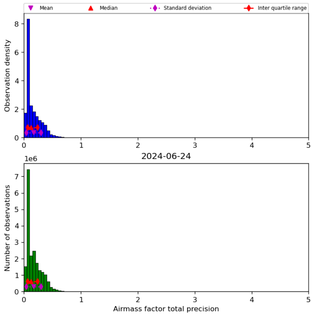
Figure 41: Histogram of “Airmass factor total precision” for 2024-06-24 to 2024-06-25
