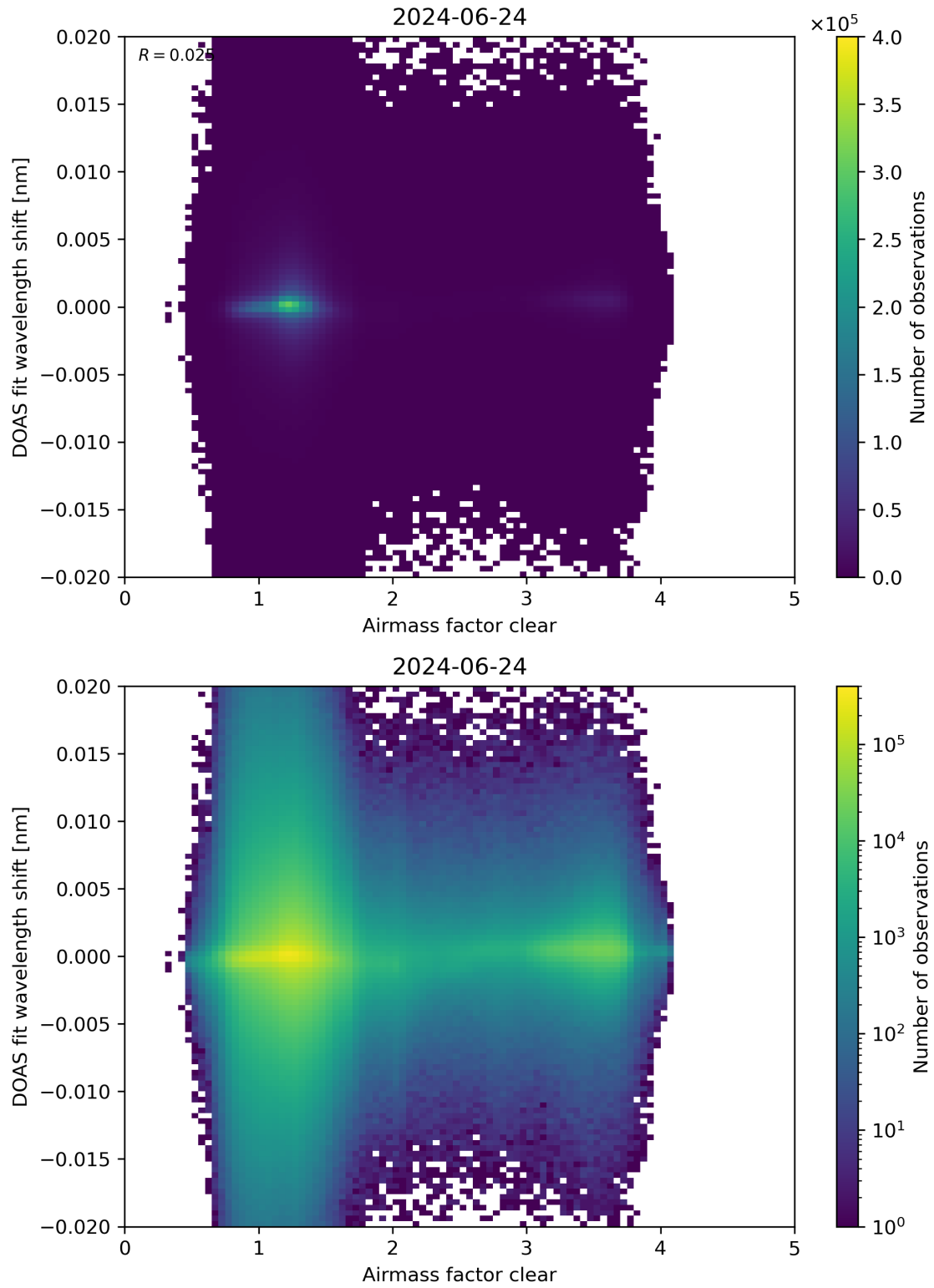
Figure 72: Scatter density plot of “Airmass factor clear” against “DOAS fit wavelength shift” for 2024-06-24 to 2024-06-25.
