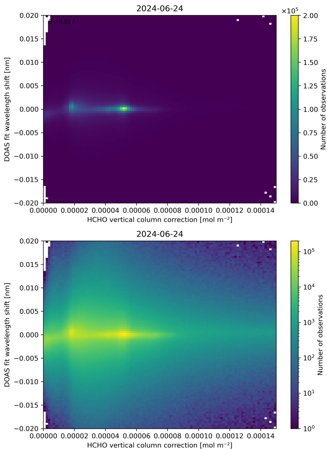
Figure 113: Scatter density plot of “HCHO vertical column correction” against “DOAS fit wavelength shift” for 2024-06-24 to 2024-06-25.
