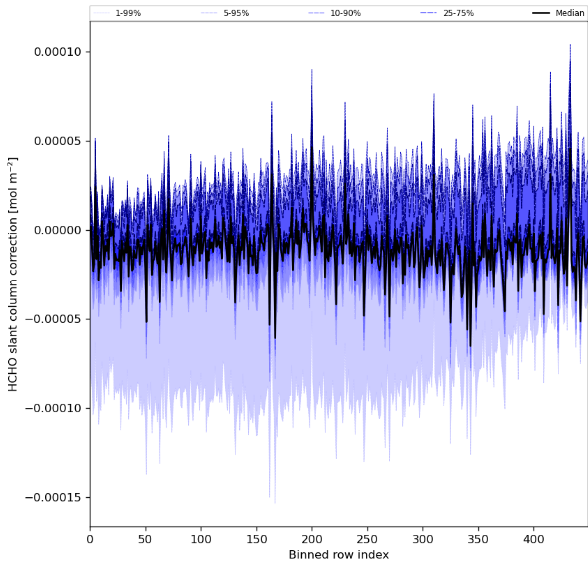
Figure 61: Along track statistics of “HCHO slant column correction” for 2024-06-24 to 2024-06-25
