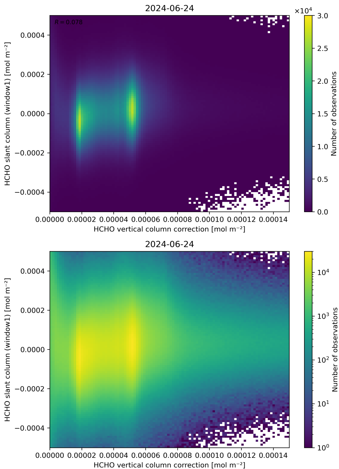
Figure 118: Scatter density plot of “HCHO vertical column correction” against “HCHO slant column (window1)” for 2024-06-24 to 2024-06-25.
