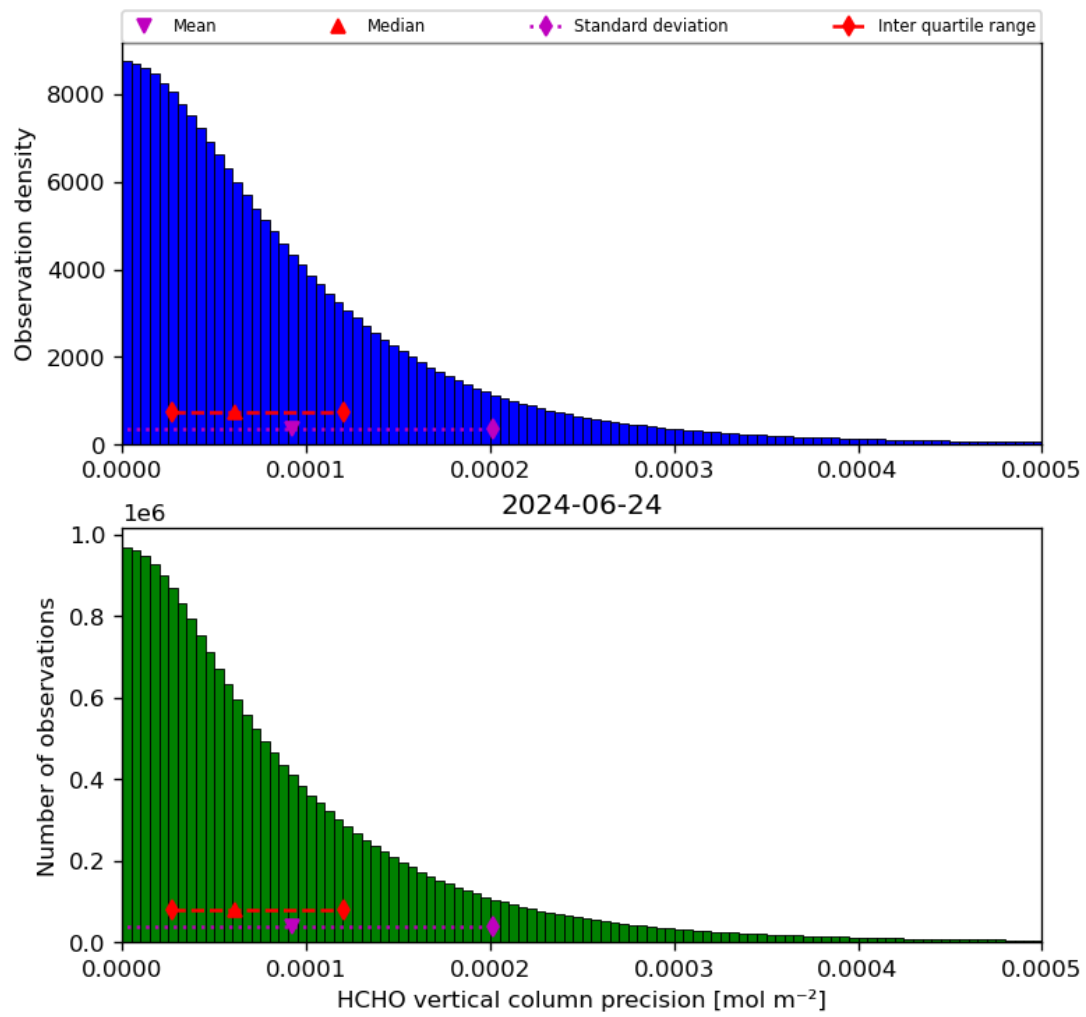
Figure 36: Histogram of “HCHO vertical column precision” for 2024-06-24 to 2024-06-25
