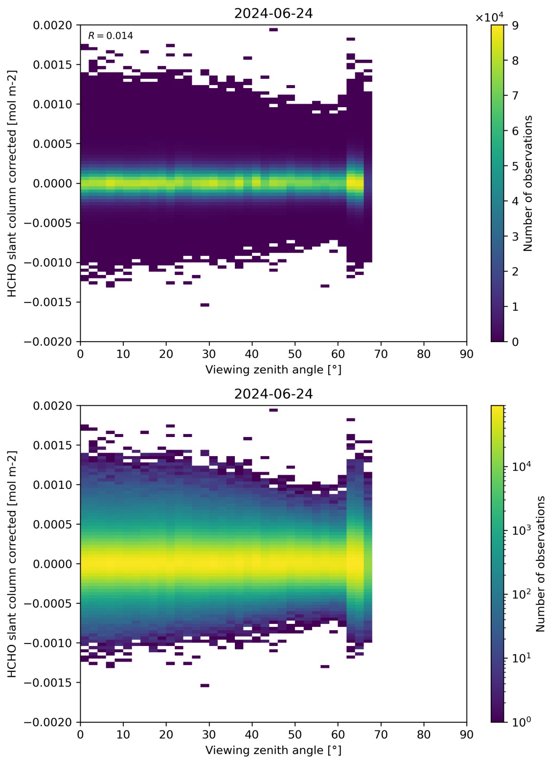
Figure 186: Scatter density plot of “Viewing zenith angle” against “HCHO slant column corrected” for 2024-06-24 to 2024-06-25.
