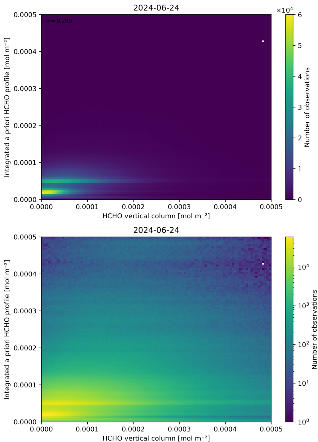
Figure 135: Scatter density plot of “HCHO vertical column” against “Integrated a priori HCHO profile” for 2024-06-24 to 2024-06-25.
