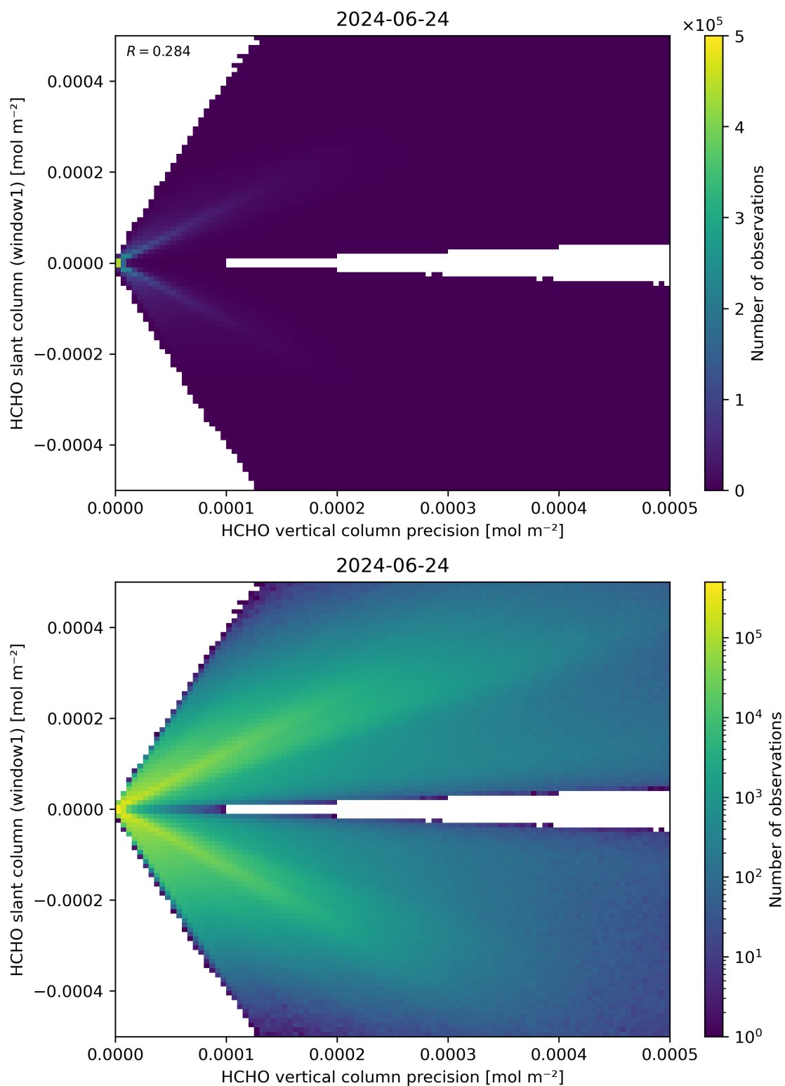
Figure 142: Scatter density plot of “HCHO vertical column precision” against “HCHO slant column (window1)” for 2024-06-24 to 2024-06-25.
