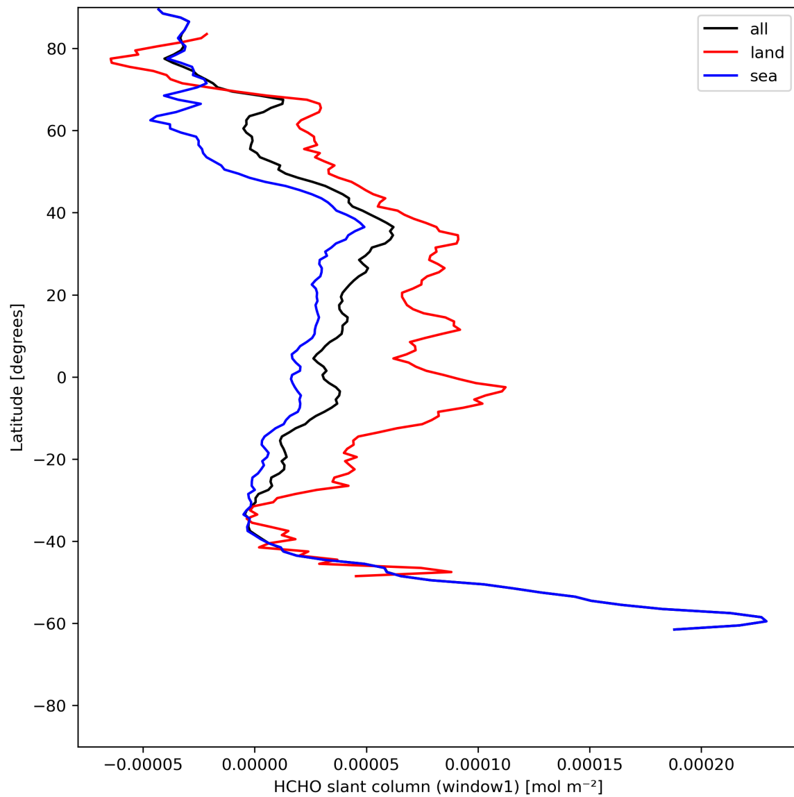
Figure 24: Zonal average of “HCHO slant column (window1)” for 2024-06-24 to 2024-06-25.
