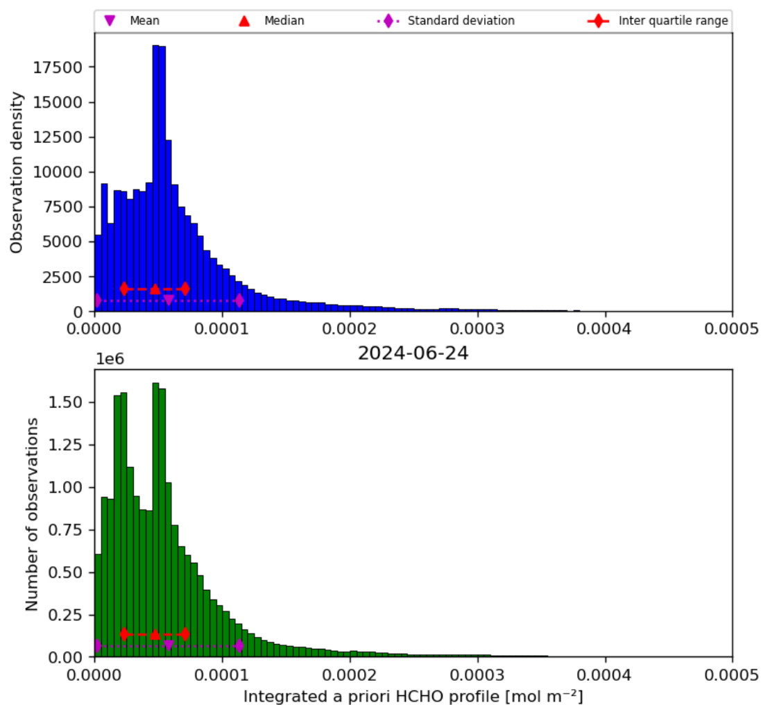
Figure 43: Histogram of “Integrated a priori HCHO profile” for 2024-06-24 to 2024-06-25
