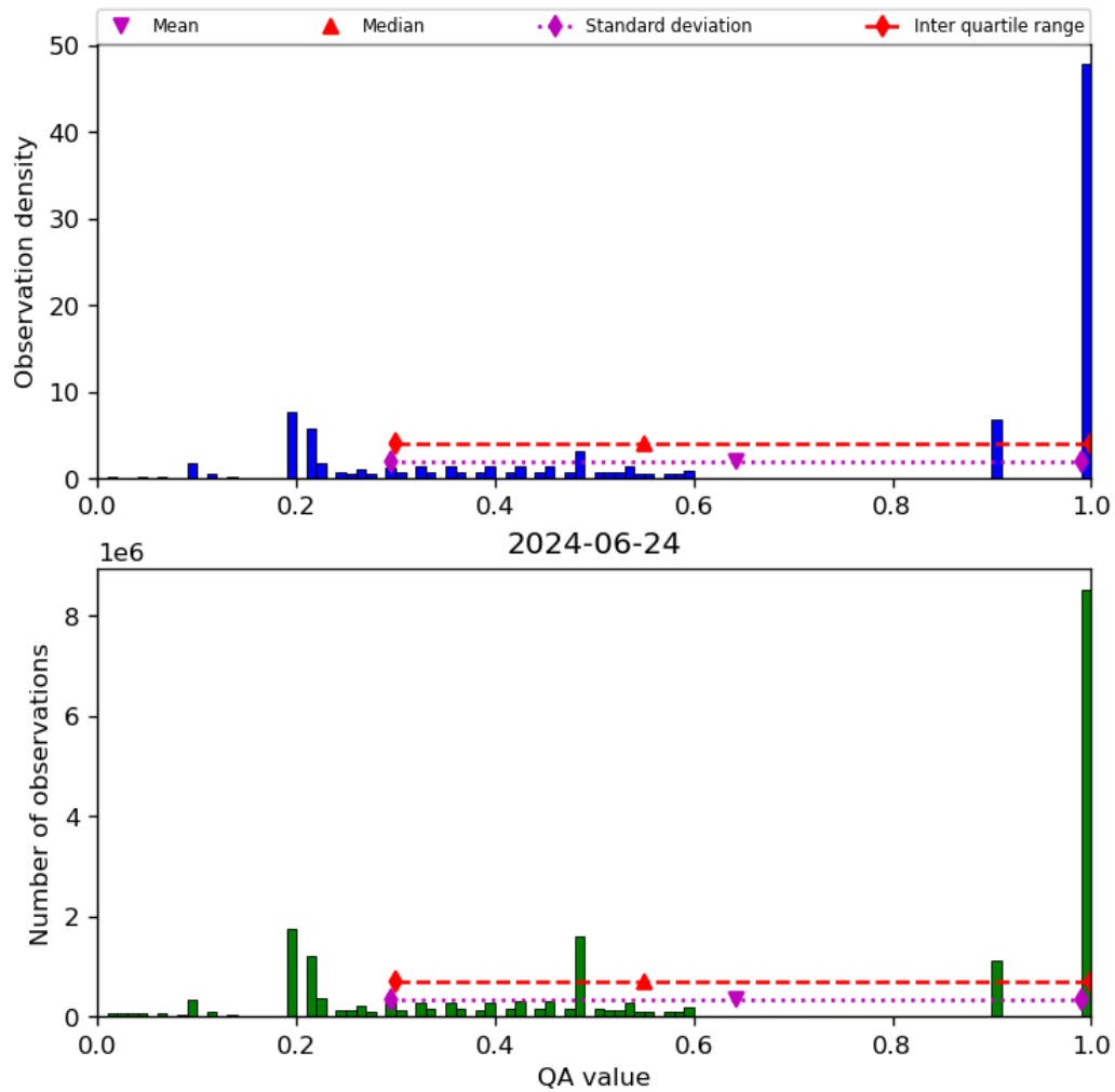
Figure 34: Histogram of “QA value” for 2024-06-24 to 2024-06-25
