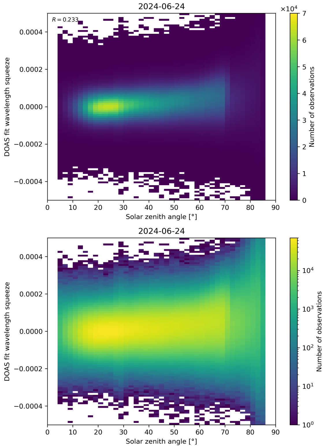
Figure 169: Scatter density plot of “Solar zenith angle” against “DOAS fit wavelength squeeze” for 2024-06-24 to 2024-06-25.
