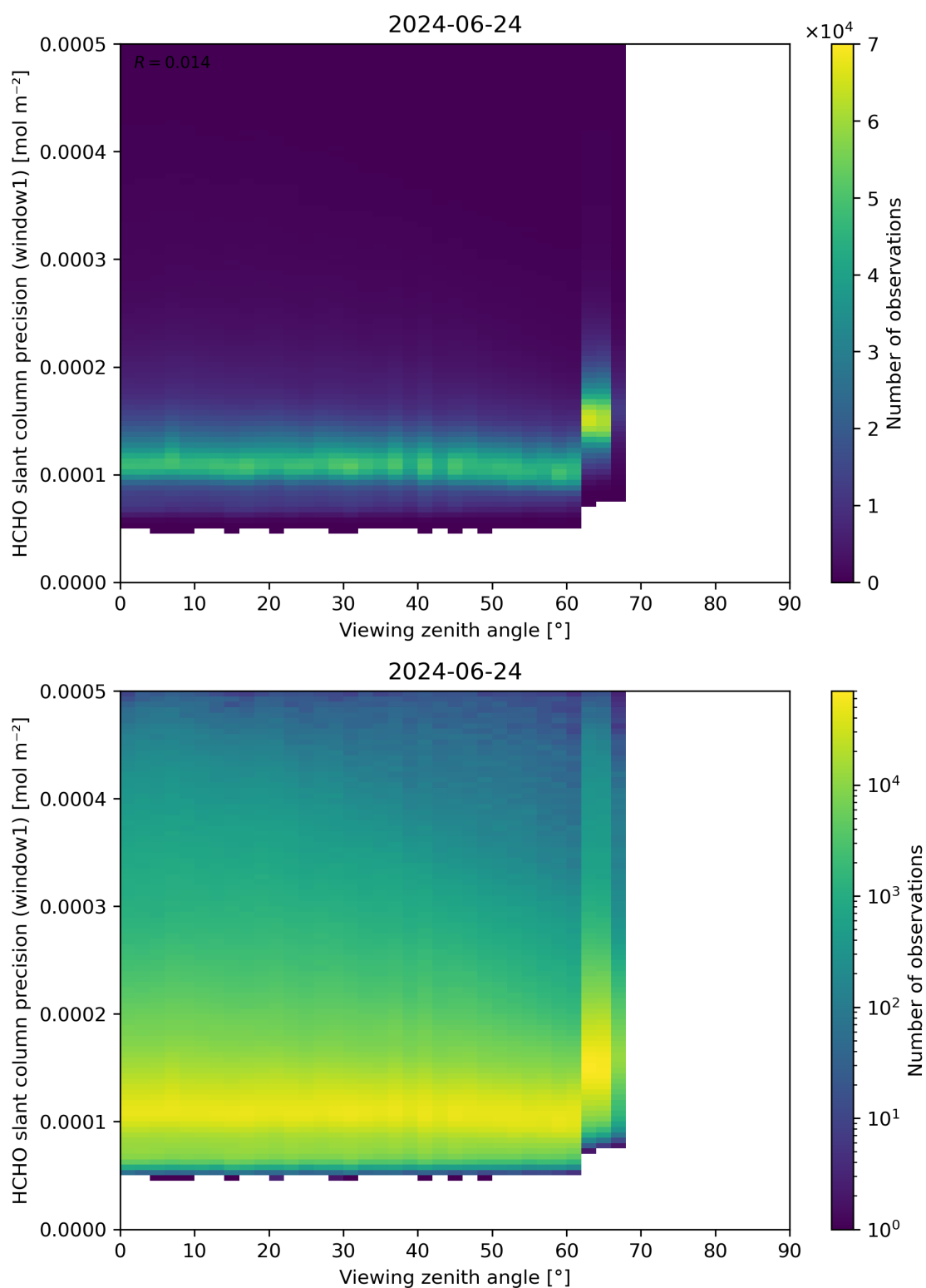
Figure 189: Scatter density plot of “Viewing zenith angle” against “HCHO slant column precision (window1)” for 2024-06-24 to 2024-06-25.
