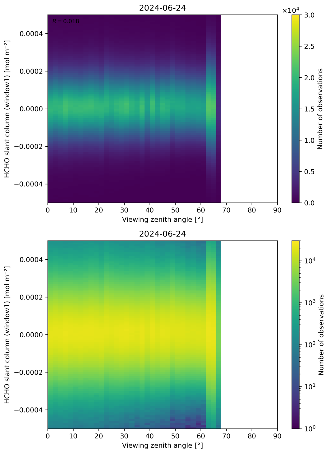
Figure 188: Scatter density plot of “Viewing zenith angle” against “HCHO slant column (window1)” for 2024-06-24 to 2024-06-25.
