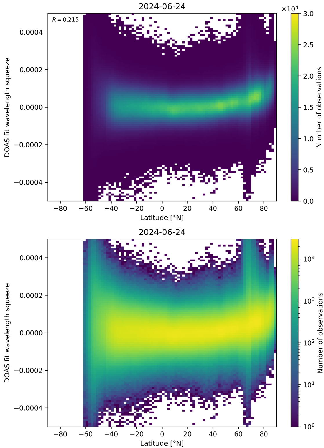
Figure 155: Scatter density plot of “Latitude” against “DOAS fit wavelength squeeze” for 2024-06-24 to 2024-06-25.
