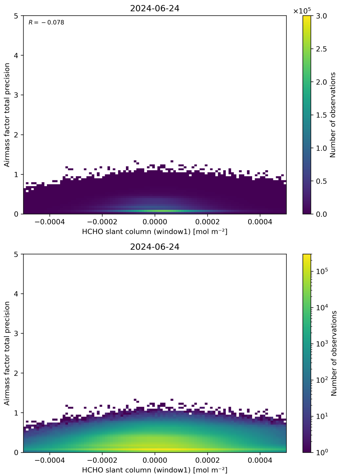
Figure 86: Scatter density plot of “HCHO slant column (window1)” against “Airmass factor total precision” for 2024-06-24 to 2024-06-25.
