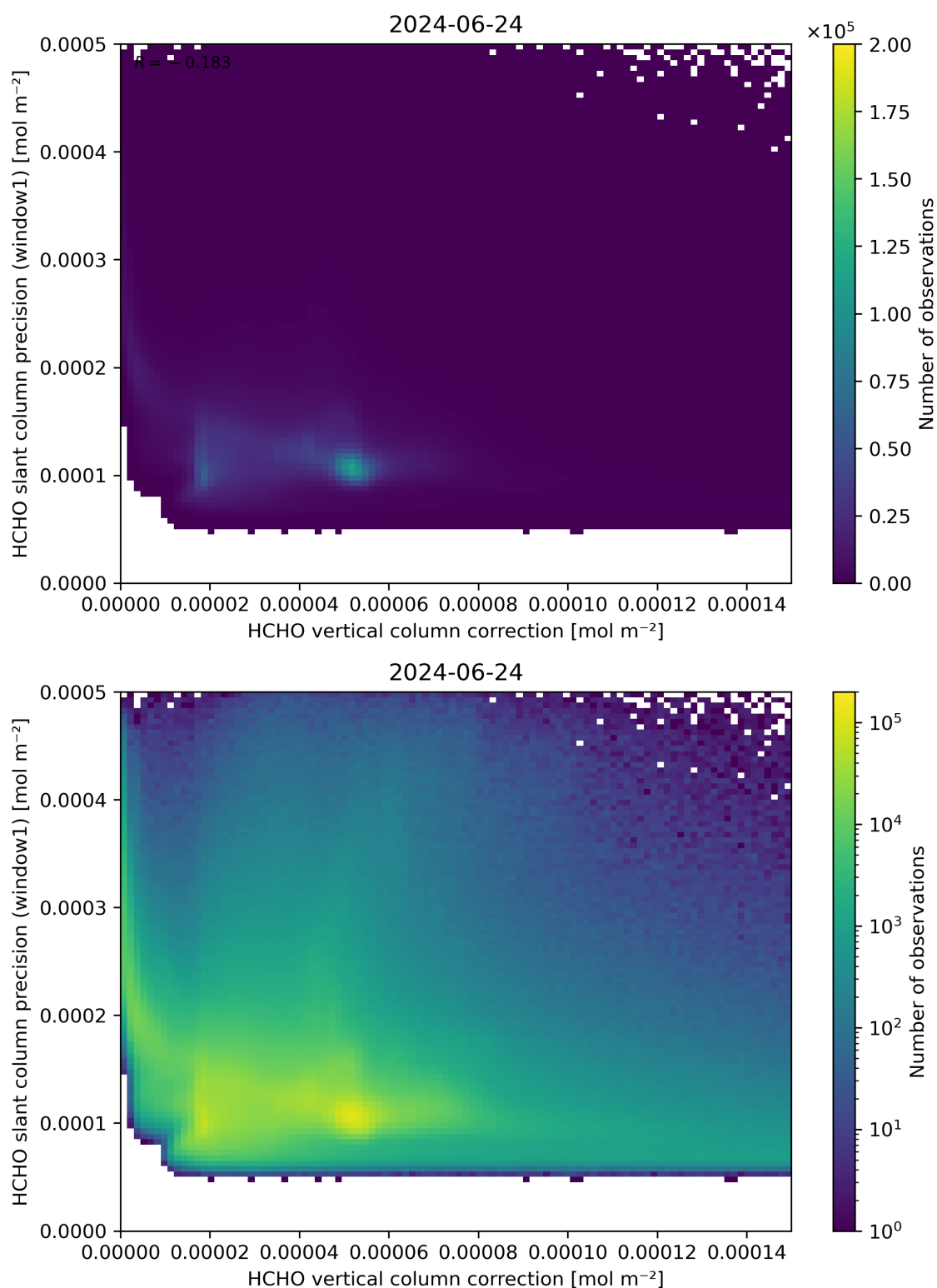
Figure 119: Scatter density plot of “HCHO vertical column correction” against “HCHO slant column precision (window1)” for 2024-06-24 to 2024-06-25.
