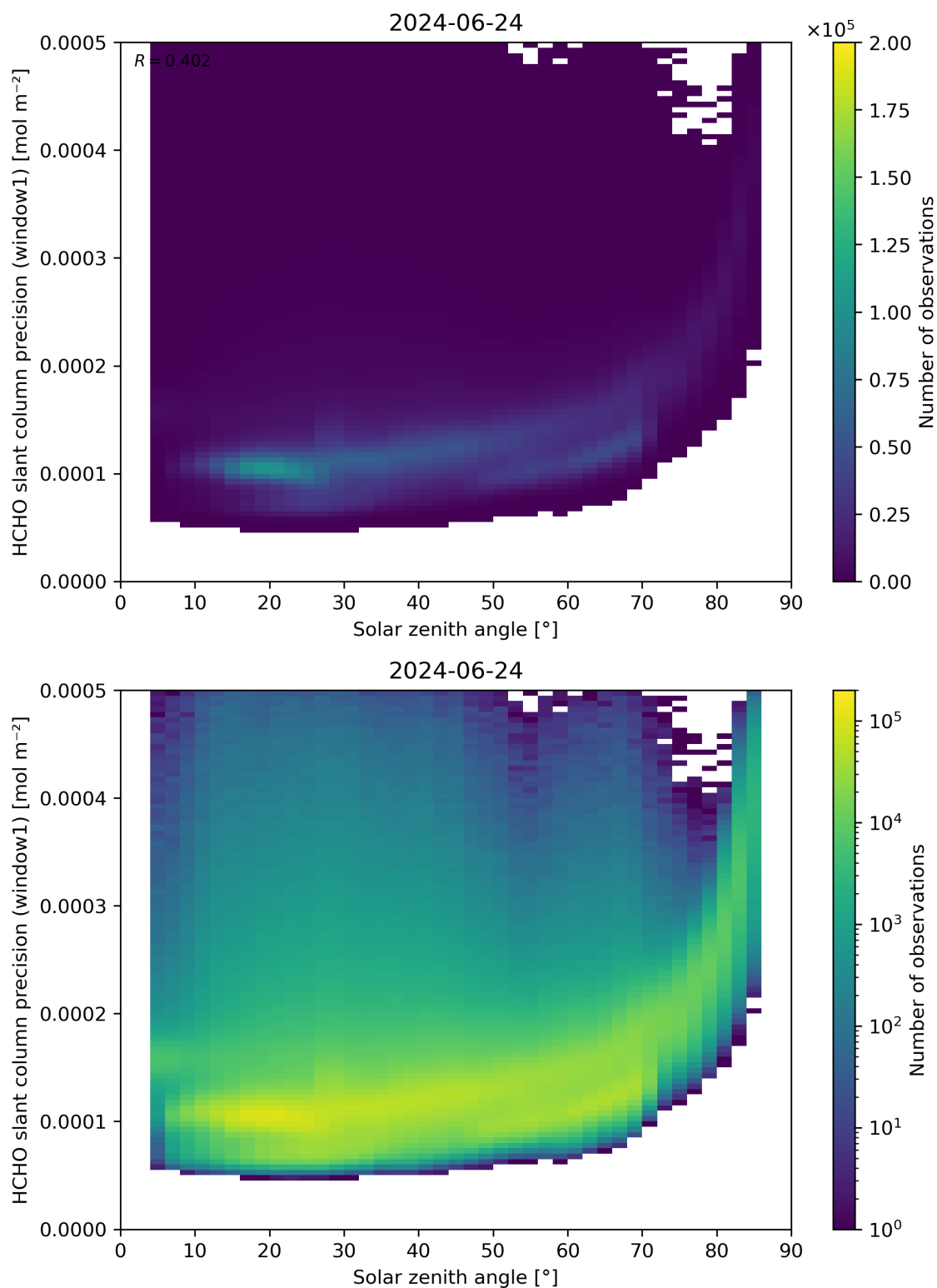
Figure 174: Scatter density plot of “Solar zenith angle” against “HCHO slant column precision (window1)” for 2024-06-24 to 2024-06-25.
