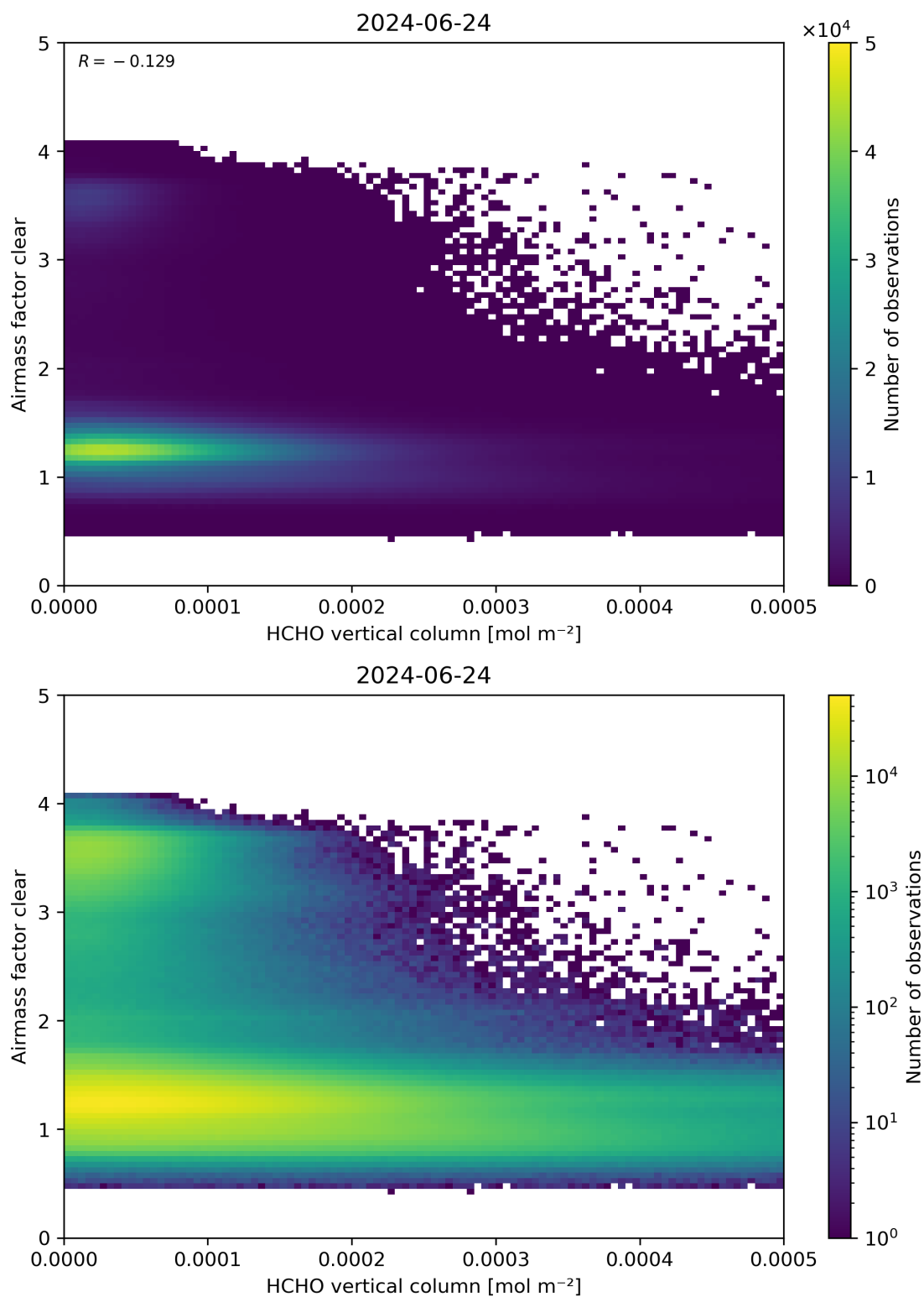
Figure 126: Scatter density plot of “HCHO vertical column” against “Airmass factor clear” for 2024-06-24 to 2024-06-25.
