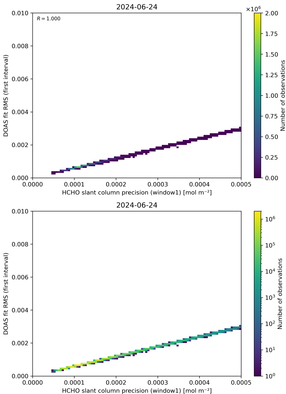
Figure 88: Scatter density plot of “HCHO slant column precision (window1)” against “DOAS fit RMS (first interval)” for 2024-06-24 to 2024-06-25.
