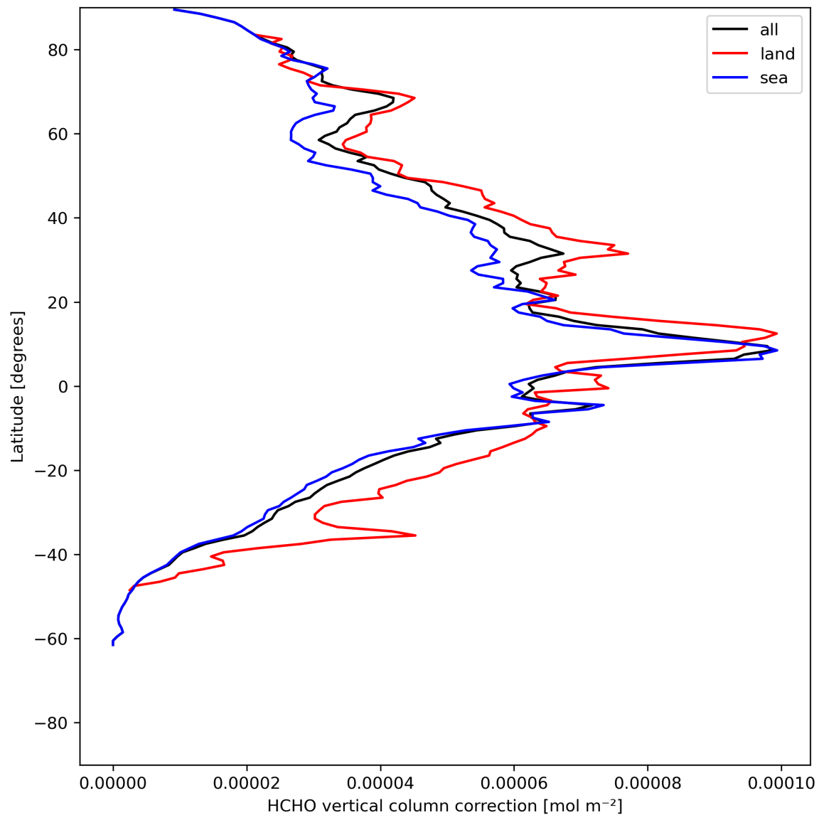
Figure 23: Zonal average of “HCHO vertical column correction” for 2024-06-24 to 2024-06-25.
