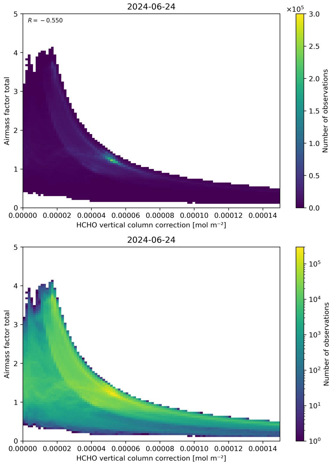
Figure 120: Scatter density plot of “HCHO vertical column correction” against “Airmass factor total” for 2024-06-24 to 2024-06-25.
