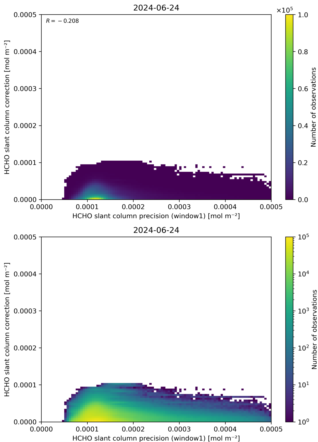
Figure 93: Scatter density plot of “HCHO slant column precision (window1)” against “HCHO slant column correction” for 2024-06-24 to 2024-06-25.
