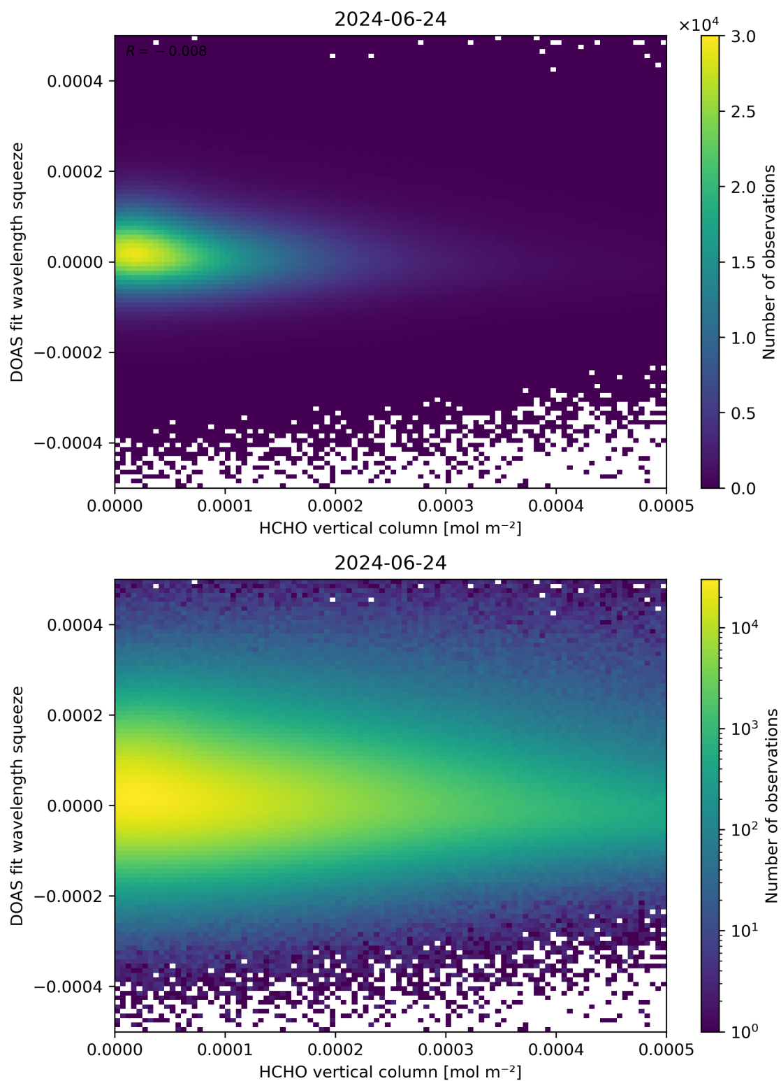
Figure 125: Scatter density plot of “HCHO vertical column” against “DOAS fit wavelength squeeze” for 2024-06-24 to 2024-06-25.
