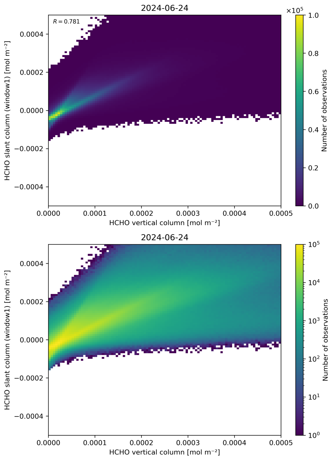
Figure 129: Scatter density plot of “HCHO vertical column” against “HCHO slant column (window1)” for 2024-06-24 to 2024-06-25.
