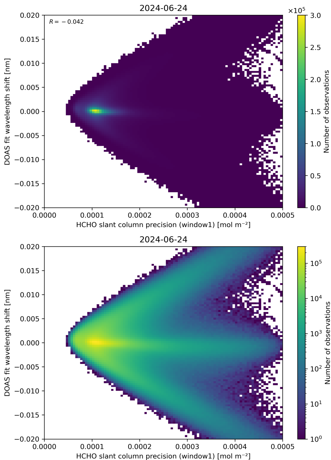
Figure 89: Scatter density plot of “HCHO slant column precision (window1)” against “DOAS fit wavelength shift” for 2024-06-24 to 2024-06-25.
