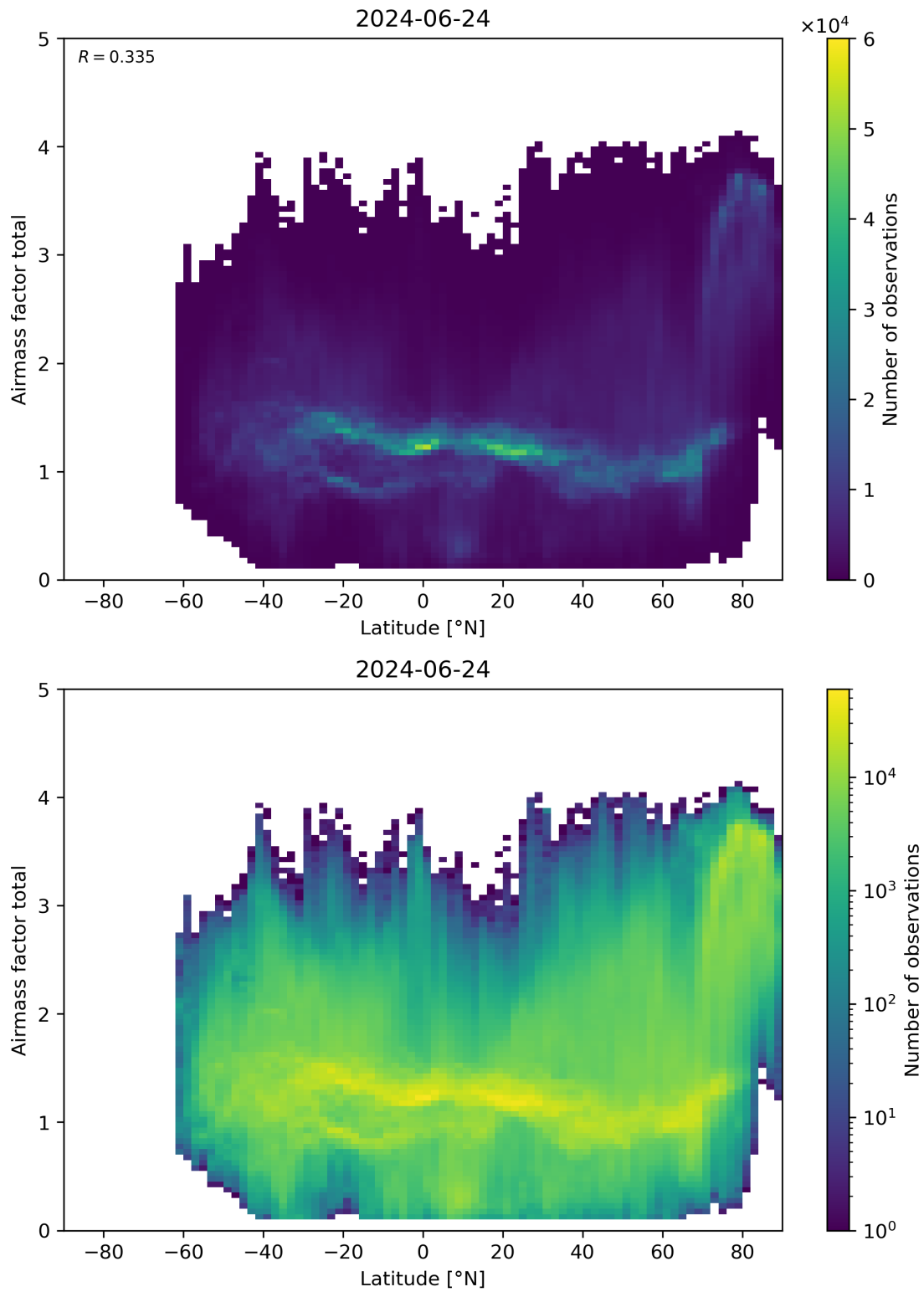
Figure 161: Scatter density plot of “Latitude” against “Airmass factor total” for 2024-06-24 to 2024-06-25.
