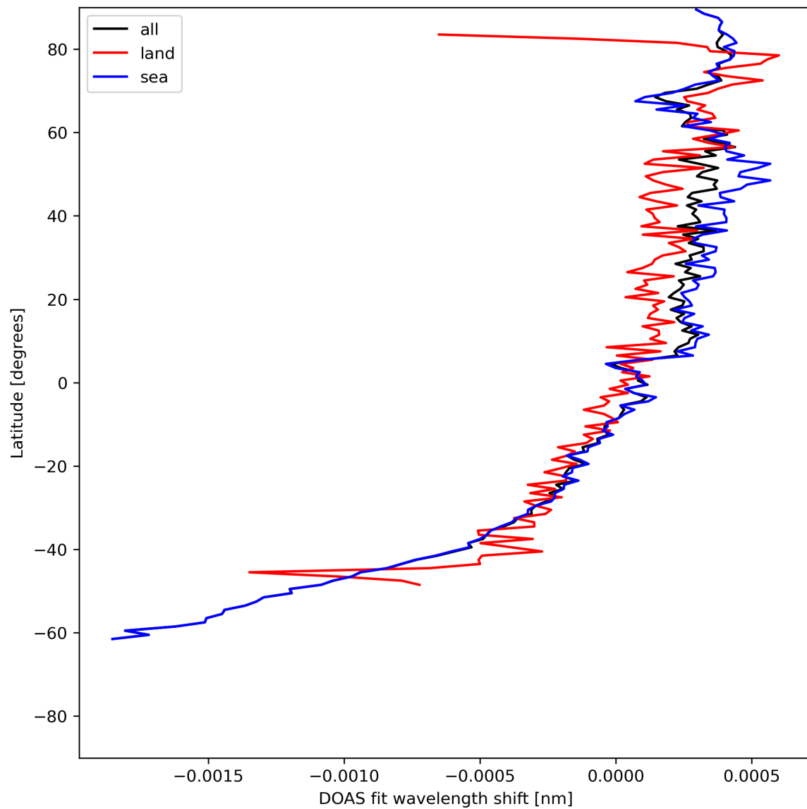
Figure 30: Zonal average of "DOAS fit wavelength shift" for 2024-06-24 to 2024-06-25.
