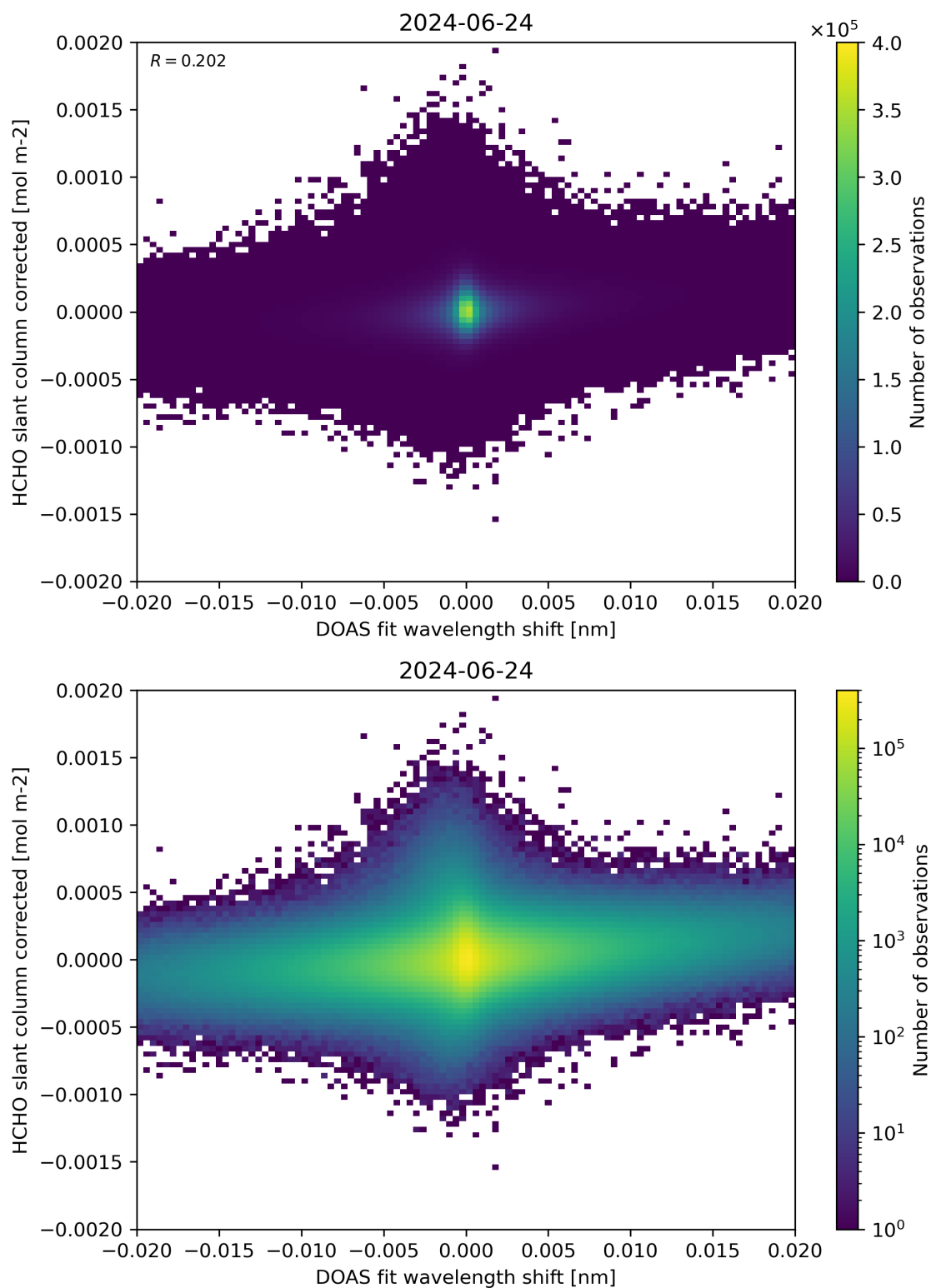
Figure 66: Scatter density plot of “DOAS fit wavelength shift” against “HCHO slant column corrected” for 2024-06-24 to 2024-06-25.
