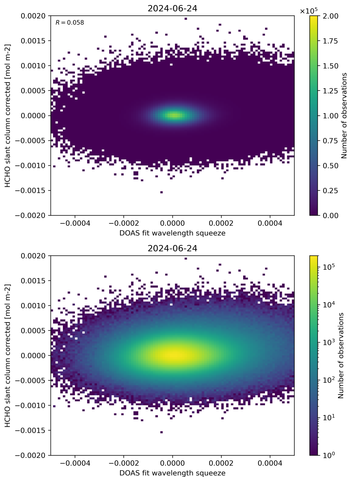
Figure 69: Scatter density plot of “DOAS fit wavelength squeeze” against “HCHO slant column corrected” for 2024-06-24 to 2024-06-25.
