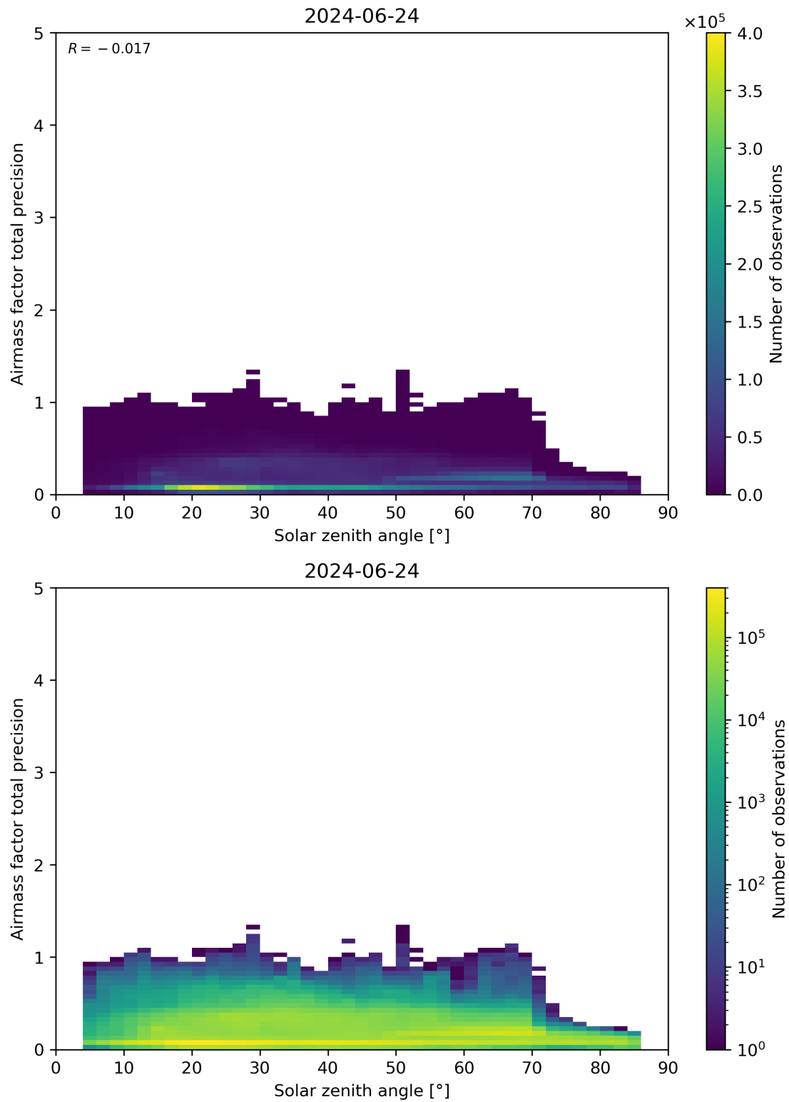
Figure 176: Scatter density plot of “Solar zenith angle” against “Airmass factor total precision” for 2024-06-24 to 2024-06-25.
