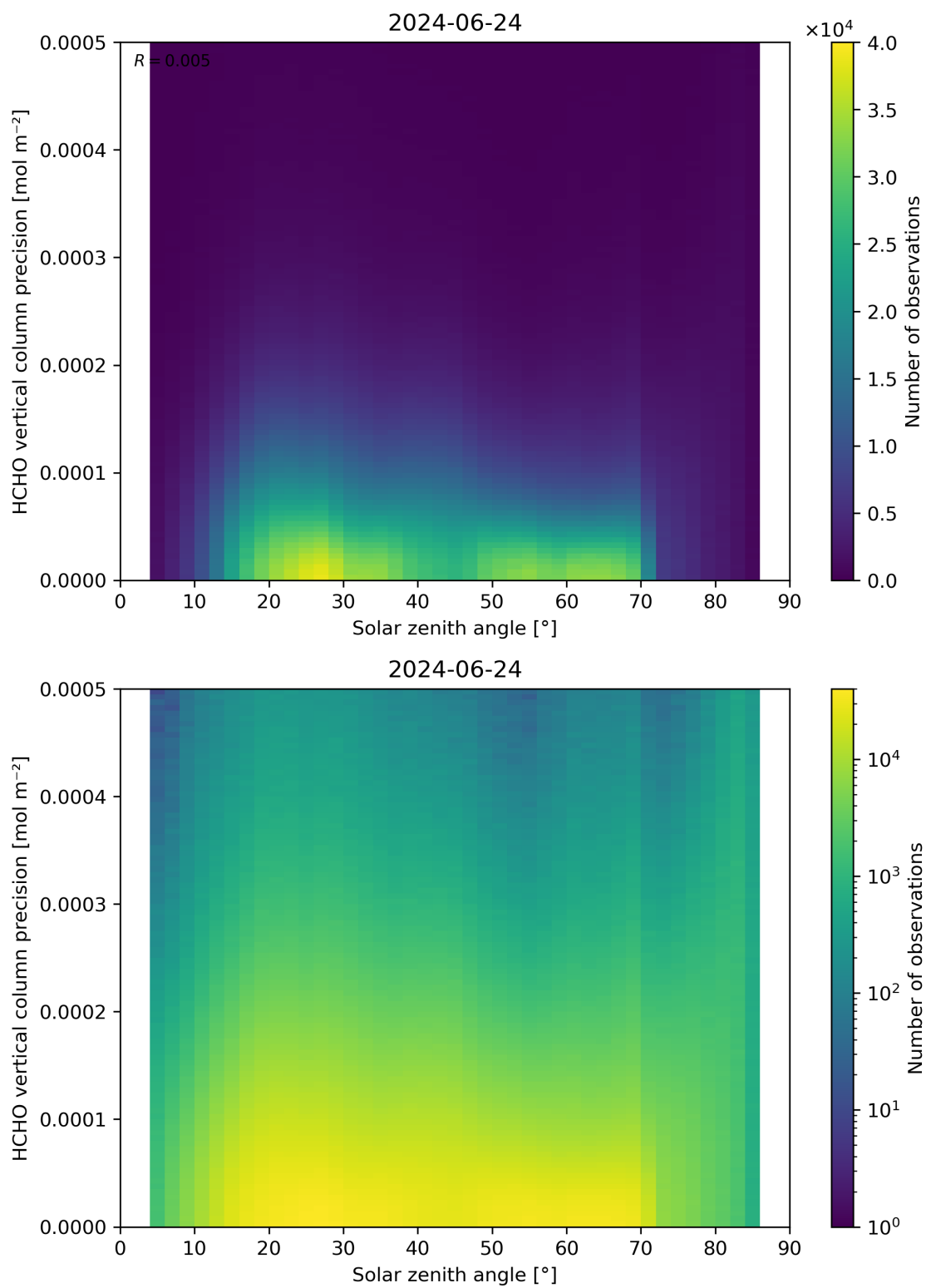
Figure 179: Scatter density plot of “Solar zenith angle” against “HCHO vertical column precision” for 2024-06-24 to 2024-06-25.
