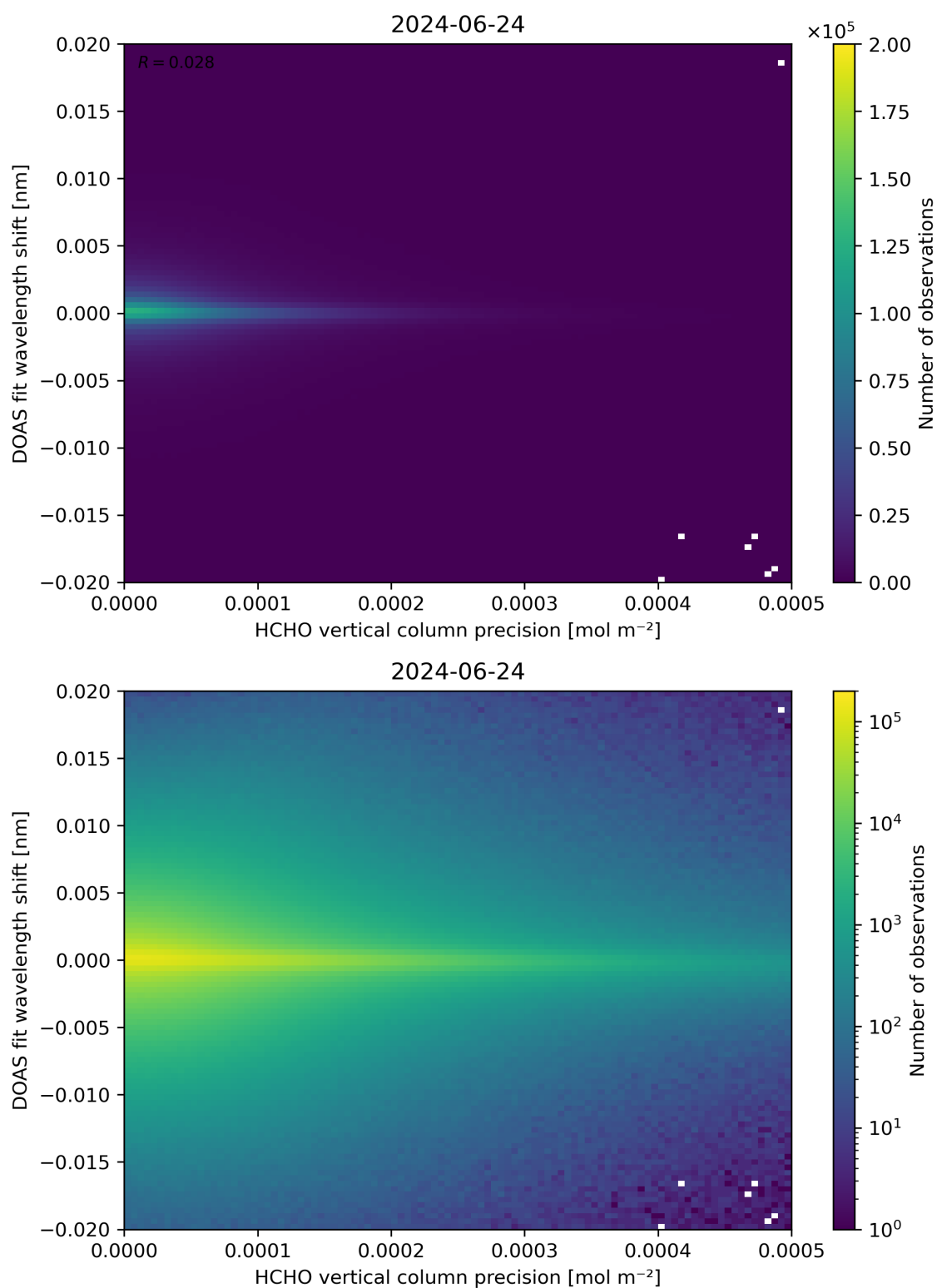
Figure 137: Scatter density plot of “HCHO vertical column precision” against “DOAS fit wavelength shift” for 2024-06-24 to 2024-06-25.
