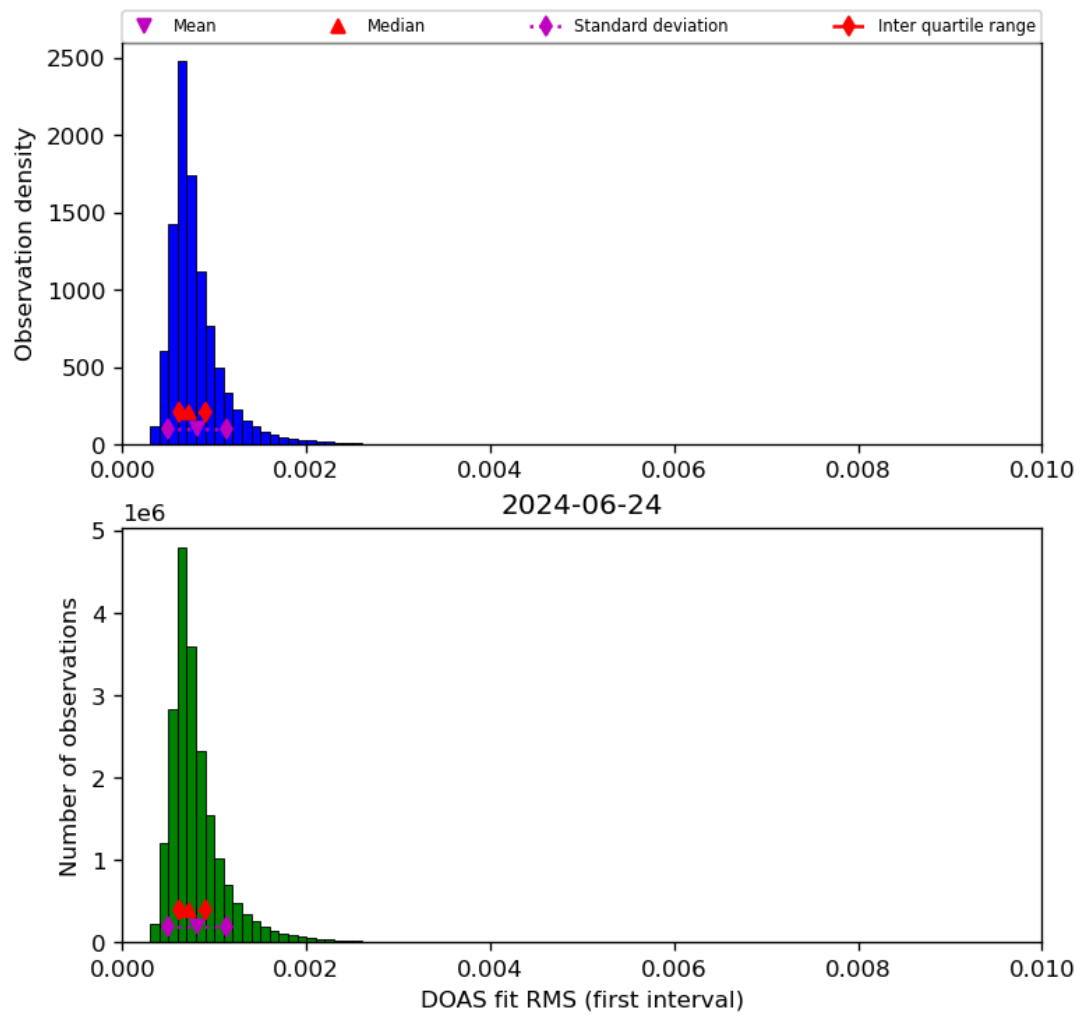
Figure 46: Histogram of “DOAS fit RMS (first interval)” for 2024-06-24 to 2024-06-25
