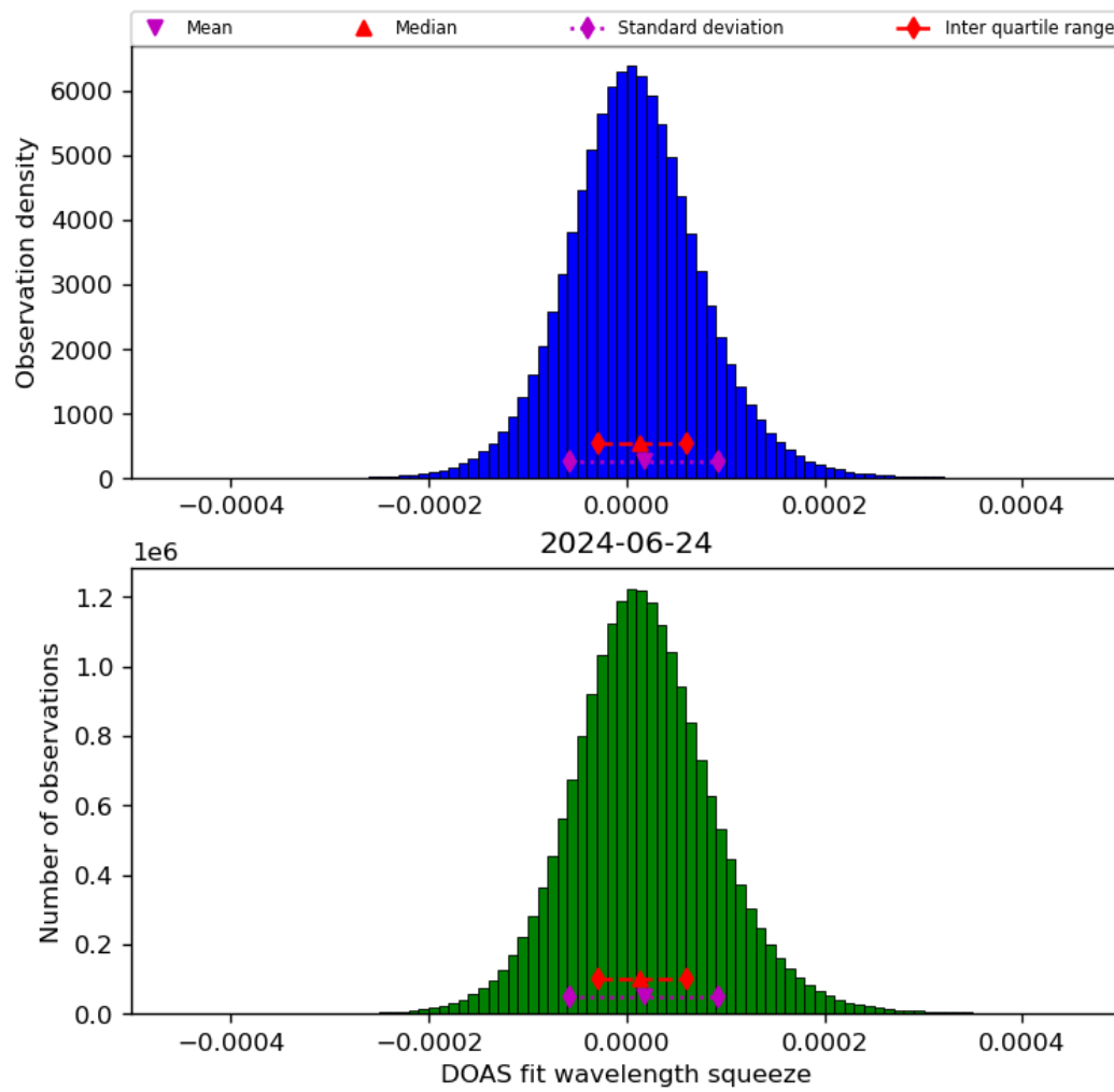
Figure 45: Histogram of “DOAS fit wavelength squeeze” for 2024-06-24 to 2024-06-25
