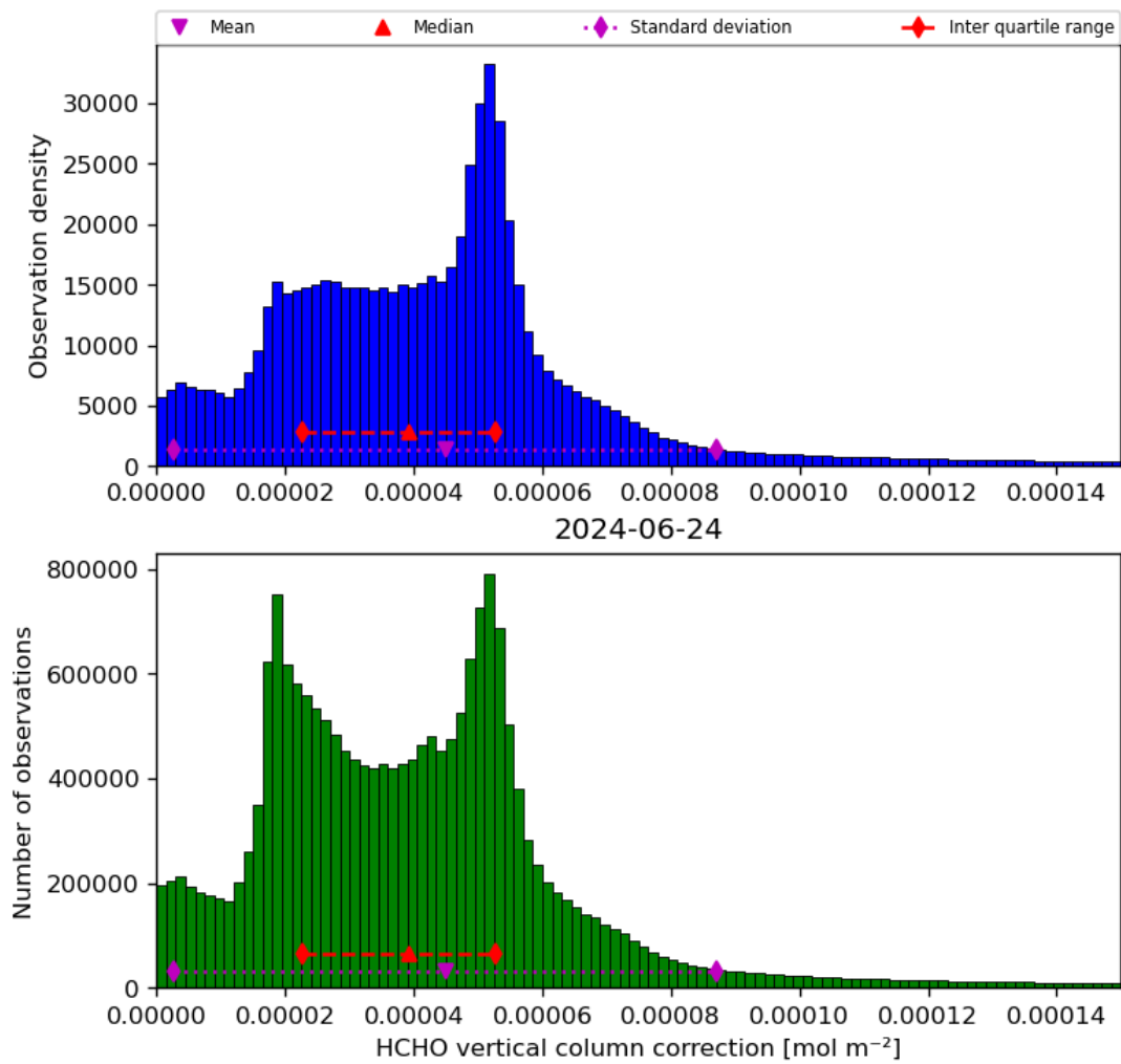
Figure 37: Histogram of “HCHO vertical column correction” for 2024-06-24 to 2024-06-25
