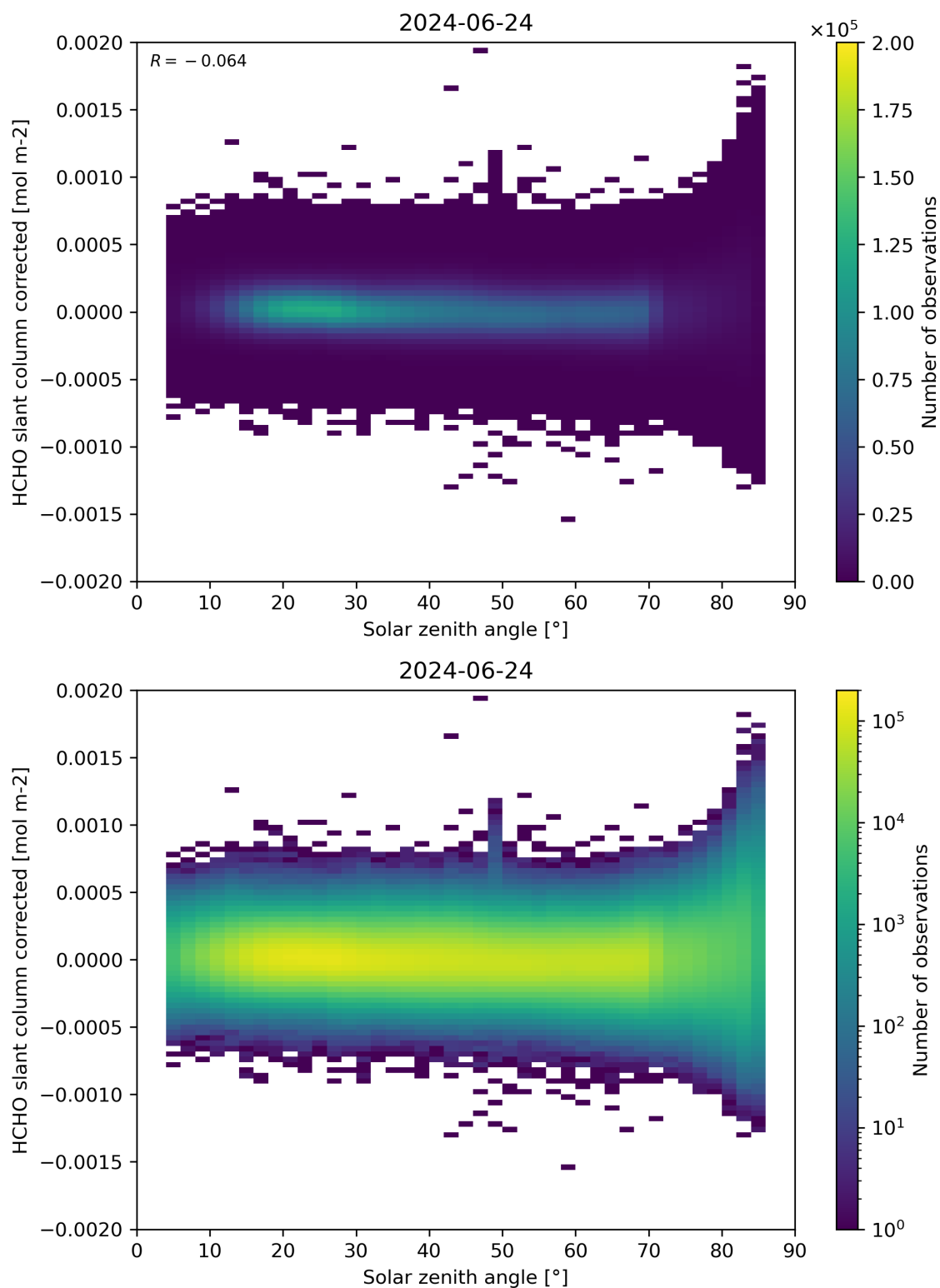
Figure 171: Scatter density plot of “Solar zenith angle” against “HCHO slant column corrected” for 2024-06-24 to 2024-06-25.
