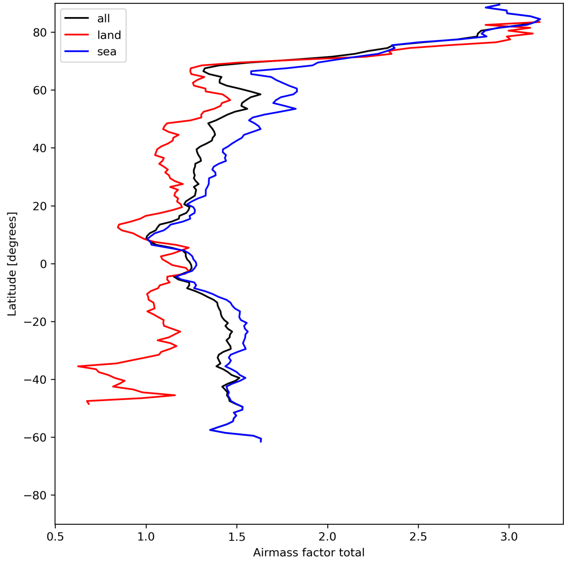
Figure 26: Zonal average of “Airmass factor total” for 2024-06-24 to 2024-06-25.
