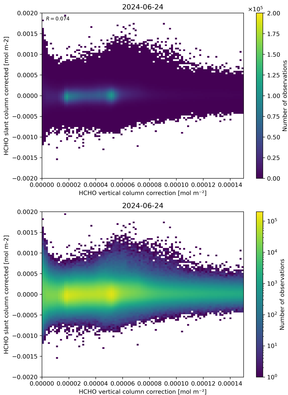
Figure 116: Scatter density plot of “HCHO vertical column correction” against “HCHO slant column corrected” for 2024-06-24 to 2024-06-25.
