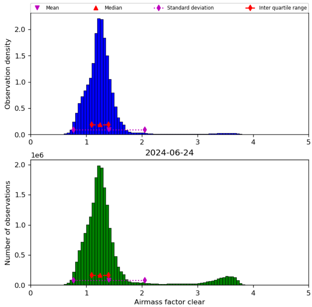
Figure 42: Histogram of “Airmass factor clear” for 2024-06-24 to 2024-06-25
