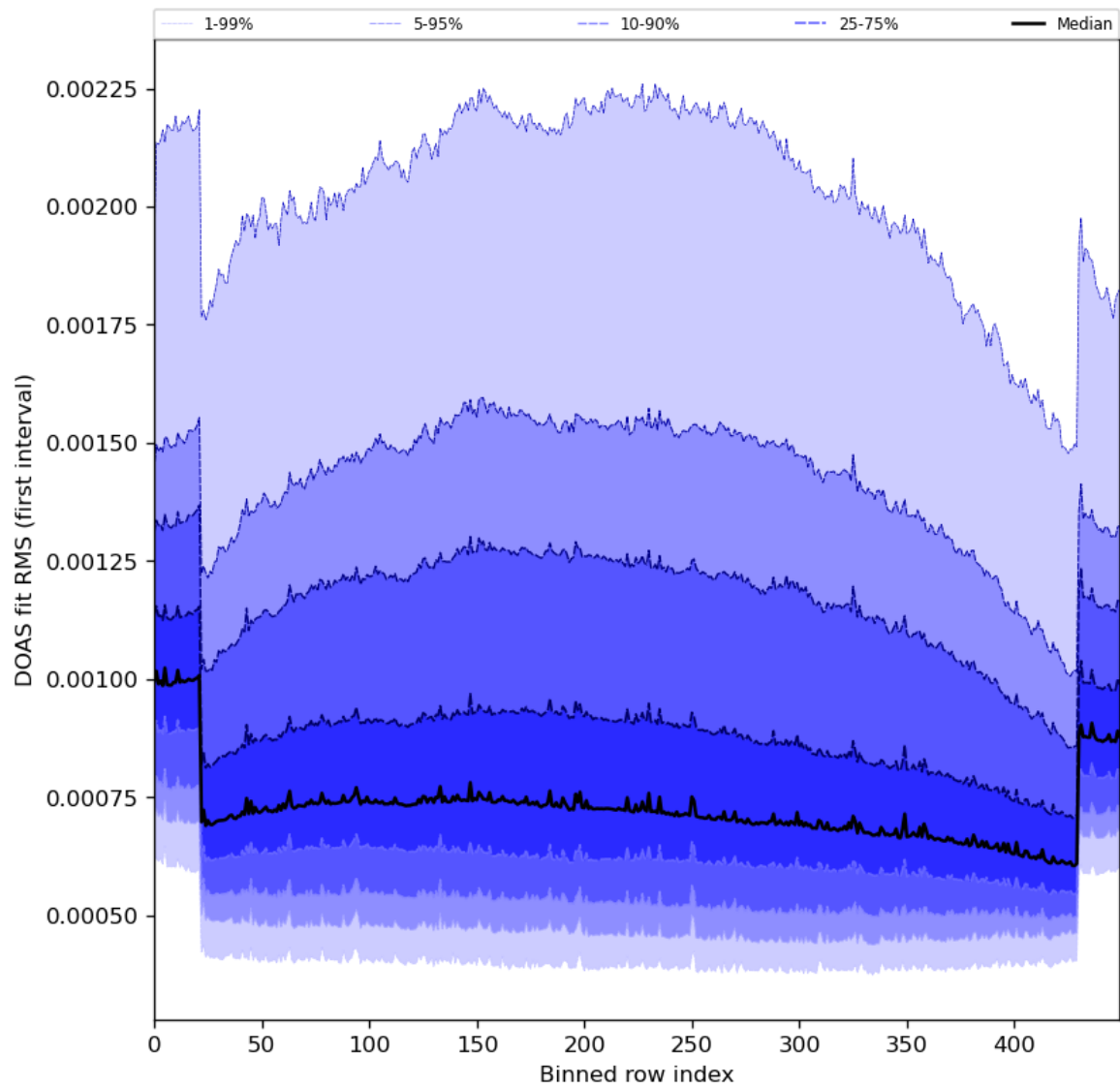
Figure 60: Along track statistics of “DOAS fit RMS (first interval)” for 2024-06-24 to 2024-06-25
