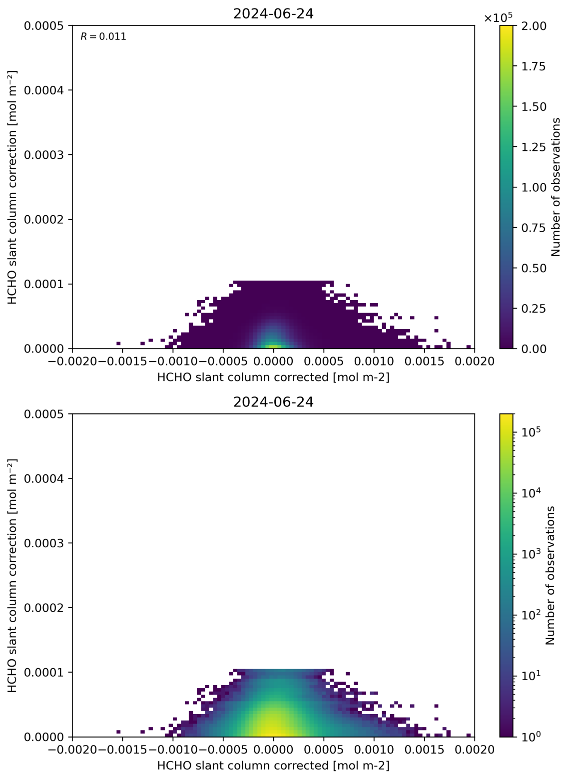
Figure 77: Scatter density plot of “HCHO slant column corrected” against “HCHO slant column correction” for 2024-06-24 to 2024-06-25.
