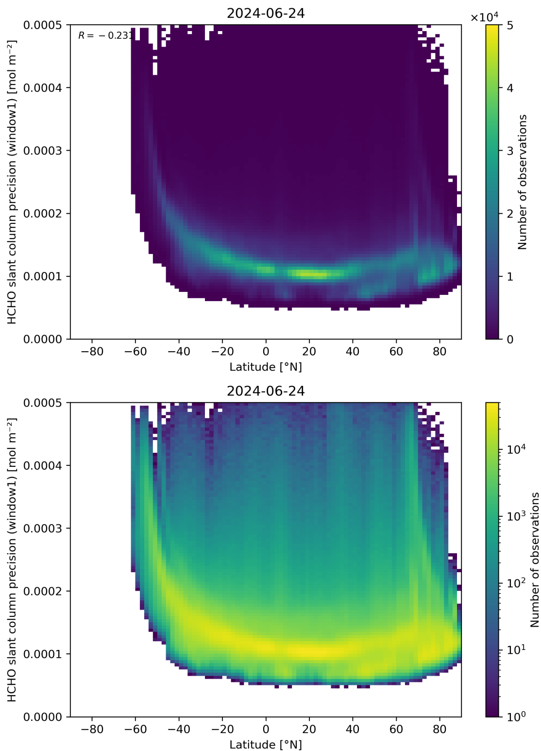
Figure 160: Scatter density plot of “Latitude” against “HCHO slant column precision (window1)” for 2024-06-24 to 2024-06-25.
