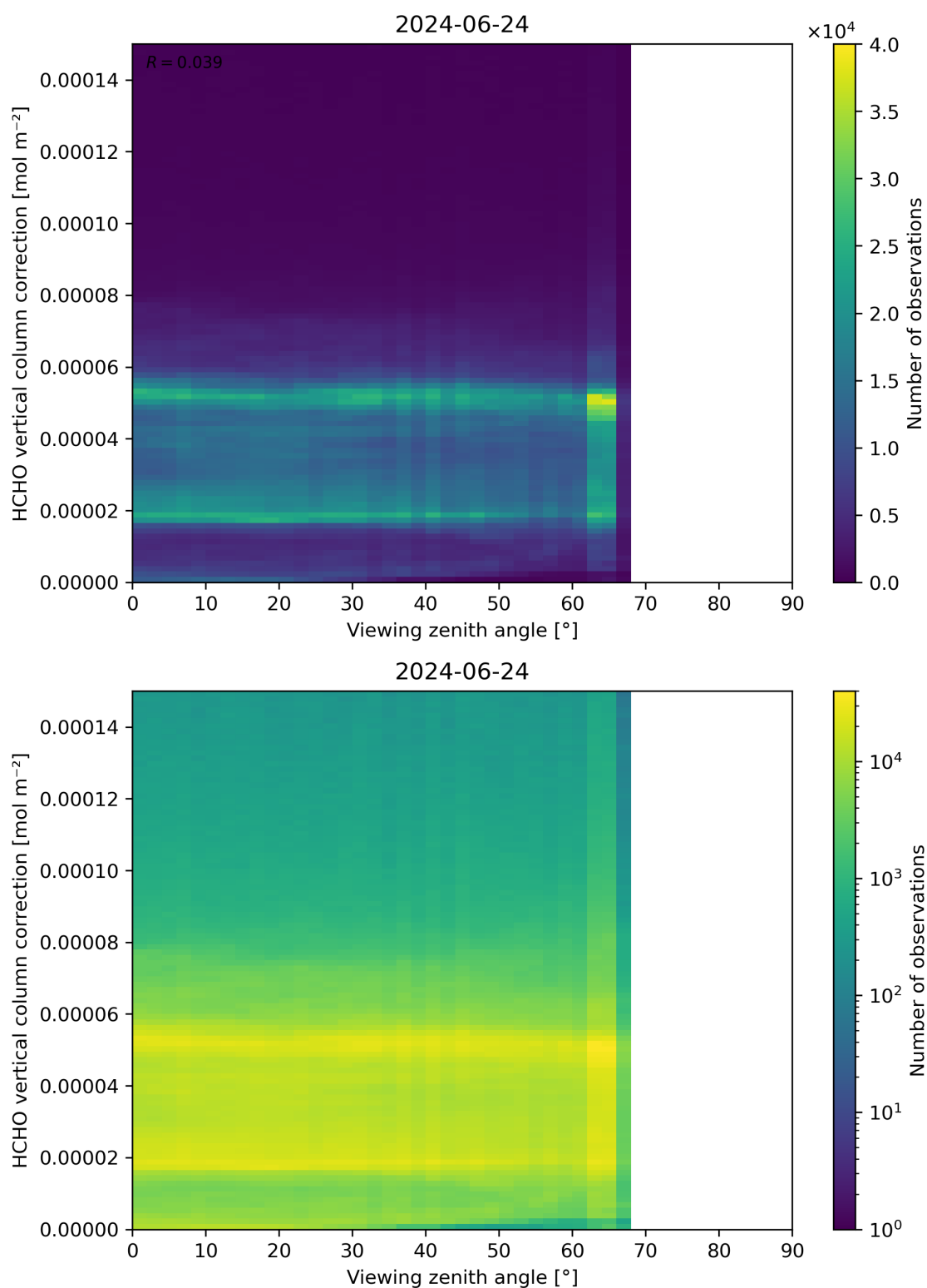
Figure 193: Scatter density plot of “Viewing zenith angle” against “HCHO vertical column correction” for 2024-06-24 to 2024-06-25.
