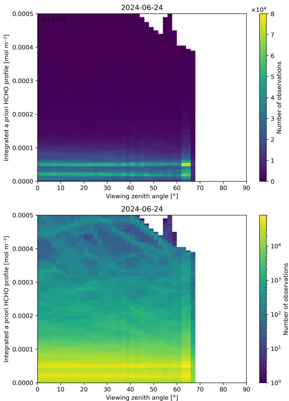
Figure 195: Scatter density plot of “Viewing zenith angle” against “Integrated a priori HCHO profile” for 2024-06-24 to 2024-06-25.
