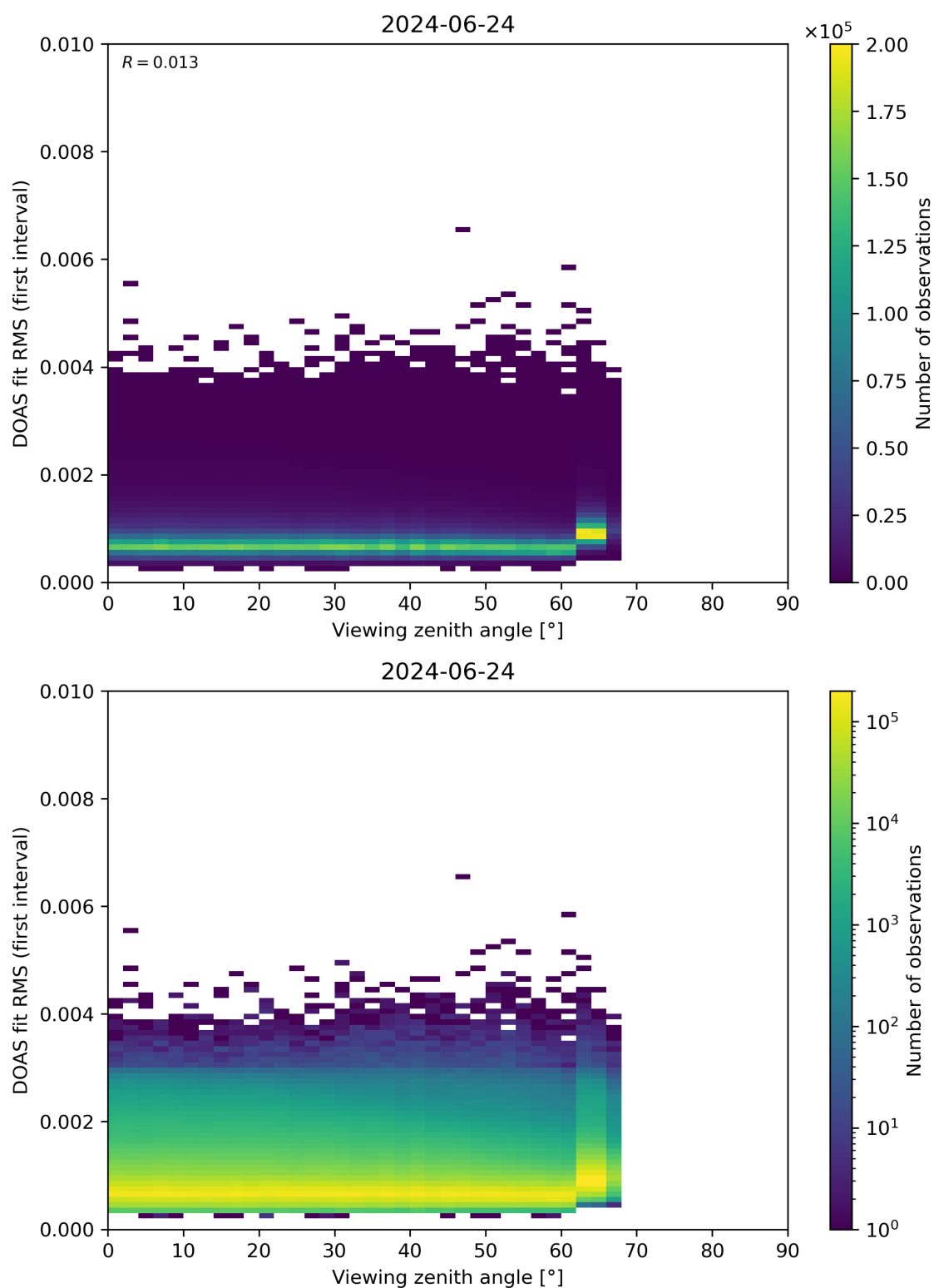
Figure 182: Scatter density plot of “Viewing zenith angle” against “DOAS fit RMS (first interval)” for 2024-06-24 to 2024-06-25.
