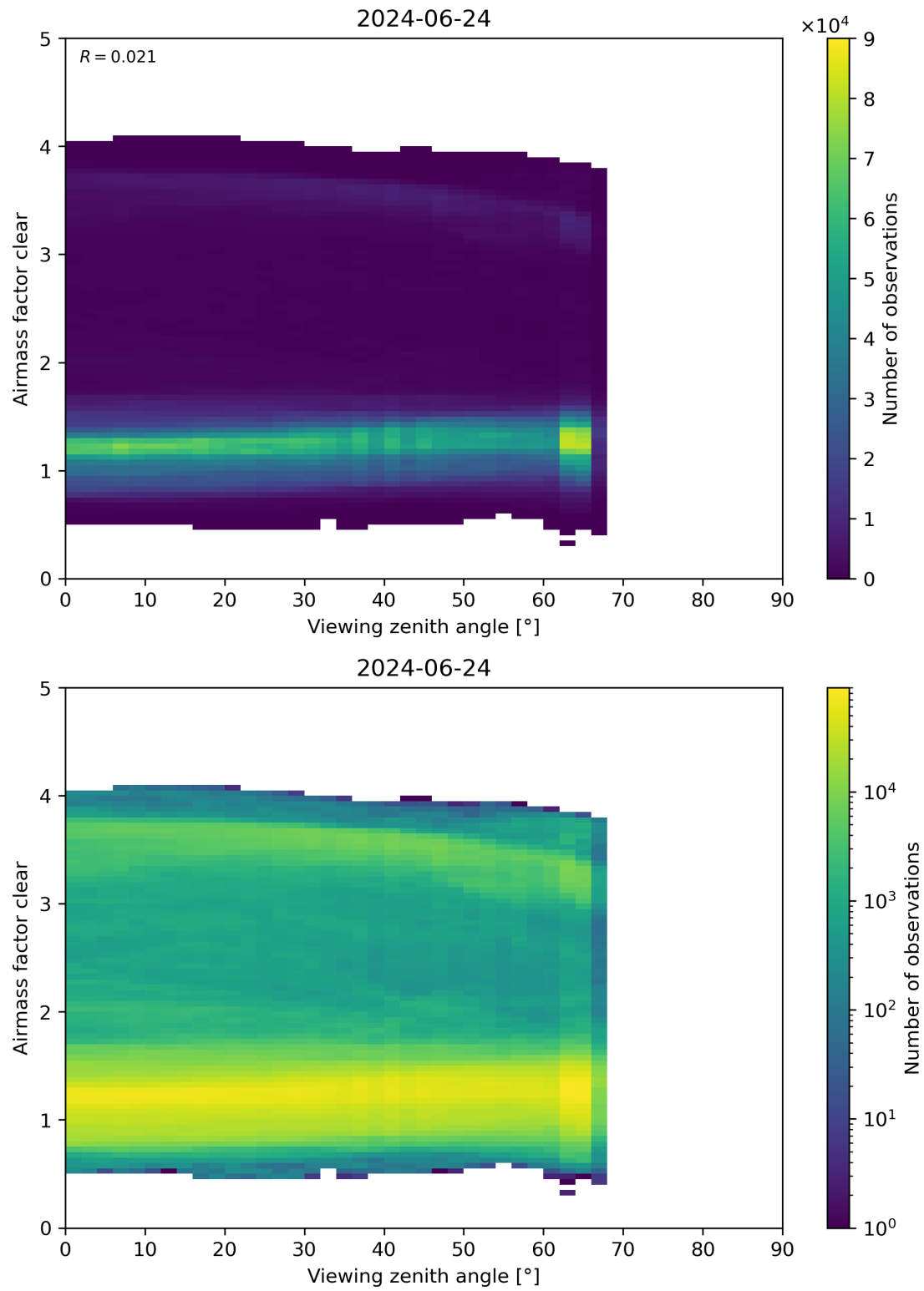
Figure 185: Scatter density plot of “Viewing zenith angle” against “Airmass factor clear” for 2024-06-24 to 2024-06-25.
