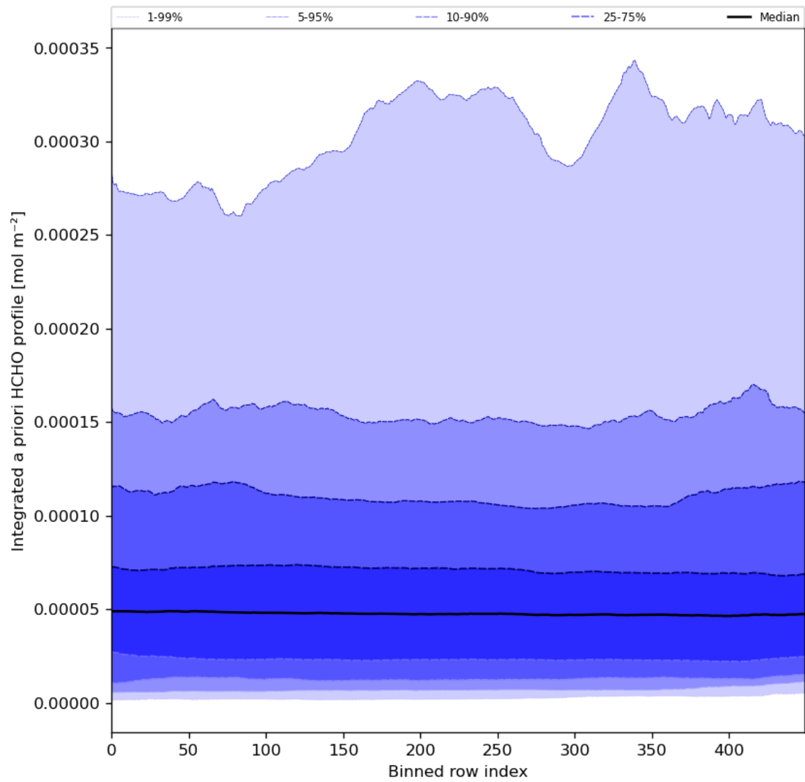
Figure 57: Along track statistics of "Integrated a priori HCHO profile" for 2024-06-24 to 2024-06-25
