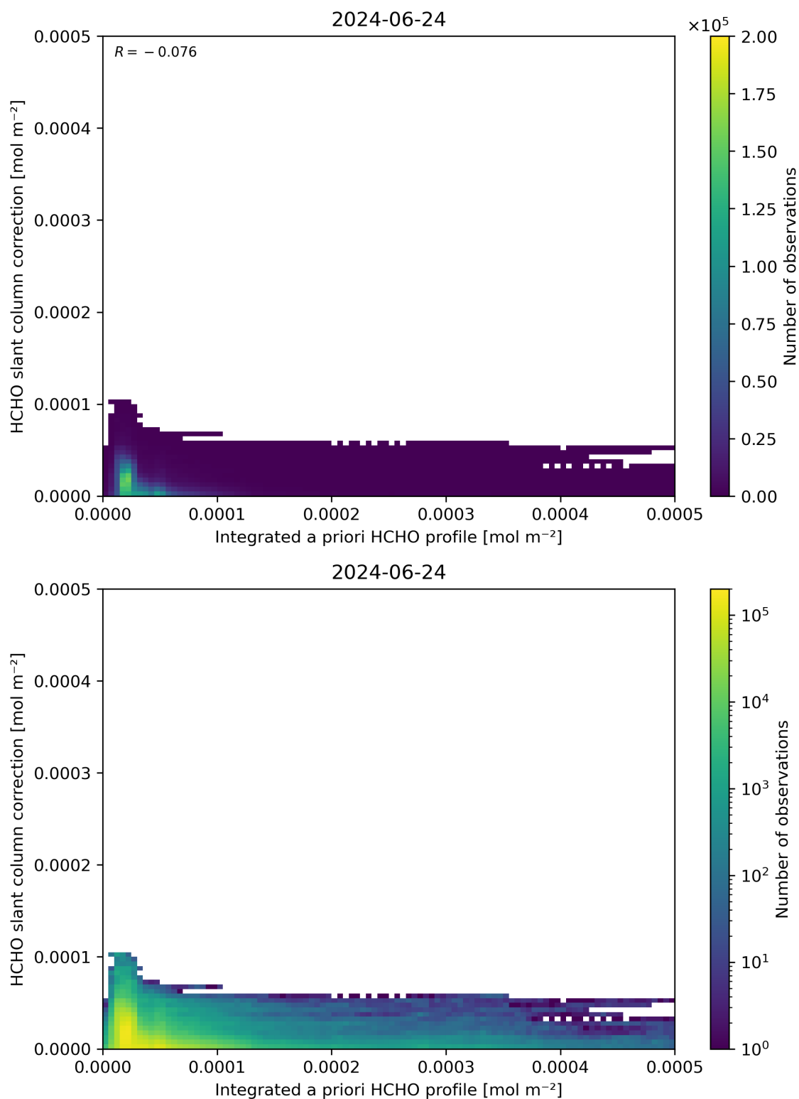
Figure 152: Scatter density plot of “Integrated a priori HCHO profile” against “HCHO slant column correction” for 2024-06-24 to 2024-06-25.
