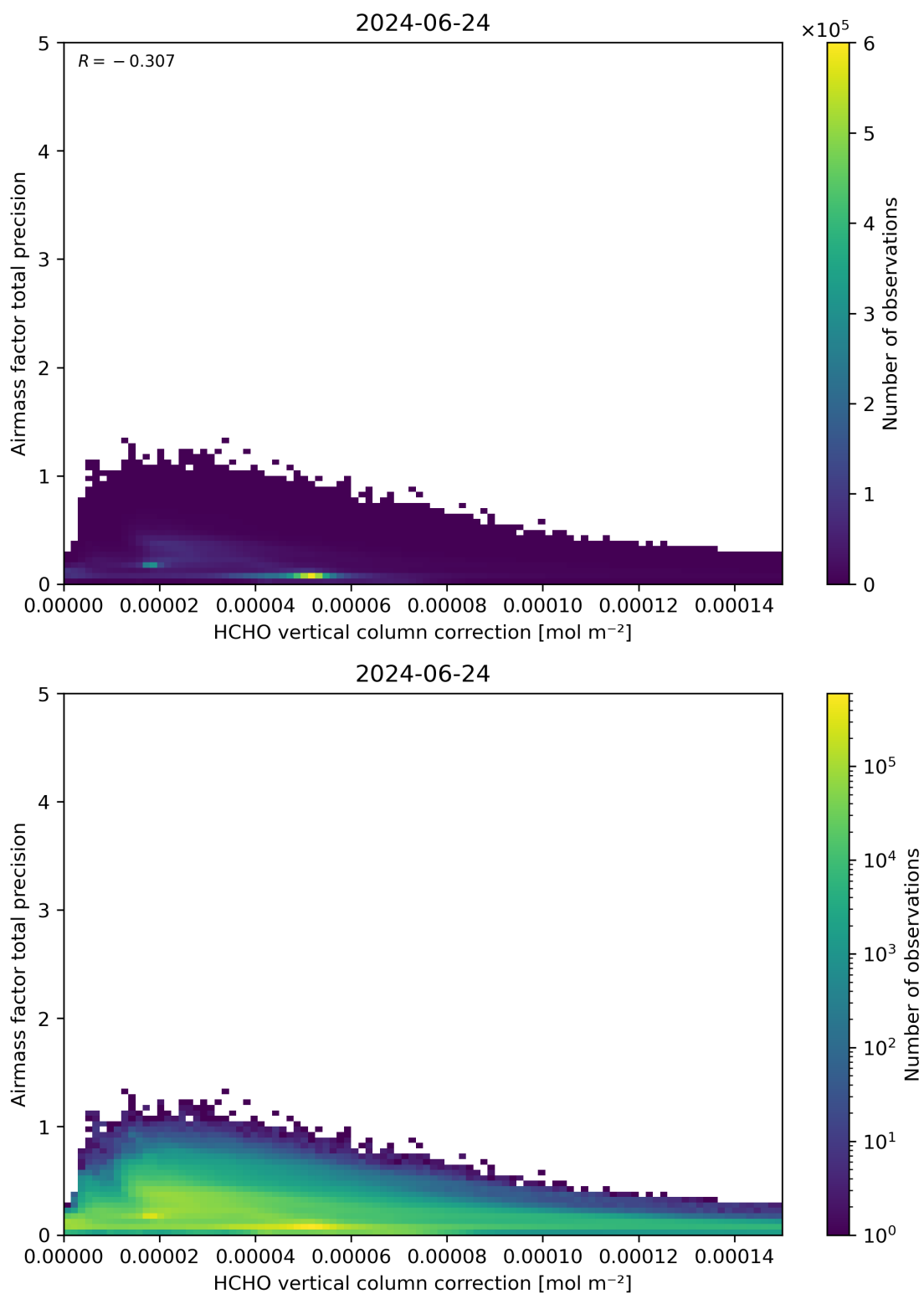
Figure 121: Scatter density plot of “HCHO vertical column correction” against “Airmass factor total precision” for 2024-06-24 to 2024-06-25.
