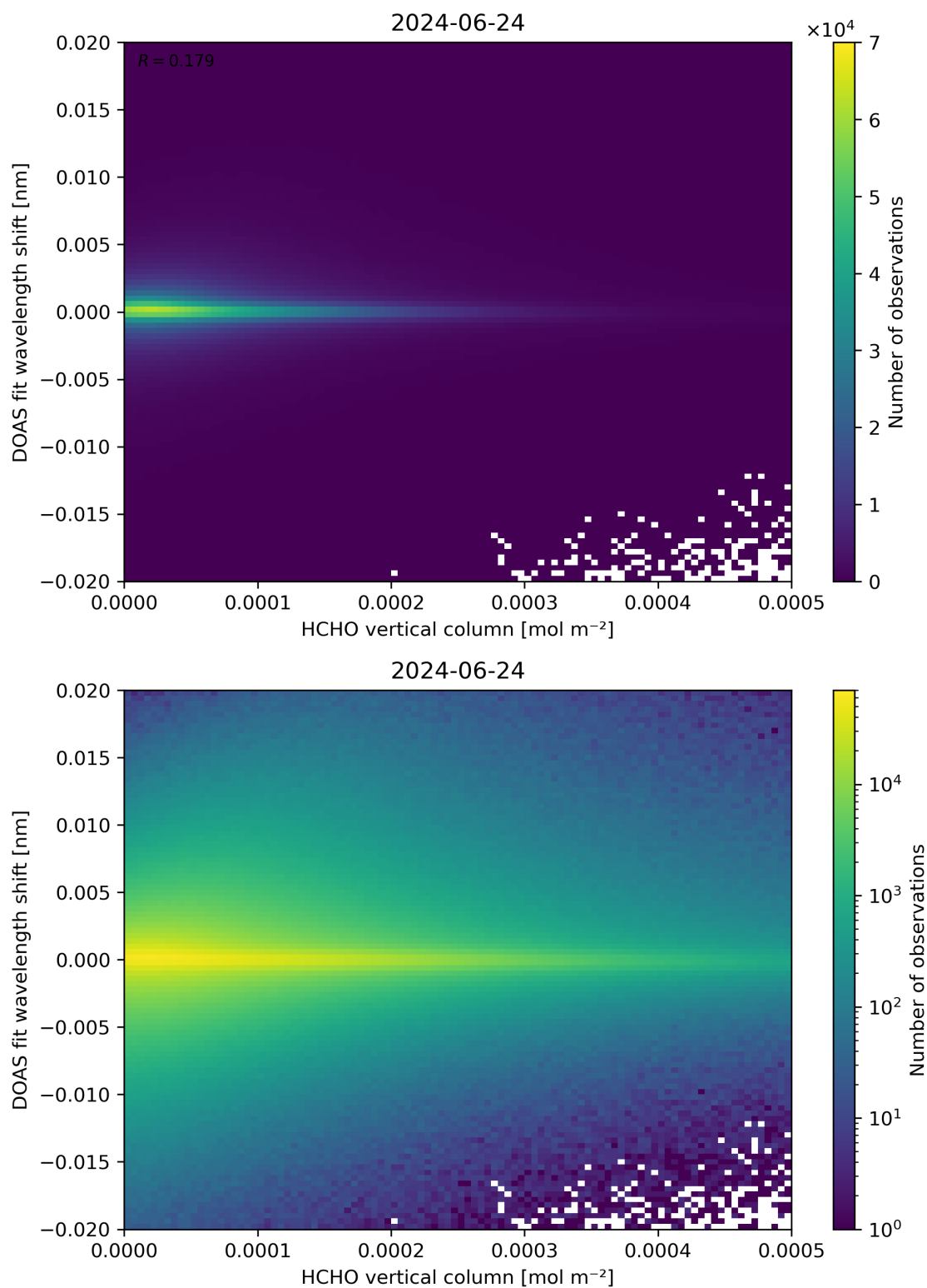
Figure 124: Scatter density plot of “HCHO vertical column” against “DOAS fit wavelength shift” for 2024-06-24 to 2024-06-25.
