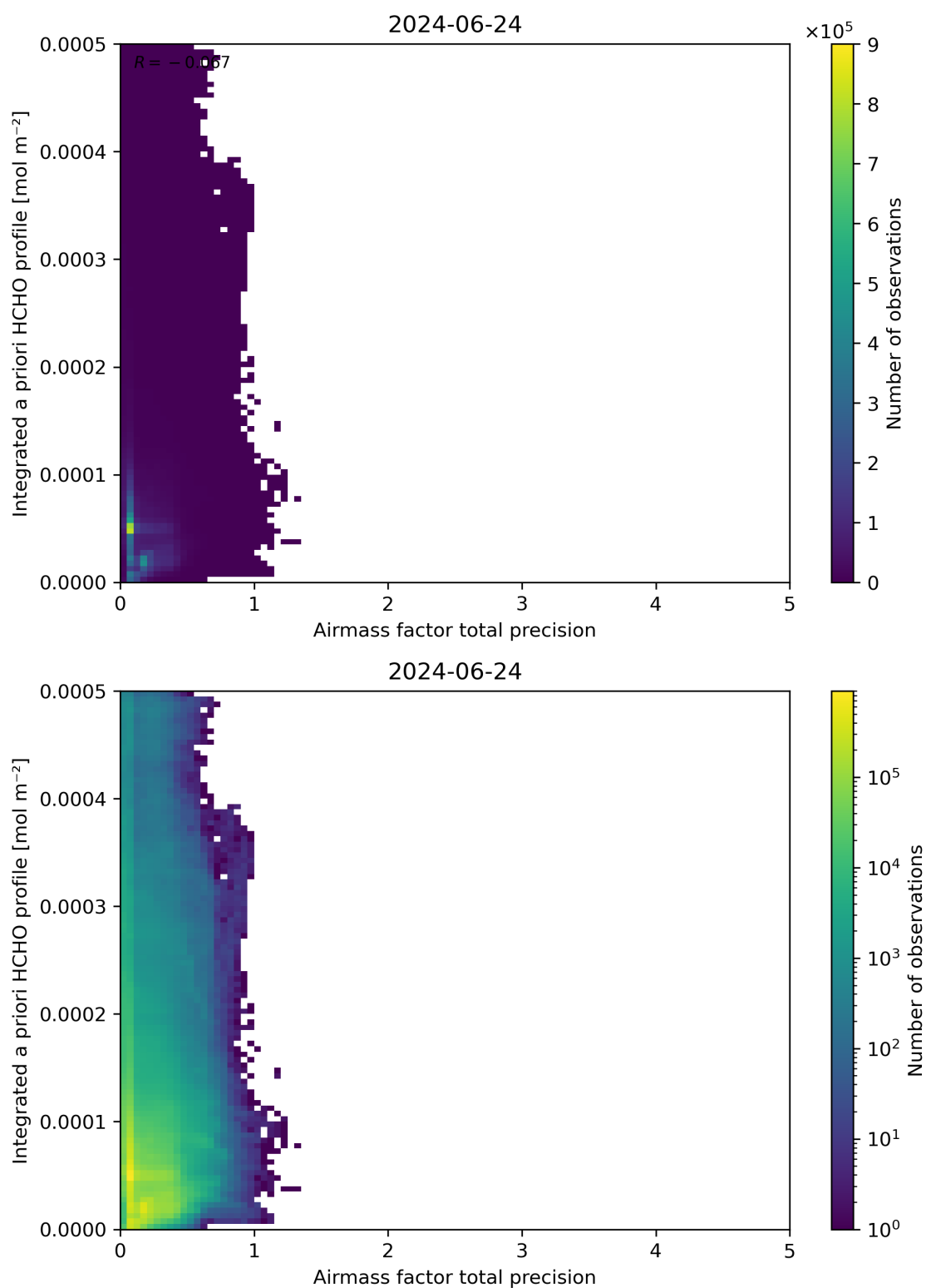
Figure 111: Scatter density plot of “Airmass factor total precision” against “Integrated a priori HCHO profile” for 2024-06-24 to 2024-06-25.
