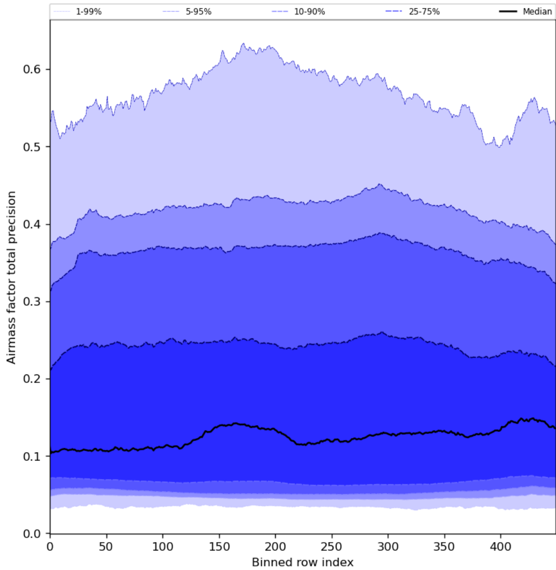
Figure 55: Along track statistics of “Airmass factor total precision” for 2024-06-24 to 2024-06-25
