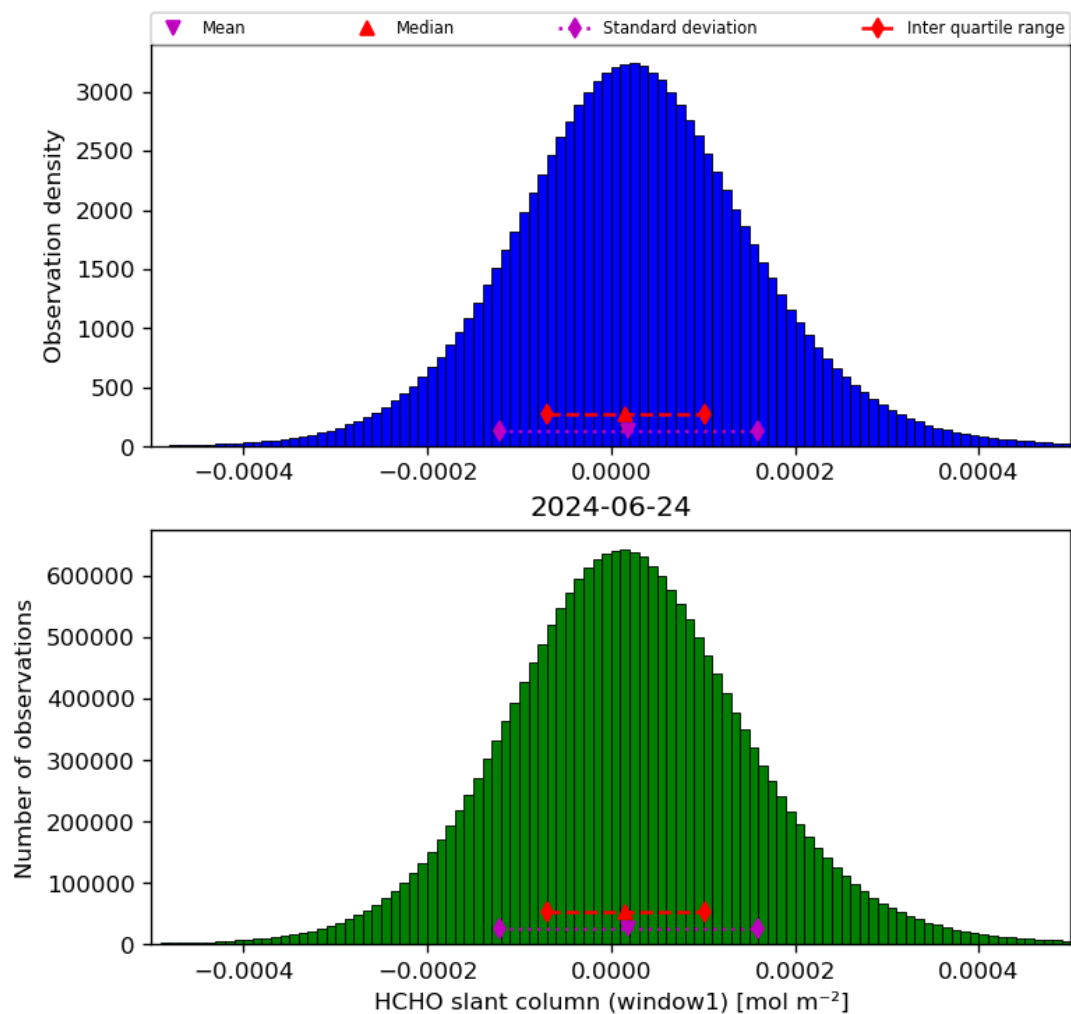
Figure 38: Histogram of “HCHO slant column (window1)” for 2024-06-24 to 2024-06-25
