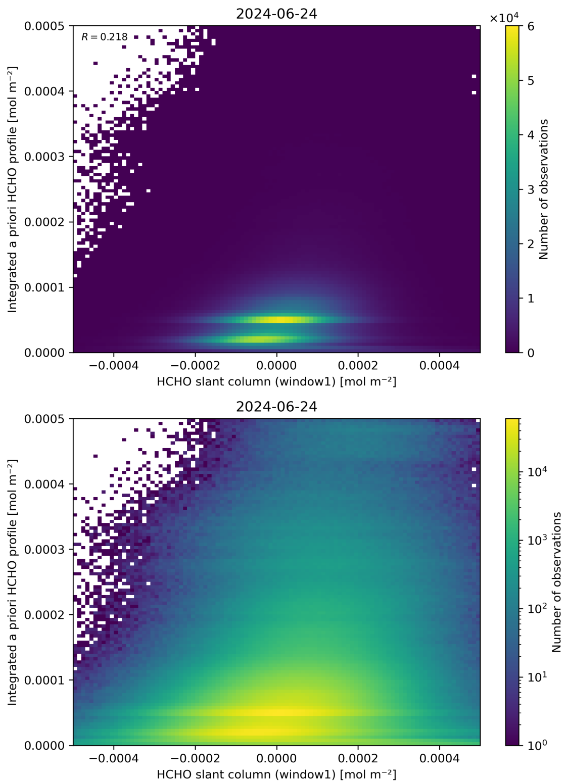
Figure 87: Scatter density plot of “HCHO slant column (window1)” against “Integrated a priori HCHO profile” for 2024-06-24 to 2024-06-25.
