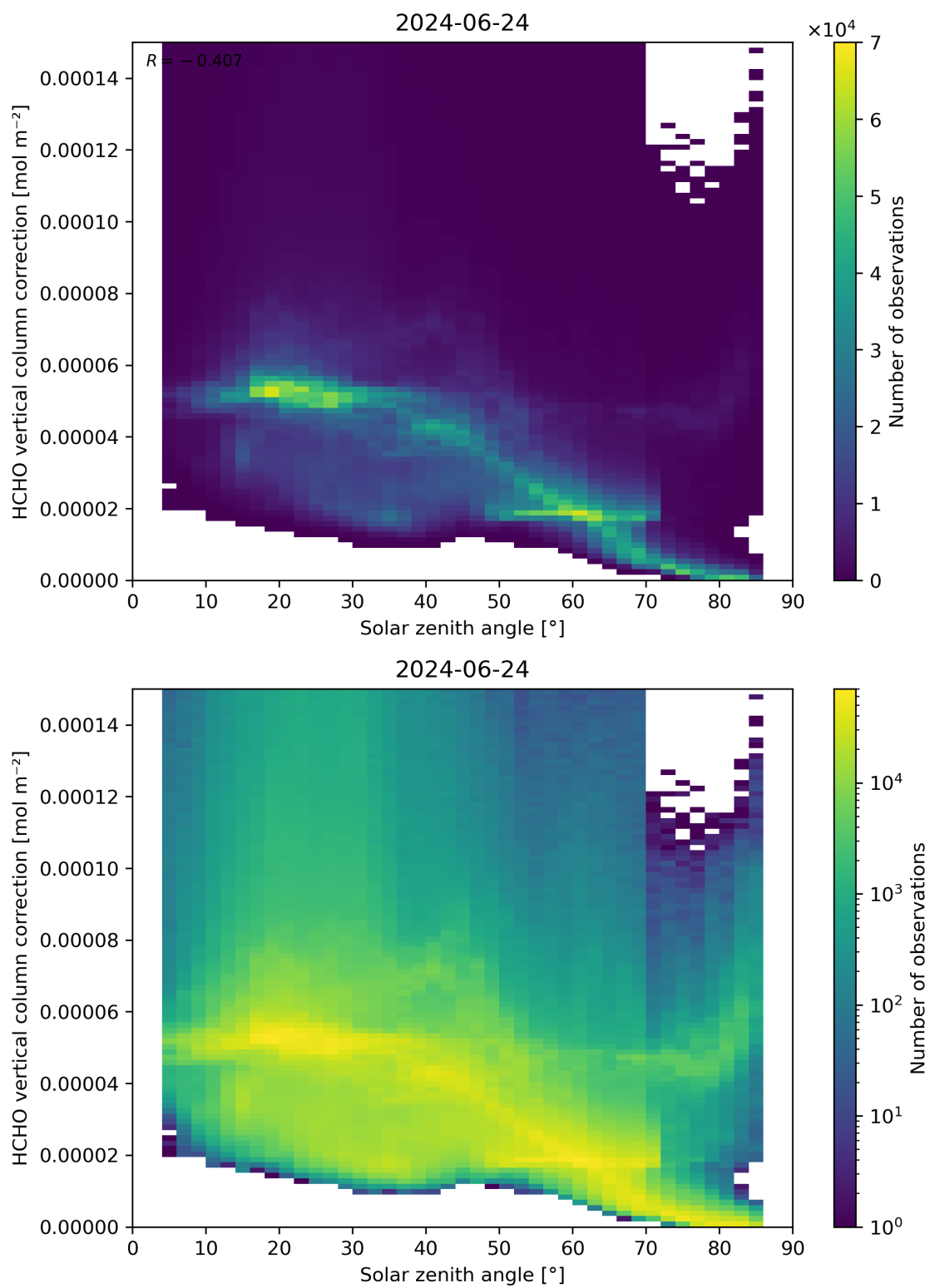
Figure 178: Scatter density plot of “Solar zenith angle” against “HCHO vertical column correction” for 2024-06-24 to 2024-06-25.
