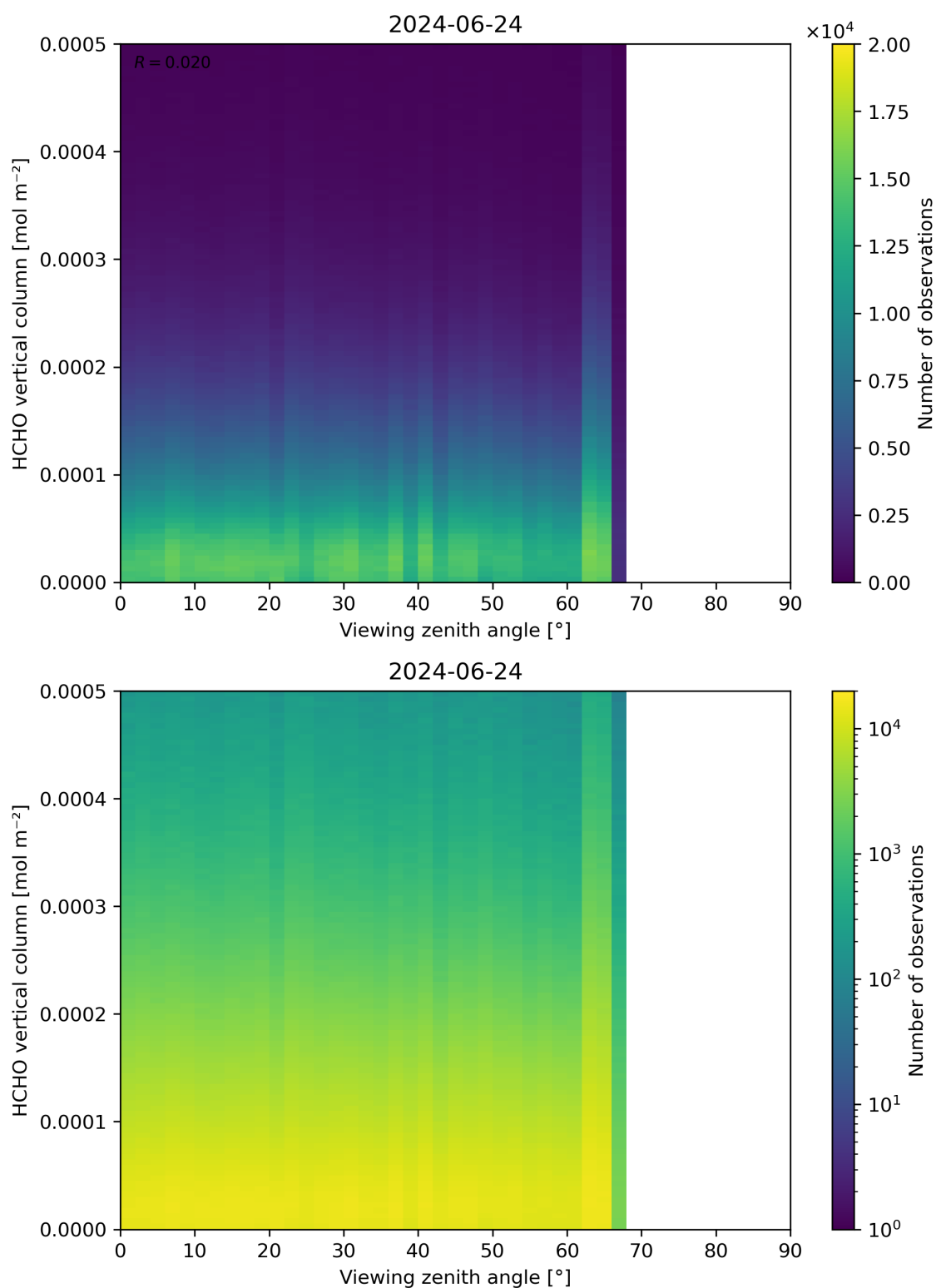
Figure 192: Scatter density plot of “Viewing zenith angle” against “HCHO vertical column” for 2024-06-24 to 2024-06-25.
