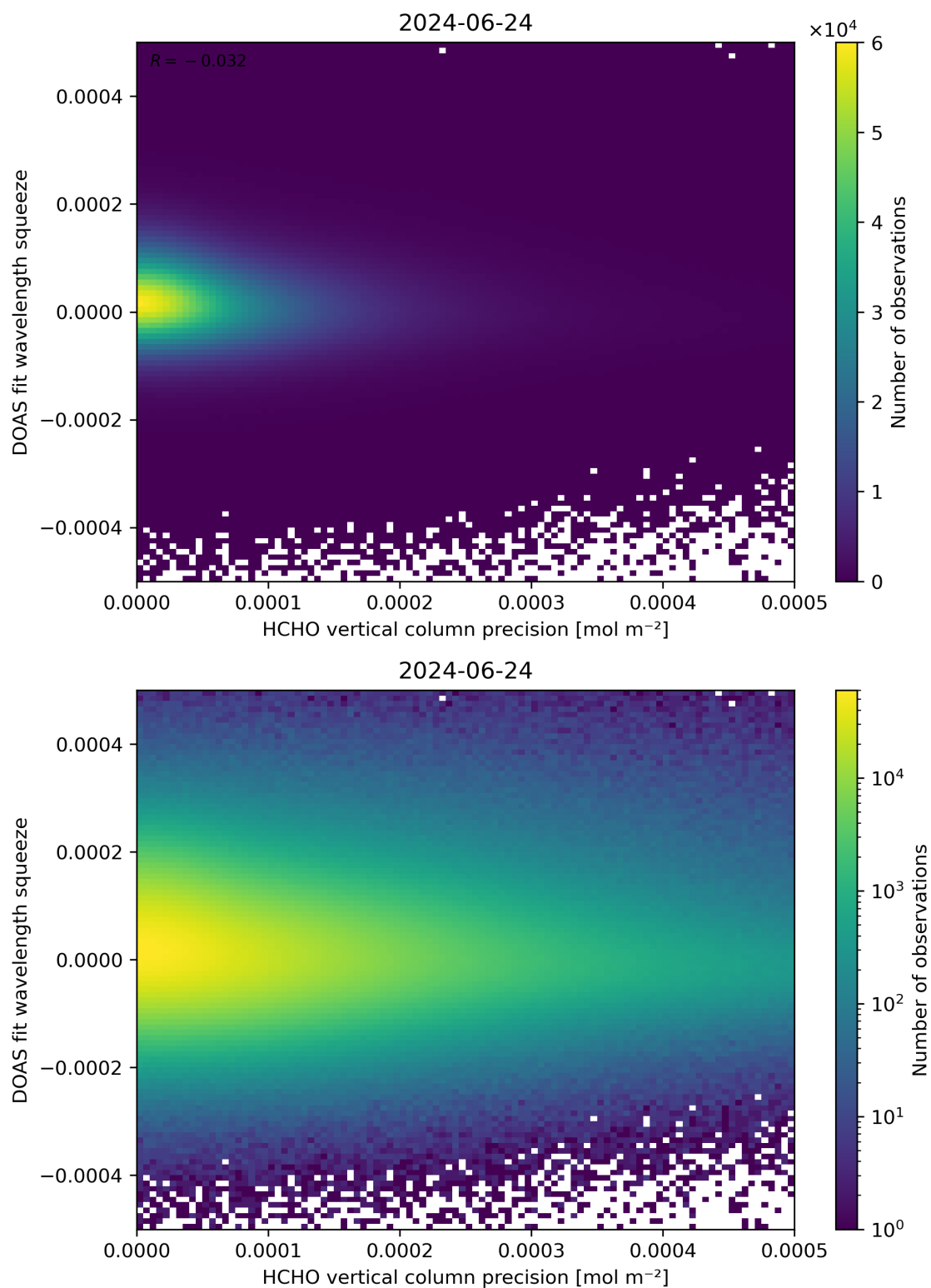
Figure 138: Scatter density plot of “HCHO vertical column precision” against “DOAS fit wavelength squeeze” for 2024-06-24 to 2024-06-25.
