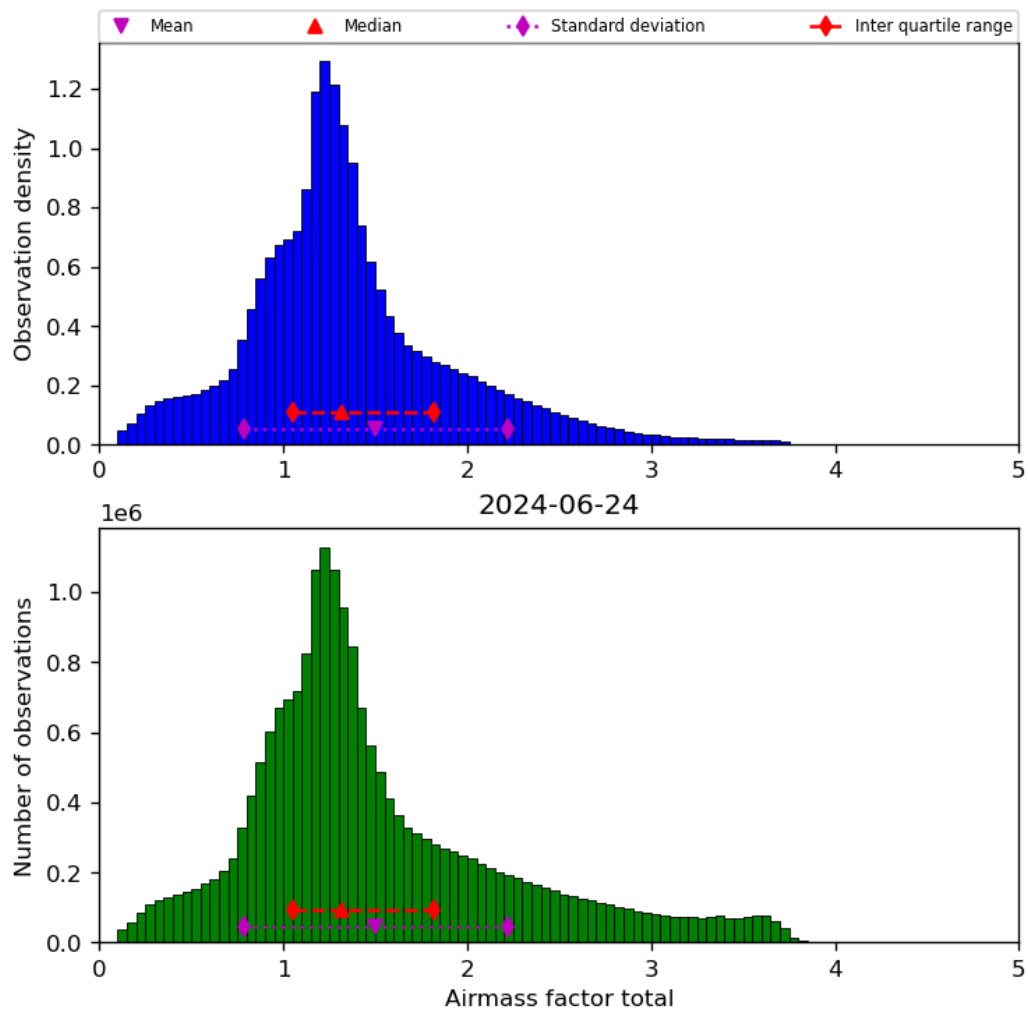
Figure 40: Histogram of “Airmass factor total” for 2024-06-24 to 2024-06-25
