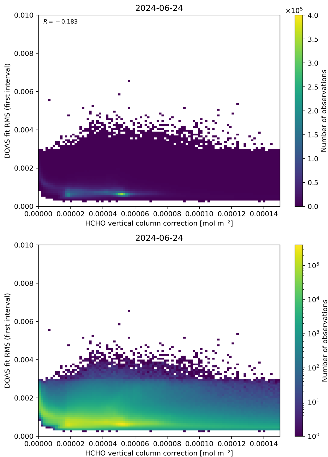
Figure 112: Scatter density plot of “HCHO vertical column correction” against “DOAS fit RMS (first interval)” for 2024-06-24 to 2024-06-25.
