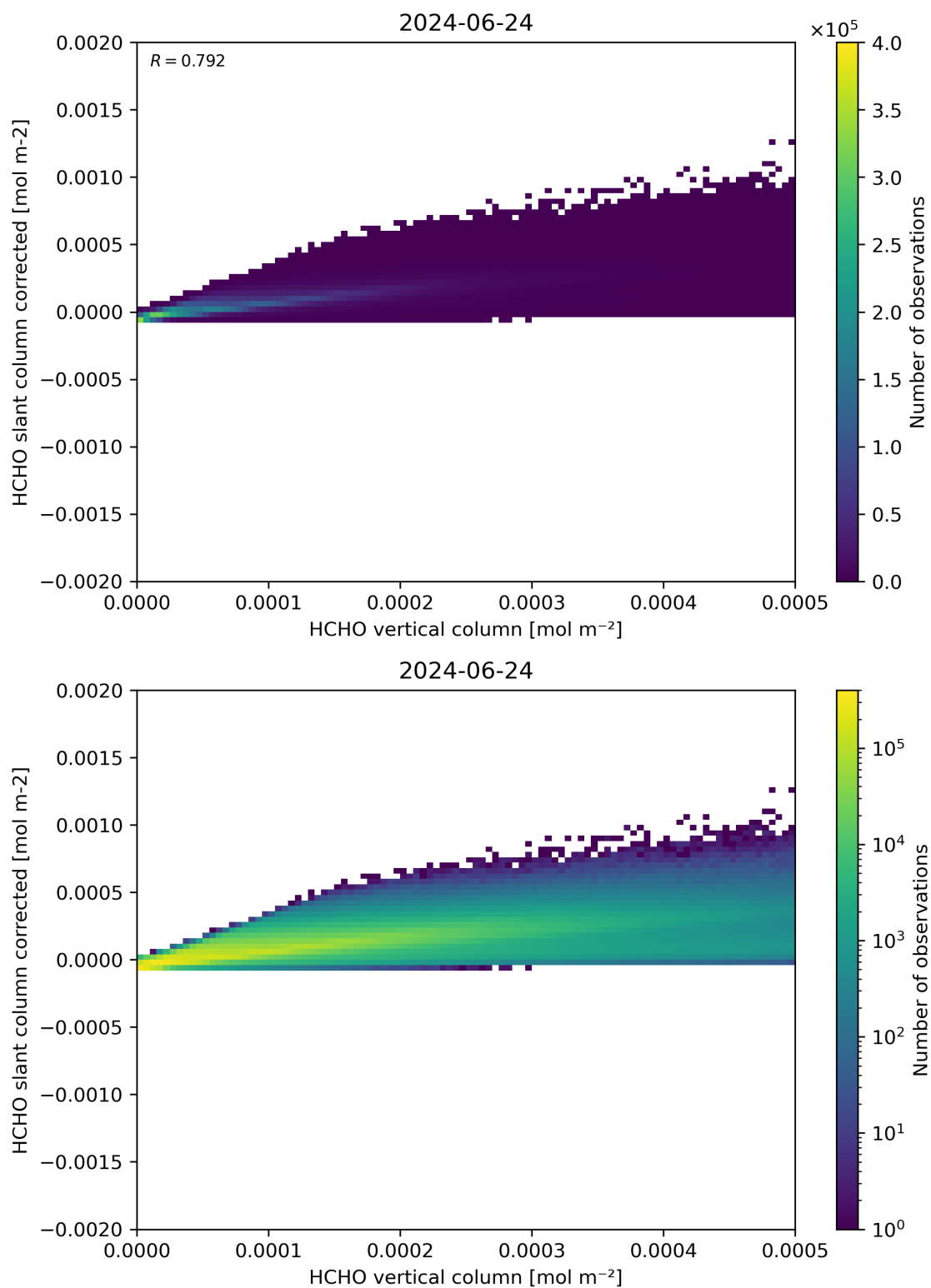
Figure 127: Scatter density plot of “HCHO vertical column” against “HCHO slant column corrected” for 2024-06-24 to 2024-06-25.
