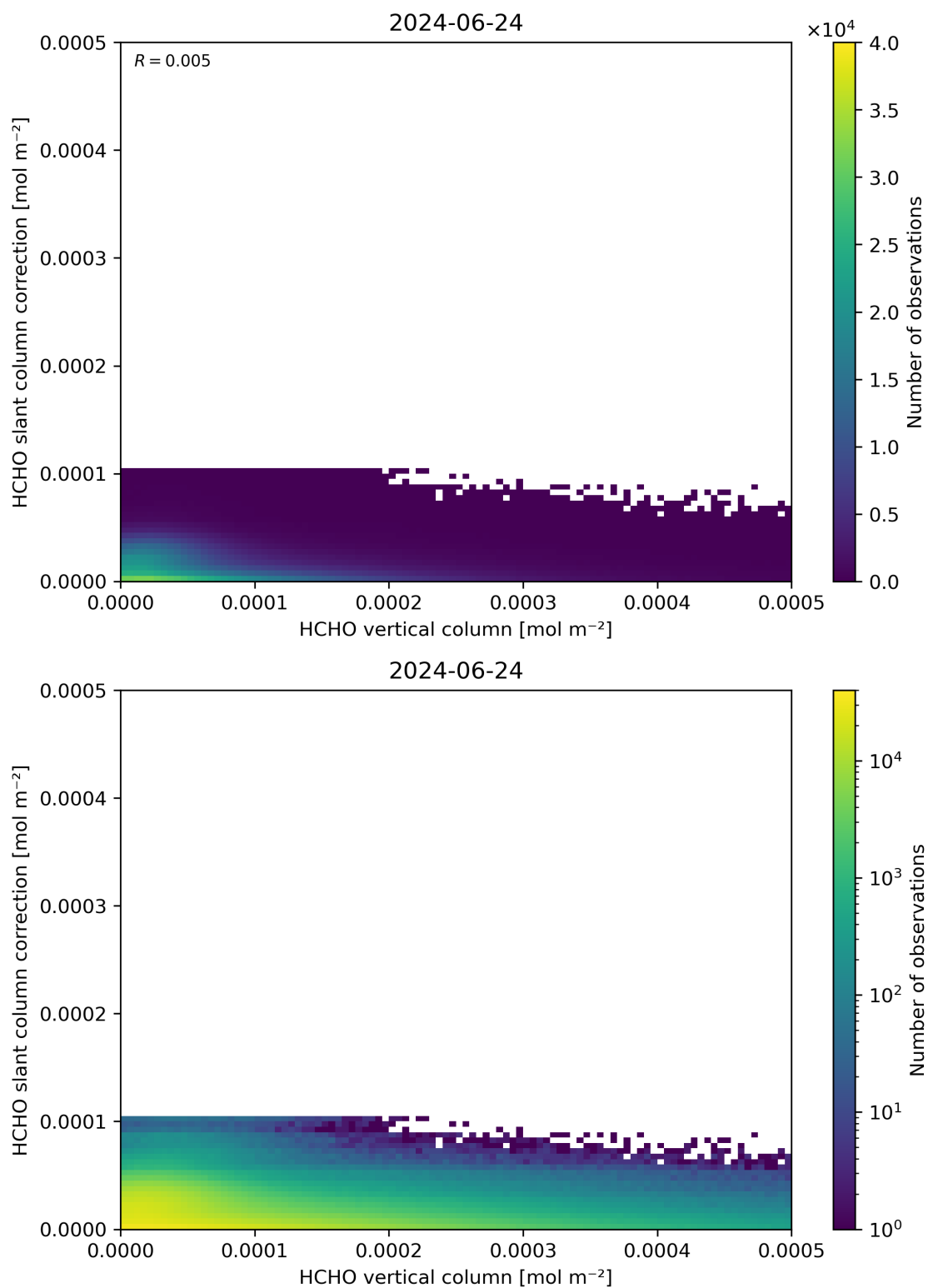
Figure 128: Scatter density plot of “HCHO vertical column” against “HCHO slant column correction” for 2024-06-24 to 2024-06-25.
