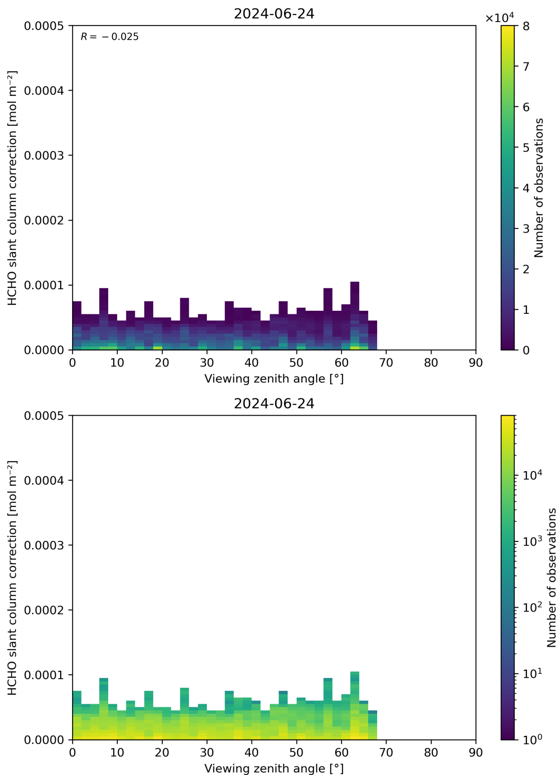
Figure 187: Scatter density plot of “Viewing zenith angle” against “HCHO slant column correction” for 2024-06-24 to 2024-06-25.
