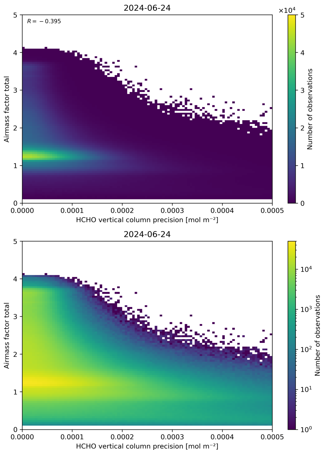
Figure 144: Scatter density plot of “HCHO vertical column precision” against “Airmass factor total” for 2024-06-24 to 2024-06-25.
