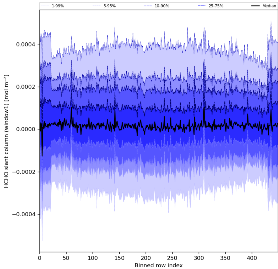
Figure 52: Along track statistics of “HCHO slant column (window1)” for 2024-06-24 to 2024-06-25
