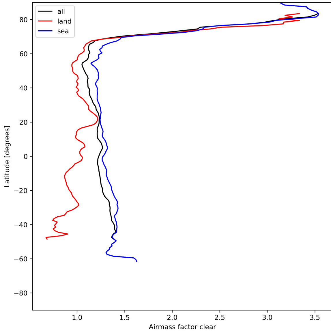
Figure 28: Zonal average of “Airmass factor clear” for 2024-06-24 to 2024-06-25.
