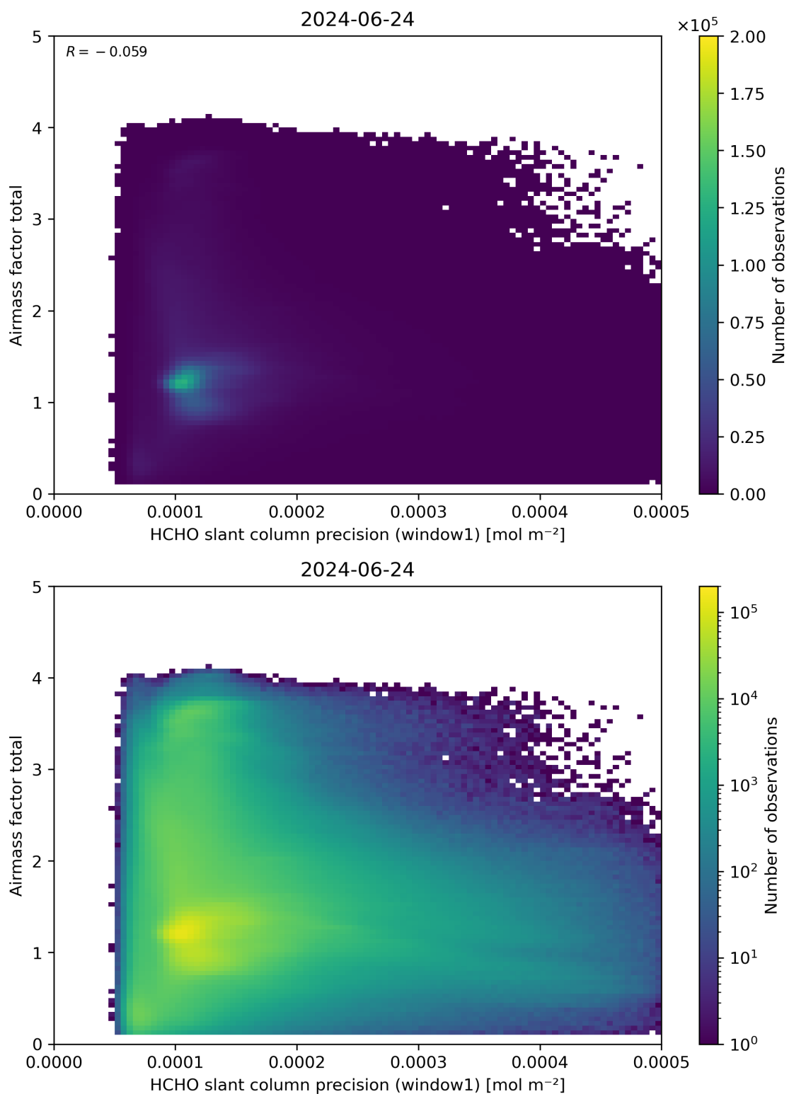
Figure 94: Scatter density plot of “HCHO slant column precision (window1)” against “Airmass factor total” for 2024-06-24 to 2024-06-25.
