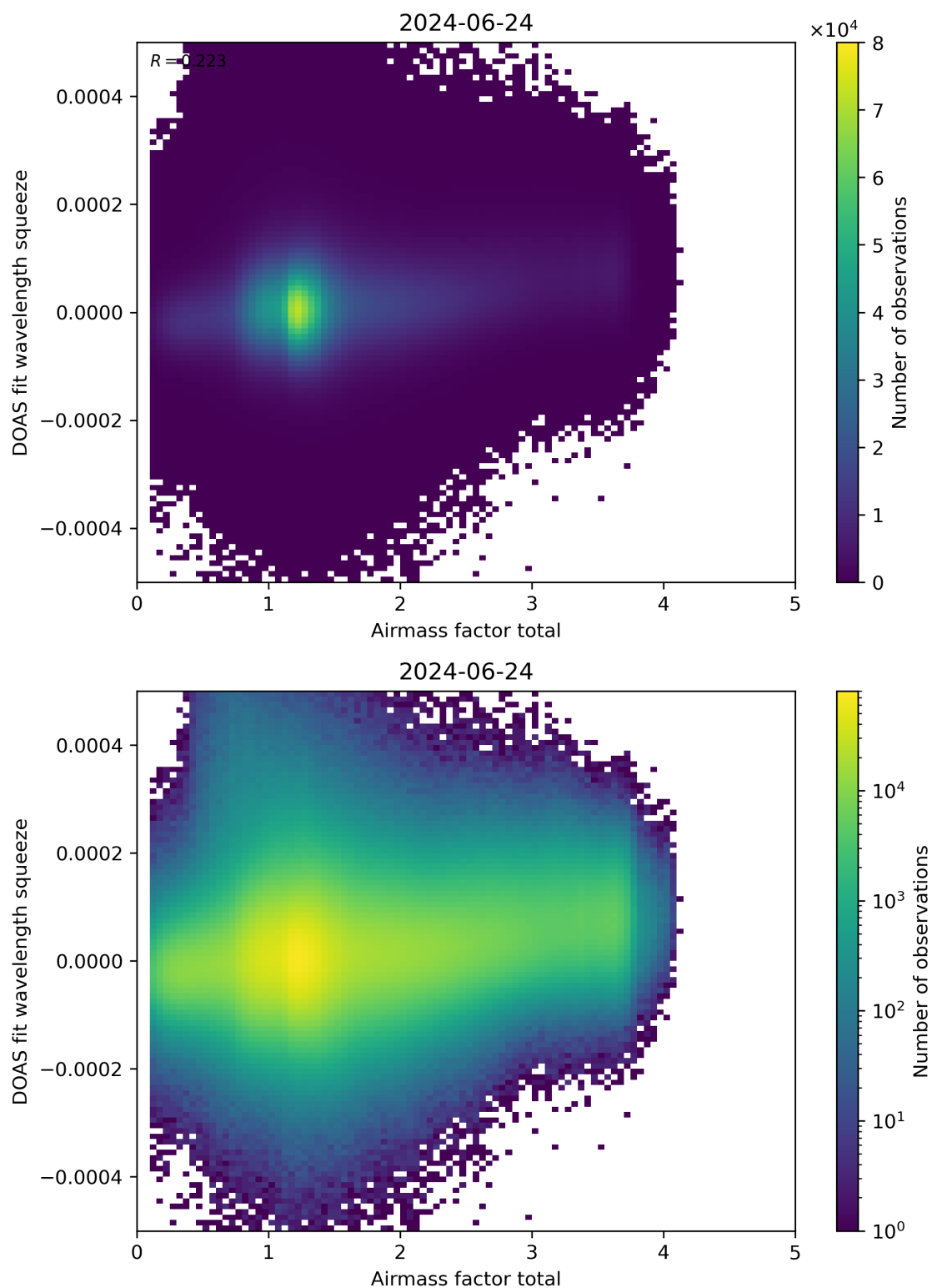
Figure 99: Scatter density plot of “Airmass factor total” against “DOAS fit wavelength squeeze” for 2024-06-24 to 2024-06-25.
