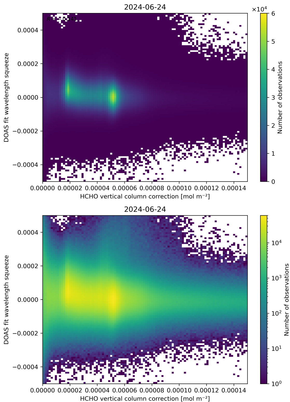
Figure 114: Scatter density plot of “HCHO vertical column correction” against “DOAS fit wavelength squeeze” for 2024-06-24 to 2024-06-25.
