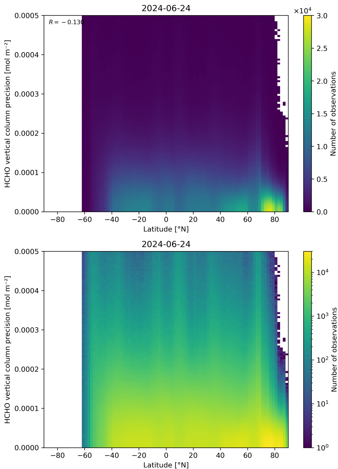
Figure 165: Scatter density plot of “Latitude” against “HCHO vertical column precision” for 2024-06-24 to 2024-06-25.
