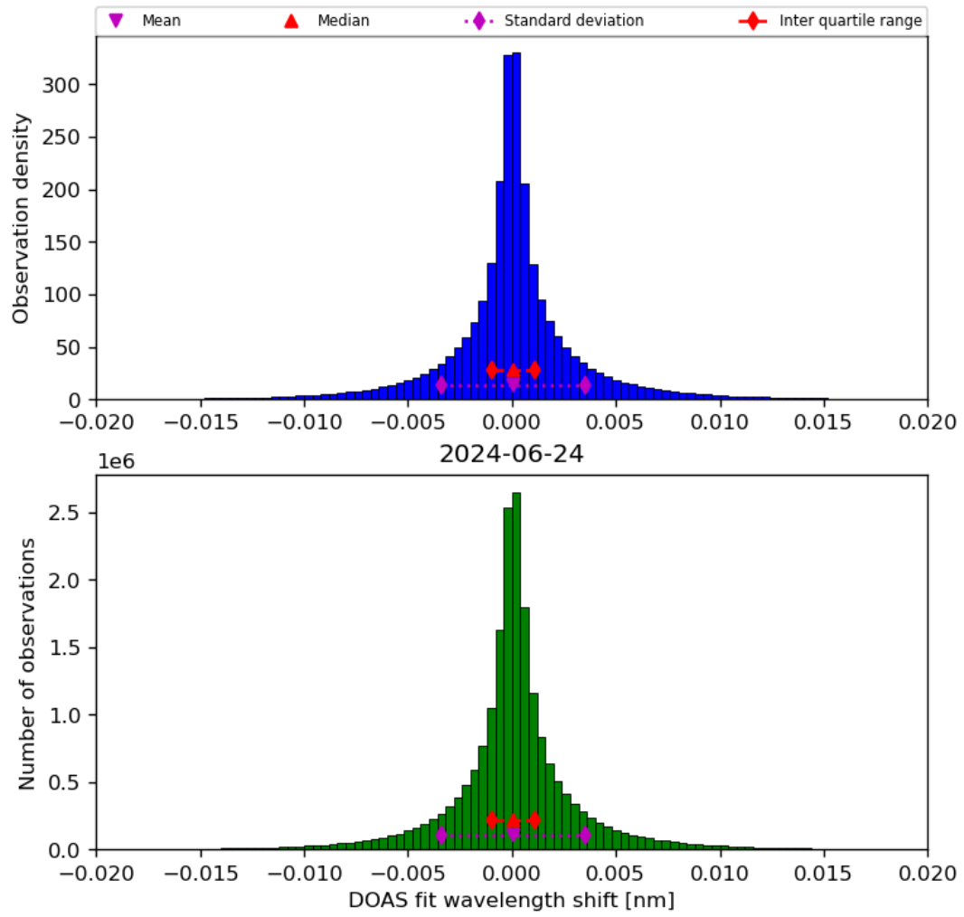
Figure 44: Histogram of “DOAS fit wavelength shift” for 2024-06-24 to 2024-06-25
