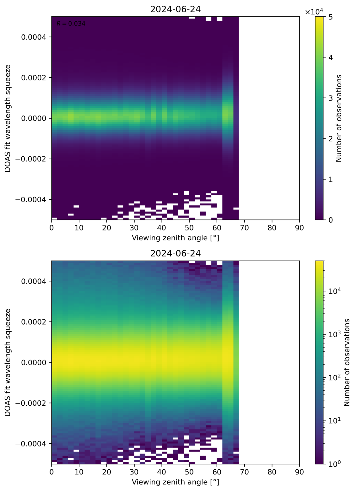
Figure 184: Scatter density plot of “Viewing zenith angle” against “DOAS fit wavelength squeeze” for 2024-06-24 to 2024-06-25.
