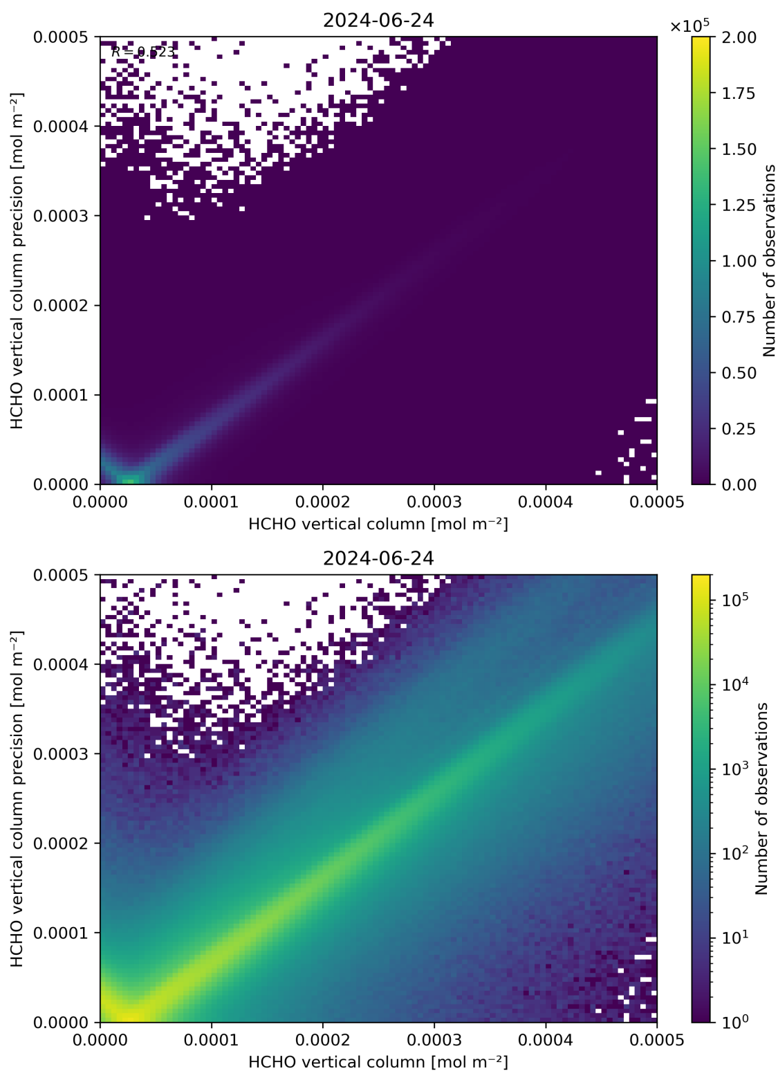
Figure 134: Scatter density plot of “HCHO vertical column” against “HCHO vertical column precision” for 2024-06-24 to 2024-06-25.
