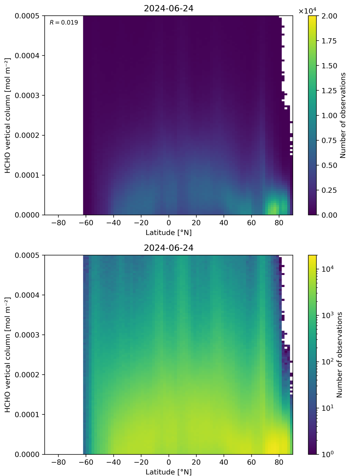
Figure 163: Scatter density plot of “Latitude” against “HCHO vertical column” for 2024-06-24 to 2024-06-25.
