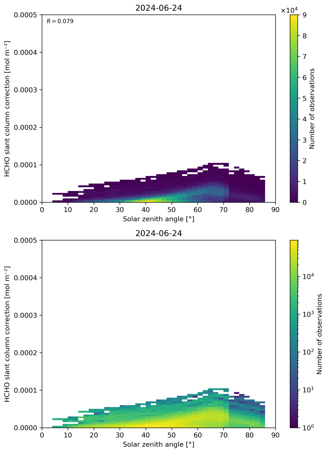
Figure 172: Scatter density plot of “Solar zenith angle” against “HCHO slant column correction” for 2024-06-24 to 2024-06-25.
