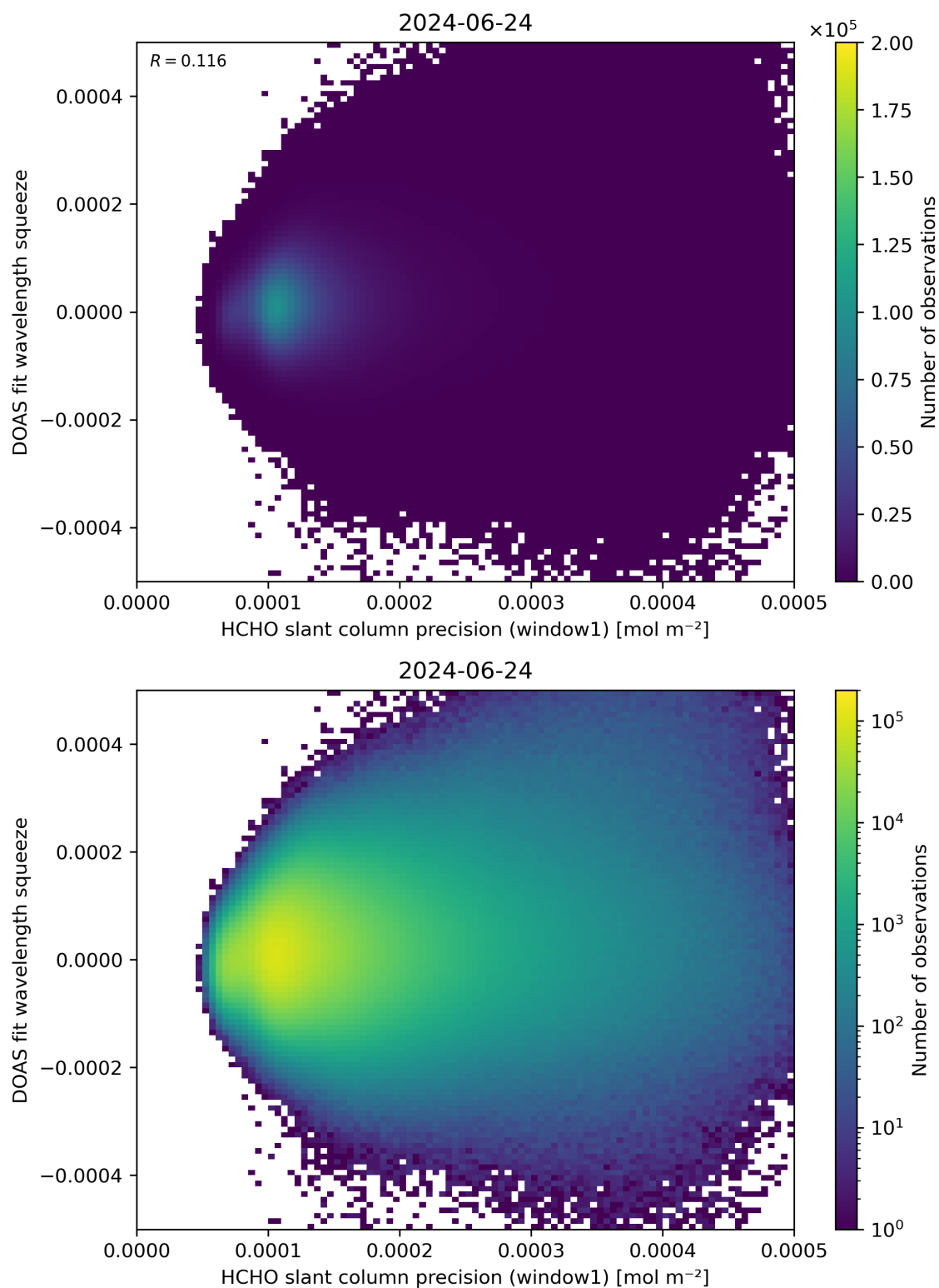
Figure 90: Scatter density plot of “HCHO slant column precision (window1)” against “DOAS fit wavelength squeeze” for 2024-06-24 to 2024-06-25.
