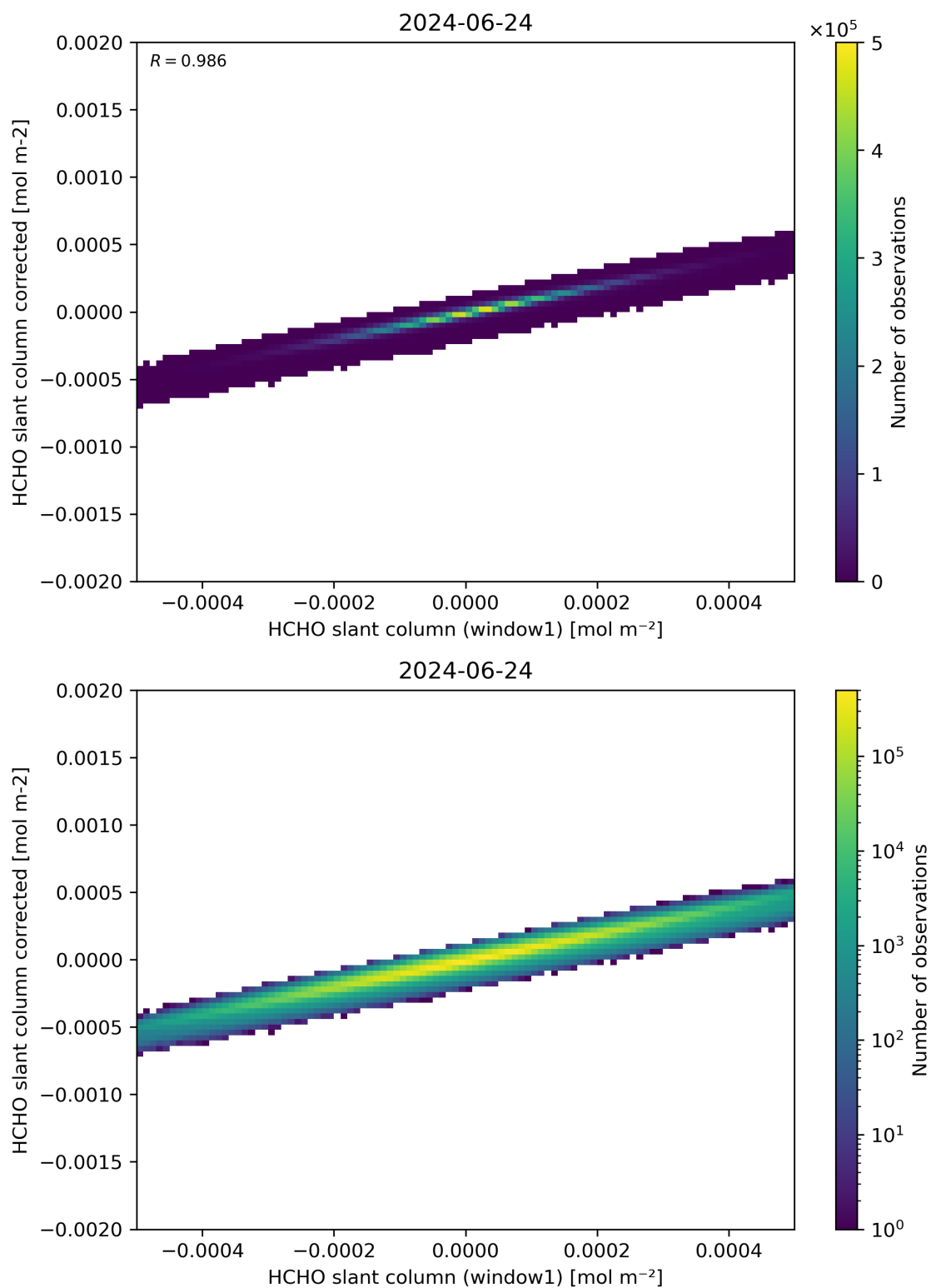
Figure 82: Scatter density plot of “HCHO slant column (window1)” against “HCHO slant column corrected” for 2024-06-24 to 2024-06-25.
