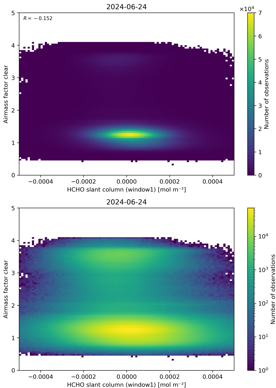
Figure 81: Scatter density plot of “HCHO slant column (window1)” against “Airmass factor clear” for 2024-06-24 to 2024-06-25.
