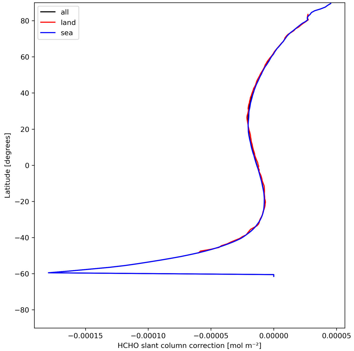
Figure 33: Zonal average of “HCHO slant column correction” for 2024-06-24 to 2024-06-25.
