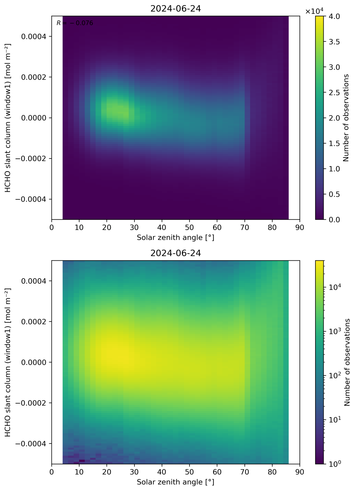
Figure 173: Scatter density plot of “Solar zenith angle” against “HCHO slant column (window1)” for 2024-06-24 to 2024-06-25.
