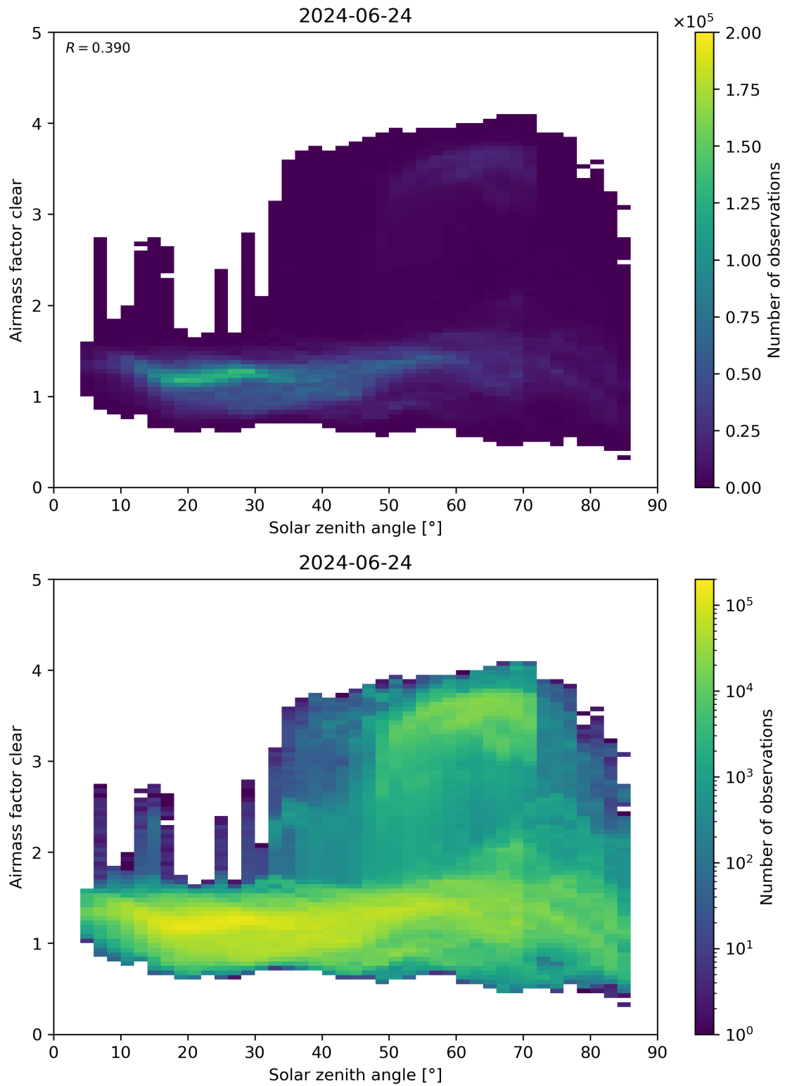
Figure 170: Scatter density plot of “Solar zenith angle” against “Airmass factor clear” for 2024-06-24 to 2024-06-25.
