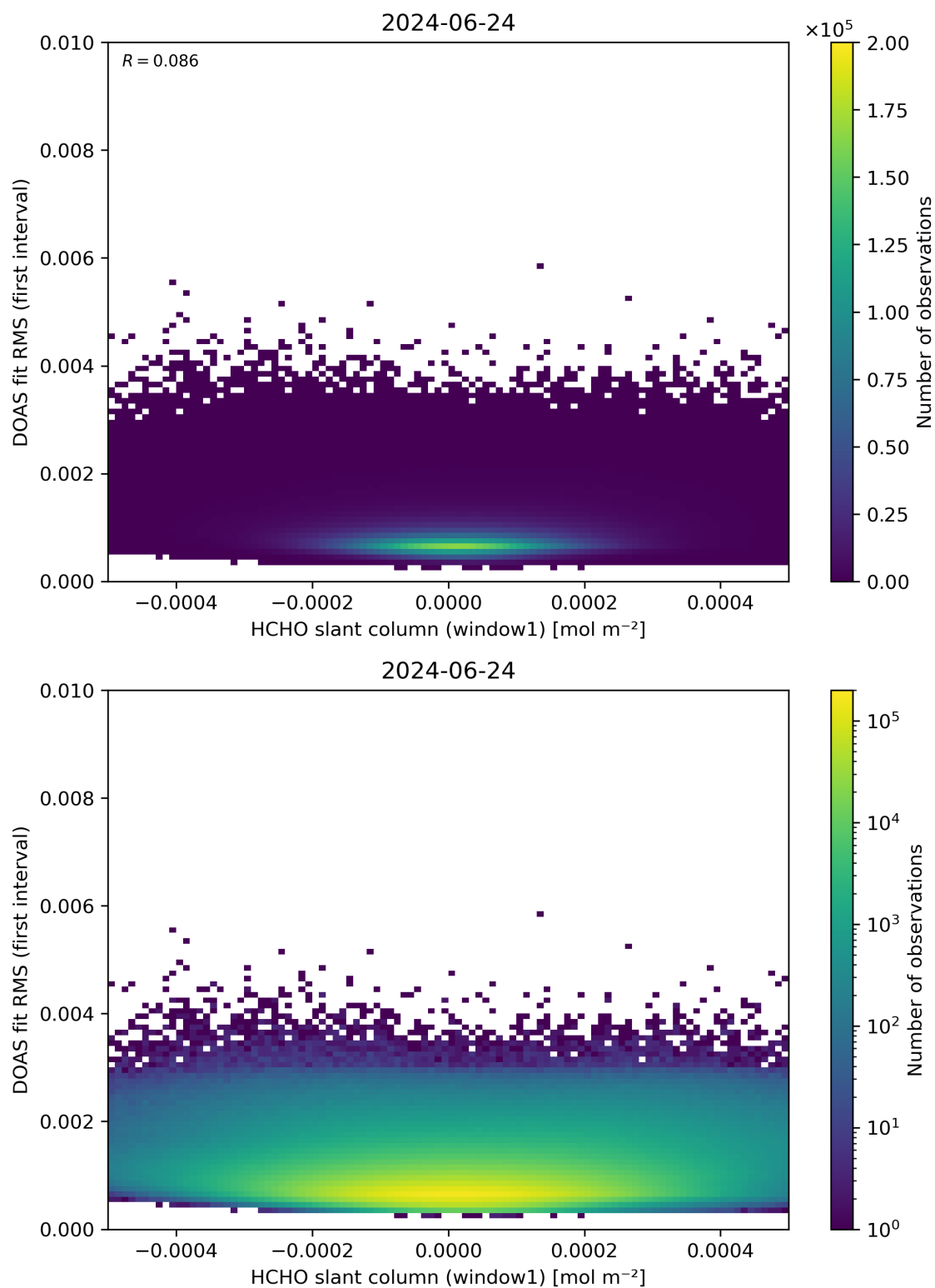
Figure 78: Scatter density plot of “HCHO slant column (window1)” against “DOAS fit RMS (first interval)” for 2024-06-24 to 2024-06-25.
