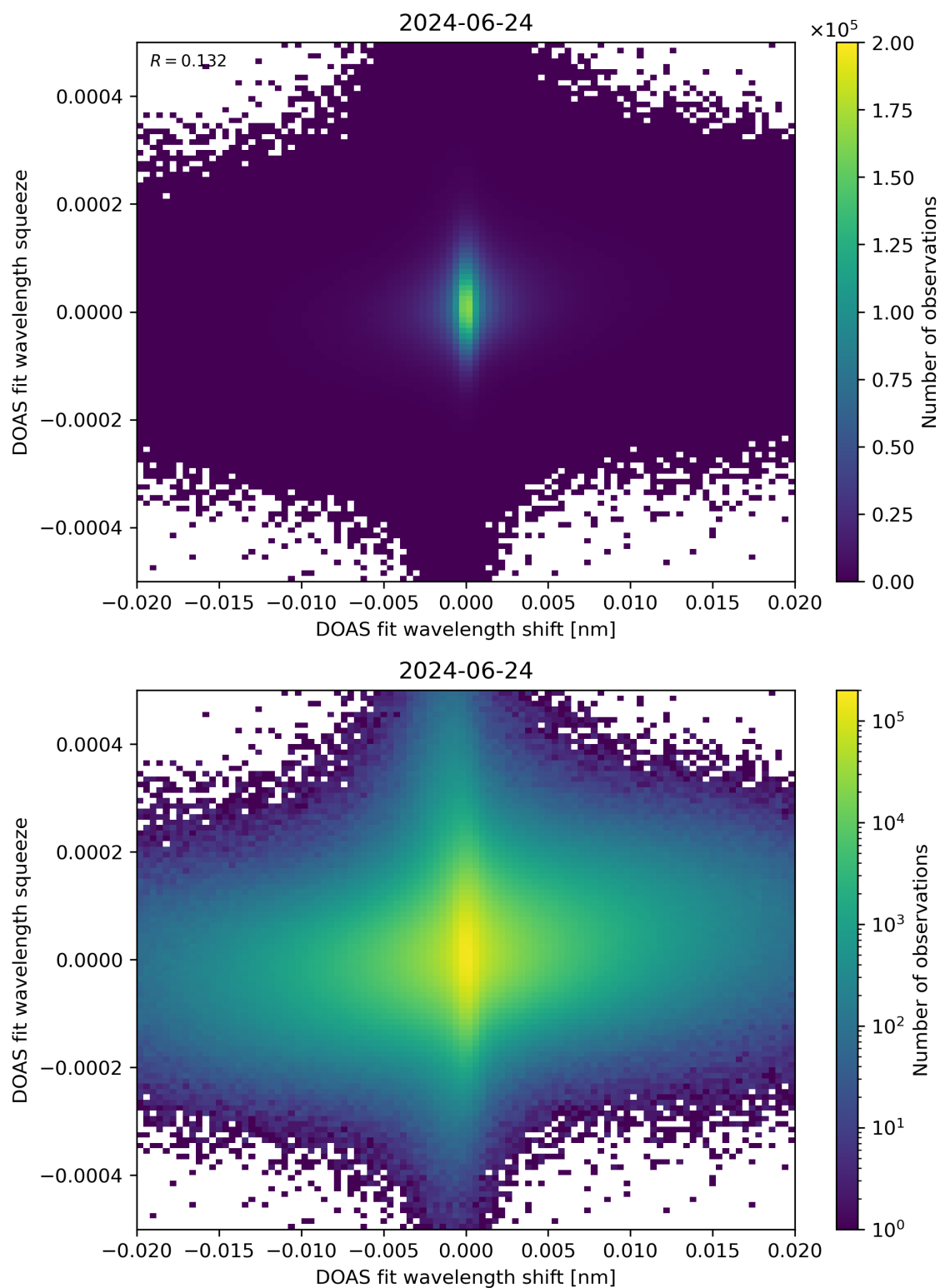
Figure 65: Scatter density plot of “DOAS fit wavelength shift” against “DOAS fit wavelength squeeze” for 2024-06-24 to 2024-06-25.
