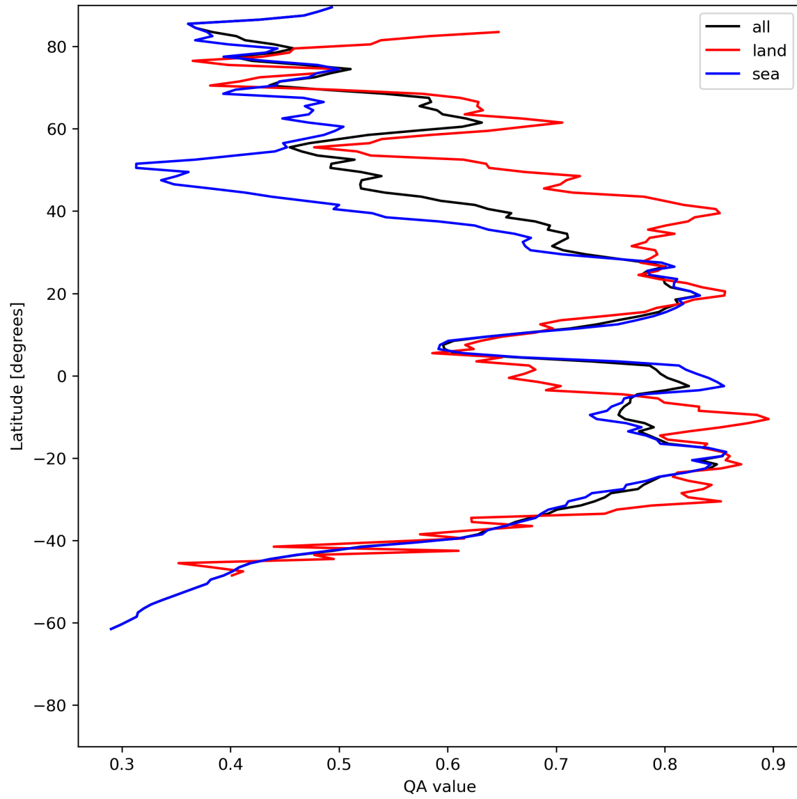
Figure 20: Zonal average of “QA value” for 2024-06-24 to 2024-06-25.
