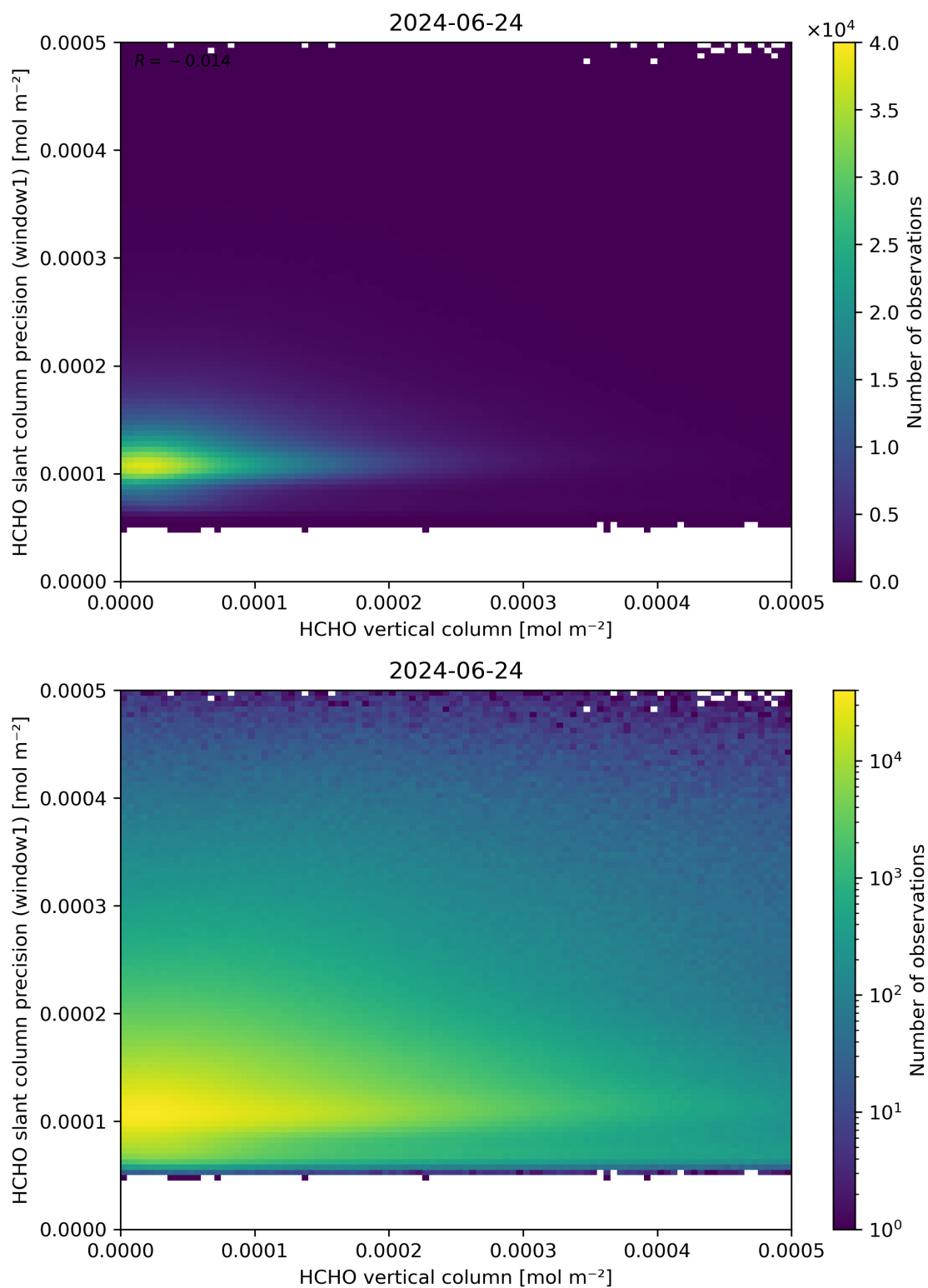
Figure 130: Scatter density plot of “HCHO vertical column” against “HCHO slant column precision (window1)” for 2024-06-24 to 2024-06-25.
