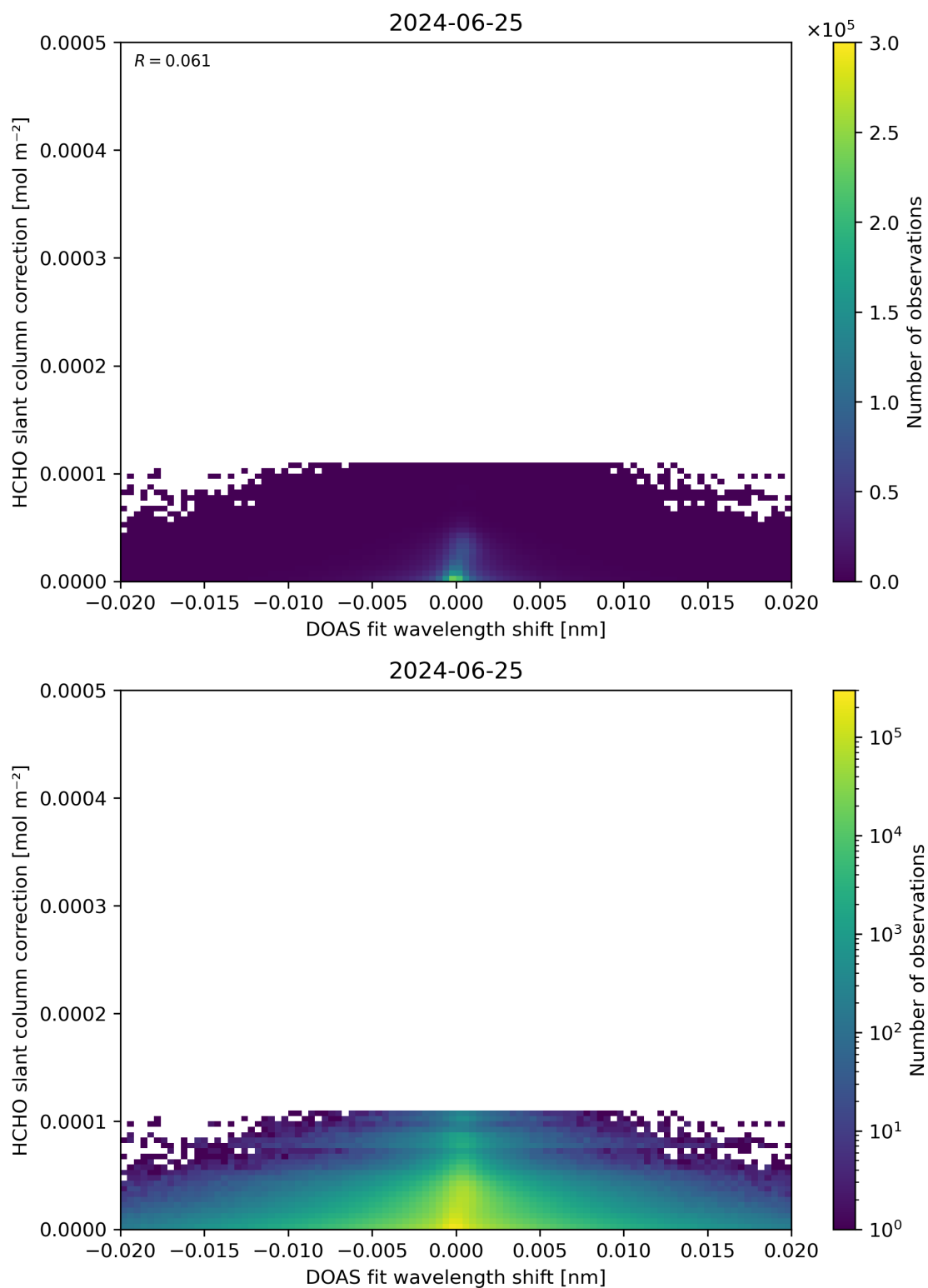
Figure 67: Scatter density plot of “DOAS fit wavelength shift” against “HCHO slant column correction” for 2024-06-24 to 2024-06-26.
