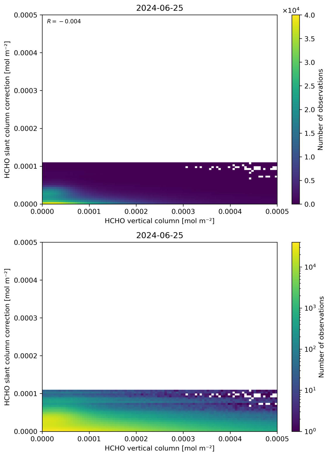
Figure 128: Scatter density plot of “HCHO vertical column” against “HCHO slant column correction” for 2024-06-24 to 2024-06-26.
