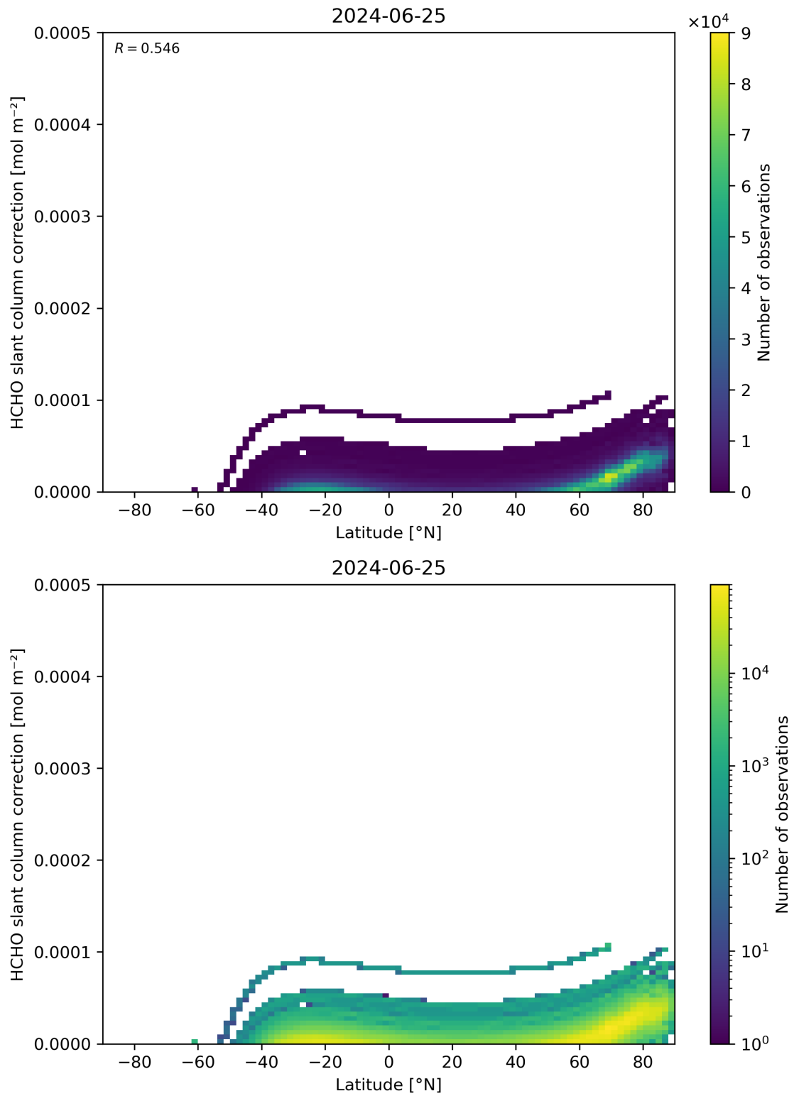
Figure 158: Scatter density plot of “Latitude” against “HCHO slant column correction” for 2024-06-24 to 2024-06-26.
