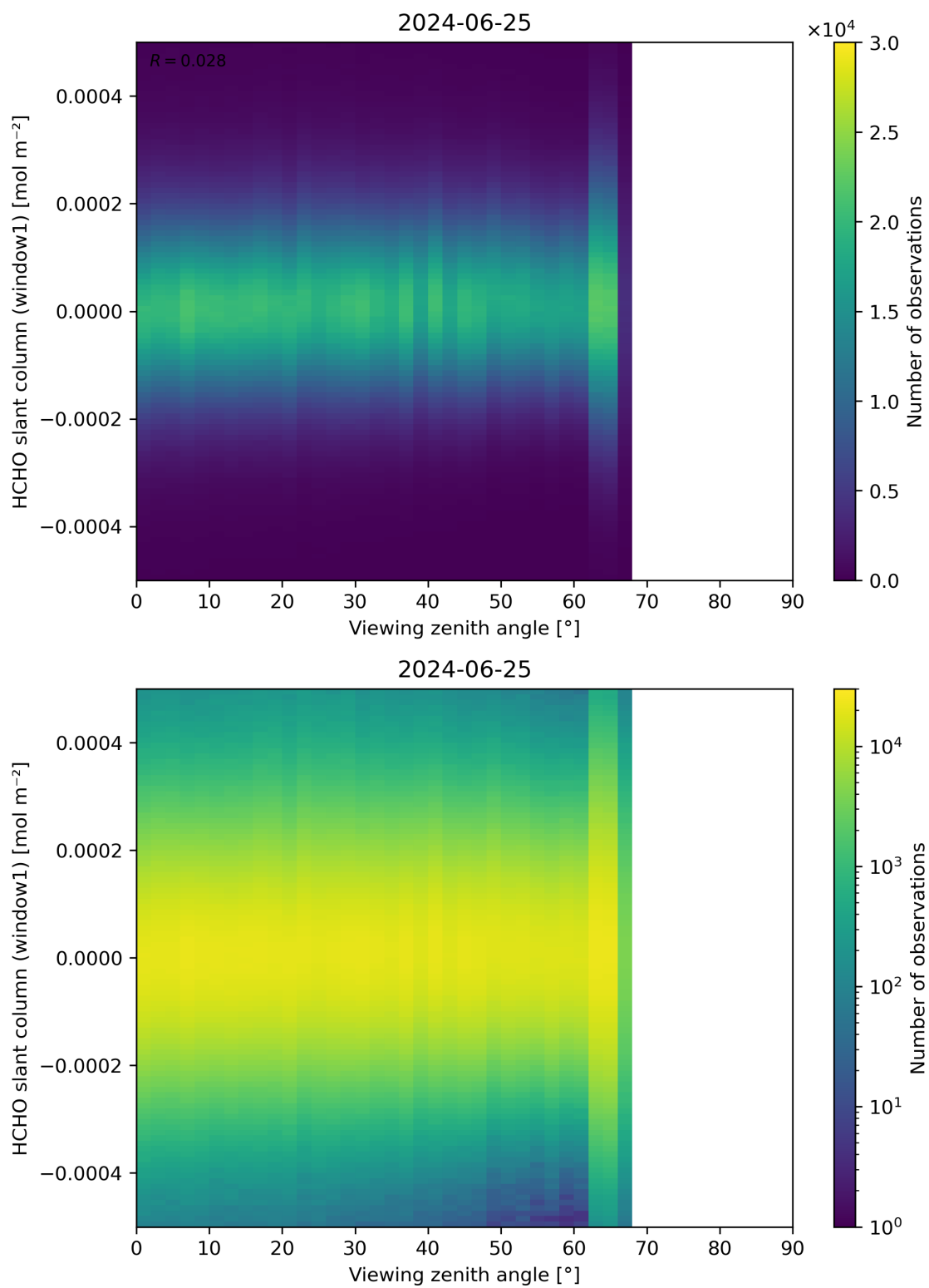
Figure 188: Scatter density plot of “Viewing zenith angle” against “HCHO slant column (window1)” for 2024-06-24 to 2024-06-26.
