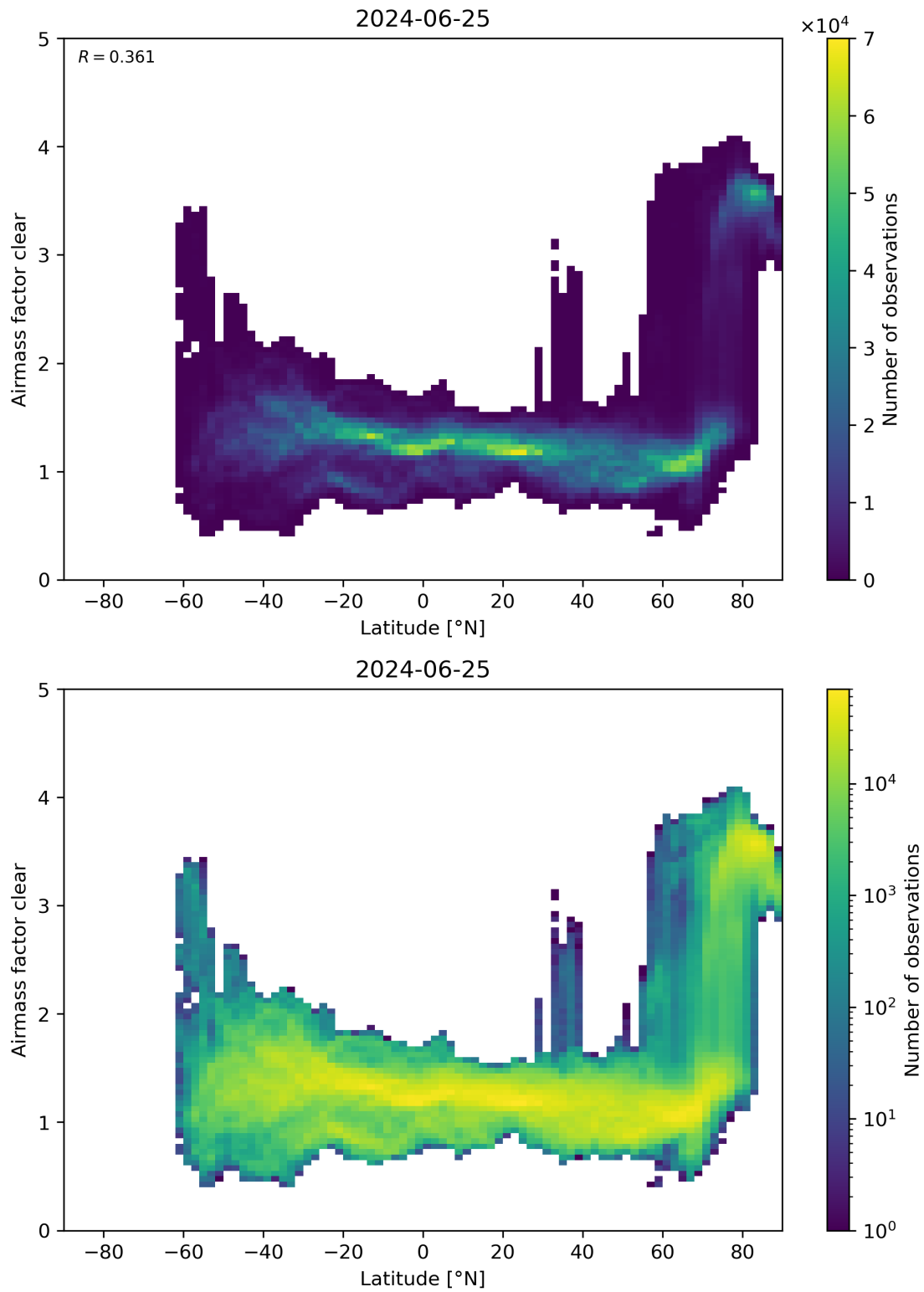
Figure 156: Scatter density plot of “Latitude” against “Airmass factor clear” for 2024-06-24 to 2024-06-26.
