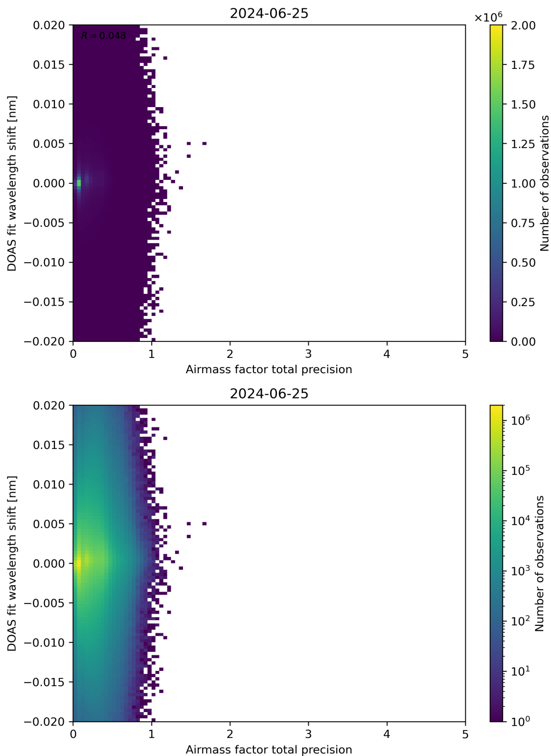
Figure 106: Scatter density plot of “Airmass factor total precision” against “DOAS fit wavelength shift” for 2024-06-24 to 2024-06-26.
