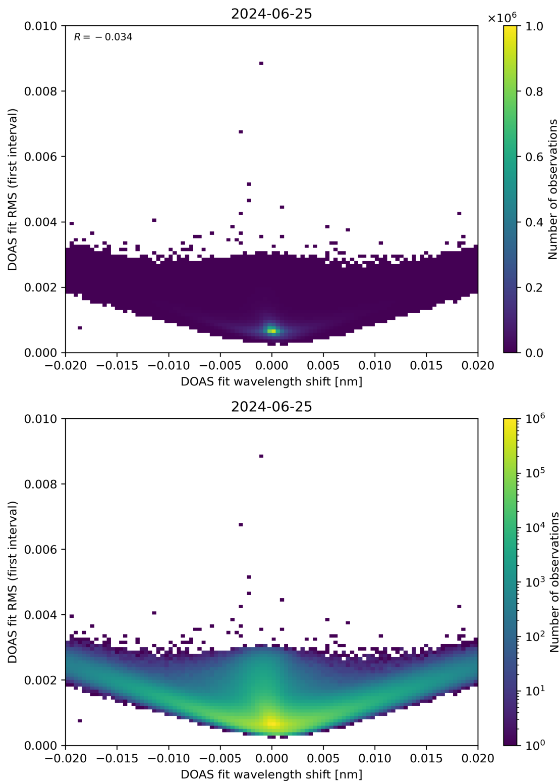
Figure 64: Scatter density plot of “DOAS fit wavelength shift” against “DOAS fit RMS (first interval)” for 2024-06-24 to 2024-06-26.
