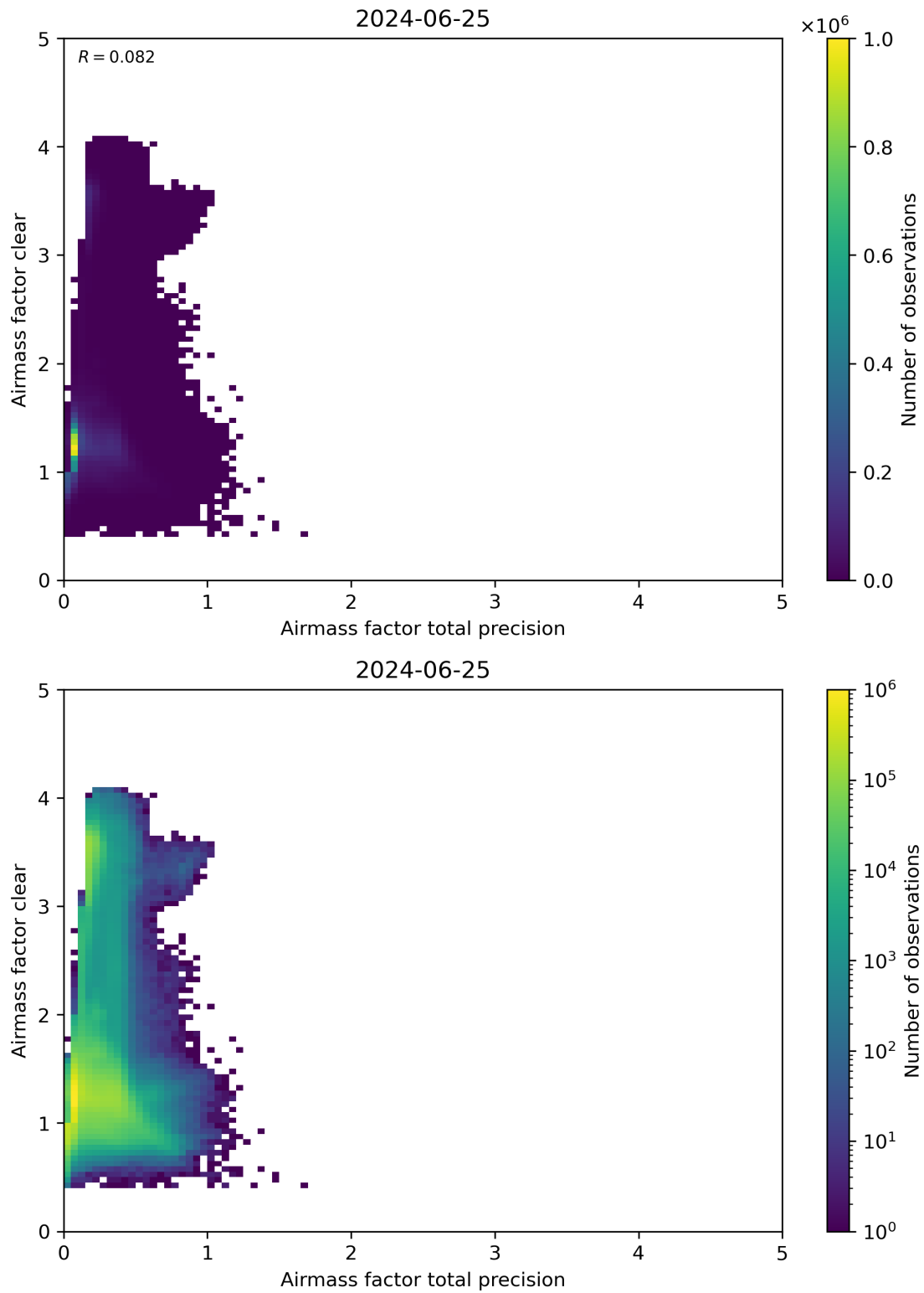
Figure 108: Scatter density plot of “Airmass factor total precision” against “Airmass factor clear” for 2024-06-24 to 2024-06-26.
