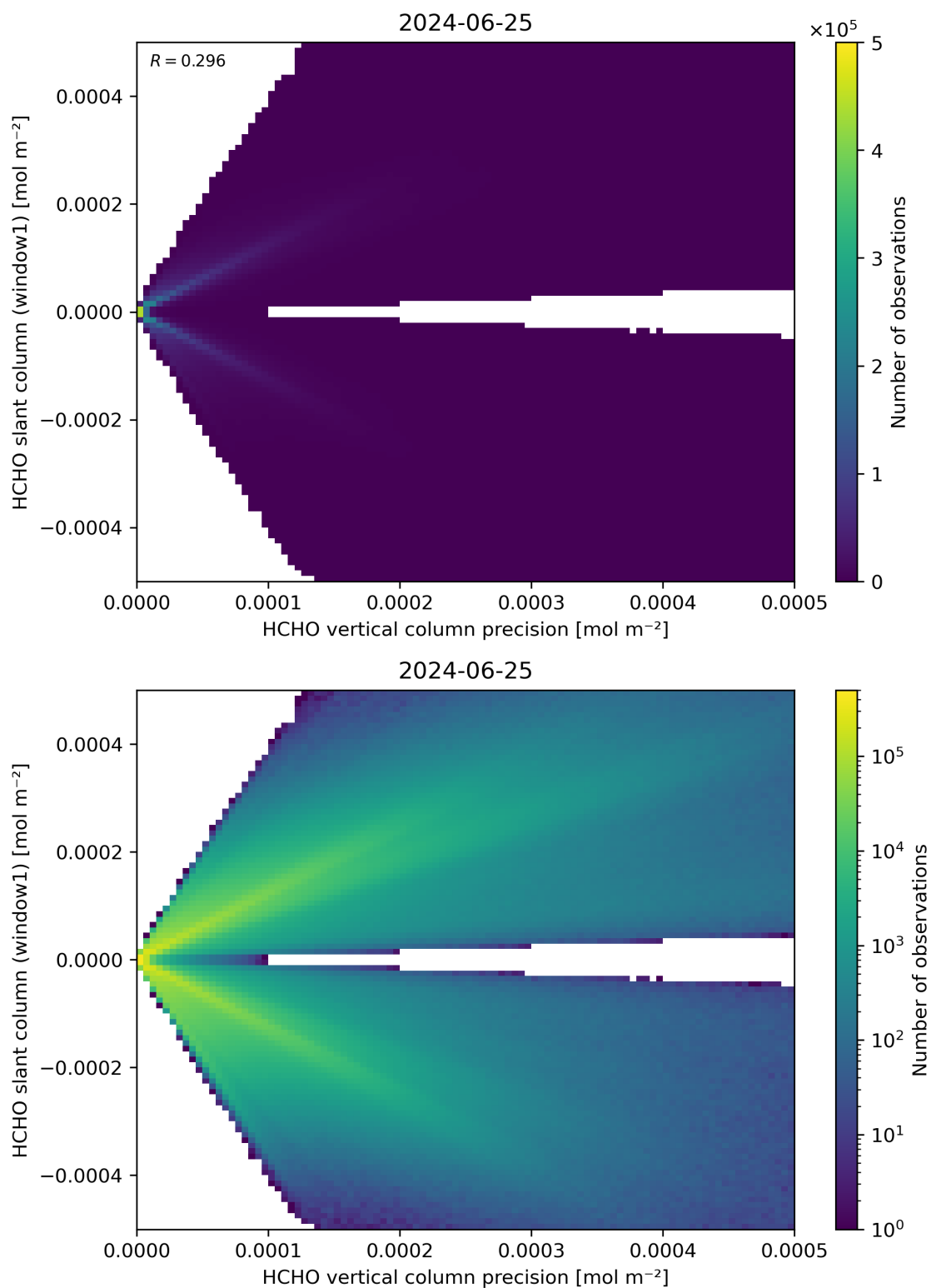
Figure 142: Scatter density plot of “HCHO vertical column precision” against “HCHO slant column (window1)” for 2024-06-24 to 2024-06-26.
