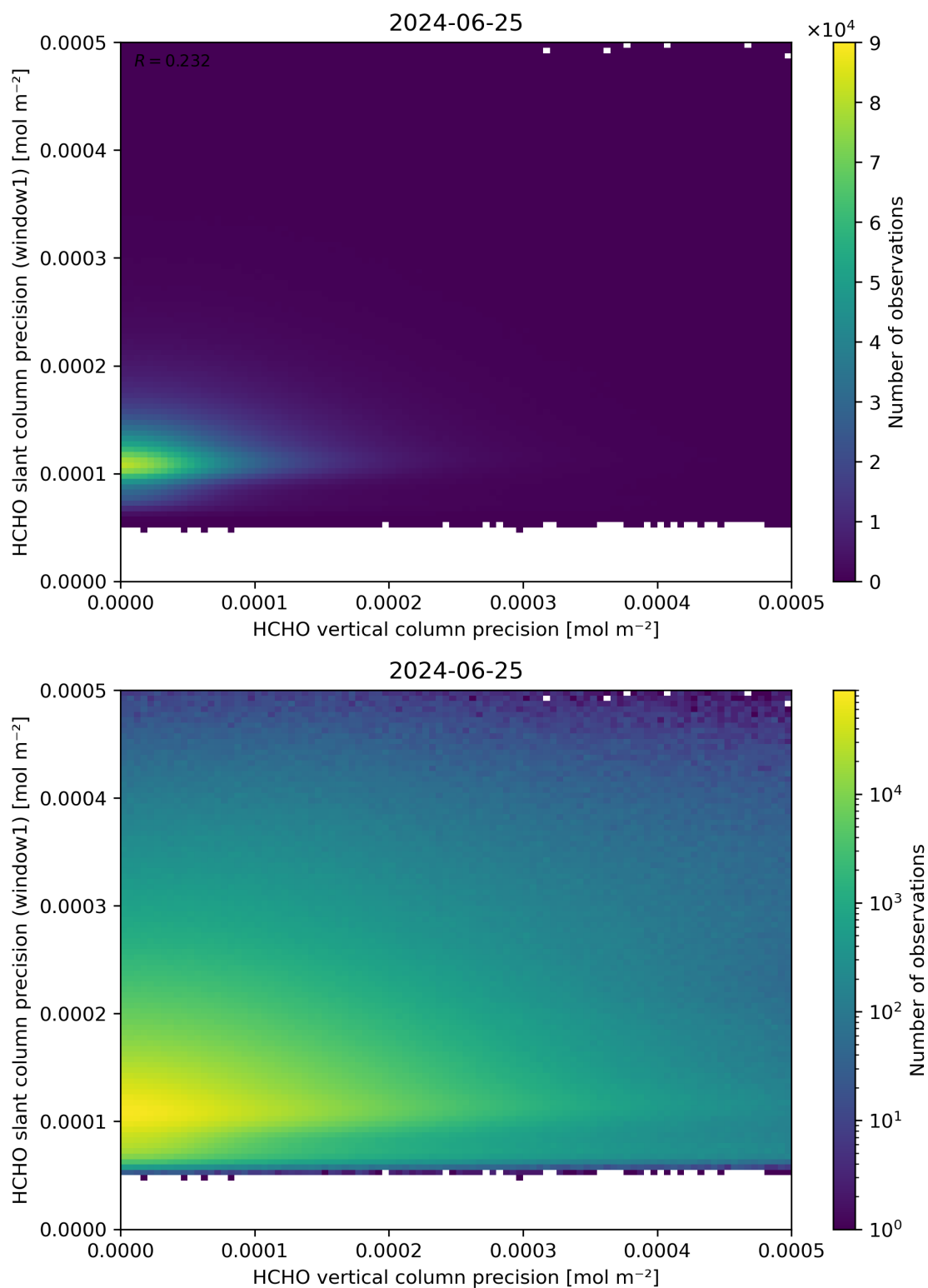
Figure 143: Scatter density plot of “HCHO vertical column precision” against “HCHO slant column precision (window1)” for 2024-06-24 to 2024-06-26.
