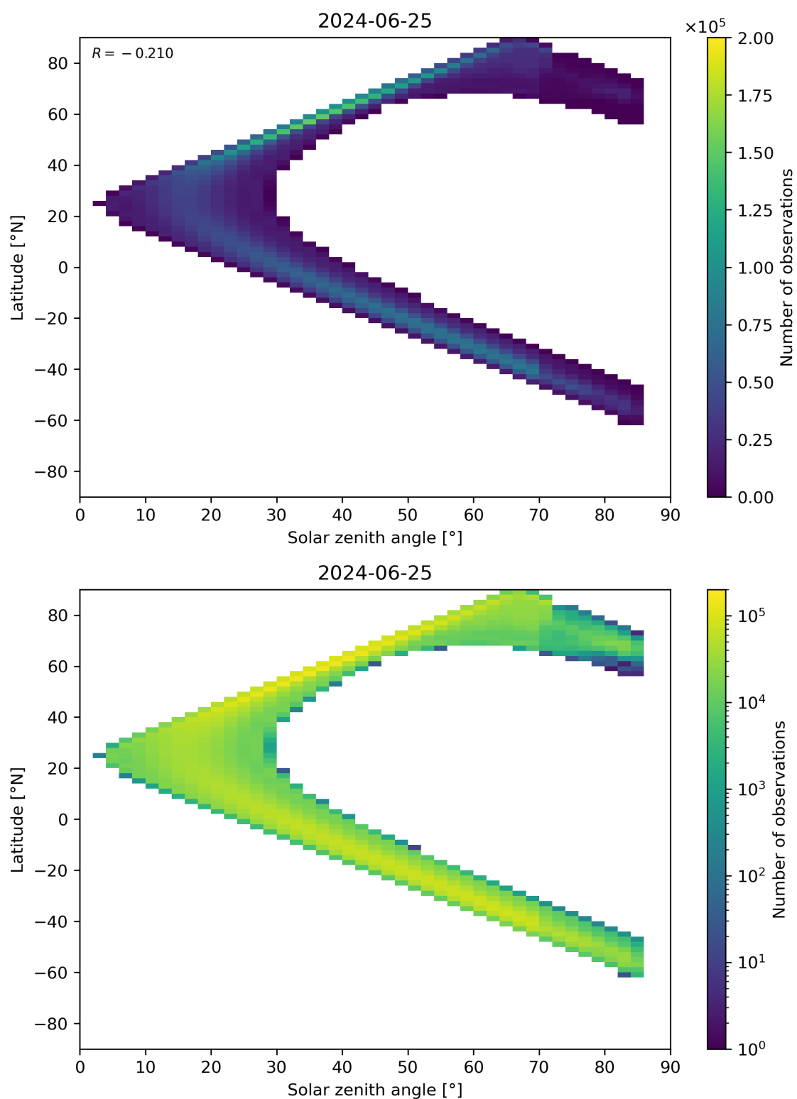
Figure 181: Scatter density plot of “Solar zenith angle” against “Latitude” for 2024-06-24 to 2024-06-26.
