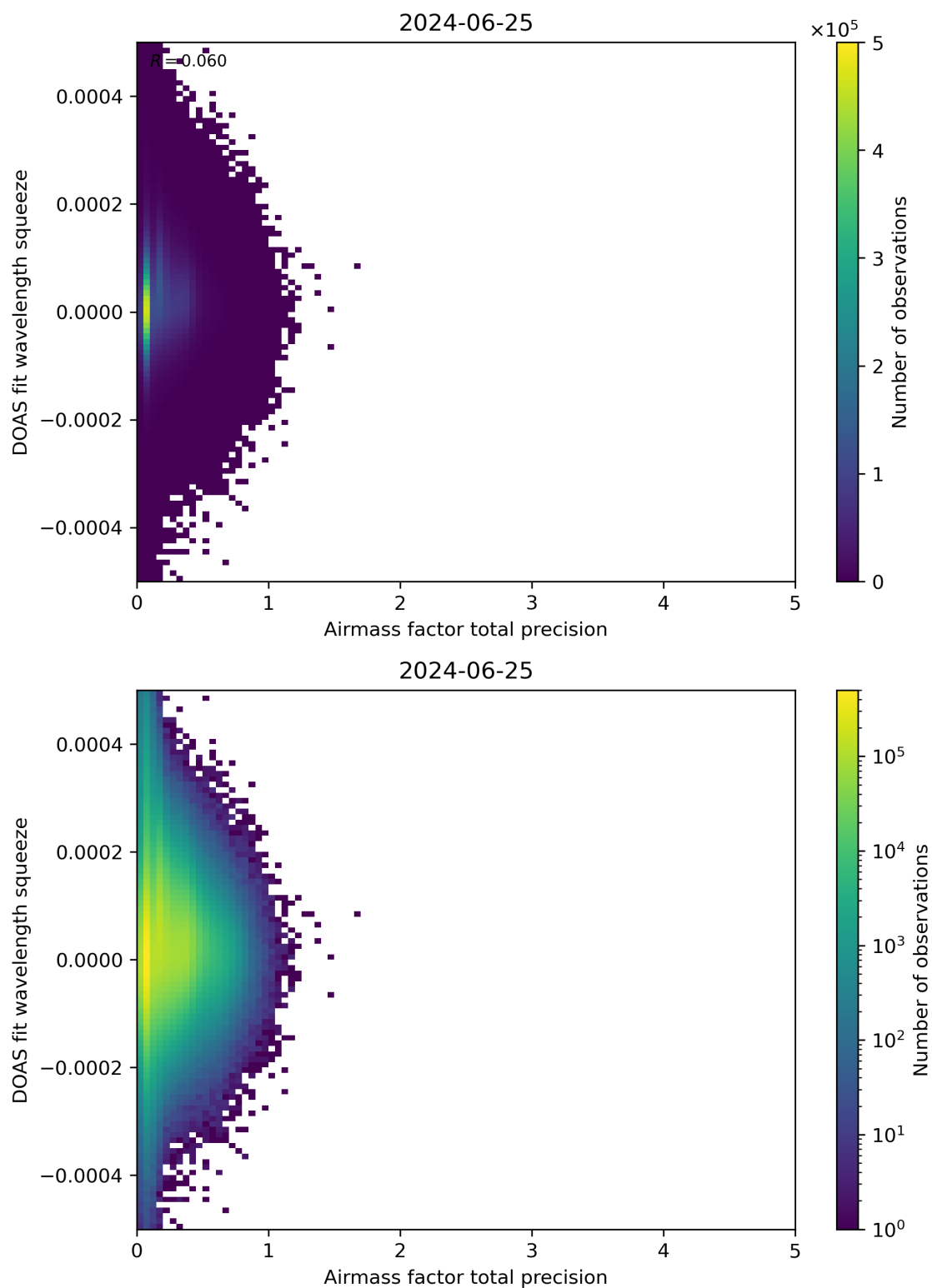
Figure 107: Scatter density plot of “Airmass factor total precision” against “DOAS fit wavelength squeeze” for 2024-06-24 to 2024-06-26.
