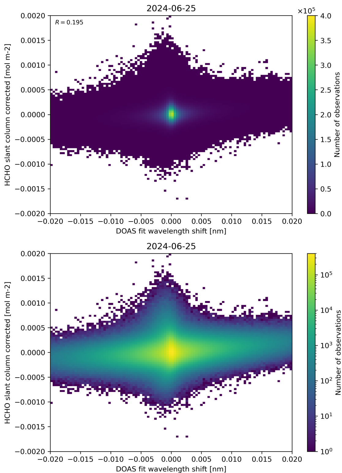
Figure 66: Scatter density plot of “DOAS fit wavelength shift” against “HCHO slant column corrected” for 2024-06-24 to 2024-06-26.
