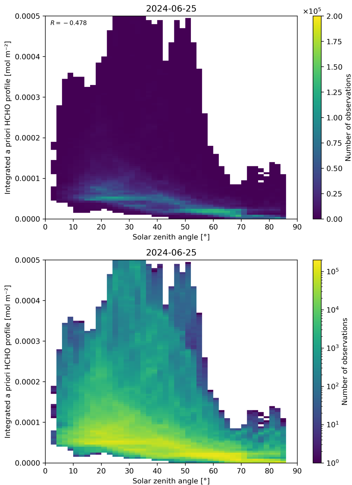
Figure 180: Scatter density plot of “Solar zenith angle” against “Integrated a priori HCHO profile” for 2024-06-24 to 2024-06-26.
