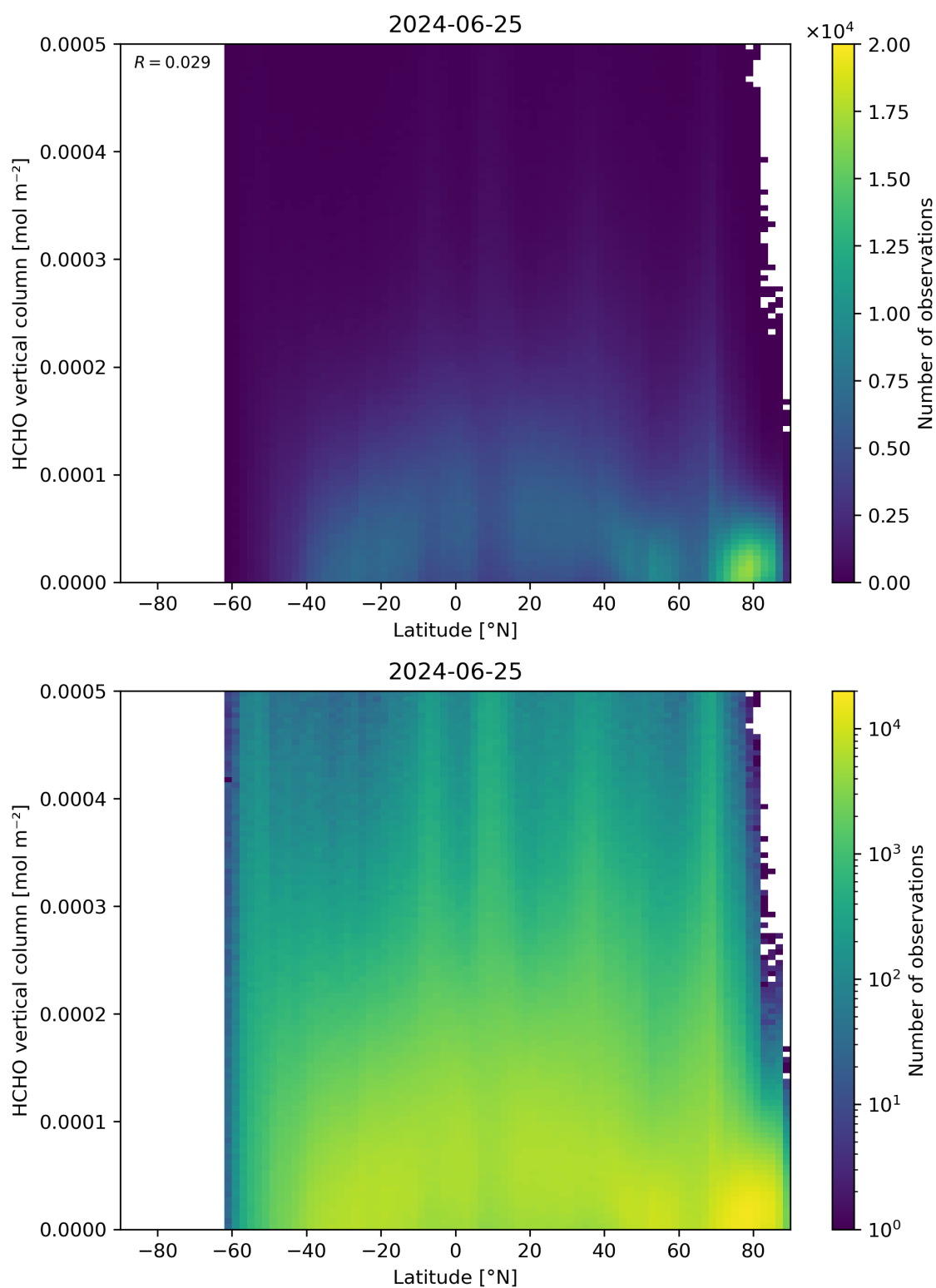
Figure 163: Scatter density plot of “Latitude” against “HCHO vertical column” for 2024-06-24 to 2024-06-26.
