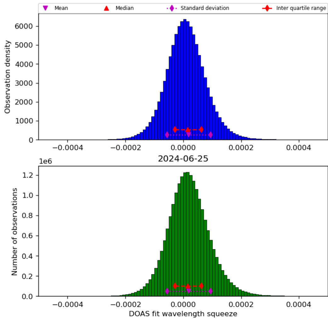
Figure 45: Histogram of “DOAS fit wavelength squeeze” for 2024-06-24 to 2024-06-26
