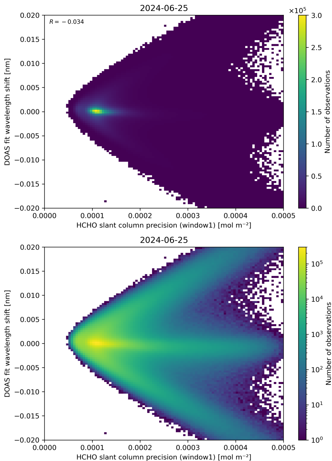
Figure 89: Scatter density plot of “HCHO slant column precision (window1)” against “DOAS fit wavelength shift” for 2024-06-24 to 2024-06-26.
