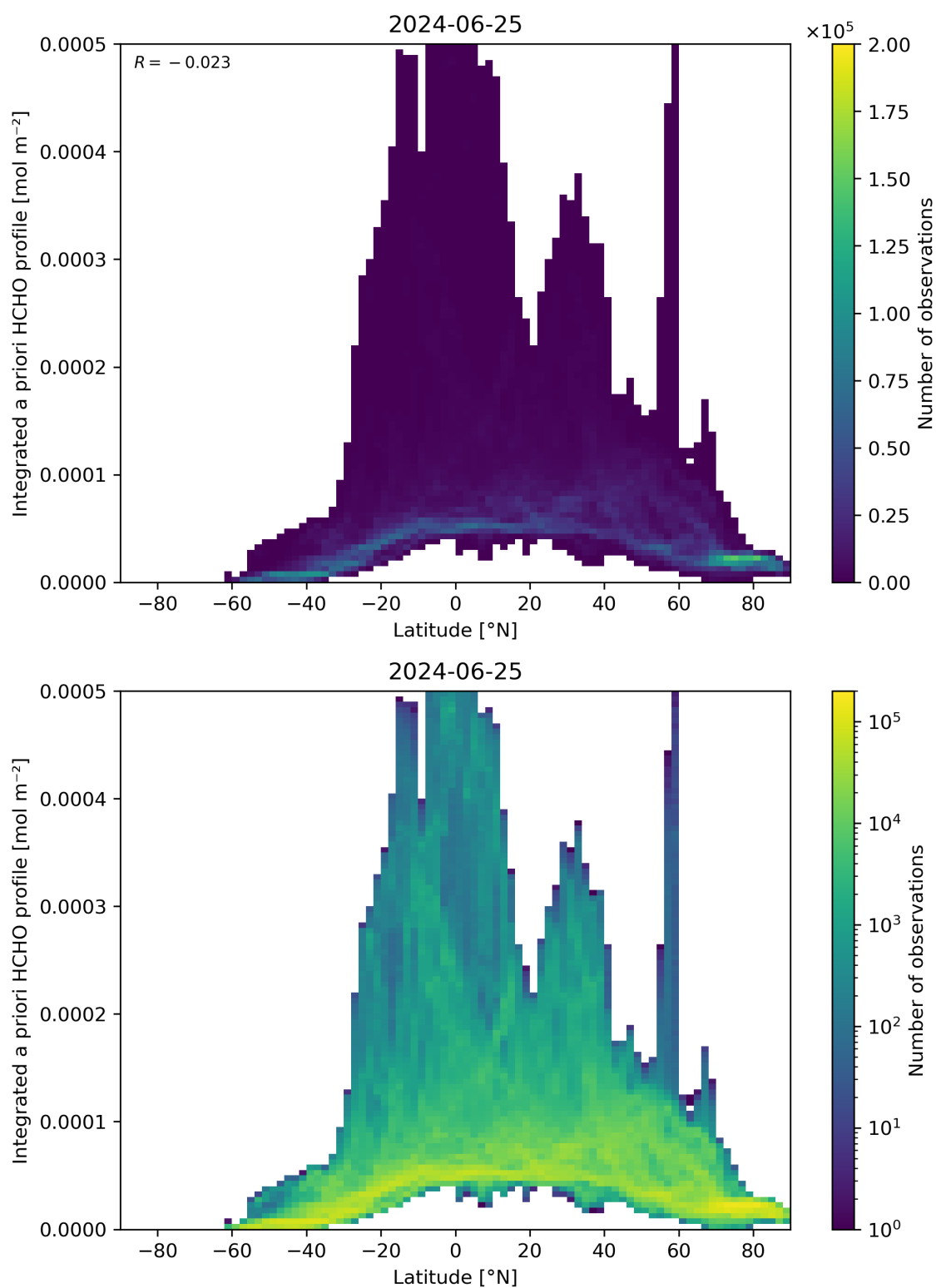
Figure 166: Scatter density plot of “Latitude” against “Integrated a priori HCHO profile” for 2024-06-24 to 2024-06-26.
