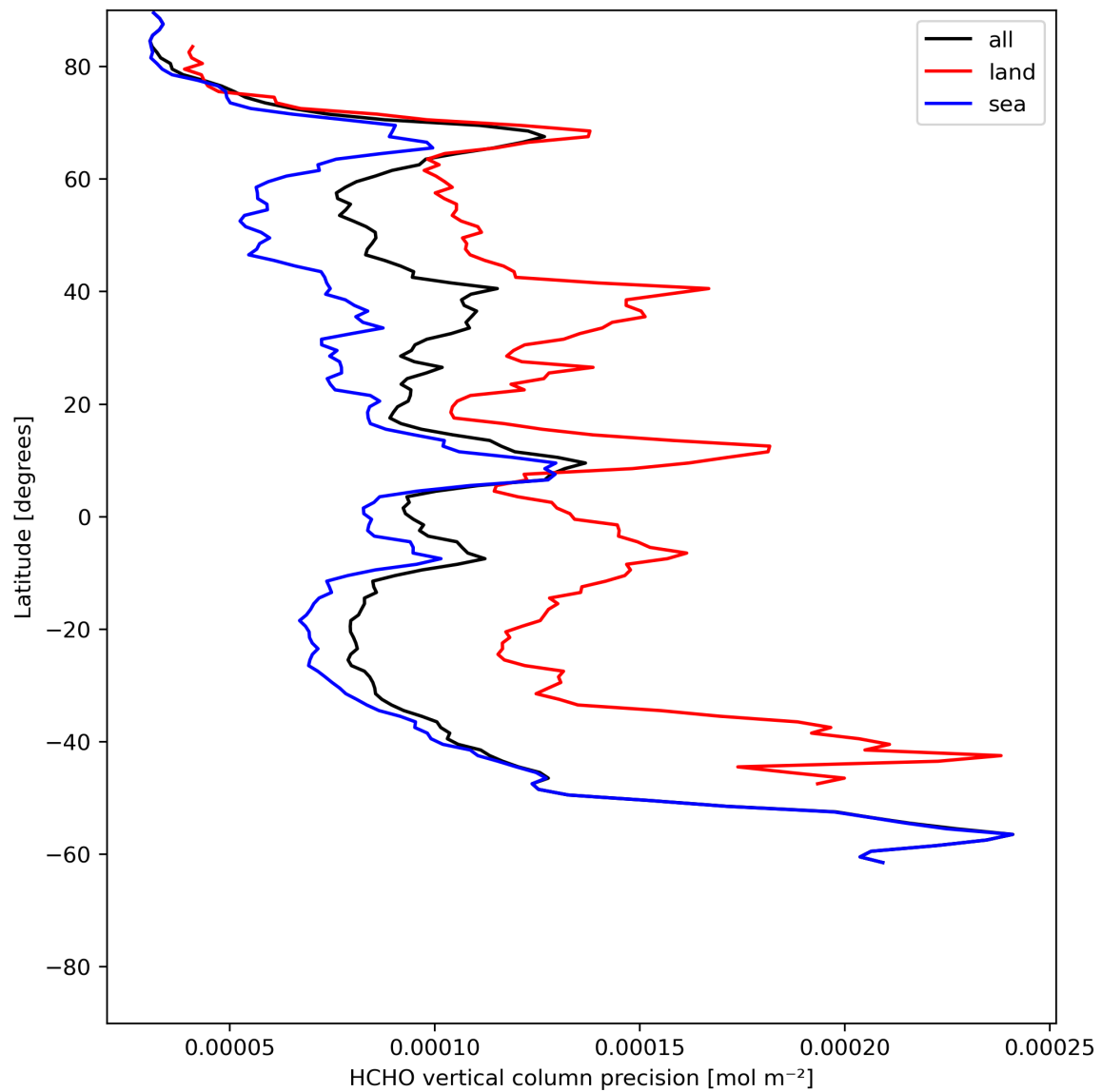
Figure 22: Zonal average of “HCHO vertical column precision” for 2024-06-24 to 2024-06-26.
