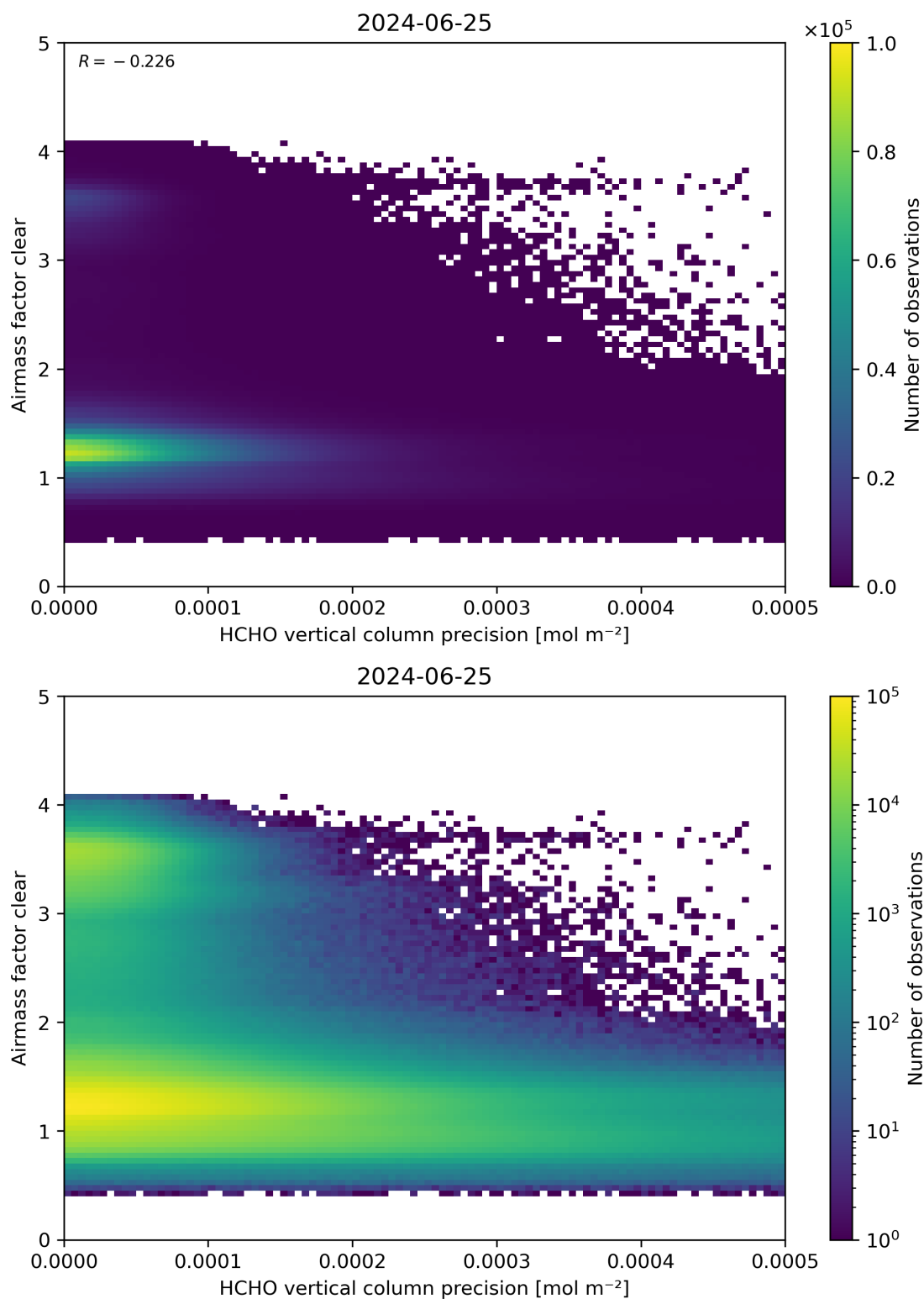
Figure 139: Scatter density plot of “HCHO vertical column precision” against “Airmass factor clear” for 2024-06-24 to 2024-06-26.
