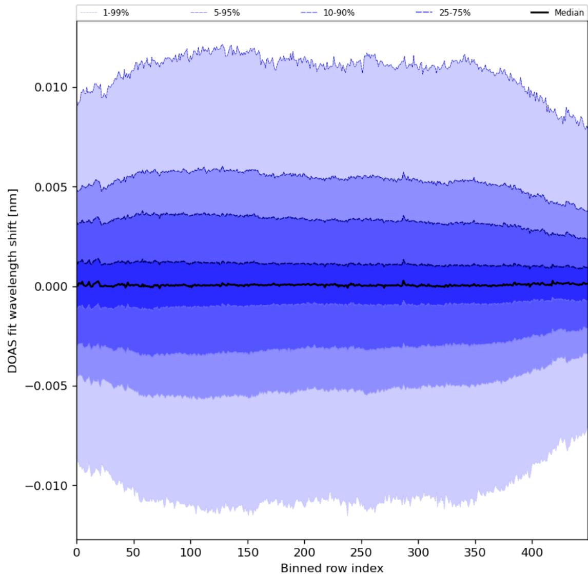
Figure 58: Along track statistics of “DOAS fit wavelength shift” for 2024-06-24 to 2024-06-26
