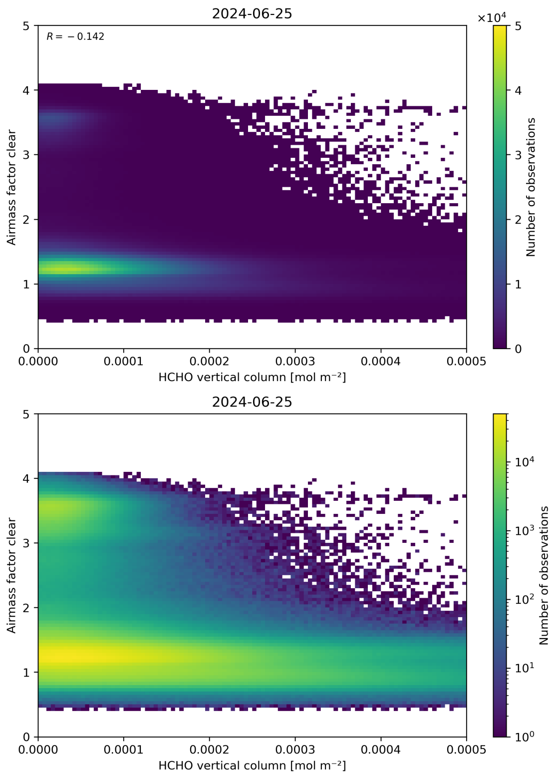
Figure 126: Scatter density plot of “HCHO vertical column” against “Airmass factor clear” for 2024-06-24 to 2024-06-26.
