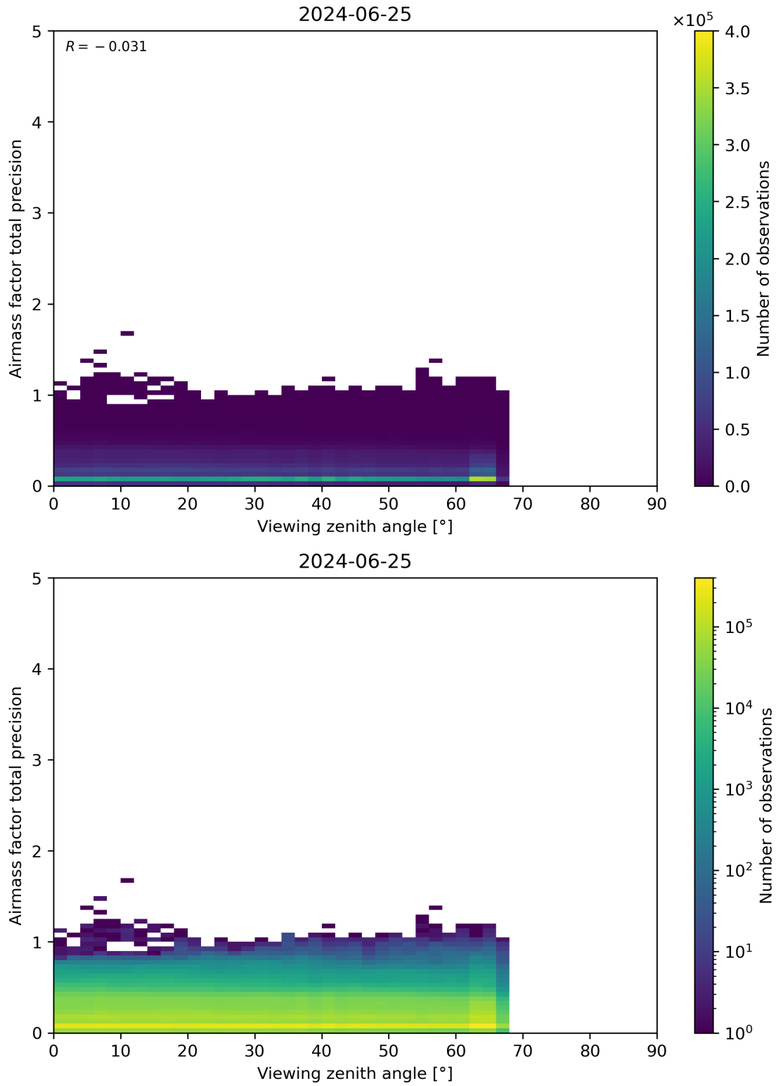
Figure 191: Scatter density plot of “Viewing zenith angle” against “Airmass factor total precision” for 2024-06-24 to 2024-06-26.
