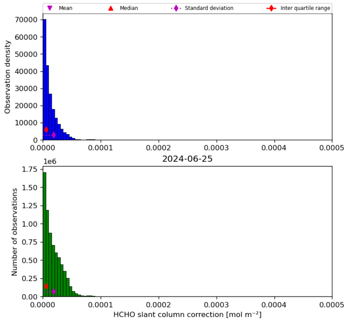
Figure 47: Histogram of “HCHO slant column correction” for 2024-06-24 to 2024-06-26
