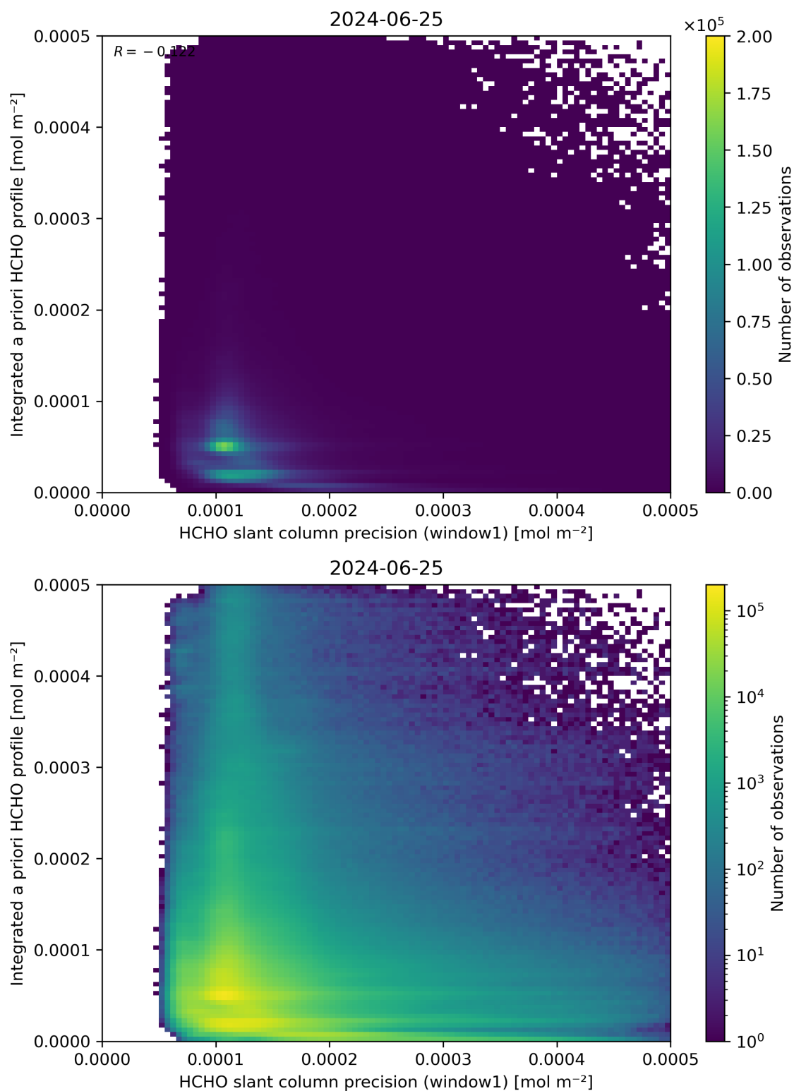
Figure 96: Scatter density plot of “HCHO slant column precision (window1)” against “Integrated a priori HCHO profile” for 2024-06-24 to 2024-06-26.
