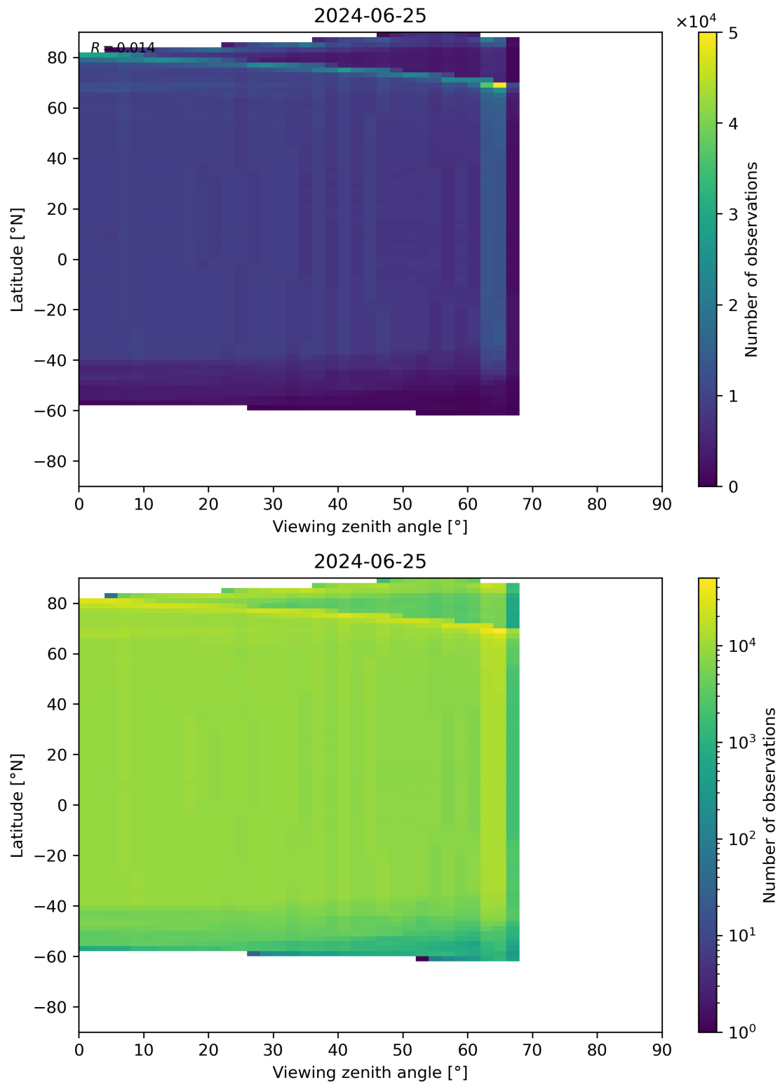
Figure 196: Scatter density plot of “Viewing zenith angle” against “Latitude” for 2024-06-24 to 2024-06-26.
