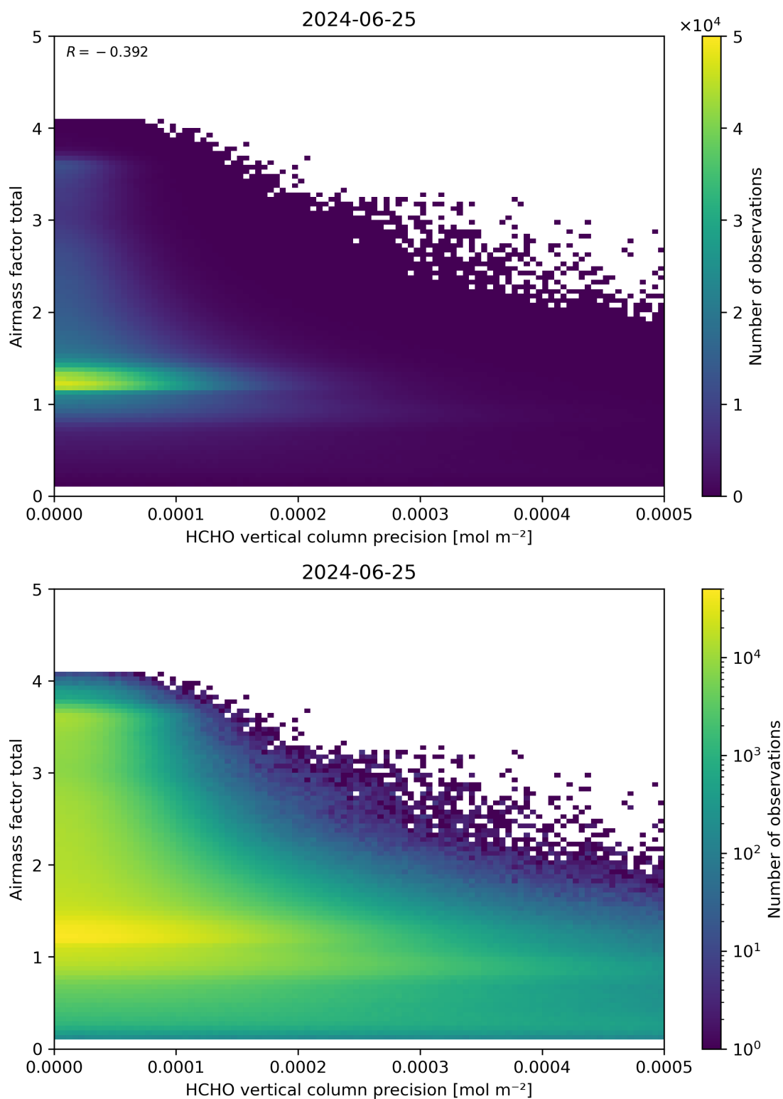
Figure 144: Scatter density plot of “HCHO vertical column precision” against “Airmass factor total” for 2024-06-24 to 2024-06-26.
