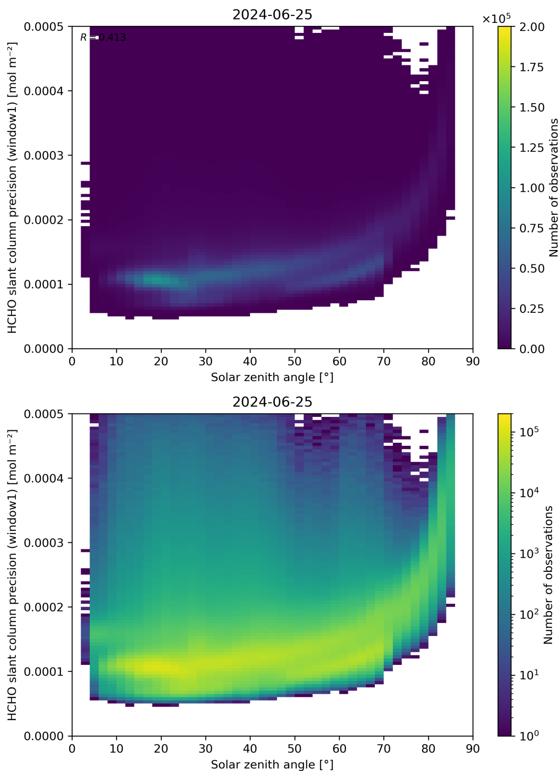
Figure 174: Scatter density plot of “Solar zenith angle” against “HCHO slant column precision (window1)” for 2024-06-24 to 2024-06-26.
