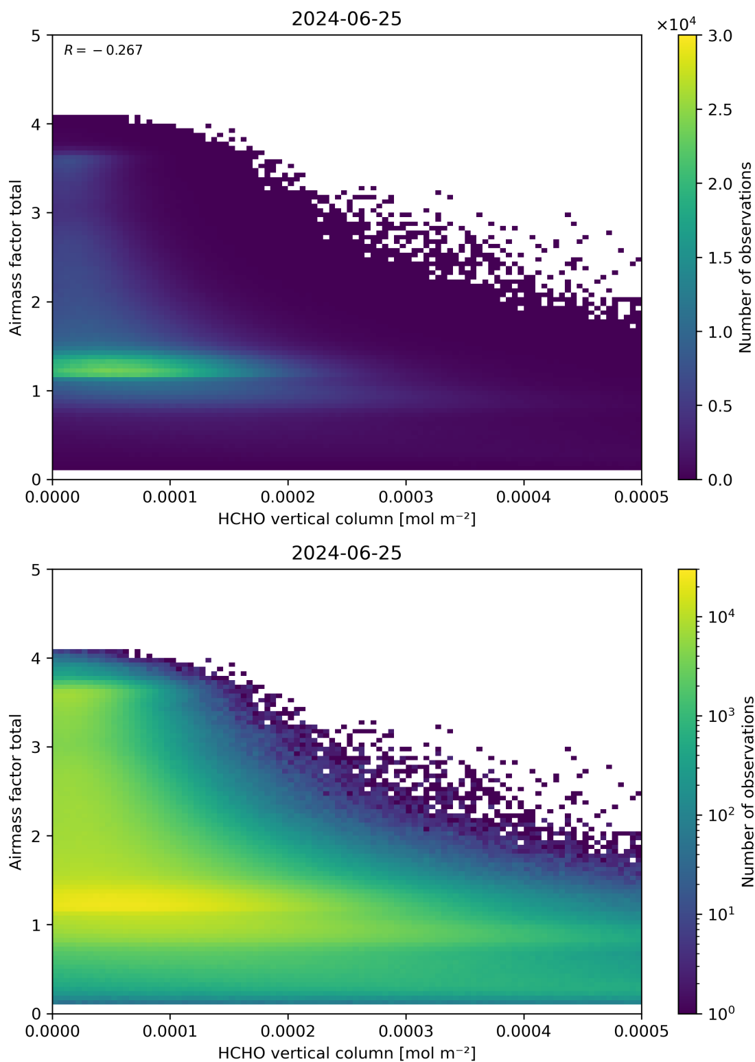
Figure 131: Scatter density plot of “HCHO vertical column” against “Airmass factor total” for 2024-06-24 to 2024-06-26.
