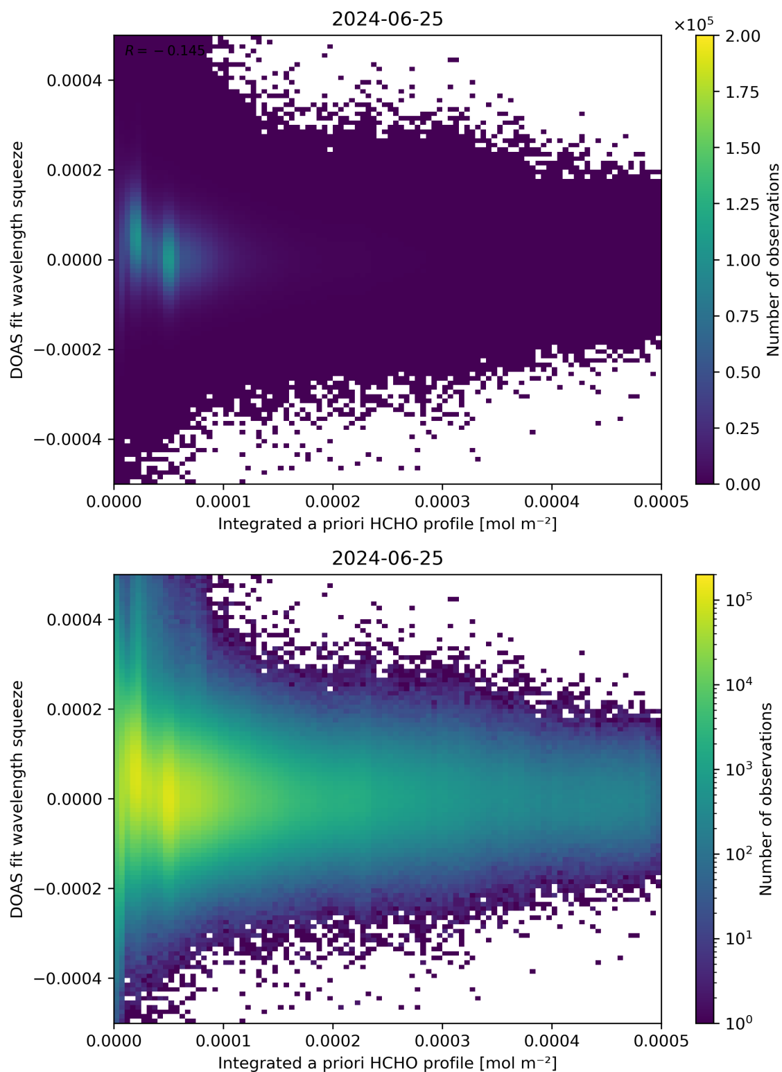
Figure 150: Scatter density plot of “Integrated a priori HCHO profile” against “DOAS fit wavelength squeeze” for 2024-06-24 to 2024-06-26.
