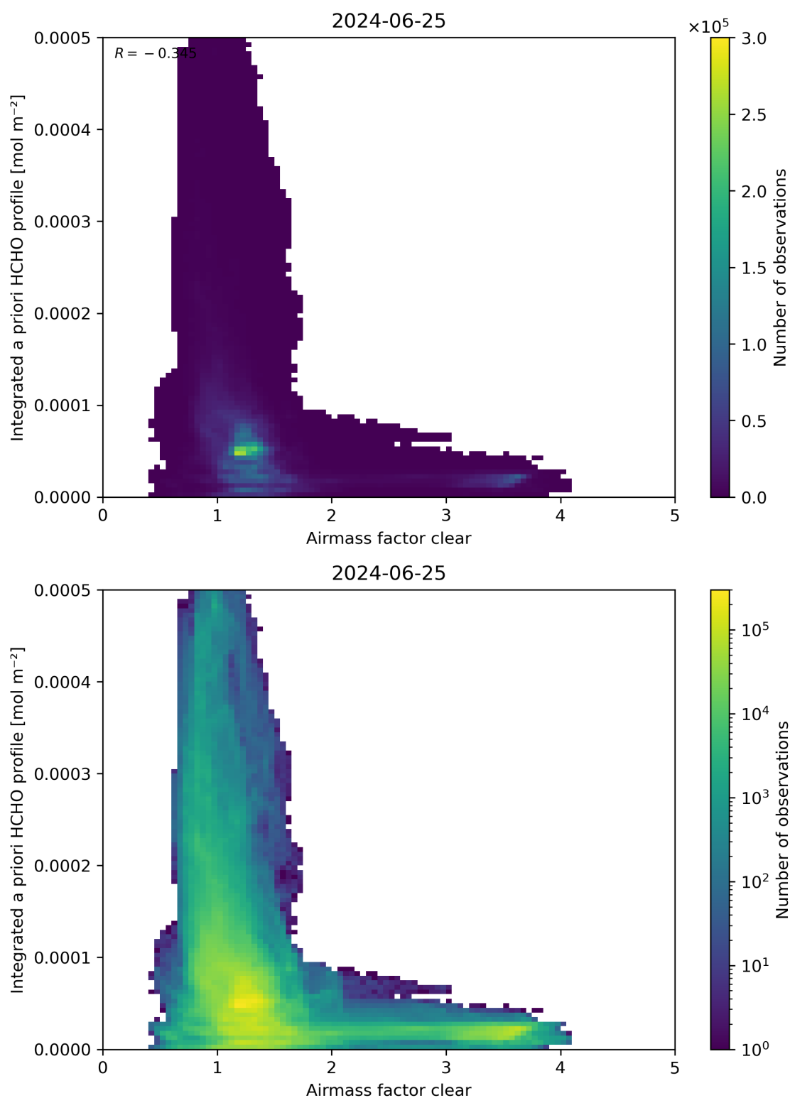
Figure 76: Scatter density plot of “Airmass factor clear” against “Integrated a priori HCHO profile” for 2024-06-24 to 2024-06-26.
