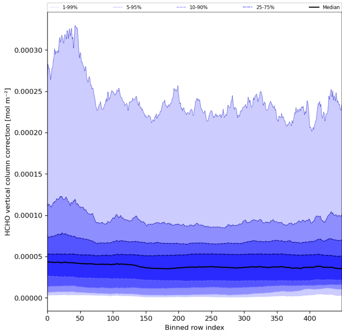
Figure 51: Along track statistics of “HCHO vertical column correction” for 2024-06-24 to 2024-06-26
