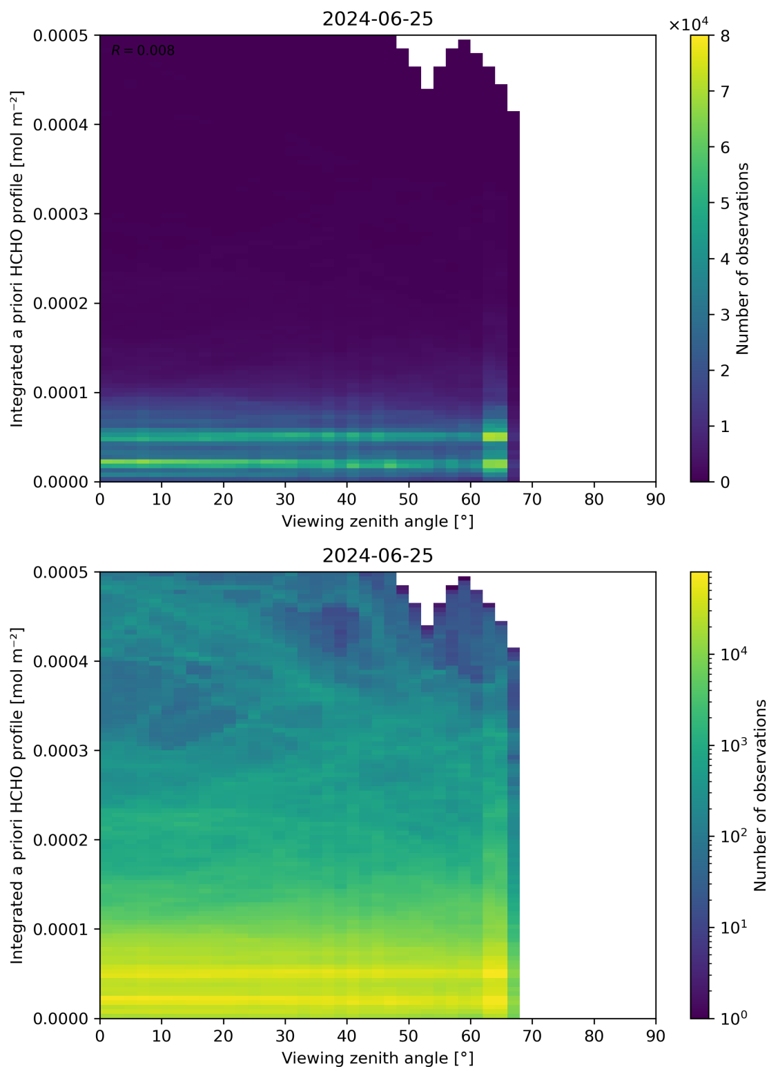
Figure 195: Scatter density plot of “Viewing zenith angle” against “Integrated a priori HCHO profile” for 2024-06-24 to 2024-06-26.
