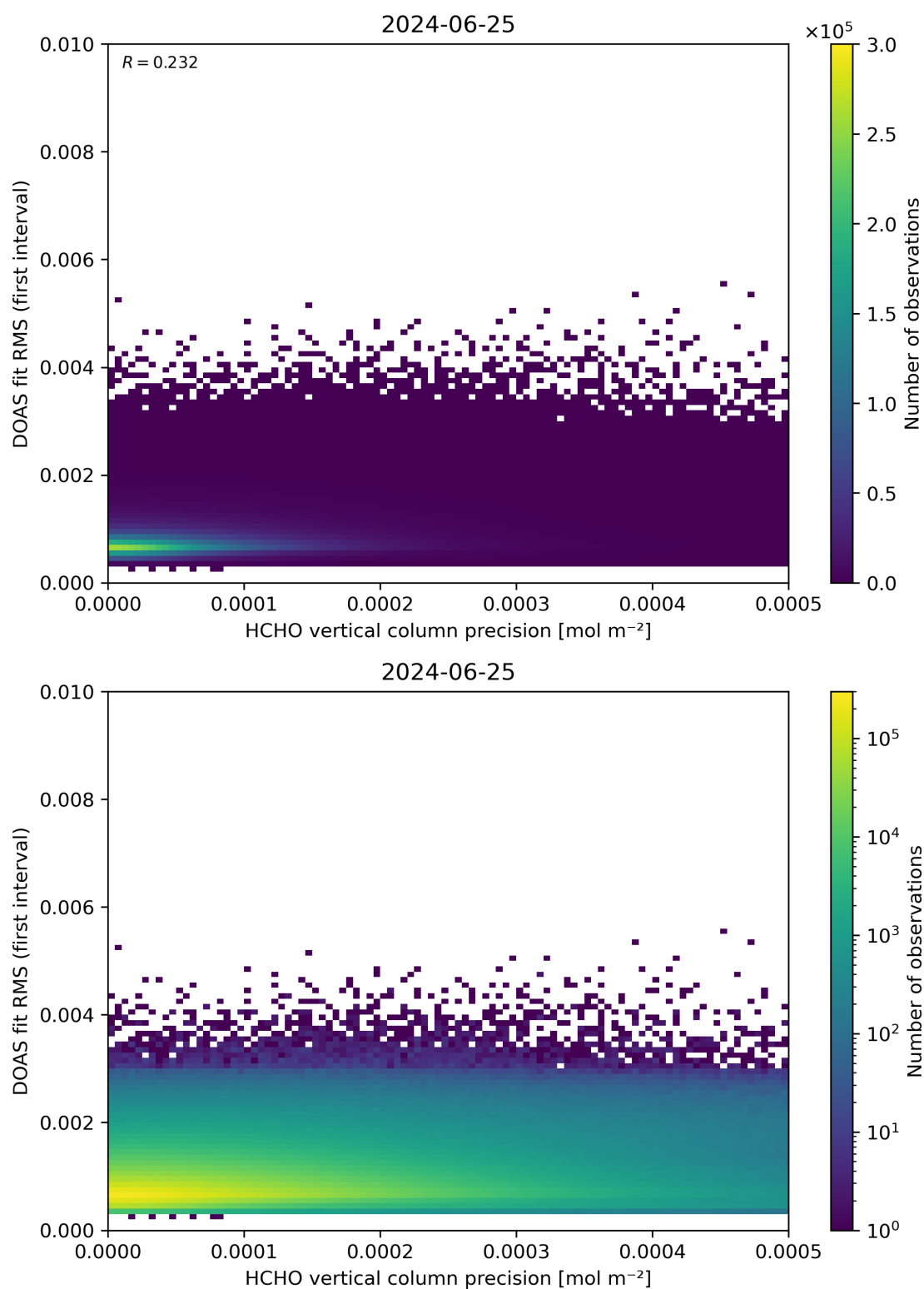
Figure 136: Scatter density plot of “HCHO vertical column precision” against “DOAS fit RMS (first interval)” for 2024-06-24 to 2024-06-26.
