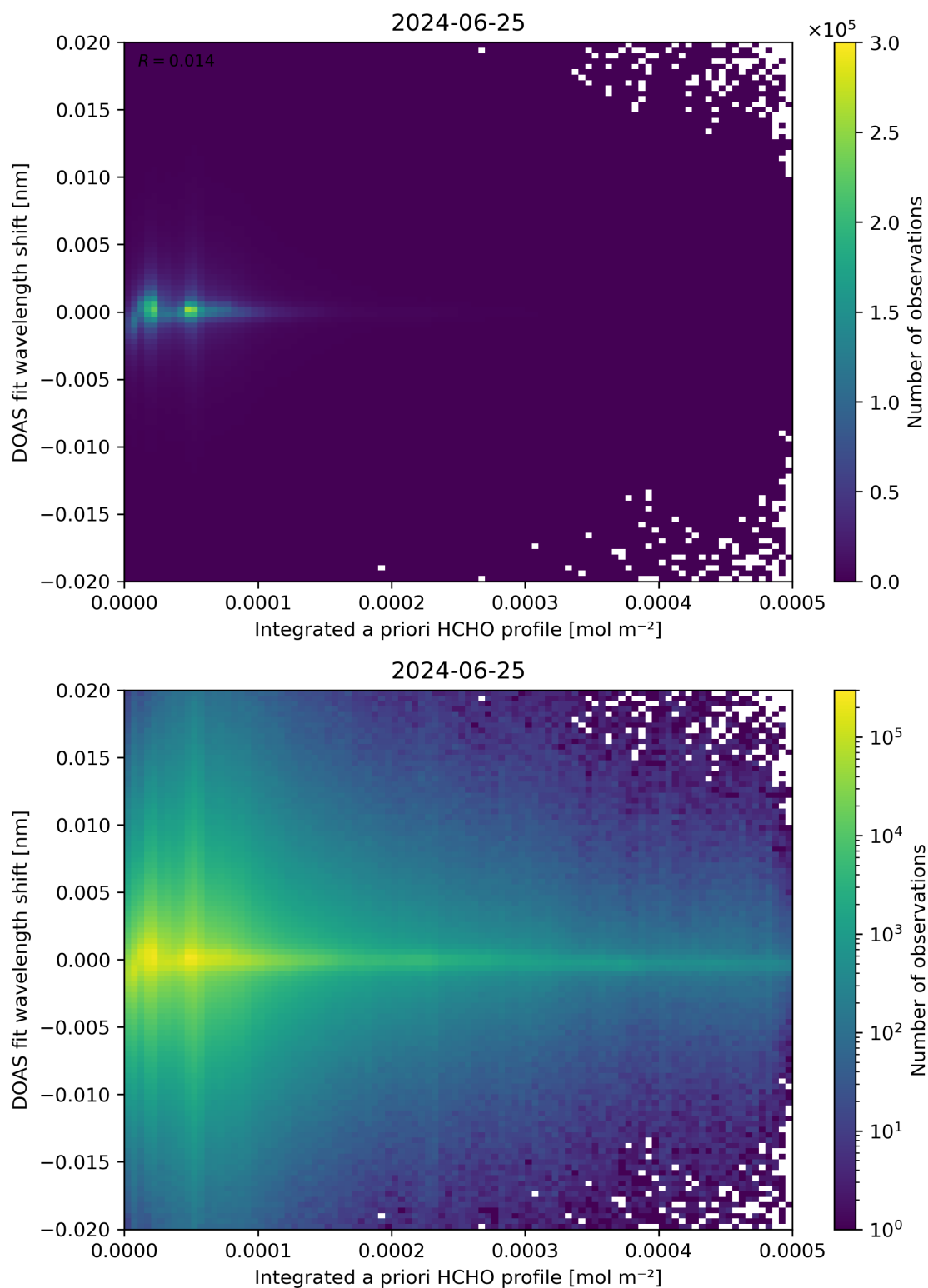
Figure 149: Scatter density plot of “Integrated a priori HCHO profile” against “DOAS fit wavelength shift” for 2024-06-24 to 2024-06-26.
