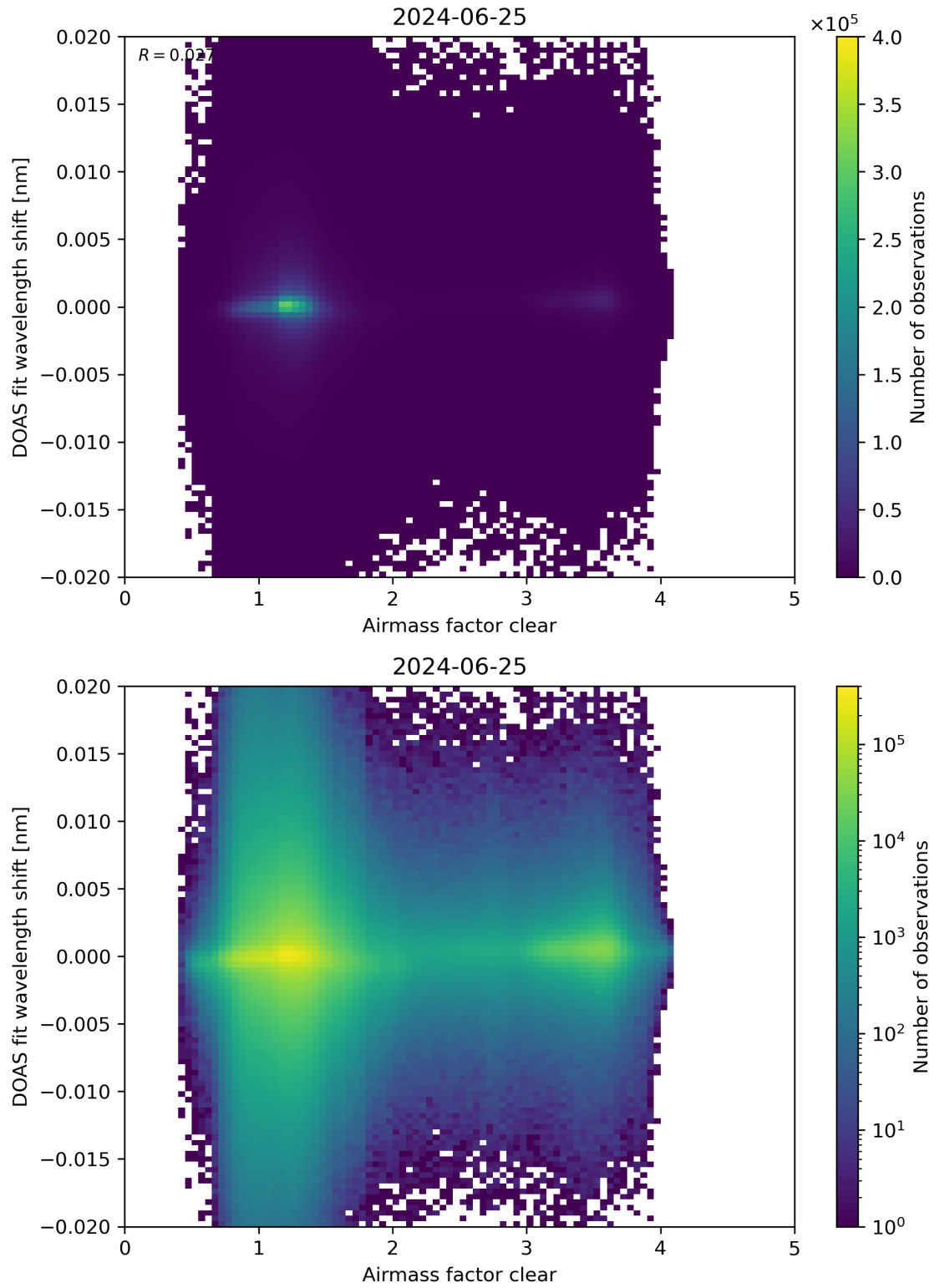
Figure 72: Scatter density plot of “Airmass factor clear” against “DOAS fit wavelength shift” for 2024-06-24 to 2024-06-26.
