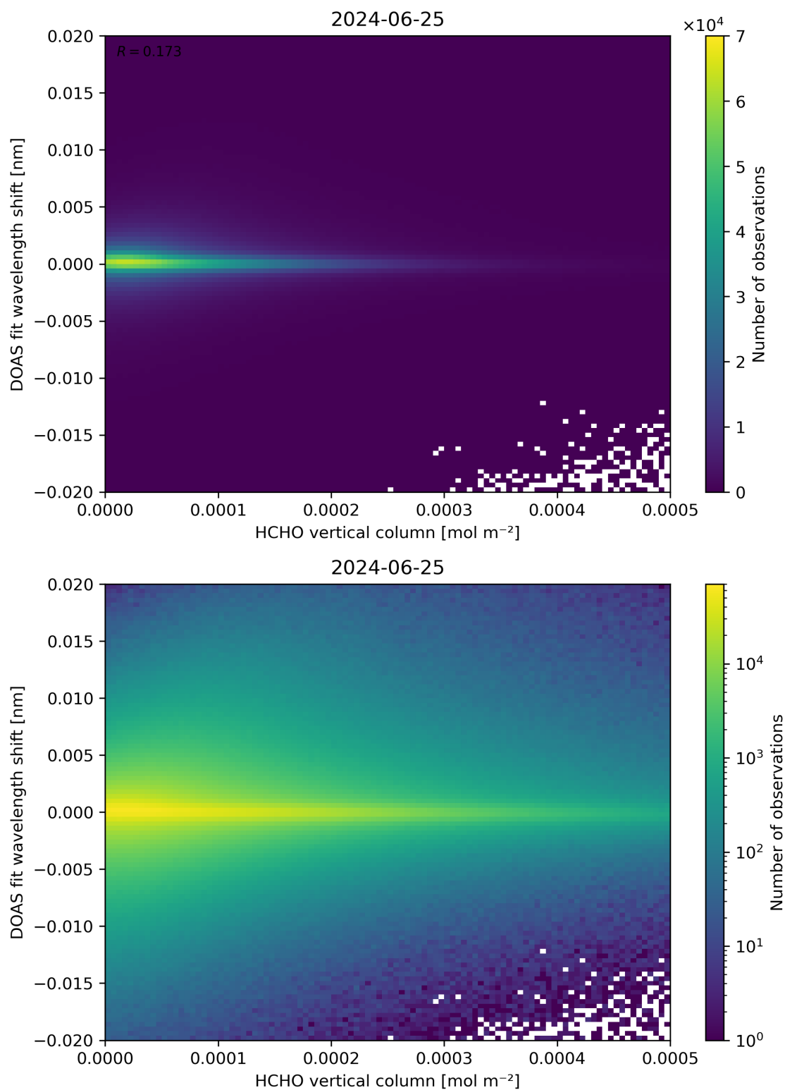
Figure 124: Scatter density plot of “HCHO vertical column” against “DOAS fit wavelength shift” for 2024-06-24 to 2024-06-26.
