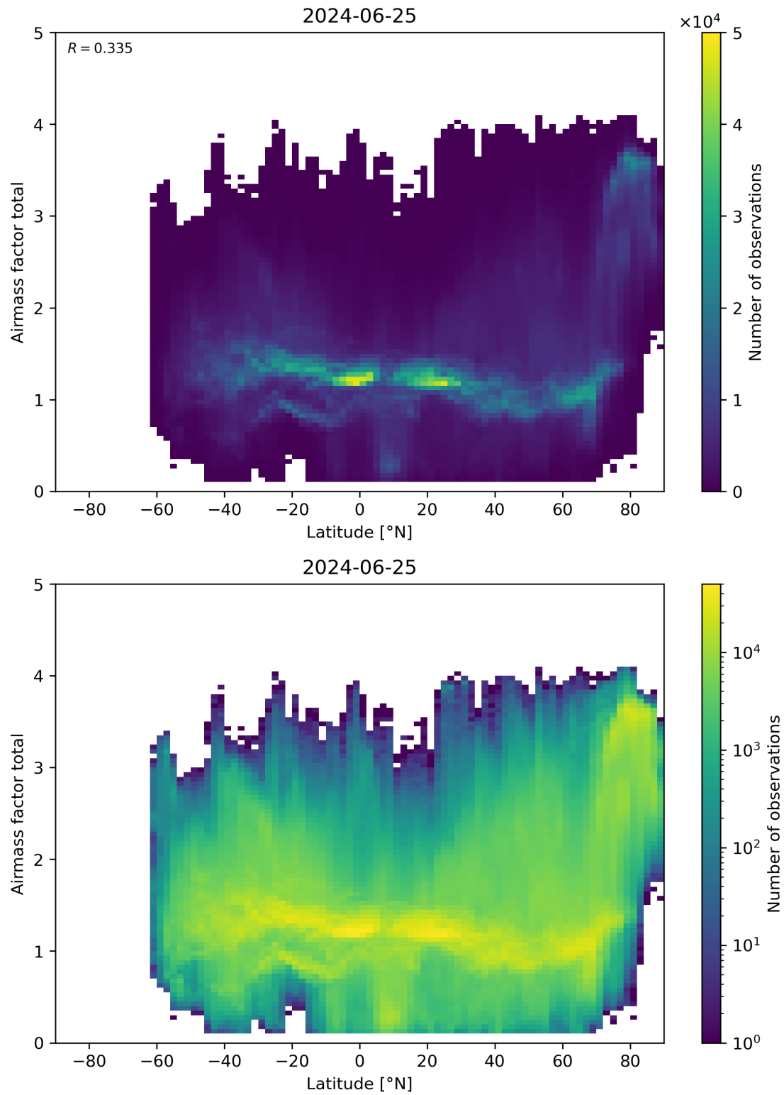
Figure 161: Scatter density plot of “Latitude” against “Airmass factor total” for 2024-06-24 to 2024-06-26.
