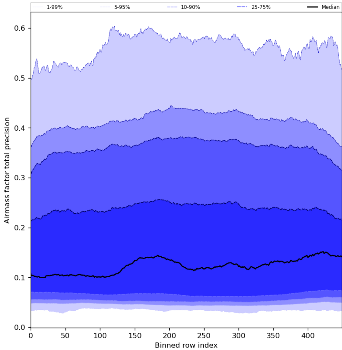
Figure 55: Along track statistics of “Airmass factor total precision” for 2024-06-24 to 2024-06-26
