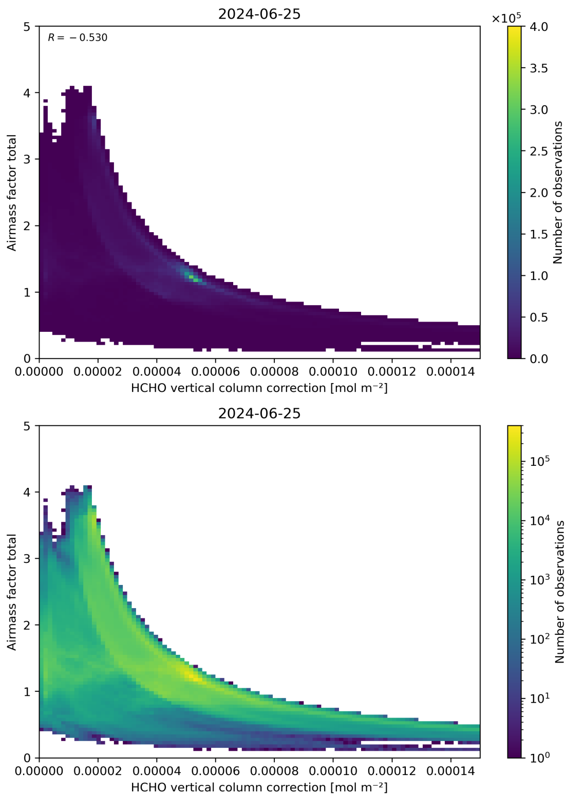
Figure 120: Scatter density plot of “HCHO vertical column correction” against “Airmass factor total” for 2024-06-24 to 2024-06-26.
