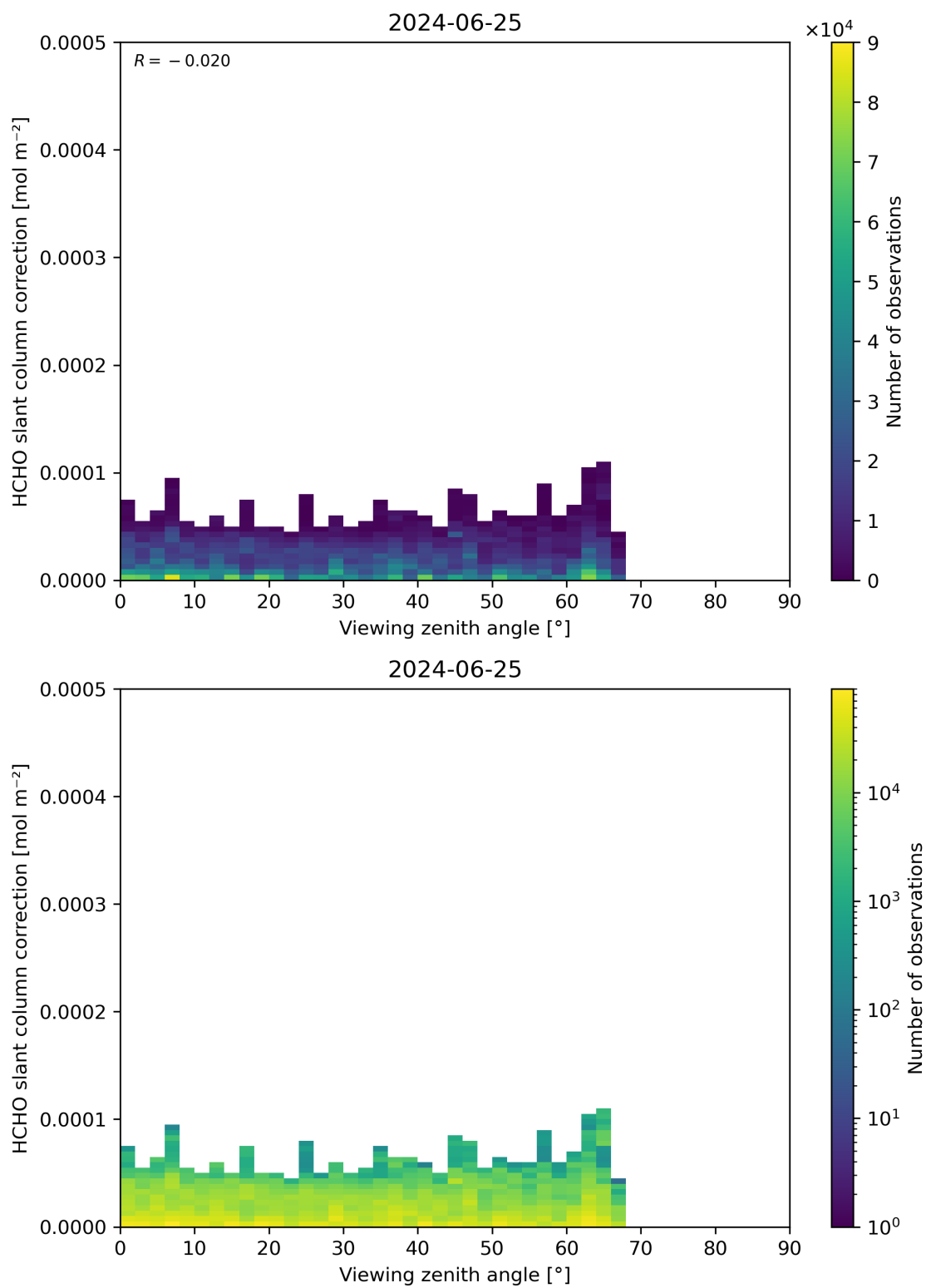
Figure 187: Scatter density plot of “Viewing zenith angle” against “HCHO slant column correction” for 2024-06-24 to 2024-06-26.
