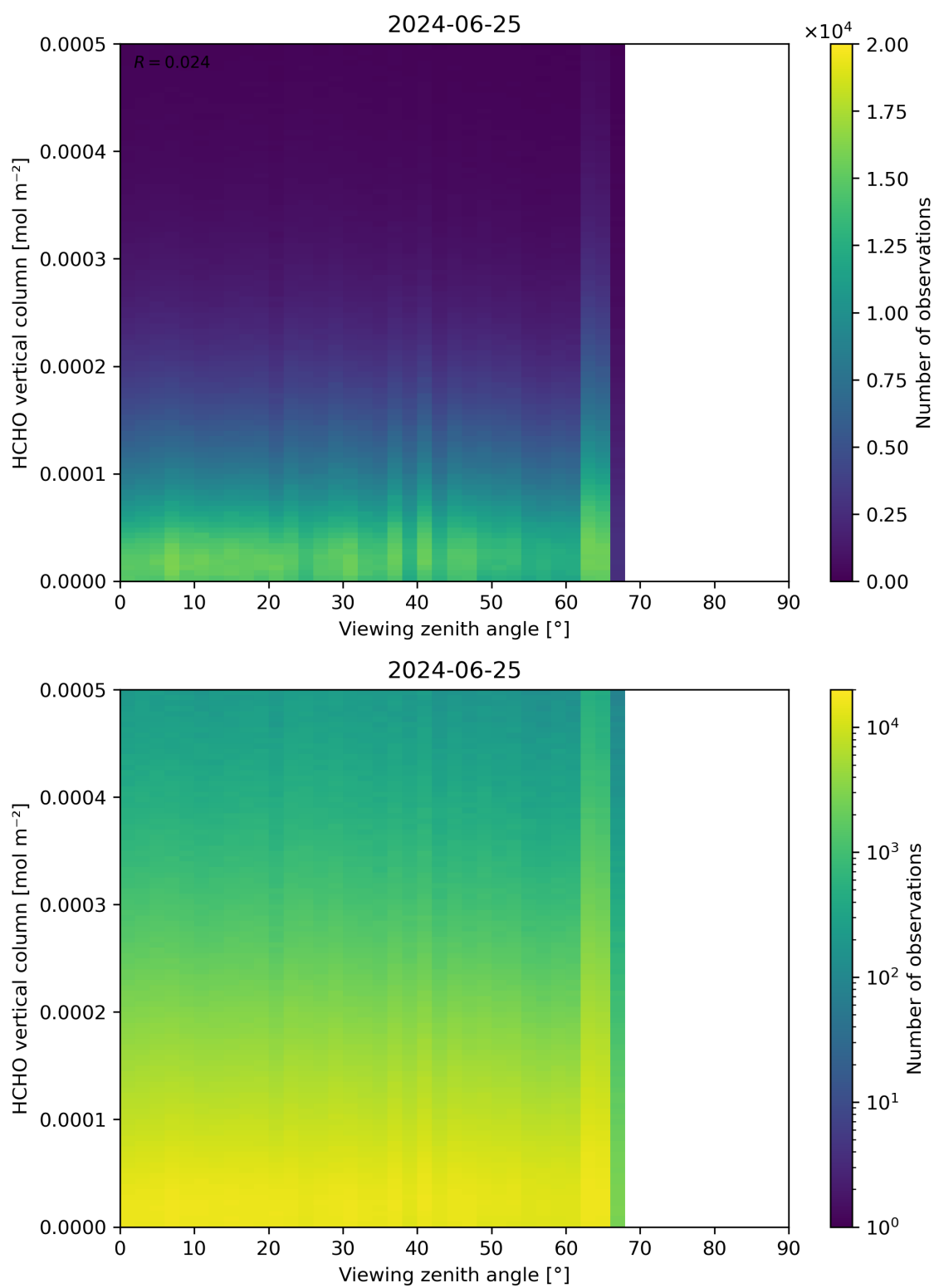
Figure 192: Scatter density plot of “Viewing zenith angle” against “HCHO vertical column” for 2024-06-24 to 2024-06-26.
