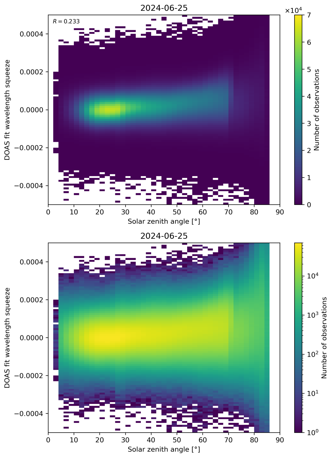
Figure 169: Scatter density plot of “Solar zenith angle” against “DOAS fit wavelength squeeze” for 2024-06-24 to 2024-06-26.
