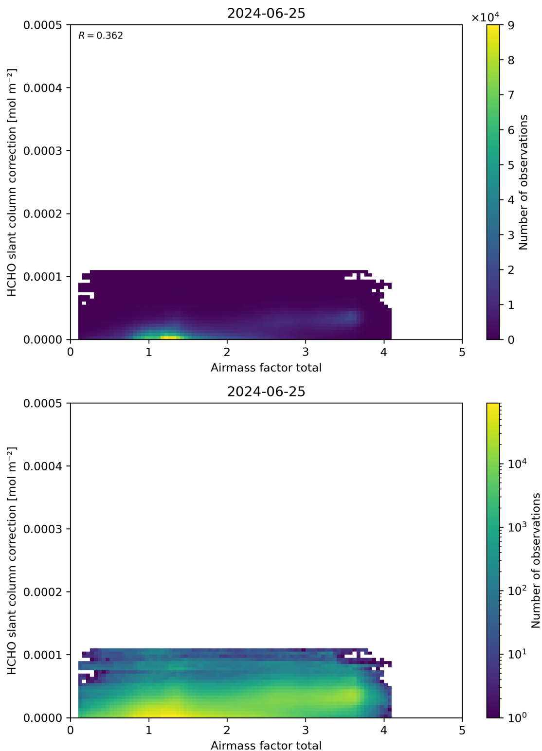
Figure 102: Scatter density plot of “Airmass factor total” against “HCHO slant column correction” for 2024-06-24 to 2024-06-26.
