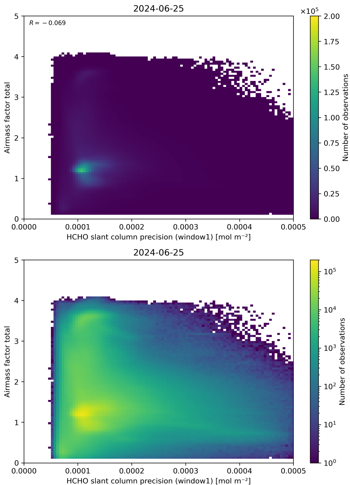
Figure 94: Scatter density plot of “HCHO slant column precision (window1)” against “Airmass factor total” for 2024-06-24 to 2024-06-26.
