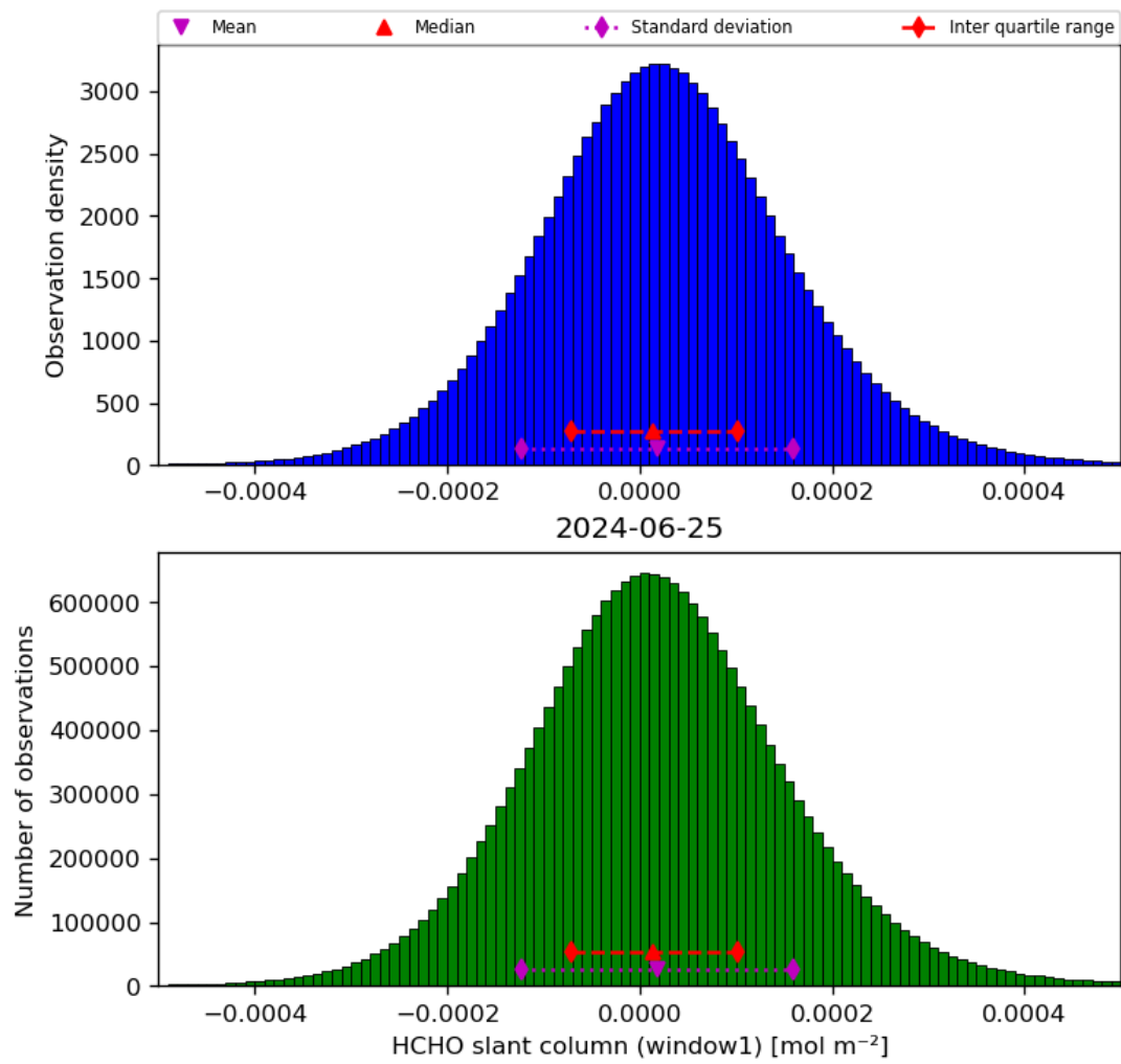
Figure 38: Histogram of “HCHO slant column (window1)” for 2024-06-24 to 2024-06-26
