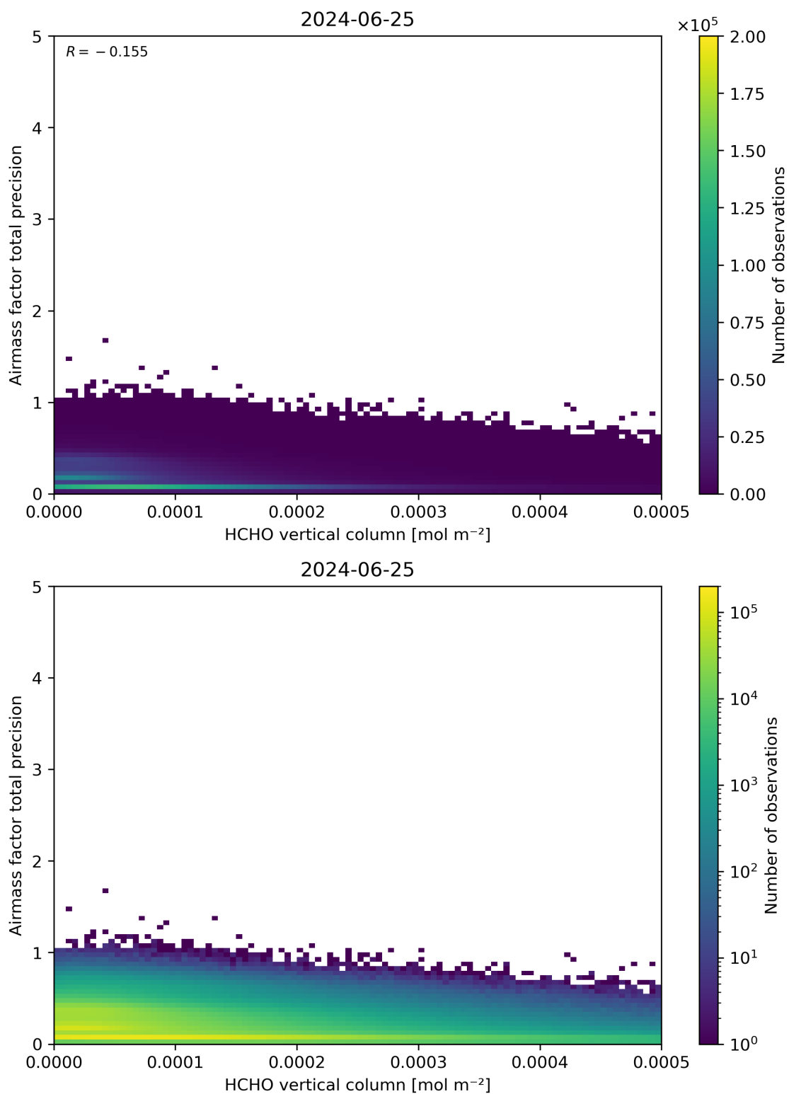
Figure 132: Scatter density plot of “HCHO vertical column” against “Airmass factor total precision” for 2024-06-24 to 2024-06-26.
