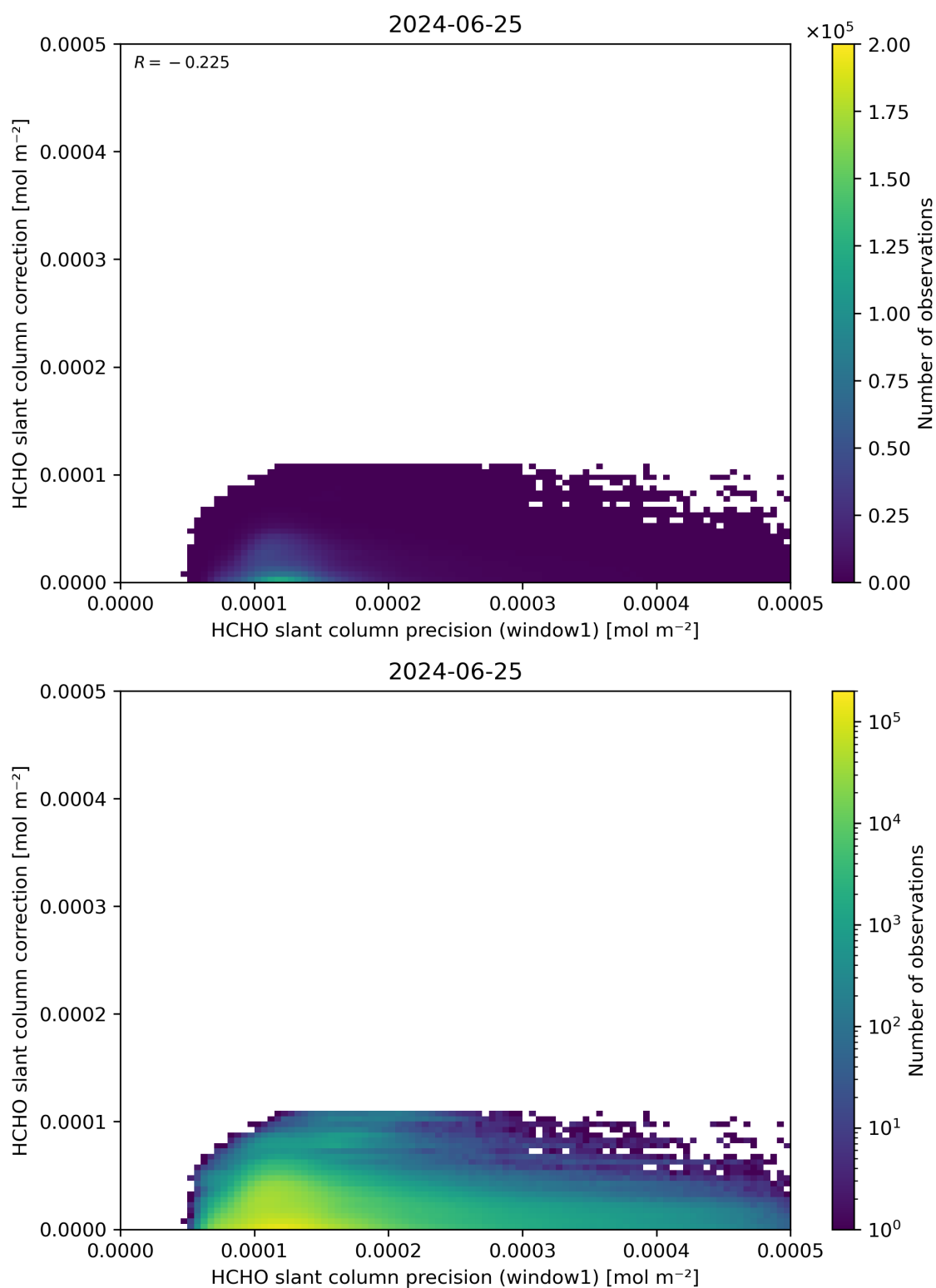
Figure 93: Scatter density plot of “HCHO slant column precision (window1)” against “HCHO slant column correction” for 2024-06-24 to 2024-06-26.
