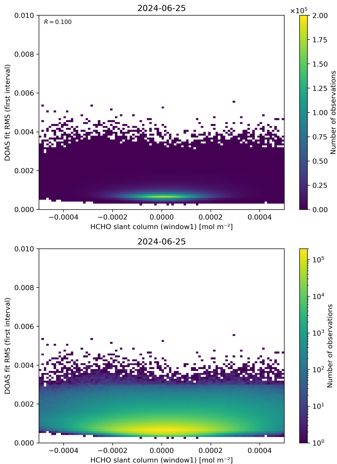
Figure 78: Scatter density plot of “HCHO slant column (window1)” against “DOAS fit RMS (first interval)” for 2024-06-24 to 2024-06-26.
