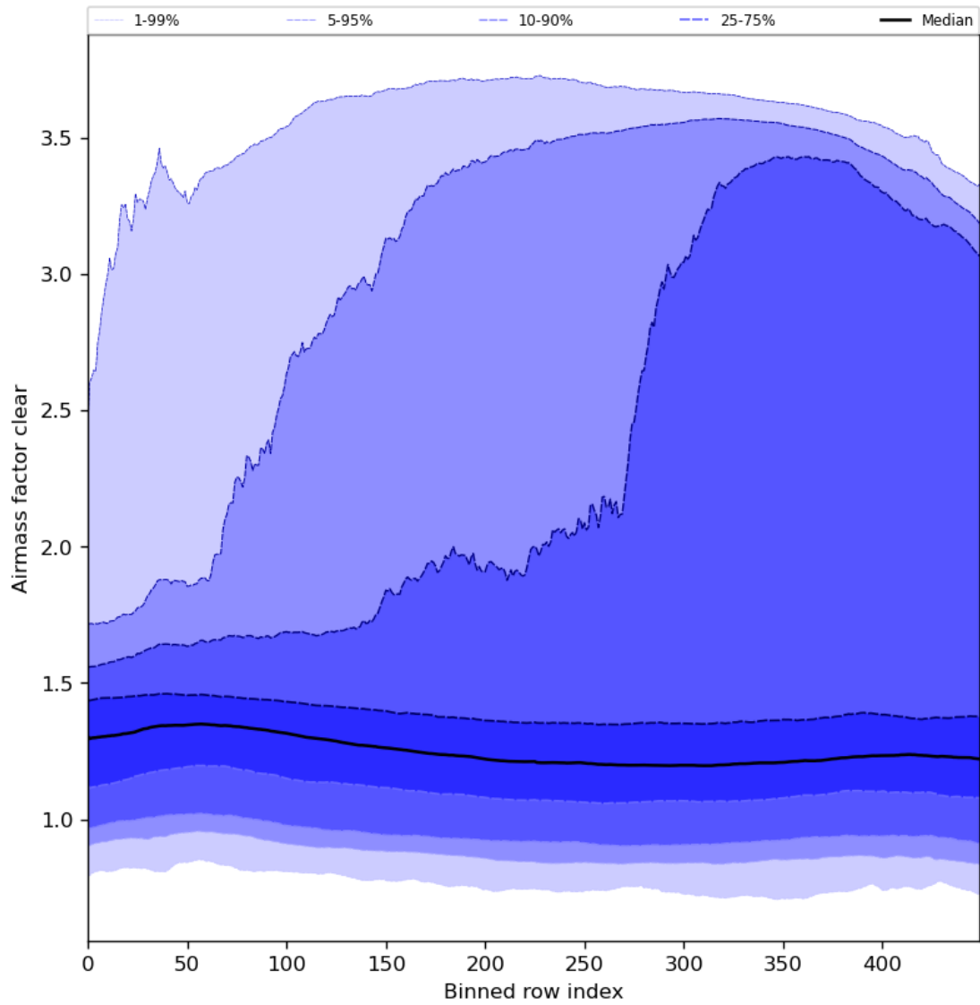
Figure 56: Along track statistics of “Airmass factor clear” for 2024-06-24 to 2024-06-26
