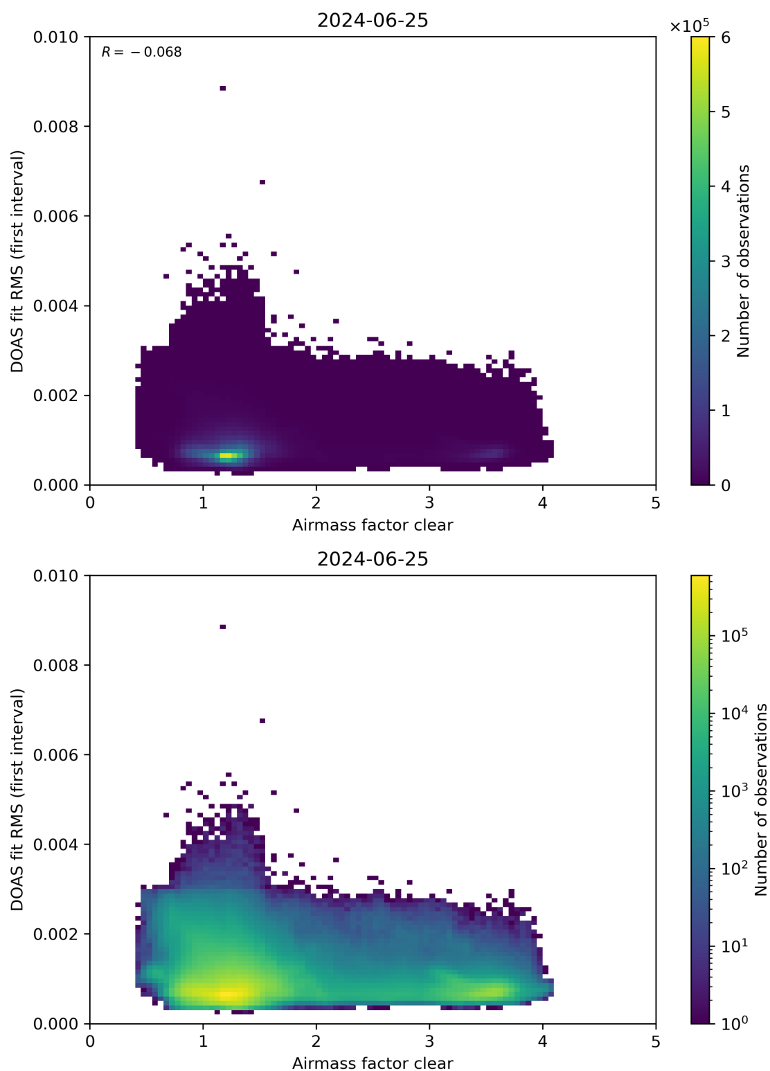
Figure 71: Scatter density plot of “Airmass factor clear” against “DOAS fit RMS (first interval)” for 2024-06-24 to 2024-06-26.
