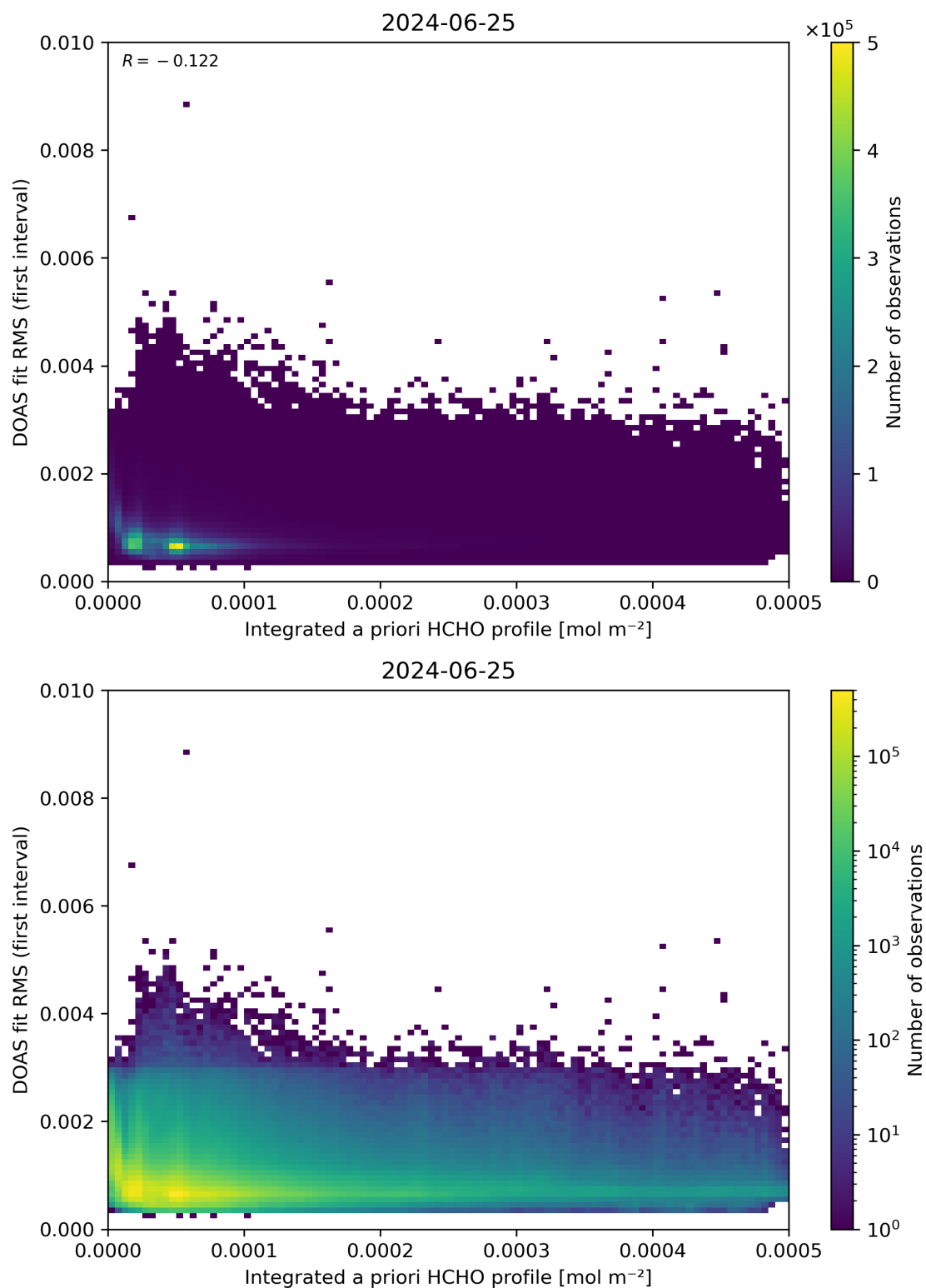
Figure 148: Scatter density plot of “Integrated a priori HCHO profile” against “DOAS fit RMS (first interval)” for 2024-06-24 to 2024-06-26.
