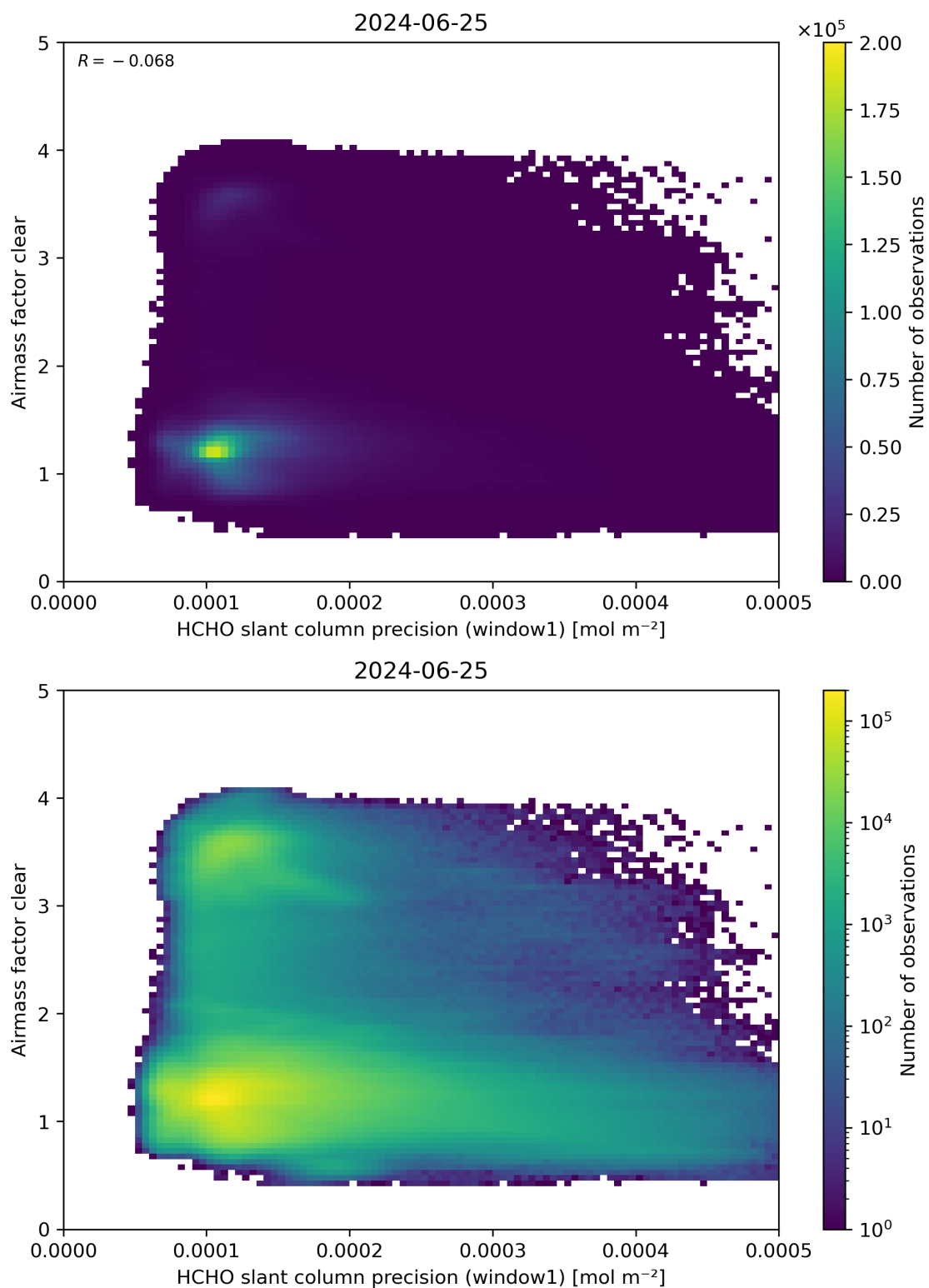
Figure 91: Scatter density plot of “HCHO slant column precision (window1)” against “Airmass factor clear” for 2024-06-24 to 2024-06-26.
