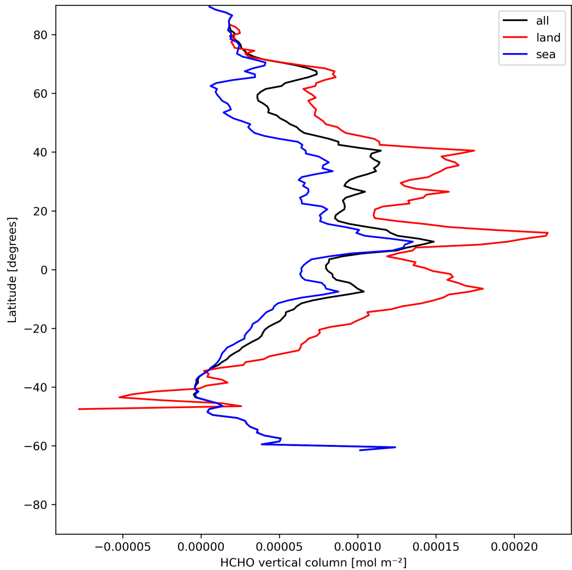
Figure 21: Zonal average of “HCHO vertical column” for 2024-06-24 to 2024-06-26.
