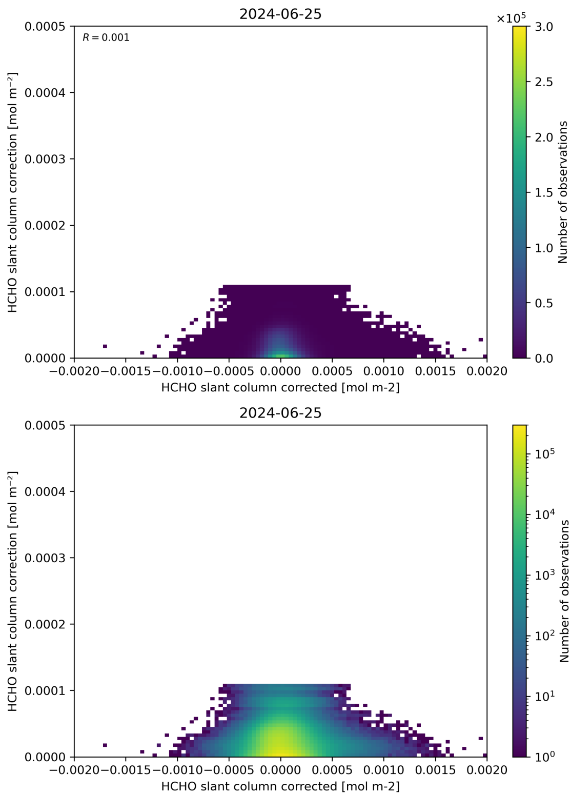
Figure 77: Scatter density plot of “HCHO slant column corrected” against “HCHO slant column correction” for 2024-06-24 to 2024-06-26.
