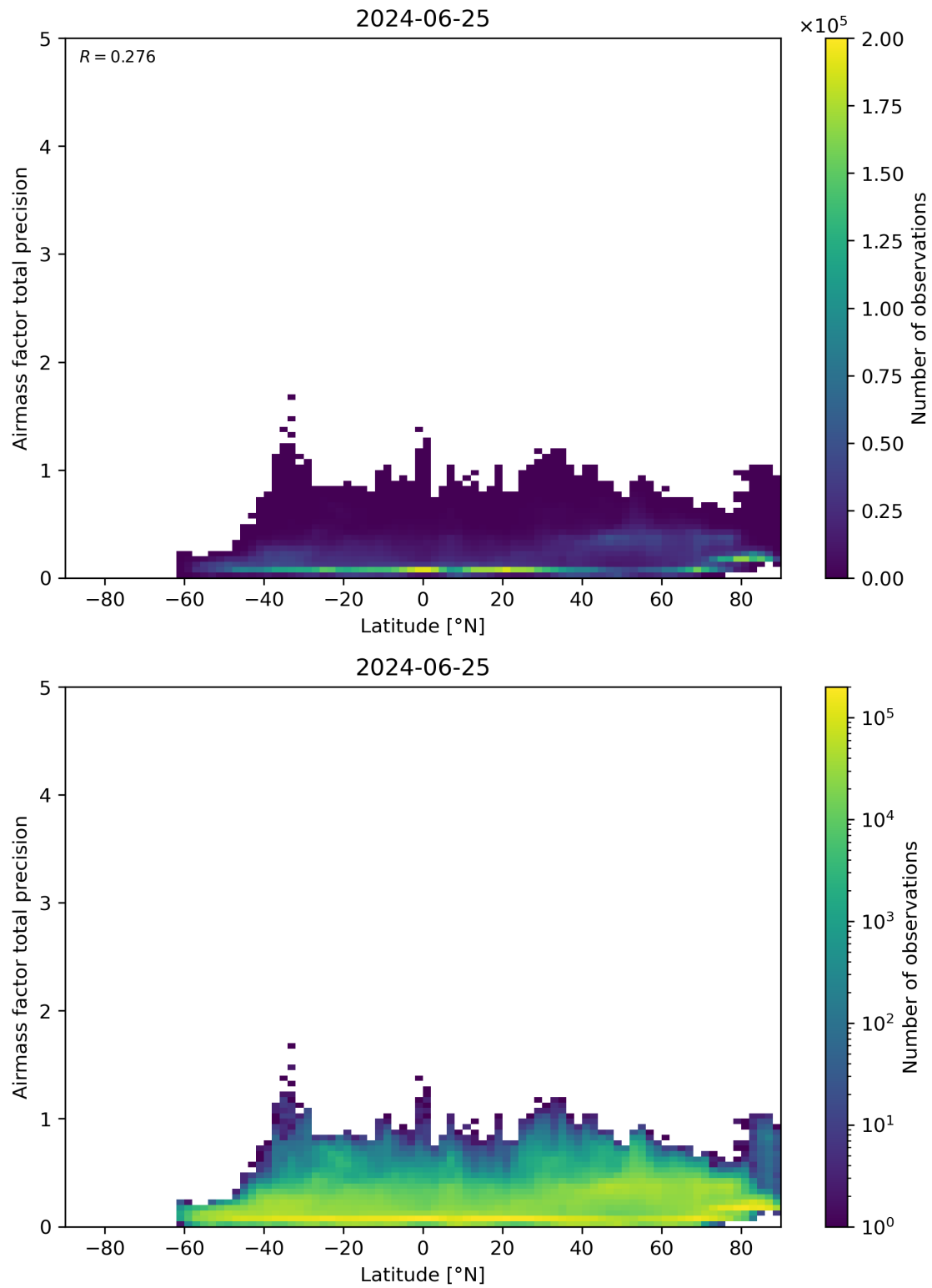
Figure 162: Scatter density plot of “Latitude” against “Airmass factor total precision” for 2024-06-24 to 2024-06-26.
