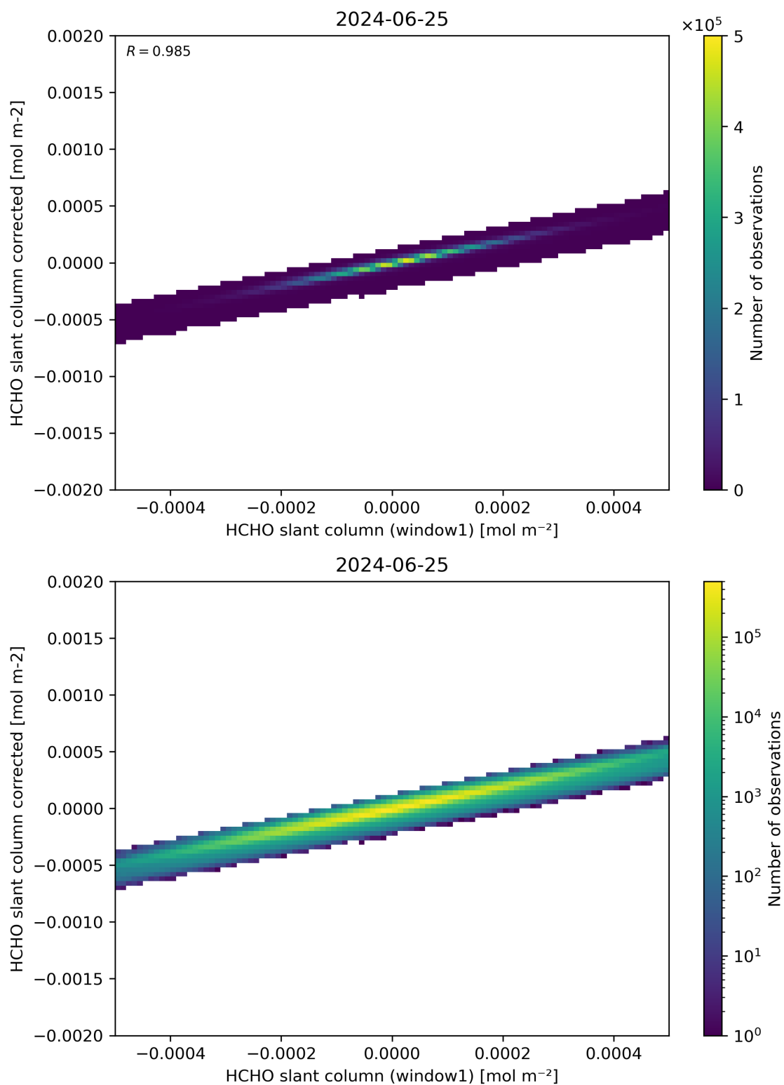
Figure 82: Scatter density plot of “HCHO slant column (window1)” against “HCHO slant column corrected” for 2024-06-24 to 2024-06-26.
