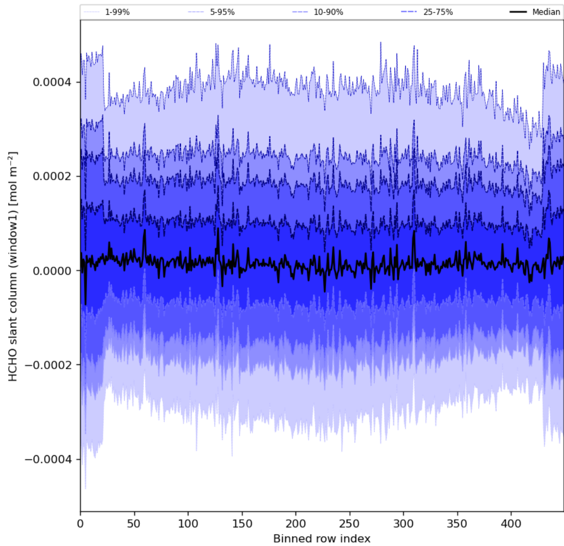
Figure 52: Along track statistics of “HCHO slant column (window1)” for 2024-06-24 to 2024-06-26
