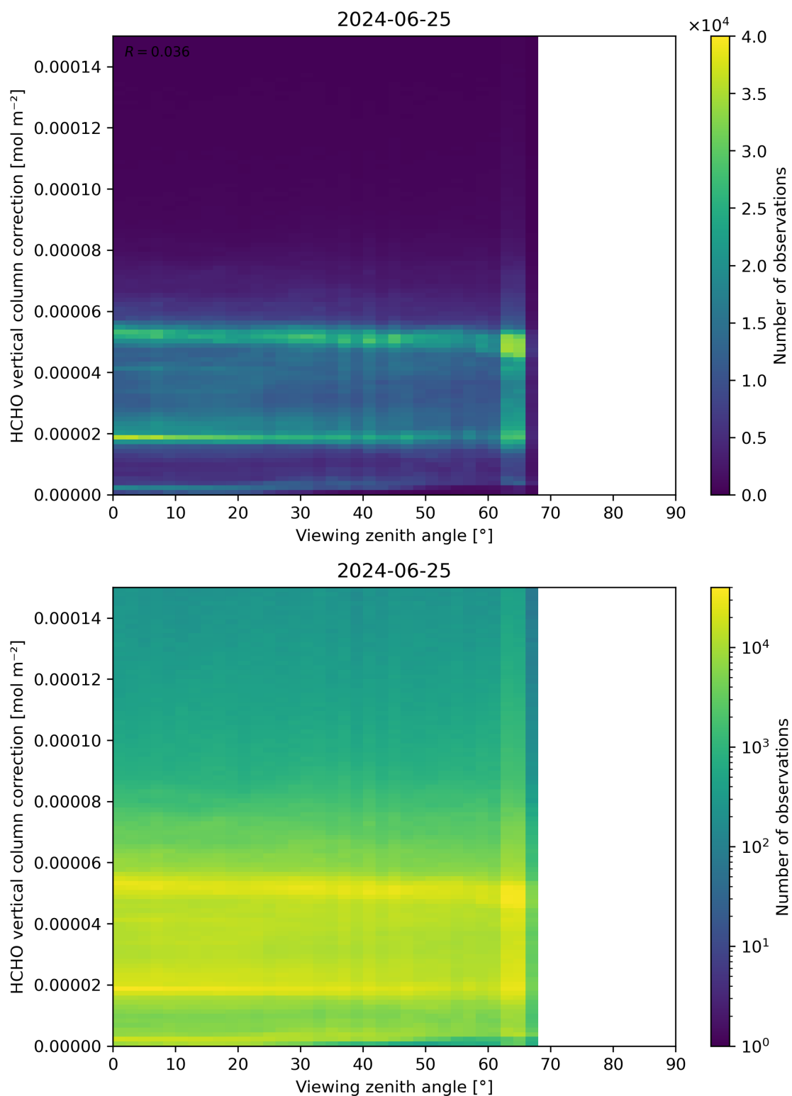
Figure 193: Scatter density plot of “Viewing zenith angle” against “HCHO vertical column correction” for 2024-06-24 to 2024-06-26.
