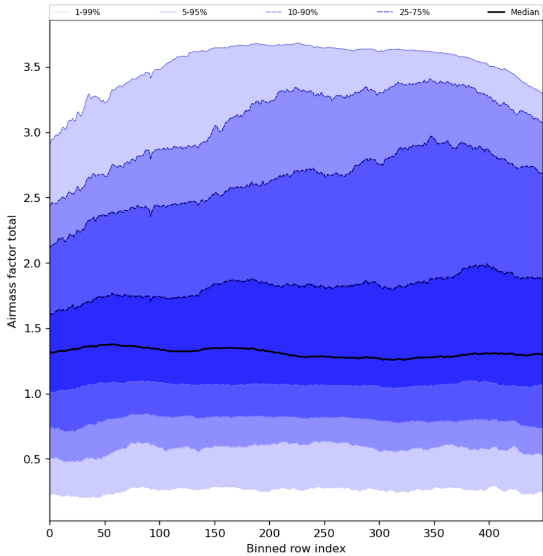
Figure 54: Along track statistics of “Airmass factor total” for 2024-06-24 to 2024-06-26
