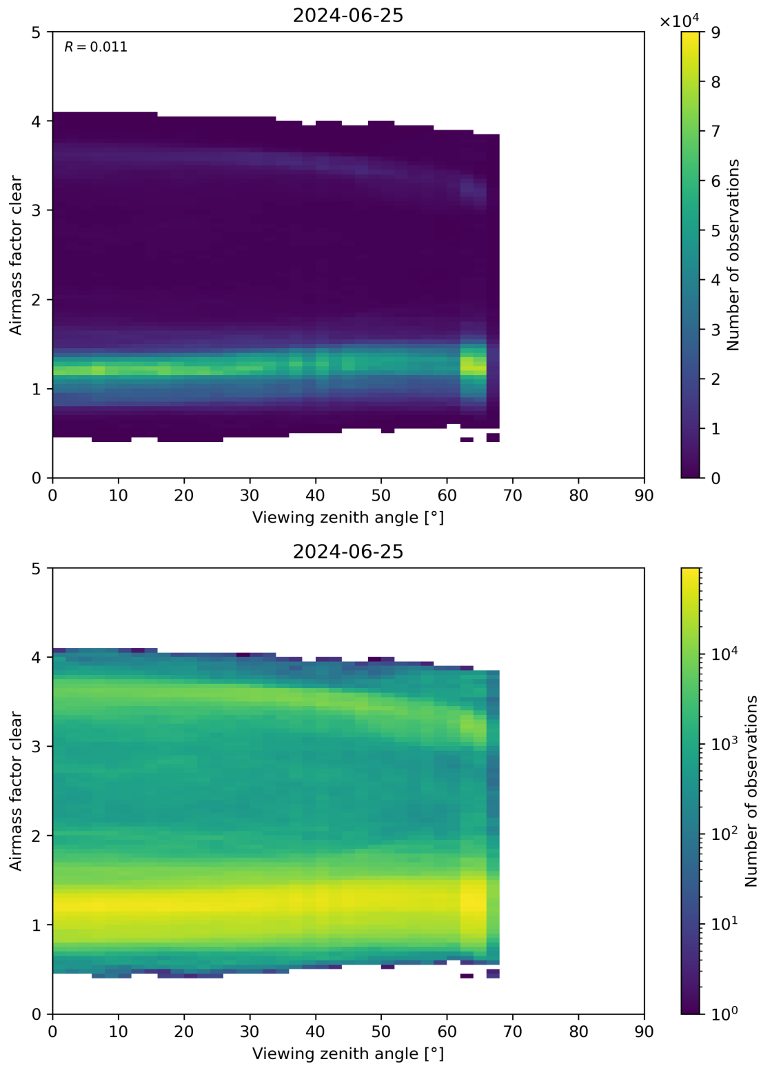
Figure 185: Scatter density plot of “Viewing zenith angle” against “Airmass factor clear” for 2024-06-24 to 2024-06-26.
