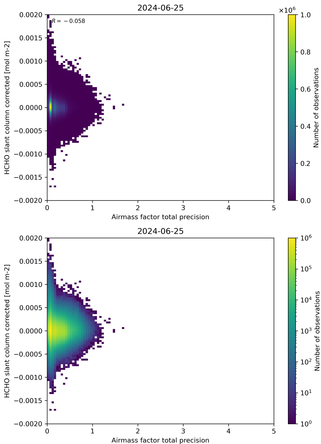
Figure 109: Scatter density plot of “Airmass factor total precision” against “HCHO slant column corrected” for 2024-06-24 to 2024-06-26.
