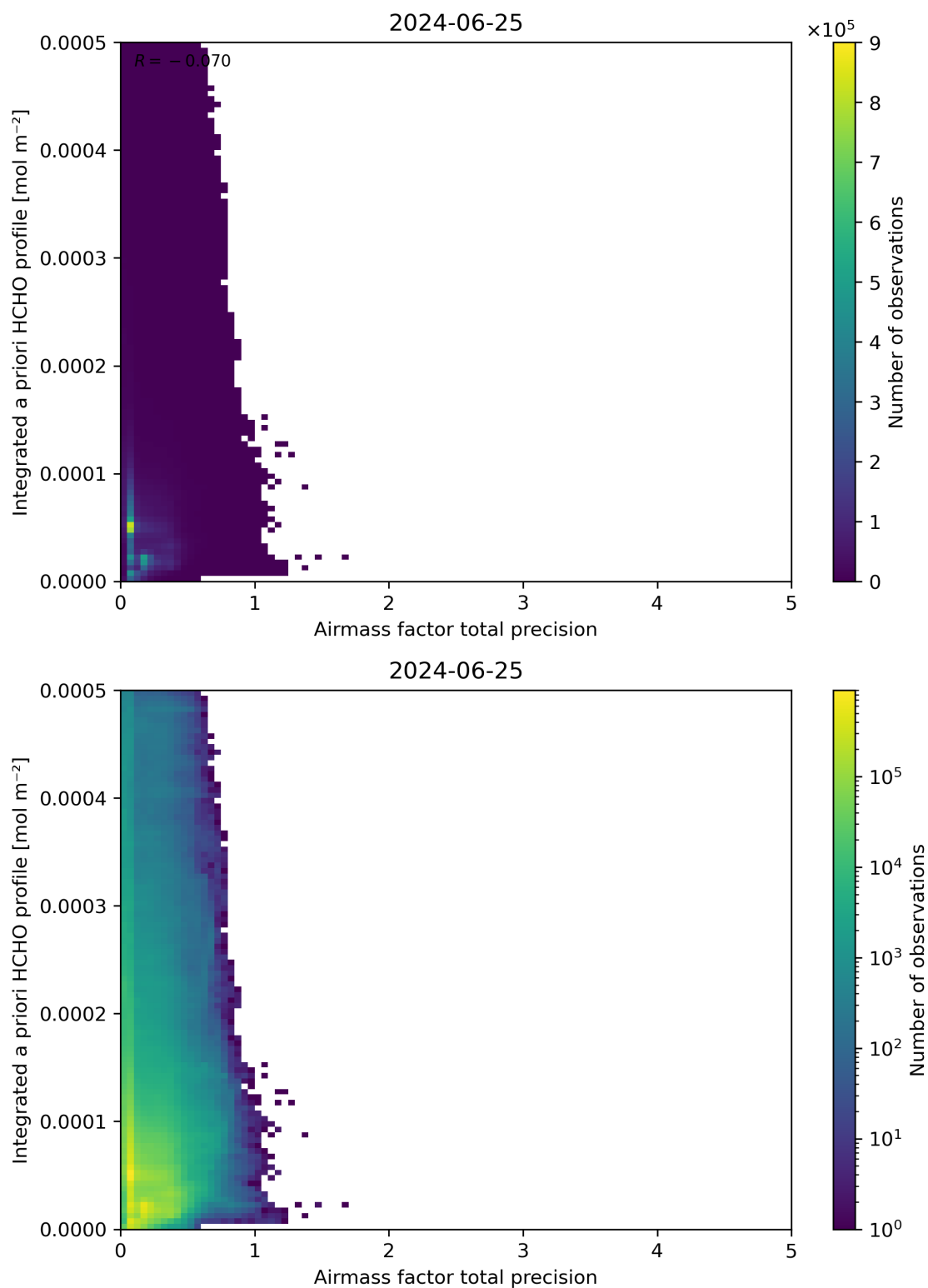
Figure 111: Scatter density plot of “Airmass factor total precision” against “Integrated a priori HCHO profile” for 2024-06-24 to 2024-06-26.
