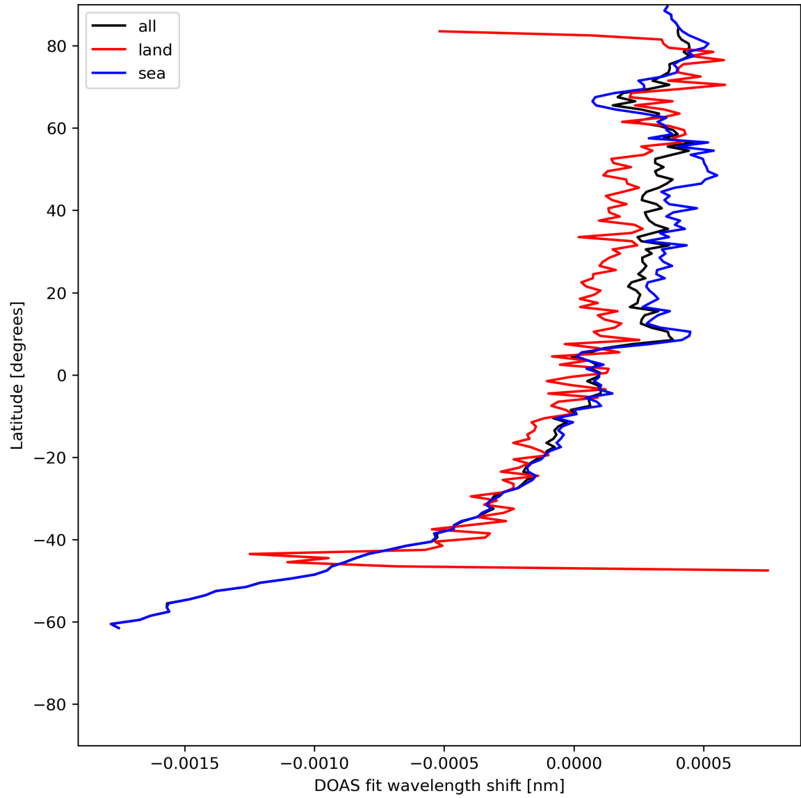
Figure 30: Zonal average of “DOAS fit wavelength shift” for 2024-06-24 to 2024-06-26.
