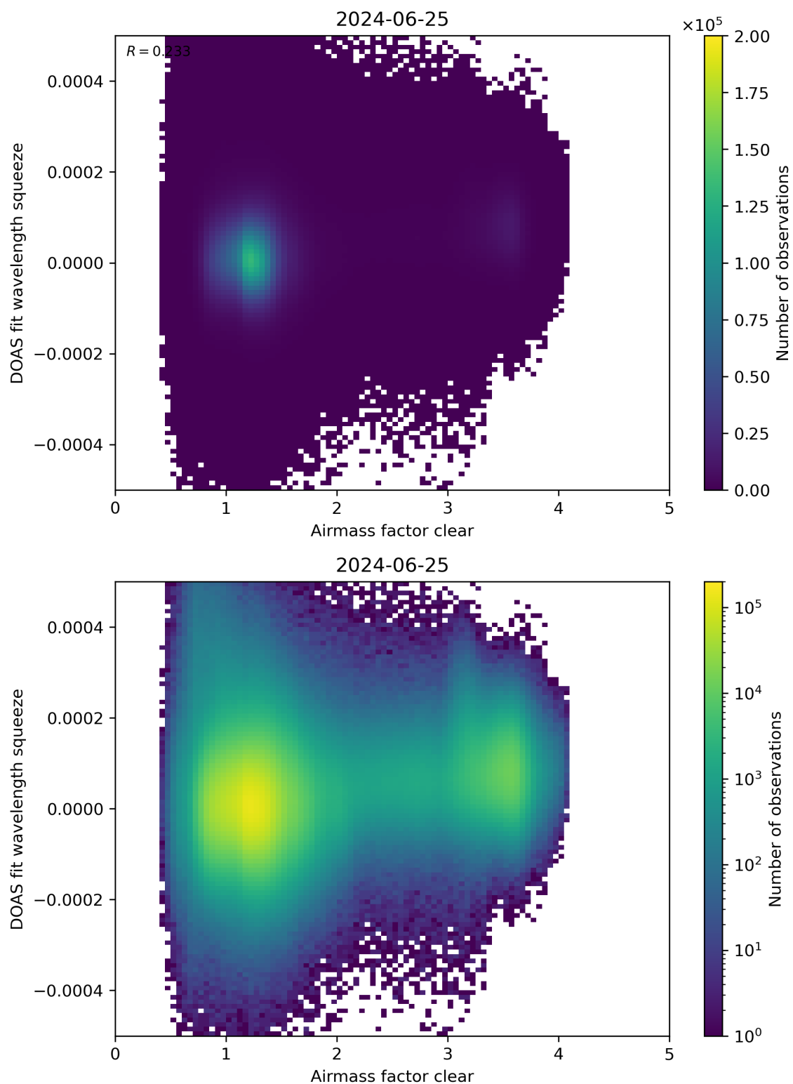
Figure 73: Scatter density plot of “Airmass factor clear” against “DOAS fit wavelength squeeze” for 2024-06-24 to 2024-06-26.
