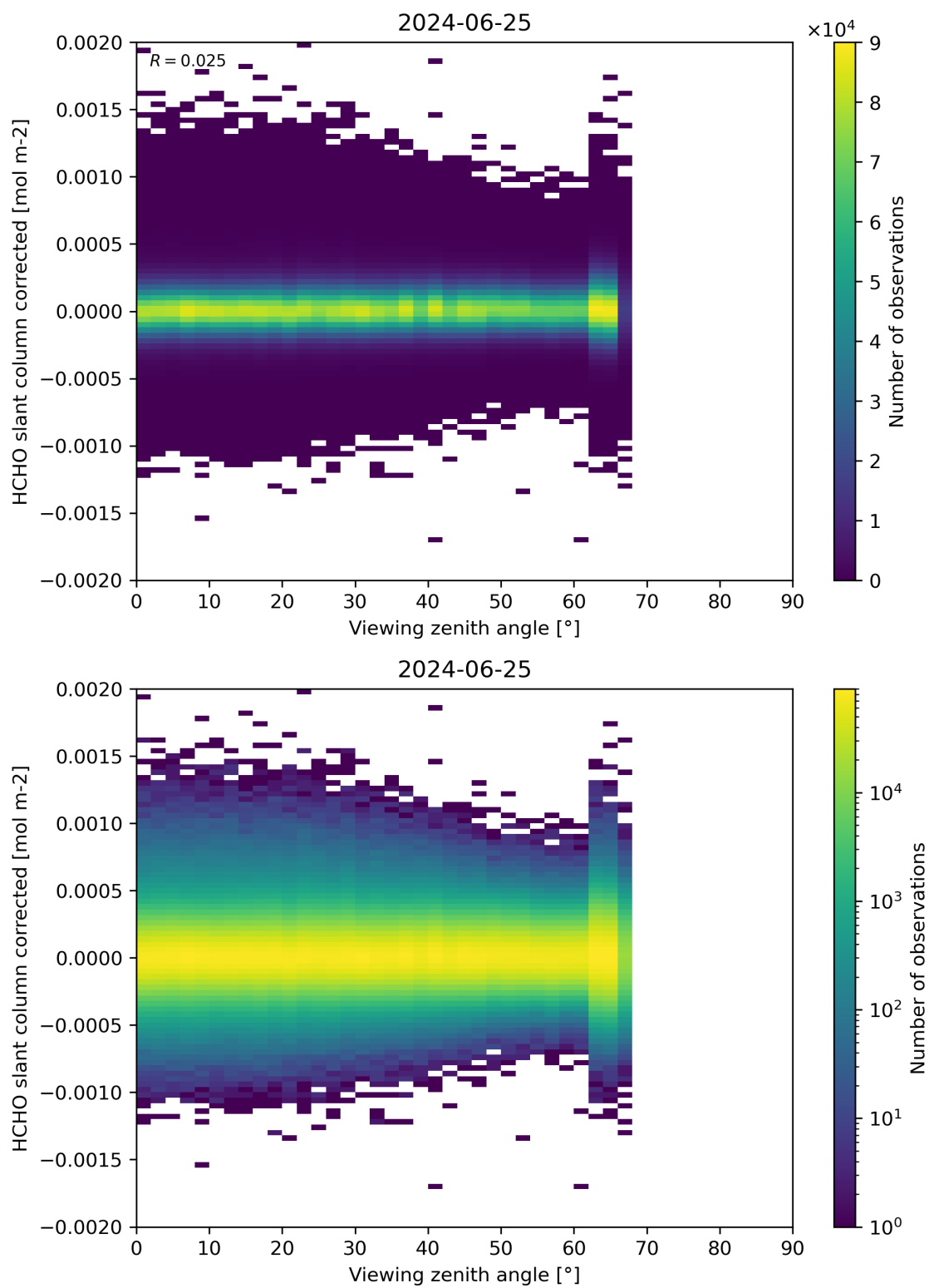
Figure 186: Scatter density plot of “Viewing zenith angle” against “HCHO slant column corrected” for 2024-06-24 to 2024-06-26.
