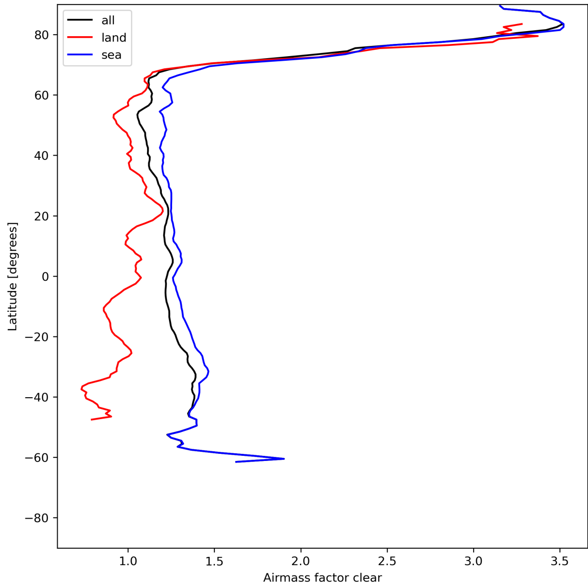
Figure 28: Zonal average of “Airmass factor clear” for 2024-06-24 to 2024-06-26.
