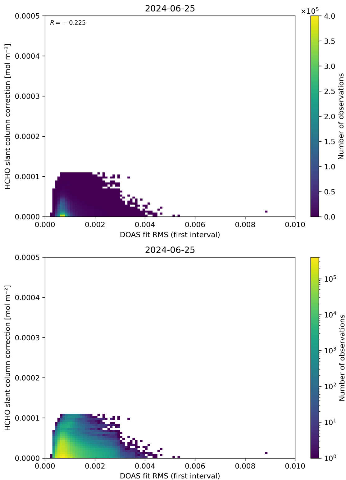
Figure 63: Scatter density plot of “DOAS fit RMS (first interval)” against “HCHO slant column correction” for 2024-06-24 to 2024-06-26.
