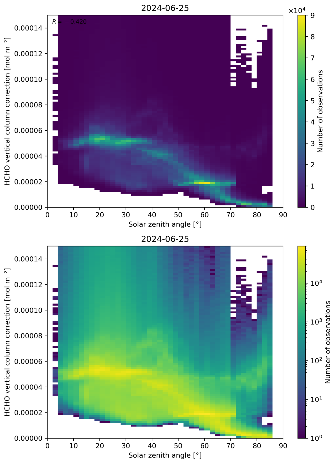
Figure 178: Scatter density plot of “Solar zenith angle” against “HCHO vertical column correction” for 2024-06-24 to 2024-06-26.
