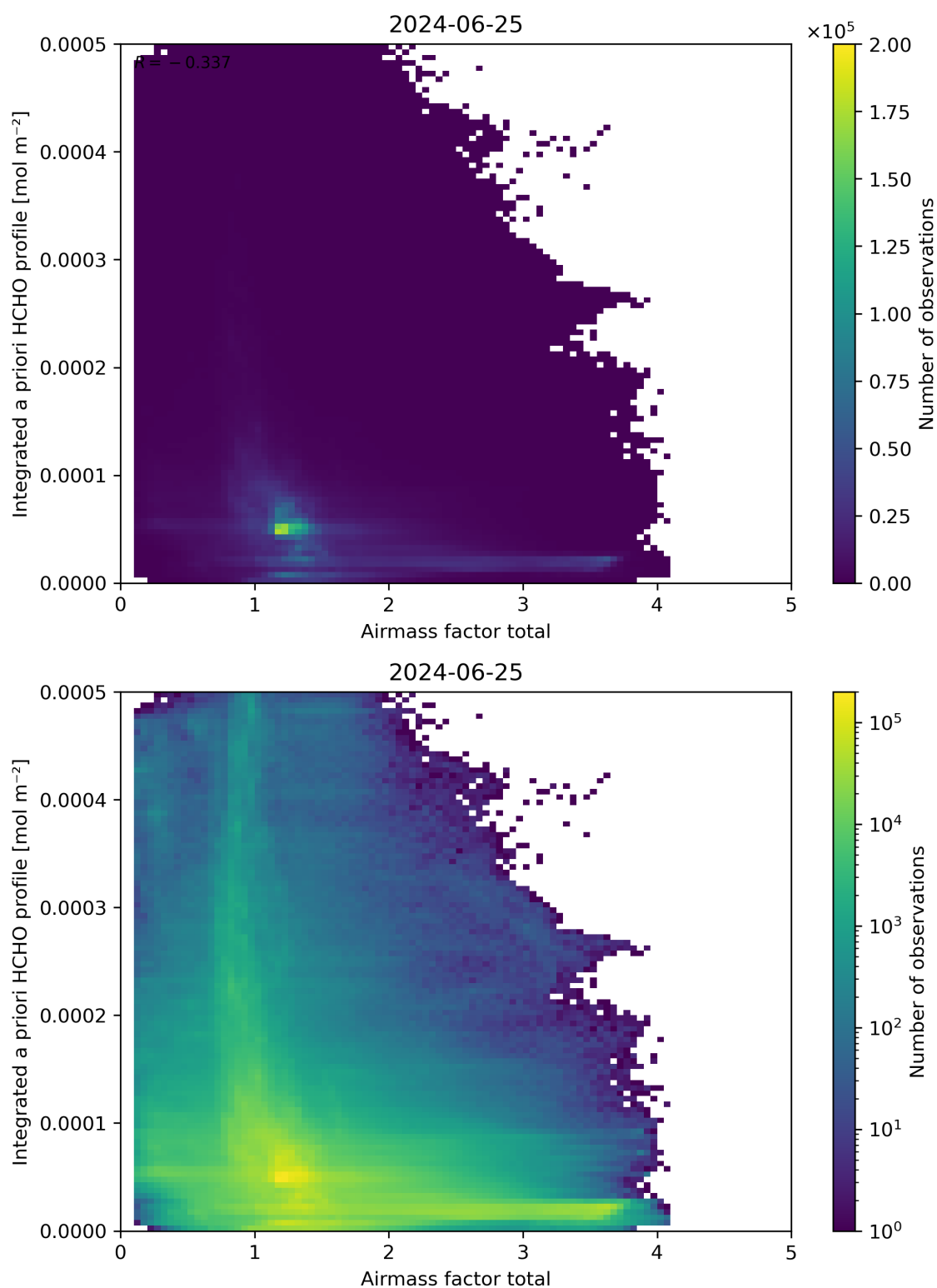
Figure 104: Scatter density plot of “Airmass factor total” against “Integrated a priori HCHO profile” for 2024-06-24 to 2024-06-26.
