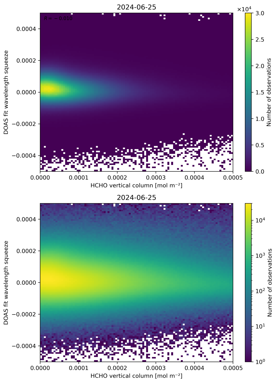
Figure 125: Scatter density plot of “HCHO vertical column” against “DOAS fit wavelength squeeze” for 2024-06-24 to 2024-06-26.
