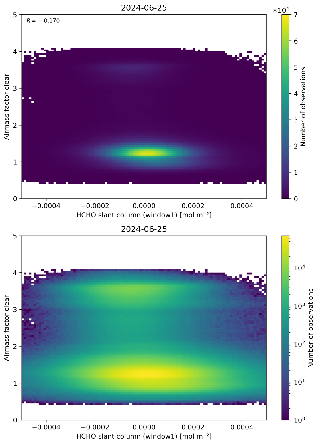
Figure 81: Scatter density plot of “HCHO slant column (window1)” against “Airmass factor clear” for 2024-06-24 to 2024-06-26.
