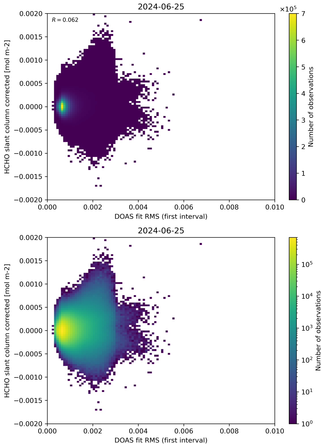
Figure 62: Scatter density plot of “DOAS fit RMS (first interval)” against “HCHO slant column corrected” for 2024-06-24 to 2024-06-26.
