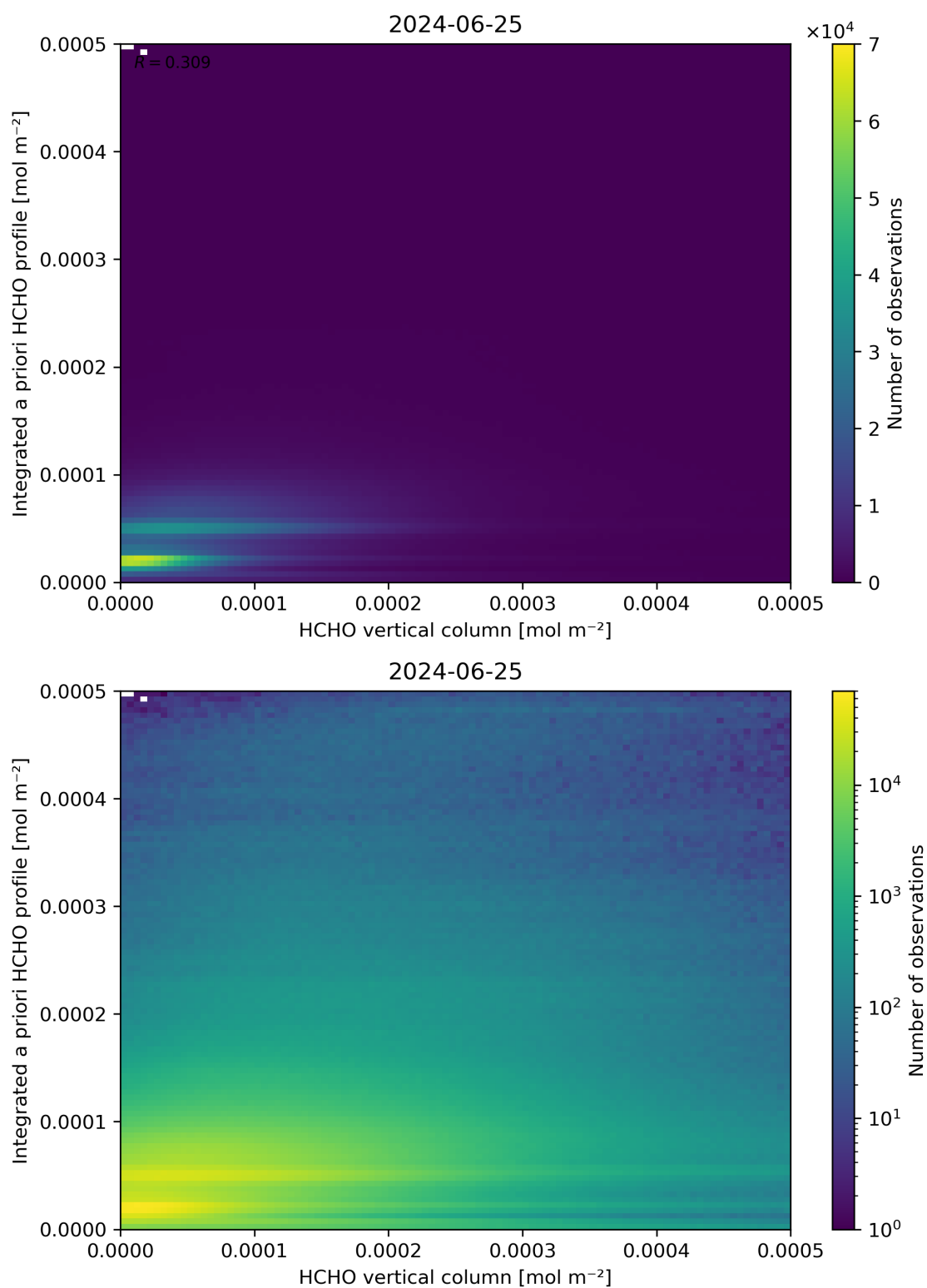
Figure 135: Scatter density plot of “HCHO vertical column” against “Integrated a priori HCHO profile” for 2024-06-24 to 2024-06-26.
