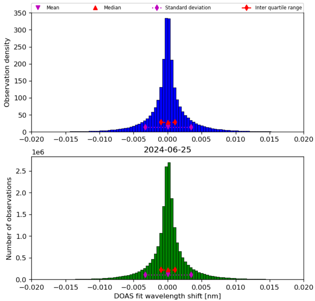
Figure 44: Histogram of “DOAS fit wavelength shift” for 2024-06-24 to 2024-06-26
