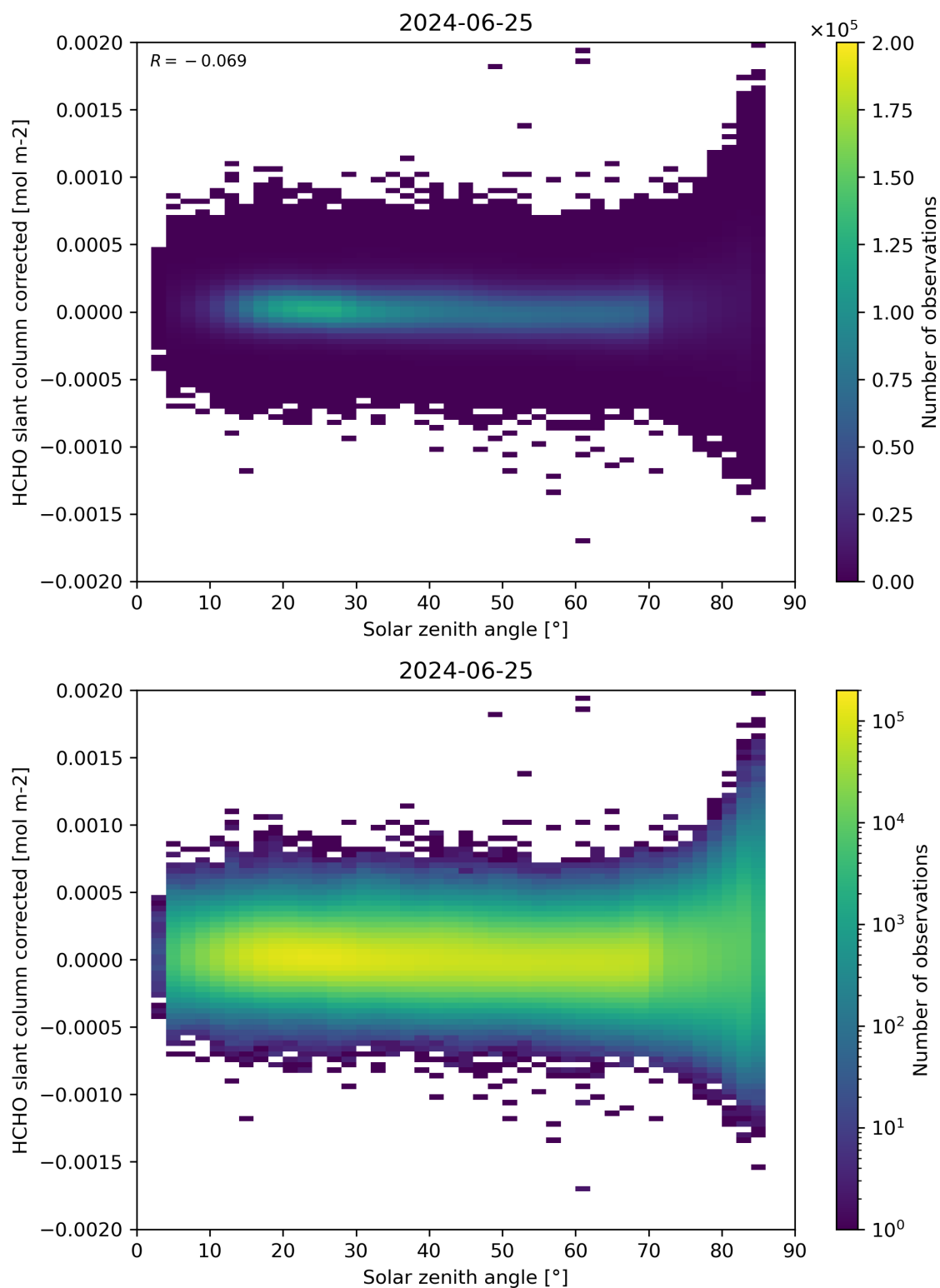
Figure 171: Scatter density plot of “Solar zenith angle” against “HCHO slant column corrected” for 2024-06-24 to 2024-06-26.
