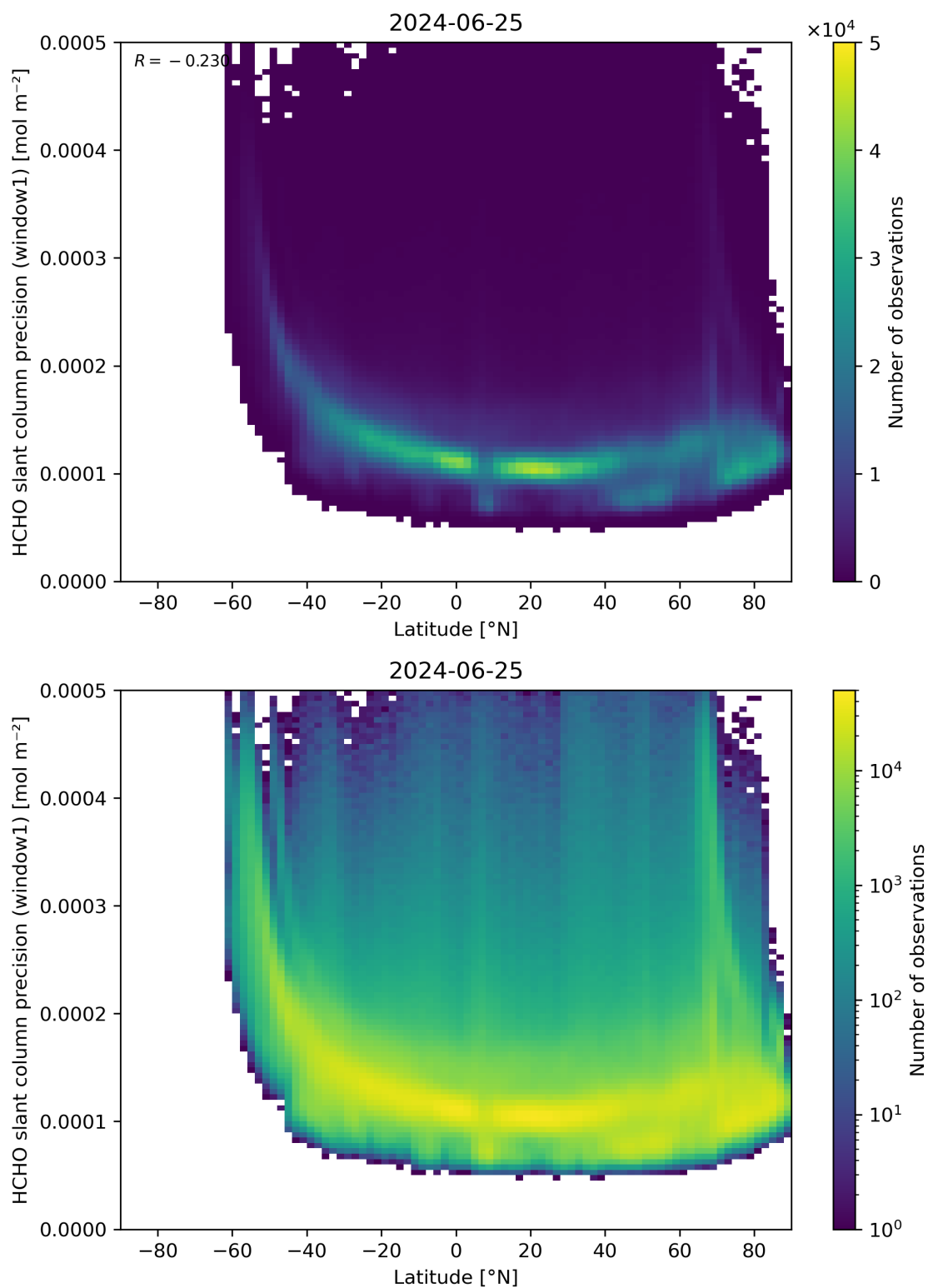
Figure 160: Scatter density plot of “Latitude” against “HCHO slant column precision (window1)” for 2024-06-24 to 2024-06-26.
