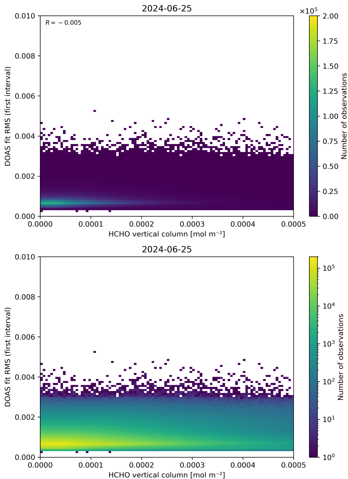
Figure 123: Scatter density plot of “HCHO vertical column” against “DOAS fit RMS (first interval)” for 2024-06-24 to 2024-06-26.
