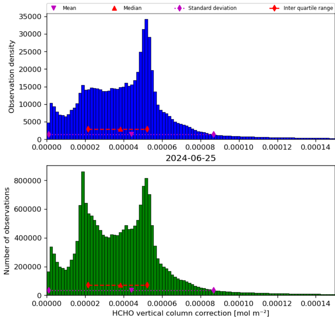
Figure 37: Histogram of “HCHO vertical column correction” for 2024-06-24 to 2024-06-26
