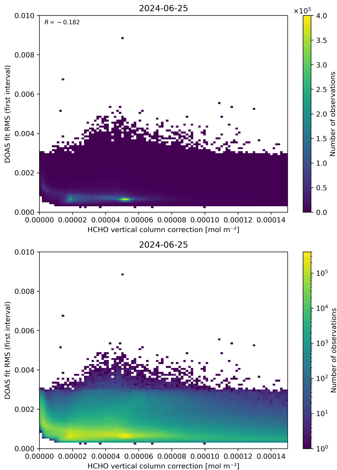
Figure 112: Scatter density plot of “HCHO vertical column correction” against “DOAS fit RMS (first interval)” for 2024-06-24 to 2024-06-26.
