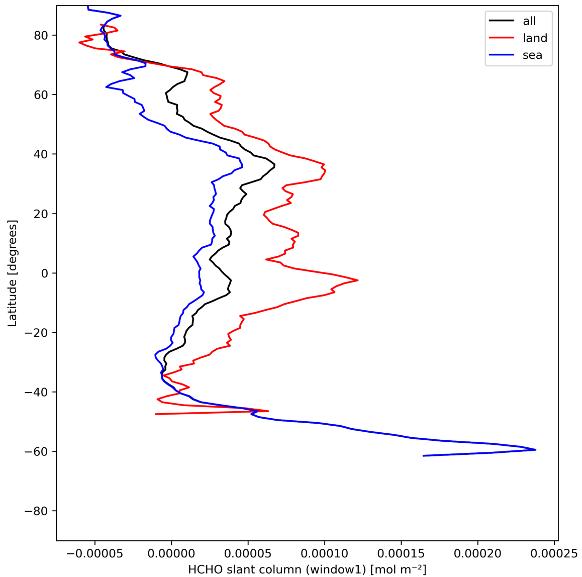
Figure 24: Zonal average of “HCHO slant column (window1)” for 2024-06-24 to 2024-06-26.
