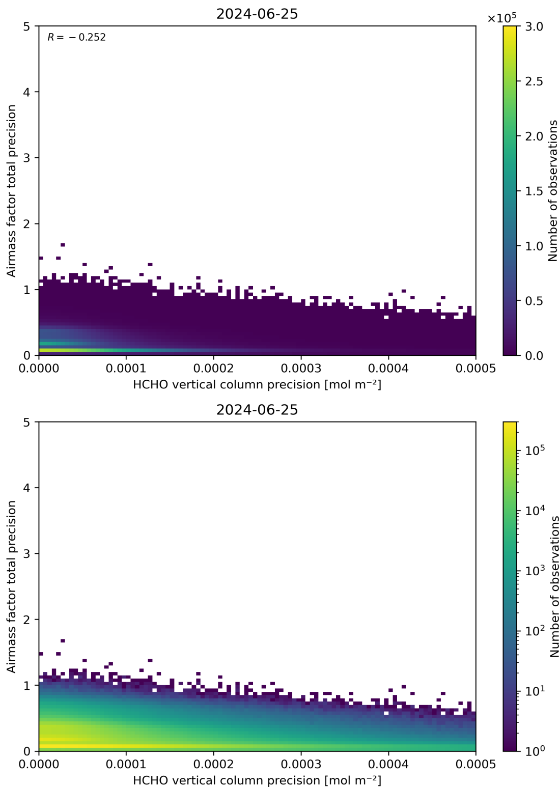
Figure 145: Scatter density plot of “HCHO vertical column precision” against “Airmass factor total precision” for 2024-06-24 to 2024-06-26.
