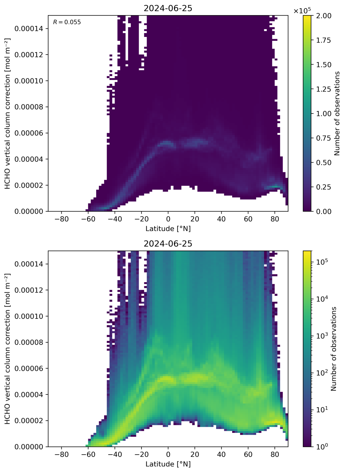
Figure 164: Scatter density plot of “Latitude” against “HCHO vertical column correction” for 2024-06-24 to 2024-06-26.
