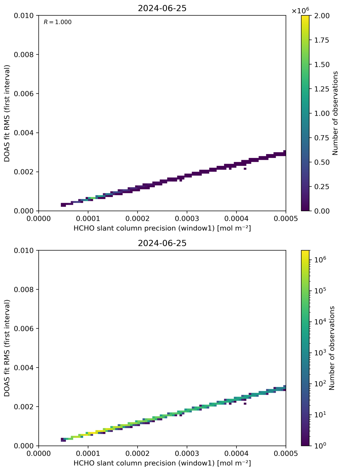
Figure 88: Scatter density plot of “HCHO slant column precision (window1)” against “DOAS fit RMS (first interval)” for 2024-06-24 to 2024-06-26.
