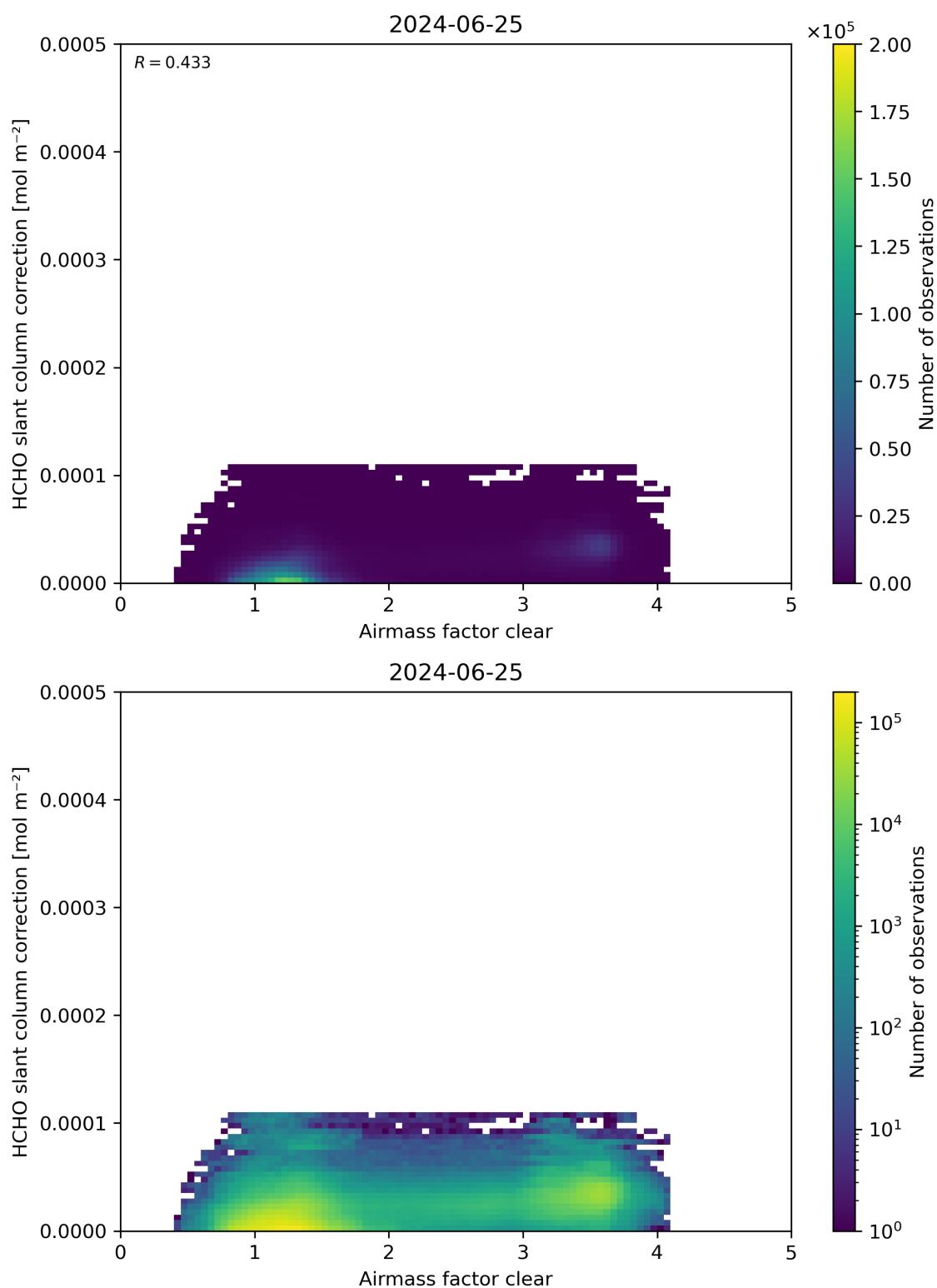
Figure 75: Scatter density plot of “Airmass factor clear” against “HCHO slant column correction” for 2024-06-24 to 2024-06-26.
