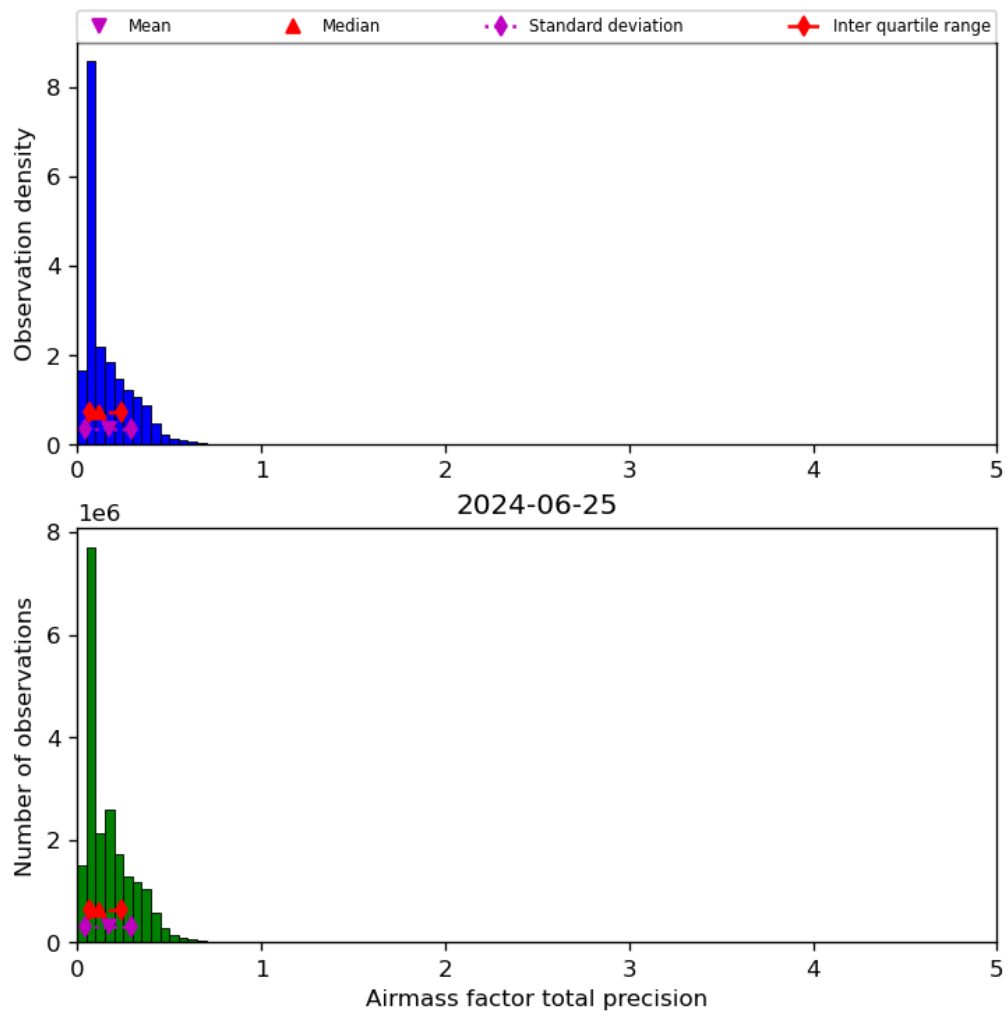
Figure 41: Histogram of “Airmass factor total precision” for 2024-06-24 to 2024-06-26
