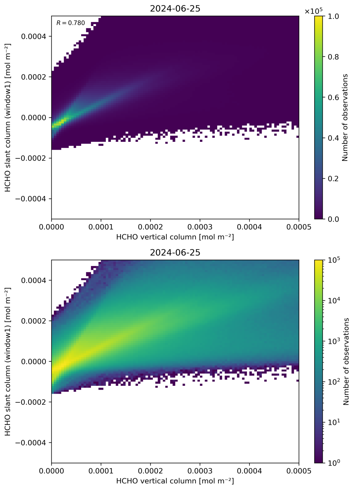
Figure 129: Scatter density plot of “HCHO vertical column” against “HCHO slant column (window1)” for 2024-06-24 to 2024-06-26.
