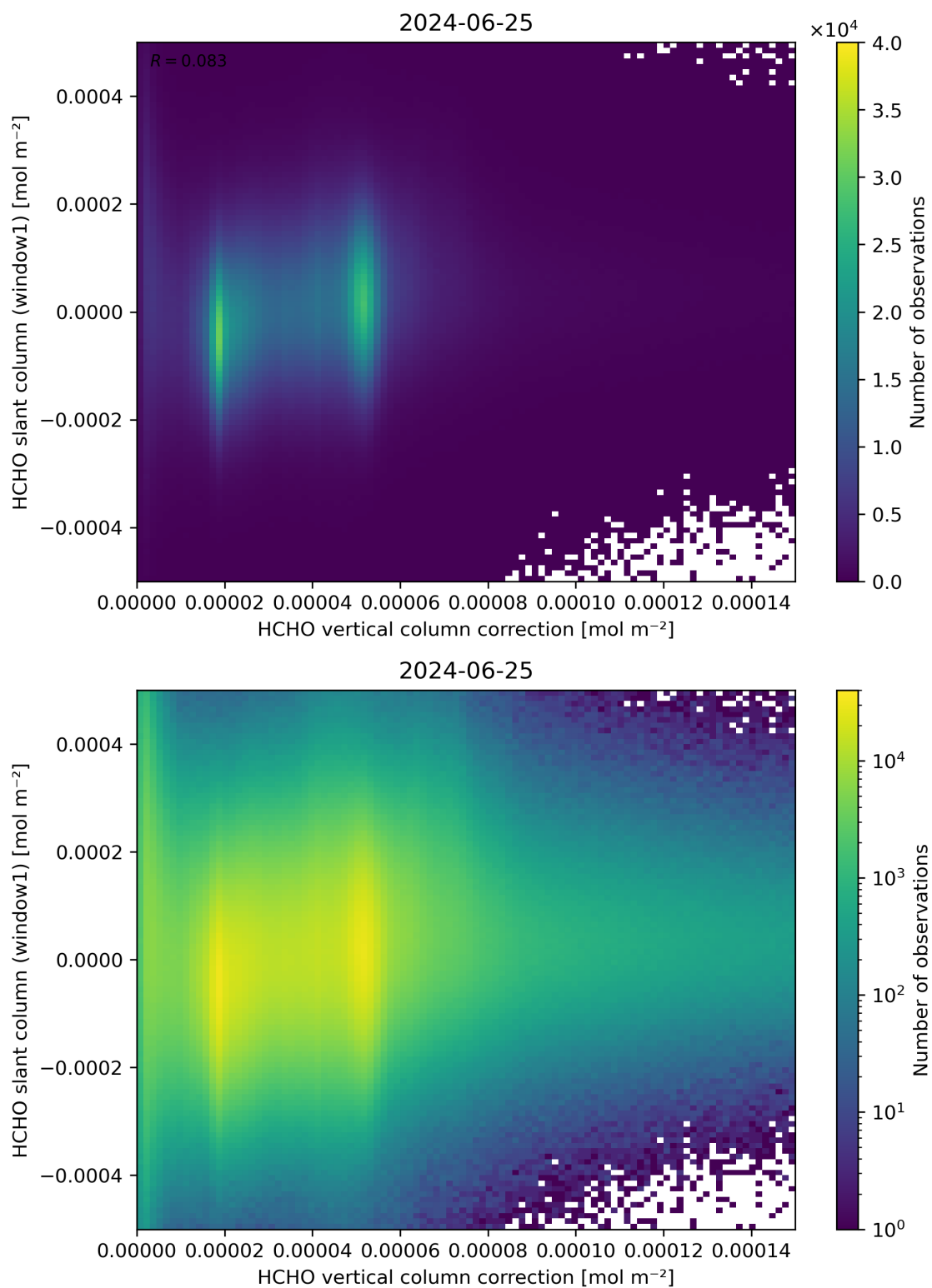
Figure 118: Scatter density plot of “HCHO vertical column correction” against “HCHO slant column (window1)” for 2024-06-24 to 2024-06-26.
