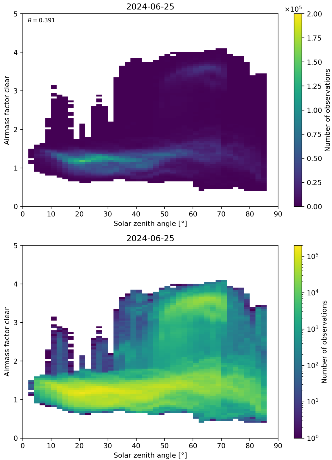
Figure 170: Scatter density plot of “Solar zenith angle” against “Airmass factor clear” for 2024-06-24 to 2024-06-26.
