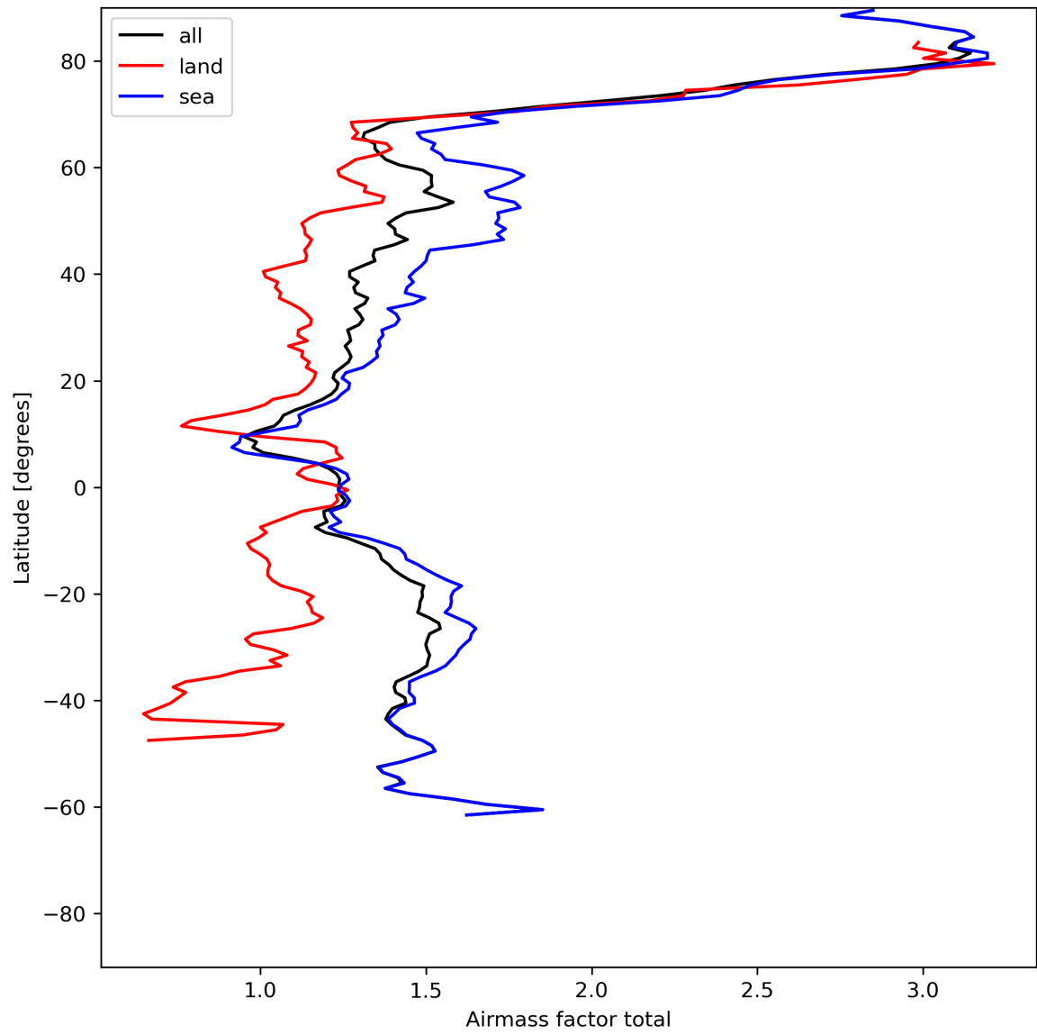
Figure 26: Zonal average of “Airmass factor total” for 2024-06-24 to 2024-06-26.
