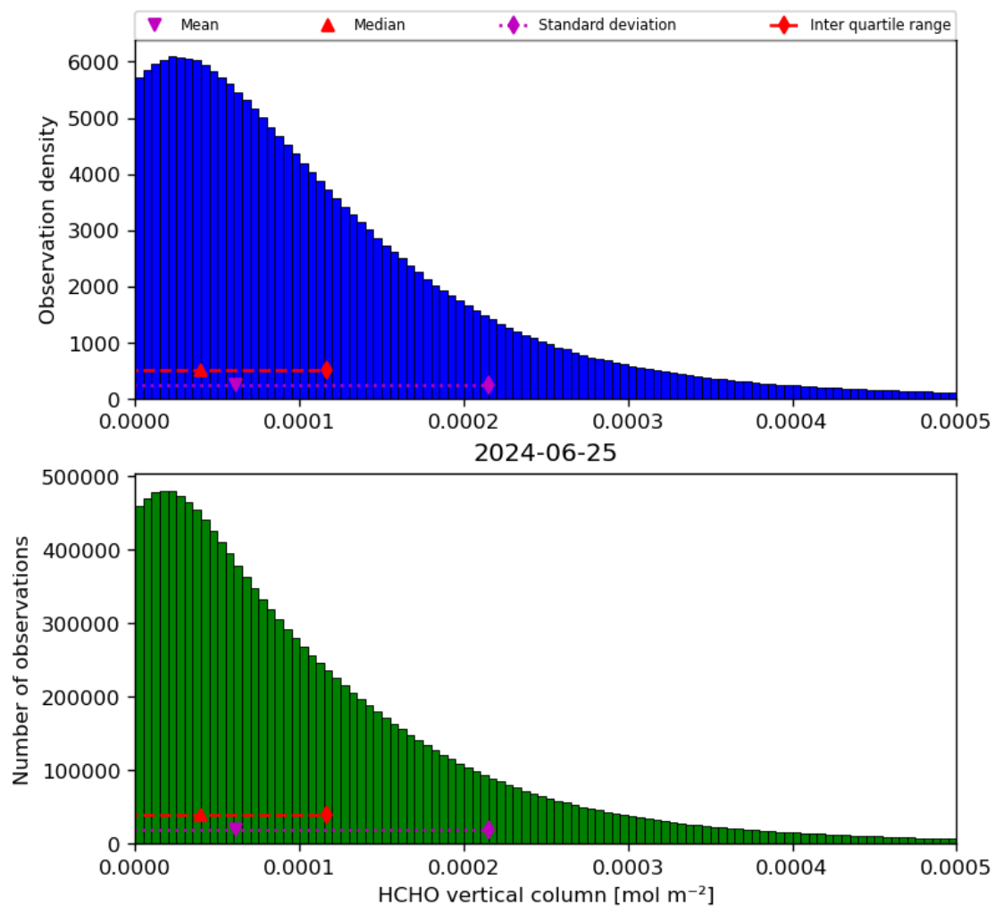
Figure 35: Histogram of “HCHO vertical column” for 2024-06-24 to 2024-06-26
