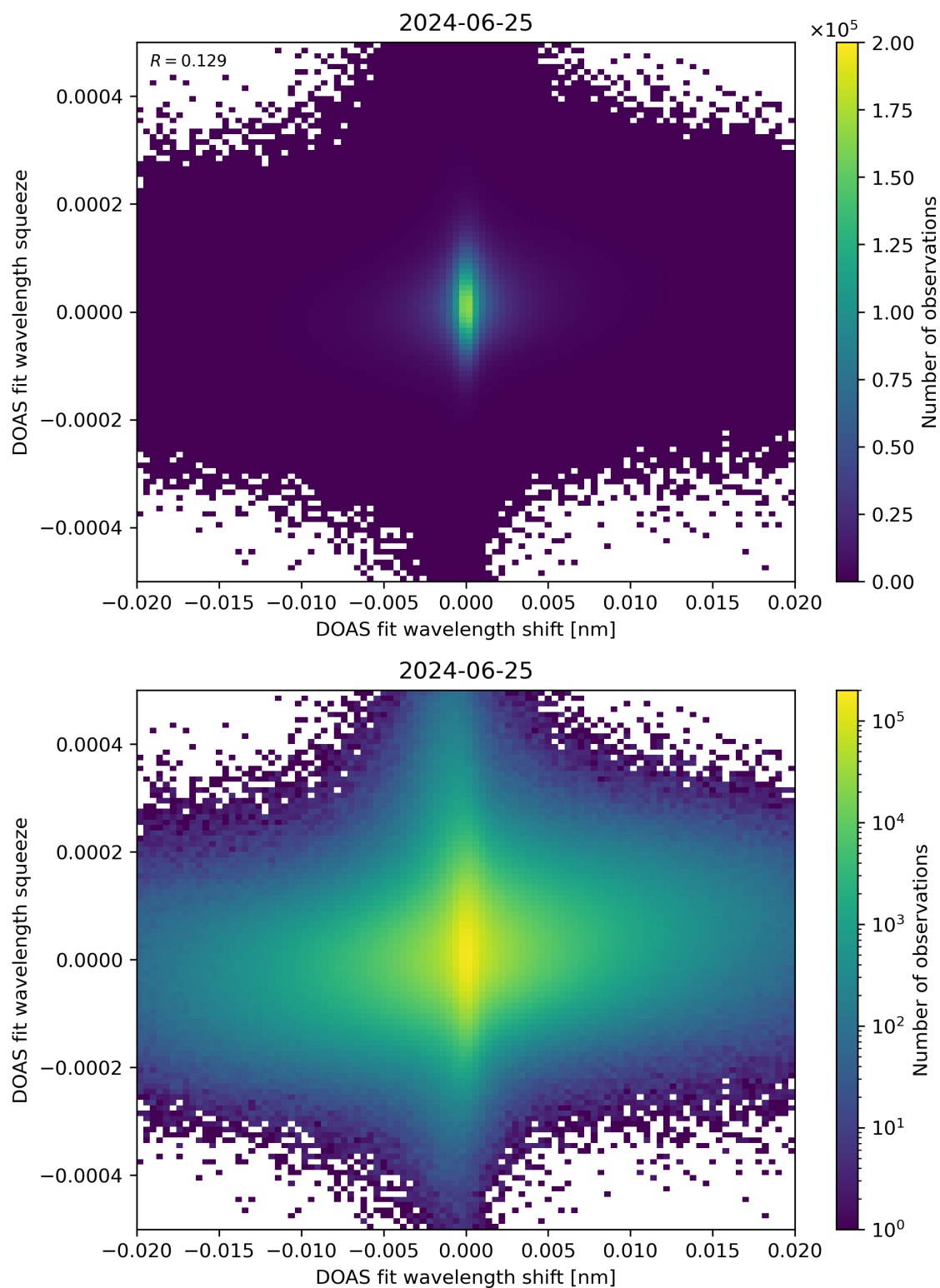
Figure 65: Scatter density plot of “DOAS fit wavelength shift” against “DOAS fit wavelength squeeze” for 2024-06-24 to 2024-06-26.
