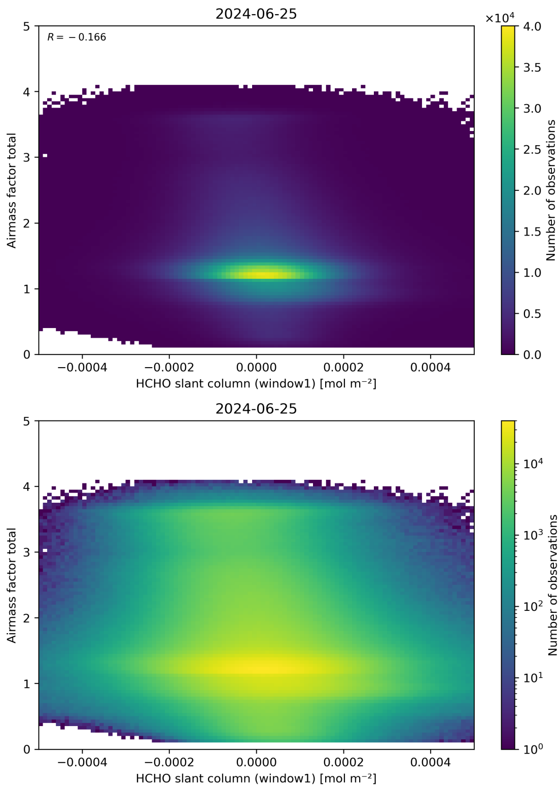
Figure 85: Scatter density plot of “HCHO slant column (window1)” against “Airmass factor total” for 2024-06-24 to 2024-06-26.
