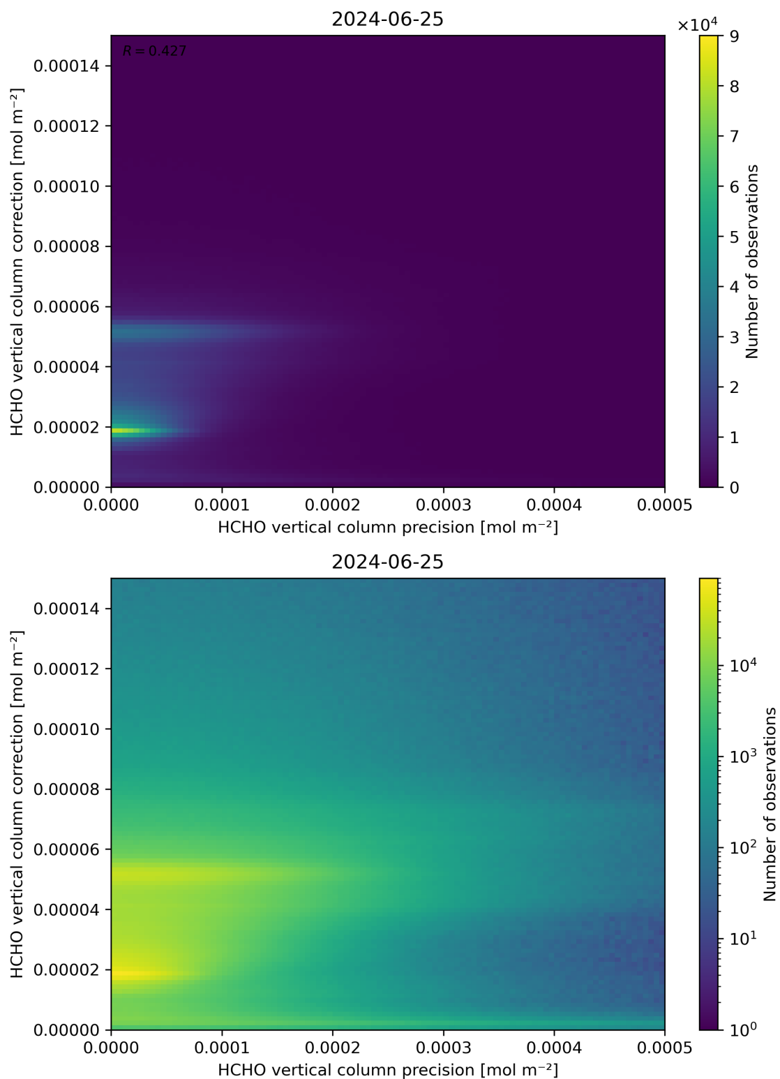
Figure 146: Scatter density plot of “HCHO vertical column precision” against “HCHO vertical column correction” for 2024-06-24 to 2024-06-26.
