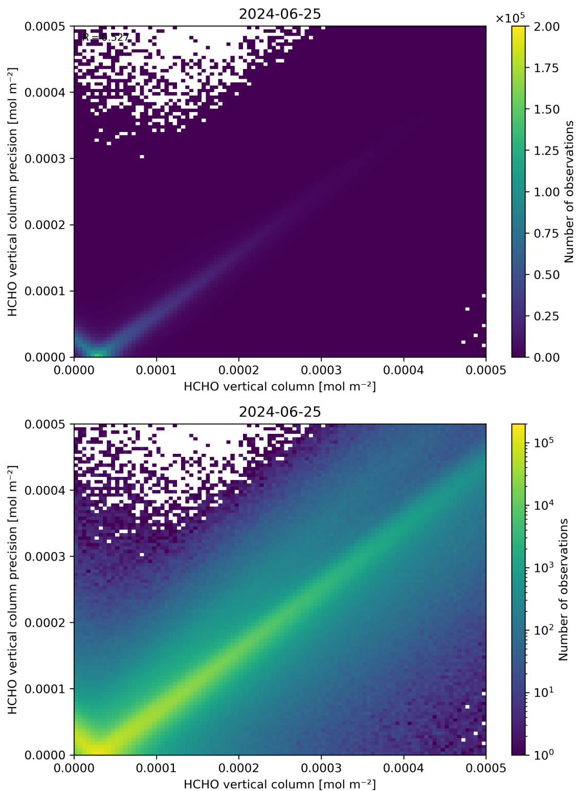
Figure 134: Scatter density plot of “HCHO vertical column” against “HCHO vertical column precision” for 2024-06-24 to 2024-06-26.
