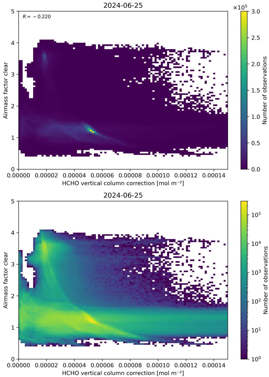
Figure 115: Scatter density plot of “HCHO vertical column correction” against “Airmass factor clear” for 2024-06-24 to 2024-06-26.
