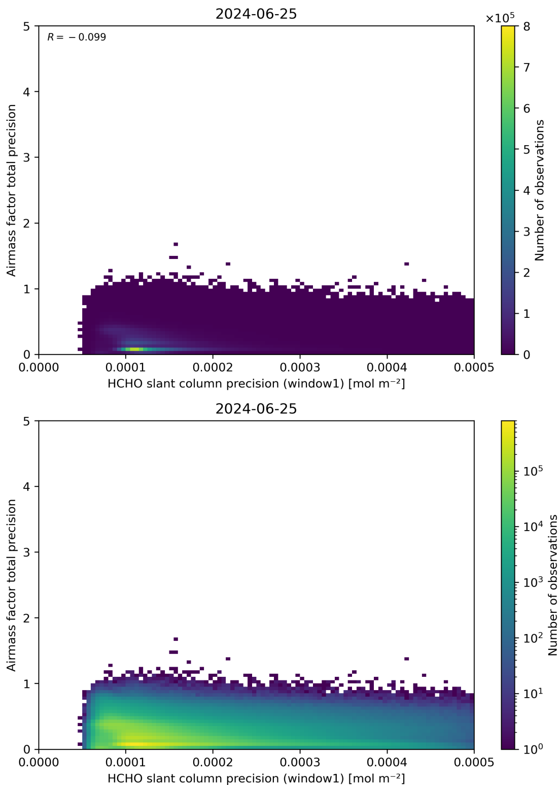
Figure 95: Scatter density plot of “HCHO slant column precision (window1)” against “Airmass factor total precision” for 2024-06-24 to 2024-06-26.
