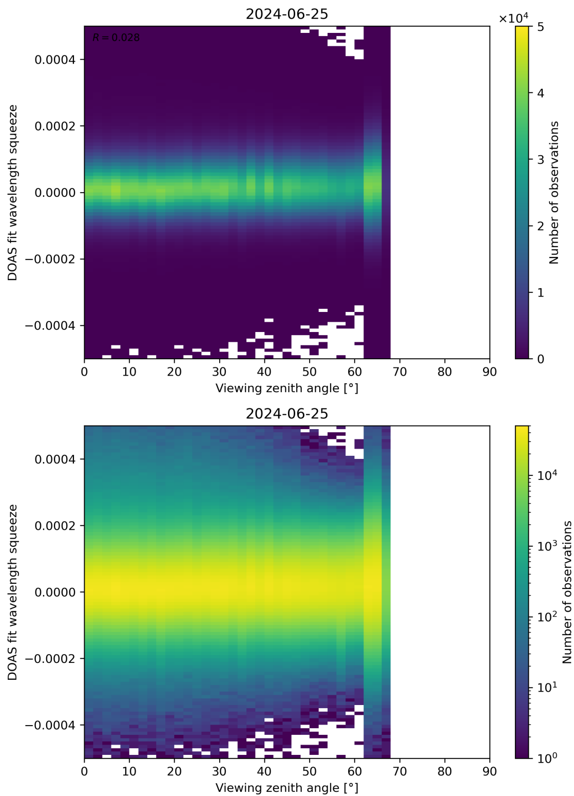
Figure 184: Scatter density plot of “Viewing zenith angle” against “DOAS fit wavelength squeeze” for 2024-06-24 to 2024-06-26.
