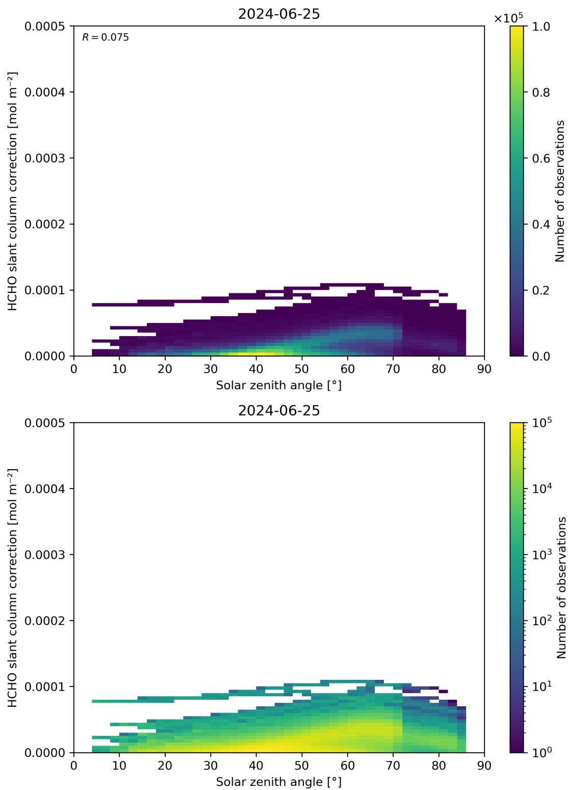
Figure 172: Scatter density plot of “Solar zenith angle” against “HCHO slant column correction” for 2024-06-24 to 2024-06-26.
