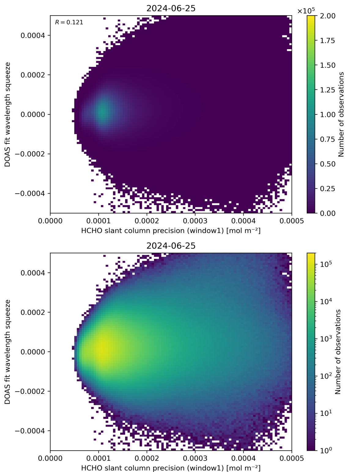
Figure 90: Scatter density plot of “HCHO slant column precision (window1)” against “DOAS fit wavelength squeeze” for 2024-06-24 to 2024-06-26.
