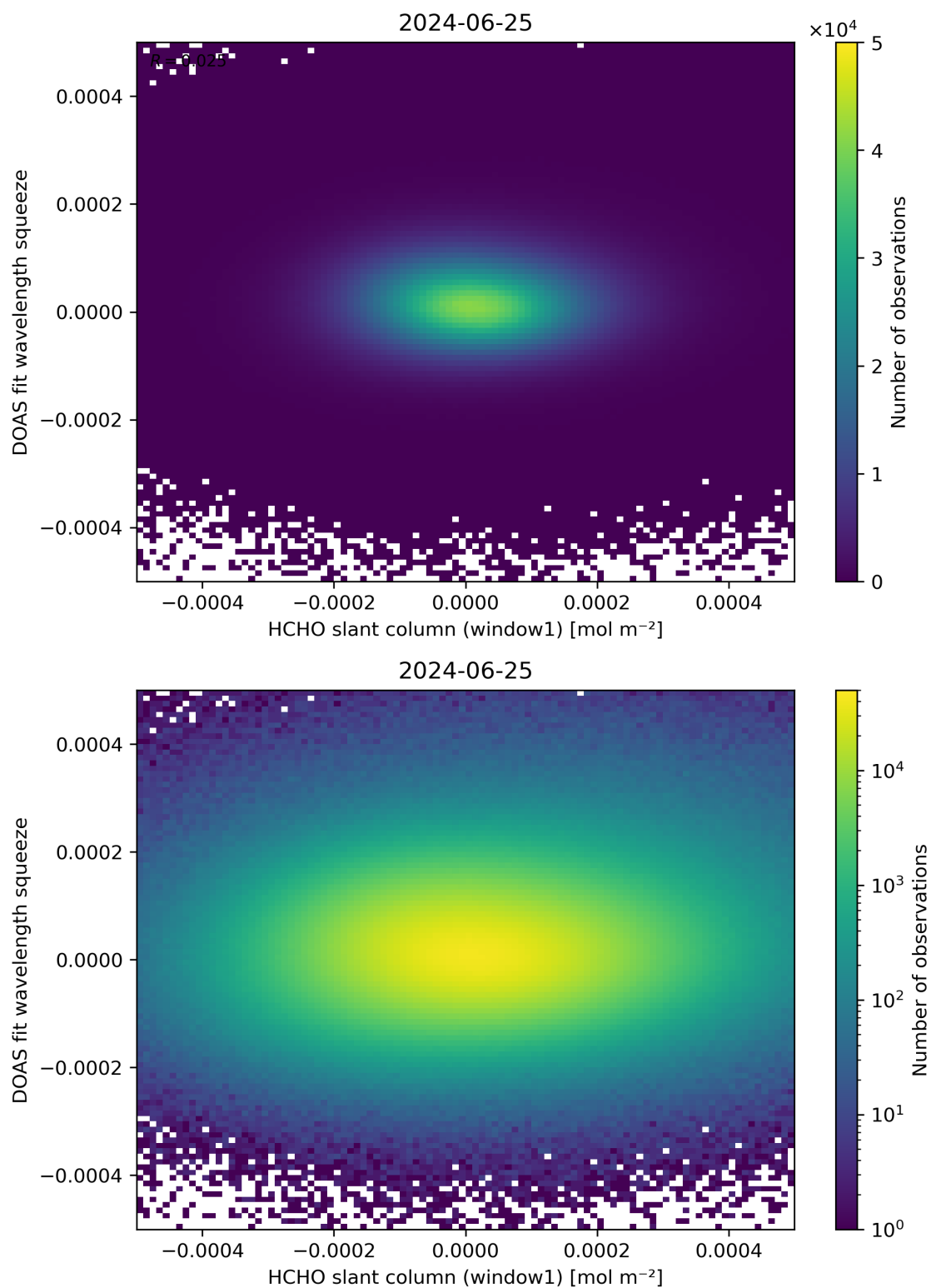
Figure 80: Scatter density plot of “HCHO slant column (window1)” against “DOAS fit wavelength squeeze” for 2024-06-24 to 2024-06-26.
