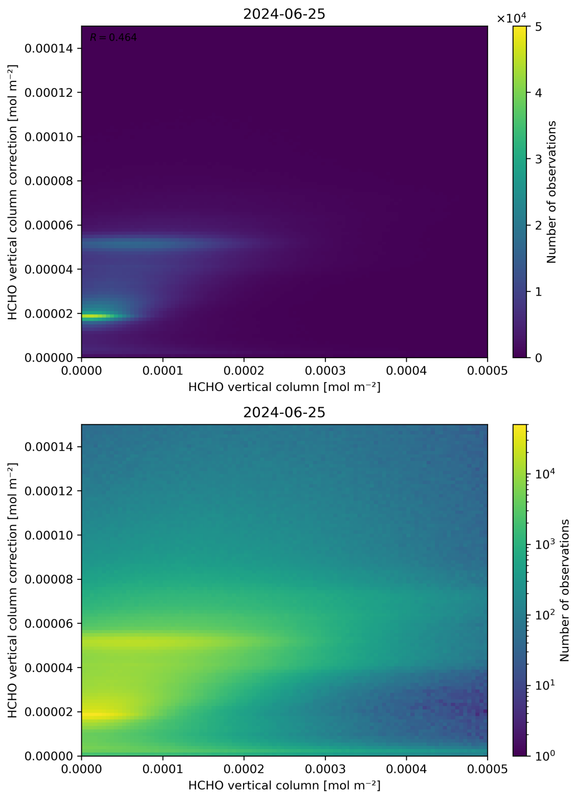
Figure 133: Scatter density plot of “HCHO vertical column” against “HCHO vertical column correction” for 2024-06-24 to 2024-06-26.
