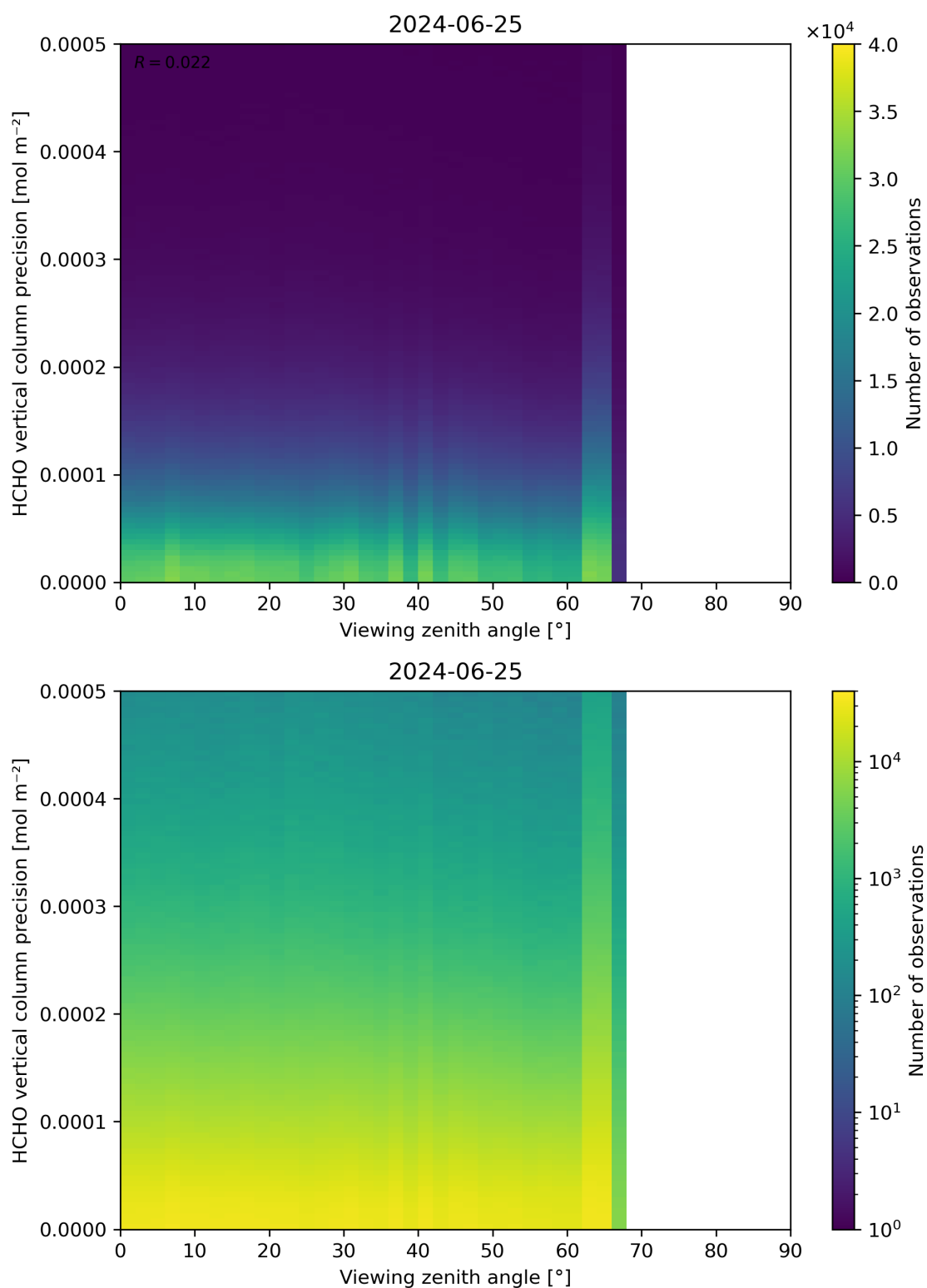
Figure 194: Scatter density plot of “Viewing zenith angle” against “HCHO vertical column precision” for 2024-06-24 to 2024-06-26.
