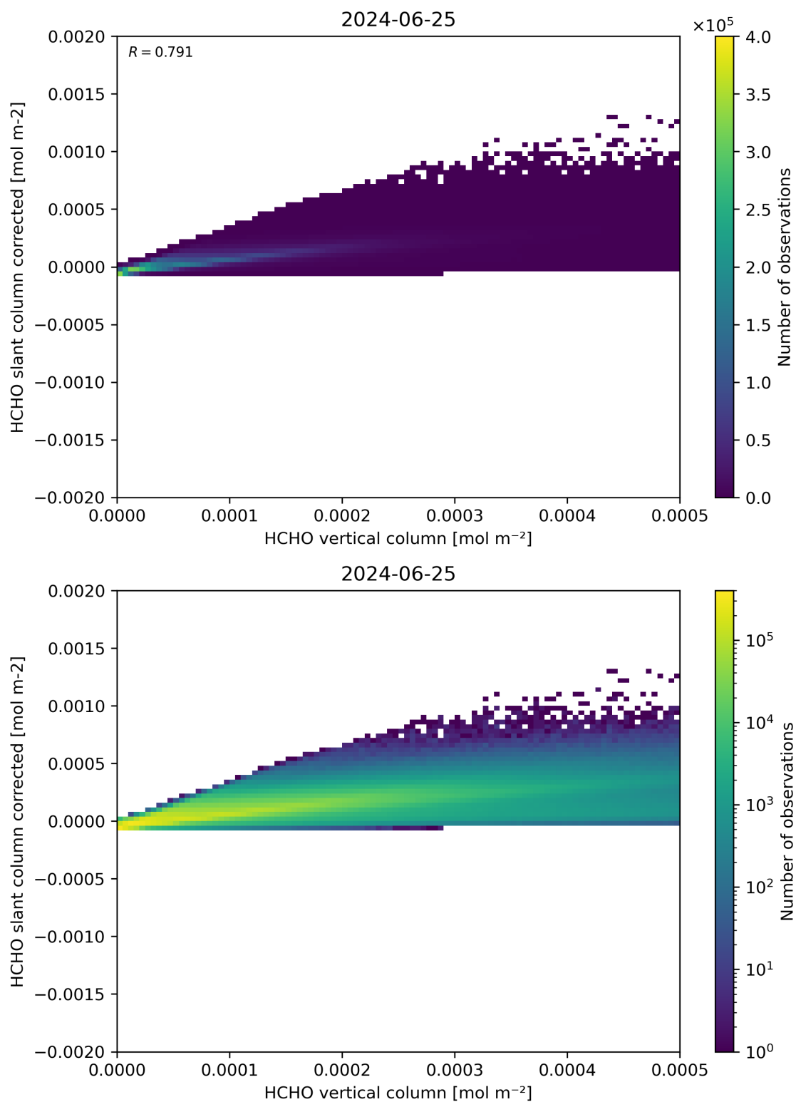
Figure 127: Scatter density plot of “HCHO vertical column” against “HCHO slant column corrected” for 2024-06-24 to 2024-06-26.
