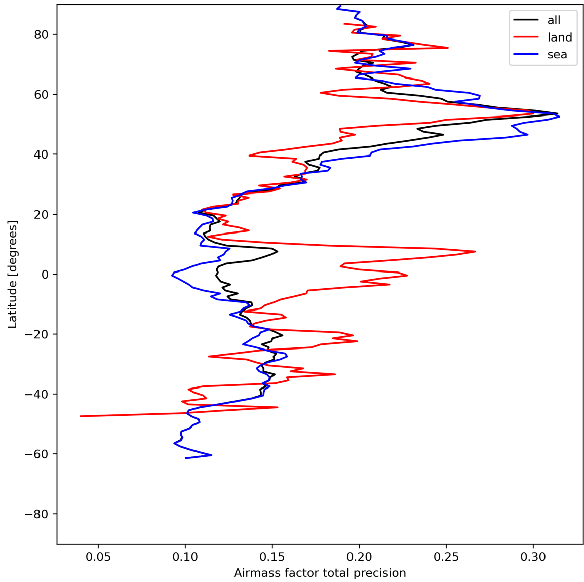
Figure 27: Zonal average of “Airmass factor total precision” for 2024-06-24 to 2024-06-26.
