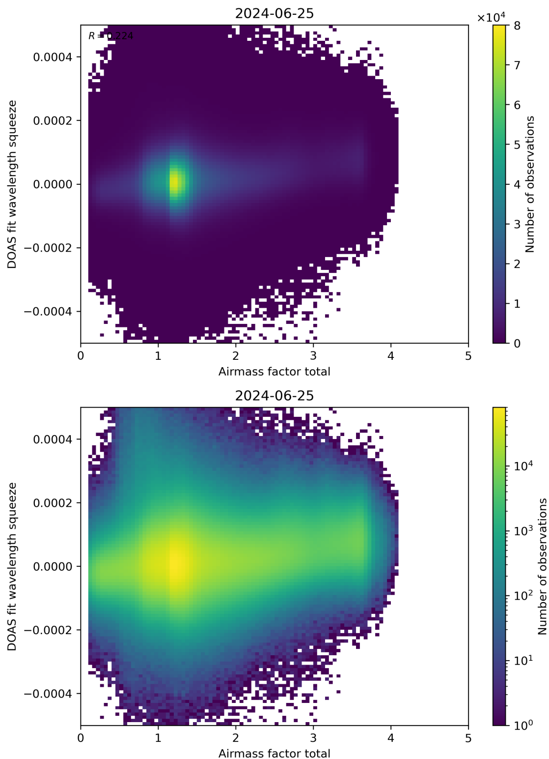
Figure 99: Scatter density plot of “Airmass factor total” against “DOAS fit wavelength squeeze” for 2024-06-24 to 2024-06-26.
