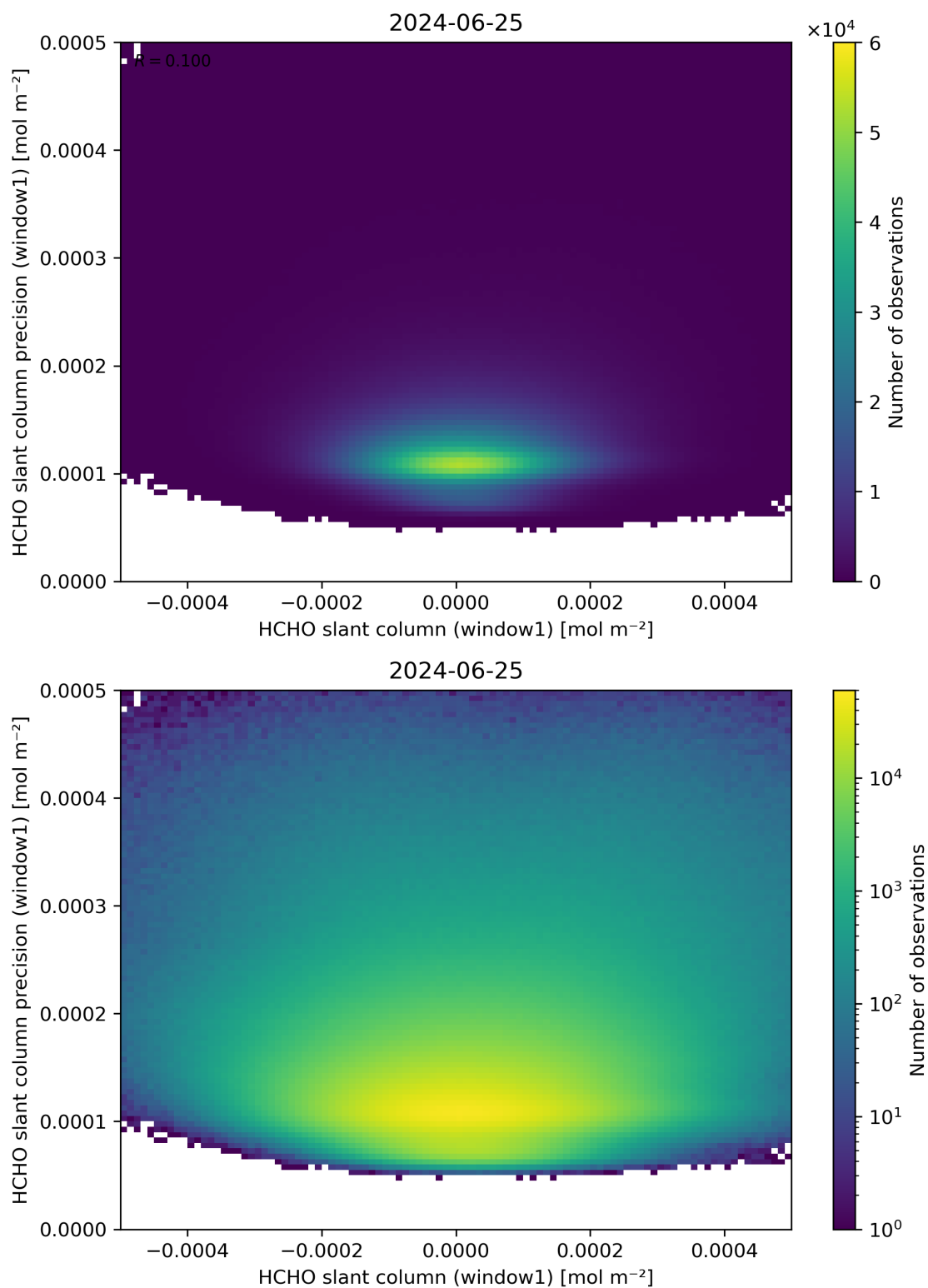
Figure 84: Scatter density plot of “HCHO slant column (window1)” against “HCHO slant column precision (window1)” for 2024-06-24 to 2024-06-26.
