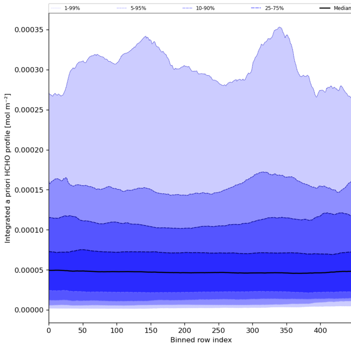
Figure 57: Along track statistics of “Integrated a priori HCHO profile” for 2024-06-24 to 2024-06-26
