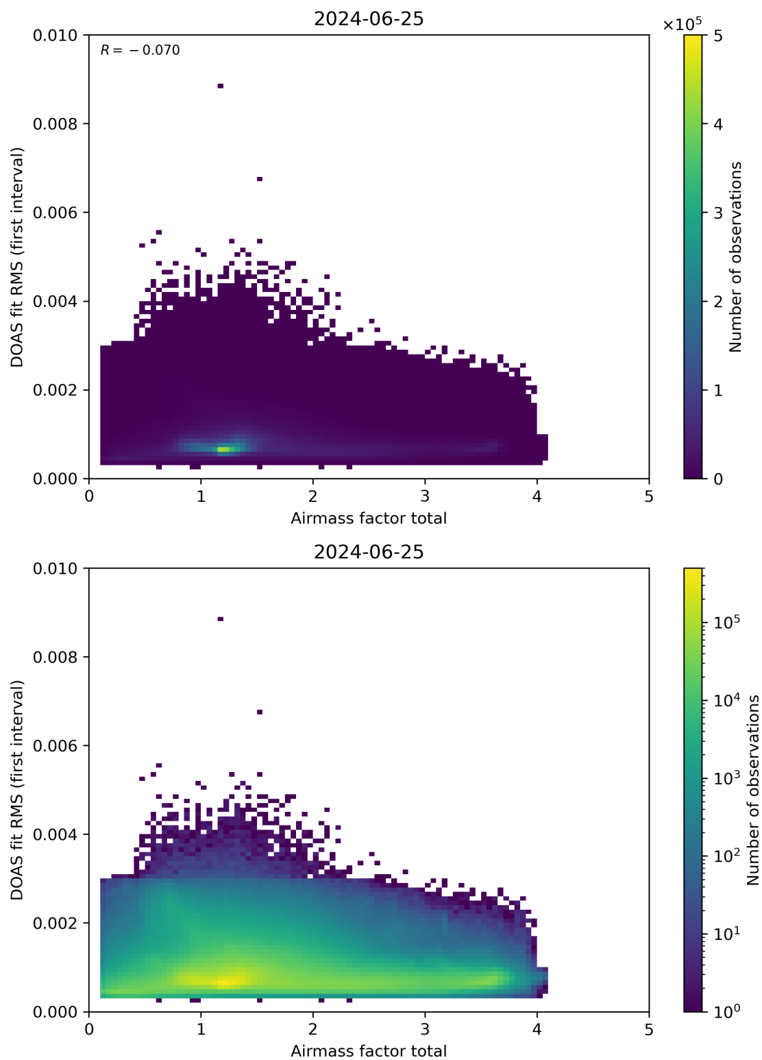
Figure 97: Scatter density plot of “Airmass factor total” against “DOAS fit RMS (first interval)” for 2024-06-24 to 2024-06-26.
