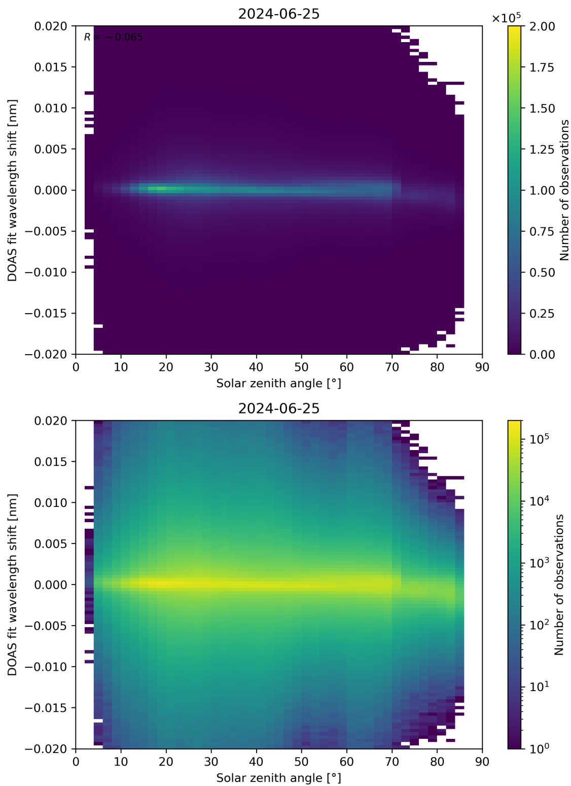
Figure 168: Scatter density plot of “Solar zenith angle” against “DOAS fit wavelength shift” for 2024-06-24 to 2024-06-26.
