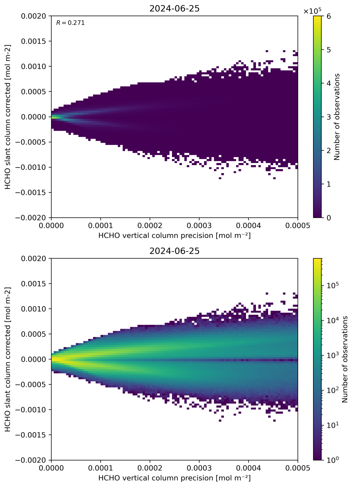
Figure 140: Scatter density plot of “HCHO vertical column precision” against “HCHO slant column corrected” for 2024-06-24 to 2024-06-26.
