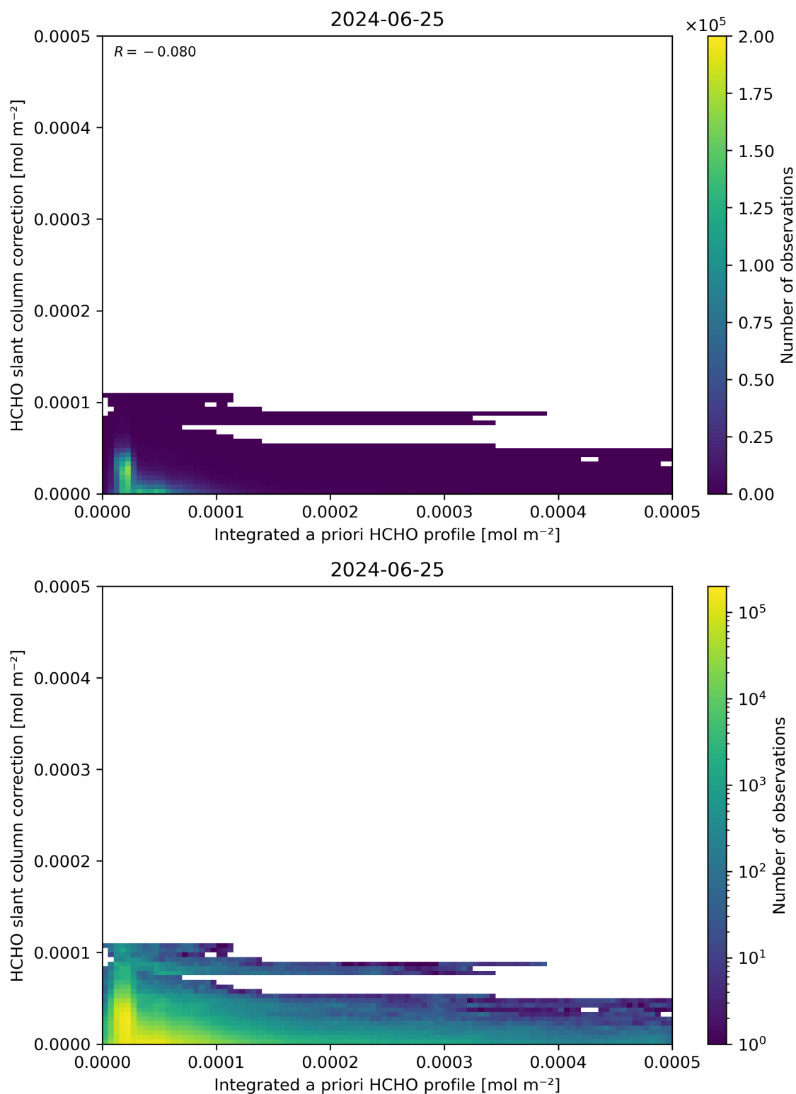
Figure 152: Scatter density plot of “Integrated a priori HCHO profile” against “HCHO slant column correction” for 2024-06-24 to 2024-06-26.
