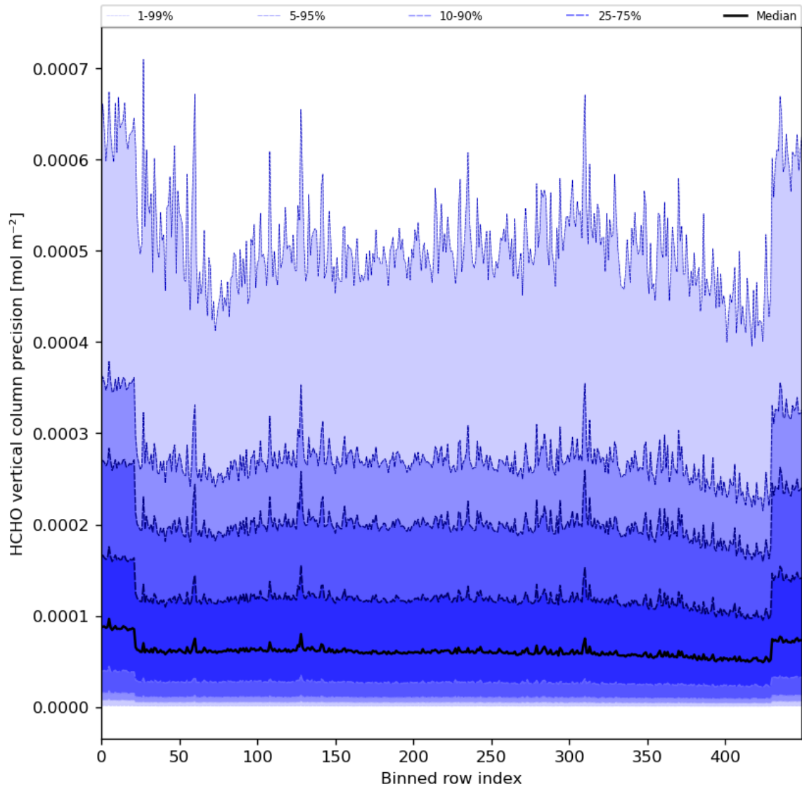
Figure 50: Along track statistics of “HCHO vertical column precision” for 2024-06-24 to 2024-06-26
