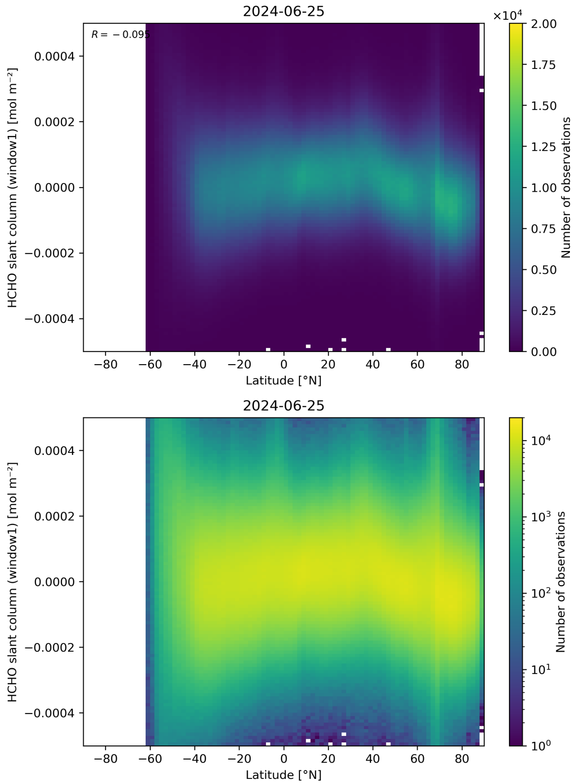
Figure 159: Scatter density plot of “Latitude” against “HCHO slant column (window1)” for 2024-06-24 to 2024-06-26.
