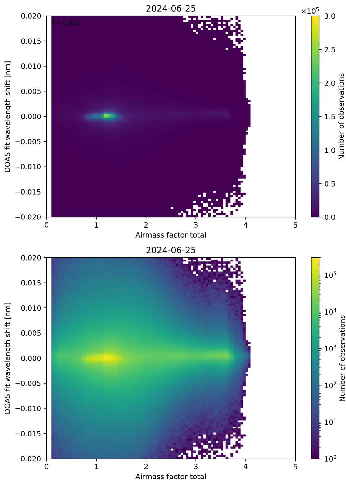
Figure 98: Scatter density plot of “Airmass factor total” against “DOAS fit wavelength shift” for 2024-06-24 to 2024-06-26.
