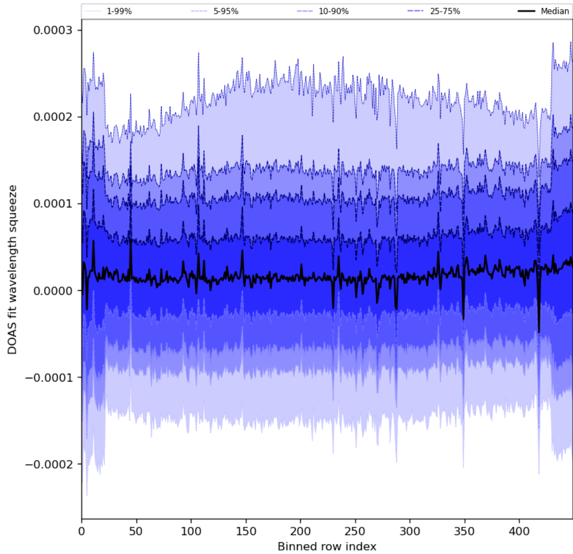
Figure 59: Along track statistics of “DOAS fit wavelength squeeze” for 2024-06-24 to 2024-06-26
