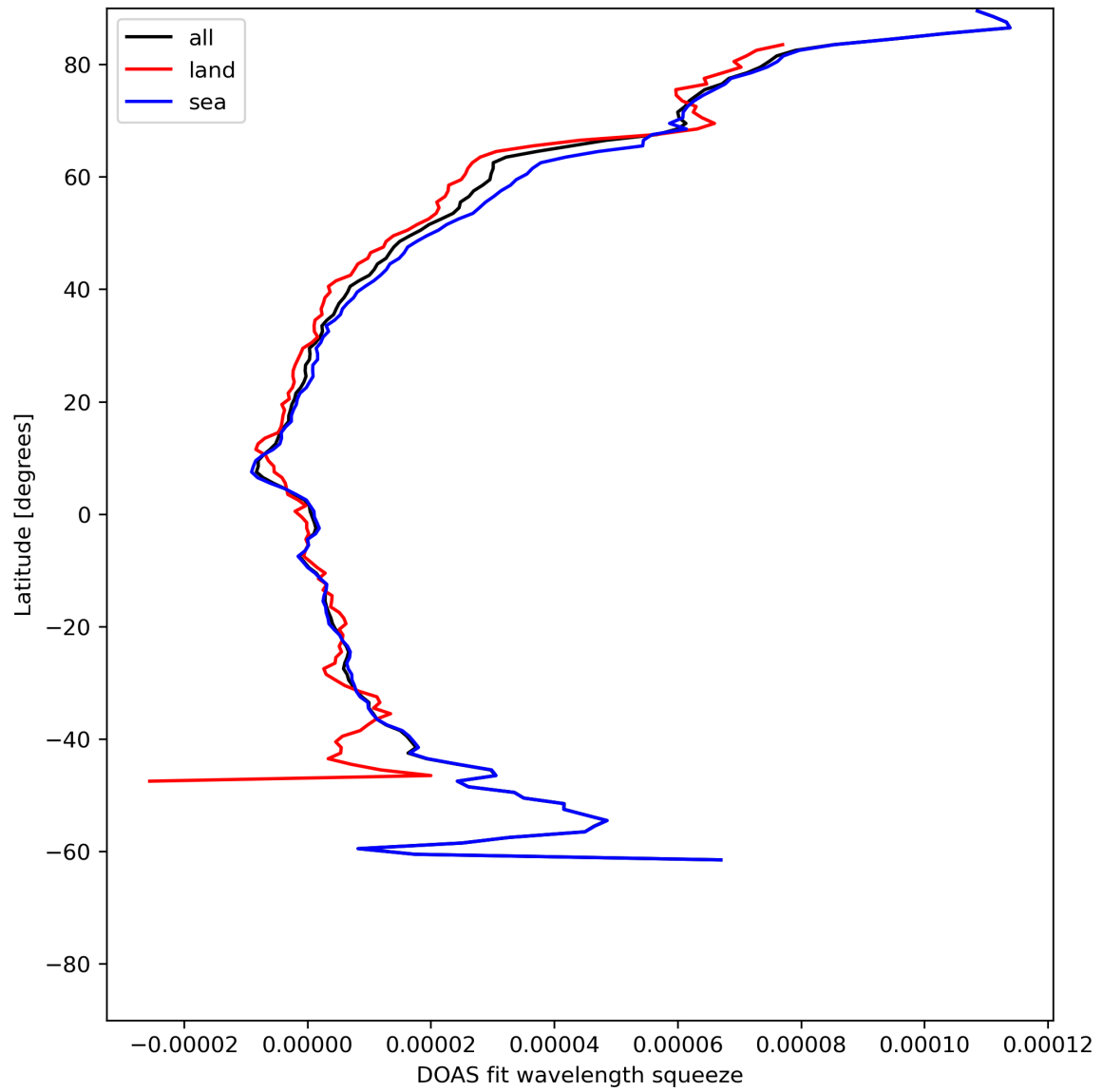
Figure 31: Zonal average of “DOAS fit wavelength squeeze” for 2024-06-24 to 2024-06-26.
