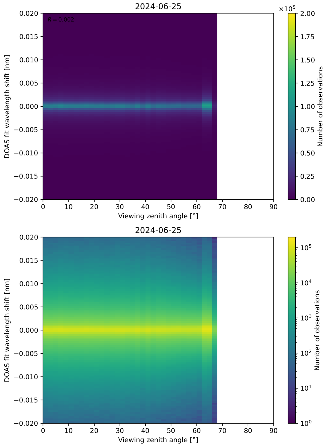
Figure 183: Scatter density plot of “Viewing zenith angle” against “DOAS fit wavelength shift” for 2024-06-24 to 2024-06-26.
