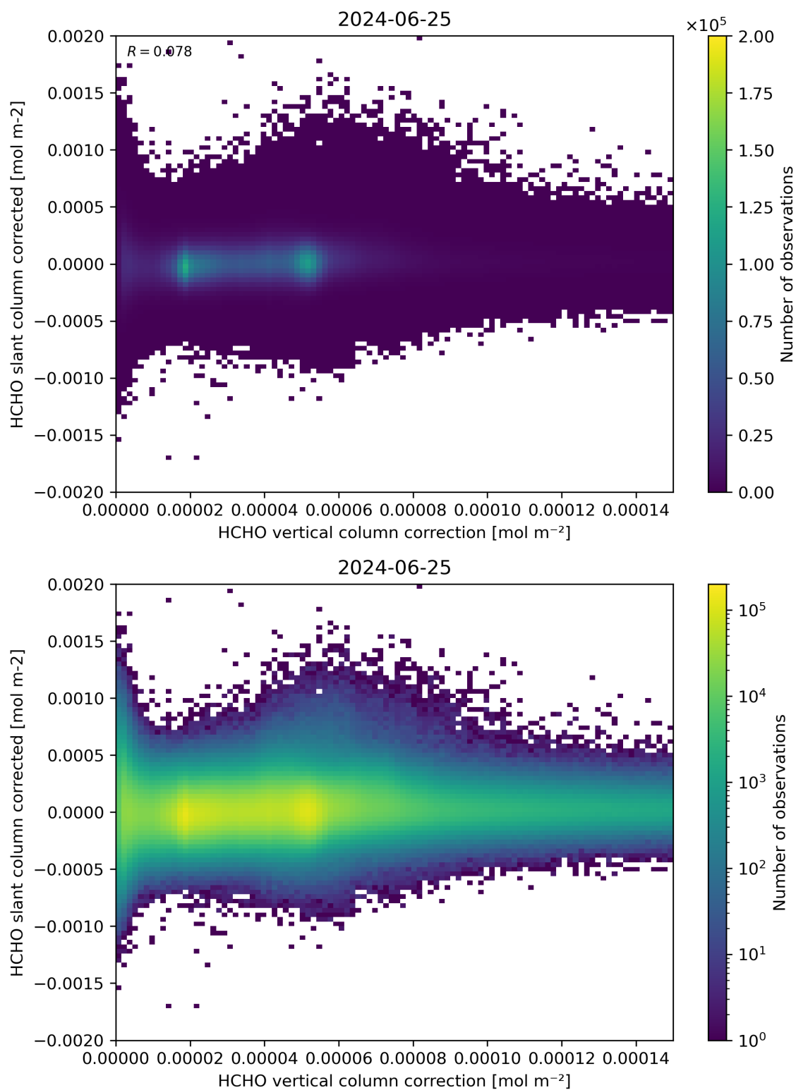
Figure 116: Scatter density plot of “HCHO vertical column correction” against “HCHO slant column corrected” for 2024-06-24 to 2024-06-26.
