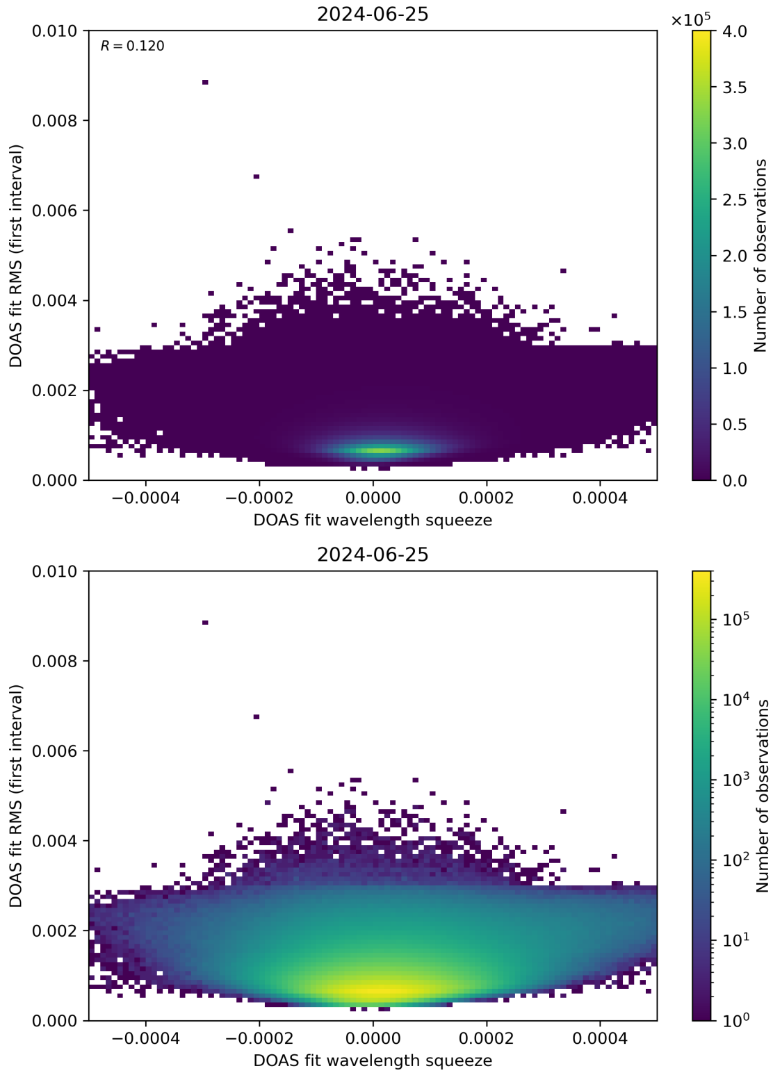
Figure 68: Scatter density plot of “DOAS fit wavelength squeeze” against “DOAS fit RMS (first interval)” for 2024-06-24 to 2024-06-26.
