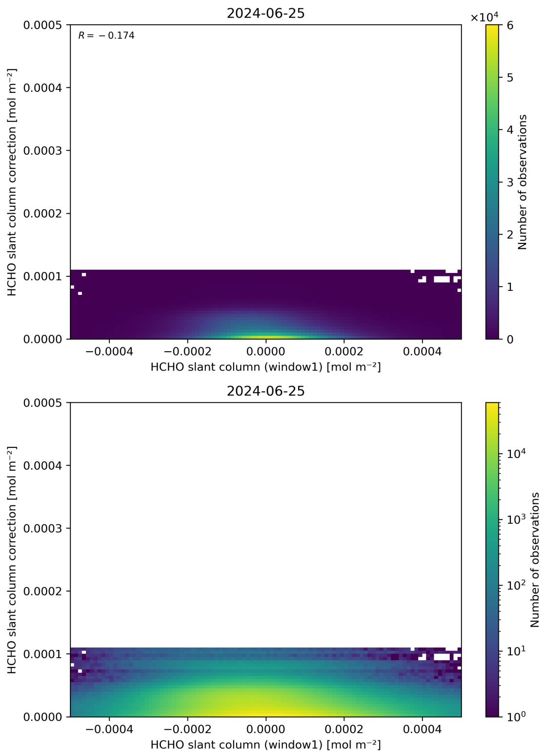
Figure 83: Scatter density plot of “HCHO slant column (window1)” against “HCHO slant column correction” for 2024-06-24 to 2024-06-26.
