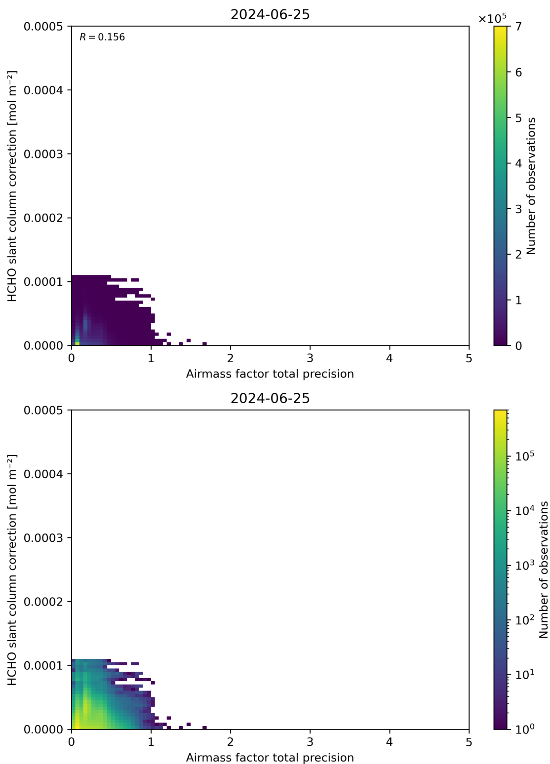
Figure 110: Scatter density plot of “Airmass factor total precision” against “HCHO slant column correction” for 2024-06-24 to 2024-06-26.
