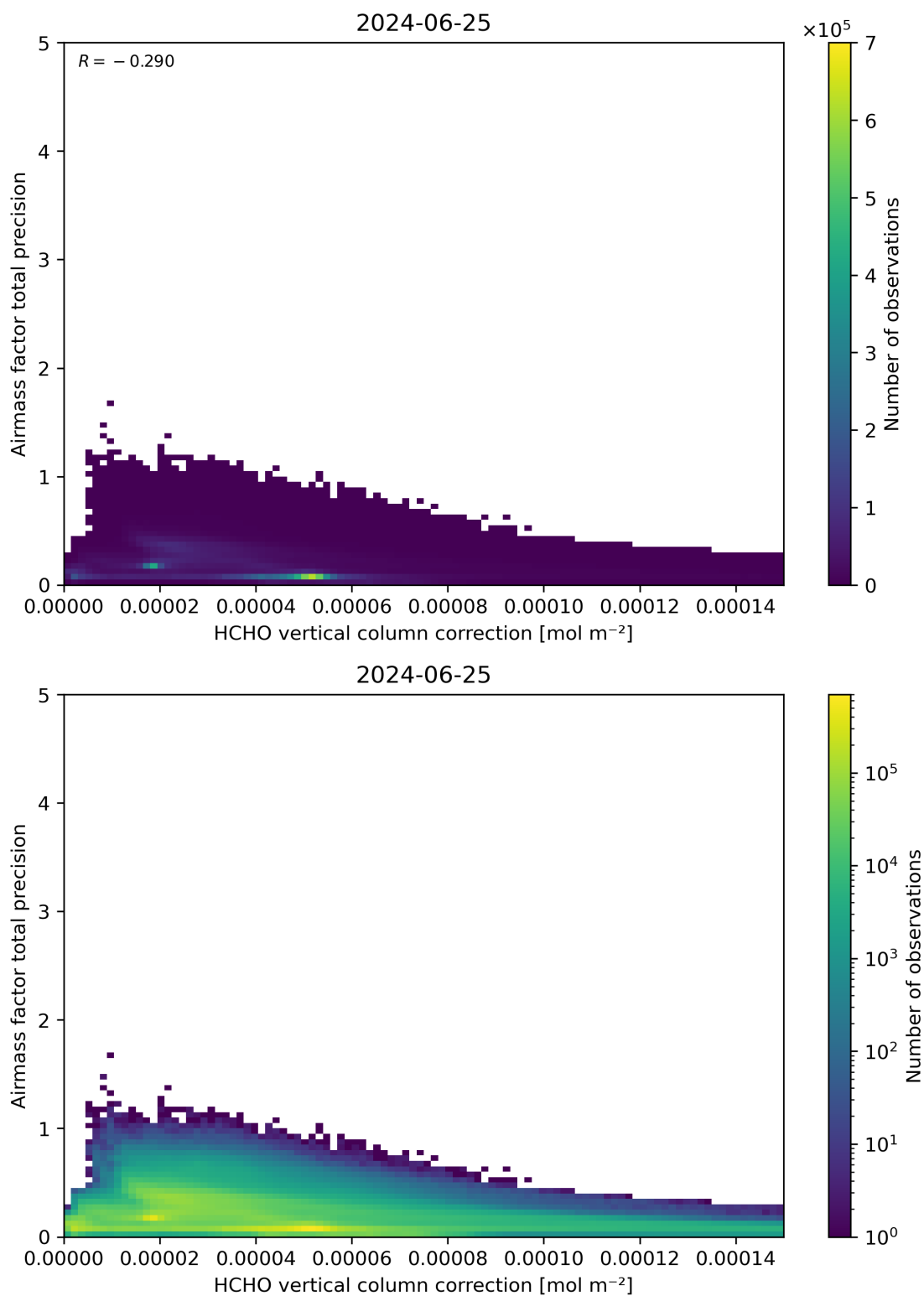
Figure 121: Scatter density plot of “HCHO vertical column correction” against “Airmass factor total precision” for 2024-06-24 to 2024-06-26.
