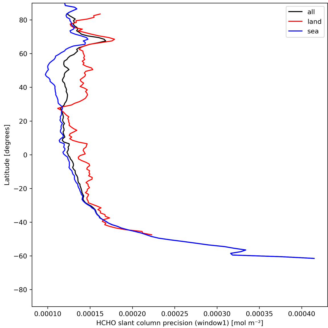
Figure 25: Zonal average of “HCHO slant column precision (window1)” for 2024-06-24 to 2024-06-26.
