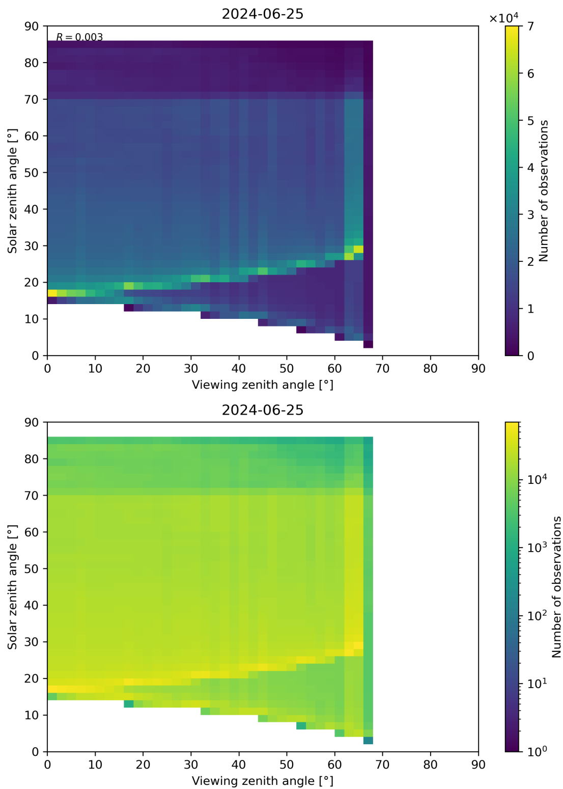
Figure 197: Scatter density plot of “Viewing zenith angle” against “Solar zenith angle” for 2024-06-24 to 2024-06-26.
