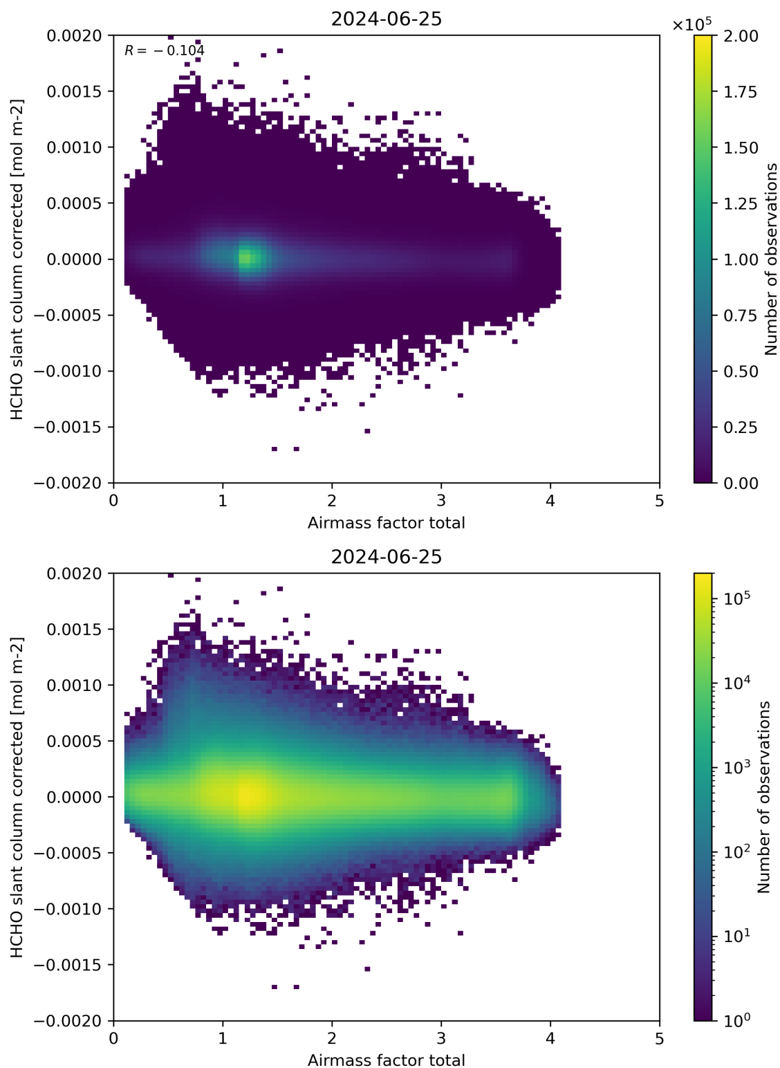
Figure 101: Scatter density plot of “Airmass factor total” against “HCHO slant column corrected” for 2024-06-24 to 2024-06-26.
