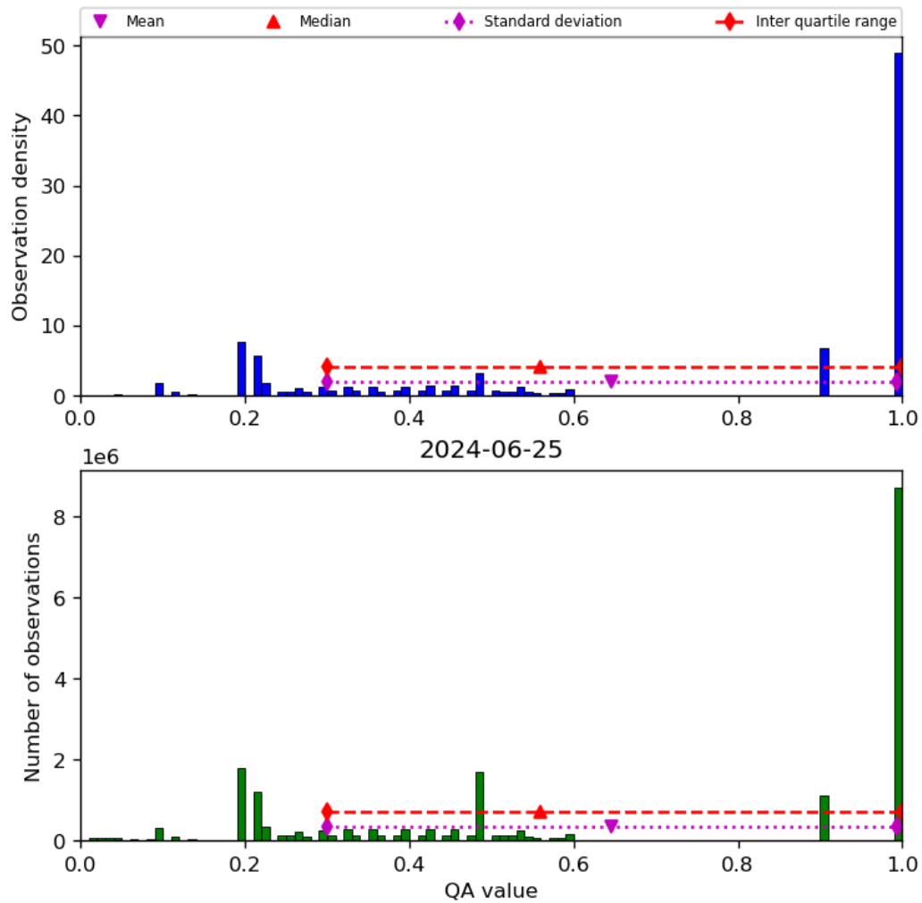
Figure 34: Histogram of “QA value” for 2024-06-24 to 2024-06-26
