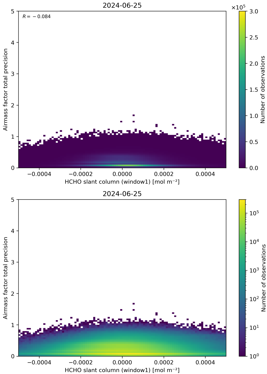
Figure 86: Scatter density plot of “HCHO slant column (window1)” against “Airmass factor total precision” for 2024-06-24 to 2024-06-26.
