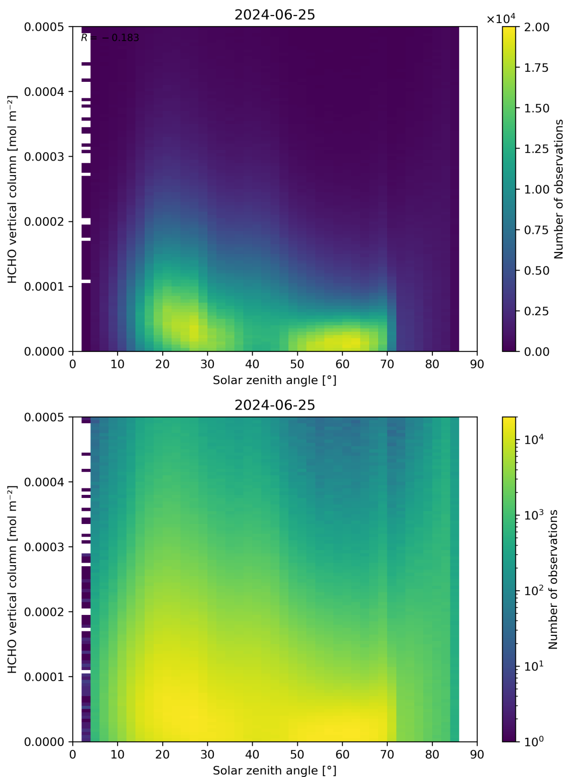
Figure 177: Scatter density plot of “Solar zenith angle” against “HCHO vertical column” for 2024-06-24 to 2024-06-26.
