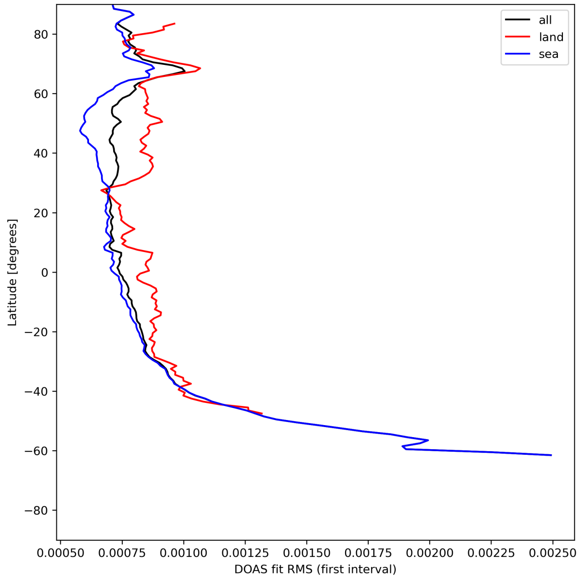
Figure 32: Zonal average of "DOAS fit RMS (first interval)" for 2024-06-24 to 2024-06-26.
