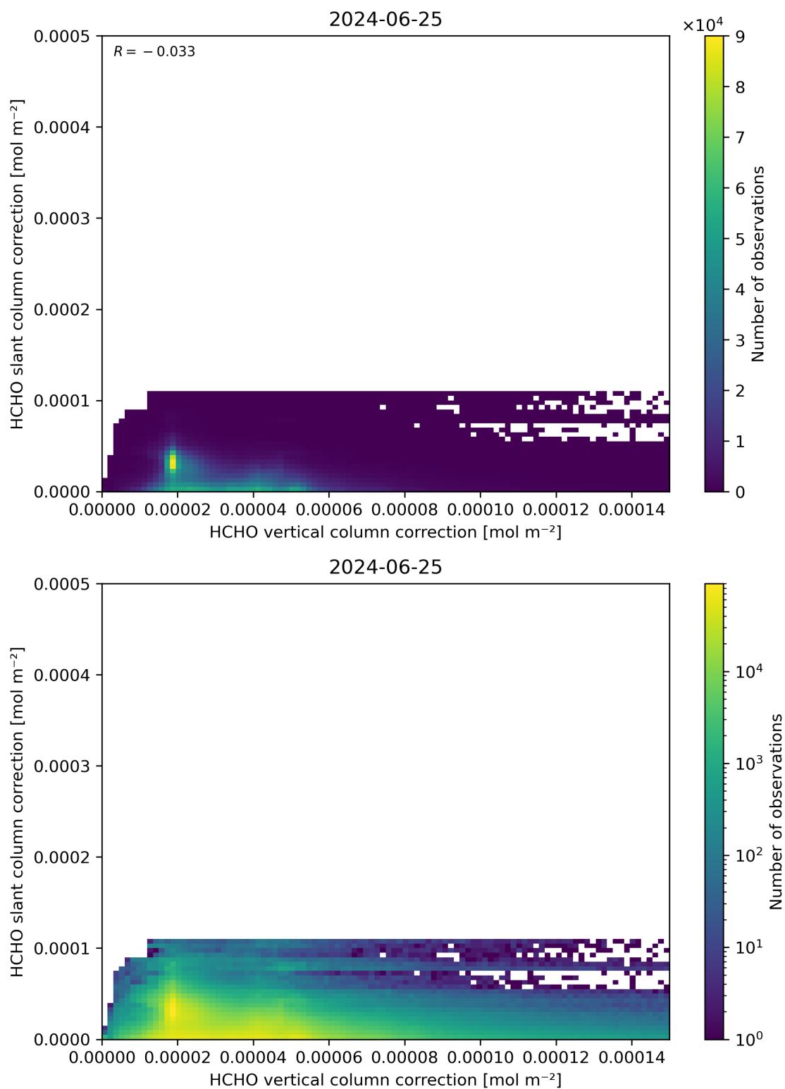
Figure 117: Scatter density plot of “HCHO vertical column correction” against “HCHO slant column correction” for 2024-06-24 to 2024-06-26.
