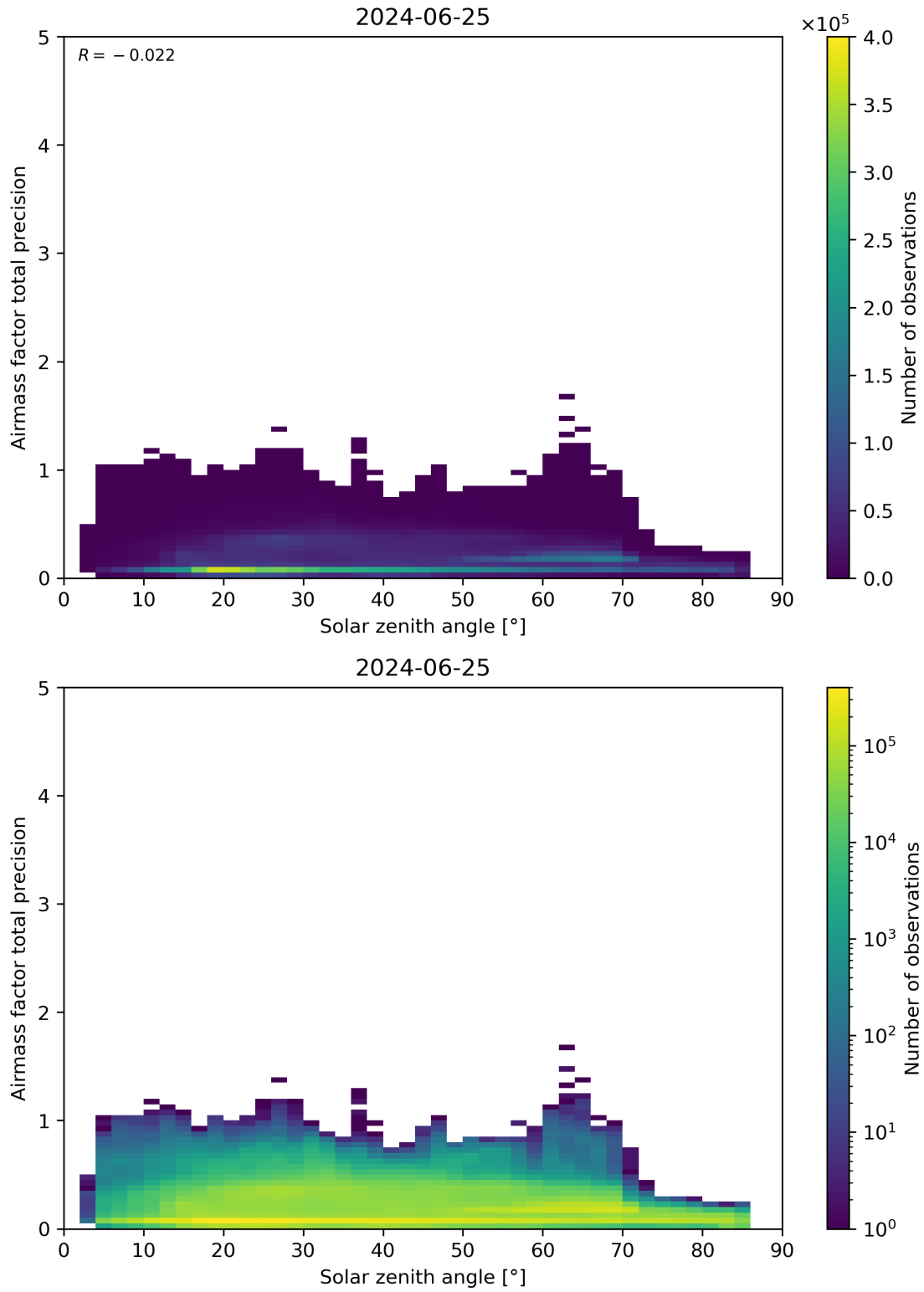
Figure 176: Scatter density plot of “Solar zenith angle” against “Airmass factor total precision” for 2024-06-24 to 2024-06-26.
