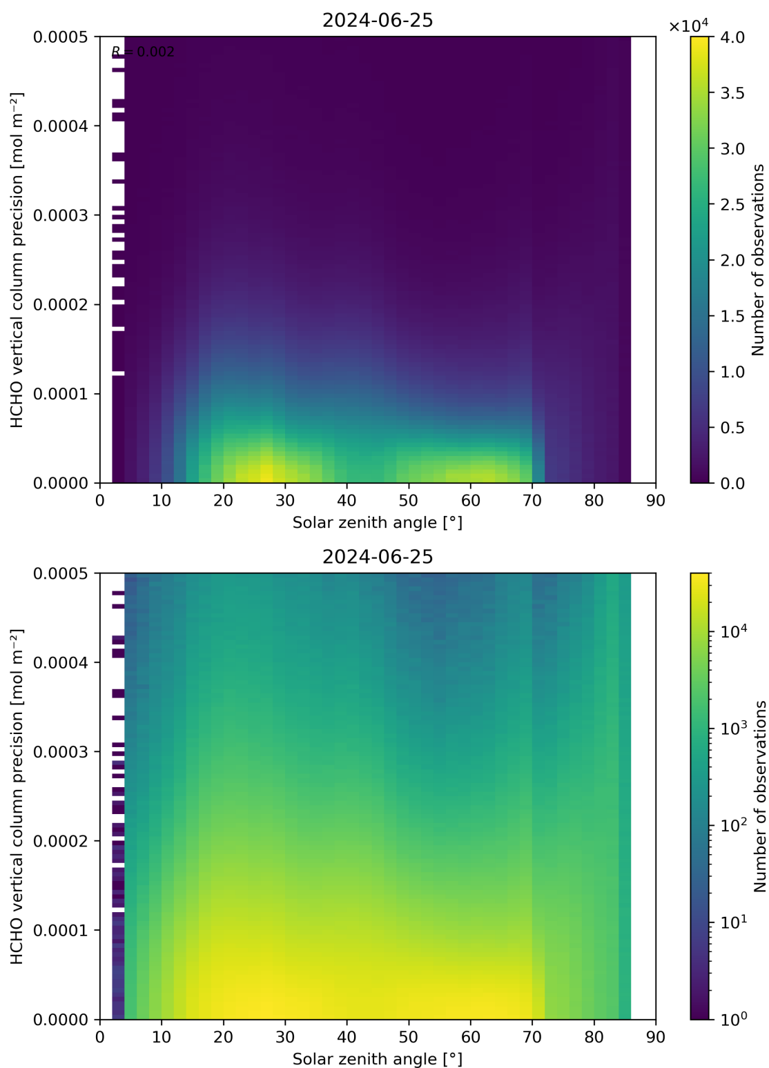
Figure 179: Scatter density plot of “Solar zenith angle” against “HCHO vertical column precision” for 2024-06-24 to 2024-06-26.
