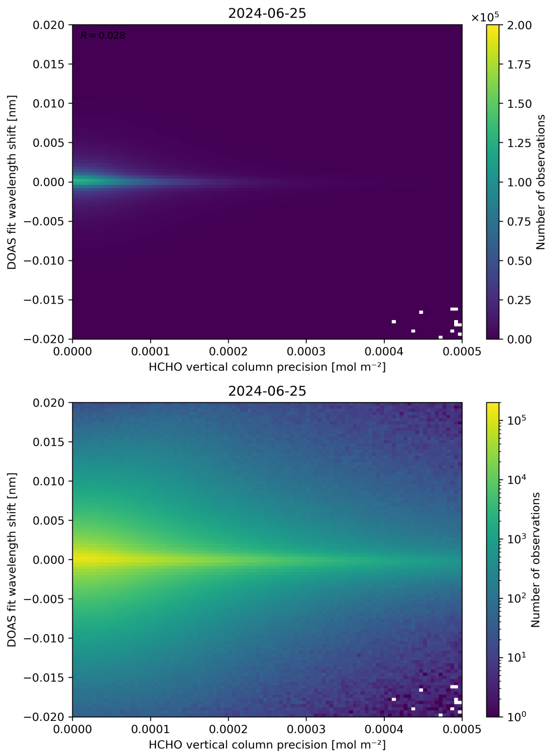
Figure 137: Scatter density plot of “HCHO vertical column precision” against “DOAS fit wavelength shift” for 2024-06-24 to 2024-06-26.
