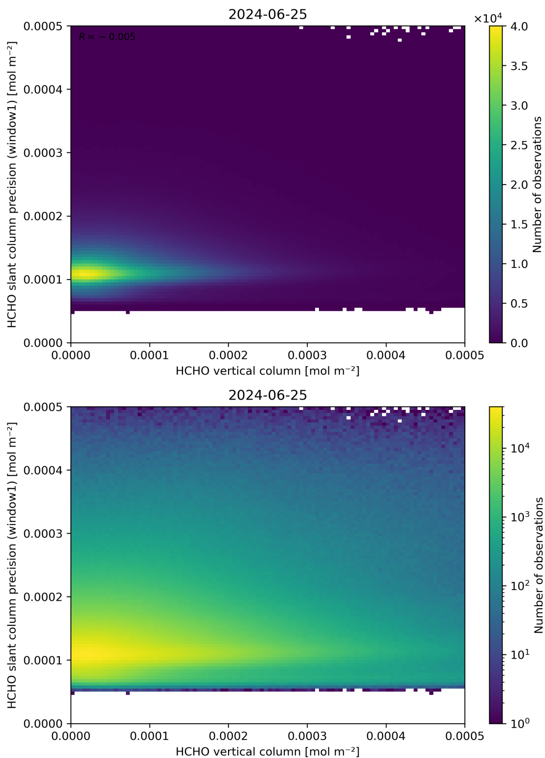
Figure 130: Scatter density plot of “HCHO vertical column” against “HCHO slant column precision (window1)” for 2024-06-24 to 2024-06-26.
