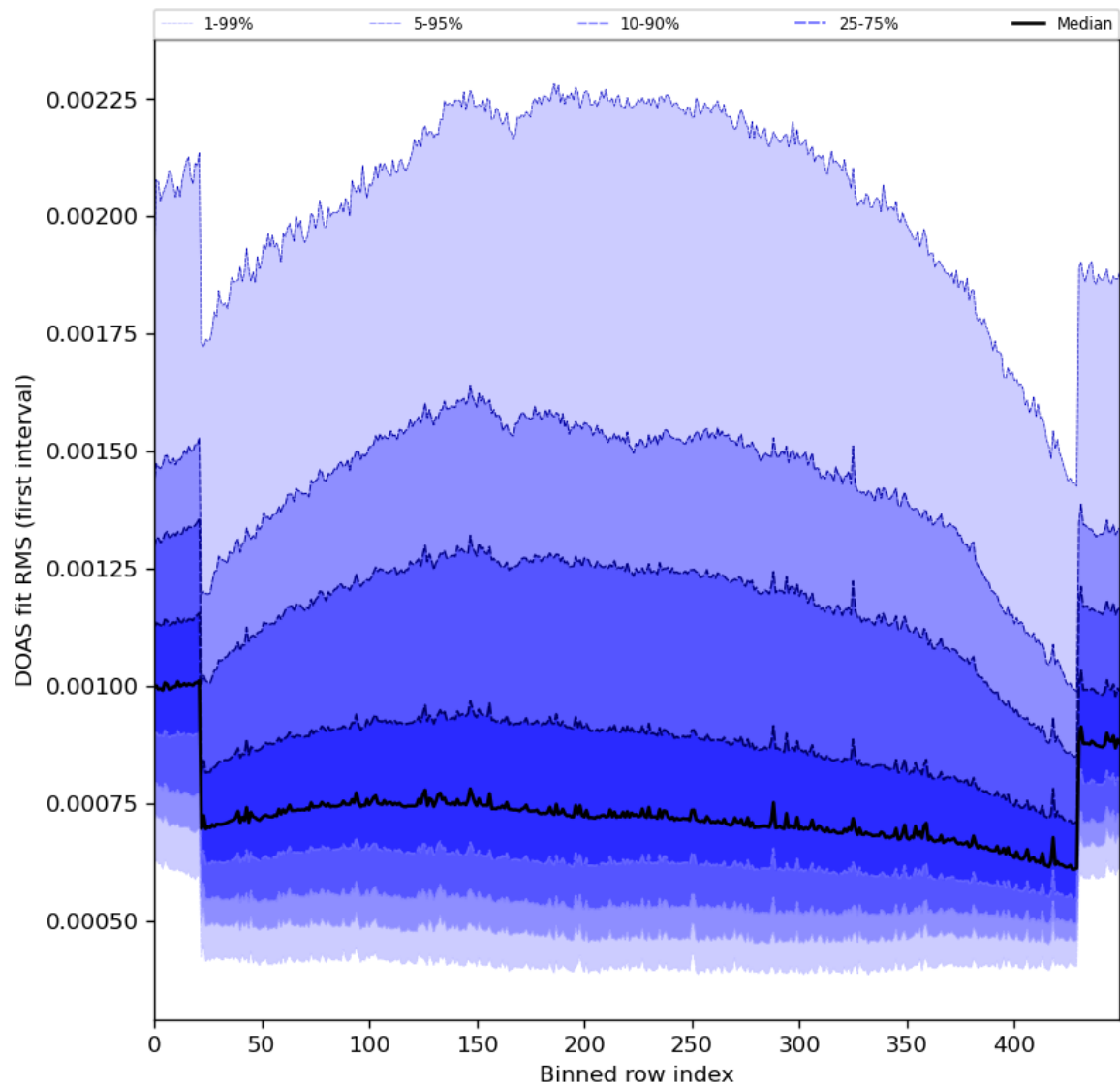
Figure 60: Along track statistics of “DOAS fit RMS (first interval)” for 2024-06-24 to 2024-06-26
