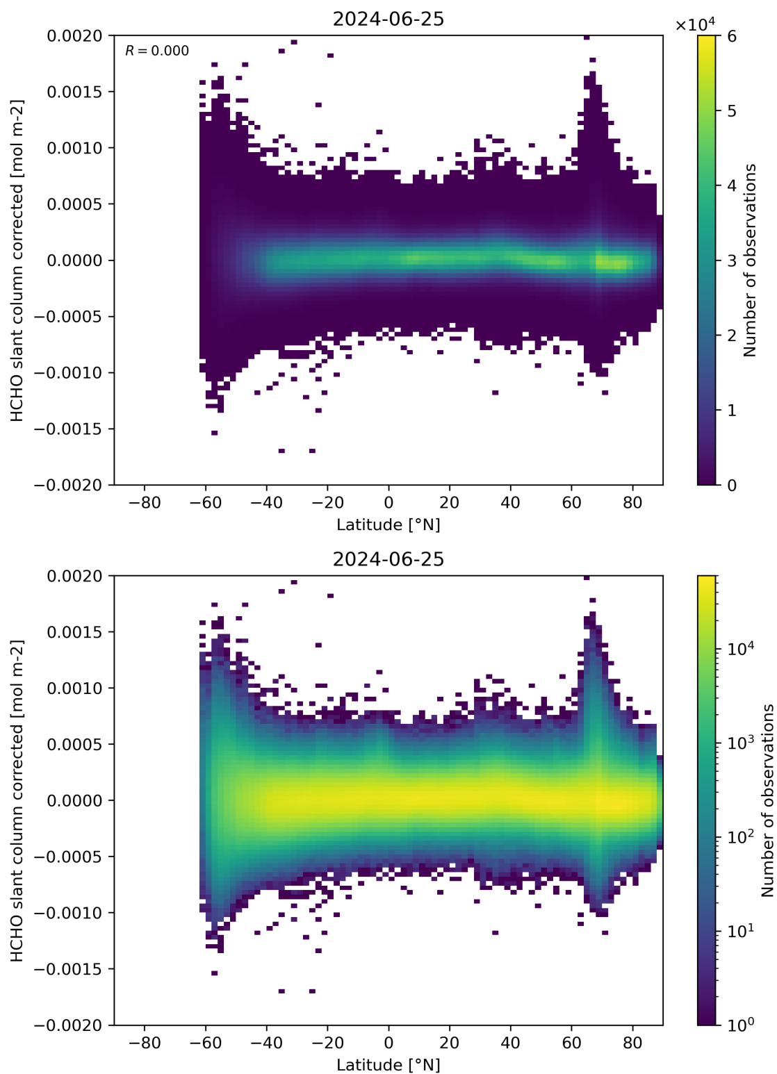
Figure 157: Scatter density plot of “Latitude” against “HCHO slant column corrected” for 2024-06-24 to 2024-06-26.
