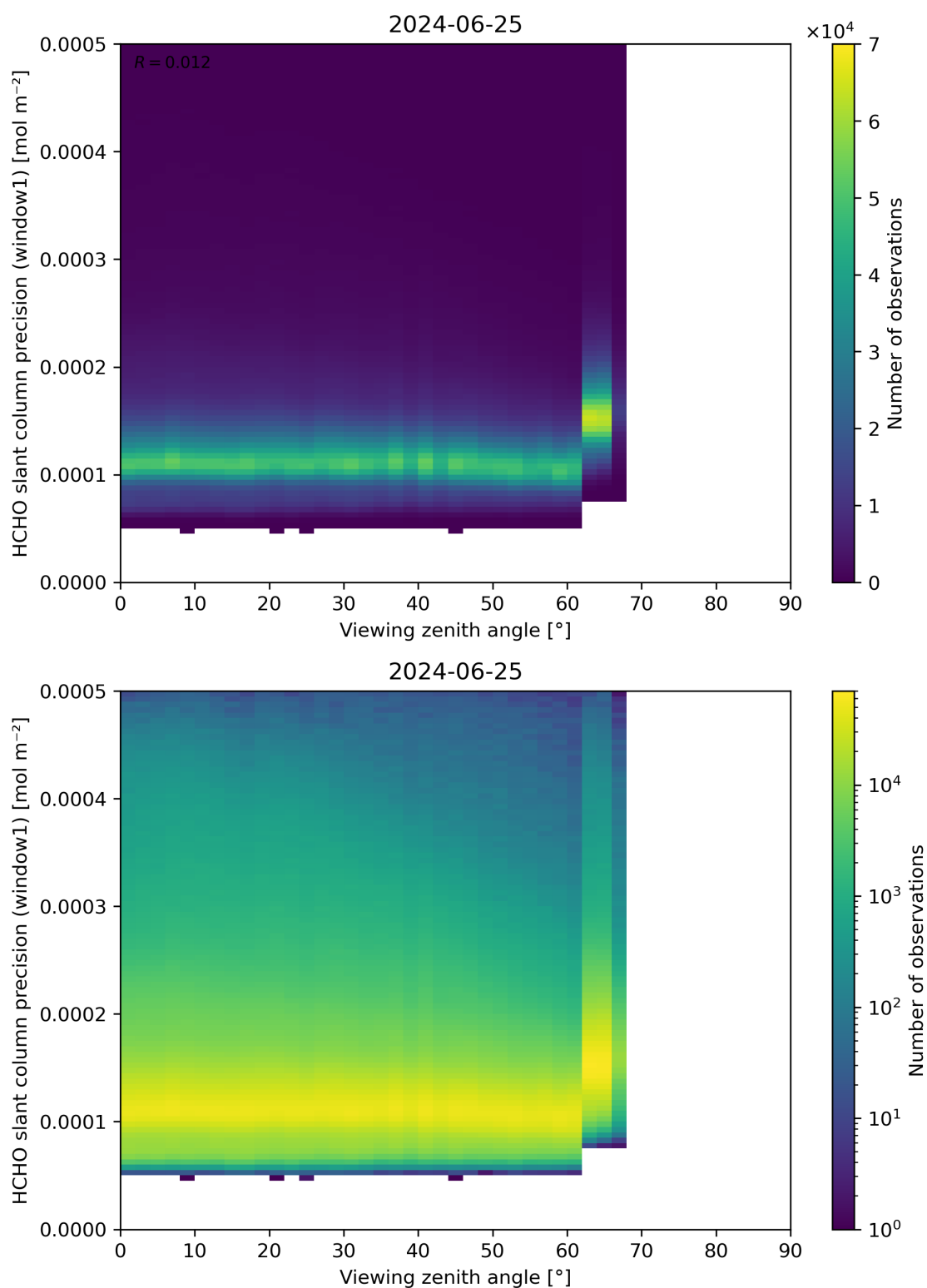
Figure 189: Scatter density plot of “Viewing zenith angle” against “HCHO slant column precision (window1)” for 2024-06-24 to 2024-06-26.
