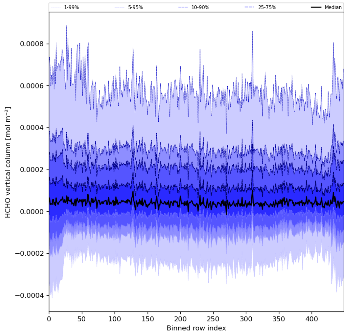
Figure 49: Along track statistics of “HCHO vertical column” for 2024-06-24 to 2024-06-26
