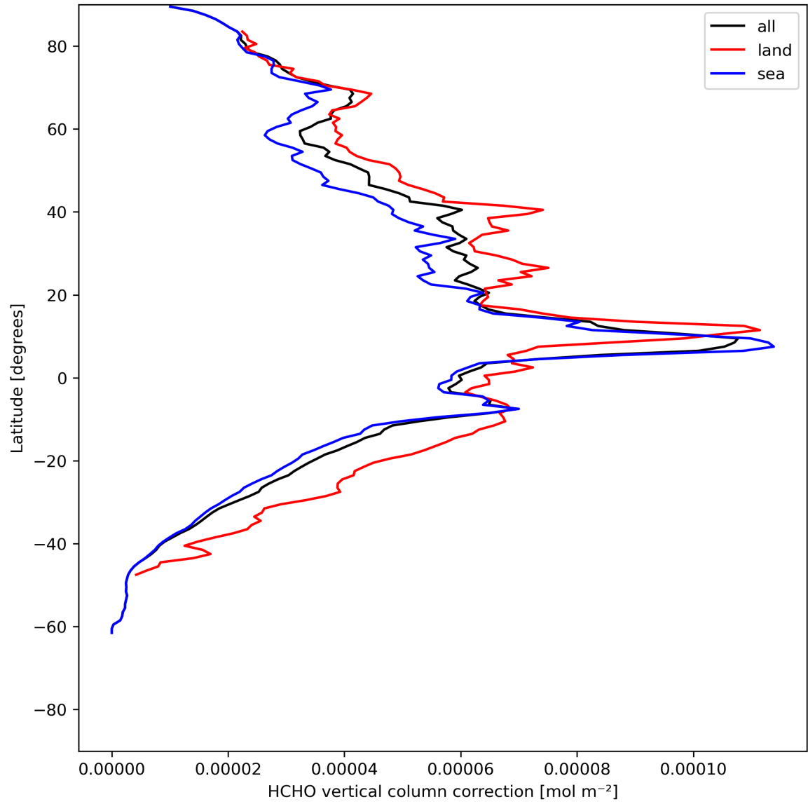
Figure 23: Zonal average of “HCHO vertical column correction” for 2024-06-24 to 2024-06-26.
