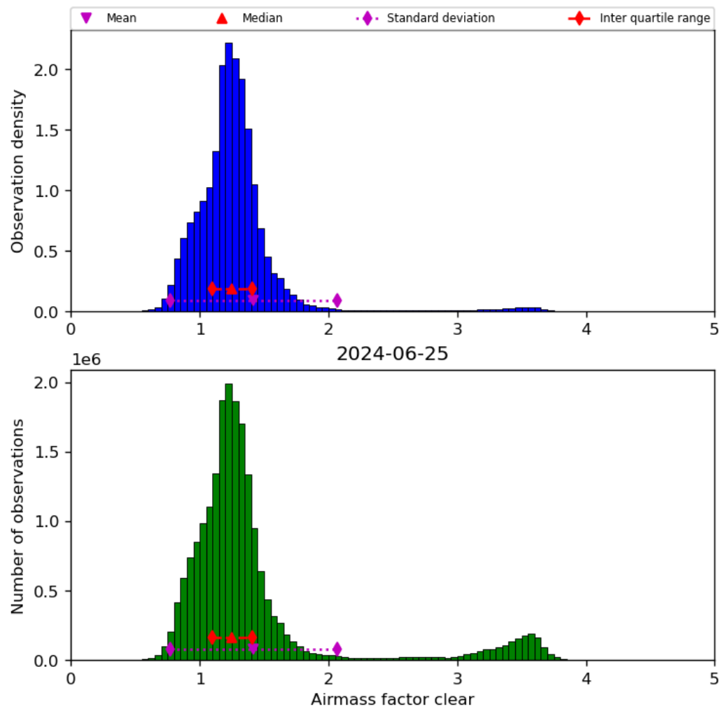
Figure 42: Histogram of “Airmass factor clear” for 2024-06-24 to 2024-06-26
