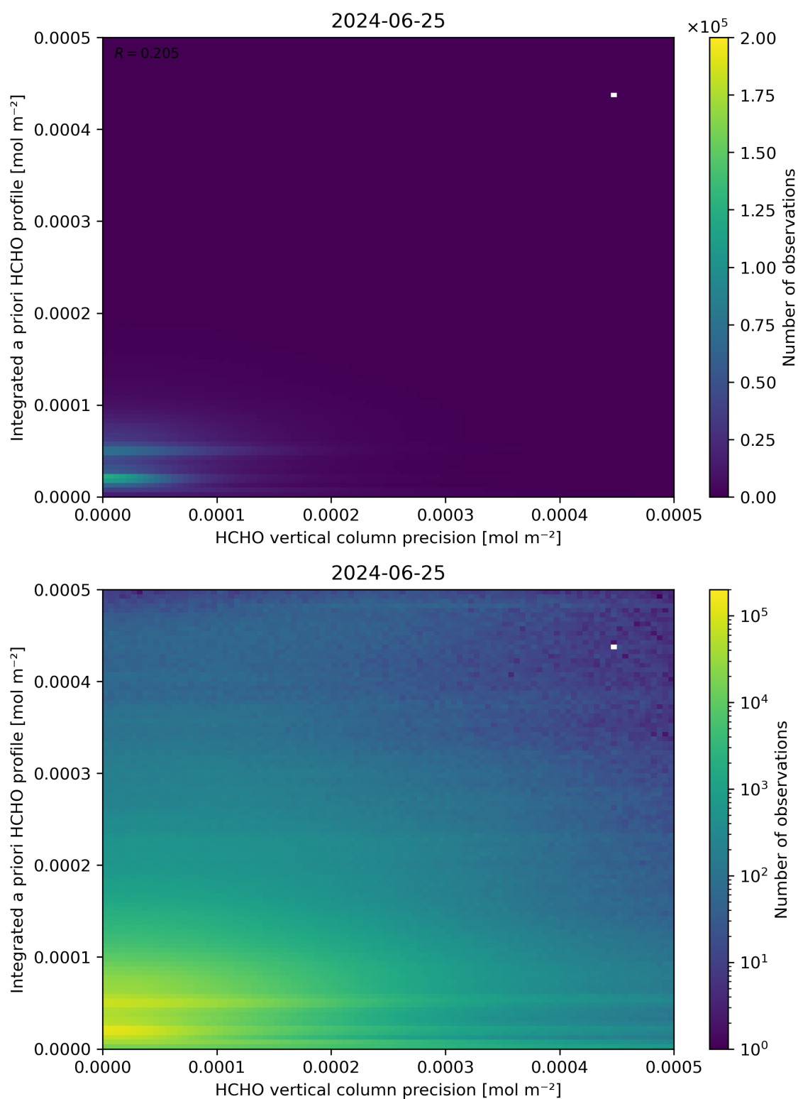
Figure 147: Scatter density plot of “HCHO vertical column precision” against “Integrated a priori HCHO profile” for 2024-06-24 to 2024-06-26.
