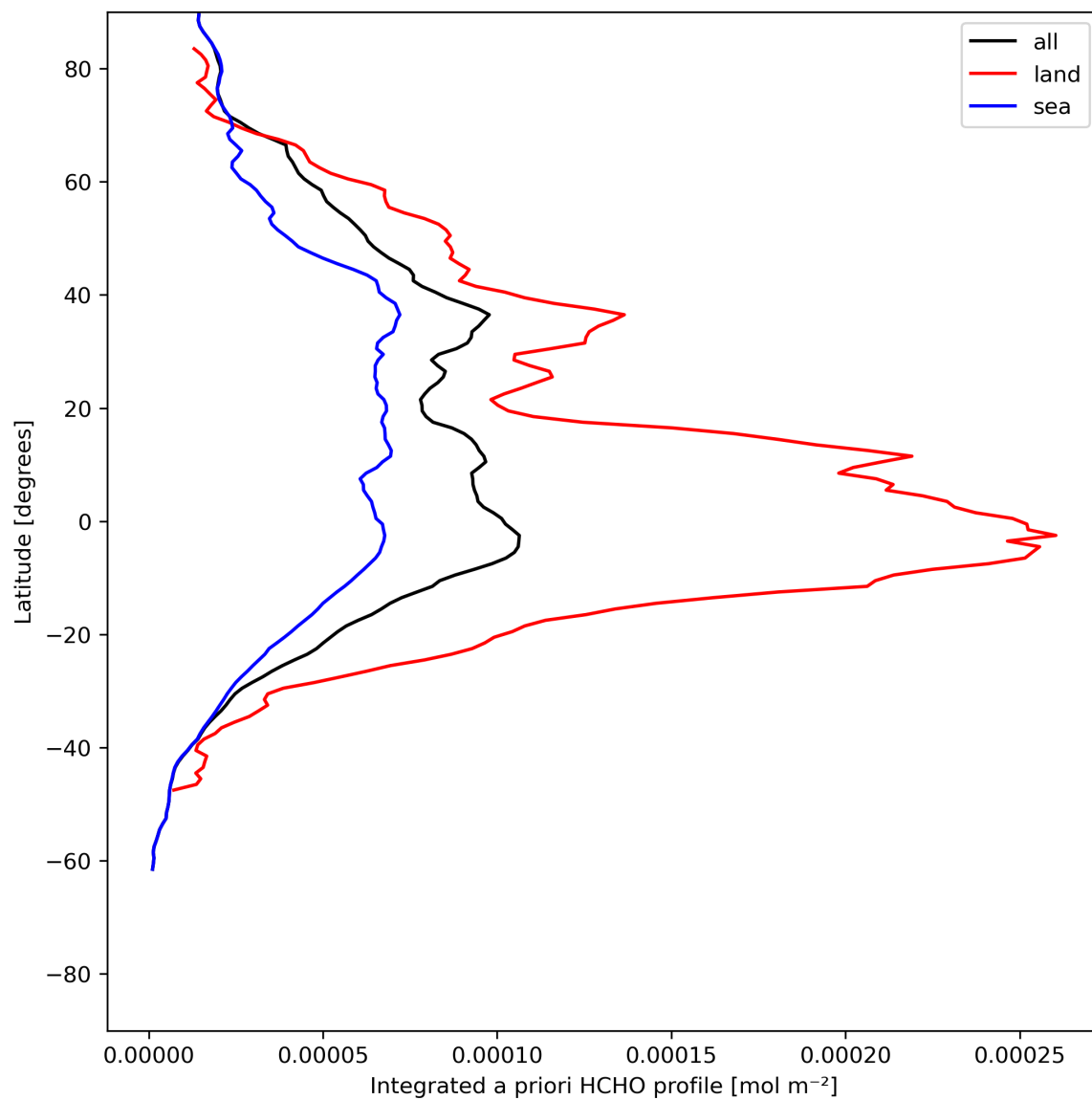
Figure 29: Zonal average of “Integrated a priori HCHO profile” for 2024-06-24 to 2024-06-26.
