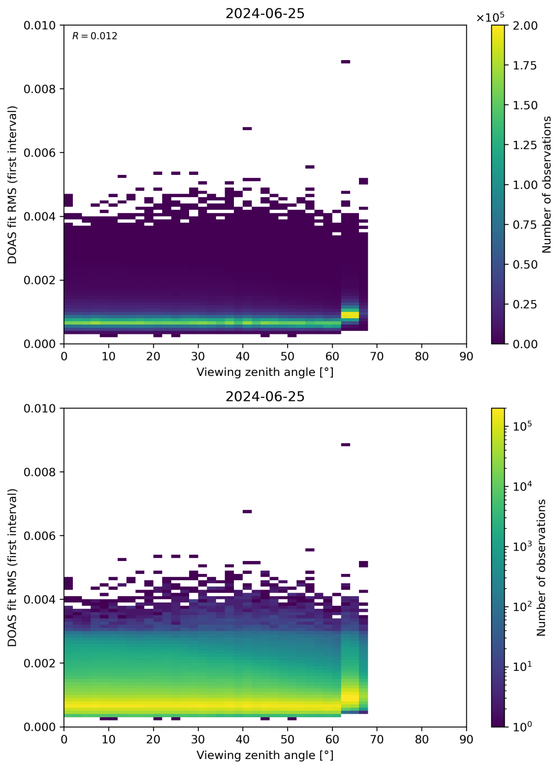
Figure 182: Scatter density plot of “Viewing zenith angle” against “DOAS fit RMS (first interval)” for 2024-06-24 to 2024-06-26.
