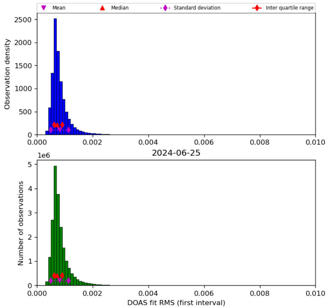
Figure 46: Histogram of “DOAS fit RMS (first interval)” for 2024-06-24 to 2024-06-26
