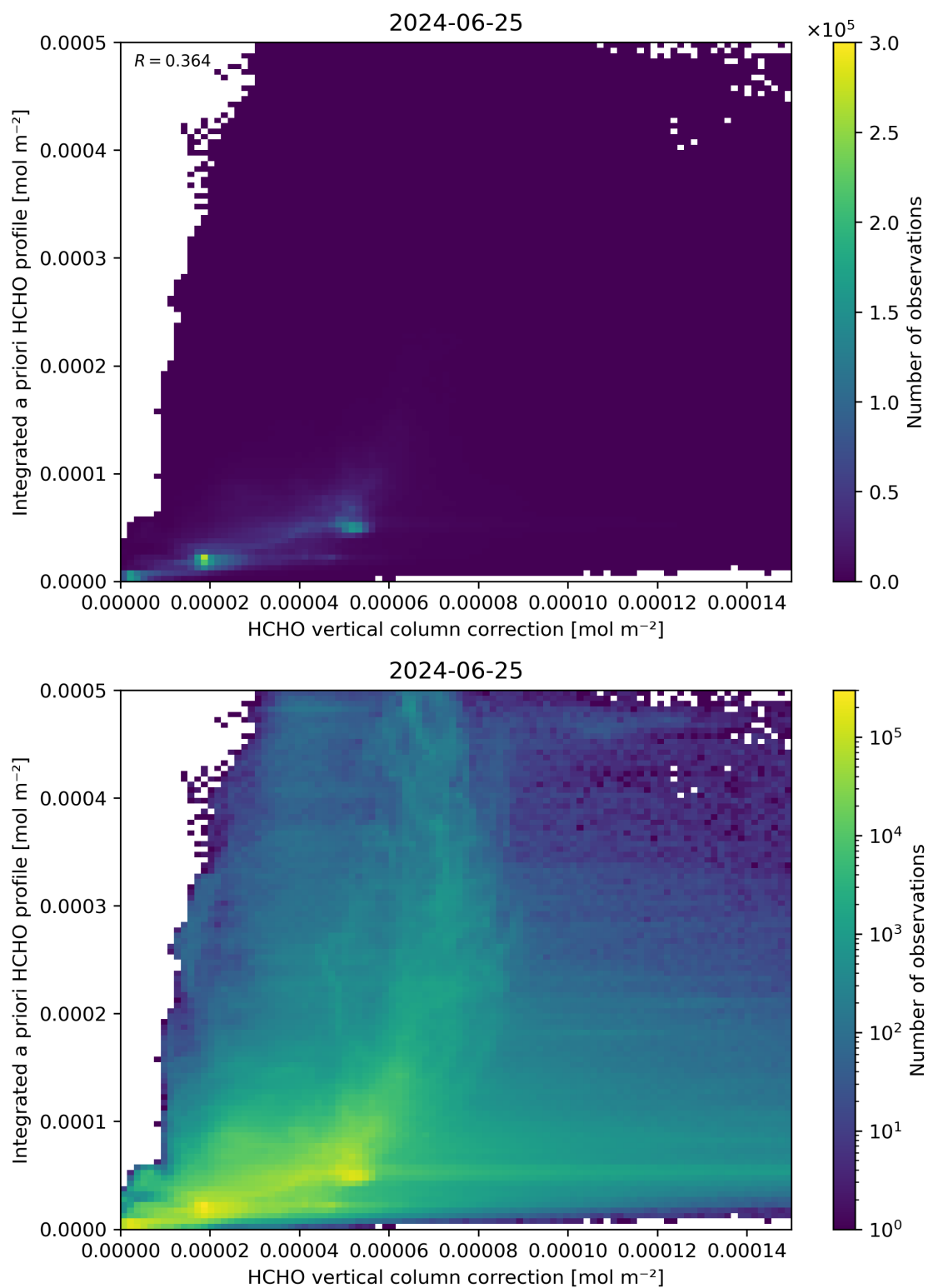
Figure 122: Scatter density plot of “HCHO vertical column correction” against “Integrated a priori HCHO profile” for 2024-06-24 to 2024-06-26.
