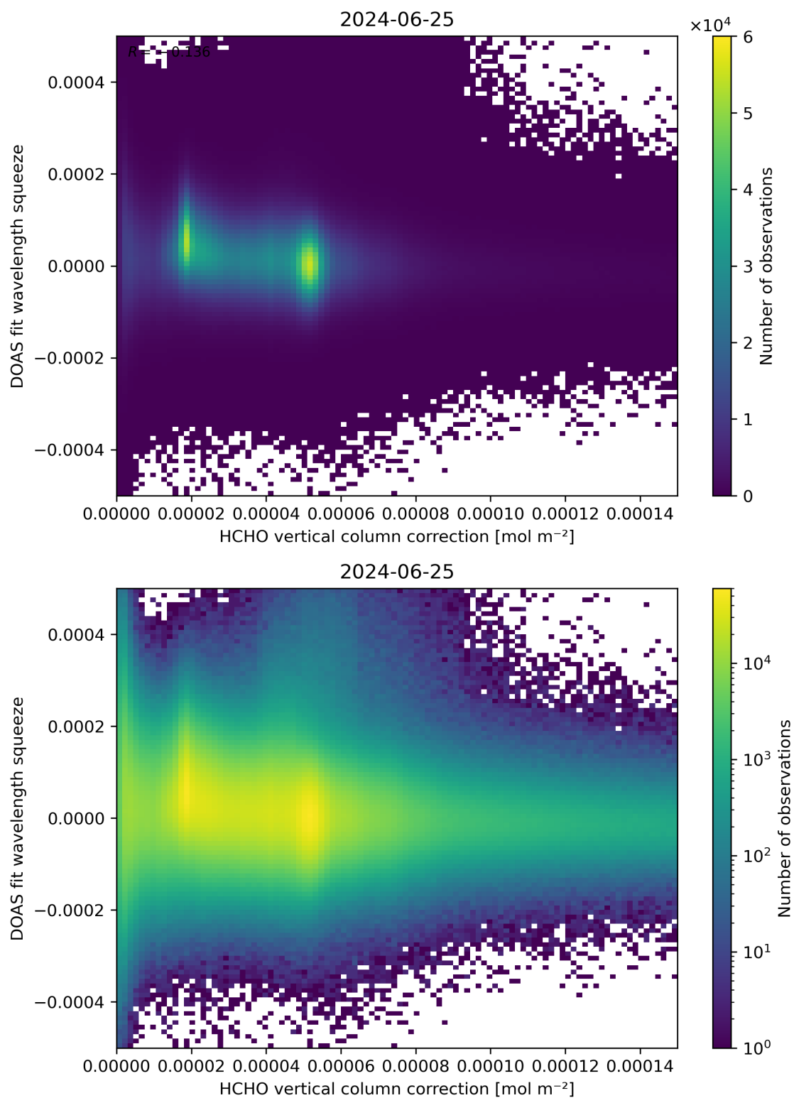
Figure 114: Scatter density plot of “HCHO vertical column correction” against “DOAS fit wavelength squeeze” for 2024-06-24 to 2024-06-26.
