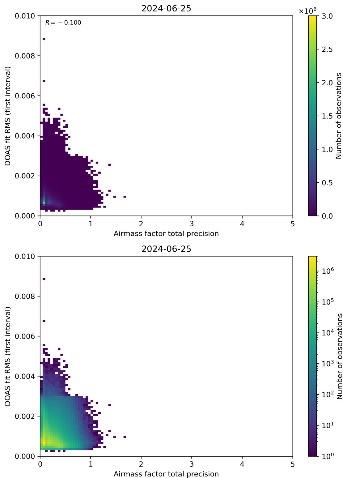
Figure 105: Scatter density plot of “Airmass factor total precision” against “DOAS fit RMS (first interval)” for 2024-06-24 to 2024-06-26.
