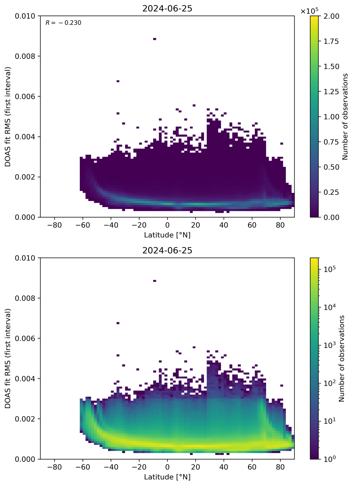
Figure 153: Scatter density plot of “Latitude” against “DOAS fit RMS (first interval)” for 2024-06-24 to 2024-06-26.
