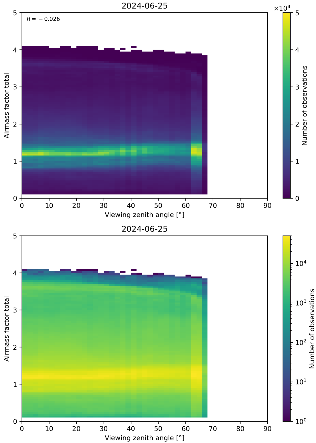
Figure 190: Scatter density plot of “Viewing zenith angle” against “Airmass factor total” for 2024-06-24 to 2024-06-26.
