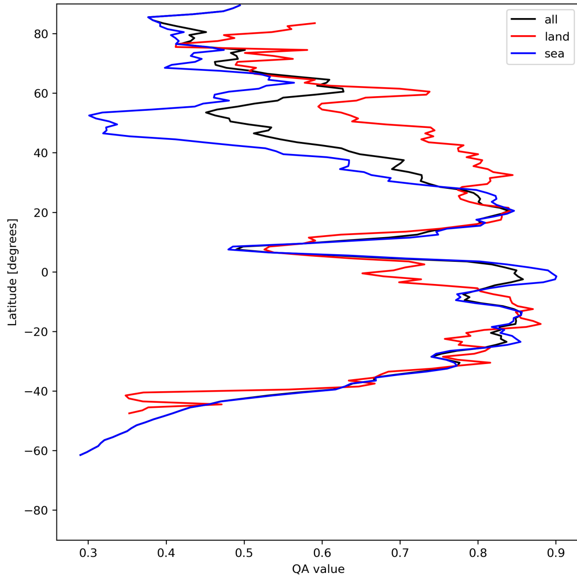
Figure 20: Zonal average of “QA value” for 2024-06-24 to 2024-06-26.
