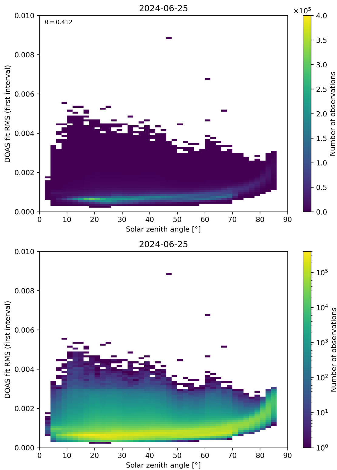
Figure 167: Scatter density plot of “Solar zenith angle” against “DOAS fit RMS (first interval)” for 2024-06-24 to 2024-06-26.
