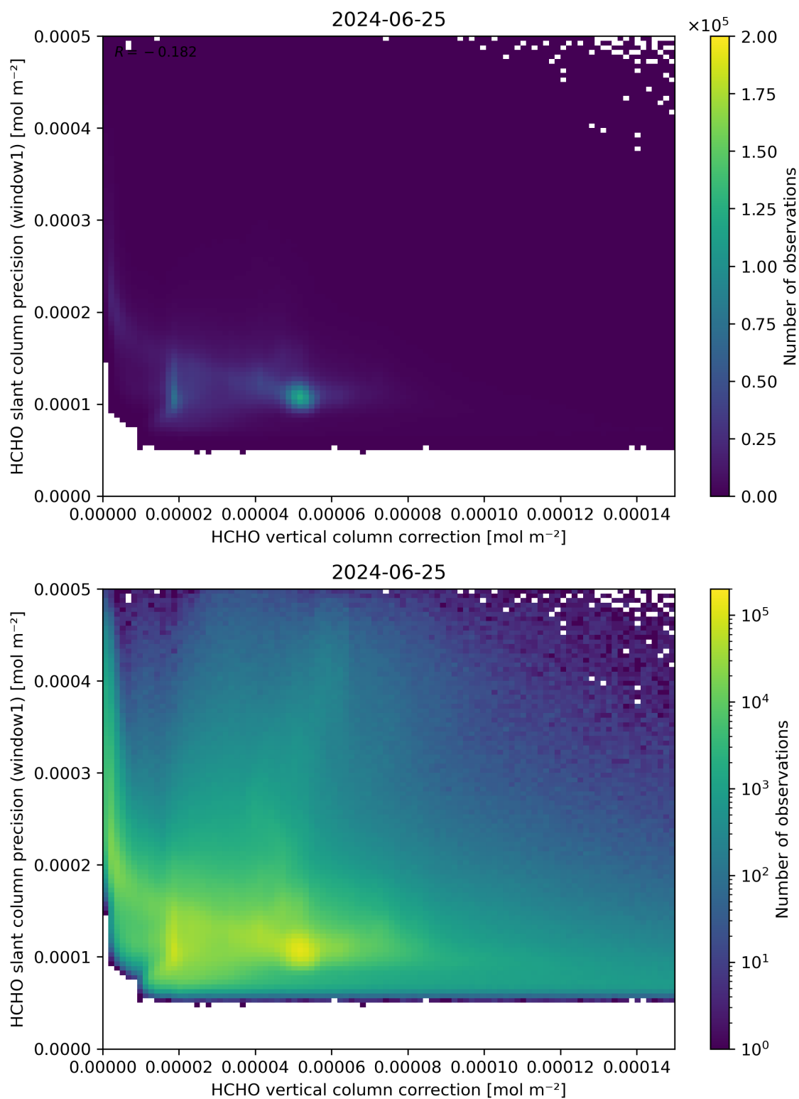
Figure 119: Scatter density plot of “HCHO vertical column correction” against “HCHO slant column precision (window1)” for 2024-06-24 to 2024-06-26.
