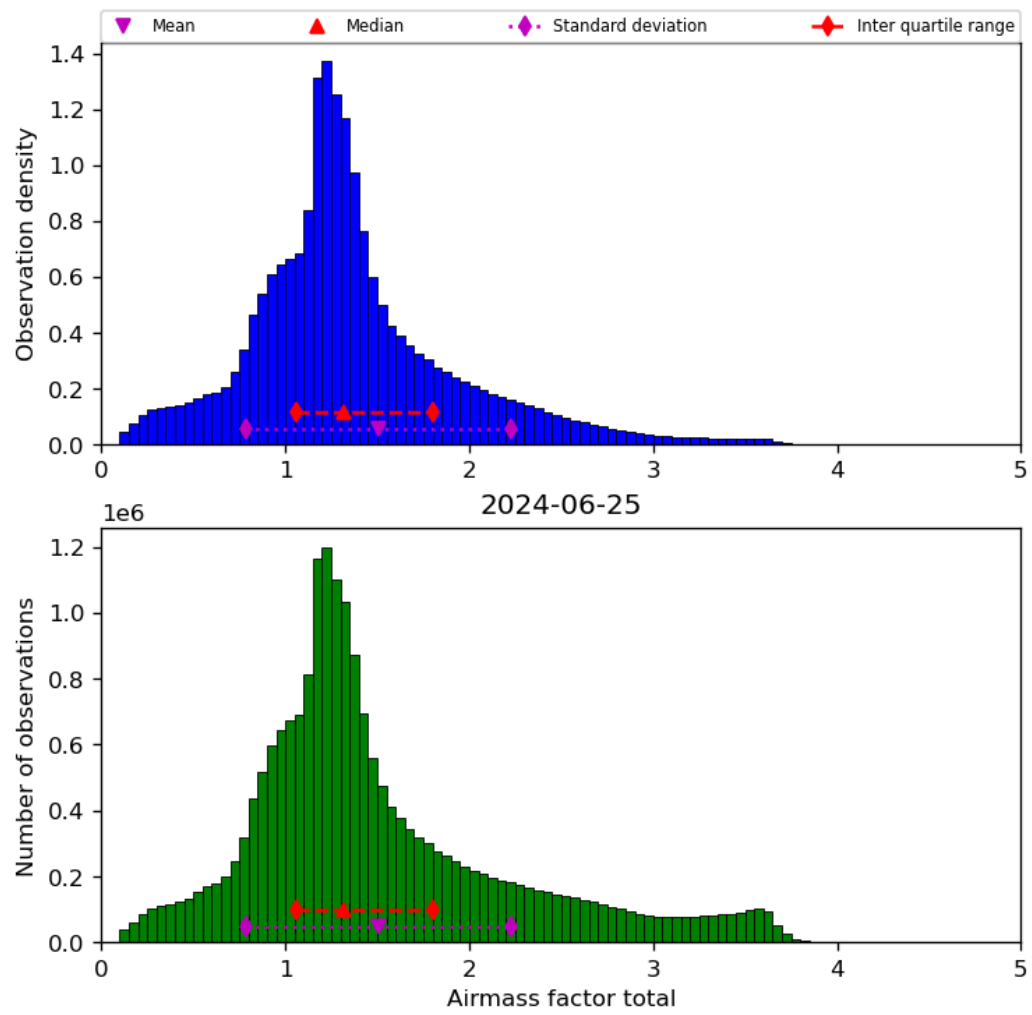
Figure 40: Histogram of “Airmass factor total” for 2024-06-24 to 2024-06-26
