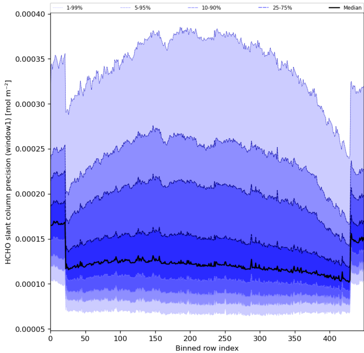
Figure 53: Along track statistics of “HCHO slant column precision (window1)” for 2024-06-24 to 2024-06-26
