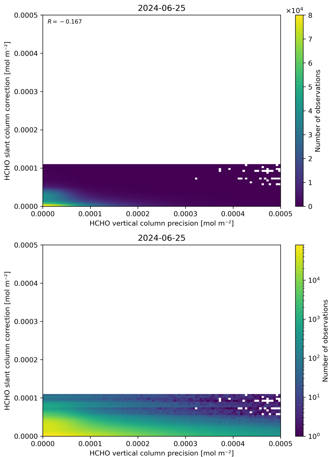
Figure 141: Scatter density plot of “HCHO vertical column precision” against “HCHO slant column correction” for 2024-06-24 to 2024-06-26.
