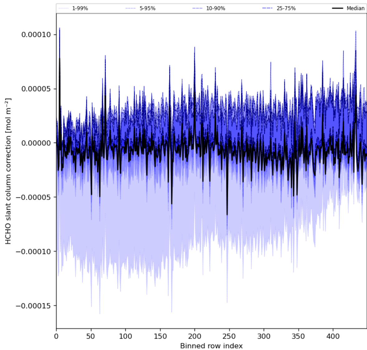
Figure 61: Along track statistics of "HCHO slant column correction" for 2024-06-24 to 2024-06-26
