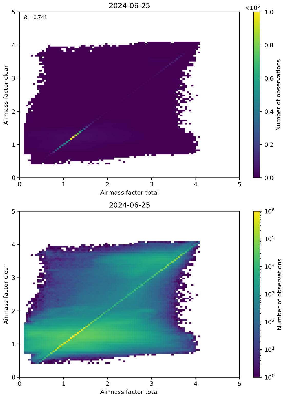
Figure 100: Scatter density plot of “Airmass factor total” against “Airmass factor clear” for 2024-06-24 to 2024-06-26.
