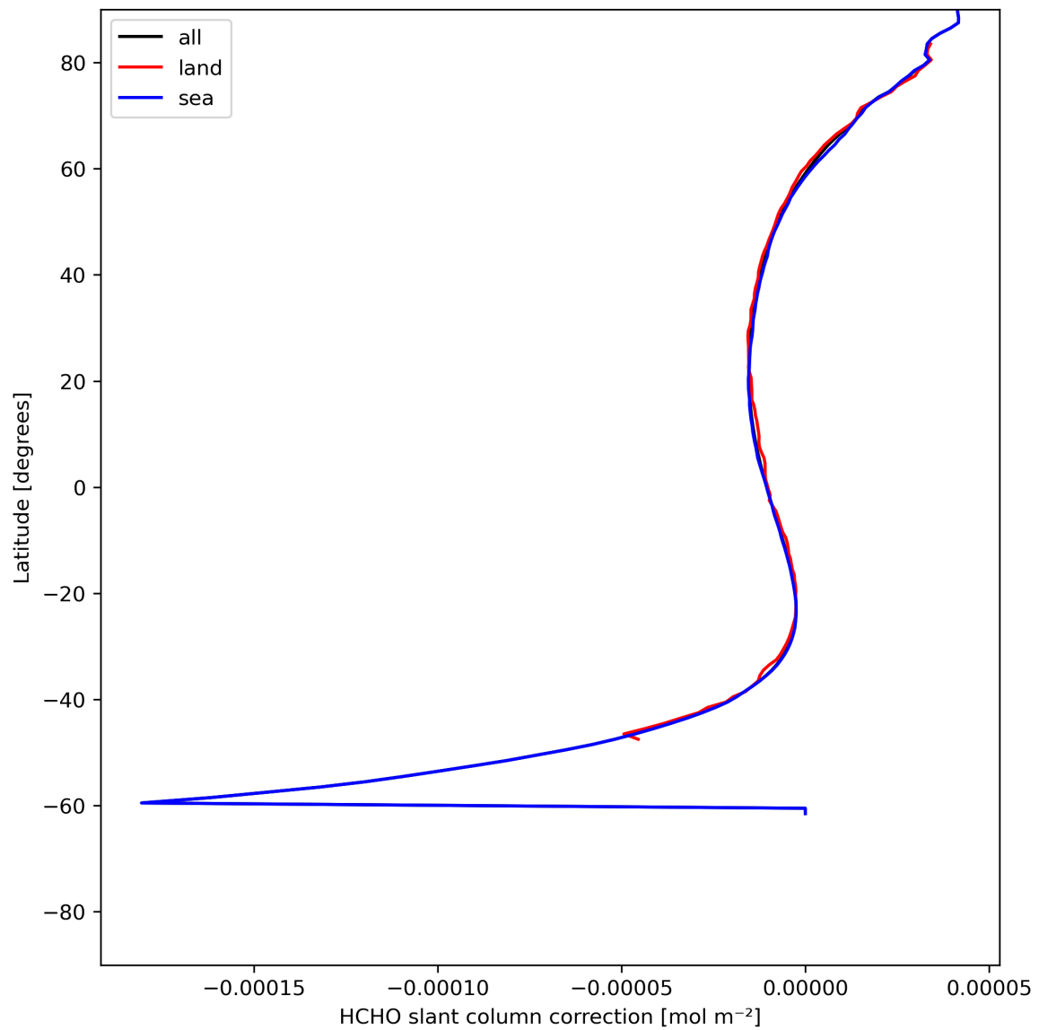
Figure 33: Zonal average of “HCHO slant column correction” for 2024-06-24 to 2024-06-26.
