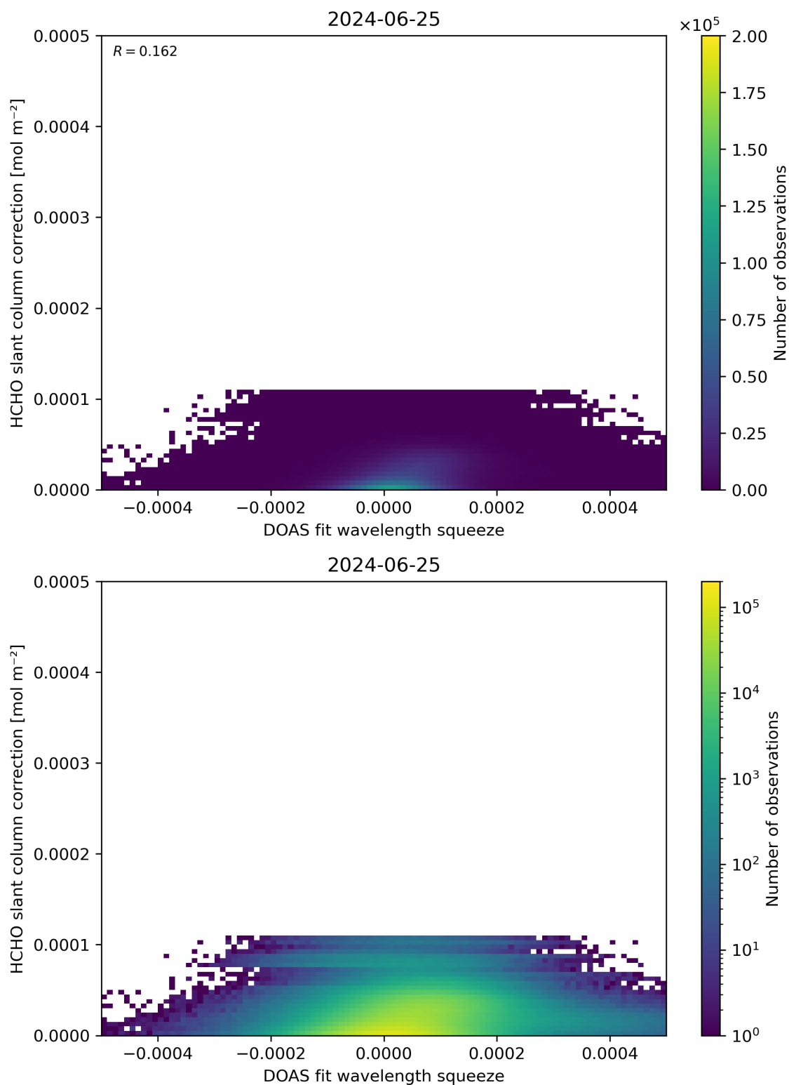
Figure 70: Scatter density plot of “DOAS fit wavelength squeeze” against “HCHO slant column correction” for 2024-06-24 to 2024-06-26.
