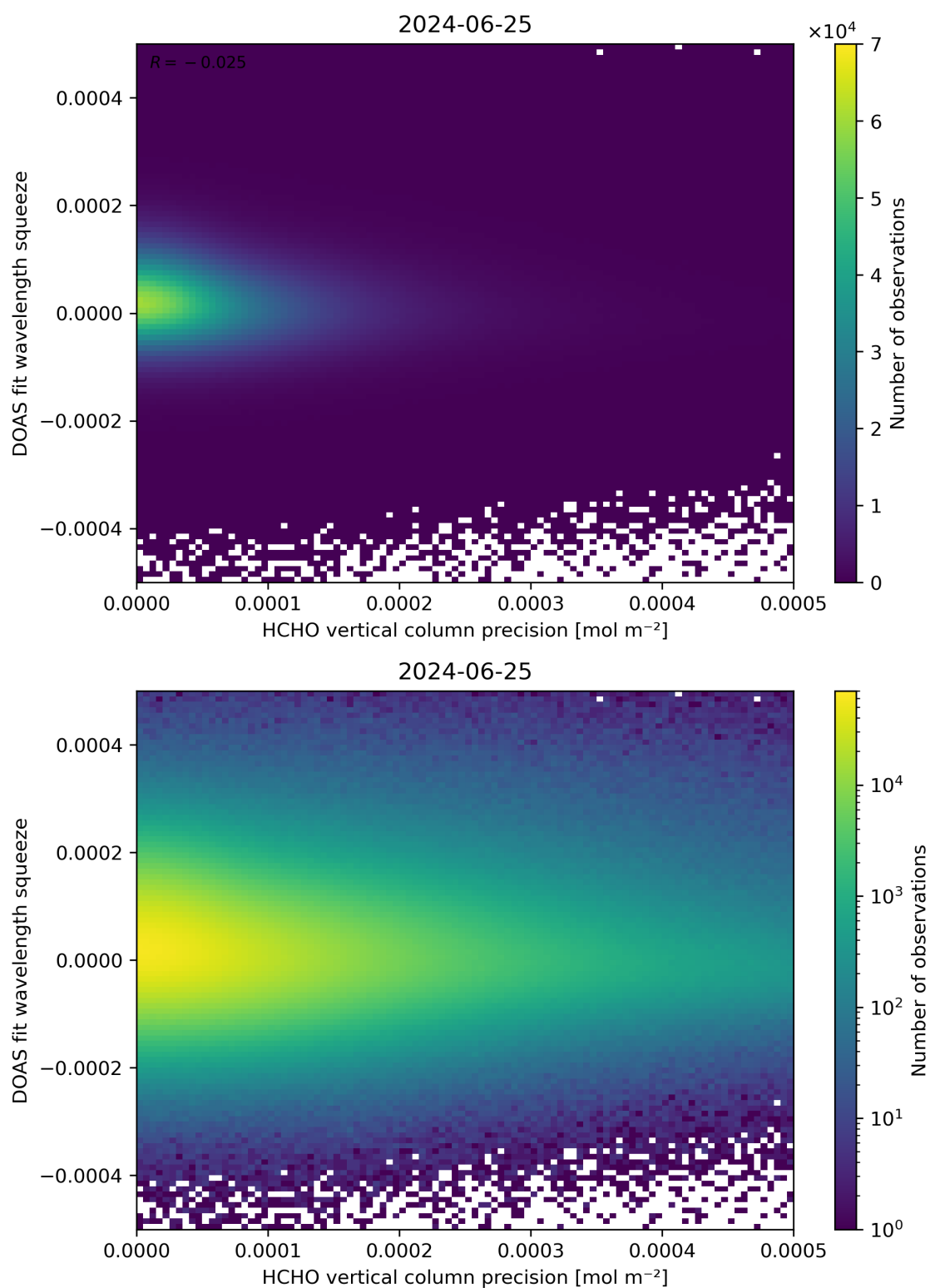
Figure 138: Scatter density plot of “HCHO vertical column precision” against “DOAS fit wavelength squeeze” for 2024-06-24 to 2024-06-26.
