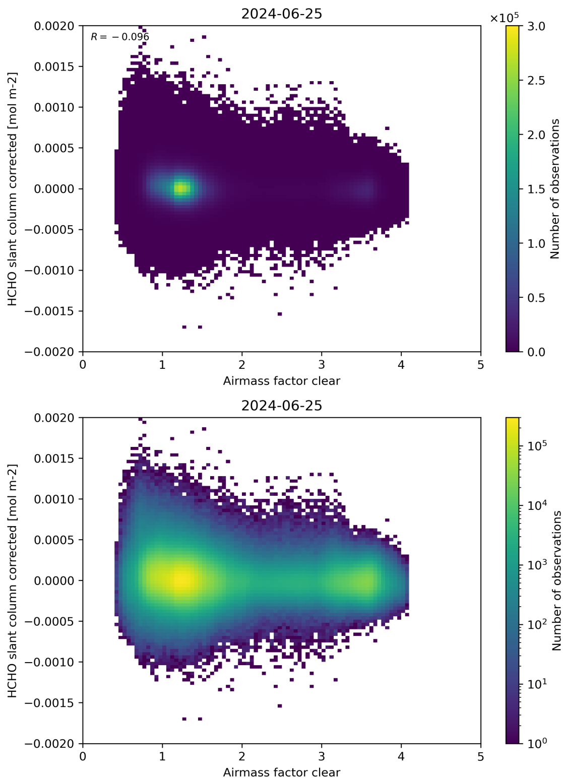
Figure 74: Scatter density plot of “Airmass factor clear” against “HCHO slant column corrected” for 2024-06-24 to 2024-06-26.
