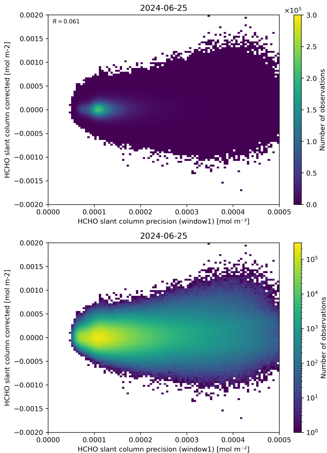
Figure 92: Scatter density plot of “HCHO slant column precision (window1)” against “HCHO slant column corrected” for 2024-06-24 to 2024-06-26.
