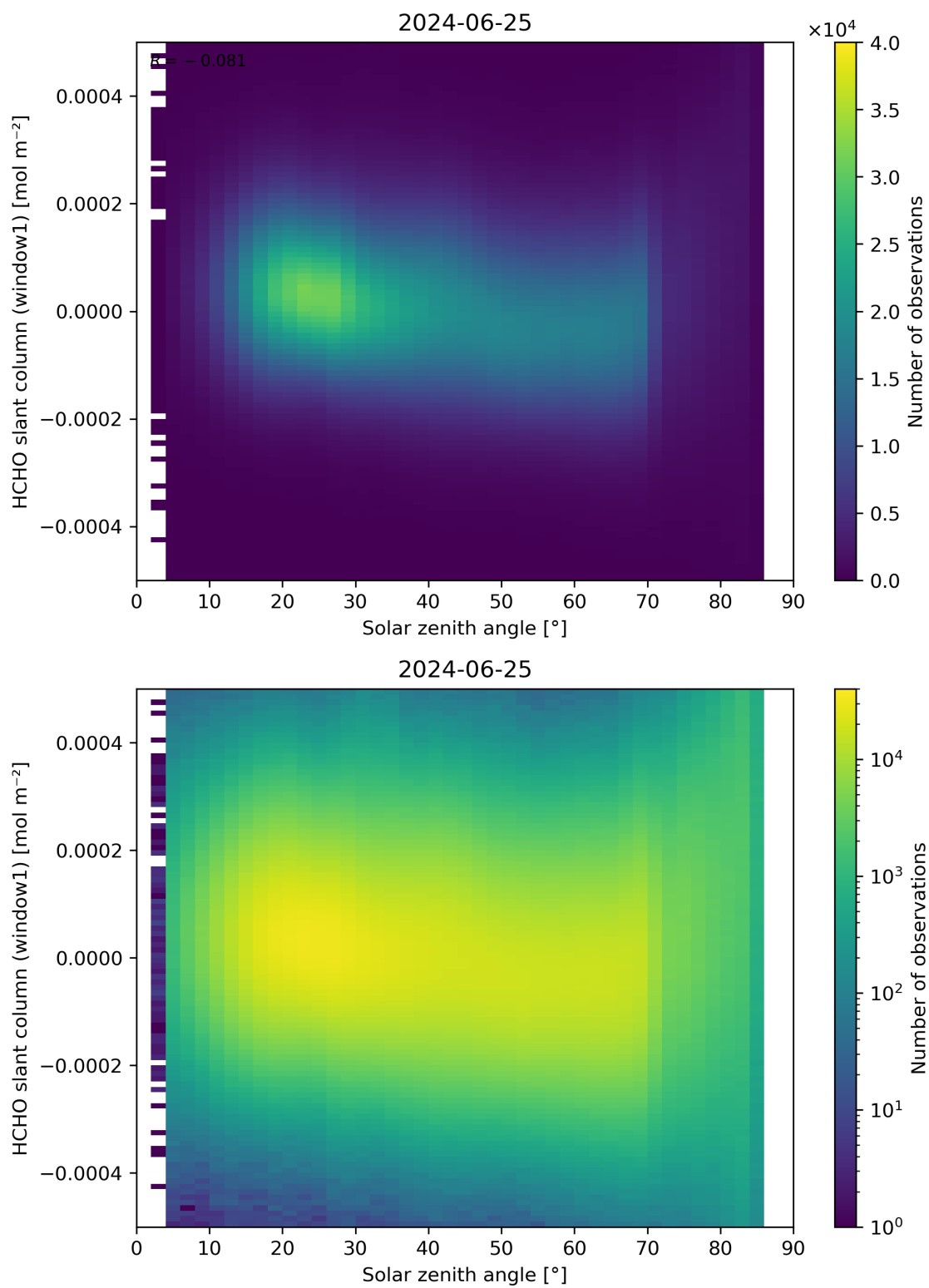
Figure 173: Scatter density plot of “Solar zenith angle” against “HCHO slant column (window1)” for 2024-06-24 to 2024-06-26.
