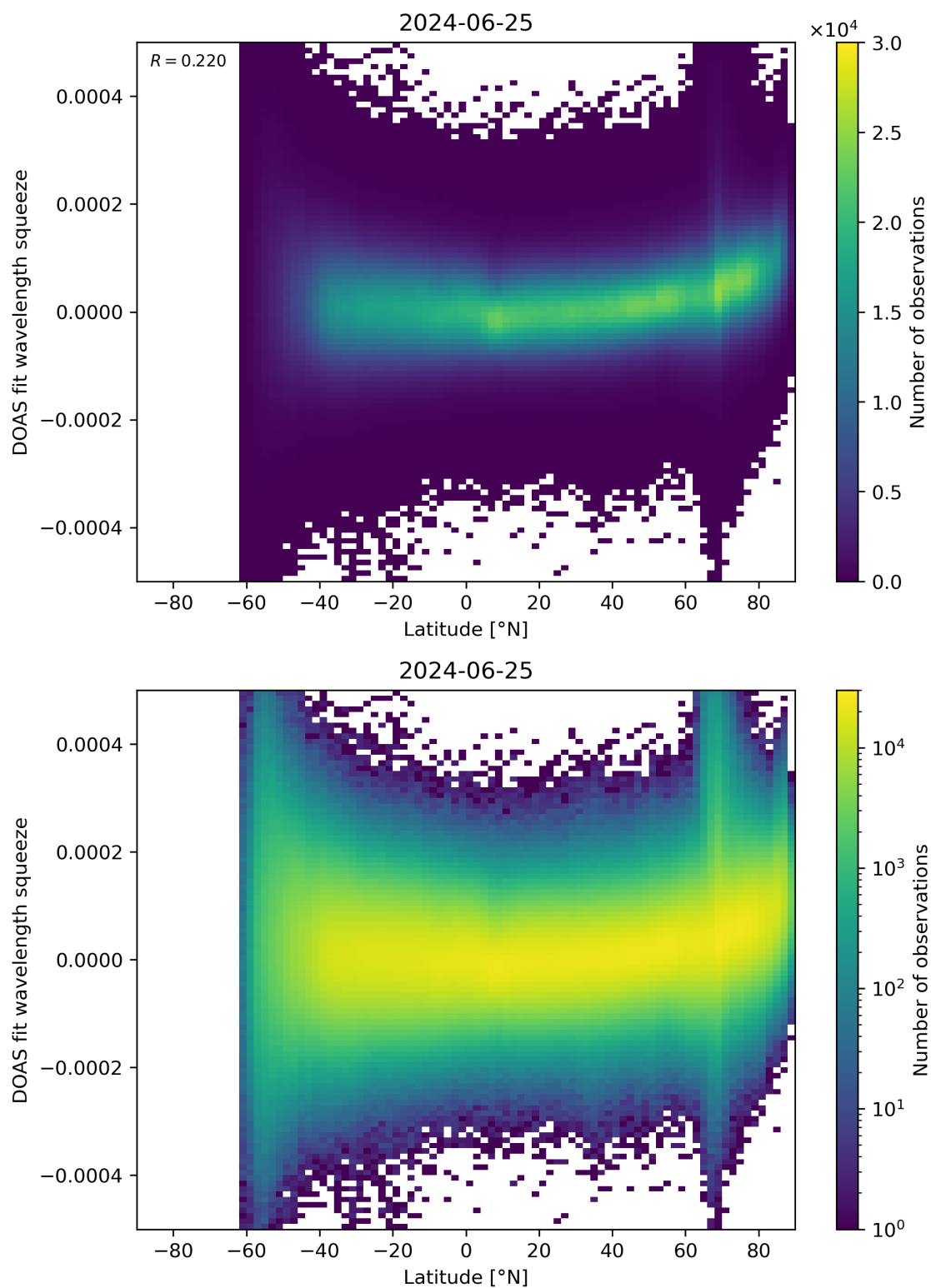
Figure 155: Scatter density plot of “Latitude” against “DOAS fit wavelength squeeze” for 2024-06-24 to 2024-06-26.
