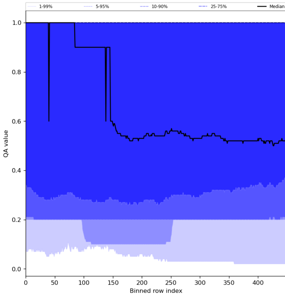
Figure 48: Along track statistics of “QA value” for 2024-06-24 to 2024-06-26
