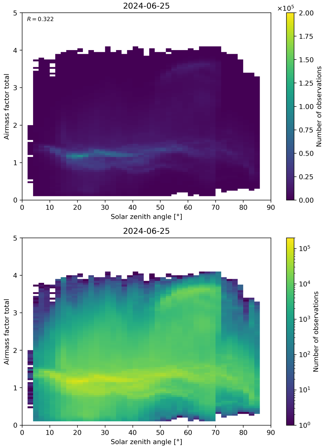
Figure 175: Scatter density plot of “Solar zenith angle” against “Airmass factor total” for 2024-06-24 to 2024-06-26.
