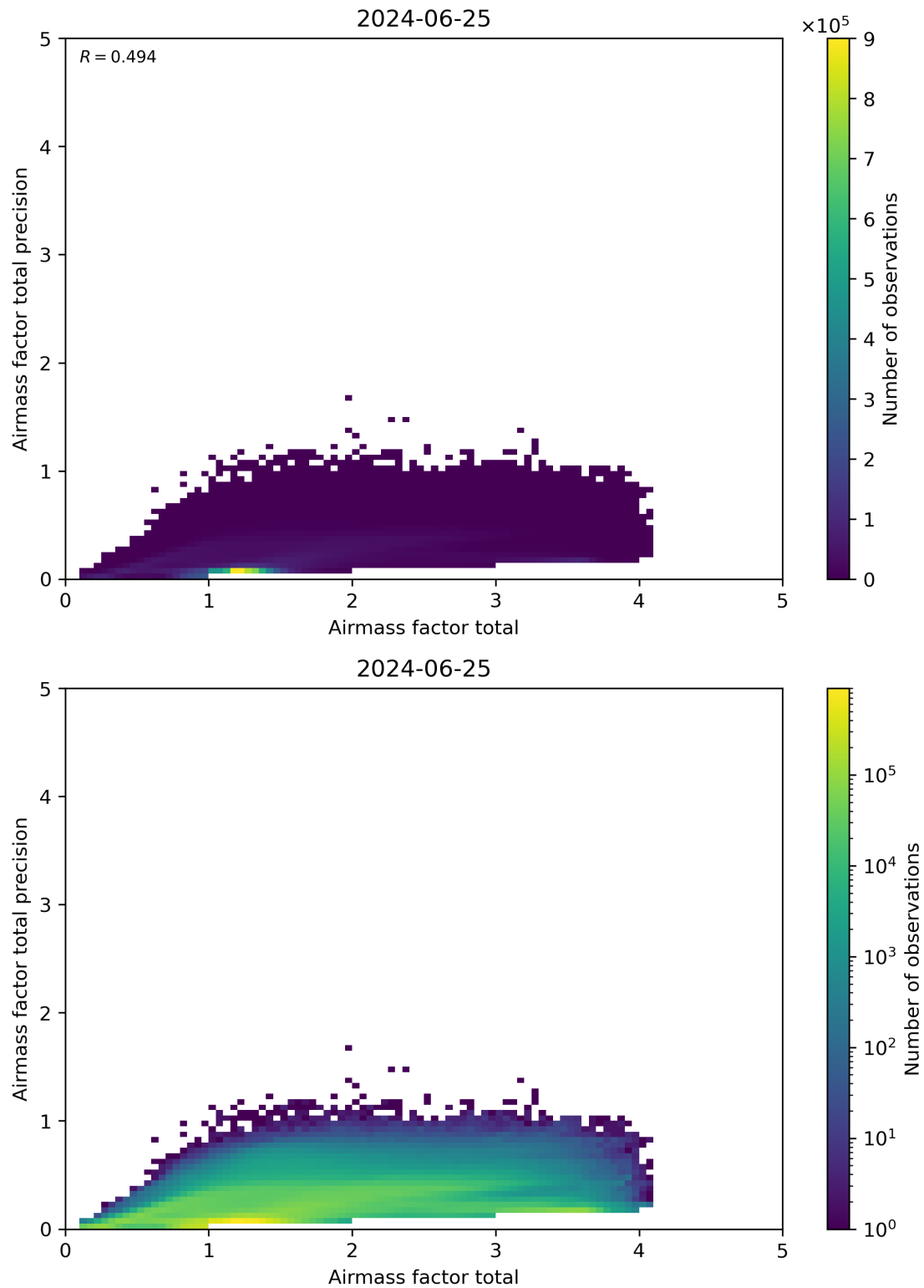
Figure 103: Scatter density plot of “Airmass factor total” against “Airmass factor total precision” for 2024-06-24 to 2024-06-26.
