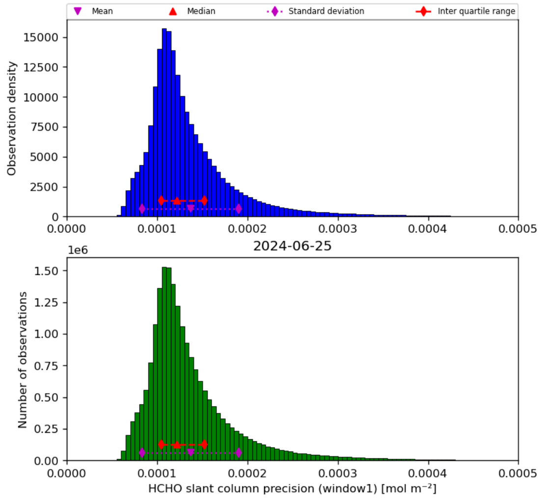
Figure 39: Histogram of “HCHO slant column precision (window1)” for 2024-06-24 to 2024-06-26
