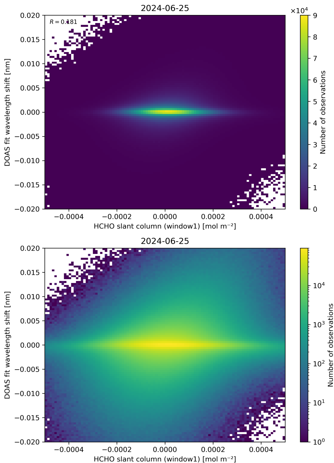
Figure 79: Scatter density plot of “HCHO slant column (window1)” against “DOAS fit wavelength shift” for 2024-06-24 to 2024-06-26.
