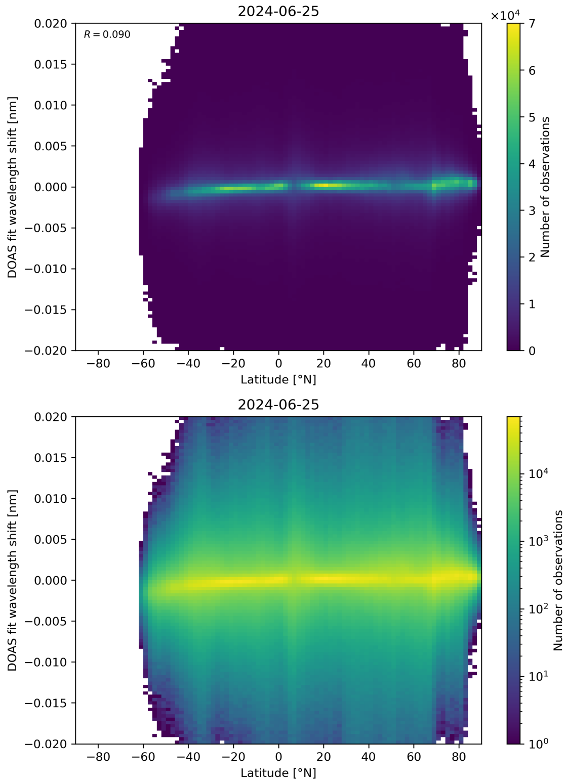
Figure 154: Scatter density plot of “Latitude” against “DOAS fit wavelength shift” for 2024-06-24 to 2024-06-26.
