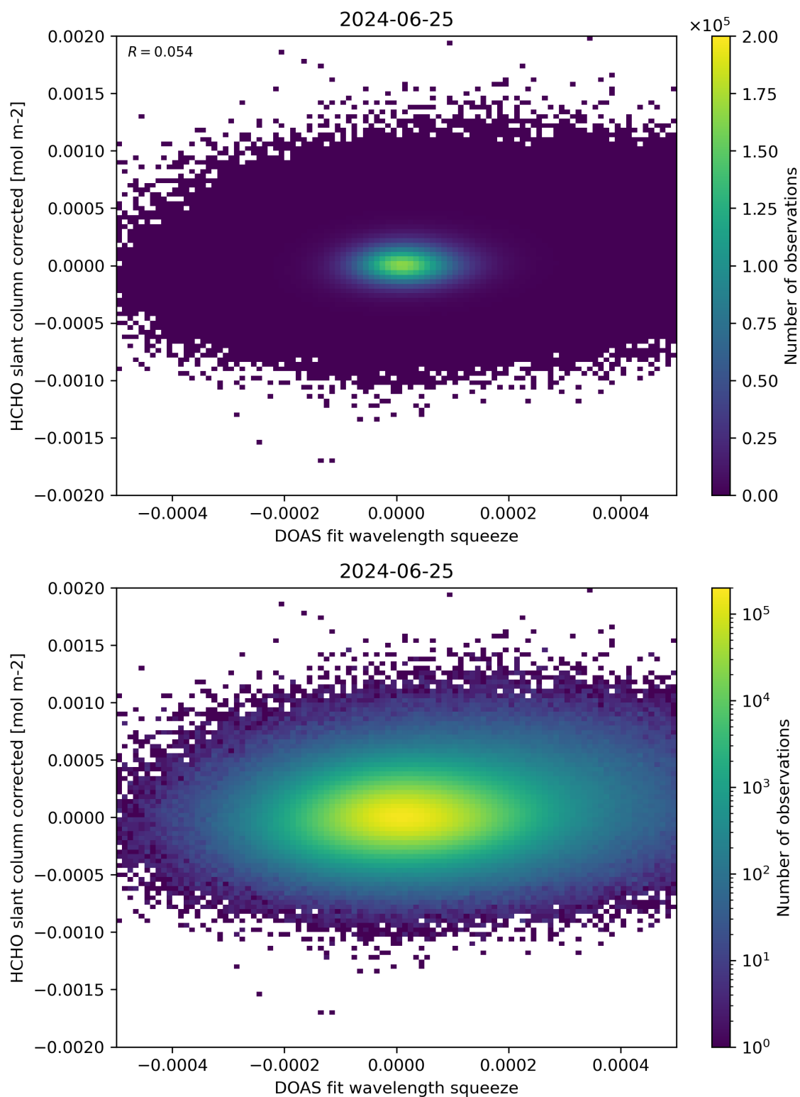
Figure 69: Scatter density plot of “DOAS fit wavelength squeeze” against “HCHO slant column corrected” for 2024-06-24 to 2024-06-26.
