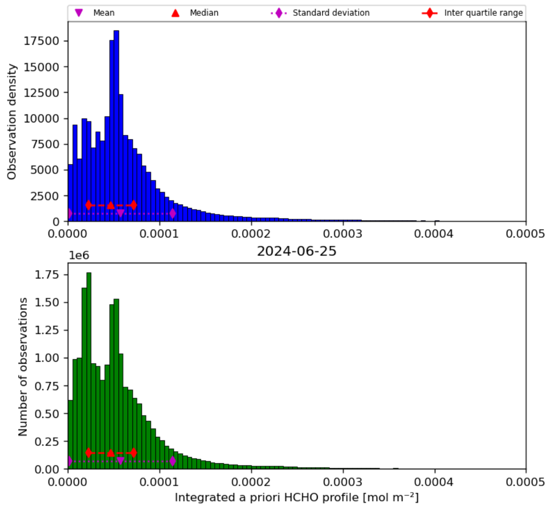
Figure 43: Histogram of “Integrated a priori HCHO profile” for 2024-06-24 to 2024-06-26
