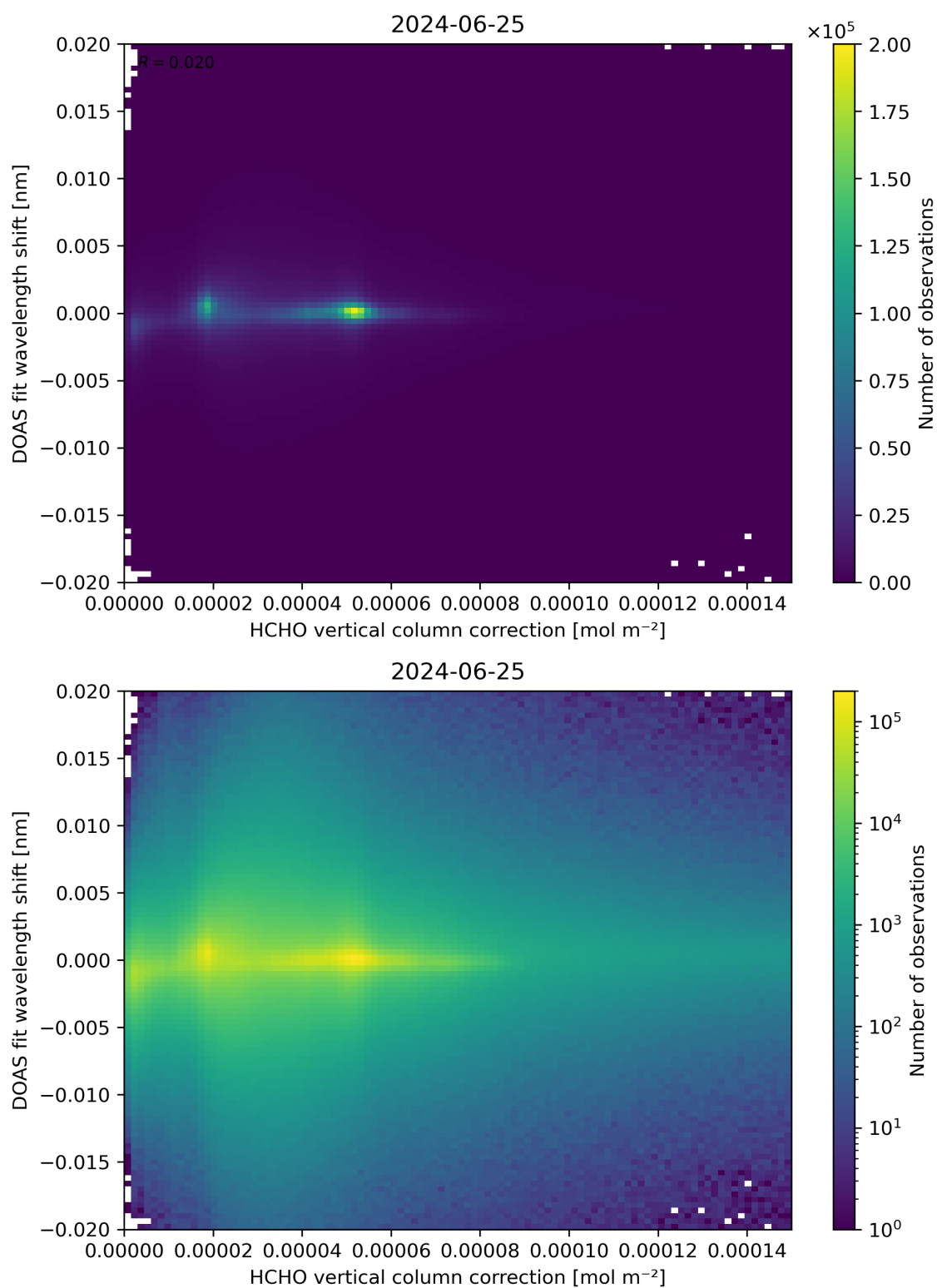
Figure 113: Scatter density plot of “HCHO vertical column correction” against “DOAS fit wavelength shift” for 2024-06-24 to 2024-06-26.
