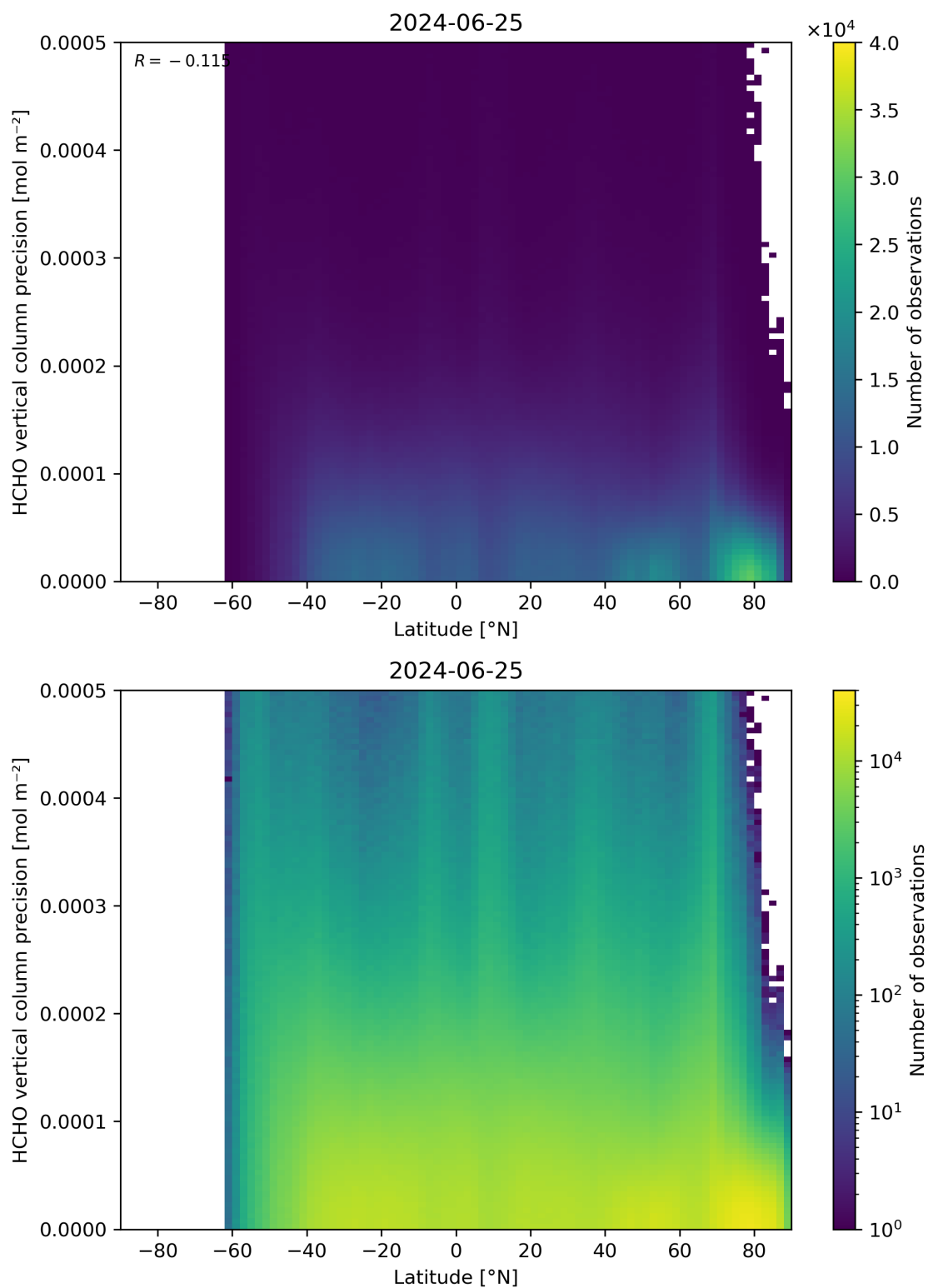
Figure 165: Scatter density plot of “Latitude” against “HCHO vertical column precision” for 2024-06-24 to 2024-06-26.
