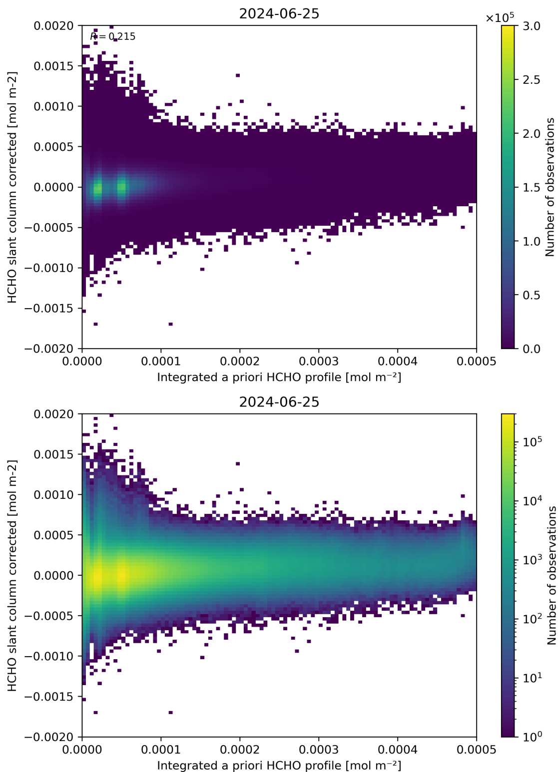
Figure 151: Scatter density plot of “Integrated a priori HCHO profile” against “HCHO slant column corrected” for 2024-06-24 to 2024-06-26.
