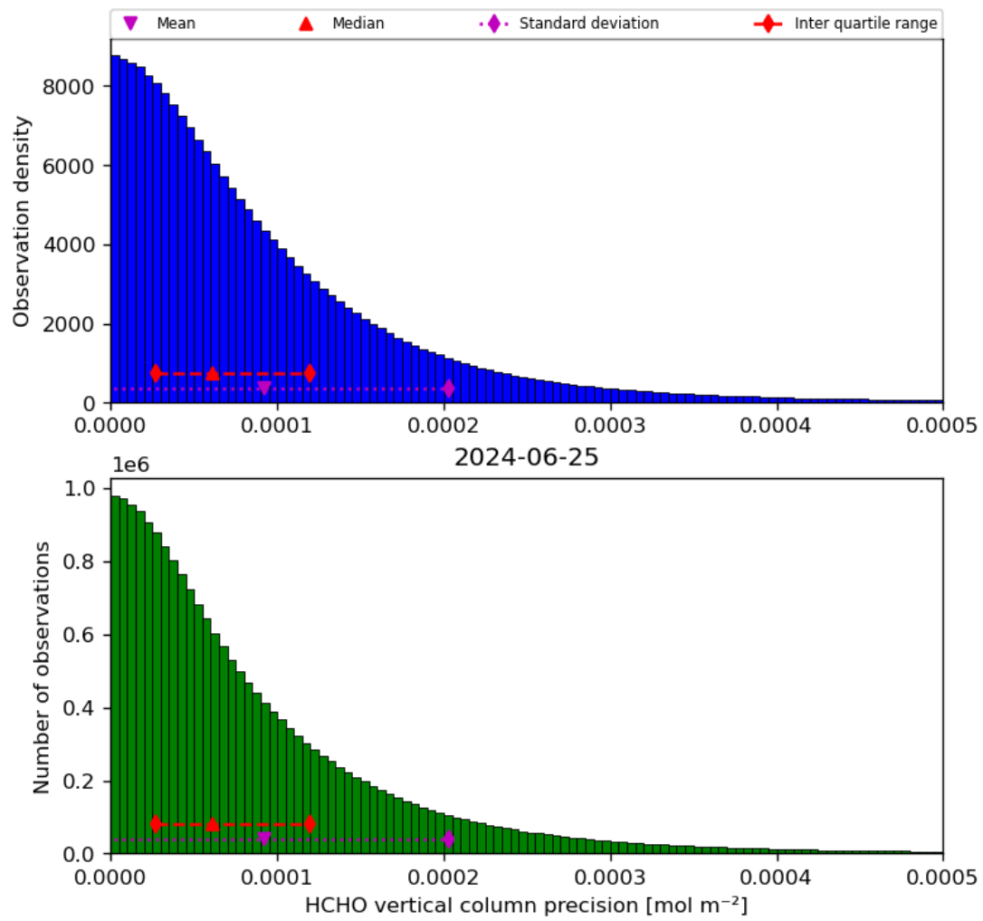
Figure 36: Histogram of “HCHO vertical column precision” for 2024-06-24 to 2024-06-26
