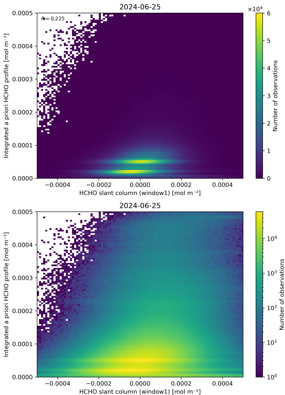
Figure 87: Scatter density plot of “HCHO slant column (window1)” against “Integrated a priori HCHO profile” for 2024-06-24 to 2024-06-26.
