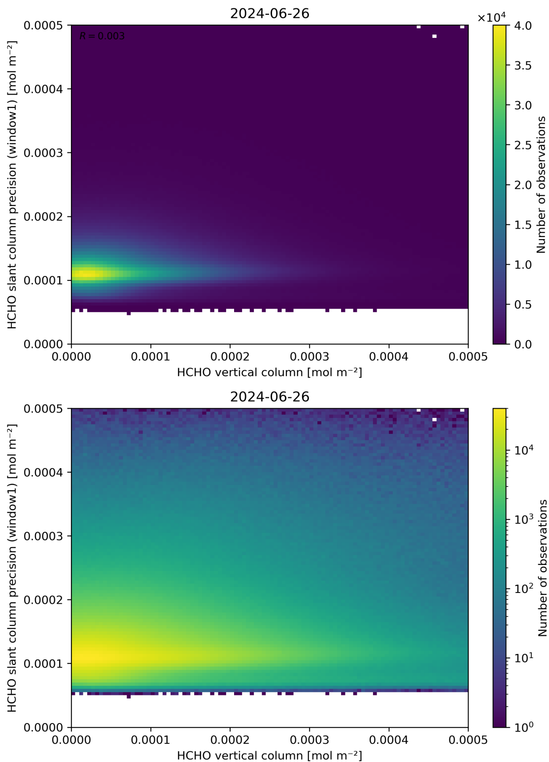
Figure 130: Scatter density plot of “HCHO vertical column” against “HCHO slant column precision (window1)” for 2024-06-25 to 2024-06-27.
