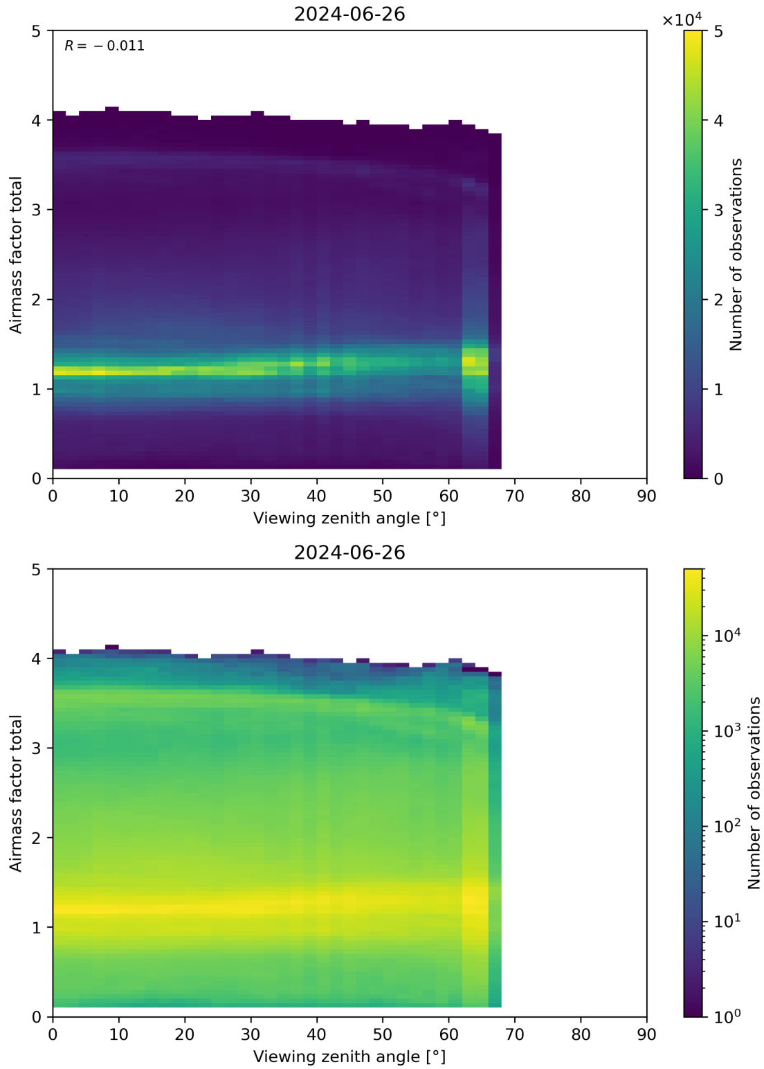
Figure 190: Scatter density plot of “Viewing zenith angle” against “Airmass factor total” for 2024-06-25 to 2024-06-27.
