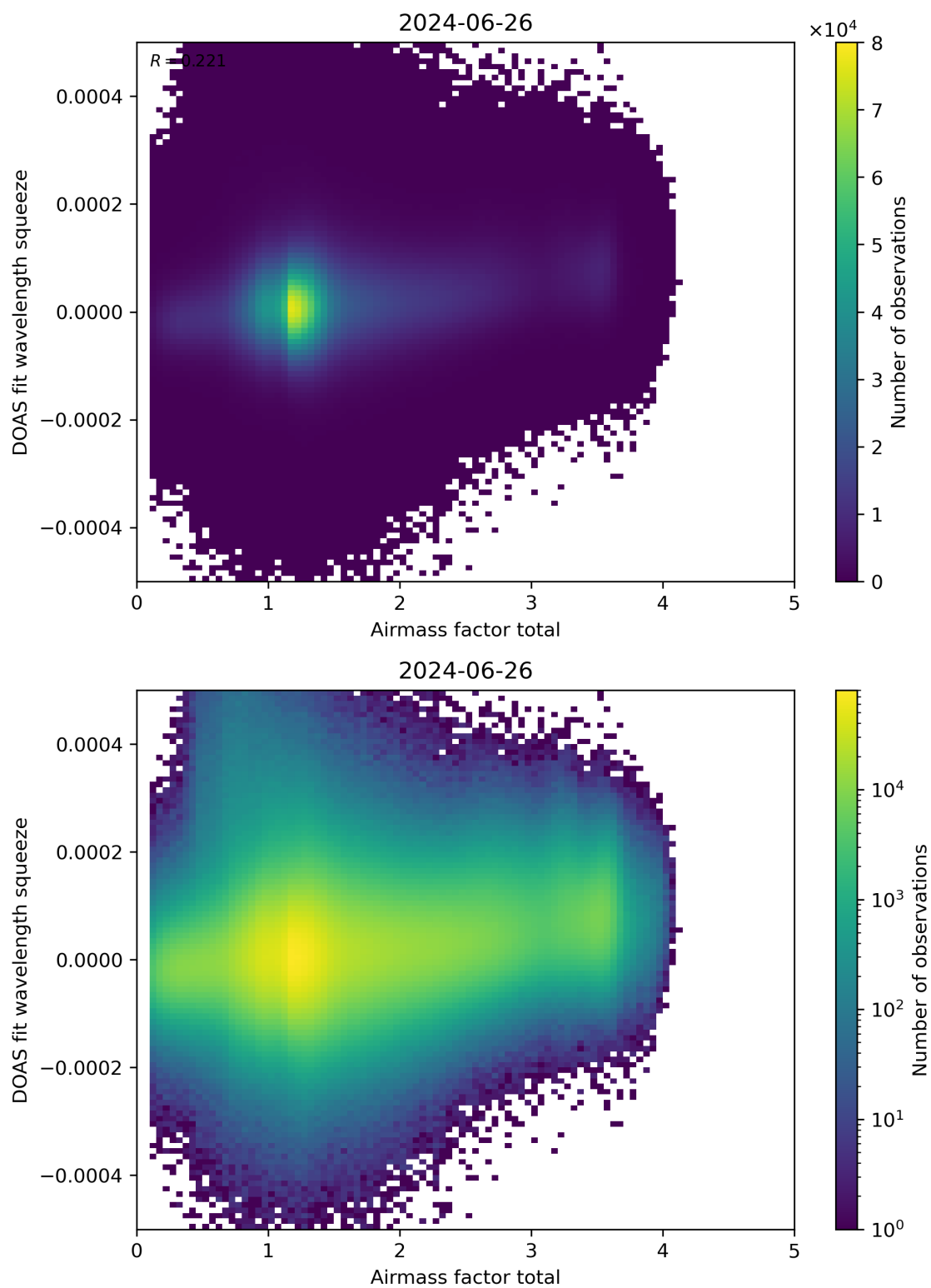
Figure 99: Scatter density plot of “Airmass factor total” against “DOAS fit wavelength squeeze” for 2024-06-25 to 2024-06-27.
