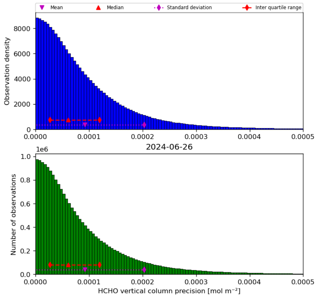
Figure 36: Histogram of “HCHO vertical column precision” for 2024-06-25 to 2024-06-27
