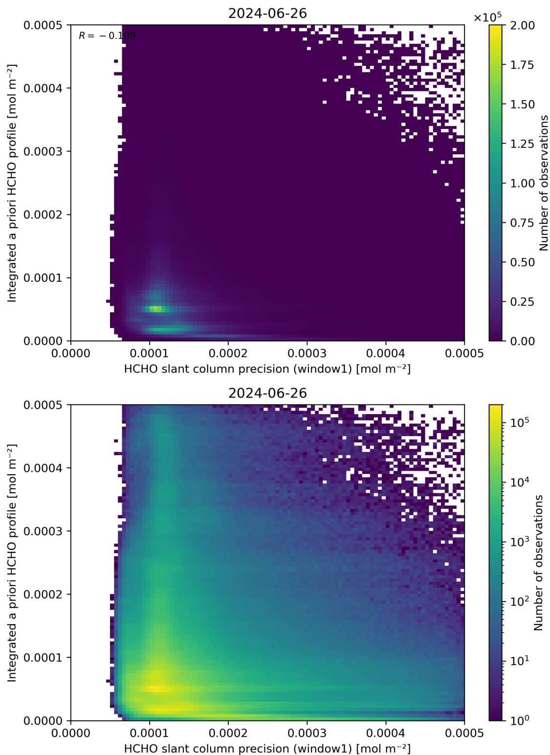
Figure 96: Scatter density plot of “HCHO slant column precision (window1)” against “Integrated a priori HCHO profile” for 2024-06-25 to 2024-06-27.
