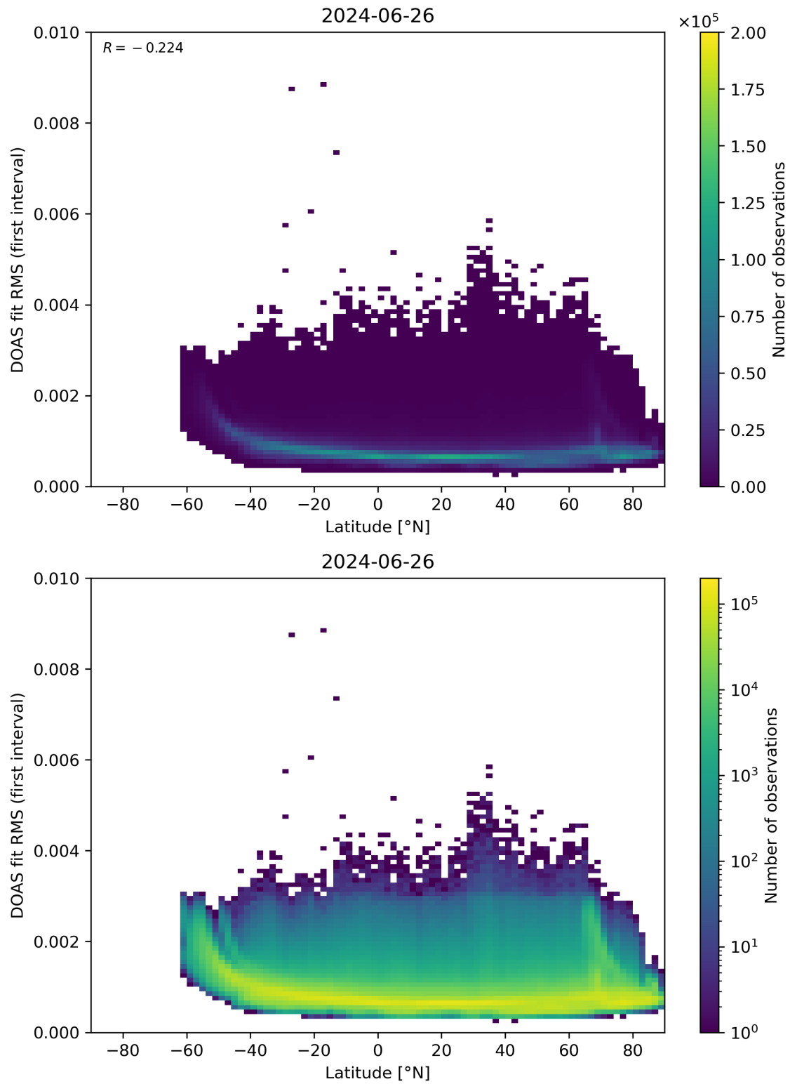
Figure 153: Scatter density plot of “Latitude” against “DOAS fit RMS (first interval)” for 2024-06-25 to 2024-06-27.
