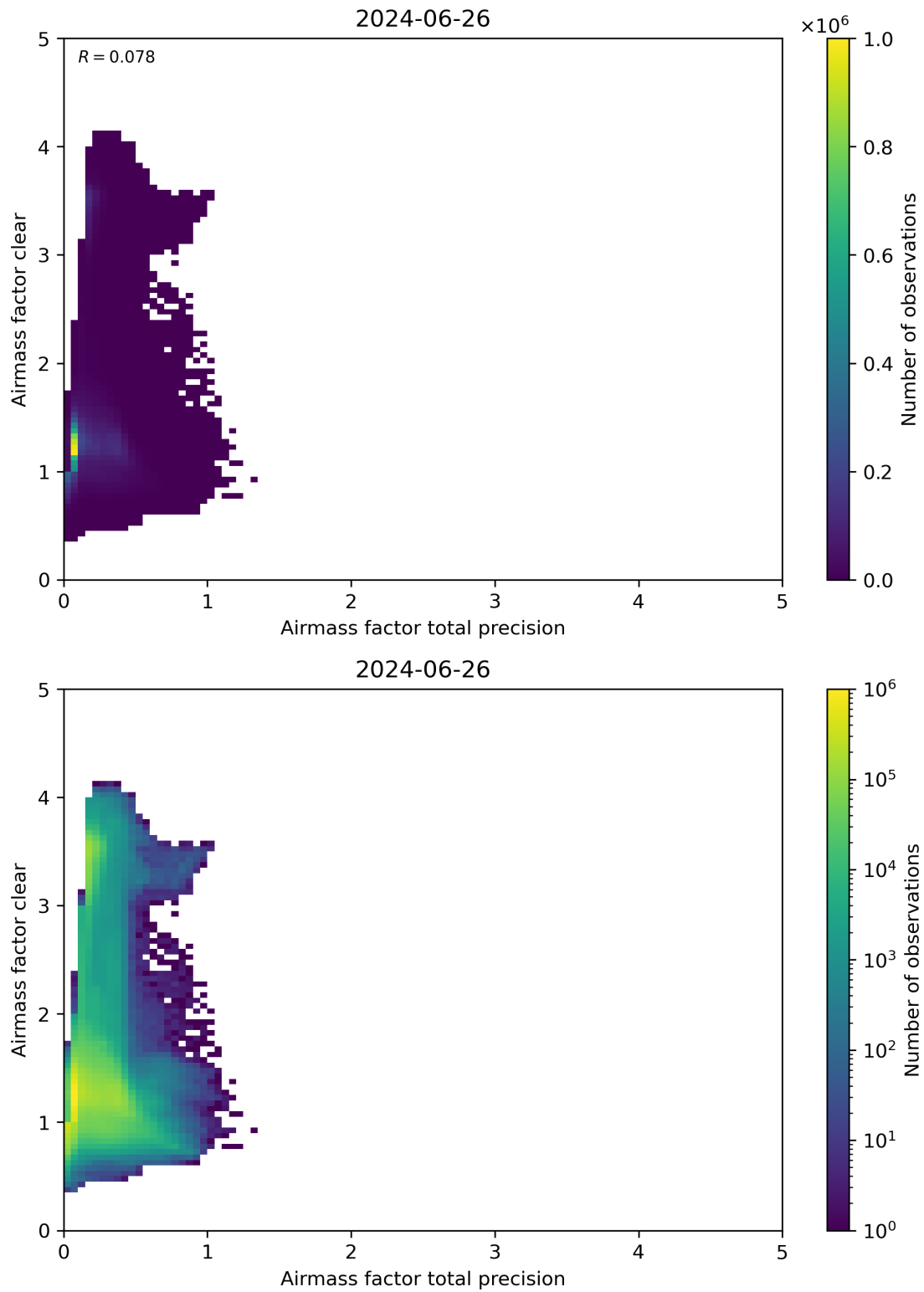
Figure 108: Scatter density plot of “Airmass factor total precision” against “Airmass factor clear” for 2024-06-25 to 2024-06-27.
