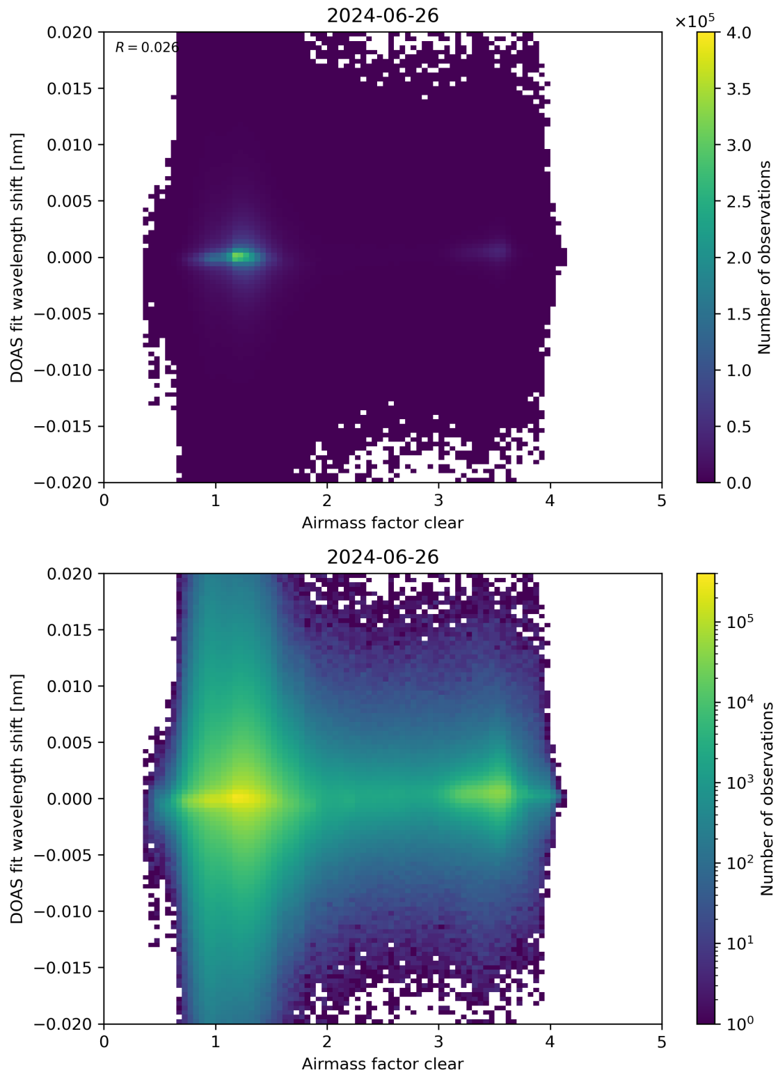
Figure 72: Scatter density plot of “Airmass factor clear” against “DOAS fit wavelength shift” for 2024-06-25 to 2024-06-27.
