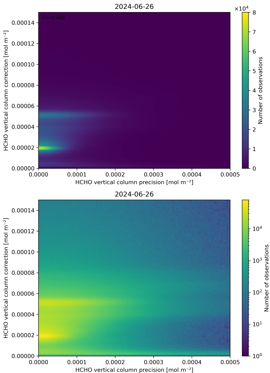
Figure 146: Scatter density plot of “HCHO vertical column precision” against “HCHO vertical column correction” for 2024-06-25 to 2024-06-27.
