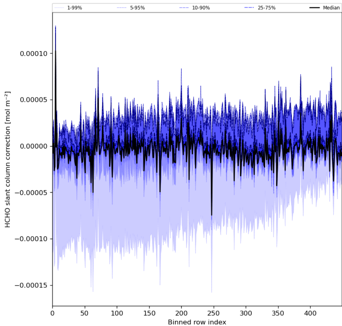
Figure 61: Along track statistics of “HCHO slant column correction” for 2024-06-25 to 2024-06-27
