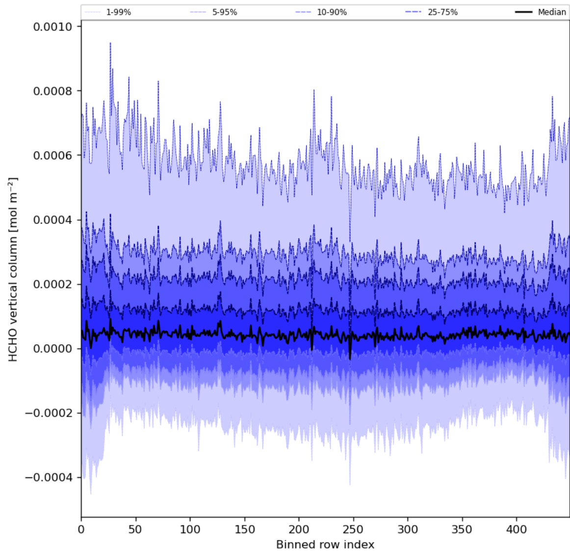
Figure 49: Along track statistics of “HCHO vertical column” for 2024-06-25 to 2024-06-27
