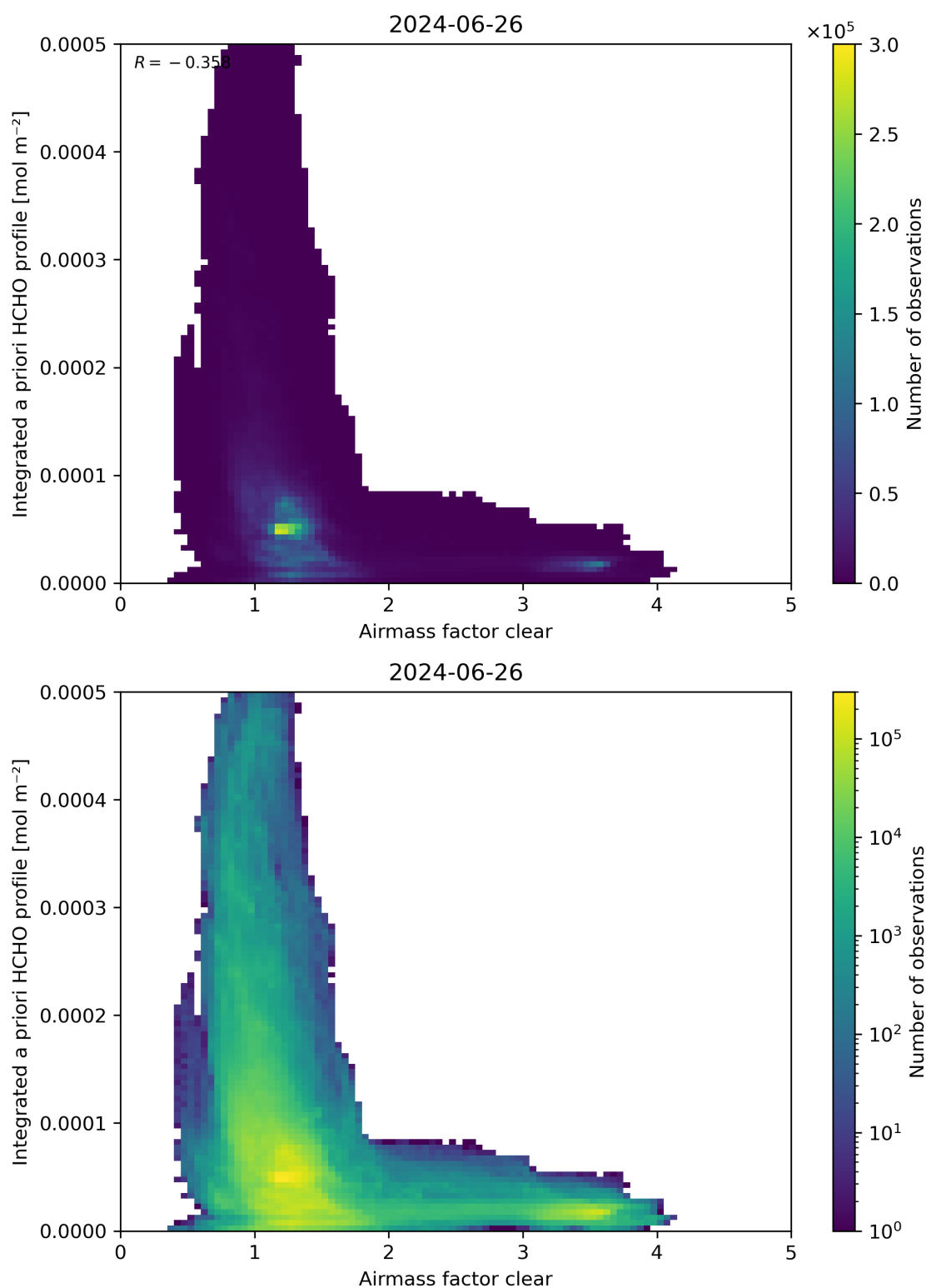
Figure 76: Scatter density plot of “Airmass factor clear” against “Integrated a priori HCHO profile” for 2024-06-25 to 2024-06-27.
