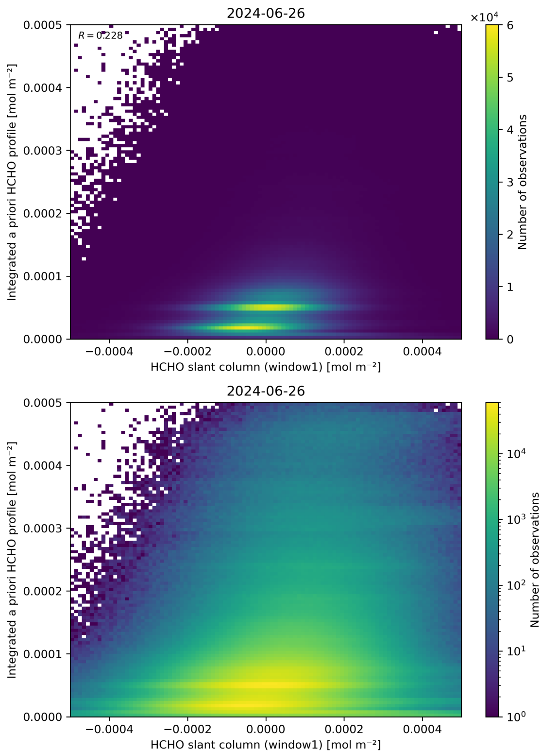
Figure 87: Scatter density plot of “HCHO slant column (window1)” against “Integrated a priori HCHO profile” for 2024-06-25 to 2024-06-27.
