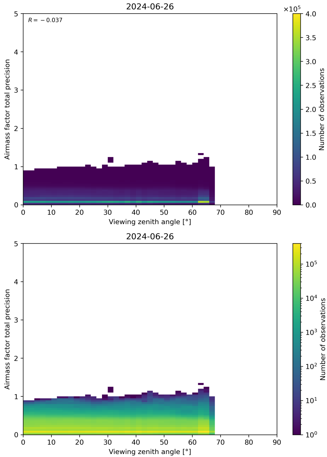
Figure 191: Scatter density plot of “Viewing zenith angle” against “Airmass factor total precision” for 2024-06-25 to 2024-06-27.
