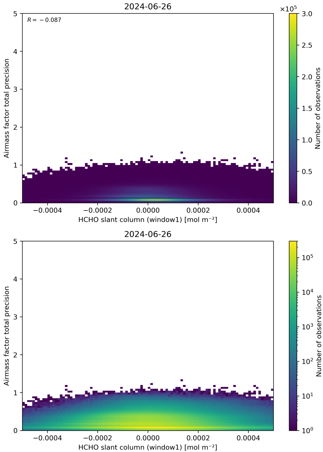
Figure 86: Scatter density plot of “HCHO slant column (window1)” against “Airmass factor total precision” for 2024-06-25 to 2024-06-27.
