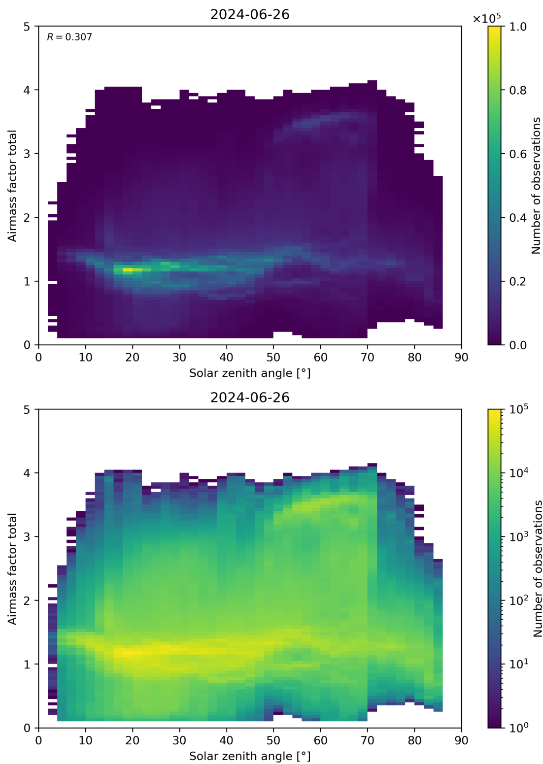
Figure 175: Scatter density plot of “Solar zenith angle” against “Airmass factor total” for 2024-06-25 to 2024-06-27.
