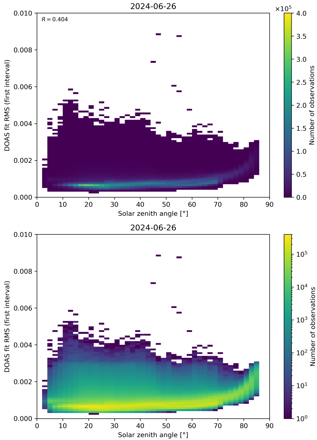
Figure 167: Scatter density plot of “Solar zenith angle” against “DOAS fit RMS (first interval)” for 2024-06-25 to 2024-06-27.
