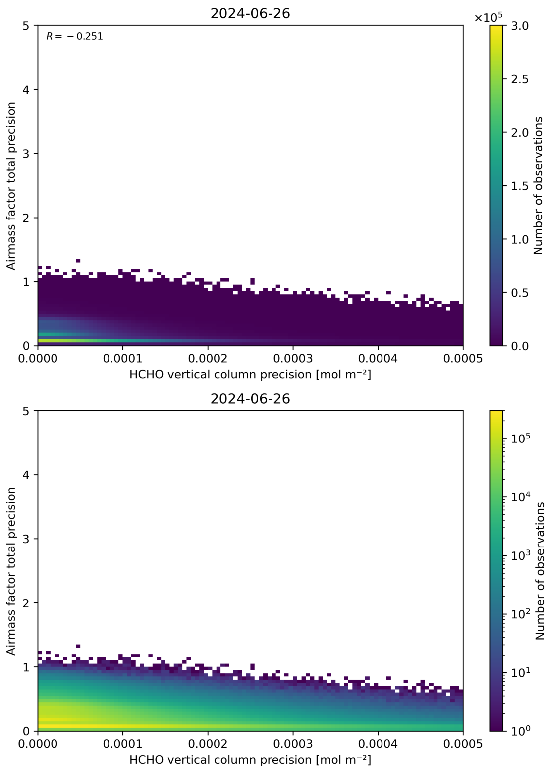
Figure 145: Scatter density plot of “HCHO vertical column precision” against “Airmass factor total precision” for 2024-06-25 to 2024-06-27.
