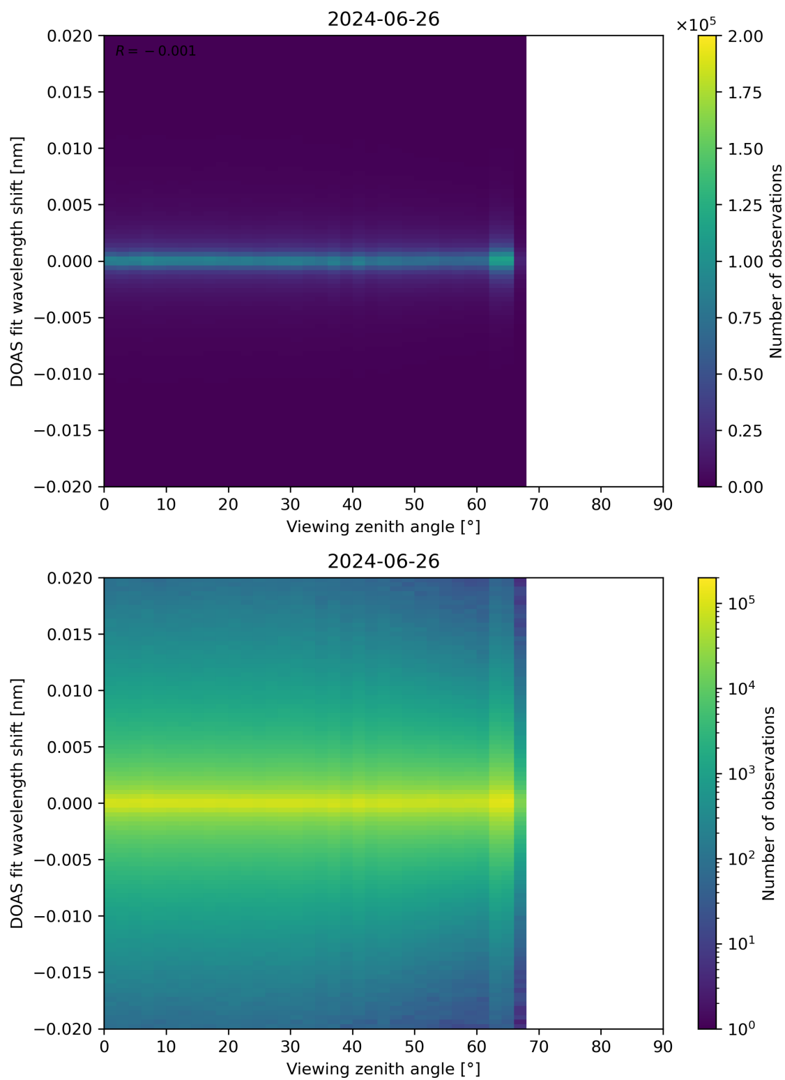
Figure 183: Scatter density plot of “Viewing zenith angle” against “DOAS fit wavelength shift” for 2024-06-25 to 2024-06-27.
