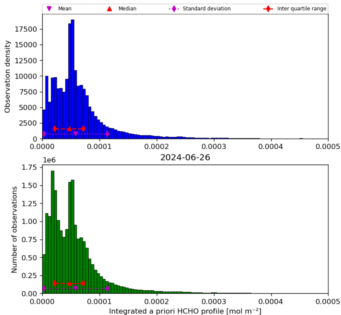
Figure 43: Histogram of “Integrated a priori HCHO profile” for 2024-06-25 to 2024-06-27
