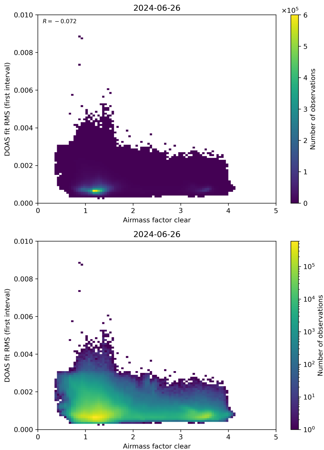
Figure 71: Scatter density plot of “Airmass factor clear” against “DOAS fit RMS (first interval)” for 2024-06-25 to 2024-06-27.
