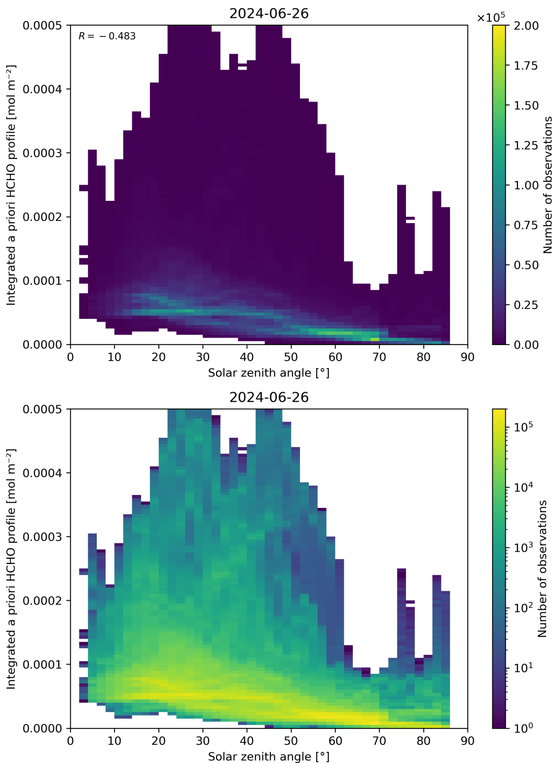
Figure 180: Scatter density plot of “Solar zenith angle” against “Integrated a priori HCHO profile” for 2024-06-25 to 2024-06-27.
