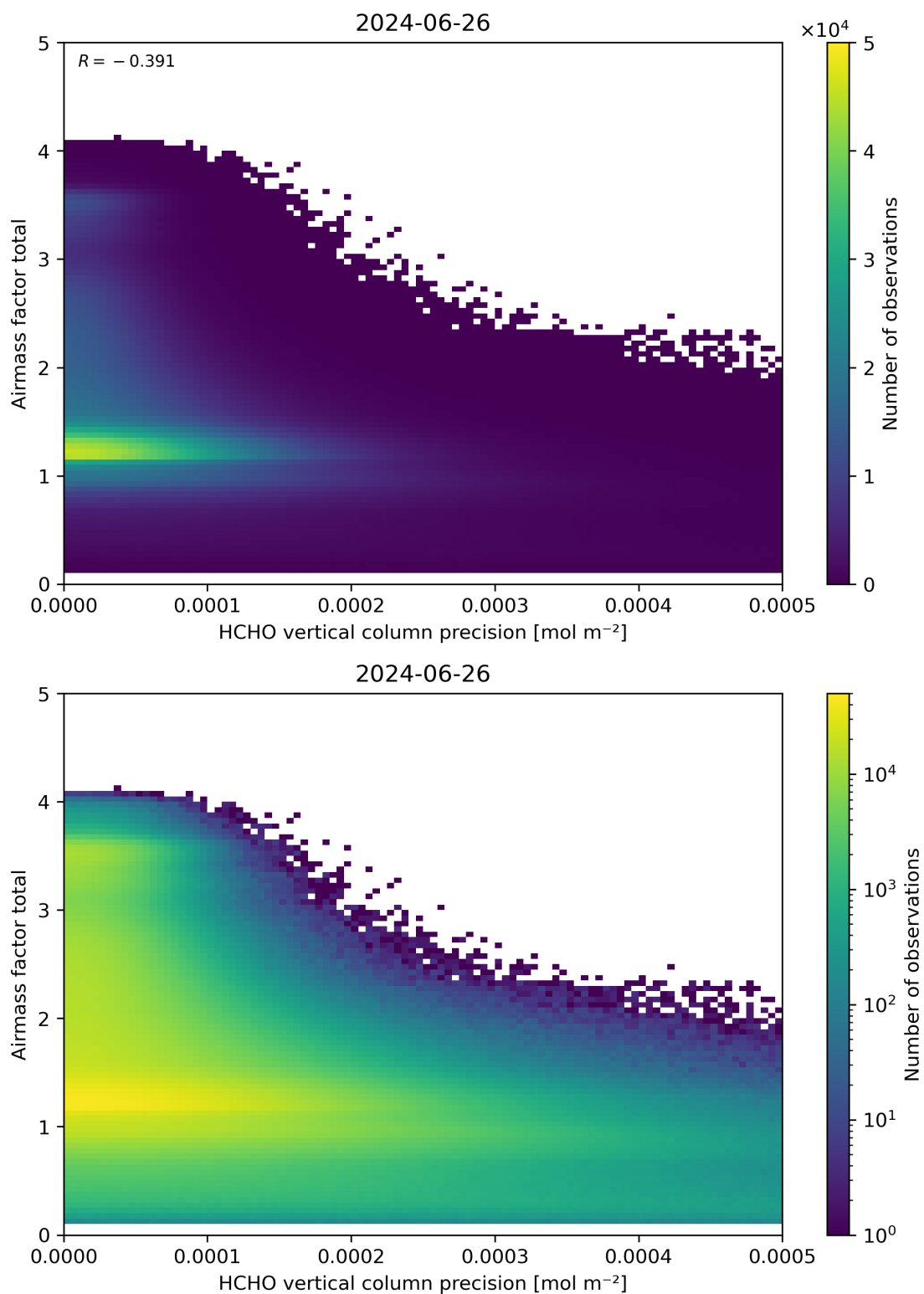
Figure 144: Scatter density plot of “HCHO vertical column precision” against “Airmass factor total” for 2024-06-25 to 2024-06-27.
