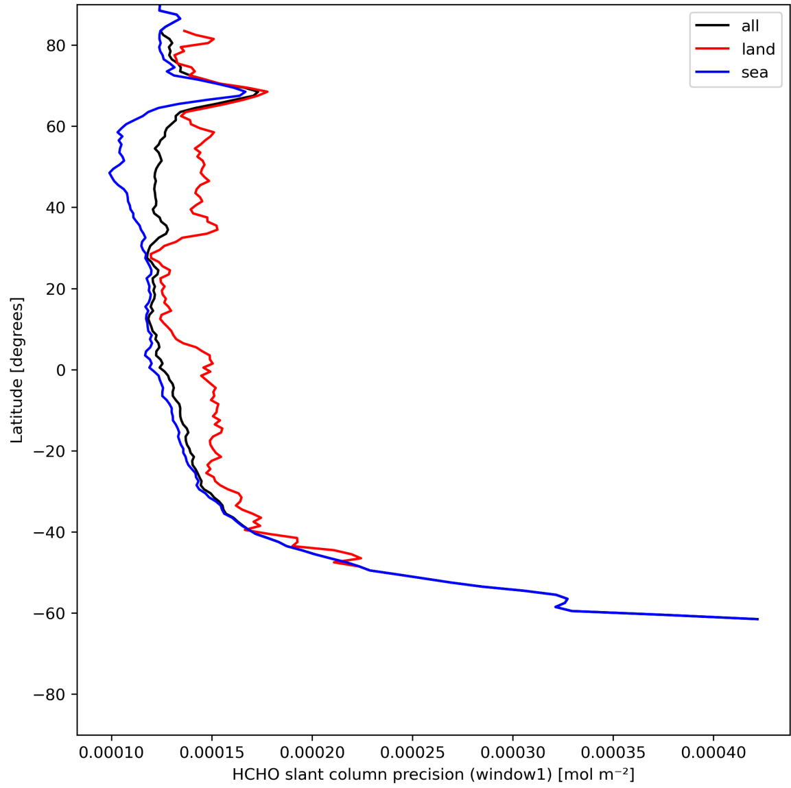
Figure 25: Zonal average of “HCHO slant column precision (window1)” for 2024-06-25 to 2024-06-27.
