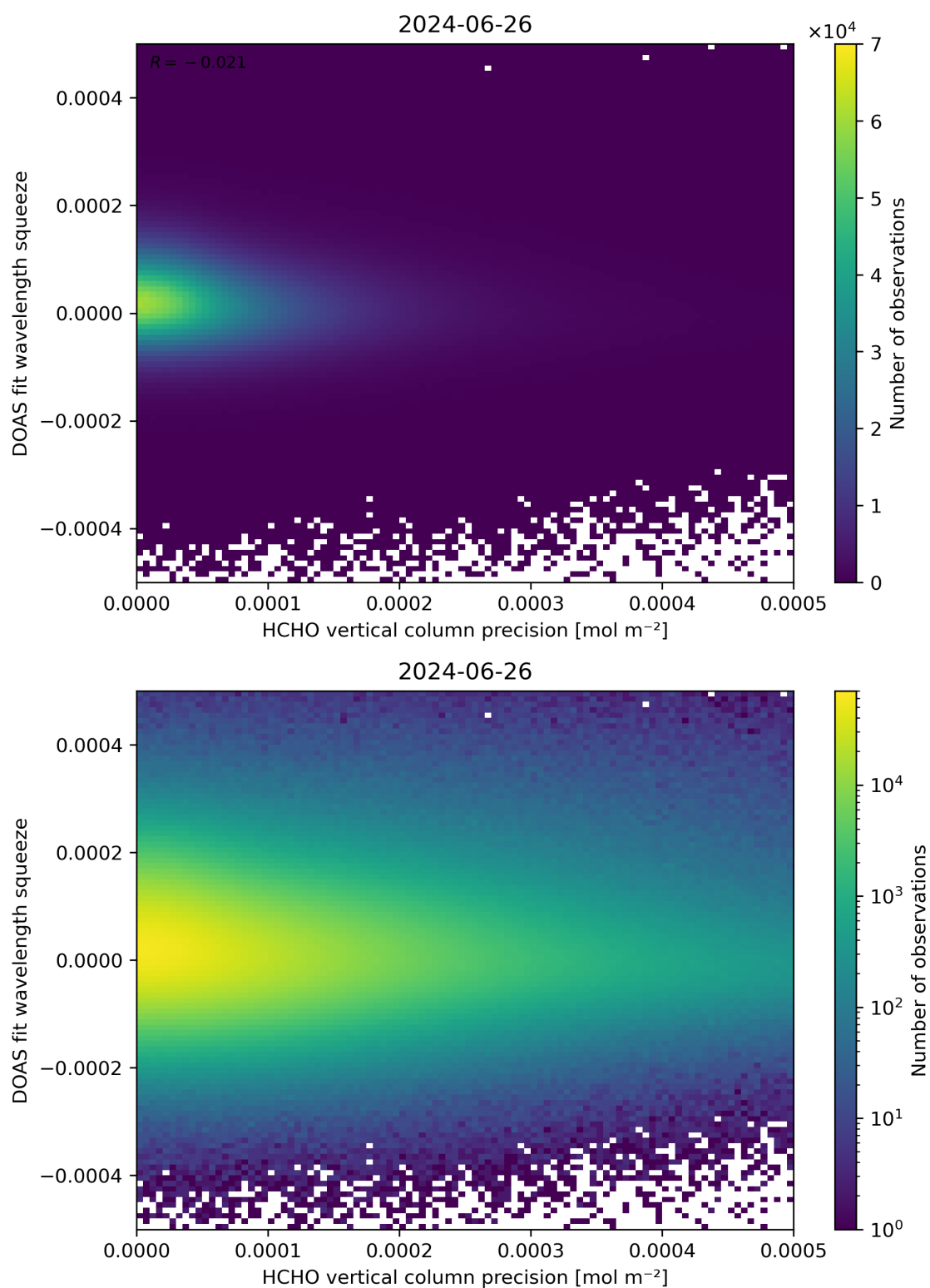
Figure 138: Scatter density plot of “HCHO vertical column precision” against “DOAS fit wavelength squeeze” for 2024-06-25 to 2024-06-27.
