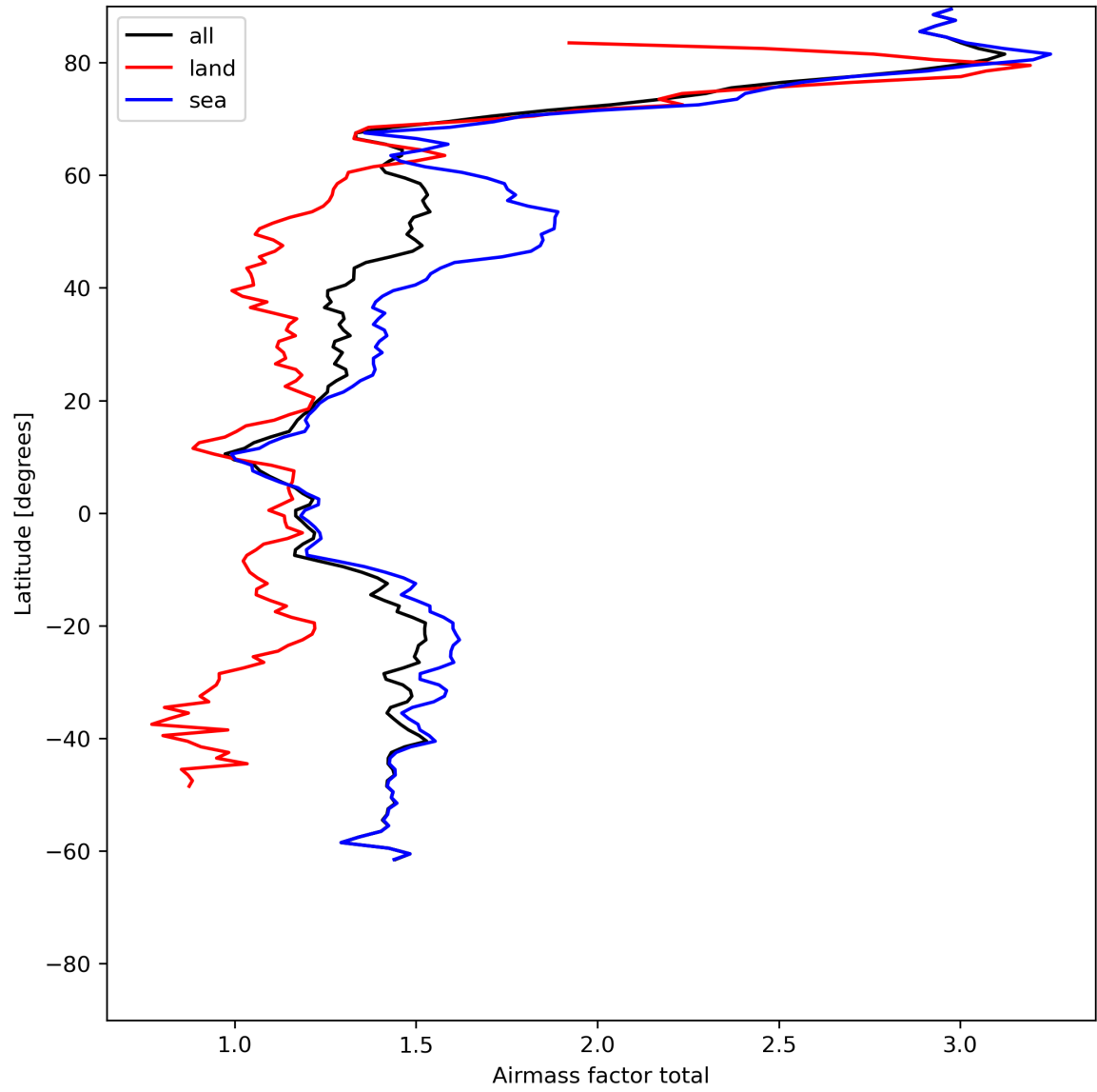
Figure 26: Zonal average of “Airmass factor total” for 2024-06-25 to 2024-06-27.
