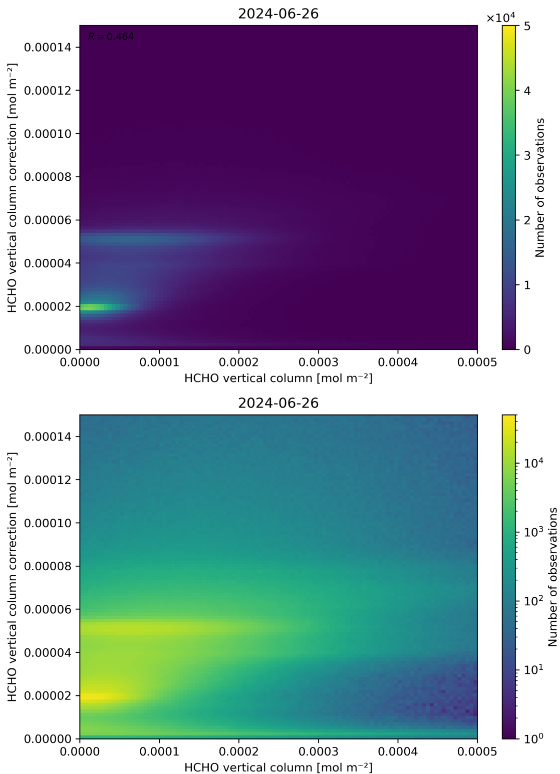
Figure 133: Scatter density plot of “HCHO vertical column” against “HCHO vertical column correction” for 2024-06-25 to 2024-06-27.
