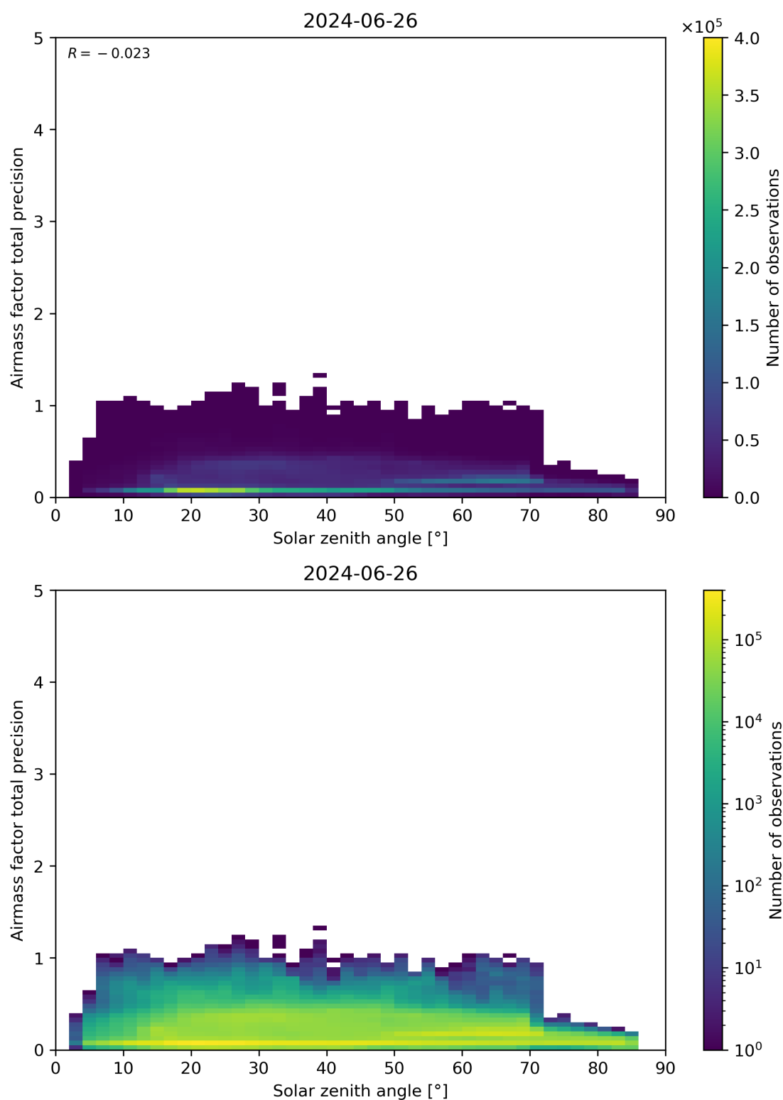
Figure 176: Scatter density plot of “Solar zenith angle” against “Airmass factor total precision” for 2024-06-25 to 2024-06-27.
