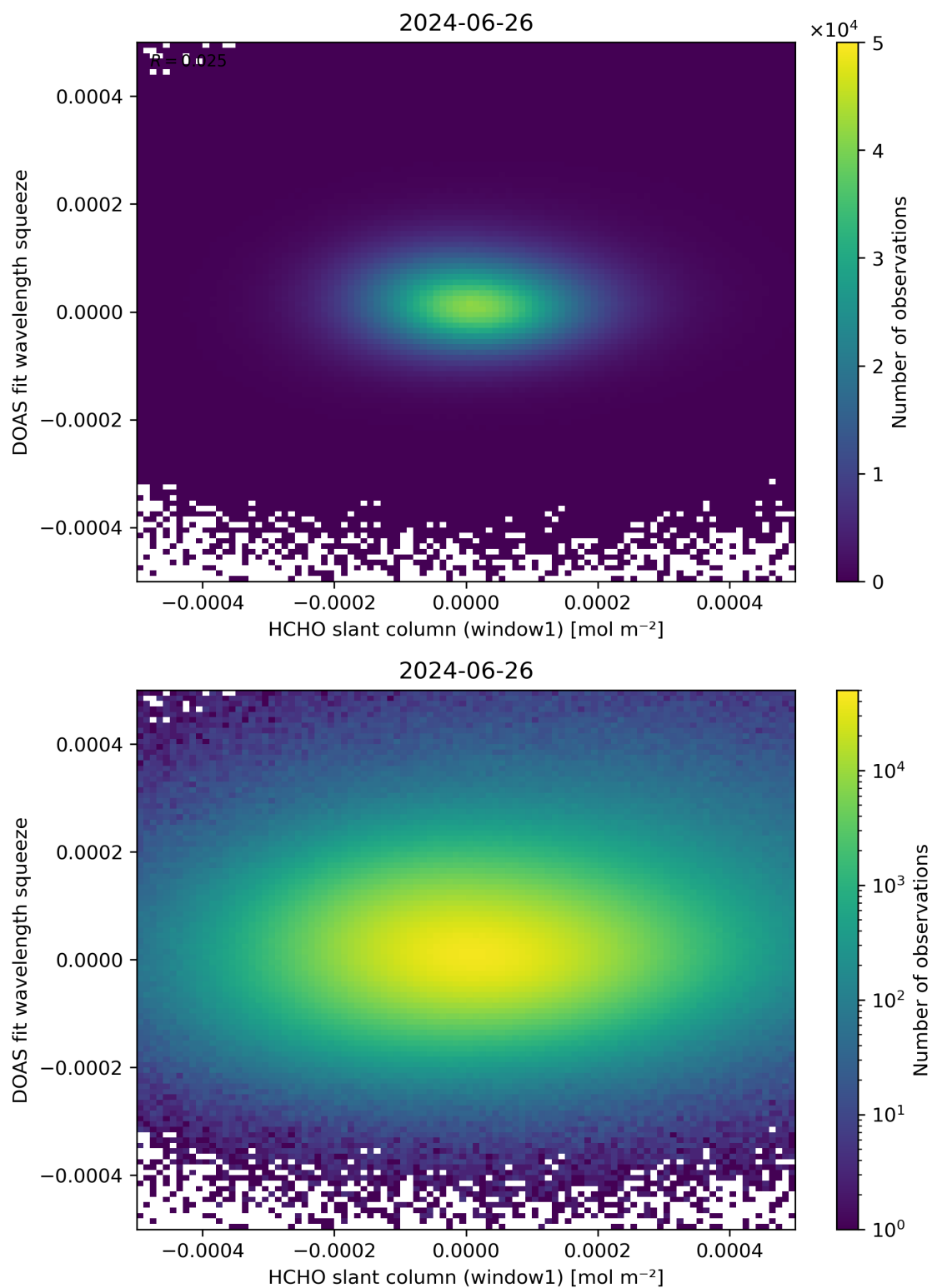
Figure 80: Scatter density plot of “HCHO slant column (window1)” against “DOAS fit wavelength squeeze” for 2024-06-25 to 2024-06-27.
