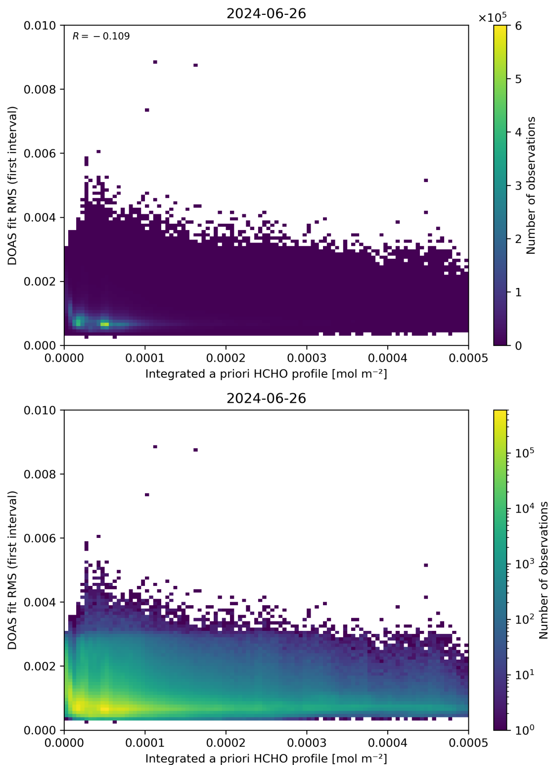
Figure 148: Scatter density plot of “Integrated a priori HCHO profile” against “DOAS fit RMS (first interval)” for 2024-06-25 to 2024-06-27.
