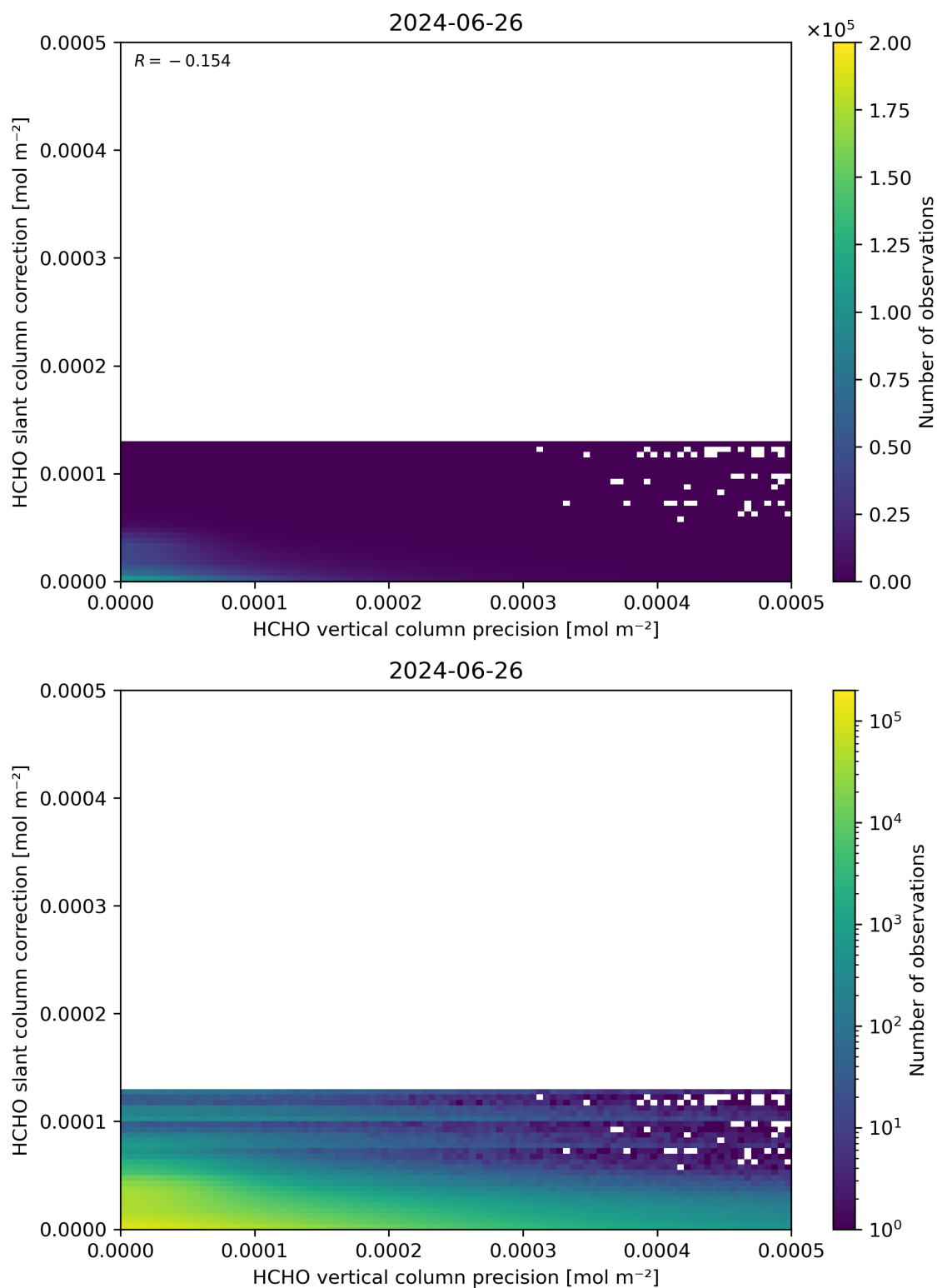
Figure 141: Scatter density plot of “HCHO vertical column precision” against “HCHO slant column correction” for 2024-06-25 to 2024-06-27.
