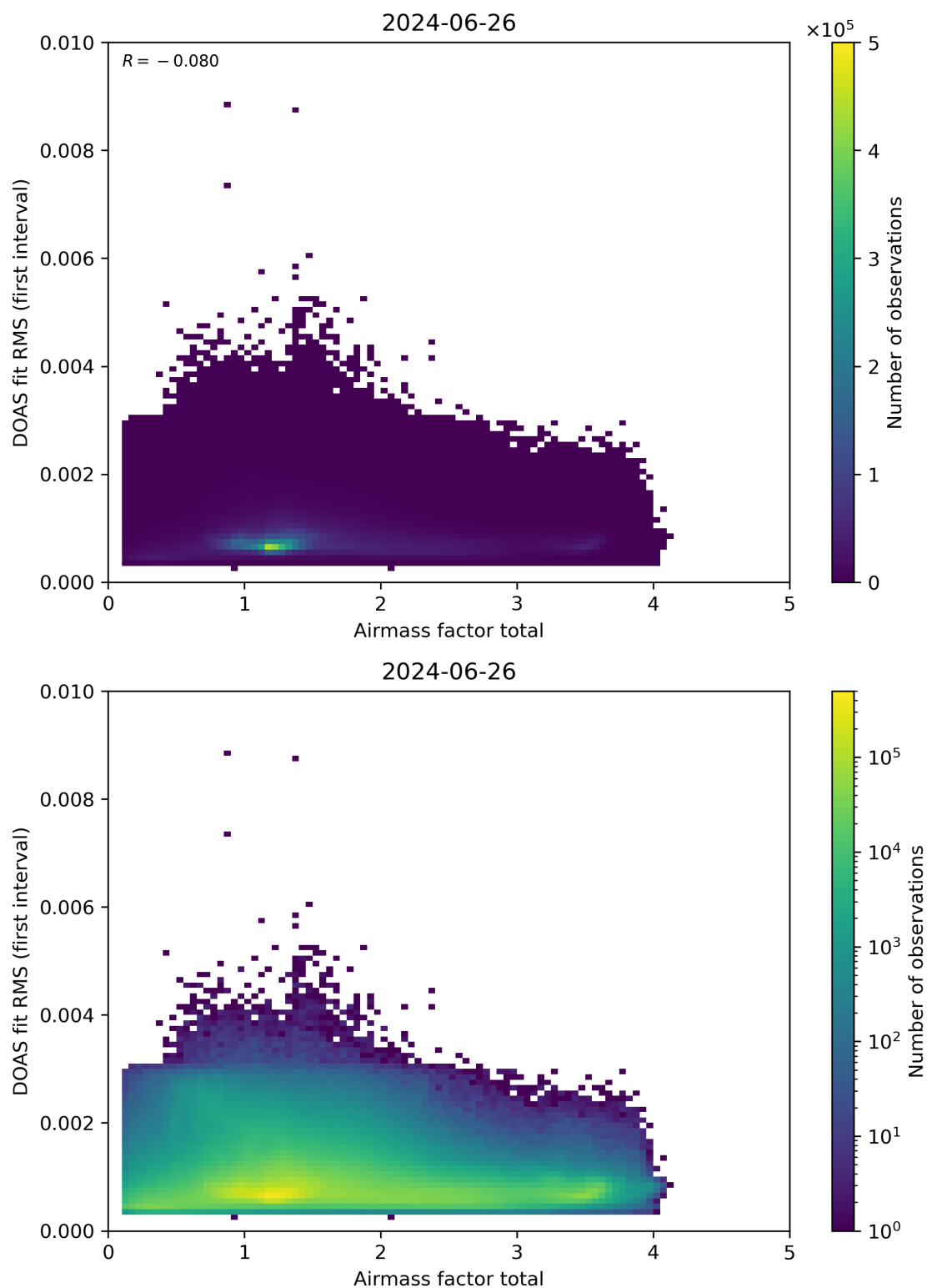
Figure 97: Scatter density plot of “Airmass factor total” against “DOAS fit RMS (first interval)” for 2024-06-25 to 2024-06-27.
