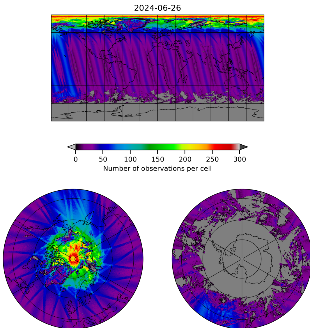
Figure 19: Map of the number of observations for 2024-06-25 to 2024-06-27
