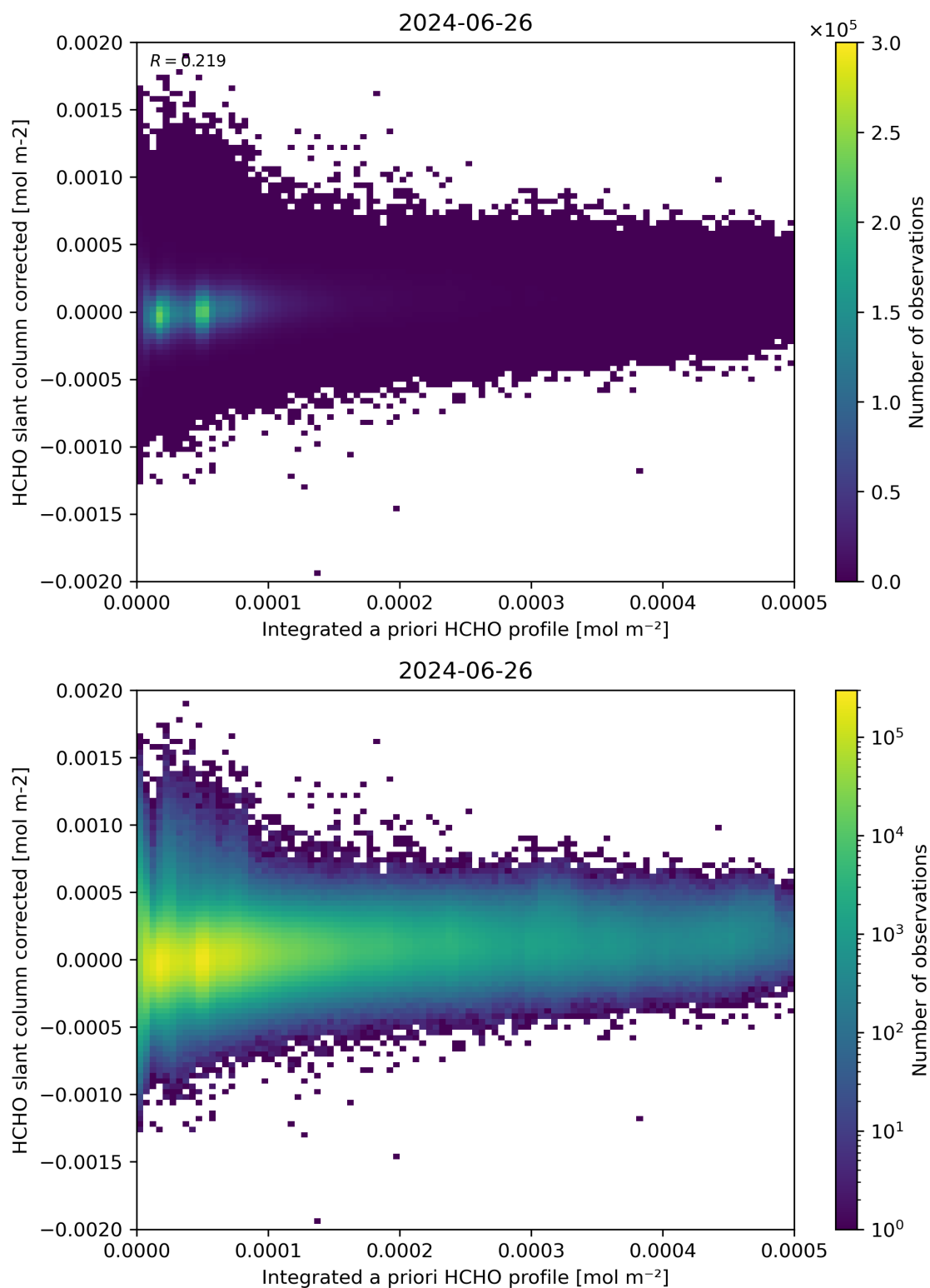
Figure 151: Scatter density plot of “Integrated a priori HCHO profile” against “HCHO slant column corrected” for 2024-06-25 to 2024-06-27.
