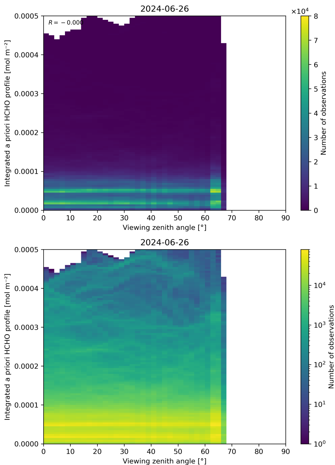
Figure 195: Scatter density plot of “Viewing zenith angle” against “Integrated a priori HCHO profile” for 2024-06-25 to 2024-06-27.
