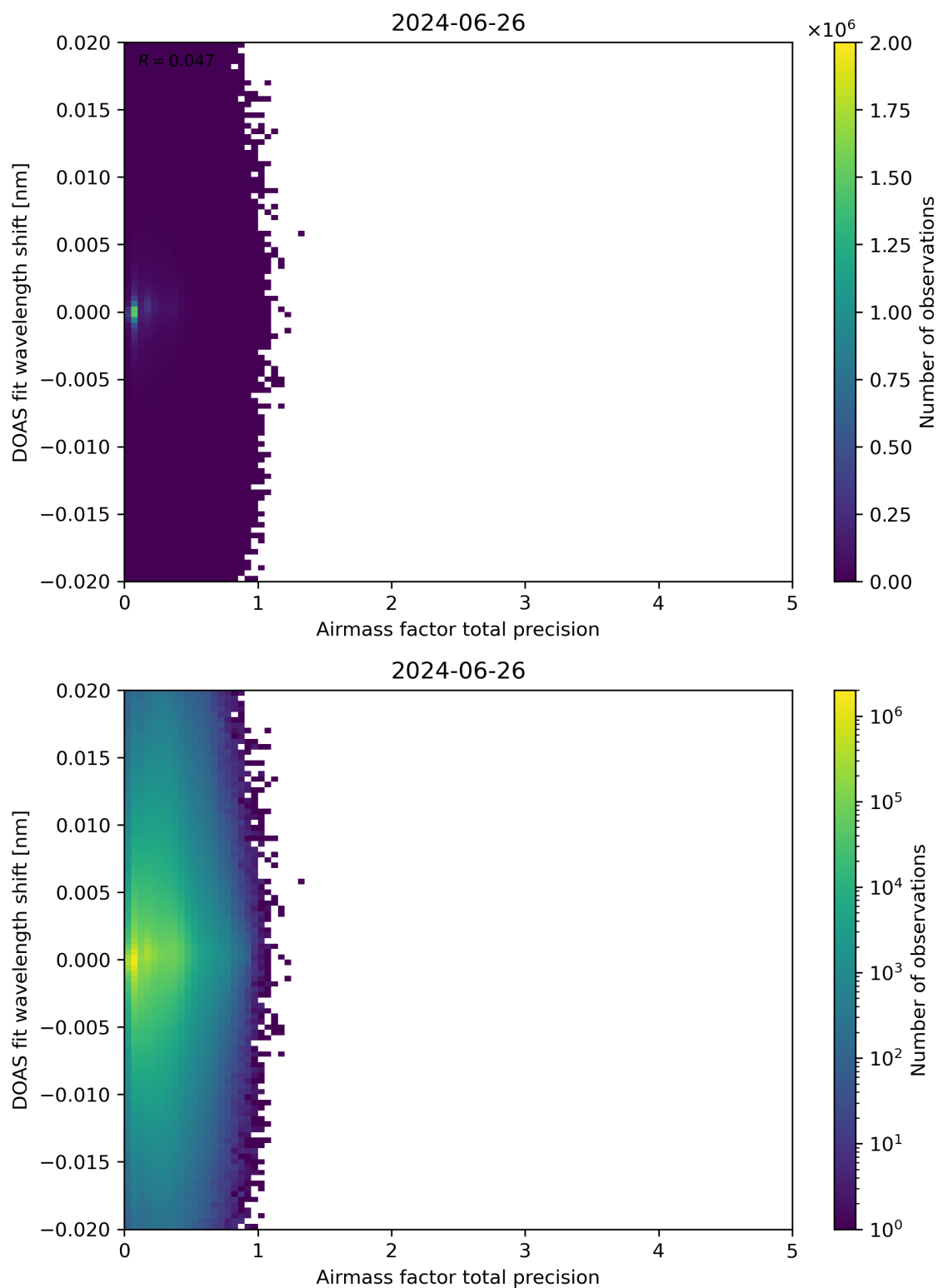
Figure 106: Scatter density plot of “Airmass factor total precision” against “DOAS fit wavelength shift” for 2024-06-25 to 2024-06-27.
