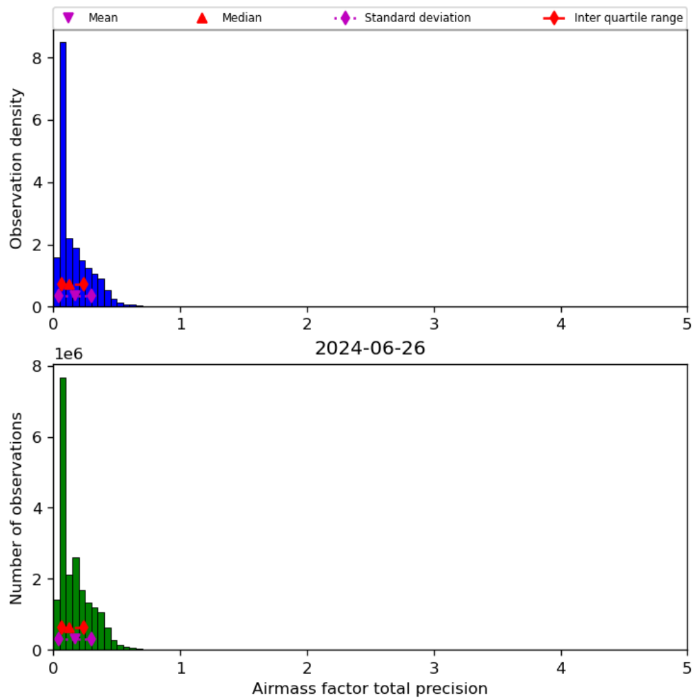
Figure 41: Histogram of “Airmass factor total precision” for 2024-06-25 to 2024-06-27
