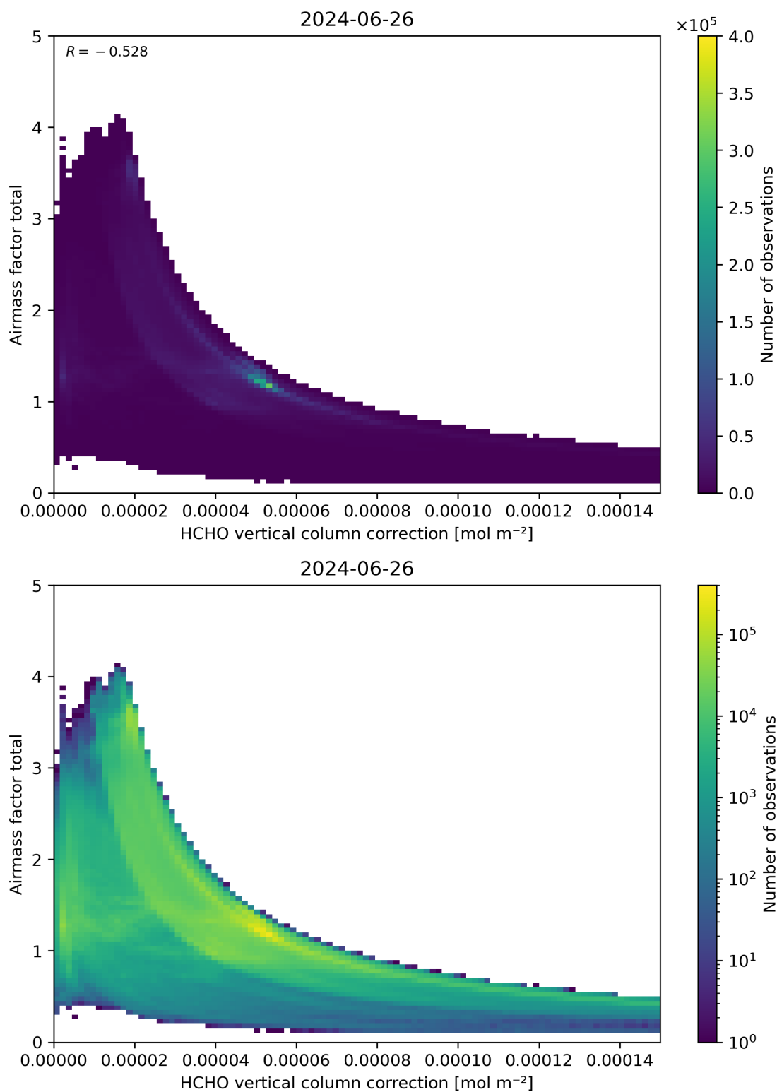
Figure 120: Scatter density plot of “HCHO vertical column correction” against “Airmass factor total” for 2024-06-25 to 2024-06-27.
