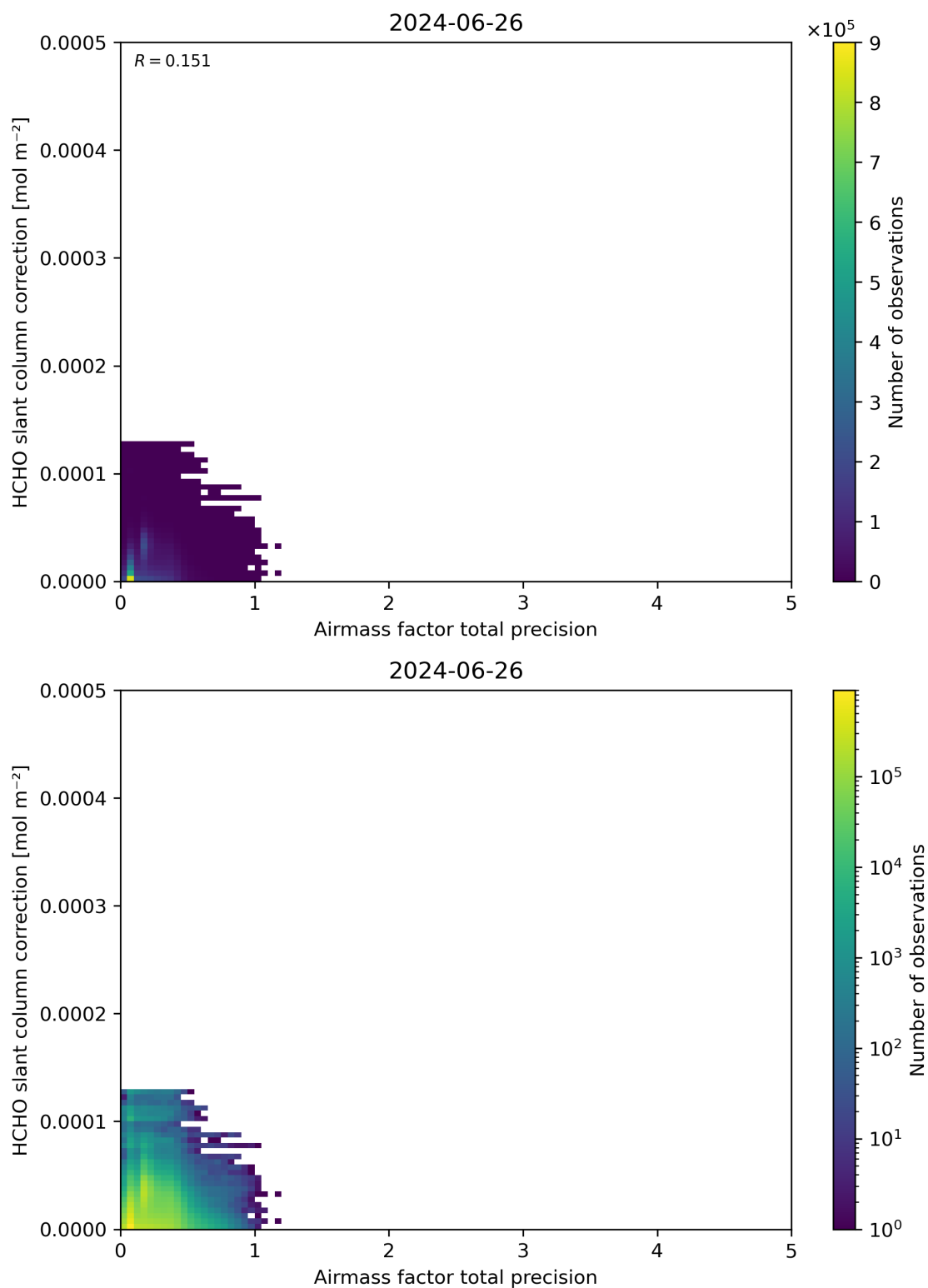
Figure 110: Scatter density plot of “Airmass factor total precision” against “HCHO slant column correction” for 2024-06-25 to 2024-06-27.
