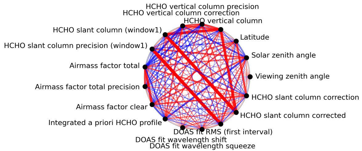
Figure 1: Map of correlation graph for 2024-06-25 to 2024-06-27.
