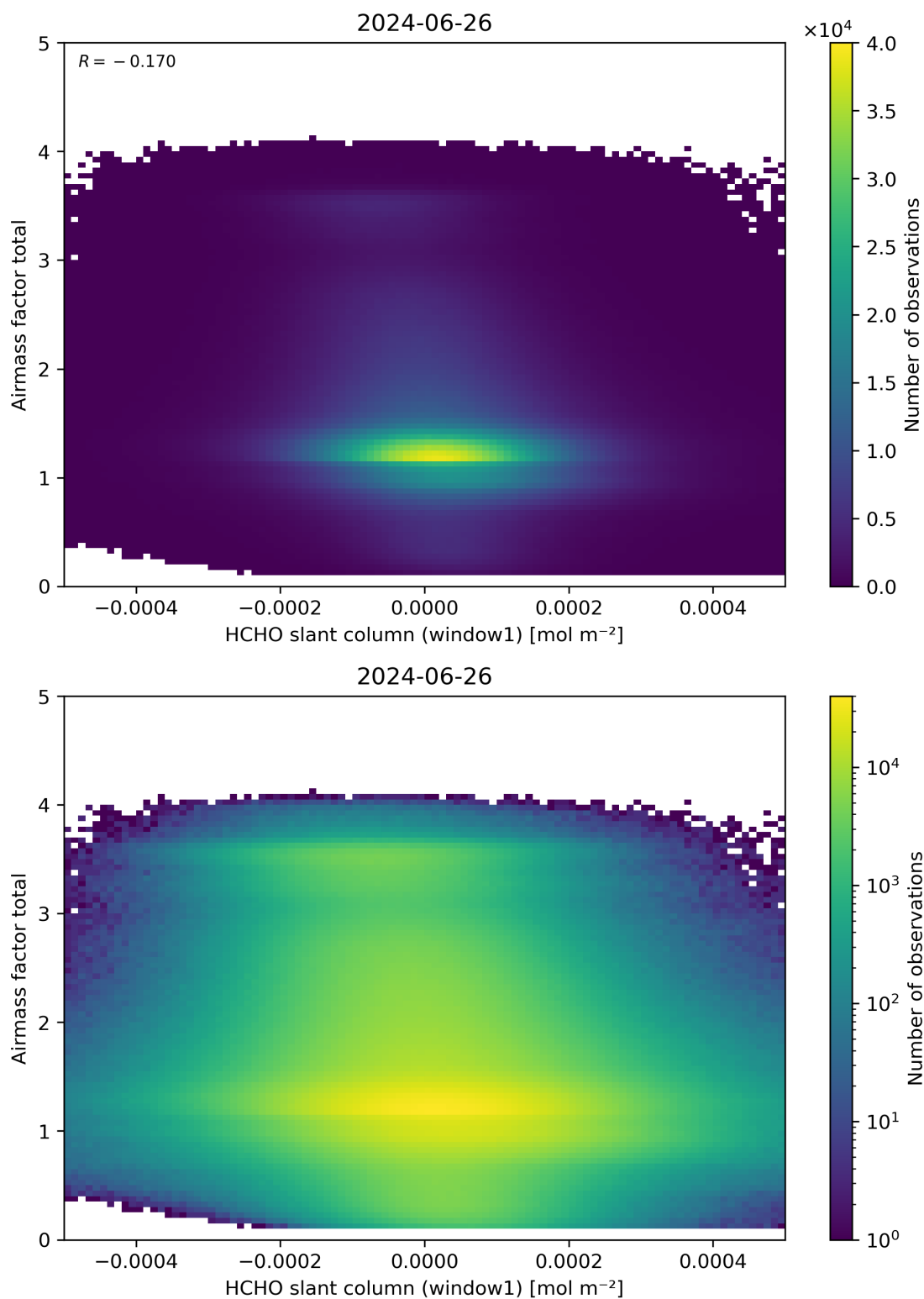
Figure 85: Scatter density plot of “HCHO slant column (window1)” against “Airmass factor total” for 2024-06-25 to 2024-06-27.
