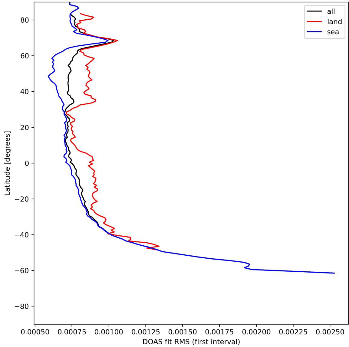
Figure 32: Zonal average of “DOAS fit RMS (first interval)” for 2024-06-25 to 2024-06-27.
