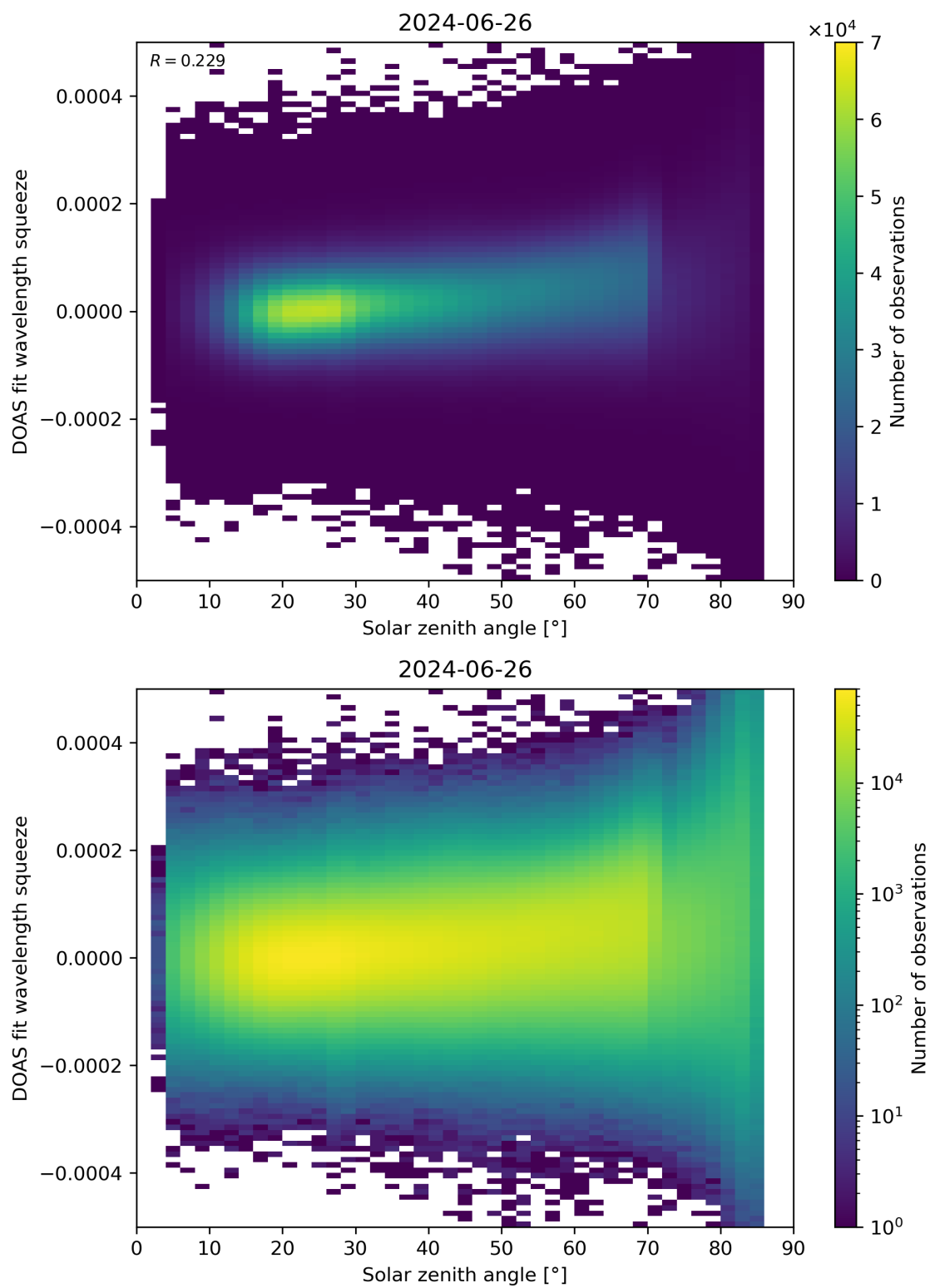
Figure 169: Scatter density plot of “Solar zenith angle” against “DOAS fit wavelength squeeze” for 2024-06-25 to 2024-06-27.
