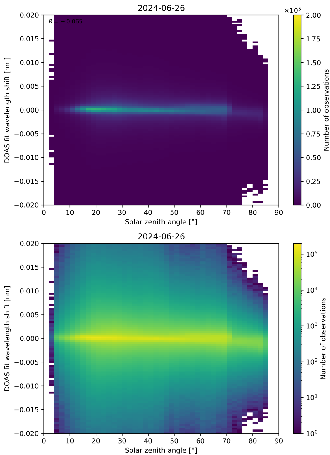
Figure 168: Scatter density plot of “Solar zenith angle” against “DOAS fit wavelength shift” for 2024-06-25 to 2024-06-27.
