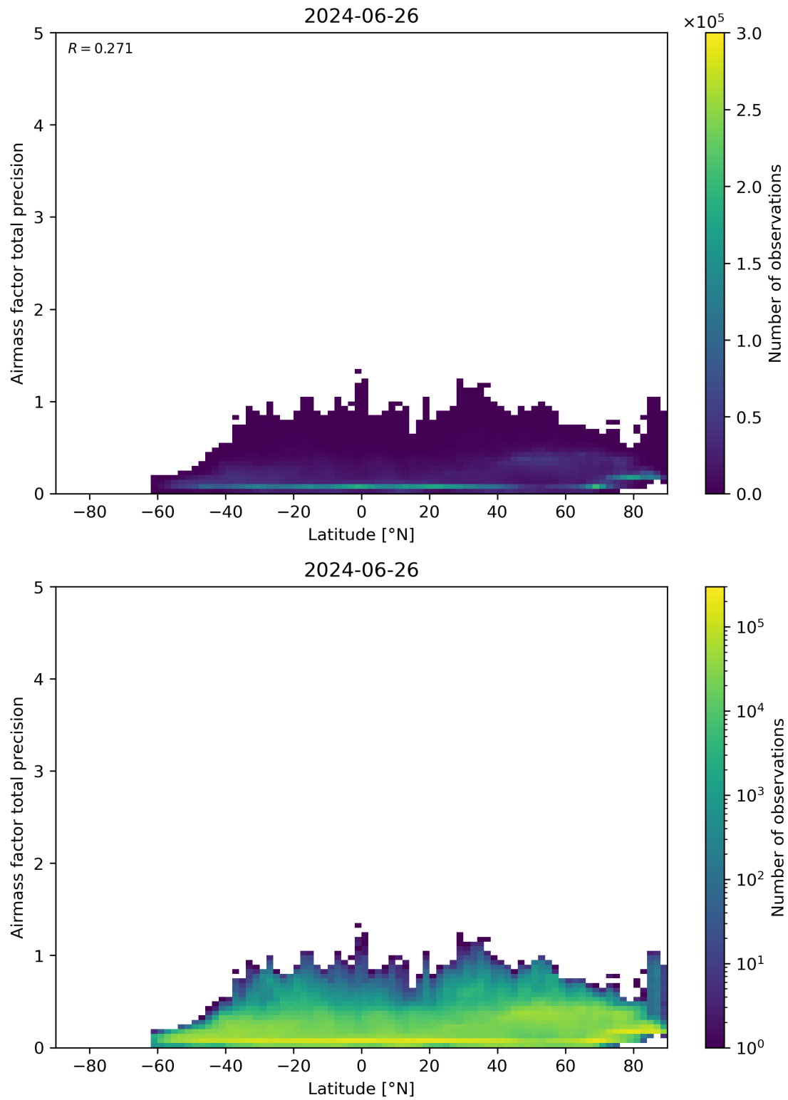
Figure 162: Scatter density plot of “Latitude” against “Airmass factor total precision” for 2024-06-25 to 2024-06-27.
