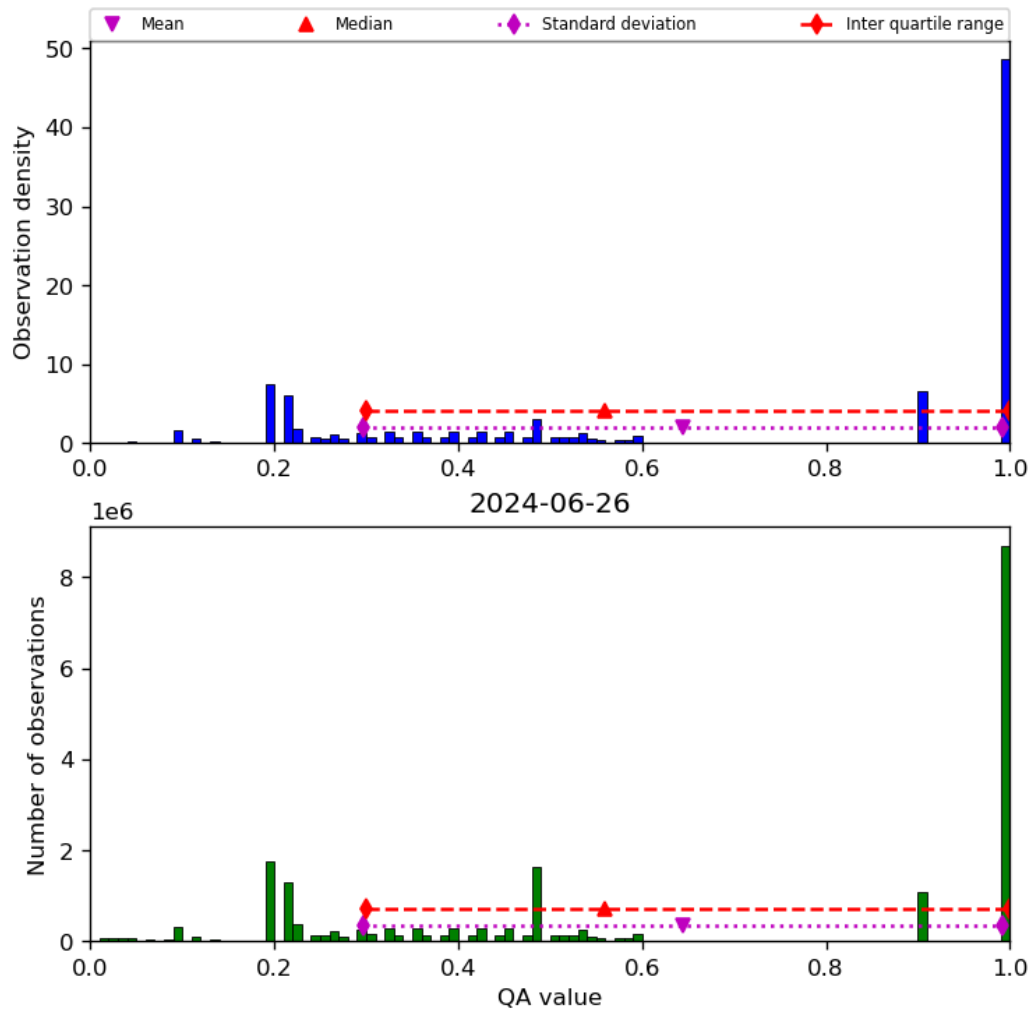
Figure 34: Histogram of “QA value” for 2024-06-25 to 2024-06-27
