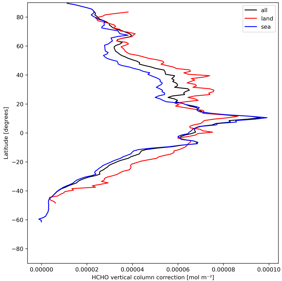
Figure 23: Zonal average of “HCHO vertical column correction” for 2024-06-25 to 2024-06-27.
