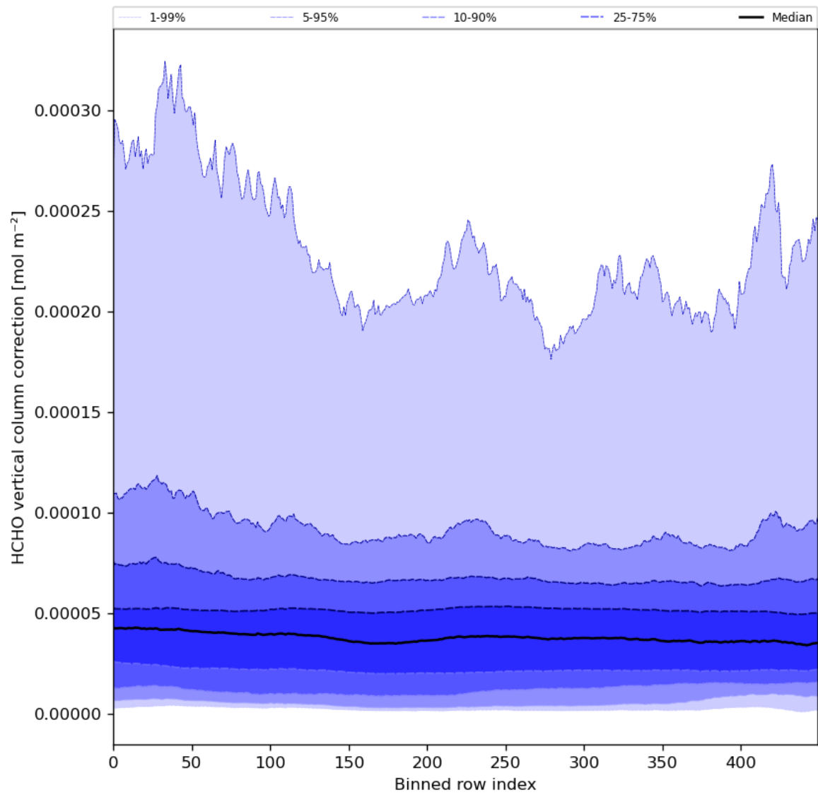
Figure 51: Along track statistics of “HCHO vertical column correction” for 2024-06-25 to 2024-06-27
