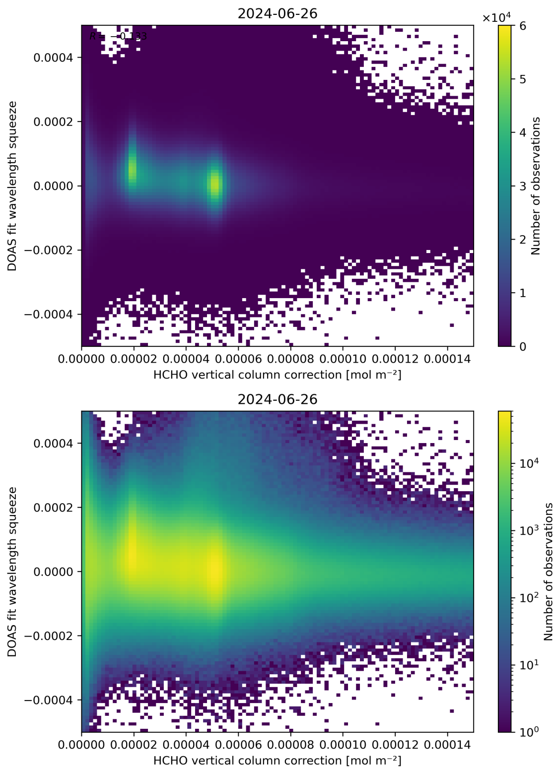
Figure 114: Scatter density plot of “HCHO vertical column correction” against “DOAS fit wavelength squeeze” for 2024-06-25 to 2024-06-27.
