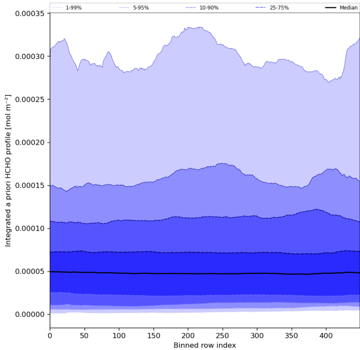
Figure 57: Along track statistics of “Integrated a priori HCHO profile” for 2024-06-25 to 2024-06-27
