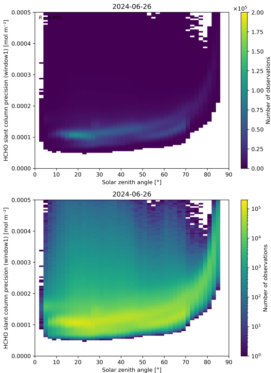
Figure 174: Scatter density plot of “Solar zenith angle” against “HCHO slant column precision (window1)” for 2024-06-25 to 2024-06-27.
