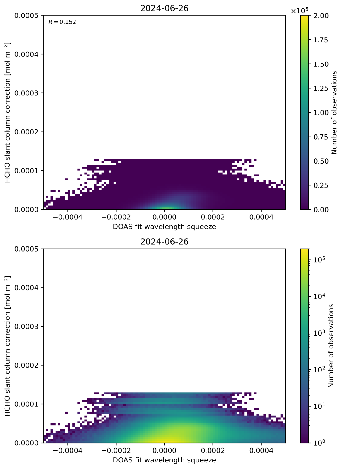
Figure 70: Scatter density plot of “DOAS fit wavelength squeeze” against “HCHO slant column correction” for 2024-06-25 to 2024-06-27.
