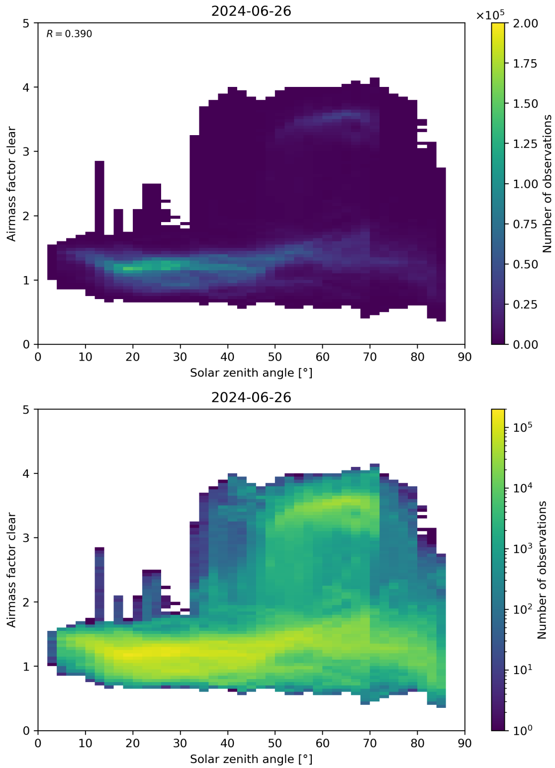
Figure 170: Scatter density plot of “Solar zenith angle” against “Airmass factor clear” for 2024-06-25 to 2024-06-27.
