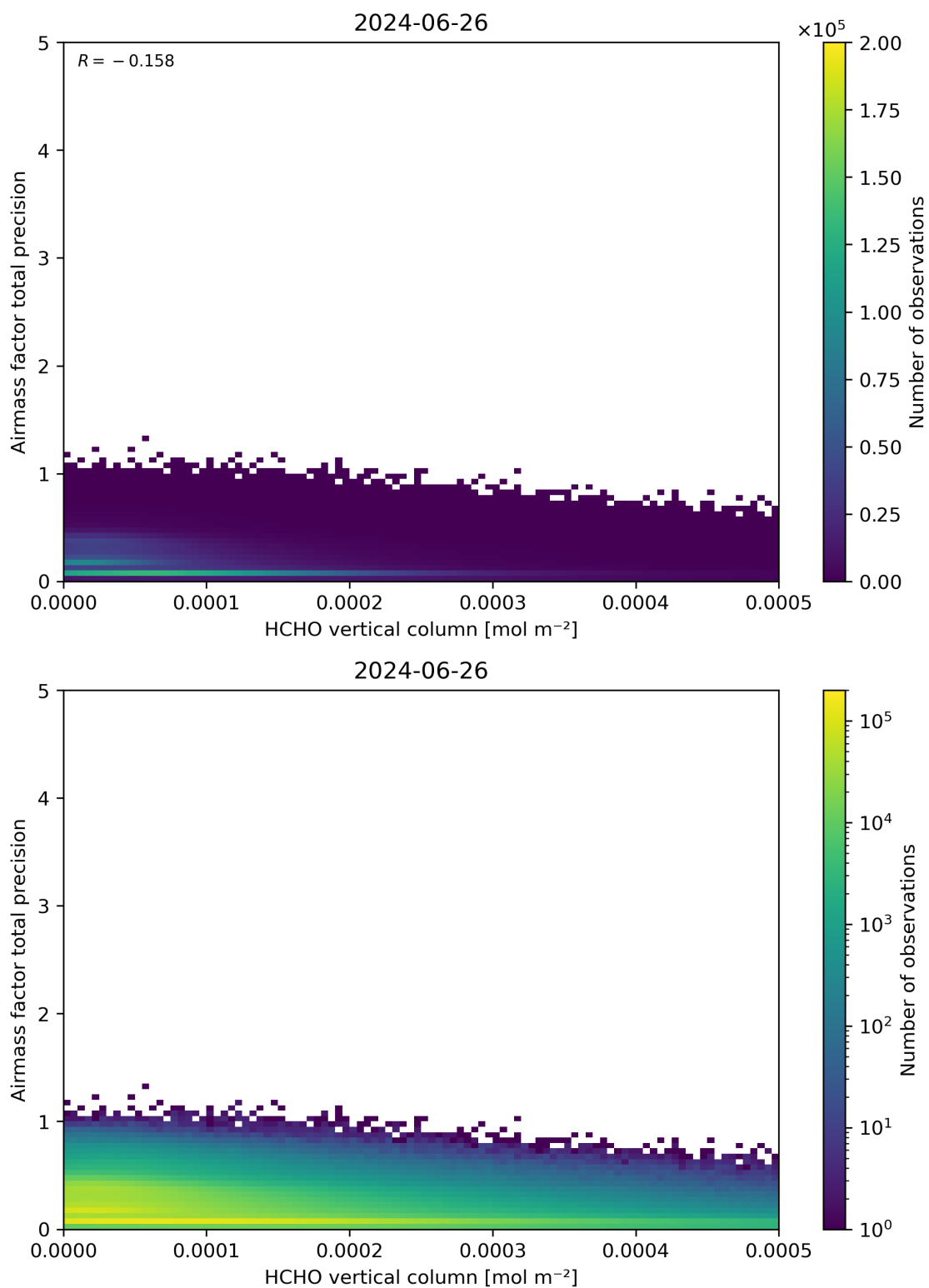
Figure 132: Scatter density plot of “HCHO vertical column” against “Airmass factor total precision” for 2024-06-25 to 2024-06-27.
