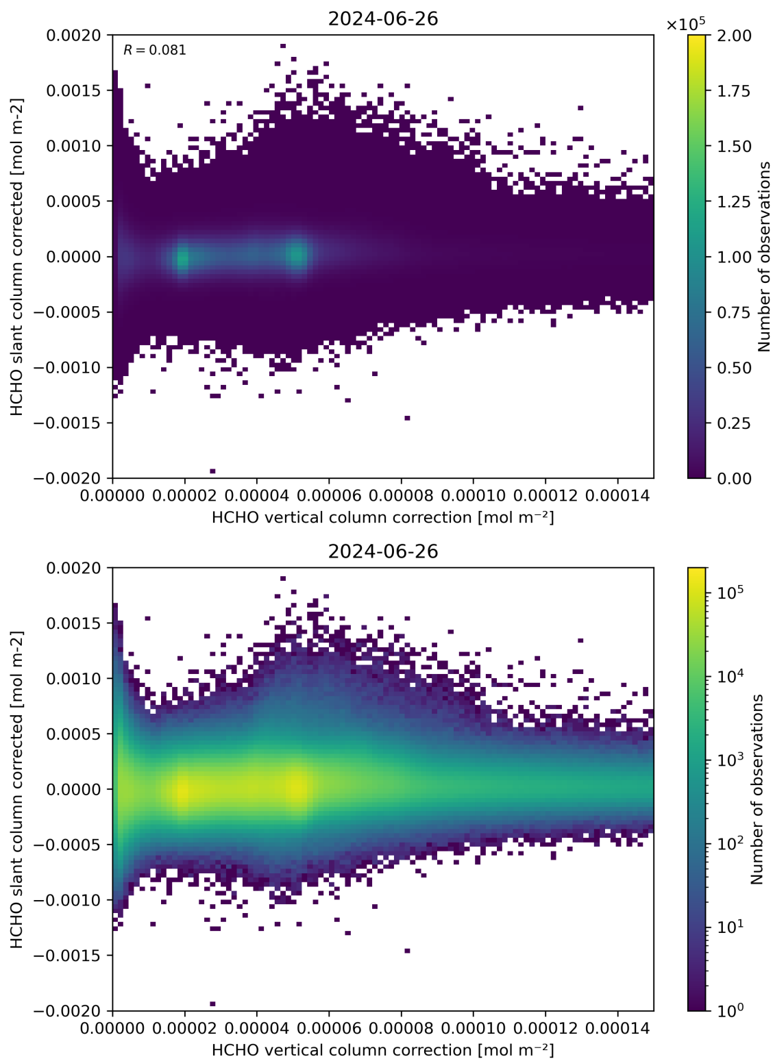
Figure 116: Scatter density plot of “HCHO vertical column correction” against “HCHO slant column corrected” for 2024-06-25 to 2024-06-27.
