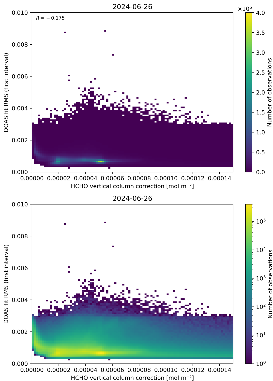
Figure 112: Scatter density plot of “HCHO vertical column correction” against “DOAS fit RMS (first interval)” for 2024-06-25 to 2024-06-27.
