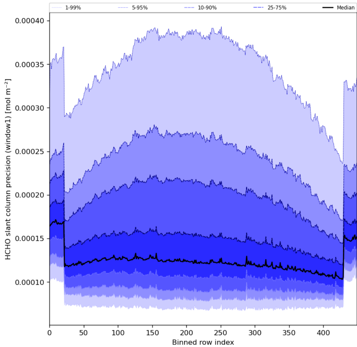
Figure 53: Along track statistics of “HCHO slant column precision (window1)” for 2024-06-25 to 2024-06-27
