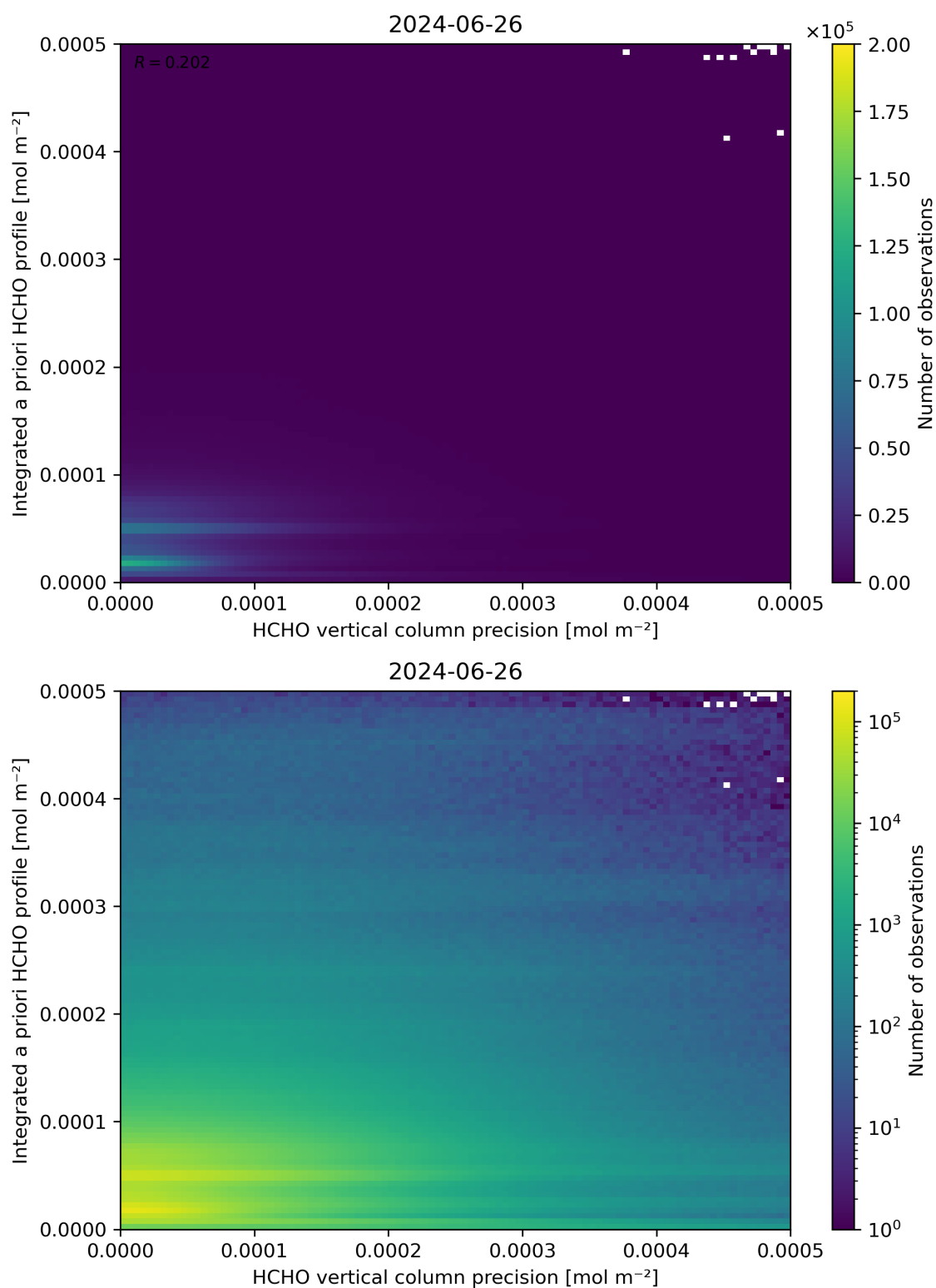
Figure 147: Scatter density plot of “HCHO vertical column precision” against “Integrated a priori HCHO profile” for 2024-06-25 to 2024-06-27.
