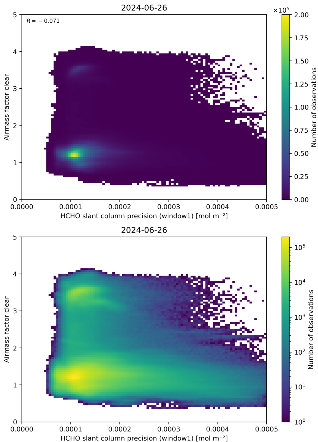
Figure 91: Scatter density plot of “HCHO slant column precision (window1)” against “Airmass factor clear” for 2024-06-25 to 2024-06-27.
