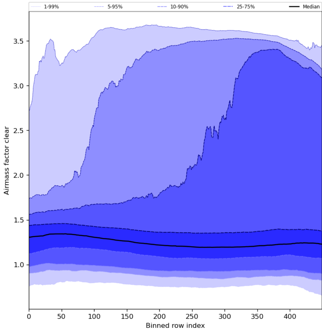
Figure 56: Along track statistics of “Airmass factor clear” for 2024-06-25 to 2024-06-27
