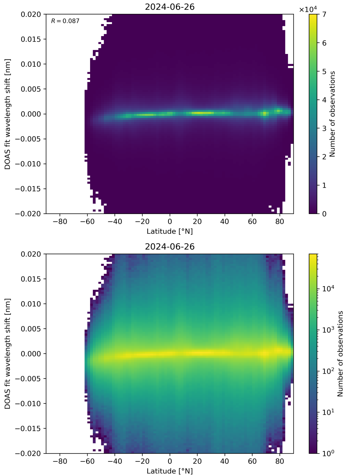
Figure 154: Scatter density plot of “Latitude” against “DOAS fit wavelength shift” for 2024-06-25 to 2024-06-27.
