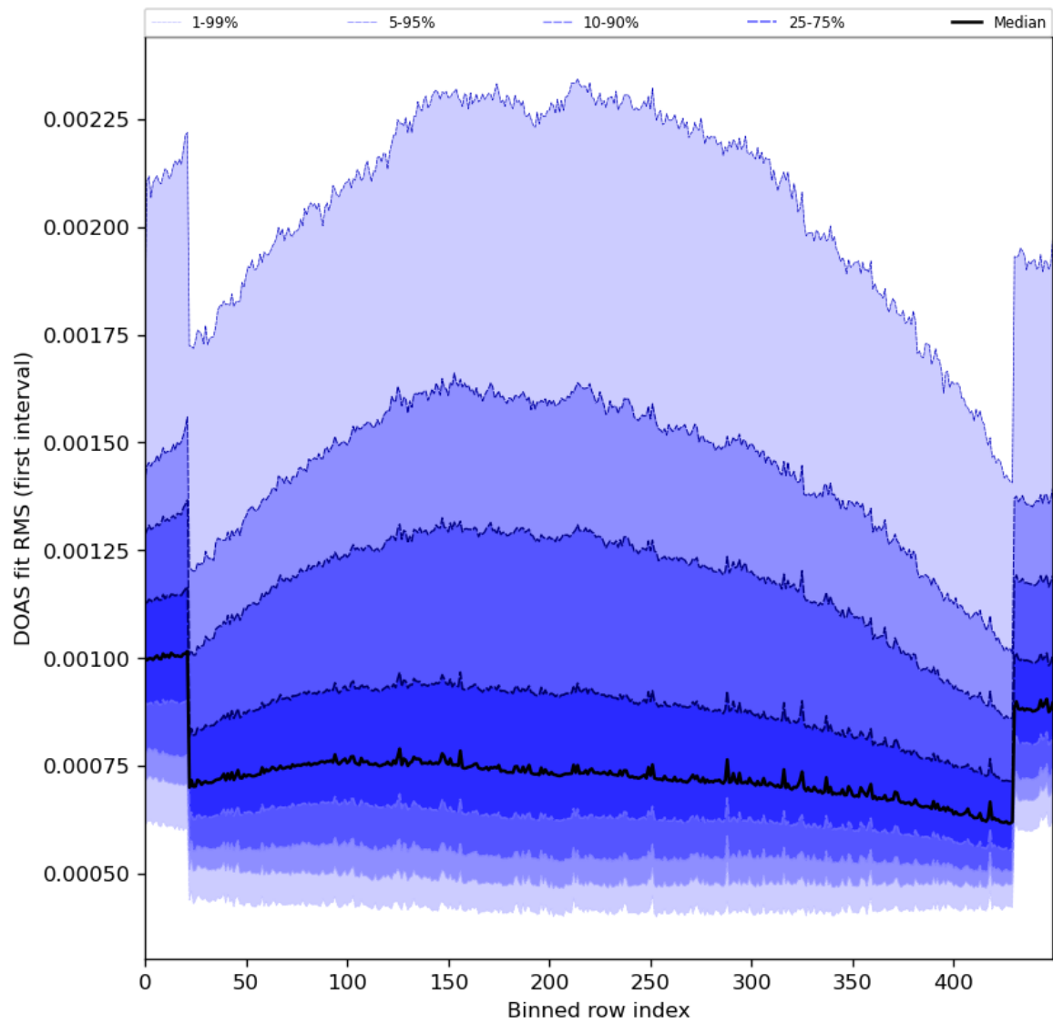
Figure 60: Along track statistics of “DOAS fit RMS (first interval)” for 2024-06-25 to 2024-06-27
