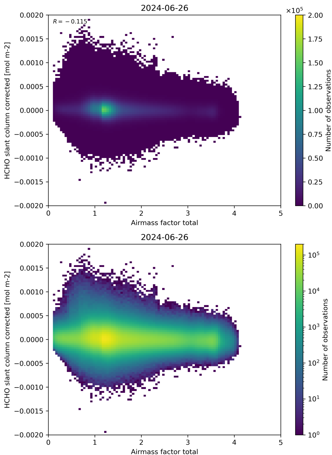
Figure 101: Scatter density plot of “Airmass factor total” against “HCHO slant column corrected” for 2024-06-25 to 2024-06-27.
