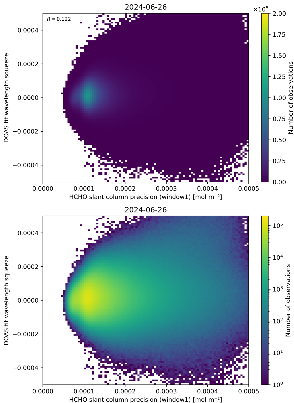
Figure 90: Scatter density plot of “HCHO slant column precision (window1)” against “DOAS fit wavelength squeeze” for 2024-06-25 to 2024-06-27.
