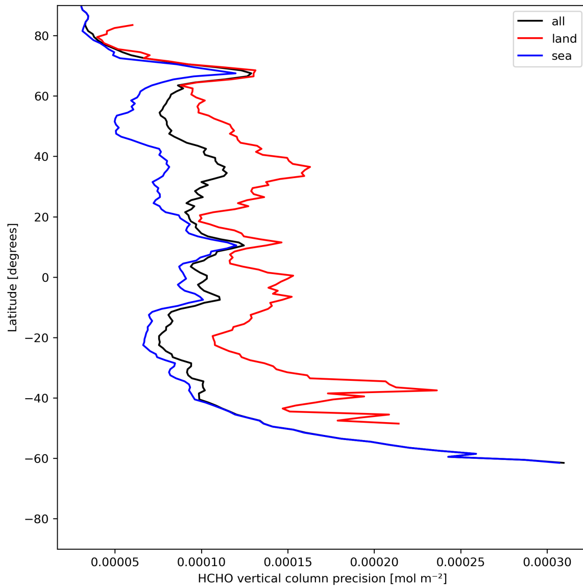
Figure 22: Zonal average of “HCHO vertical column precision” for 2024-06-25 to 2024-06-27.
