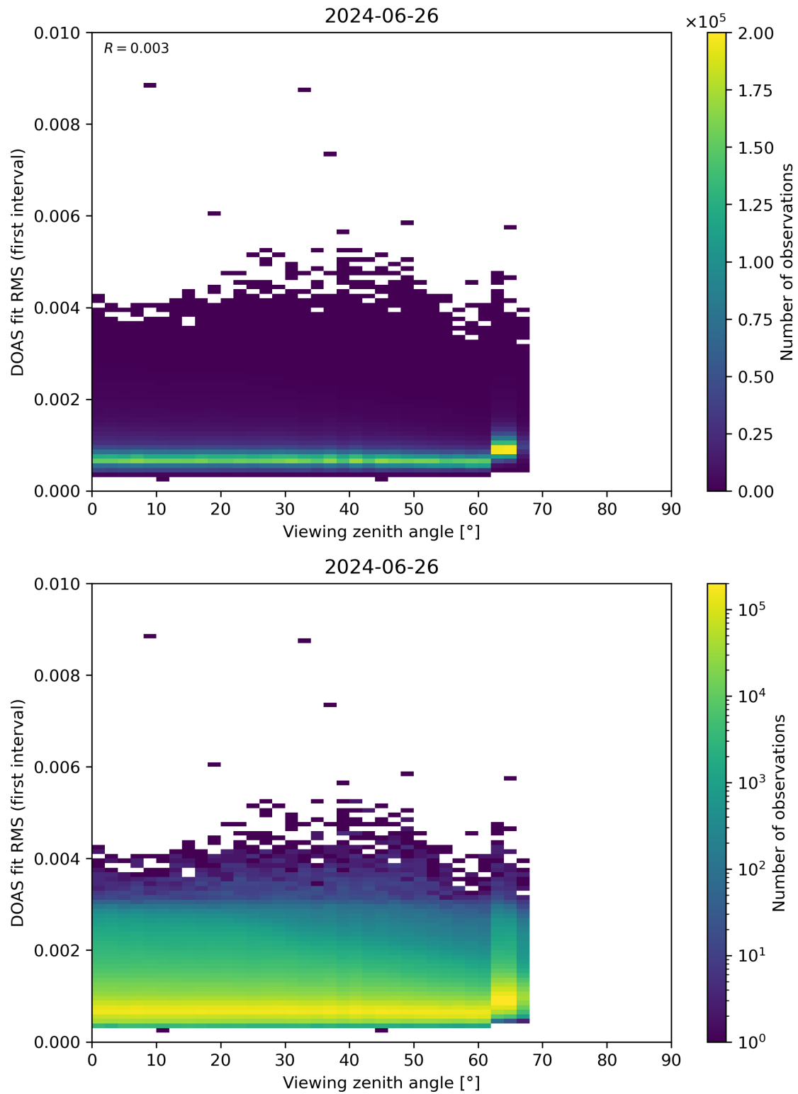
Figure 182: Scatter density plot of “Viewing zenith angle” against “DOAS fit RMS (first interval)” for 2024-06-25 to 2024-06-27.
