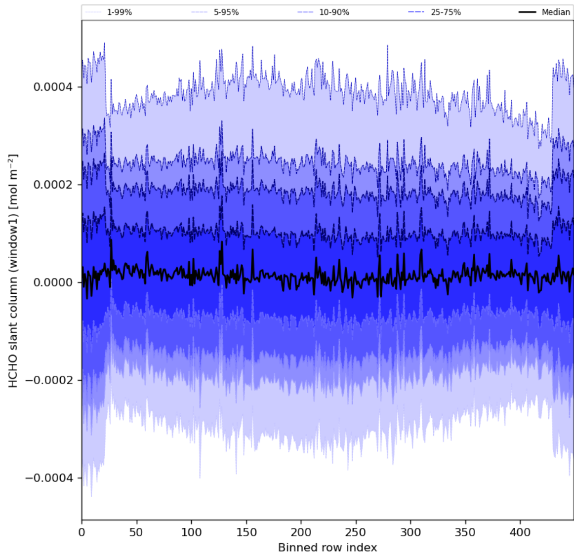
Figure 52: Along track statistics of “HCHO slant column (window1)” for 2024-06-25 to 2024-06-27
