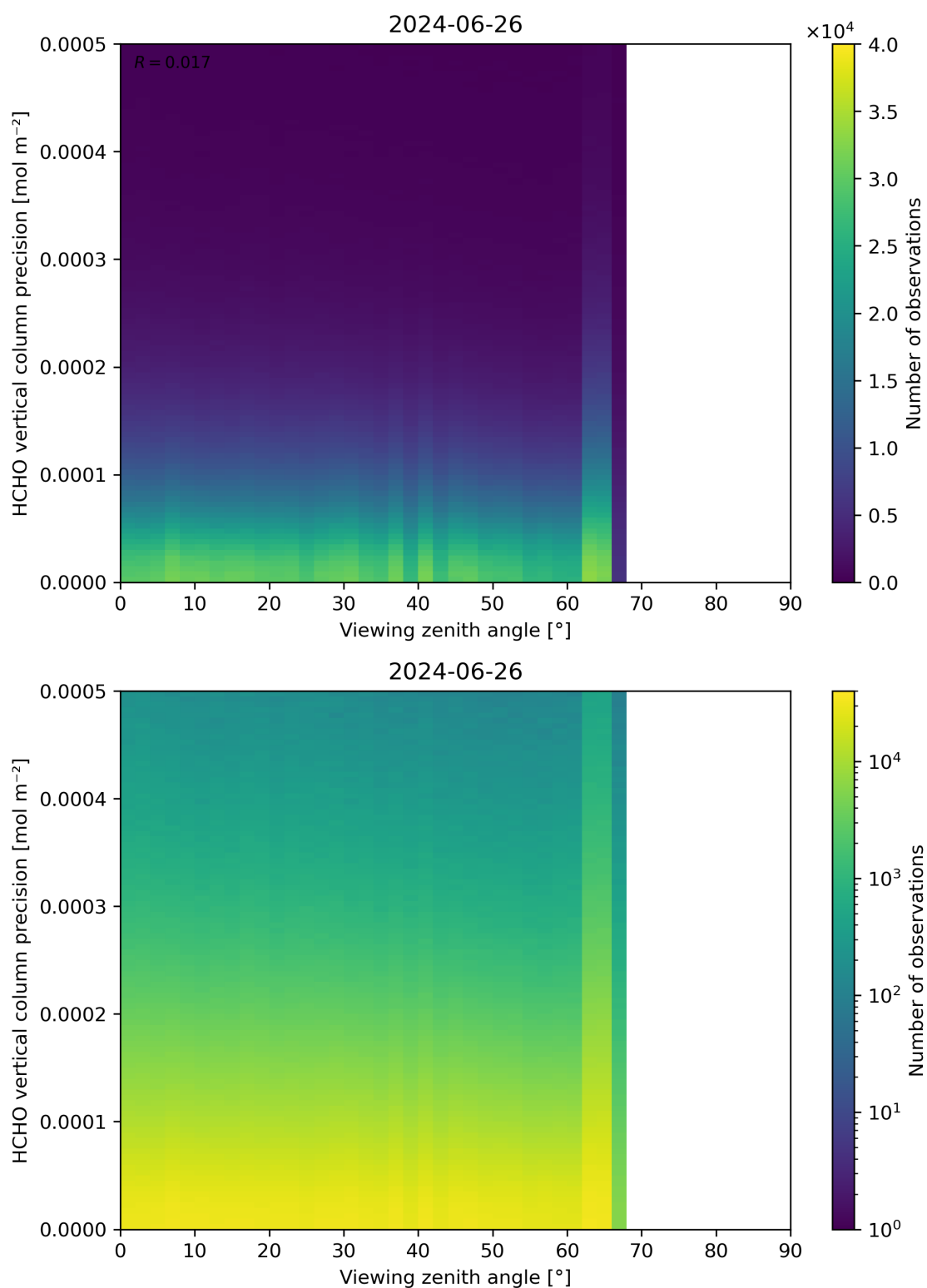
Figure 194: Scatter density plot of “Viewing zenith angle” against “HCHO vertical column precision” for 2024-06-25 to 2024-06-27.
