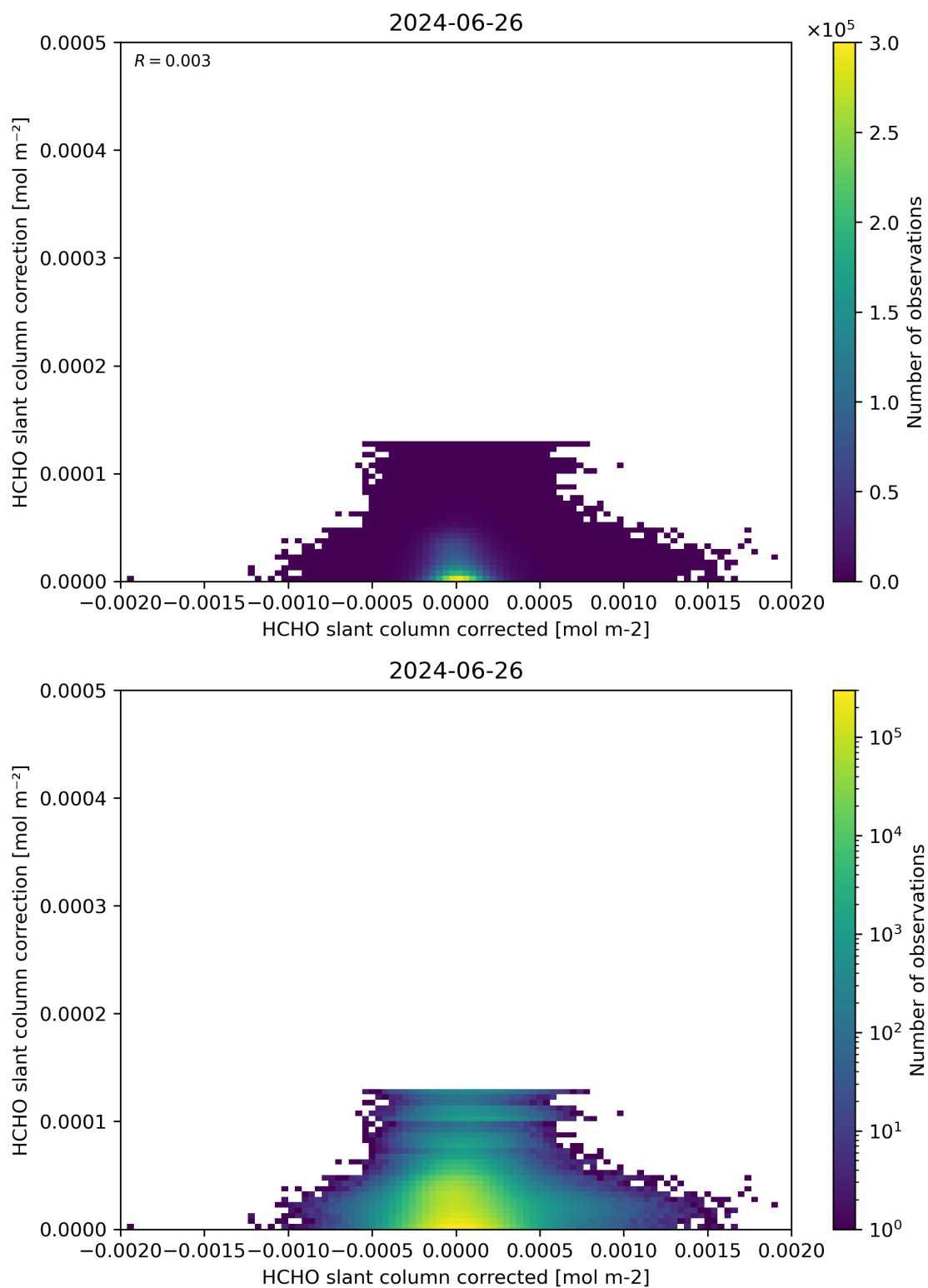
Figure 77: Scatter density plot of “HCHO slant column corrected” against “HCHO slant column correction” for 2024-06-25 to 2024-06-27.
