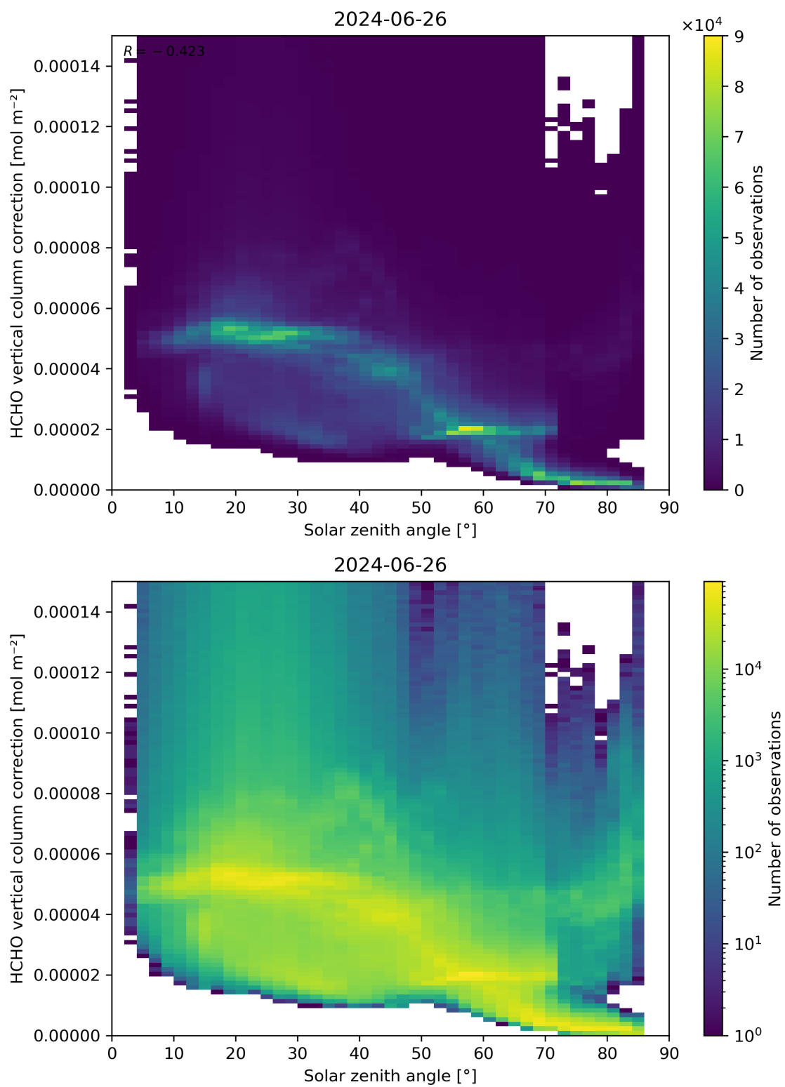
Figure 178: Scatter density plot of “Solar zenith angle” against “HCHO vertical column correction” for 2024-06-25 to 2024-06-27.
