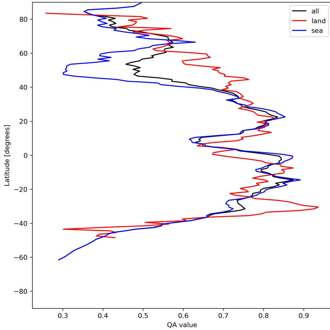
Figure 20: Zonal average of “QA value” for 2024-06-25 to 2024-06-27.
