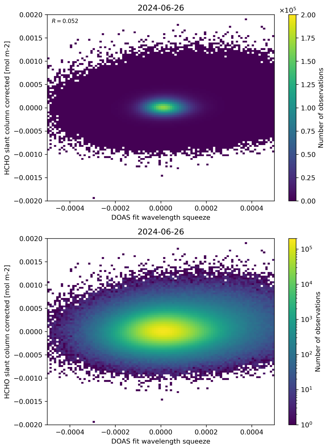
Figure 69: Scatter density plot of “DOAS fit wavelength squeeze” against “HCHO slant column corrected” for 2024-06-25 to 2024-06-27.
