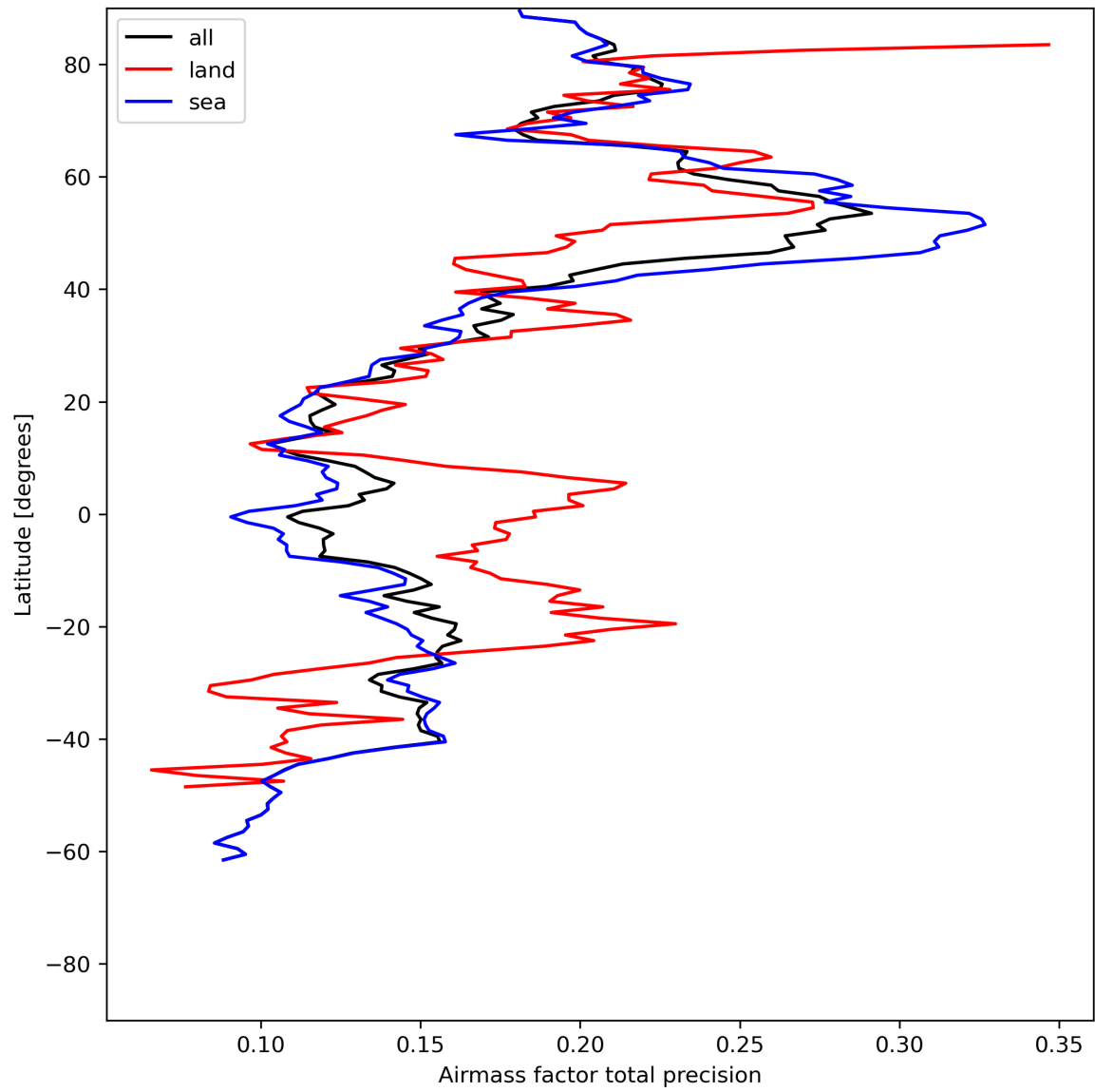
Figure 27: Zonal average of “Airmass factor total precision” for 2024-06-25 to 2024-06-27.
