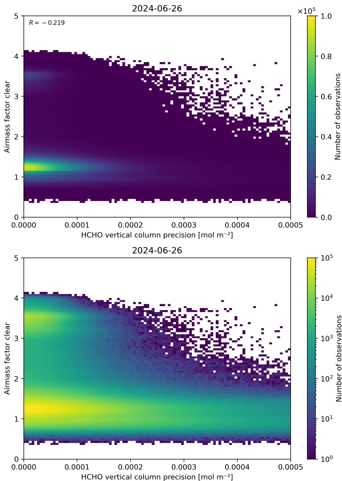
Figure 139: Scatter density plot of “HCHO vertical column precision” against “Airmass factor clear” for 2024-06-25 to 2024-06-27.
