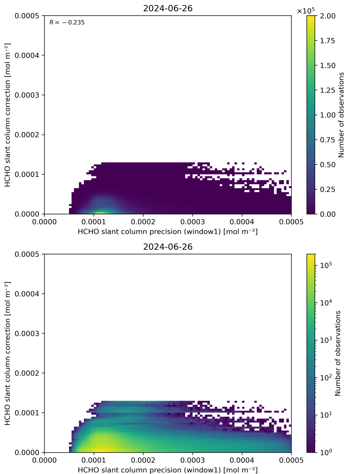
Figure 93: Scatter density plot of “HCHO slant column precision (window1)” against “HCHO slant column correction” for 2024-06-25 to 2024-06-27.
