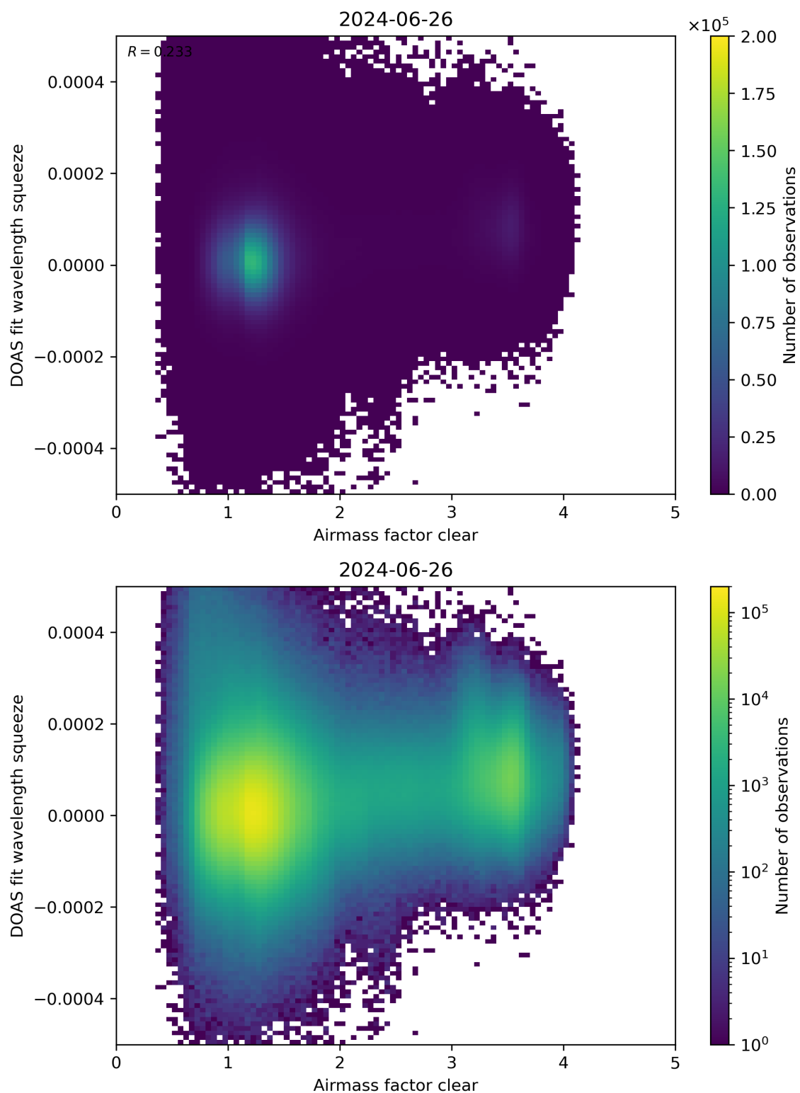
Figure 73: Scatter density plot of “Airmass factor clear” against “DOAS fit wavelength squeeze” for 2024-06-25 to 2024-06-27.
