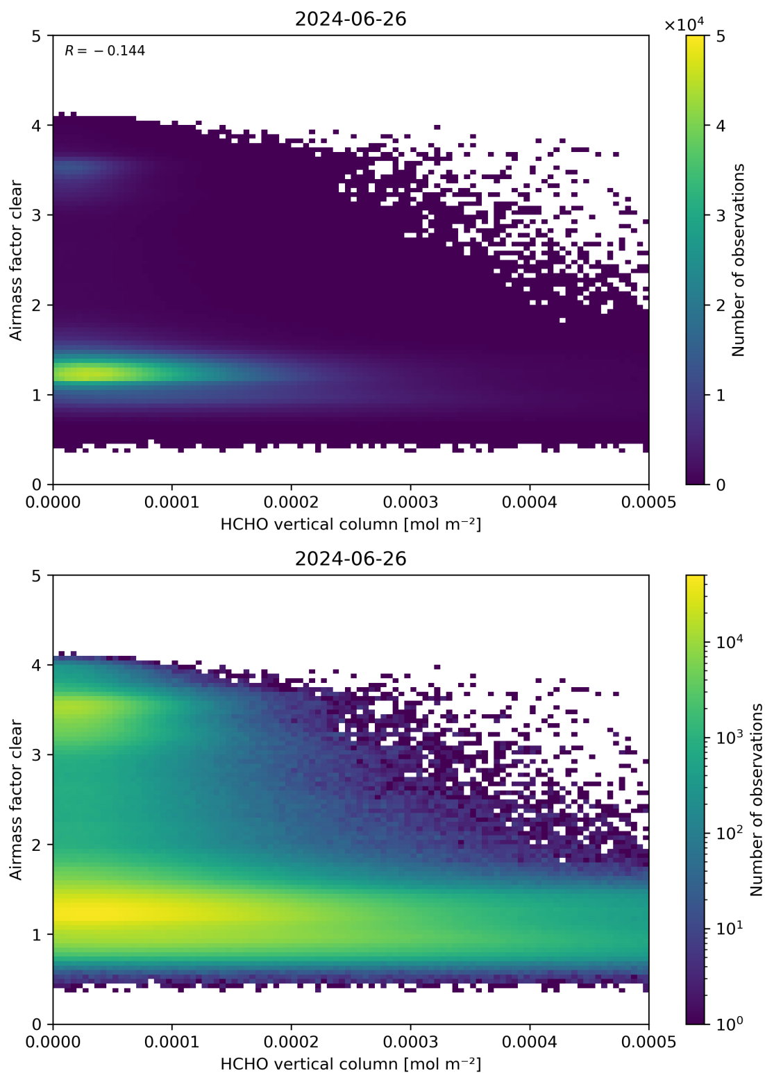
Figure 126: Scatter density plot of “HCHO vertical column” against “Airmass factor clear” for 2024-06-25 to 2024-06-27.
