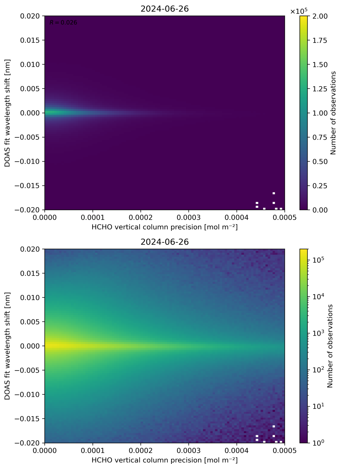
Figure 137: Scatter density plot of “HCHO vertical column precision” against “DOAS fit wavelength shift” for 2024-06-25 to 2024-06-27.
