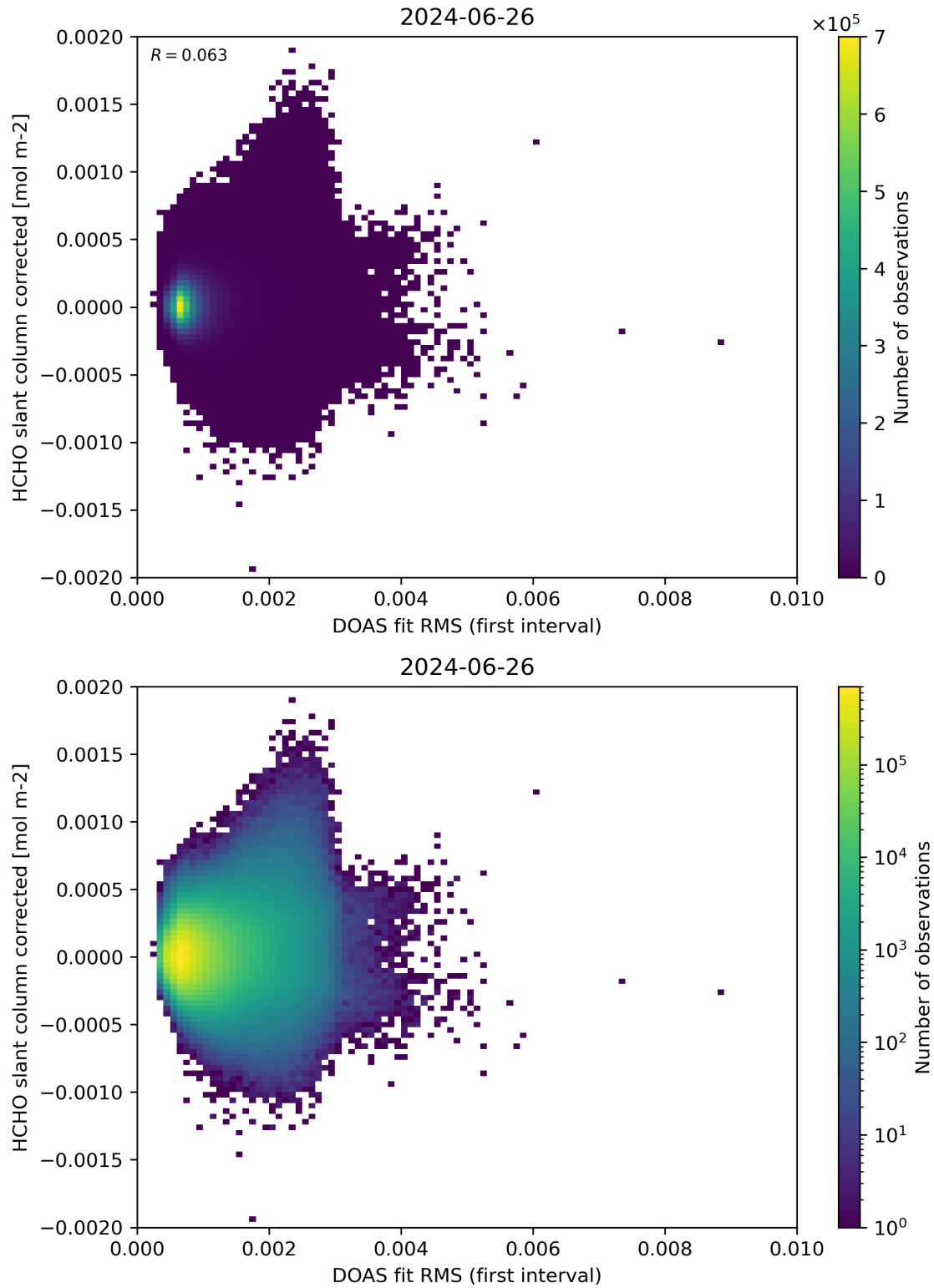
Figure 62: Scatter density plot of “DOAS fit RMS (first interval)” against “HCHO slant column corrected” for 2024-06-25 to 2024-06-27.
