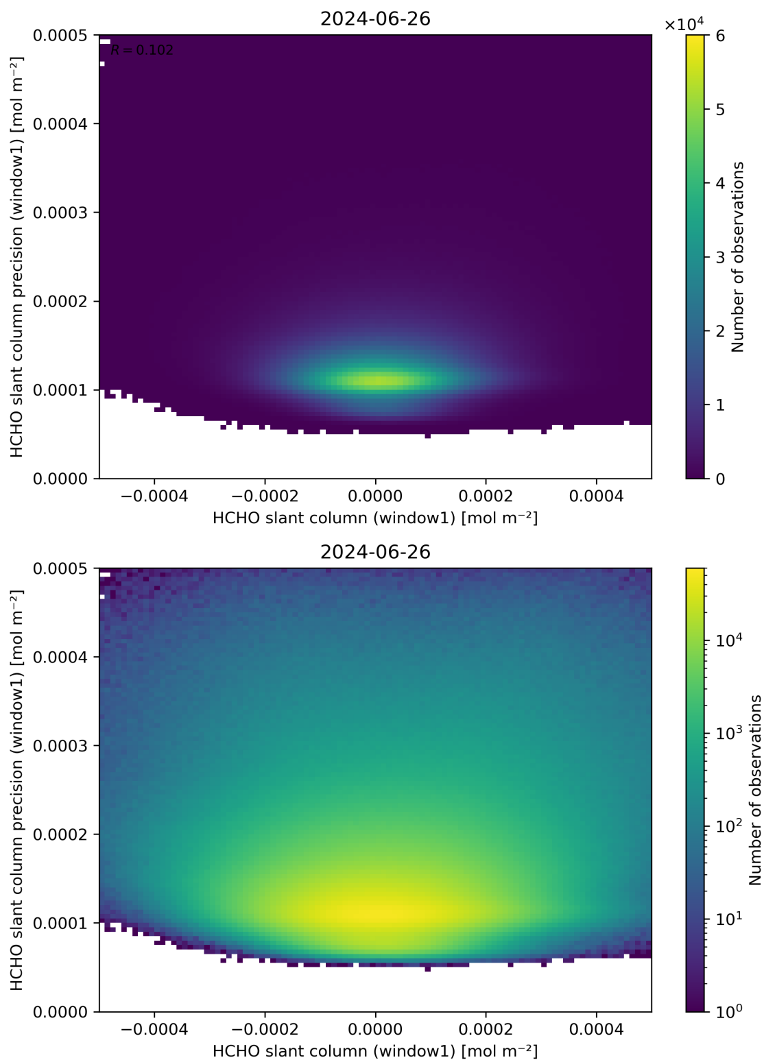
Figure 84: Scatter density plot of “HCHO slant column (window1)” against “HCHO slant column precision (window1)” for 2024-06-25 to 2024-06-27.
