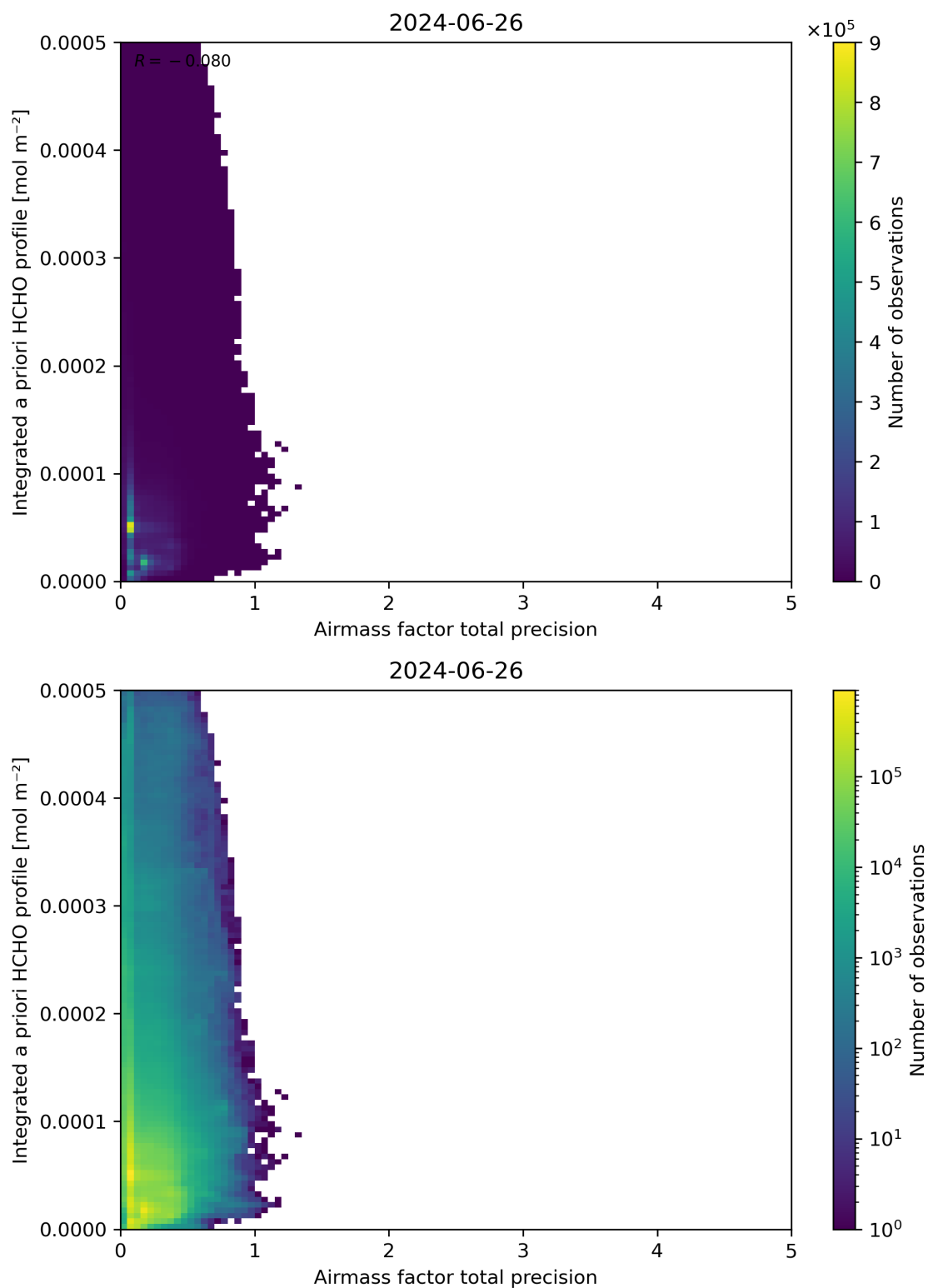
Figure 111: Scatter density plot of “Airmass factor total precision” against “Integrated a priori HCHO profile” for 2024-06-25 to 2024-06-27.
