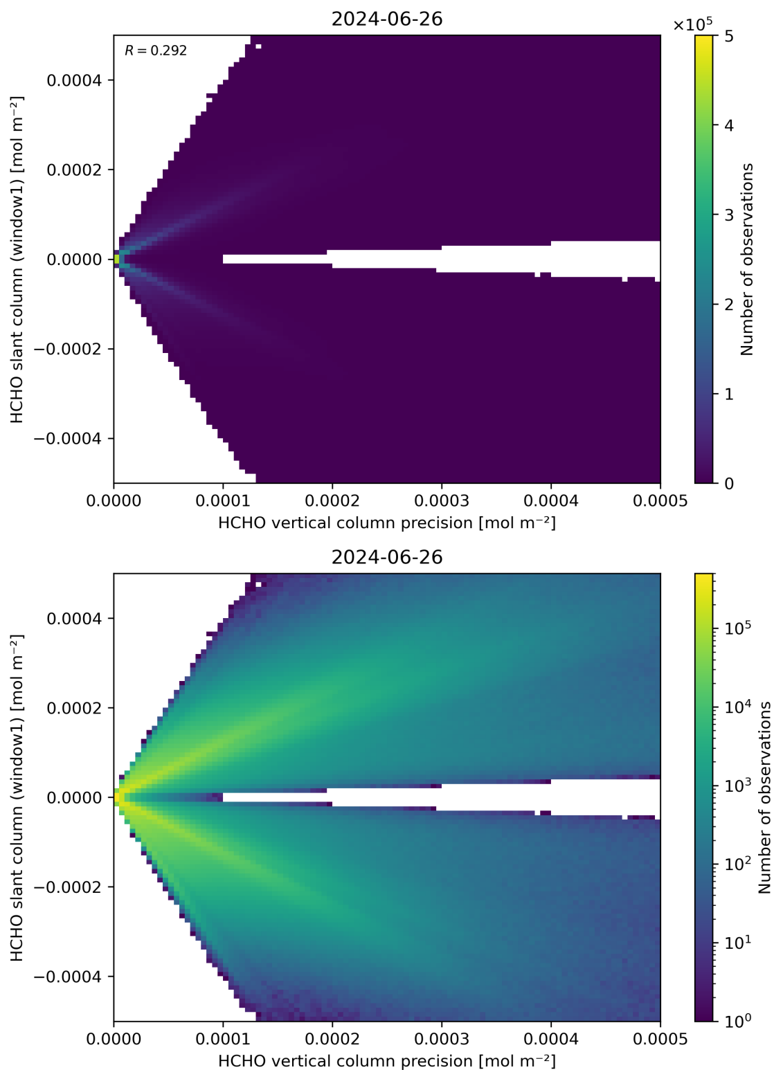
Figure 142: Scatter density plot of “HCHO vertical column precision” against “HCHO slant column (window1)” for 2024-06-25 to 2024-06-27.
