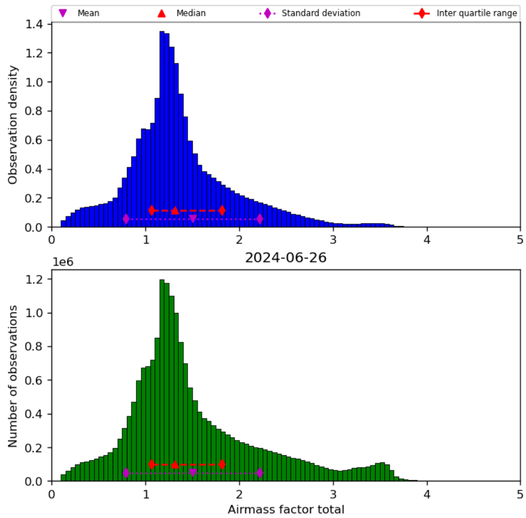
Figure 40: Histogram of “Airmass factor total” for 2024-06-25 to 2024-06-27
