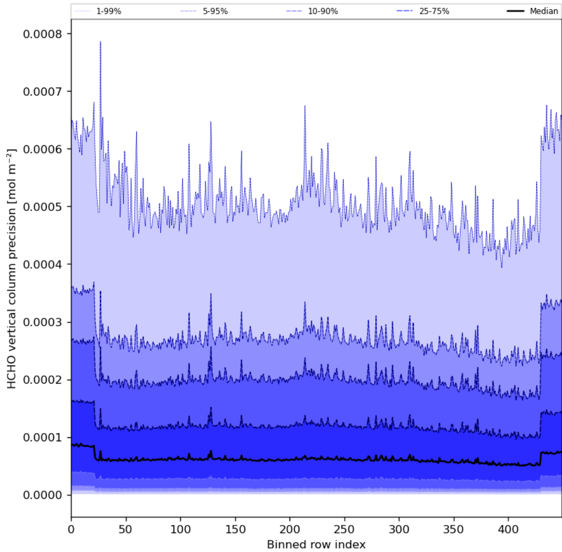
Figure 50: Along track statistics of “HCHO vertical column precision” for 2024-06-25 to 2024-06-27
