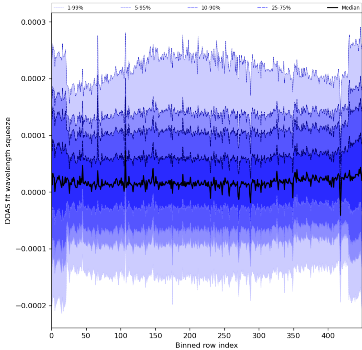
Figure 59: Along track statistics of “DOAS fit wavelength squeeze” for 2024-06-25 to 2024-06-27
