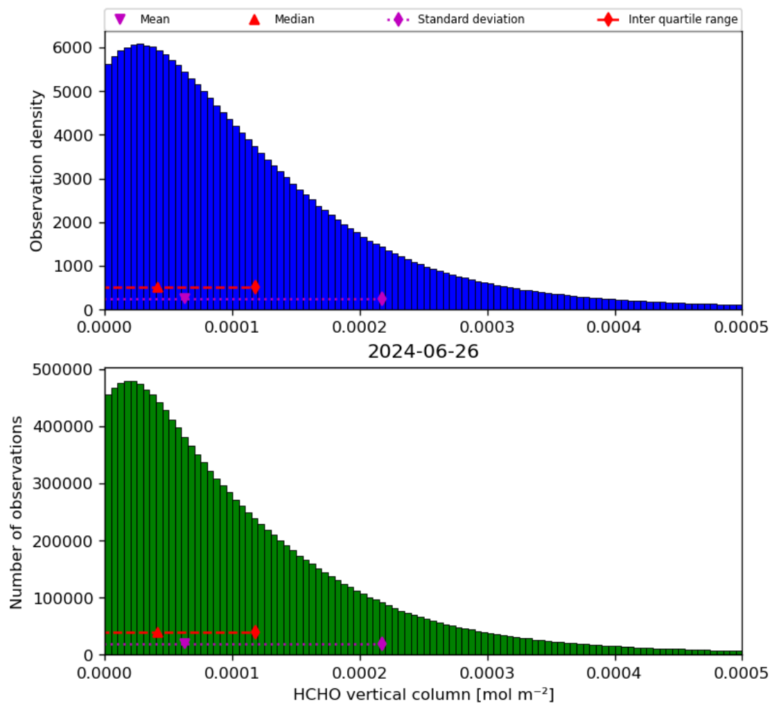
Figure 35: Histogram of “HCHO vertical column” for 2024-06-25 to 2024-06-27
