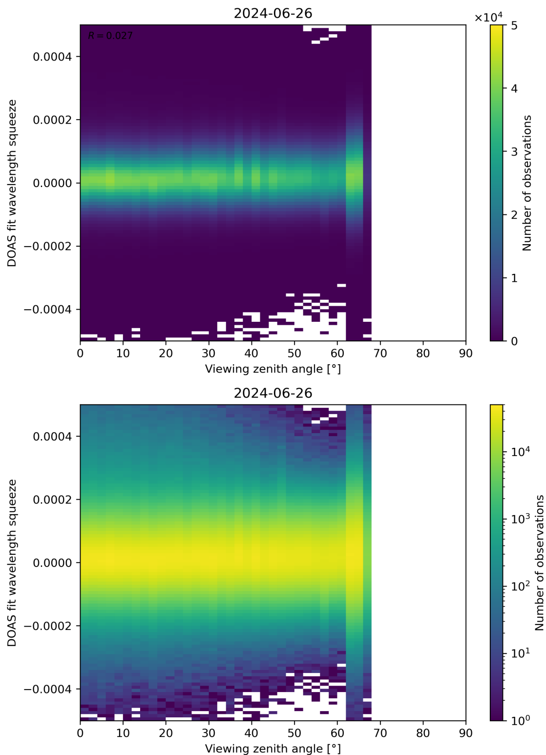
Figure 184: Scatter density plot of “Viewing zenith angle” against “DOAS fit wavelength squeeze” for 2024-06-25 to 2024-06-27.
