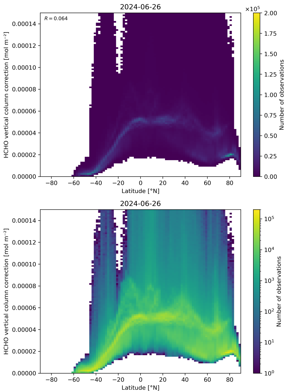
Figure 164: Scatter density plot of “Latitude” against “HCHO vertical column correction” for 2024-06-25 to 2024-06-27.
