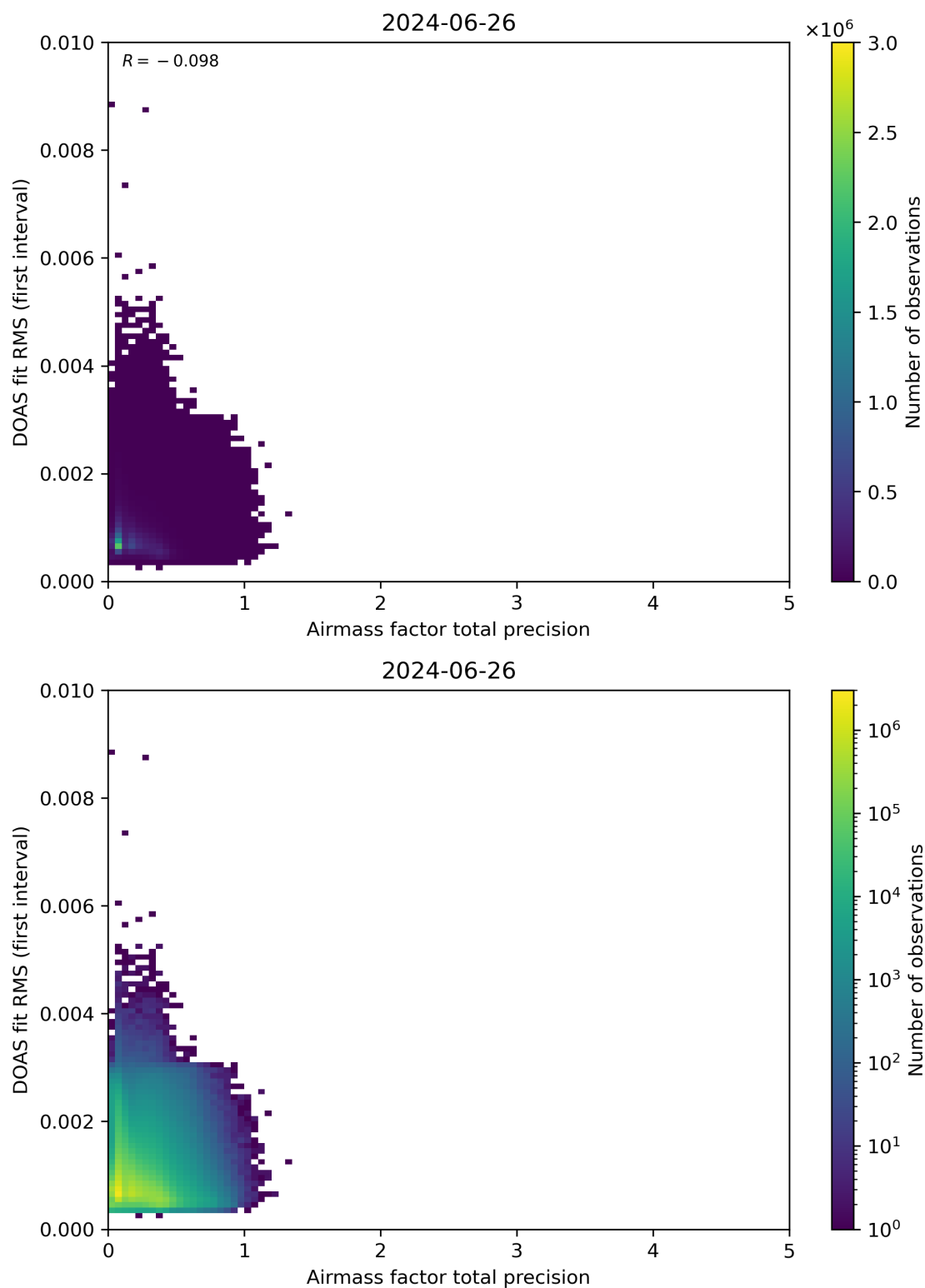
Figure 105: Scatter density plot of “Airmass factor total precision” against “DOAS fit RMS (first interval)” for 2024-06-25 to 2024-06-27.
