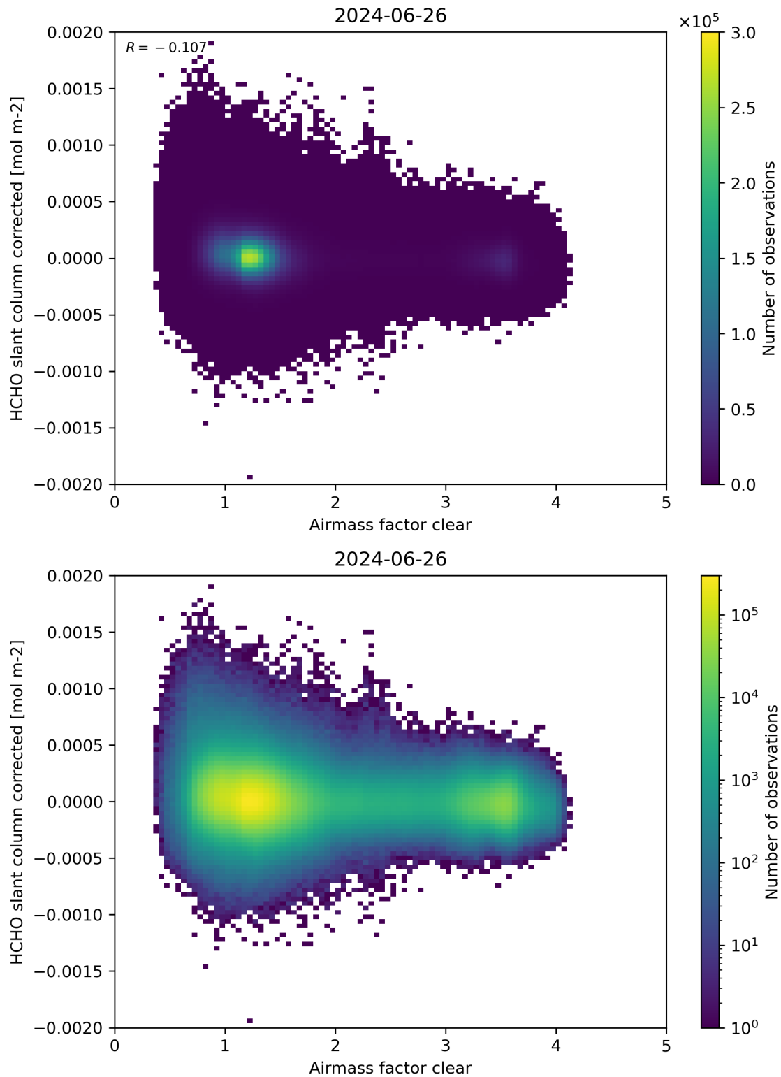
Figure 74: Scatter density plot of “Airmass factor clear” against “HCHO slant column corrected” for 2024-06-25 to 2024-06-27.
