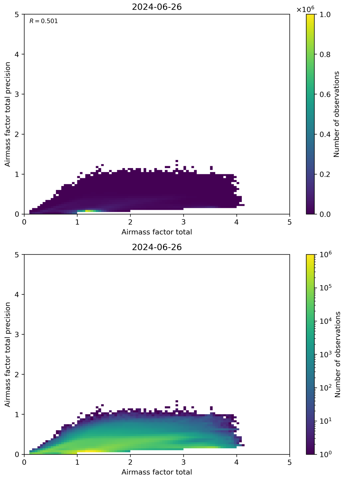
Figure 103: Scatter density plot of “Airmass factor total” against “Airmass factor total precision” for 2024-06-25 to 2024-06-27.
