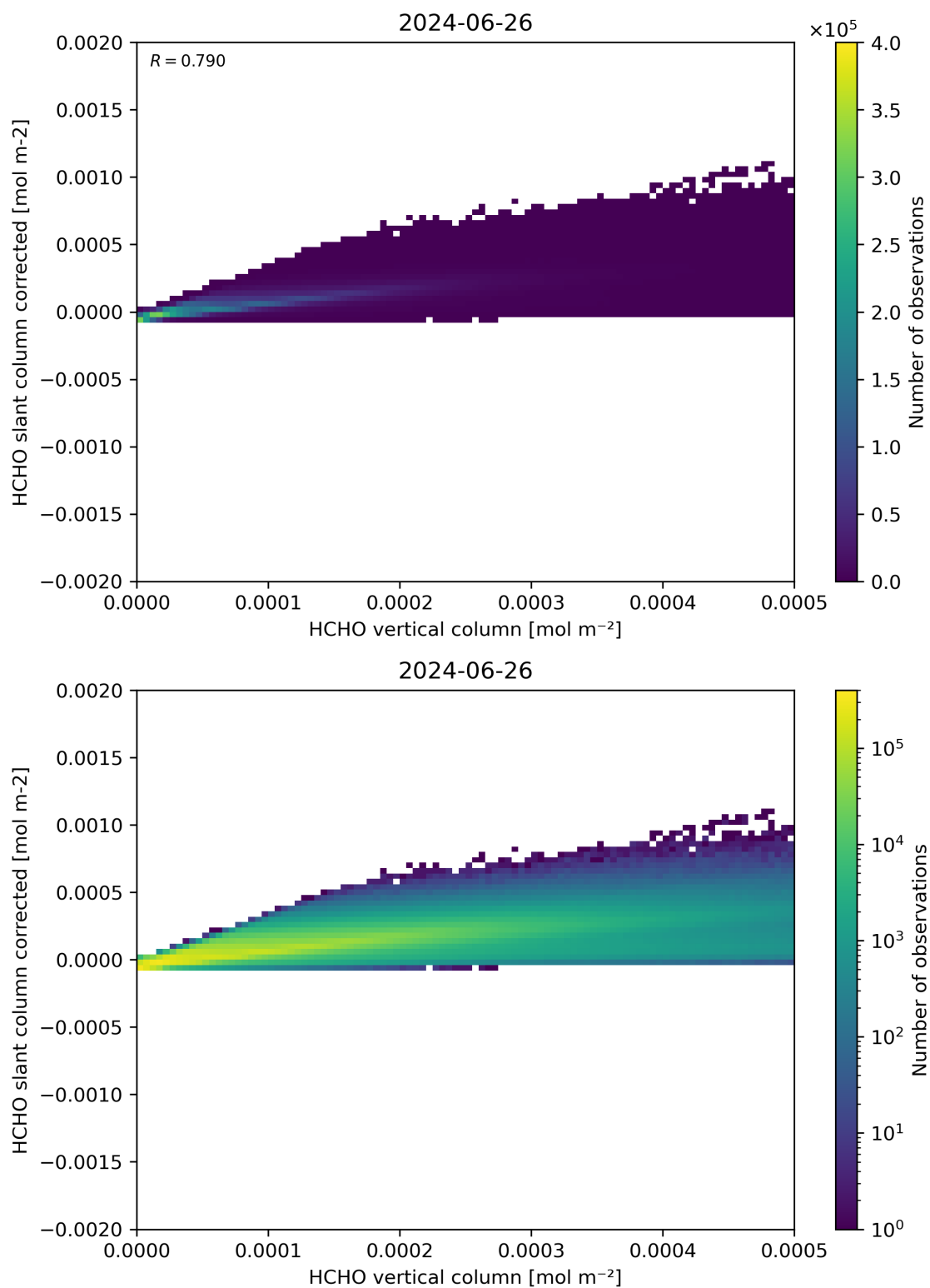
Figure 127: Scatter density plot of “HCHO vertical column” against “HCHO slant column corrected” for 2024-06-25 to 2024-06-27.
