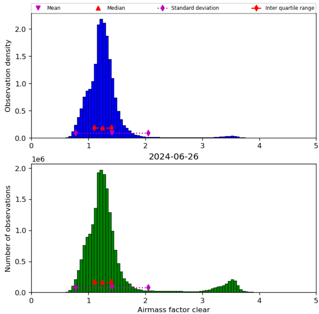
Figure 42: Histogram of “Airmass factor clear” for 2024-06-25 to 2024-06-27
