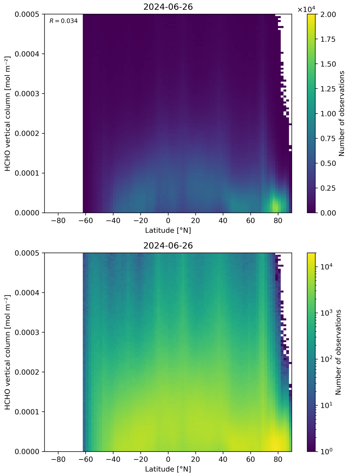
Figure 163: Scatter density plot of “Latitude” against “HCHO vertical column” for 2024-06-25 to 2024-06-27.
