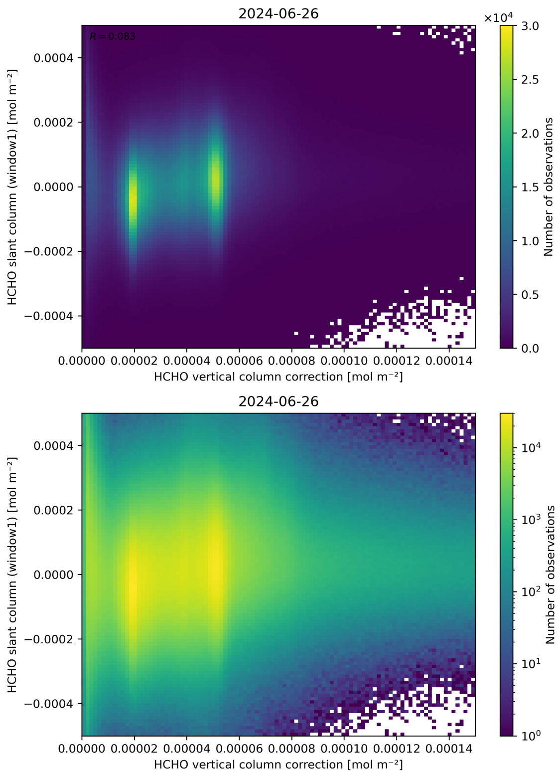
Figure 118: Scatter density plot of “HCHO vertical column correction” against “HCHO slant column (window1)” for 2024-06-25 to 2024-06-27.
