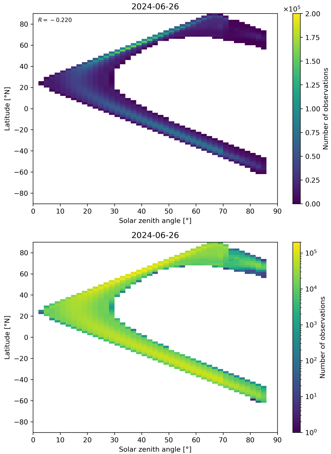
Figure 181: Scatter density plot of “Solar zenith angle” against “Latitude” for 2024-06-25 to 2024-06-27.
