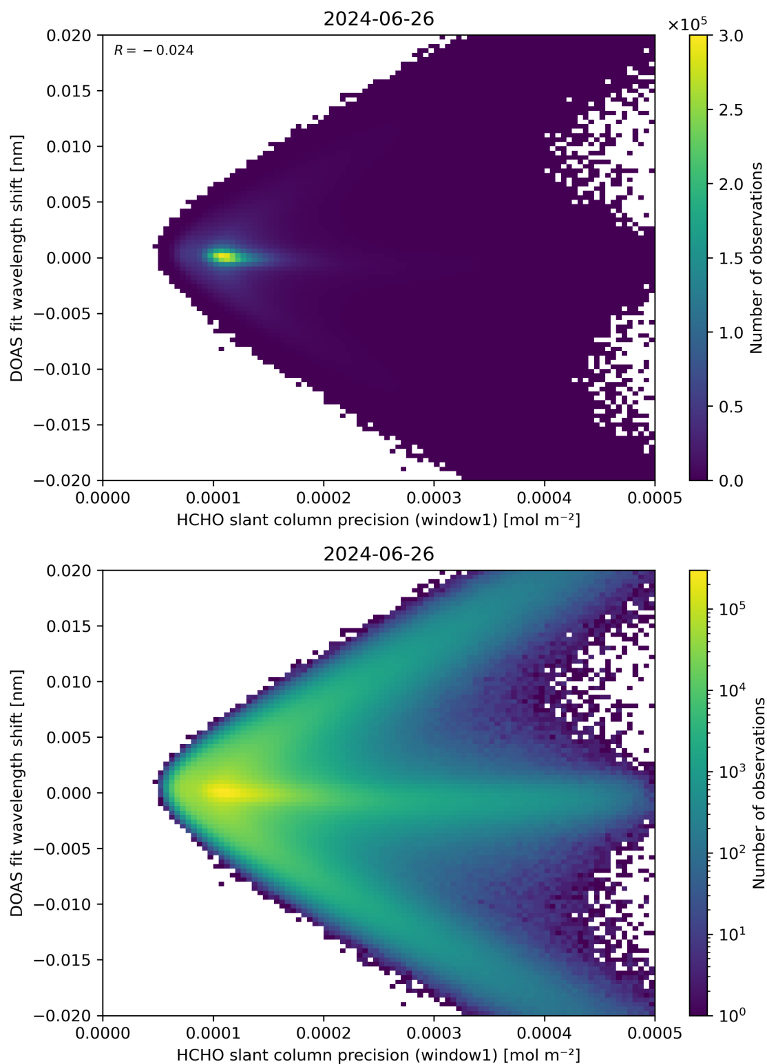
Figure 89: Scatter density plot of “HCHO slant column precision (window1)” against “DOAS fit wavelength shift” for 2024-06-25 to 2024-06-27.
