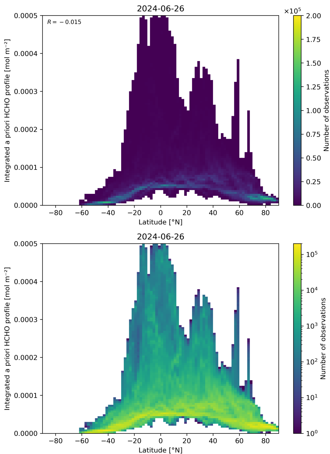
Figure 166: Scatter density plot of “Latitude” against “Integrated a priori HCHO profile” for 2024-06-25 to 2024-06-27.
