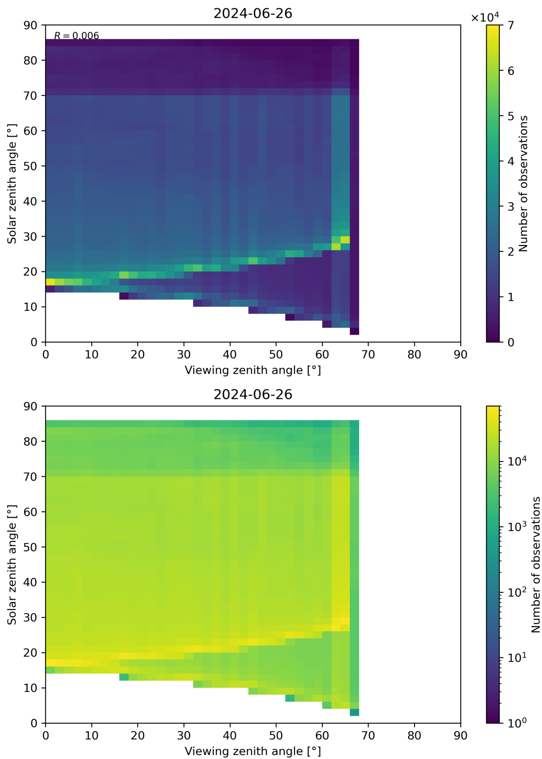
Figure 197: Scatter density plot of “Viewing zenith angle” against “Solar zenith angle” for 2024-06-25 to 2024-06-27.
