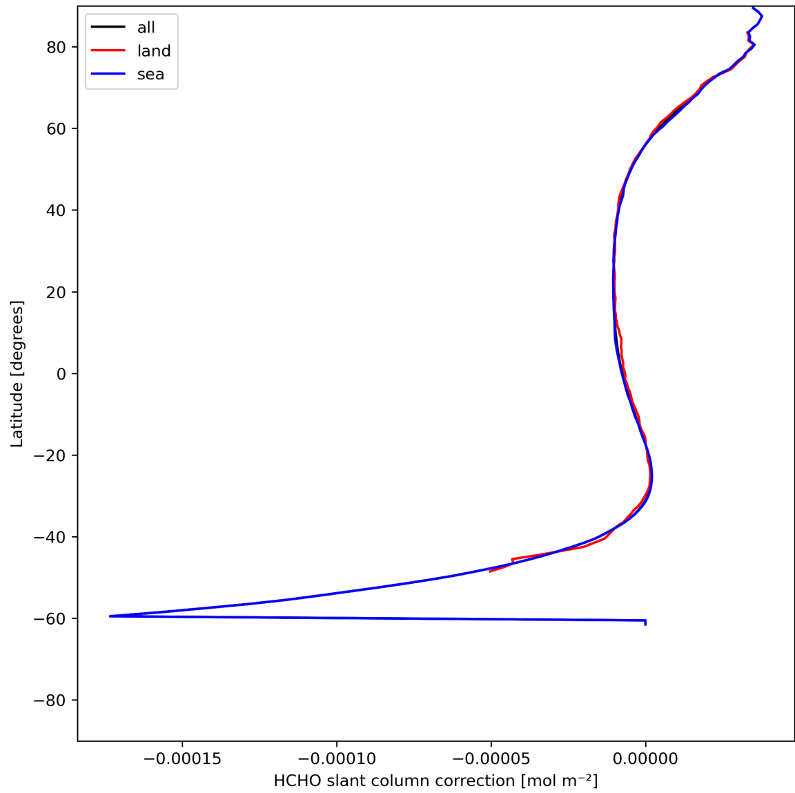
Figure 33: Zonal average of “HCHO slant column correction” for 2024-06-25 to 2024-06-27.
