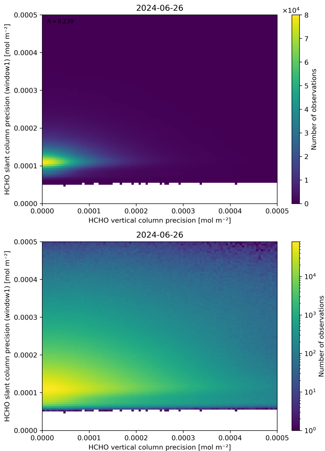
Figure 143: Scatter density plot of “HCHO vertical column precision” against “HCHO slant column precision (window1)” for 2024-06-25 to 2024-06-27.
