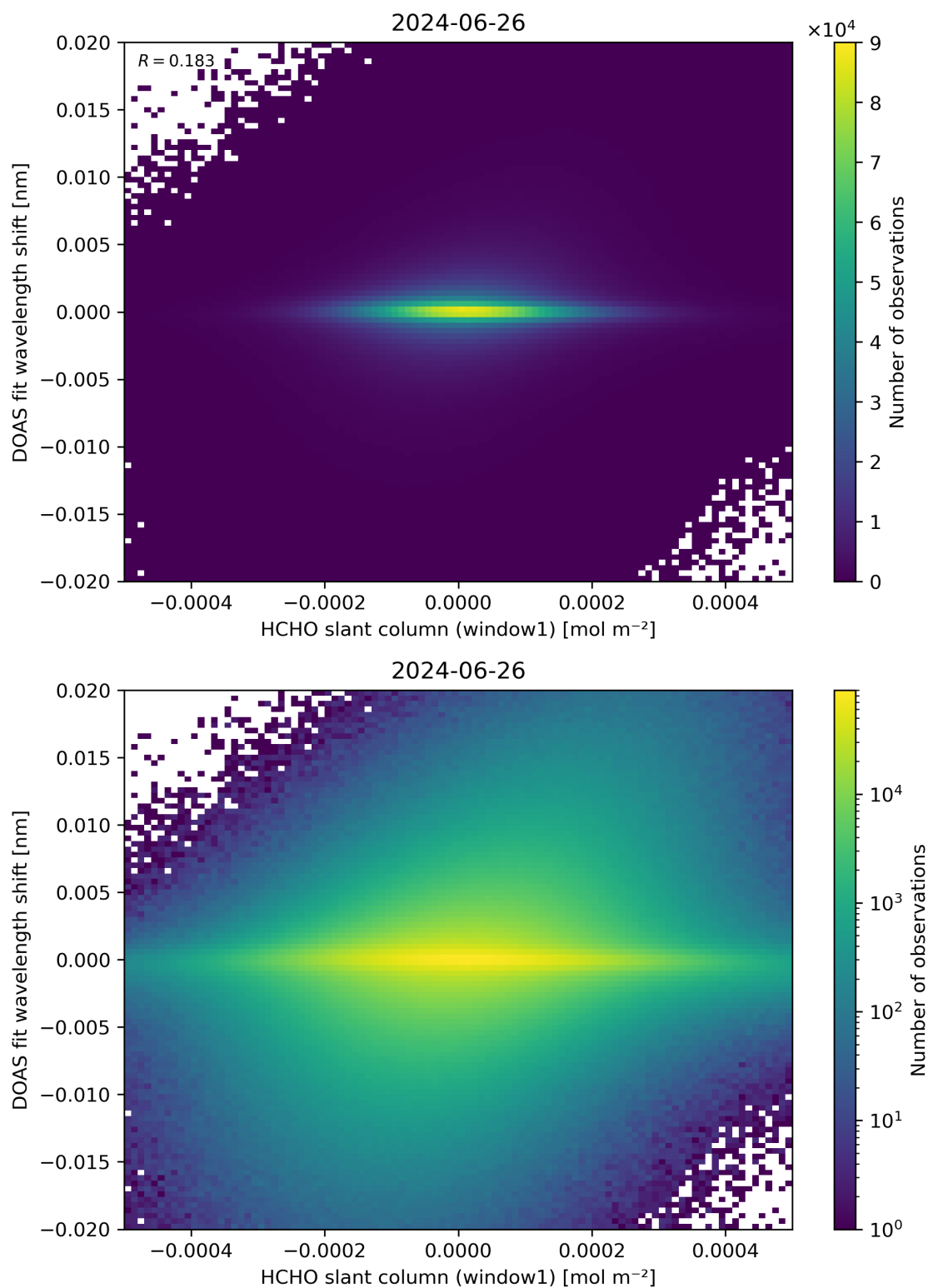
Figure 79: Scatter density plot of “HCHO slant column (window1)” against “DOAS fit wavelength shift” for 2024-06-25 to 2024-06-27.
