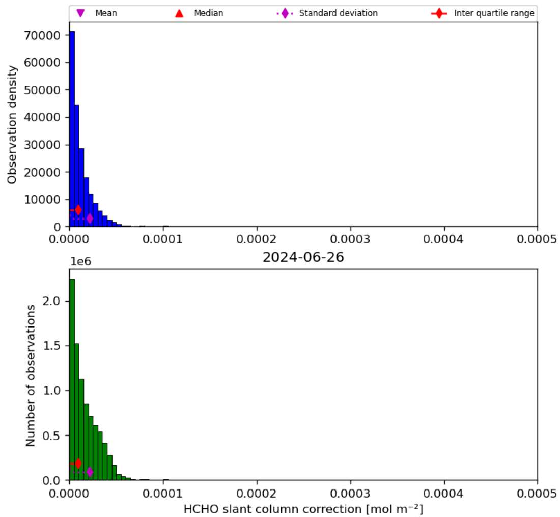
Figure 47: Histogram of “HCHO slant column correction” for 2024-06-25 to 2024-06-27
