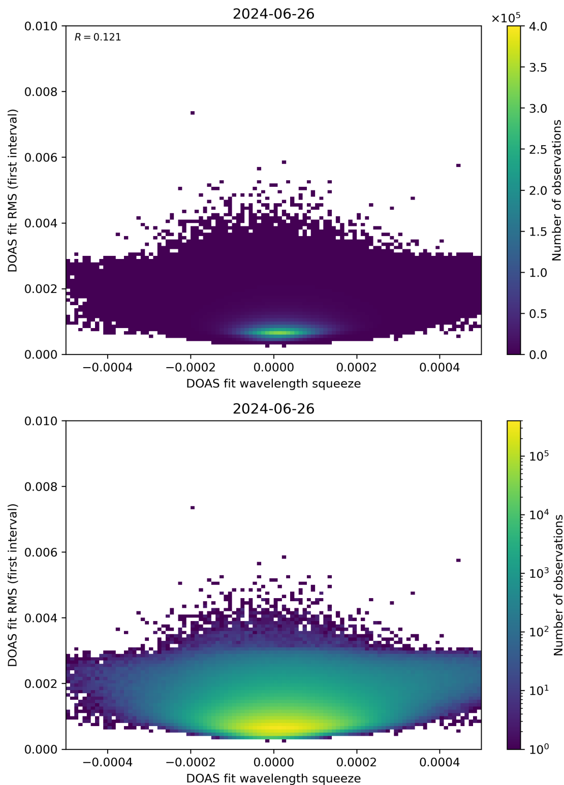
Figure 68: Scatter density plot of “DOAS fit wavelength squeeze” against “DOAS fit RMS (first interval)” for 2024-06-25 to 2024-06-27.
