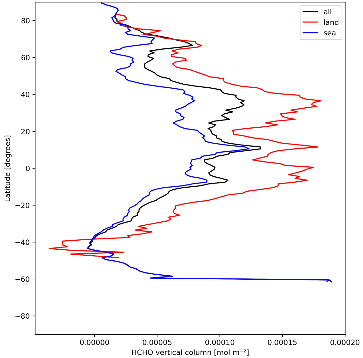
Figure 21: Zonal average of “HCHO vertical column” for 2024-06-25 to 2024-06-27.
