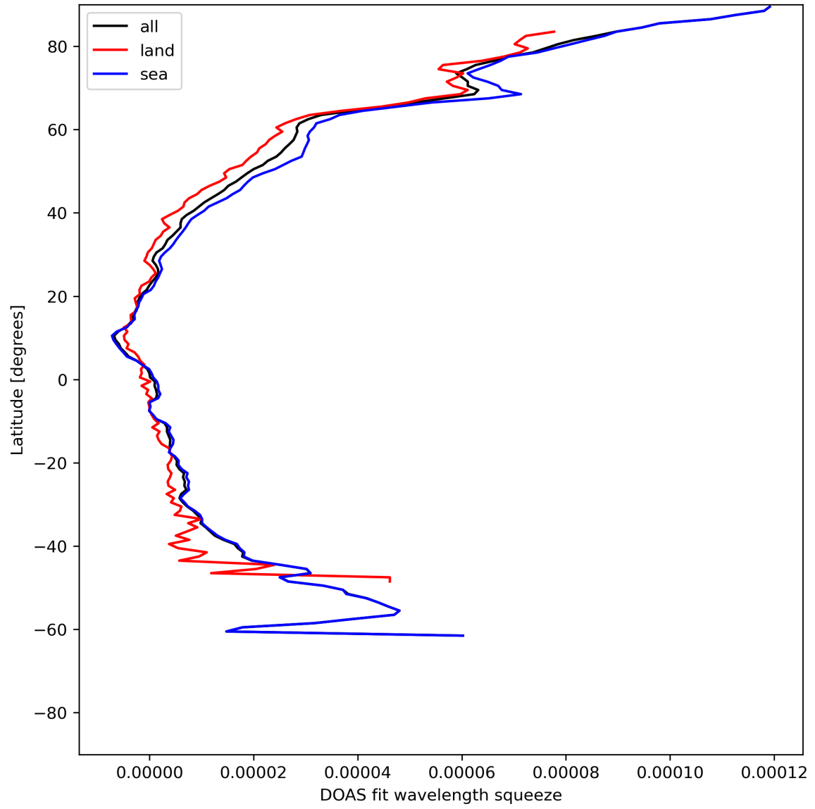
Figure 31: Zonal average of “DOAS fit wavelength squeeze” for 2024-06-25 to 2024-06-27.
