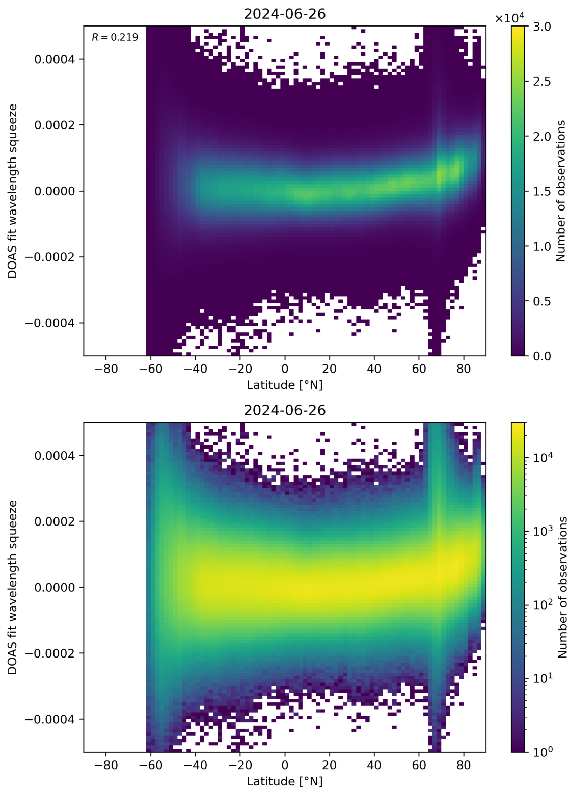
Figure 155: Scatter density plot of “Latitude” against “DOAS fit wavelength squeeze” for 2024-06-25 to 2024-06-27.
