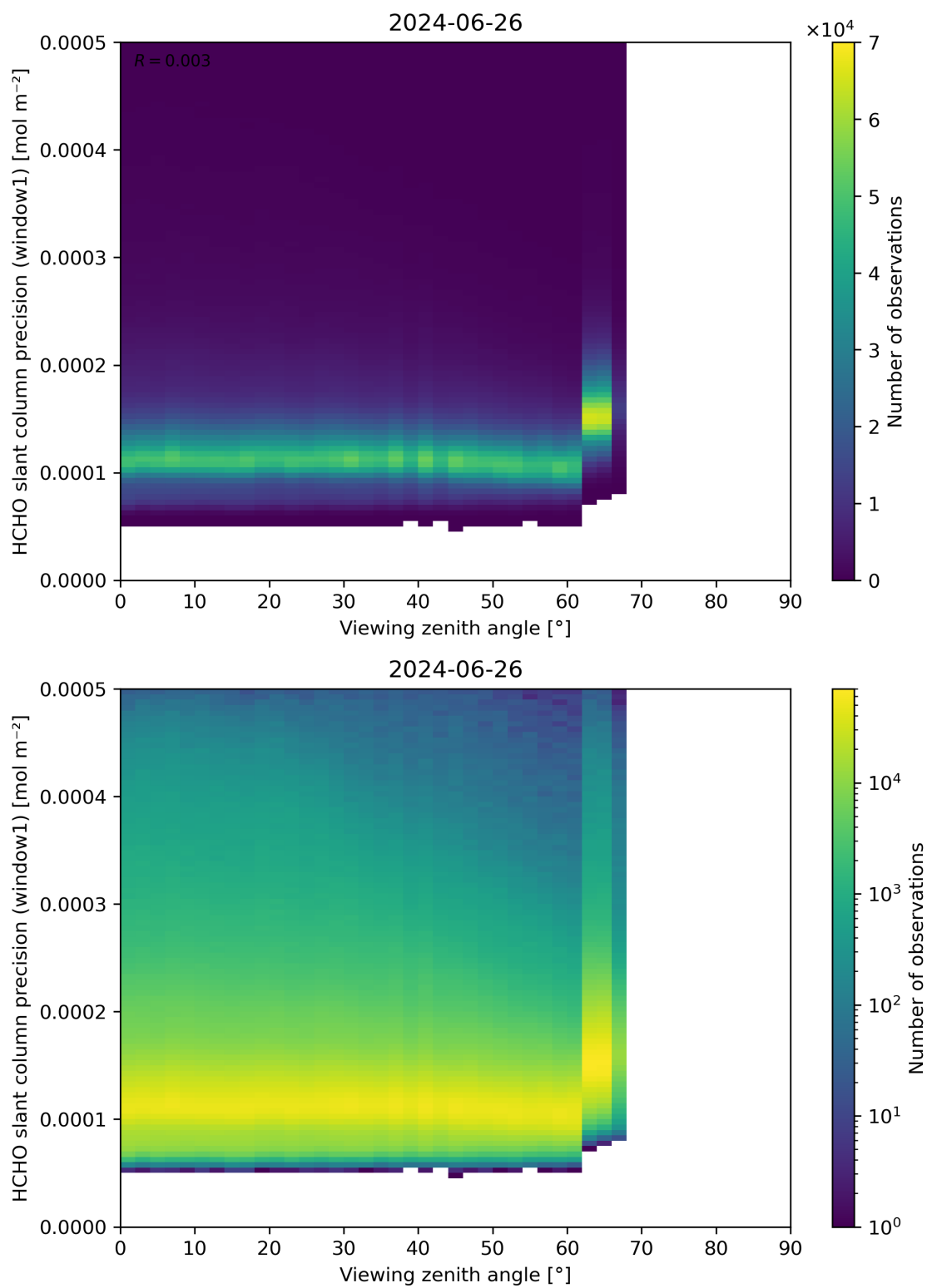
Figure 189: Scatter density plot of “Viewing zenith angle” against “HCHO slant column precision (window1)” for 2024-06-25 to 2024-06-27.
