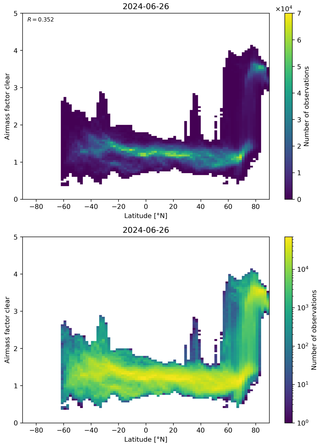
Figure 156: Scatter density plot of “Latitude” against “Airmass factor clear” for 2024-06-25 to 2024-06-27.
