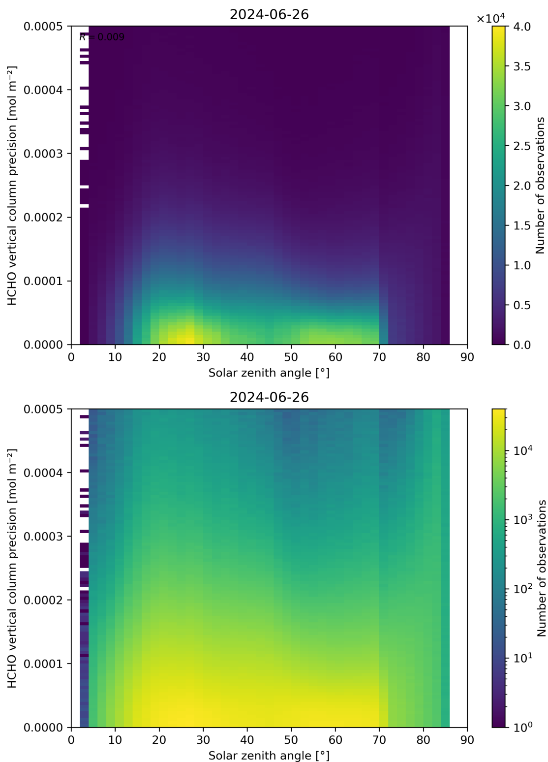
Figure 179: Scatter density plot of “Solar zenith angle” against “HCHO vertical column precision” for 2024-06-25 to 2024-06-27.
