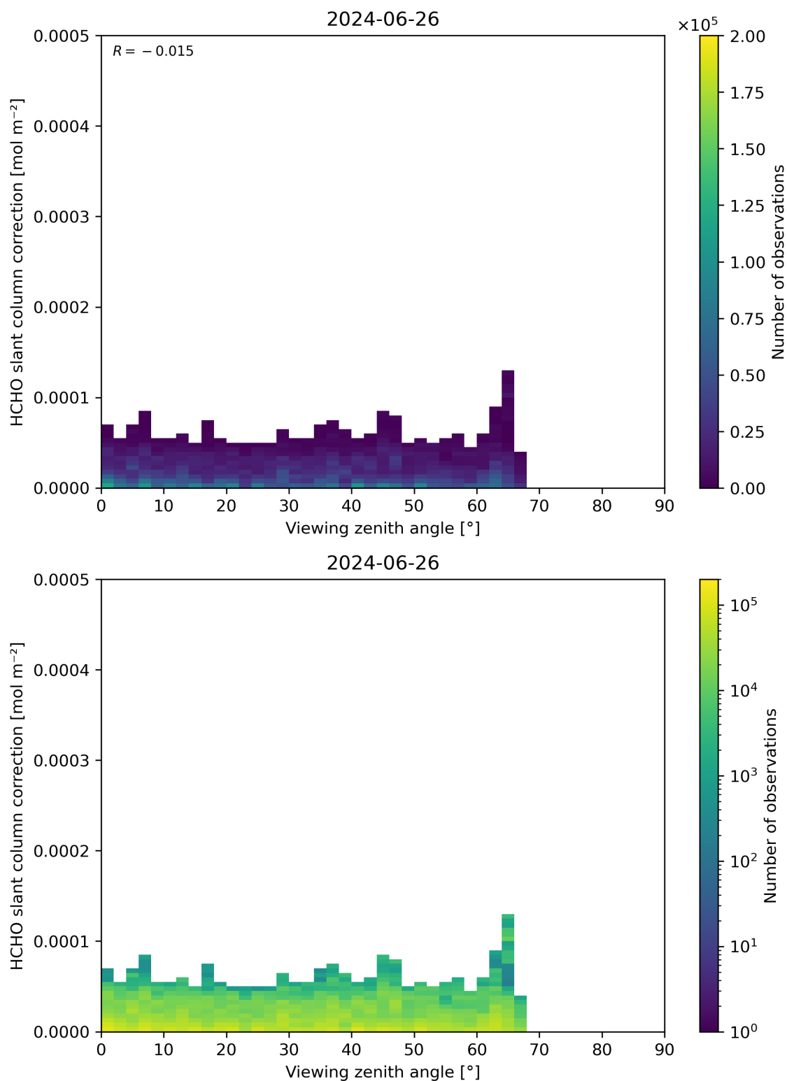
Figure 187: Scatter density plot of “Viewing zenith angle” against “HCHO slant column correction” for 2024-06-25 to 2024-06-27.
