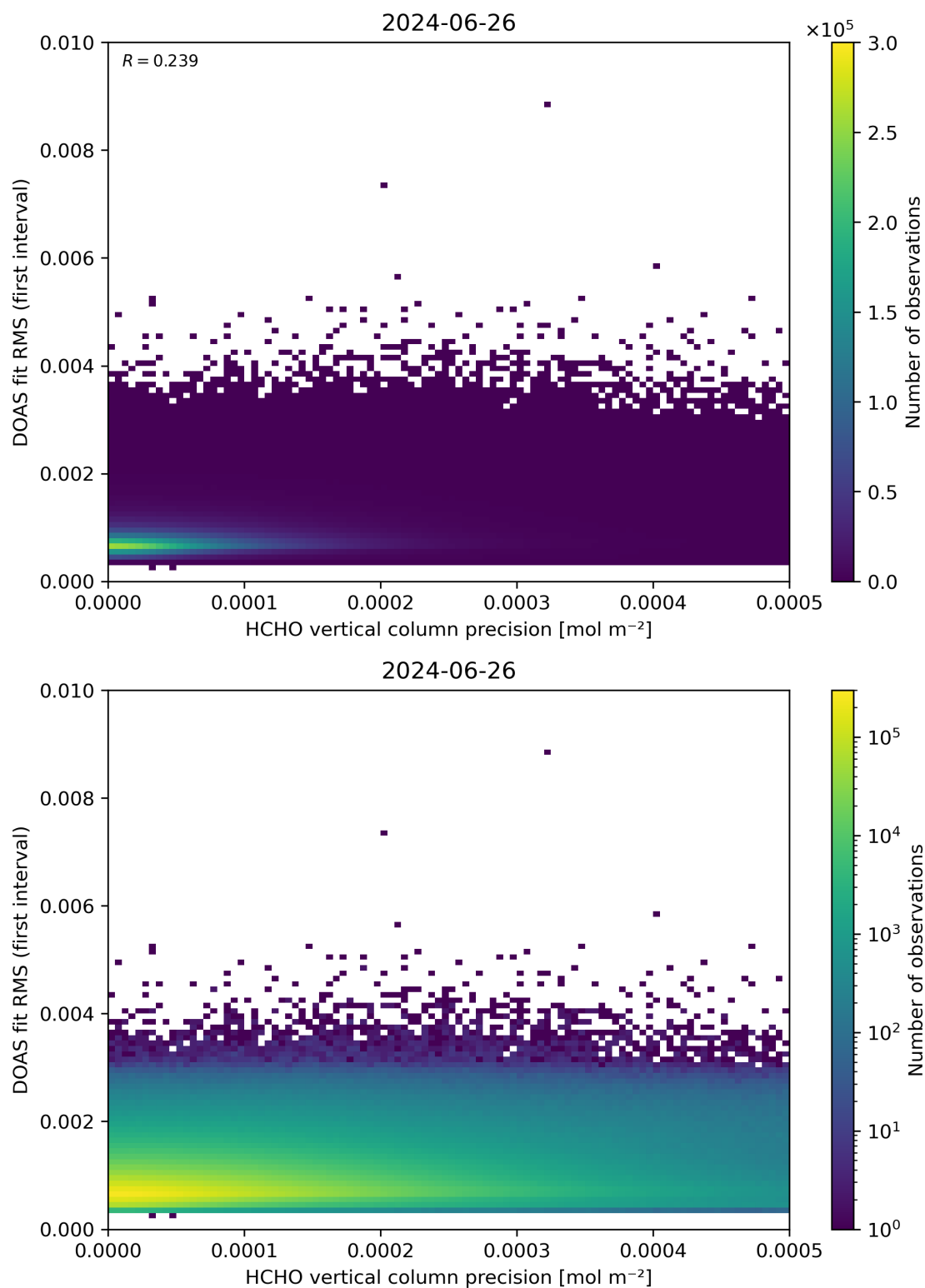
Figure 136: Scatter density plot of “HCHO vertical column precision” against “DOAS fit RMS (first interval)” for 2024-06-25 to 2024-06-27.
