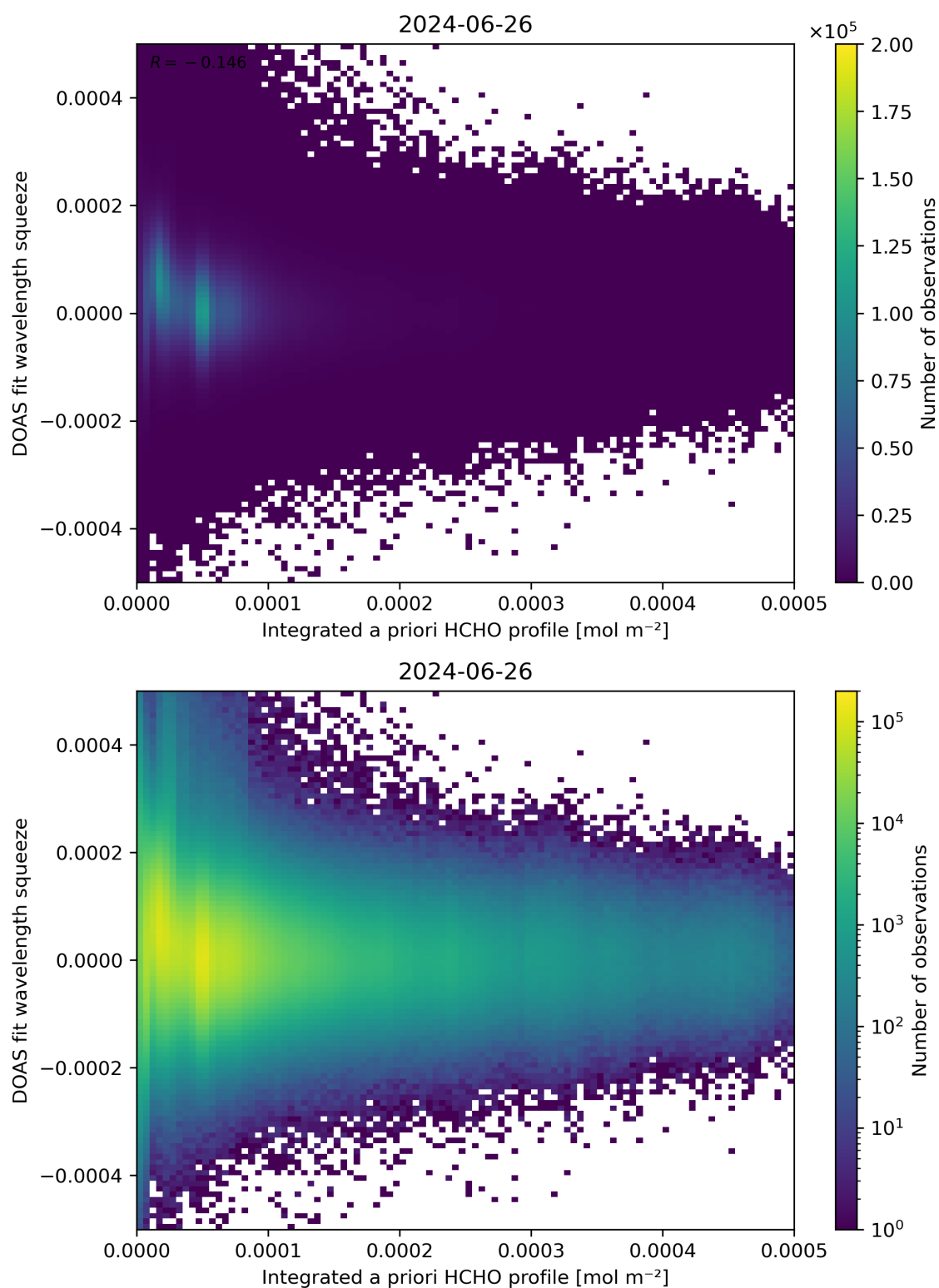
Figure 150: Scatter density plot of “Integrated a priori HCHO profile” against “DOAS fit wavelength squeeze” for 2024-06-25 to 2024-06-27.
