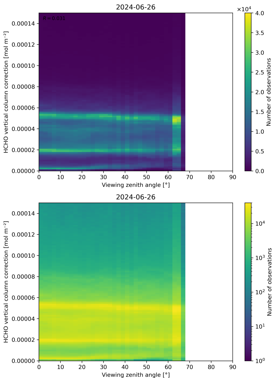
Figure 193: Scatter density plot of “Viewing zenith angle” against “HCHO vertical column correction” for 2024-06-25 to 2024-06-27.
