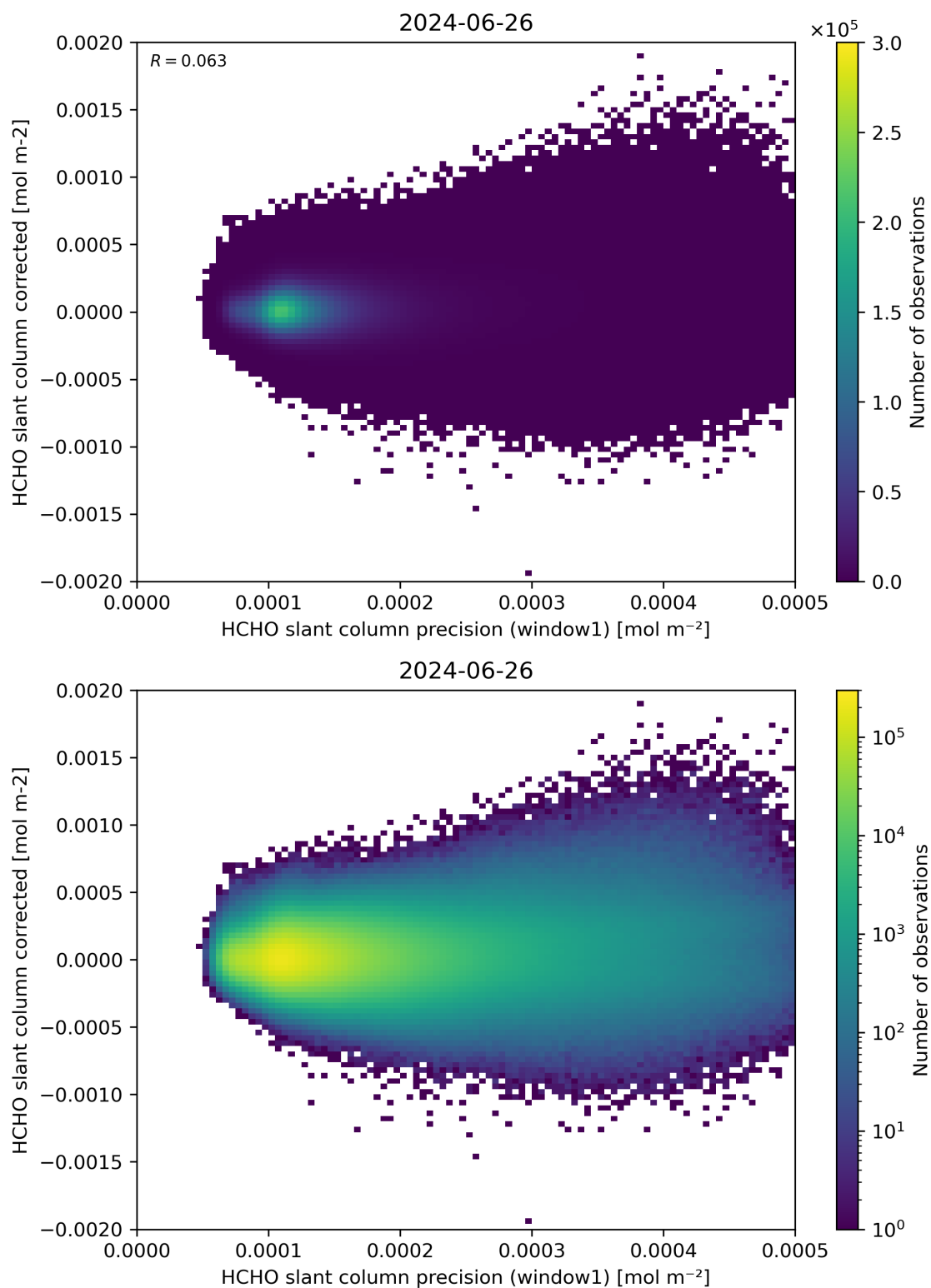
Figure 92: Scatter density plot of “HCHO slant column precision (window1)” against “HCHO slant column corrected” for 2024-06-25 to 2024-06-27.
