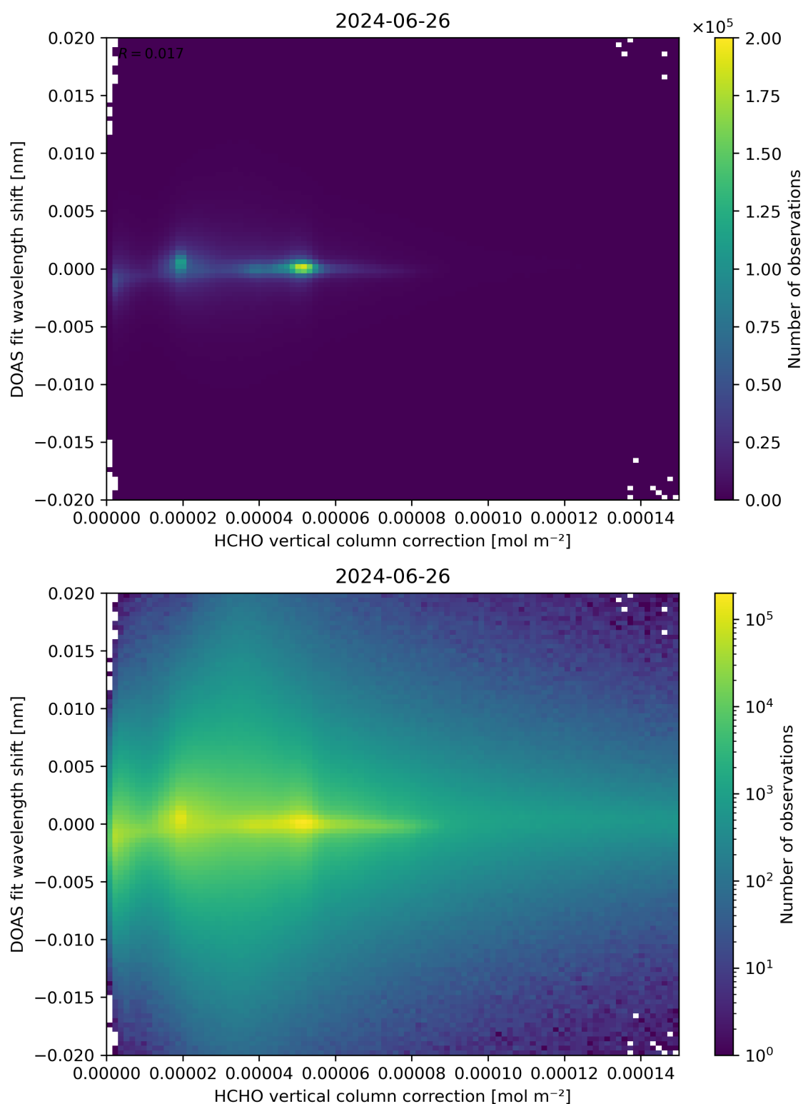
Figure 113: Scatter density plot of “HCHO vertical column correction” against “DOAS fit wavelength shift” for 2024-06-25 to 2024-06-27.
