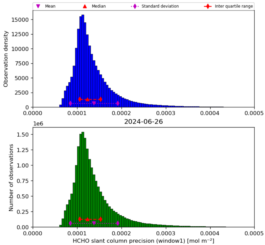
Figure 39: Histogram of “HCHO slant column precision (window1)” for 2024-06-25 to 2024-06-27
