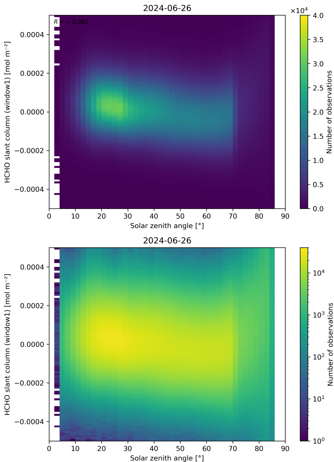
Figure 173: Scatter density plot of “Solar zenith angle” against “HCHO slant column (window1)” for 2024-06-25 to 2024-06-27.
