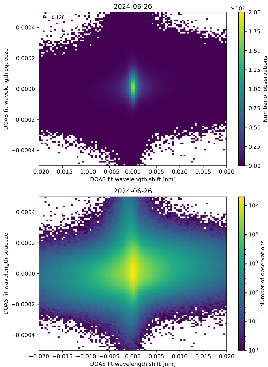
Figure 65: Scatter density plot of “DOAS fit wavelength shift” against “DOAS fit wavelength squeeze” for 2024-06-25 to 2024-06-27.
