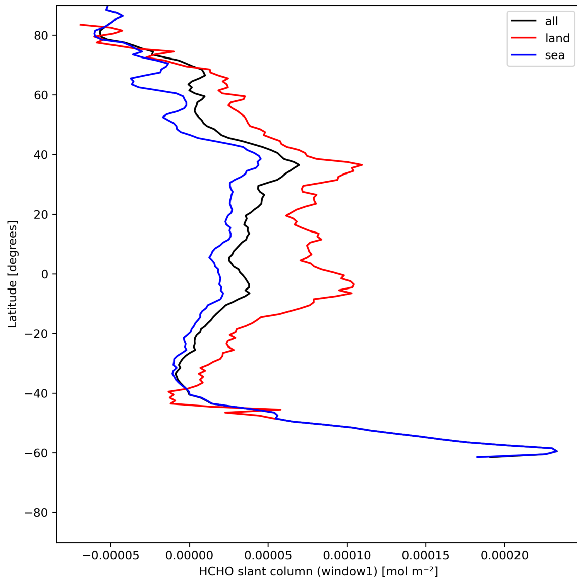
Figure 24: Zonal average of “HCHO slant column (window1)” for 2024-06-25 to 2024-06-27.
