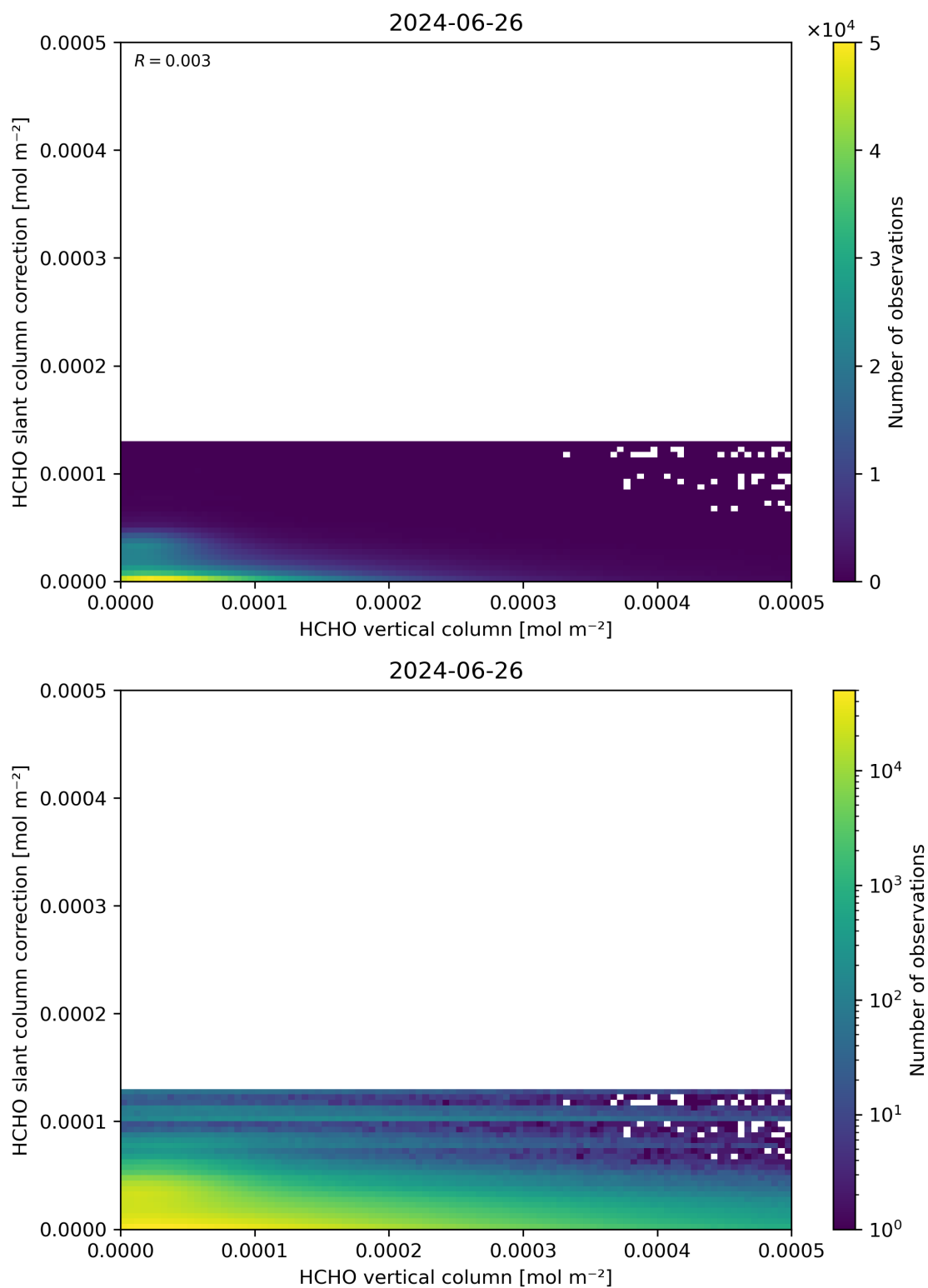
Figure 128: Scatter density plot of “HCHO vertical column” against “HCHO slant column correction” for 2024-06-25 to 2024-06-27.
