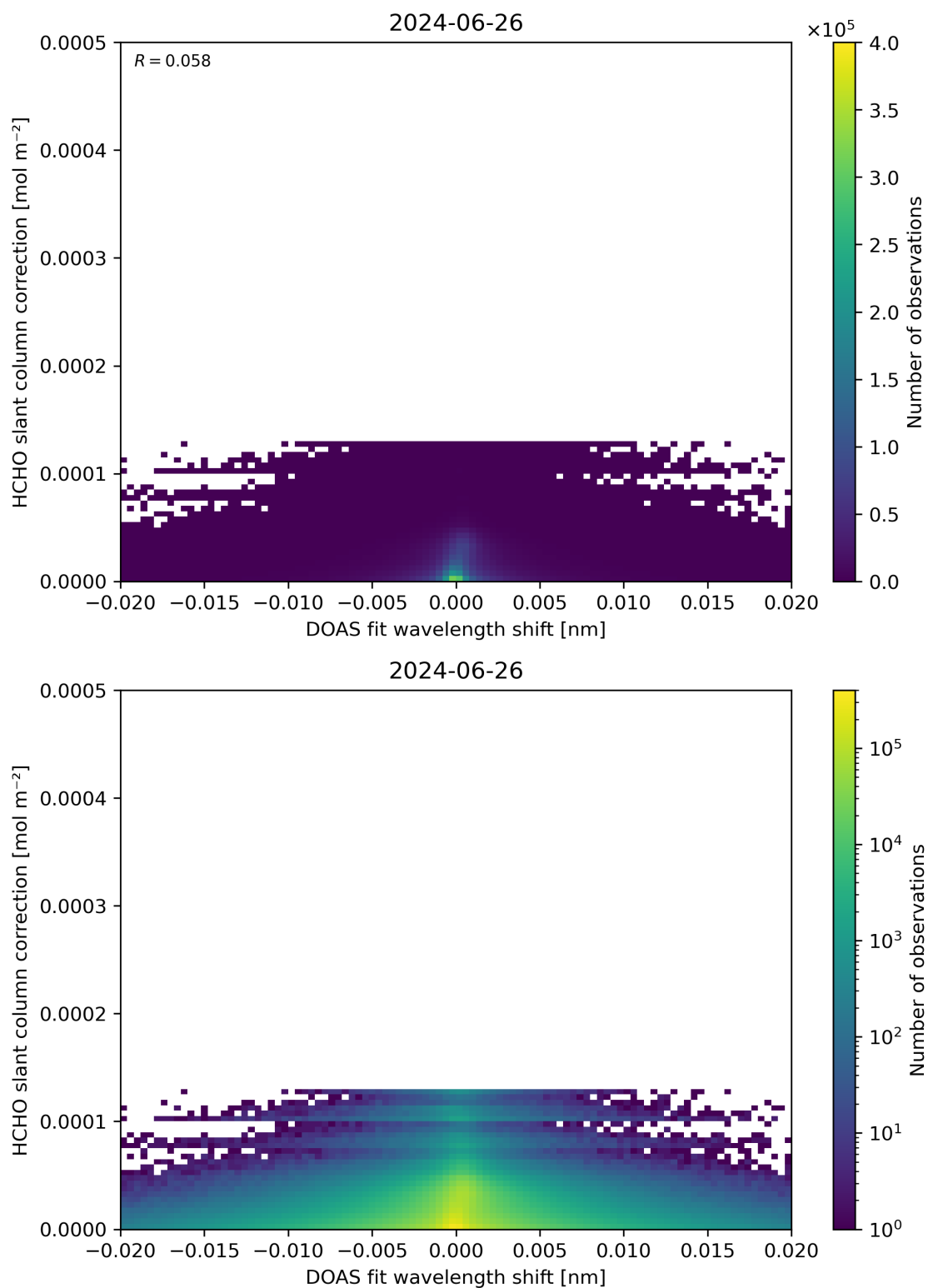
Figure 67: Scatter density plot of “DOAS fit wavelength shift” against “HCHO slant column correction” for 2024-06-25 to 2024-06-27.
