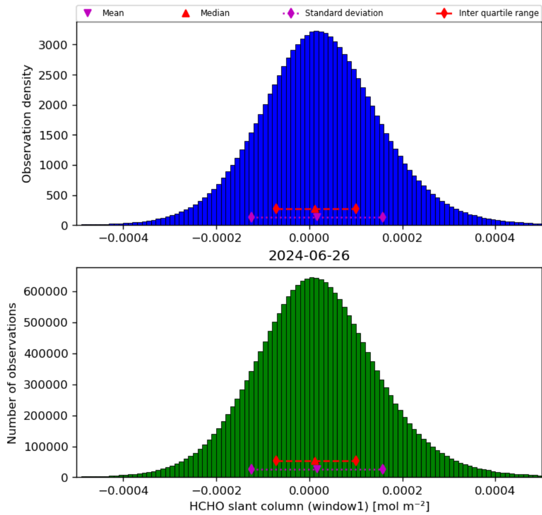
Figure 38: Histogram of “HCHO slant column (window1)” for 2024-06-25 to 2024-06-27
