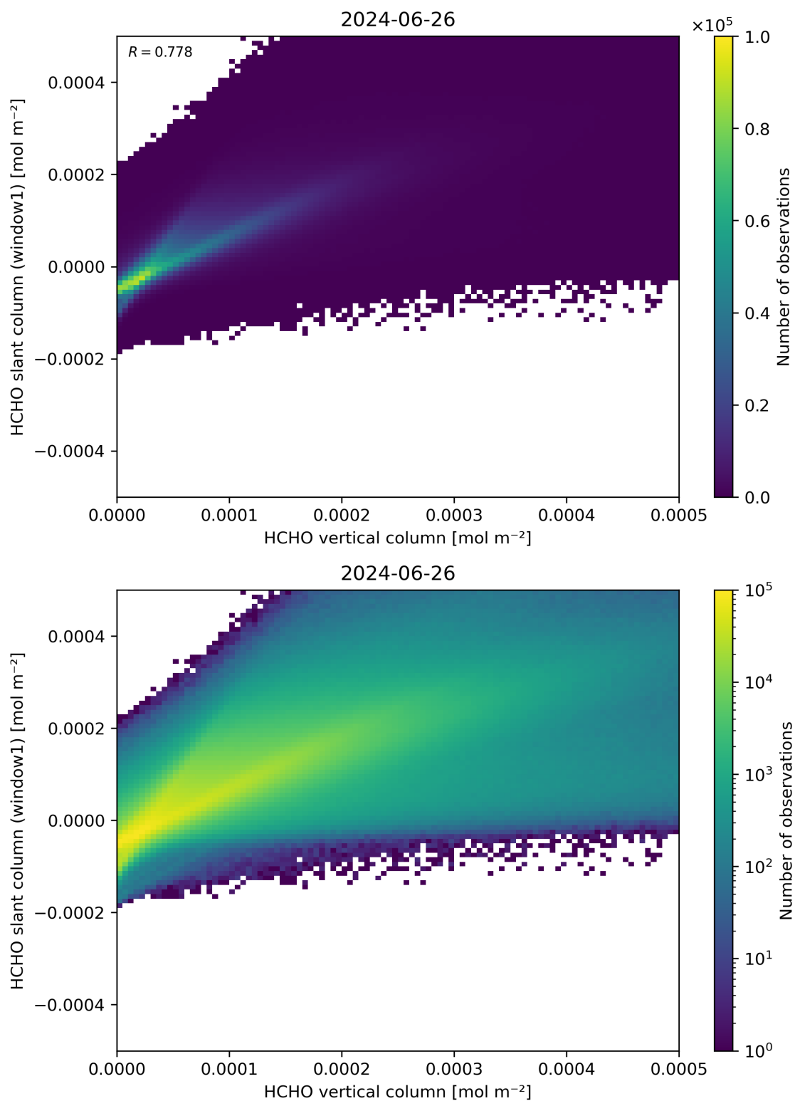
Figure 129: Scatter density plot of “HCHO vertical column” against “HCHO slant column (window1)” for 2024-06-25 to 2024-06-27.
