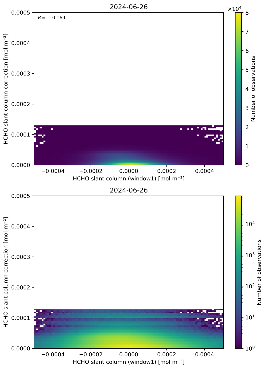
Figure 83: Scatter density plot of “HCHO slant column (window1)” against “HCHO slant column correction” for 2024-06-25 to 2024-06-27.
