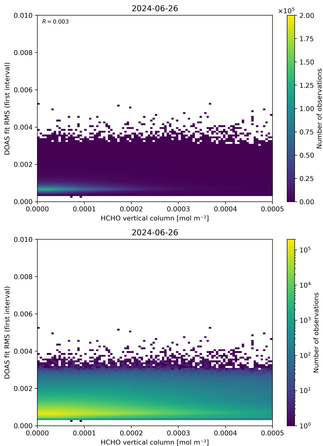
Figure 123: Scatter density plot of “HCHO vertical column” against “DOAS fit RMS (first interval)” for 2024-06-25 to 2024-06-27.
