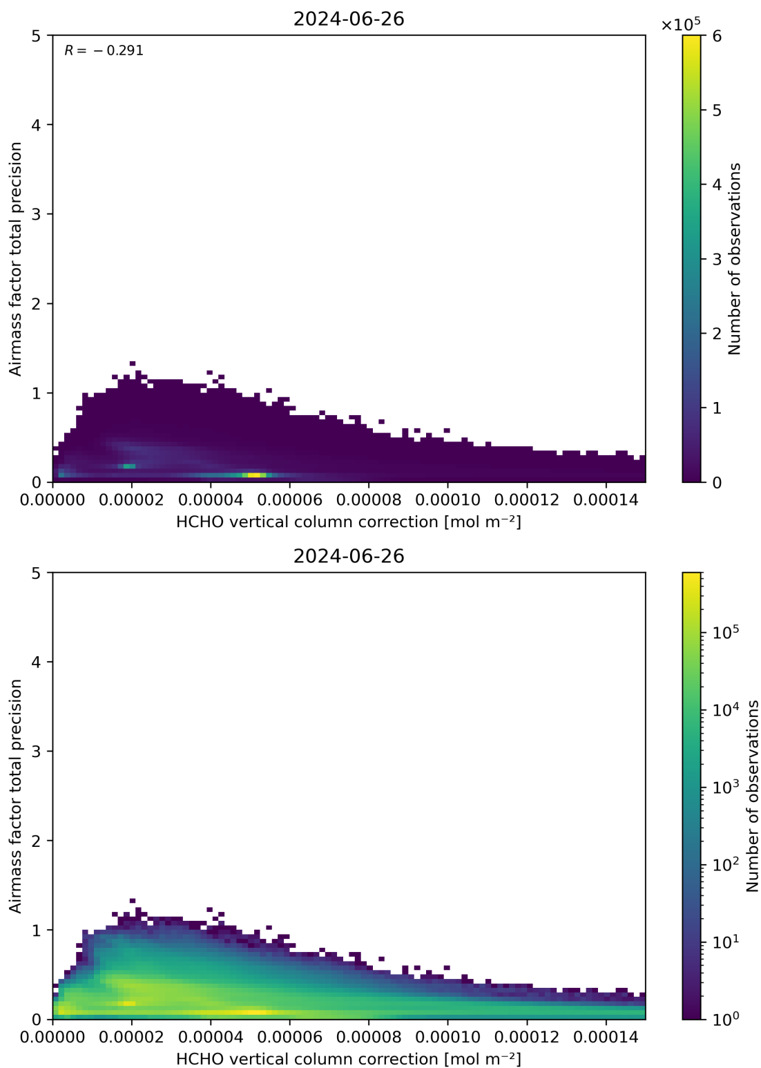
Figure 121: Scatter density plot of “HCHO vertical column correction” against “Airmass factor total precision” for 2024-06-25 to 2024-06-27.
