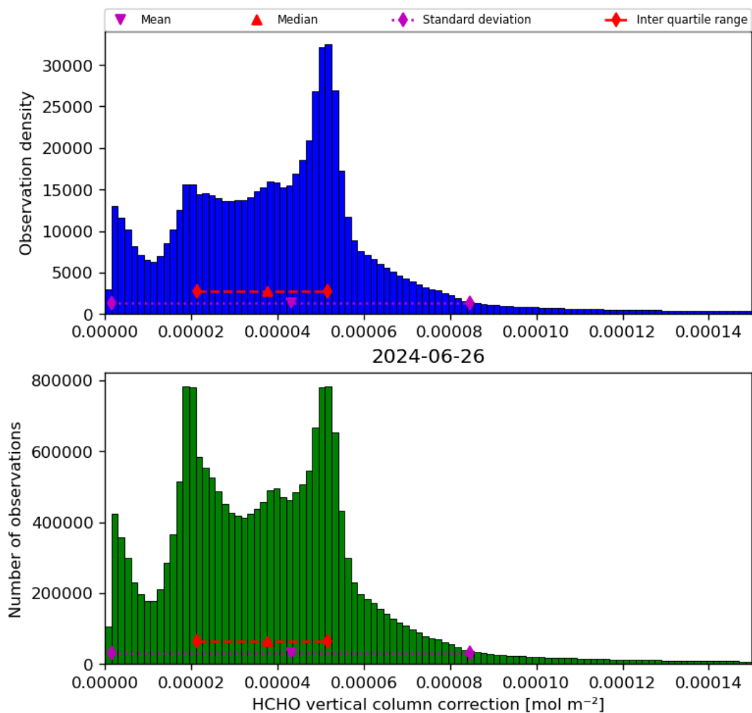
Figure 37: Histogram of “HCHO vertical column correction” for 2024-06-25 to 2024-06-27
