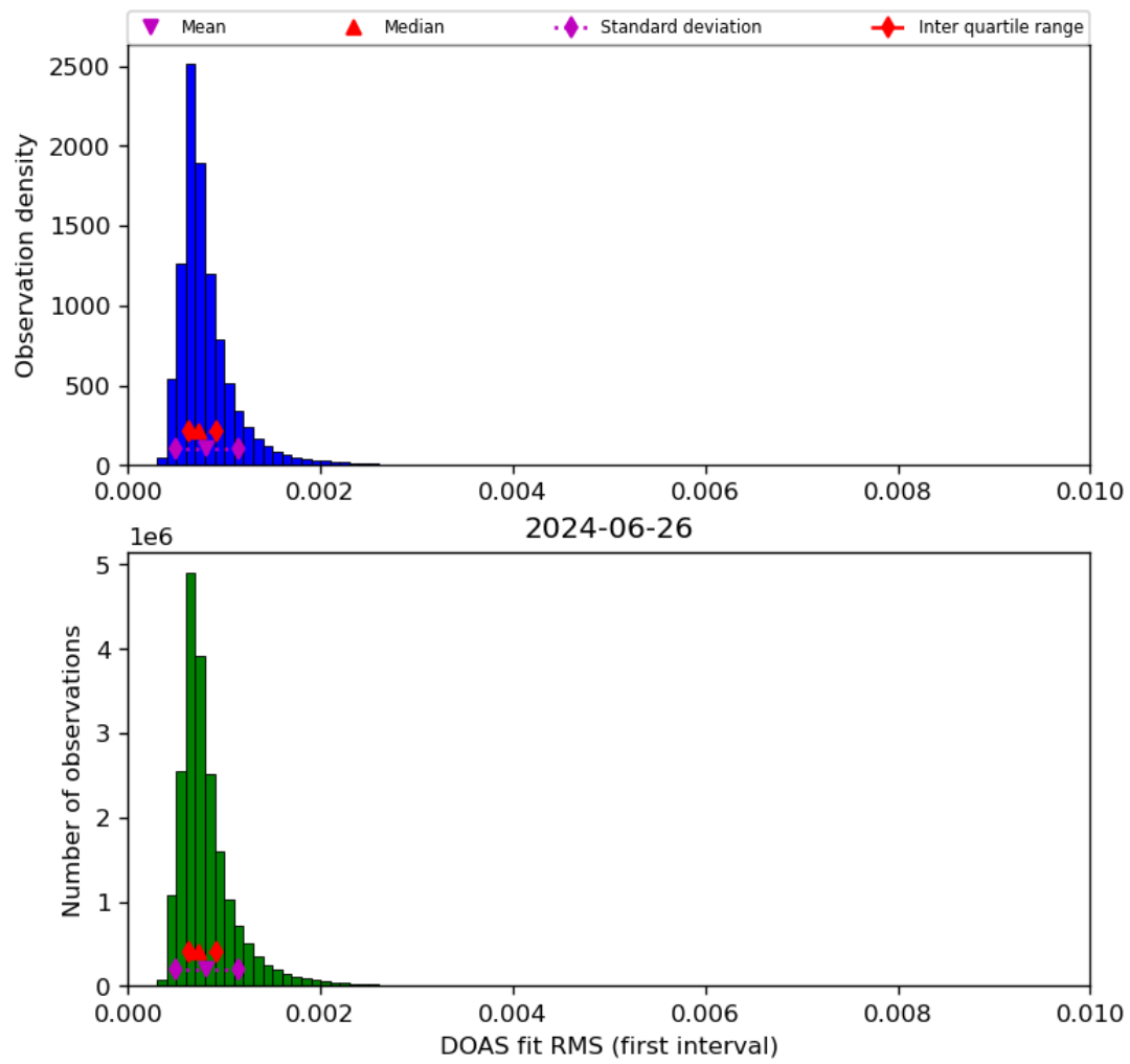
Figure 46: Histogram of “DOAS fit RMS (first interval)” for 2024-06-25 to 2024-06-27
