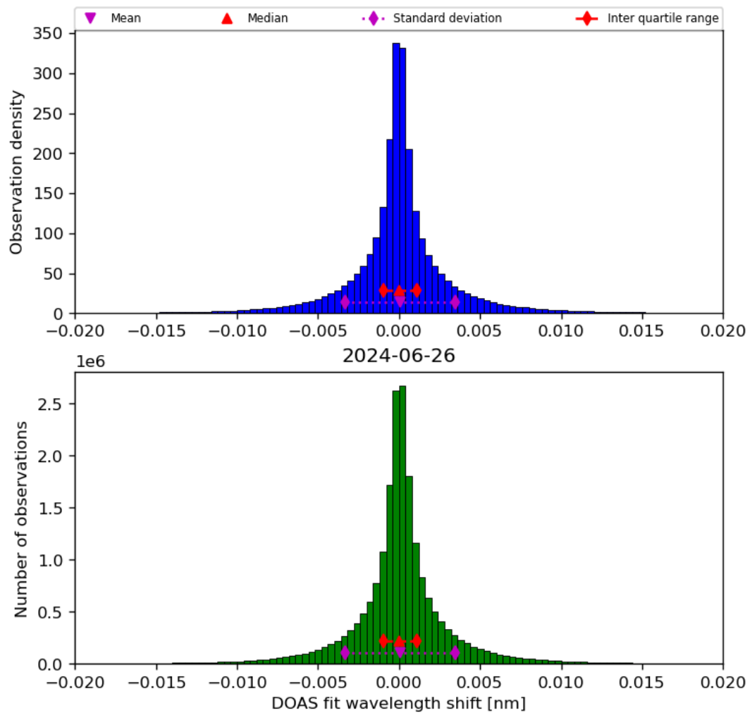
Figure 44: Histogram of “DOAS fit wavelength shift” for 2024-06-25 to 2024-06-27
