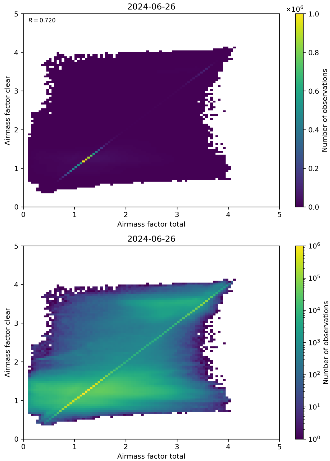
Figure 100: Scatter density plot of “Airmass factor total” against “Airmass factor clear” for 2024-06-25 to 2024-06-27.
