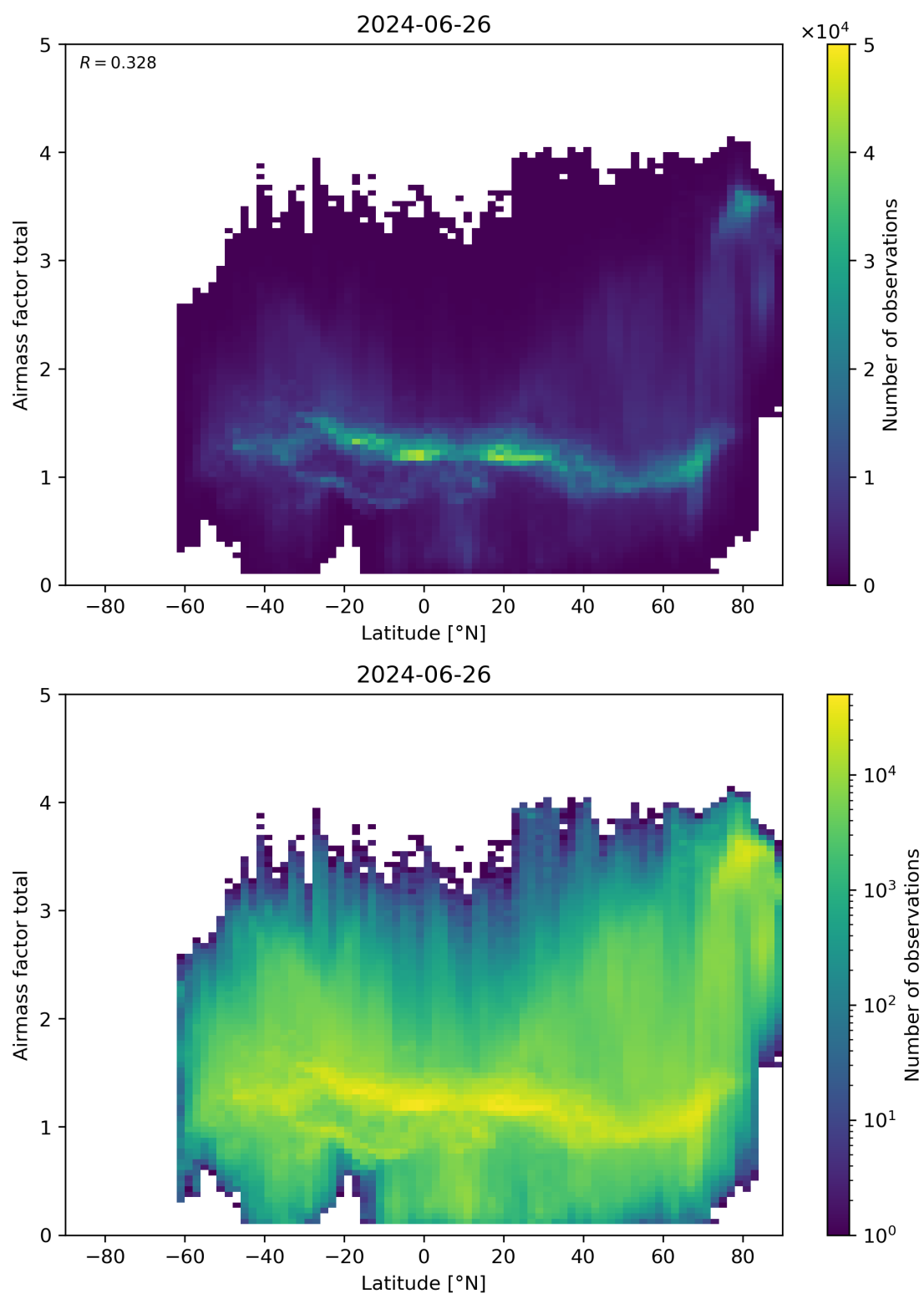
Figure 161: Scatter density plot of “Latitude” against “Airmass factor total” for 2024-06-25 to 2024-06-27.
