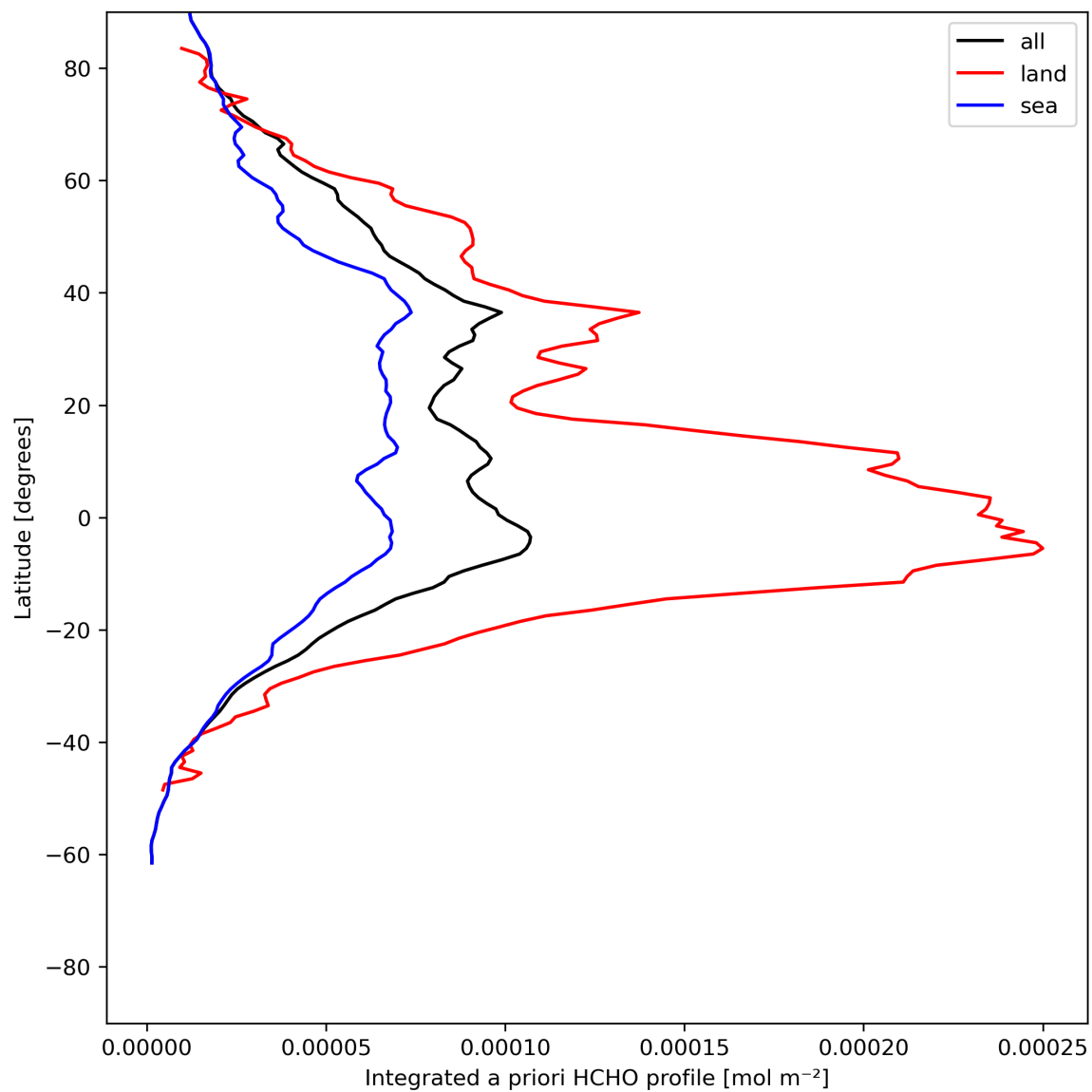
Figure 29: Zonal average of “Integrated a priori HCHO profile” for 2024-06-25 to 2024-06-27.
