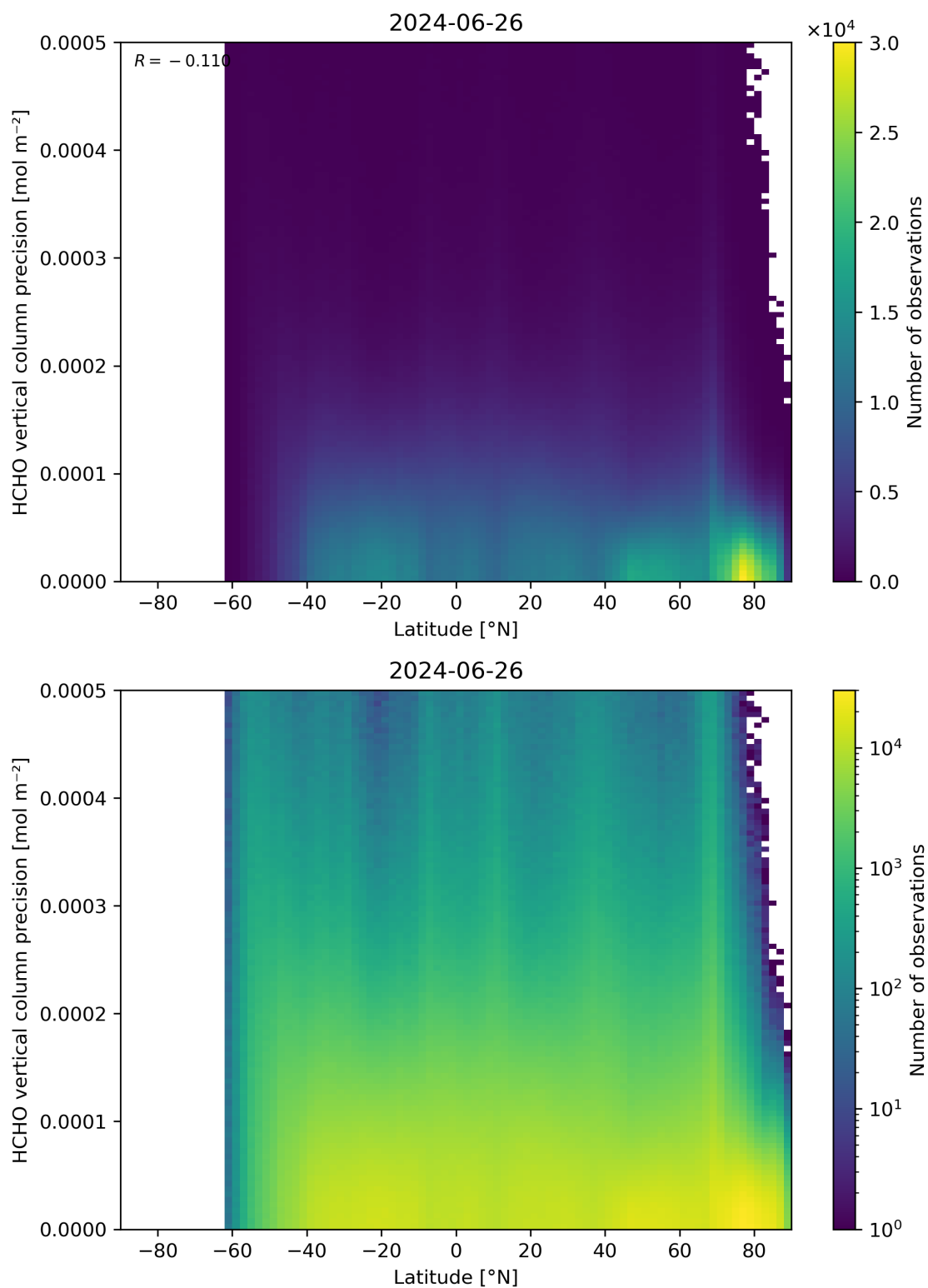
Figure 165: Scatter density plot of “Latitude” against “HCHO vertical column precision” for 2024-06-25 to 2024-06-27.
