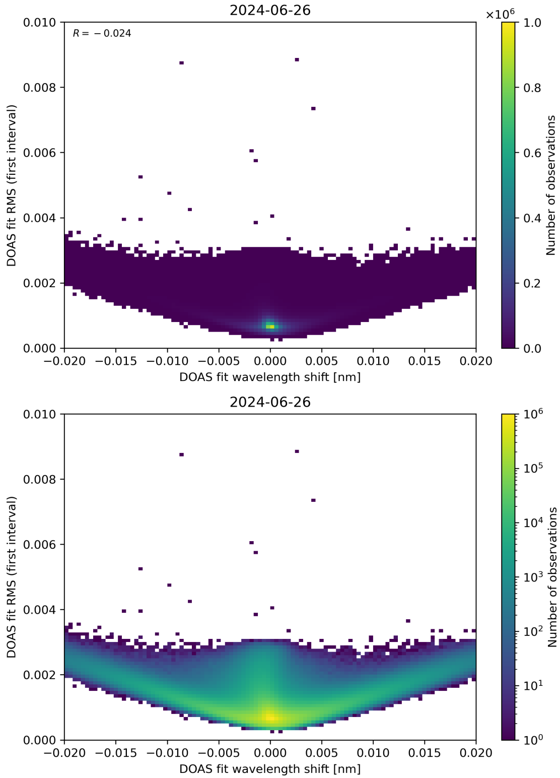
Figure 64: Scatter density plot of “DOAS fit wavelength shift” against “DOAS fit RMS (first interval)” for 2024-06-25 to 2024-06-27.
