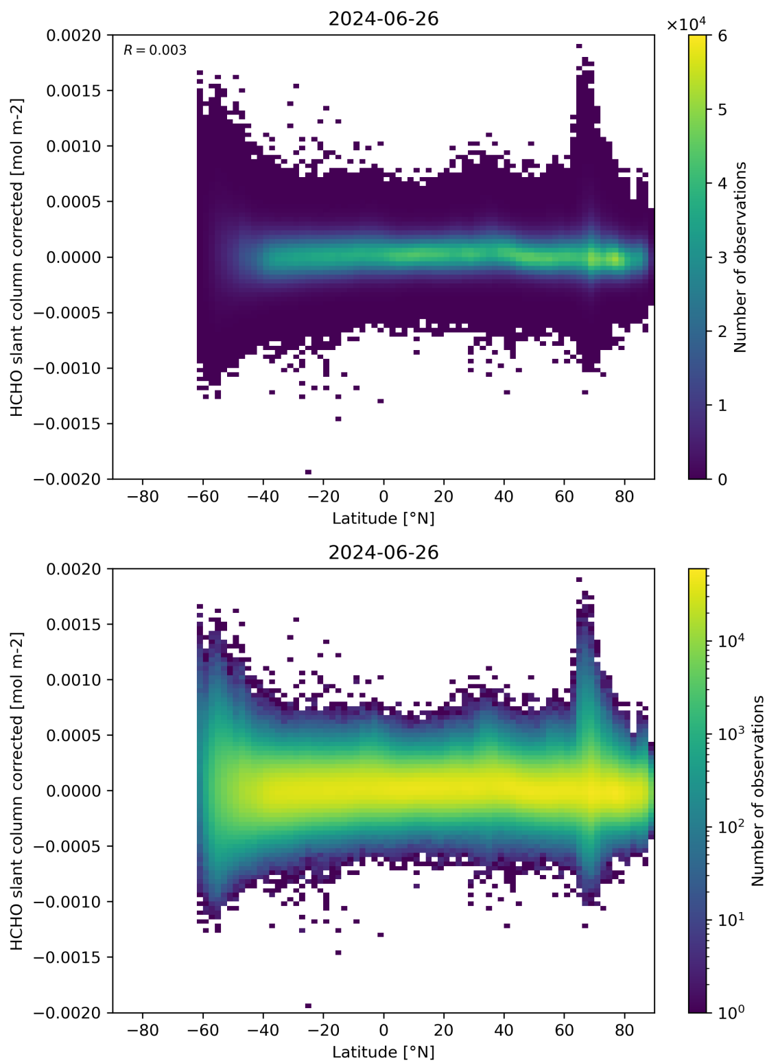
Figure 157: Scatter density plot of “Latitude” against “HCHO slant column corrected” for 2024-06-25 to 2024-06-27.
