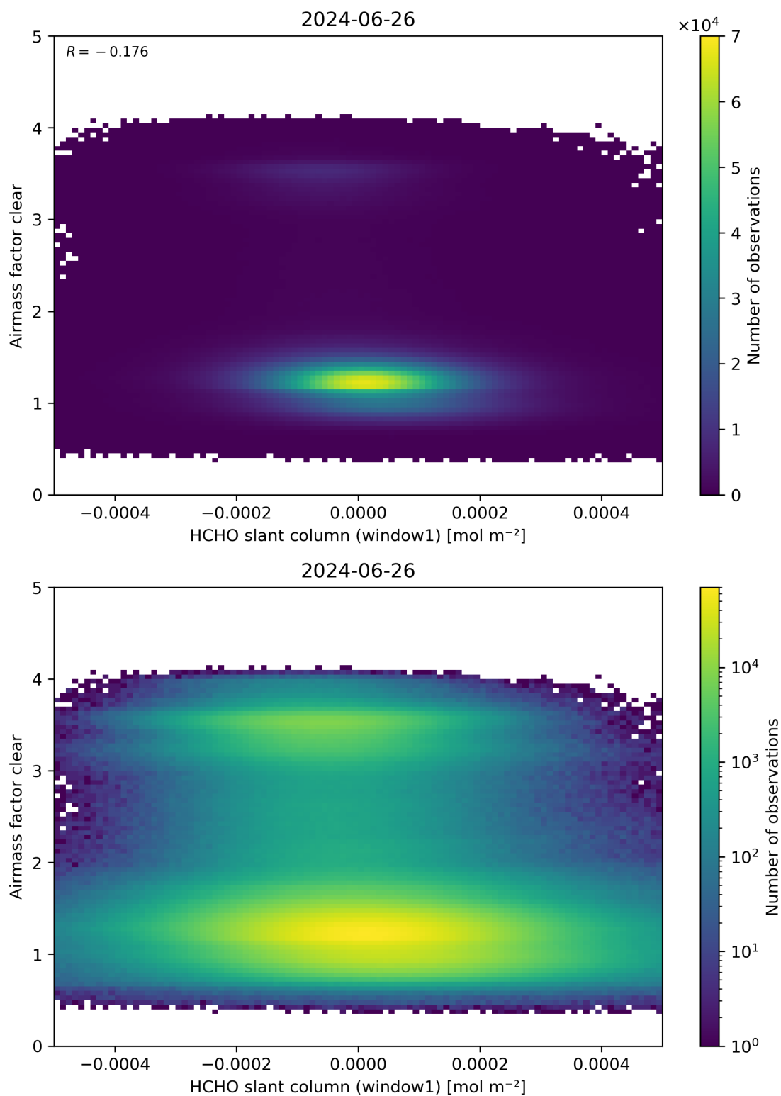
Figure 81: Scatter density plot of “HCHO slant column (window1)” against “Airmass factor clear” for 2024-06-25 to 2024-06-27.
