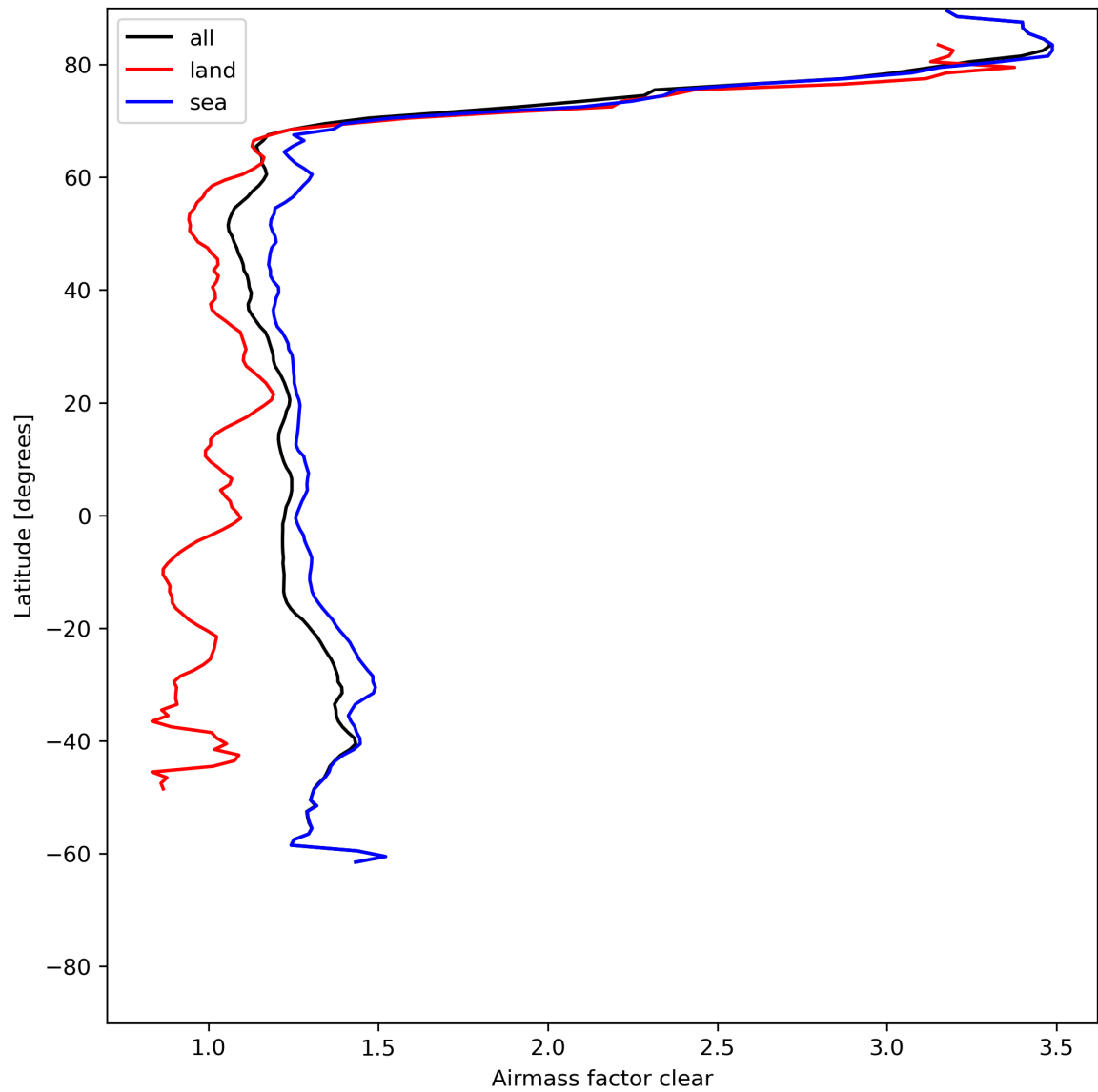
Figure 28: Zonal average of “Airmass factor clear” for 2024-06-25 to 2024-06-27.
