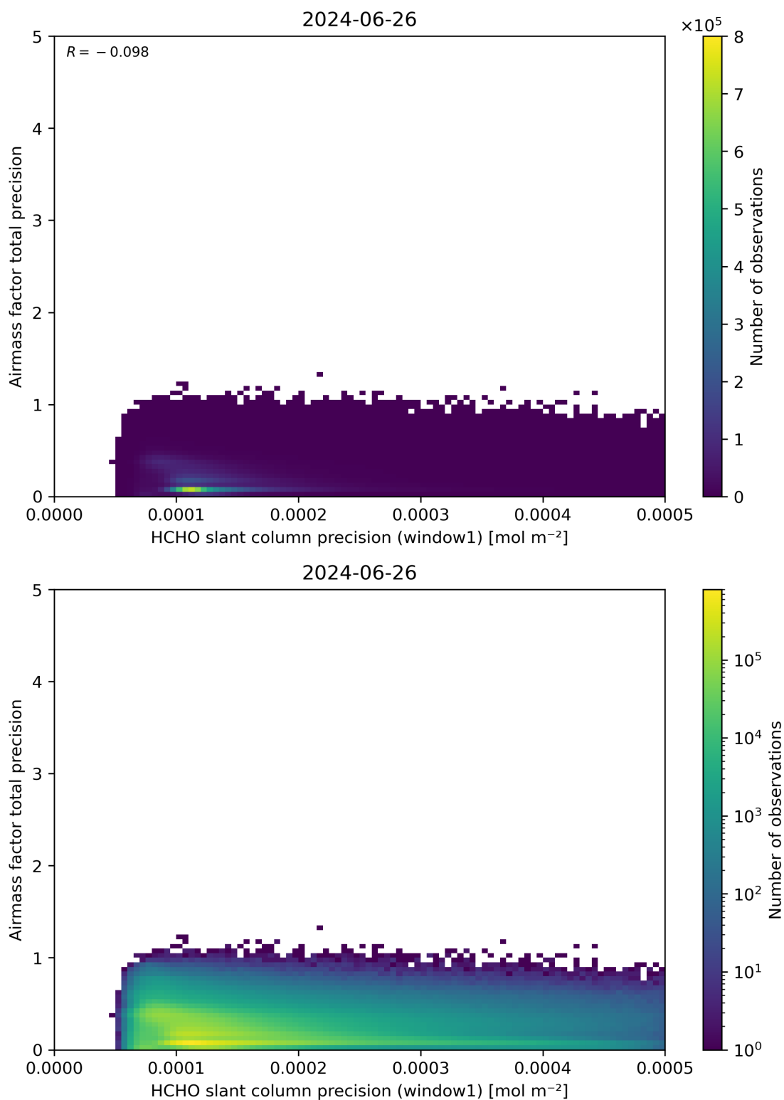
Figure 95: Scatter density plot of “HCHO slant column precision (window1)” against “Airmass factor total precision” for 2024-06-25 to 2024-06-27.
