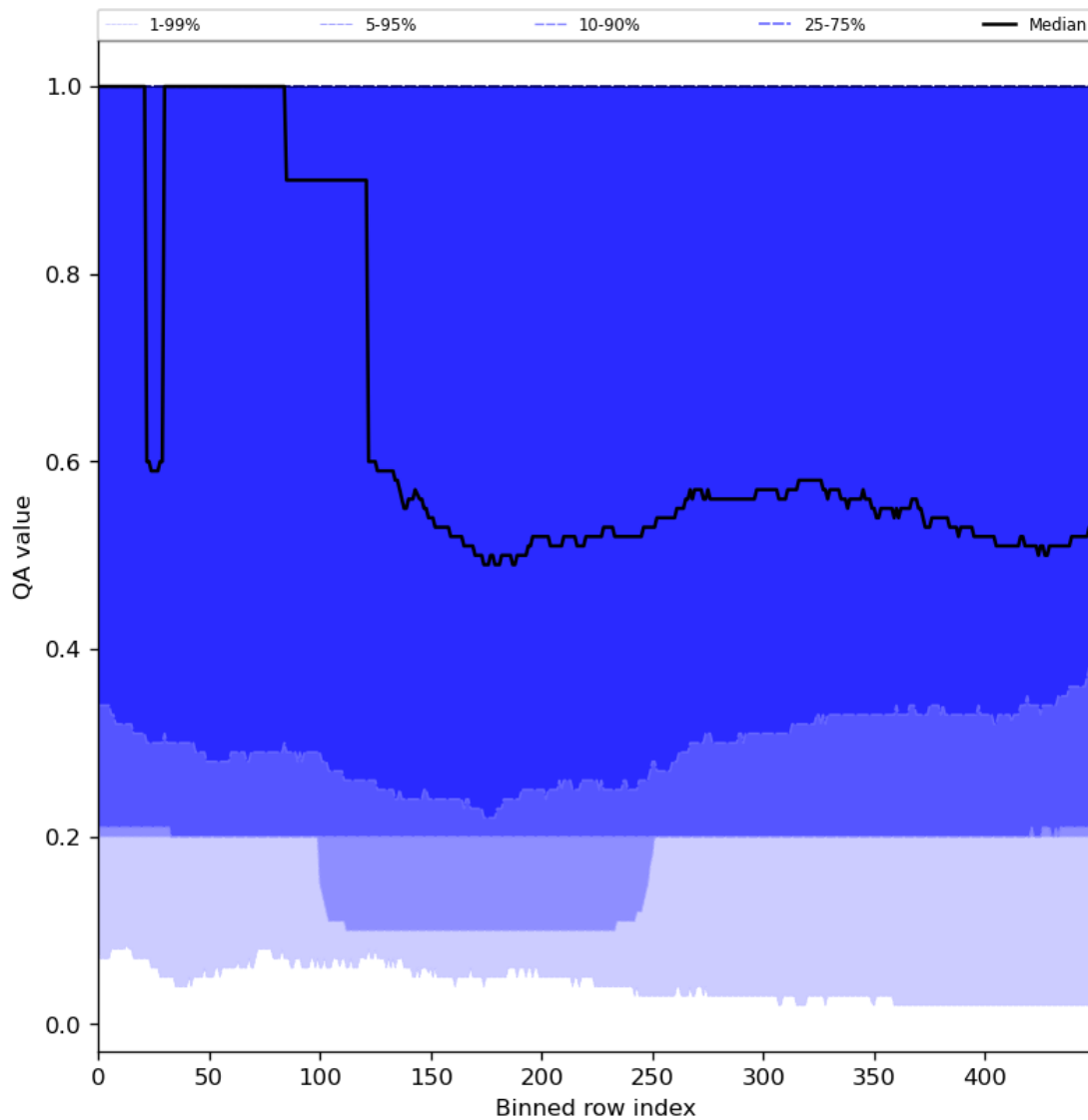
Figure 48: Along track statistics of “QA value” for 2024-06-25 to 2024-06-27
