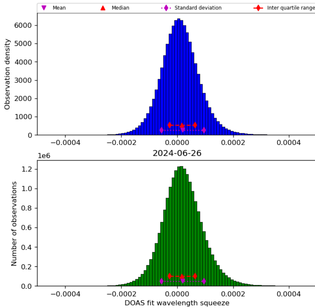
Figure 45: Histogram of “DOAS fit wavelength squeeze” for 2024-06-25 to 2024-06-27
