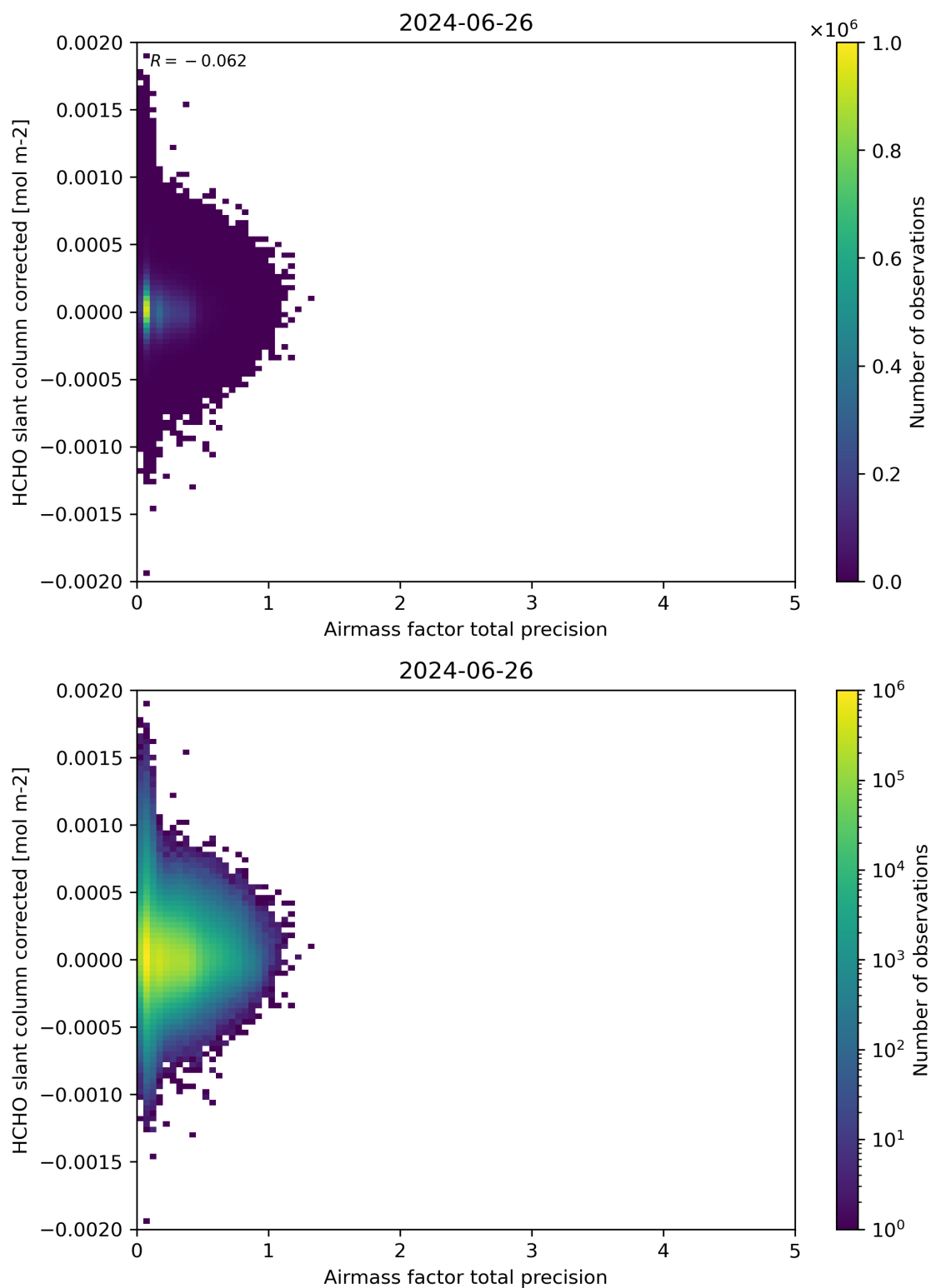
Figure 109: Scatter density plot of “Airmass factor total precision” against “HCHO slant column corrected” for 2024-06-25 to 2024-06-27.
