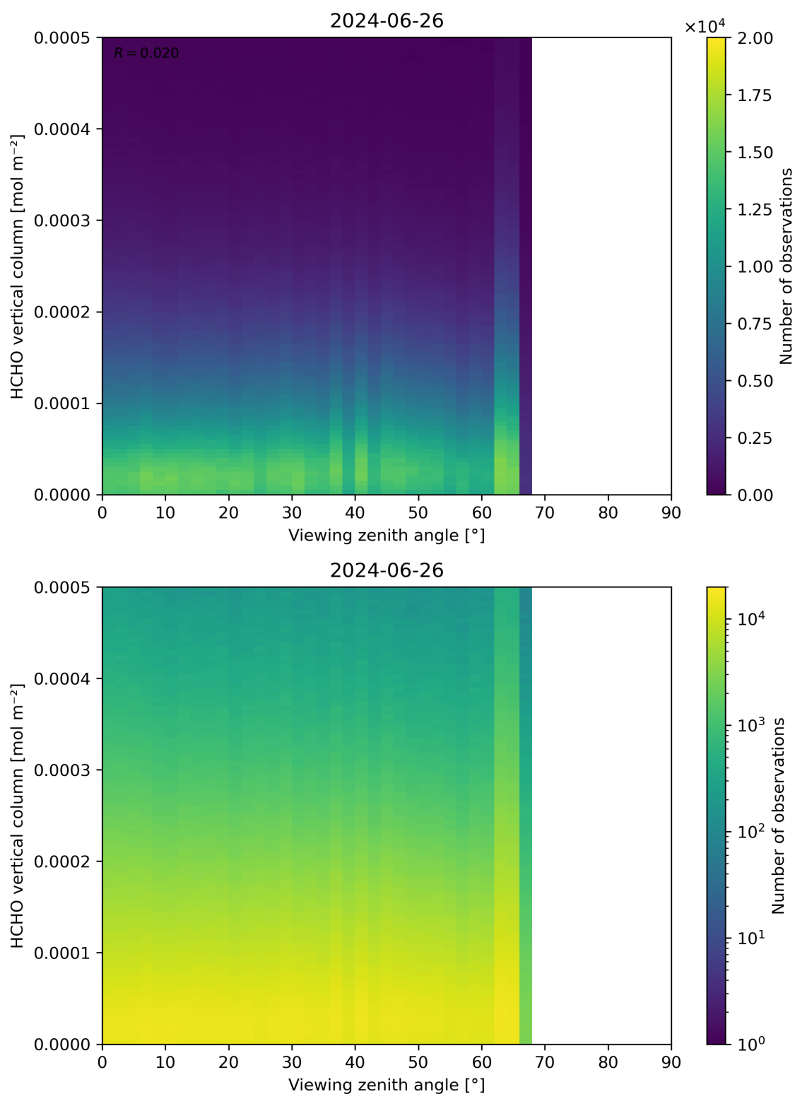
Figure 192: Scatter density plot of “Viewing zenith angle” against “HCHO vertical column” for 2024-06-25 to 2024-06-27.
