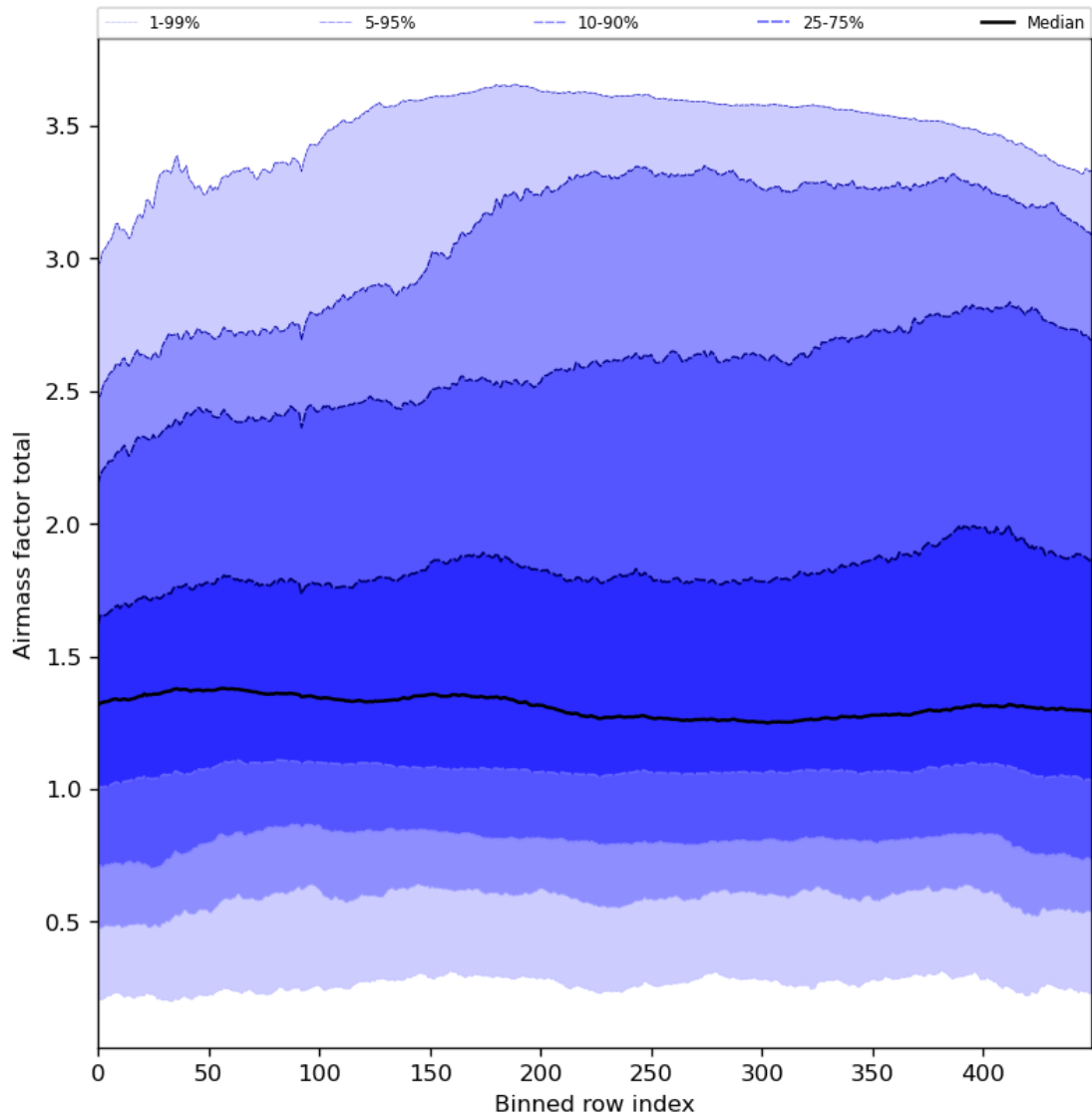
Figure 54: Along track statistics of “Airmass factor total” for 2024-06-25 to 2024-06-27
