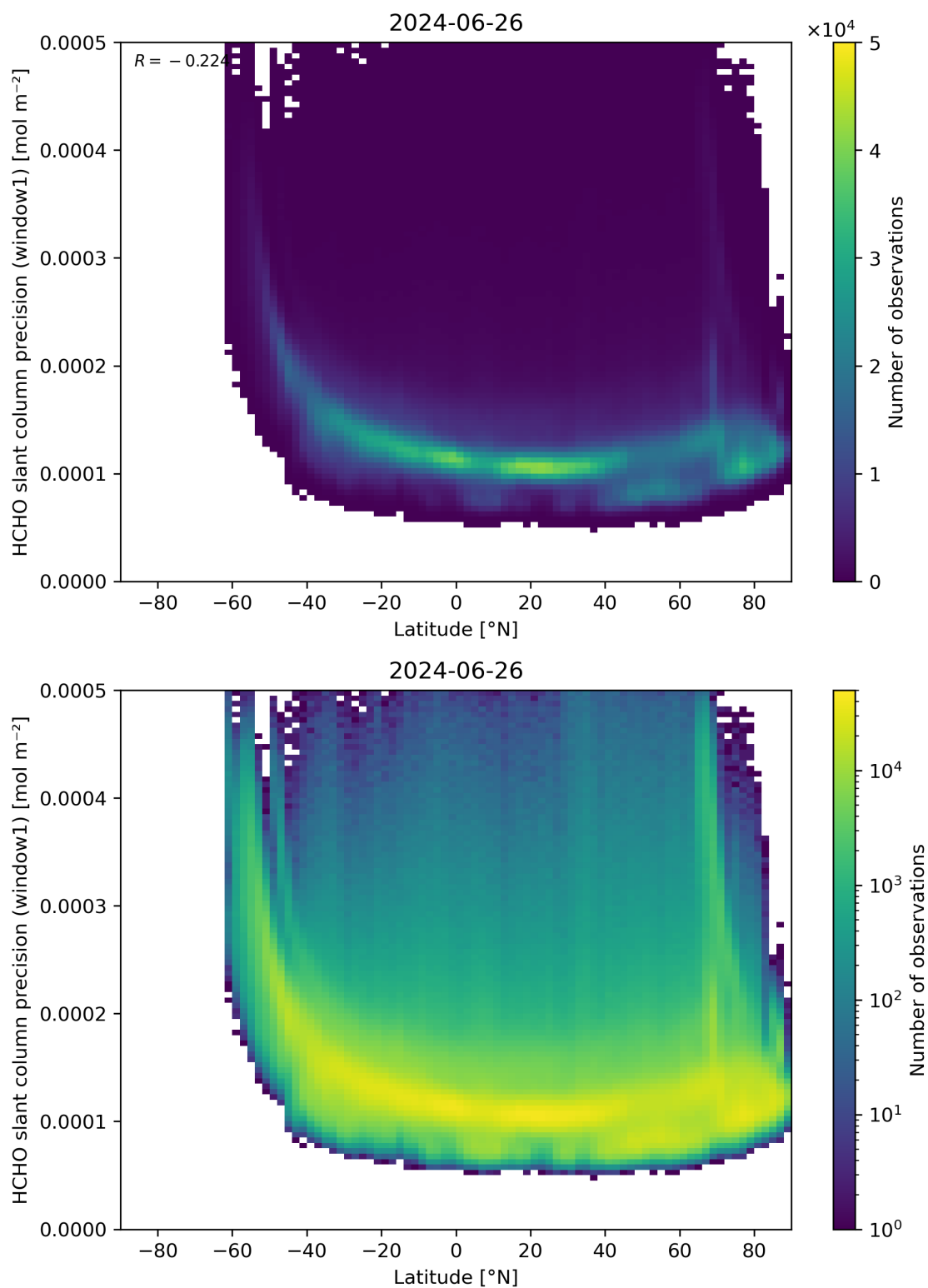
Figure 160: Scatter density plot of “Latitude” against “HCHO slant column precision (window1)” for 2024-06-25 to 2024-06-27.
