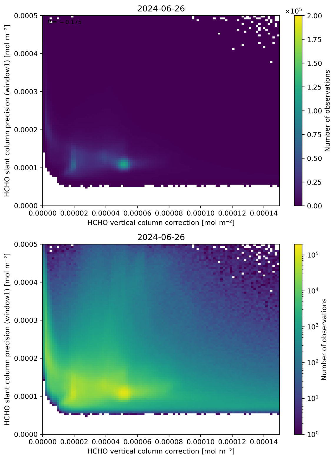
Figure 119: Scatter density plot of “HCHO vertical column correction” against “HCHO slant column precision (window1)” for 2024-06-25 to 2024-06-27.
