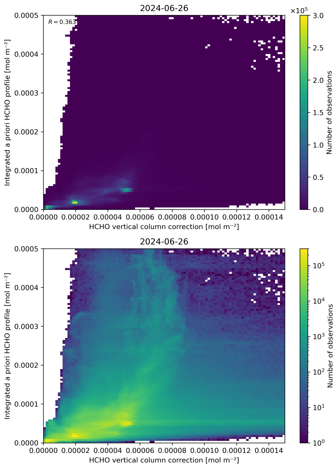
Figure 122: Scatter density plot of “HCHO vertical column correction” against “Integrated a priori HCHO profile” for 2024-06-25 to 2024-06-27.
