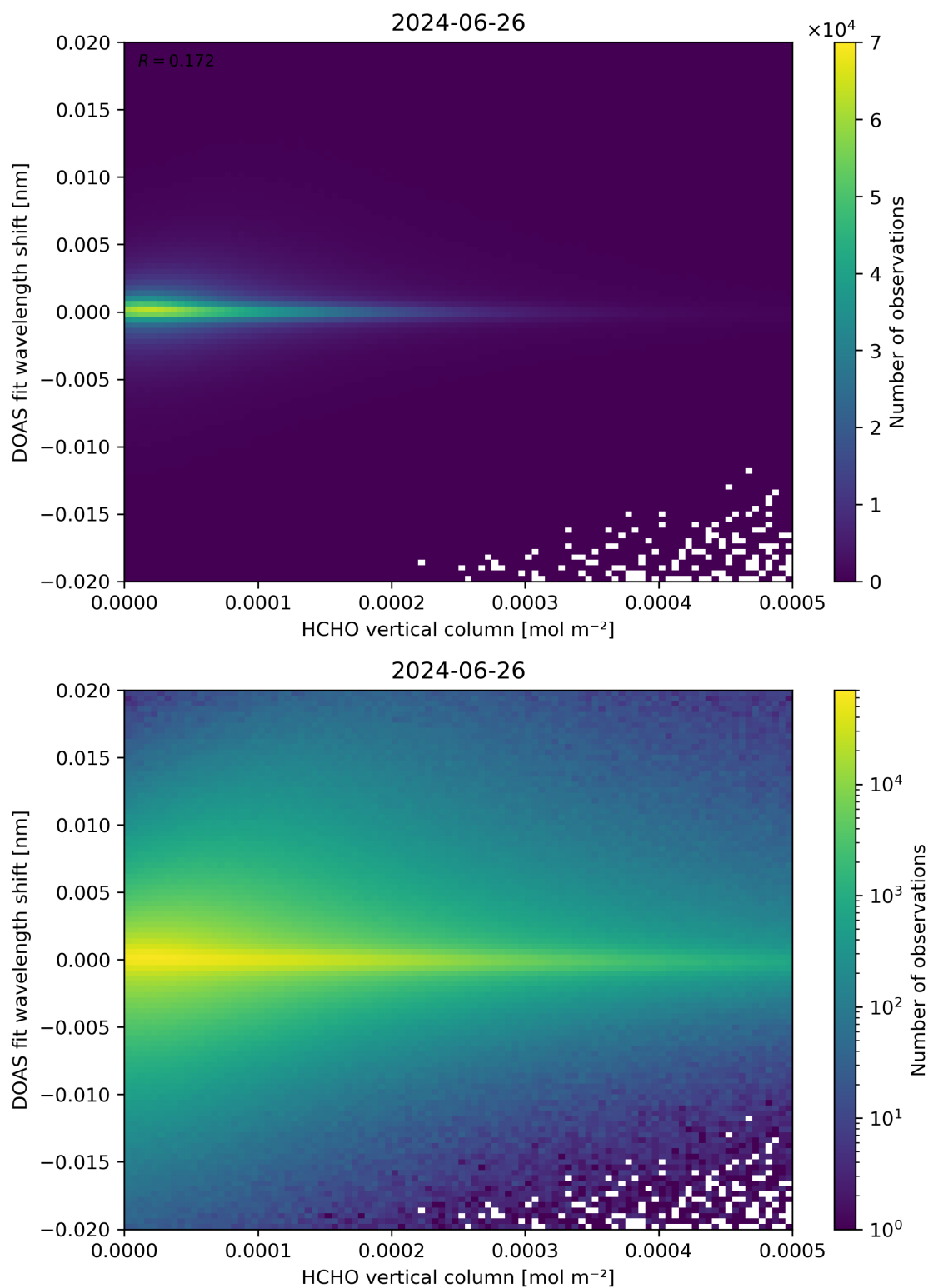
Figure 124: Scatter density plot of “HCHO vertical column” against “DOAS fit wavelength shift” for 2024-06-25 to 2024-06-27.
