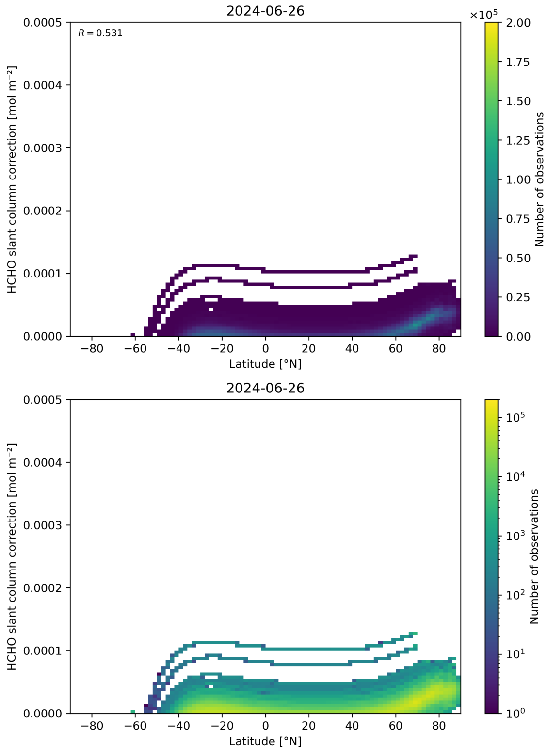
Figure 158: Scatter density plot of “Latitude” against “HCHO slant column correction” for 2024-06-25 to 2024-06-27.
