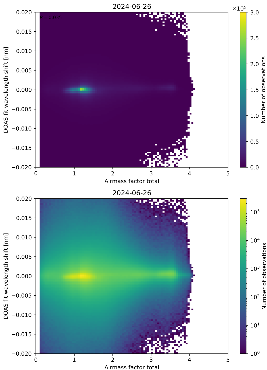
Figure 98: Scatter density plot of “Airmass factor total” against “DOAS fit wavelength shift” for 2024-06-25 to 2024-06-27.
