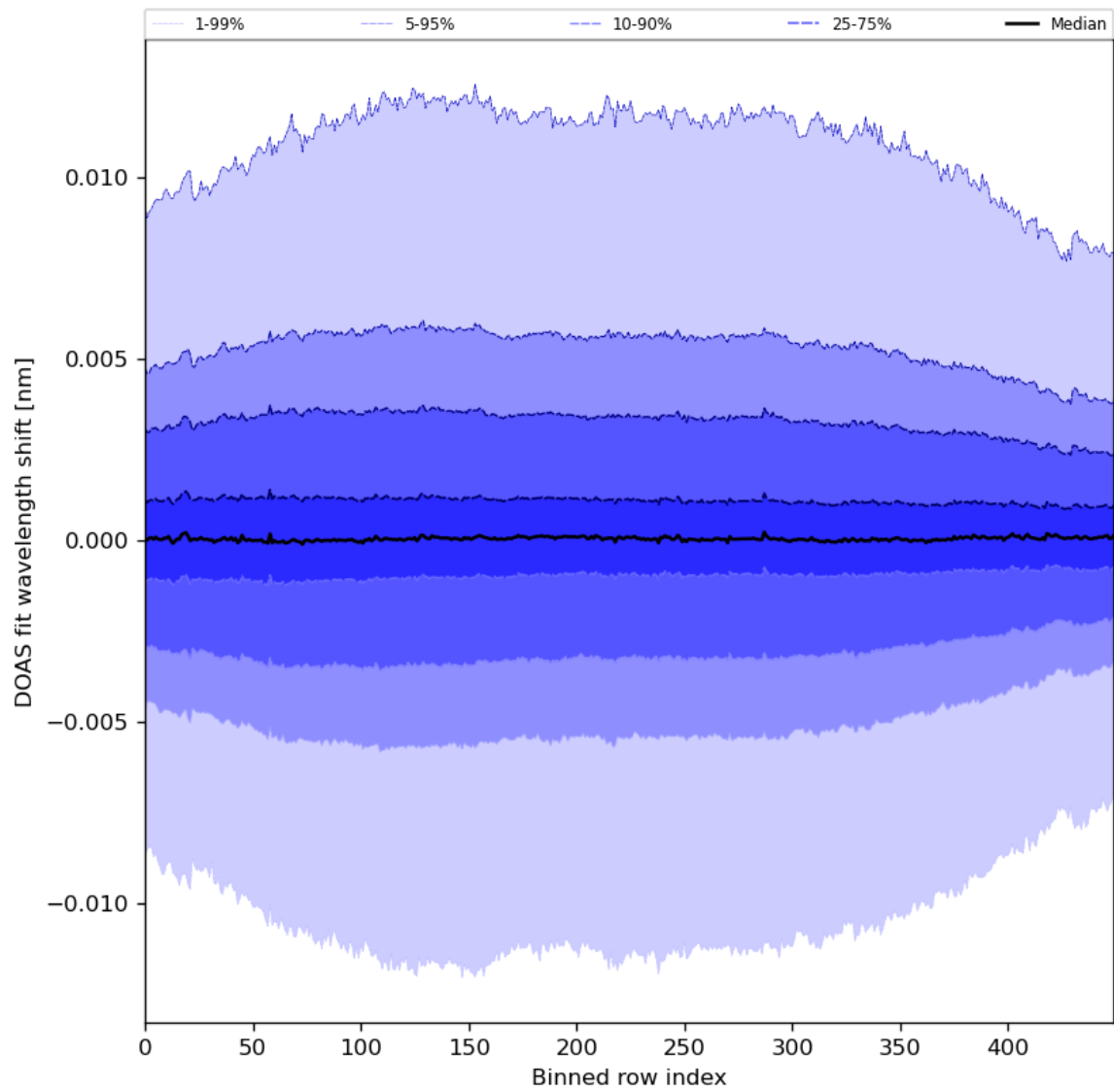
Figure 58: Along track statistics of “DOAS fit wavelength shift” for 2024-06-25 to 2024-06-27
