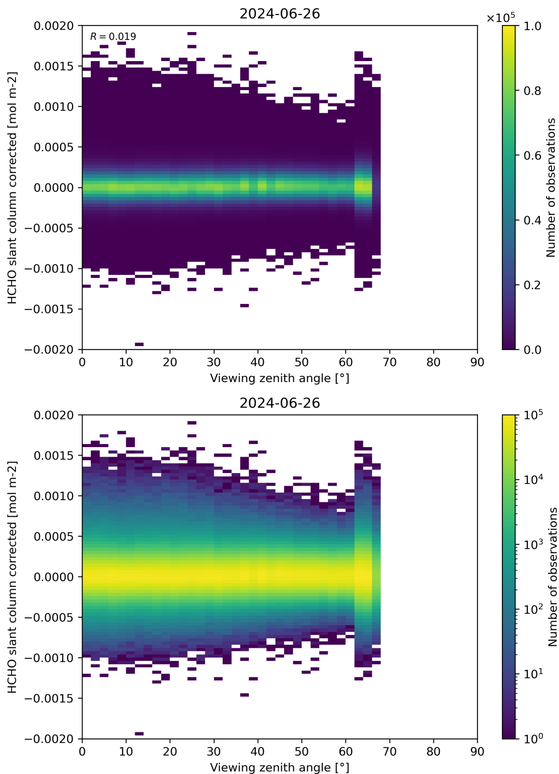
Figure 186: Scatter density plot of “Viewing zenith angle” against “HCHO slant column corrected” for 2024-06-25 to 2024-06-27.
