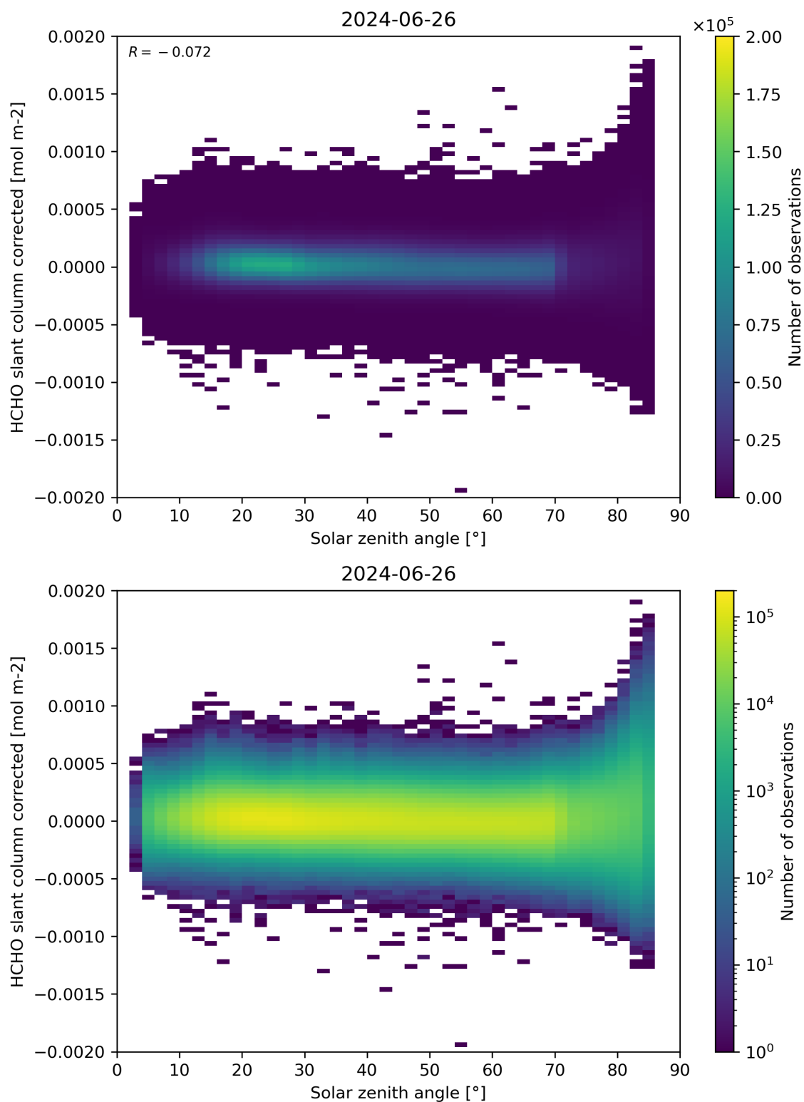
Figure 171: Scatter density plot of “Solar zenith angle” against “HCHO slant column corrected” for 2024-06-25 to 2024-06-27.
