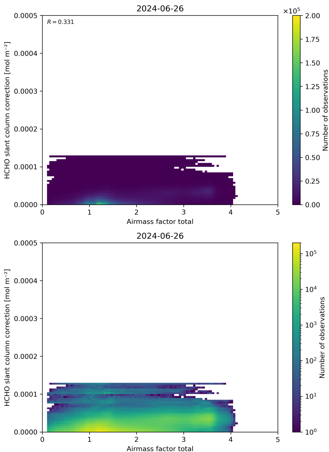
Figure 102: Scatter density plot of “Airmass factor total” against “HCHO slant column correction” for 2024-06-25 to 2024-06-27.
