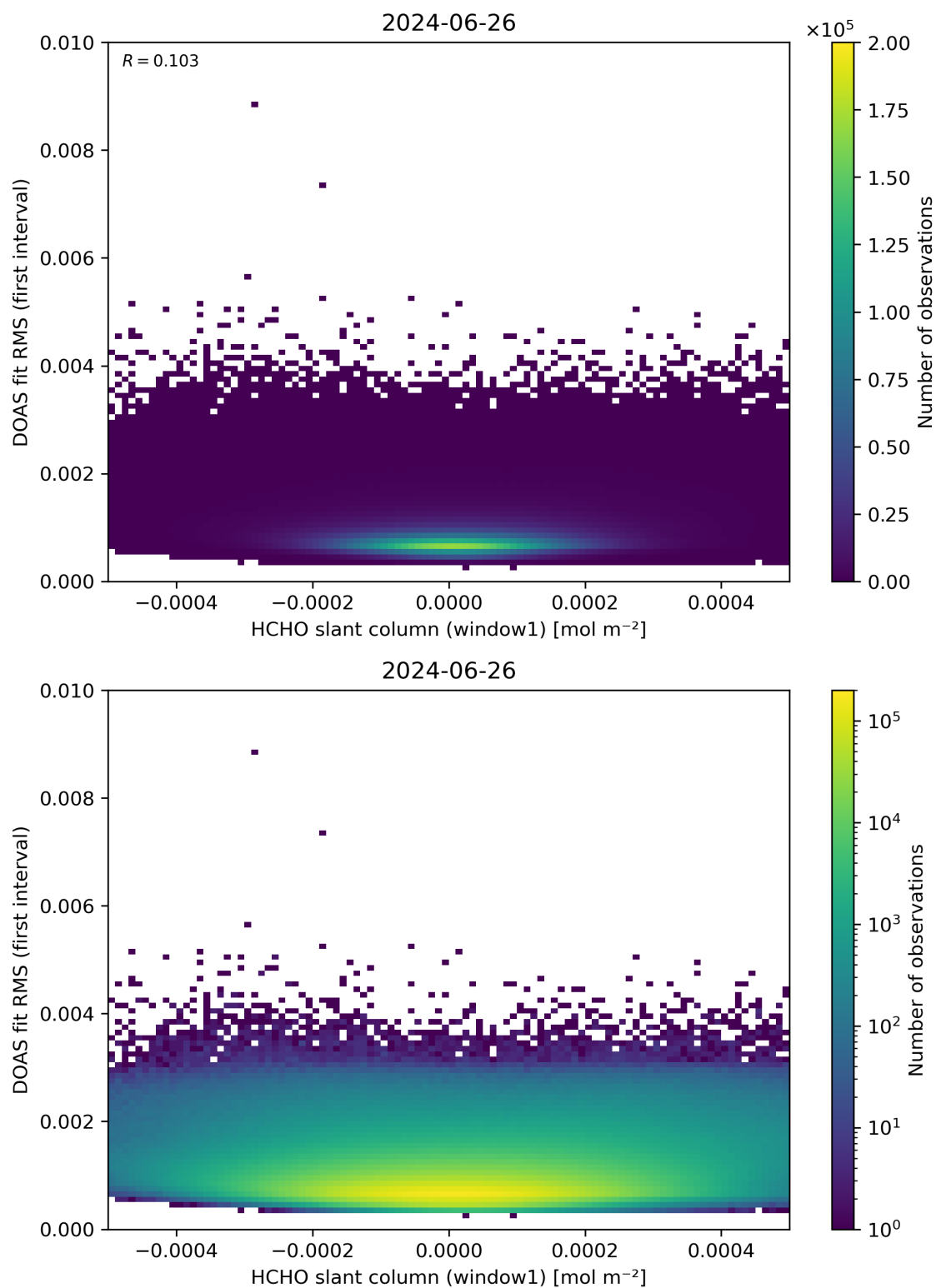
Figure 78: Scatter density plot of “HCHO slant column (window1)” against “DOAS fit RMS (first interval)” for 2024-06-25 to 2024-06-27.
