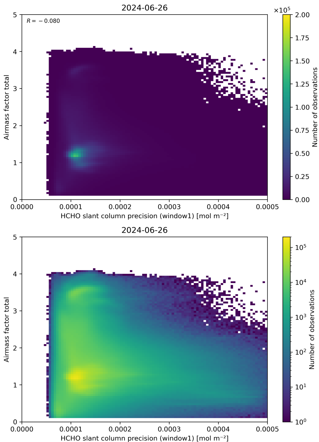
Figure 94: Scatter density plot of “HCHO slant column precision (window1)” against “Airmass factor total” for 2024-06-25 to 2024-06-27.
