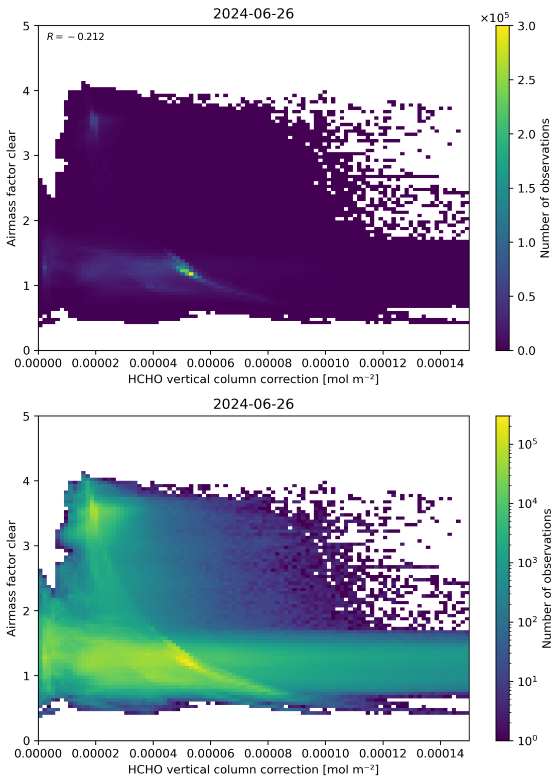
Figure 115: Scatter density plot of “HCHO vertical column correction” against “Airmass factor clear” for 2024-06-25 to 2024-06-27.
