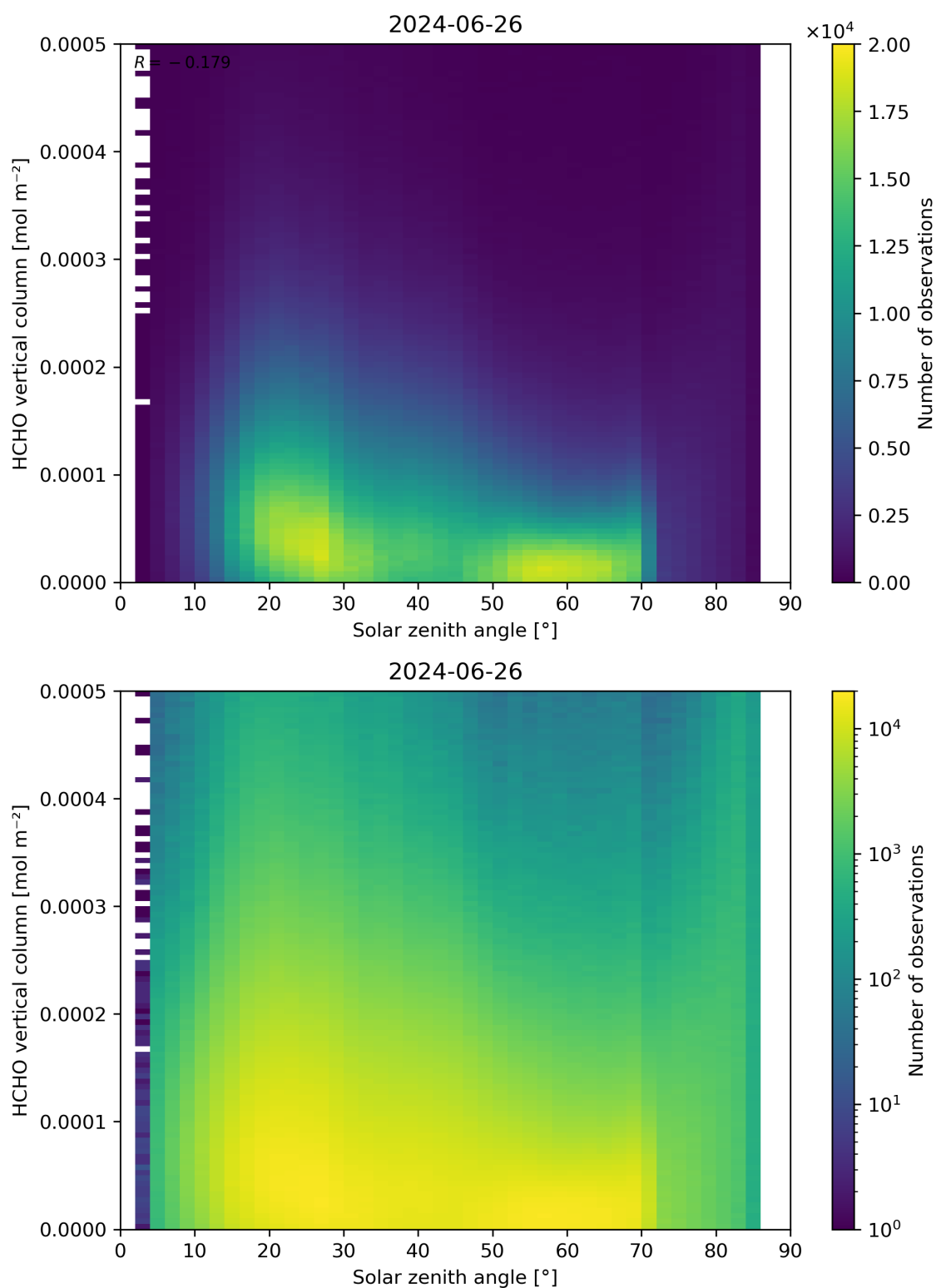
Figure 177: Scatter density plot of “Solar zenith angle” against “HCHO vertical column” for 2024-06-25 to 2024-06-27.
