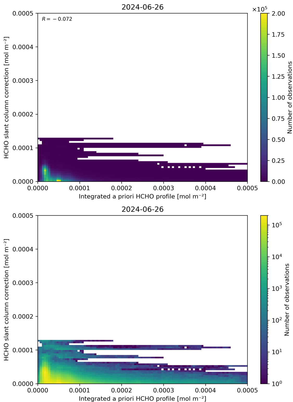
Figure 152: Scatter density plot of “Integrated a priori HCHO profile” against “HCHO slant column correction” for 2024-06-25 to 2024-06-27.
