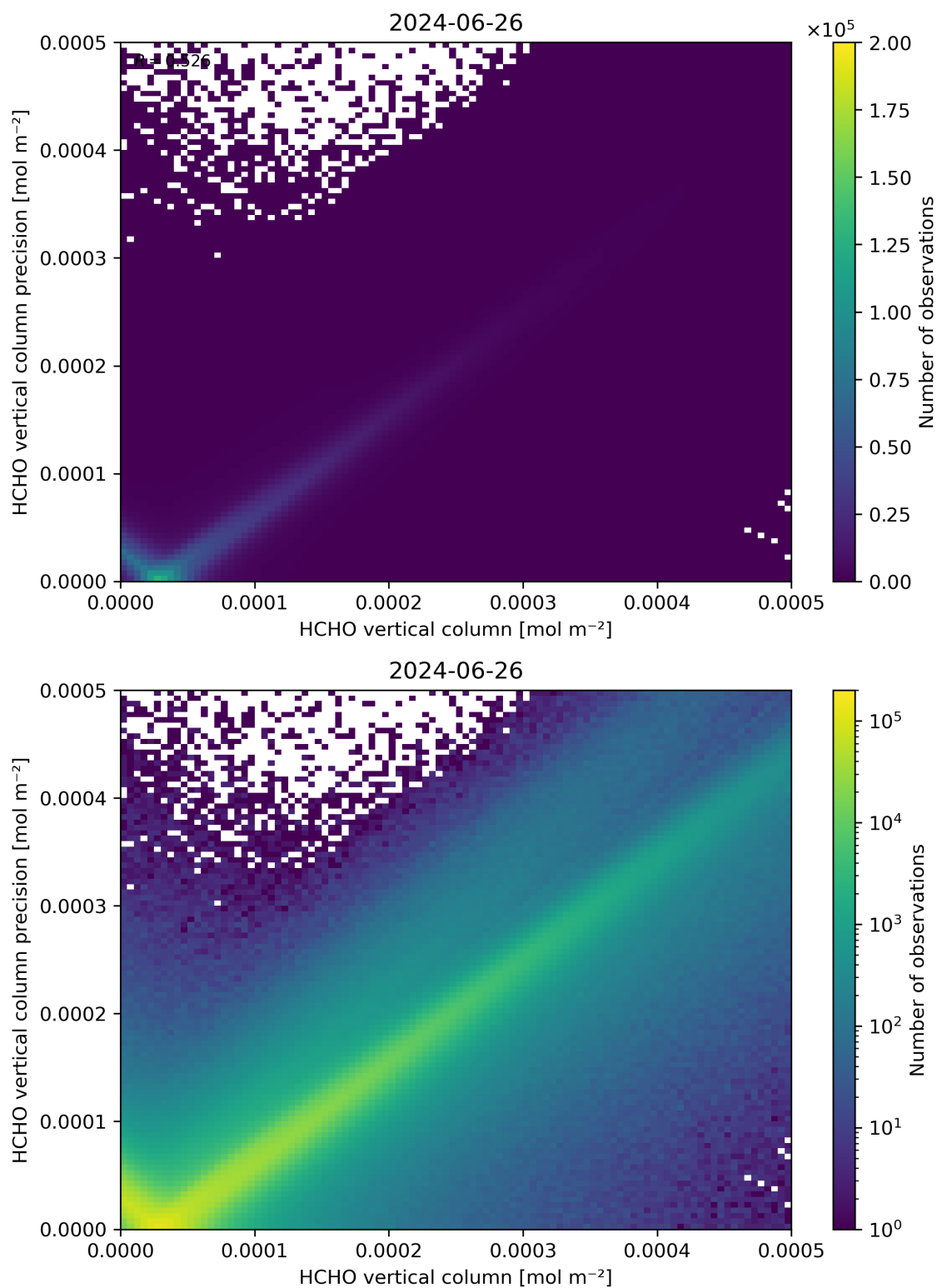
Figure 134: Scatter density plot of “HCHO vertical column” against “HCHO vertical column precision” for 2024-06-25 to 2024-06-27.
