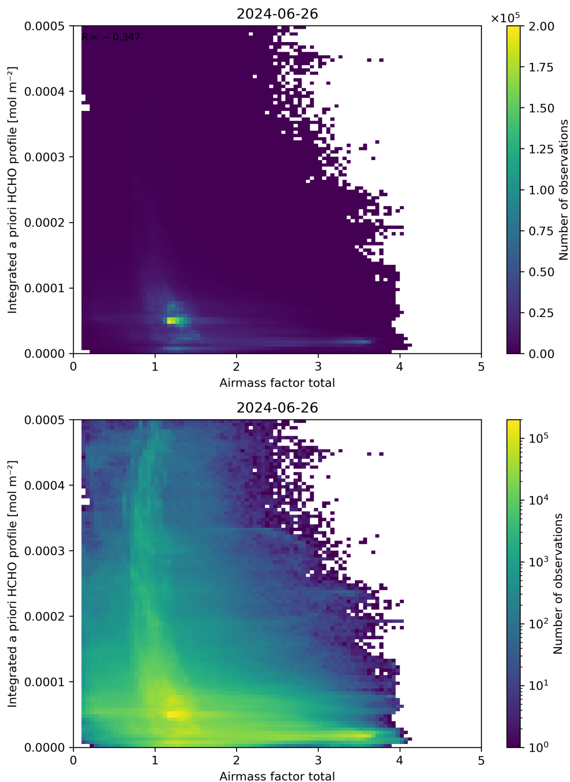
Figure 104: Scatter density plot of “Airmass factor total” against “Integrated a priori HCHO profile” for 2024-06-25 to 2024-06-27.
