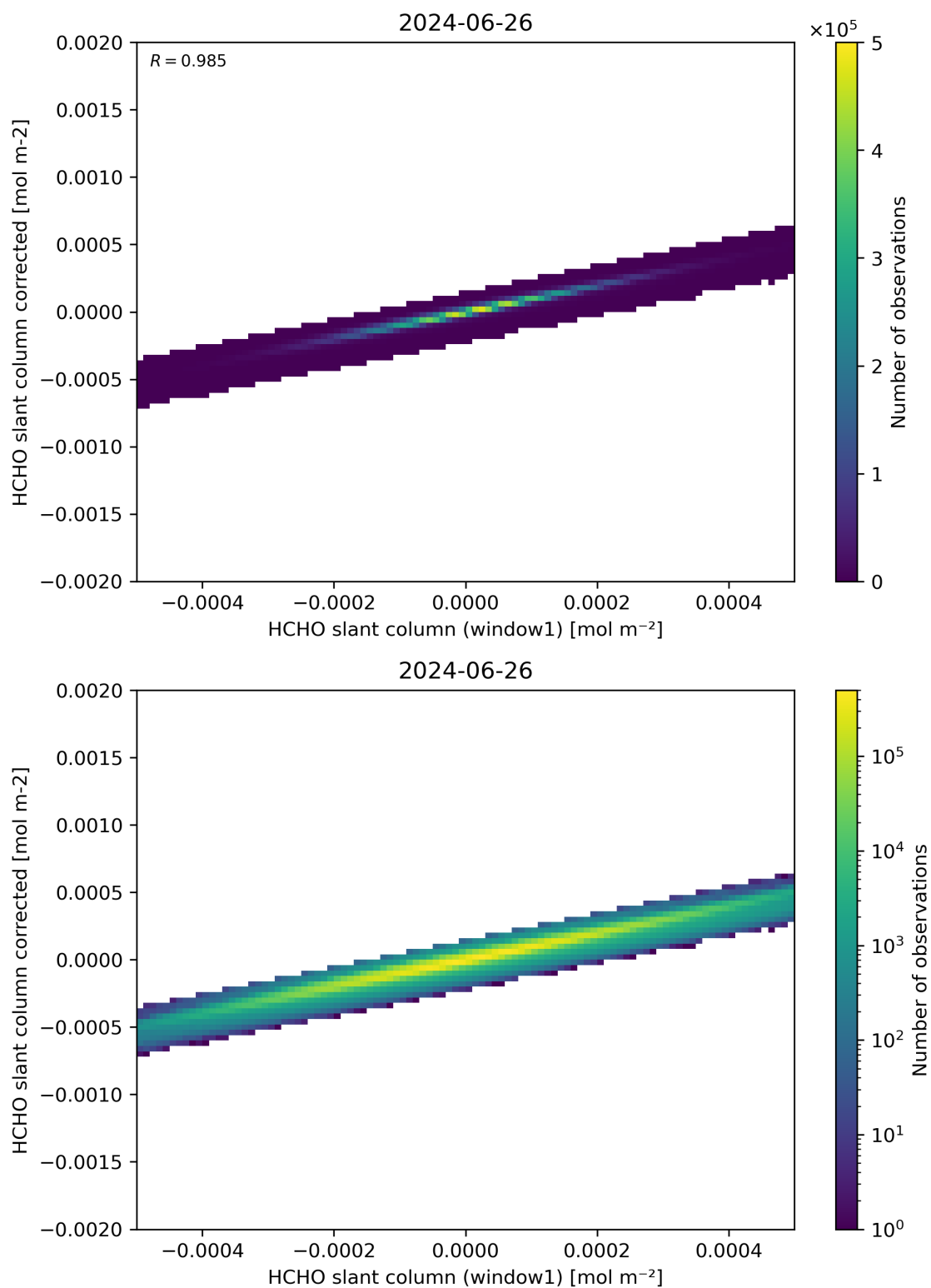
Figure 82: Scatter density plot of “HCHO slant column (window1)” against “HCHO slant column corrected” for 2024-06-25 to 2024-06-27.
