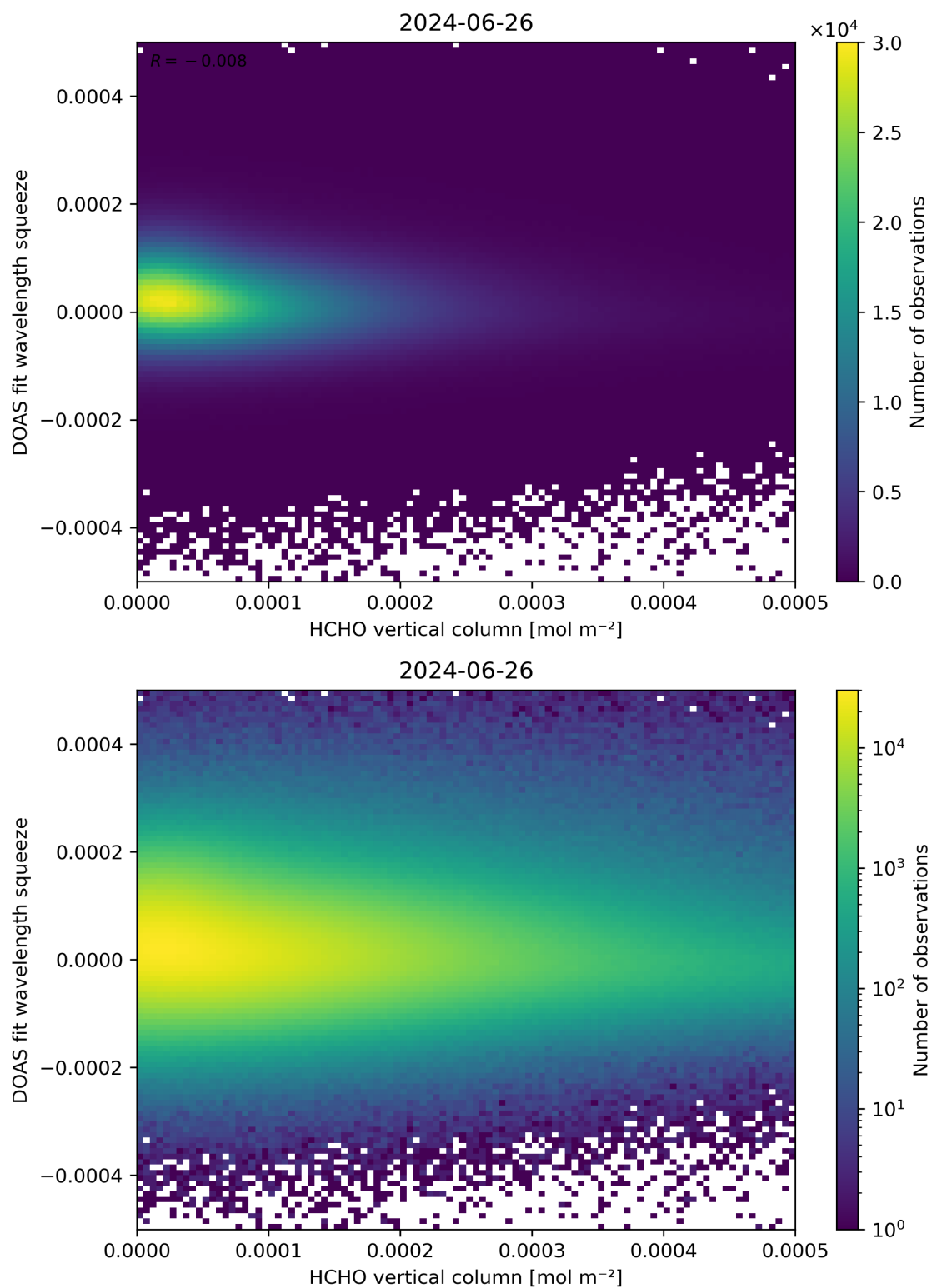
Figure 125: Scatter density plot of “HCHO vertical column” against “DOAS fit wavelength squeeze” for 2024-06-25 to 2024-06-27.
