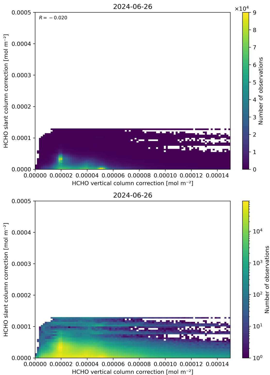
Figure 117: Scatter density plot of “HCHO vertical column correction” against “HCHO slant column correction” for 2024-06-25 to 2024-06-27.
