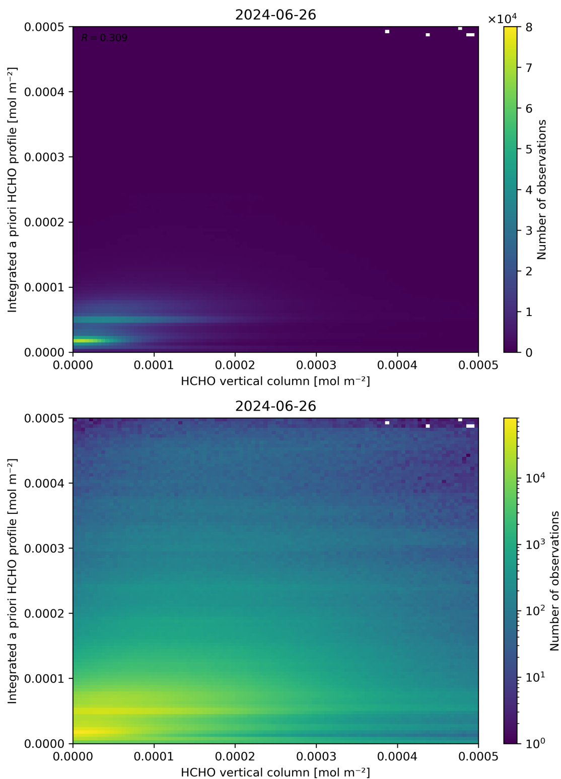
Figure 135: Scatter density plot of “HCHO vertical column” against “Integrated a priori HCHO profile” for 2024-06-25 to 2024-06-27.
