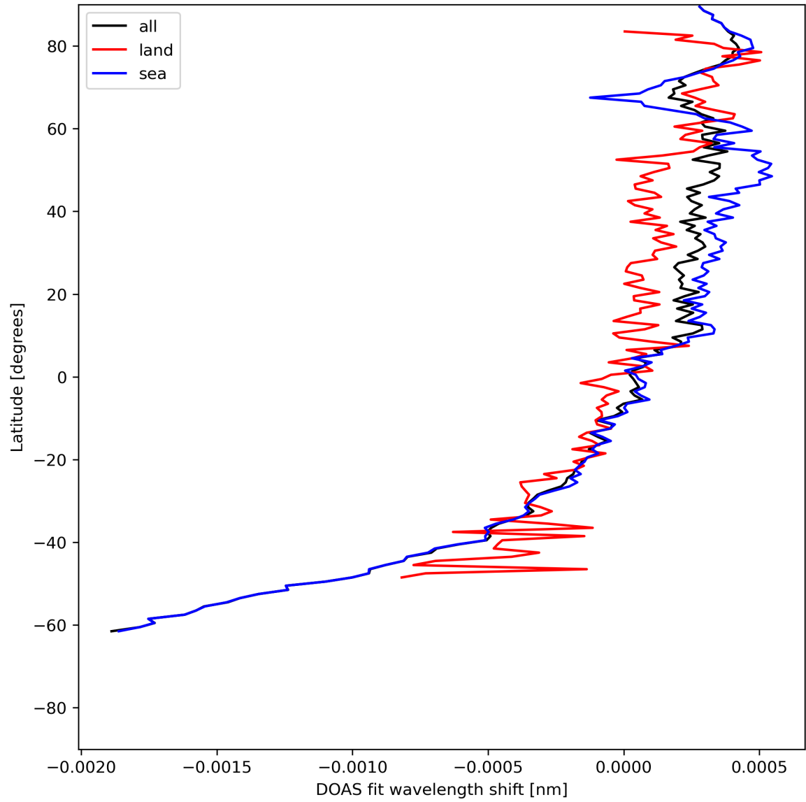
Figure 30: Zonal average of “DOAS fit wavelength shift” for 2024-06-25 to 2024-06-27.
