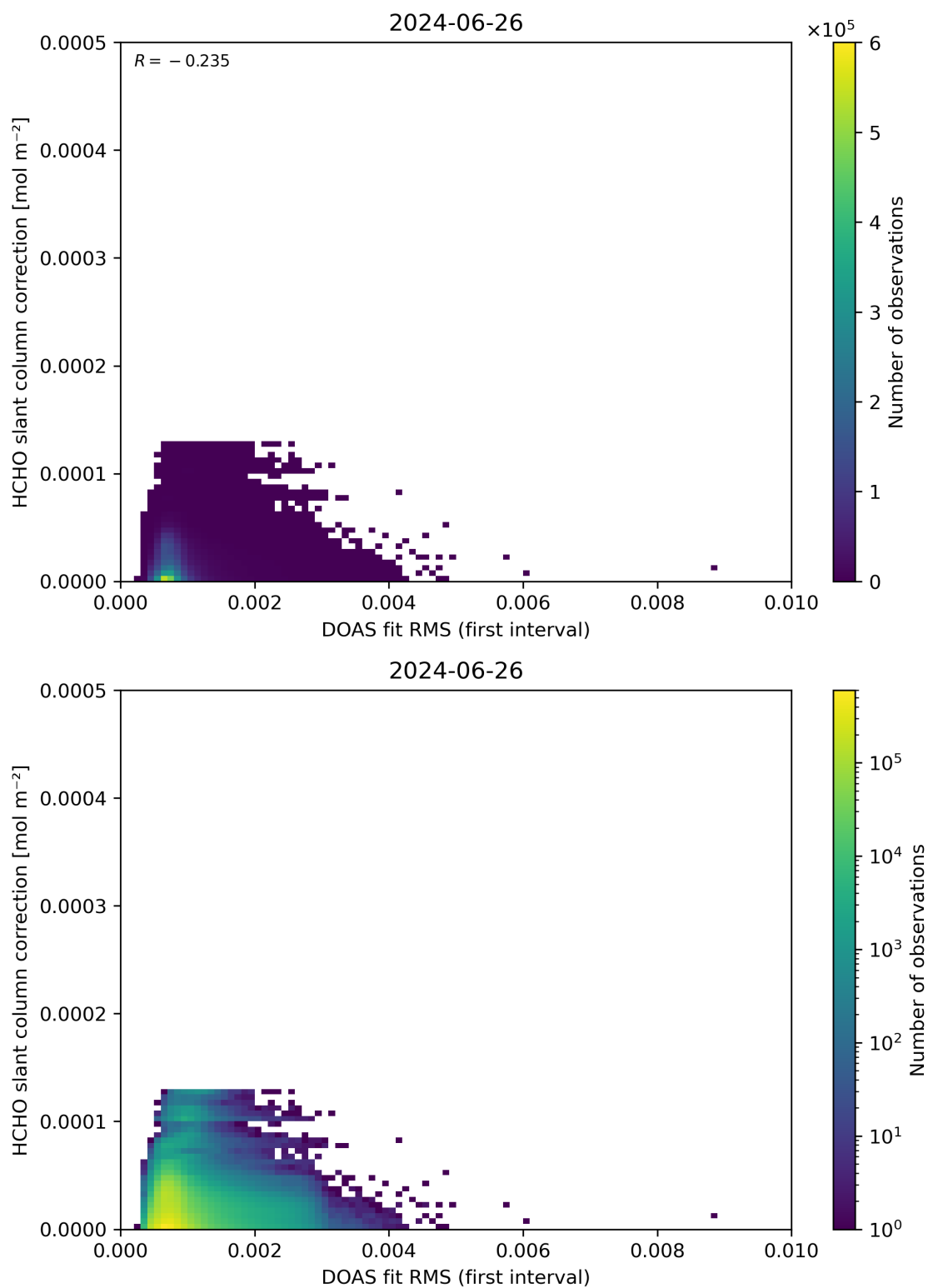
Figure 63: Scatter density plot of “DOAS fit RMS (first interval)” against “HCHO slant column correction” for 2024-06-25 to 2024-06-27.
