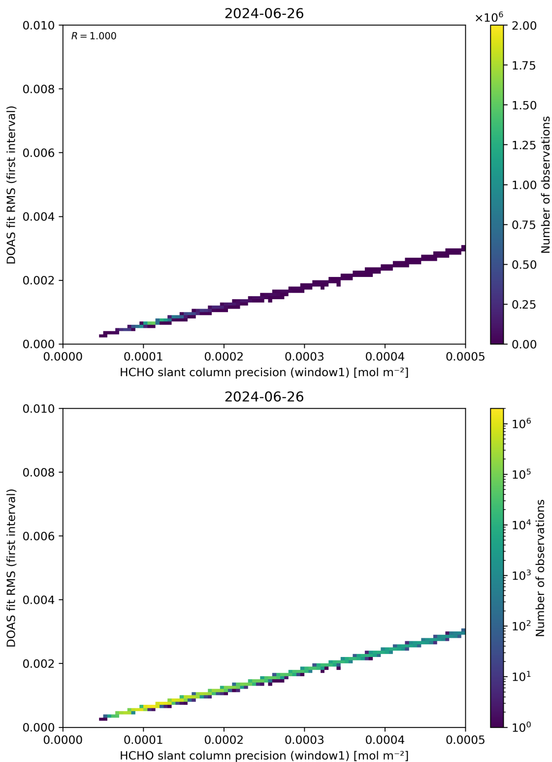
Figure 88: Scatter density plot of “HCHO slant column precision (window1)” against “DOAS fit RMS (first interval)” for 2024-06-25 to 2024-06-27.
