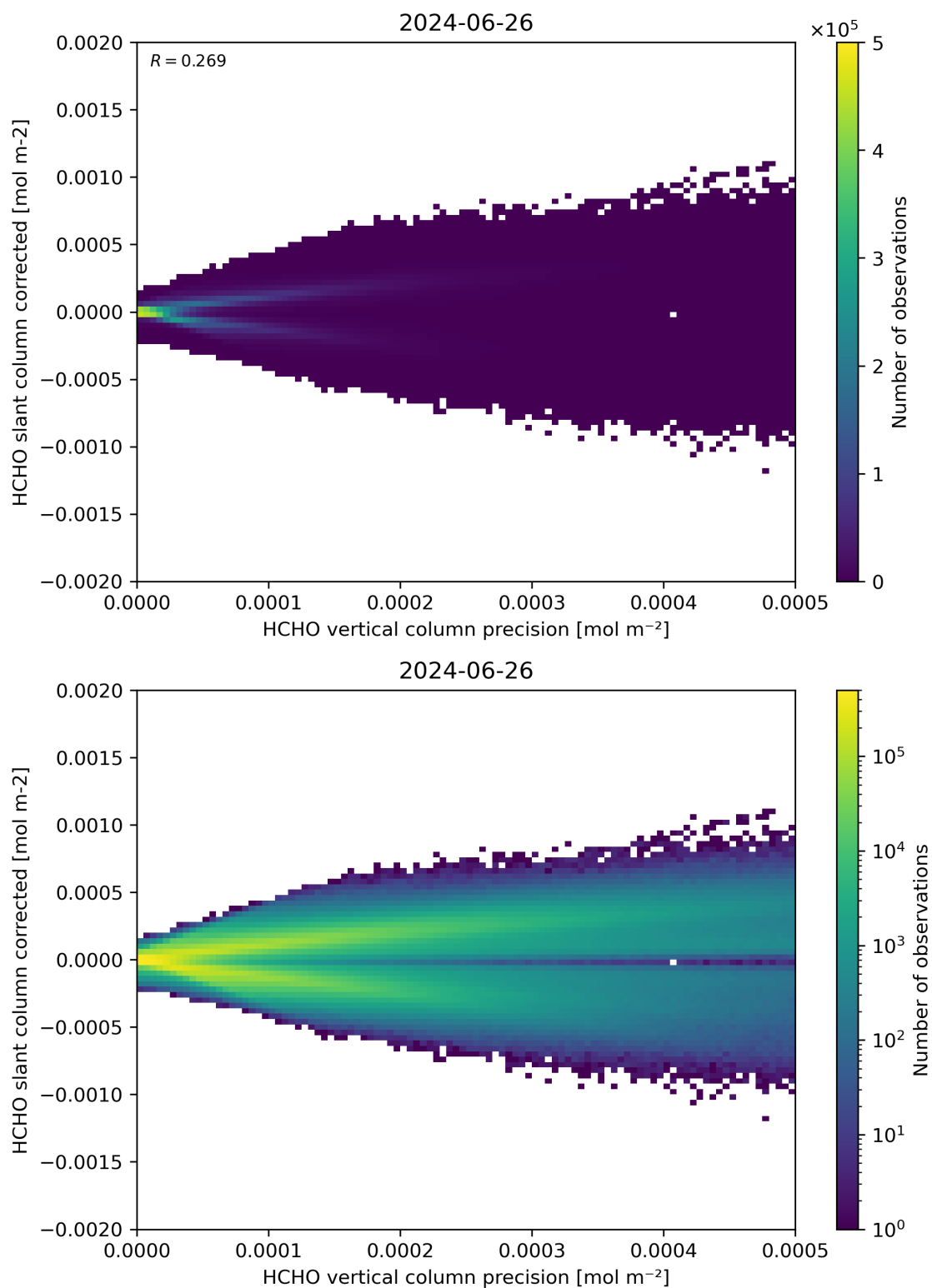
Figure 140: Scatter density plot of “HCHO vertical column precision” against “HCHO slant column corrected” for 2024-06-25 to 2024-06-27.
