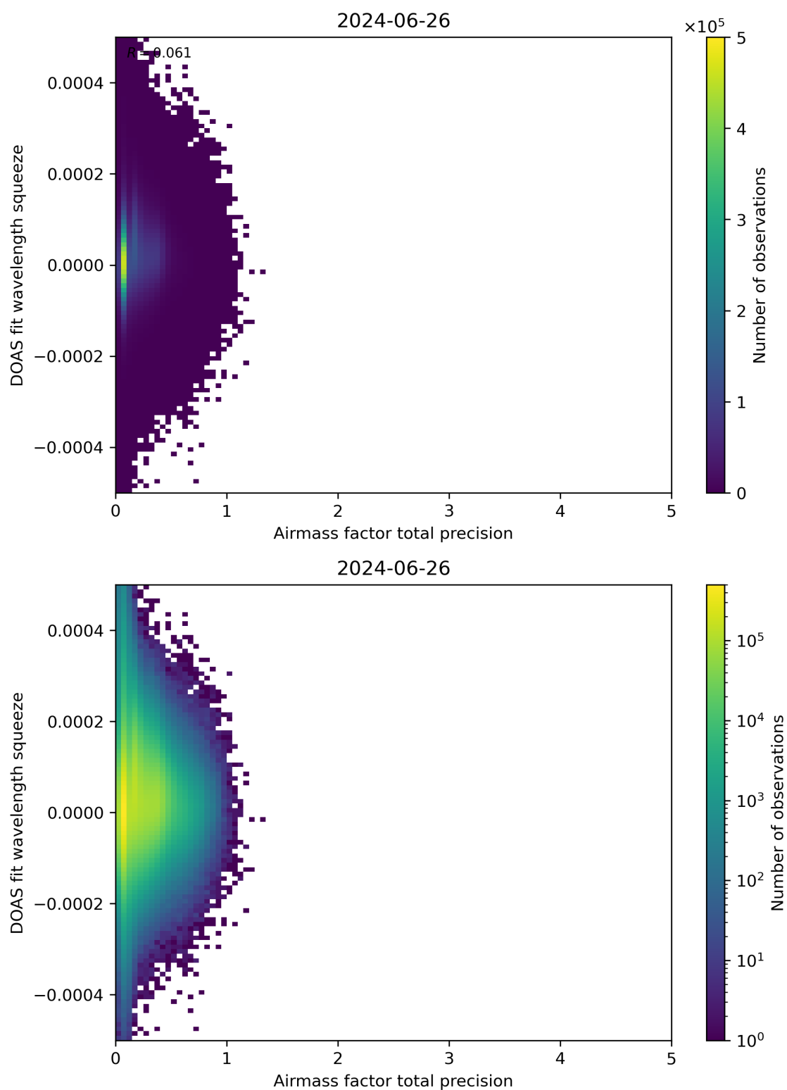
Figure 107: Scatter density plot of “Airmass factor total precision” against “DOAS fit wavelength squeeze” for 2024-06-25 to 2024-06-27.
