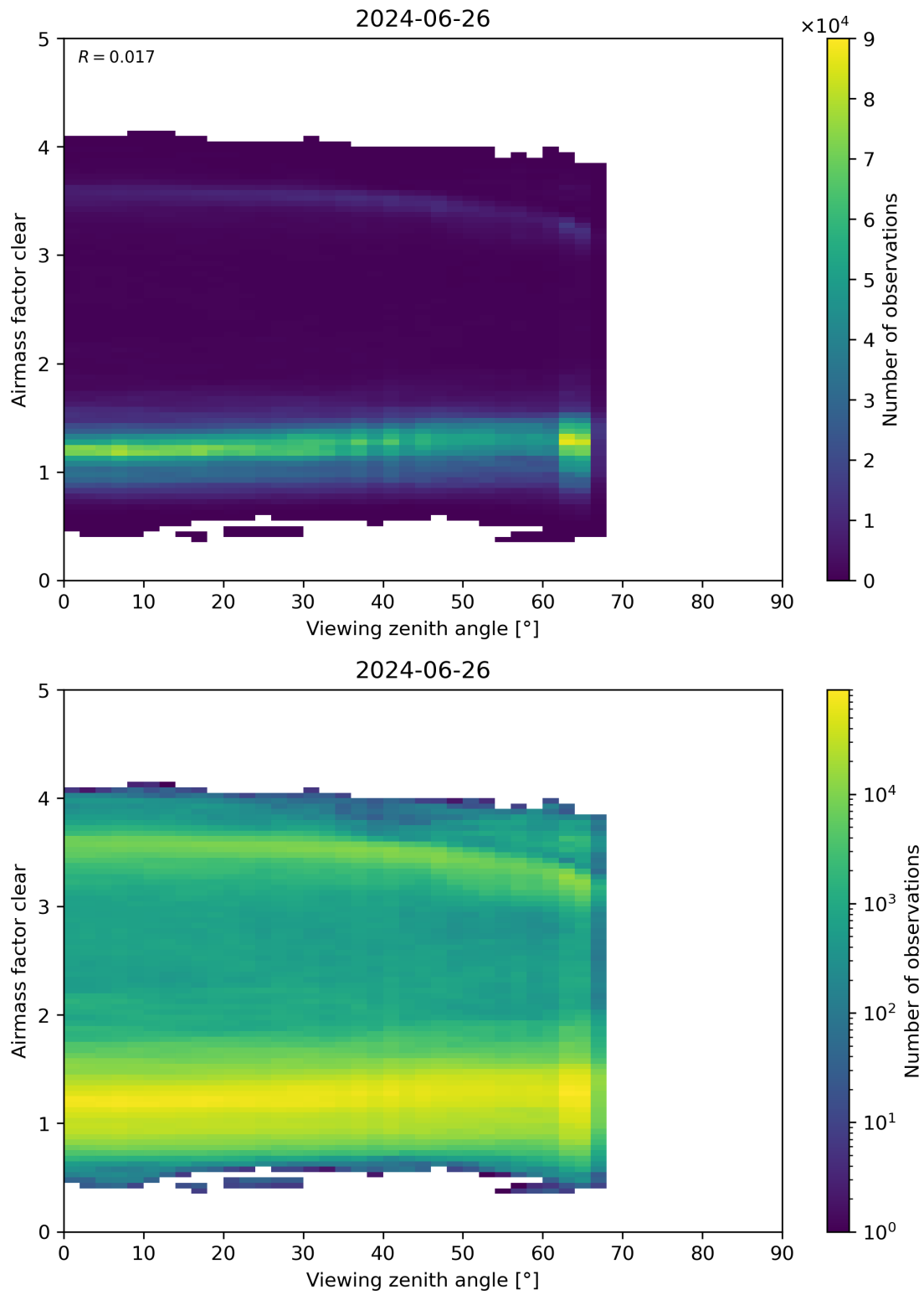
Figure 185: Scatter density plot of “Viewing zenith angle” against “Airmass factor clear” for 2024-06-25 to 2024-06-27.
