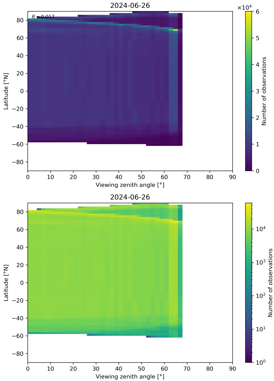
Figure 196: Scatter density plot of “Viewing zenith angle” against “Latitude” for 2024-06-25 to 2024-06-27.
