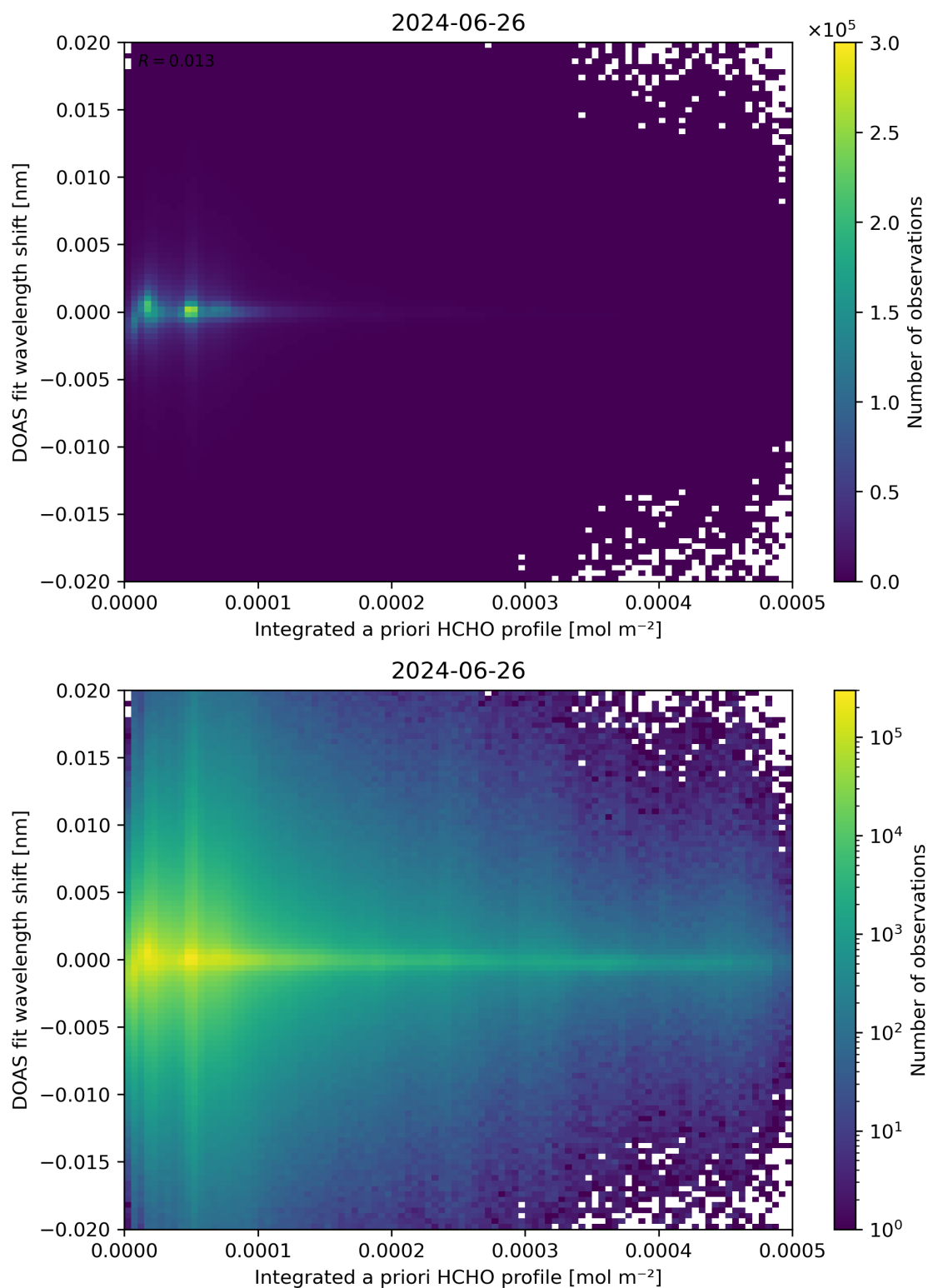
Figure 149: Scatter density plot of “Integrated a priori HCHO profile” against “DOAS fit wavelength shift” for 2024-06-25 to 2024-06-27.
