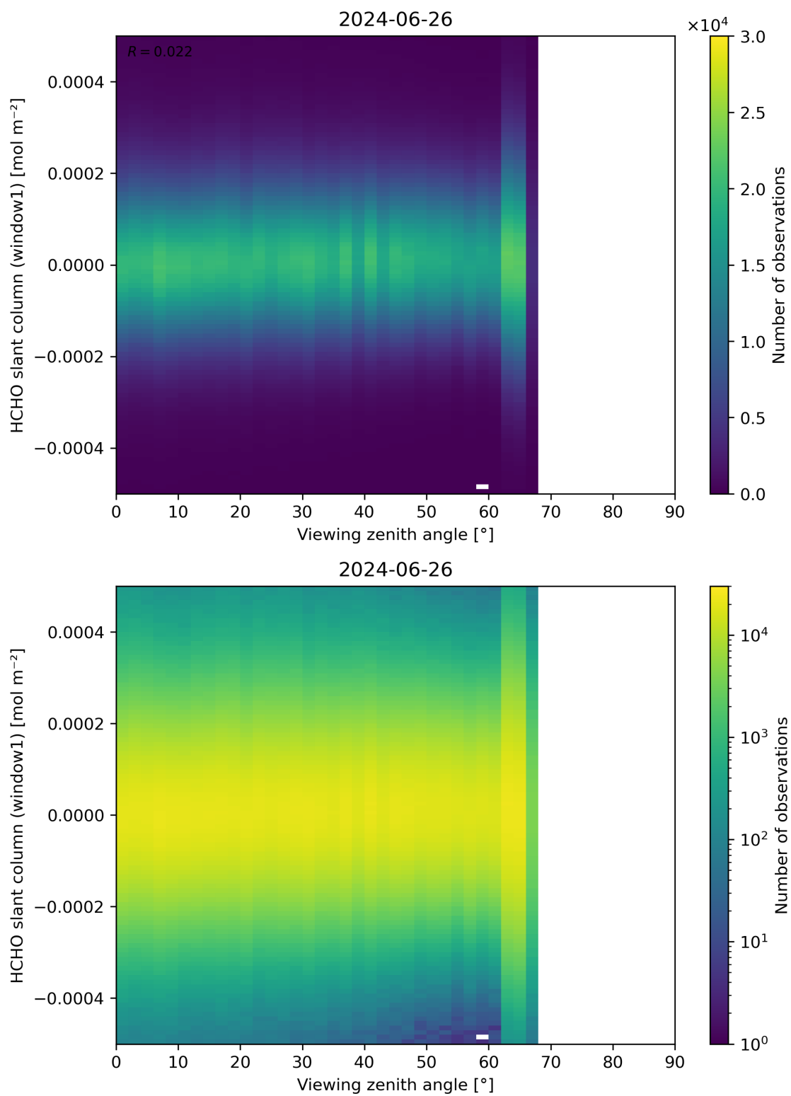
Figure 188: Scatter density plot of “Viewing zenith angle” against “HCHO slant column (window1)” for 2024-06-25 to 2024-06-27.
