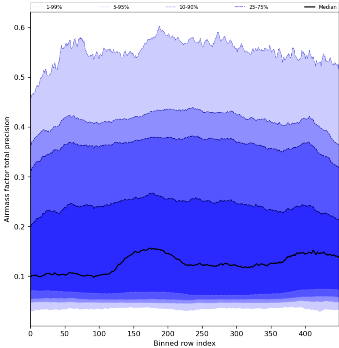
Figure 55: Along track statistics of “Airmass factor total precision” for 2024-06-25 to 2024-06-27
