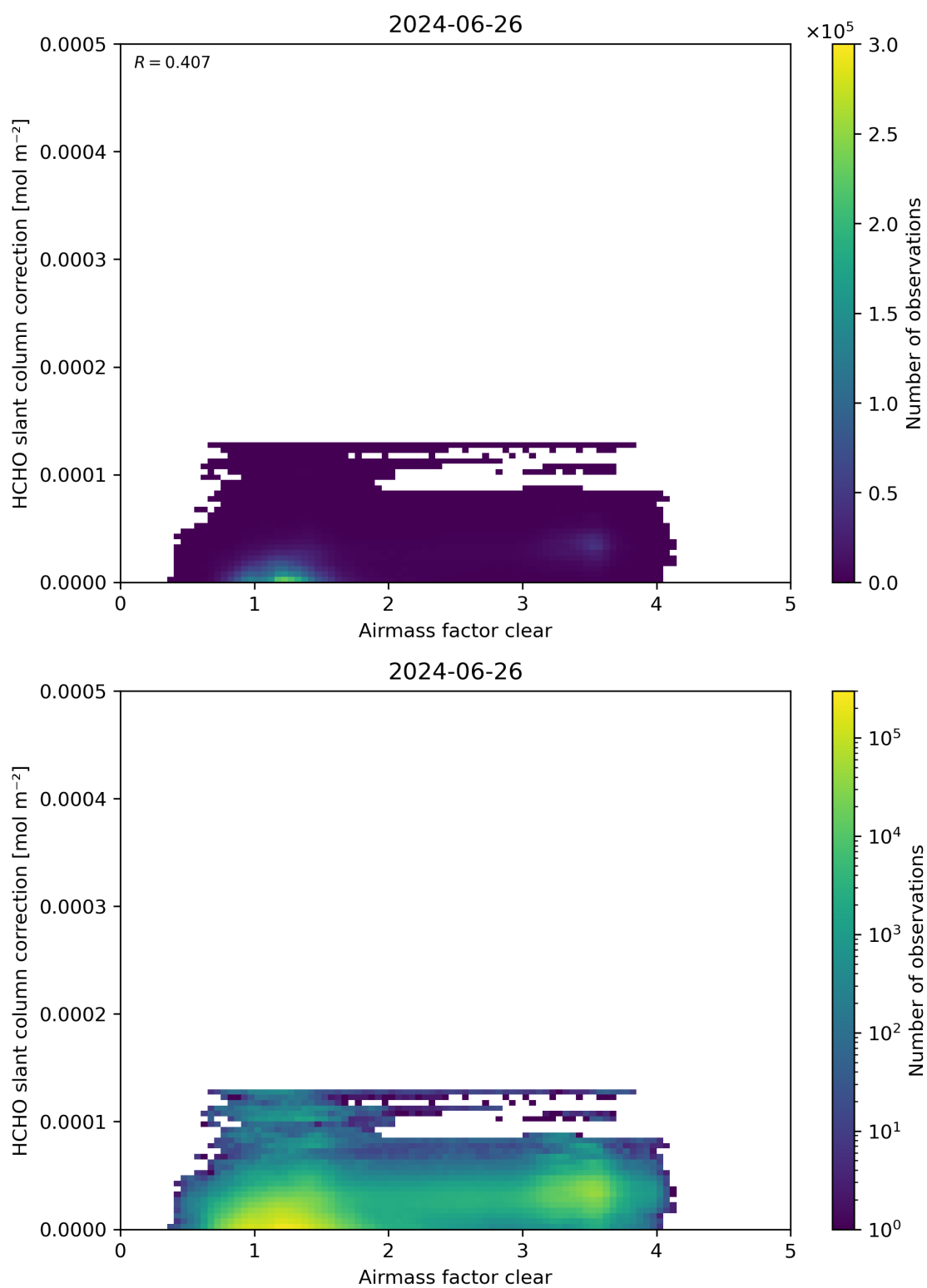
Figure 75: Scatter density plot of “Airmass factor clear” against “HCHO slant column correction” for 2024-06-25 to 2024-06-27.
