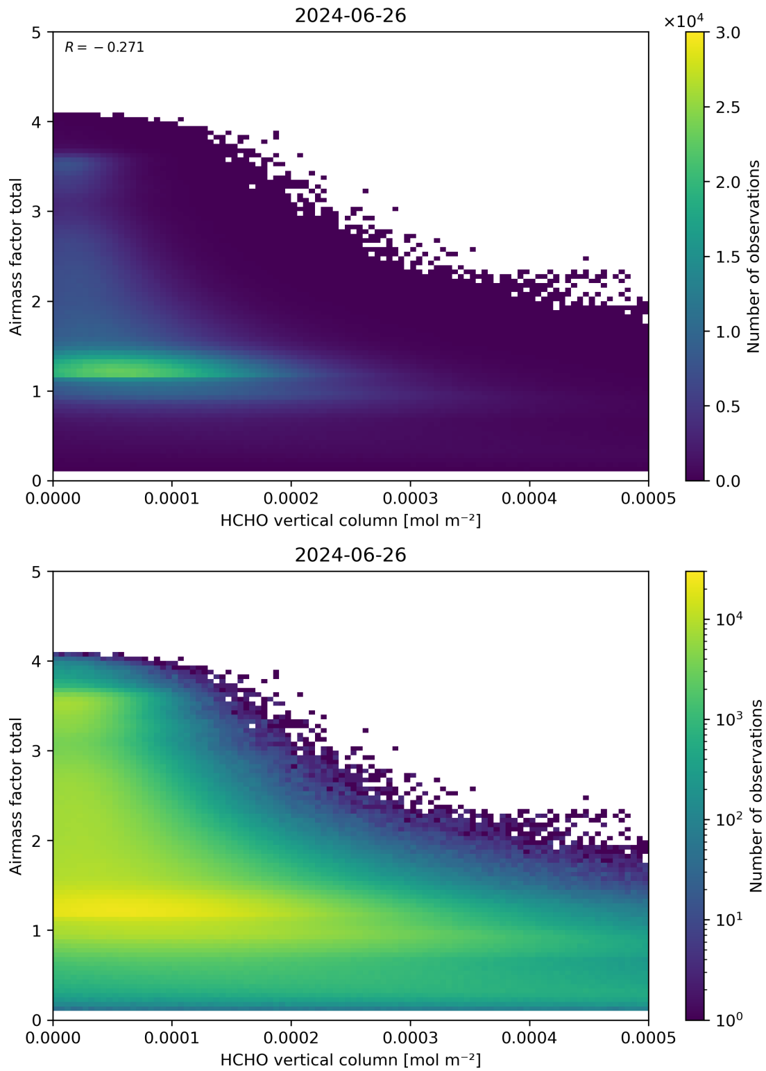
Figure 131: Scatter density plot of “HCHO vertical column” against “Airmass factor total” for 2024-06-25 to 2024-06-27.
