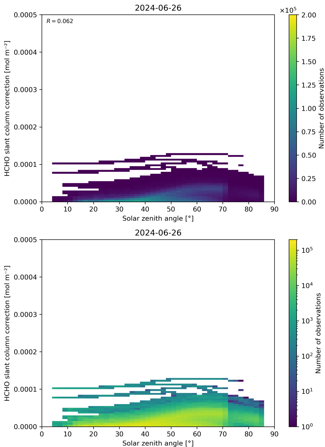
Figure 172: Scatter density plot of “Solar zenith angle” against “HCHO slant column correction” for 2024-06-25 to 2024-06-27.
