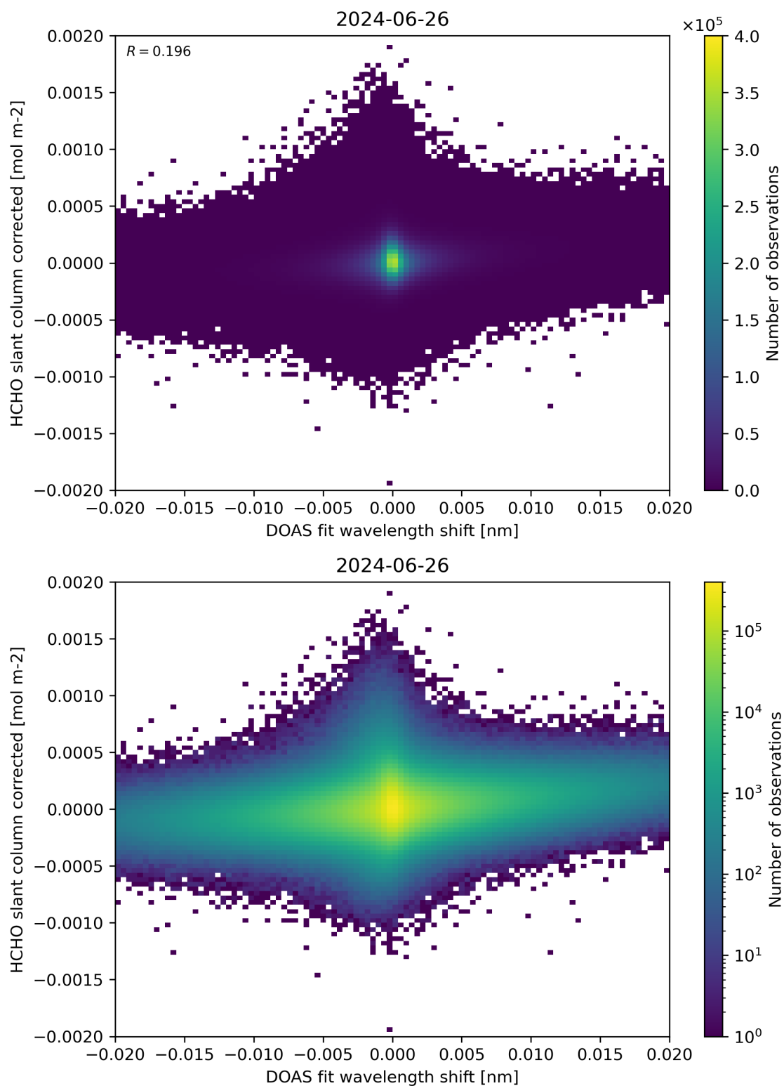
Figure 66: Scatter density plot of “DOAS fit wavelength shift” against “HCHO slant column corrected” for 2024-06-25 to 2024-06-27.
