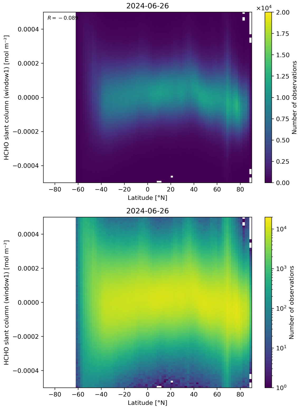
Figure 159: Scatter density plot of “Latitude” against “HCHO slant column (window1)” for 2024-06-25 to 2024-06-27.
