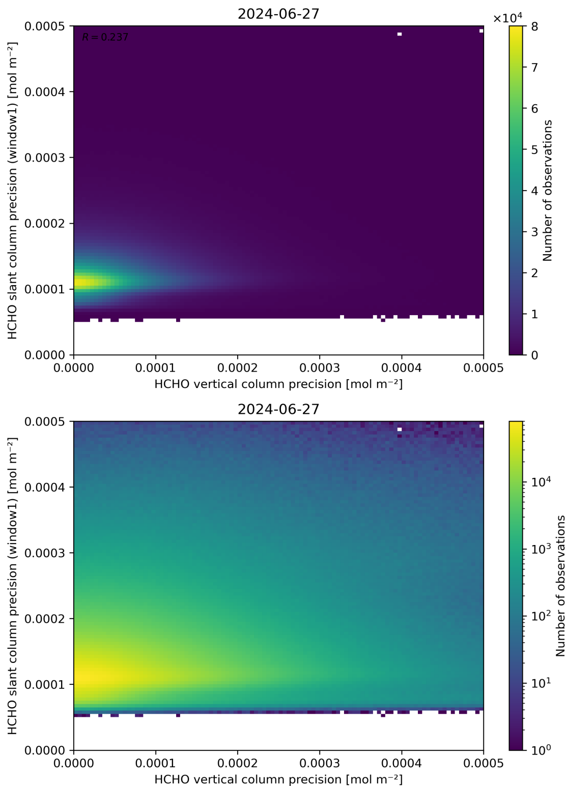
Figure 143: Scatter density plot of “HCHO vertical column precision” against “HCHO slant column precision (window1)” for 2024-06-26 to 2024-06-28.
