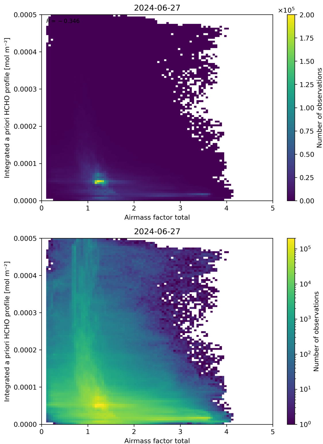
Figure 104: Scatter density plot of “Airmass factor total” against “Integrated a priori HCHO profile” for 2024-06-26 to 2024-06-28.
