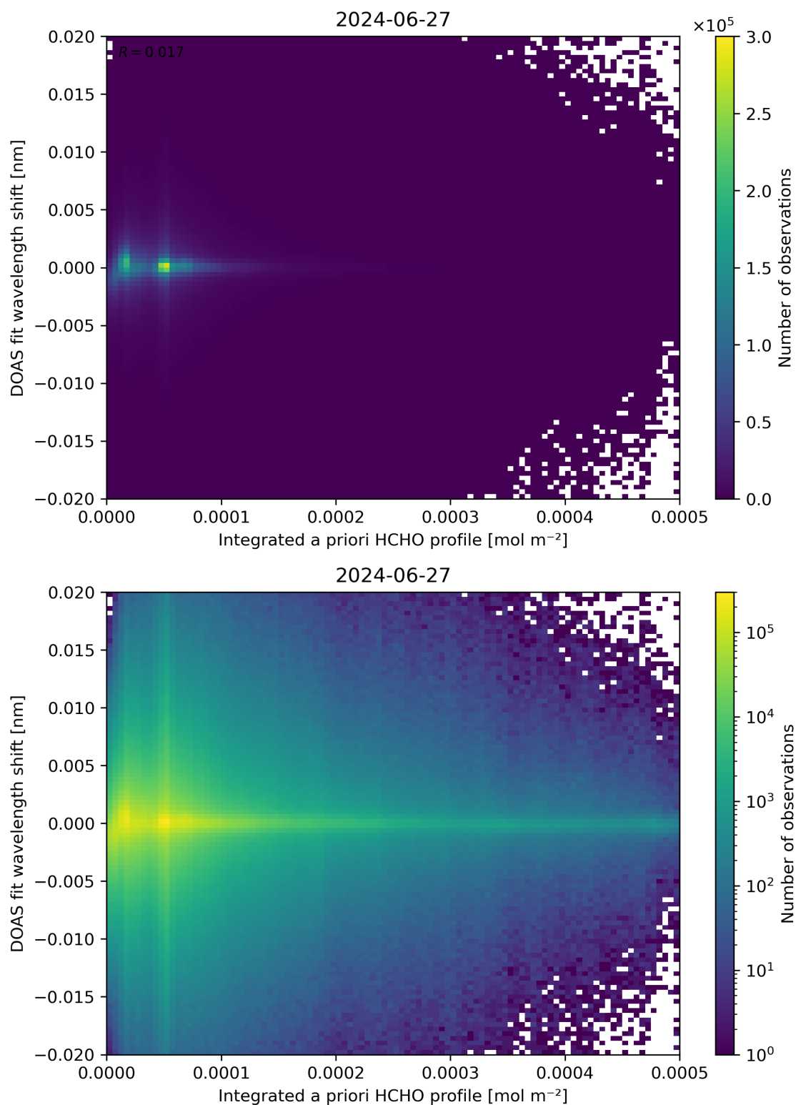
Figure 149: Scatter density plot of “Integrated a priori HCHO profile” against “DOAS fit wavelength shift” for 2024-06-26 to 2024-06-28.
