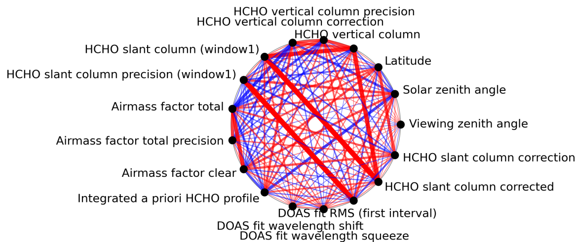
Figure 1: Map of correlation graph for 2024-06-26 to 2024-06-28.
