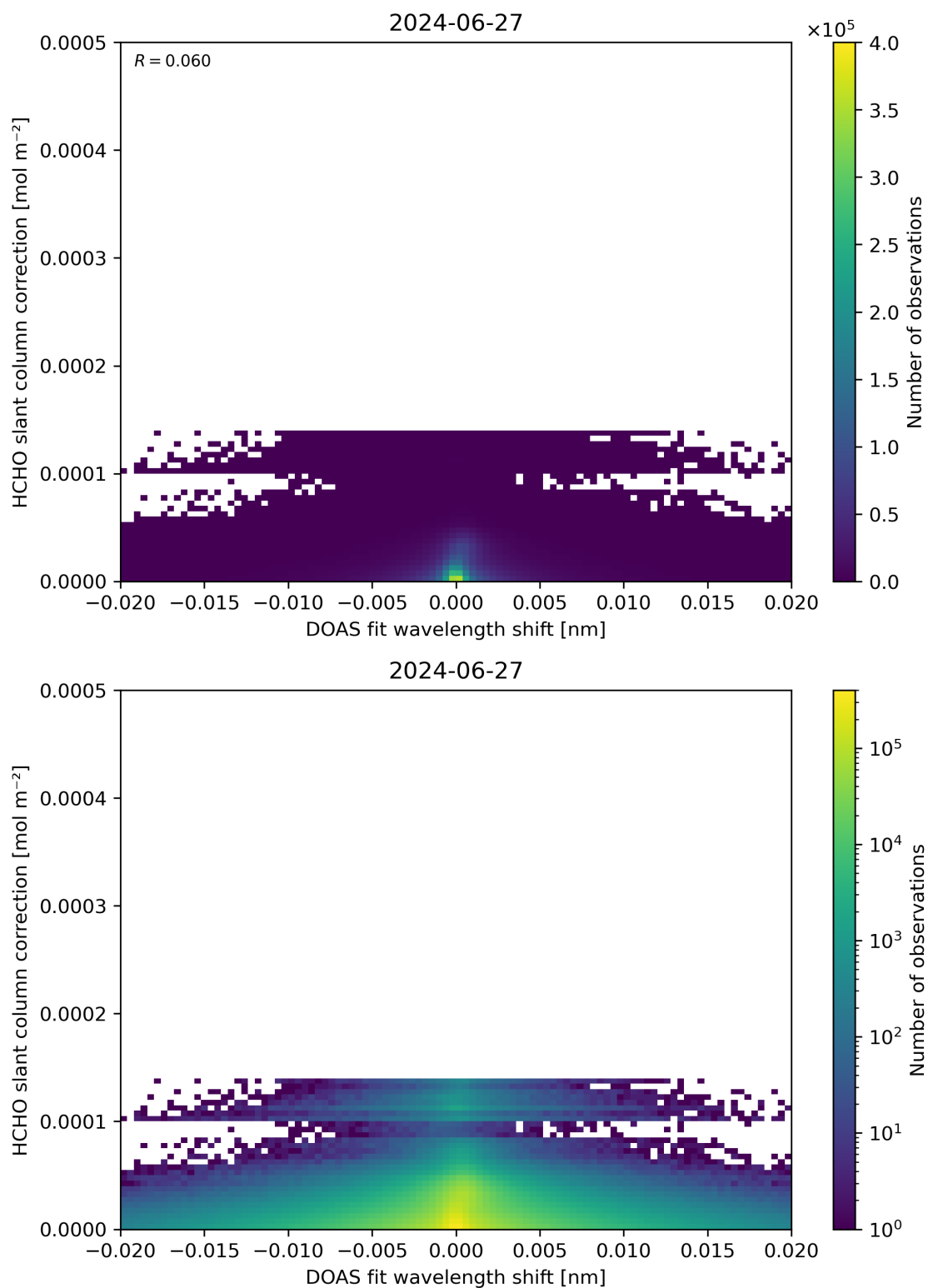
Figure 67: Scatter density plot of “DOAS fit wavelength shift” against “HCHO slant column correction” for 2024-06-26 to 2024-06-28.
