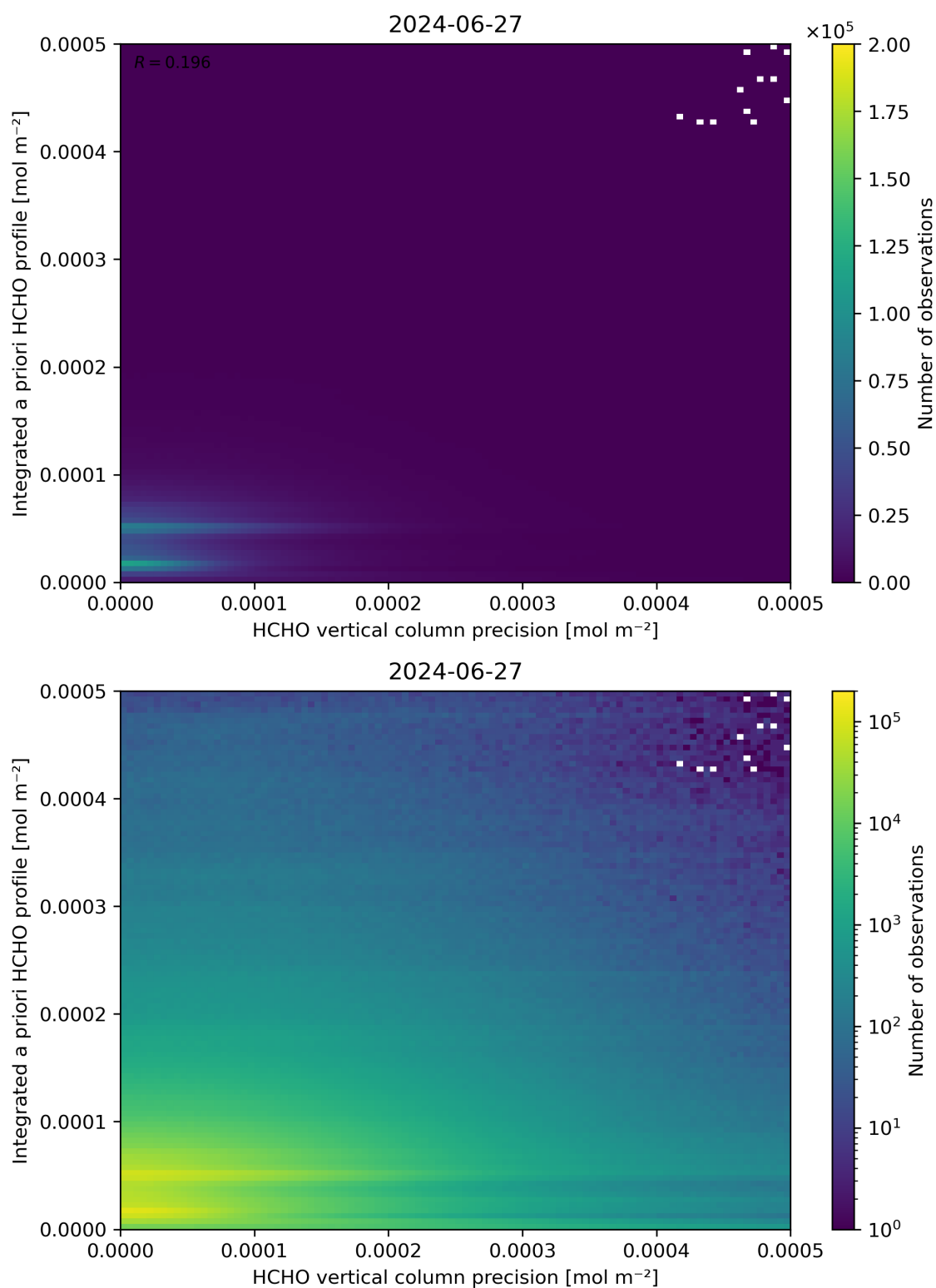
Figure 147: Scatter density plot of “HCHO vertical column precision” against “Integrated a priori HCHO profile” for 2024-06-26 to 2024-06-28.
