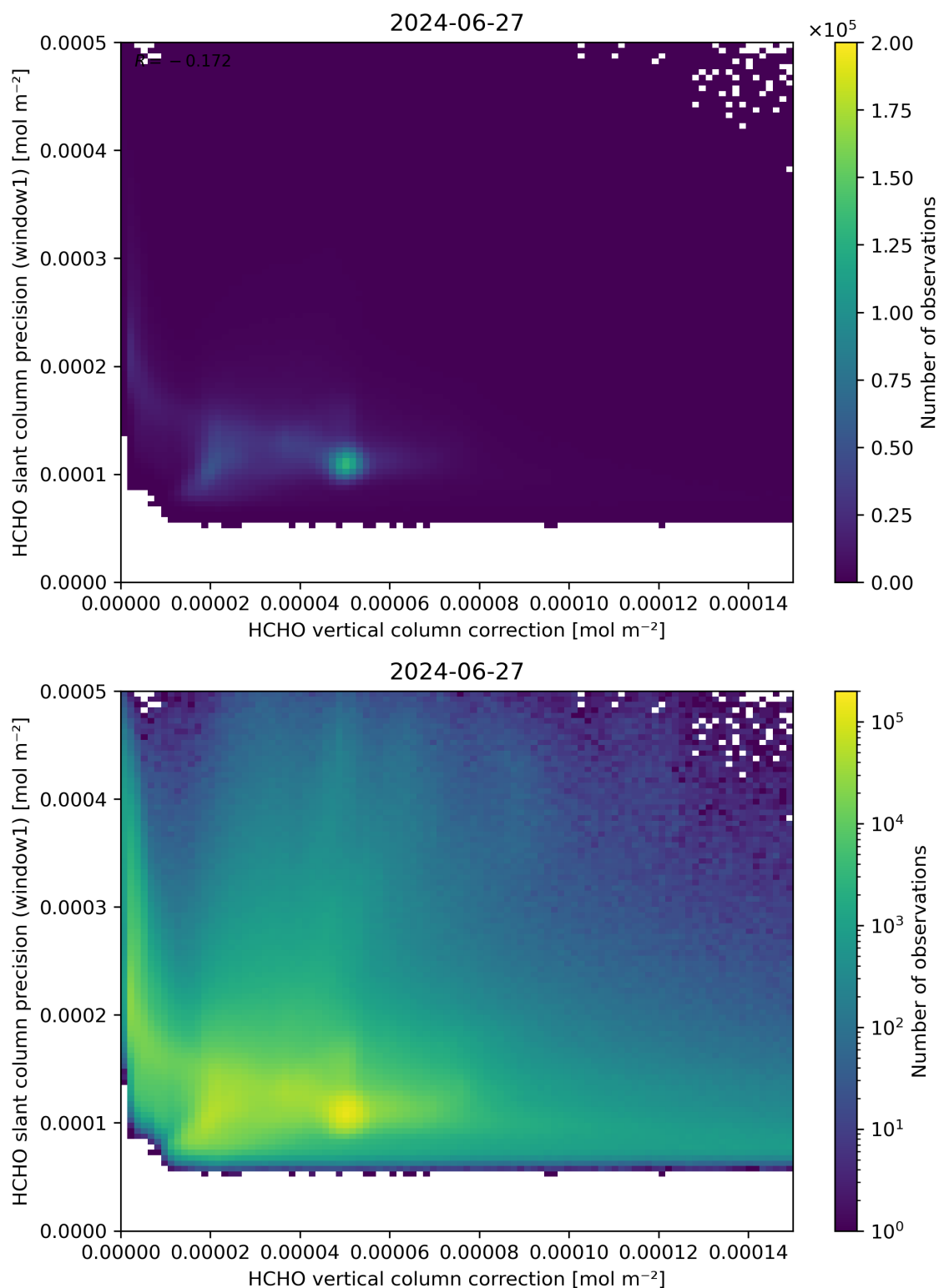
Figure 119: Scatter density plot of “HCHO vertical column correction” against “HCHO slant column precision (window1)” for 2024-06-26 to 2024-06-28.
