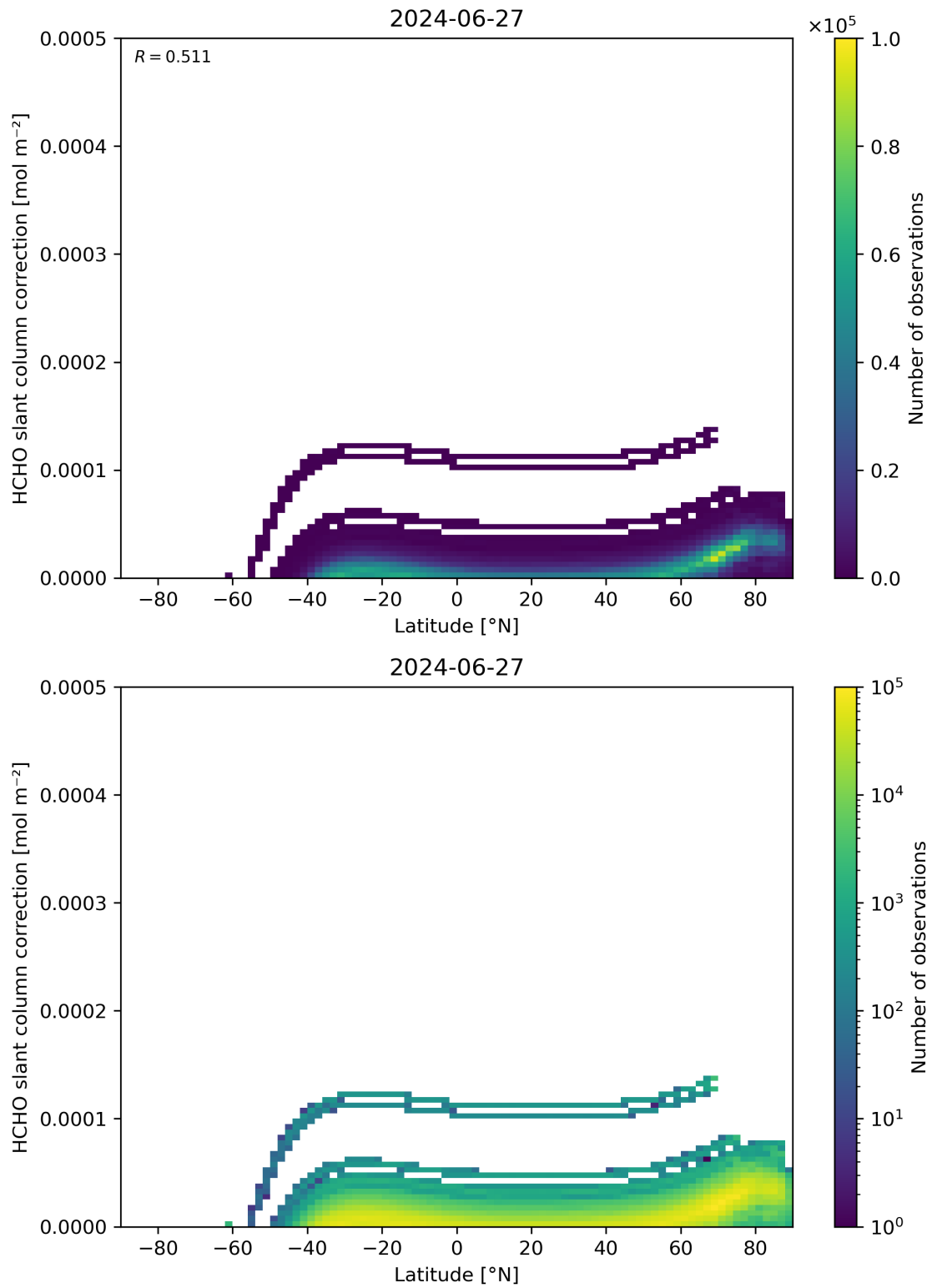
Figure 158: Scatter density plot of “Latitude” against “HCHO slant column correction” for 2024-06-26 to 2024-06-28.
