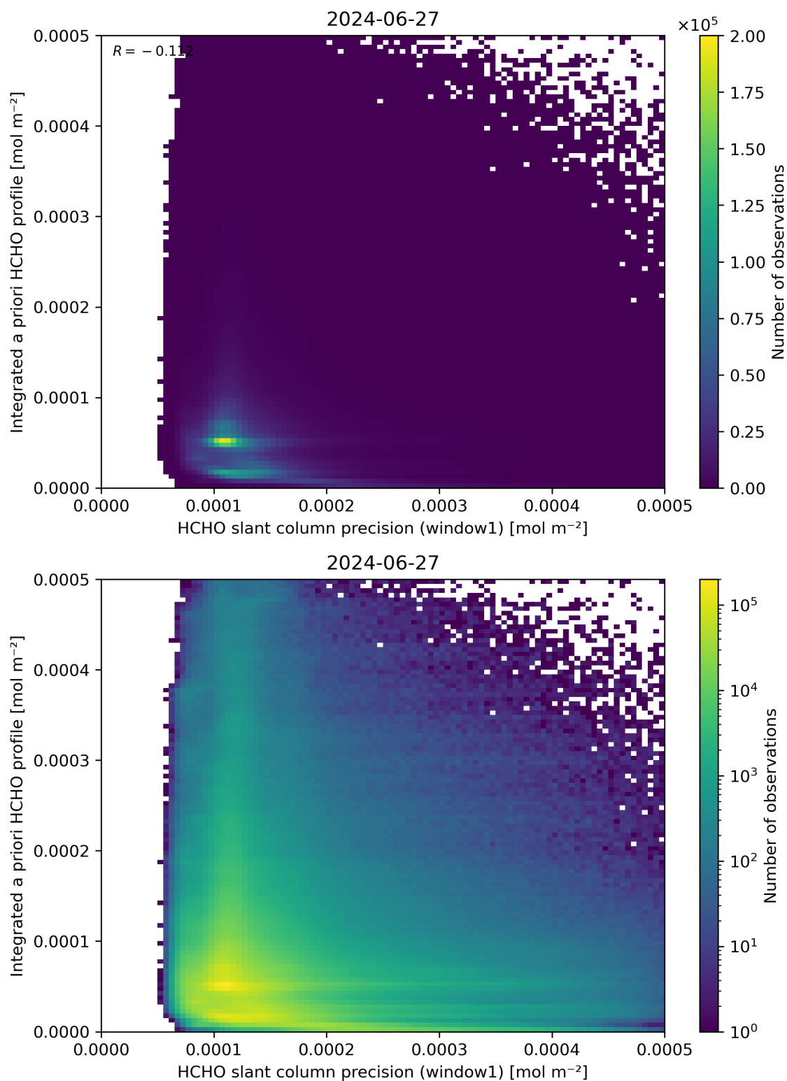
Figure 96: Scatter density plot of “HCHO slant column precision (window1)” against “Integrated a priori HCHO profile” for 2024-06-26 to 2024-06-28.
