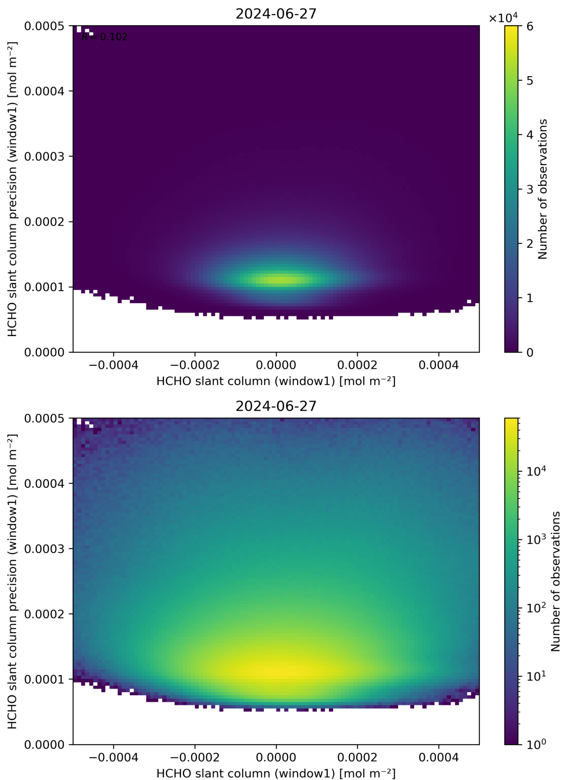
Figure 84: Scatter density plot of “HCHO slant column (window1)” against “HCHO slant column precision (window1)” for 2024-06-26 to 2024-06-28.
