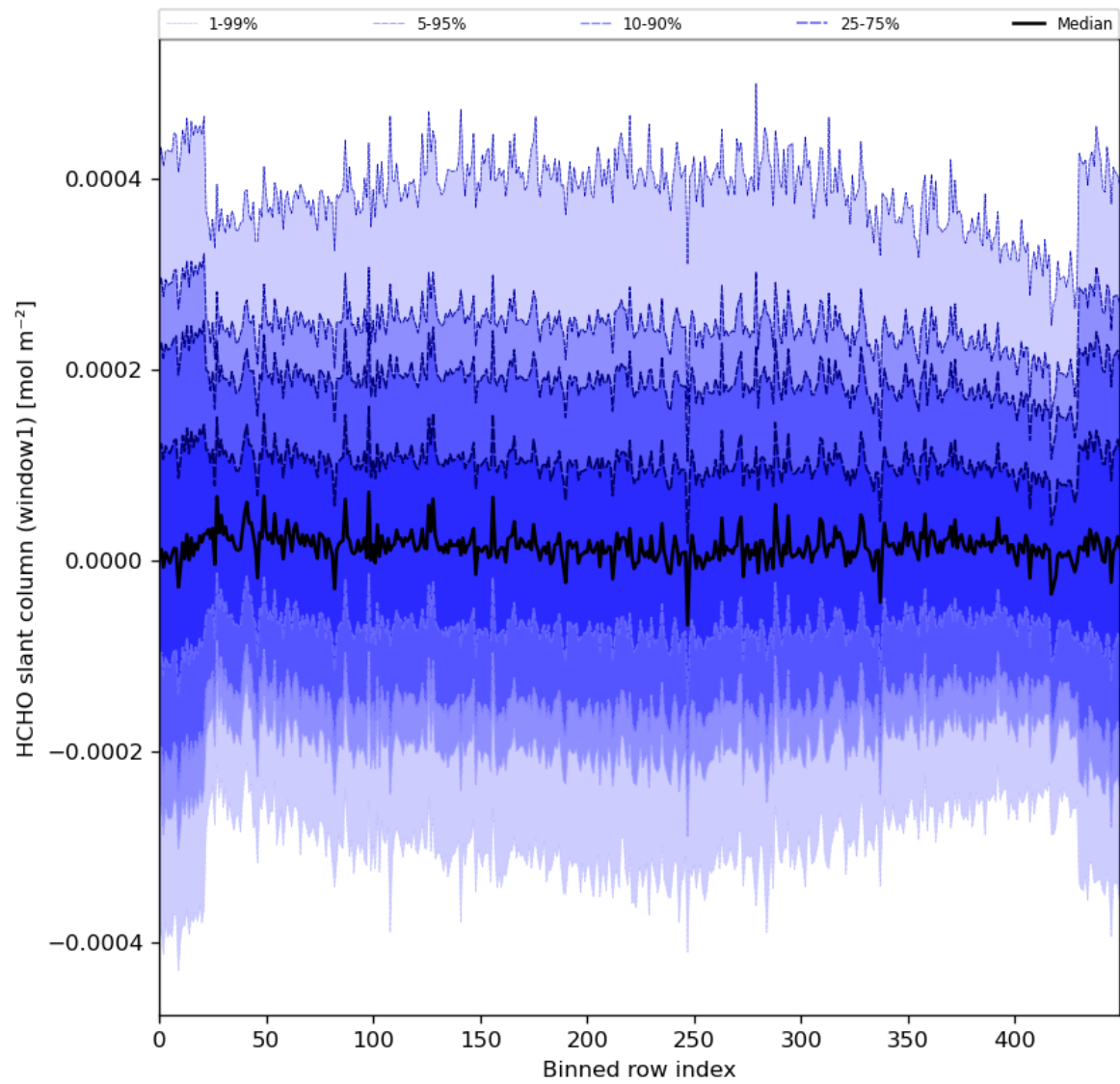
Figure 52: Along track statistics of “HCHO slant column (window1)” for 2024-06-26 to 2024-06-28
