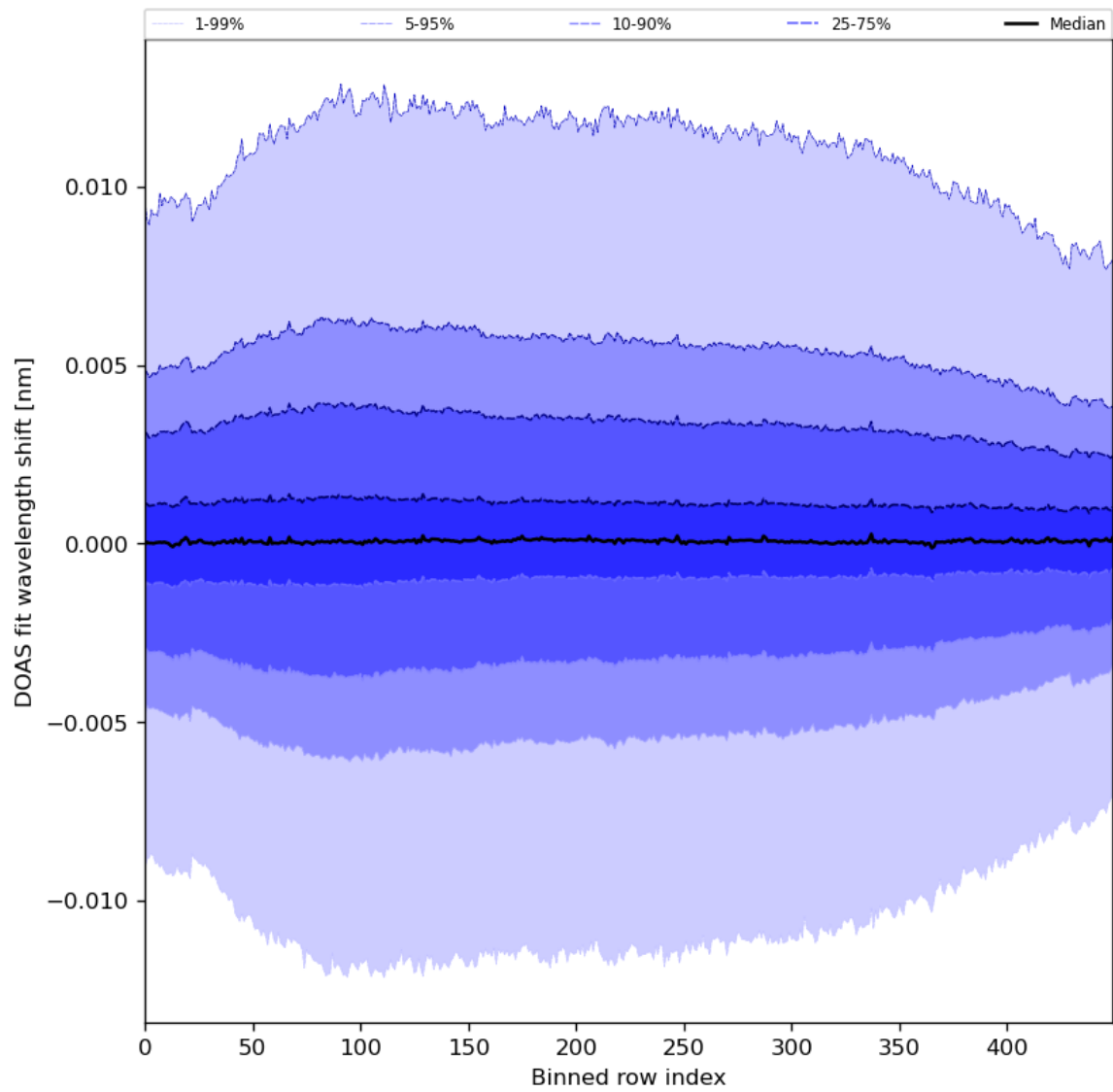
Figure 58: Along track statistics of “DOAS fit wavelength shift” for 2024-06-26 to 2024-06-28
