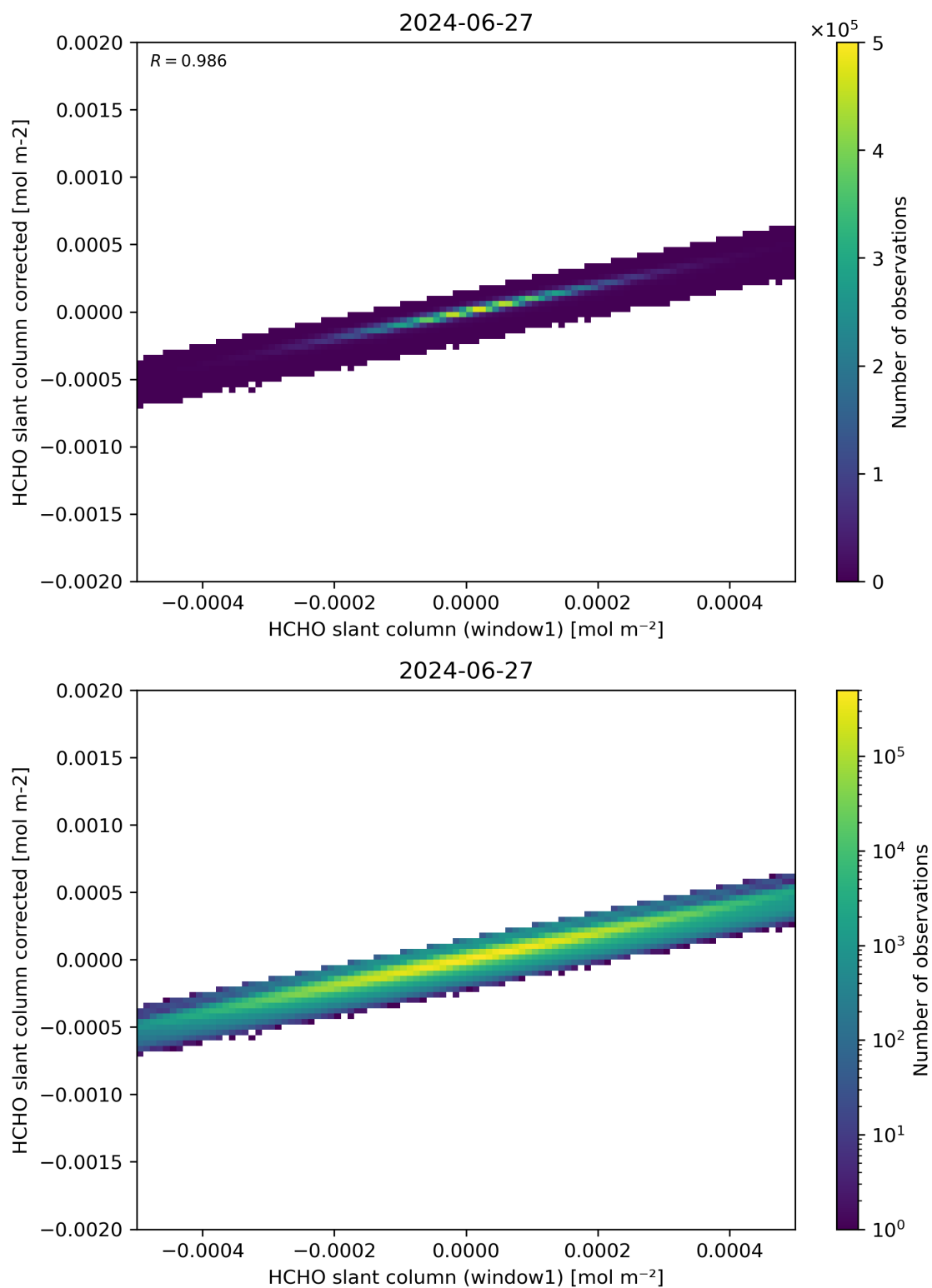
Figure 82: Scatter density plot of “HCHO slant column (window1)” against “HCHO slant column corrected” for 2024-06-26 to 2024-06-28.
