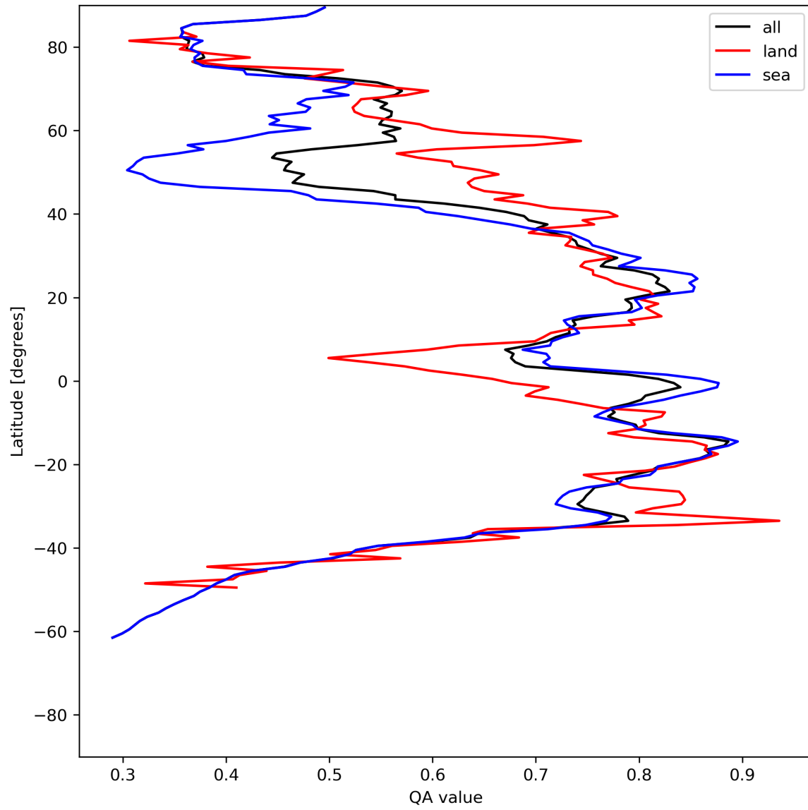
Figure 20: Zonal average of “QA value” for 2024-06-26 to 2024-06-28.
