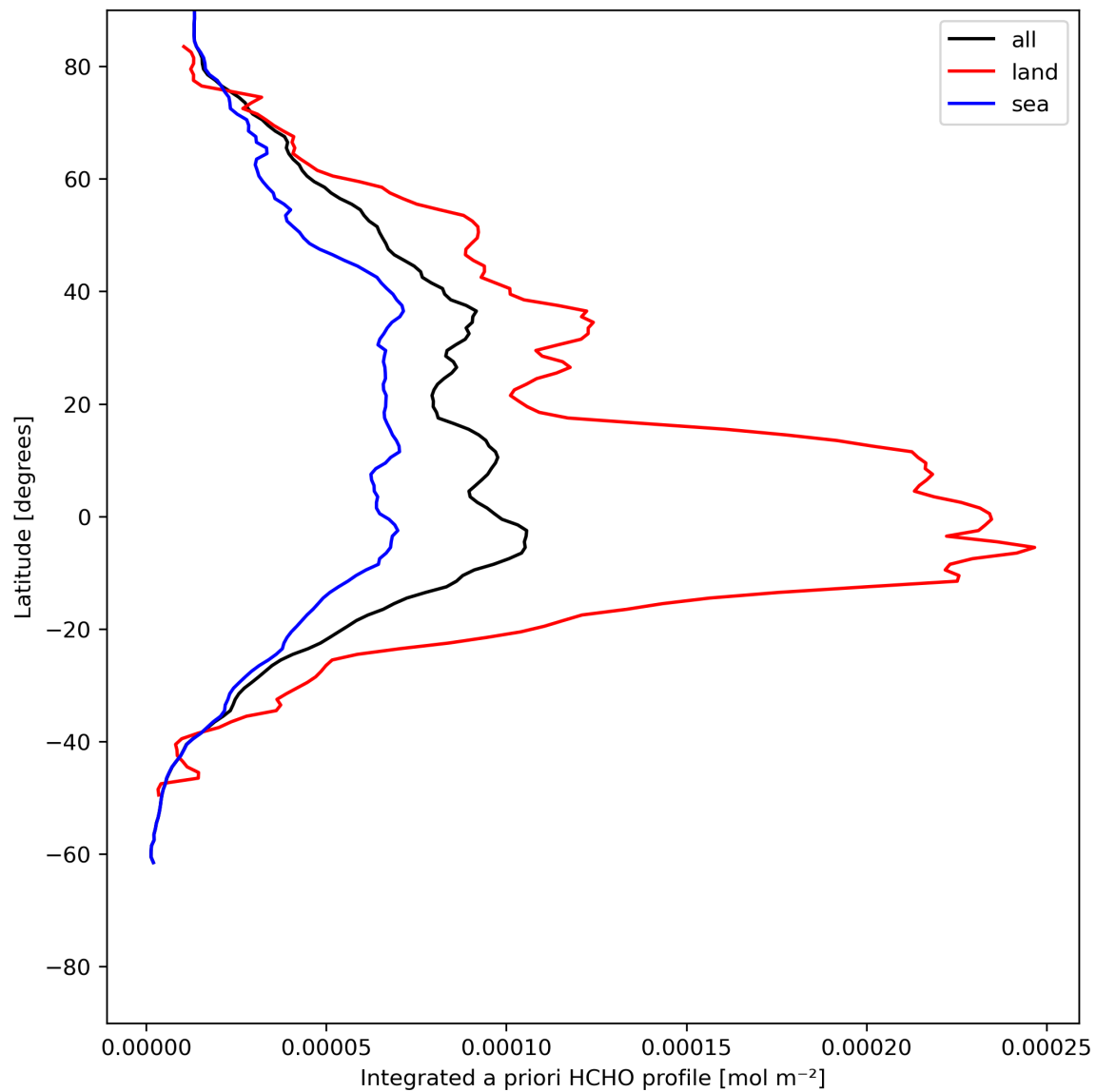
Figure 29: Zonal average of “Integrated a priori HCHO profile” for 2024-06-26 to 2024-06-28.
