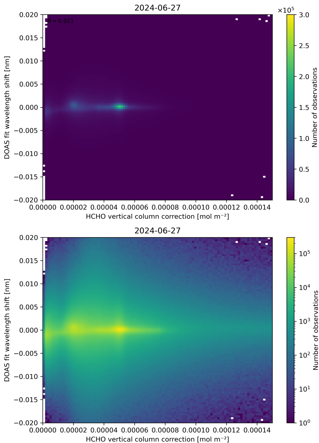
Figure 113: Scatter density plot of “HCHO vertical column correction” against “DOAS fit wavelength shift” for 2024-06-26 to 2024-06-28.
