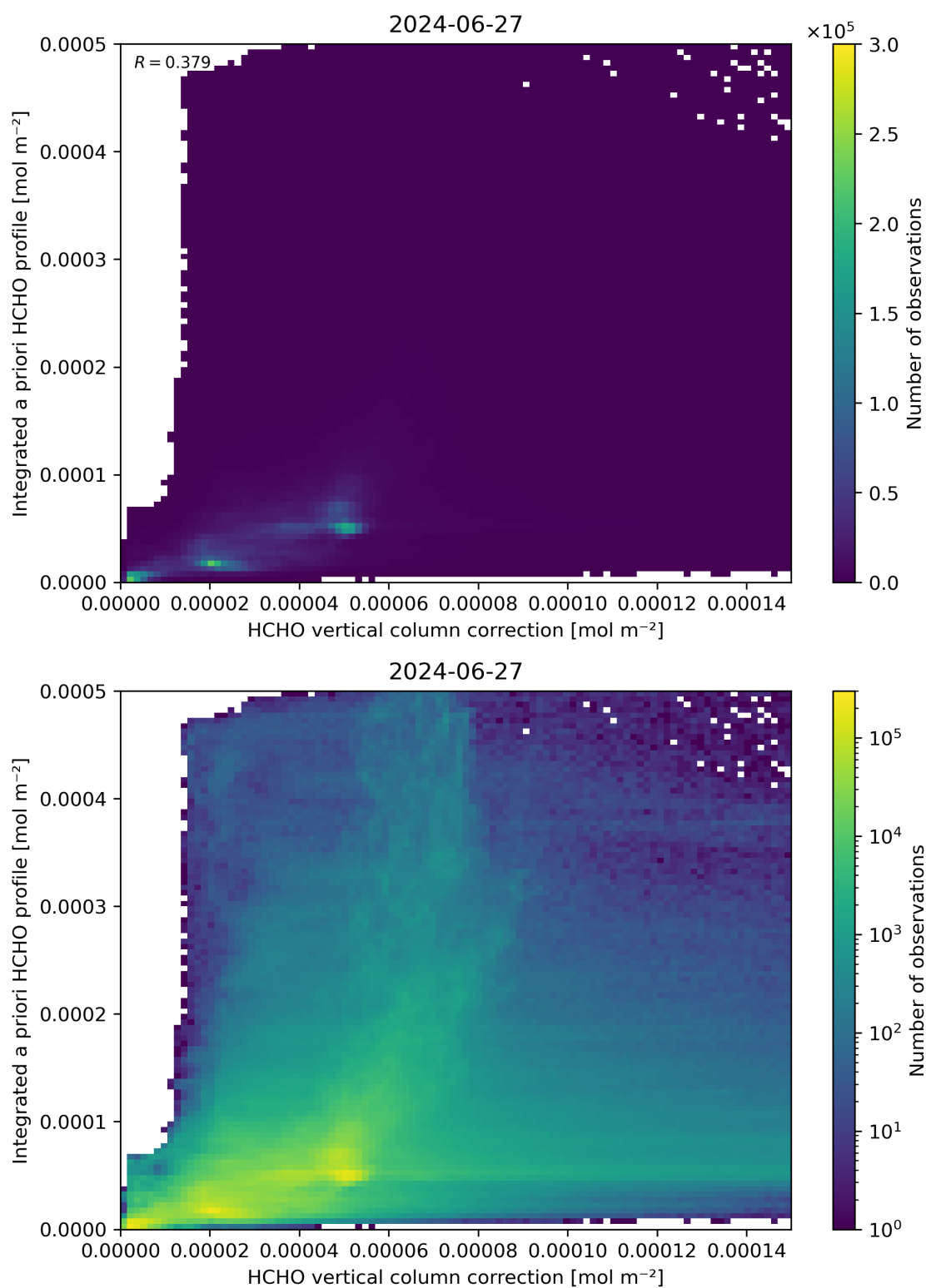
Figure 122: Scatter density plot of “HCHO vertical column correction” against “Integrated a priori HCHO profile” for 2024-06-26 to 2024-06-28.
