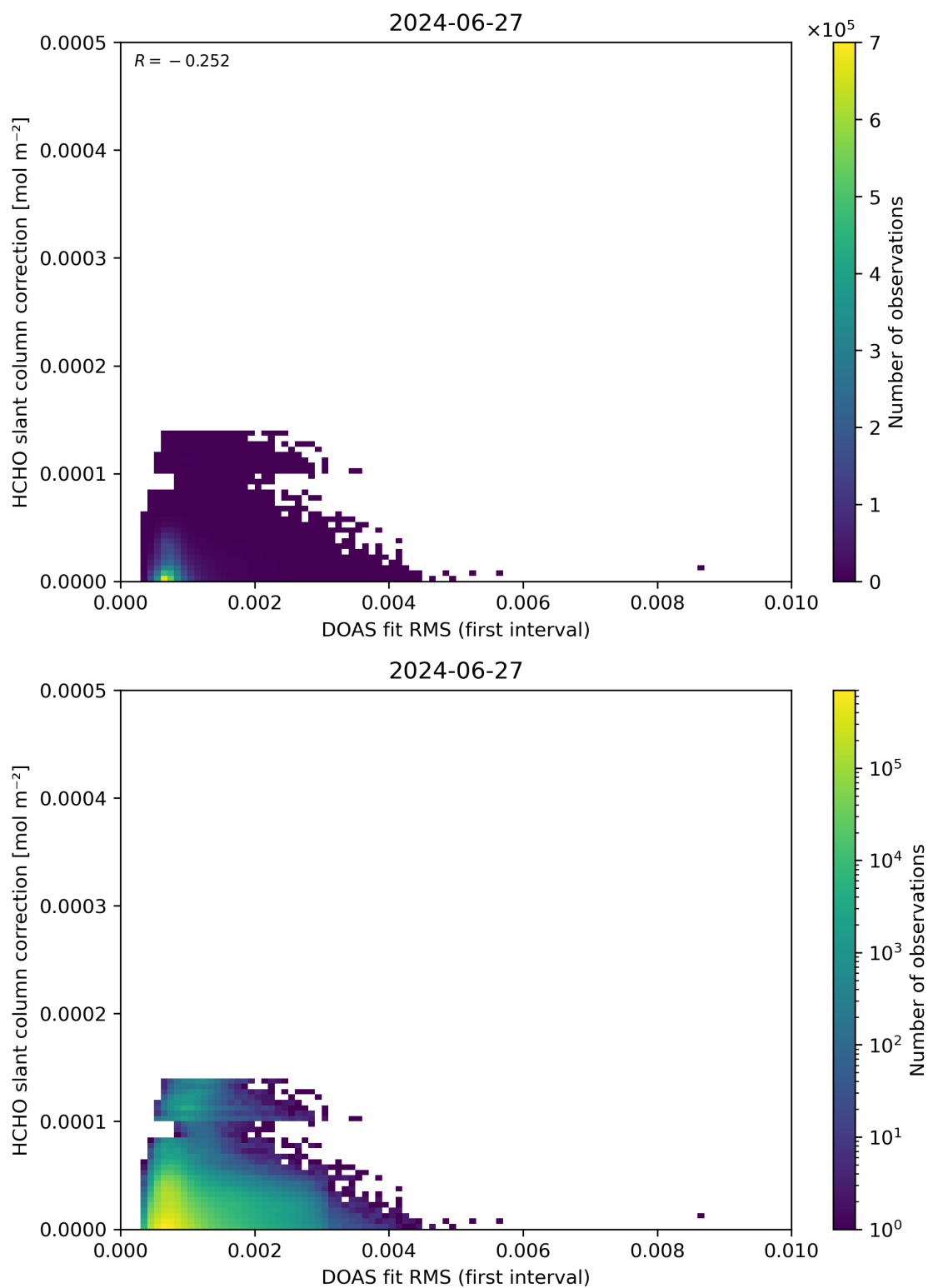
Figure 63: Scatter density plot of “DOAS fit RMS (first interval)” against “HCHO slant column correction” for 2024-06-26 to 2024-06-28.
