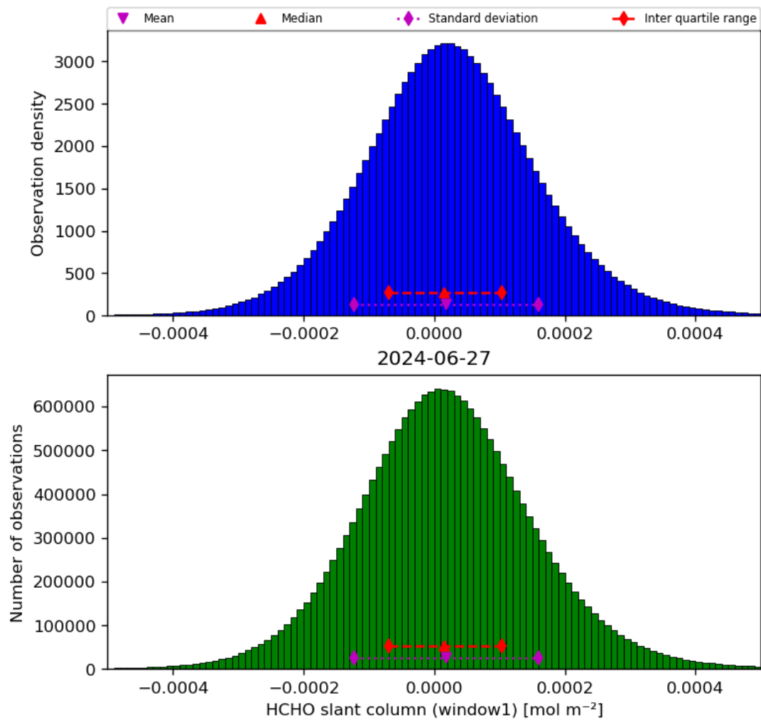
Figure 38: Histogram of “HCHO slant column (window1)” for 2024-06-26 to 2024-06-28
