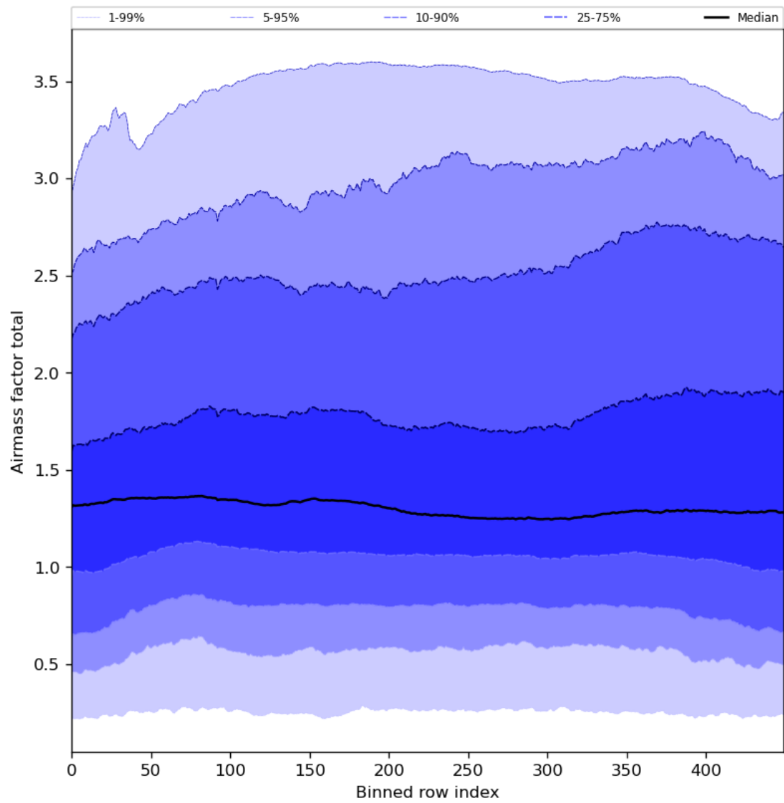
Figure 54: Along track statistics of “Airmass factor total” for 2024-06-26 to 2024-06-28
