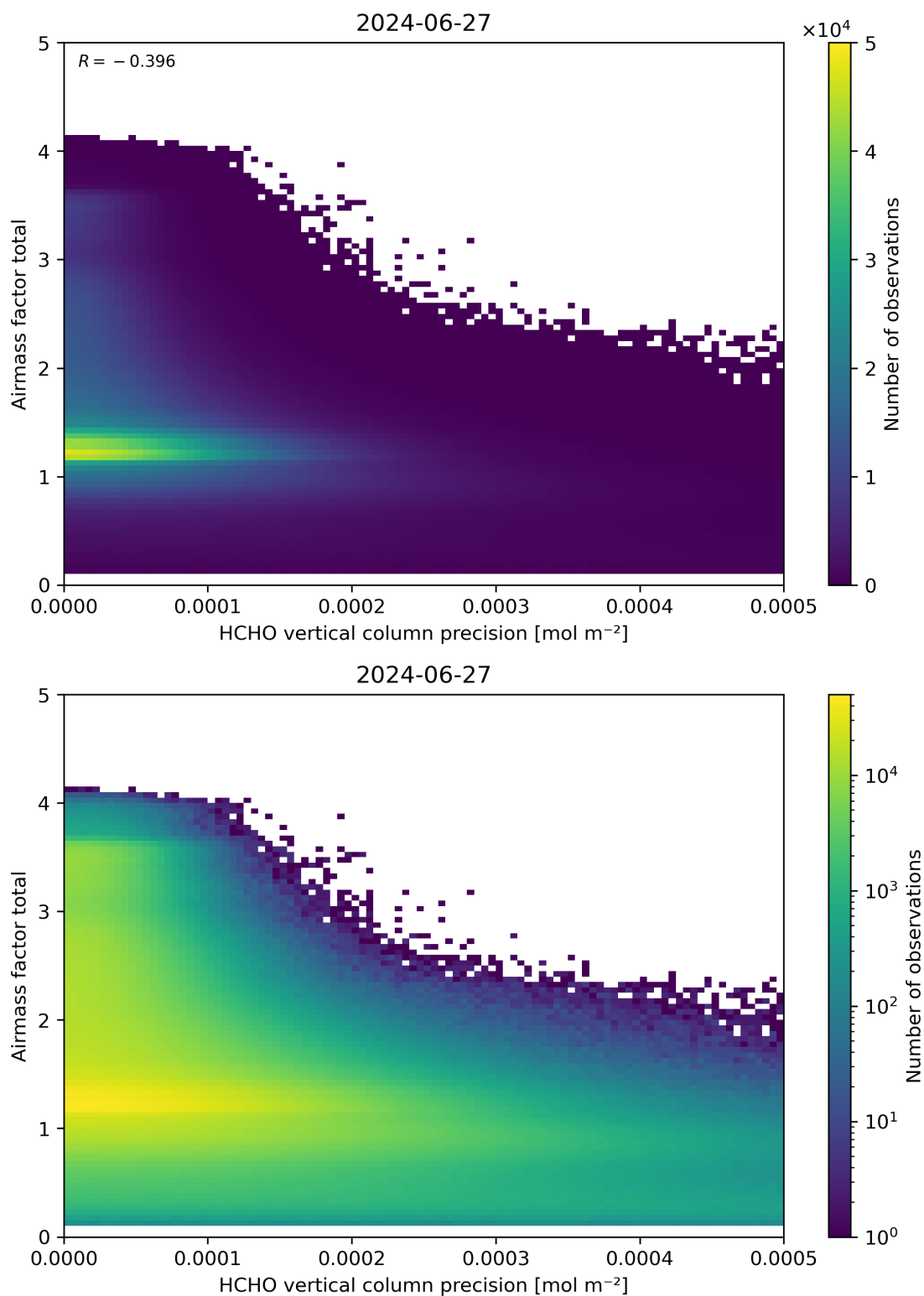
Figure 144: Scatter density plot of “HCHO vertical column precision” against “Airmass factor total” for 2024-06-26 to 2024-06-28.
