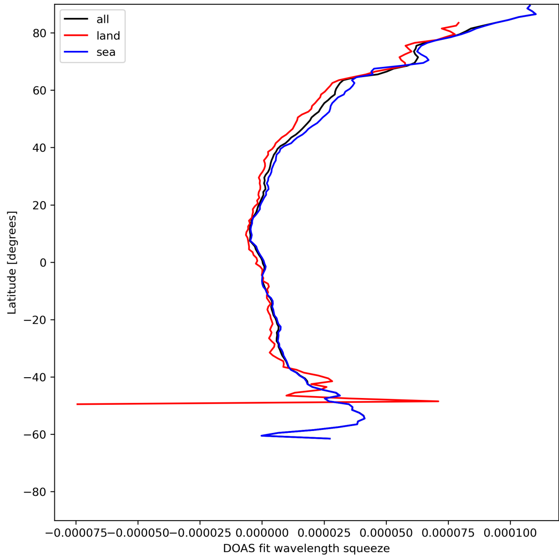
Figure 31: Zonal average of “DOAS fit wavelength squeeze” for 2024-06-26 to 2024-06-28.
