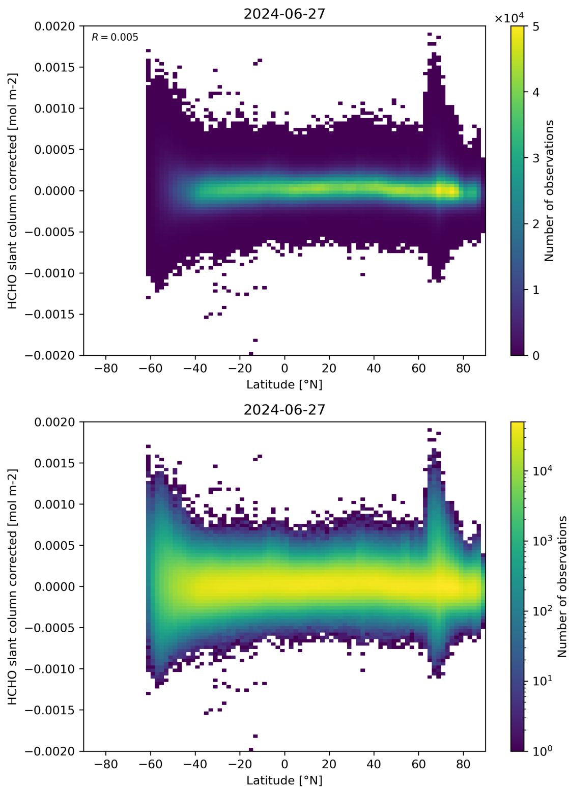
Figure 157: Scatter density plot of “Latitude” against “HCHO slant column corrected” for 2024-06-26 to 2024-06-28.
