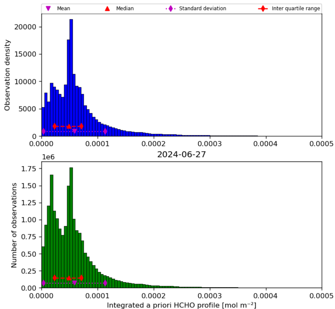
Figure 43: Histogram of “Integrated a priori HCHO profile” for 2024-06-26 to 2024-06-28
