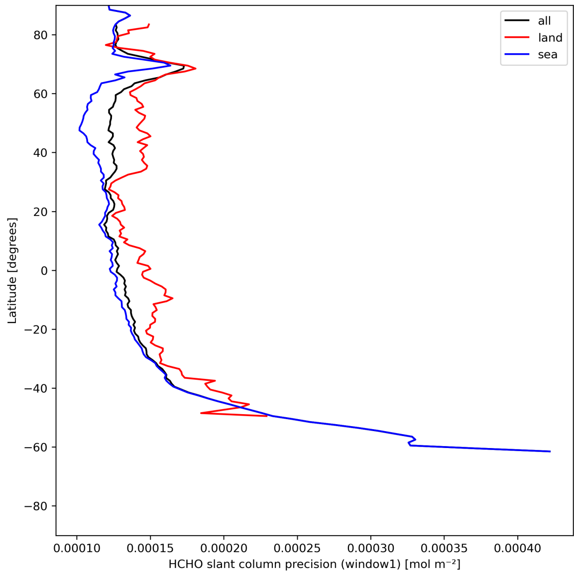
Figure 25: Zonal average of “HCHO slant column precision (window1)” for 2024-06-26 to 2024-06-28.
