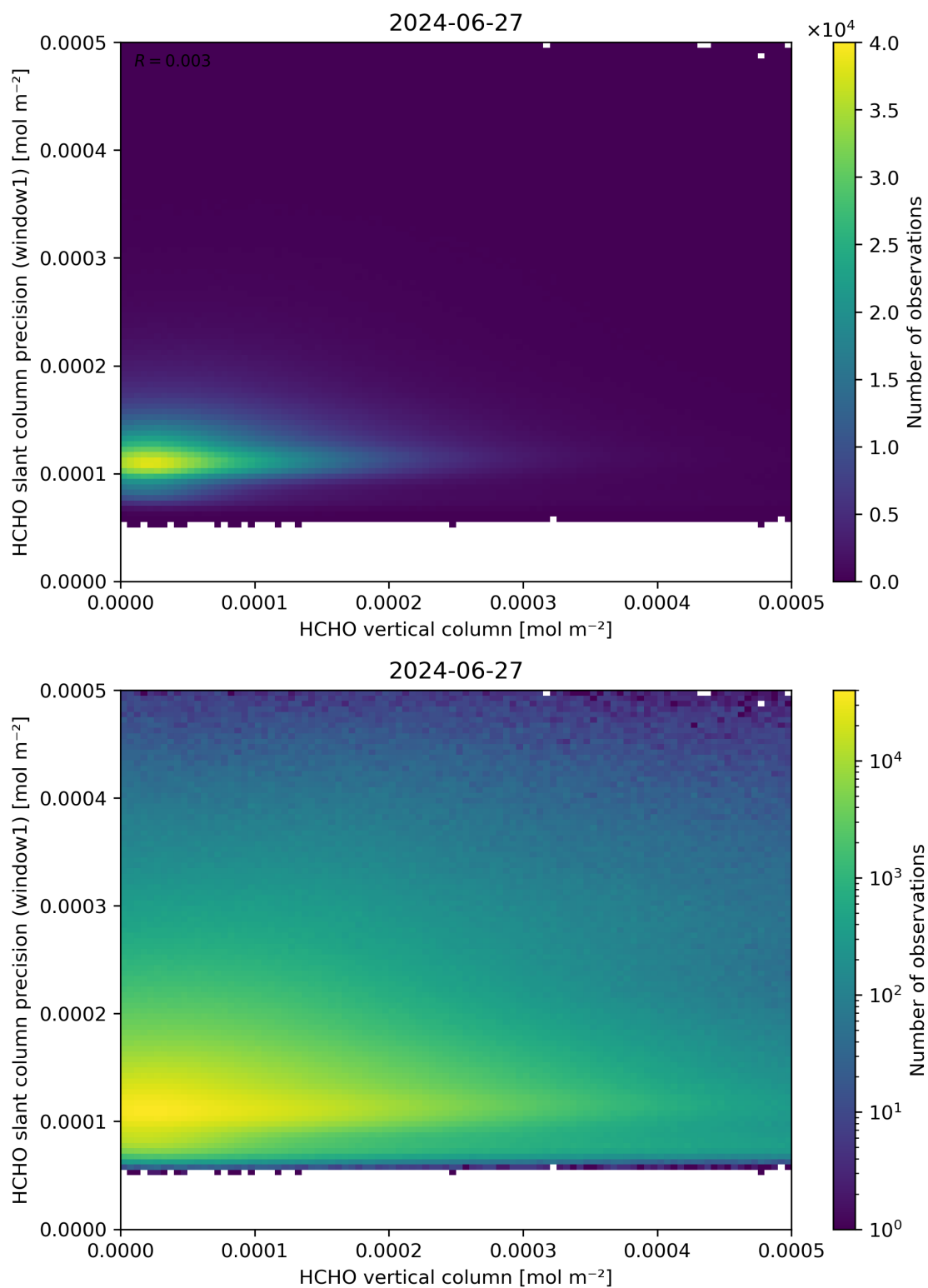
Figure 130: Scatter density plot of “HCHO vertical column” against “HCHO slant column precision (window1)” for 2024-06-26 to 2024-06-28.
