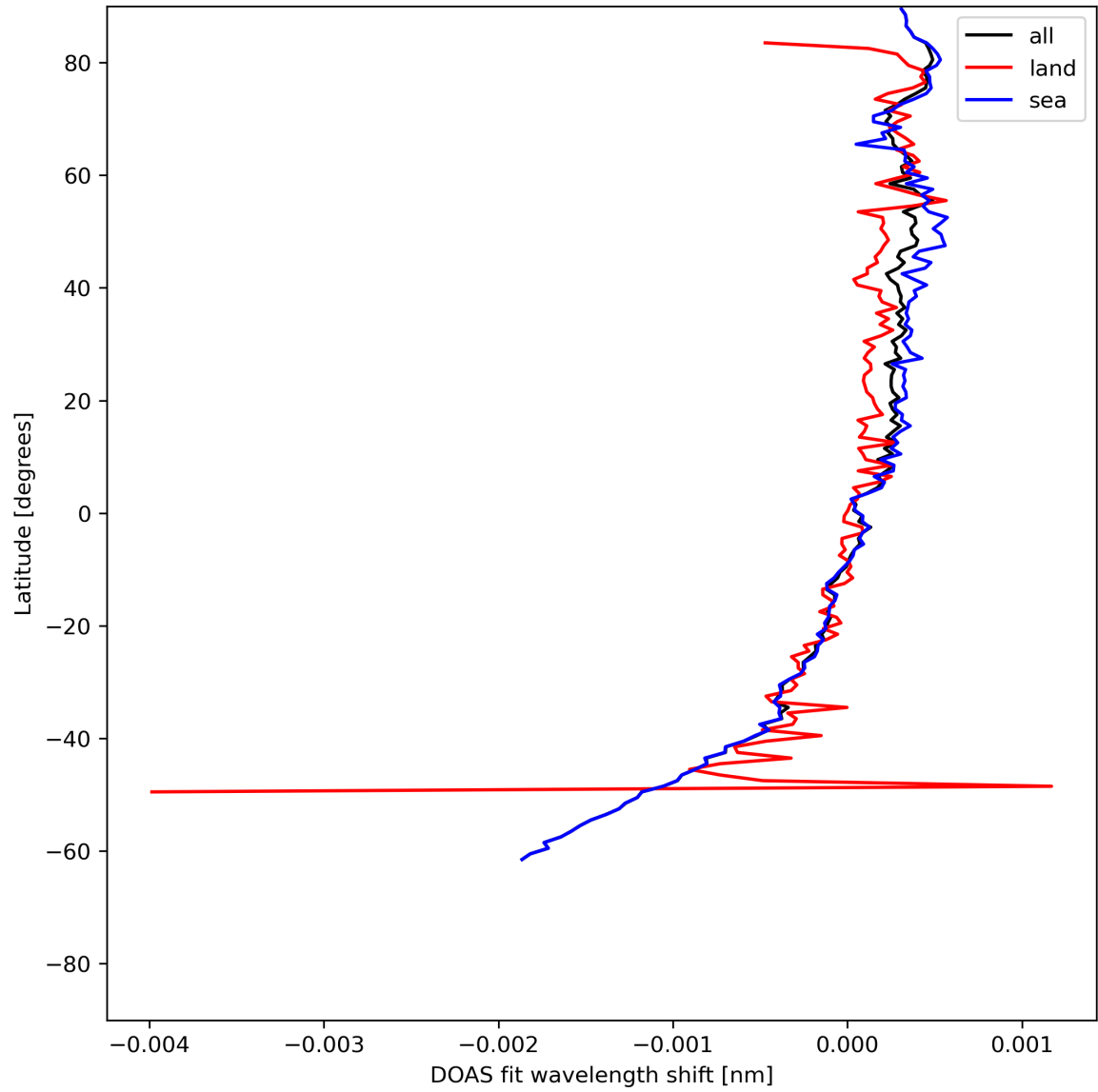
Figure 30: Zonal average of “DOAS fit wavelength shift” for 2024-06-26 to 2024-06-28.
