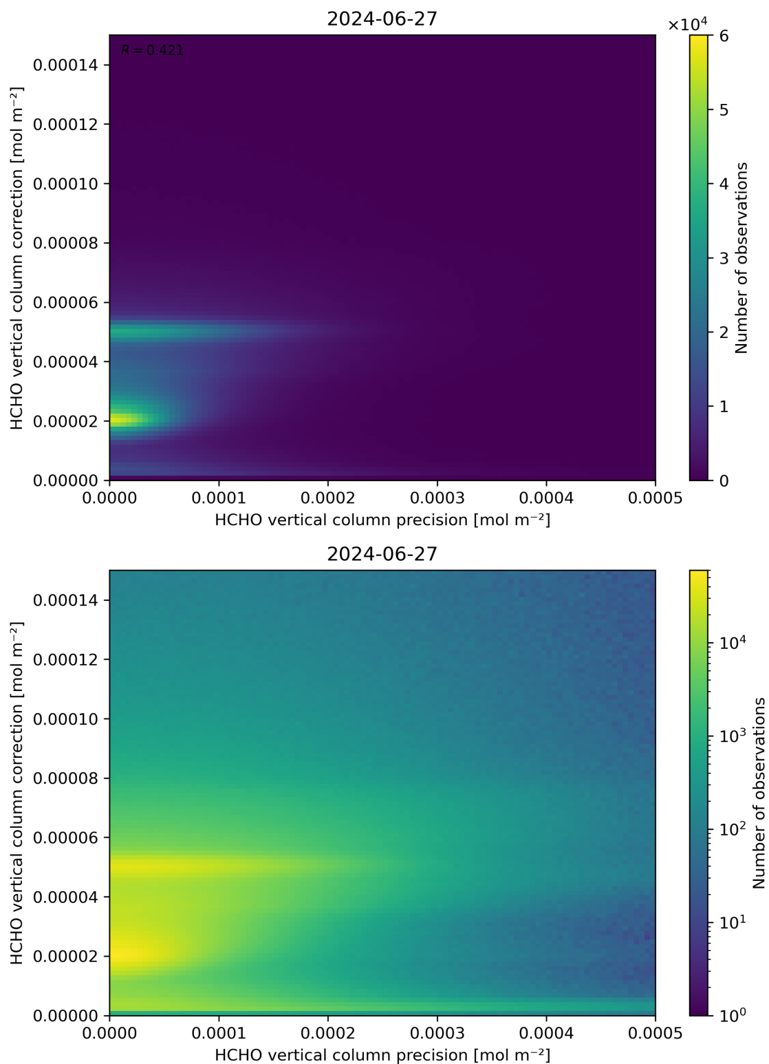
Figure 146: Scatter density plot of “HCHO vertical column precision” against “HCHO vertical column correction” for 2024-06-26 to 2024-06-28.
