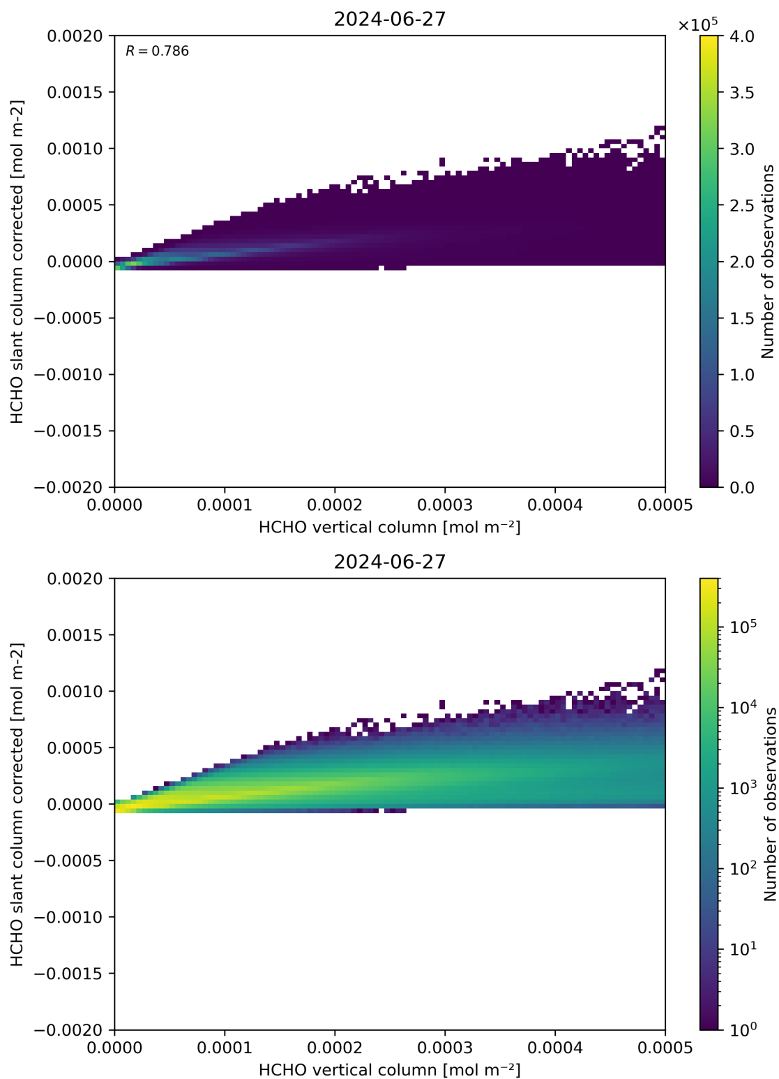
Figure 127: Scatter density plot of “HCHO vertical column” against “HCHO slant column corrected” for 2024-06-26 to 2024-06-28.
