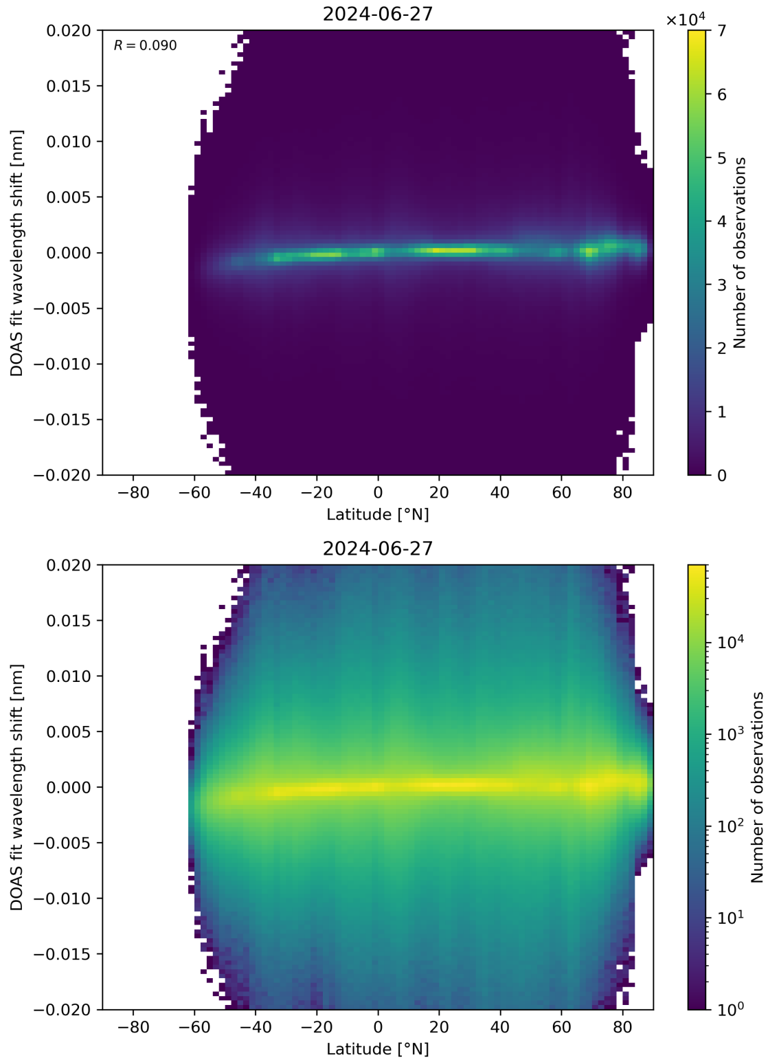
Figure 154: Scatter density plot of “Latitude” against “DOAS fit wavelength shift” for 2024-06-26 to 2024-06-28.
