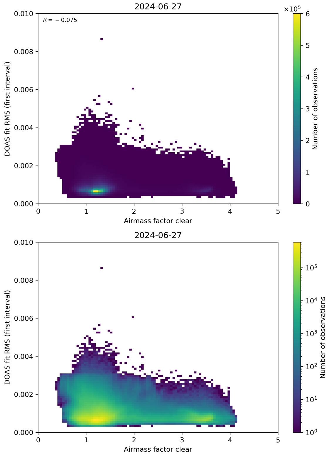
Figure 71: Scatter density plot of “Airmass factor clear” against “DOAS fit RMS (first interval)” for 2024-06-26 to 2024-06-28.
