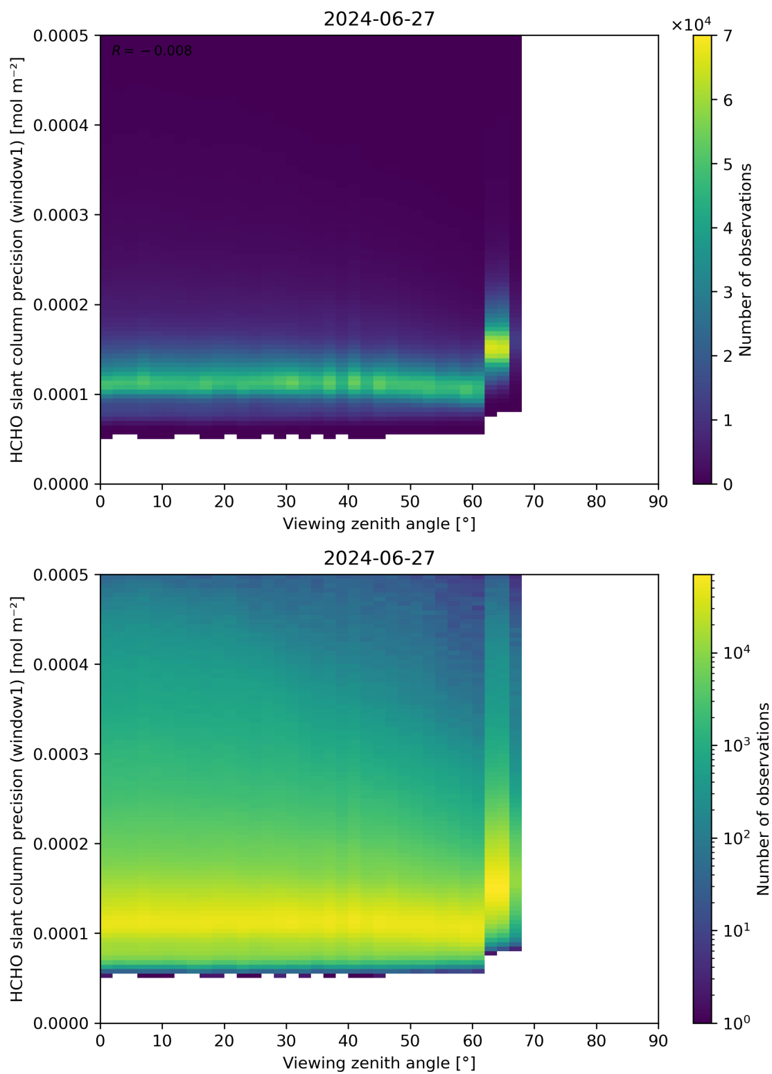
Figure 189: Scatter density plot of “Viewing zenith angle” against “HCHO slant column precision (window1)” for 2024-06-26 to 2024-06-28.
