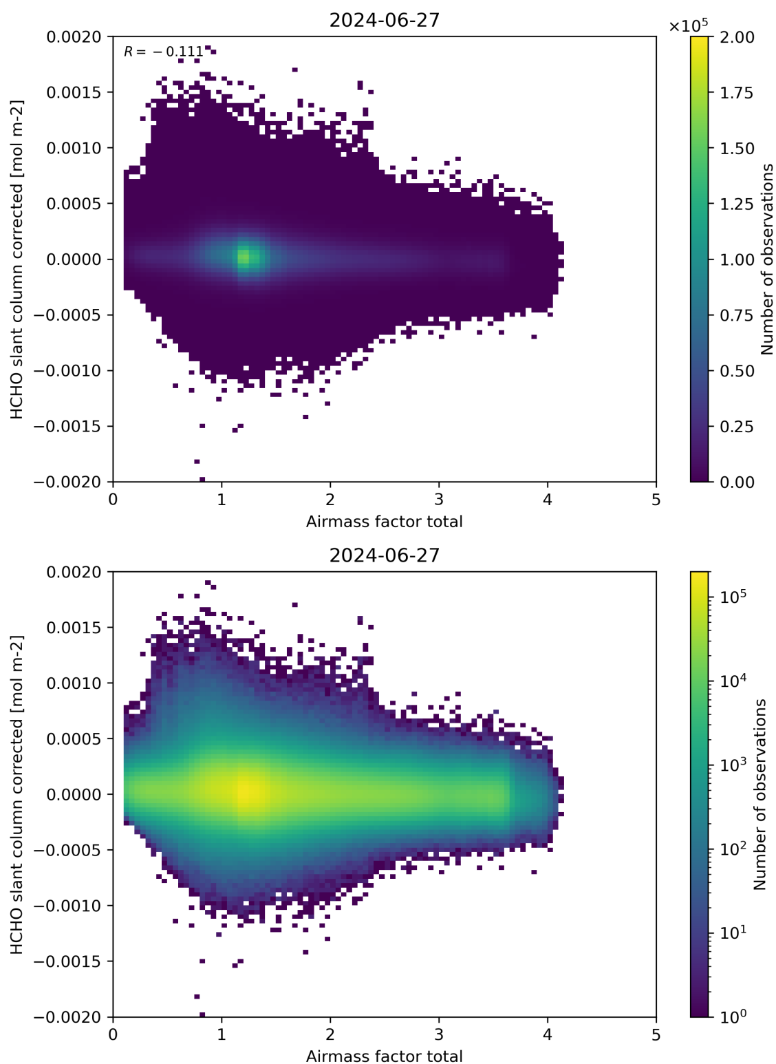
Figure 101: Scatter density plot of “Airmass factor total” against “HCHO slant column corrected” for 2024-06-26 to 2024-06-28.
