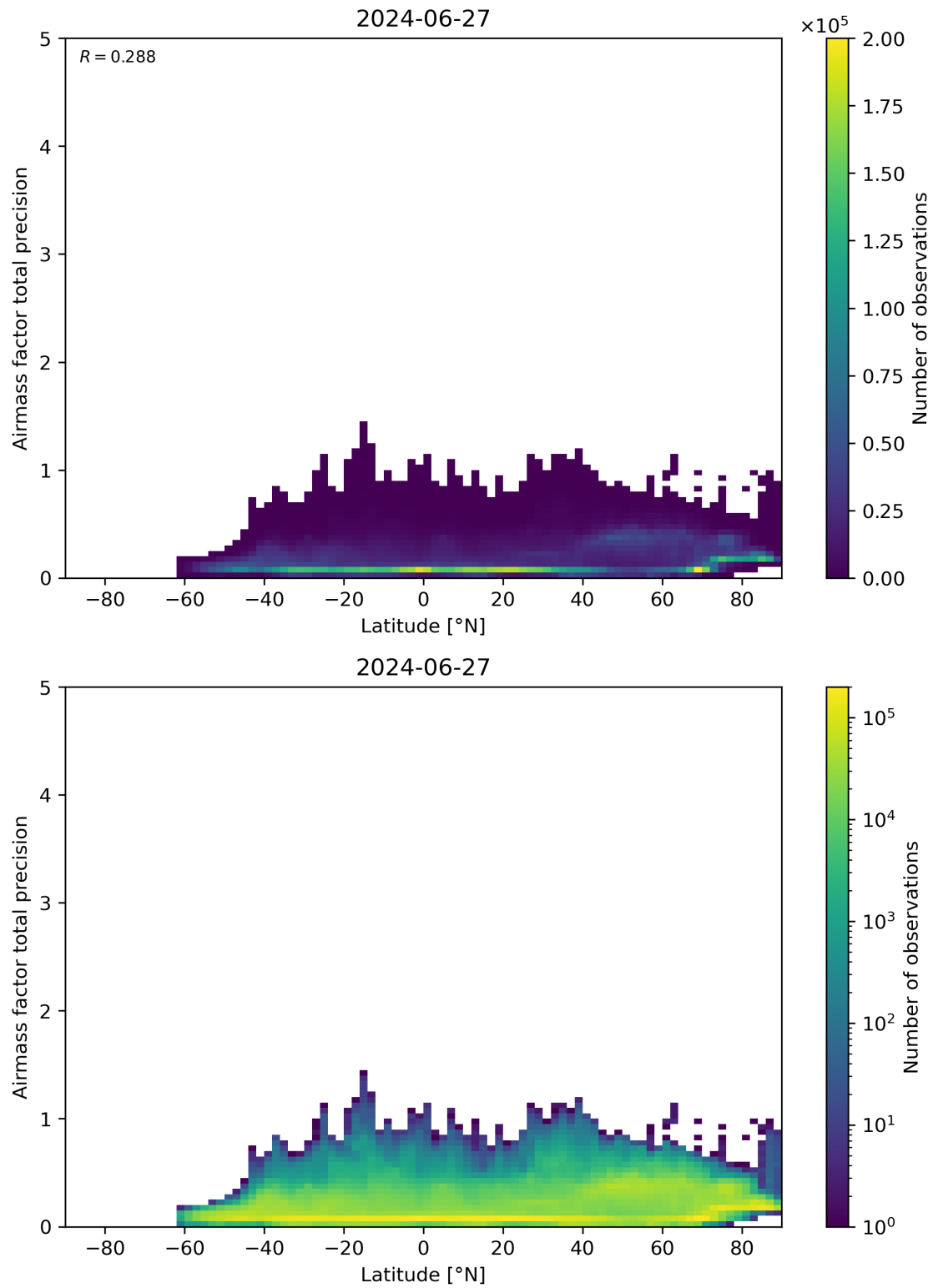
Figure 162: Scatter density plot of “Latitude” against “Airmass factor total precision” for 2024-06-26 to 2024-06-28.
