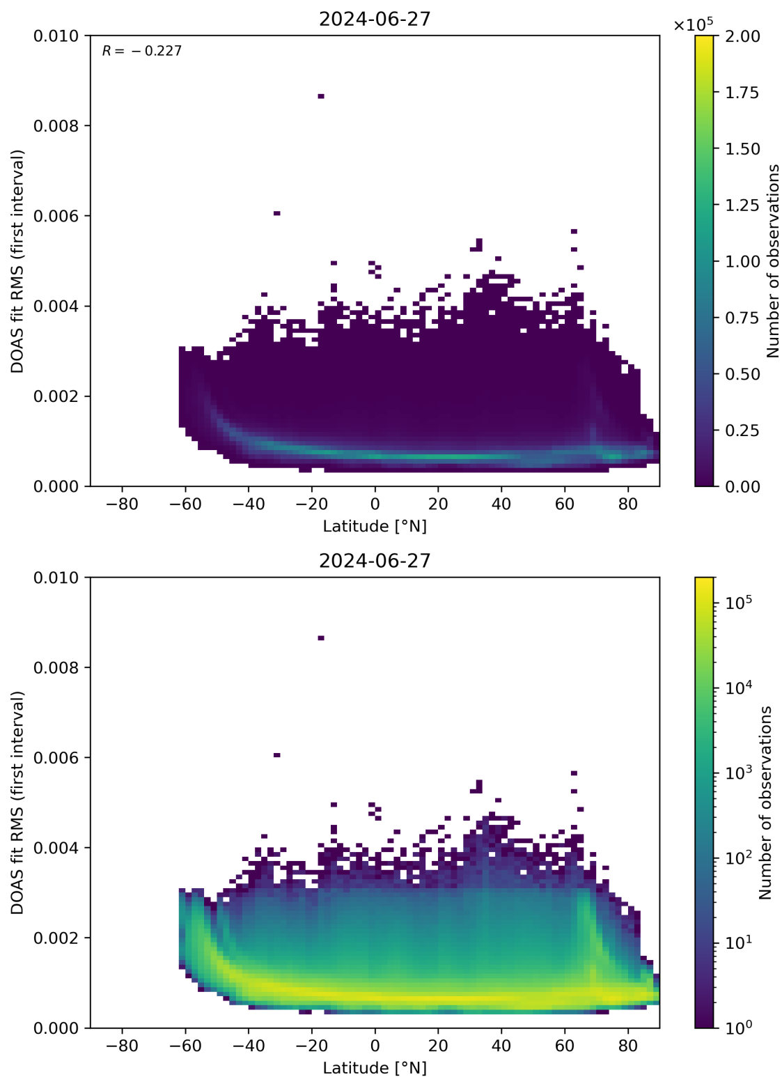
Figure 153: Scatter density plot of “Latitude” against “DOAS fit RMS (first interval)” for 2024-06-26 to 2024-06-28.
