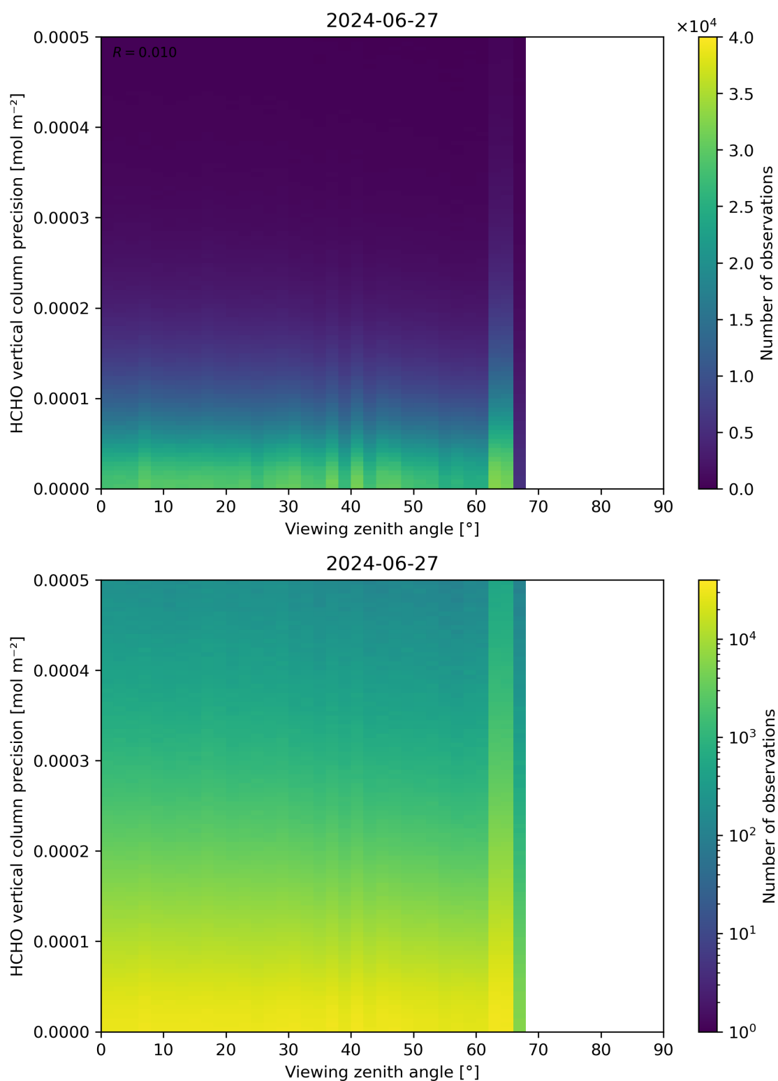
Figure 194: Scatter density plot of “Viewing zenith angle” against “HCHO vertical column precision” for 2024-06-26 to 2024-06-28.
