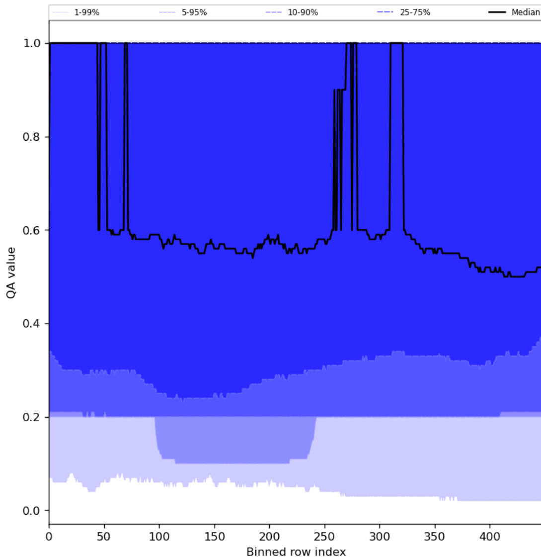
Figure 48: Along track statistics of “QA value” for 2024-06-26 to 2024-06-28
