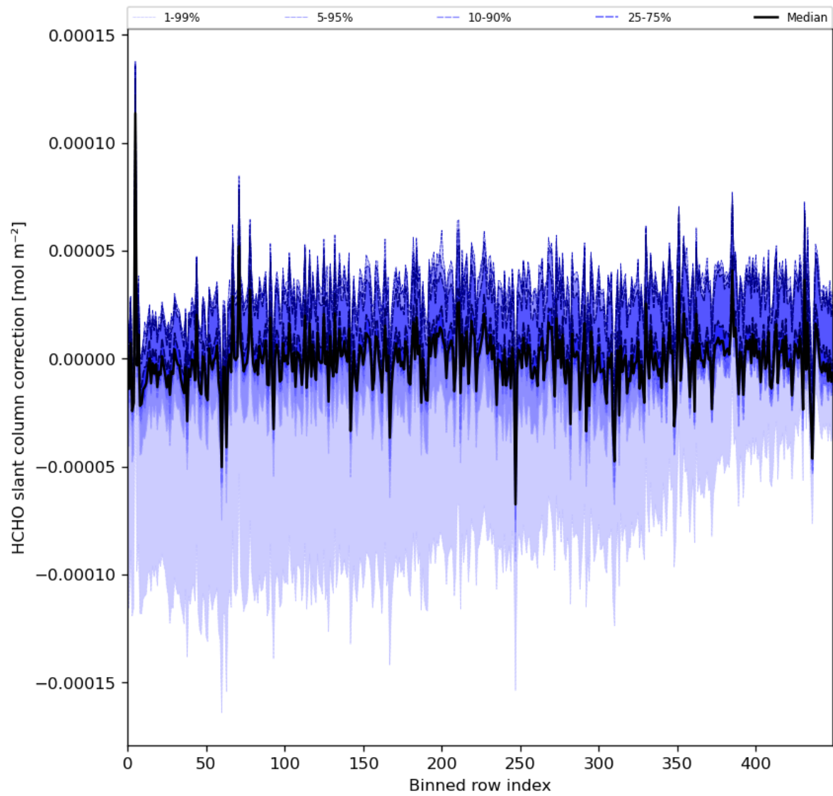
Figure 61: Along track statistics of “HCHO slant column correction” for 2024-06-26 to 2024-06-28
