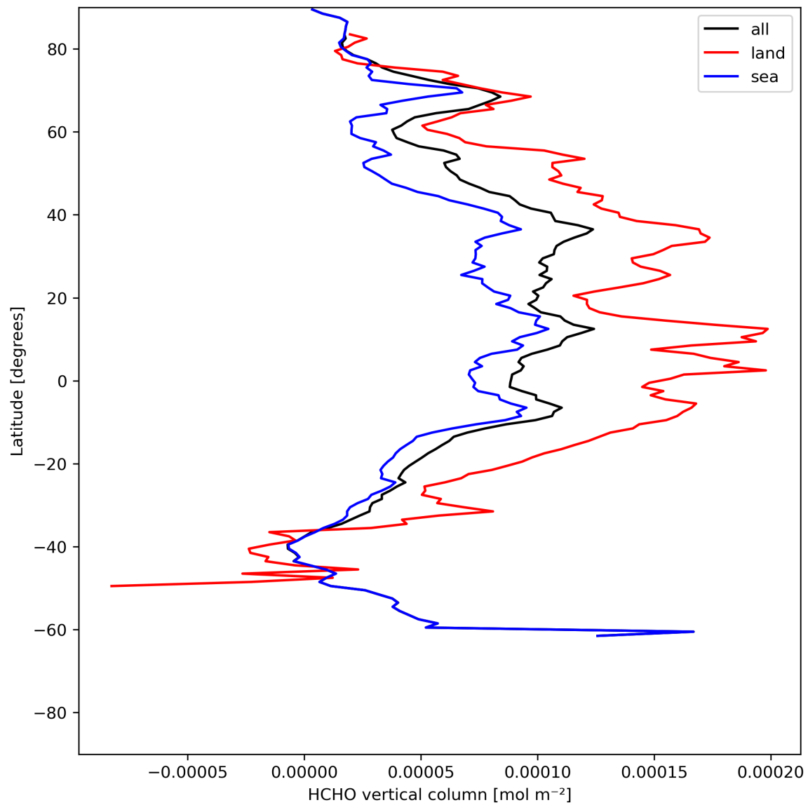
Figure 21: Zonal average of “HCHO vertical column” for 2024-06-26 to 2024-06-28.
