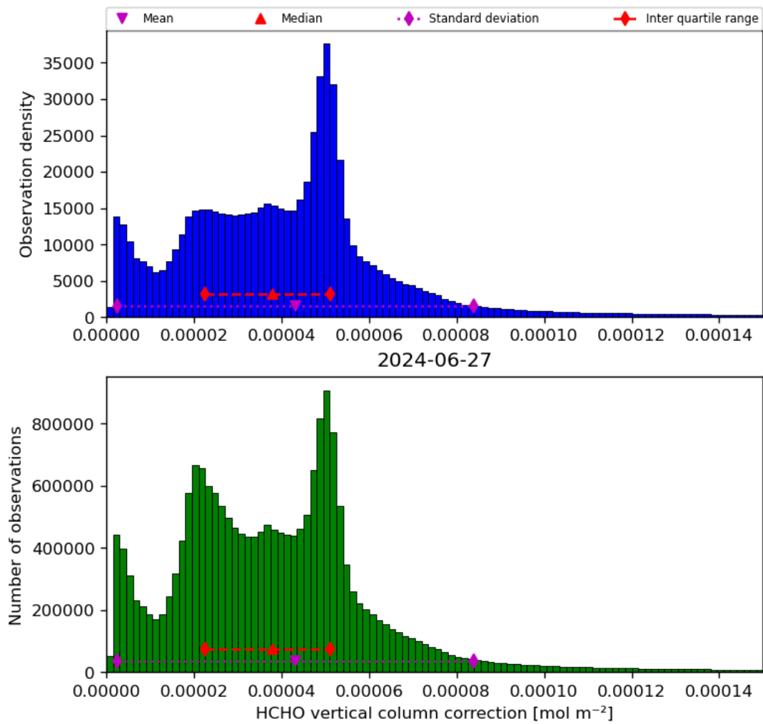
Figure 37: Histogram of “HCHO vertical column correction” for 2024-06-26 to 2024-06-28
