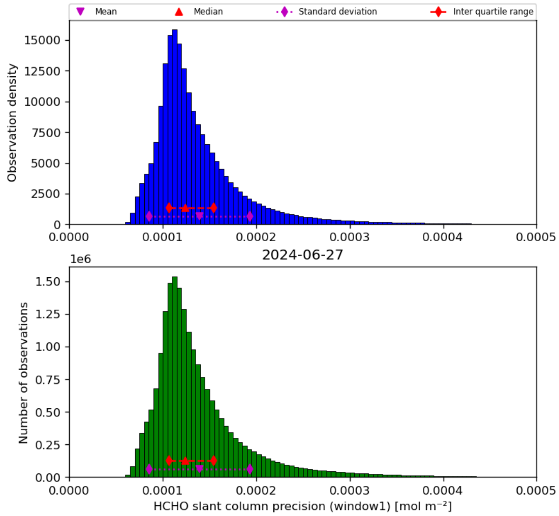
Figure 39: Histogram of “HCHO slant column precision (window1)” for 2024-06-26 to 2024-06-28
