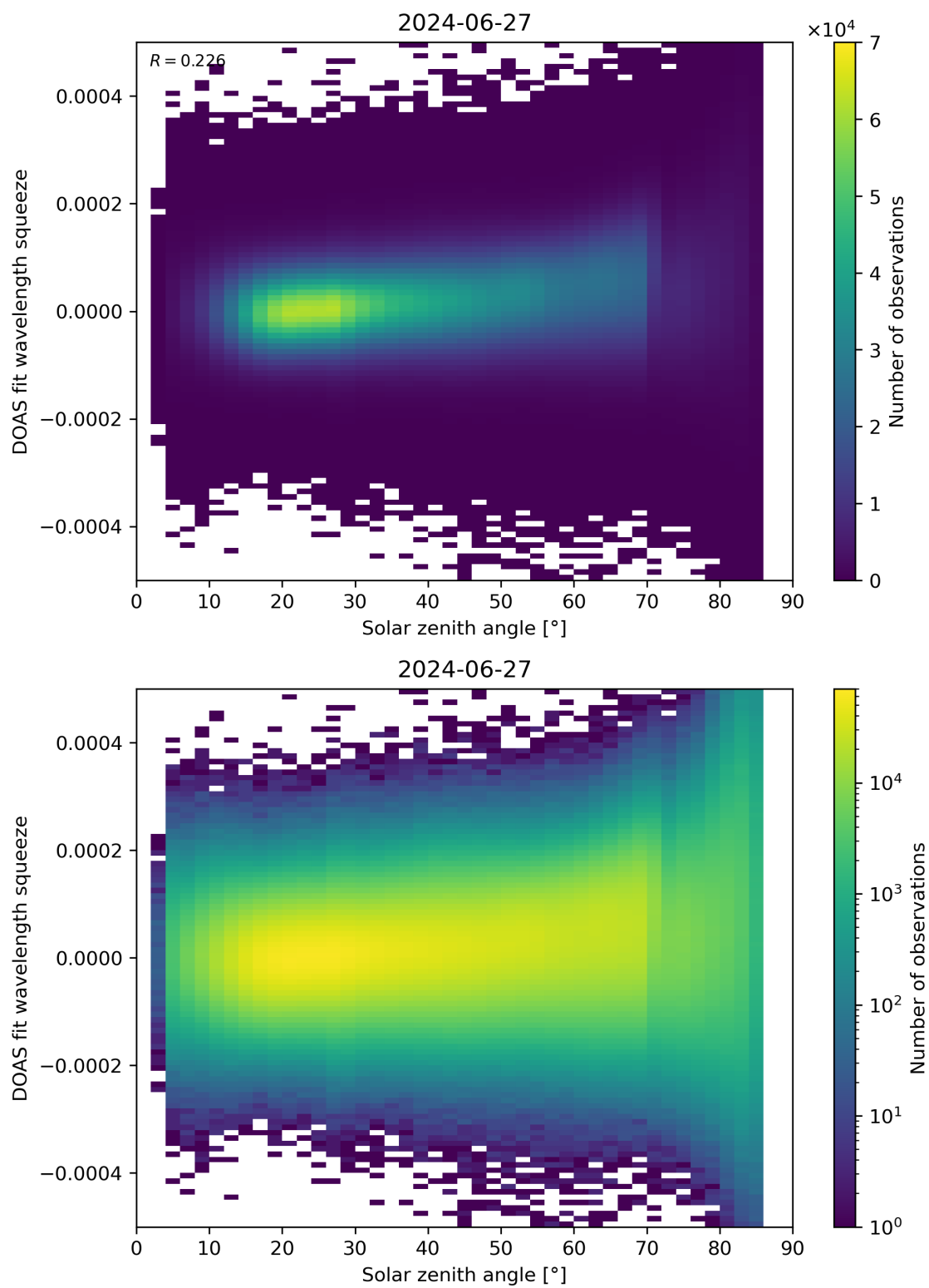
Figure 169: Scatter density plot of “Solar zenith angle” against “DOAS fit wavelength squeeze” for 2024-06-26 to 2024-06-28.
