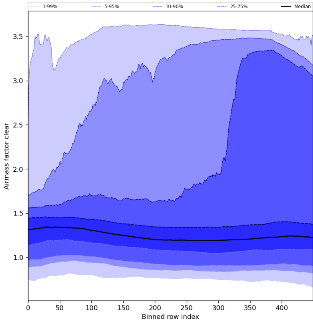
Figure 56: Along track statistics of “Airmass factor clear” for 2024-06-26 to 2024-06-28
