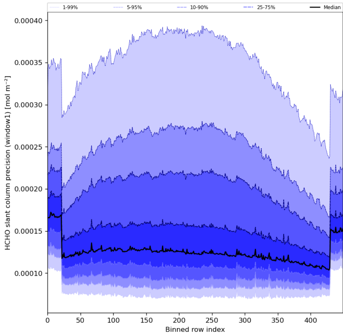
Figure 53: Along track statistics of “HCHO slant column precision (window1)” for 2024-06-26 to 2024-06-28
