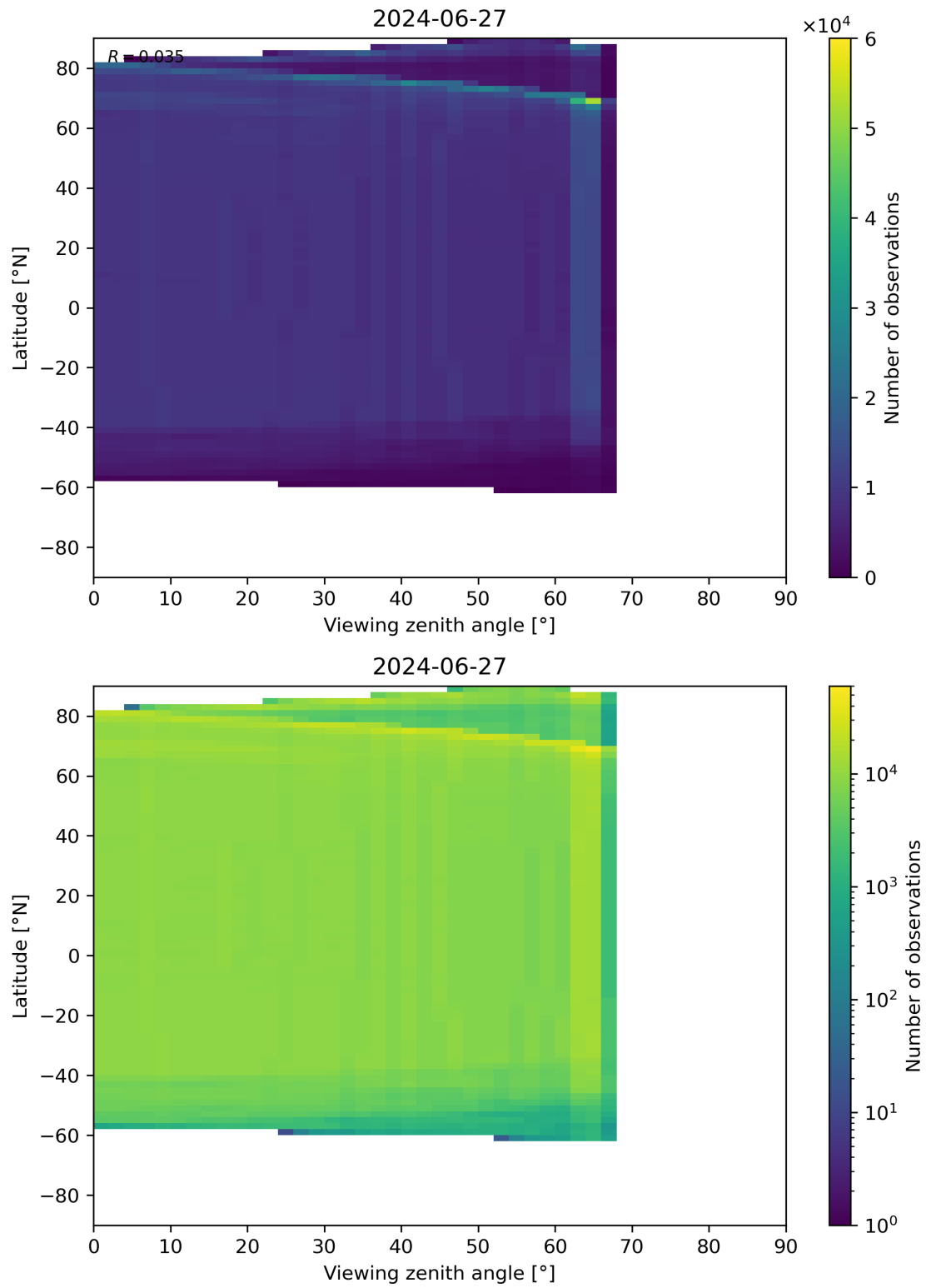
Figure 196: Scatter density plot of “Viewing zenith angle” against “Latitude” for 2024-06-26 to 2024-06-28.
