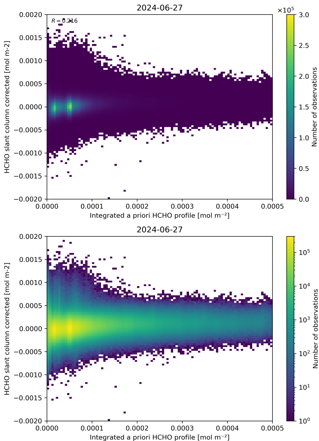
Figure 151: Scatter density plot of “Integrated a priori HCHO profile” against “HCHO slant column corrected” for 2024-06-26 to 2024-06-28.
