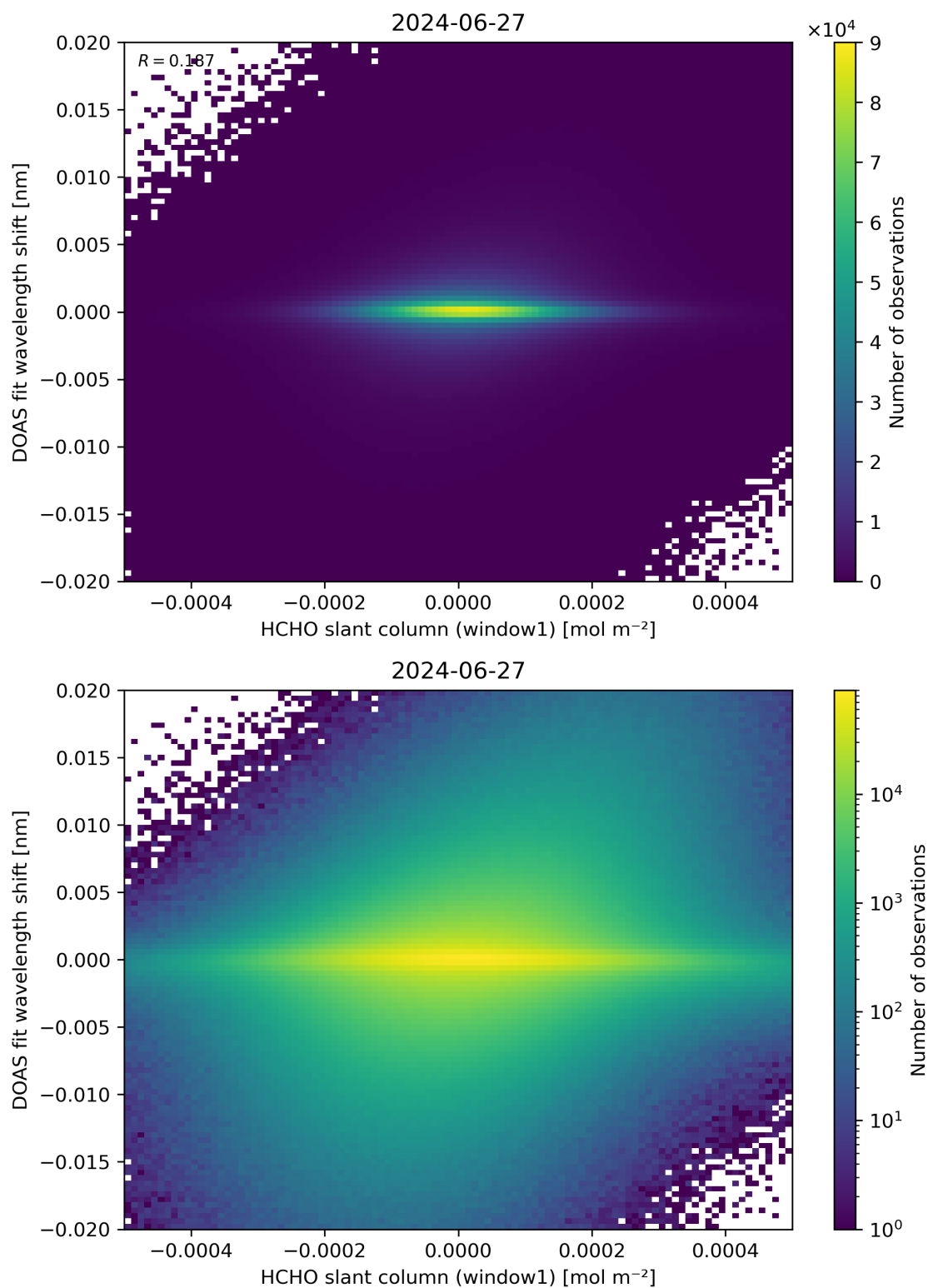
Figure 79: Scatter density plot of “HCHO slant column (window1)” against “DOAS fit wavelength shift” for 2024-06-26 to 2024-06-28.
