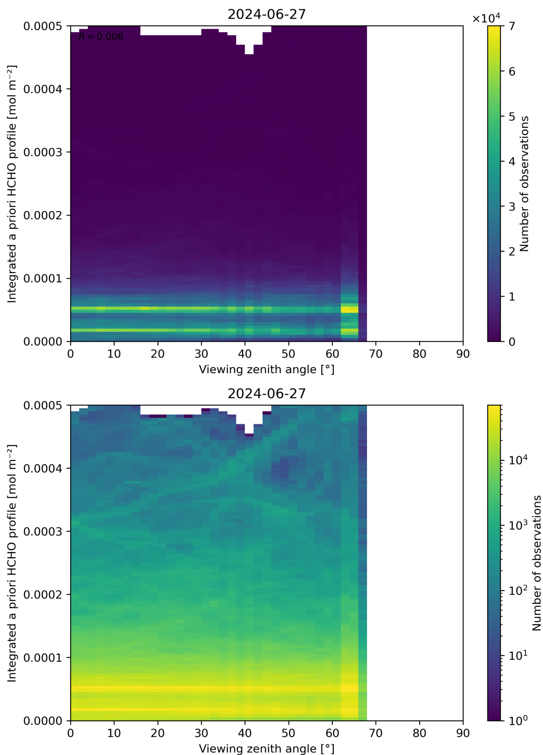
Figure 195: Scatter density plot of “Viewing zenith angle” against “Integrated a priori HCHO profile” for 2024-06-26 to 2024-06-28.
