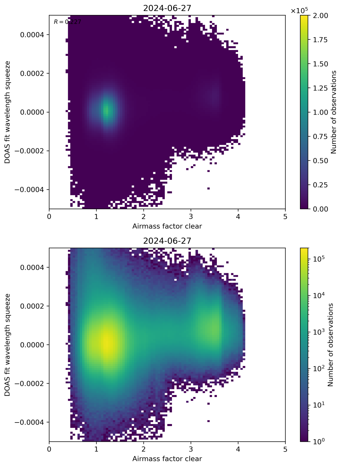
Figure 73: Scatter density plot of “Airmass factor clear” against “DOAS fit wavelength squeeze” for 2024-06-26 to 2024-06-28.
