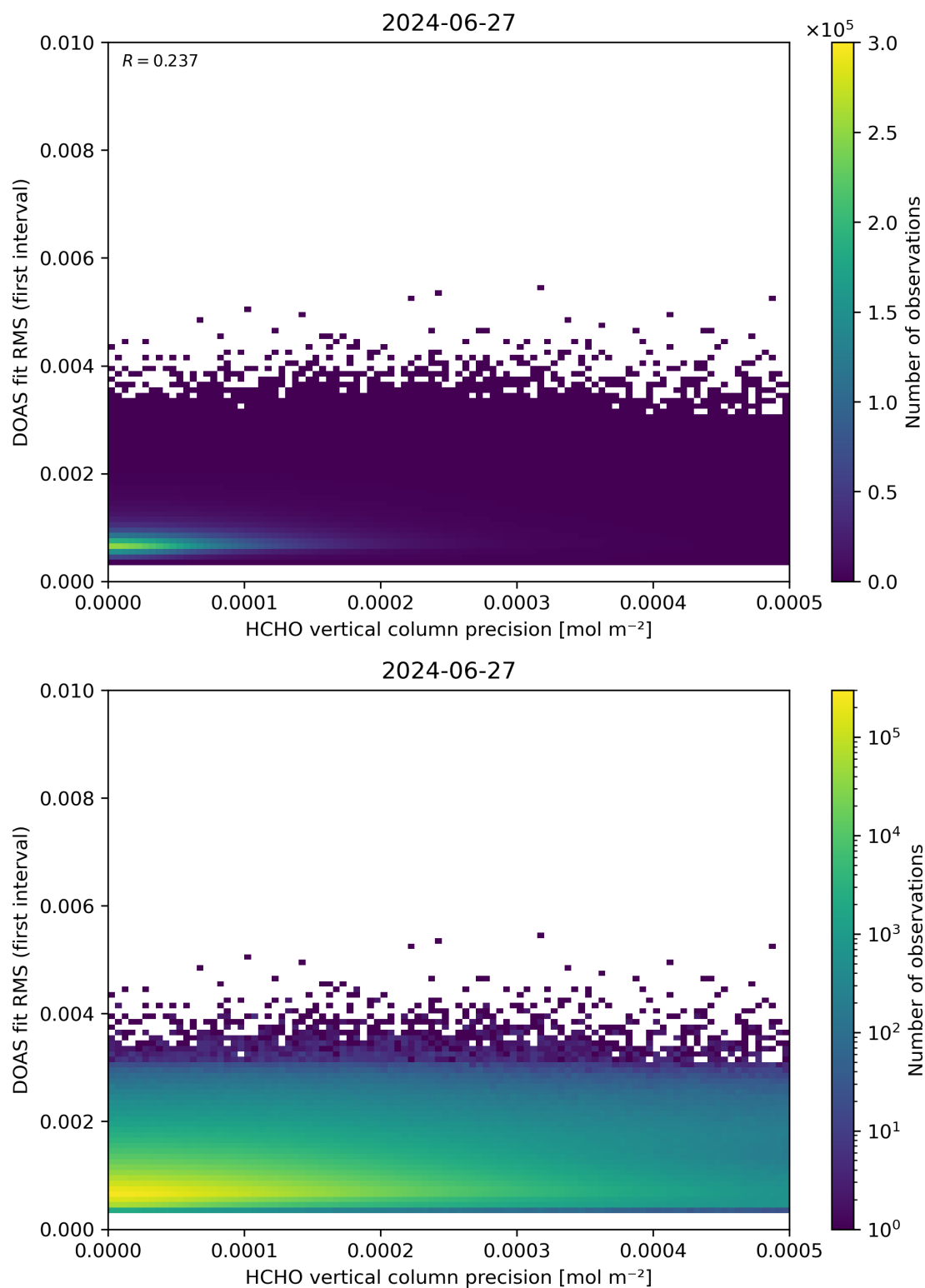
Figure 136: Scatter density plot of “HCHO vertical column precision” against “DOAS fit RMS (first interval)” for 2024-06-26 to 2024-06-28.
