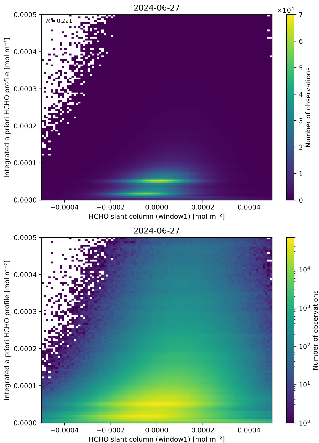
Figure 87: Scatter density plot of “HCHO slant column (window1)” against “Integrated a priori HCHO profile” for 2024-06-26 to 2024-06-28.
