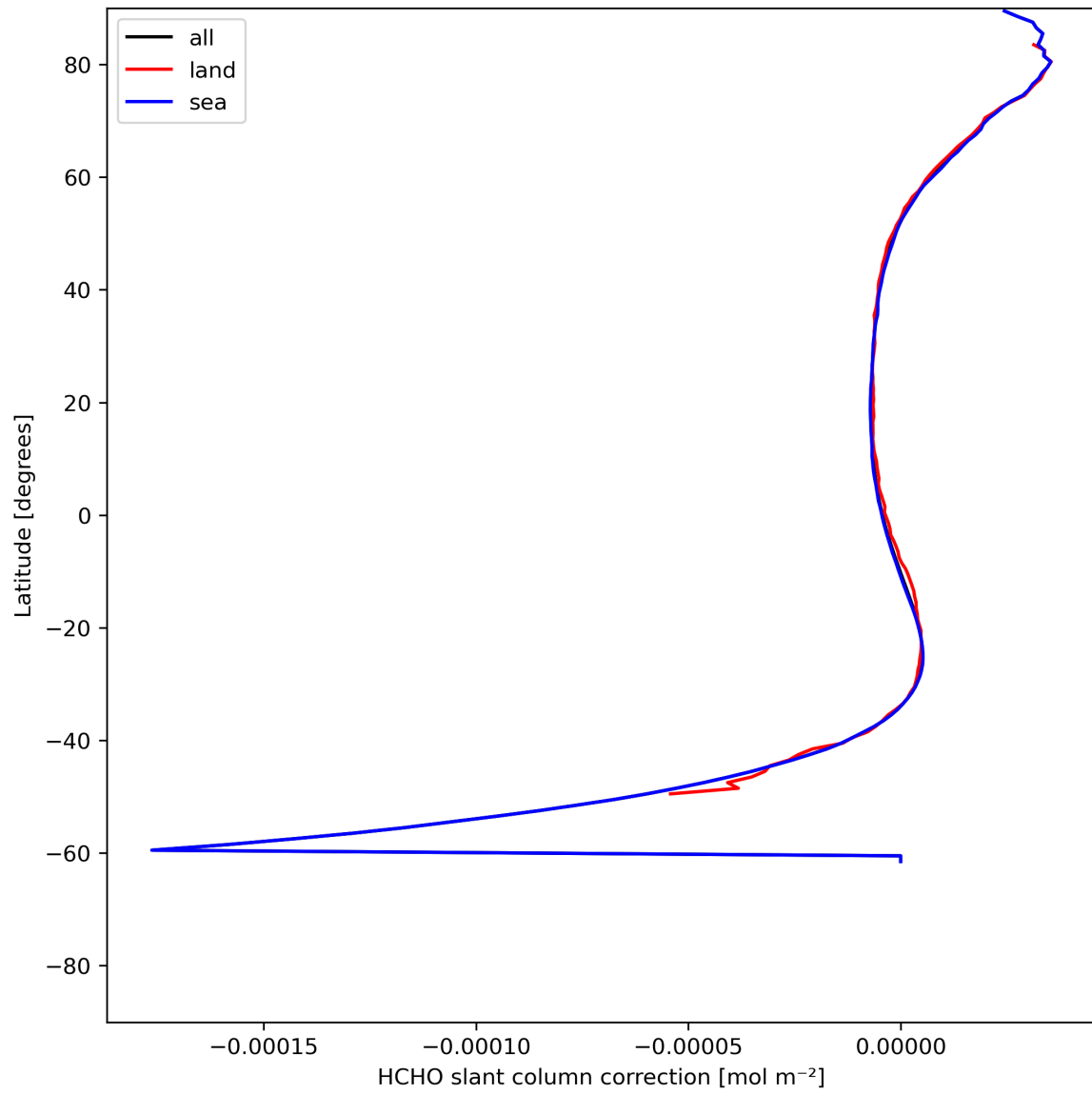
Figure 33: Zonal average of “HCHO slant column correction” for 2024-06-26 to 2024-06-28.
