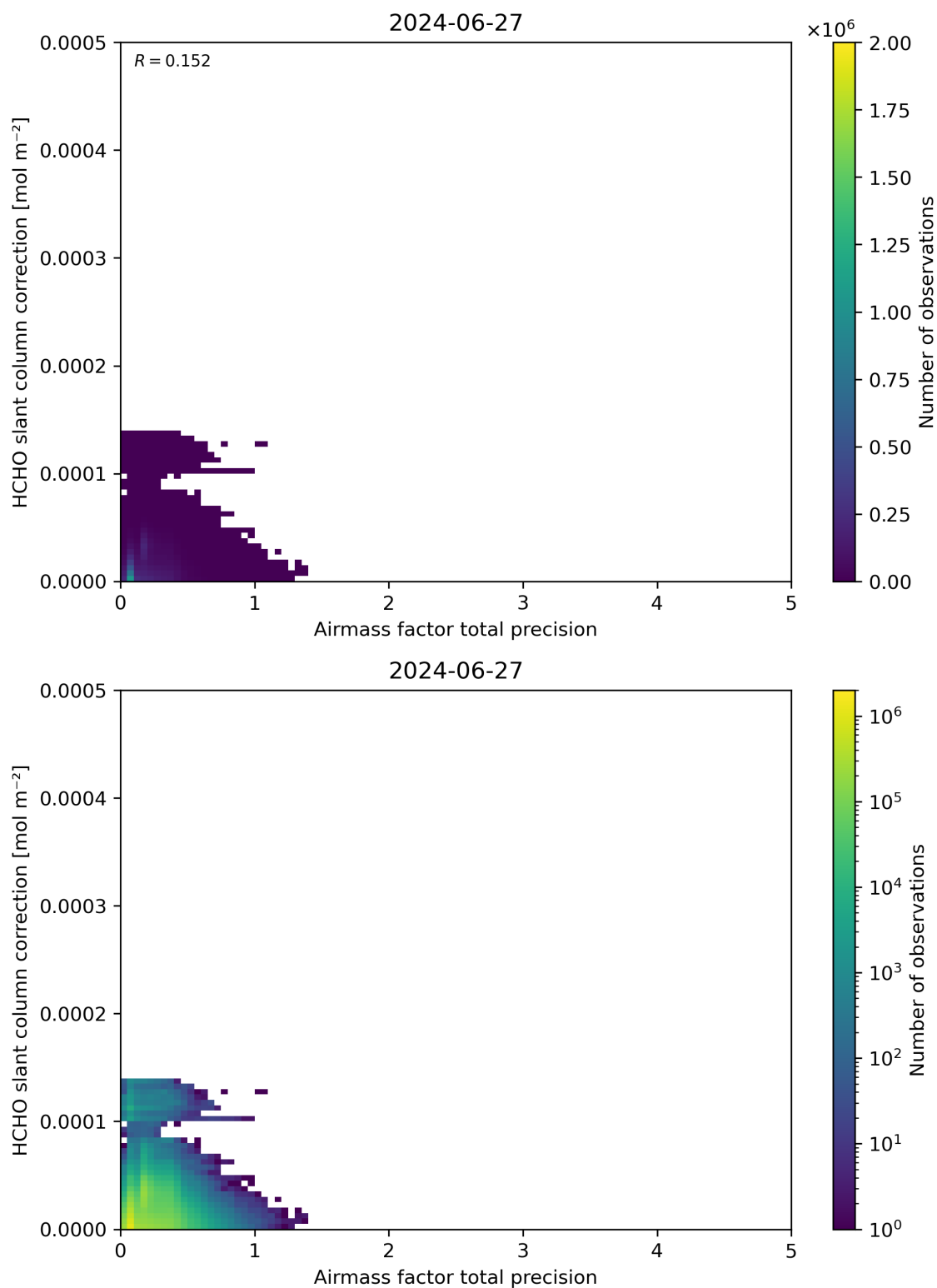
Figure 110: Scatter density plot of “Airmass factor total precision” against “HCHO slant column correction” for 2024-06-26 to 2024-06-28.
