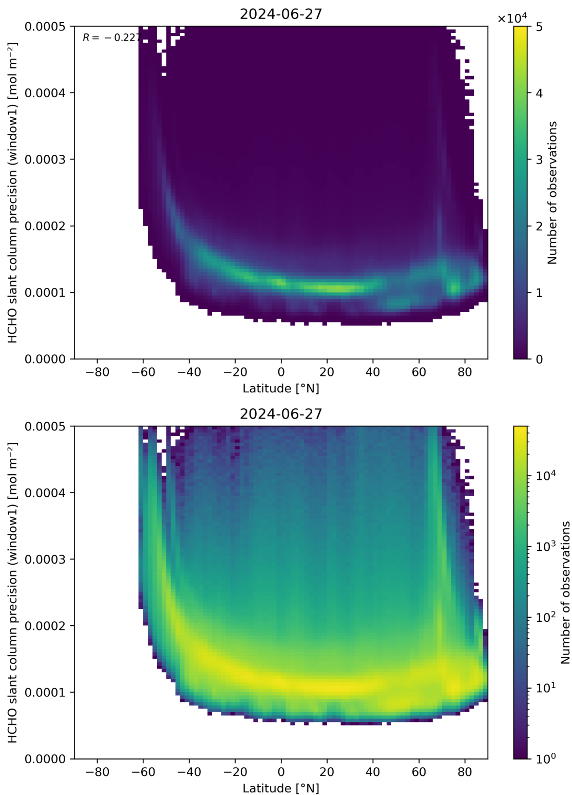
Figure 160: Scatter density plot of “Latitude” against “HCHO slant column precision (window1)” for 2024-06-26 to 2024-06-28.
