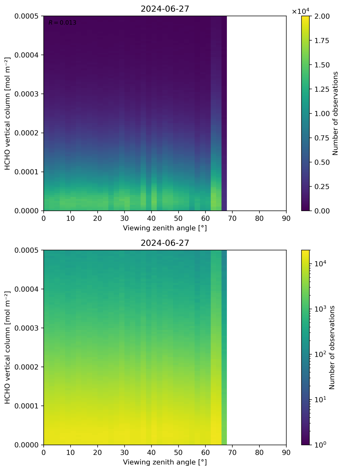
Figure 192: Scatter density plot of “Viewing zenith angle” against “HCHO vertical column” for 2024-06-26 to 2024-06-28.
