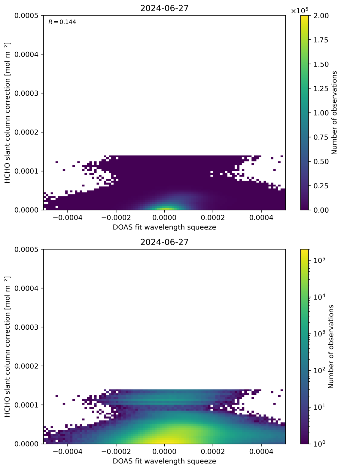
Figure 70: Scatter density plot of “DOAS fit wavelength squeeze” against “HCHO slant column correction” for 2024-06-26 to 2024-06-28.
