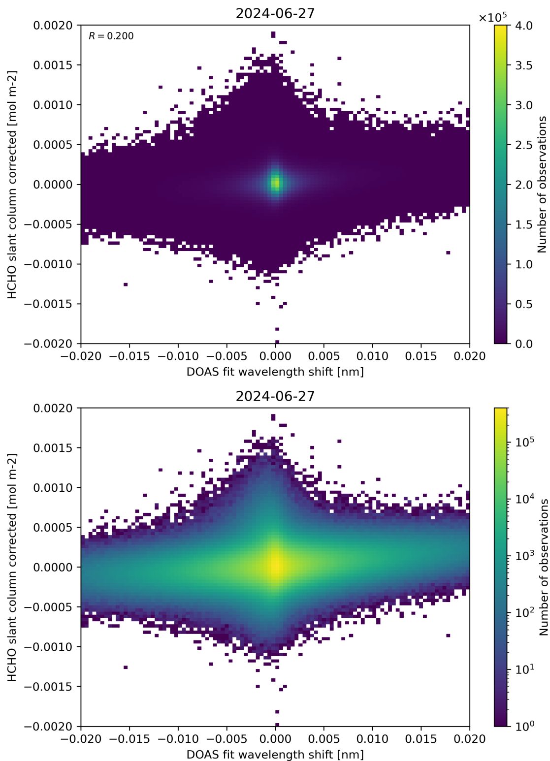
Figure 66: Scatter density plot of “DOAS fit wavelength shift” against “HCHO slant column corrected” for 2024-06-26 to 2024-06-28.
