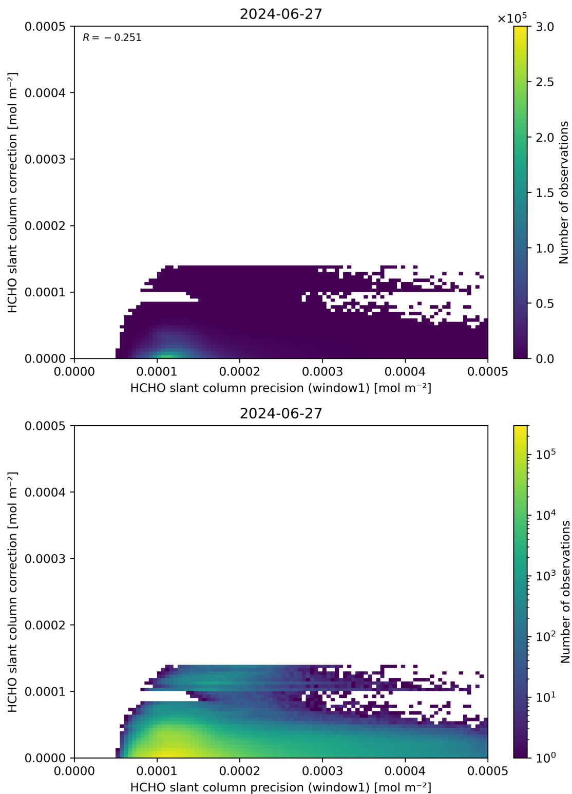
Figure 93: Scatter density plot of “HCHO slant column precision (window1)” against “HCHO slant column correction” for 2024-06-26 to 2024-06-28.
