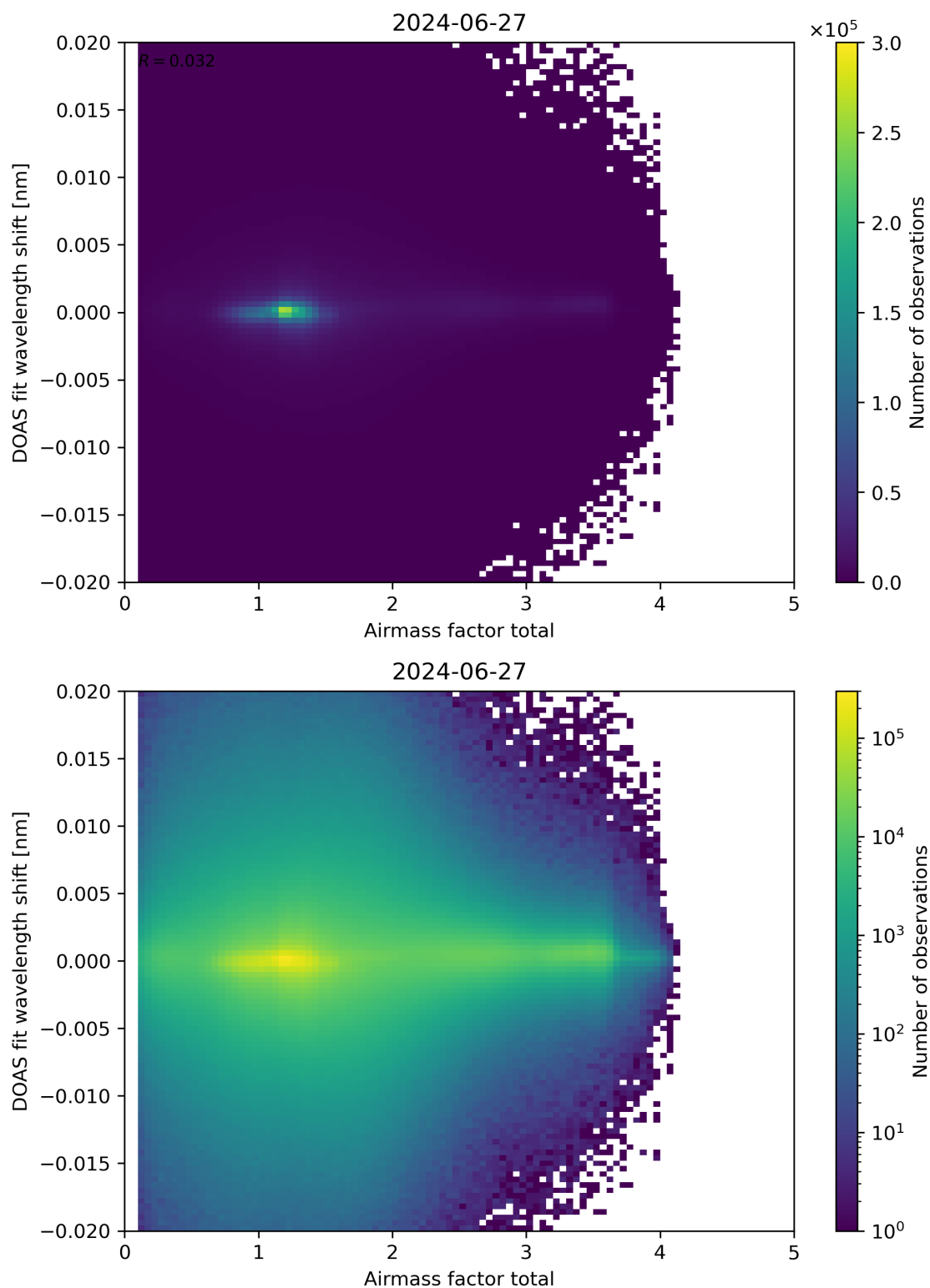
Figure 98: Scatter density plot of “Airmass factor total” against “DOAS fit wavelength shift” for 2024-06-26 to 2024-06-28.
