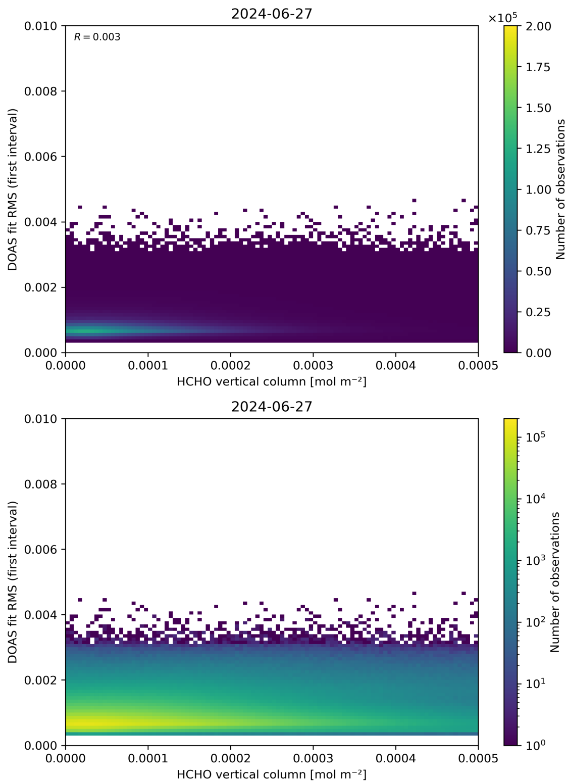
Figure 123: Scatter density plot of “HCHO vertical column” against “DOAS fit RMS (first interval)” for 2024-06-26 to 2024-06-28.
