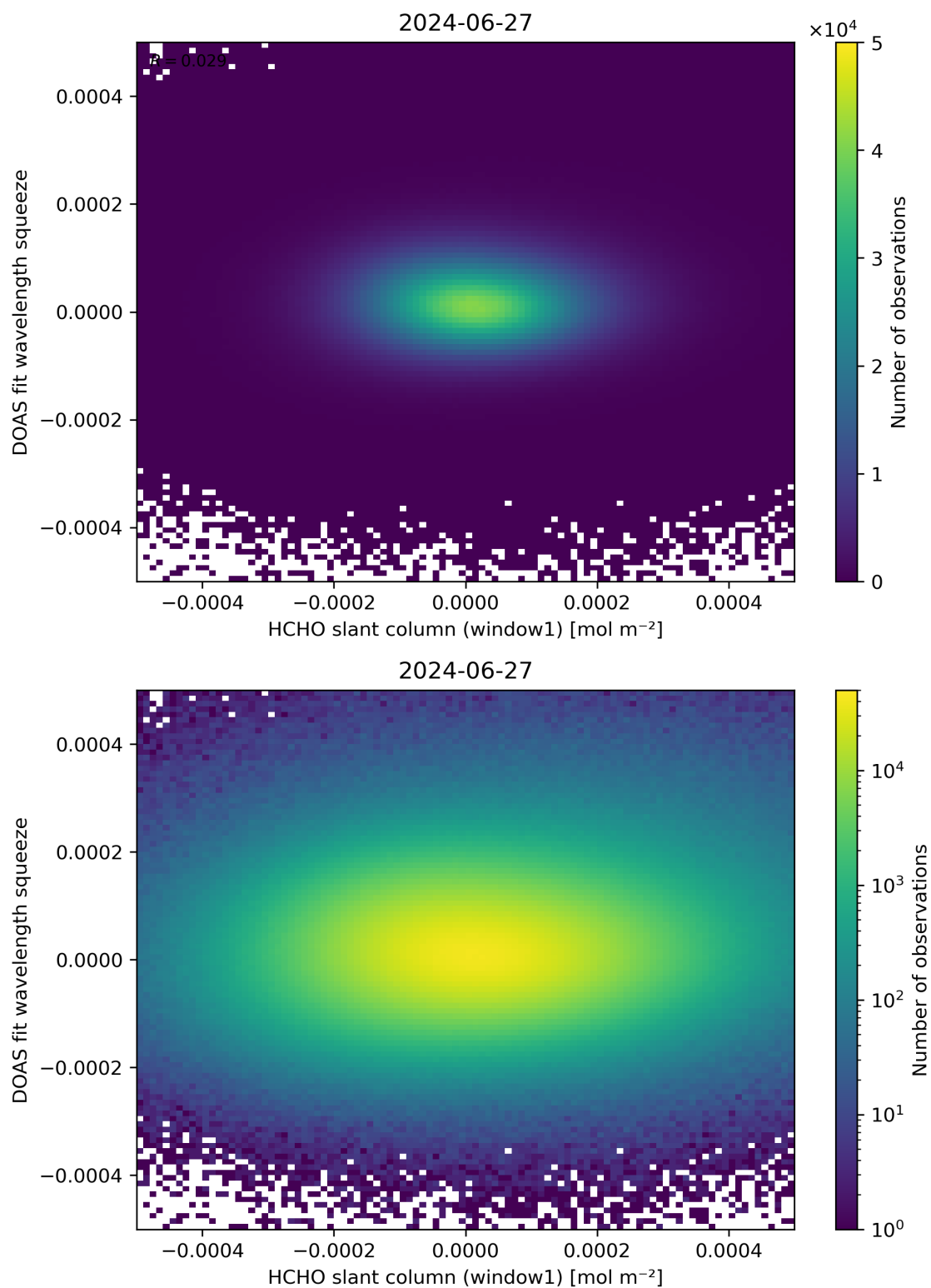
Figure 80: Scatter density plot of “HCHO slant column (window1)” against “DOAS fit wavelength squeeze” for 2024-06-26 to 2024-06-28.
