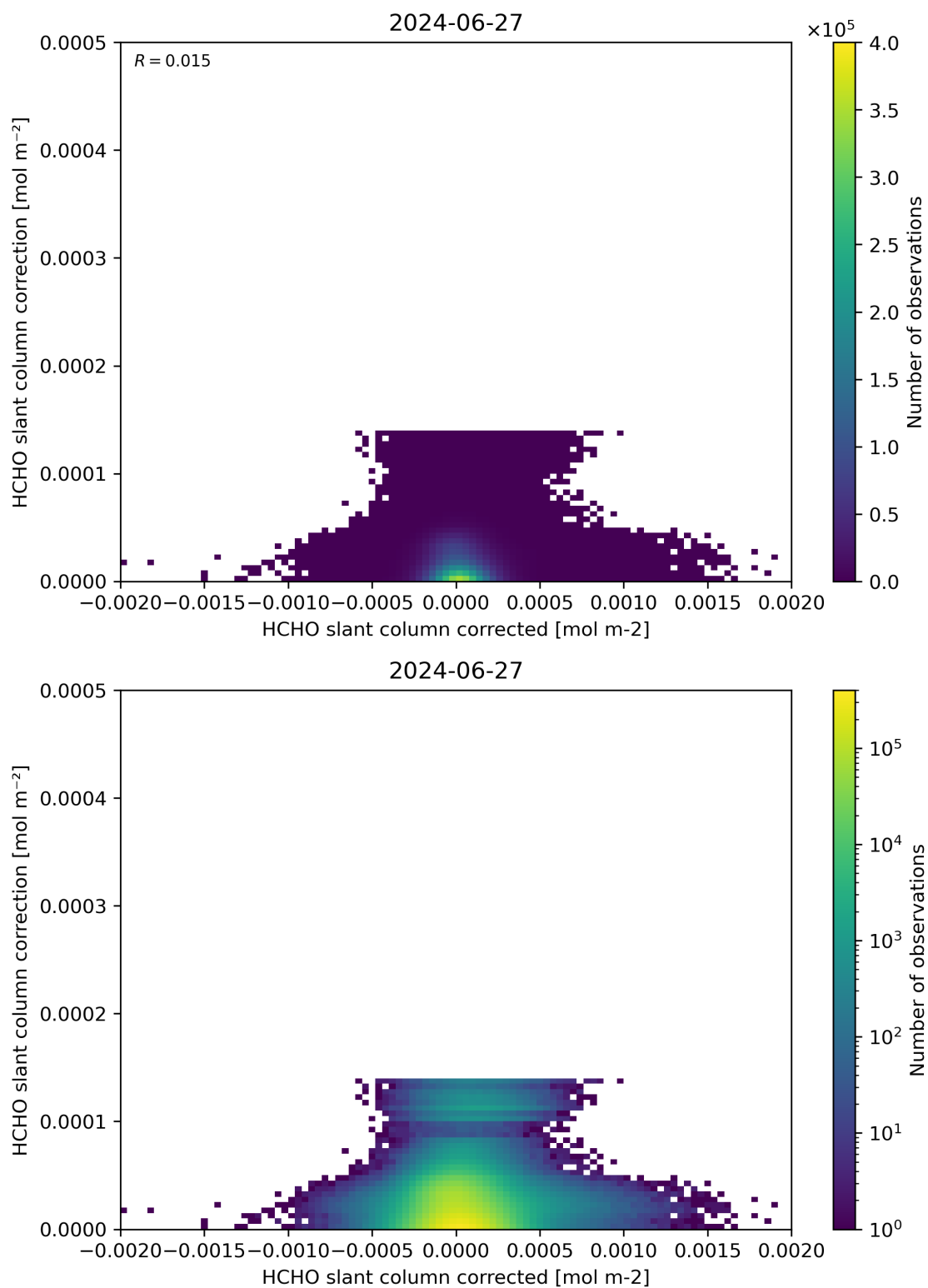
Figure 77: Scatter density plot of “HCHO slant column corrected” against “HCHO slant column correction” for 2024-06-26 to 2024-06-28.
