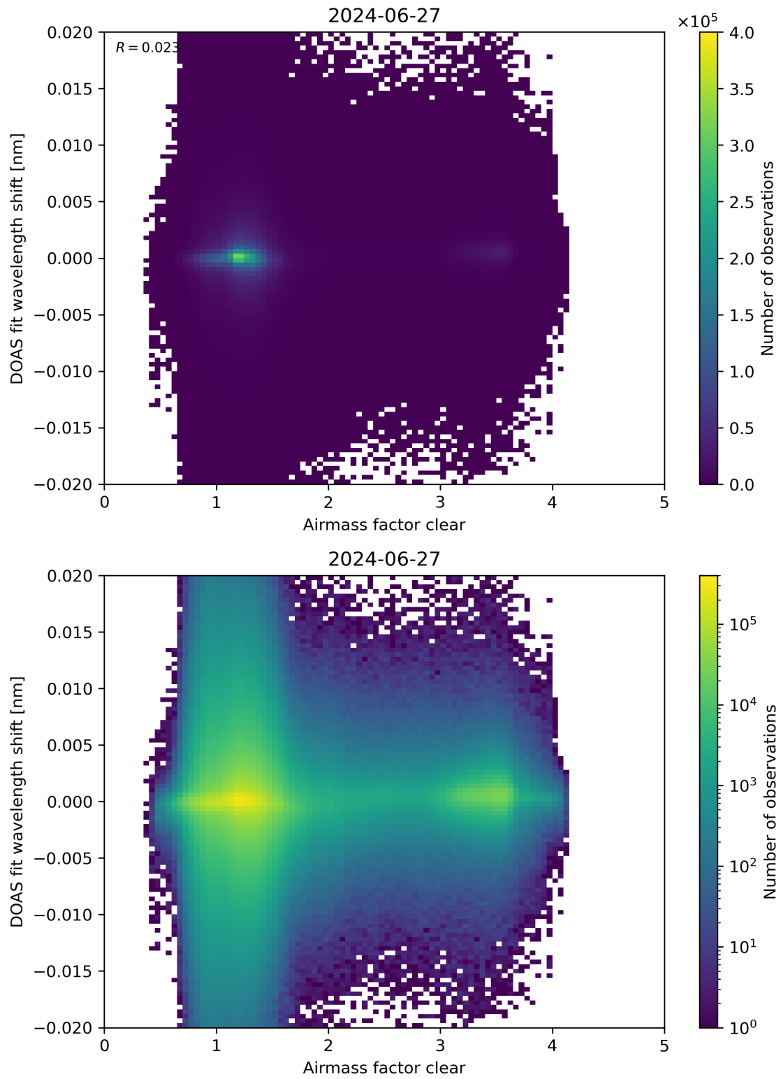
Figure 72: Scatter density plot of “Airmass factor clear” against “DOAS fit wavelength shift” for 2024-06-26 to 2024-06-28.
