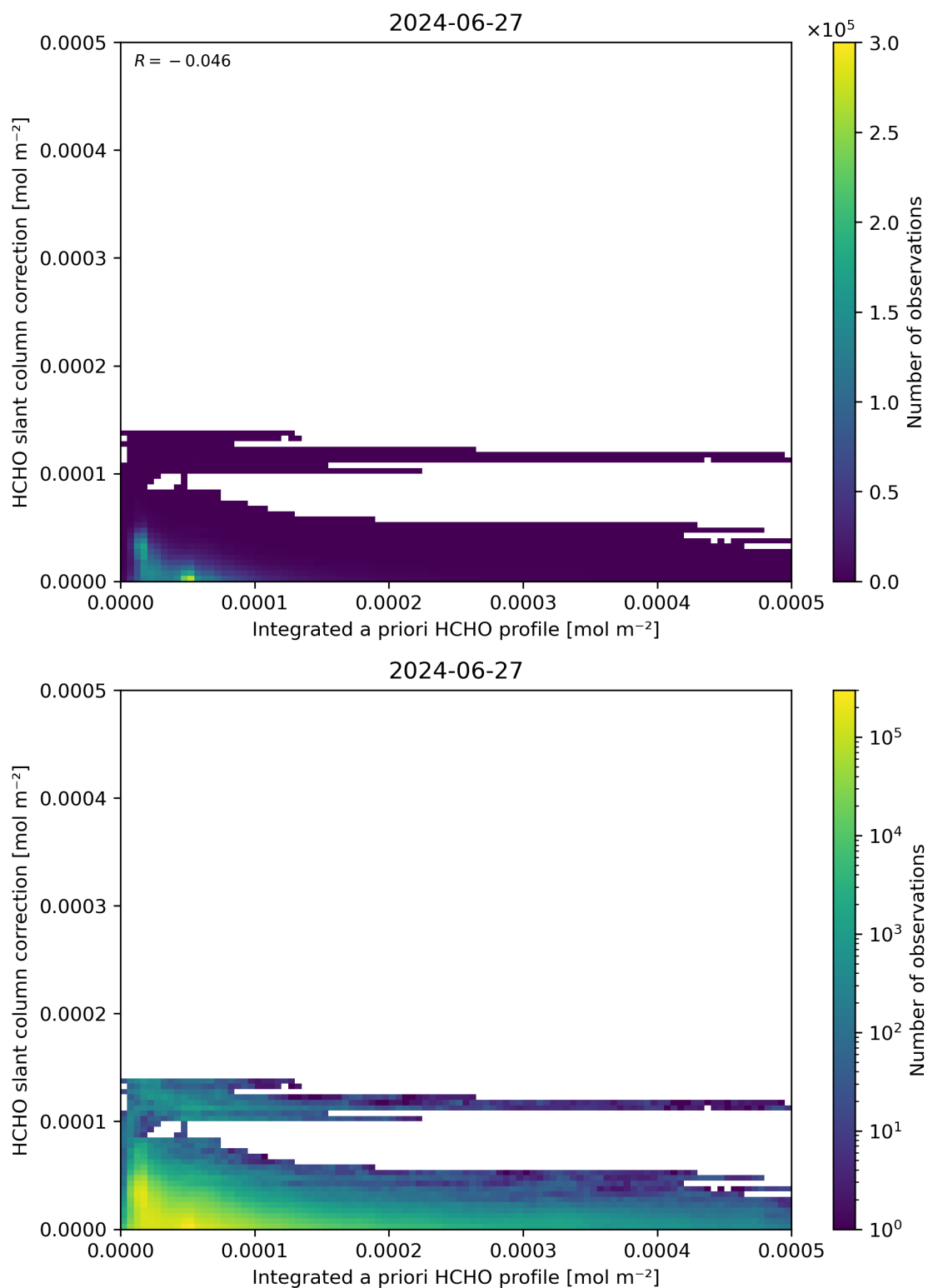
Figure 152: Scatter density plot of “Integrated a priori HCHO profile” against “HCHO slant column correction” for 2024-06-26 to 2024-06-28.
