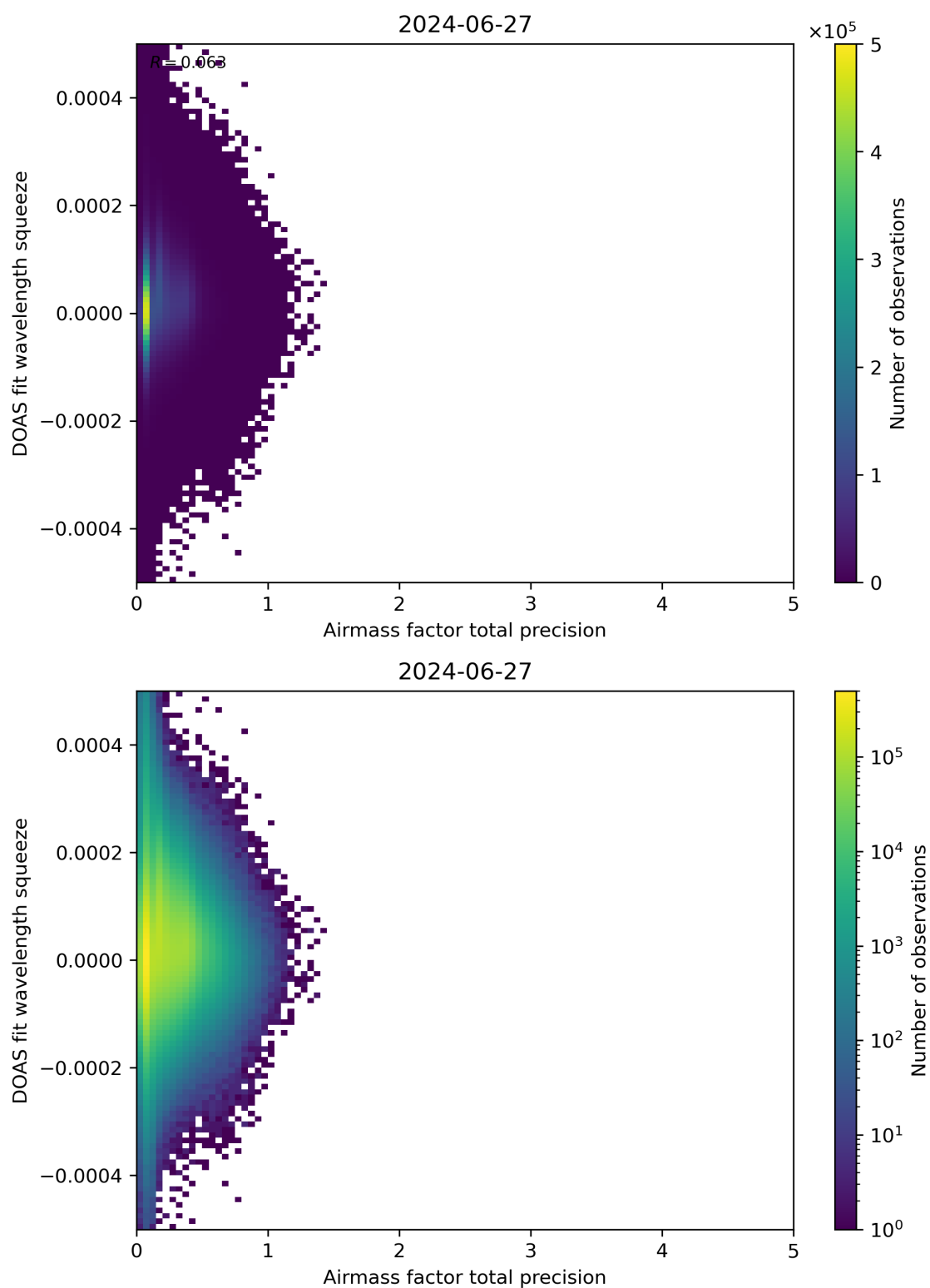
Figure 107: Scatter density plot of “Airmass factor total precision” against “DOAS fit wavelength squeeze” for 2024-06-26 to 2024-06-28.
