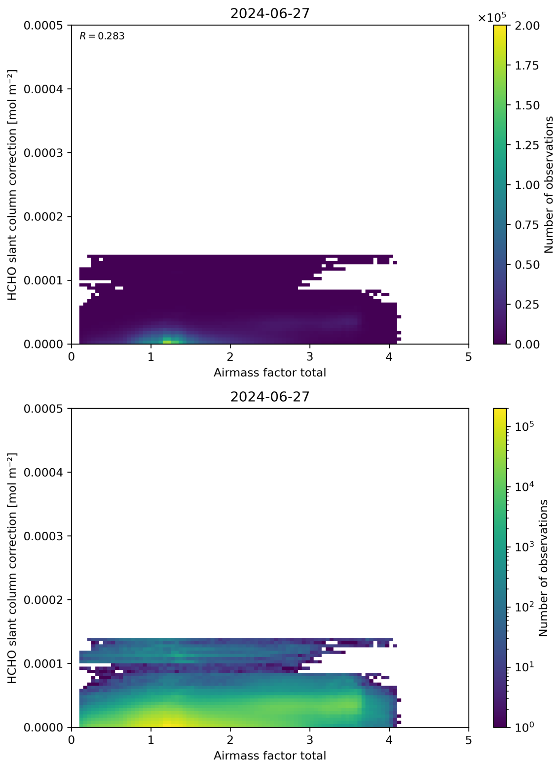
Figure 102: Scatter density plot of “Airmass factor total” against “HCHO slant column correction” for 2024-06-26 to 2024-06-28.
