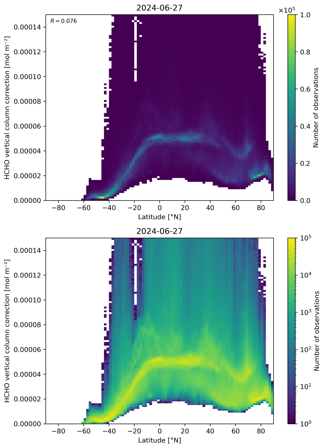
Figure 164: Scatter density plot of “Latitude” against “HCHO vertical column correction” for 2024-06-26 to 2024-06-28.
