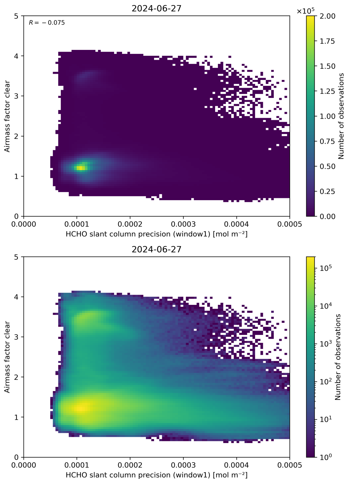
Figure 91: Scatter density plot of “HCHO slant column precision (window1)” against “Airmass factor clear” for 2024-06-26 to 2024-06-28.
