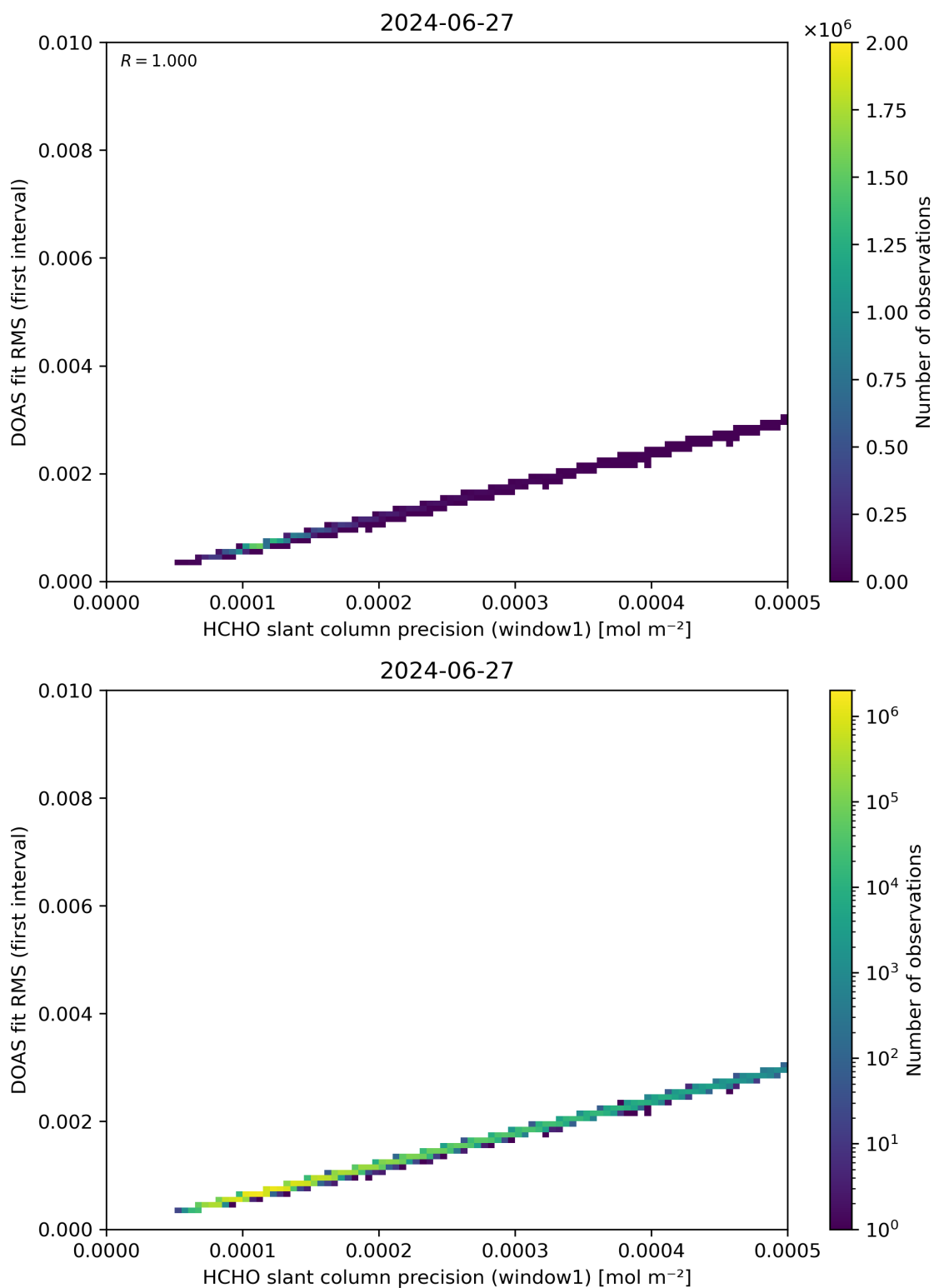
Figure 88: Scatter density plot of “HCHO slant column precision (window1)” against “DOAS fit RMS (first interval)” for 2024-06-26 to 2024-06-28.
