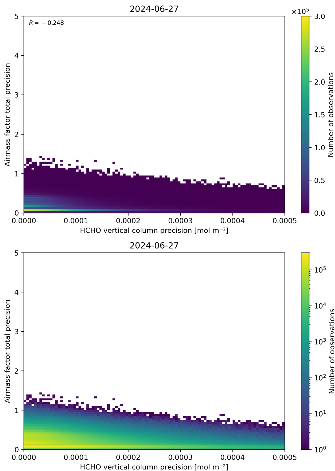
Figure 145: Scatter density plot of “HCHO vertical column precision” against “Airmass factor total precision” for 2024-06-26 to 2024-06-28.
