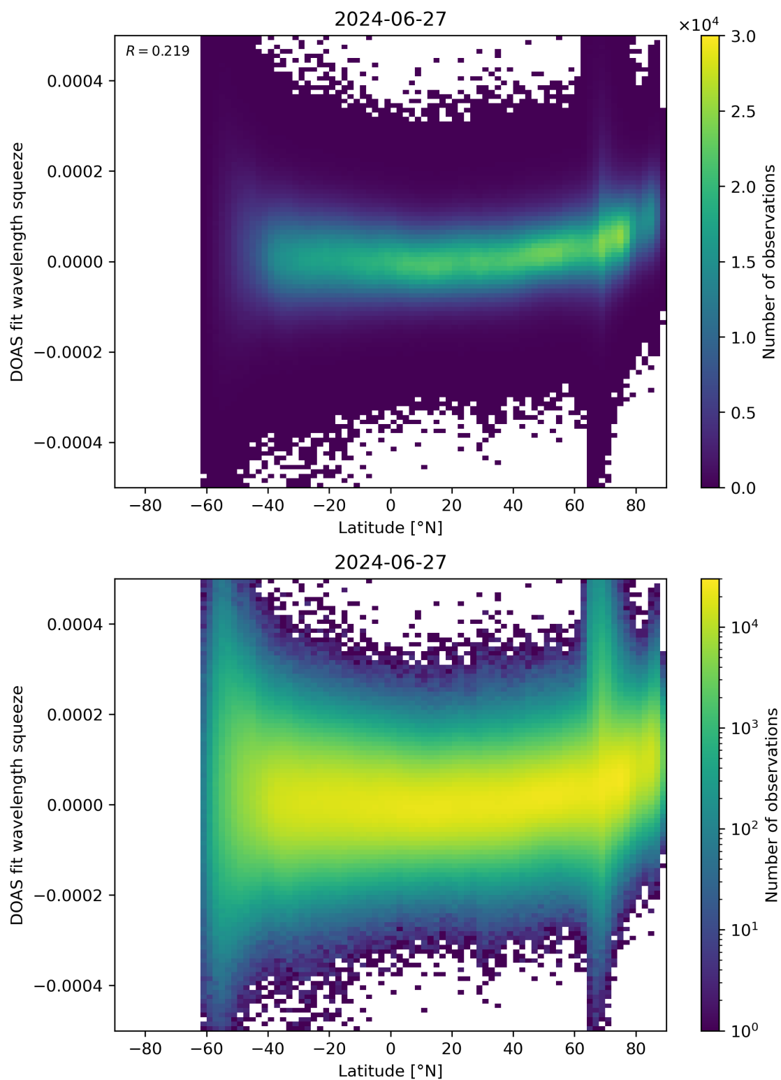
Figure 155: Scatter density plot of “Latitude” against “DOAS fit wavelength squeeze” for 2024-06-26 to 2024-06-28.
