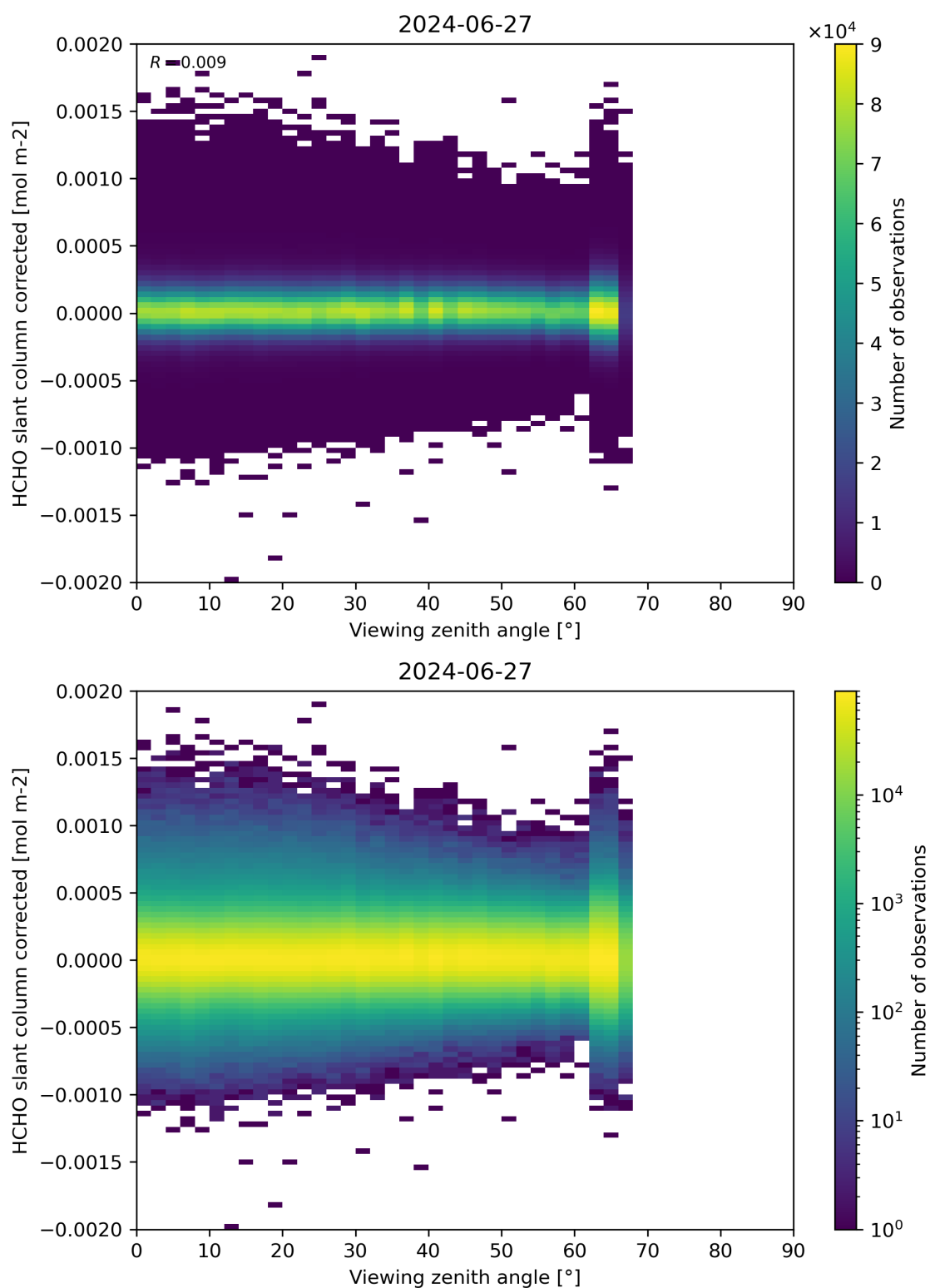
Figure 186: Scatter density plot of “Viewing zenith angle” against “HCHO slant column corrected” for 2024-06-26 to 2024-06-28.
