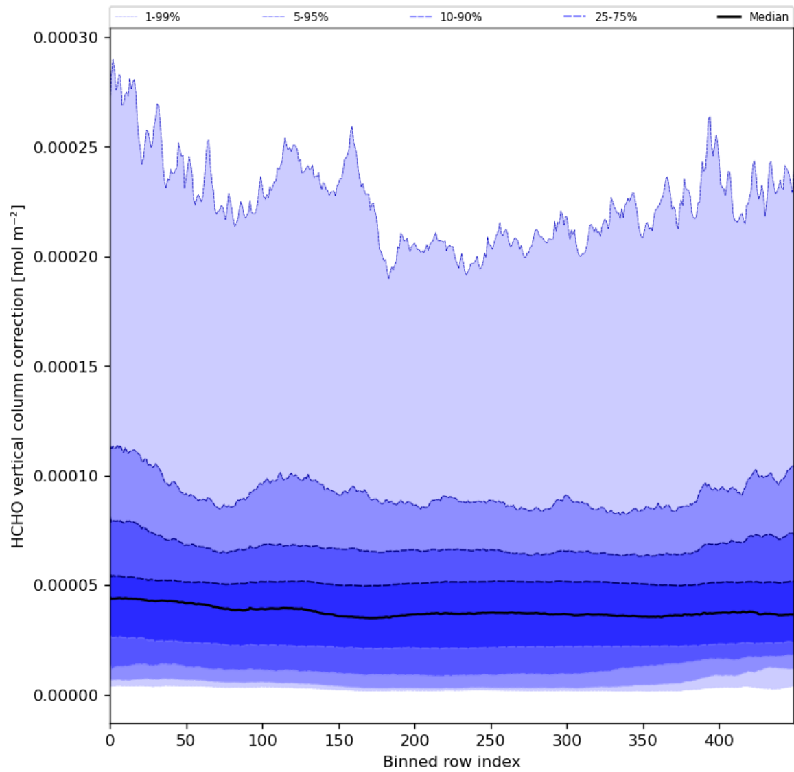
Figure 51: Along track statistics of “HCHO vertical column correction” for 2024-06-26 to 2024-06-28
