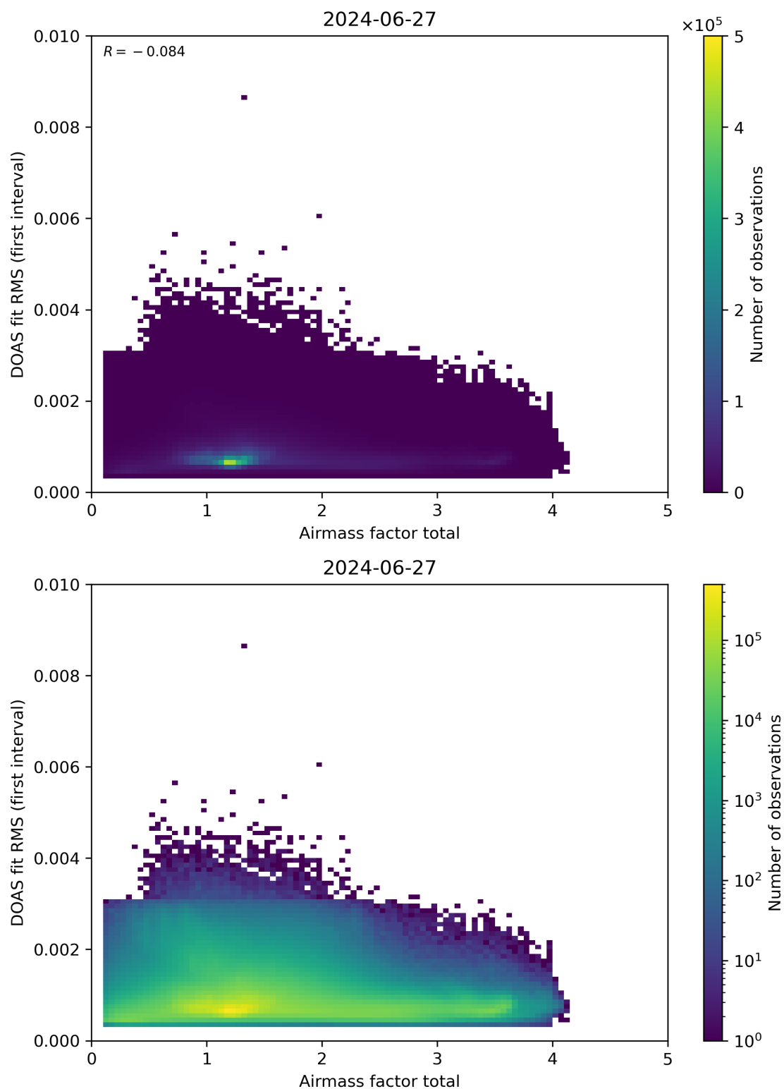
Figure 97: Scatter density plot of “Airmass factor total” against “DOAS fit RMS (first interval)” for 2024-06-26 to 2024-06-28.
