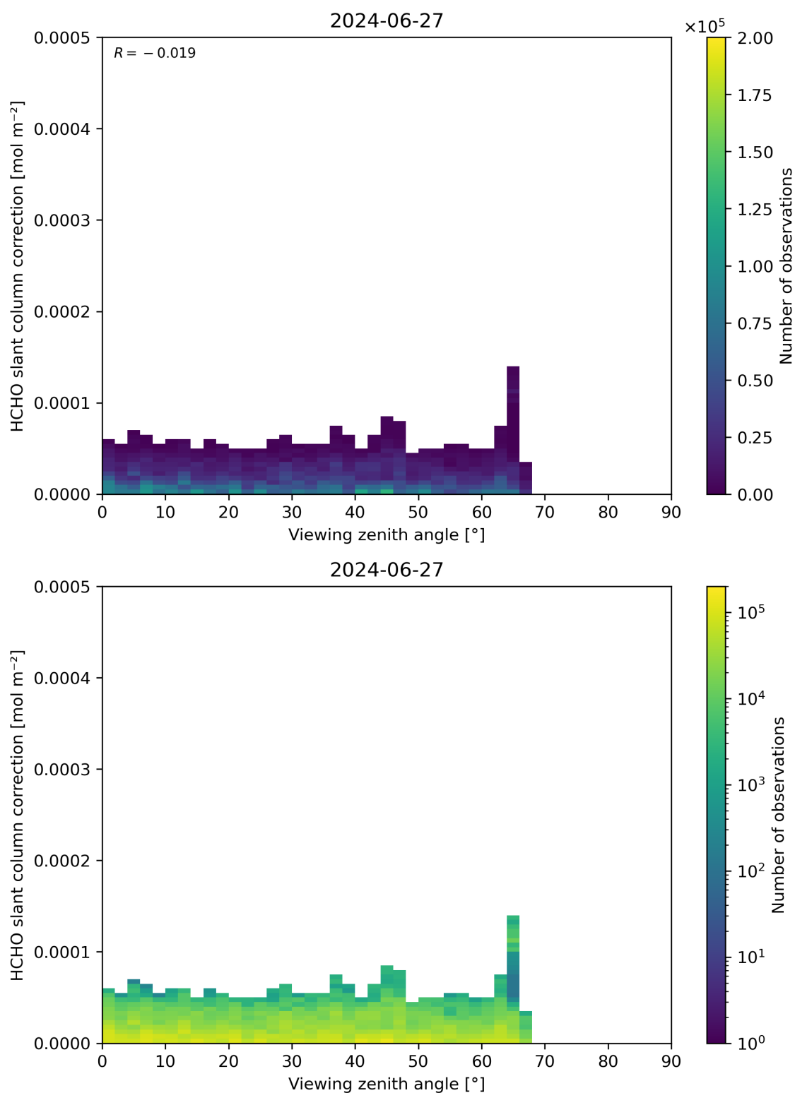
Figure 187: Scatter density plot of “Viewing zenith angle” against “HCHO slant column correction” for 2024-06-26 to 2024-06-28.
