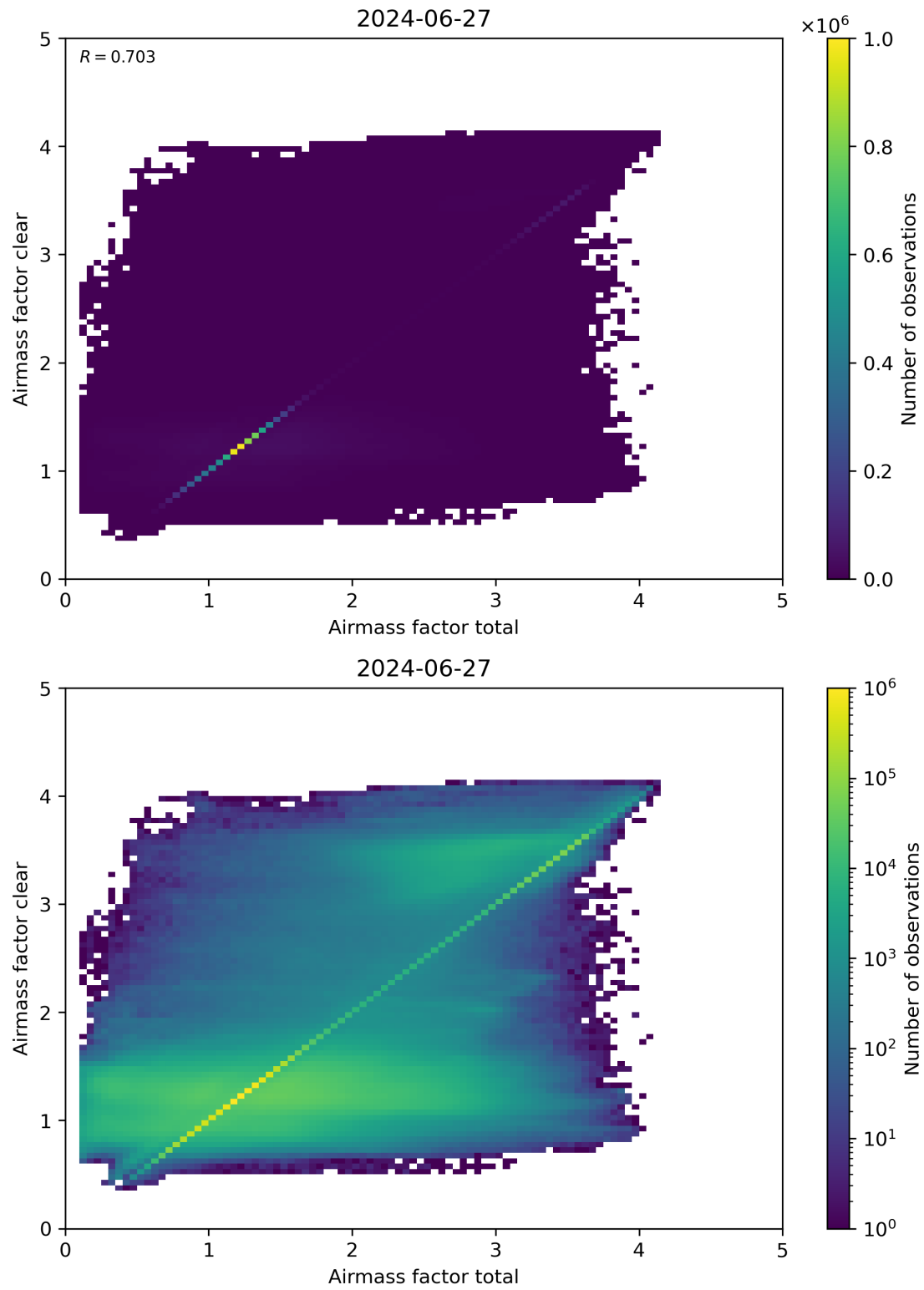
Figure 100: Scatter density plot of “Airmass factor total” against “Airmass factor clear” for 2024-06-26 to 2024-06-28.
