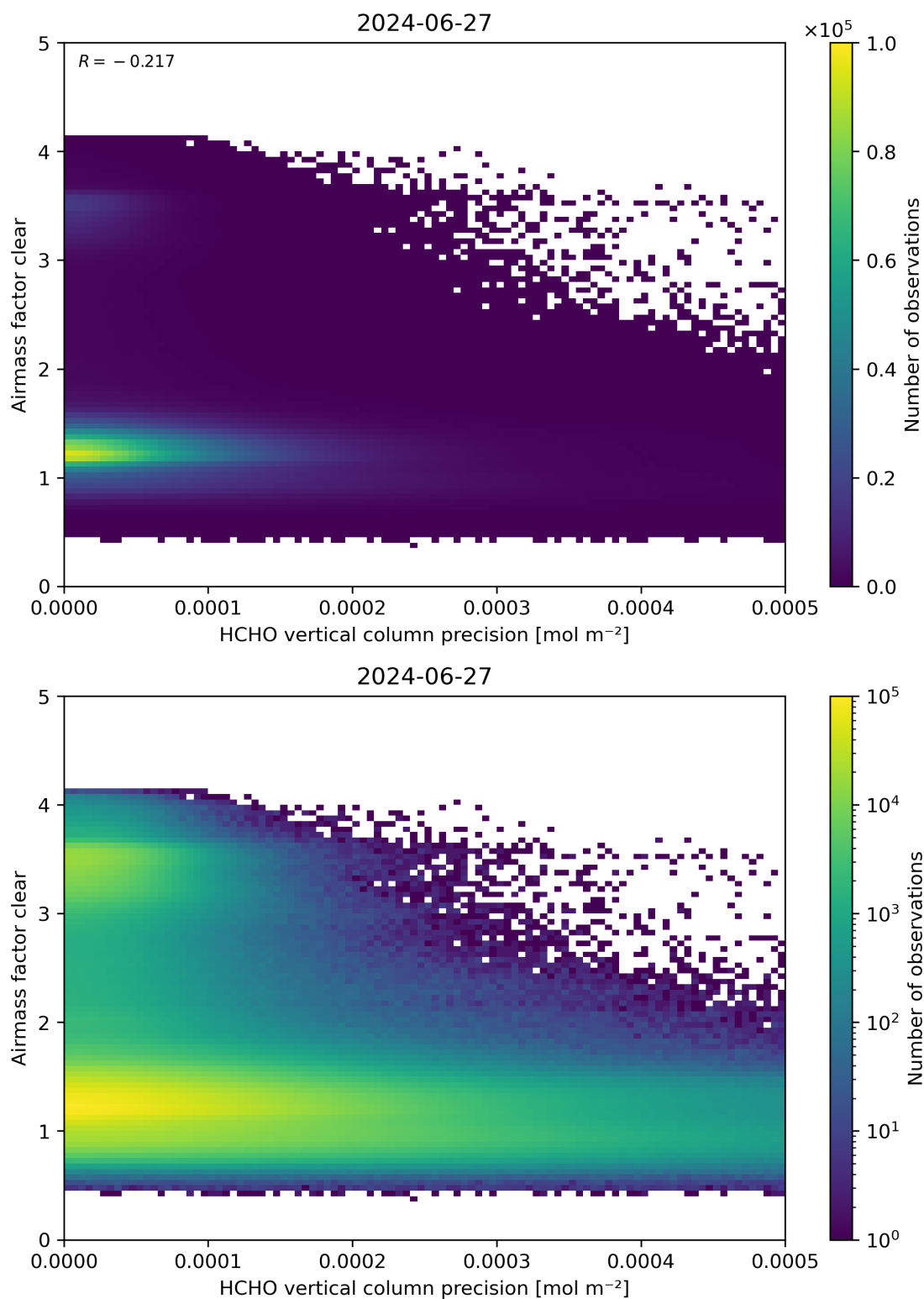
Figure 139: Scatter density plot of “HCHO vertical column precision” against “Airmass factor clear” for 2024-06-26 to 2024-06-28.
