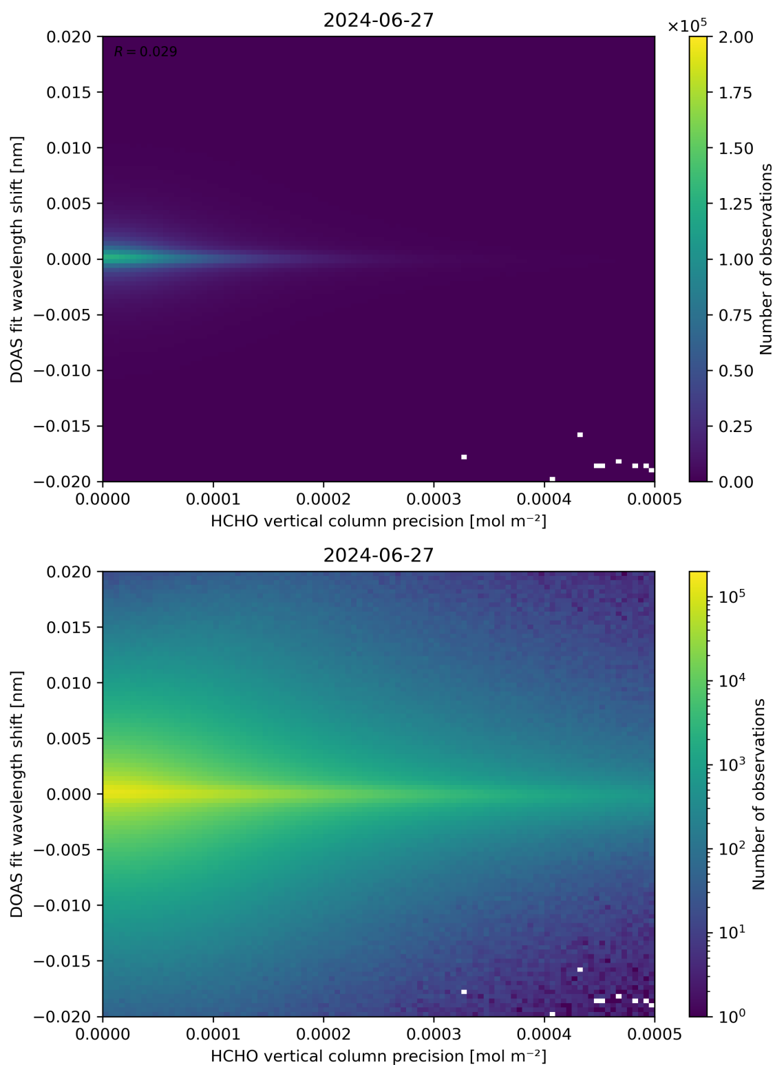
Figure 137: Scatter density plot of “HCHO vertical column precision” against “DOAS fit wavelength shift” for 2024-06-26 to 2024-06-28.
