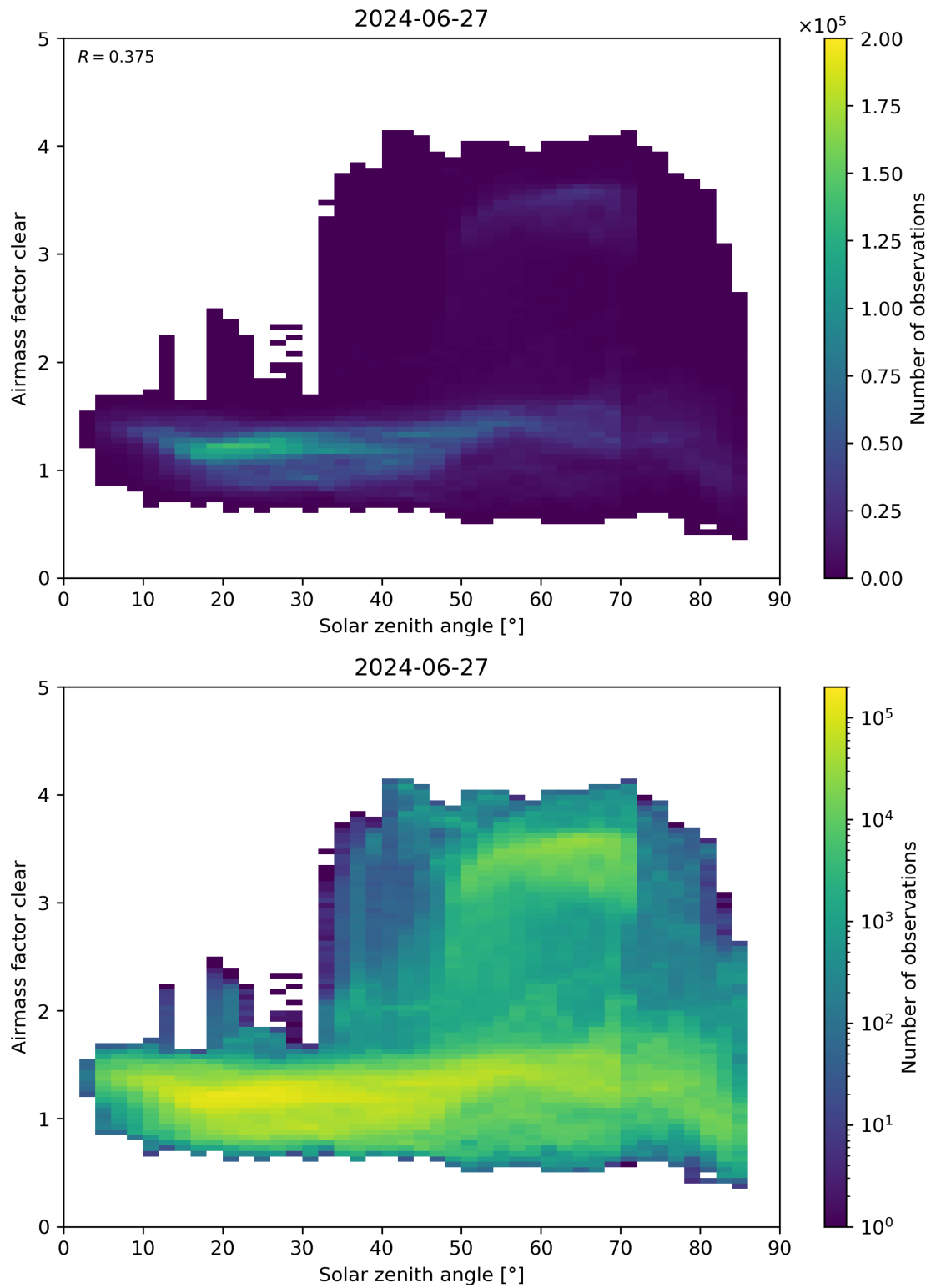
Figure 170: Scatter density plot of “Solar zenith angle” against “Airmass factor clear” for 2024-06-26 to 2024-06-28.
