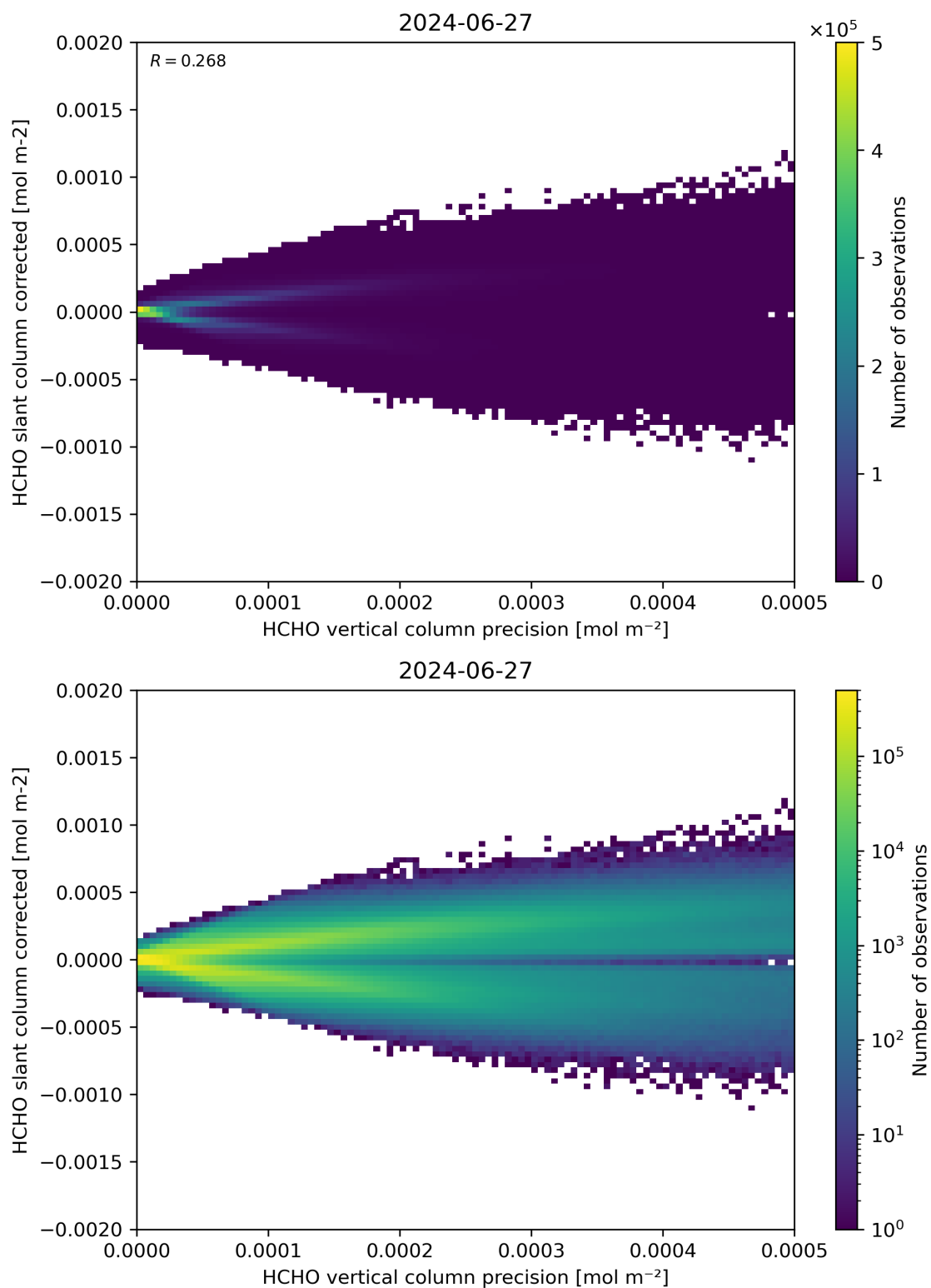
Figure 140: Scatter density plot of “HCHO vertical column precision” against “HCHO slant column corrected” for 2024-06-26 to 2024-06-28.
