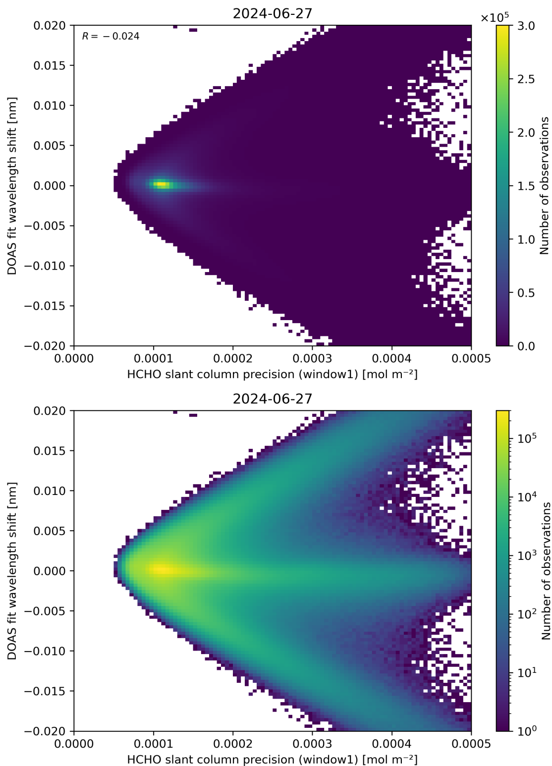
Figure 89: Scatter density plot of “HCHO slant column precision (window1)” against “DOAS fit wavelength shift” for 2024-06-26 to 2024-06-28.
