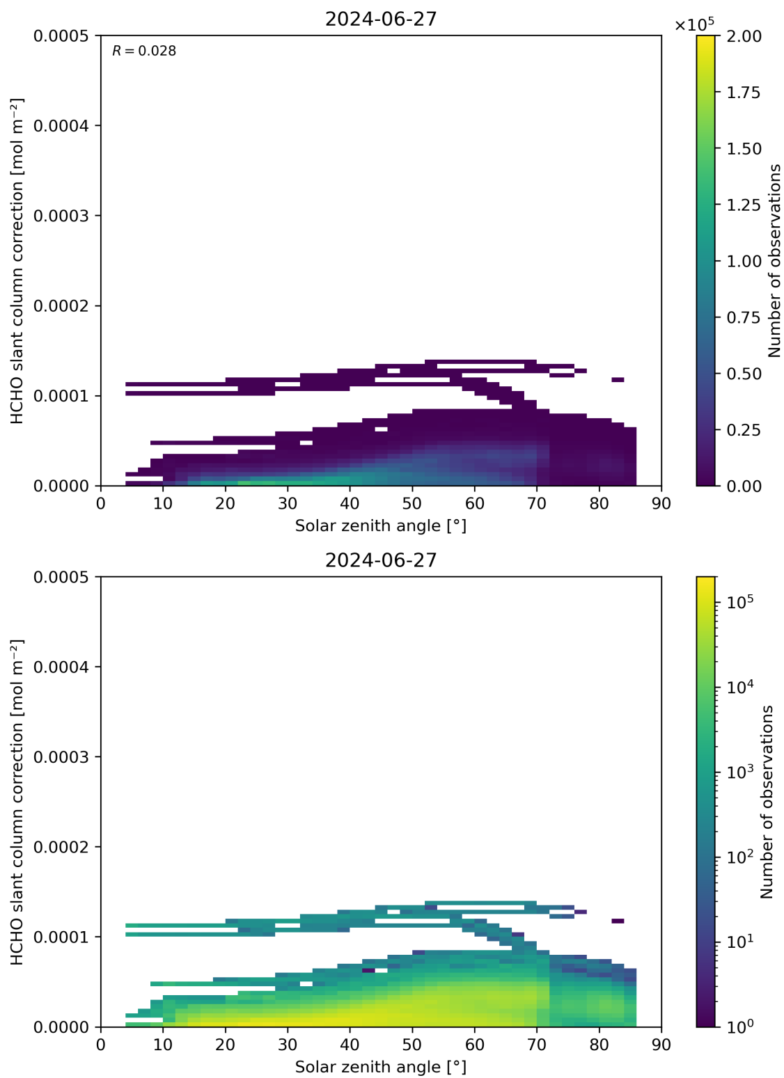
Figure 172: Scatter density plot of “Solar zenith angle” against “HCHO slant column correction” for 2024-06-26 to 2024-06-28.
