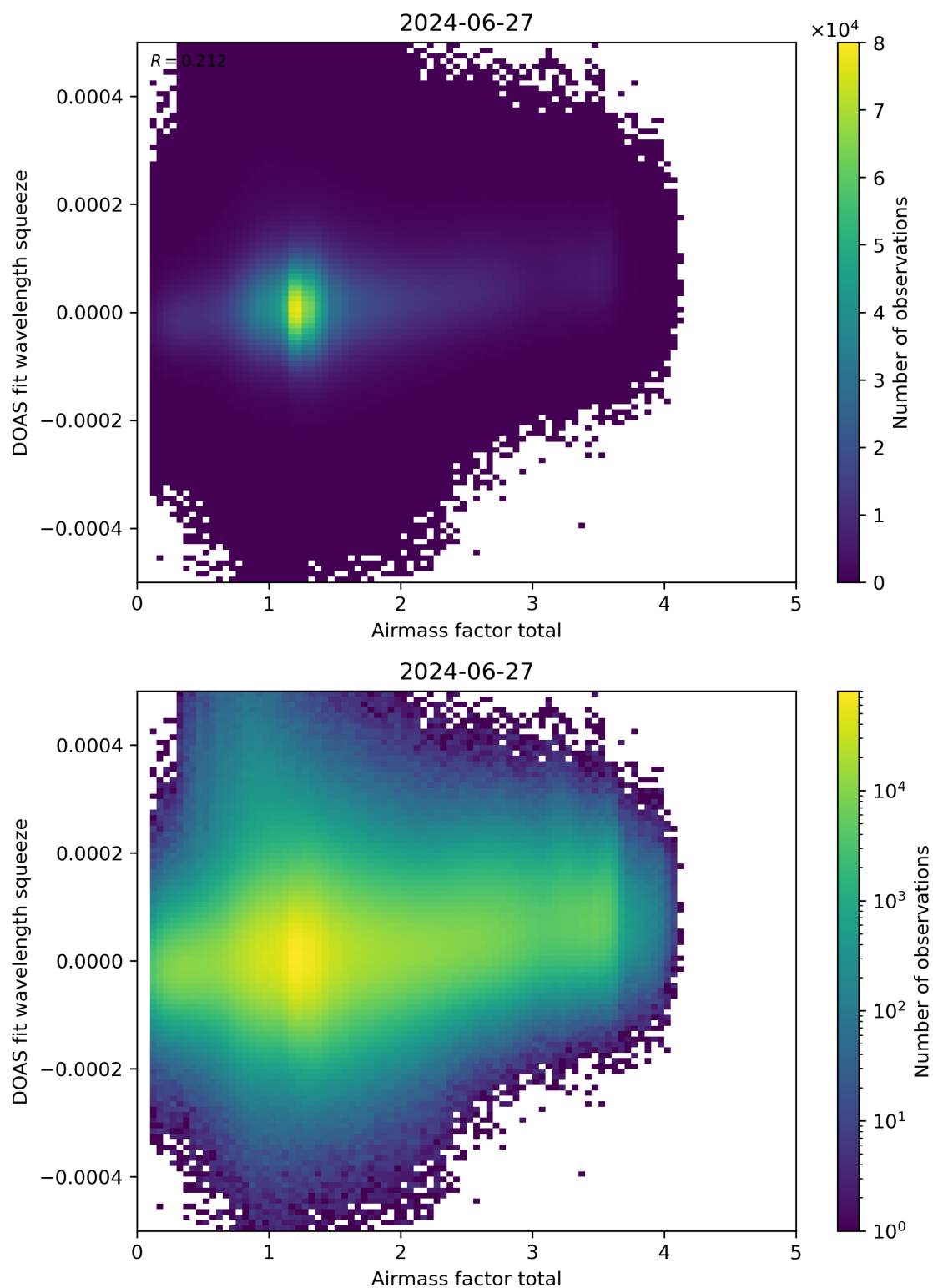
Figure 99: Scatter density plot of “Airmass factor total” against “DOAS fit wavelength squeeze” for 2024-06-26 to 2024-06-28.
