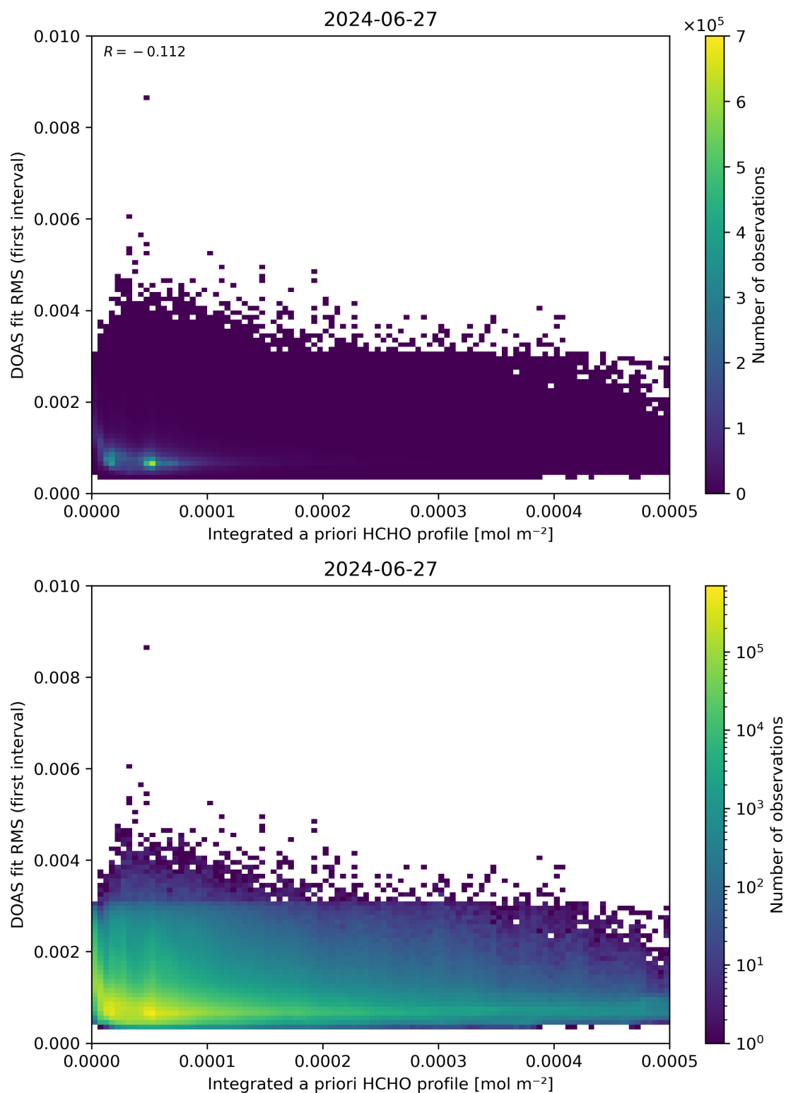
Figure 148: Scatter density plot of “Integrated a priori HCHO profile” against “DOAS fit RMS (first interval)” for 2024-06-26 to 2024-06-28.
