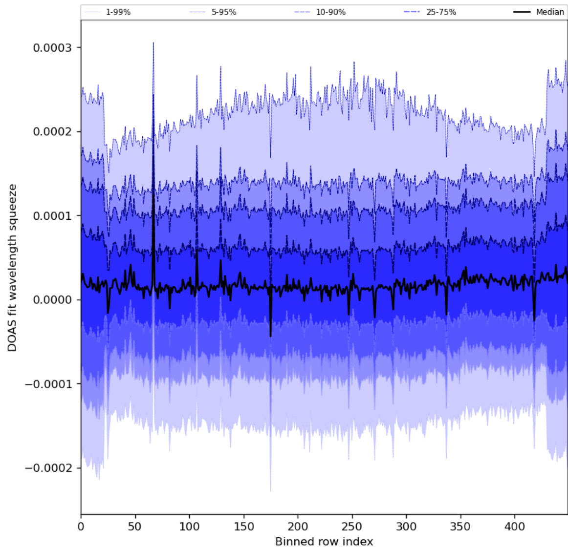
Figure 59: Along track statistics of “DOAS fit wavelength squeeze” for 2024-06-26 to 2024-06-28
