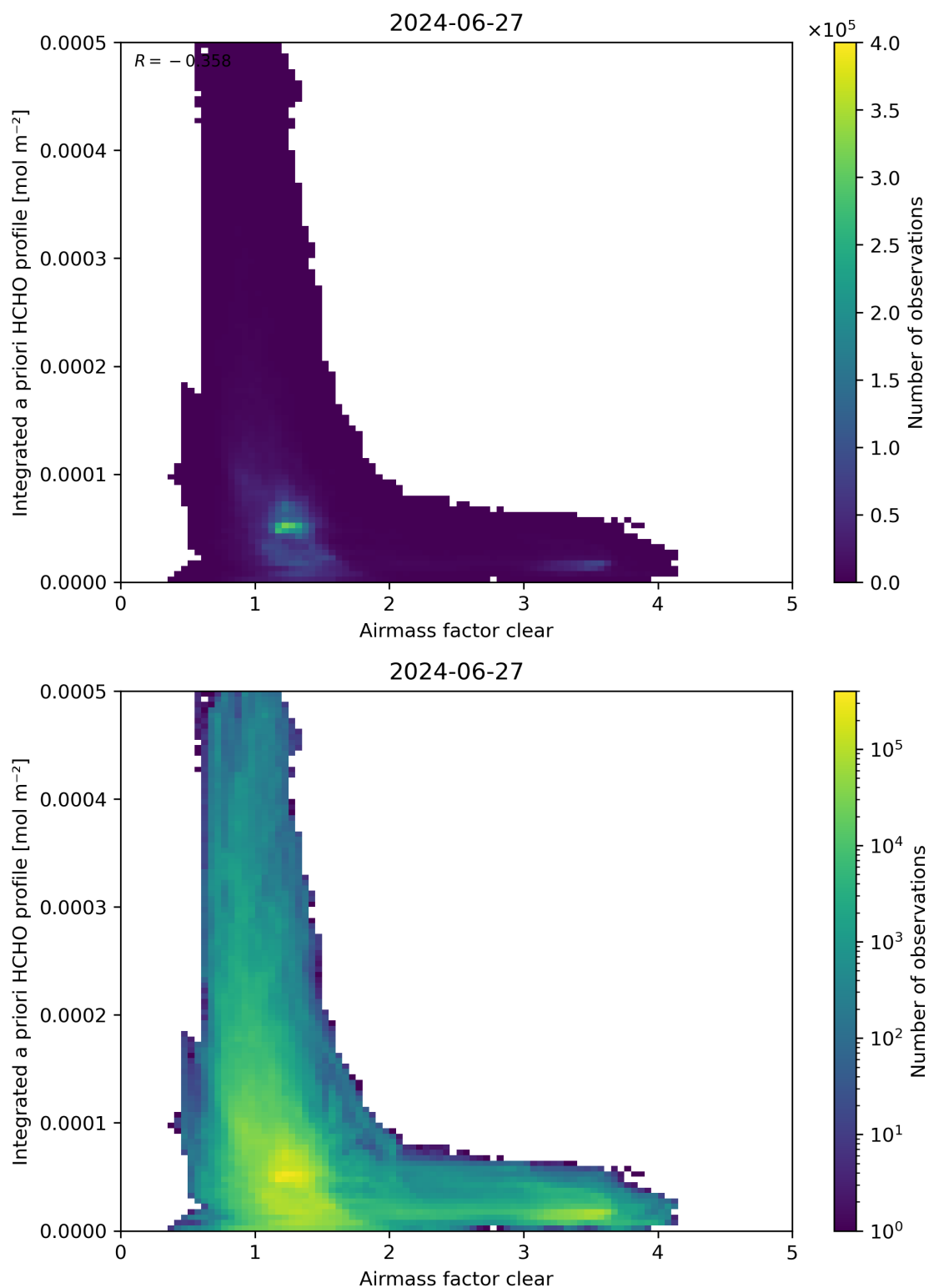
Figure 76: Scatter density plot of “Airmass factor clear” against “Integrated a priori HCHO profile” for 2024-06-26 to 2024-06-28.
