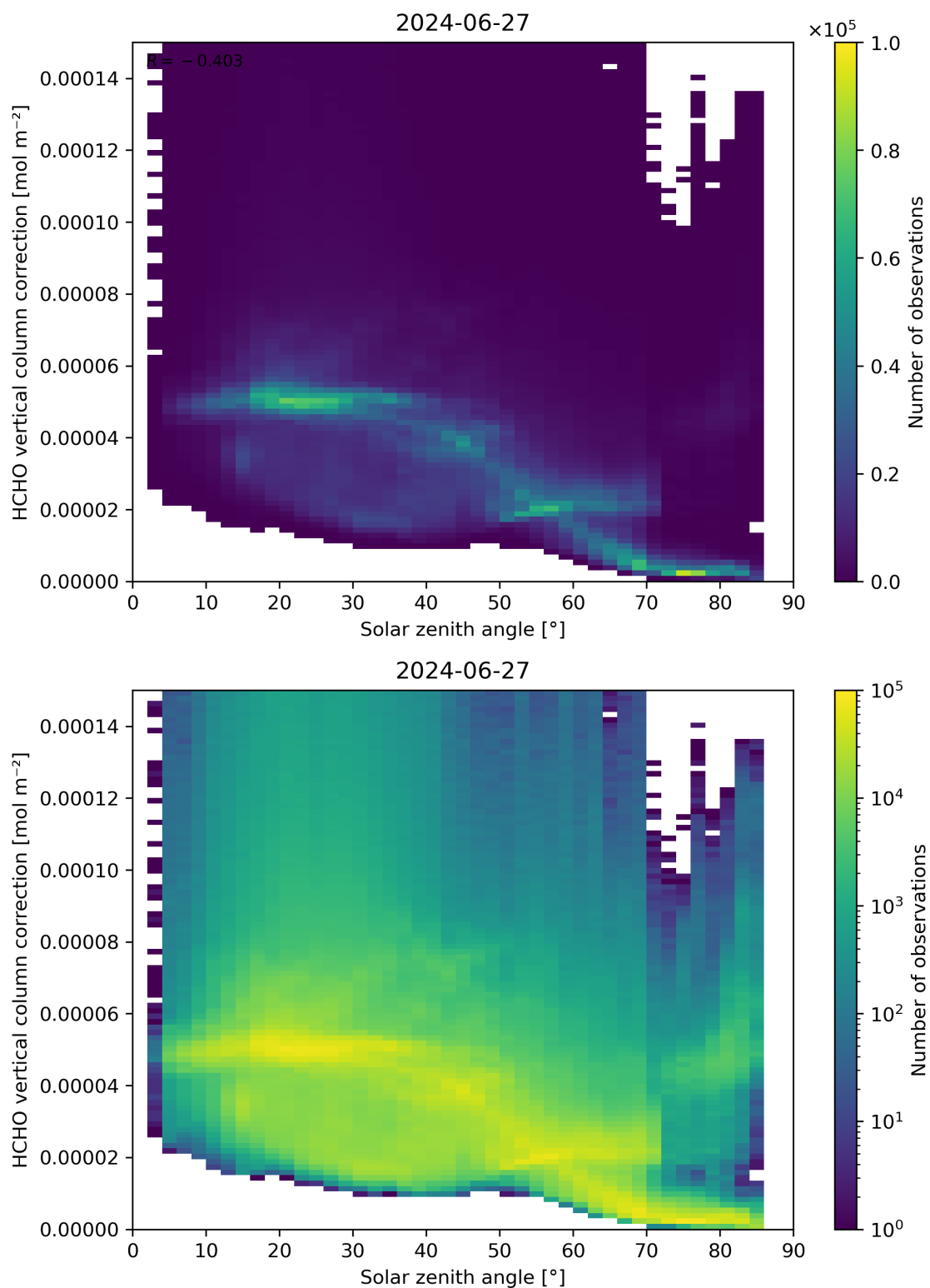
Figure 178: Scatter density plot of “Solar zenith angle” against “HCHO vertical column correction” for 2024-06-26 to 2024-06-28.
