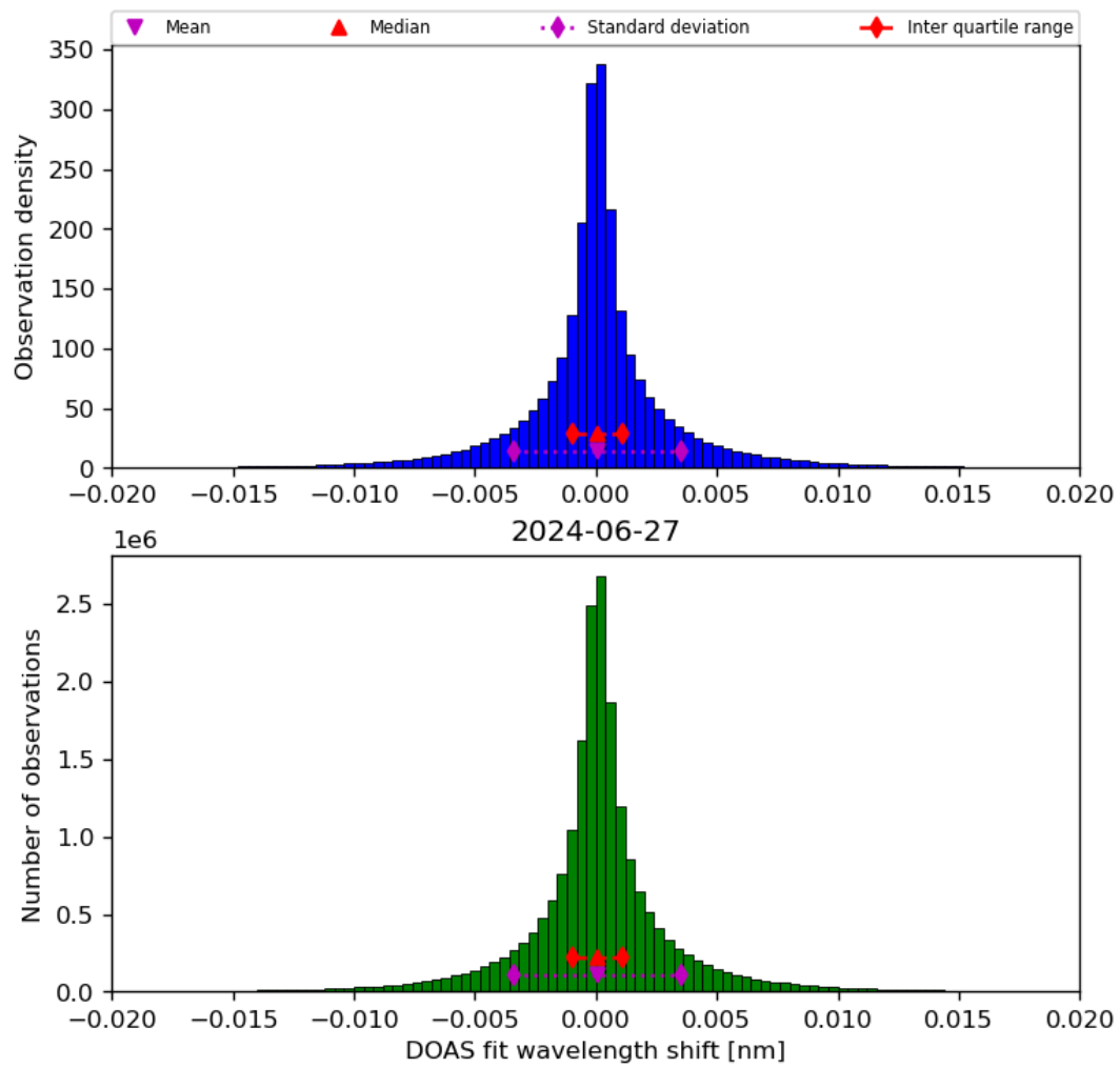
Figure 44: Histogram of “DOAS fit wavelength shift” for 2024-06-26 to 2024-06-28
