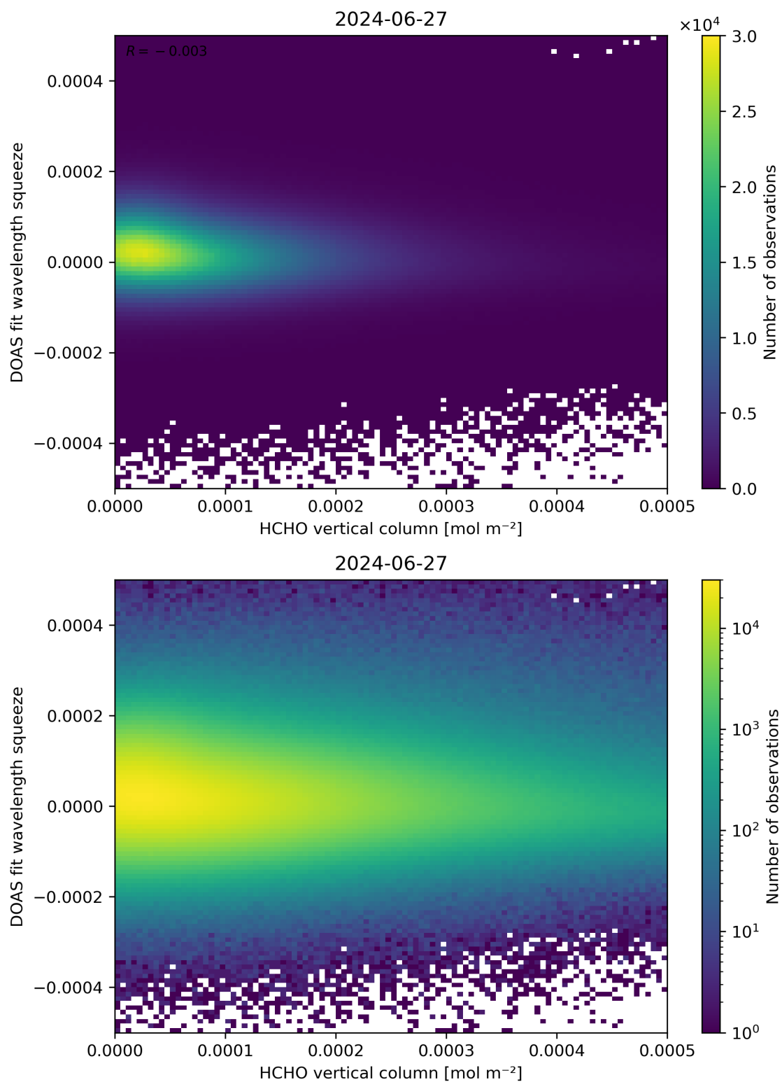
Figure 125: Scatter density plot of “HCHO vertical column” against “DOAS fit wavelength squeeze” for 2024-06-26 to 2024-06-28.
