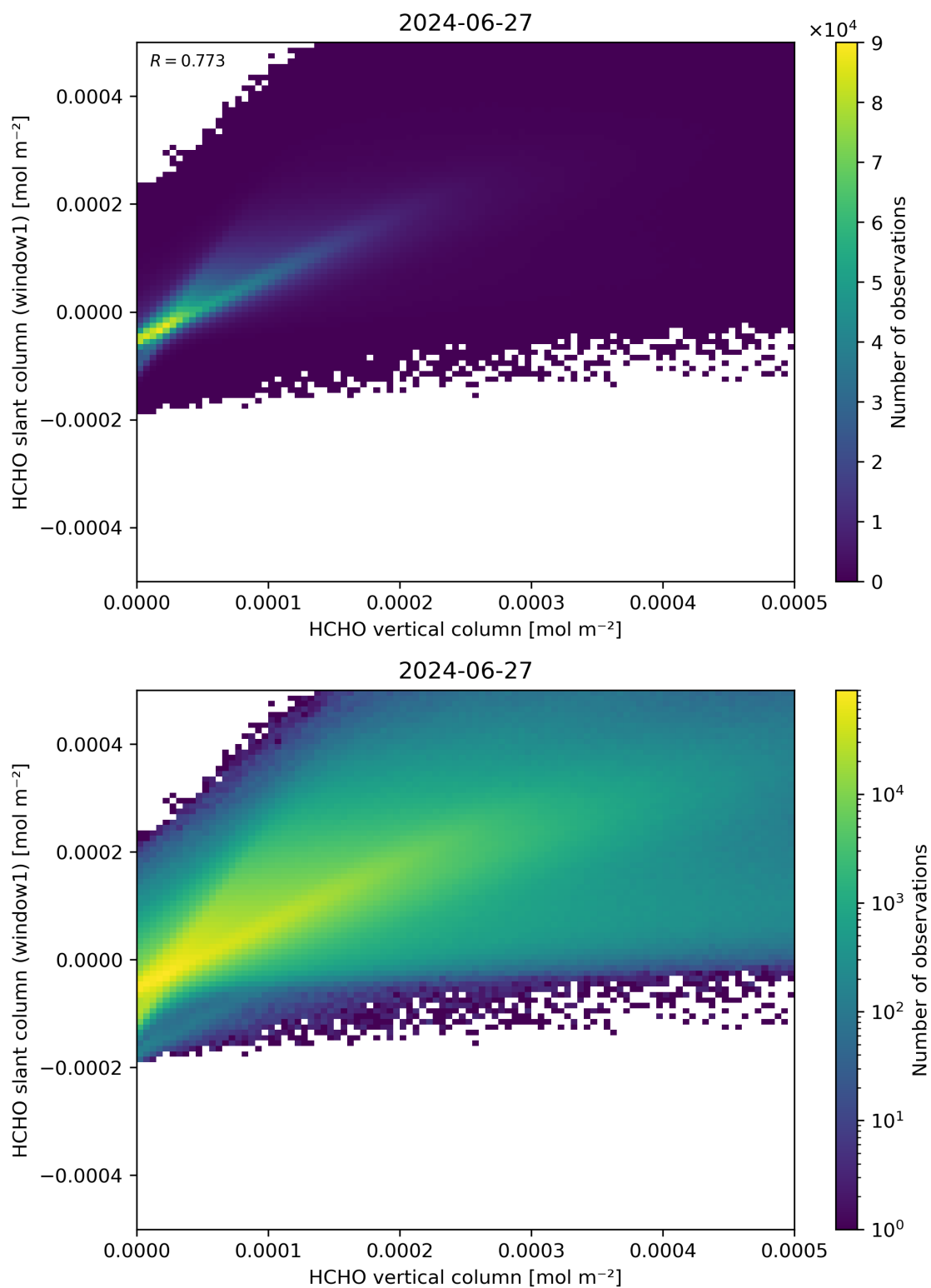
Figure 129: Scatter density plot of “HCHO vertical column” against “HCHO slant column (window1)” for 2024-06-26 to 2024-06-28.
