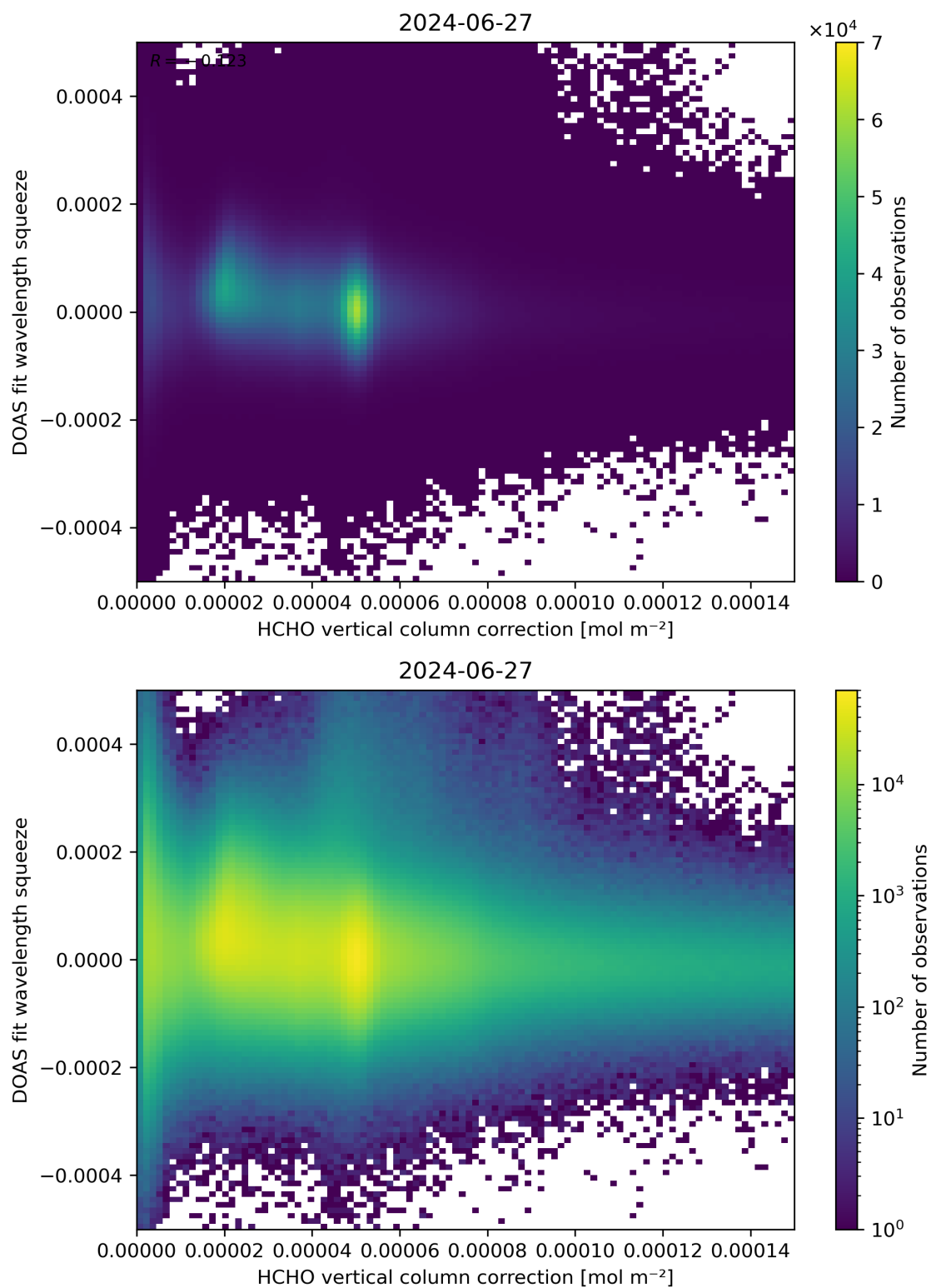
Figure 114: Scatter density plot of “HCHO vertical column correction” against “DOAS fit wavelength squeeze” for 2024-06-26 to 2024-06-28.
