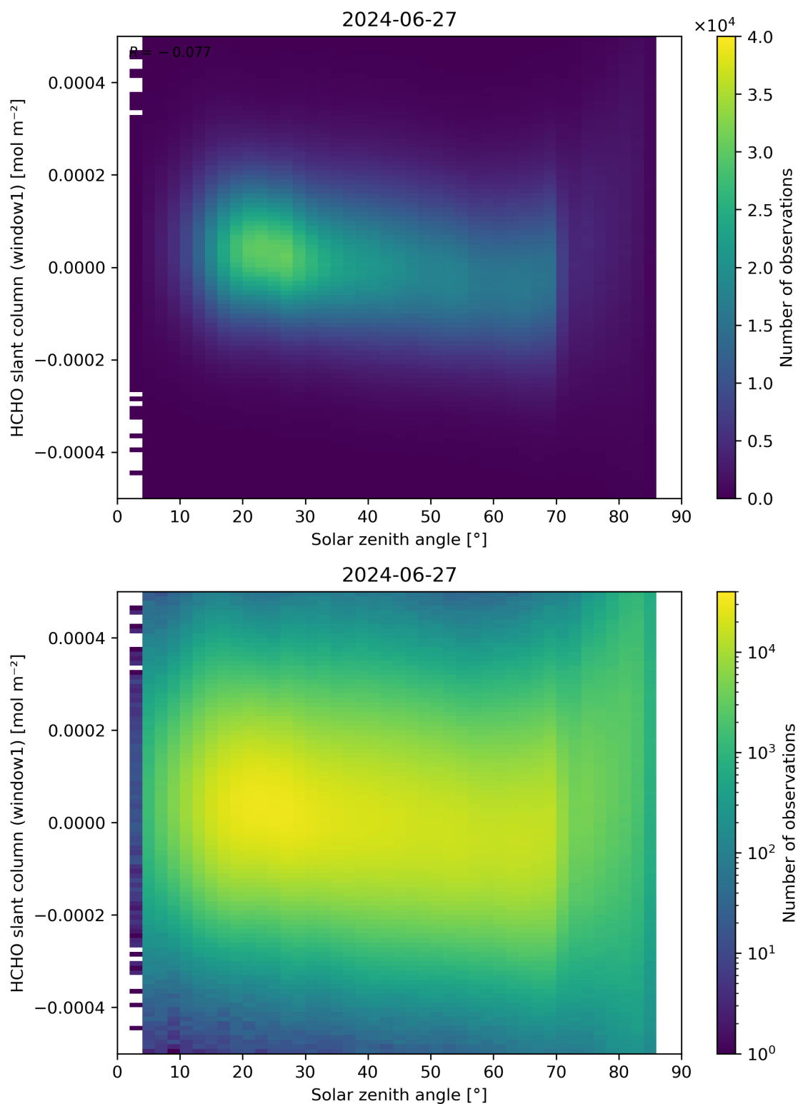
Figure 173: Scatter density plot of “Solar zenith angle” against “HCHO slant column (window1)” for 2024-06-26 to 2024-06-28.
