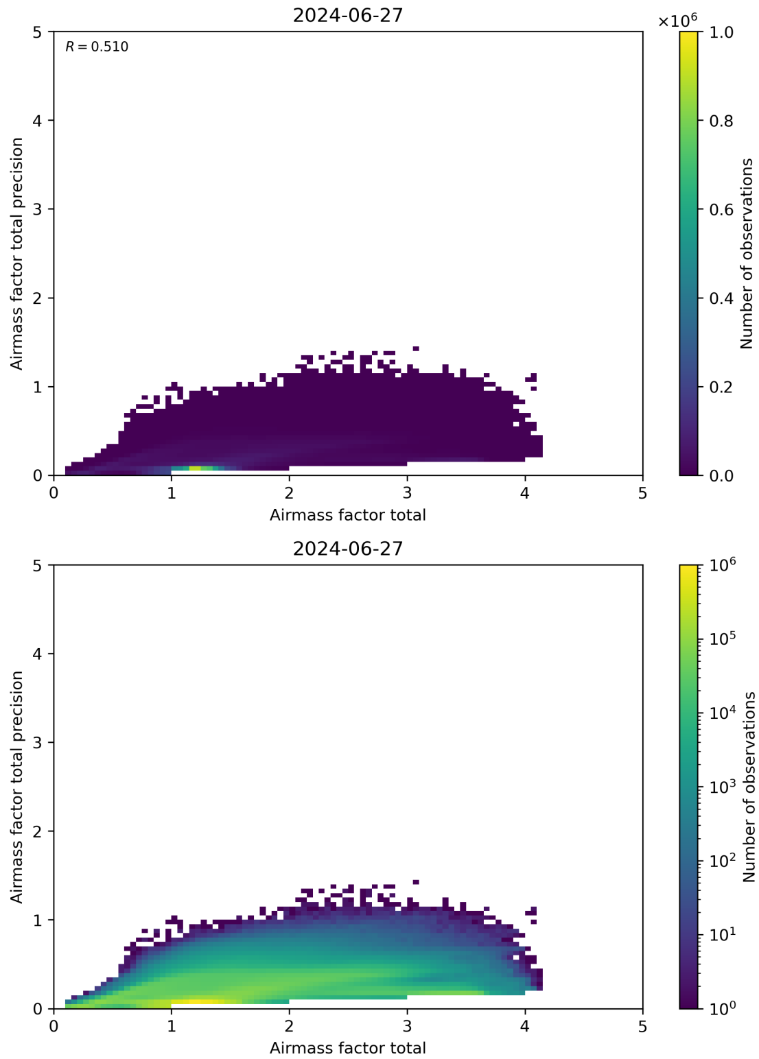
Figure 103: Scatter density plot of “Airmass factor total” against “Airmass factor total precision” for 2024-06-26 to 2024-06-28.
