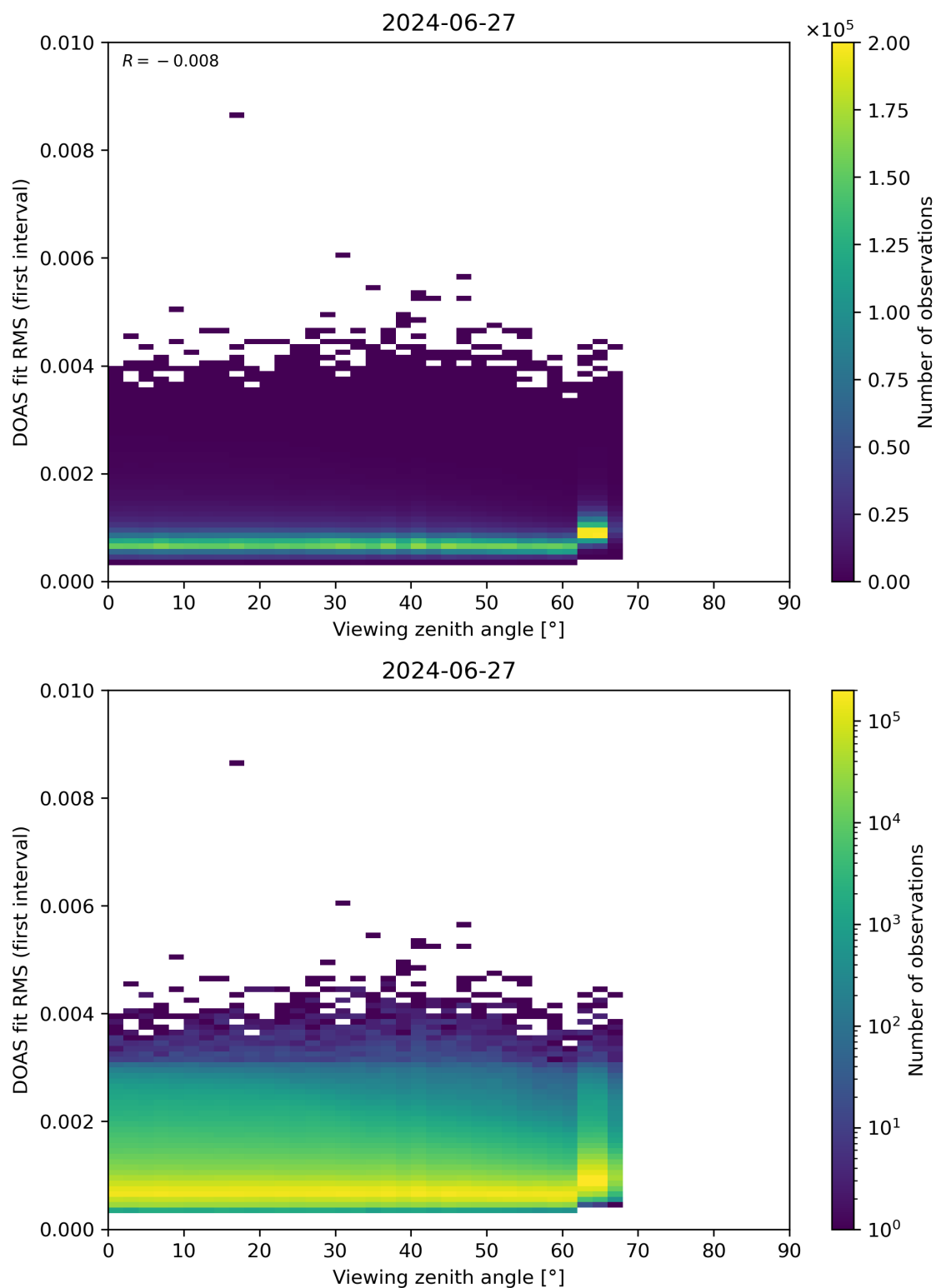
Figure 182: Scatter density plot of “Viewing zenith angle” against “DOAS fit RMS (first interval)” for 2024-06-26 to 2024-06-28.
