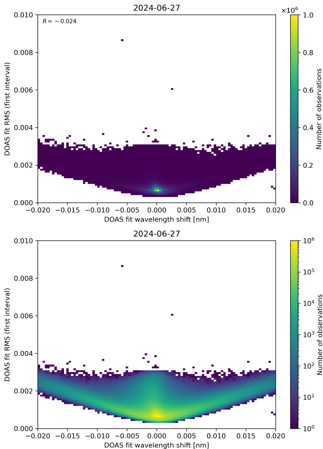
Figure 64: Scatter density plot of “DOAS fit wavelength shift” against “DOAS fit RMS (first interval)” for 2024-06-26 to 2024-06-28.
