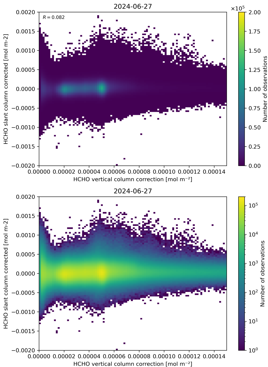
Figure 116: Scatter density plot of “HCHO vertical column correction” against “HCHO slant column corrected” for 2024-06-26 to 2024-06-28.
