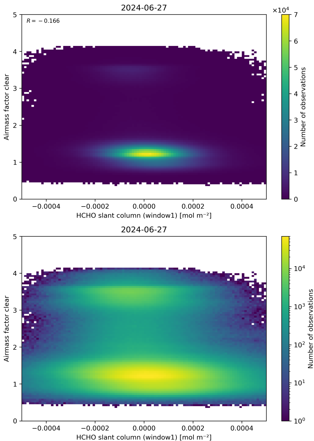
Figure 81: Scatter density plot of “HCHO slant column (window1)” against “Airmass factor clear” for 2024-06-26 to 2024-06-28.
