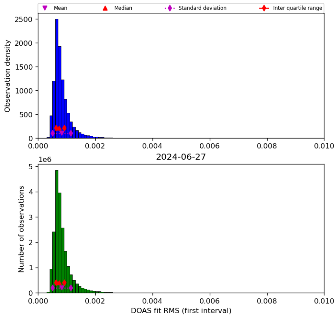
Figure 46: Histogram of “DOAS fit RMS (first interval)” for 2024-06-26 to 2024-06-28
