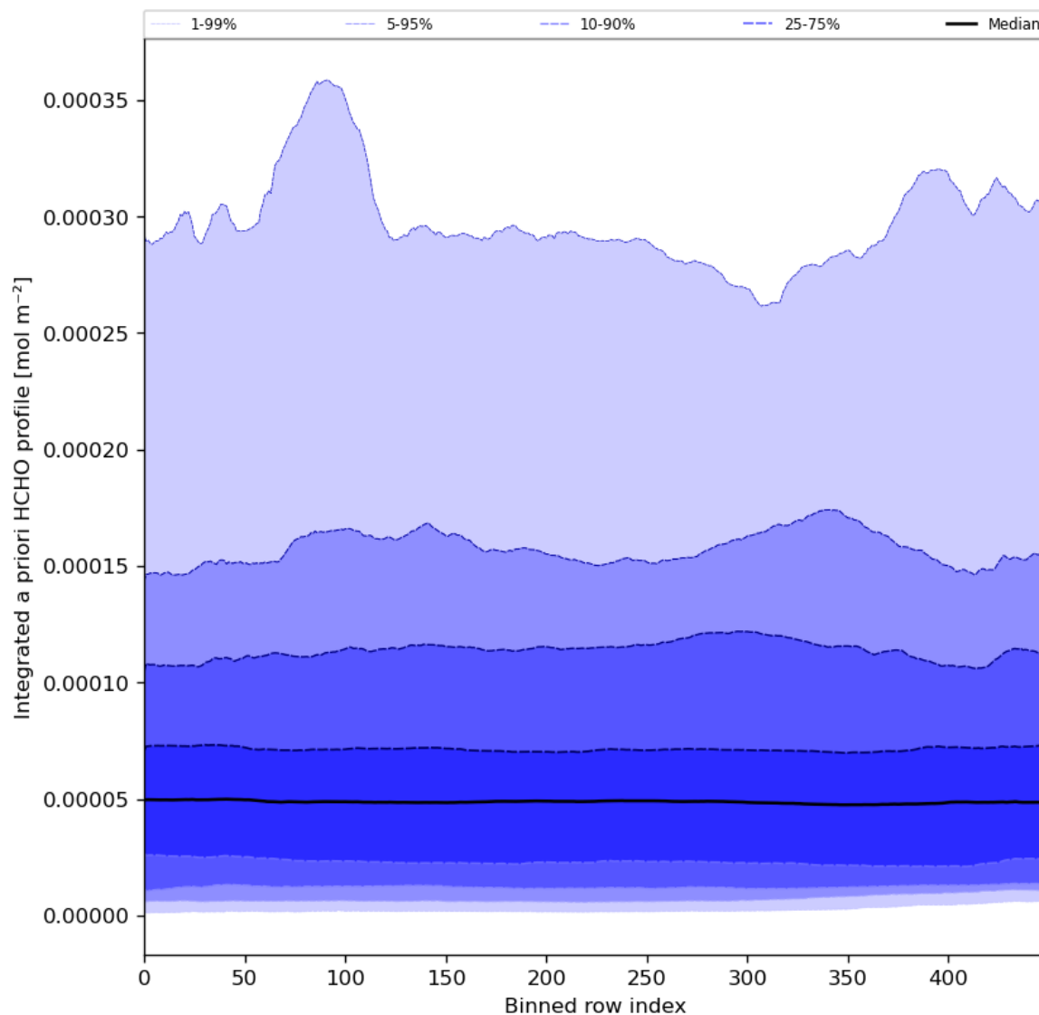
Figure 57: Along track statistics of “Integrated a priori HCHO profile” for 2024-06-26 to 2024-06-28
