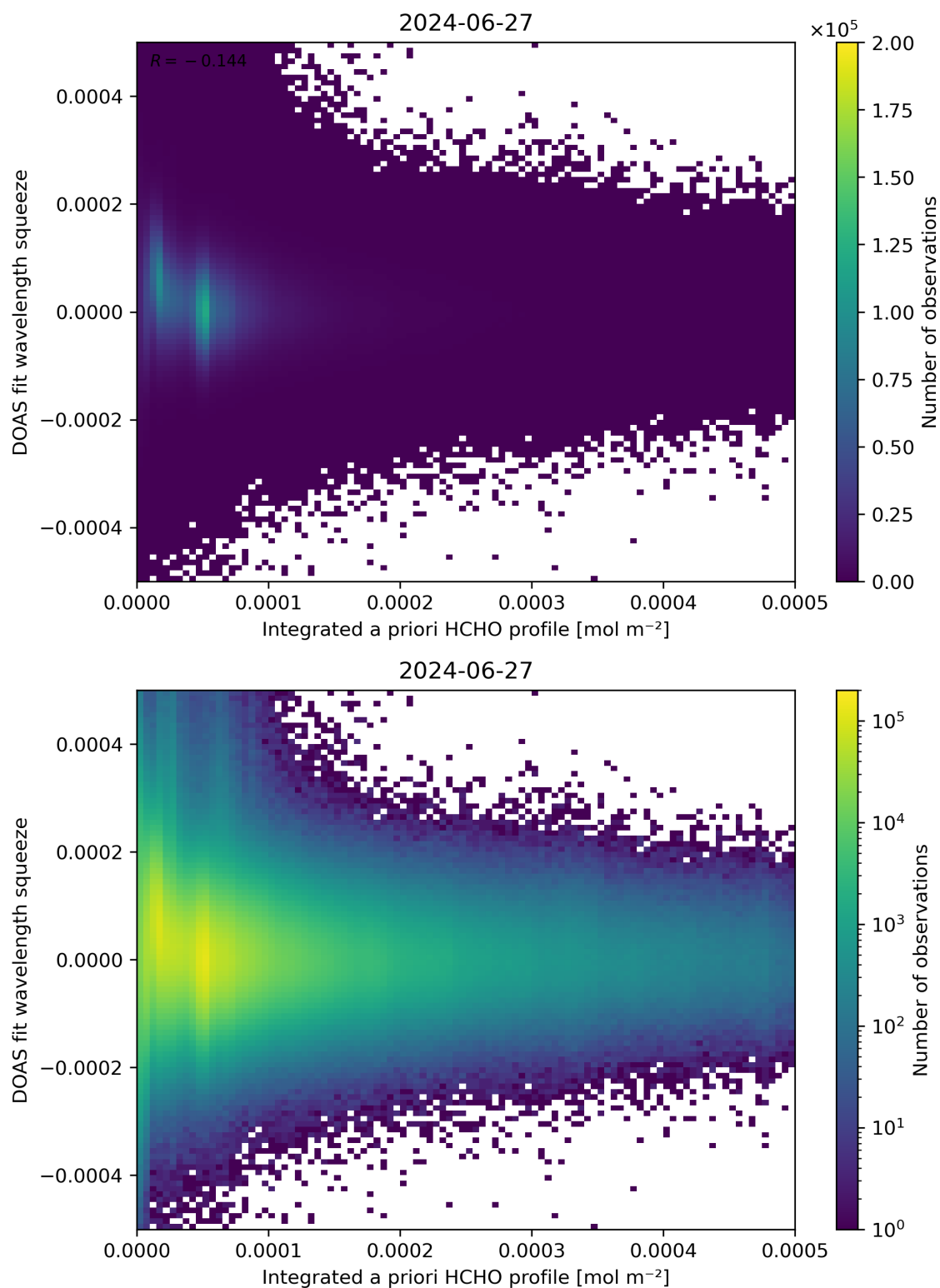
Figure 150: Scatter density plot of “Integrated a priori HCHO profile” against “DOAS fit wavelength squeeze” for 2024-06-26 to 2024-06-28.
