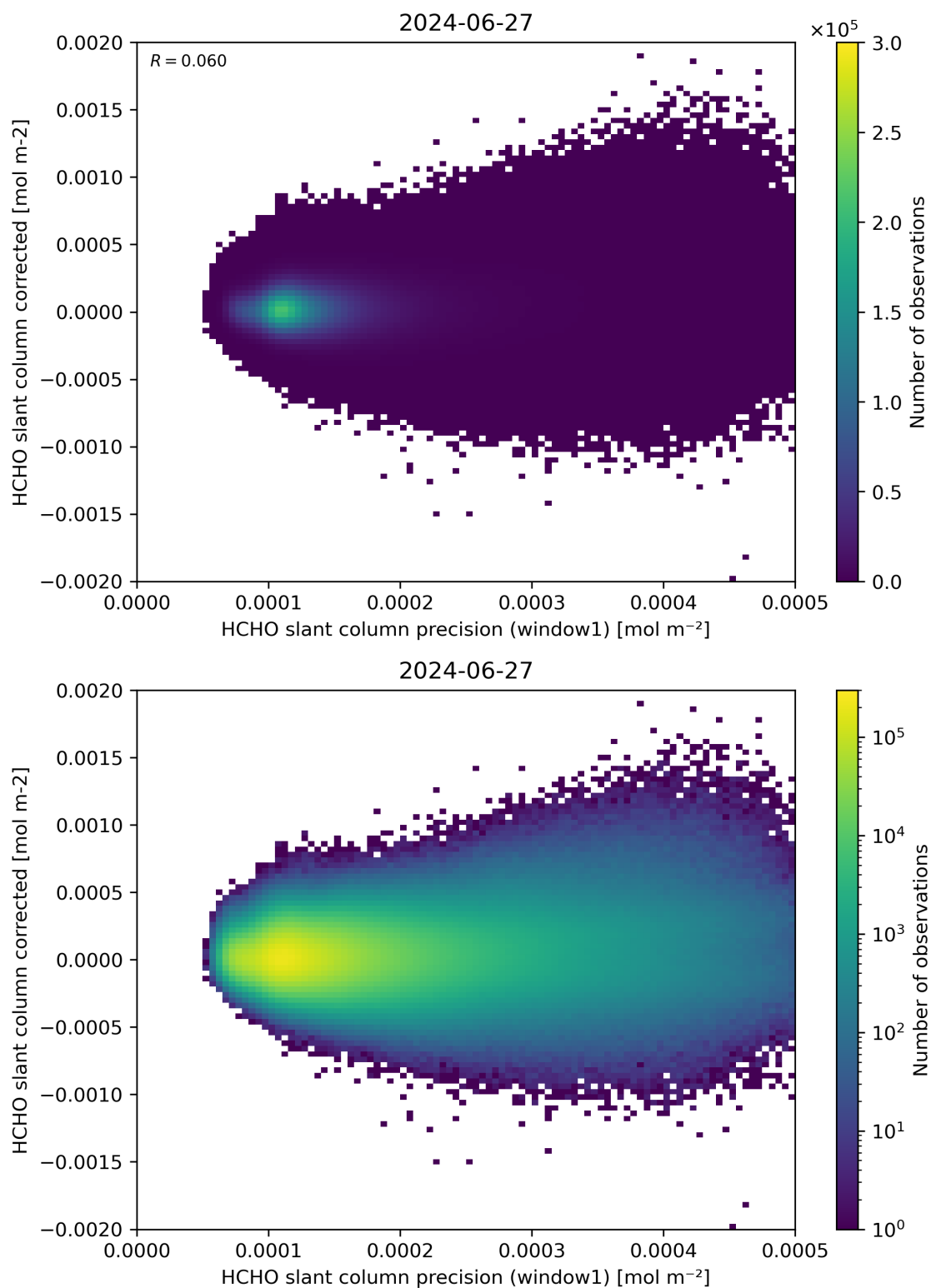
Figure 92: Scatter density plot of “HCHO slant column precision (window1)” against “HCHO slant column corrected” for 2024-06-26 to 2024-06-28.
