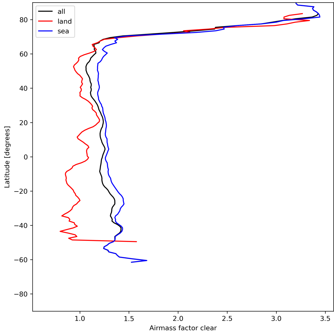
Figure 28: Zonal average of “Airmass factor clear” for 2024-06-26 to 2024-06-28.
