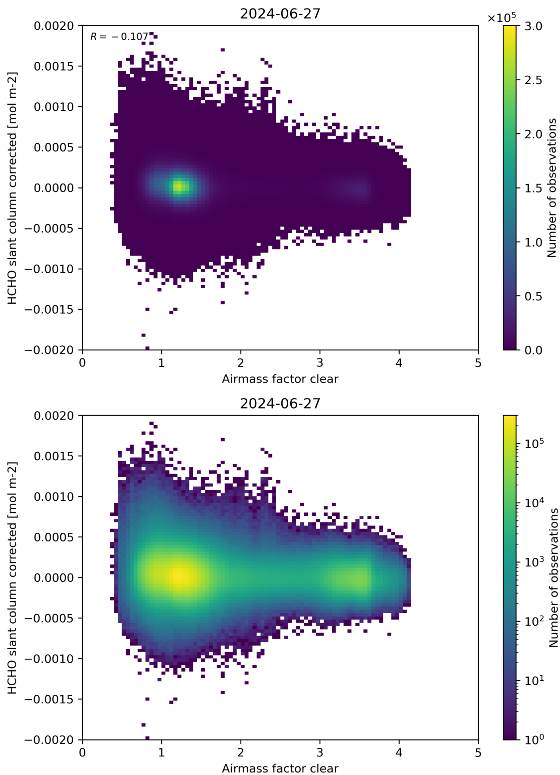
Figure 74: Scatter density plot of “Airmass factor clear” against “HCHO slant column corrected” for 2024-06-26 to 2024-06-28.
