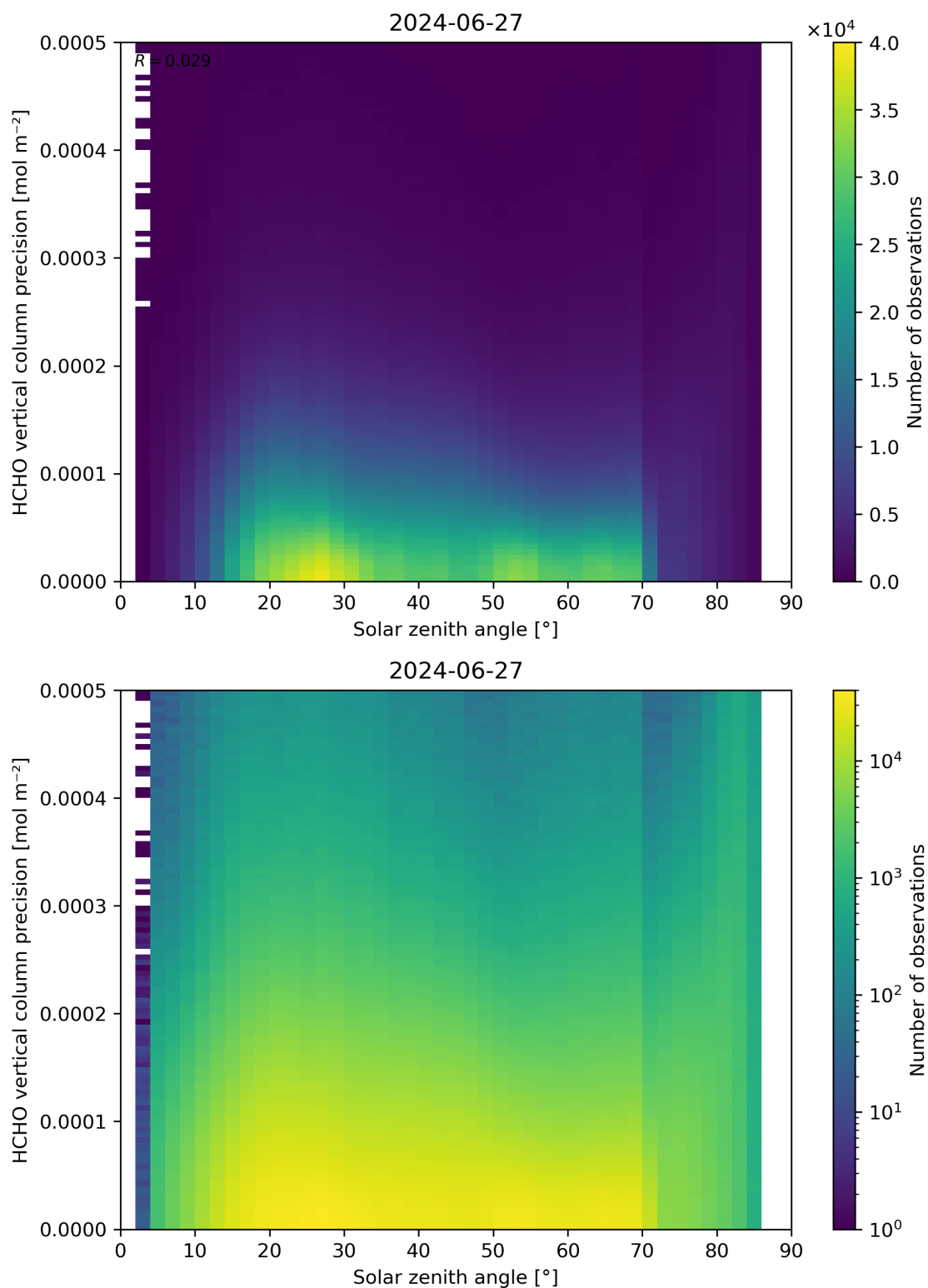
Figure 179: Scatter density plot of “Solar zenith angle” against “HCHO vertical column precision” for 2024-06-26 to 2024-06-28.
