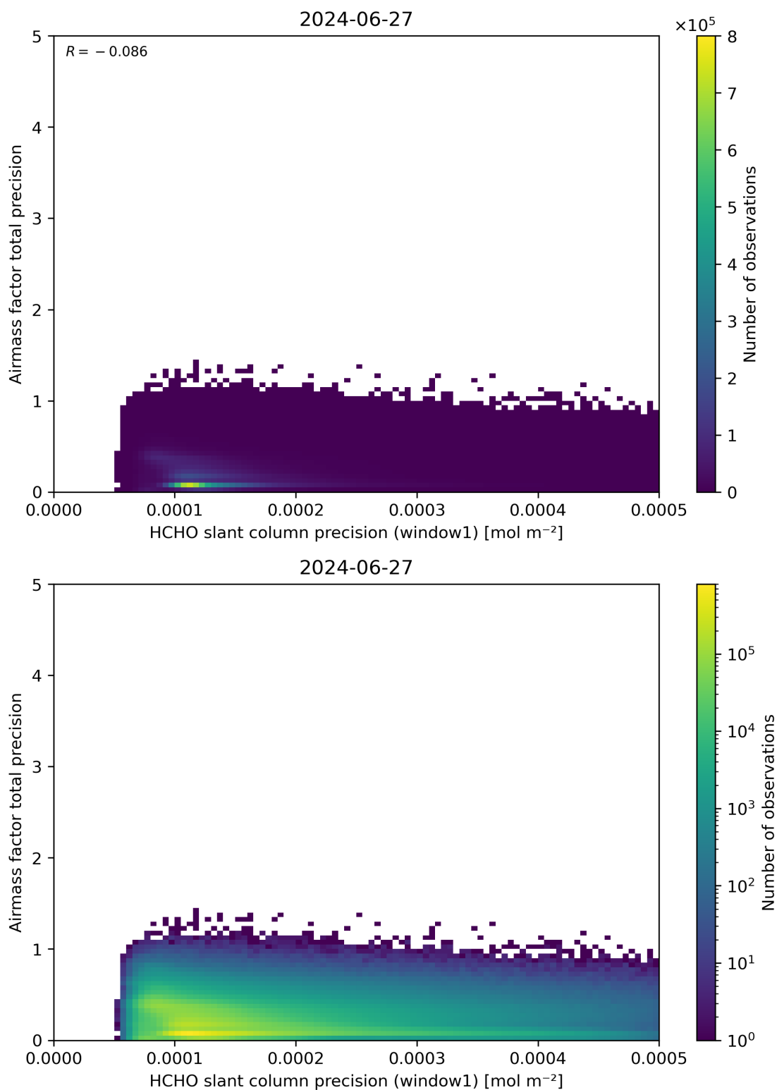
Figure 95: Scatter density plot of “HCHO slant column precision (window1)” against “Airmass factor total precision” for 2024-06-26 to 2024-06-28.
