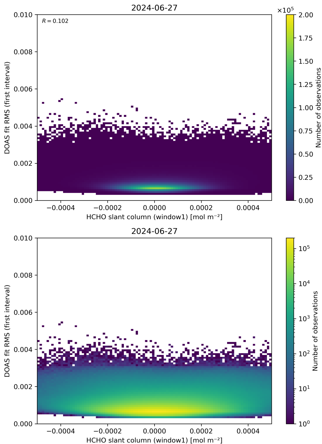
Figure 78: Scatter density plot of “HCHO slant column (window1)” against “DOAS fit RMS (first interval)” for 2024-06-26 to 2024-06-28.
