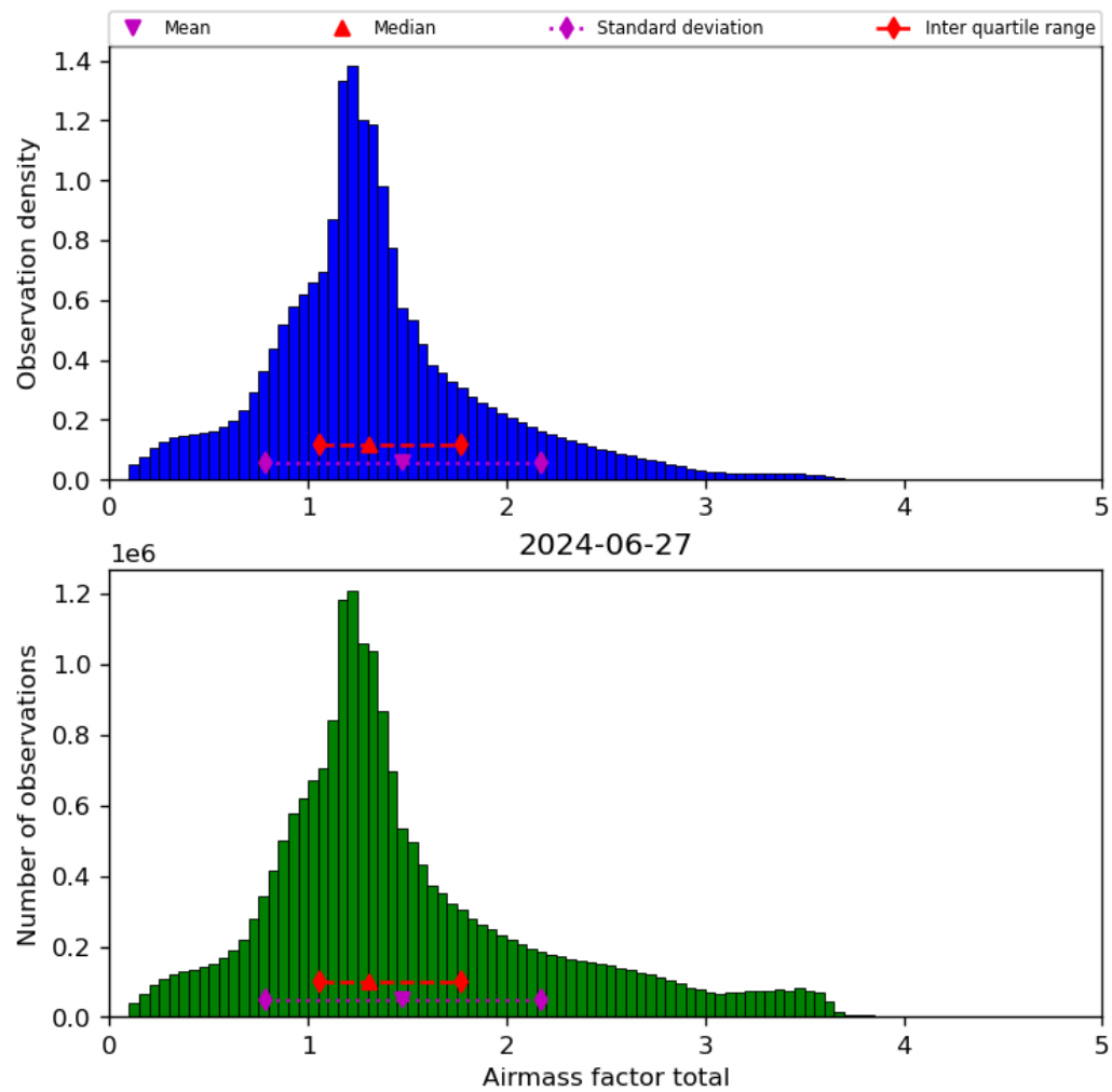
Figure 40: Histogram of “Airmass factor total” for 2024-06-26 to 2024-06-28
