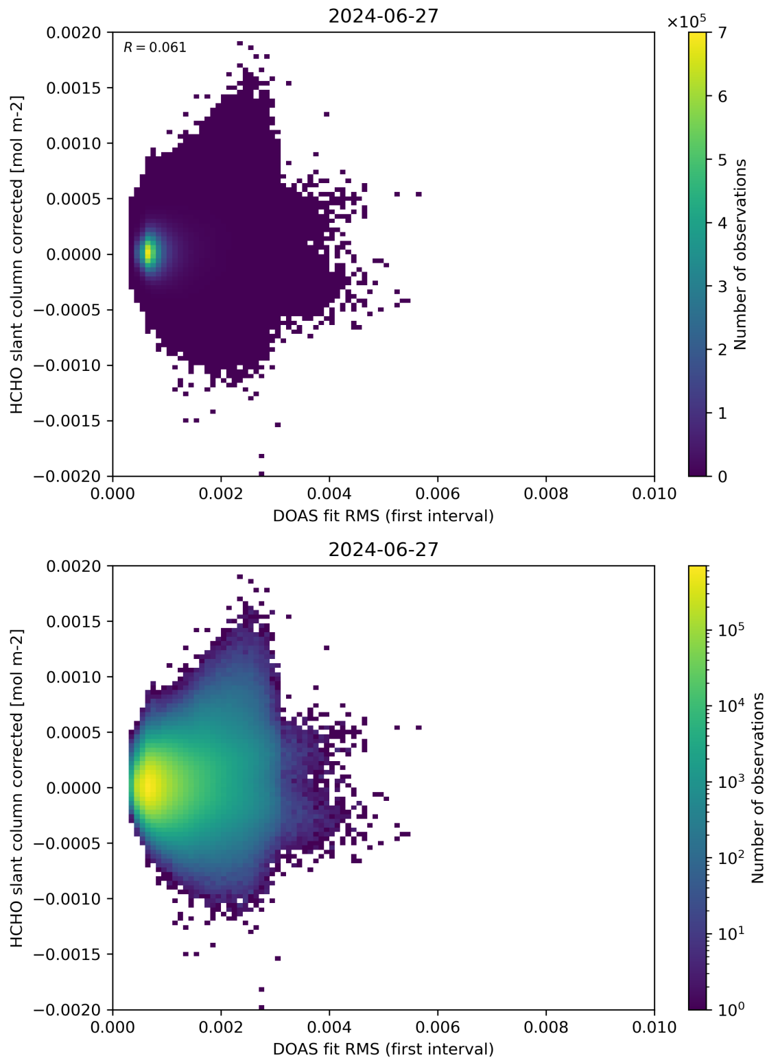
Figure 62: Scatter density plot of “DOAS fit RMS (first interval)” against “HCHO slant column corrected” for 2024-06-26 to 2024-06-28.
