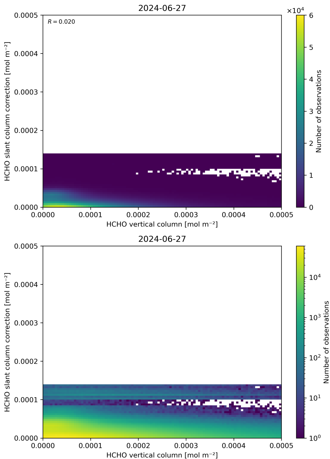
Figure 128: Scatter density plot of “HCHO vertical column” against “HCHO slant column correction” for 2024-06-26 to 2024-06-28.
