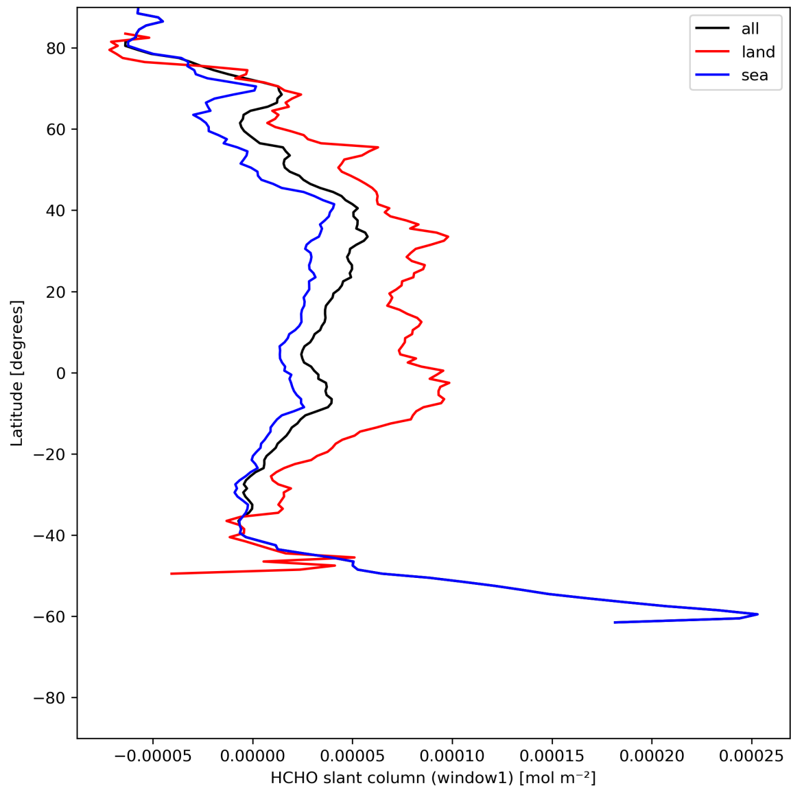
Figure 24: Zonal average of “HCHO slant column (window1)” for 2024-06-26 to 2024-06-28.
