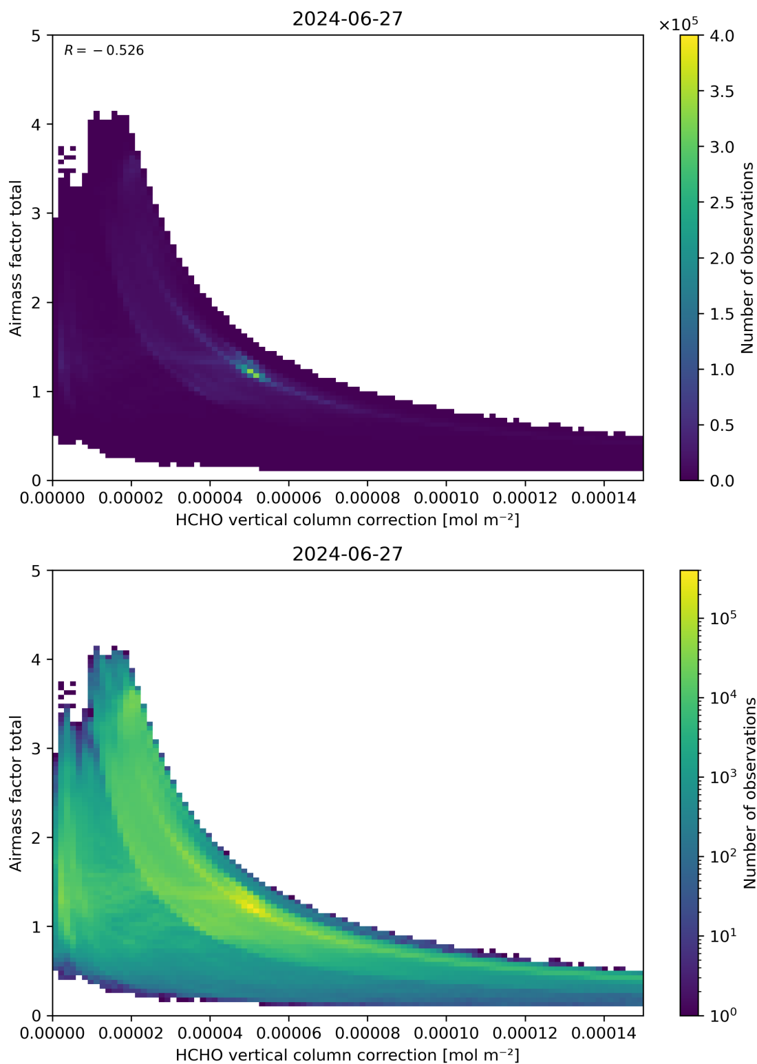
Figure 120: Scatter density plot of “HCHO vertical column correction” against “Airmass factor total” for 2024-06-26 to 2024-06-28.
