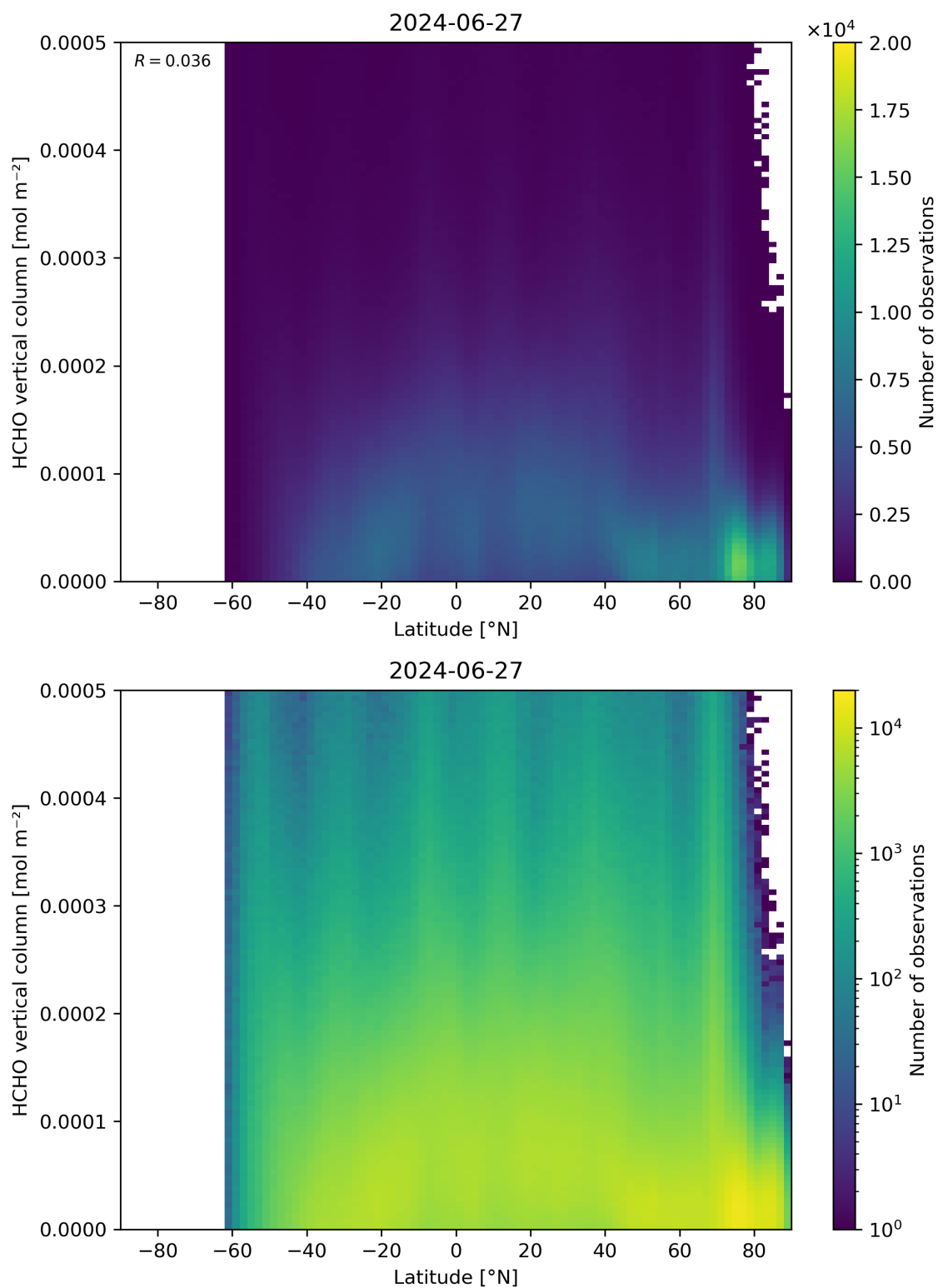
Figure 163: Scatter density plot of “Latitude” against “HCHO vertical column” for 2024-06-26 to 2024-06-28.
