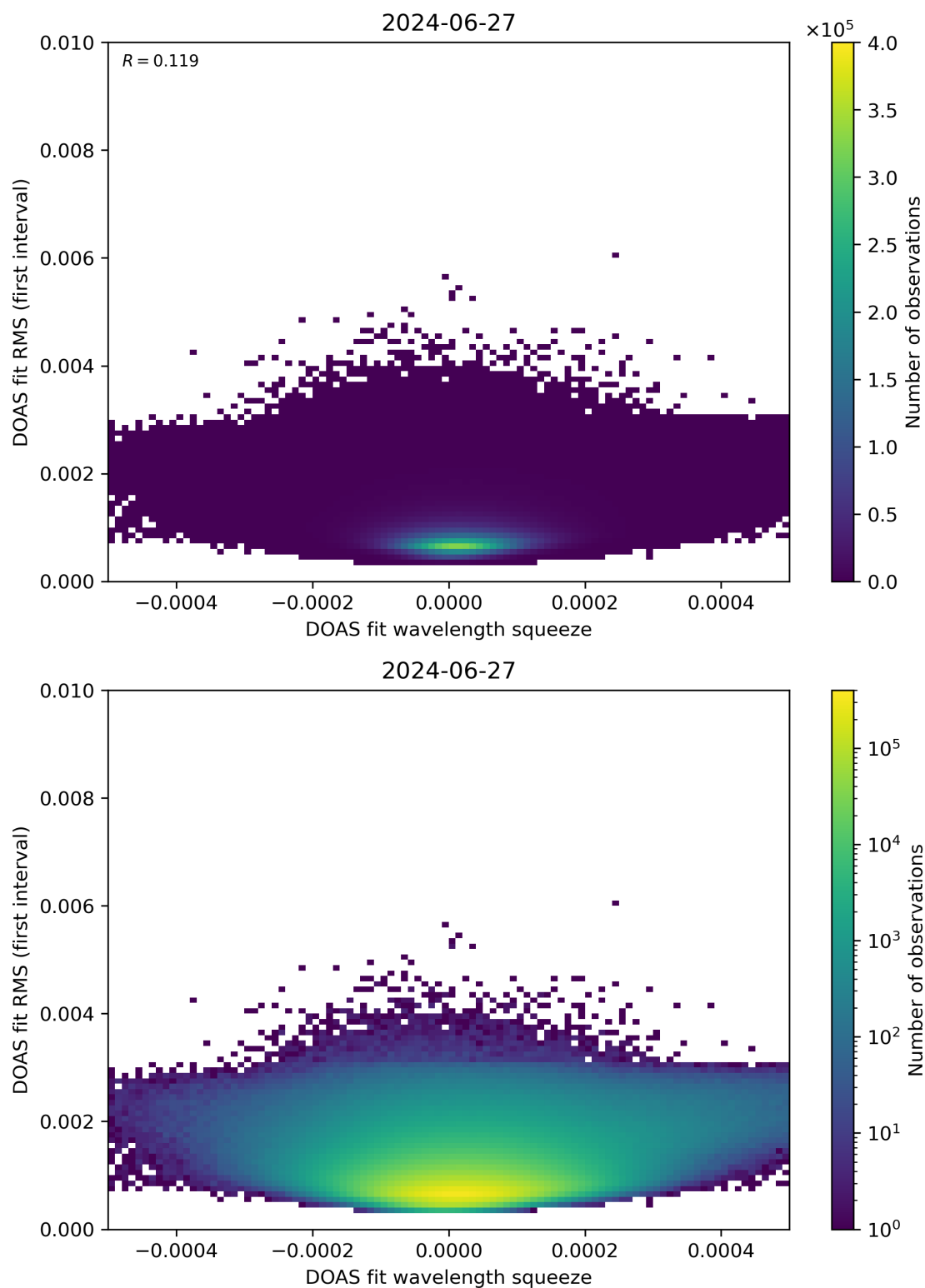
Figure 68: Scatter density plot of “DOAS fit wavelength squeeze” against “DOAS fit RMS (first interval)” for 2024-06-26 to 2024-06-28.
