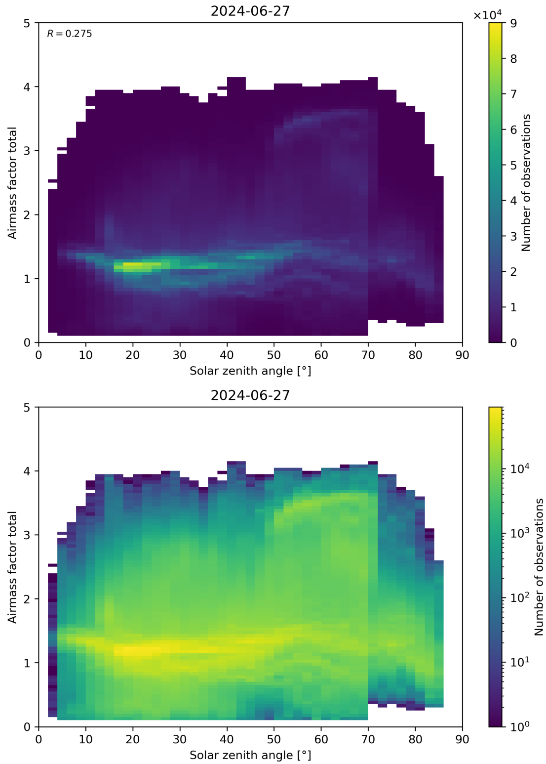
Figure 175: Scatter density plot of “Solar zenith angle” against “Airmass factor total” for 2024-06-26 to 2024-06-28.
