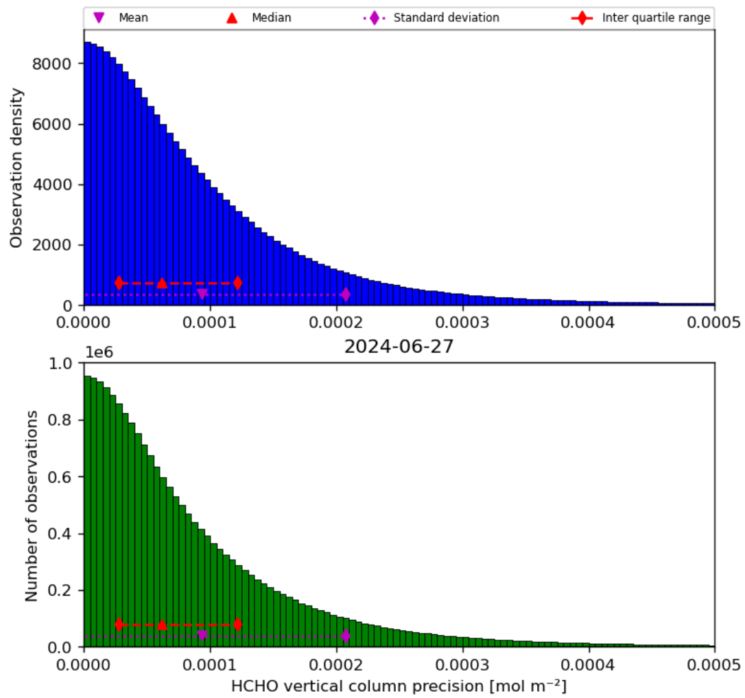
Figure 36: Histogram of “HCHO vertical column precision” for 2024-06-26 to 2024-06-28
