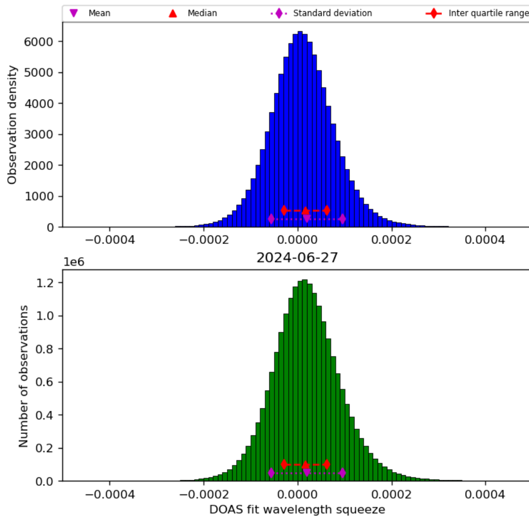
Figure 45: Histogram of “DOAS fit wavelength squeeze” for 2024-06-26 to 2024-06-28
