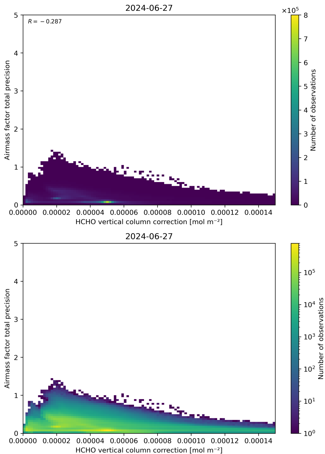
Figure 121: Scatter density plot of “HCHO vertical column correction” against “Airmass factor total precision” for 2024-06-26 to 2024-06-28.
