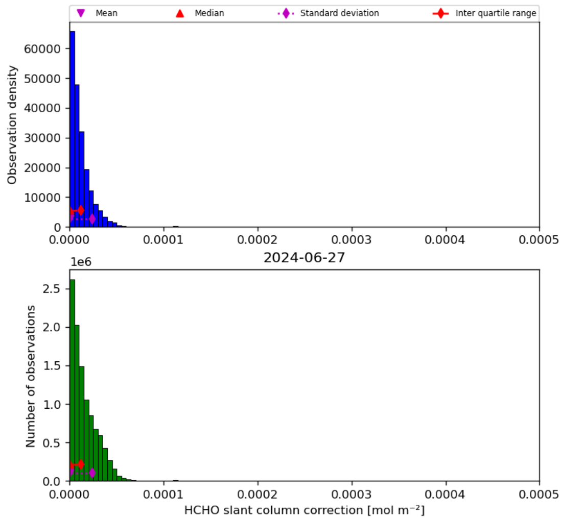
Figure 47: Histogram of “HCHO slant column correction” for 2024-06-26 to 2024-06-28
