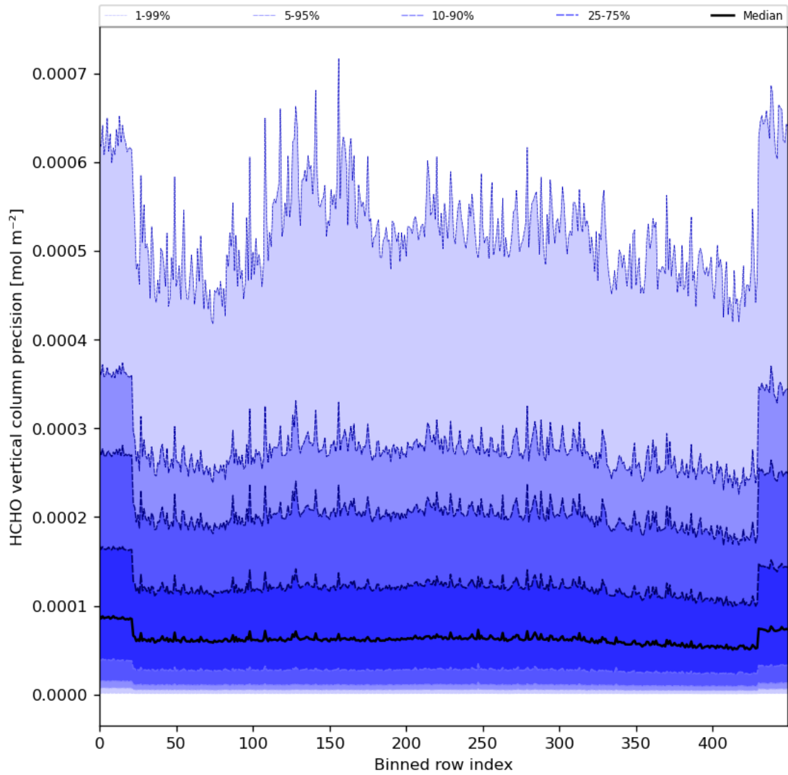
Figure 50: Along track statistics of “HCHO vertical column precision” for 2024-06-26 to 2024-06-28
