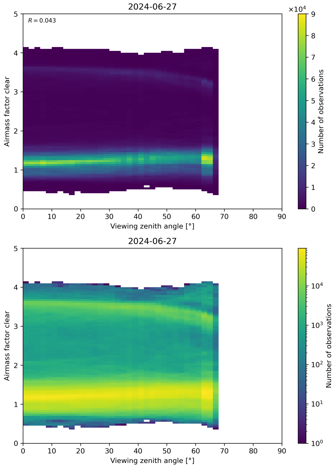
Figure 185: Scatter density plot of “Viewing zenith angle” against “Airmass factor clear” for 2024-06-26 to 2024-06-28.
