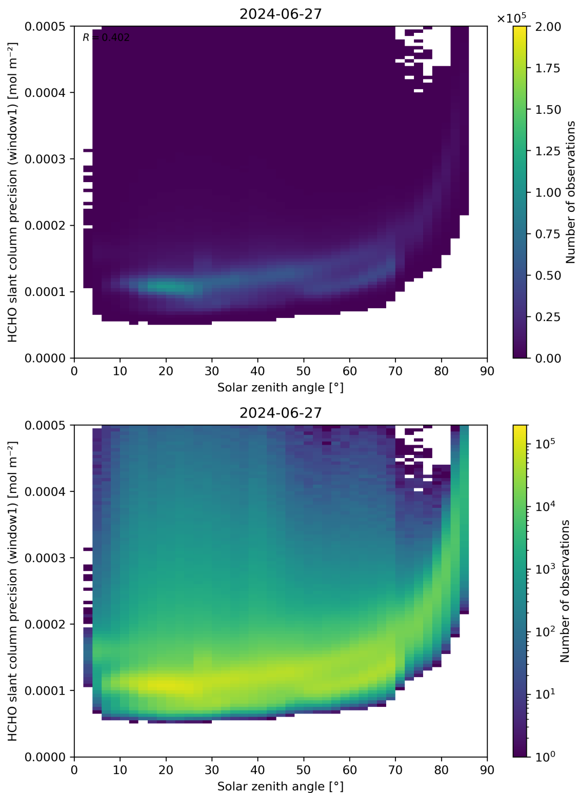
Figure 174: Scatter density plot of “Solar zenith angle” against “HCHO slant column precision (window1)” for 2024-06-26 to 2024-06-28.
