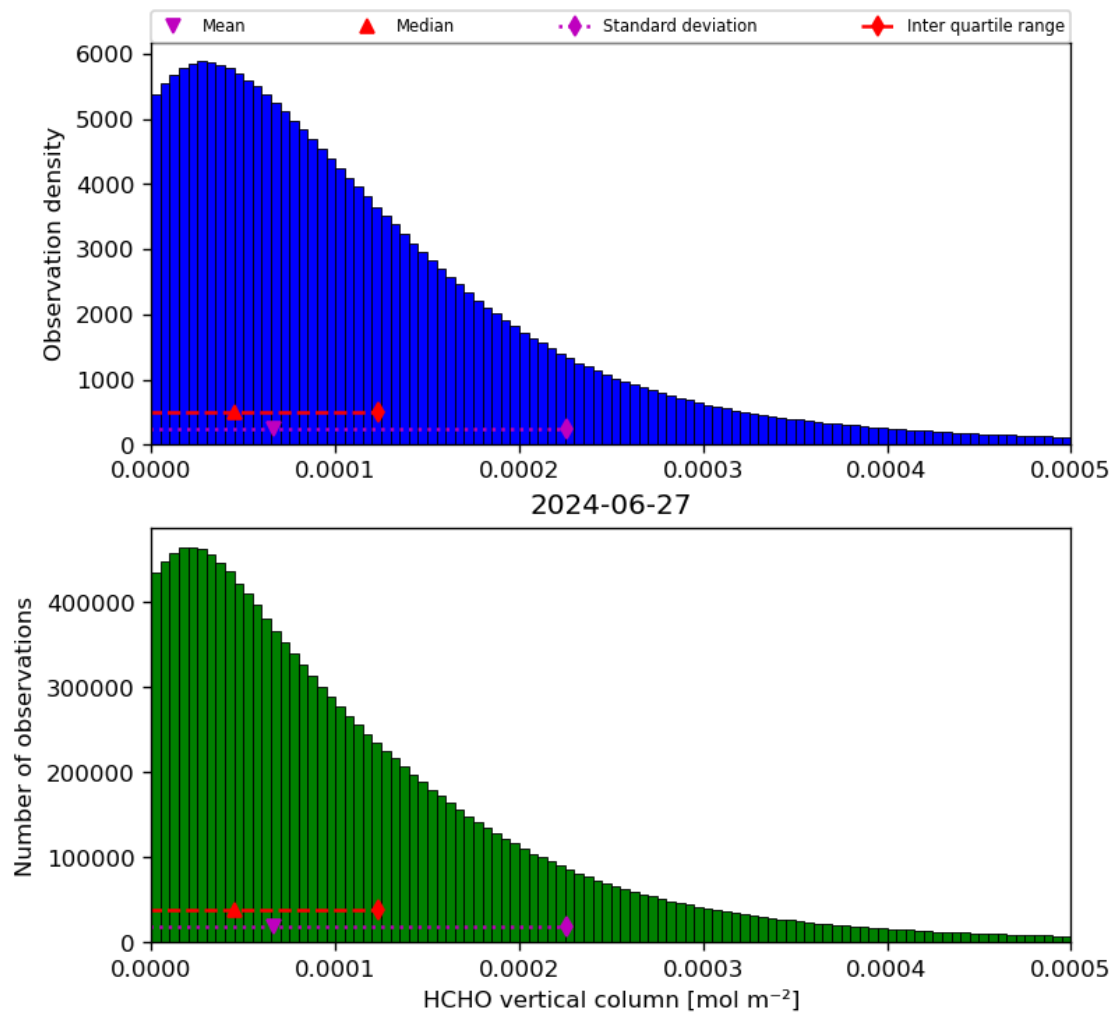
Figure 35: Histogram of “HCHO vertical column” for 2024-06-26 to 2024-06-28
