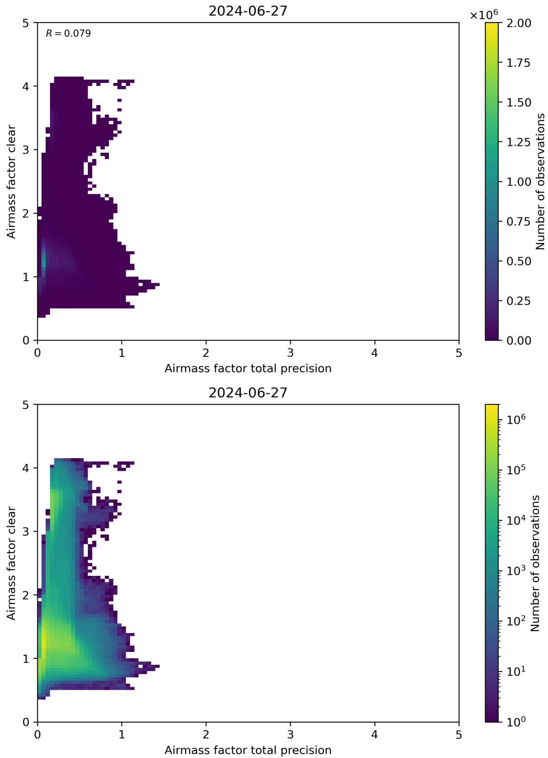
Figure 108: Scatter density plot of “Airmass factor total precision” against “Airmass factor clear” for 2024-06-26 to 2024-06-28.
