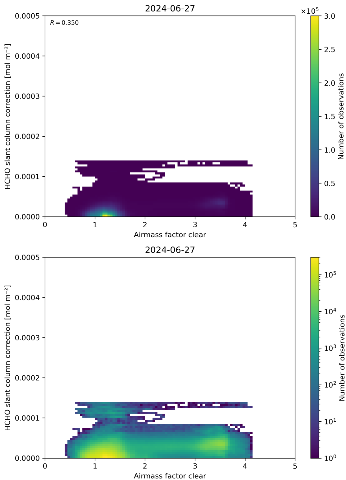
Figure 75: Scatter density plot of “Airmass factor clear” against “HCHO slant column correction” for 2024-06-26 to 2024-06-28.
