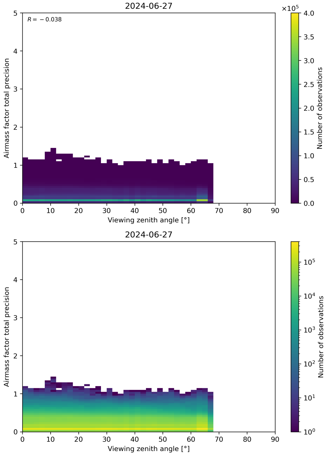
Figure 191: Scatter density plot of “Viewing zenith angle” against “Airmass factor total precision” for 2024-06-26 to 2024-06-28.
