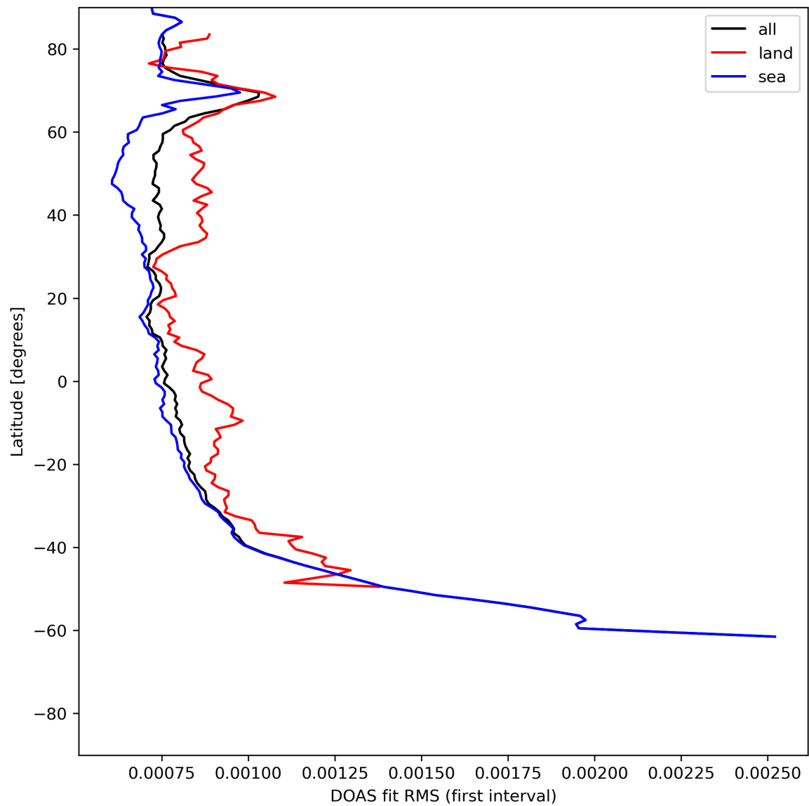
Figure 32: Zonal average of “DOAS fit RMS (first interval)” for 2024-06-26 to 2024-06-28.
