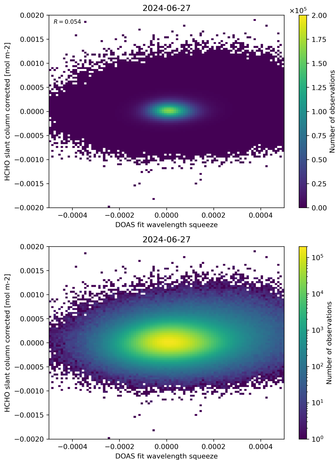
Figure 69: Scatter density plot of “DOAS fit wavelength squeeze” against “HCHO slant column corrected” for 2024-06-26 to 2024-06-28.
