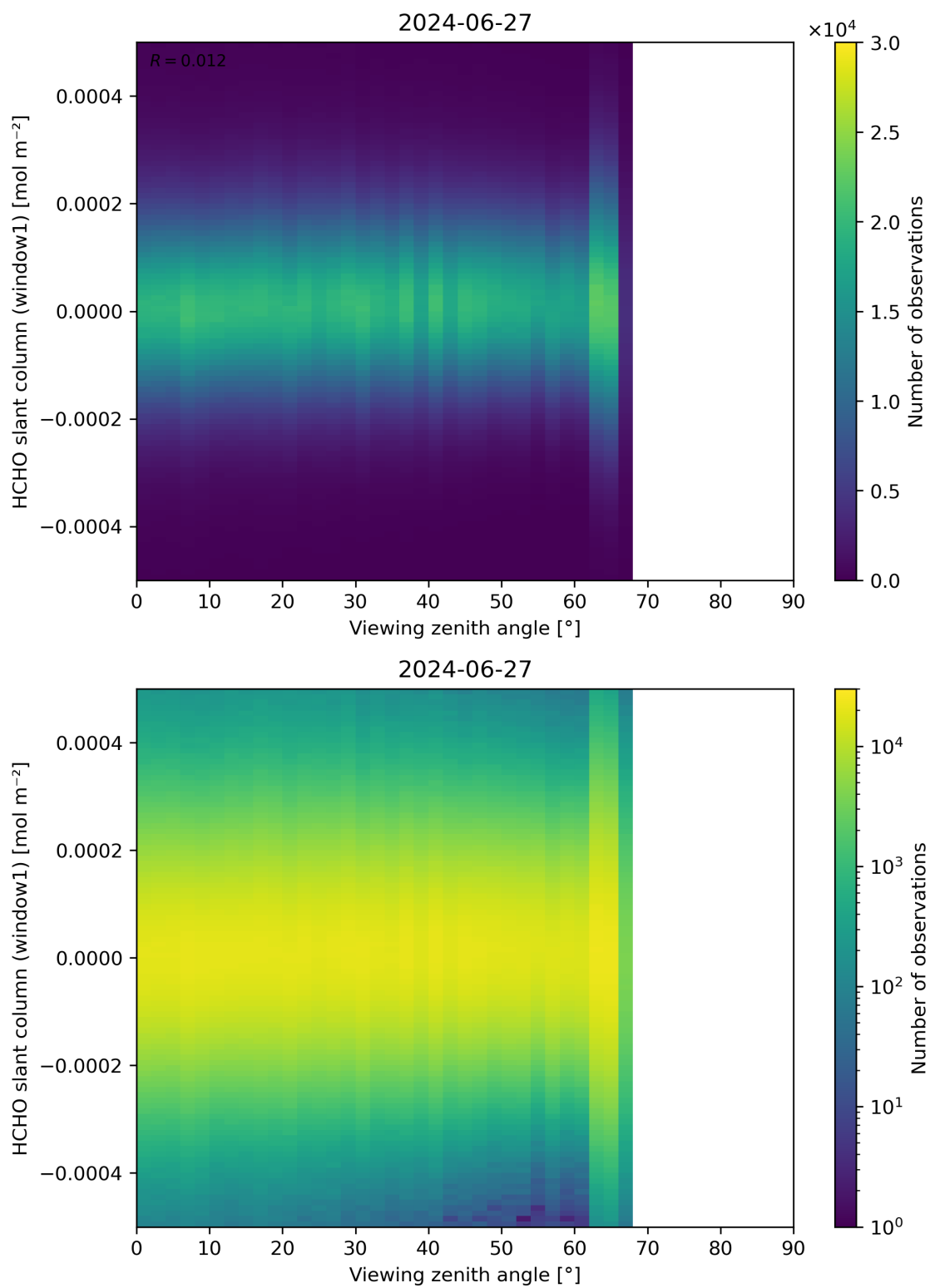
Figure 188: Scatter density plot of “Viewing zenith angle” against “HCHO slant column (window1)” for 2024-06-26 to 2024-06-28.
