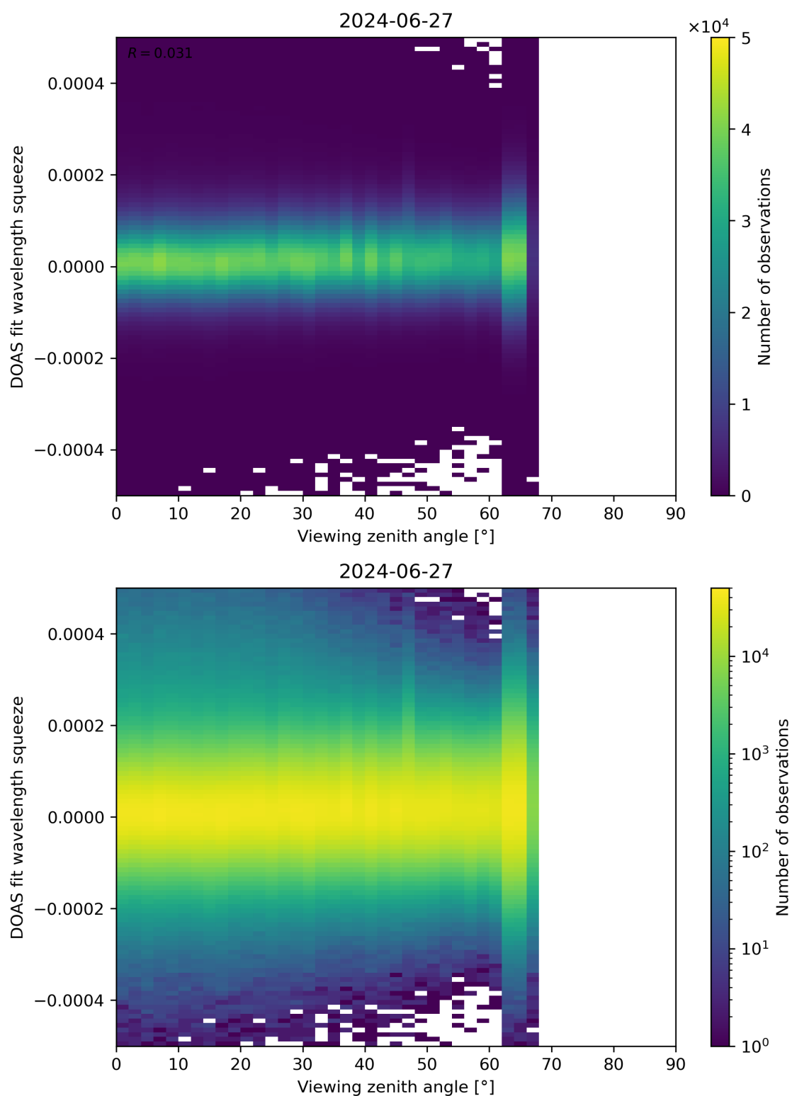
Figure 184: Scatter density plot of “Viewing zenith angle” against “DOAS fit wavelength squeeze” for 2024-06-26 to 2024-06-28.
