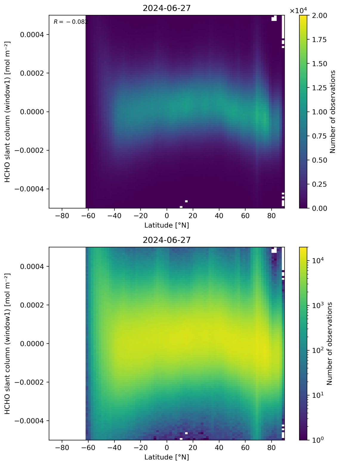
Figure 159: Scatter density plot of “Latitude” against “HCHO slant column (window1)” for 2024-06-26 to 2024-06-28.
