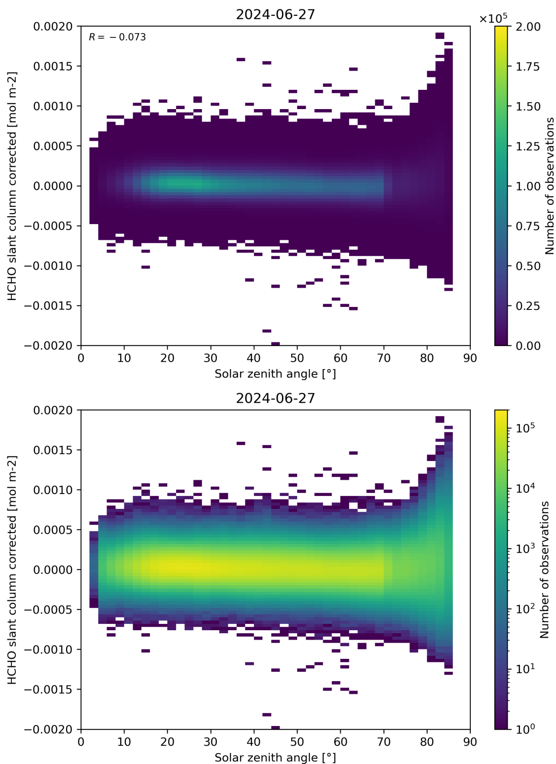
Figure 171: Scatter density plot of “Solar zenith angle” against “HCHO slant column corrected” for 2024-06-26 to 2024-06-28.
