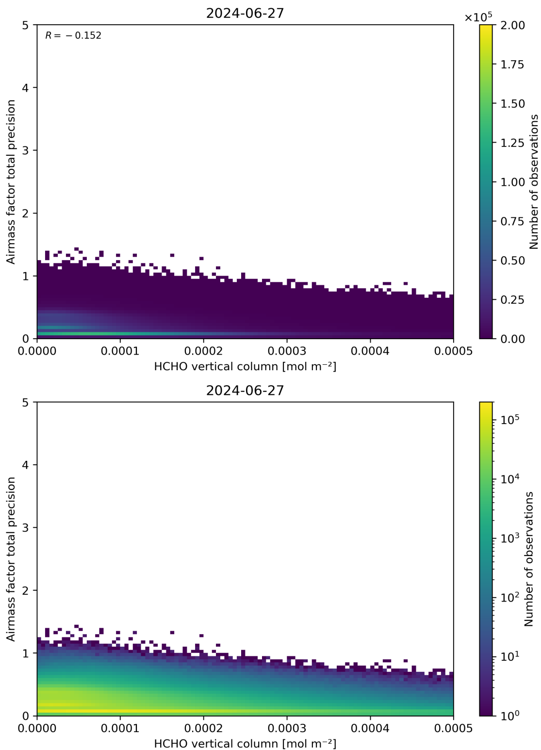
Figure 132: Scatter density plot of “HCHO vertical column” against “Airmass factor total precision” for 2024-06-26 to 2024-06-28.
