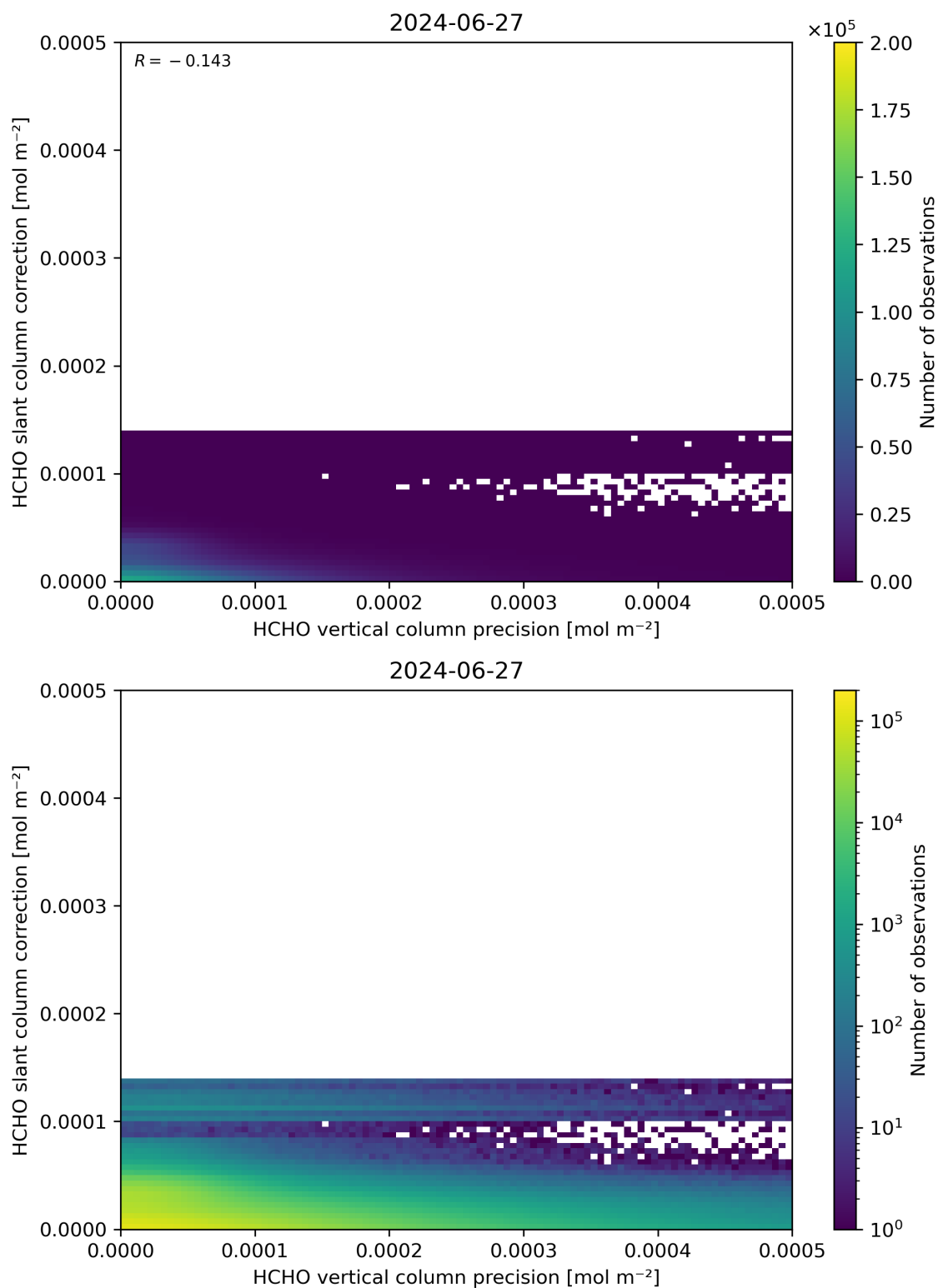
Figure 141: Scatter density plot of “HCHO vertical column precision” against “HCHO slant column correction” for 2024-06-26 to 2024-06-28.
