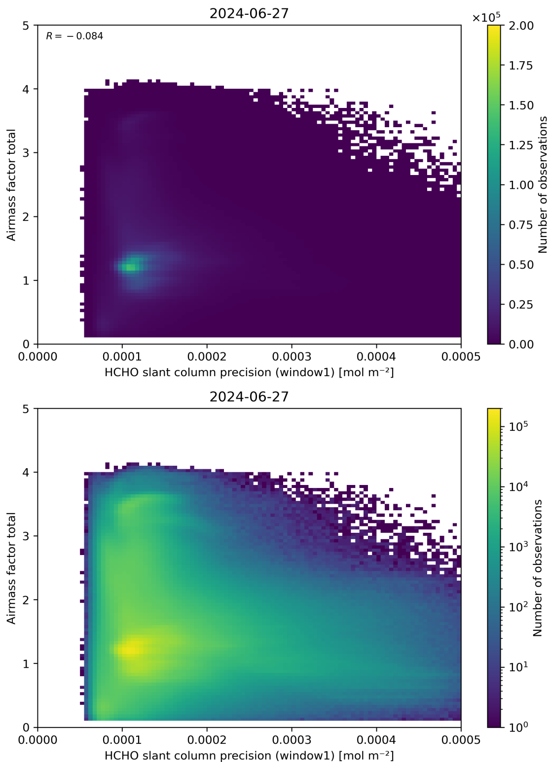
Figure 94: Scatter density plot of “HCHO slant column precision (window1)” against “Airmass factor total” for 2024-06-26 to 2024-06-28.
