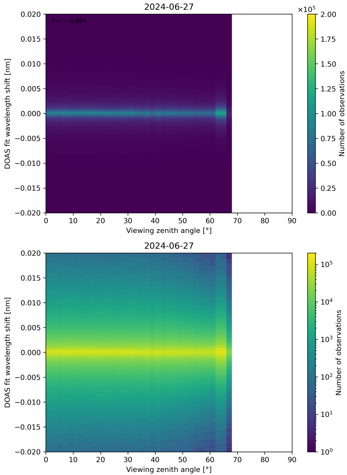
Figure 183: Scatter density plot of “Viewing zenith angle” against “DOAS fit wavelength shift” for 2024-06-26 to 2024-06-28.
