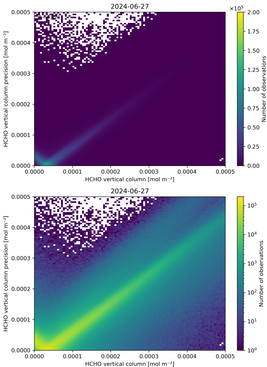
Figure 134: Scatter density plot of “HCHO vertical column” against “HCHO vertical column precision” for 2024-06-26 to 2024-06-28.
