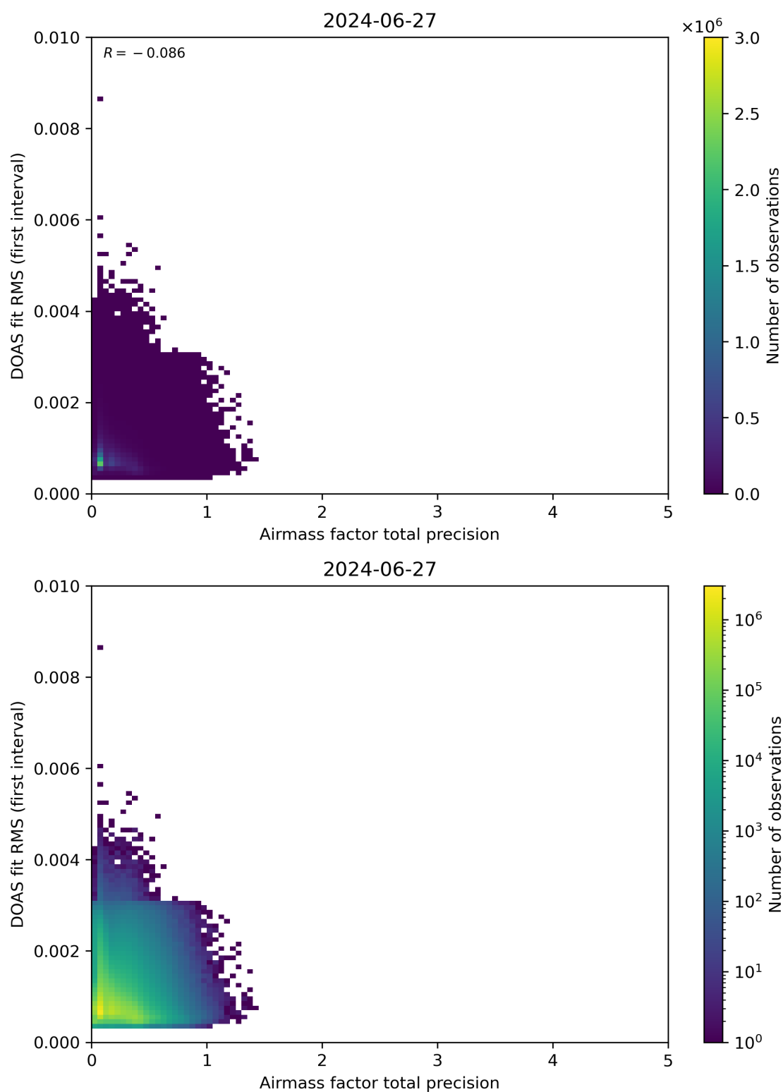
Figure 105: Scatter density plot of “Airmass factor total precision” against “DOAS fit RMS (first interval)” for 2024-06-26 to 2024-06-28.
