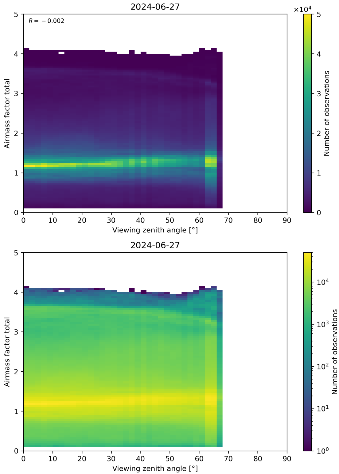
Figure 190: Scatter density plot of “Viewing zenith angle” against “Airmass factor total” for 2024-06-26 to 2024-06-28.
