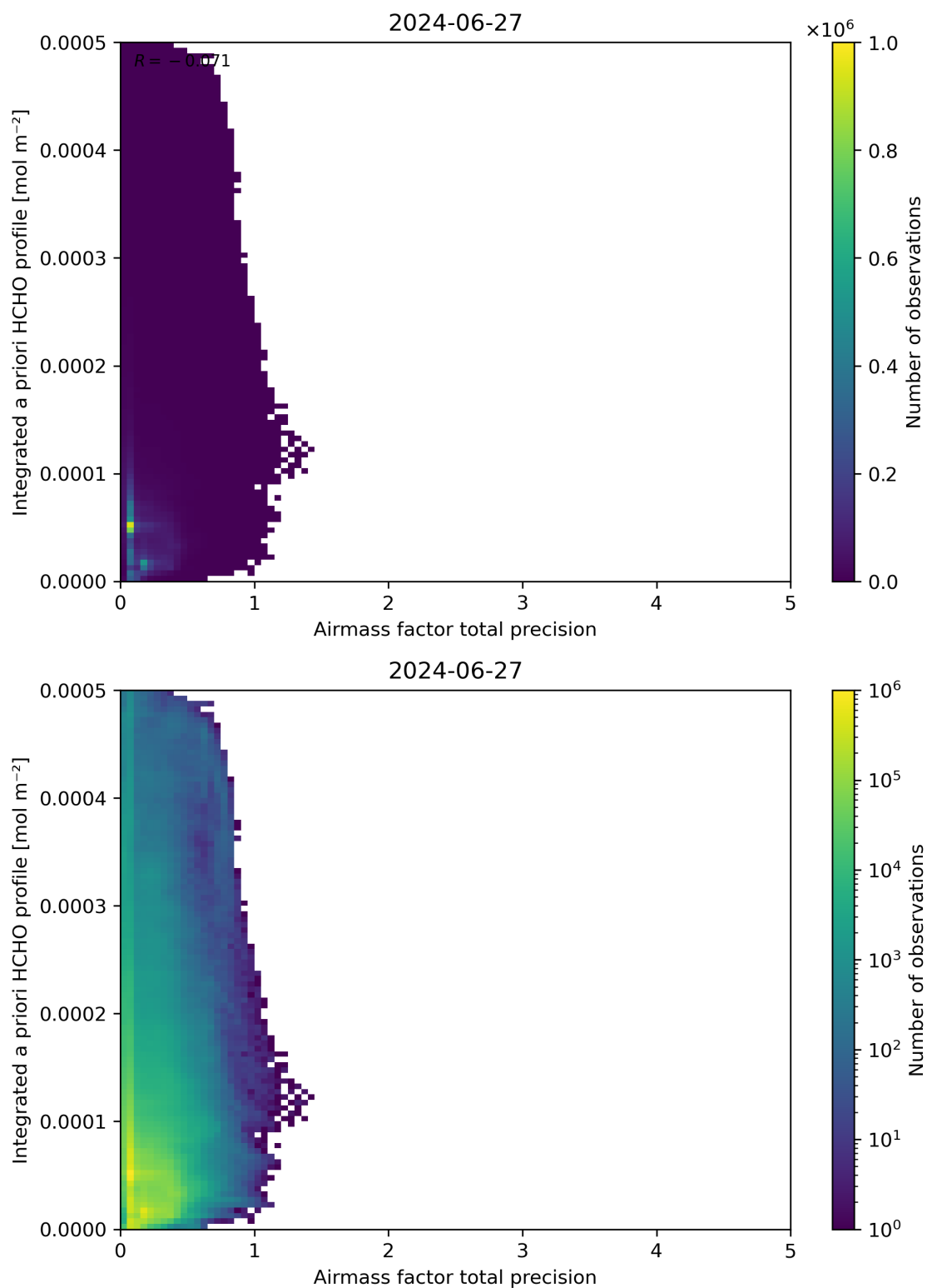
Figure 111: Scatter density plot of “Airmass factor total precision” against “Integrated a priori HCHO profile” for 2024-06-26 to 2024-06-28.
