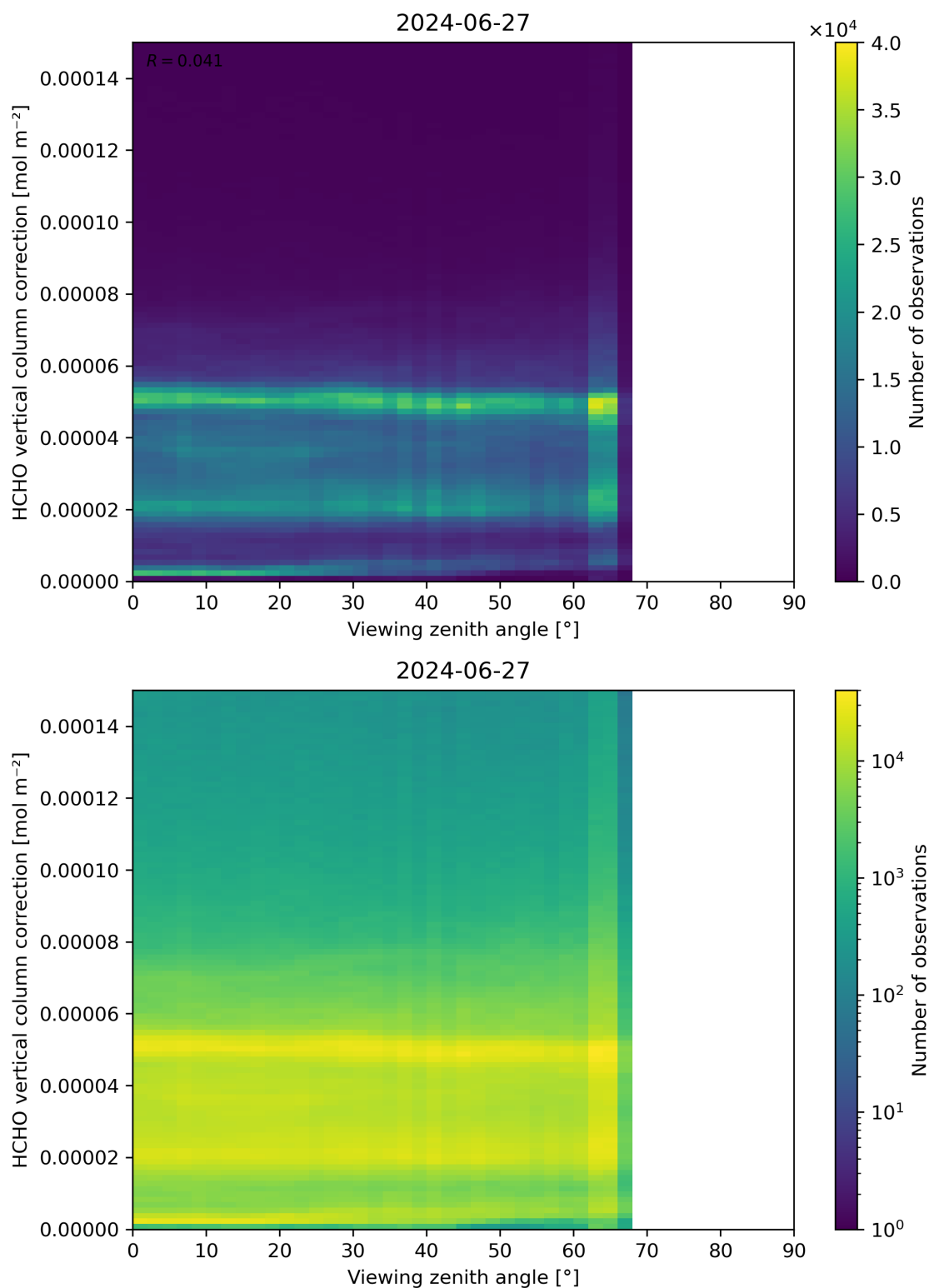
Figure 193: Scatter density plot of “Viewing zenith angle” against “HCHO vertical column correction” for 2024-06-26 to 2024-06-28.
