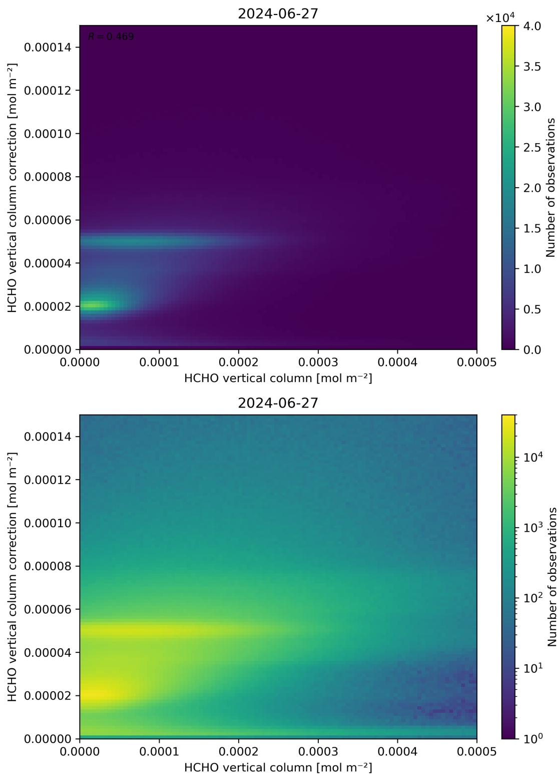
Figure 133: Scatter density plot of “HCHO vertical column” against “HCHO vertical column correction” for 2024-06-26 to 2024-06-28.
