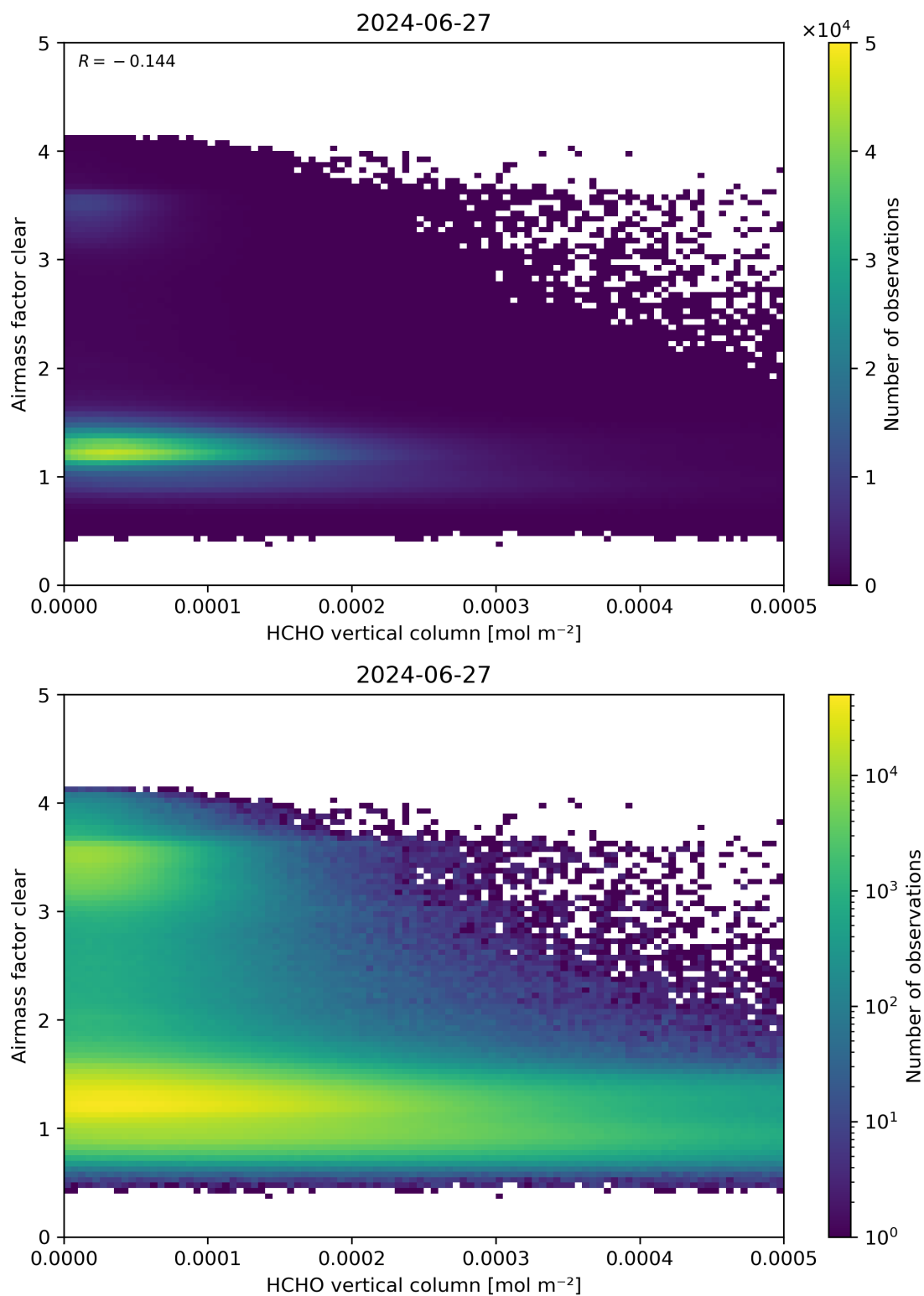
Figure 126: Scatter density plot of “HCHO vertical column” against “Airmass factor clear” for 2024-06-26 to 2024-06-28.
