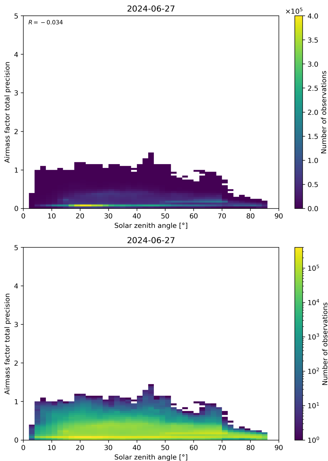
Figure 176: Scatter density plot of “Solar zenith angle” against “Airmass factor total precision” for 2024-06-26 to 2024-06-28.
