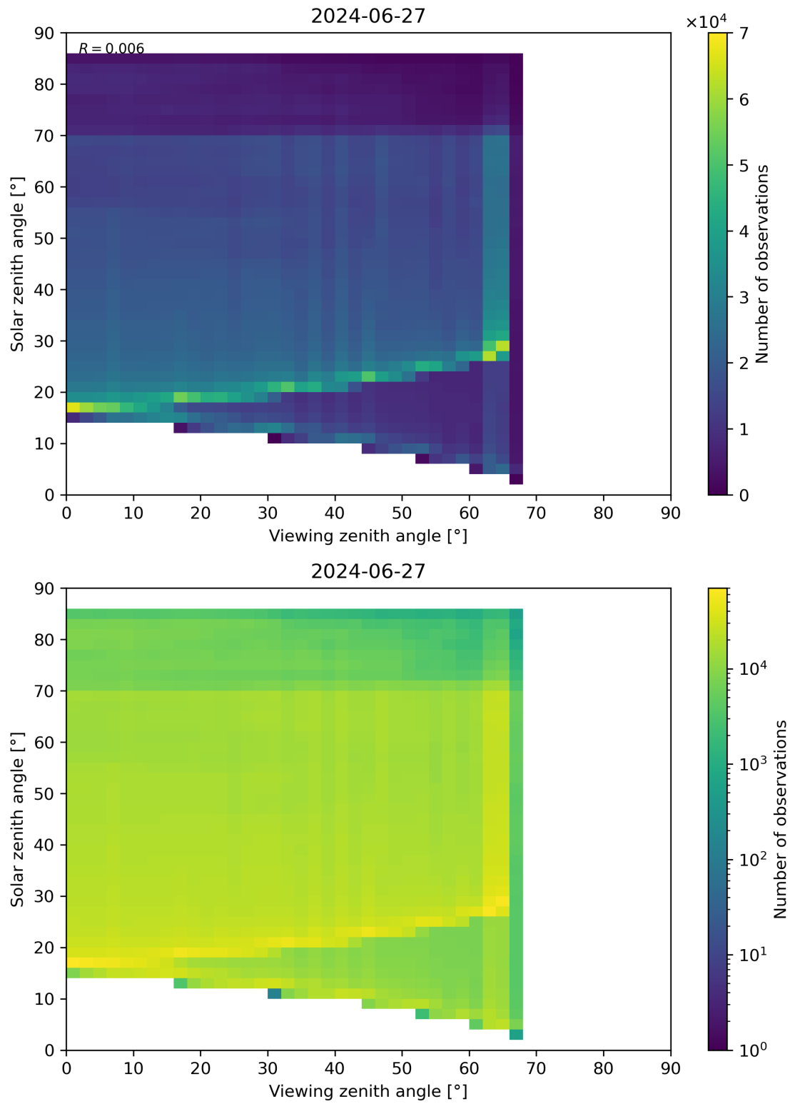
Figure 197: Scatter density plot of “Viewing zenith angle” against “Solar zenith angle” for 2024-06-26 to 2024-06-28.
