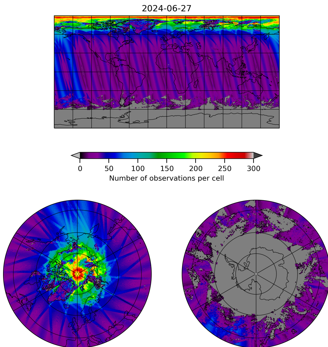
Figure 19: Map of the number of observations for 2024-06-26 to 2024-06-28
