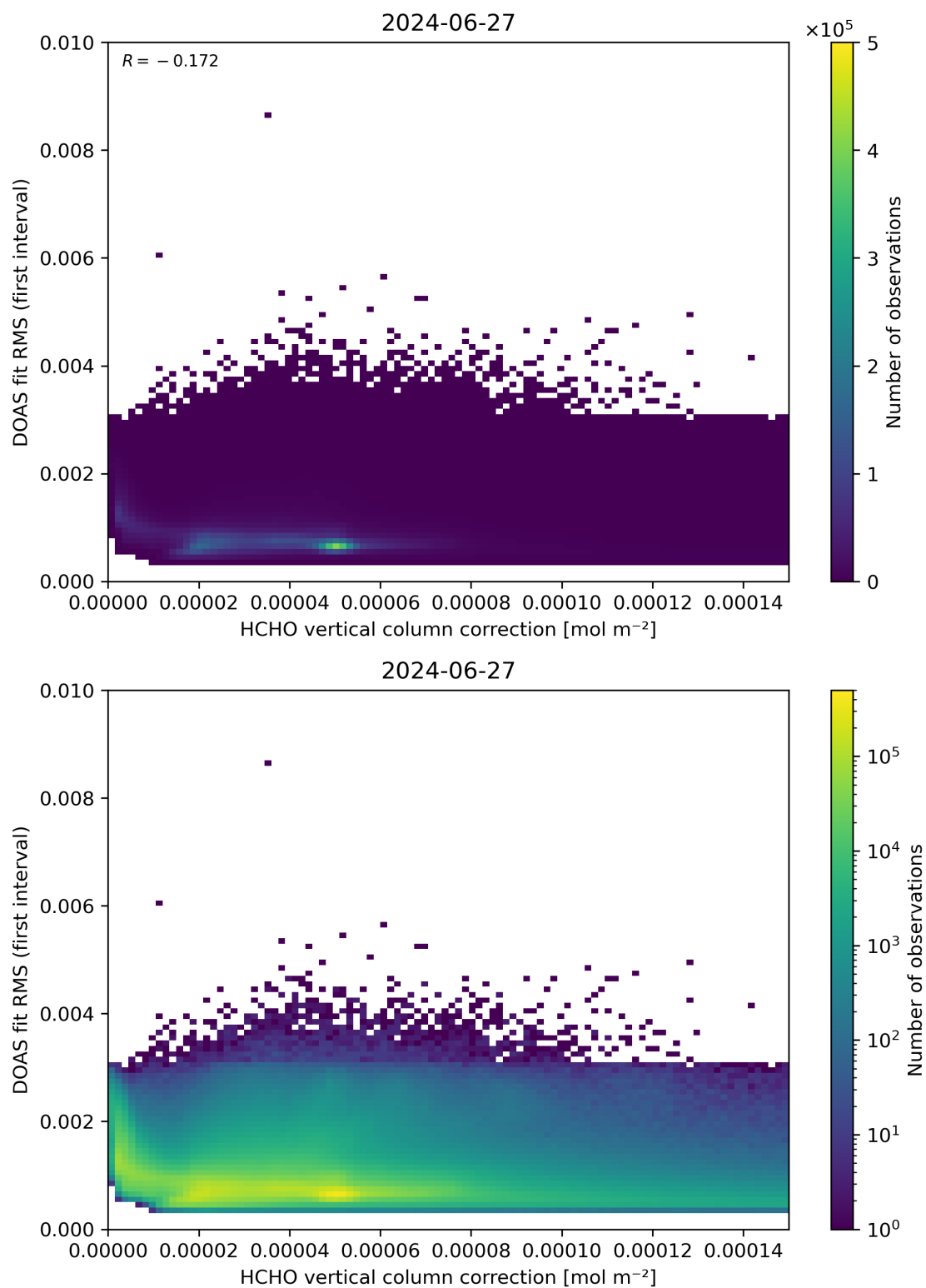
Figure 112: Scatter density plot of “HCHO vertical column correction” against “DOAS fit RMS (first interval)” for 2024-06-26 to 2024-06-28.
