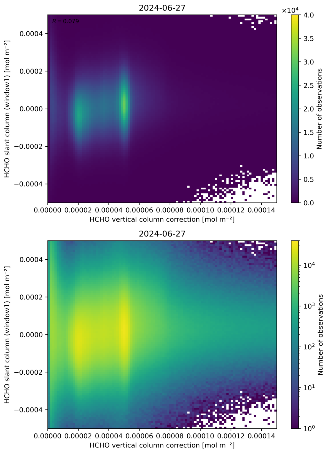
Figure 118: Scatter density plot of “HCHO vertical column correction” against “HCHO slant column (window1)” for 2024-06-26 to 2024-06-28.
