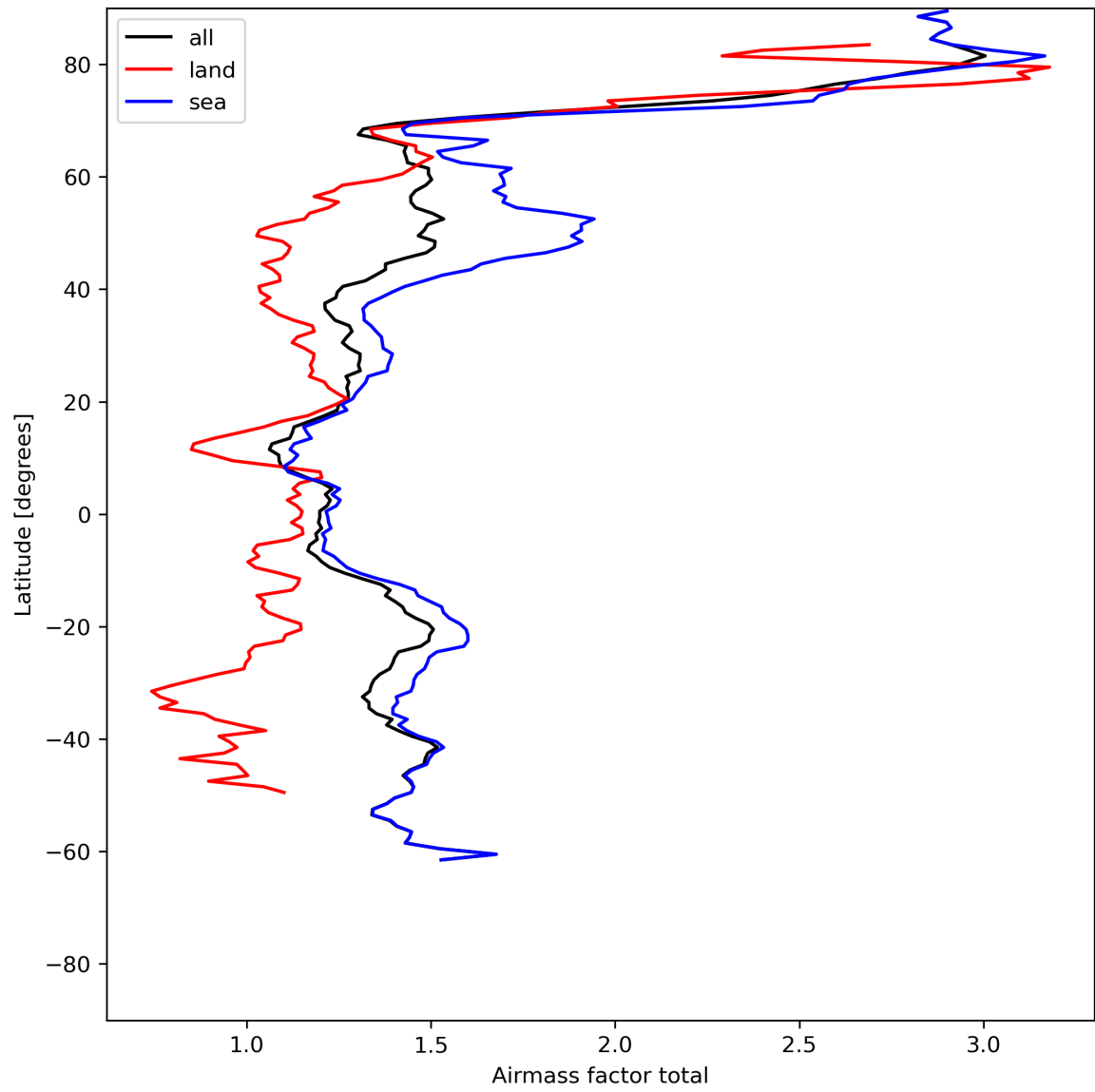
Figure 26: Zonal average of “Airmass factor total” for 2024-06-26 to 2024-06-28.
