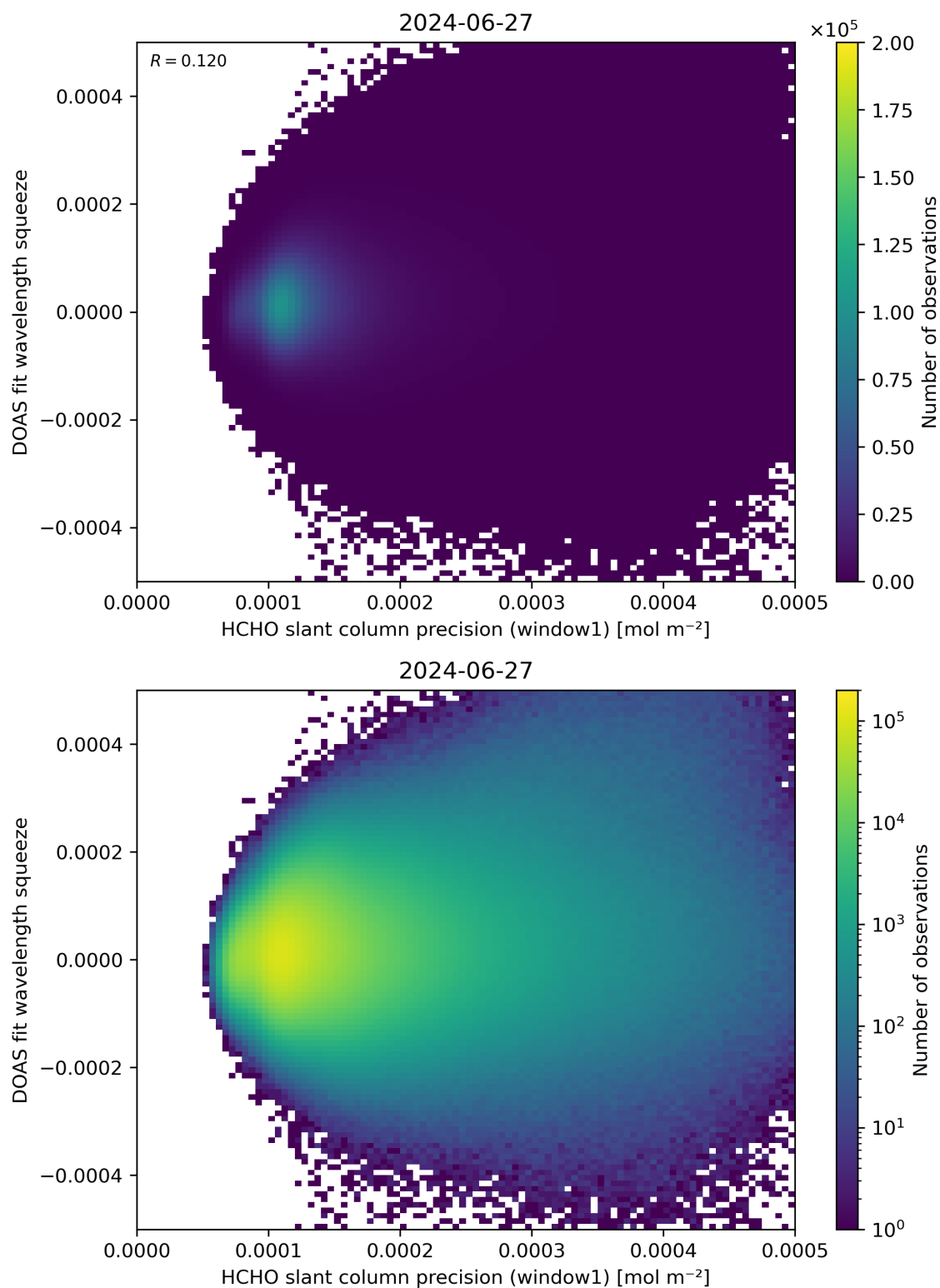
Figure 90: Scatter density plot of “HCHO slant column precision (window1)” against “DOAS fit wavelength squeeze” for 2024-06-26 to 2024-06-28.
