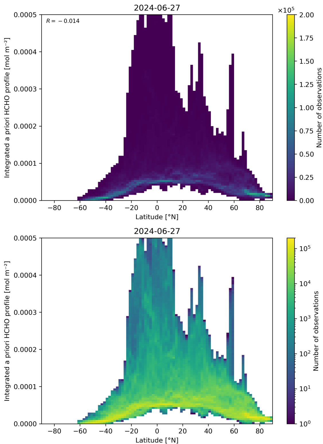
Figure 166: Scatter density plot of “Latitude” against “Integrated a priori HCHO profile” for 2024-06-26 to 2024-06-28.
