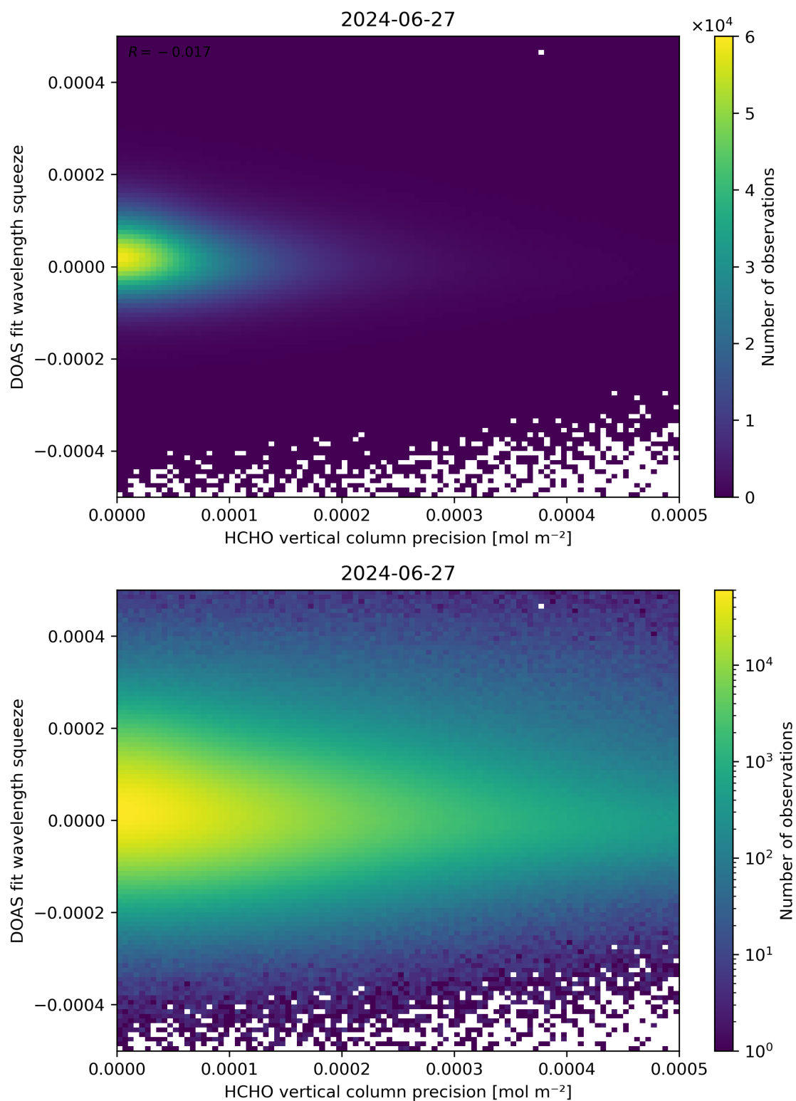
Figure 138: Scatter density plot of “HCHO vertical column precision” against “DOAS fit wavelength squeeze” for 2024-06-26 to 2024-06-28.
