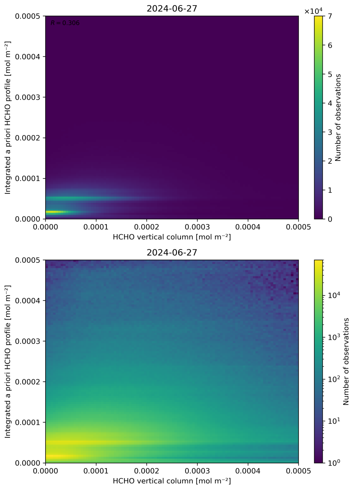
Figure 135: Scatter density plot of “HCHO vertical column” against “Integrated a priori HCHO profile” for 2024-06-26 to 2024-06-28.
