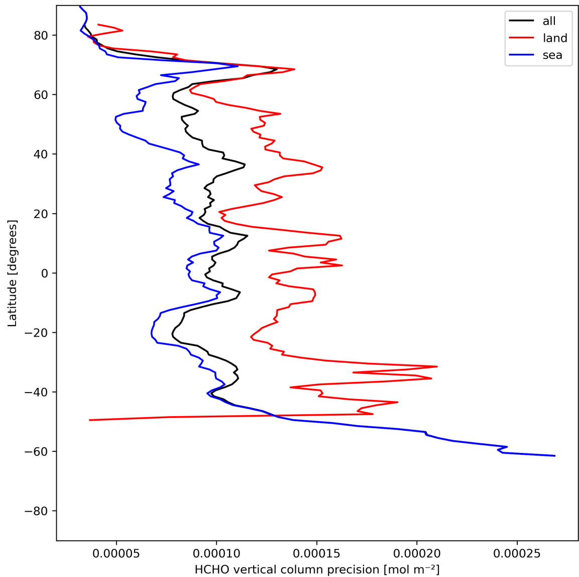
Figure 22: Zonal average of “HCHO vertical column precision” for 2024-06-26 to 2024-06-28.
