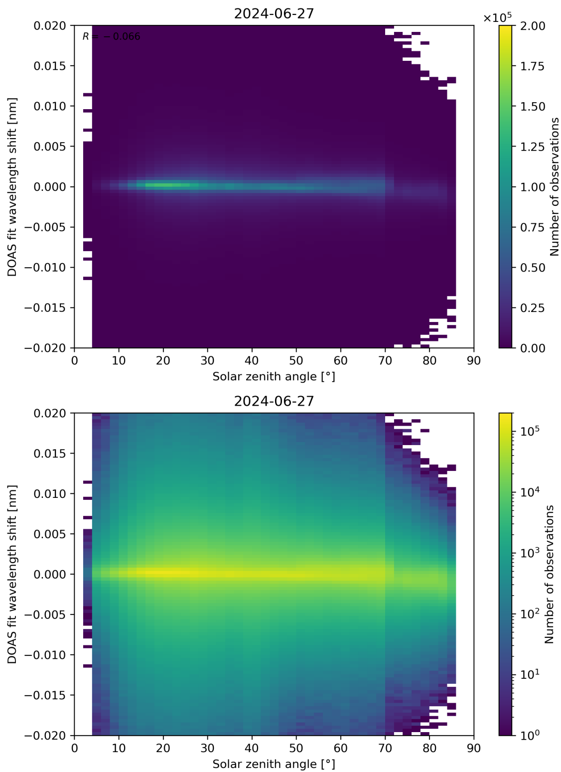
Figure 168: Scatter density plot of “Solar zenith angle” against “DOAS fit wavelength shift” for 2024-06-26 to 2024-06-28.
