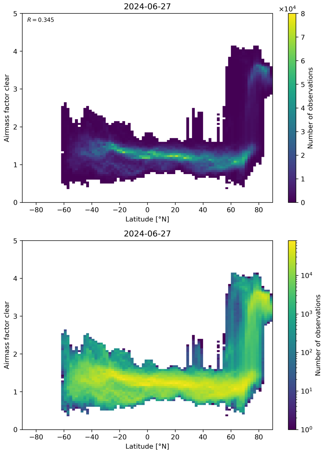
Figure 156: Scatter density plot of “Latitude” against “Airmass factor clear” for 2024-06-26 to 2024-06-28.
