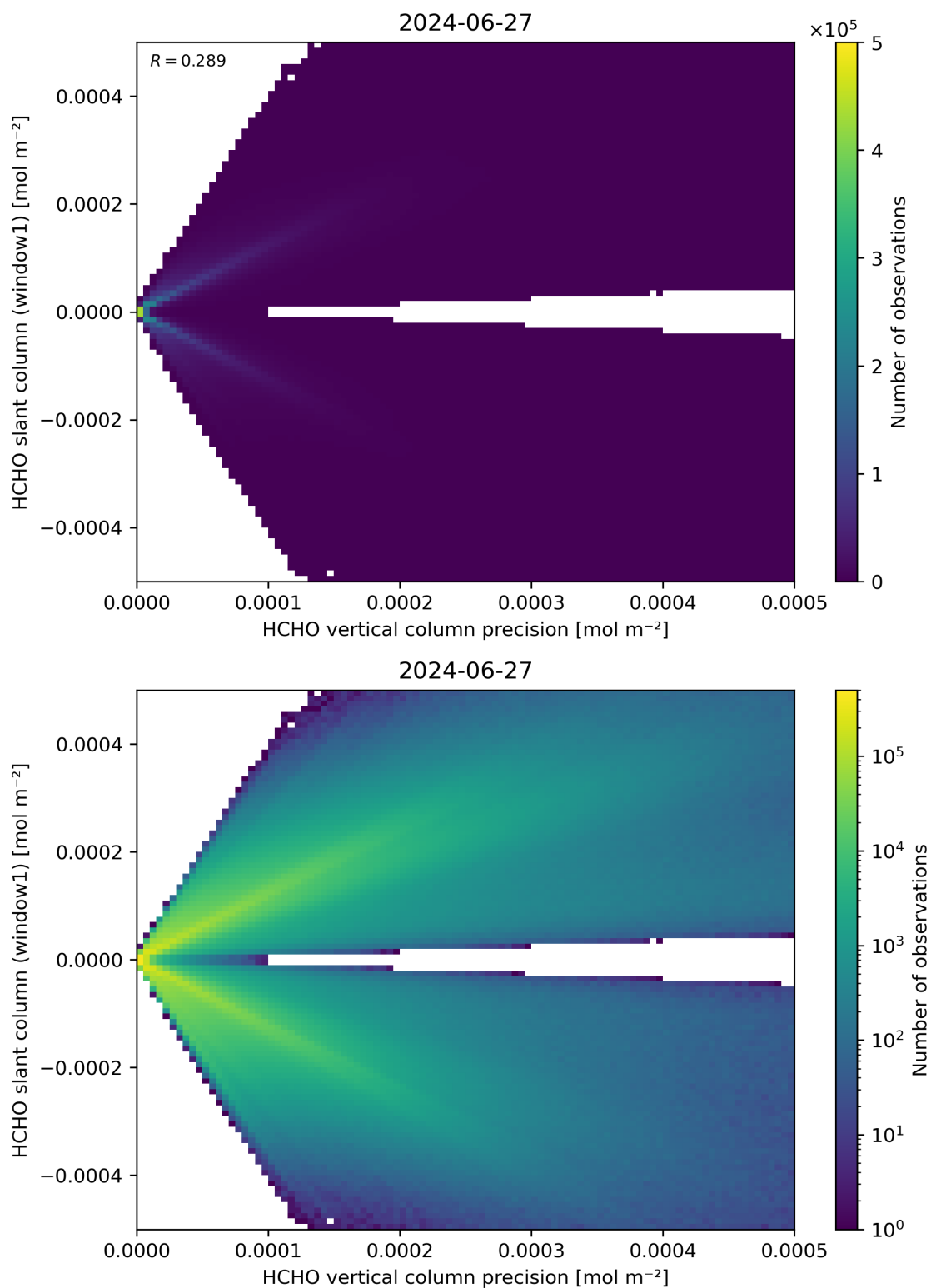
Figure 142: Scatter density plot of “HCHO vertical column precision” against “HCHO slant column (window1)” for 2024-06-26 to 2024-06-28.
