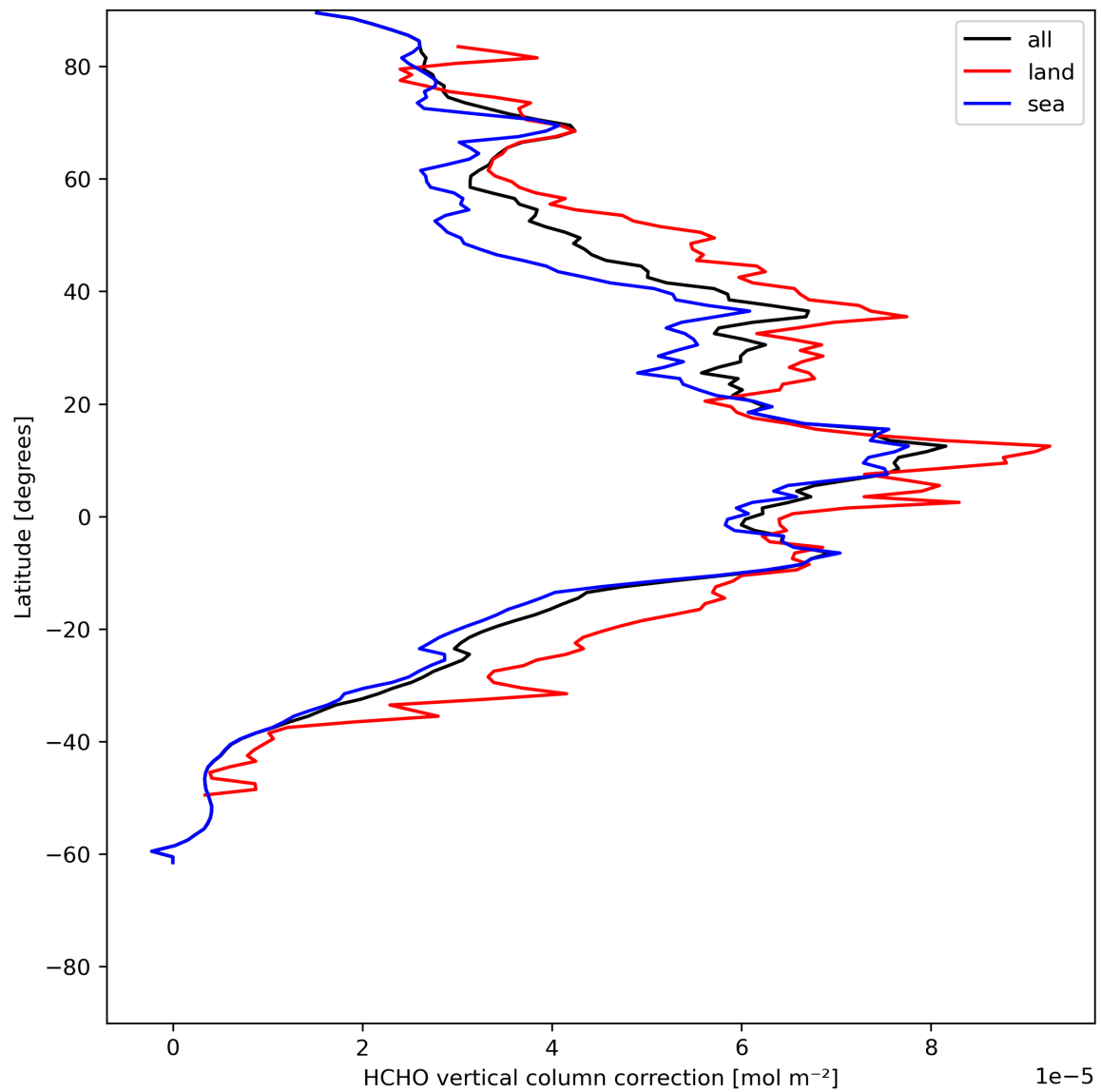
Figure 23: Zonal average of “HCHO vertical column correction” for 2024-06-26 to 2024-06-28.
