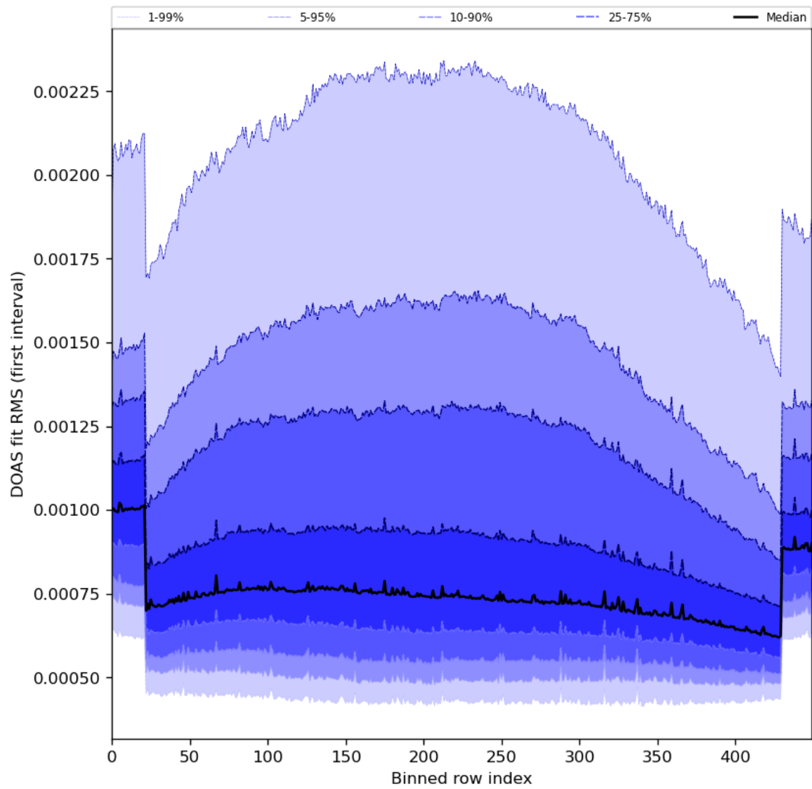
Figure 60: Along track statistics of “DOAS fit RMS (first interval)” for 2024-06-26 to 2024-06-28
