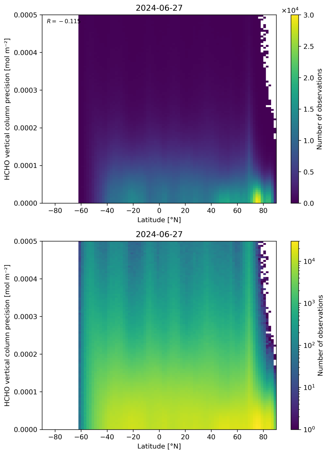
Figure 165: Scatter density plot of “Latitude” against “HCHO vertical column precision” for 2024-06-26 to 2024-06-28.
