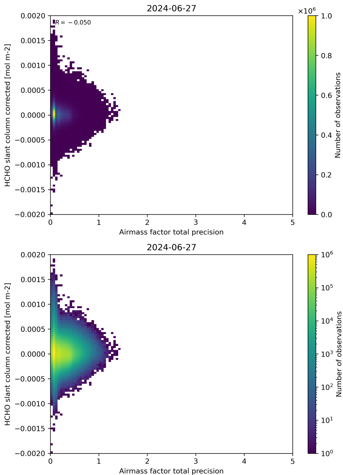
Figure 109: Scatter density plot of “Airmass factor total precision” against “HCHO slant column corrected” for 2024-06-26 to 2024-06-28.
