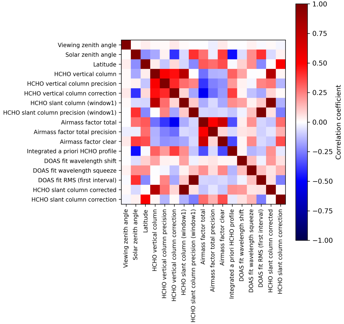
Figure 2: Map of correlation matrix for 2024-06-26 to 2024-06-28.
