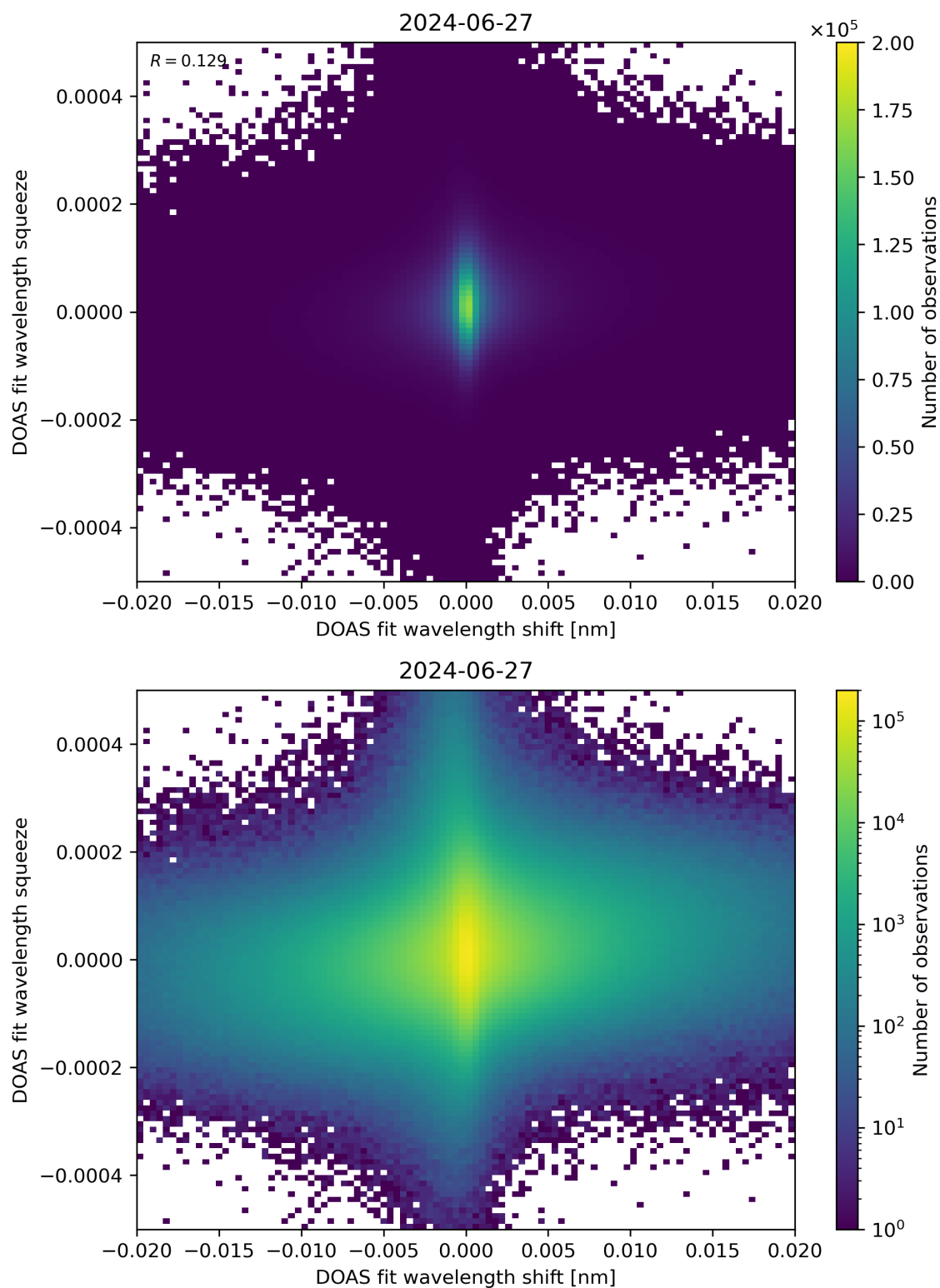
Figure 65: Scatter density plot of “DOAS fit wavelength shift” against “DOAS fit wavelength squeeze” for 2024-06-26 to 2024-06-28.
