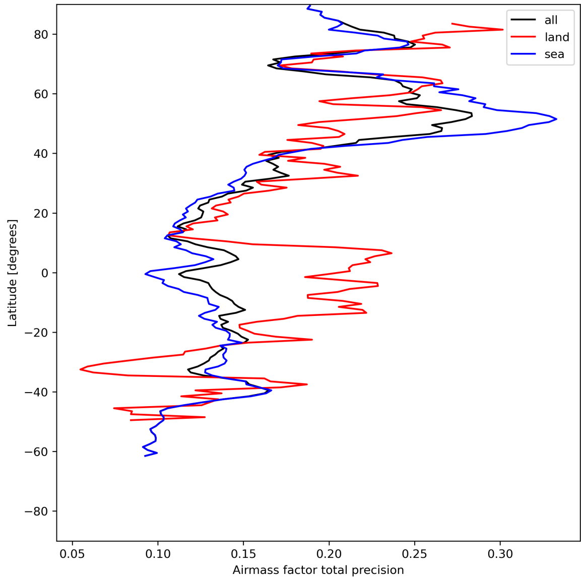
Figure 27: Zonal average of “Airmass factor total precision” for 2024-06-26 to 2024-06-28.
