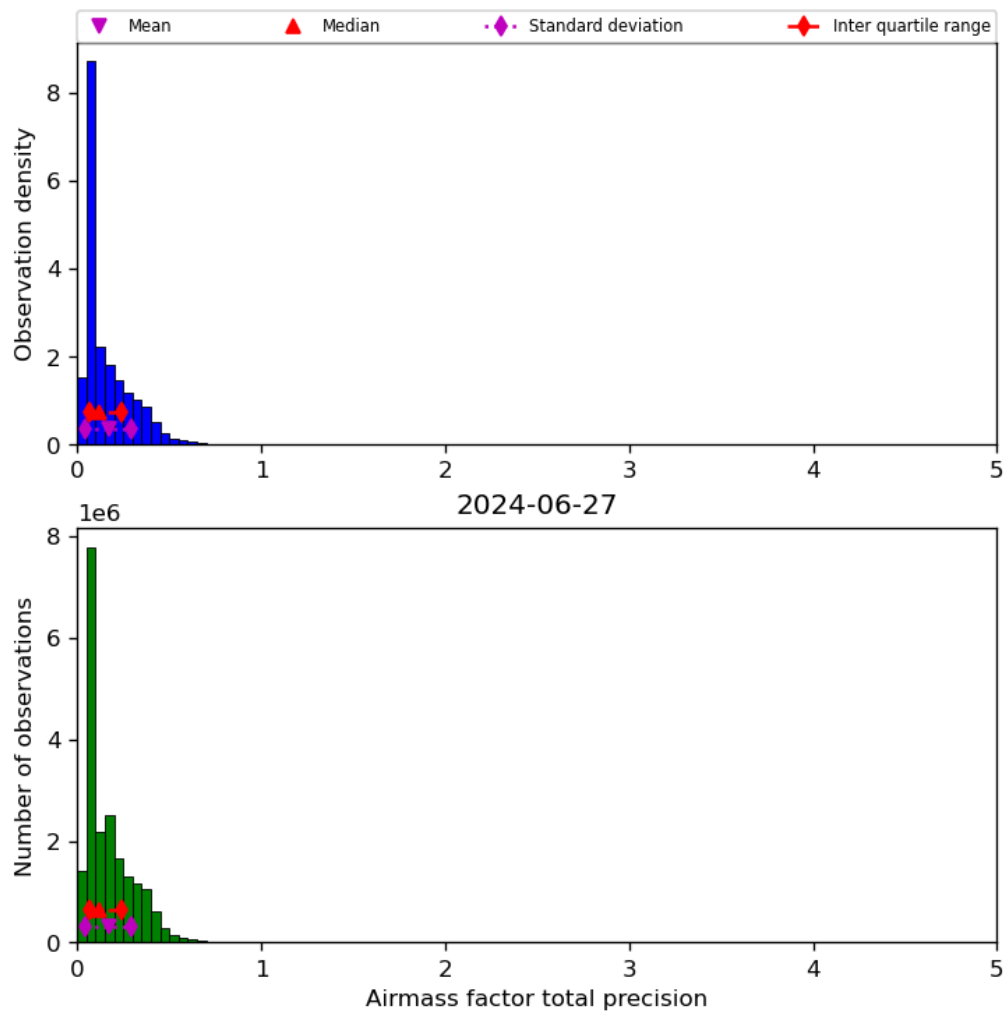
Figure 41: Histogram of “Airmass factor total precision” for 2024-06-26 to 2024-06-28
