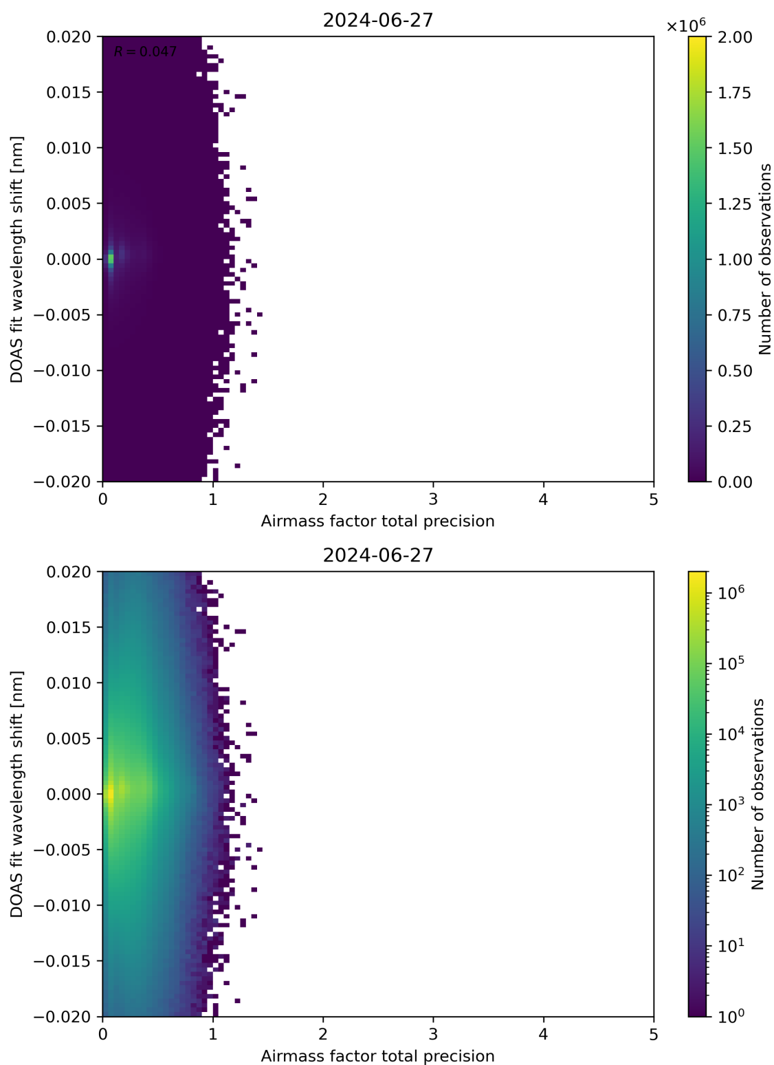
Figure 106: Scatter density plot of “Airmass factor total precision” against “DOAS fit wavelength shift” for 2024-06-26 to 2024-06-28.
