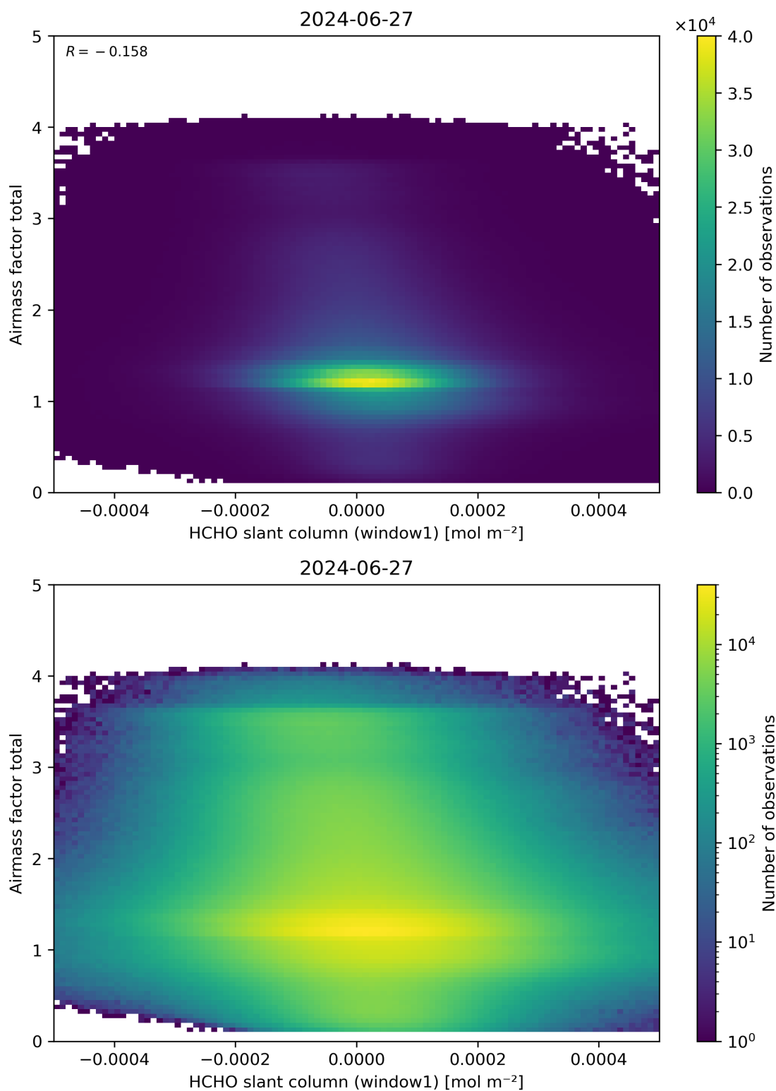
Figure 85: Scatter density plot of “HCHO slant column (window1)” against “Airmass factor total” for 2024-06-26 to 2024-06-28.
