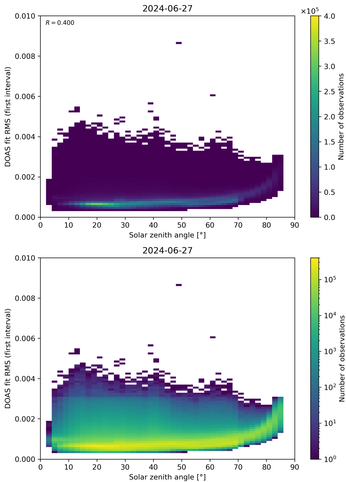
Figure 167: Scatter density plot of “Solar zenith angle” against “DOAS fit RMS (first interval)” for 2024-06-26 to 2024-06-28.
