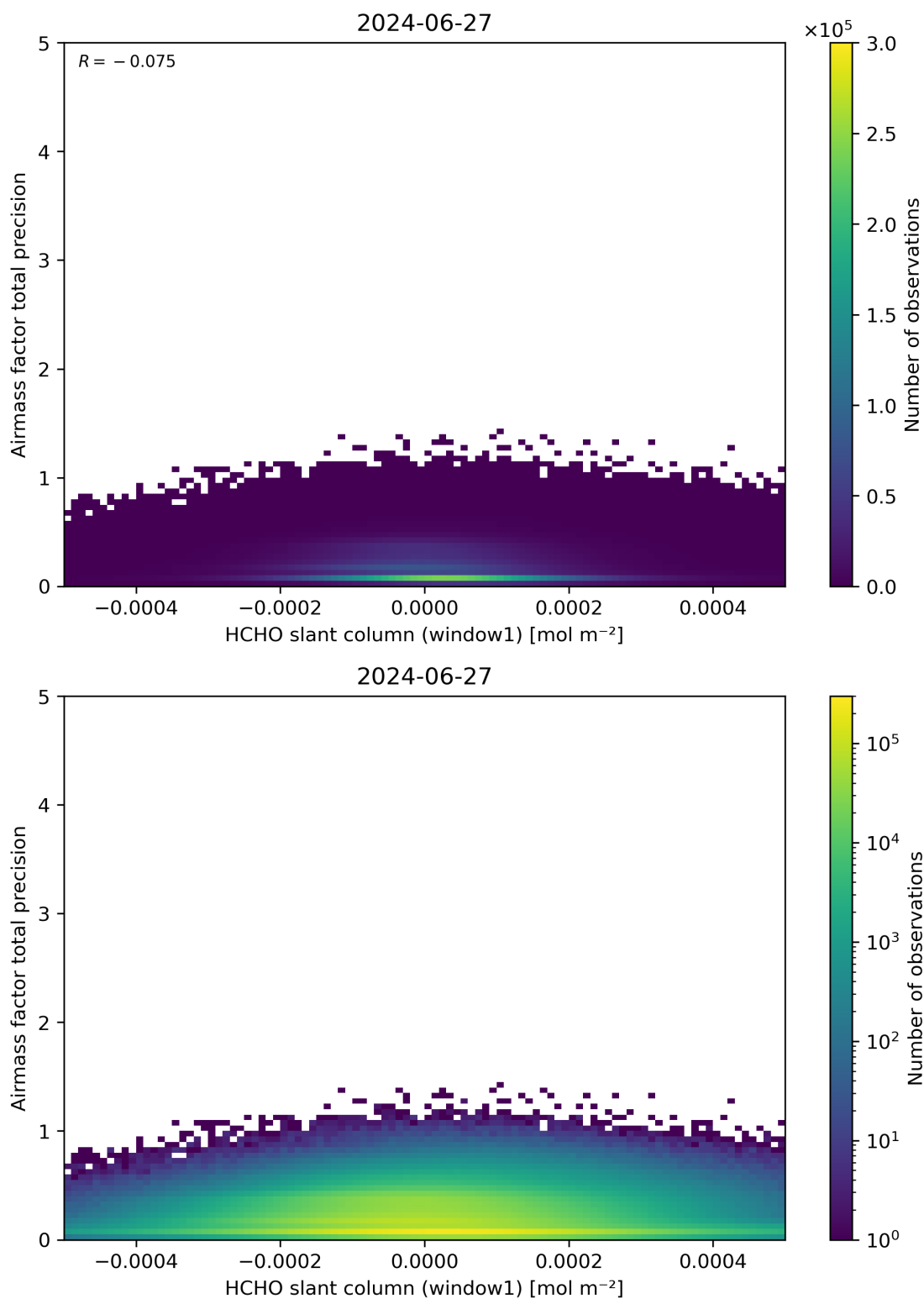
Figure 86: Scatter density plot of “HCHO slant column (window1)” against “Airmass factor total precision” for 2024-06-26 to 2024-06-28.
