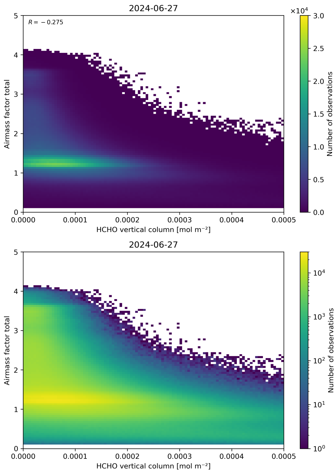
Figure 131: Scatter density plot of “HCHO vertical column” against “Airmass factor total” for 2024-06-26 to 2024-06-28.
