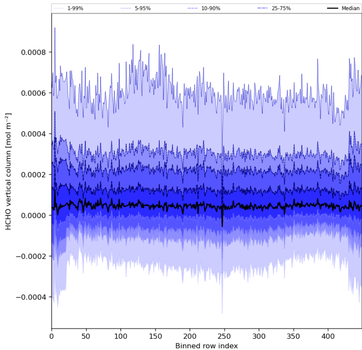
Figure 49: Along track statistics of “HCHO vertical column” for 2024-06-26 to 2024-06-28
