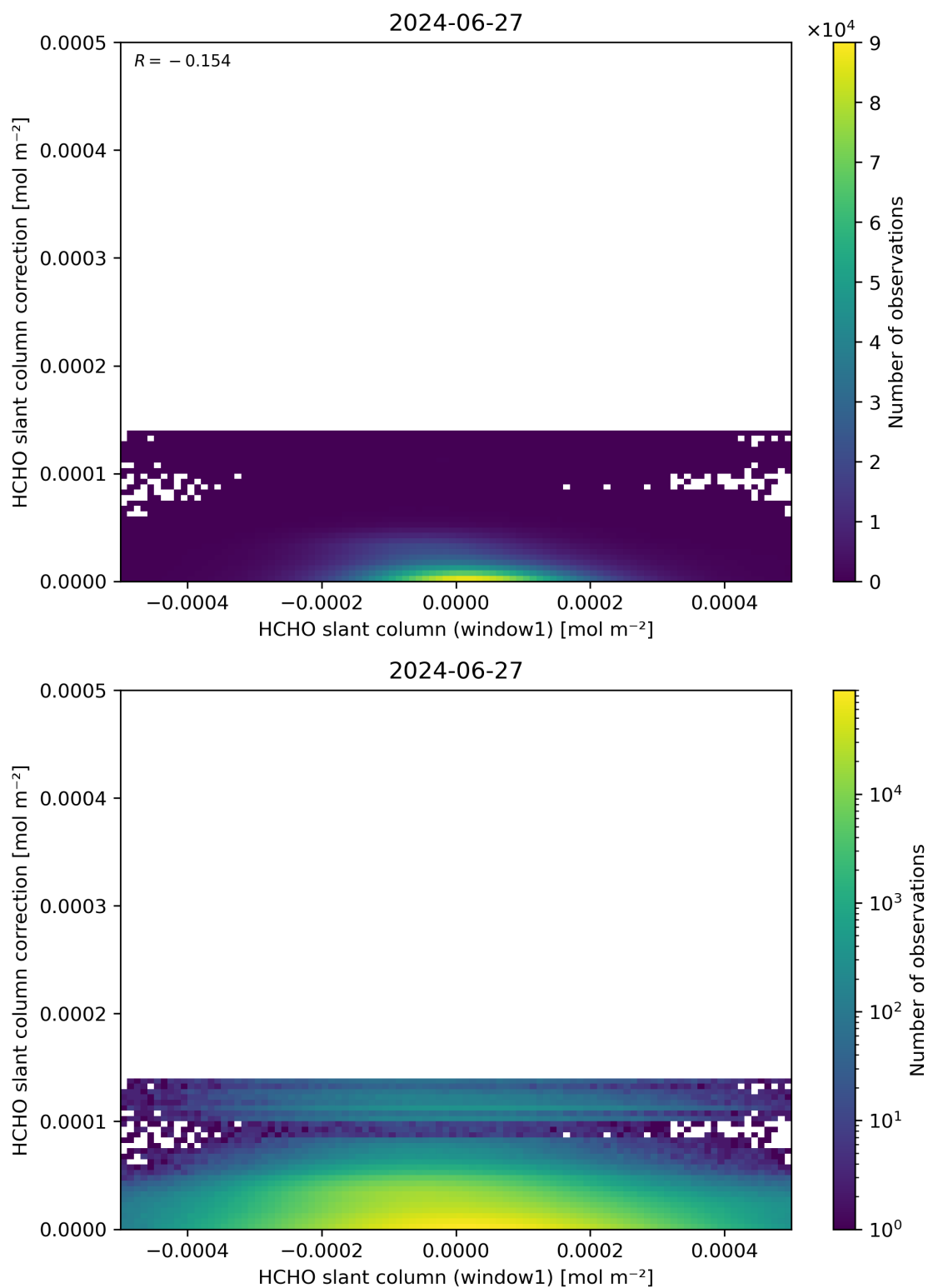
Figure 83: Scatter density plot of “HCHO slant column (window1)” against “HCHO slant column correction” for 2024-06-26 to 2024-06-28.
