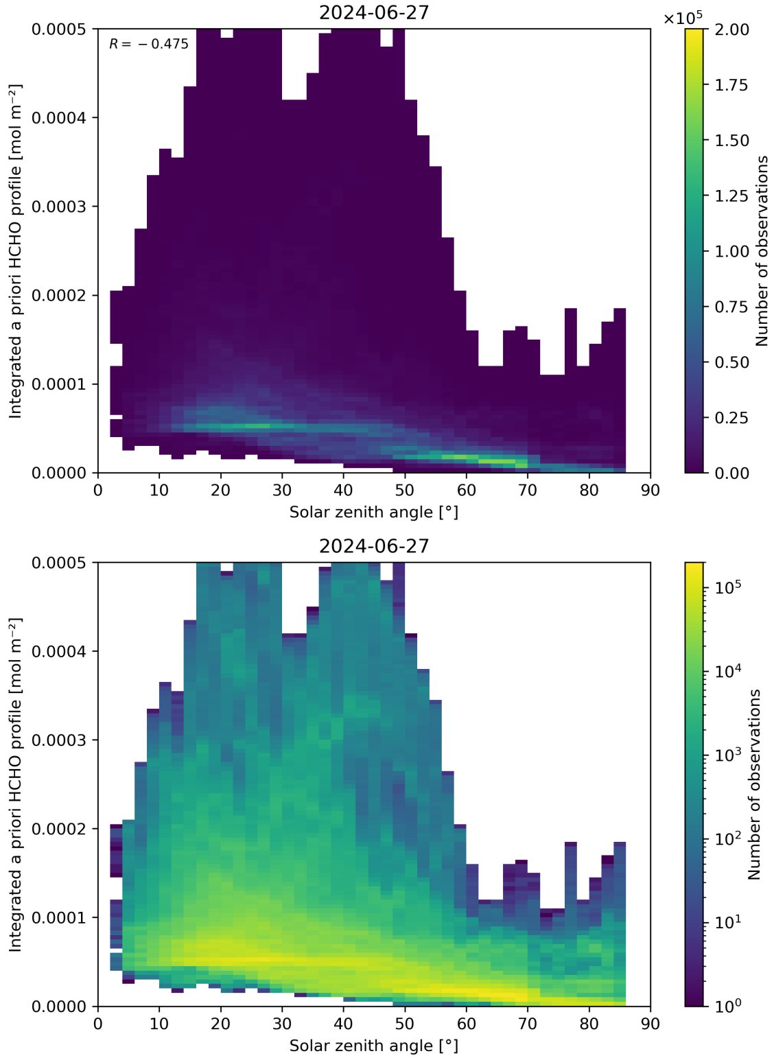
Figure 180: Scatter density plot of “Solar zenith angle” against “Integrated a priori HCHO profile” for 2024-06-26 to 2024-06-28.
