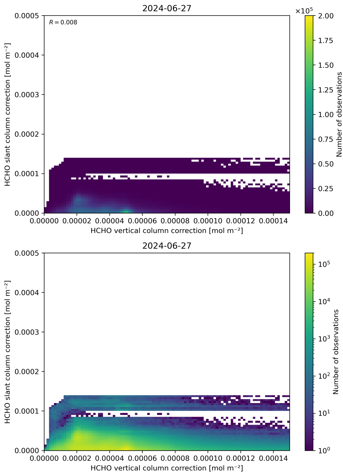
Figure 117: Scatter density plot of “HCHO vertical column correction” against “HCHO slant column correction” for 2024-06-26 to 2024-06-28.
