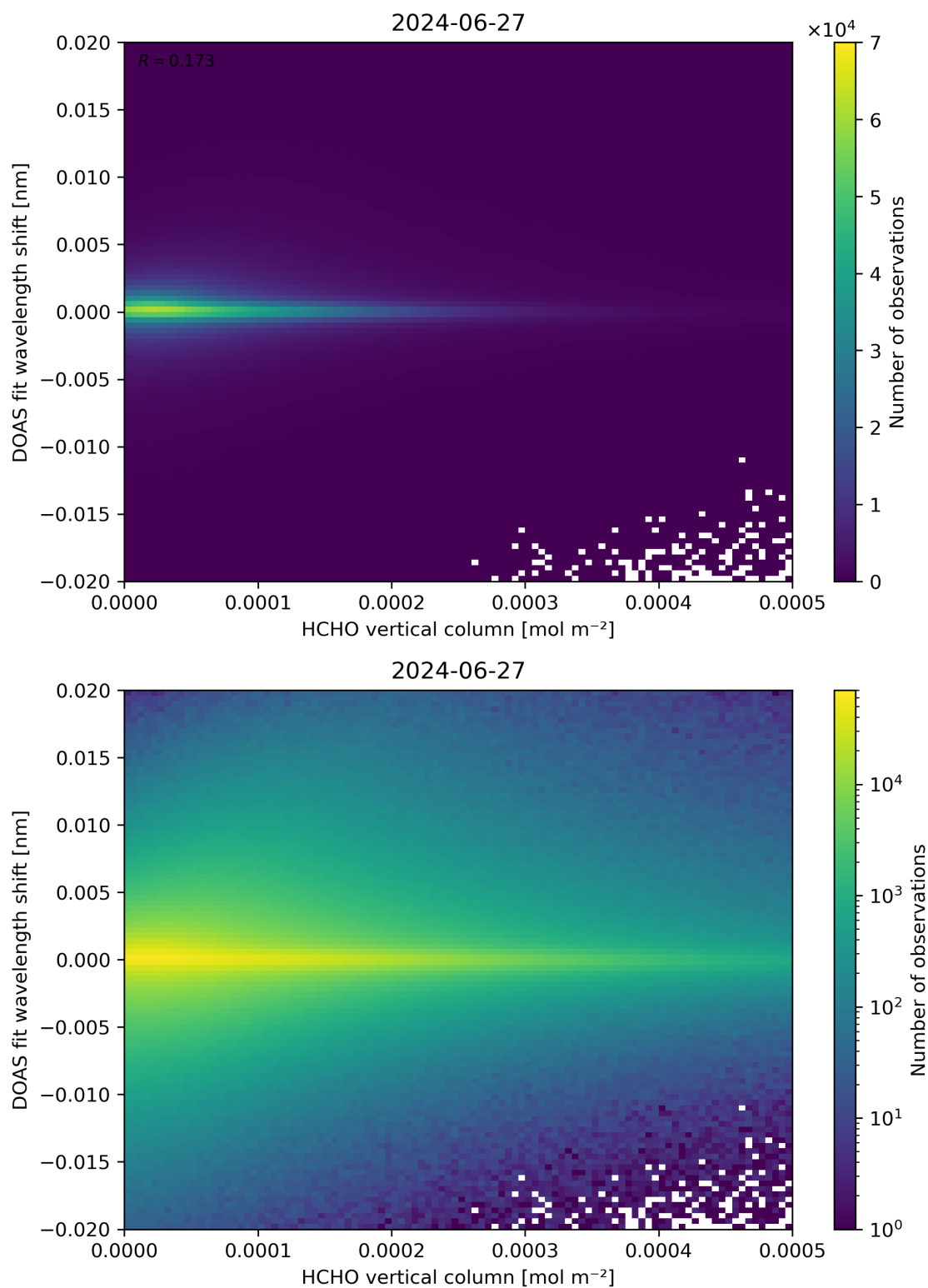
Figure 124: Scatter density plot of “HCHO vertical column” against “DOAS fit wavelength shift” for 2024-06-26 to 2024-06-28.
