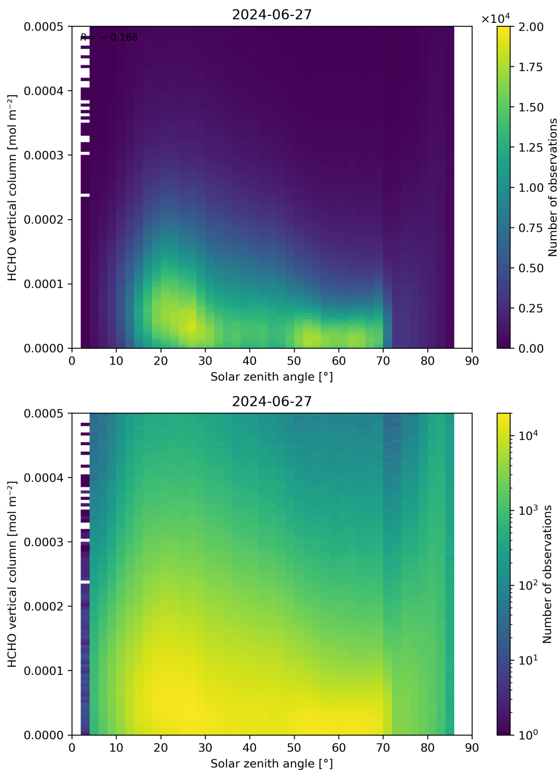
Figure 177: Scatter density plot of “Solar zenith angle” against “HCHO vertical column” for 2024-06-26 to 2024-06-28.
