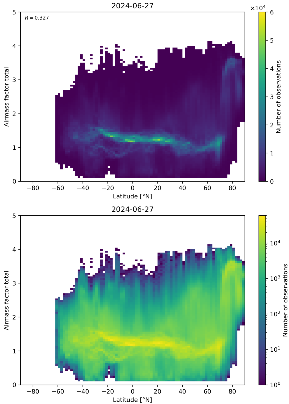
Figure 161: Scatter density plot of “Latitude” against “Airmass factor total” for 2024-06-26 to 2024-06-28.
