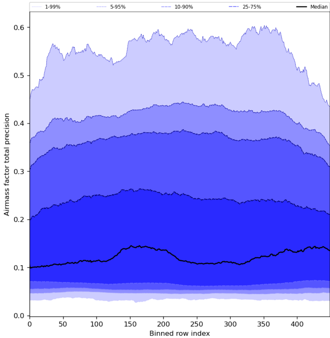
Figure 55: Along track statistics of “Airmass factor total precision” for 2024-06-26 to 2024-06-28
