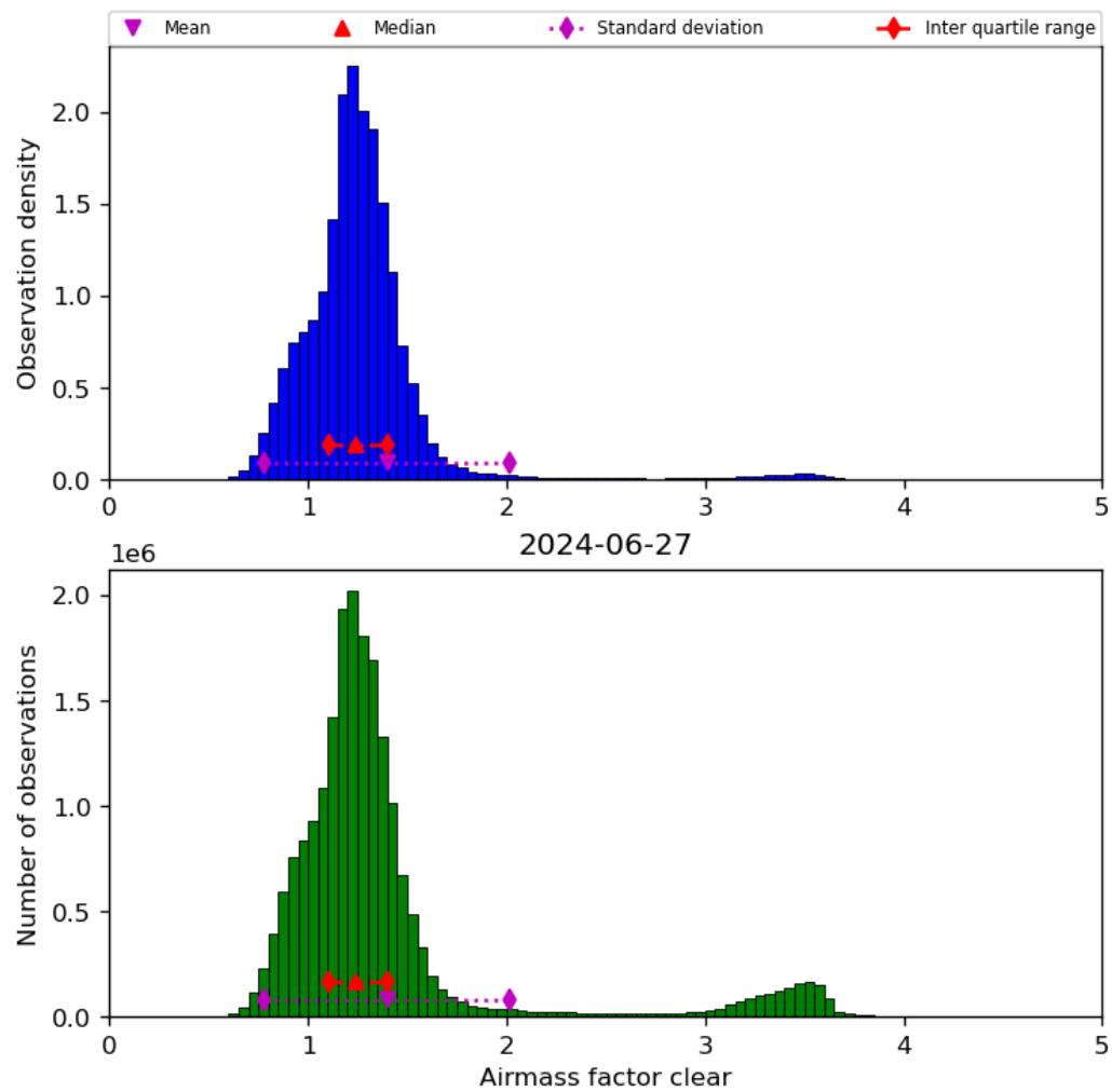
Figure 42: Histogram of “Airmass factor clear” for 2024-06-26 to 2024-06-28
