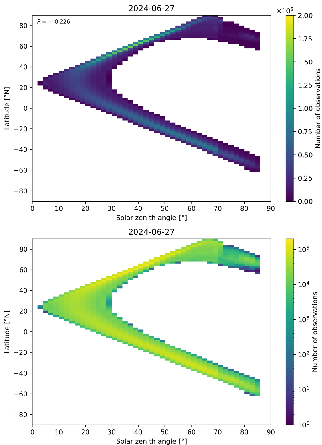
Figure 181: Scatter density plot of “Solar zenith angle” against “Latitude” for 2024-06-26 to 2024-06-28.
