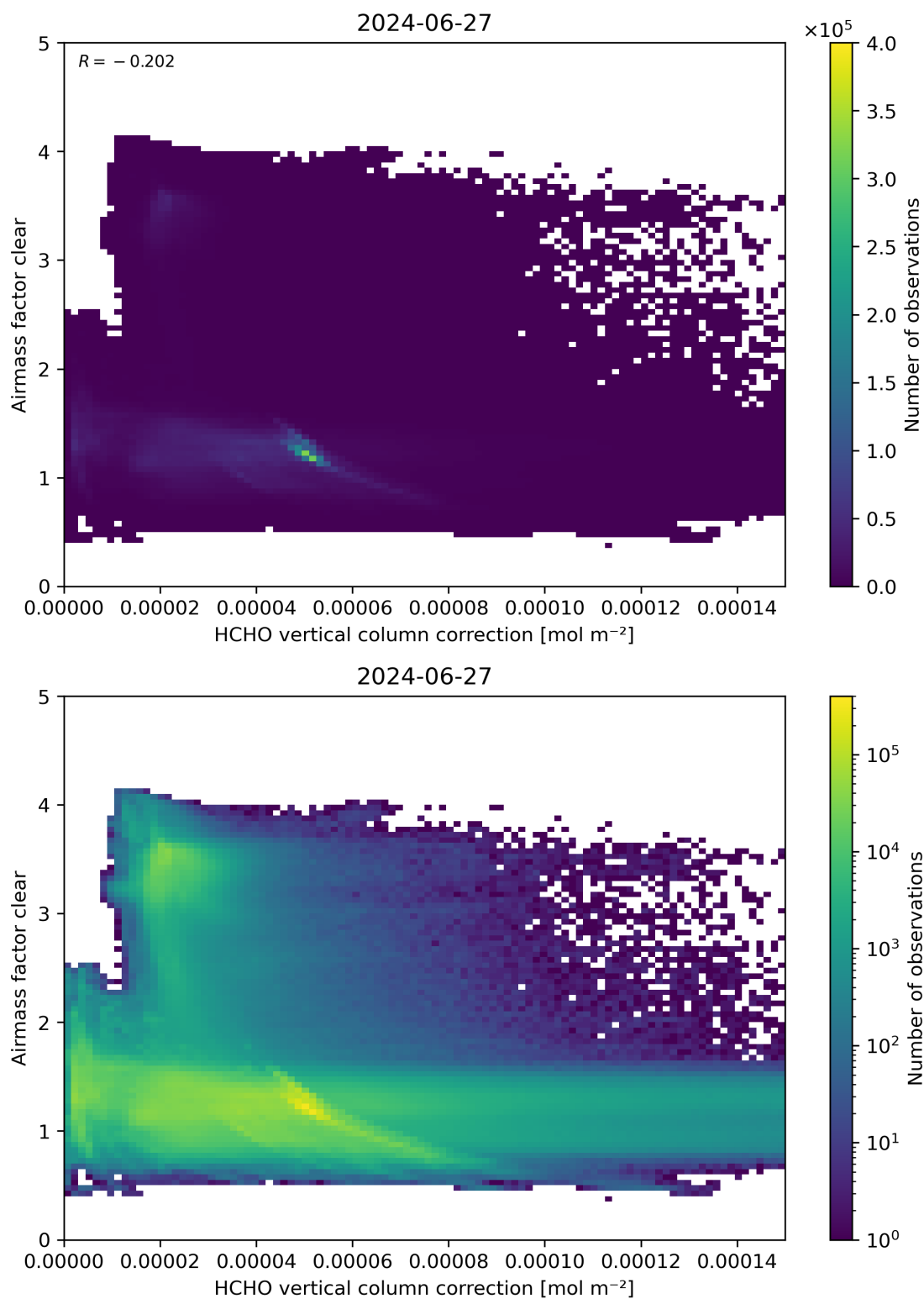
Figure 115: Scatter density plot of “HCHO vertical column correction” against “Airmass factor clear” for 2024-06-26 to 2024-06-28.
