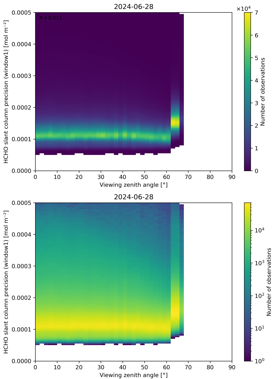
Figure 189: Scatter density plot of “Viewing zenith angle” against “HCHO slant column precision (window1)” for 2024-06-27 to 2024-06-29.
