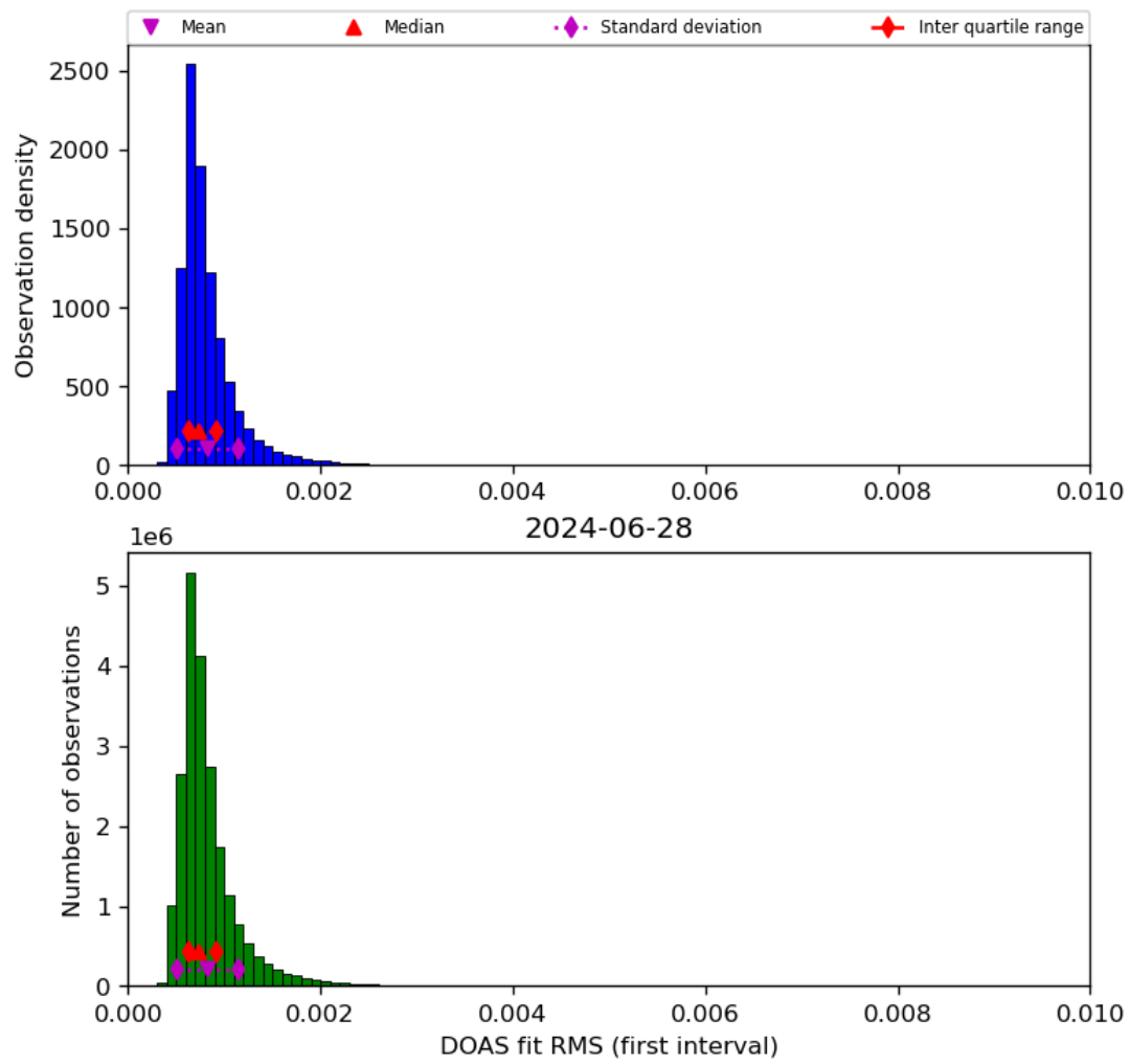
Figure 46: Histogram of “DOAS fit RMS (first interval)” for 2024-06-27 to 2024-06-29
