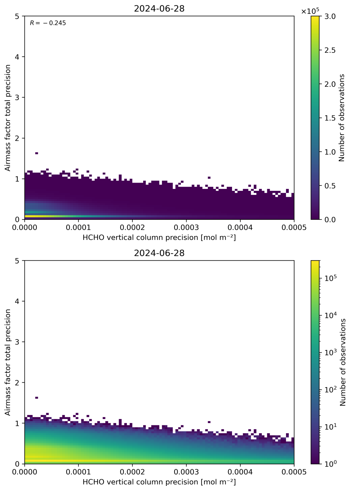
Figure 145: Scatter density plot of “HCHO vertical column precision” against “Airmass factor total precision” for 2024-06-27 to 2024-06-29.
