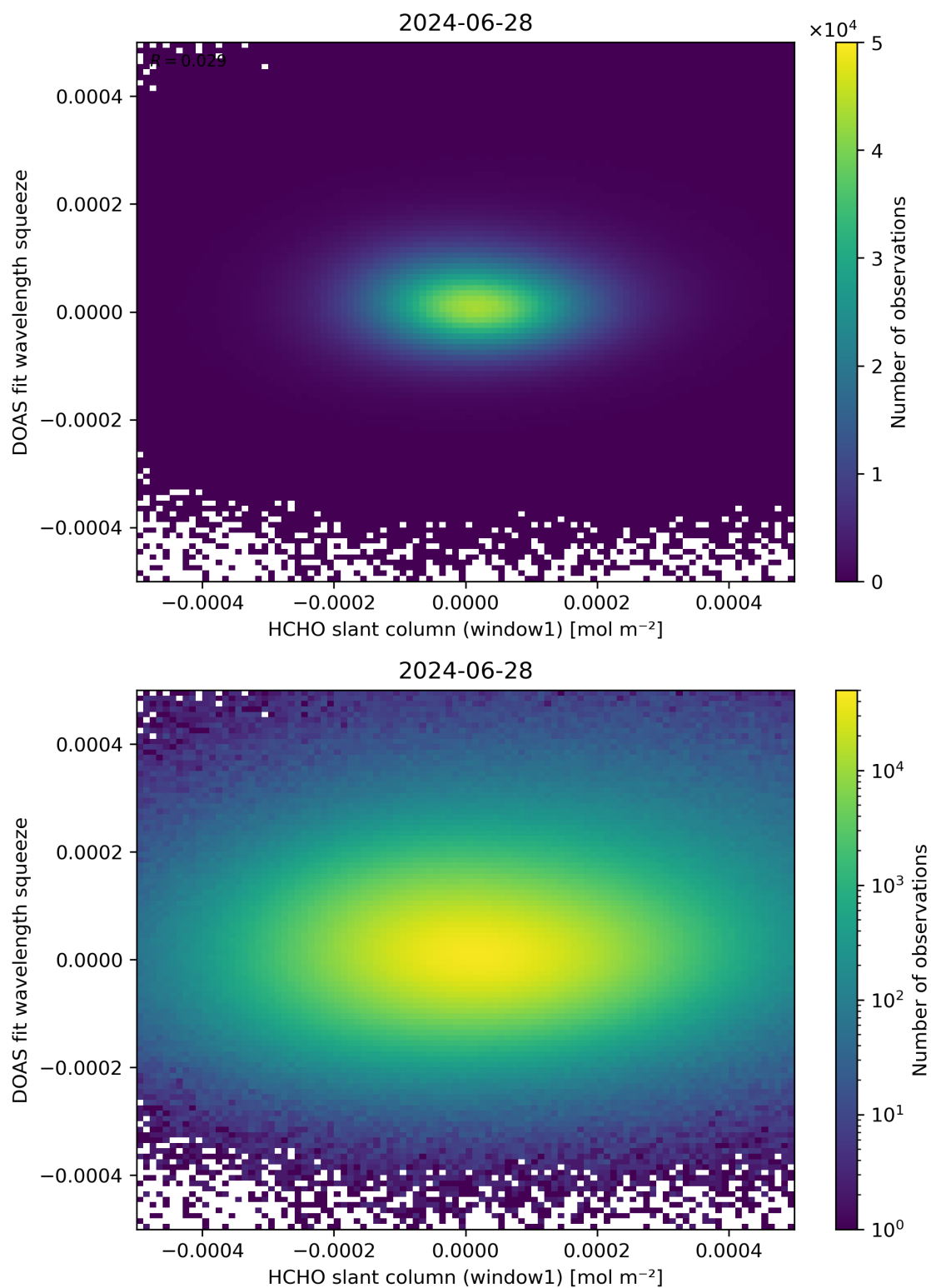
Figure 80: Scatter density plot of “HCHO slant column (window1)” against “DOAS fit wavelength squeeze” for 2024-06-27 to 2024-06-29.
