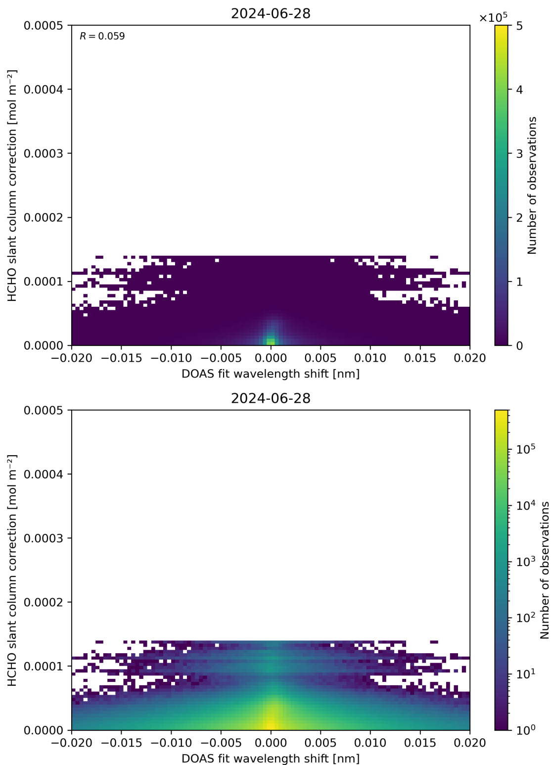
Figure 67: Scatter density plot of “DOAS fit wavelength shift” against “HCHO slant column correction” for 2024-06-27 to 2024-06-29.
