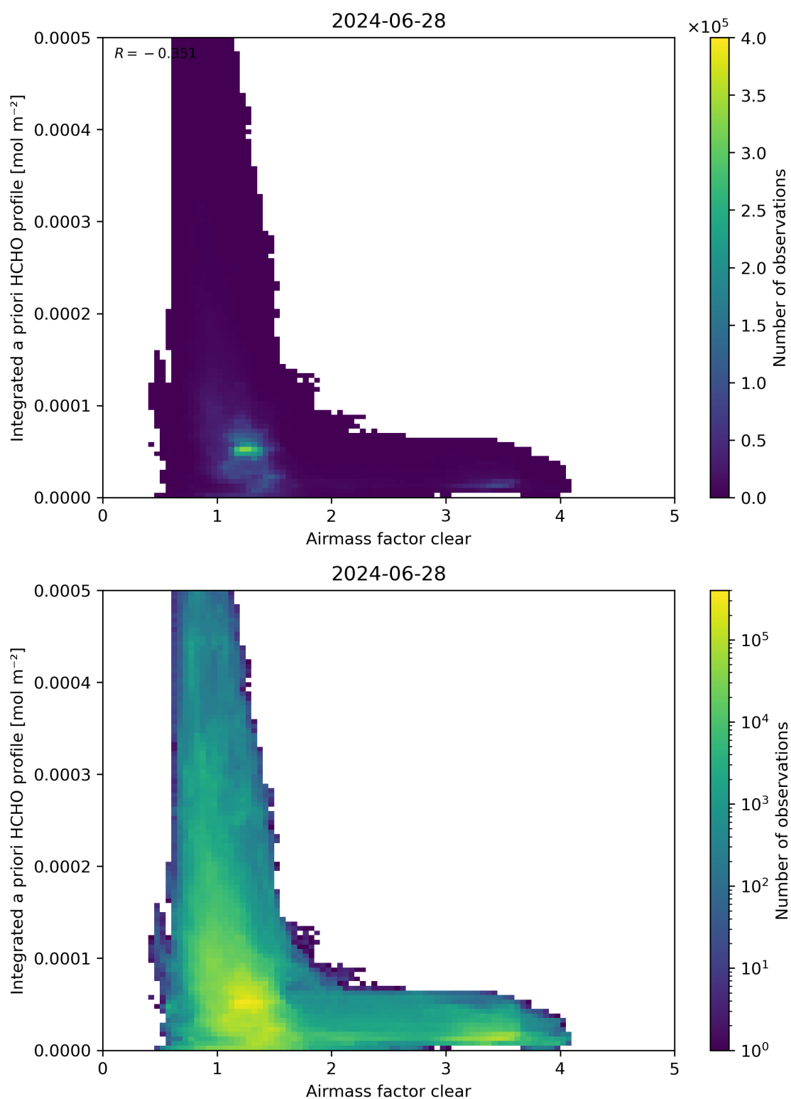
Figure 76: Scatter density plot of “Airmass factor clear” against “Integrated a priori HCHO profile” for 2024-06-27 to 2024-06-29.
