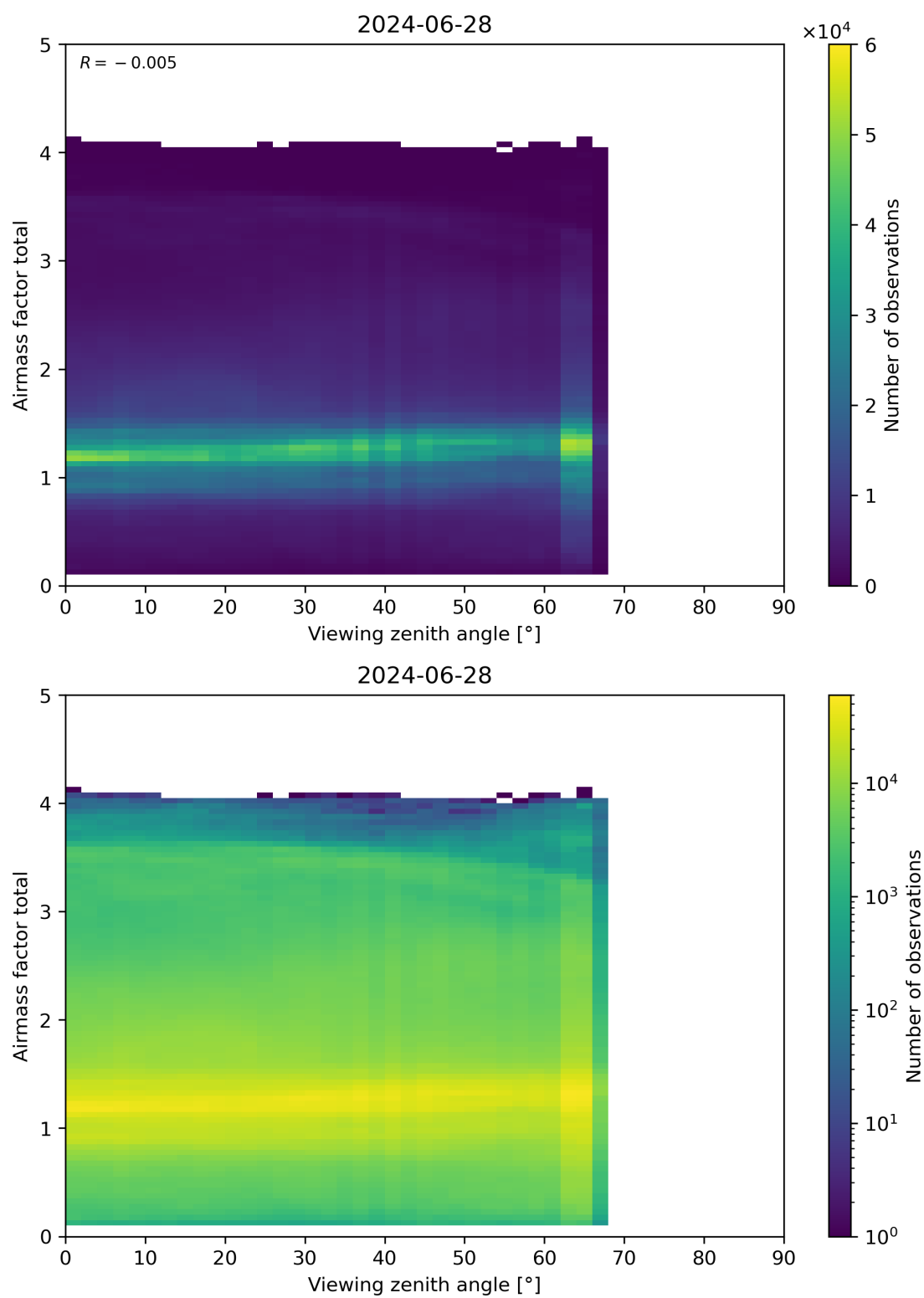
Figure 190: Scatter density plot of “Viewing zenith angle” against “Airmass factor total” for 2024-06-27 to 2024-06-29.
