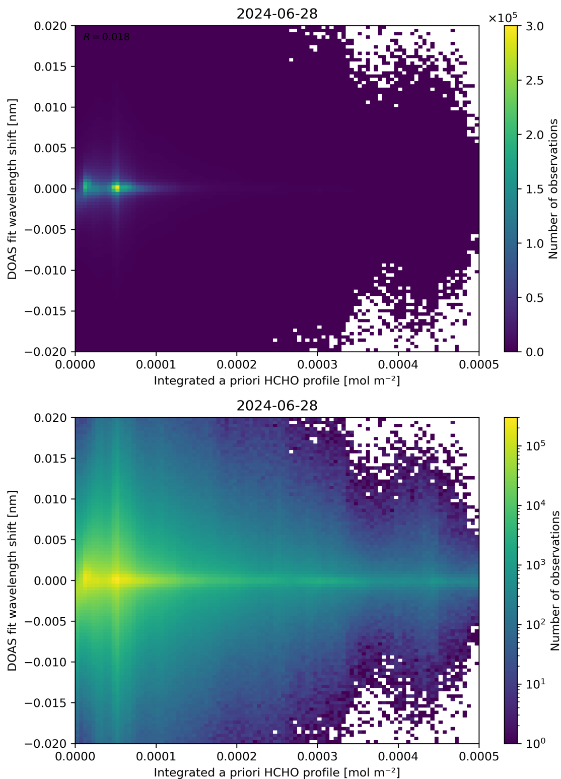
Figure 149: Scatter density plot of “Integrated a priori HCHO profile” against “DOAS fit wavelength shift” for 2024-06-27 to 2024-06-29.
