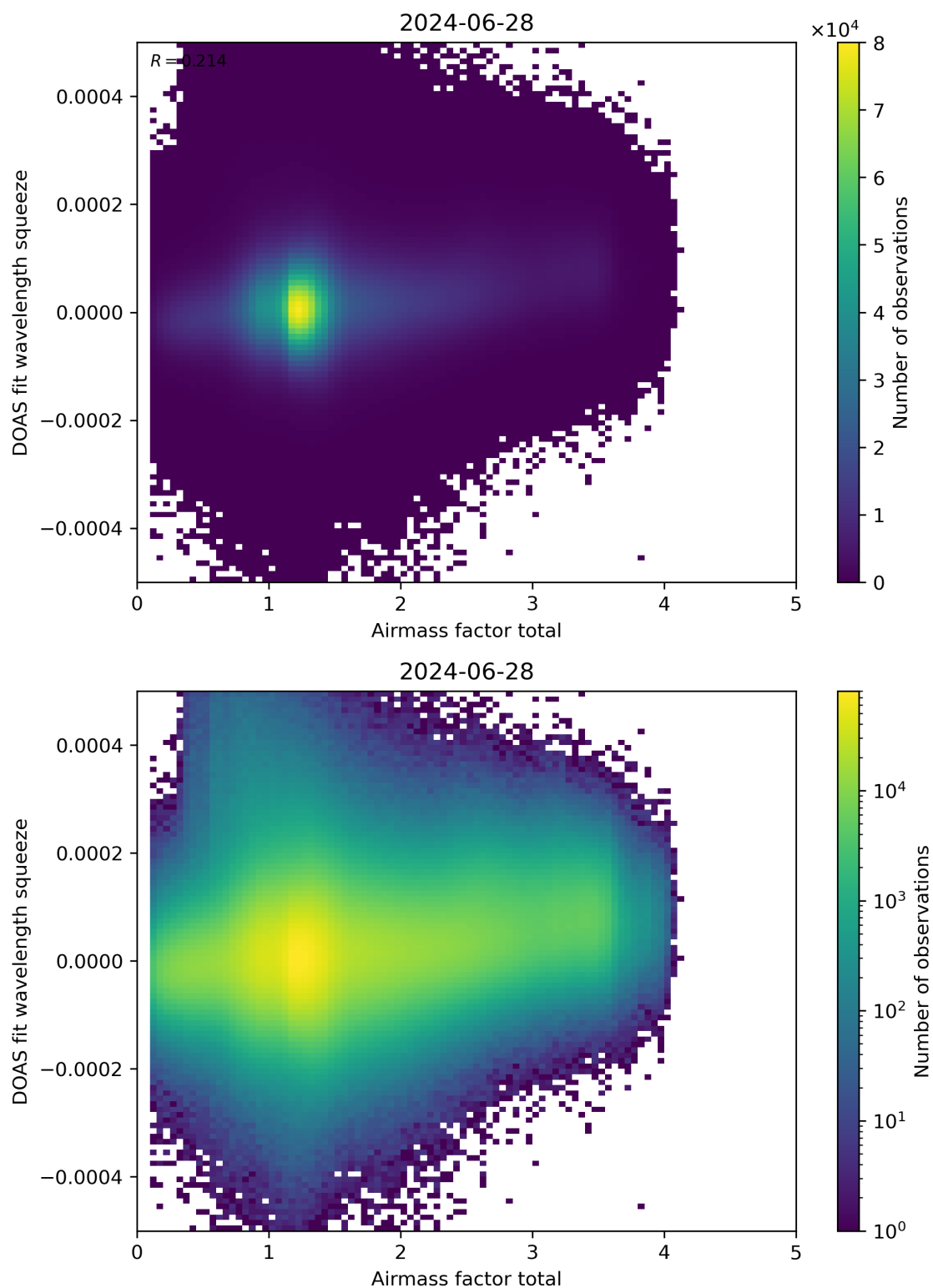
Figure 99: Scatter density plot of “Airmass factor total” against “DOAS fit wavelength squeeze” for 2024-06-27 to 2024-06-29.
