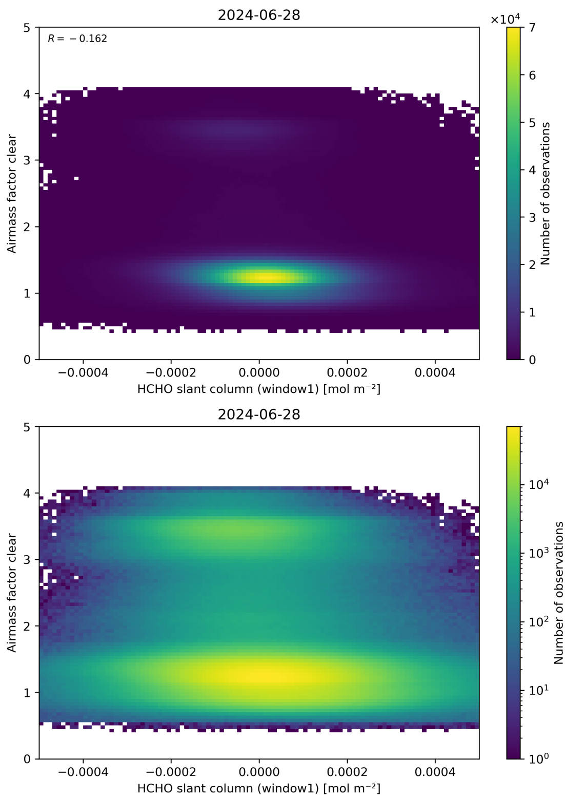
Figure 81: Scatter density plot of “HCHO slant column (window1)” against “Airmass factor clear” for 2024-06-27 to 2024-06-29.
