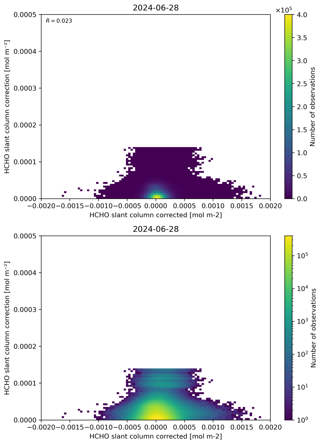
Figure 77: Scatter density plot of “HCHO slant column corrected” against “HCHO slant column correction” for 2024-06-27 to 2024-06-29.
