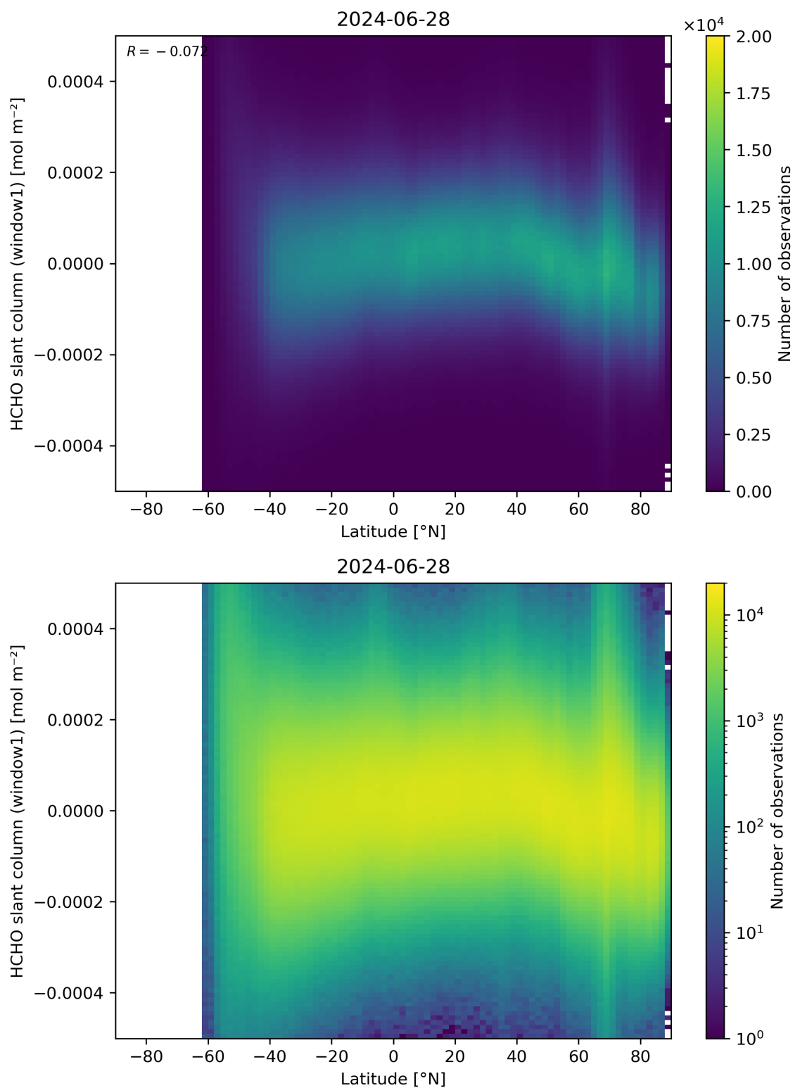
Figure 159: Scatter density plot of “Latitude” against “HCHO slant column (window1)” for 2024-06-27 to 2024-06-29.
