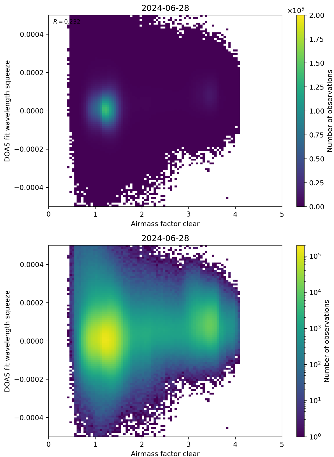
Figure 73: Scatter density plot of “Airmass factor clear” against “DOAS fit wavelength squeeze” for 2024-06-27 to 2024-06-29.
