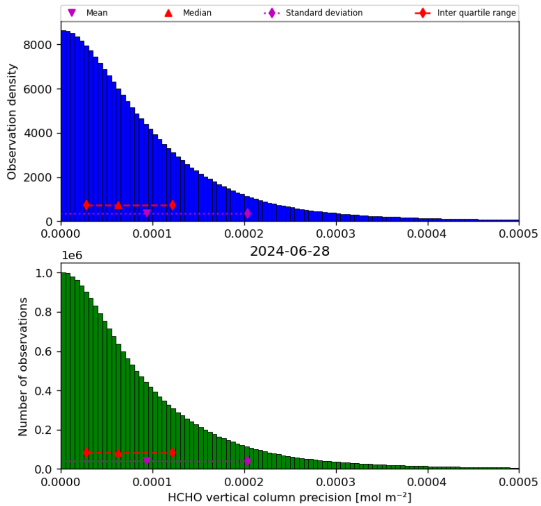
Figure 36: Histogram of “HCHO vertical column precision” for 2024-06-27 to 2024-06-29
