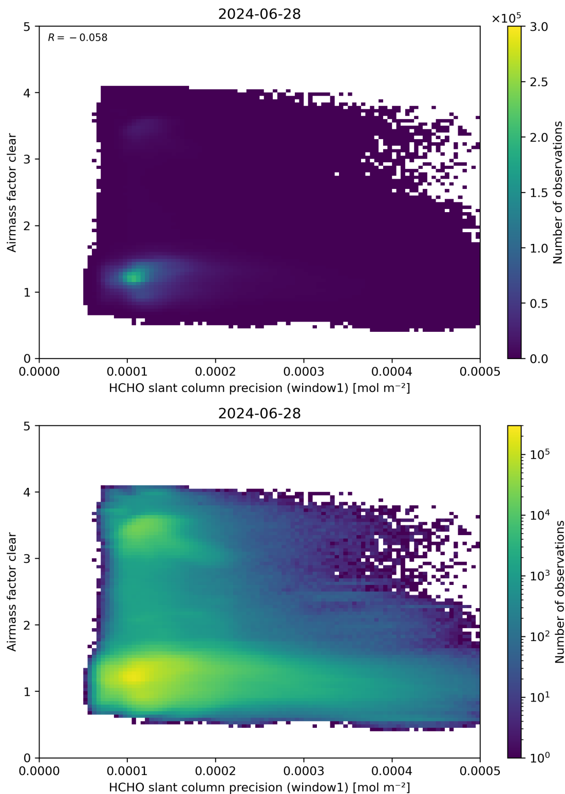
Figure 91: Scatter density plot of “HCHO slant column precision (window1)” against “Airmass factor clear” for 2024-06-27 to 2024-06-29.
