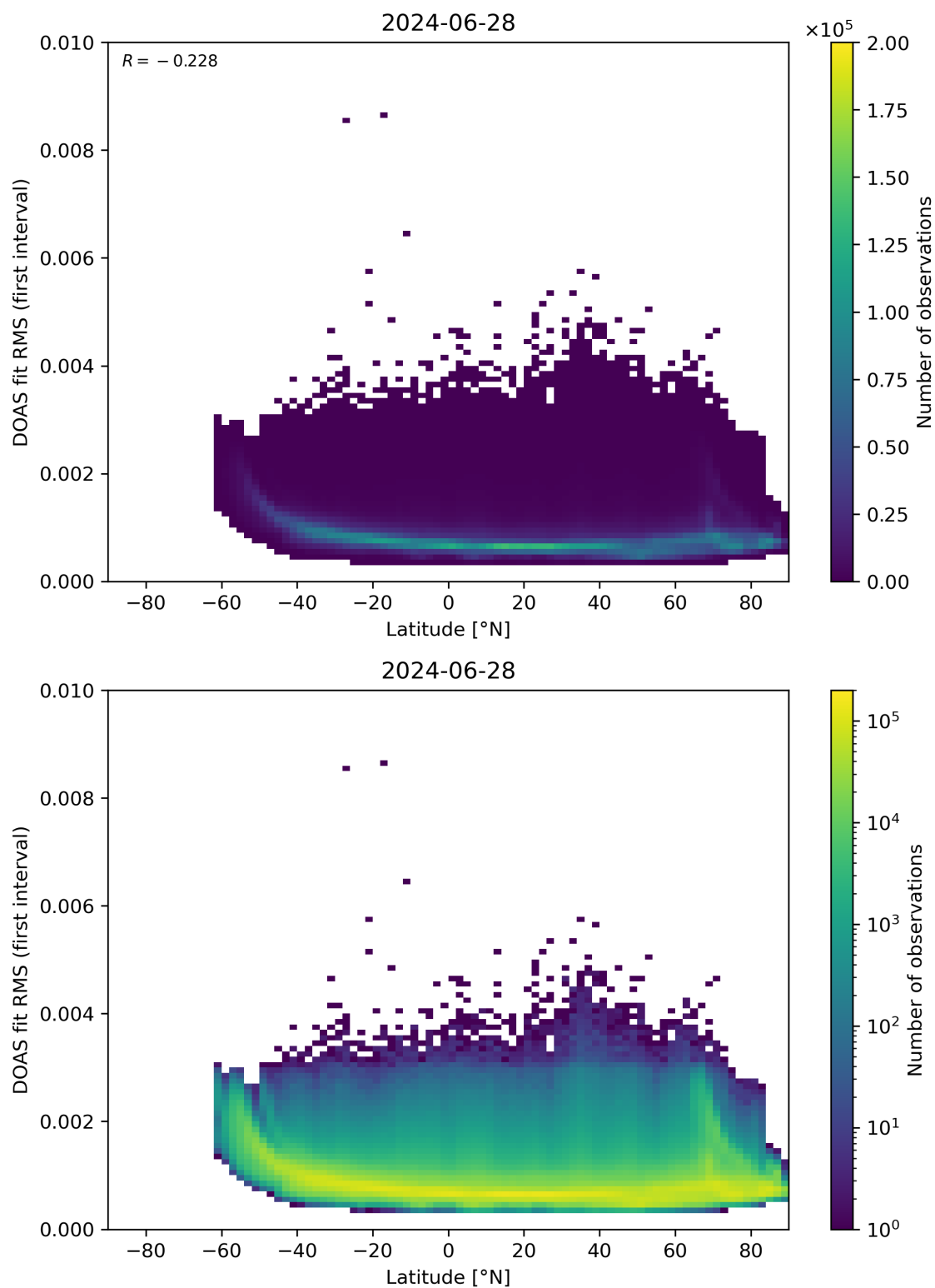
Figure 153: Scatter density plot of “Latitude” against “DOAS fit RMS (first interval)” for 2024-06-27 to 2024-06-29.
