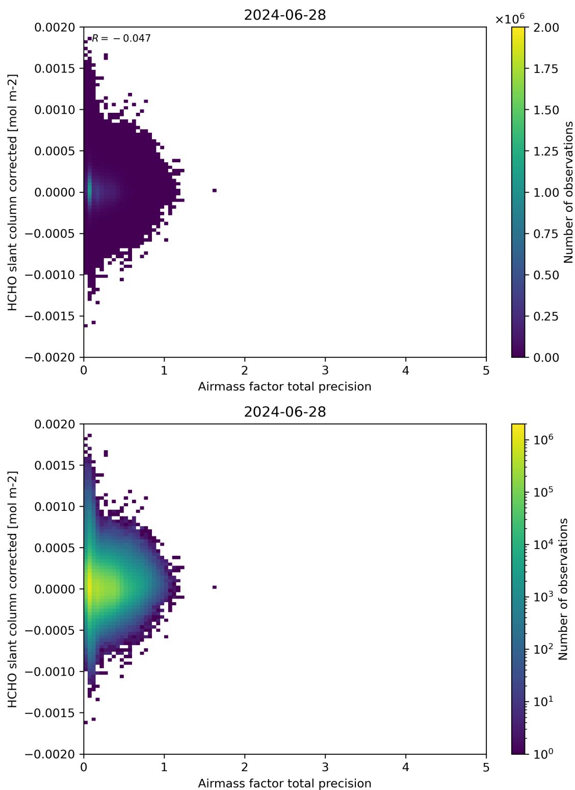
Figure 109: Scatter density plot of “Airmass factor total precision” against “HCHO slant column corrected” for 2024-06-27 to 2024-06-29.
