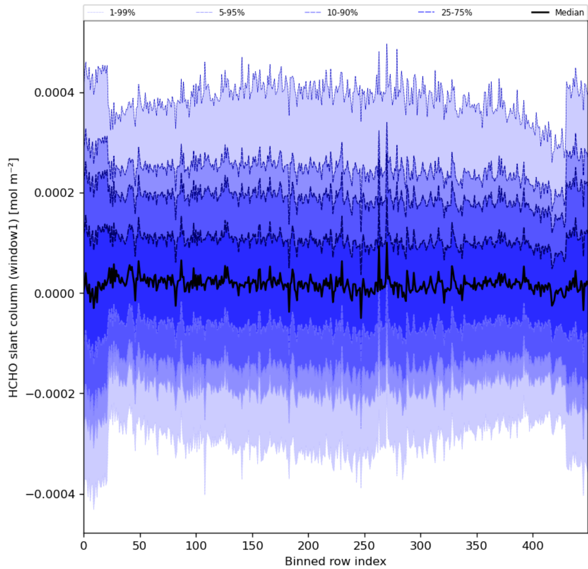
Figure 52: Along track statistics of “HCHO slant column (window1)” for 2024-06-27 to 2024-06-29
