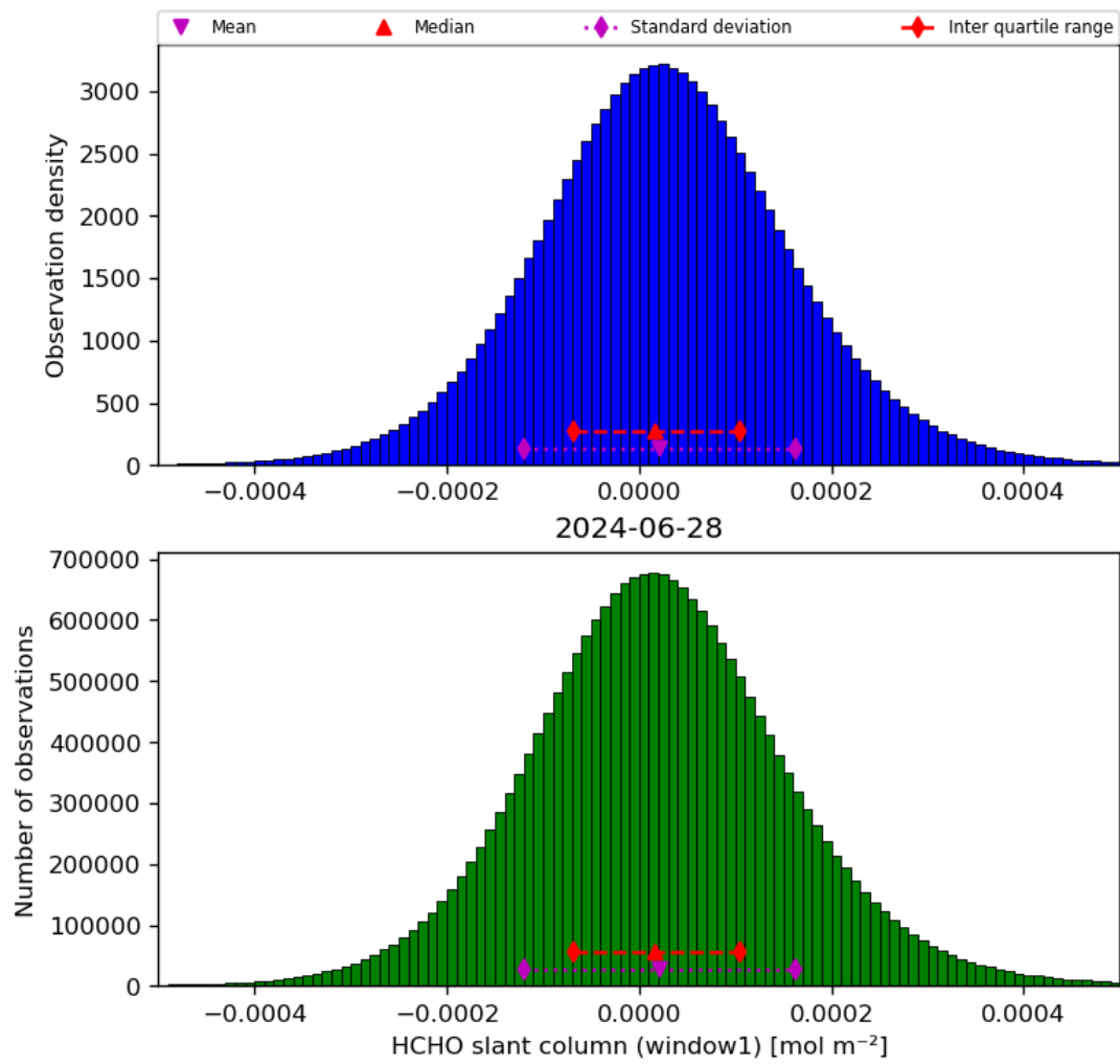
Figure 38: Histogram of “HCHO slant column (window1)” for 2024-06-27 to 2024-06-29
