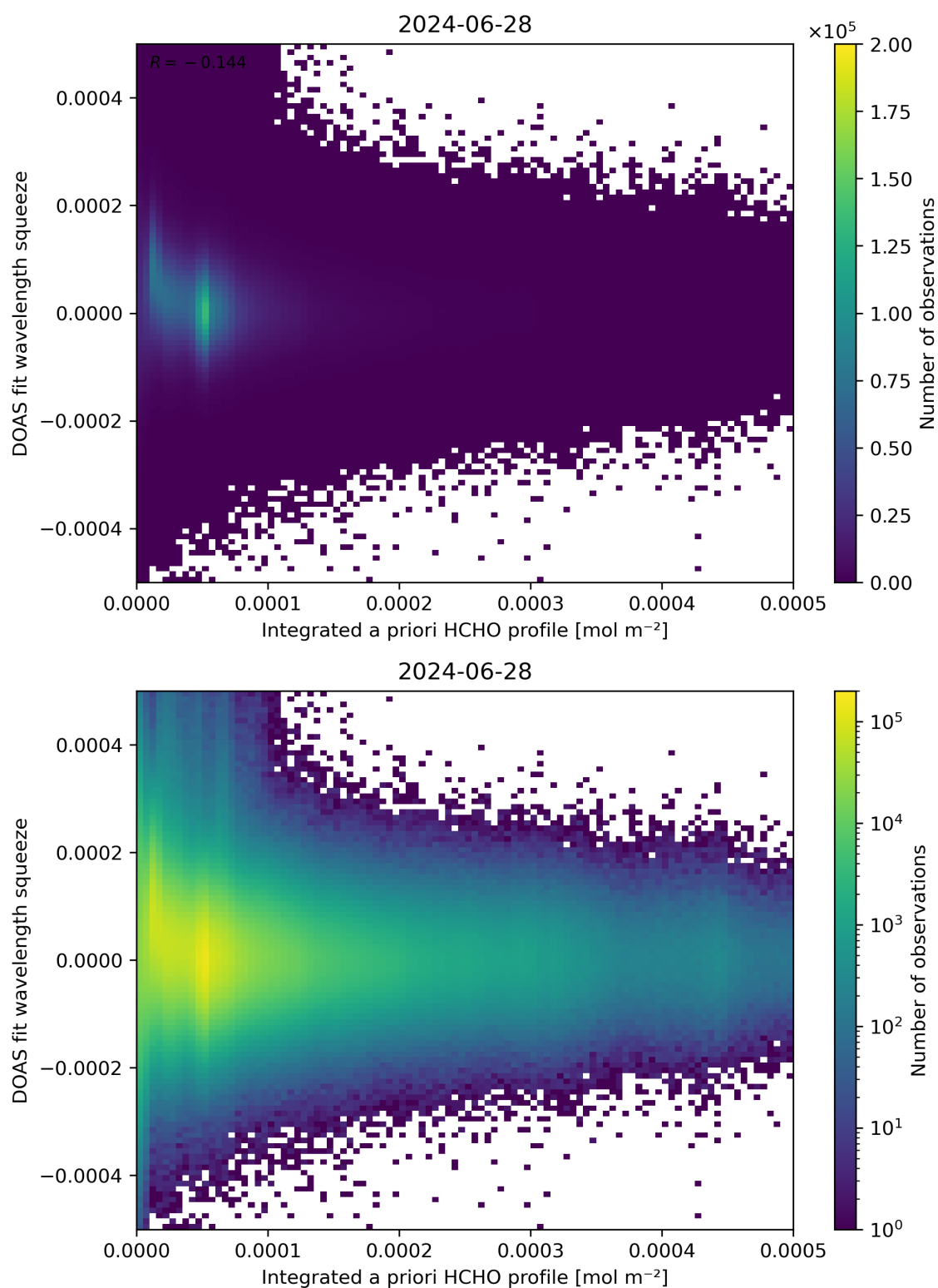
Figure 150: Scatter density plot of “Integrated a priori HCHO profile” against “DOAS fit wavelength squeeze” for 2024-06-27 to 2024-06-29.
