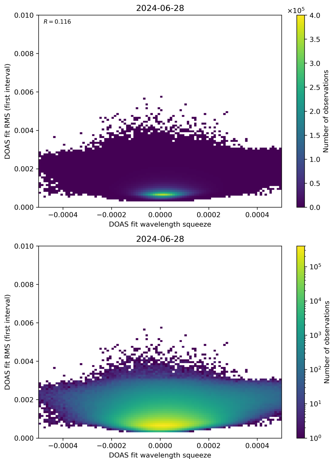
Figure 68: Scatter density plot of “DOAS fit wavelength squeeze” against “DOAS fit RMS (first interval)” for 2024-06-27 to 2024-06-29.
