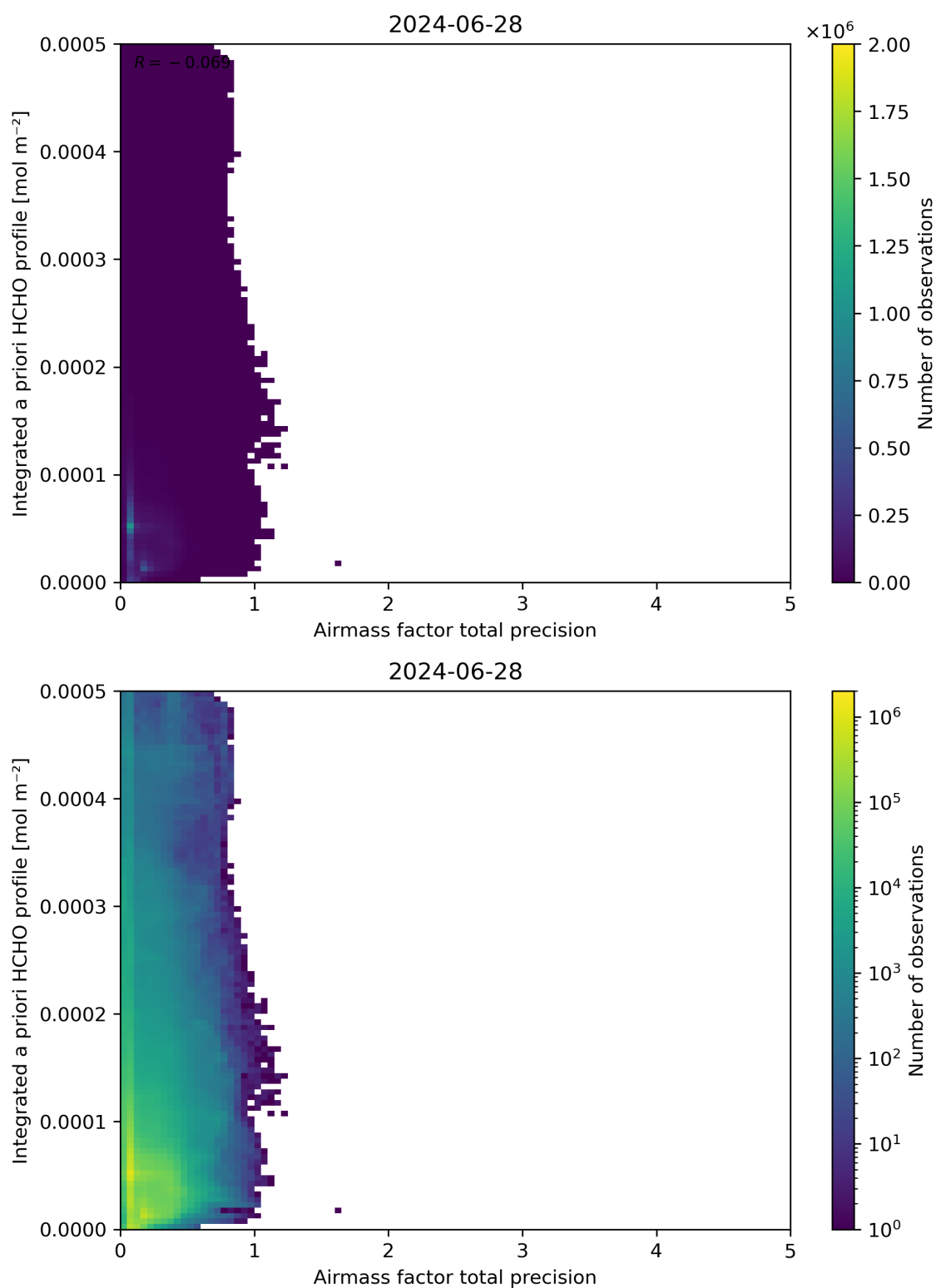
Figure 111: Scatter density plot of “Airmass factor total precision” against “Integrated a priori HCHO profile” for 2024-06-27 to 2024-06-29.
