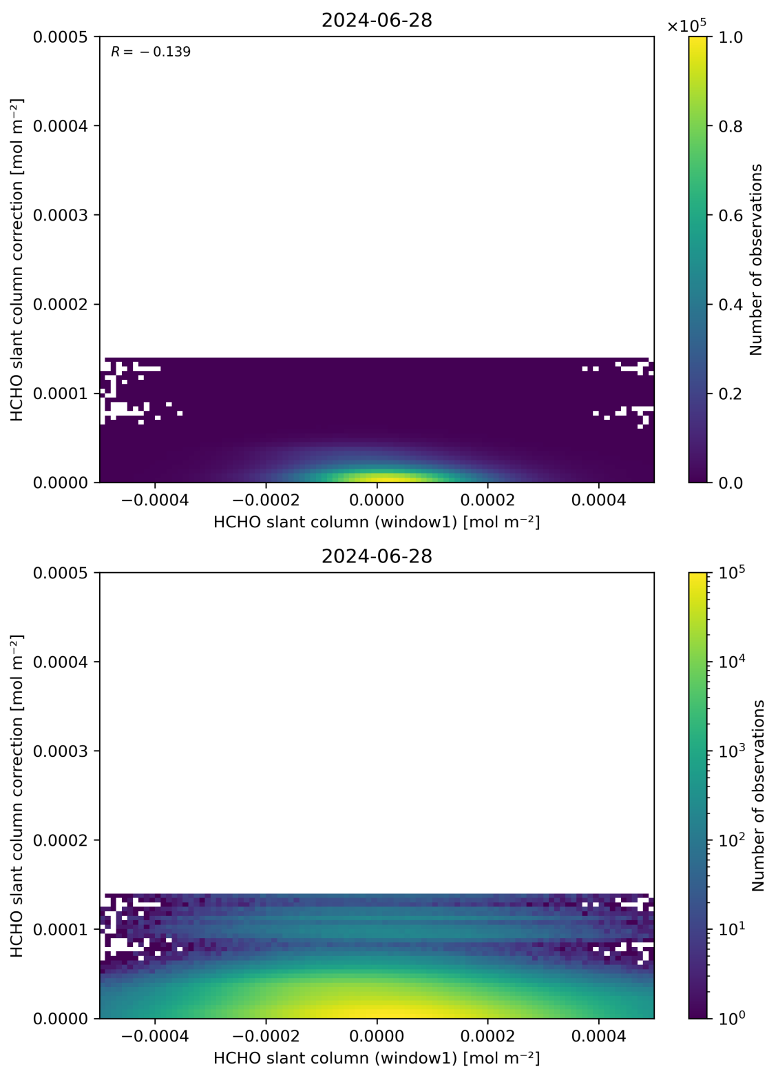
Figure 83: Scatter density plot of “HCHO slant column (window1)” against “HCHO slant column correction” for 2024-06-27 to 2024-06-29.
