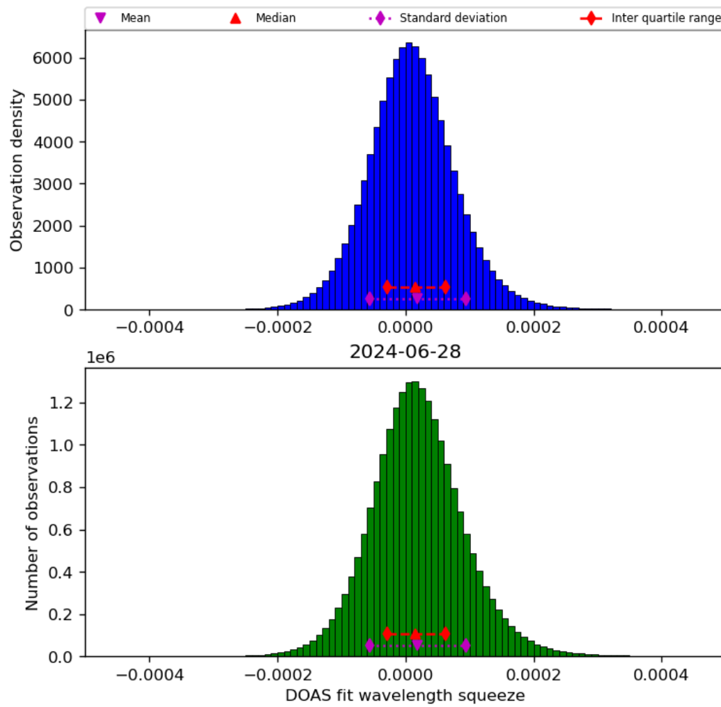
Figure 45: Histogram of “DOAS fit wavelength squeeze” for 2024-06-27 to 2024-06-29
