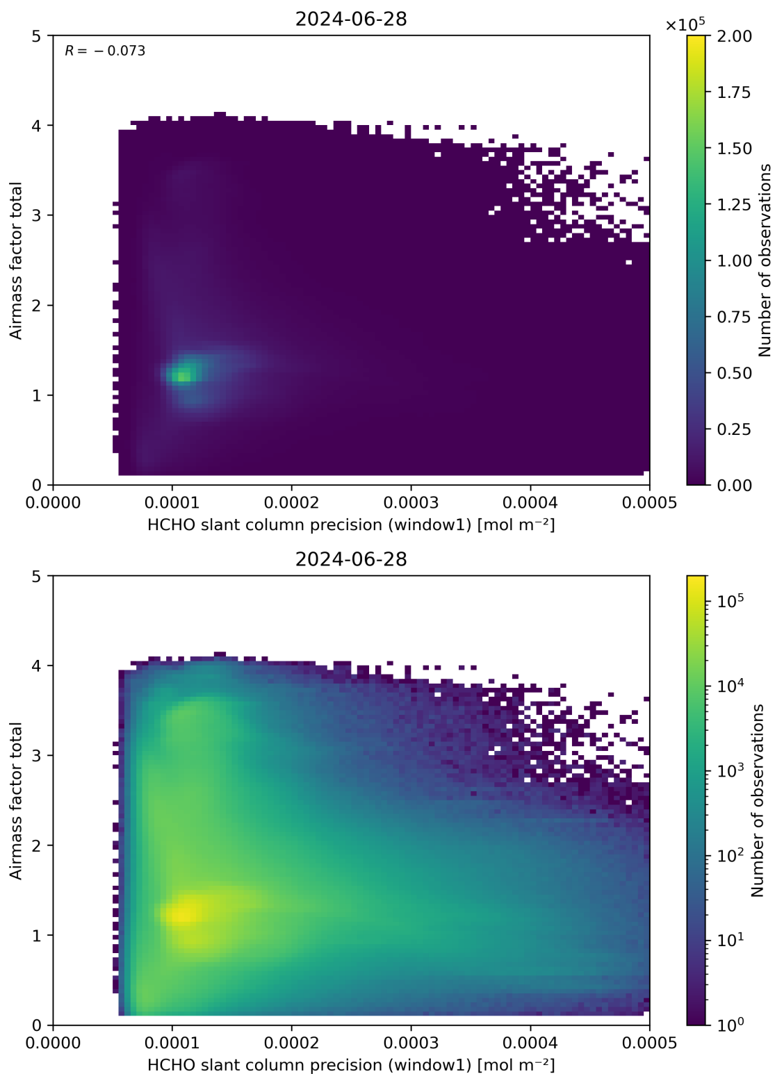
Figure 94: Scatter density plot of “HCHO slant column precision (window1)” against “Airmass factor total” for 2024-06-27 to 2024-06-29.
