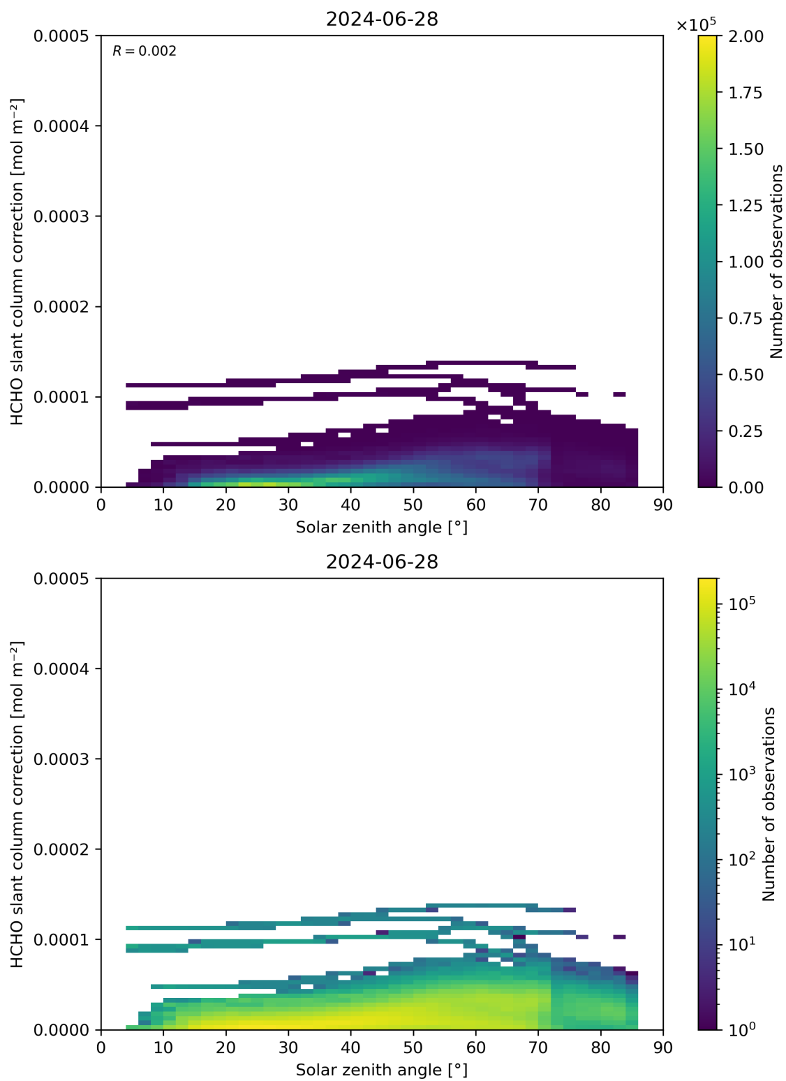
Figure 172: Scatter density plot of “Solar zenith angle” against “HCHO slant column correction” for 2024-06-27 to 2024-06-29.
