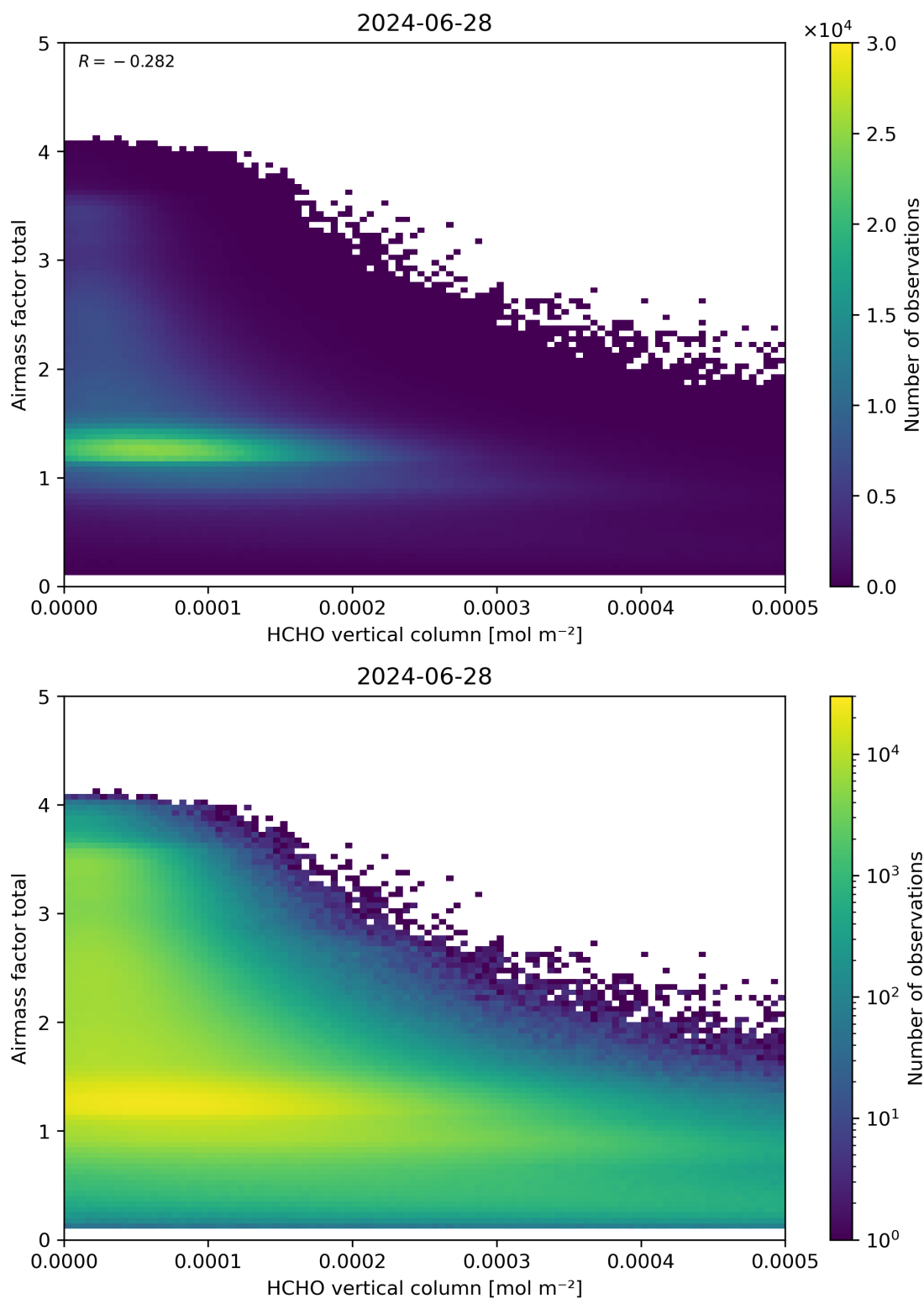
Figure 131: Scatter density plot of “HCHO vertical column” against “Airmass factor total” for 2024-06-27 to 2024-06-29.
