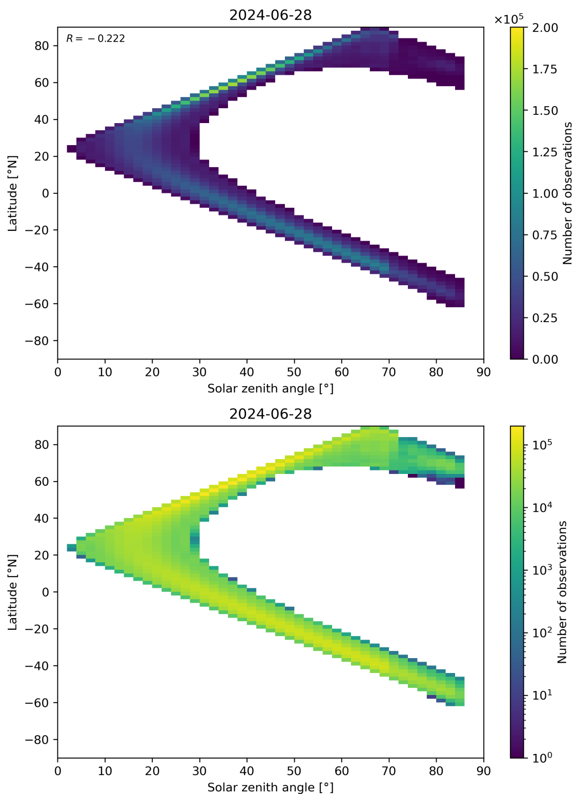
Figure 181: Scatter density plot of “Solar zenith angle” against “Latitude” for 2024-06-27 to 2024-06-29.
