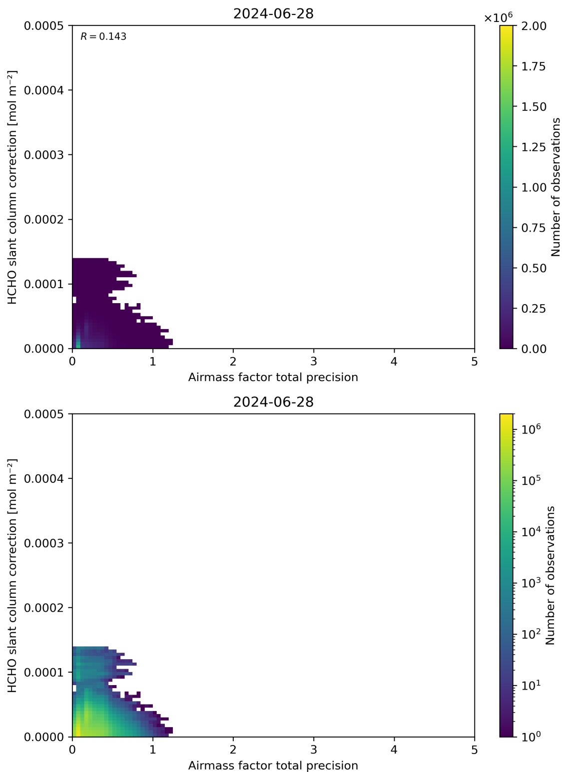
Figure 110: Scatter density plot of “Airmass factor total precision” against “HCHO slant column correction” for 2024-06-27 to 2024-06-29.
