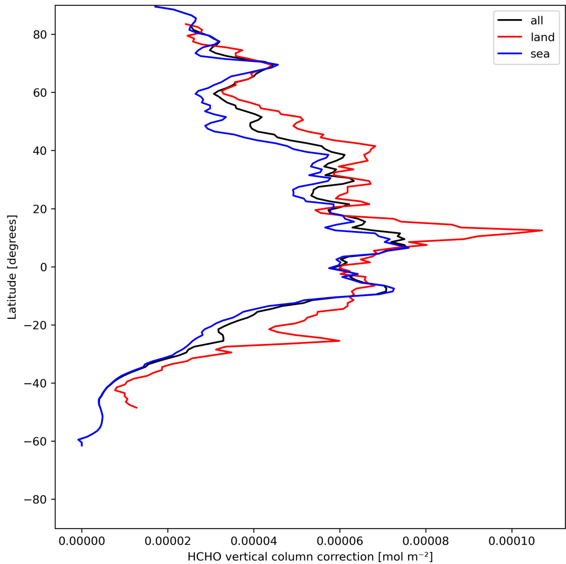
Figure 23: Zonal average of “HCHO vertical column correction” for 2024-06-27 to 2024-06-29.
