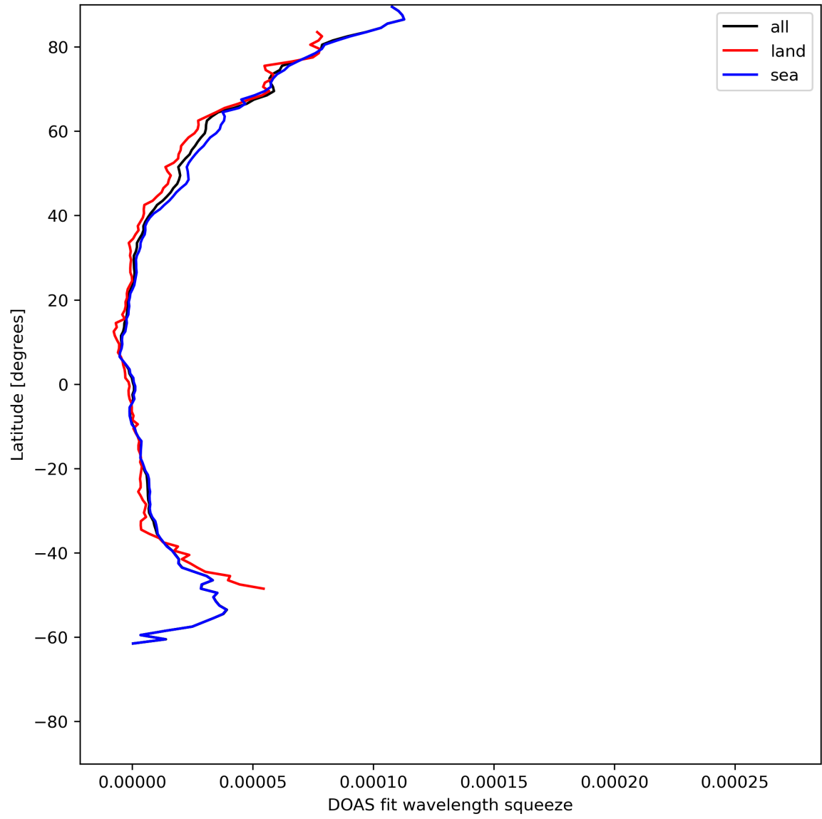
Figure 31: Zonal average of “DOAS fit wavelength squeeze” for 2024-06-27 to 2024-06-29.
