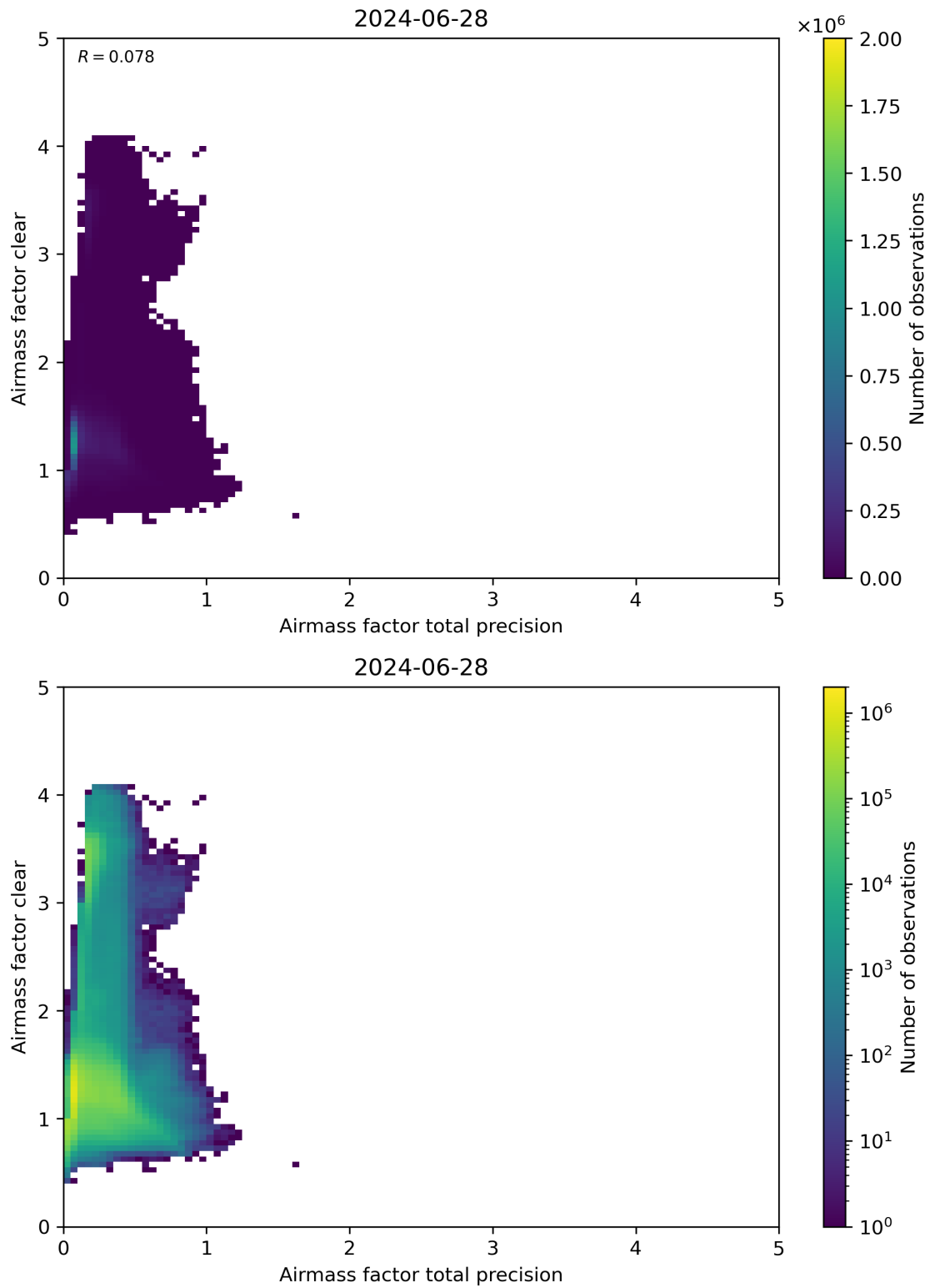
Figure 108: Scatter density plot of “Airmass factor total precision” against “Airmass factor clear” for 2024-06-27 to 2024-06-29.
