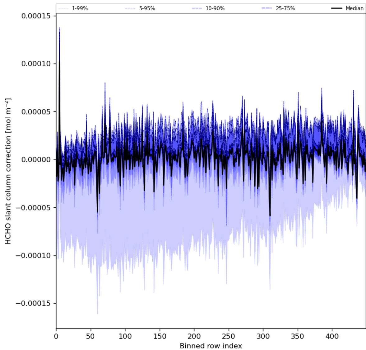
Figure 61: Along track statistics of “HCHO slant column correction” for 2024-06-27 to 2024-06-29
