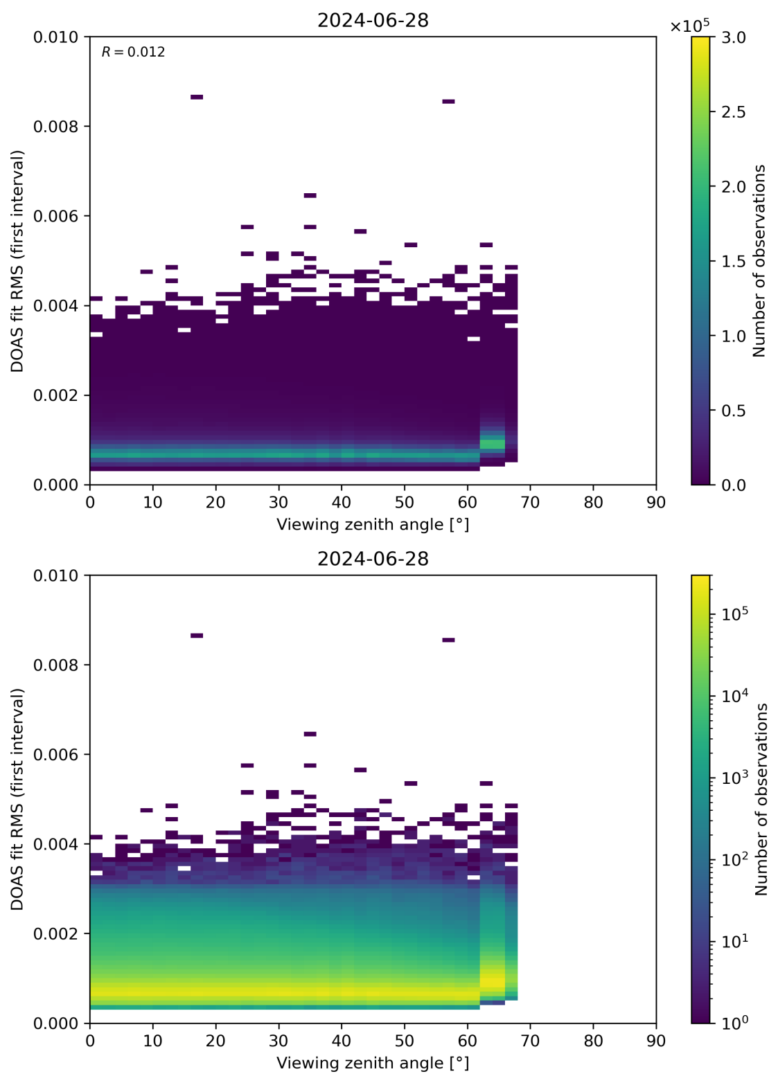
Figure 182: Scatter density plot of “Viewing zenith angle” against “DOAS fit RMS (first interval)” for 2024-06-27 to 2024-06-29.
