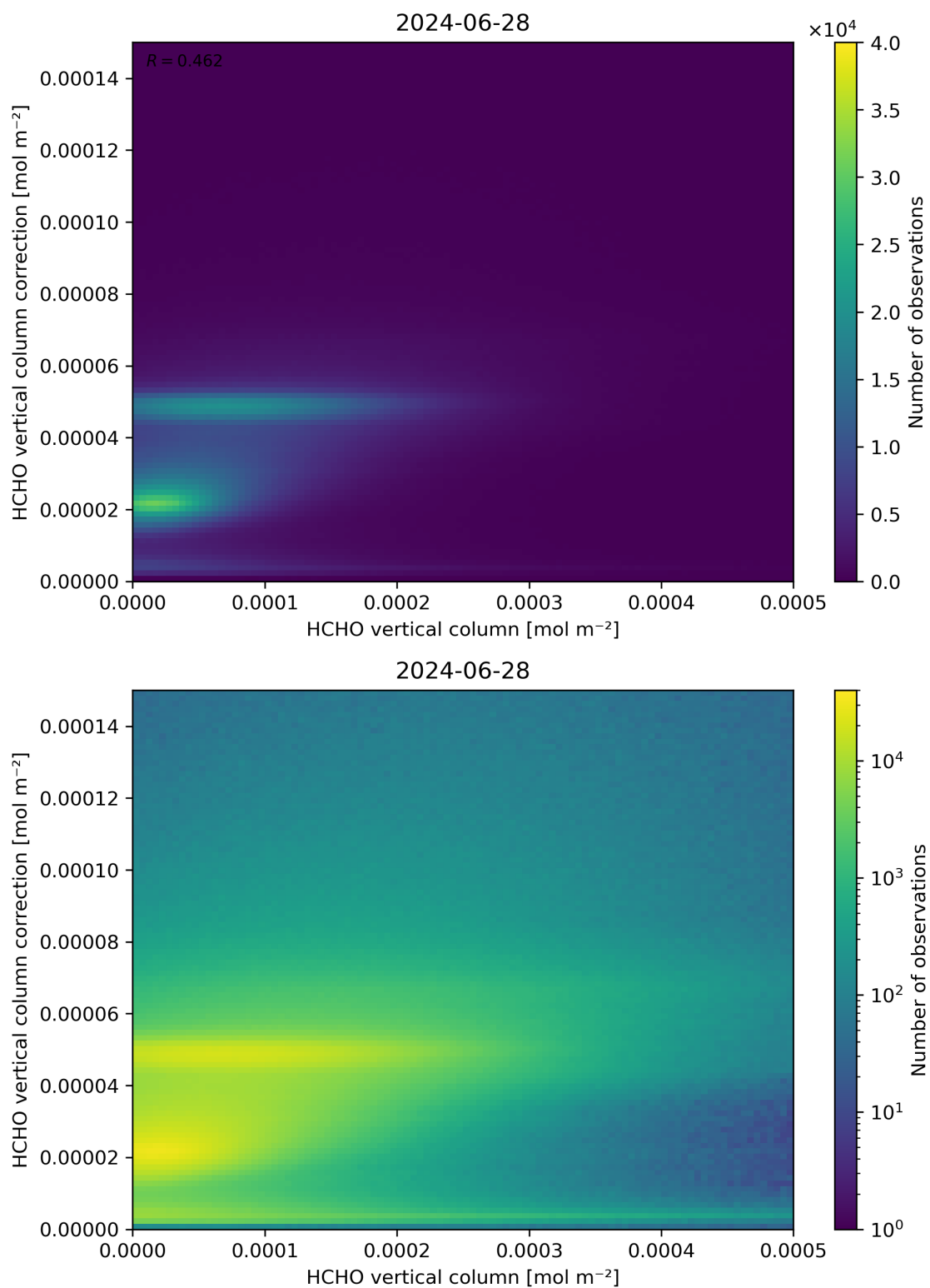
Figure 133: Scatter density plot of “HCHO vertical column” against “HCHO vertical column correction” for 2024-06-27 to 2024-06-29.
