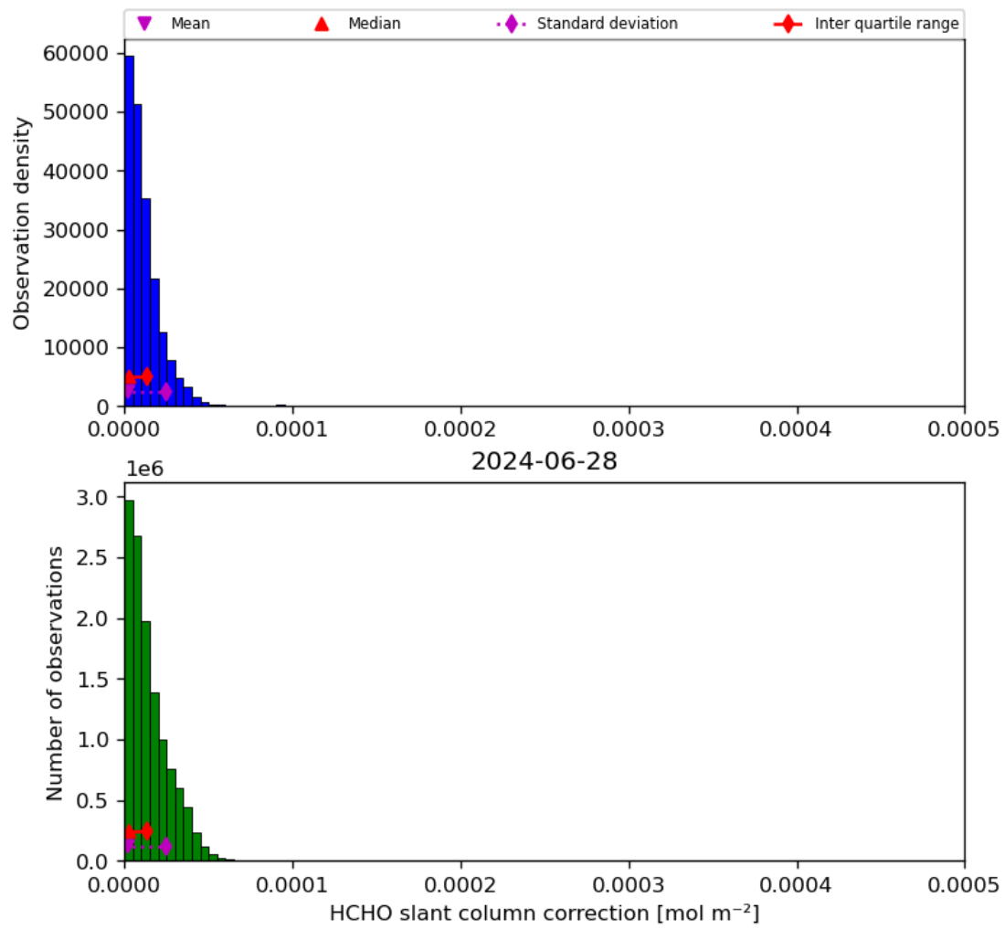
Figure 47: Histogram of “HCHO slant column correction” for 2024-06-27 to 2024-06-29
