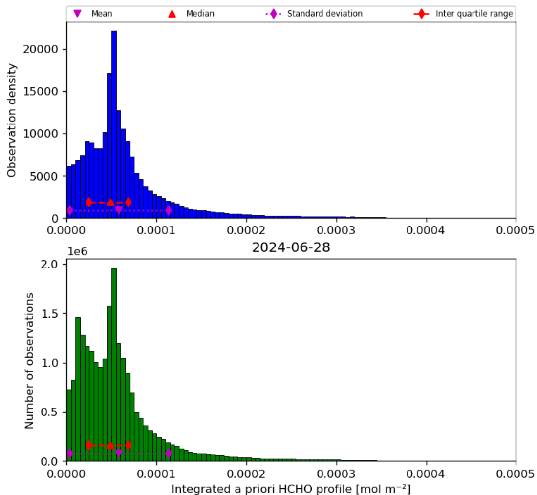
Figure 43: Histogram of “Integrated a priori HCHO profile” for 2024-06-27 to 2024-06-29
