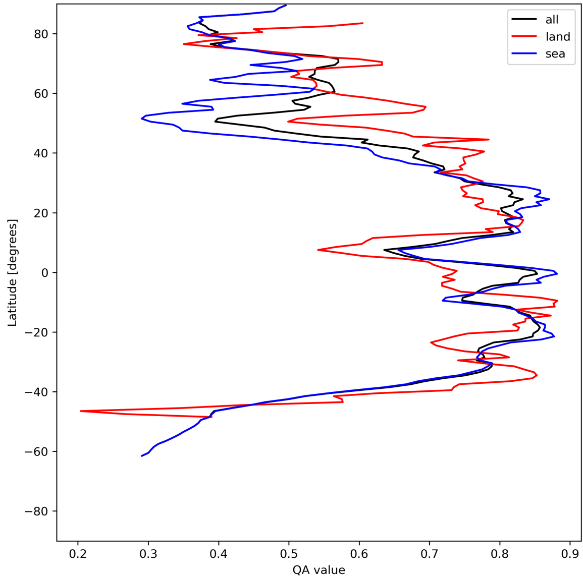
Figure 20: Zonal average of “QA value” for 2024-06-27 to 2024-06-29.
