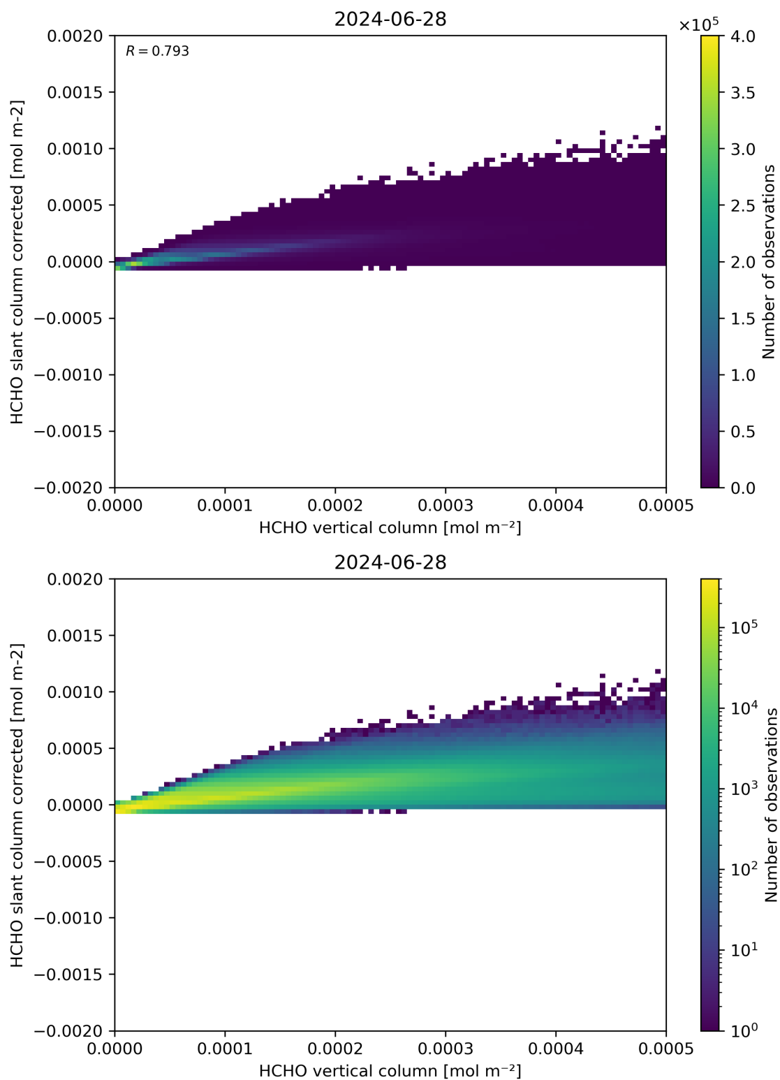
Figure 127: Scatter density plot of “HCHO vertical column” against “HCHO slant column corrected” for 2024-06-27 to 2024-06-29.
