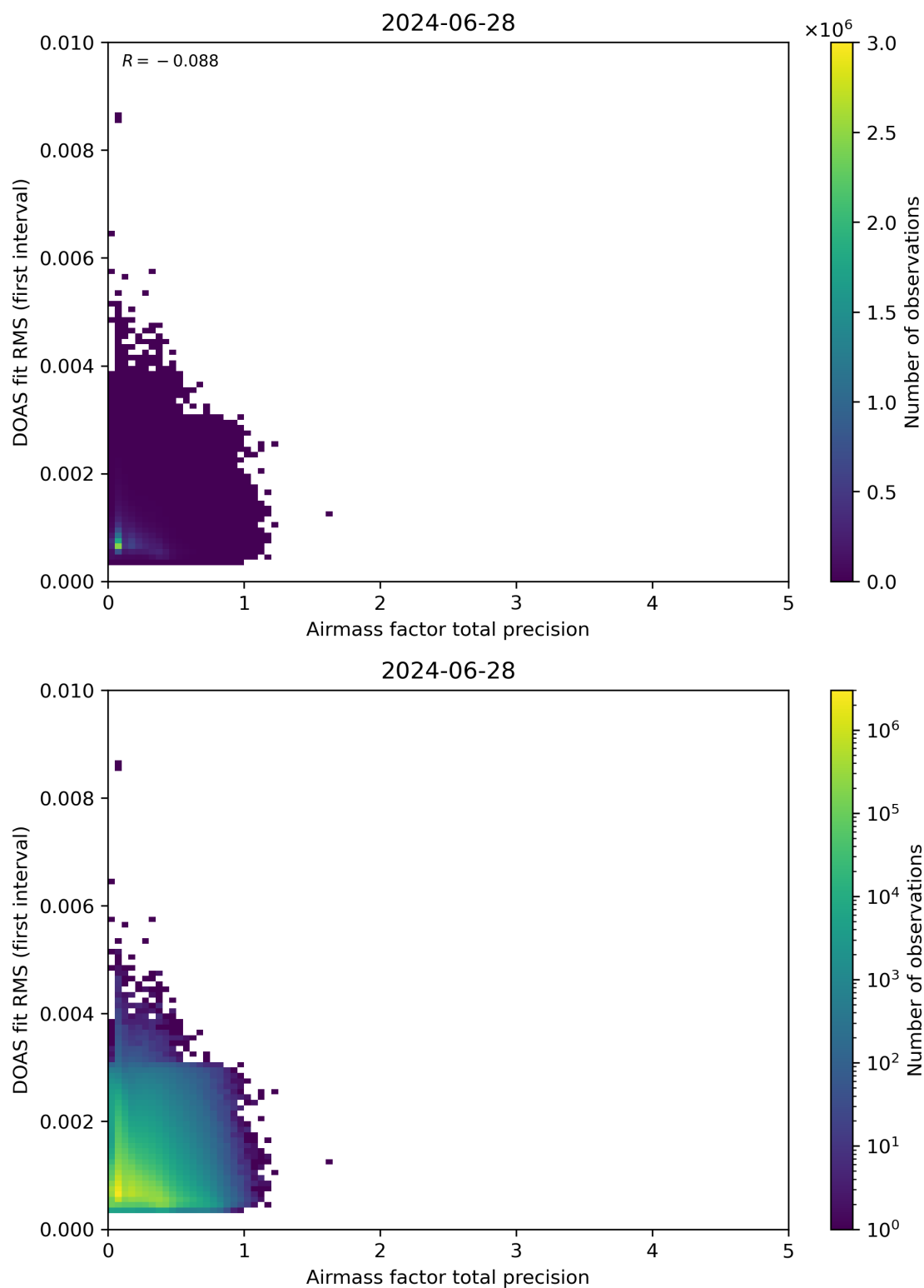
Figure 105: Scatter density plot of “Airmass factor total precision” against “DOAS fit RMS (first interval)” for 2024-06-27 to 2024-06-29.
