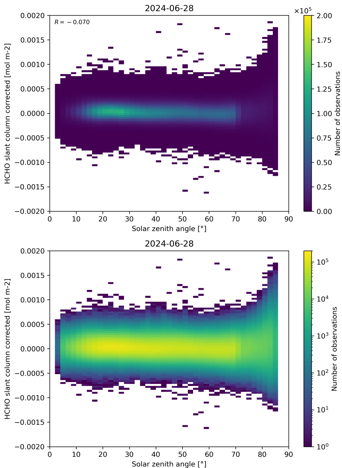
Figure 171: Scatter density plot of “Solar zenith angle” against “HCHO slant column corrected” for 2024-06-27 to 2024-06-29.
