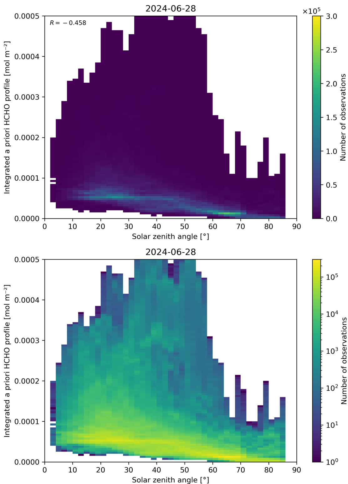
Figure 180: Scatter density plot of “Solar zenith angle” against “Integrated a priori HCHO profile” for 2024-06-27 to 2024-06-29.
