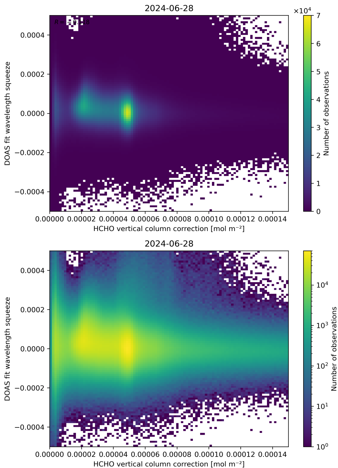
Figure 114: Scatter density plot of “HCHO vertical column correction” against “DOAS fit wavelength squeeze” for 2024-06-27 to 2024-06-29.
