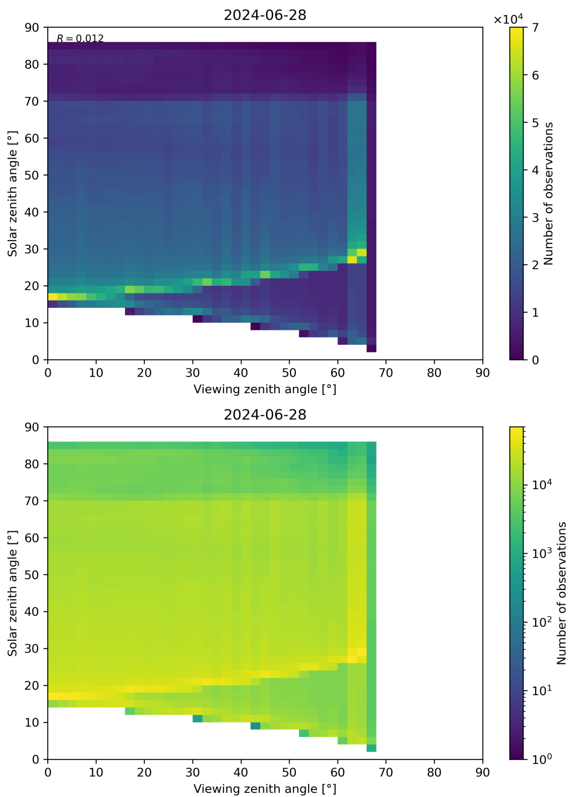
Figure 197: Scatter density plot of “Viewing zenith angle” against “Solar zenith angle” for 2024-06-27 to 2024-06-29.
