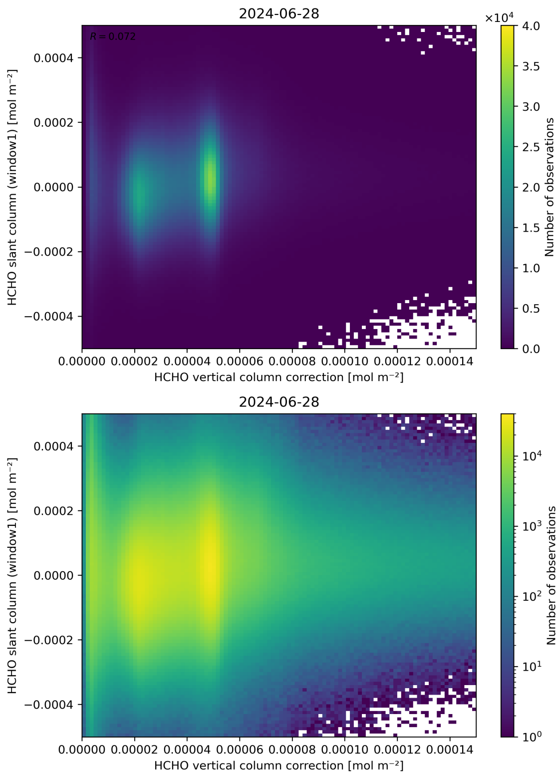
Figure 118: Scatter density plot of “HCHO vertical column correction” against “HCHO slant column (window1)” for 2024-06-27 to 2024-06-29.
