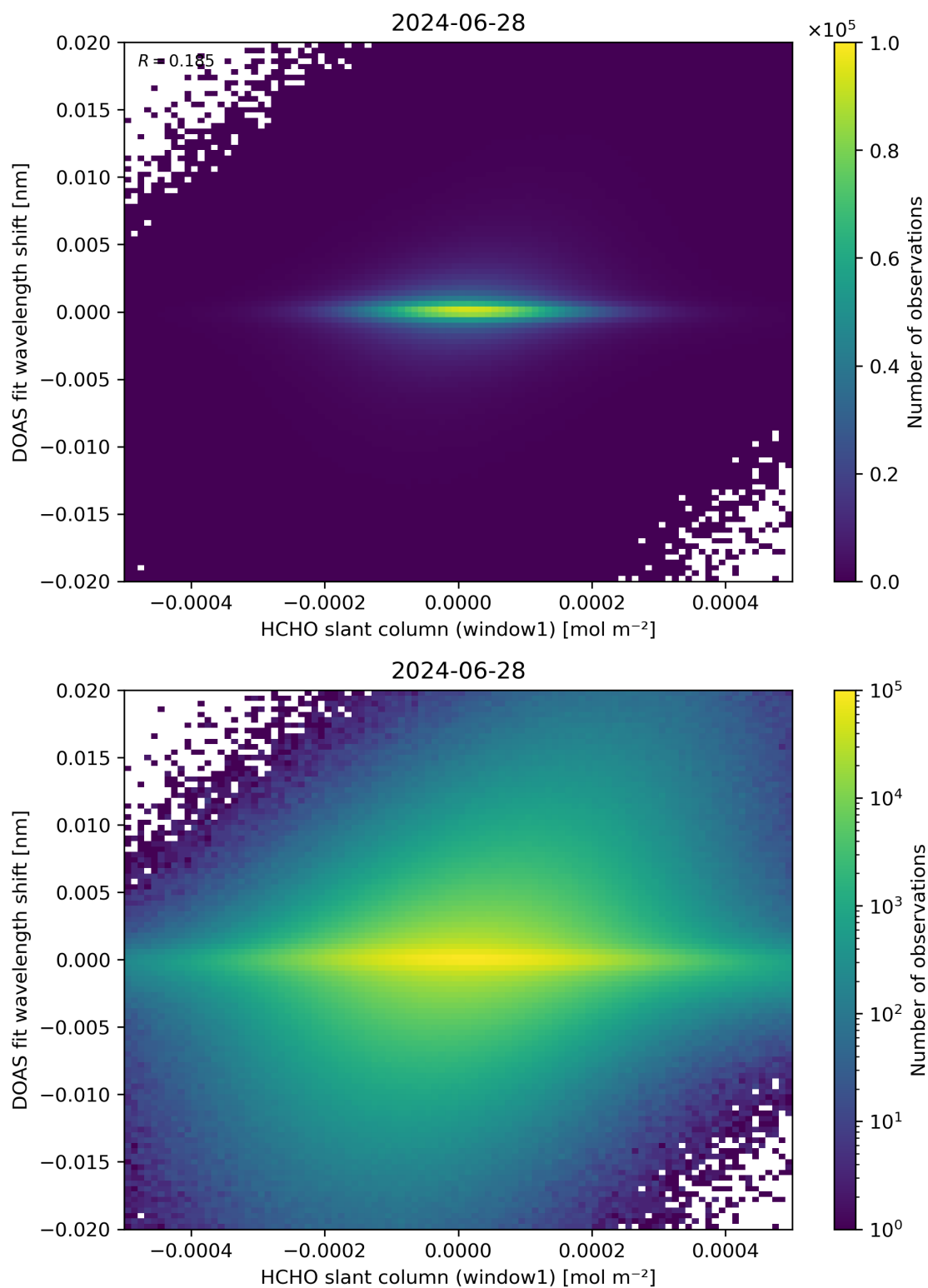
Figure 79: Scatter density plot of “HCHO slant column (window1)” against “DOAS fit wavelength shift” for 2024-06-27 to 2024-06-29.
