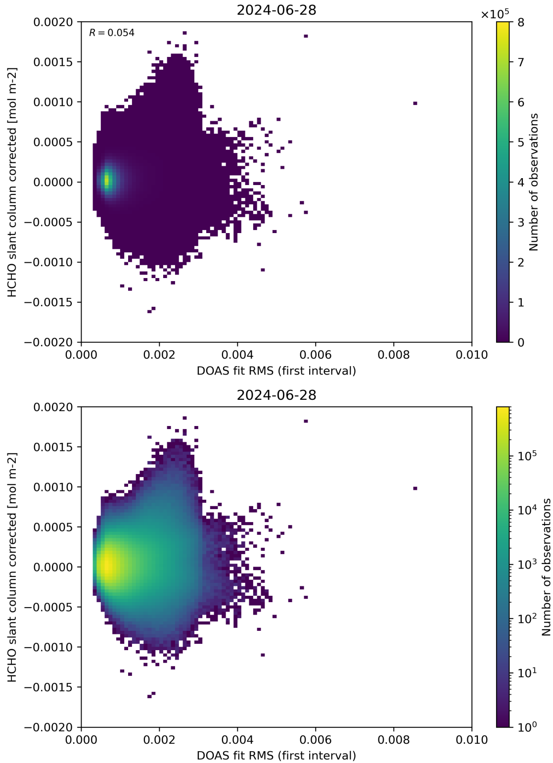
Figure 62: Scatter density plot of “DOAS fit RMS (first interval)” against “HCHO slant column corrected” for 2024-06-27 to 2024-06-29.
