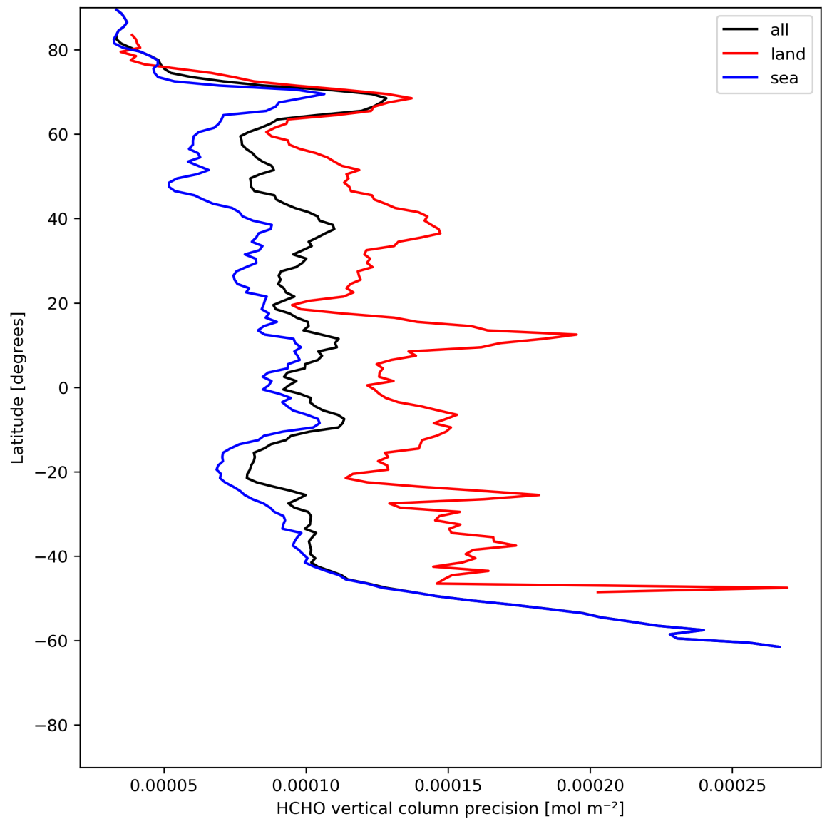
Figure 22: Zonal average of “HCHO vertical column precision” for 2024-06-27 to 2024-06-29.
