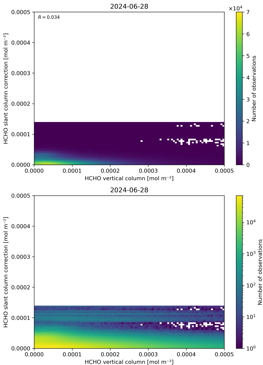
Figure 128: Scatter density plot of “HCHO vertical column” against “HCHO slant column correction” for 2024-06-27 to 2024-06-29.
