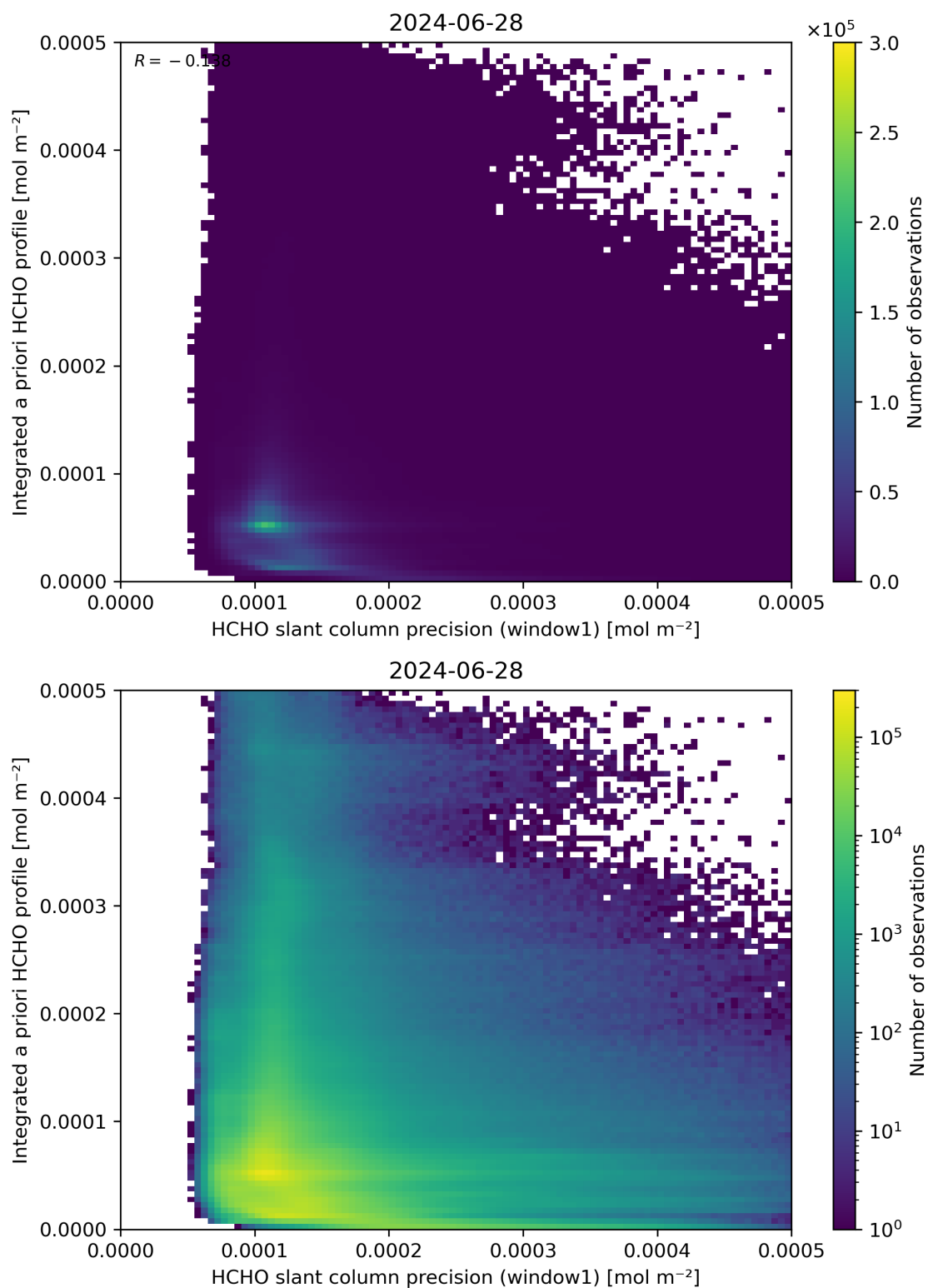
Figure 96: Scatter density plot of “HCHO slant column precision (window1)” against “Integrated a priori HCHO profile” for 2024-06-27 to 2024-06-29.
