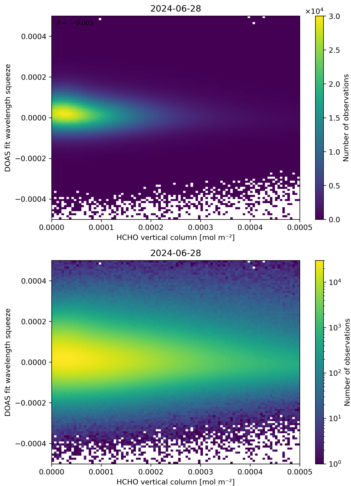
Figure 125: Scatter density plot of “HCHO vertical column” against “DOAS fit wavelength squeeze” for 2024-06-27 to 2024-06-29.
