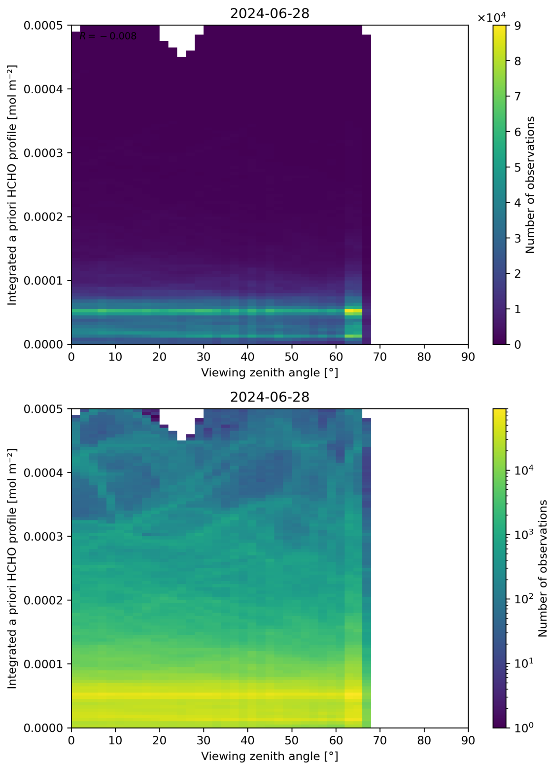
Figure 195: Scatter density plot of “Viewing zenith angle” against “Integrated a priori HCHO profile” for 2024-06-27 to 2024-06-29.
