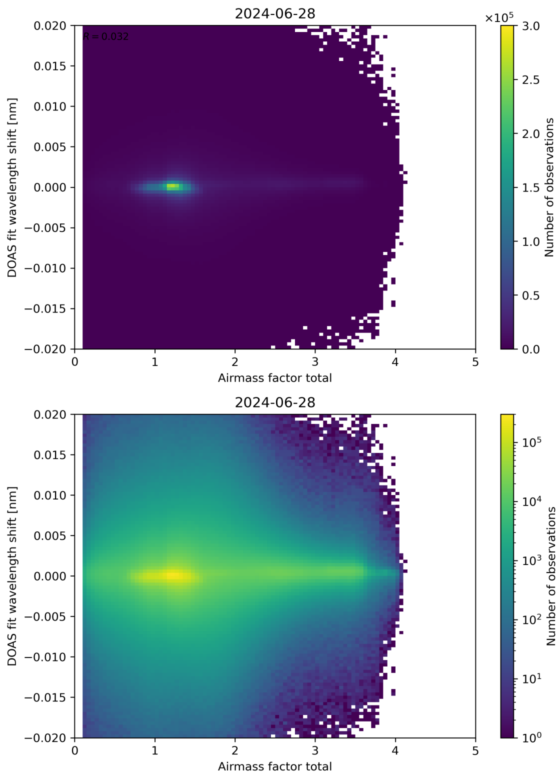
Figure 98: Scatter density plot of “Airmass factor total” against “DOAS fit wavelength shift” for 2024-06-27 to 2024-06-29.
