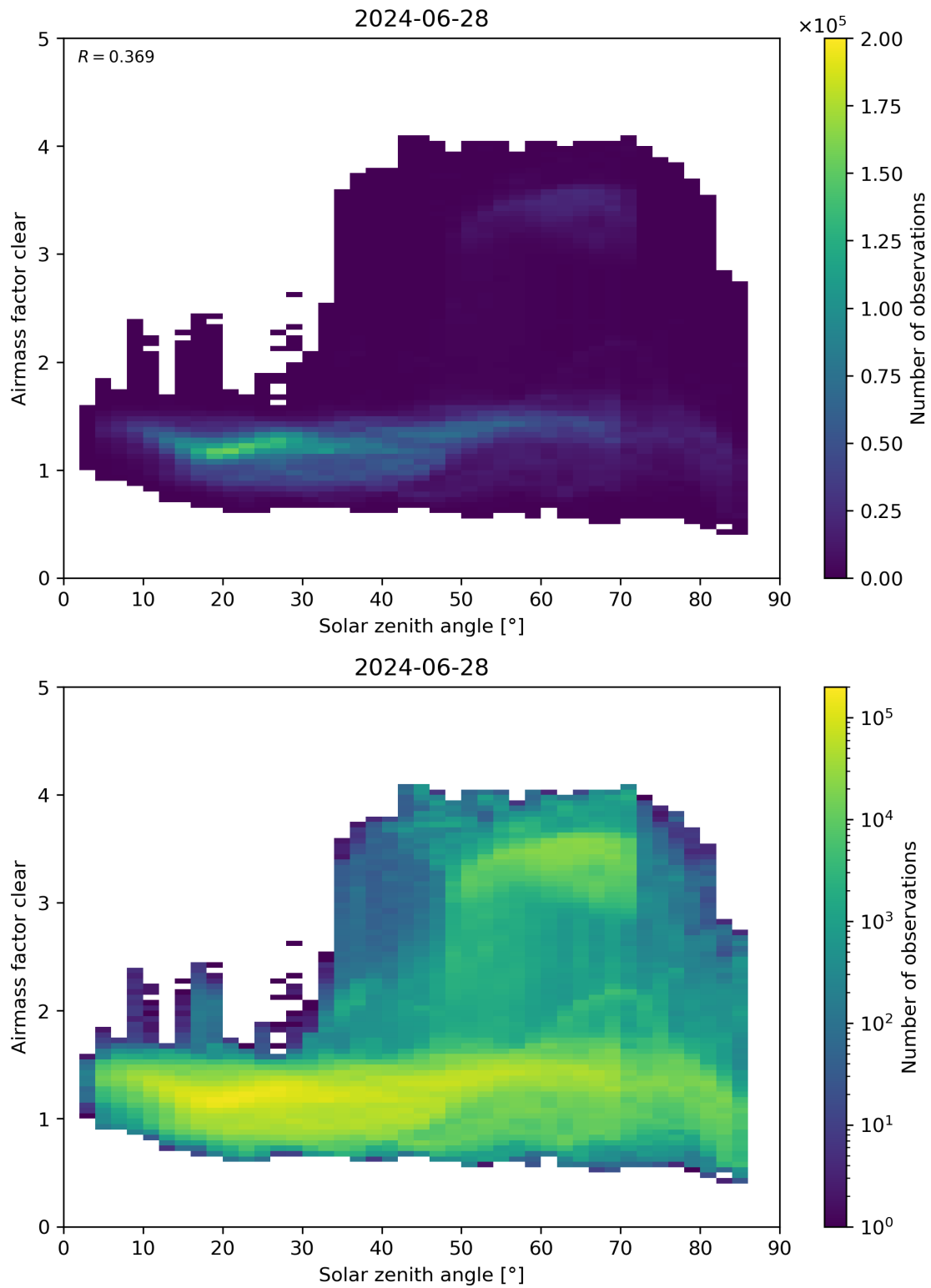
Figure 170: Scatter density plot of “Solar zenith angle” against “Airmass factor clear” for 2024-06-27 to 2024-06-29.
