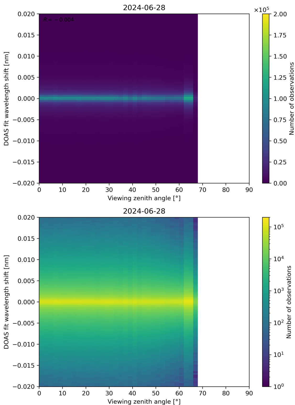
Figure 183: Scatter density plot of “Viewing zenith angle” against “DOAS fit wavelength shift” for 2024-06-27 to 2024-06-29.
