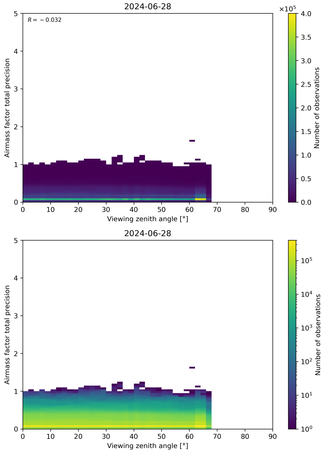
Figure 191: Scatter density plot of “Viewing zenith angle” against “Airmass factor total precision” for 2024-06-27 to 2024-06-29.
