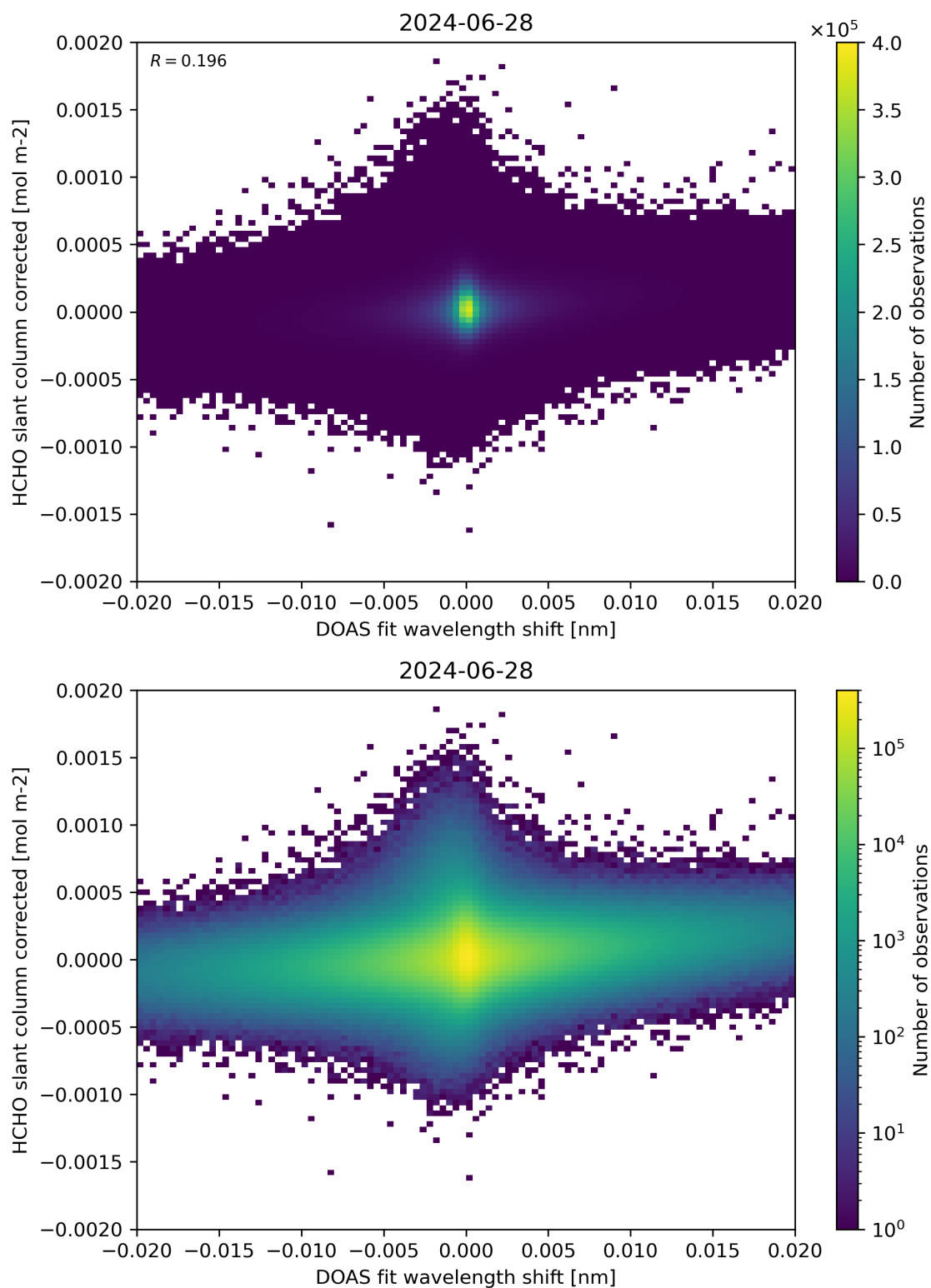
Figure 66: Scatter density plot of “DOAS fit wavelength shift” against “HCHO slant column corrected” for 2024-06-27 to 2024-06-29.
