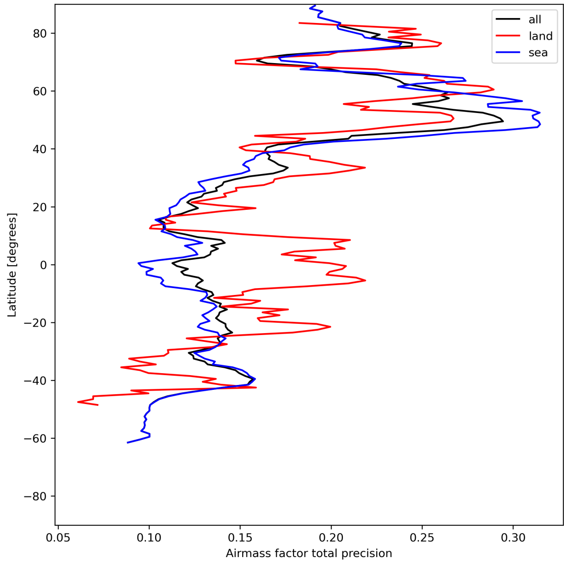
Figure 27: Zonal average of “Airmass factor total precision” for 2024-06-27 to 2024-06-29.
