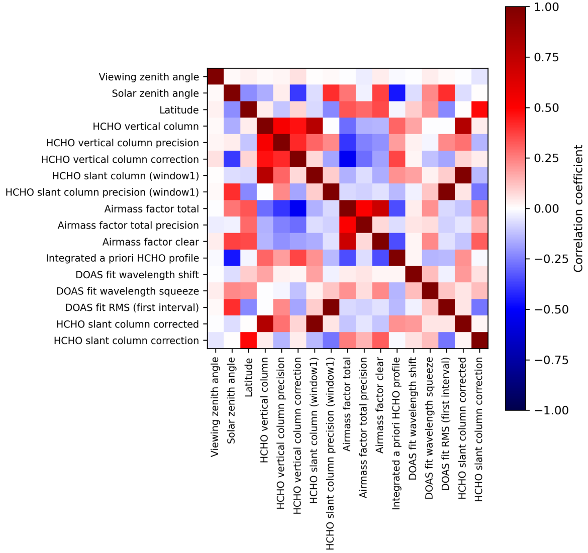
Figure 2: Map of correlation matrix for 2024-06-27 to 2024-06-29.
