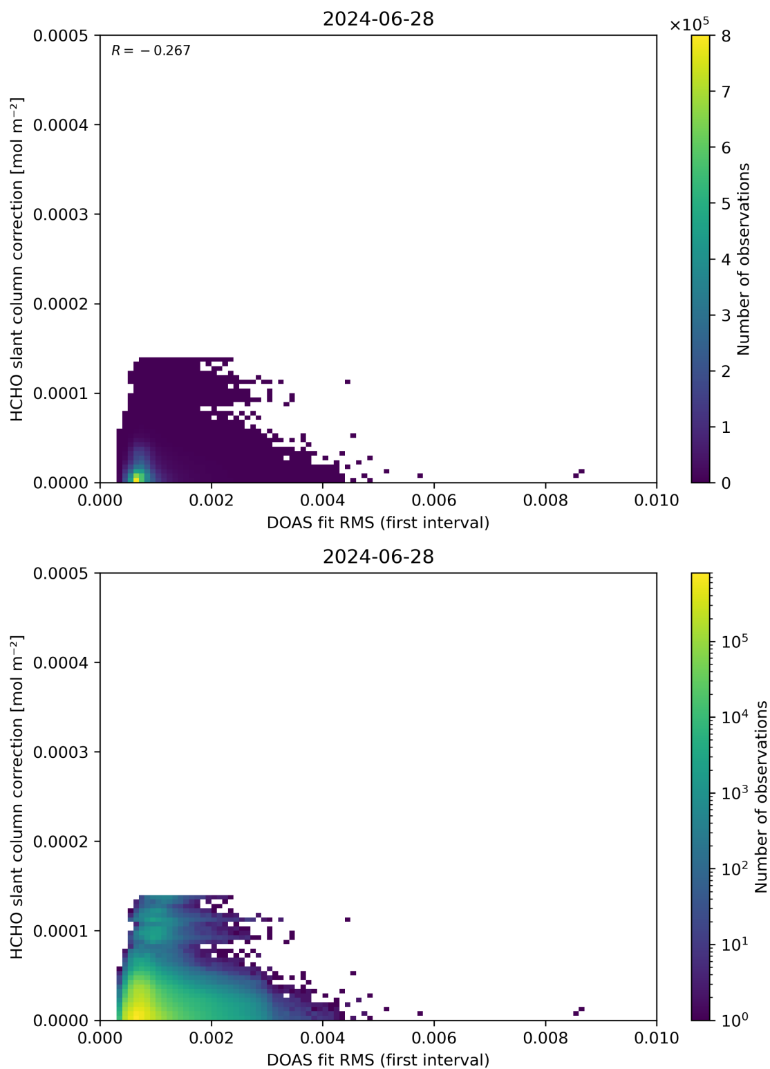
Figure 63: Scatter density plot of “DOAS fit RMS (first interval)” against “HCHO slant column correction” for 2024-06-27 to 2024-06-29.
