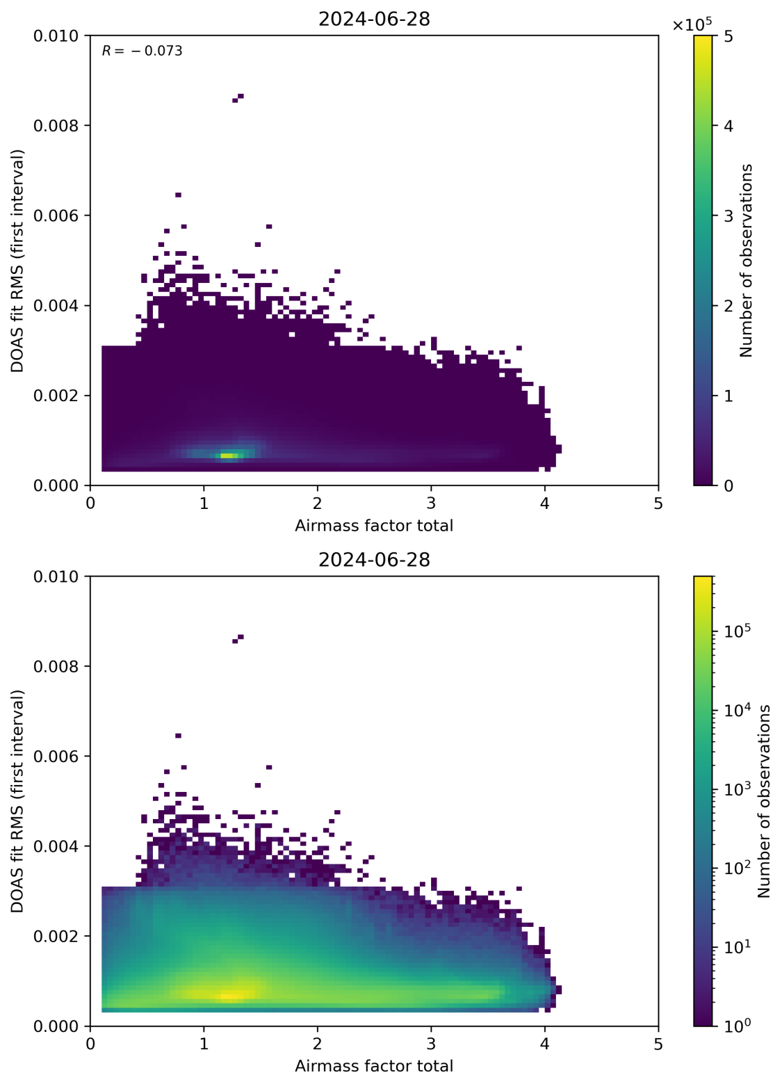
Figure 97: Scatter density plot of “Airmass factor total” against “DOAS fit RMS (first interval)” for 2024-06-27 to 2024-06-29.
