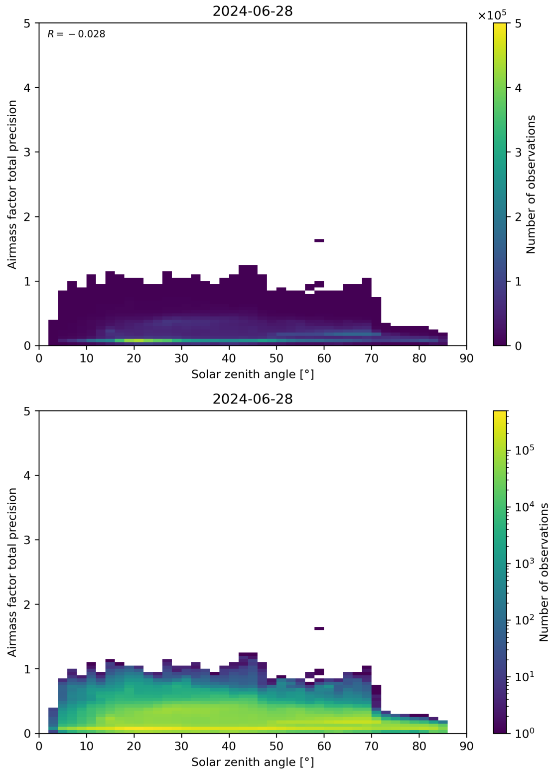
Figure 176: Scatter density plot of “Solar zenith angle” against “Airmass factor total precision” for 2024-06-27 to 2024-06-29.
