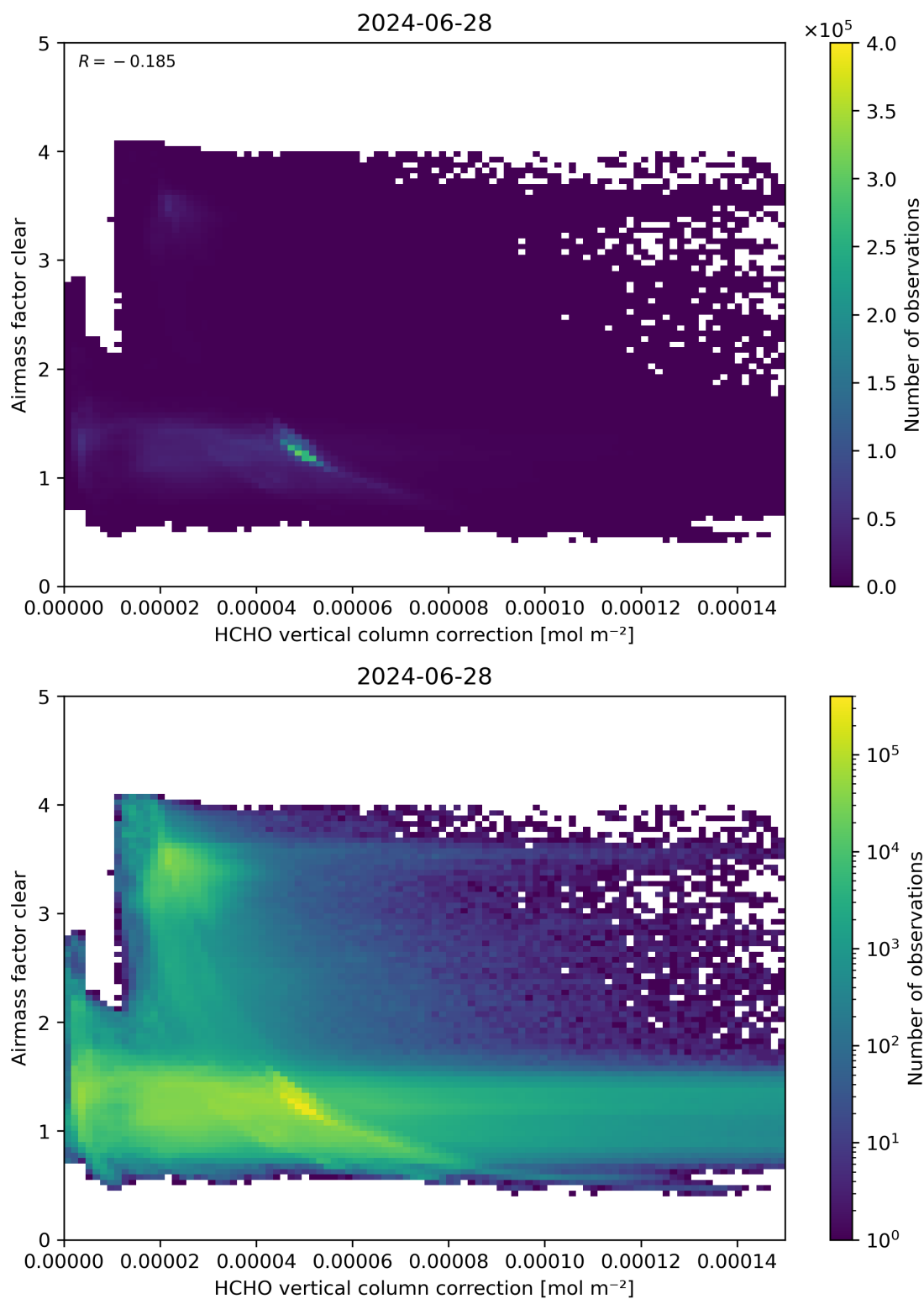
Figure 115: Scatter density plot of “HCHO vertical column correction” against “Airmass factor clear” for 2024-06-27 to 2024-06-29.
