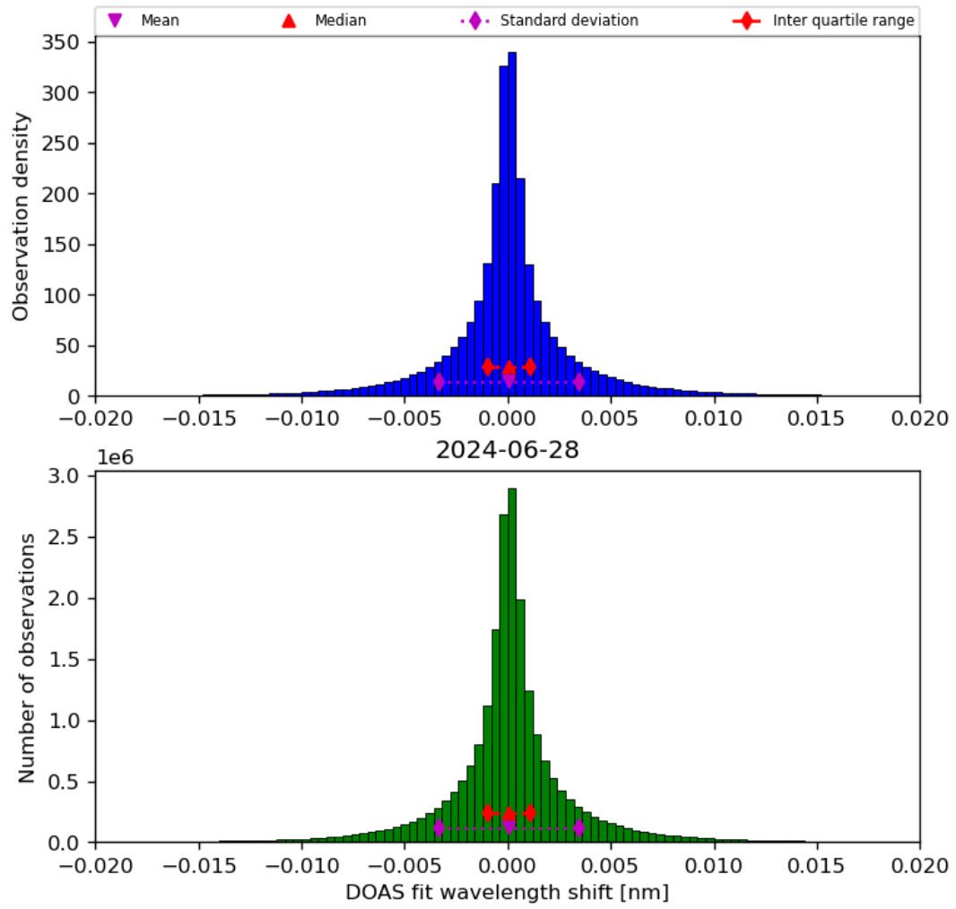
Figure 44: Histogram of “DOAS fit wavelength shift” for 2024-06-27 to 2024-06-29
