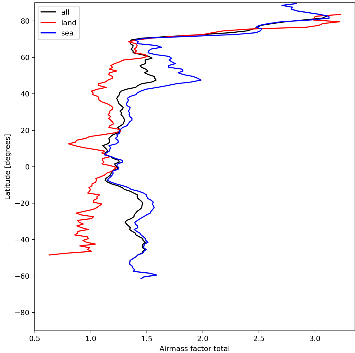
Figure 26: Zonal average of “Airmass factor total” for 2024-06-27 to 2024-06-29.
