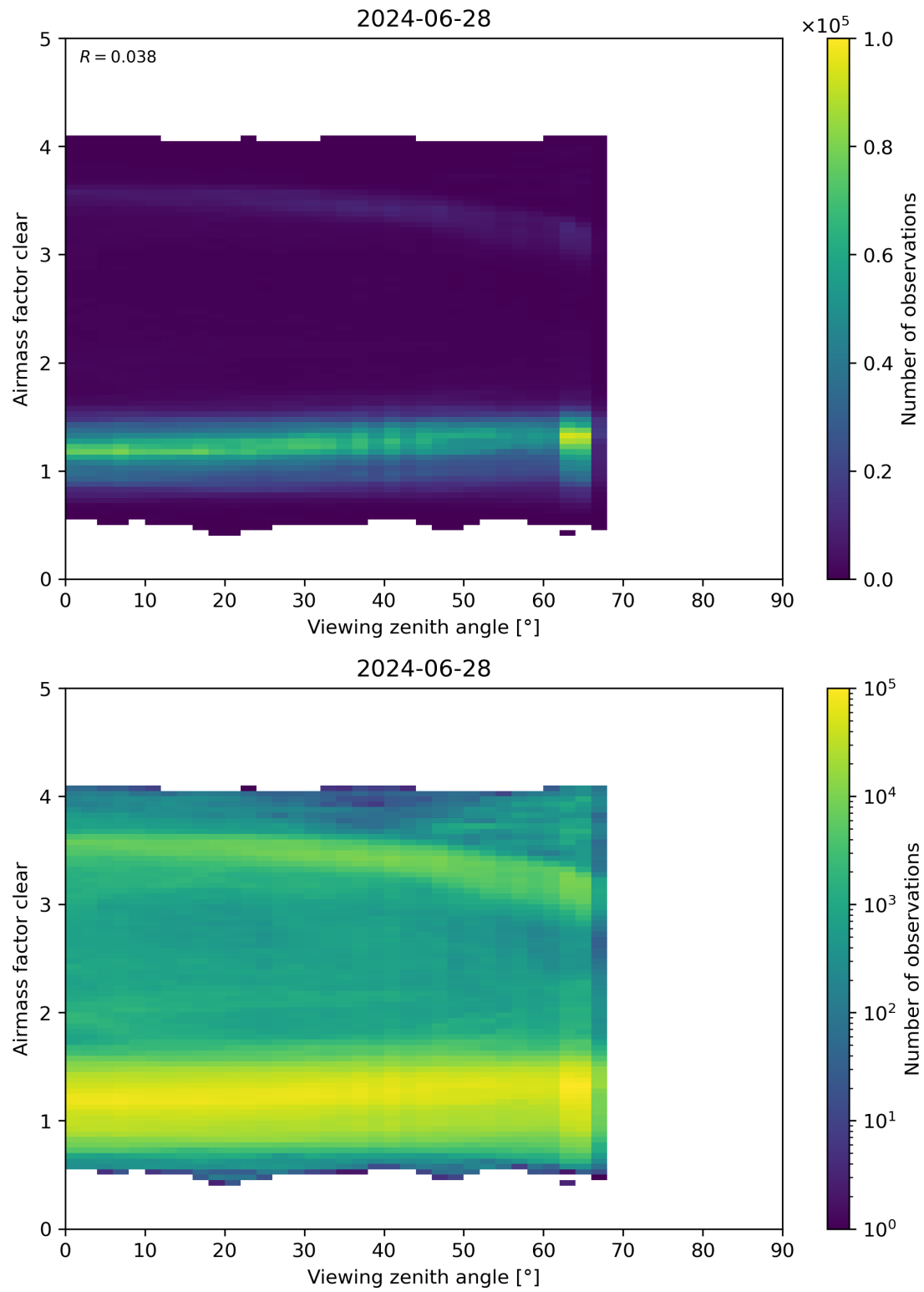
Figure 185: Scatter density plot of “Viewing zenith angle” against “Airmass factor clear” for 2024-06-27 to 2024-06-29.
