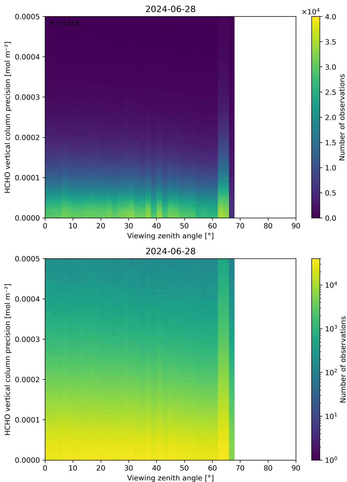
Figure 194: Scatter density plot of “Viewing zenith angle” against “HCHO vertical column precision” for 2024-06-27 to 2024-06-29.
