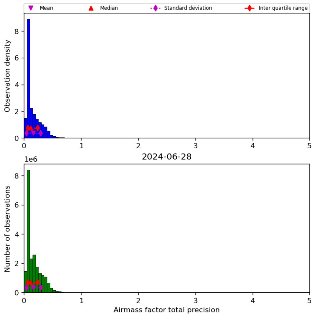
Figure 41: Histogram of “Airmass factor total precision” for 2024-06-27 to 2024-06-29
