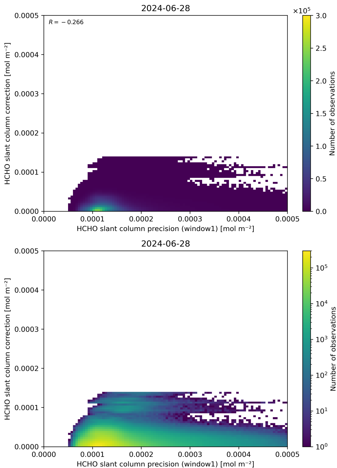
Figure 93: Scatter density plot of “HCHO slant column precision (window1)” against “HCHO slant column correction” for 2024-06-27 to 2024-06-29.
