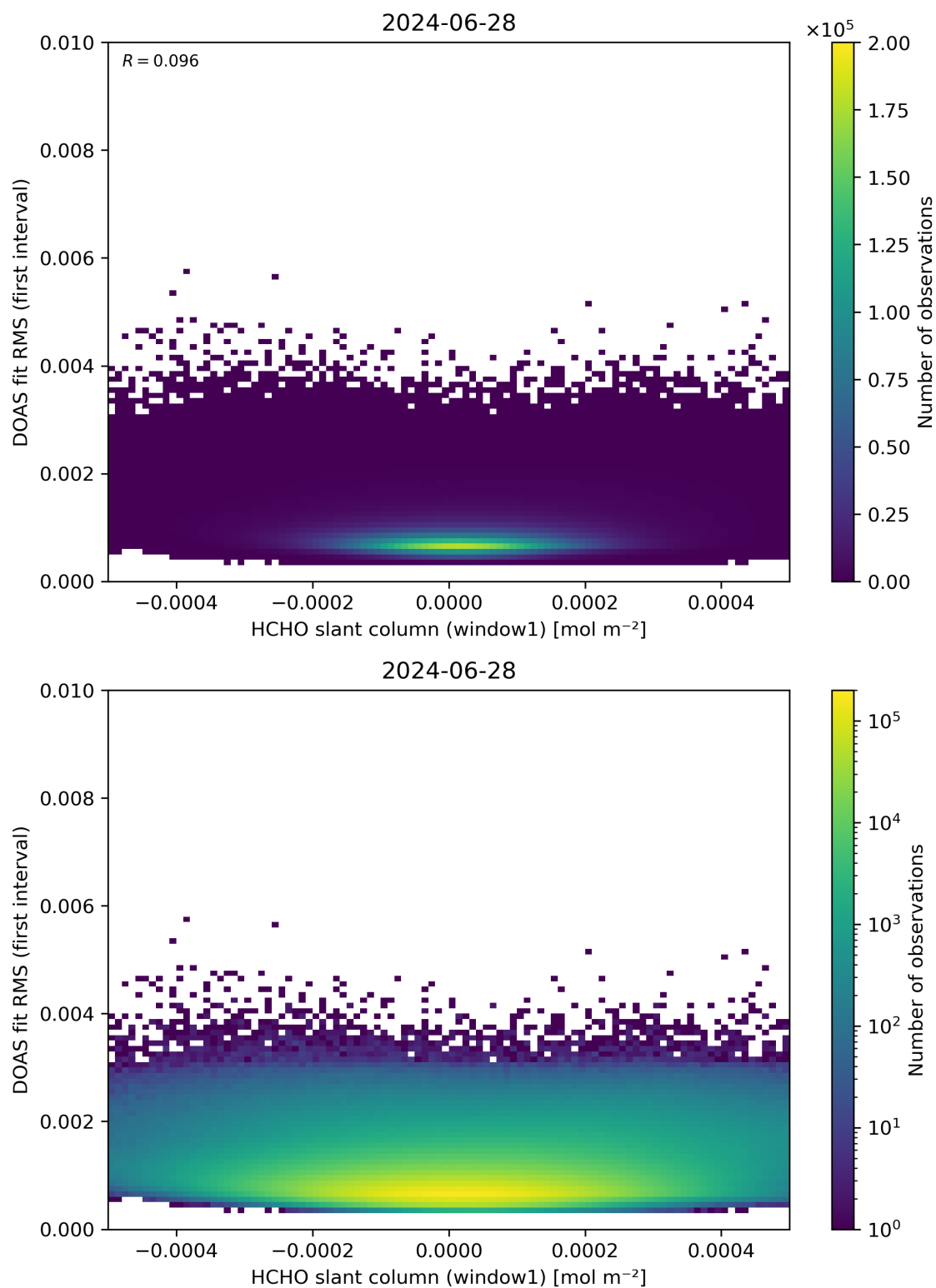
Figure 78: Scatter density plot of “HCHO slant column (window1)” against “DOAS fit RMS (first interval)” for 2024-06-27 to 2024-06-29.
