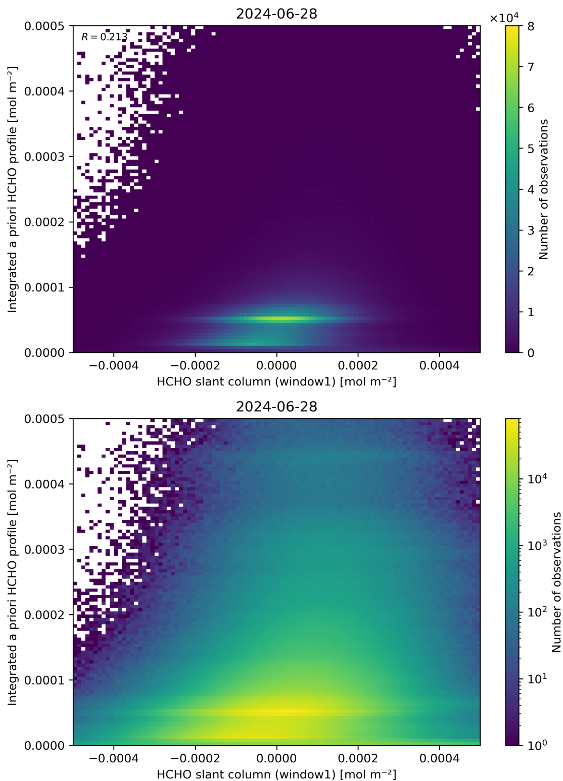
Figure 87: Scatter density plot of “HCHO slant column (window1)” against “Integrated a priori HCHO profile” for 2024-06-27 to 2024-06-29.
