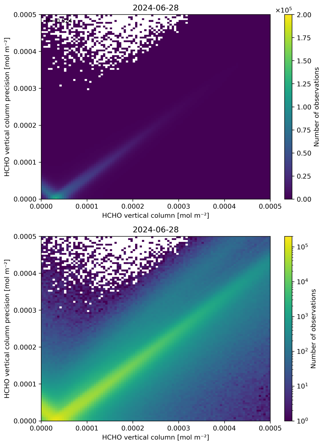
Figure 134: Scatter density plot of “HCHO vertical column” against “HCHO vertical column precision” for 2024-06-27 to 2024-06-29.
