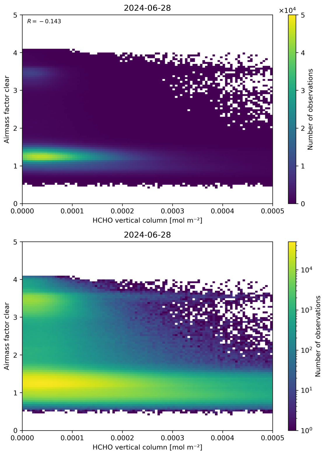
Figure 126: Scatter density plot of “HCHO vertical column” against “Airmass factor clear” for 2024-06-27 to 2024-06-29.
