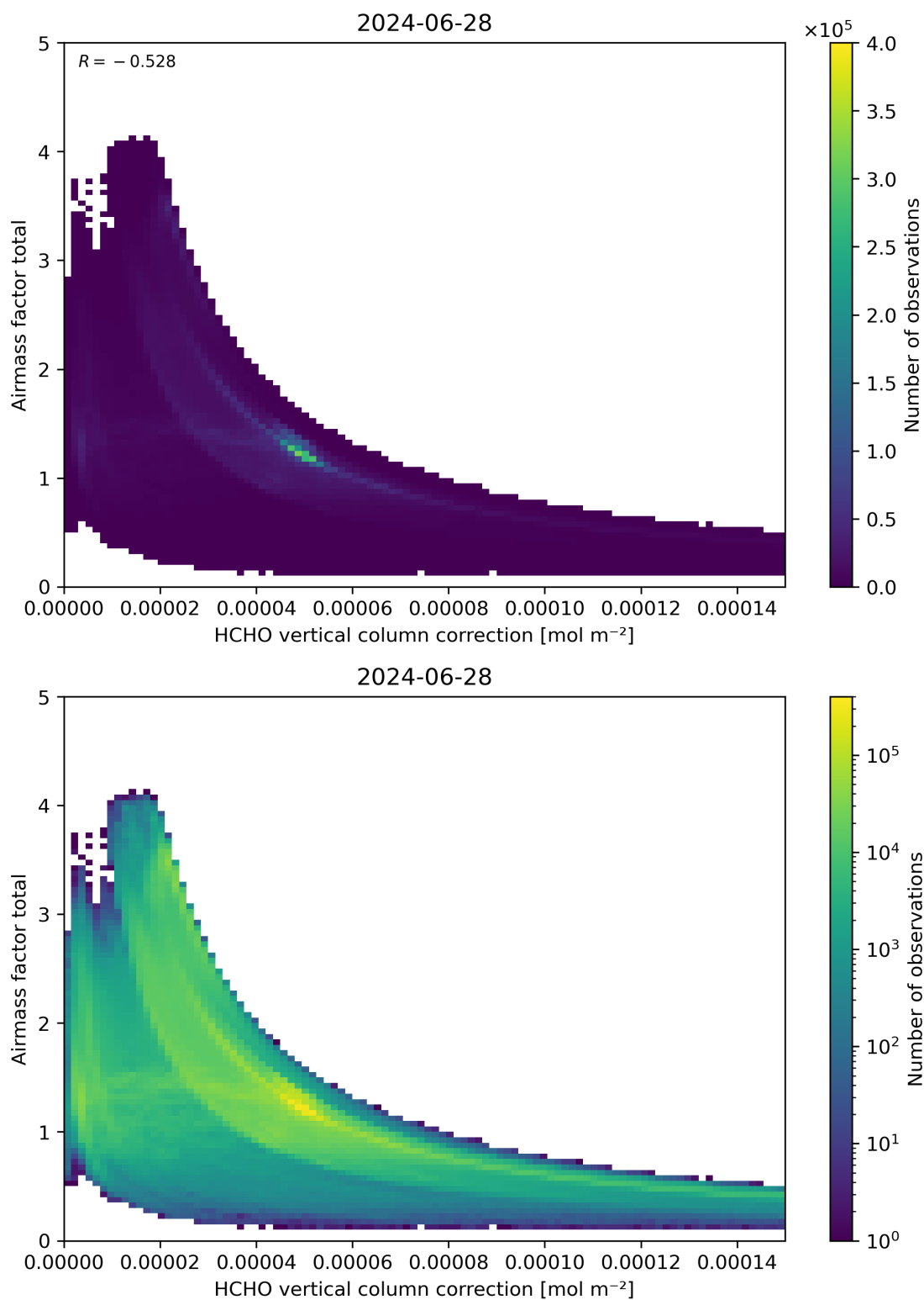
Figure 120: Scatter density plot of “HCHO vertical column correction” against “Airmass factor total” for 2024-06-27 to 2024-06-29.
