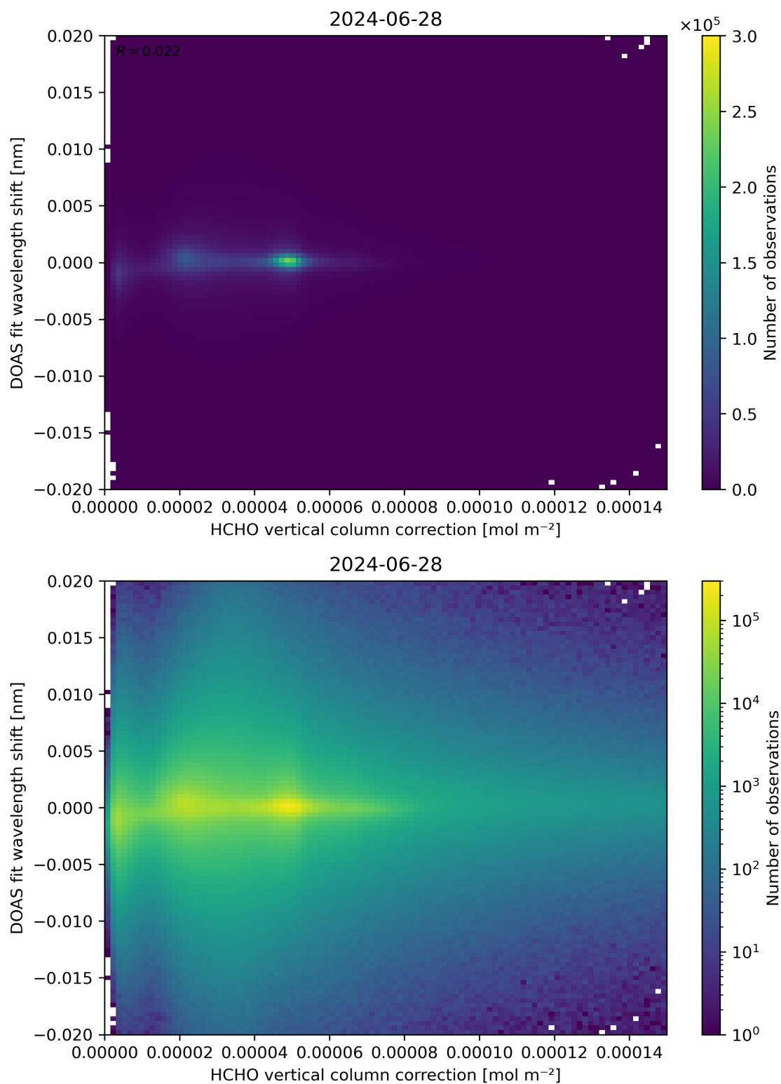
Figure 113: Scatter density plot of “HCHO vertical column correction” against “DOAS fit wavelength shift” for 2024-06-27 to 2024-06-29.
