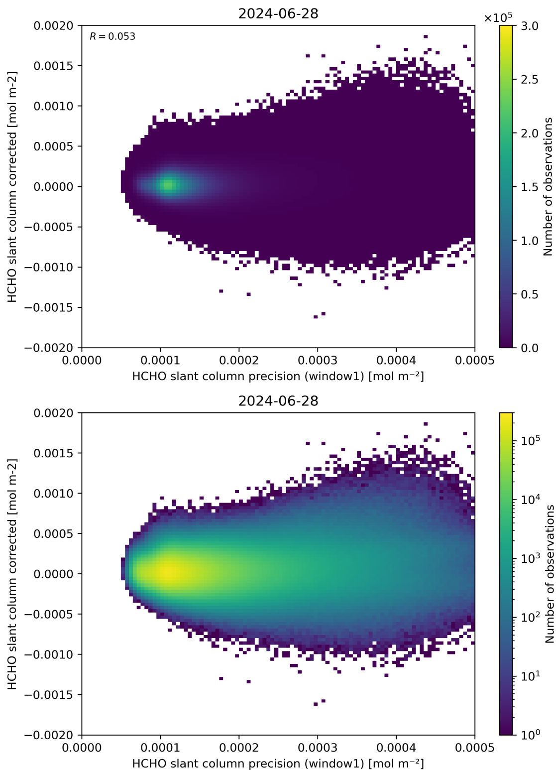
Figure 92: Scatter density plot of “HCHO slant column precision (window1)” against “HCHO slant column corrected” for 2024-06-27 to 2024-06-29.
