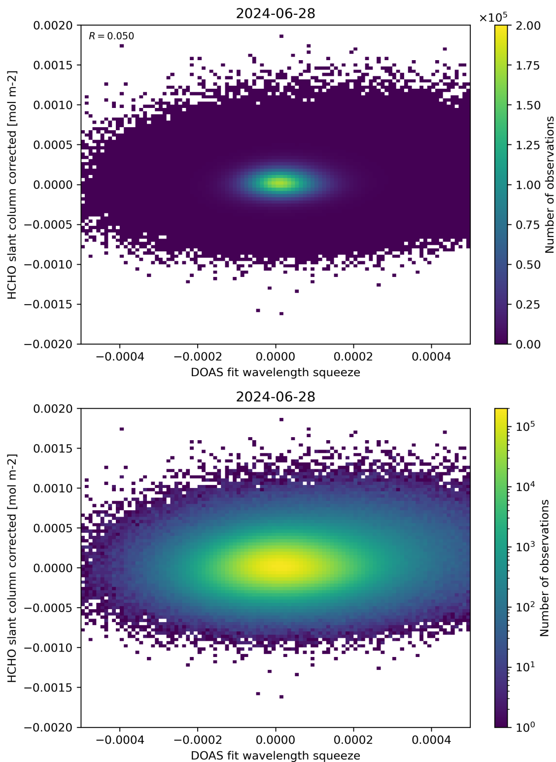
Figure 69: Scatter density plot of “DOAS fit wavelength squeeze” against “HCHO slant column corrected” for 2024-06-27 to 2024-06-29.
