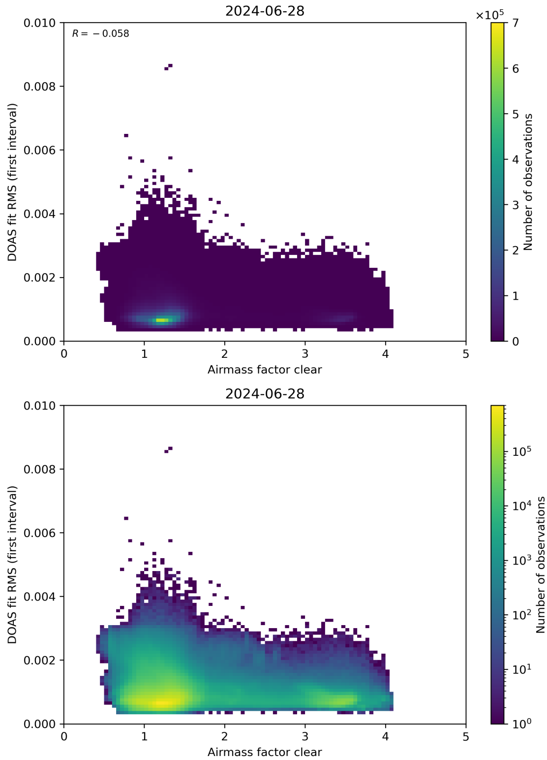
Figure 71: Scatter density plot of “Airmass factor clear” against “DOAS fit RMS (first interval)” for 2024-06-27 to 2024-06-29.
