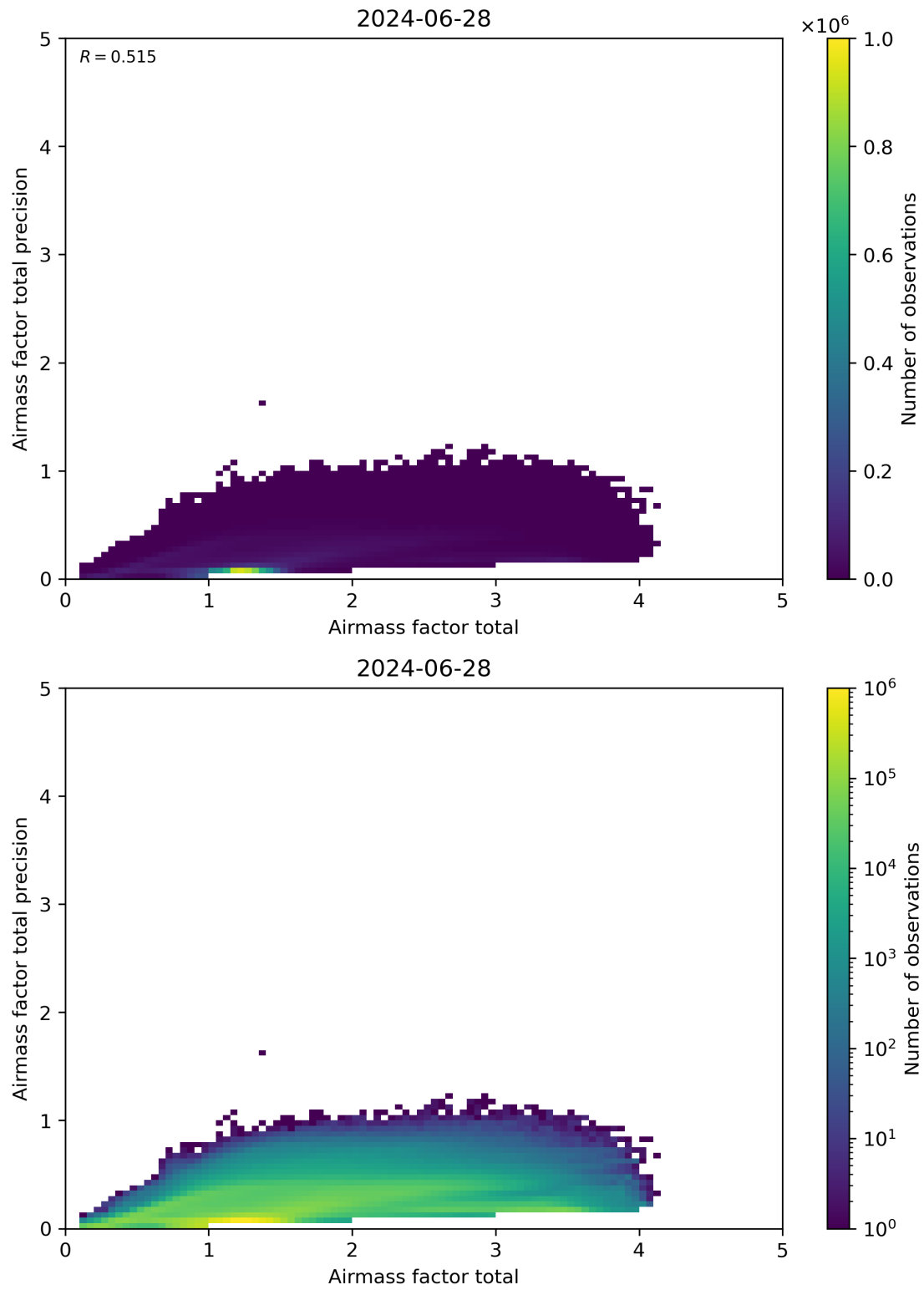
Figure 103: Scatter density plot of “Airmass factor total” against “Airmass factor total precision” for 2024-06-27 to 2024-06-29.
