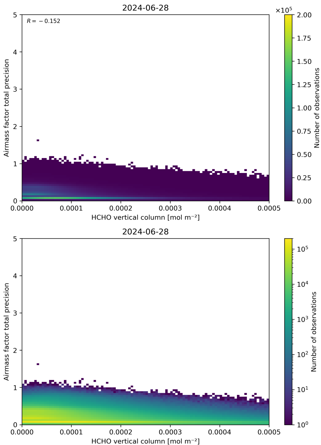
Figure 132: Scatter density plot of “HCHO vertical column” against “Airmass factor total precision” for 2024-06-27 to 2024-06-29.
