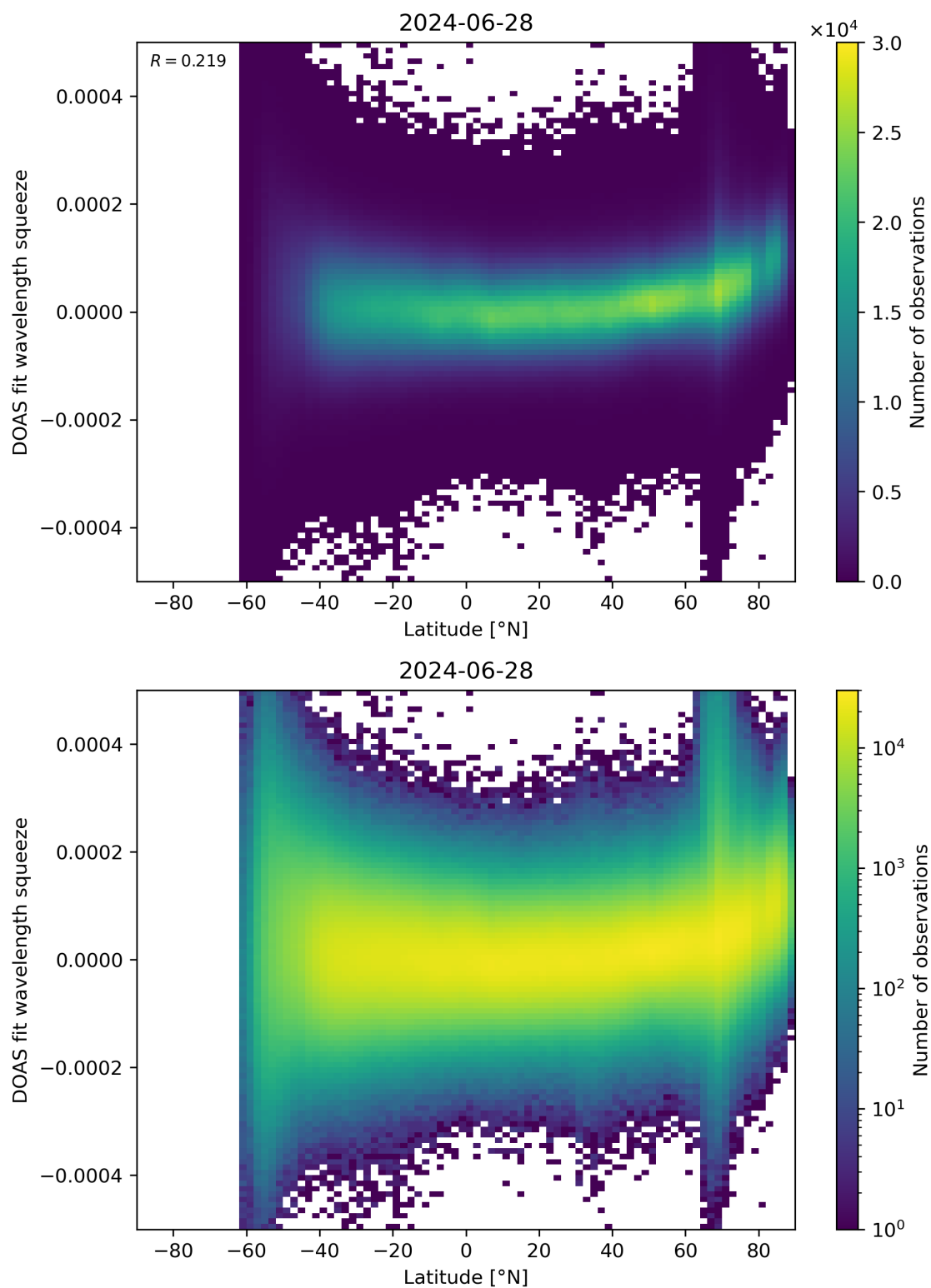
Figure 155: Scatter density plot of “Latitude” against “DOAS fit wavelength squeeze” for 2024-06-27 to 2024-06-29.
