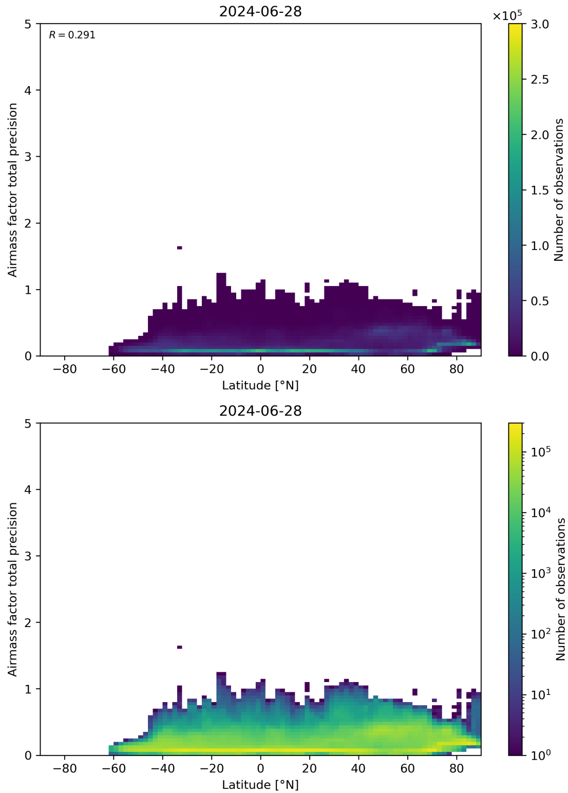
Figure 162: Scatter density plot of “Latitude” against “Airmass factor total precision” for 2024-06-27 to 2024-06-29.
