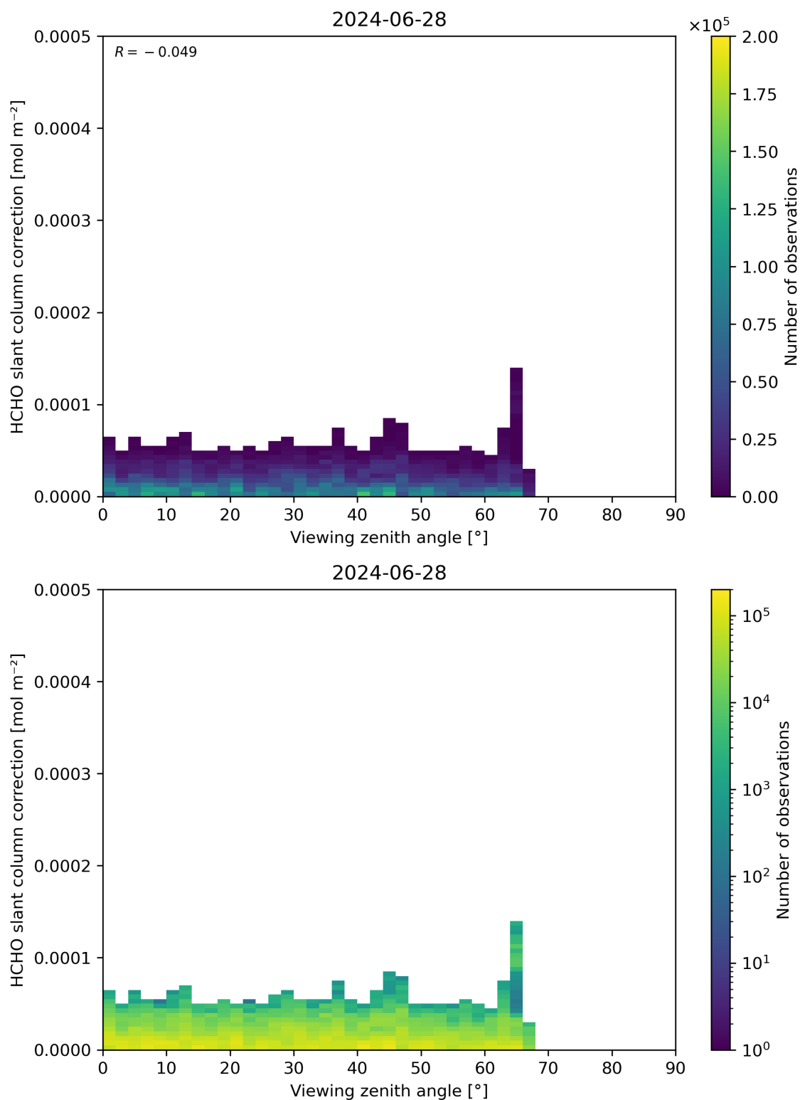
Figure 187: Scatter density plot of “Viewing zenith angle” against “HCHO slant column correction” for 2024-06-27 to 2024-06-29.
