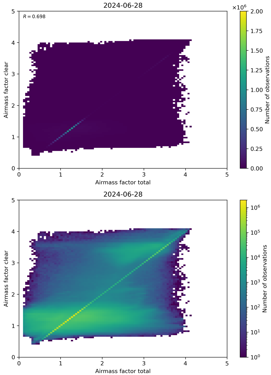
Figure 100: Scatter density plot of “Airmass factor total” against “Airmass factor clear” for 2024-06-27 to 2024-06-29.
