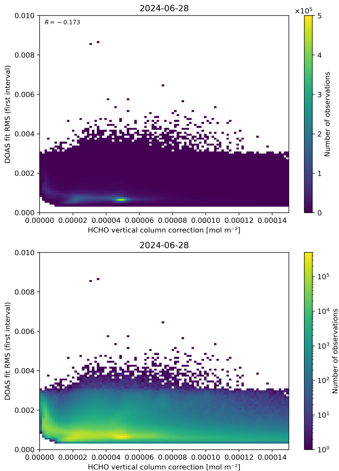
Figure 112: Scatter density plot of “HCHO vertical column correction” against “DOAS fit RMS (first interval)” for 2024-06-27 to 2024-06-29.
