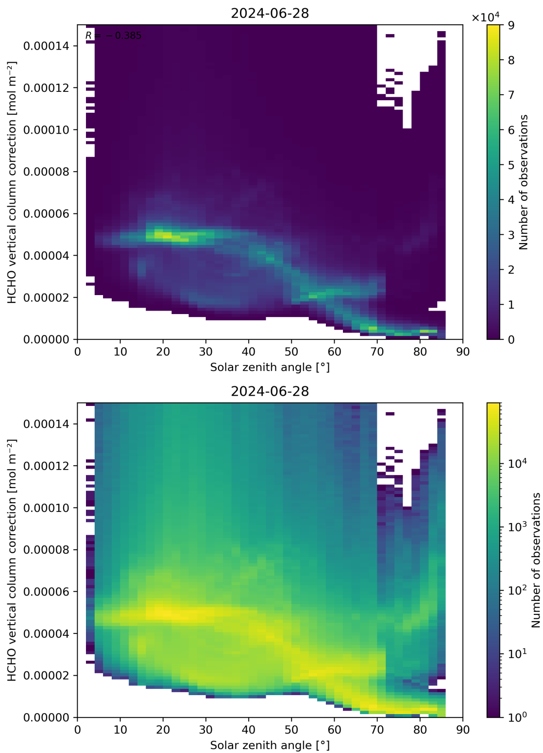
Figure 178: Scatter density plot of “Solar zenith angle” against “HCHO vertical column correction” for 2024-06-27 to 2024-06-29.
