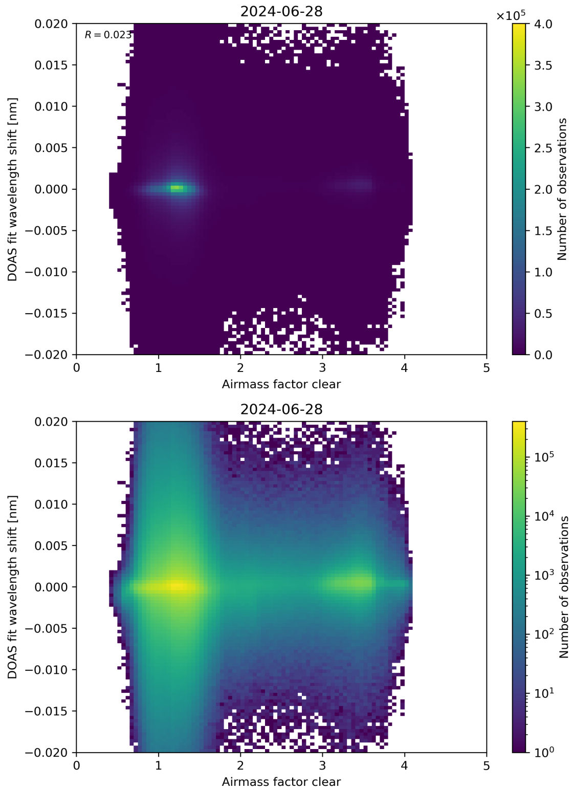
Figure 72: Scatter density plot of “Airmass factor clear” against “DOAS fit wavelength shift” for 2024-06-27 to 2024-06-29.
