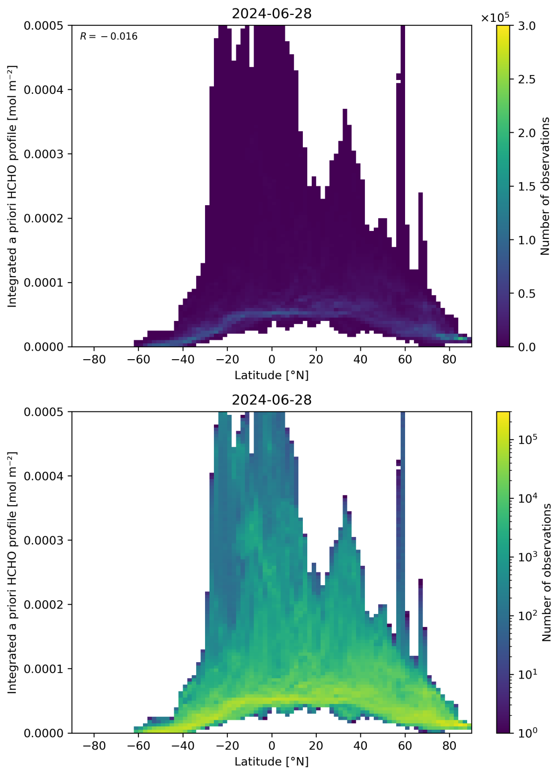
Figure 166: Scatter density plot of “Latitude” against “Integrated a priori HCHO profile” for 2024-06-27 to 2024-06-29.
