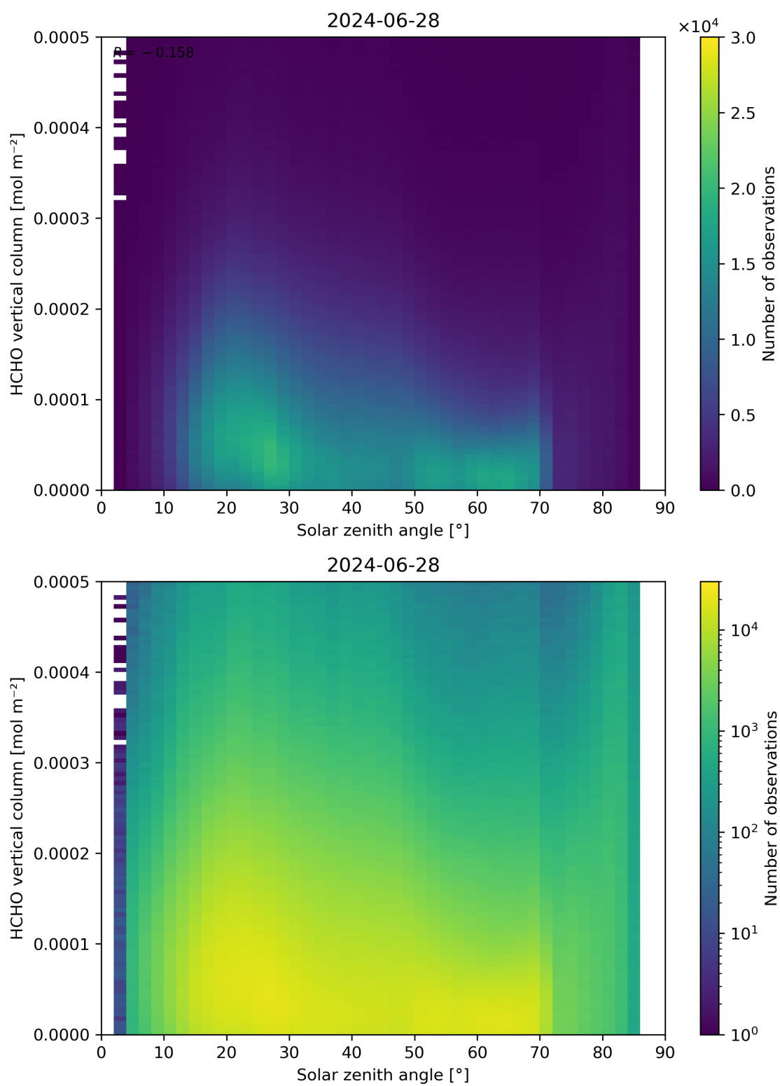
Figure 177: Scatter density plot of “Solar zenith angle” against “HCHO vertical column” for 2024-06-27 to 2024-06-29.
