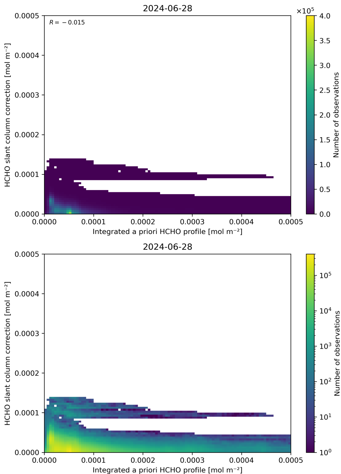
Figure 152: Scatter density plot of “Integrated a priori HCHO profile” against “HCHO slant column correction” for 2024-06-27 to 2024-06-29.
