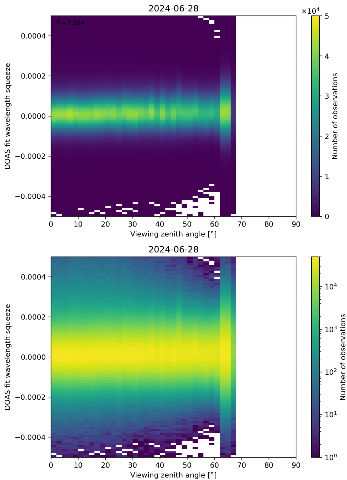
Figure 184: Scatter density plot of “Viewing zenith angle” against “DOAS fit wavelength squeeze” for 2024-06-27 to 2024-06-29.
