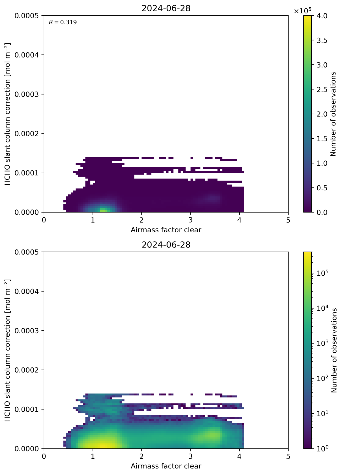
Figure 75: Scatter density plot of “Airmass factor clear” against “HCHO slant column correction” for 2024-06-27 to 2024-06-29.
