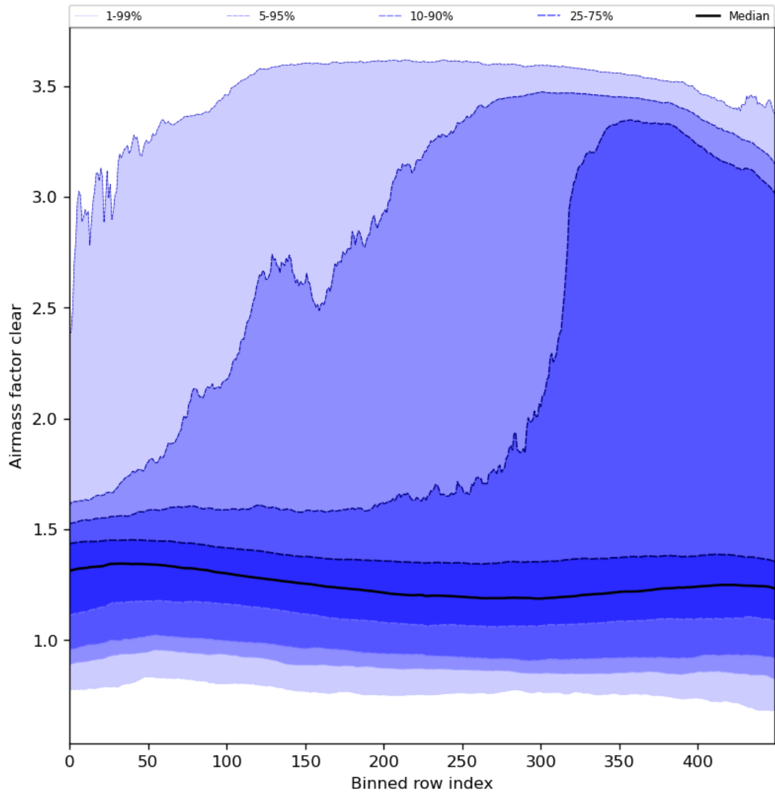
Figure 56: Along track statistics of “Airmass factor clear” for 2024-06-27 to 2024-06-29
