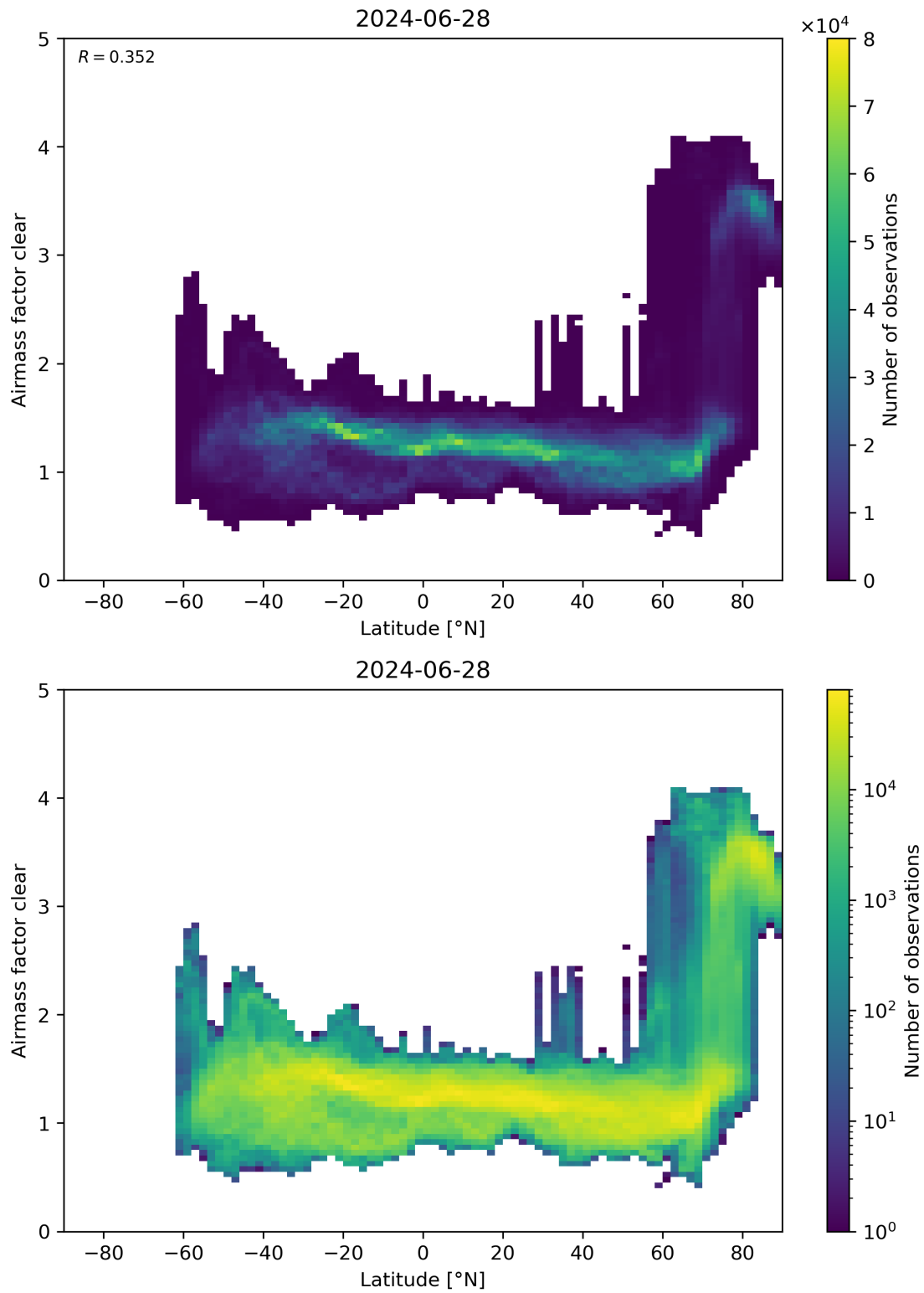
Figure 156: Scatter density plot of “Latitude” against “Airmass factor clear” for 2024-06-27 to 2024-06-29.
