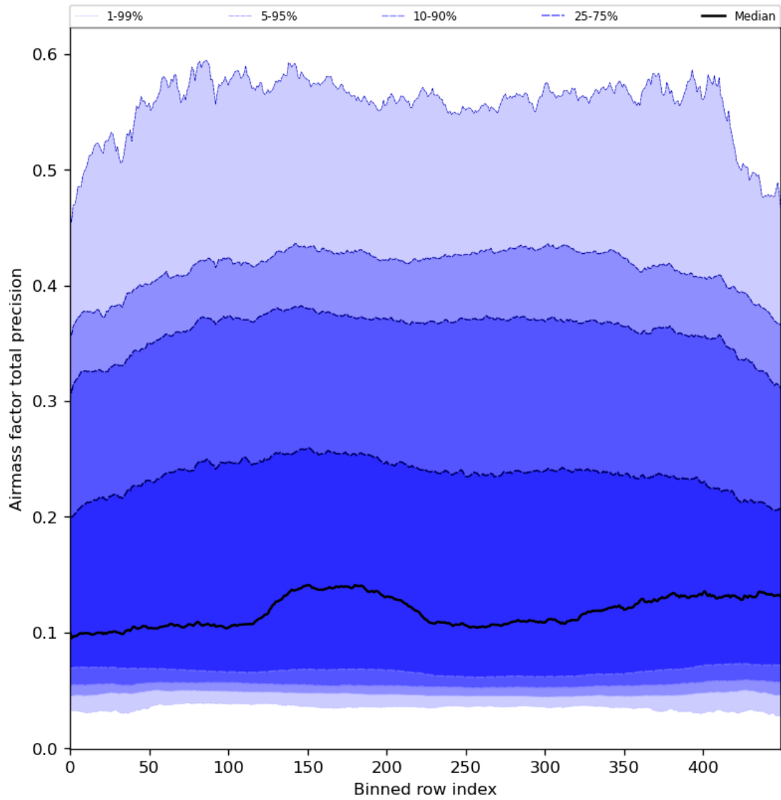
Figure 55: Along track statistics of “Airmass factor total precision” for 2024-06-27 to 2024-06-29
