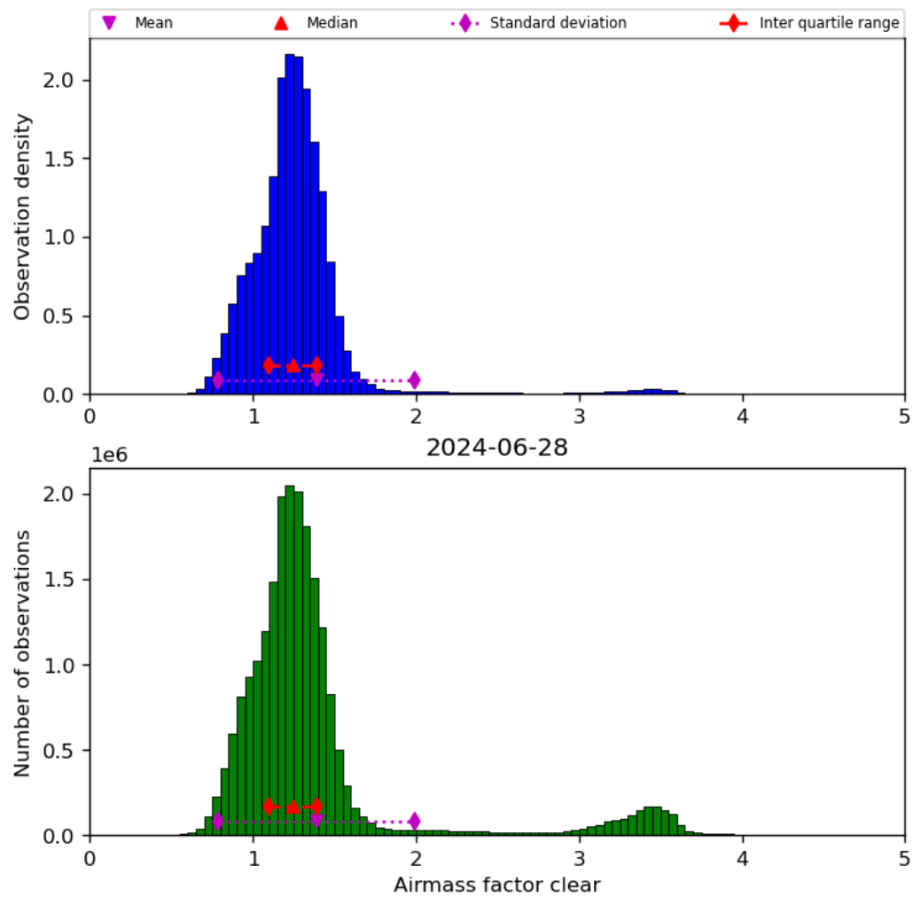
Figure 42: Histogram of “Airmass factor clear” for 2024-06-27 to 2024-06-29
