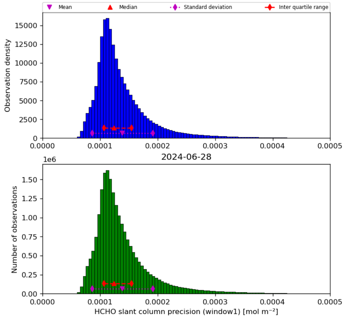
Figure 39: Histogram of “HCHO slant column precision (window1)” for 2024-06-27 to 2024-06-29
