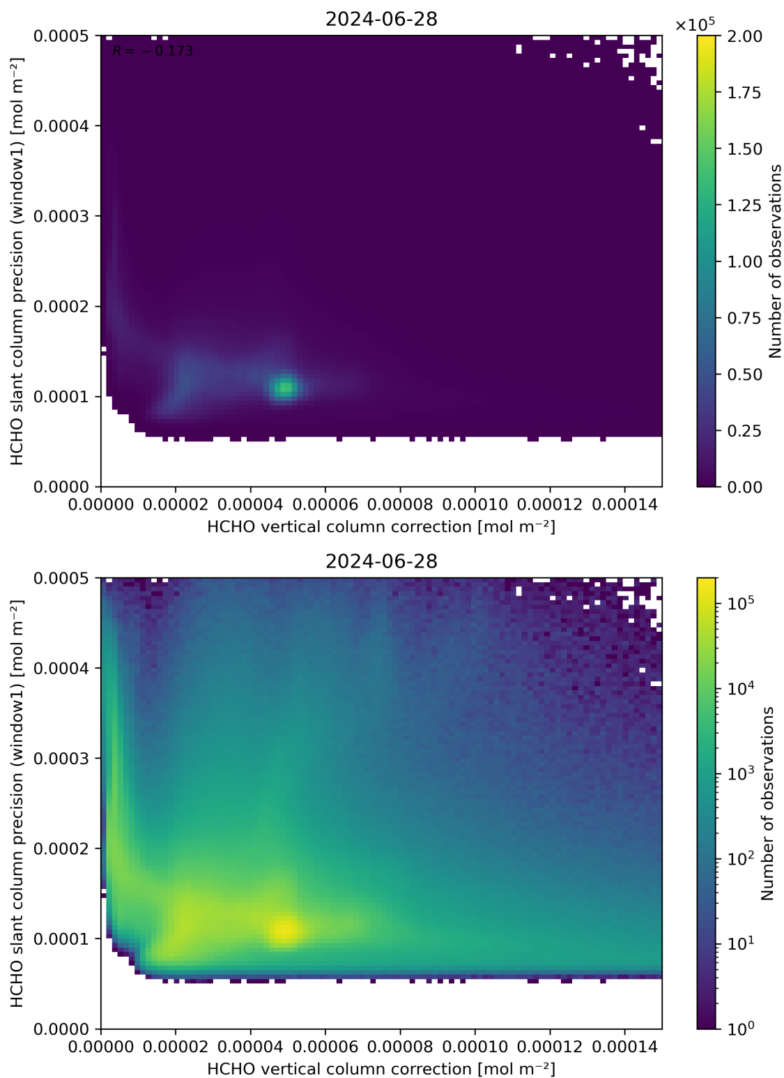
Figure 119: Scatter density plot of “HCHO vertical column correction” against “HCHO slant column precision (window1)” for 2024-06-27 to 2024-06-29.
