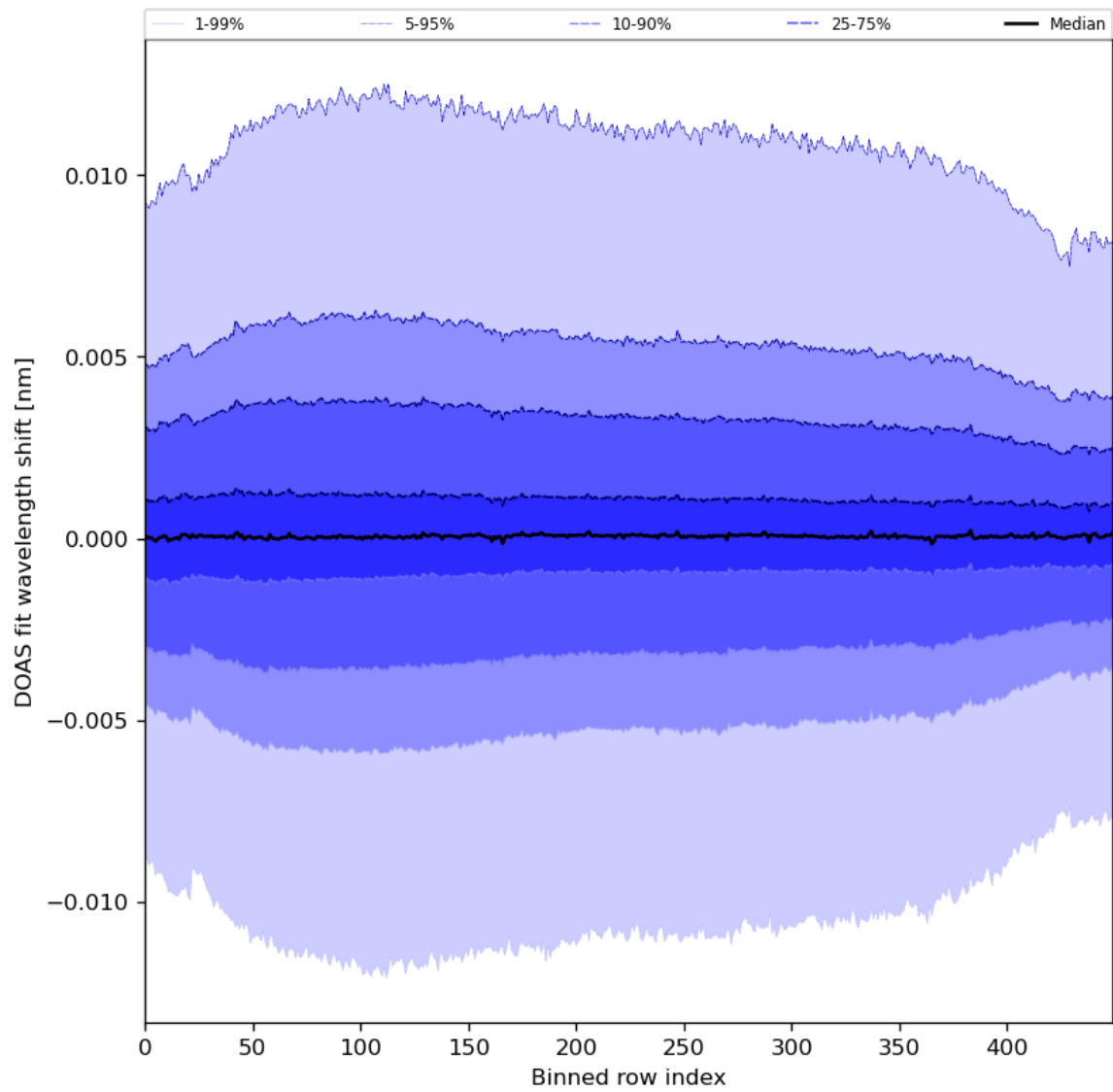
Figure 58: Along track statistics of “DOAS fit wavelength shift” for 2024-06-27 to 2024-06-29
