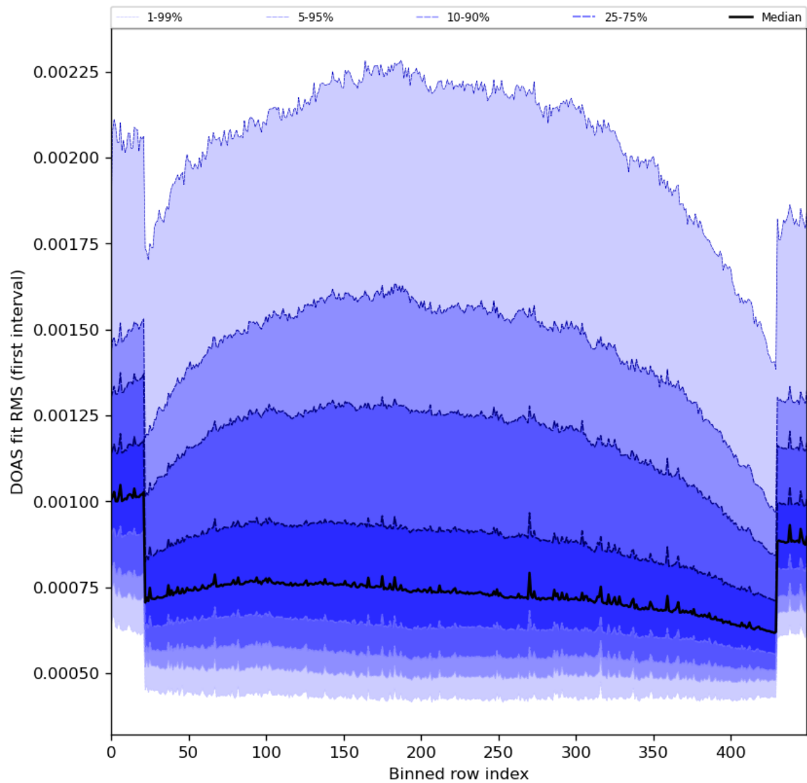
Figure 60: Along track statistics of “DOAS fit RMS (first interval)” for 2024-06-27 to 2024-06-29
