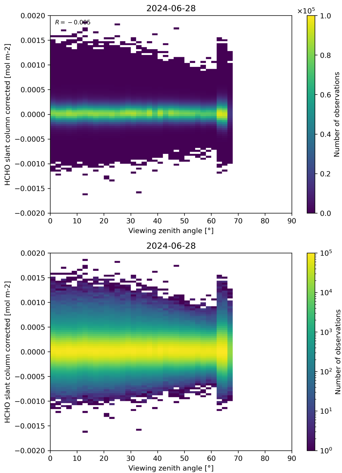
Figure 186: Scatter density plot of “Viewing zenith angle” against “HCHO slant column corrected” for 2024-06-27 to 2024-06-29.
