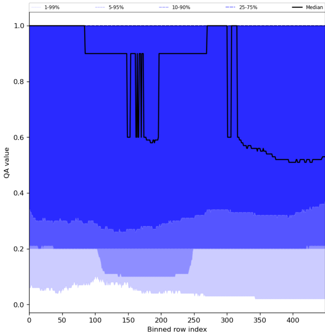
Figure 48: Along track statistics of “QA value” for 2024-06-27 to 2024-06-29
