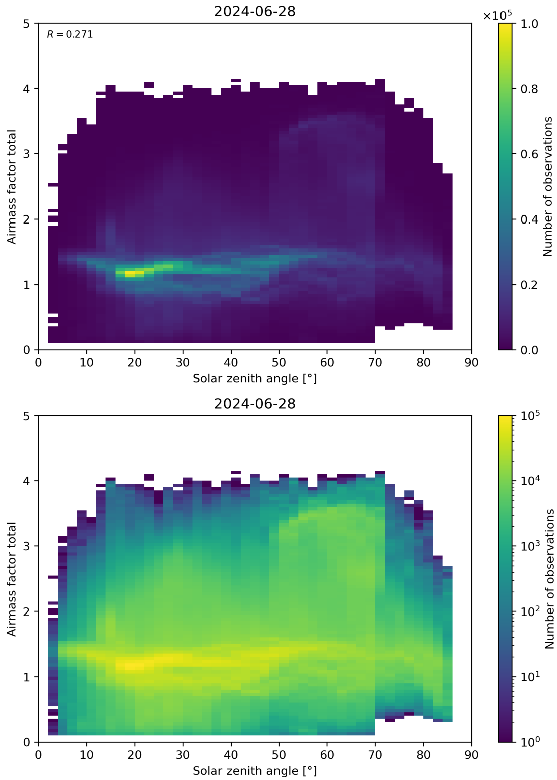
Figure 175: Scatter density plot of “Solar zenith angle” against “Airmass factor total” for 2024-06-27 to 2024-06-29.
