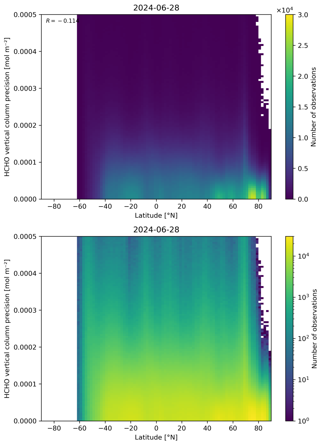
Figure 165: Scatter density plot of “Latitude” against “HCHO vertical column precision” for 2024-06-27 to 2024-06-29.
