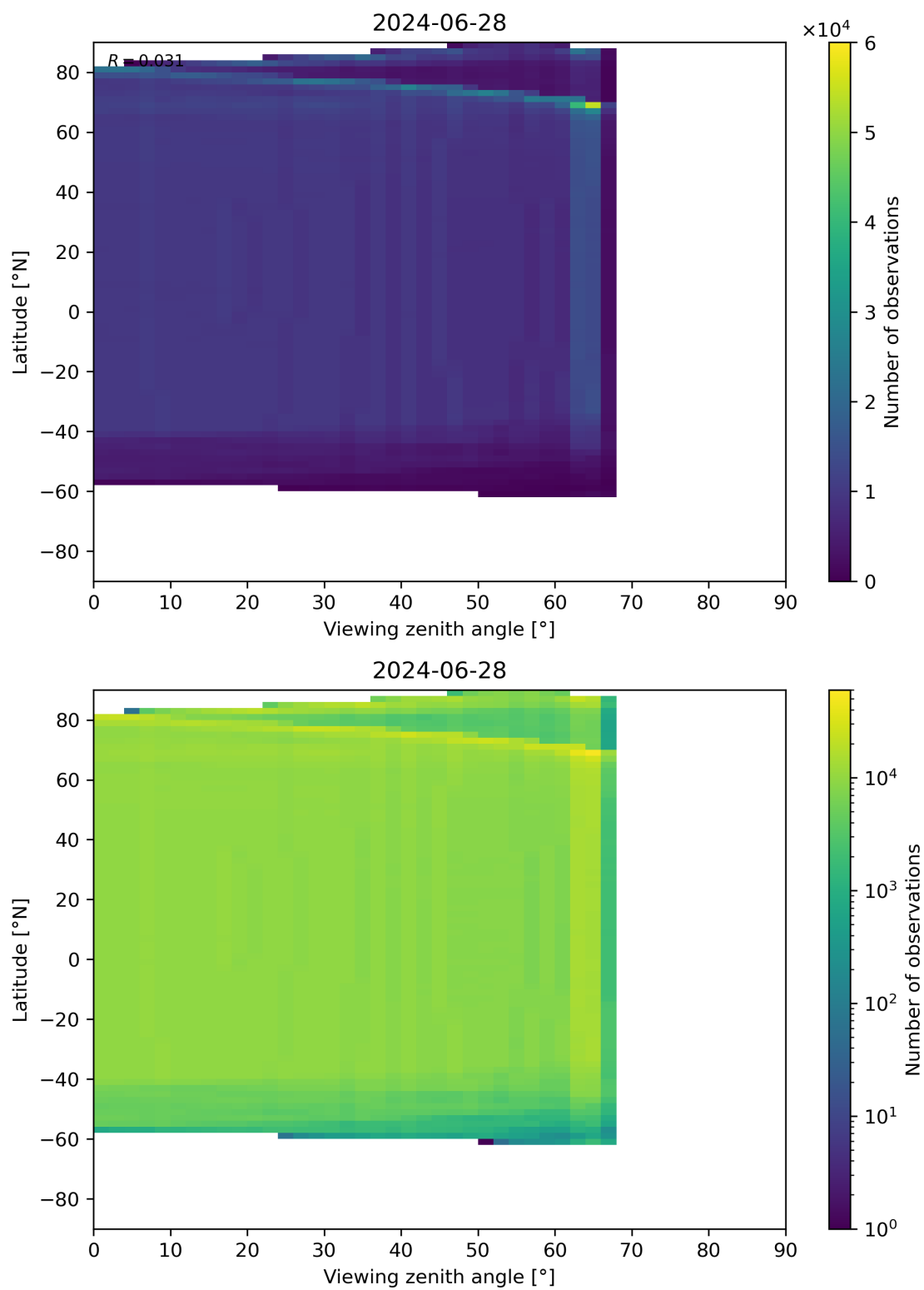
Figure 196: Scatter density plot of “Viewing zenith angle” against “Latitude” for 2024-06-27 to 2024-06-29.
