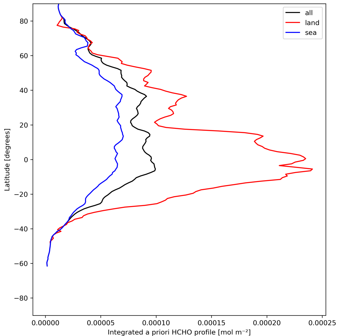
Figure 29: Zonal average of “Integrated a priori HCHO profile” for 2024-06-27 to 2024-06-29.
