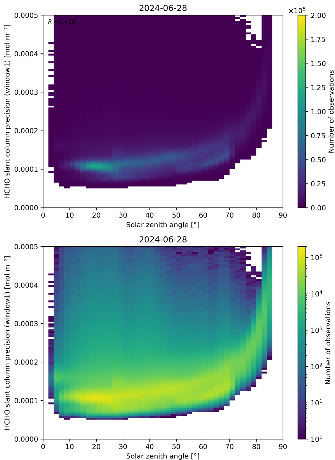
Figure 174: Scatter density plot of “Solar zenith angle” against “HCHO slant column precision (window1)” for 2024-06-27 to 2024-06-29.
