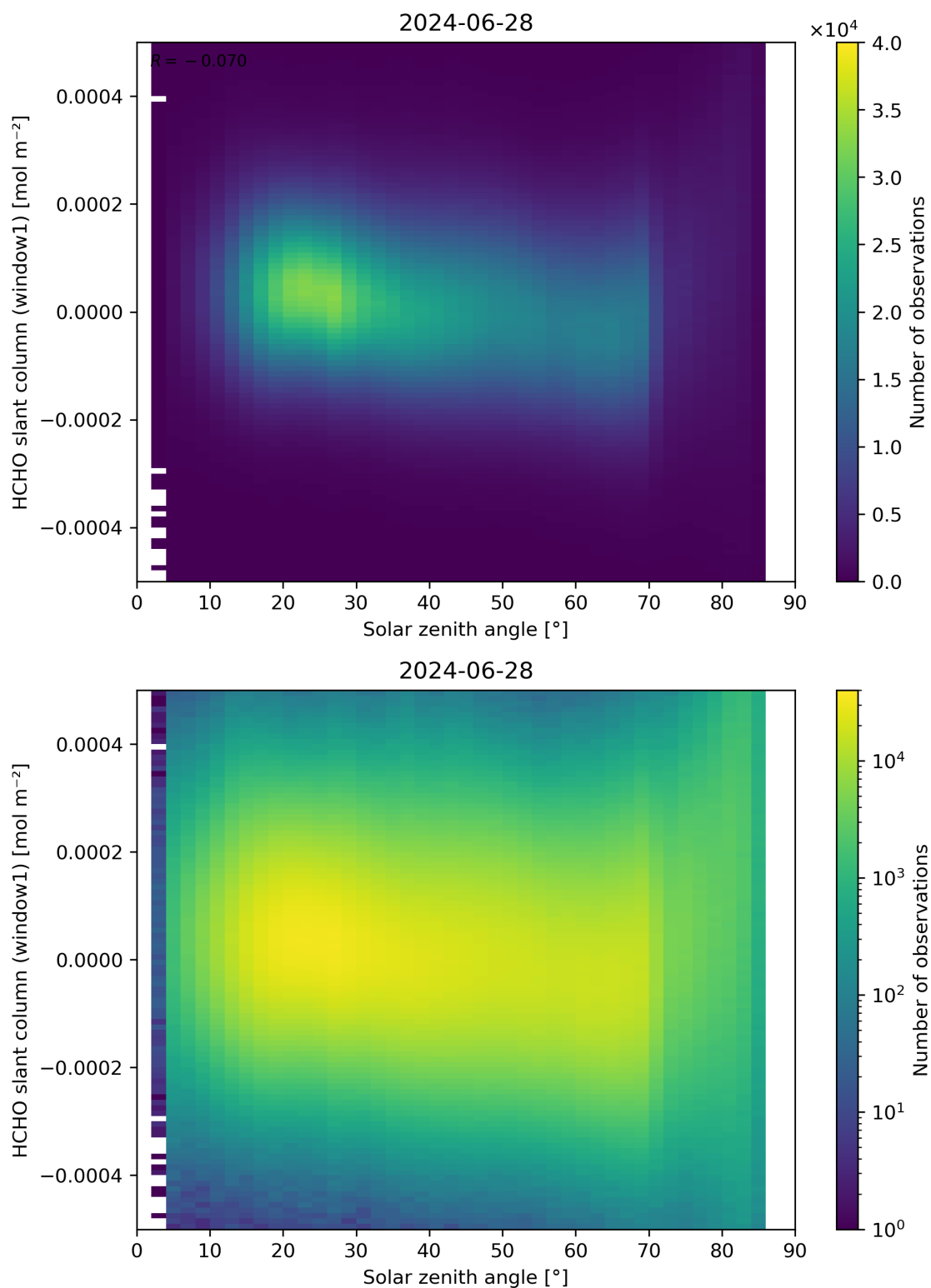
Figure 173: Scatter density plot of “Solar zenith angle” against “HCHO slant column (window1)” for 2024-06-27 to 2024-06-29.
