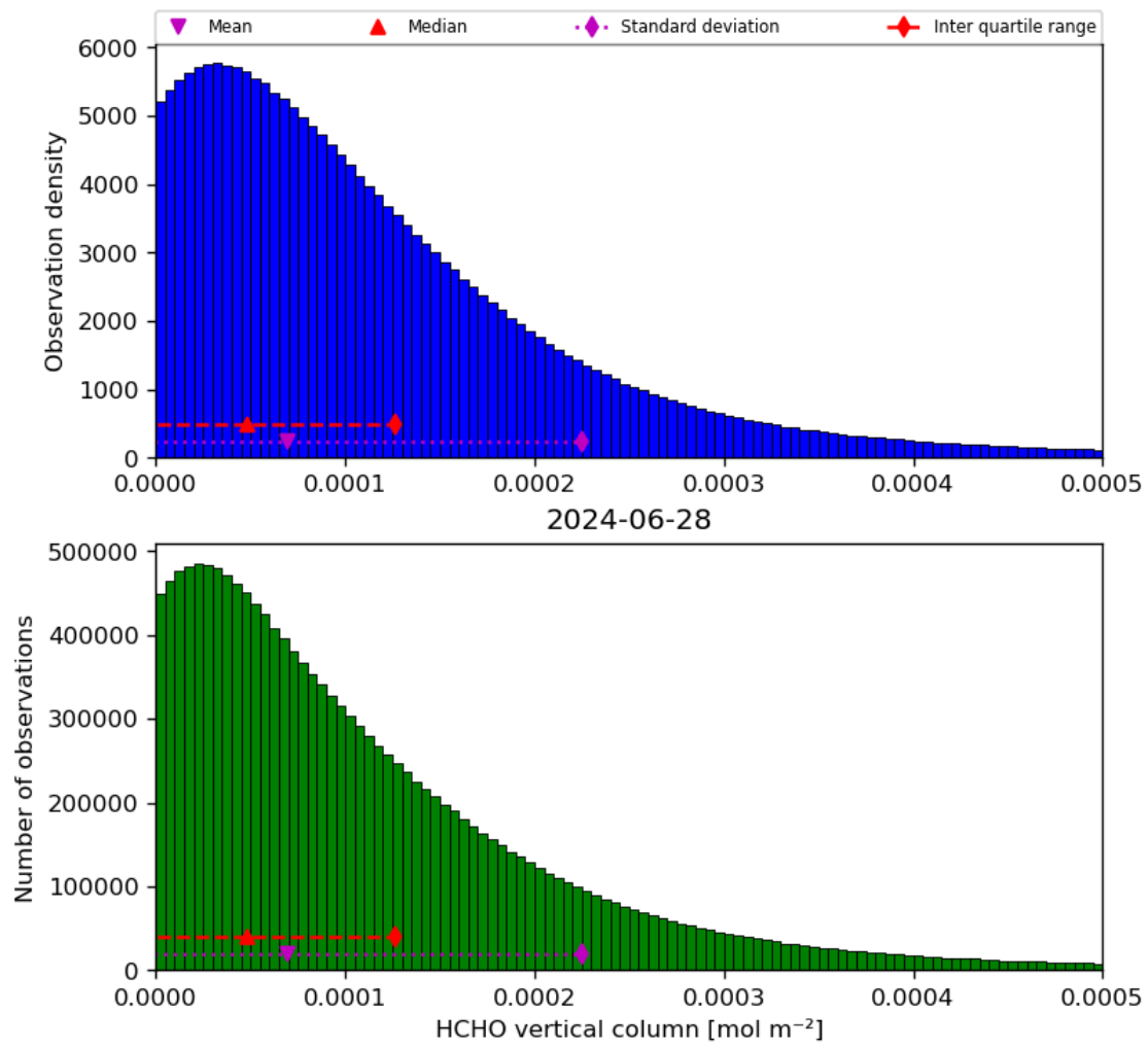
Figure 35: Histogram of “HCHO vertical column” for 2024-06-27 to 2024-06-29
