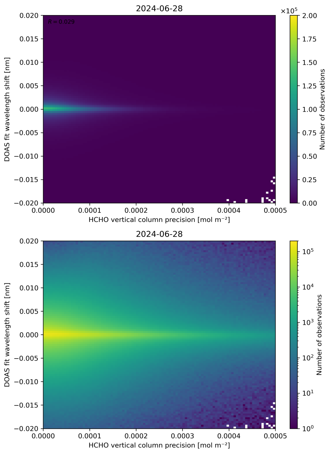
Figure 137: Scatter density plot of “HCHO vertical column precision” against “DOAS fit wavelength shift” for 2024-06-27 to 2024-06-29.
