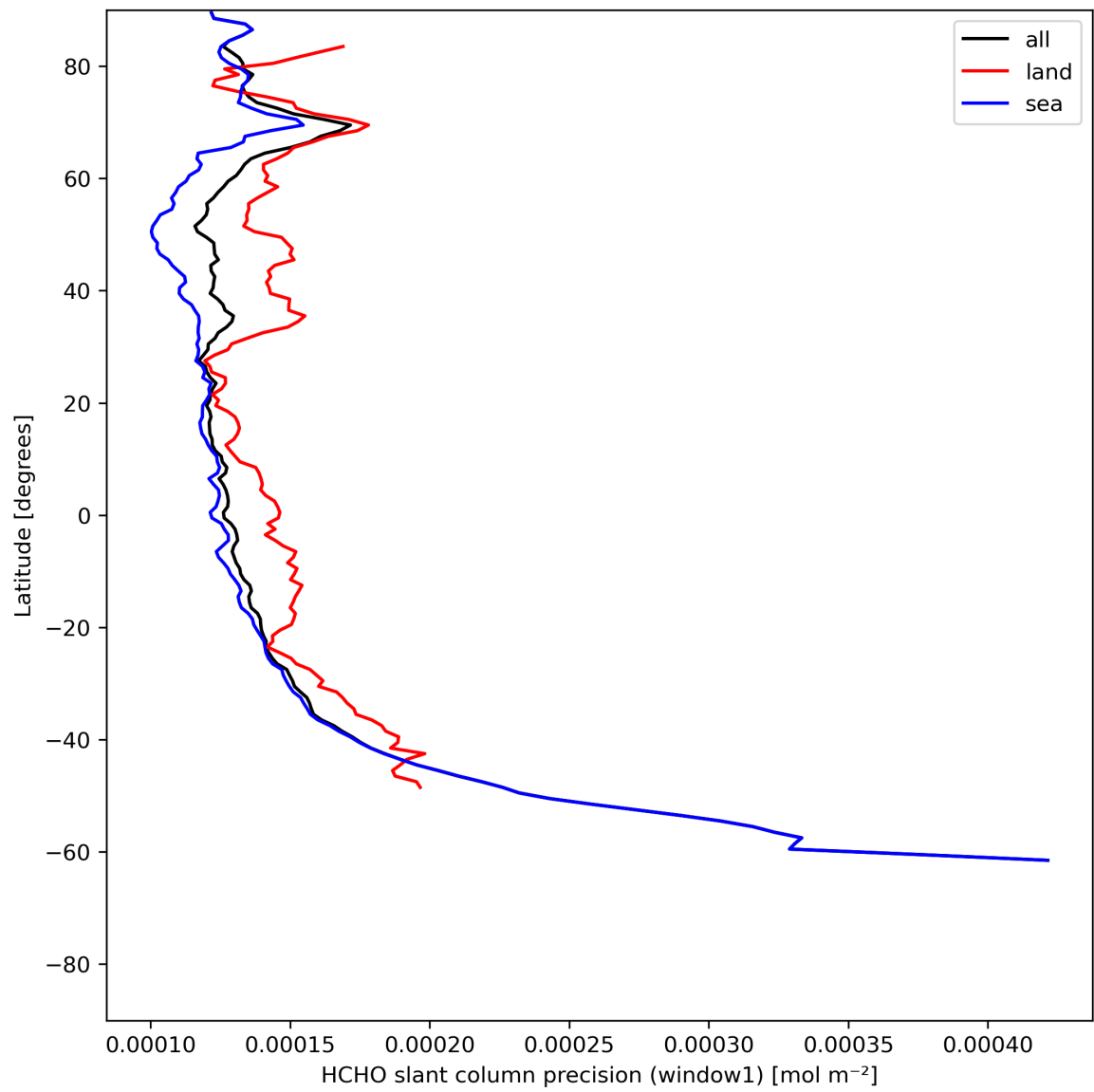
Figure 25: Zonal average of “HCHO slant column precision (window1)” for 2024-06-27 to 2024-06-29.
