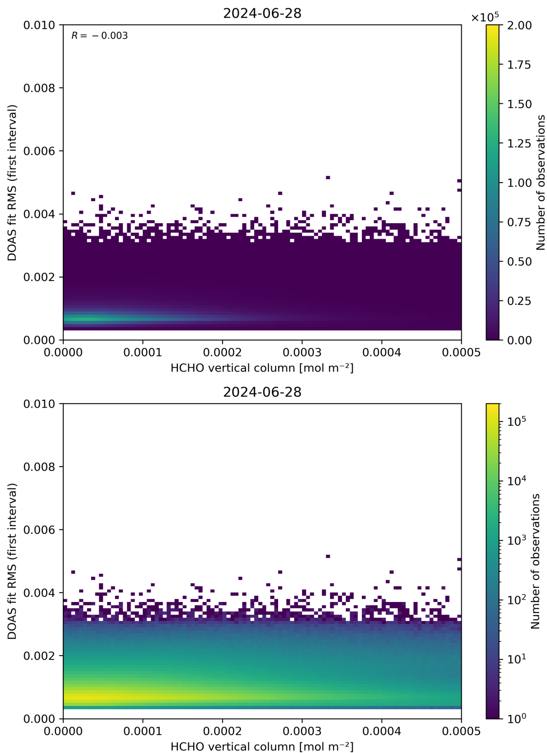
Figure 123: Scatter density plot of “HCHO vertical column” against “DOAS fit RMS (first interval)” for 2024-06-27 to 2024-06-29.
