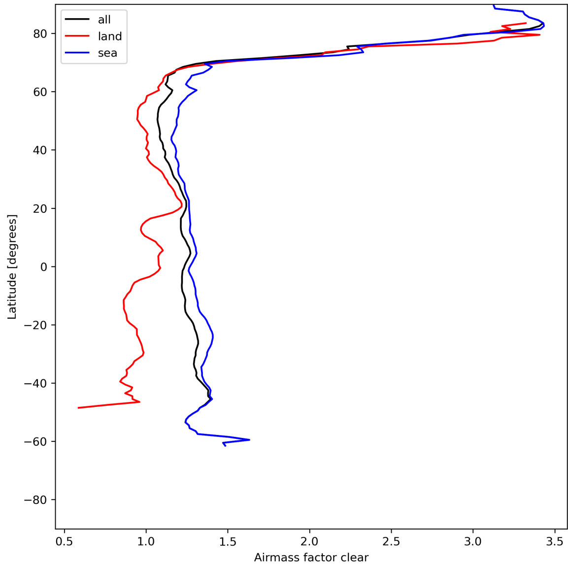
Figure 28: Zonal average of “Airmass factor clear” for 2024-06-27 to 2024-06-29.
