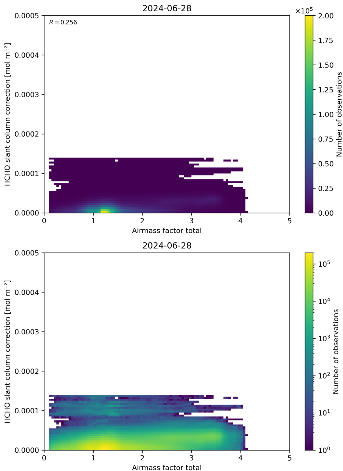
Figure 102: Scatter density plot of “Airmass factor total” against “HCHO slant column correction” for 2024-06-27 to 2024-06-29.
