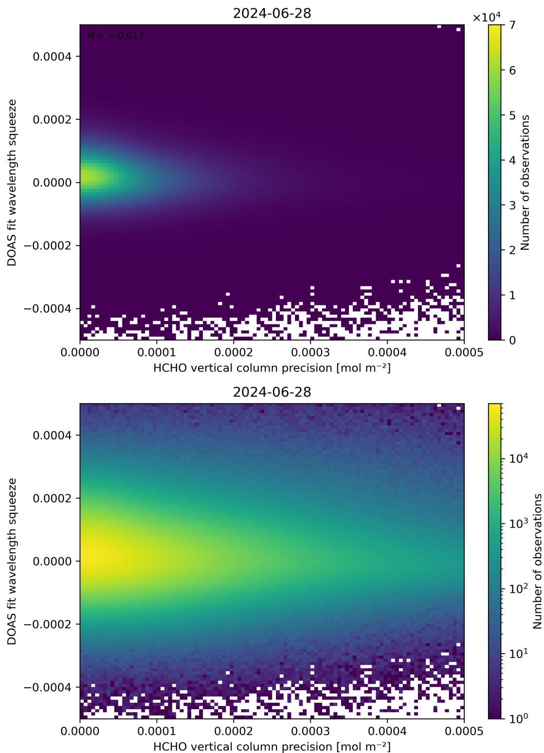
Figure 138: Scatter density plot of “HCHO vertical column precision” against “DOAS fit wavelength squeeze” for 2024-06-27 to 2024-06-29.
