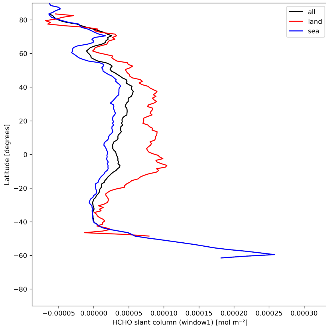
Figure 24: Zonal average of “HCHO slant column (window1)” for 2024-06-27 to 2024-06-29.
