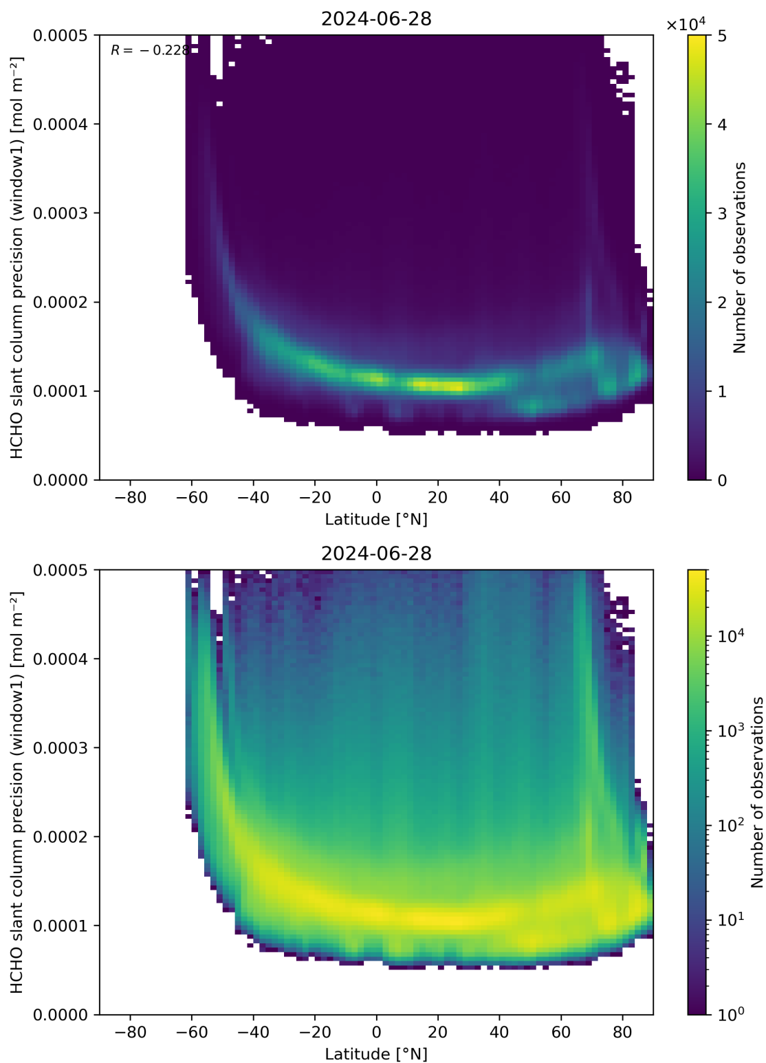
Figure 160: Scatter density plot of “Latitude” against “HCHO slant column precision (window1)” for 2024-06-27 to 2024-06-29.
