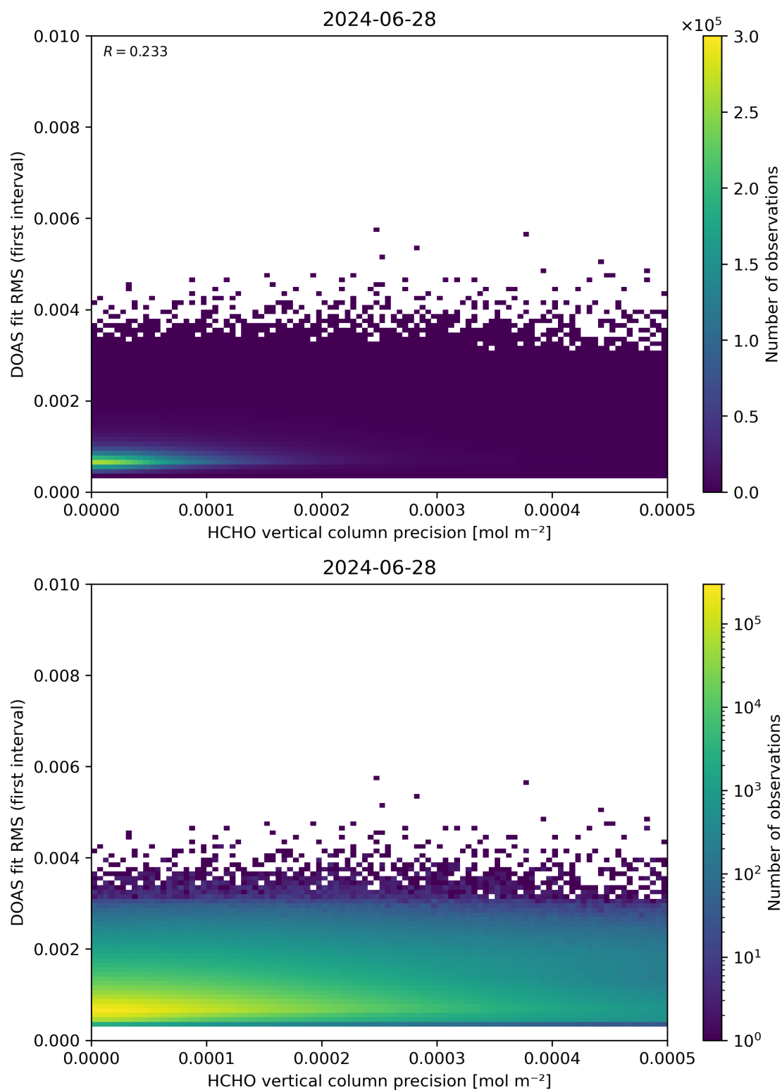
Figure 136: Scatter density plot of “HCHO vertical column precision” against “DOAS fit RMS (first interval)” for 2024-06-27 to 2024-06-29.
