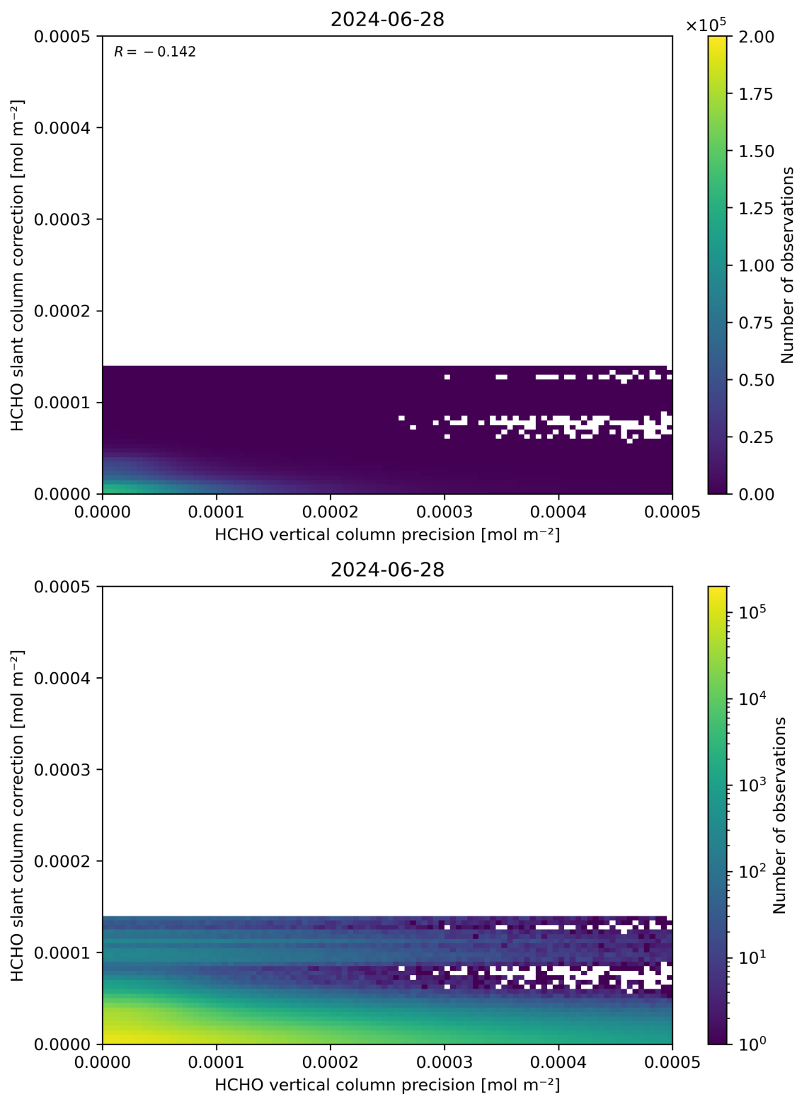
Figure 141: Scatter density plot of “HCHO vertical column precision” against “HCHO slant column correction” for 2024-06-27 to 2024-06-29.
