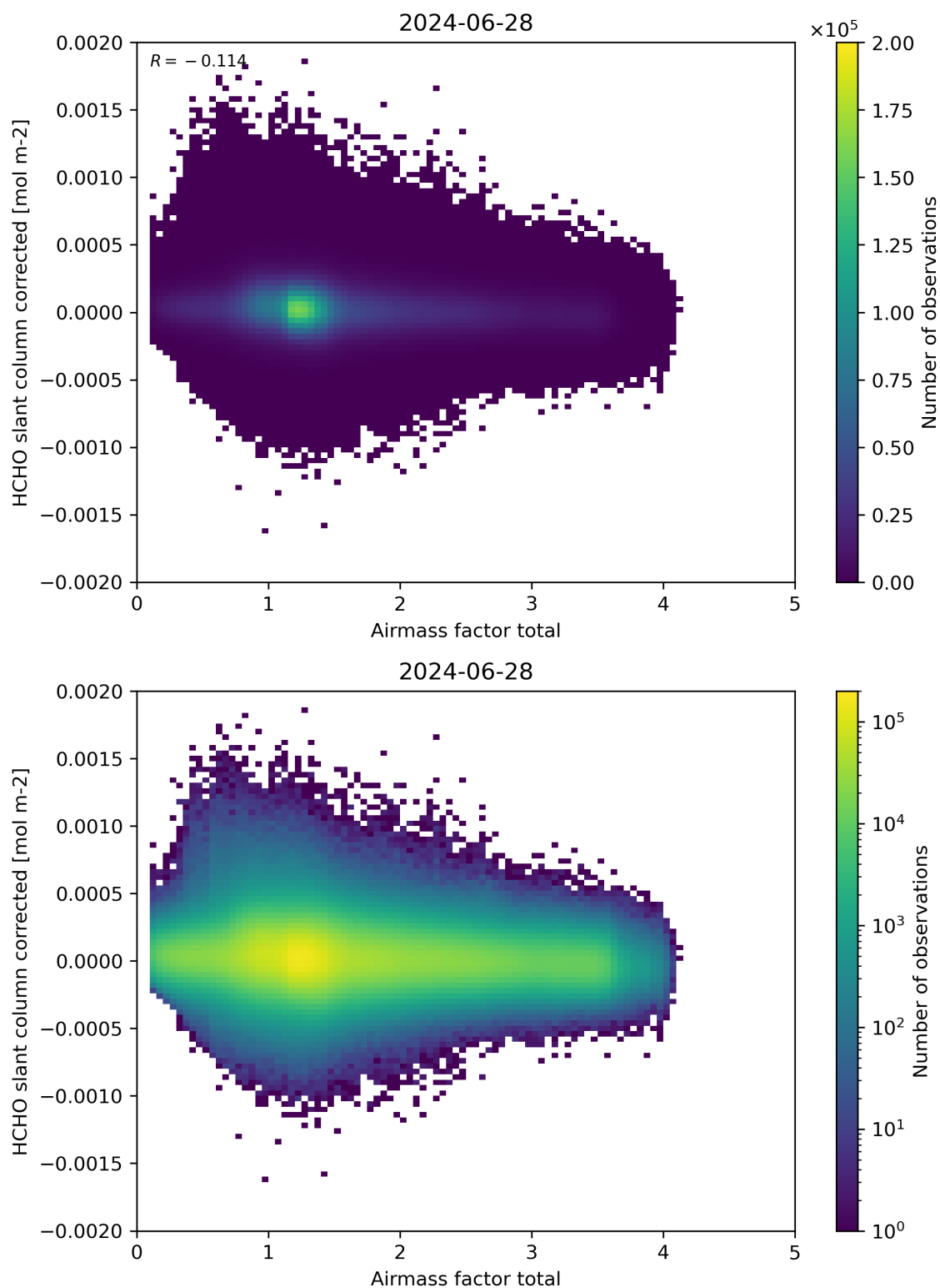
Figure 101: Scatter density plot of “Airmass factor total” against “HCHO slant column corrected” for 2024-06-27 to 2024-06-29.
