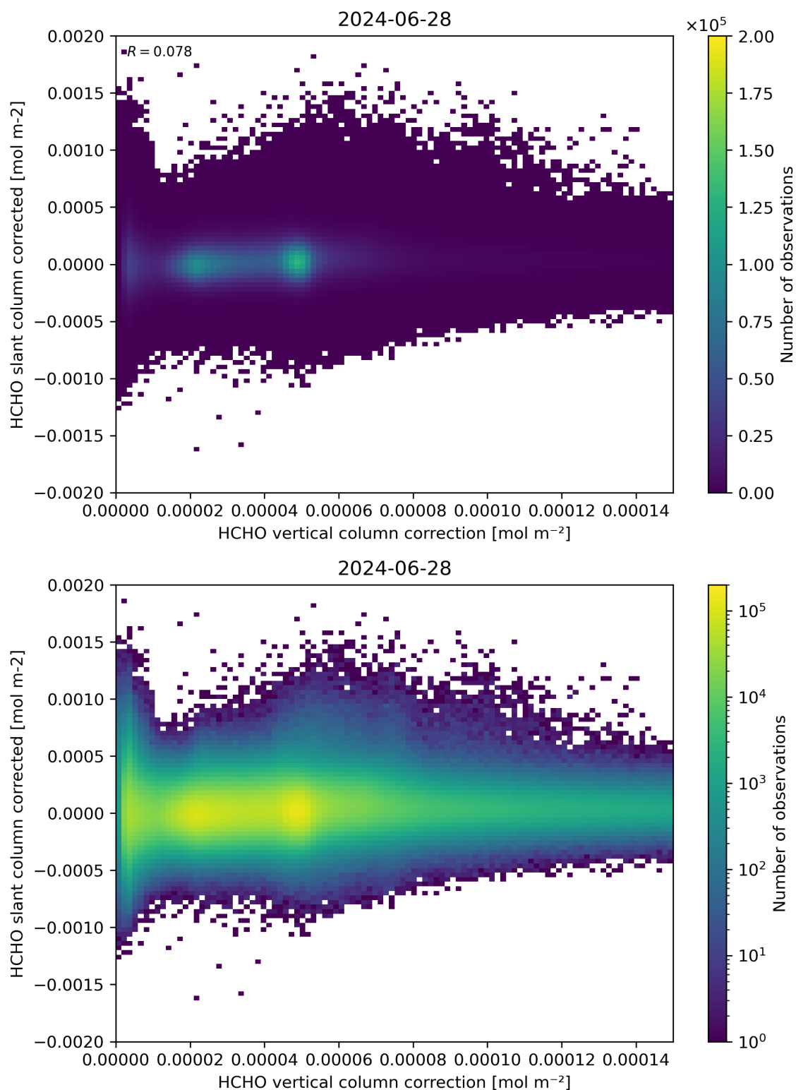
Figure 116: Scatter density plot of “HCHO vertical column correction” against “HCHO slant column corrected” for 2024-06-27 to 2024-06-29.
