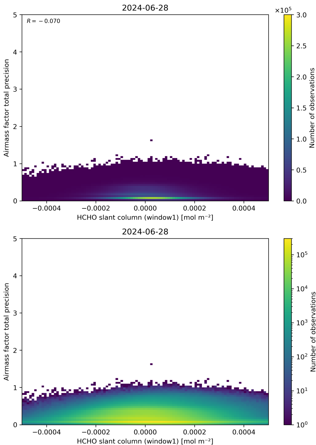
Figure 86: Scatter density plot of “HCHO slant column (window1)” against “Airmass factor total precision” for 2024-06-27 to 2024-06-29.
