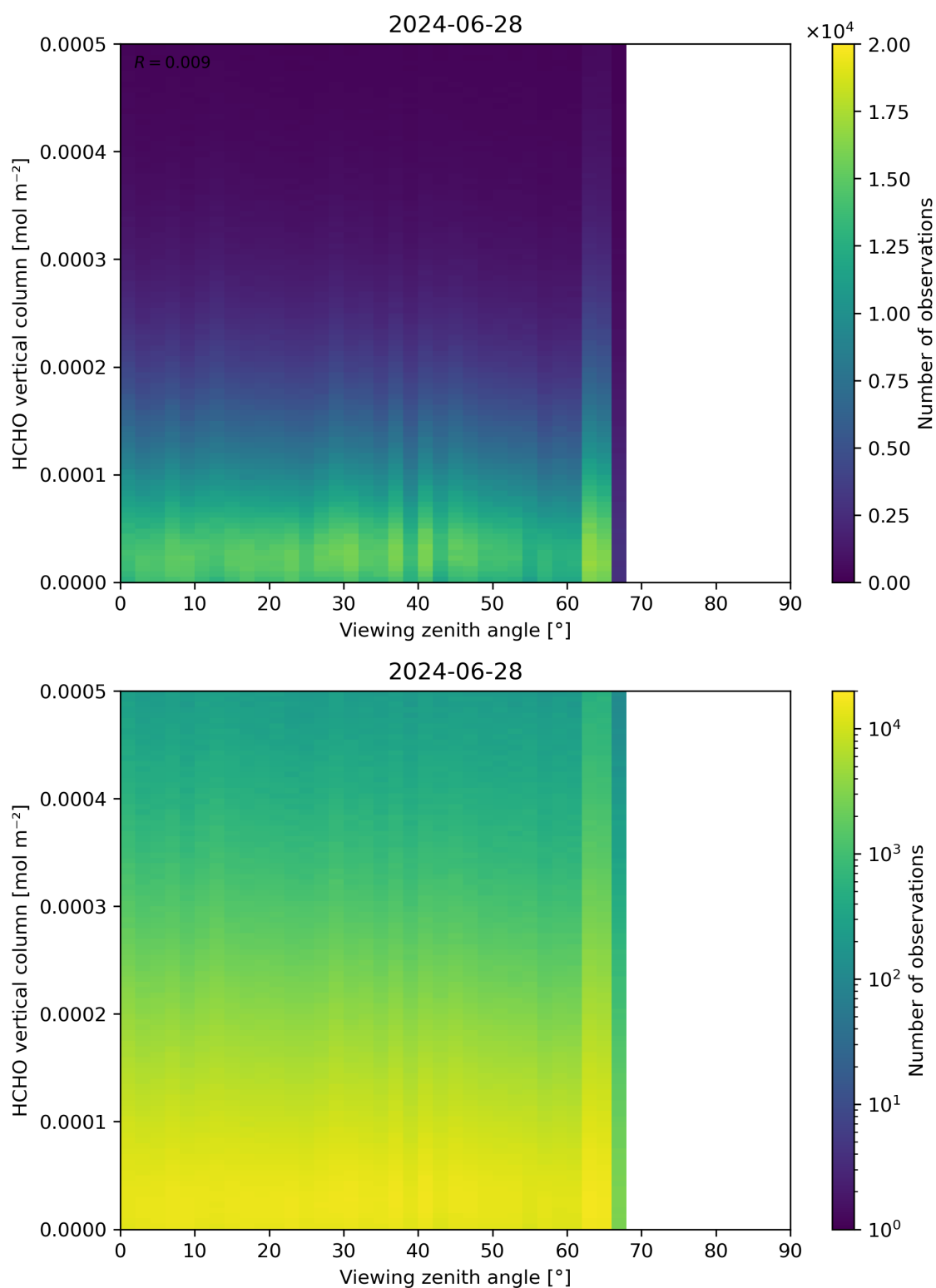
Figure 192: Scatter density plot of “Viewing zenith angle” against “HCHO vertical column” for 2024-06-27 to 2024-06-29.
