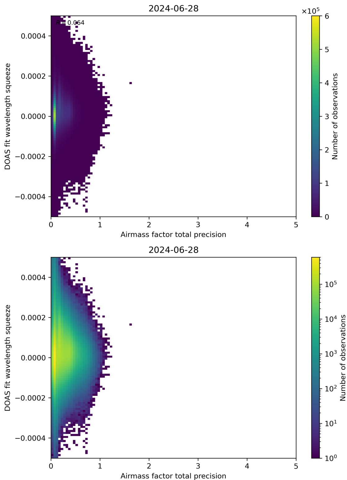
Figure 107: Scatter density plot of “Airmass factor total precision” against “DOAS fit wavelength squeeze” for 2024-06-27 to 2024-06-29.
