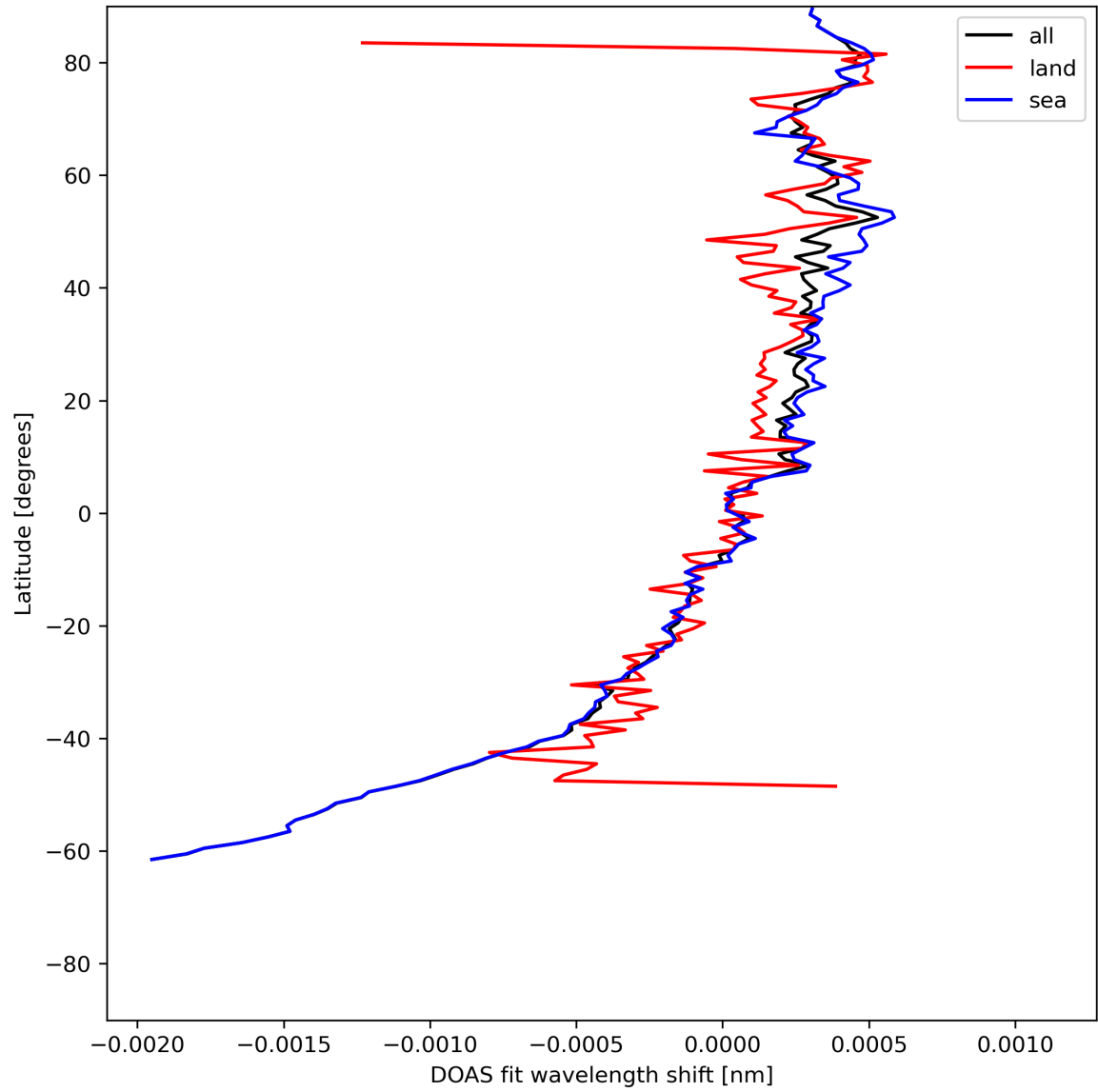
Figure 30: Zonal average of “DOAS fit wavelength shift” for 2024-06-27 to 2024-06-29.
