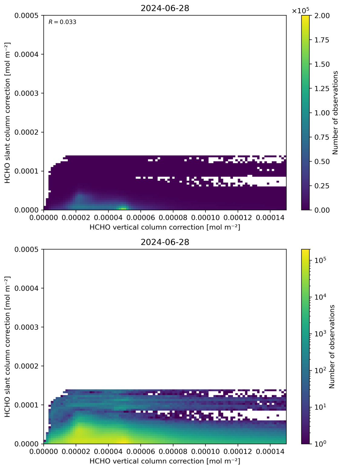
Figure 117: Scatter density plot of “HCHO vertical column correction” against “HCHO slant column correction” for 2024-06-27 to 2024-06-29.
