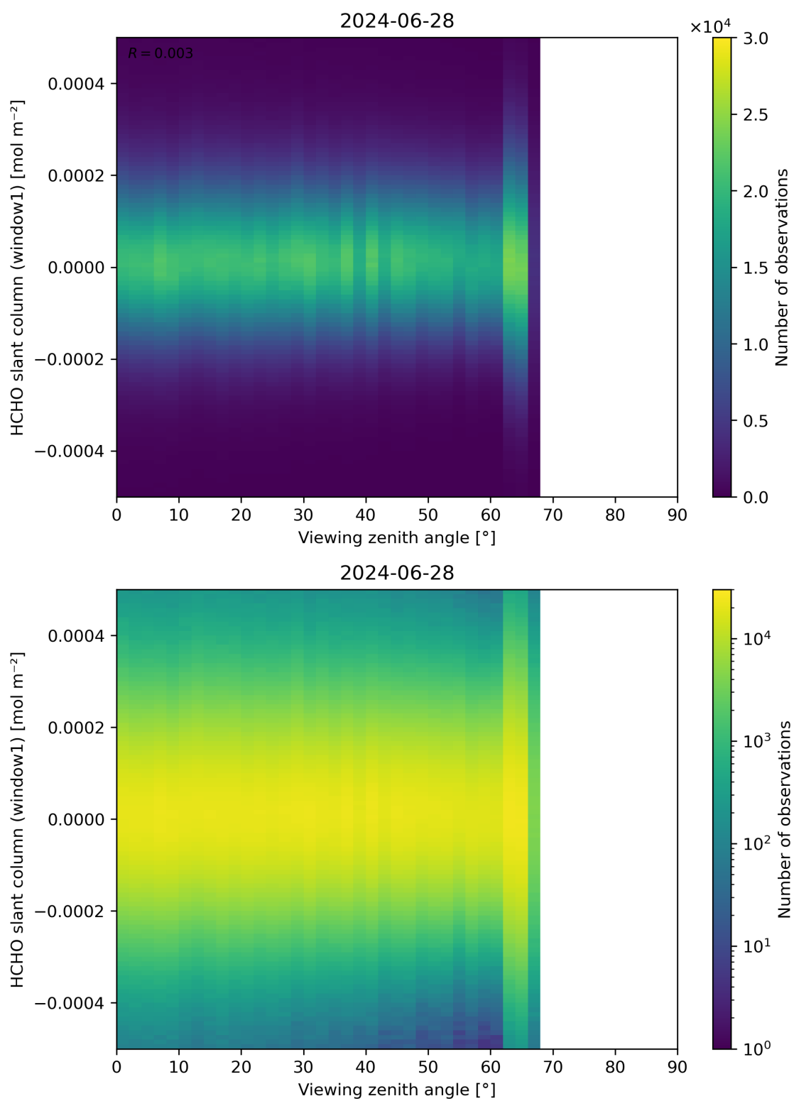
Figure 188: Scatter density plot of “Viewing zenith angle” against “HCHO slant column (window1)” for 2024-06-27 to 2024-06-29.
