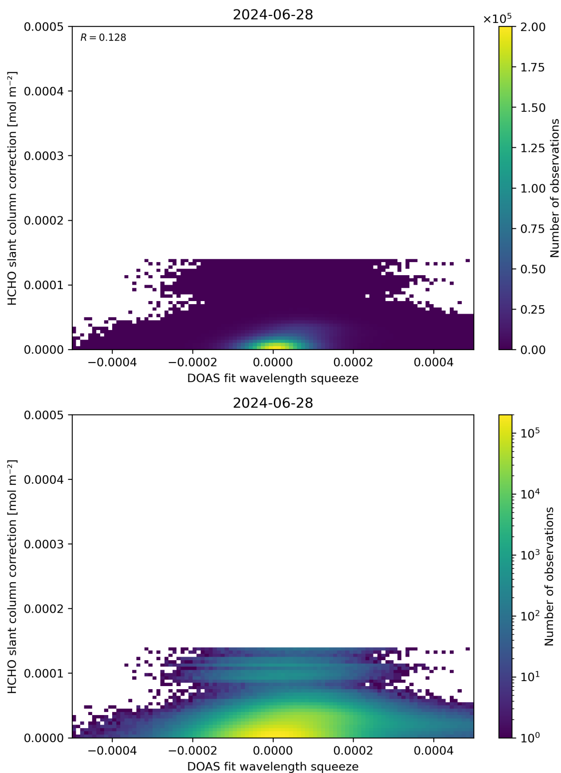
Figure 70: Scatter density plot of “DOAS fit wavelength squeeze” against “HCHO slant column correction” for 2024-06-27 to 2024-06-29.
