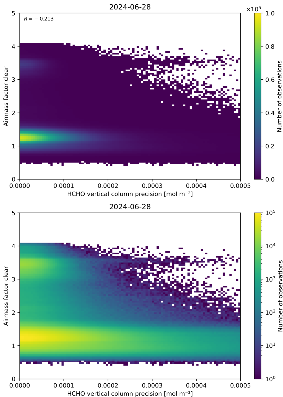
Figure 139: Scatter density plot of “HCHO vertical column precision” against “Airmass factor clear” for 2024-06-27 to 2024-06-29.
