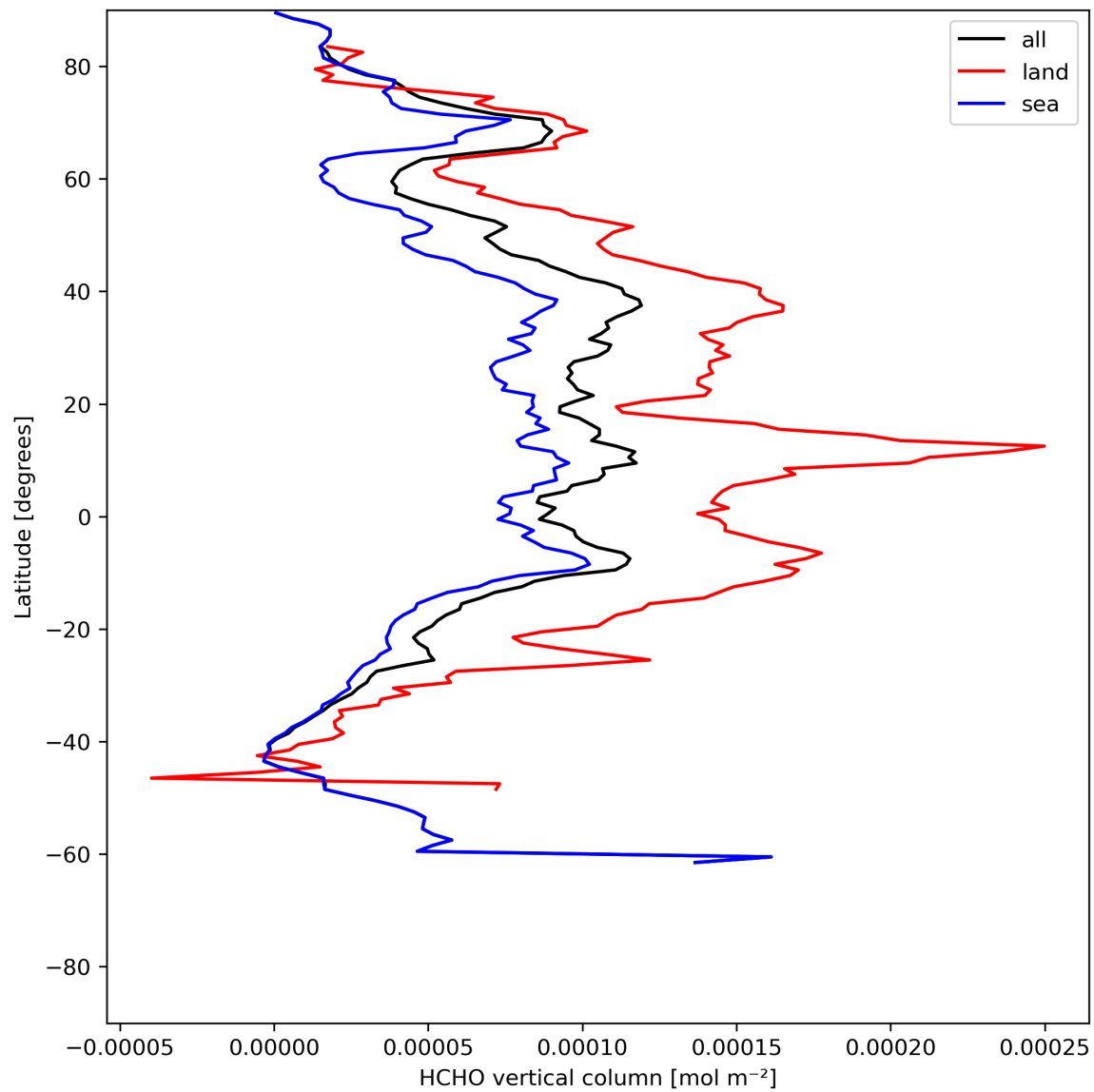
Figure 21: Zonal average of “HCHO vertical column” for 2024-06-27 to 2024-06-29.
