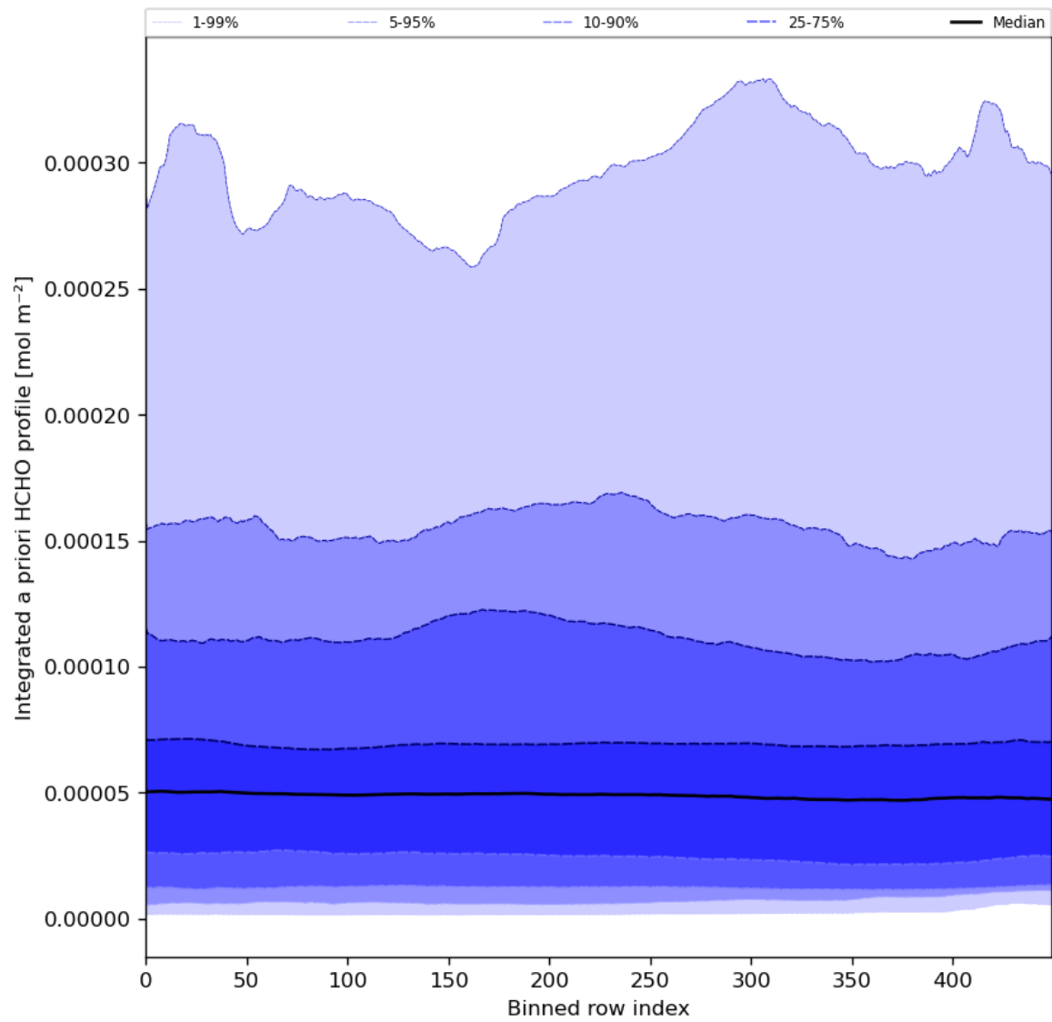
Figure 57: Along track statistics of "Integrated a priori HCHO profile" for 2024-06-27 to 2024-06-29
