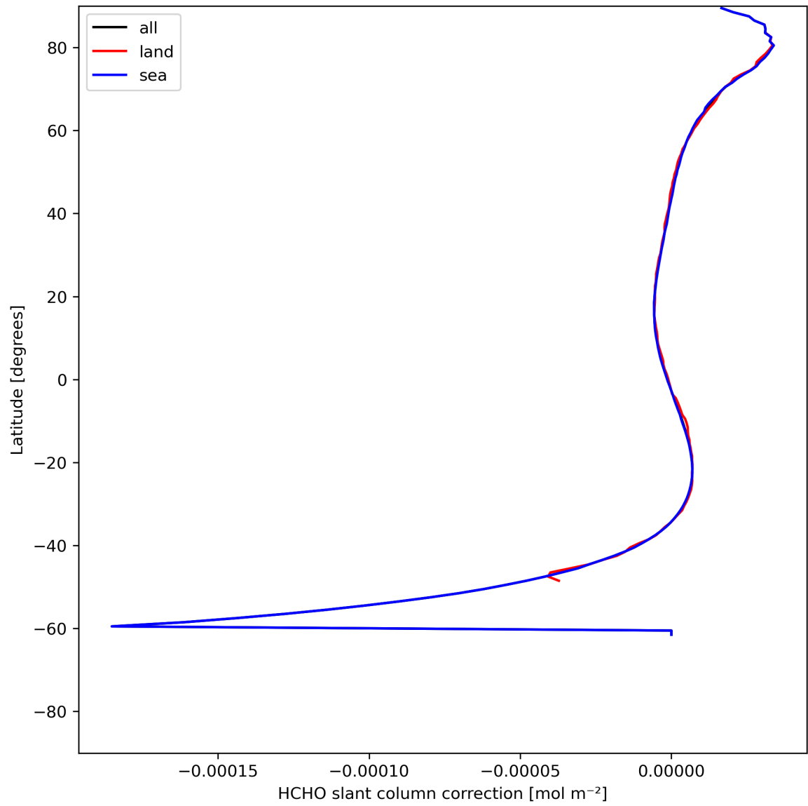
Figure 33: Zonal average of “HCHO slant column correction” for 2024-06-27 to 2024-06-29.
