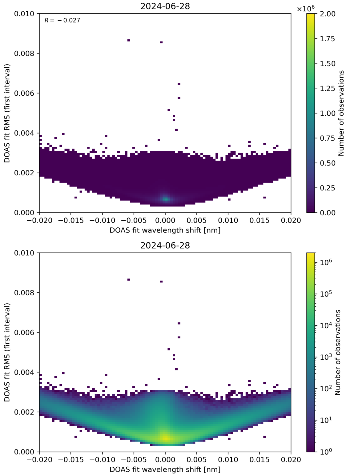
Figure 64: Scatter density plot of “DOAS fit wavelength shift” against “DOAS fit RMS (first interval)” for 2024-06-27 to 2024-06-29.
