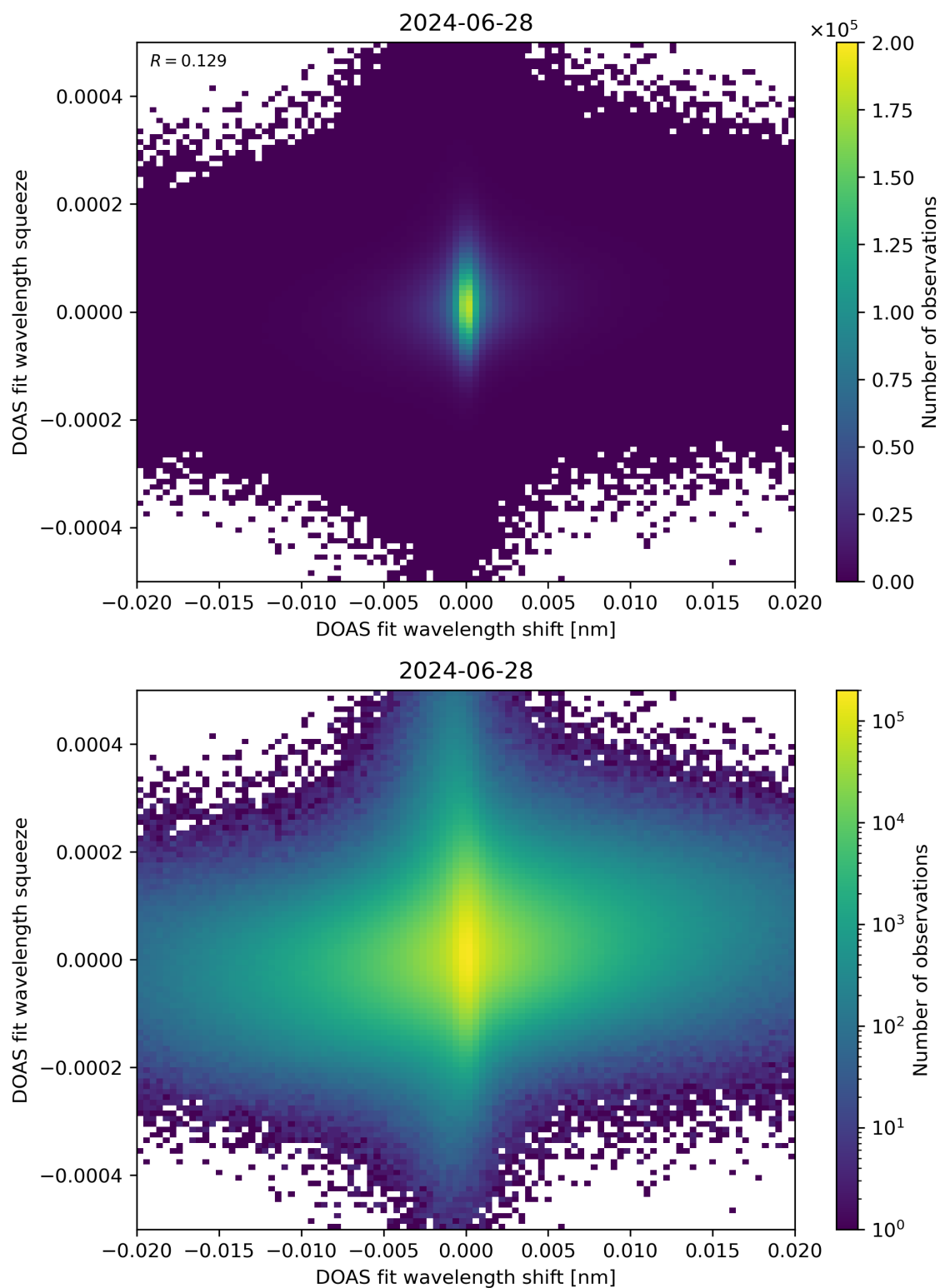
Figure 65: Scatter density plot of “DOAS fit wavelength shift” against “DOAS fit wavelength squeeze” for 2024-06-27 to 2024-06-29.
