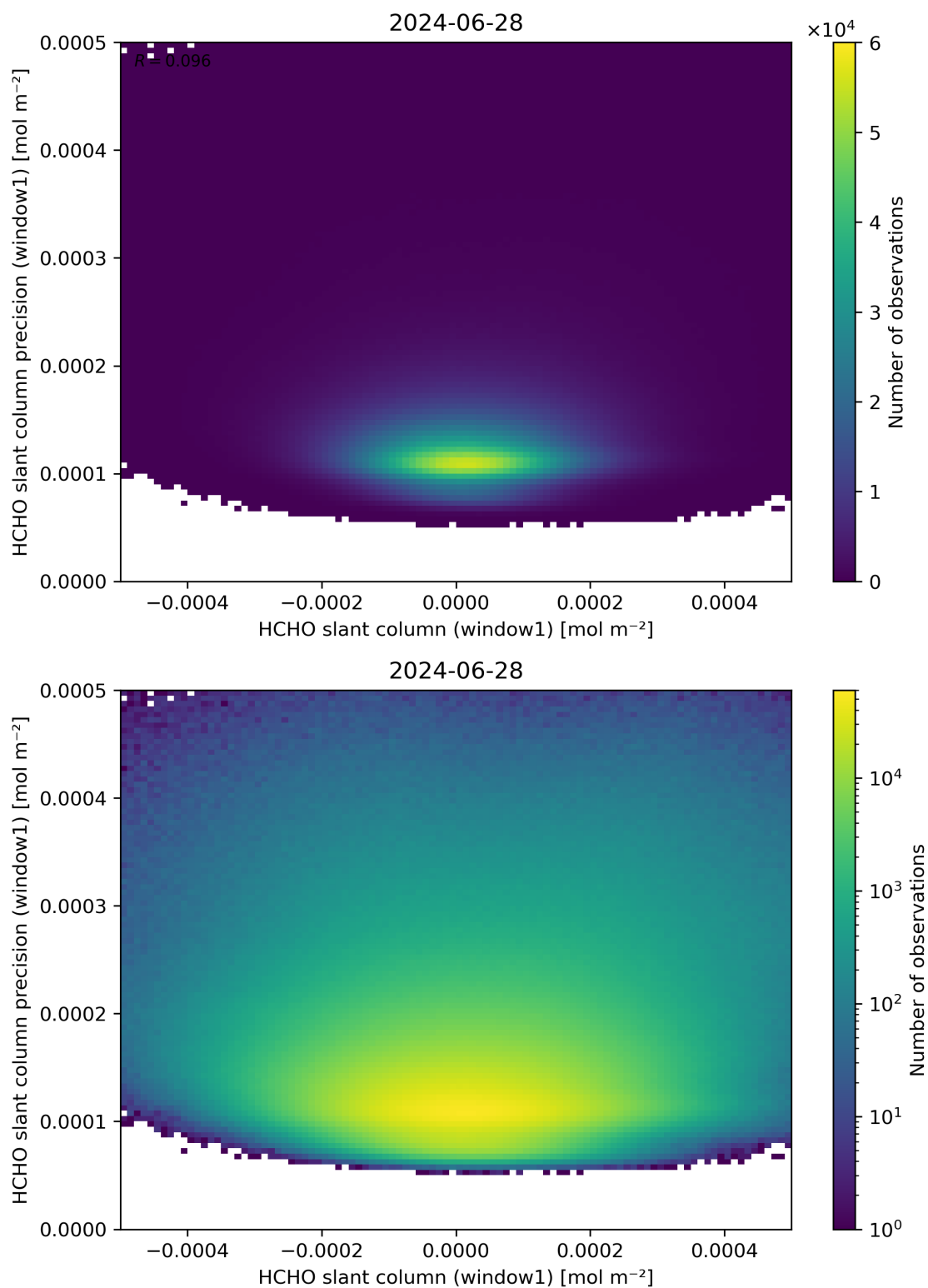
Figure 84: Scatter density plot of “HCHO slant column (window1)” against “HCHO slant column precision (window1)” for 2024-06-27 to 2024-06-29.
