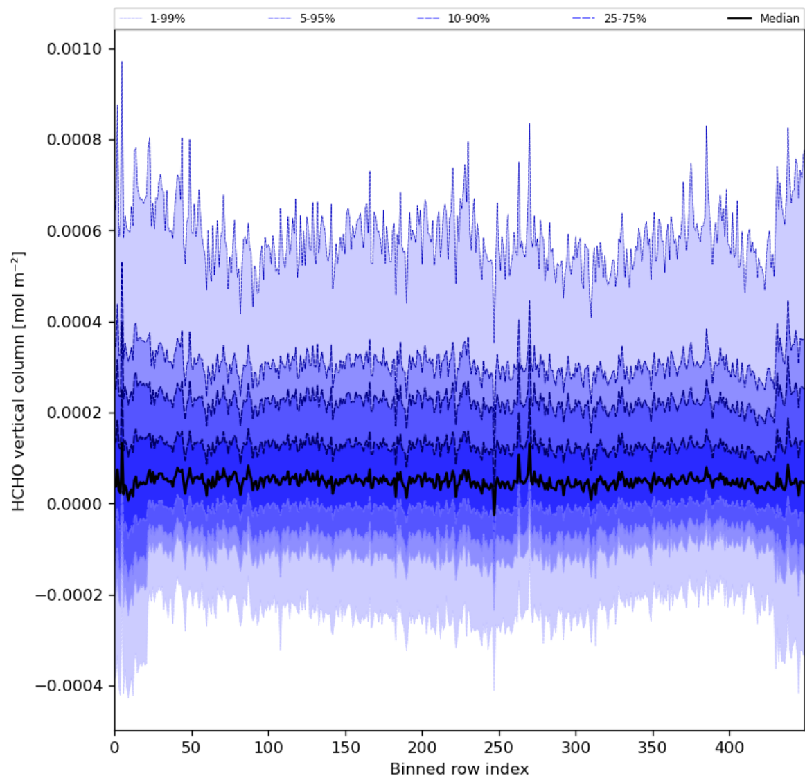
Figure 49: Along track statistics of “HCHO vertical column” for 2024-06-27 to 2024-06-29
