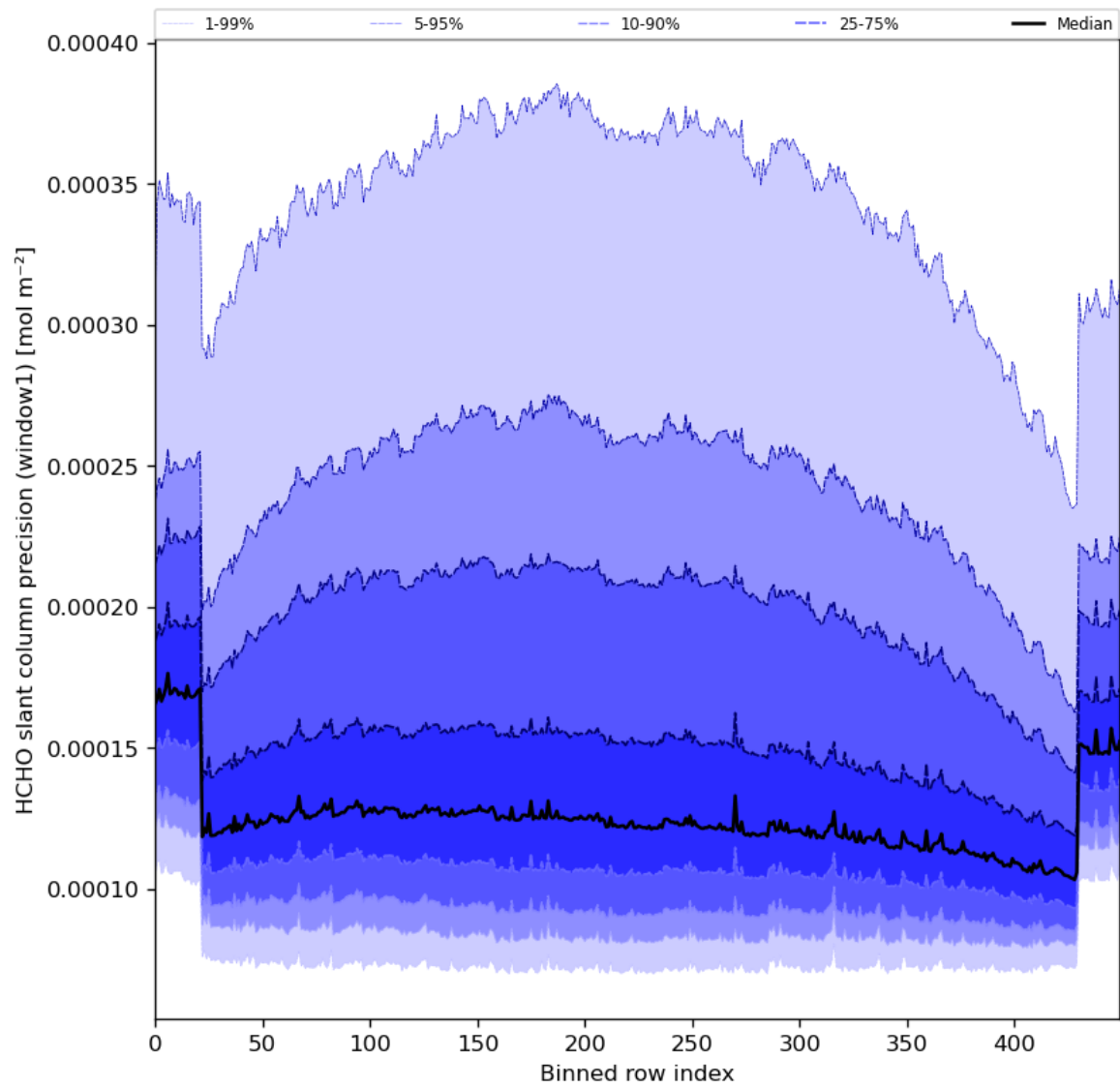
Figure 53: Along track statistics of “HCHO slant column precision (window1)” for 2024-06-27 to 2024-06-29
