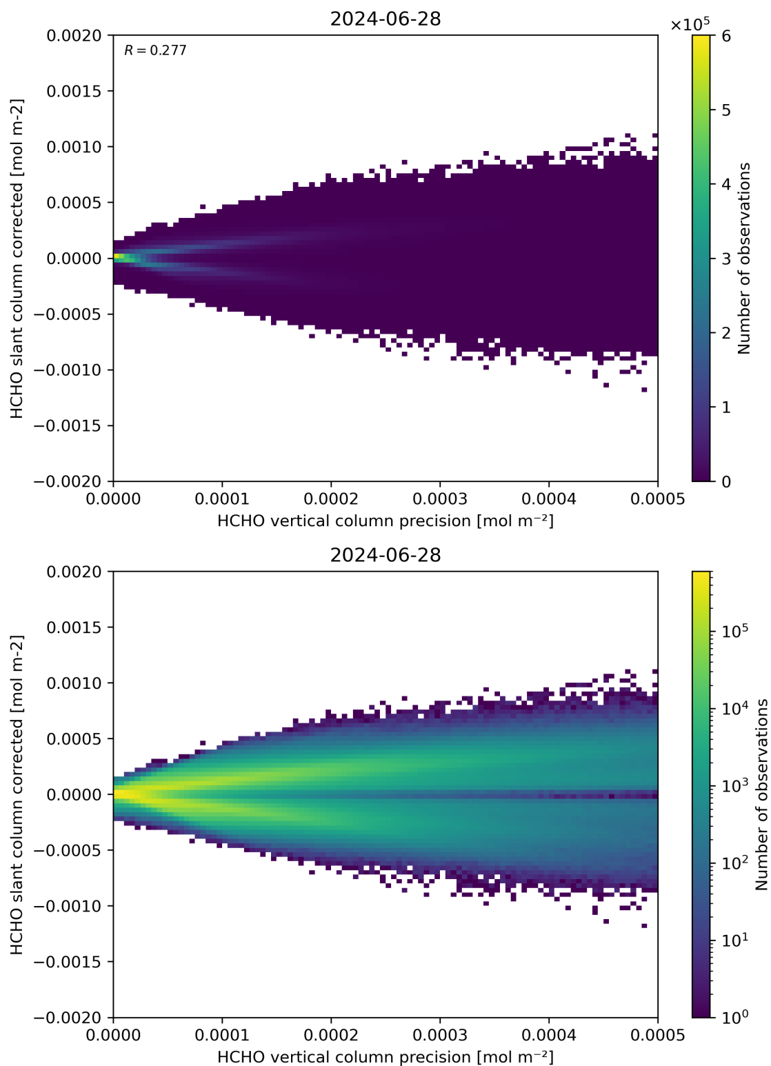
Figure 140: Scatter density plot of “HCHO vertical column precision” against “HCHO slant column corrected” for 2024-06-27 to 2024-06-29.
