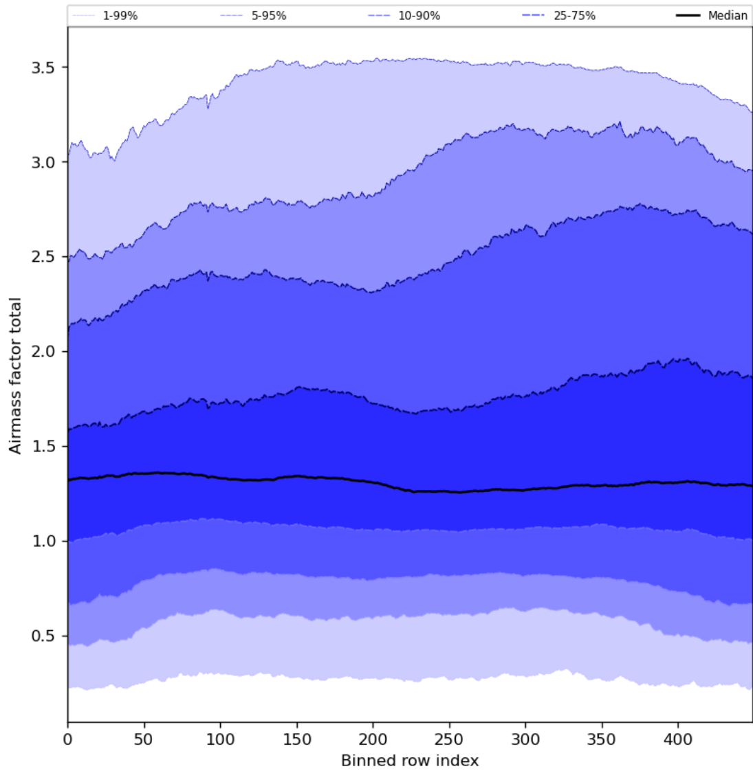
Figure 54: Along track statistics of “Airmass factor total” for 2024-06-27 to 2024-06-29
