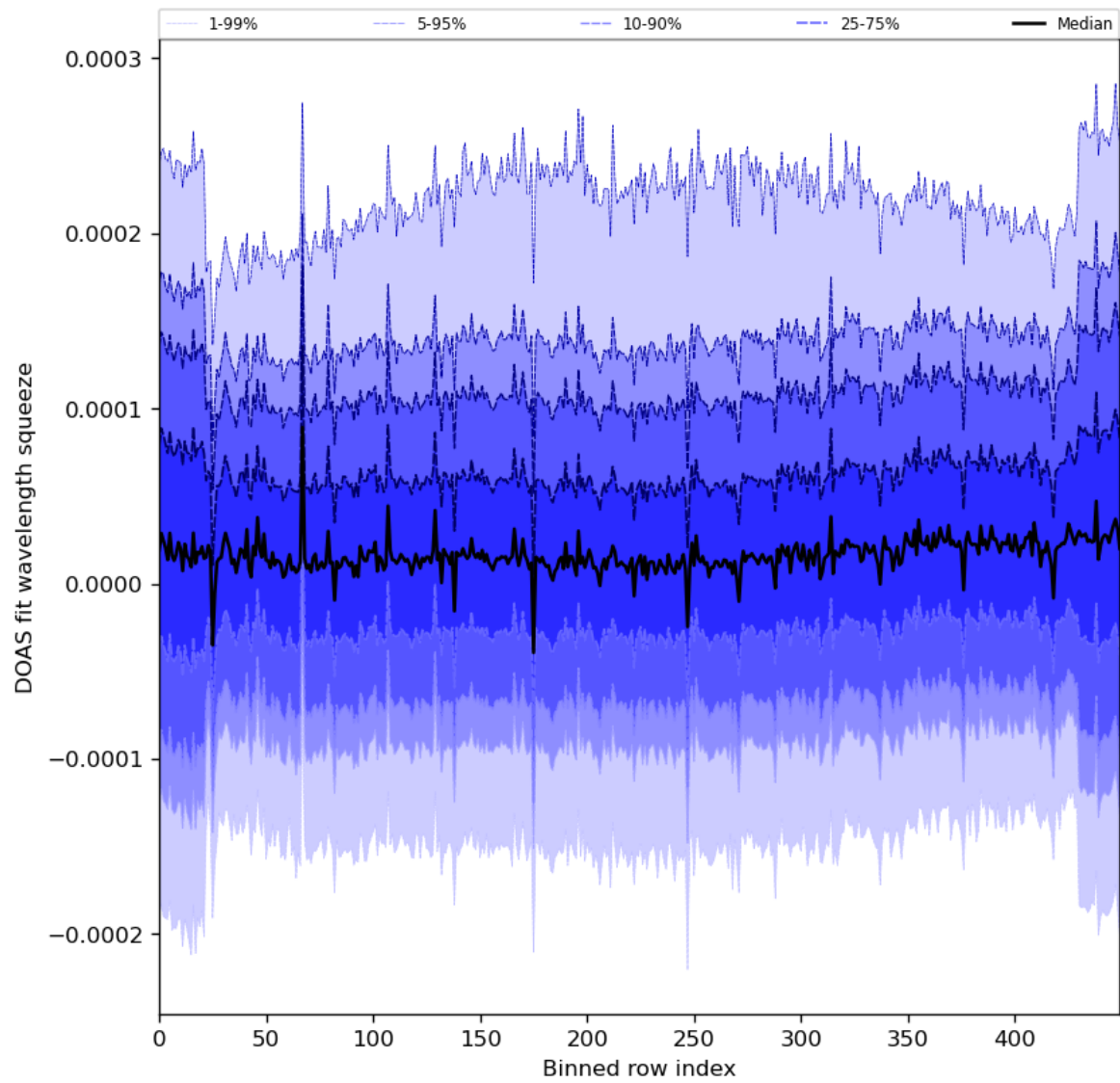
Figure 59: Along track statistics of “DOAS fit wavelength squeeze” for 2024-06-27 to 2024-06-29
