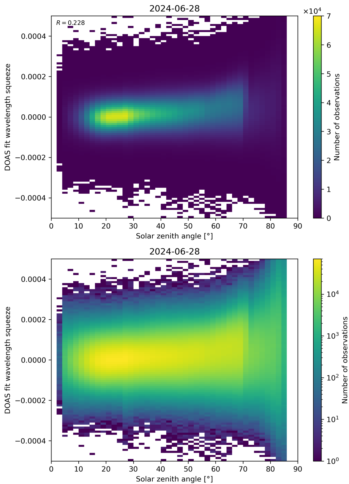
Figure 169: Scatter density plot of “Solar zenith angle” against “DOAS fit wavelength squeeze” for 2024-06-27 to 2024-06-29.
