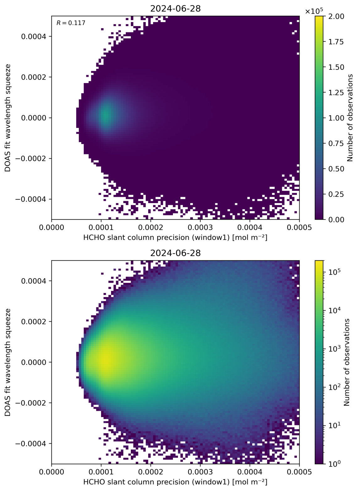
Figure 90: Scatter density plot of “HCHO slant column precision (window1)” against “DOAS fit wavelength squeeze” for 2024-06-27 to 2024-06-29.
