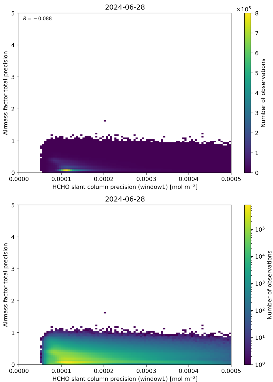
Figure 95: Scatter density plot of “HCHO slant column precision (window1)” against “Airmass factor total precision” for 2024-06-27 to 2024-06-29.
