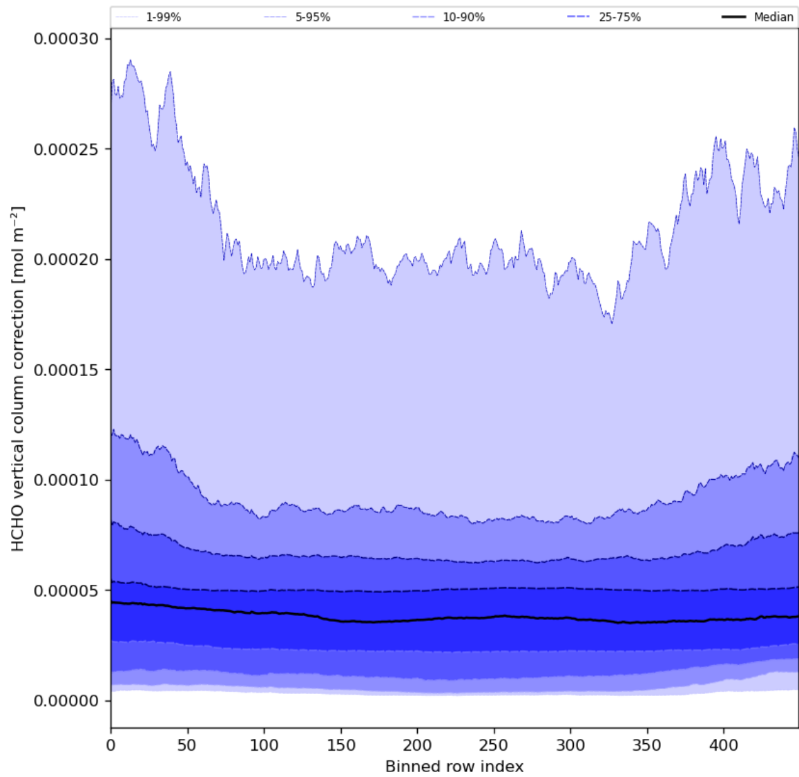
Figure 51: Along track statistics of “HCHO vertical column correction” for 2024-06-27 to 2024-06-29
