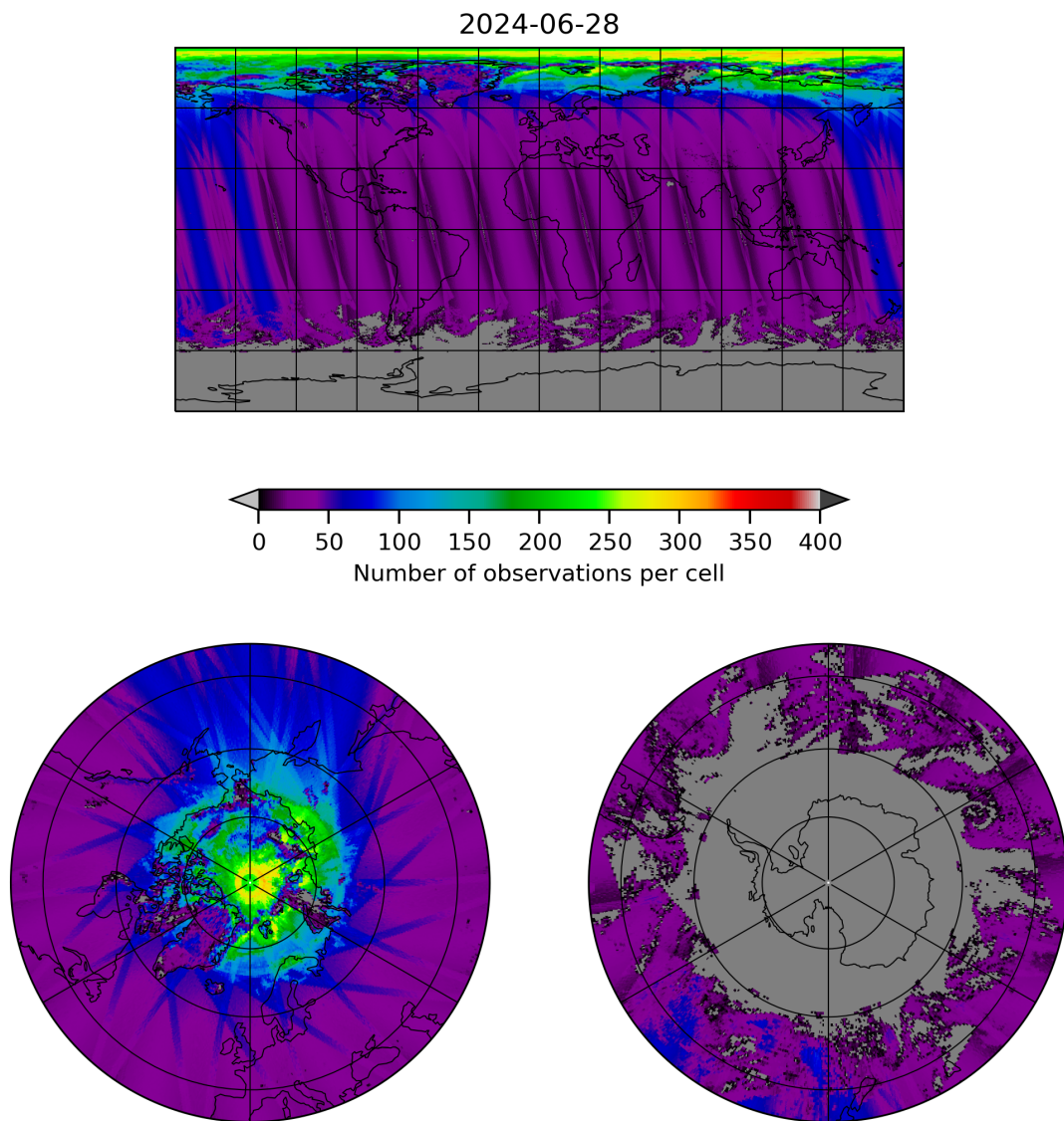
Figure 19: Map of the number of observations for 2024-06-27 to 2024-06-29
