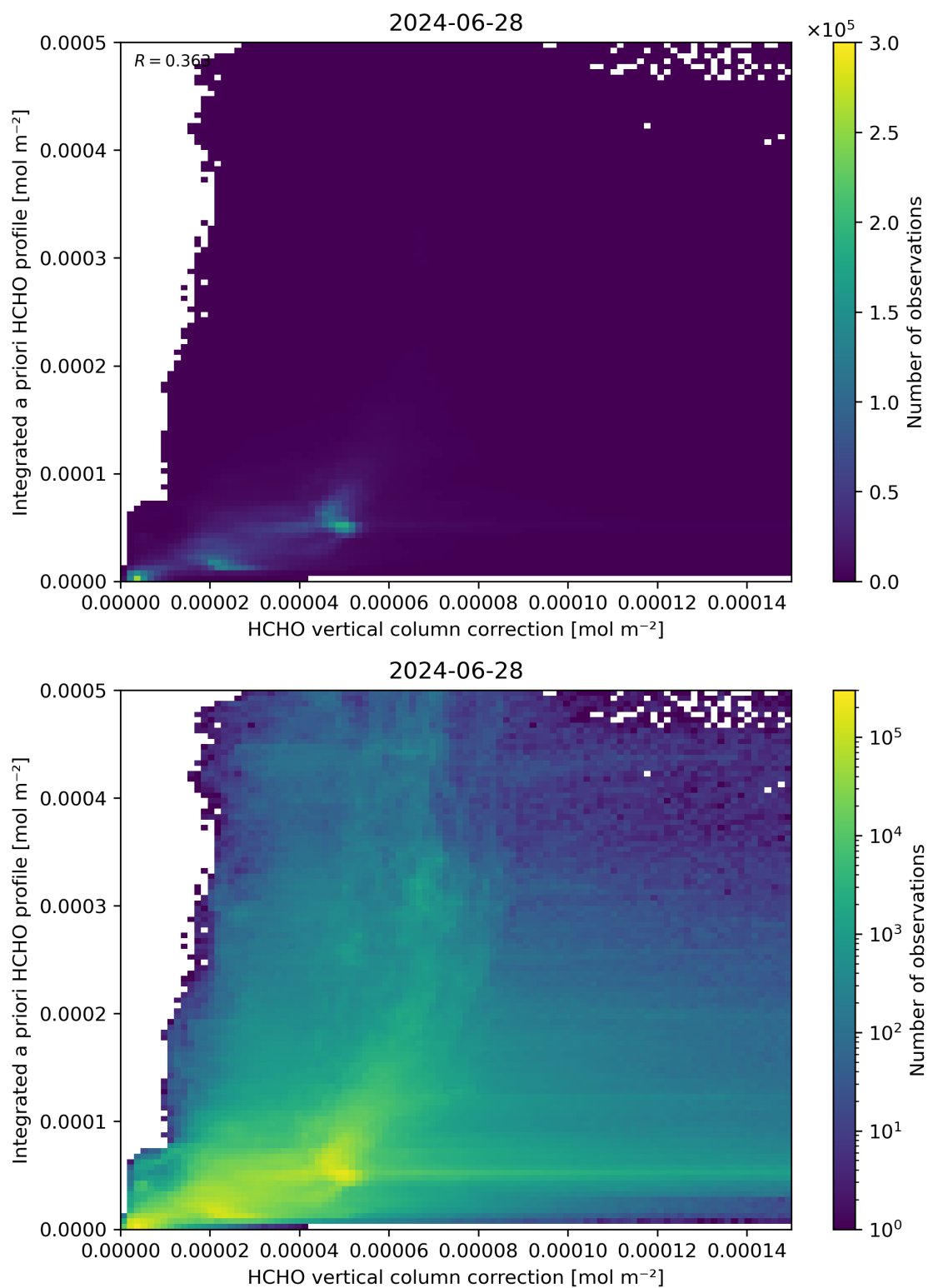
Figure 122: Scatter density plot of “HCHO vertical column correction” against “Integrated a priori HCHO profile” for 2024-06-27 to 2024-06-29.
