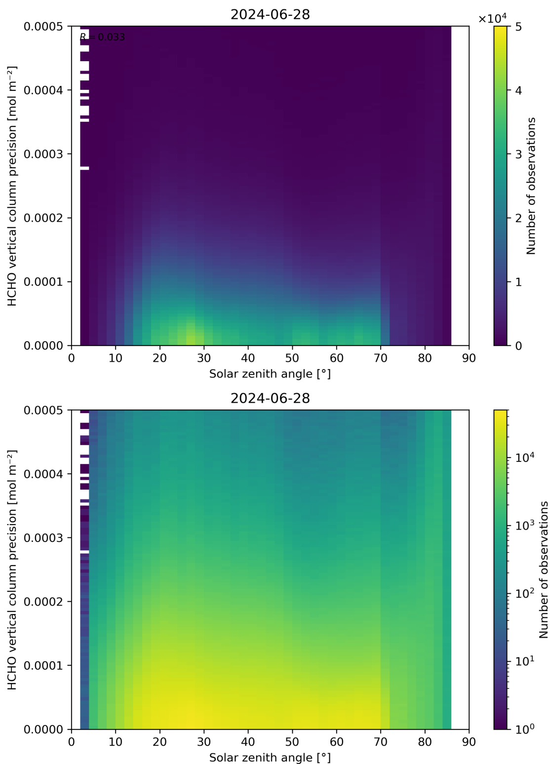
Figure 179: Scatter density plot of “Solar zenith angle” against “HCHO vertical column precision” for 2024-06-27 to 2024-06-29.
