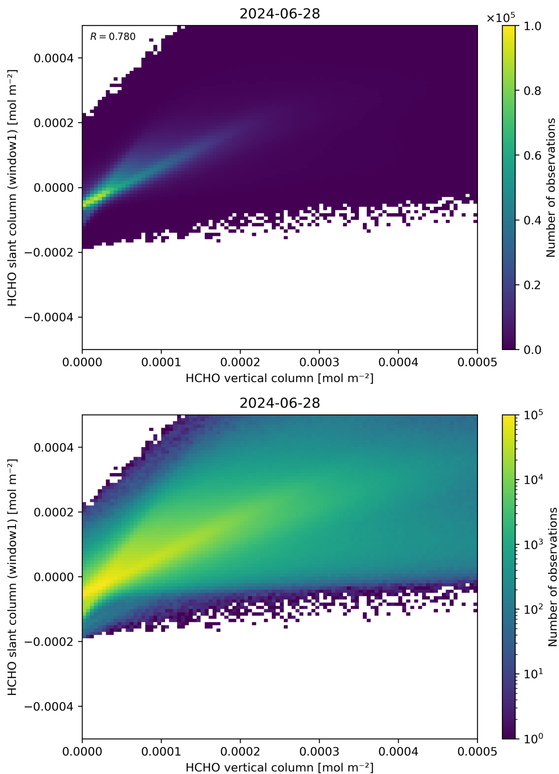
Figure 129: Scatter density plot of “HCHO vertical column” against “HCHO slant column (window1)” for 2024-06-27 to 2024-06-29.
