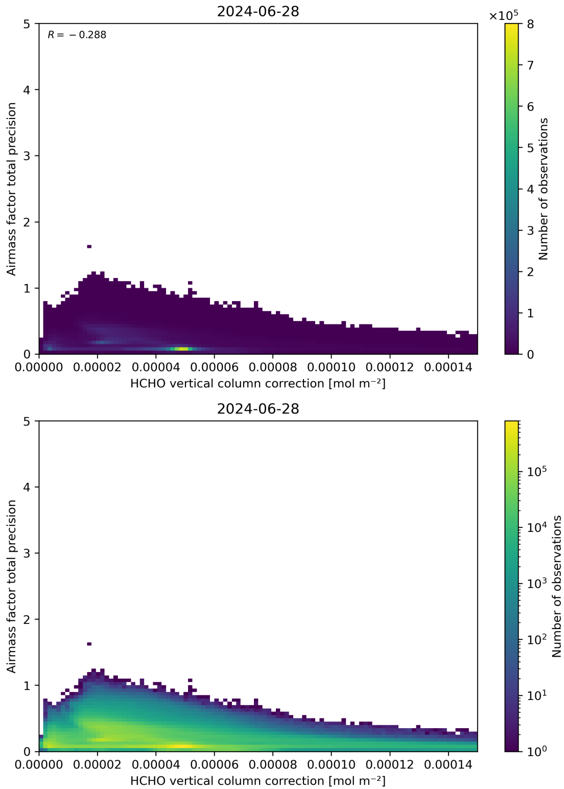
Figure 121: Scatter density plot of “HCHO vertical column correction” against “Airmass factor total precision” for 2024-06-27 to 2024-06-29.
