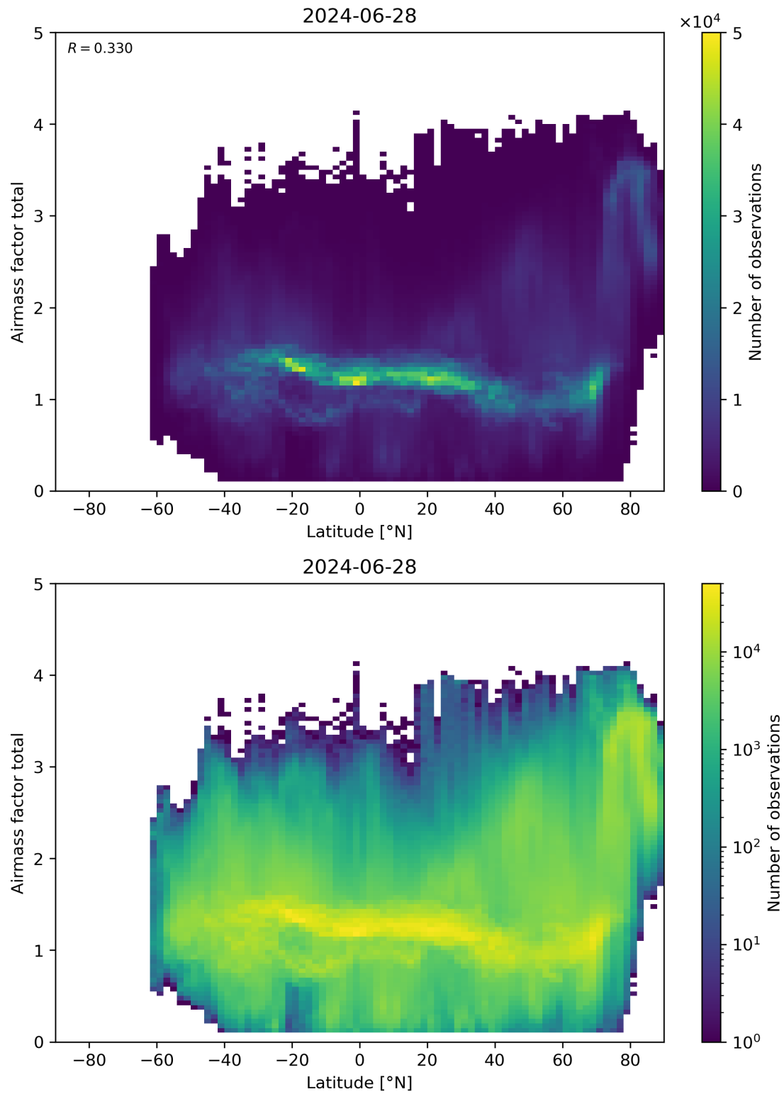
Figure 161: Scatter density plot of “Latitude” against “Airmass factor total” for 2024-06-27 to 2024-06-29.
