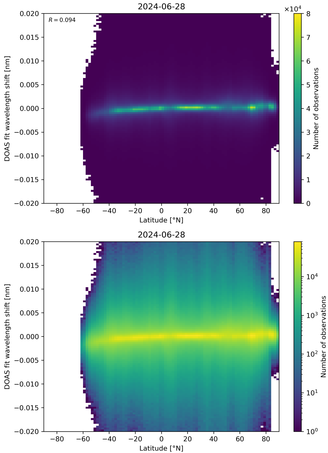
Figure 154: Scatter density plot of “Latitude” against “DOAS fit wavelength shift” for 2024-06-27 to 2024-06-29.
