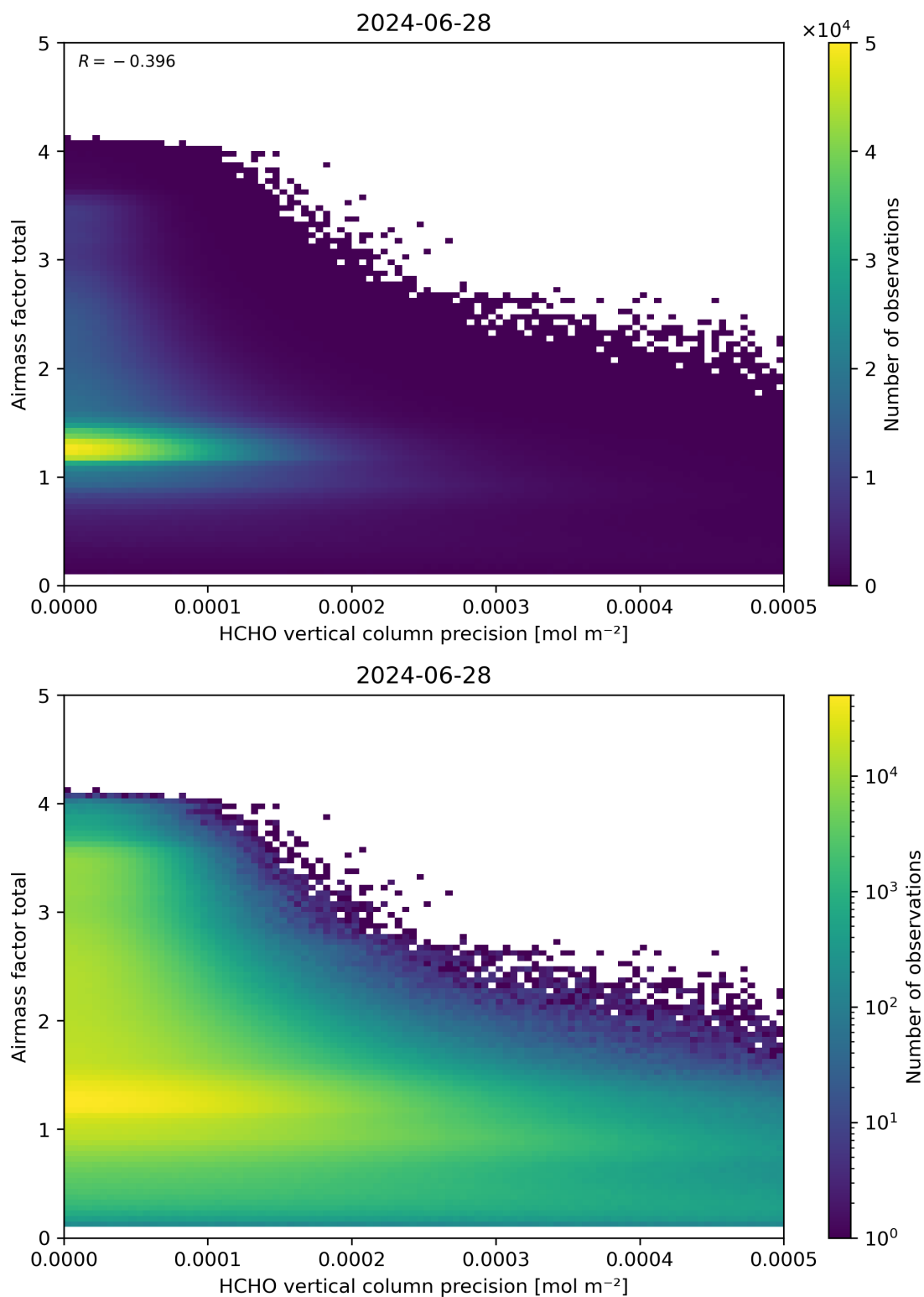
Figure 144: Scatter density plot of “HCHO vertical column precision” against “Airmass factor total” for 2024-06-27 to 2024-06-29.
