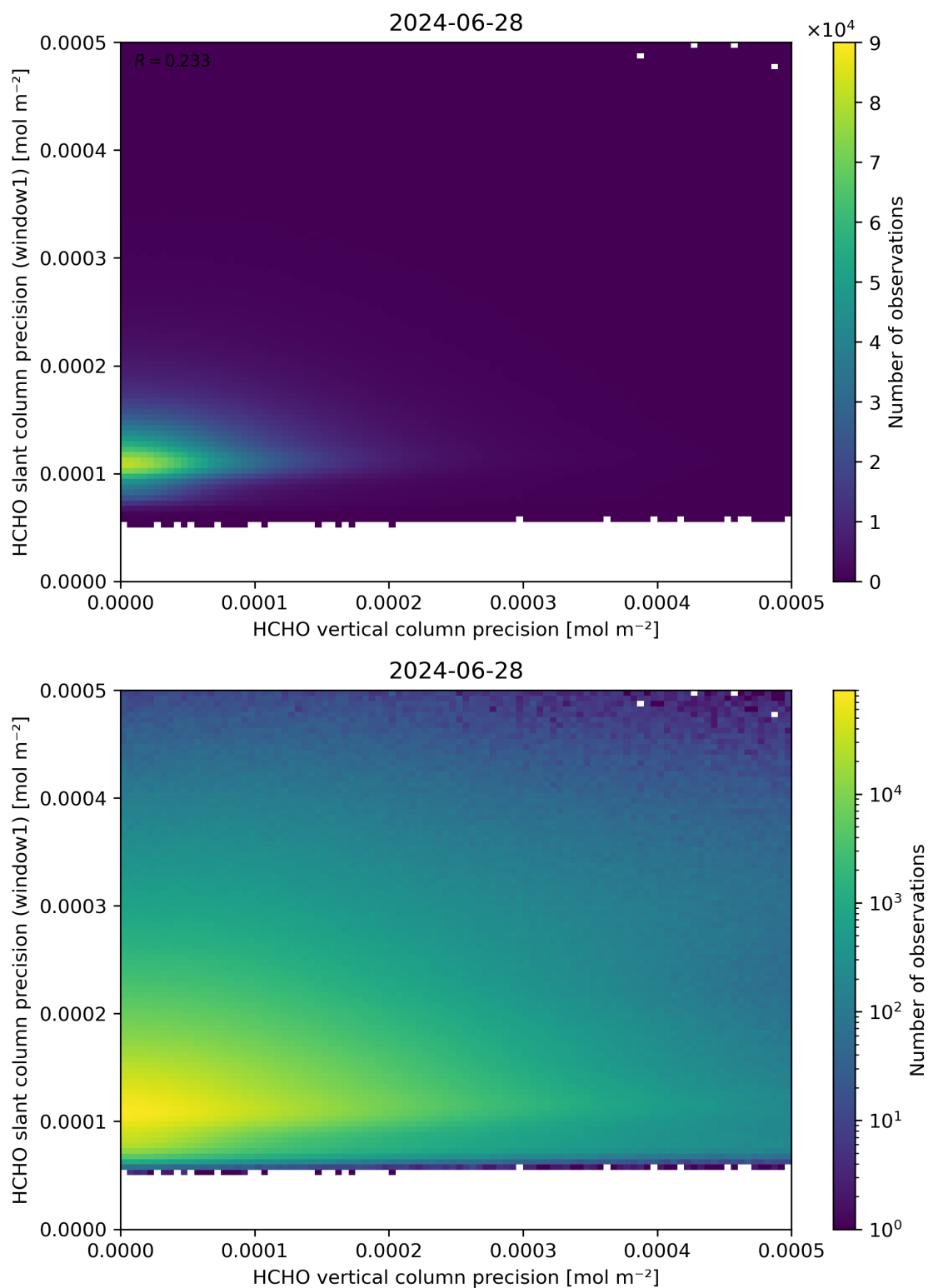
Figure 143: Scatter density plot of “HCHO vertical column precision” against “HCHO slant column precision (window1)” for 2024-06-27 to 2024-06-29.
