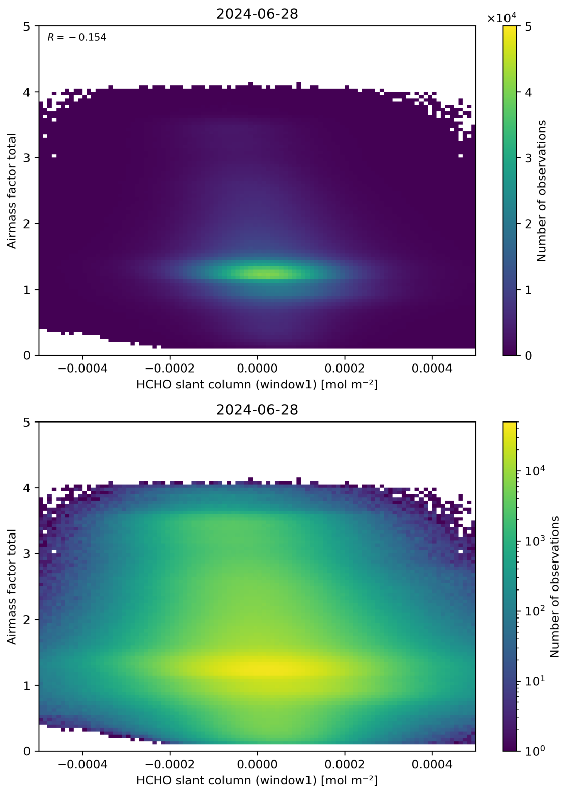
Figure 85: Scatter density plot of “HCHO slant column (window1)” against “Airmass factor total” for 2024-06-27 to 2024-06-29.
