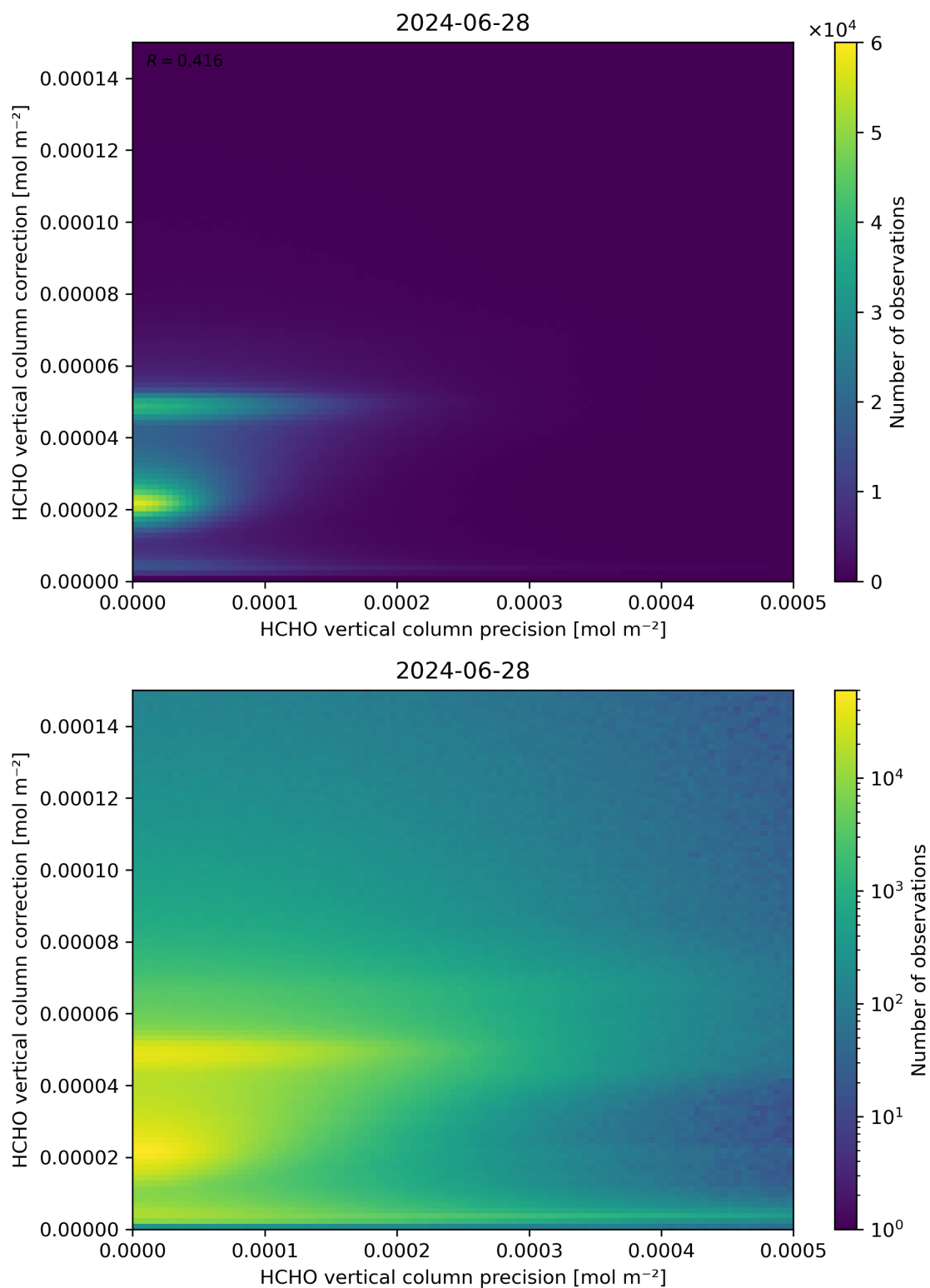
Figure 146: Scatter density plot of “HCHO vertical column precision” against “HCHO vertical column correction” for 2024-06-27 to 2024-06-29.
