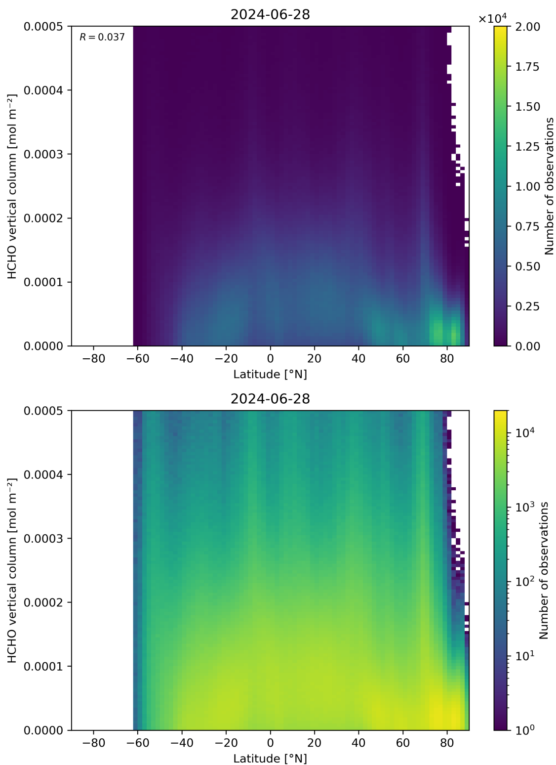
Figure 163: Scatter density plot of “Latitude” against “HCHO vertical column” for 2024-06-27 to 2024-06-29.
