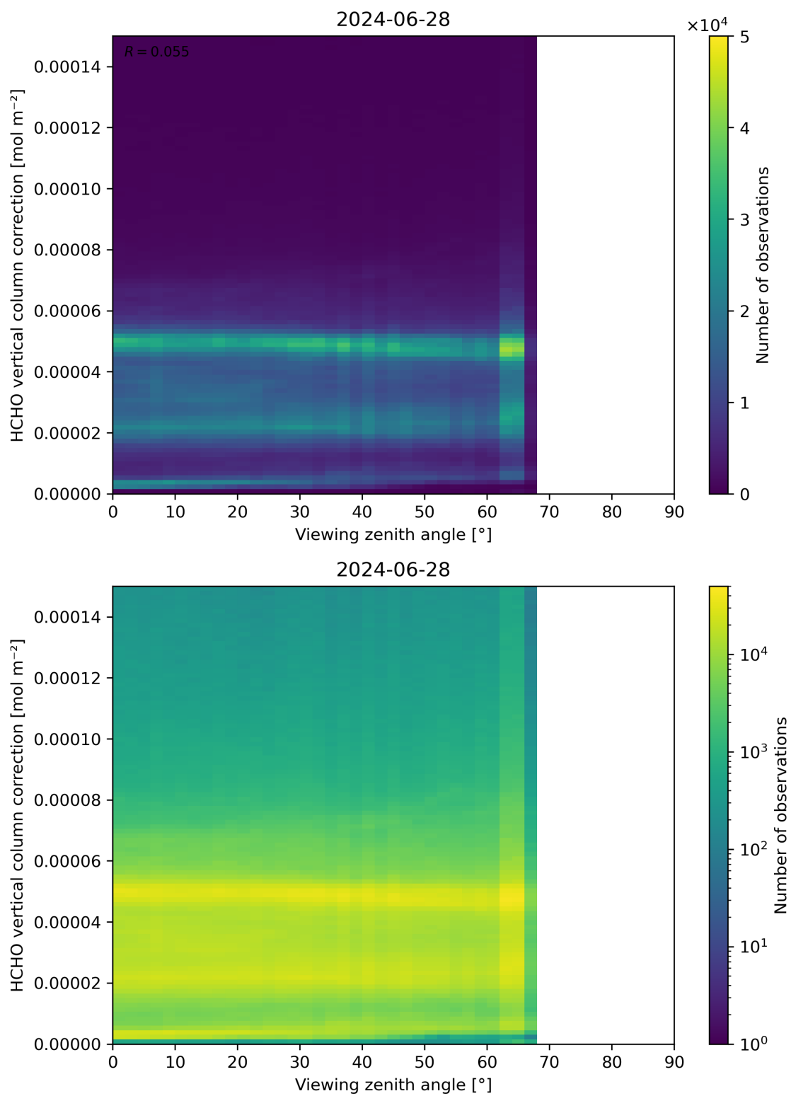
Figure 193: Scatter density plot of “Viewing zenith angle” against “HCHO vertical column correction” for 2024-06-27 to 2024-06-29.
