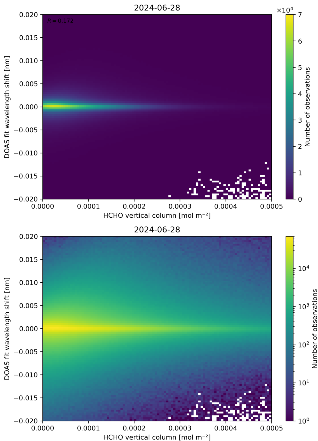
Figure 124: Scatter density plot of “HCHO vertical column” against “DOAS fit wavelength shift” for 2024-06-27 to 2024-06-29.
