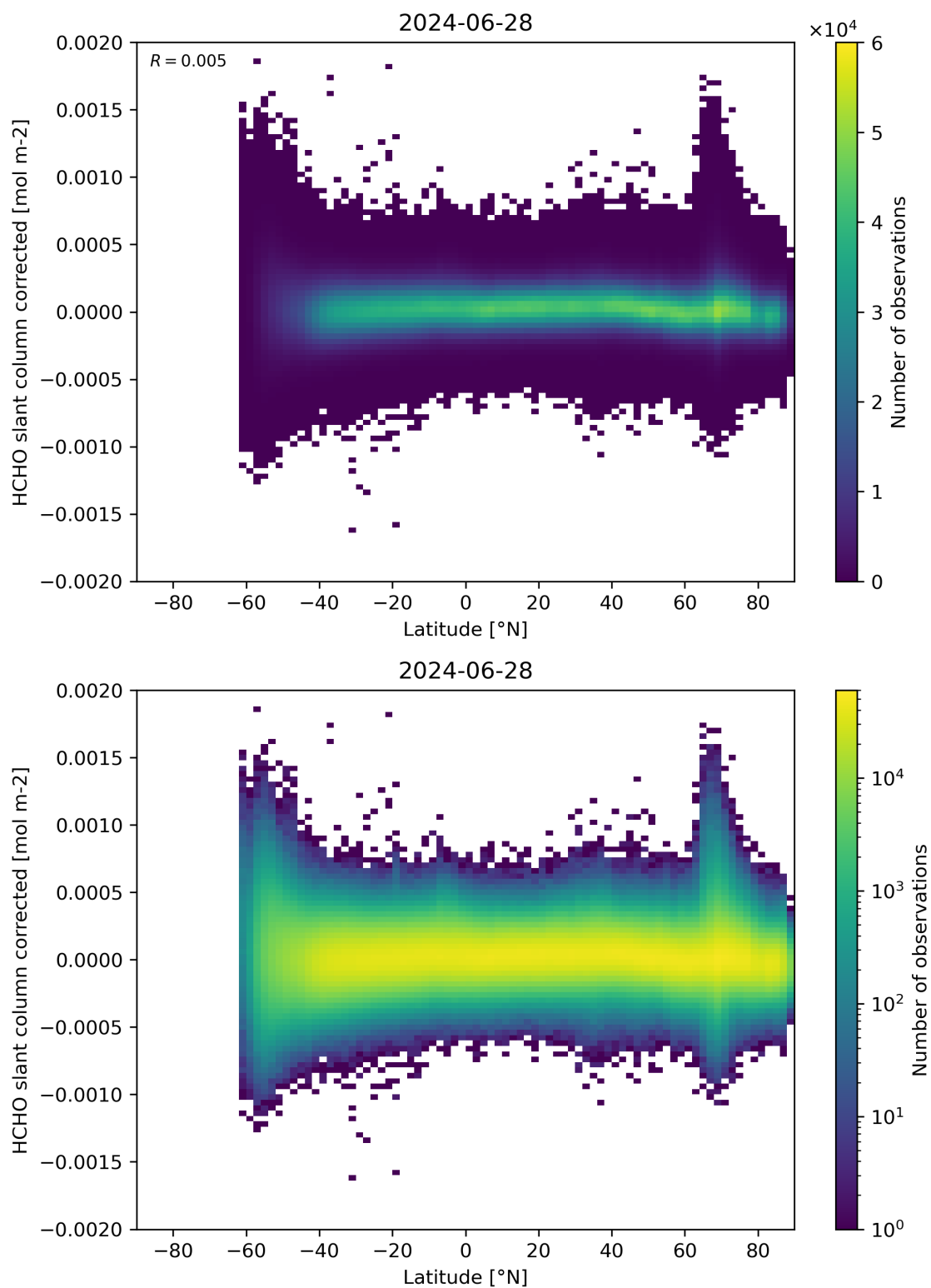
Figure 157: Scatter density plot of “Latitude” against “HCHO slant column corrected” for 2024-06-27 to 2024-06-29.
