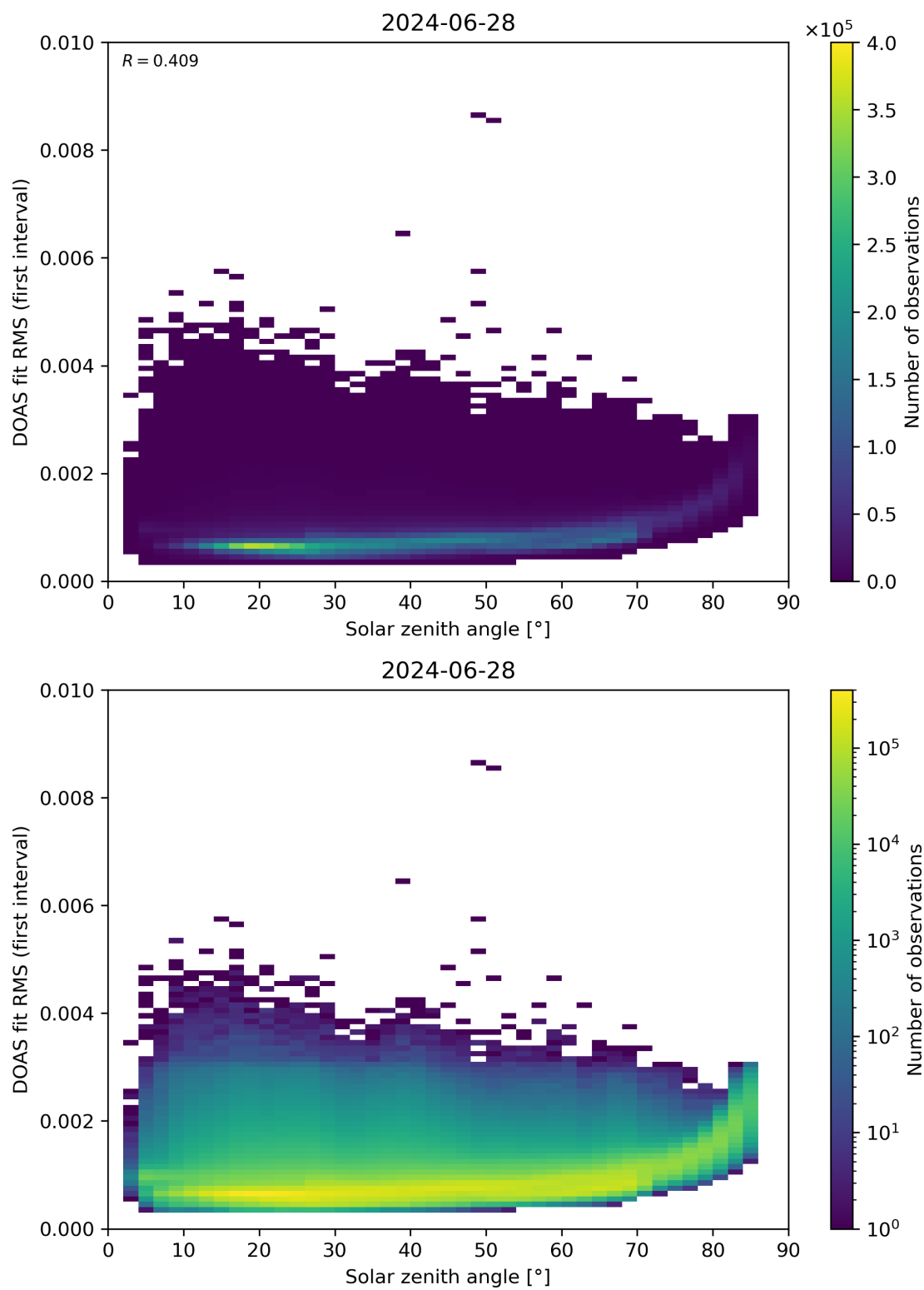
Figure 167: Scatter density plot of “Solar zenith angle” against “DOAS fit RMS (first interval)” for 2024-06-27 to 2024-06-29.
