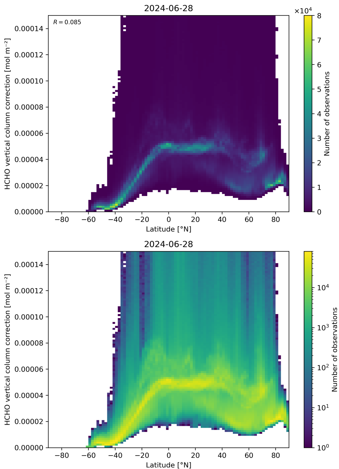
Figure 164: Scatter density plot of “Latitude” against “HCHO vertical column correction” for 2024-06-27 to 2024-06-29.
