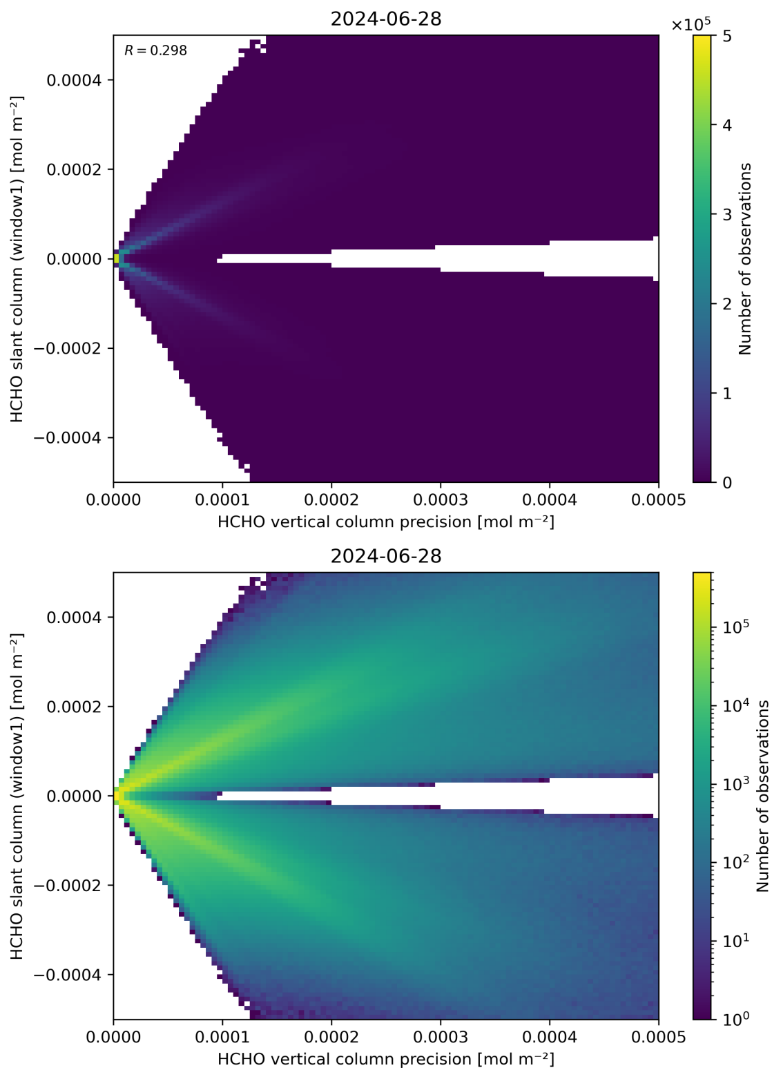
Figure 142: Scatter density plot of “HCHO vertical column precision” against “HCHO slant column (window1)” for 2024-06-27 to 2024-06-29.
