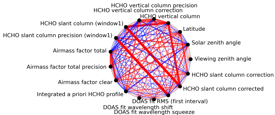
Figure 1: Map of correlation graph for 2024-06-27 to 2024-06-29.
