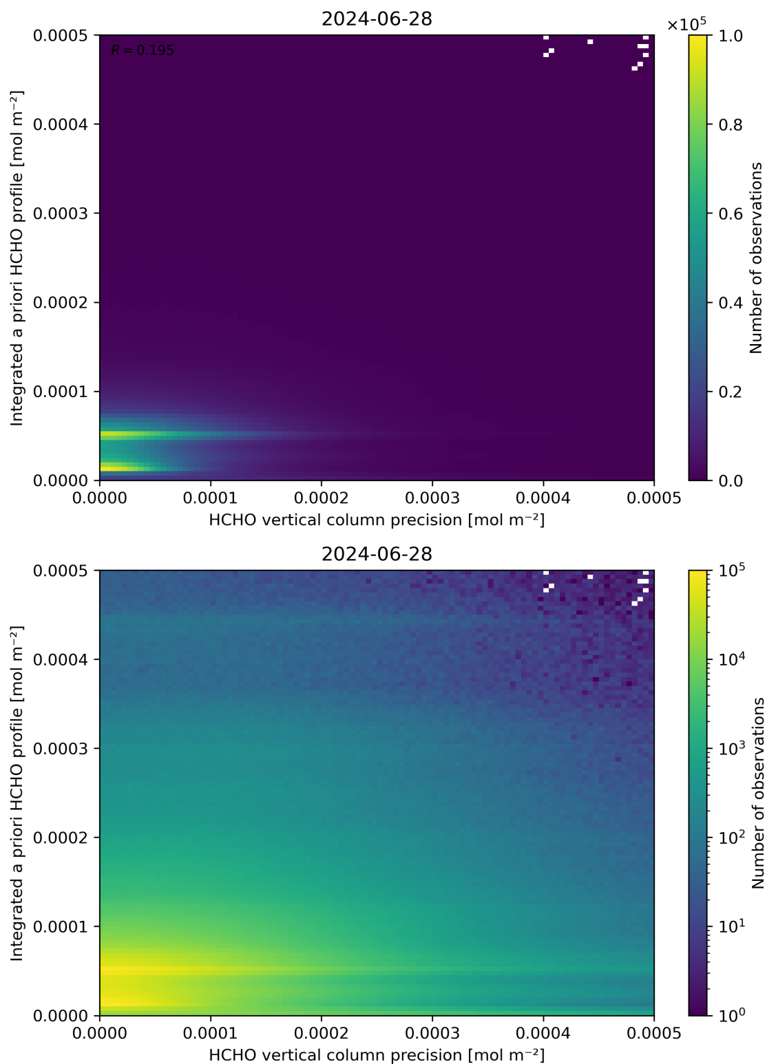
Figure 147: Scatter density plot of “HCHO vertical column precision” against “Integrated a priori HCHO profile” for 2024-06-27 to 2024-06-29.
