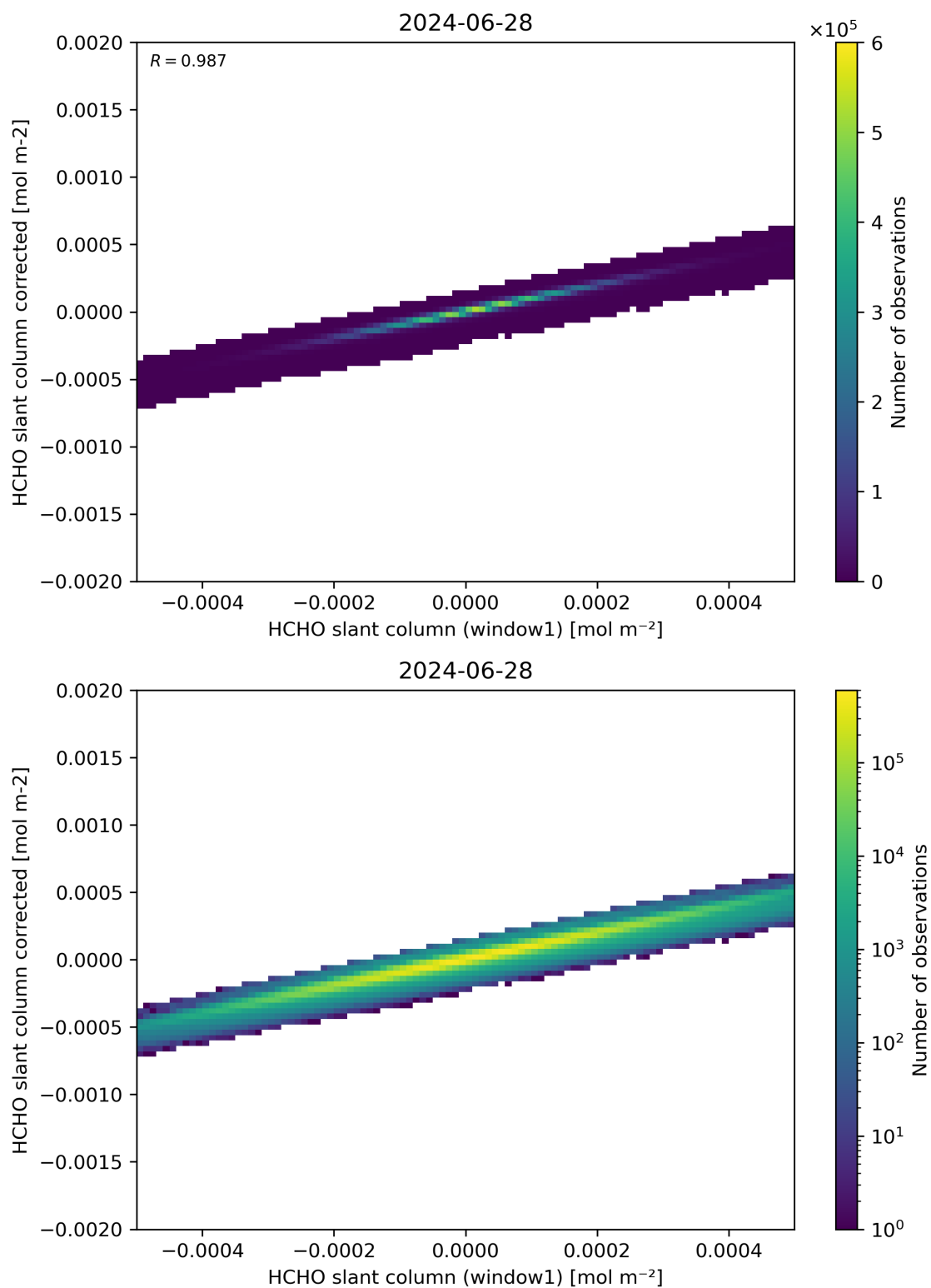
Figure 82: Scatter density plot of “HCHO slant column (window1)” against “HCHO slant column corrected” for 2024-06-27 to 2024-06-29.
