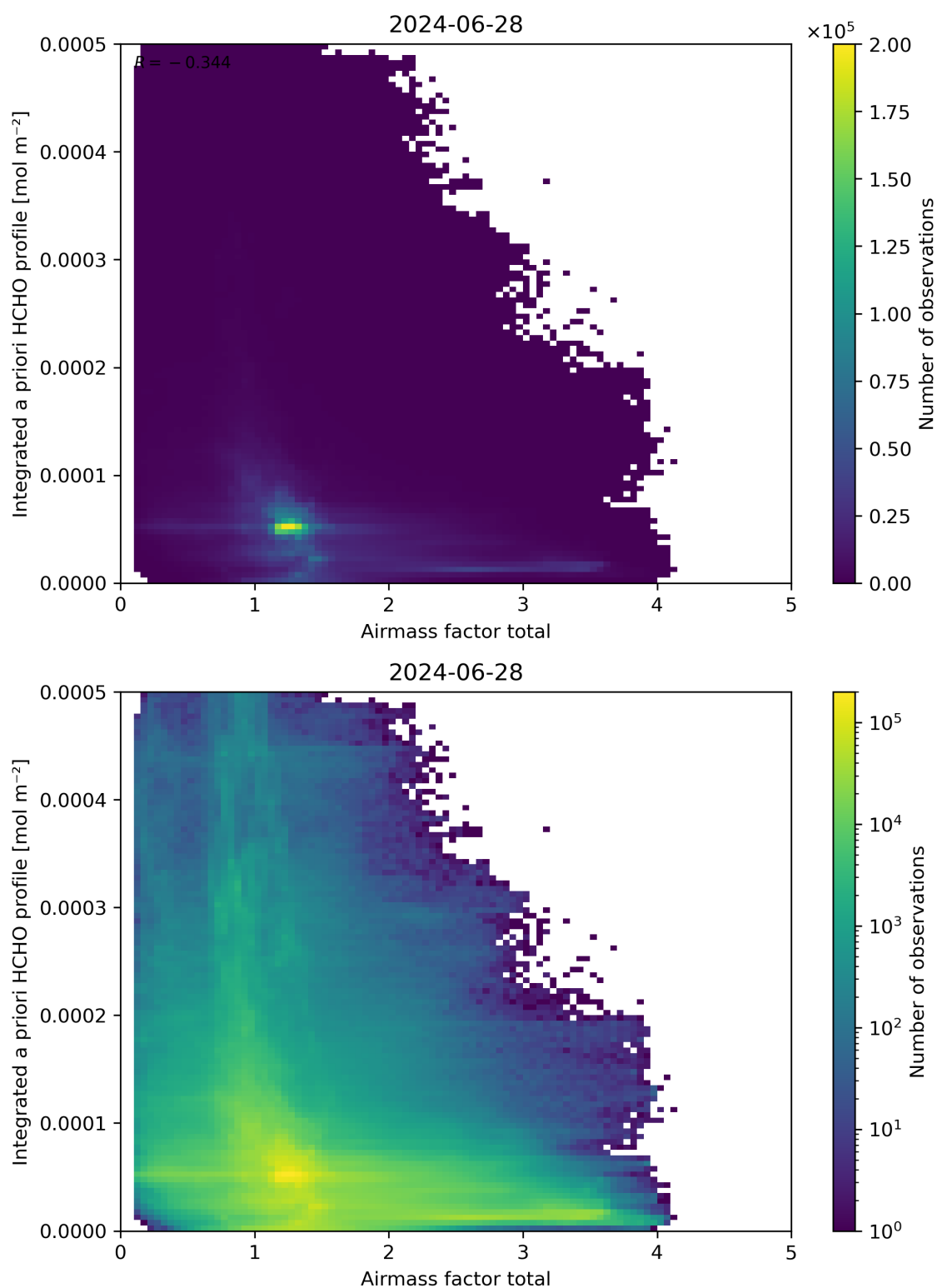
Figure 104: Scatter density plot of “Airmass factor total” against “Integrated a priori HCHO profile” for 2024-06-27 to 2024-06-29.
