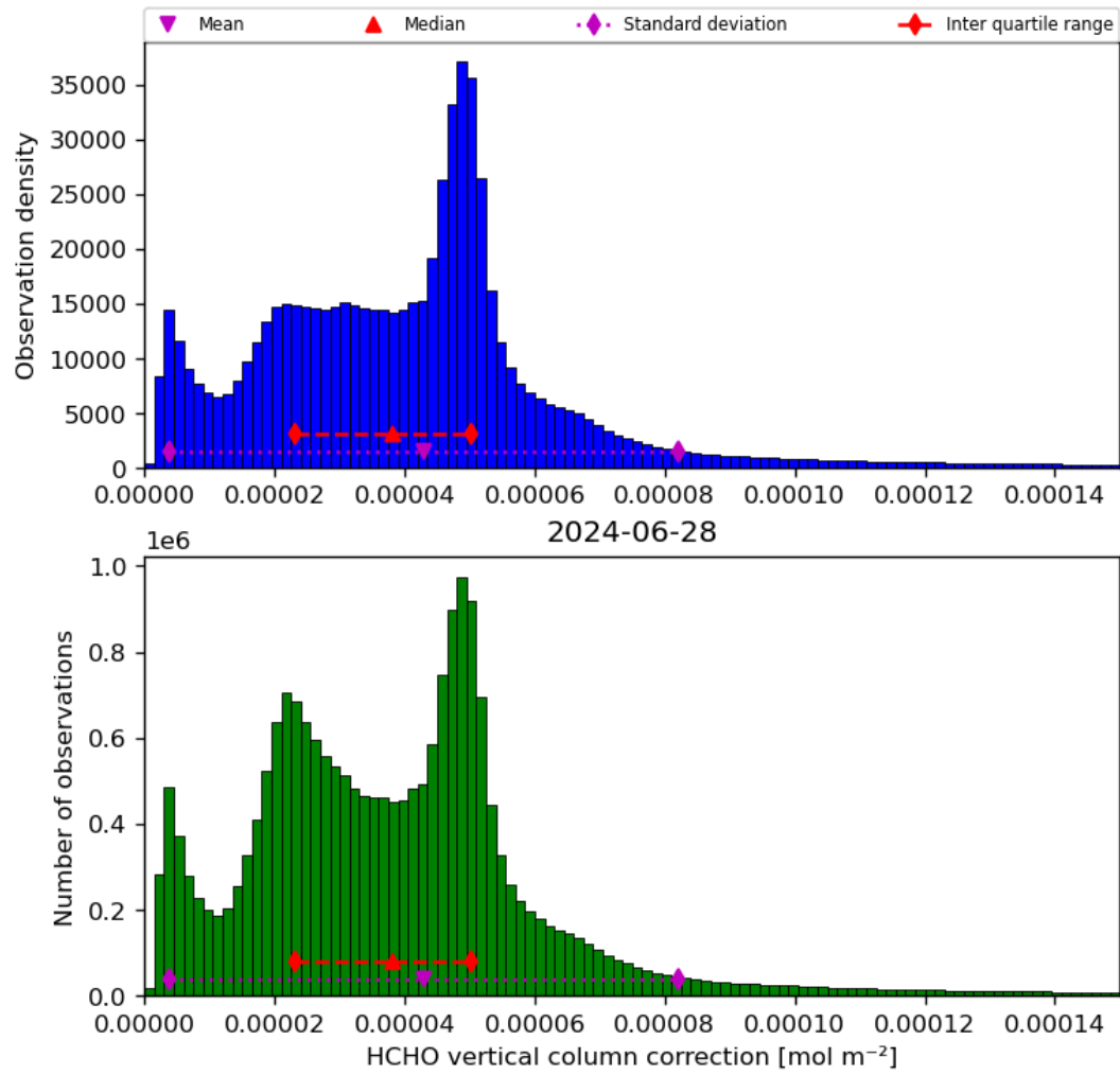
Figure 37: Histogram of “HCHO vertical column correction” for 2024-06-27 to 2024-06-29
