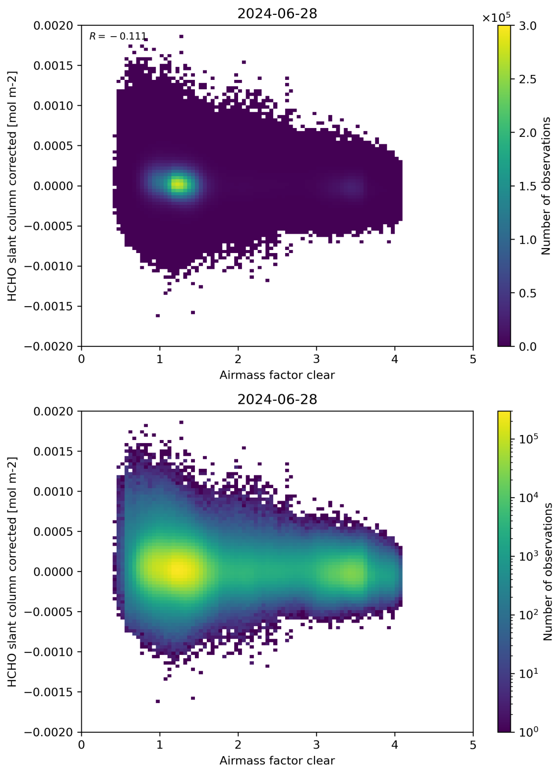
Figure 74: Scatter density plot of “Airmass factor clear” against “HCHO slant column corrected” for 2024-06-27 to 2024-06-29.
