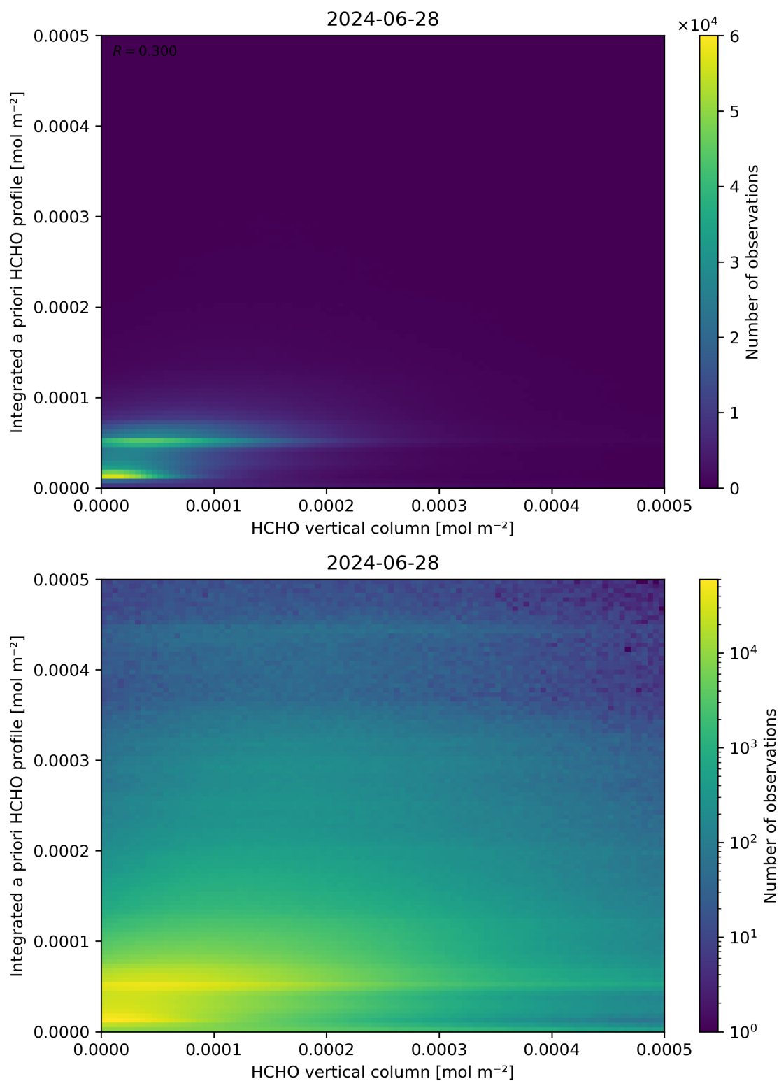
Figure 135: Scatter density plot of “HCHO vertical column” against “Integrated a priori HCHO profile” for 2024-06-27 to 2024-06-29.
