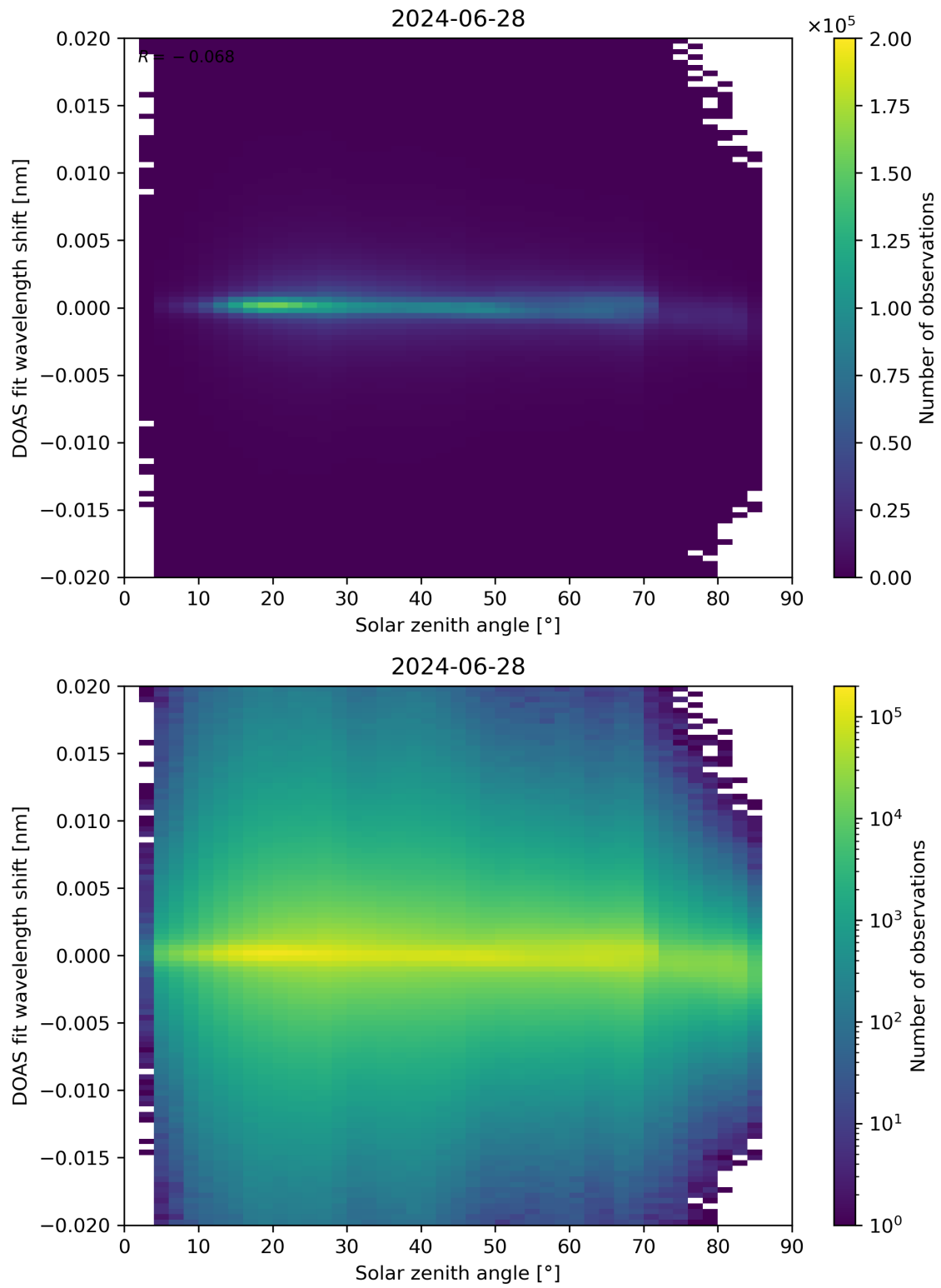
Figure 168: Scatter density plot of “Solar zenith angle” against “DOAS fit wavelength shift” for 2024-06-27 to 2024-06-29.
