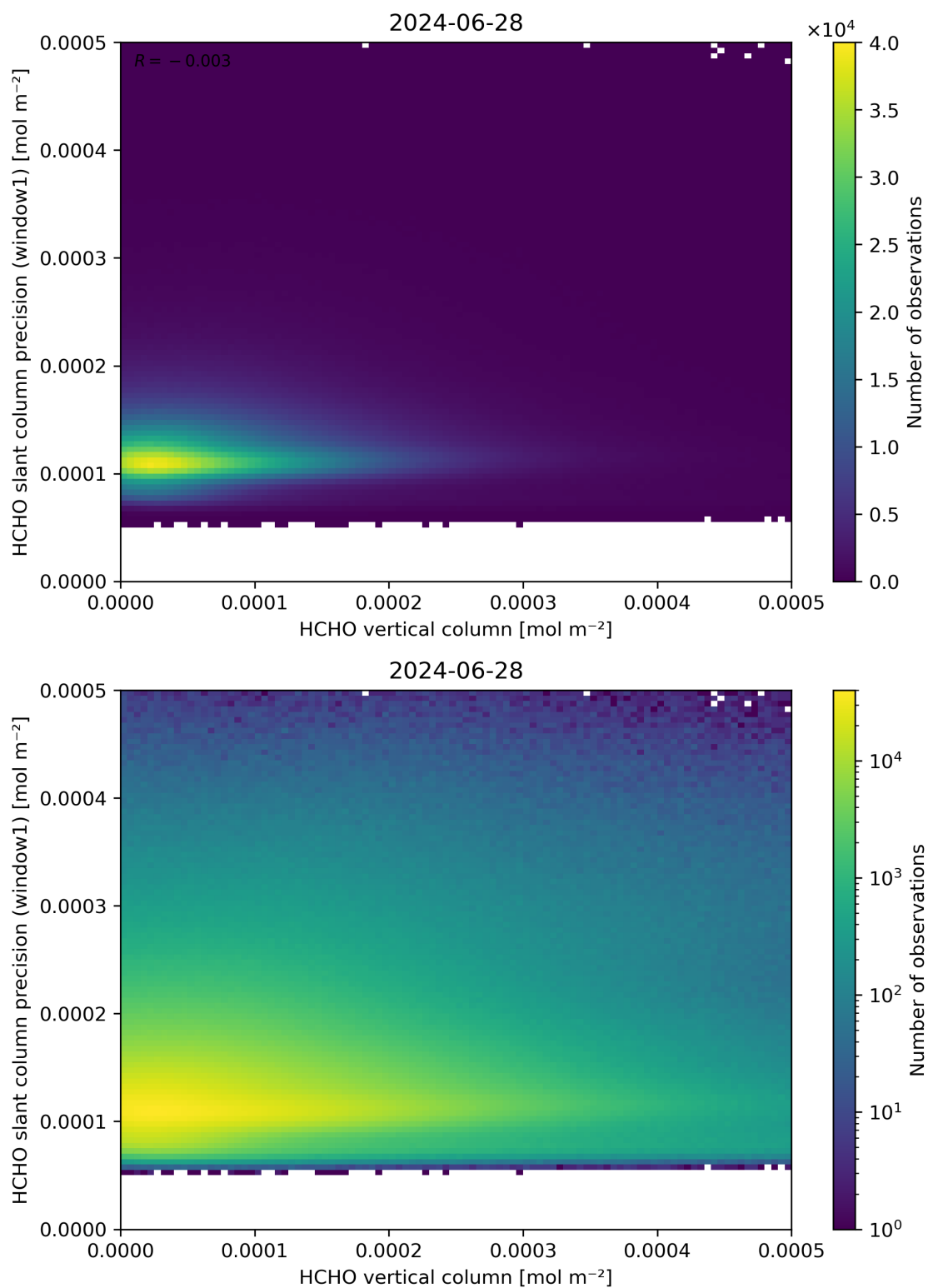
Figure 130: Scatter density plot of “HCHO vertical column” against “HCHO slant column precision (window1)” for 2024-06-27 to 2024-06-29.
