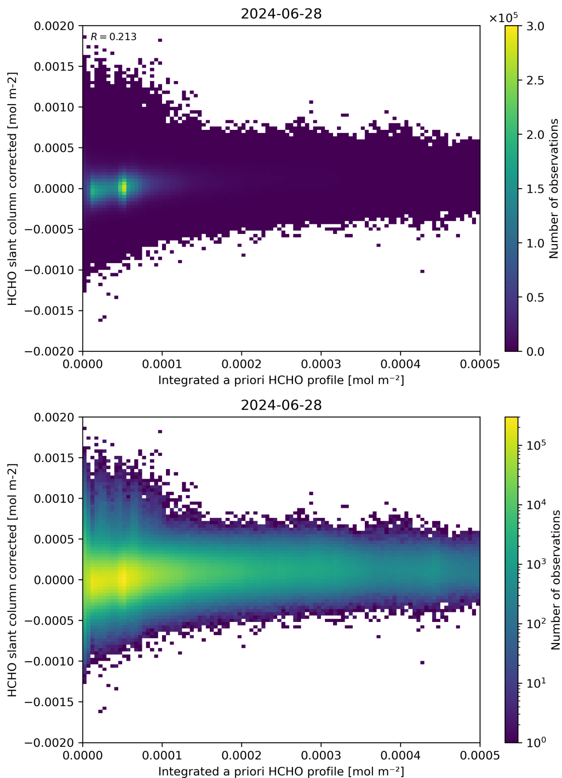
Figure 151: Scatter density plot of “Integrated a priori HCHO profile” against “HCHO slant column corrected” for 2024-06-27 to 2024-06-29.
