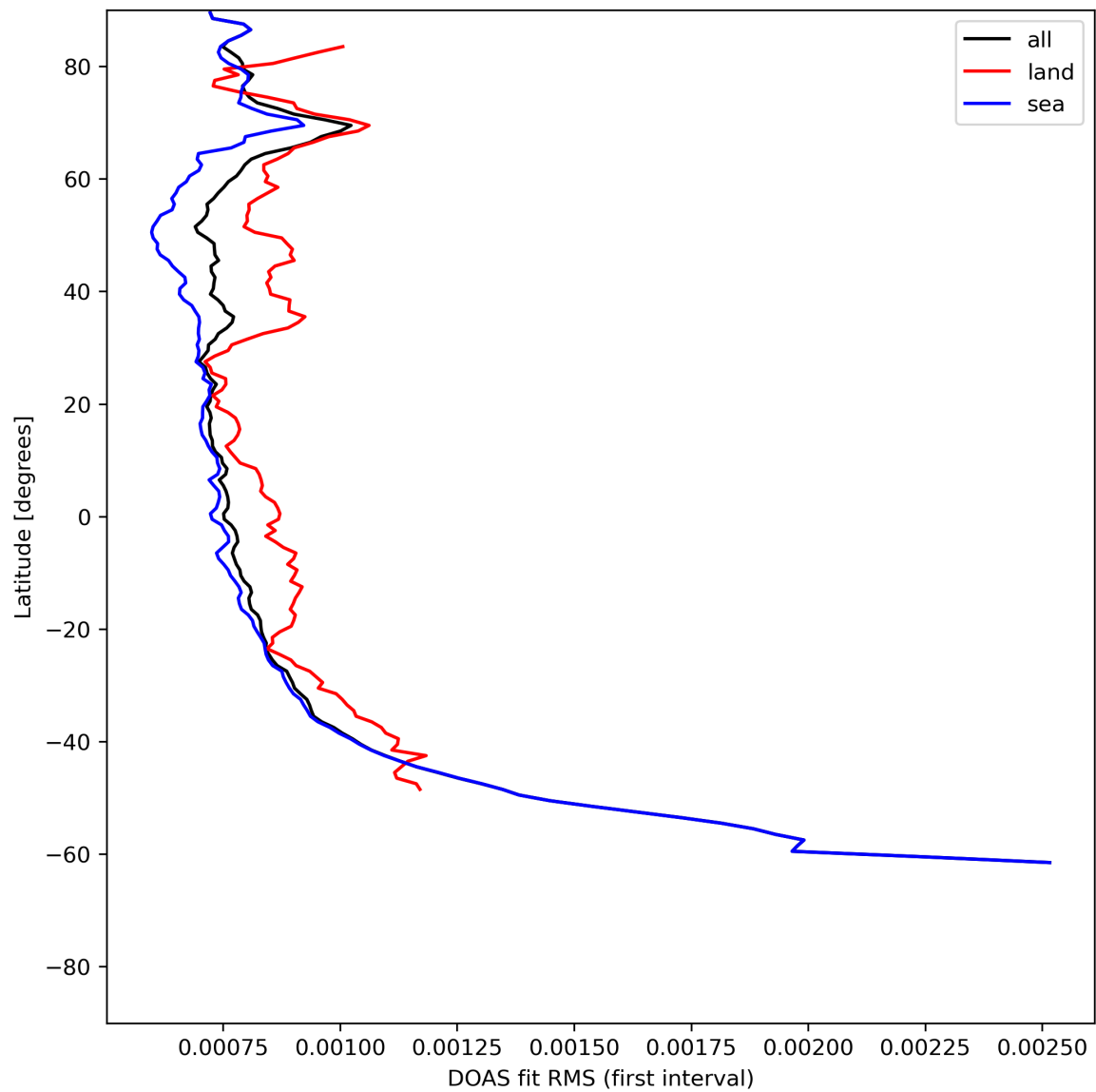
Figure 32: Zonal average of “DOAS fit RMS (first interval)” for 2024-06-27 to 2024-06-29.
