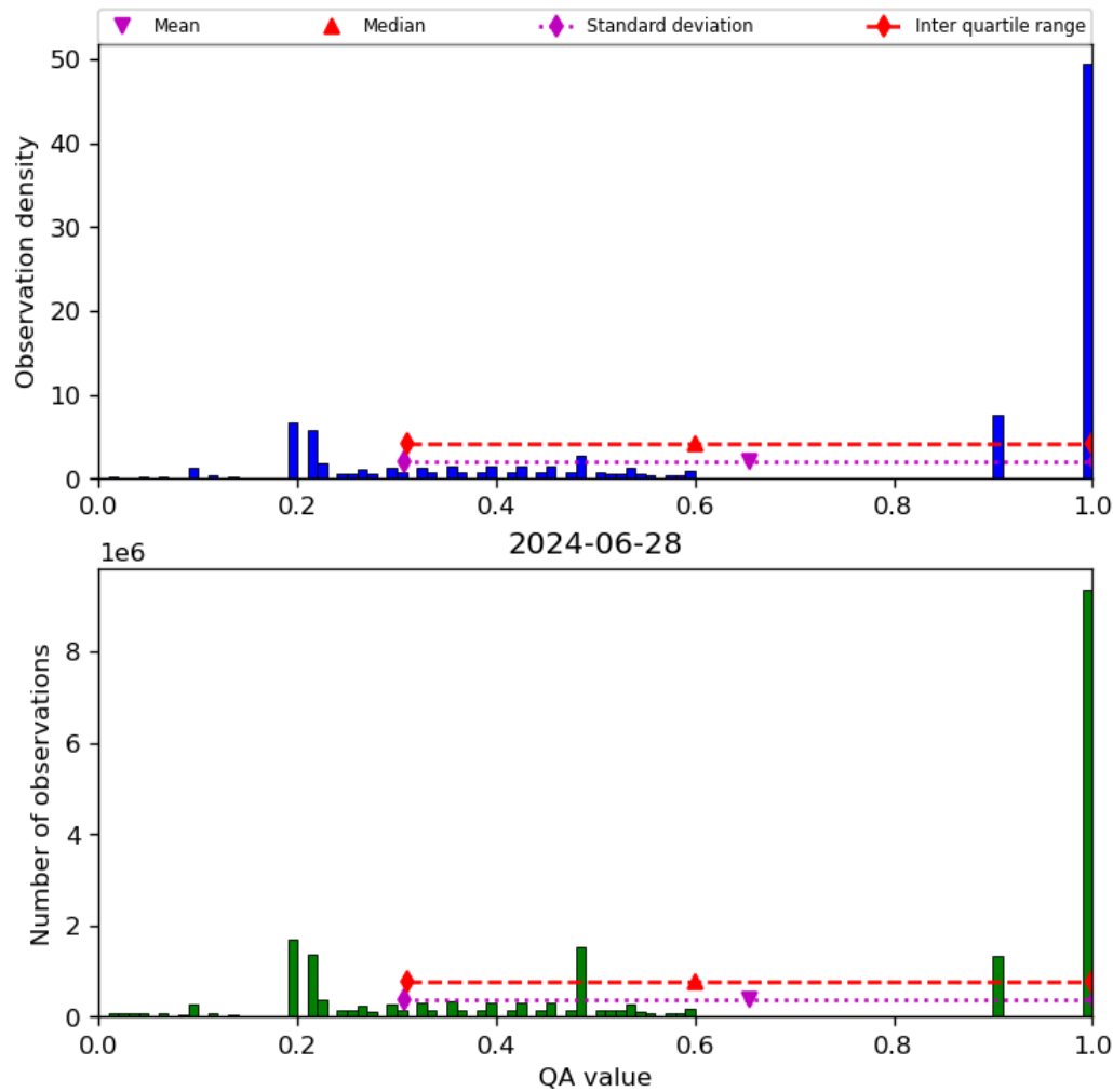
Figure 34: Histogram of “QA value” for 2024-06-27 to 2024-06-29
