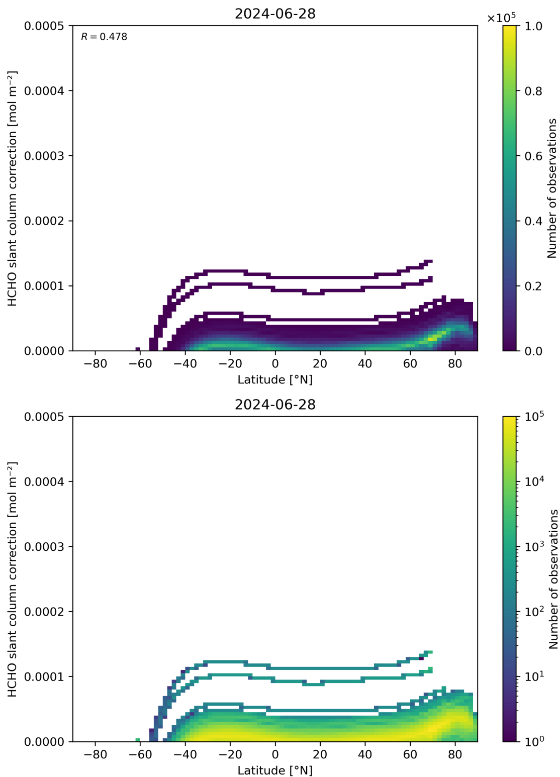
Figure 158: Scatter density plot of “Latitude” against “HCHO slant column correction” for 2024-06-27 to 2024-06-29.
