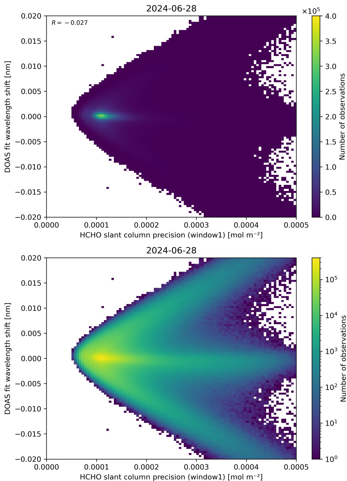
Figure 89: Scatter density plot of “HCHO slant column precision (window1)” against “DOAS fit wavelength shift” for 2024-06-27 to 2024-06-29.
