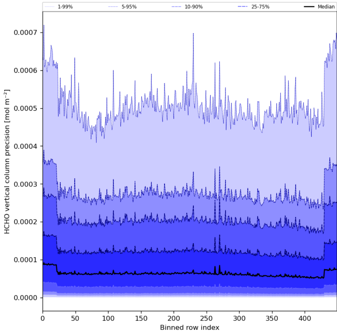
Figure 50: Along track statistics of “HCHO vertical column precision” for 2024-06-27 to 2024-06-29
