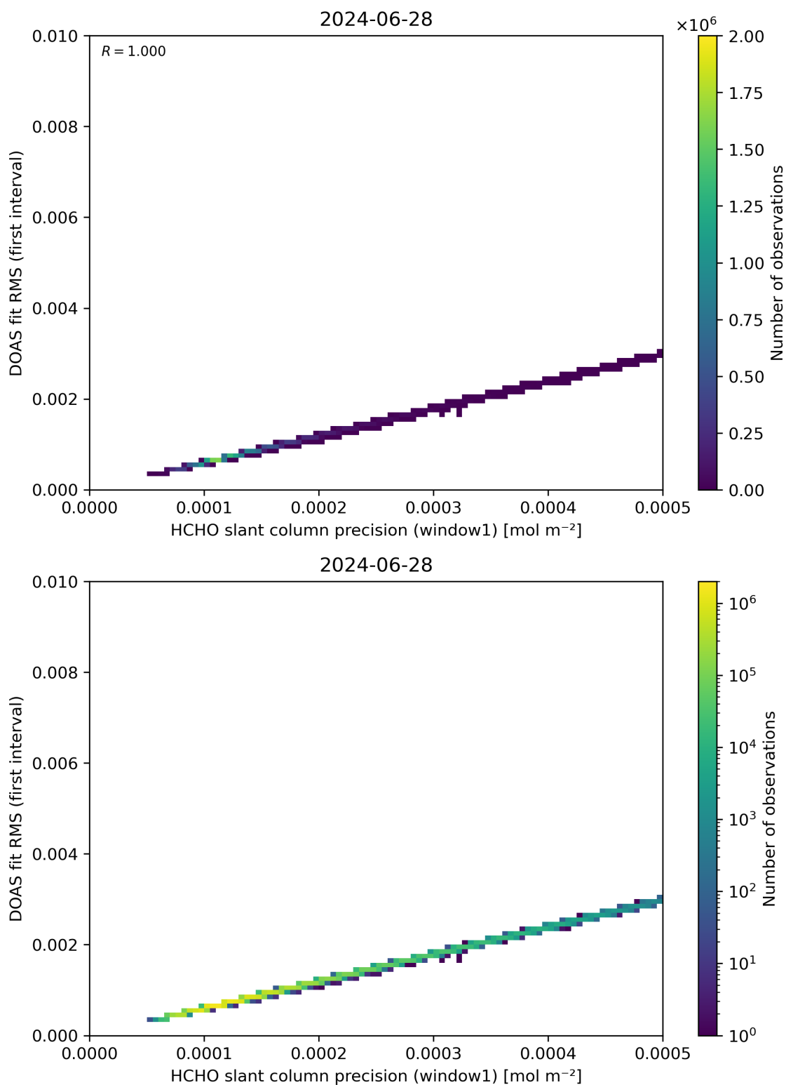
Figure 88: Scatter density plot of “HCHO slant column precision (window1)” against “DOAS fit RMS (first interval)” for 2024-06-27 to 2024-06-29.
