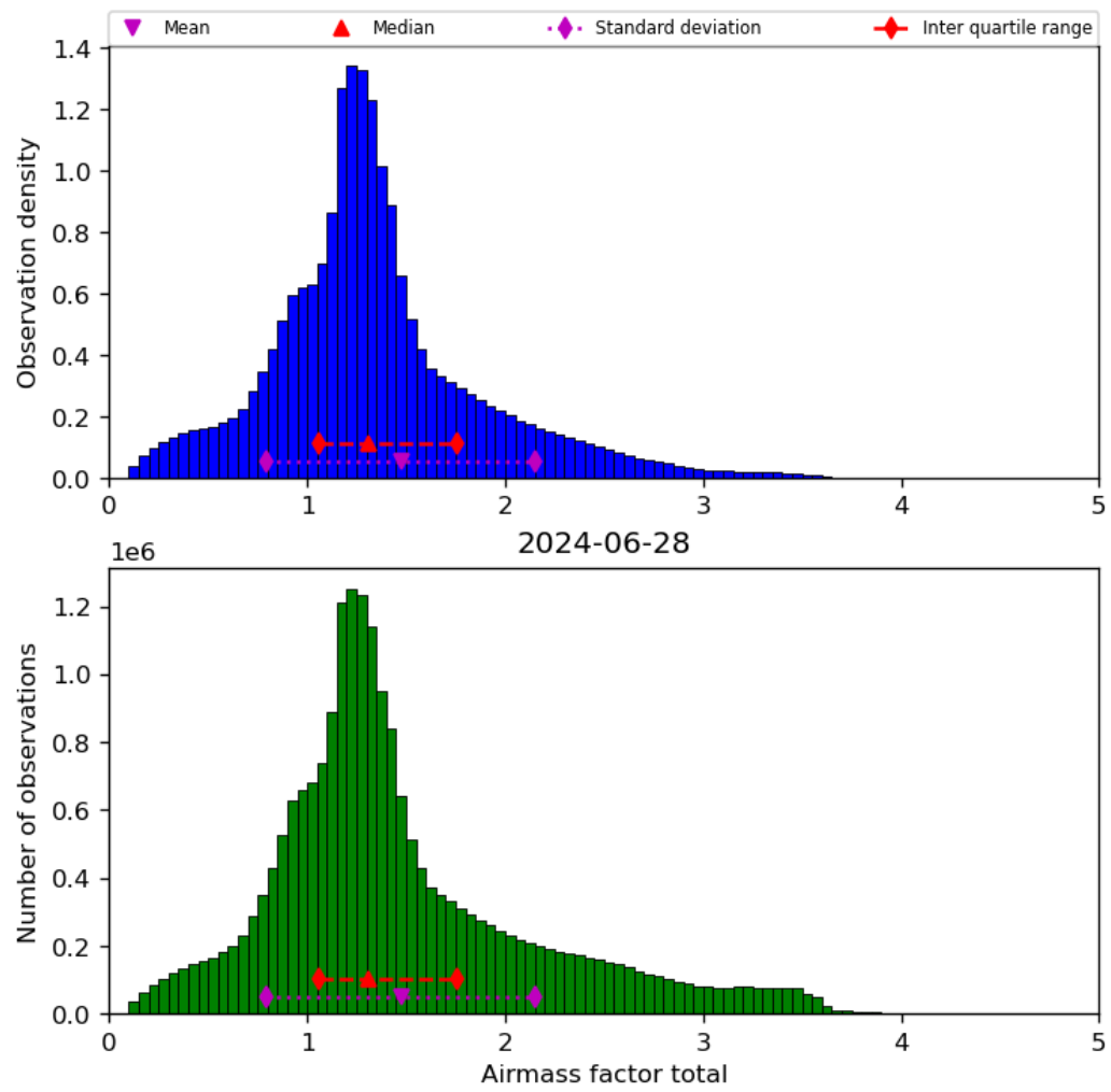
Figure 40: Histogram of “Airmass factor total” for 2024-06-27 to 2024-06-29
