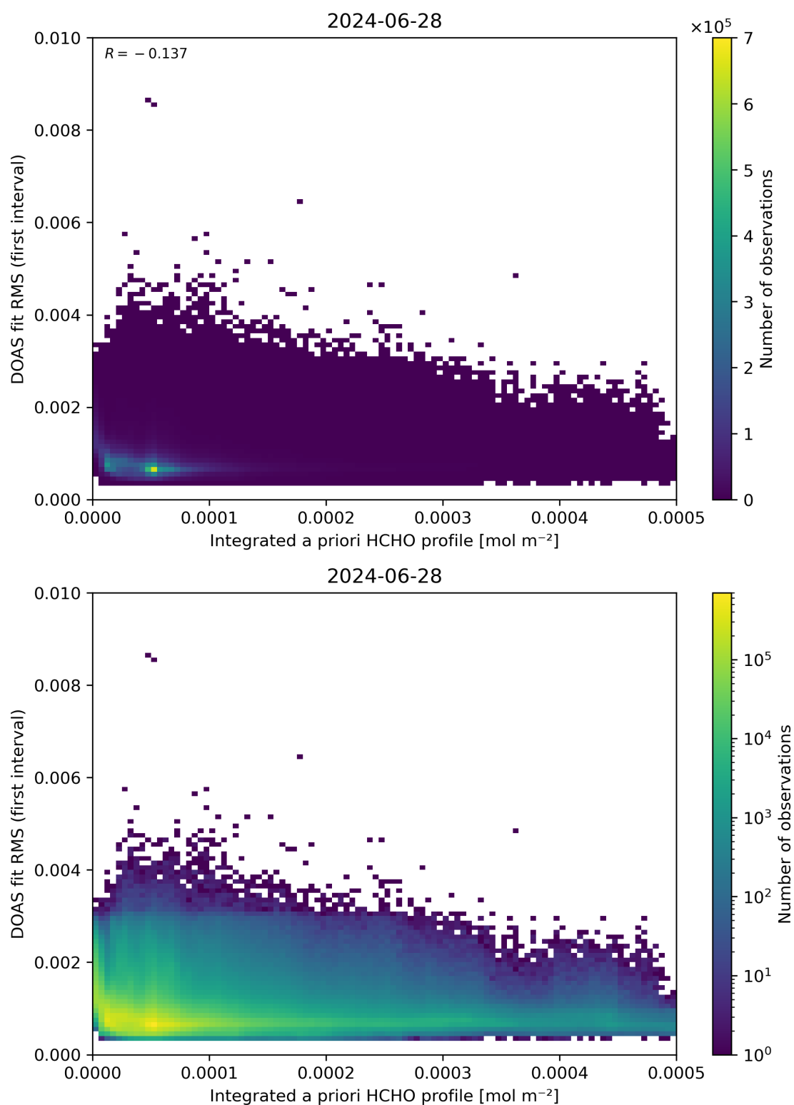
Figure 148: Scatter density plot of “Integrated a priori HCHO profile” against “DOAS fit RMS (first interval)” for 2024-06-27 to 2024-06-29.
