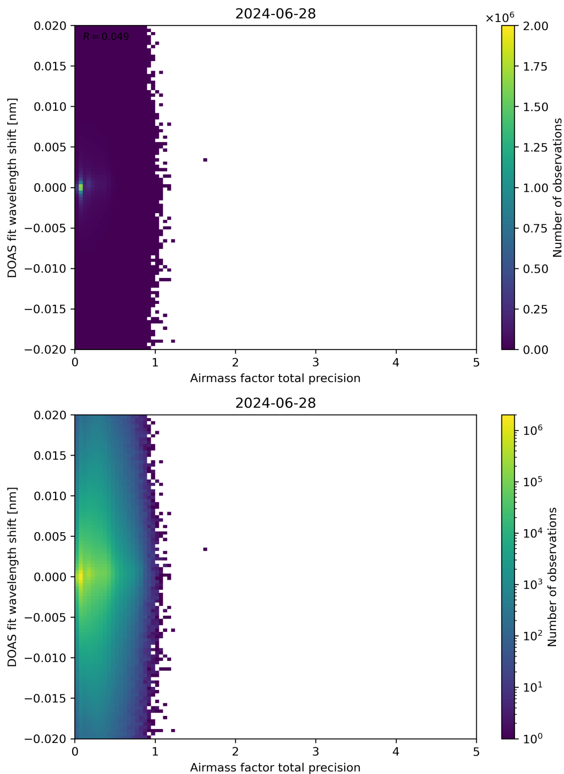
Figure 106: Scatter density plot of “Airmass factor total precision” against “DOAS fit wavelength shift” for 2024-06-27 to 2024-06-29.
