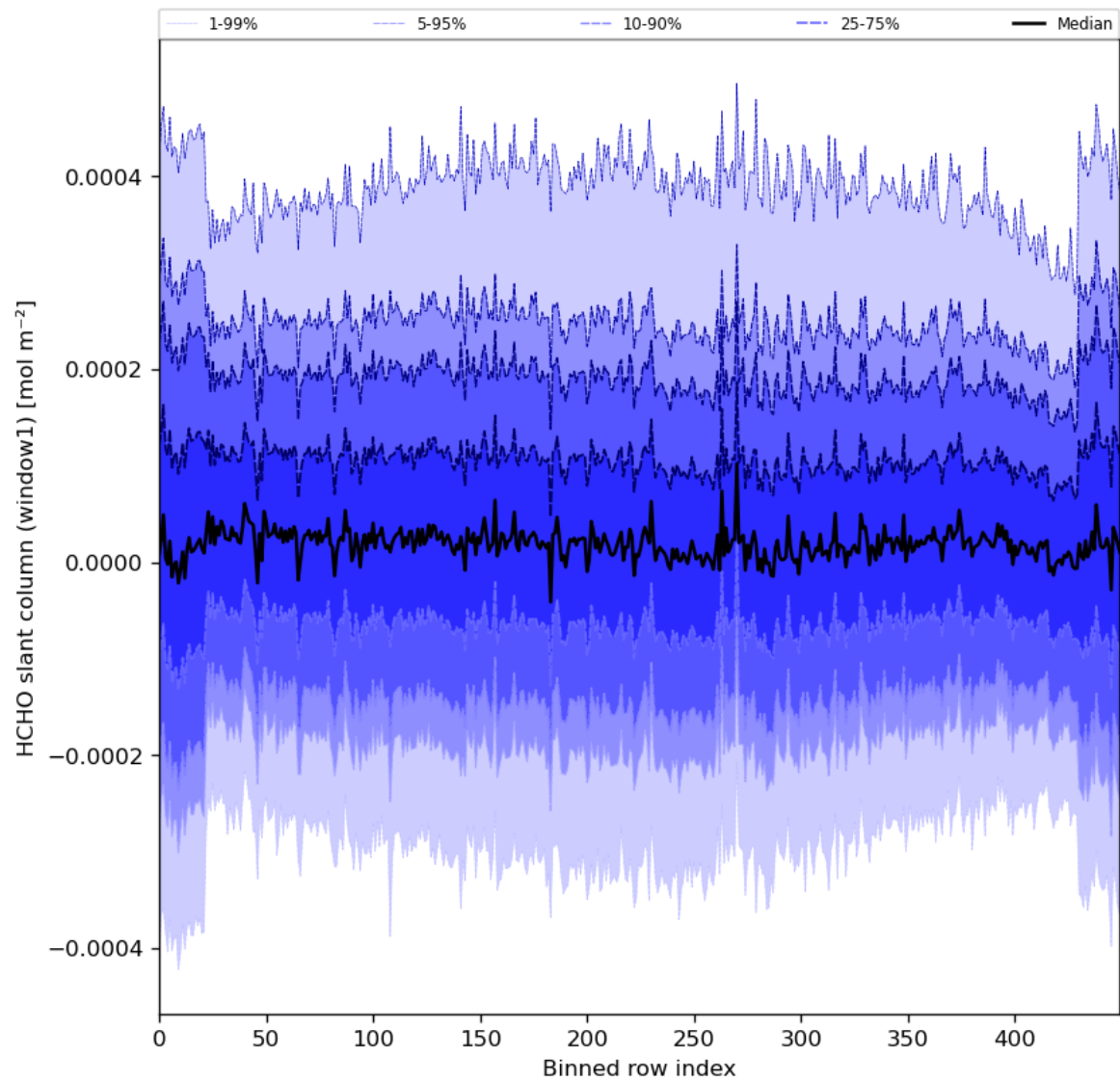
Figure 52: Along track statistics of “HCHO slant column (window1)” for 2024-06-29 to 2024-06-30
