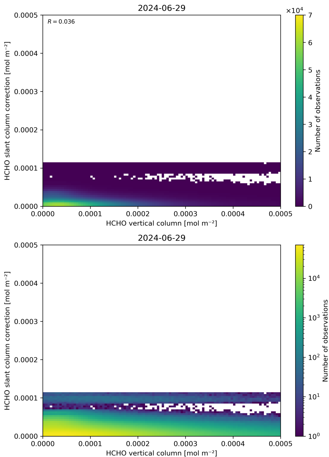
Figure 128: Scatter density plot of “HCHO vertical column” against “HCHO slant column correction” for 2024-06-29 to 2024-06-30.
