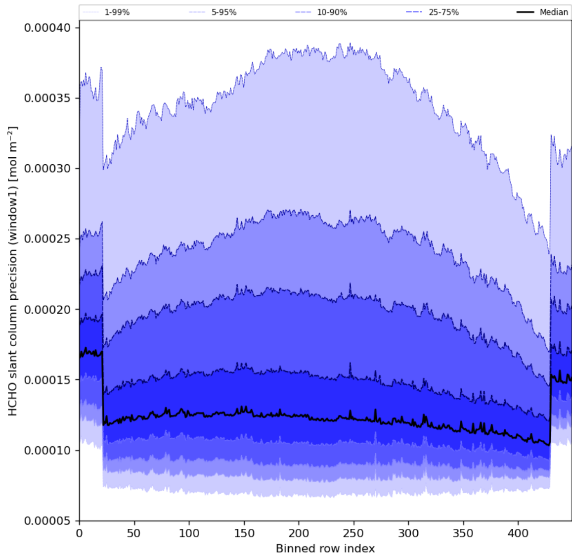
Figure 53: Along track statistics of “HCHO slant column precision (window1)” for 2024-06-29 to 2024-06-30
