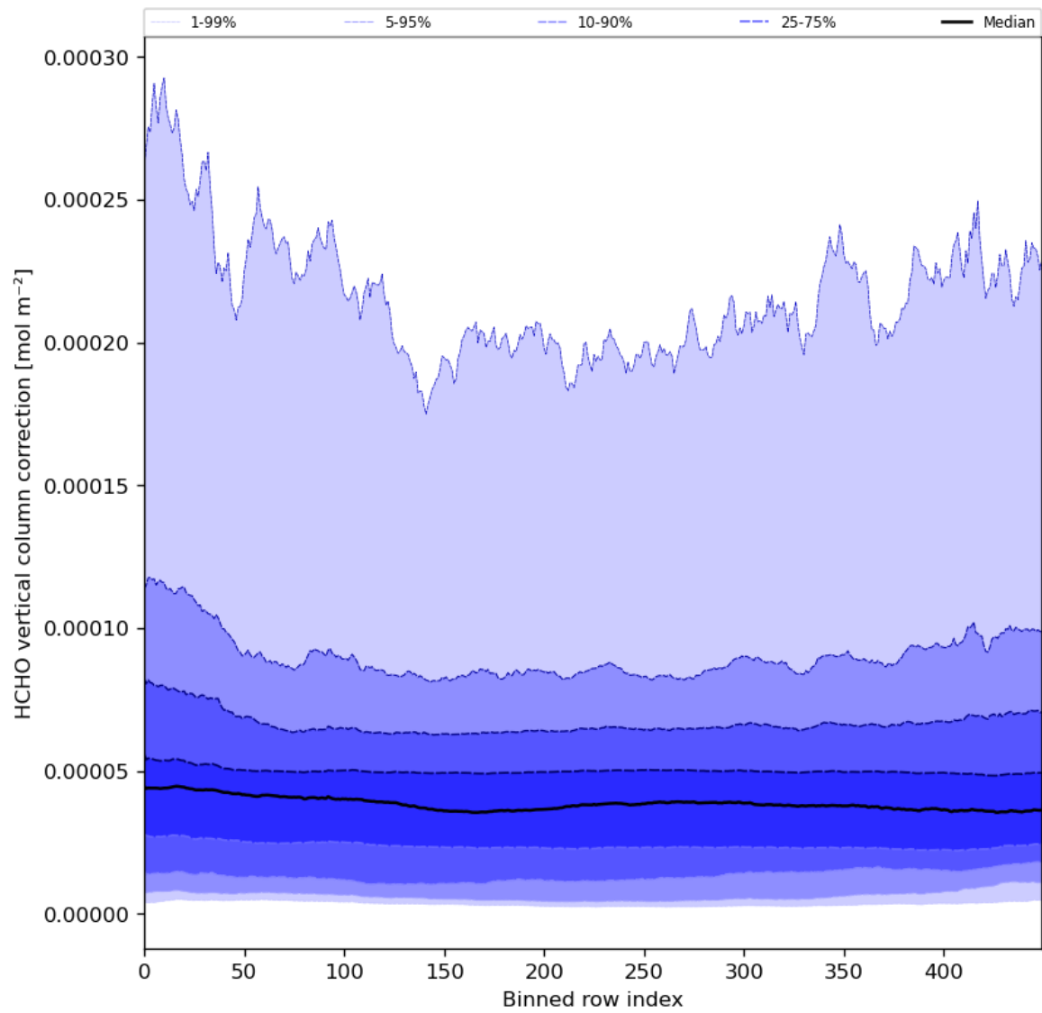
Figure 51: Along track statistics of “HCHO vertical column correction” for 2024-06-29 to 2024-06-30
