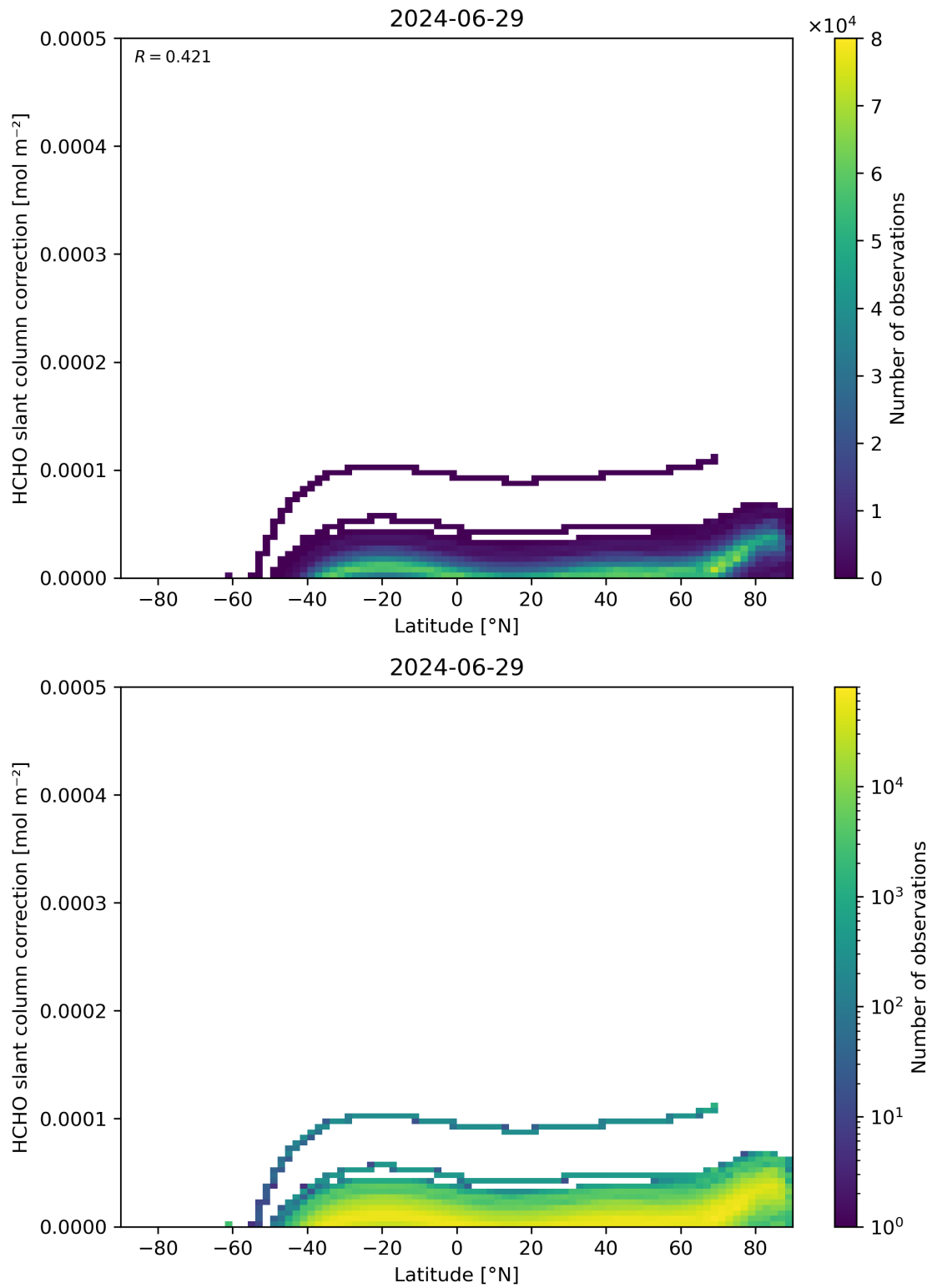
Figure 158: Scatter density plot of “Latitude” against “HCHO slant column correction” for 2024-06-29 to 2024-06-30.
