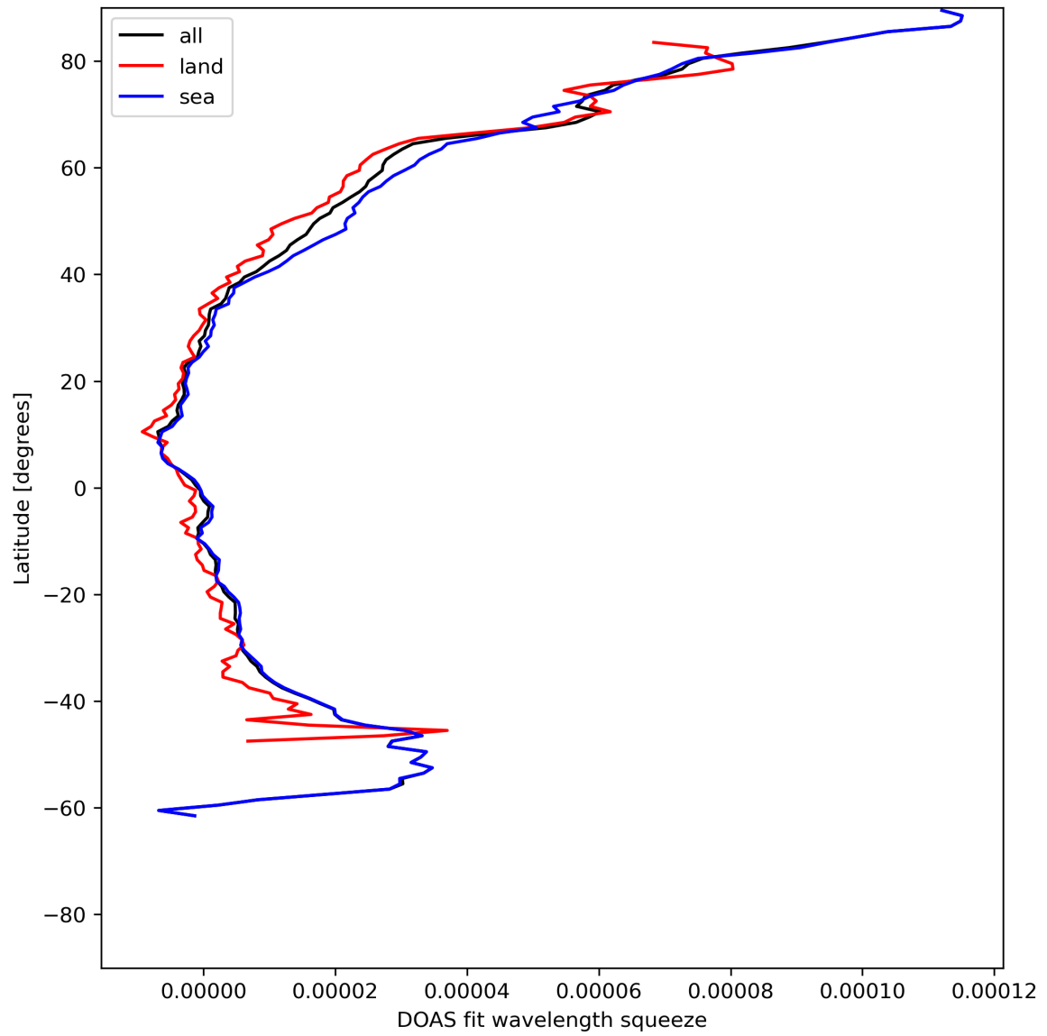
Figure 31: Zonal average of "DOAS fit wavelength squeeze" for 2024-06-29 to 2024-06-30.
