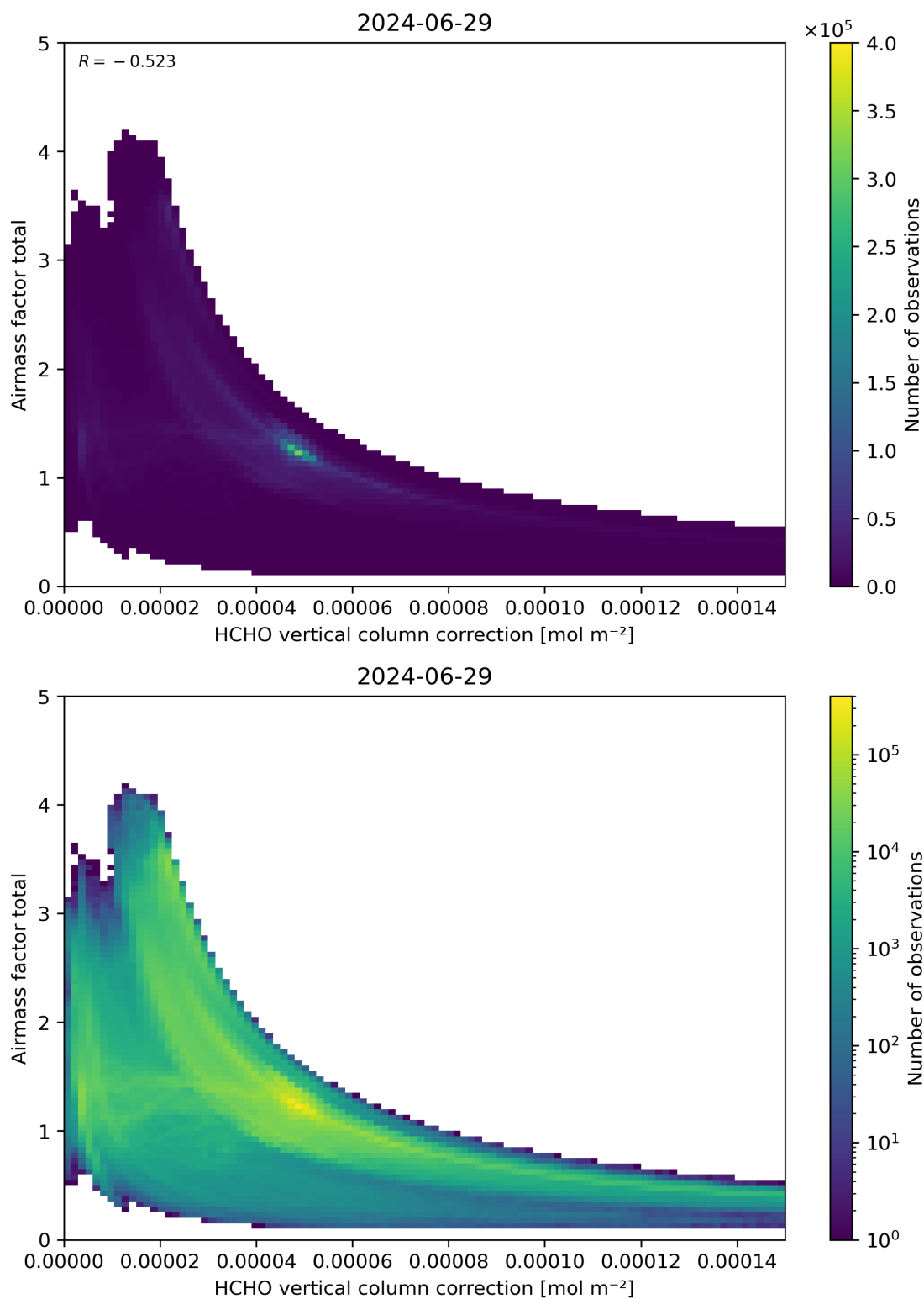
Figure 120: Scatter density plot of “HCHO vertical column correction” against “Airmass factor total” for 2024-06-29 to 2024-06-30.
