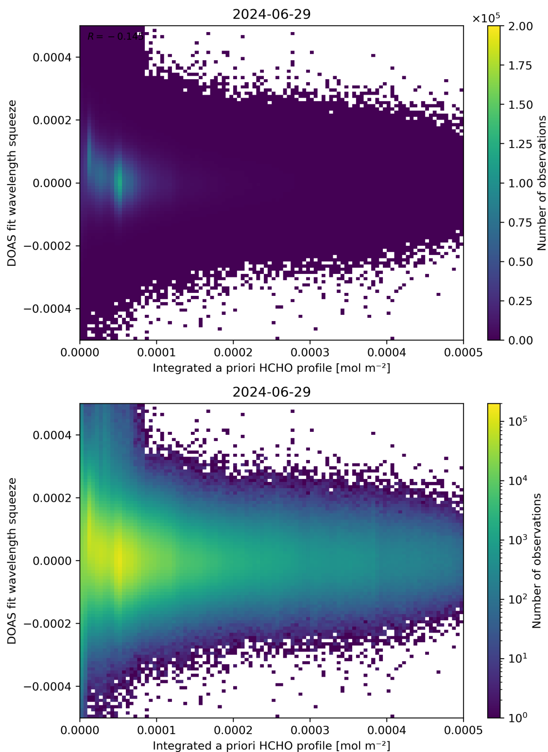
Figure 150: Scatter density plot of “Integrated a priori HCHO profile” against “DOAS fit wavelength squeeze” for 2024-06-29 to 2024-06-30.
