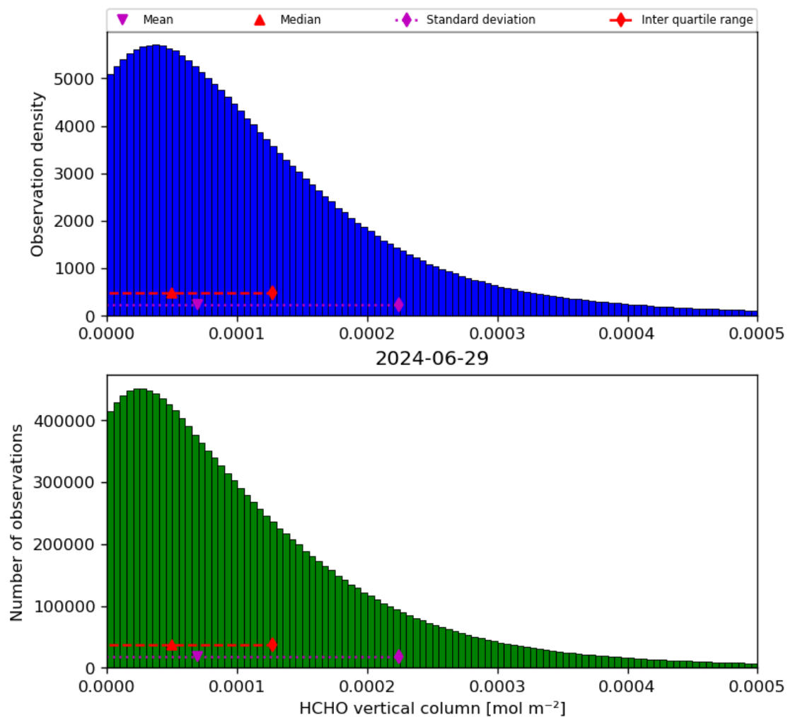
Figure 35: Histogram of “HCHO vertical column” for 2024-06-29 to 2024-06-30
