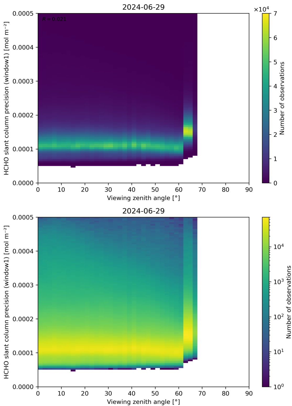
Figure 189: Scatter density plot of “Viewing zenith angle” against “HCHO slant column precision (window1)” for 2024-06-29 to 2024-06-30.
