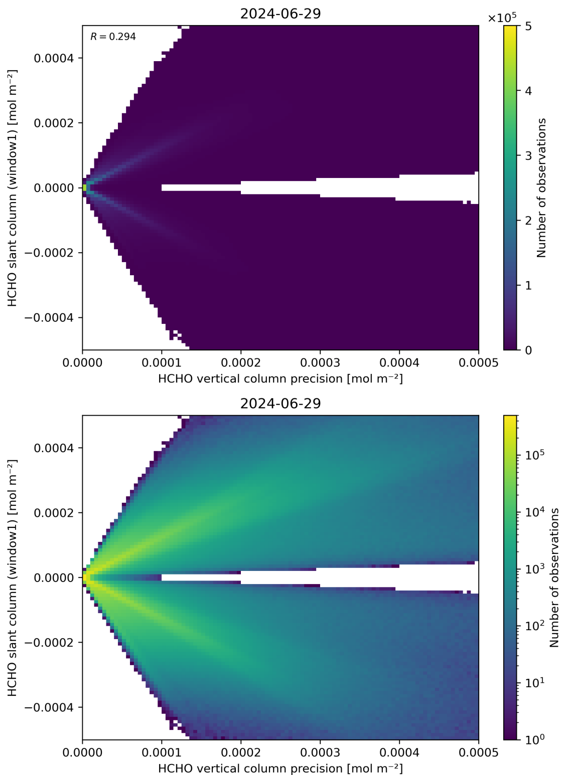
Figure 142: Scatter density plot of “HCHO vertical column precision” against “HCHO slant column (window1)” for 2024-06-29 to 2024-06-30.
