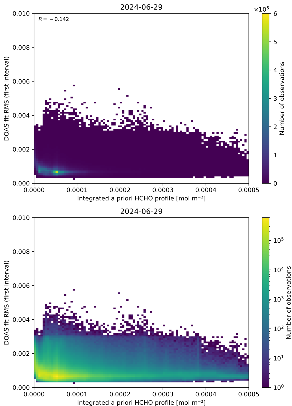
Figure 148: Scatter density plot of “Integrated a priori HCHO profile” against “DOAS fit RMS (first interval)” for 2024-06-29 to 2024-06-30.
