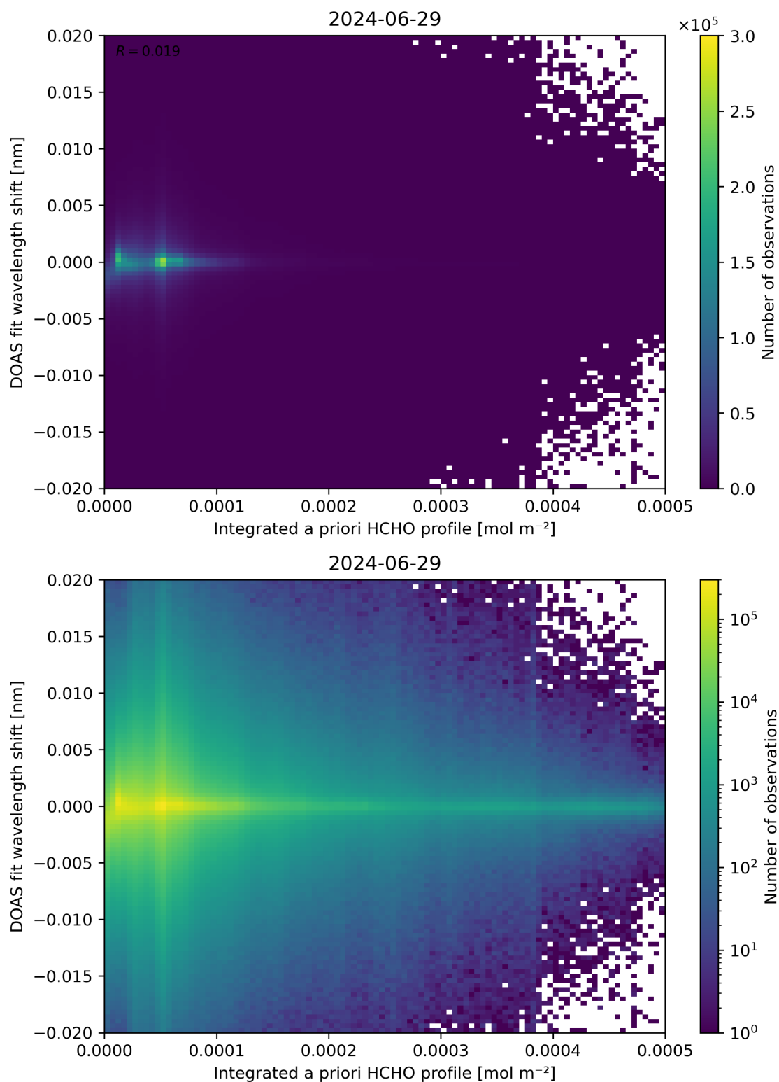
Figure 149: Scatter density plot of “Integrated a priori HCHO profile” against “DOAS fit wavelength shift” for 2024-06-29 to 2024-06-30.
