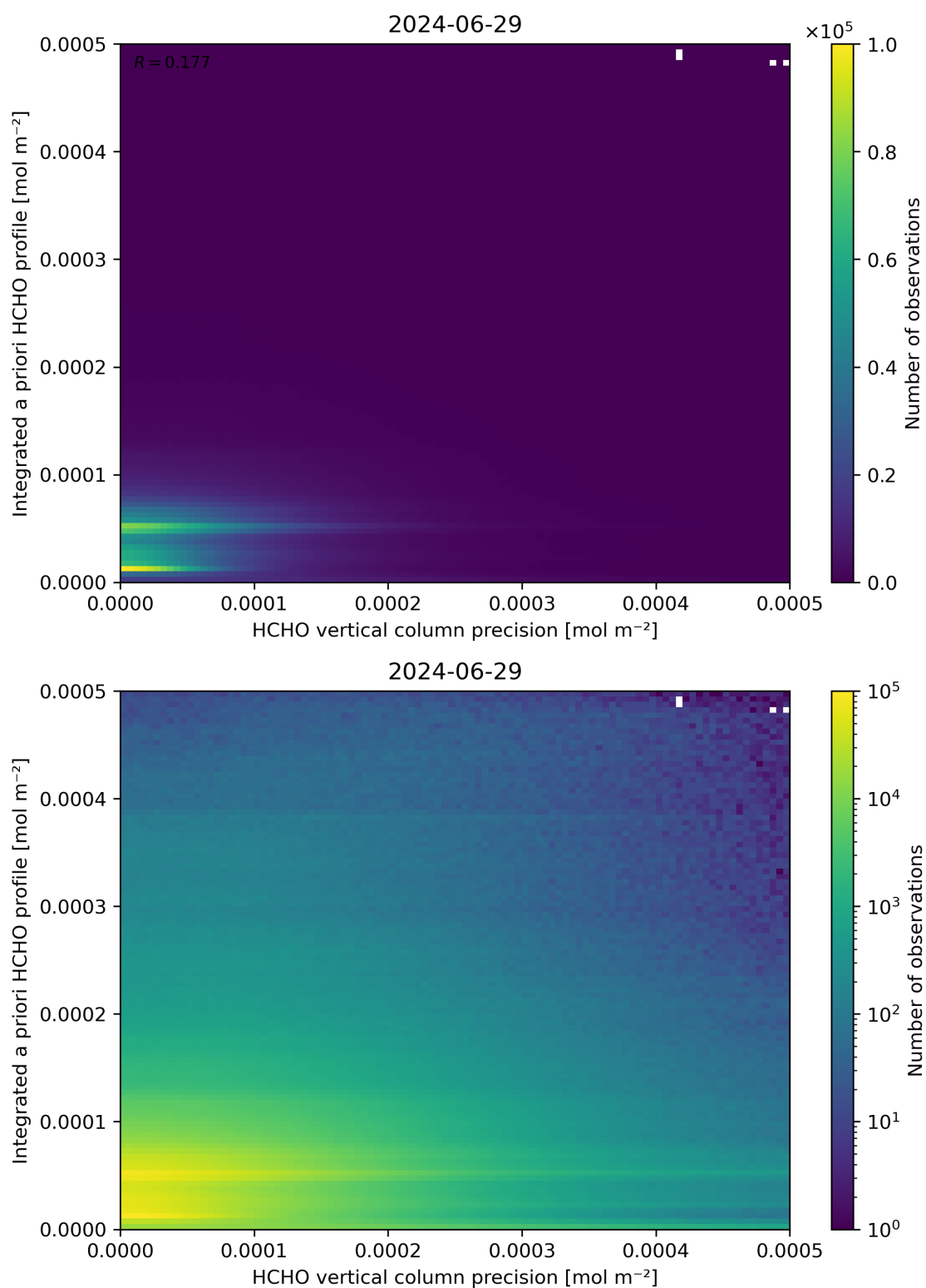
Figure 147: Scatter density plot of “HCHO vertical column precision” against “Integrated a priori HCHO profile” for 2024-06-29 to 2024-06-30.
