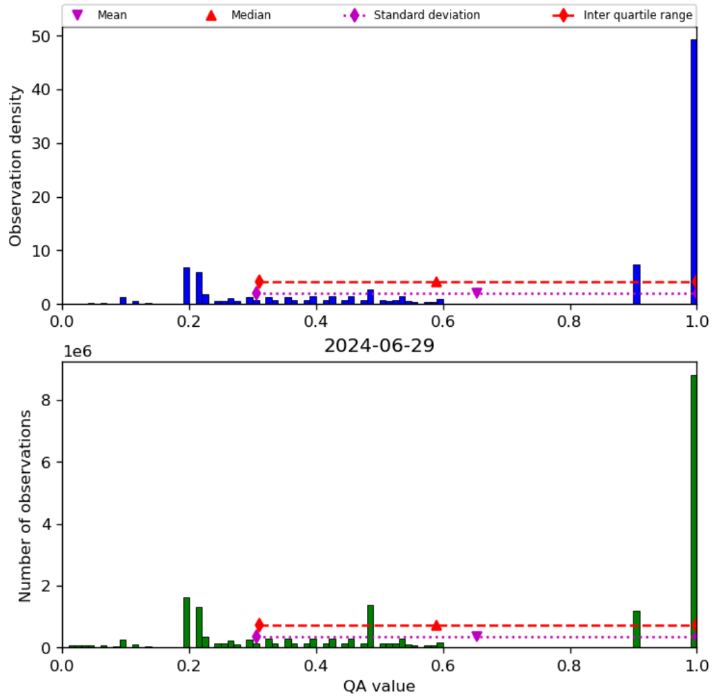
Figure 34: Histogram of “QA value” for 2024-06-29 to 2024-06-30
