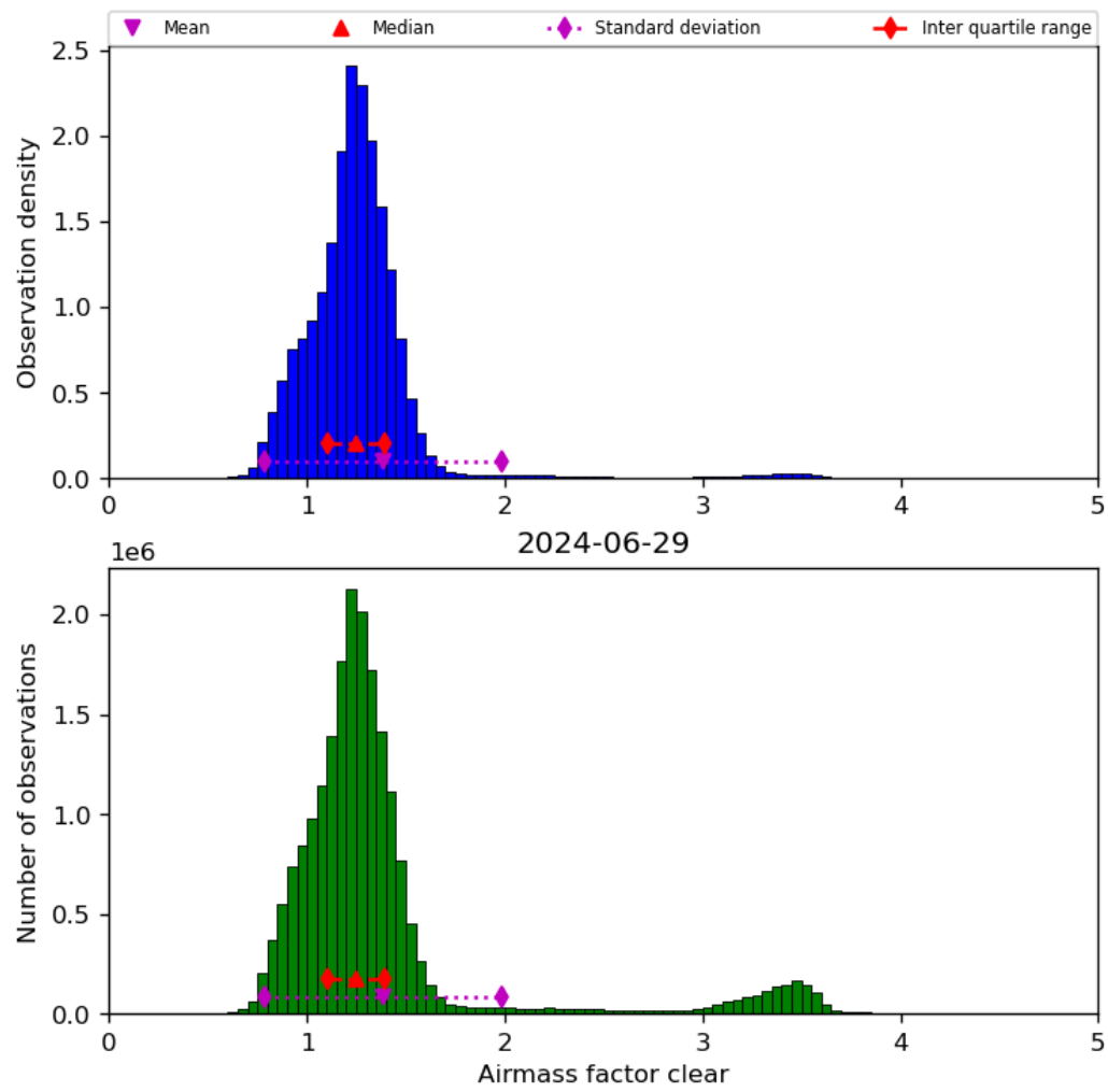
Figure 42: Histogram of “Airmass factor clear” for 2024-06-29 to 2024-06-30
