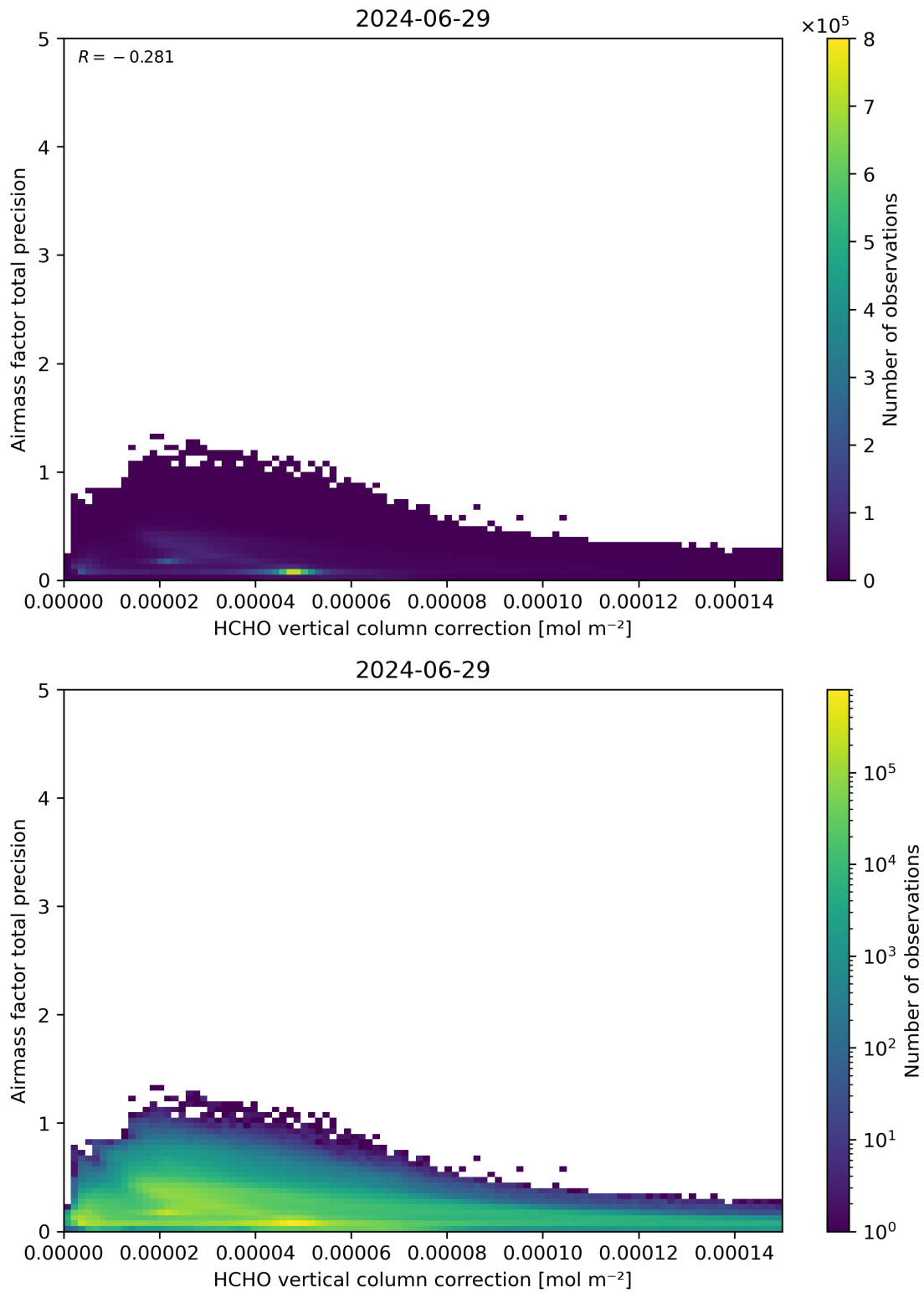
Figure 121: Scatter density plot of “HCHO vertical column correction” against “Airmass factor total precision” for 2024-06-29 to 2024-06-30.
