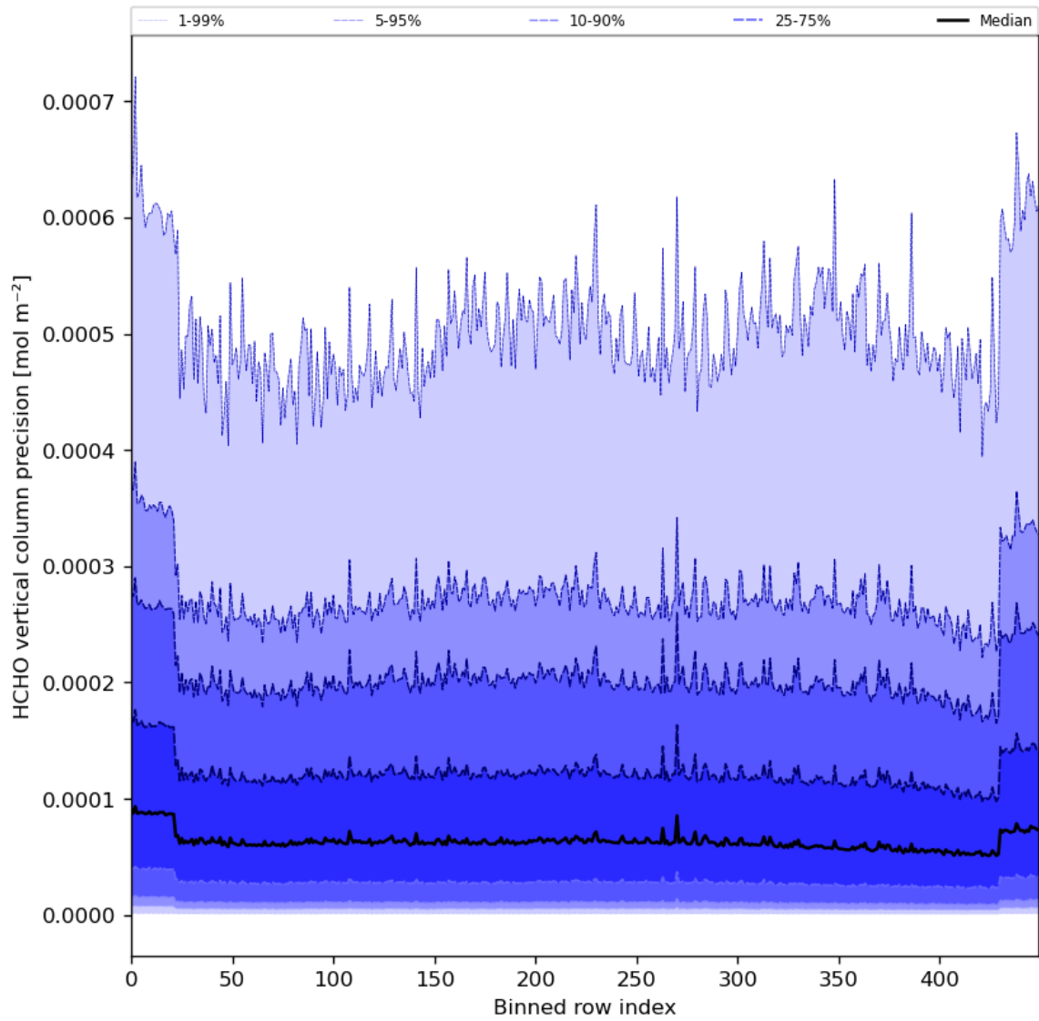
Figure 50: Along track statistics of “HCHO vertical column precision” for 2024-06-29 to 2024-06-30
