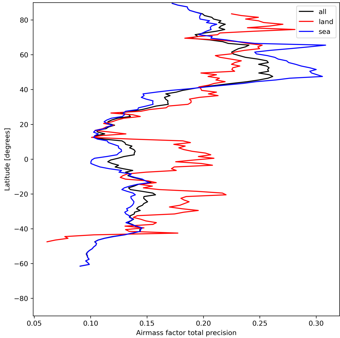
Figure 27: Zonal average of “Airmass factor total precision” for 2024-06-29 to 2024-06-30.
