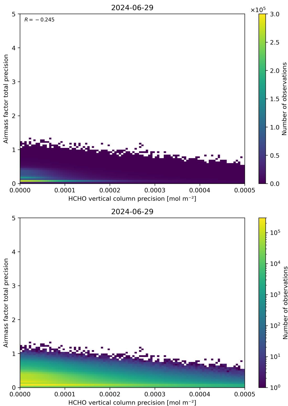
Figure 145: Scatter density plot of “HCHO vertical column precision” against “Airmass factor total precision” for 2024-06-29 to 2024-06-30.
