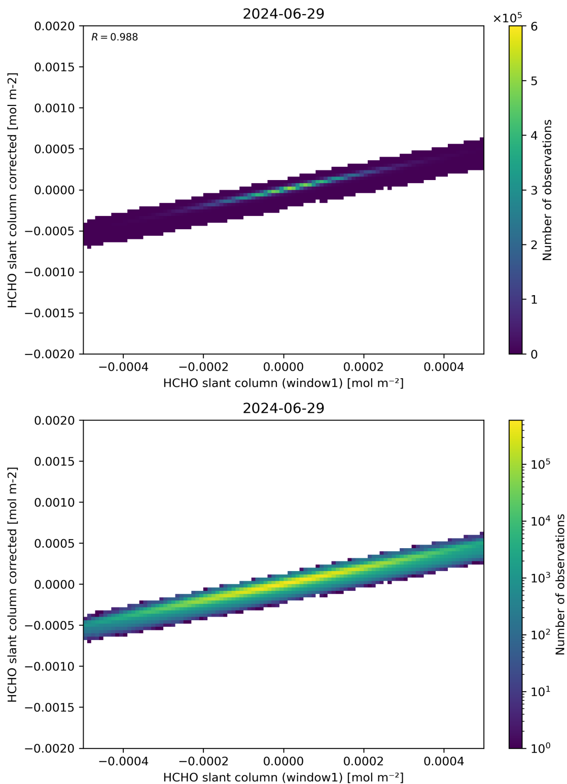
Figure 82: Scatter density plot of “HCHO slant column (window1)” against “HCHO slant column corrected” for 2024-06-29 to 2024-06-30.
