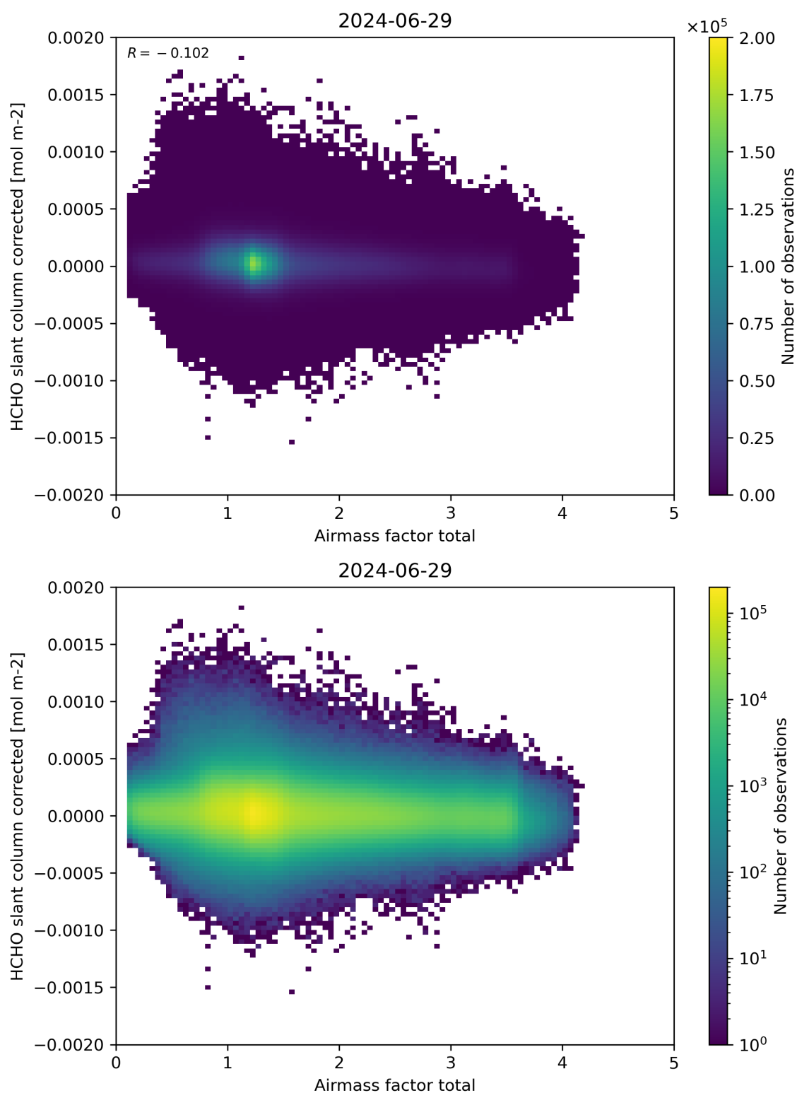
Figure 101: Scatter density plot of “Airmass factor total” against “HCHO slant column corrected” for 2024-06-29 to 2024-06-30.
