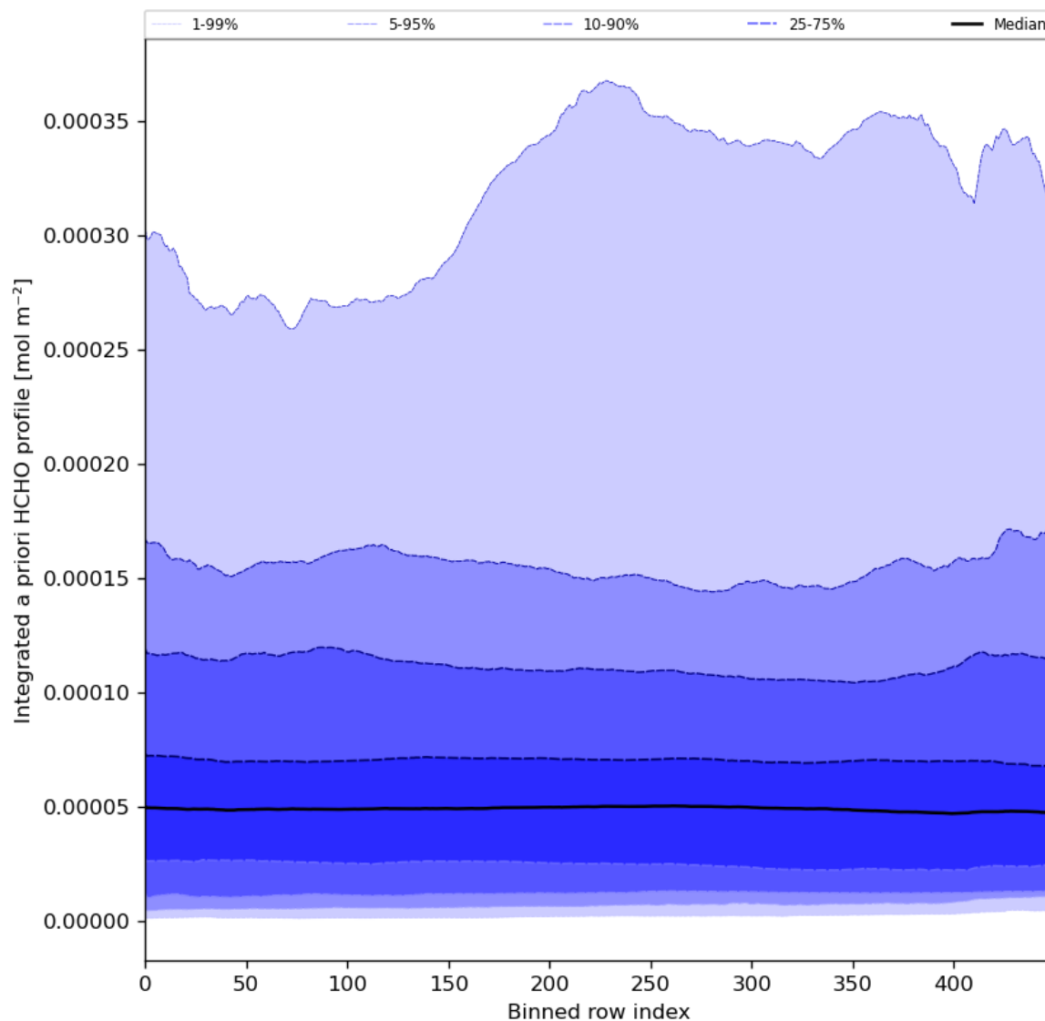
Figure 57: Along track statistics of "Integrated a priori HCHO profile" for 2024-06-29 to 2024-06-30
