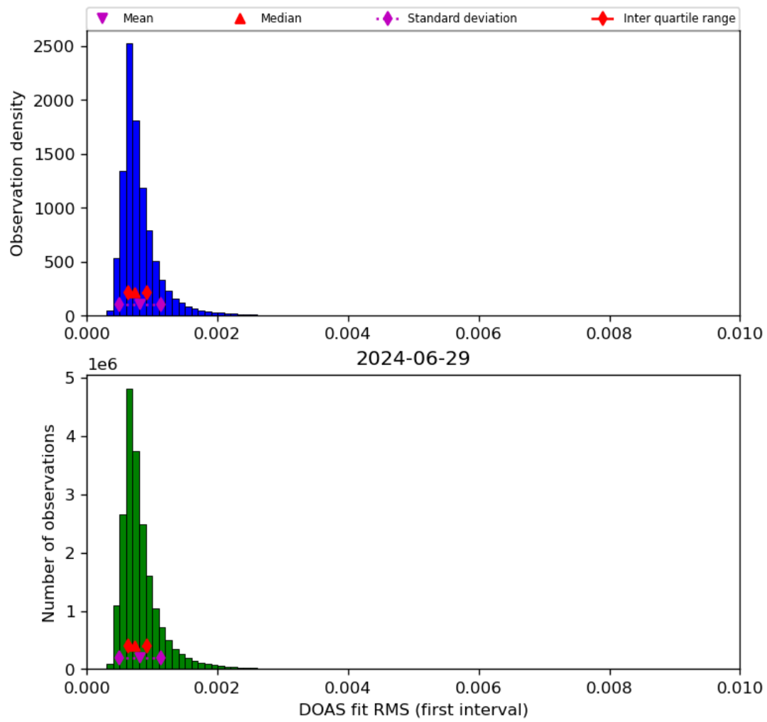
Figure 46: Histogram of “DOAS fit RMS (first interval)” for 2024-06-29 to 2024-06-30
