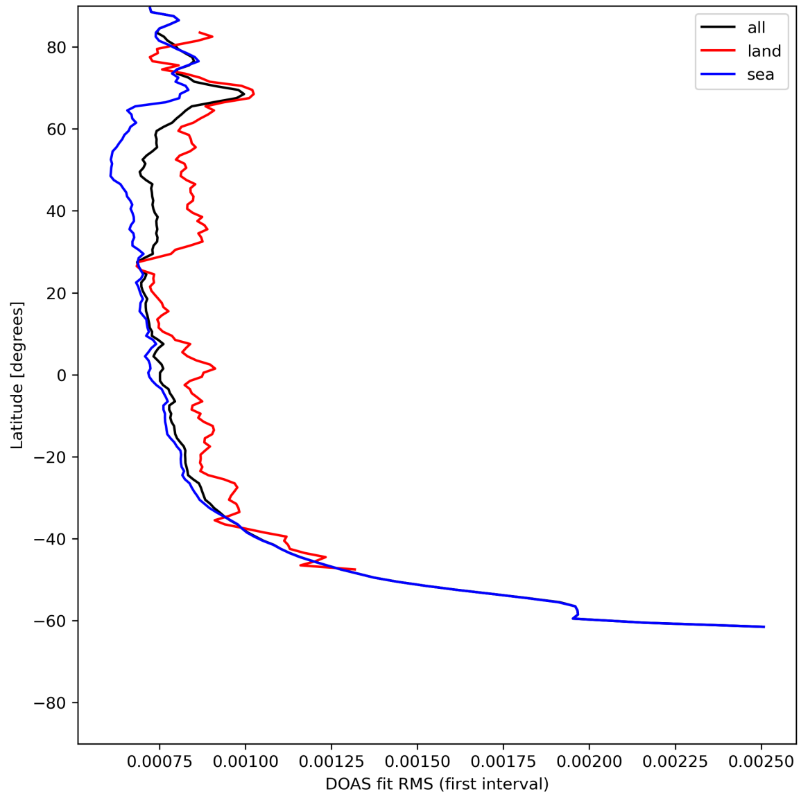
Figure 32: Zonal average of “DOAS fit RMS (first interval)” for 2024-06-29 to 2024-06-30.
