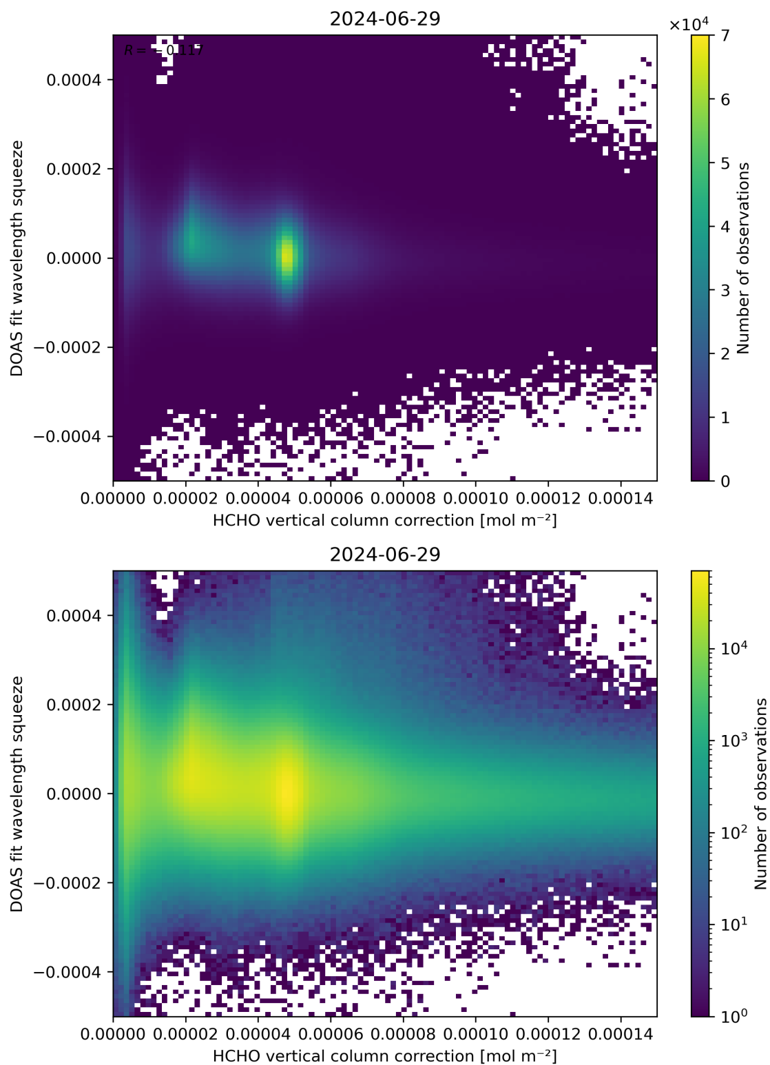
Figure 114: Scatter density plot of “HCHO vertical column correction” against “DOAS fit wavelength squeeze” for 2024-06-29 to 2024-06-30.
