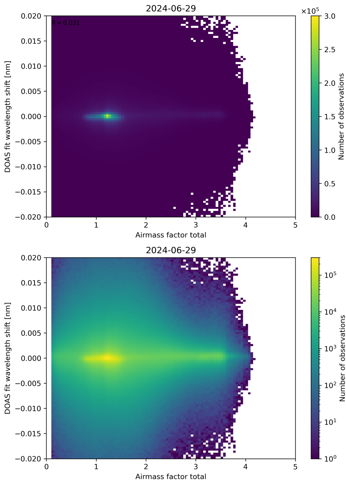
Figure 98: Scatter density plot of “Airmass factor total” against “DOAS fit wavelength shift” for 2024-06-29 to 2024-06-30.
