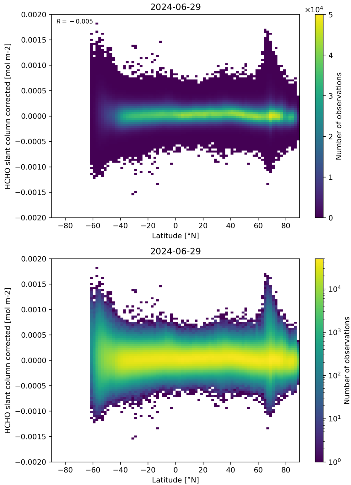
Figure 157: Scatter density plot of “Latitude” against “HCHO slant column corrected” for 2024-06-29 to 2024-06-30.
