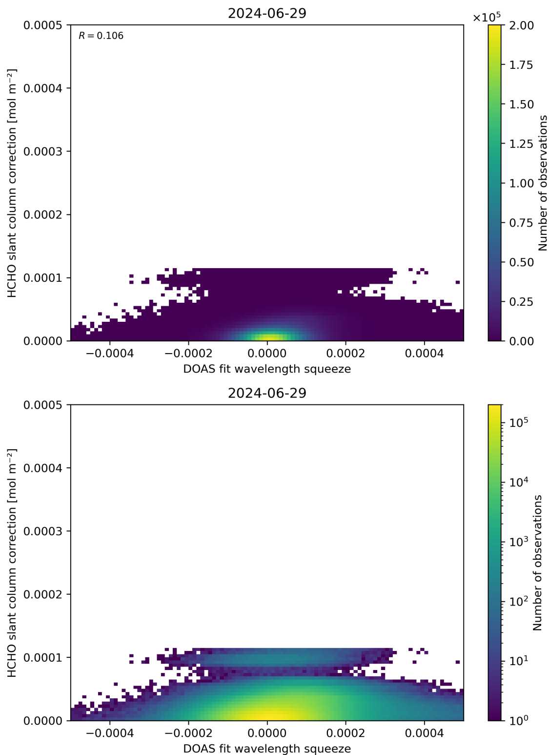
Figure 70: Scatter density plot of “DOAS fit wavelength squeeze” against “HCHO slant column correction” for 2024-06-29 to 2024-06-30.
