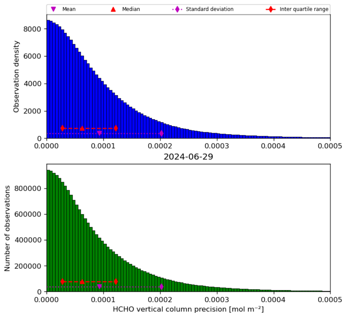
Figure 36: Histogram of “HCHO vertical column precision” for 2024-06-29 to 2024-06-30
