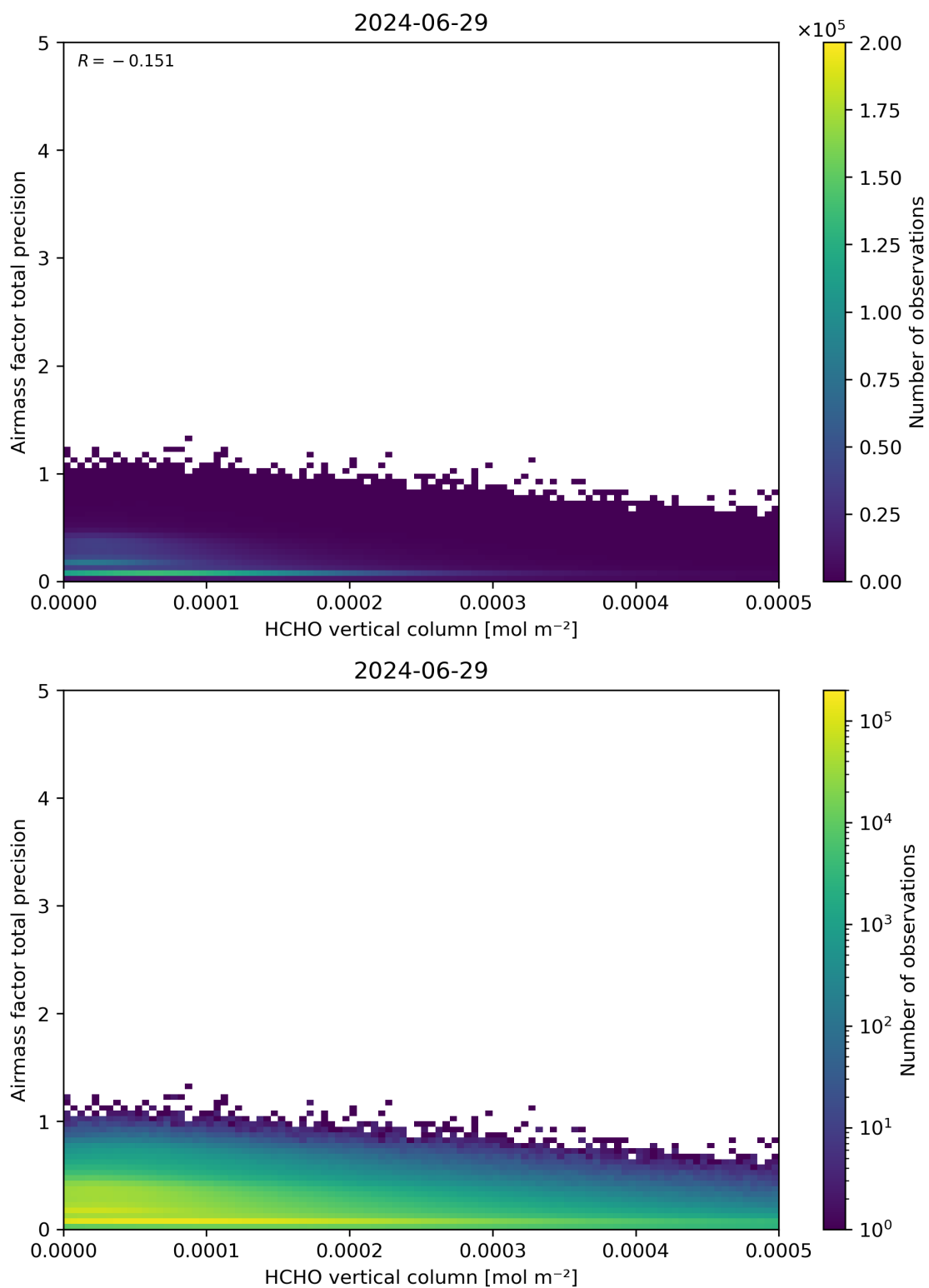
Figure 132: Scatter density plot of “HCHO vertical column” against “Airmass factor total precision” for 2024-06-29 to 2024-06-30.
