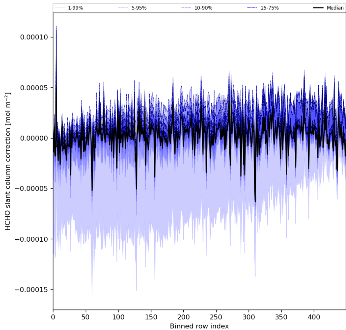
Figure 61: Along track statistics of “HCHO slant column correction” for 2024-06-29 to 2024-06-30
