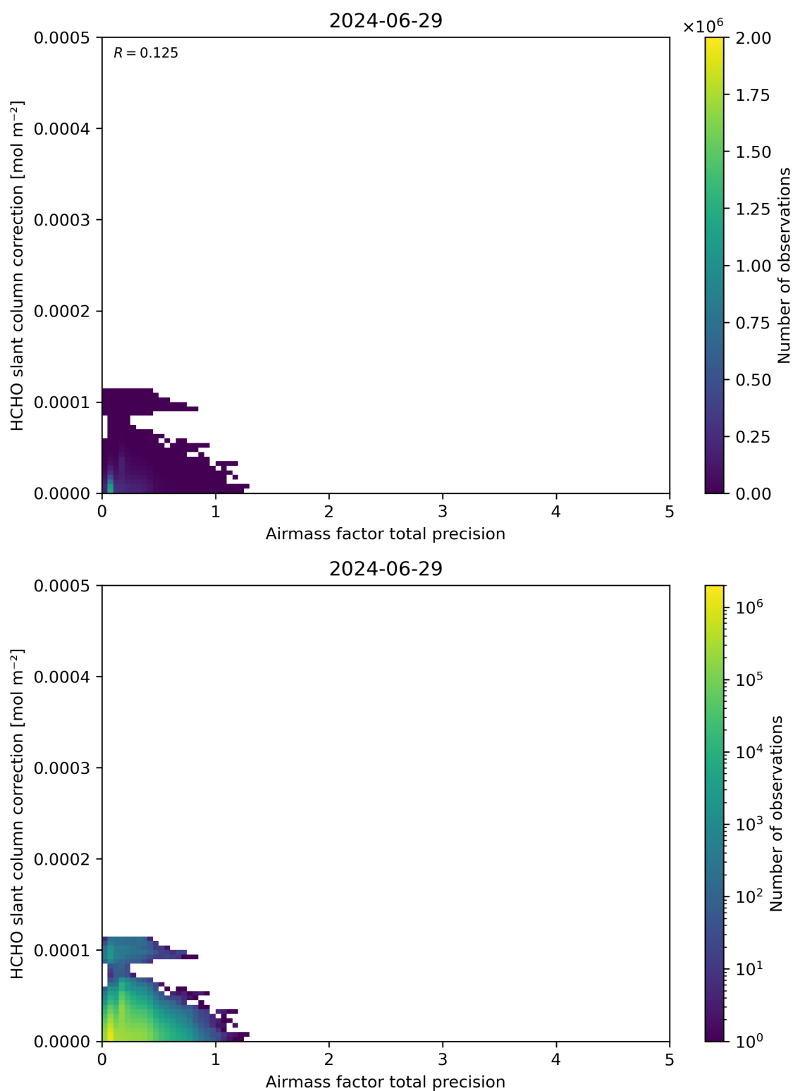
Figure 110: Scatter density plot of “Airmass factor total precision” against “HCHO slant column correction” for 2024-06-29 to 2024-06-30.
