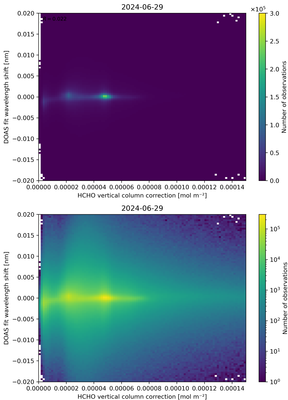
Figure 113: Scatter density plot of “HCHO vertical column correction” against “DOAS fit wavelength shift” for 2024-06-29 to 2024-06-30.
