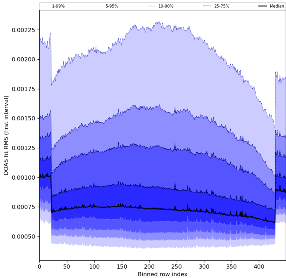
Figure 60: Along track statistics of “DOAS fit RMS (first interval)” for 2024-06-29 to 2024-06-30
