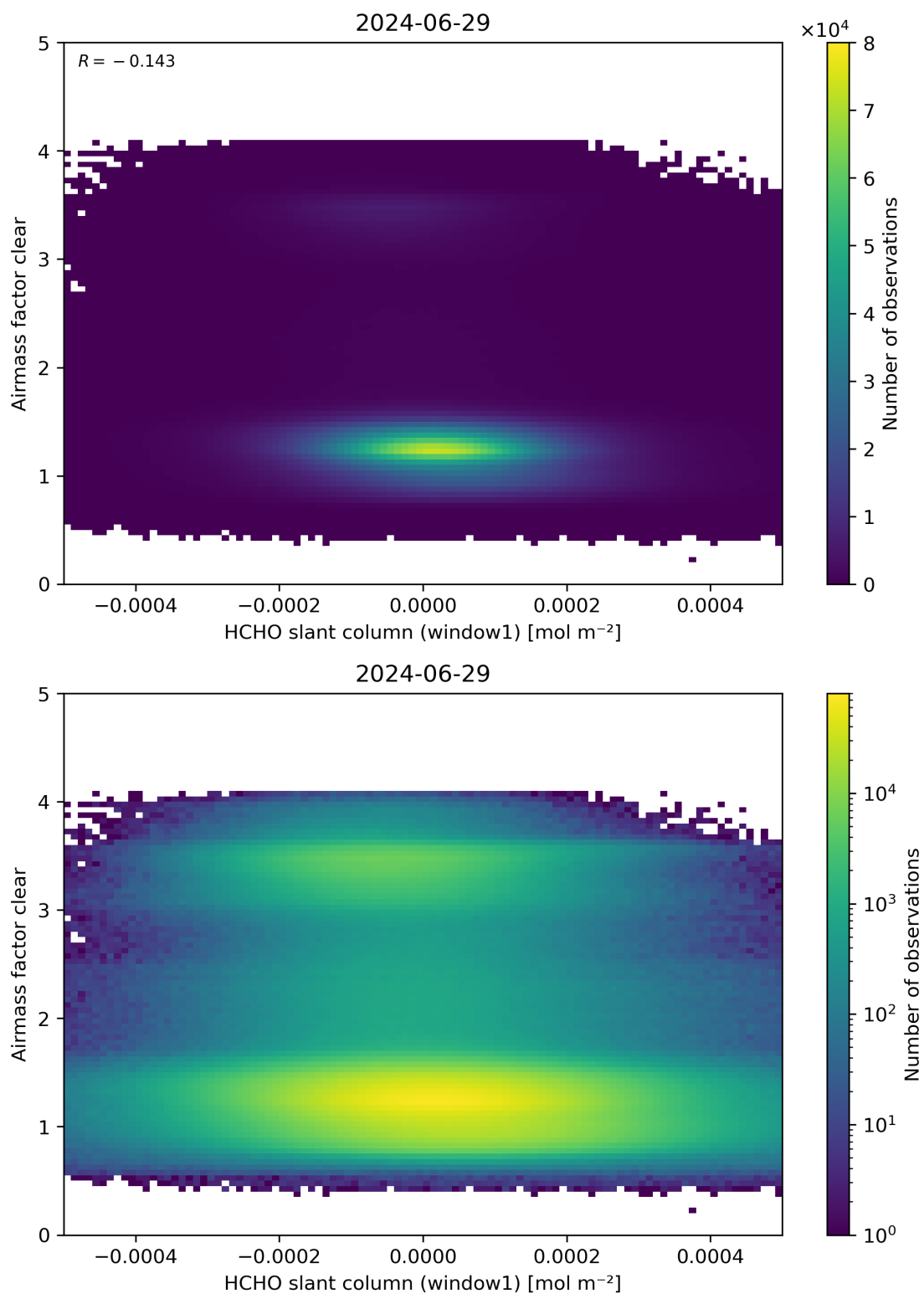
Figure 81: Scatter density plot of “HCHO slant column (window1)” against “Airmass factor clear” for 2024-06-29 to 2024-06-30.
