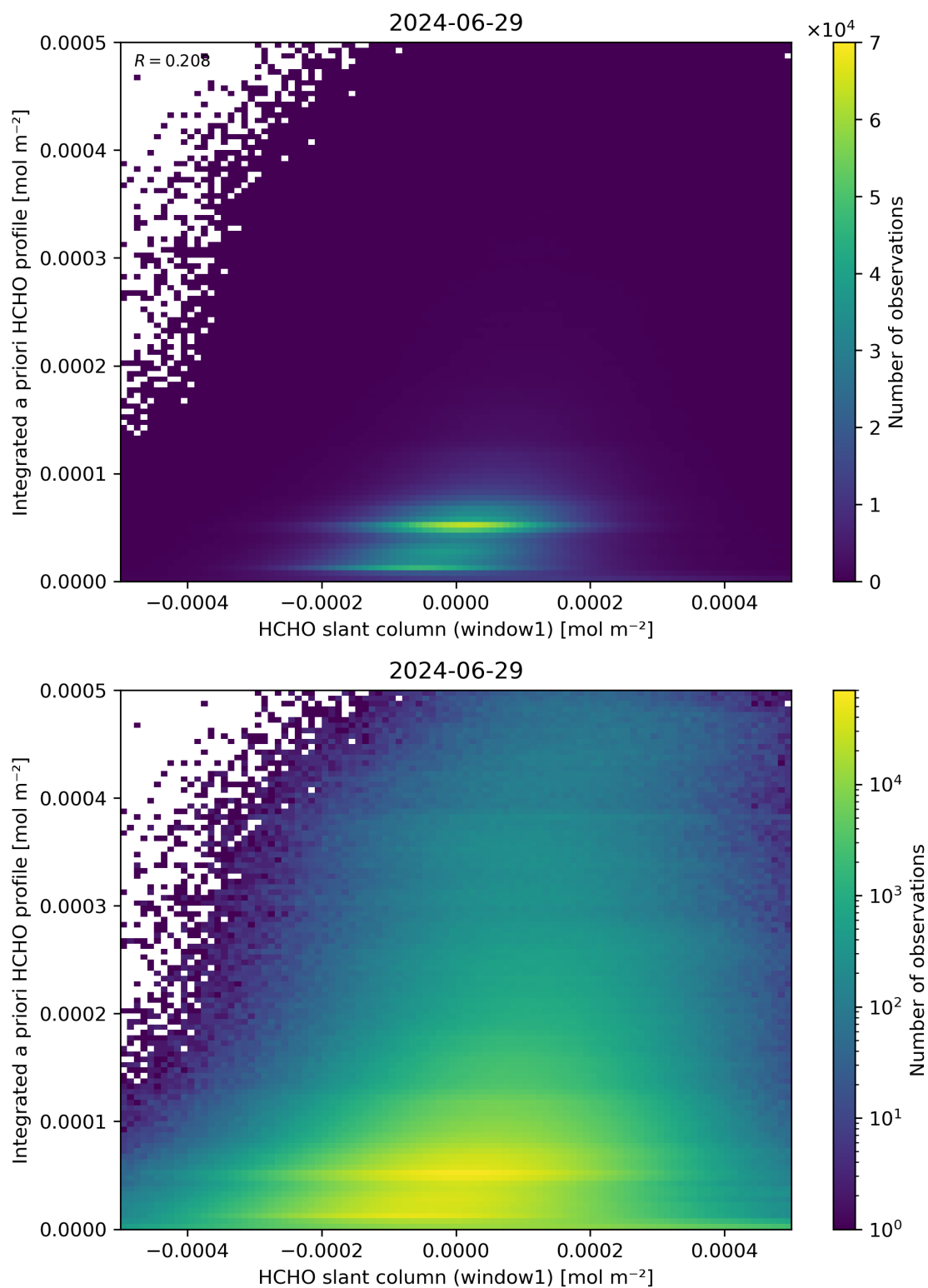
Figure 87: Scatter density plot of “HCHO slant column (window1)” against “Integrated a priori HCHO profile” for 2024-06-29 to 2024-06-30.
