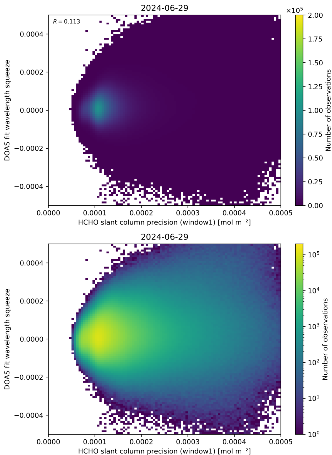
Figure 90: Scatter density plot of “HCHO slant column precision (window1)” against “DOAS fit wavelength squeeze” for 2024-06-29 to 2024-06-30.
