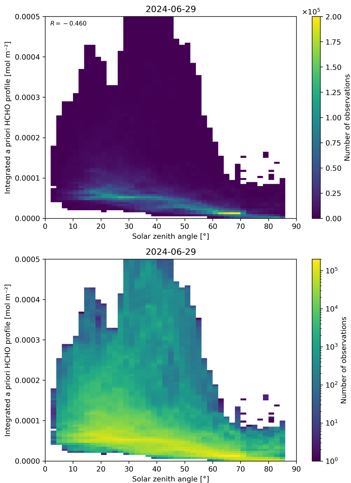
Figure 180: Scatter density plot of “Solar zenith angle” against “Integrated a priori HCHO profile” for 2024-06-29 to 2024-06-30.
