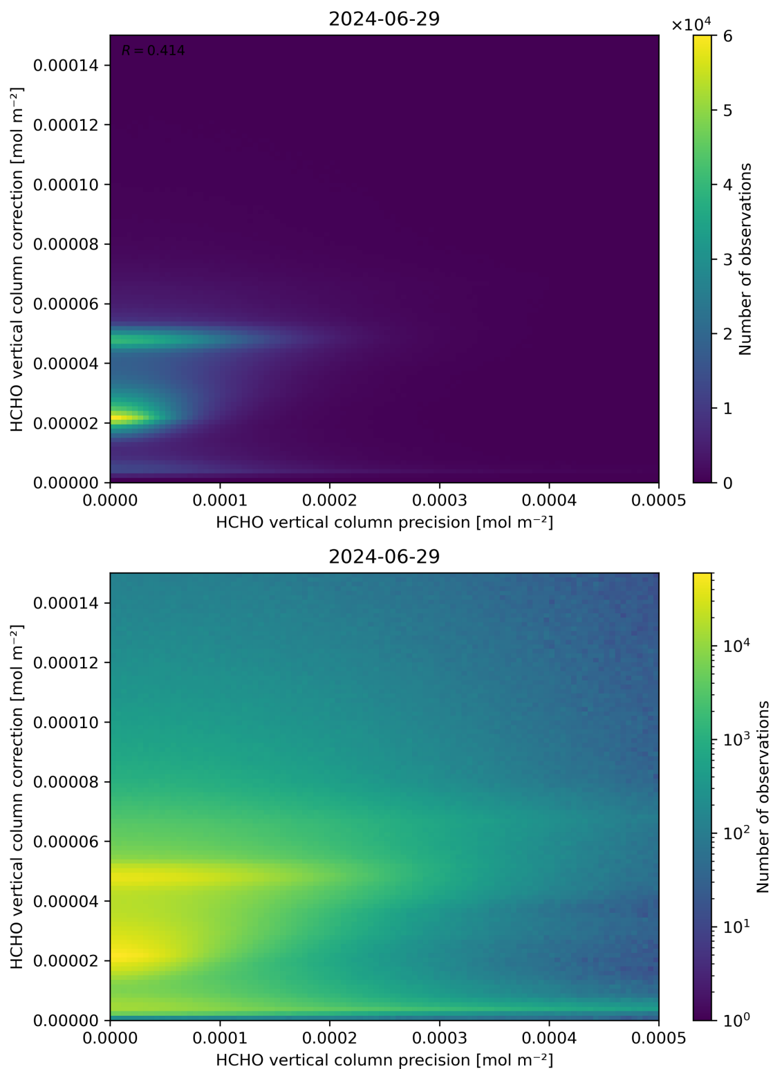
Figure 146: Scatter density plot of “HCHO vertical column precision” against “HCHO vertical column correction” for 2024-06-29 to 2024-06-30.
