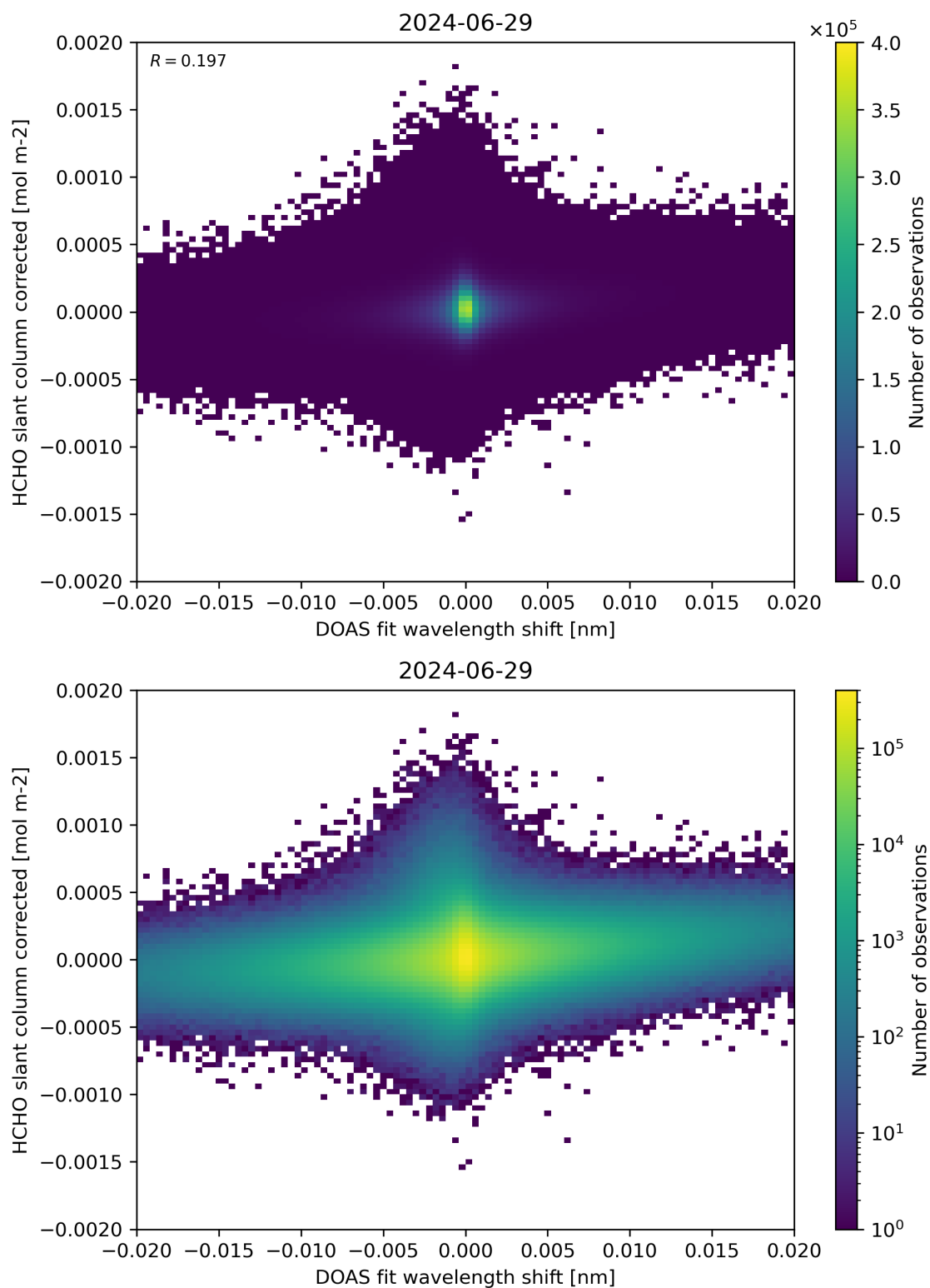
Figure 66: Scatter density plot of “DOAS fit wavelength shift” against “HCHO slant column corrected” for 2024-06-29 to 2024-06-30.
