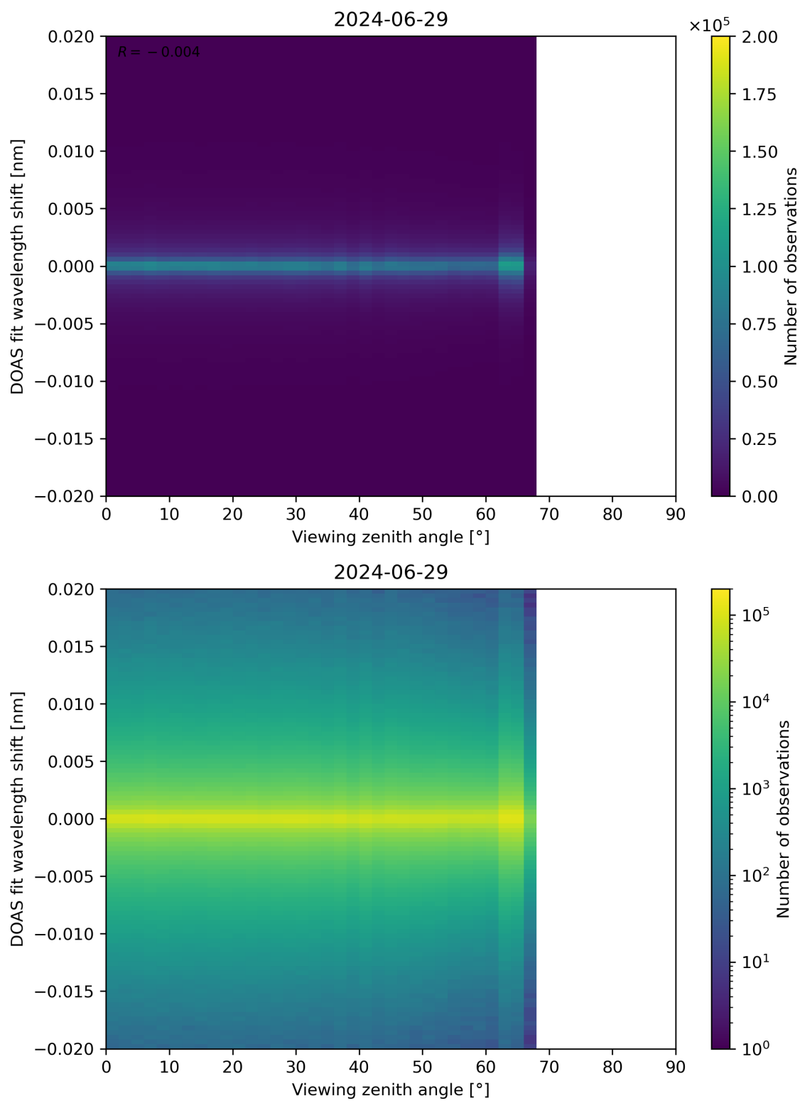
Figure 183: Scatter density plot of “Viewing zenith angle” against “DOAS fit wavelength shift” for 2024-06-29 to 2024-06-30.
