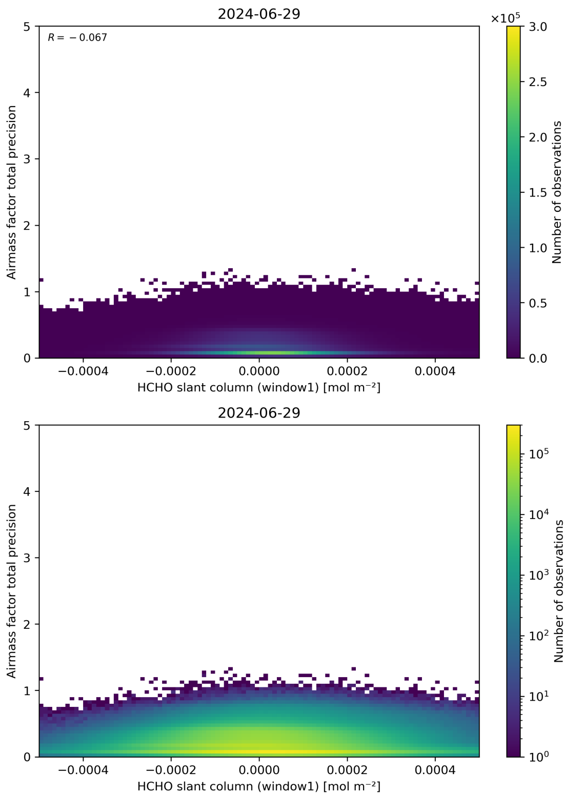
Figure 86: Scatter density plot of “HCHO slant column (window1)” against “Airmass factor total precision” for 2024-06-29 to 2024-06-30.
