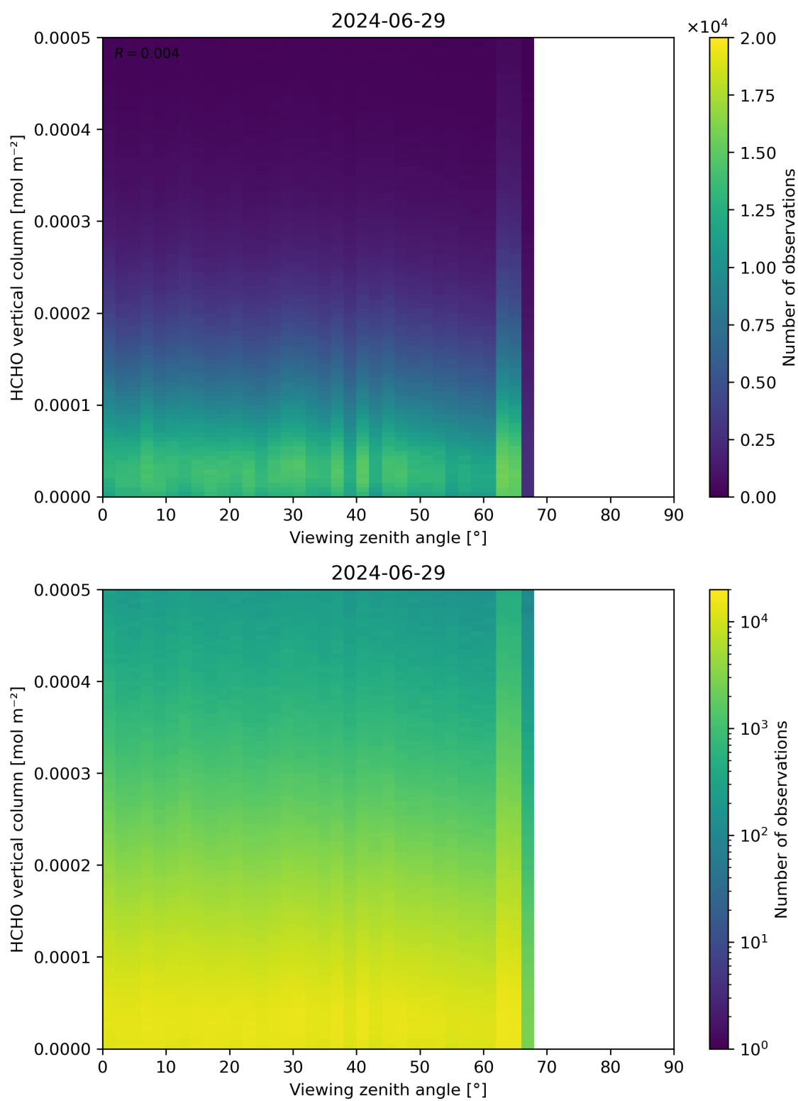
Figure 192: Scatter density plot of “Viewing zenith angle” against “HCHO vertical column” for 2024-06-29 to 2024-06-30.
