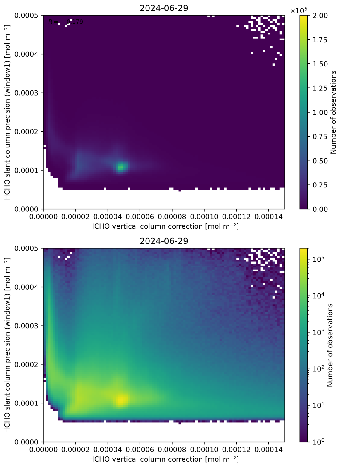
Figure 119: Scatter density plot of “HCHO vertical column correction” against “HCHO slant column precision (window1)” for 2024-06-29 to 2024-06-30.
