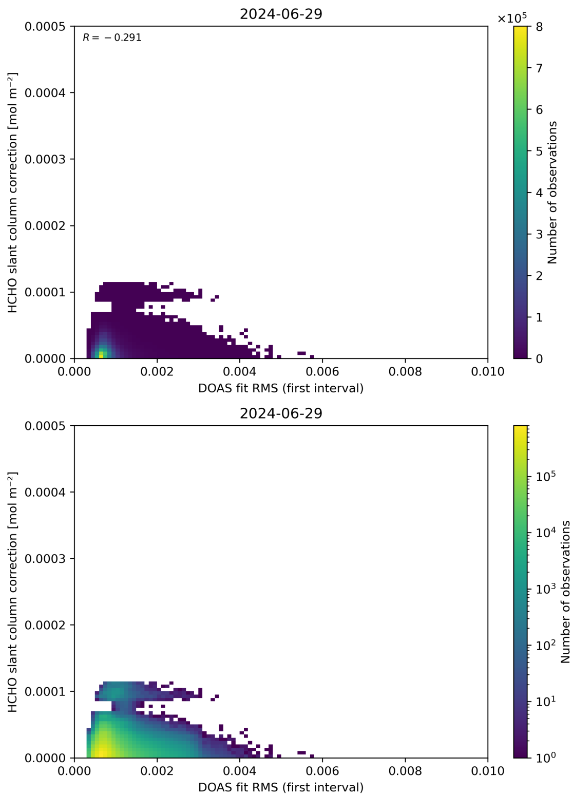
Figure 63: Scatter density plot of “DOAS fit RMS (first interval)” against “HCHO slant column correction” for 2024-06-29 to 2024-06-30.
