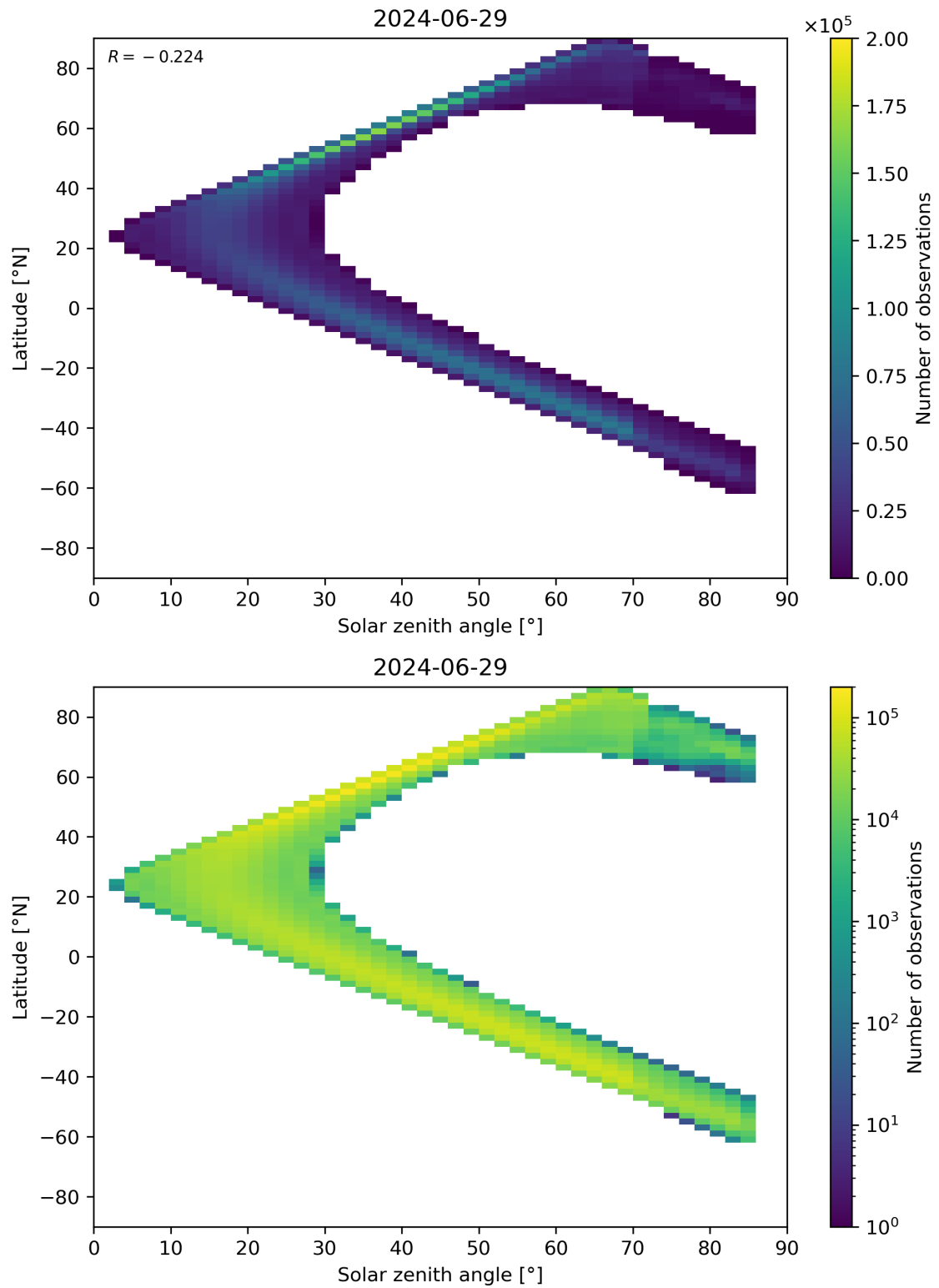
Figure 181: Scatter density plot of “Solar zenith angle” against “Latitude” for 2024-06-29 to 2024-06-30.
