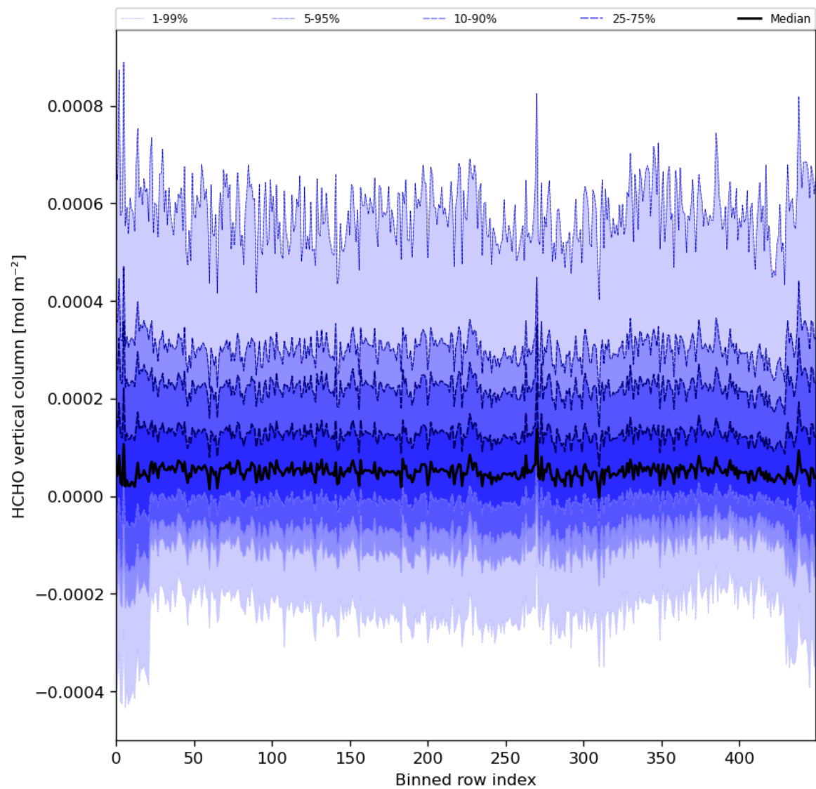
Figure 49: Along track statistics of “HCHO vertical column” for 2024-06-29 to 2024-06-30
