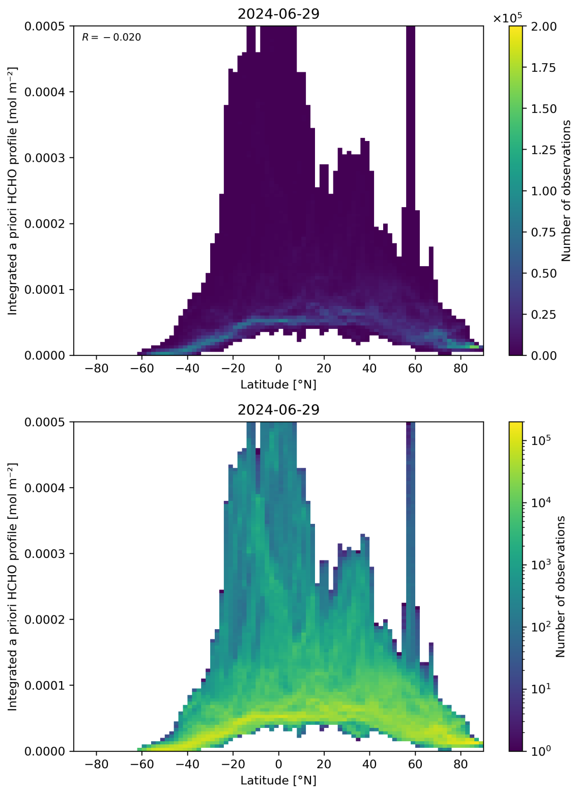
Figure 166: Scatter density plot of “Latitude” against “Integrated a priori HCHO profile” for 2024-06-29 to 2024-06-30.
