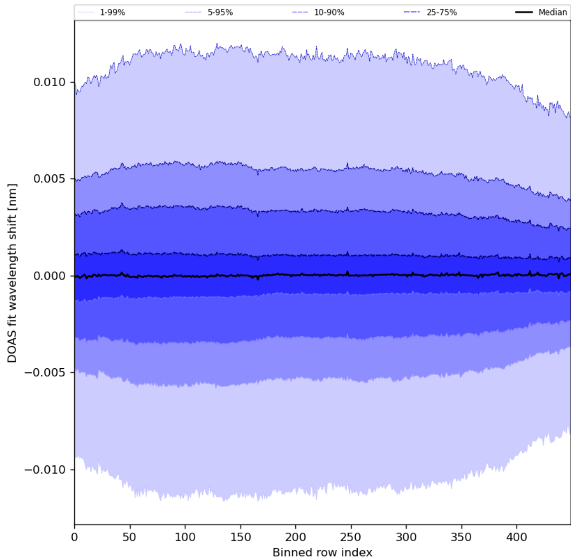
Figure 58: Along track statistics of “DOAS fit wavelength shift” for 2024-06-29 to 2024-06-30
