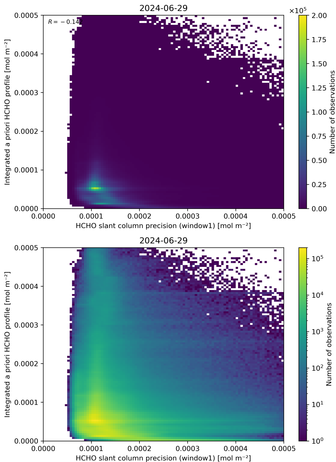
Figure 96: Scatter density plot of “HCHO slant column precision (window1)” against “Integrated a priori HCHO profile” for 2024-06-29 to 2024-06-30.
