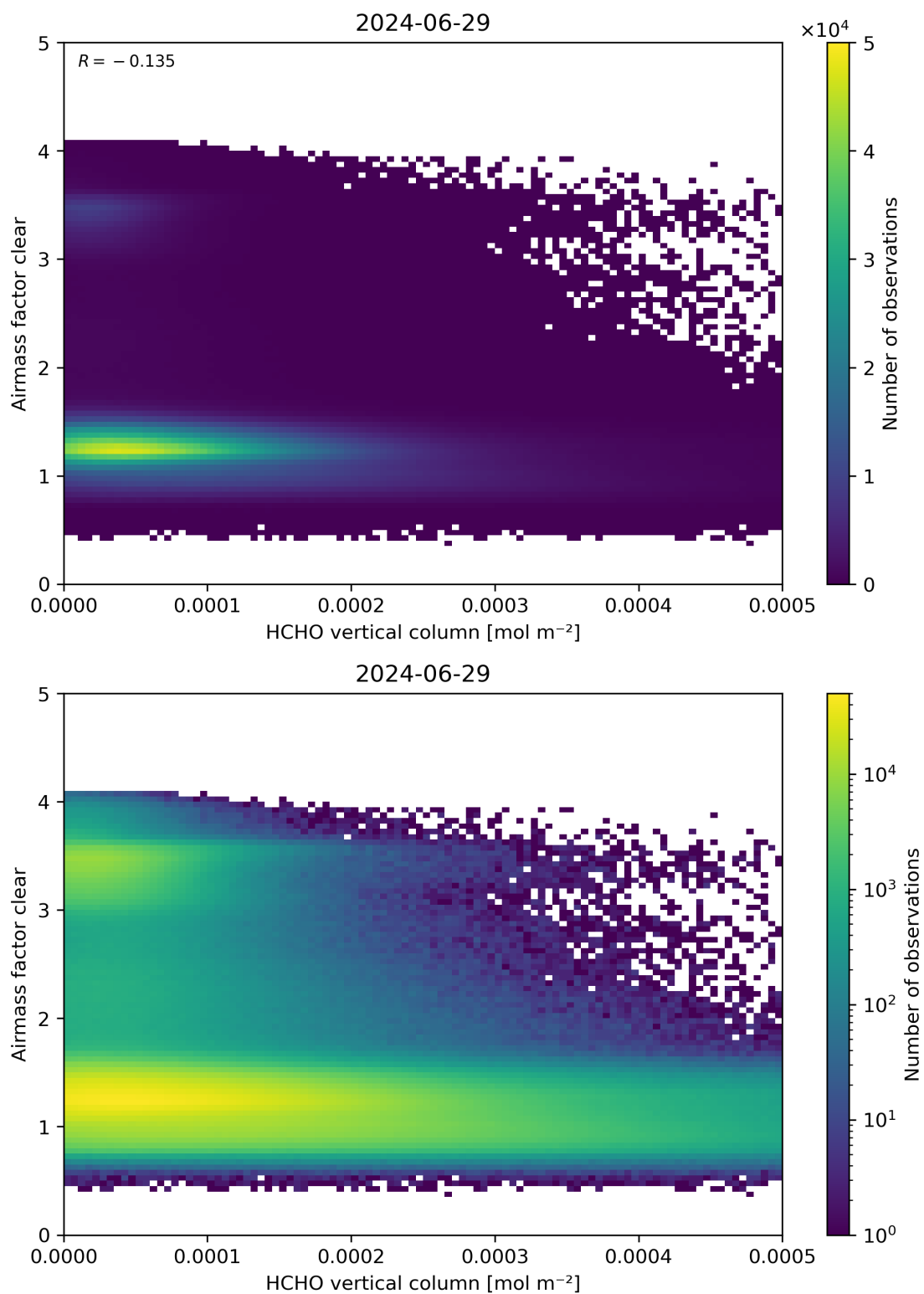
Figure 126: Scatter density plot of “HCHO vertical column” against “Airmass factor clear” for 2024-06-29 to 2024-06-30.
