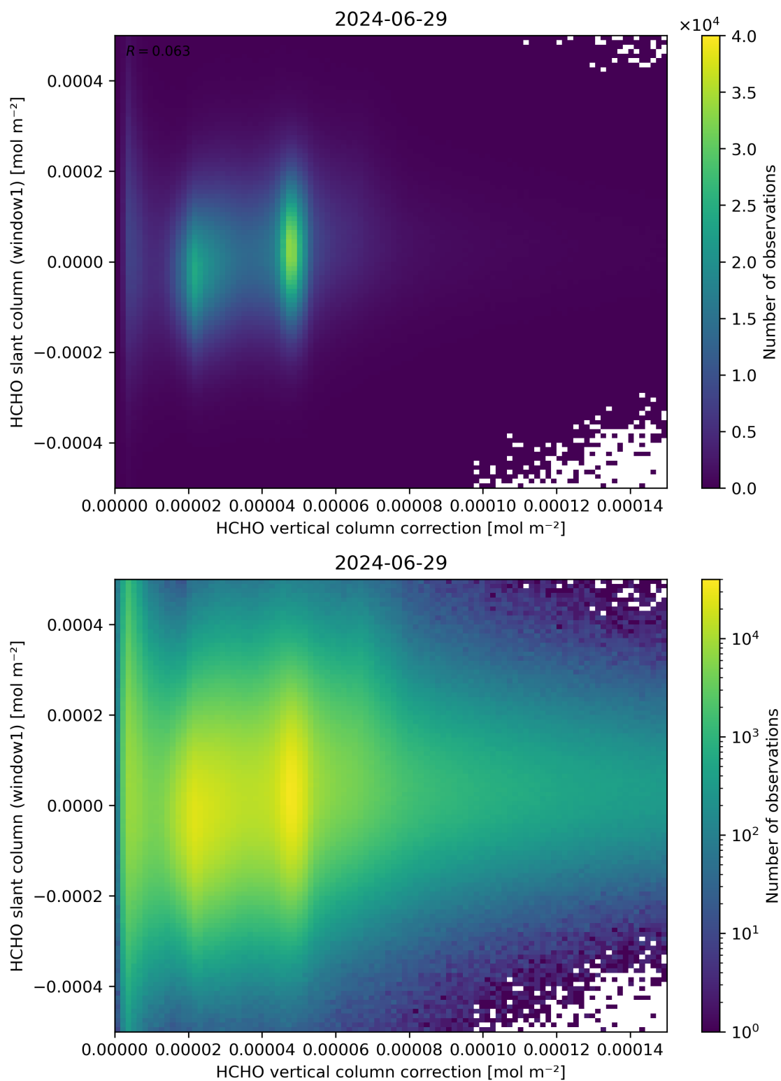
Figure 118: Scatter density plot of “HCHO vertical column correction” against “HCHO slant column (window1)” for 2024-06-29 to 2024-06-30.
