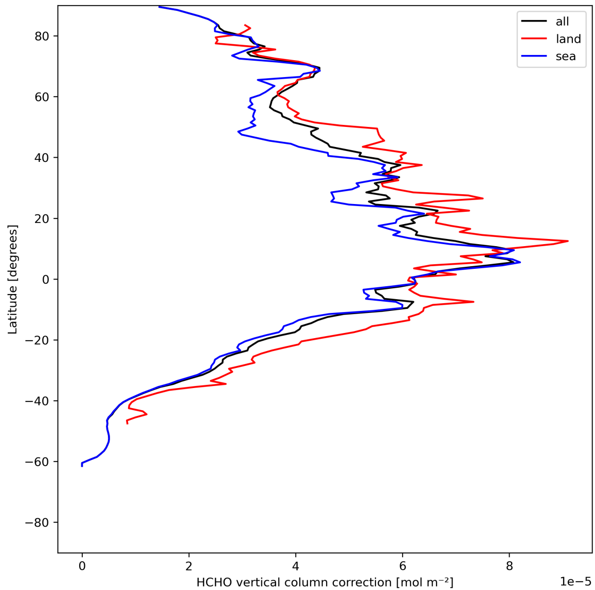
Figure 23: Zonal average of “HCHO vertical column correction” for 2024-06-29 to 2024-06-30.
