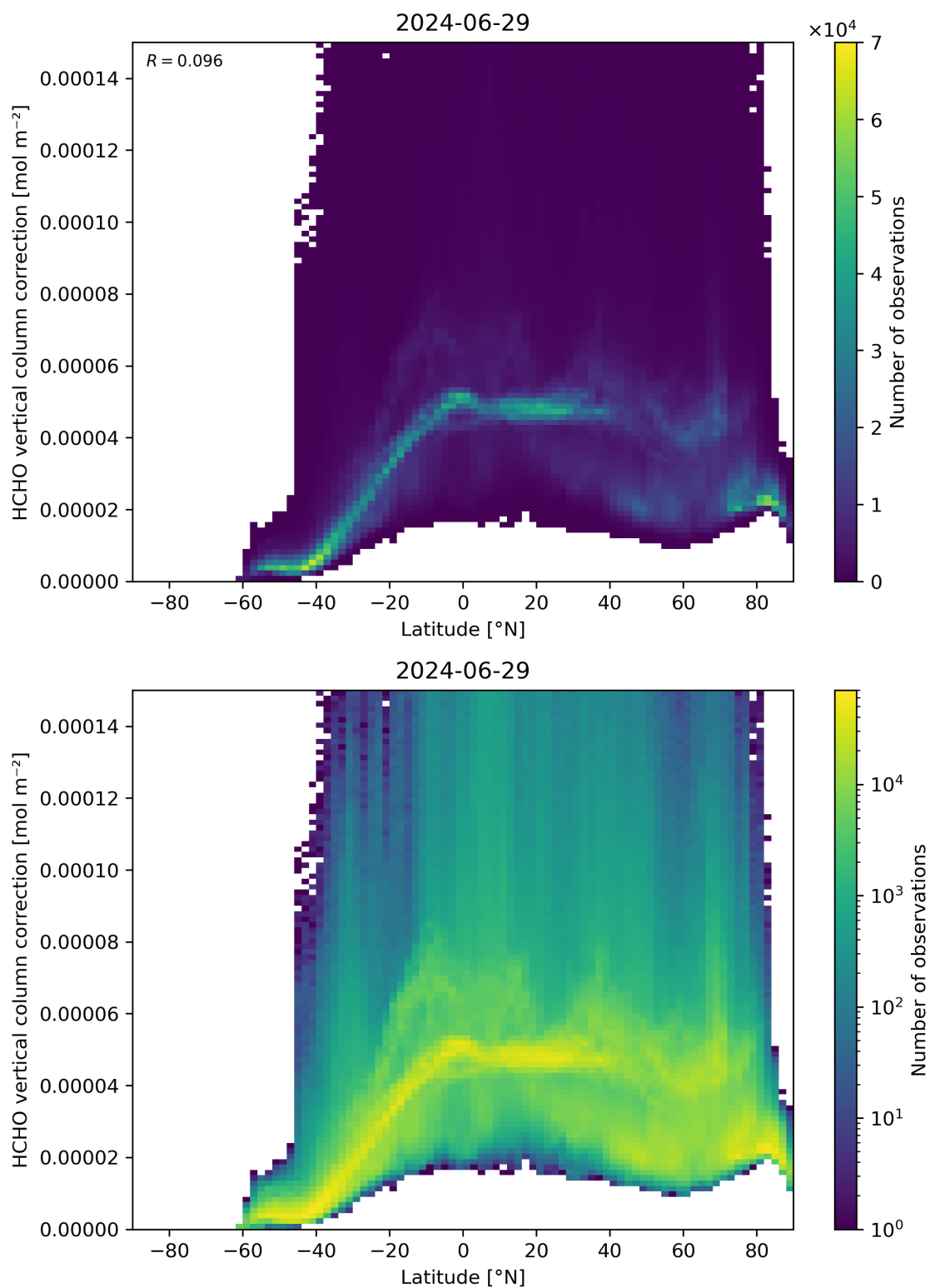
Figure 164: Scatter density plot of “Latitude” against “HCHO vertical column correction” for 2024-06-29 to 2024-06-30.
