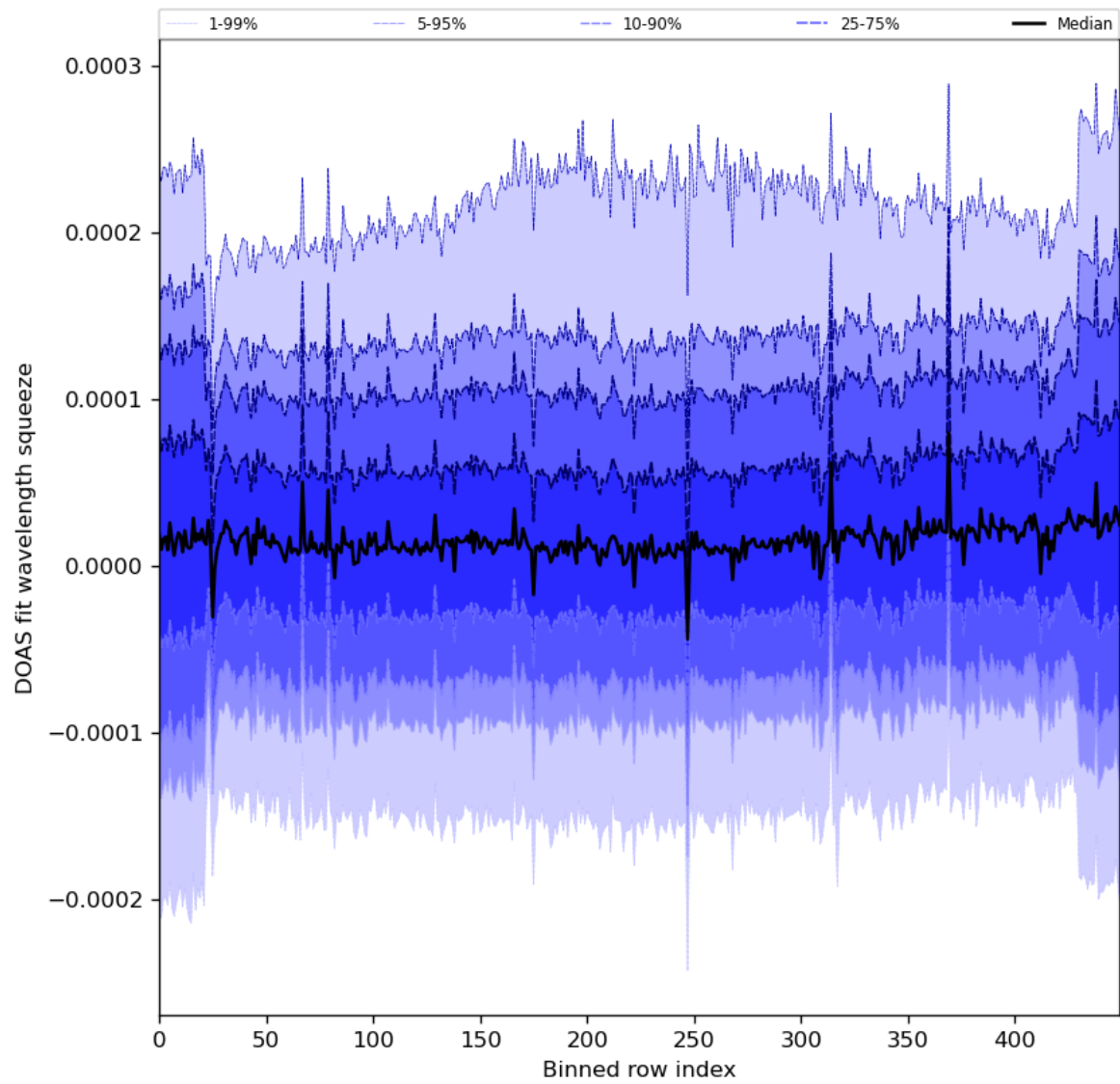
Figure 59: Along track statistics of “DOAS fit wavelength squeeze” for 2024-06-29 to 2024-06-30
