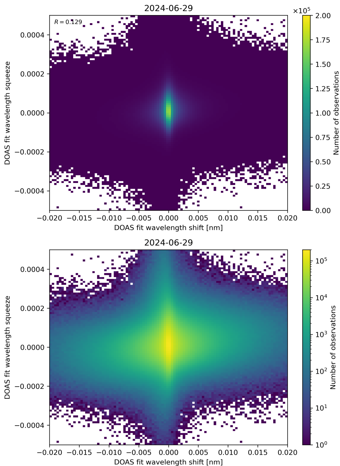
Figure 65: Scatter density plot of “DOAS fit wavelength shift” against “DOAS fit wavelength squeeze” for 2024-06-29 to 2024-06-30.
