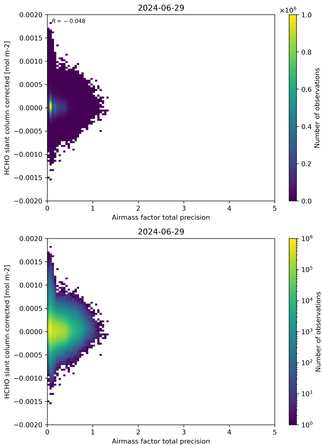
Figure 109: Scatter density plot of “Airmass factor total precision” against “HCHO slant column corrected” for 2024-06-29 to 2024-06-30.
