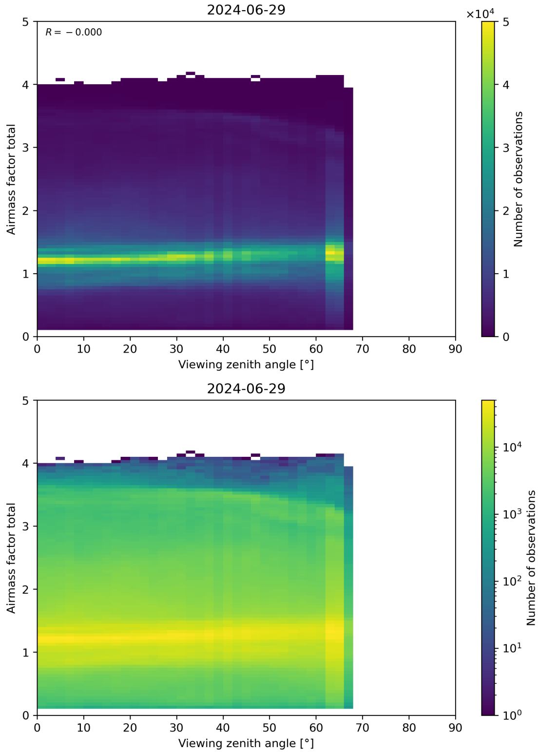
Figure 190: Scatter density plot of “Viewing zenith angle” against “Airmass factor total” for 2024-06-29 to 2024-06-30.
