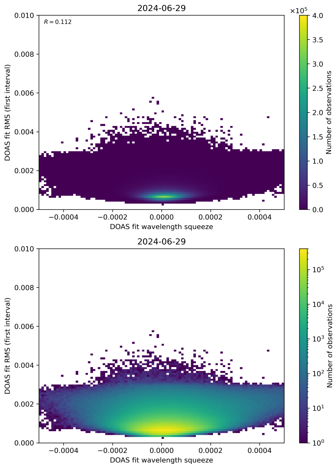
Figure 68: Scatter density plot of “DOAS fit wavelength squeeze” against “DOAS fit RMS (first interval)” for 2024-06-29 to 2024-06-30.
