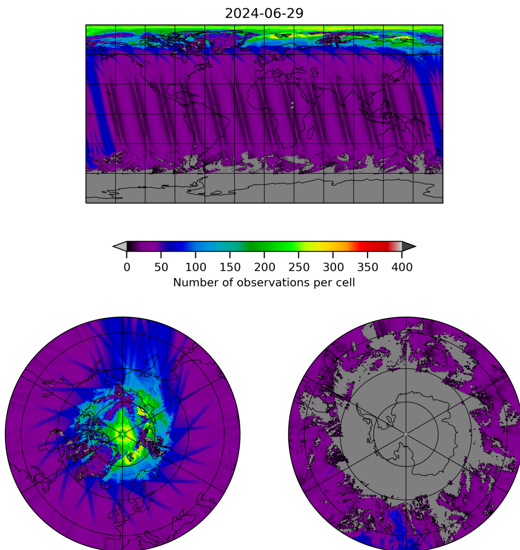
Figure 19: Map of the number of observations for 2024-06-29 to 2024-06-30
