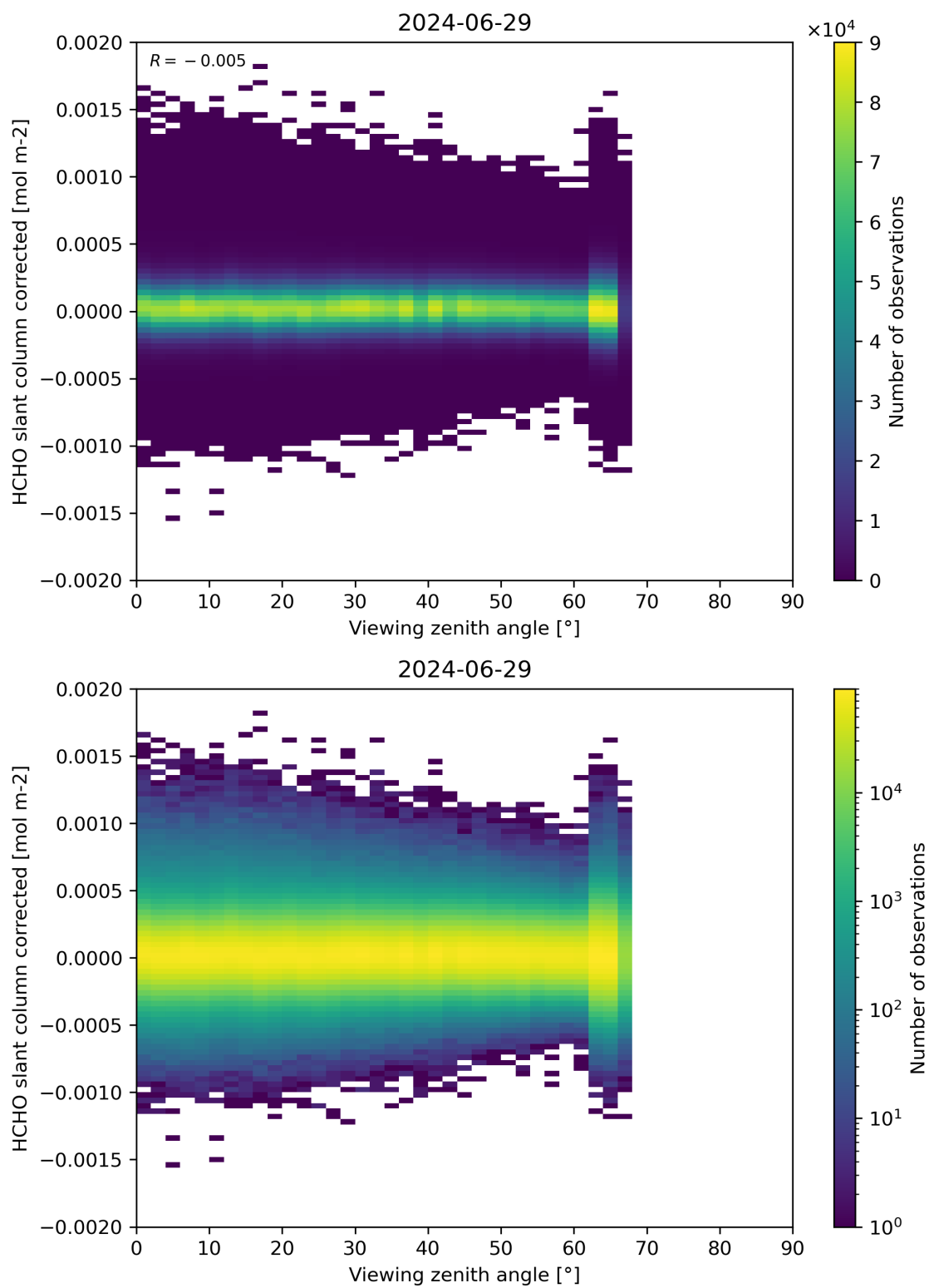
Figure 186: Scatter density plot of “Viewing zenith angle” against “HCHO slant column corrected” for 2024-06-29 to 2024-06-30.
