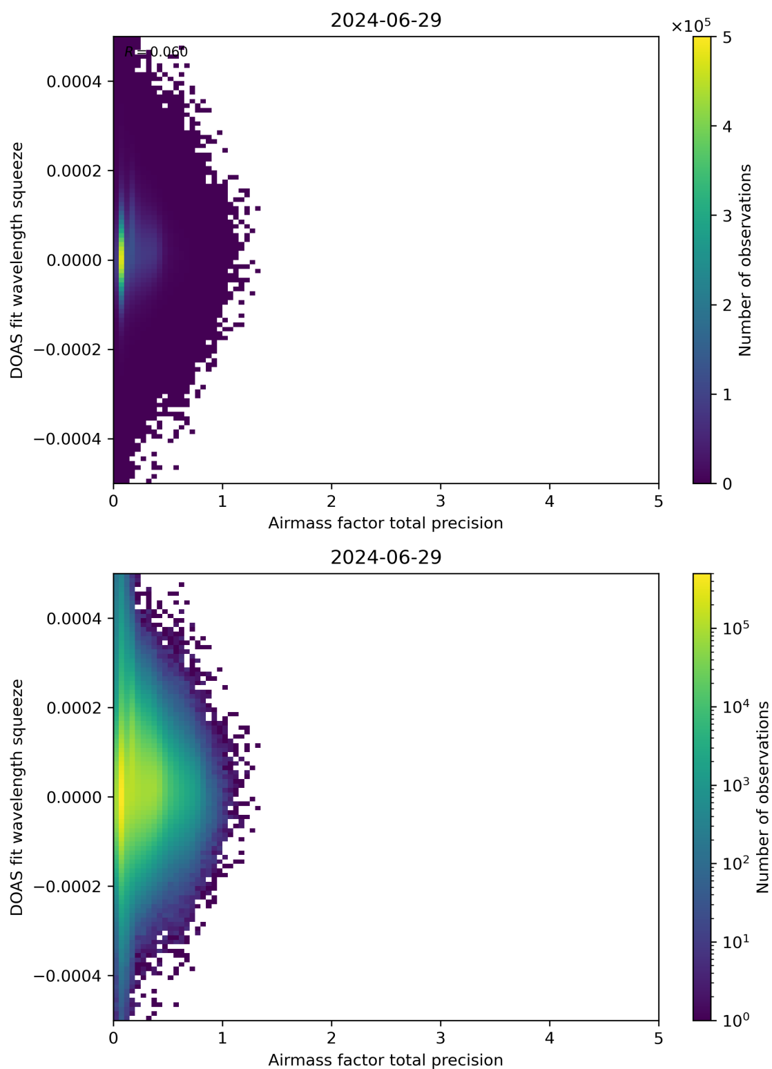
Figure 107: Scatter density plot of “Airmass factor total precision” against “DOAS fit wavelength squeeze” for 2024-06-29 to 2024-06-30.
