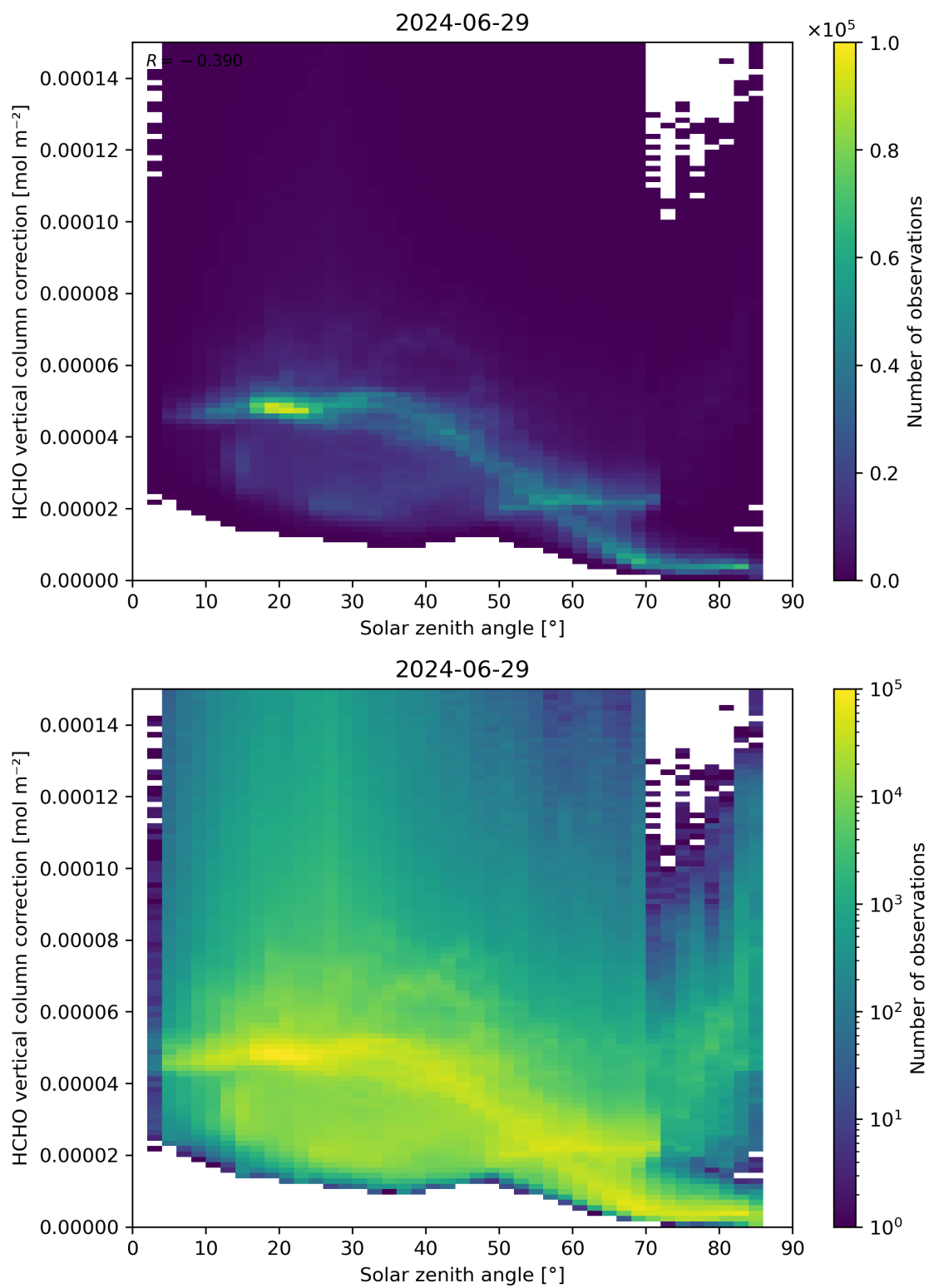
Figure 178: Scatter density plot of “Solar zenith angle” against “HCHO vertical column correction” for 2024-06-29 to 2024-06-30.
