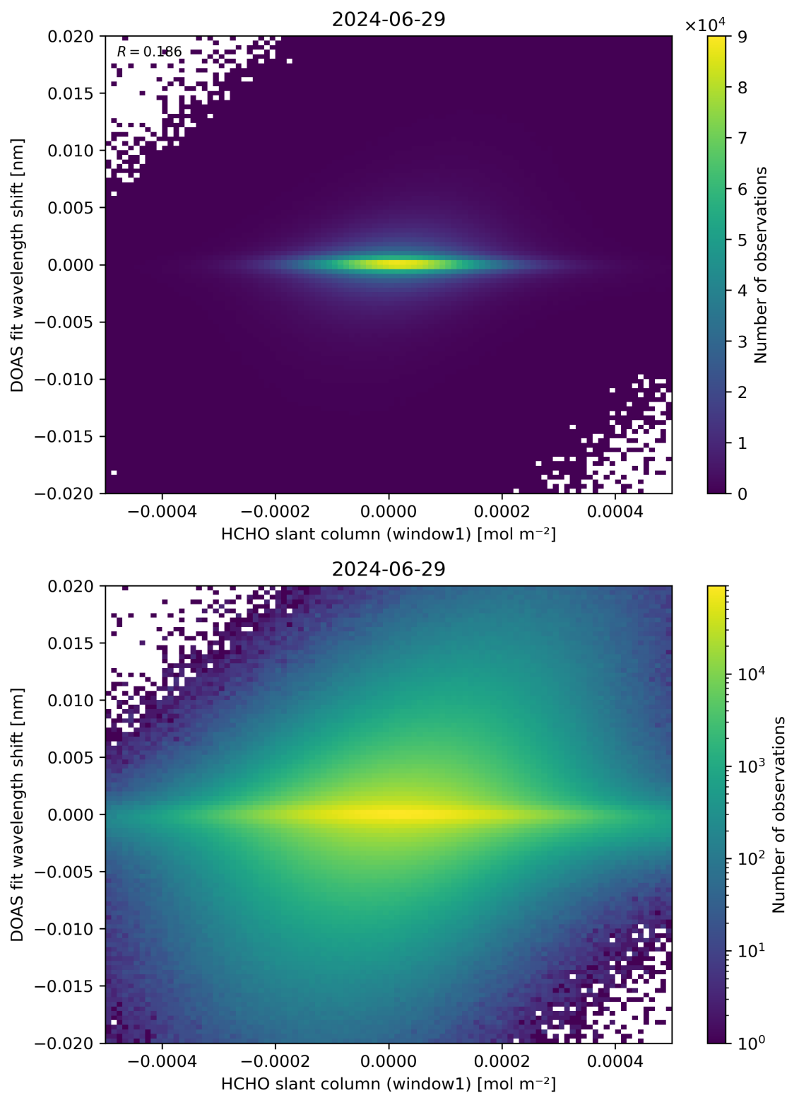
Figure 79: Scatter density plot of “HCHO slant column (window1)” against “DOAS fit wavelength shift” for 2024-06-29 to 2024-06-30.
