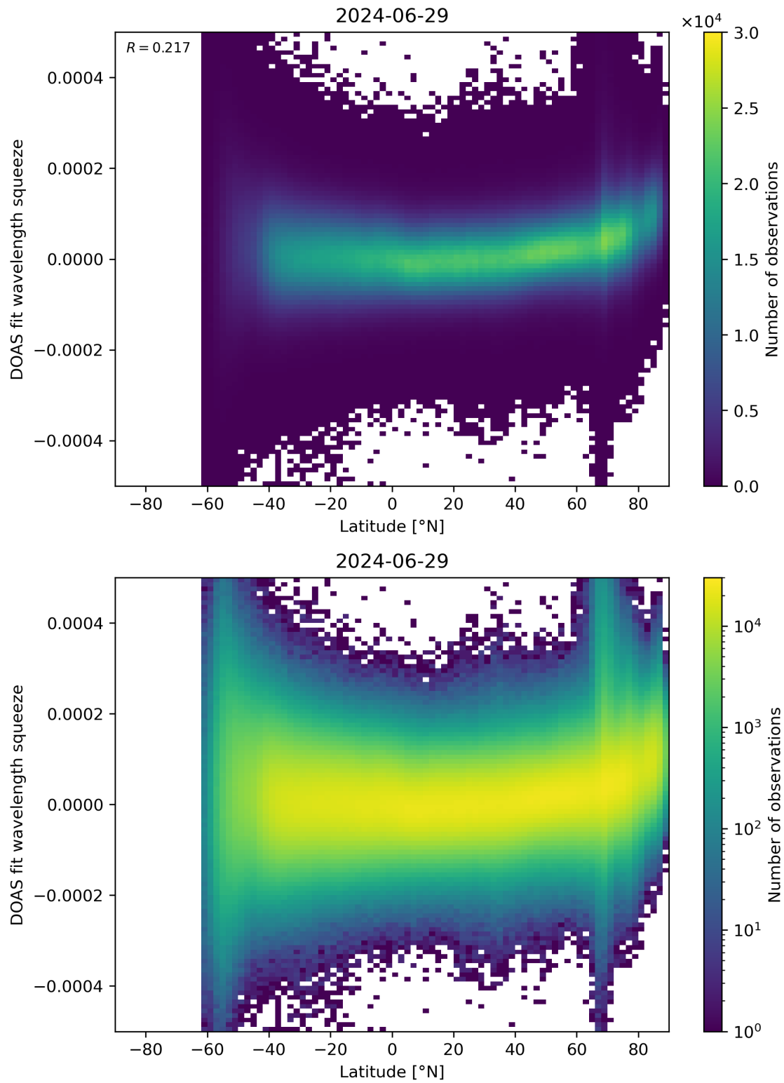
Figure 155: Scatter density plot of “Latitude” against “DOAS fit wavelength squeeze” for 2024-06-29 to 2024-06-30.
