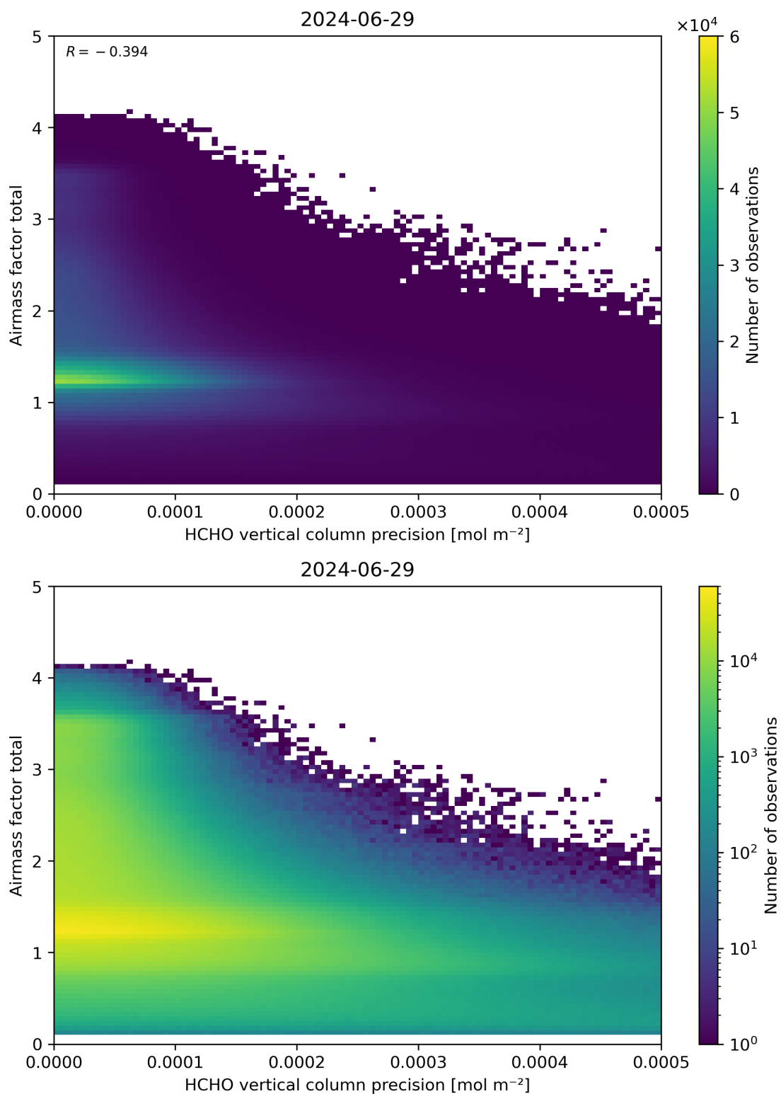
Figure 144: Scatter density plot of “HCHO vertical column precision” against “Airmass factor total” for 2024-06-29 to 2024-06-30.
