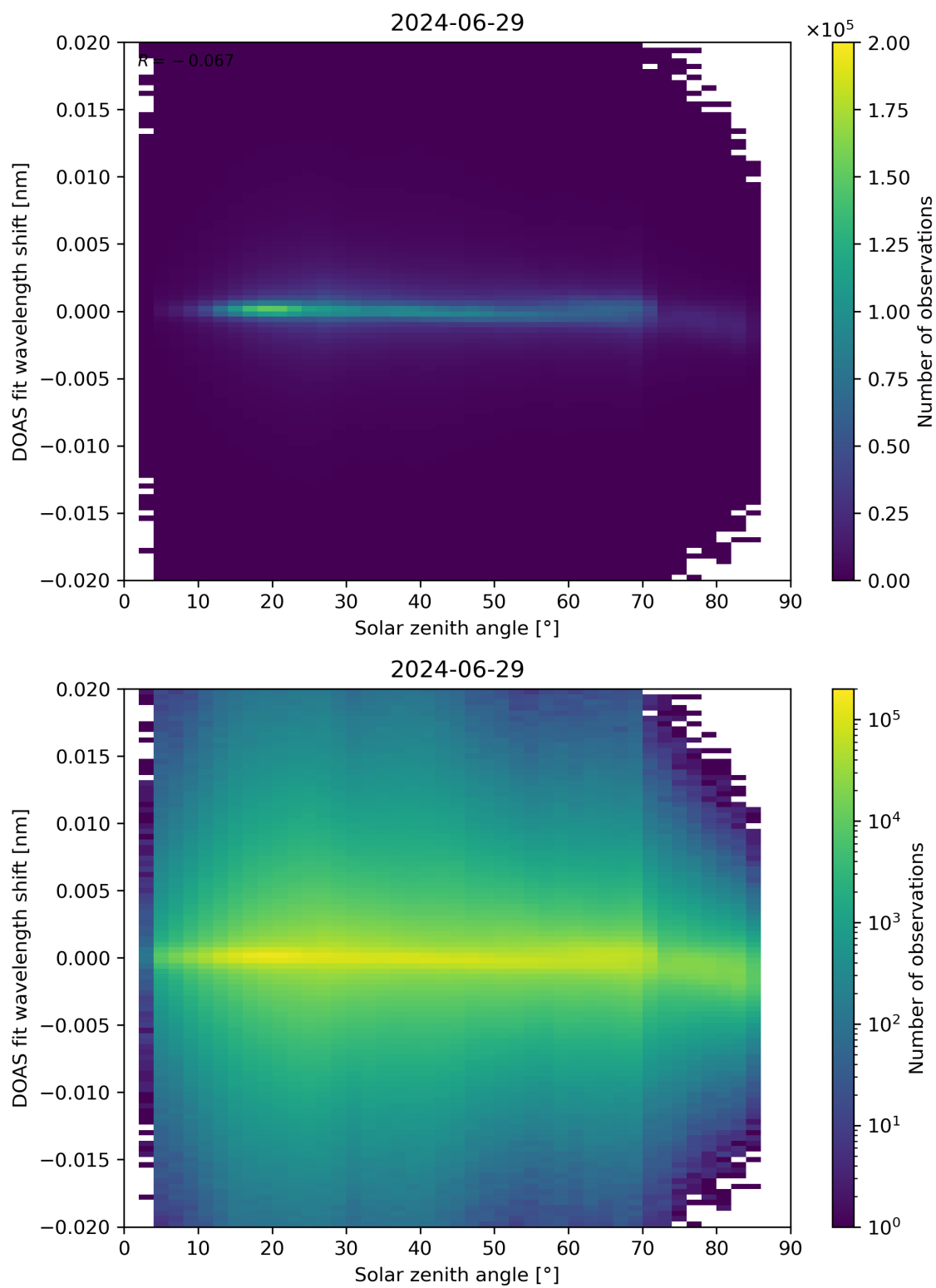
Figure 168: Scatter density plot of “Solar zenith angle” against “DOAS fit wavelength shift” for 2024-06-29 to 2024-06-30.
