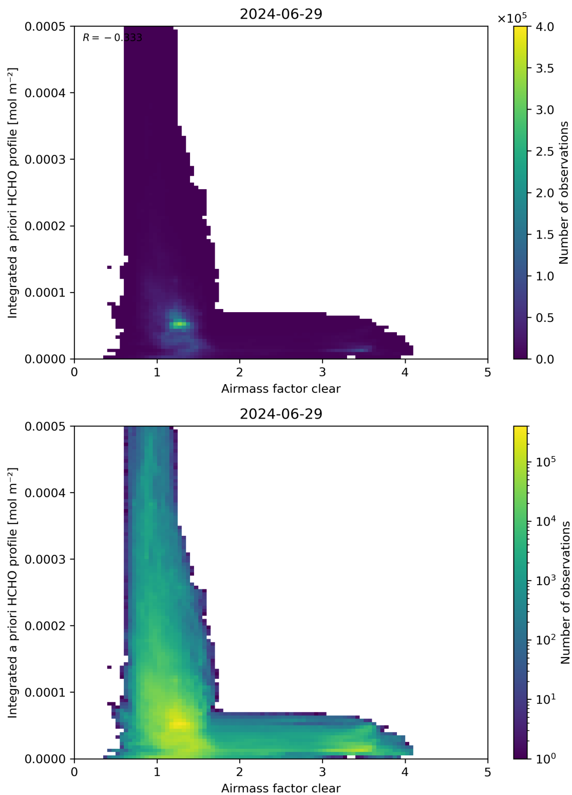
Figure 76: Scatter density plot of “Airmass factor clear” against “Integrated a priori HCHO profile” for 2024-06-29 to 2024-06-30.
