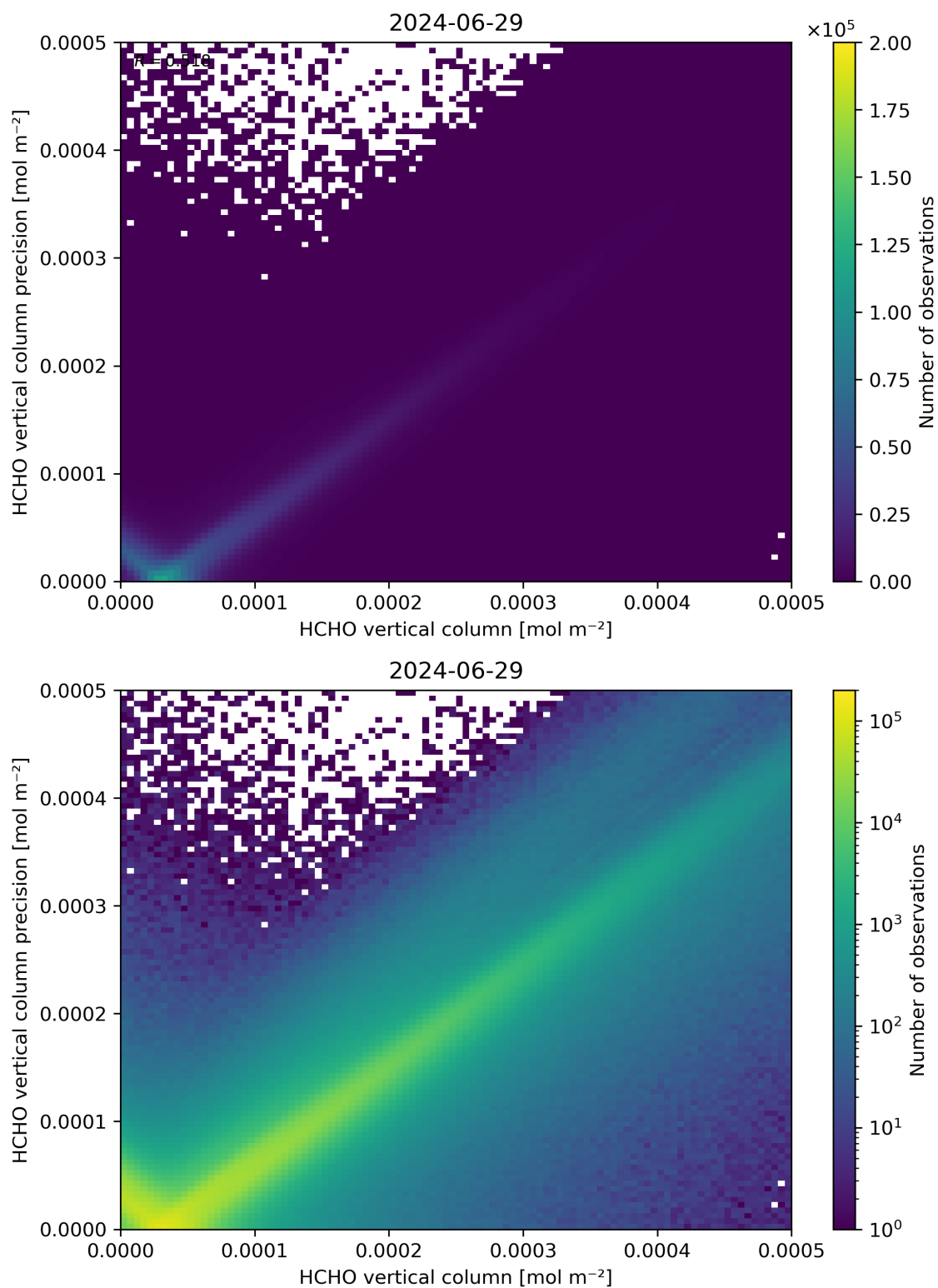
Figure 134: Scatter density plot of “HCHO vertical column” against “HCHO vertical column precision” for 2024-06-29 to 2024-06-30.
