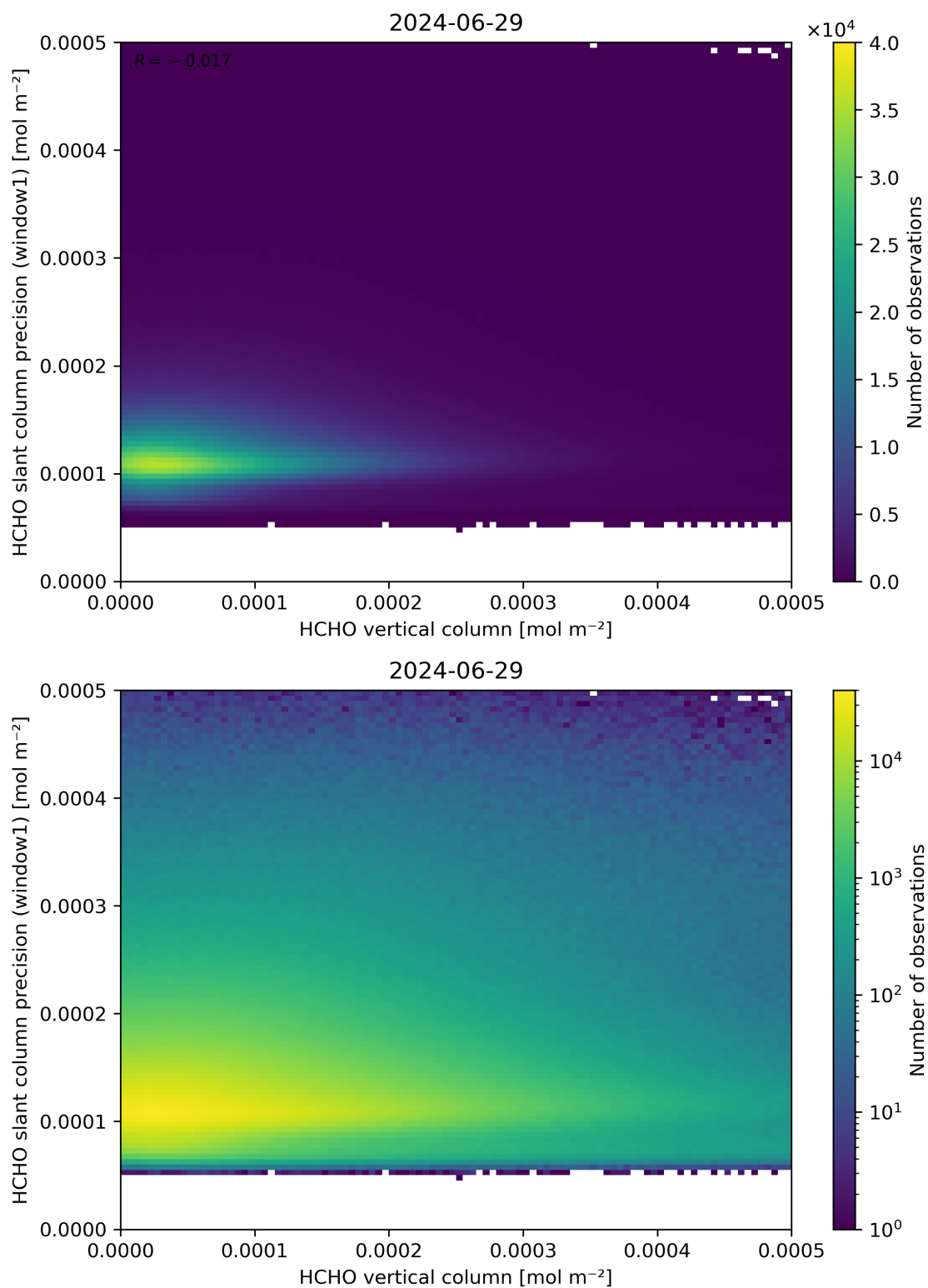
Figure 130: Scatter density plot of “HCHO vertical column” against “HCHO slant column precision (window1)” for 2024-06-29 to 2024-06-30.
