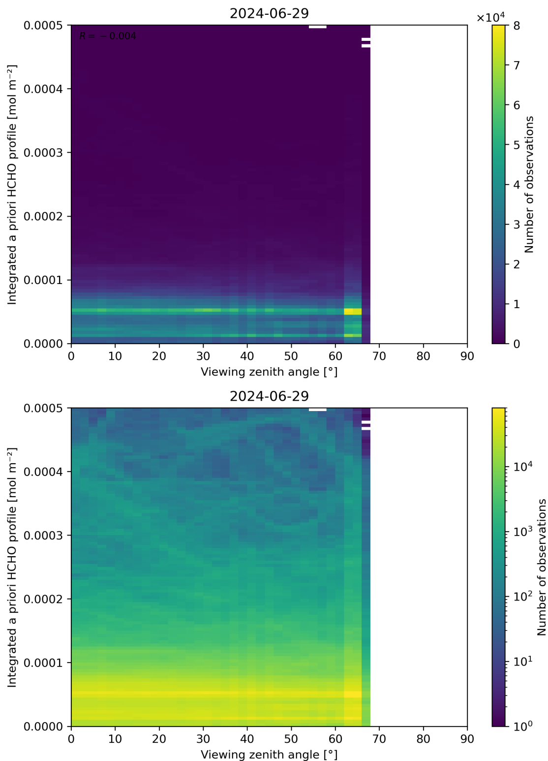
Figure 195: Scatter density plot of “Viewing zenith angle” against “Integrated a priori HCHO profile” for 2024-06-29 to 2024-06-30.
