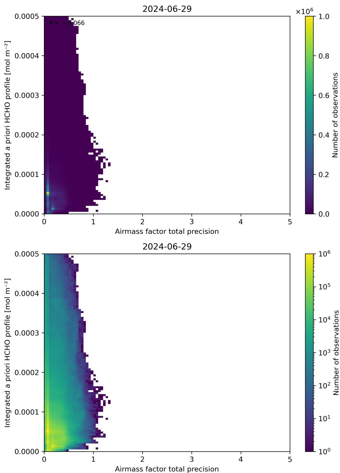
Figure 111: Scatter density plot of “Airmass factor total precision” against “Integrated a priori HCHO profile” for 2024-06-29 to 2024-06-30.
