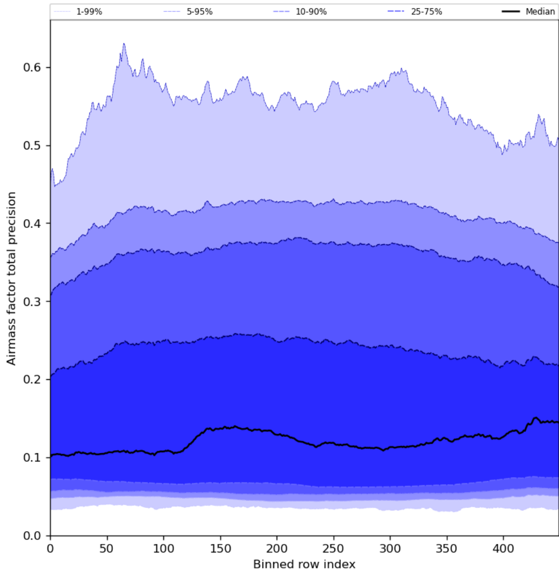
Figure 55: Along track statistics of “Airmass factor total precision” for 2024-06-29 to 2024-06-30
