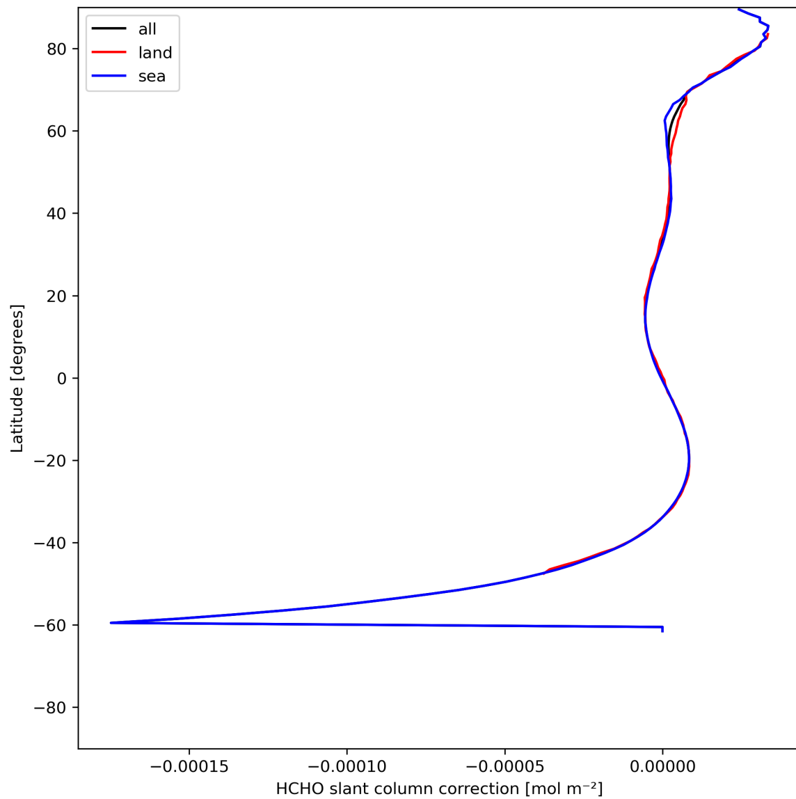
Figure 33: Zonal average of “HCHO slant column correction” for 2024-06-29 to 2024-06-30.
