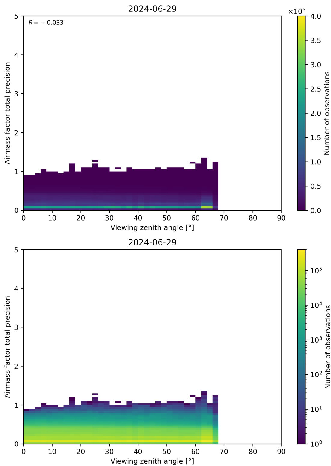
Figure 191: Scatter density plot of “Viewing zenith angle” against “Airmass factor total precision” for 2024-06-29 to 2024-06-30.
