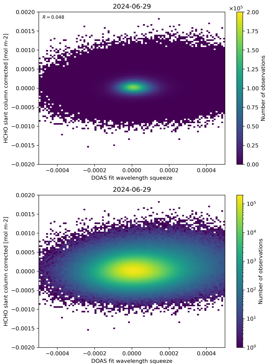
Figure 69: Scatter density plot of “DOAS fit wavelength squeeze” against “HCHO slant column corrected” for 2024-06-29 to 2024-06-30.
