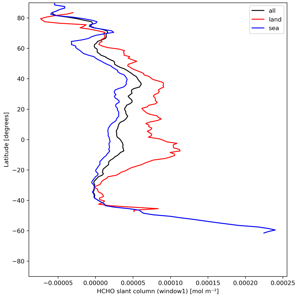
Figure 24: Zonal average of “HCHO slant column (window1)” for 2024-06-29 to 2024-06-30.
