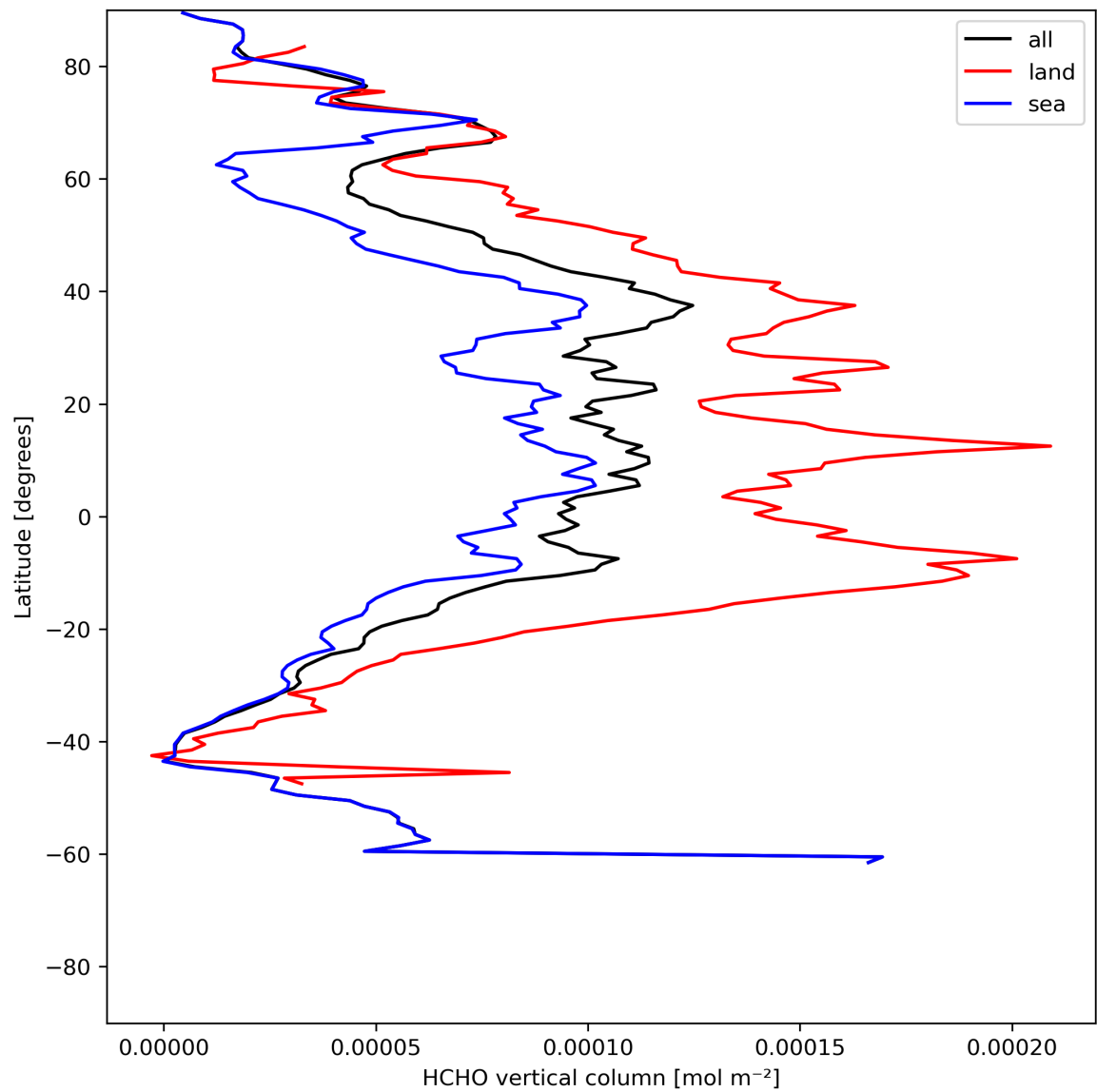
Figure 21: Zonal average of “HCHO vertical column” for 2024-06-29 to 2024-06-30.
