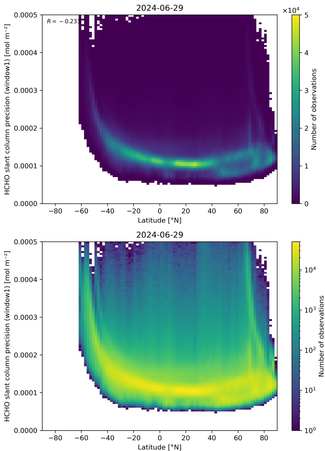
Figure 160: Scatter density plot of “Latitude” against “HCHO slant column precision (window1)” for 2024-06-29 to 2024-06-30.
