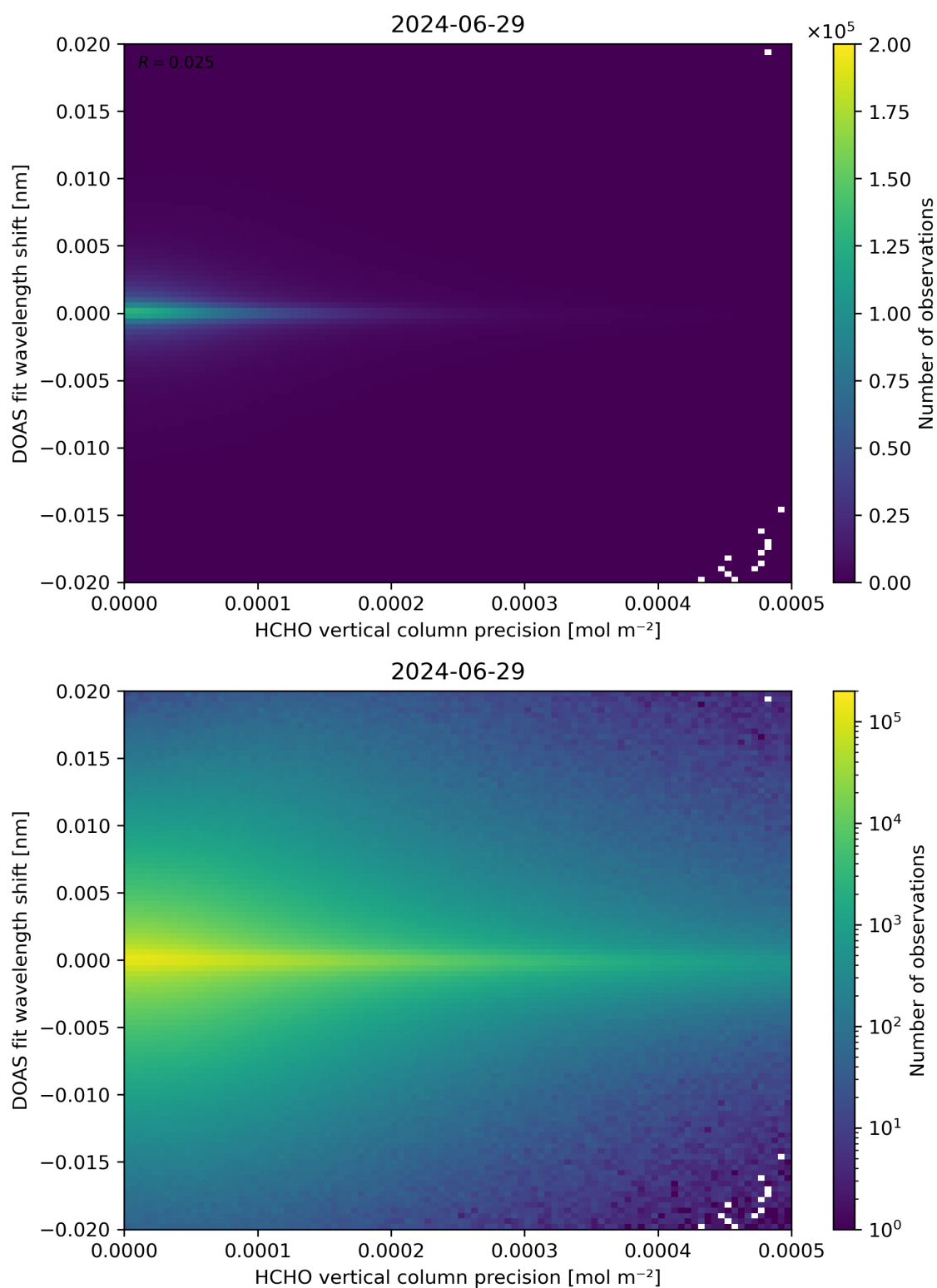
Figure 137: Scatter density plot of “HCHO vertical column precision” against “DOAS fit wavelength shift” for 2024-06-29 to 2024-06-30.
