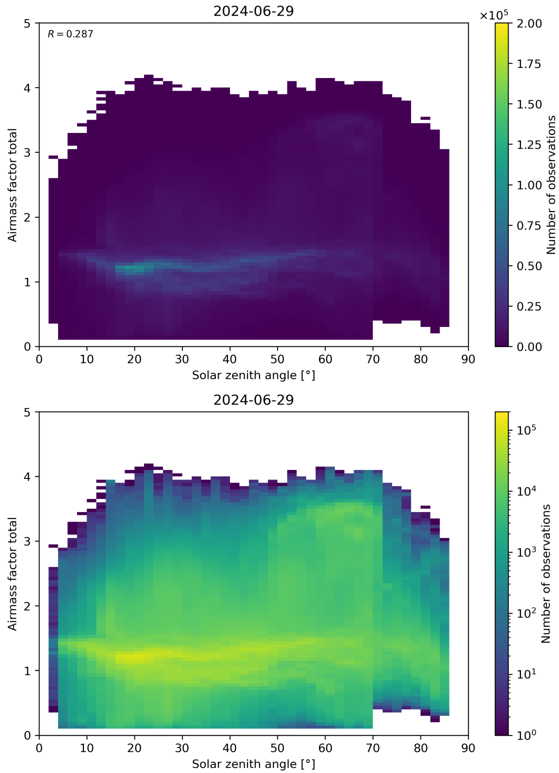
Figure 175: Scatter density plot of “Solar zenith angle” against “Airmass factor total” for 2024-06-29 to 2024-06-30.
