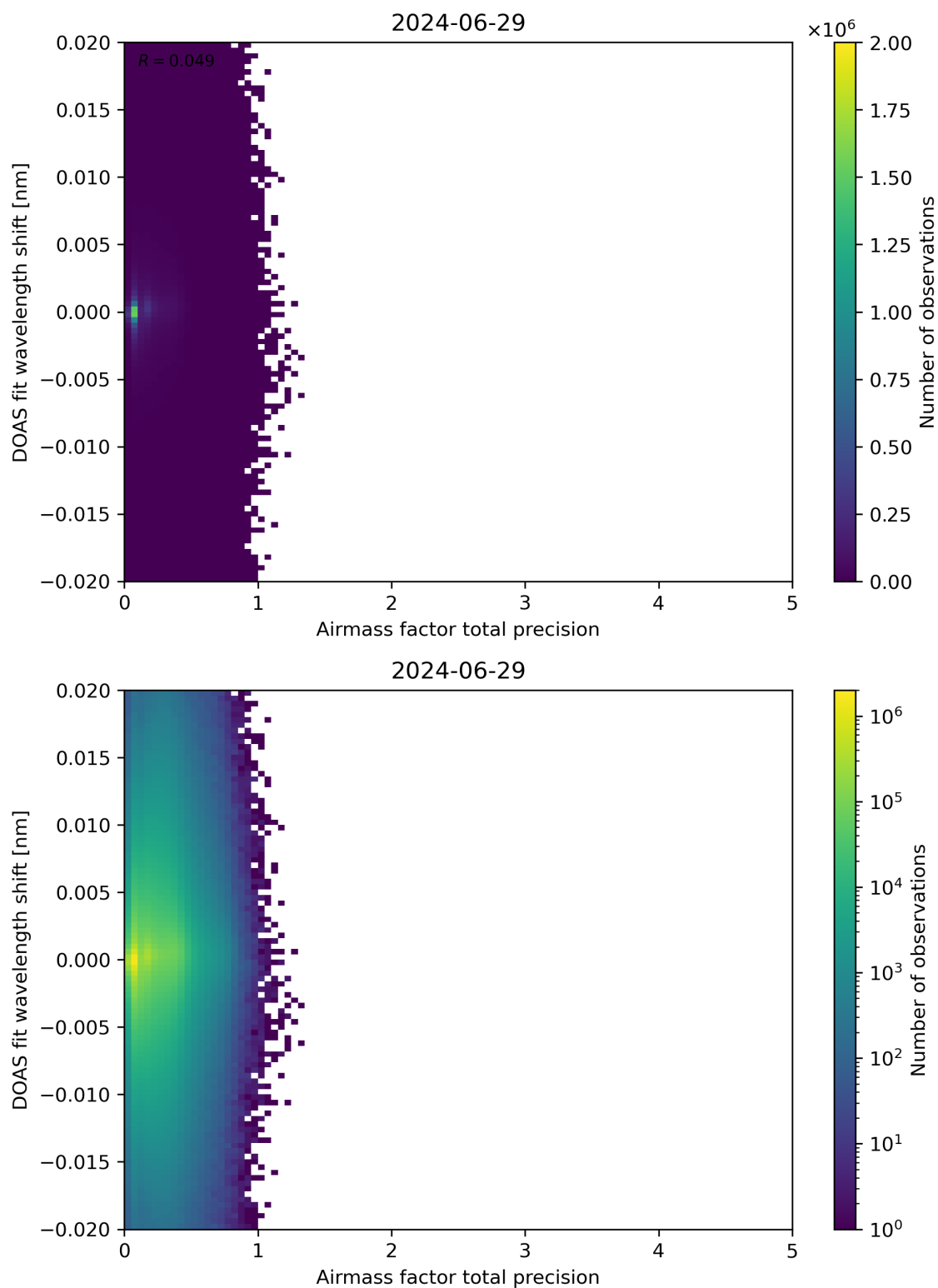
Figure 106: Scatter density plot of “Airmass factor total precision” against “DOAS fit wavelength shift” for 2024-06-29 to 2024-06-30.
