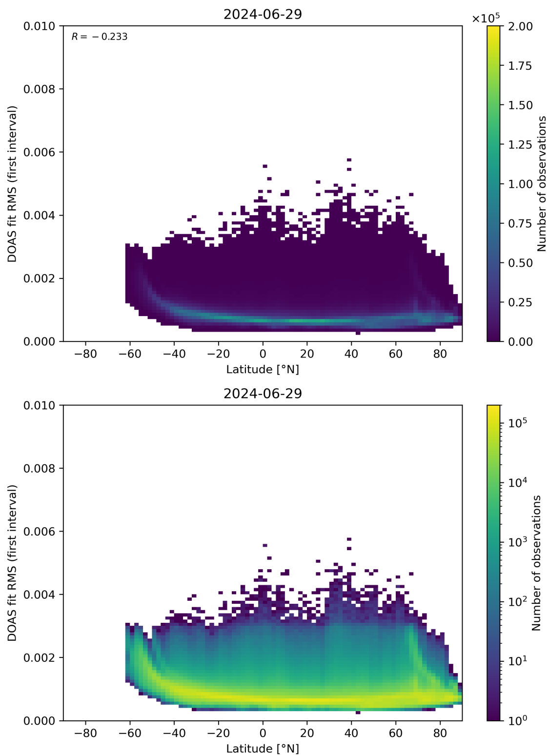
Figure 153: Scatter density plot of “Latitude” against “DOAS fit RMS (first interval)” for 2024-06-29 to 2024-06-30.
