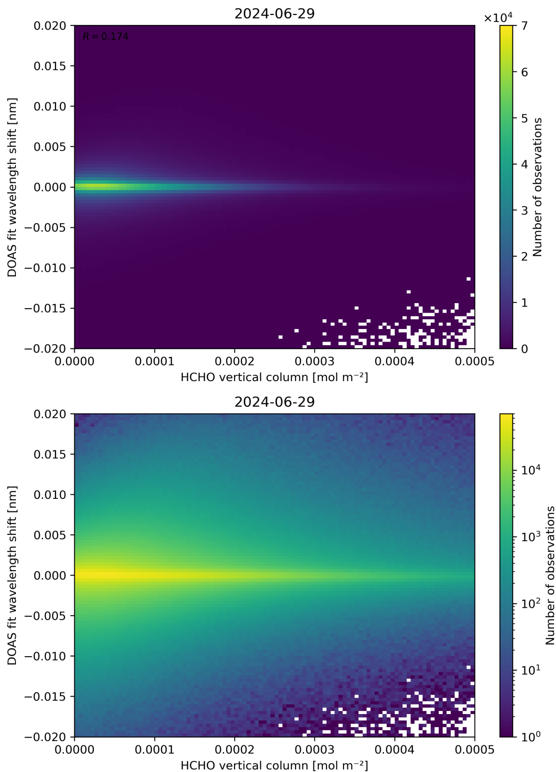
Figure 124: Scatter density plot of “HCHO vertical column” against “DOAS fit wavelength shift” for 2024-06-29 to 2024-06-30.
