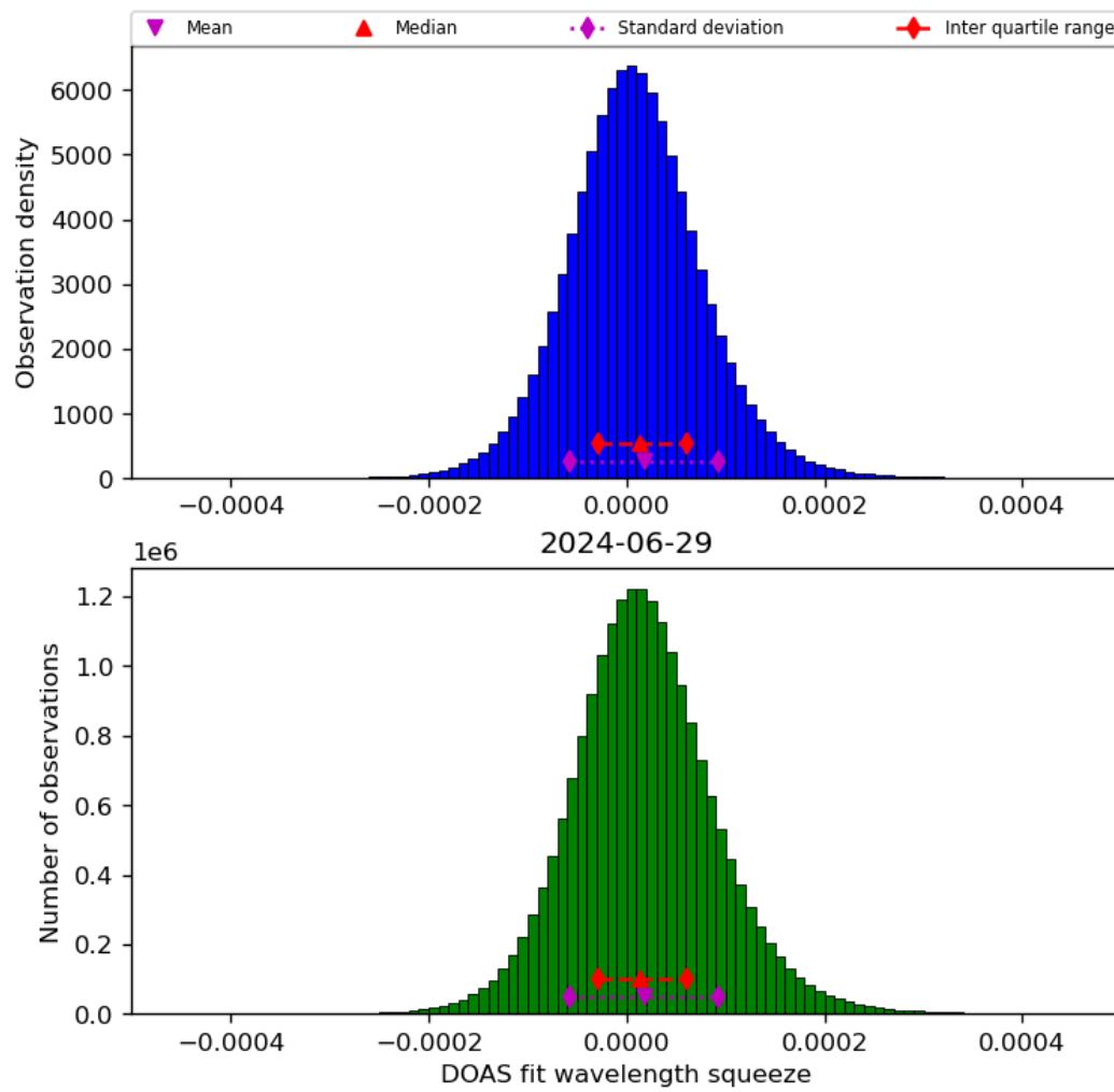
Figure 45: Histogram of “DOAS fit wavelength squeeze” for 2024-06-29 to 2024-06-30
