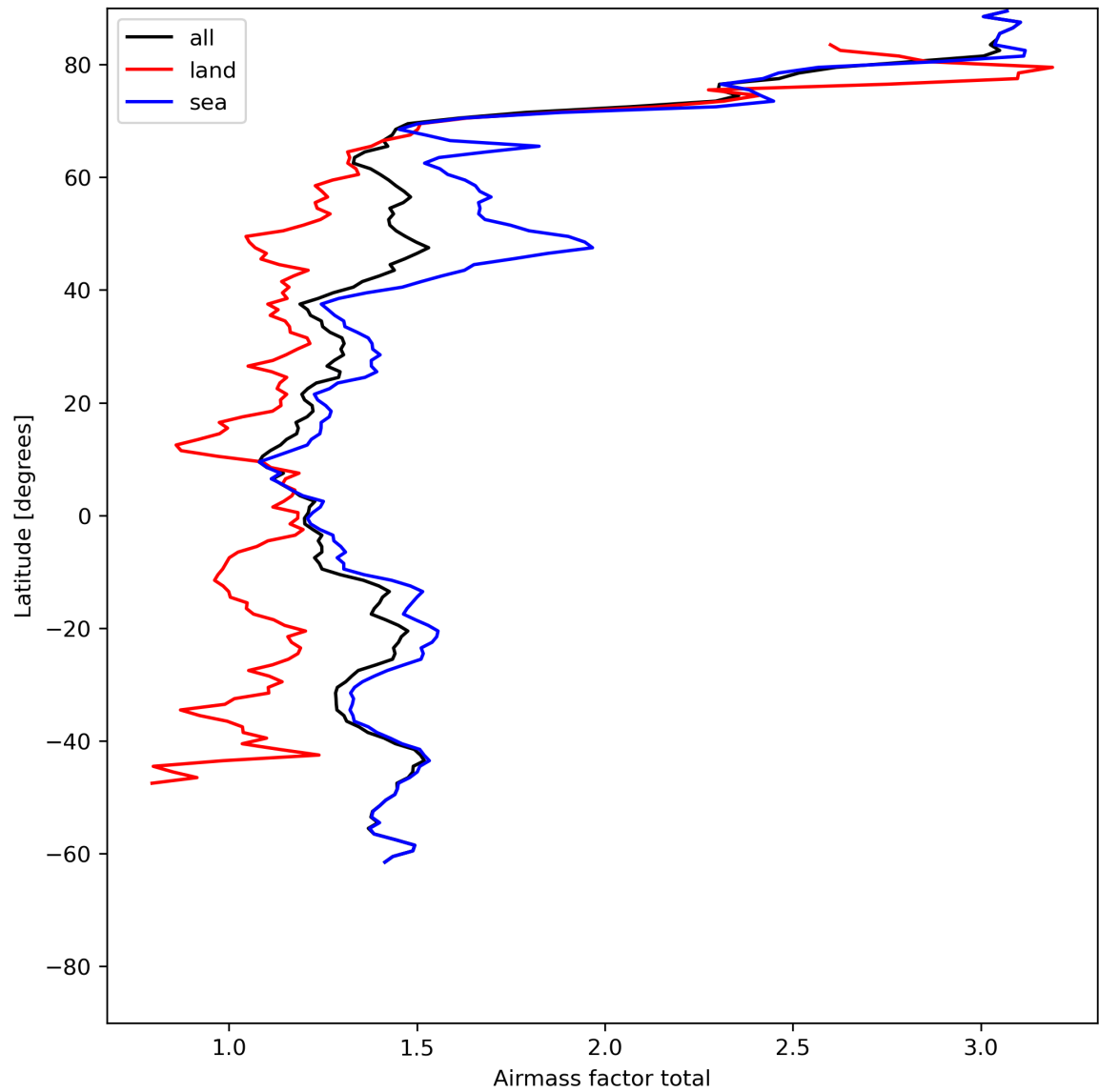
Figure 26: Zonal average of “Airmass factor total” for 2024-06-29 to 2024-06-30.
