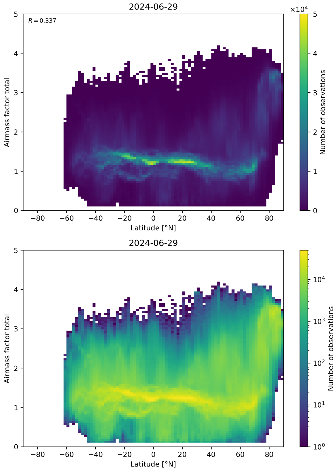
Figure 161: Scatter density plot of “Latitude” against “Airmass factor total” for 2024-06-29 to 2024-06-30.
