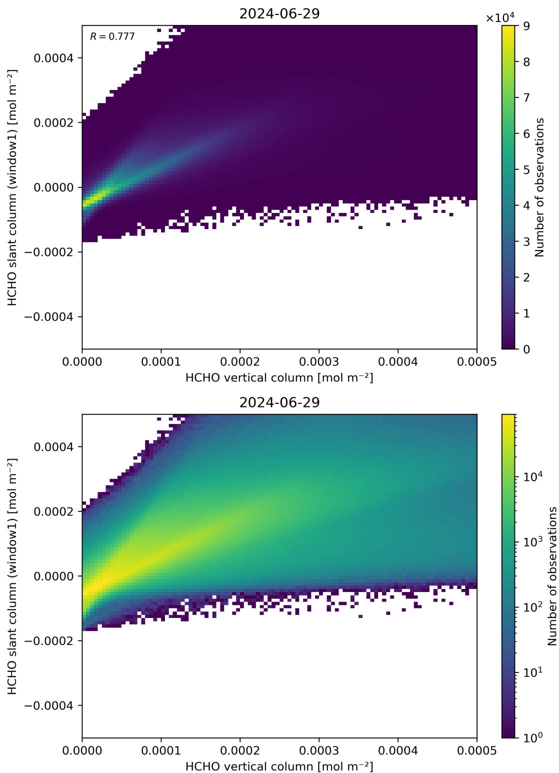
Figure 129: Scatter density plot of “HCHO vertical column” against “HCHO slant column (window1)” for 2024-06-29 to 2024-06-30.
