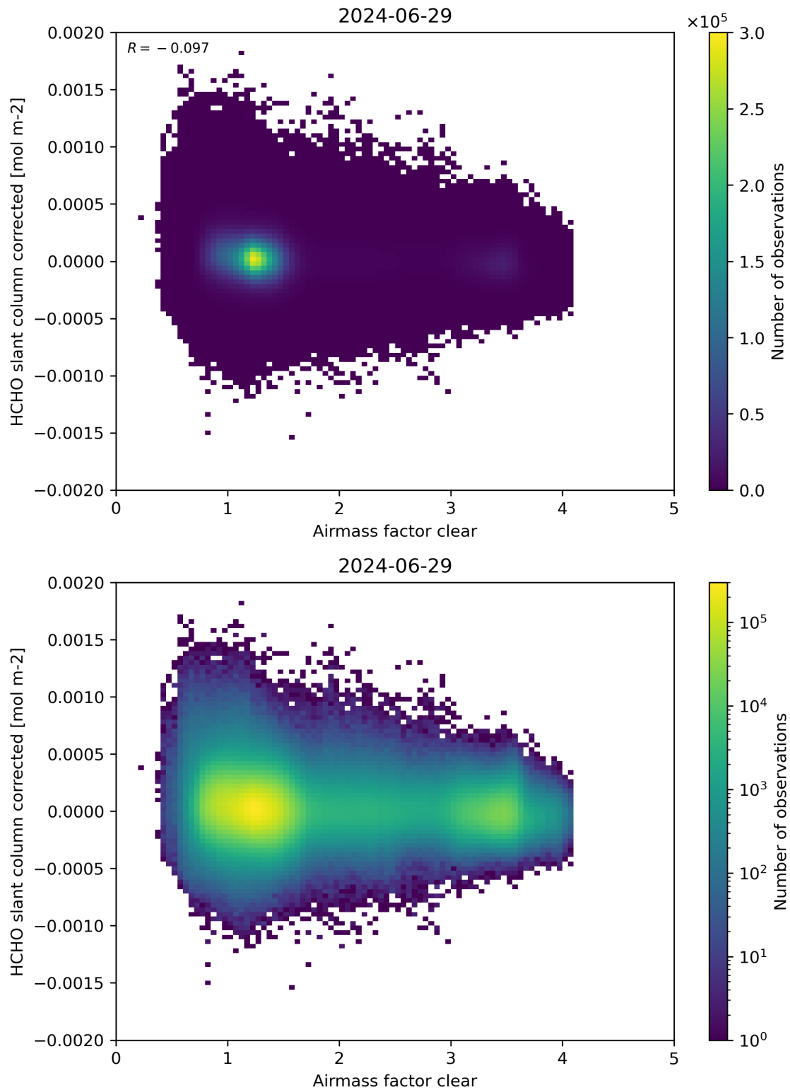
Figure 74: Scatter density plot of “Airmass factor clear” against “HCHO slant column corrected” for 2024-06-29 to 2024-06-30.
