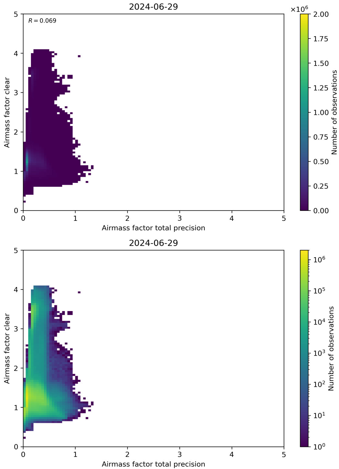
Figure 108: Scatter density plot of “Airmass factor total precision” against “Airmass factor clear” for 2024-06-29 to 2024-06-30.
