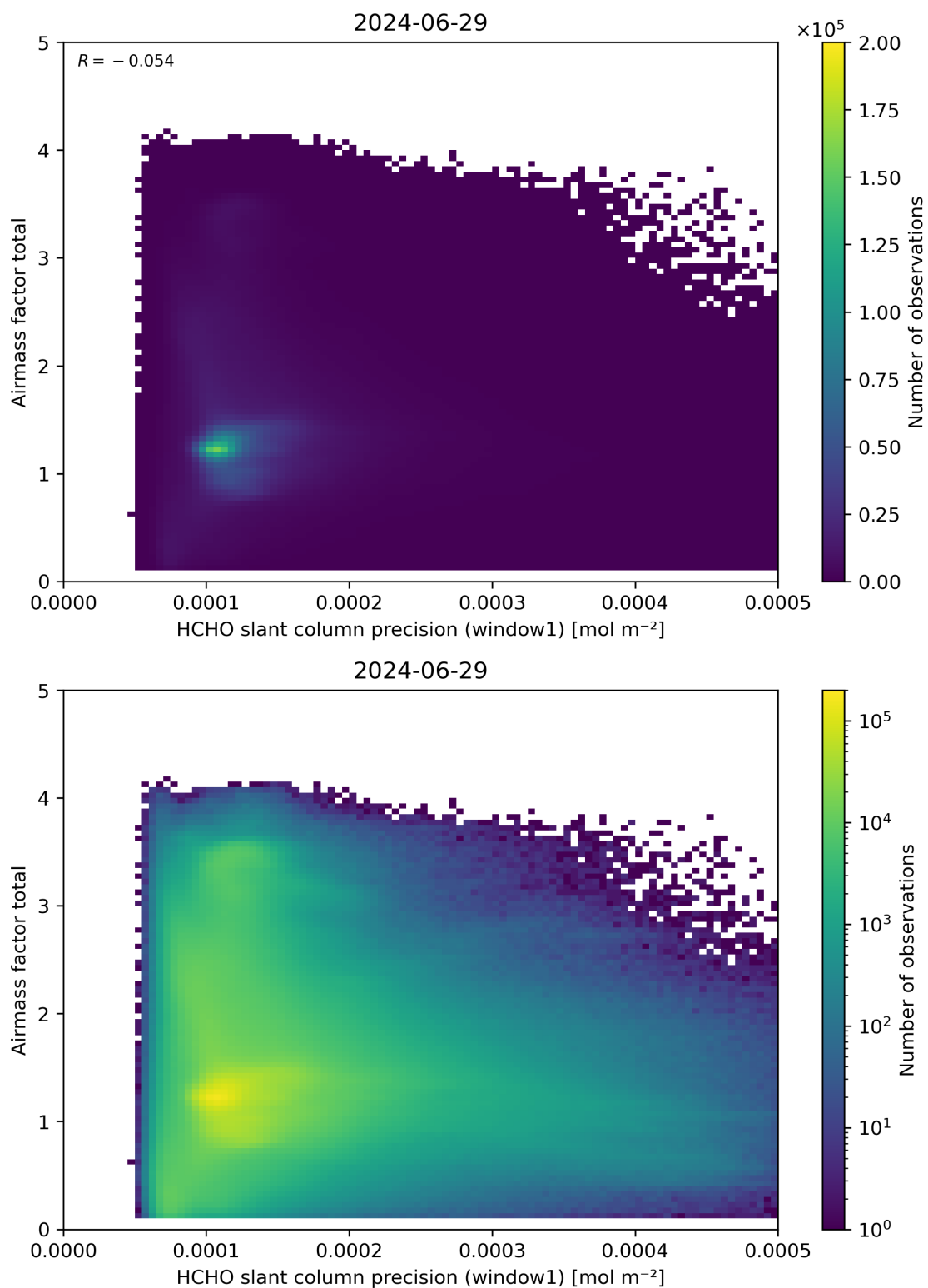
Figure 94: Scatter density plot of “HCHO slant column precision (window1)” against “Airmass factor total” for 2024-06-29 to 2024-06-30.
