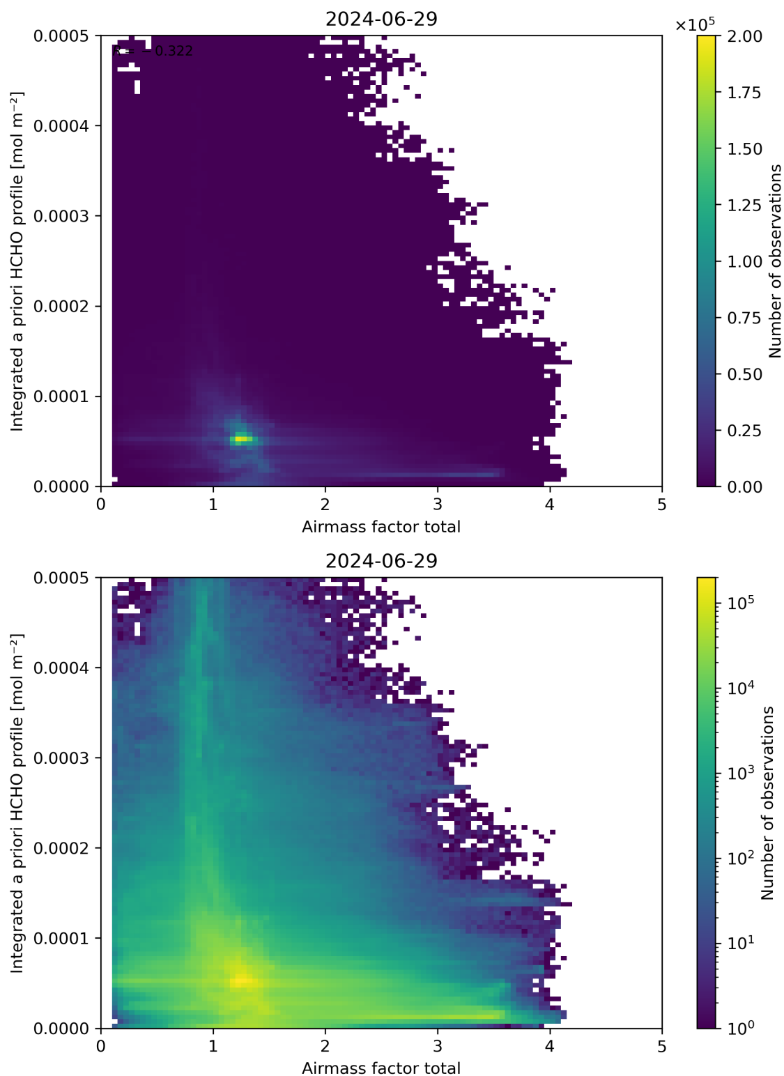
Figure 104: Scatter density plot of “Airmass factor total” against “Integrated a priori HCHO profile” for 2024-06-29 to 2024-06-30.
