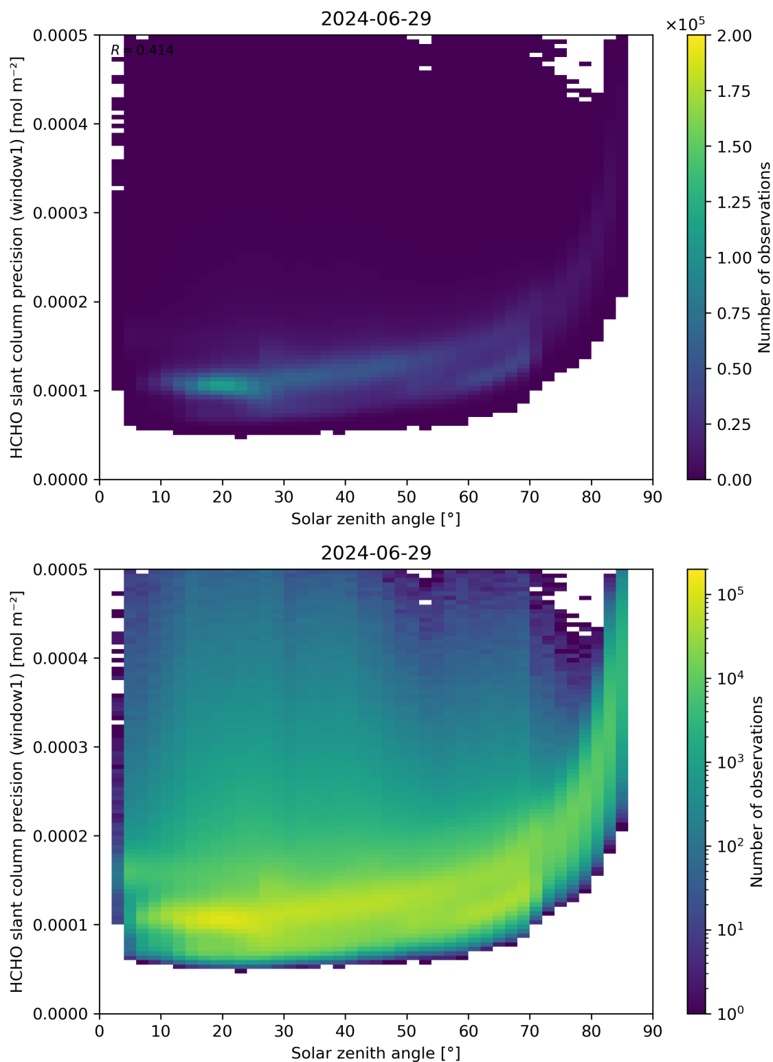
Figure 174: Scatter density plot of “Solar zenith angle” against “HCHO slant column precision (window1)” for 2024-06-29 to 2024-06-30.
