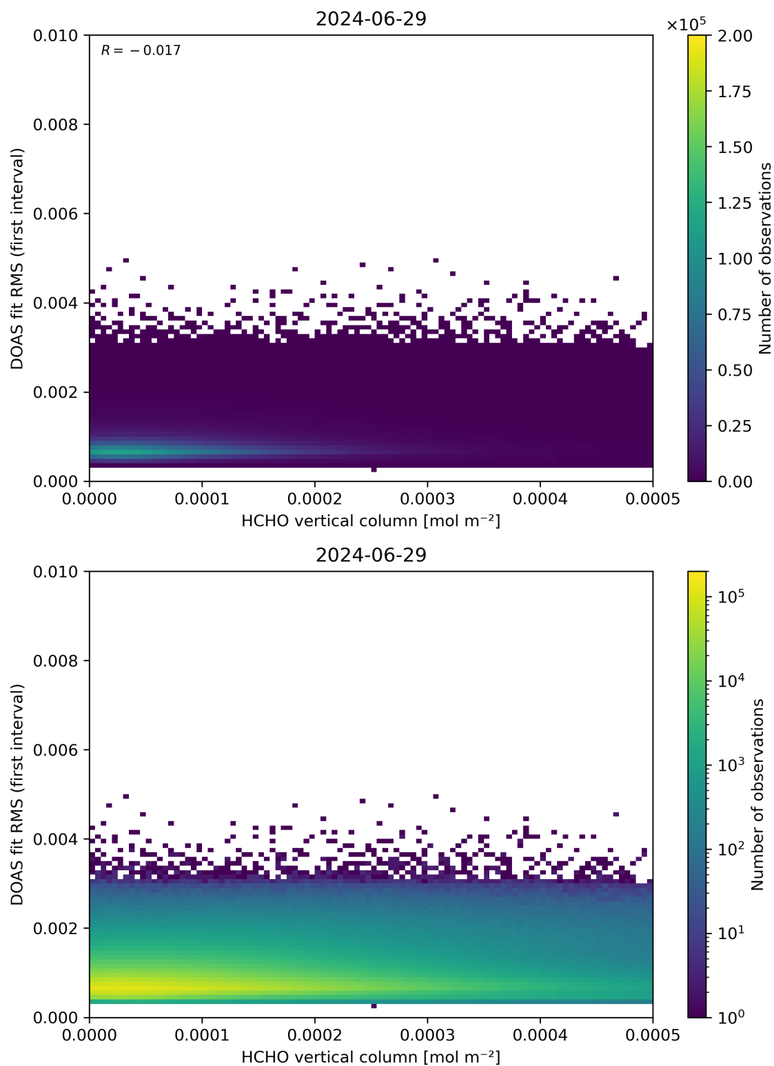
Figure 123: Scatter density plot of “HCHO vertical column” against “DOAS fit RMS (first interval)” for 2024-06-29 to 2024-06-30.
