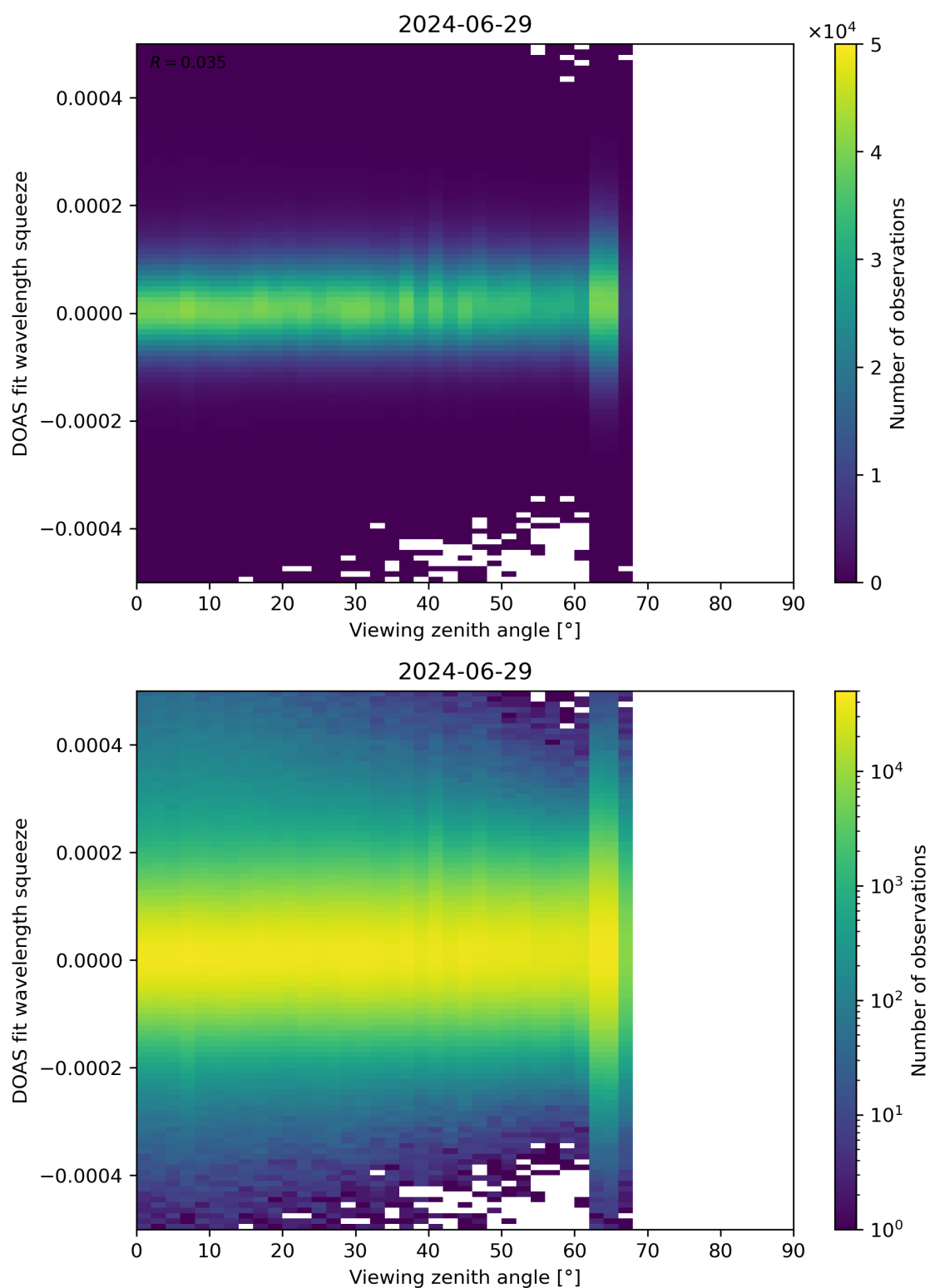
Figure 184: Scatter density plot of “Viewing zenith angle” against “DOAS fit wavelength squeeze” for 2024-06-29 to 2024-06-30.
