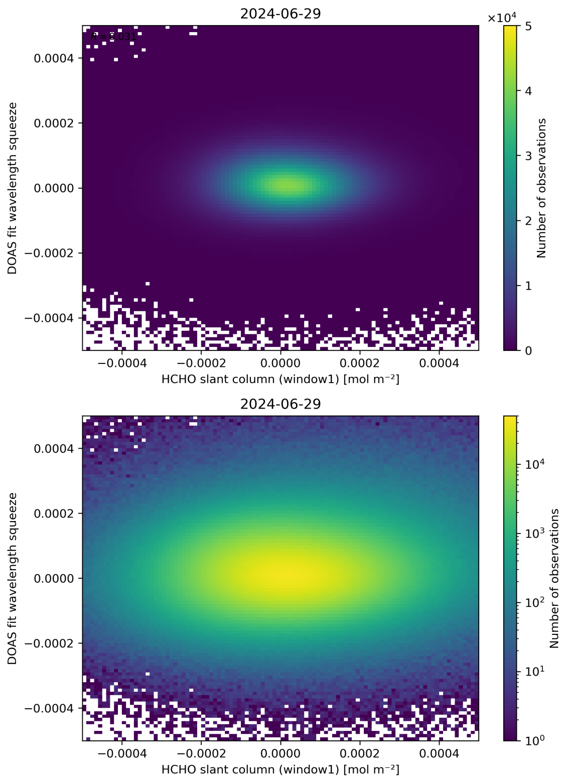
Figure 80: Scatter density plot of “HCHO slant column (window1)” against “DOAS fit wavelength squeeze” for 2024-06-29 to 2024-06-30.
