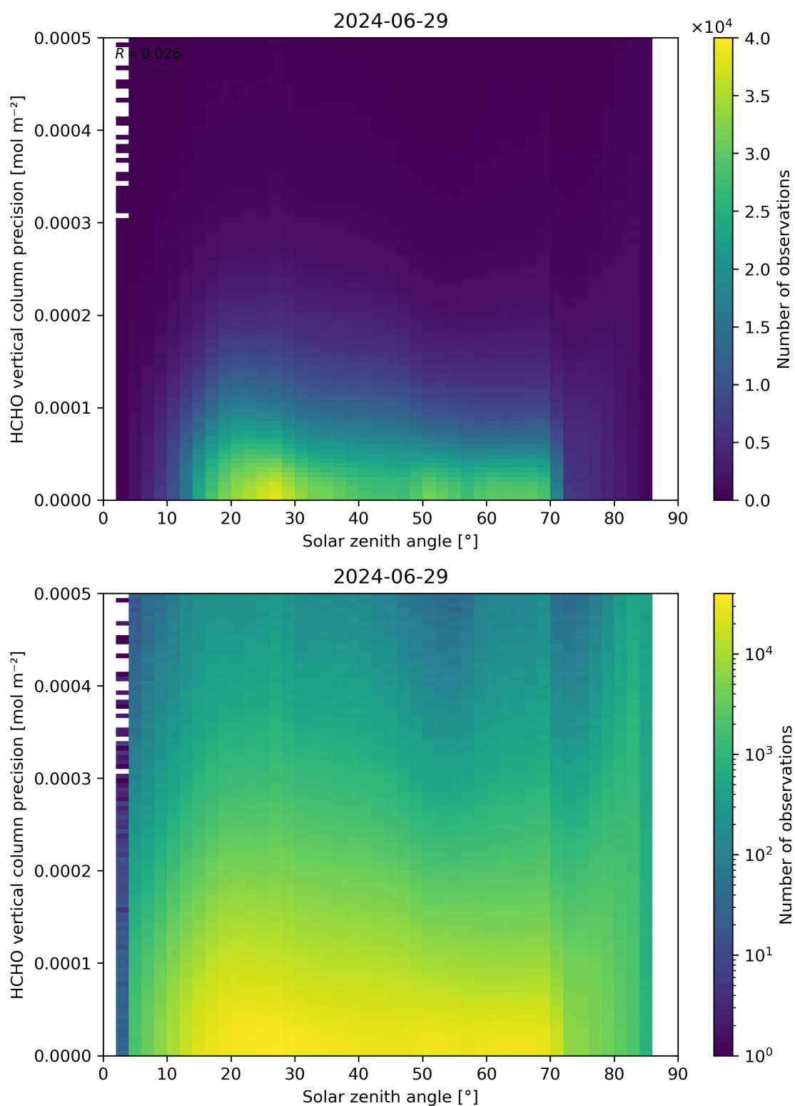
Figure 179: Scatter density plot of “Solar zenith angle” against “HCHO vertical column precision” for 2024-06-29 to 2024-06-30.
