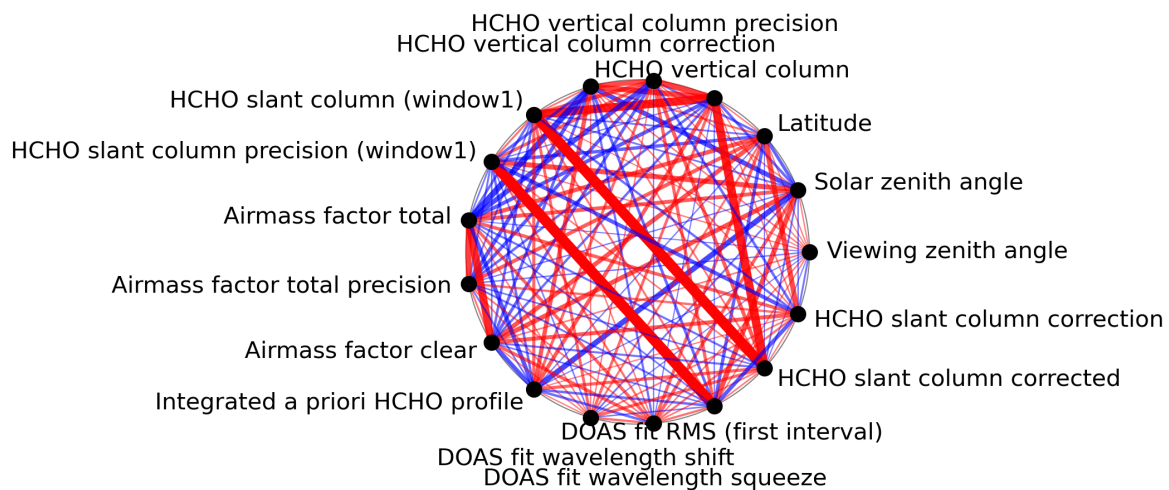
Figure 1: Map of correlation graph for 2024-06-29 to 2024-06-30.
