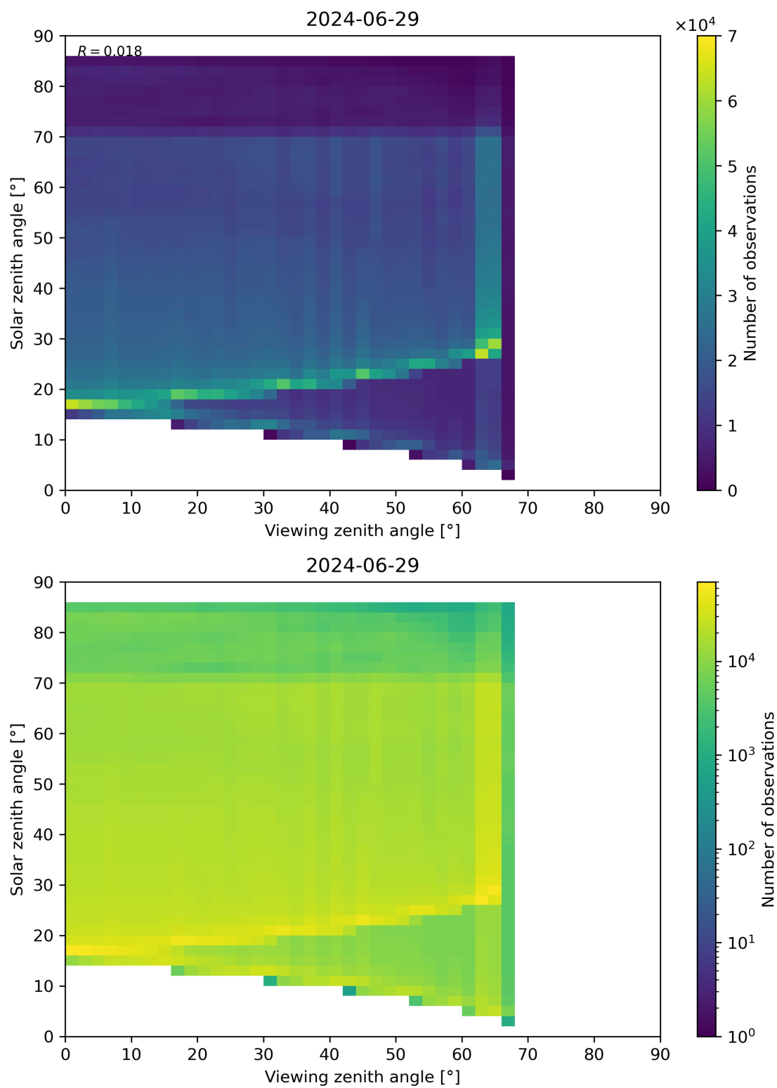
Figure 197: Scatter density plot of “Viewing zenith angle” against “Solar zenith angle” for 2024-06-29 to 2024-06-30.
