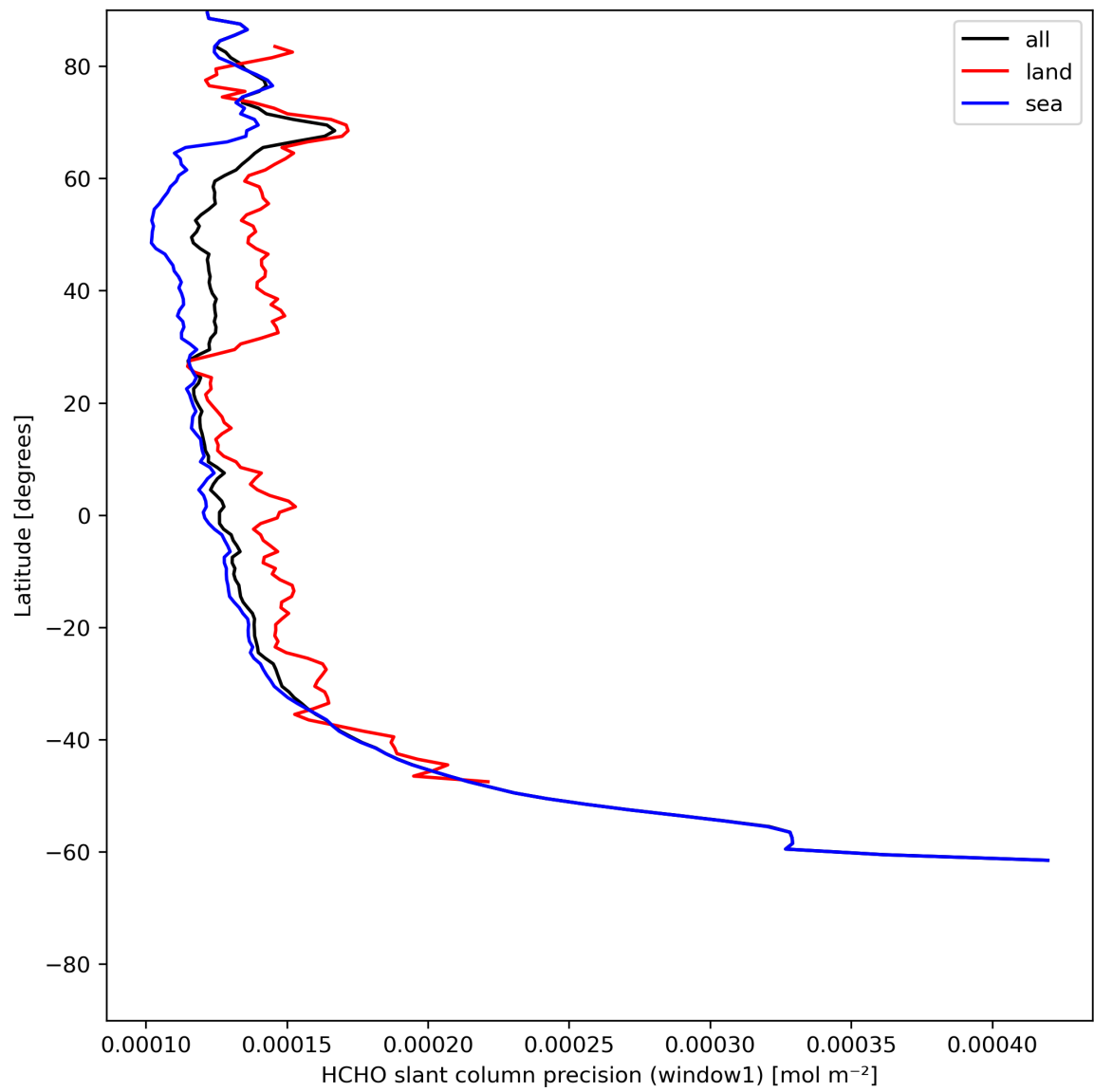
Figure 25: Zonal average of “HCHO slant column precision (window1)” for 2024-06-29 to 2024-06-30.
