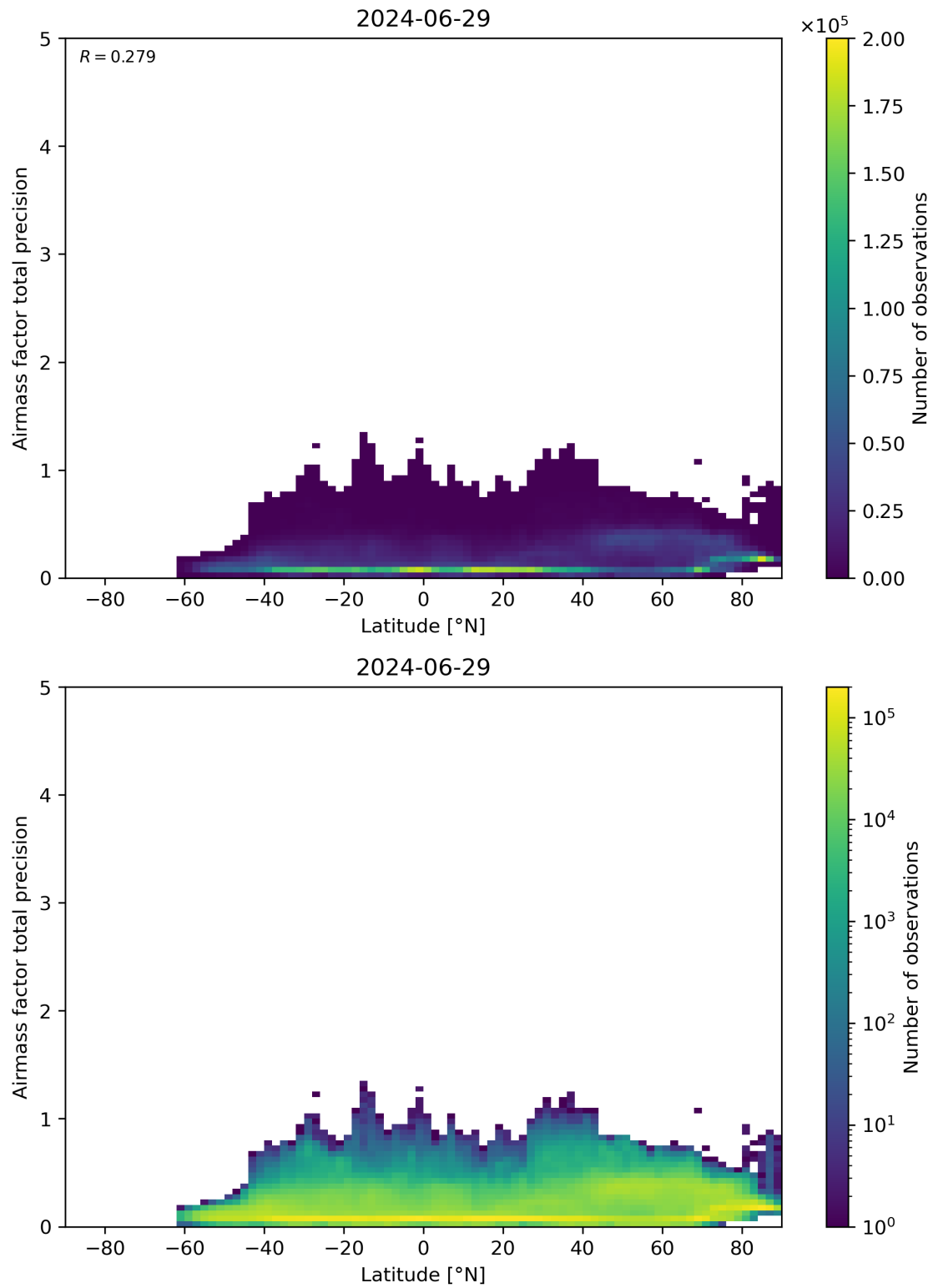
Figure 162: Scatter density plot of “Latitude” against “Airmass factor total precision” for 2024-06-29 to 2024-06-30.
