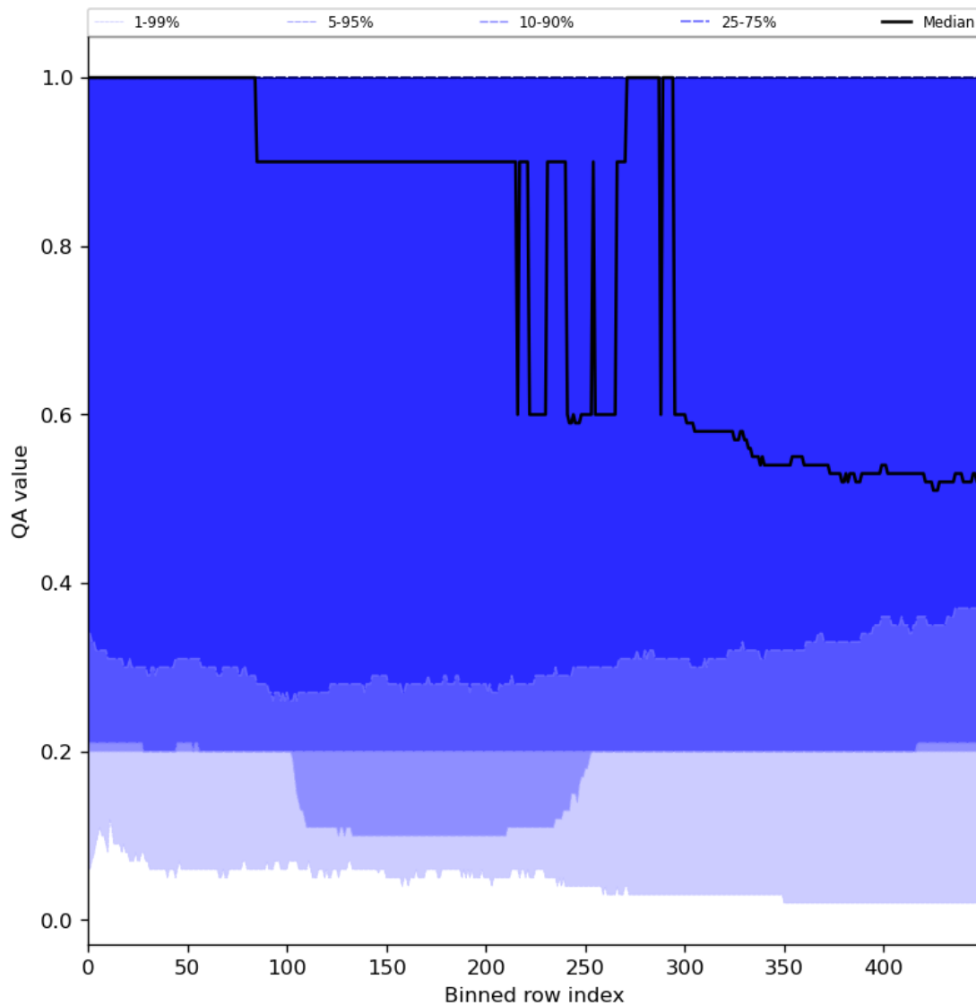
Figure 48: Along track statistics of “QA value” for 2024-06-29 to 2024-06-30
