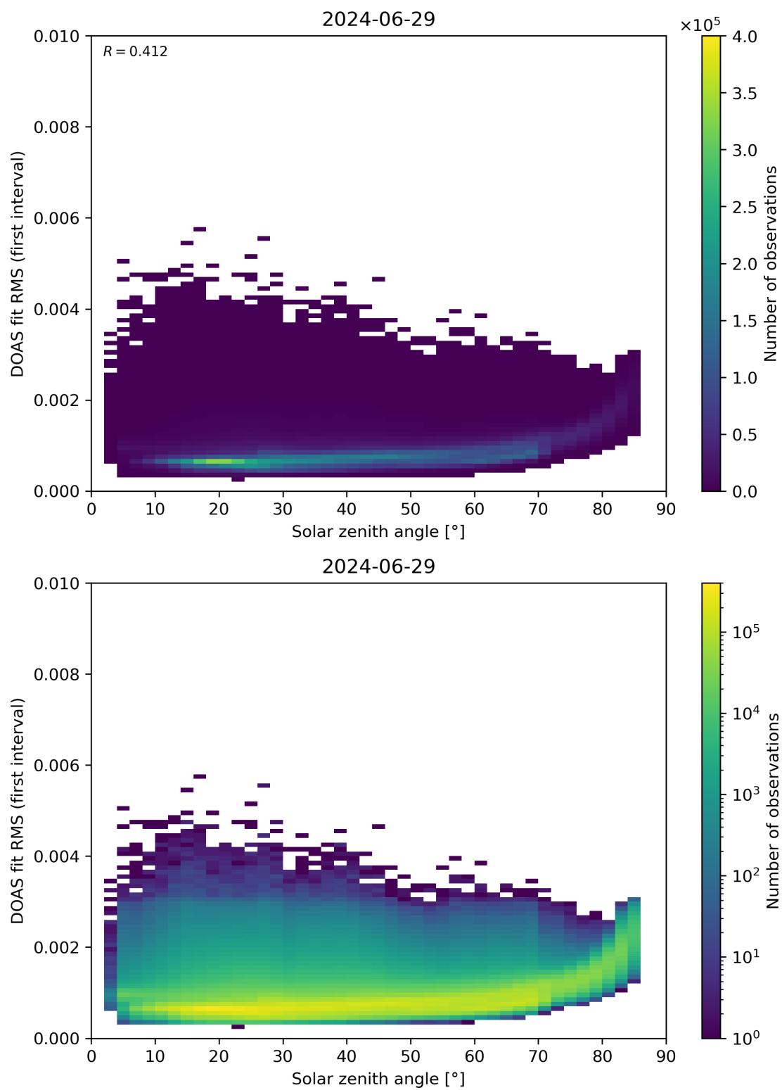
Figure 167: Scatter density plot of “Solar zenith angle” against “DOAS fit RMS (first interval)” for 2024-06-29 to 2024-06-30.
