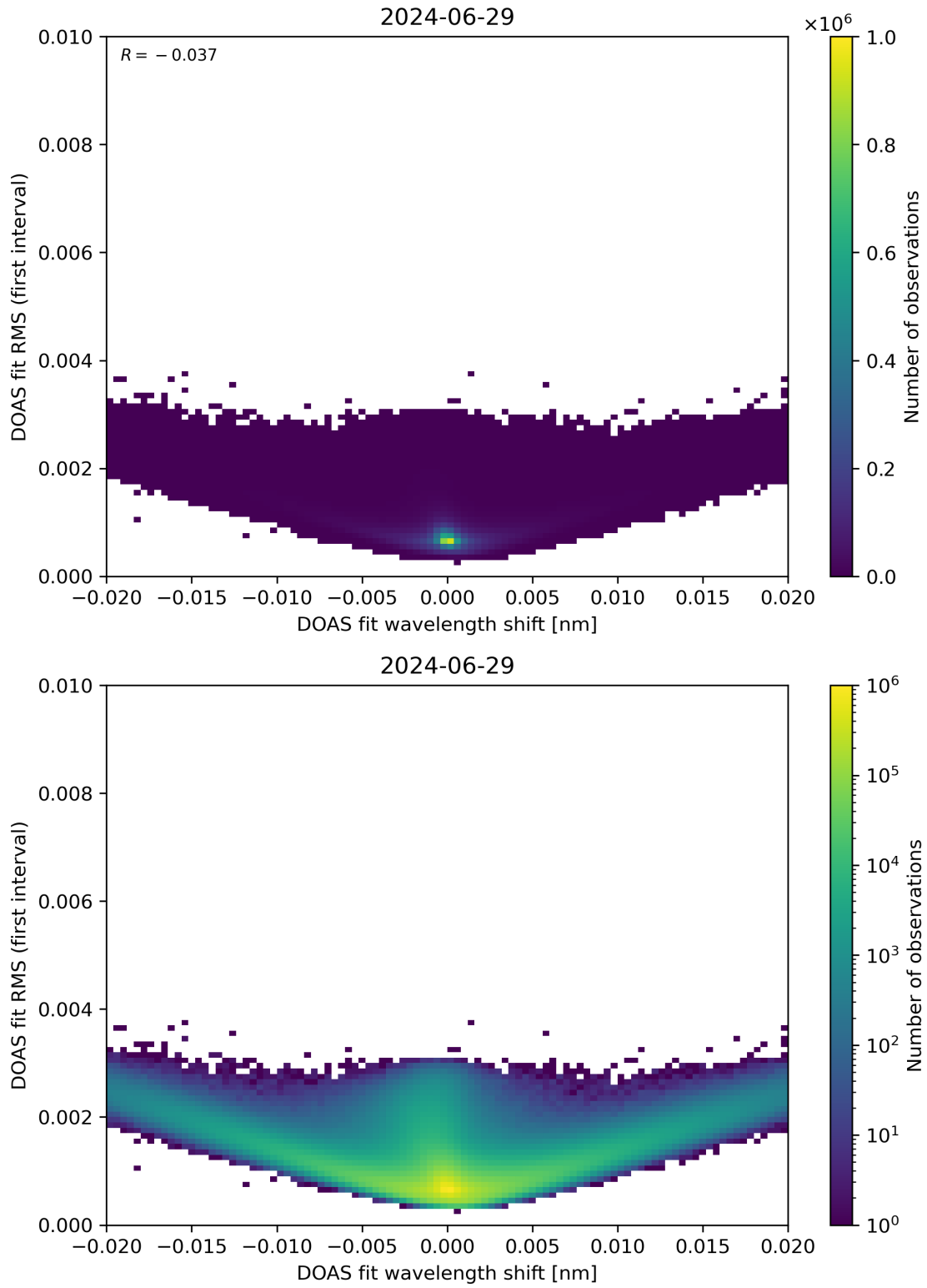
Figure 64: Scatter density plot of “DOAS fit wavelength shift” against “DOAS fit RMS (first interval)” for 2024-06-29 to 2024-06-30.
