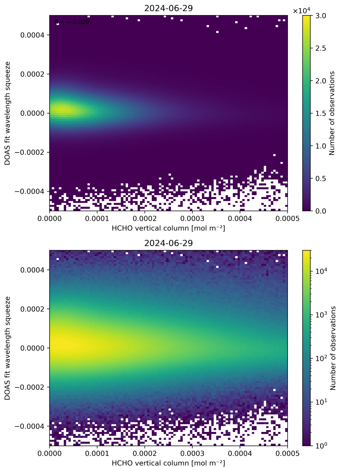
Figure 125: Scatter density plot of “HCHO vertical column” against “DOAS fit wavelength squeeze” for 2024-06-29 to 2024-06-30.
