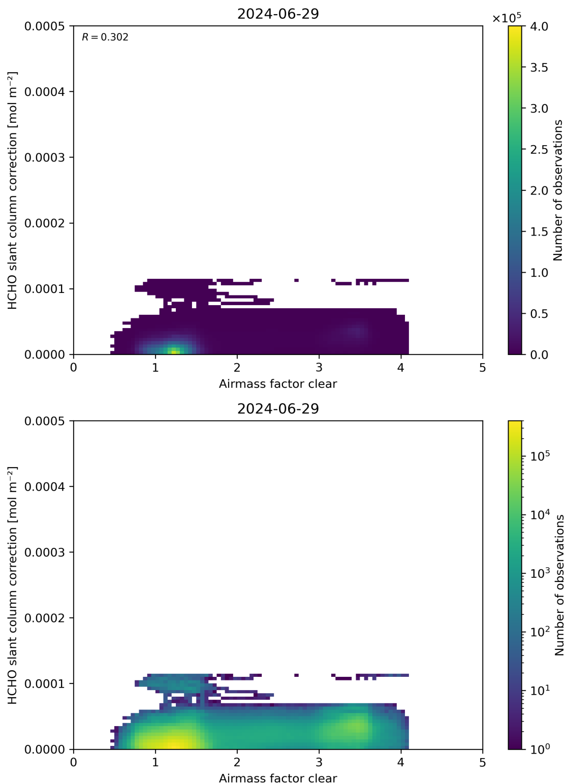
Figure 75: Scatter density plot of “Airmass factor clear” against “HCHO slant column correction” for 2024-06-29 to 2024-06-30.
