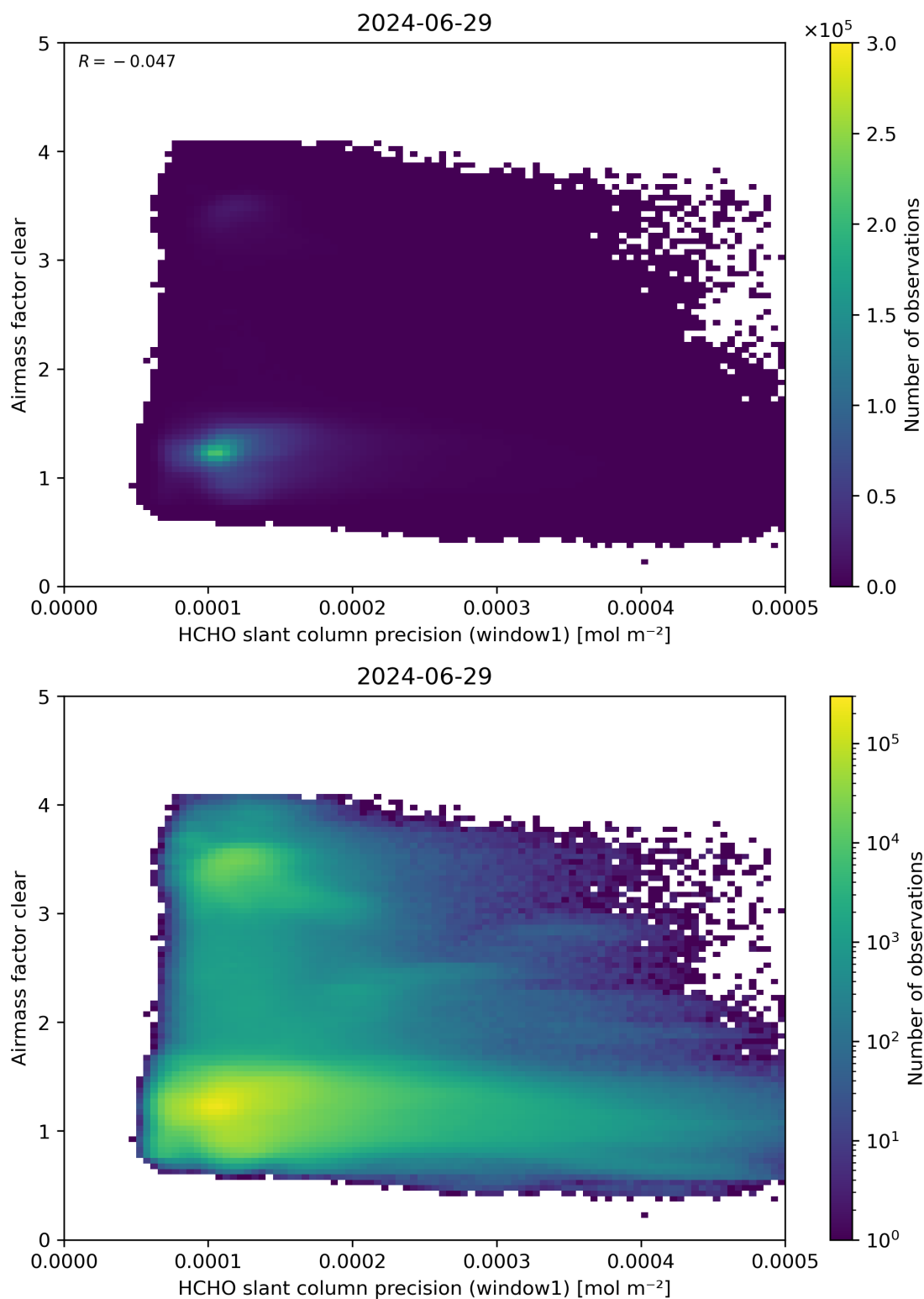
Figure 91: Scatter density plot of “HCHO slant column precision (window1)” against “Airmass factor clear” for 2024-06-29 to 2024-06-30.
