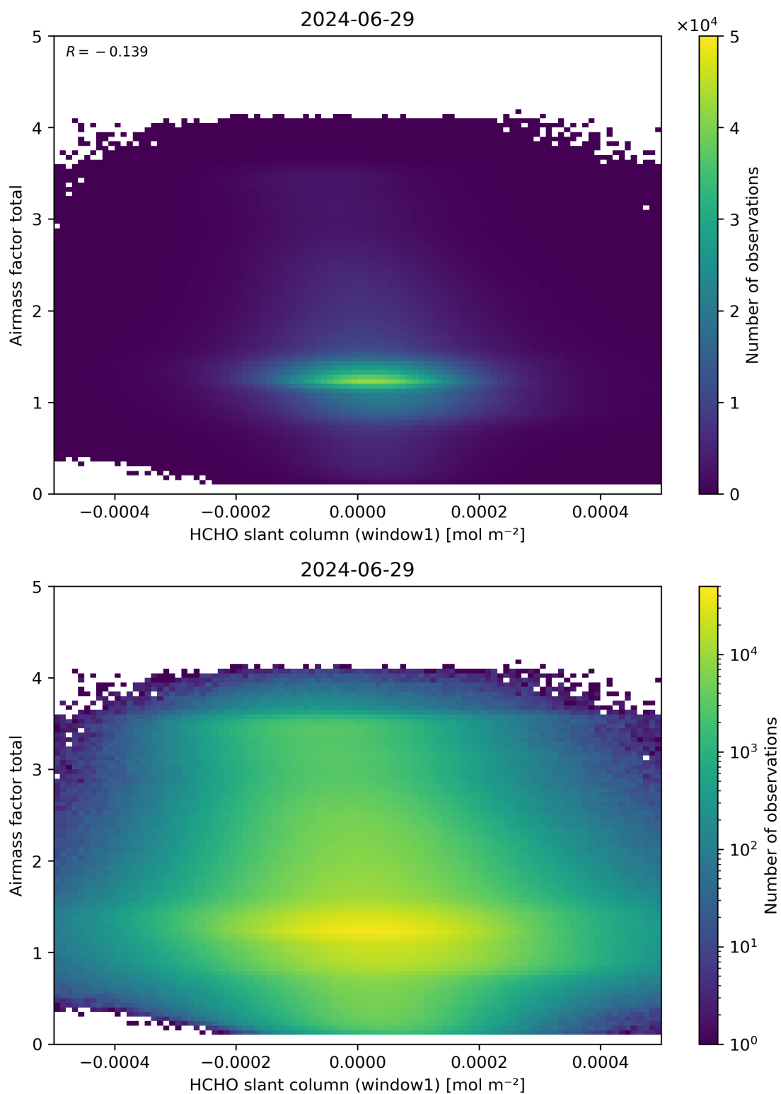
Figure 85: Scatter density plot of “HCHO slant column (window1)” against “Airmass factor total” for 2024-06-29 to 2024-06-30.
