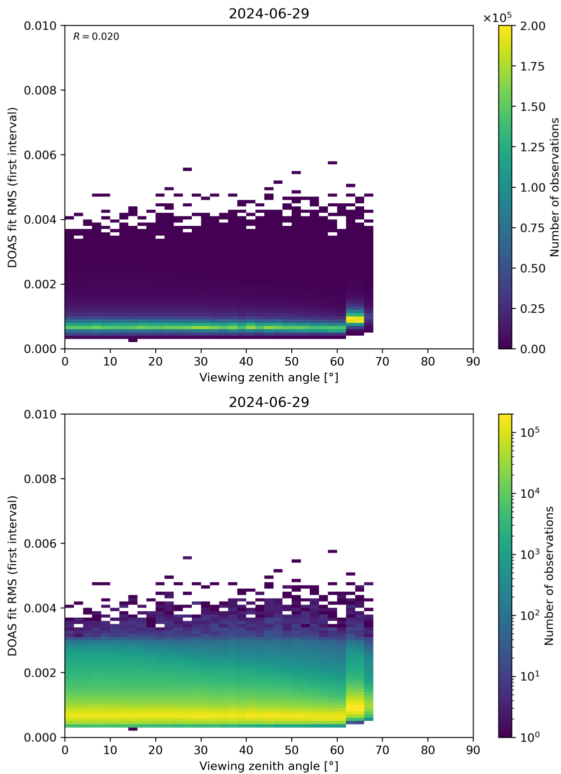
Figure 182: Scatter density plot of “Viewing zenith angle” against “DOAS fit RMS (first interval)” for 2024-06-29 to 2024-06-30.
