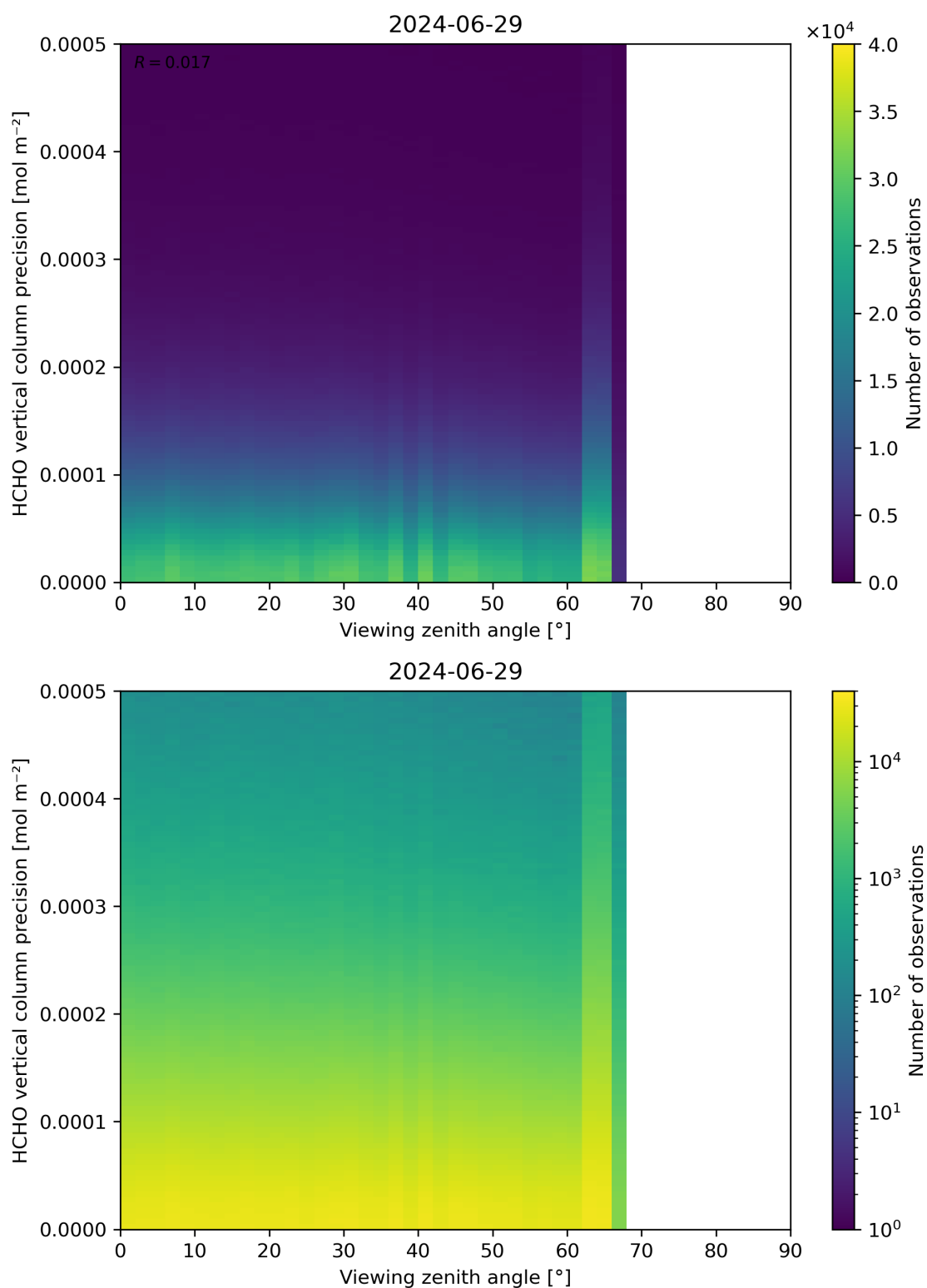
Figure 194: Scatter density plot of “Viewing zenith angle” against “HCHO vertical column precision” for 2024-06-29 to 2024-06-30.
