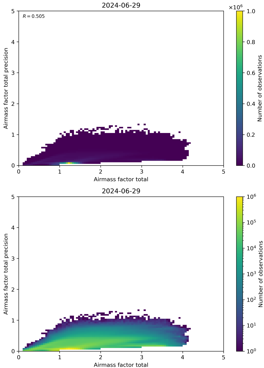
Figure 103: Scatter density plot of “Airmass factor total” against “Airmass factor total precision” for 2024-06-29 to 2024-06-30.
