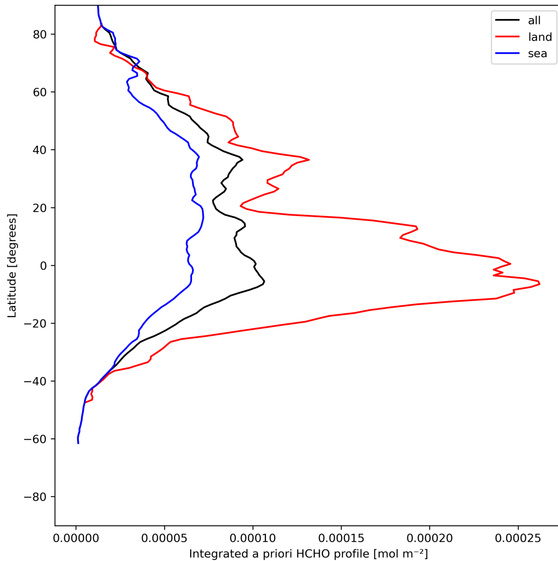
Figure 29: Zonal average of “Integrated a priori HCHO profile” for 2024-06-29 to 2024-06-30.
