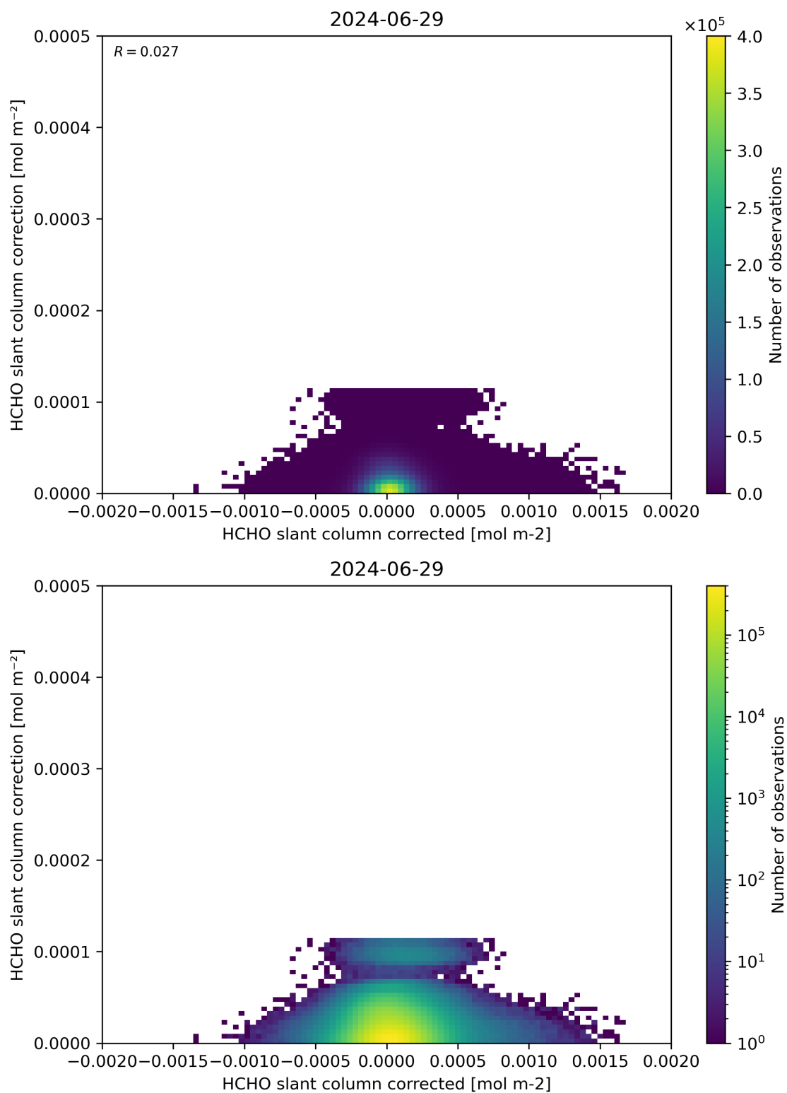
Figure 77: Scatter density plot of “HCHO slant column corrected” against “HCHO slant column correction” for 2024-06-29 to 2024-06-30.
