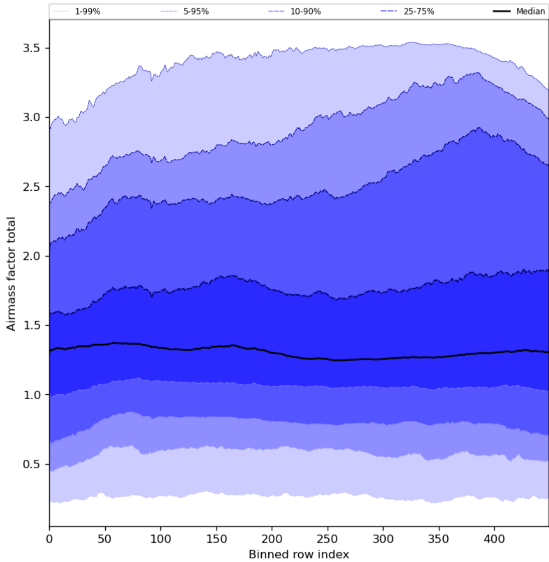
Figure 54: Along track statistics of “Airmass factor total” for 2024-06-29 to 2024-06-30
