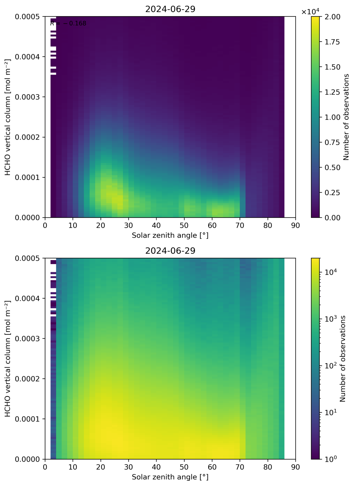
Figure 177: Scatter density plot of “Solar zenith angle” against “HCHO vertical column” for 2024-06-29 to 2024-06-30.
