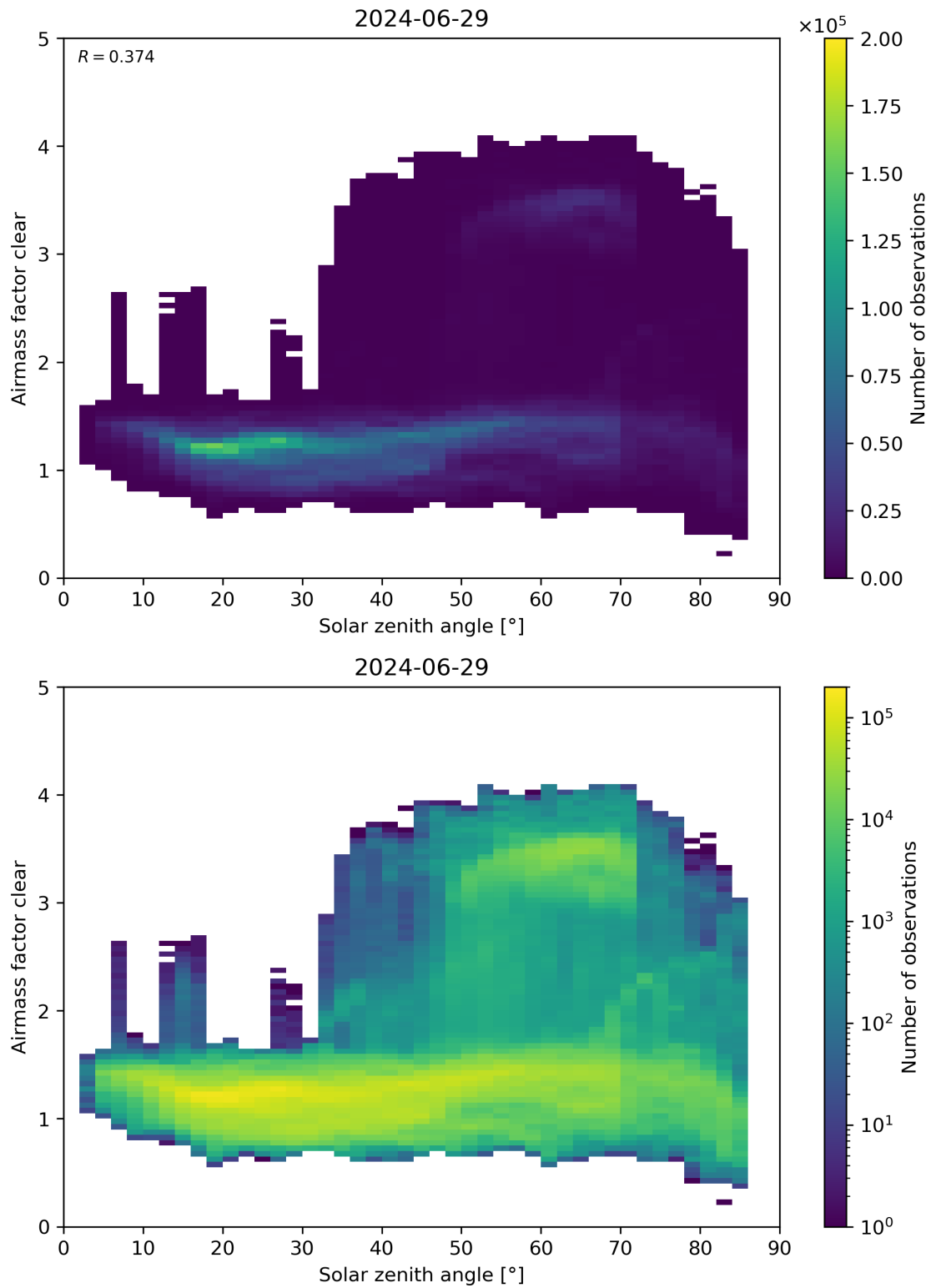
Figure 170: Scatter density plot of “Solar zenith angle” against “Airmass factor clear” for 2024-06-29 to 2024-06-30.
