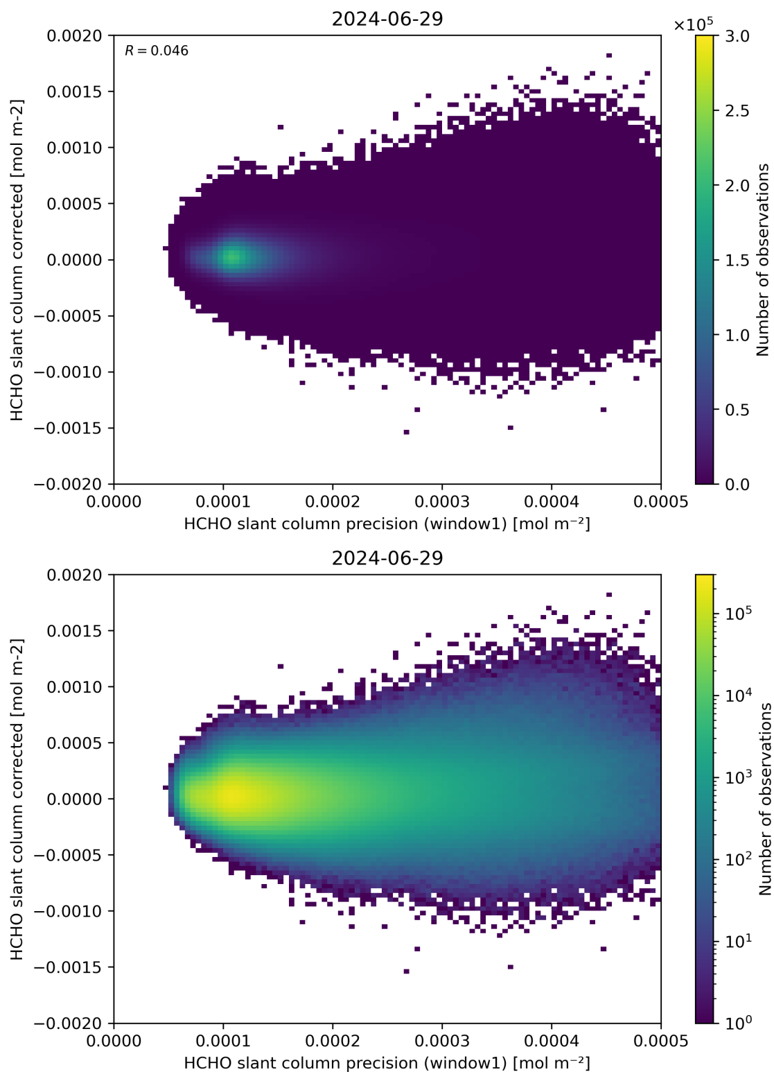
Figure 92: Scatter density plot of “HCHO slant column precision (window1)” against “HCHO slant column corrected” for 2024-06-29 to 2024-06-30.
