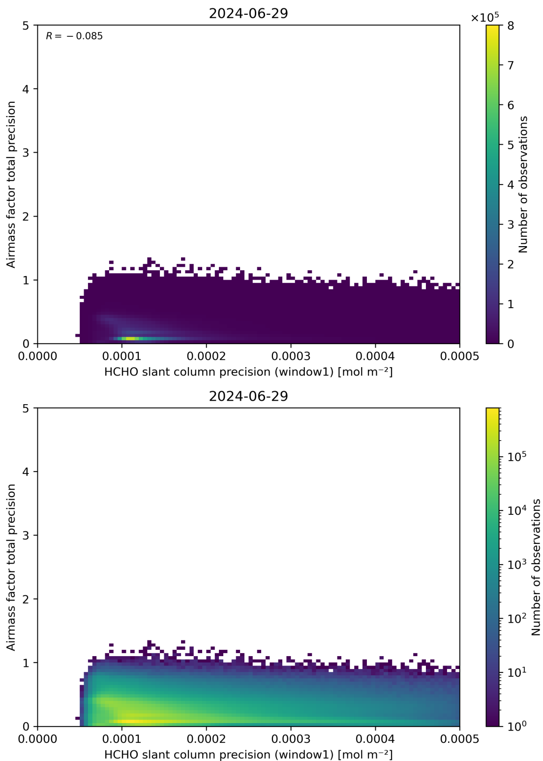
Figure 95: Scatter density plot of “HCHO slant column precision (window1)” against “Airmass factor total precision” for 2024-06-29 to 2024-06-30.
