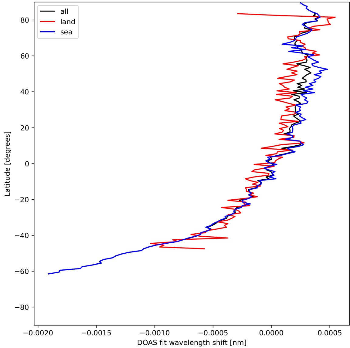
Figure 30: Zonal average of “DOAS fit wavelength shift” for 2024-06-29 to 2024-06-30.
