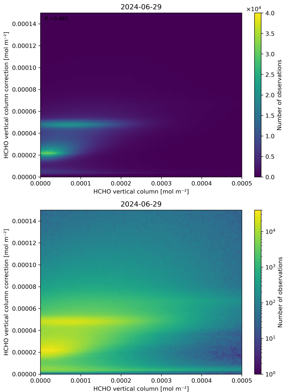
Figure 133: Scatter density plot of “HCHO vertical column” against “HCHO vertical column correction” for 2024-06-29 to 2024-06-30.
