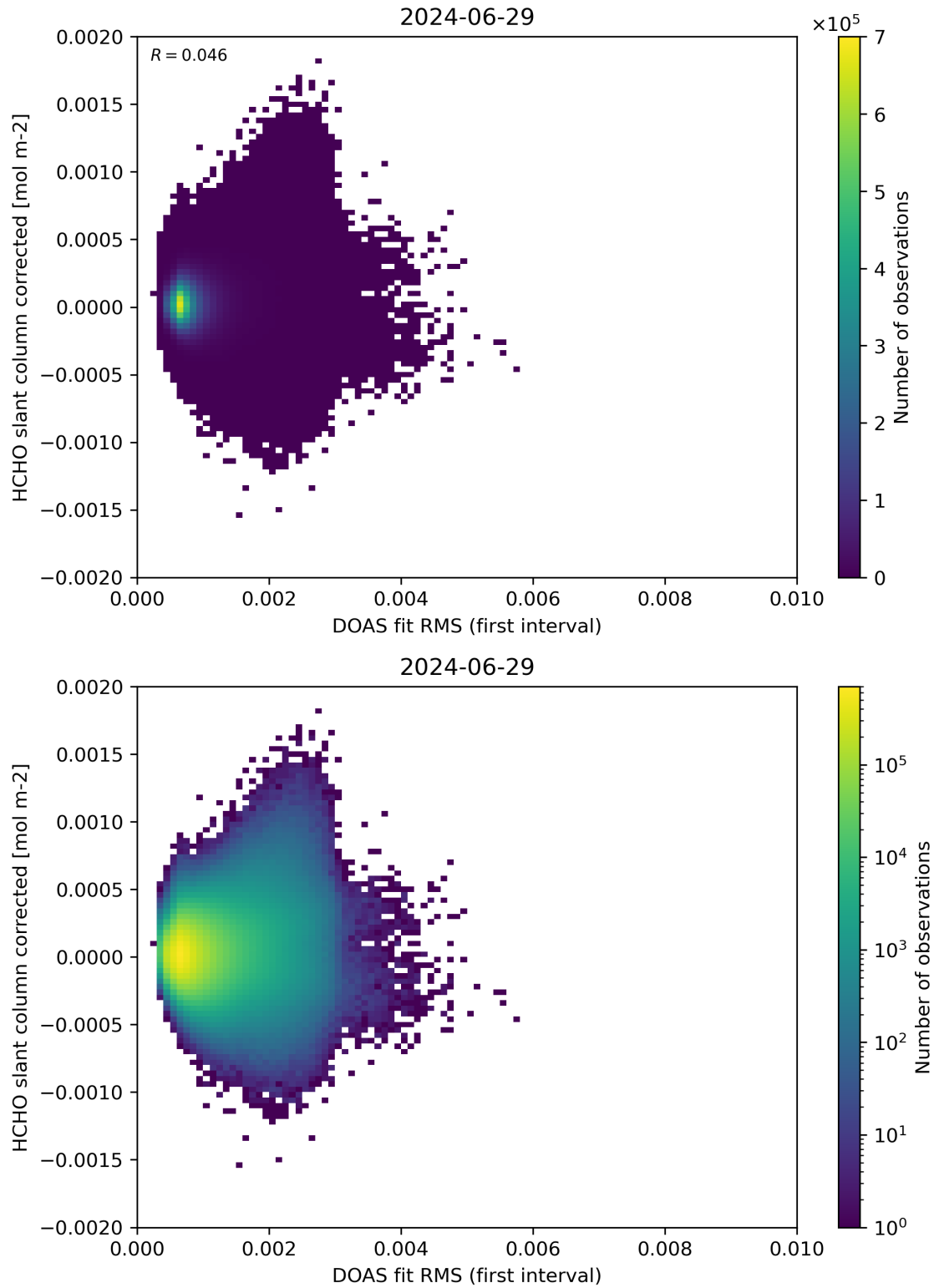
Figure 62: Scatter density plot of “DOAS fit RMS (first interval)” against “HCHO slant column corrected” for 2024-06-29 to 2024-06-30.
