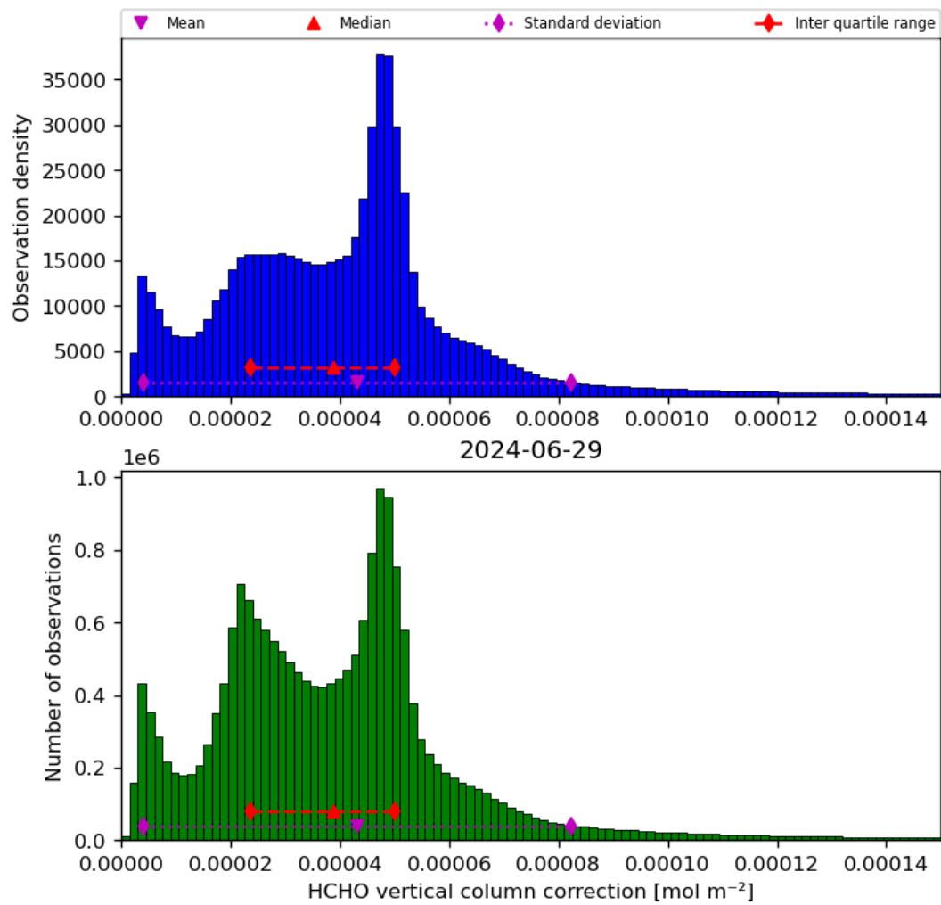
Figure 37: Histogram of “HCHO vertical column correction” for 2024-06-29 to 2024-06-30
