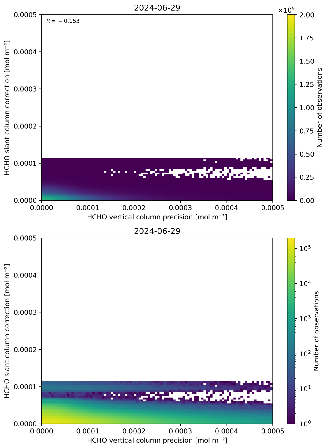
Figure 141: Scatter density plot of “HCHO vertical column precision” against “HCHO slant column correction” for 2024-06-29 to 2024-06-30.
