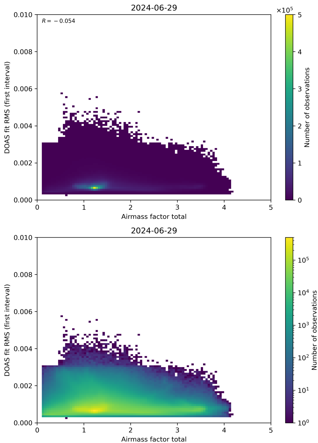
Figure 97: Scatter density plot of “Airmass factor total” against “DOAS fit RMS (first interval)” for 2024-06-29 to 2024-06-30.
