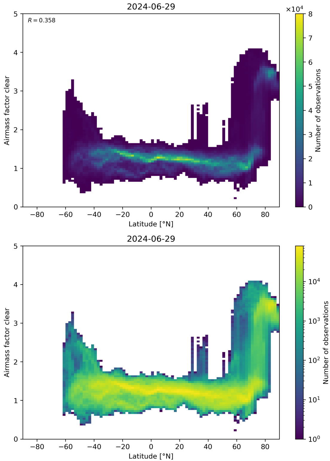
Figure 156: Scatter density plot of “Latitude” against “Airmass factor clear” for 2024-06-29 to 2024-06-30.
