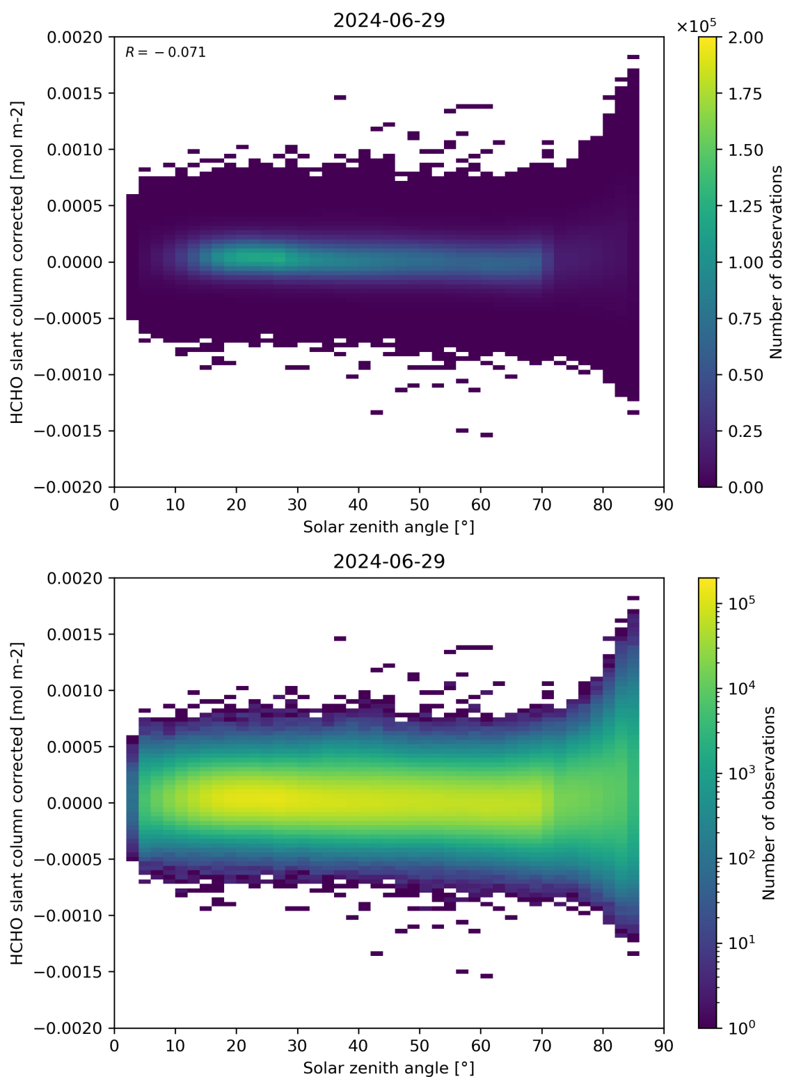
Figure 171: Scatter density plot of “Solar zenith angle” against “HCHO slant column corrected” for 2024-06-29 to 2024-06-30.
