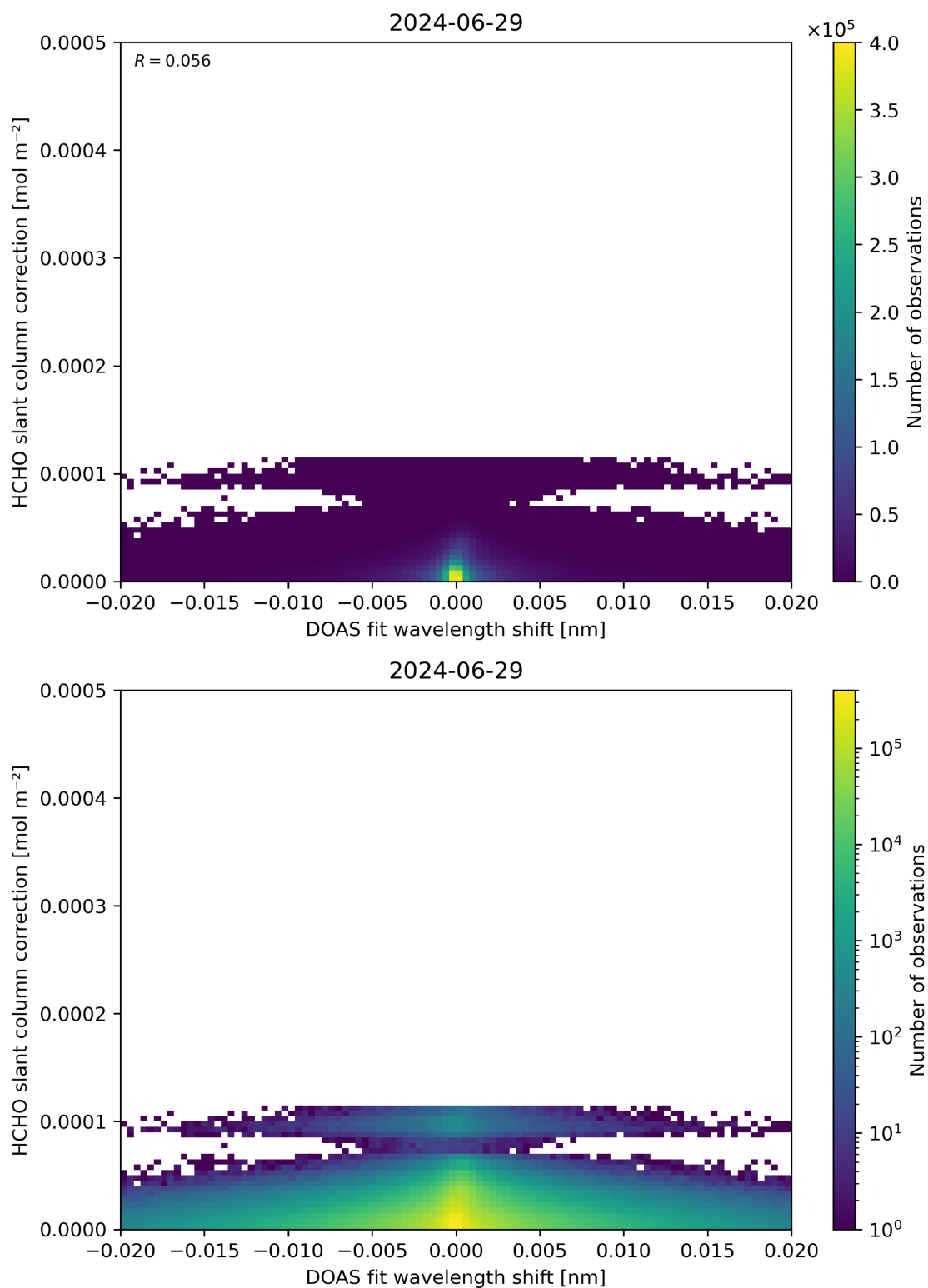
Figure 67: Scatter density plot of “DOAS fit wavelength shift” against “HCHO slant column correction” for 2024-06-29 to 2024-06-30.
