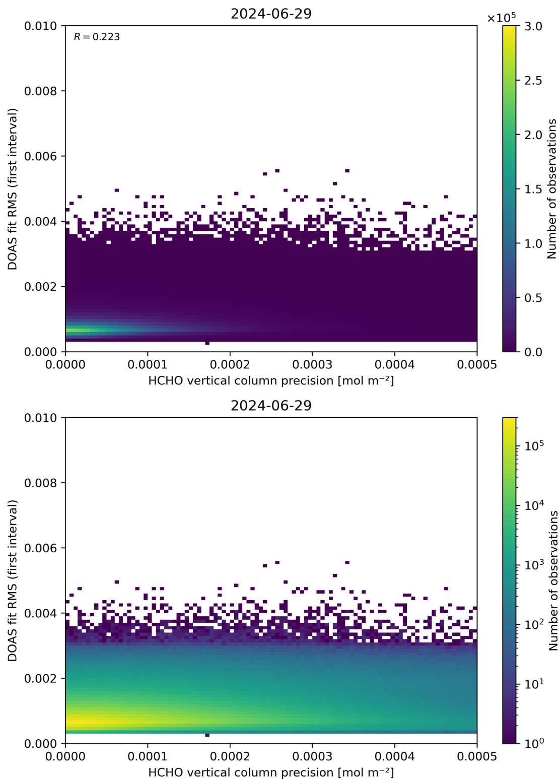
Figure 136: Scatter density plot of “HCHO vertical column precision” against “DOAS fit RMS (first interval)” for 2024-06-29 to 2024-06-30.
