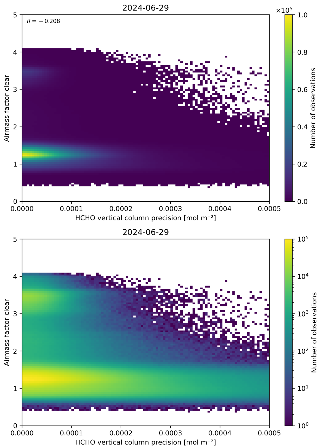
Figure 139: Scatter density plot of “HCHO vertical column precision” against “Airmass factor clear” for 2024-06-29 to 2024-06-30.
