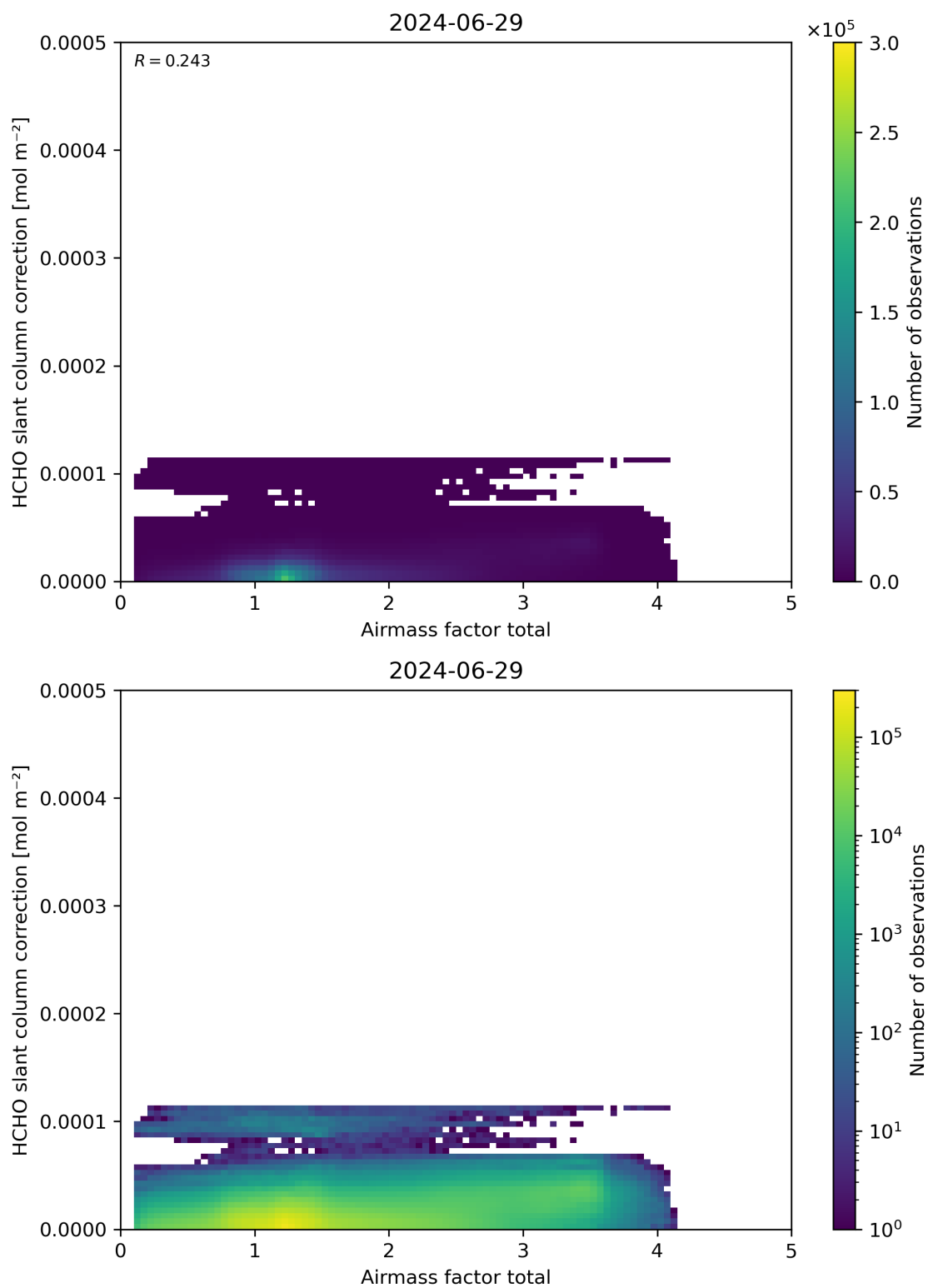
Figure 102: Scatter density plot of “Airmass factor total” against “HCHO slant column correction” for 2024-06-29 to 2024-06-30.
