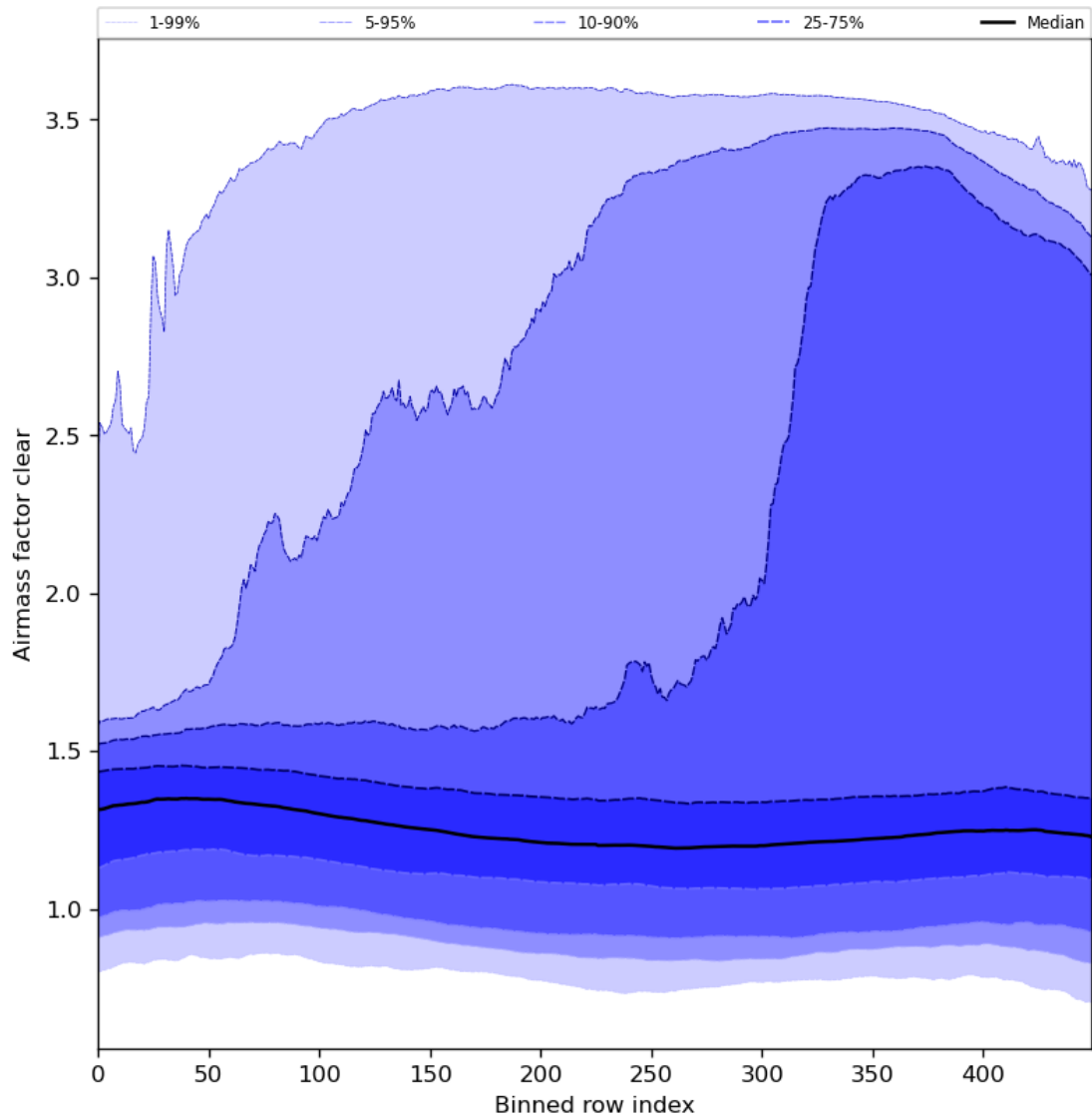
Figure 56: Along track statistics of “Airmass factor clear” for 2024-06-29 to 2024-06-30
