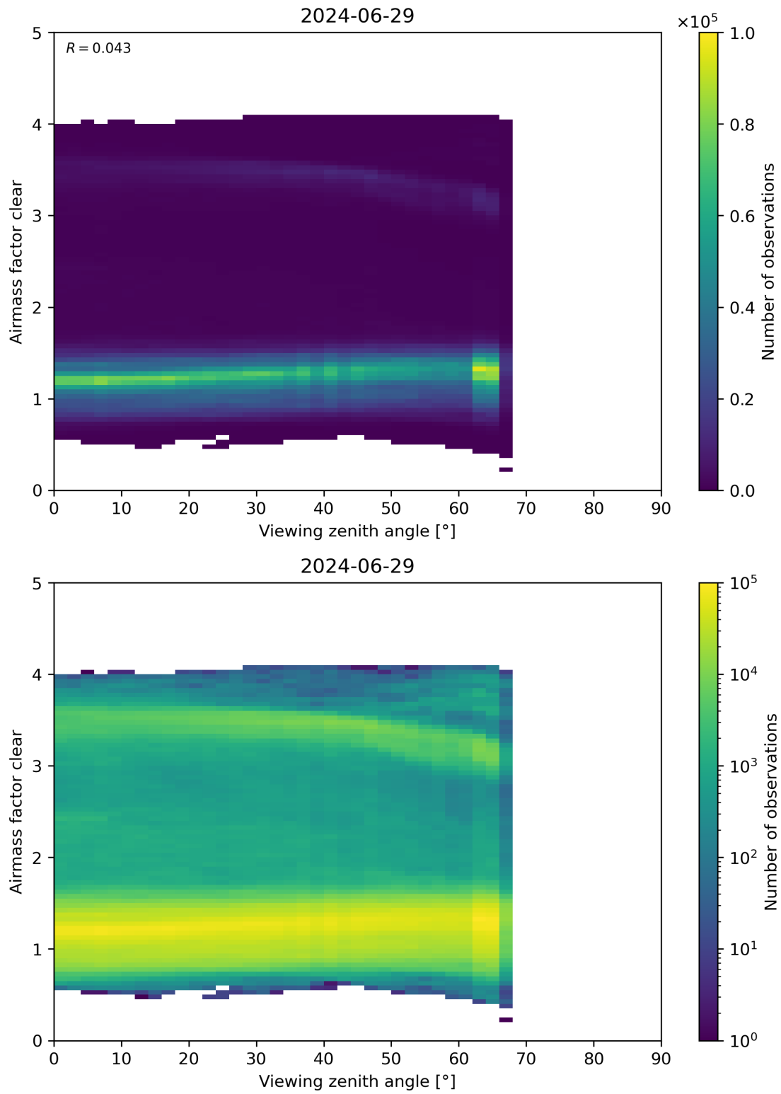
Figure 185: Scatter density plot of “Viewing zenith angle” against “Airmass factor clear” for 2024-06-29 to 2024-06-30.
