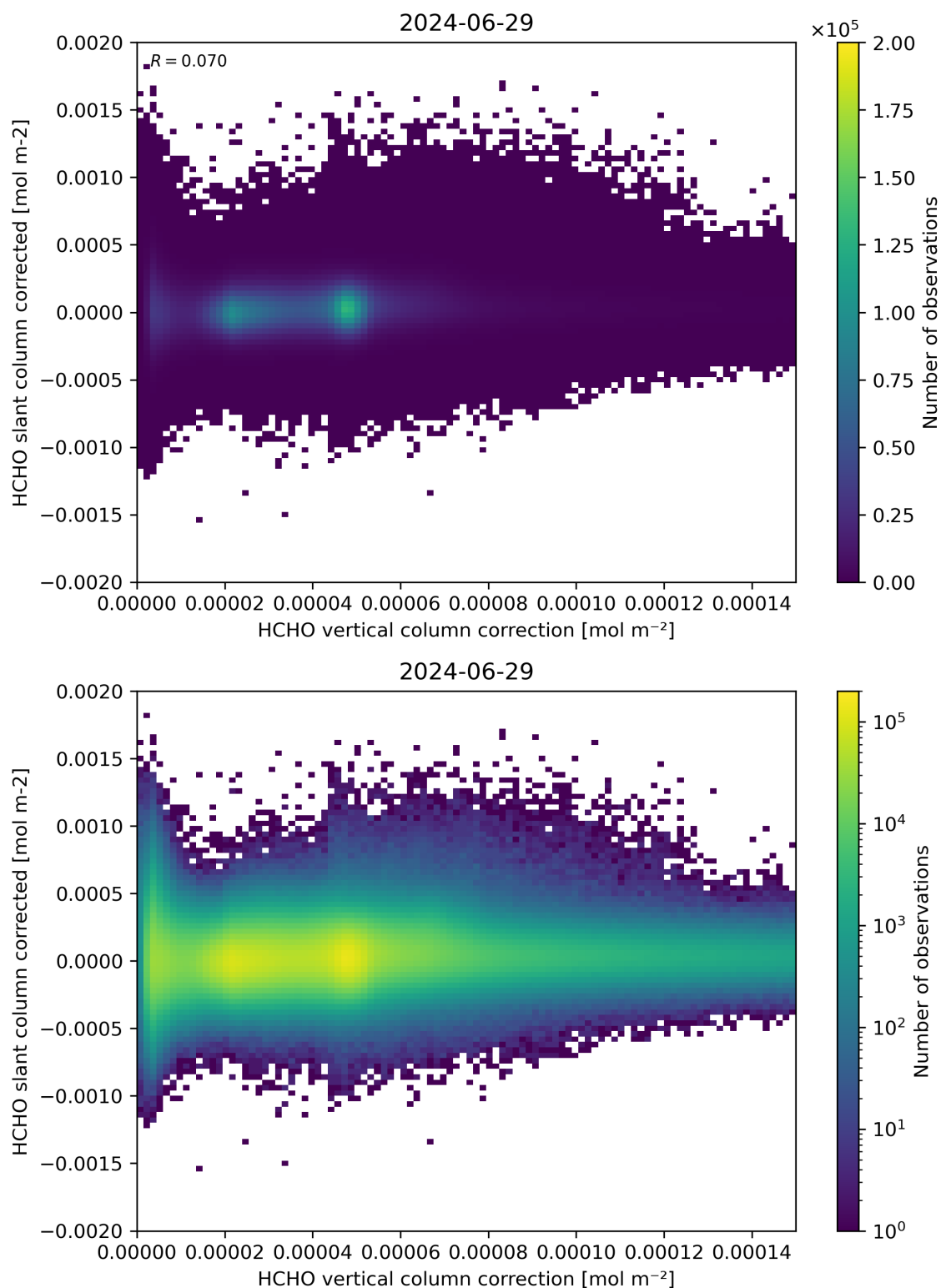
Figure 116: Scatter density plot of “HCHO vertical column correction” against “HCHO slant column corrected” for 2024-06-29 to 2024-06-30.
