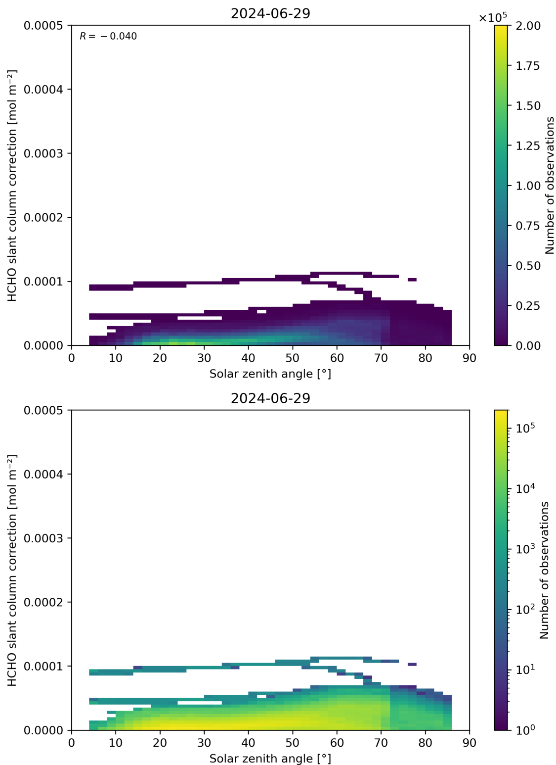
Figure 172: Scatter density plot of “Solar zenith angle” against “HCHO slant column correction” for 2024-06-29 to 2024-06-30.
