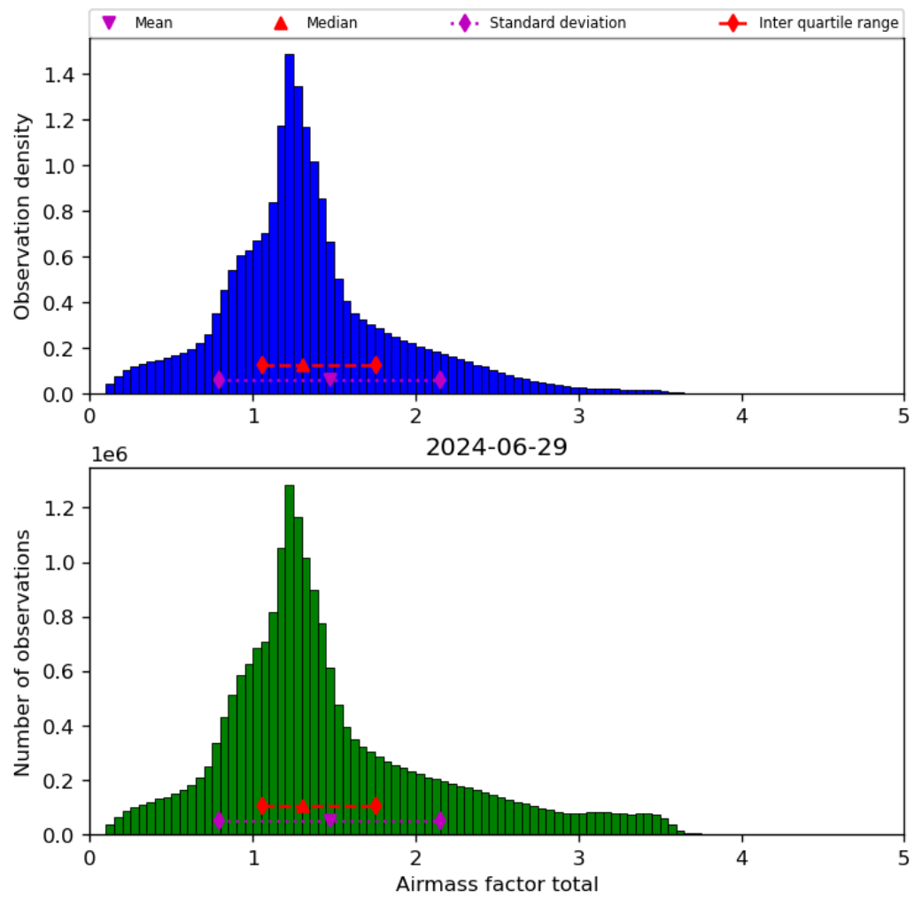
Figure 40: Histogram of “Airmass factor total” for 2024-06-29 to 2024-06-30
