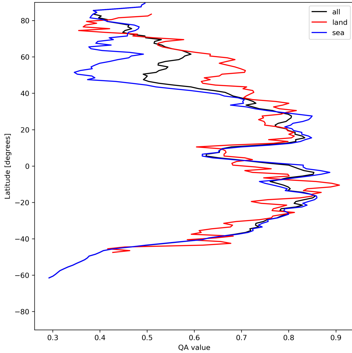
Figure 20: Zonal average of “QA value” for 2024-06-29 to 2024-06-30.
