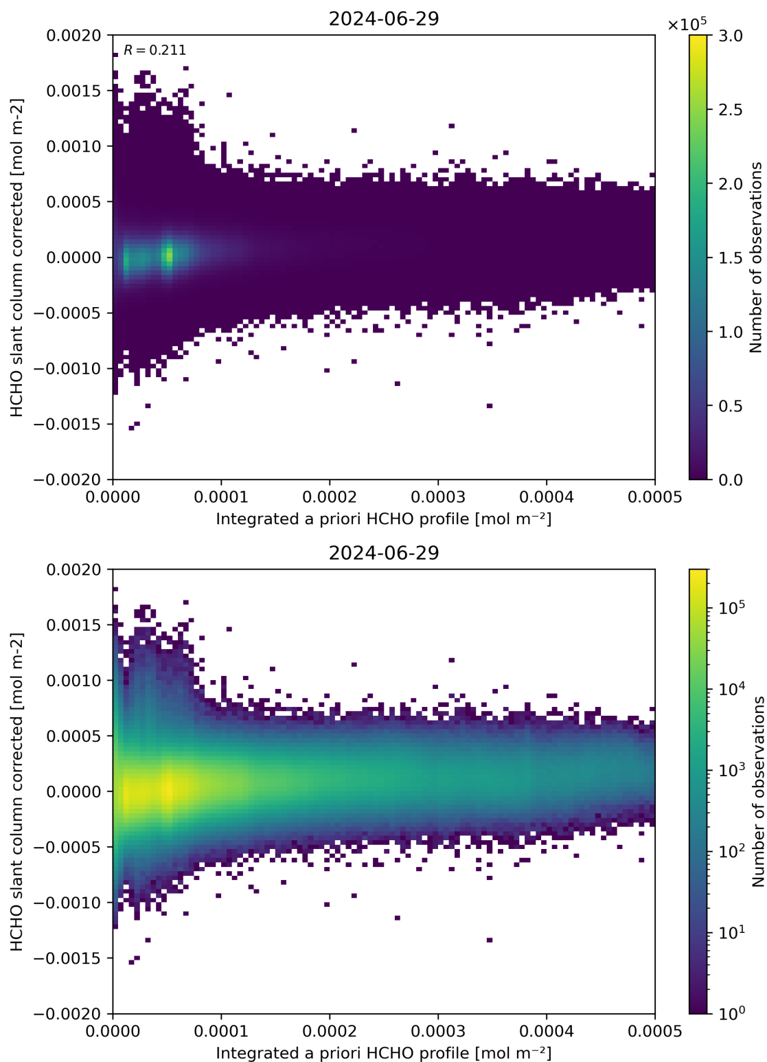
Figure 151: Scatter density plot of “Integrated a priori HCHO profile” against “HCHO slant column corrected” for 2024-06-29 to 2024-06-30.
