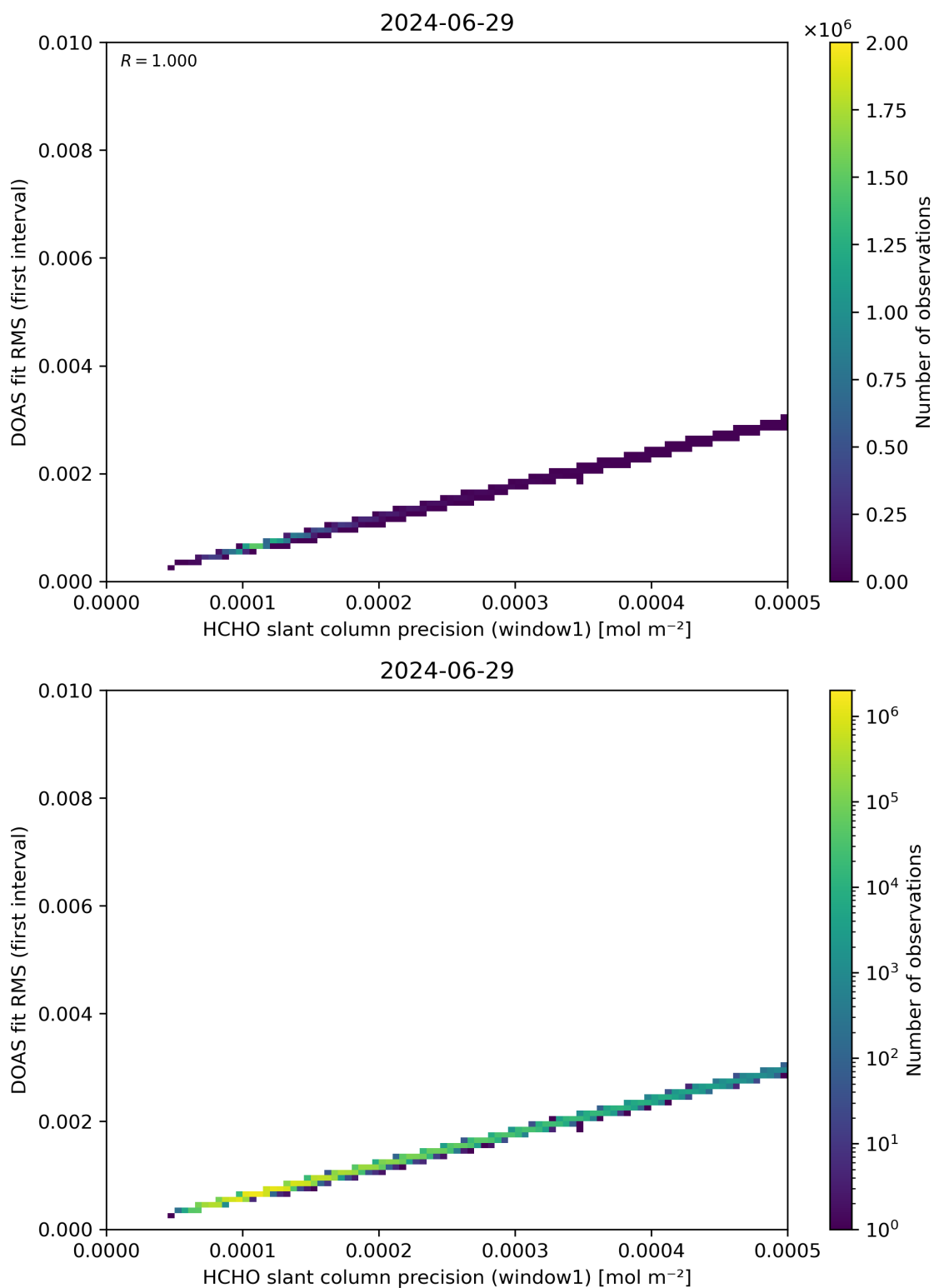
Figure 88: Scatter density plot of “HCHO slant column precision (window1)” against “DOAS fit RMS (first interval)” for 2024-06-29 to 2024-06-30.
