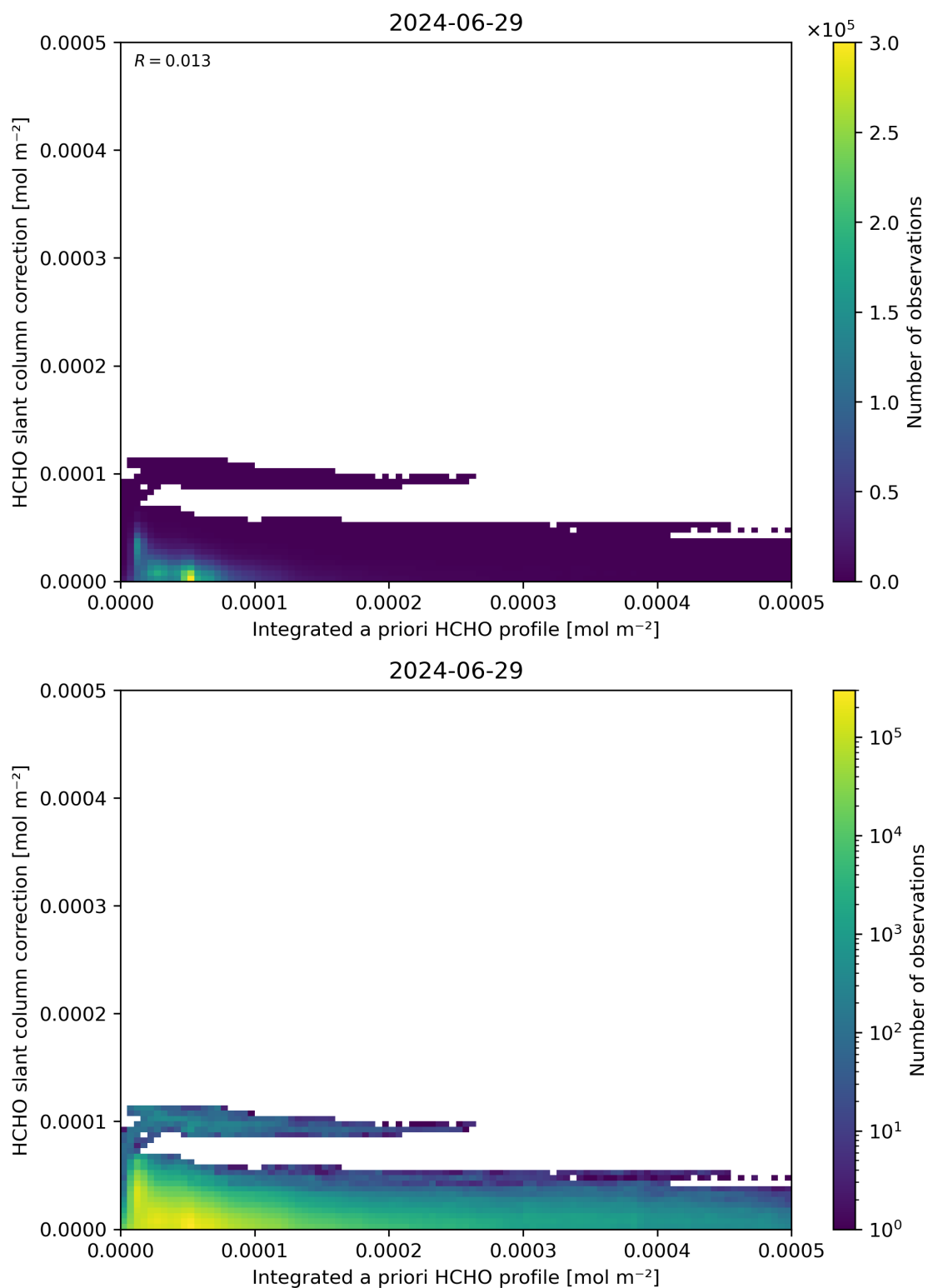
Figure 152: Scatter density plot of “Integrated a priori HCHO profile” against “HCHO slant column correction” for 2024-06-29 to 2024-06-30.
