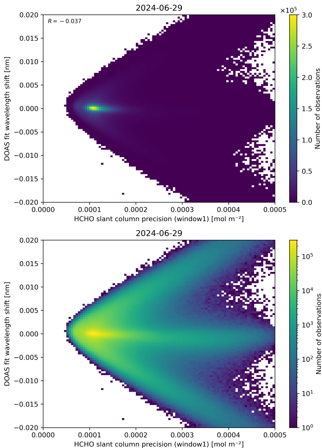
Figure 89: Scatter density plot of “HCHO slant column precision (window1)” against “DOAS fit wavelength shift” for 2024-06-29 to 2024-06-30.
