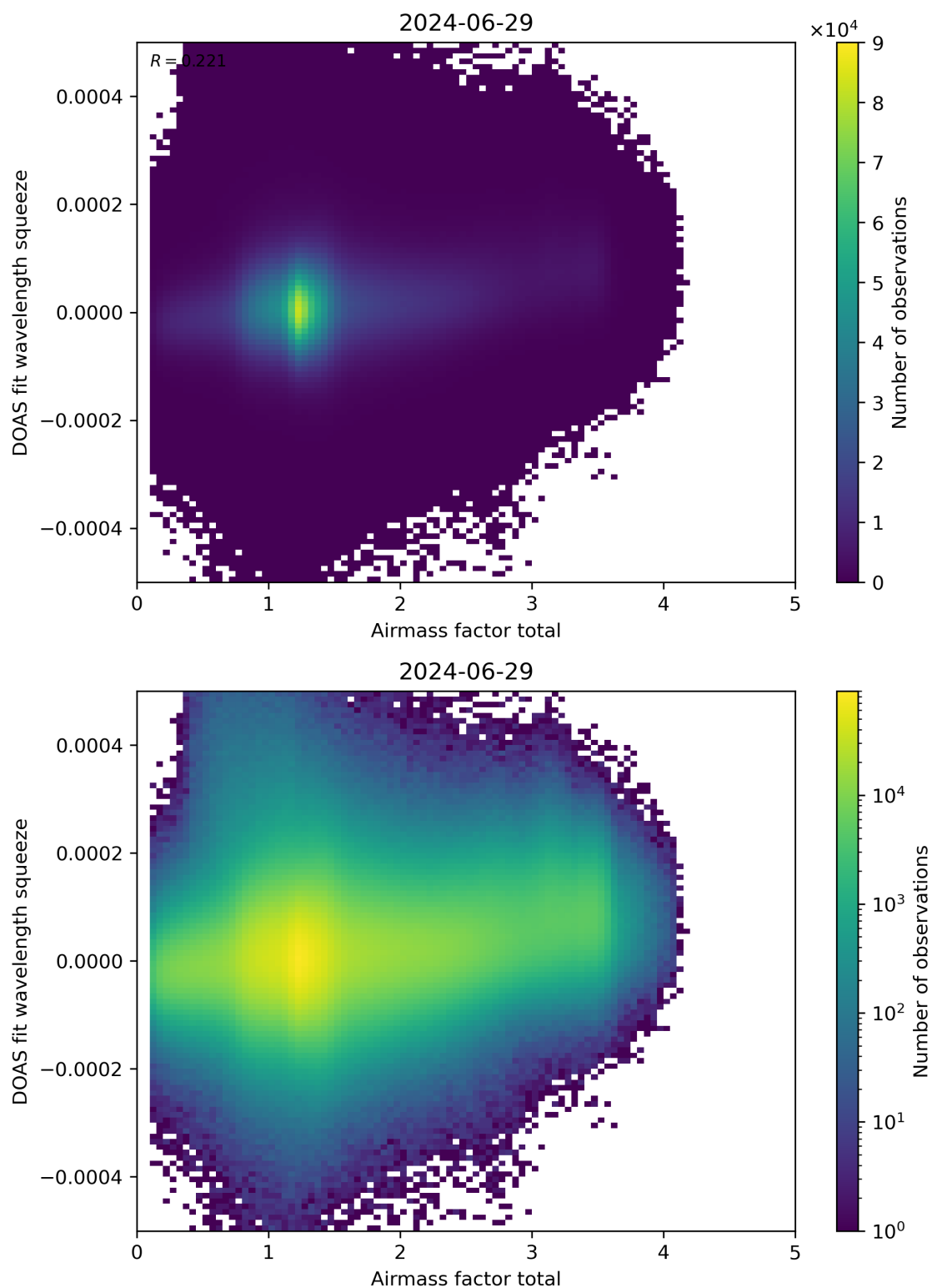
Figure 99: Scatter density plot of “Airmass factor total” against “DOAS fit wavelength squeeze” for 2024-06-29 to 2024-06-30.
