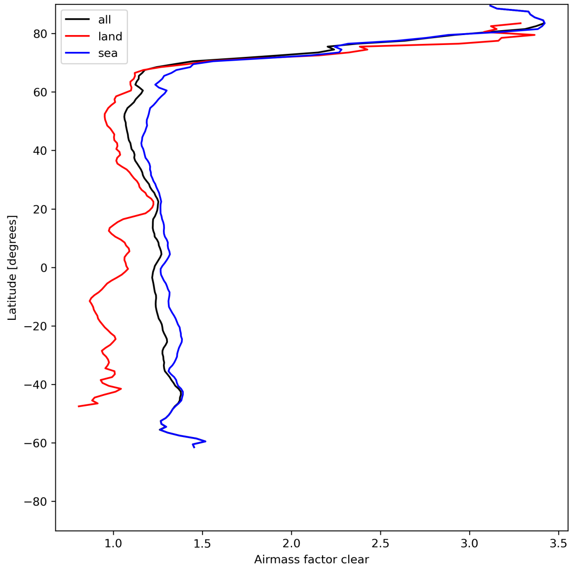
Figure 28: Zonal average of “Airmass factor clear” for 2024-06-29 to 2024-06-30.
