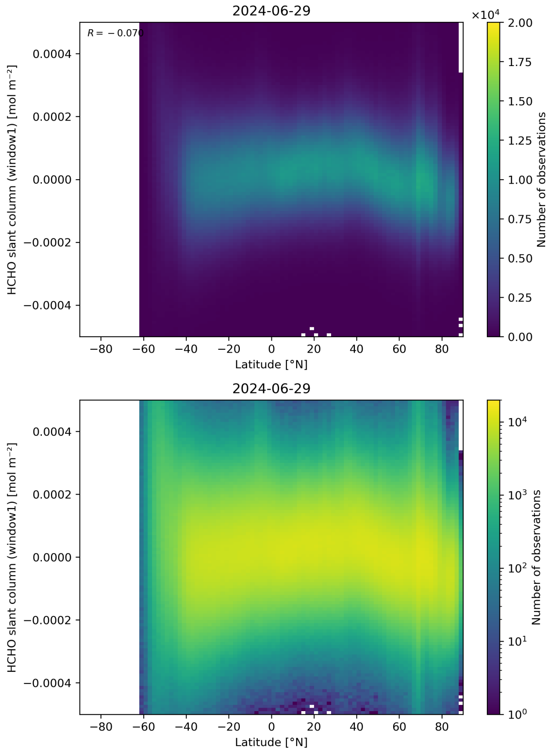
Figure 159: Scatter density plot of “Latitude” against “HCHO slant column (window1)” for 2024-06-29 to 2024-06-30.
