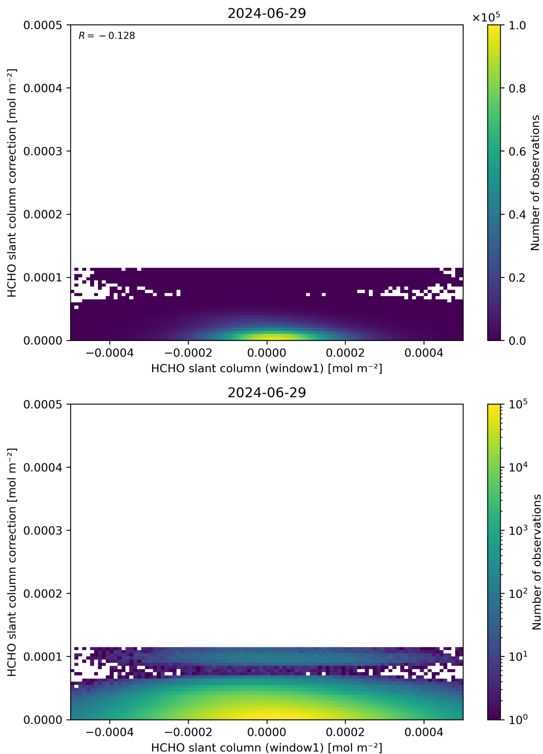
Figure 83: Scatter density plot of “HCHO slant column (window1)” against “HCHO slant column correction” for 2024-06-29 to 2024-06-30.
