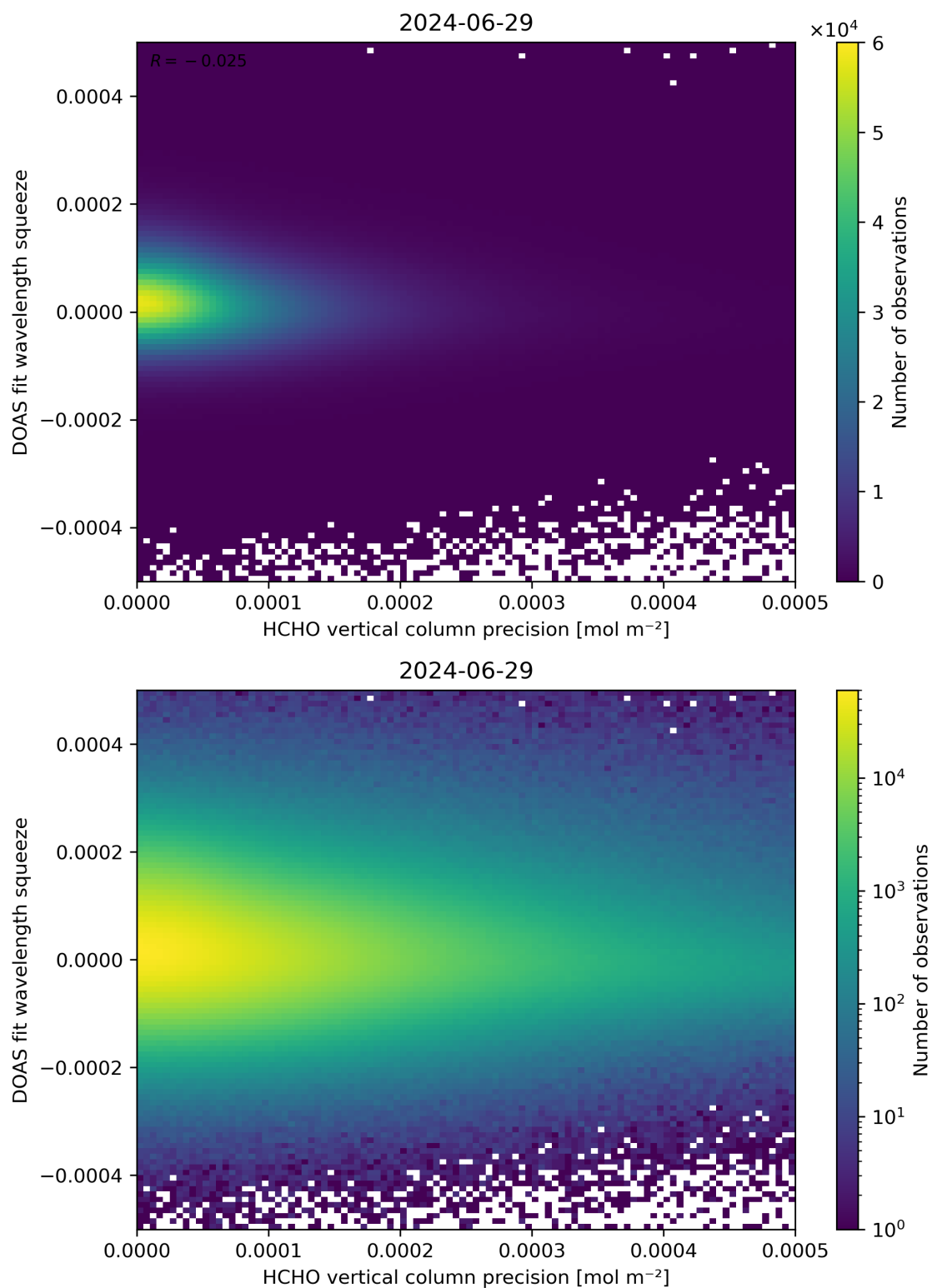
Figure 138: Scatter density plot of “HCHO vertical column precision” against “DOAS fit wavelength squeeze” for 2024-06-29 to 2024-06-30.
