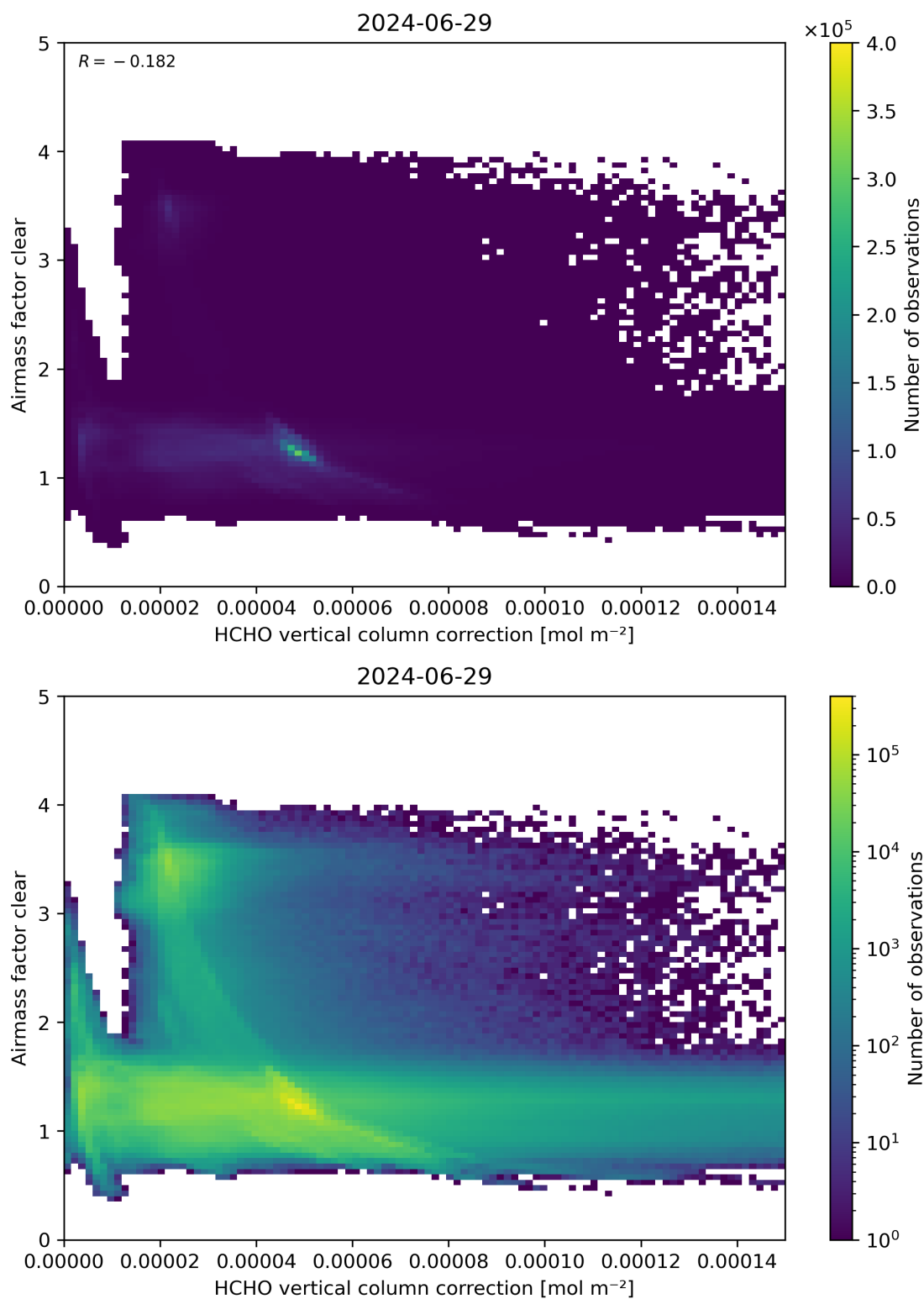
Figure 115: Scatter density plot of “HCHO vertical column correction” against “Airmass factor clear” for 2024-06-29 to 2024-06-30.
