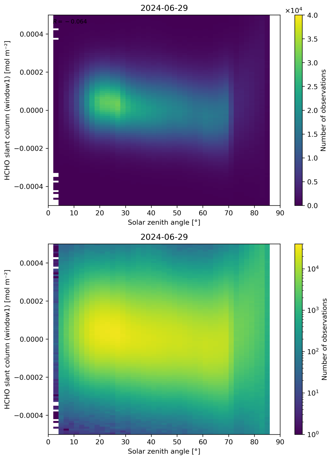
Figure 173: Scatter density plot of “Solar zenith angle” against “HCHO slant column (window1)” for 2024-06-29 to 2024-06-30.
