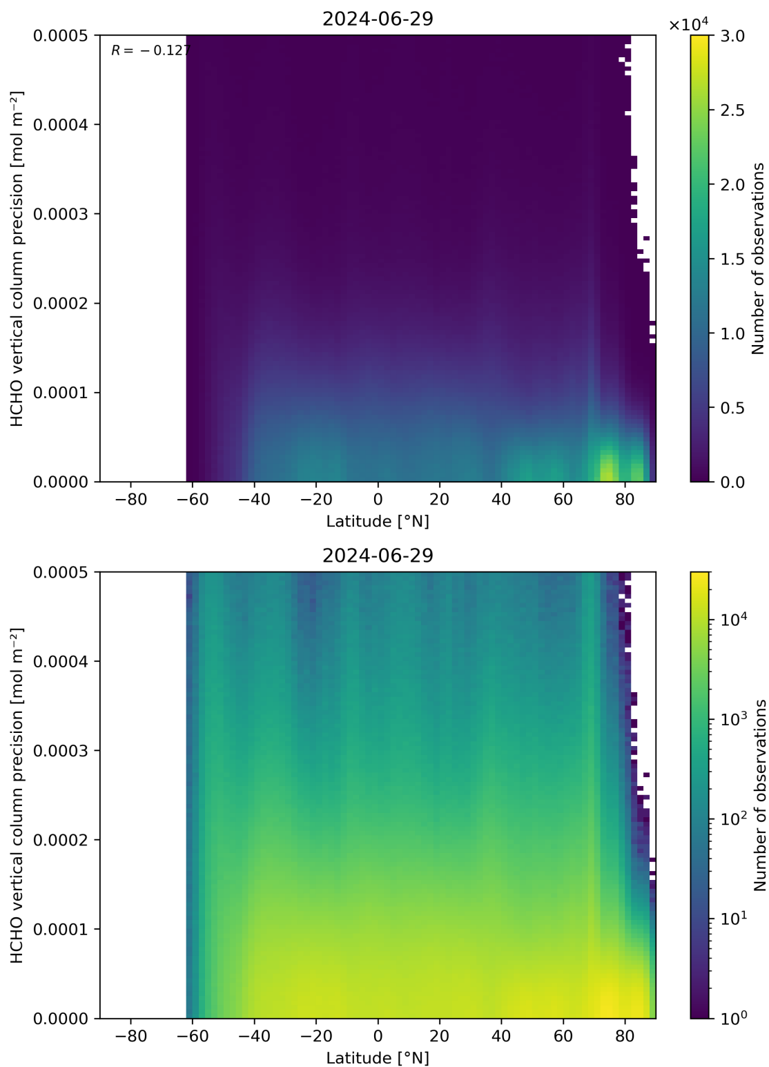
Figure 165: Scatter density plot of “Latitude” against “HCHO vertical column precision” for 2024-06-29 to 2024-06-30.
