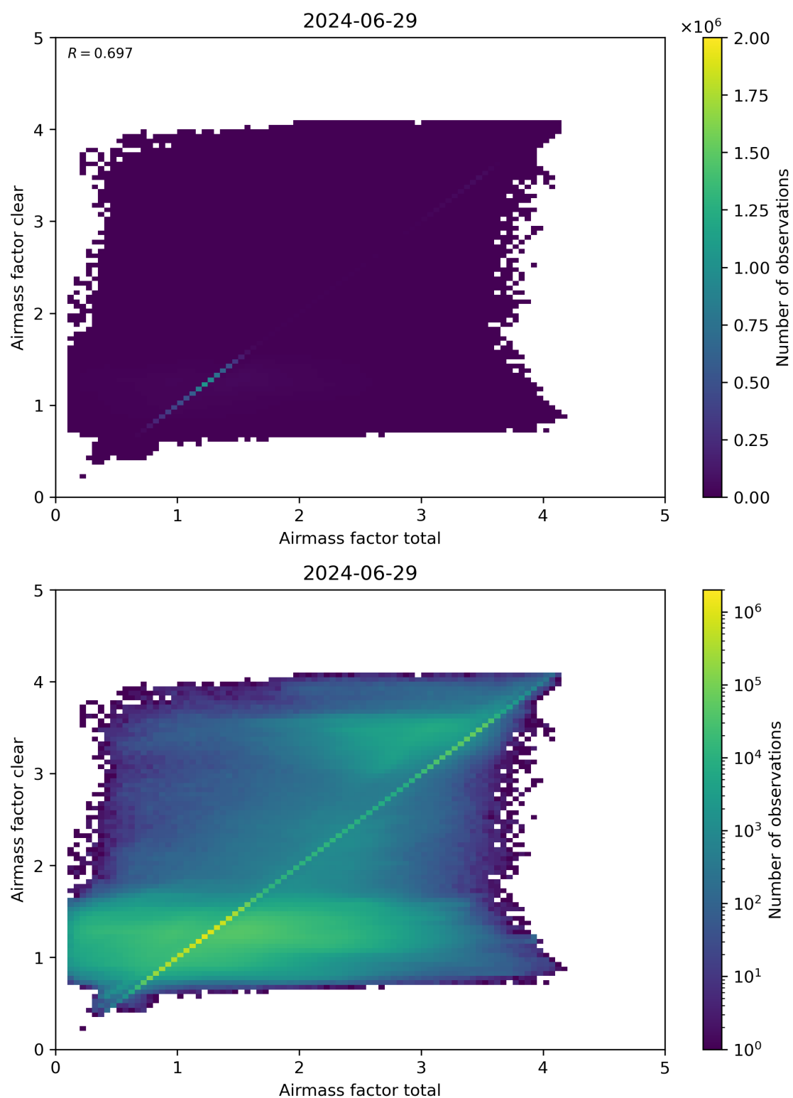
Figure 100: Scatter density plot of “Airmass factor total” against “Airmass factor clear” for 2024-06-29 to 2024-06-30.
