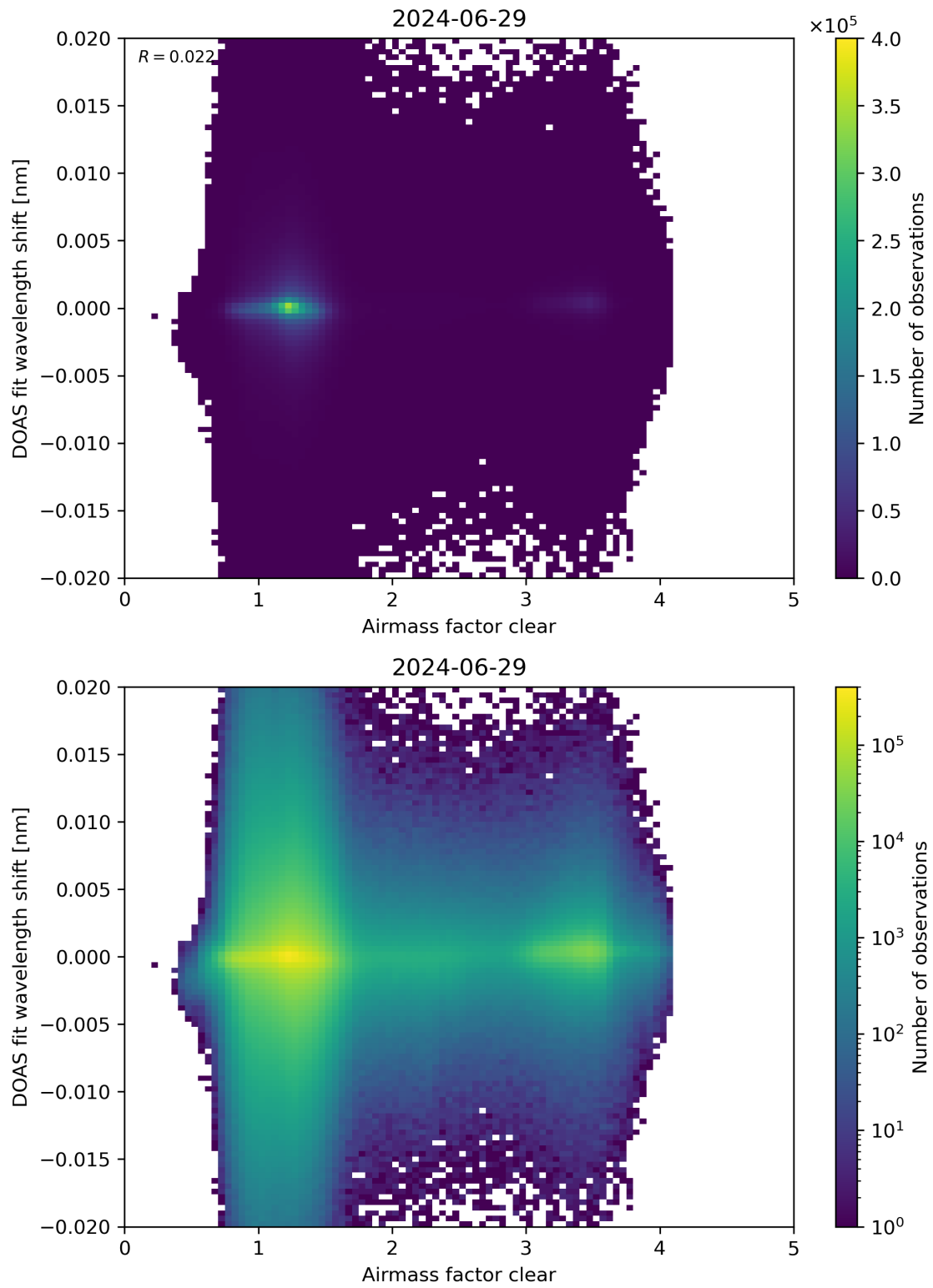
Figure 72: Scatter density plot of “Airmass factor clear” against “DOAS fit wavelength shift” for 2024-06-29 to 2024-06-30.
