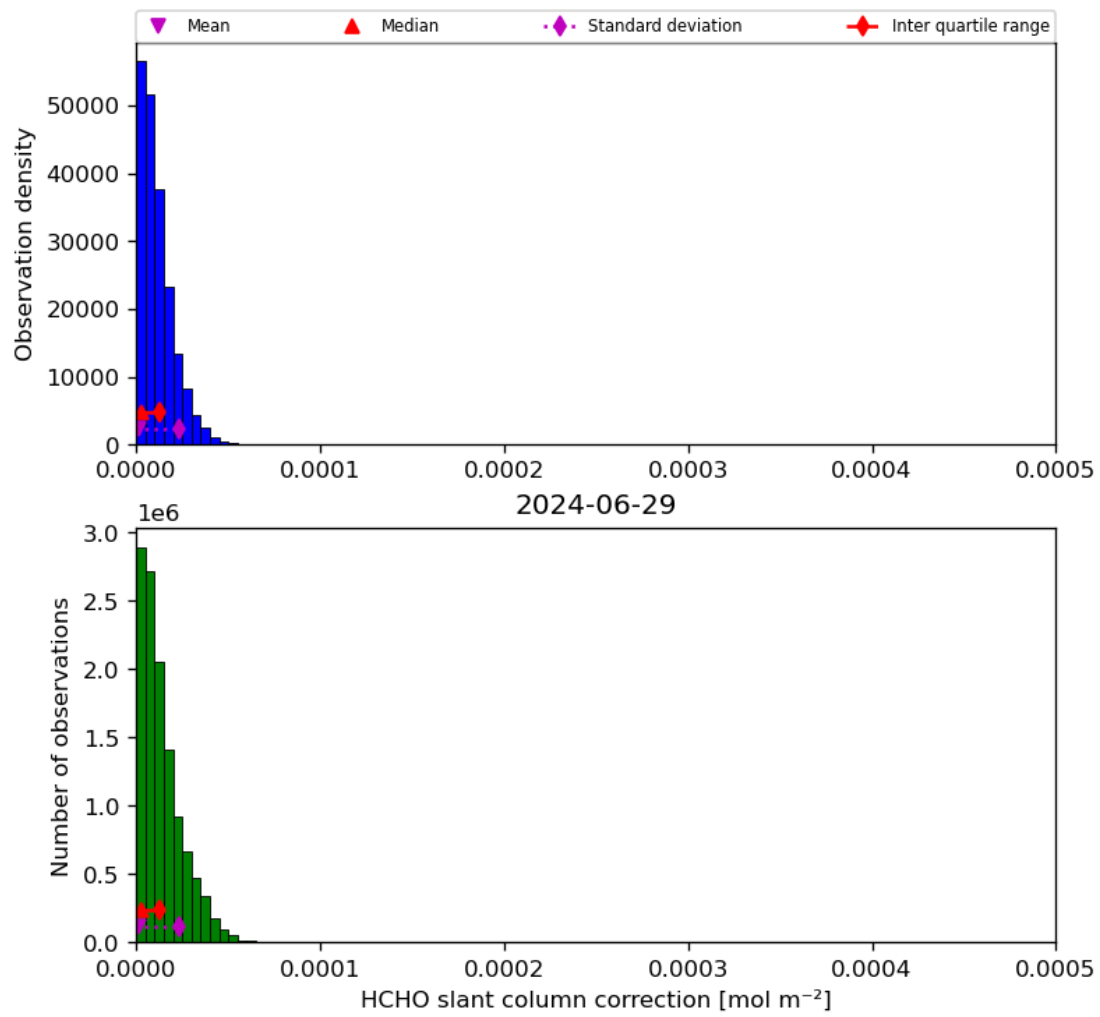
Figure 47: Histogram of “HCHO slant column correction” for 2024-06-29 to 2024-06-30
