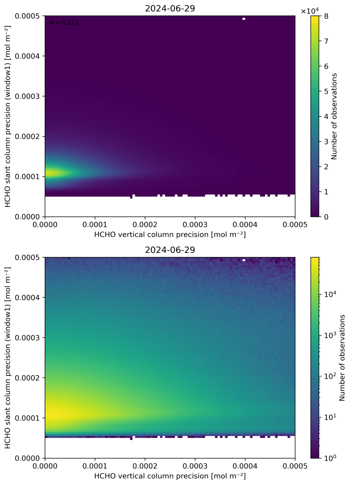
Figure 143: Scatter density plot of “HCHO vertical column precision” against “HCHO slant column precision (window1)” for 2024-06-29 to 2024-06-30.
