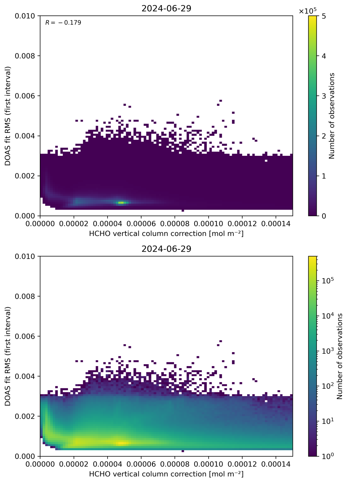
Figure 112: Scatter density plot of “HCHO vertical column correction” against “DOAS fit RMS (first interval)” for 2024-06-29 to 2024-06-30.
