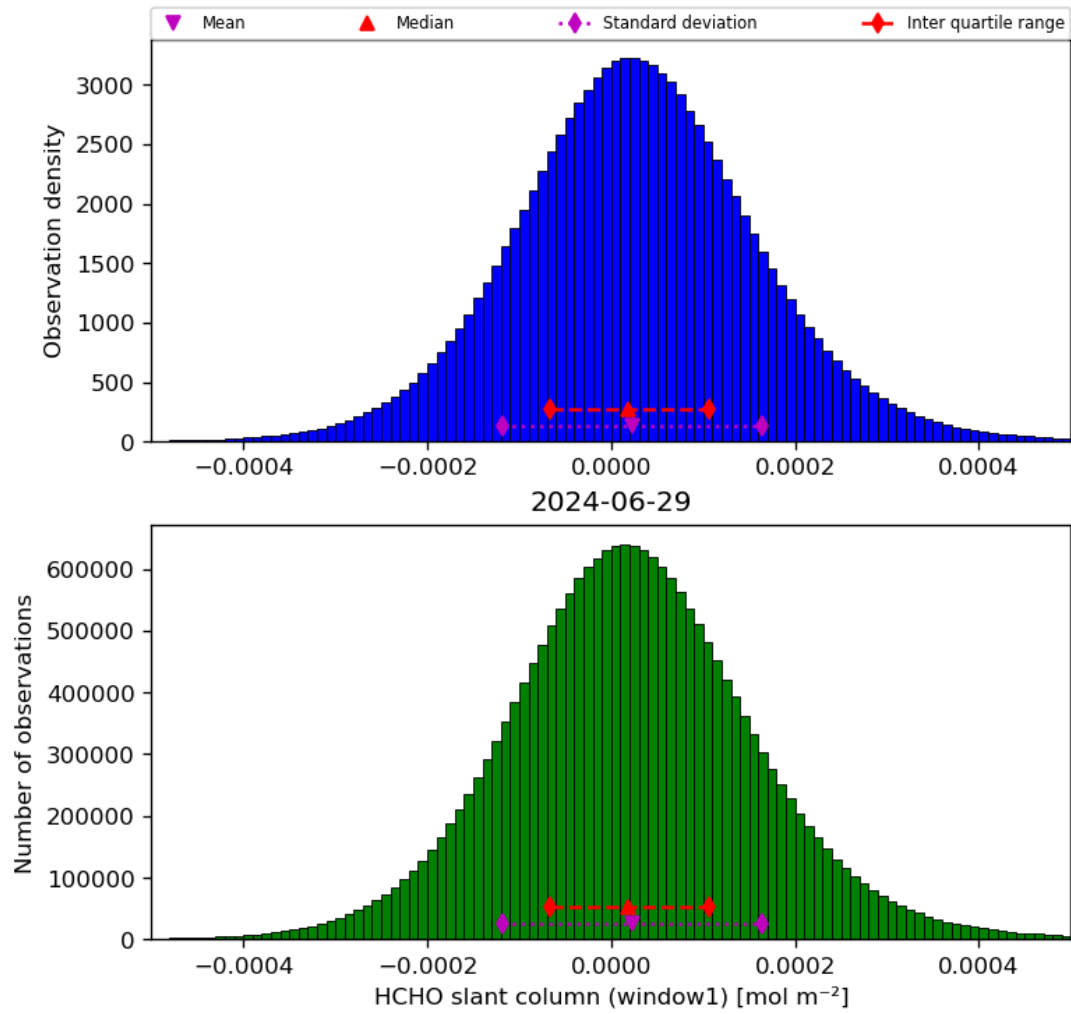
Figure 38: Histogram of “HCHO slant column (window1)” for 2024-06-29 to 2024-06-30
