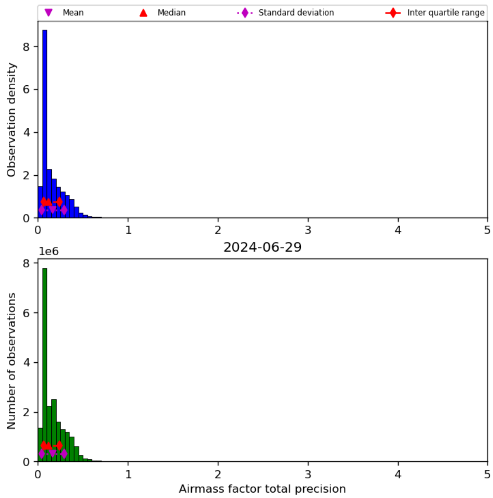
Figure 41: Histogram of “Airmass factor total precision” for 2024-06-29 to 2024-06-30
