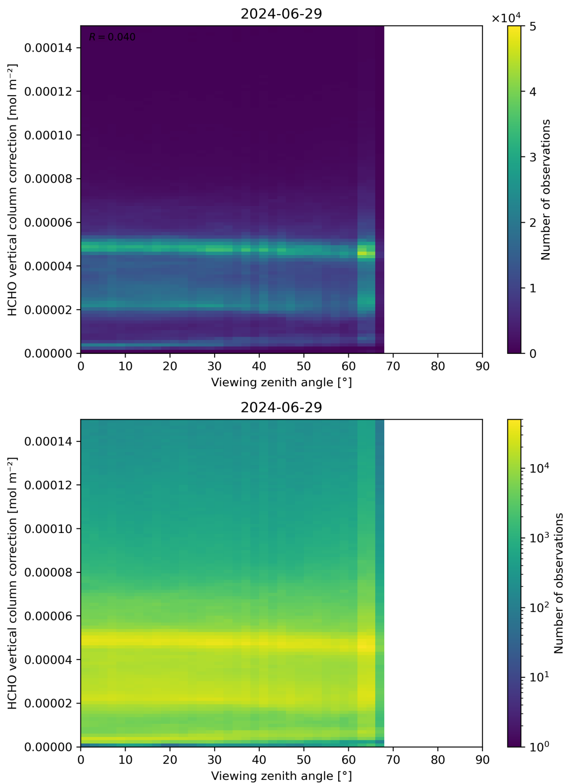
Figure 193: Scatter density plot of “Viewing zenith angle” against “HCHO vertical column correction” for 2024-06-29 to 2024-06-30.
