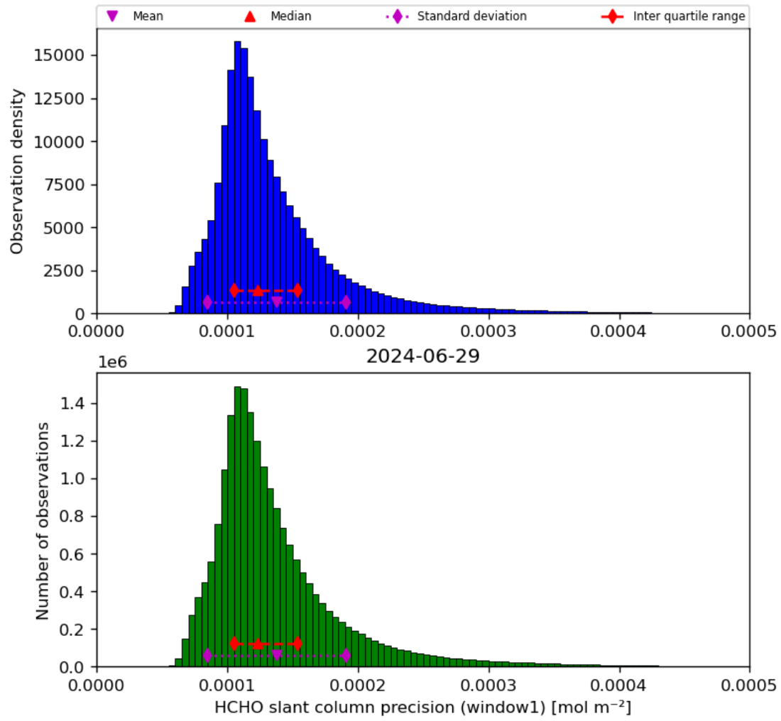
Figure 39: Histogram of “HCHO slant column precision (window1)” for 2024-06-29 to 2024-06-30
