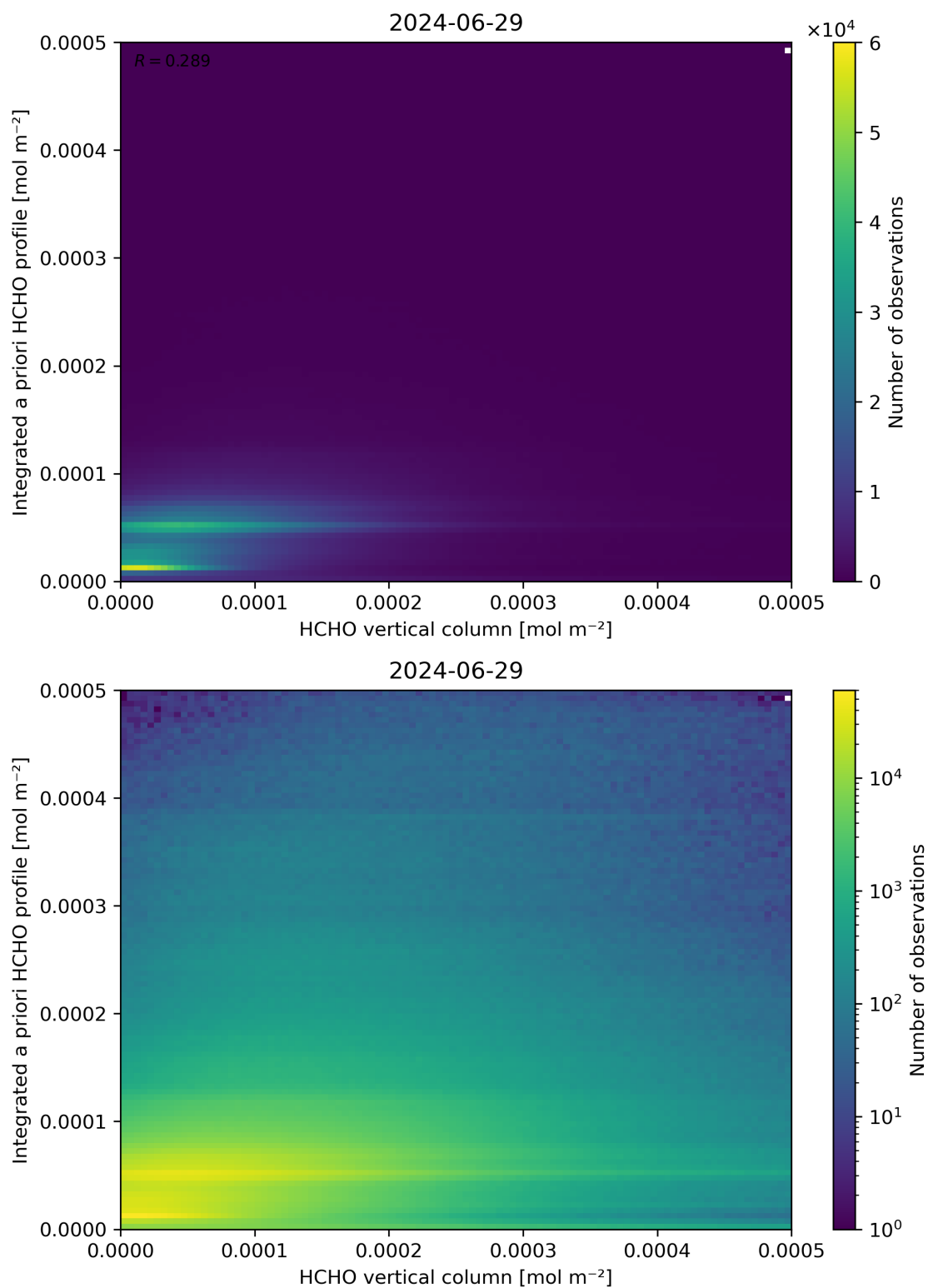
Figure 135: Scatter density plot of “HCHO vertical column” against “Integrated a priori HCHO profile” for 2024-06-29 to 2024-06-30.
