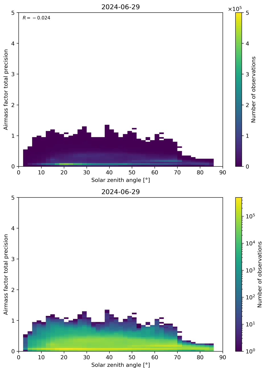
Figure 176: Scatter density plot of “Solar zenith angle” against “Airmass factor total precision” for 2024-06-29 to 2024-06-30.
