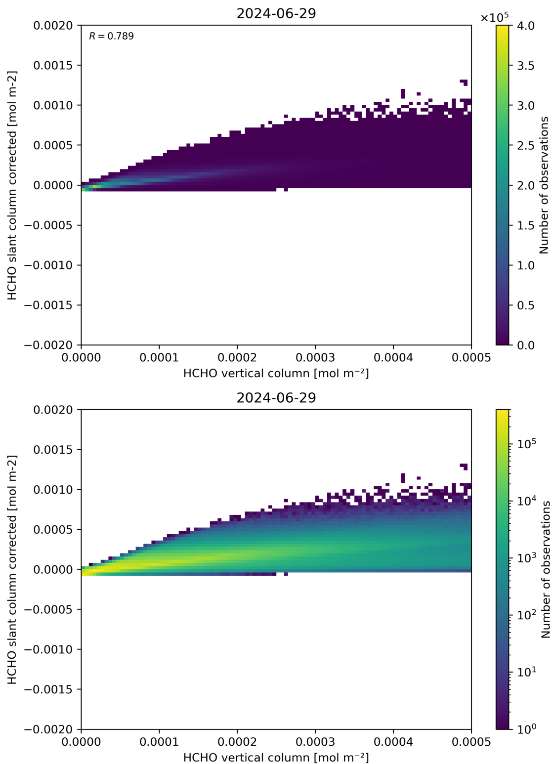
Figure 127: Scatter density plot of “HCHO vertical column” against “HCHO slant column corrected” for 2024-06-29 to 2024-06-30.
