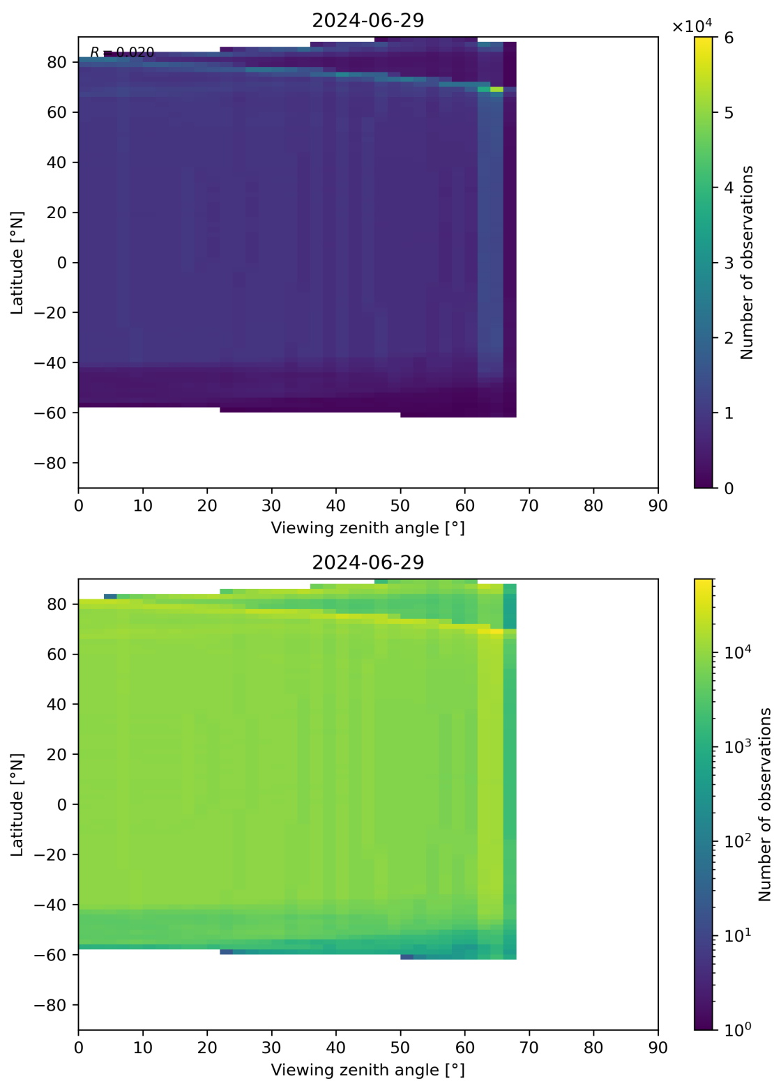
Figure 196: Scatter density plot of “Viewing zenith angle” against “Latitude” for 2024-06-29 to 2024-06-30.
