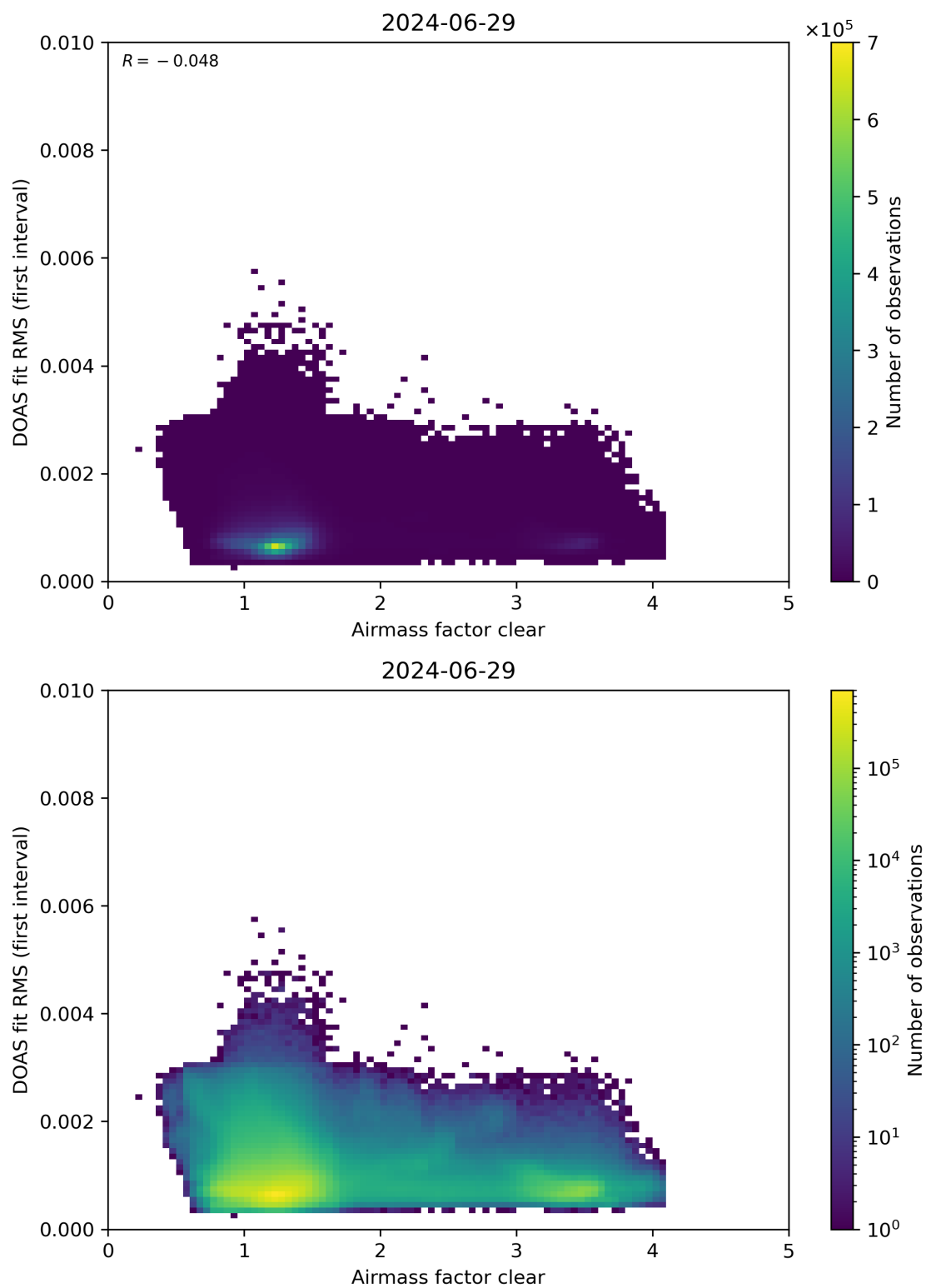
Figure 71: Scatter density plot of “Airmass factor clear” against “DOAS fit RMS (first interval)” for 2024-06-29 to 2024-06-30.
