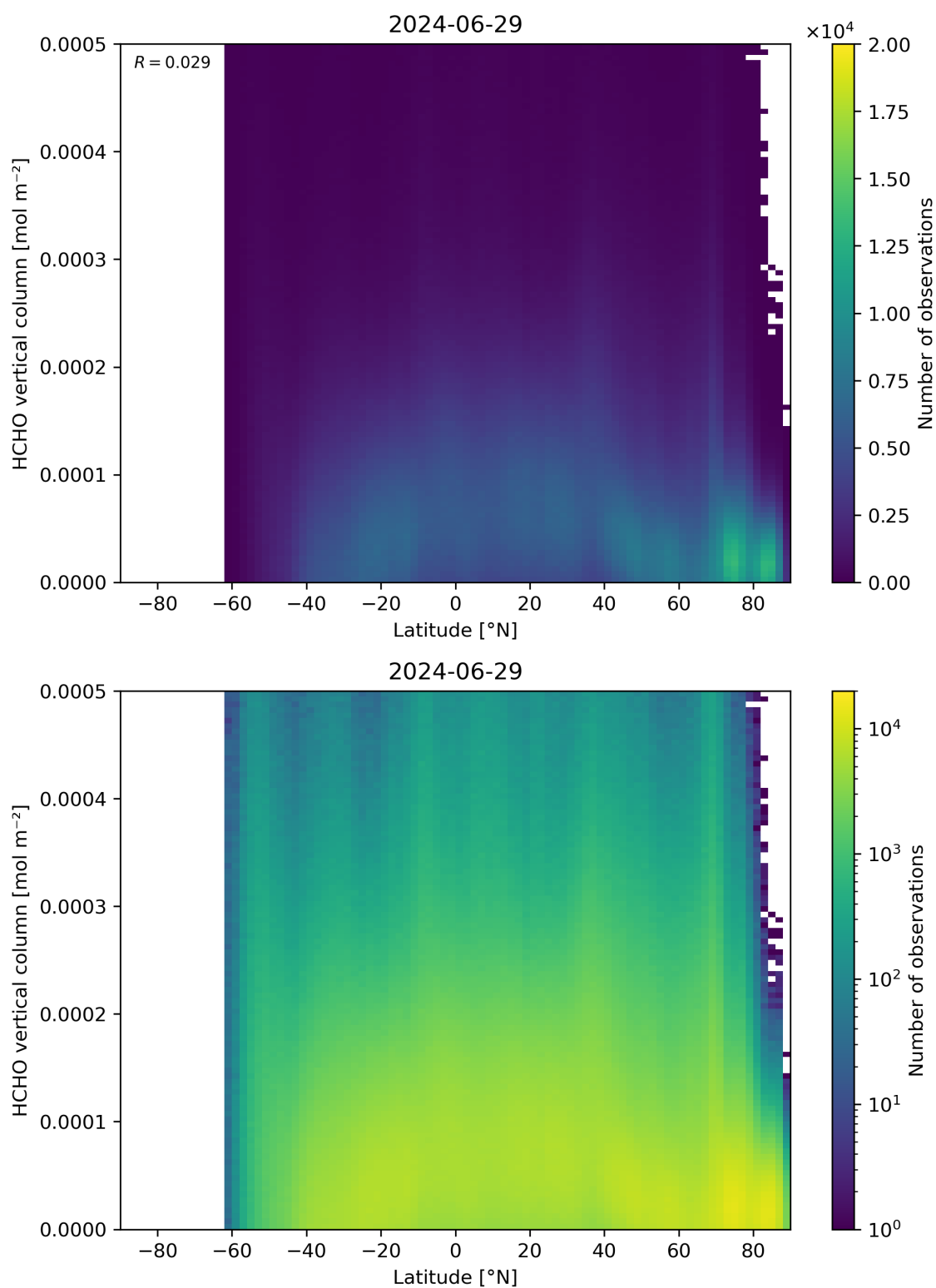
Figure 163: Scatter density plot of “Latitude” against “HCHO vertical column” for 2024-06-29 to 2024-06-30.
