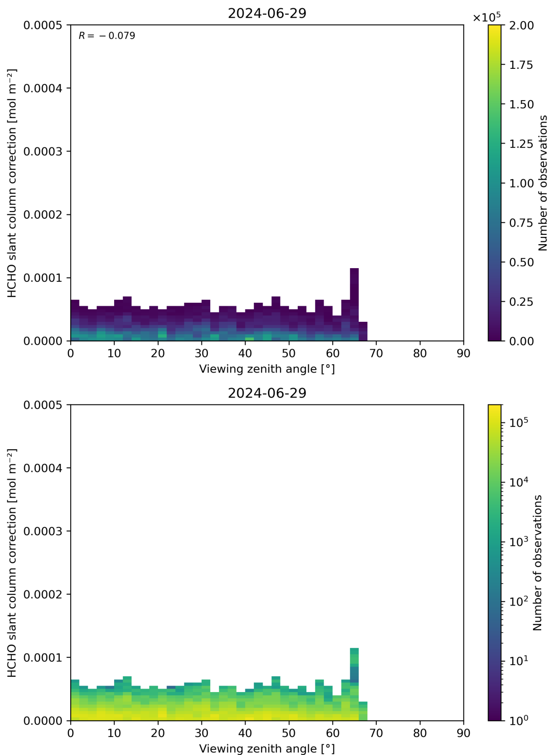
Figure 187: Scatter density plot of “Viewing zenith angle” against “HCHO slant column correction” for 2024-06-29 to 2024-06-30.
