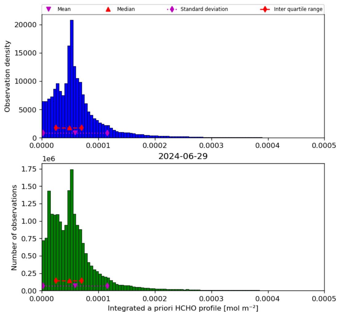
Figure 43: Histogram of “Integrated a priori HCHO profile” for 2024-06-29 to 2024-06-30
