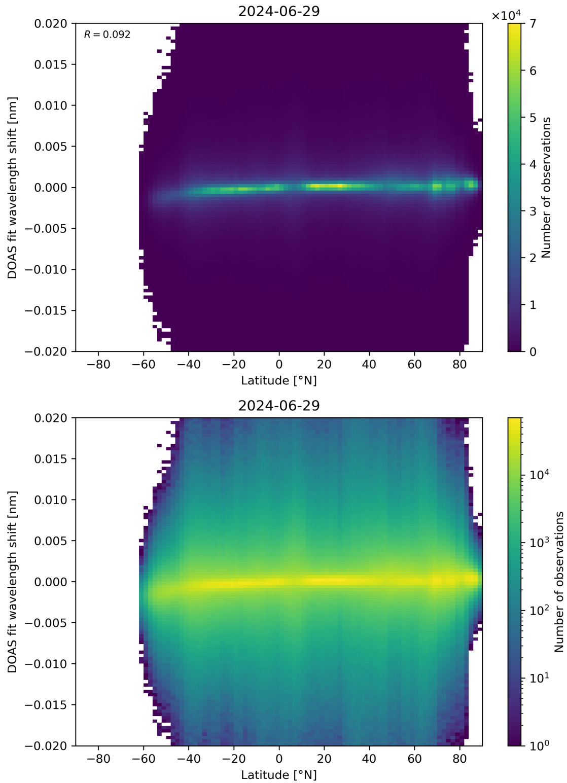
Figure 154: Scatter density plot of “Latitude” against “DOAS fit wavelength shift” for 2024-06-29 to 2024-06-30.
