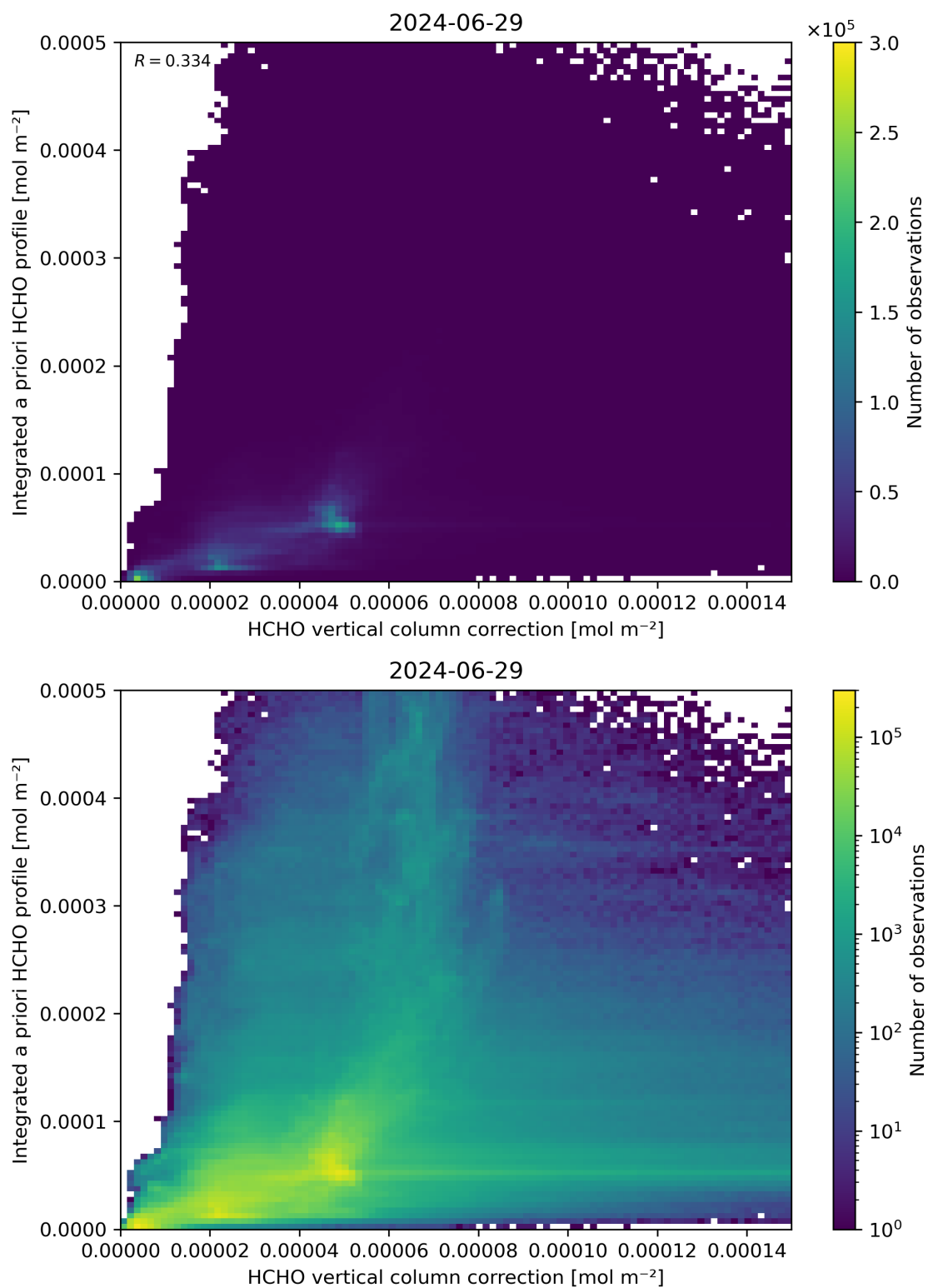
Figure 122: Scatter density plot of “HCHO vertical column correction” against “Integrated a priori HCHO profile” for 2024-06-29 to 2024-06-30.
