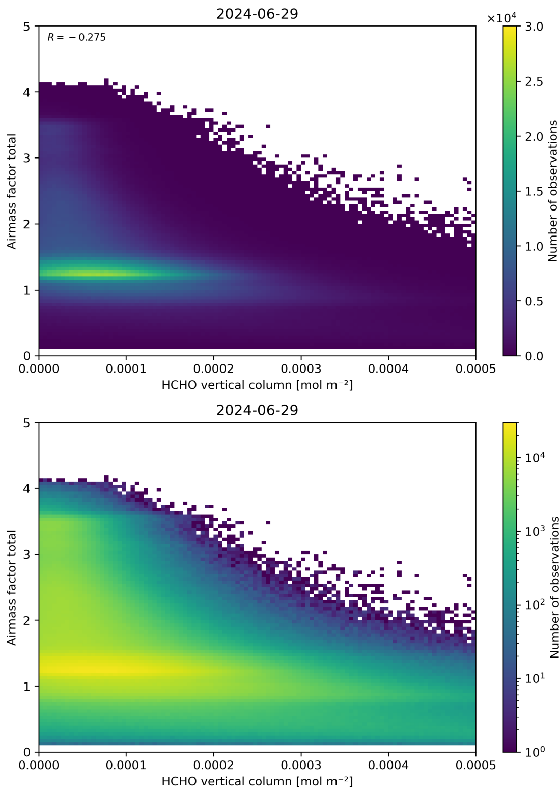
Figure 131: Scatter density plot of “HCHO vertical column” against “Airmass factor total” for 2024-06-29 to 2024-06-30.
