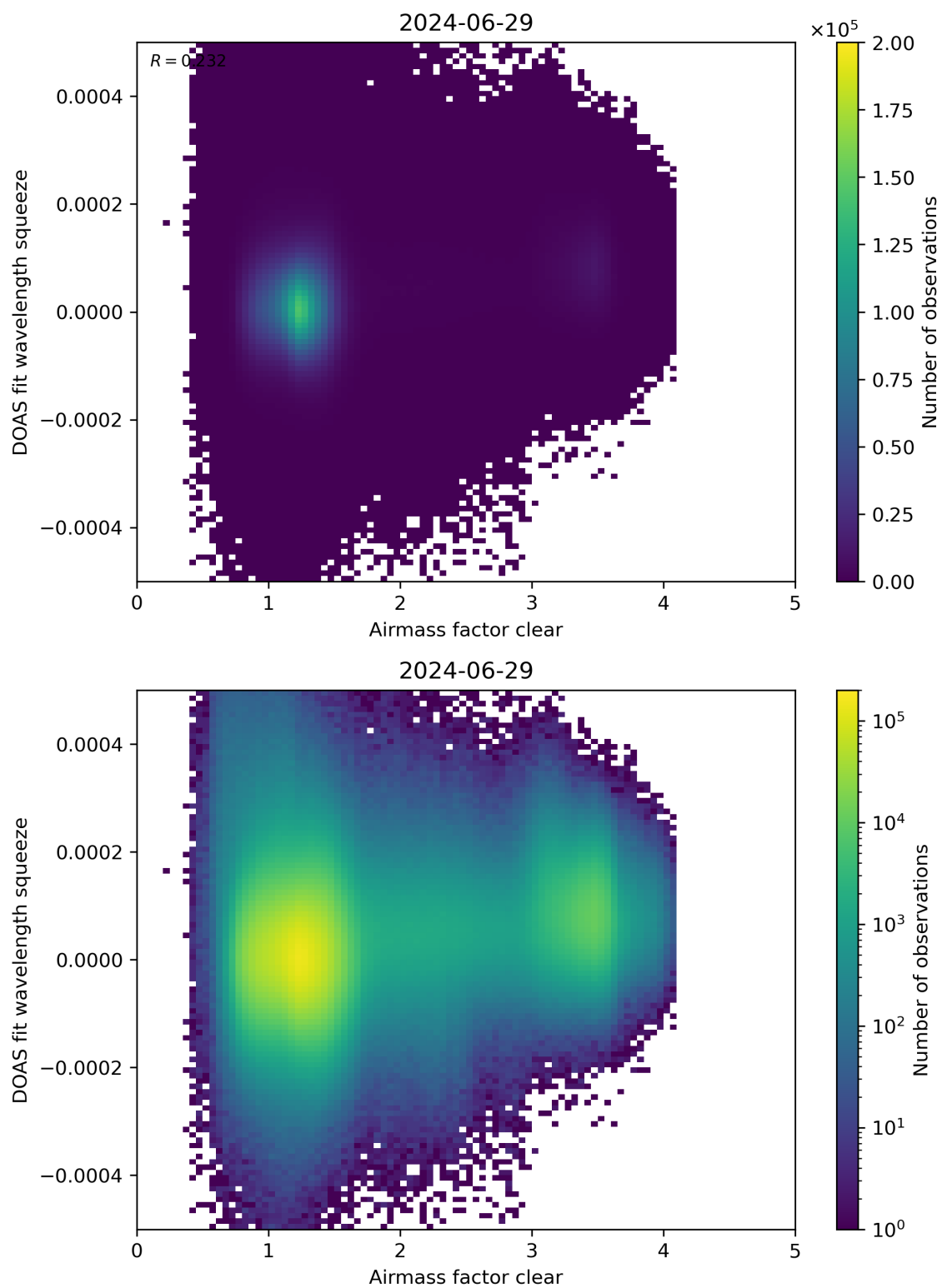
Figure 73: Scatter density plot of “Airmass factor clear” against “DOAS fit wavelength squeeze” for 2024-06-29 to 2024-06-30.
