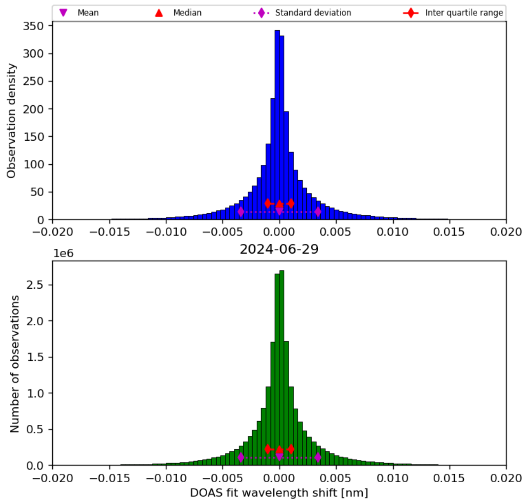
Figure 44: Histogram of “DOAS fit wavelength shift” for 2024-06-29 to 2024-06-30
