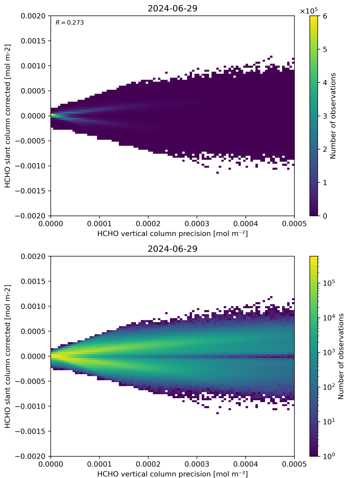
Figure 140: Scatter density plot of “HCHO vertical column precision” against “HCHO slant column corrected” for 2024-06-29 to 2024-06-30.
