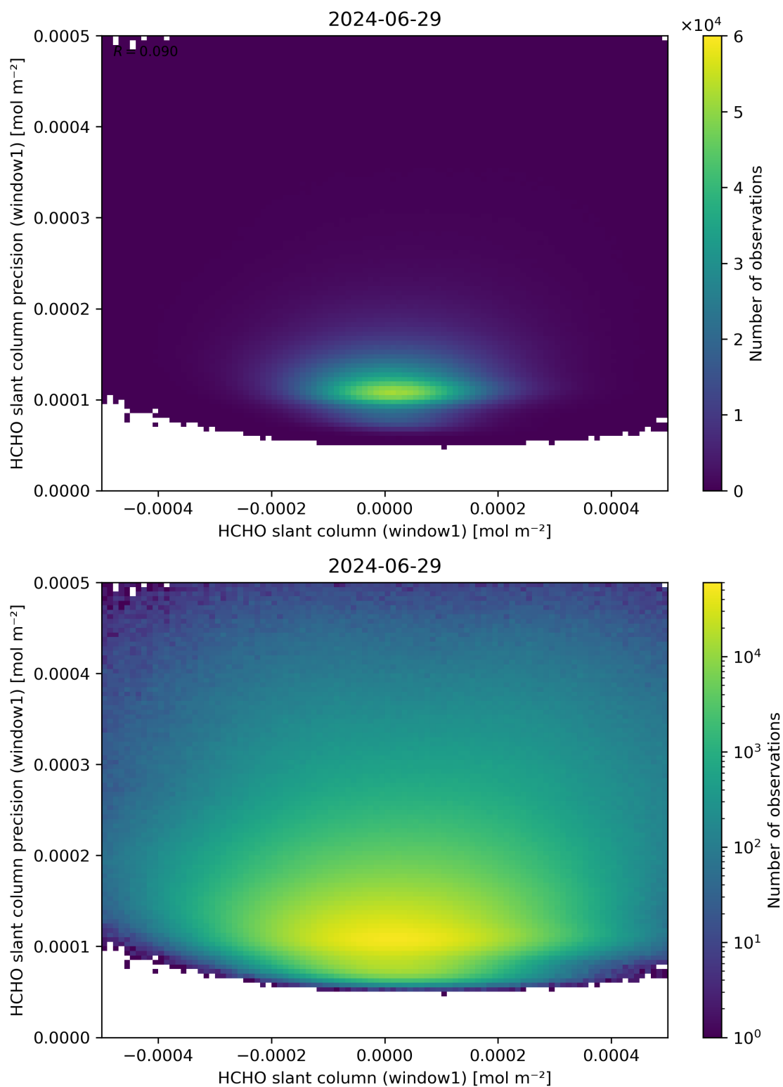
Figure 84: Scatter density plot of “HCHO slant column (window1)” against “HCHO slant column precision (window1)” for 2024-06-29 to 2024-06-30.
