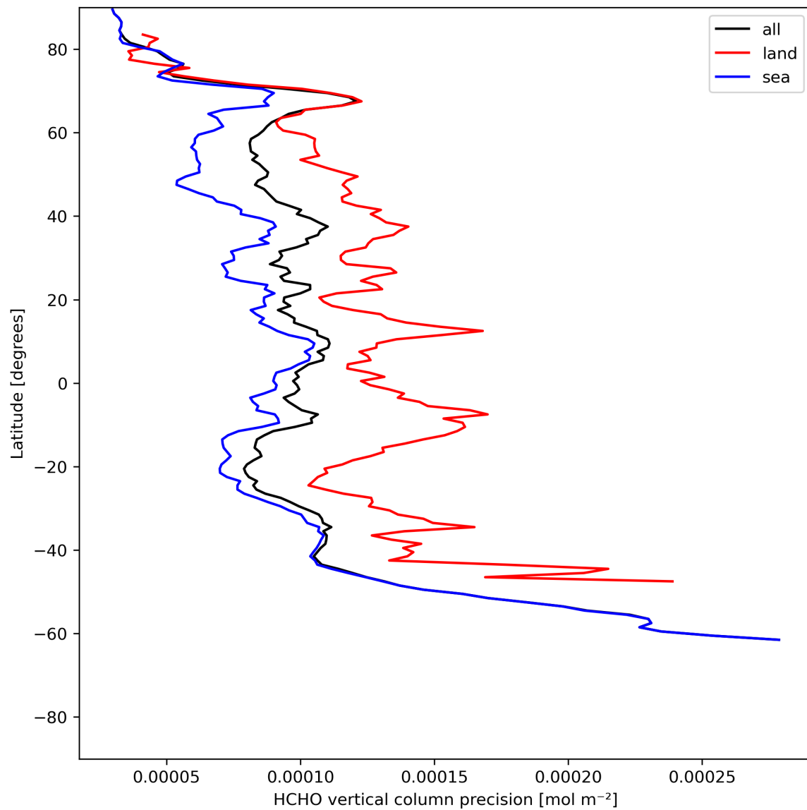
Figure 22: Zonal average of “HCHO vertical column precision” for 2024-06-29 to 2024-06-30.
