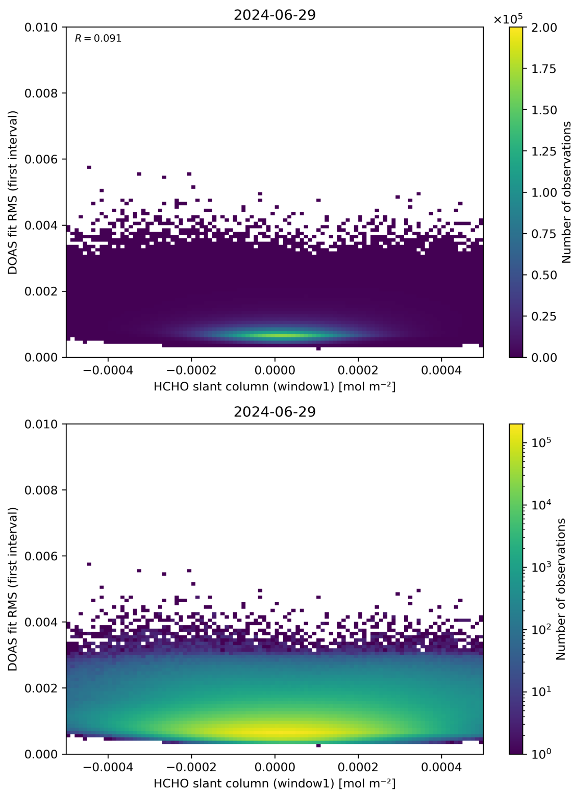
Figure 78: Scatter density plot of “HCHO slant column (window1)” against “DOAS fit RMS (first interval)” for 2024-06-29 to 2024-06-30.
