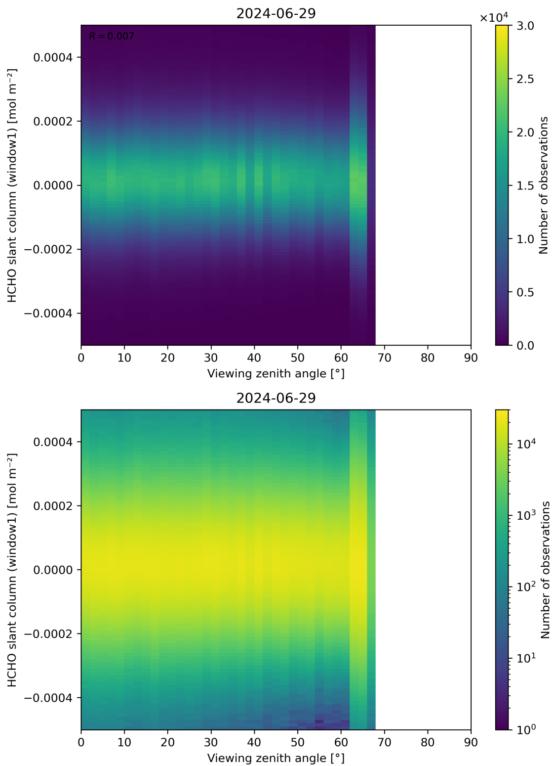
Figure 188: Scatter density plot of “Viewing zenith angle” against “HCHO slant column (window1)” for 2024-06-29 to 2024-06-30.
