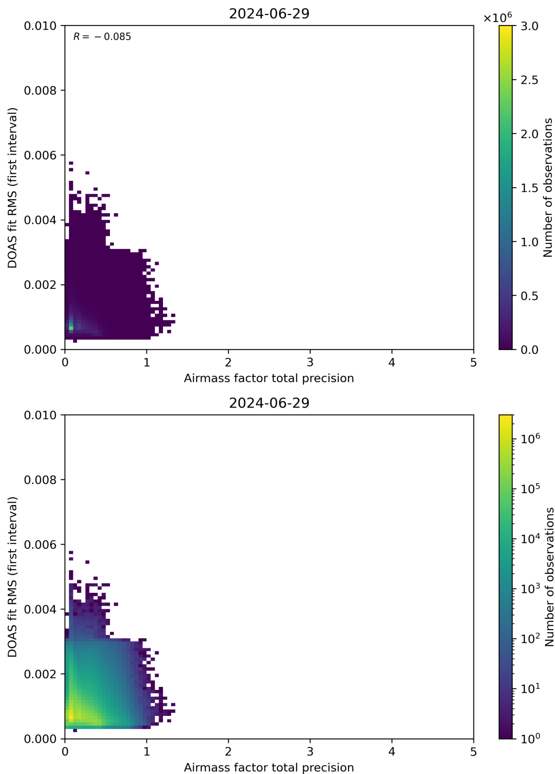
Figure 105: Scatter density plot of “Airmass factor total precision” against “DOAS fit RMS (first interval)” for 2024-06-29 to 2024-06-30.
