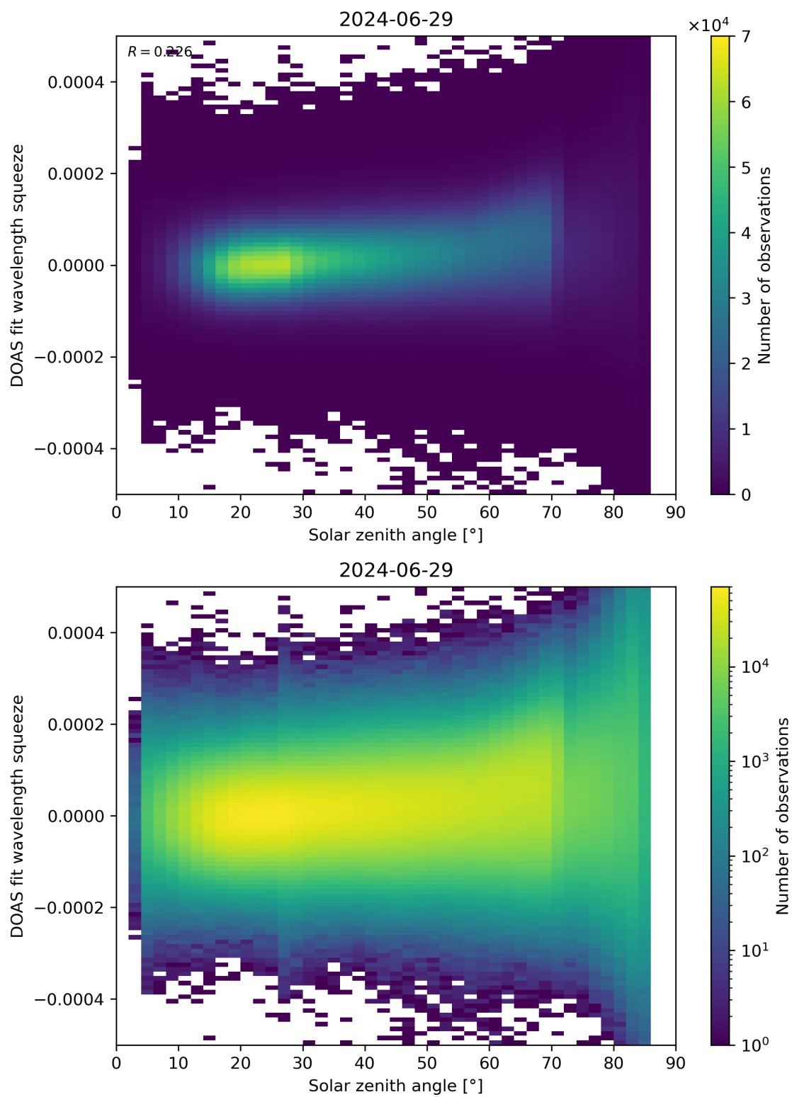
Figure 169: Scatter density plot of “Solar zenith angle” against “DOAS fit wavelength squeeze” for 2024-06-29 to 2024-06-30.
