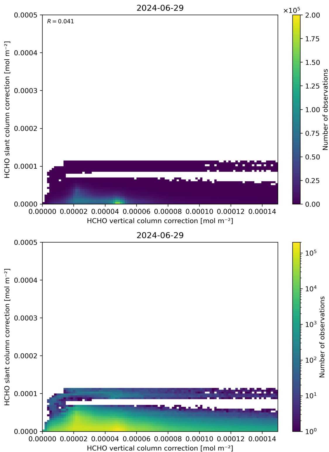
Figure 117: Scatter density plot of “HCHO vertical column correction” against “HCHO slant column correction” for 2024-06-29 to 2024-06-30.
