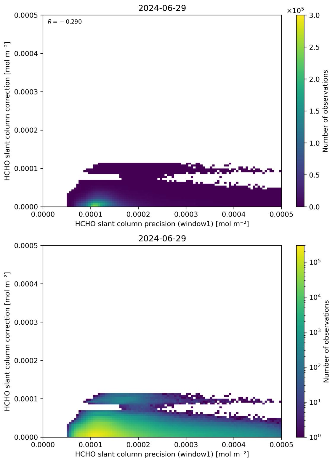
Figure 93: Scatter density plot of “HCHO slant column precision (window1)” against “HCHO slant column correction” for 2024-06-29 to 2024-06-30.
