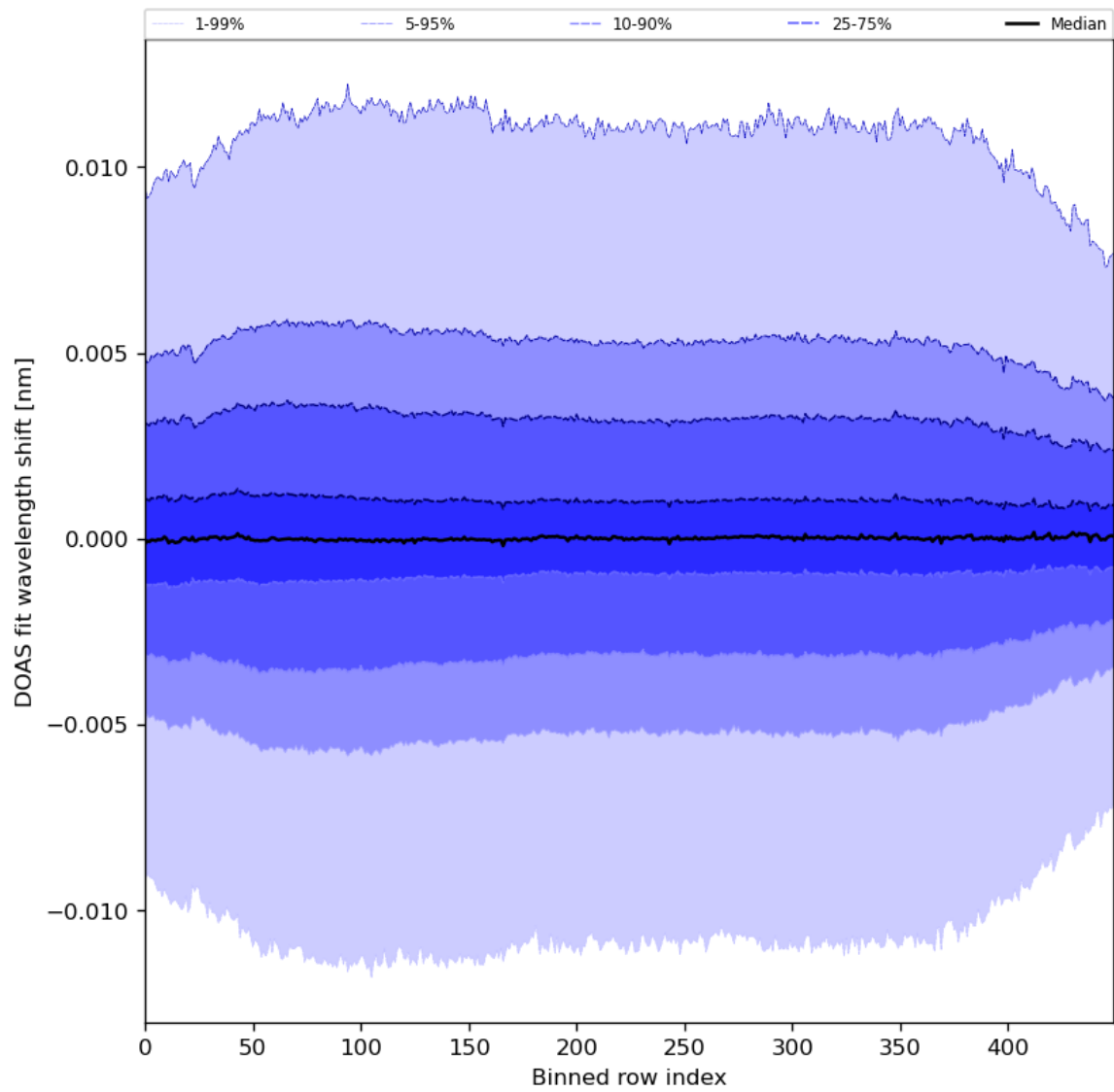
Figure 58: Along track statistics of “DOAS fit wavelength shift” for 2024-06-29 to 2024-07-01
