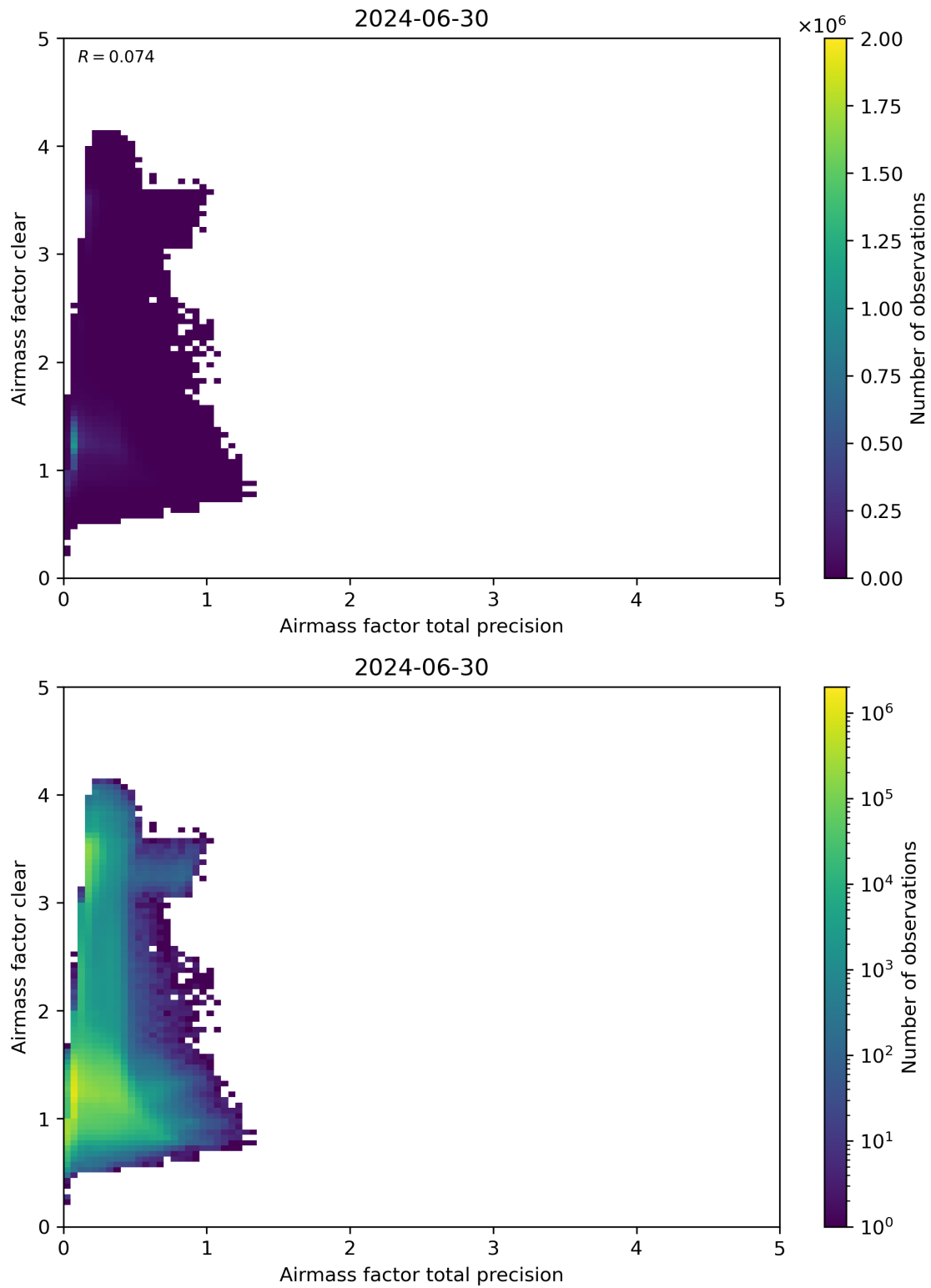
Figure 108: Scatter density plot of “Airmass factor total precision” against “Airmass factor clear” for 2024-06-29 to 2024-07-01.
