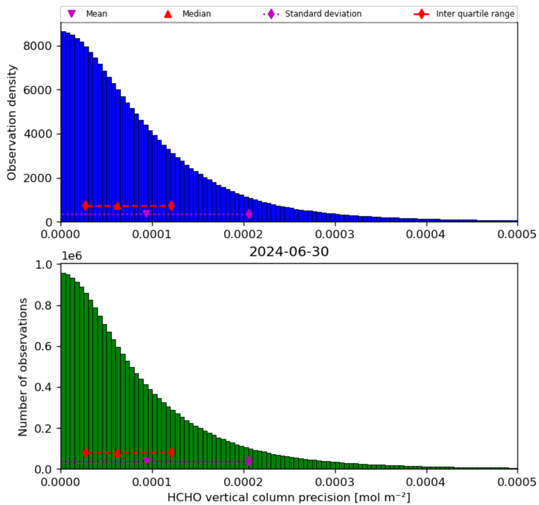
Figure 36: Histogram of “HCHO vertical column precision” for 2024-06-29 to 2024-07-01
