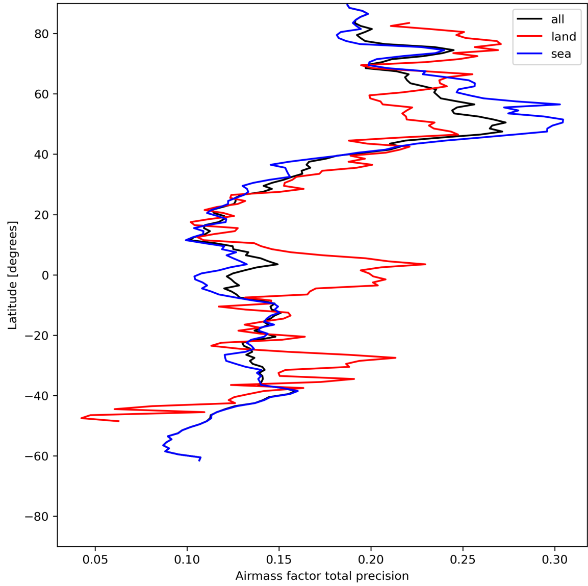
Figure 27: Zonal average of “Airmass factor total precision” for 2024-06-29 to 2024-07-01.
