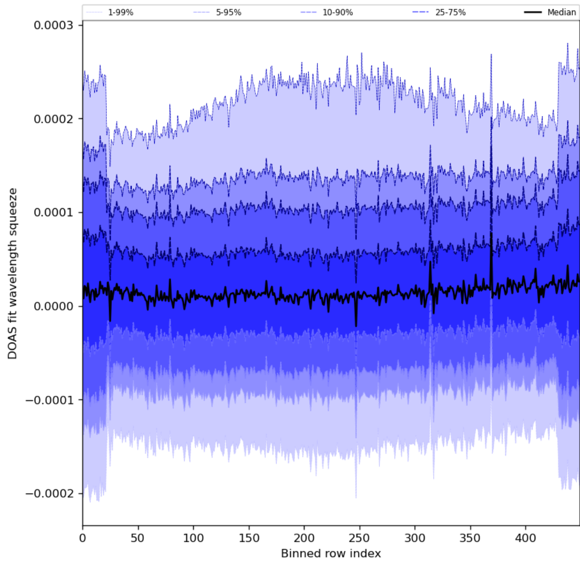
Figure 59: Along track statistics of “DOAS fit wavelength squeeze” for 2024-06-29 to 2024-07-01
