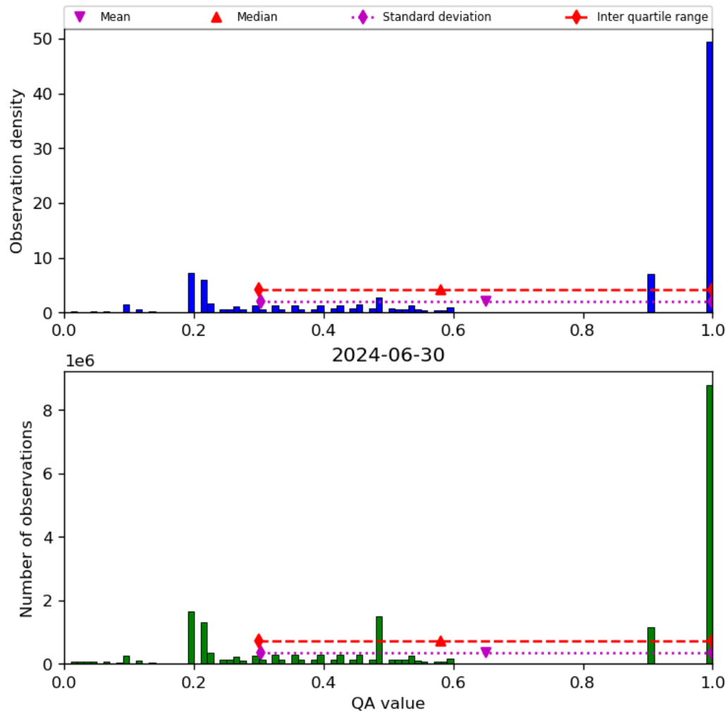
Figure 34: Histogram of “QA value” for 2024-06-29 to 2024-07-01
