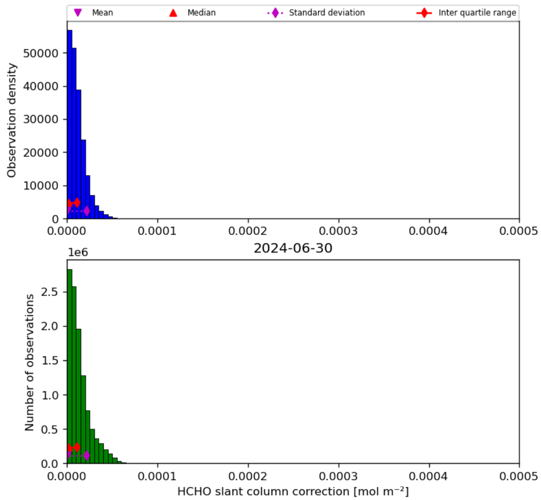
Figure 47: Histogram of “HCHO slant column correction” for 2024-06-29 to 2024-07-01
