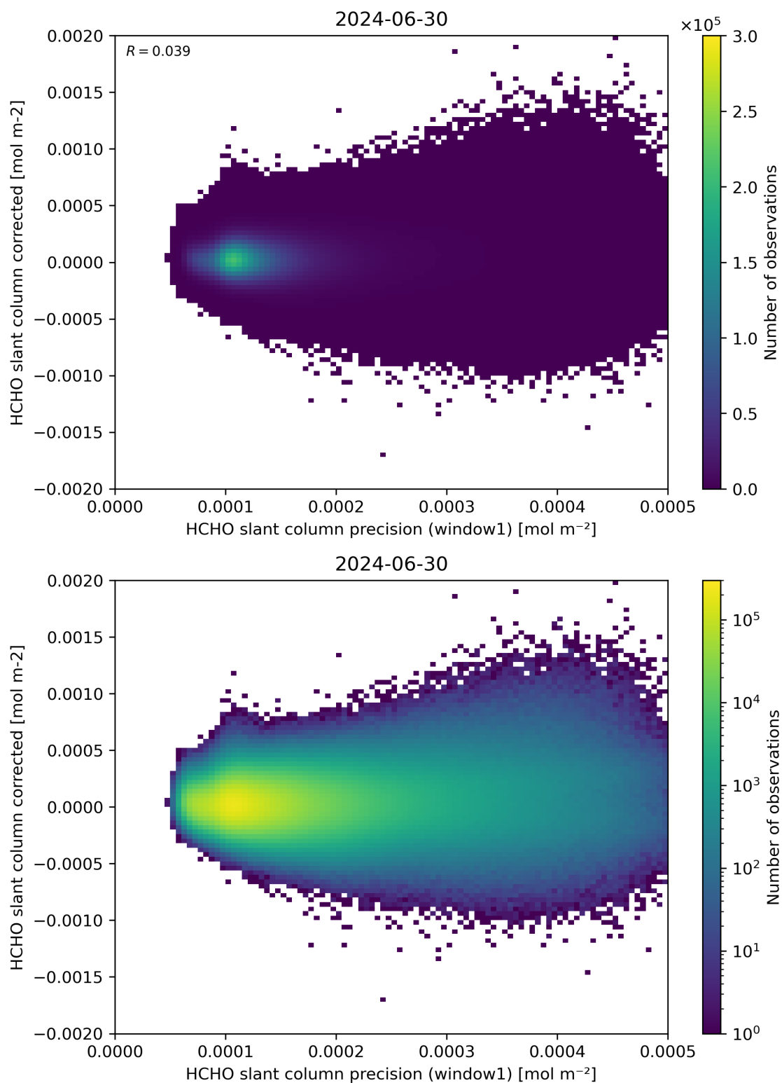
Figure 92: Scatter density plot of “HCHO slant column precision (window1)” against “HCHO slant column corrected” for 2024-06-29 to 2024-07-01.
