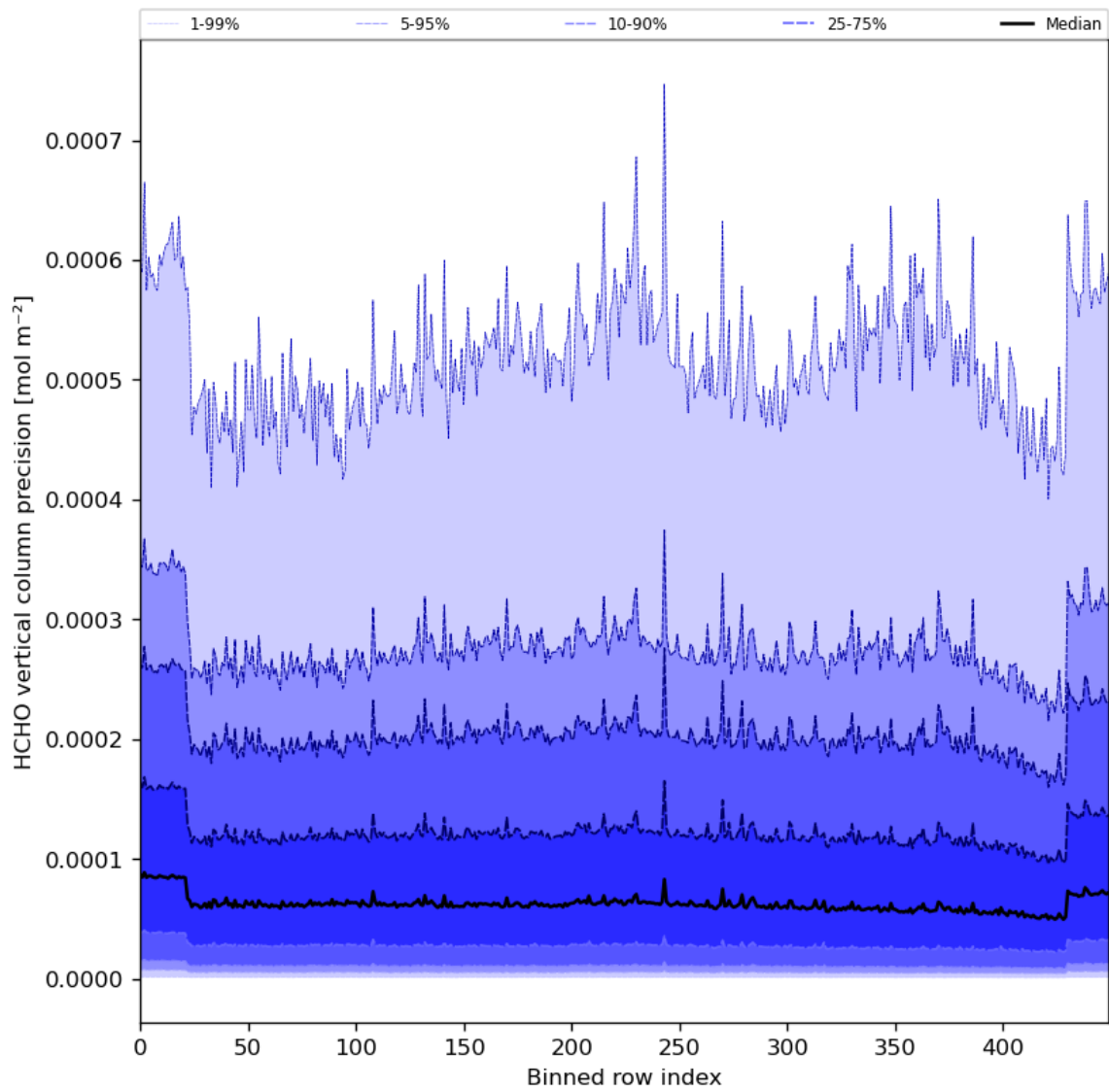
Figure 50: Along track statistics of “HCHO vertical column precision” for 2024-06-29 to 2024-07-01
