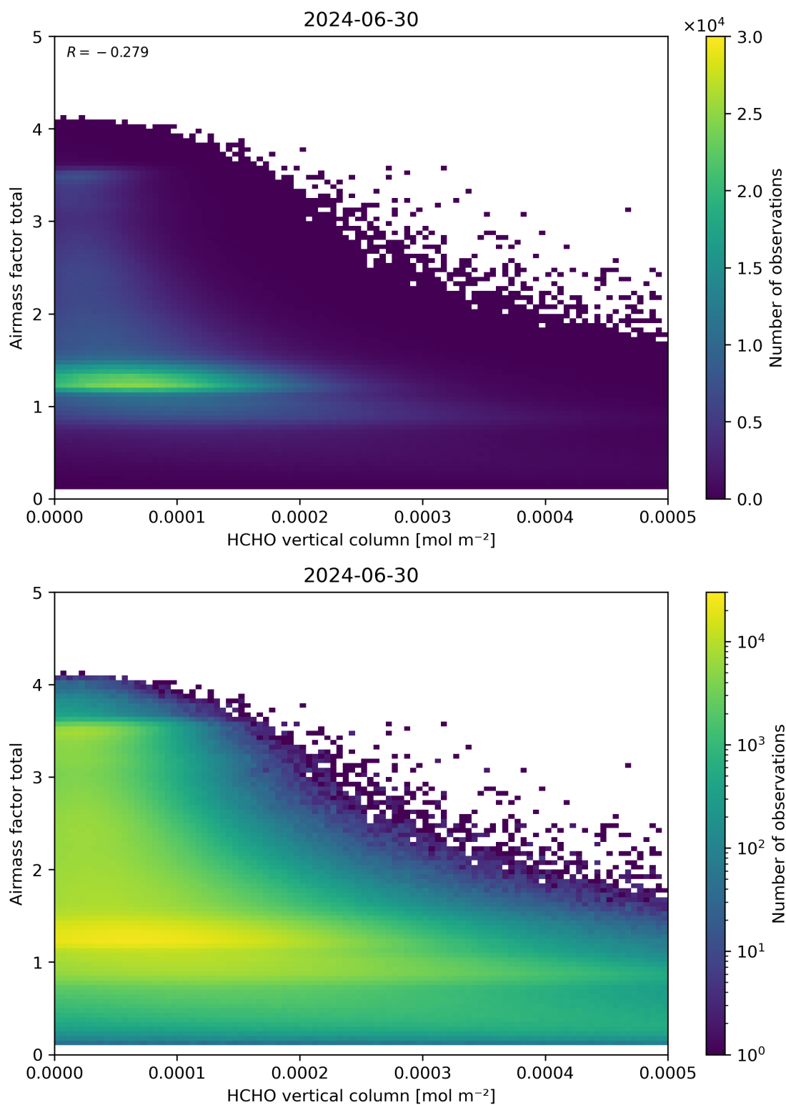
Figure 131: Scatter density plot of “HCHO vertical column” against “Airmass factor total” for 2024-06-29 to 2024-07-01.
