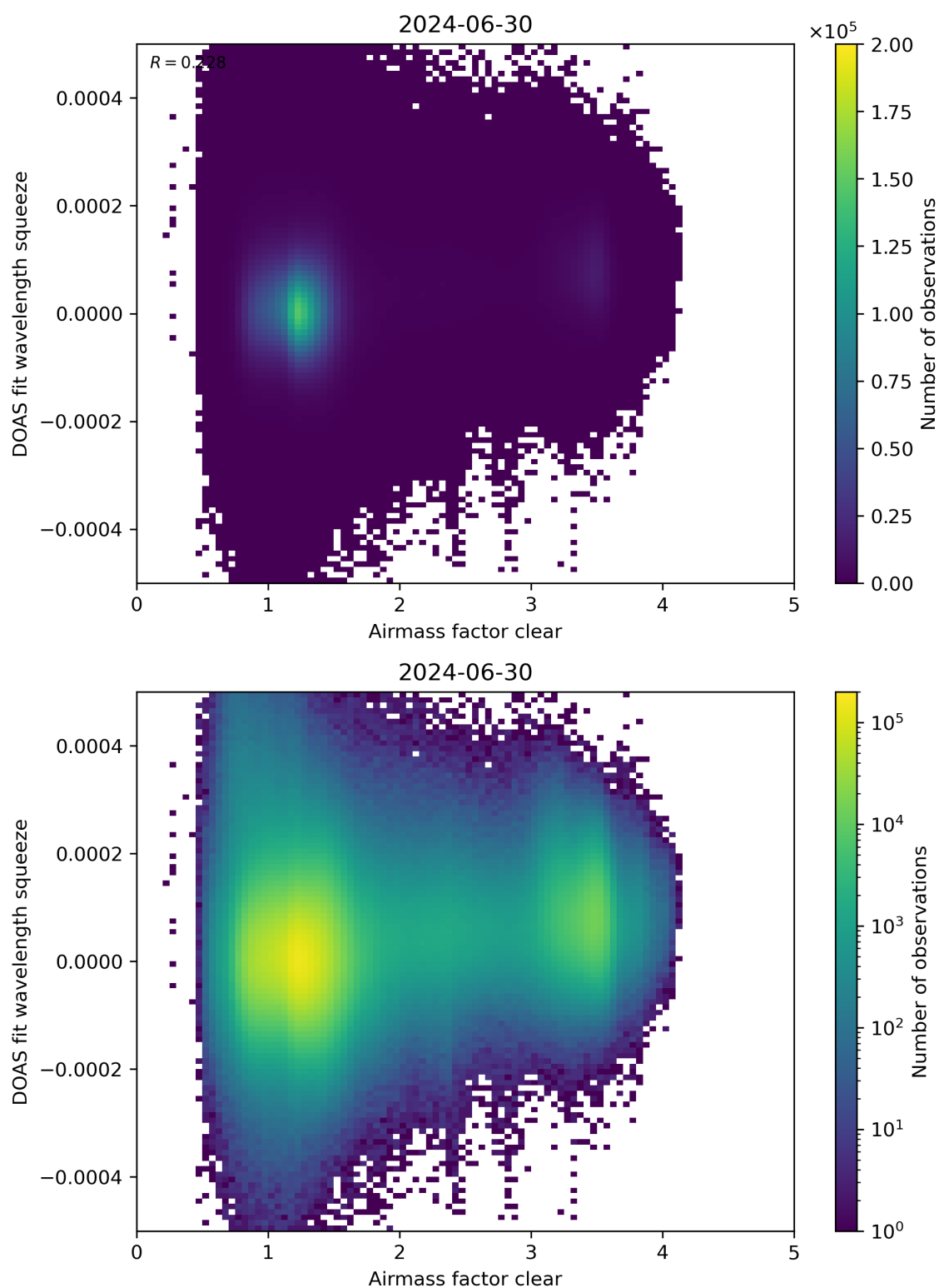
Figure 73: Scatter density plot of “Airmass factor clear” against “DOAS fit wavelength squeeze” for 2024-06-29 to 2024-07-01.
