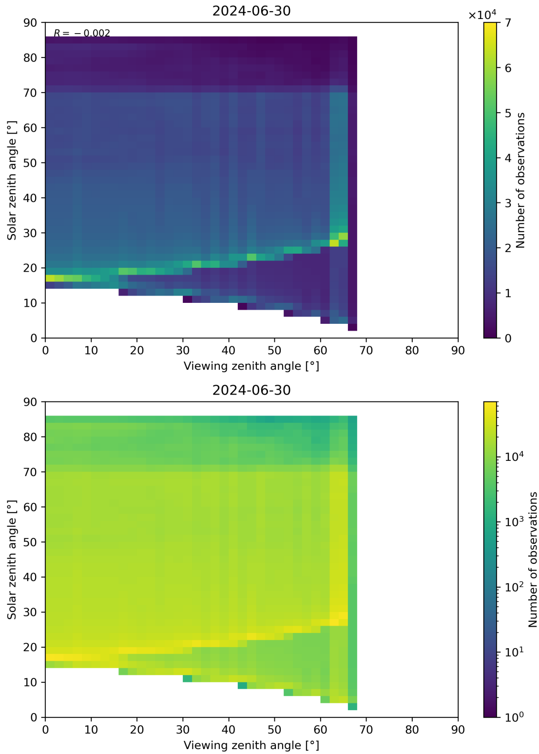
Figure 197: Scatter density plot of “Viewing zenith angle” against “Solar zenith angle” for 2024-06-29 to 2024-07-01.
