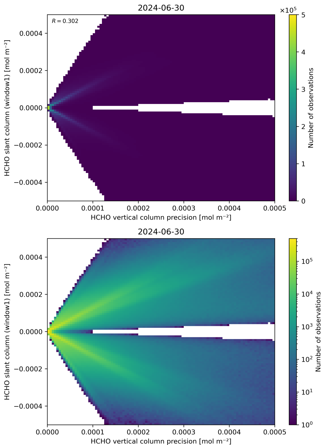
Figure 142: Scatter density plot of “HCHO vertical column precision” against “HCHO slant column (window1)” for 2024-06-29 to 2024-07-01.
