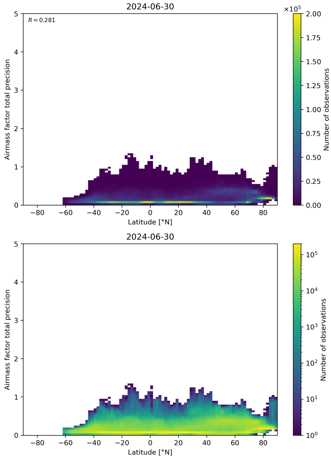
Figure 162: Scatter density plot of “Latitude” against “Airmass factor total precision” for 2024-06-29 to 2024-07-01.
