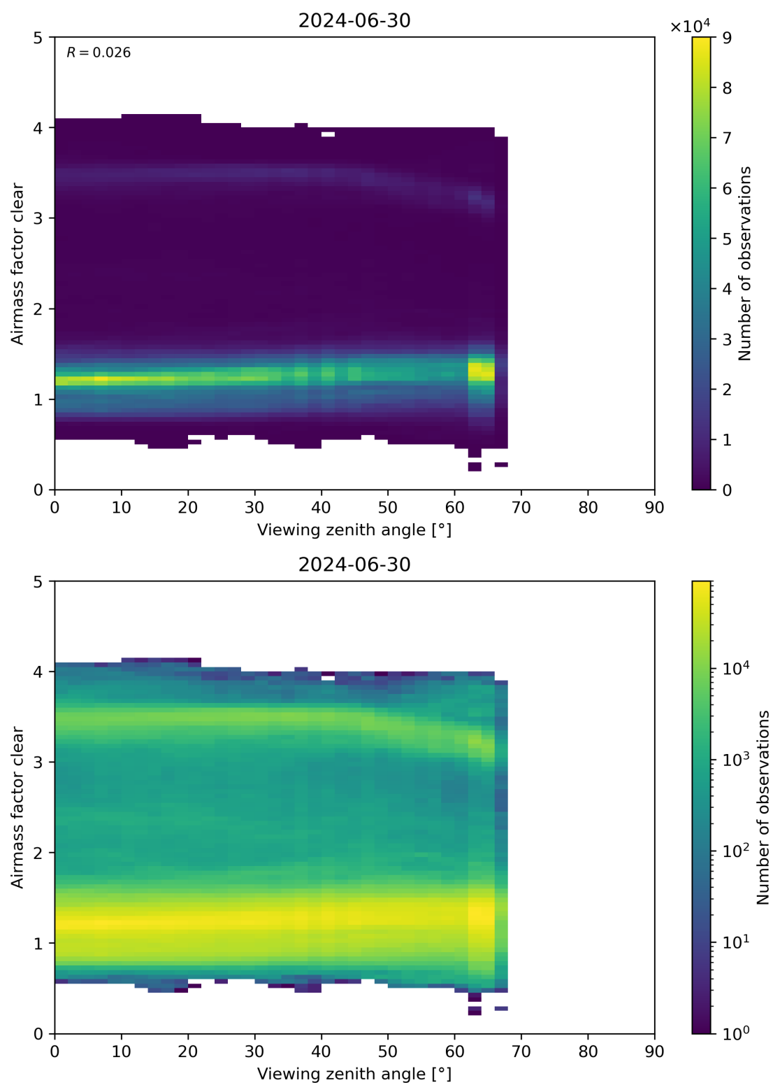
Figure 185: Scatter density plot of “Viewing zenith angle” against “Airmass factor clear” for 2024-06-29 to 2024-07-01.
