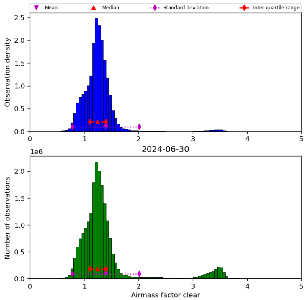
Figure 42: Histogram of “Airmass factor clear” for 2024-06-29 to 2024-07-01
