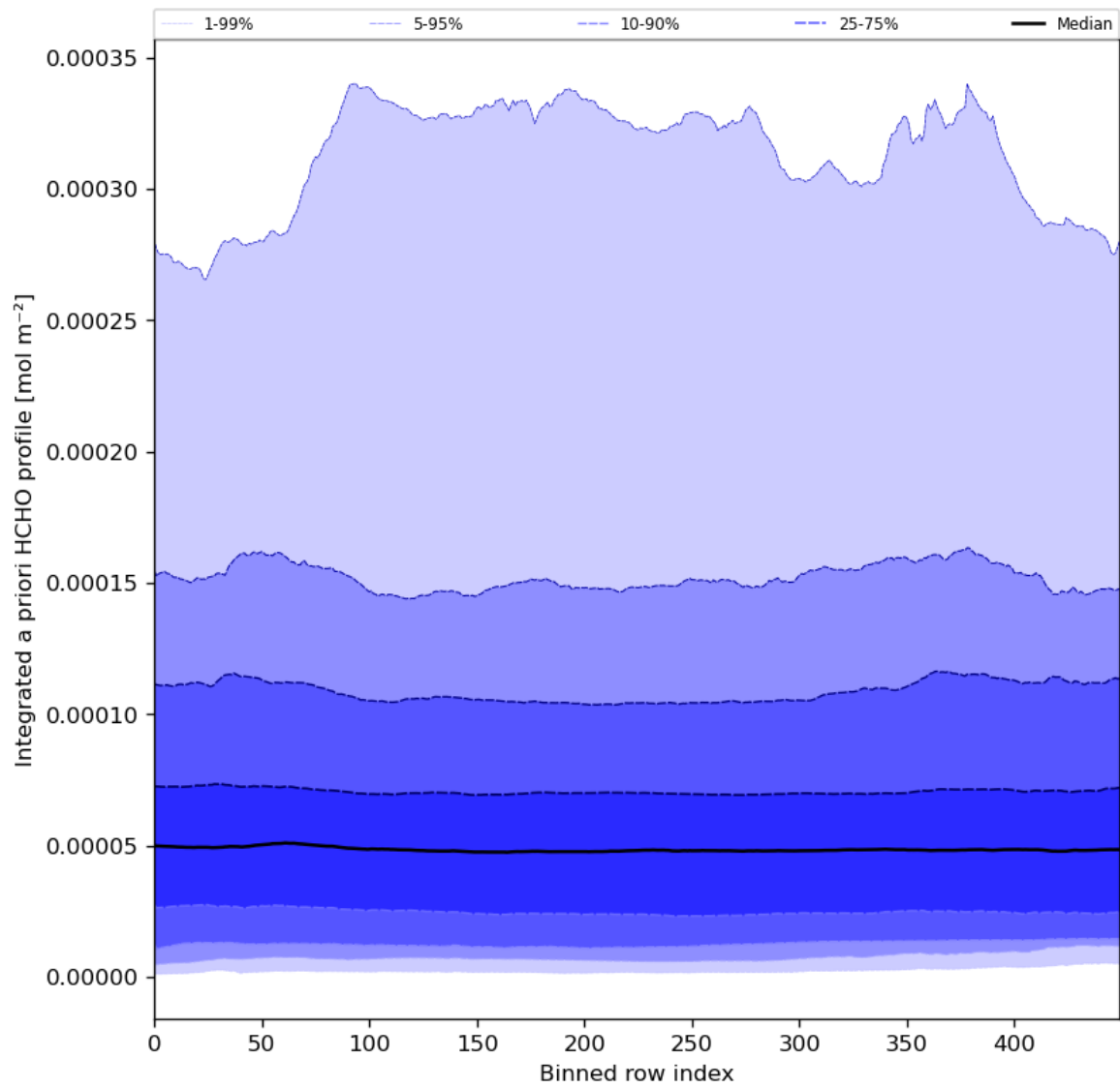
Figure 57: Along track statistics of “Integrated a priori HCHO profile” for 2024-06-29 to 2024-07-01
