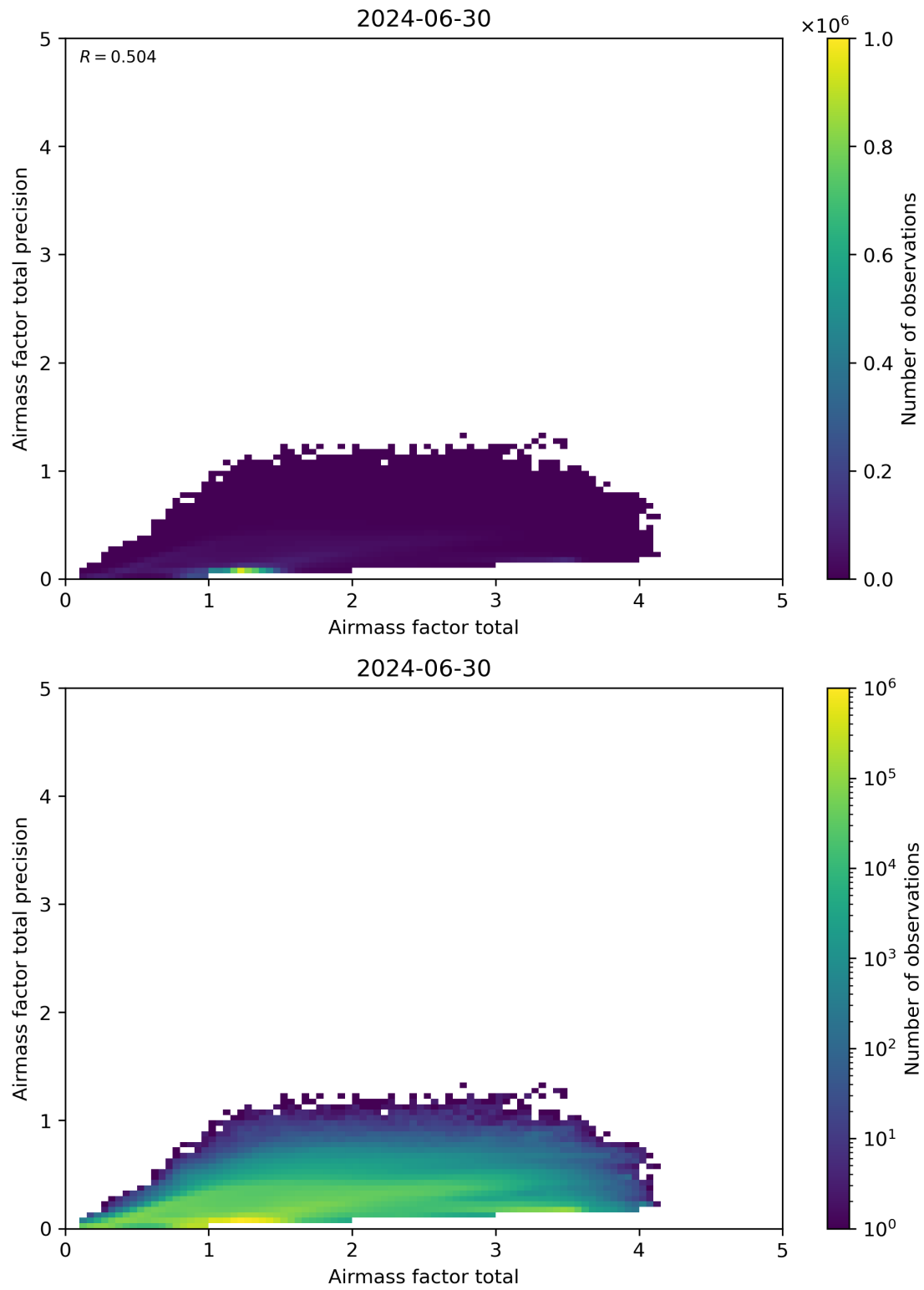
Figure 103: Scatter density plot of “Airmass factor total” against “Airmass factor total precision” for 2024-06-29 to 2024-07-01.
