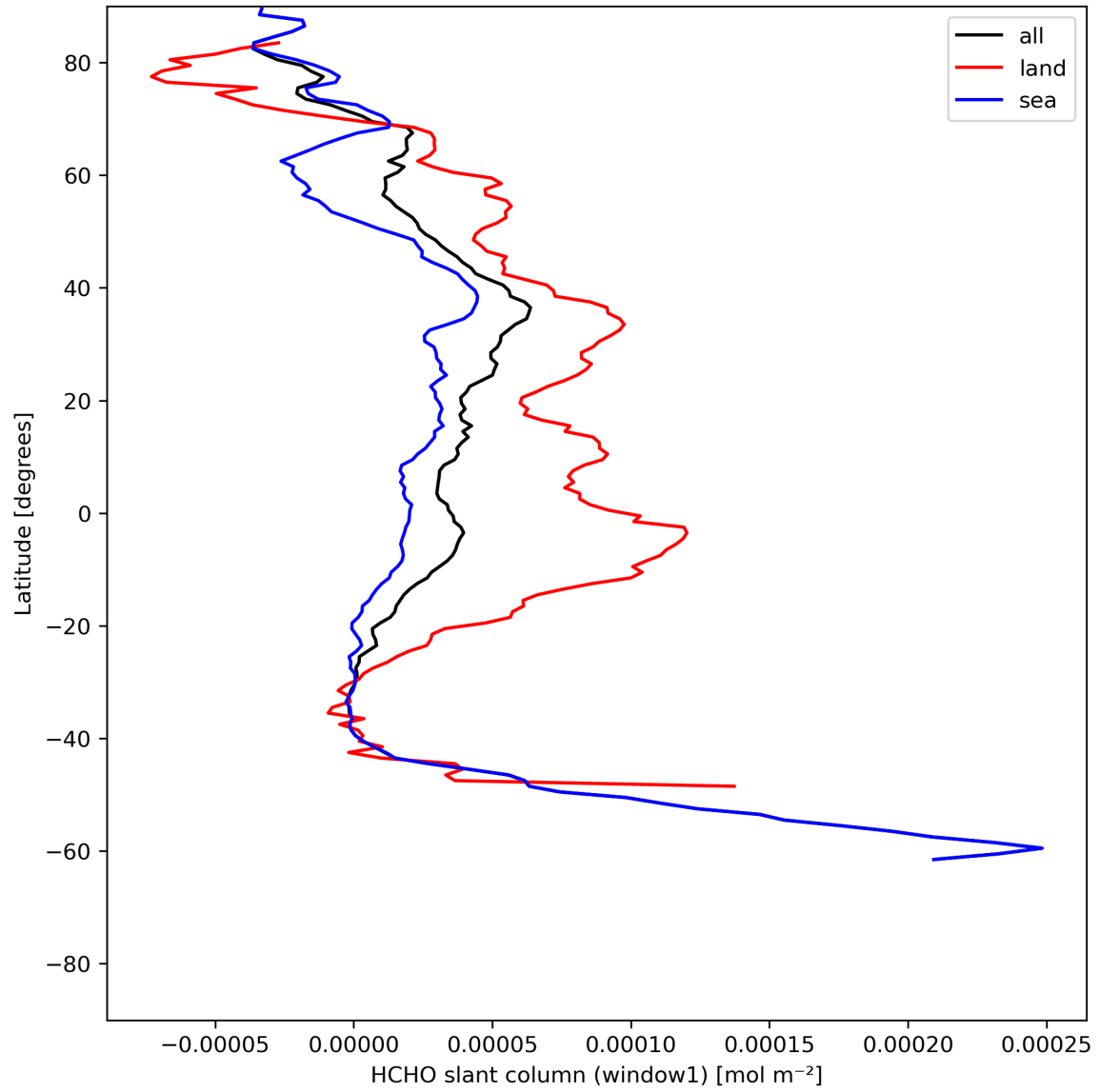
Figure 24: Zonal average of “HCHO slant column (window1)” for 2024-06-29 to 2024-07-01.
