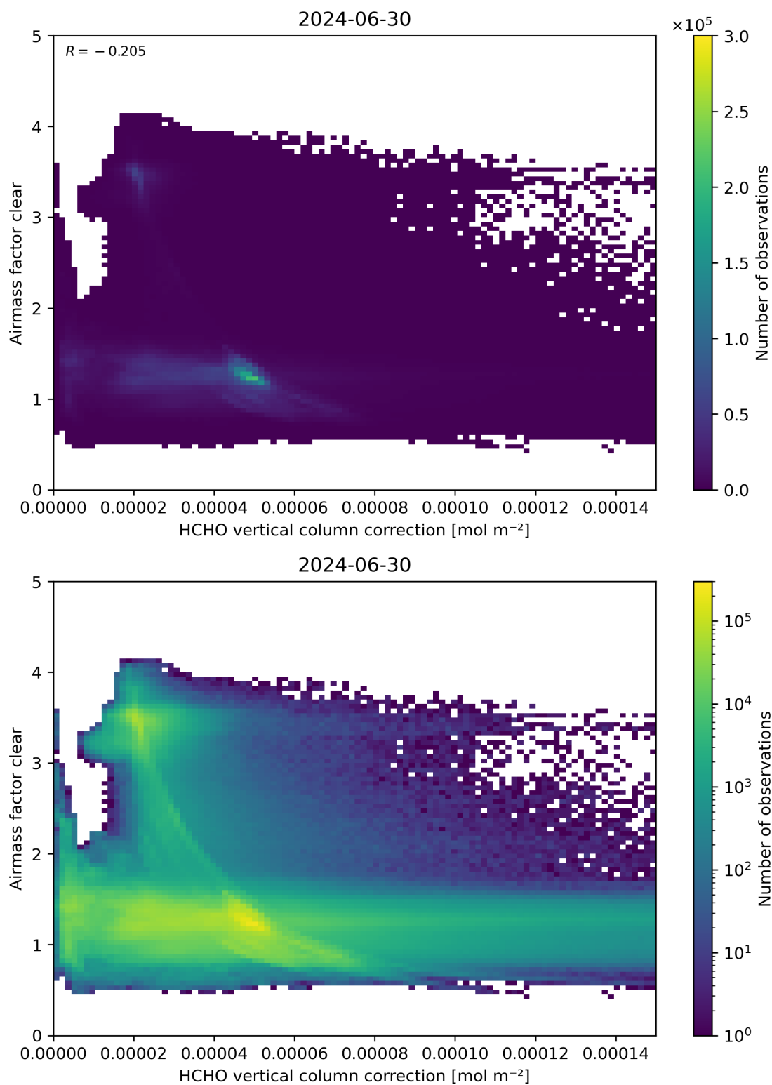
Figure 115: Scatter density plot of “HCHO vertical column correction” against “Airmass factor clear” for 2024-06-29 to 2024-07-01.
