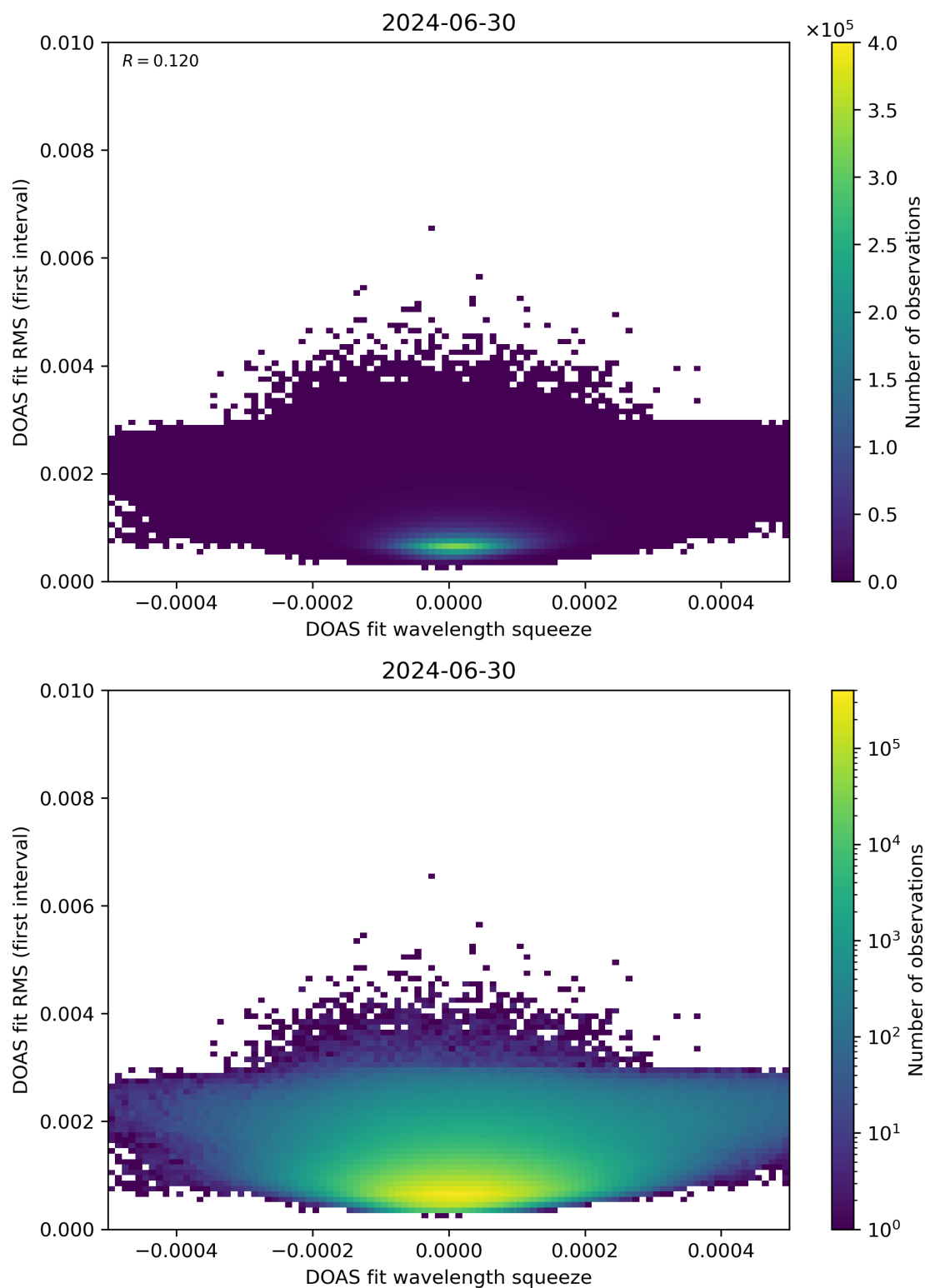
Figure 68: Scatter density plot of “DOAS fit wavelength squeeze” against “DOAS fit RMS (first interval)” for 2024-06-29 to 2024-07-01.
