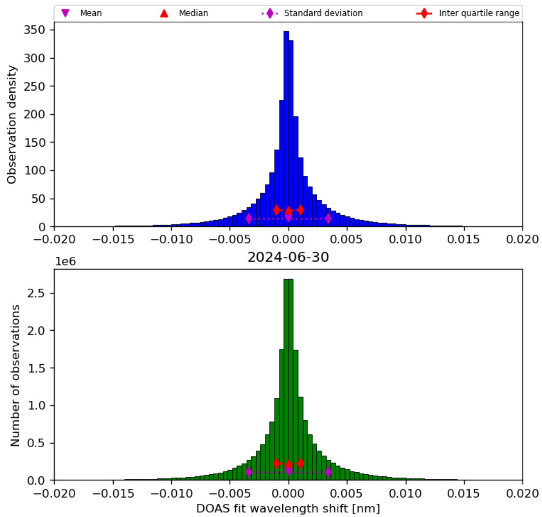
Figure 44: Histogram of “DOAS fit wavelength shift” for 2024-06-29 to 2024-07-01
