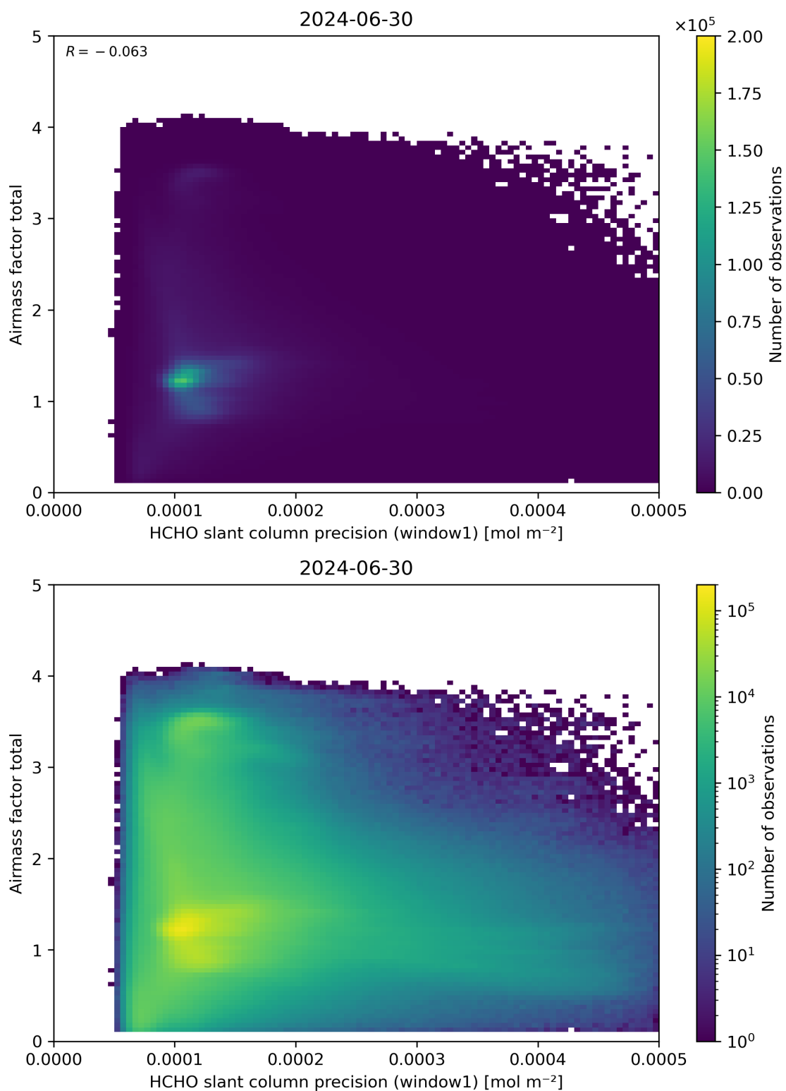
Figure 94: Scatter density plot of “HCHO slant column precision (window1)” against “Airmass factor total” for 2024-06-29 to 2024-07-01.
