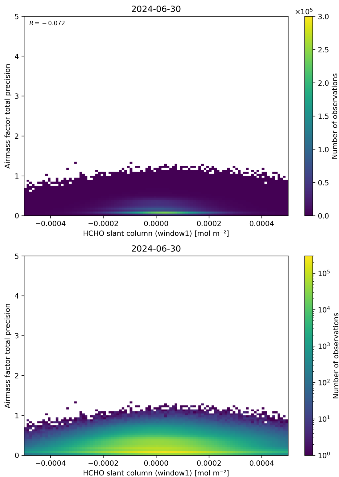
Figure 86: Scatter density plot of “HCHO slant column (window1)” against “Airmass factor total precision” for 2024-06-29 to 2024-07-01.
