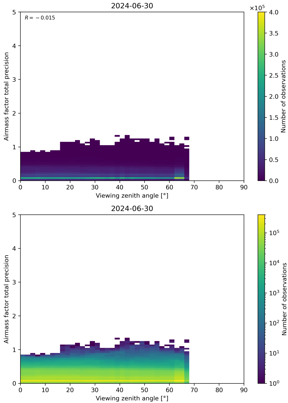
Figure 191: Scatter density plot of “Viewing zenith angle” against “Airmass factor total precision” for 2024-06-29 to 2024-07-01.
