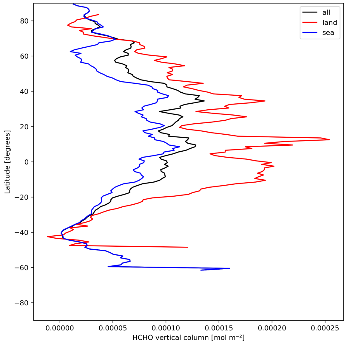
Figure 21: Zonal average of “HCHO vertical column” for 2024-06-29 to 2024-07-01.
