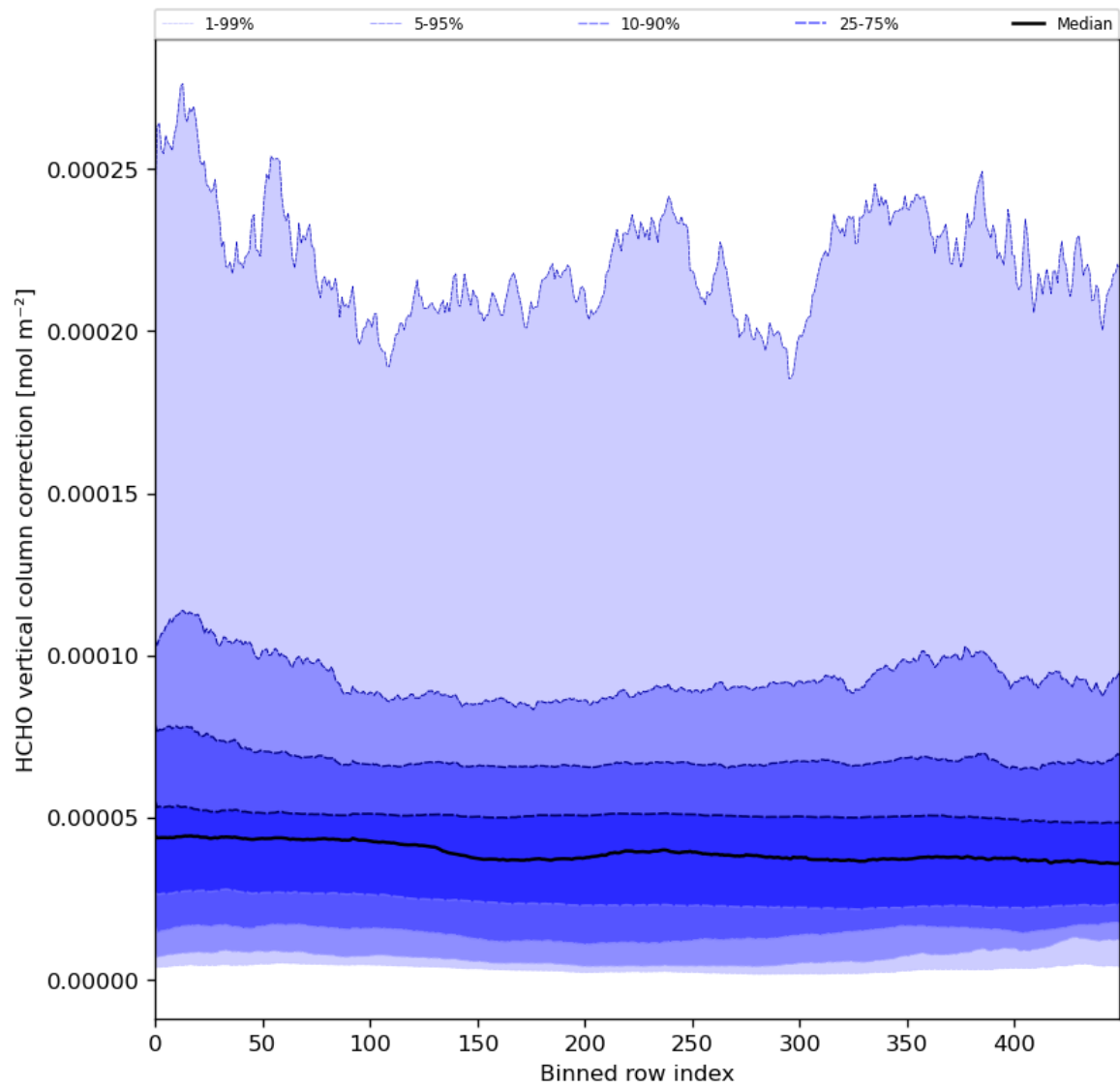
Figure 51: Along track statistics of “HCHO vertical column correction” for 2024-06-29 to 2024-07-01
