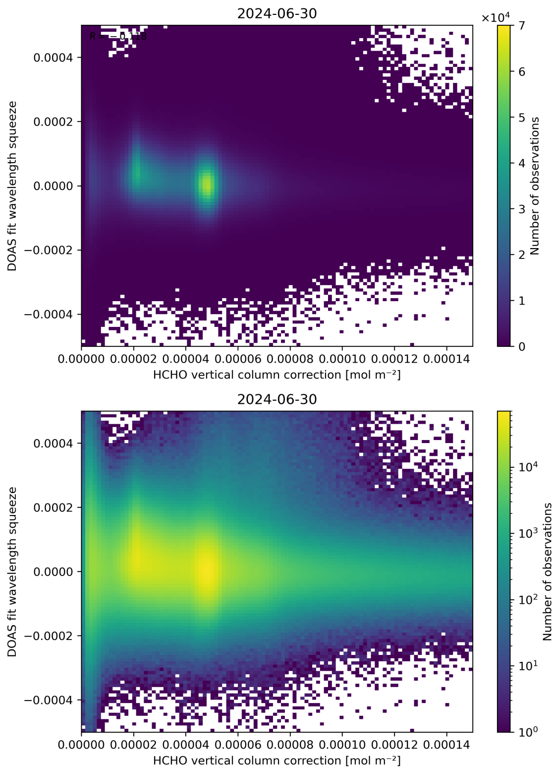
Figure 114: Scatter density plot of “HCHO vertical column correction” against “DOAS fit wavelength squeeze” for 2024-06-29 to 2024-07-01.
