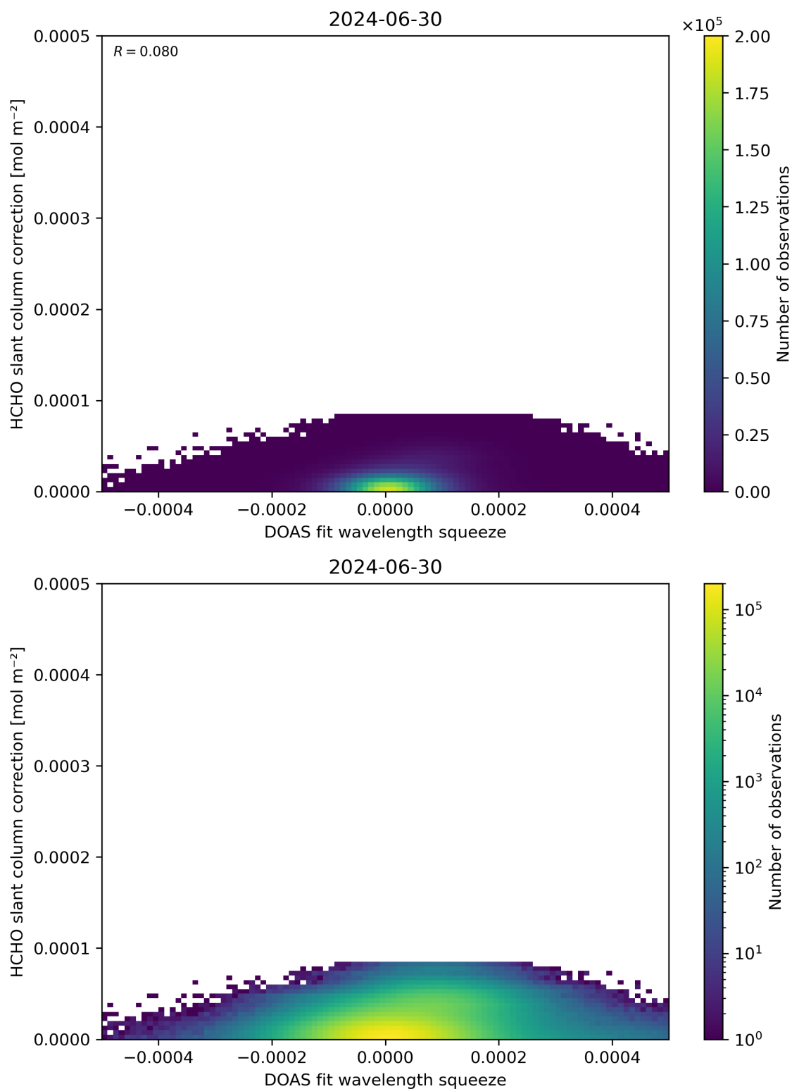
Figure 70: Scatter density plot of “DOAS fit wavelength squeeze” against “HCHO slant column correction” for 2024-06-29 to 2024-07-01.
