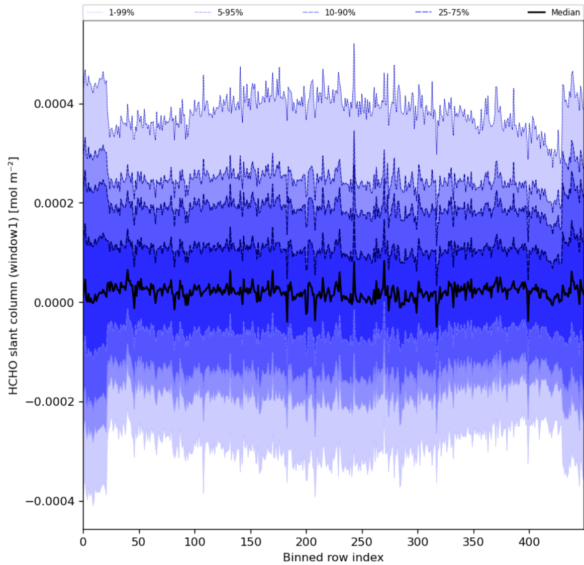
Figure 52: Along track statistics of “HCHO slant column (window1)” for 2024-06-29 to 2024-07-01
