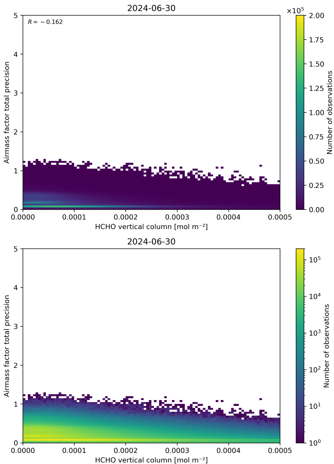
Figure 132: Scatter density plot of “HCHO vertical column” against “Airmass factor total precision” for 2024-06-29 to 2024-07-01.
