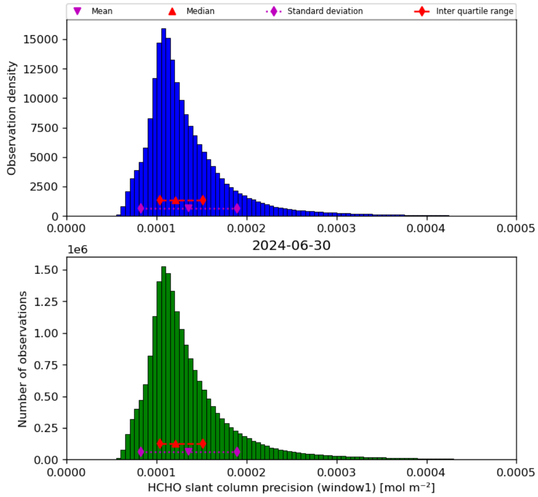
Figure 39: Histogram of “HCHO slant column precision (window1)” for 2024-06-29 to 2024-07-01
