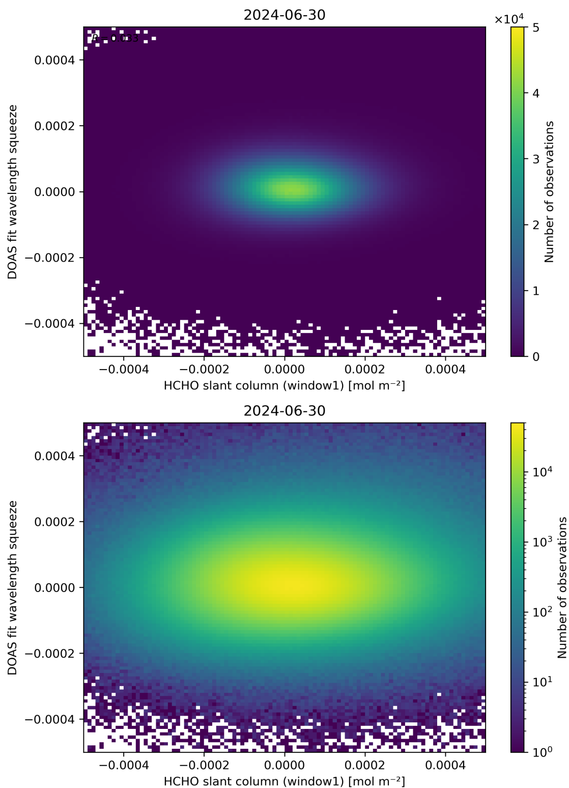
Figure 80: Scatter density plot of “HCHO slant column (window1)” against “DOAS fit wavelength squeeze” for 2024-06-29 to 2024-07-01.
