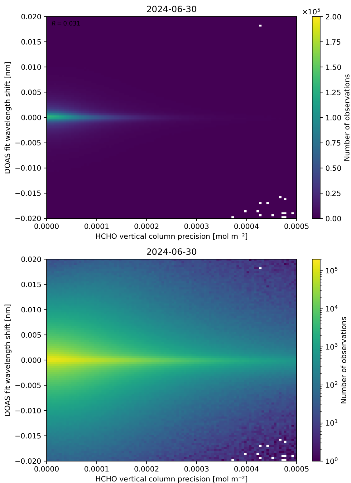
Figure 137: Scatter density plot of “HCHO vertical column precision” against “DOAS fit wavelength shift” for 2024-06-29 to 2024-07-01.
