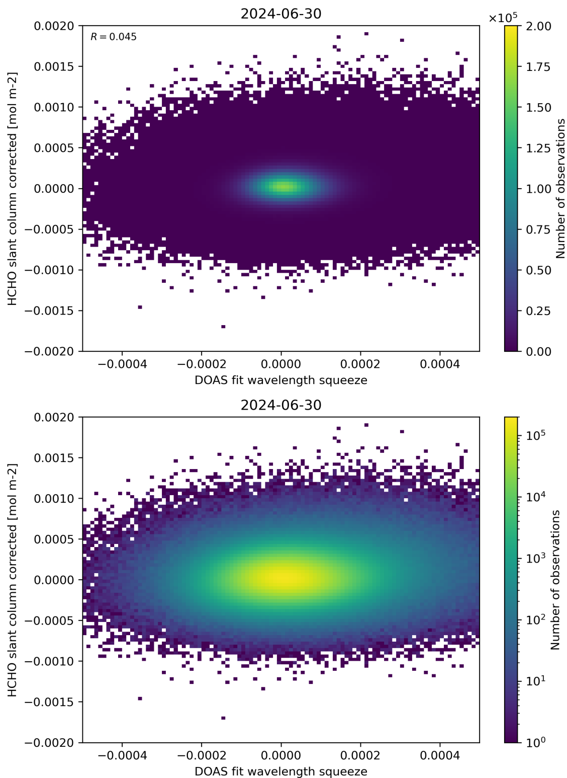
Figure 69: Scatter density plot of “DOAS fit wavelength squeeze” against “HCHO slant column corrected” for 2024-06-29 to 2024-07-01.
