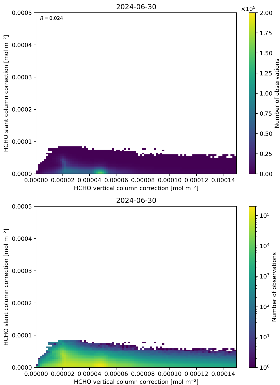
Figure 117: Scatter density plot of “HCHO vertical column correction” against “HCHO slant column correction” for 2024-06-29 to 2024-07-01.
