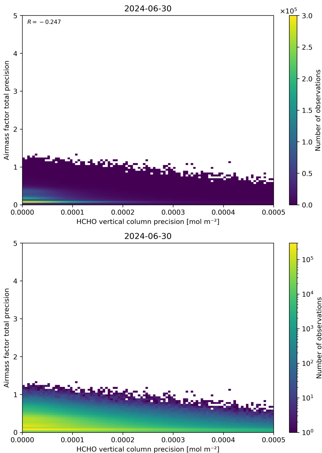
Figure 145: Scatter density plot of “HCHO vertical column precision” against “Airmass factor total precision” for 2024-06-29 to 2024-07-01.
