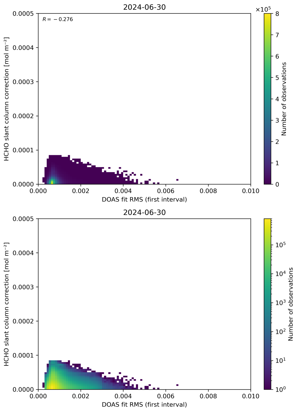
Figure 63: Scatter density plot of “DOAS fit RMS (first interval)” against “HCHO slant column correction” for 2024-06-29 to 2024-07-01.
