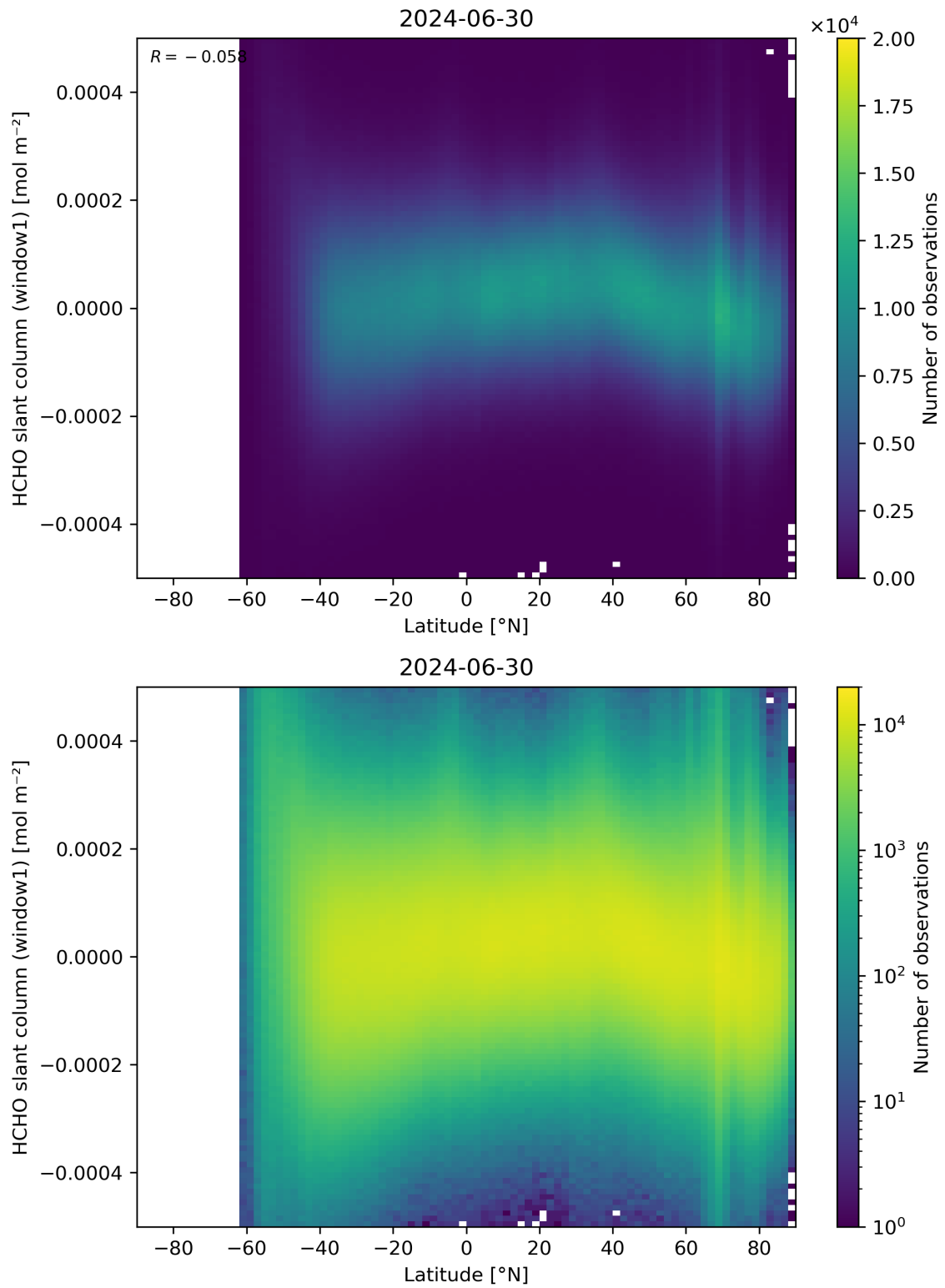
Figure 159: Scatter density plot of “Latitude” against “HCHO slant column (window1)” for 2024-06-29 to 2024-07-01.
