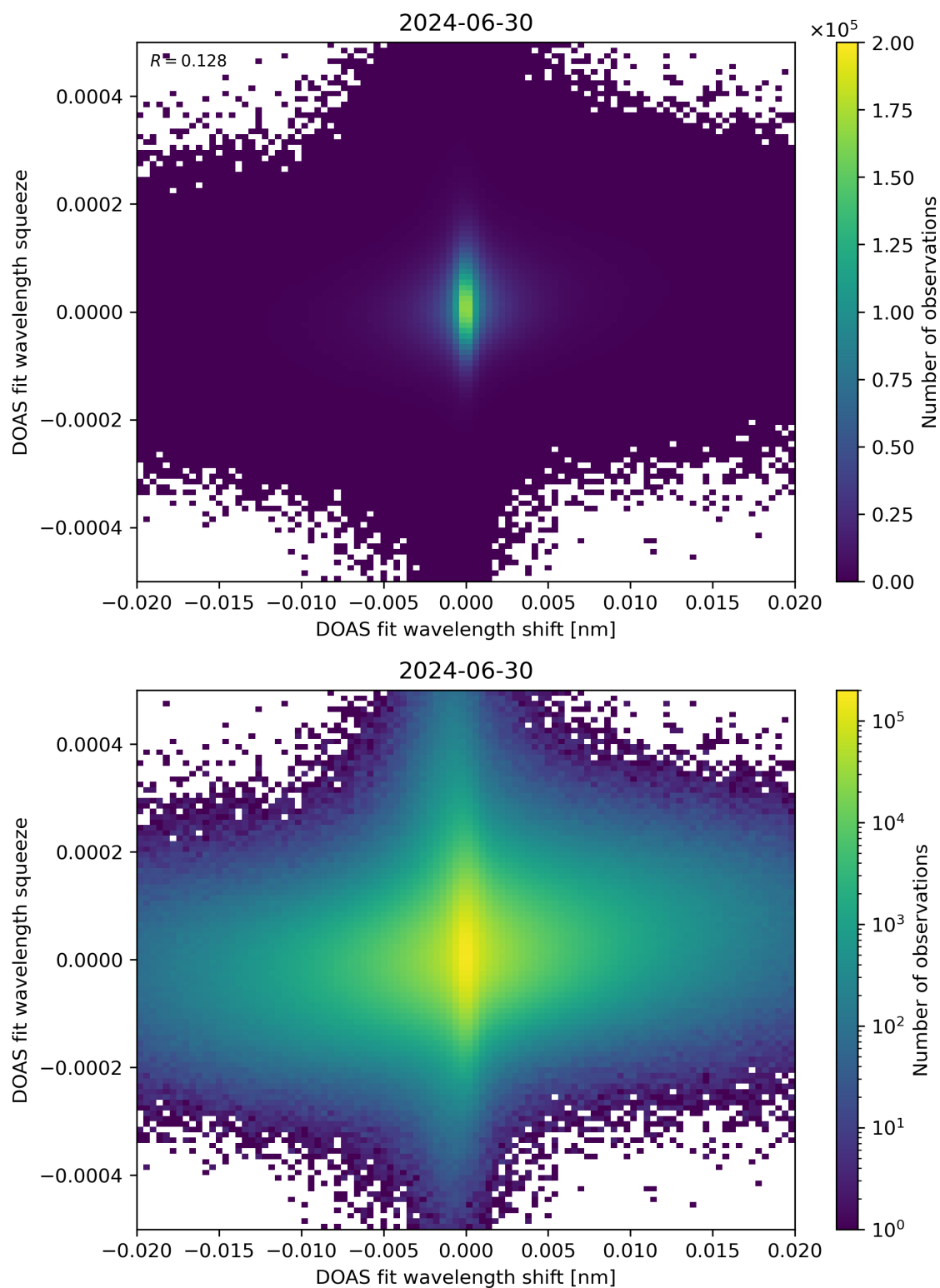
Figure 65: Scatter density plot of “DOAS fit wavelength shift” against “DOAS fit wavelength squeeze” for 2024-06-29 to 2024-07-01.
