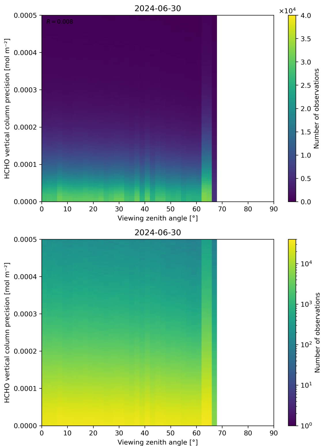
Figure 194: Scatter density plot of “Viewing zenith angle” against “HCHO vertical column precision” for 2024-06-29 to 2024-07-01.
