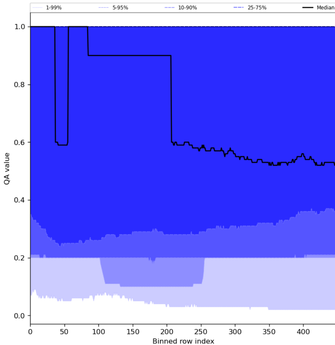
Figure 48: Along track statistics of “QA value” for 2024-06-29 to 2024-07-01
