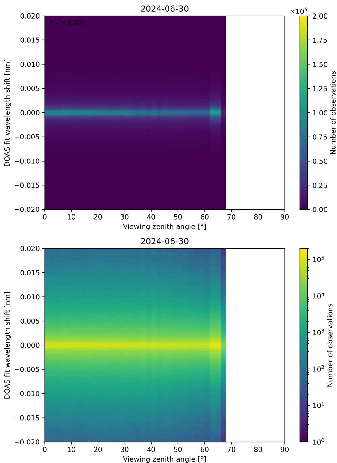
Figure 183: Scatter density plot of “Viewing zenith angle” against “DOAS fit wavelength shift” for 2024-06-29 to 2024-07-01.
