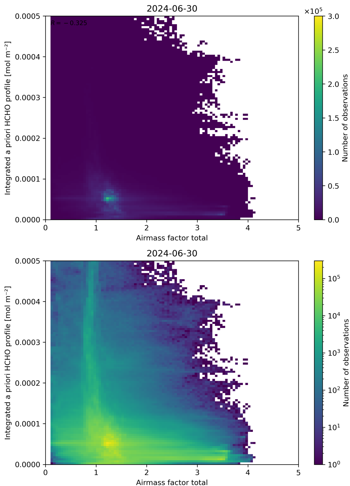
Figure 104: Scatter density plot of “Air mass factor total” against “Integrated a priori HCHO profile” for 2024-06-29 to 2024-07-01.
