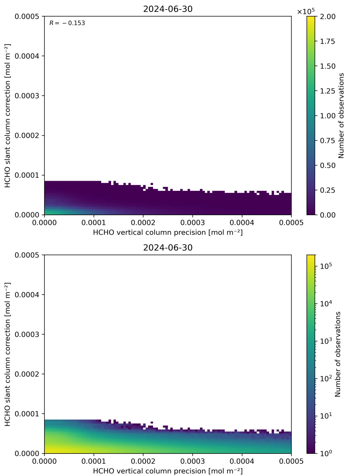
Figure 141: Scatter density plot of “HCHO vertical column precision” against “HCHO slant column correction” for 2024-06-29 to 2024-07-01.
