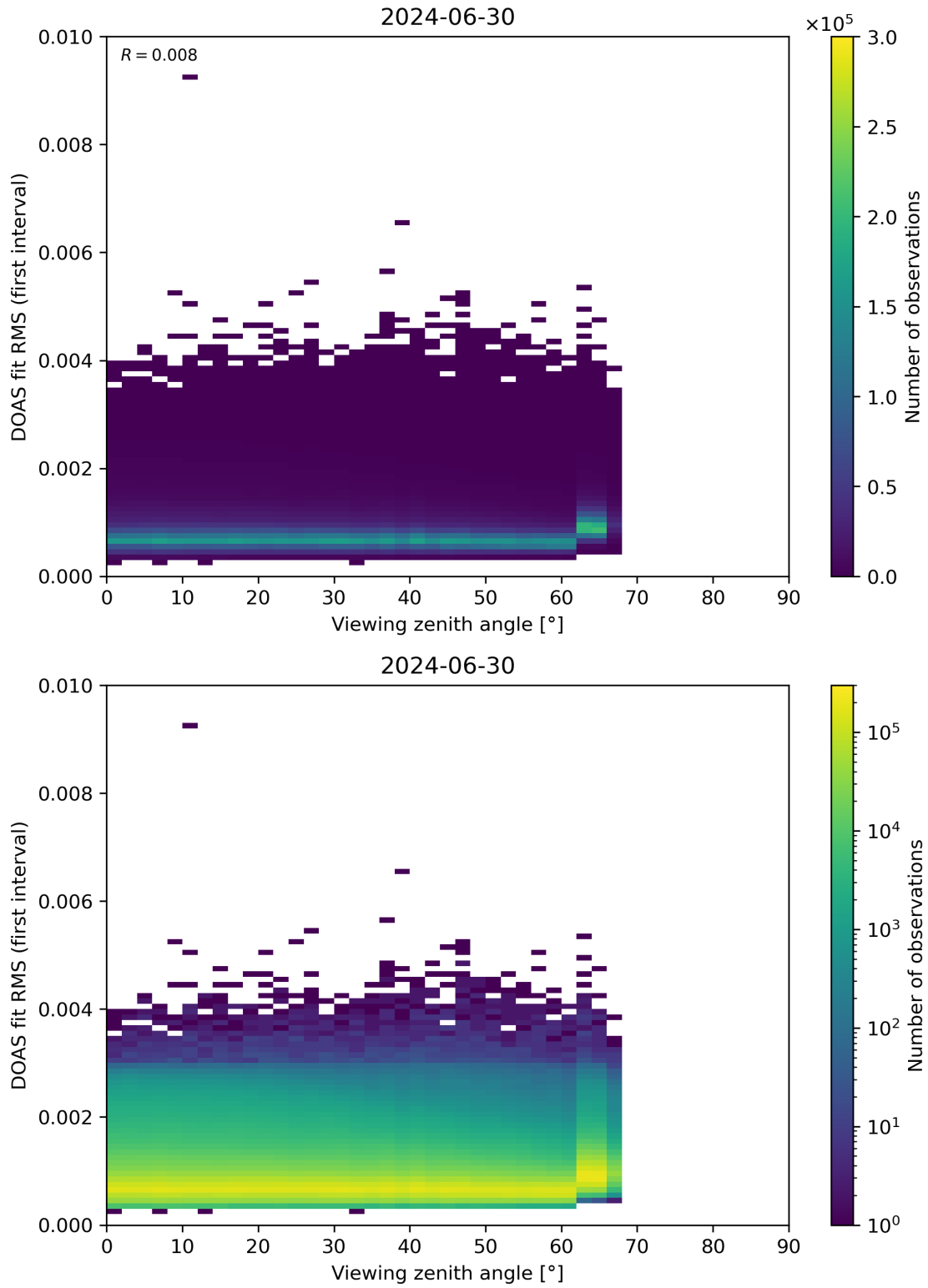
Figure 182: Scatter density plot of “Viewing zenith angle” against “DOAS fit RMS (first interval)” for 2024-06-29 to 2024-07-01.
