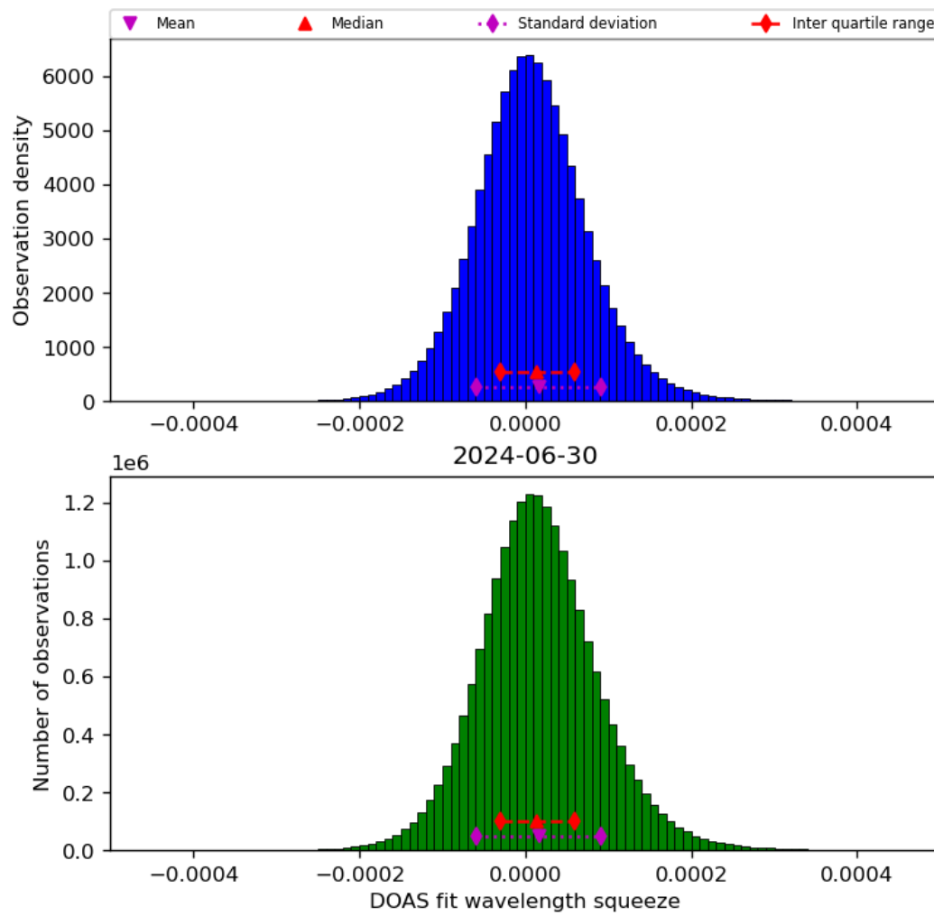
Figure 45: Histogram of “DOAS fit wavelength squeeze” for 2024-06-29 to 2024-07-01
