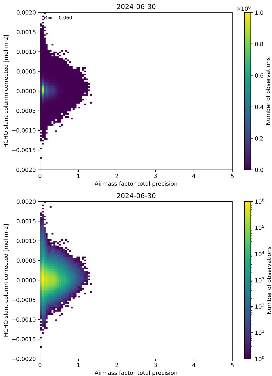
Figure 109: Scatter density plot of “Airmass factor total precision” against “HCHO slant column corrected” for 2024-06-29 to 2024-07-01.
