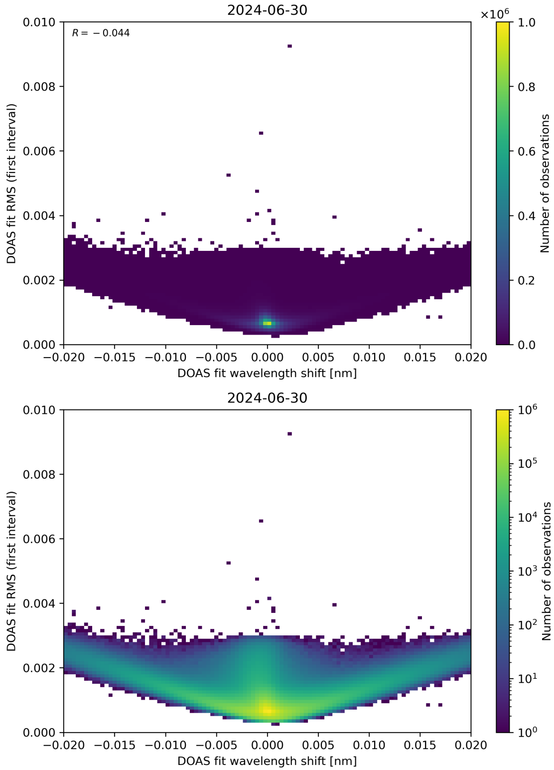
Figure 64: Scatter density plot of “DOAS fit wavelength shift” against “DOAS fit RMS (first interval)” for 2024-06-29 to 2024-07-01.
