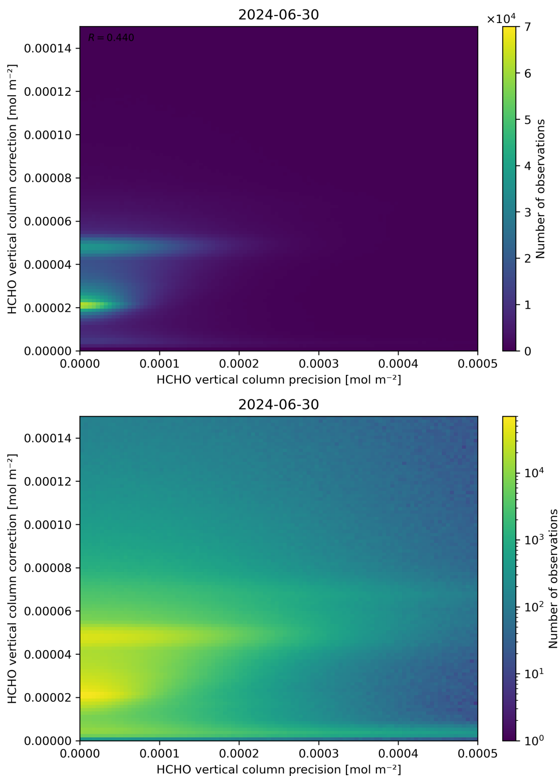
Figure 146: Scatter density plot of “HCHO vertical column precision” against “HCHO vertical column correction” for 2024-06-29 to 2024-07-01.
