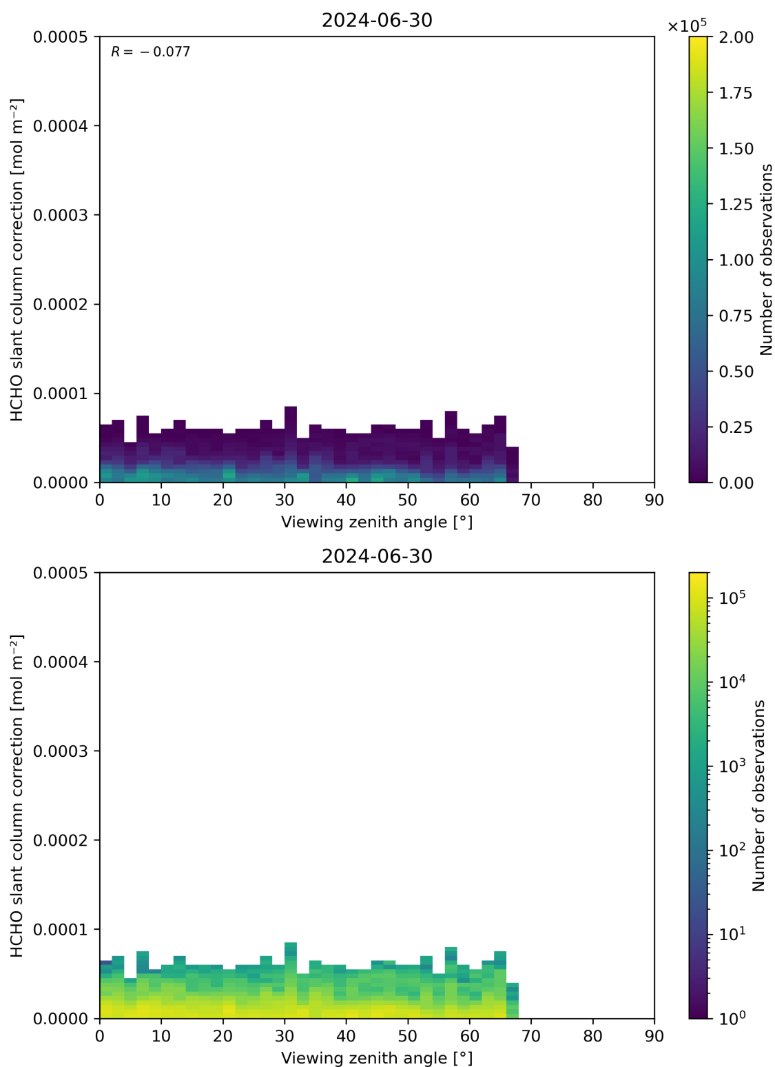
Figure 187: Scatter density plot of “Viewing zenith angle” against “HCHO slant column correction” for 2024-06-29 to 2024-07-01.
