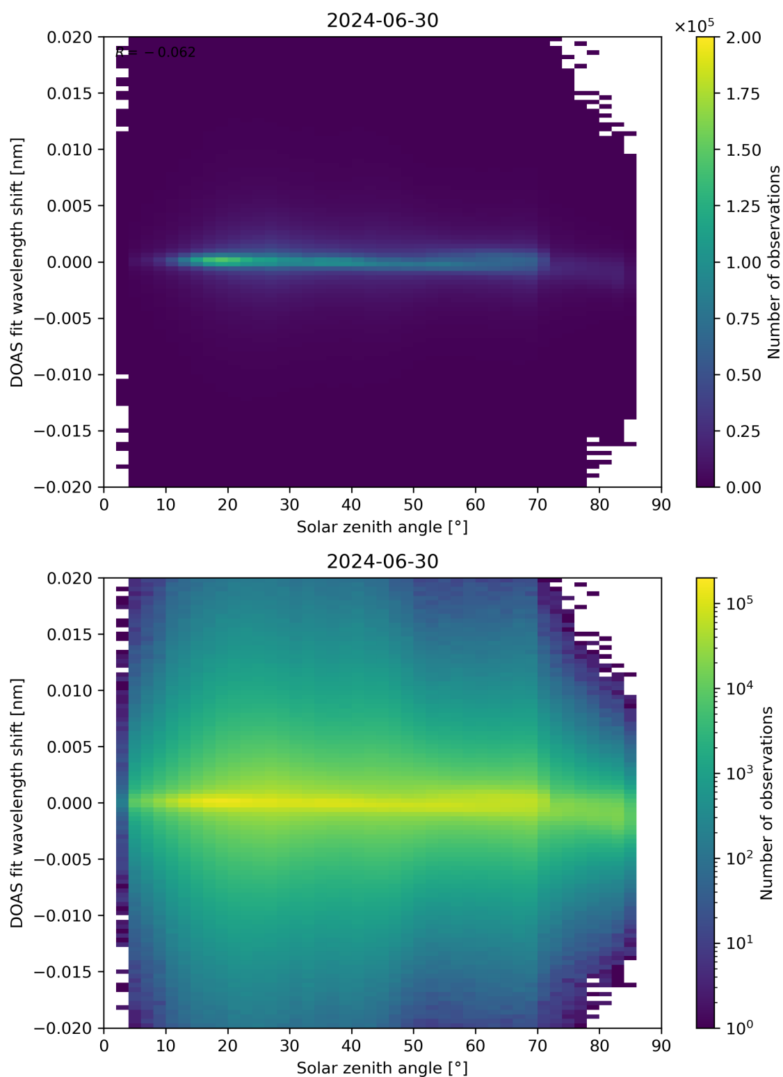
Figure 168: Scatter density plot of “Solar zenith angle” against “DOAS fit wavelength shift” for 2024-06-29 to 2024-07-01.
