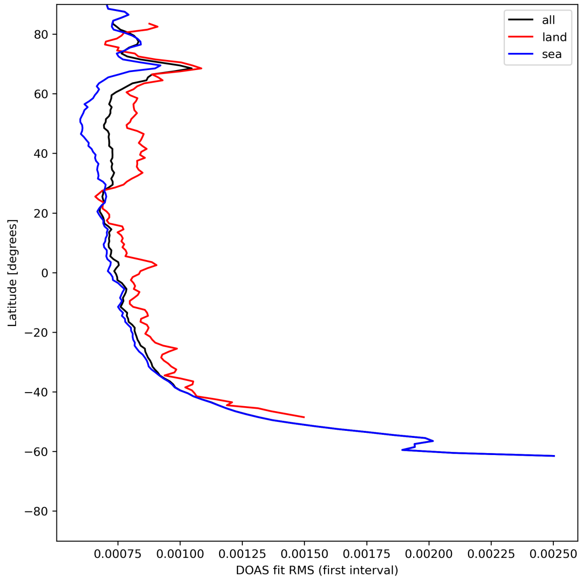
Figure 32: Zonal average of “DOAS fit RMS (first interval)” for 2024-06-29 to 2024-07-01.
