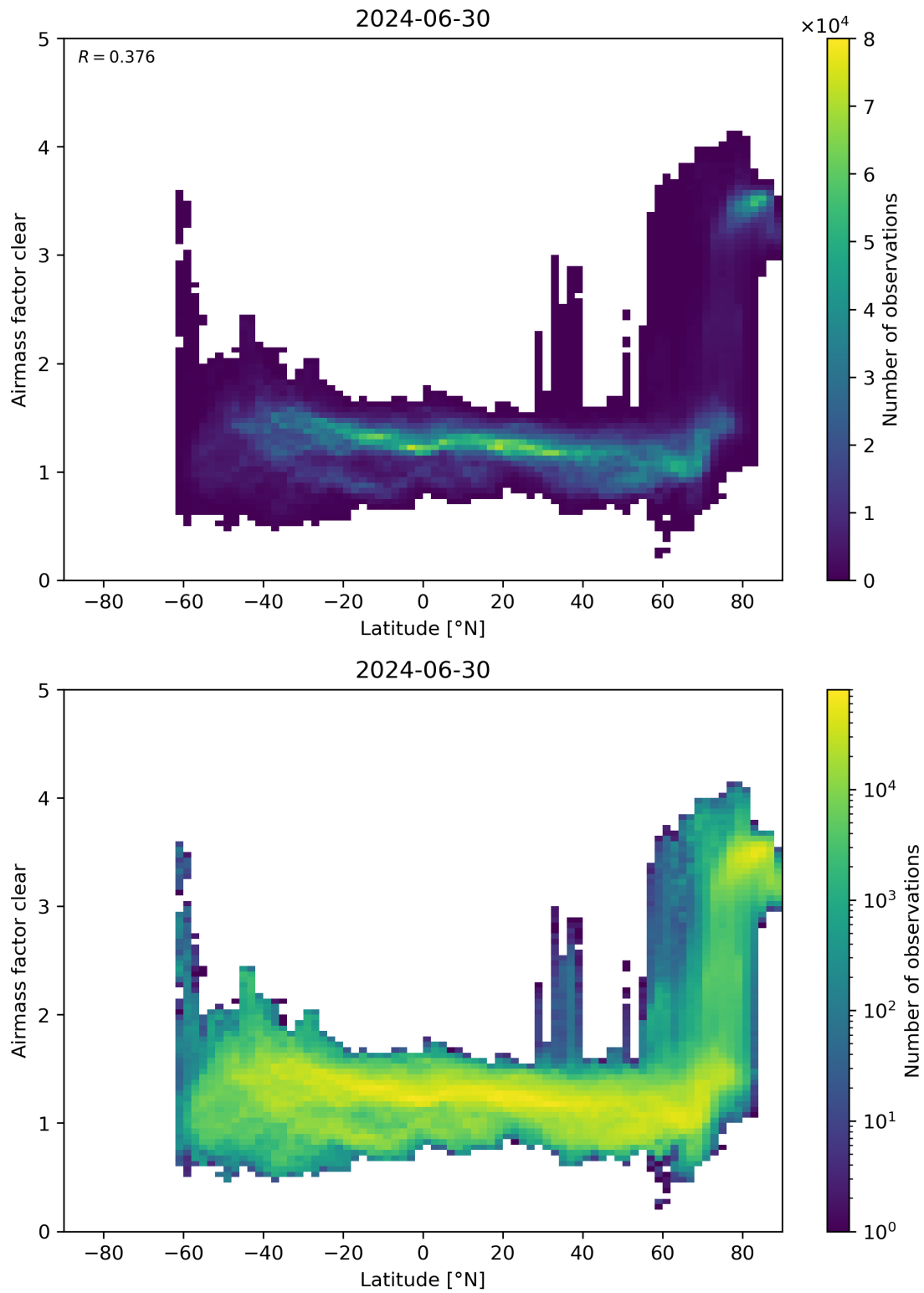
Figure 156: Scatter density plot of “Latitude” against “Airmass factor clear” for 2024-06-29 to 2024-07-01.
