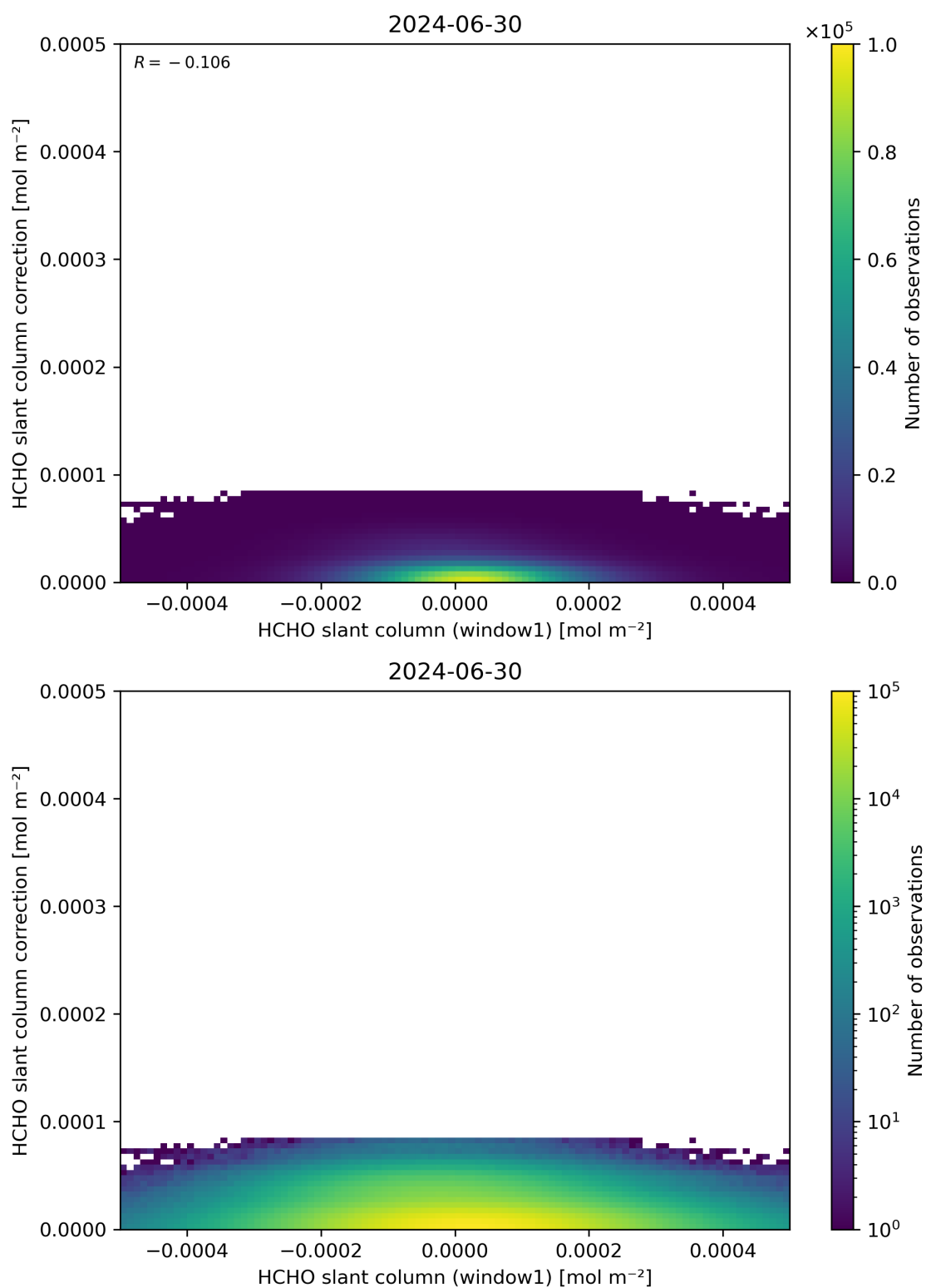
Figure 83: Scatter density plot of “HCHO slant column (window1)” against “HCHO slant column correction” for 2024-06-29 to 2024-07-01.
