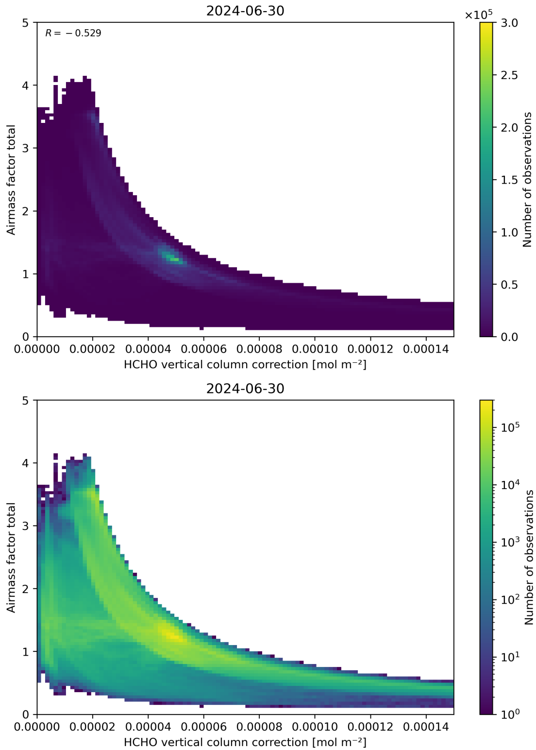
Figure 120: Scatter density plot of “HCHO vertical column correction” against “Airmass factor total” for 2024-06-29 to 2024-07-01.
