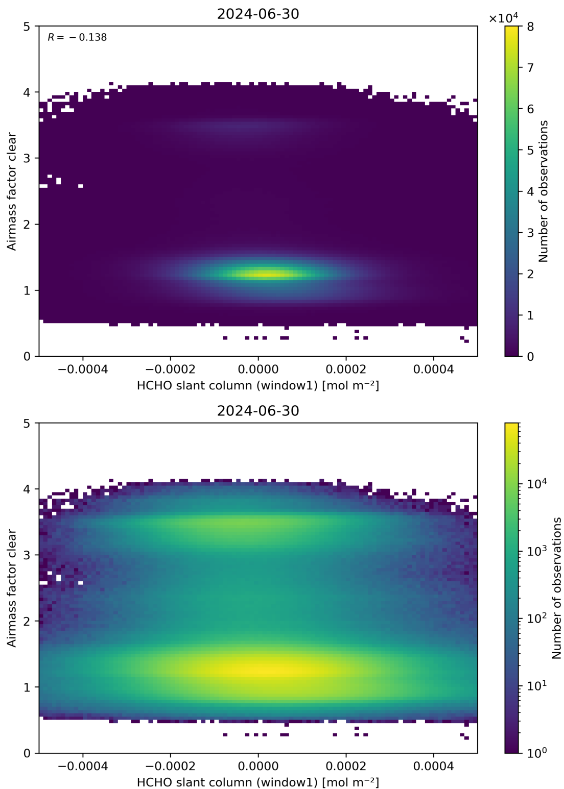
Figure 81: Scatter density plot of “HCHO slant column (window1)” against “Airmass factor clear” for 2024-06-29 to 2024-07-01.
