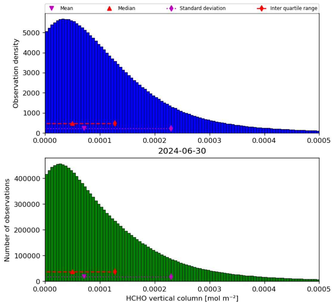
Figure 35: Histogram of “HCHO vertical column” for 2024-06-29 to 2024-07-01
