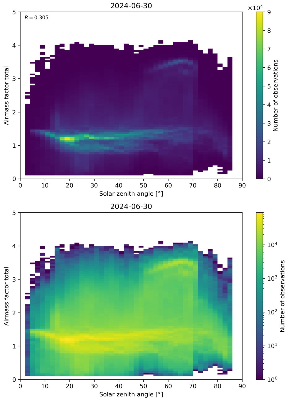
Figure 175: Scatter density plot of “Solar zenith angle” against “Airmass factor total” for 2024-06-29 to 2024-07-01.
