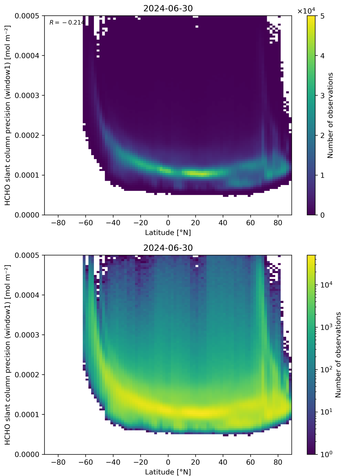
Figure 160: Scatter density plot of “Latitude” against “HCHO slant column precision (window1)” for 2024-06-29 to 2024-07-01.
