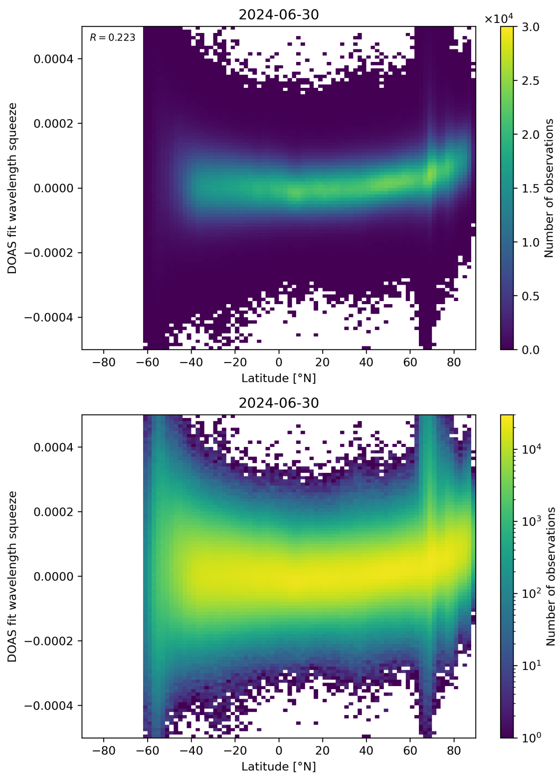
Figure 155: Scatter density plot of “Latitude” against “DOAS fit wavelength squeeze” for 2024-06-29 to 2024-07-01.
