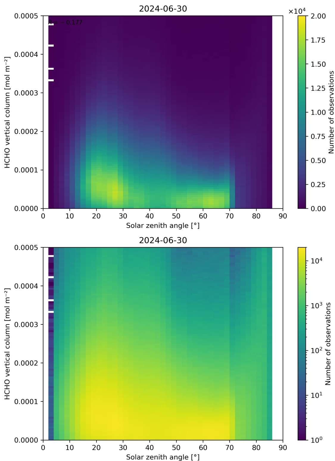
Figure 177: Scatter density plot of “Solar zenith angle” against “HCHO vertical column” for 2024-06-29 to 2024-07-01.
