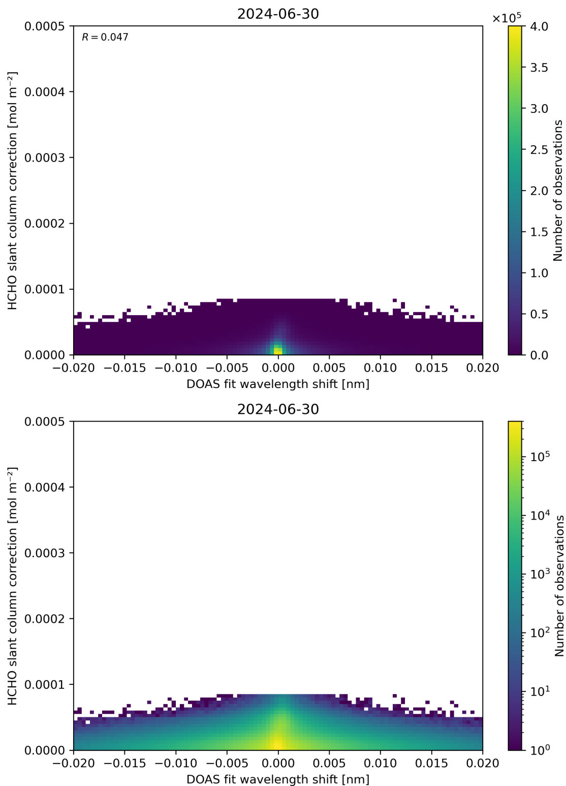
Figure 67: Scatter density plot of “DOAS fit wavelength shift” against “HCHO slant column correction” for 2024-06-29 to 2024-07-01.
