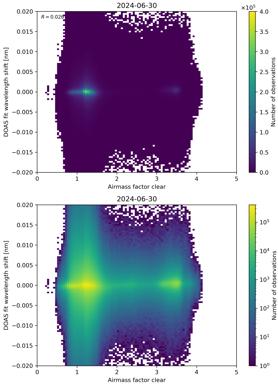
Figure 72: Scatter density plot of “Airmass factor clear” against “DOAS fit wavelength shift” for 2024-06-29 to 2024-07-01.
