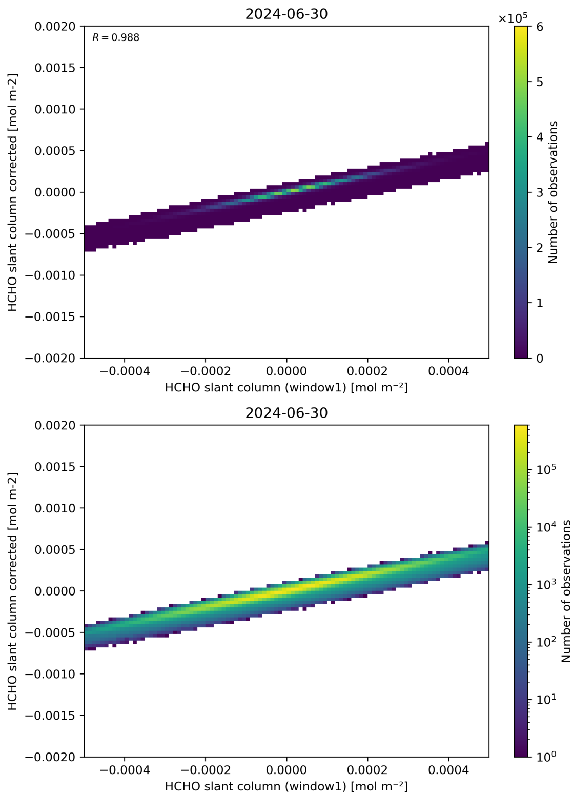
Figure 82: Scatter density plot of “HCHO slant column (window1)” against “HCHO slant column corrected” for 2024-06-29 to 2024-07-01.
