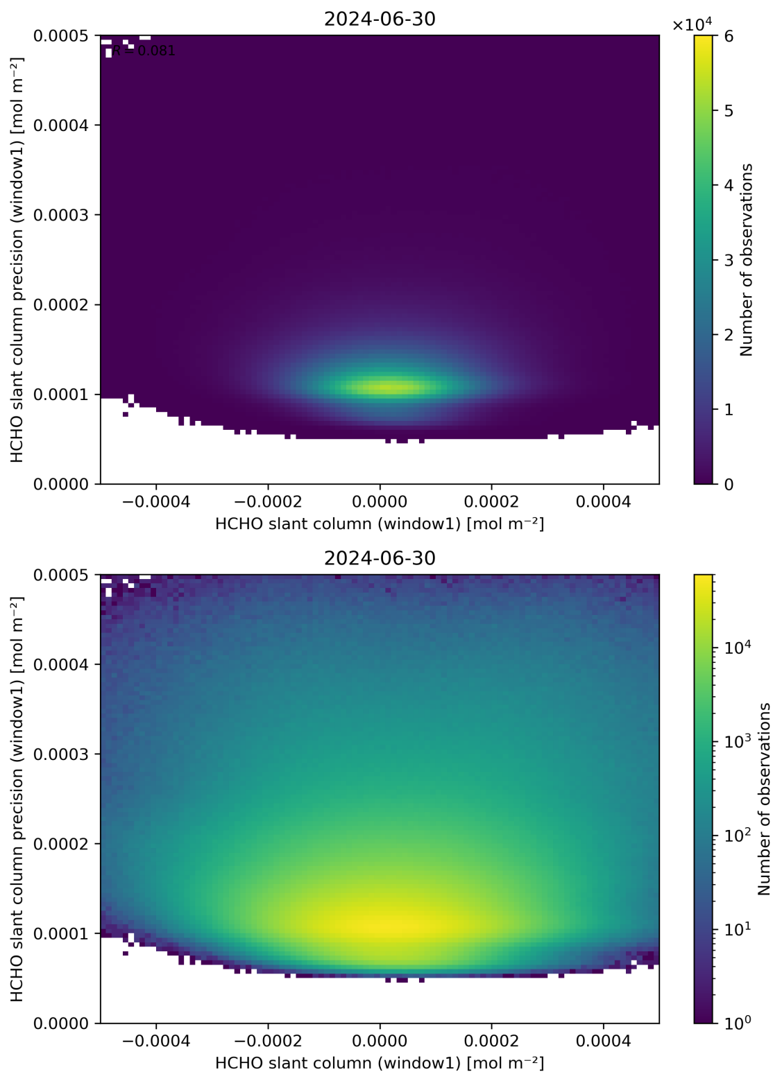
Figure 84: Scatter density plot of “HCHO slant column (window1)” against “HCHO slant column precision (window1)” for 2024-06-29 to 2024-07-01.
