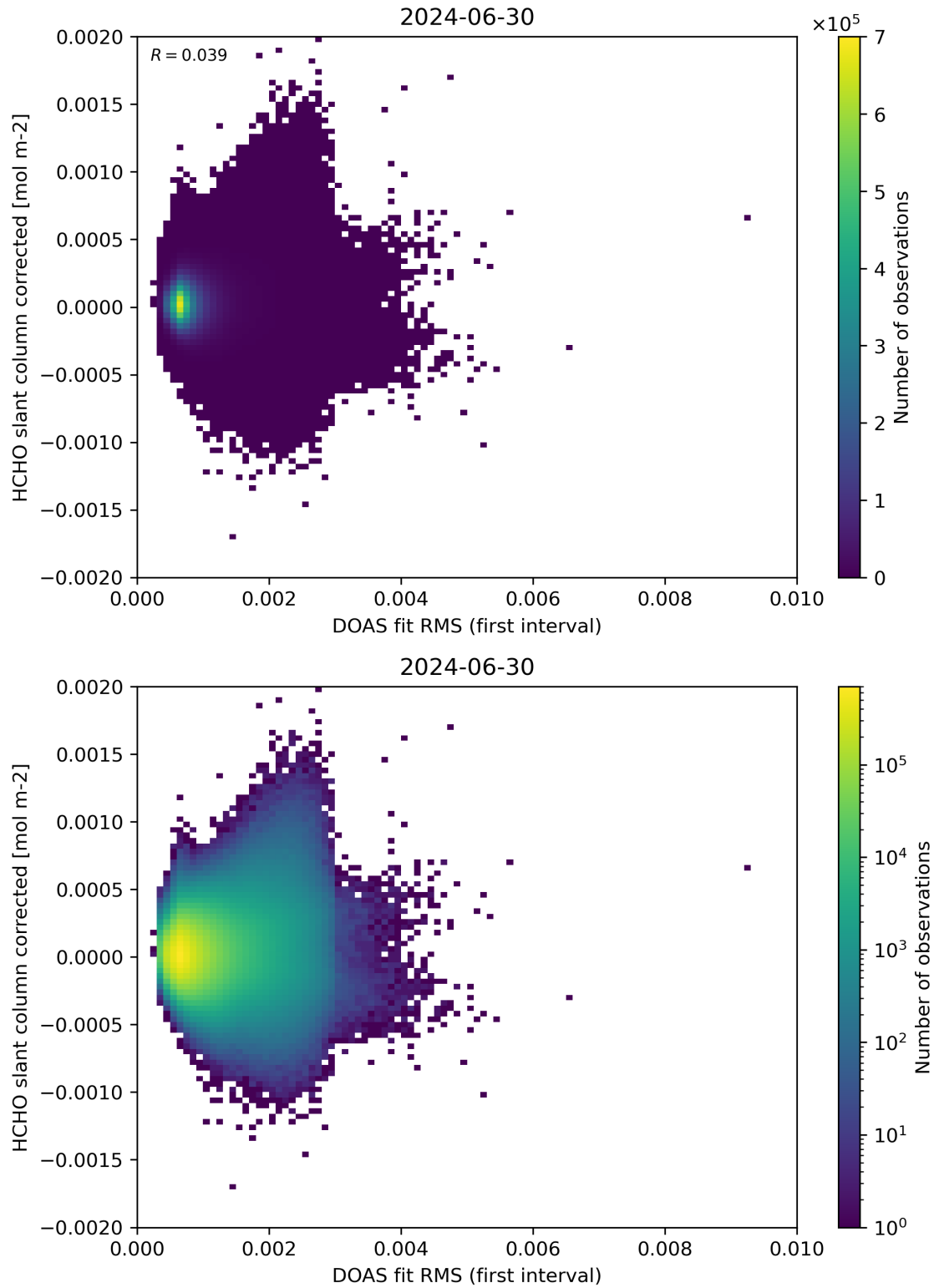
Figure 62: Scatter density plot of “DOAS fit RMS (first interval)” against “HCHO slant column corrected” for 2024-06-29 to 2024-07-01.
