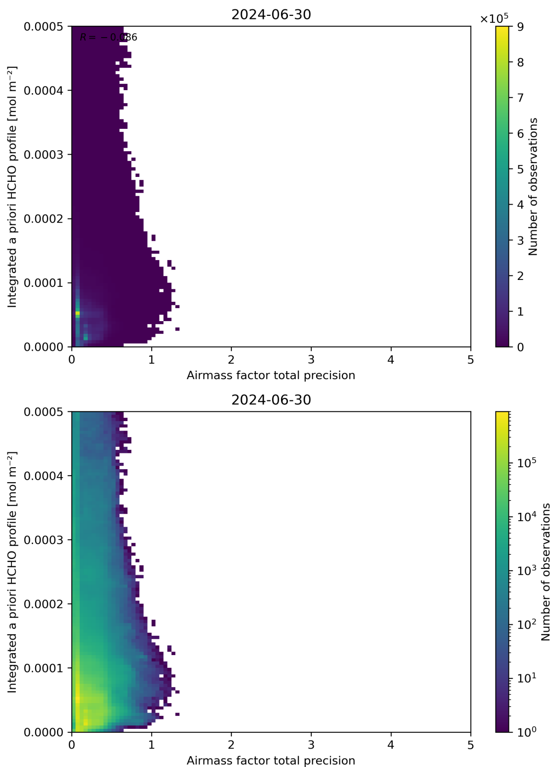
Figure 111: Scatter density plot of “Airmass factor total precision” against “Integrated a priori HCHO profile” for 2024-06-29 to 2024-07-01.
