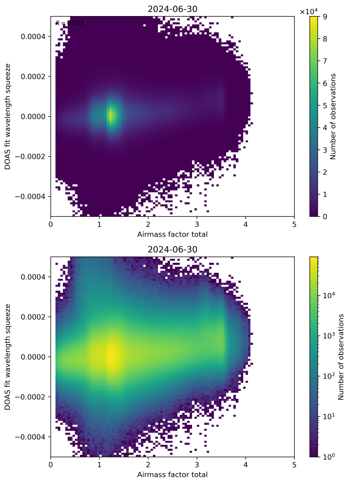
Figure 99: Scatter density plot of “Airmass factor total” against “DOAS fit wavelength squeeze” for 2024-06-29 to 2024-07-01.
