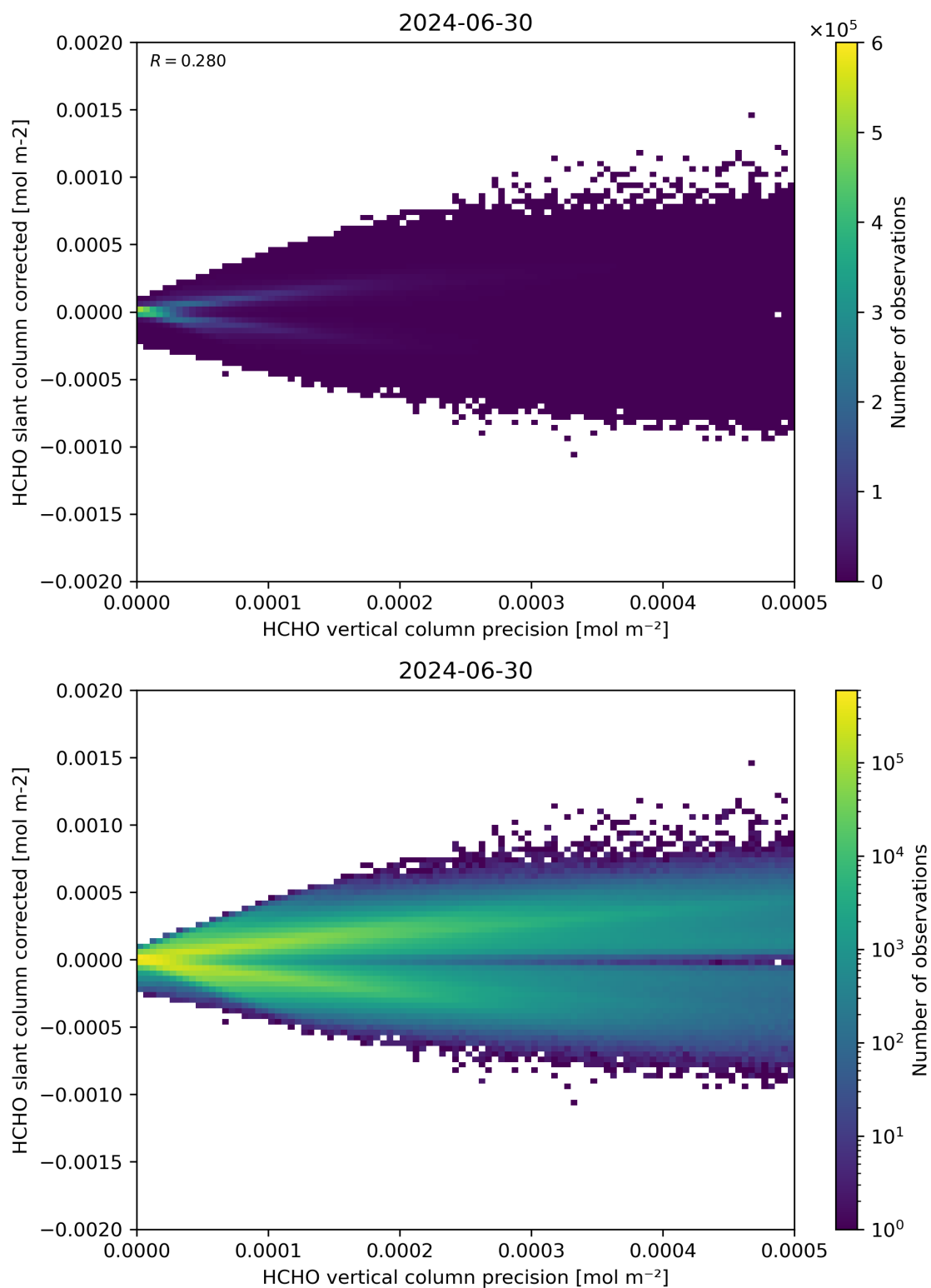
Figure 140: Scatter density plot of “HCHO vertical column precision” against “HCHO slant column corrected” for 2024-06-29 to 2024-07-01.
