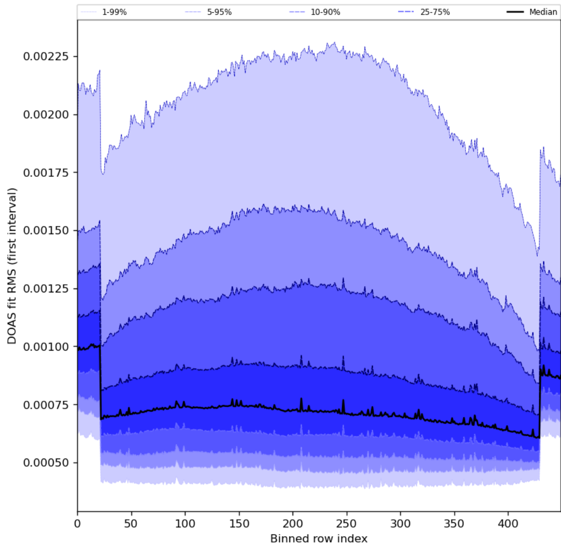
Figure 60: Along track statistics of “DOAS fit RMS (first interval)” for 2024-06-29 to 2024-07-01
