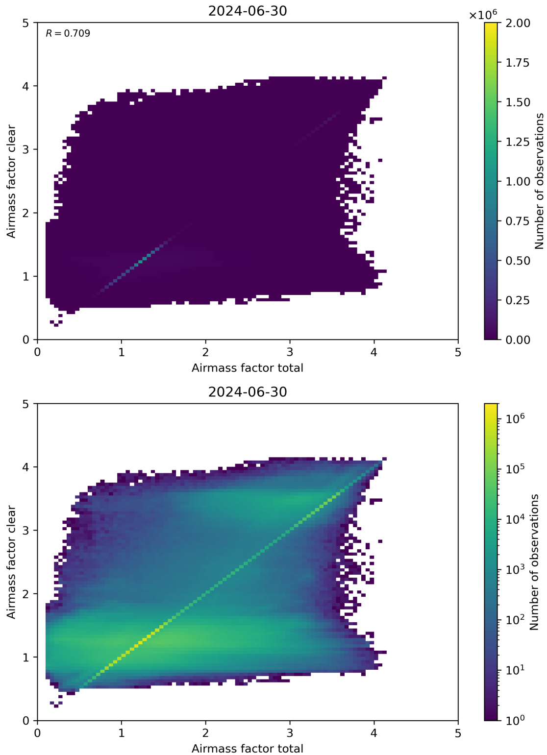
Figure 100: Scatter density plot of “Airmass factor total” against “Airmass factor clear” for 2024-06-29 to 2024-07-01.
