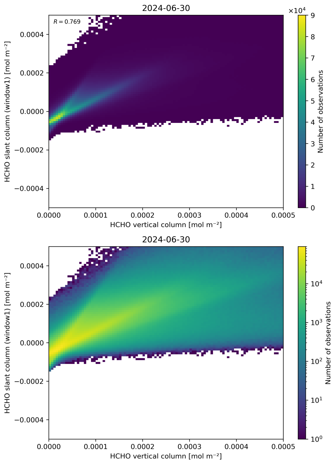
Figure 129: Scatter density plot of “HCHO vertical column” against “HCHO slant column (window1)” for 2024-06-29 to 2024-07-01.
