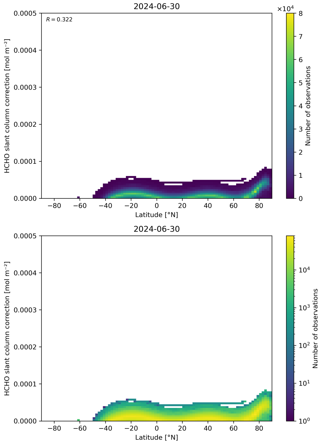
Figure 158: Scatter density plot of “Latitude” against “HCHO slant column correction” for 2024-06-29 to 2024-07-01.
