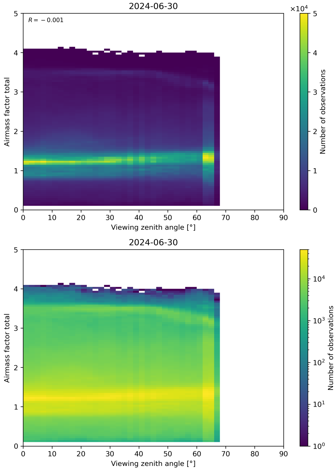
Figure 190: Scatter density plot of “Viewing zenith angle” against “Airmass factor total” for 2024-06-29 to 2024-07-01.
