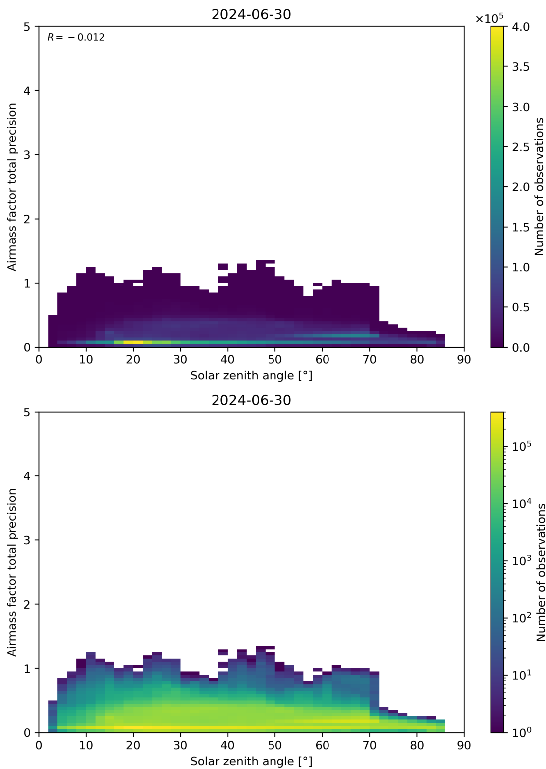
Figure 176: Scatter density plot of “Solar zenith angle” against “Airmass factor total precision” for 2024-06-29 to 2024-07-01.
