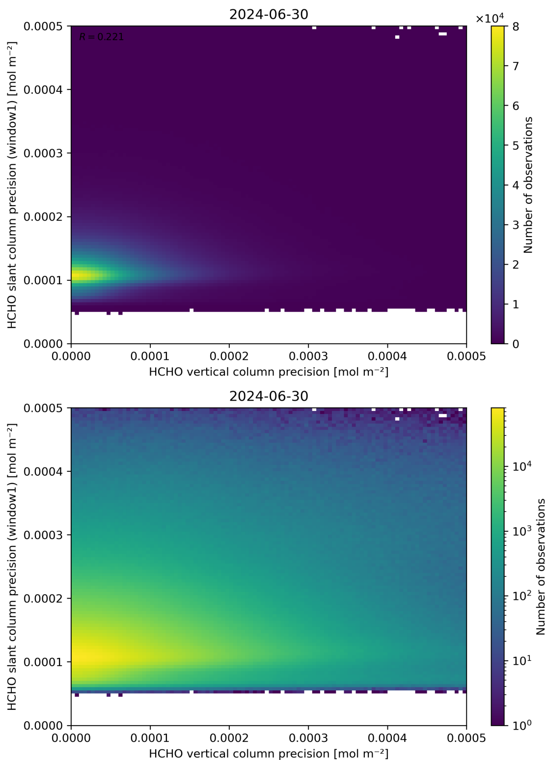
Figure 143: Scatter density plot of “HCHO vertical column precision” against “HCHO slant column precision (window1)” for 2024-06-29 to 2024-07-01.
