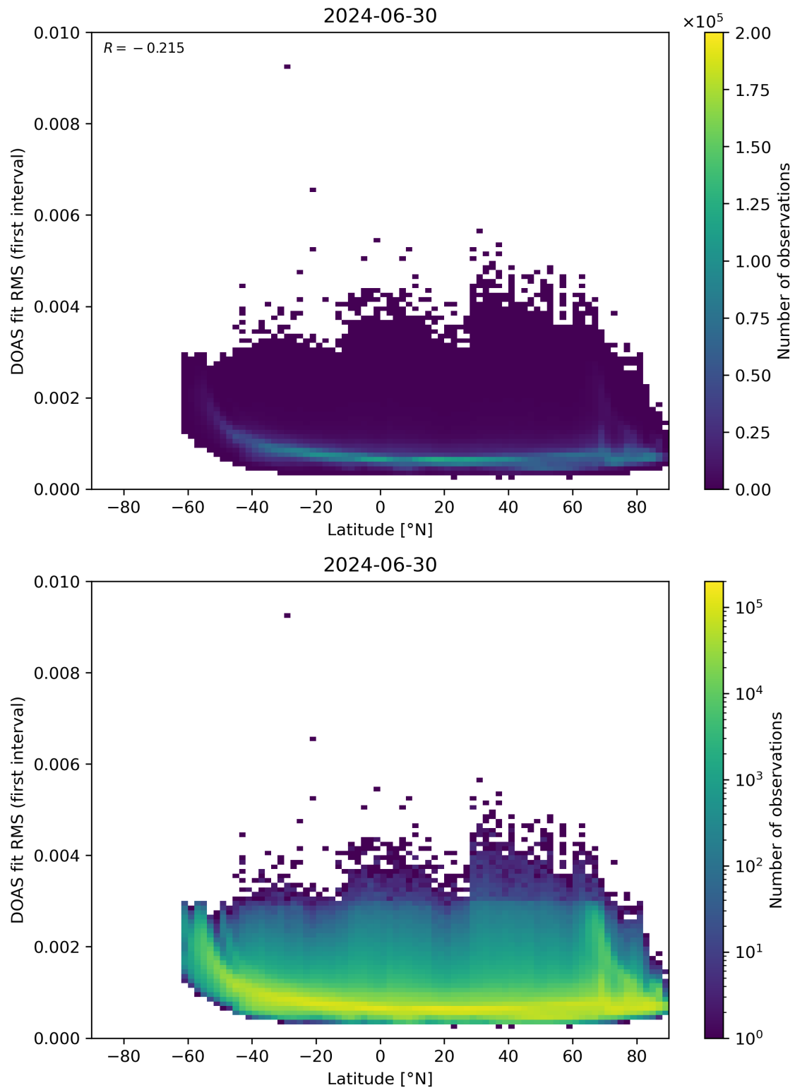
Figure 153: Scatter density plot of “Latitude” against “DOAS fit RMS (first interval)” for 2024-06-29 to 2024-07-01.
