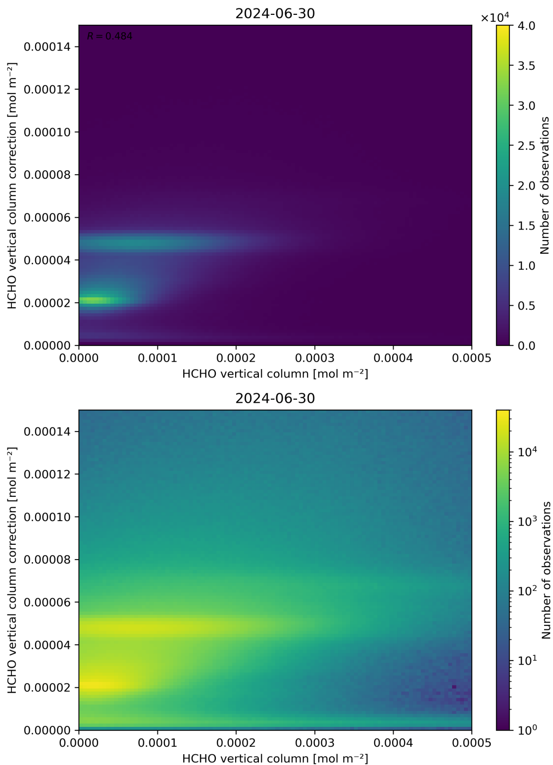
Figure 133: Scatter density plot of “HCHO vertical column” against “HCHO vertical column correction” for 2024-06-29 to 2024-07-01.
