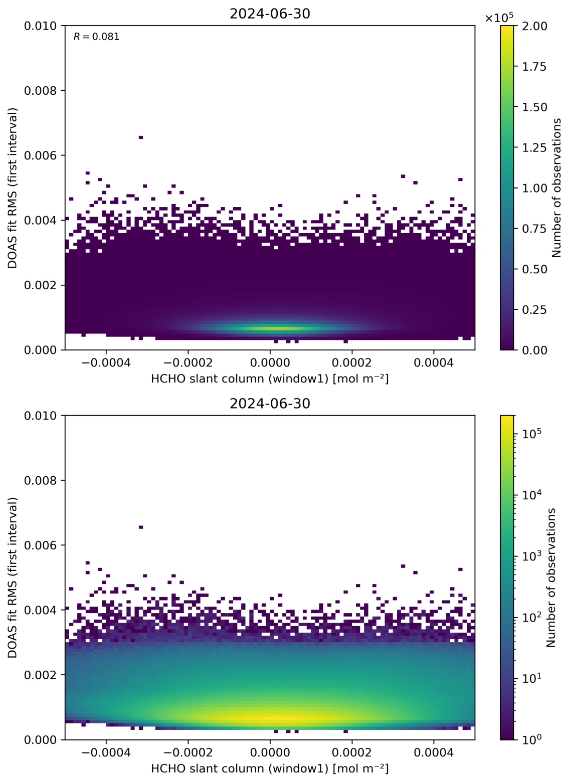
Figure 78: Scatter density plot of “HCHO slant column (window1)” against “DOAS fit RMS (first interval)” for 2024-06-29 to 2024-07-01.
