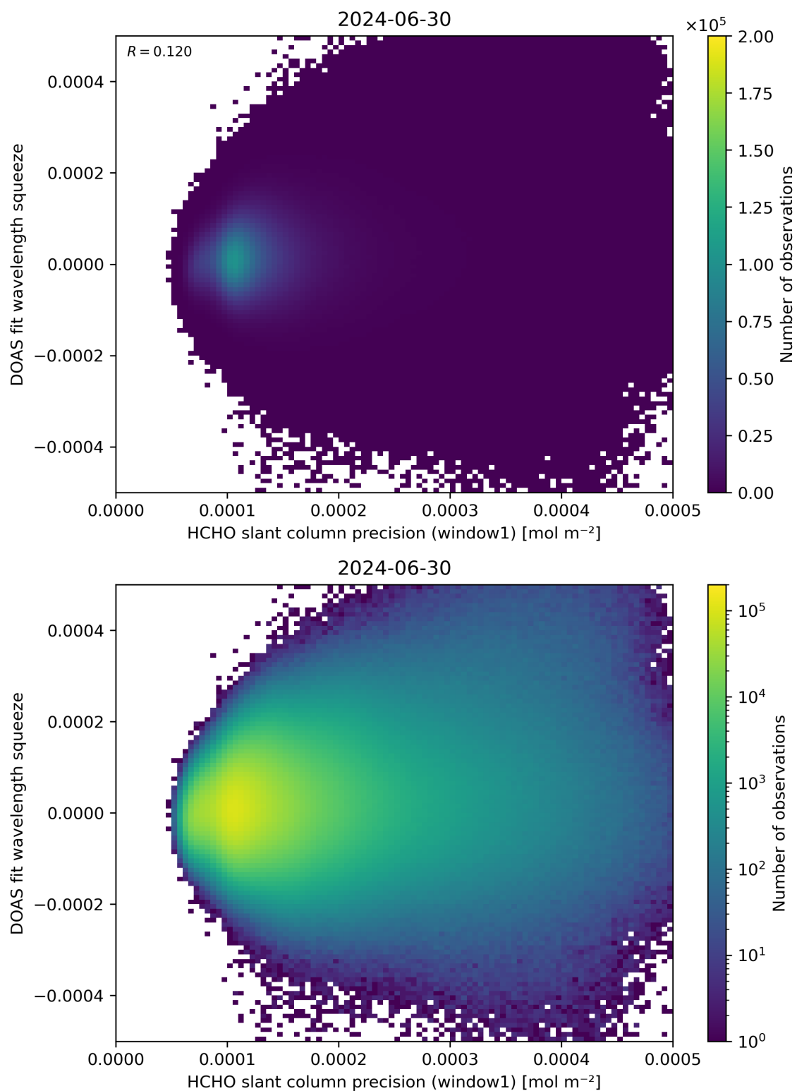
Figure 90: Scatter density plot of “HCHO slant column precision (window1)” against “DOAS fit wavelength squeeze” for 2024-06-29 to 2024-07-01.
