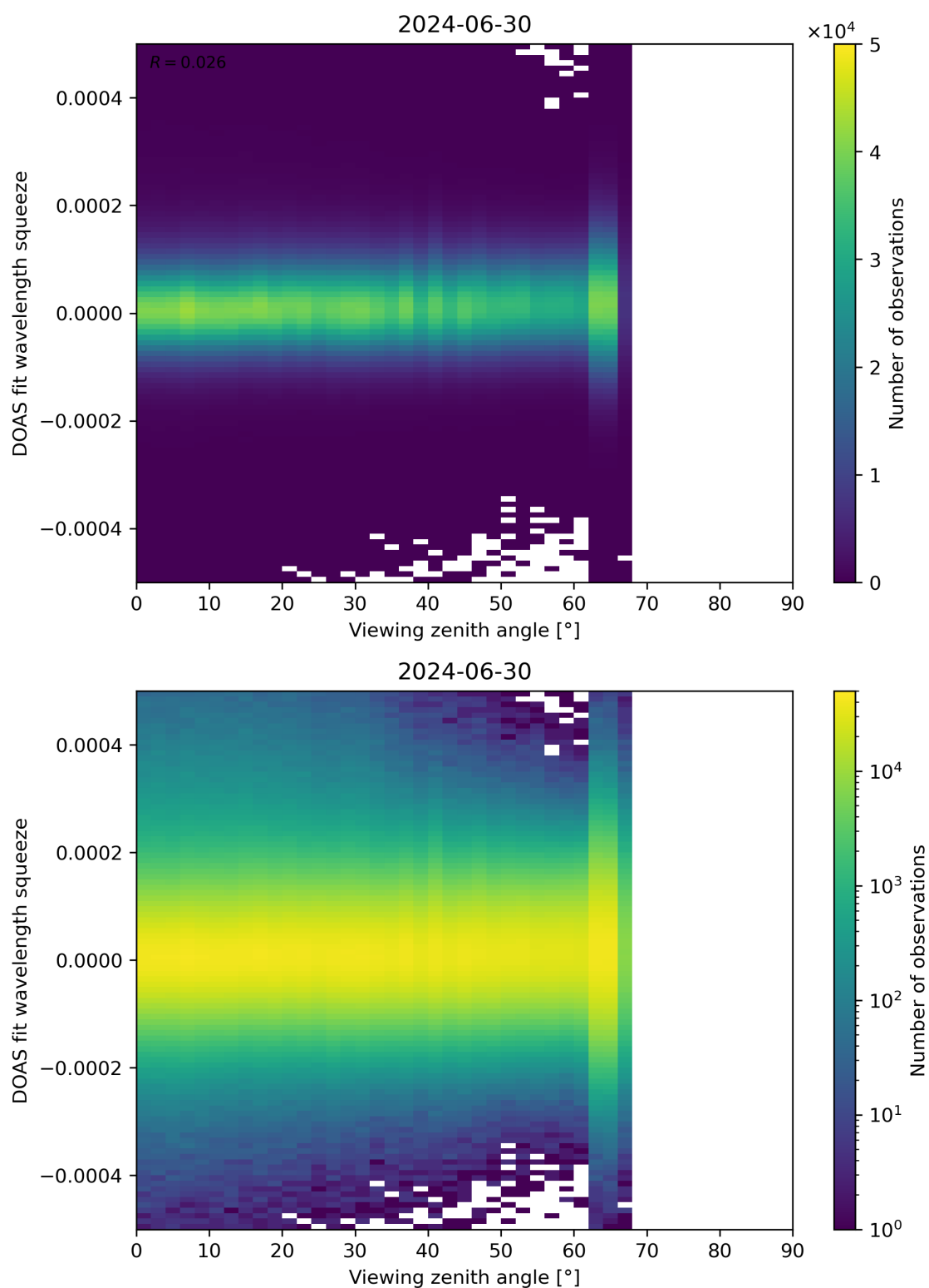
Figure 184: Scatter density plot of “Viewing zenith angle” against “DOAS fit wavelength squeeze” for 2024-06-29 to 2024-07-01.
