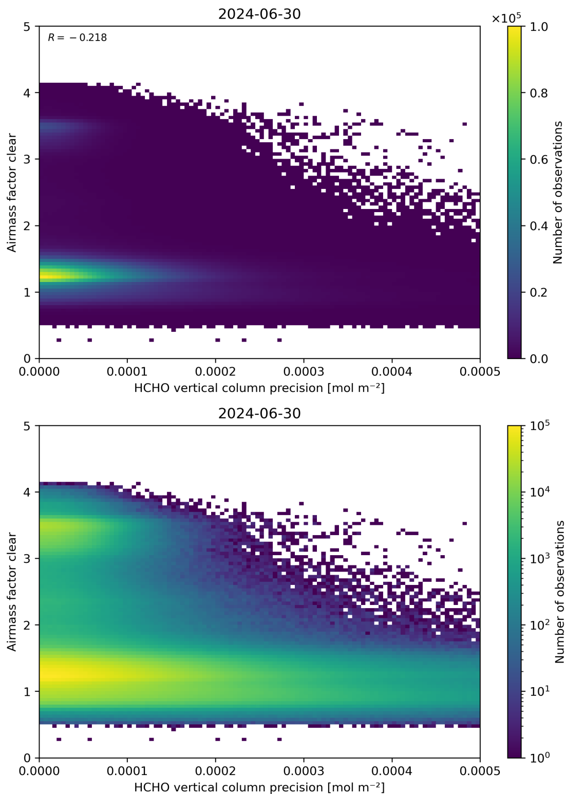
Figure 139: Scatter density plot of “HCHO vertical column precision” against “Airmass factor clear” for 2024-06-29 to 2024-07-01.
