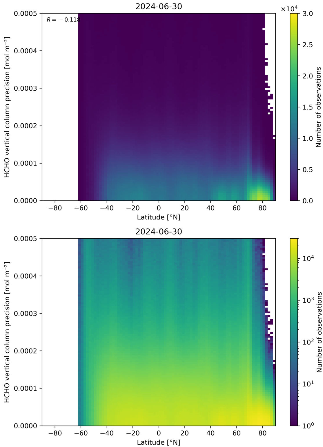
Figure 165: Scatter density plot of “Latitude” against “HCHO vertical column precision” for 2024-06-29 to 2024-07-01.
