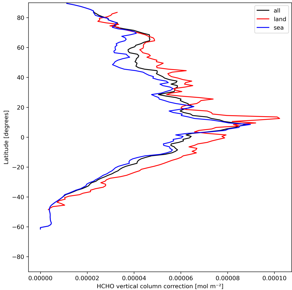
Figure 23: Zonal average of “HCHO vertical column correction” for 2024-06-29 to 2024-07-01.
