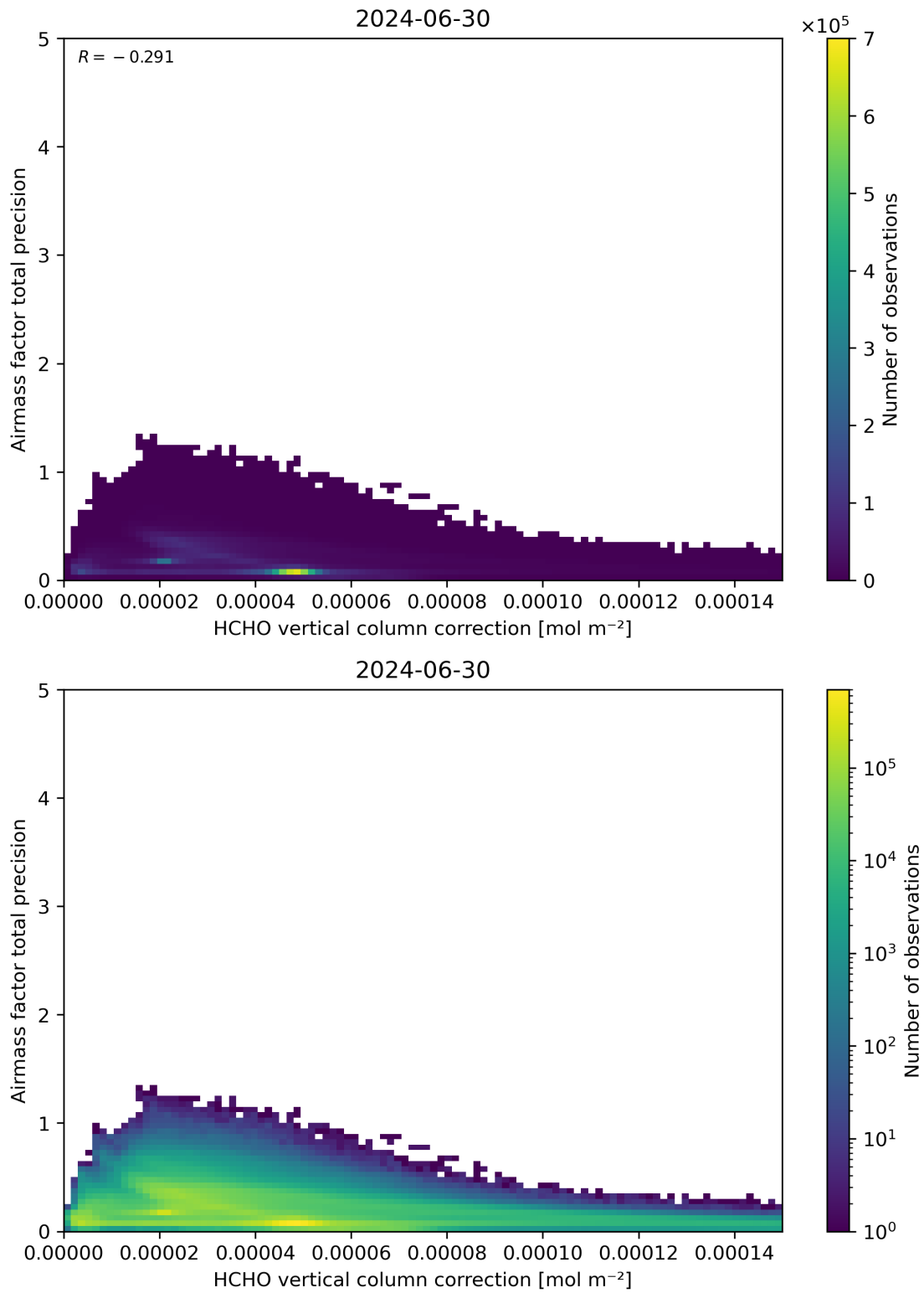
Figure 121: Scatter density plot of “HCHO vertical column correction” against “Airmass factor total precision” for 2024-06-29 to 2024-07-01.
