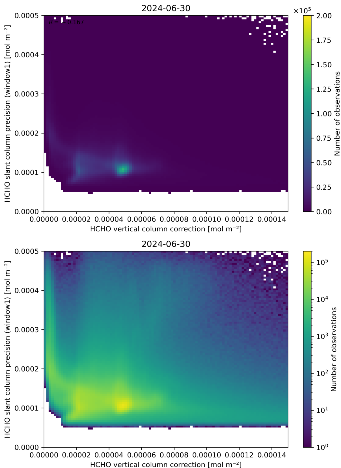
Figure 119: Scatter density plot of “HCHO vertical column correction” against “HCHO slant column precision (window1)” for 2024-06-29 to 2024-07-01.
