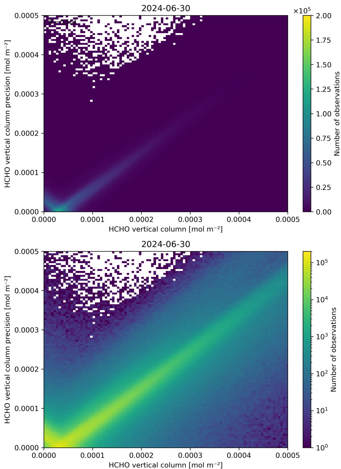
Figure 134: Scatter density plot of “HCHO vertical column” against “HCHO vertical column precision” for 2024-06-29 to 2024-07-01.
