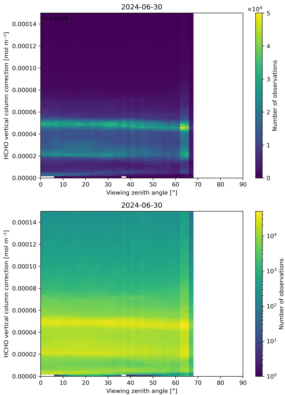
Figure 193: Scatter density plot of “Viewing zenith angle” against “HCHO vertical column correction” for 2024-06-29 to 2024-07-01.
