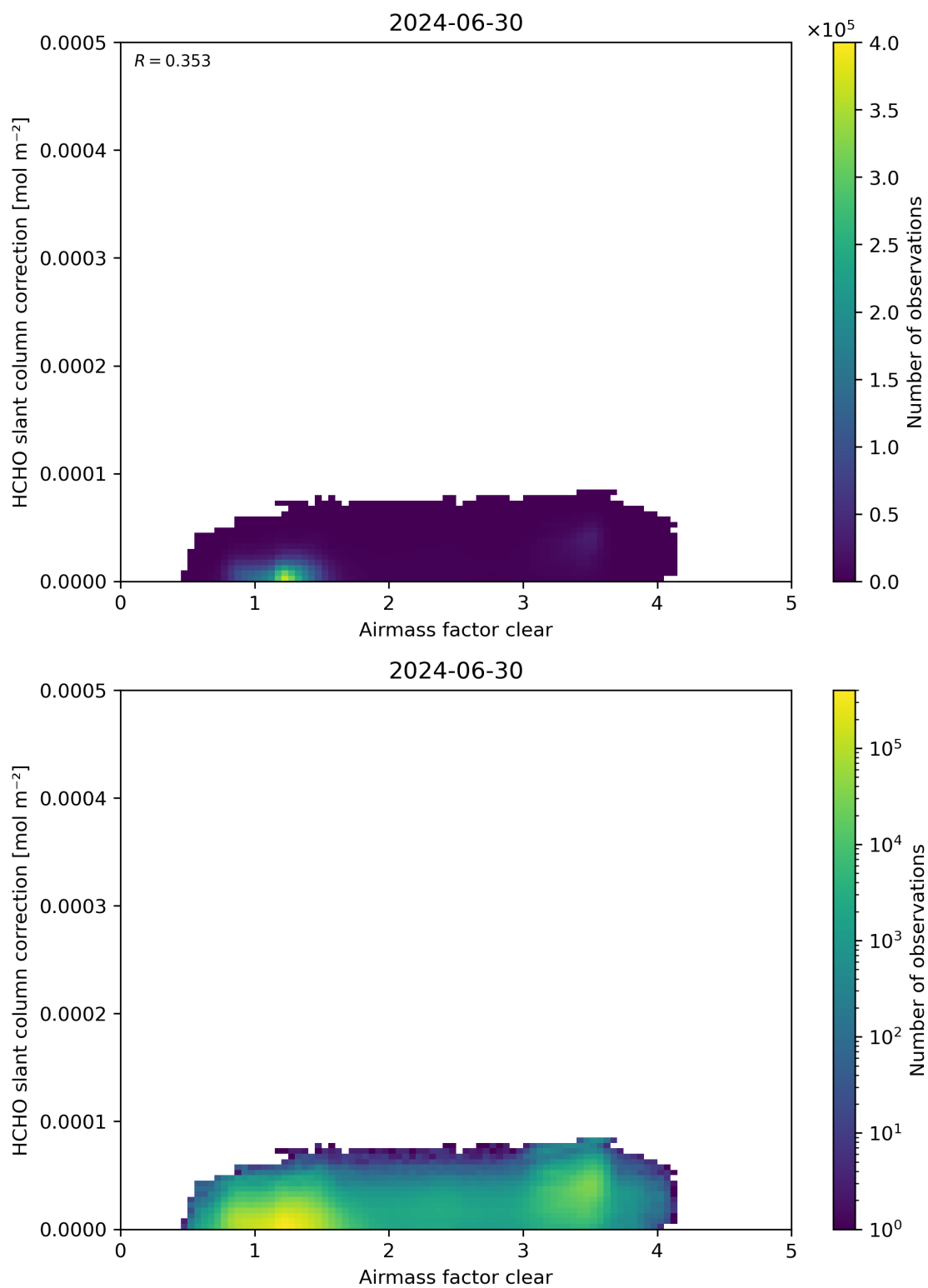
Figure 75: Scatter density plot of “Airmass factor clear” against “HCHO slant column correction” for 2024-06-29 to 2024-07-01.
