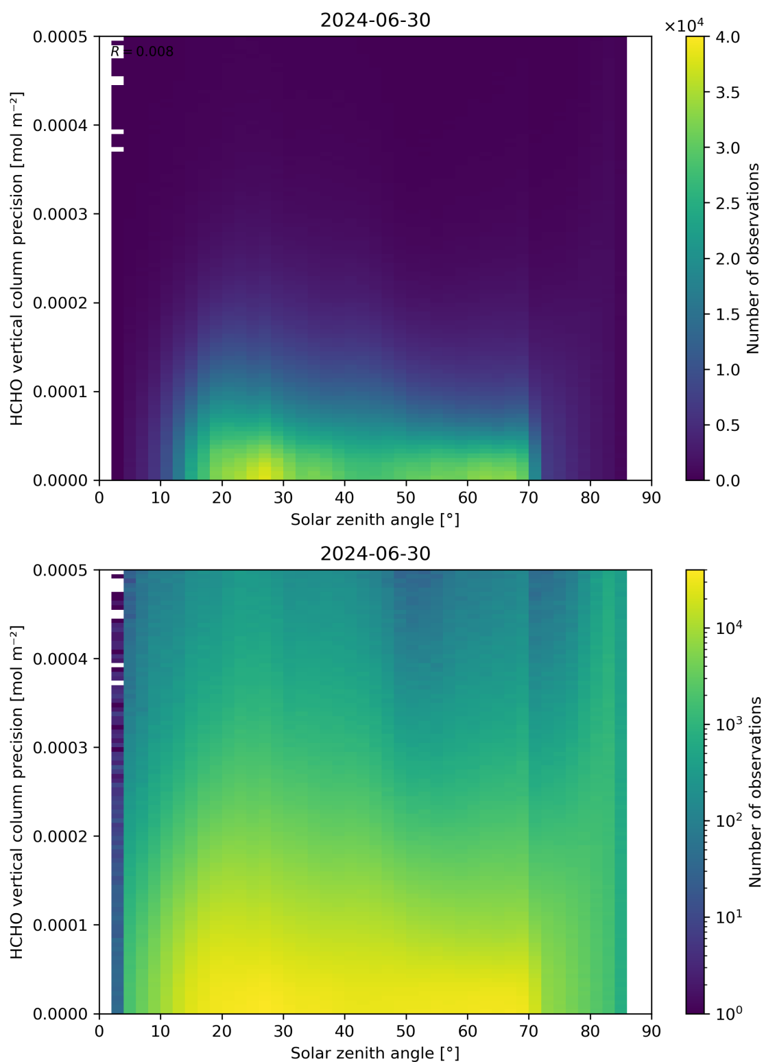
Figure 179: Scatter density plot of “Solar zenith angle” against “HCHO vertical column precision” for 2024-06-29 to 2024-07-01.
