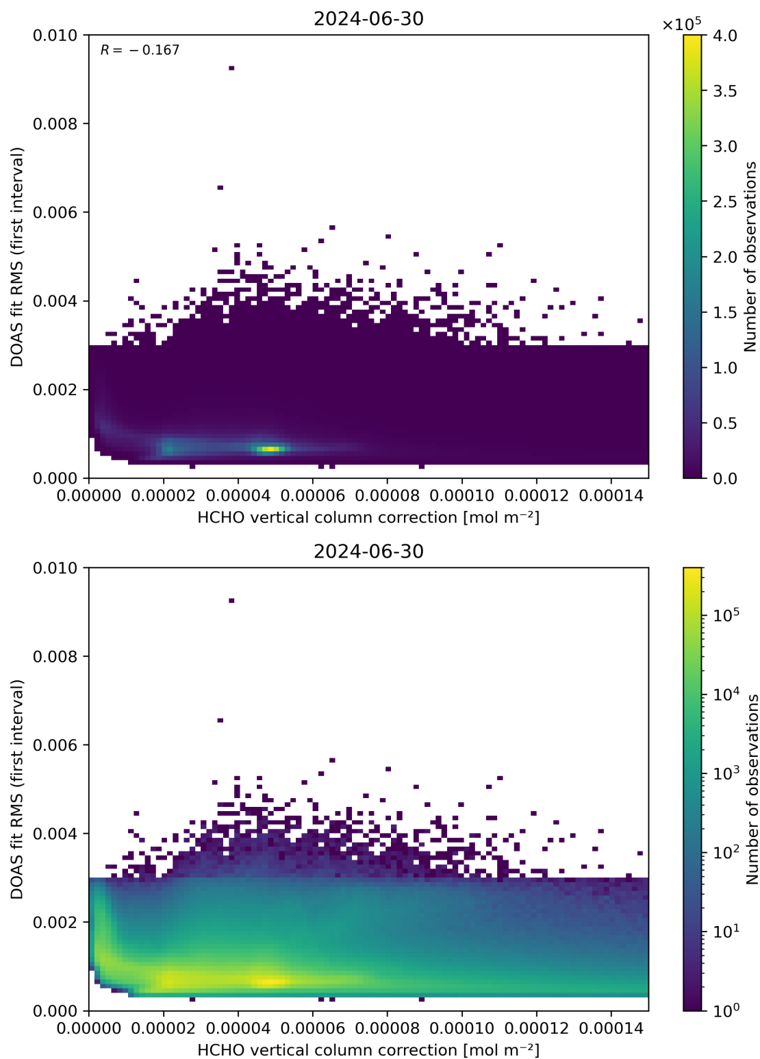
Figure 112: Scatter density plot of “HCHO vertical column correction” against “DOAS fit RMS (first interval)” for 2024-06-29 to 2024-07-01.
