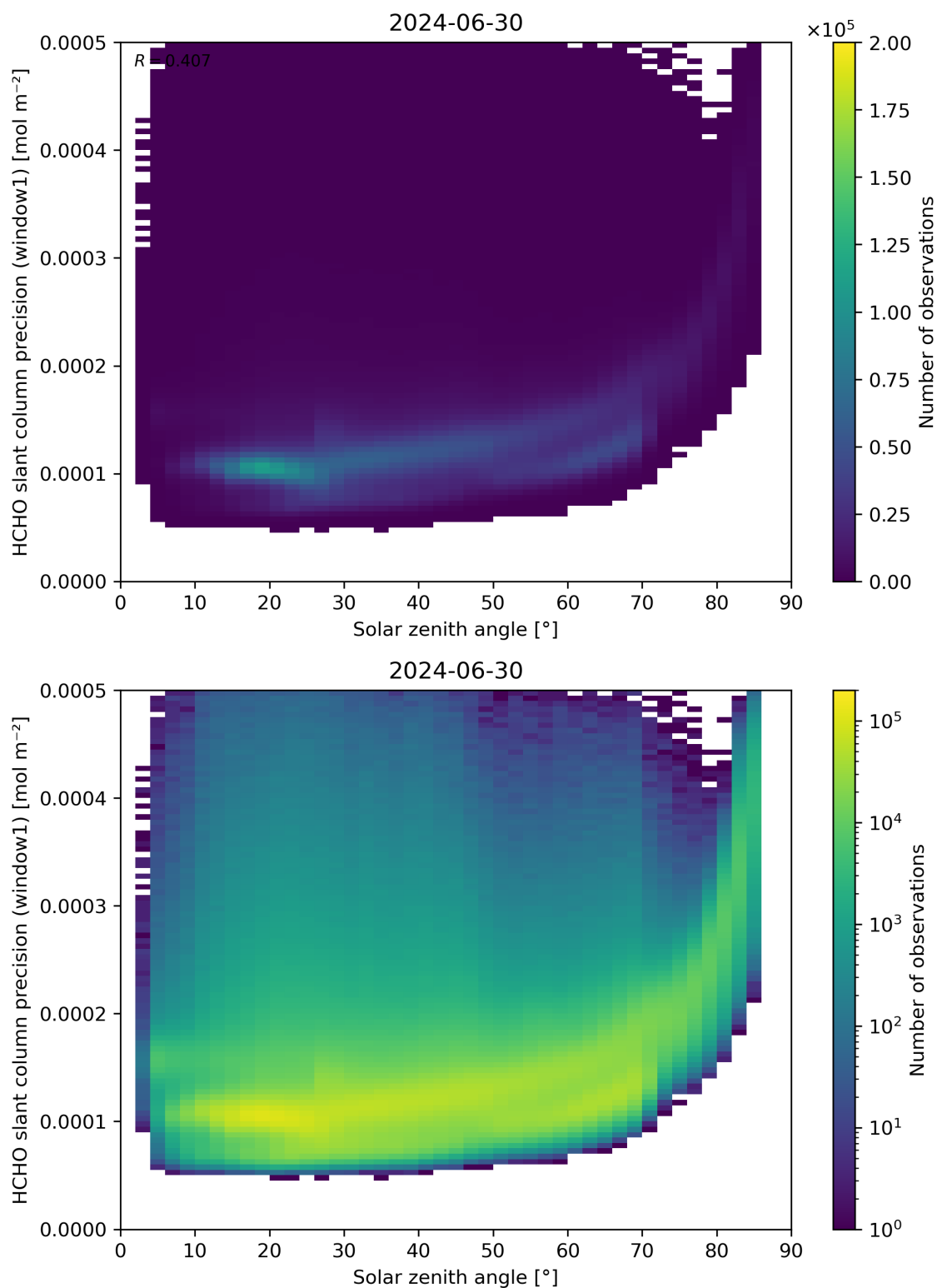
Figure 174: Scatter density plot of “Solar zenith angle” against “HCHO slant column precision (window1)” for 2024-06-29 to 2024-07-01.
