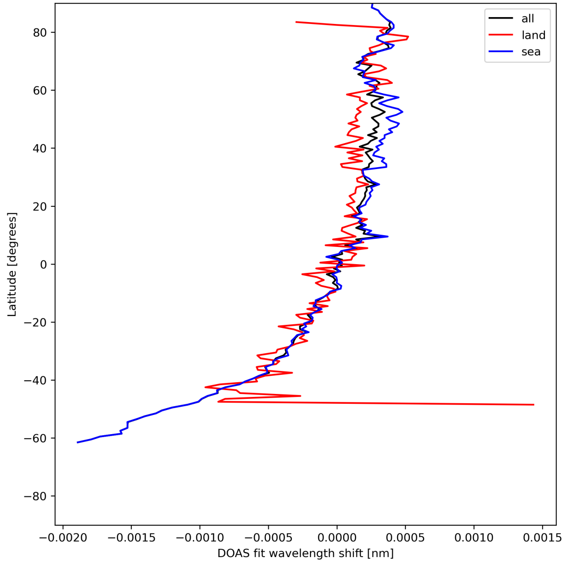
Figure 30: Zonal average of "DOAS fit wavelength shift" for 2024-06-29 to 2024-07-01.
