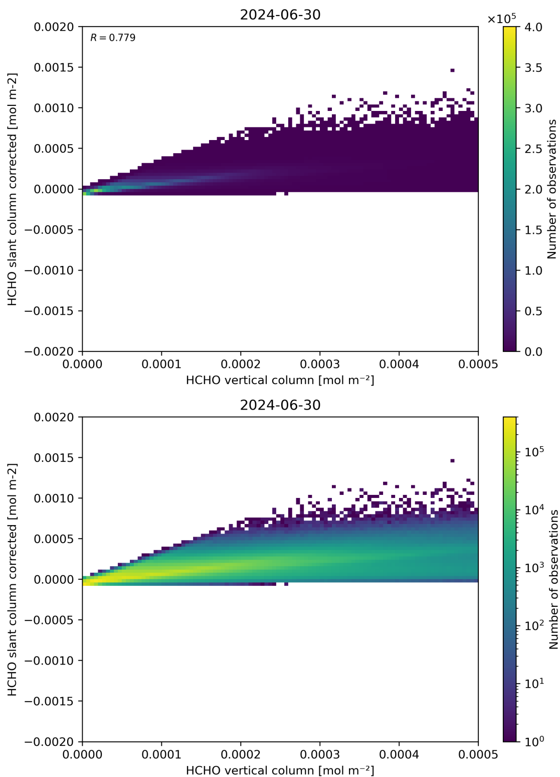
Figure 127: Scatter density plot of “HCHO vertical column” against “HCHO slant column corrected” for 2024-06-29 to 2024-07-01.
