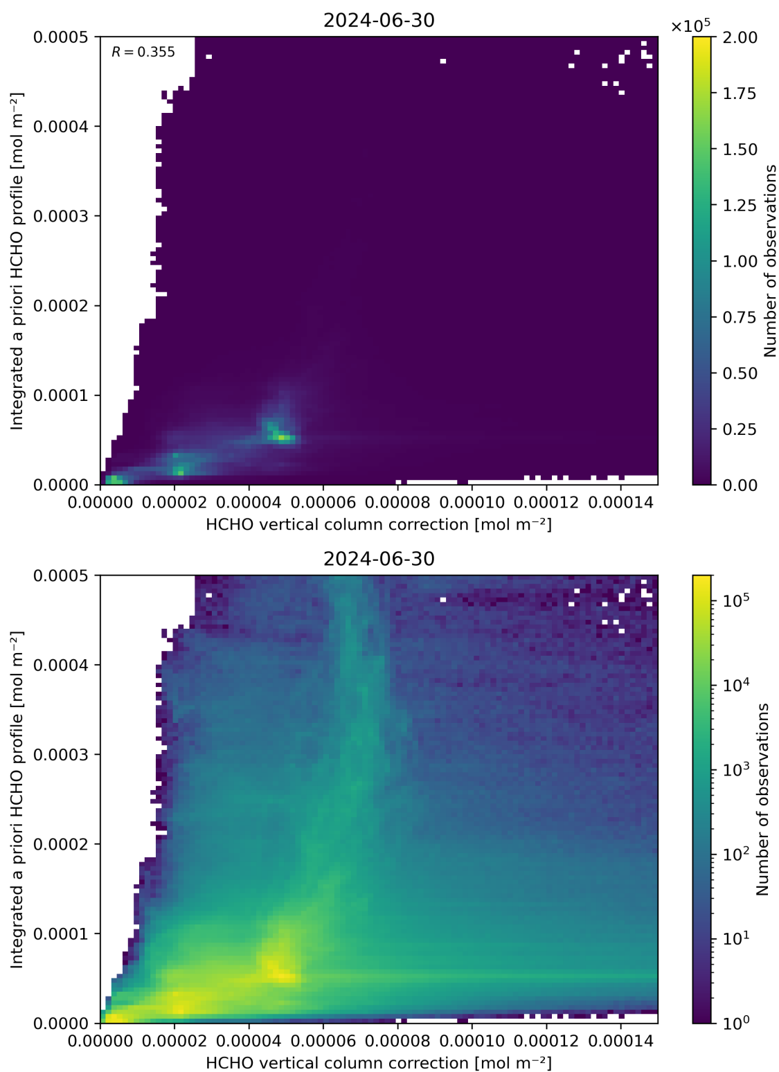
Figure 122: Scatter density plot of “HCHO vertical column correction” against “Integrated a priori HCHO profile” for 2024-06-29 to 2024-07-01.
