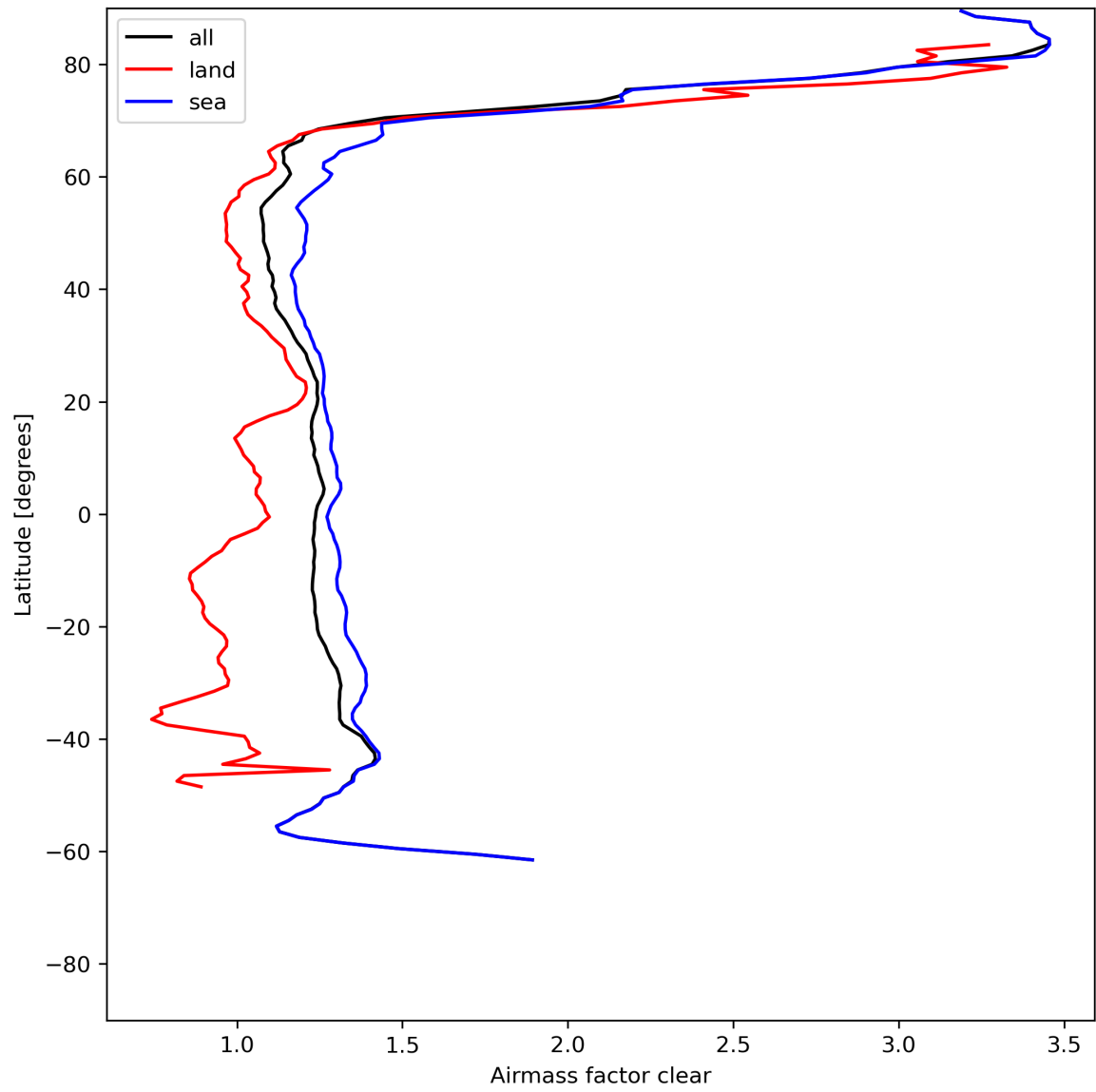
Figure 28: Zonal average of “Airmass factor clear” for 2024-06-29 to 2024-07-01.
