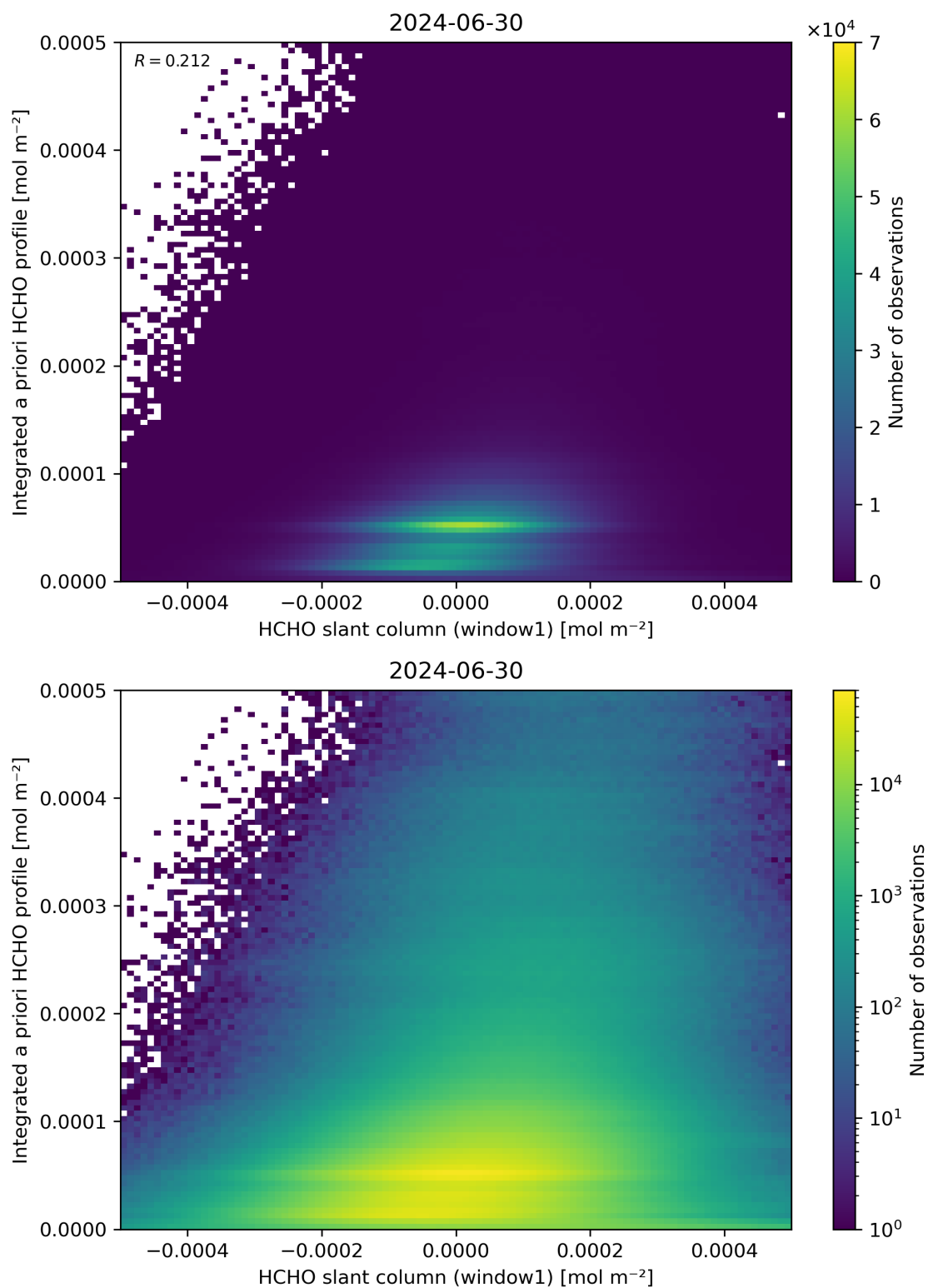
Figure 87: Scatter density plot of “HCHO slant column (window1)” against “Integrated a priori HCHO profile” for 2024-06-29 to 2024-07-01.
