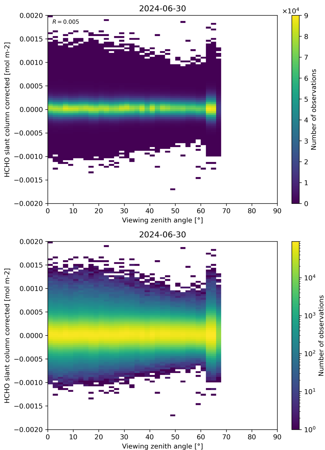
Figure 186: Scatter density plot of “Viewing zenith angle” against “HCHO slant column corrected” for 2024-06-29 to 2024-07-01.
