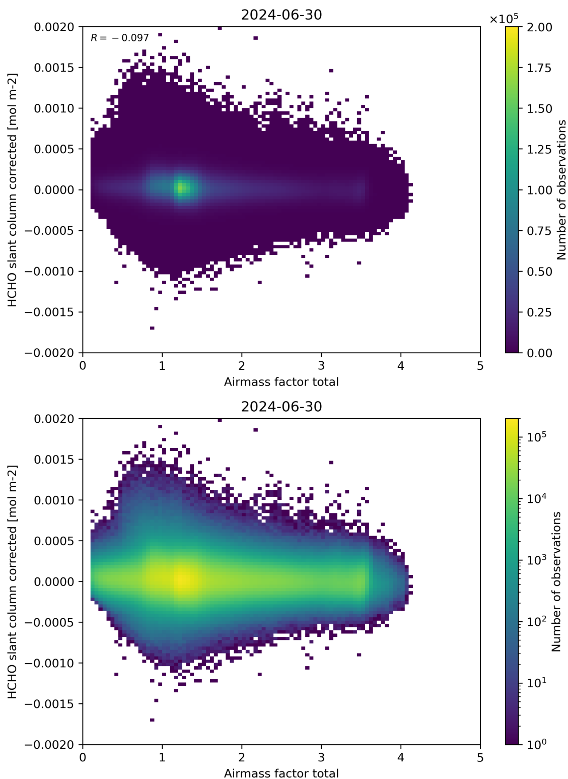
Figure 101: Scatter density plot of “Airmass factor total” against “HCHO slant column corrected” for 2024-06-29 to 2024-07-01.
