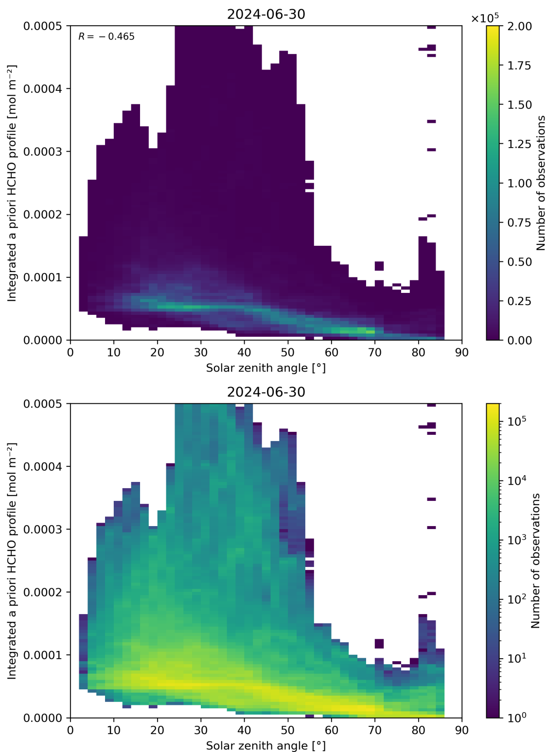
Figure 180: Scatter density plot of “Solar zenith angle” against “Integrated a priori HCHO profile” for 2024-06-29 to 2024-07-01.
