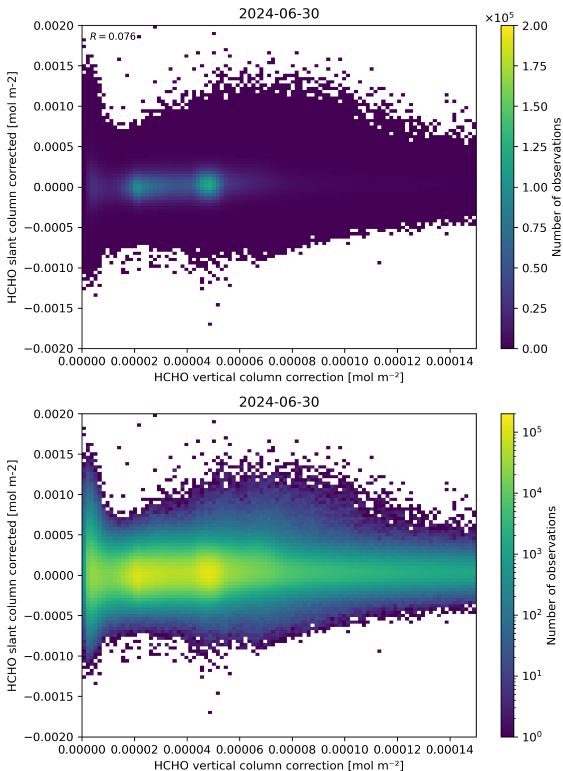
Figure 116: Scatter density plot of “HCHO vertical column correction” against “HCHO slant column corrected” for 2024-06-29 to 2024-07-01.
