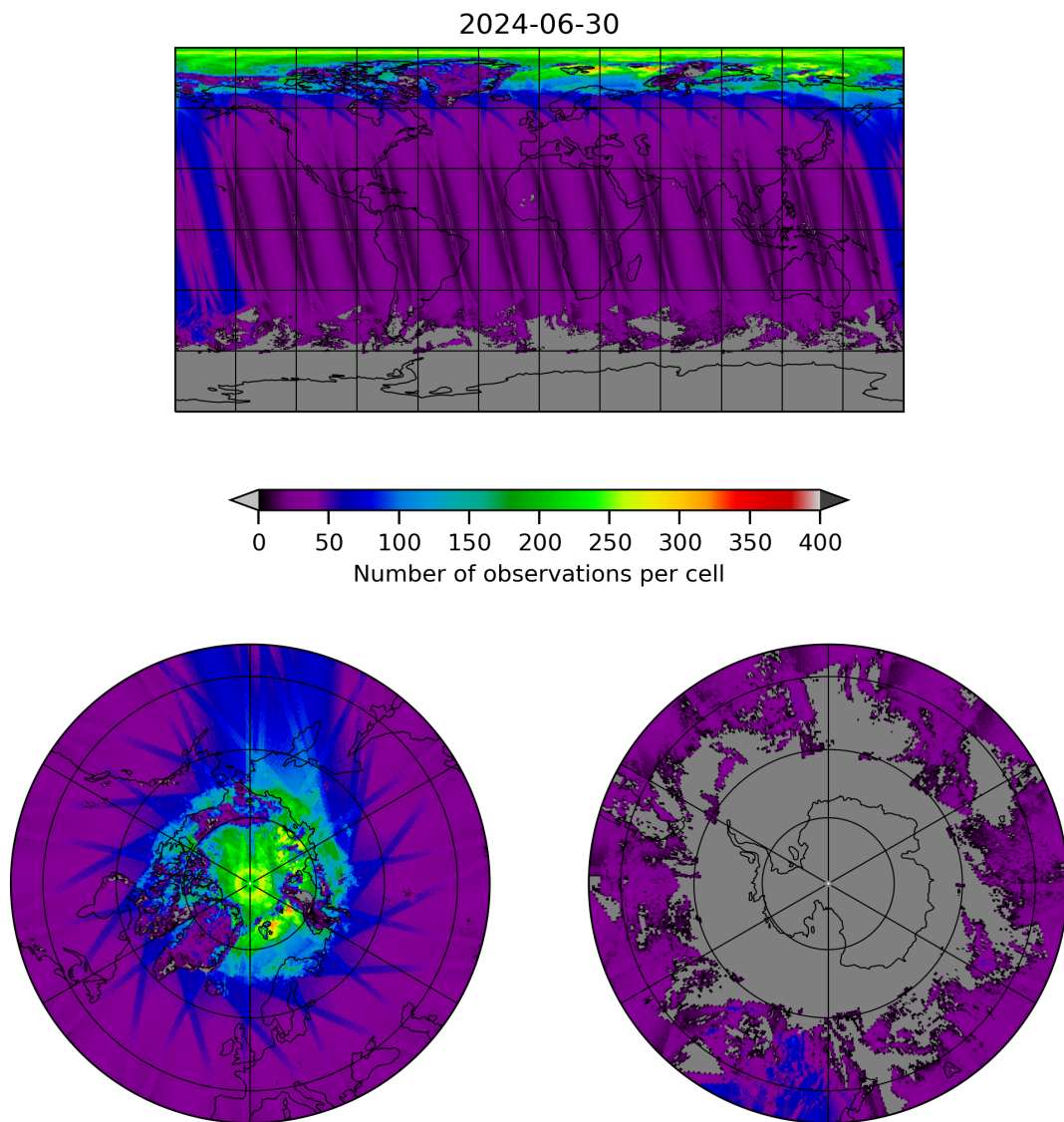
Figure 19: Map of the number of observations for 2024-06-29 to 2024-07-01
