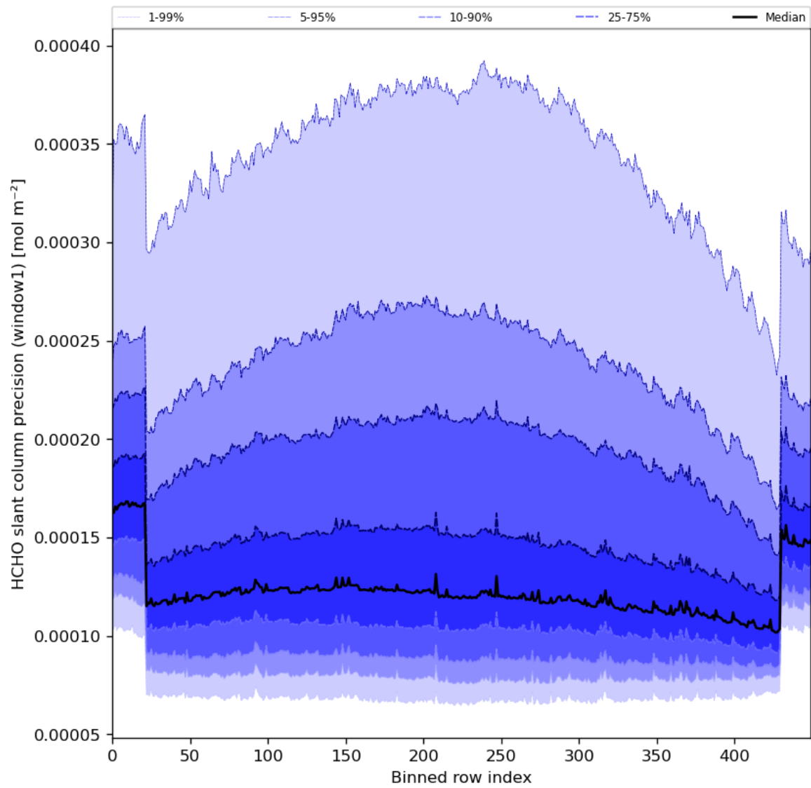
Figure 53: Along track statistics of “HCHO slant column precision (window1)” for 2024-06-29 to 2024-07-01
