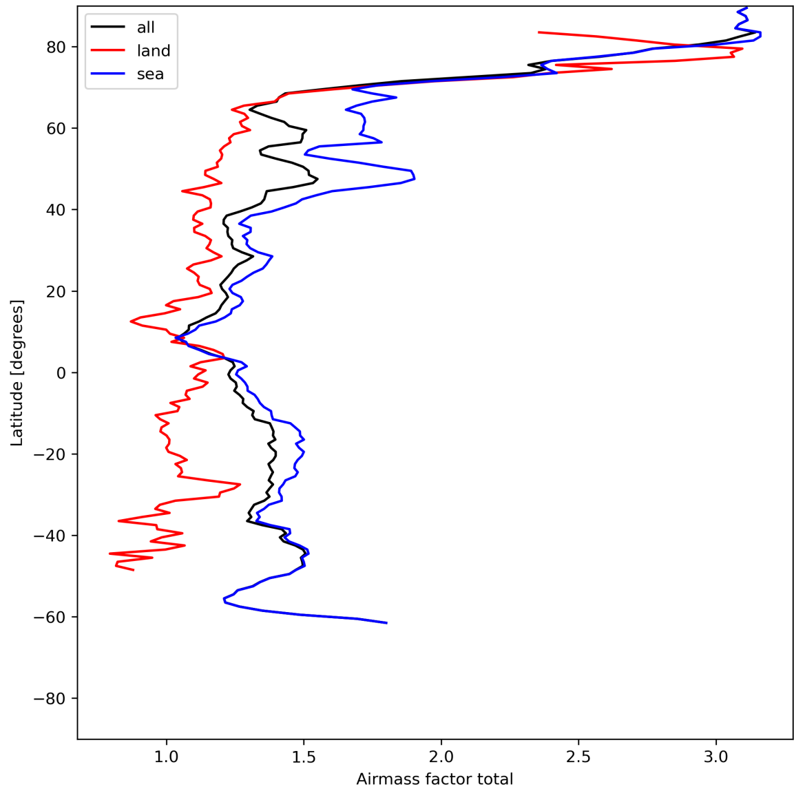
Figure 26: Zonal average of “Airmass factor total” for 2024-06-29 to 2024-07-01.
