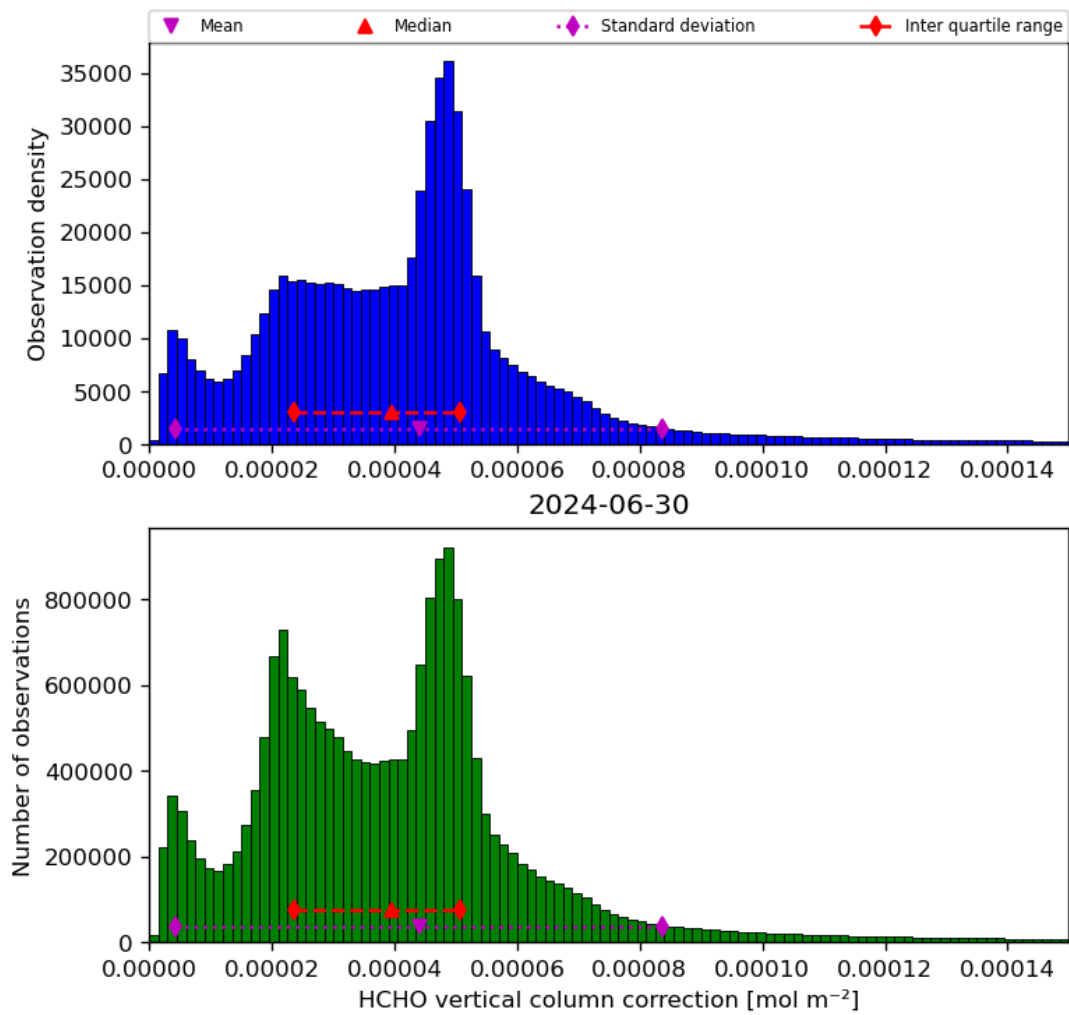
Figure 37: Histogram of “HCHO vertical column correction” for 2024-06-29 to 2024-07-01
