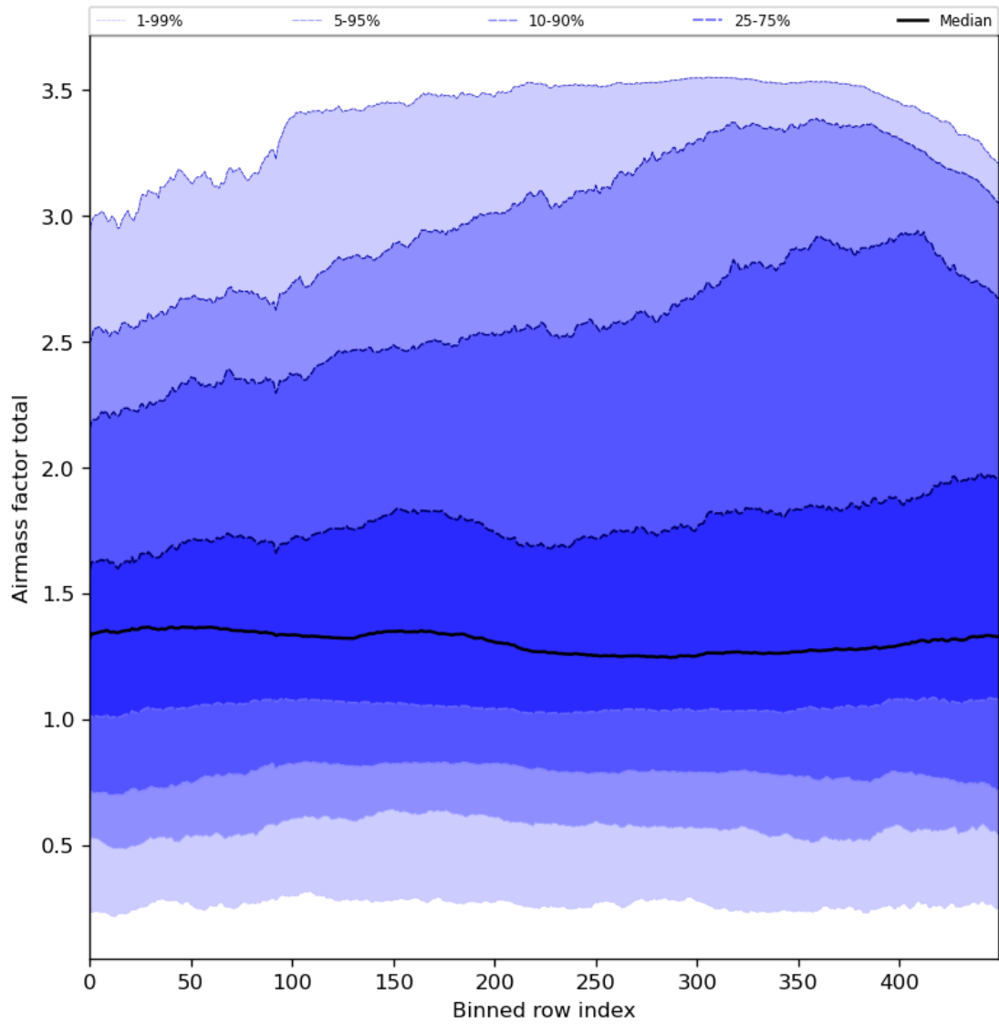
Figure 54: Along track statistics of “Airmass factor total” for 2024-06-29 to 2024-07-01
