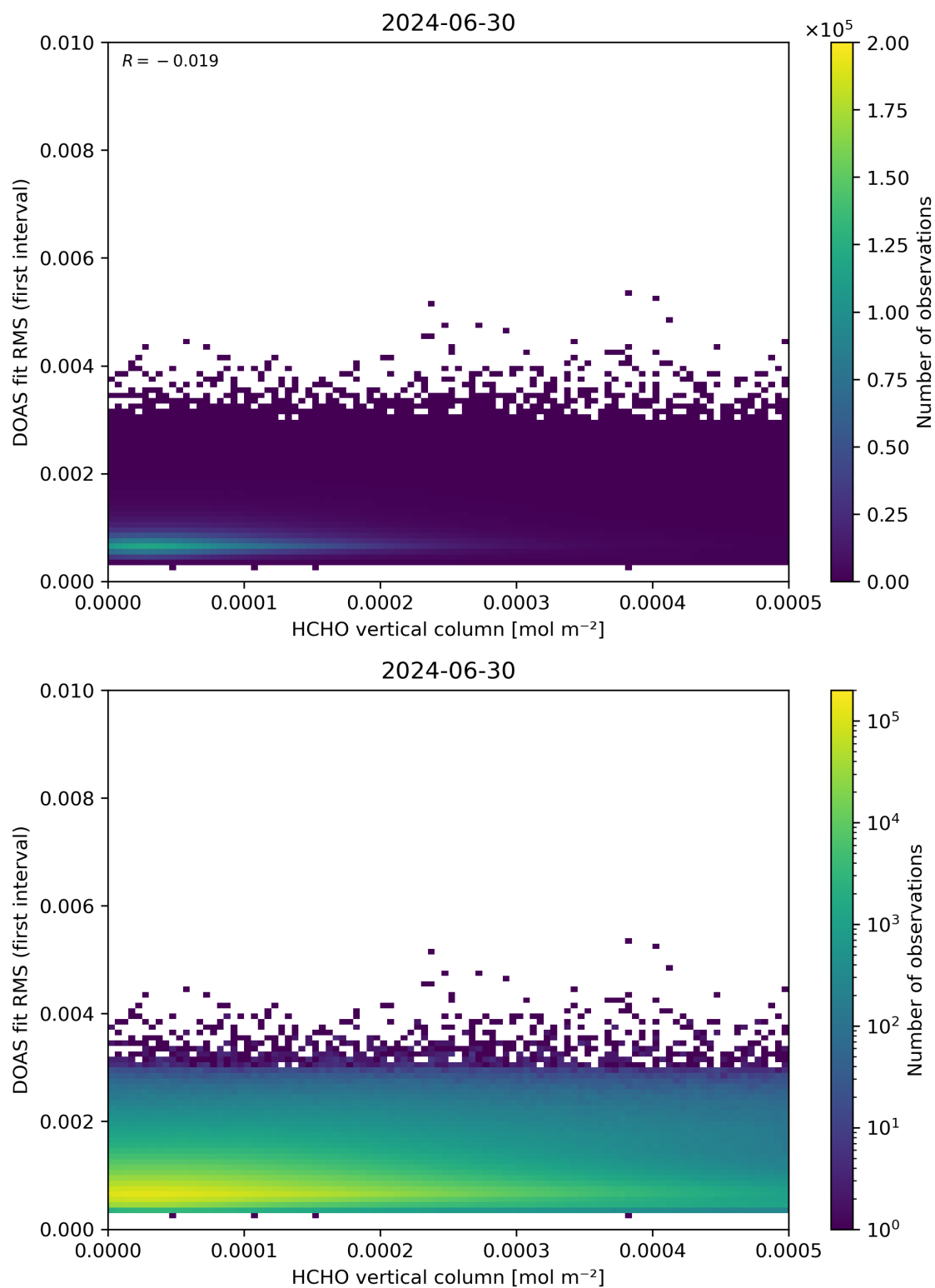
Figure 123: Scatter density plot of “HCHO vertical column” against “DOAS fit RMS (first interval)” for 2024-06-29 to 2024-07-01.
