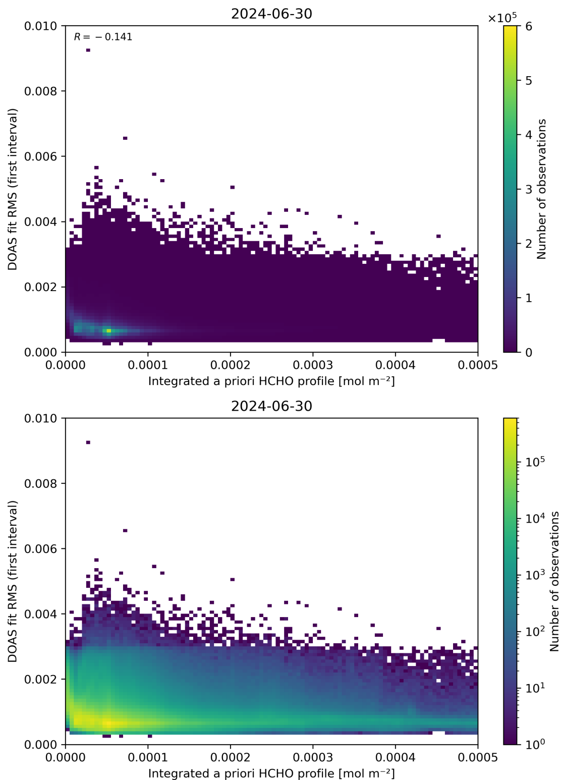
Figure 148: Scatter density plot of “Integrated a priori HCHO profile” against “DOAS fit RMS (first interval)” for 2024-06-29 to 2024-07-01.
