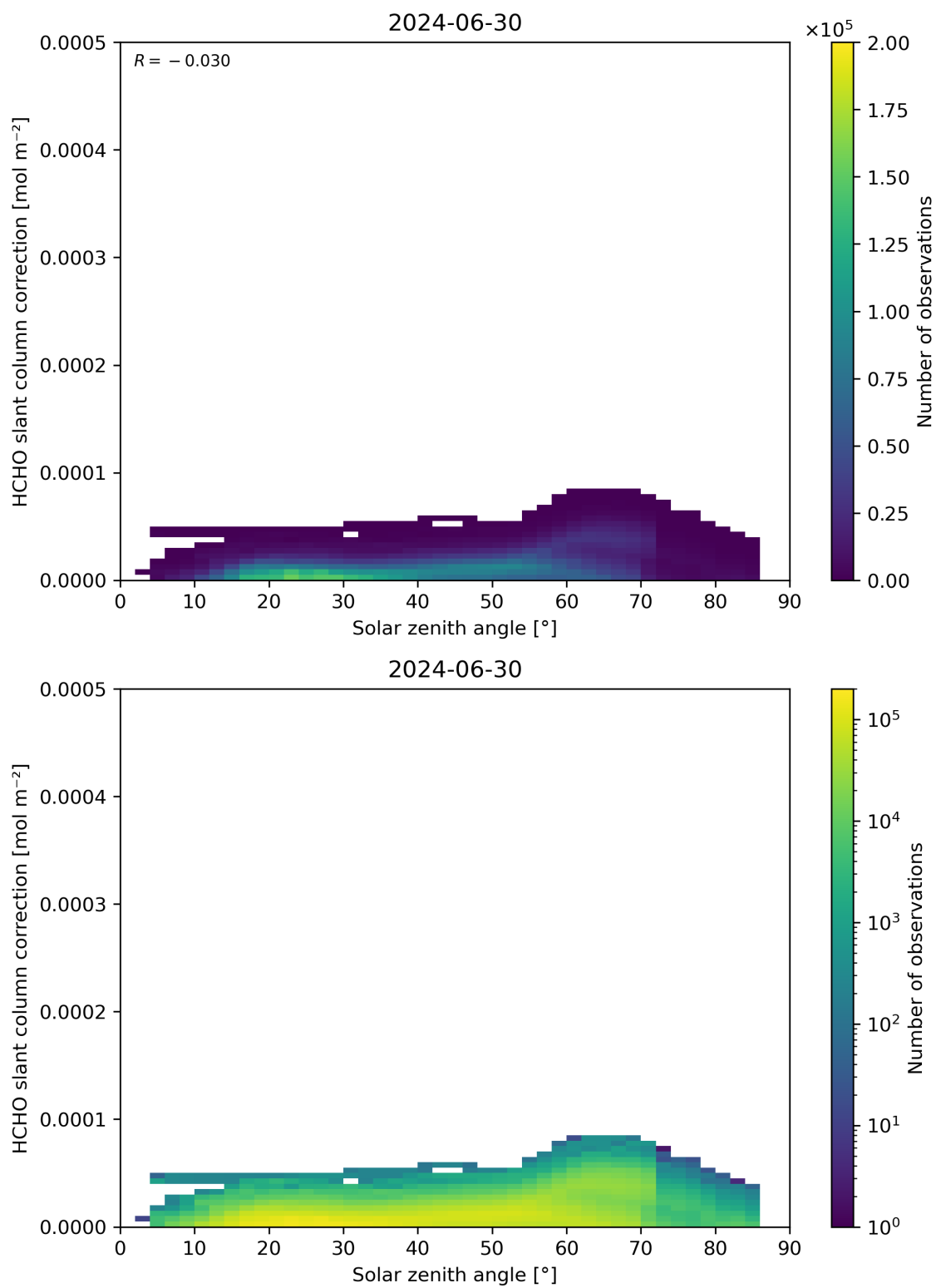
Figure 172: Scatter density plot of “Solar zenith angle” against “HCHO slant column correction” for 2024-06-29 to 2024-07-01.
