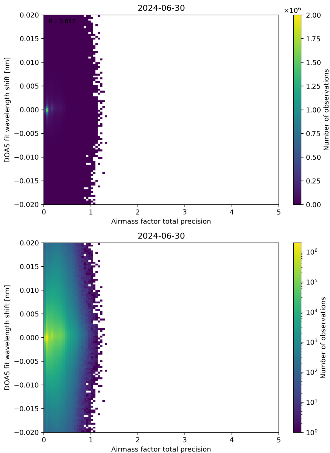
Figure 106: Scatter density plot of “Airmass factor total precision” against “DOAS fit wavelength shift” for 2024-06-29 to 2024-07-01.
