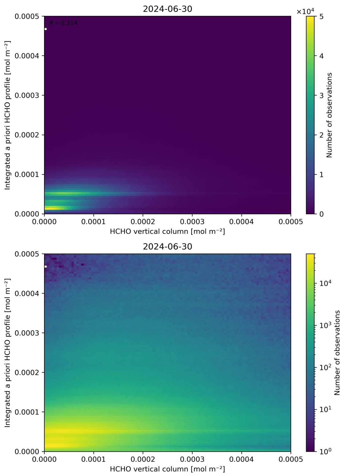
Figure 135: Scatter density plot of “HCHO vertical column” against “Integrated a priori HCHO profile” for 2024-06-29 to 2024-07-01.
