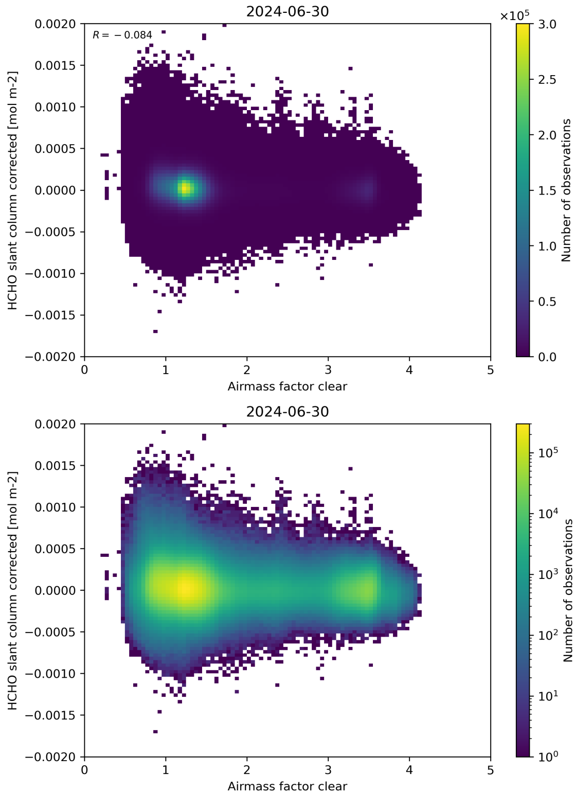
Figure 74: Scatter density plot of “Airmass factor clear” against “HCHO slant column corrected” for 2024-06-29 to 2024-07-01.
