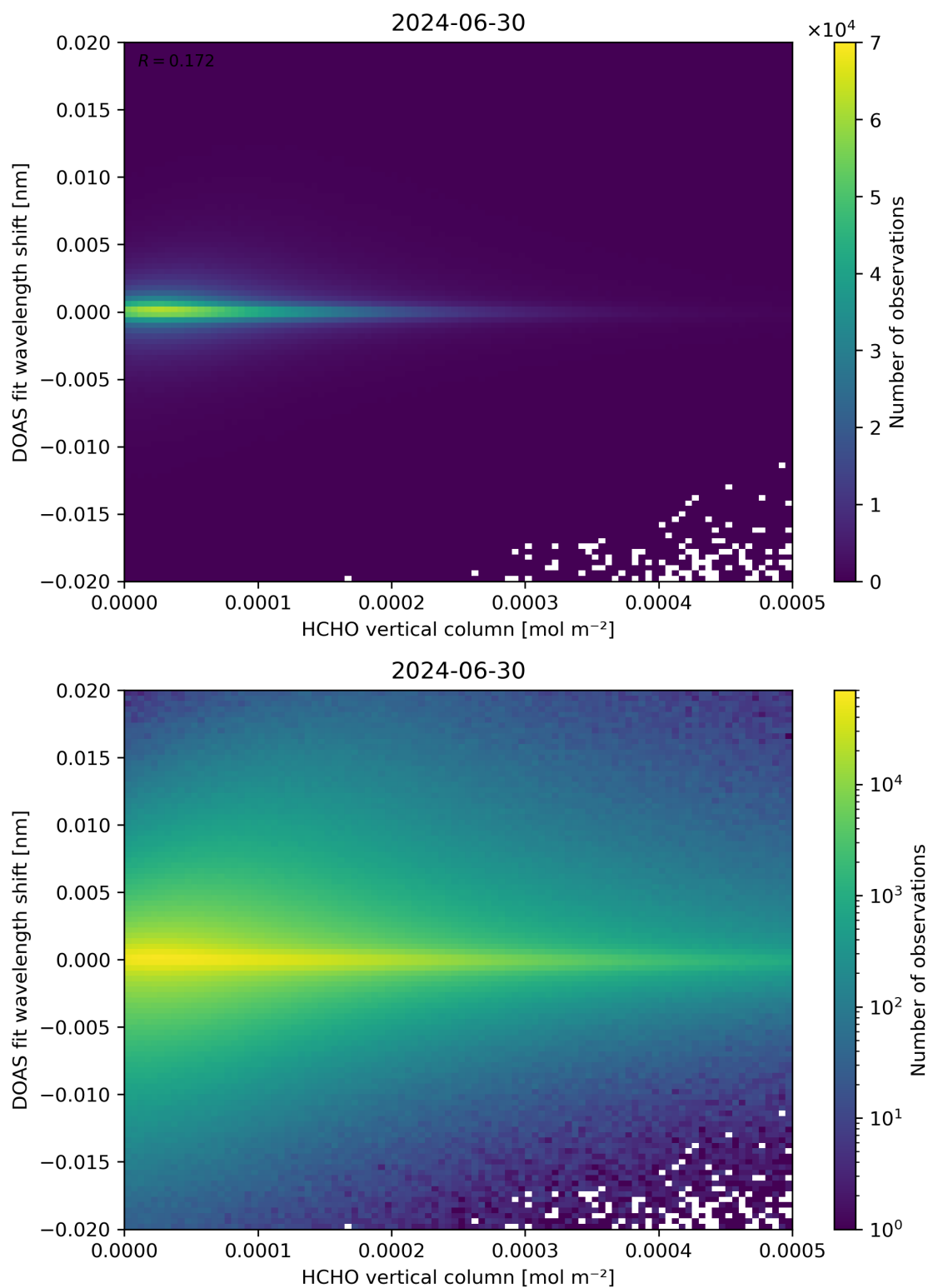
Figure 124: Scatter density plot of “HCHO vertical column” against “DOAS fit wavelength shift” for 2024-06-29 to 2024-07-01.
