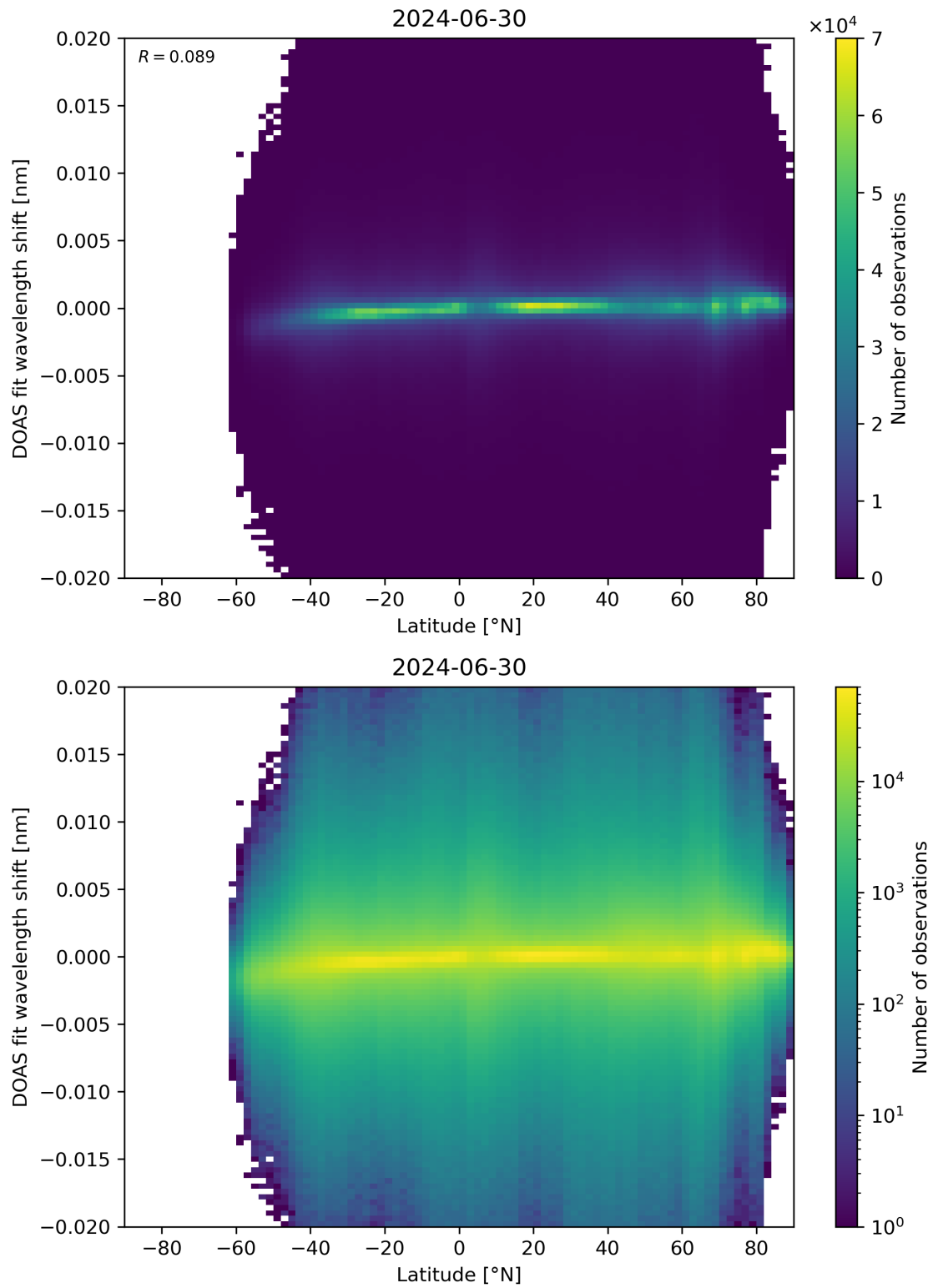
Figure 154: Scatter density plot of “Latitude” against “DOAS fit wavelength shift” for 2024-06-29 to 2024-07-01.
