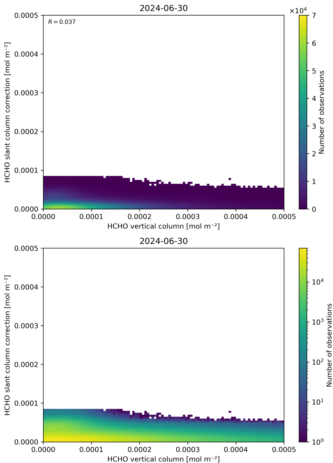
Figure 128: Scatter density plot of “HCHO vertical column” against “HCHO slant column correction” for 2024-06-29 to 2024-07-01.
