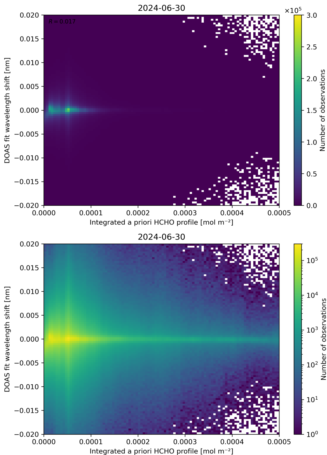
Figure 149: Scatter density plot of “Integrated a priori HCHO profile” against “DOAS fit wavelength shift” for 2024-06-29 to 2024-07-01.
