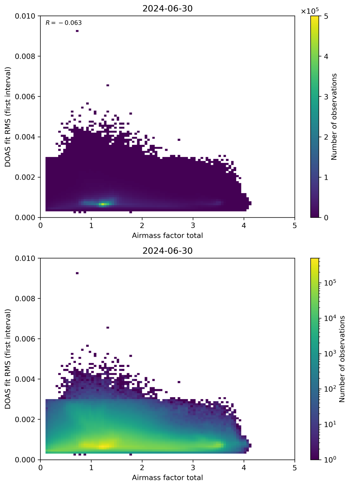
Figure 97: Scatter density plot of “Airmass factor total” against “DOAS fit RMS (first interval)” for 2024-06-29 to 2024-07-01.
