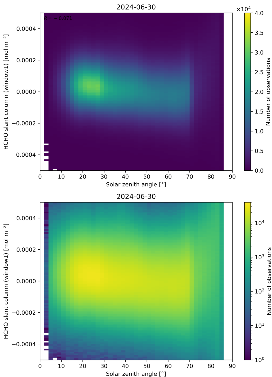
Figure 173: Scatter density plot of “Solar zenith angle” against “HCHO slant column (window1)” for 2024-06-29 to 2024-07-01.
