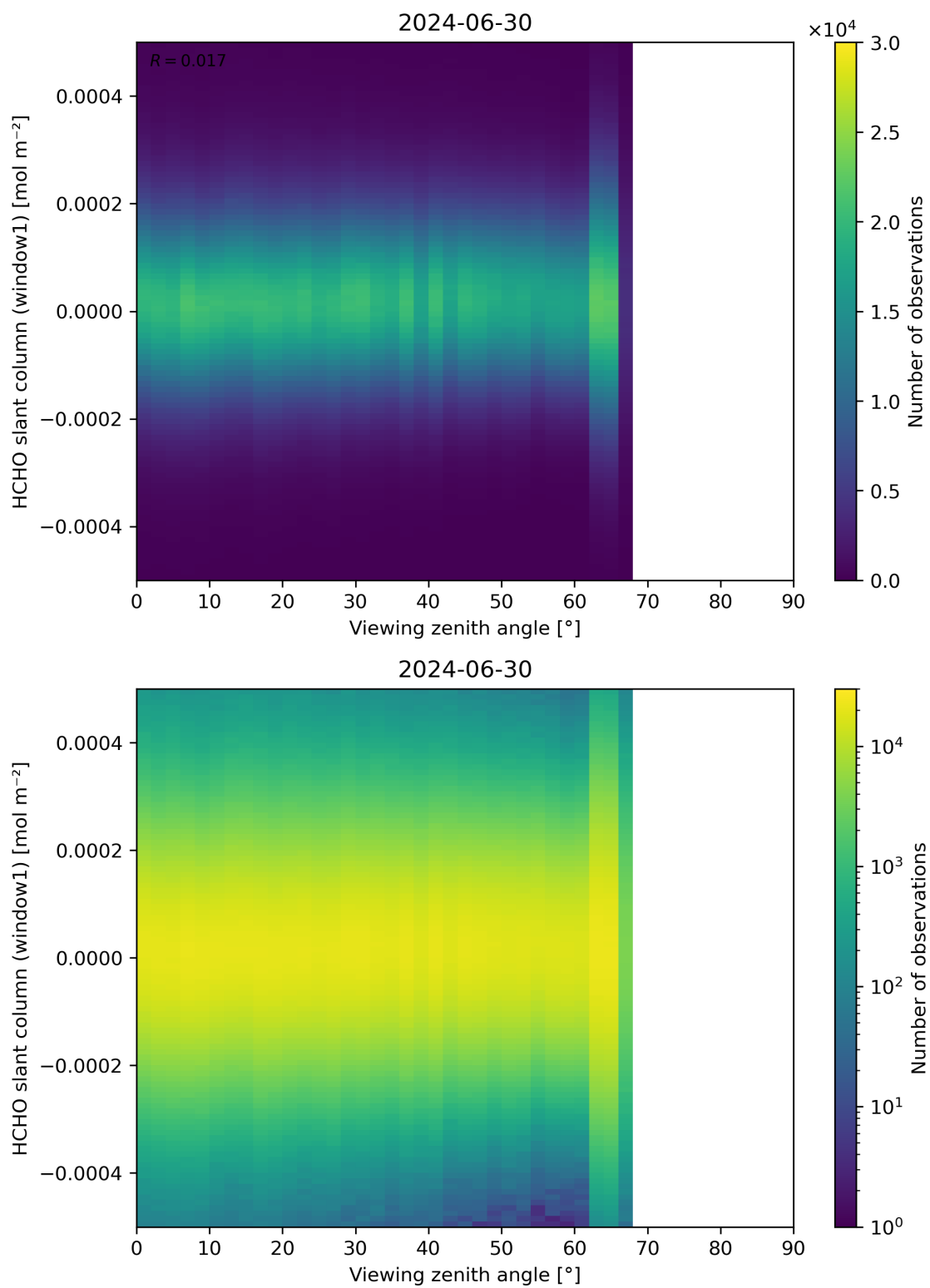
Figure 188: Scatter density plot of “Viewing zenith angle” against “HCHO slant column (window1)” for 2024-06-29 to 2024-07-01.
