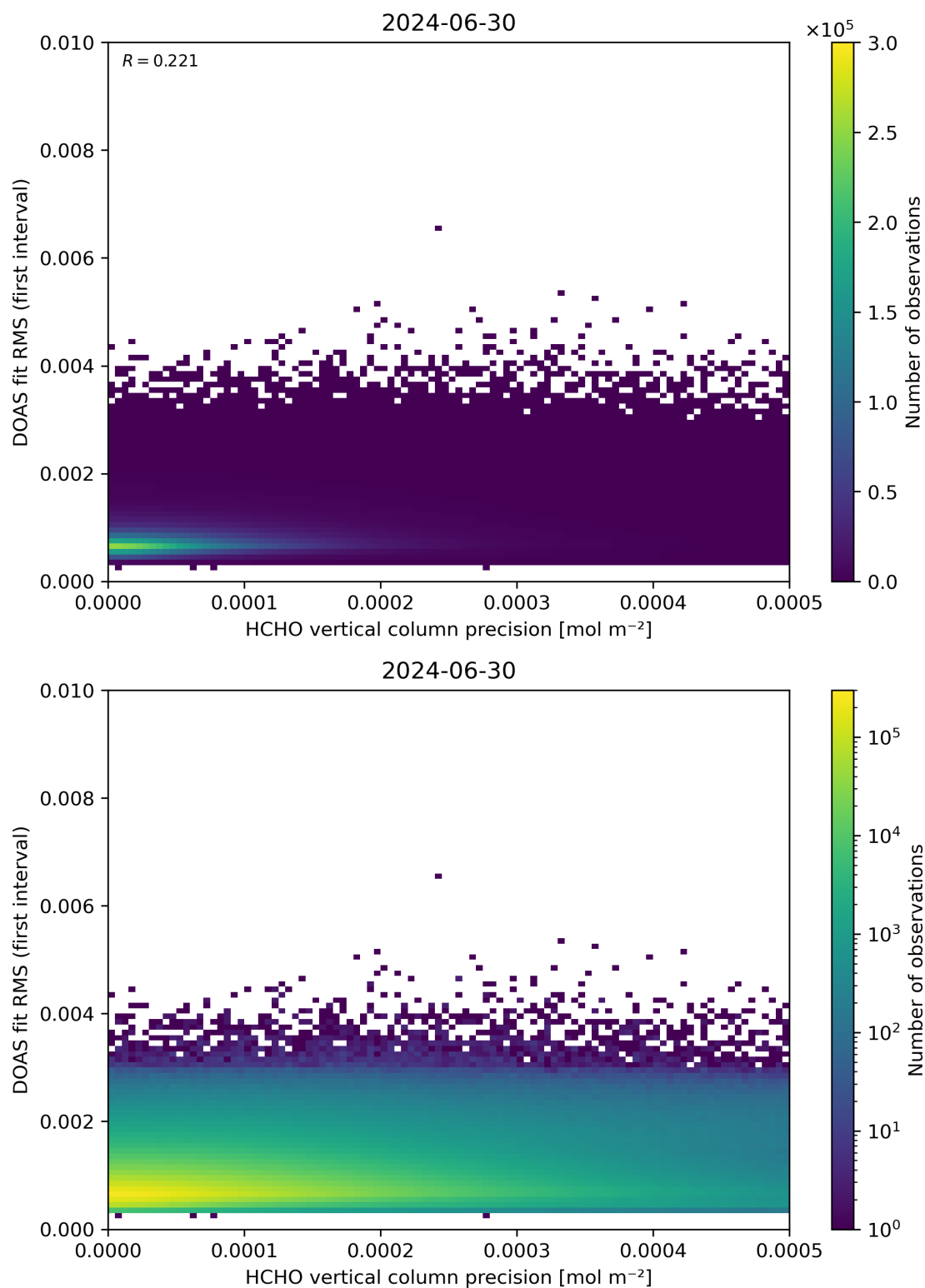
Figure 136: Scatter density plot of “HCHO vertical column precision” against “DOAS fit RMS (first interval)” for 2024-06-29 to 2024-07-01.
