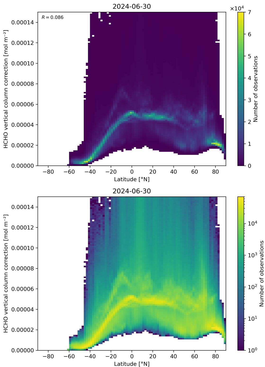
Figure 164: Scatter density plot of “Latitude” against “HCHO vertical column correction” for 2024-06-29 to 2024-07-01.
