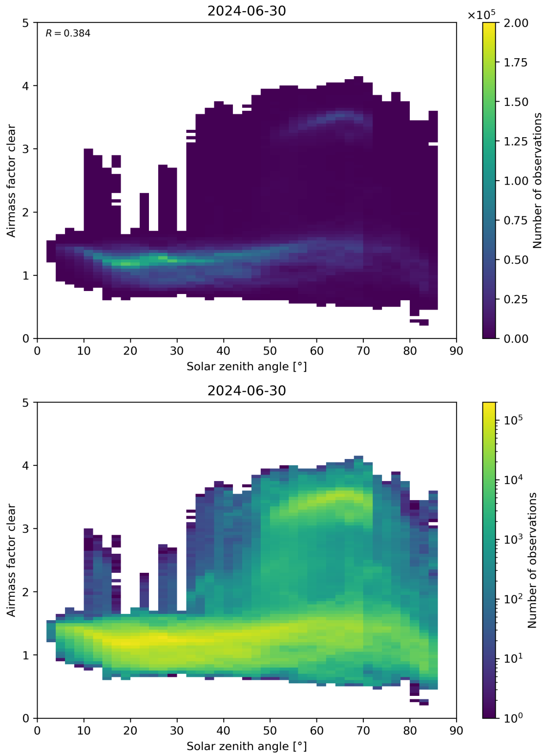
Figure 170: Scatter density plot of “Solar zenith angle” against “Airmass factor clear” for 2024-06-29 to 2024-07-01.
