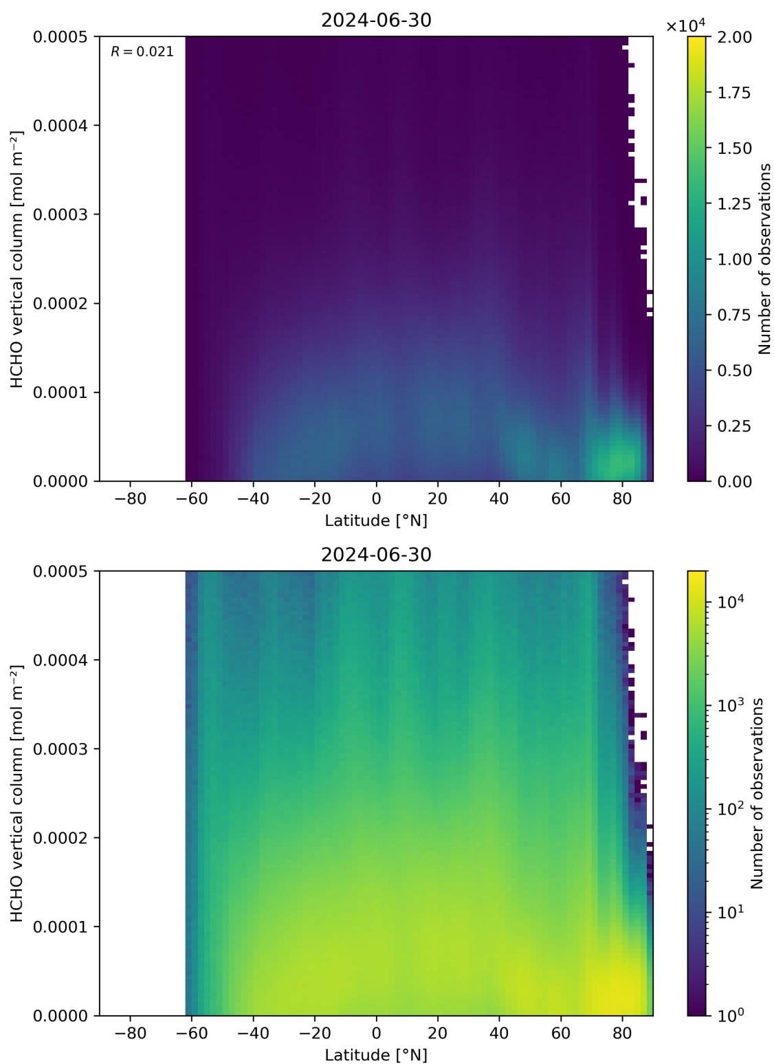
Figure 163: Scatter density plot of “Latitude” against “HCHO vertical column” for 2024-06-29 to 2024-07-01.
