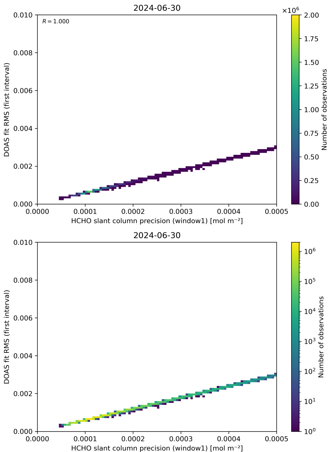
Figure 88: Scatter density plot of “HCHO slant column precision (window1)” against “DOAS fit RMS (first interval)” for 2024-06-29 to 2024-07-01.
