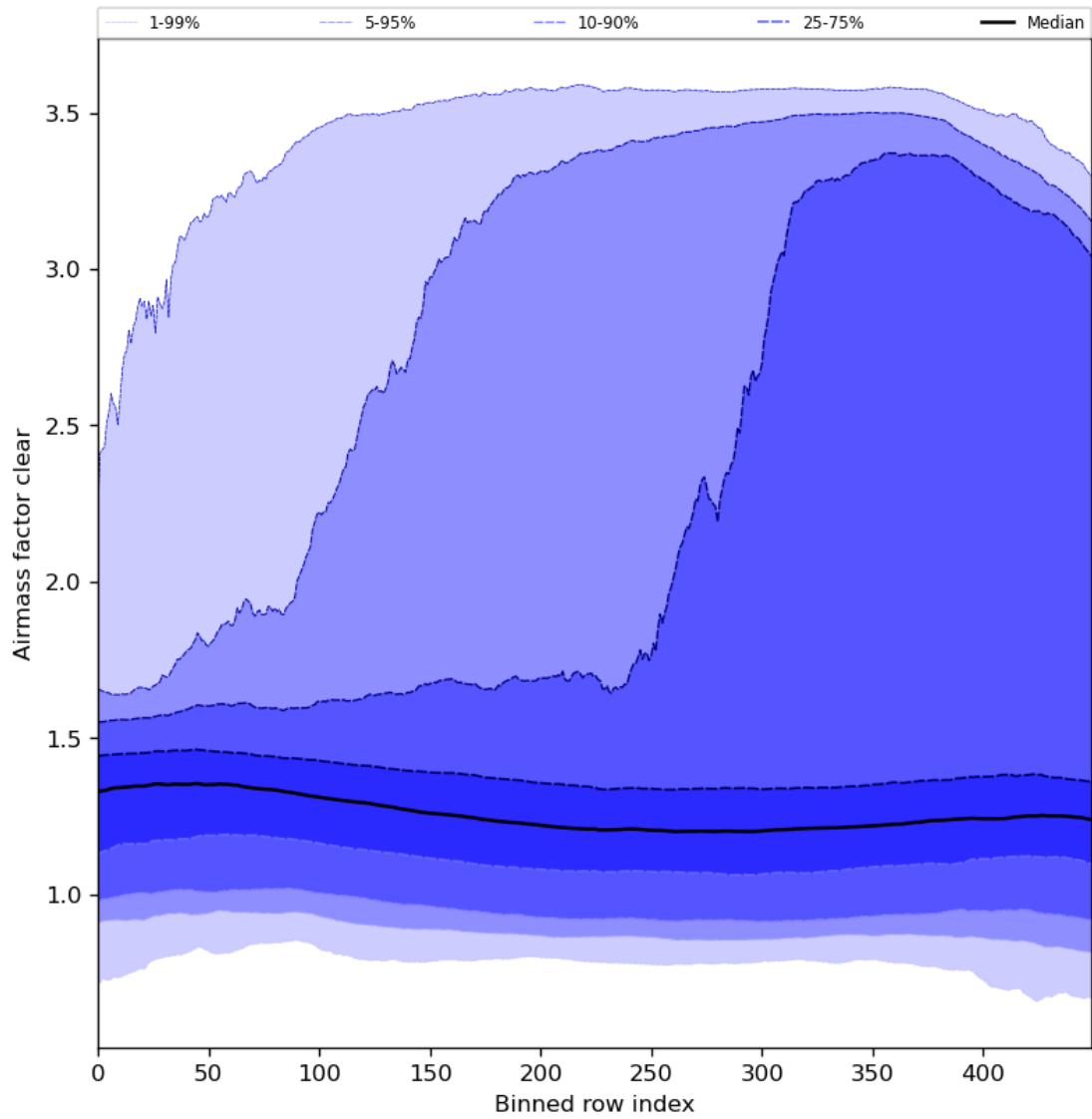
Figure 56: Along track statistics of “Airmass factor clear” for 2024-06-29 to 2024-07-01
