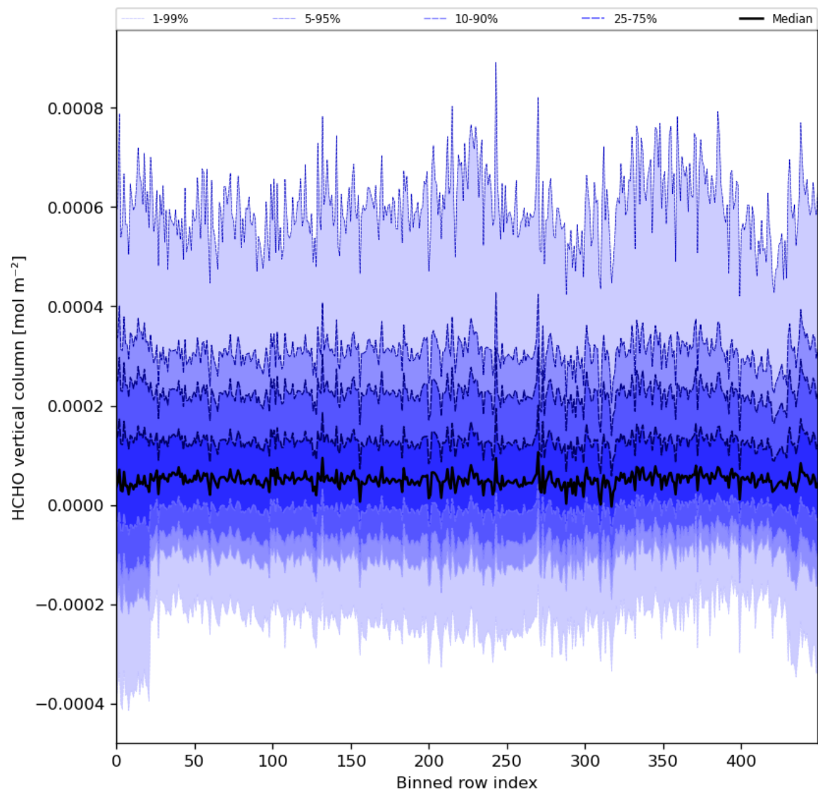
Figure 49: Along track statistics of “HCHO vertical column” for 2024-06-29 to 2024-07-01
