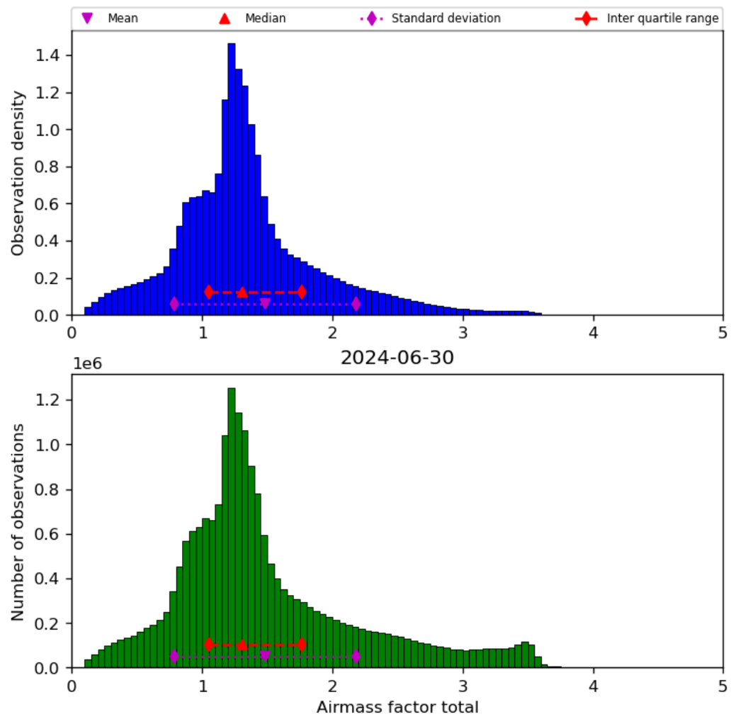
Figure 40: Histogram of "Airmass factor total" for 2024-06-29 to 2024-07-01
