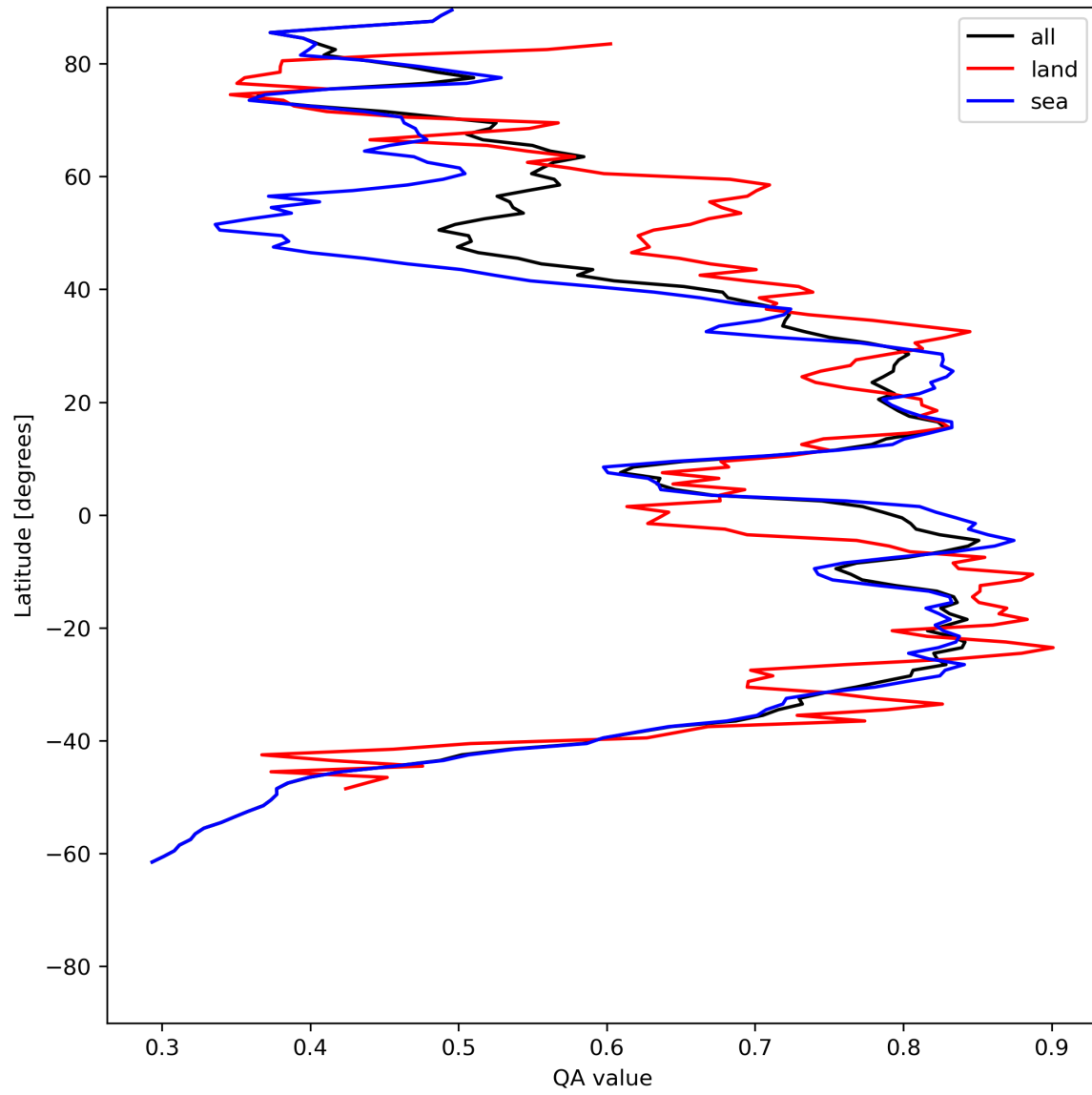
Figure 20: Zonal average of “QA value” for 2024-06-29 to 2024-07-01.
