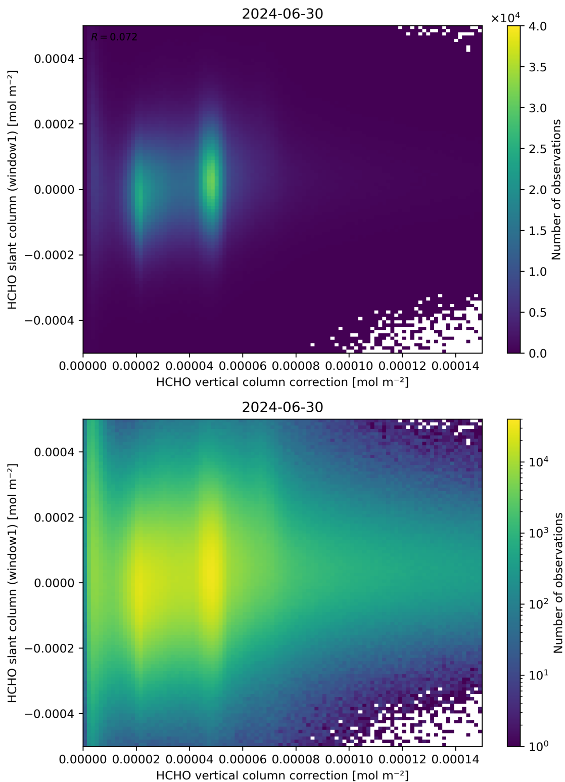
Figure 118: Scatter density plot of “HCHO vertical column correction” against “HCHO slant column (window1)” for 2024-06-29 to 2024-07-01.
