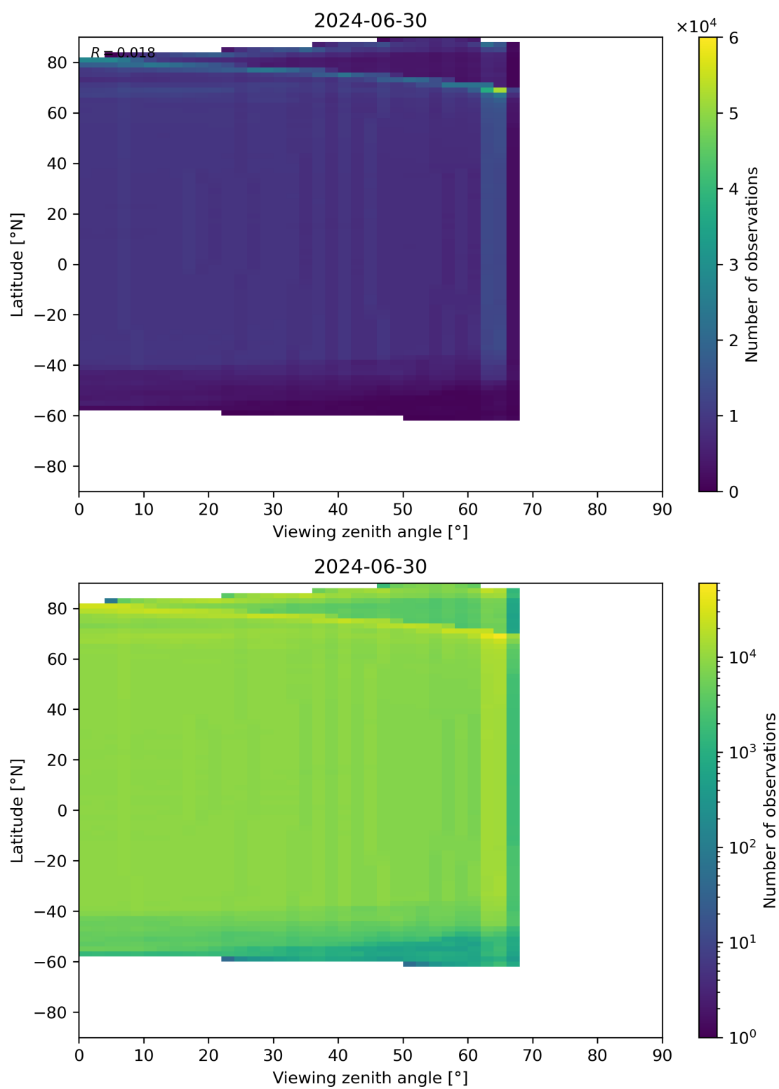
Figure 196: Scatter density plot of “Viewing zenith angle” against “Latitude” for 2024-06-29 to 2024-07-01.
