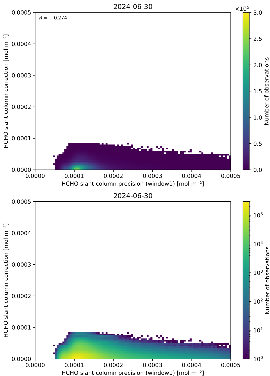
Figure 93: Scatter density plot of “HCHO slant column precision (window1)” against “HCHO slant column correction” for 2024-06-29 to 2024-07-01.
