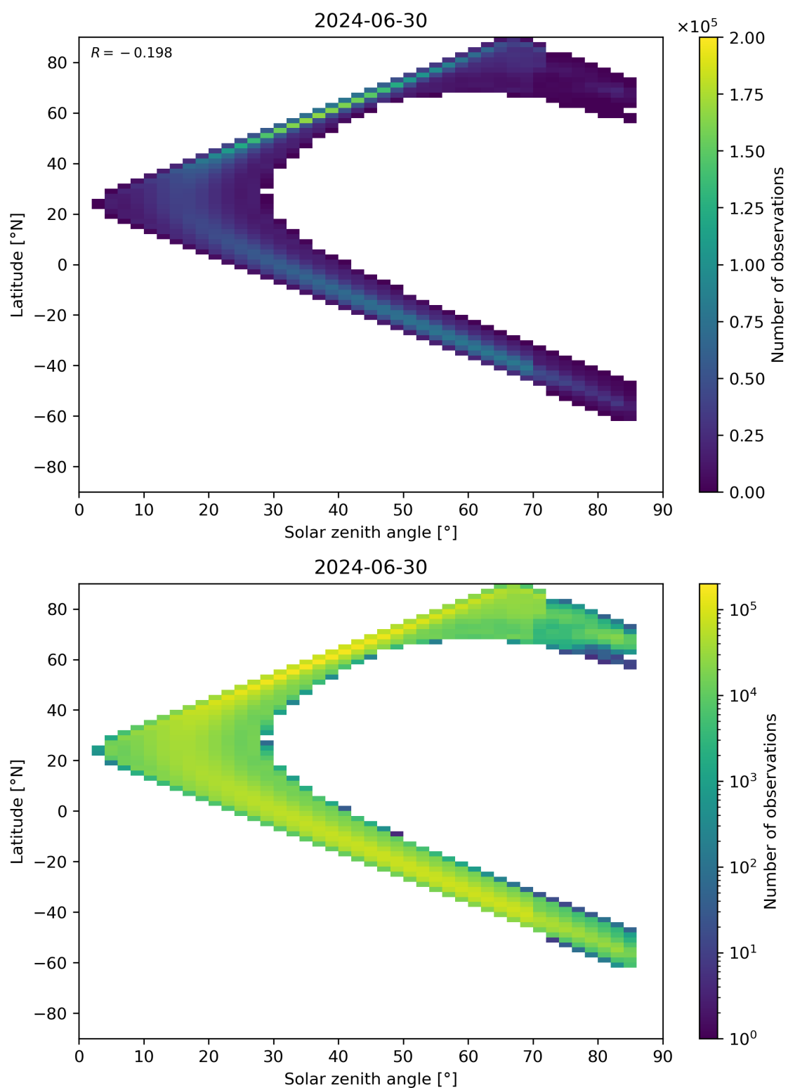
Figure 181: Scatter density plot of “Solar zenith angle” against “Latitude” for 2024-06-29 to 2024-07-01.
