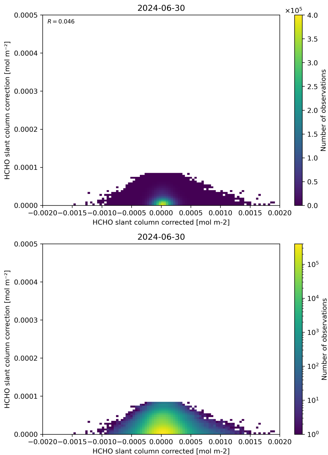
Figure 77: Scatter density plot of “HCHO slant column corrected” against “HCHO slant column correction” for 2024-06-29 to 2024-07-01.
