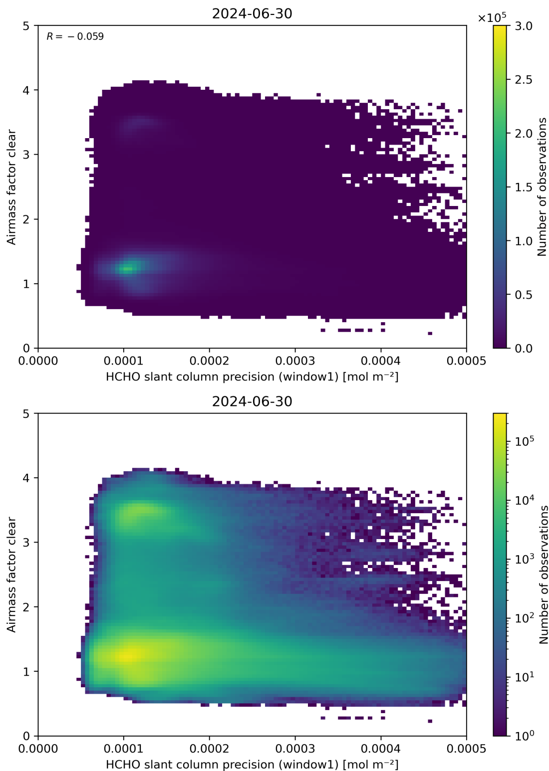
Figure 91: Scatter density plot of “HCHO slant column precision (window1)” against “Airmass factor clear” for 2024-06-29 to 2024-07-01.
