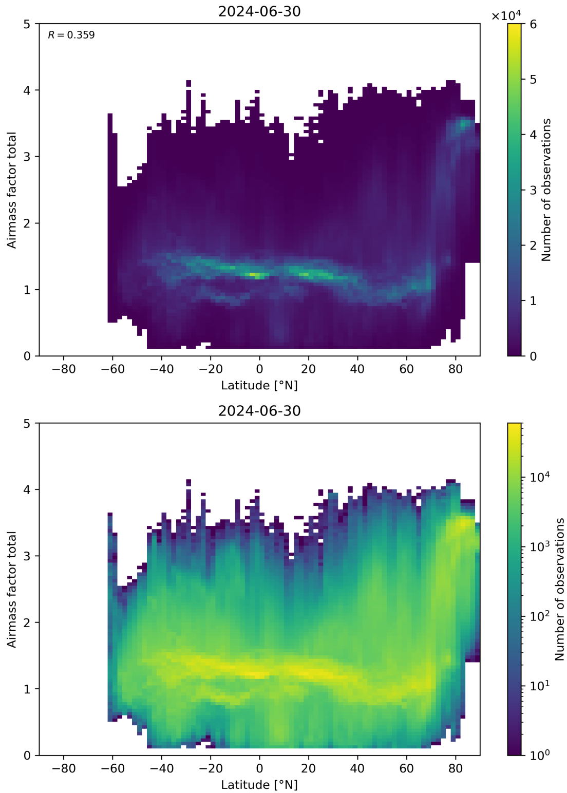
Figure 161: Scatter density plot of “Latitude” against “Airmass factor total” for 2024-06-29 to 2024-07-01.
