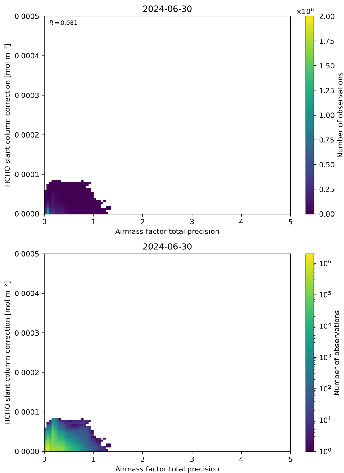
Figure 110: Scatter density plot of “Airmass factor total precision” against “HCHO slant column correction” for 2024-06-29 to 2024-07-01.
