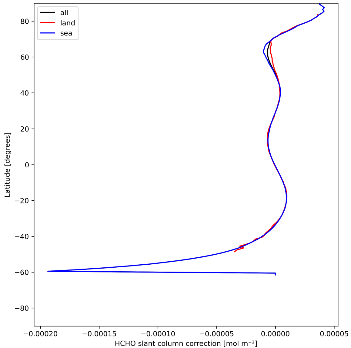
Figure 33: Zonal average of “HCHO slant column correction” for 2024-06-29 to 2024-07-01.
