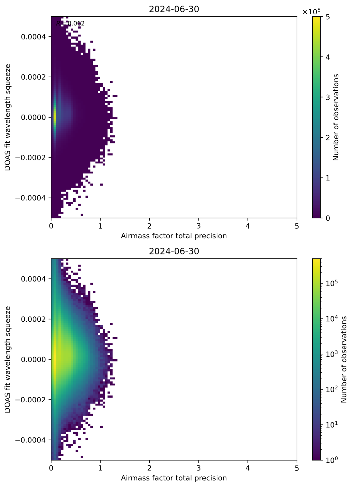
Figure 107: Scatter density plot of “Airmass factor total precision” against “DOAS fit wavelength squeeze” for 2024-06-29 to 2024-07-01.
