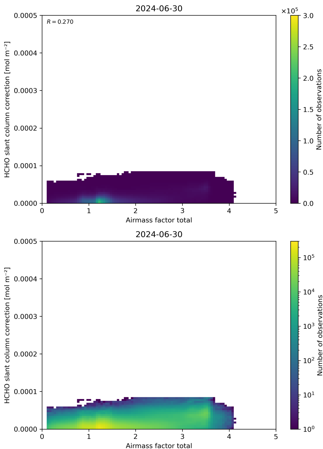
Figure 102: Scatter density plot of “Airmass factor total” against “HCHO slant column correction” for 2024-06-29 to 2024-07-01.
