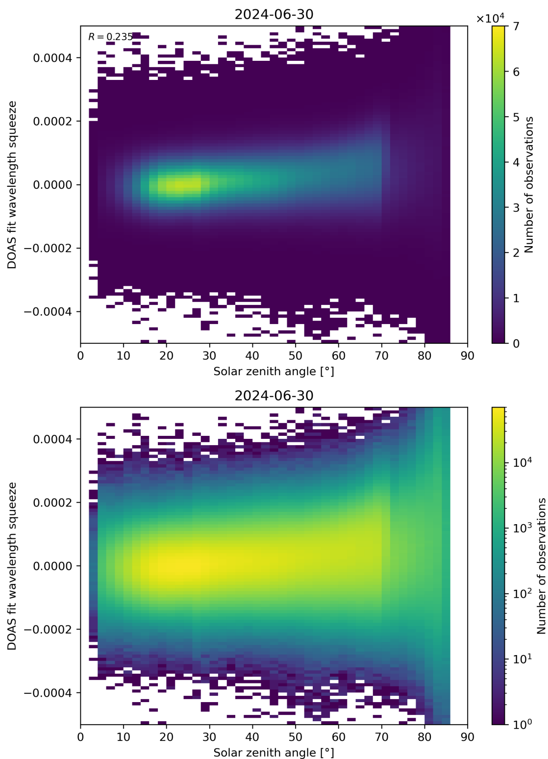
Figure 169: Scatter density plot of “Solar zenith angle” against “DOAS fit wavelength squeeze” for 2024-06-29 to 2024-07-01.
