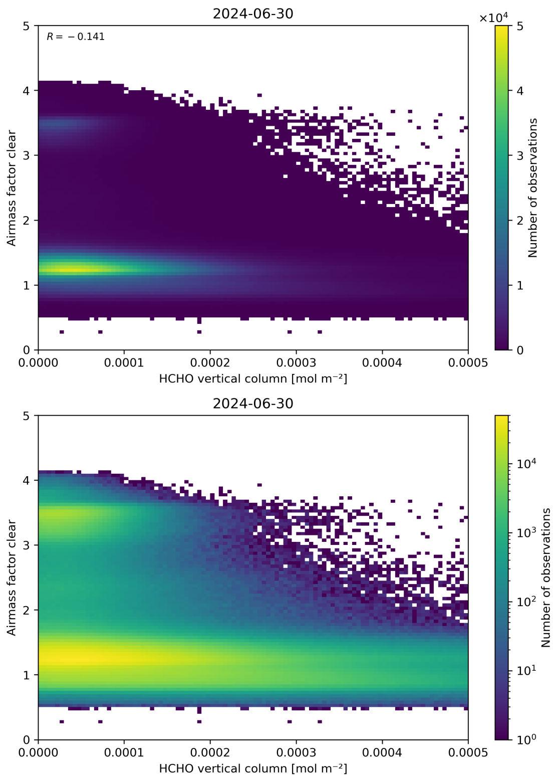
Figure 126: Scatter density plot of “HCHO vertical column” against “Airmass factor clear” for 2024-06-29 to 2024-07-01.
