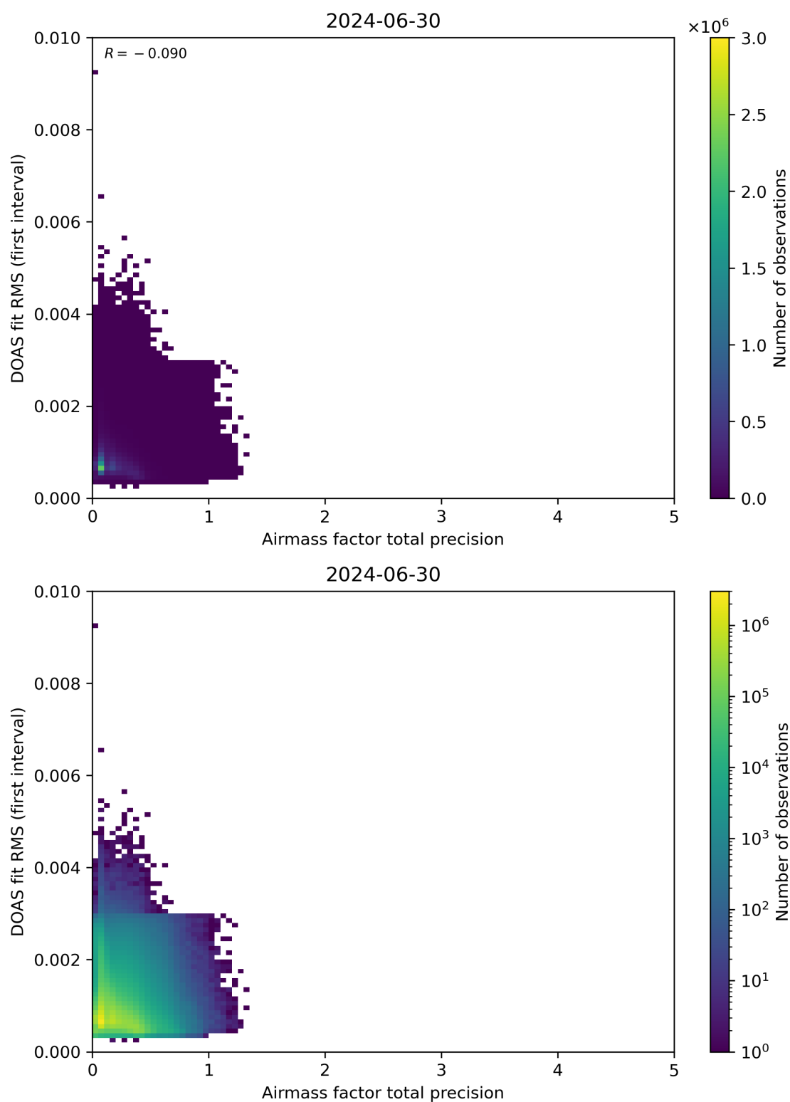
Figure 105: Scatter density plot of “Airmass factor total precision” against “DOAS fit RMS (first interval)” for 2024-06-29 to 2024-07-01.
