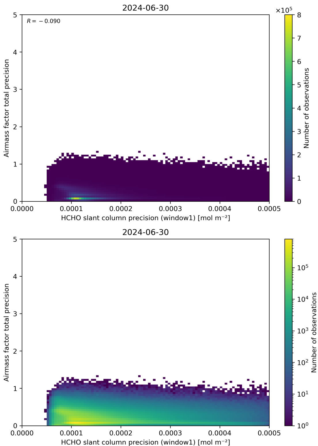
Figure 95: Scatter density plot of “HCHO slant column precision (window1)” against “Airmass factor total precision” for 2024-06-29 to 2024-07-01.
