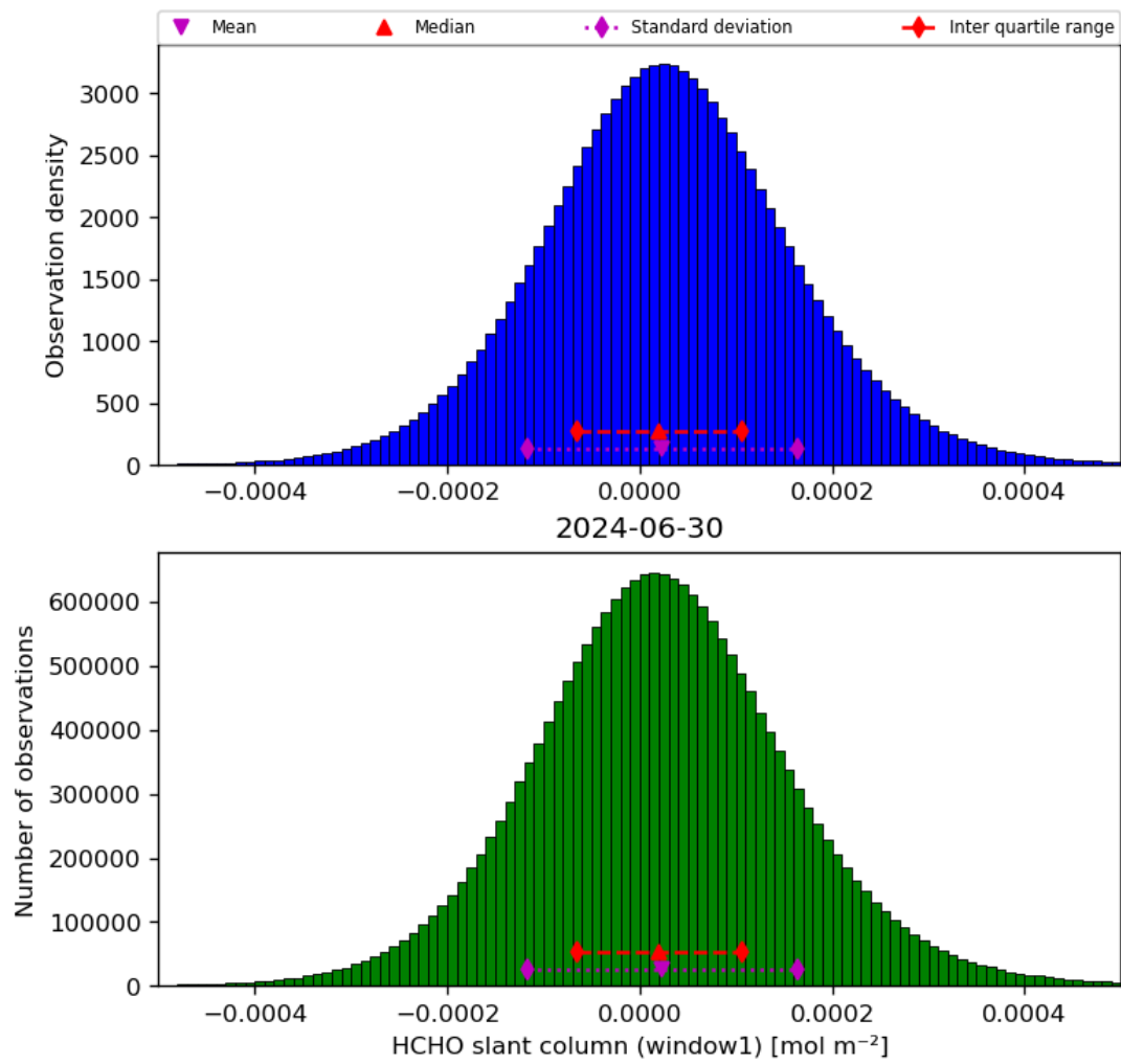
Figure 38: Histogram of “HCHO slant column (window1)” for 2024-06-29 to 2024-07-01
