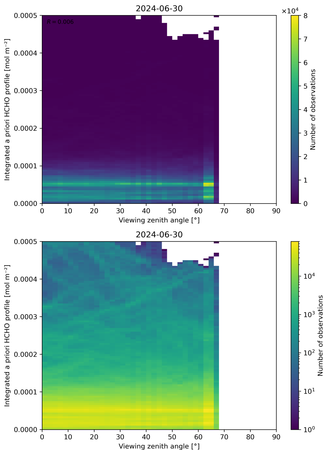
Figure 195: Scatter density plot of “Viewing zenith angle” against “Integrated a priori HCHO profile” for 2024-06-29 to 2024-07-01.
