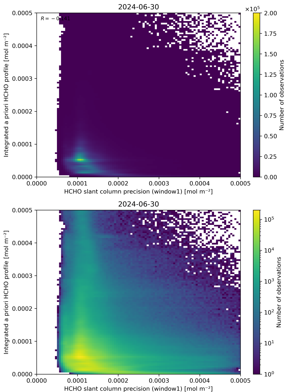
Figure 96: Scatter density plot of “HCHO slant column precision (window1)” against “Integrated a priori HCHO profile” for 2024-06-29 to 2024-07-01.
