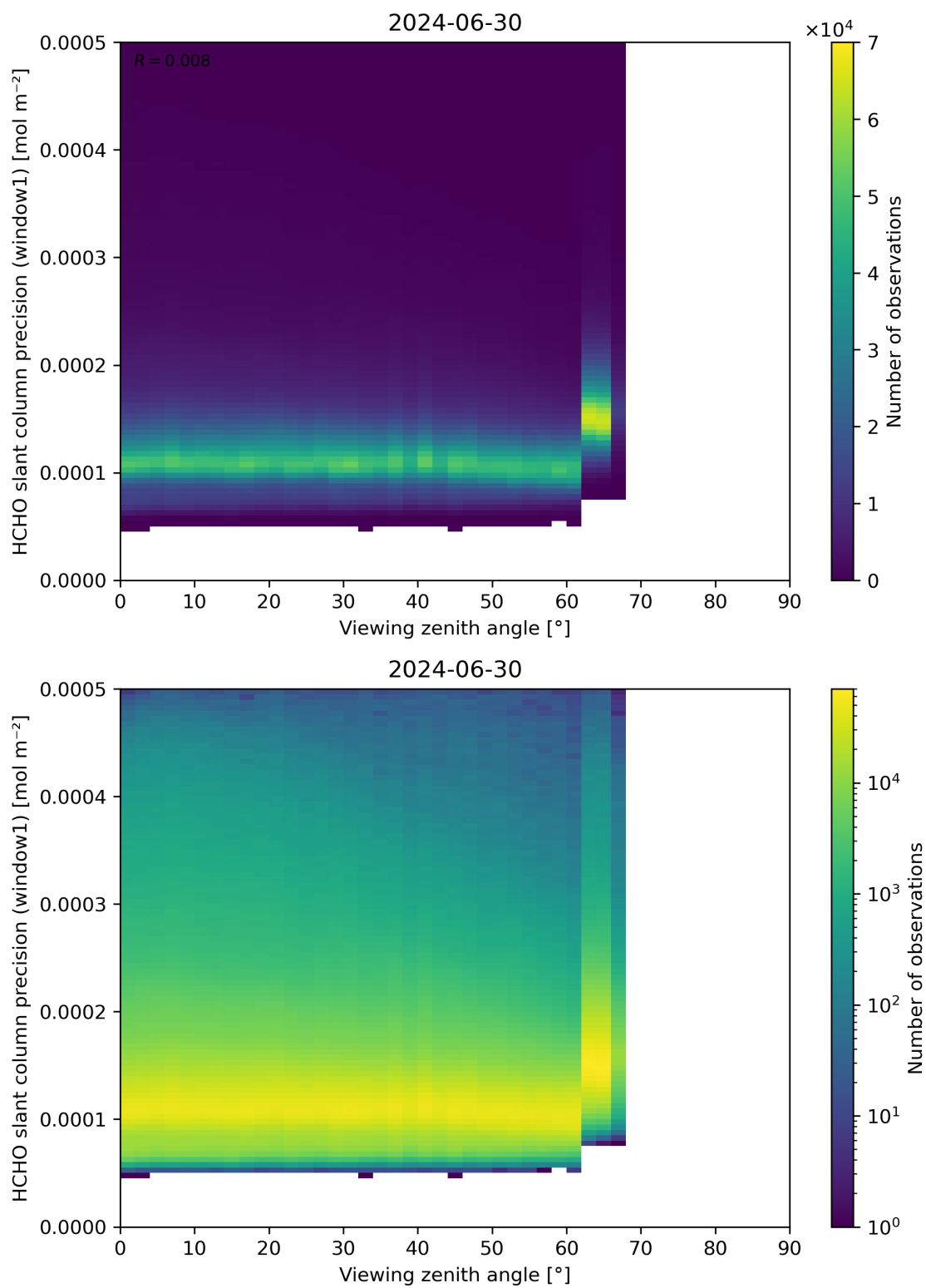
Figure 189: Scatter density plot of “Viewing zenith angle” against “HCHO slant column precision (window1)” for 2024-06-29 to 2024-07-01.
