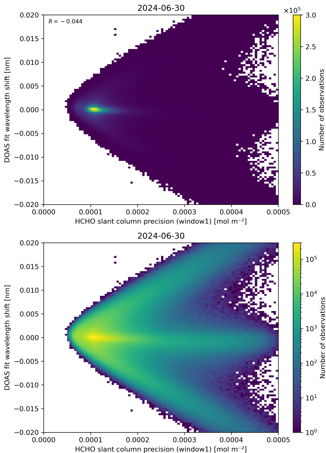
Figure 89: Scatter density plot of “HCHO slant column precision (window1)” against “DOAS fit wavelength shift” for 2024-06-29 to 2024-07-01.
