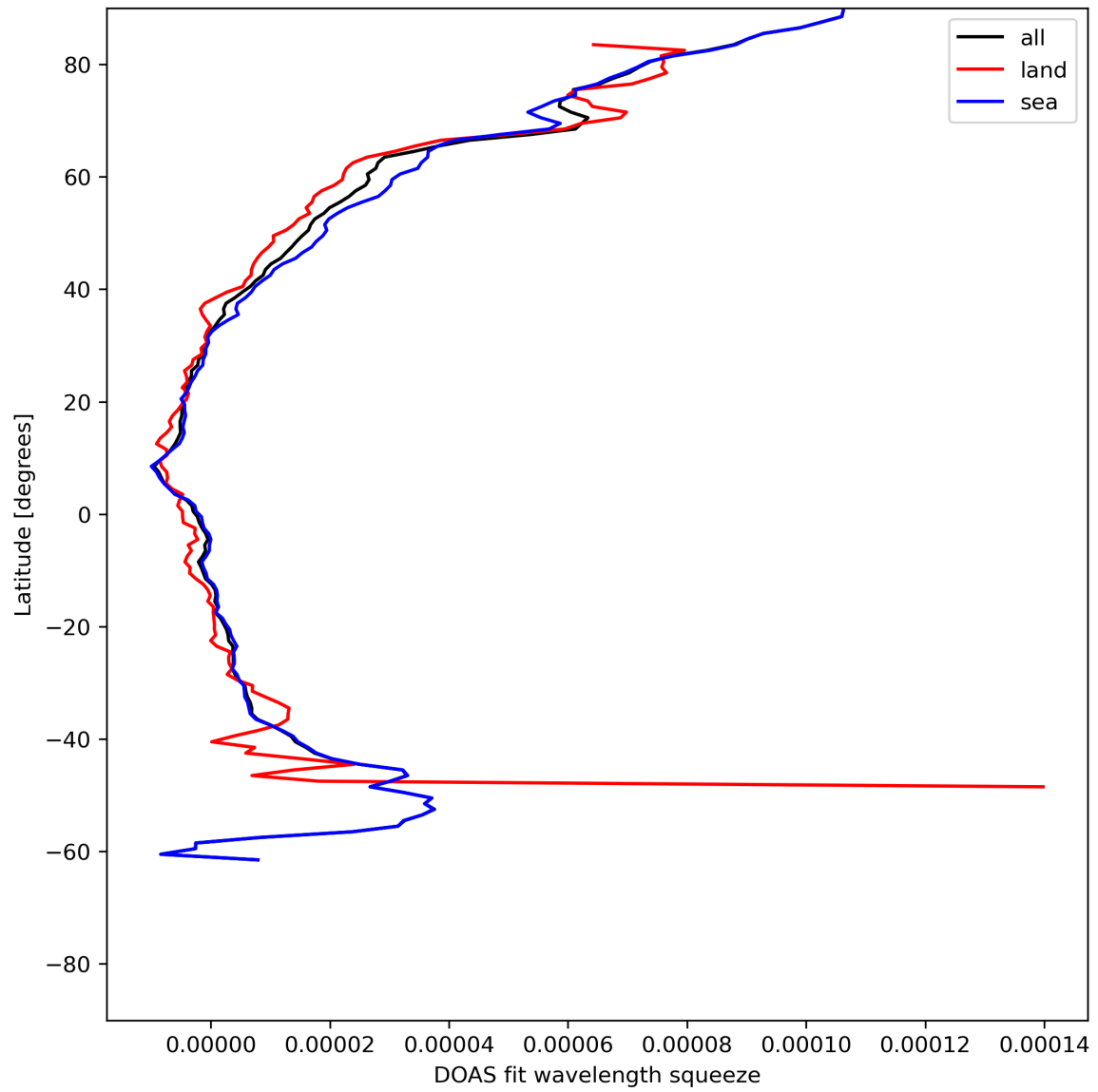
Figure 31: Zonal average of “DOAS fit wavelength squeeze” for 2024-06-29 to 2024-07-01.
