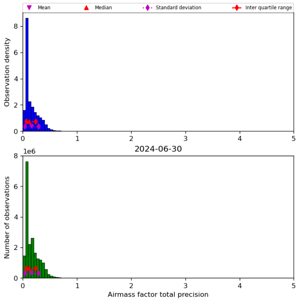
Figure 41: Histogram of “Airmass factor total precision” for 2024-06-29 to 2024-07-01
