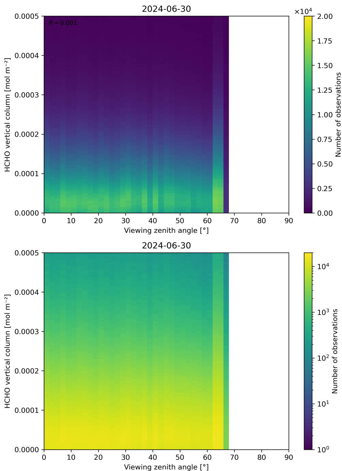
Figure 192: Scatter density plot of “Viewing zenith angle” against “HCHO vertical column” for 2024-06-29 to 2024-07-01.
