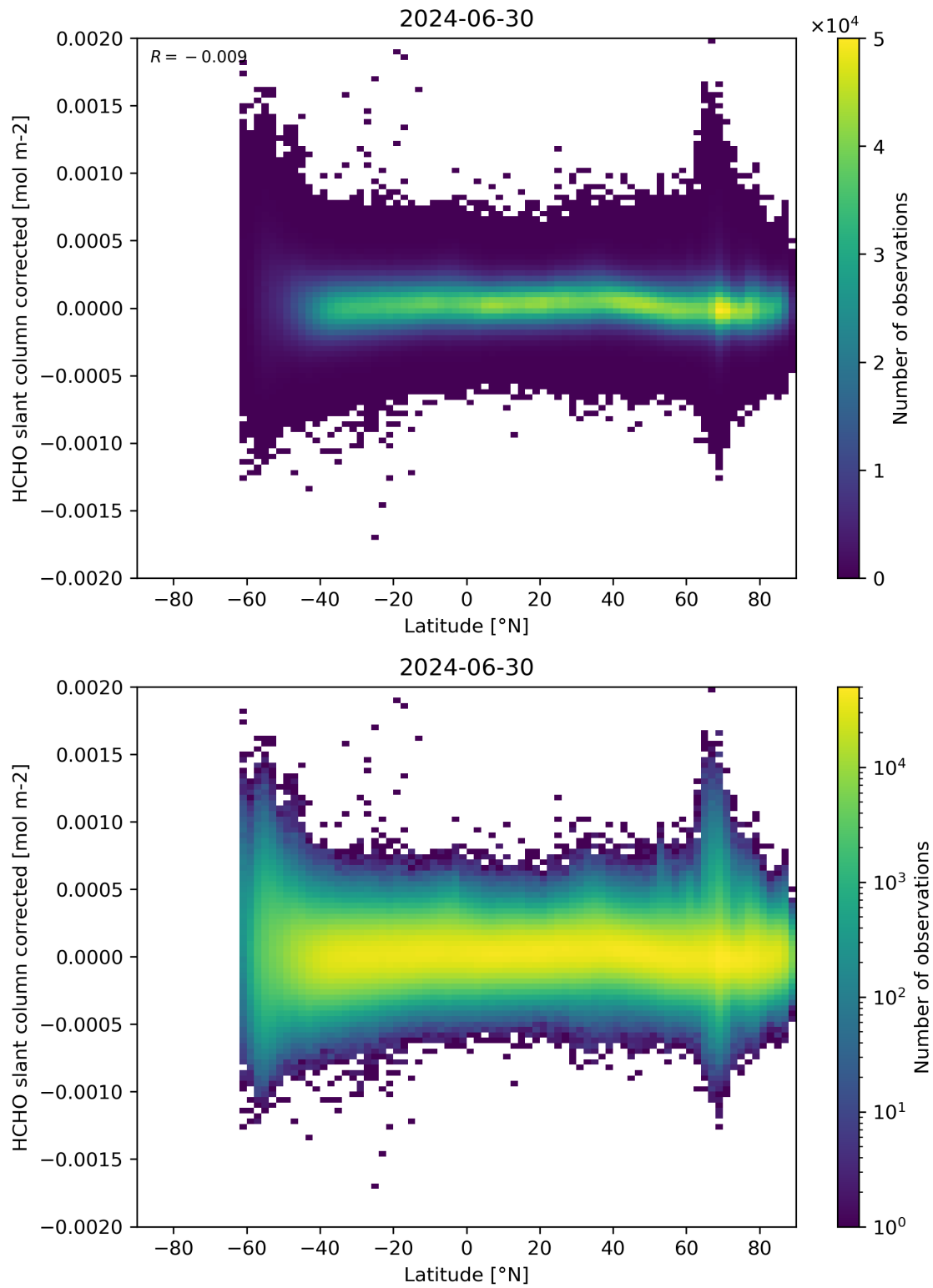
Figure 157: Scatter density plot of “Latitude” against “HCHO slant column corrected” for 2024-06-29 to 2024-07-01.
