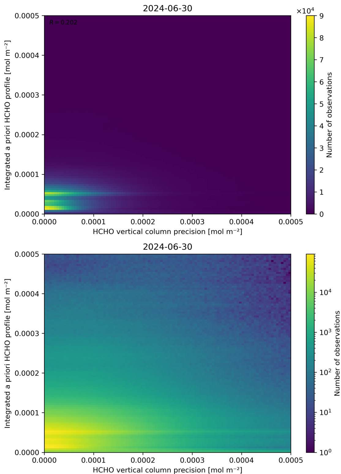
Figure 147: Scatter density plot of “HCHO vertical column precision” against “Integrated a priori HCHO profile” for 2024-06-29 to 2024-07-01.
