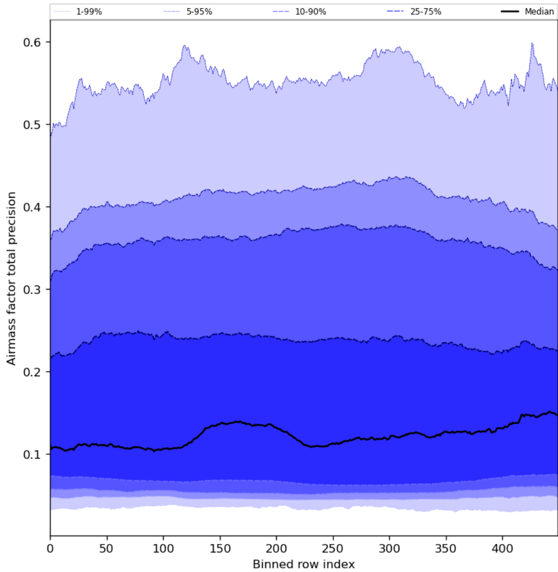
Figure 55: Along track statistics of “Airmass factor total precision” for 2024-06-29 to 2024-07-01
