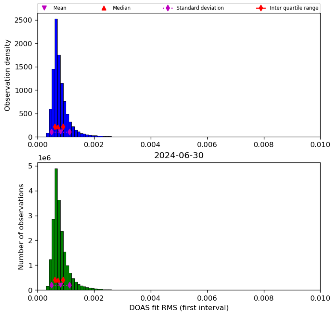
Figure 46: Histogram of “DOAS fit RMS (first interval)” for 2024-06-29 to 2024-07-01
