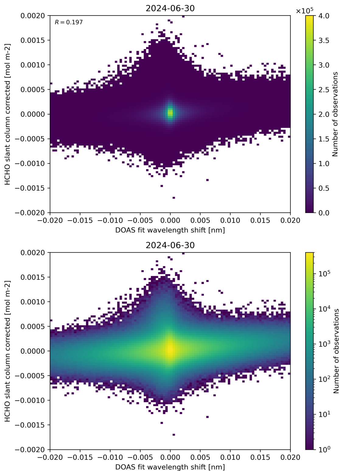
Figure 66: Scatter density plot of “DOAS fit wavelength shift” against “HCHO slant column corrected” for 2024-06-29 to 2024-07-01.
