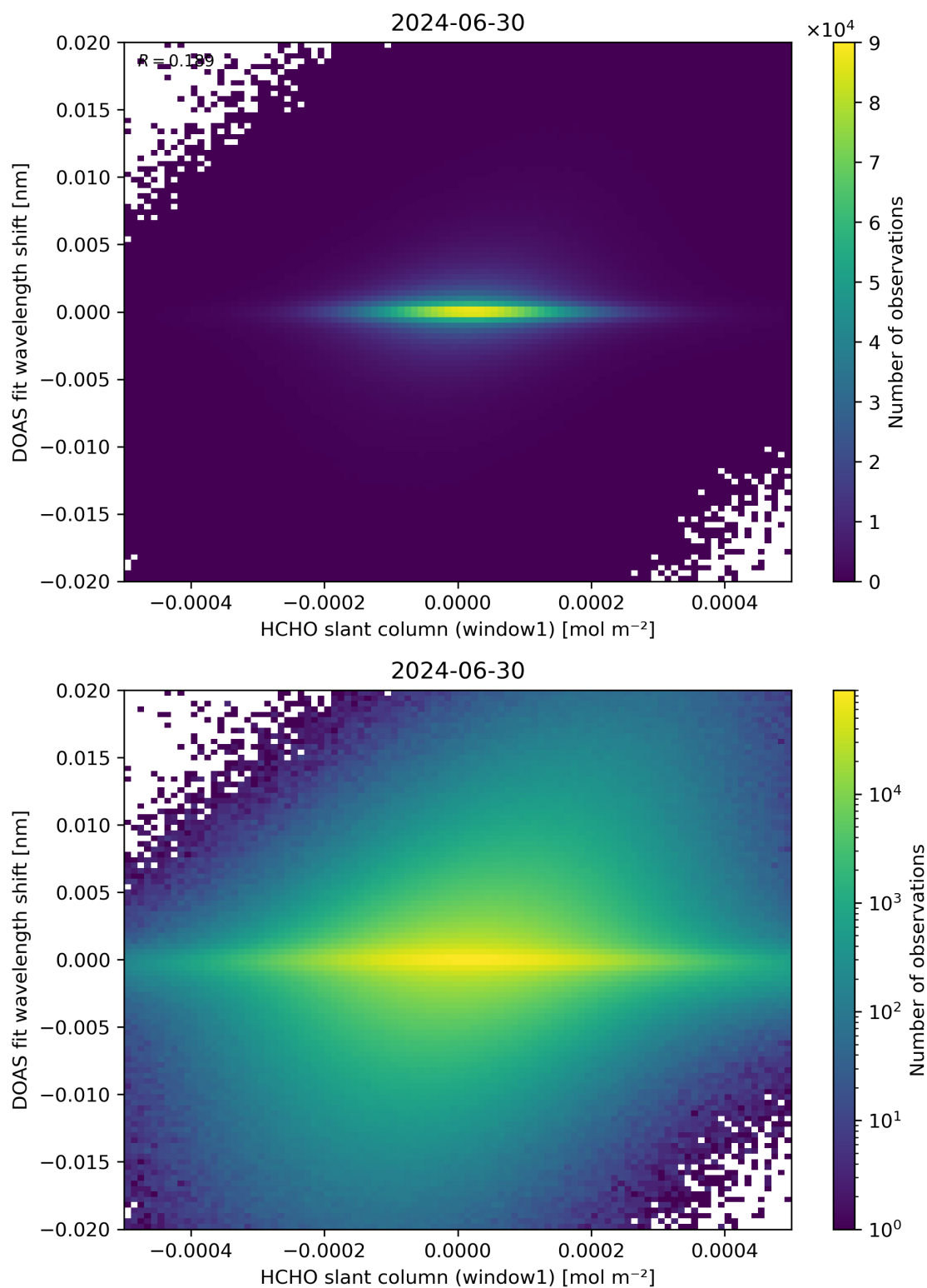
Figure 79: Scatter density plot of “HCHO slant column (window1)” against “DOAS fit wavelength shift” for 2024-06-29 to 2024-07-01.
