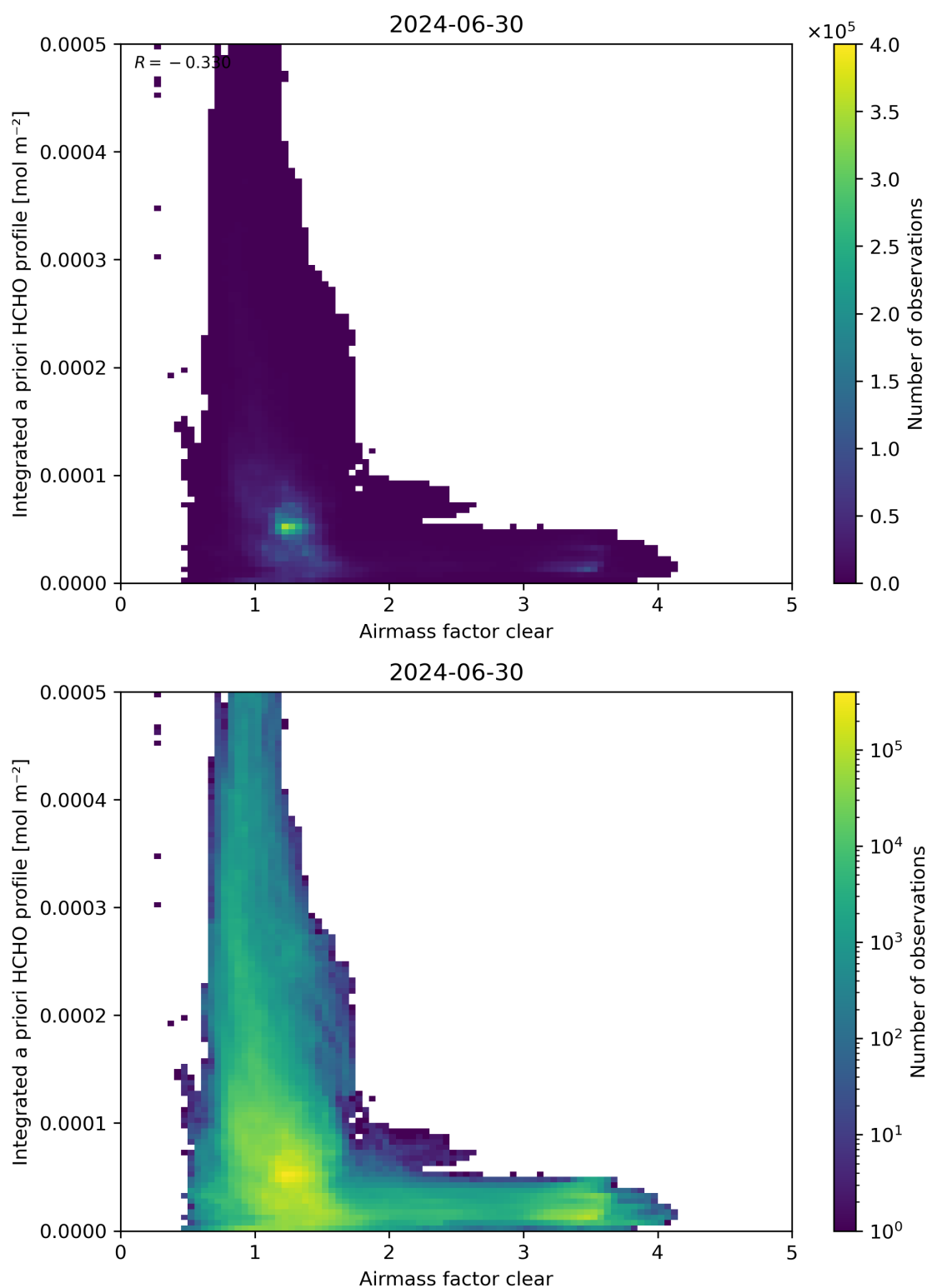
Figure 76: Scatter density plot of “Airmass factor clear” against “Integrated a priori HCHO profile” for 2024-06-29 to 2024-07-01.
