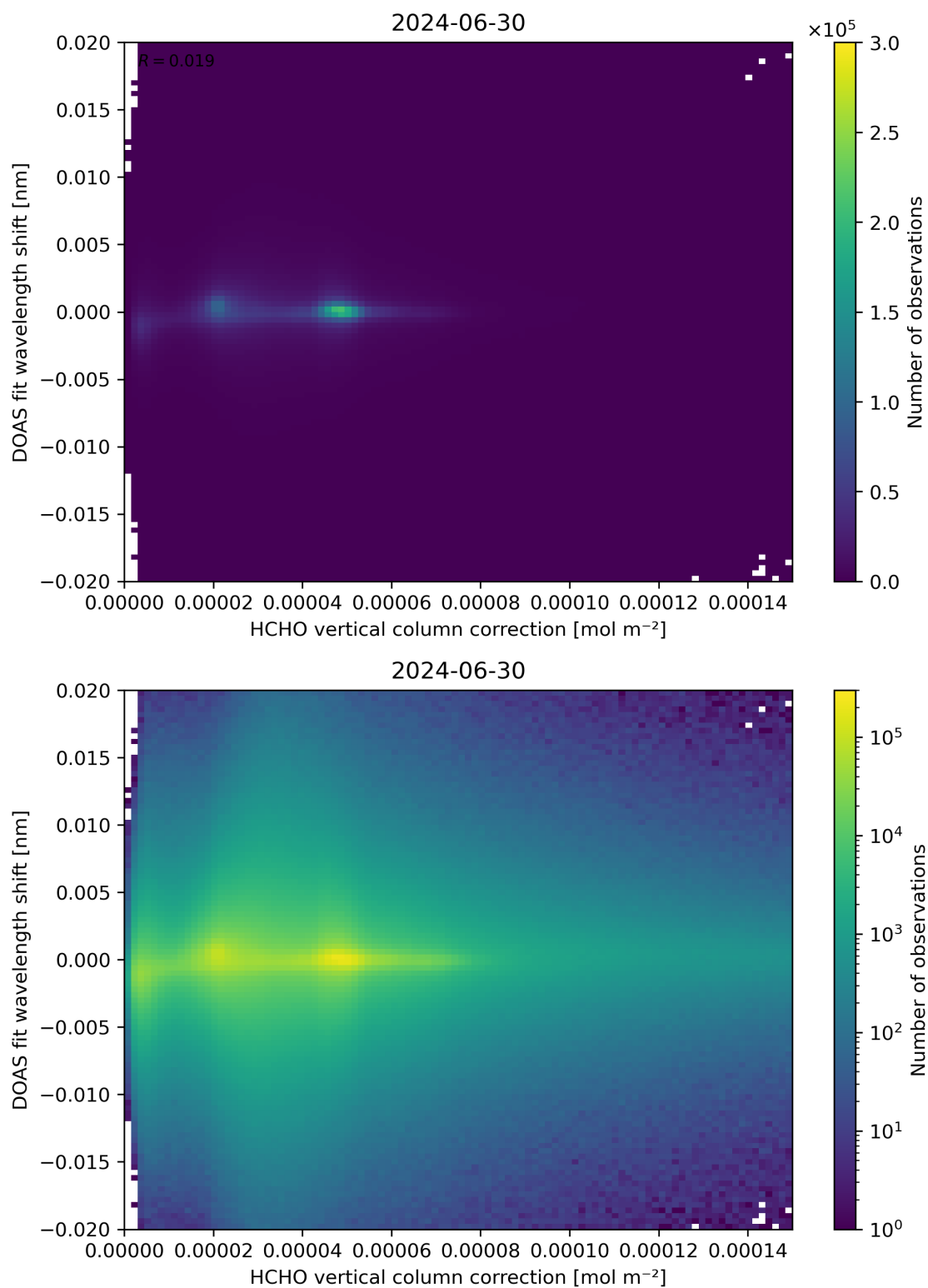
Figure 113: Scatter density plot of “HCHO vertical column correction” against “DOAS fit wavelength shift” for 2024-06-29 to 2024-07-01.
