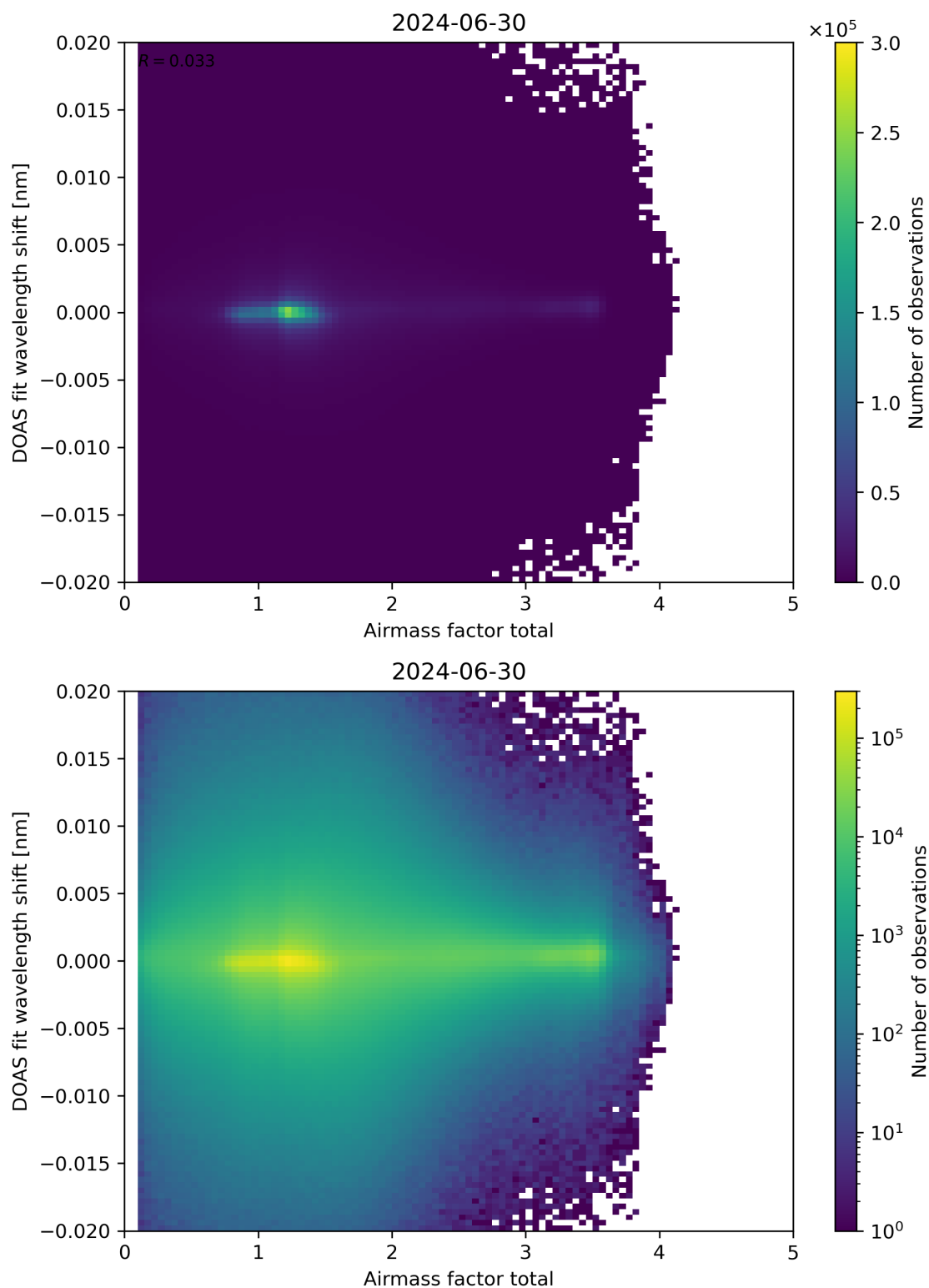
Figure 98: Scatter density plot of “Airmass factor total” against “DOAS fit wavelength shift” for 2024-06-29 to 2024-07-01.
