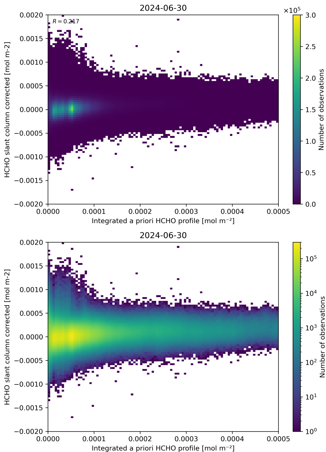
Figure 151: Scatter density plot of “Integrated a priori HCHO profile” against “HCHO slant column corrected” for 2024-06-29 to 2024-07-01.
