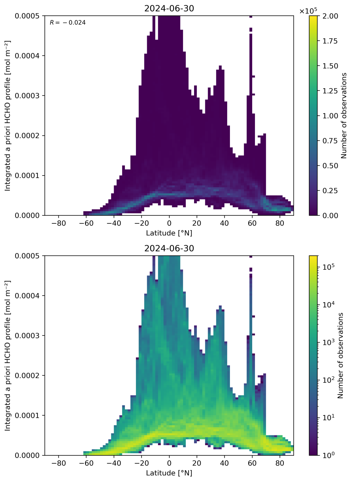
Figure 166: Scatter density plot of “Latitude” against “Integrated a priori HCHO profile” for 2024-06-29 to 2024-07-01.
