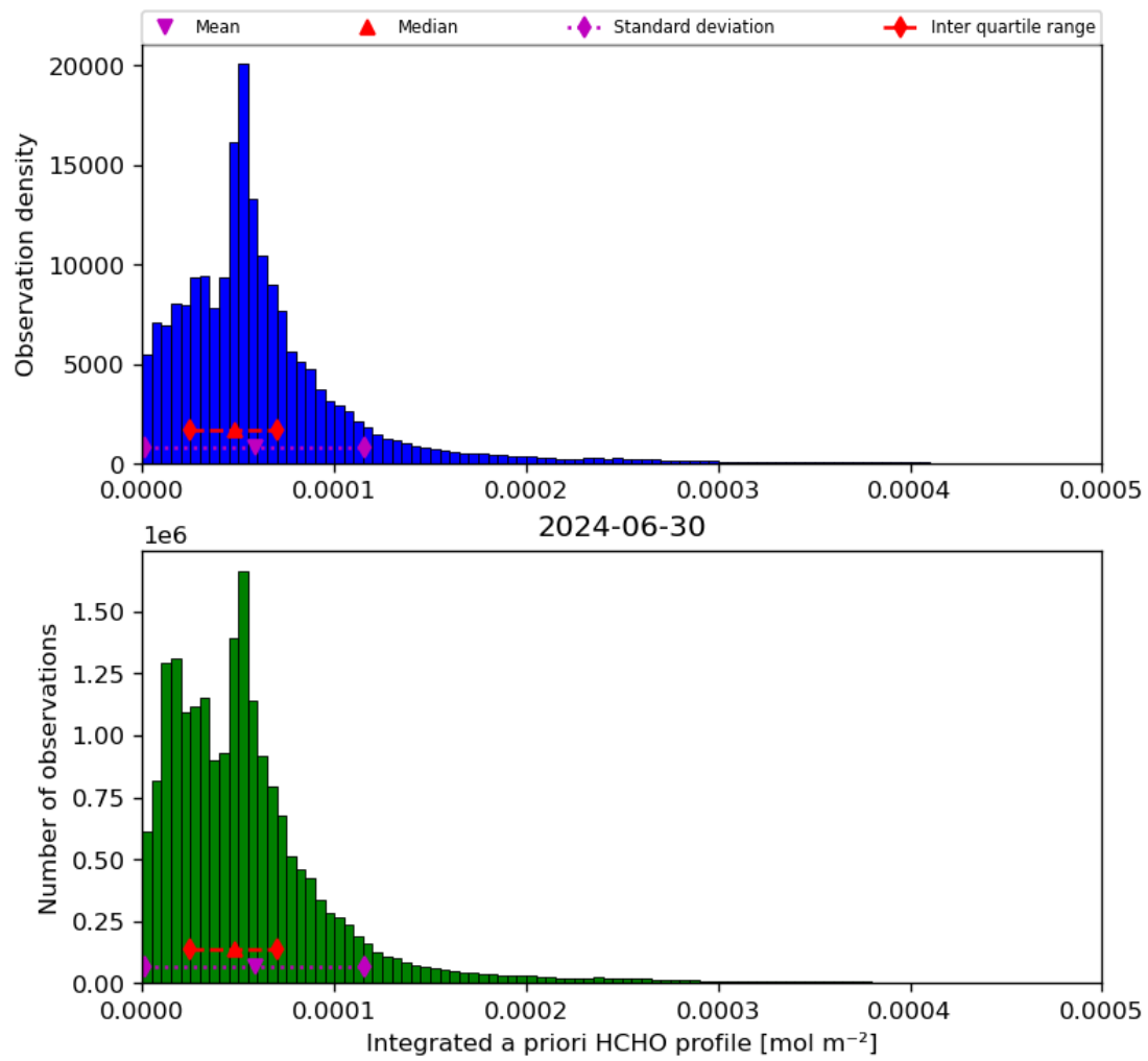
Figure 43: Histogram of “Integrated a priori HCHO profile” for 2024-06-29 to 2024-07-01
