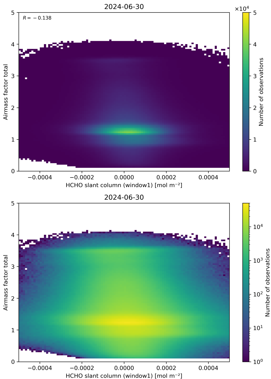
Figure 85: Scatter density plot of “HCHO slant column (window1)” against “Airmass factor total” for 2024-06-29 to 2024-07-01.
