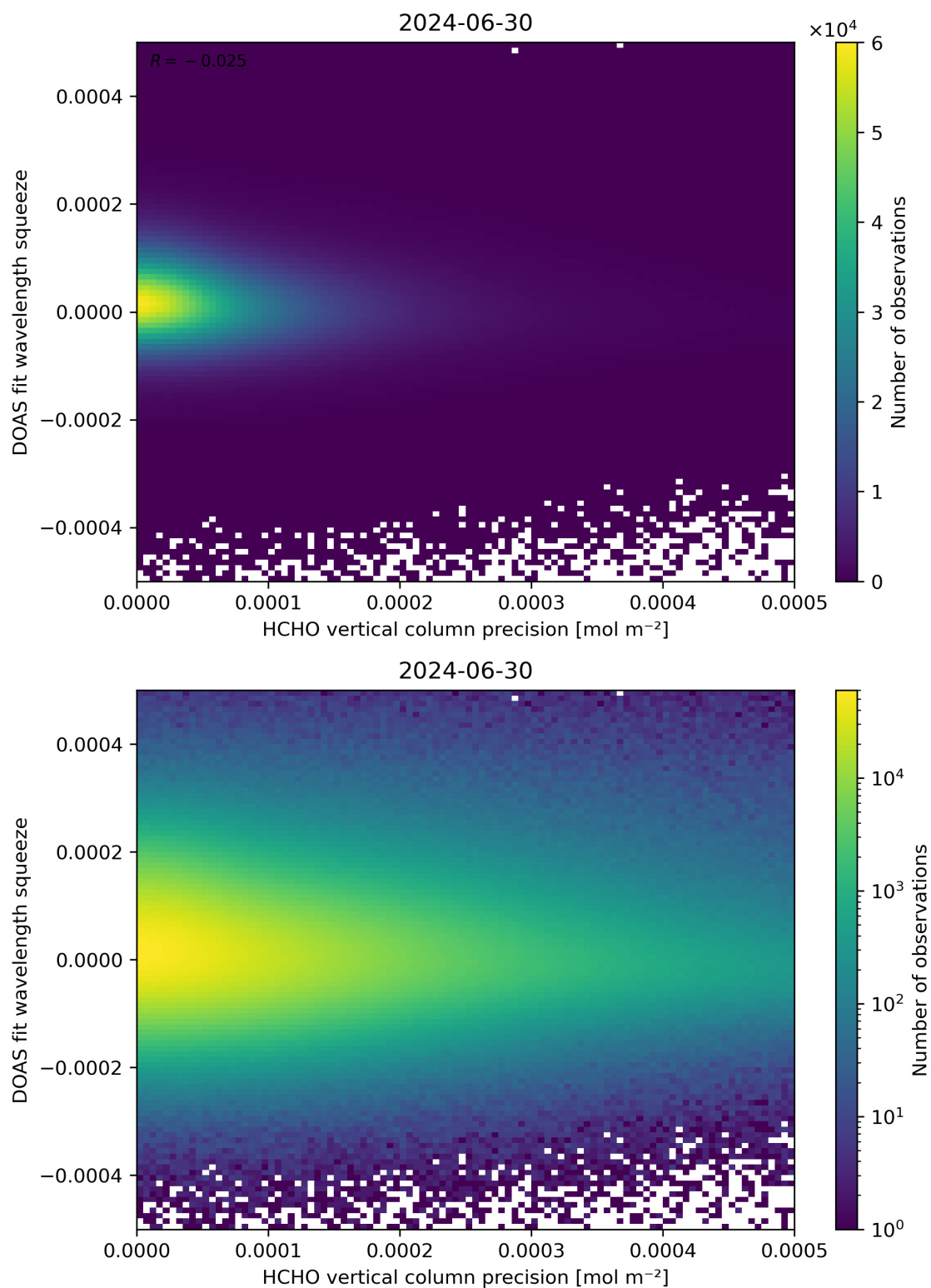
Figure 138: Scatter density plot of “HCHO vertical column precision” against “DOAS fit wavelength squeeze” for 2024-06-29 to 2024-07-01.
