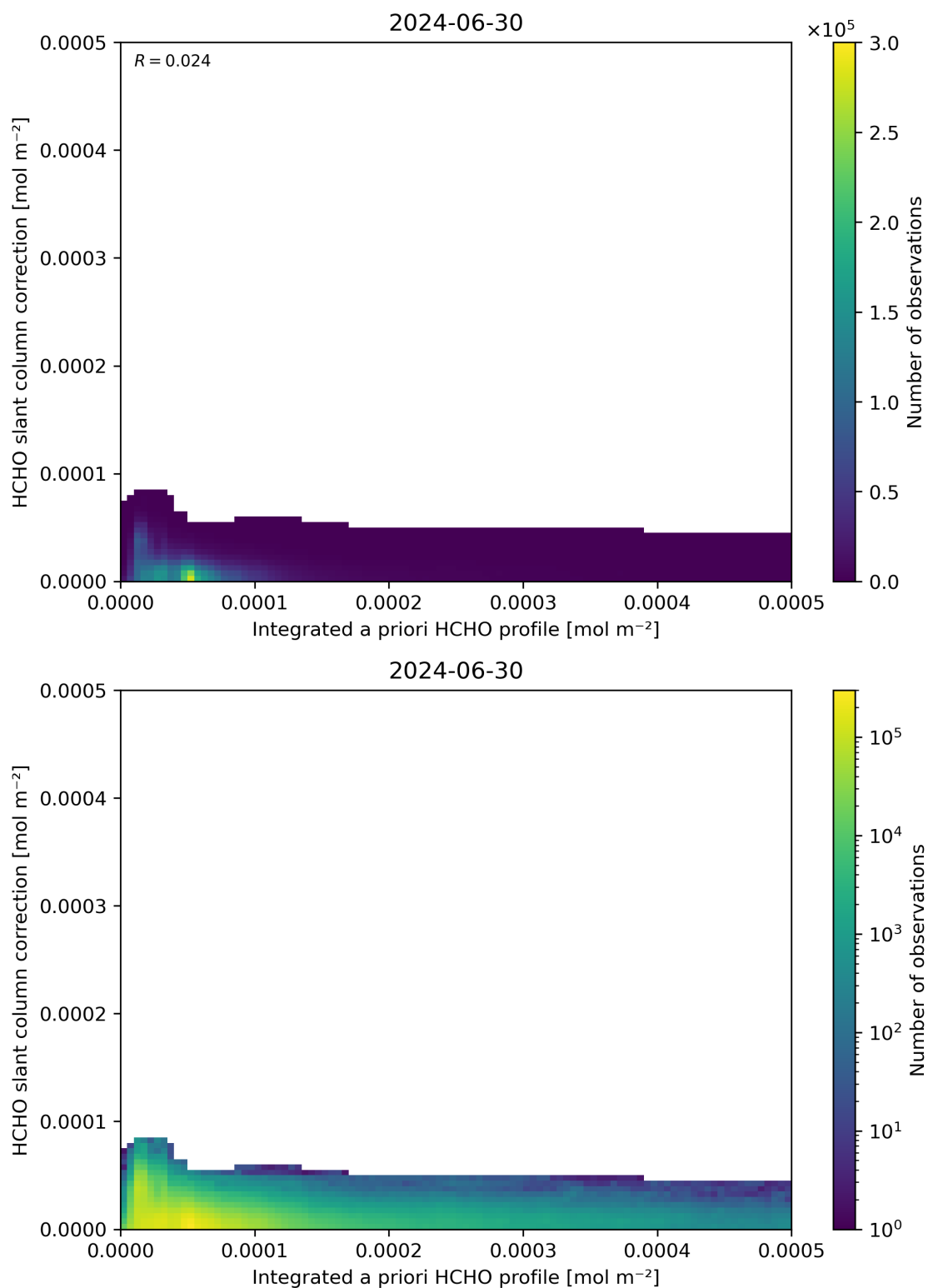
Figure 152: Scatter density plot of “Integrated a priori HCHO profile” against “HCHO slant column correction” for 2024-06-29 to 2024-07-01.
