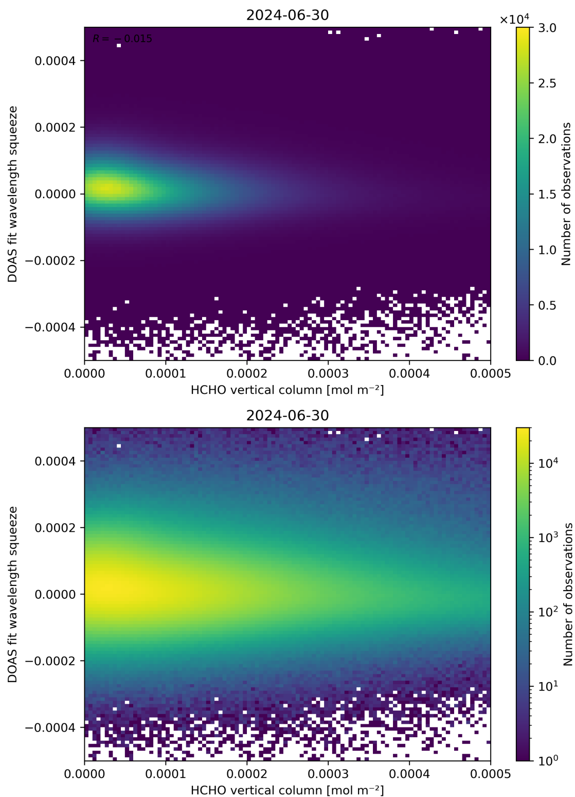
Figure 125: Scatter density plot of “HCHO vertical column” against “DOAS fit wavelength squeeze” for 2024-06-29 to 2024-07-01.
