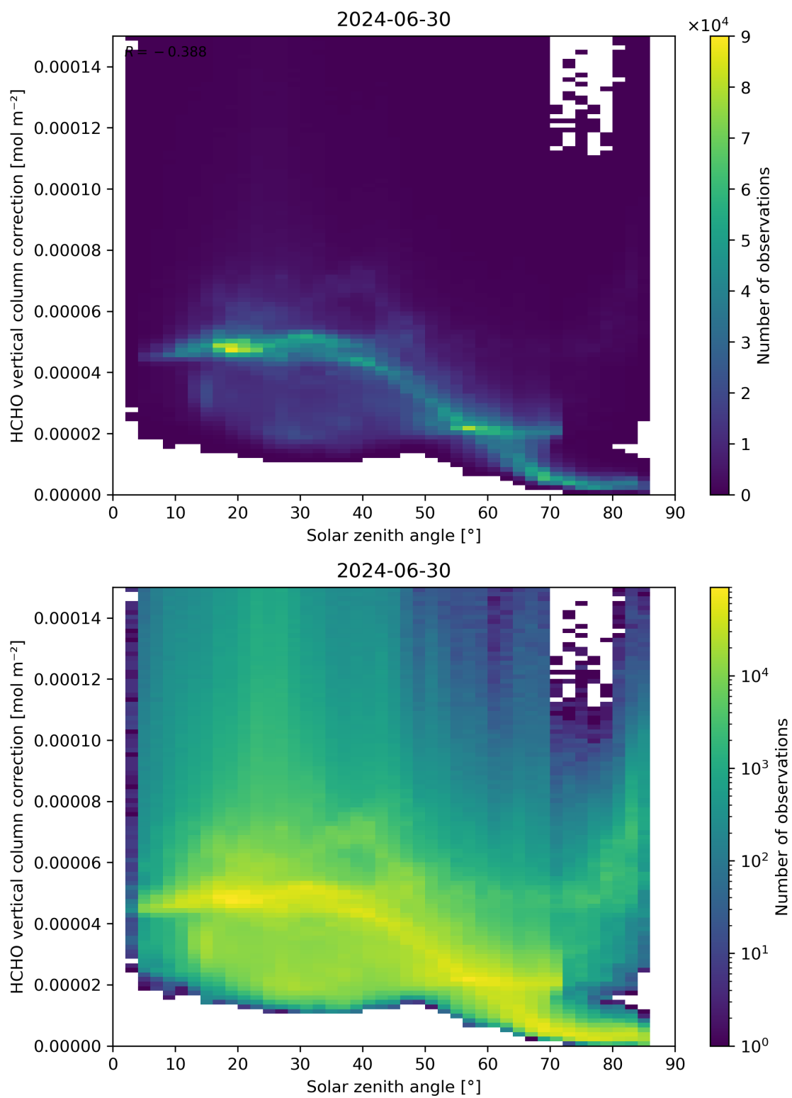
Figure 178: Scatter density plot of “Solar zenith angle” against “HCHO vertical column correction” for 2024-06-29 to 2024-07-01.
