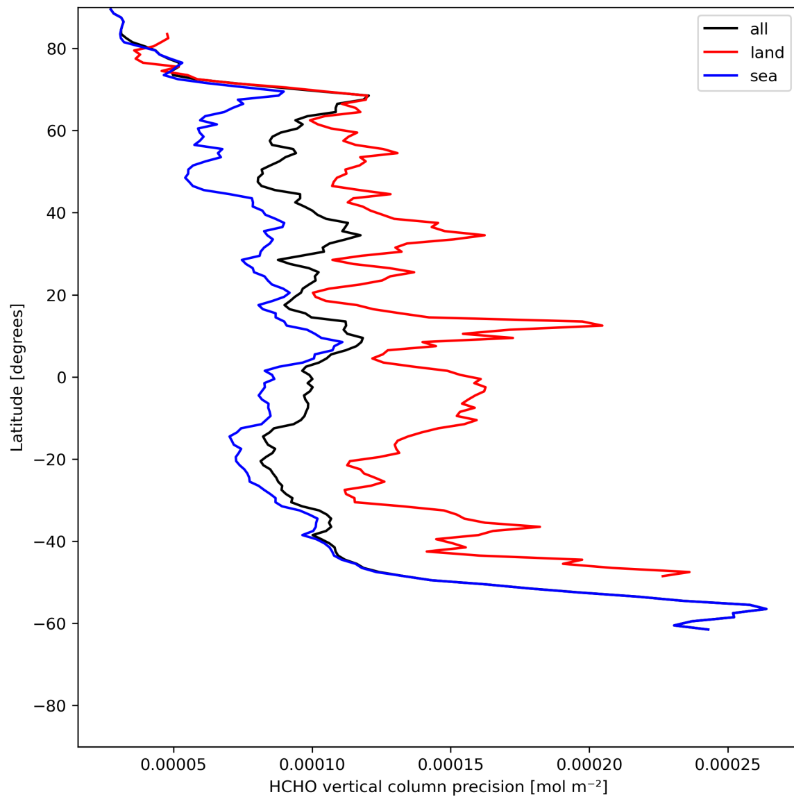
Figure 22: Zonal average of “HCHO vertical column precision” for 2024-06-29 to 2024-07-01.
