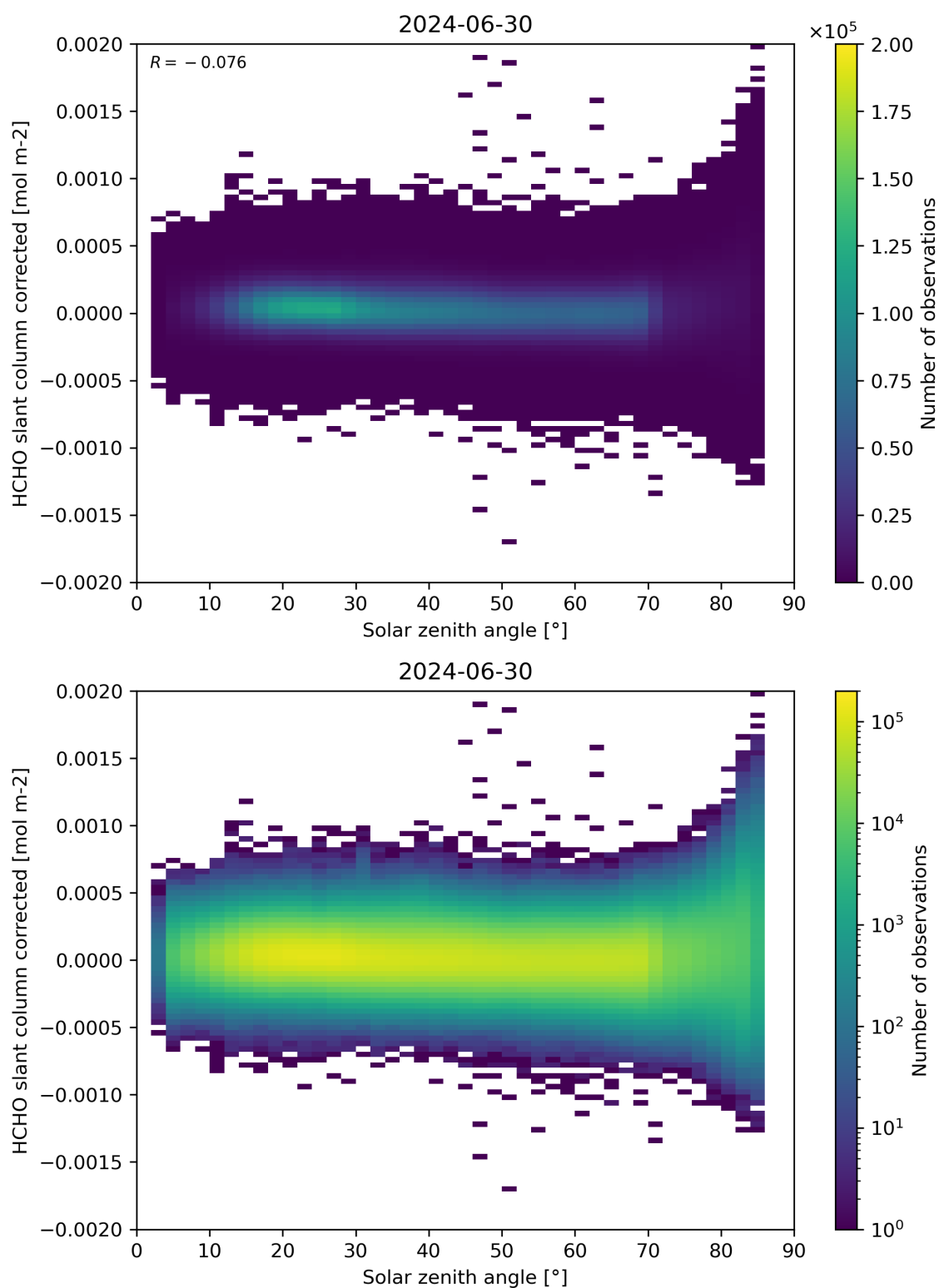
Figure 171: Scatter density plot of “Solar zenith angle” against “HCHO slant column corrected” for 2024-06-29 to 2024-07-01.
