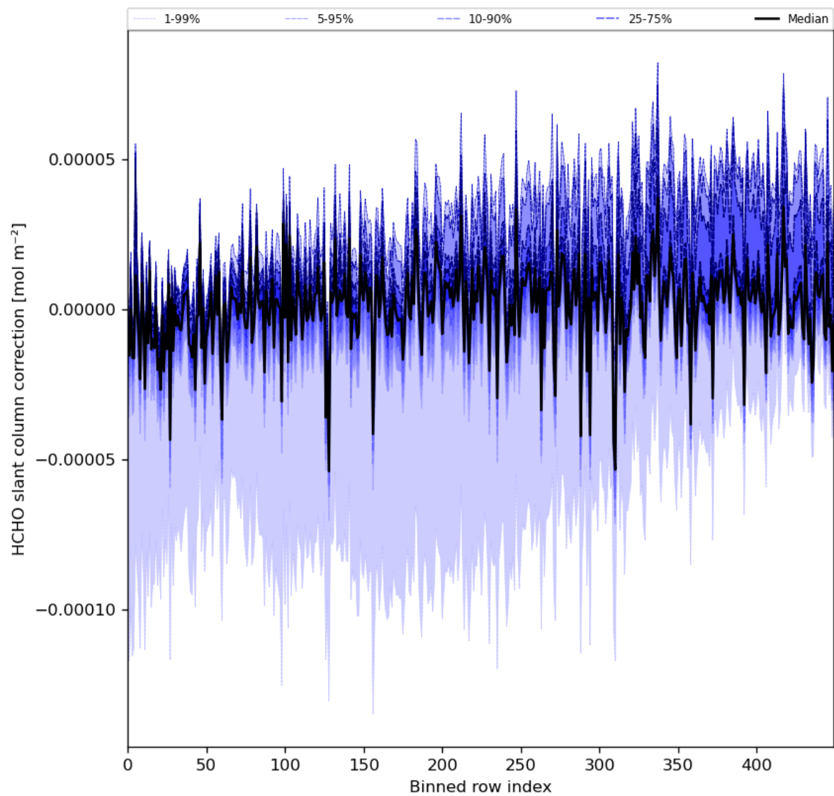
Figure 61: Along track statistics of “HCHO slant column correction” for 2024-06-29 to 2024-07-01
