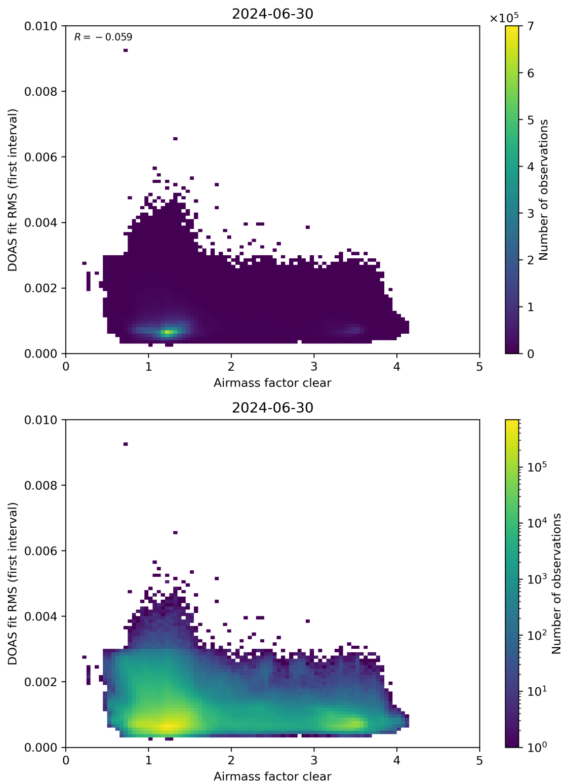
Figure 71: Scatter density plot of “Airmass factor clear” against “DOAS fit RMS (first interval)” for 2024-06-29 to 2024-07-01.
