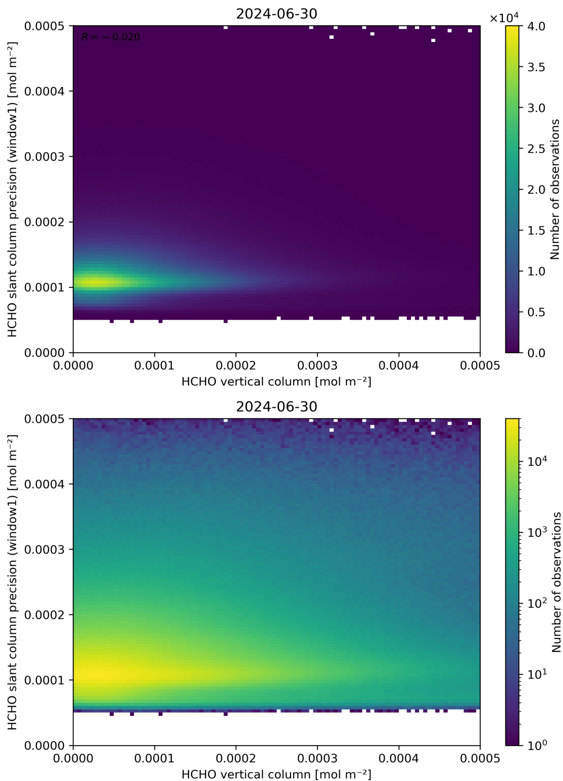
Figure 130: Scatter density plot of “HCHO vertical column” against “HCHO slant column precision (window1)” for 2024-06-29 to 2024-07-01.
