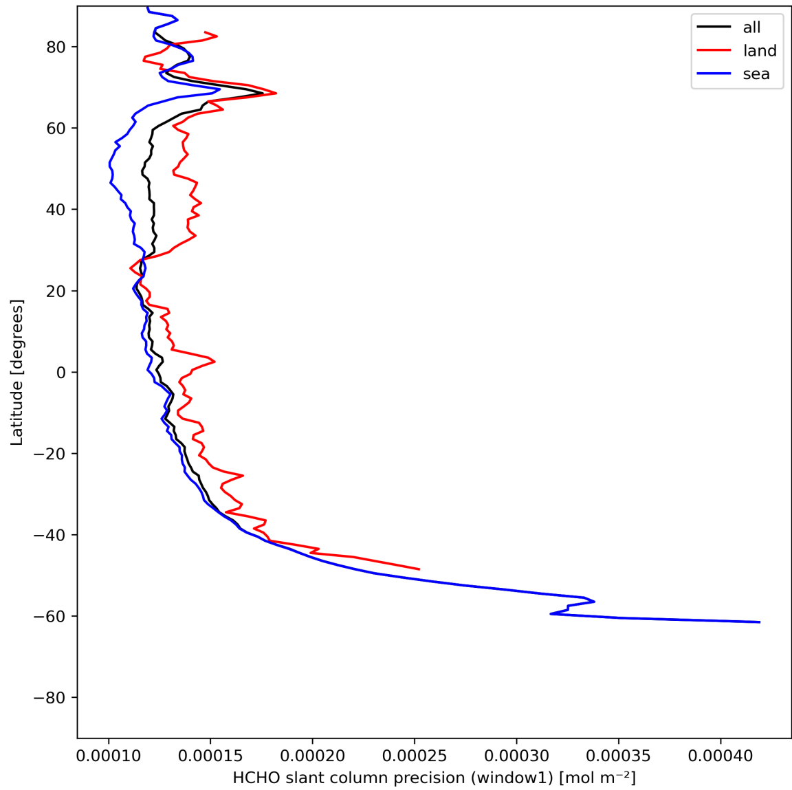
Figure 25: Zonal average of "HCHO slant column precision (window1)" for 2024-06-29 to 2024-07-01.
