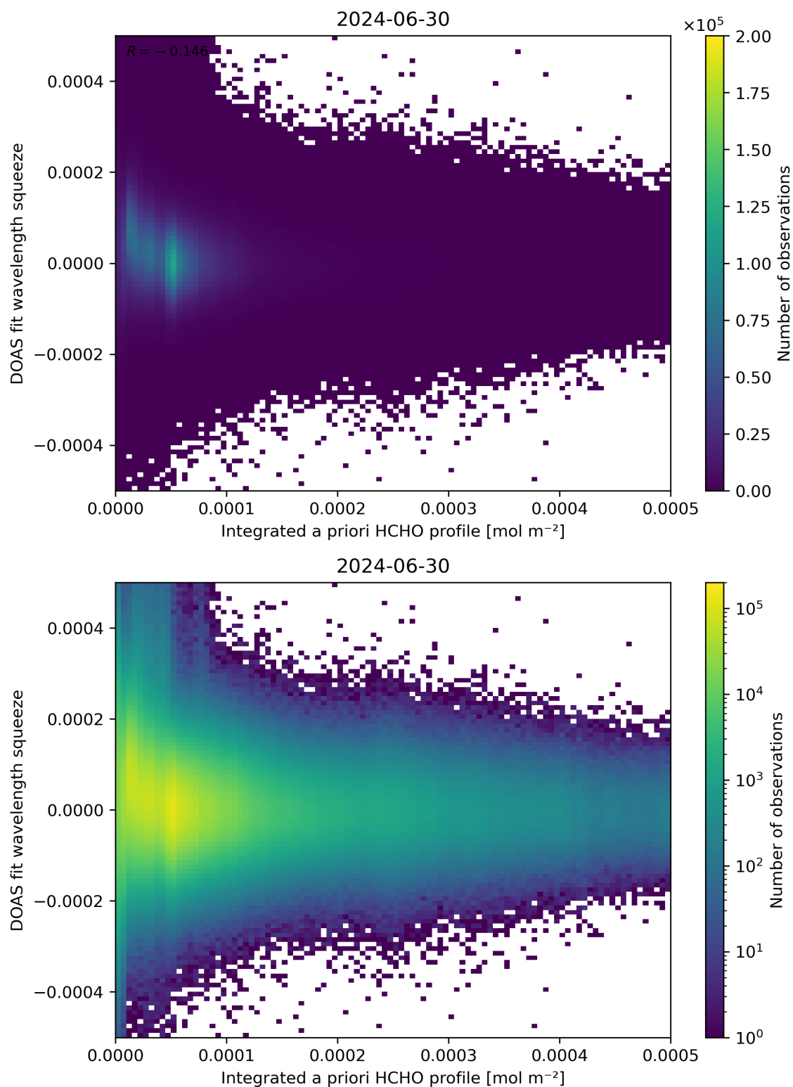
Figure 150: Scatter density plot of “Integrated a priori HCHO profile” against “DOAS fit wavelength squeeze” for 2024-06-29 to 2024-07-01.
