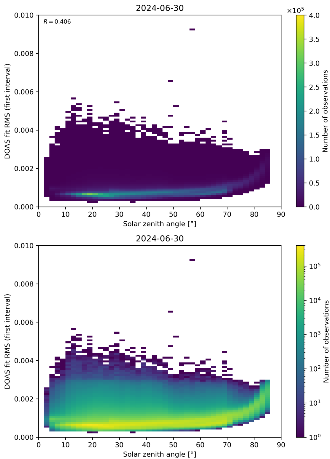
Figure 167: Scatter density plot of “Solar zenith angle” against “DOAS fit RMS (first interval)” for 2024-06-29 to 2024-07-01.
