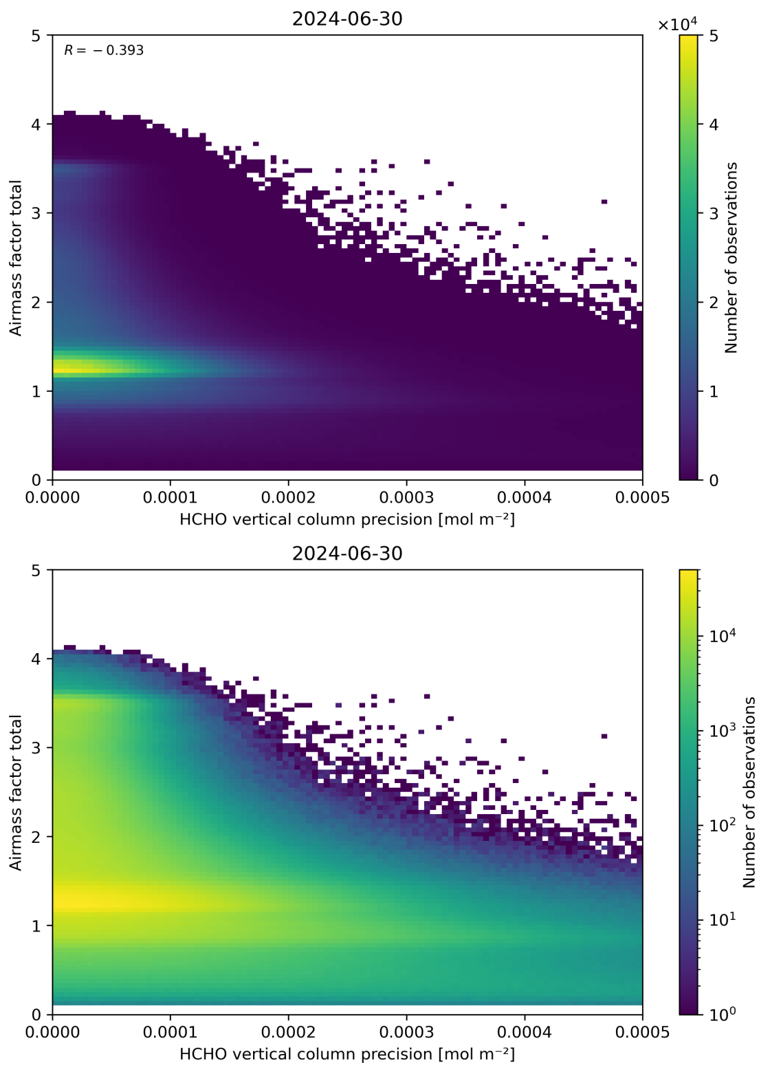
Figure 144: Scatter density plot of “HCHO vertical column precision” against “Airmass factor total” for 2024-06-29 to 2024-07-01.
