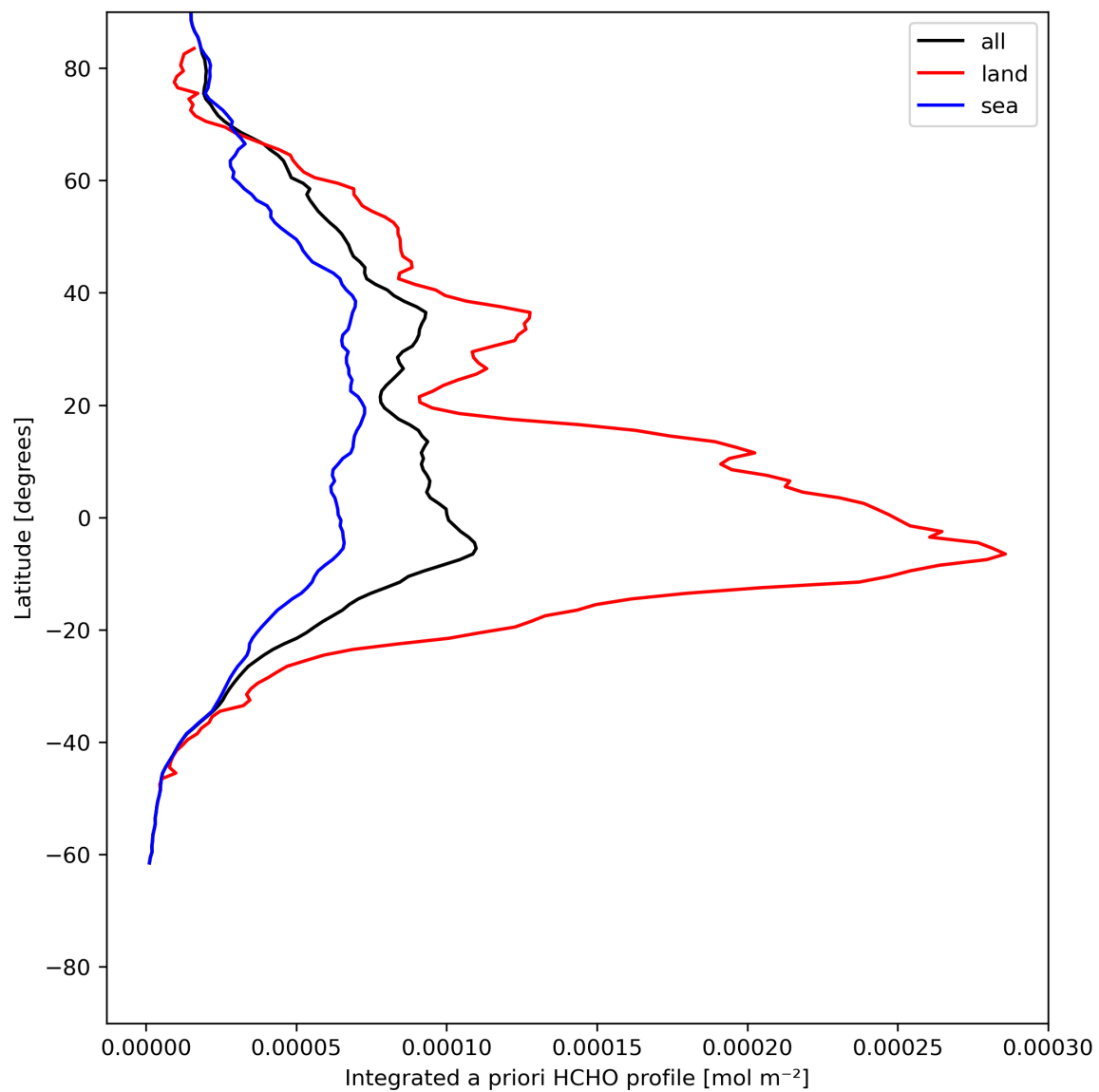
Figure 29: Zonal average of “Integrated a priori HCHO profile” for 2024-06-29 to 2024-07-01.
