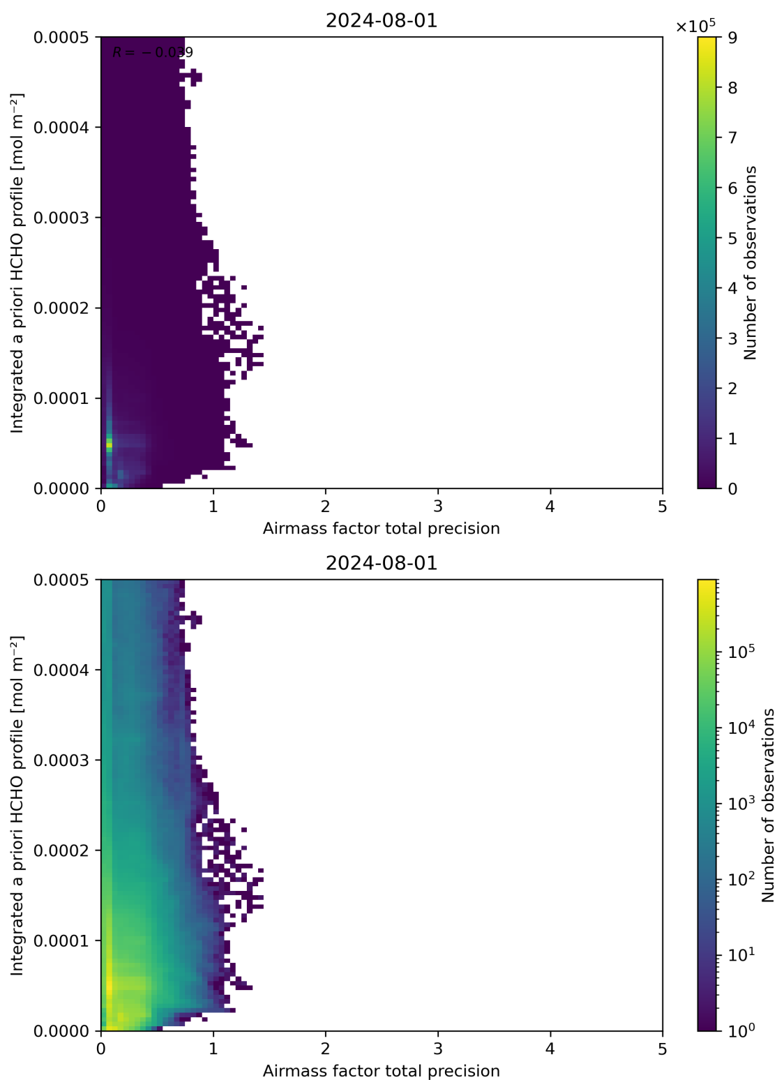
Figure 111: Scatter density plot of “Airmass factor total precision” against “Integrated a priori HCHO profile” for 2024-07-31 to 2024-08-02.
