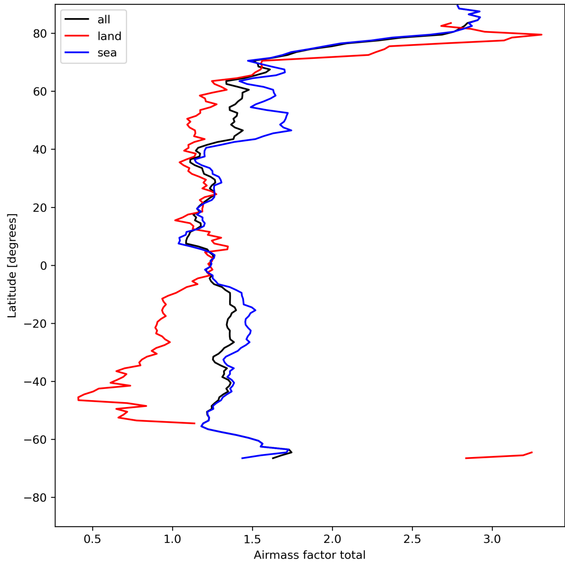
Figure 26: Zonal average of “Airmass factor total” for 2024-07-31 to 2024-08-02.
