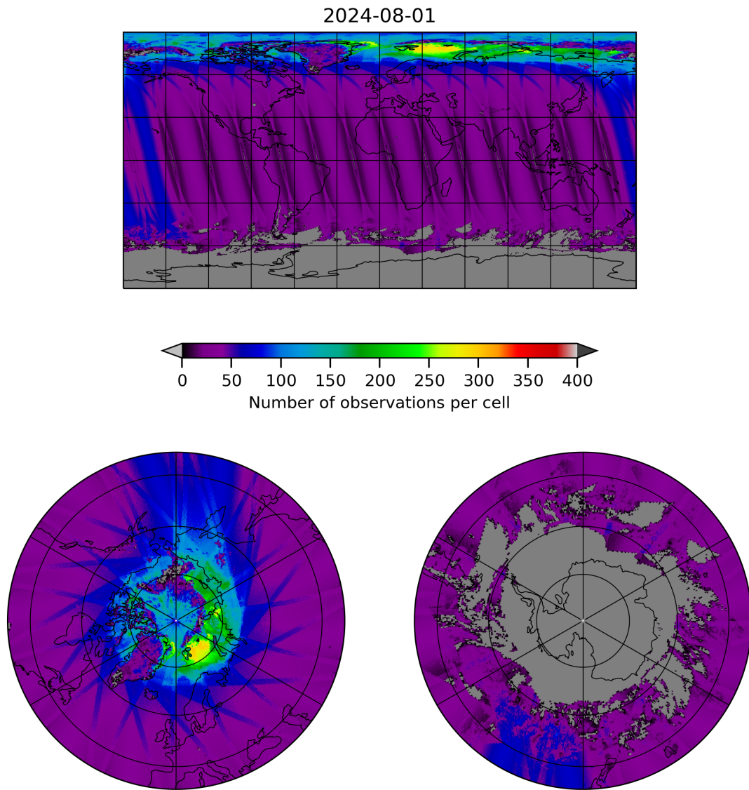
Figure 19: Map of the number of observations for 2024-07-31 to 2024-08-02
