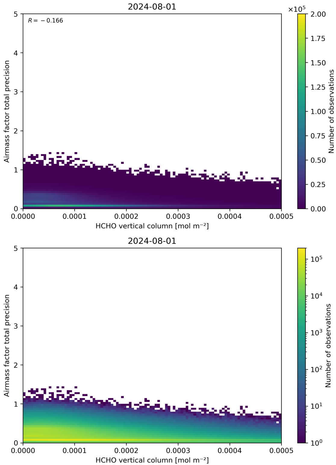
Figure 132: Scatter density plot of “HCHO vertical column” against “Airmass factor total precision” for 2024-07-31 to 2024-08-02.
