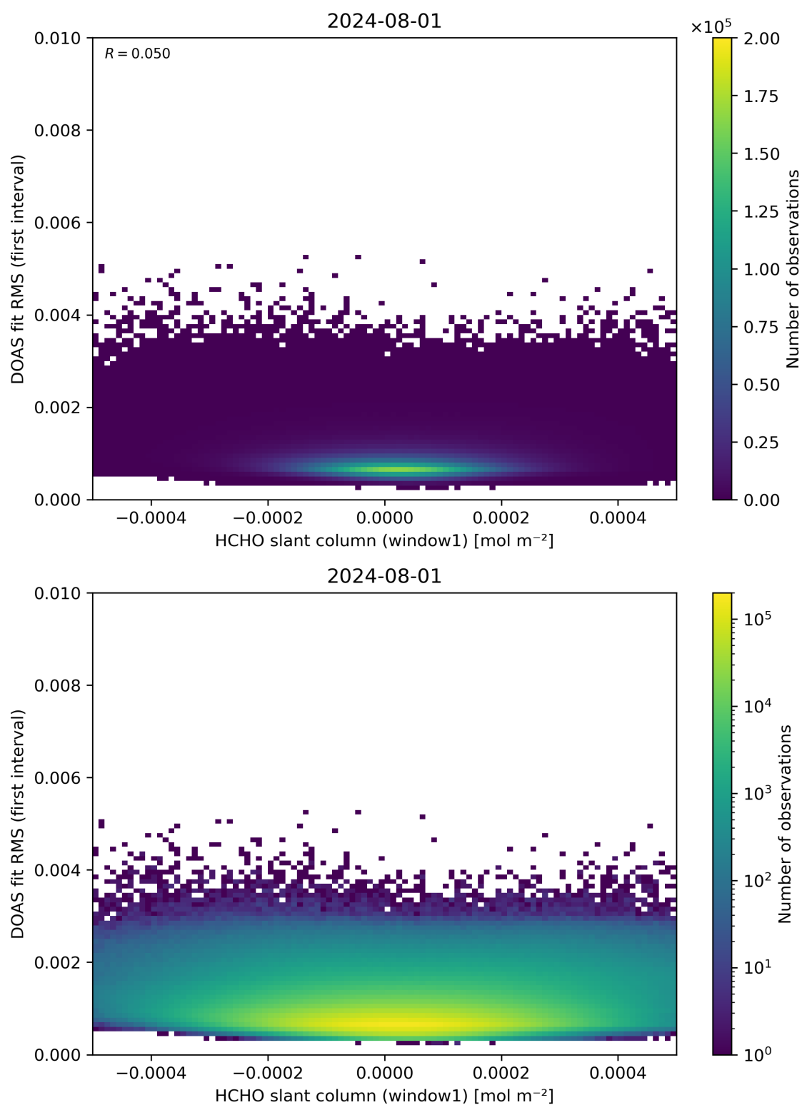
Figure 78: Scatter density plot of “HCHO slant column (window1)” against “DOAS fit RMS (first interval)” for 2024-07-31 to 2024-08-02.
