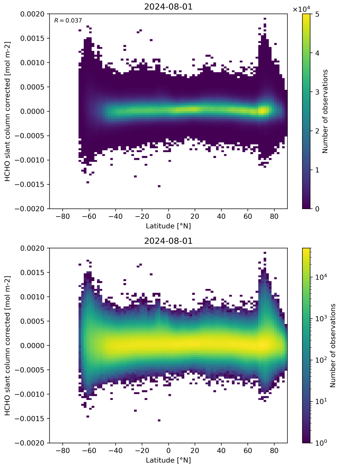
Figure 157: Scatter density plot of “Latitude” against “HCHO slant column corrected” for 2024-07-31 to 2024-08-02.
