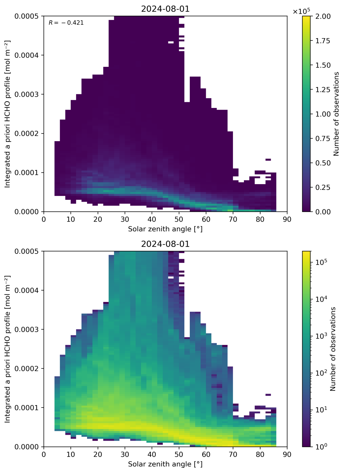
Figure 180: Scatter density plot of “Solar zenith angle” against “Integrated a priori HCHO profile” for 2024-07-31 to 2024-08-02.
