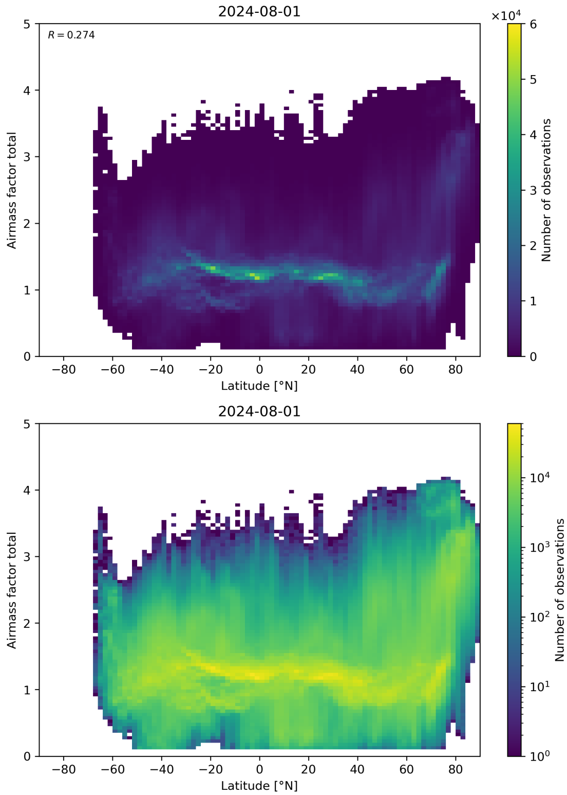
Figure 161: Scatter density plot of “Latitude” against “Airmass factor total” for 2024-07-31 to 2024-08-02.
