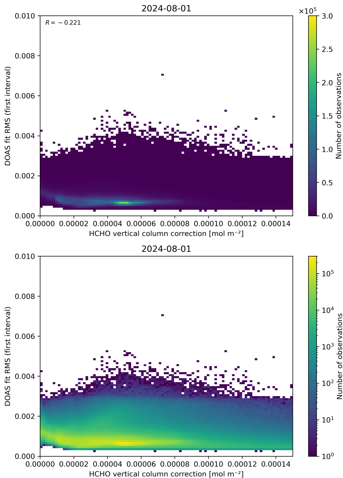
Figure 112: Scatter density plot of “HCHO vertical column correction” against “DOAS fit RMS (first interval)” for 2024-07-31 to 2024-08-02.
