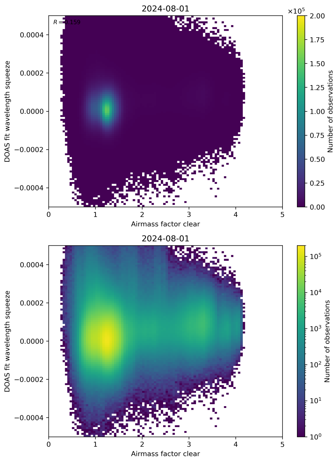
Figure 73: Scatter density plot of “Airmass factor clear” against “DOAS fit wavelength squeeze” for 2024-07-31 to 2024-08-02.
