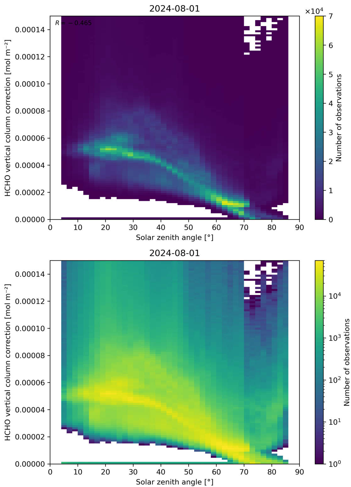
Figure 178: Scatter density plot of “Solar zenith angle” against “HCHO vertical column correction” for 2024-07-31 to 2024-08-02.
