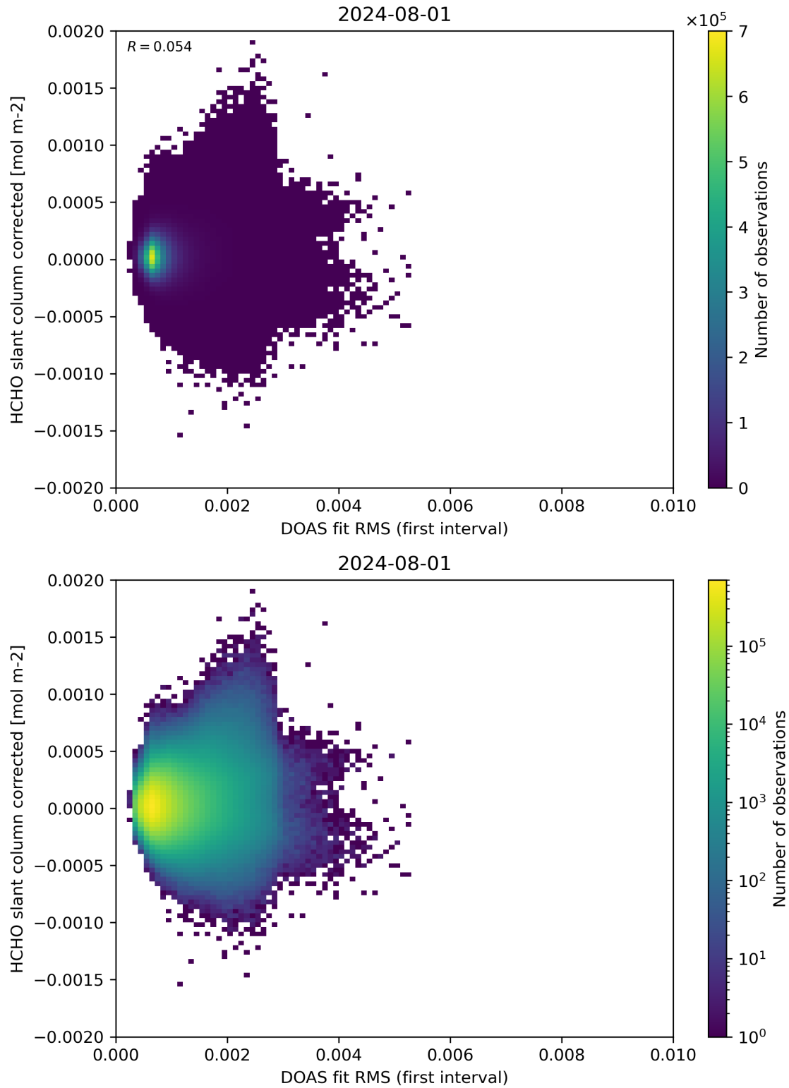
Figure 62: Scatter density plot of “DOAS fit RMS (first interval)” against “HCHO slant column corrected” for 2024-07-31 to 2024-08-02.
