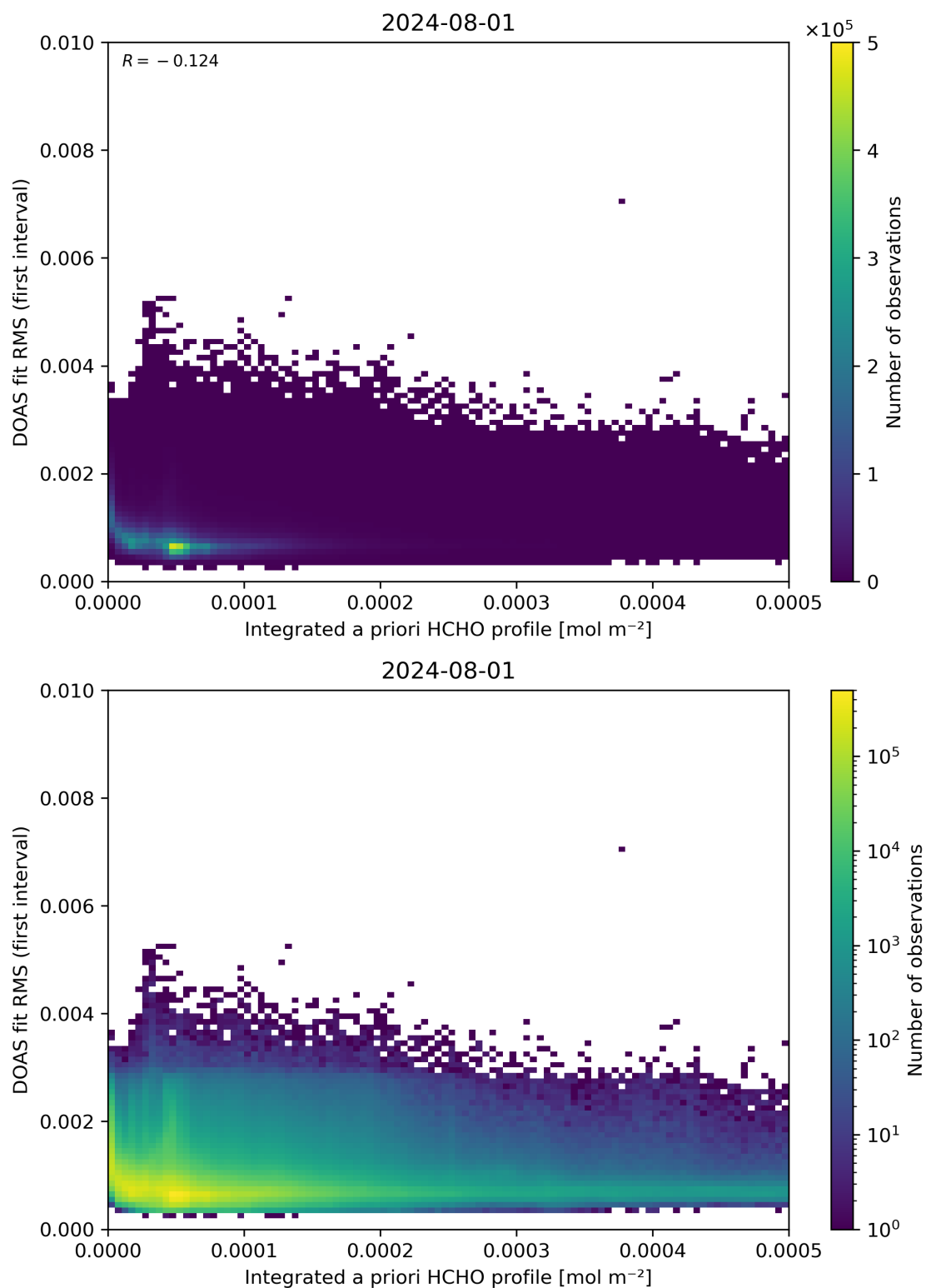
Figure 148: Scatter density plot of “Integrated a priori HCHO profile” against “DOAS fit RMS (first interval)” for 2024-07-31 to 2024-08-02.
