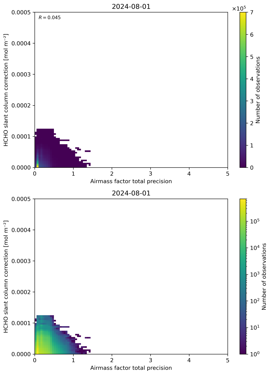
Figure 110: Scatter density plot of “Airmass factor total precision” against “HCHO slant column correction” for 2024-07-31 to 2024-08-02.
