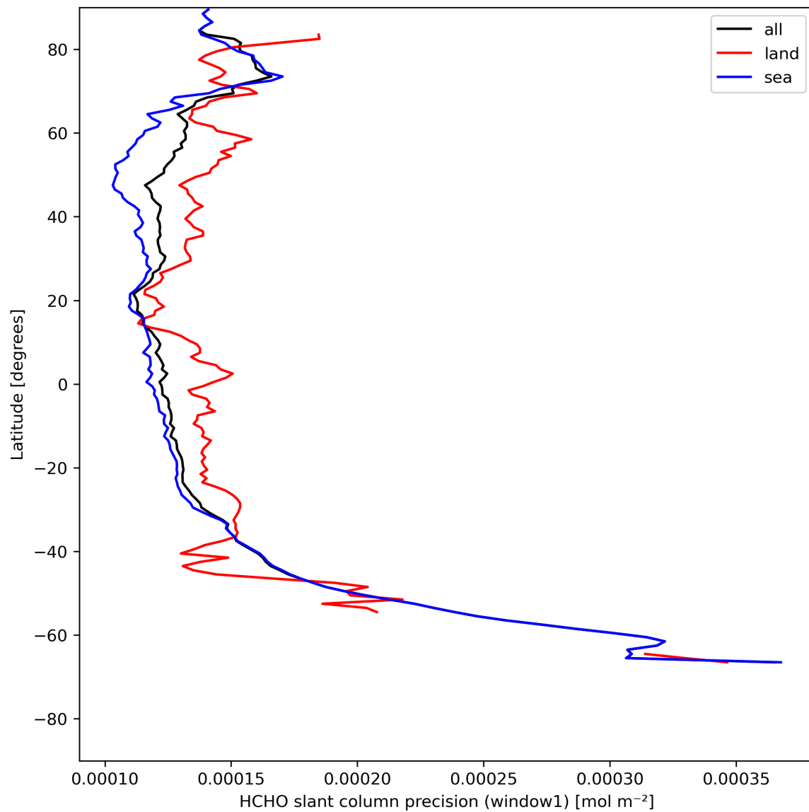
Figure 25: Zonal average of “HCHO slant column precision (window1)” for 2024-07-31 to 2024-08-02.
