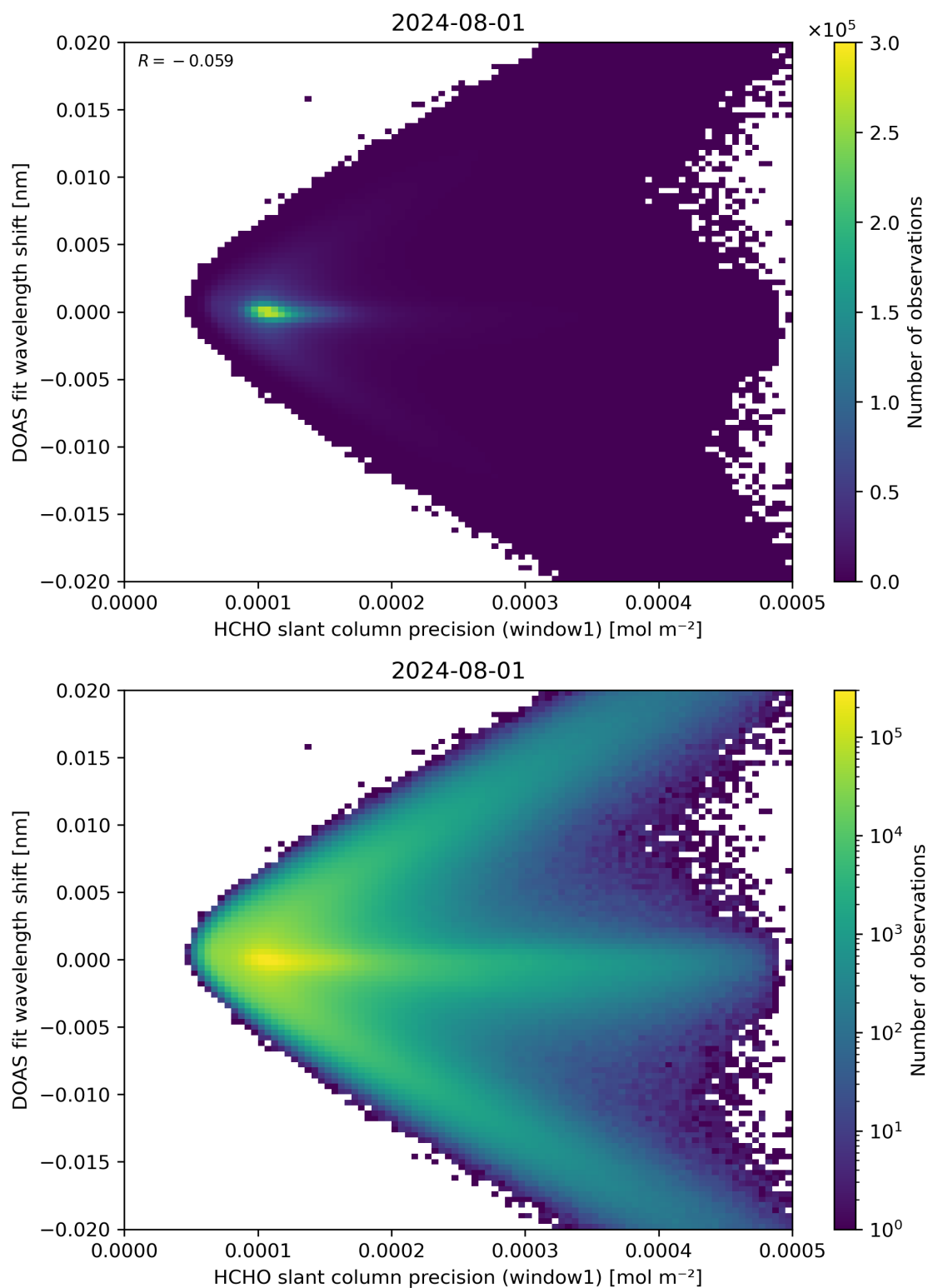
Figure 89: Scatter density plot of “HCHO slant column precision (window1)” against “DOAS fit wavelength shift” for 2024-07-31 to 2024-08-02.
