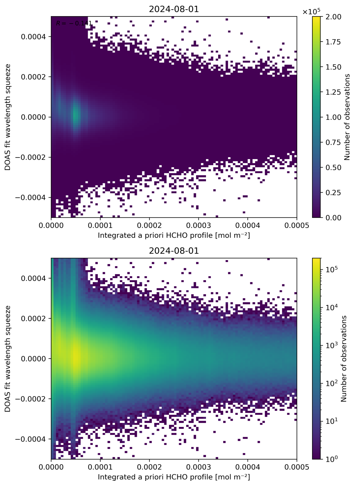
Figure 150: Scatter density plot of “Integrated a priori HCHO profile” against “DOAS fit wavelength squeeze” for 2024-07-31 to 2024-08-02.
