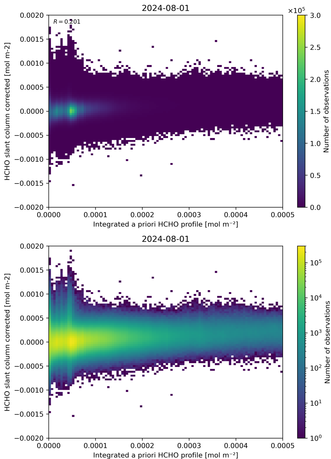
Figure 151: Scatter density plot of “Integrated a priori HCHO profile” against “HCHO slant column corrected” for 2024-07-31 to 2024-08-02.
