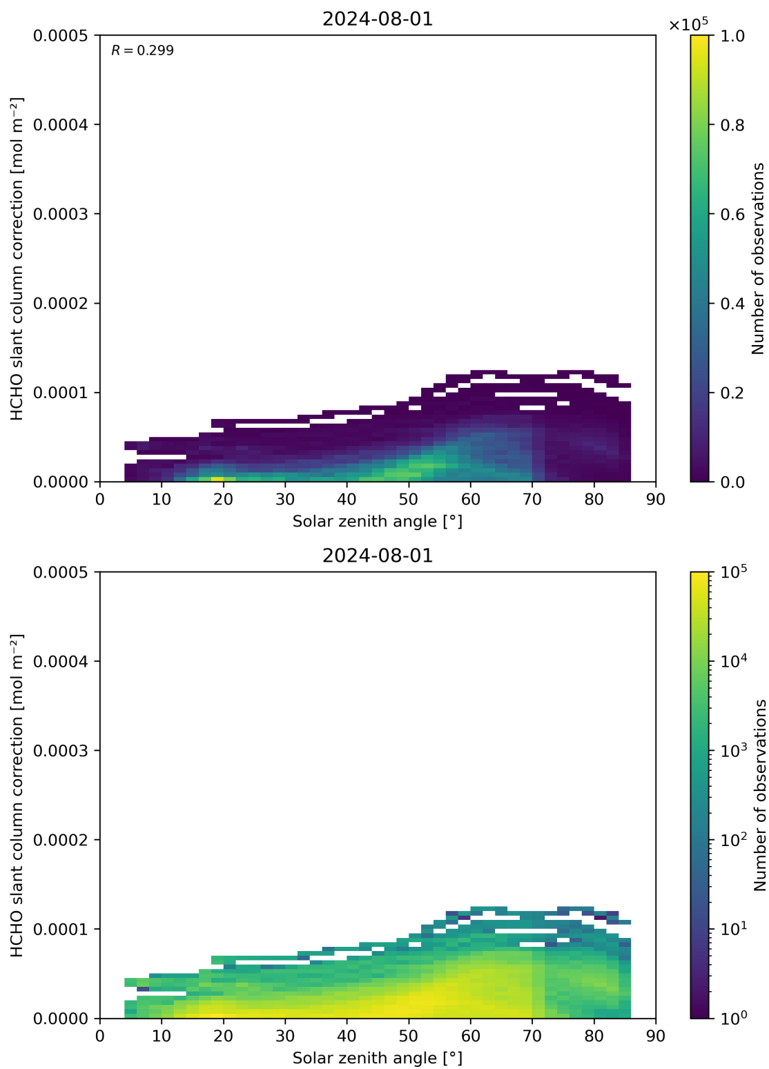
Figure 172: Scatter density plot of “Solar zenith angle” against “HCHO slant column correction” for 2024-07-31 to 2024-08-02.
