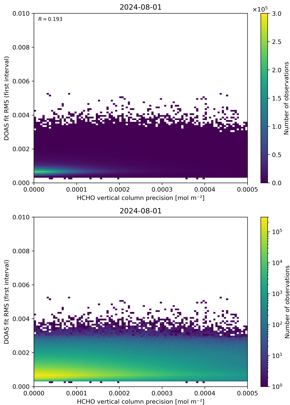
Figure 136: Scatter density plot of “HCHO vertical column precision” against “DOAS fit RMS (first interval)” for 2024-07-31 to 2024-08-02.
