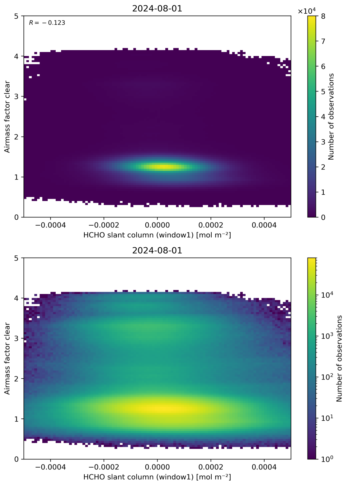
Figure 81: Scatter density plot of “HCHO slant column (window1)” against “Airmass factor clear” for 2024-07-31 to 2024-08-02.
