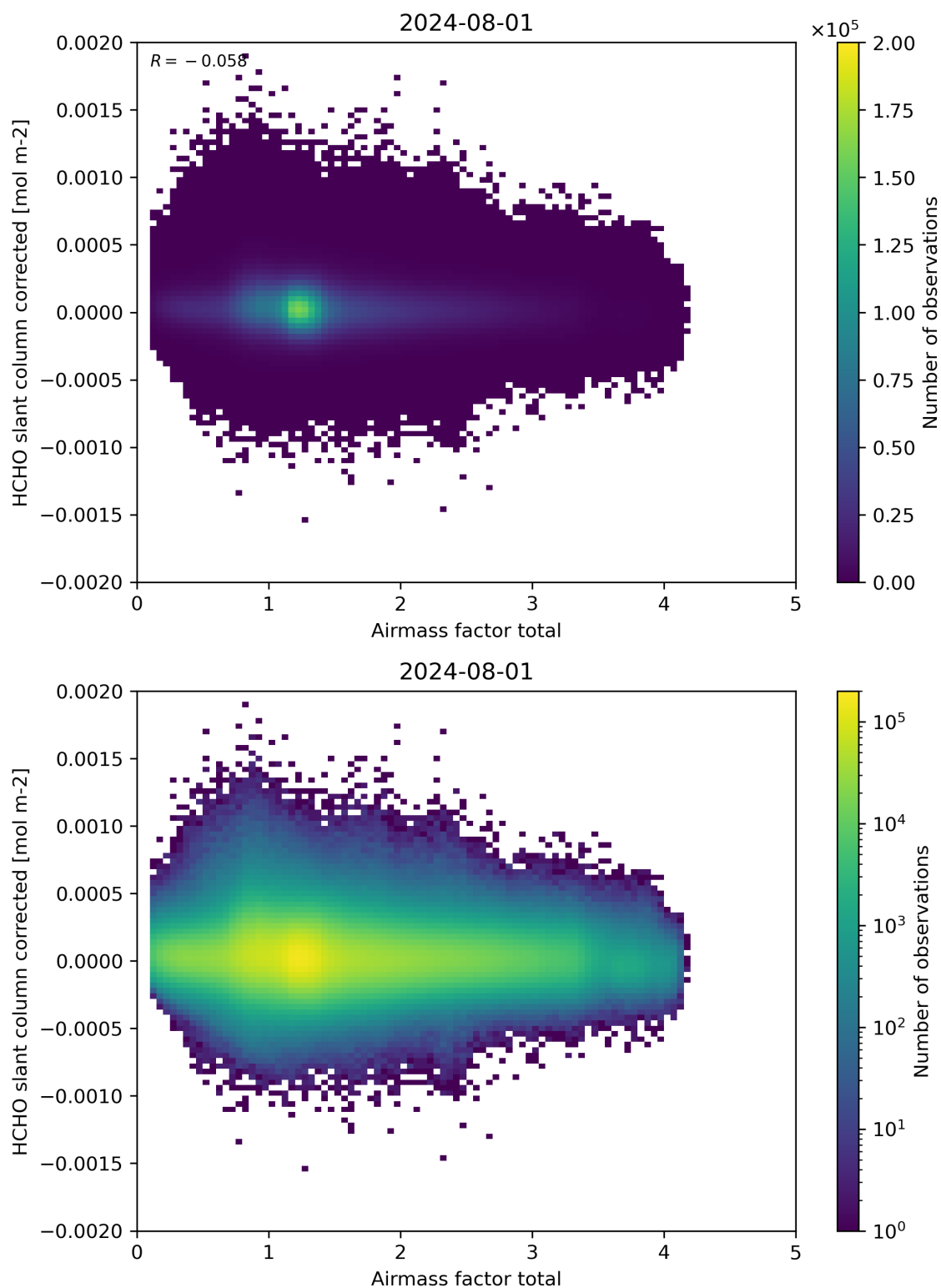
Figure 101: Scatter density plot of “Airmass factor total” against “HCHO slant column corrected” for 2024-07-31 to 2024-08-02.
