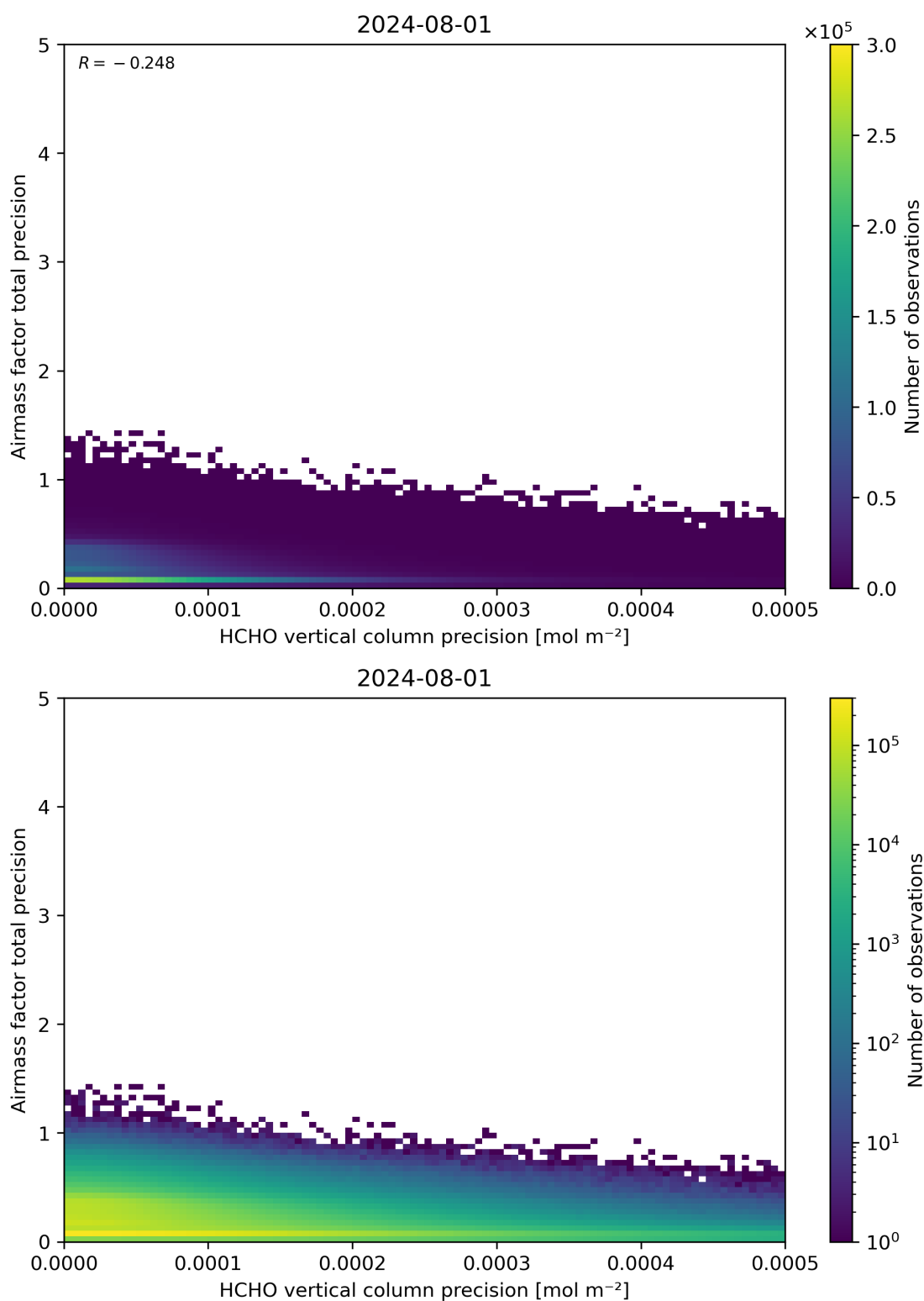
Figure 145: Scatter density plot of “HCHO vertical column precision” against “Airmass factor total precision” for 2024-07-31 to 2024-08-02.
