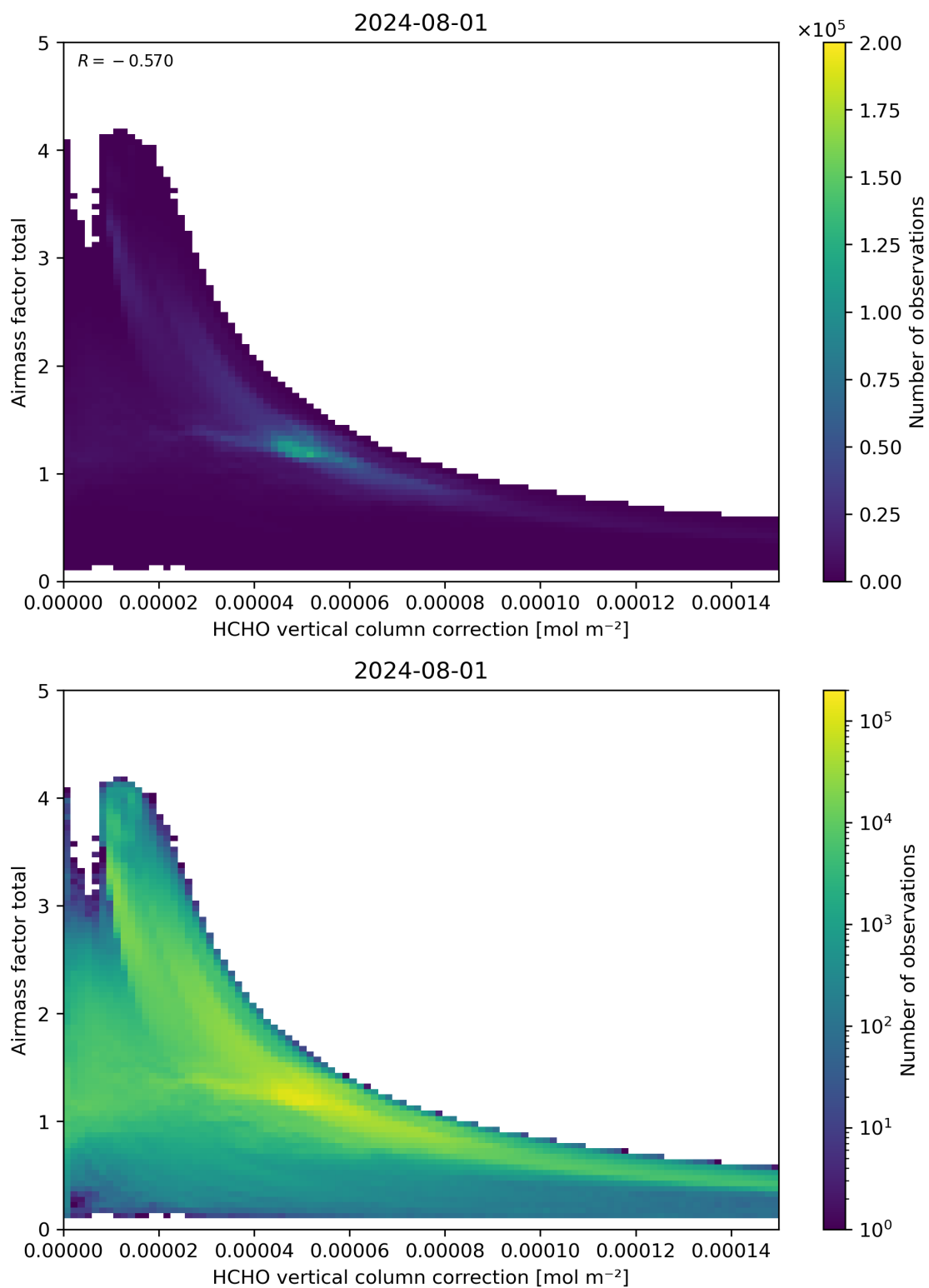
Figure 120: Scatter density plot of “HCHO vertical column correction” against “Airmass factor total” for 2024-07-31 to 2024-08-02.
