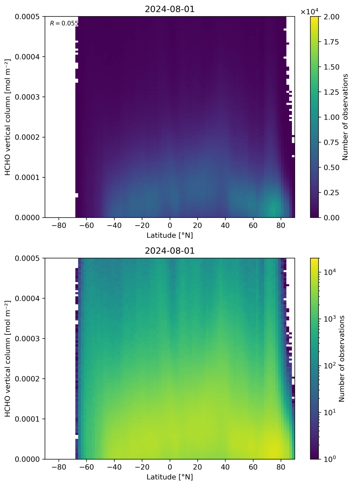
Figure 163: Scatter density plot of “Latitude” against “HCHO vertical column” for 2024-07-31 to 2024-08-02.
