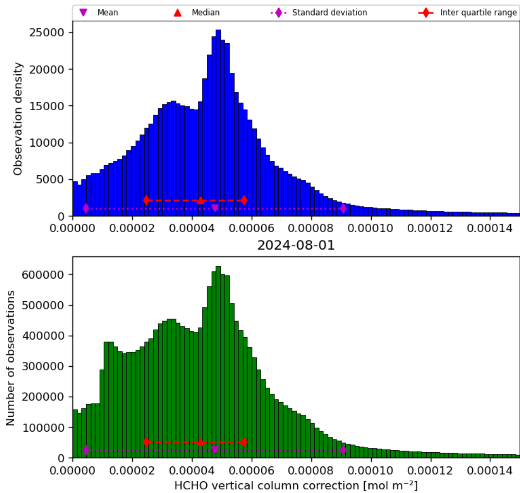
Figure 37: Histogram of “HCHO vertical column correction” for 2024-07-31 to 2024-08-02
