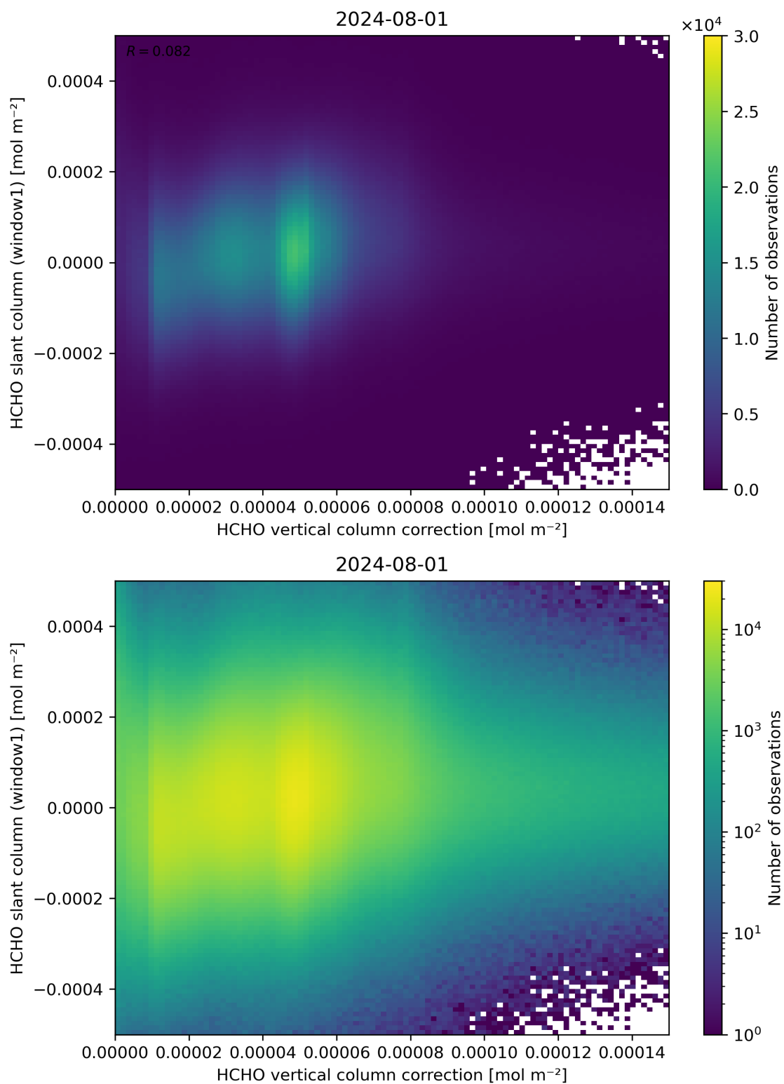
Figure 118: Scatter density plot of “HCHO vertical column correction” against “HCHO slant column (window1)” for 2024-07-31 to 2024-08-02.
