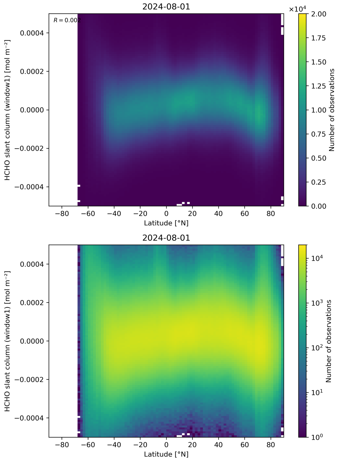
Figure 159: Scatter density plot of “Latitude” against “HCHO slant column (window1)” for 2024-07-31 to 2024-08-02.
