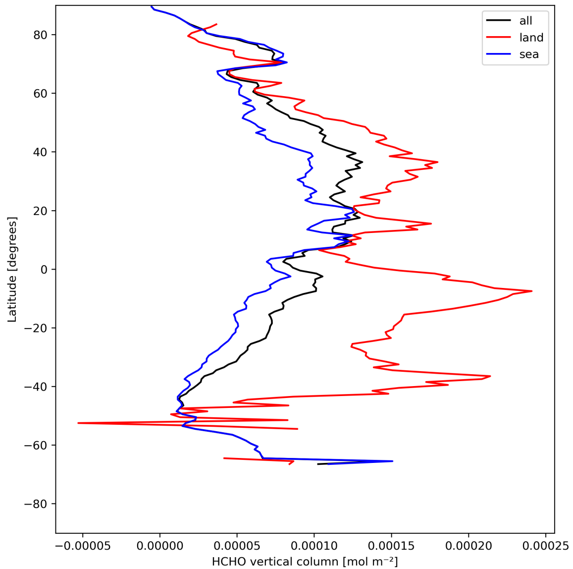
Figure 21: Zonal average of “HCHO vertical column” for 2024-07-31 to 2024-08-02.
