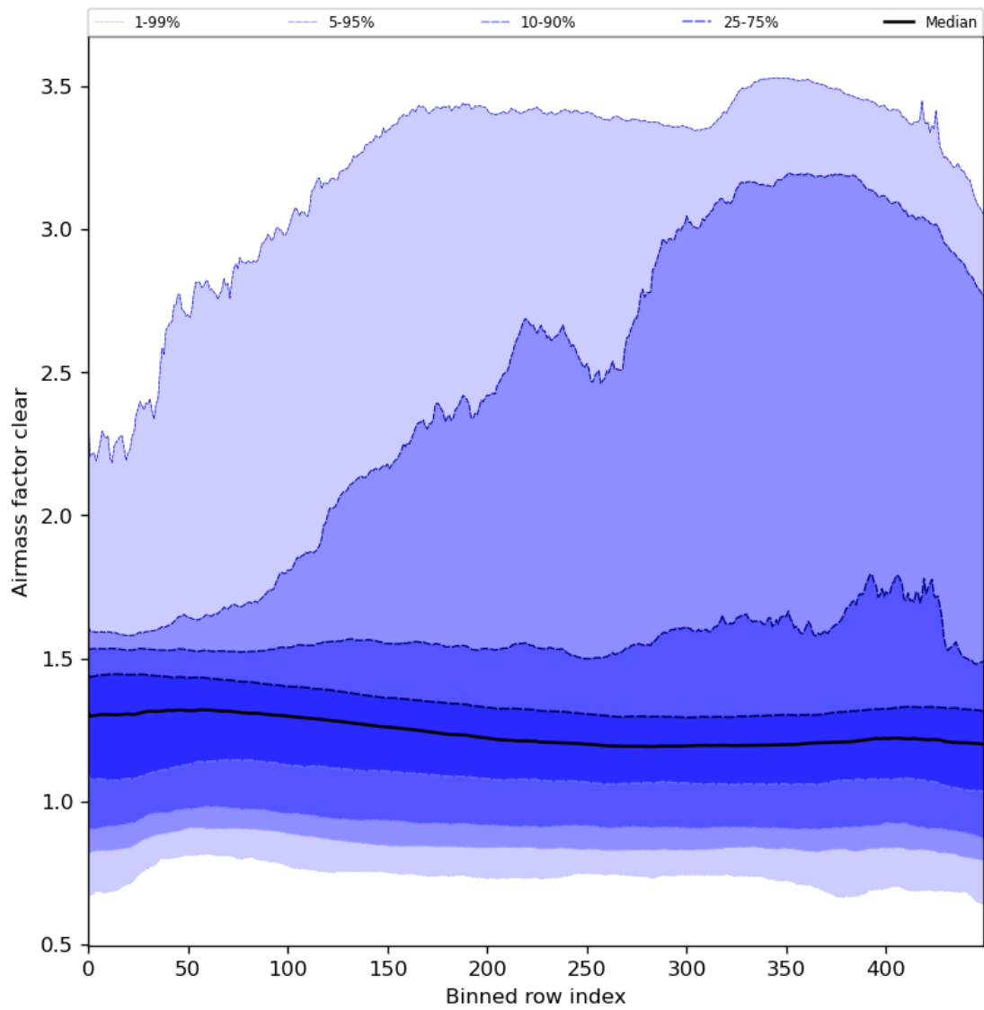
Figure 56: Along track statistics of “Air mass factor clear” for 2024-07-31 to 2024-08-02
