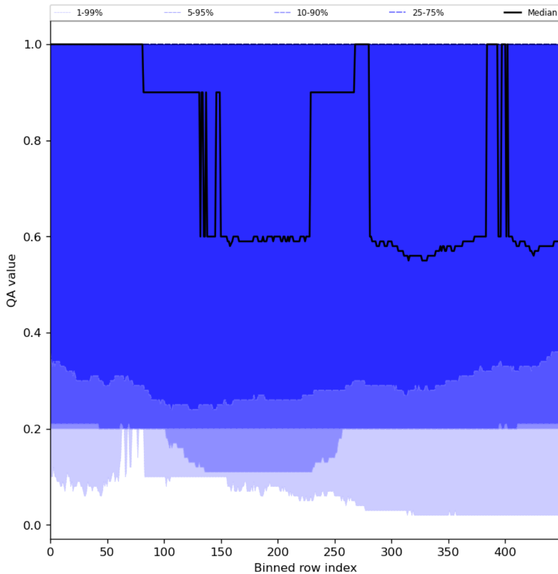
Figure 48: Along track statistics of “QA value” for 2024-07-31 to 2024-08-02
