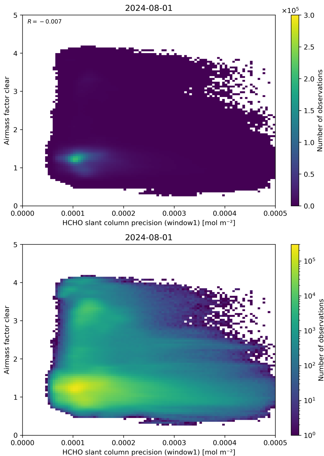
Figure 91: Scatter density plot of “HCHO slant column precision (window1)” against “Airmass factor clear” for 2024-07-31 to 2024-08-02.
