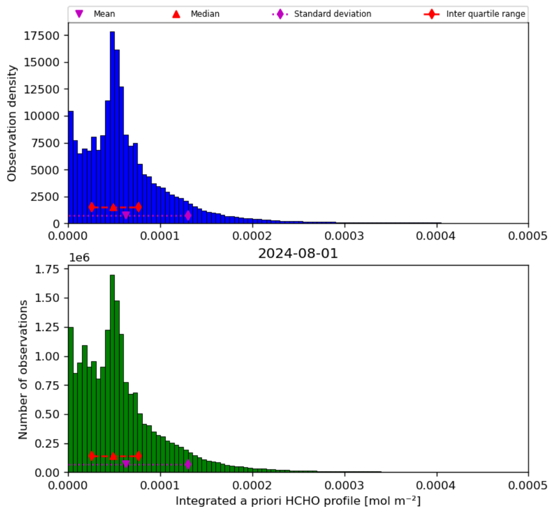
Figure 43: Histogram of “Integrated a priori HCHO profile” for 2024-07-31 to 2024-08-02
