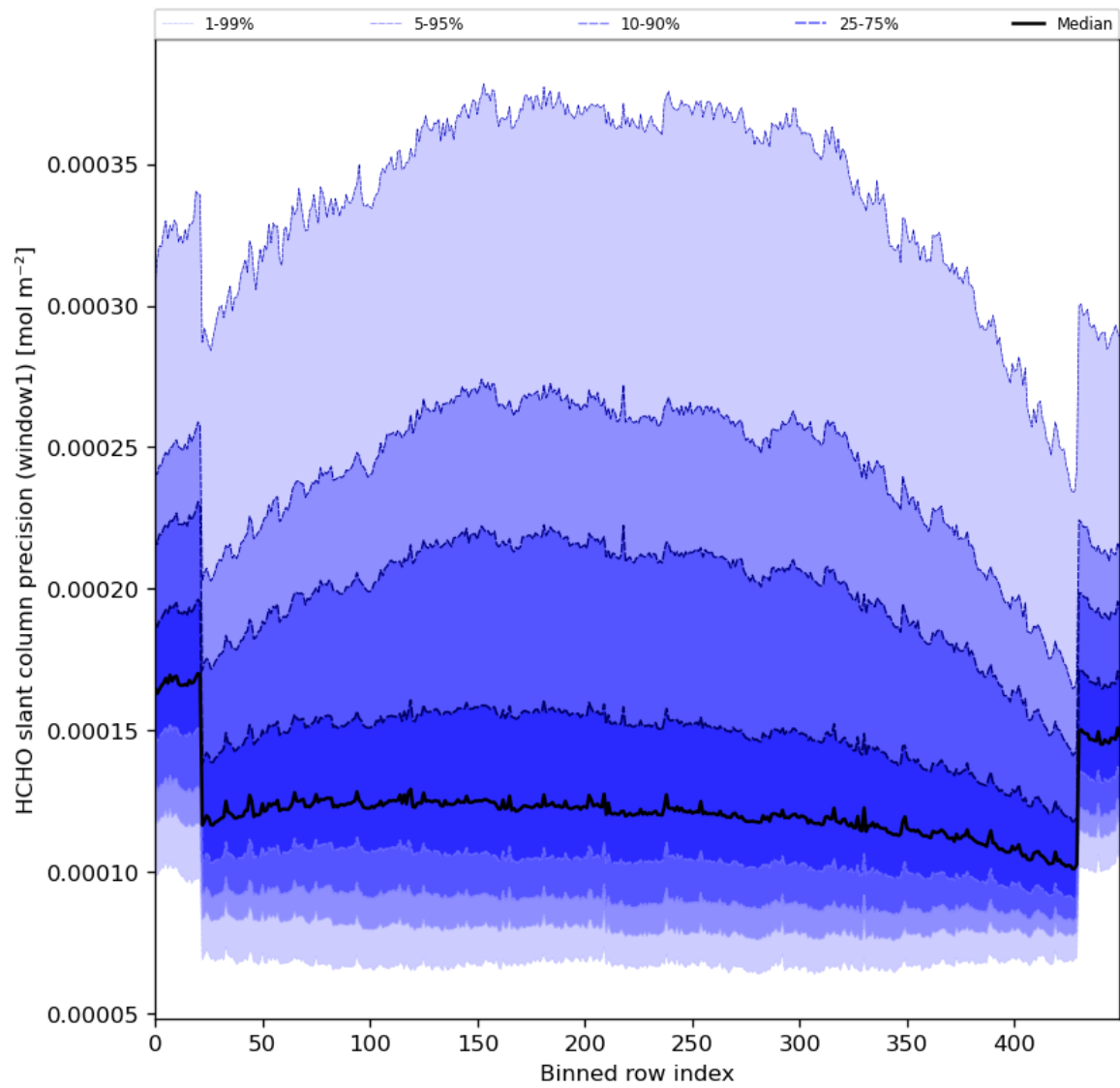
Figure 53: Along track statistics of “HCHO slant column precision (window1)” for 2024-07-31 to 2024-08-02
