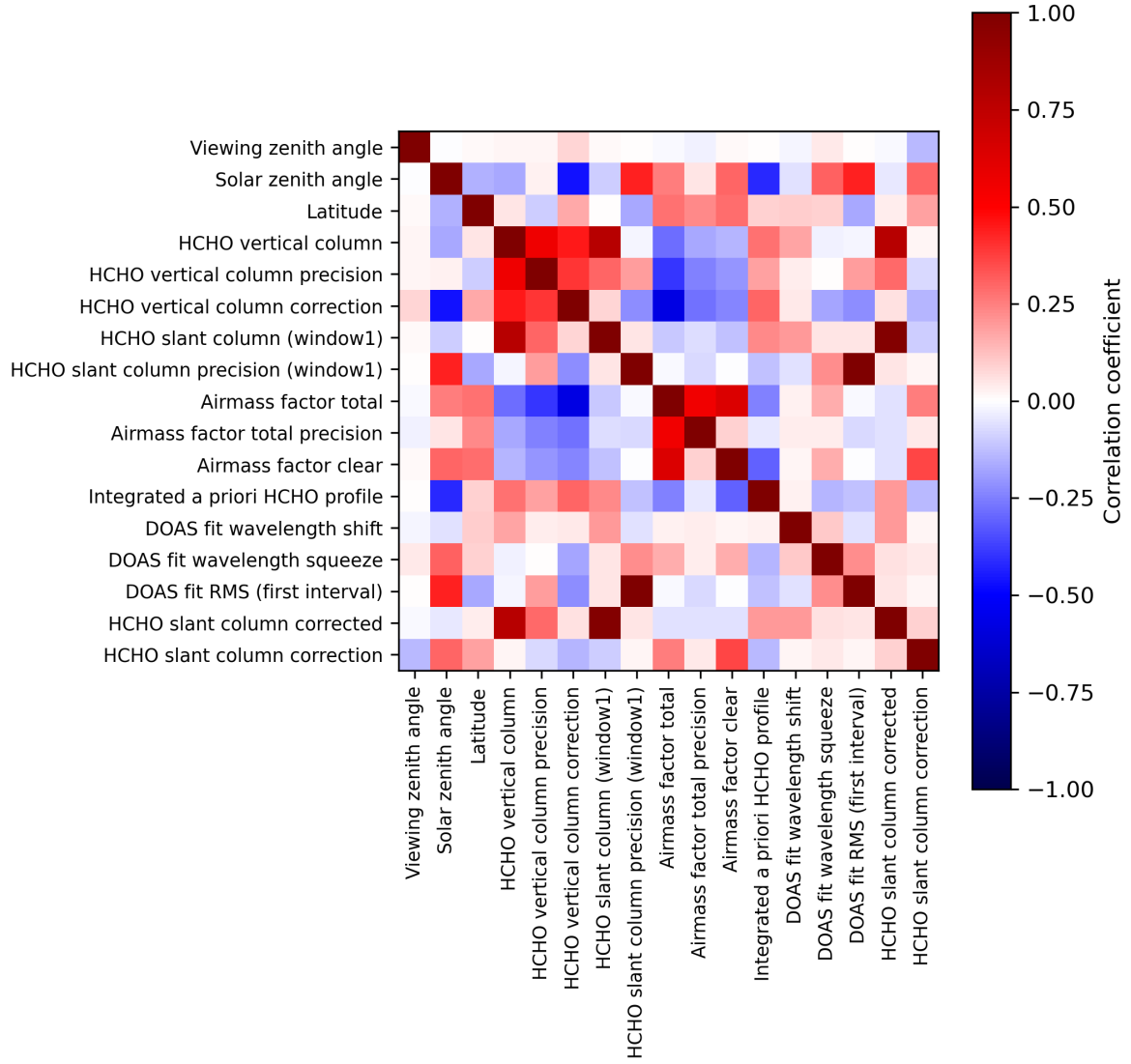
Figure 2: Map of correlation matrix for 2024-07-31 to 2024-08-02.
