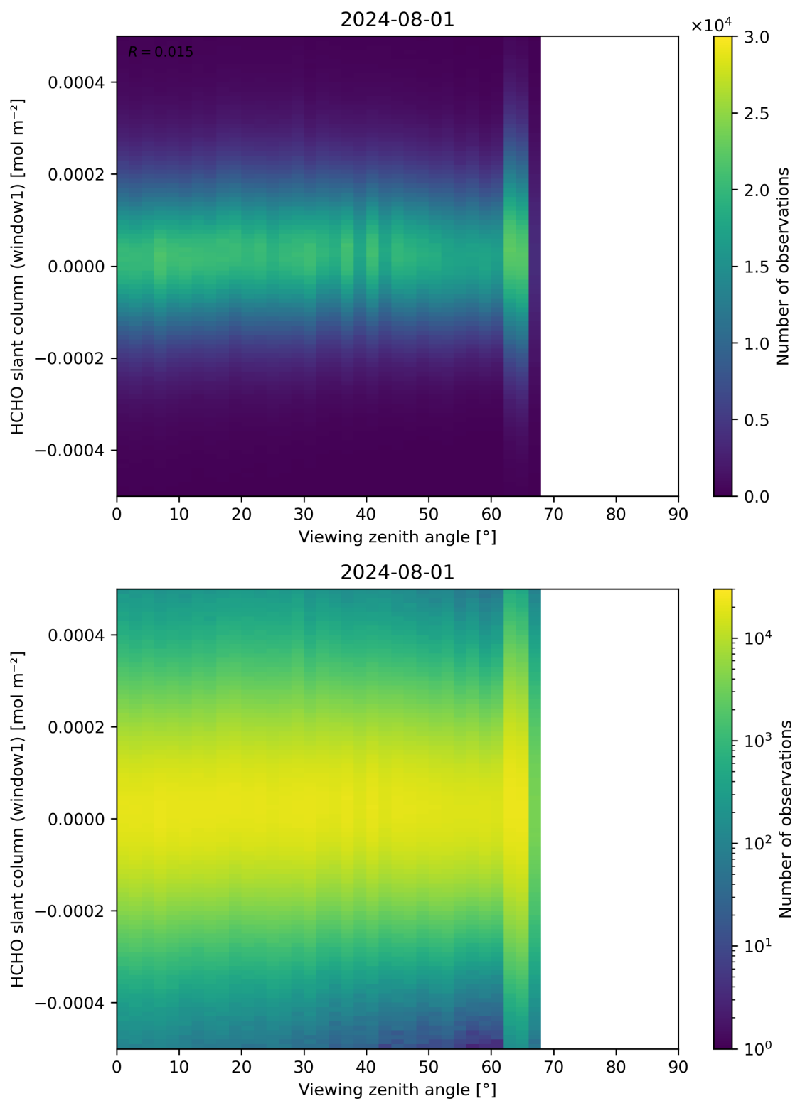
Figure 188: Scatter density plot of “Viewing zenith angle” against “HCHO slant column (window1)” for 2024-07-31 to 2024-08-02.
