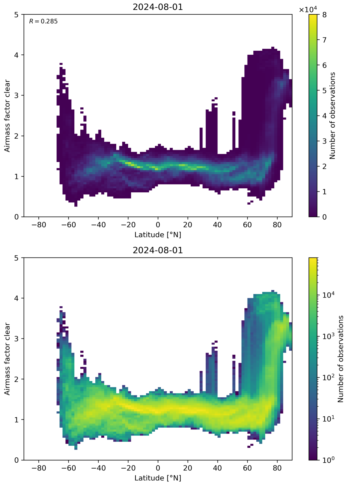
Figure 156: Scatter density plot of “Latitude” against “Airmass factor clear” for 2024-07-31 to 2024-08-02.
