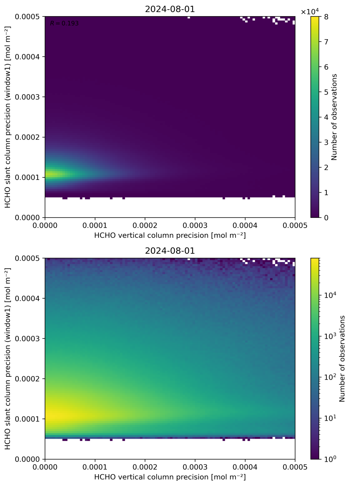
Figure 143: Scatter density plot of “HCHO vertical column precision” against “HCHO slant column precision (window1)” for 2024-07-31 to 2024-08-02.
