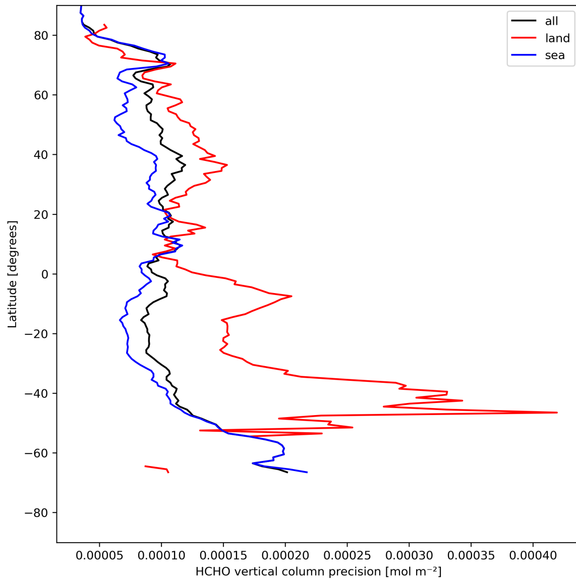
Figure 22: Zonal average of “HCHO vertical column precision” for 2024-07-31 to 2024-08-02.
