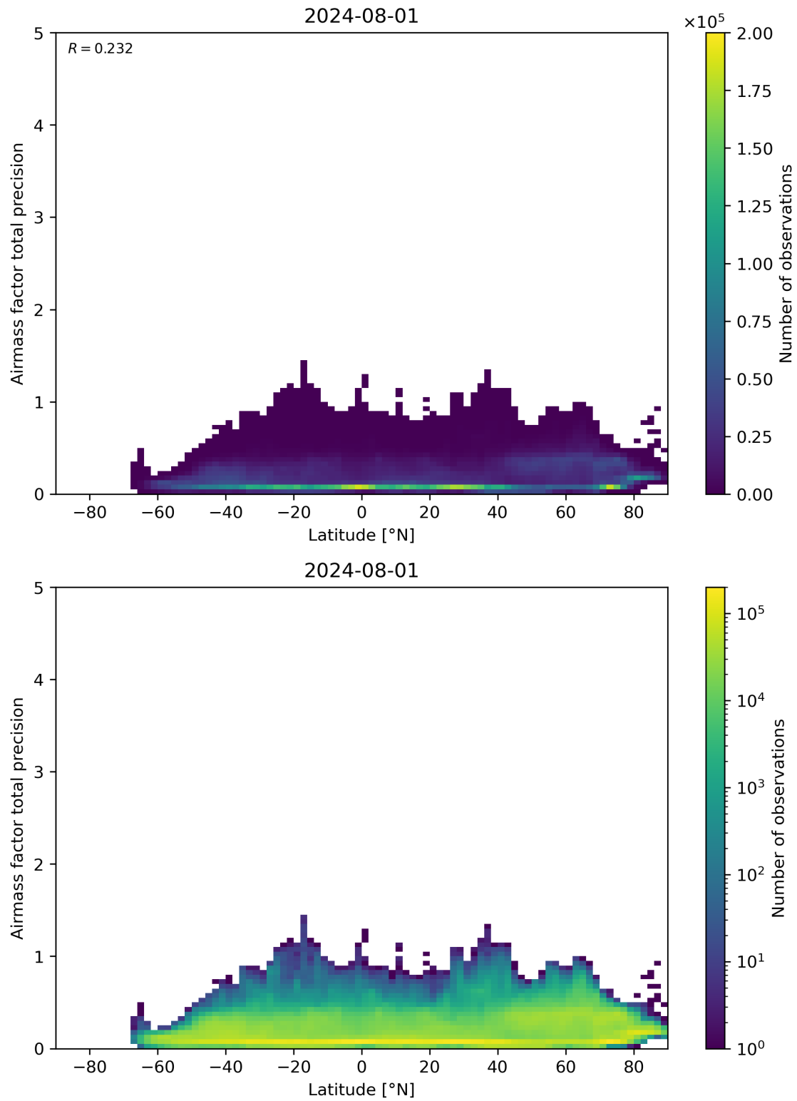
Figure 162: Scatter density plot of “Latitude” against “Airmass factor total precision” for 2024-07-31 to 2024-08-02.
