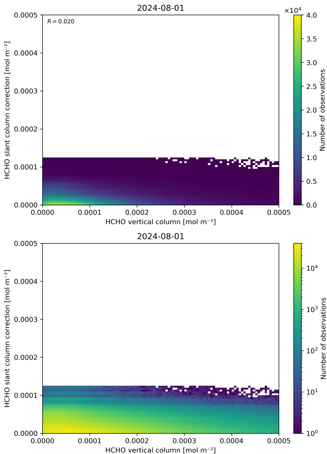
Figure 128: Scatter density plot of “HCHO vertical column” against “HCHO slant column correction” for 2024-07-31 to 2024-08-02.
