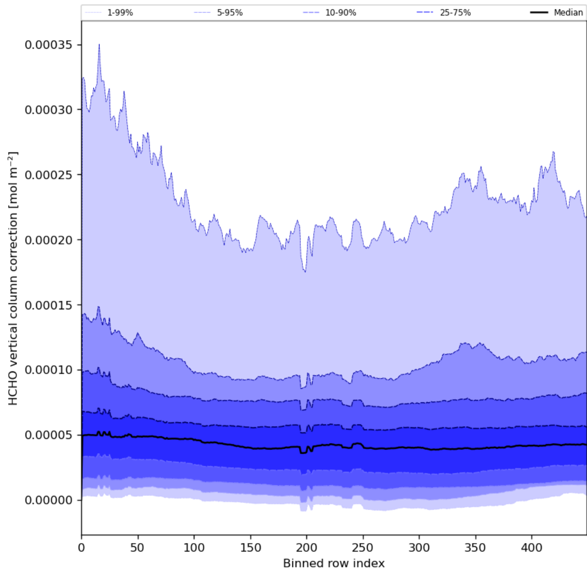
Figure 51: Along track statistics of “HCHO vertical column correction” for 2024-07-31 to 2024-08-02
