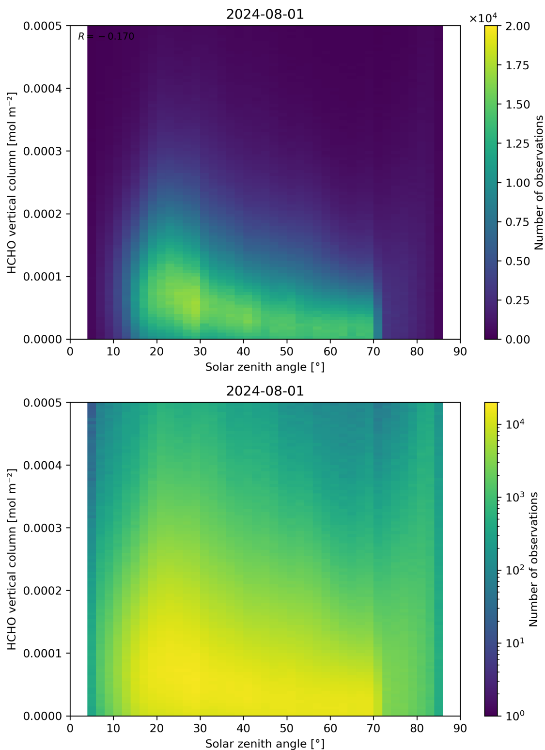
Figure 177: Scatter density plot of “Solar zenith angle” against “HCHO vertical column” for 2024-07-31 to 2024-08-02.
