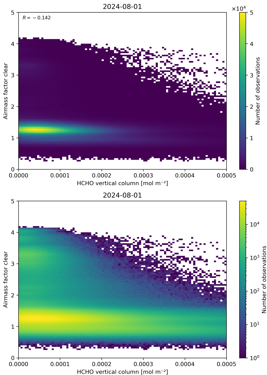
Figure 126: Scatter density plot of “HCHO vertical column” against “Airmass factor clear” for 2024-07-31 to 2024-08-02.
