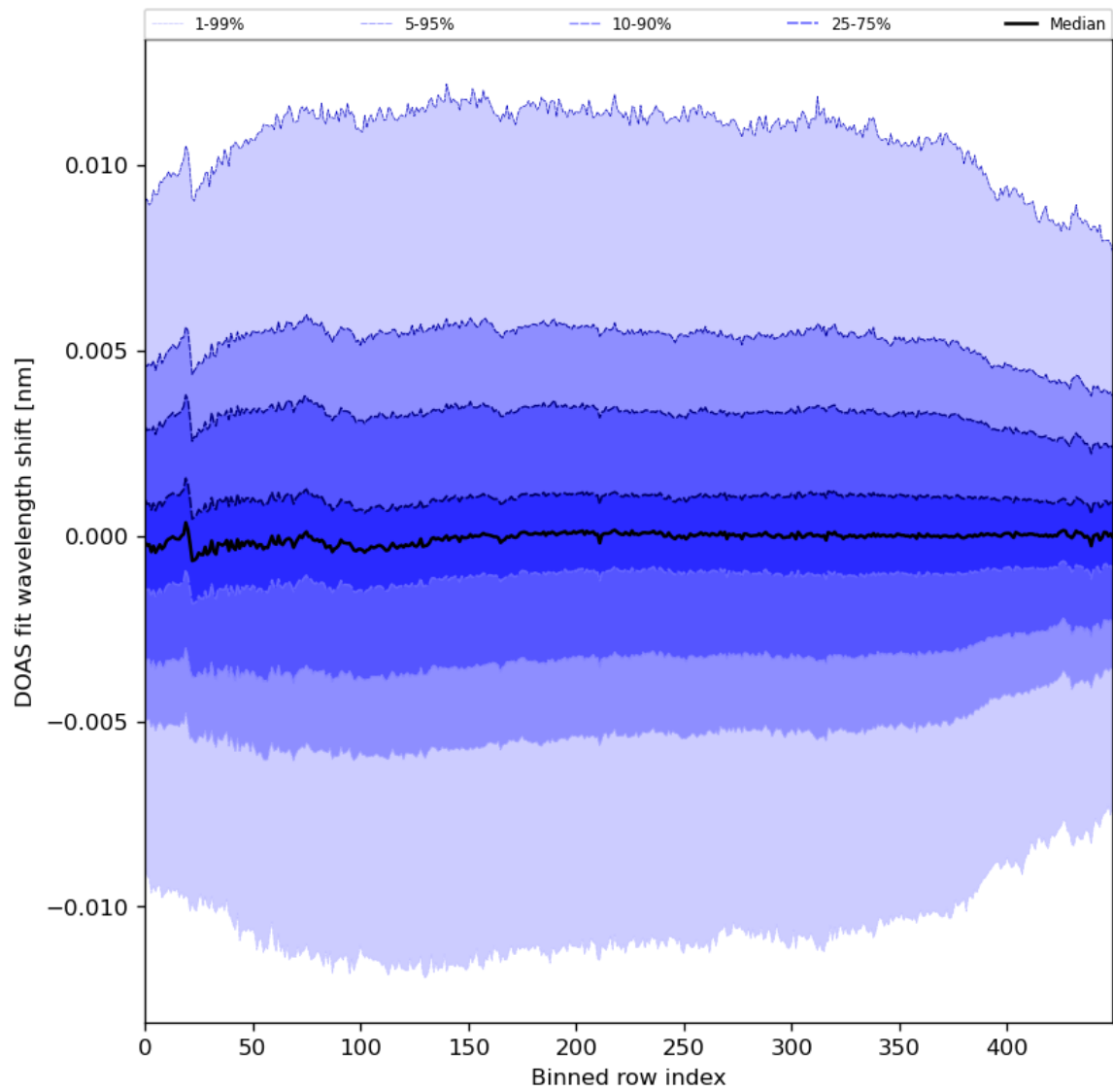
Figure 58: Along track statistics of “DOAS fit wavelength shift” for 2024-07-31 to 2024-08-02
