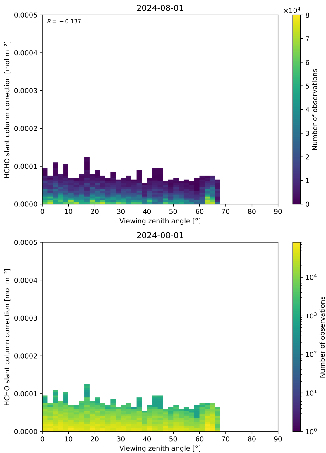
Figure 187: Scatter density plot of “Viewing zenith angle” against “HCHO slant column correction” for 2024-07-31 to 2024-08-02.
