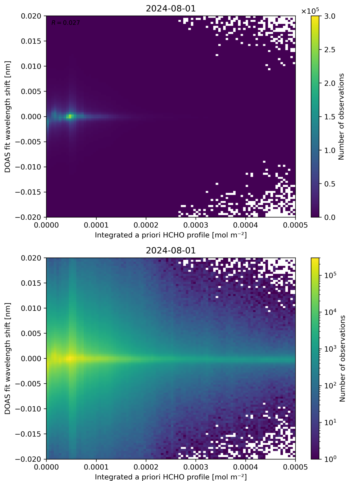
Figure 149: Scatter density plot of “Integrated a priori HCHO profile” against “DOAS fit wavelength shift” for 2024-07-31 to 2024-08-02.
