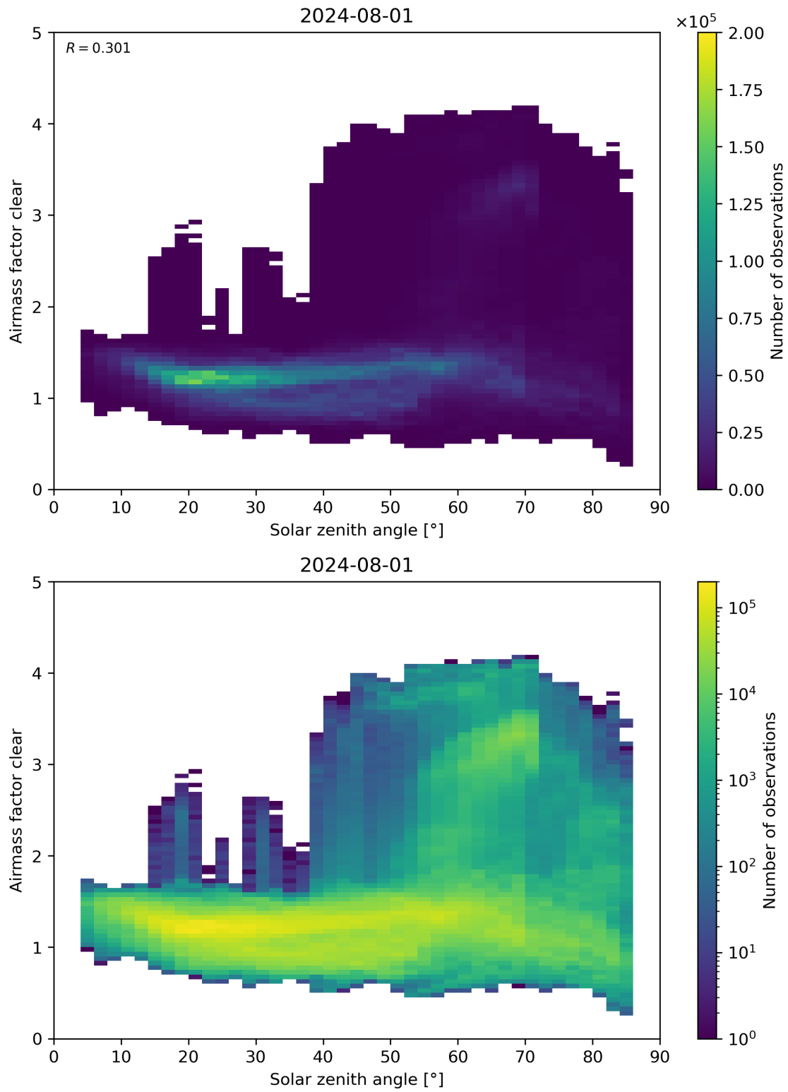
Figure 170: Scatter density plot of “Solar zenith angle” against “Airmass factor clear” for 2024-07-31 to 2024-08-02.
