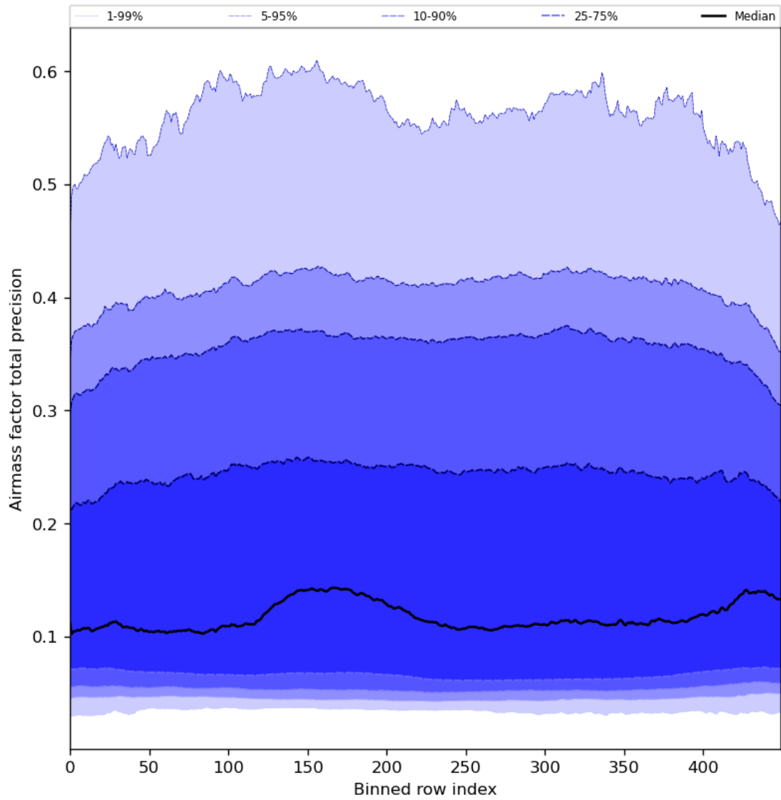
Figure 55: Along track statistics of “Airmass factor total precision” for 2024-07-31 to 2024-08-02
