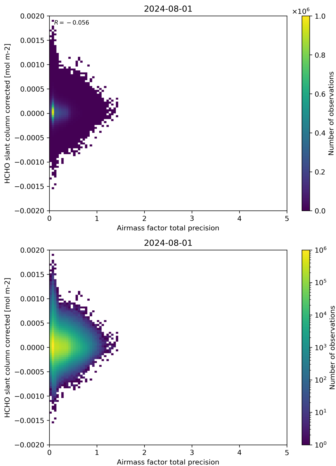
Figure 109: Scatter density plot of “Airmass factor total precision” against “HCHO slant column corrected” for 2024-07-31 to 2024-08-02.
