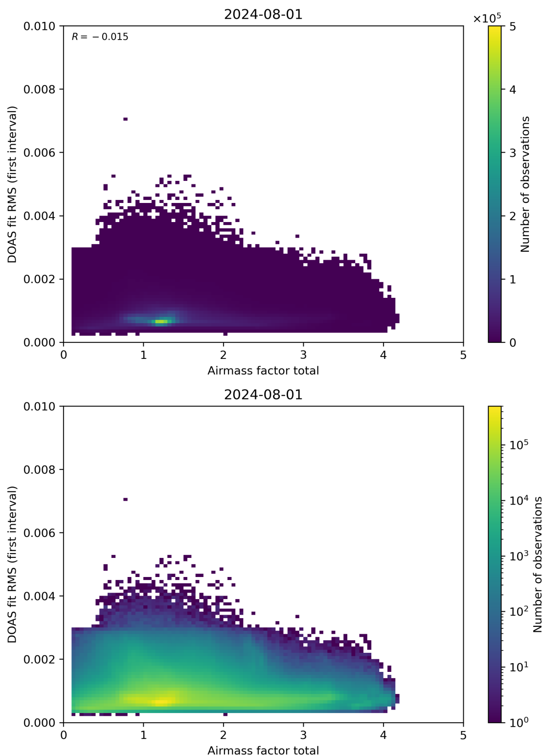
Figure 97: Scatter density plot of “Airmass factor total” against “DOAS fit RMS (first interval)” for 2024-07-31 to 2024-08-02.
