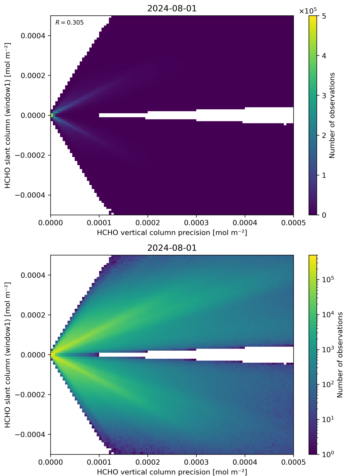
Figure 142: Scatter density plot of “HCHO vertical column precision” against “HCHO slant column (window1)” for 2024-07-31 to 2024-08-02.
