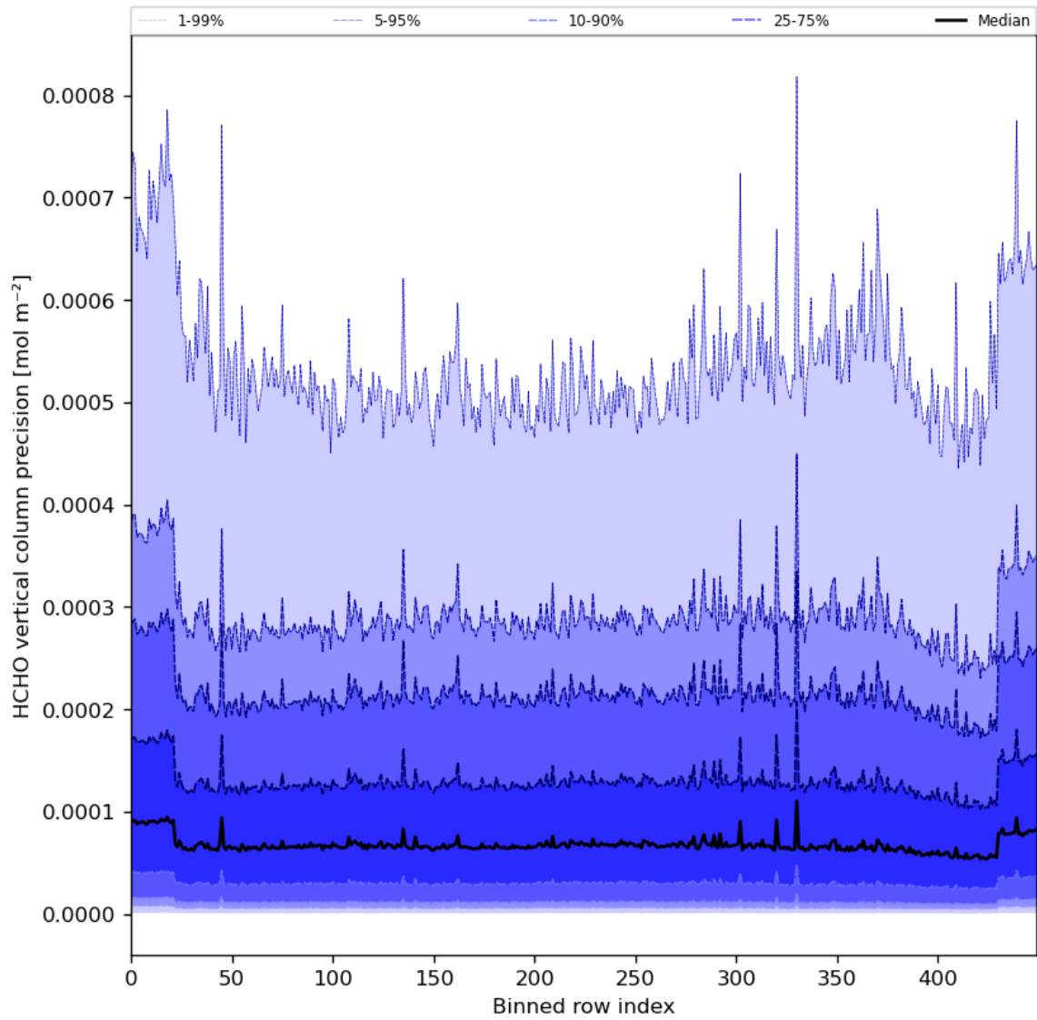
Figure 50: Along track statistics of “HCHO vertical column precision” for 2024-07-31 to 2024-08-02
