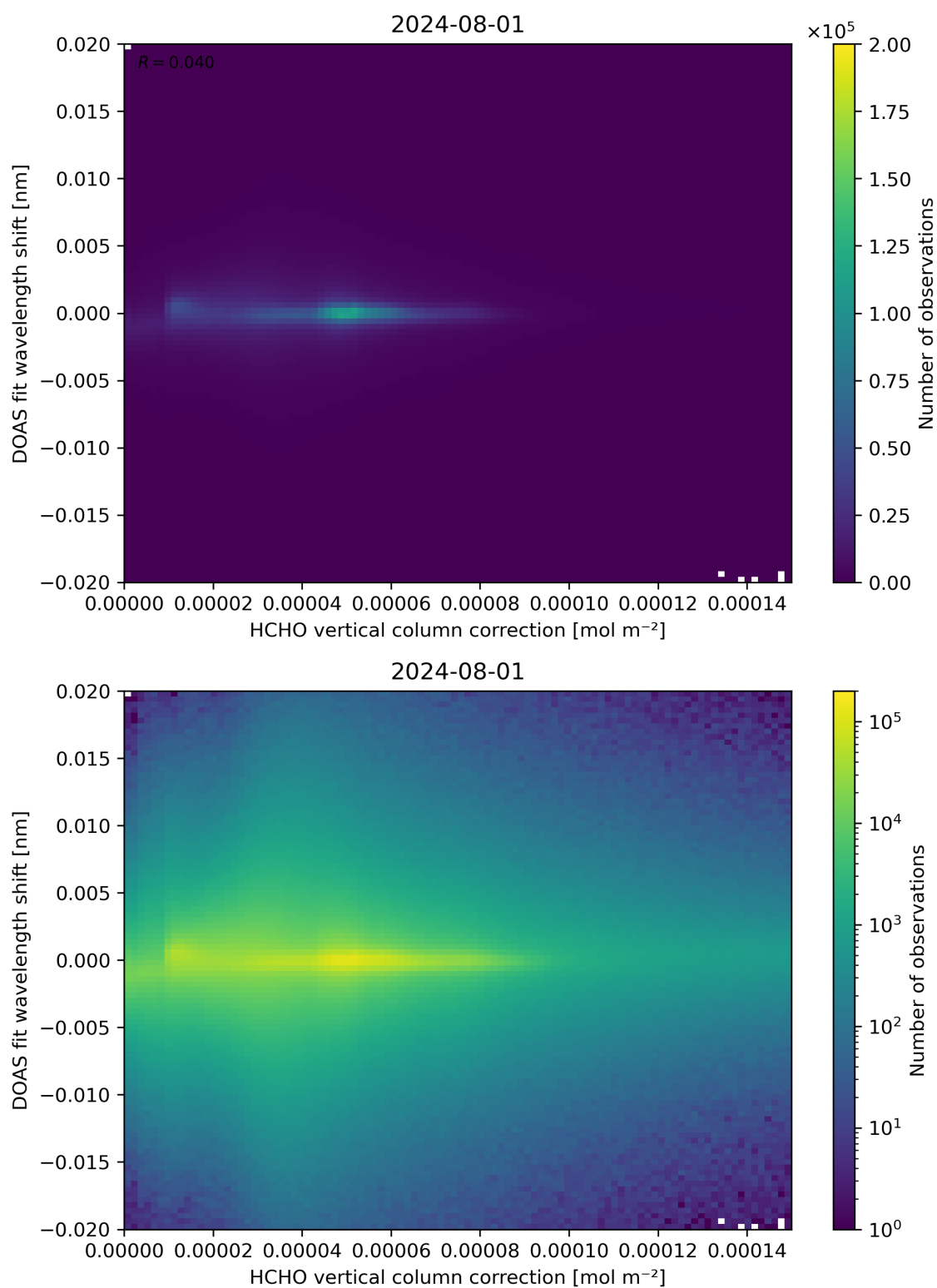
Figure 113: Scatter density plot of “HCHO vertical column correction” against “DOAS fit wavelength shift” for 2024-07-31 to 2024-08-02.
