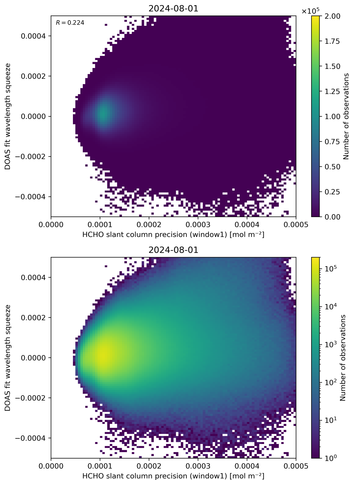
Figure 90: Scatter density plot of “HCHO slant column precision (window1)” against “DOAS fit wavelength squeeze” for 2024-07-31 to 2024-08-02.
