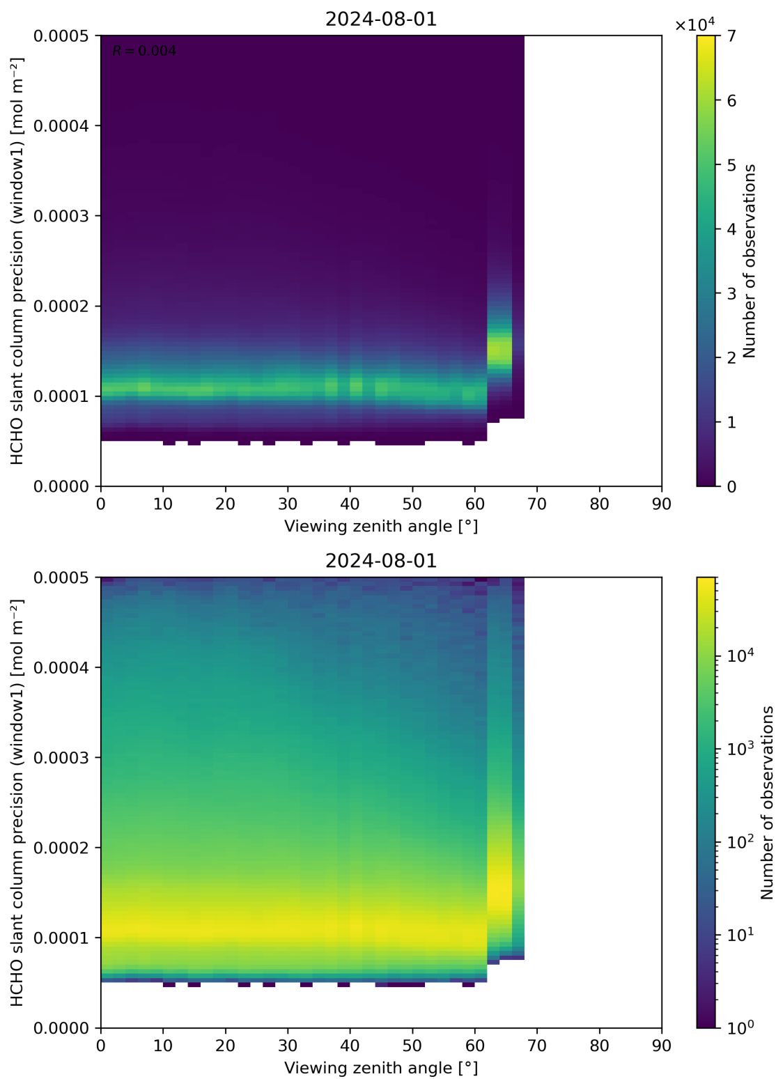
Figure 189: Scatter density plot of “Viewing zenith angle” against “HCHO slant column precision (window1)” for 2024-07-31 to 2024-08-02.
