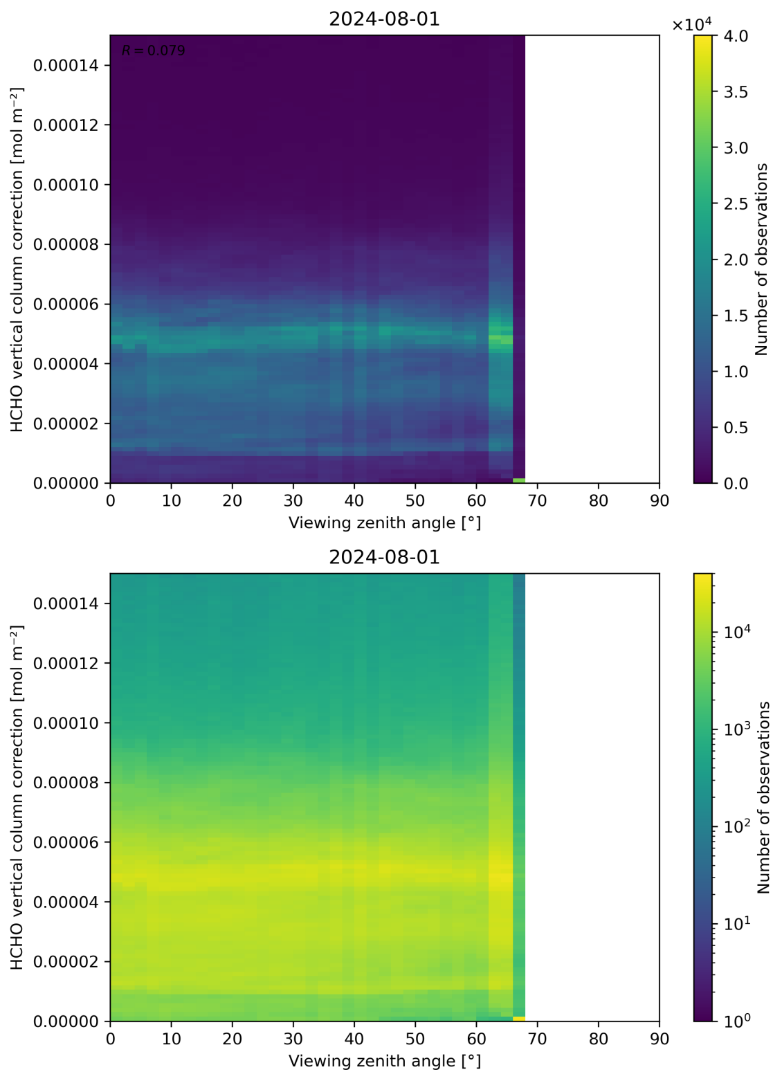
Figure 193: Scatter density plot of “Viewing zenith angle” against “HCHO vertical column correction” for 2024-07-31 to 2024-08-02.
