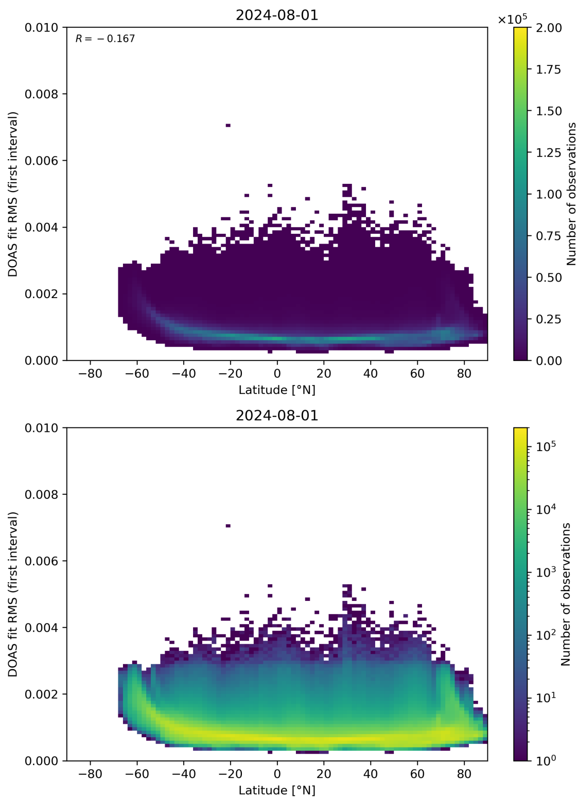
Figure 153: Scatter density plot of “Latitude” against “DOAS fit RMS (first interval)” for 2024-07-31 to 2024-08-02.
