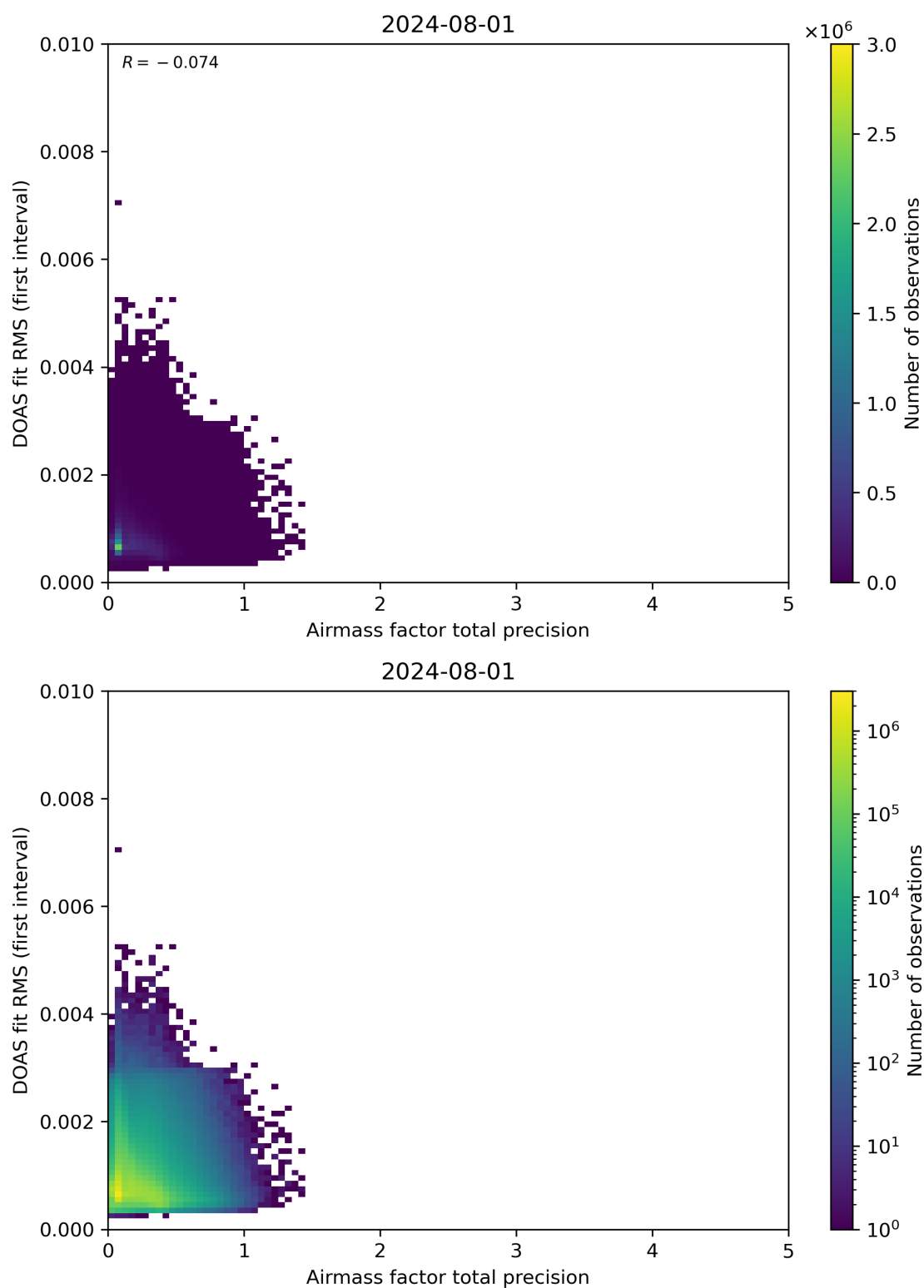
Figure 105: Scatter density plot of “Airmass factor total precision” against “DOAS fit RMS (first interval)” for 2024-07-31 to 2024-08-02.
