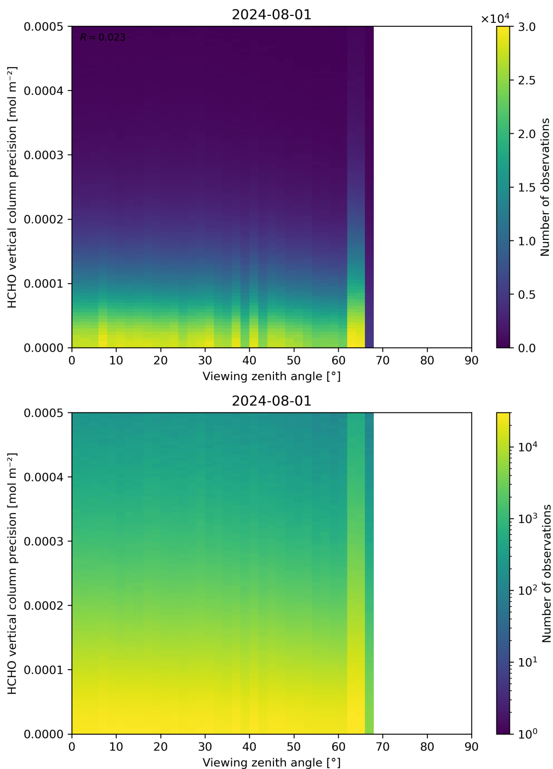
Figure 194: Scatter density plot of “Viewing zenith angle” against “HCHO vertical column precision” for 2024-07-31 to 2024-08-02.
