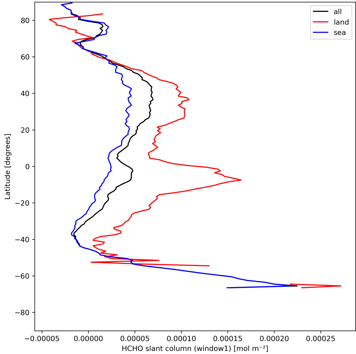
Figure 24: Zonal average of “HCHO slant column (window1)” for 2024-07-31 to 2024-08-02.
