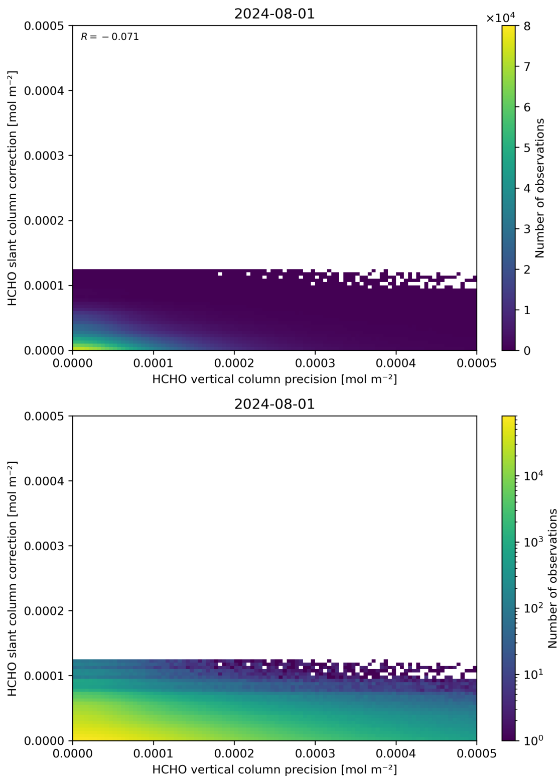
Figure 141: Scatter density plot of “HCHO vertical column precision” against “HCHO slant column correction” for 2024-07-31 to 2024-08-02.
