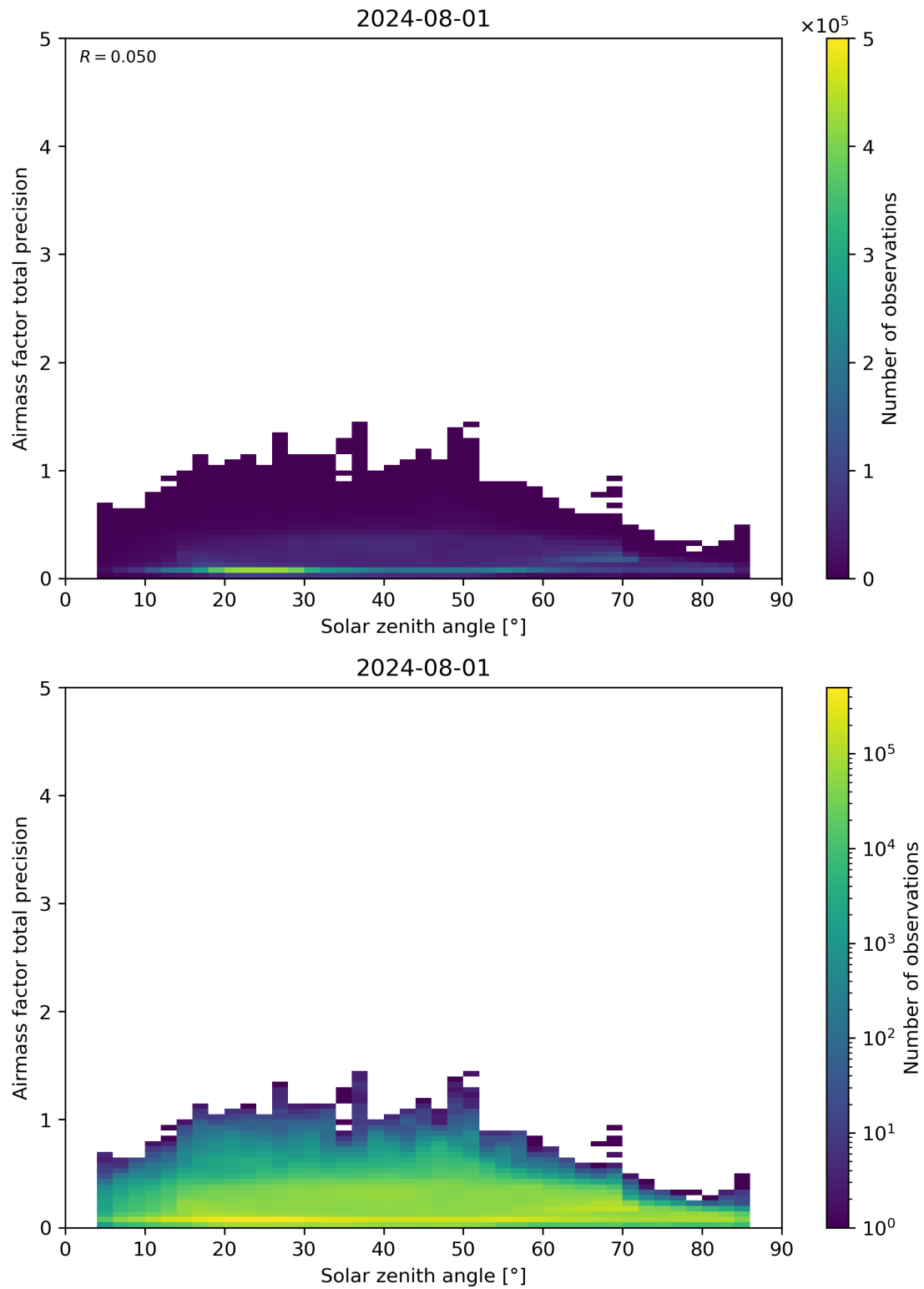
Figure 176: Scatter density plot of “Solar zenith angle” against “Airmass factor total precision” for 2024-07-31 to 2024-08-02.
