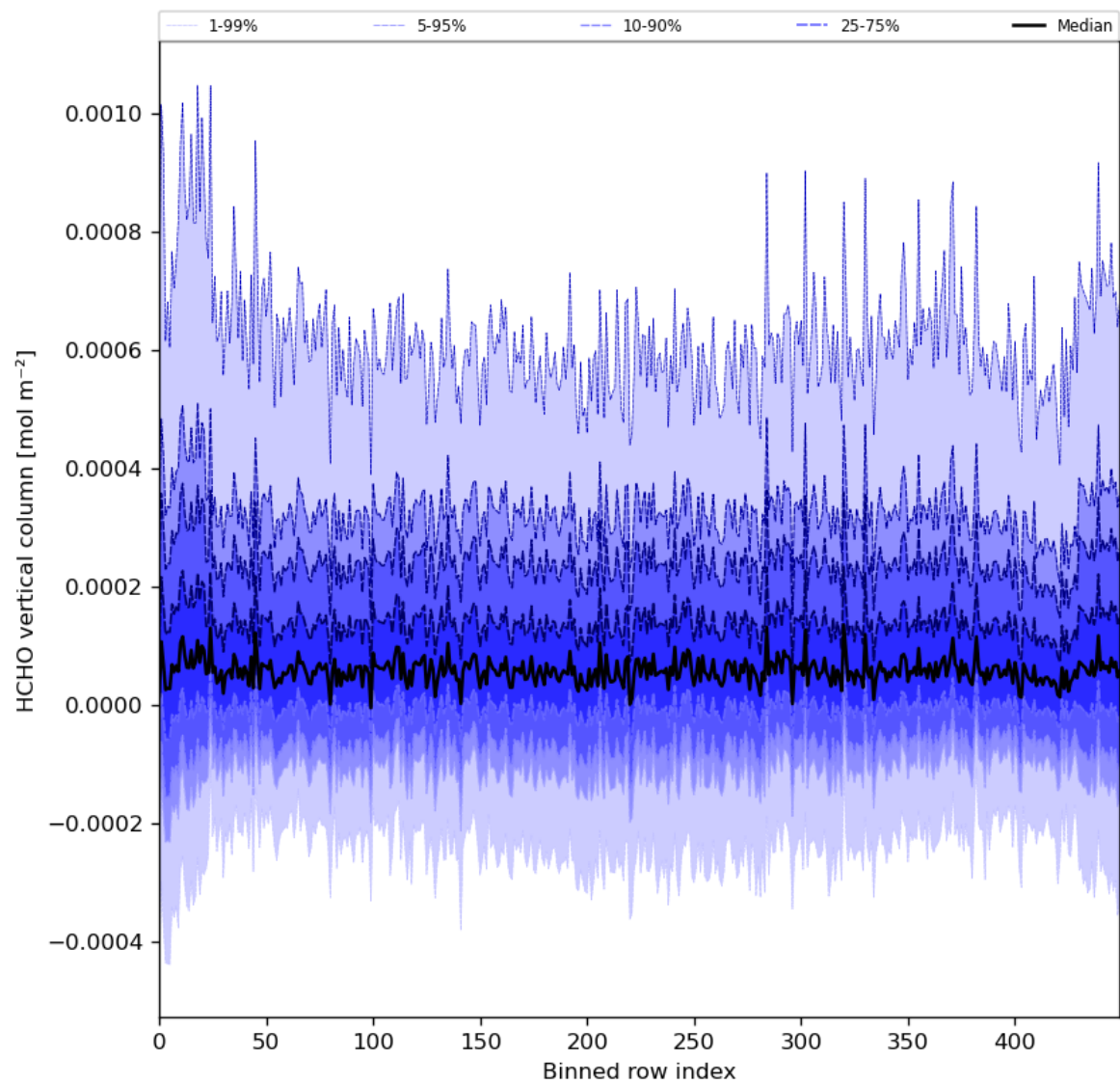
Figure 49: Along track statistics of “HCHO vertical column” for 2024-07-31 to 2024-08-02
