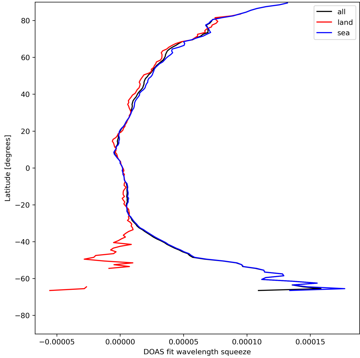
Figure 31: Zonal average of “DOAS fit wavelength squeeze” for 2024-07-31 to 2024-08-02.
