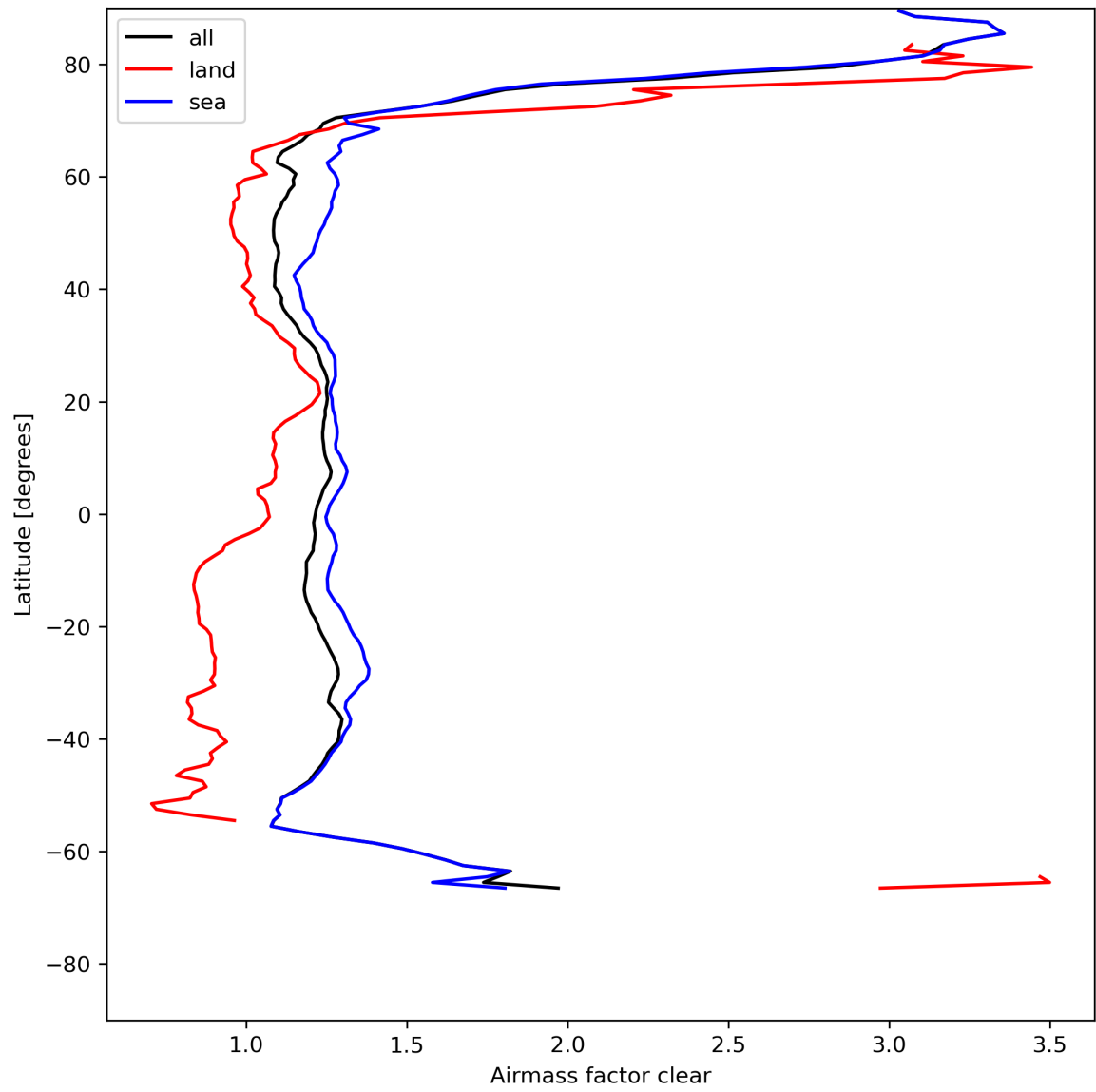
Figure 28: Zonal average of “Airmass factor clear” for 2024-07-31 to 2024-08-02.
