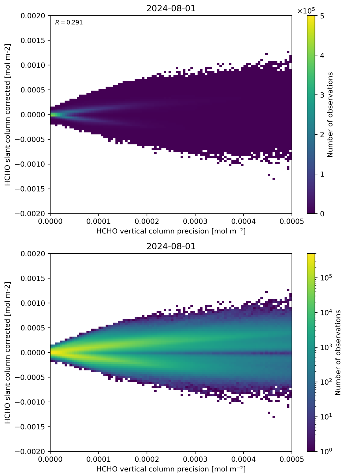
Figure 140: Scatter density plot of “HCHO vertical column precision” against “HCHO slant column corrected” for 2024-07-31 to 2024-08-02.
