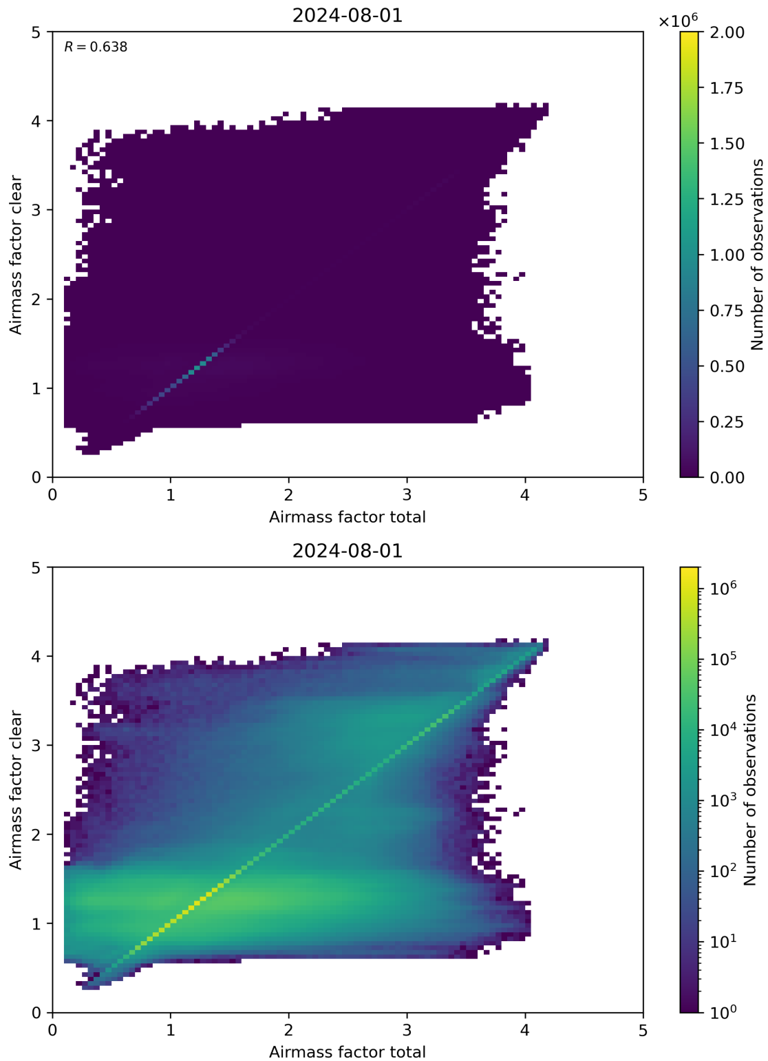
Figure 100: Scatter density plot of “Airmass factor total” against “Airmass factor clear” for 2024-07-31 to 2024-08-02.
