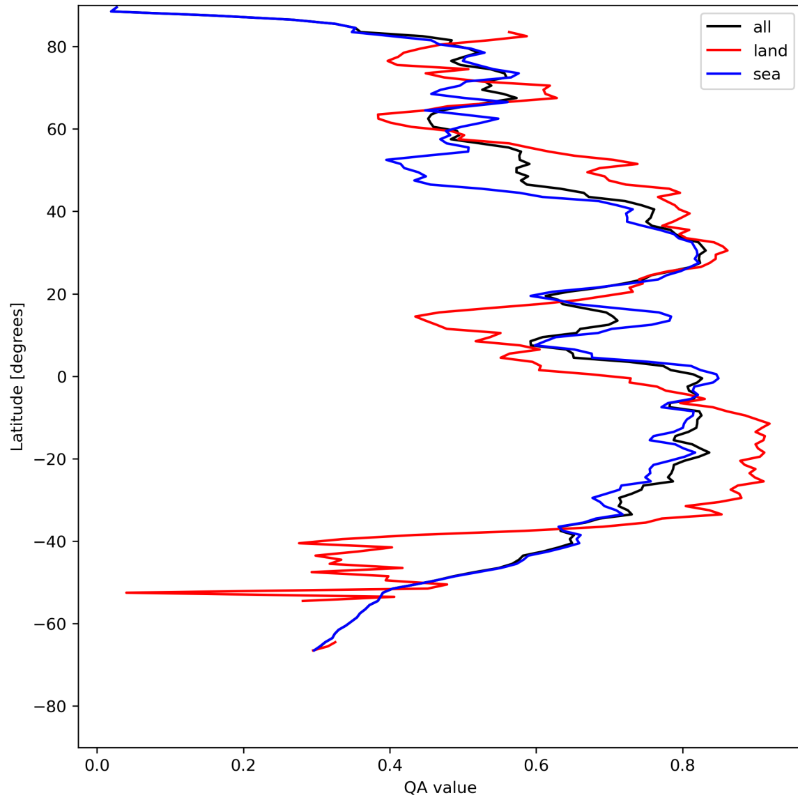
Figure 20: Zonal average of “QA value” for 2024-07-31 to 2024-08-02.
