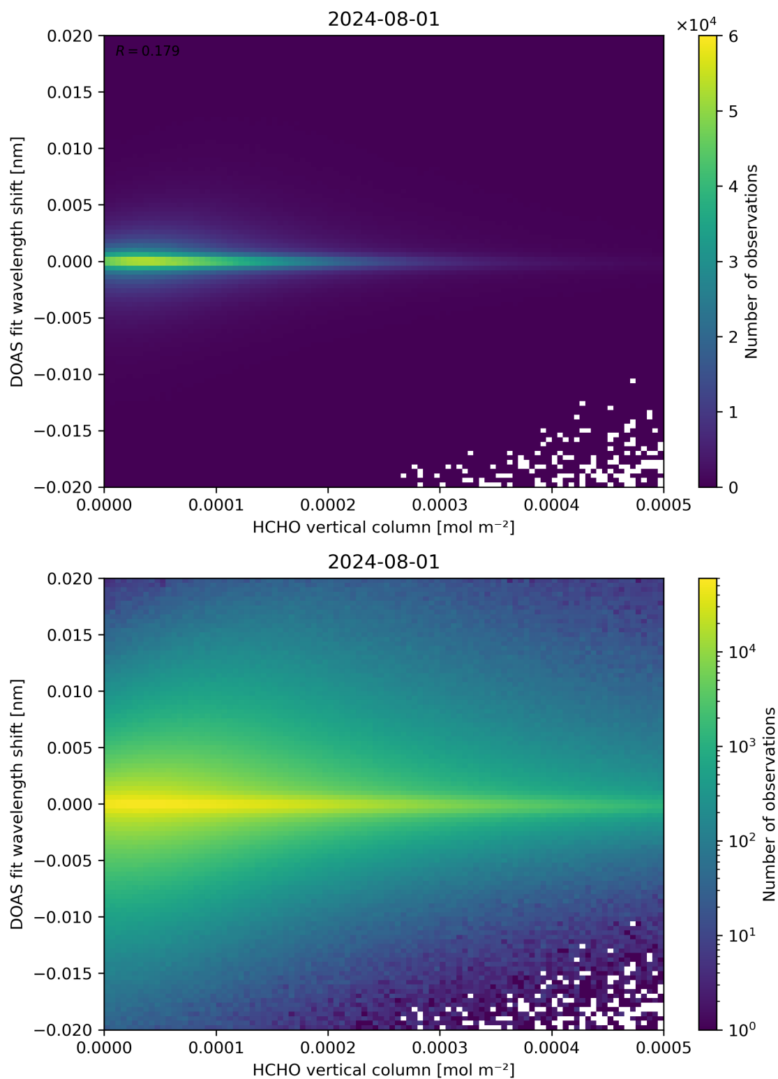
Figure 124: Scatter density plot of “HCHO vertical column” against “DOAS fit wavelength shift” for 2024-07-31 to 2024-08-02.
