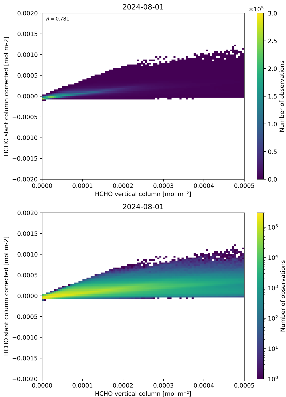
Figure 127: Scatter density plot of “HCHO vertical column” against “HCHO slant column corrected” for 2024-07-31 to 2024-08-02.
