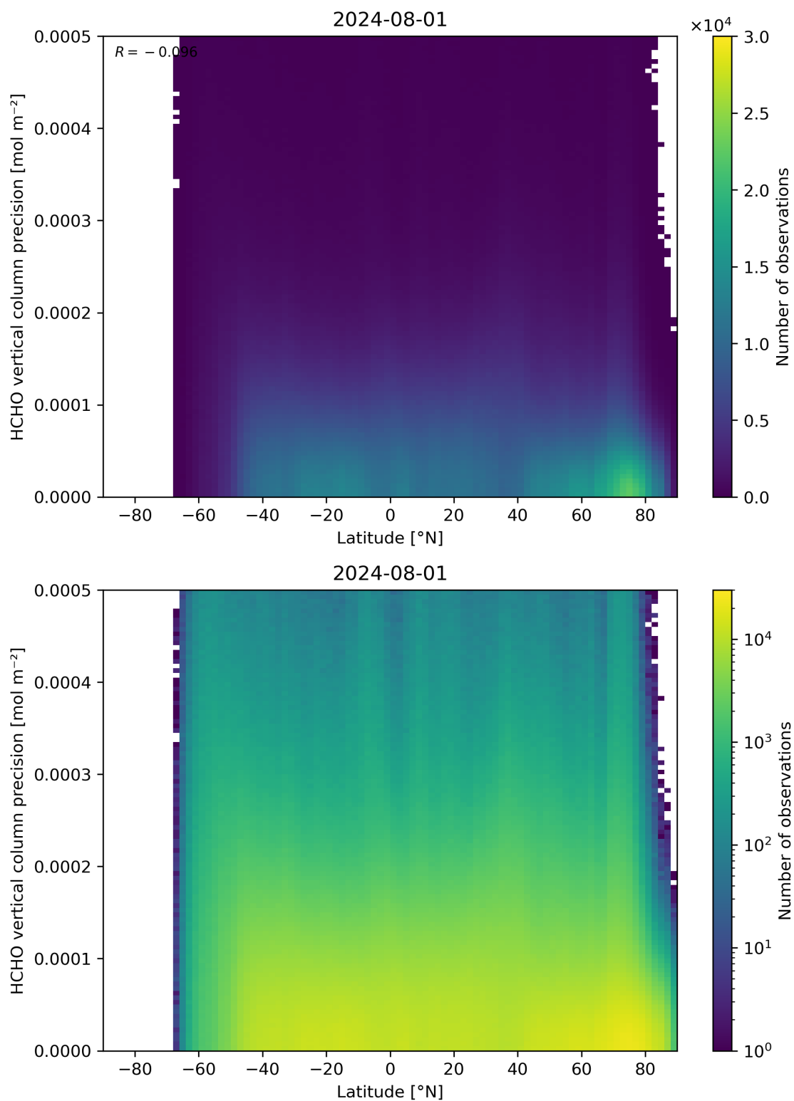
Figure 165: Scatter density plot of “Latitude” against “HCHO vertical column precision” for 2024-07-31 to 2024-08-02.
