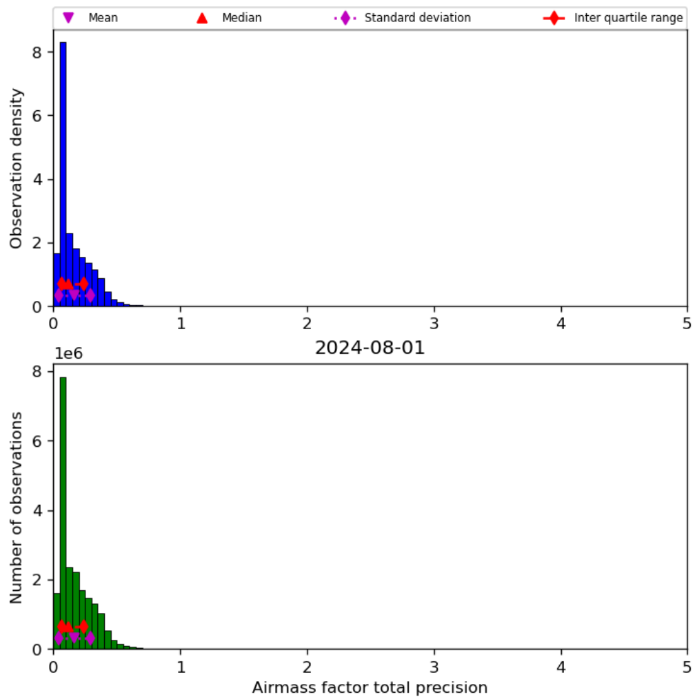
Figure 41: Histogram of “Airmass factor total precision” for 2024-07-31 to 2024-08-02
