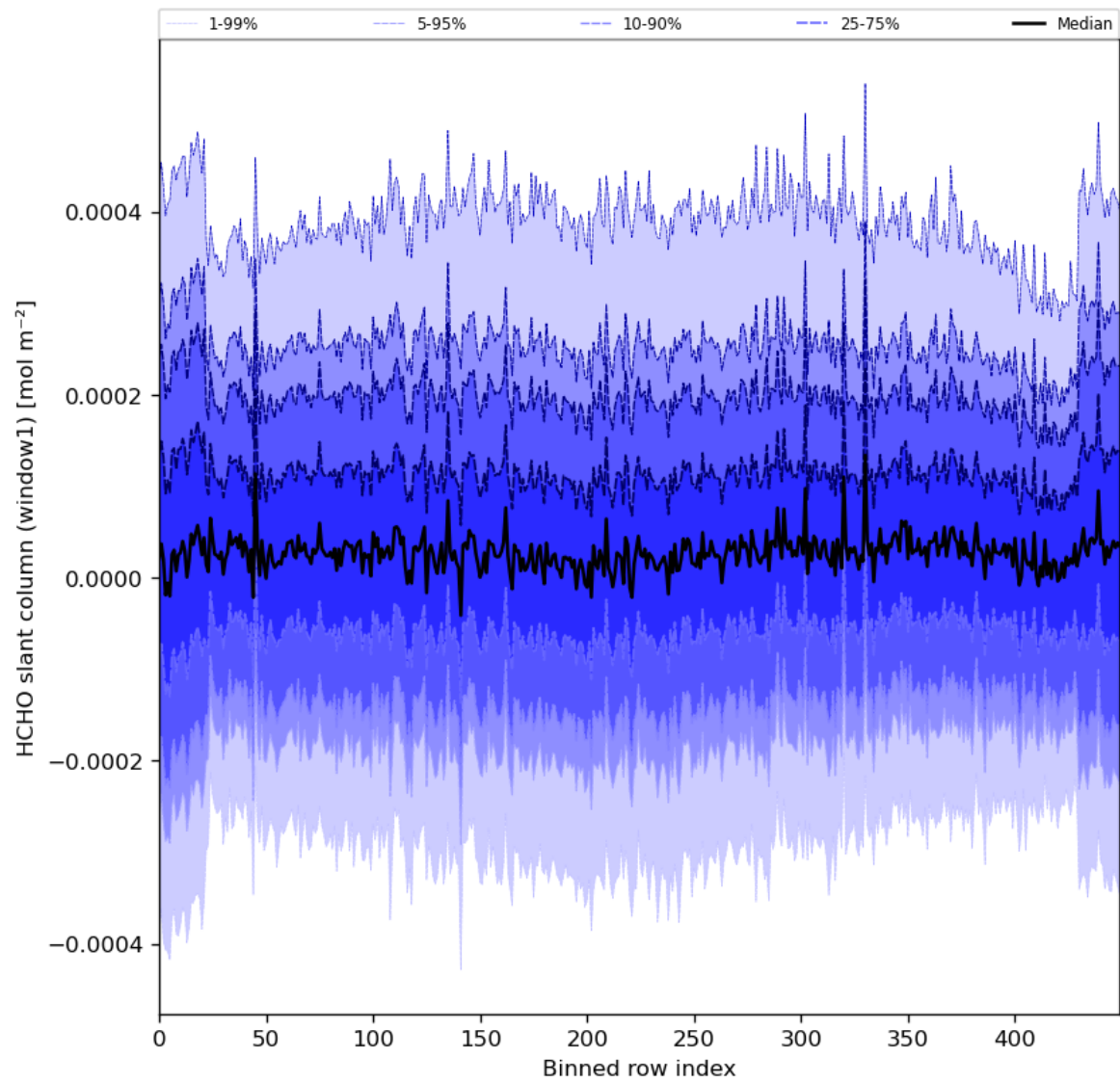
Figure 52: Along track statistics of “HCHO slant column (window1)” for 2024-07-31 to 2024-08-02
