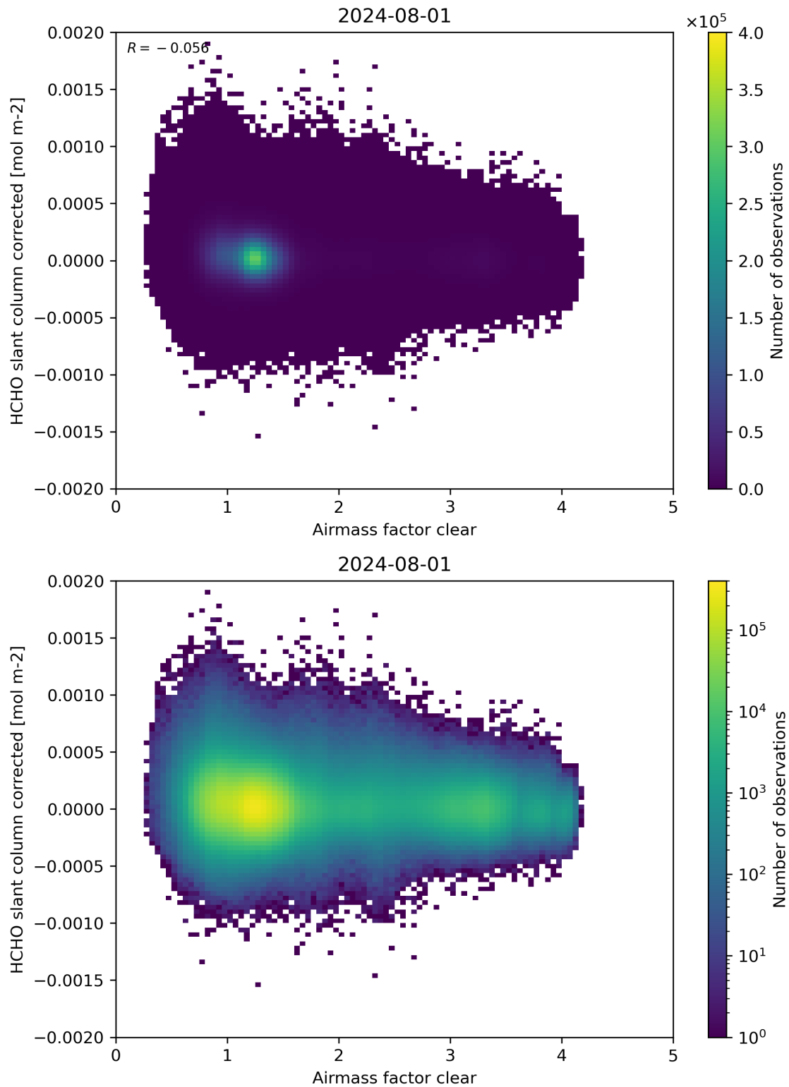
Figure 74: Scatter density plot of “Airmass factor clear” against “HCHO slant column corrected” for 2024-07-31 to 2024-08-02.
