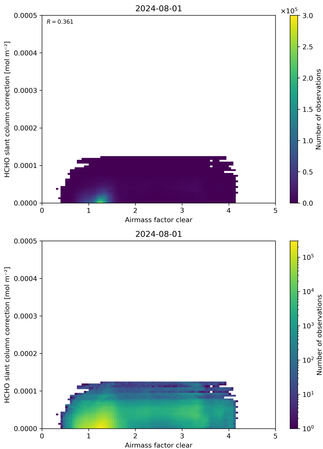
Figure 75: Scatter density plot of “Airmass factor clear” against “HCHO slant column correction” for 2024-07-31 to 2024-08-02.
