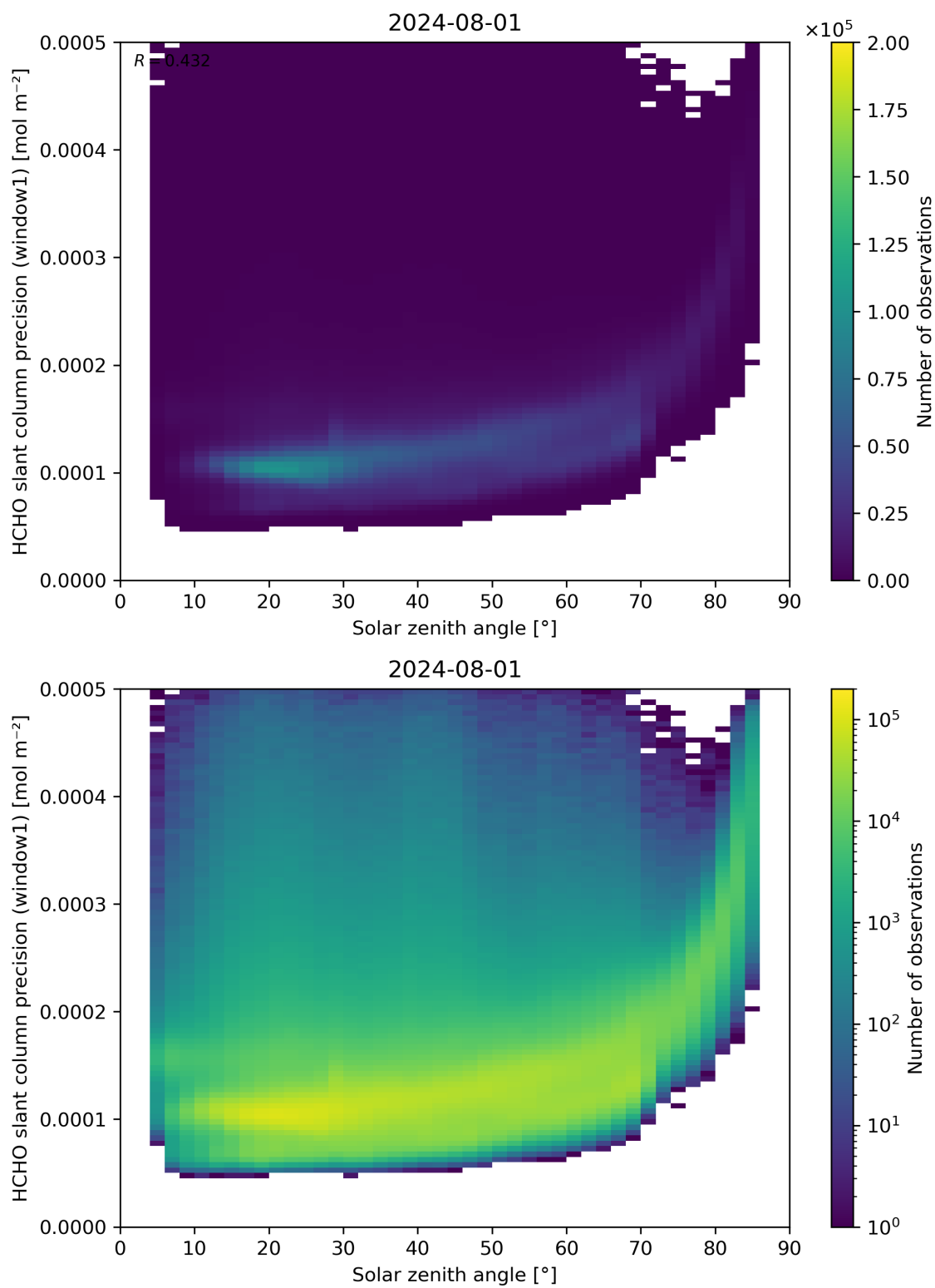
Figure 174: Scatter density plot of “Solar zenith angle” against “HCHO slant column precision (window1)” for 2024-07-31 to 2024-08-02.
