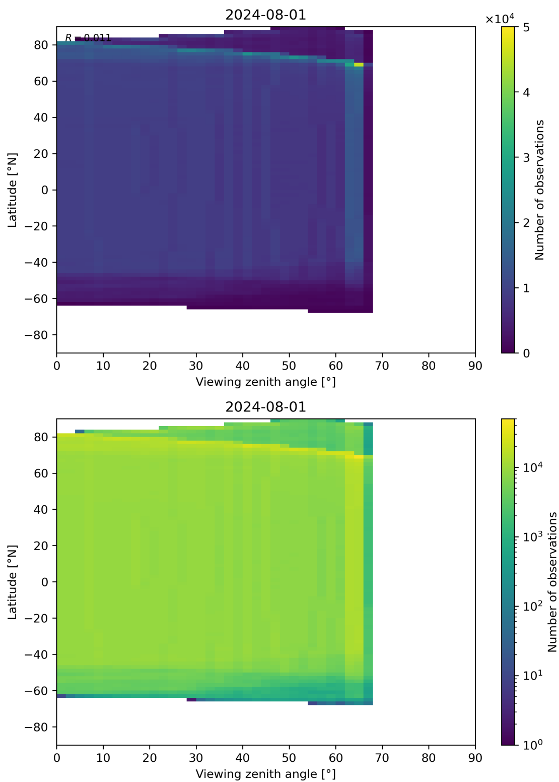
Figure 196: Scatter density plot of “Viewing zenith angle” against “Latitude” for 2024-07-31 to 2024-08-02.
