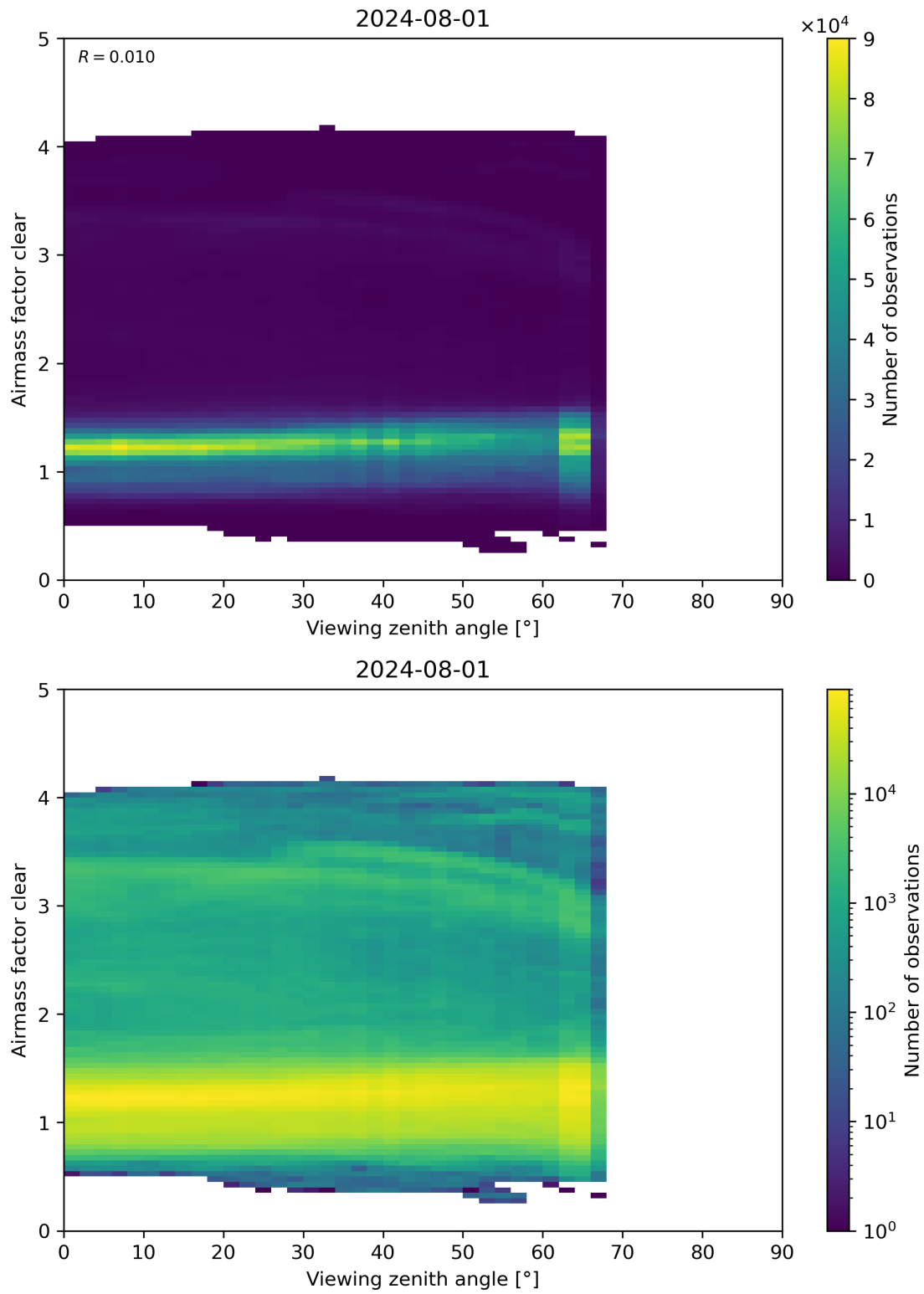
Figure 185: Scatter density plot of “Viewing zenith angle” against “Airmass factor clear” for 2024-07-31 to 2024-08-02.
