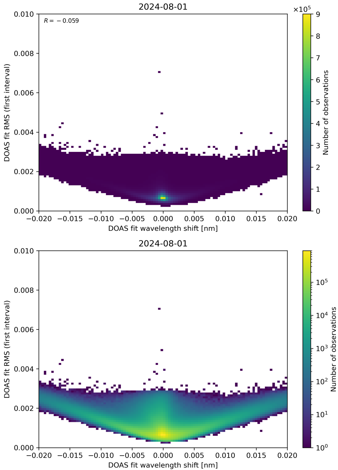
Figure 64: Scatter density plot of “DOAS fit wavelength shift” against “DOAS fit RMS (first interval)” for 2024-07-31 to 2024-08-02.
