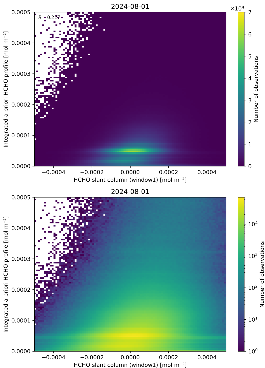
Figure 87: Scatter density plot of “HCHO slant column (window1)” against “Integrated a priori HCHO profile” for 2024-07-31 to 2024-08-02.
