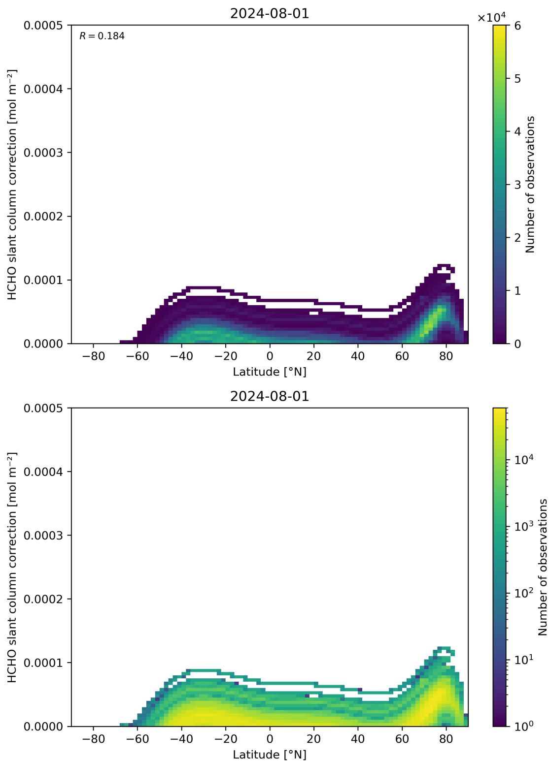
Figure 158: Scatter density plot of “Latitude” against “HCHO slant column correction” for 2024-07-31 to 2024-08-02.
