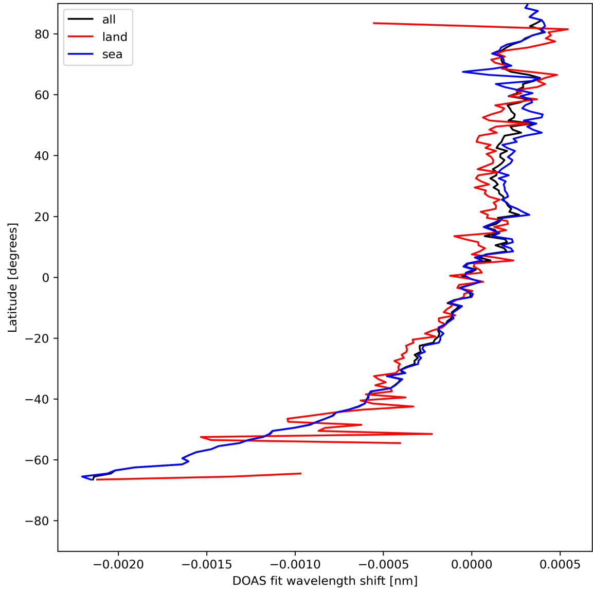
Figure 30: Zonal average of "DOAS fit wavelength shift" for 2024-07-31 to 2024-08-02.
