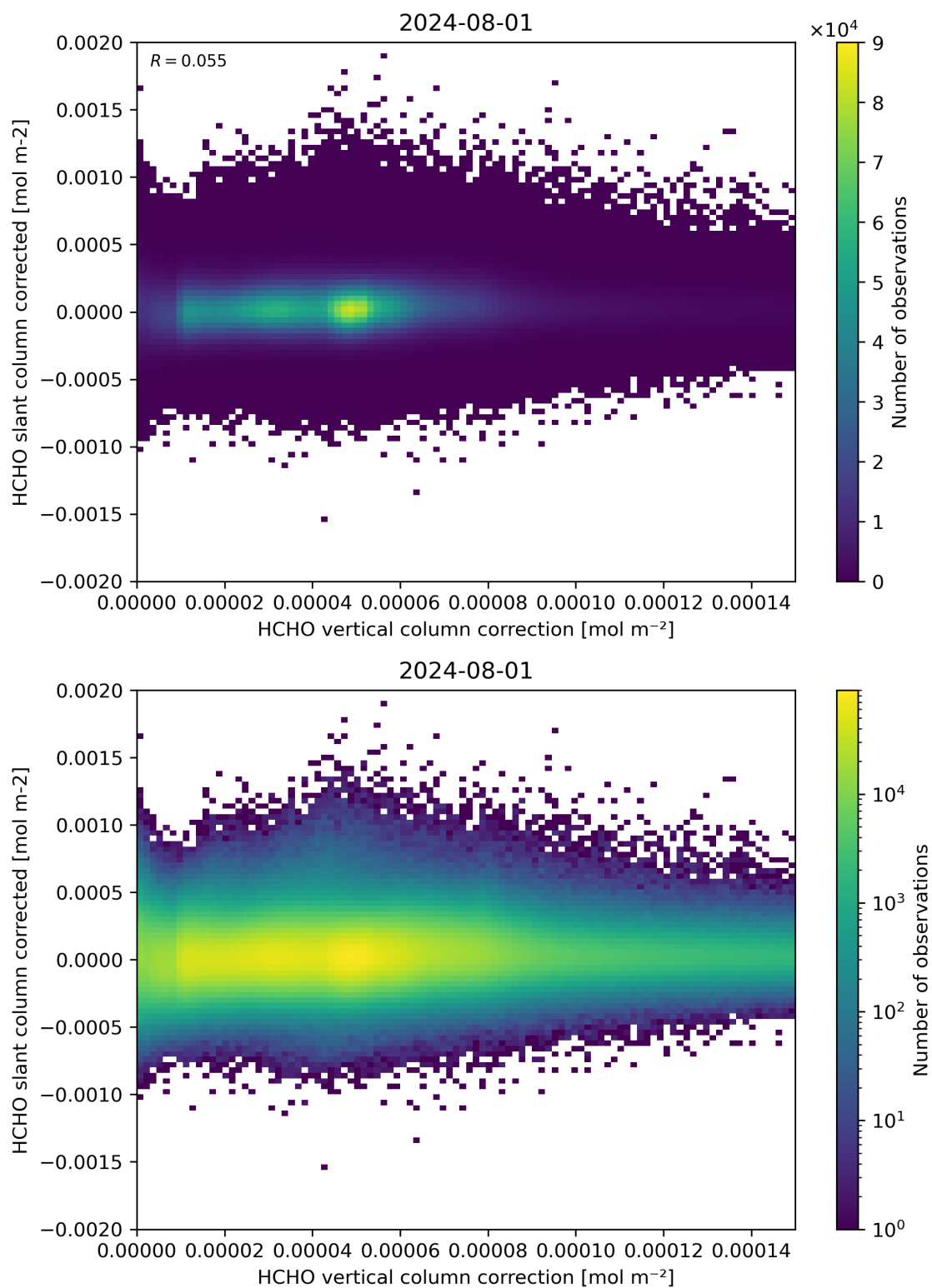
Figure 116: Scatter density plot of “HCHO vertical column correction” against “HCHO slant column corrected” for 2024-07-31 to 2024-08-02.
