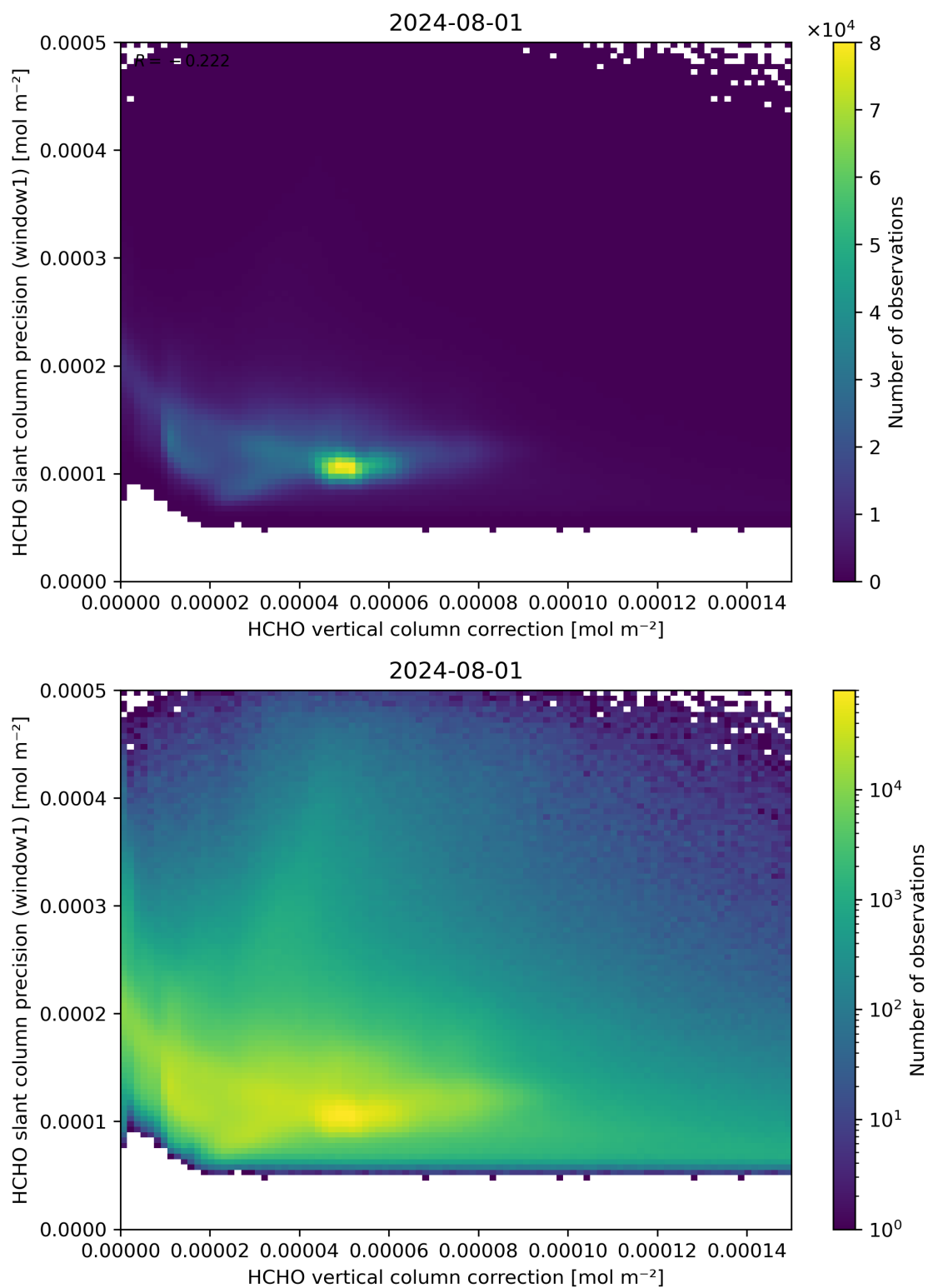
Figure 119: Scatter density plot of “HCHO vertical column correction” against “HCHO slant column precision (window1)” for 2024-07-31 to 2024-08-02.
