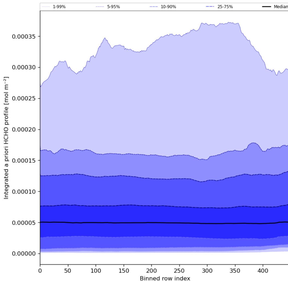
Figure 57: Along track statistics of “Integrated a priori HCHO profile” for 2024-07-31 to 2024-08-02
