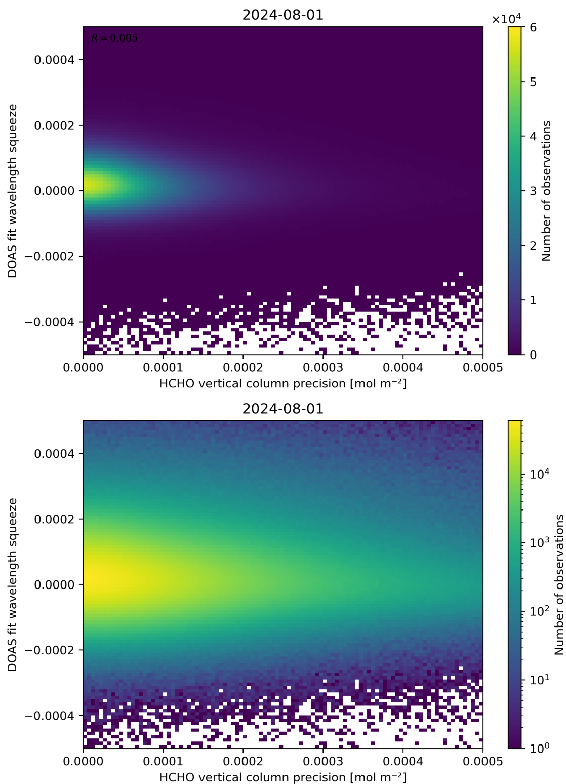
Figure 138: Scatter density plot of “HCHO vertical column precision” against “DOAS fit wavelength squeeze” for 2024-07-31 to 2024-08-02.
