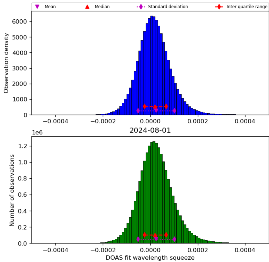
Figure 45: Histogram of “DOAS fit wavelength squeeze” for 2024-07-31 to 2024-08-02
