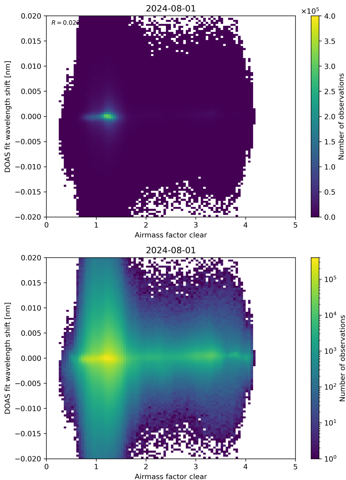
Figure 72: Scatter density plot of “Airmass factor clear” against “DOAS fit wavelength shift” for 2024-07-31 to 2024-08-02.
