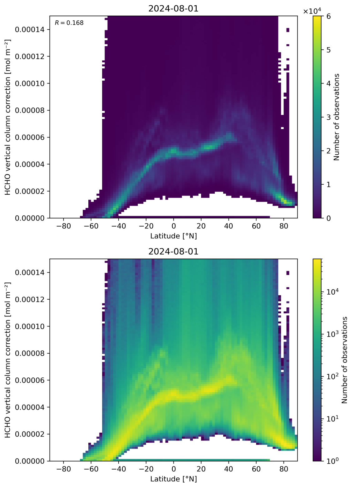
Figure 164: Scatter density plot of “Latitude” against “HCHO vertical column correction” for 2024-07-31 to 2024-08-02.
