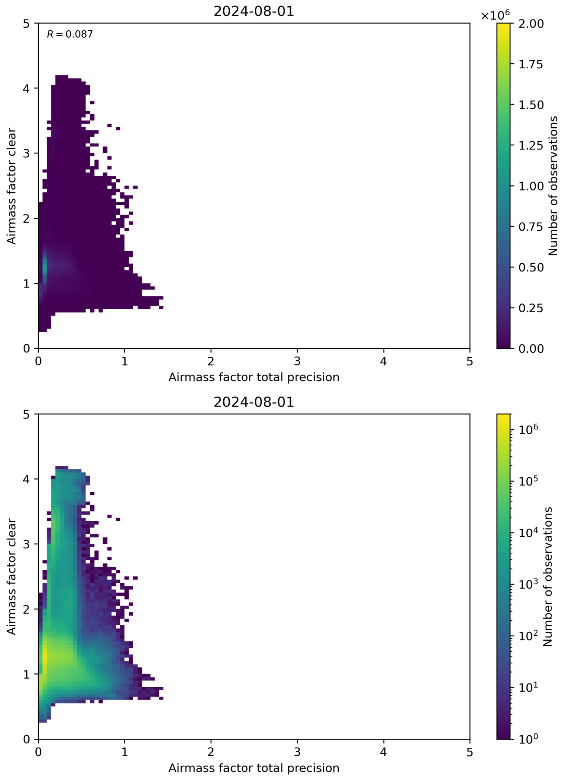
Figure 108: Scatter density plot of “Airmass factor total precision” against “Airmass factor clear” for 2024-07-31 to 2024-08-02.
