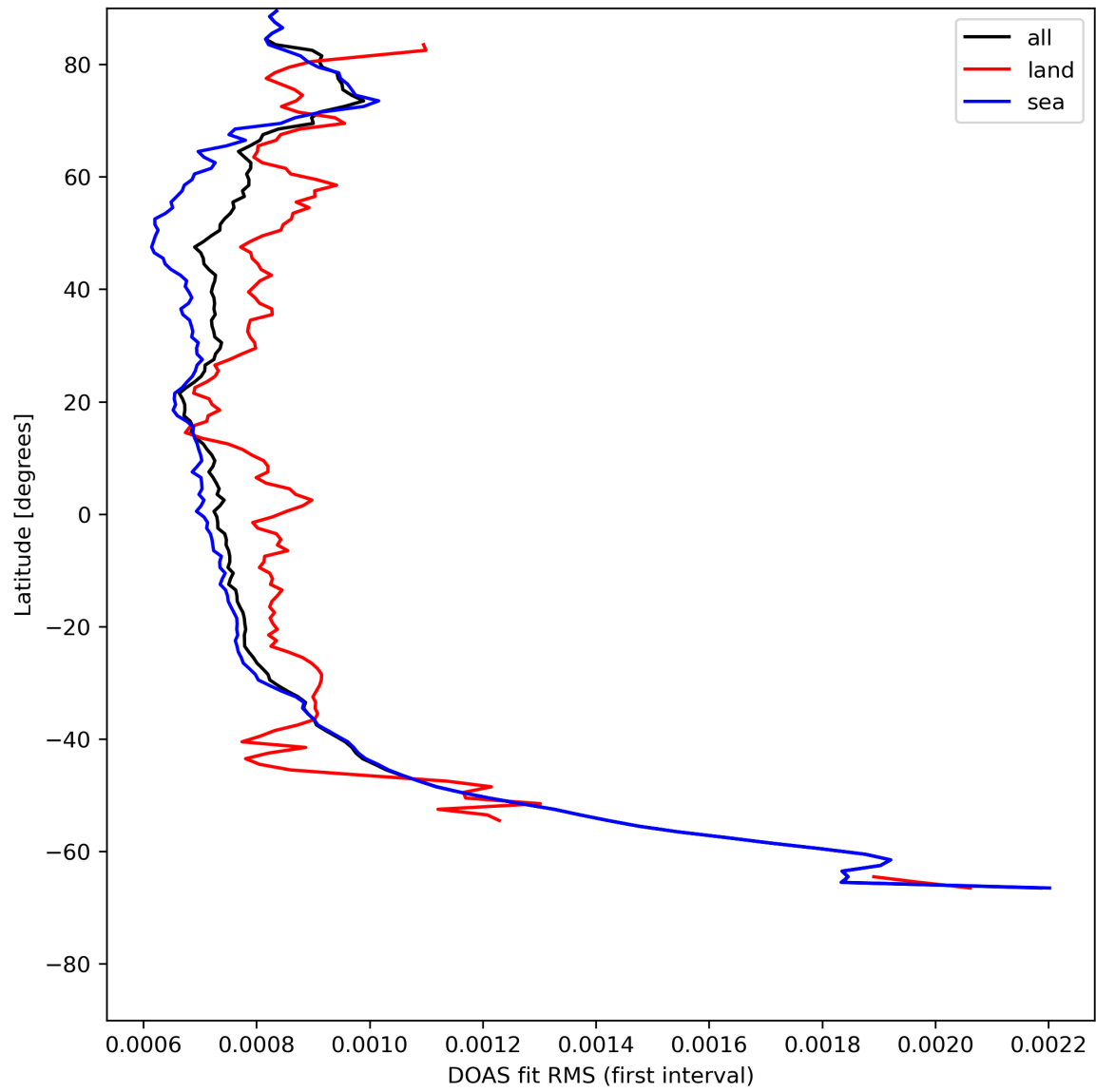
Figure 32: Zonal average of "DOAS fit RMS (first interval)" for 2024-07-31 to 2024-08-02.
