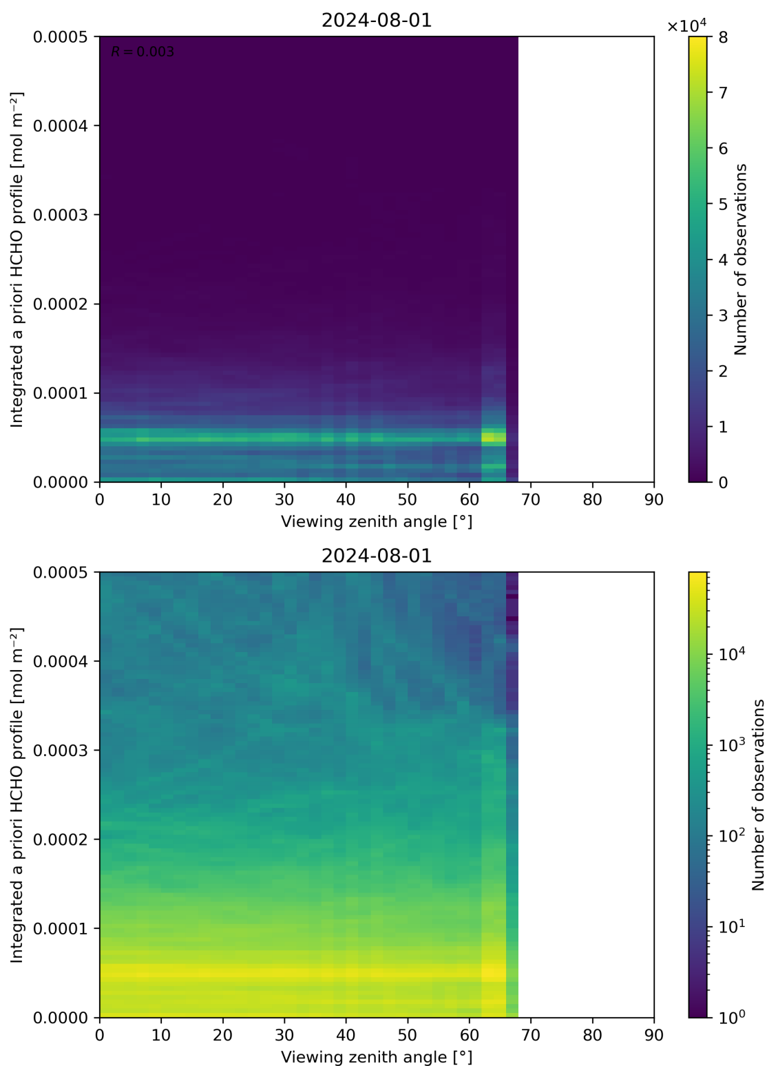
Figure 195: Scatter density plot of “Viewing zenith angle” against “Integrated a priori HCHO profile” for 2024-07-31 to 2024-08-02.
