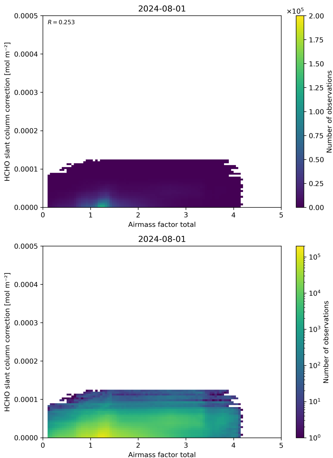
Figure 102: Scatter density plot of “Airmass factor total” against “HCHO slant column correction” for 2024-07-31 to 2024-08-02.
