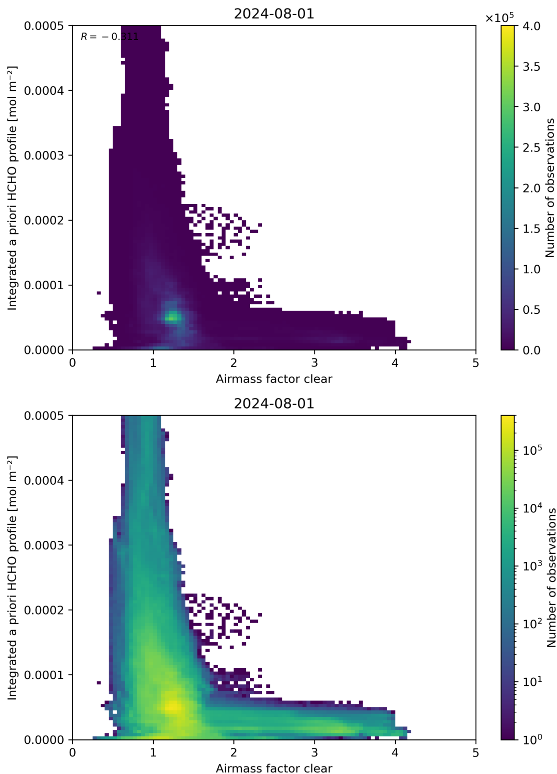
Figure 76: Scatter density plot of “Airmass factor clear” against “Integrated a priori HCHO profile” for 2024-07-31 to 2024-08-02.
