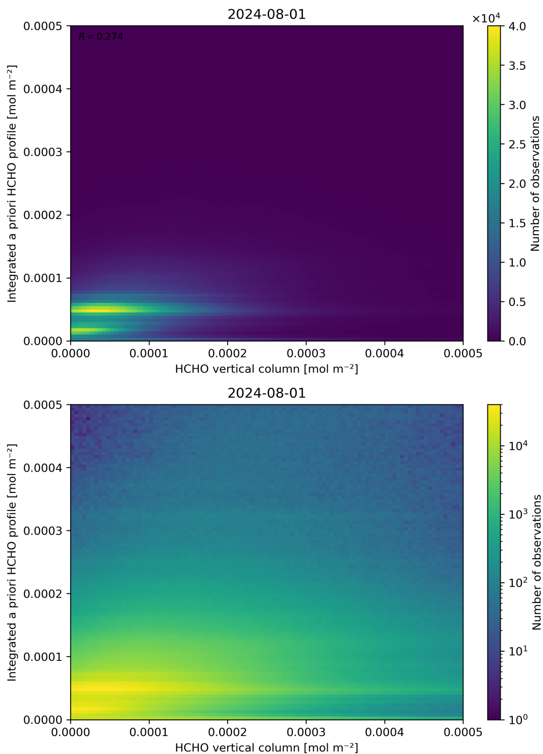
Figure 135: Scatter density plot of “HCHO vertical column” against “Integrated a priori HCHO profile” for 2024-07-31 to 2024-08-02.
