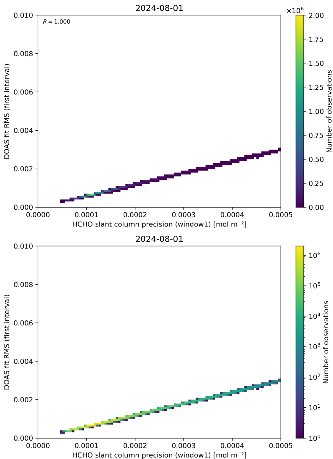
Figure 88: Scatter density plot of “HCHO slant column precision (window1)” against “DOAS fit RMS (first interval)” for 2024-07-31 to 2024-08-02.
