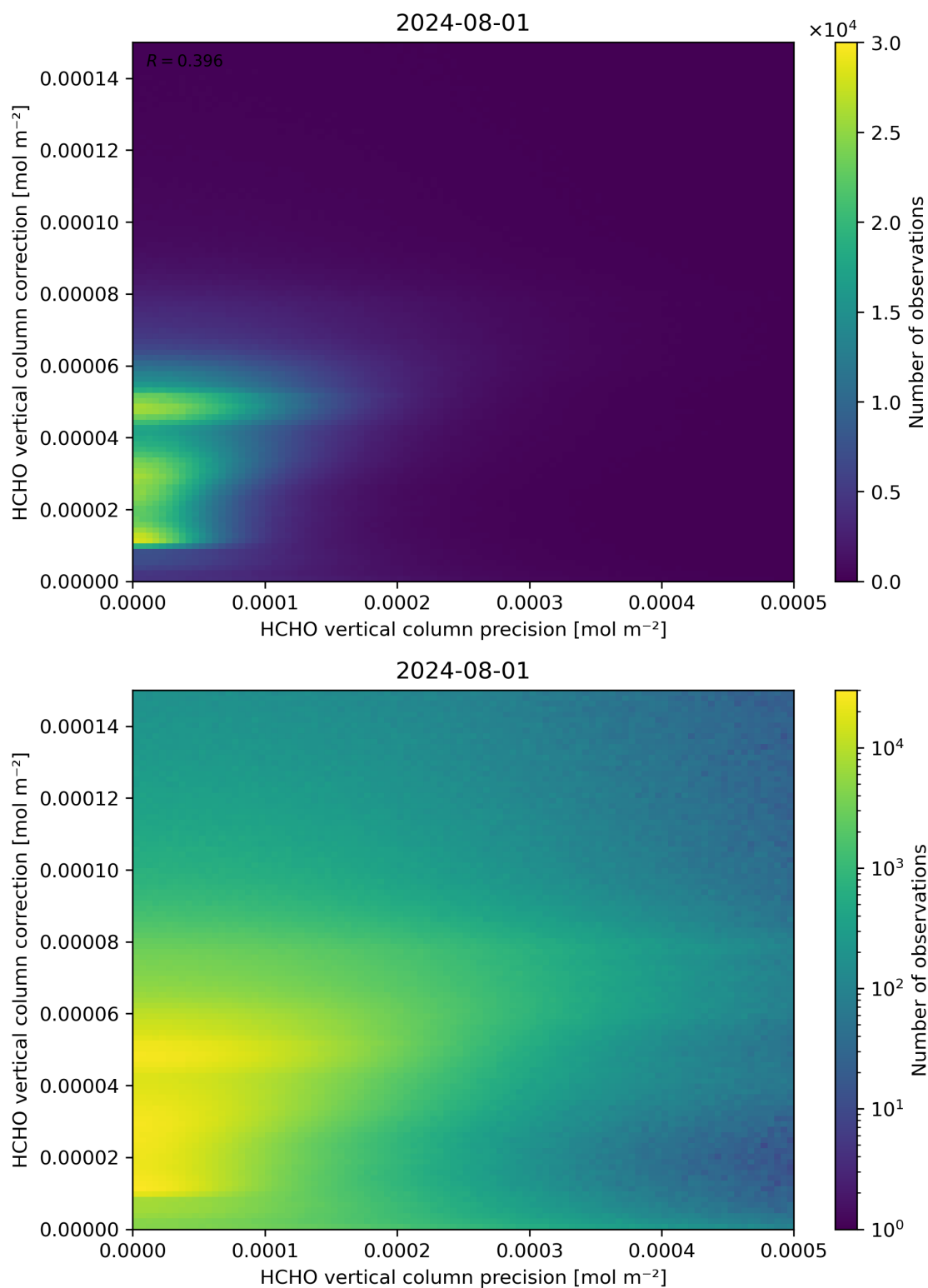
Figure 146: Scatter density plot of “HCHO vertical column precision” against “HCHO vertical column correction” for 2024-07-31 to 2024-08-02.
