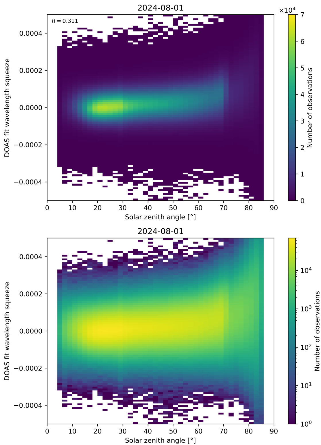
Figure 169: Scatter density plot of “Solar zenith angle” against “DOAS fit wavelength squeeze” for 2024-07-31 to 2024-08-02.
