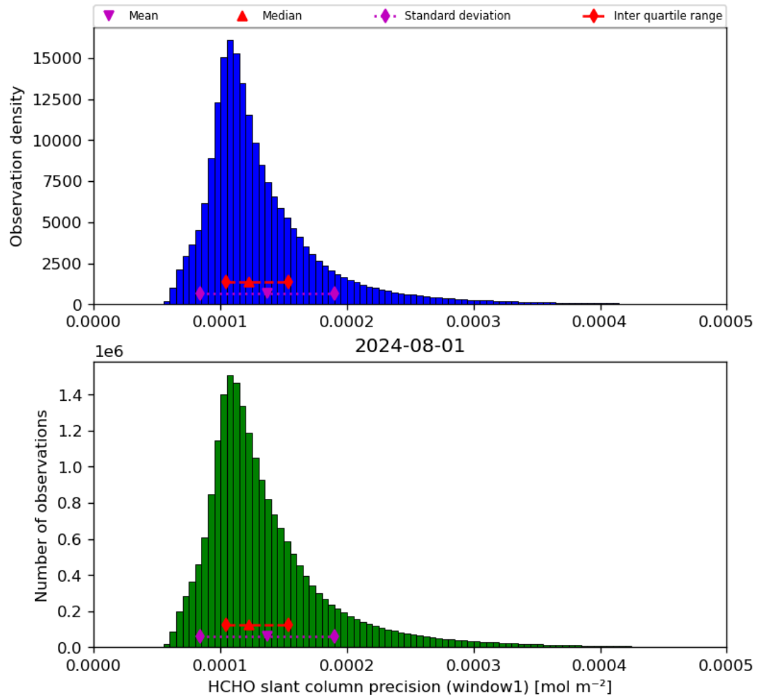
Figure 39: Histogram of “HCHO slant column precision (window1)” for 2024-07-31 to 2024-08-02
