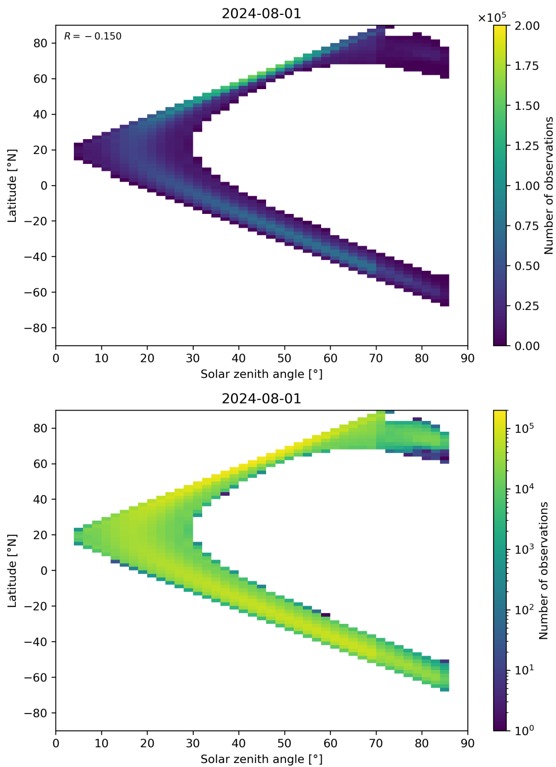
Figure 181: Scatter density plot of “Solar zenith angle” against “Latitude” for 2024-07-31 to 2024-08-02.
