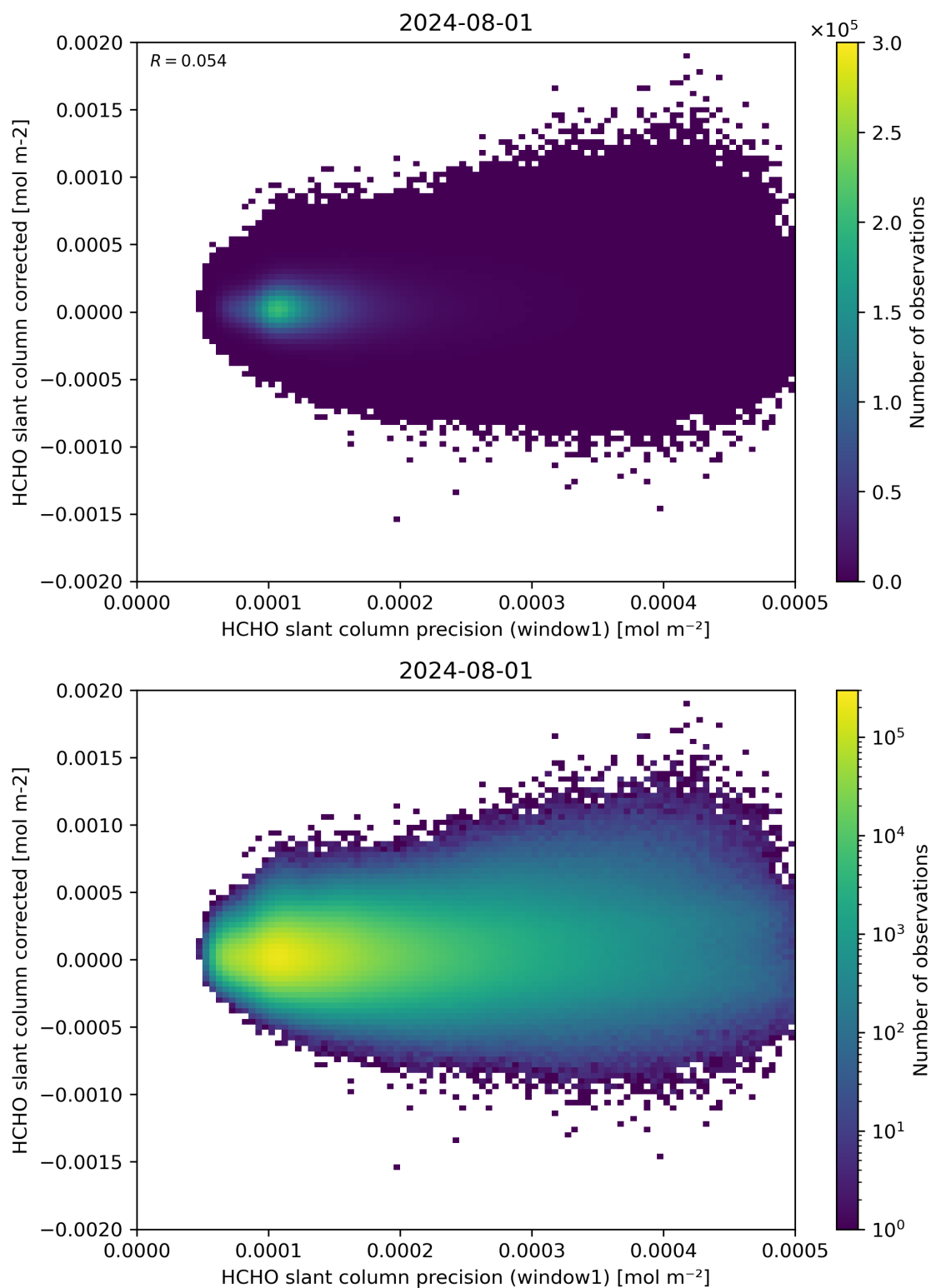
Figure 92: Scatter density plot of “HCHO slant column precision (window1)” against “HCHO slant column corrected” for 2024-07-31 to 2024-08-02.
