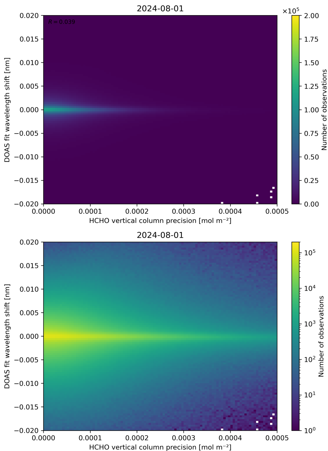
Figure 137: Scatter density plot of “HCHO vertical column precision” against “DOAS fit wavelength shift” for 2024-07-31 to 2024-08-02.
