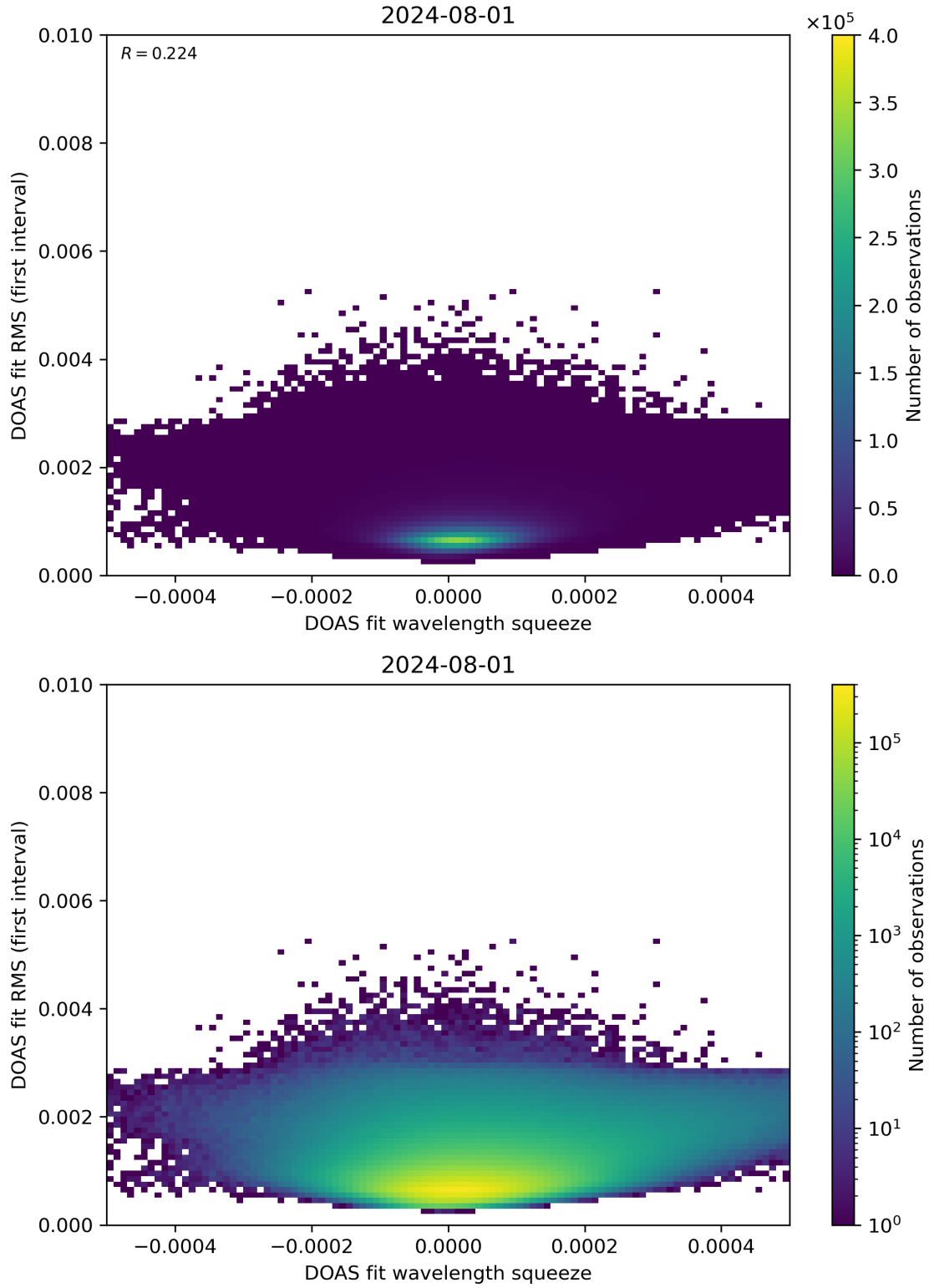
Figure 68: Scatter density plot of “DOAS fit wavelength squeeze” against “DOAS fit RMS (first interval)” for 2024-07-31 to 2024-08-02.
