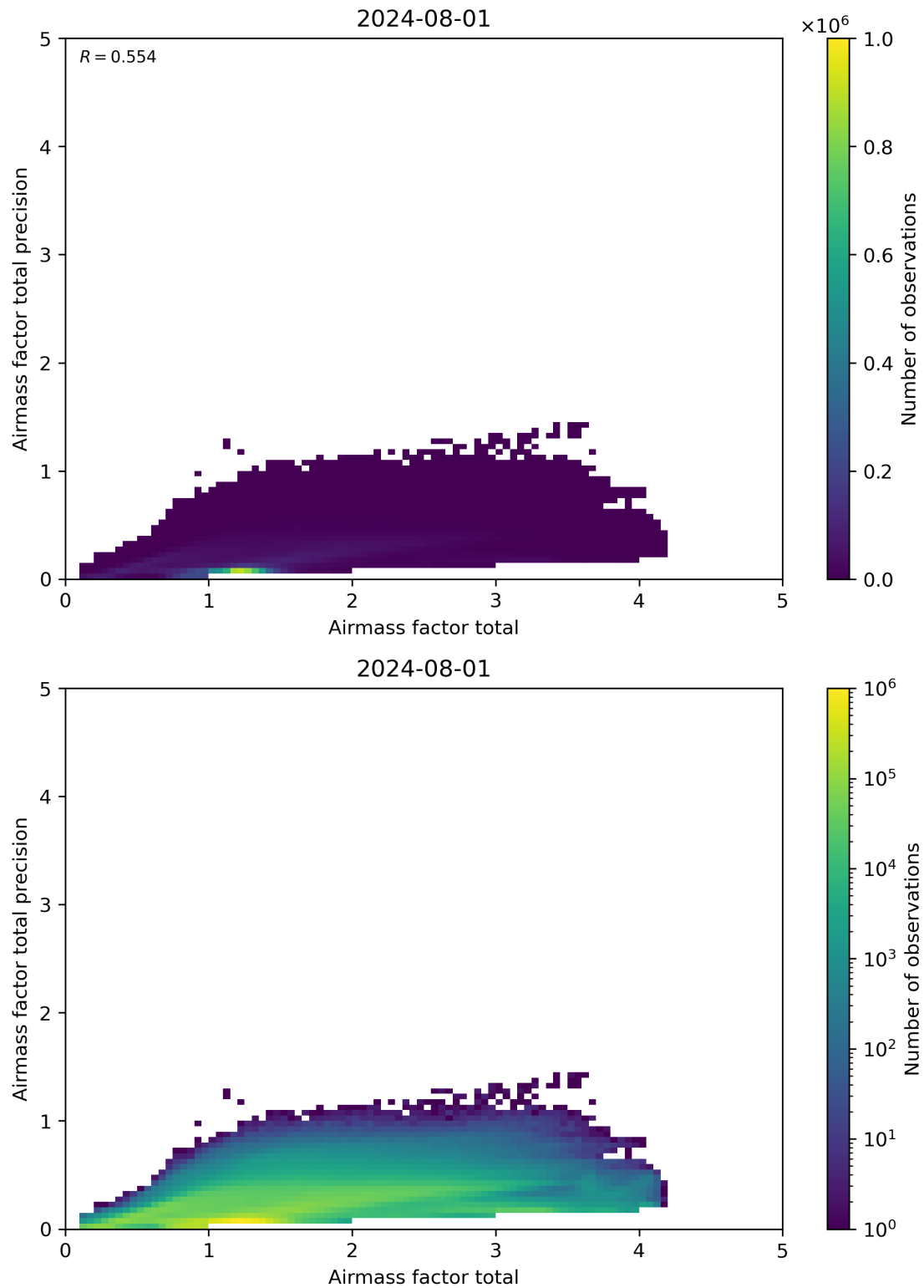
Figure 103: Scatter density plot of “Airmass factor total” against “Airmass factor total precision” for 2024-07-31 to 2024-08-02.
