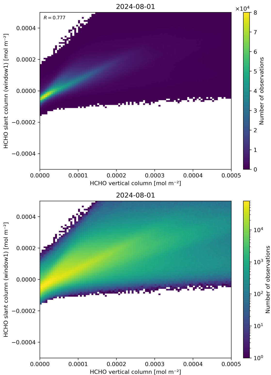
Figure 129: Scatter density plot of “HCHO vertical column” against “HCHO slant column (window1)” for 2024-07-31 to 2024-08-02.
