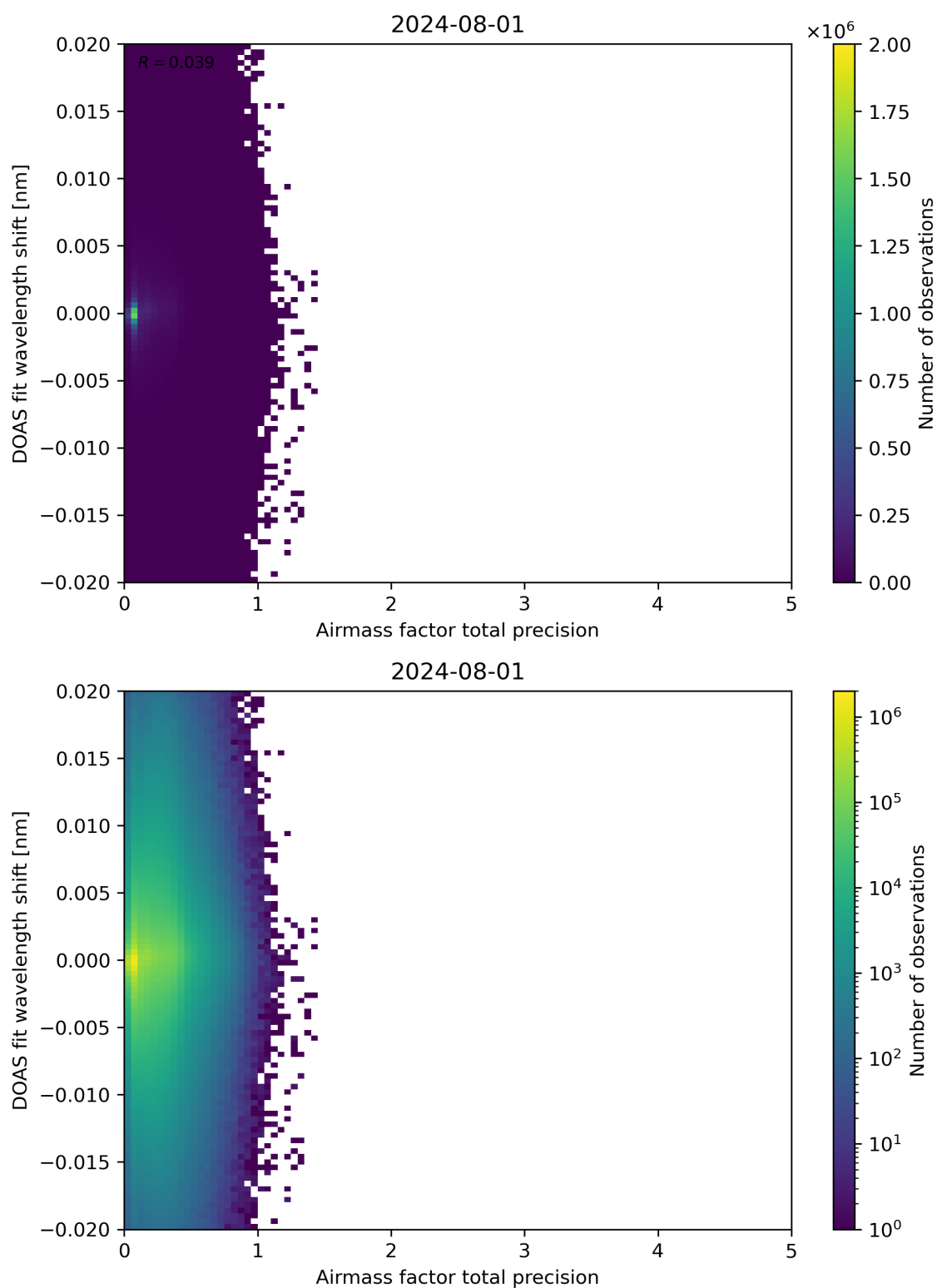
Figure 106: Scatter density plot of “Airmass factor total precision” against “DOAS fit wavelength shift” for 2024-07-31 to 2024-08-02.
