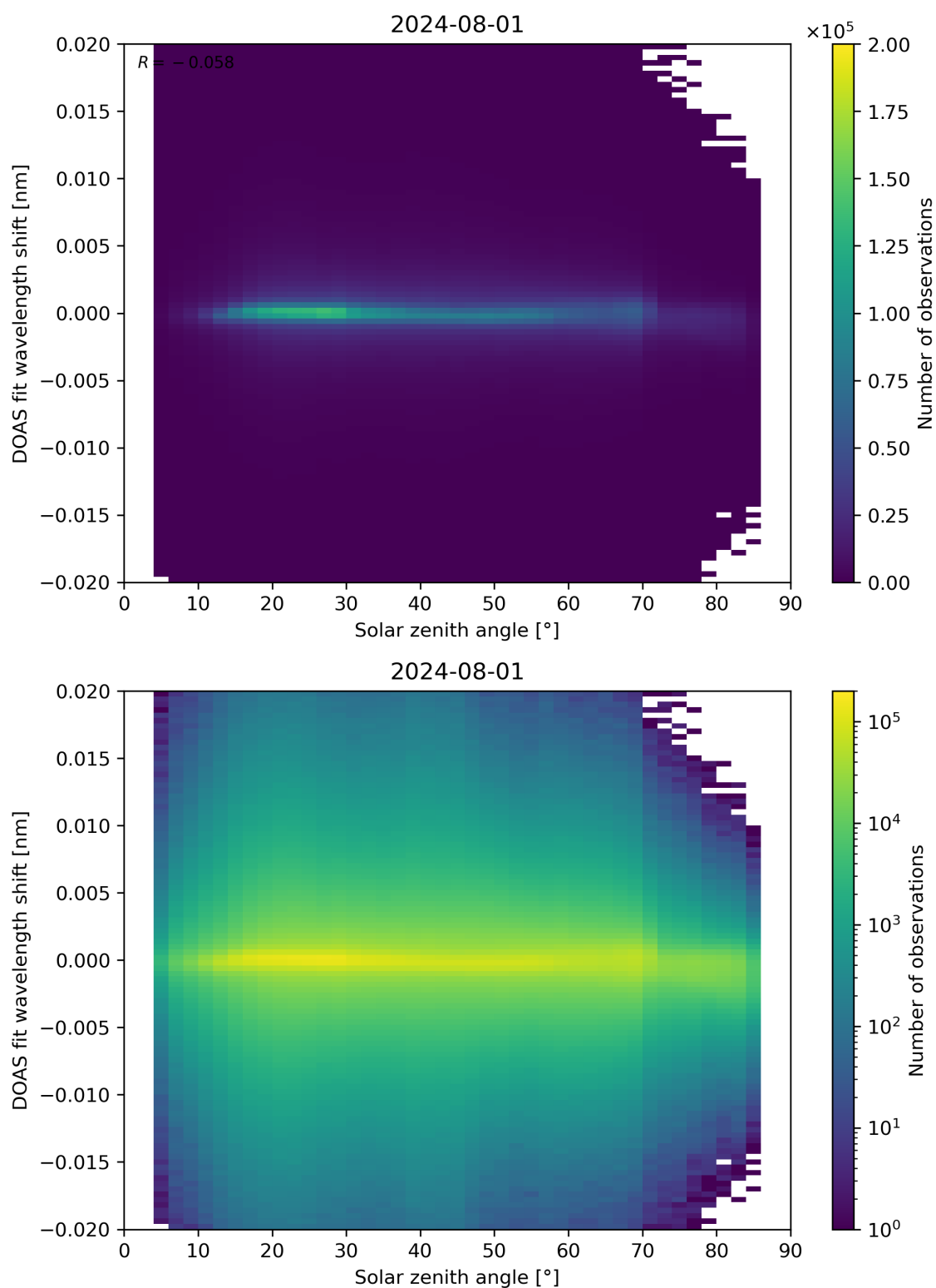
Figure 168: Scatter density plot of “Solar zenith angle” against “DOAS fit wavelength shift” for 2024-07-31 to 2024-08-02.
