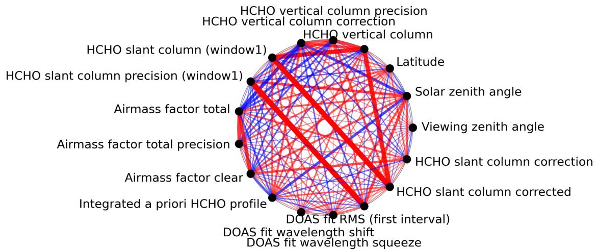
Figure 1: Map of correlation graph for 2024-07-31 to 2024-08-02.
