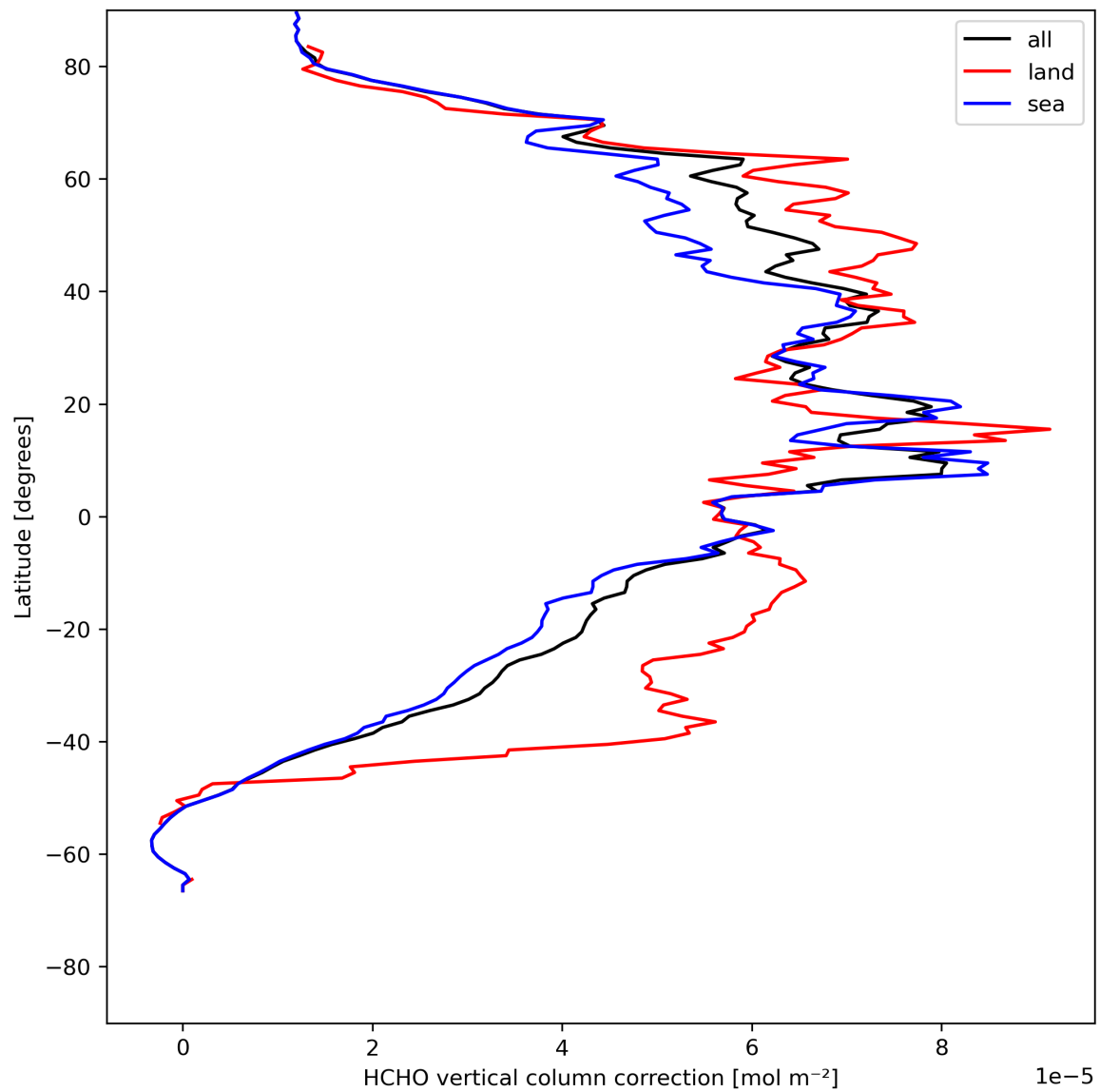
Figure 23: Zonal average of “HCHO vertical column correction” for 2024-07-31 to 2024-08-02.
