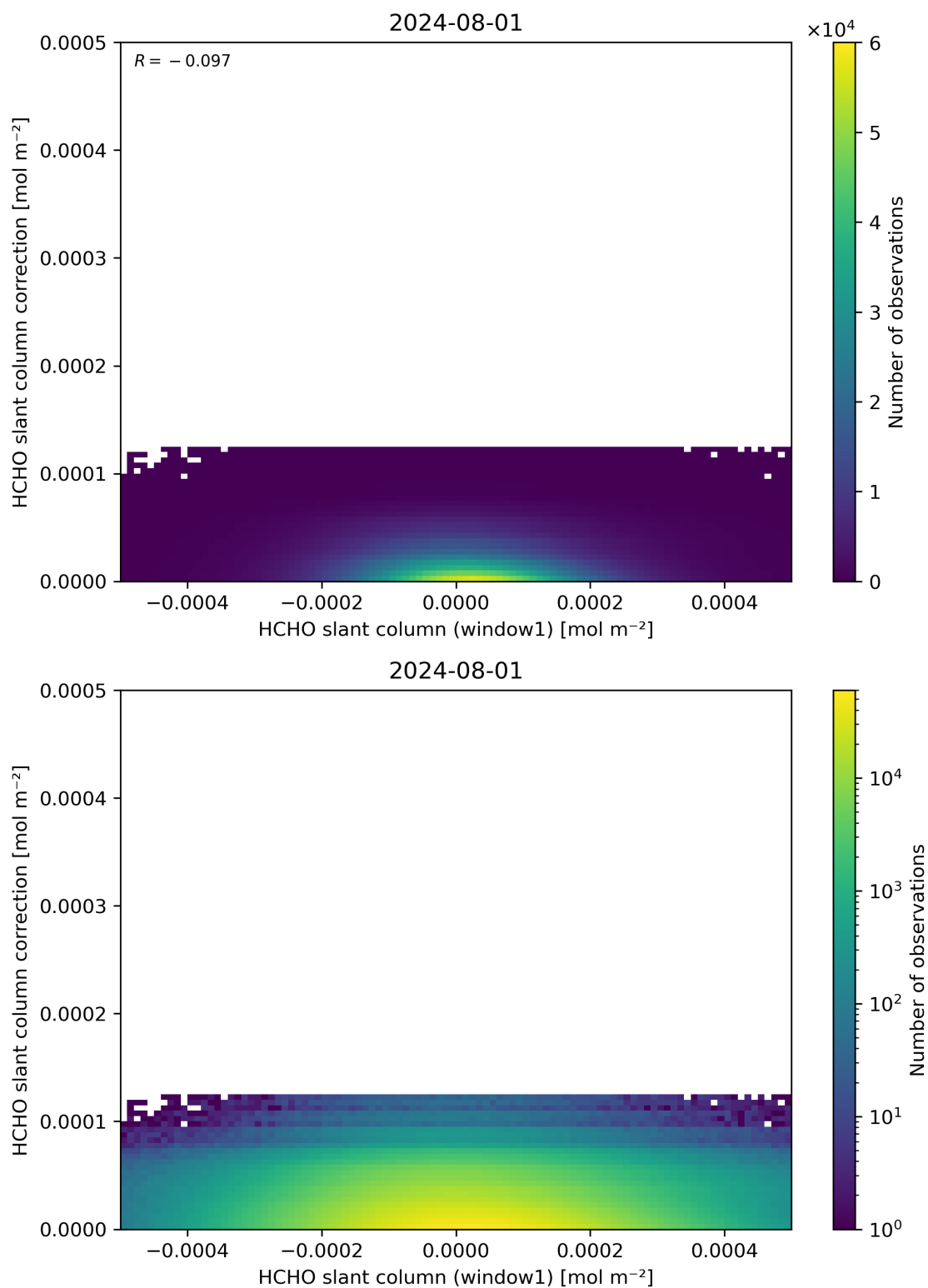
Figure 83: Scatter density plot of “HCHO slant column (window1)” against “HCHO slant column correction” for 2024-07-31 to 2024-08-02.
