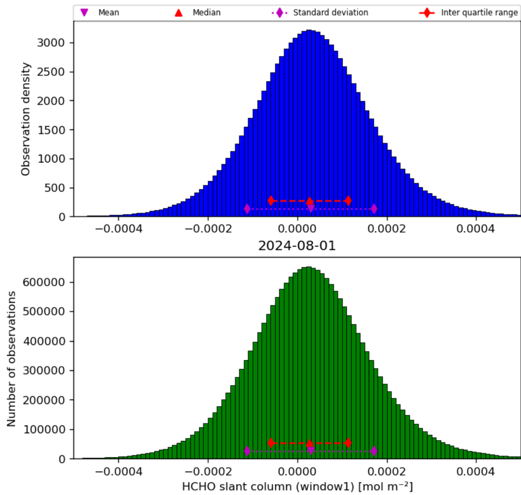
Figure 38: Histogram of “HCHO slant column (window1)” for 2024-07-31 to 2024-08-02
