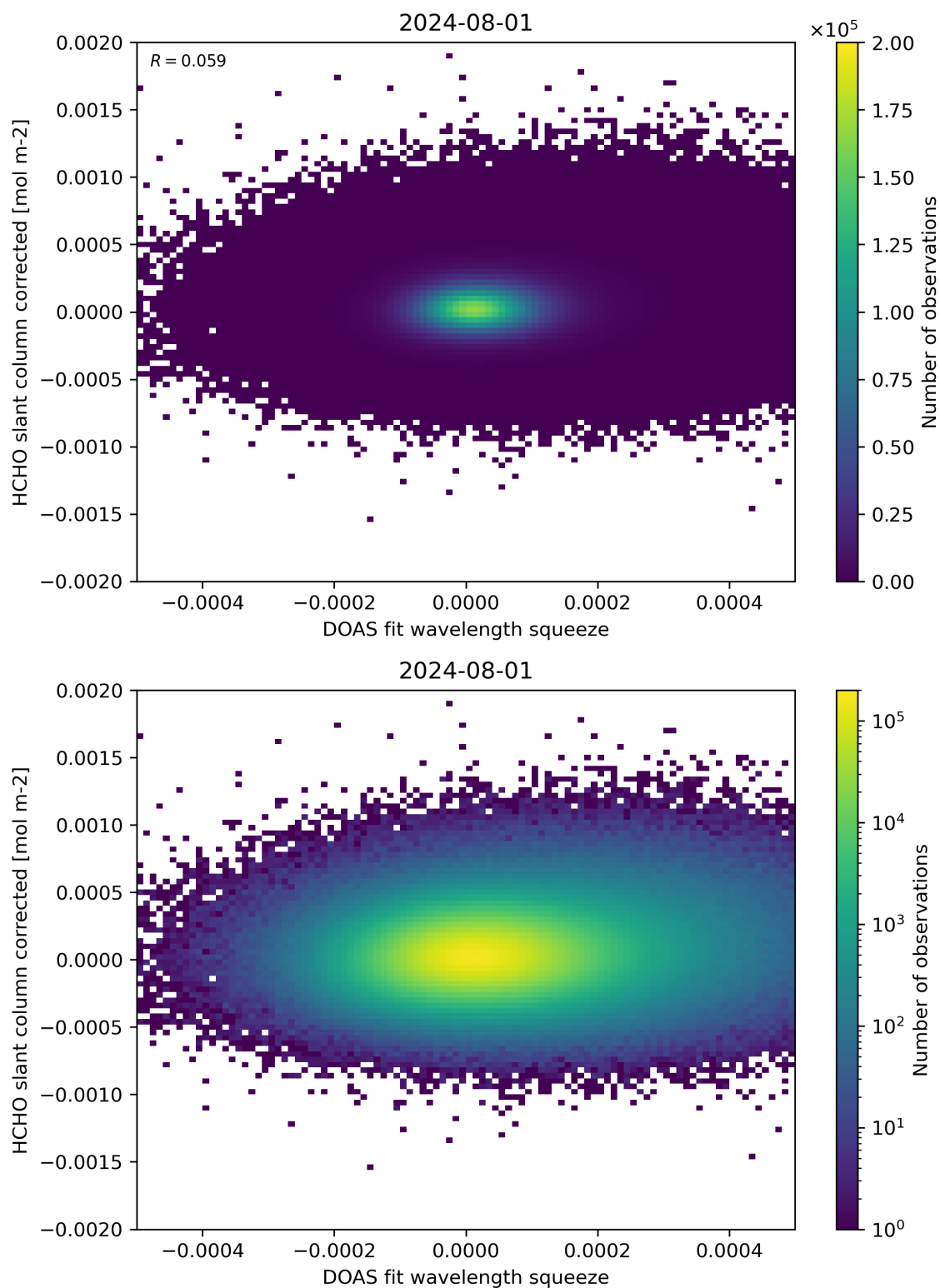
Figure 69: Scatter density plot of “DOAS fit wavelength squeeze” against “HCHO slant column corrected” for 2024-07-31 to 2024-08-02.
