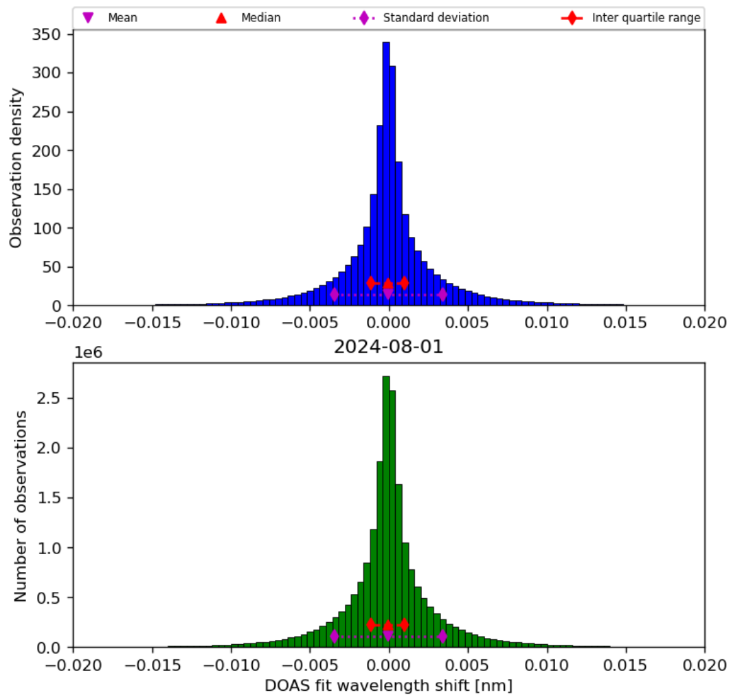
Figure 44: Histogram of “DOAS fit wavelength shift” for 2024-07-31 to 2024-08-02
