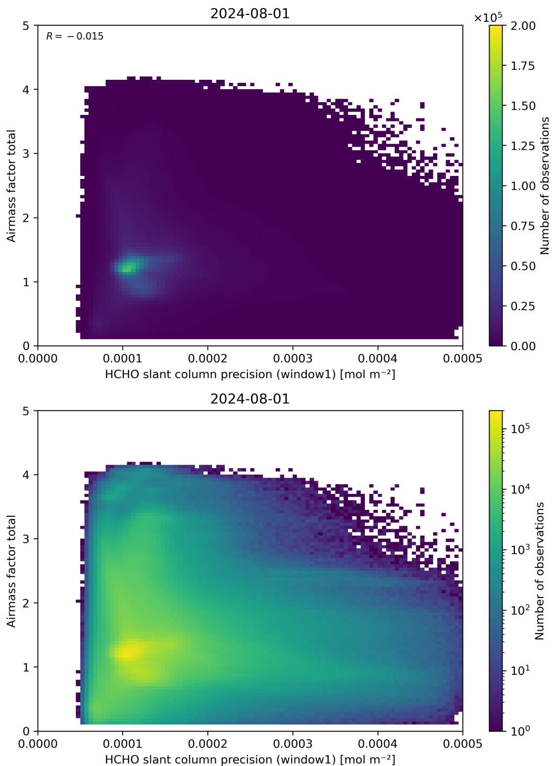
Figure 94: Scatter density plot of “HCHO slant column precision (window1)” against “Airmass factor total” for 2024-07-31 to 2024-08-02.
