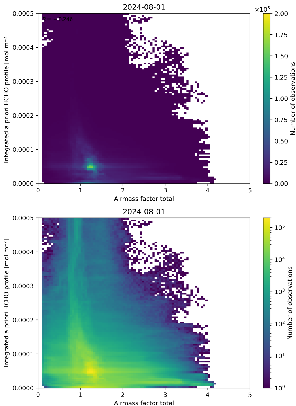
Figure 104: Scatter density plot of “Airmass factor total” against “Integrated a priori HCHO profile” for 2024-07-31 to 2024-08-02.
