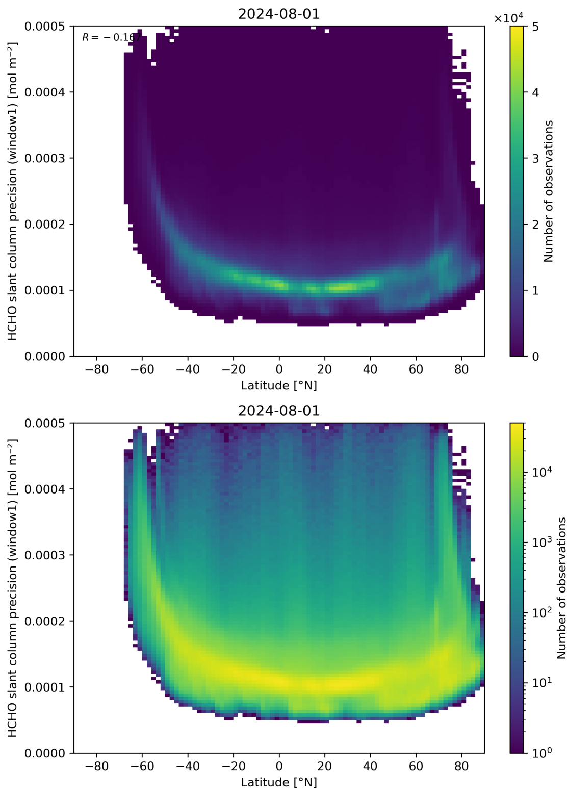
Figure 160: Scatter density plot of “Latitude” against “HCHO slant column precision (window1)” for 2024-07-31 to 2024-08-02.
