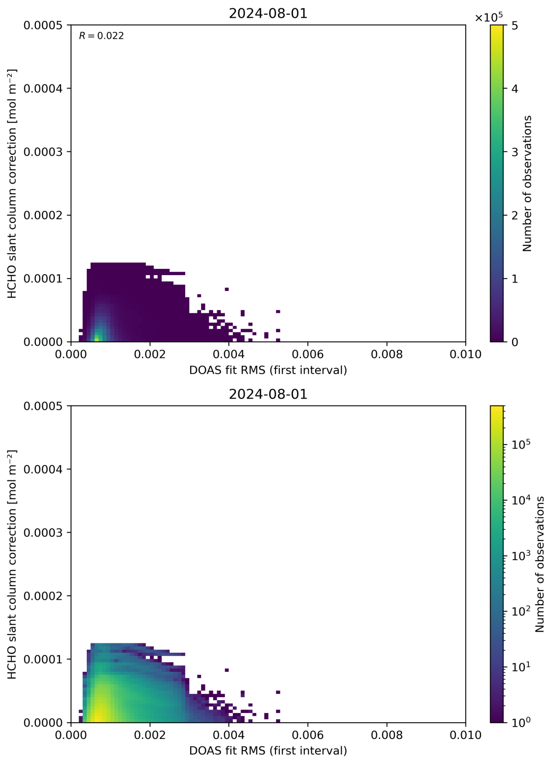
Figure 63: Scatter density plot of “DOAS fit RMS (first interval)” against “HCHO slant column correction” for 2024-07-31 to 2024-08-02.
