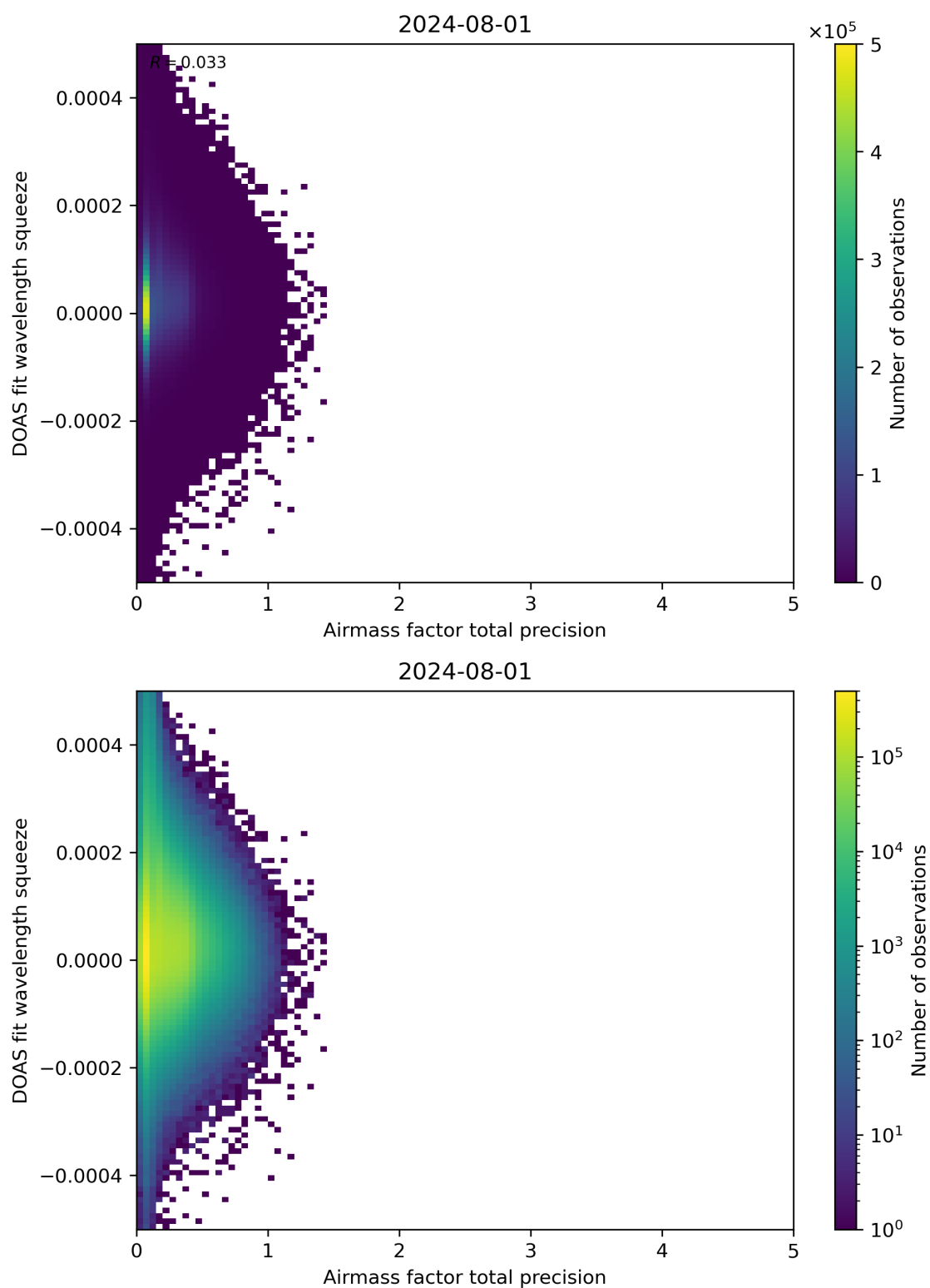
Figure 107: Scatter density plot of “Airmass factor total precision” against “DOAS fit wavelength squeeze” for 2024-07-31 to 2024-08-02.
