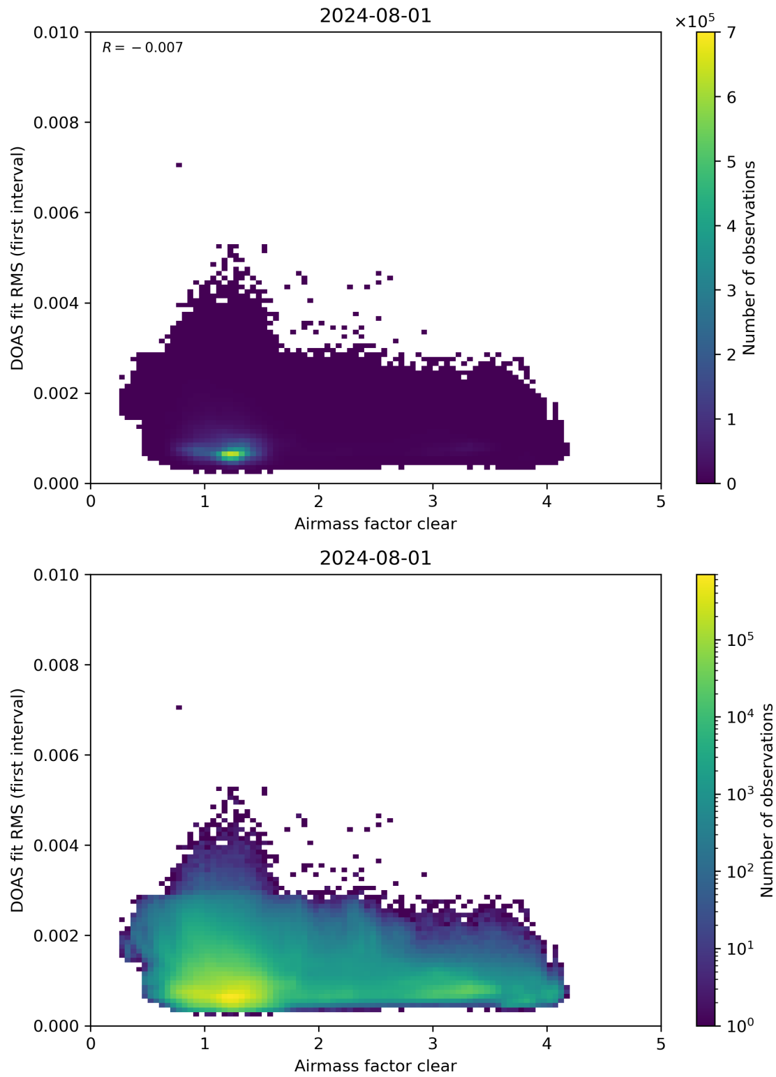
Figure 71: Scatter density plot of “Airmass factor clear” against “DOAS fit RMS (first interval)” for 2024-07-31 to 2024-08-02.
