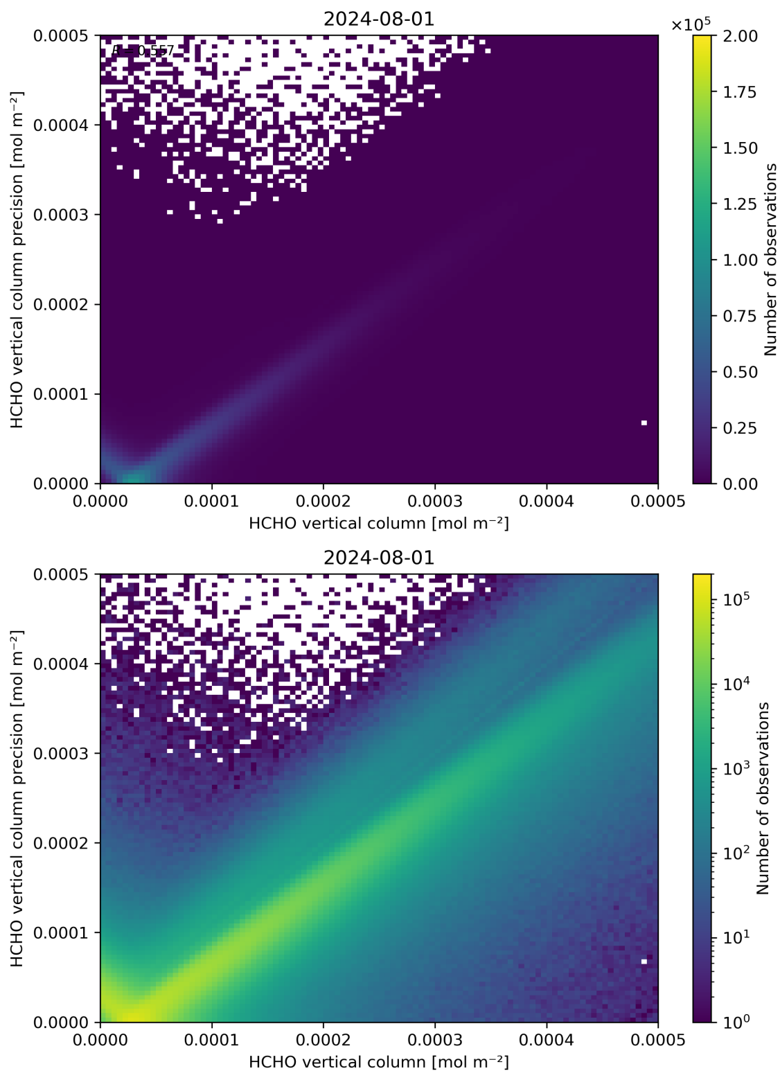
Figure 134: Scatter density plot of “HCHO vertical column” against “HCHO vertical column precision” for 2024-07-31 to 2024-08-02.
