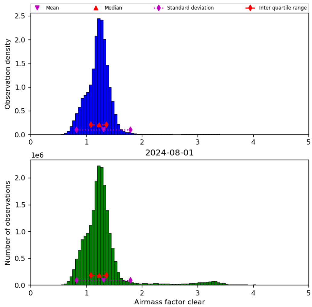
Figure 42: Histogram of “Airmass factor clear” for 2024-07-31 to 2024-08-02
