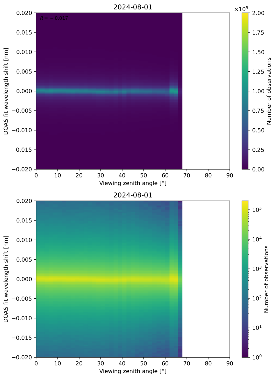
Figure 183: Scatter density plot of “Viewing zenith angle” against “DOAS fit wavelength shift” for 2024-07-31 to 2024-08-02.
