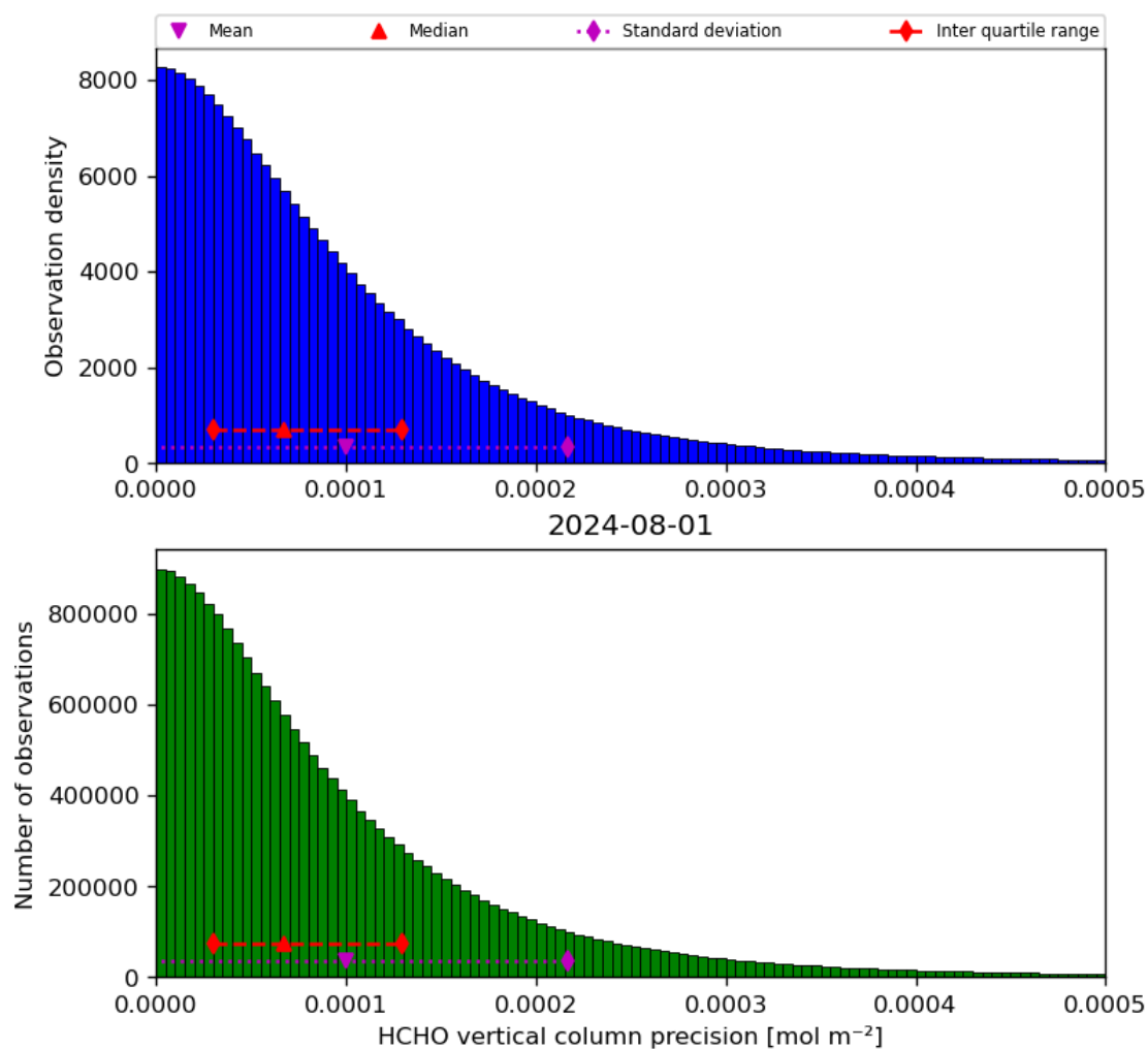
Figure 36: Histogram of “HCHO vertical column precision” for 2024-07-31 to 2024-08-02
