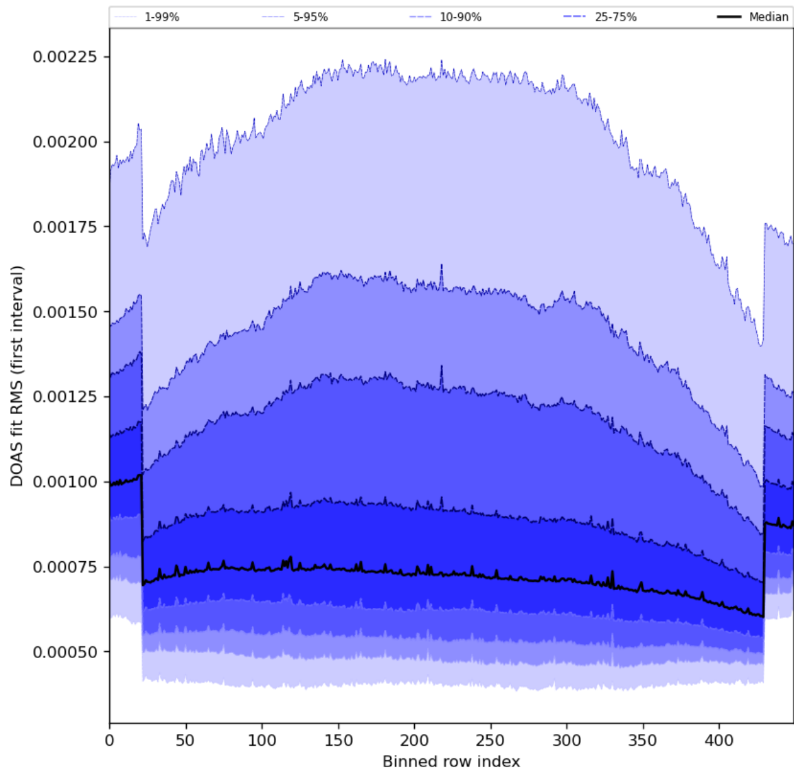
Figure 60: Along track statistics of “DOAS fit RMS (first interval)” for 2024-07-31 to 2024-08-02
