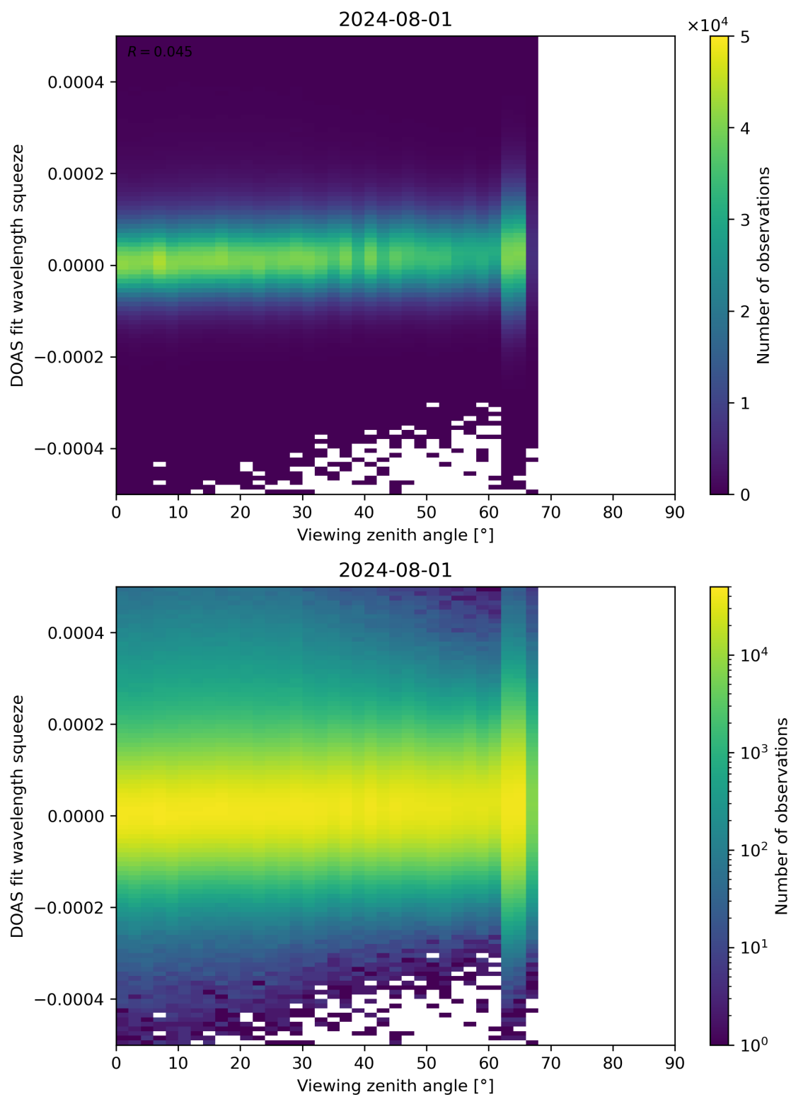
Figure 184: Scatter density plot of “Viewing zenith angle” against “DOAS fit wavelength squeeze” for 2024-07-31 to 2024-08-02.
