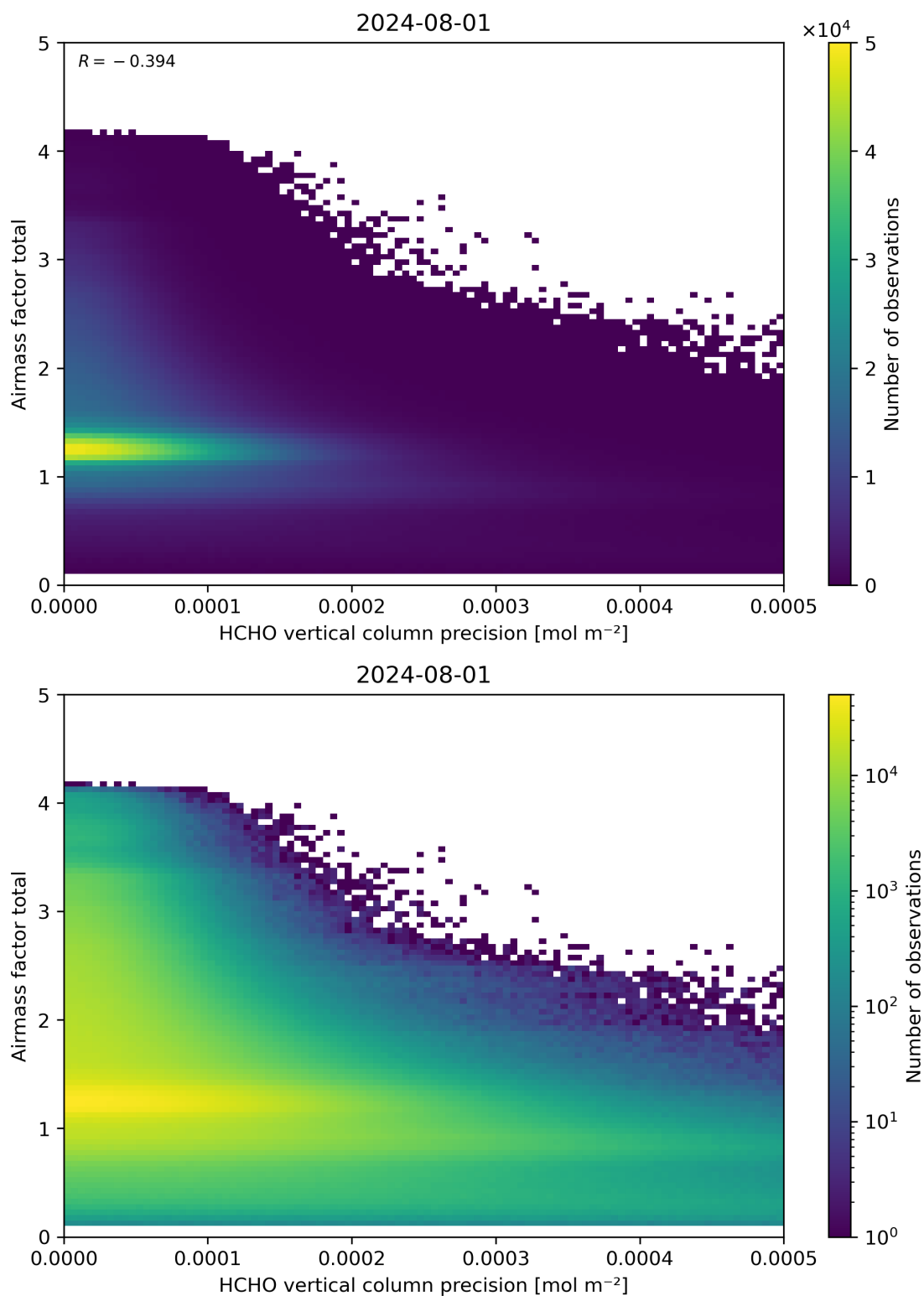
Figure 144: Scatter density plot of “HCHO vertical column precision” against “Airmass factor total” for 2024-07-31 to 2024-08-02.
