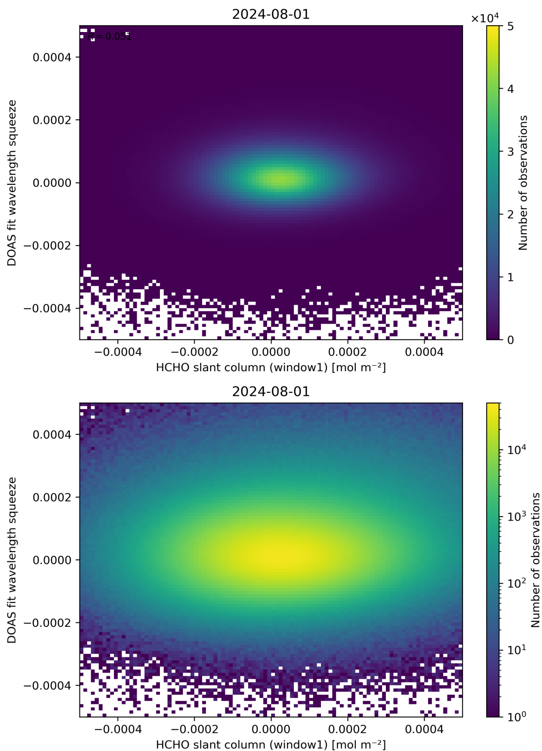
Figure 80: Scatter density plot of “HCHO slant column (window1)” against “DOAS fit wavelength squeeze” for 2024-07-31 to 2024-08-02.
