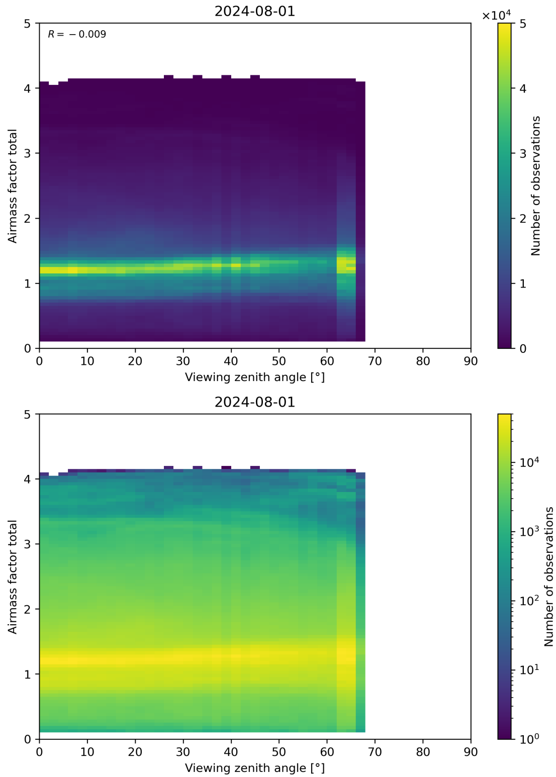
Figure 190: Scatter density plot of “Viewing zenith angle” against “Airmass factor total” for 2024-07-31 to 2024-08-02.
