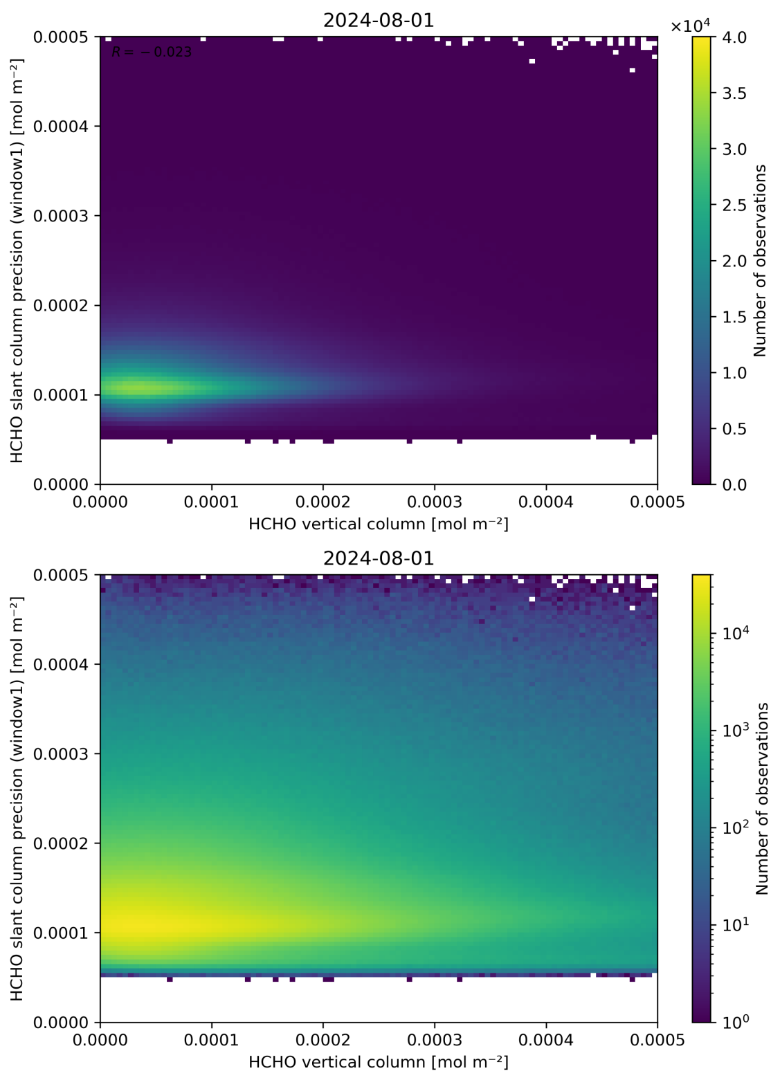
Figure 130: Scatter density plot of “HCHO vertical column” against “HCHO slant column precision (window1)” for 2024-07-31 to 2024-08-02.
