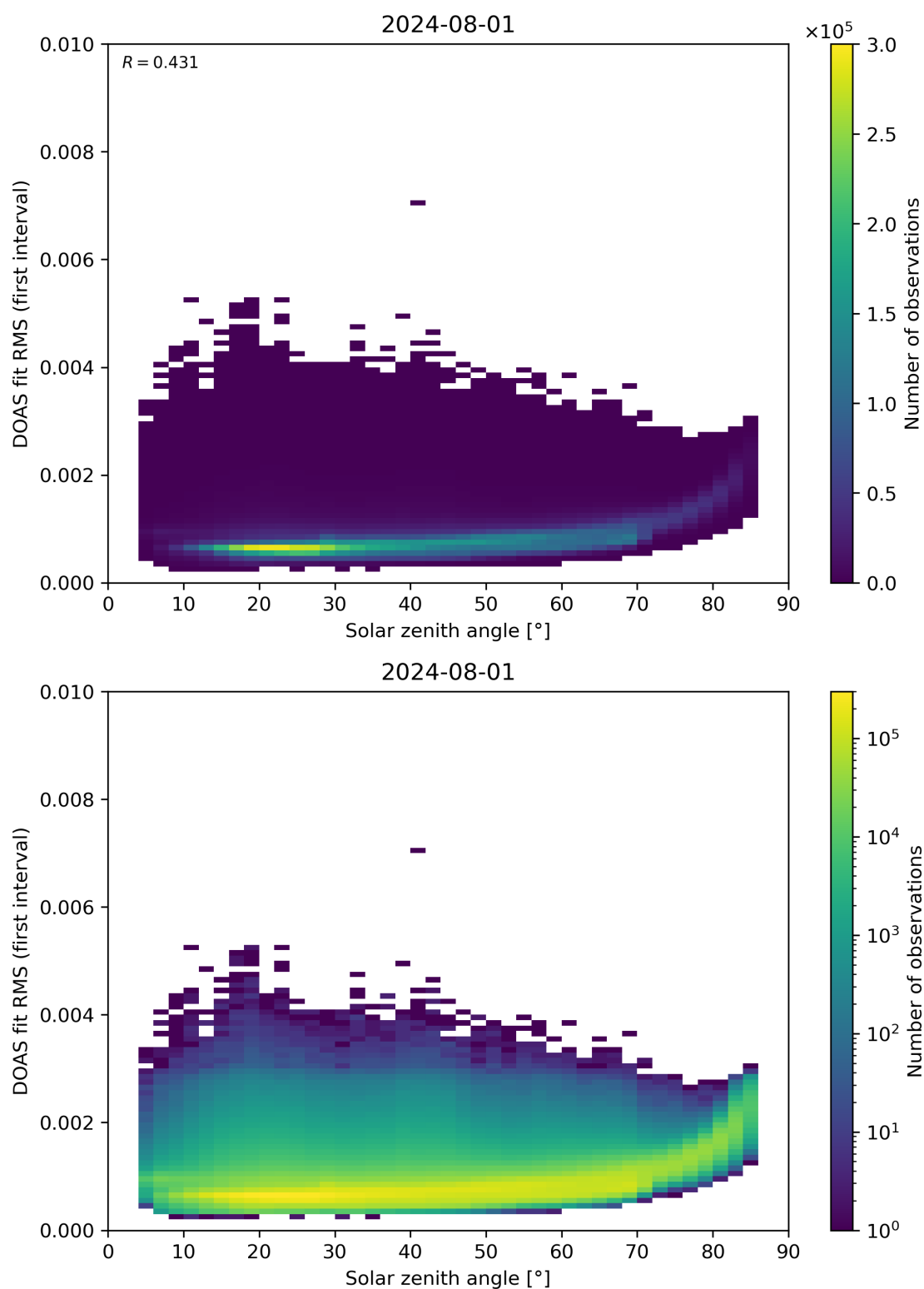
Figure 167: Scatter density plot of “Solar zenith angle” against “DOAS fit RMS (first interval)” for 2024-07-31 to 2024-08-02.
