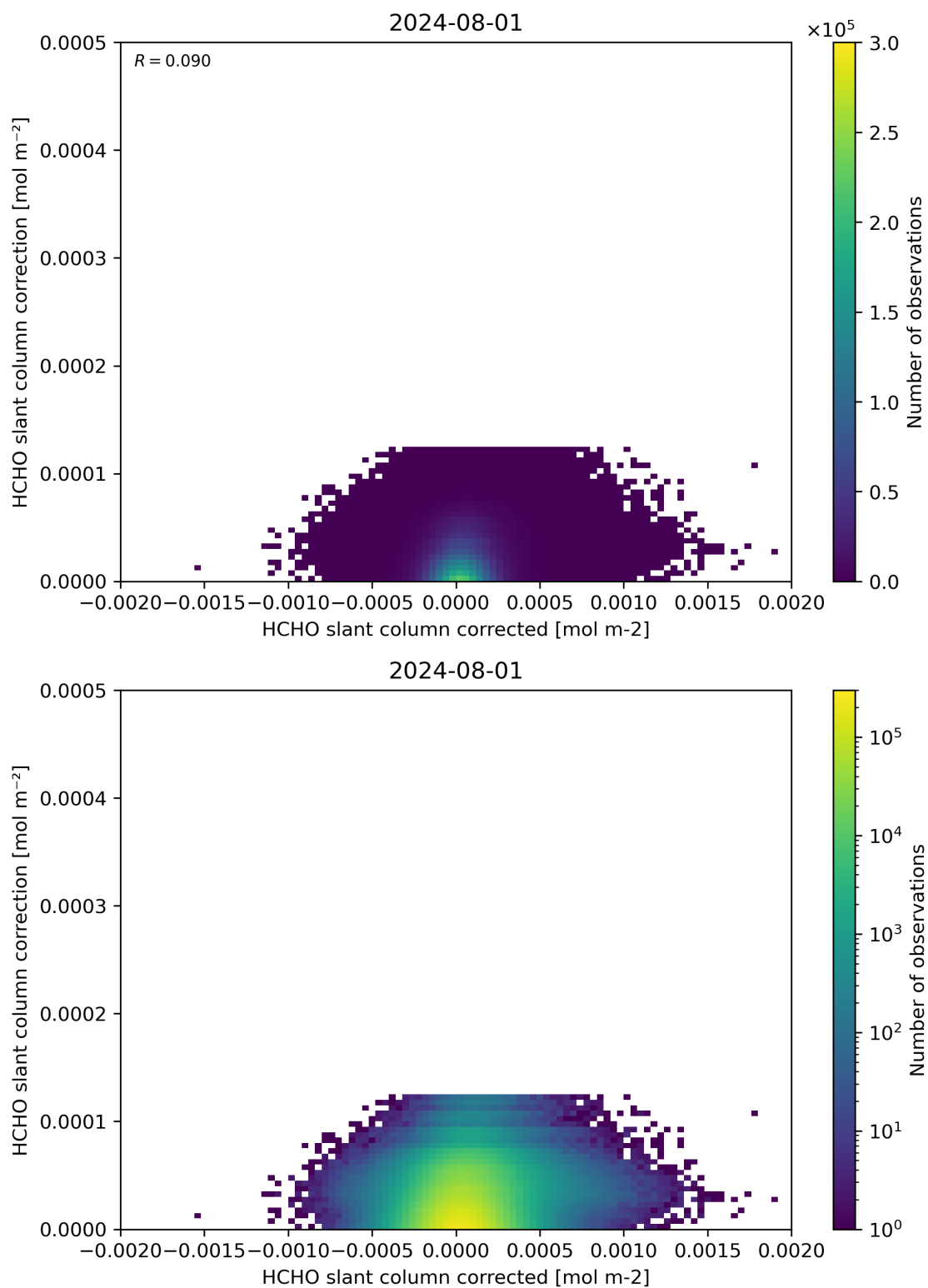
Figure 77: Scatter density plot of “HCHO slant column corrected” against “HCHO slant column correction” for 2024-07-31 to 2024-08-02.
