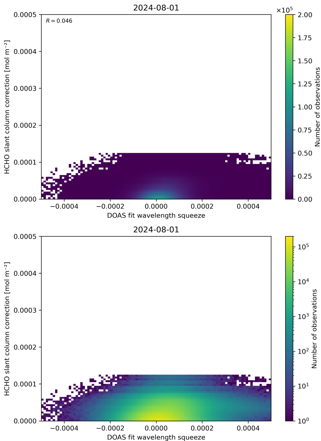
Figure 70: Scatter density plot of “DOAS fit wavelength squeeze” against “HCHO slant column correction” for 2024-07-31 to 2024-08-02.
