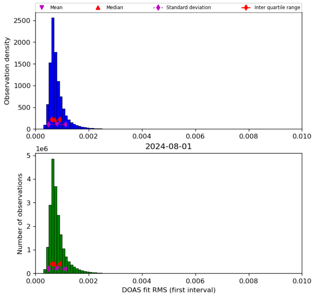
Figure 46: Histogram of “DOAS fit RMS (first interval)” for 2024-07-31 to 2024-08-02
