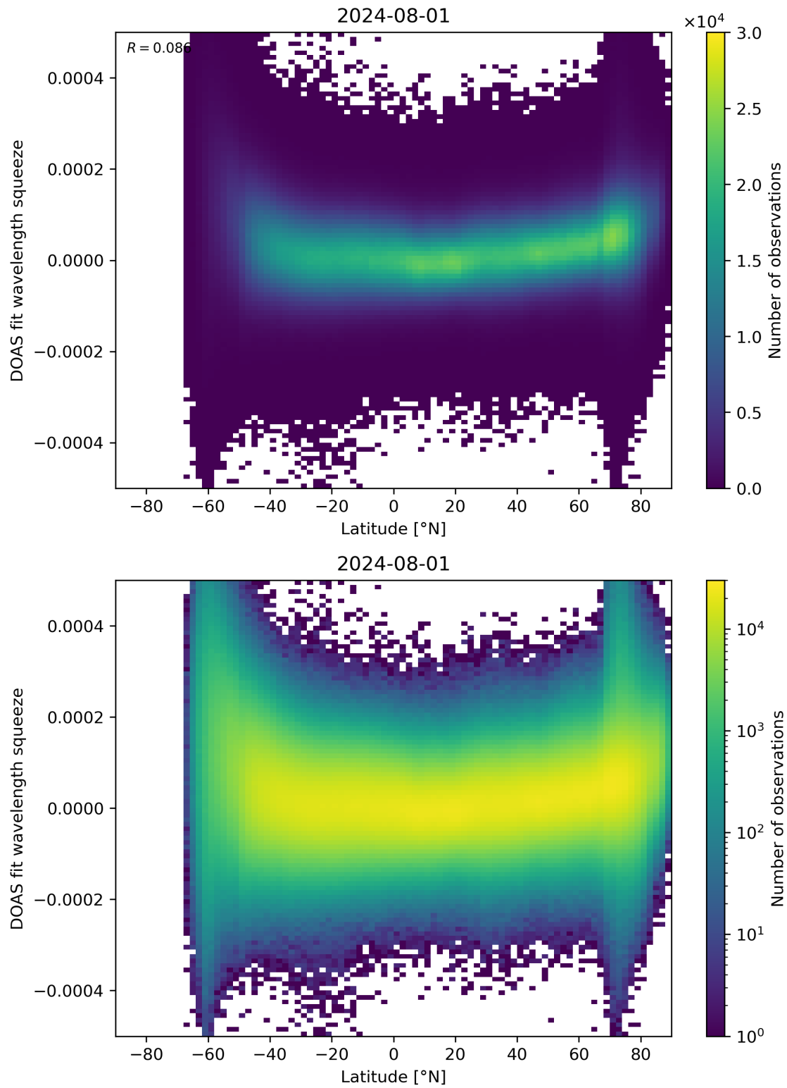
Figure 155: Scatter density plot of “Latitude” against “DOAS fit wavelength squeeze” for 2024-07-31 to 2024-08-02.
