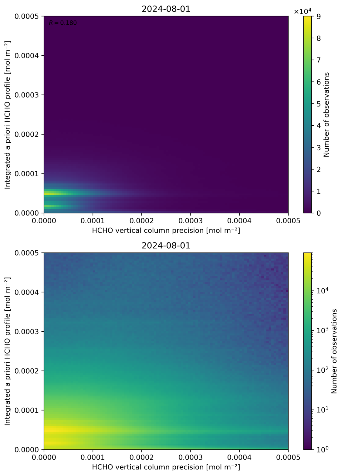
Figure 147: Scatter density plot of “HCHO vertical column precision” against “Integrated a priori HCHO profile” for 2024-07-31 to 2024-08-02.
