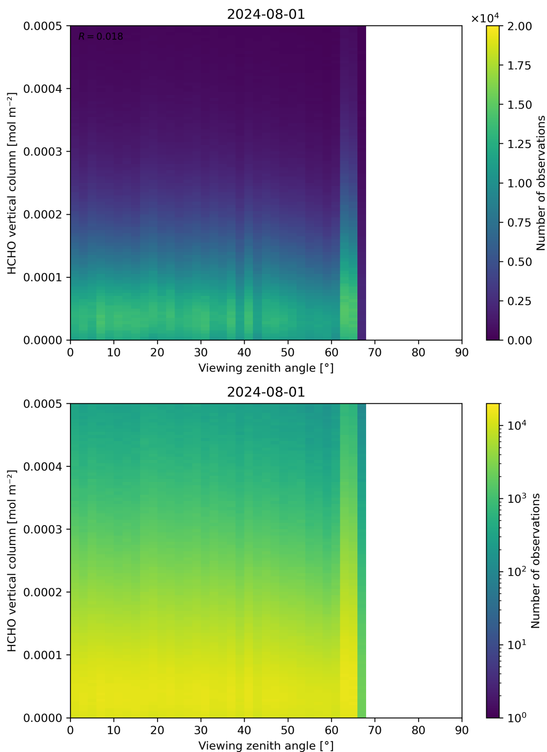
Figure 192: Scatter density plot of “Viewing zenith angle” against “HCHO vertical column” for 2024-07-31 to 2024-08-02.
