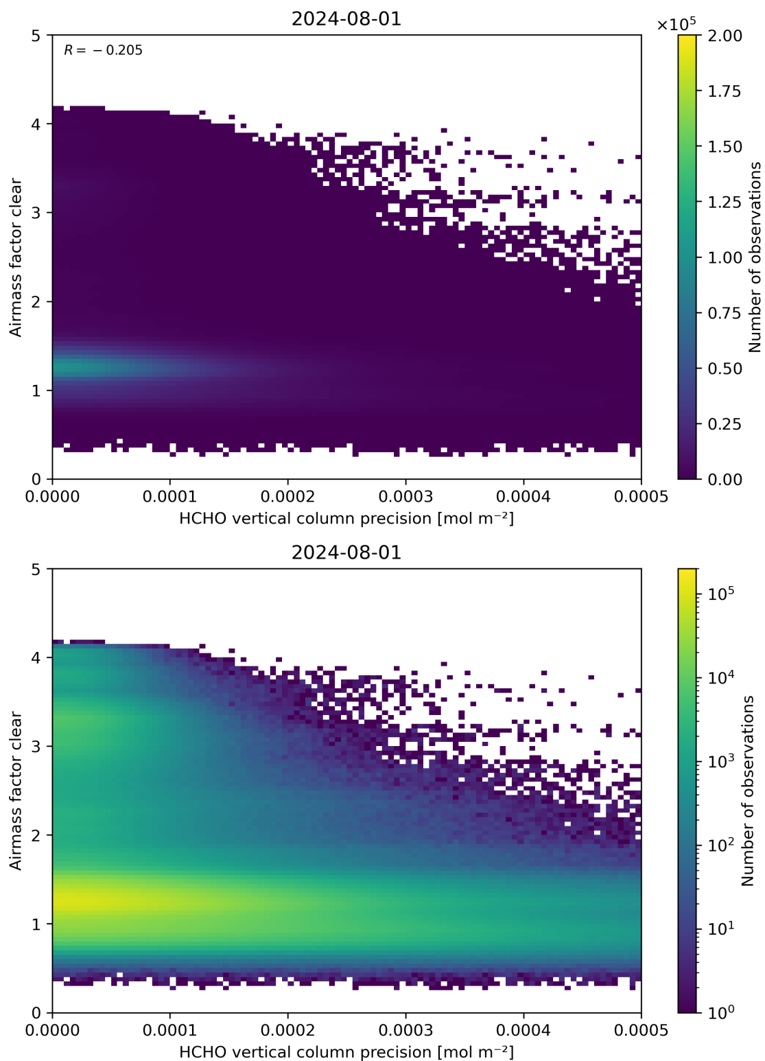
Figure 139: Scatter density plot of “HCHO vertical column precision” against “Airmass factor clear” for 2024-07-31 to 2024-08-02.
