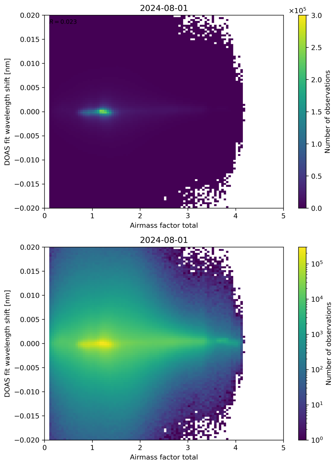
Figure 98: Scatter density plot of “Airmass factor total” against “DOAS fit wavelength shift” for 2024-07-31 to 2024-08-02.
