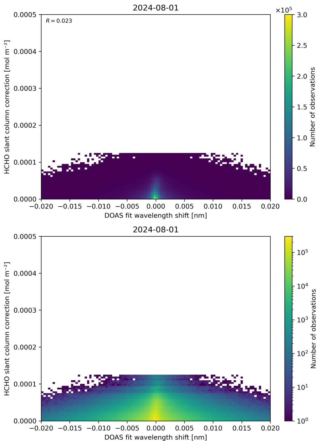
Figure 67: Scatter density plot of “DOAS fit wavelength shift” against “HCHO slant column correction” for 2024-07-31 to 2024-08-02.
