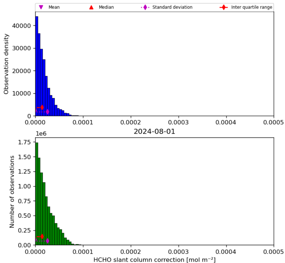
Figure 47: Histogram of “HCHO slant column correction” for 2024-07-31 to 2024-08-02
