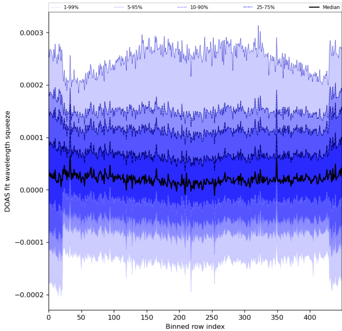
Figure 59: Along track statistics of “DOAS fit wavelength squeeze” for 2024-07-31 to 2024-08-02
