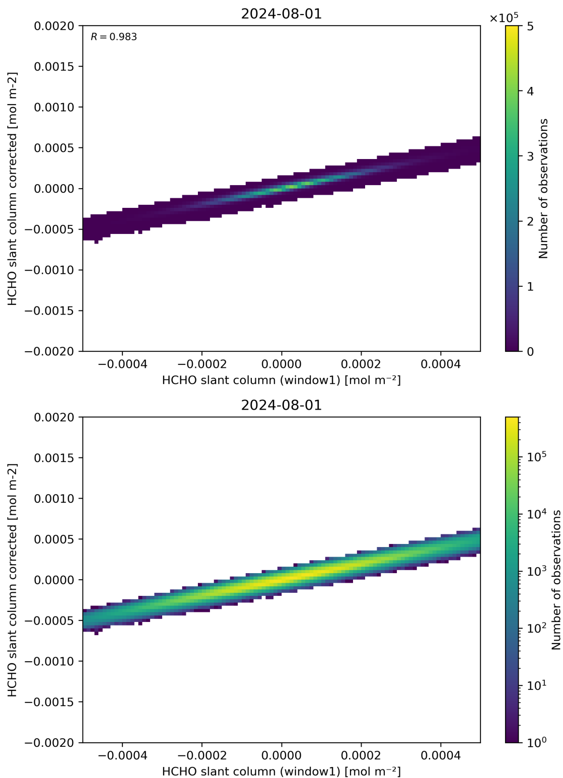
Figure 82: Scatter density plot of “HCHO slant column (window1)” against “HCHO slant column corrected” for 2024-07-31 to 2024-08-02.
