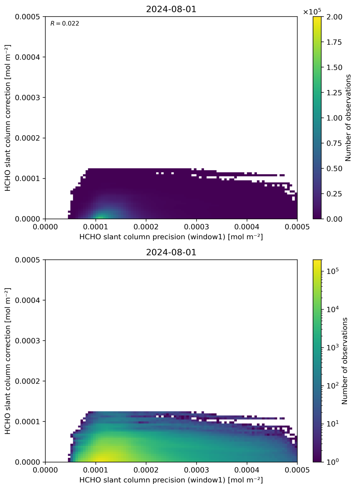
Figure 93: Scatter density plot of “HCHO slant column precision (window1)” against “HCHO slant column correction” for 2024-07-31 to 2024-08-02.
