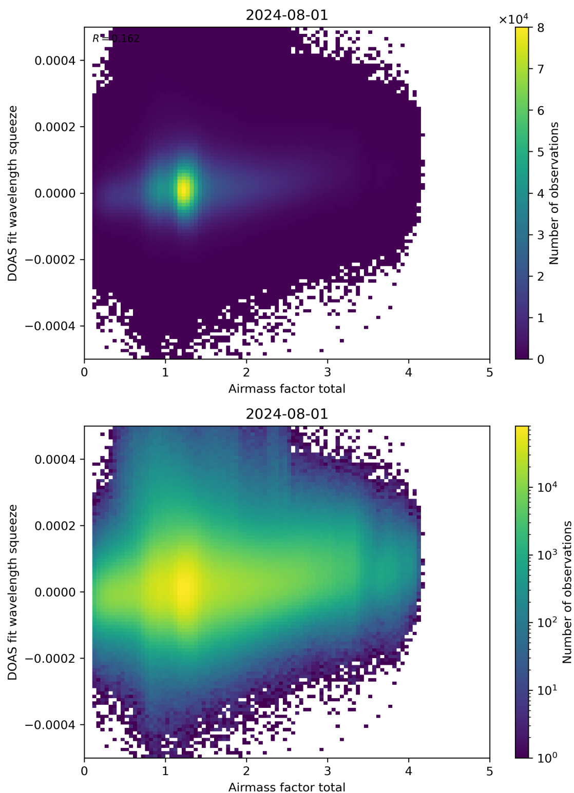
Figure 99: Scatter density plot of “Airmass factor total” against “DOAS fit wavelength squeeze” for 2024-07-31 to 2024-08-02.
