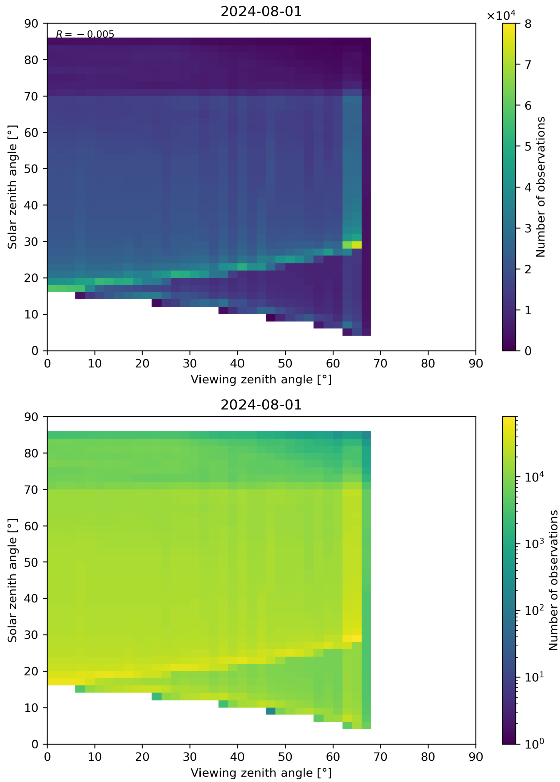
Figure 197: Scatter density plot of “Viewing zenith angle” against “Solar zenith angle” for 2024-07-31 to 2024-08-02.
