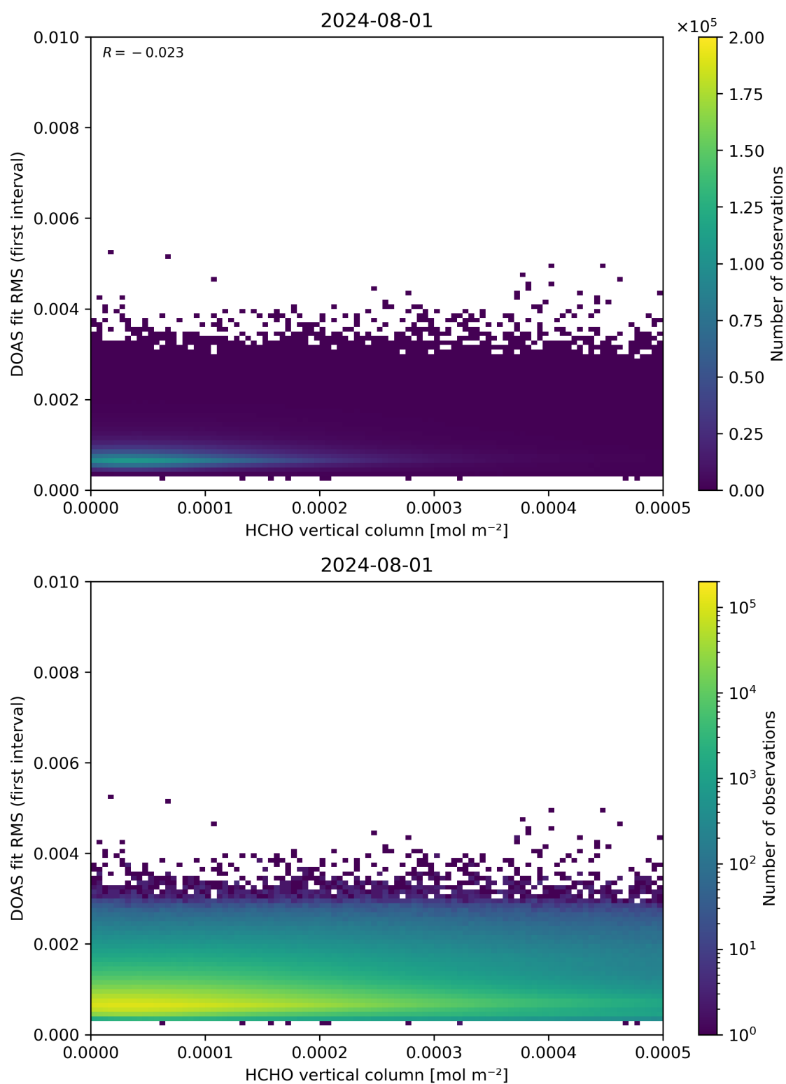
Figure 123: Scatter density plot of “HCHO vertical column” against “DOAS fit RMS (first interval)” for 2024-07-31 to 2024-08-02.
