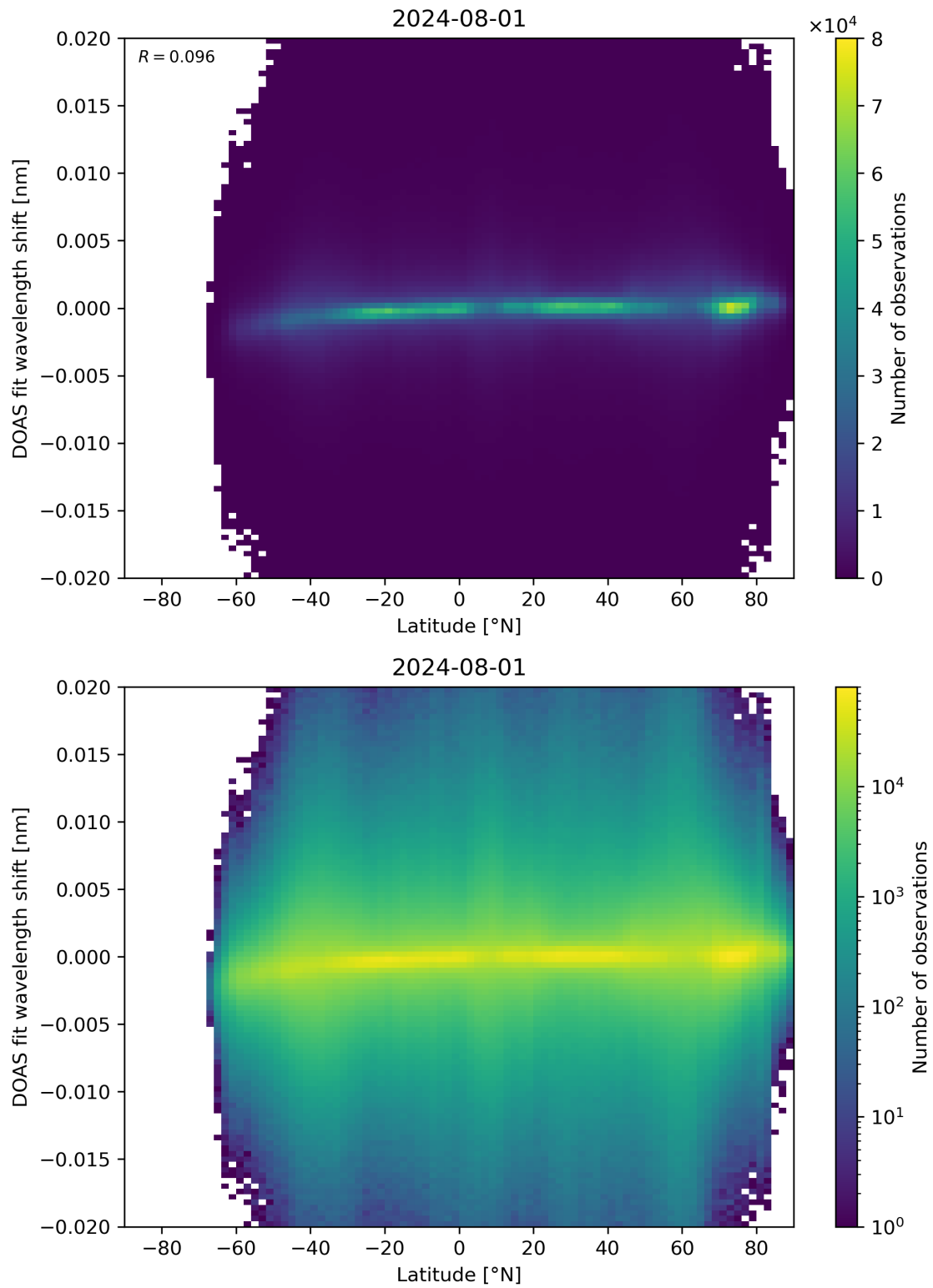
Figure 154: Scatter density plot of “Latitude” against “DOAS fit wavelength shift” for 2024-07-31 to 2024-08-02.
