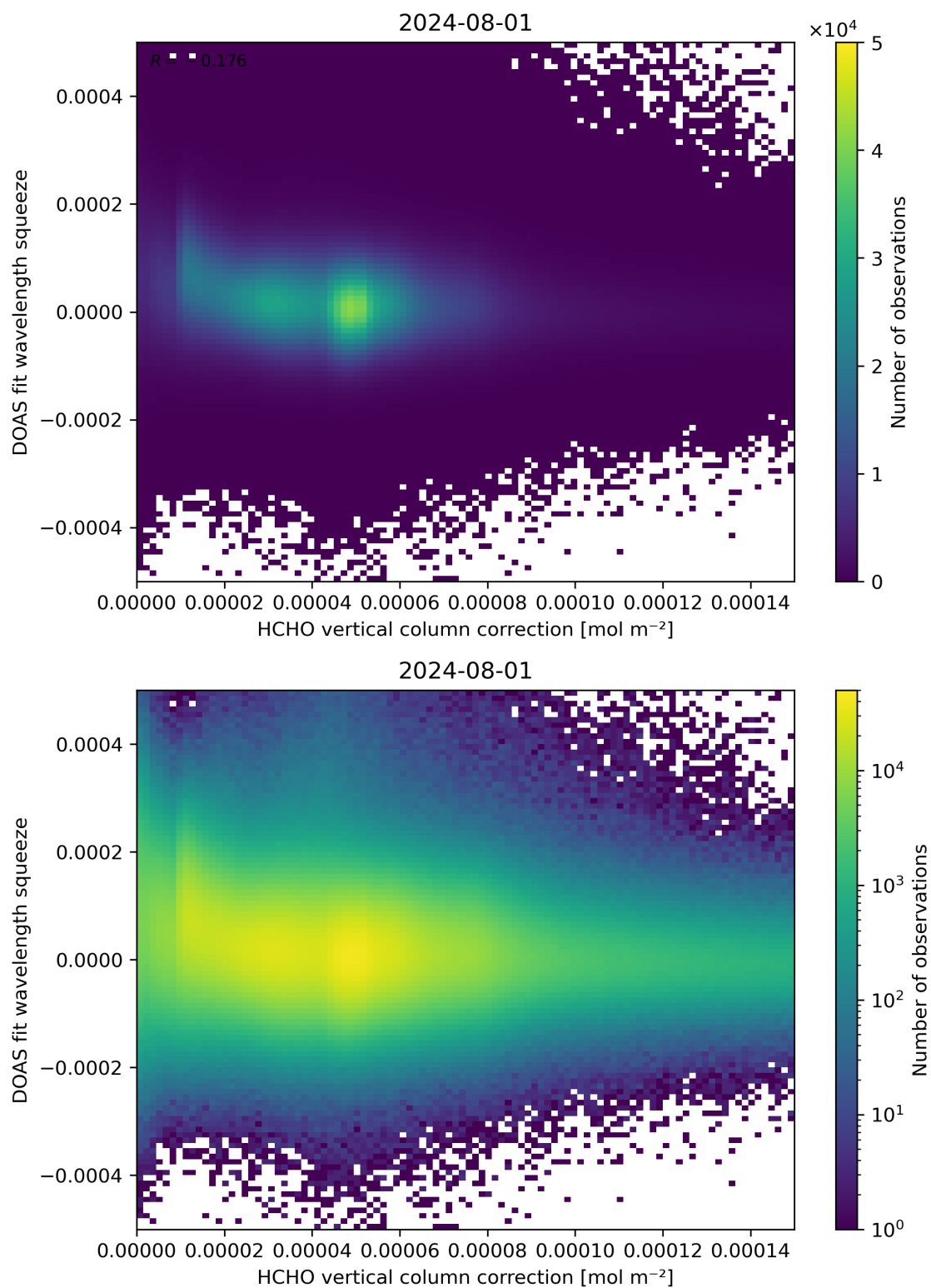
Figure 114: Scatter density plot of “HCHO vertical column correction” against “DOAS fit wavelength squeeze” for 2024-07-31 to 2024-08-02.
