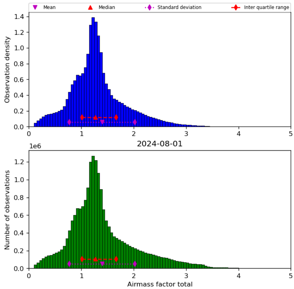
Figure 40: Histogram of “Airmass factor total” for 2024-07-31 to 2024-08-02
