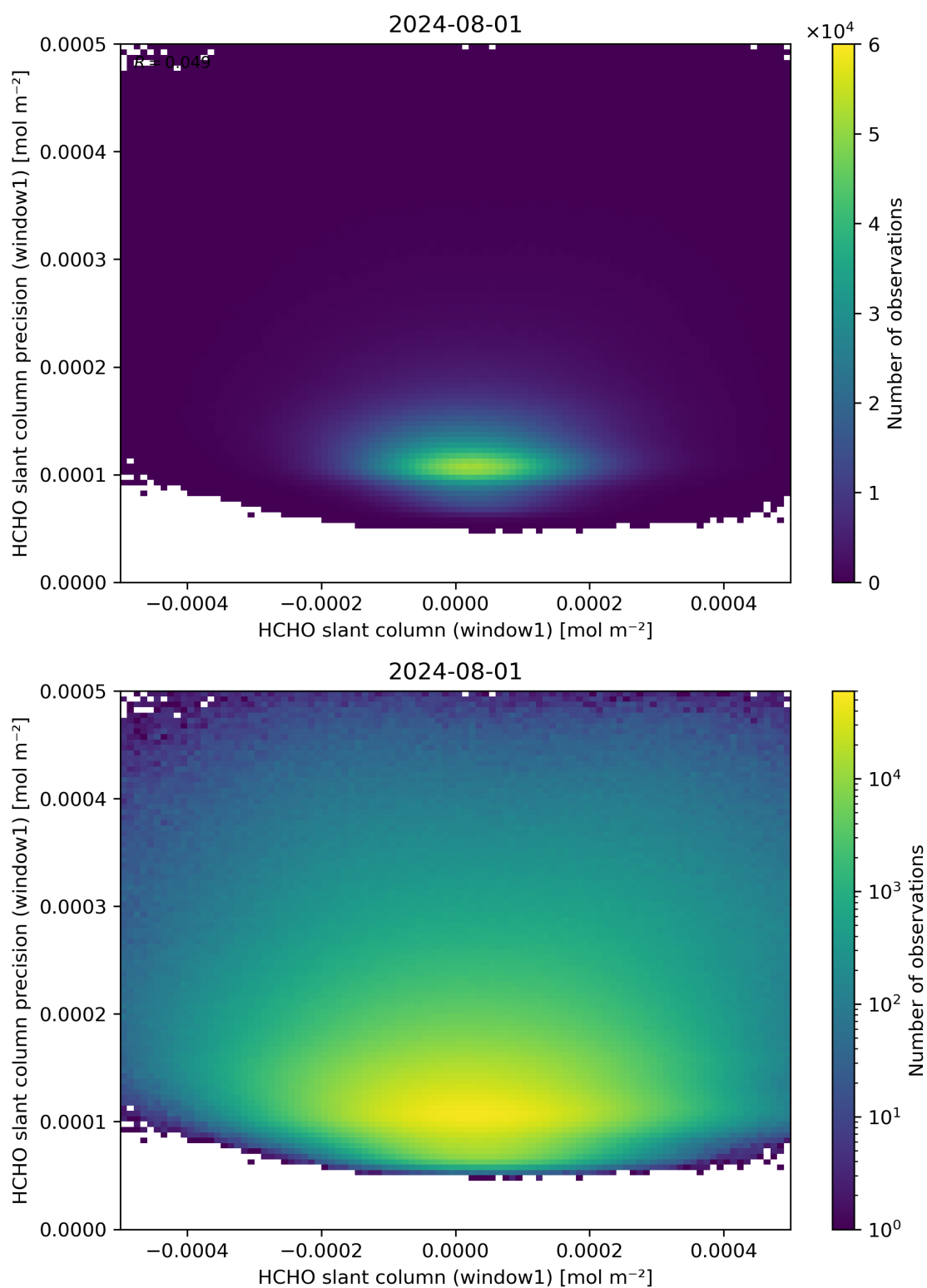
Figure 84: Scatter density plot of “HCHO slant column (window1)” against “HCHO slant column precision (window1)” for 2024-07-31 to 2024-08-02.
