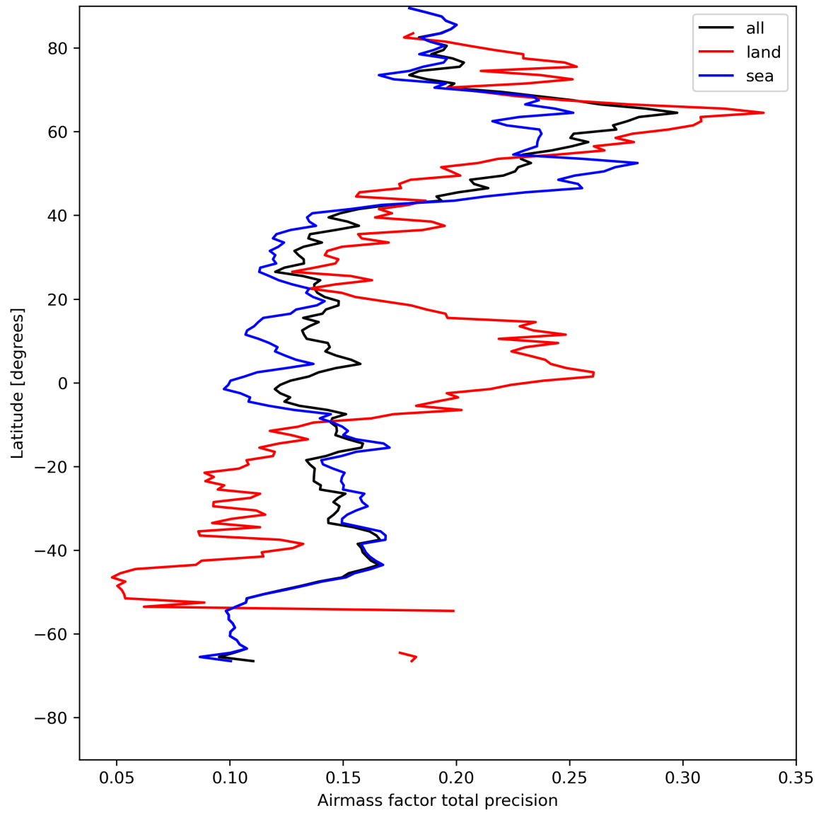
Figure 27: Zonal average of “Airmass factor total precision” for 2024-07-31 to 2024-08-02.
