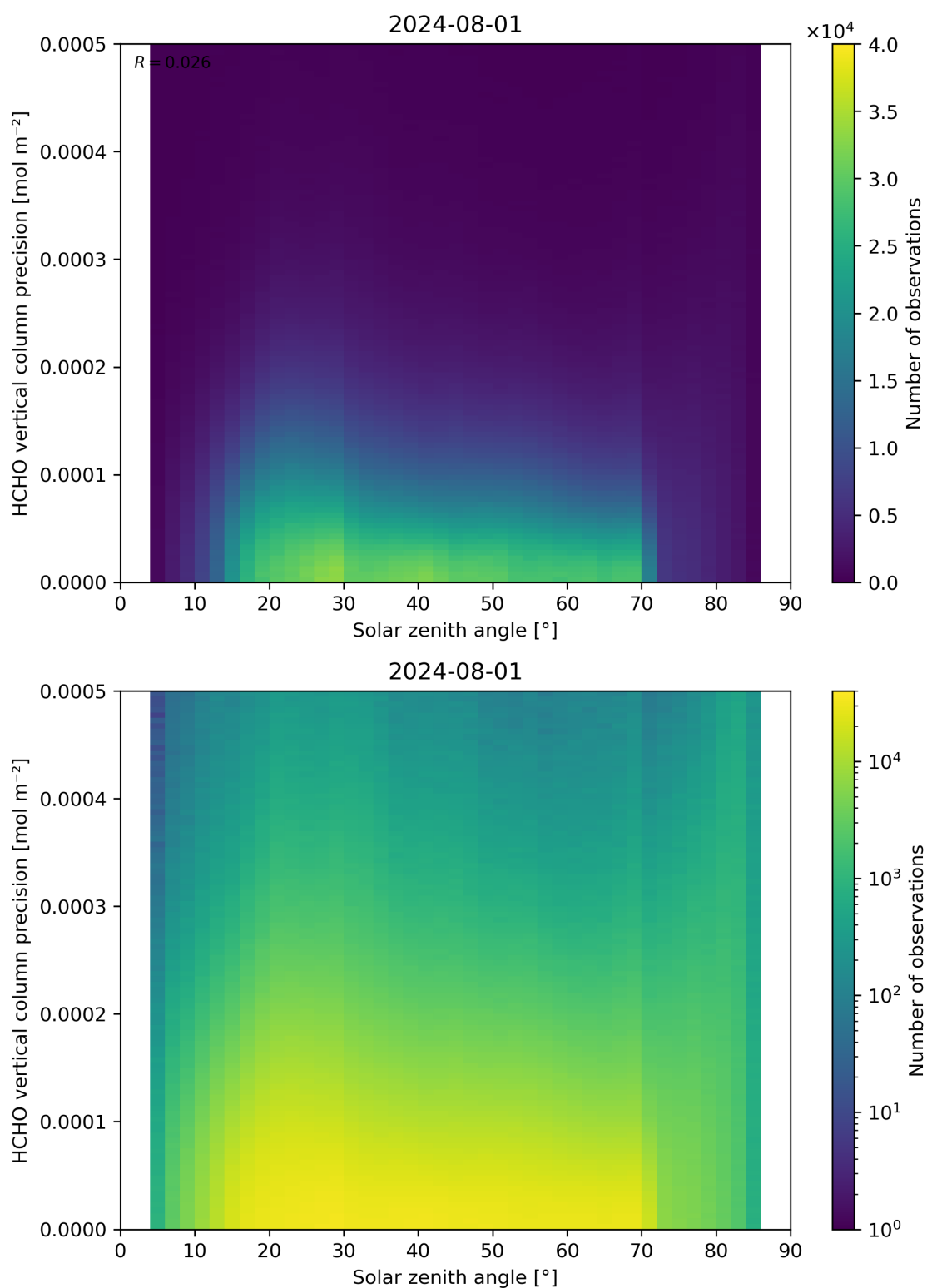
Figure 179: Scatter density plot of “Solar zenith angle” against “HCHO vertical column precision” for 2024-07-31 to 2024-08-02.
