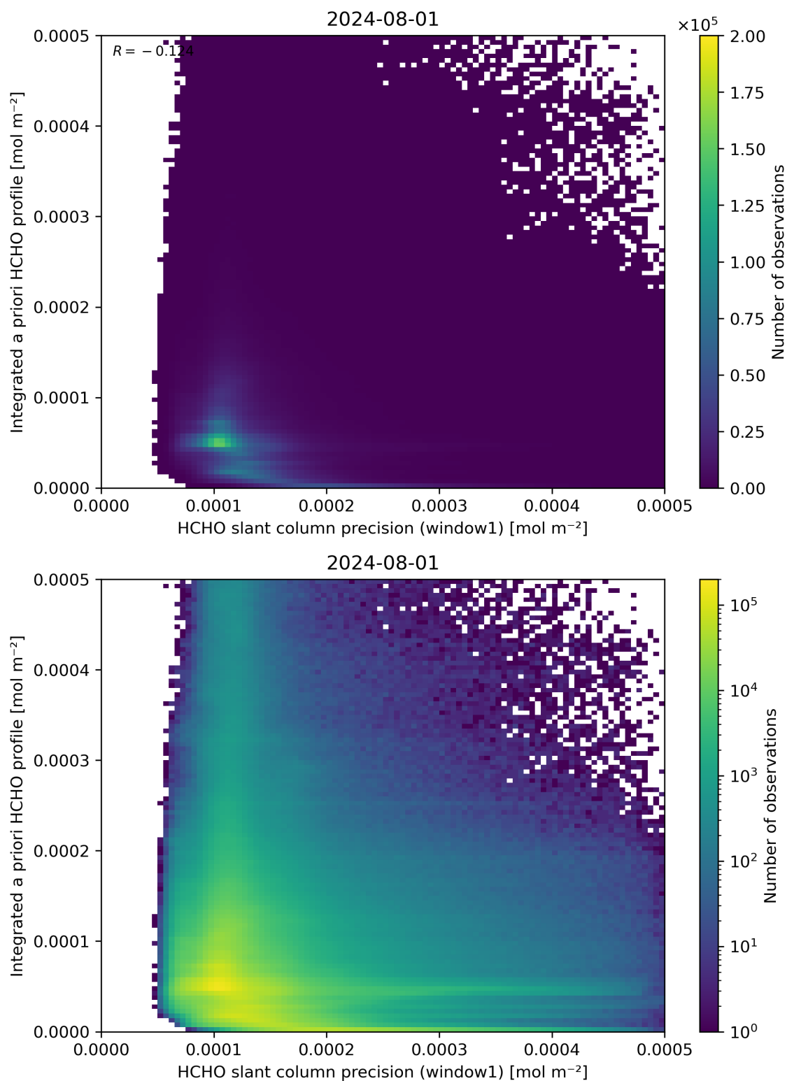
Figure 96: Scatter density plot of “HCHO slant column precision (window1)” against “Integrated a priori HCHO profile” for 2024-07-31 to 2024-08-02.
