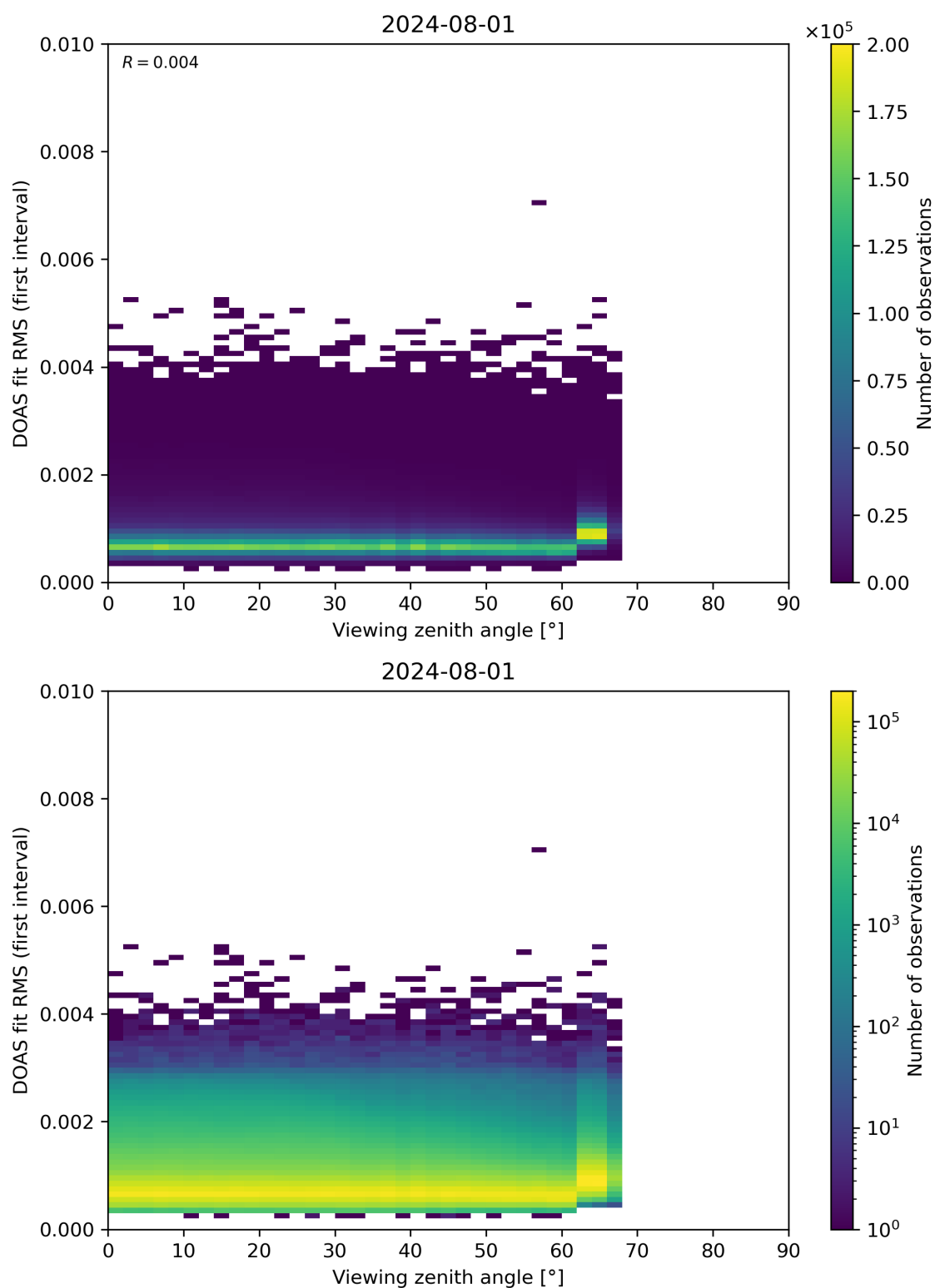
Figure 182: Scatter density plot of “Viewing zenith angle” against “DOAS fit RMS (first interval)” for 2024-07-31 to 2024-08-02.
