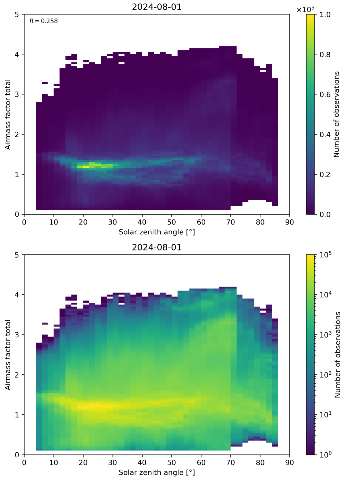
Figure 175: Scatter density plot of “Solar zenith angle” against “Airmass factor total” for 2024-07-31 to 2024-08-02.
