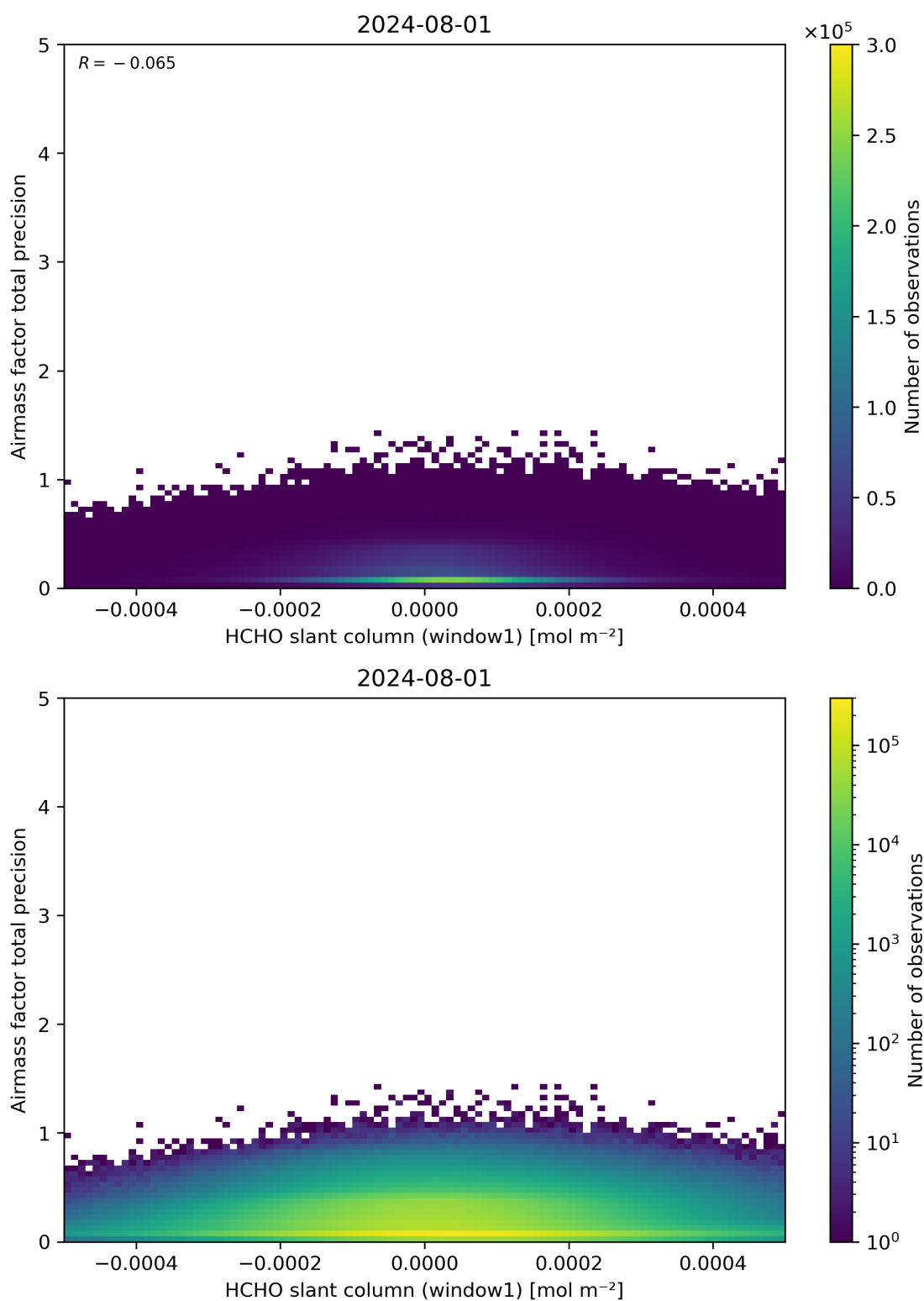
Figure 86: Scatter density plot of “HCHO slant column (window1)” against “Airmass factor total precision” for 2024-07-31 to 2024-08-02.
