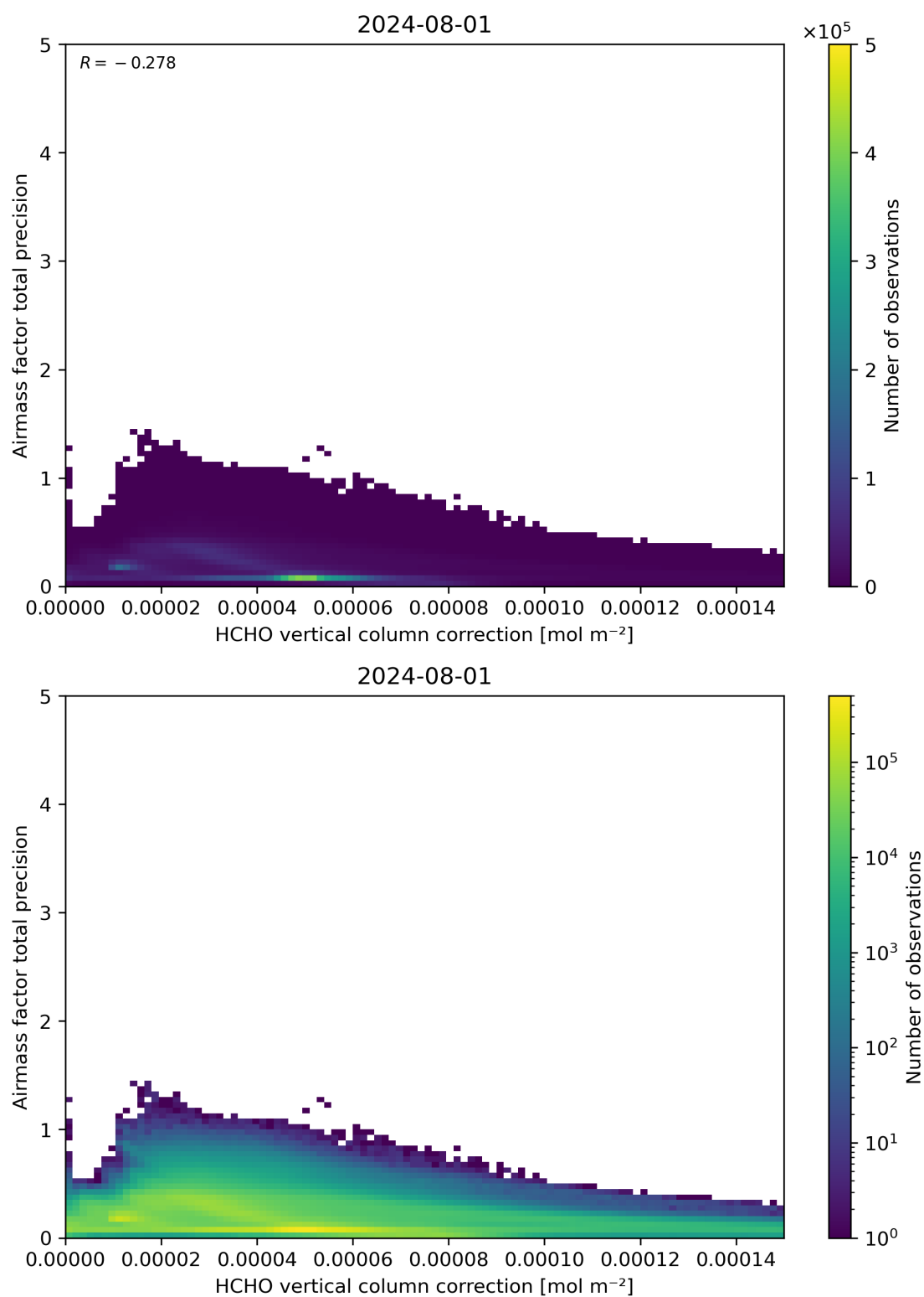
Figure 121: Scatter density plot of “HCHO vertical column correction” against “Airmass factor total precision” for 2024-07-31 to 2024-08-02.
