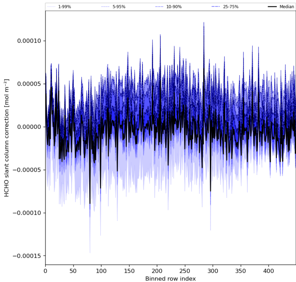
Figure 61: Along track statistics of “HCHO slant column correction” for 2024-07-31 to 2024-08-02
