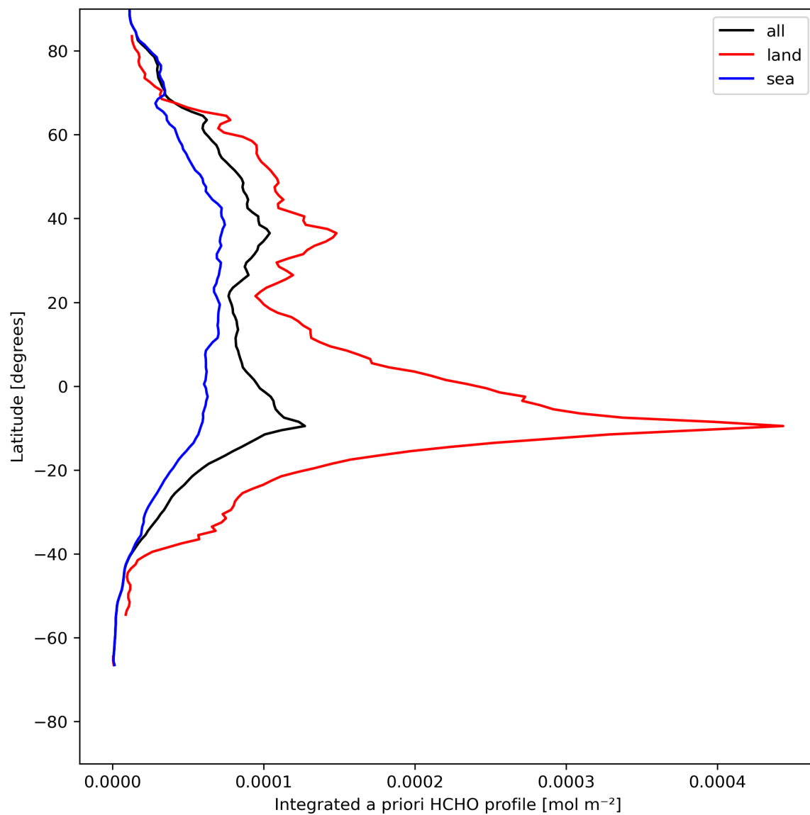
Figure 29: Zonal average of “Integrated a priori HCHO profile” for 2024-07-31 to 2024-08-02.
