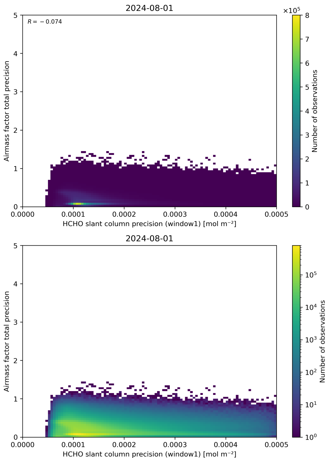
Figure 95: Scatter density plot of “HCHO slant column precision (window1)” against “Airmass factor total precision” for 2024-07-31 to 2024-08-02.
