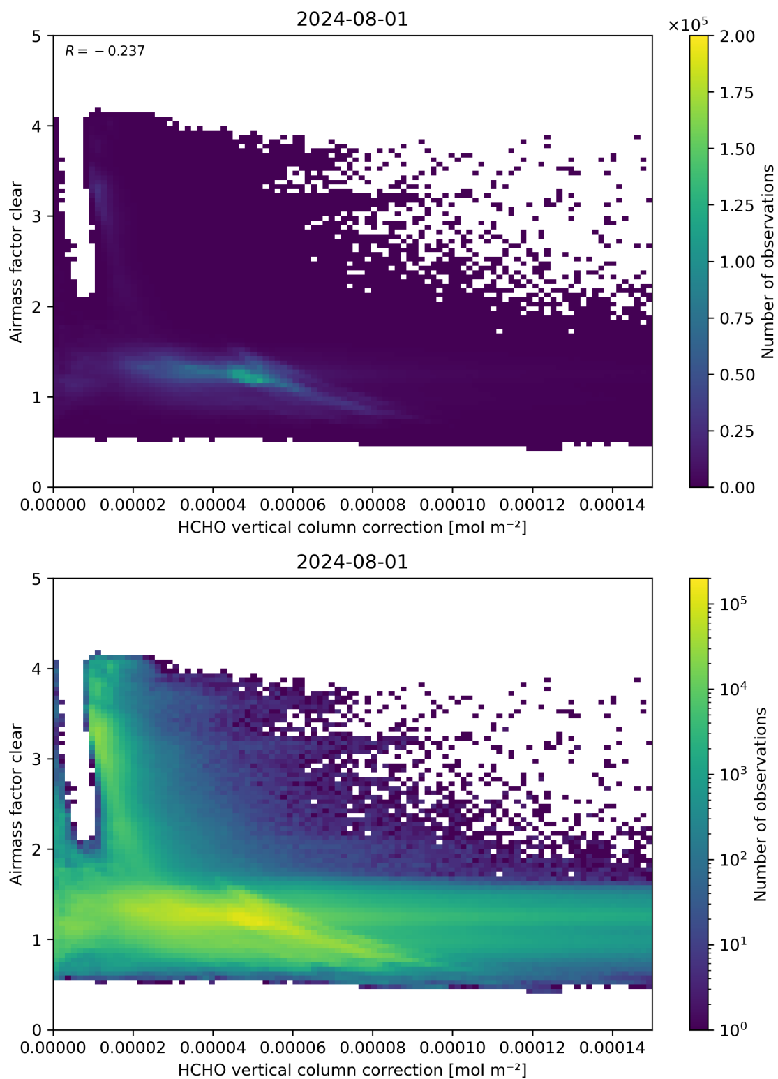
Figure 115: Scatter density plot of “HCHO vertical column correction” against “Airmass factor clear” for 2024-07-31 to 2024-08-02.
