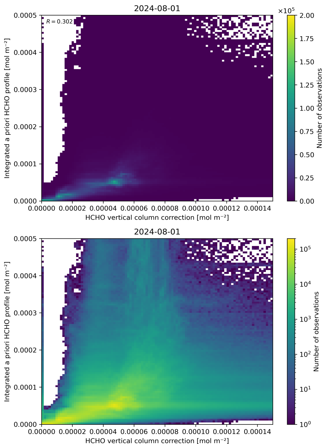
Figure 122: Scatter density plot of “HCHO vertical column correction” against “Integrated a priori HCHO profile” for 2024-07-31 to 2024-08-02.
