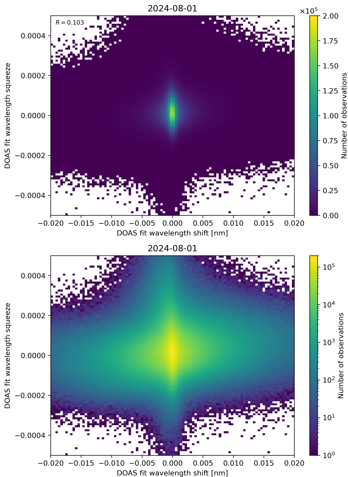
Figure 65: Scatter density plot of “DOAS fit wavelength shift” against “DOAS fit wavelength squeeze” for 2024-07-31 to 2024-08-02.
