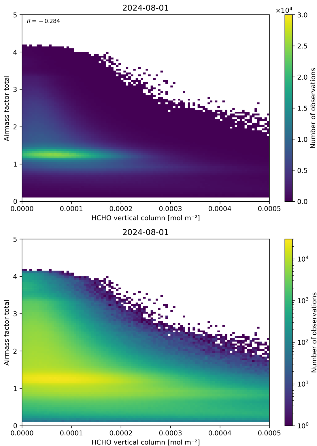
Figure 131: Scatter density plot of “HCHO vertical column” against “Airmass factor total” for 2024-07-31 to 2024-08-02.
