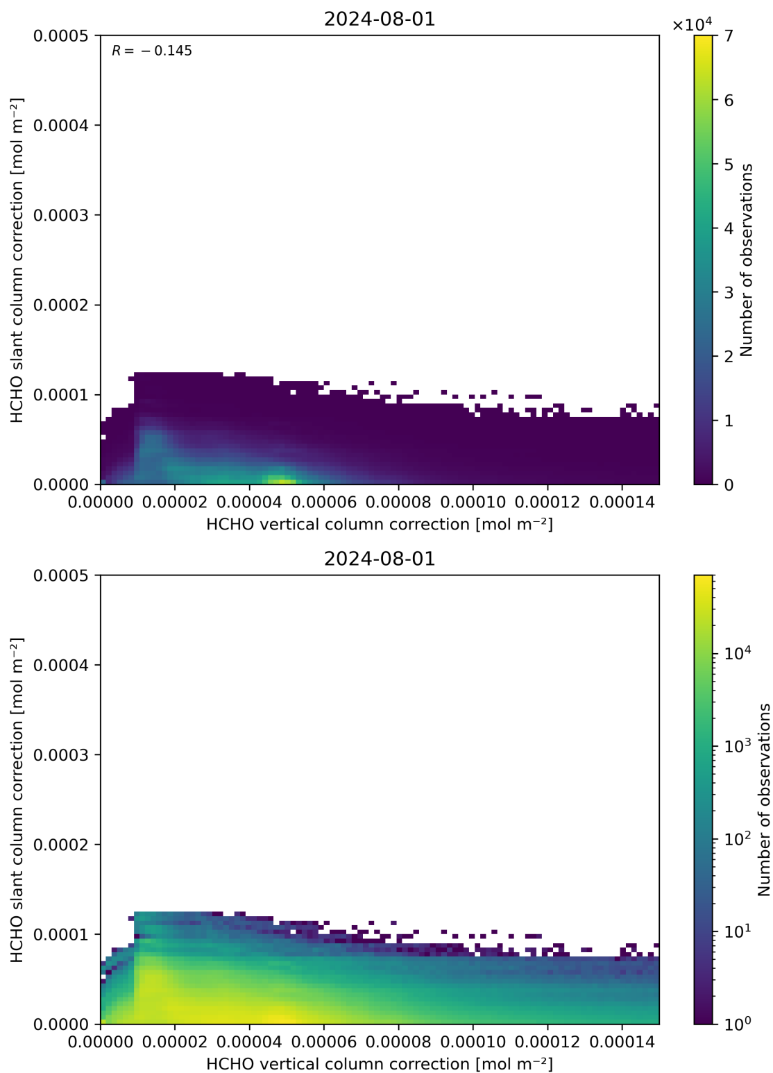
Figure 117: Scatter density plot of “HCHO vertical column correction” against “HCHO slant column correction” for 2024-07-31 to 2024-08-02.
