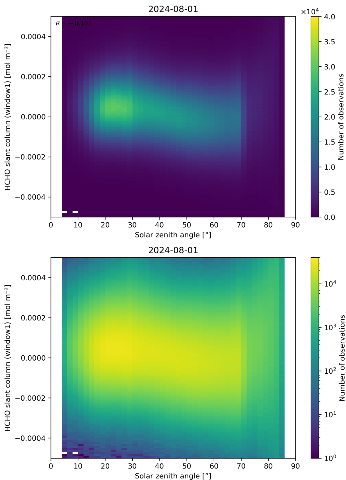
Figure 173: Scatter density plot of “Solar zenith angle” against “HCHO slant column (window1)” for 2024-07-31 to 2024-08-02.
