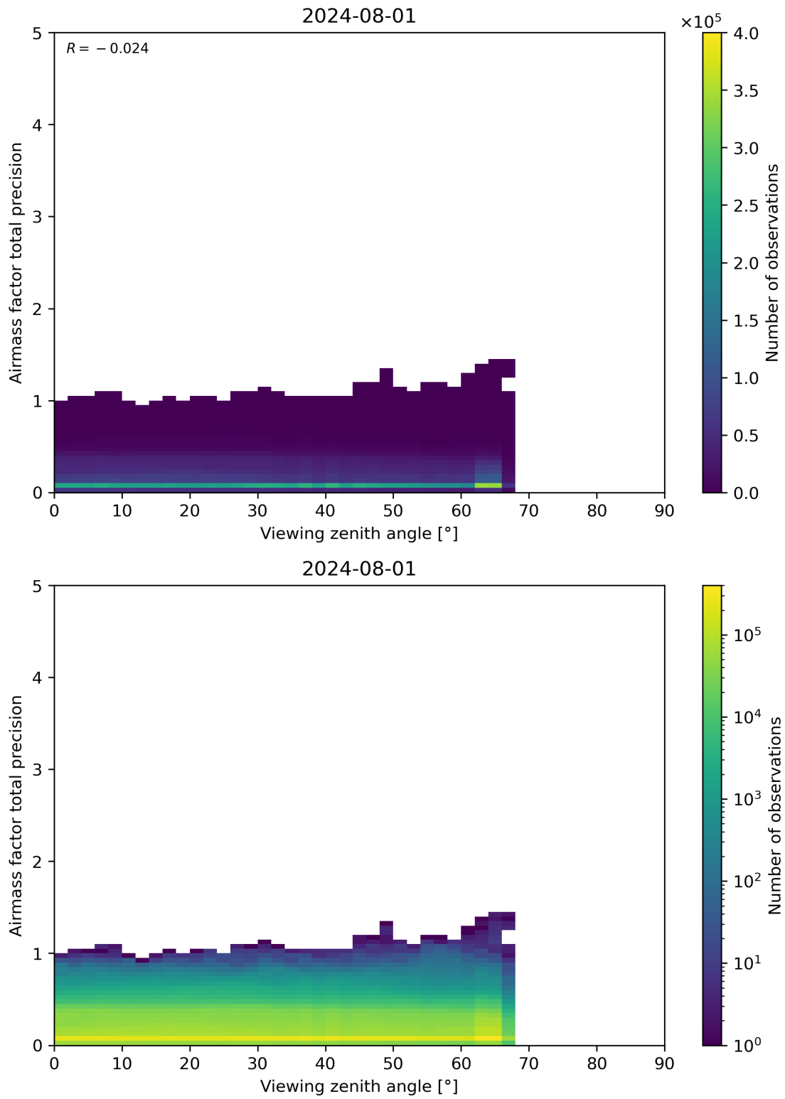
Figure 191: Scatter density plot of “Viewing zenith angle” against “Airmass factor total precision” for 2024-07-31 to 2024-08-02.
