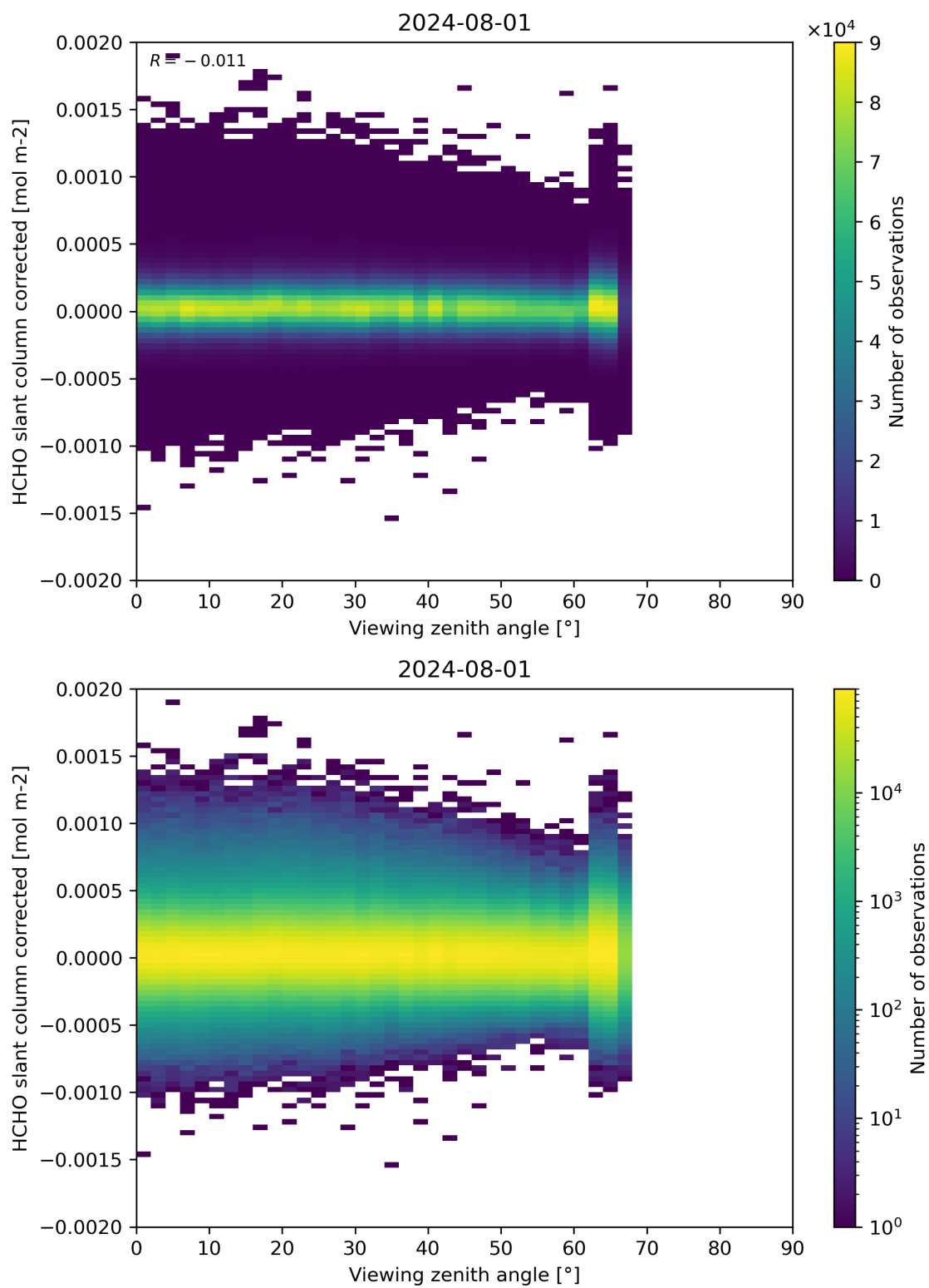
Figure 186: Scatter density plot of “Viewing zenith angle” against “HCHO slant column corrected” for 2024-07-31 to 2024-08-02.
