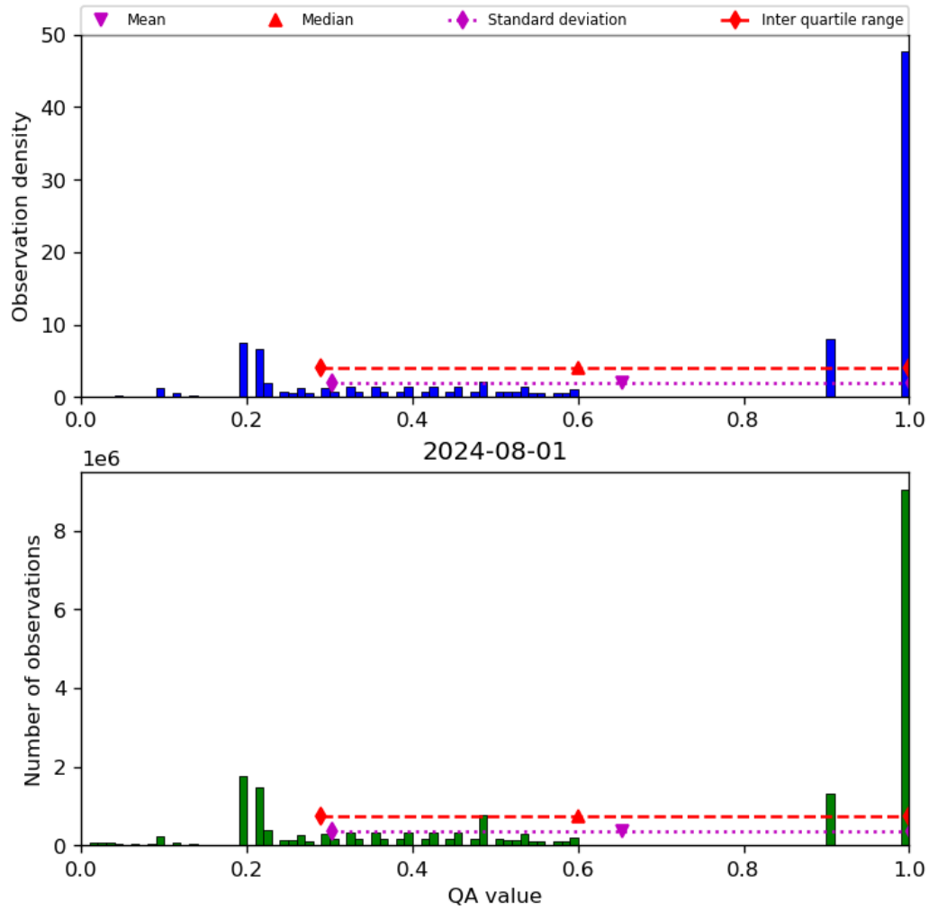
Figure 34: Histogram of “QA value” for 2024-07-31 to 2024-08-02
