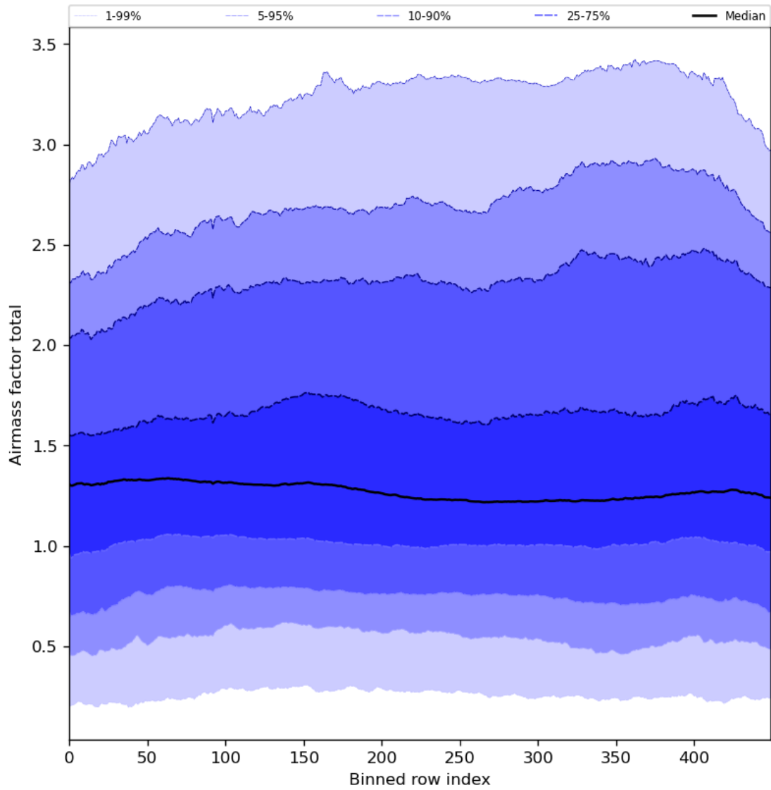
Figure 54: Along track statistics of “Airmass factor total” for 2024-07-31 to 2024-08-02
