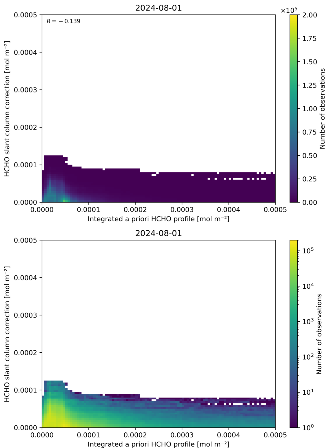
Figure 152: Scatter density plot of “Integrated a priori HCHO profile” against “HCHO slant column correction” for 2024-07-31 to 2024-08-02.
