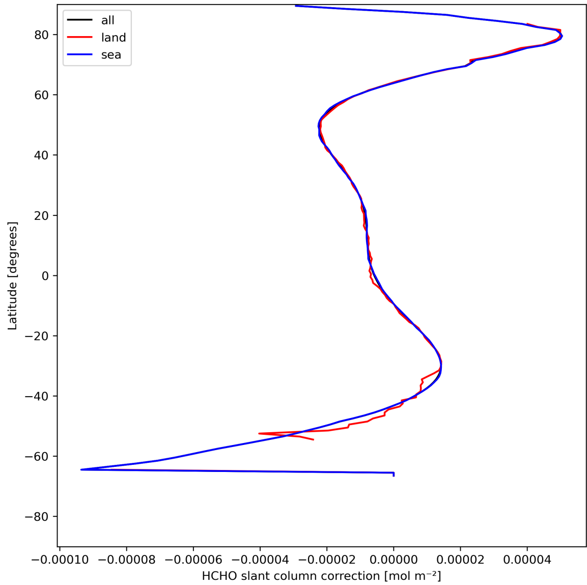
Figure 33: Zonal average of “HCHO slant column correction” for 2024-07-31 to 2024-08-02.
