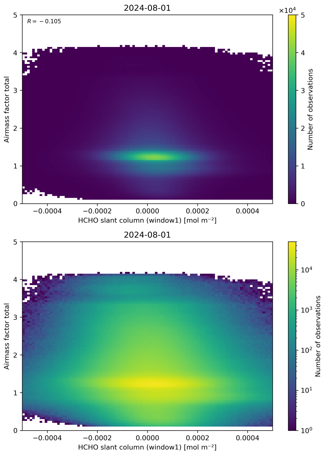
Figure 85: Scatter density plot of “HCHO slant column (window1)” against “Airmass factor total” for 2024-07-31 to 2024-08-02.
