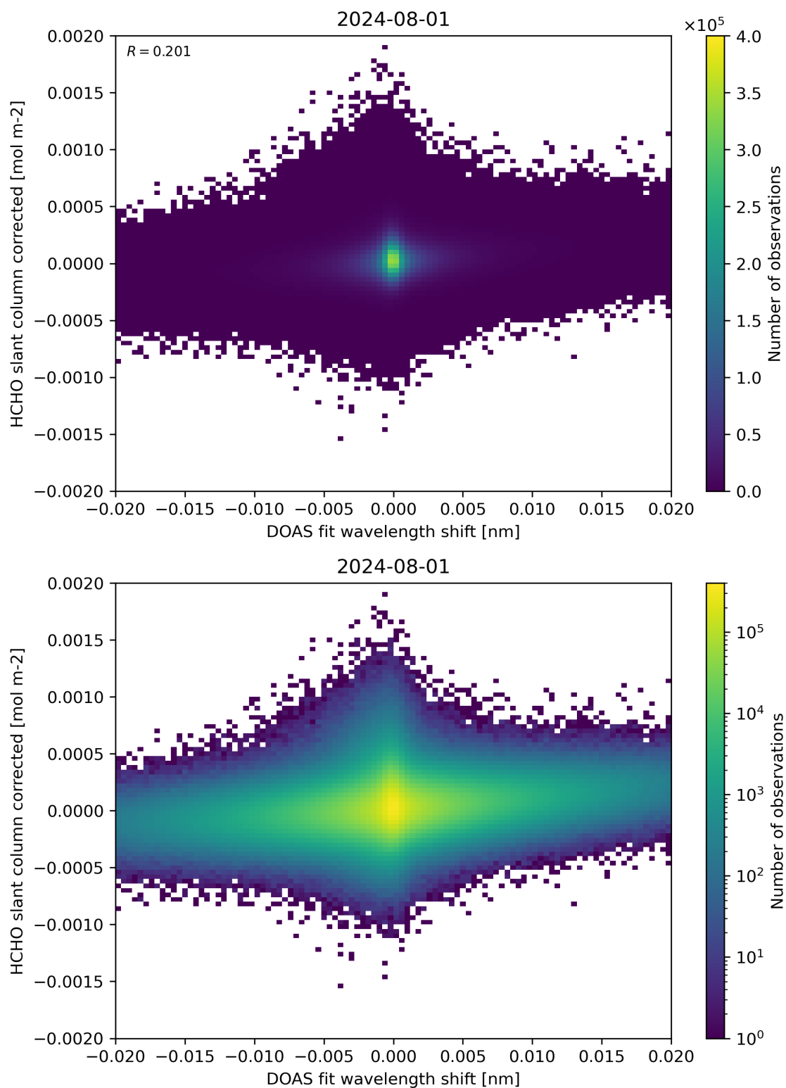
Figure 66: Scatter density plot of “DOAS fit wavelength shift” against “HCHO slant column corrected” for 2024-07-31 to 2024-08-02.
