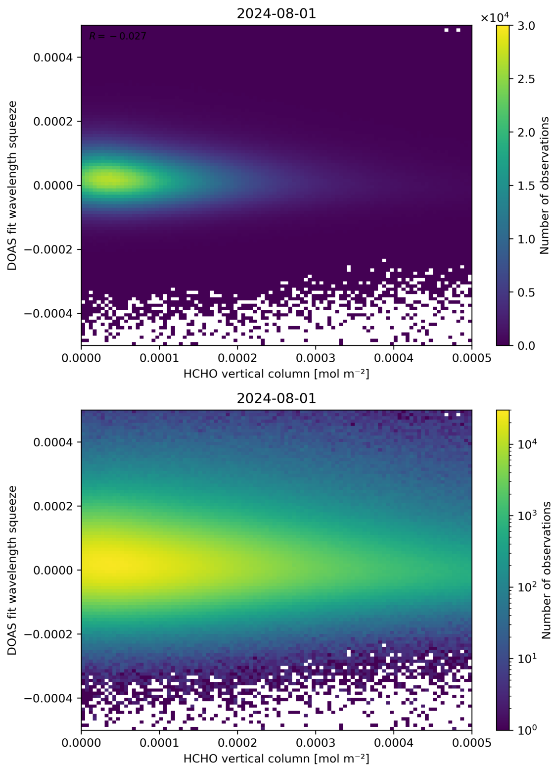
Figure 125: Scatter density plot of “HCHO vertical column” against “DOAS fit wavelength squeeze” for 2024-07-31 to 2024-08-02.
