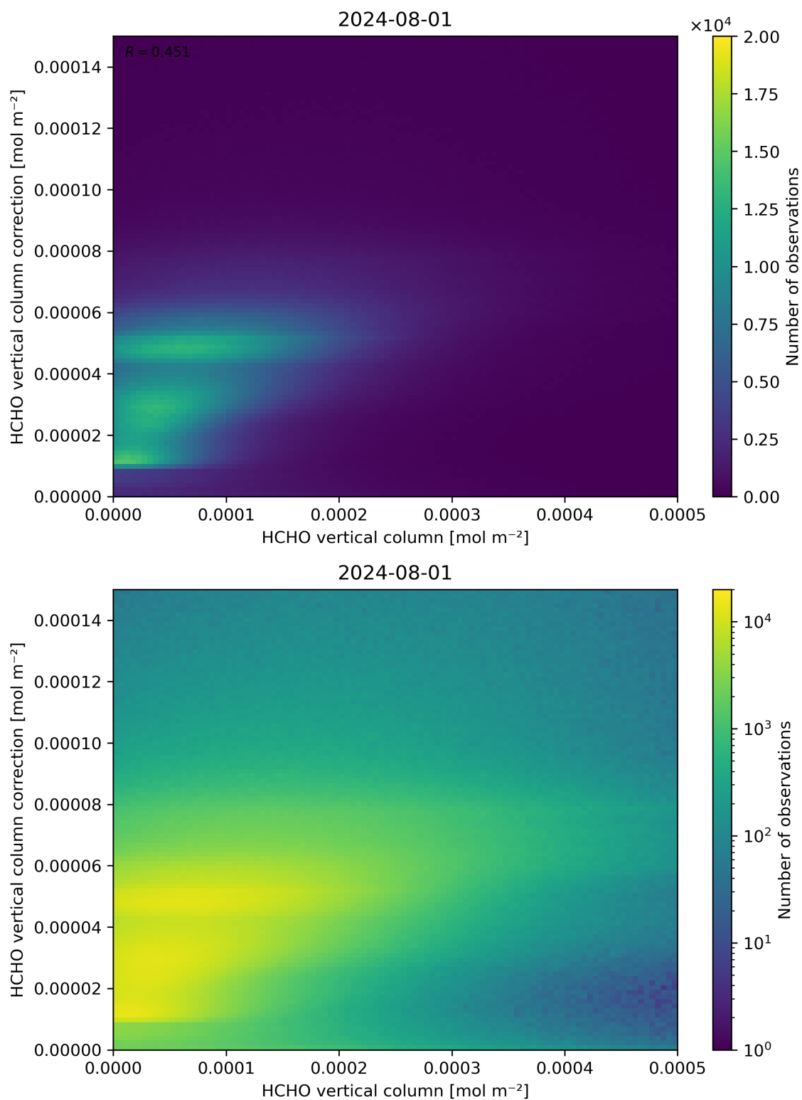
Figure 133: Scatter density plot of “HCHO vertical column” against “HCHO vertical column correction” for 2024-07-31 to 2024-08-02.
