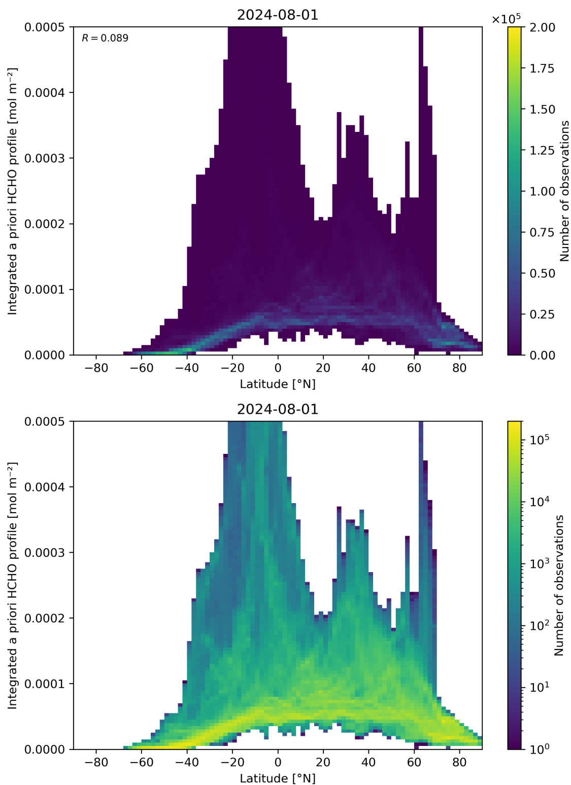
Figure 166: Scatter density plot of “Latitude” against “Integrated a priori HCHO profile” for 2024-07-31 to 2024-08-02.
