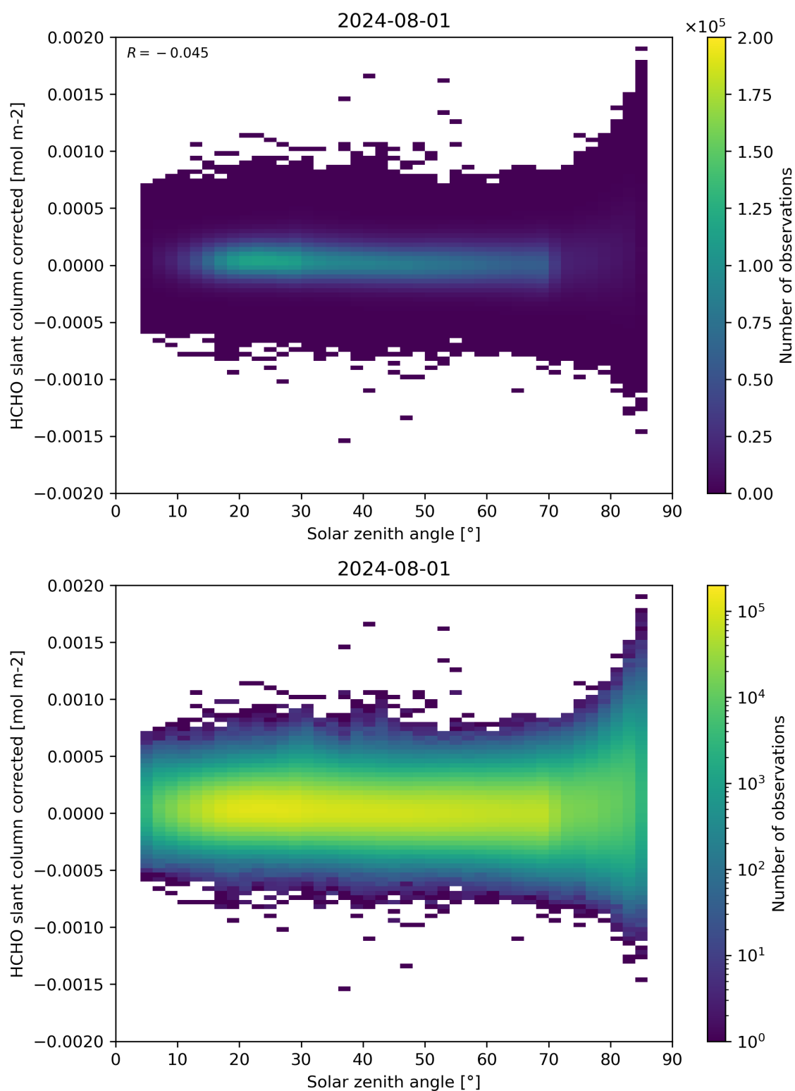
Figure 171: Scatter density plot of “Solar zenith angle” against “HCHO slant column corrected” for 2024-07-31 to 2024-08-02.
