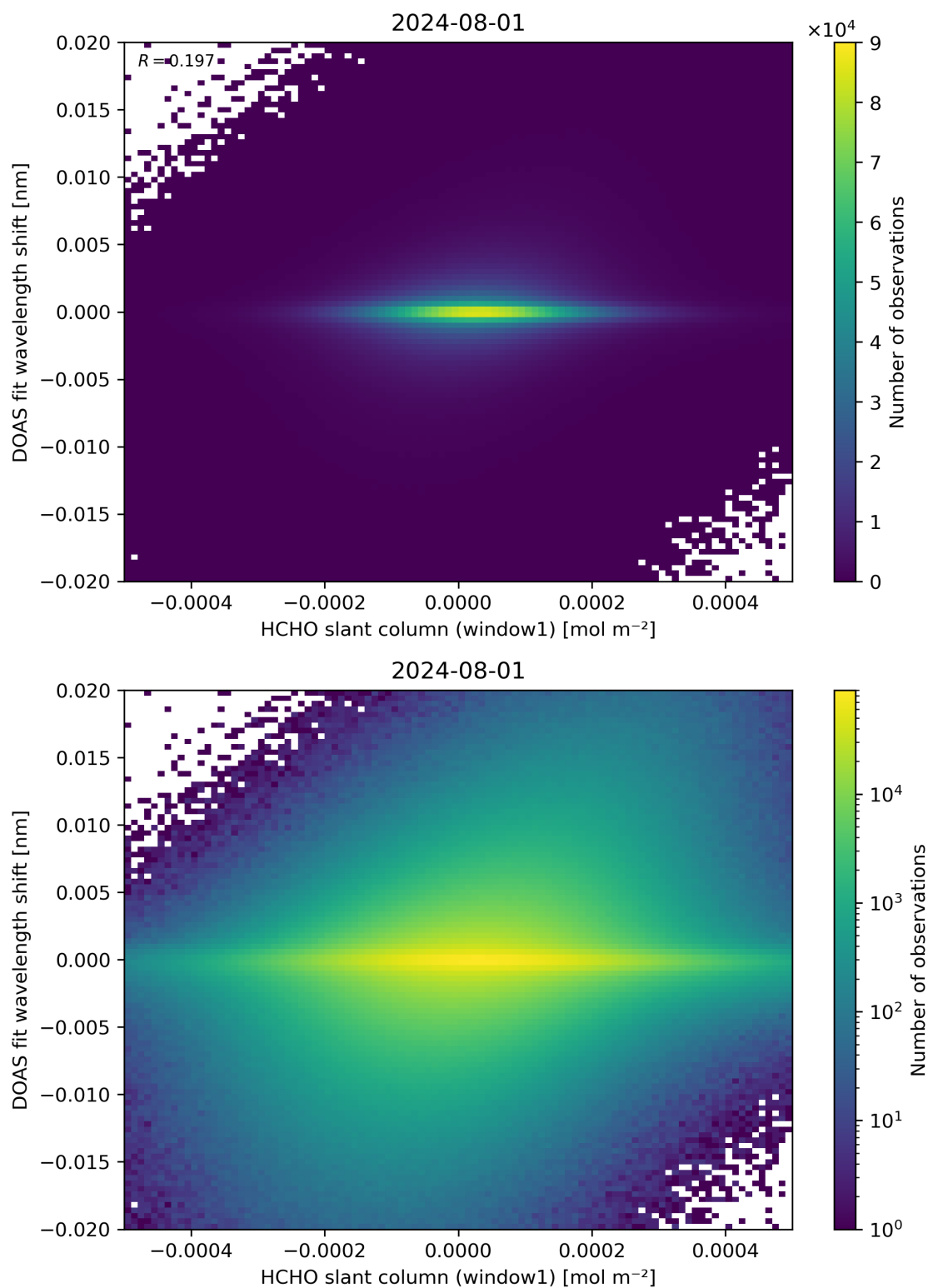
Figure 79: Scatter density plot of “HCHO slant column (window1)” against “DOAS fit wavelength shift” for 2024-07-31 to 2024-08-02.
