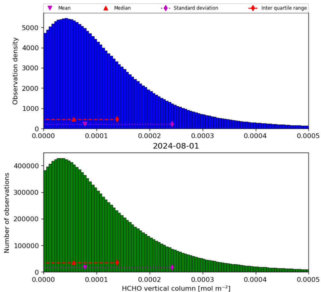
Figure 35: Histogram of “HCHO vertical column” for 2024-07-31 to 2024-08-02
