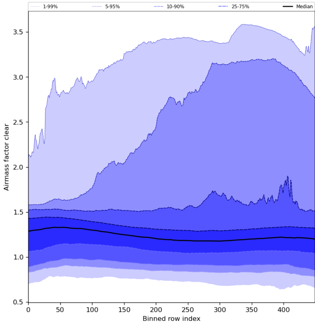
Figure 56: Along track statistics of “Airmass factor clear” for 2024-08-01 to 2024-08-03
