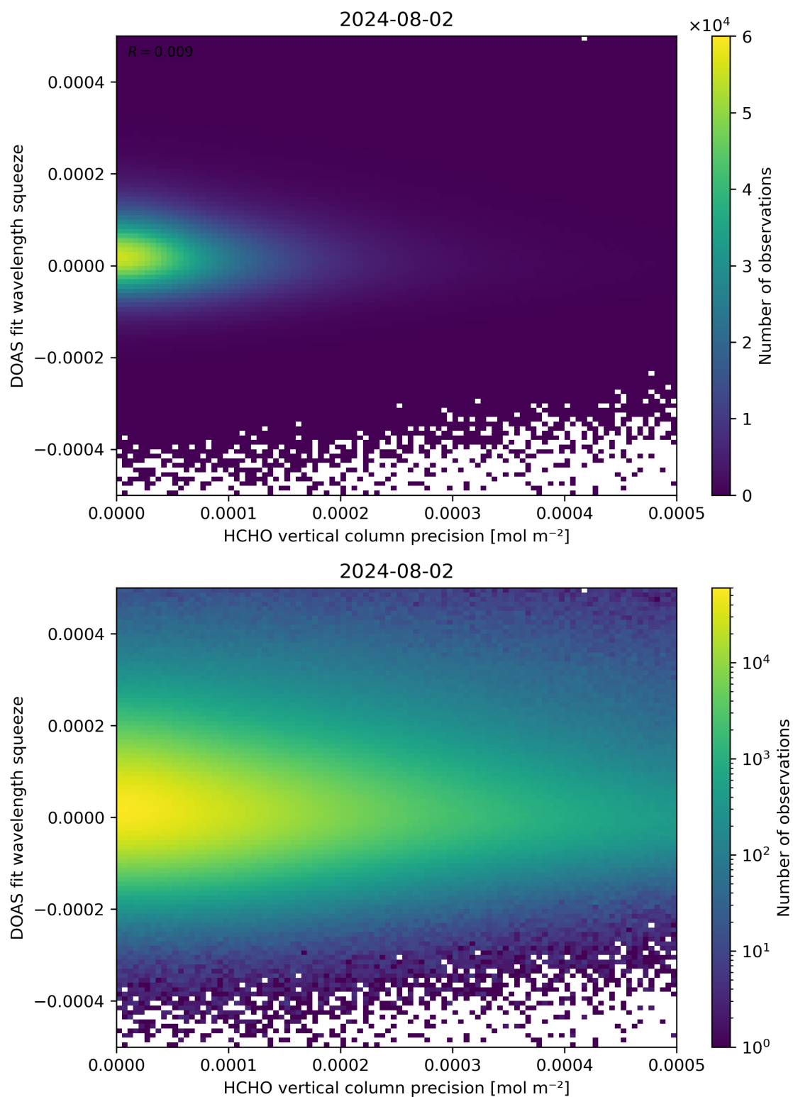
Figure 138: Scatter density plot of “HCHO vertical column precision” against “DOAS fit wavelength squeeze” for 2024-08-01 to 2024-08-03.
