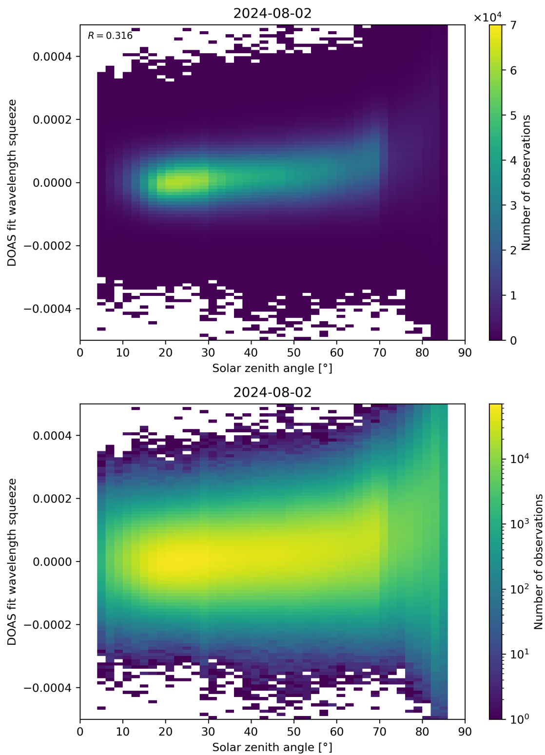
Figure 169: Scatter density plot of “Solar zenith angle” against “DOAS fit wavelength squeeze” for 2024-08-01 to 2024-08-03.
