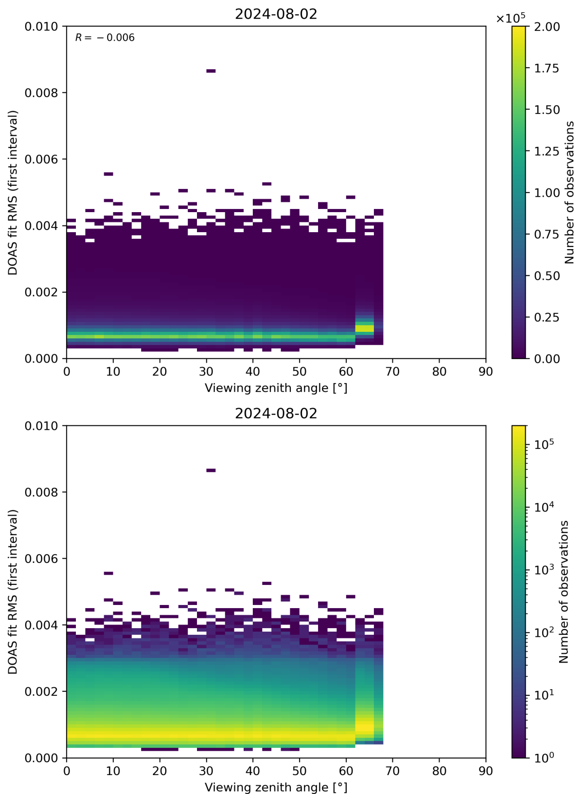
Figure 182: Scatter density plot of “Viewing zenith angle” against “DOAS fit RMS (first interval)” for 2024-08-01 to 2024-08-03.
