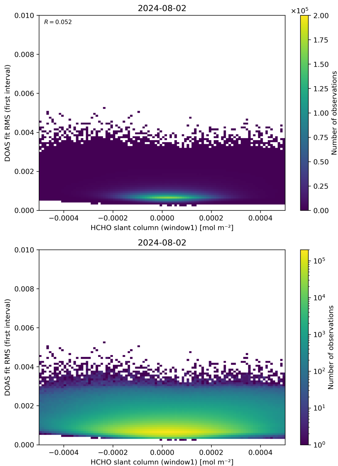
Figure 78: Scatter density plot of “HCHO slant column (window1)” against “DOAS fit RMS (first interval)” for 2024-08-01 to 2024-08-03.
