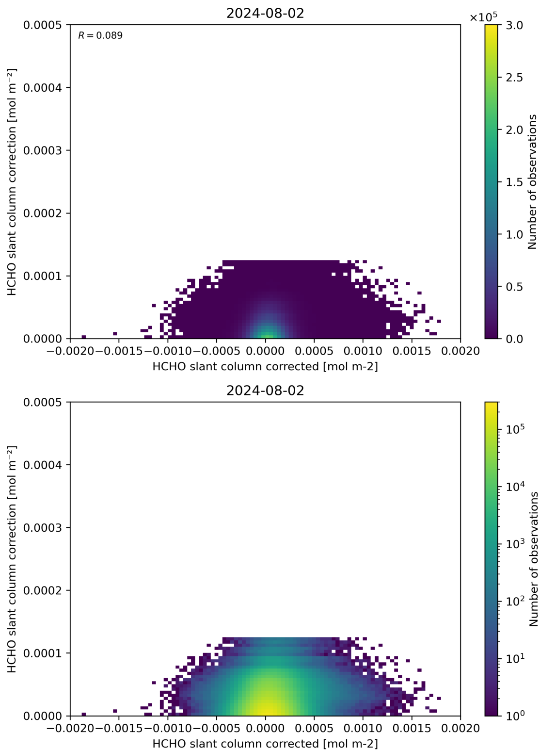
Figure 77: Scatter density plot of “HCHO slant column corrected” against “HCHO slant column correction” for 2024-08-01 to 2024-08-03.
