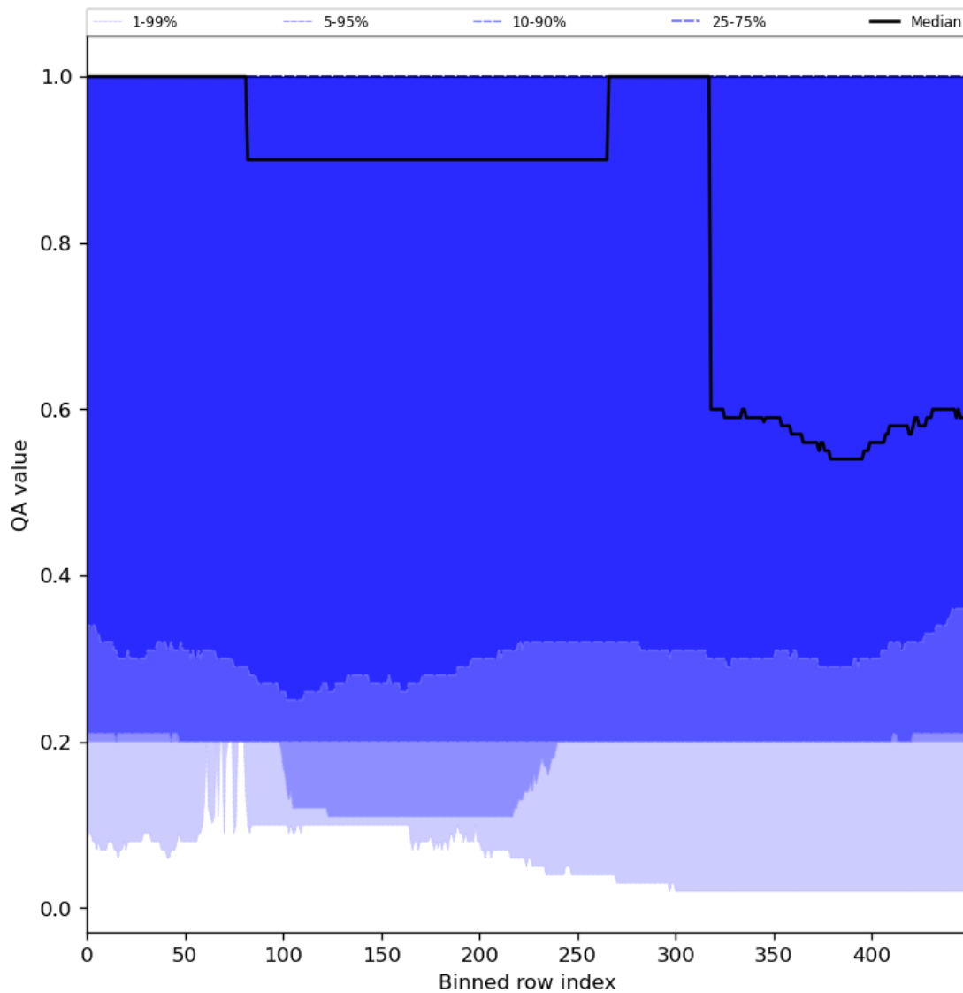
Figure 48: Along track statistics of “QA value” for 2024-08-01 to 2024-08-03
