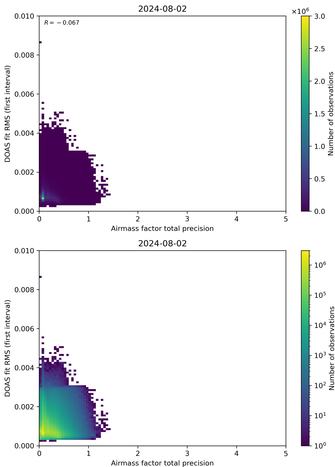
Figure 105: Scatter density plot of “Airmass factor total precision” against “DOAS fit RMS (first interval)” for 2024-08-01 to 2024-08-03.
