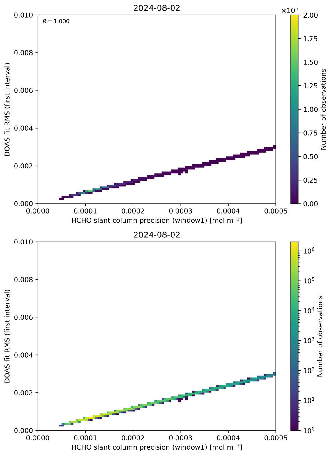
Figure 88: Scatter density plot of “HCHO slant column precision (window1)” against “DOAS fit RMS (first interval)” for 2024-08-01 to 2024-08-03.
