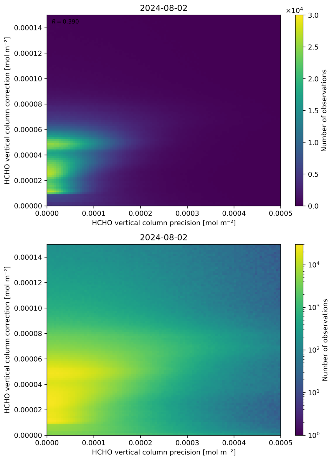
Figure 146: Scatter density plot of “HCHO vertical column precision” against “HCHO vertical column correction” for 2024-08-01 to 2024-08-03.
