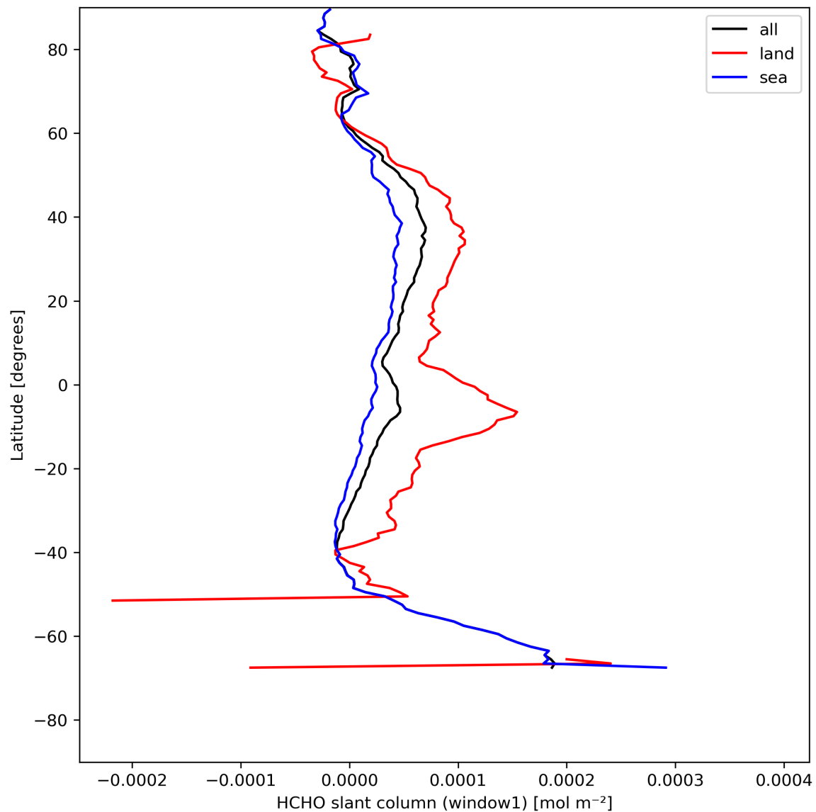
Figure 24: Zonal average of “HCHO slant column (window1)” for 2024-08-01 to 2024-08-03.
