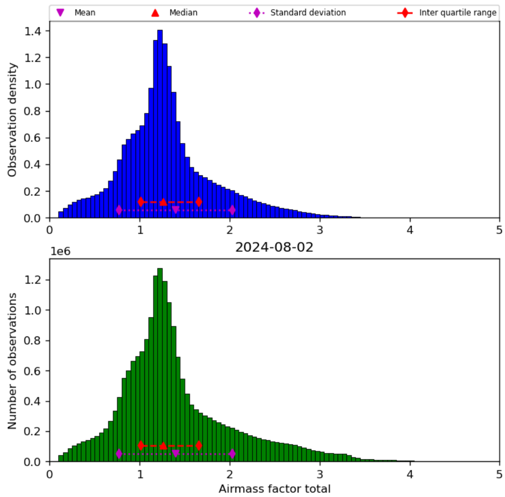
Figure 40: Histogram of “Airmass factor total” for 2024-08-01 to 2024-08-03
