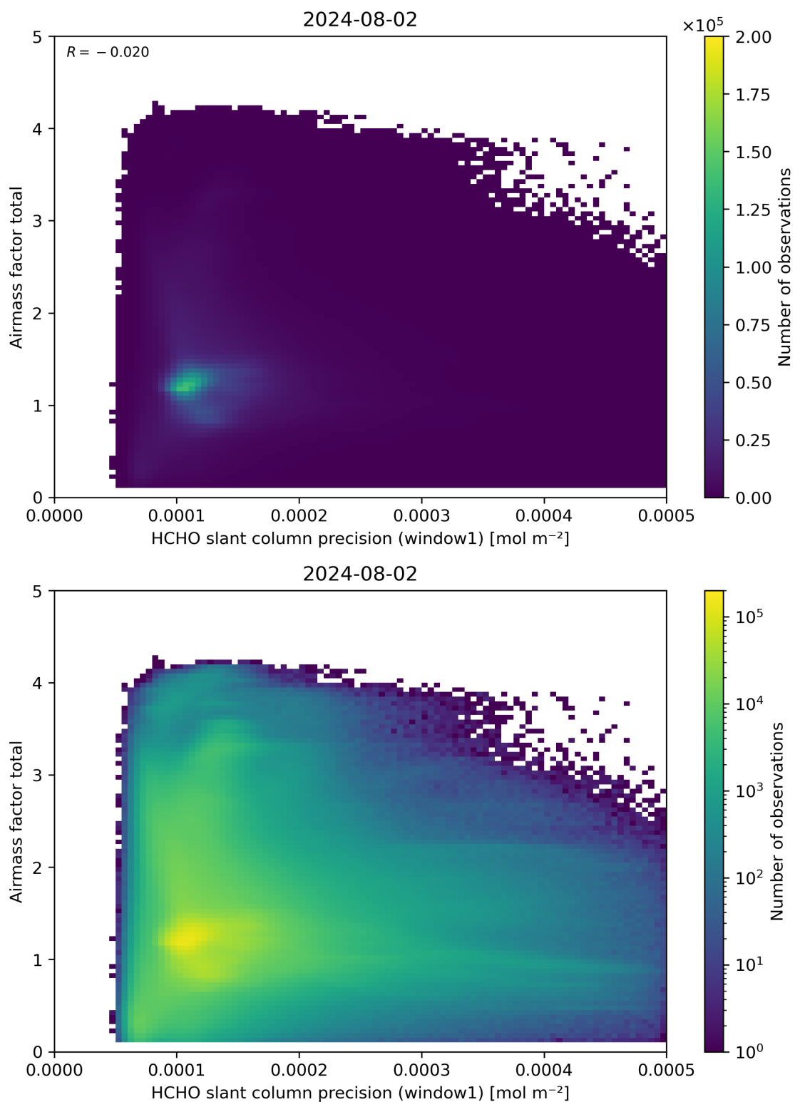
Figure 94: Scatter density plot of “HCHO slant column precision (window1)” against “Airmass factor total” for 2024-08-01 to 2024-08-03.
