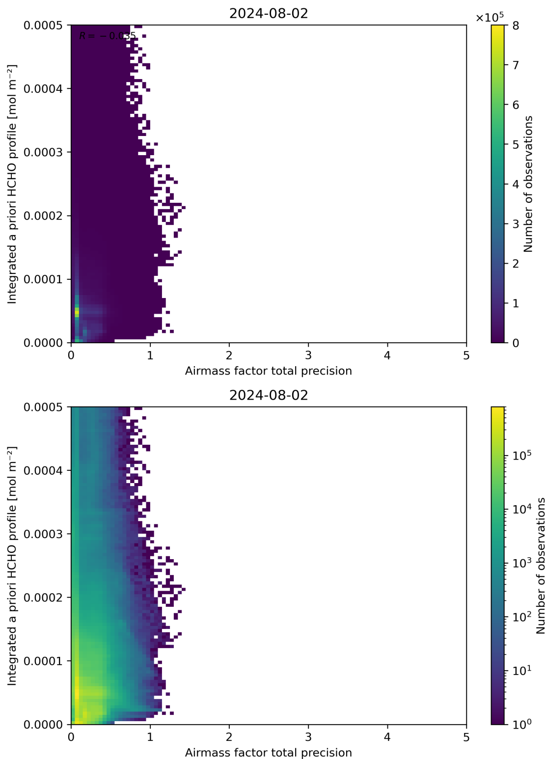
Figure 111: Scatter density plot of “Airmass factor total precision” against “Integrated a priori HCHO profile” for 2024-08-01 to 2024-08-03.
