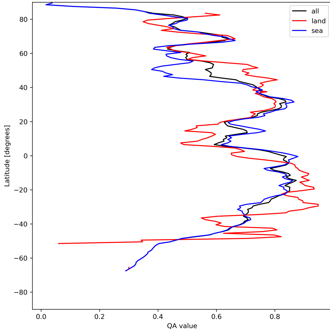
Figure 20: Zonal average of “QA value” for 2024-08-01 to 2024-08-03.
