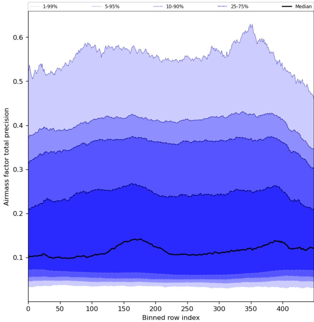
Figure 55: Along track statistics of “Airmass factor total precision” for 2024-08-01 to 2024-08-03
