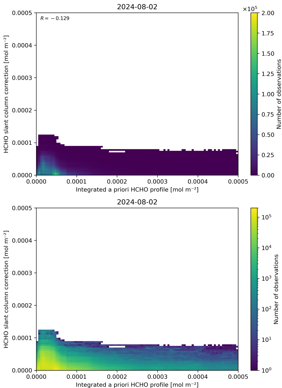
Figure 152: Scatter density plot of “Integrated a priori HCHO profile” against “HCHO slant column correction” for 2024-08-01 to 2024-08-03.
