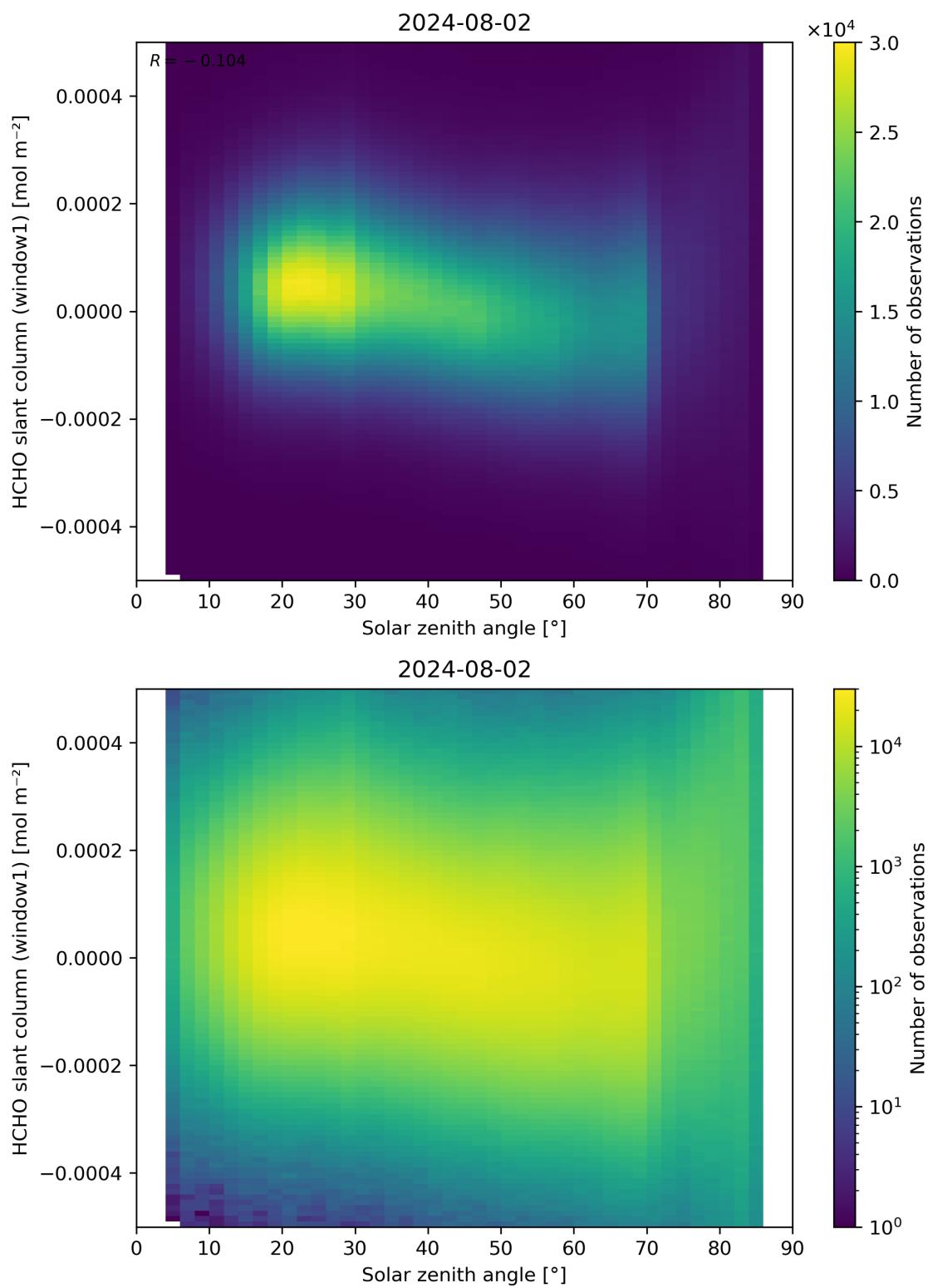
Figure 173: Scatter density plot of “Solar zenith angle” against “HCHO slant column (window1)” for 2024-08-01 to 2024-08-03.
