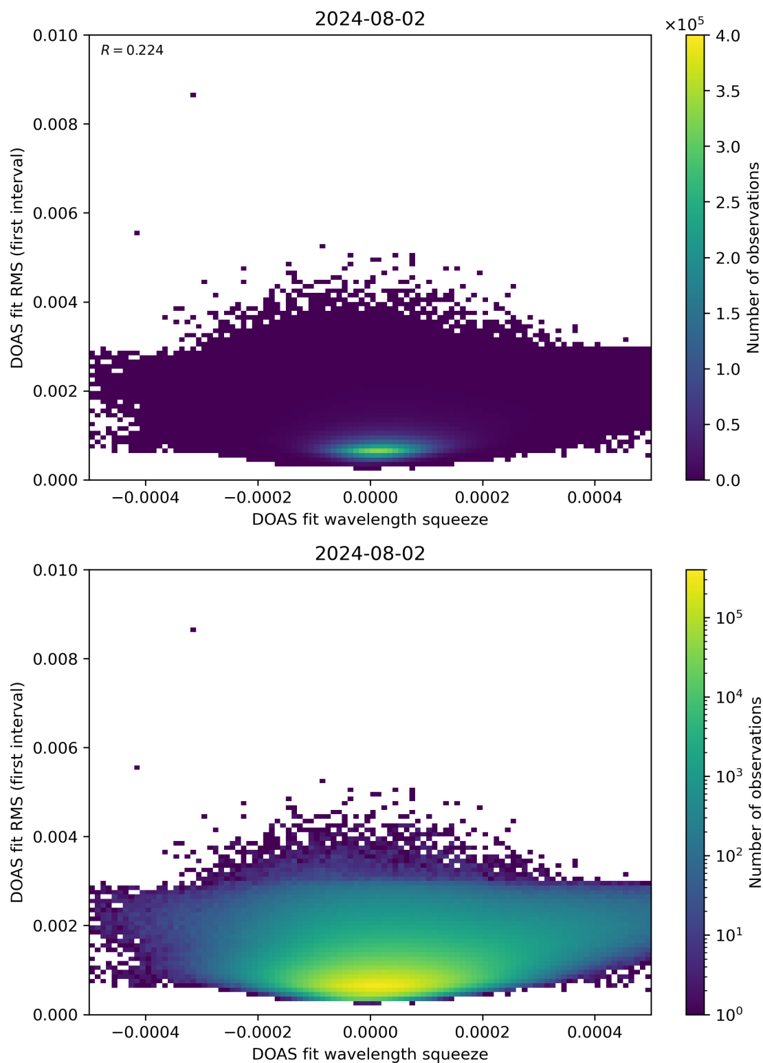
Figure 68: Scatter density plot of “DOAS fit wavelength squeeze” against “DOAS fit RMS (first interval)” for 2024-08-01 to 2024-08-03.
