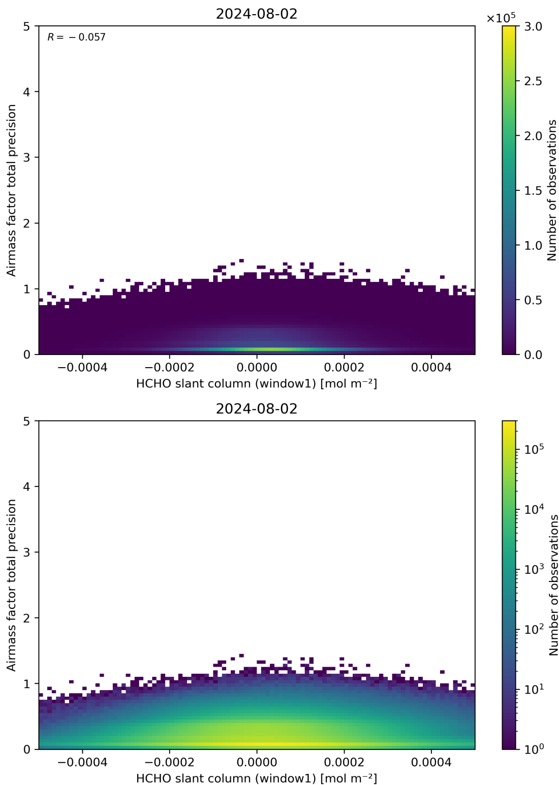
Figure 86: Scatter density plot of “HCHO slant column (window1)” against “Airmass factor total precision” for 2024-08-01 to 2024-08-03.
