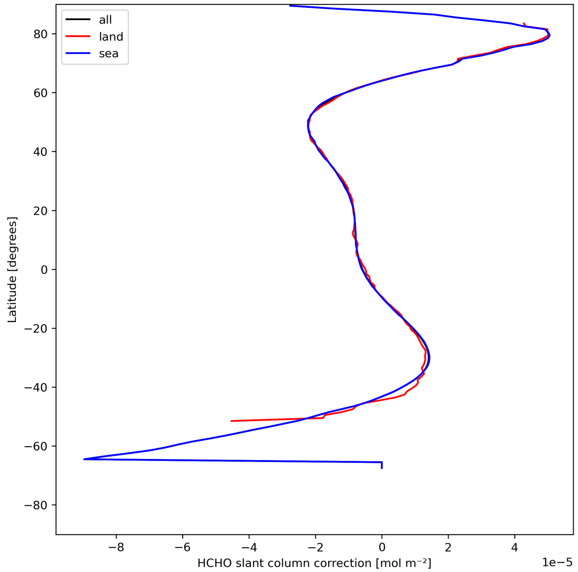
Figure 33: Zonal average of “HCHO slant column correction” for 2024-08-01 to 2024-08-03.
