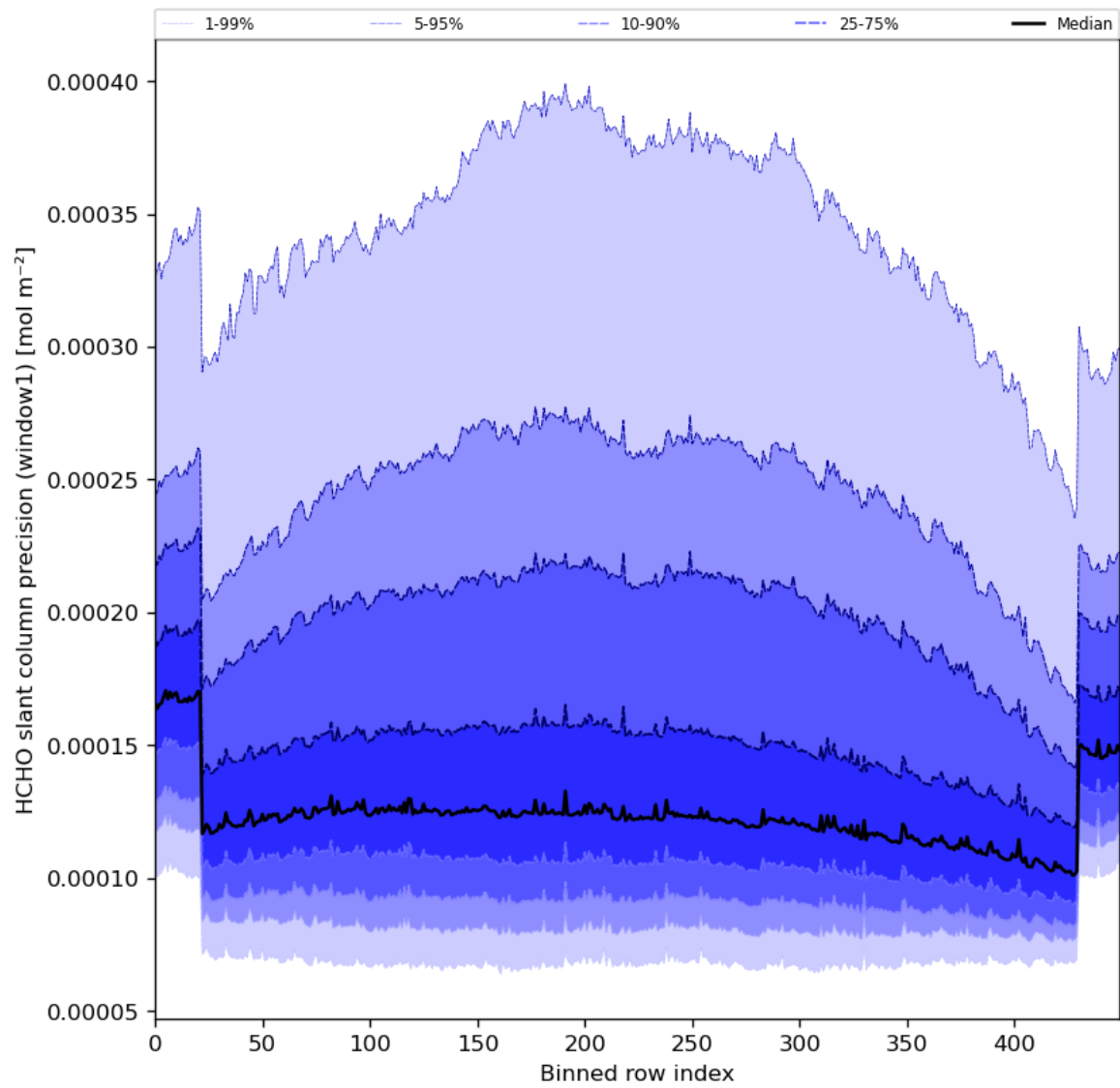
Figure 53: Along track statistics of “HCHO slant column precision (window1)” for 2024-08-01 to 2024-08-03
