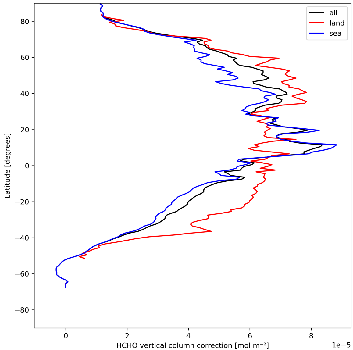
Figure 23: Zonal average of “HCHO vertical column correction” for 2024-08-01 to 2024-08-03.
