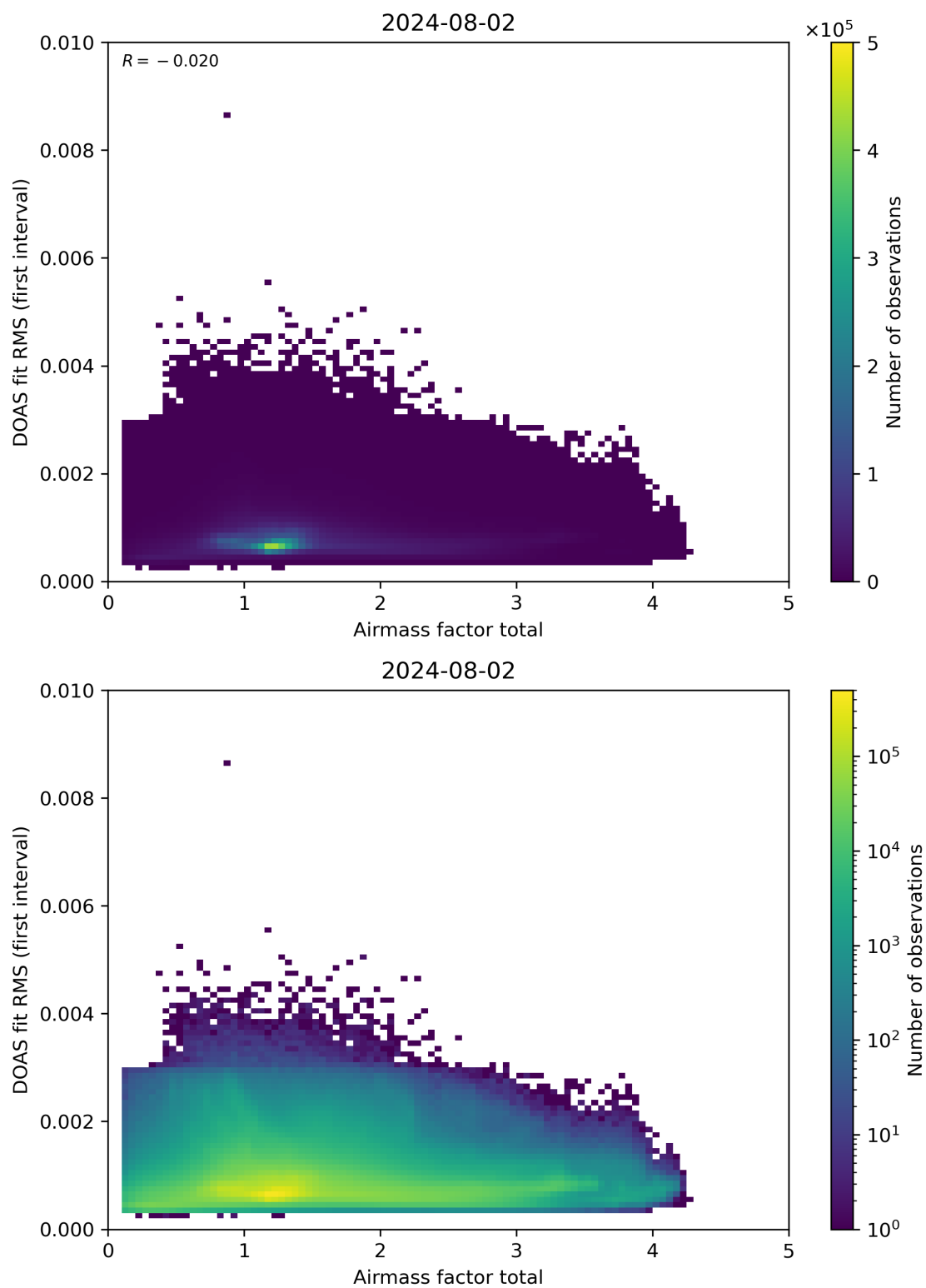
Figure 97: Scatter density plot of “Airmass factor total” against “DOAS fit RMS (first interval)” for 2024-08-01 to 2024-08-03.
