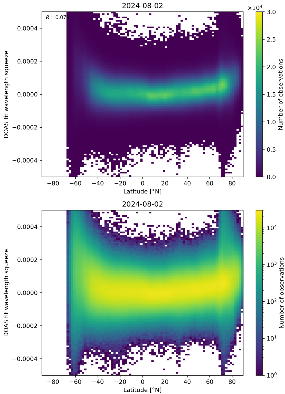
Figure 155: Scatter density plot of “Latitude” against “DOAS fit wavelength squeeze” for 2024-08-01 to 2024-08-03.
