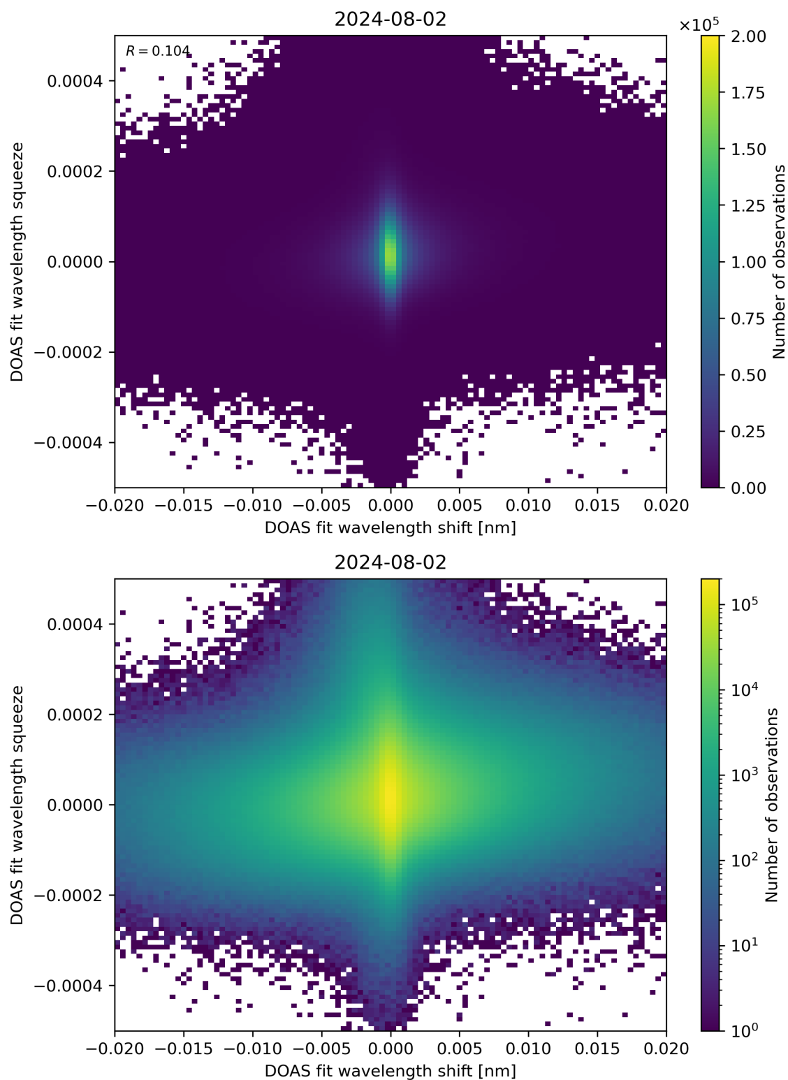
Figure 65: Scatter density plot of “DOAS fit wavelength shift” against “DOAS fit wavelength squeeze” for 2024-08-01 to 2024-08-03.
