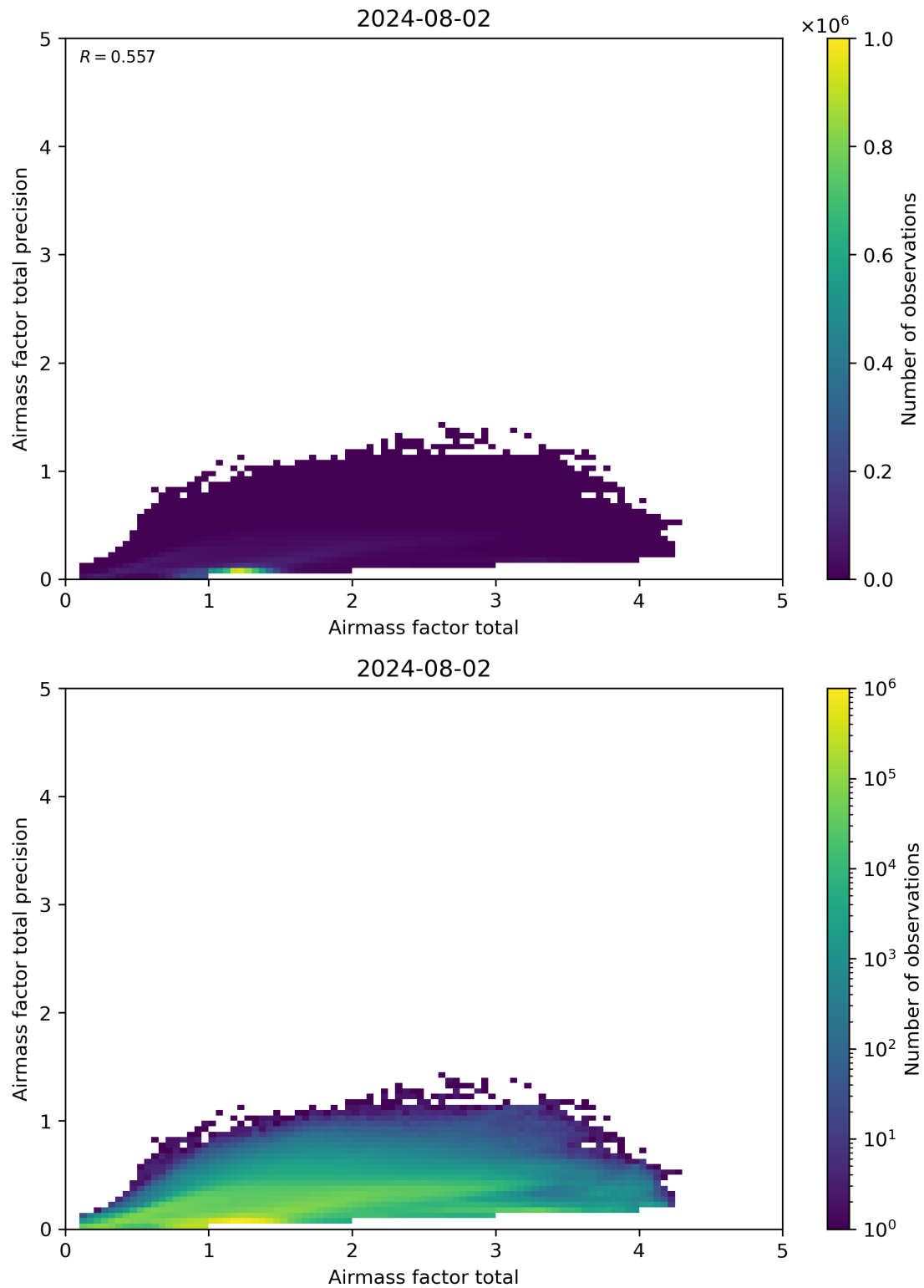
Figure 103: Scatter density plot of “Airmass factor total” against “Airmass factor total precision” for 2024-08-01 to 2024-08-03.
