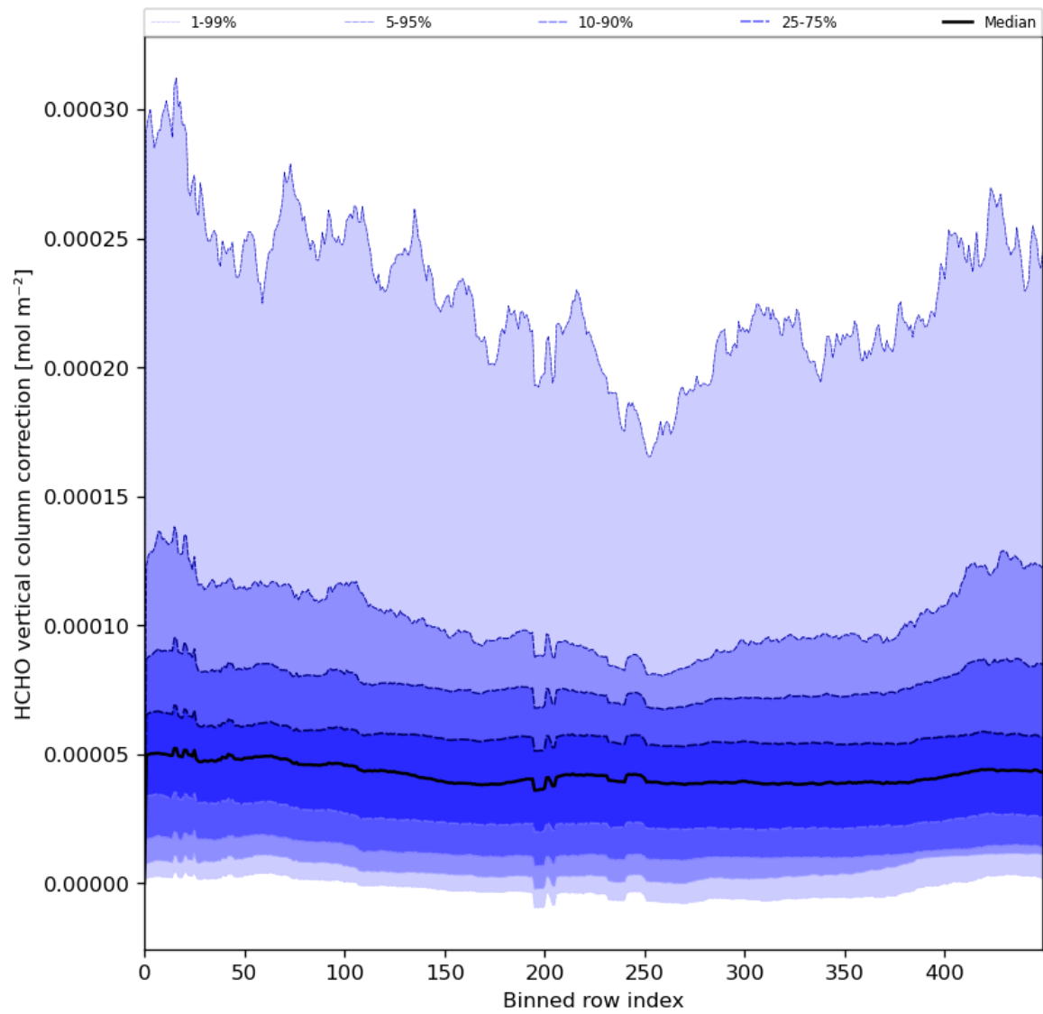
Figure 51: Along track statistics of “HCHO vertical column correction” for 2024-08-01 to 2024-08-03
