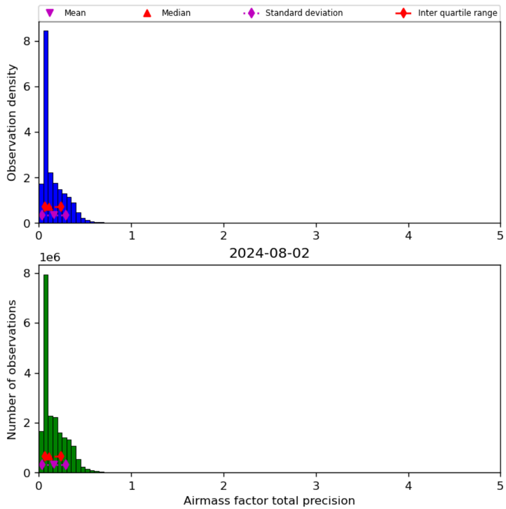
Figure 41: Histogram of "Airmass factor total precision" for 2024-08-01 to 2024-08-03
