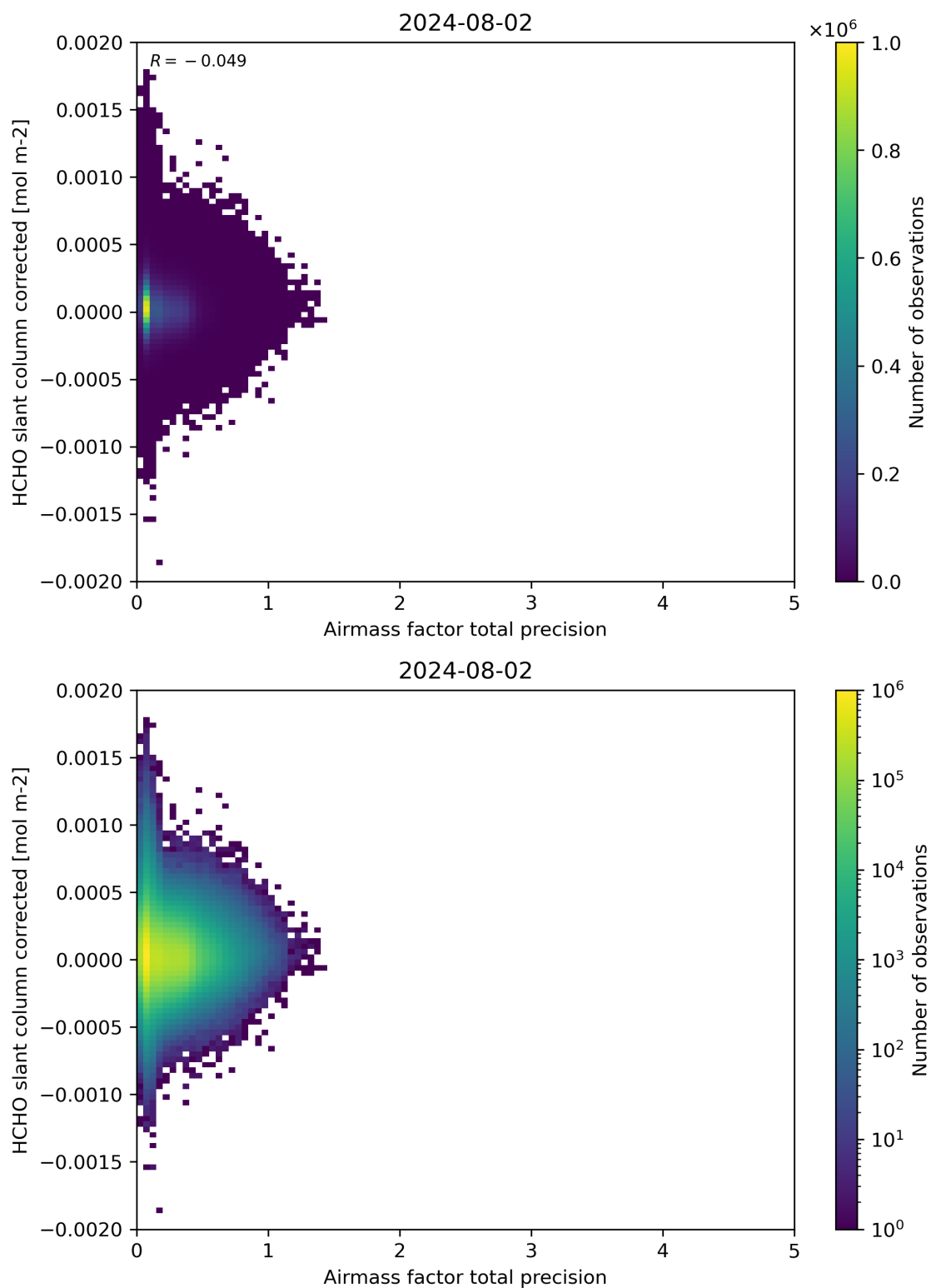
Figure 109: Scatter density plot of “Airmass factor total precision” against “HCHO slant column corrected” for 2024-08-01 to 2024-08-03.
