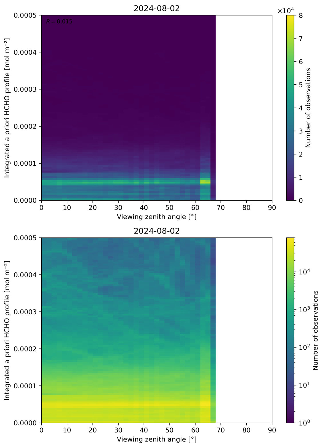
Figure 195: Scatter density plot of “Viewing zenith angle” against “Integrated a priori HCHO profile” for 2024-08-01 to 2024-08-03.
