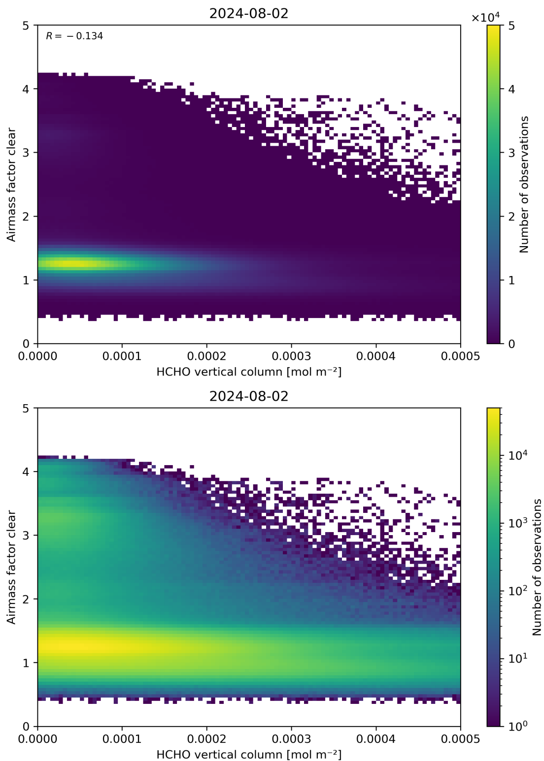
Figure 126: Scatter density plot of “HCHO vertical column” against “Airmass factor clear” for 2024-08-01 to 2024-08-03.
