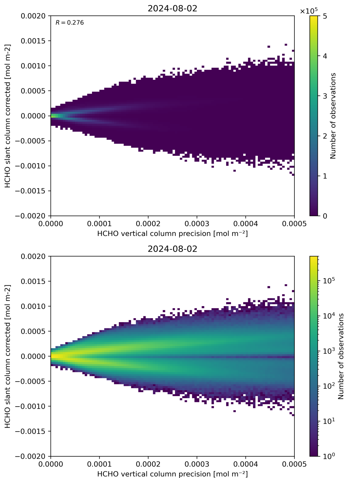
Figure 140: Scatter density plot of “HCHO vertical column precision” against “HCHO slant column corrected” for 2024-08-01 to 2024-08-03.
