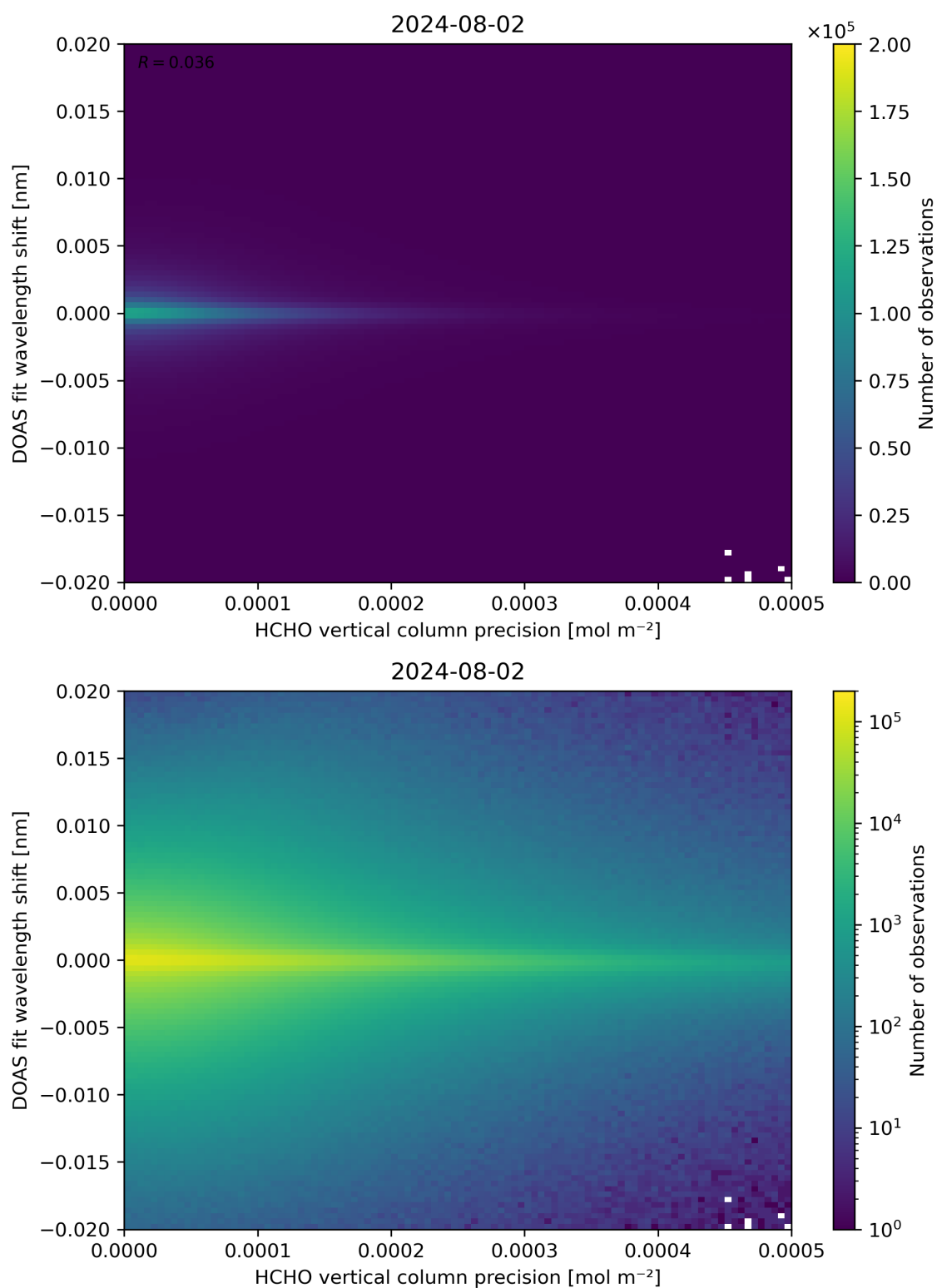
Figure 137: Scatter density plot of “HCHO vertical column precision” against “DOAS fit wavelength shift” for 2024-08-01 to 2024-08-03.
