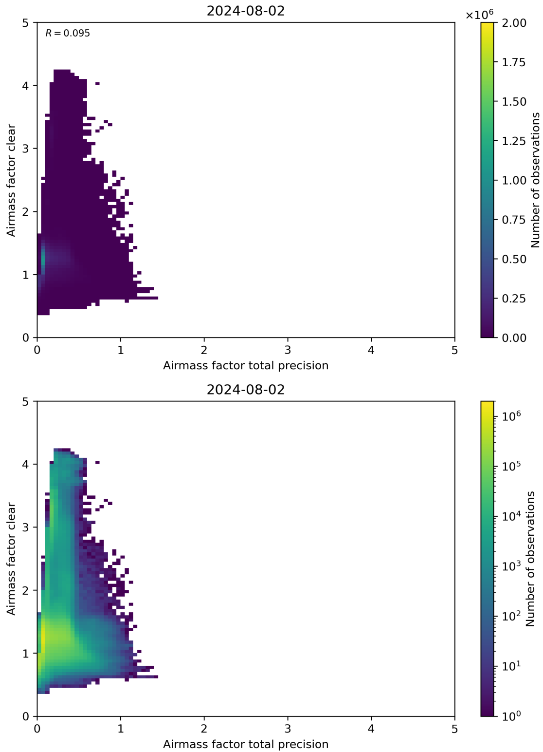
Figure 108: Scatter density plot of “Airmass factor total precision” against “Airmass factor clear” for 2024-08-01 to 2024-08-03.
