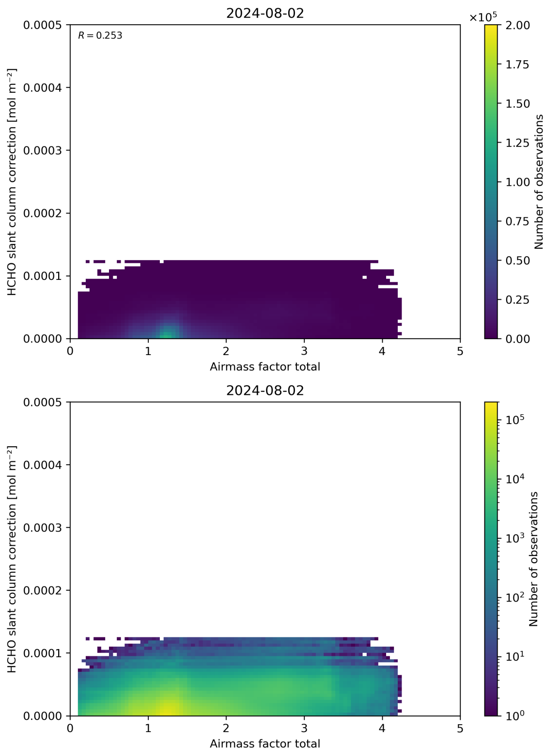
Figure 102: Scatter density plot of “Airmass factor total” against “HCHO slant column correction” for 2024-08-01 to 2024-08-03.
