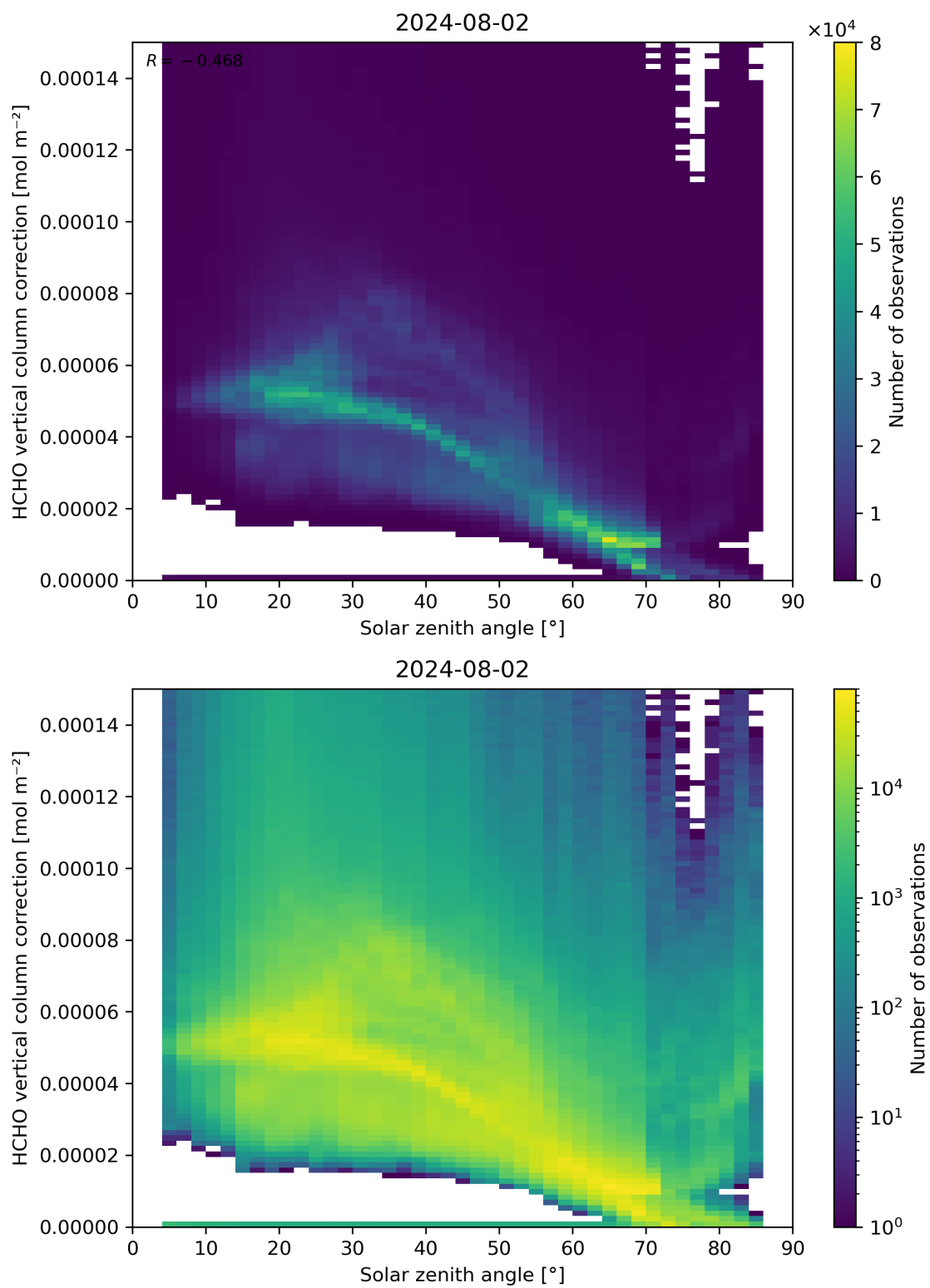
Figure 178: Scatter density plot of “Solar zenith angle” against “HCHO vertical column correction” for 2024-08-01 to 2024-08-03.
