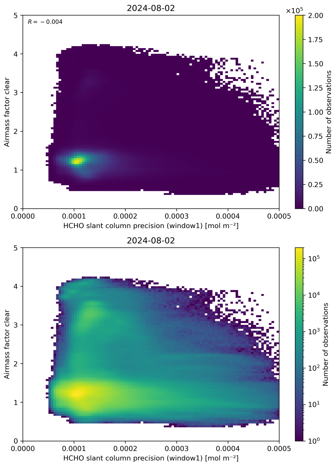
Figure 91: Scatter density plot of “HCHO slant column precision (window1)” against “Airmass factor clear” for 2024-08-01 to 2024-08-03.
