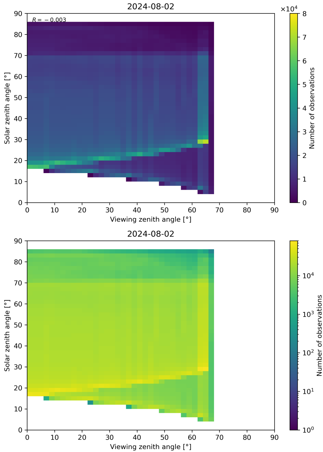
Figure 197: Scatter density plot of “Viewing zenith angle” against “Solar zenith angle” for 2024-08-01 to 2024-08-03.
