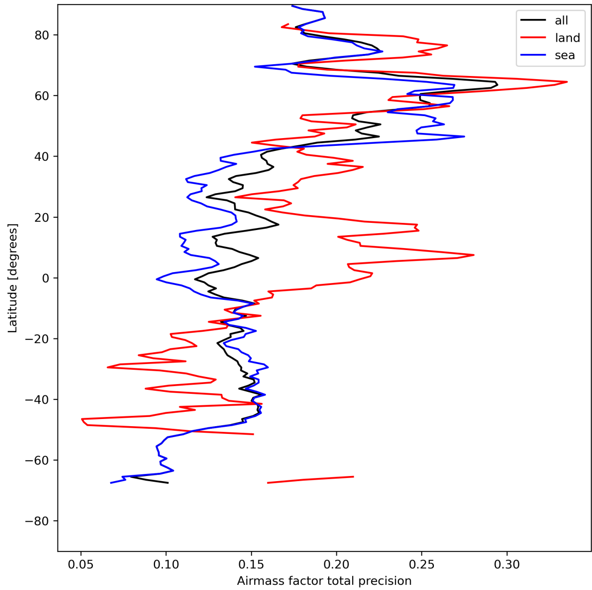
Figure 27: Zonal average of “Airmass factor total precision” for 2024-08-01 to 2024-08-03.
