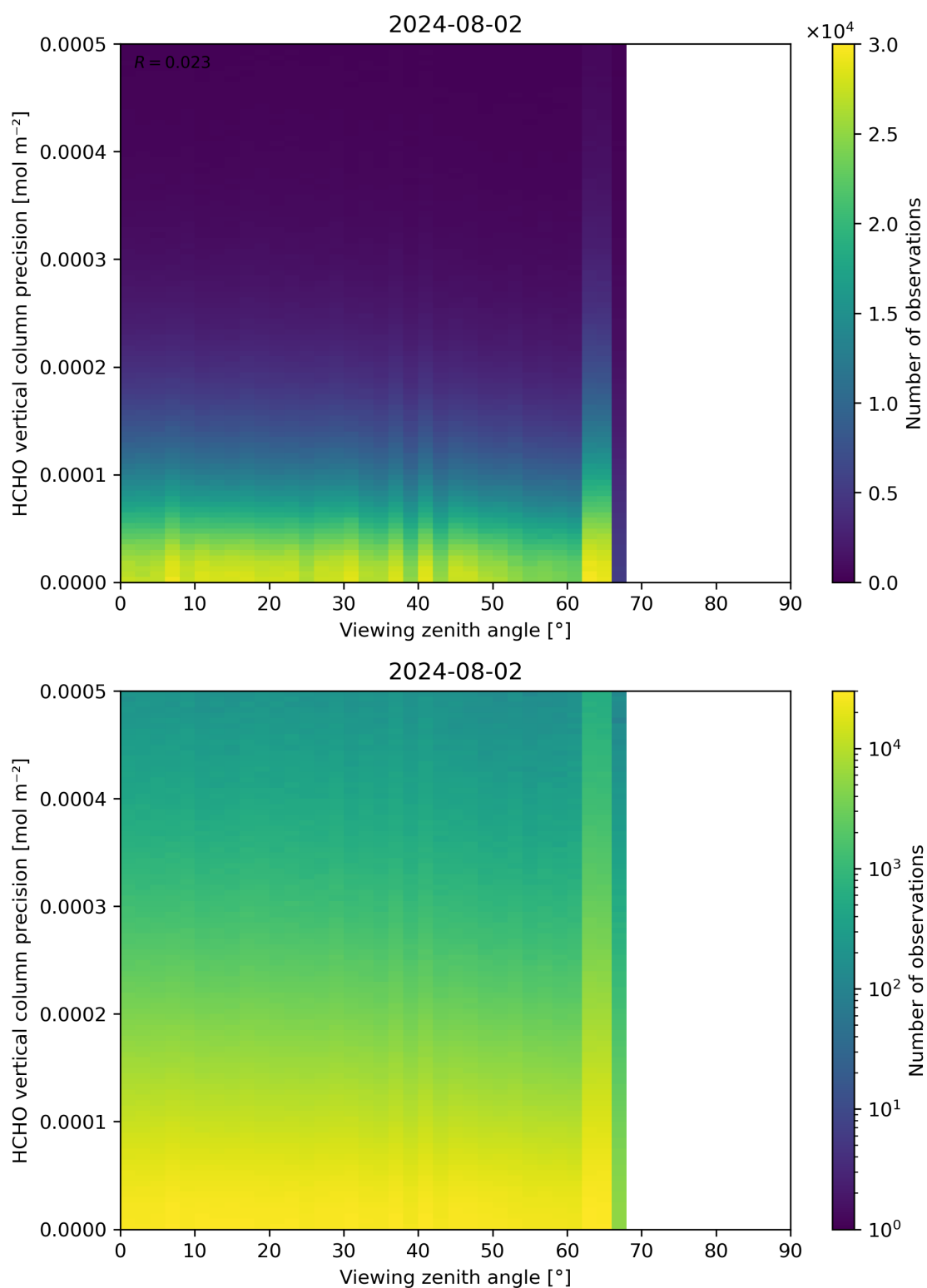
Figure 194: Scatter density plot of “Viewing zenith angle” against “HCHO vertical column precision” for 2024-08-01 to 2024-08-03.
