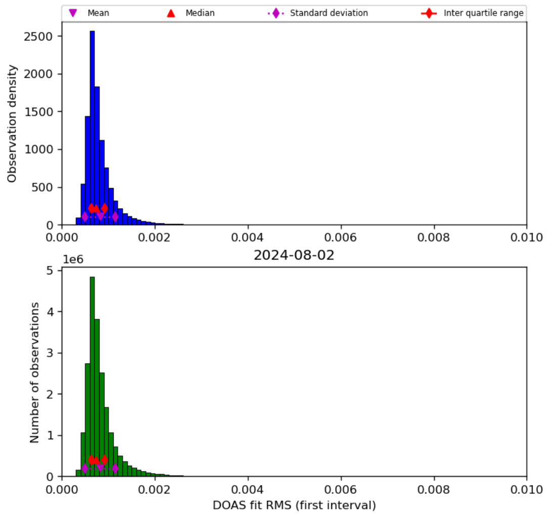
Figure 46: Histogram of “DOAS fit RMS (first interval)” for 2024-08-01 to 2024-08-03
