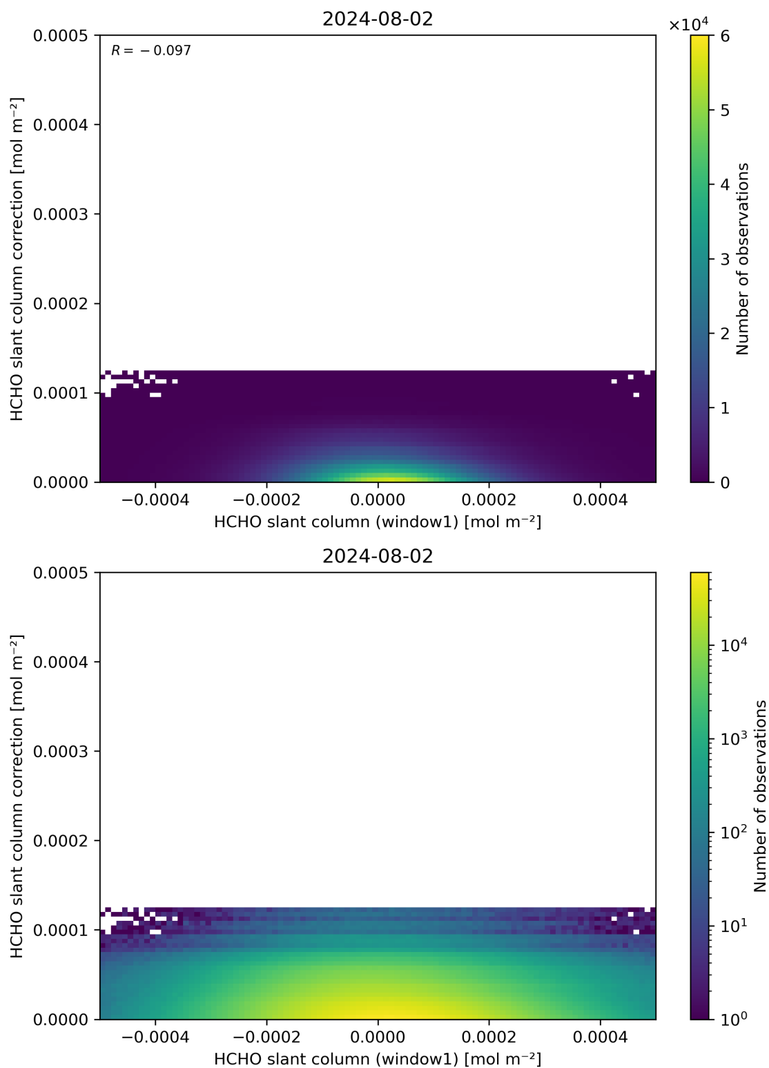
Figure 83: Scatter density plot of “HCHO slant column (window1)” against “HCHO slant column correction” for 2024-08-01 to 2024-08-03.
