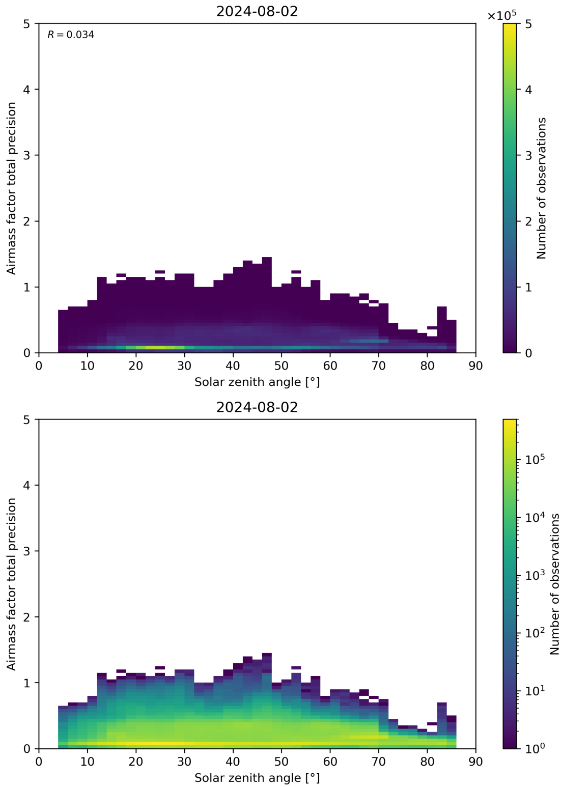
Figure 176: Scatter density plot of “Solar zenith angle” against “Airmass factor total precision” for 2024-08-01 to 2024-08-03.
