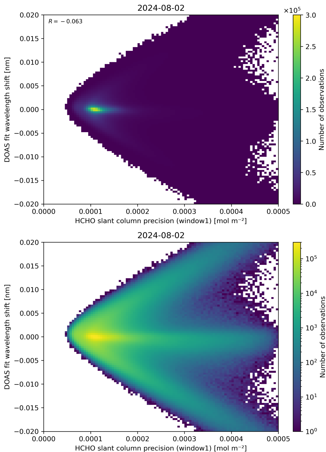
Figure 89: Scatter density plot of “HCHO slant column precision (window1)” against “DOAS fit wavelength shift” for 2024-08-01 to 2024-08-03.
