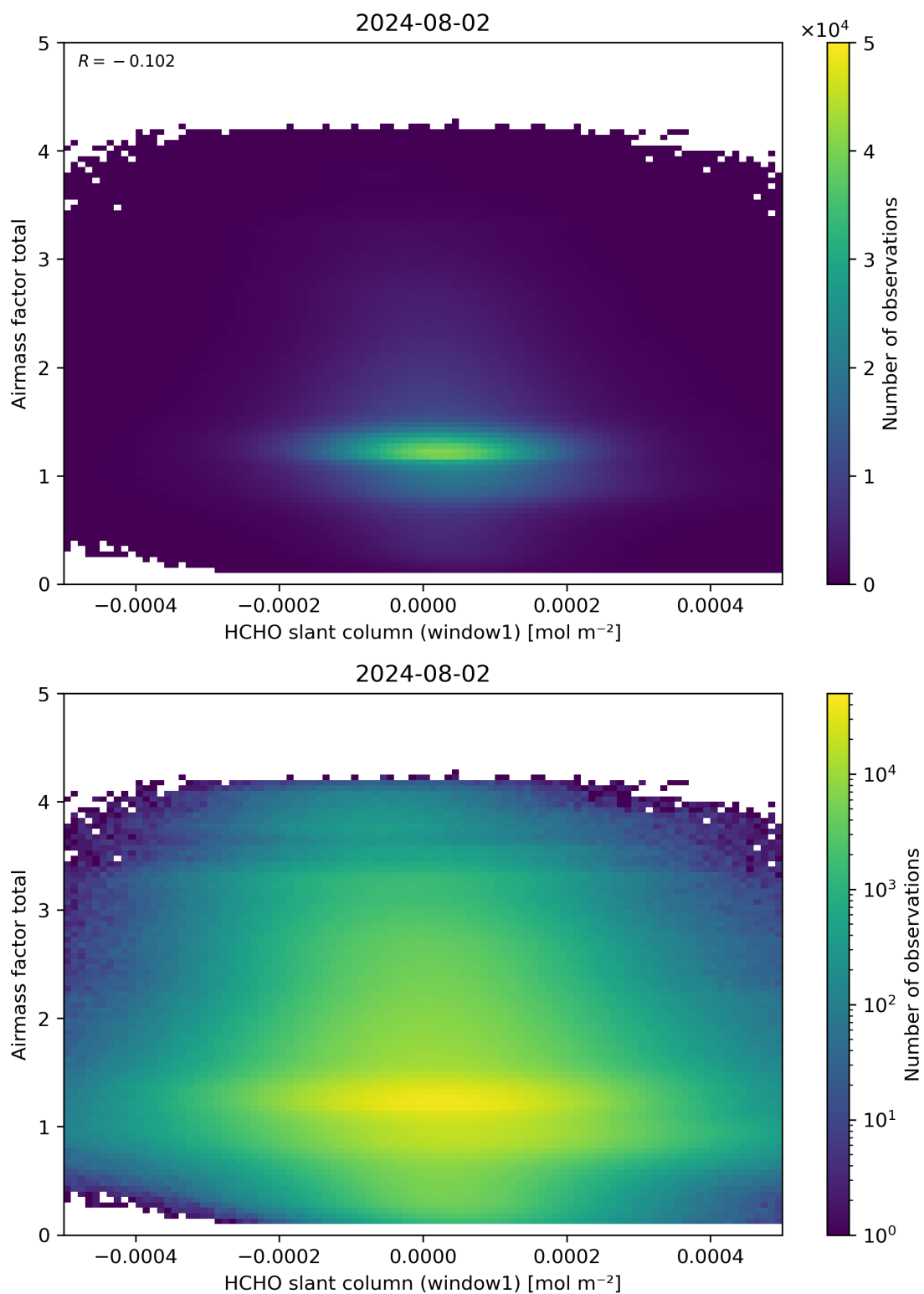
Figure 85: Scatter density plot of “HCHO slant column (window1)” against “Airmass factor total” for 2024-08-01 to 2024-08-03.
