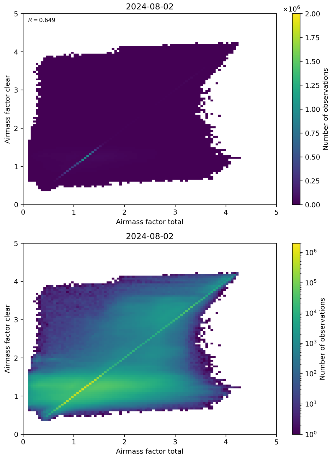
Figure 100: Scatter density plot of “Airmass factor total” against “Airmass factor clear” for 2024-08-01 to 2024-08-03.
