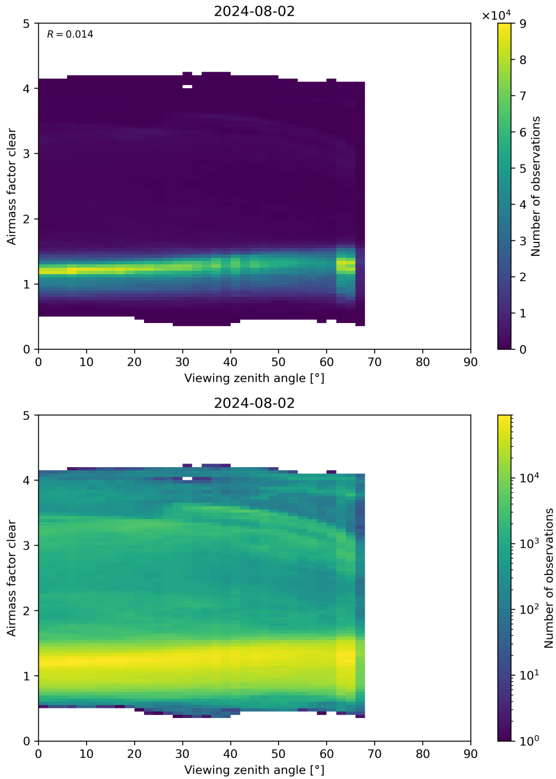
Figure 185: Scatter density plot of “Viewing zenith angle” against “Airmass factor clear” for 2024-08-01 to 2024-08-03.
