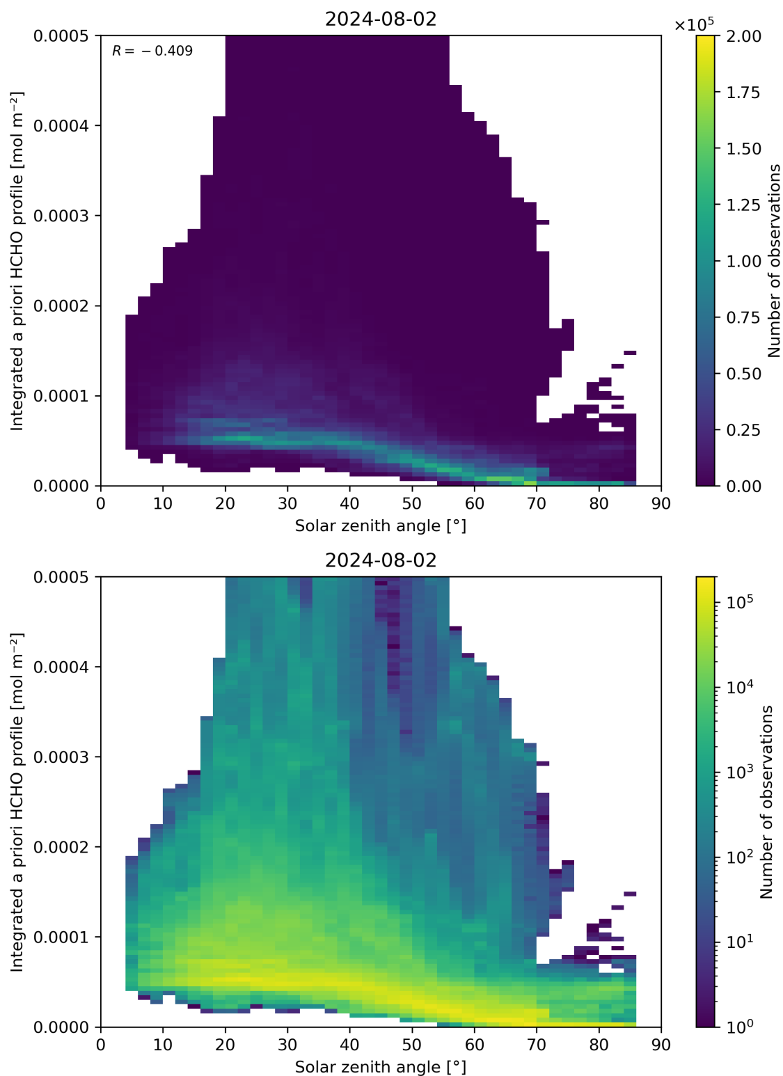
Figure 180: Scatter density plot of “Solar zenith angle” against “Integrated a priori HCHO profile” for 2024-08-01 to 2024-08-03.
