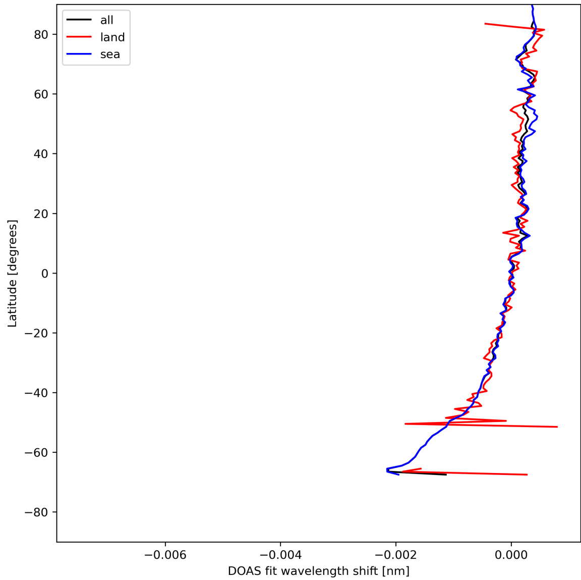
Figure 30: Zonal average of “DOAS fit wavelength shift” for 2024-08-01 to 2024-08-03.
