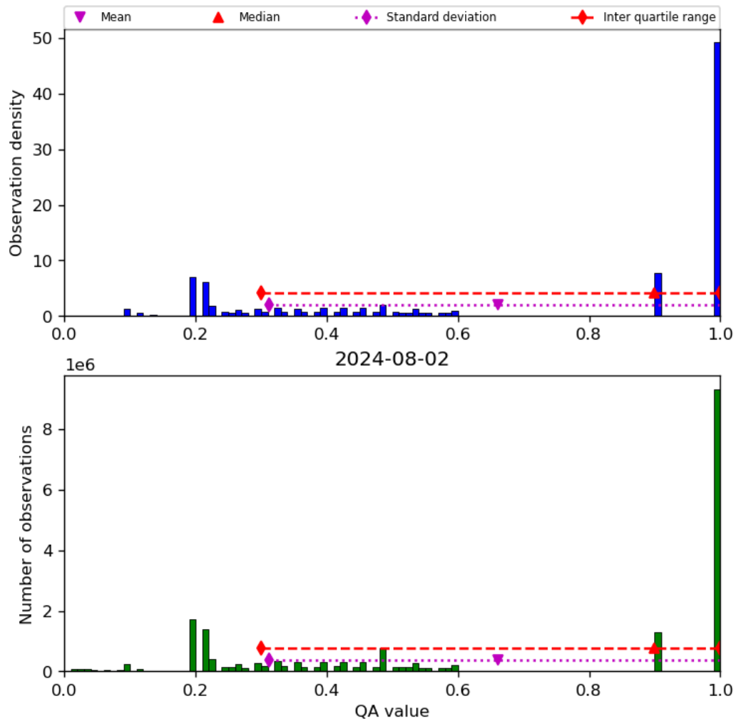
Figure 34: Histogram of “QA value” for 2024-08-01 to 2024-08-03
