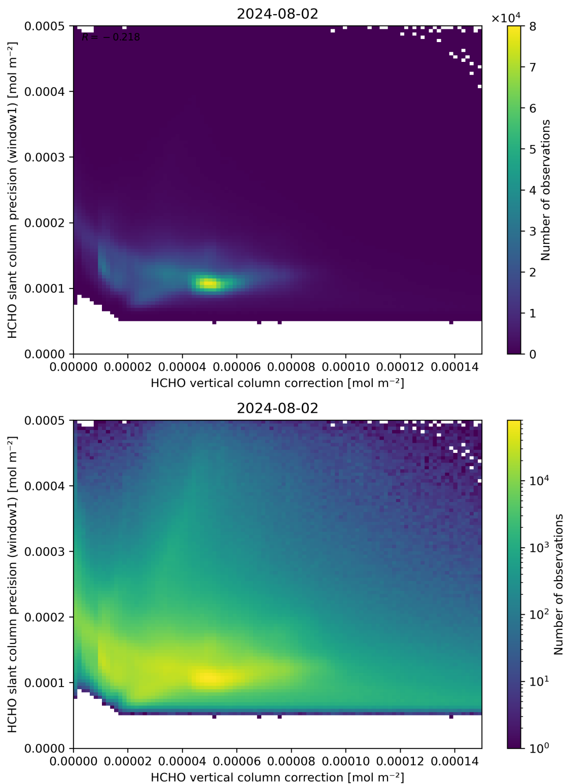
Figure 119: Scatter density plot of “HCHO vertical column correction” against “HCHO slant column precision (window1)” for 2024-08-01 to 2024-08-03.
