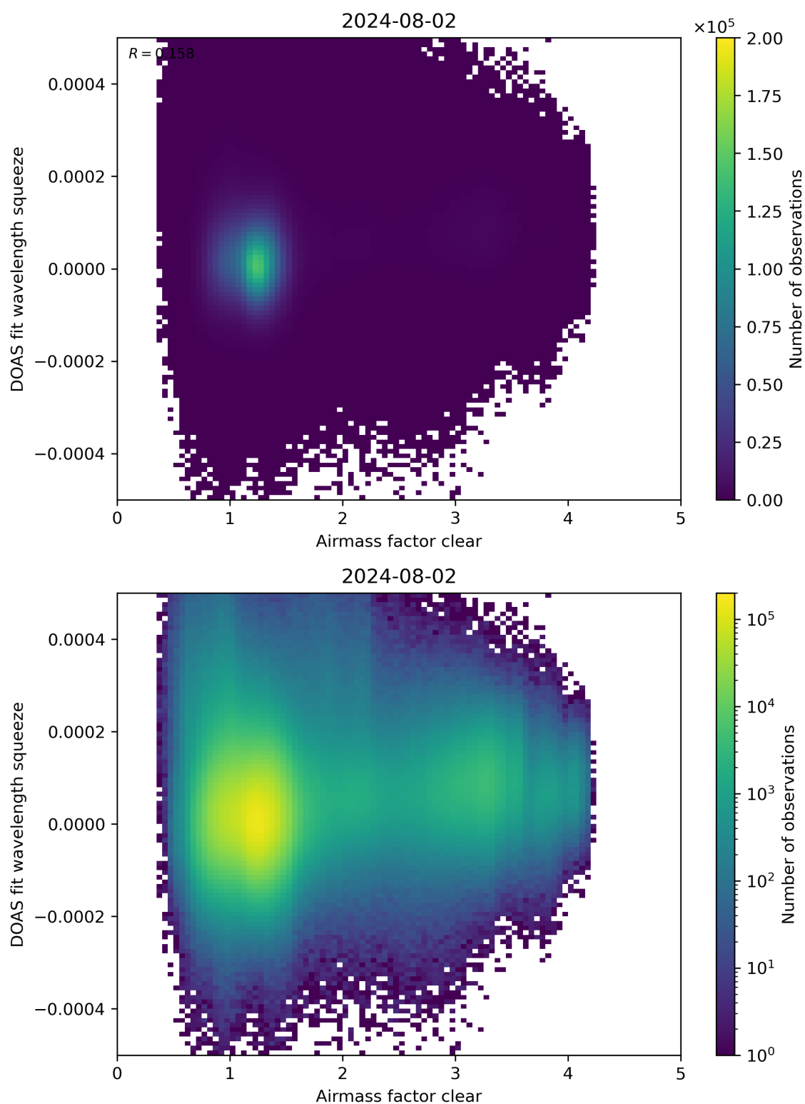
Figure 73: Scatter density plot of “Airmass factor clear” against “DOAS fit wavelength squeeze” for 2024-08-01 to 2024-08-03.
