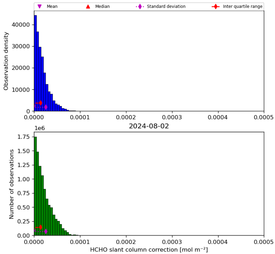
Figure 47: Histogram of “HCHO slant column correction” for 2024-08-01 to 2024-08-03
