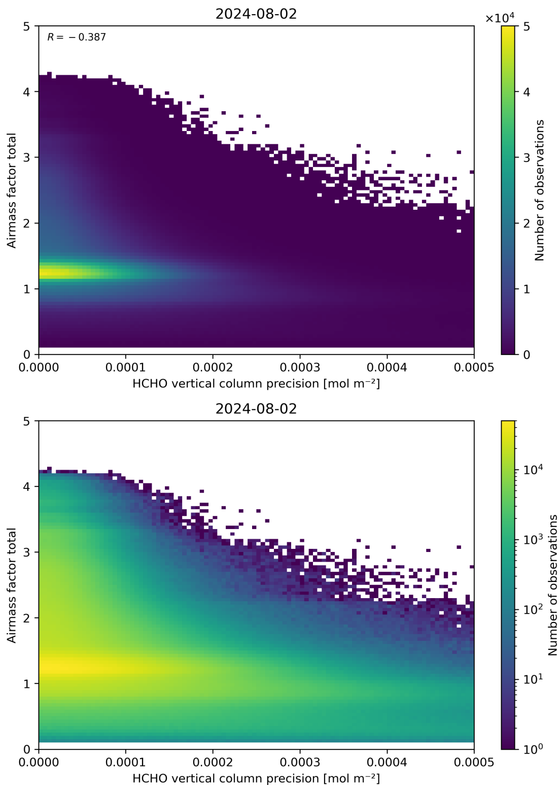
Figure 144: Scatter density plot of “HCHO vertical column precision” against “Airmass factor total” for 2024-08-01 to 2024-08-03.
