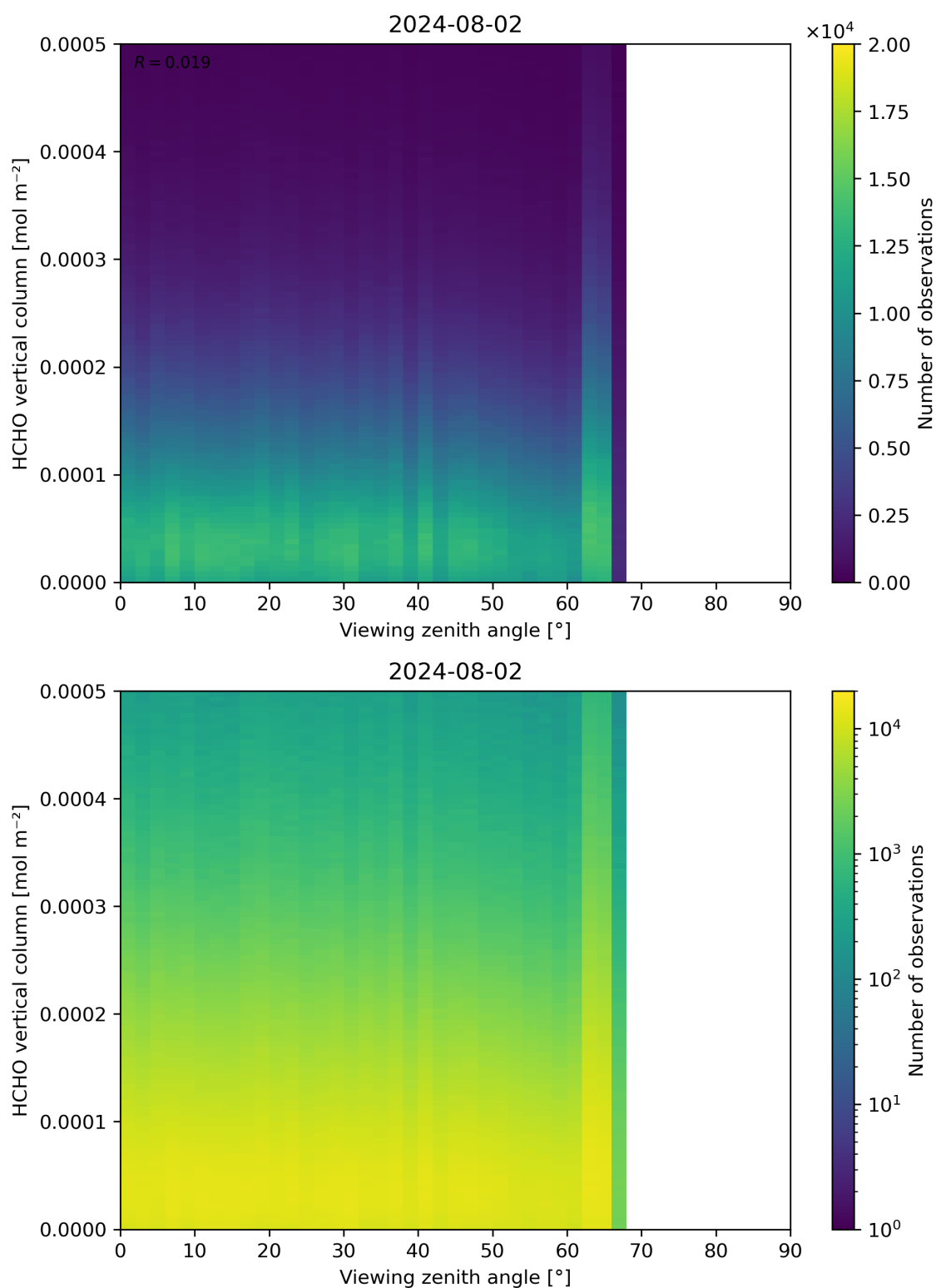
Figure 192: Scatter density plot of “Viewing zenith angle” against “HCHO vertical column” for 2024-08-01 to 2024-08-03.
