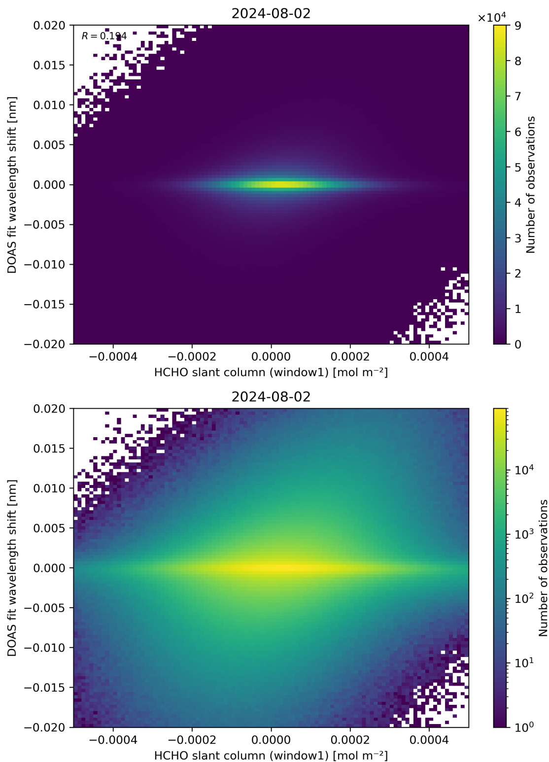
Figure 79: Scatter density plot of “HCHO slant column (window1)” against “DOAS fit wavelength shift” for 2024-08-01 to 2024-08-03.
