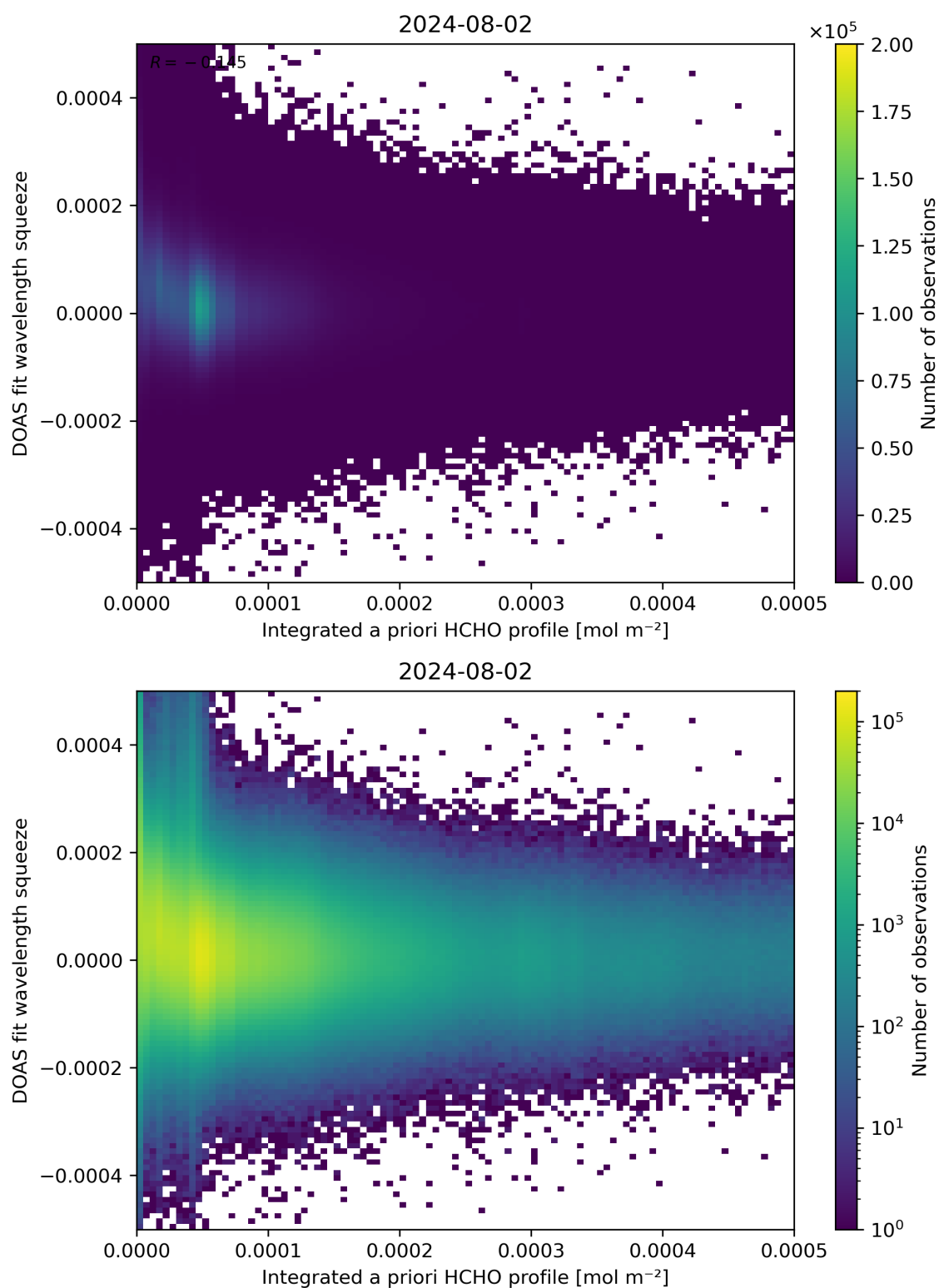
Figure 150: Scatter density plot of “Integrated a priori HCHO profile” against “DOAS fit wavelength squeeze” for 2024-08-01 to 2024-08-03.
