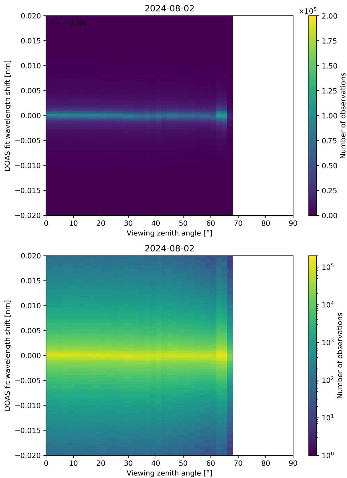
Figure 183: Scatter density plot of “Viewing zenith angle” against “DOAS fit wavelength shift” for 2024-08-01 to 2024-08-03.
