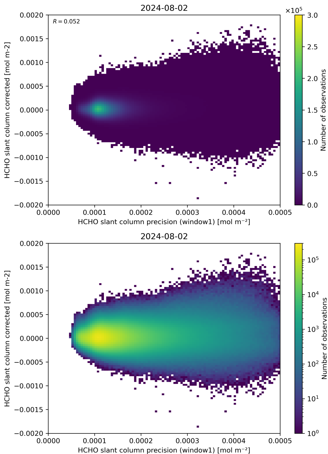
Figure 92: Scatter density plot of “HCHO slant column precision (window1)” against “HCHO slant column corrected” for 2024-08-01 to 2024-08-03.
