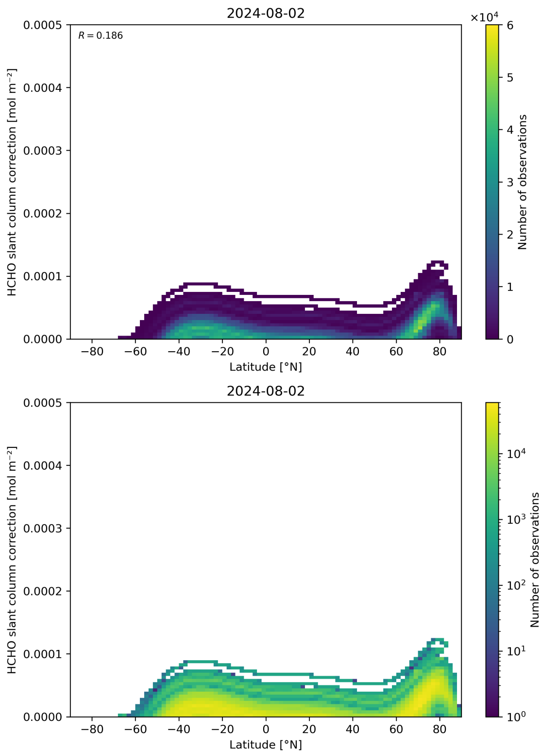
Figure 158: Scatter density plot of “Latitude” against “HCHO slant column correction” for 2024-08-01 to 2024-08-03.
