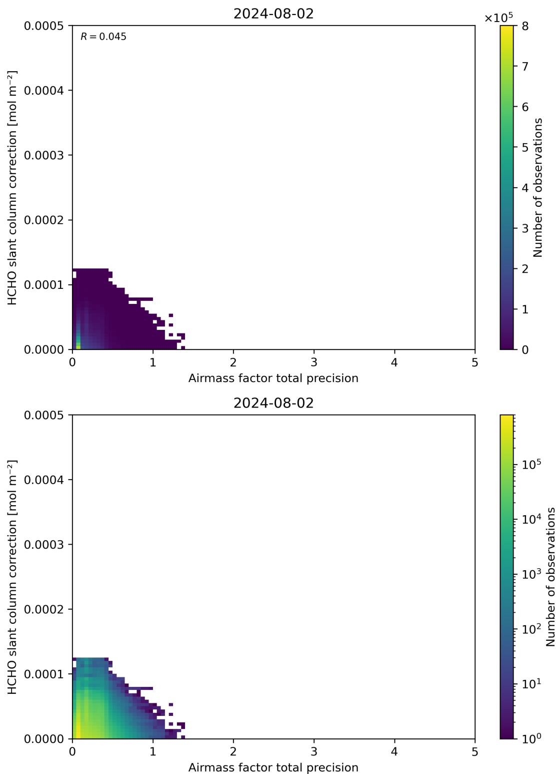
Figure 110: Scatter density plot of “Airmass factor total precision” against “HCHO slant column correction” for 2024-08-01 to 2024-08-03.
