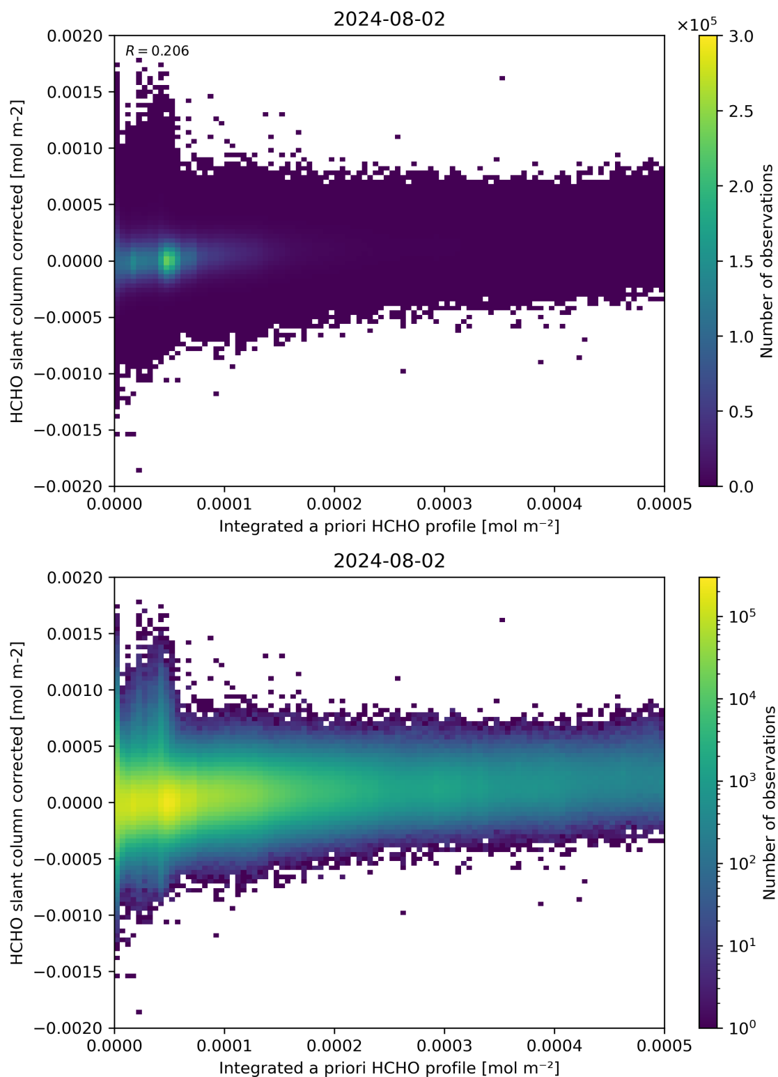
Figure 151: Scatter density plot of “Integrated a priori HCHO profile” against “HCHO slant column corrected” for 2024-08-01 to 2024-08-03.
