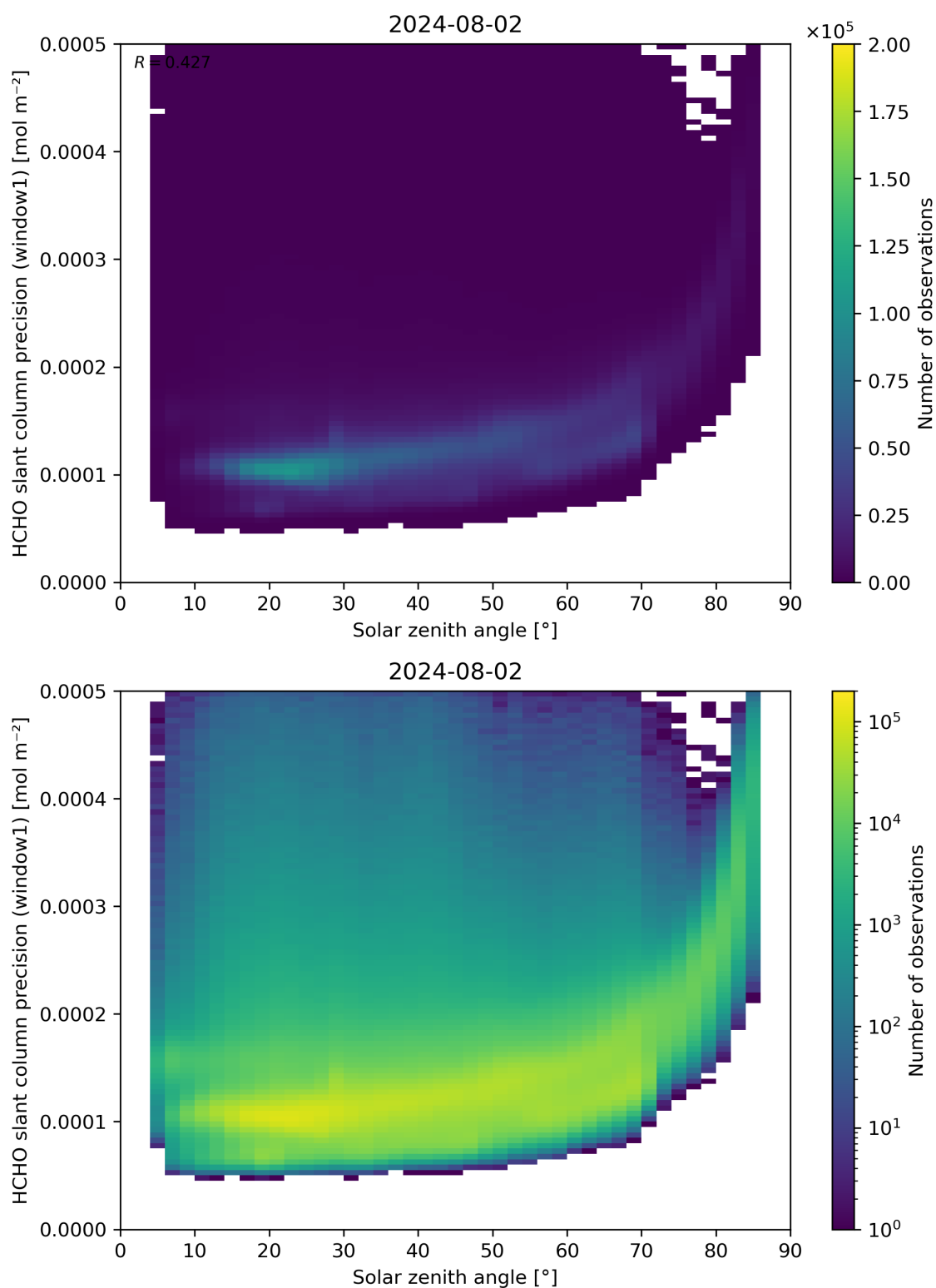
Figure 174: Scatter density plot of “Solar zenith angle” against “HCHO slant column precision (window1)” for 2024-08-01 to 2024-08-03.
