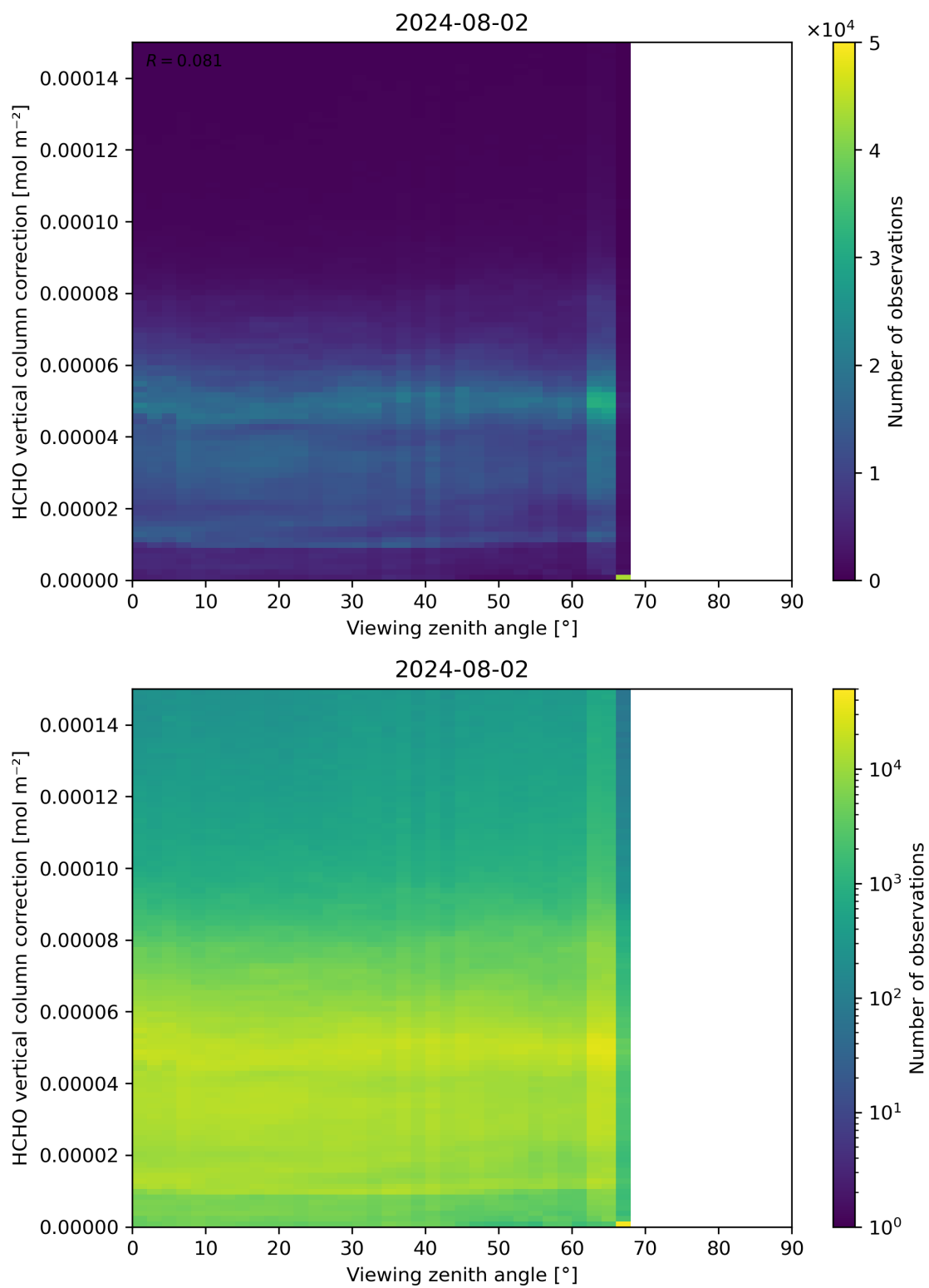
Figure 193: Scatter density plot of “Viewing zenith angle” against “HCHO vertical column correction” for 2024-08-01 to 2024-08-03.
