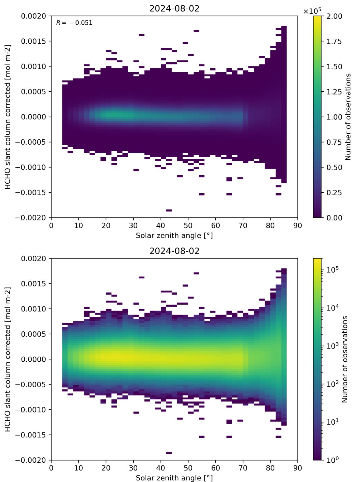
Figure 171: Scatter density plot of “Solar zenith angle” against “HCHO slant column corrected” for 2024-08-01 to 2024-08-03.
