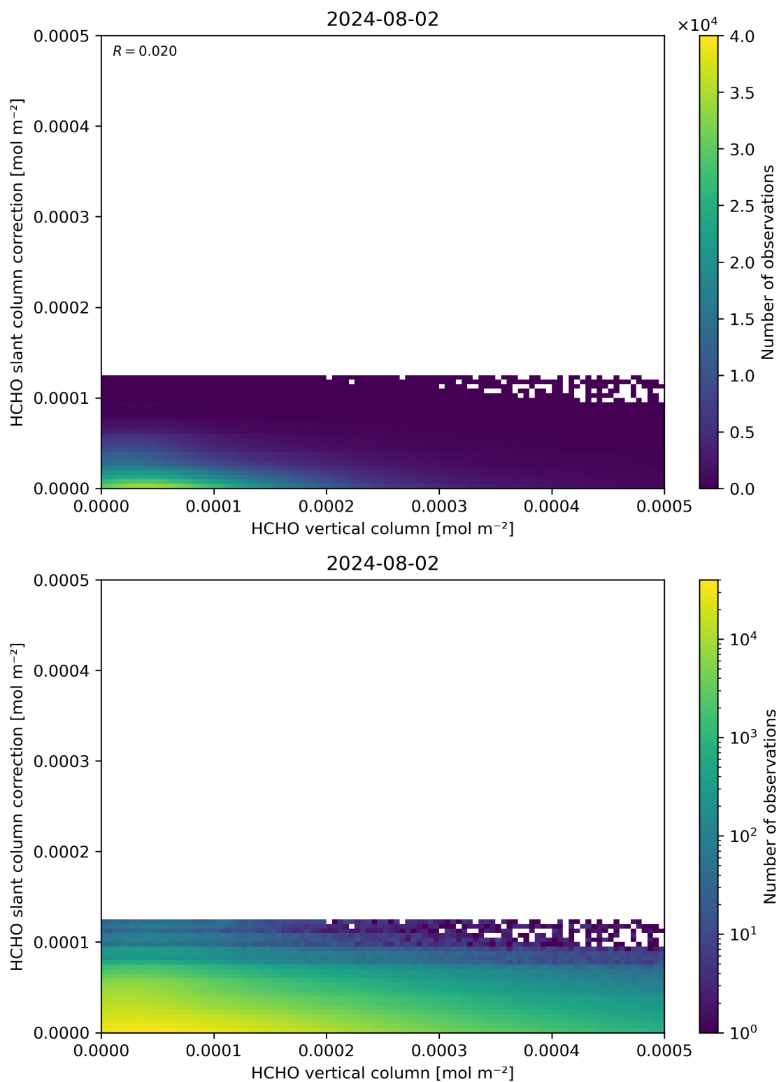
Figure 128: Scatter density plot of “HCHO vertical column” against “HCHO slant column correction” for 2024-08-01 to 2024-08-03.
