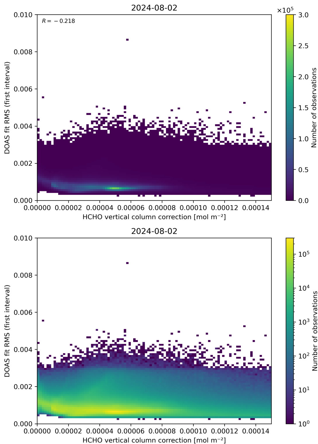
Figure 112: Scatter density plot of “HCHO vertical column correction” against “DOAS fit RMS (first interval)” for 2024-08-01 to 2024-08-03.
