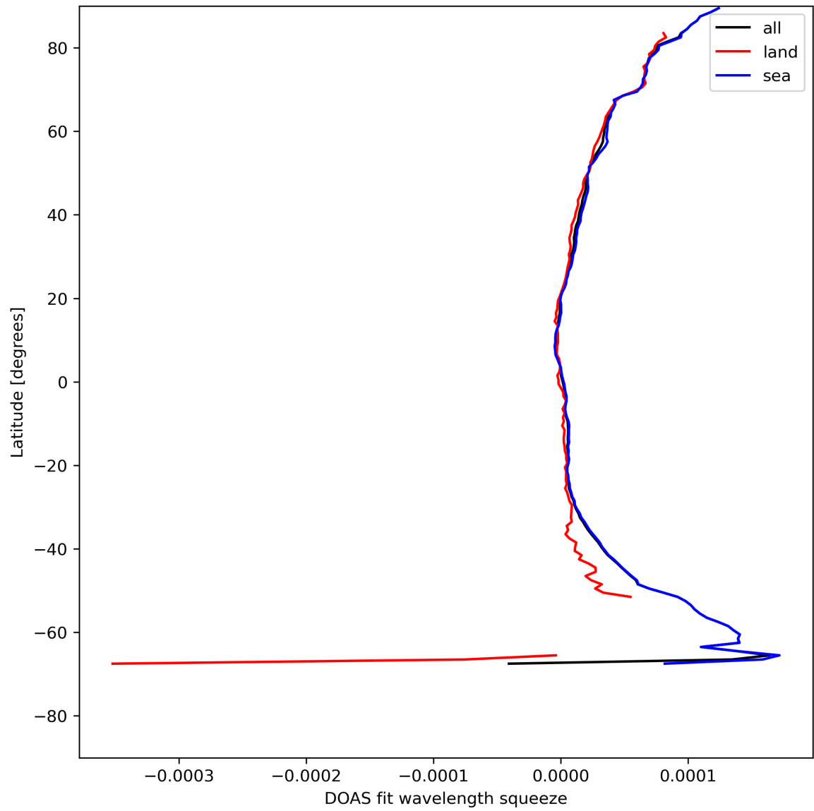
Figure 31: Zonal average of “DOAS fit wavelength squeeze” for 2024-08-01 to 2024-08-03.
