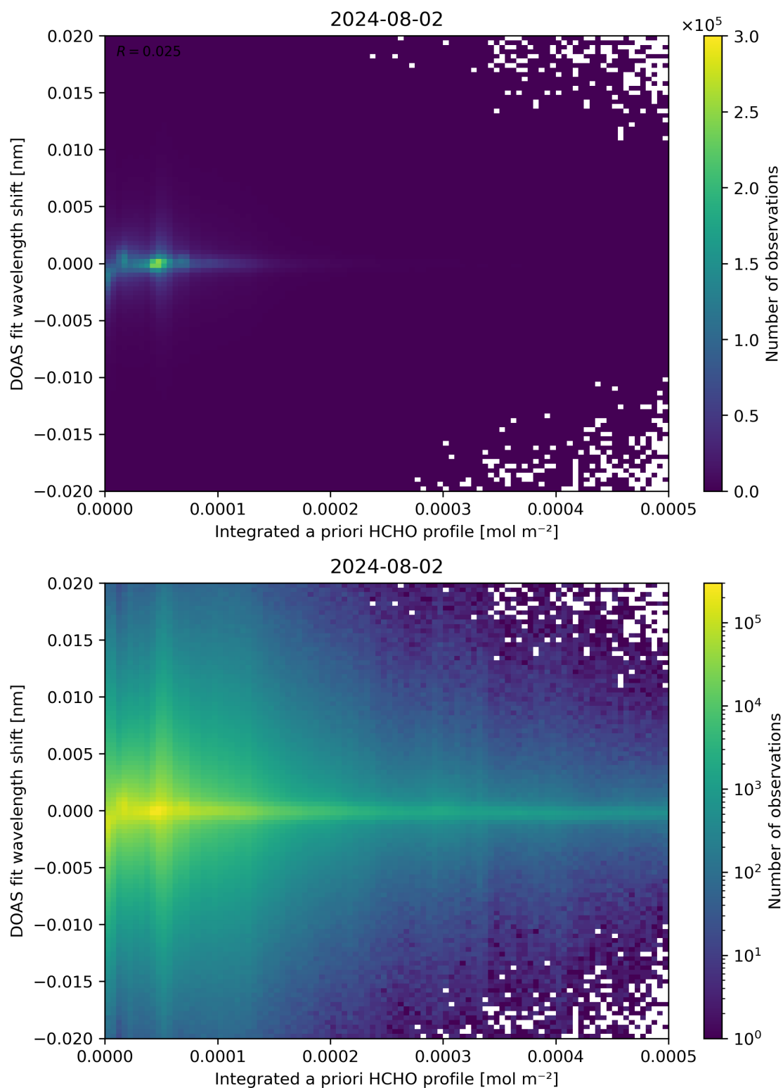
Figure 149: Scatter density plot of “Integrated a priori HCHO profile” against “DOAS fit wavelength shift” for 2024-08-01 to 2024-08-03.
