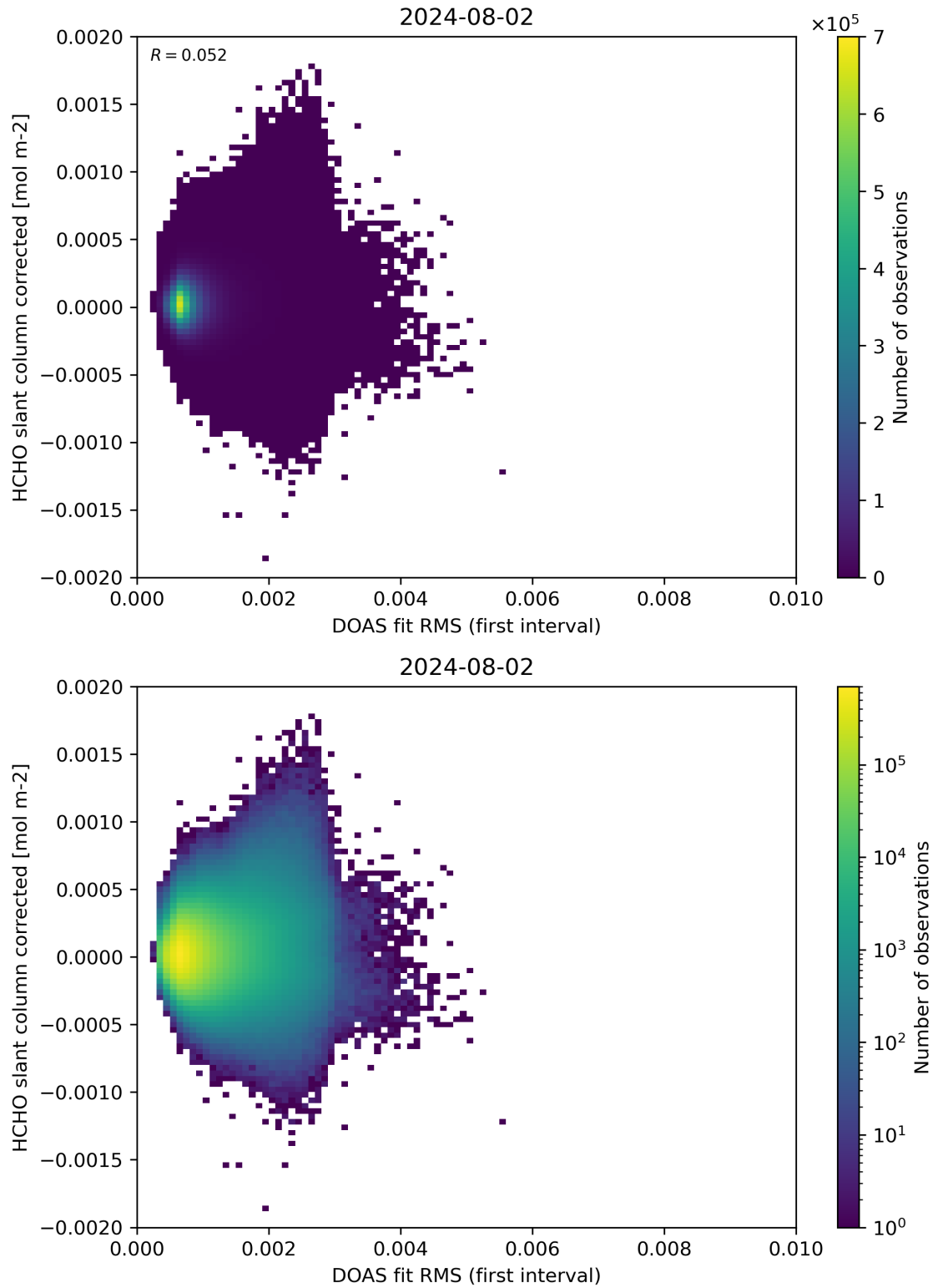
Figure 62: Scatter density plot of “DOAS fit RMS (first interval)” against “HCHO slant column corrected” for 2024-08-01 to 2024-08-03.
