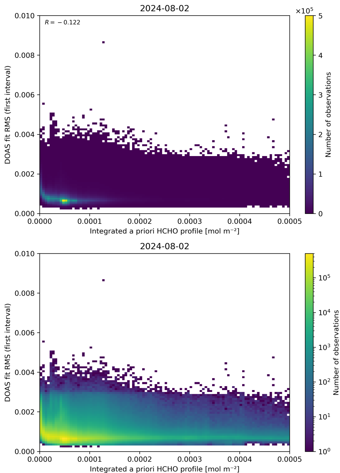
Figure 148: Scatter density plot of “Integrated a priori HCHO profile” against “DOAS fit RMS (first interval)” for 2024-08-01 to 2024-08-03.
