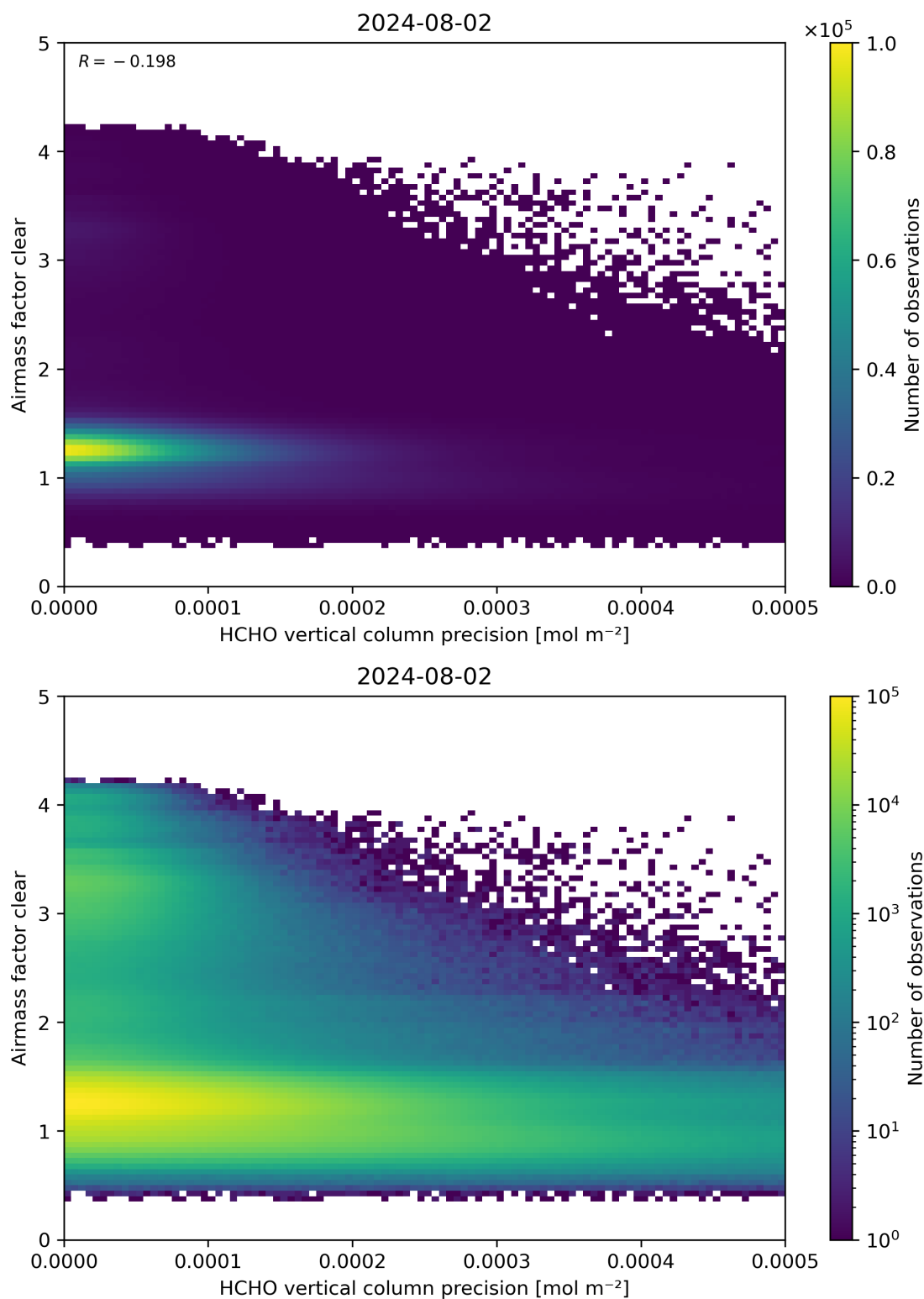
Figure 139: Scatter density plot of “HCHO vertical column precision” against “Airmass factor clear” for 2024-08-01 to 2024-08-03.
