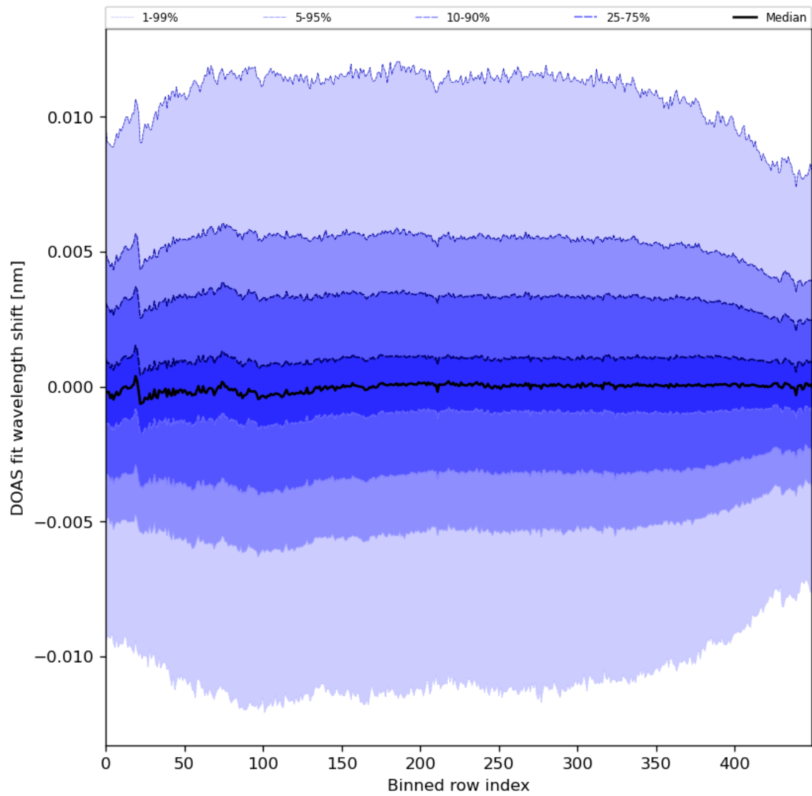
Figure 58: Along track statistics of “DOAS fit wavelength shift” for 2024-08-01 to 2024-08-03
