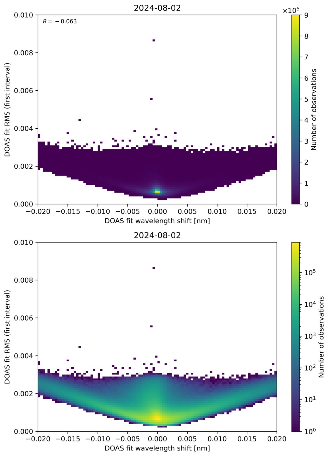
Figure 64: Scatter density plot of “DOAS fit wavelength shift” against “DOAS fit RMS (first interval)” for 2024-08-01 to 2024-08-03.
