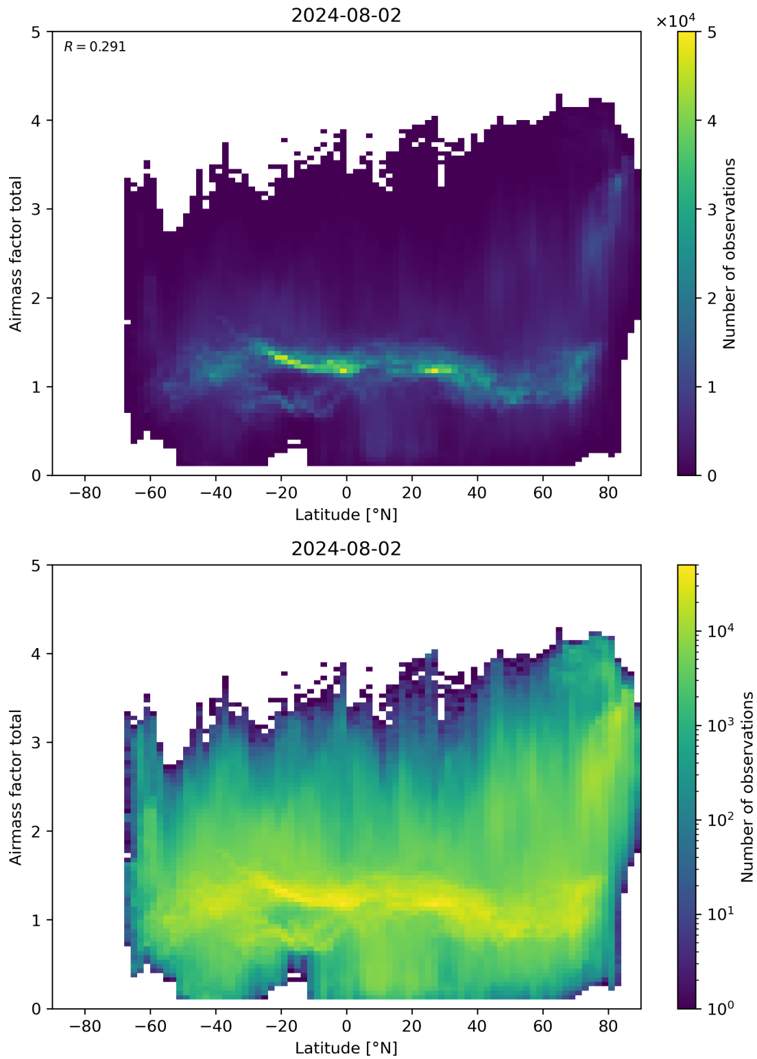
Figure 161: Scatter density plot of “Latitude” against “Airmass factor total” for 2024-08-01 to 2024-08-03.
