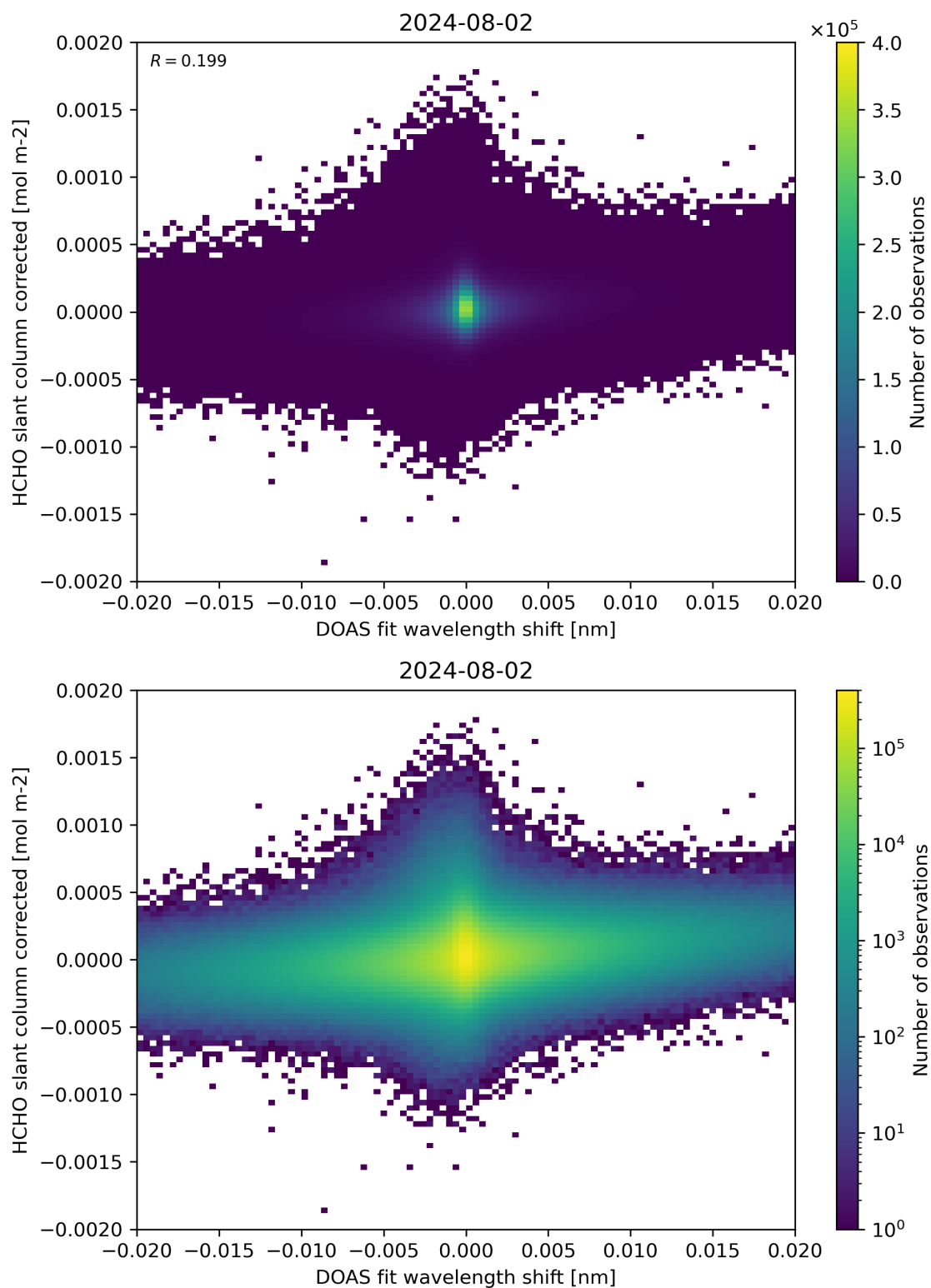
Figure 66: Scatter density plot of “DOAS fit wavelength shift” against “HCHO slant column corrected” for 2024-08-01 to 2024-08-03.
