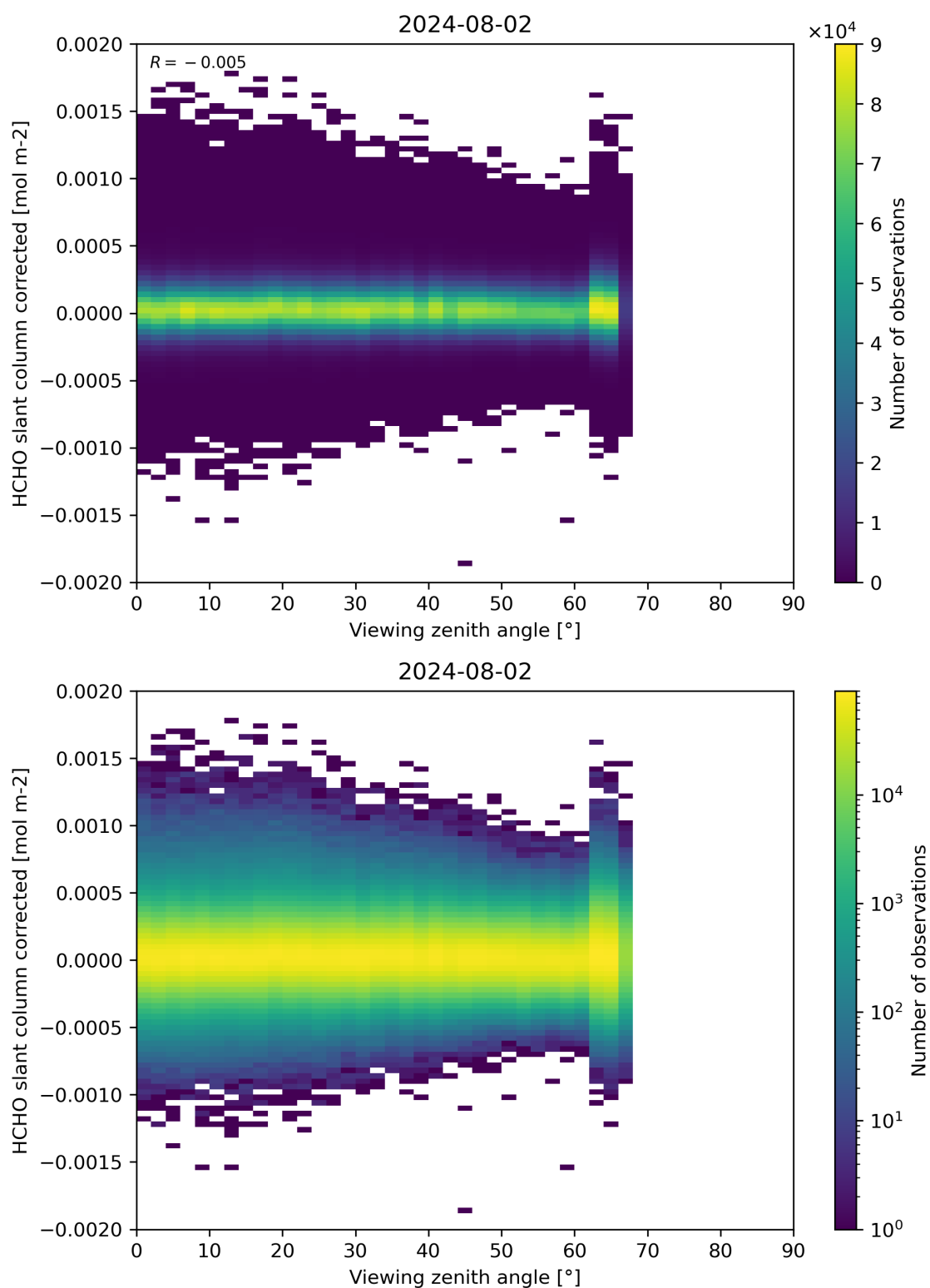
Figure 186: Scatter density plot of “Viewing zenith angle” against “HCHO slant column corrected” for 2024-08-01 to 2024-08-03.
