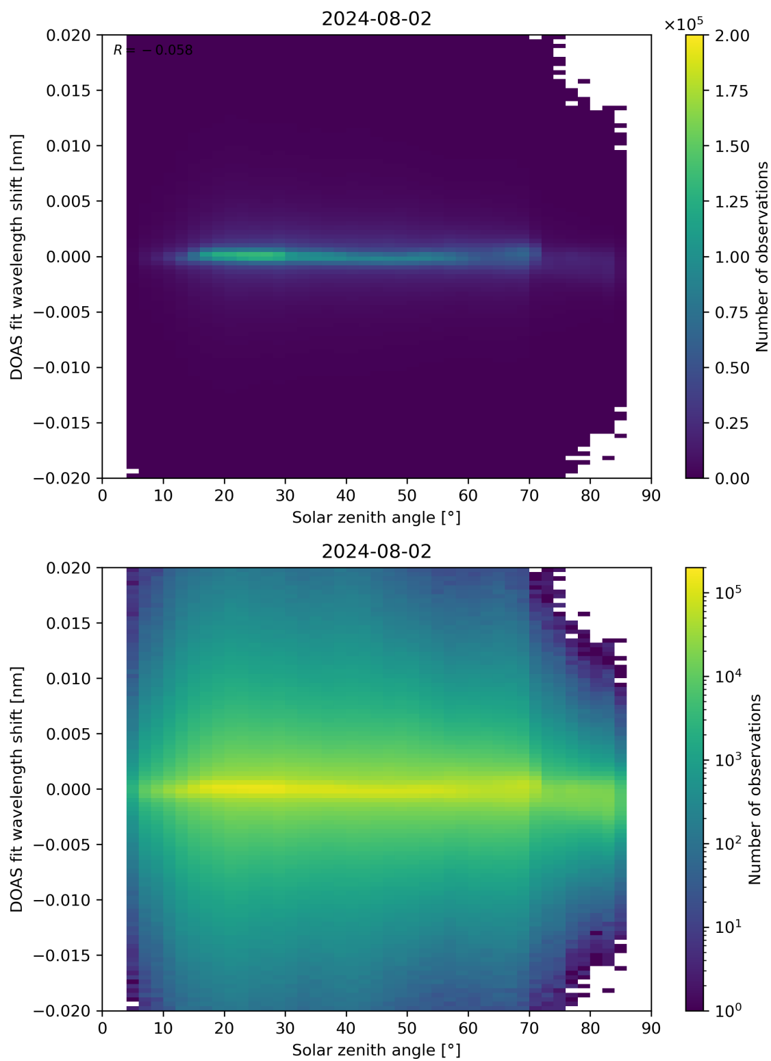
Figure 168: Scatter density plot of “Solar zenith angle” against “DOAS fit wavelength shift” for 2024-08-01 to 2024-08-03.
