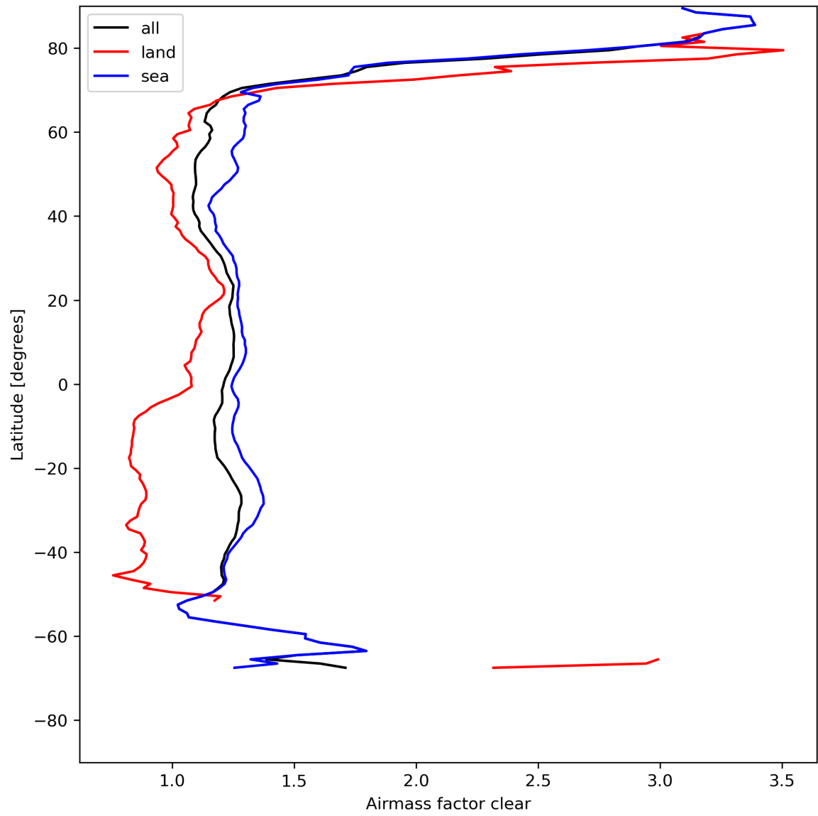
Figure 28: Zonal average of “Airmass factor clear” for 2024-08-01 to 2024-08-03.
