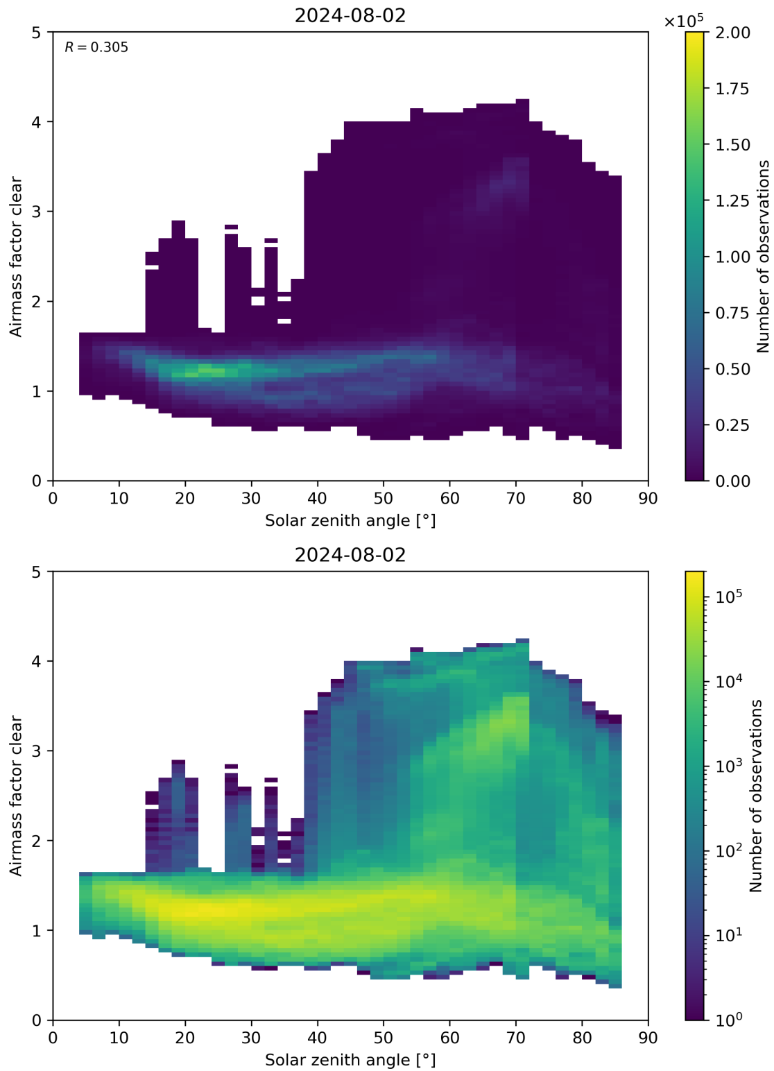
Figure 170: Scatter density plot of “Solar zenith angle” against “Airmass factor clear” for 2024-08-01 to 2024-08-03.
