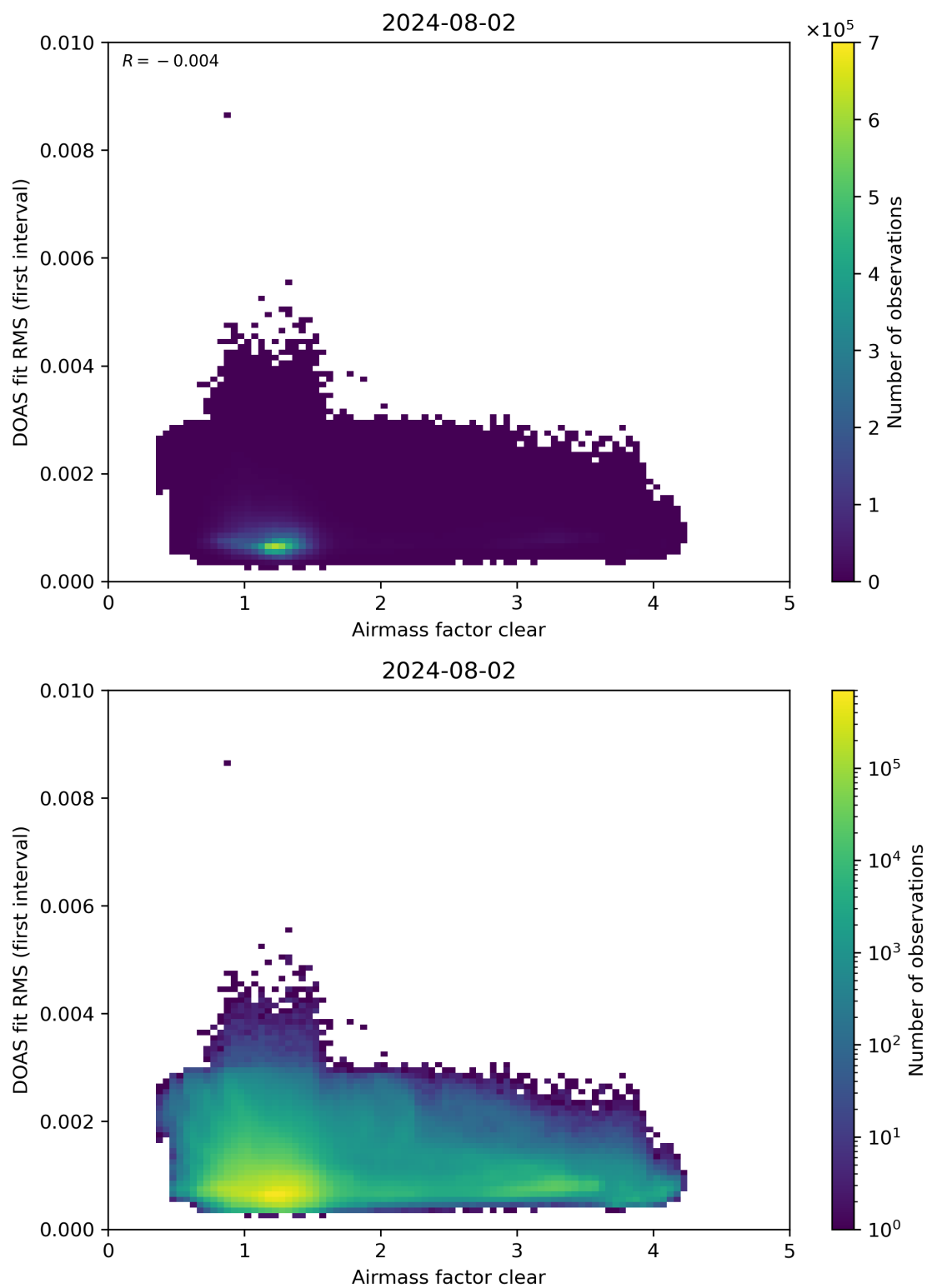
Figure 71: Scatter density plot of “Airmass factor clear” against “DOAS fit RMS (first interval)” for 2024-08-01 to 2024-08-03.
