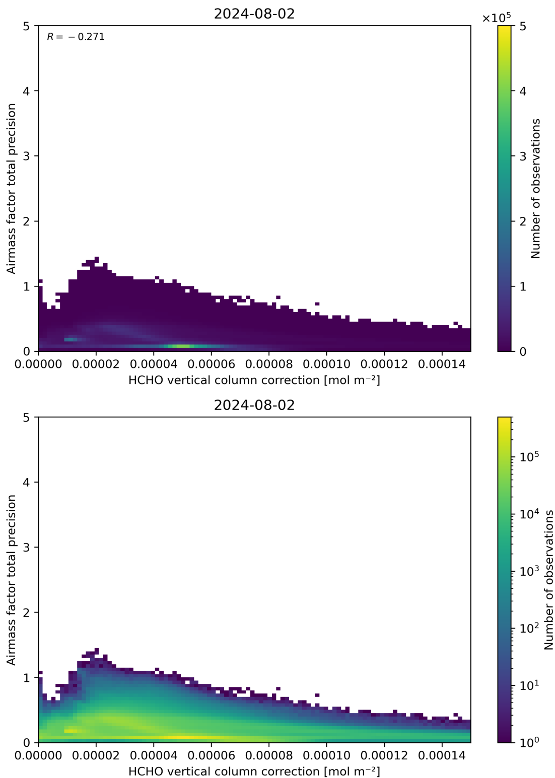
Figure 121: Scatter density plot of “HCHO vertical column correction” against “Airmass factor total precision” for 2024-08-01 to 2024-08-03.
