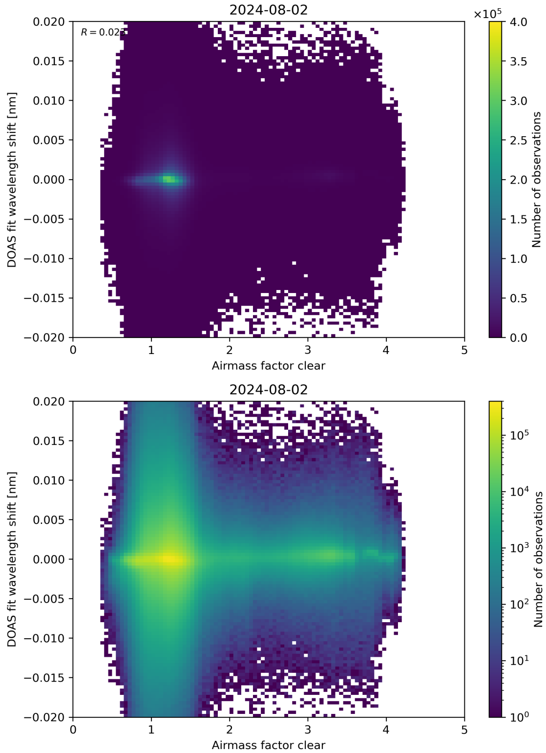
Figure 72: Scatter density plot of “Airmass factor clear” against “DOAS fit wavelength shift” for 2024-08-01 to 2024-08-03.
