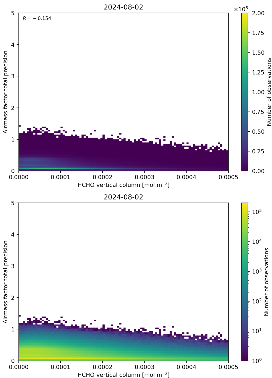
Figure 132: Scatter density plot of “HCHO vertical column” against “Airmass factor total precision” for 2024-08-01 to 2024-08-03.
