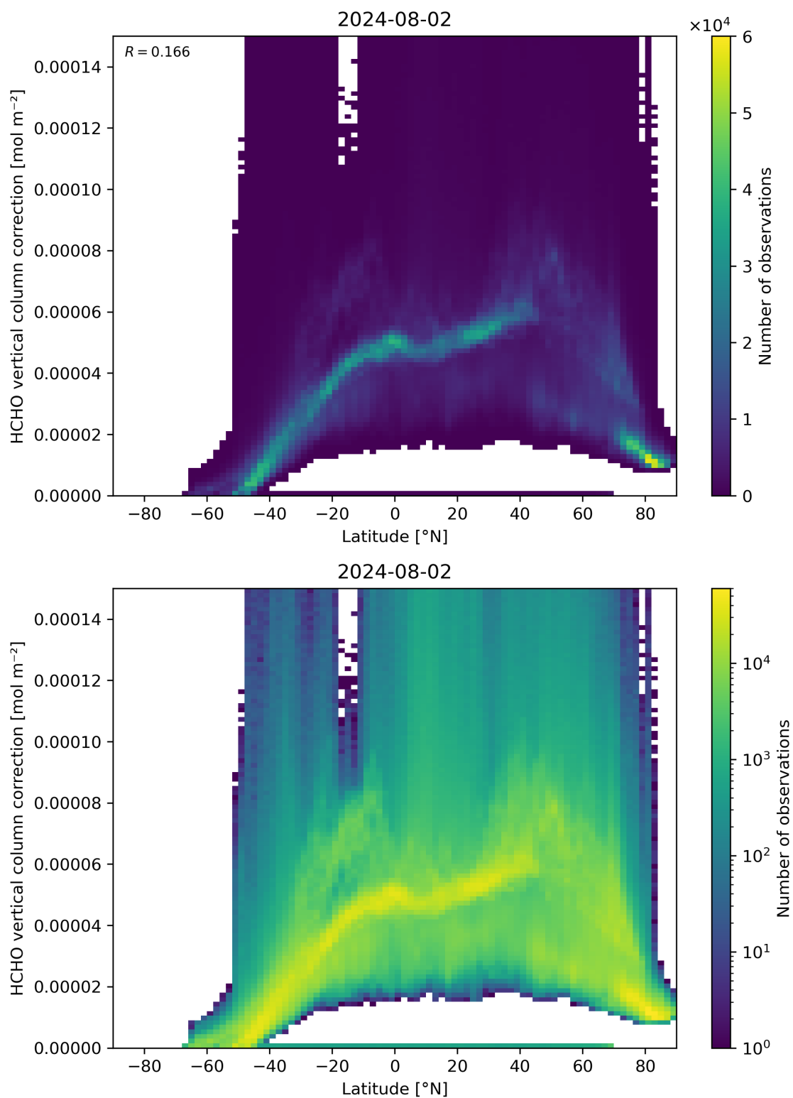
Figure 164: Scatter density plot of “Latitude” against “HCHO vertical column correction” for 2024-08-01 to 2024-08-03.
