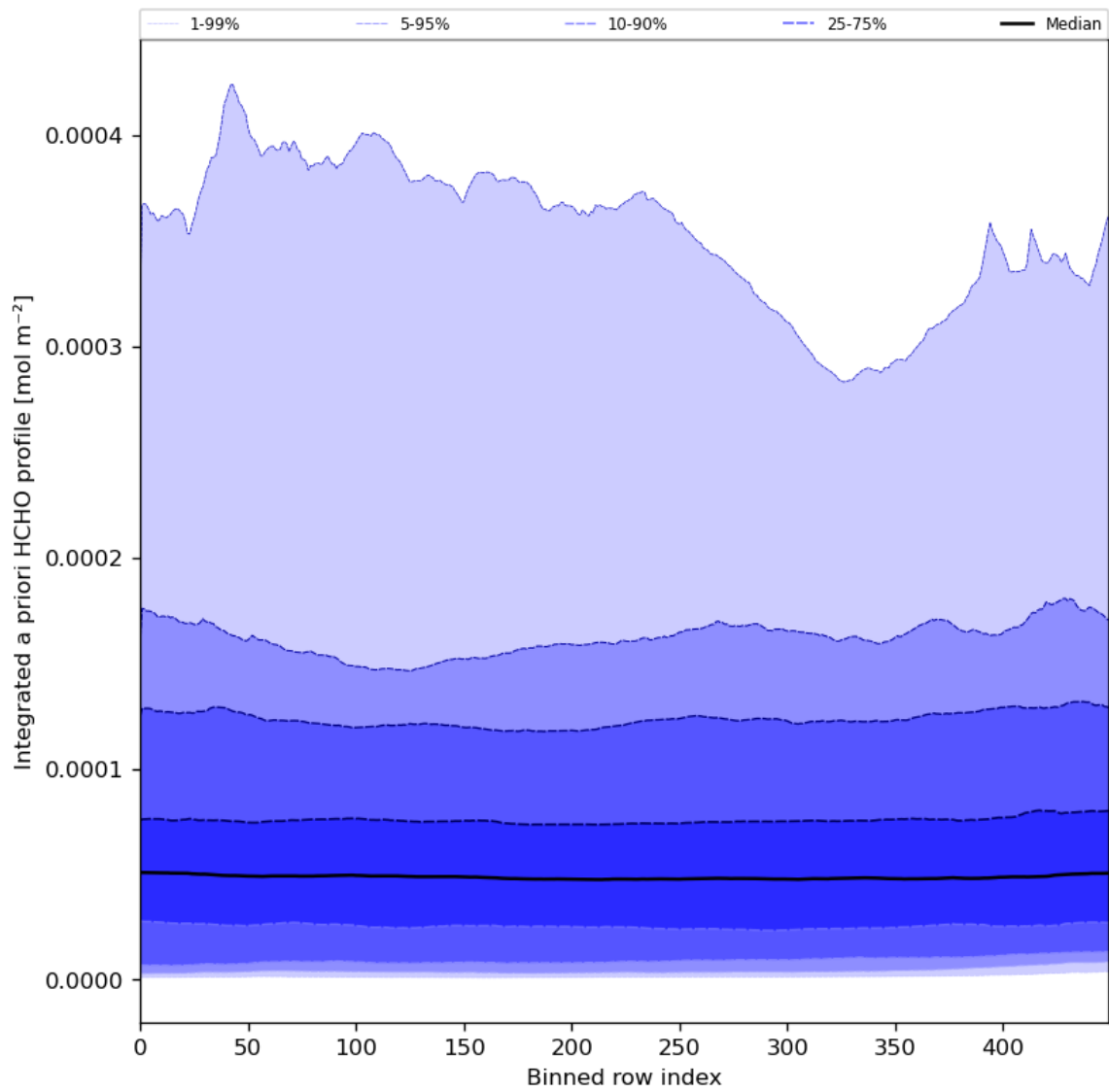
Figure 57: Along track statistics of "Integrated a priori HCHO profile" for 2024-08-01 to 2024-08-03
