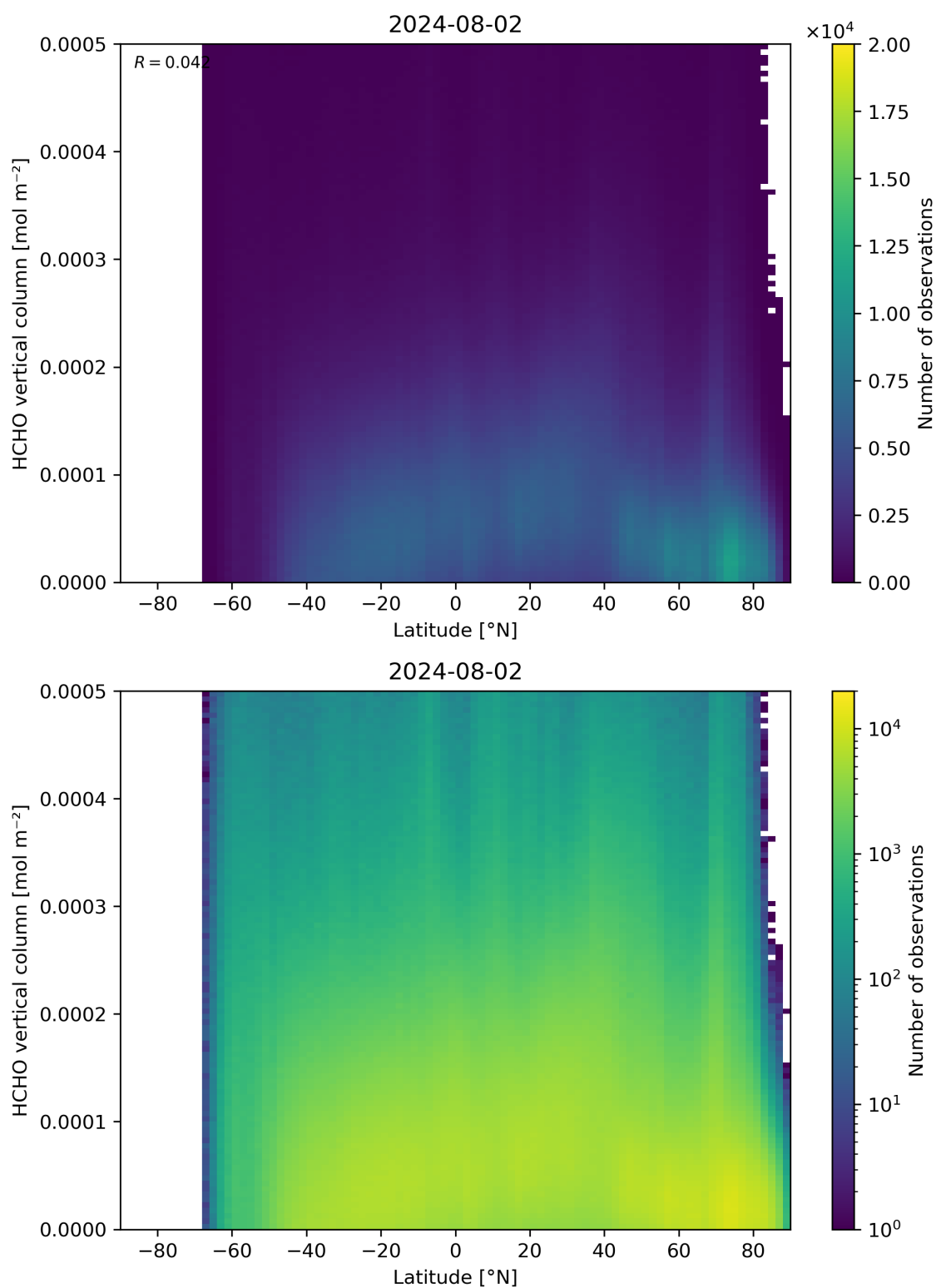
Figure 163: Scatter density plot of “Latitude” against “HCHO vertical column” for 2024-08-01 to 2024-08-03.
