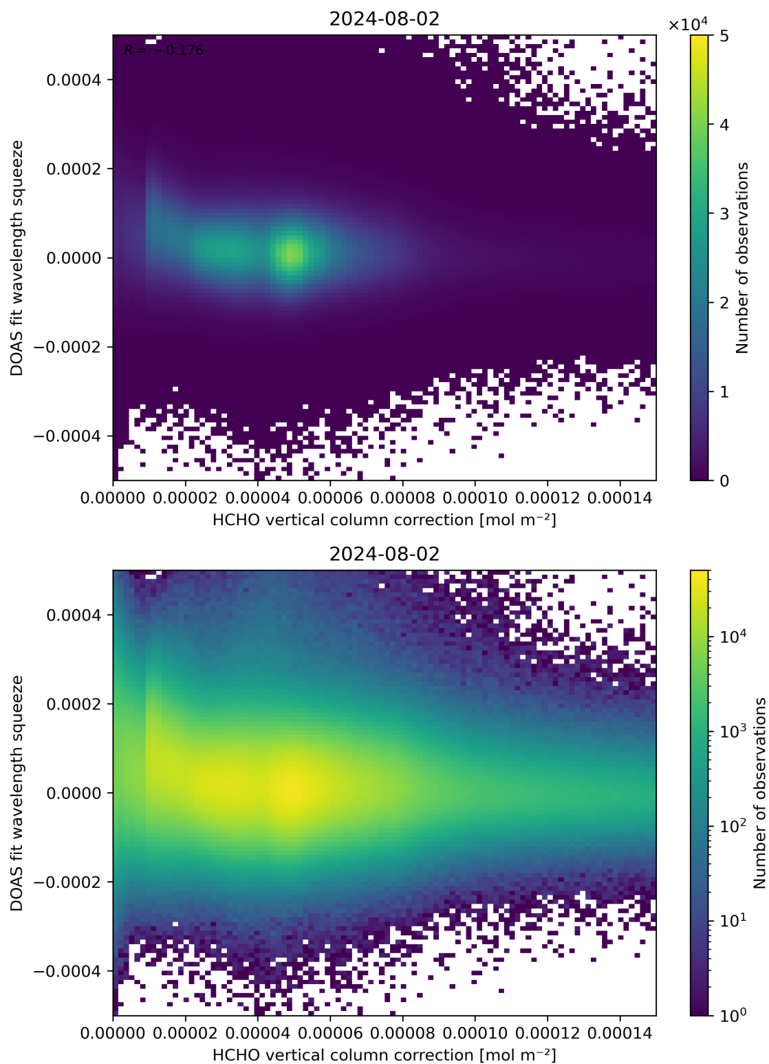
Figure 114: Scatter density plot of “HCHO vertical column correction” against “DOAS fit wavelength squeeze” for 2024-08-01 to 2024-08-03.
