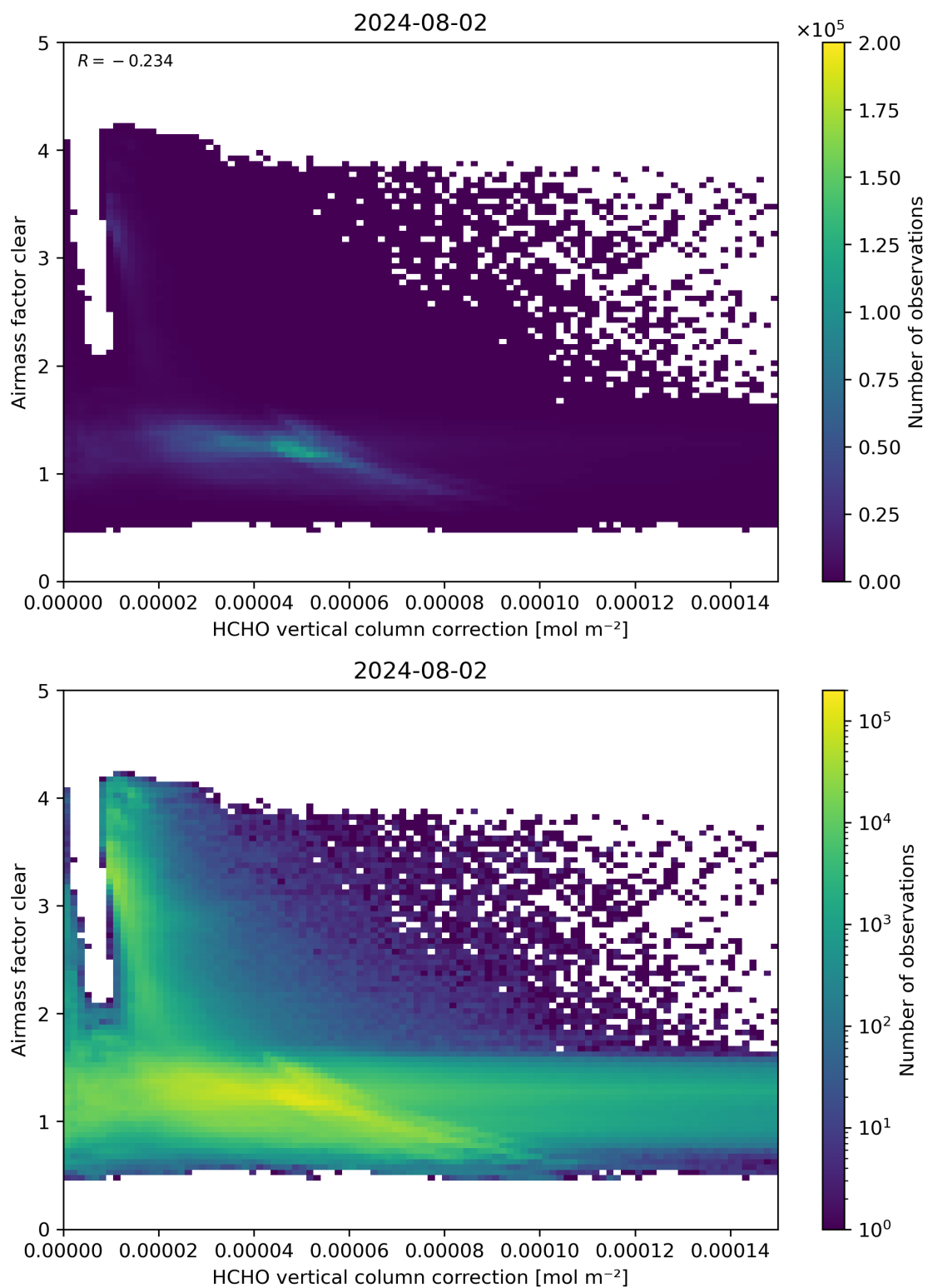
Figure 115: Scatter density plot of “HCHO vertical column correction” against “Airmass factor clear” for 2024-08-01 to 2024-08-03.
