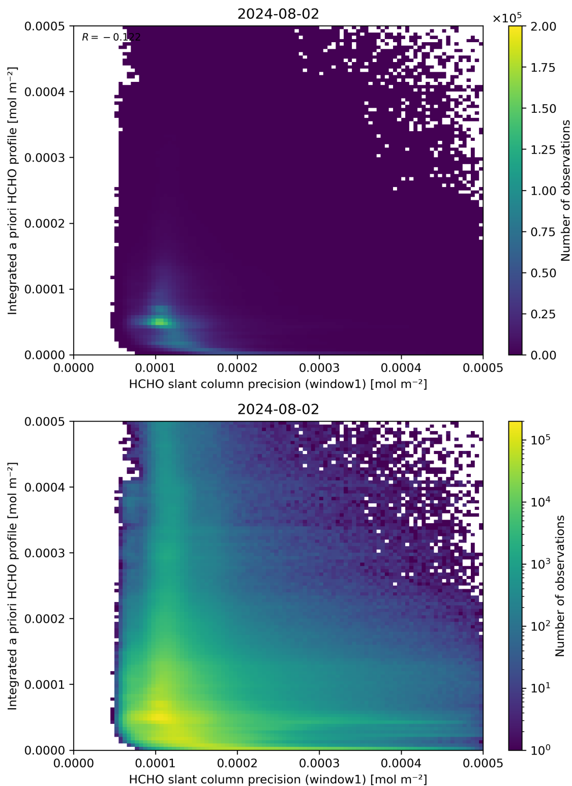
Figure 96: Scatter density plot of “HCHO slant column precision (window1)” against “Integrated a priori HCHO profile” for 2024-08-01 to 2024-08-03.
