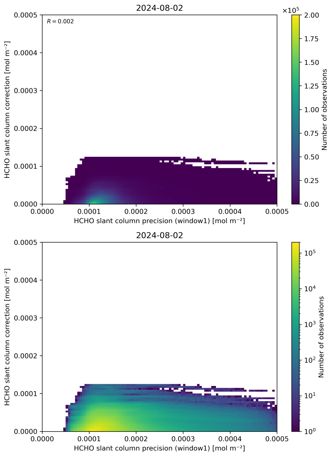
Figure 93: Scatter density plot of “HCHO slant column precision (window1)” against “HCHO slant column correction” for 2024-08-01 to 2024-08-03.
