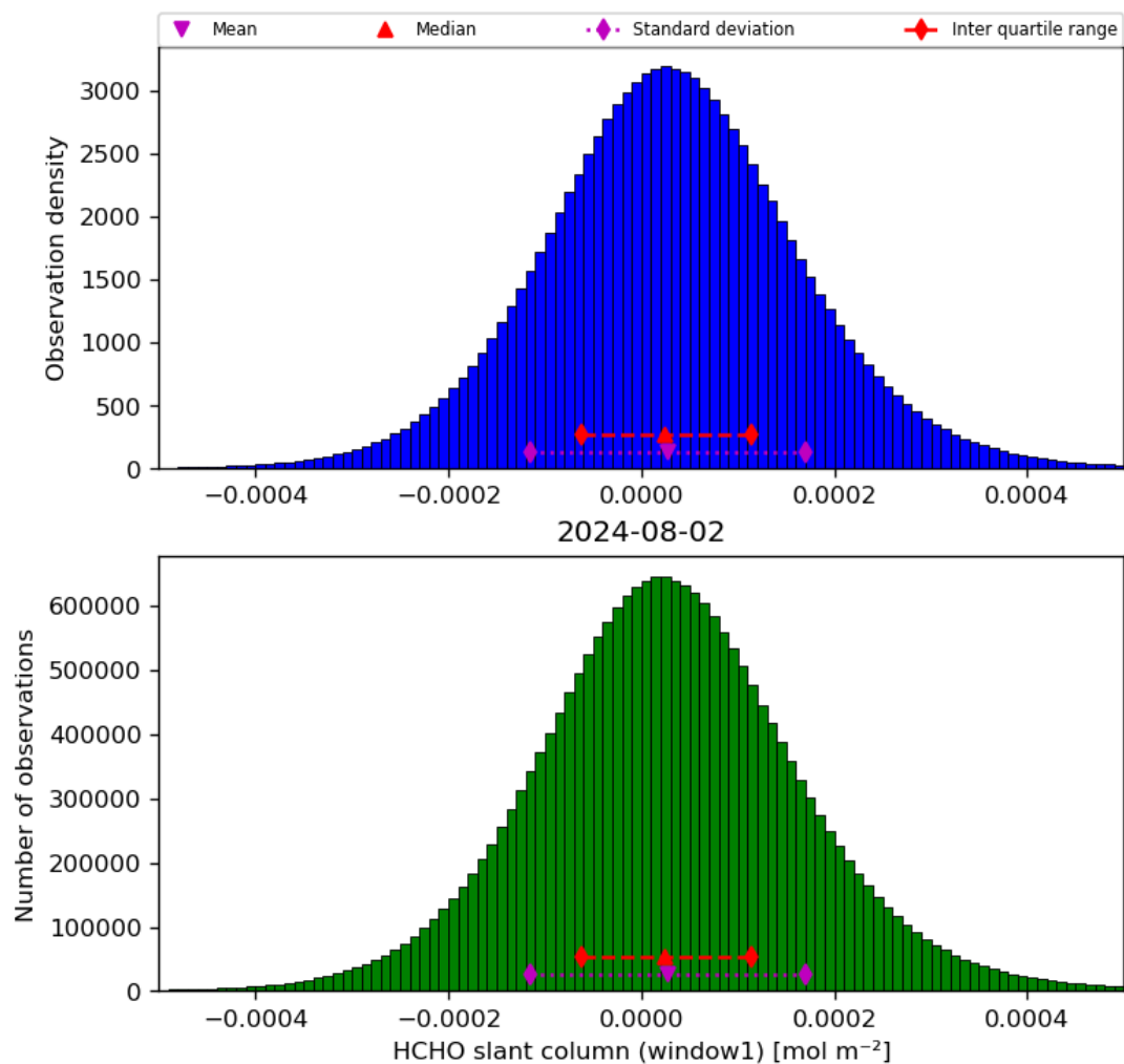
Figure 38: Histogram of “HCHO slant column (window1)” for 2024-08-01 to 2024-08-03
