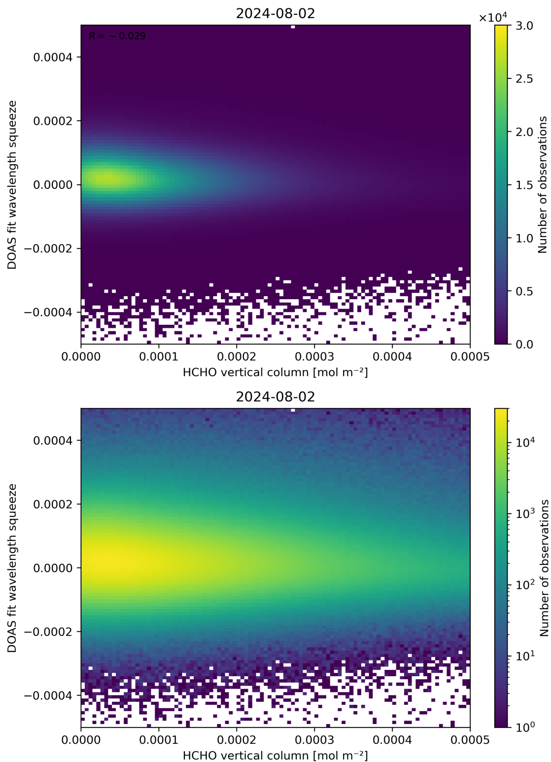
Figure 125: Scatter density plot of “HCHO vertical column” against “DOAS fit wavelength squeeze” for 2024-08-01 to 2024-08-03.
