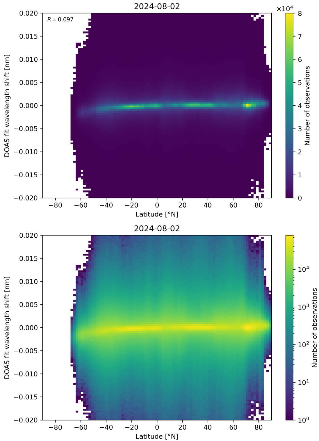
Figure 154: Scatter density plot of “Latitude” against “DOAS fit wavelength shift” for 2024-08-01 to 2024-08-03.
