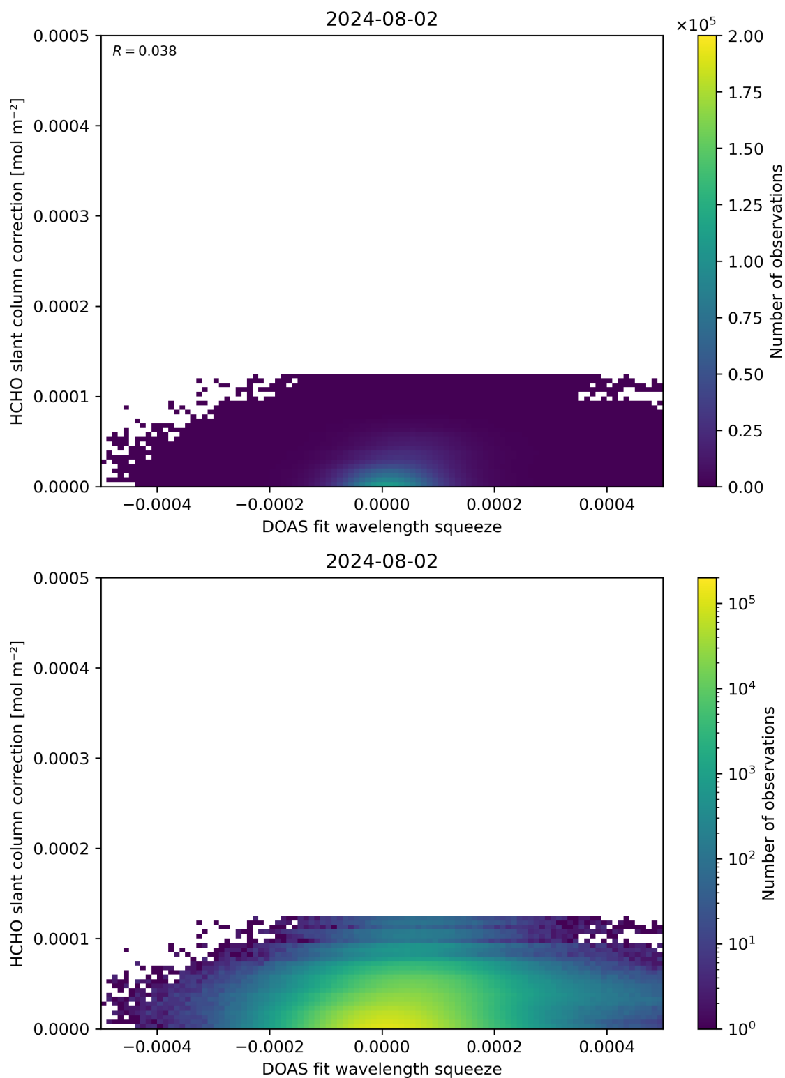
Figure 70: Scatter density plot of “DOAS fit wavelength squeeze” against “HCHO slant column correction” for 2024-08-01 to 2024-08-03.
