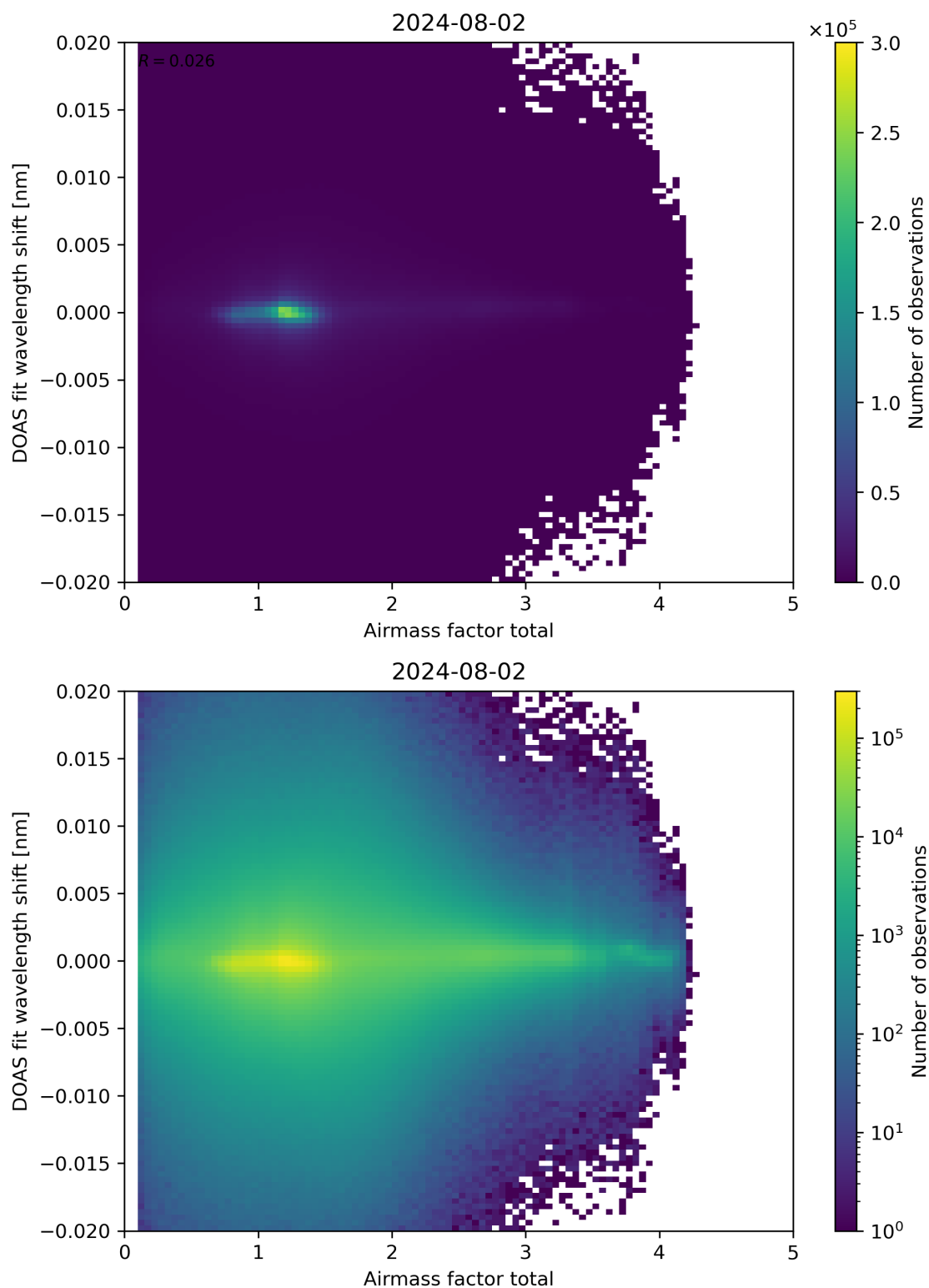
Figure 98: Scatter density plot of “Airmass factor total” against “DOAS fit wavelength shift” for 2024-08-01 to 2024-08-03.
