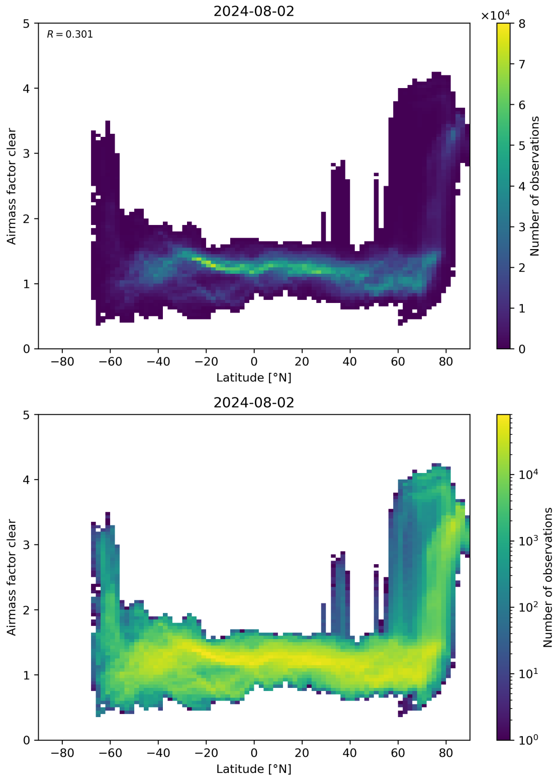
Figure 156: Scatter density plot of “Latitude” against “Airmass factor clear” for 2024-08-01 to 2024-08-03.
