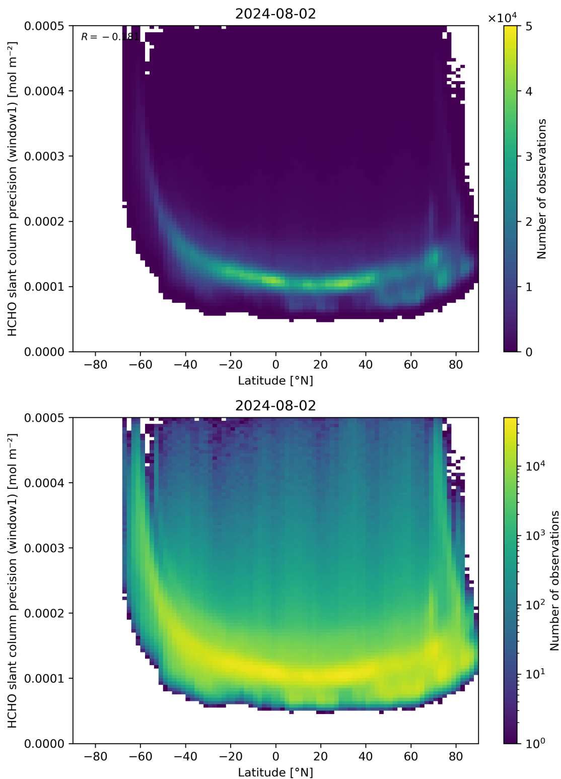
Figure 160: Scatter density plot of “Latitude” against “HCHO slant column precision (window1)” for 2024-08-01 to 2024-08-03.
