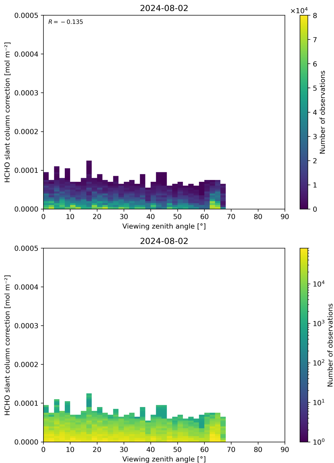
Figure 187: Scatter density plot of “Viewing zenith angle” against “HCHO slant column correction” for 2024-08-01 to 2024-08-03.
