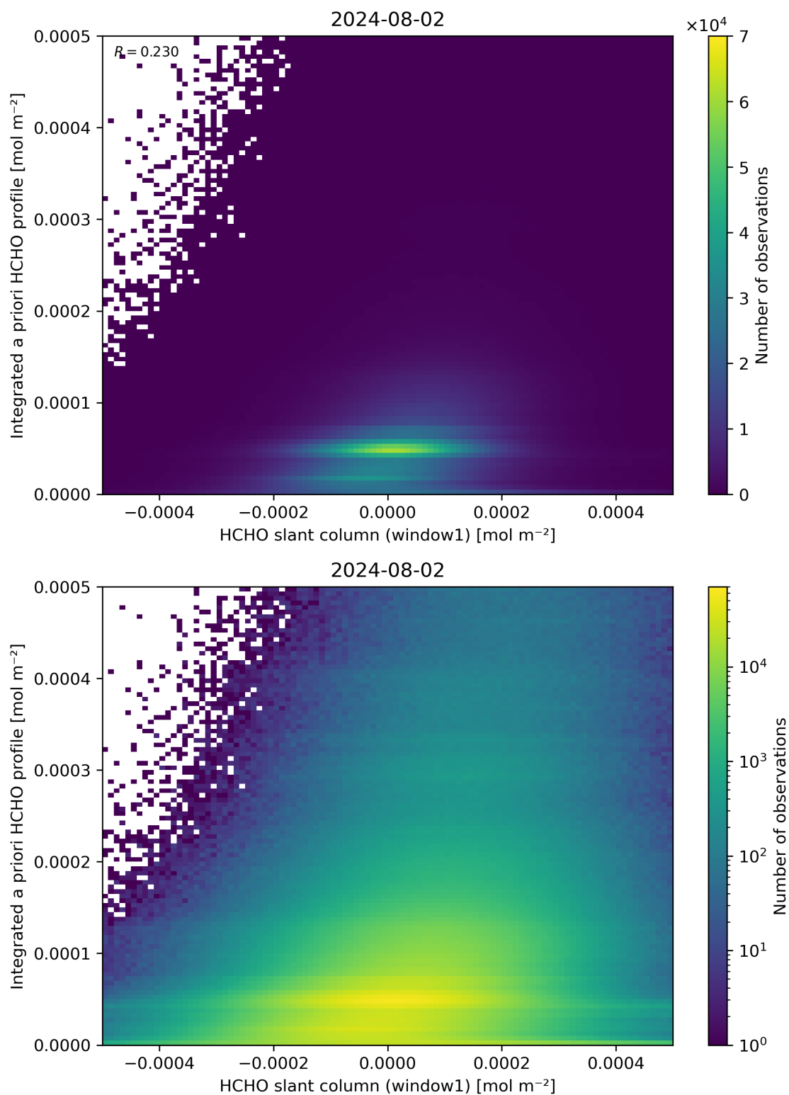
Figure 87: Scatter density plot of “HCHO slant column (window1)” against “Integrated a priori HCHO profile” for 2024-08-01 to 2024-08-03.
