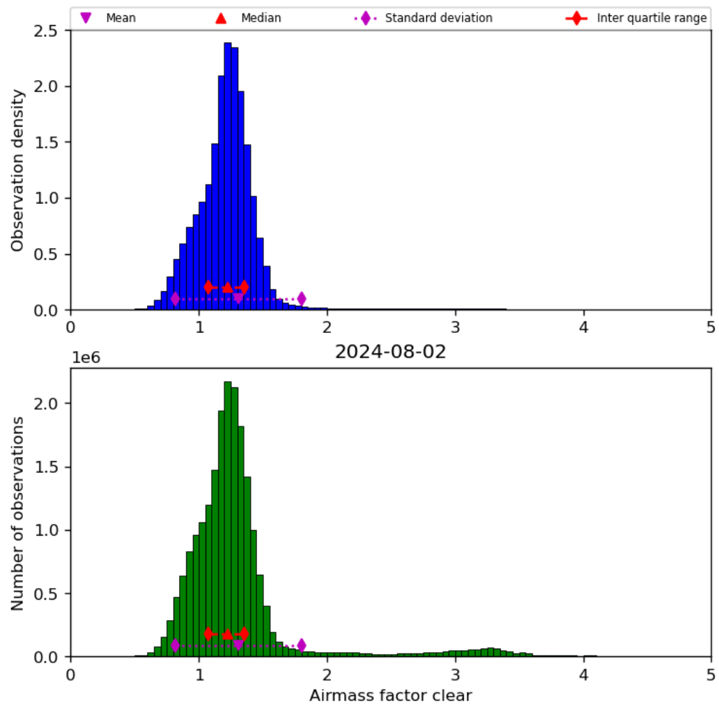
Figure 42: Histogram of “Airmass factor clear” for 2024-08-01 to 2024-08-03
