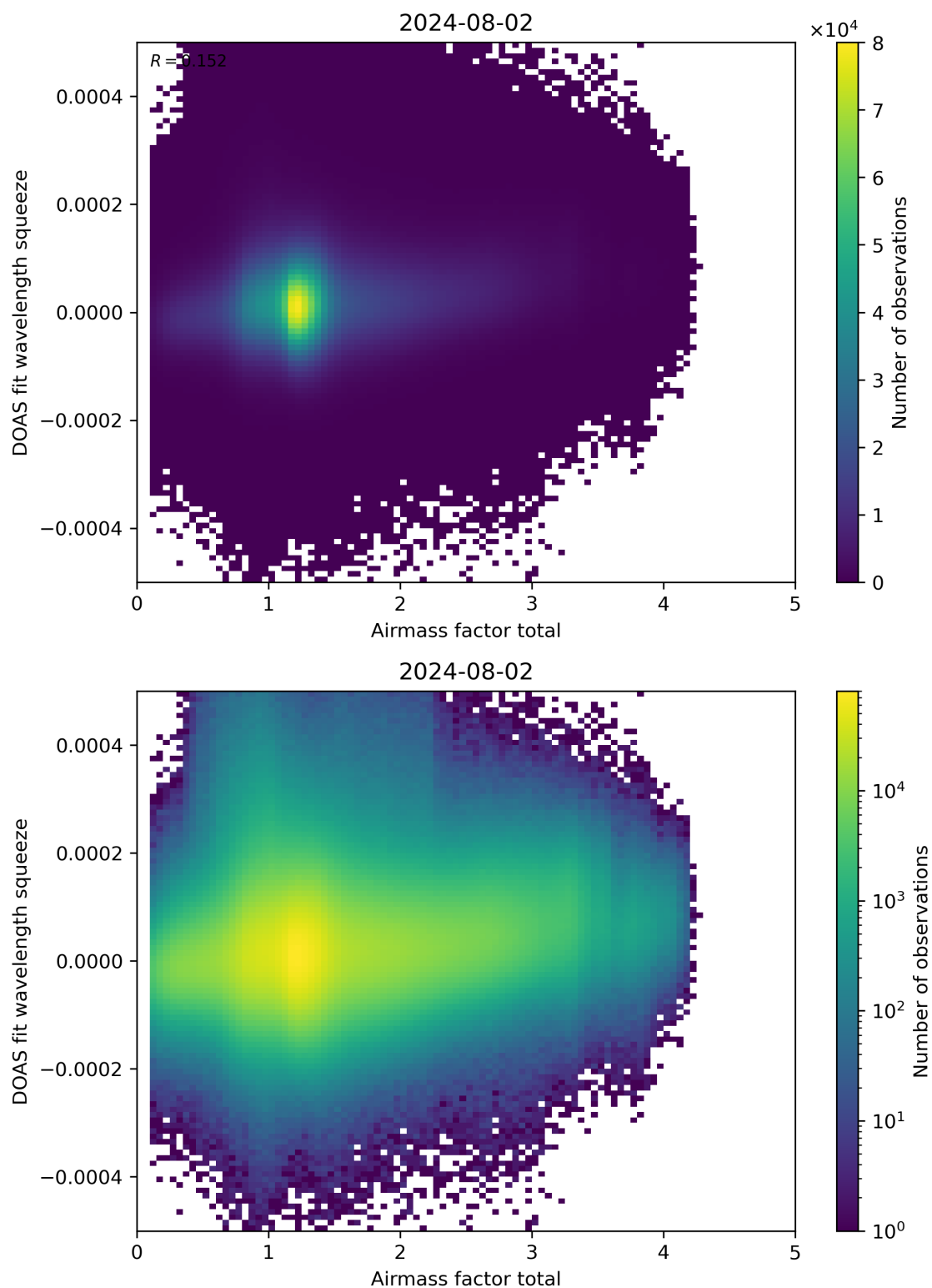
Figure 99: Scatter density plot of “Airmass factor total” against “DOAS fit wavelength squeeze” for 2024-08-01 to 2024-08-03.
