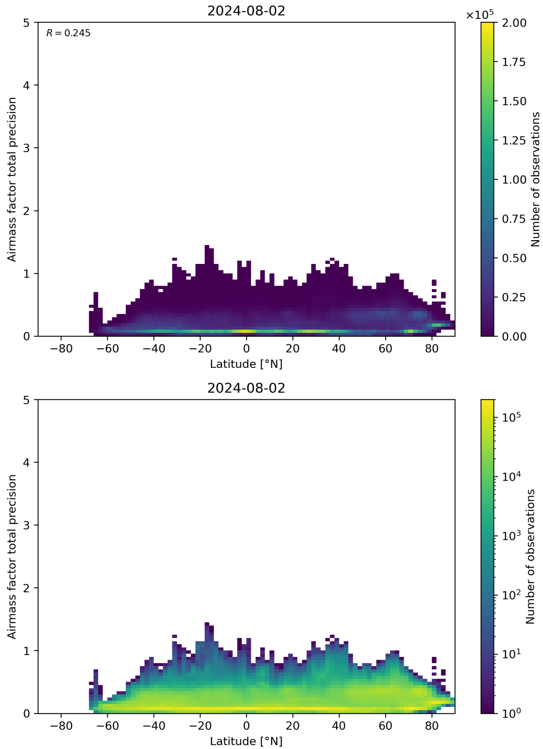
Figure 162: Scatter density plot of “Latitude” against “Airmass factor total precision” for 2024-08-01 to 2024-08-03.
