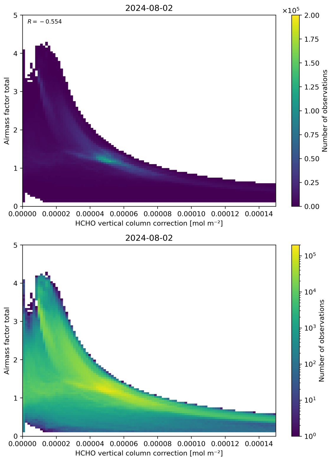
Figure 120: Scatter density plot of “HCHO vertical column correction” against “Airmass factor total” for 2024-08-01 to 2024-08-03.
