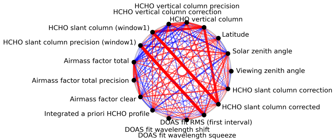
Figure 1: Map of correlation graph for 2024-08-01 to 2024-08-03.
