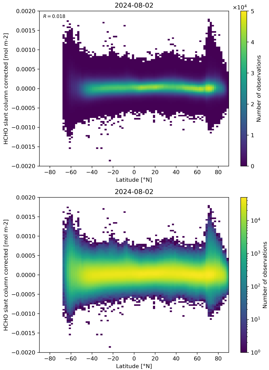
Figure 157: Scatter density plot of “Latitude” against “HCHO slant column corrected” for 2024-08-01 to 2024-08-03.
