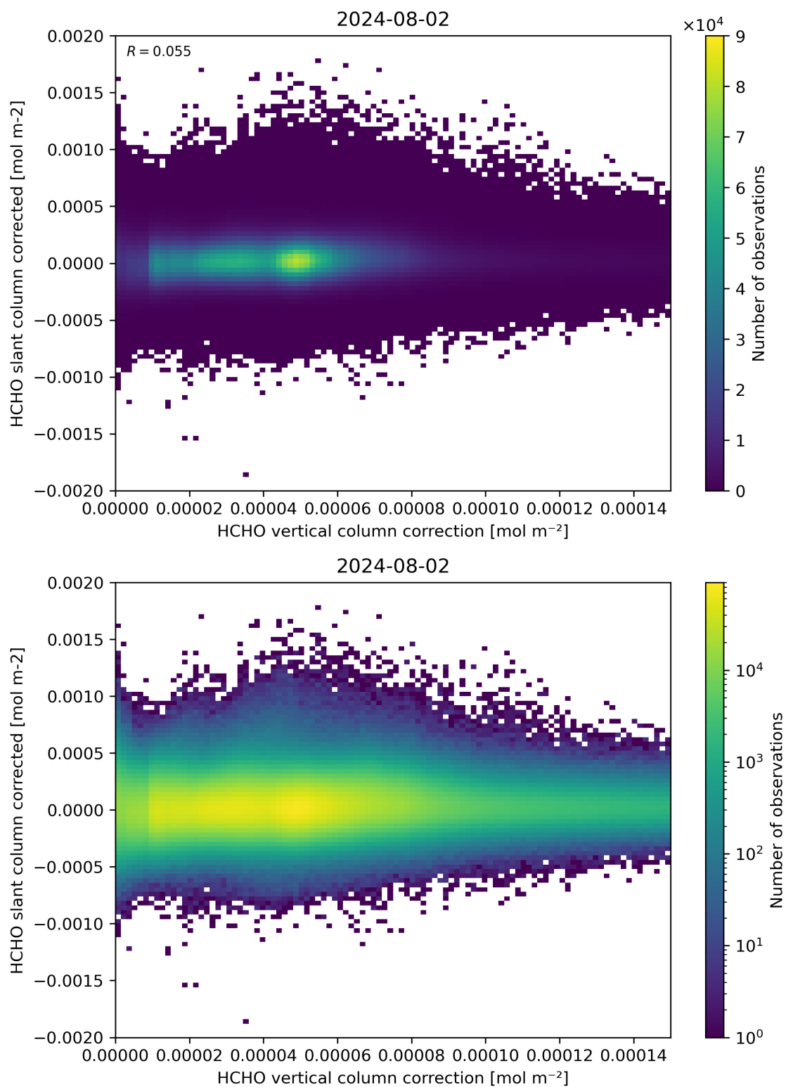
Figure 116: Scatter density plot of “HCHO vertical column correction” against “HCHO slant column corrected” for 2024-08-01 to 2024-08-03.
