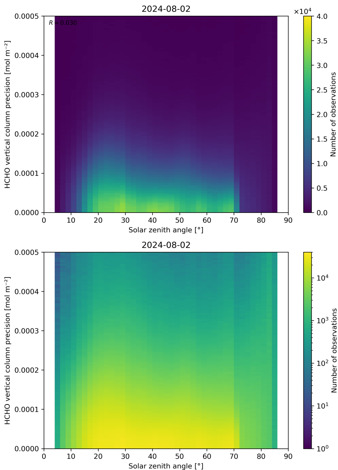
Figure 179: Scatter density plot of “Solar zenith angle” against “HCHO vertical column precision” for 2024-08-01 to 2024-08-03.
