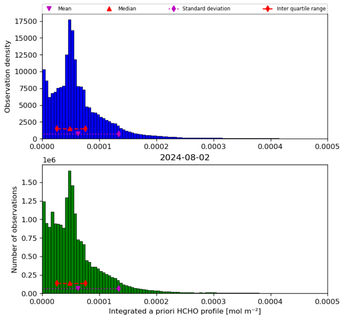
Figure 43: Histogram of “Integrated a priori HCHO profile” for 2024-08-01 to 2024-08-03
