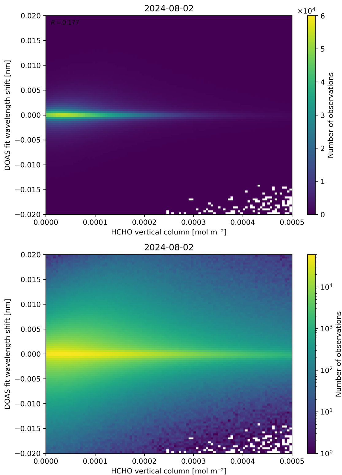
Figure 124: Scatter density plot of “HCHO vertical column” against “DOAS fit wavelength shift” for 2024-08-01 to 2024-08-03.
