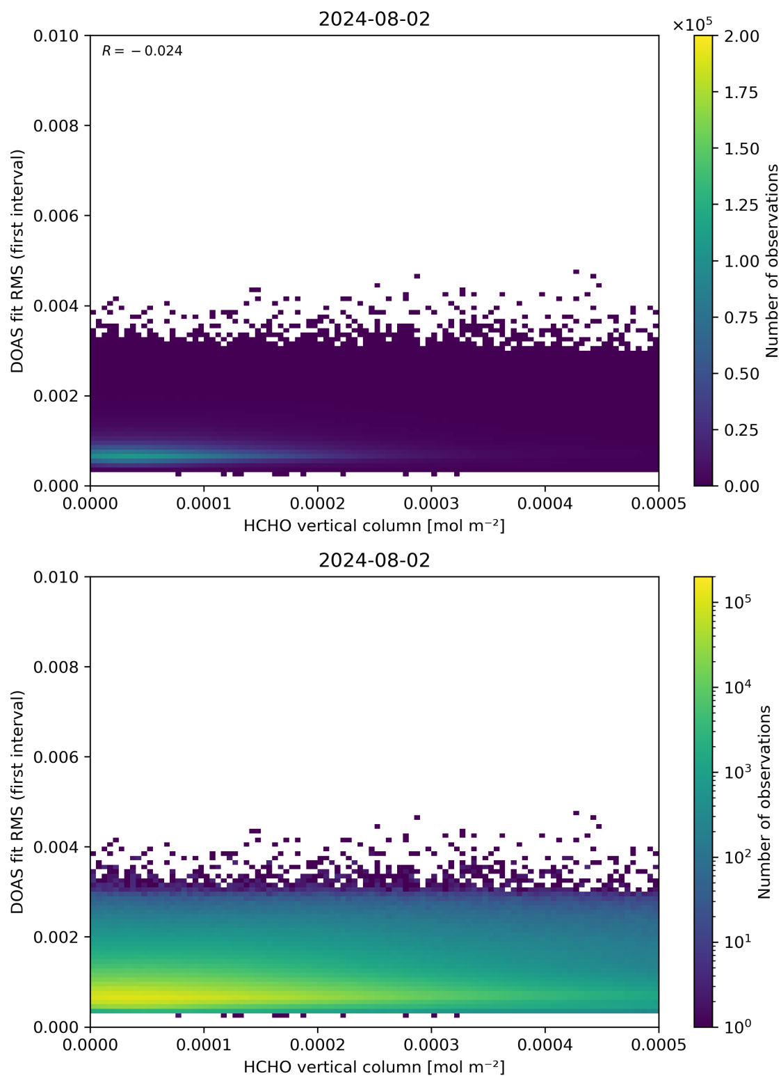
Figure 123: Scatter density plot of “HCHO vertical column” against “DOAS fit RMS (first interval)” for 2024-08-01 to 2024-08-03.
