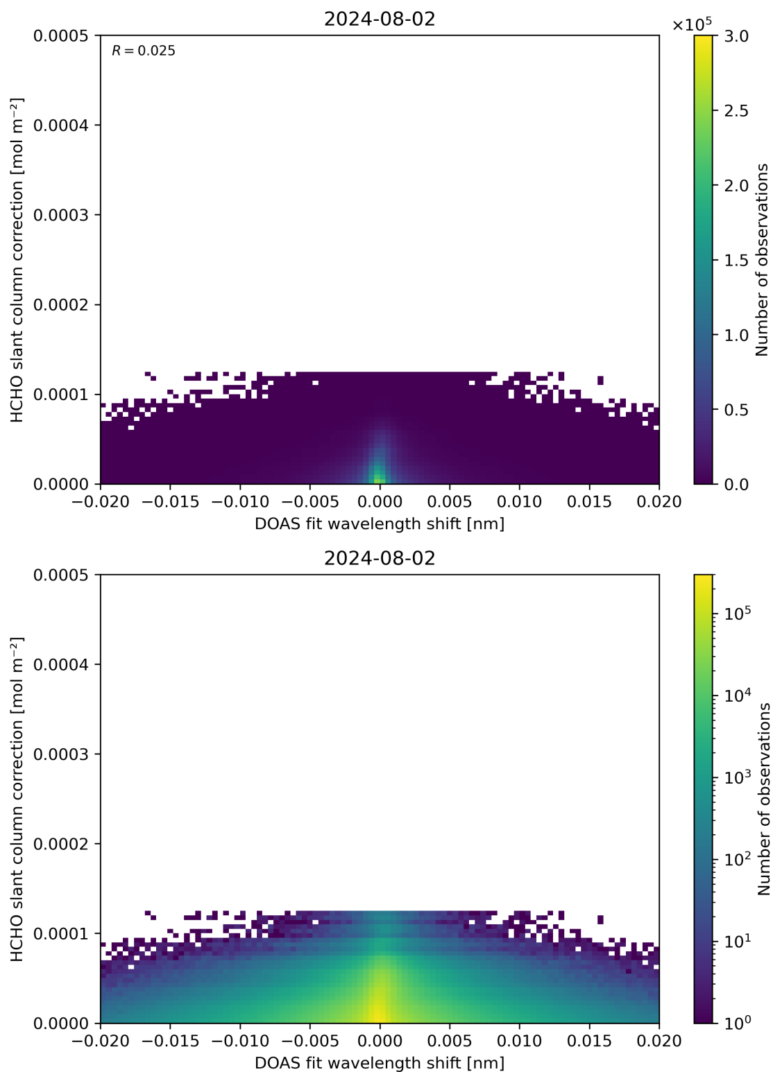
Figure 67: Scatter density plot of “DOAS fit wavelength shift” against “HCHO slant column correction” for 2024-08-01 to 2024-08-03.
