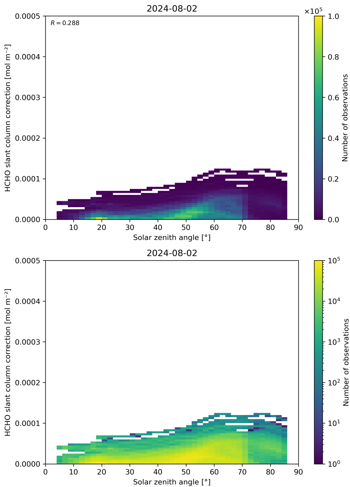
Figure 172: Scatter density plot of “Solar zenith angle” against “HCHO slant column correction” for 2024-08-01 to 2024-08-03.
