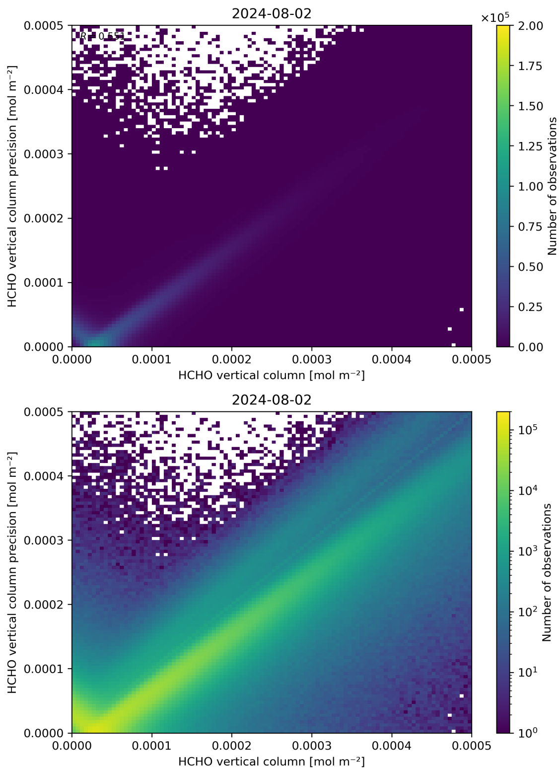
Figure 134: Scatter density plot of “HCHO vertical column” against “HCHO vertical column precision” for 2024-08-01 to 2024-08-03.
