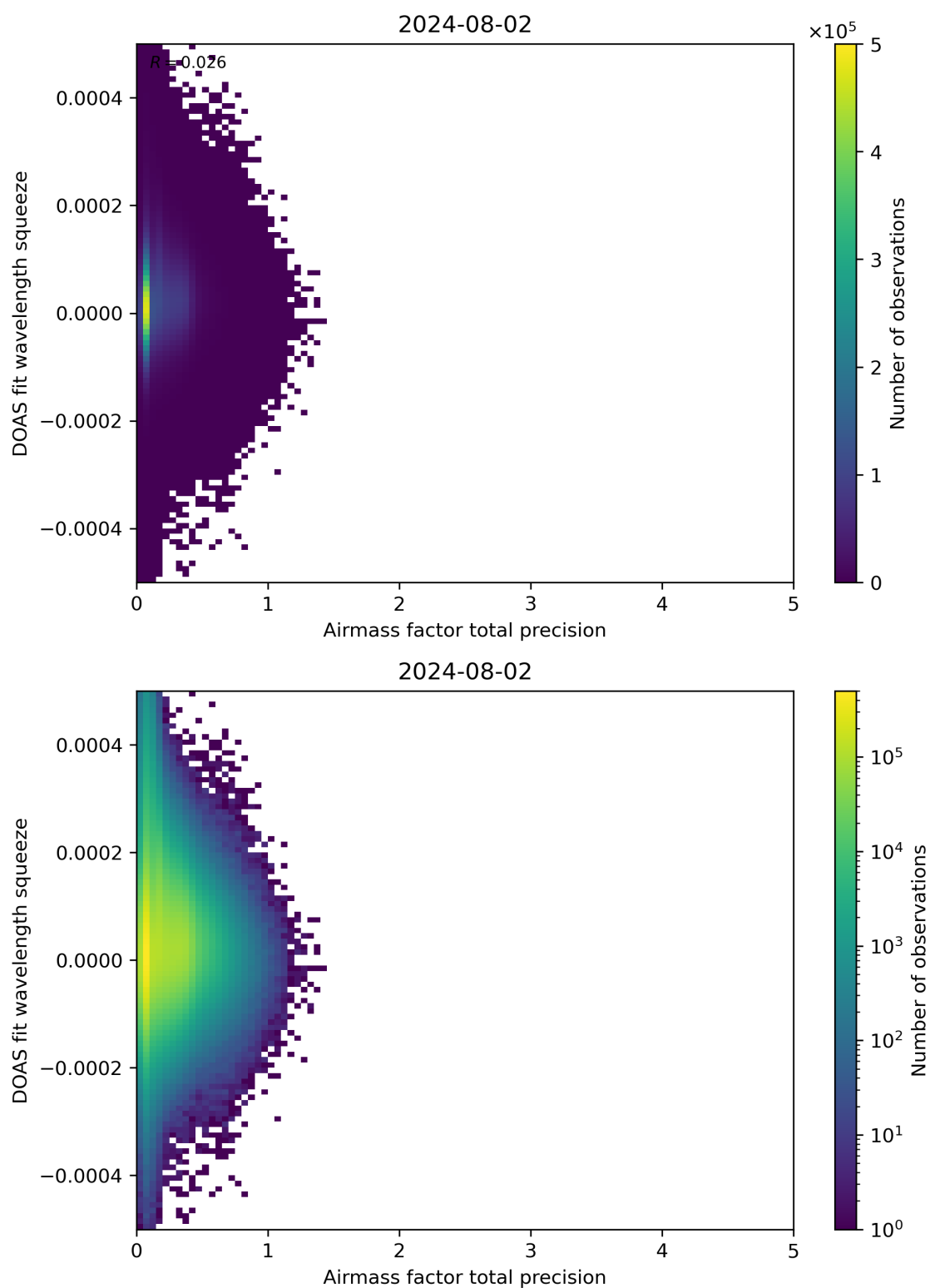
Figure 107: Scatter density plot of “Airmass factor total precision” against “DOAS fit wavelength squeeze” for 2024-08-01 to 2024-08-03.
