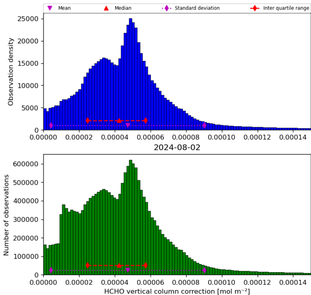
Figure 37: Histogram of “HCHO vertical column correction” for 2024-08-01 to 2024-08-03
