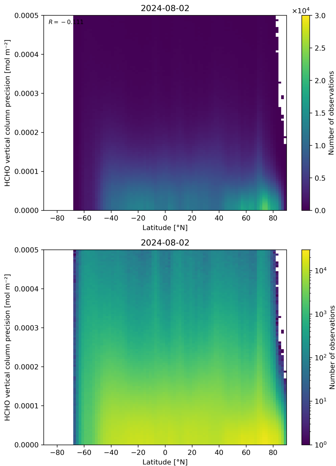
Figure 165: Scatter density plot of “Latitude” against “HCHO vertical column precision” for 2024-08-01 to 2024-08-03.
