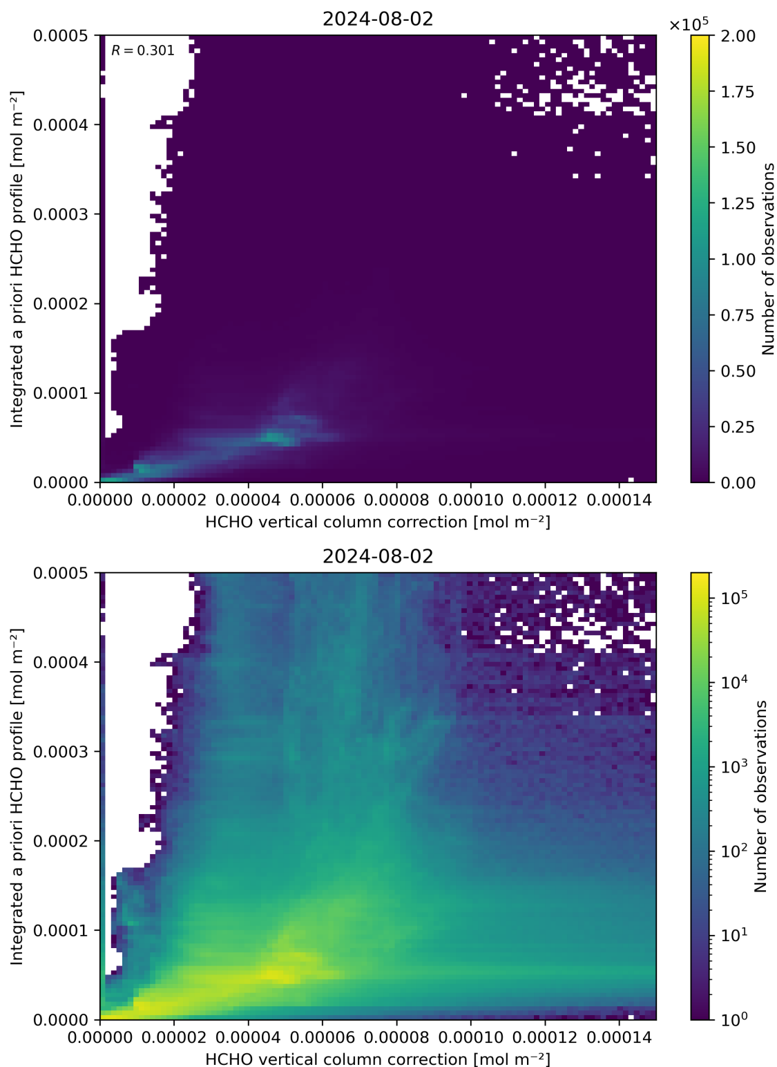
Figure 122: Scatter density plot of “HCHO vertical column correction” against “Integrated a priori HCHO profile” for 2024-08-01 to 2024-08-03.
