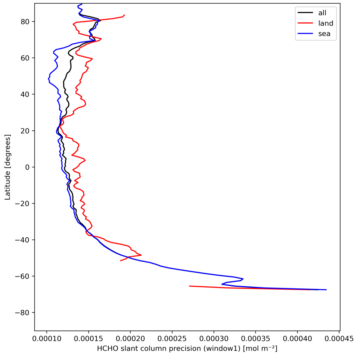
Figure 25: Zonal average of “HCHO slant column precision (window1)” for 2024-08-01 to 2024-08-03.
