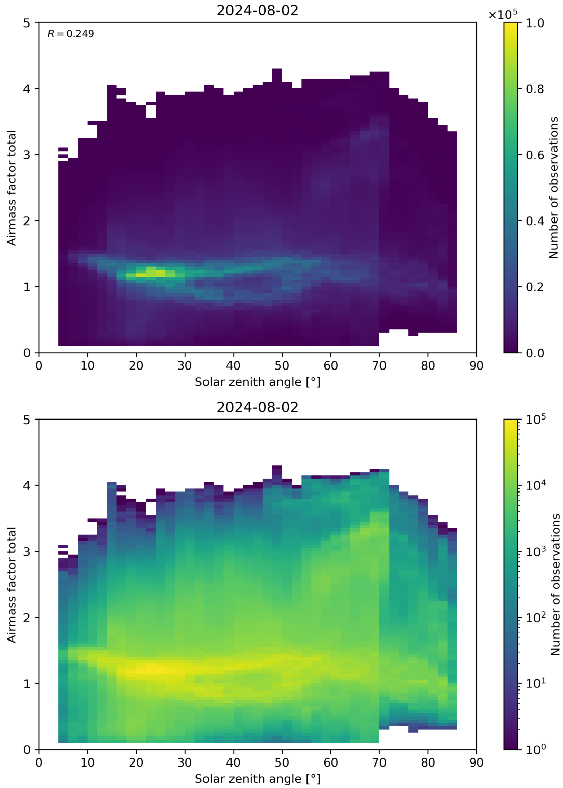
Figure 175: Scatter density plot of “Solar zenith angle” against “Airmass factor total” for 2024-08-01 to 2024-08-03.
