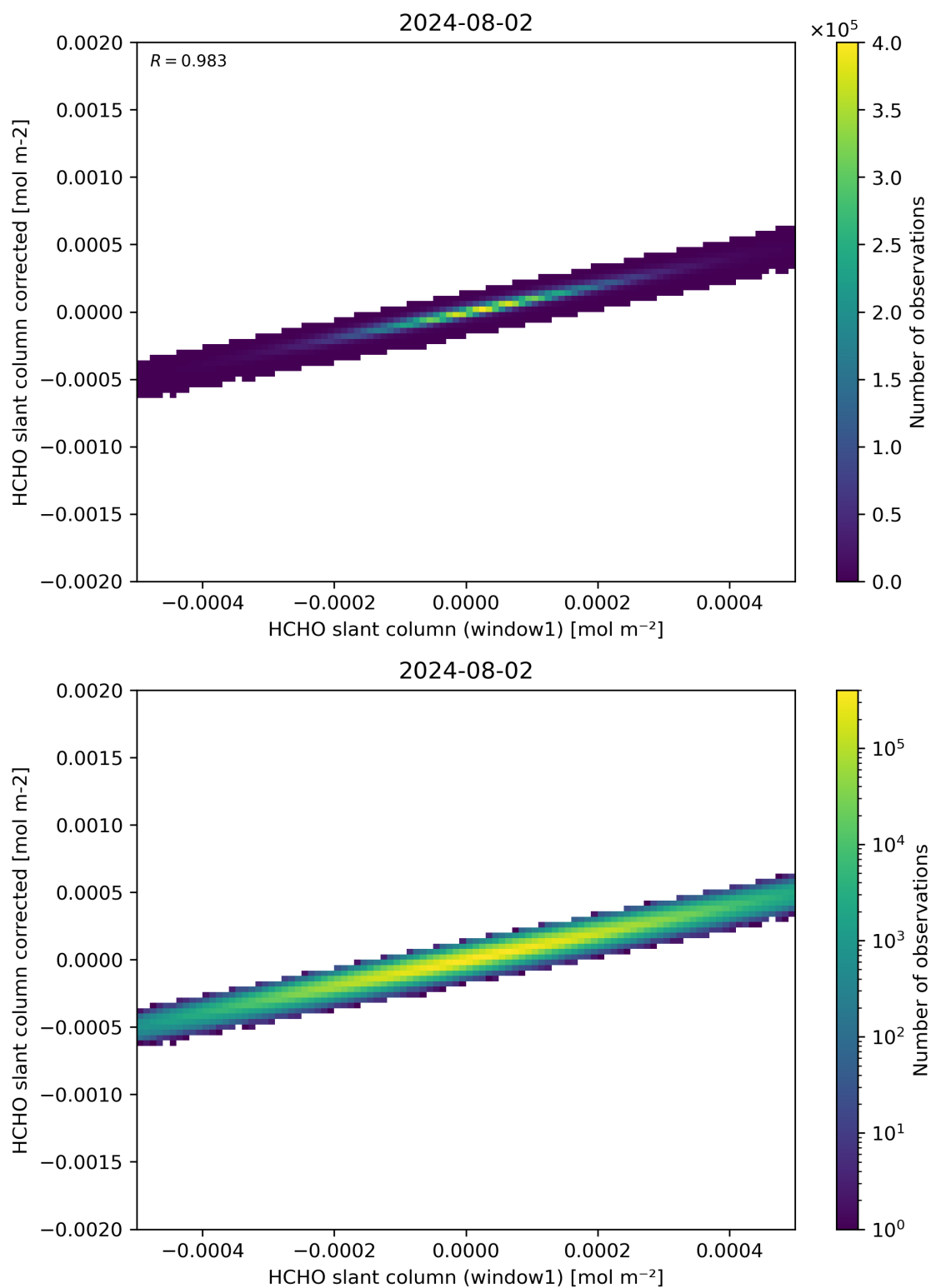
Figure 82: Scatter density plot of “HCHO slant column (window1)” against “HCHO slant column corrected” for 2024-08-01 to 2024-08-03.
