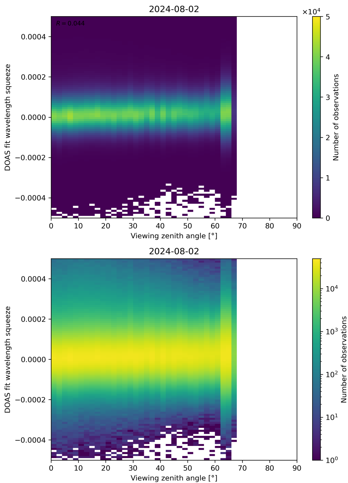
Figure 184: Scatter density plot of “Viewing zenith angle” against “DOAS fit wavelength squeeze” for 2024-08-01 to 2024-08-03.
