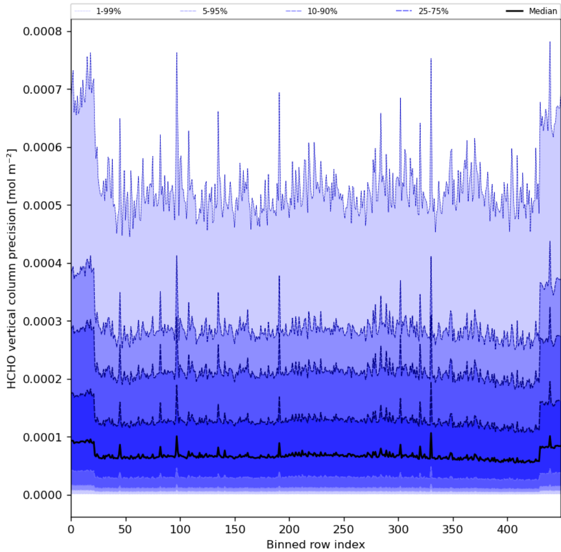
Figure 50: Along track statistics of “HCHO vertical column precision” for 2024-08-01 to 2024-08-03
