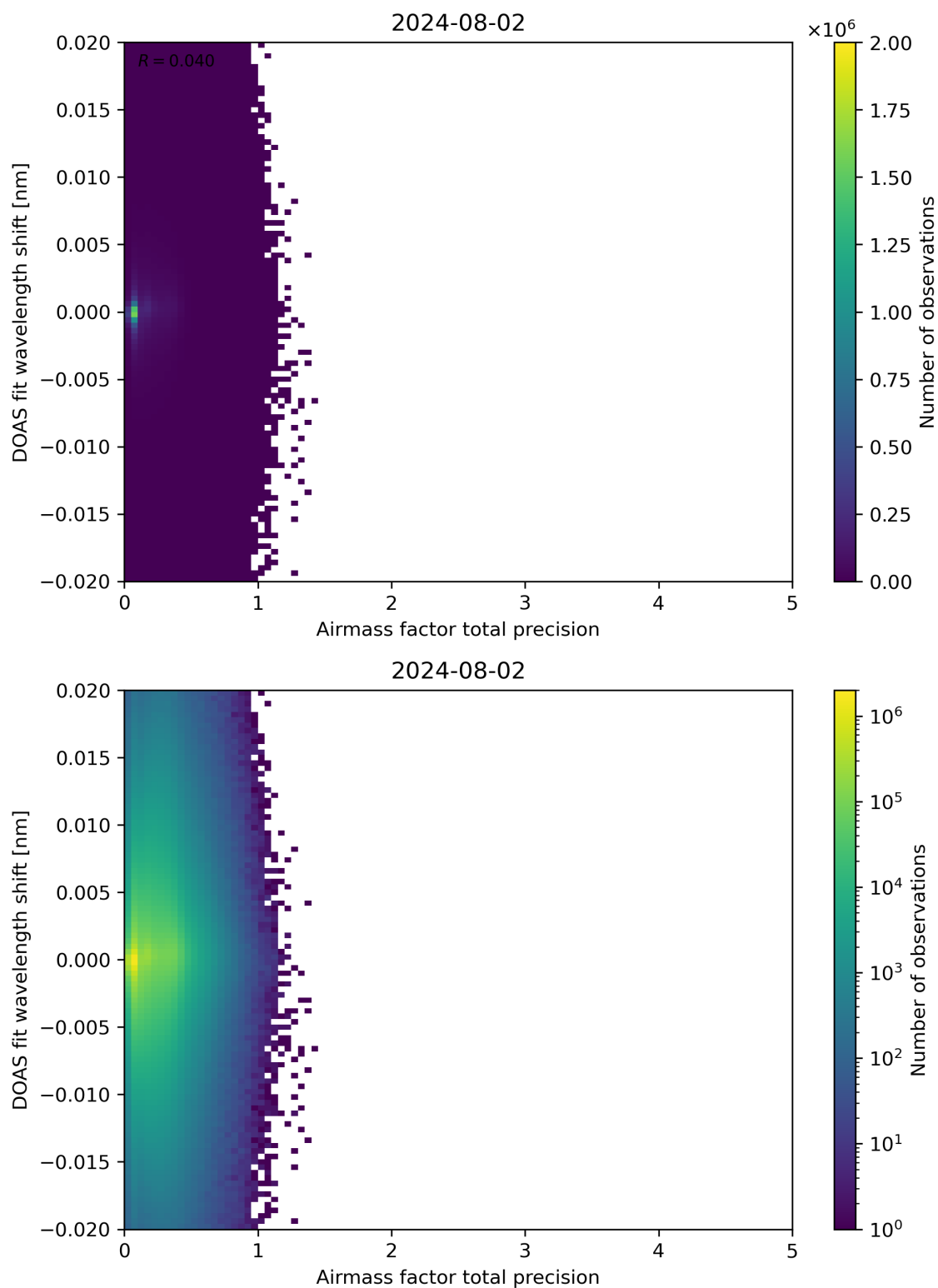
Figure 106: Scatter density plot of “Airmass factor total precision” against “DOAS fit wavelength shift” for 2024-08-01 to 2024-08-03.
