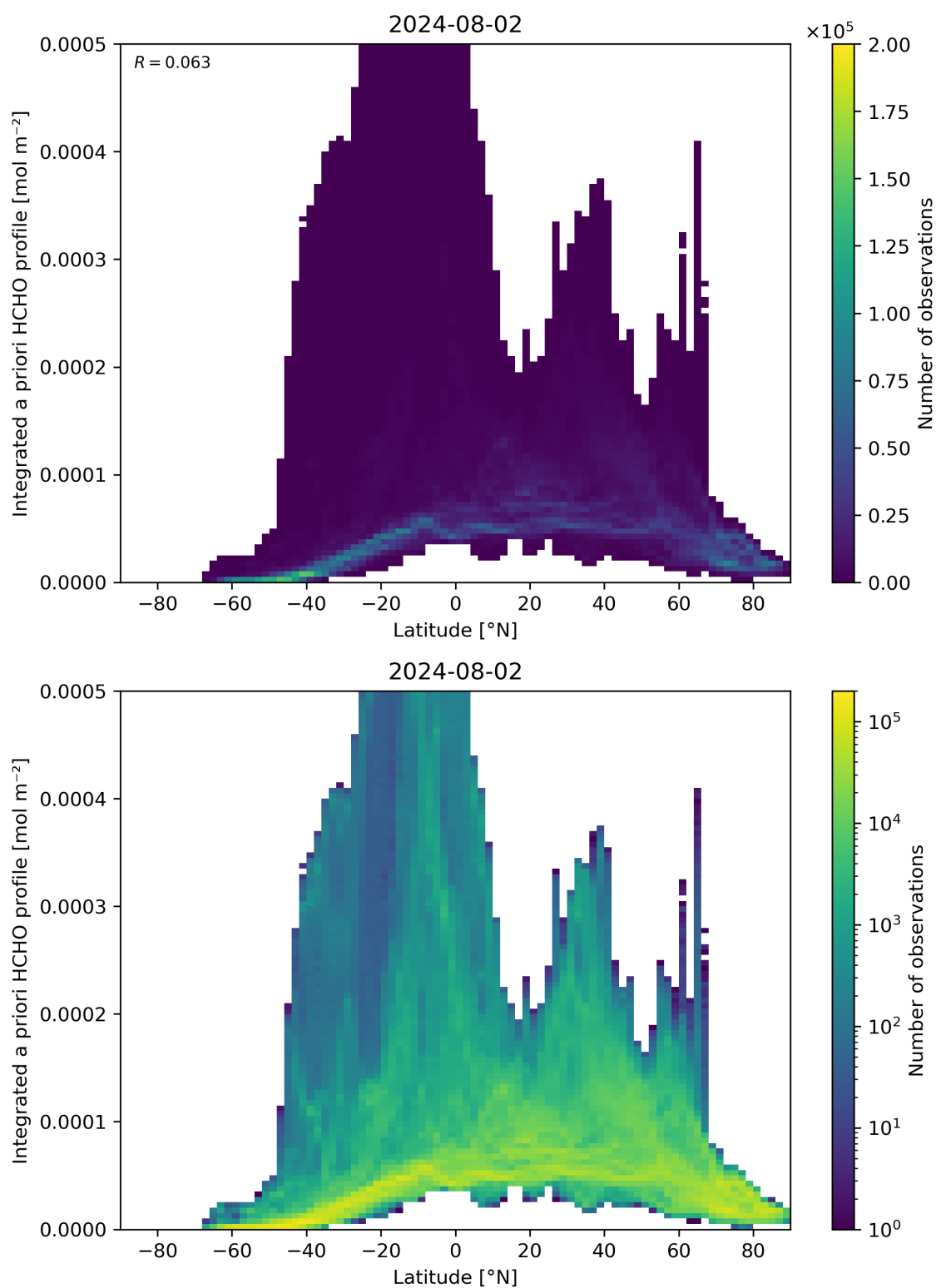
Figure 166: Scatter density plot of “Latitude” against “Integrated a priori HCHO profile” for 2024-08-01 to 2024-08-03.
