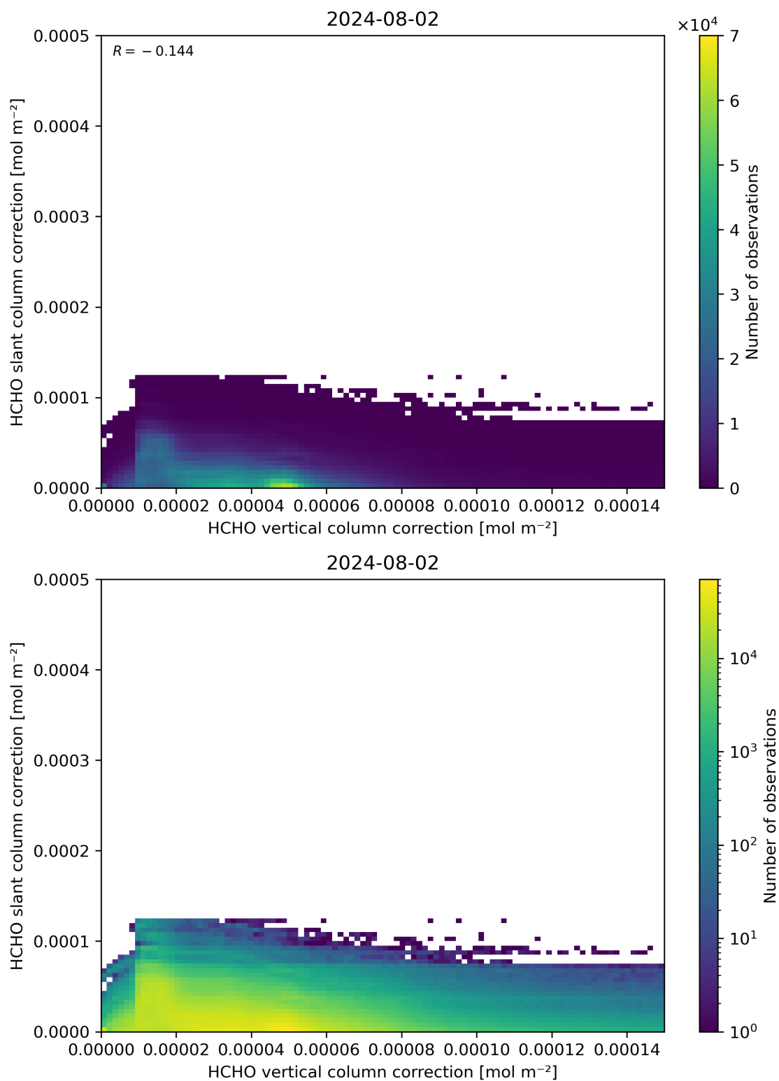
Figure 117: Scatter density plot of “HCHO vertical column correction” against “HCHO slant column correction” for 2024-08-01 to 2024-08-03.
