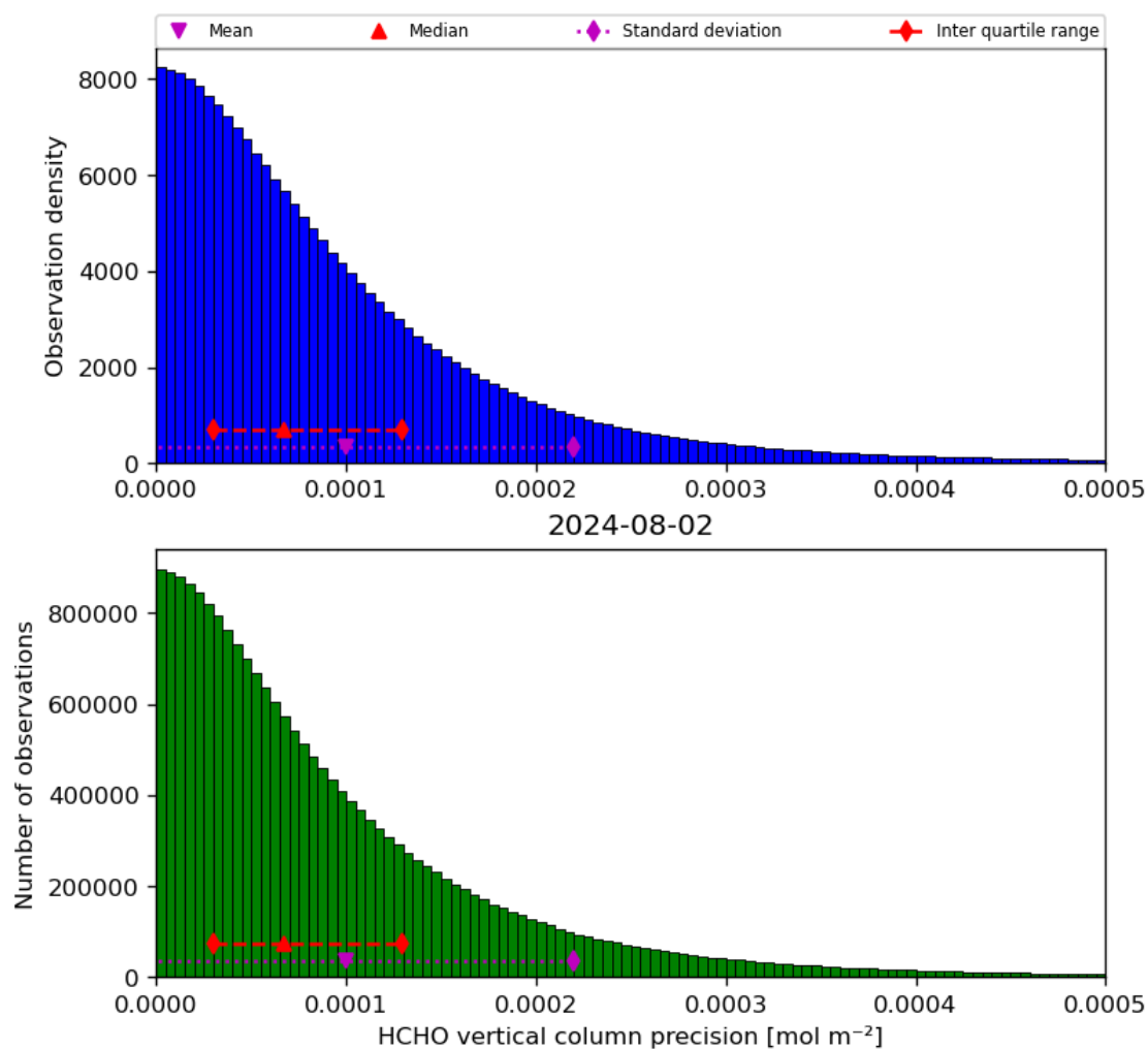
Figure 36: Histogram of “HCHO vertical column precision” for 2024-08-01 to 2024-08-03
