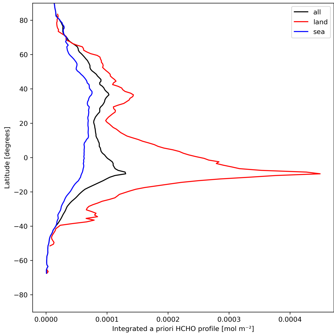
Figure 29: Zonal average of “Integrated a priori HCHO profile” for 2024-08-01 to 2024-08-03.
