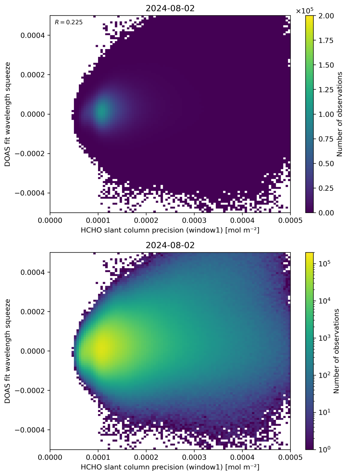
Figure 90: Scatter density plot of “HCHO slant column precision (window1)” against “DOAS fit wavelength squeeze” for 2024-08-01 to 2024-08-03.
