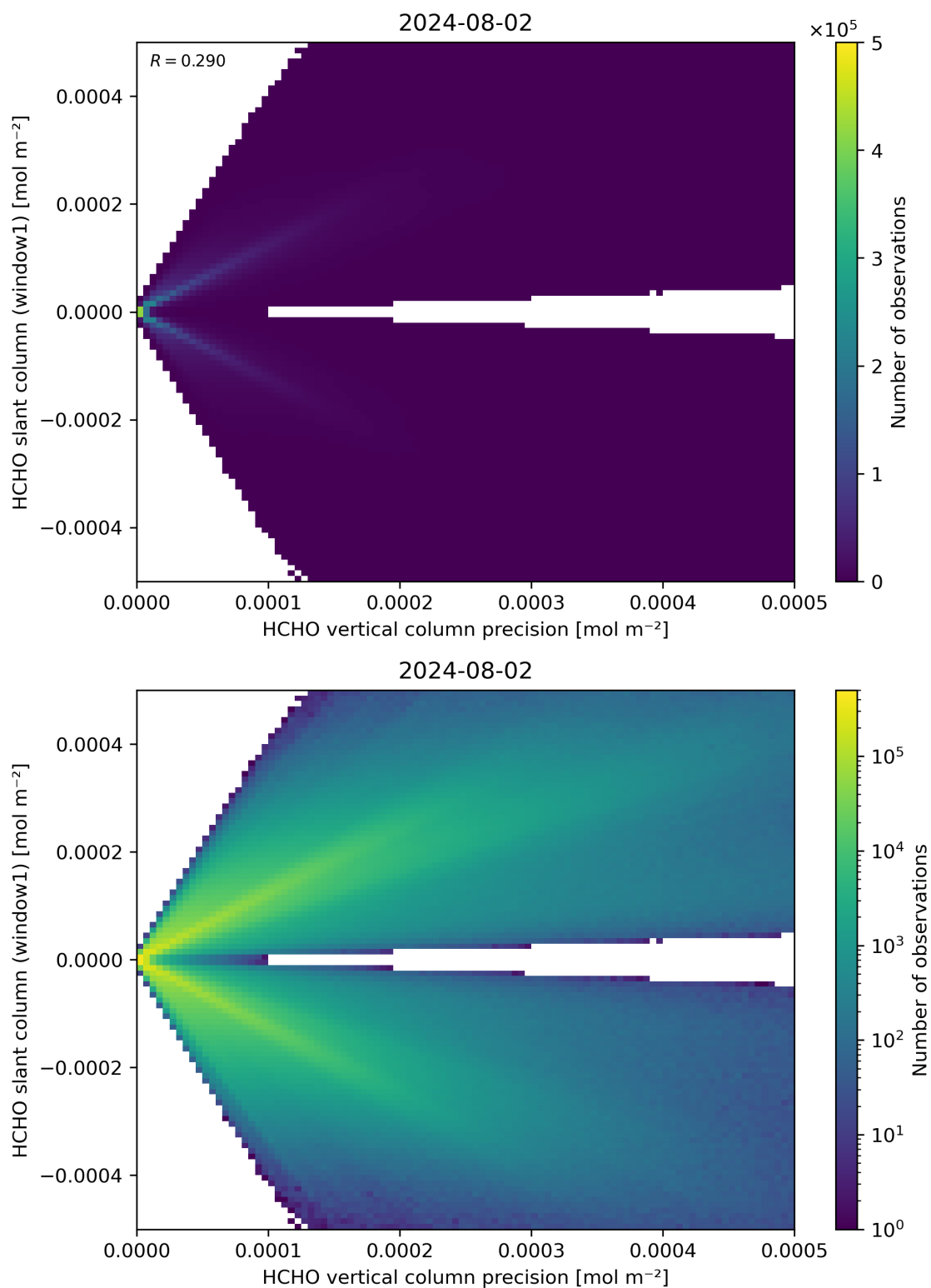
Figure 142: Scatter density plot of “HCHO vertical column precision” against “HCHO slant column (window1)” for 2024-08-01 to 2024-08-03.
