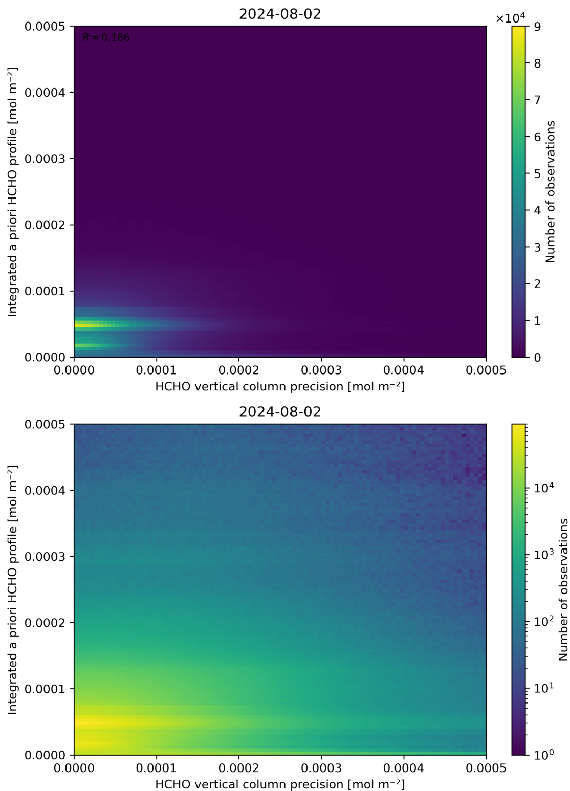
Figure 147: Scatter density plot of “HCHO vertical column precision” against “Integrated a priori HCHO profile” for 2024-08-01 to 2024-08-03.
