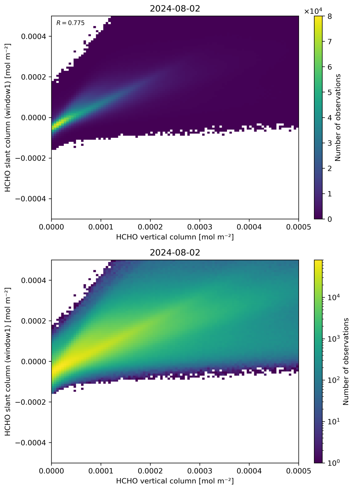
Figure 129: Scatter density plot of “HCHO vertical column” against “HCHO slant column (window1)” for 2024-08-01 to 2024-08-03.
