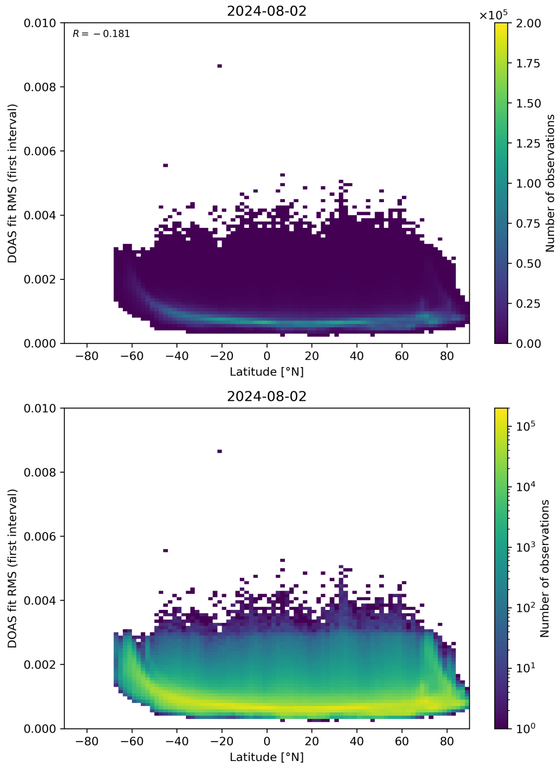
Figure 153: Scatter density plot of “Latitude” against “DOAS fit RMS (first interval)” for 2024-08-01 to 2024-08-03.
