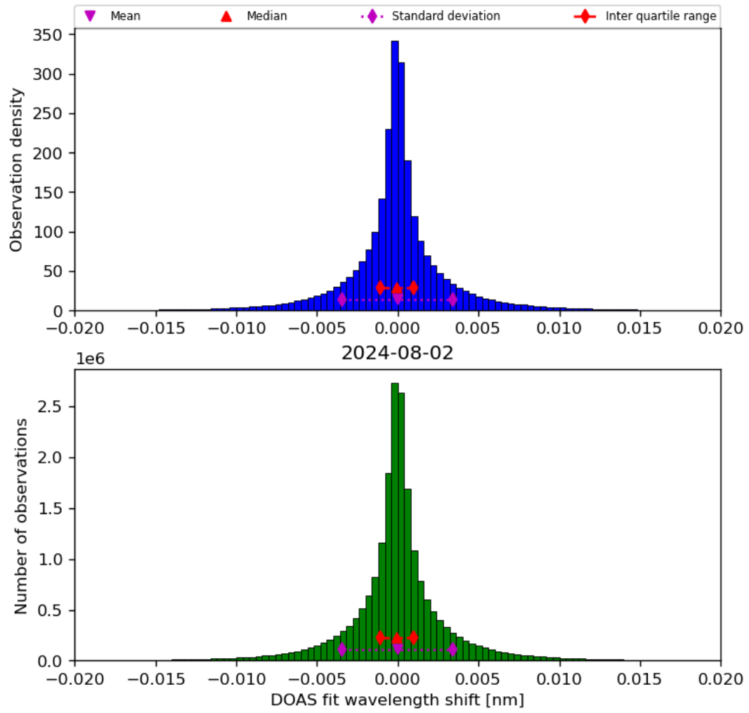
Figure 44: Histogram of “DOAS fit wavelength shift” for 2024-08-01 to 2024-08-03
