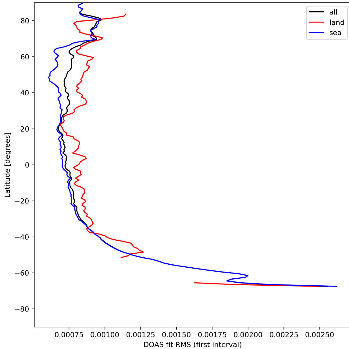
Figure 32: Zonal average of "DOAS fit RMS (first interval)" for 2024-08-01 to 2024-08-03.
