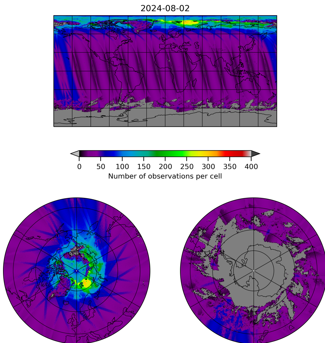
Figure 19: Map of the number of observations for 2024-08-01 to 2024-08-03
