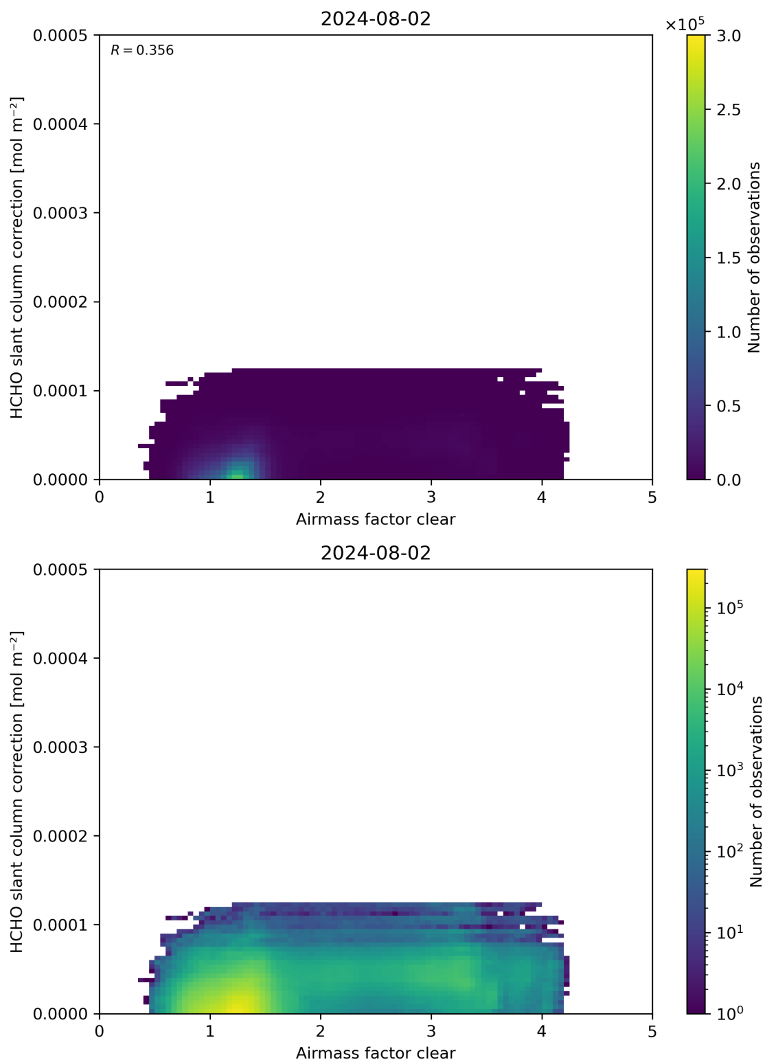
Figure 75: Scatter density plot of “Airmass factor clear” against “HCHO slant column correction” for 2024-08-01 to 2024-08-03.
