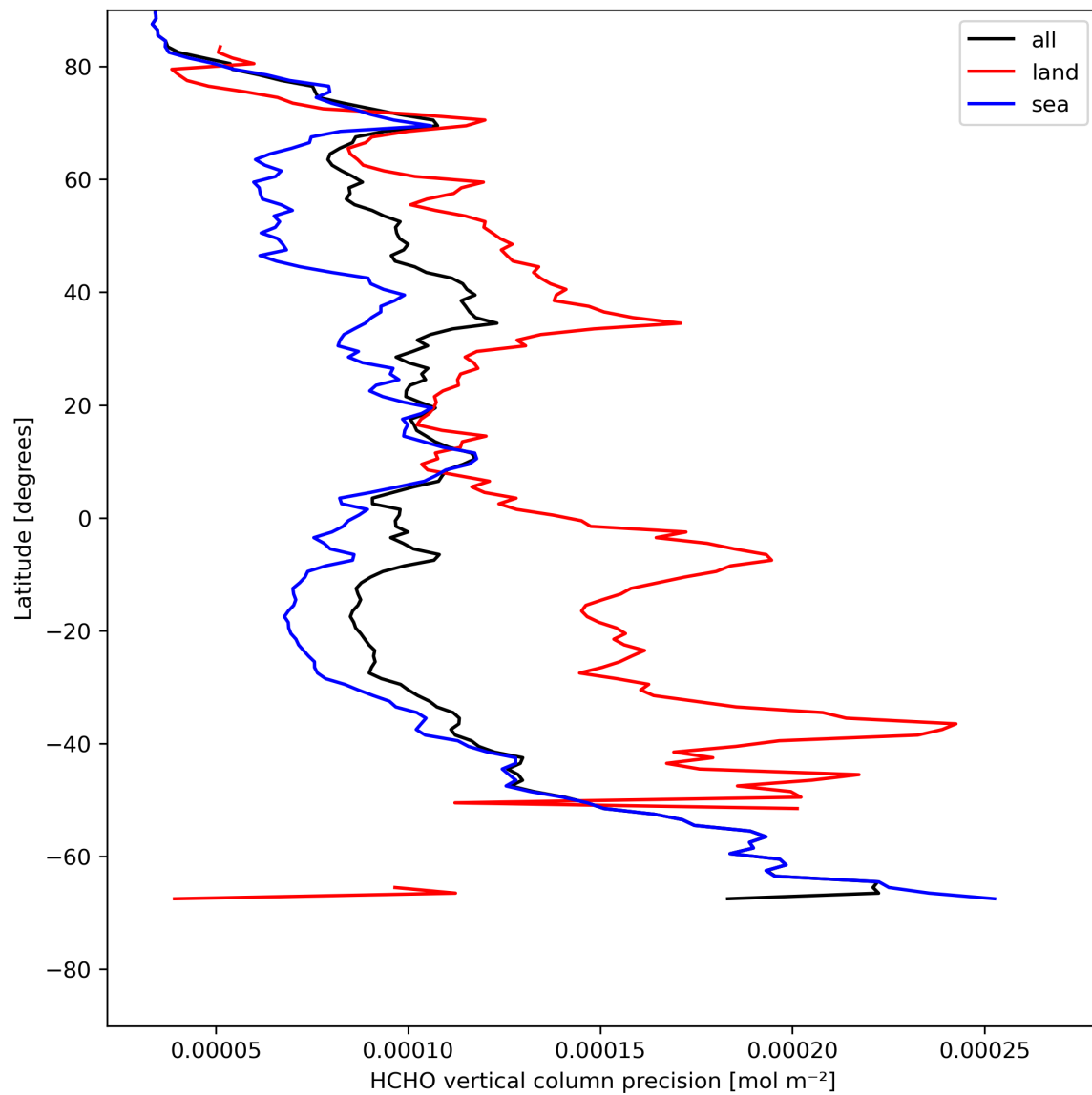
Figure 22: Zonal average of “HCHO vertical column precision” for 2024-08-01 to 2024-08-03.
