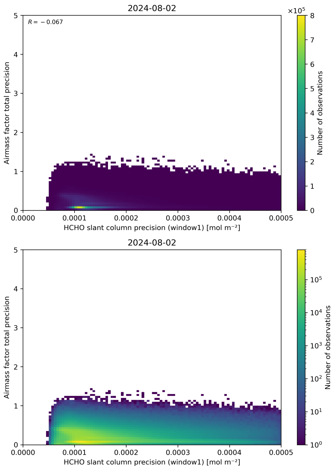
Figure 95: Scatter density plot of “HCHO slant column precision (window1)” against “Airmass factor total precision” for 2024-08-01 to 2024-08-03.
