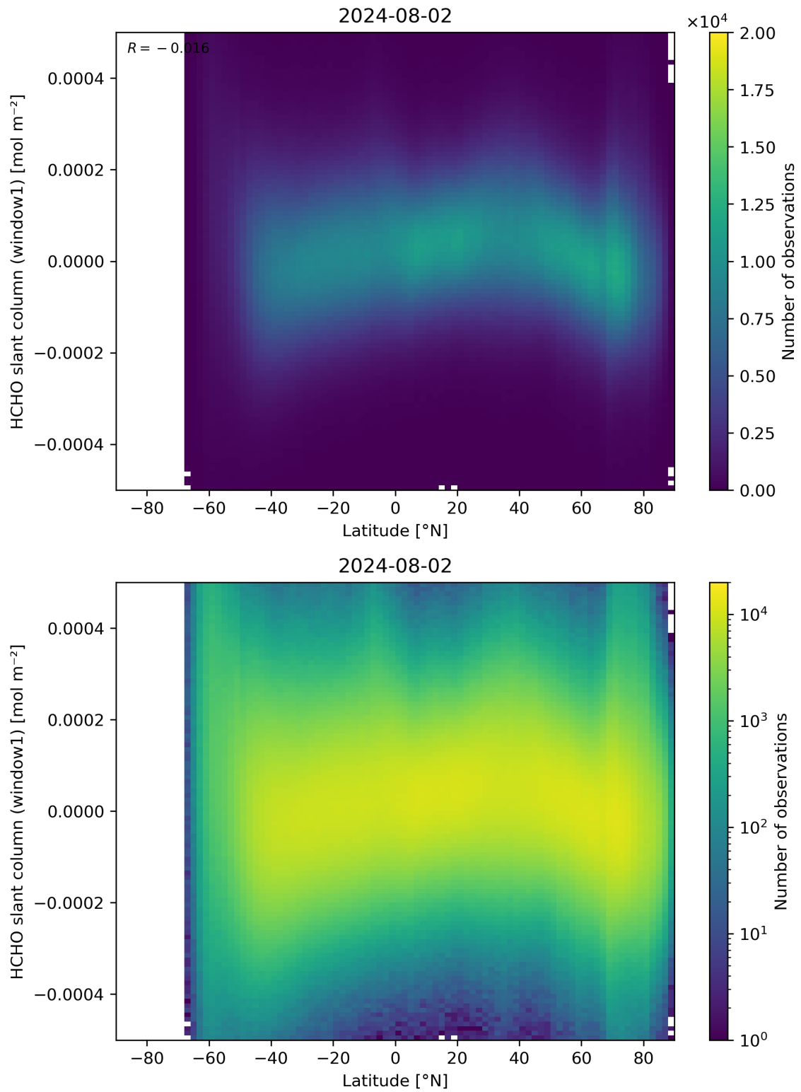
Figure 159: Scatter density plot of “Latitude” against “HCHO slant column (window1)” for 2024-08-01 to 2024-08-03.
