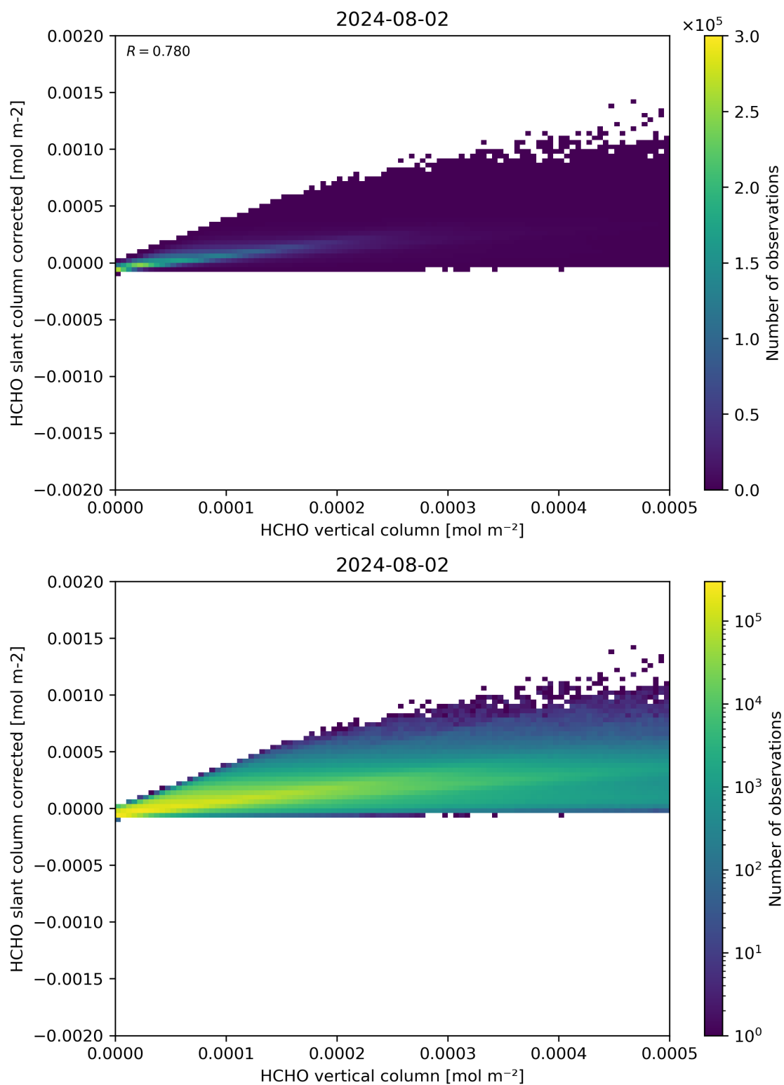
Figure 127: Scatter density plot of “HCHO vertical column” against “HCHO slant column corrected” for 2024-08-01 to 2024-08-03.
