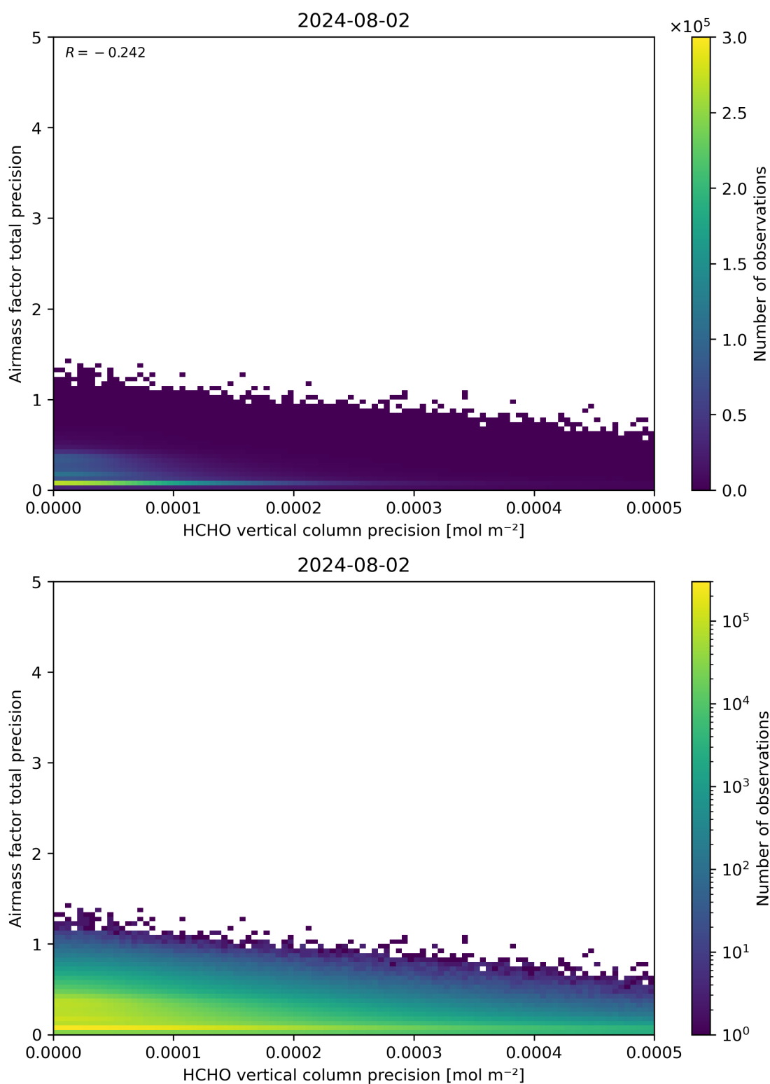
Figure 145: Scatter density plot of “HCHO vertical column precision” against “Airmass factor total precision” for 2024-08-01 to 2024-08-03.
