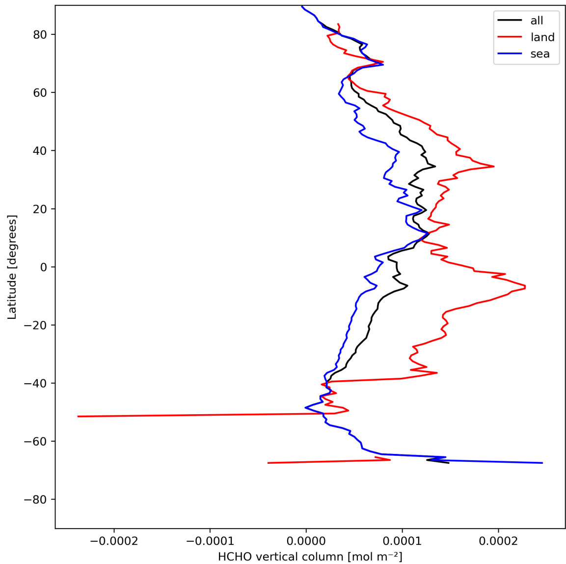
Figure 21: Zonal average of “HCHO vertical column” for 2024-08-01 to 2024-08-03.
