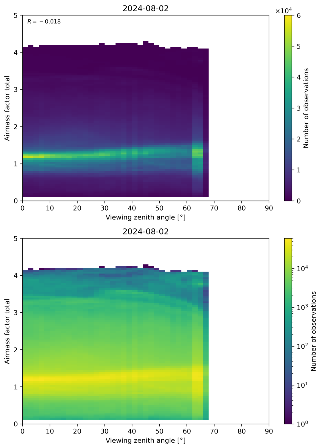
Figure 190: Scatter density plot of “Viewing zenith angle” against “Airmass factor total” for 2024-08-01 to 2024-08-03.
