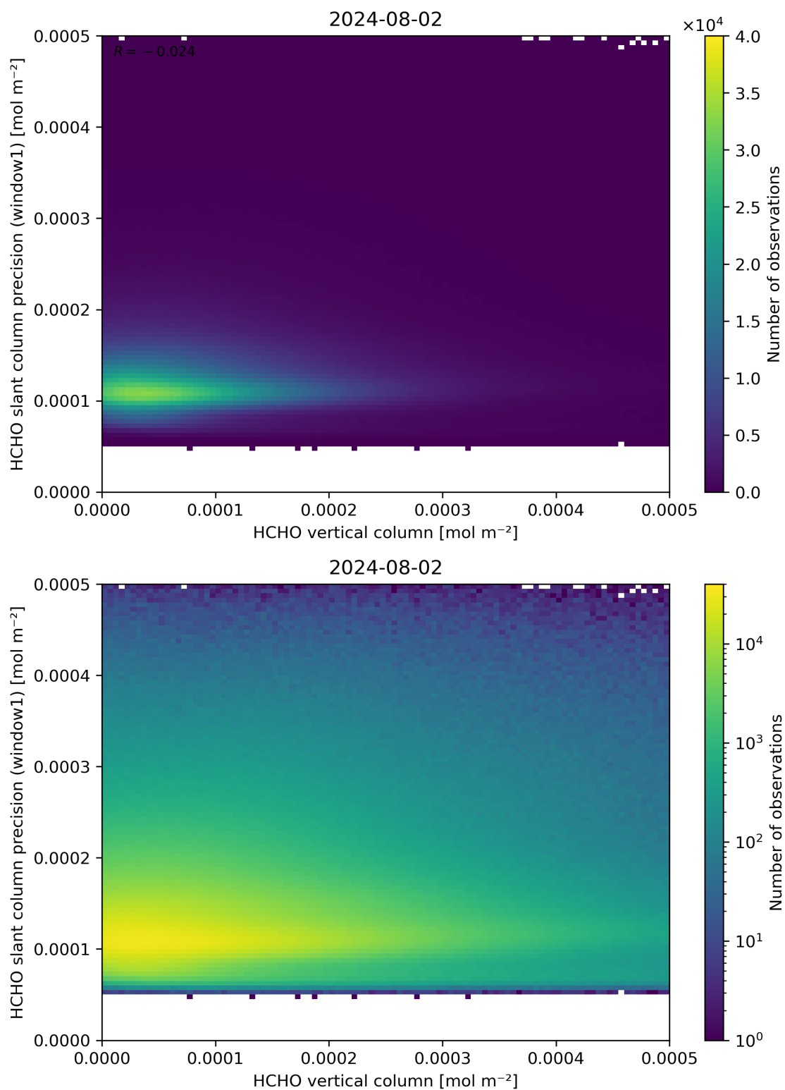
Figure 130: Scatter density plot of “HCHO vertical column” against “HCHO slant column precision (window1)” for 2024-08-01 to 2024-08-03.
