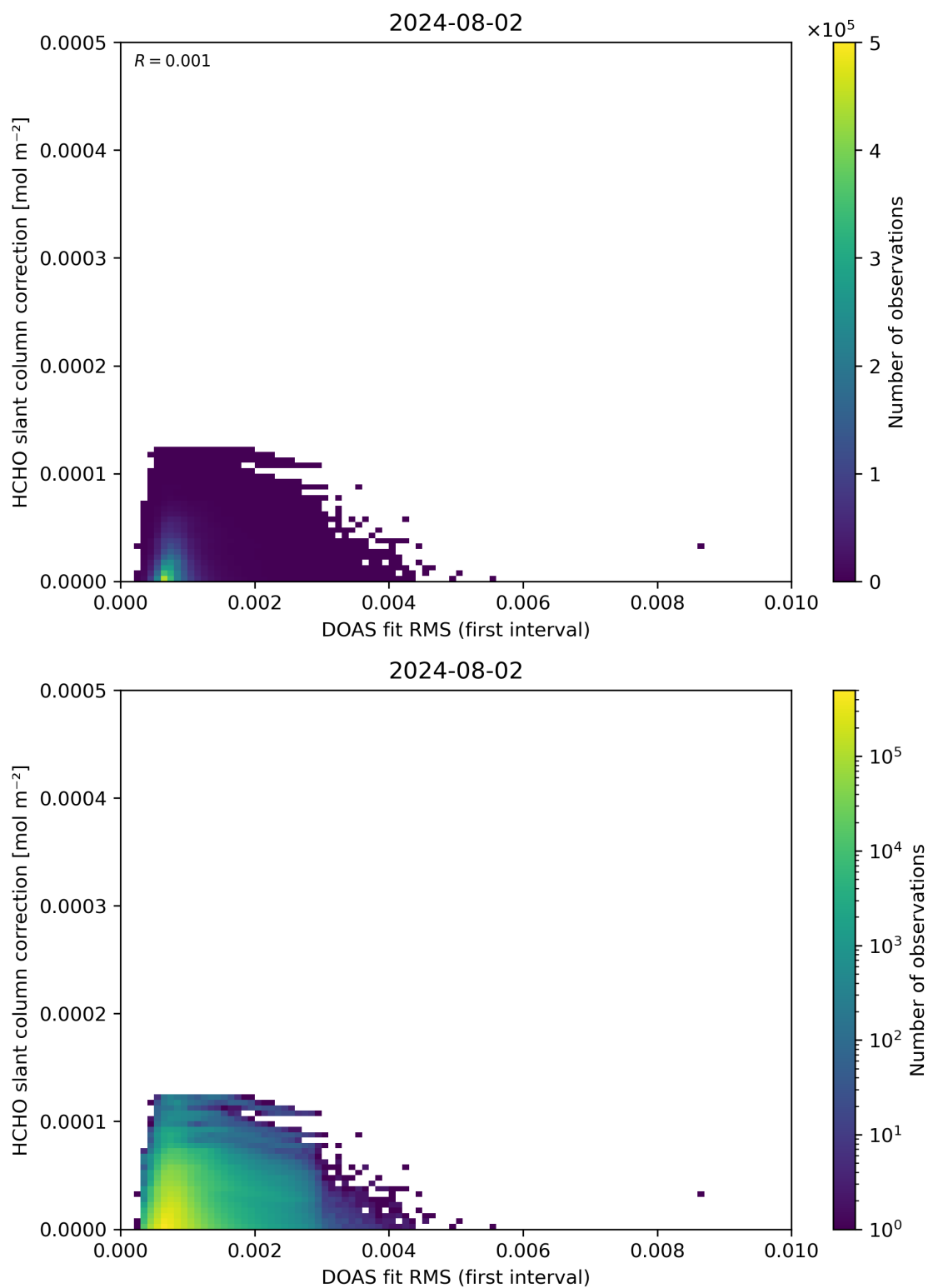
Figure 63: Scatter density plot of “DOAS fit RMS (first interval)” against “HCHO slant column correction” for 2024-08-01 to 2024-08-03.
