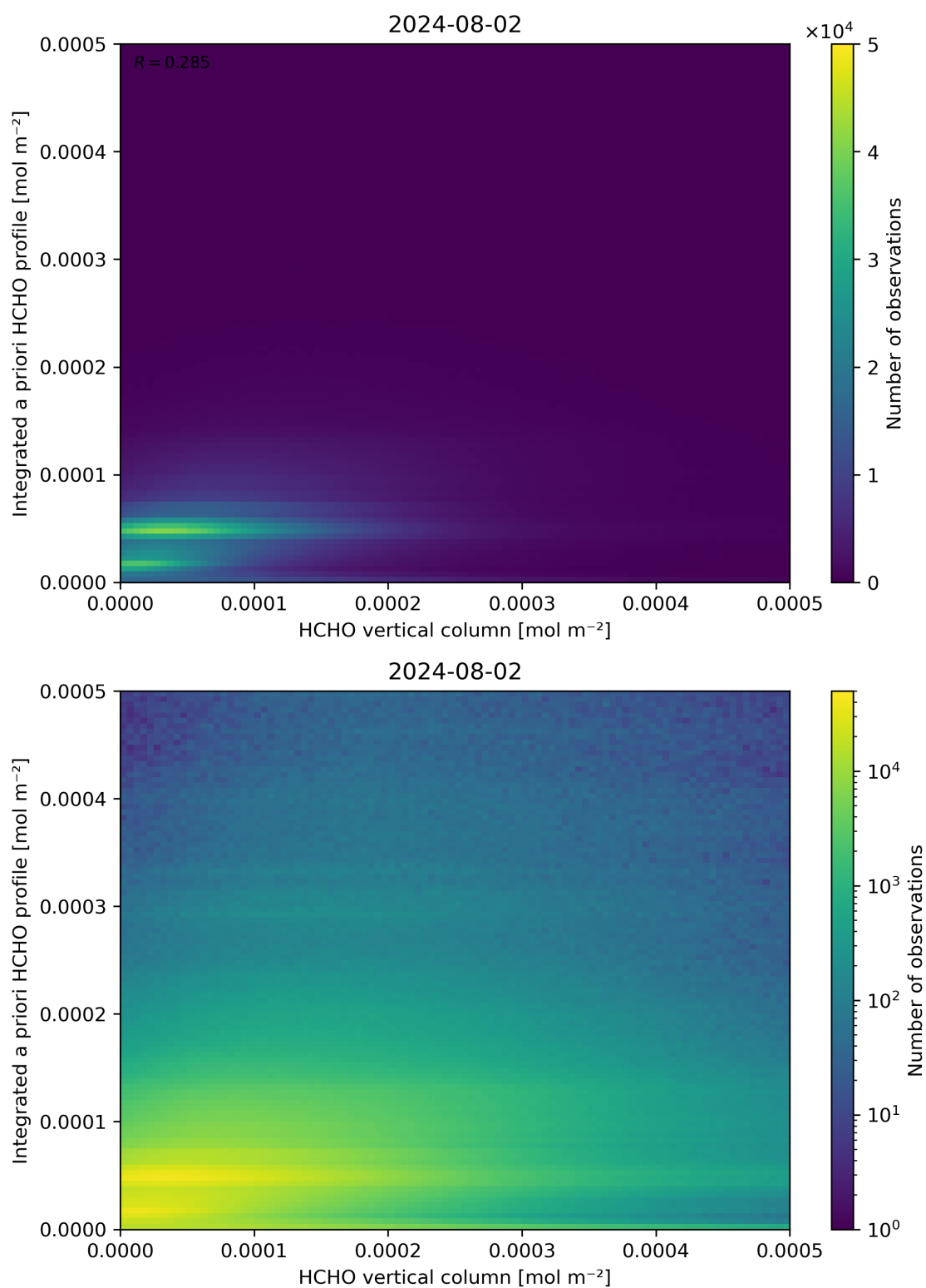
Figure 135: Scatter density plot of “HCHO vertical column” against “Integrated a priori HCHO profile” for 2024-08-01 to 2024-08-03.
