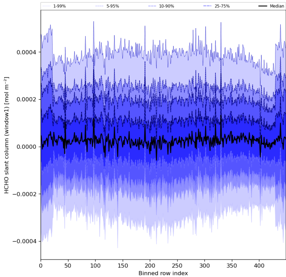
Figure 52: Along track statistics of “HCHO slant column (window1)” for 2024-08-01 to 2024-08-03
