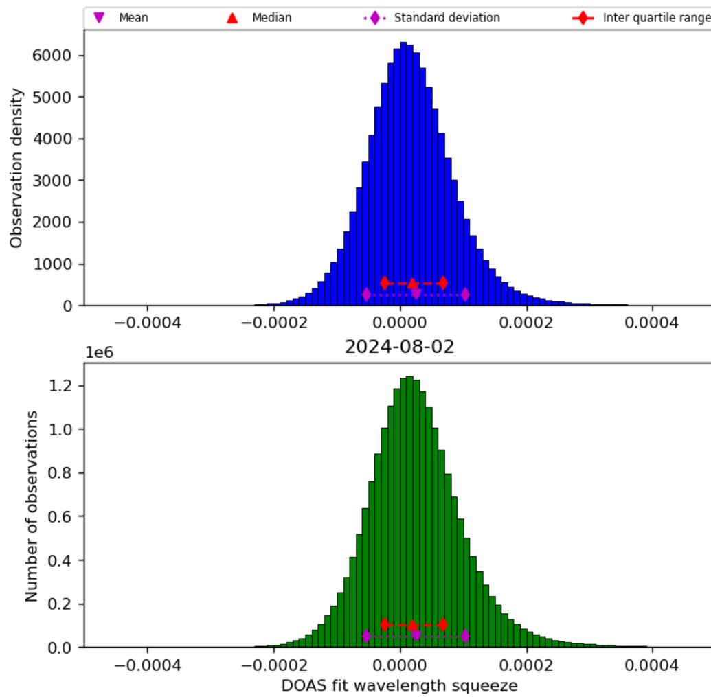
Figure 45: Histogram of “DOAS fit wavelength squeeze” for 2024-08-01 to 2024-08-03
