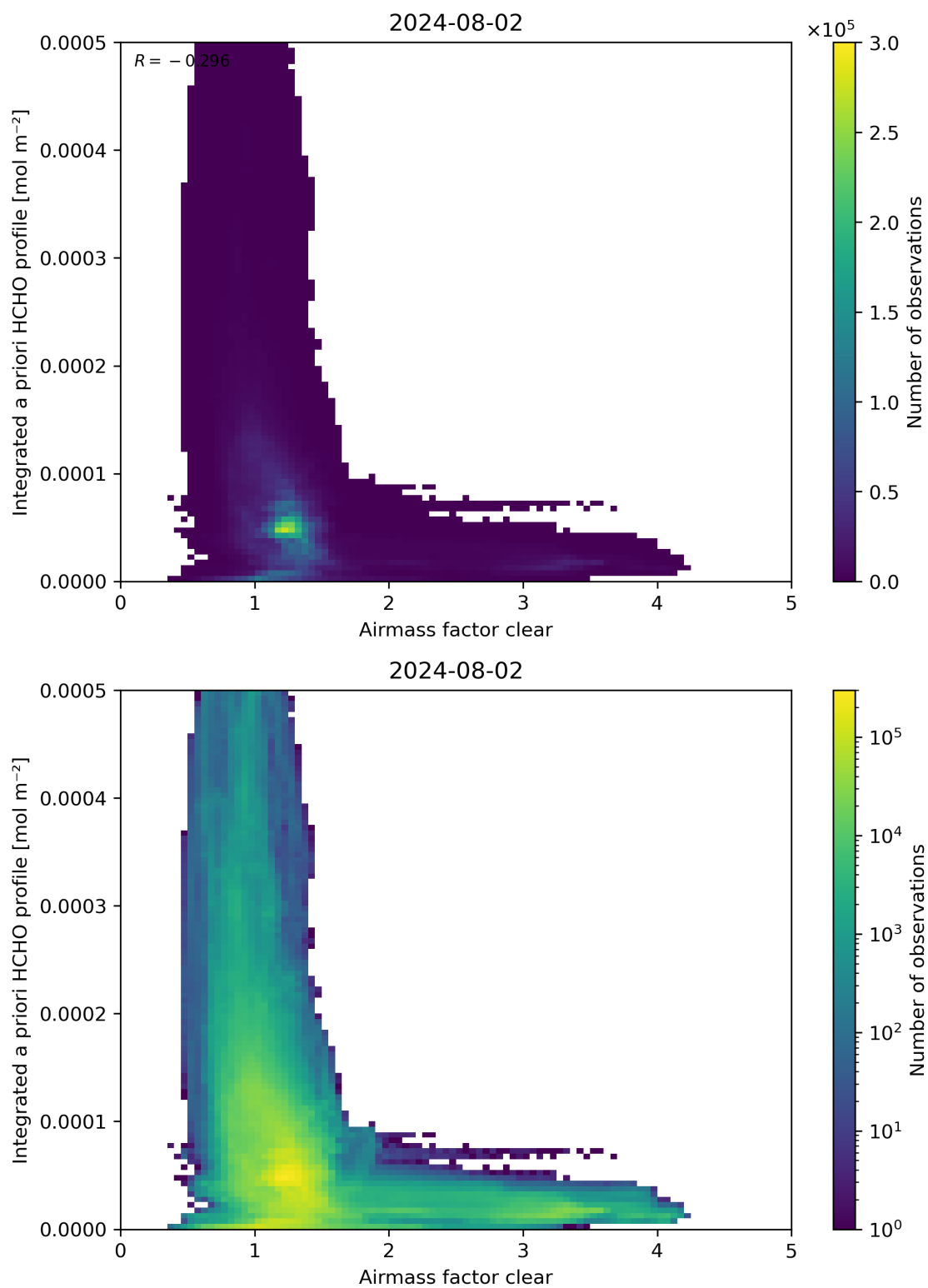
Figure 76: Scatter density plot of “Airmass factor clear” against “Integrated a priori HCHO profile” for 2024-08-01 to 2024-08-03.
