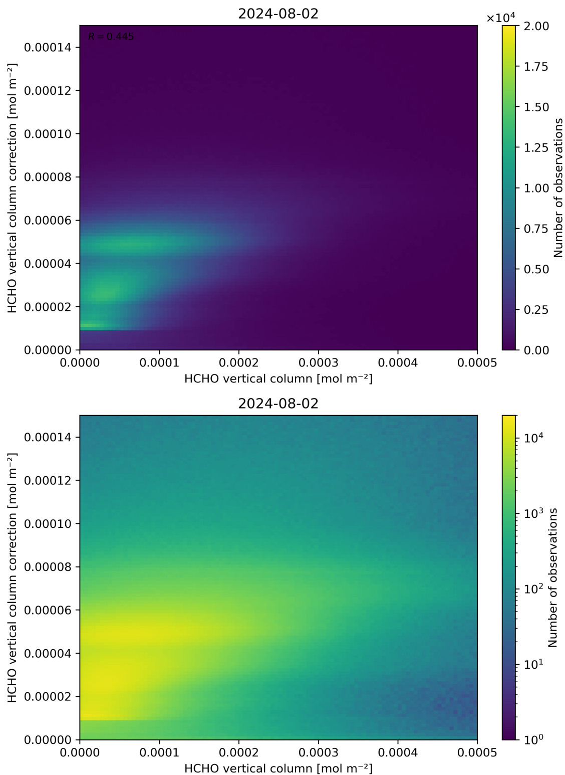
Figure 133: Scatter density plot of “HCHO vertical column” against “HCHO vertical column correction” for 2024-08-01 to 2024-08-03.
