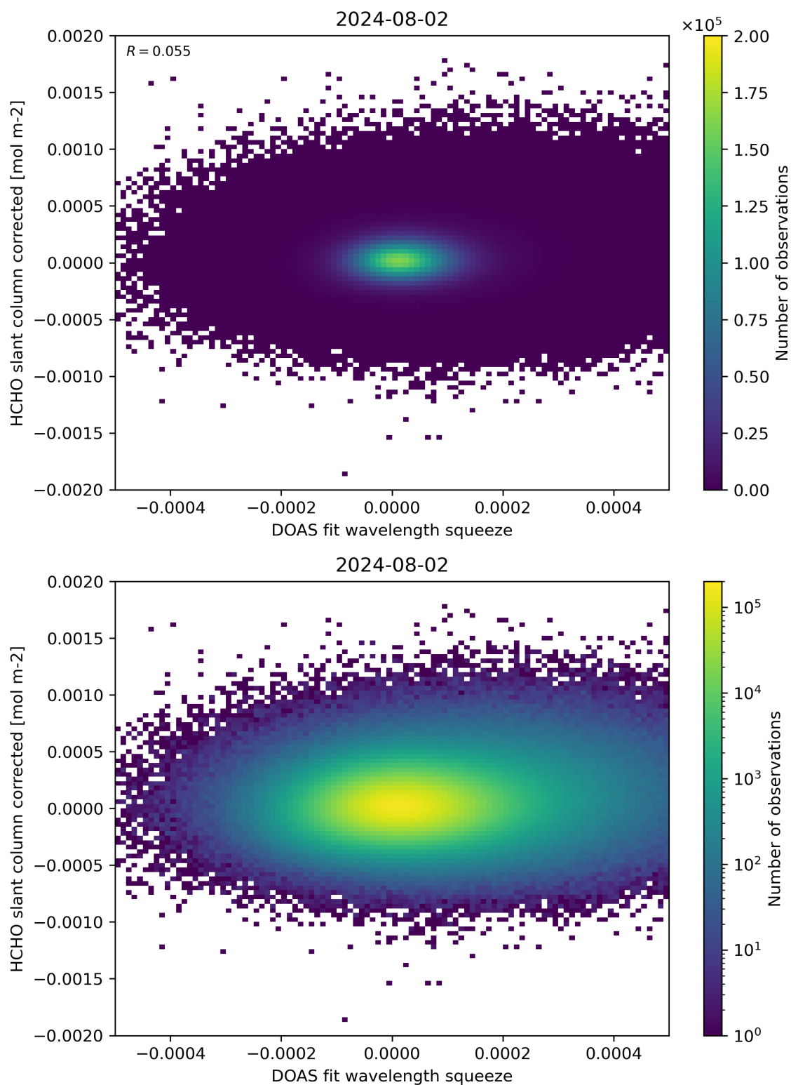
Figure 69: Scatter density plot of “DOAS fit wavelength squeeze” against “HCHO slant column corrected” for 2024-08-01 to 2024-08-03.
