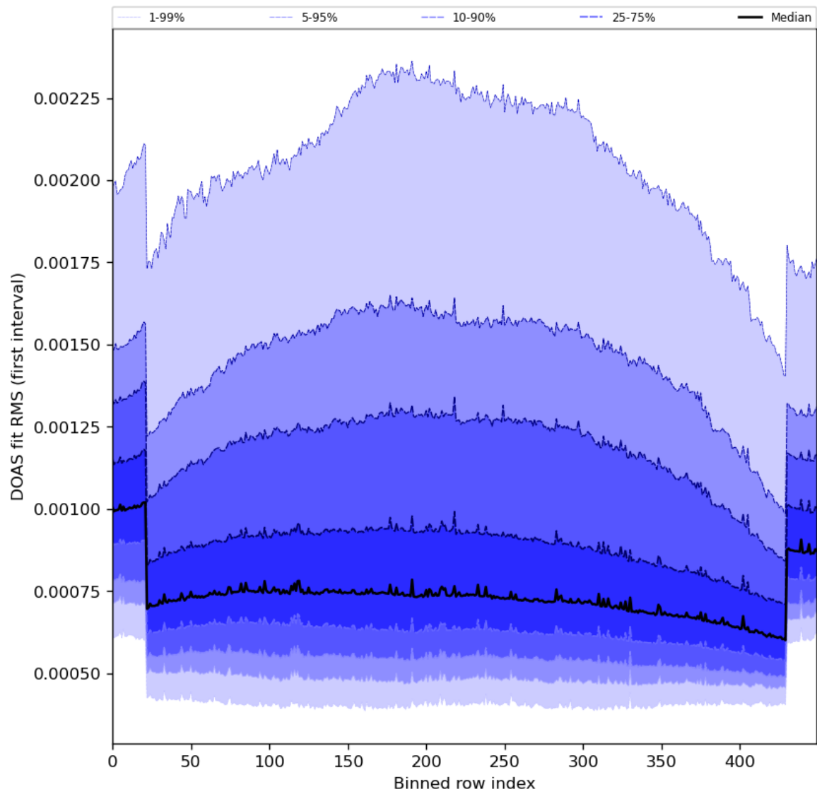
Figure 60: Along track statistics of “DOAS fit RMS (first interval)” for 2024-08-01 to 2024-08-03
