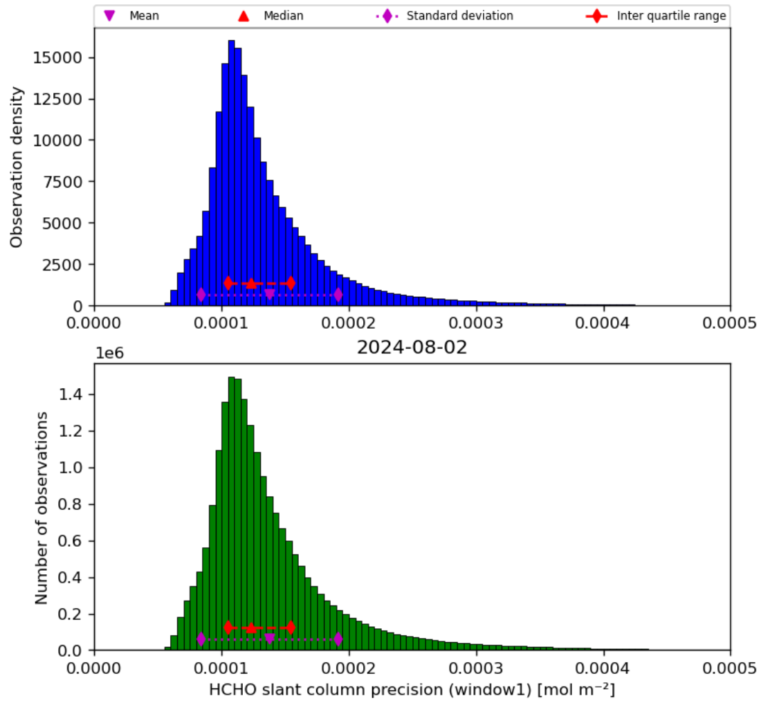
Figure 39: Histogram of “HCHO slant column precision (window1)” for 2024-08-01 to 2024-08-03
