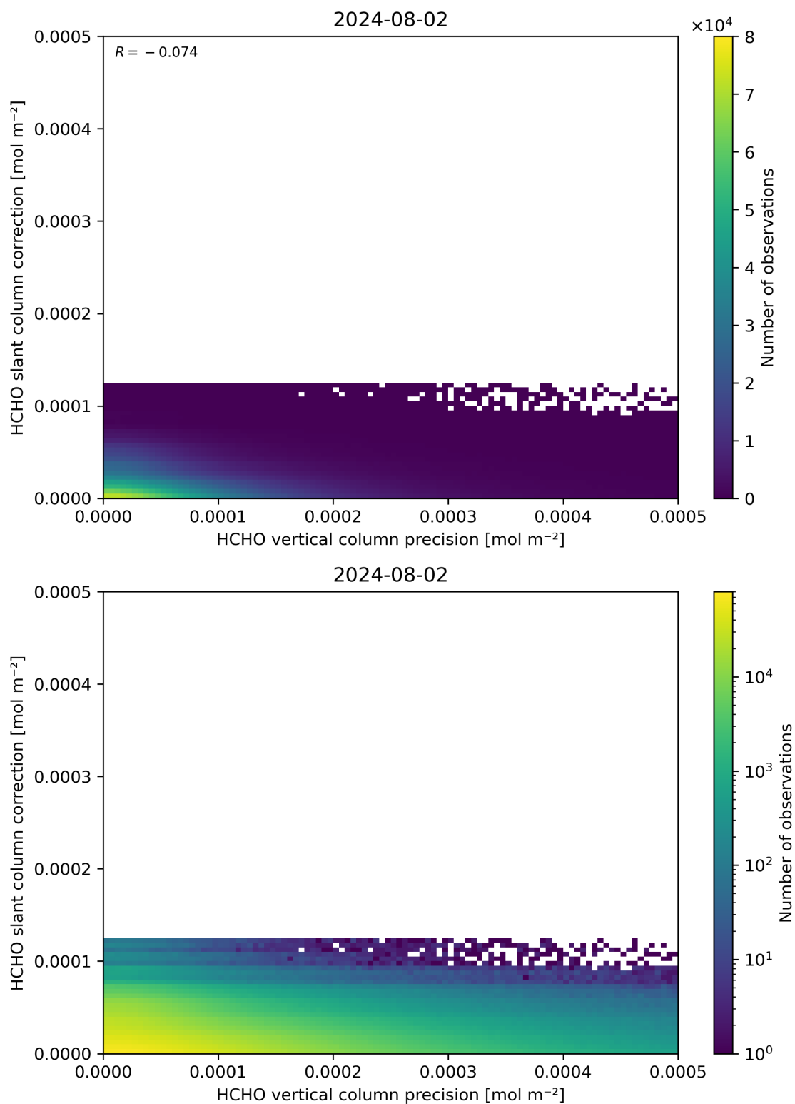
Figure 141: Scatter density plot of “HCHO vertical column precision” against “HCHO slant column correction” for 2024-08-01 to 2024-08-03.
