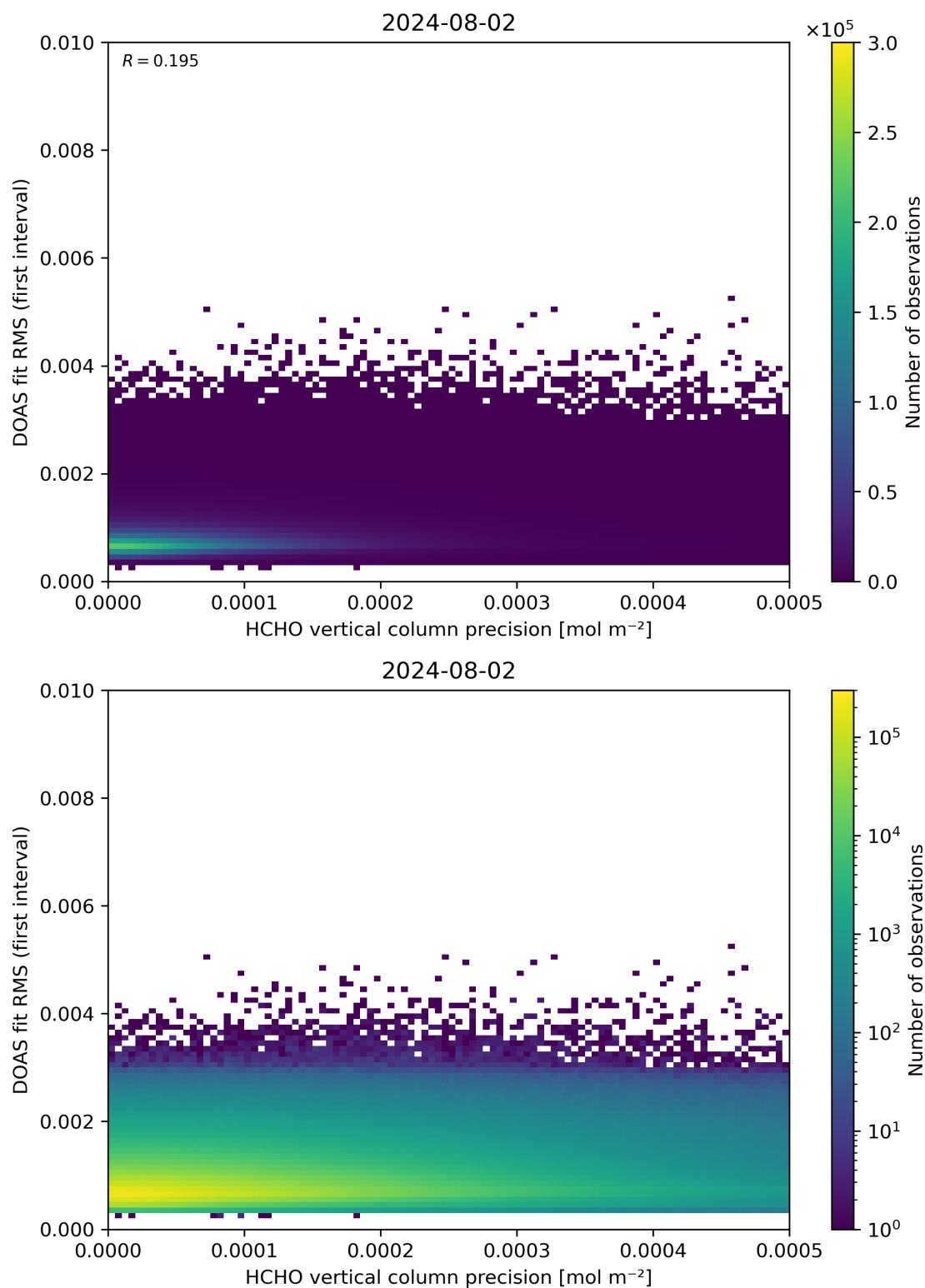
Figure 136: Scatter density plot of “HCHO vertical column precision” against “DOAS fit RMS (first interval)” for 2024-08-01 to 2024-08-03.
