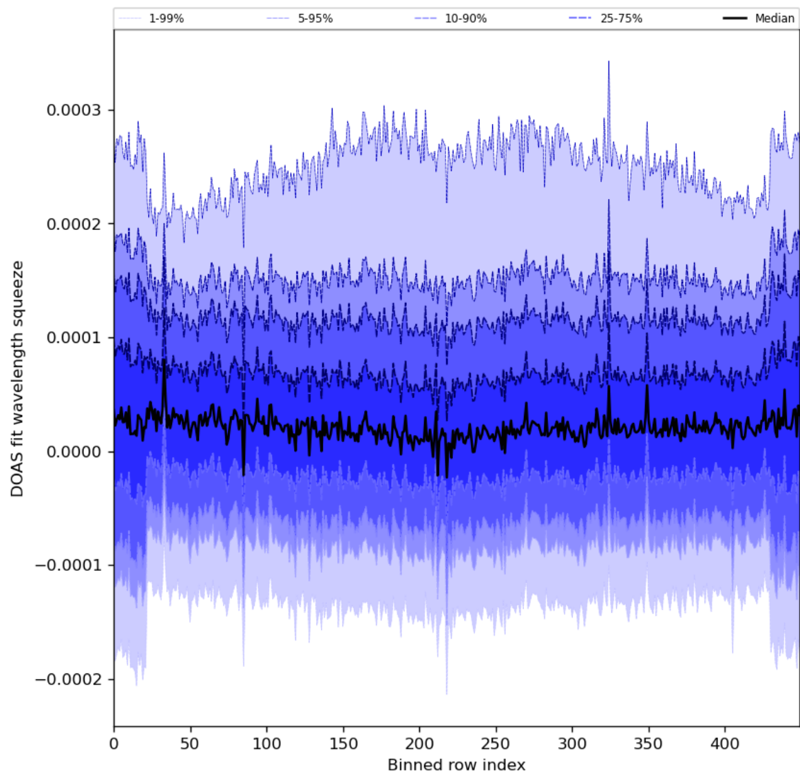
Figure 59: Along track statistics of “DOAS fit wavelength squeeze” for 2024-08-01 to 2024-08-03
