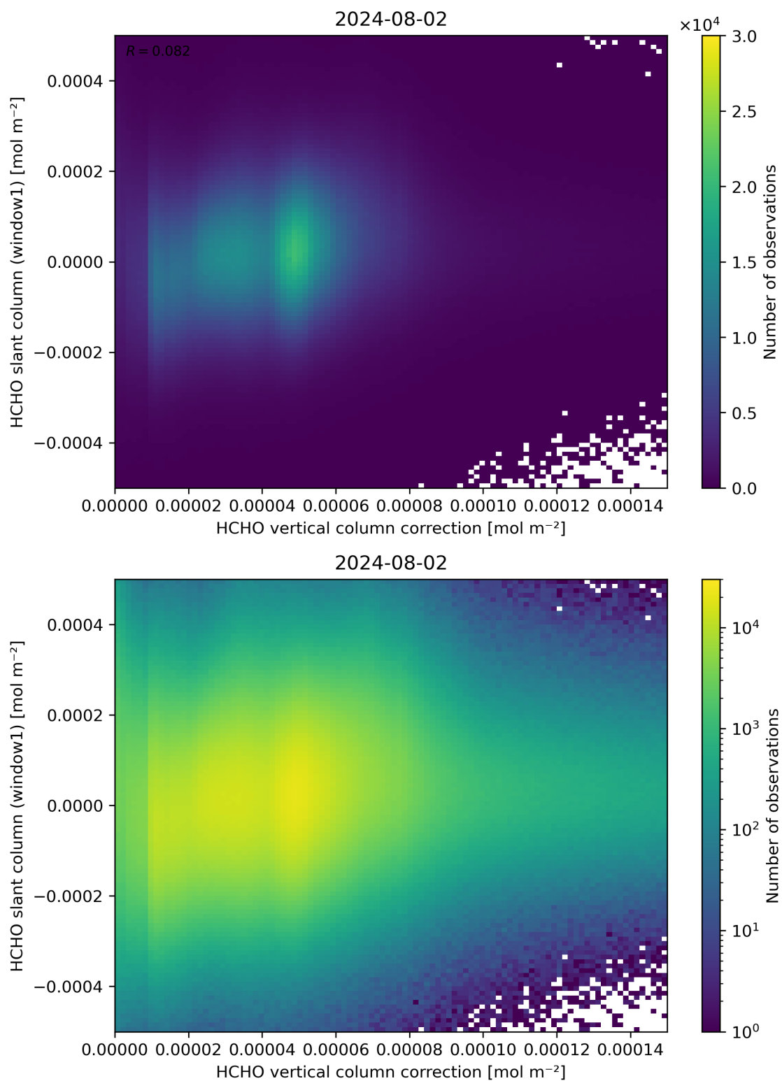
Figure 118: Scatter density plot of “HCHO vertical column correction” against “HCHO slant column (window1)” for 2024-08-01 to 2024-08-03.
