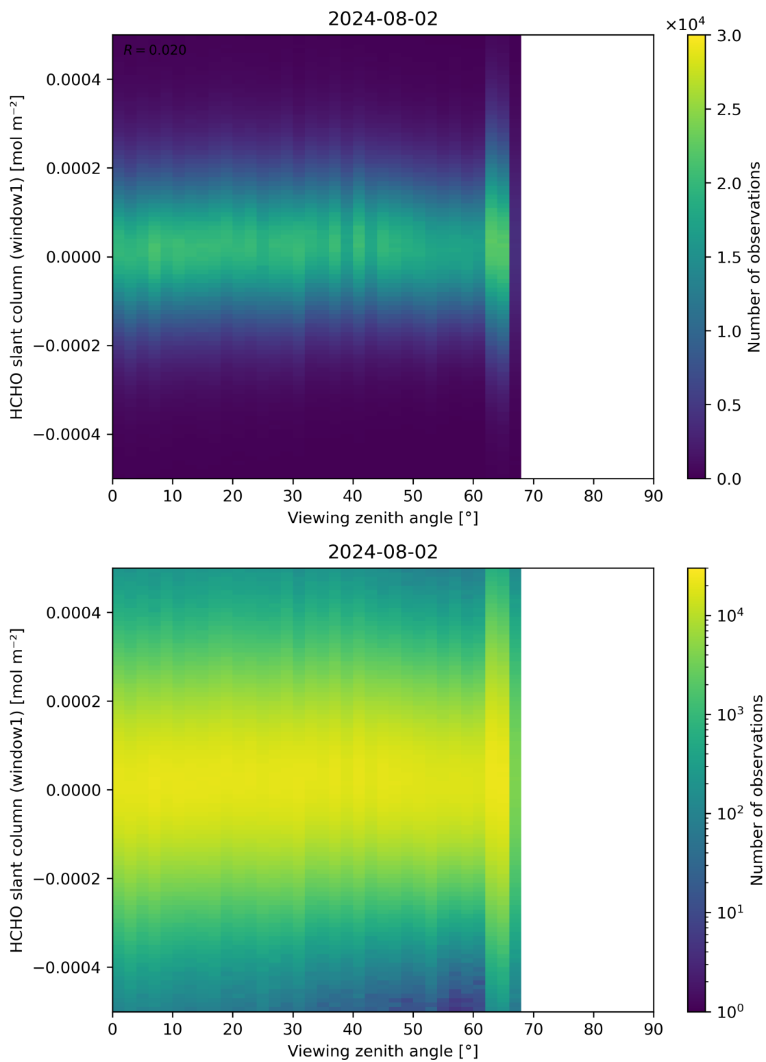
Figure 188: Scatter density plot of “Viewing zenith angle” against “HCHO slant column (window1)” for 2024-08-01 to 2024-08-03.
