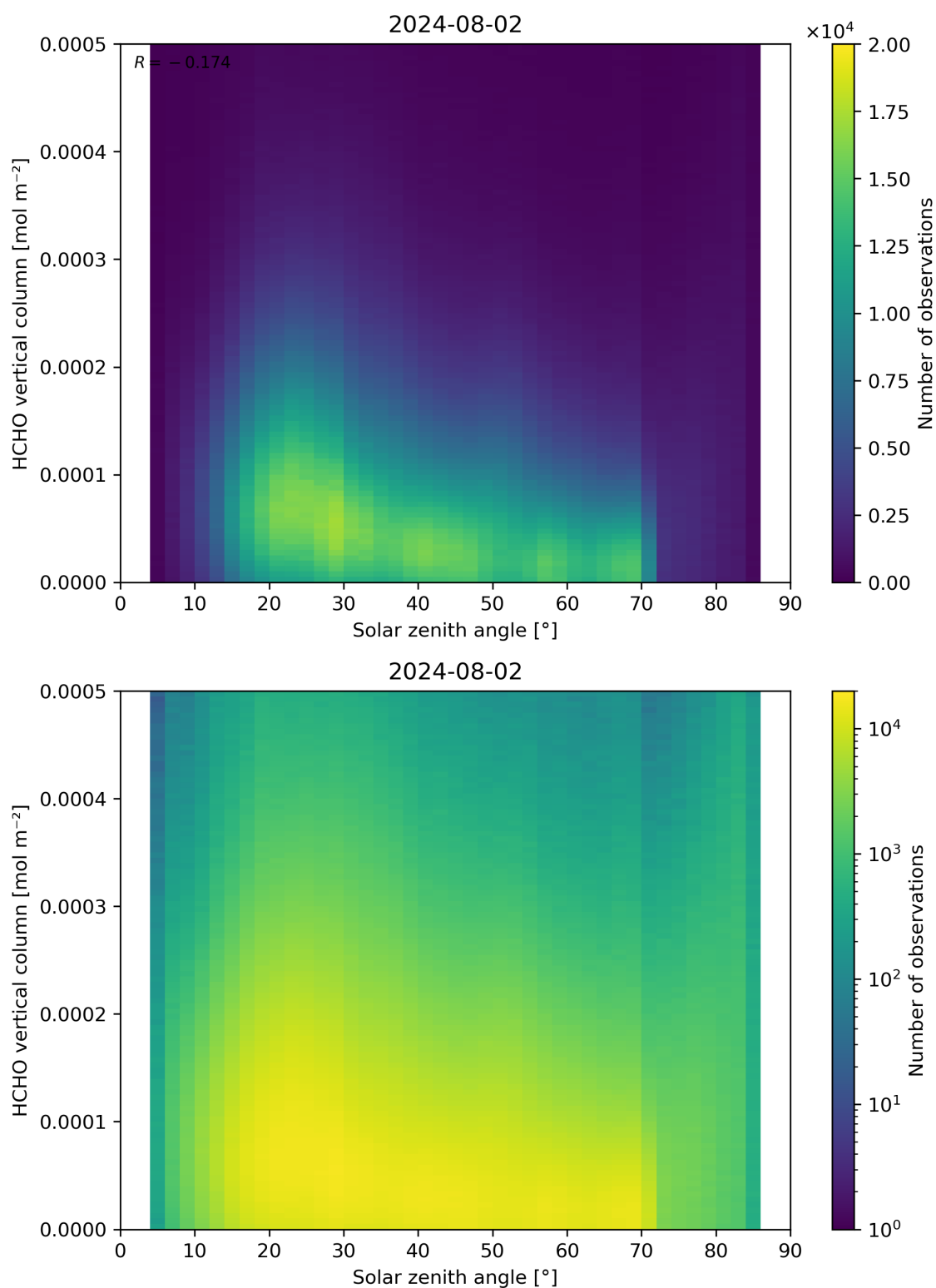
Figure 177: Scatter density plot of “Solar zenith angle” against “HCHO vertical column” for 2024-08-01 to 2024-08-03.
