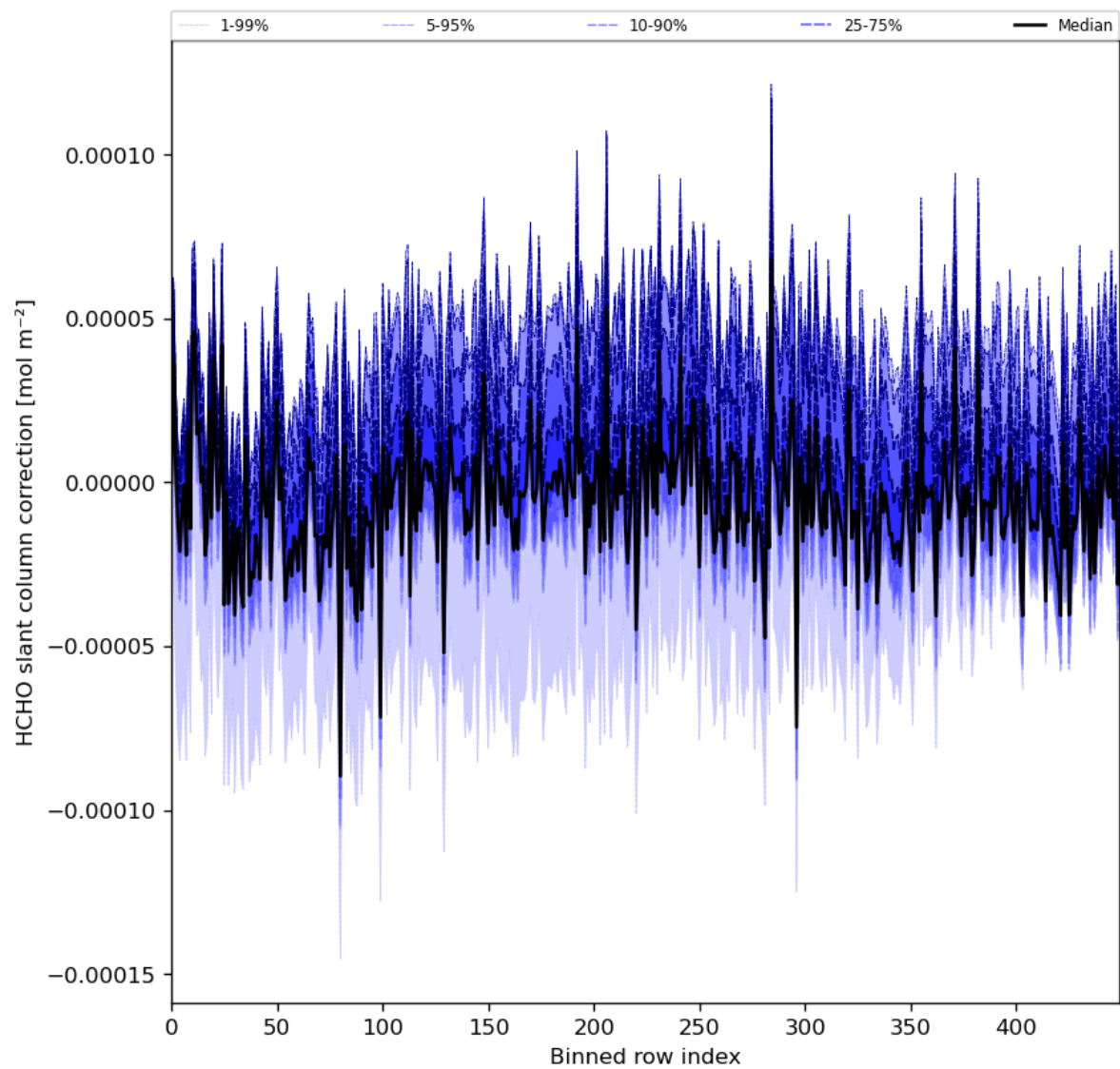
Figure 61: Along track statistics of “HCHO slant column correction” for 2024-08-01 to 2024-08-03
