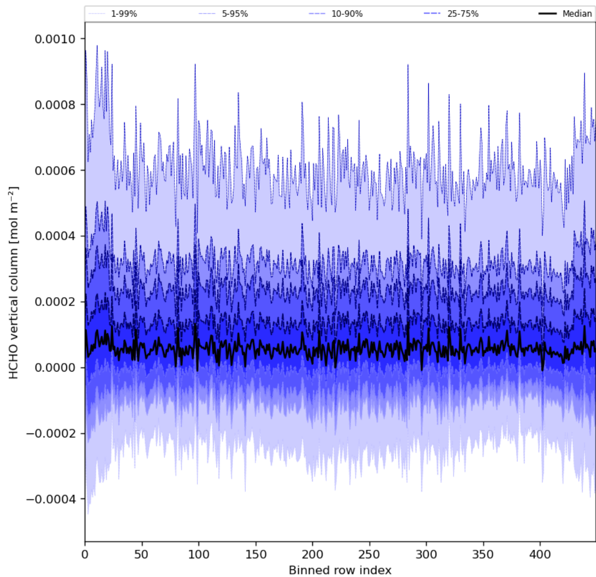
Figure 49: Along track statistics of “HCHO vertical column” for 2024-08-01 to 2024-08-03
