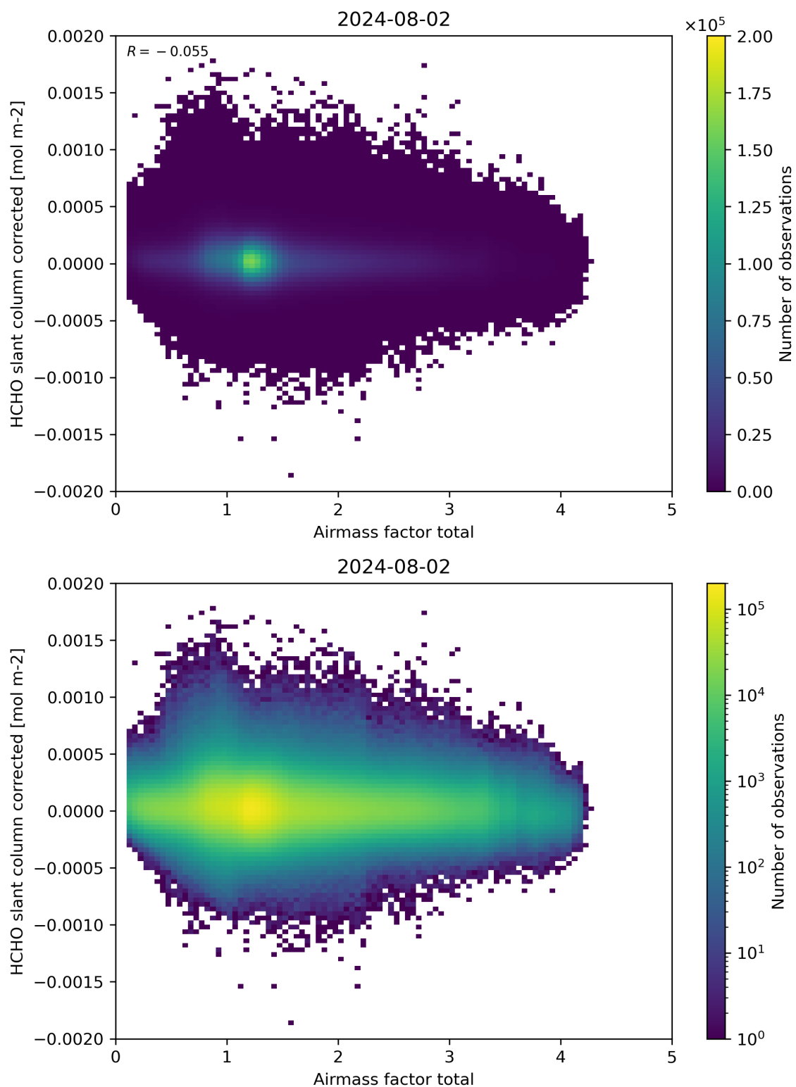
Figure 101: Scatter density plot of “Airmass factor total” against “HCHO slant column corrected” for 2024-08-01 to 2024-08-03.
