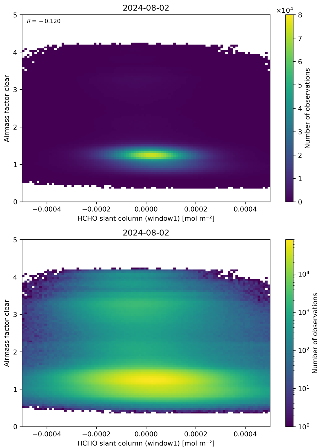
Figure 81: Scatter density plot of “HCHO slant column (window1)” against “Airmass factor clear” for 2024-08-01 to 2024-08-03.
