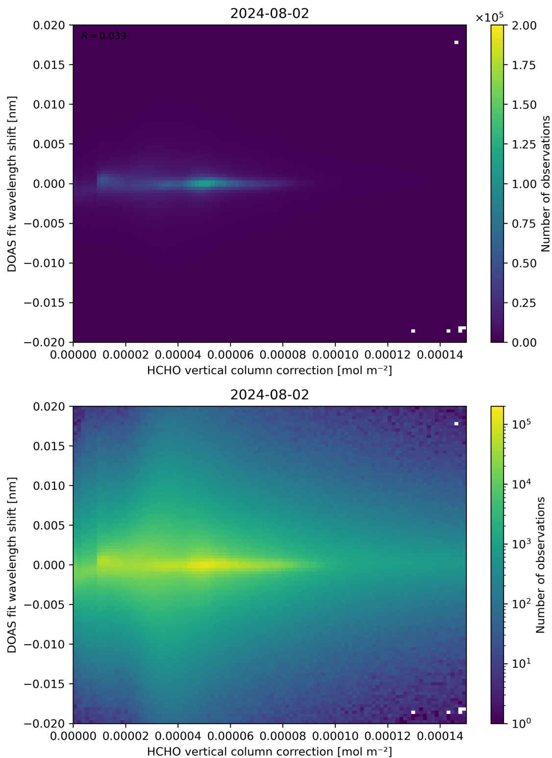
Figure 113: Scatter density plot of “HCHO vertical column correction” against “DOAS fit wavelength shift” for 2024-08-01 to 2024-08-03.
