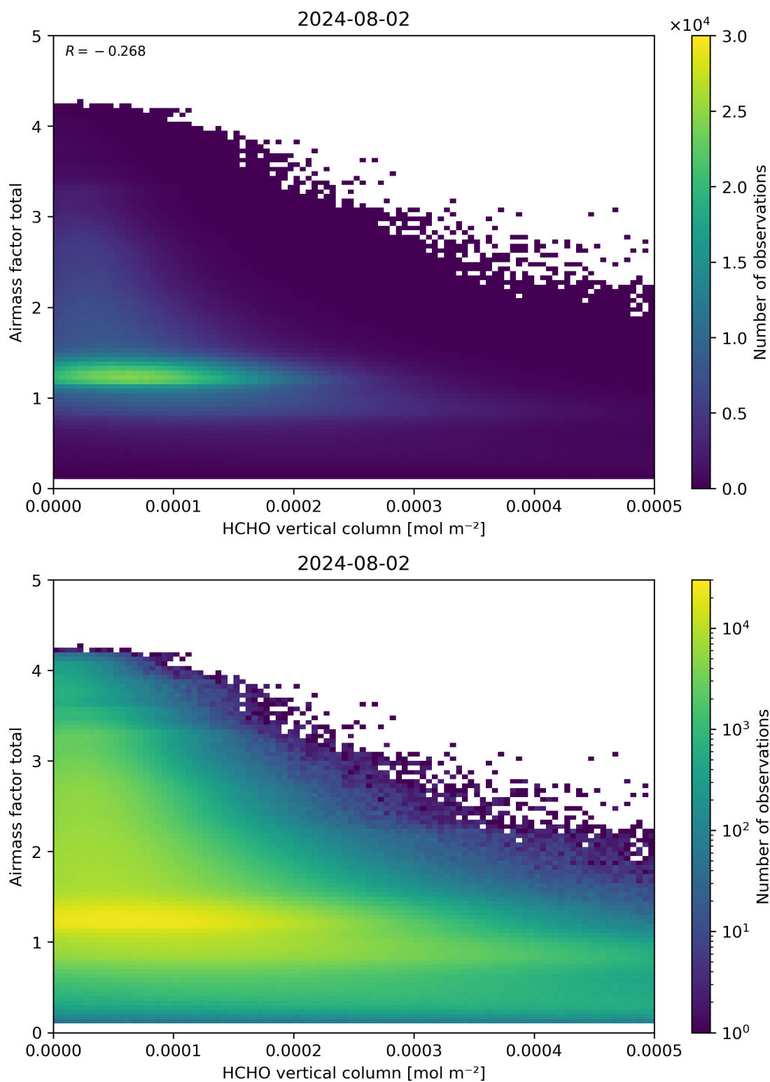
Figure 131: Scatter density plot of “HCHO vertical column” against “Airmass factor total” for 2024-08-01 to 2024-08-03.
