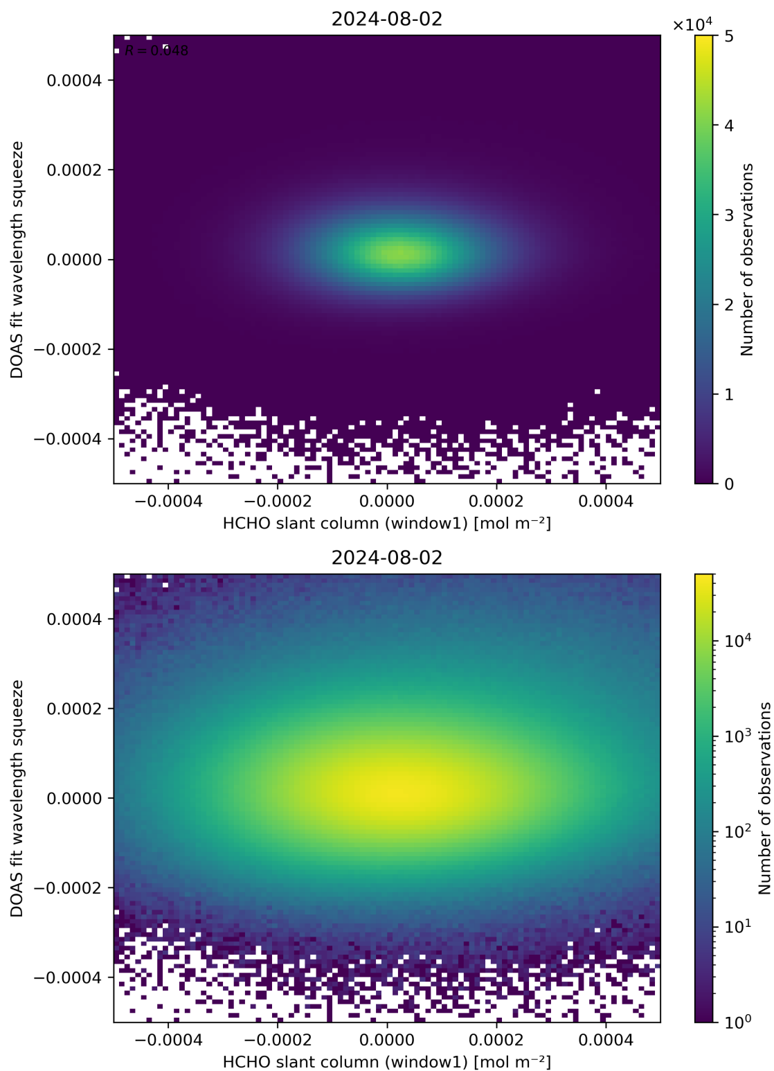
Figure 80: Scatter density plot of “HCHO slant column (window1)” against “DOAS fit wavelength squeeze” for 2024-08-01 to 2024-08-03.
