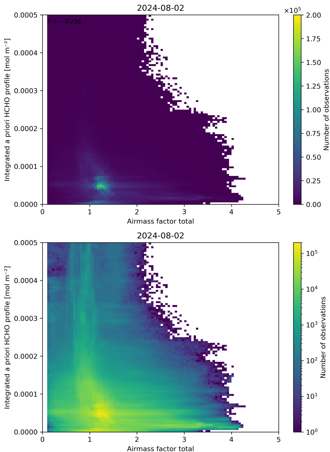
Figure 104: Scatter density plot of “Air mass factor total” against “Integrated a priori HCHO profile” for 2024-08-01 to 2024-08-03.
