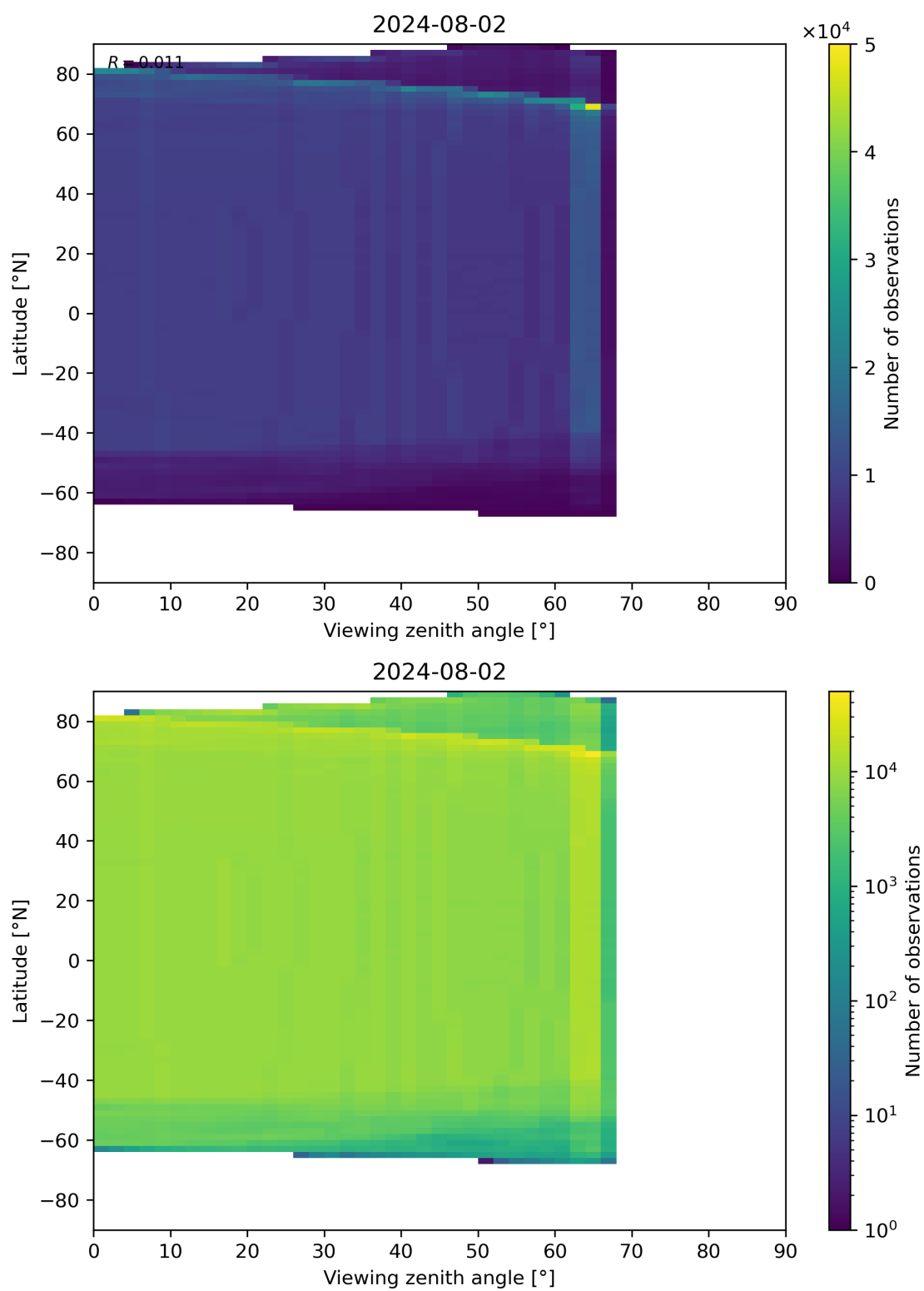
Figure 196: Scatter density plot of “Viewing zenith angle” against “Latitude” for 2024-08-01 to 2024-08-03.
