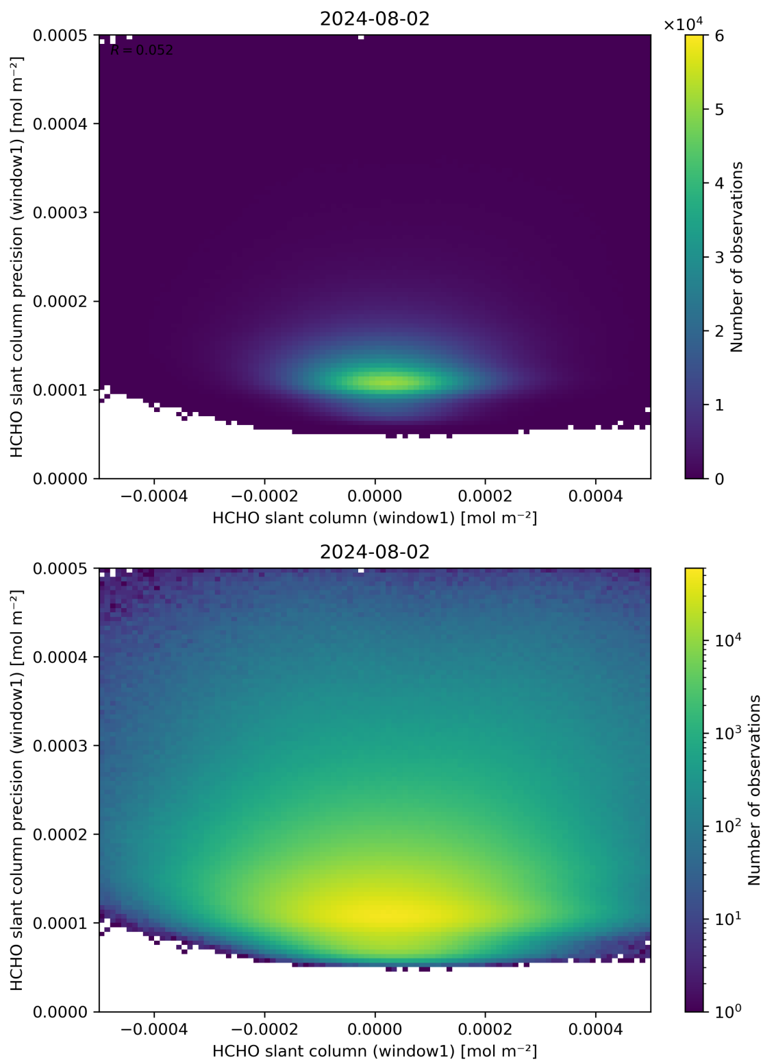
Figure 84: Scatter density plot of “HCHO slant column (window1)” against “HCHO slant column precision (window1)” for 2024-08-01 to 2024-08-03.
