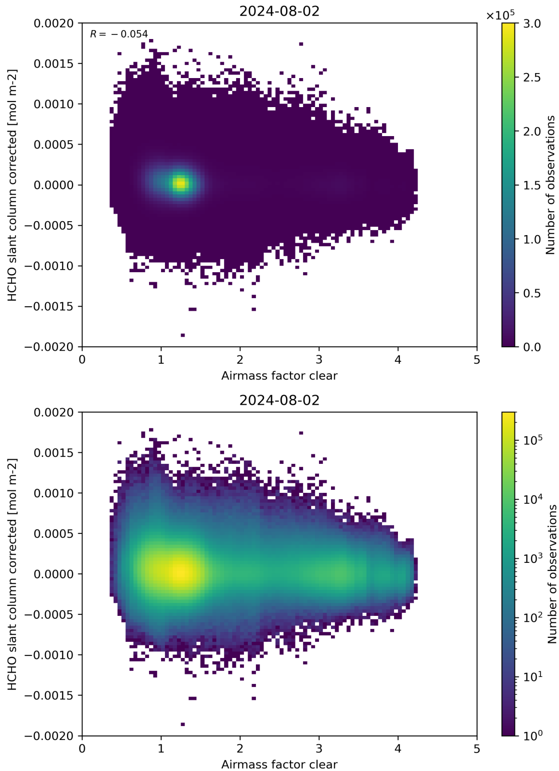
Figure 74: Scatter density plot of “Airmass factor clear” against “HCHO slant column corrected” for 2024-08-01 to 2024-08-03.
