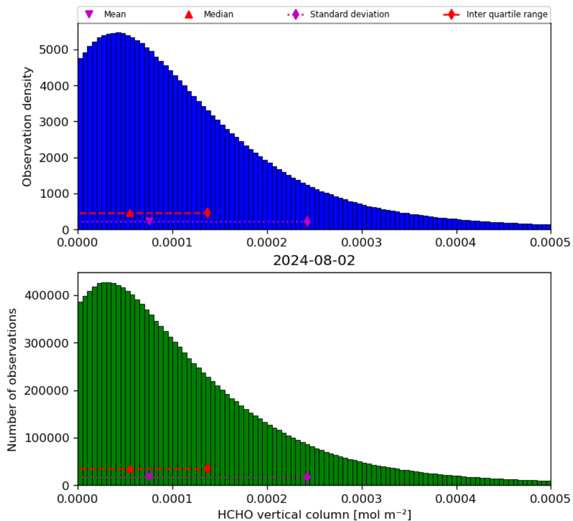
Figure 35: Histogram of “HCHO vertical column” for 2024-08-01 to 2024-08-03
