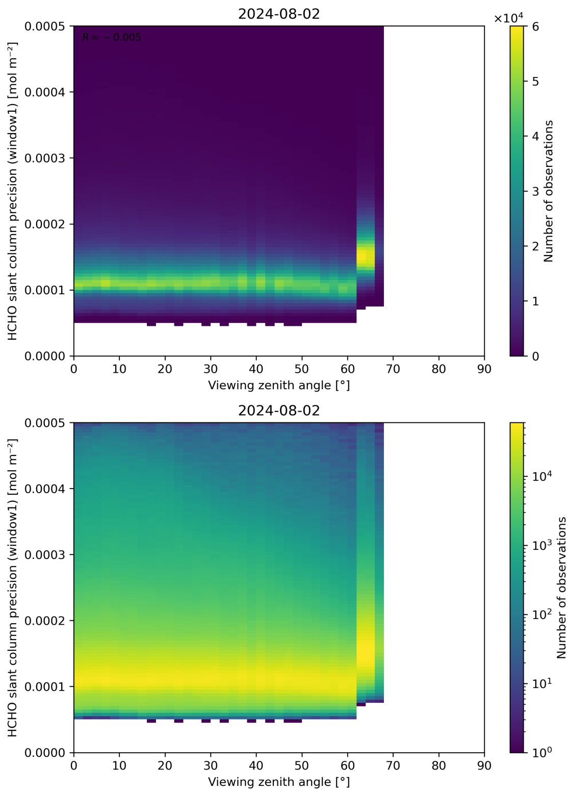
Figure 189: Scatter density plot of “Viewing zenith angle” against “HCHO slant column precision (window1)” for 2024-08-01 to 2024-08-03.
