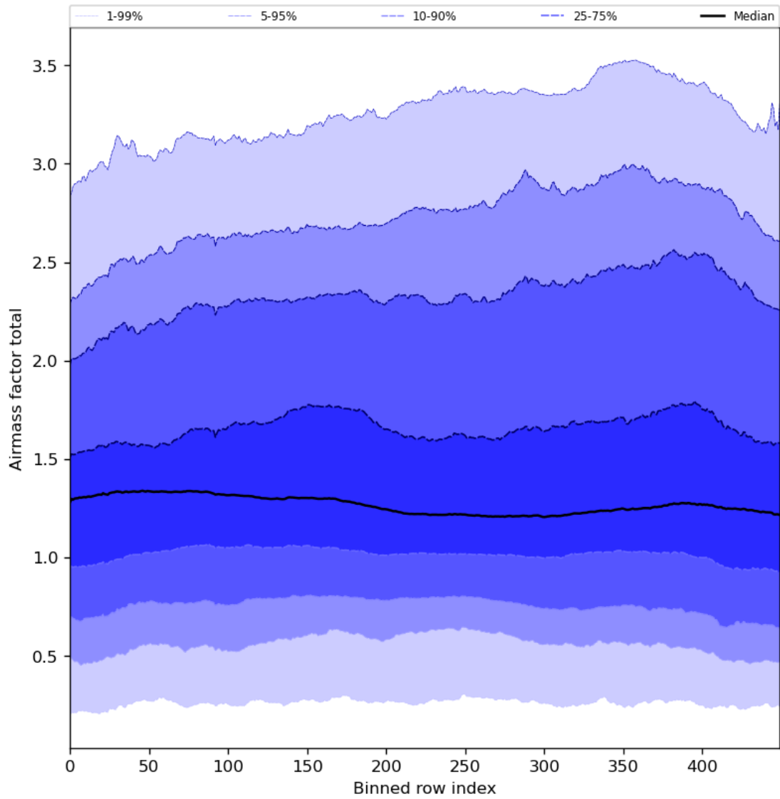
Figure 54: Along track statistics of “Airmass factor total” for 2024-08-01 to 2024-08-03
