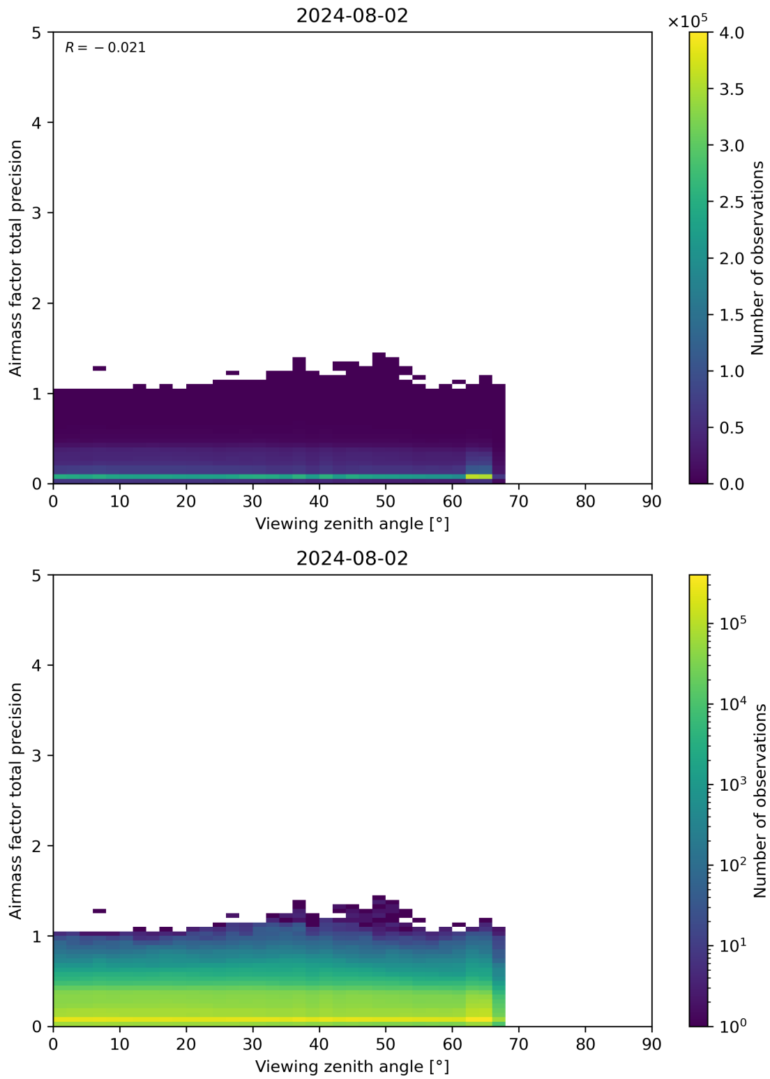
Figure 191: Scatter density plot of “Viewing zenith angle” against “Airmass factor total precision” for 2024-08-01 to 2024-08-03.
