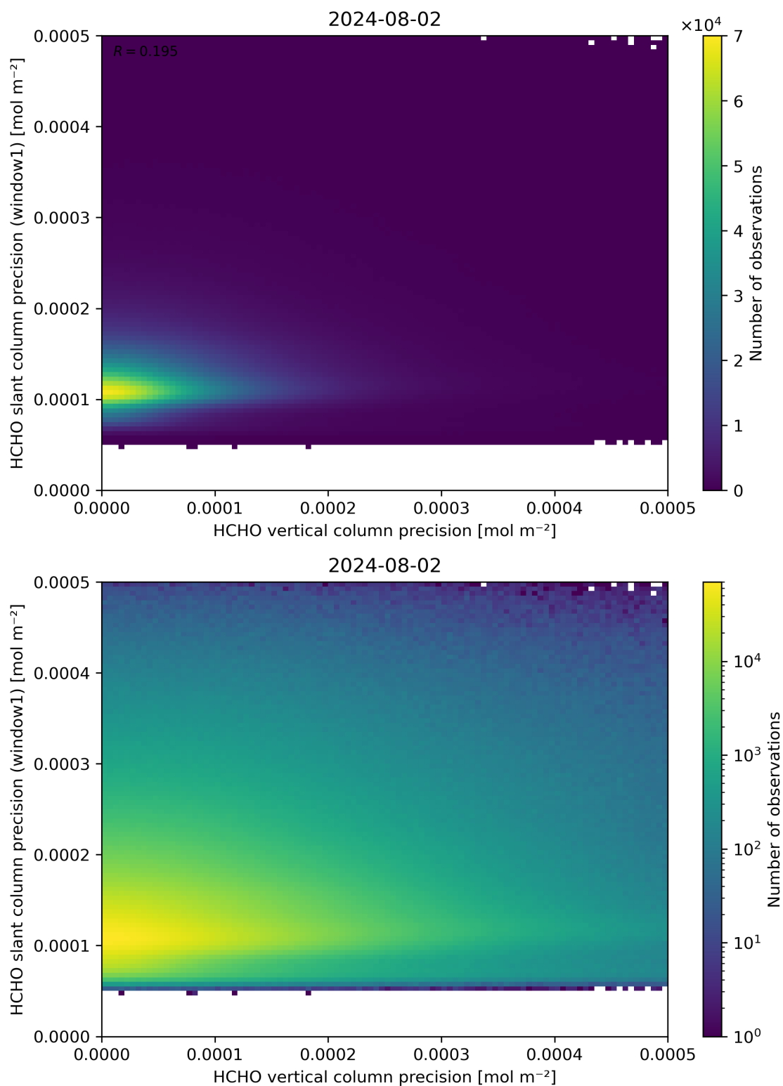
Figure 143: Scatter density plot of “HCHO vertical column precision” against “HCHO slant column precision (window1)” for 2024-08-01 to 2024-08-03.
