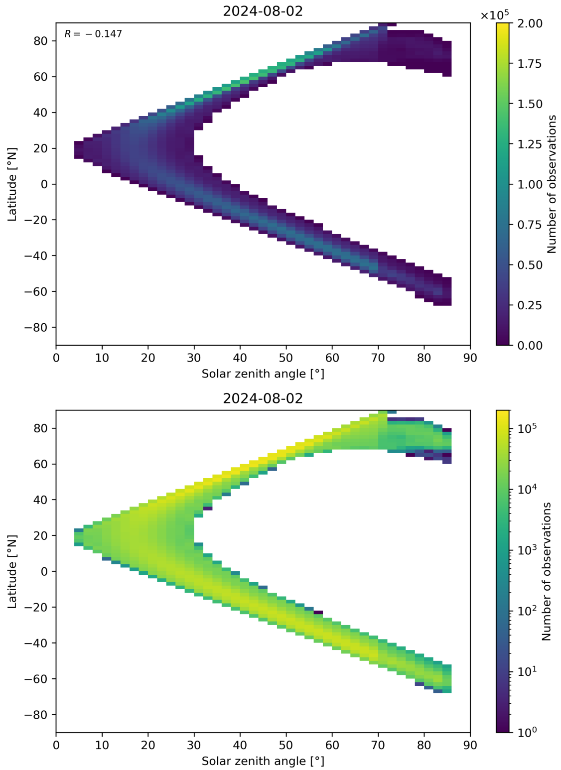
Figure 181: Scatter density plot of “Solar zenith angle” against “Latitude” for 2024-08-01 to 2024-08-03.
