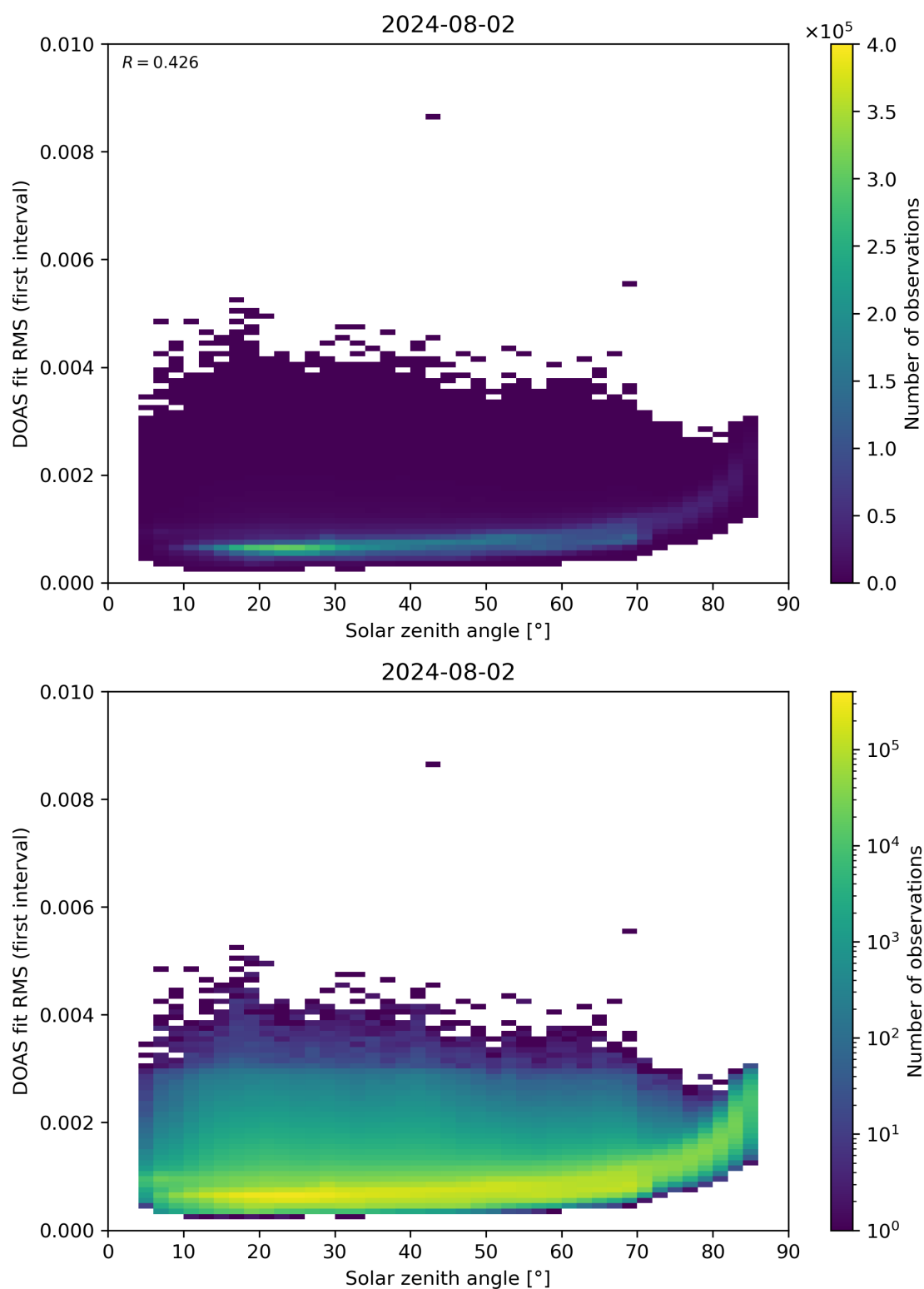
Figure 167: Scatter density plot of “Solar zenith angle” against “DOAS fit RMS (first interval)” for 2024-08-01 to 2024-08-03.
