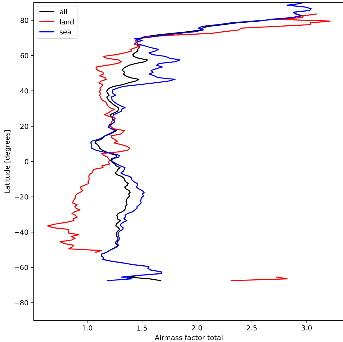
Figure 26: Zonal average of “Airmass factor total” for 2024-08-01 to 2024-08-03.
