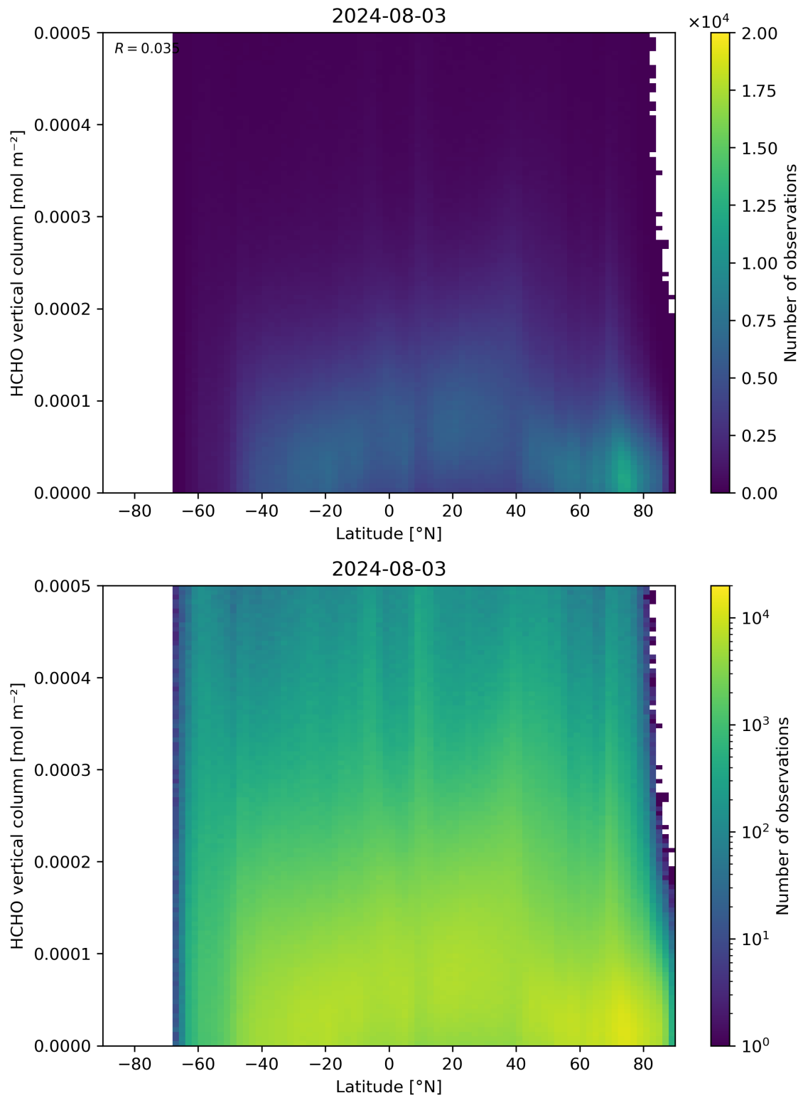
Figure 163: Scatter density plot of “Latitude” against “HCHO vertical column” for 2024-08-02 to 2024-08-04.
