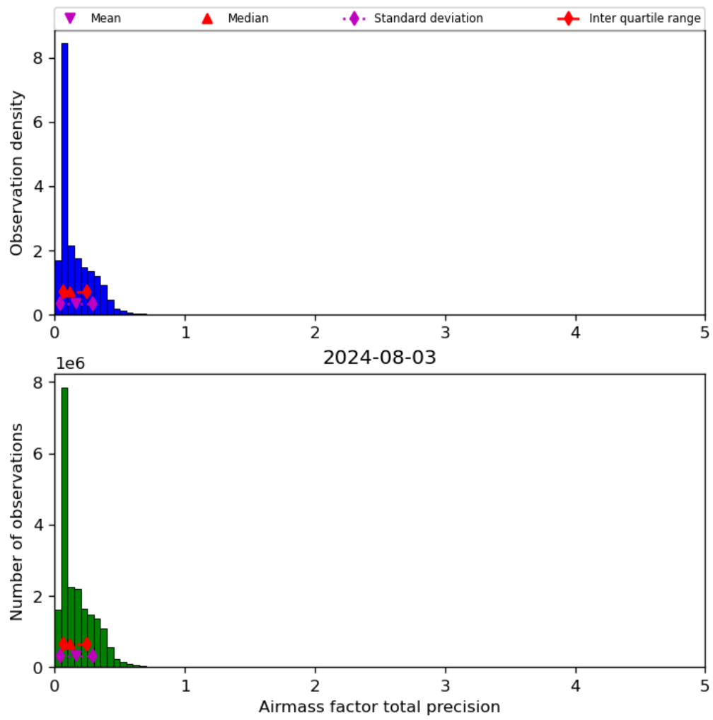
Figure 41: Histogram of “Airmass factor total precision” for 2024-08-02 to 2024-08-04
