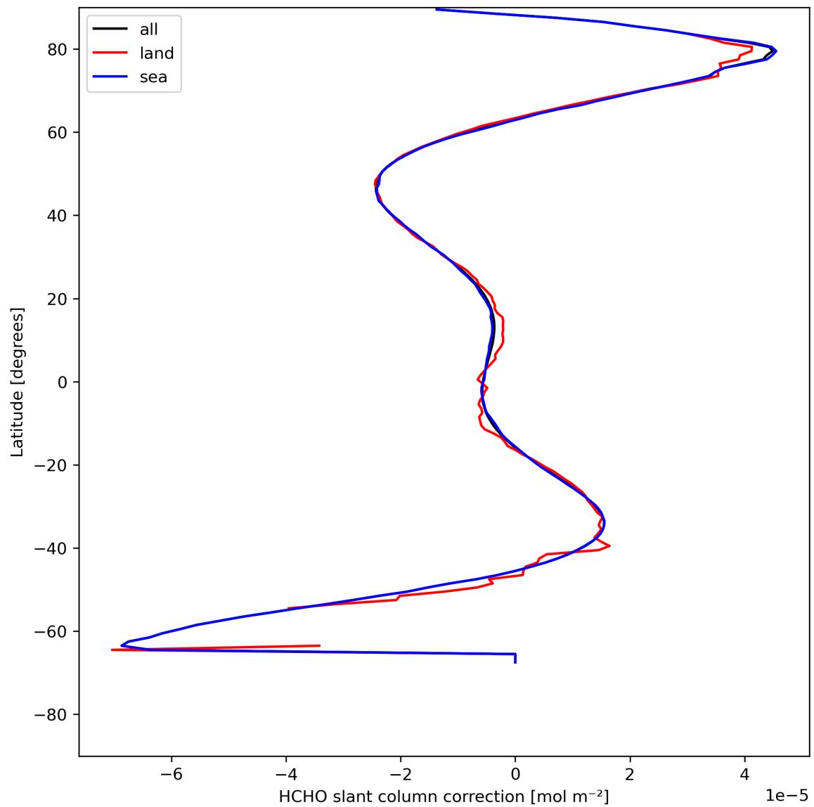
Figure 33: Zonal average of “HCHO slant column correction” for 2024-08-02 to 2024-08-04.
