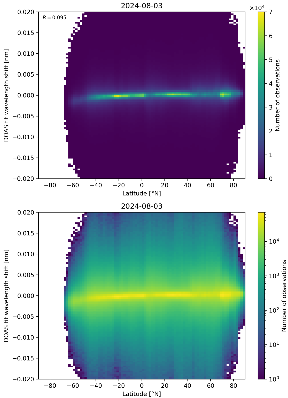
Figure 154: Scatter density plot of “Latitude” against “DOAS fit wavelength shift” for 2024-08-02 to 2024-08-04.
