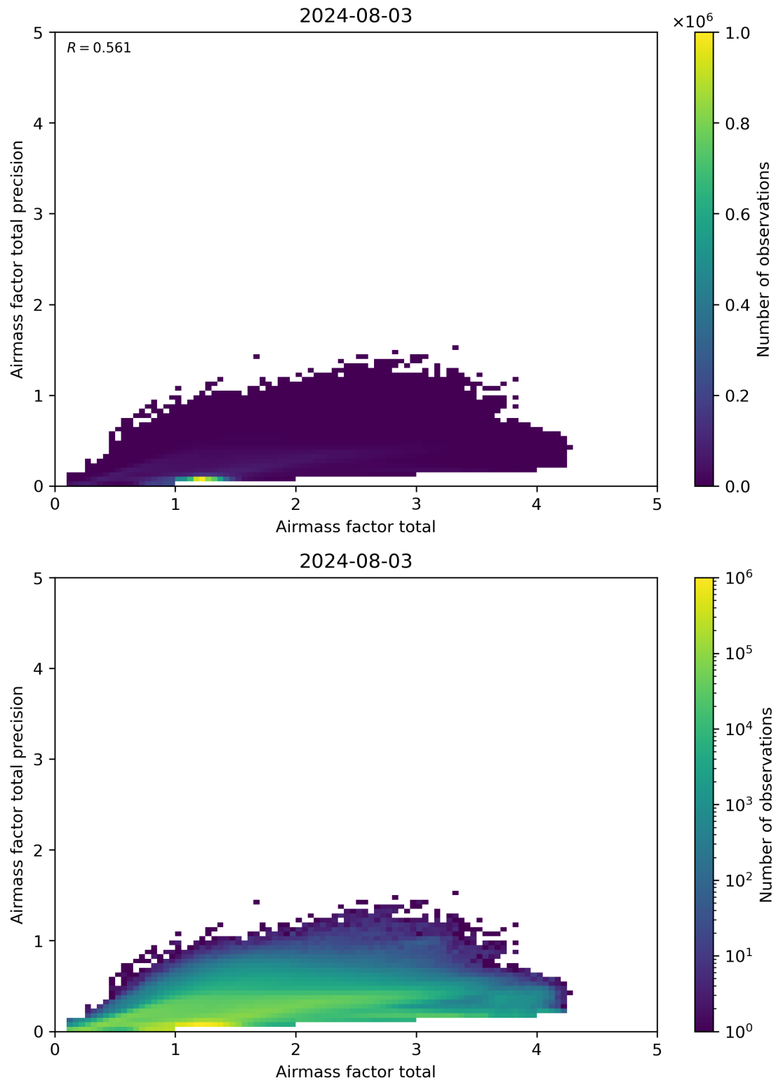
Figure 103: Scatter density plot of “Airmass factor total” against “Airmass factor total precision” for 2024-08-02 to 2024-08-04.
