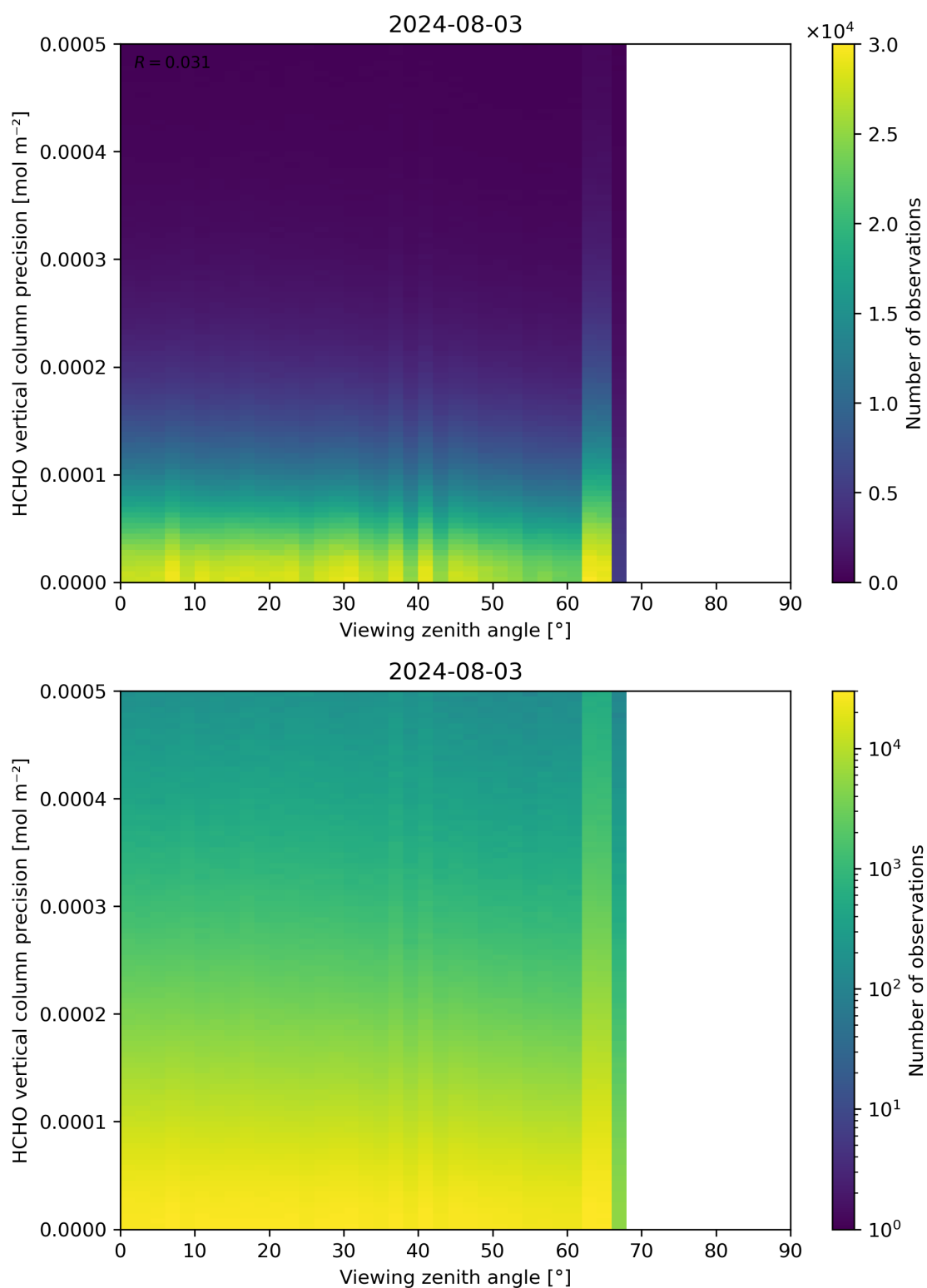
Figure 194: Scatter density plot of “Viewing zenith angle” against “HCHO vertical column precision” for 2024-08-02 to 2024-08-04.
