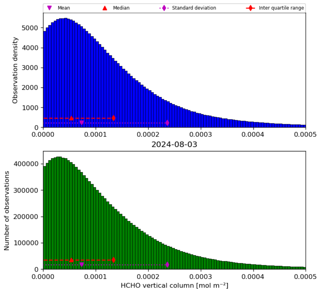
Figure 35: Histogram of “HCHO vertical column” for 2024-08-02 to 2024-08-04
