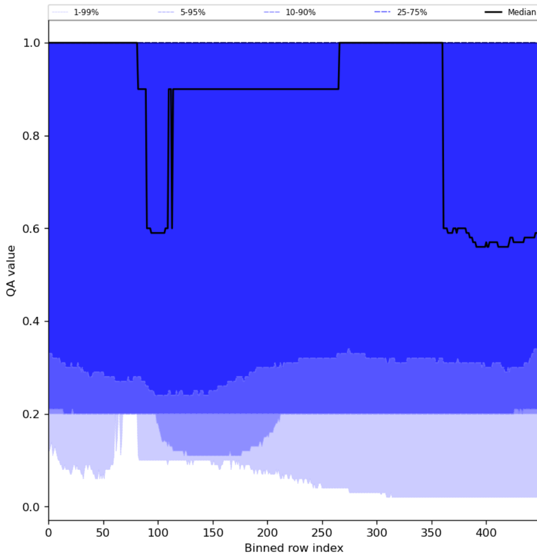
Figure 48: Along track statistics of “QA value” for 2024-08-02 to 2024-08-04
