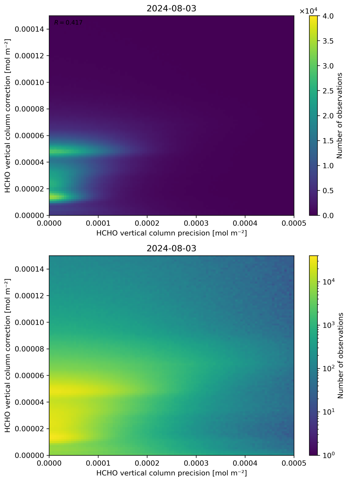
Figure 146: Scatter density plot of “HCHO vertical column precision” against “HCHO vertical column correction” for 2024-08-02 to 2024-08-04.
