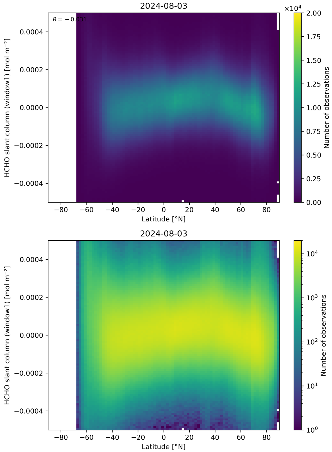
Figure 159: Scatter density plot of “Latitude” against “HCHO slant column (window1)” for 2024-08-02 to 2024-08-04.
