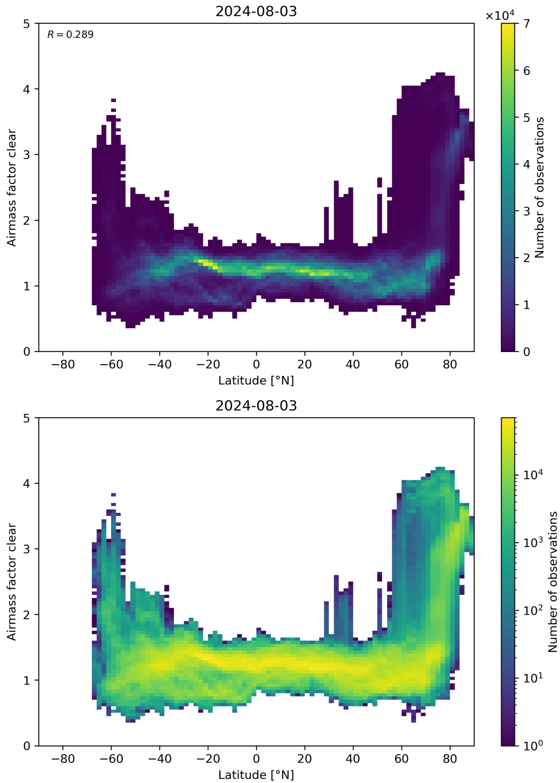
Figure 156: Scatter density plot of “Latitude” against “Airmass factor clear” for 2024-08-02 to 2024-08-04.
