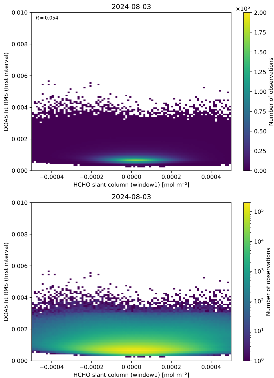
Figure 78: Scatter density plot of “HCHO slant column (window1)” against “DOAS fit RMS (first interval)” for 2024-08-02 to 2024-08-04.
