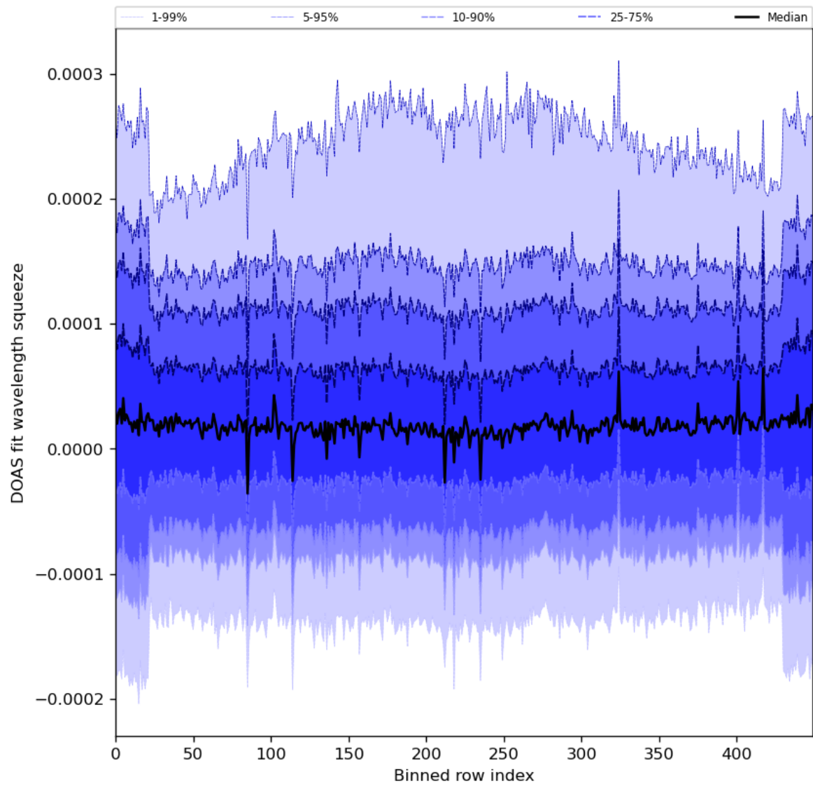
Figure 59: Along track statistics of “DOAS fit wavelength squeeze” for 2024-08-02 to 2024-08-04
