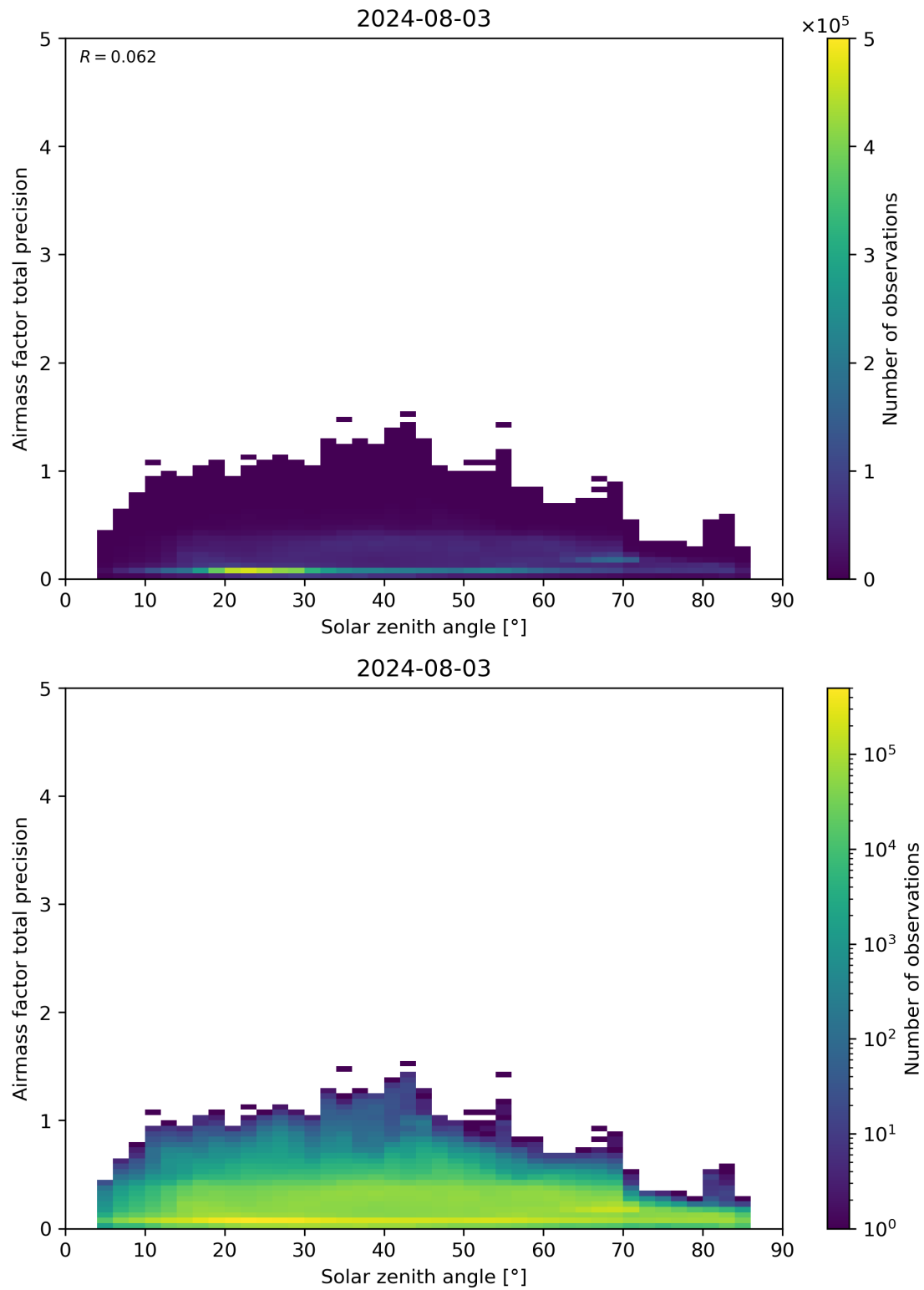
Figure 176: Scatter density plot of “Solar zenith angle” against “Airmass factor total precision” for 2024-08-02 to 2024-08-04.
