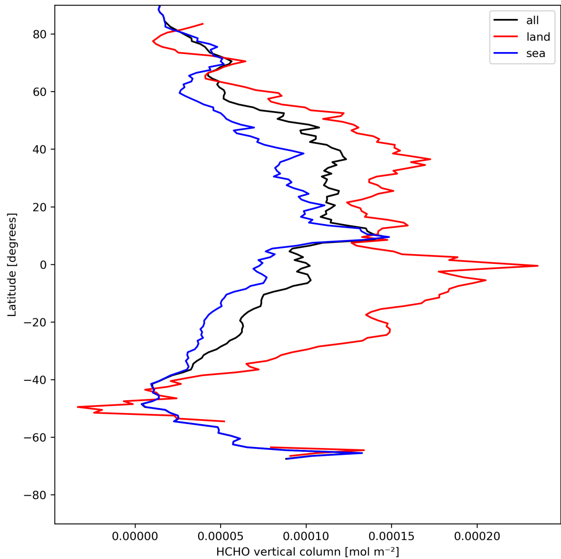
Figure 21: Zonal average of “HCHO vertical column” for 2024-08-02 to 2024-08-04.
