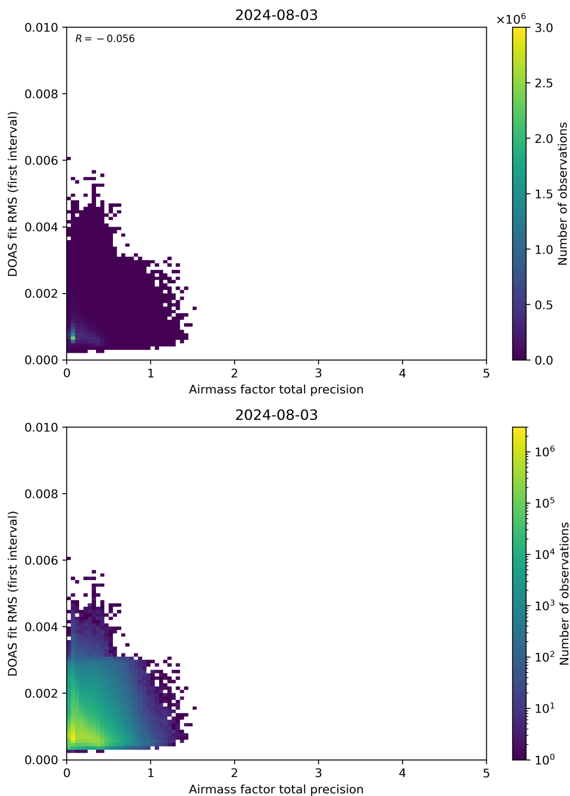
Figure 105: Scatter density plot of “Airmass factor total precision” against “DOAS fit RMS (first interval)” for 2024-08-02 to 2024-08-04.
