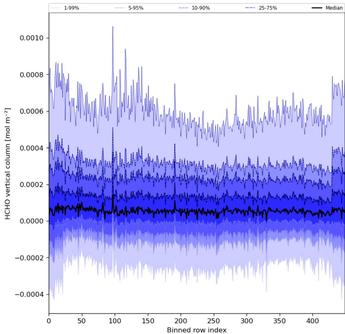
Figure 49: Along track statistics of “HCHO vertical column” for 2024-08-02 to 2024-08-04
