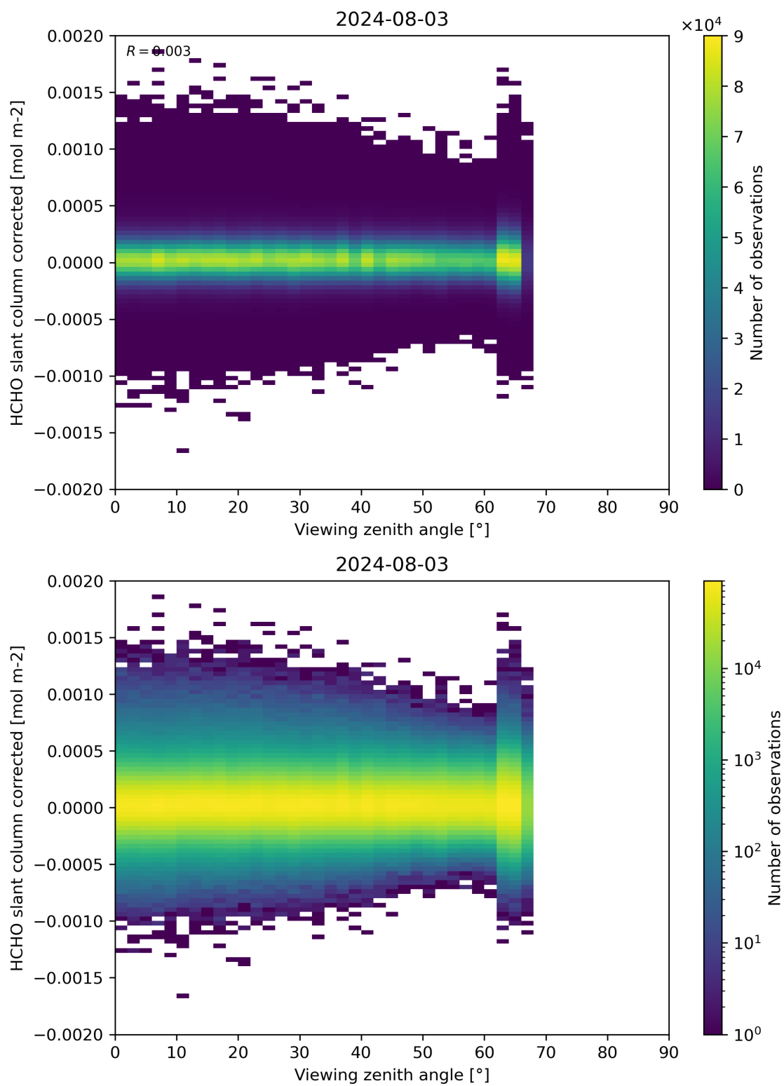
Figure 186: Scatter density plot of “Viewing zenith angle” against “HCHO slant column corrected” for 2024-08-02 to 2024-08-04.
