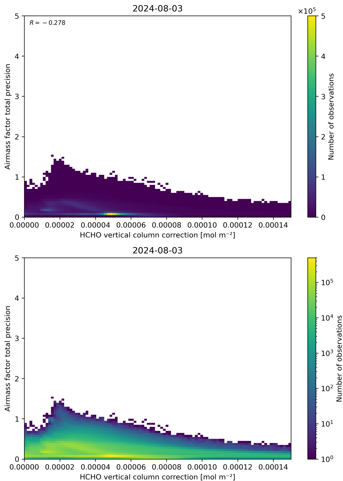
Figure 121: Scatter density plot of “HCHO vertical column correction” against “Airmass factor total precision” for 2024-08-02 to 2024-08-04.
