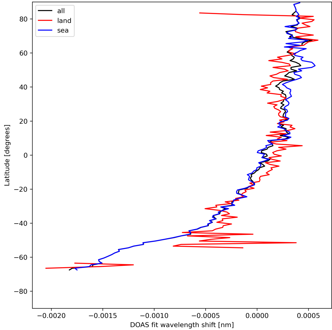
Figure 30: Zonal average of “DOAS fit wavelength shift” for 2024-08-02 to 2024-08-04.
