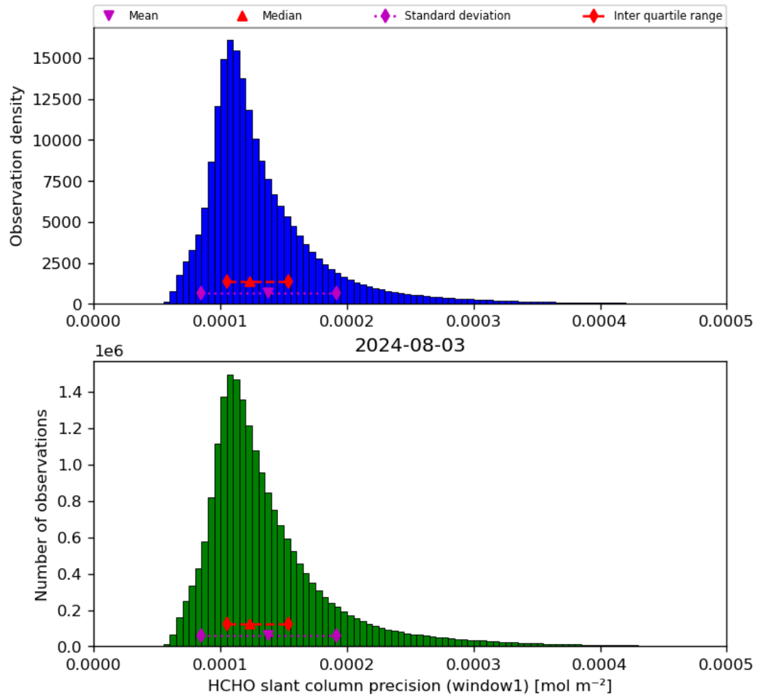
Figure 39: Histogram of “HCHO slant column precision (window1)” for 2024-08-02 to 2024-08-04
