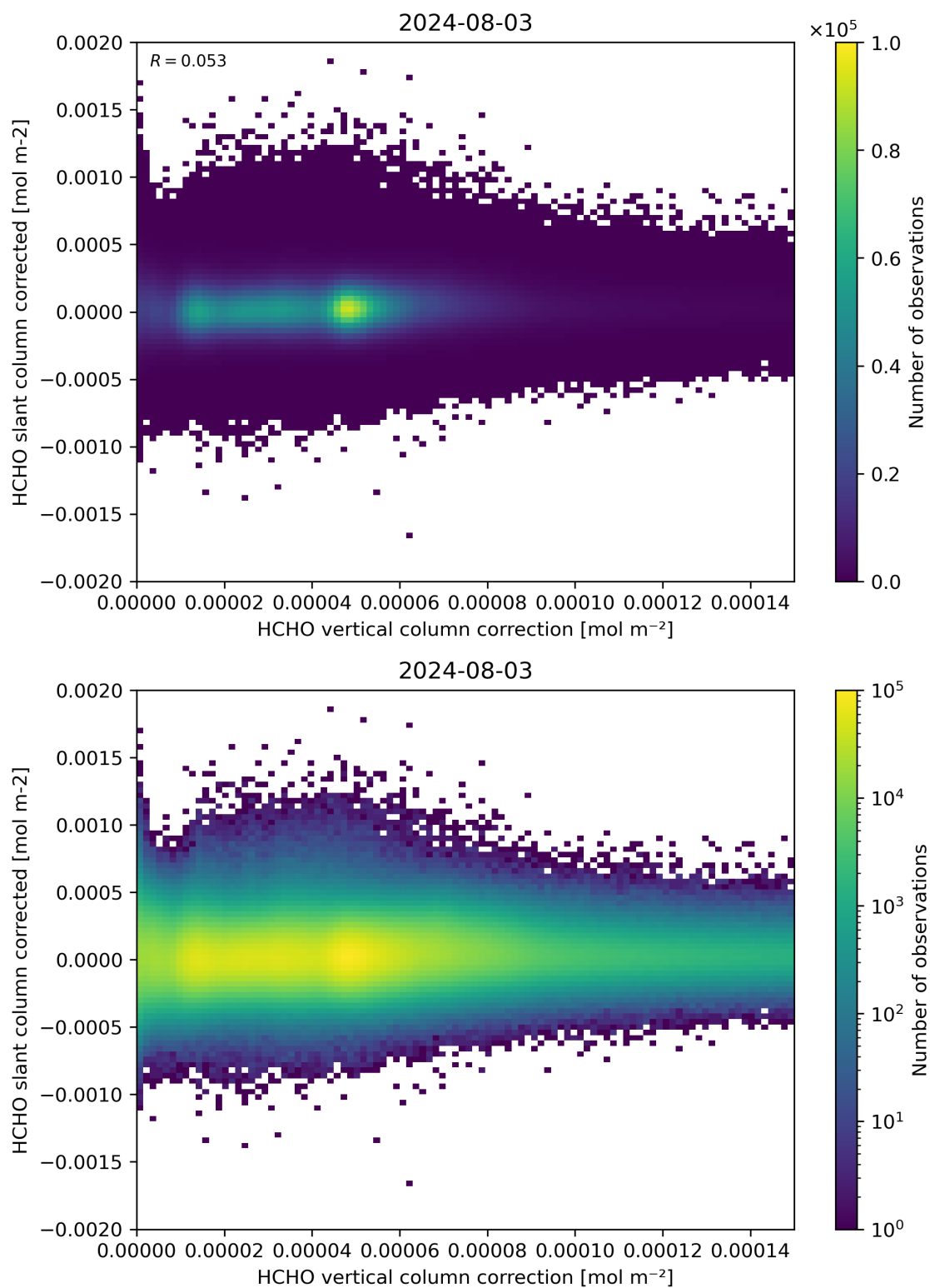
Figure 116: Scatter density plot of “HCHO vertical column correction” against “HCHO slant column corrected” for 2024-08-02 to 2024-08-04.
