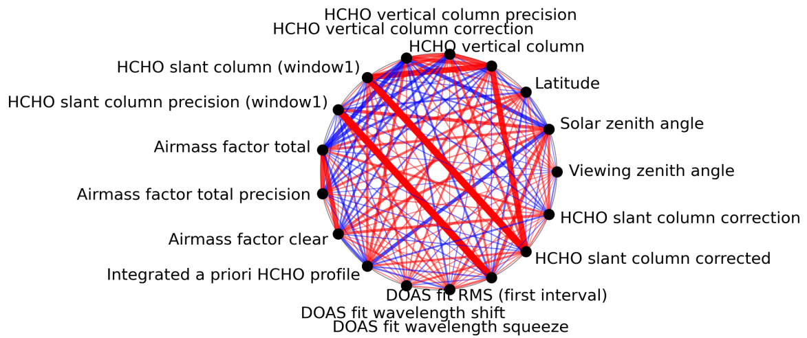
Figure 1: Map of correlation graph for 2024-08-02 to 2024-08-04.
