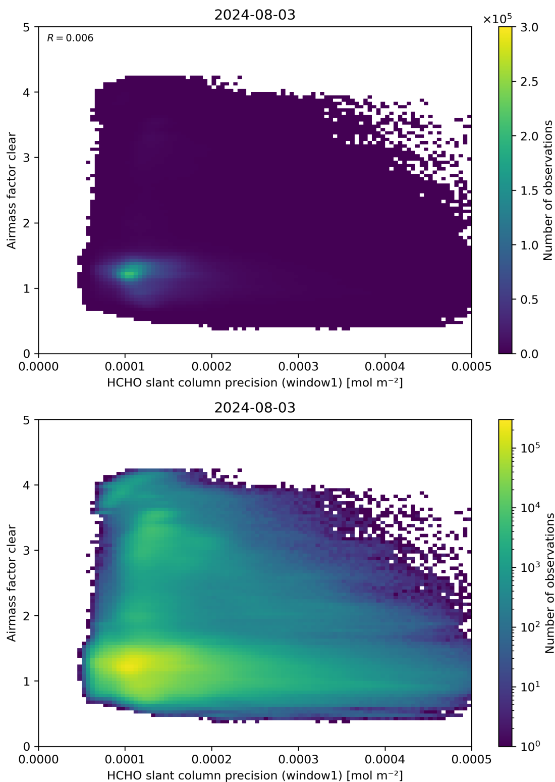
Figure 91: Scatter density plot of “HCHO slant column precision (window1)” against “Airmass factor clear” for 2024-08-02 to 2024-08-04.
