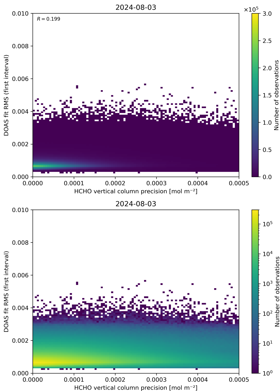
Figure 136: Scatter density plot of “HCHO vertical column precision” against “DOAS fit RMS (first interval)” for 2024-08-02 to 2024-08-04.
