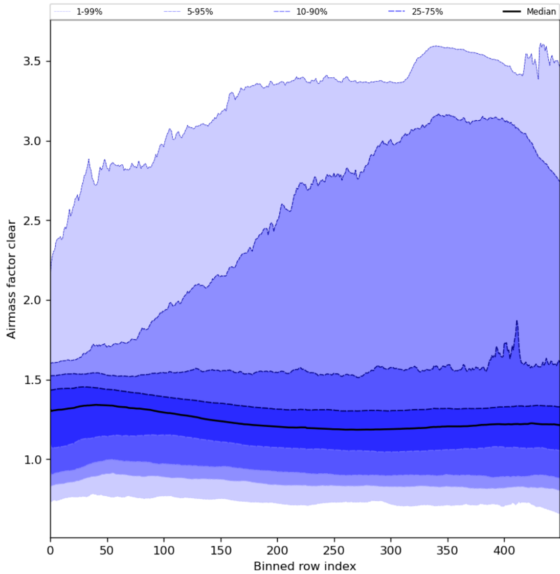
Figure 56: Along track statistics of “Airmass factor clear” for 2024-08-02 to 2024-08-04
