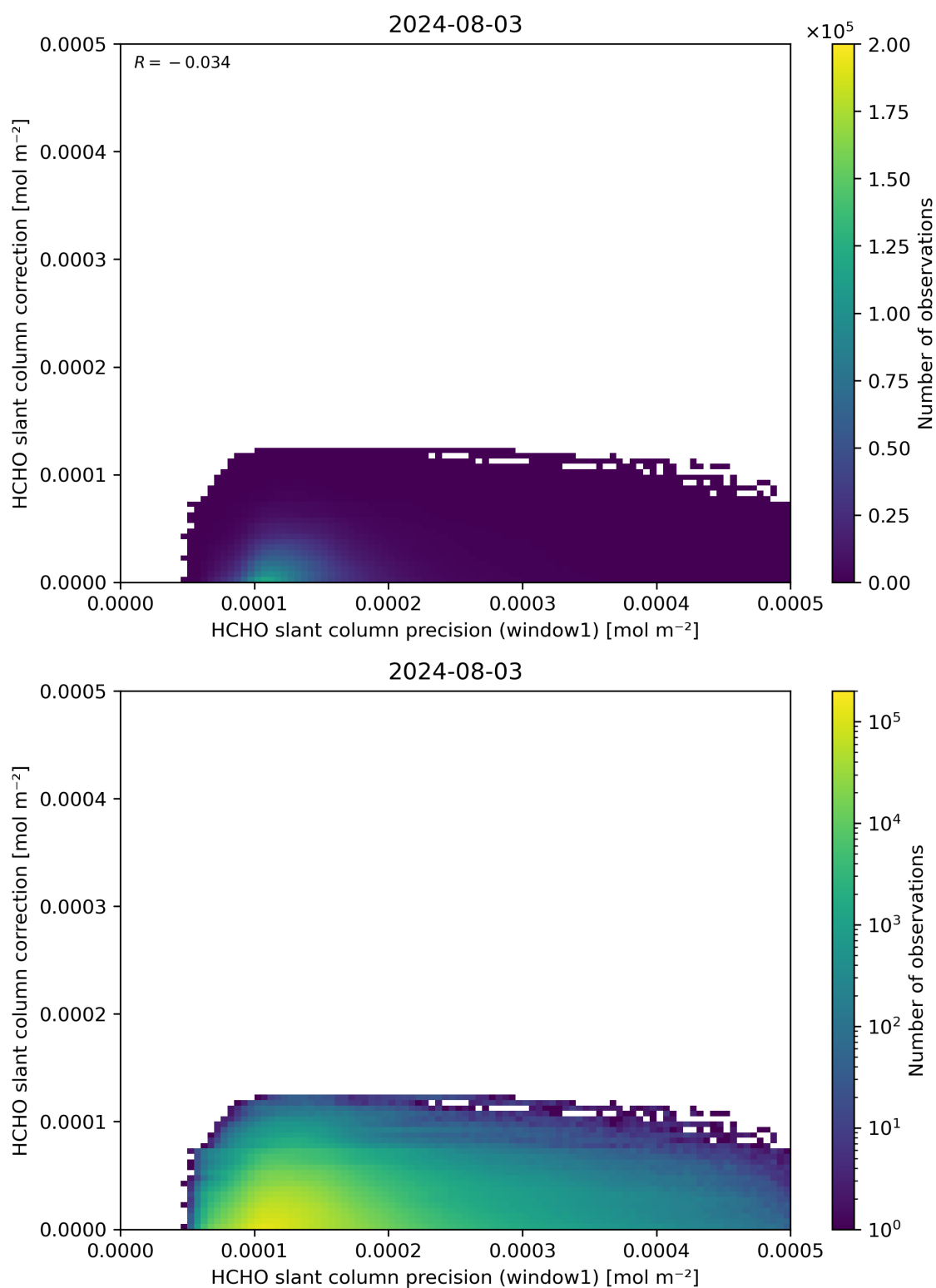
Figure 93: Scatter density plot of “HCHO slant column precision (window1)” against “HCHO slant column correction” for 2024-08-02 to 2024-08-04.
