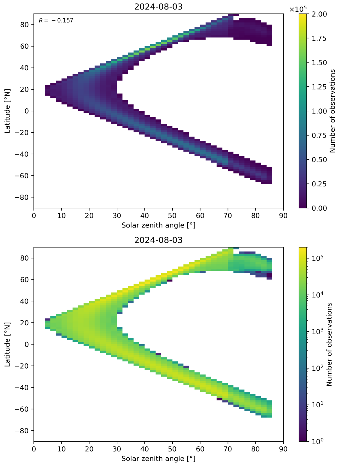
Figure 181: Scatter density plot of “Solar zenith angle” against “Latitude” for 2024-08-02 to 2024-08-04.
