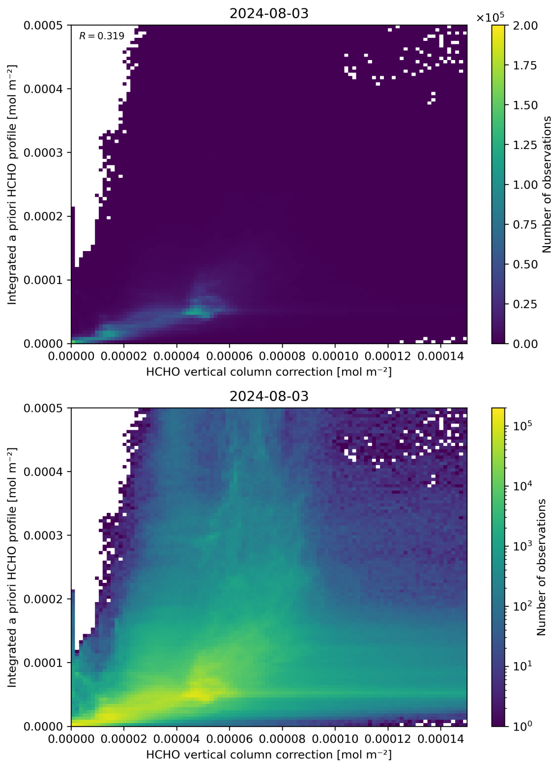
Figure 122: Scatter density plot of “HCHO vertical column correction” against “Integrated a priori HCHO profile” for 2024-08-02 to 2024-08-04.
