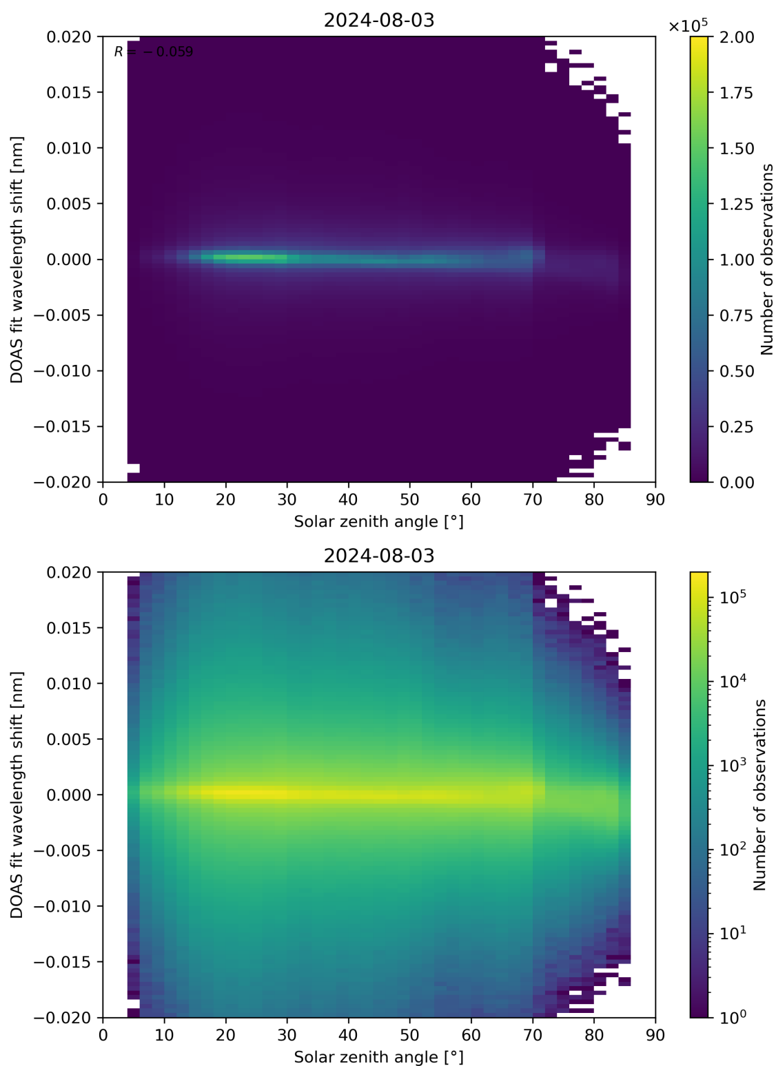
Figure 168: Scatter density plot of “Solar zenith angle” against “DOAS fit wavelength shift” for 2024-08-02 to 2024-08-04.
