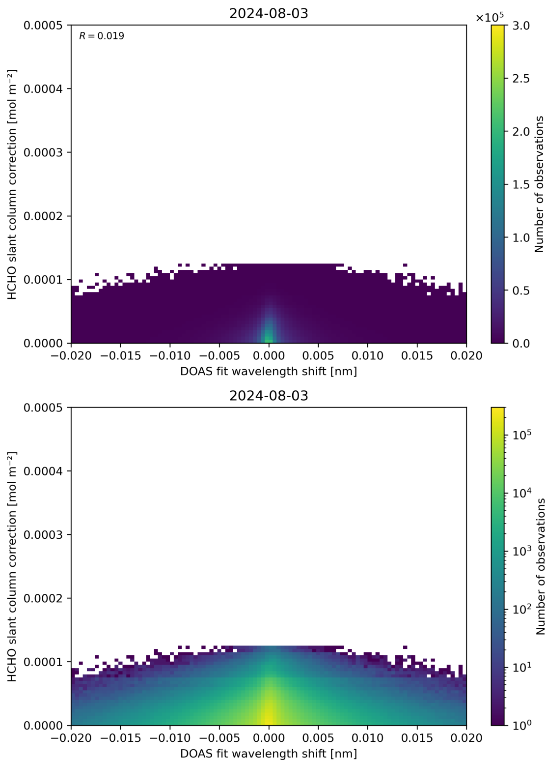
Figure 67: Scatter density plot of “DOAS fit wavelength shift” against “HCHO slant column correction” for 2024-08-02 to 2024-08-04.
