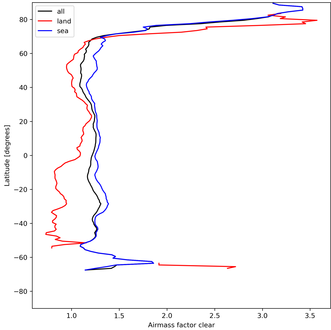
Figure 28: Zonal average of “Airmass factor clear” for 2024-08-02 to 2024-08-04.
