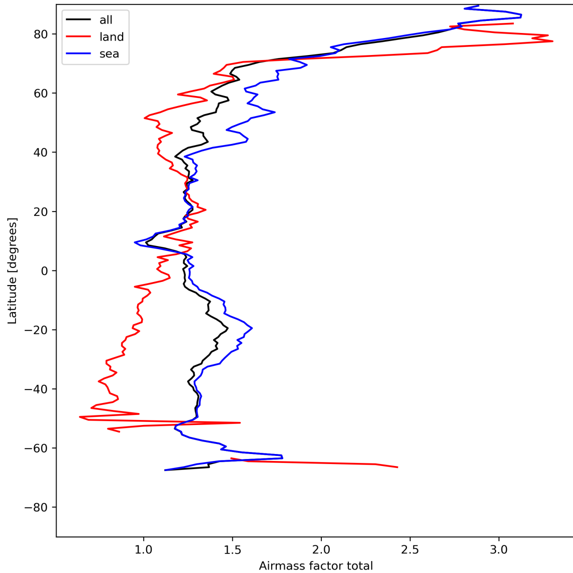
Figure 26: Zonal average of “Airmass factor total” for 2024-08-02 to 2024-08-04.
