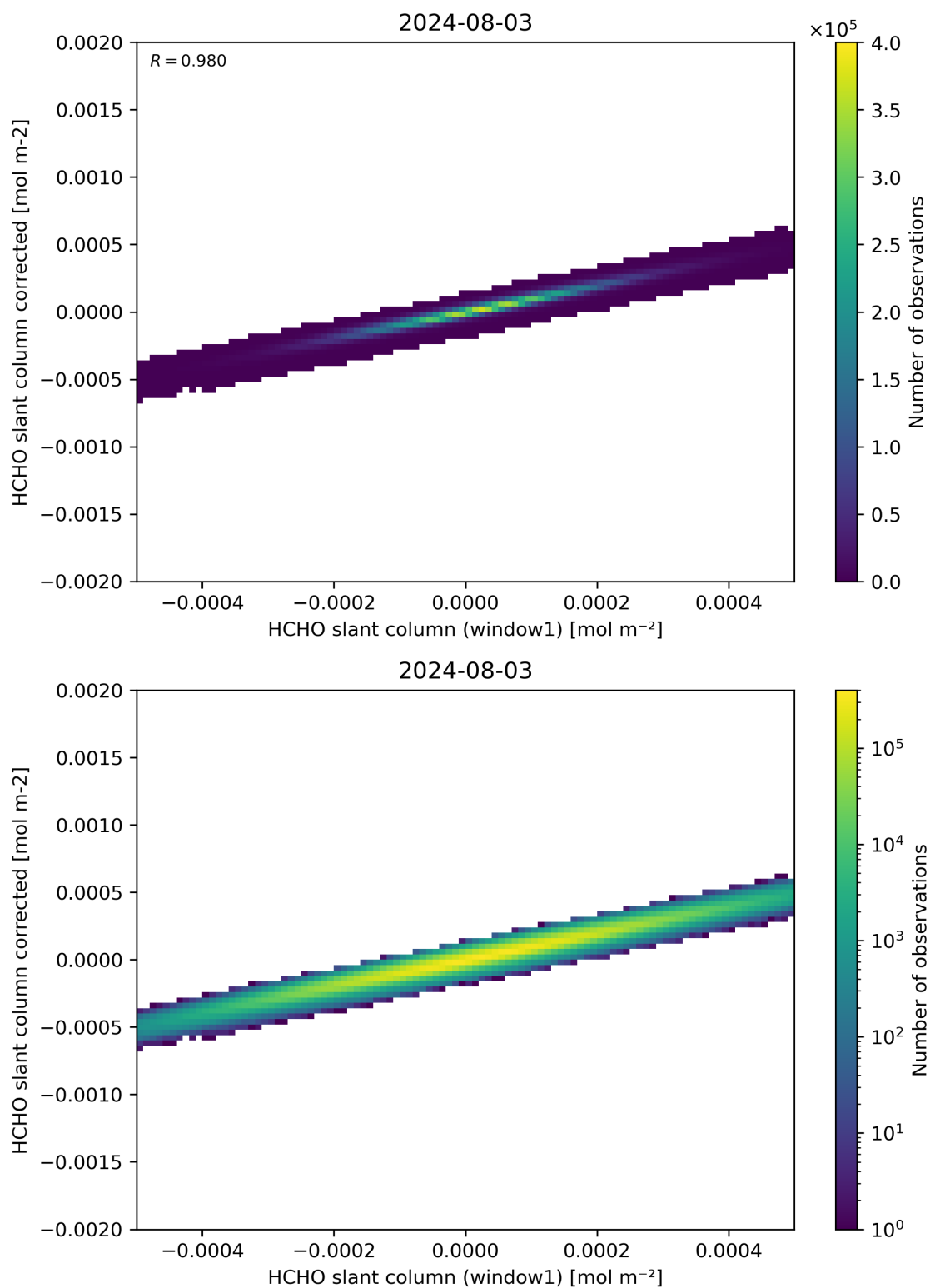
Figure 82: Scatter density plot of “HCHO slant column (window1)” against “HCHO slant column corrected” for 2024-08-02 to 2024-08-04.
