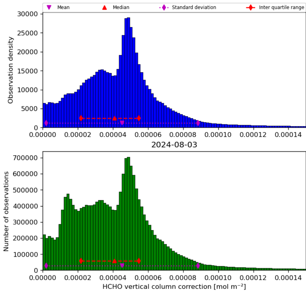
Figure 37: Histogram of “HCHO vertical column correction” for 2024-08-02 to 2024-08-04
