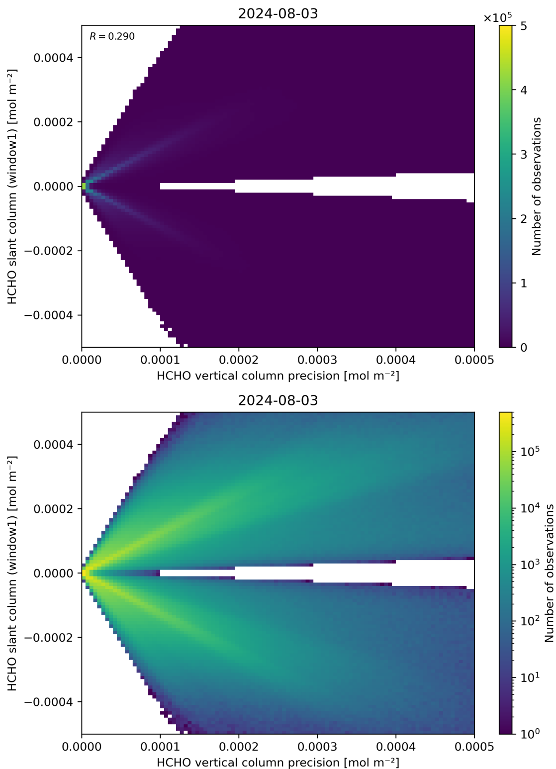
Figure 142: Scatter density plot of “HCHO vertical column precision” against “HCHO slant column (window1)” for 2024-08-02 to 2024-08-04.
