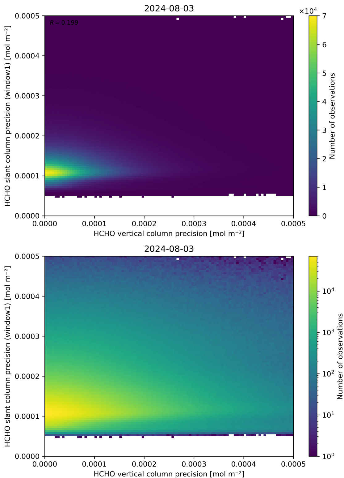
Figure 143: Scatter density plot of “HCHO vertical column precision” against “HCHO slant column precision (window1)” for 2024-08-02 to 2024-08-04.
