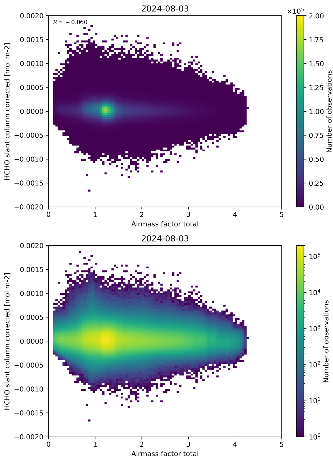
Figure 101: Scatter density plot of “Airmass factor total” against “HCHO slant column corrected” for 2024-08-02 to 2024-08-04.
