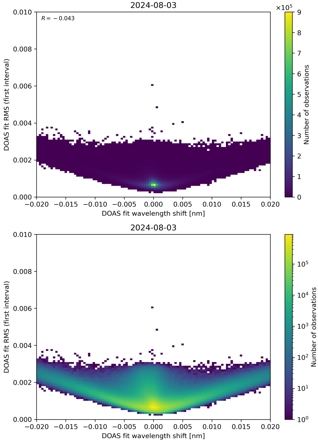
Figure 64: Scatter density plot of “DOAS fit wavelength shift” against “DOAS fit RMS (first interval)” for 2024-08-02 to 2024-08-04.
