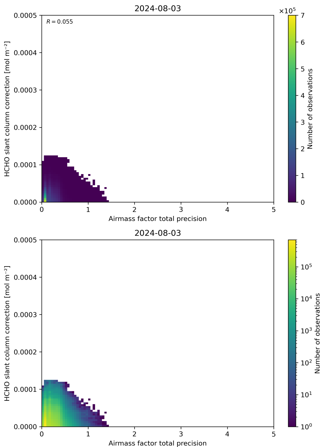
Figure 110: Scatter density plot of “Airmass factor total precision” against “HCHO slant column correction” for 2024-08-02 to 2024-08-04.
