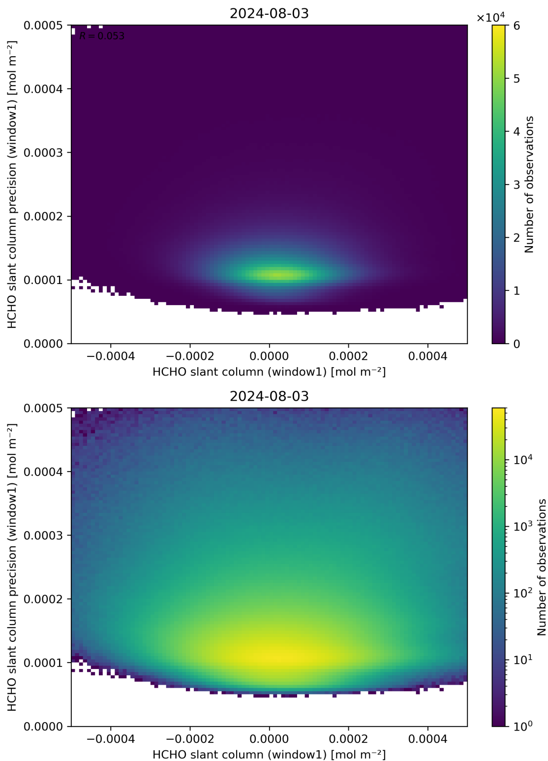
Figure 84: Scatter density plot of “HCHO slant column (window1)” against “HCHO slant column precision (window1)” for 2024-08-02 to 2024-08-04.
