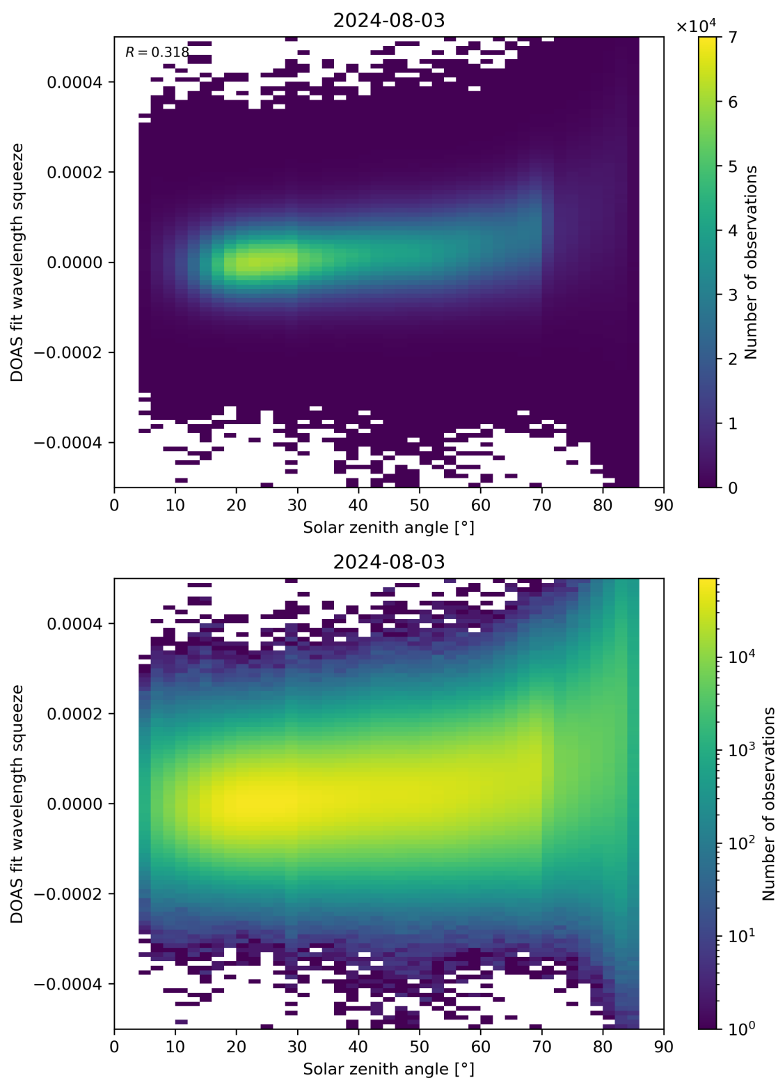
Figure 169: Scatter density plot of “Solar zenith angle” against “DOAS fit wavelength squeeze” for 2024-08-02 to 2024-08-04.
