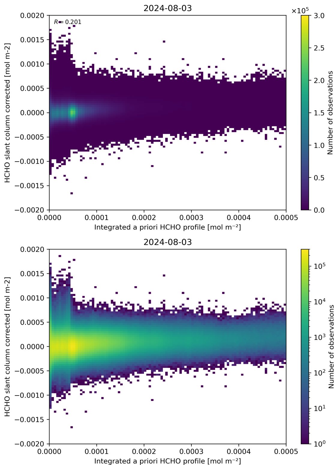
Figure 151: Scatter density plot of “Integrated a priori HCHO profile” against “HCHO slant column corrected” for 2024-08-02 to 2024-08-04.
