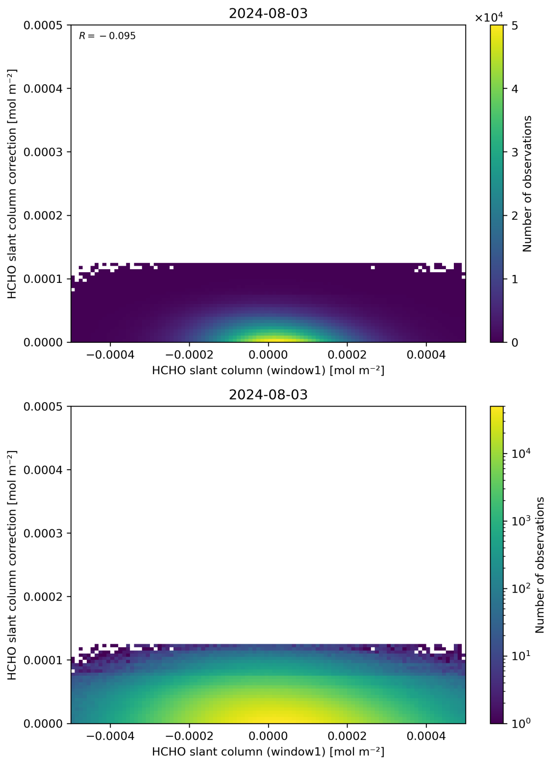
Figure 83: Scatter density plot of “HCHO slant column (window1)” against “HCHO slant column correction” for 2024-08-02 to 2024-08-04.
