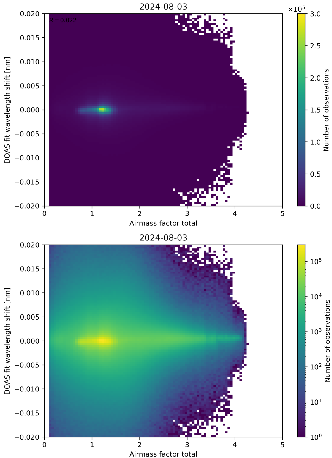
Figure 98: Scatter density plot of “Airmass factor total” against “DOAS fit wavelength shift” for 2024-08-02 to 2024-08-04.
