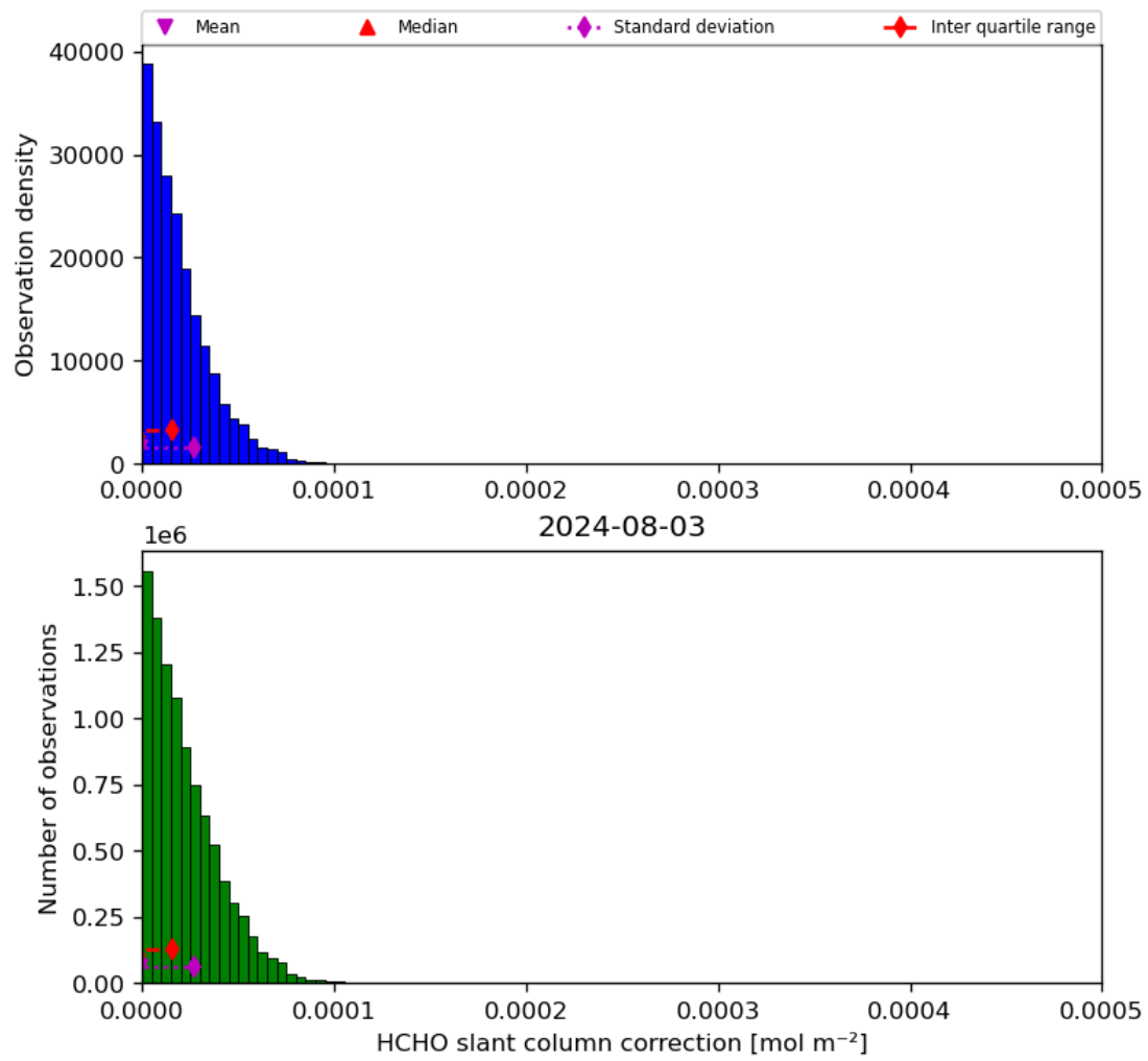
Figure 47: Histogram of “HCHO slant column correction” for 2024-08-02 to 2024-08-04
