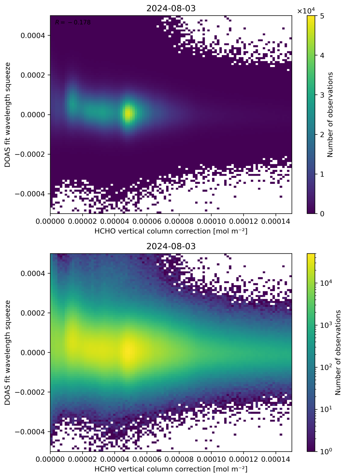
Figure 114: Scatter density plot of “HCHO vertical column correction” against “DOAS fit wavelength squeeze” for 2024-08-02 to 2024-08-04.
