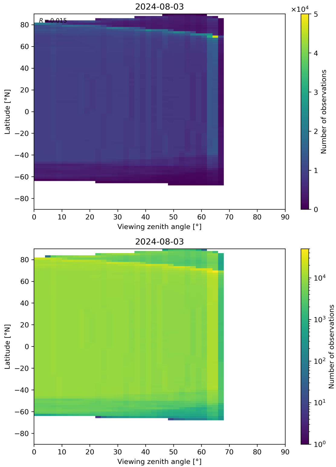
Figure 196: Scatter density plot of “Viewing zenith angle” against “Latitude” for 2024-08-02 to 2024-08-04.
