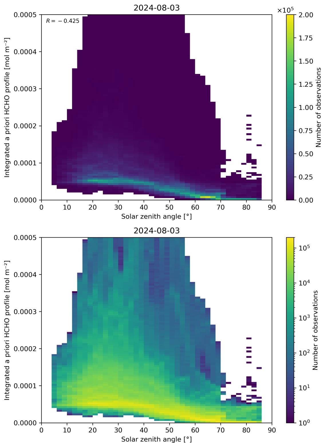
Figure 180: Scatter density plot of “Solar zenith angle” against “Integrated a priori HCHO profile” for 2024-08-02 to 2024-08-04.
