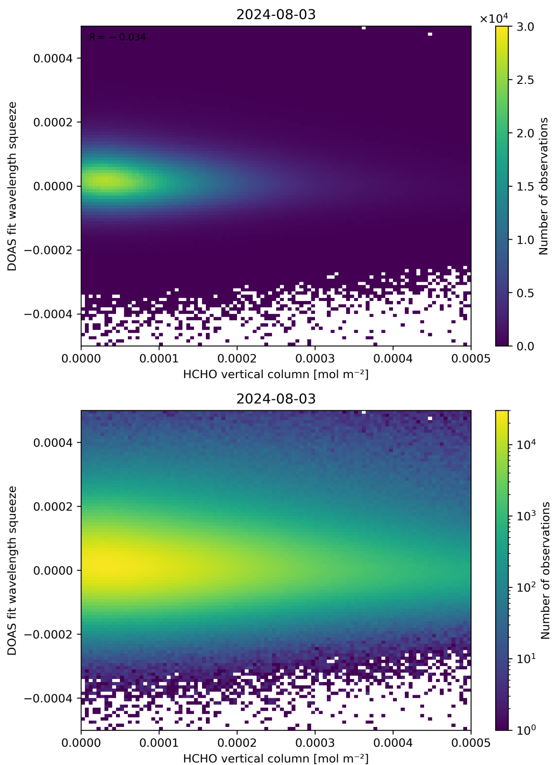
Figure 125: Scatter density plot of “HCHO vertical column” against “DOAS fit wavelength squeeze” for 2024-08-02 to 2024-08-04.
