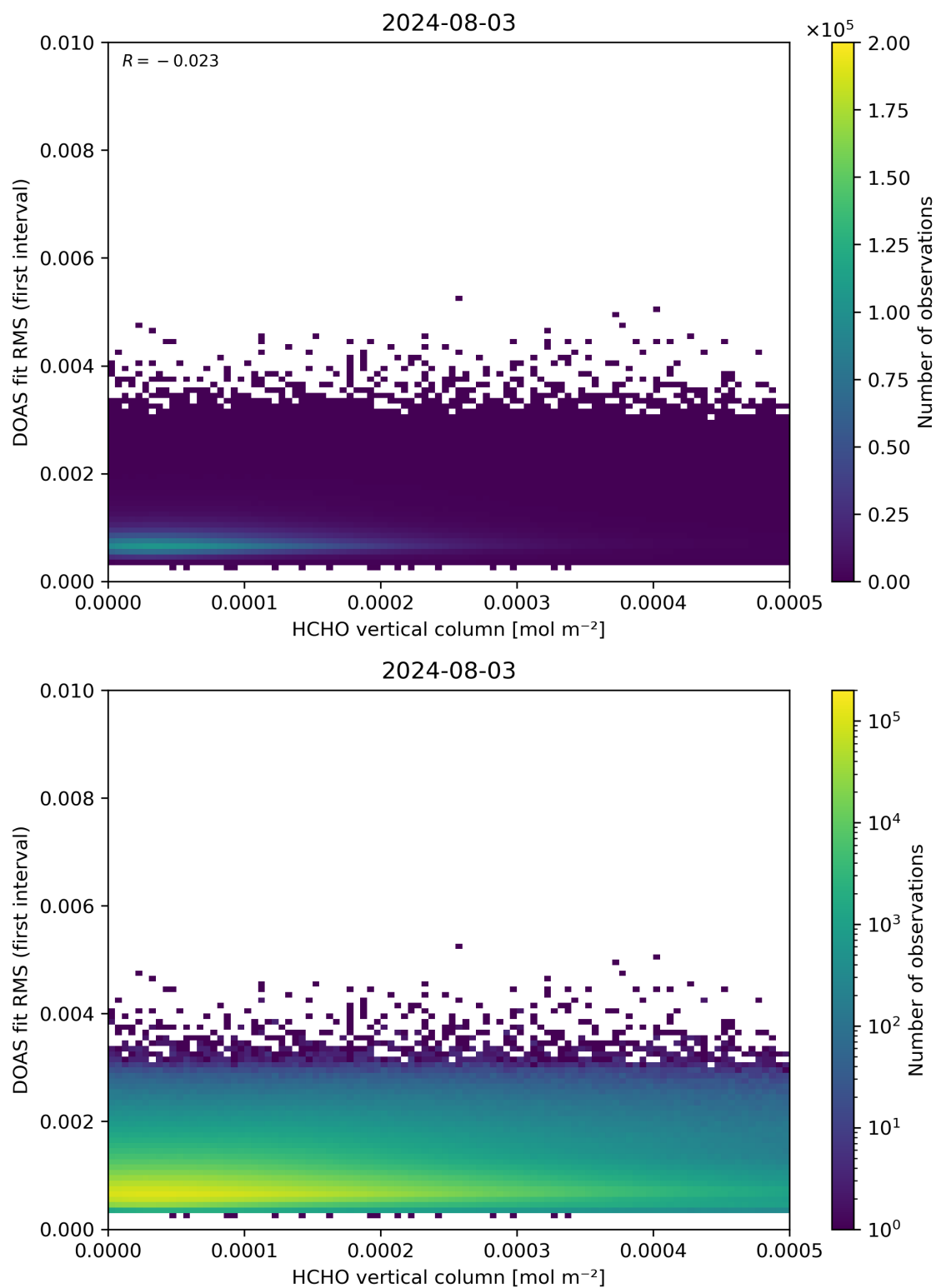
Figure 123: Scatter density plot of “HCHO vertical column” against “DOAS fit RMS (first interval)” for 2024-08-02 to 2024-08-04.
