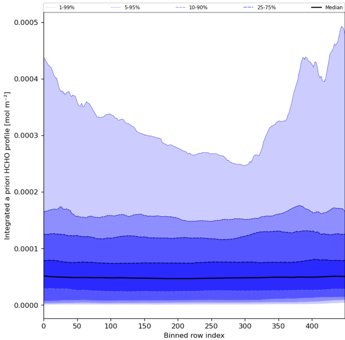
Figure 57: Along track statistics of “Integrated a priori HCHO profile” for 2024-08-02 to 2024-08-04
