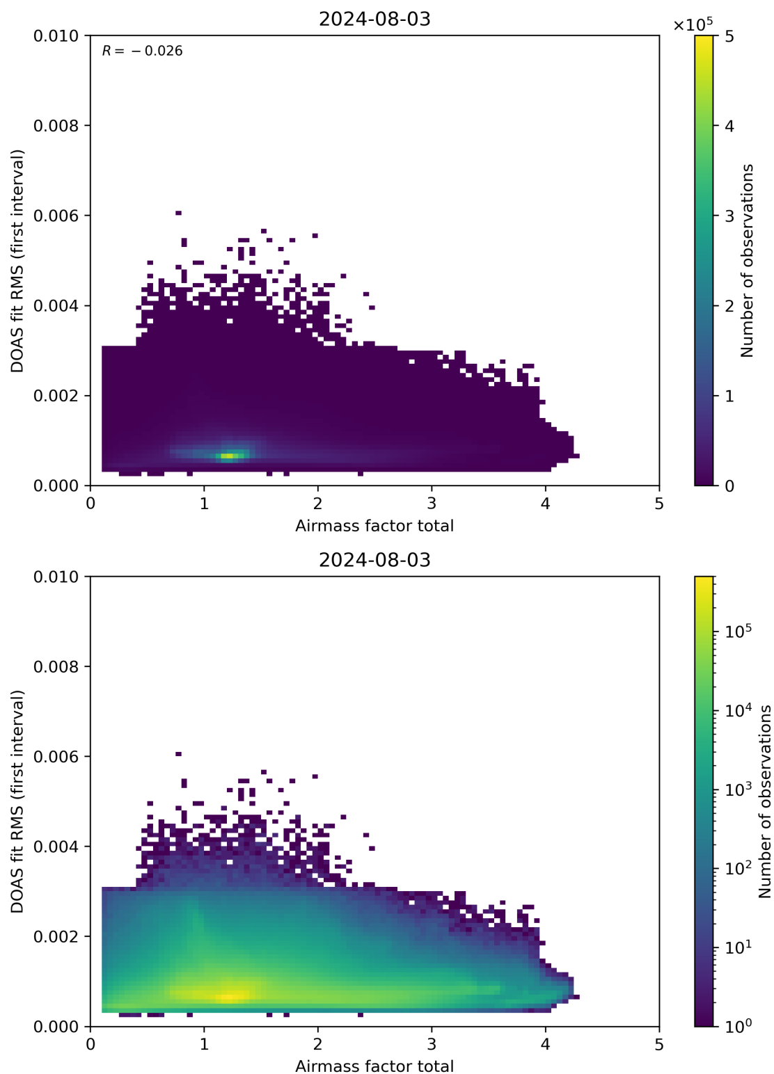
Figure 97: Scatter density plot of “Airmass factor total” against “DOAS fit RMS (first interval)” for 2024-08-02 to 2024-08-04.
