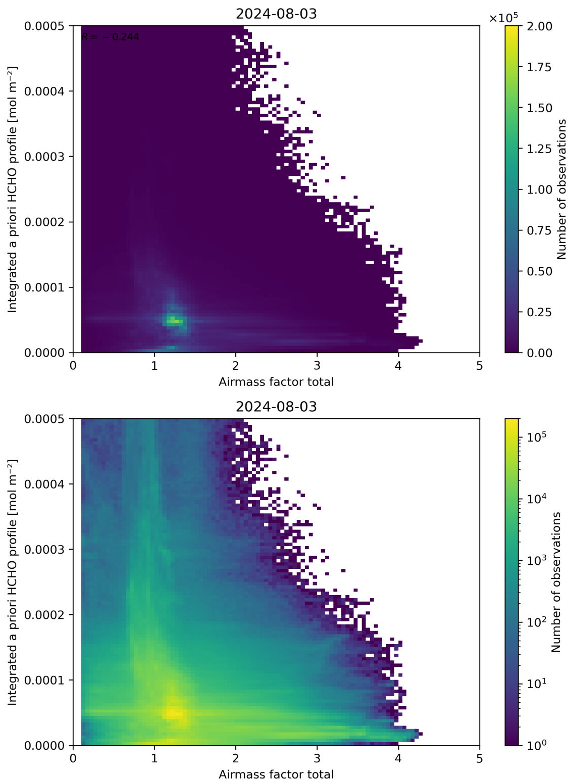
Figure 104: Scatter density plot of “Air mass factor total” against “Integrated a priori HCHO profile” for 2024-08-02 to 2024-08-04.
