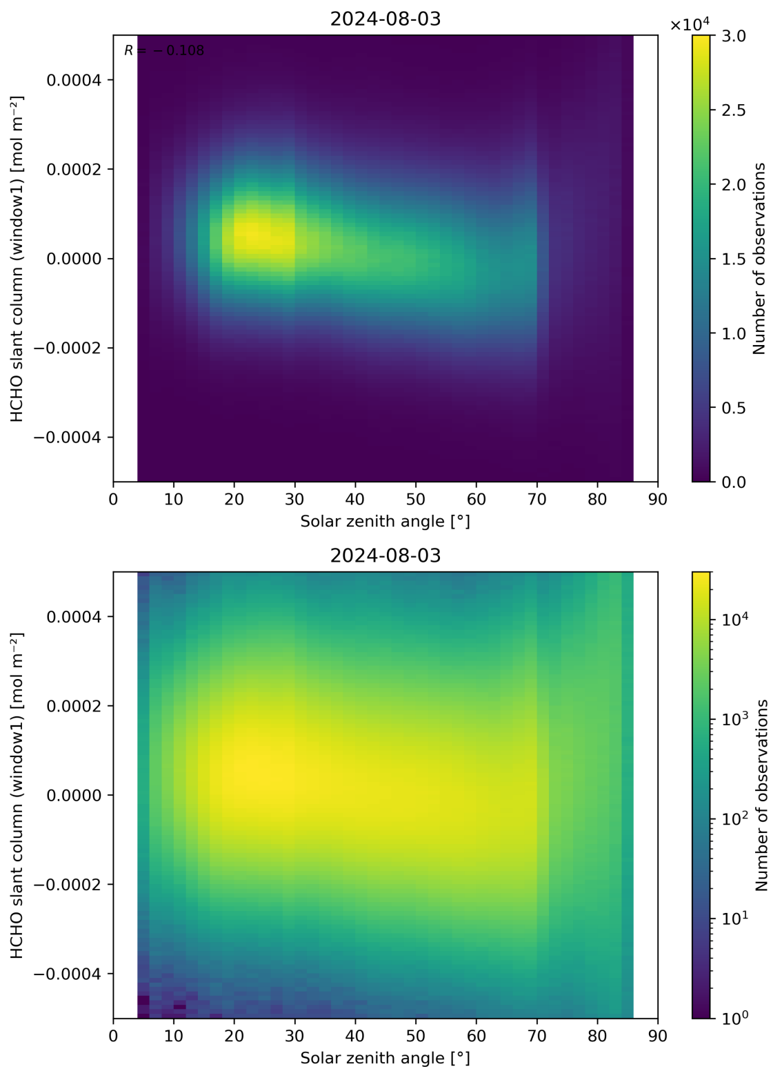
Figure 173: Scatter density plot of “Solar zenith angle” against “HCHO slant column (window1)” for 2024-08-02 to 2024-08-04.
