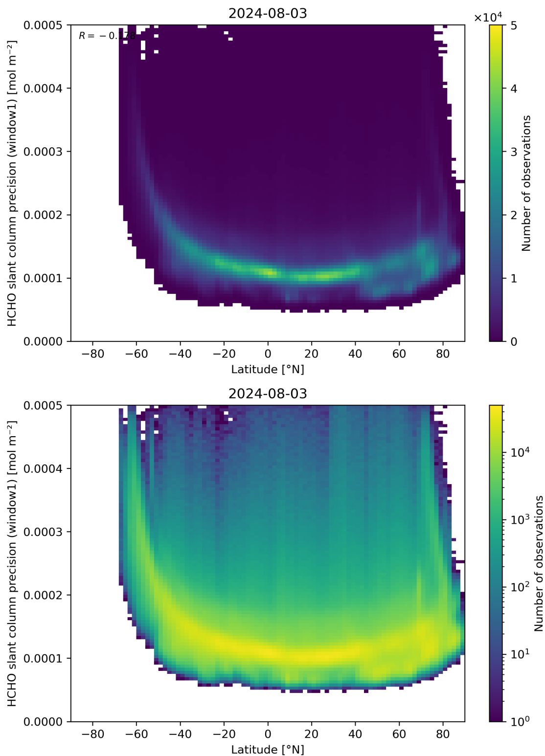
Figure 160: Scatter density plot of “Latitude” against “HCHO slant column precision (window1)” for 2024-08-02 to 2024-08-04.
