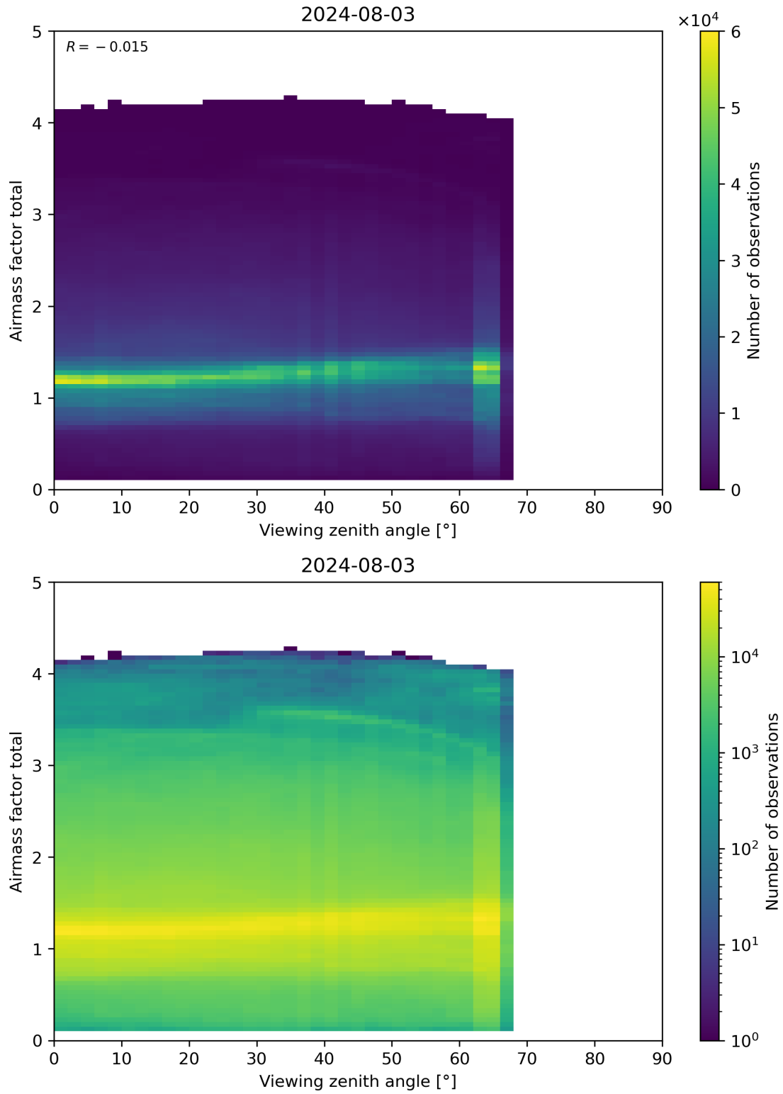
Figure 190: Scatter density plot of “Viewing zenith angle” against “Airmass factor total” for 2024-08-02 to 2024-08-04.
