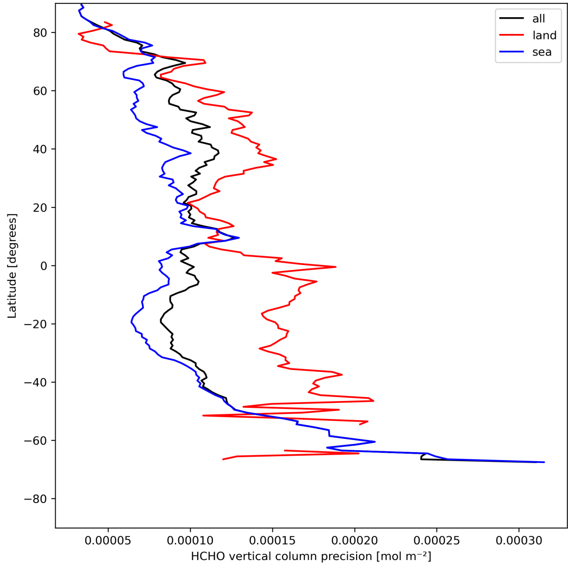
Figure 22: Zonal average of “HCHO vertical column precision” for 2024-08-02 to 2024-08-04.
