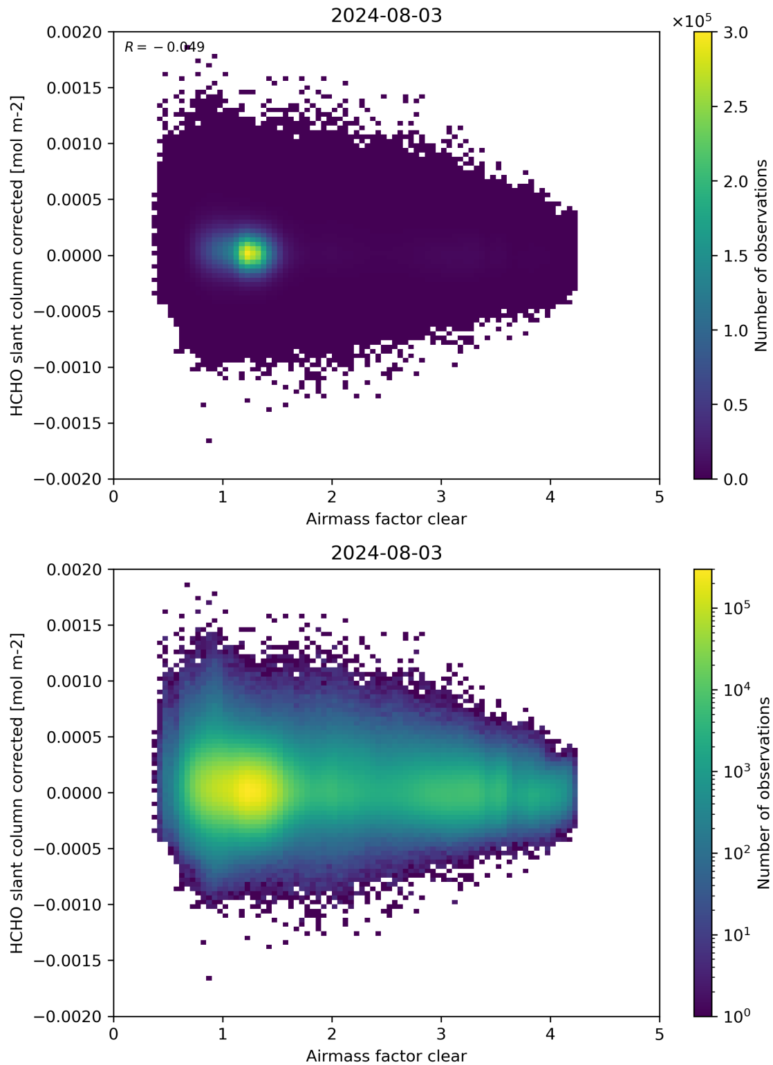
Figure 74: Scatter density plot of “Airmass factor clear” against “HCHO slant column corrected” for 2024-08-02 to 2024-08-04.
