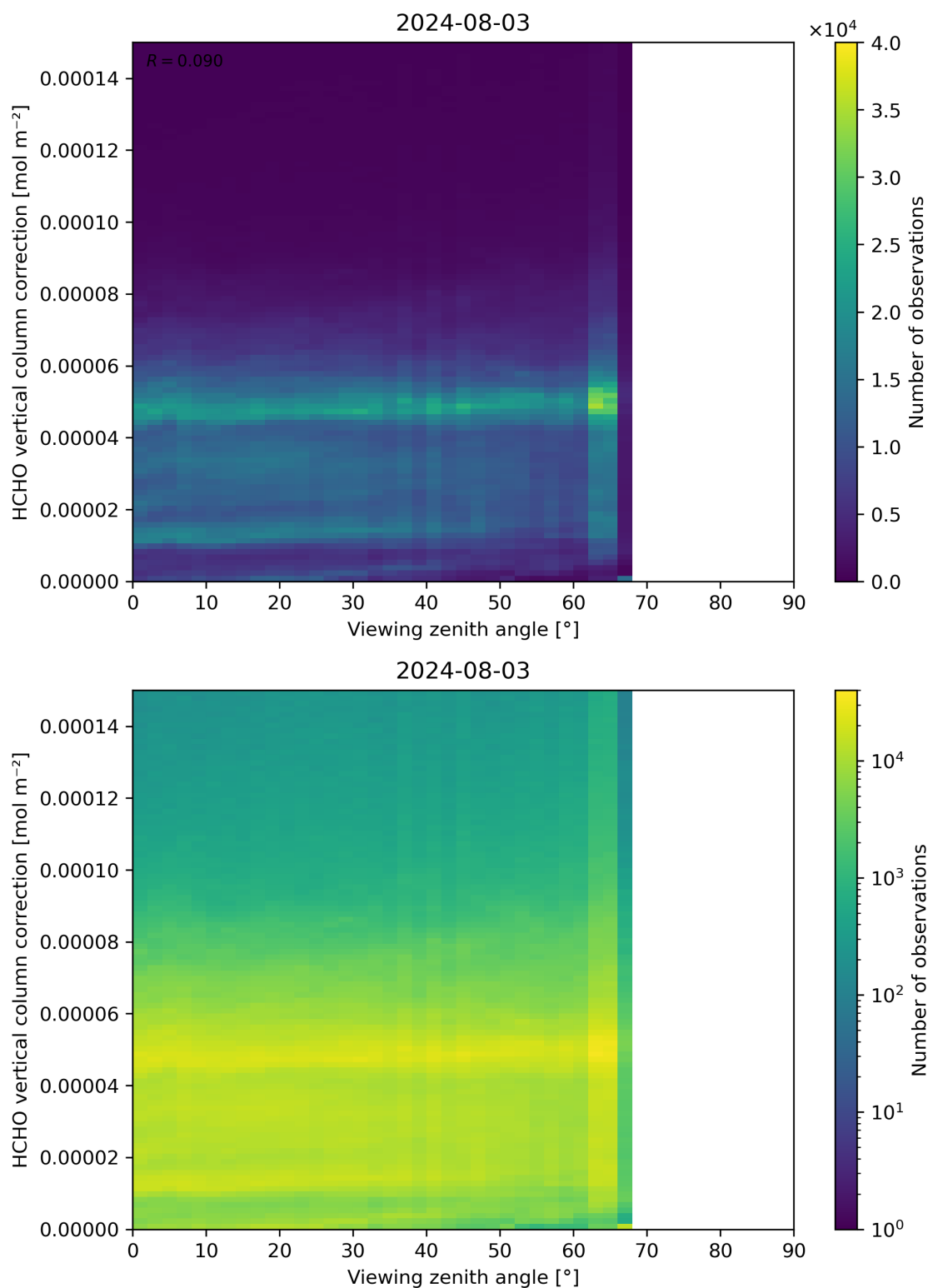
Figure 193: Scatter density plot of “Viewing zenith angle” against “HCHO vertical column correction” for 2024-08-02 to 2024-08-04.
