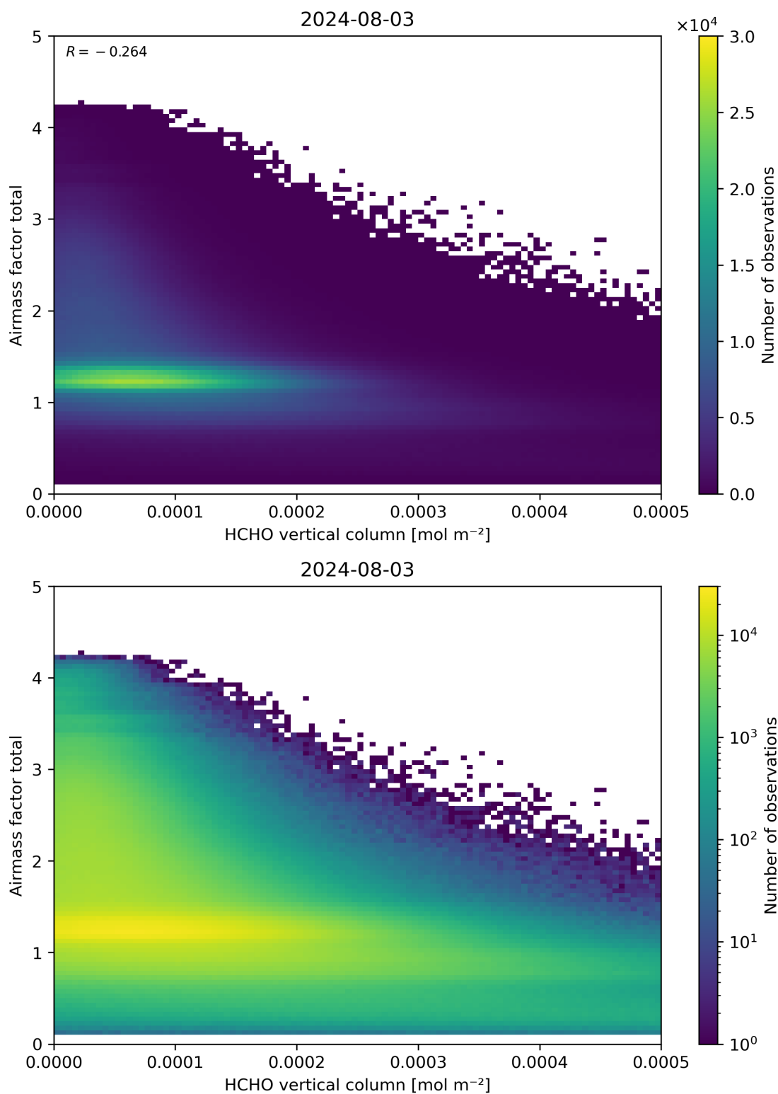
Figure 131: Scatter density plot of “HCHO vertical column” against “Airmass factor total” for 2024-08-02 to 2024-08-04.
