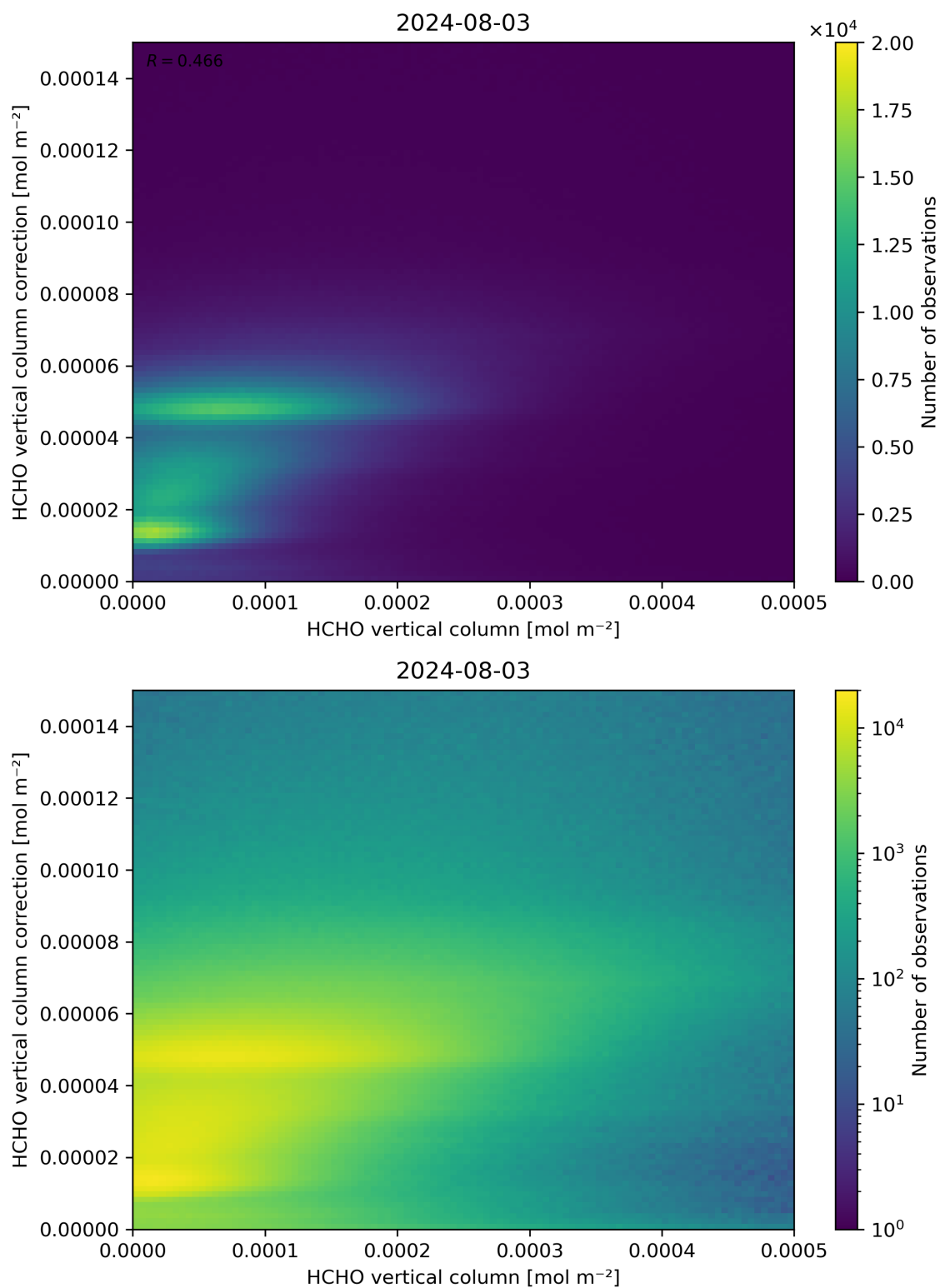
Figure 133: Scatter density plot of “HCHO vertical column” against “HCHO vertical column correction” for 2024-08-02 to 2024-08-04.
