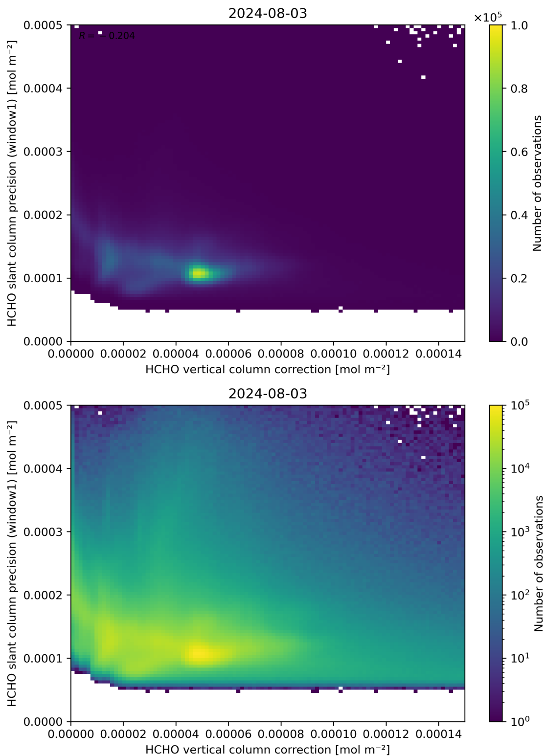
Figure 119: Scatter density plot of “HCHO vertical column correction” against “HCHO slant column precision (window1)” for 2024-08-02 to 2024-08-04.
