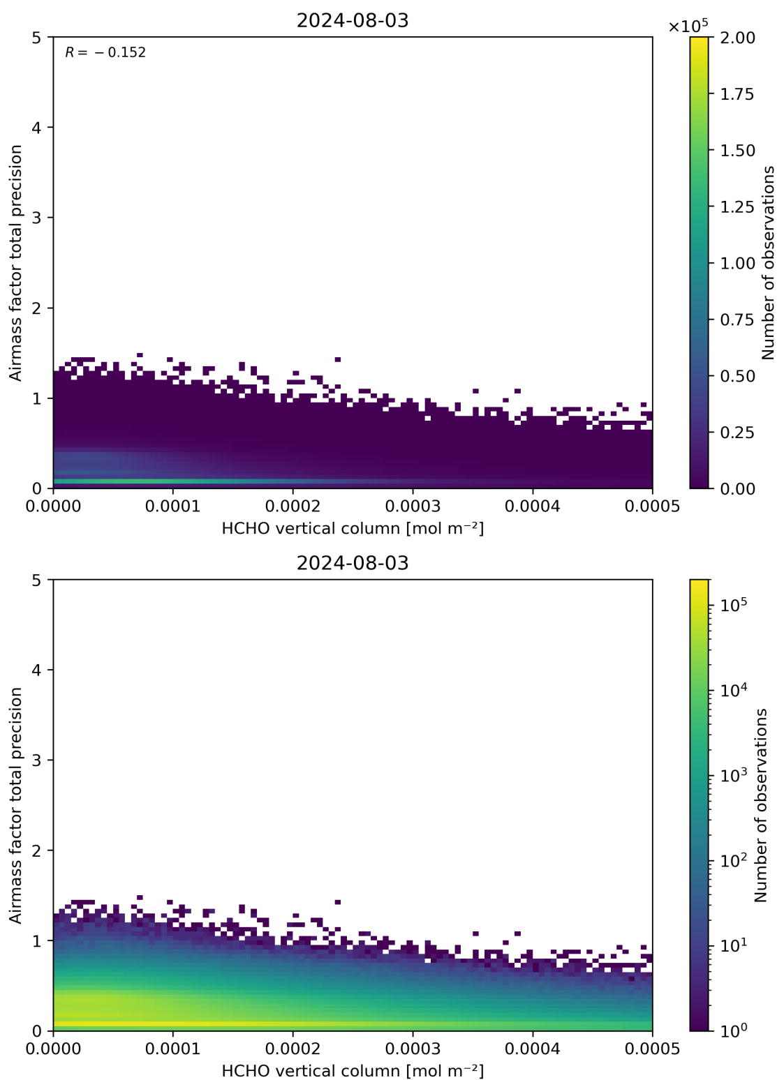
Figure 132: Scatter density plot of “HCHO vertical column” against “Airmass factor total precision” for 2024-08-02 to 2024-08-04.
