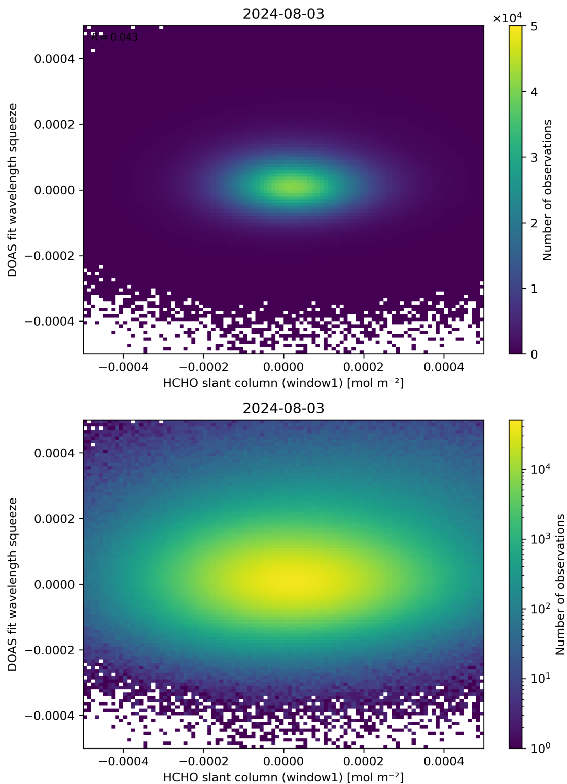
Figure 80: Scatter density plot of “HCHO slant column (window1)” against “DOAS fit wavelength squeeze” for 2024-08-02 to 2024-08-04.
