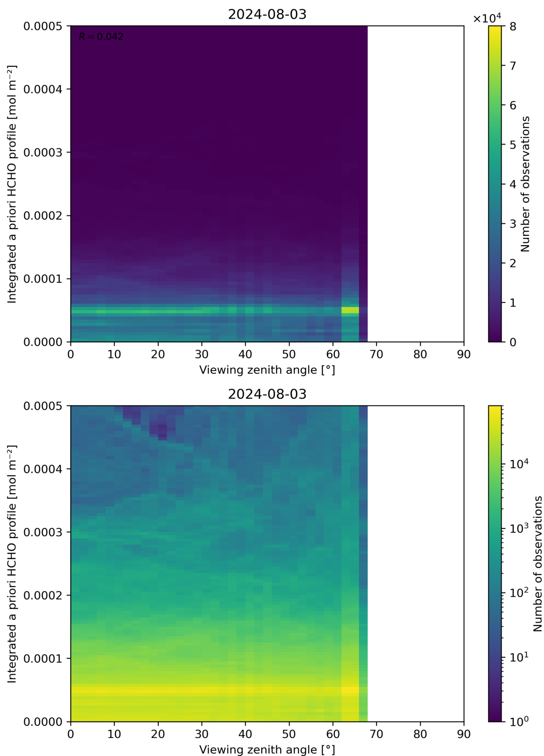
Figure 195: Scatter density plot of “Viewing zenith angle” against “Integrated a priori HCHO profile” for 2024-08-02 to 2024-08-04.
