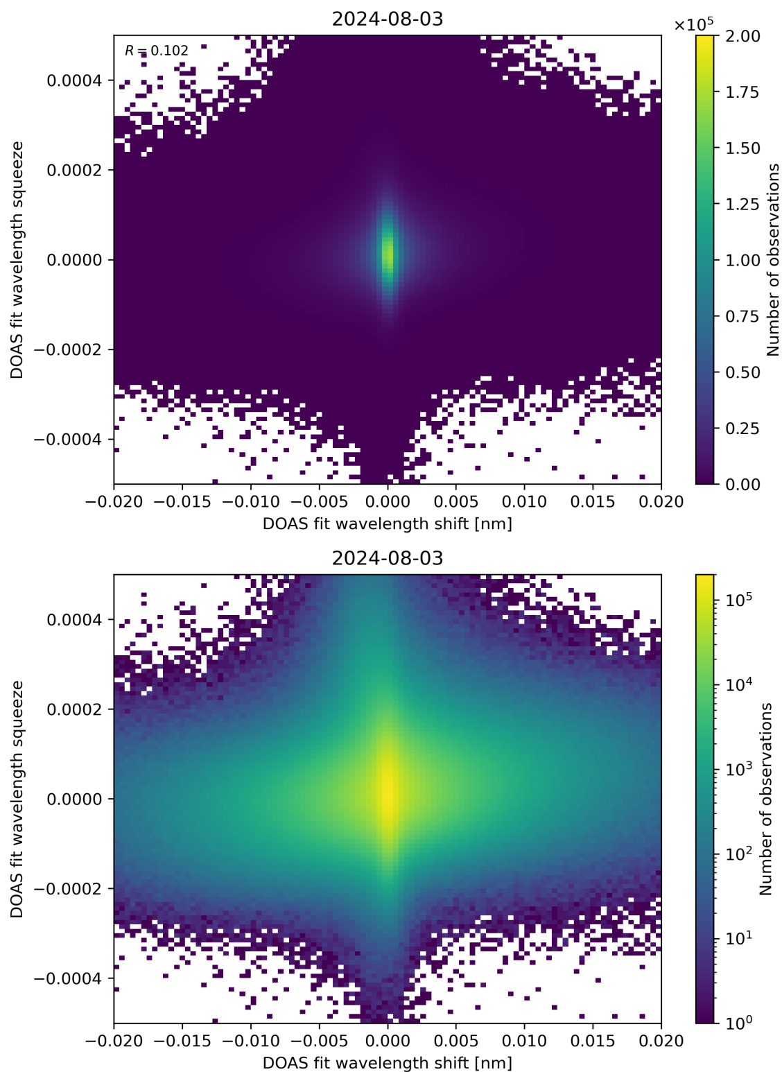
Figure 65: Scatter density plot of “DOAS fit wavelength shift” against “DOAS fit wavelength squeeze” for 2024-08-02 to 2024-08-04.
