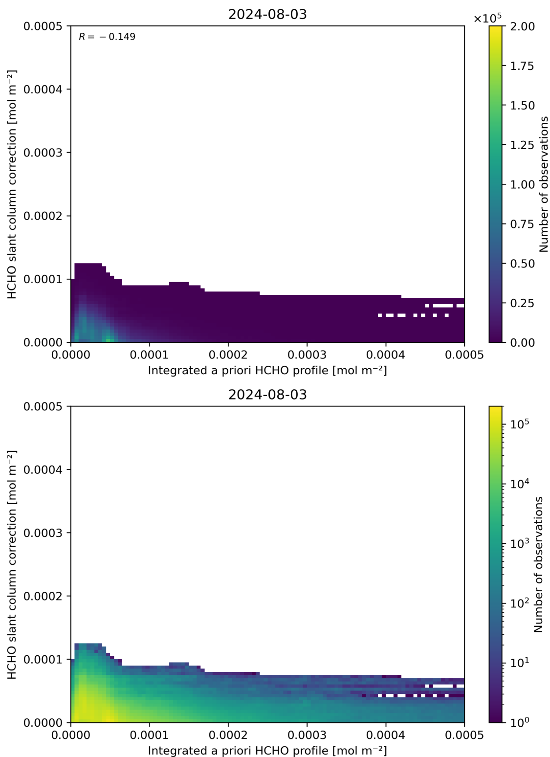
Figure 152: Scatter density plot of “Integrated a priori HCHO profile” against “HCHO slant column correction” for 2024-08-02 to 2024-08-04.
