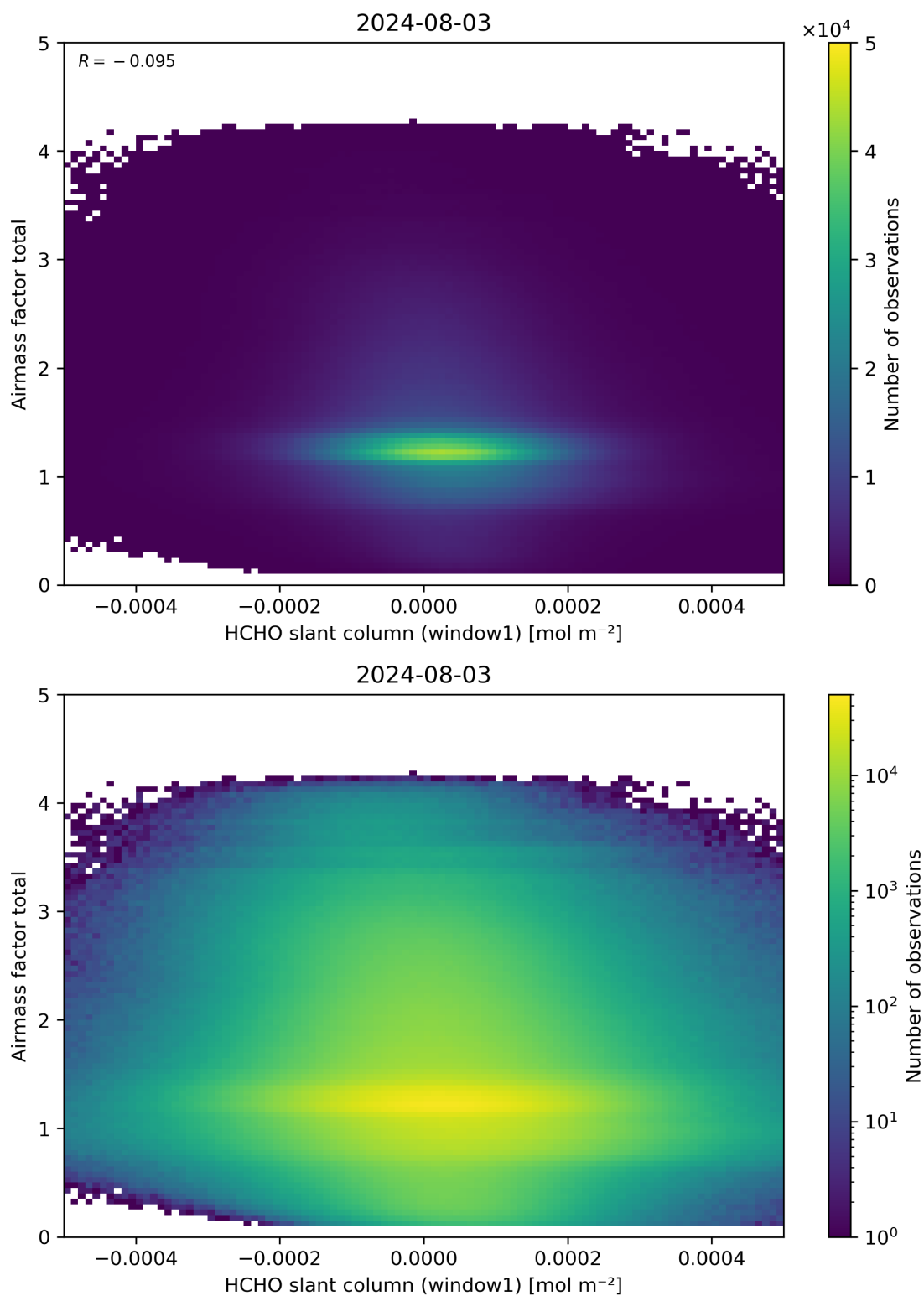
Figure 85: Scatter density plot of “HCHO slant column (window1)” against “Airmass factor total” for 2024-08-02 to 2024-08-04.
