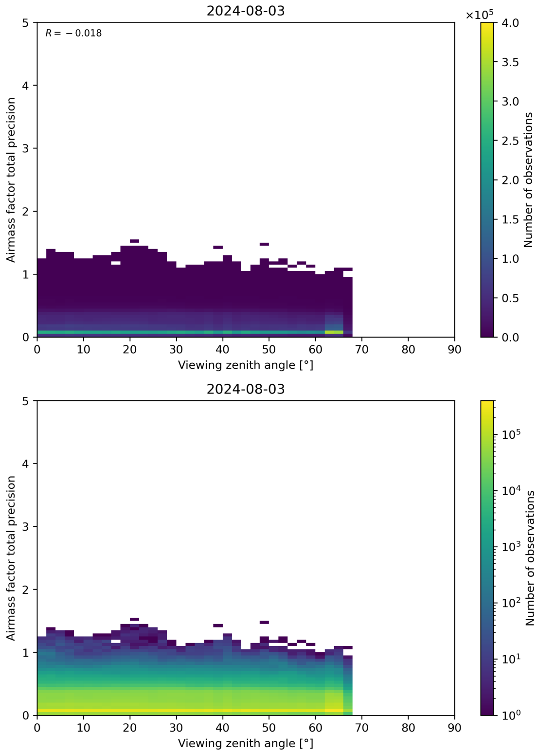
Figure 191: Scatter density plot of “Viewing zenith angle” against “Airmass factor total precision” for 2024-08-02 to 2024-08-04.
