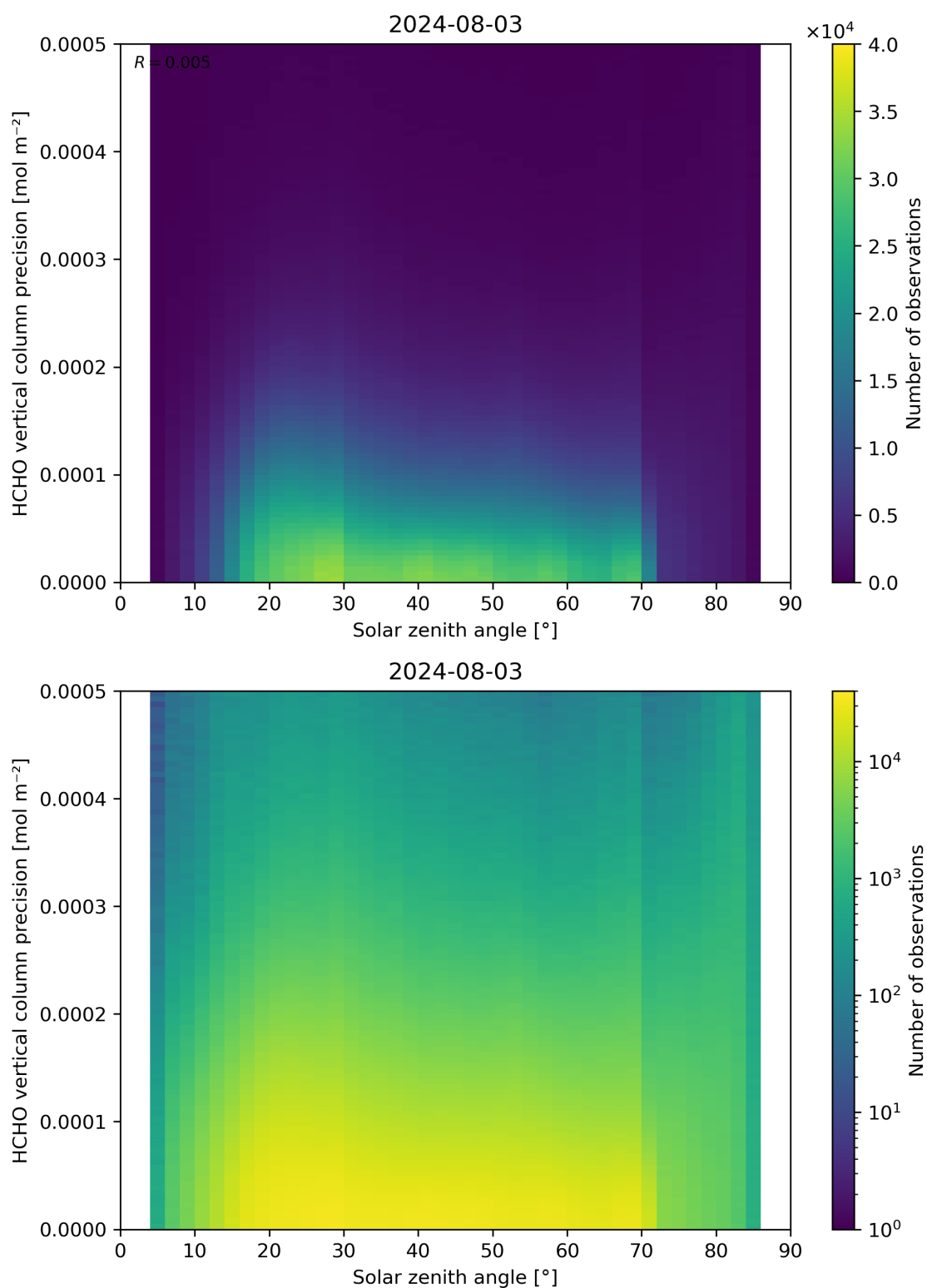
Figure 179: Scatter density plot of “Solar zenith angle” against “HCHO vertical column precision” for 2024-08-02 to 2024-08-04.
