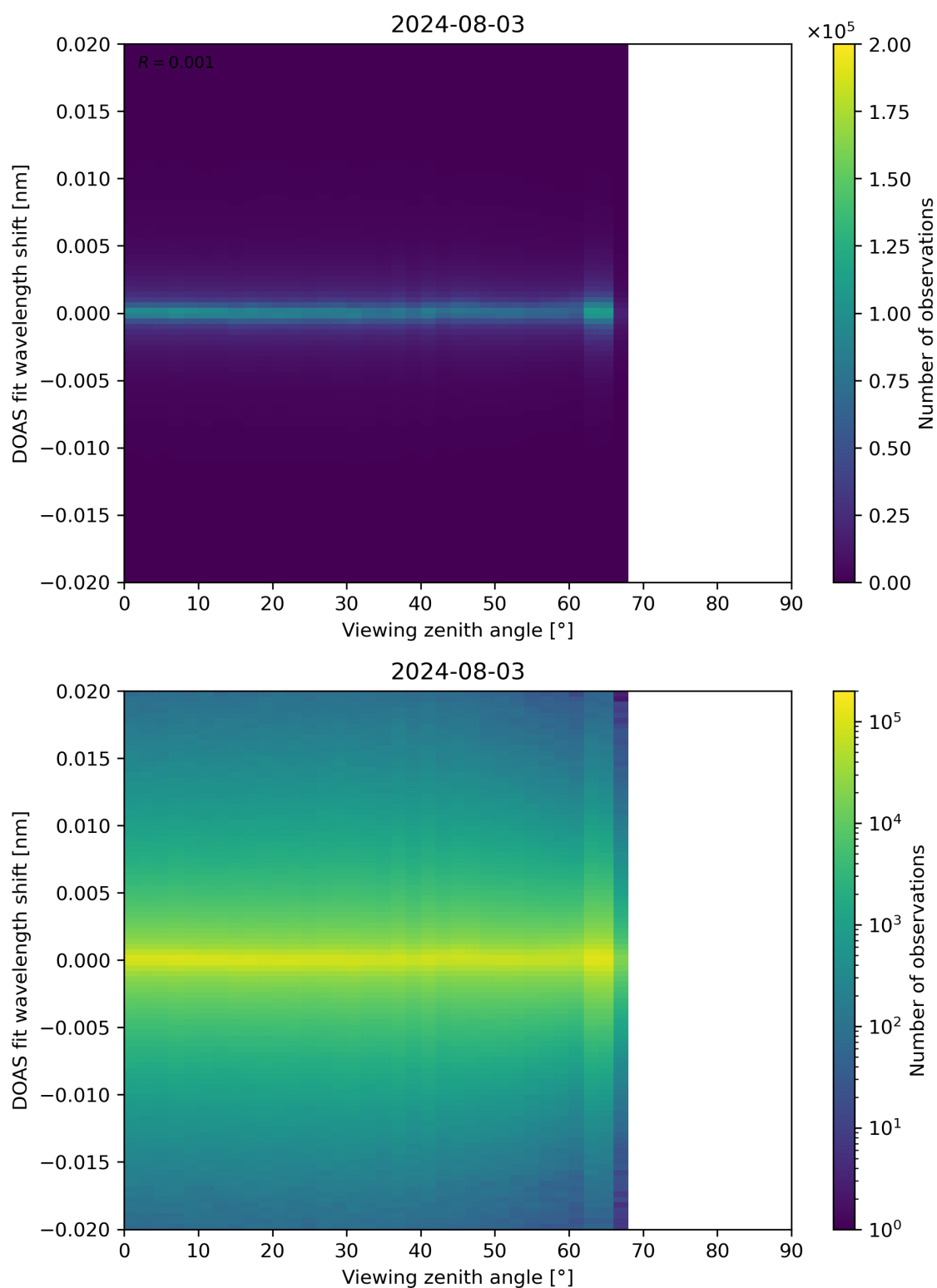
Figure 183: Scatter density plot of “Viewing zenith angle” against “DOAS fit wavelength shift” for 2024-08-02 to 2024-08-04.
