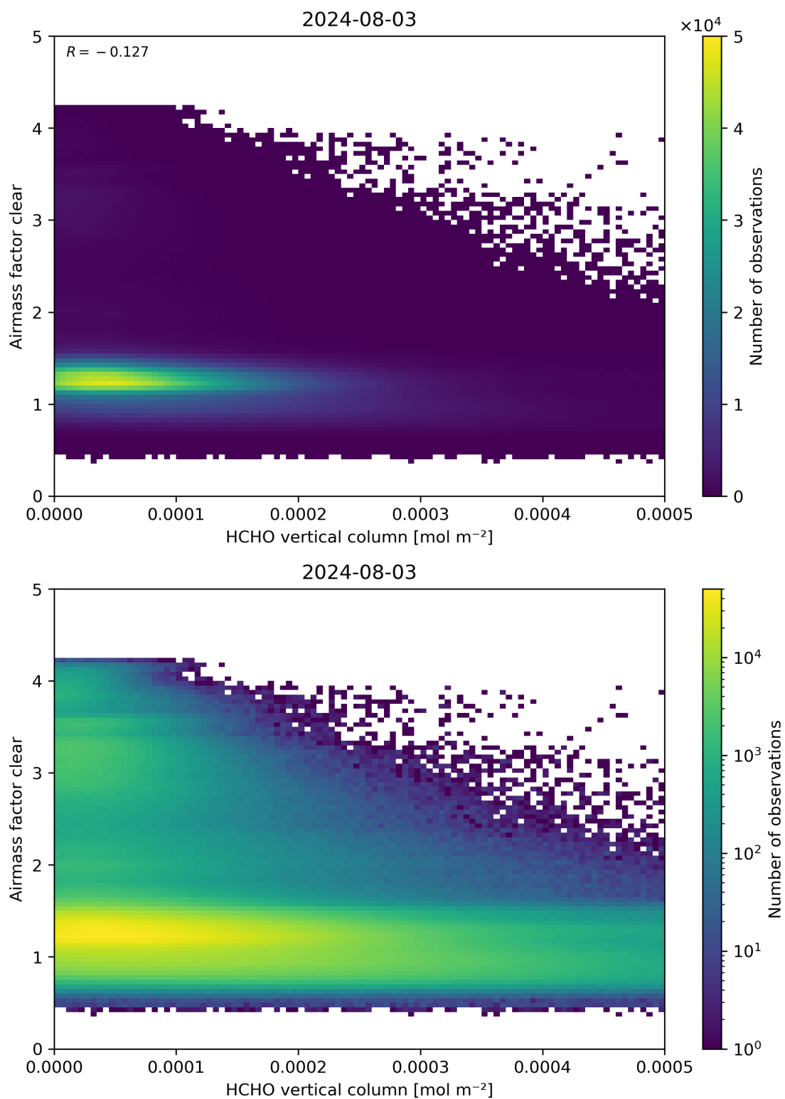
Figure 126: Scatter density plot of “HCHO vertical column” against “Airmass factor clear” for 2024-08-02 to 2024-08-04.
