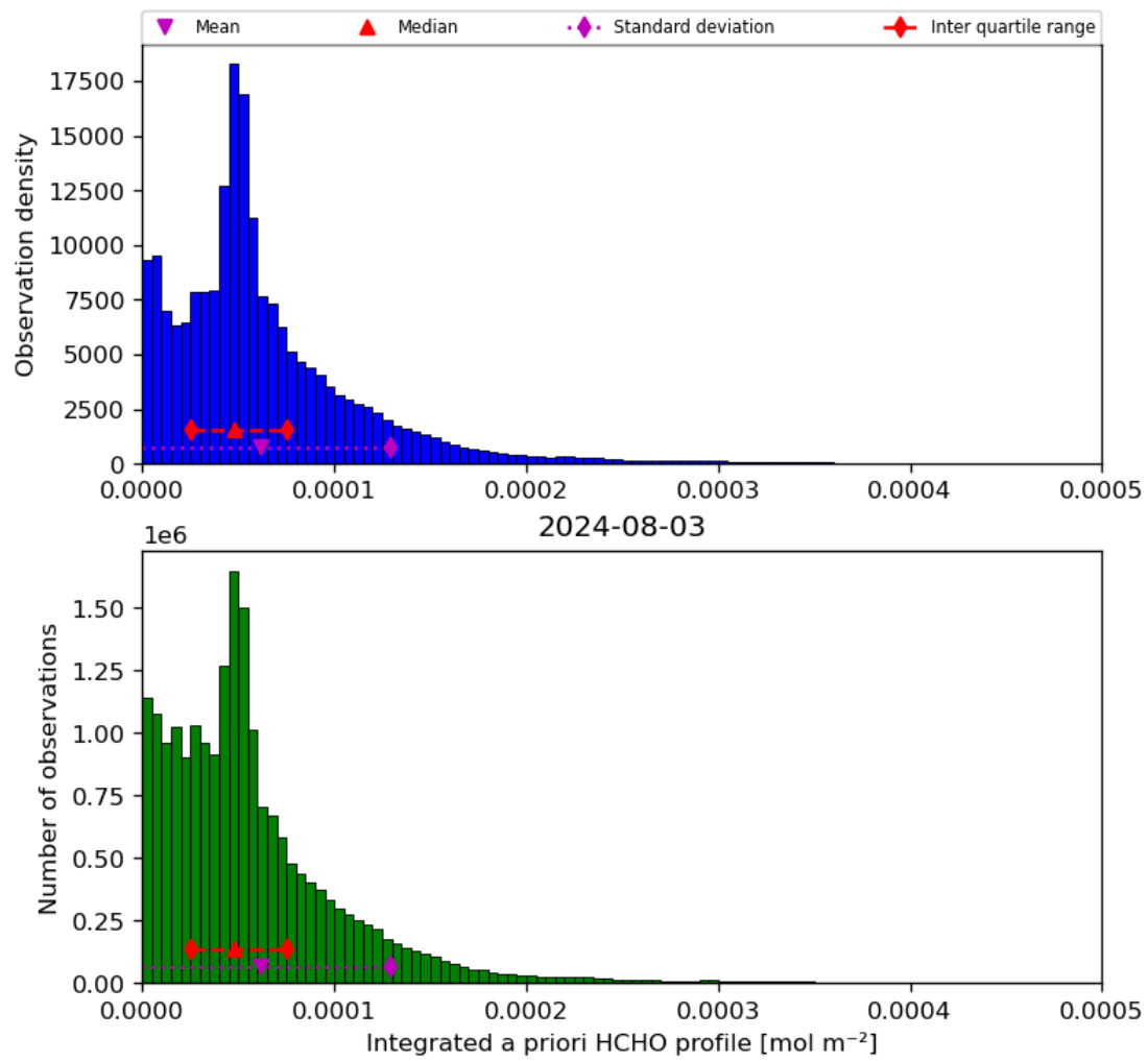
Figure 43: Histogram of “Integrated a priori HCHO profile” for 2024-08-02 to 2024-08-04
