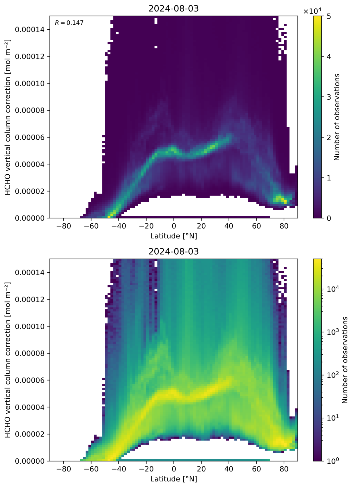
Figure 164: Scatter density plot of “Latitude” against “HCHO vertical column correction” for 2024-08-02 to 2024-08-04.
