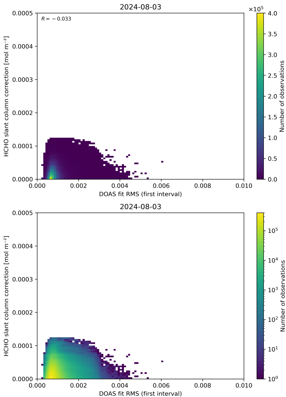
Figure 63: Scatter density plot of “DOAS fit RMS (first interval)” against “HCHO slant column correction” for 2024-08-02 to 2024-08-04.
