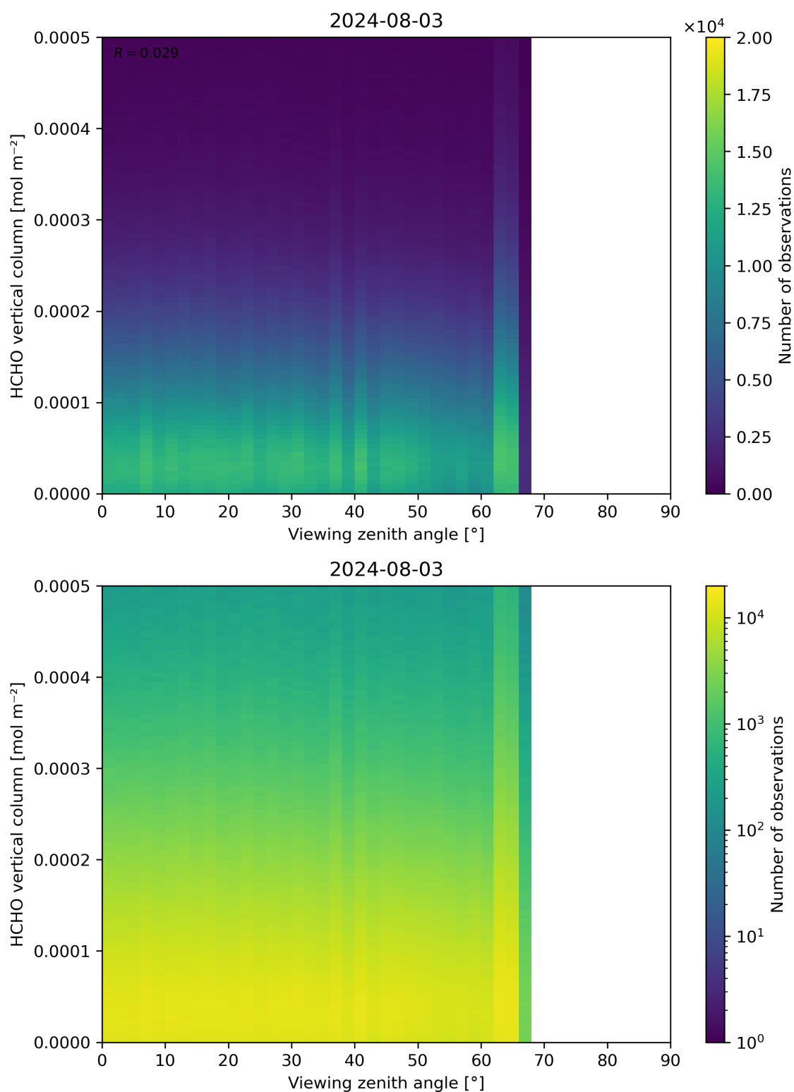
Figure 192: Scatter density plot of “Viewing zenith angle” against “HCHO vertical column” for 2024-08-02 to 2024-08-04.
