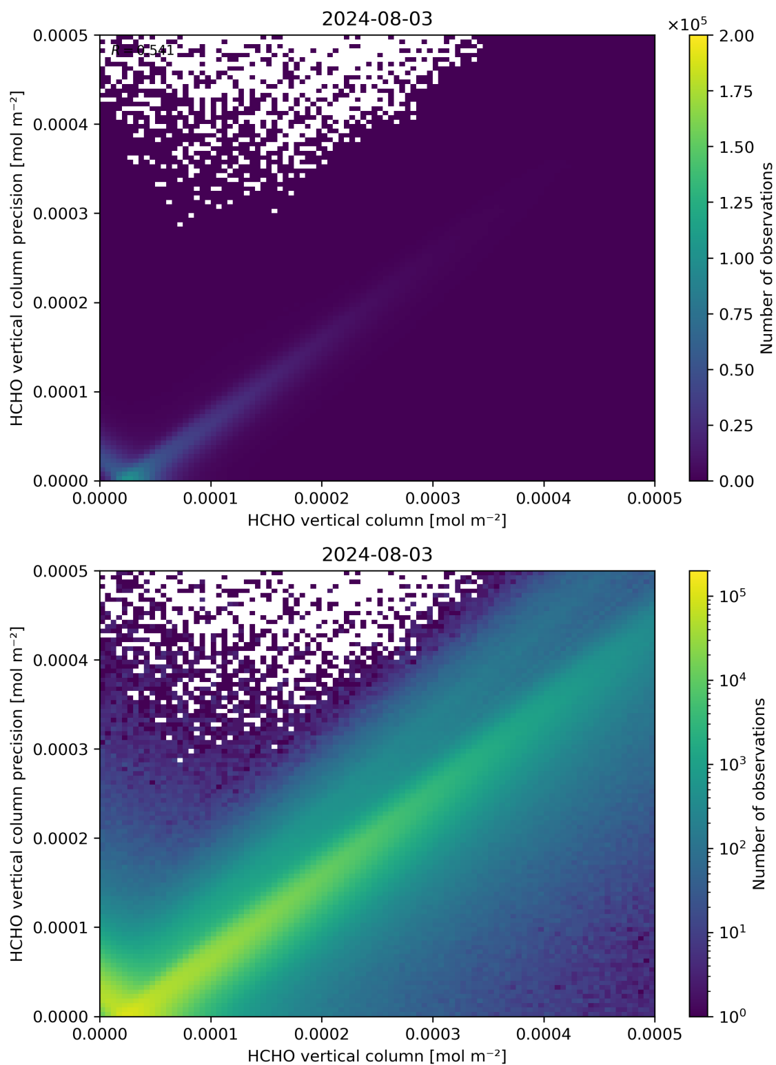
Figure 134: Scatter density plot of “HCHO vertical column” against “HCHO vertical column precision” for 2024-08-02 to 2024-08-04.
