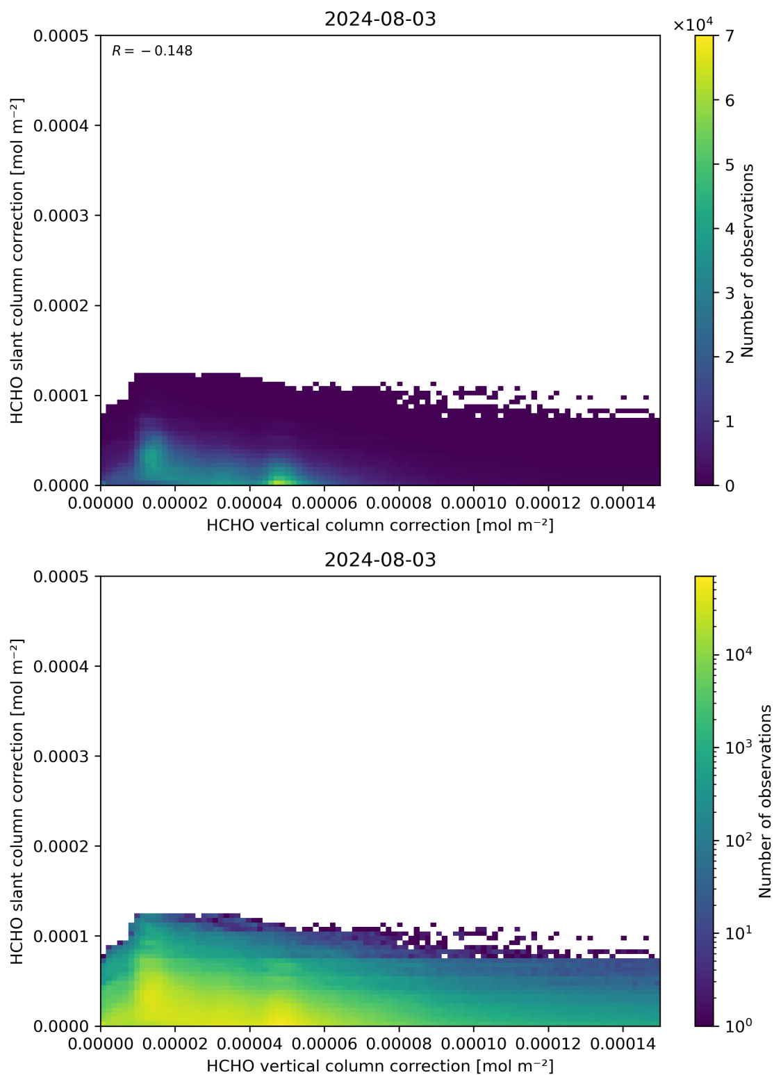
Figure 117: Scatter density plot of “HCHO vertical column correction” against “HCHO slant column correction” for 2024-08-02 to 2024-08-04.
