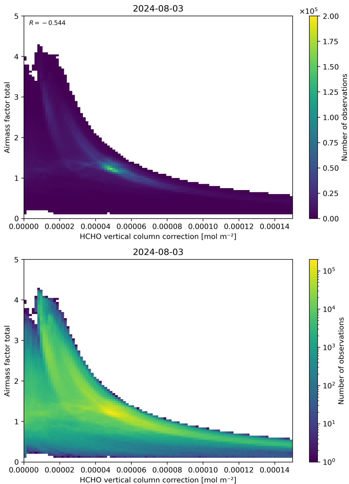
Figure 120: Scatter density plot of “HCHO vertical column correction” against “Airmass factor total” for 2024-08-02 to 2024-08-04.
