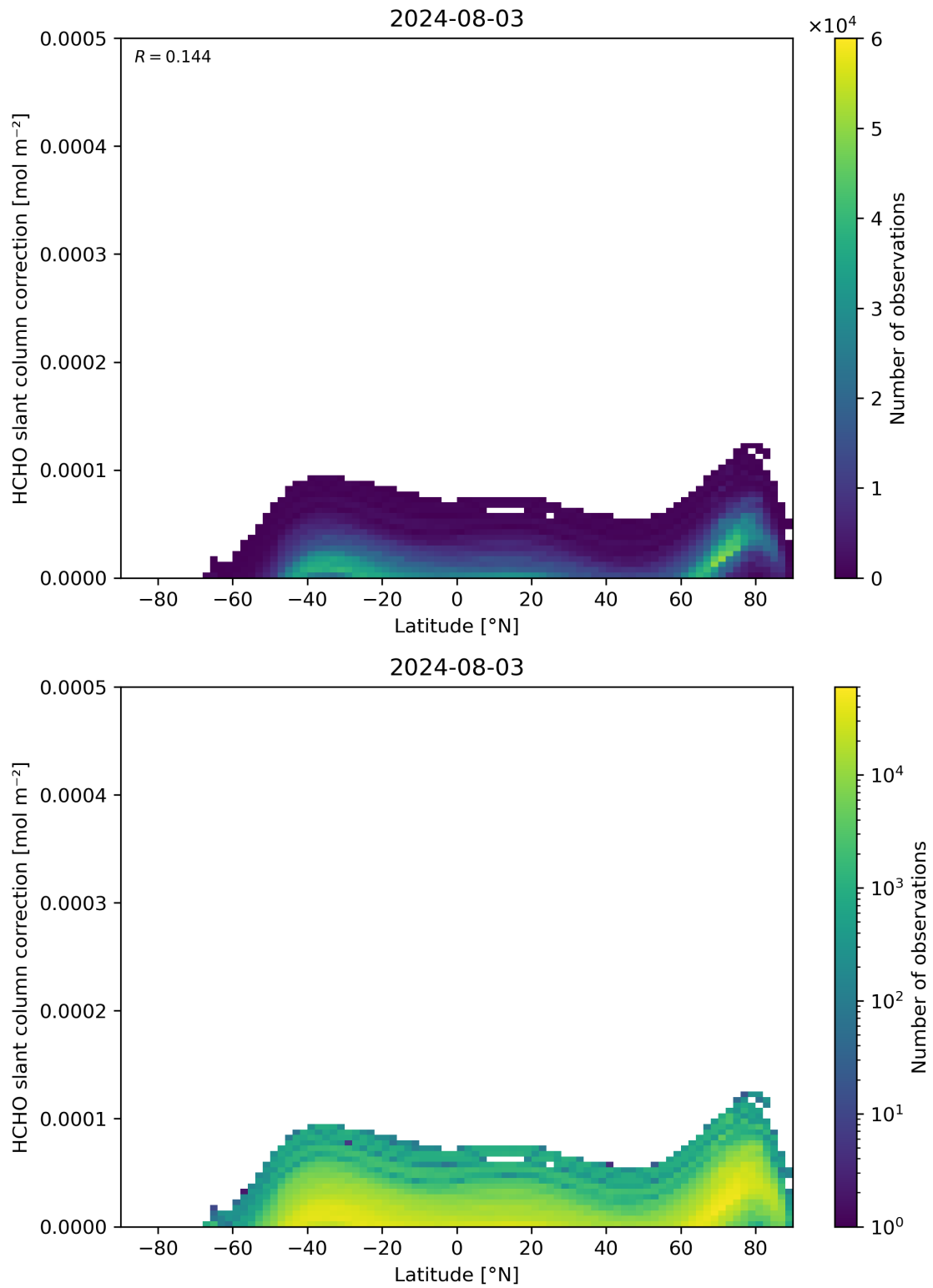
Figure 158: Scatter density plot of “Latitude” against “HCHO slant column correction” for 2024-08-02 to 2024-08-04.
