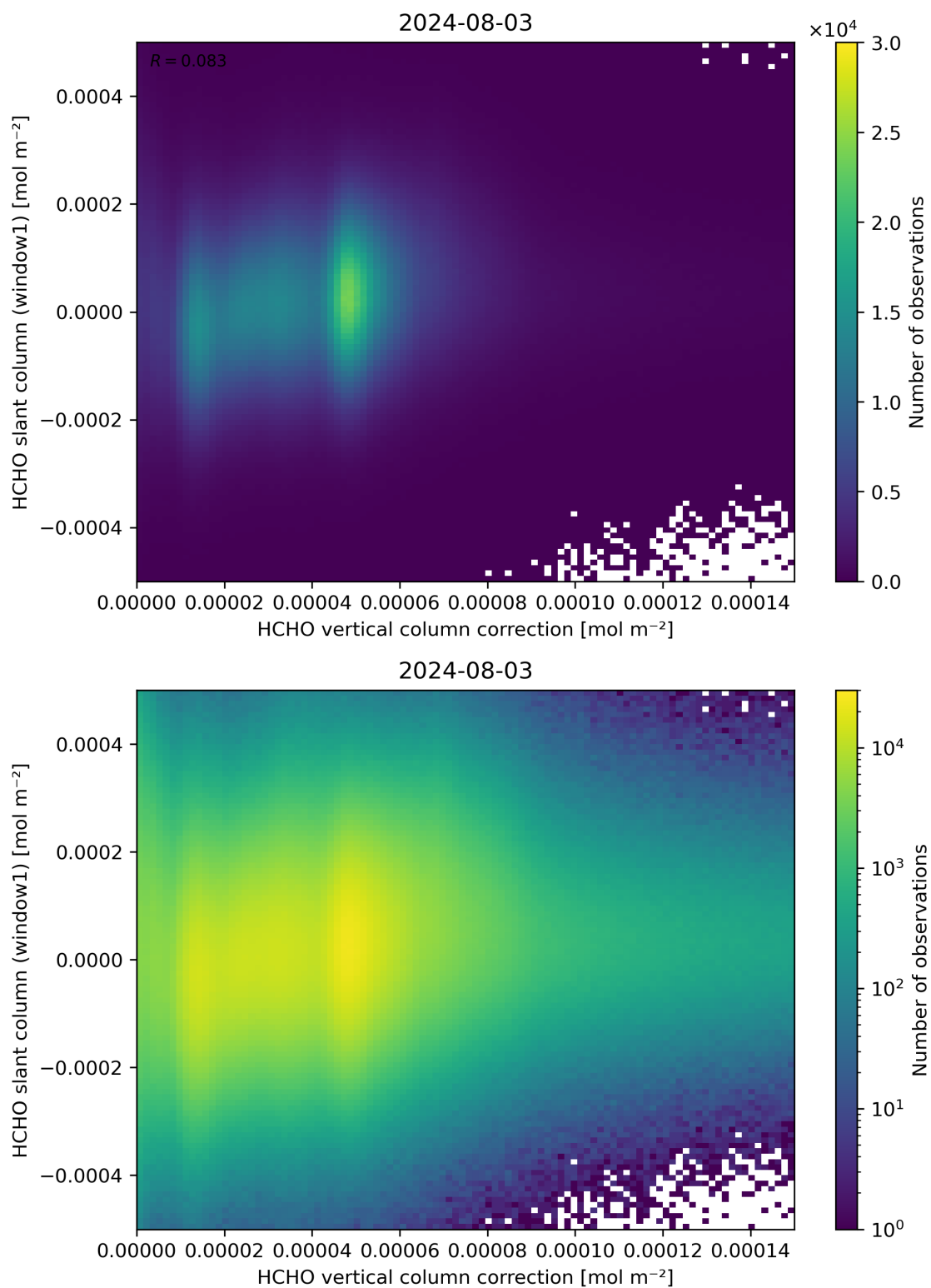
Figure 118: Scatter density plot of “HCHO vertical column correction” against “HCHO slant column (window1)” for 2024-08-02 to 2024-08-04.
