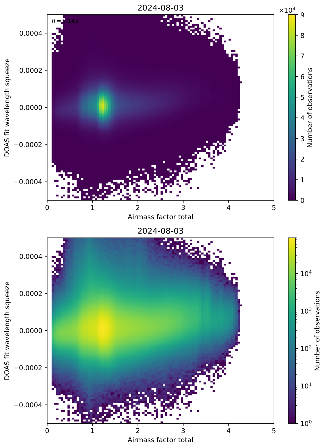
Figure 99: Scatter density plot of “Airmass factor total” against “DOAS fit wavelength squeeze” for 2024-08-02 to 2024-08-04.
