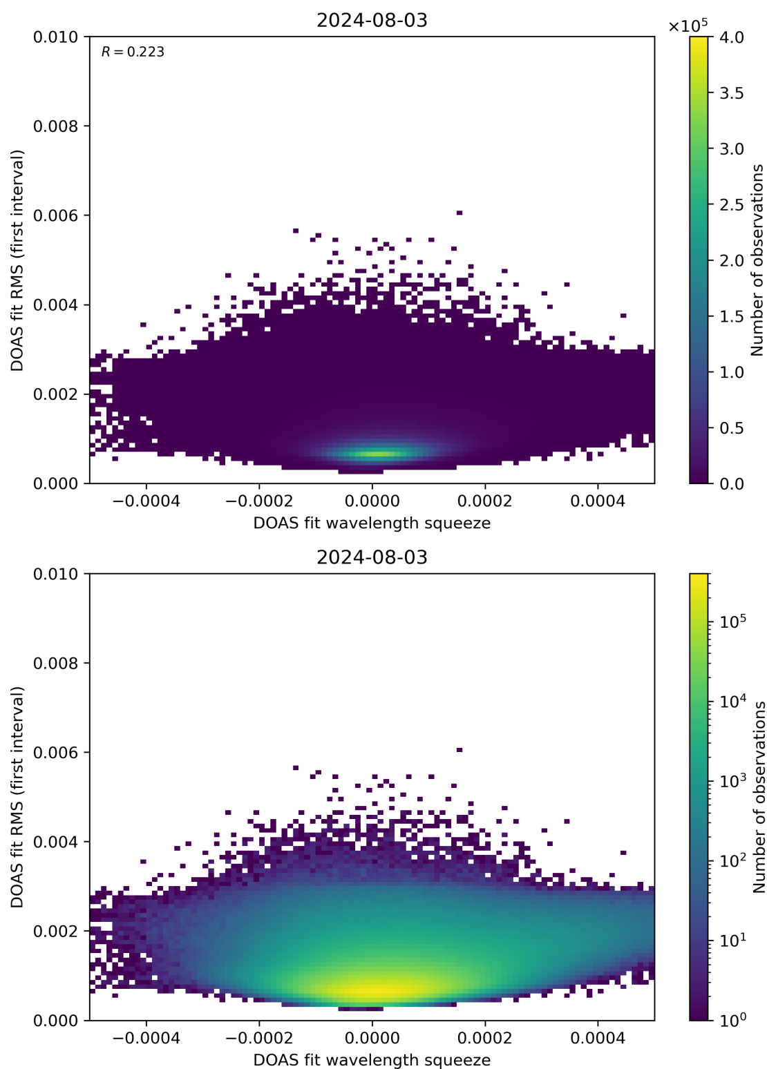
Figure 68: Scatter density plot of “DOAS fit wavelength squeeze” against “DOAS fit RMS (first interval)” for 2024-08-02 to 2024-08-04.
