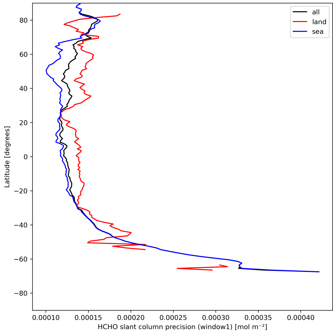
Figure 25: Zonal average of “HCHO slant column precision (window1)” for 2024-08-02 to 2024-08-04.
