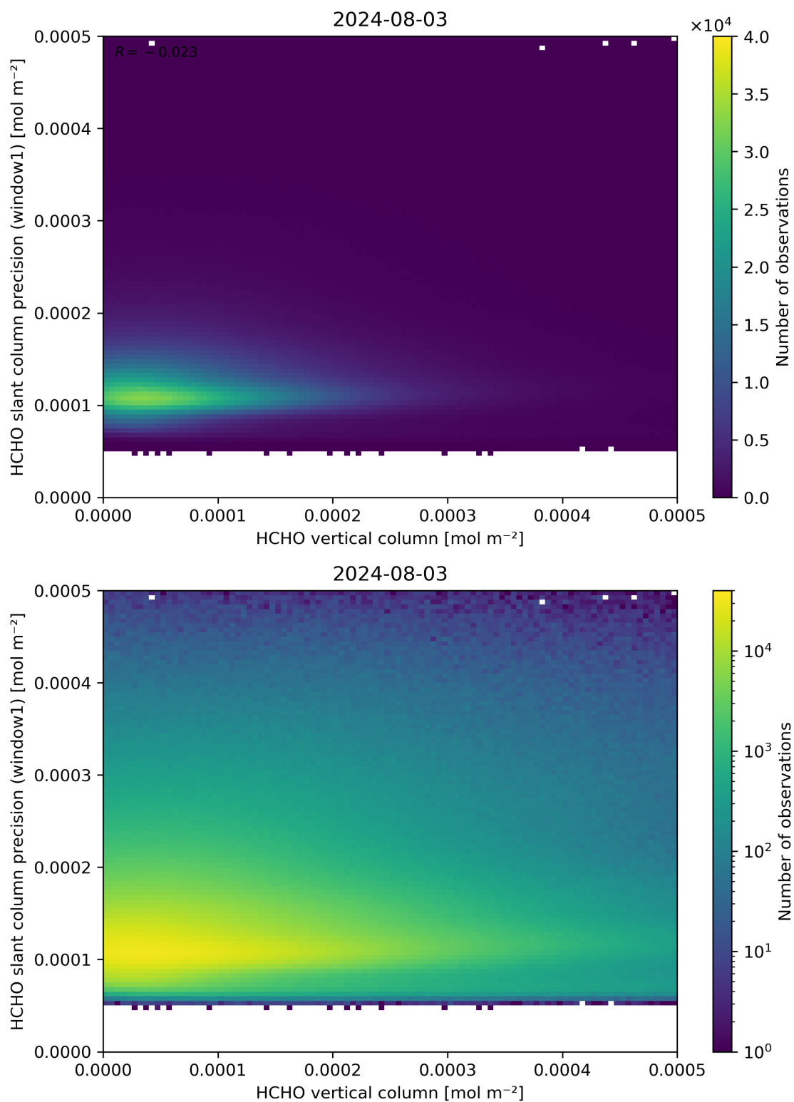
Figure 130: Scatter density plot of “HCHO vertical column” against “HCHO slant column precision (window1)” for 2024-08-02 to 2024-08-04.
