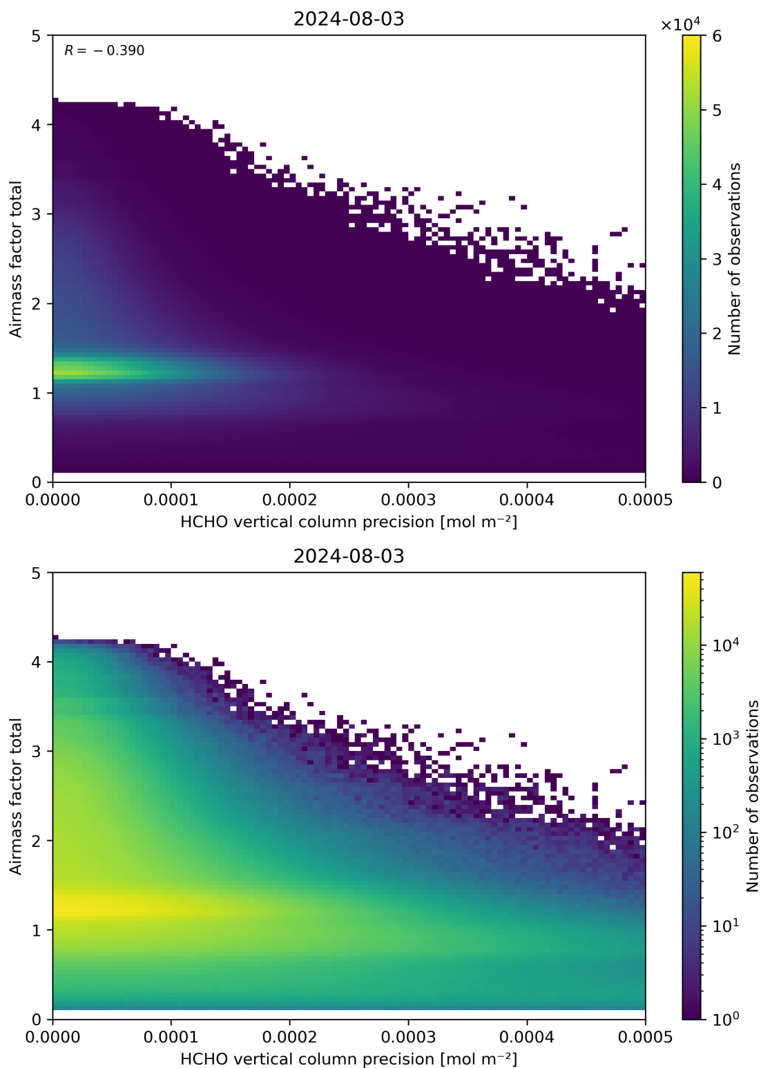
Figure 144: Scatter density plot of “HCHO vertical column precision” against “Airmass factor total” for 2024-08-02 to 2024-08-04.
