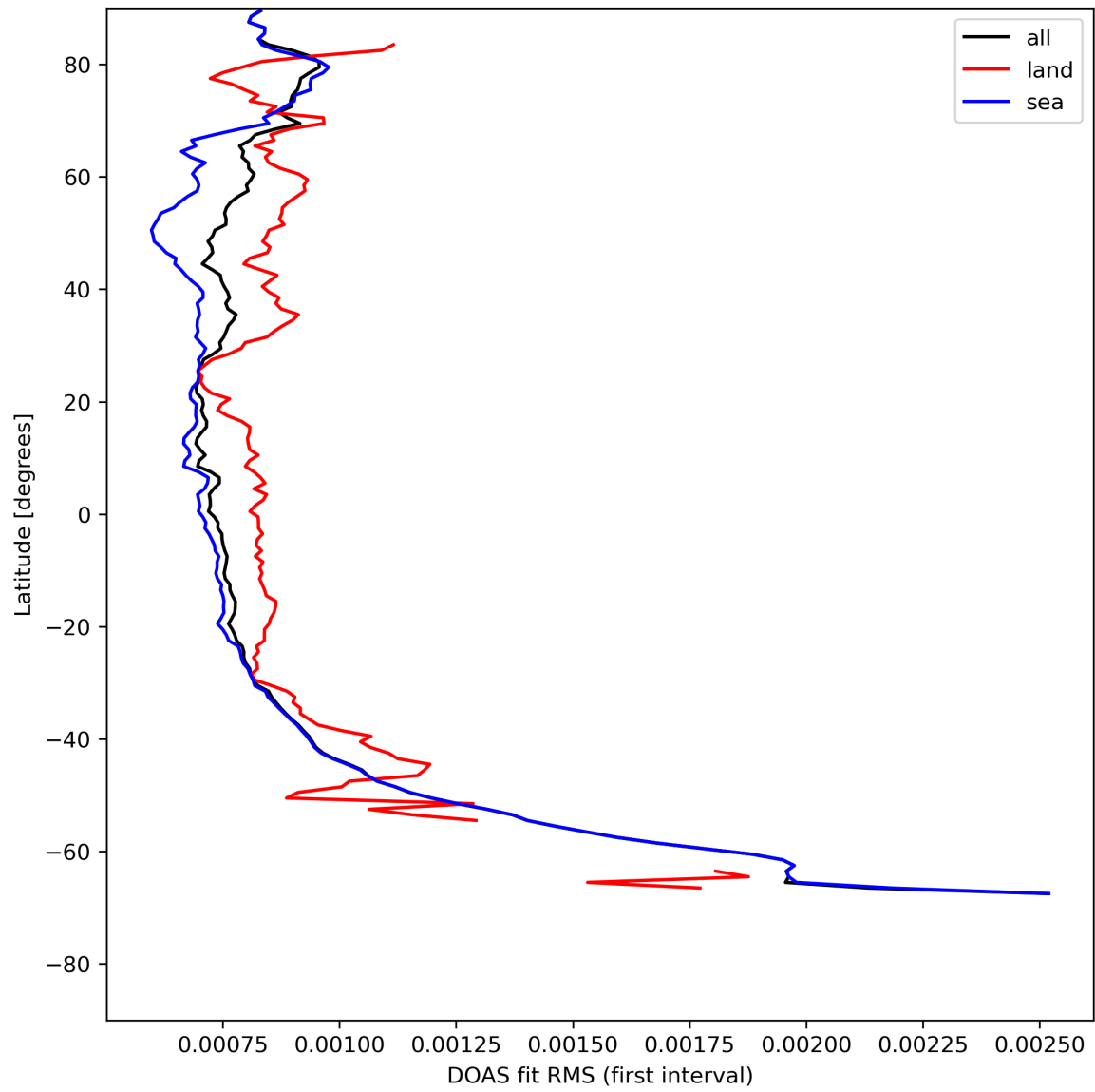
Figure 32: Zonal average of "DOAS fit RMS (first interval)" for 2024-08-02 to 2024-08-04.
