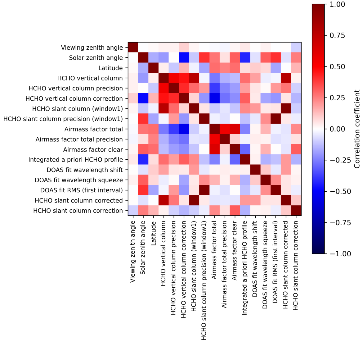
Figure 2: Map of correlation matrix for 2024-08-02 to 2024-08-04.
