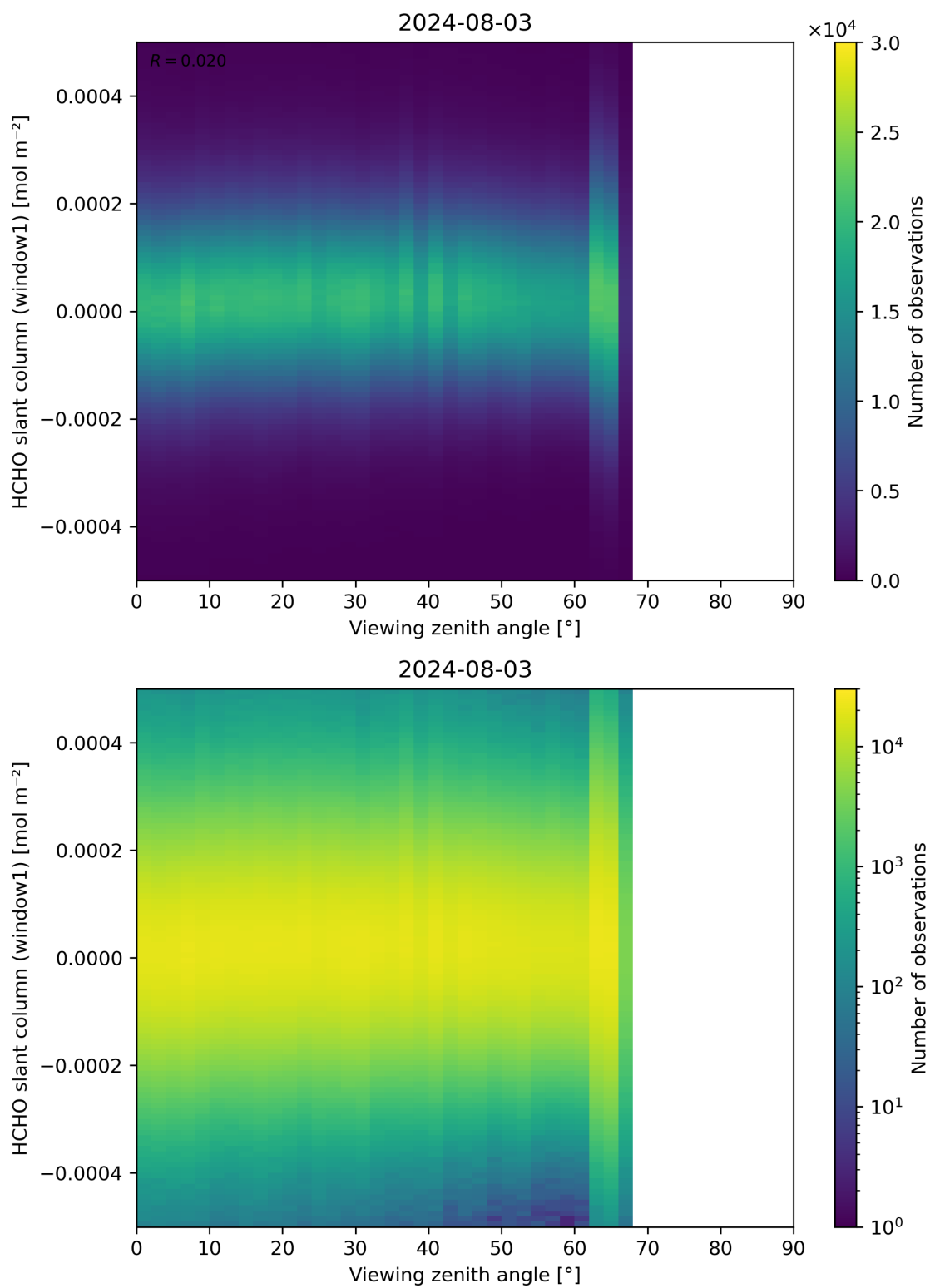
Figure 188: Scatter density plot of “Viewing zenith angle” against “HCHO slant column (window1)” for 2024-08-02 to 2024-08-04.
