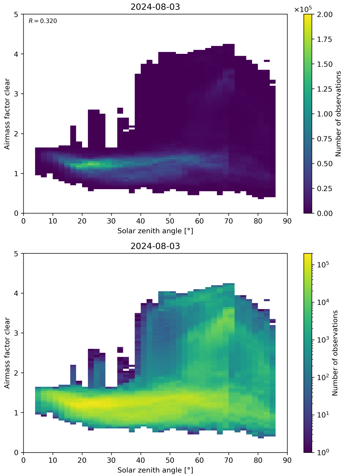
Figure 170: Scatter density plot of “Solar zenith angle” against “Airmass factor clear” for 2024-08-02 to 2024-08-04.
