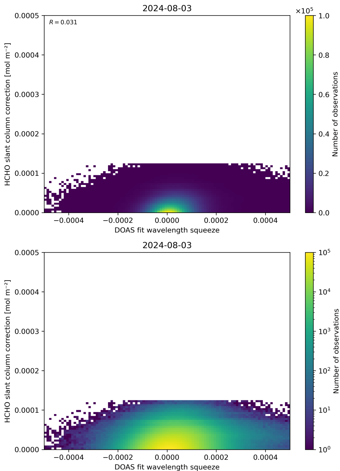
Figure 70: Scatter density plot of “DOAS fit wavelength squeeze” against “HCHO slant column correction” for 2024-08-02 to 2024-08-04.
