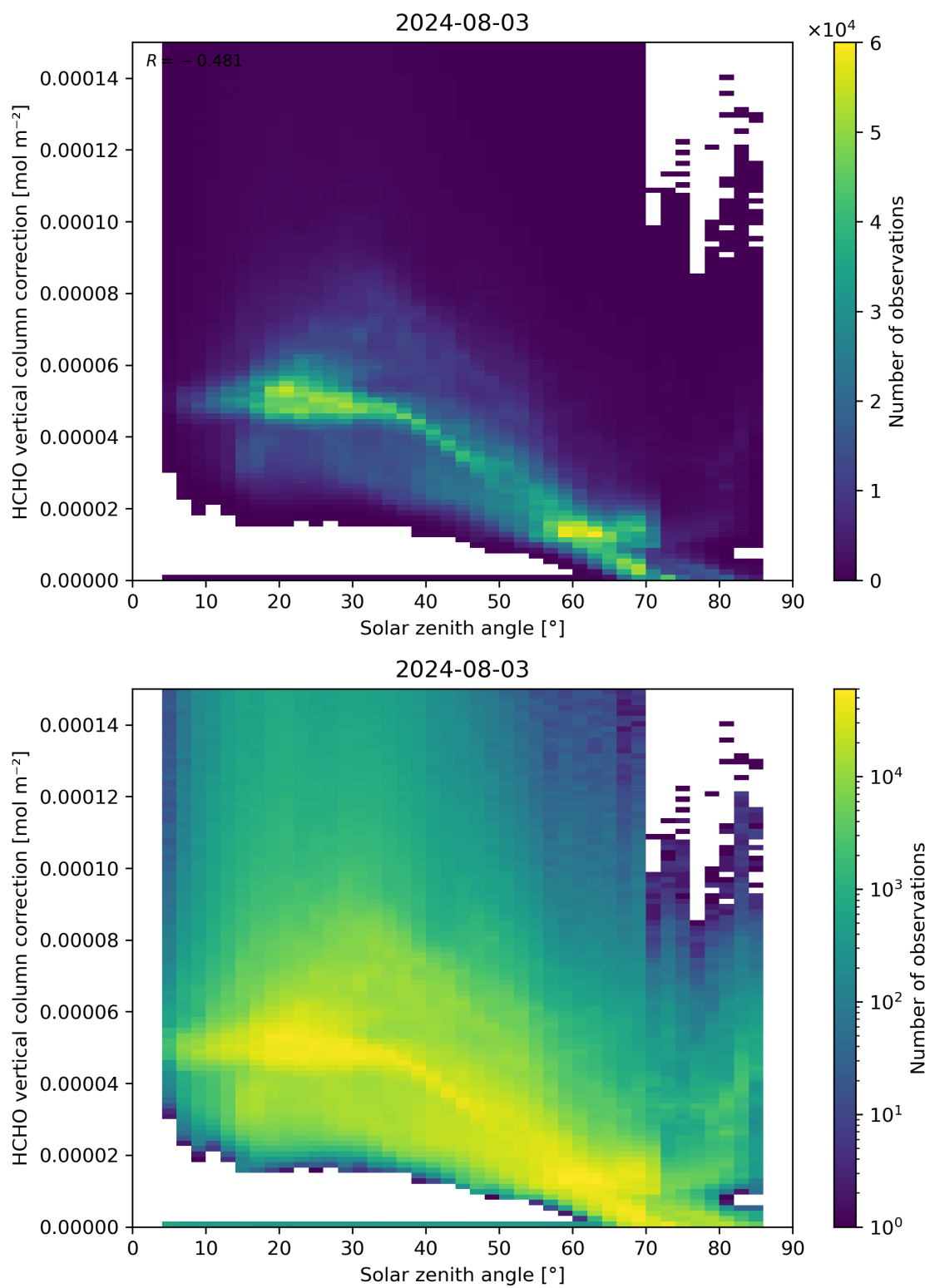
Figure 178: Scatter density plot of “Solar zenith angle” against “HCHO vertical column correction” for 2024-08-02 to 2024-08-04.
