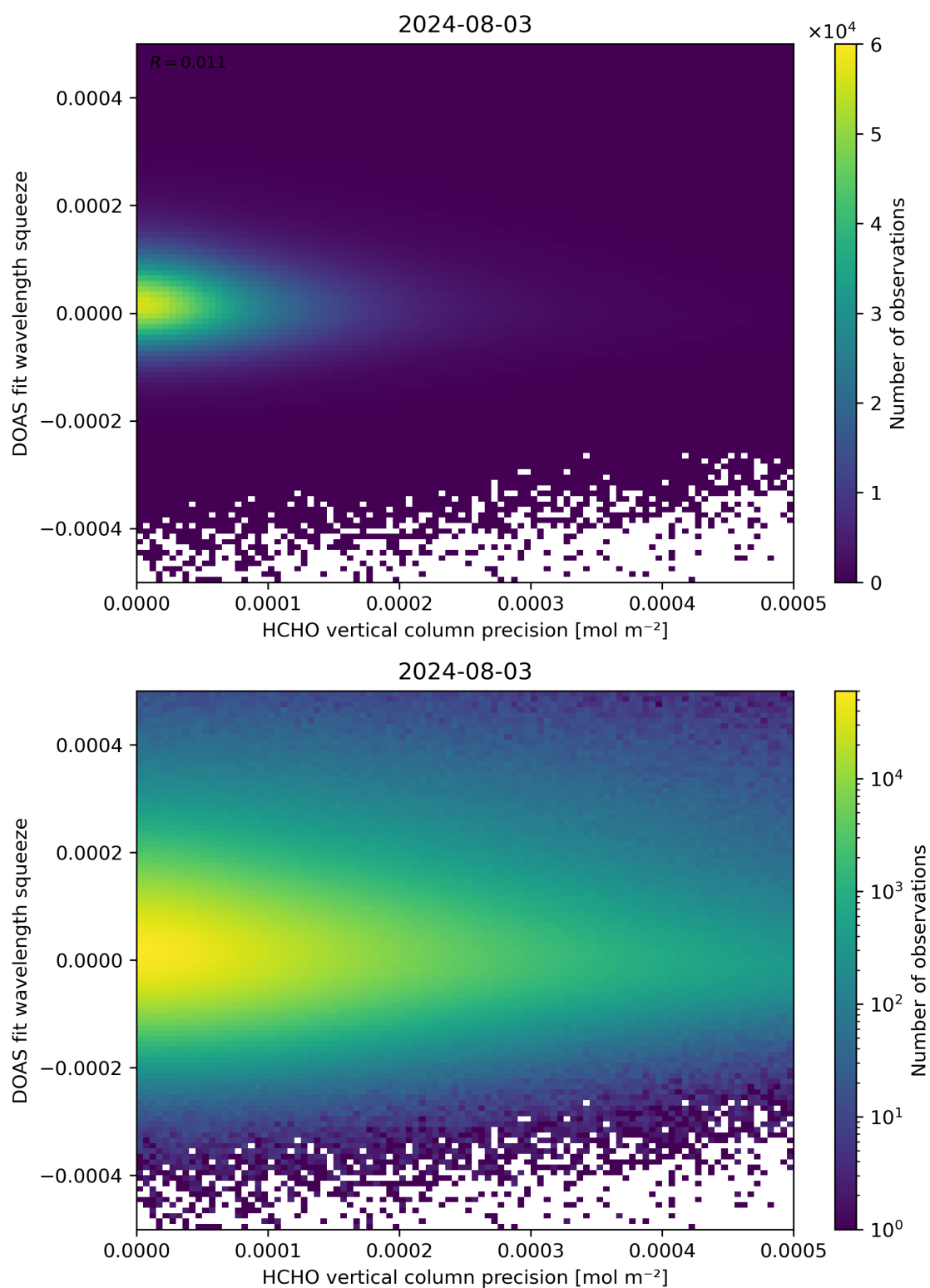
Figure 138: Scatter density plot of “HCHO vertical column precision” against “DOAS fit wavelength squeeze” for 2024-08-02 to 2024-08-04.
