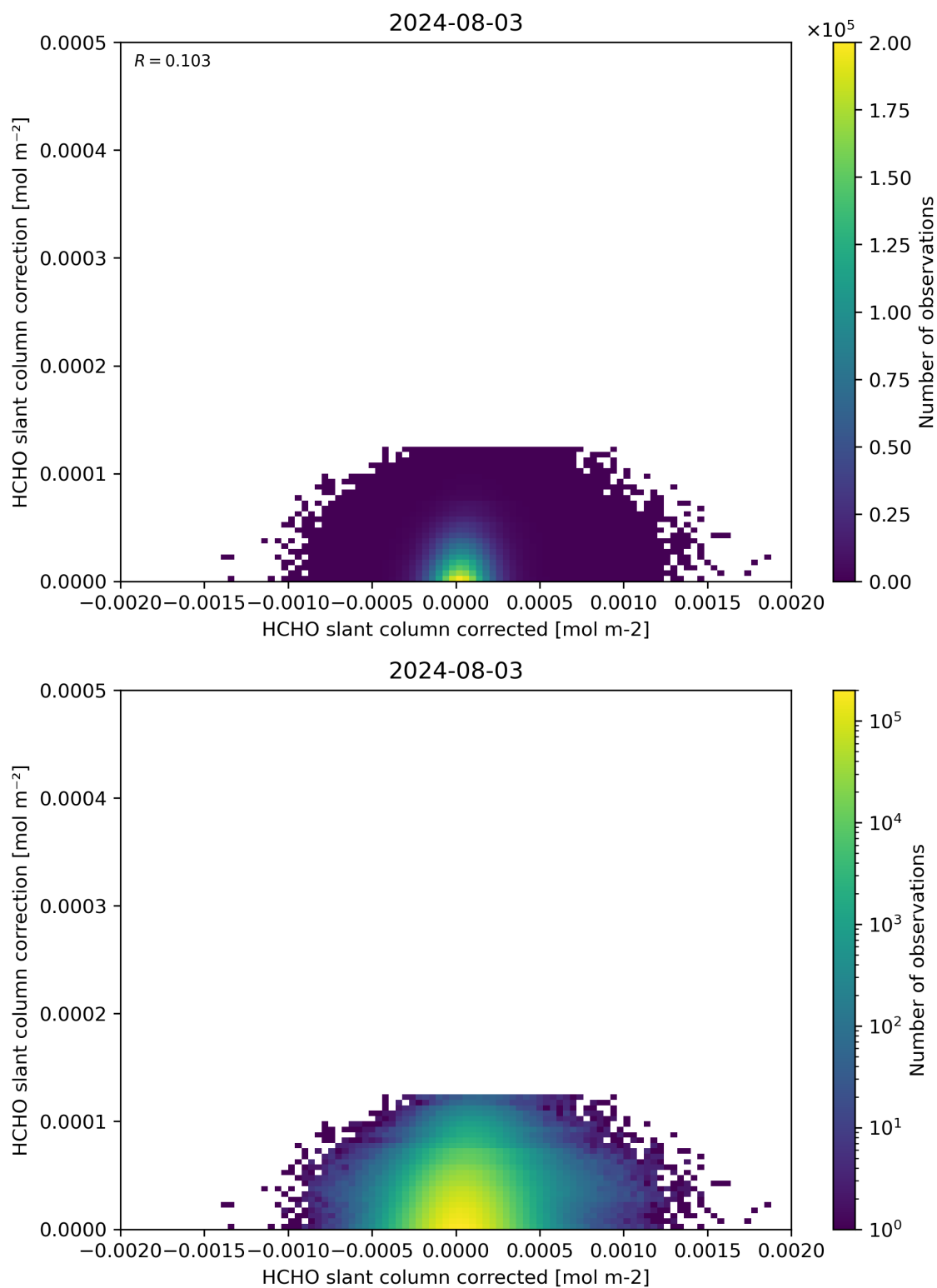
Figure 77: Scatter density plot of “HCHO slant column corrected” against “HCHO slant column correction” for 2024-08-02 to 2024-08-04.
