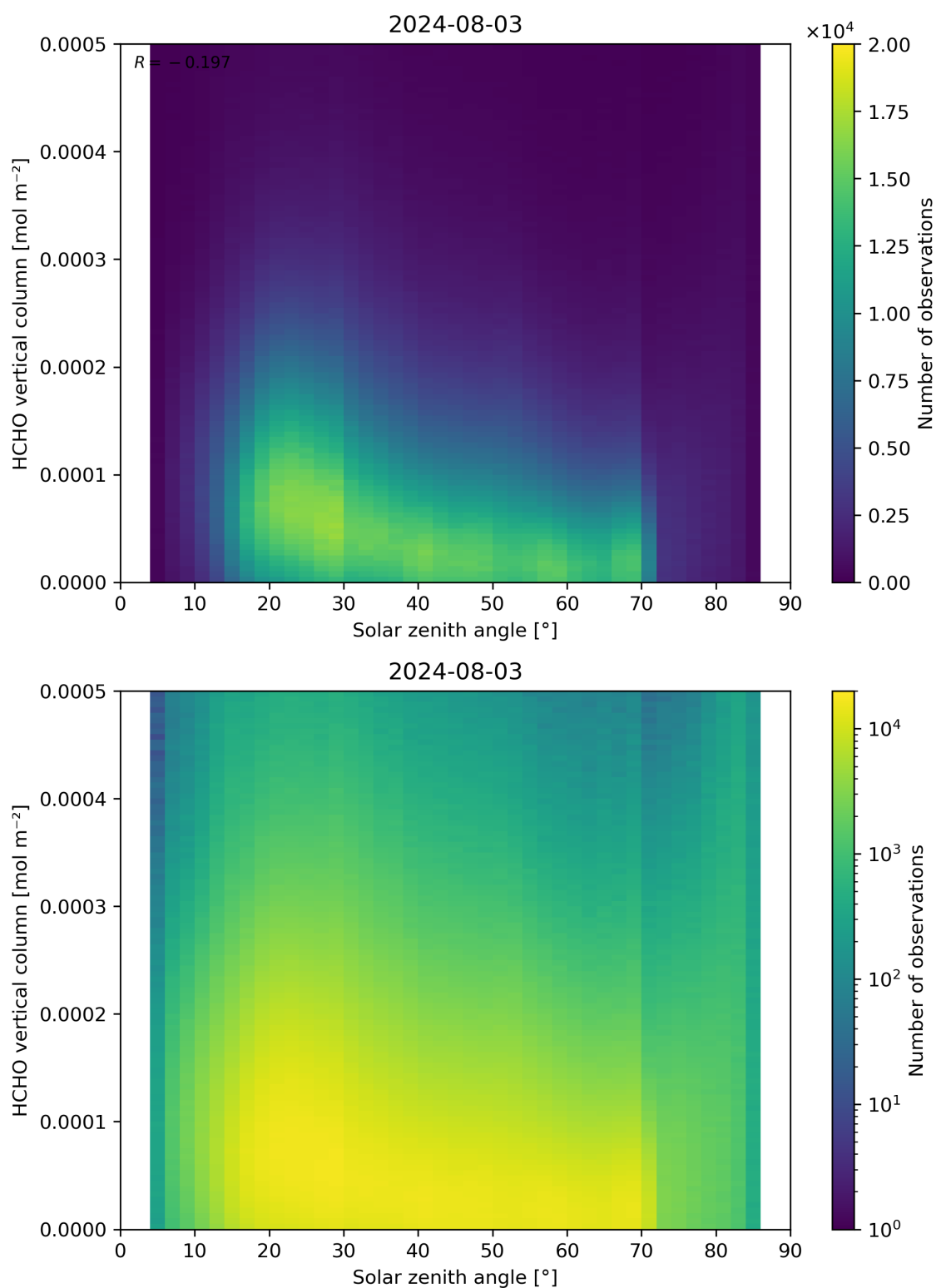
Figure 177: Scatter density plot of “Solar zenith angle” against “HCHO vertical column” for 2024-08-02 to 2024-08-04.
