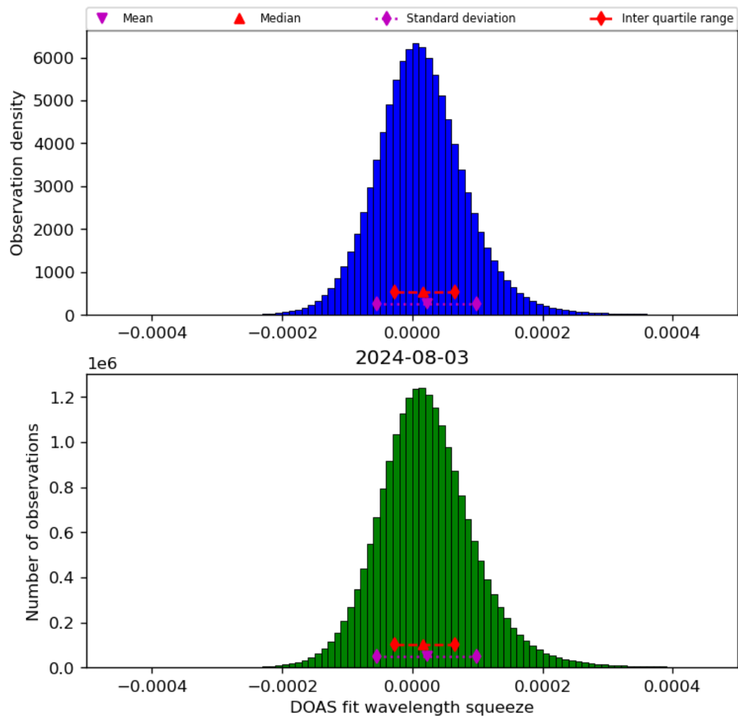
Figure 45: Histogram of “DOAS fit wavelength squeeze” for 2024-08-02 to 2024-08-04
