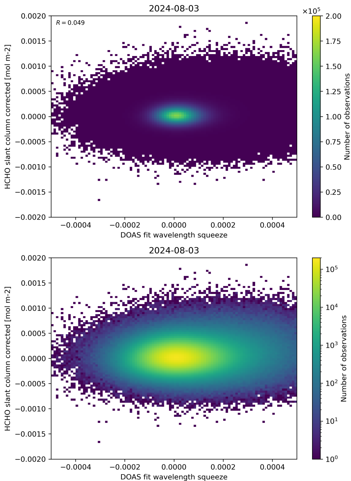
Figure 69: Scatter density plot of “DOAS fit wavelength squeeze” against “HCHO slant column corrected” for 2024-08-02 to 2024-08-04.
