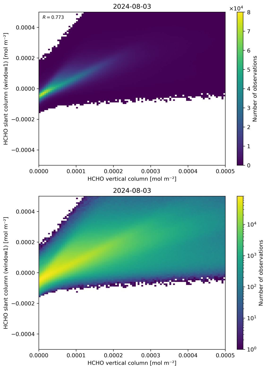
Figure 129: Scatter density plot of “HCHO vertical column” against “HCHO slant column (window1)” for 2024-08-02 to 2024-08-04.
