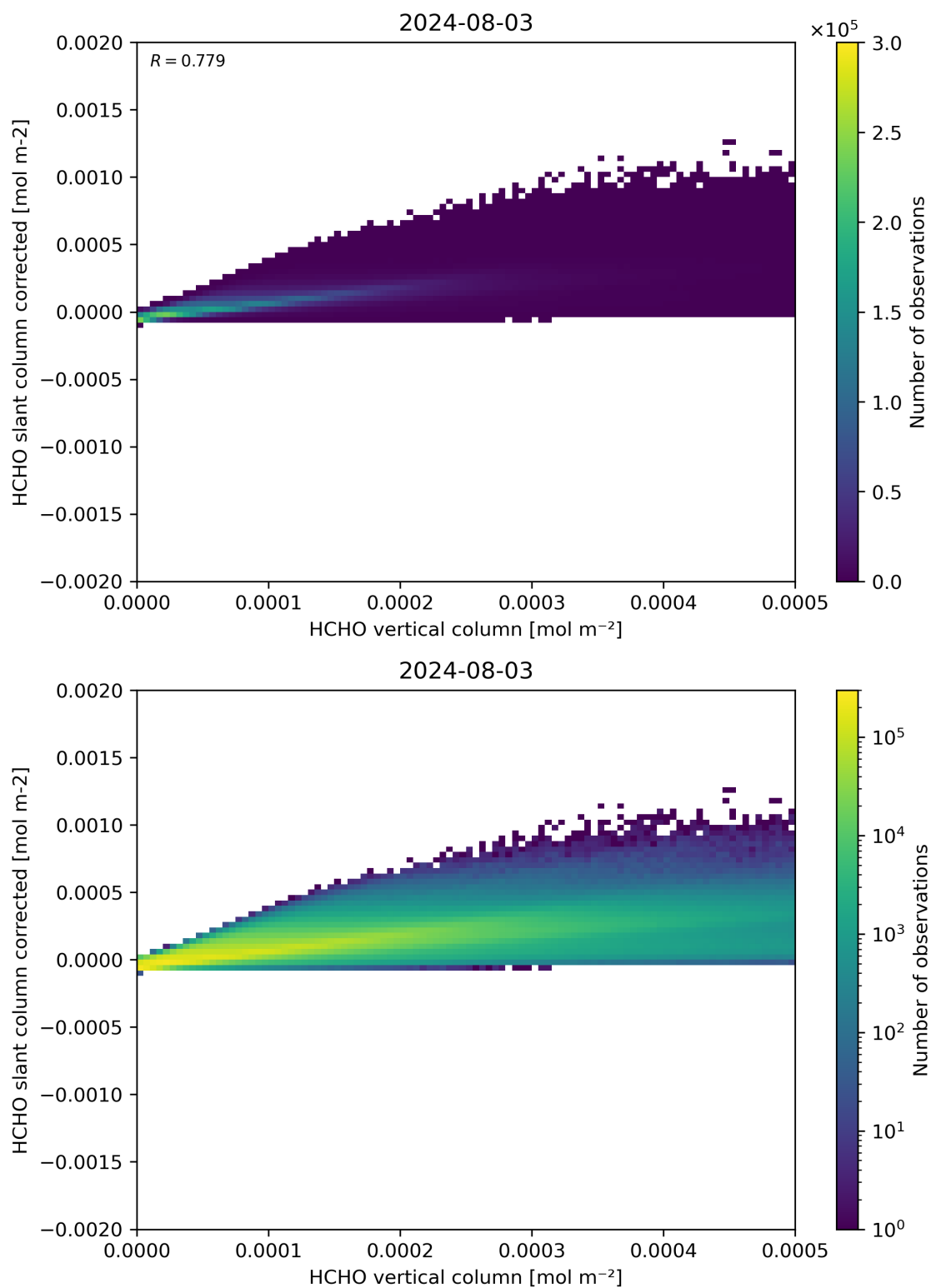
Figure 127: Scatter density plot of “HCHO vertical column” against “HCHO slant column corrected” for 2024-08-02 to 2024-08-04.
