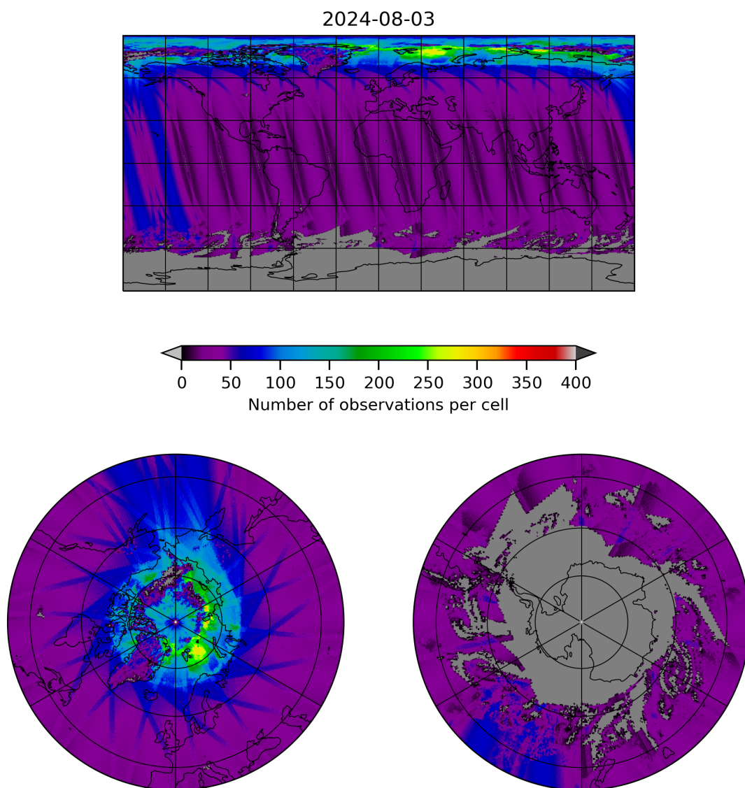
Figure 19: Map of the number of observations for 2024-08-02 to 2024-08-04
