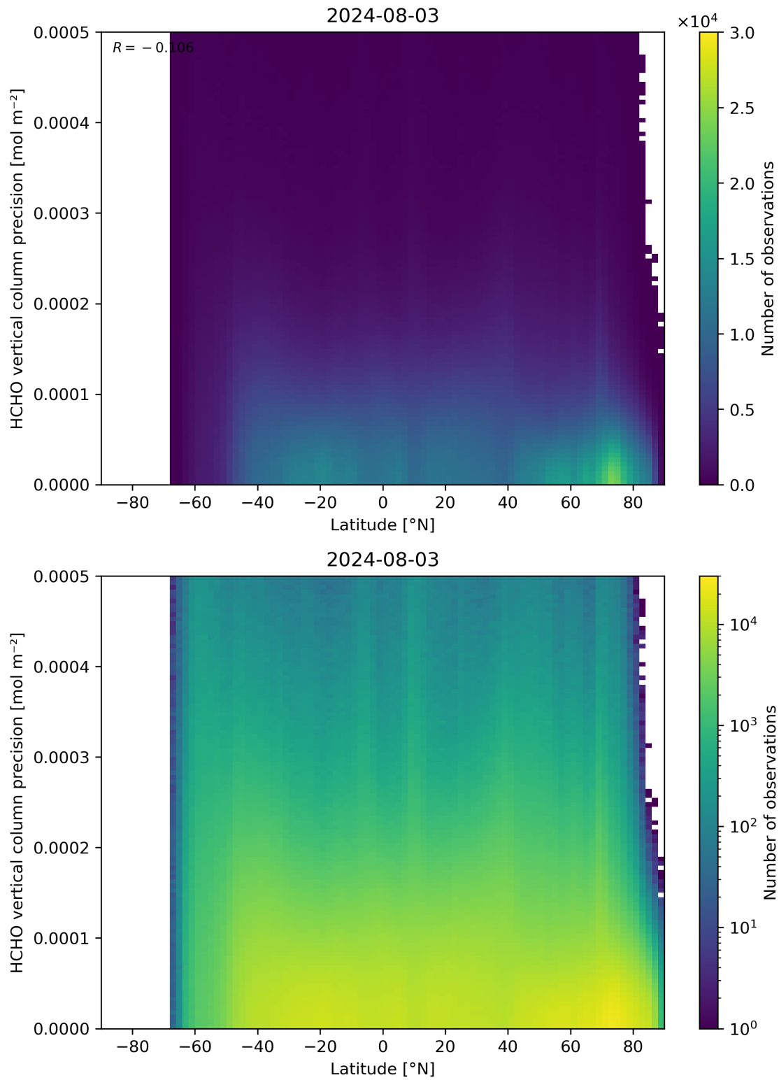
Figure 165: Scatter density plot of “Latitude” against “HCHO vertical column precision” for 2024-08-02 to 2024-08-04.
