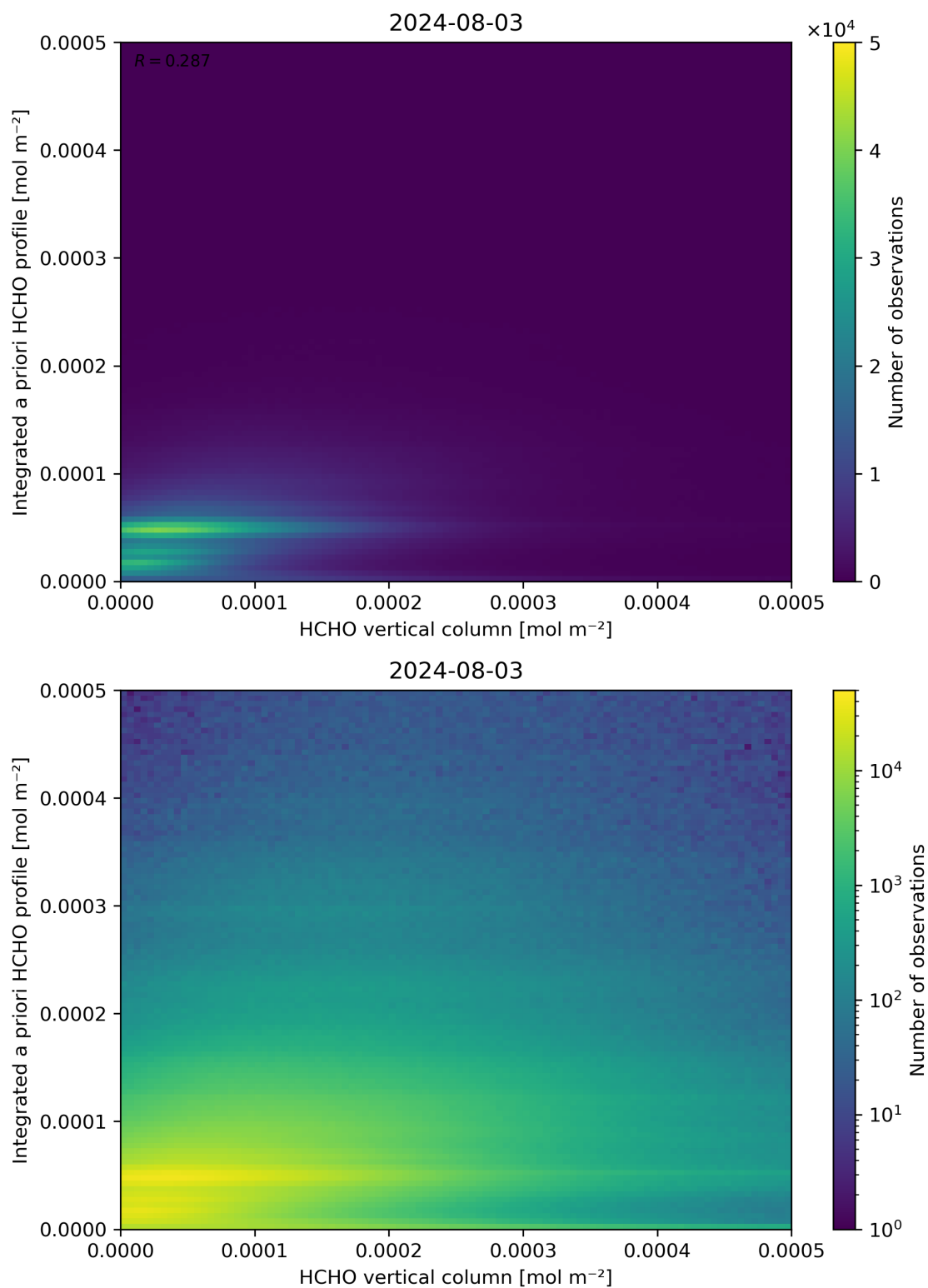
Figure 135: Scatter density plot of “HCHO vertical column” against “Integrated a priori HCHO profile” for 2024-08-02 to 2024-08-04.
