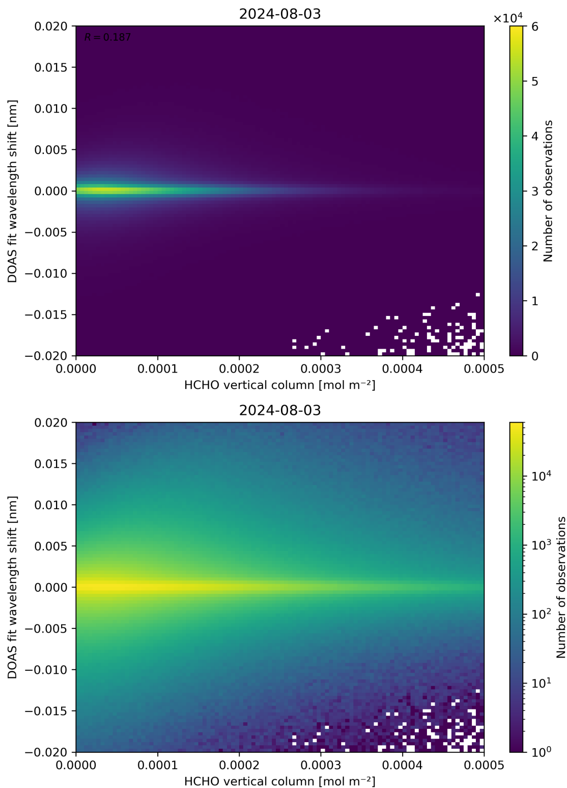
Figure 124: Scatter density plot of “HCHO vertical column” against “DOAS fit wavelength shift” for 2024-08-02 to 2024-08-04.
