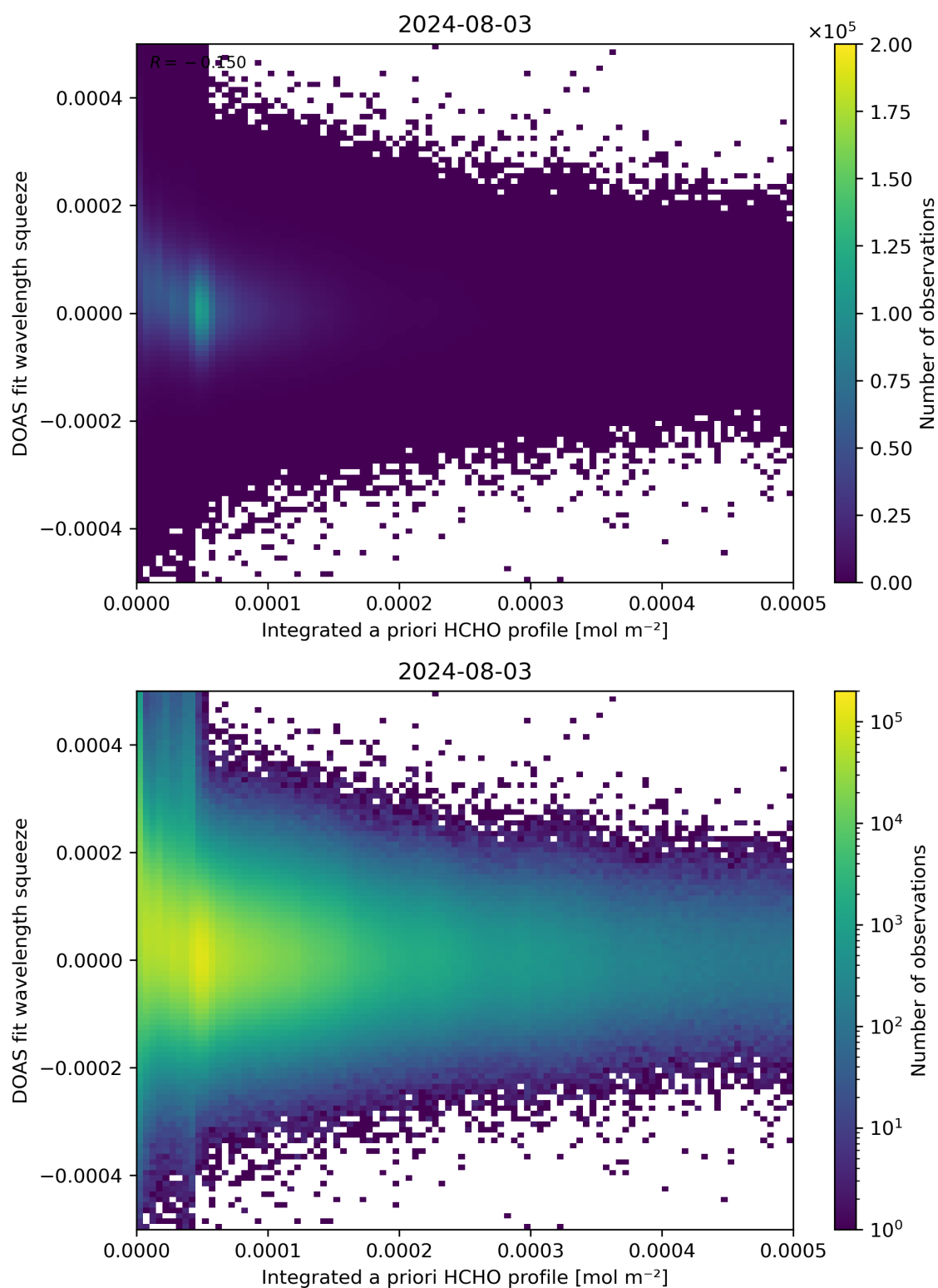
Figure 150: Scatter density plot of “Integrated a priori HCHO profile” against “DOAS fit wavelength squeeze” for 2024-08-02 to 2024-08-04.
