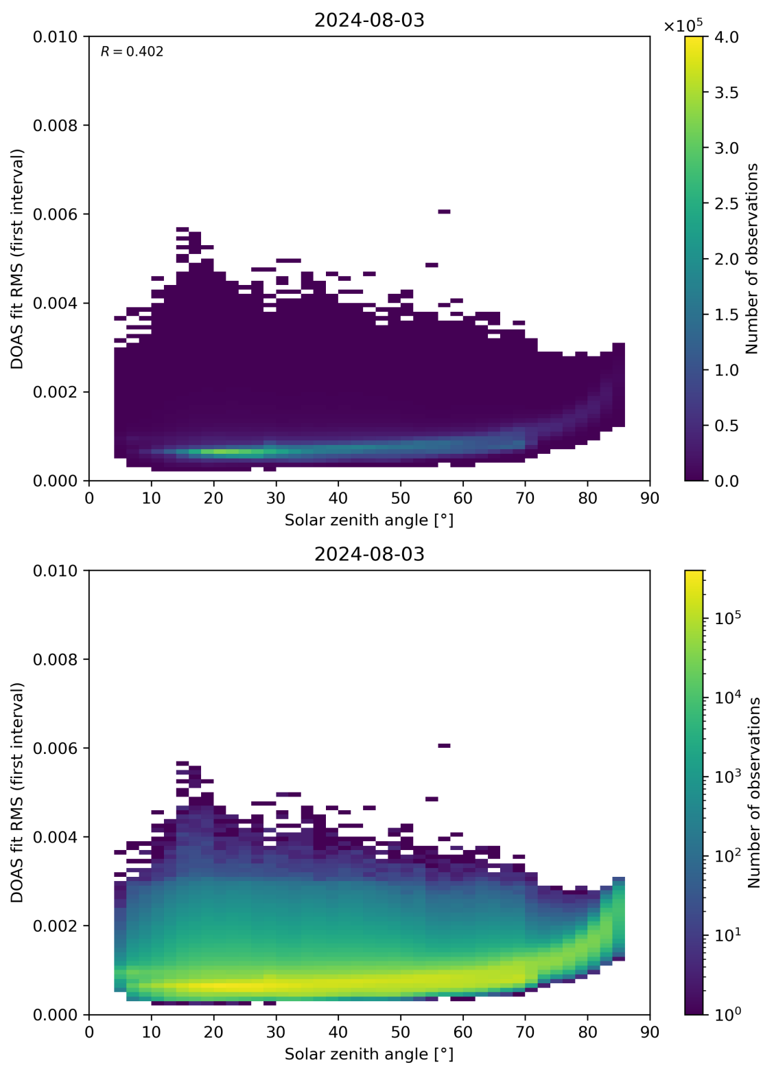
Figure 167: Scatter density plot of “Solar zenith angle” against “DOAS fit RMS (first interval)” for 2024-08-02 to 2024-08-04.
