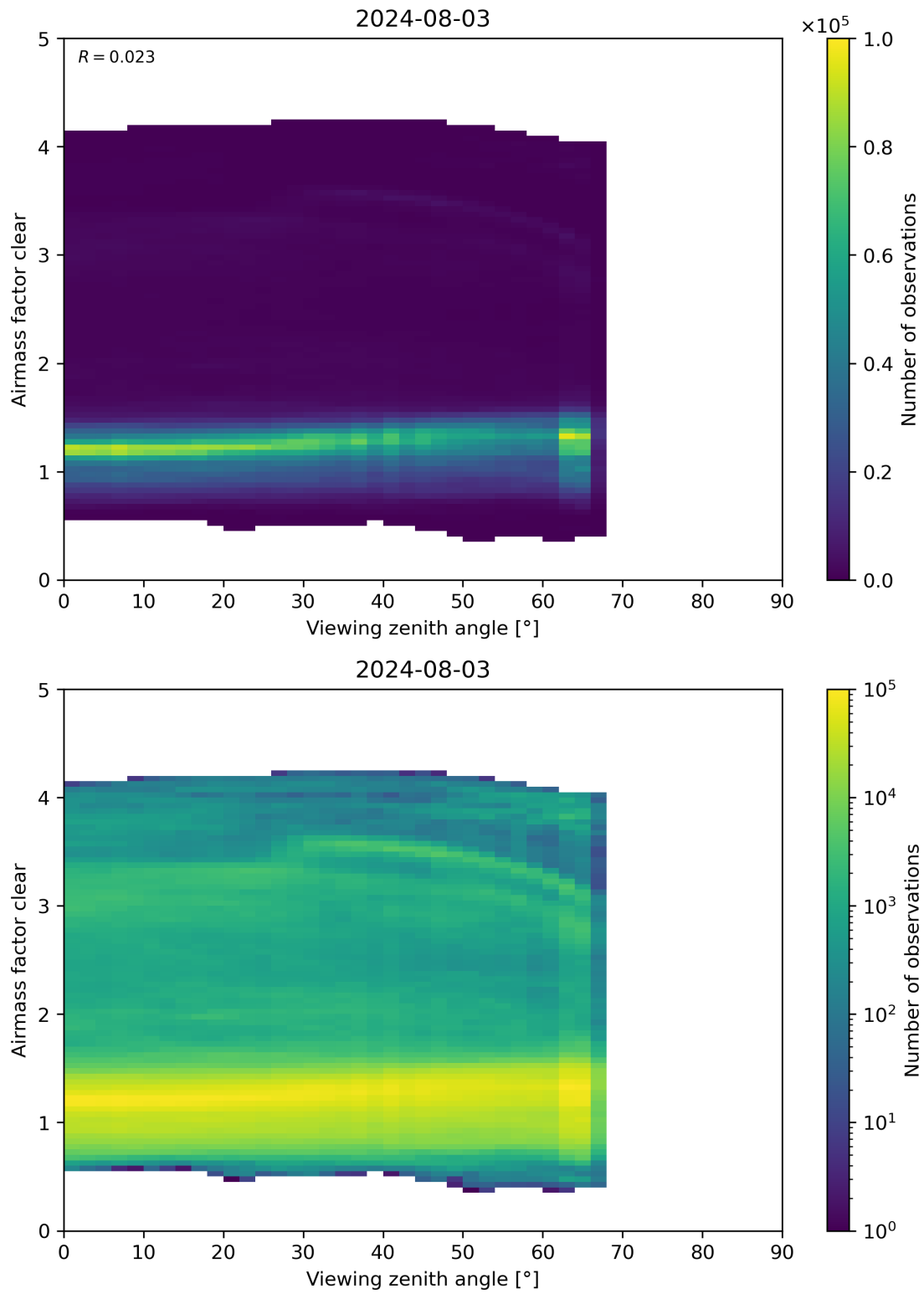
Figure 185: Scatter density plot of “Viewing zenith angle” against “Airmass factor clear” for 2024-08-02 to 2024-08-04.
