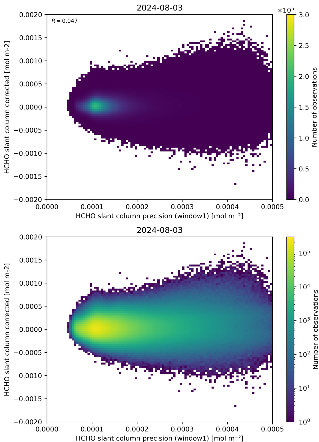
Figure 92: Scatter density plot of “HCHO slant column precision (window1)” against “HCHO slant column corrected” for 2024-08-02 to 2024-08-04.
