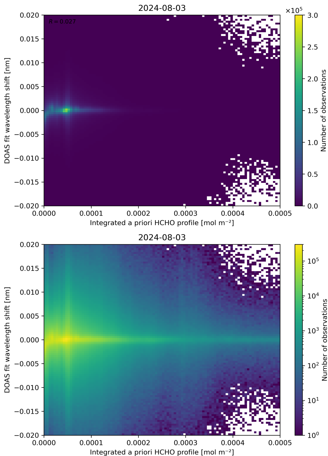
Figure 149: Scatter density plot of “Integrated a priori HCHO profile” against “DOAS fit wavelength shift” for 2024-08-02 to 2024-08-04.
