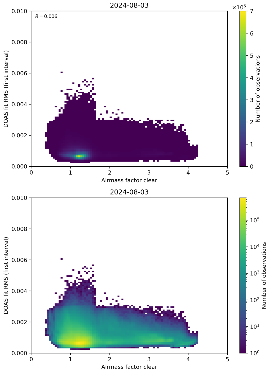
Figure 71: Scatter density plot of “Airmass factor clear” against “DOAS fit RMS (first interval)” for 2024-08-02 to 2024-08-04.
