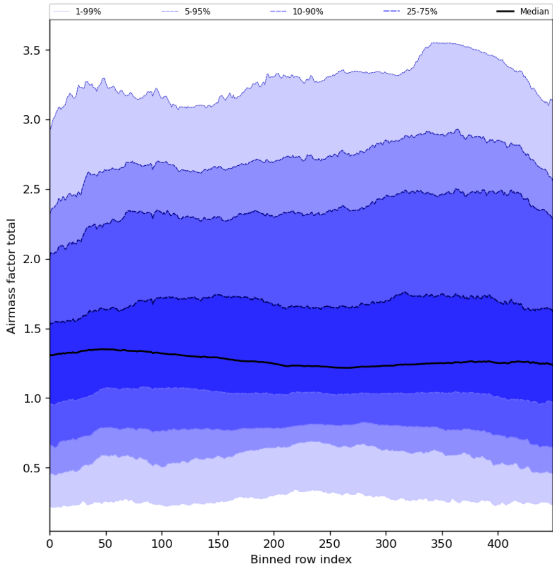
Figure 54: Along track statistics of “Airmass factor total” for 2024-08-02 to 2024-08-04
