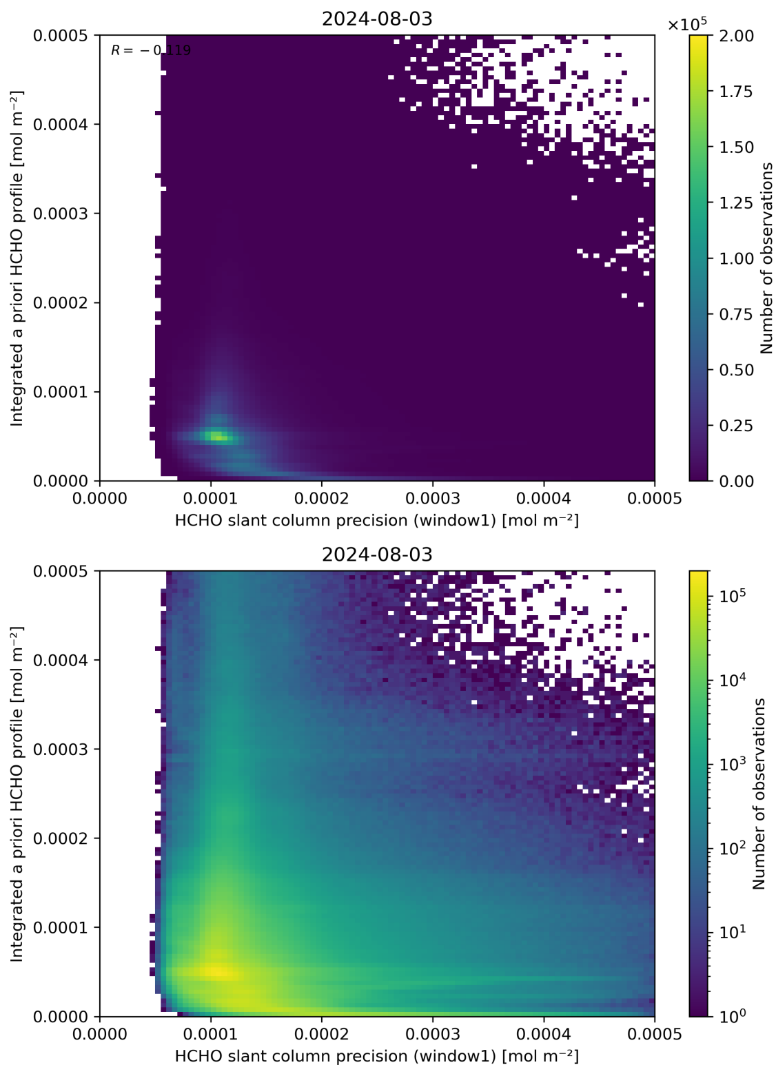
Figure 96: Scatter density plot of “HCHO slant column precision (window1)” against “Integrated a priori HCHO profile” for 2024-08-02 to 2024-08-04.
