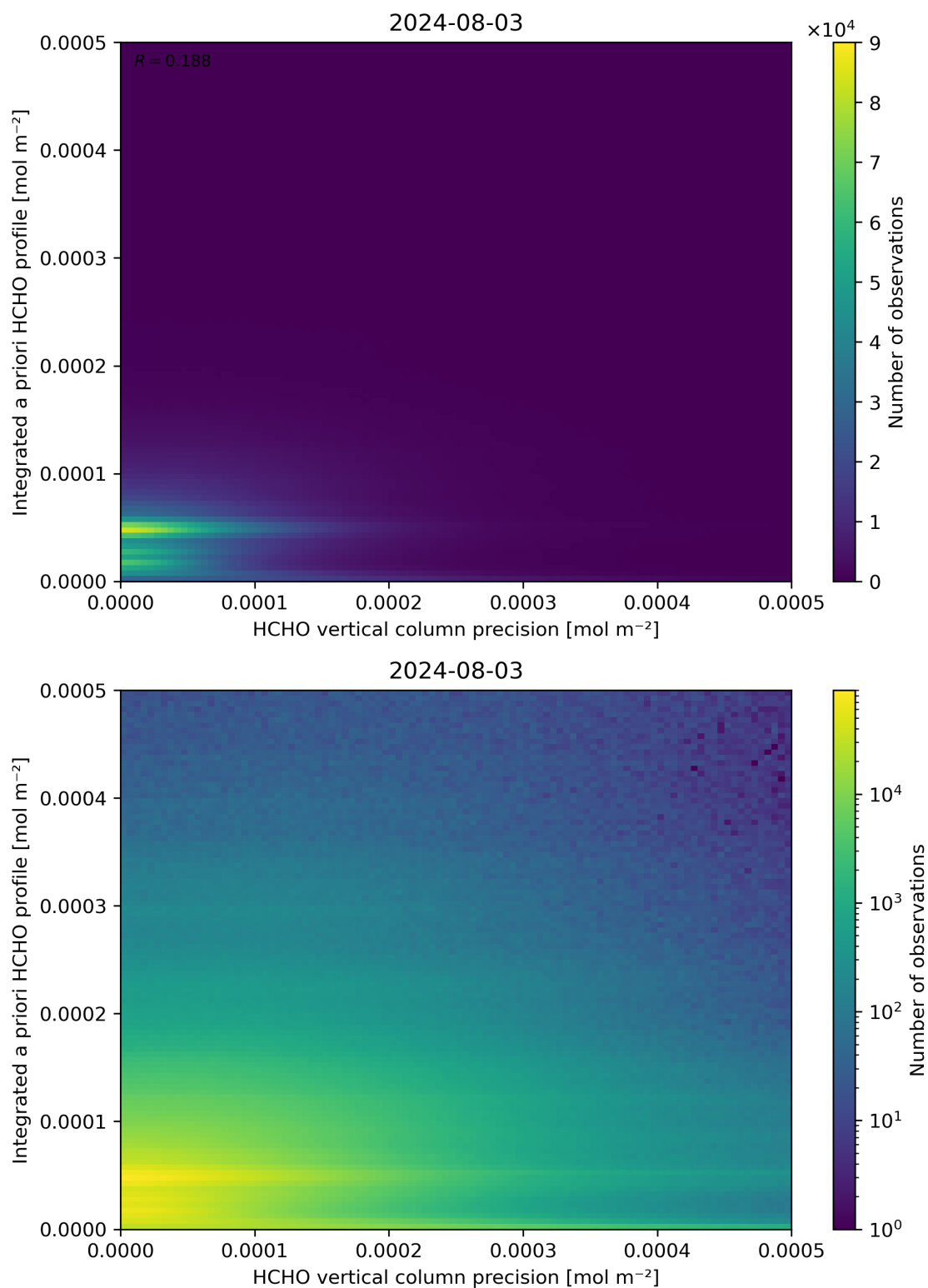
Figure 147: Scatter density plot of “HCHO vertical column precision” against “Integrated a priori HCHO profile” for 2024-08-02 to 2024-08-04.
