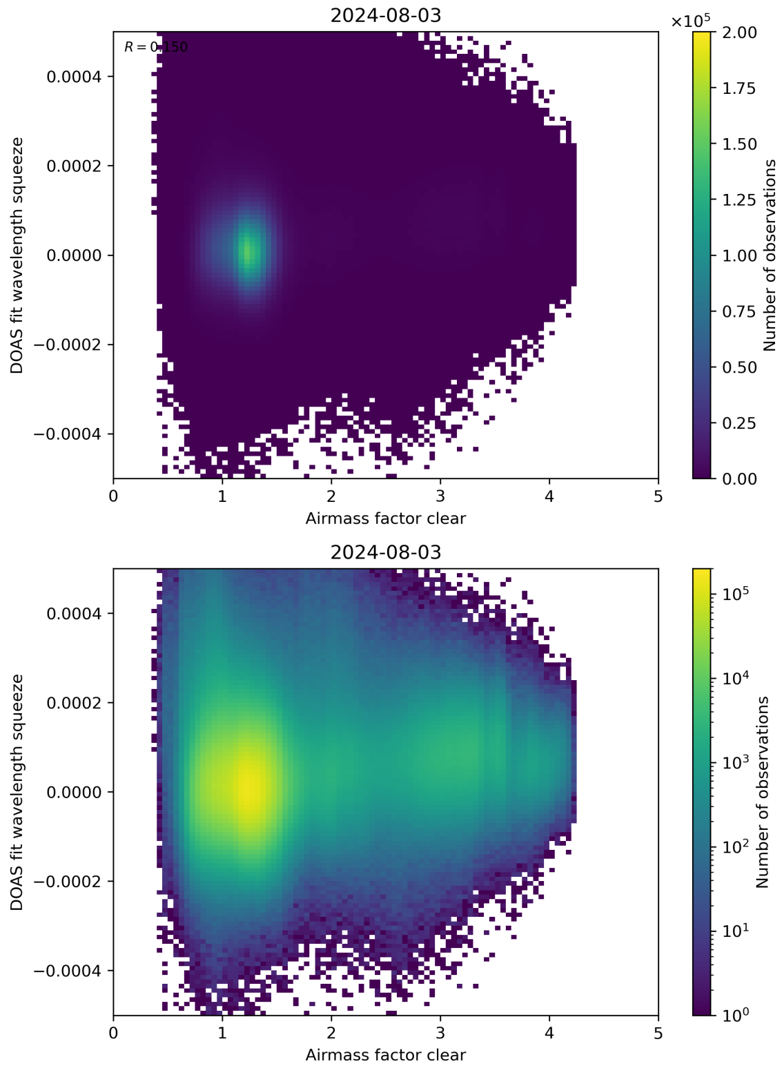
Figure 73: Scatter density plot of “Airmass factor clear” against “DOAS fit wavelength squeeze” for 2024-08-02 to 2024-08-04.
