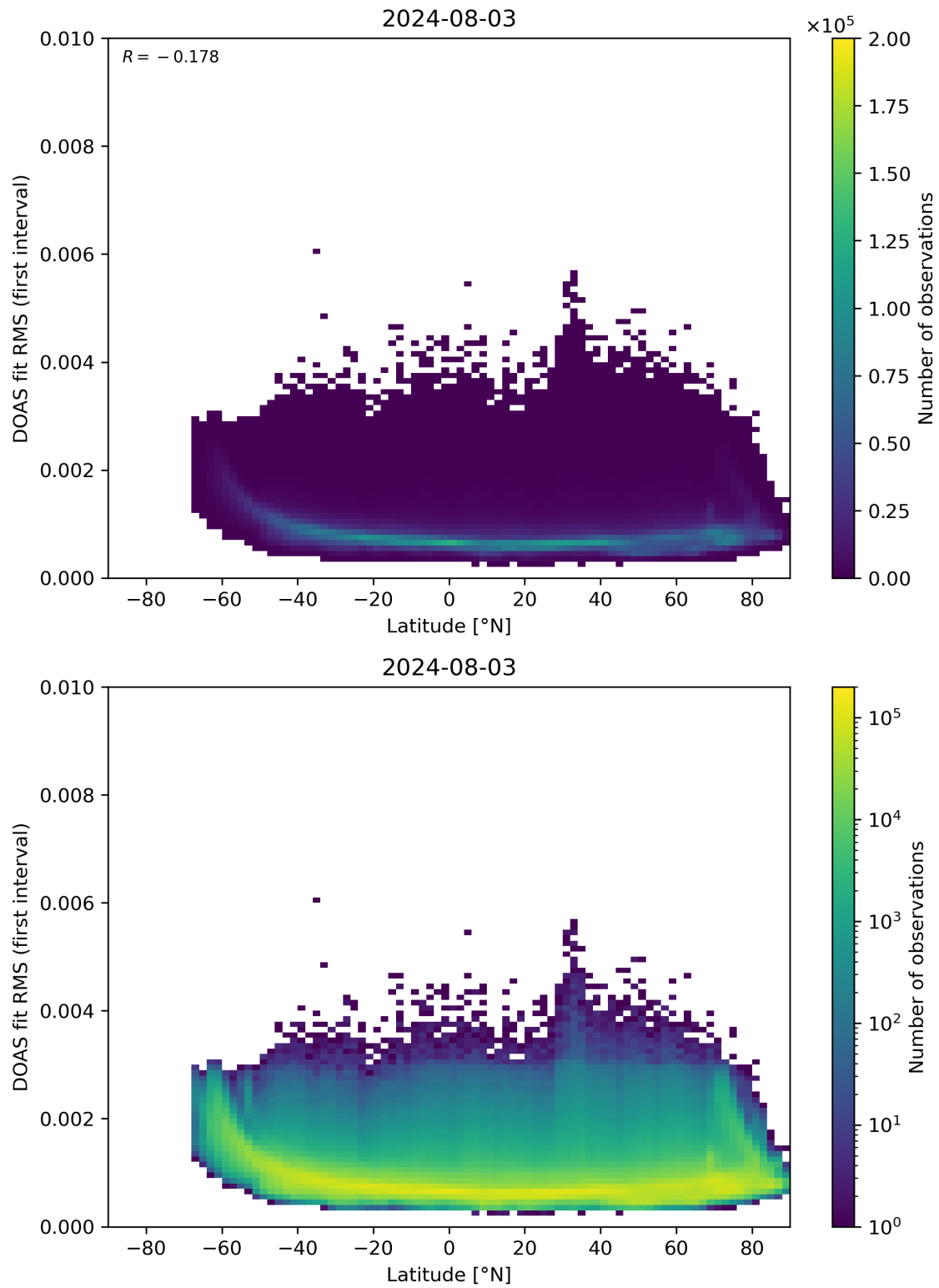
Figure 153: Scatter density plot of “Latitude” against “DOAS fit RMS (first interval)” for 2024-08-02 to 2024-08-04.
