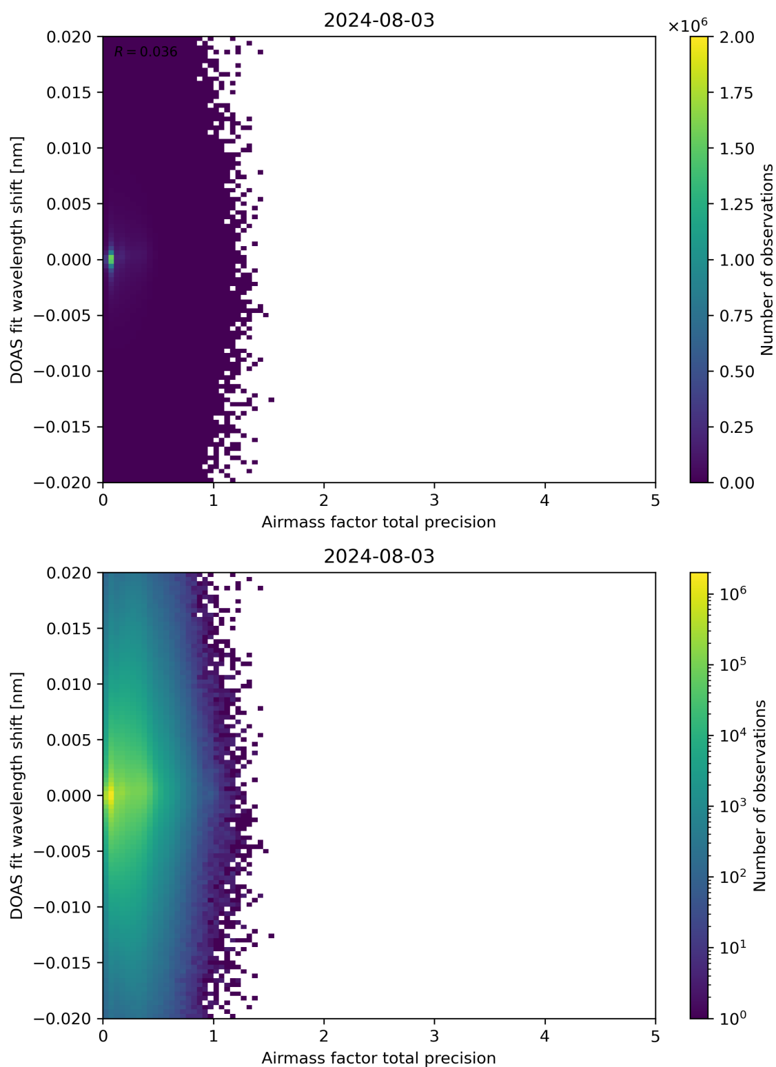
Figure 106: Scatter density plot of “Airmass factor total precision” against “DOAS fit wavelength shift” for 2024-08-02 to 2024-08-04.
