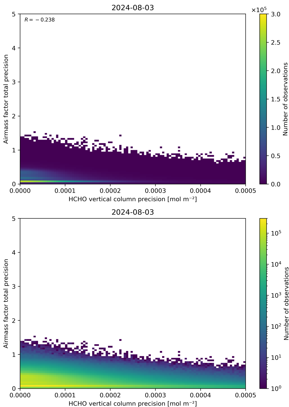
Figure 145: Scatter density plot of “HCHO vertical column precision” against “Airmass factor total precision” for 2024-08-02 to 2024-08-04.
