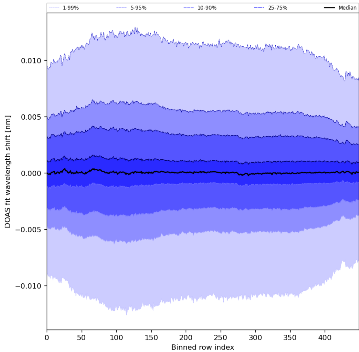
Figure 58: Along track statistics of “DOAS fit wavelength shift” for 2024-08-02 to 2024-08-04
