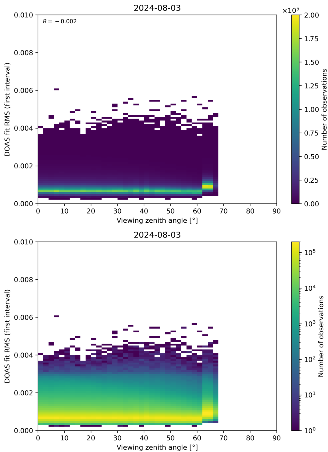
Figure 182: Scatter density plot of “Viewing zenith angle” against “DOAS fit RMS (first interval)” for 2024-08-02 to 2024-08-04.
