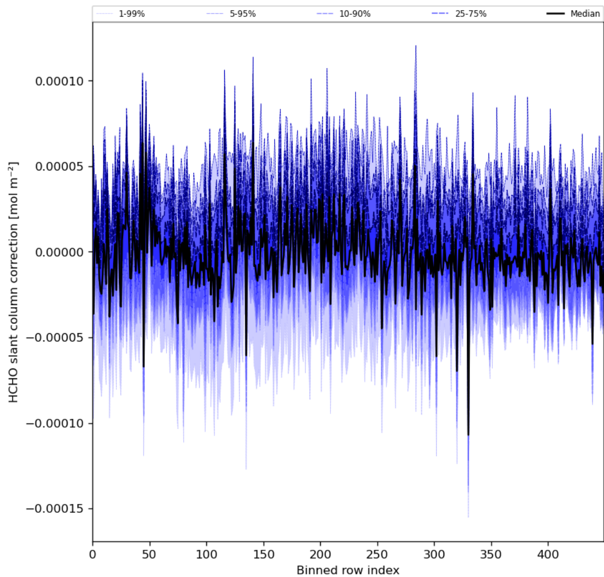
Figure 61: Along track statistics of “HCHO slant column correction” for 2024-08-02 to 2024-08-04
