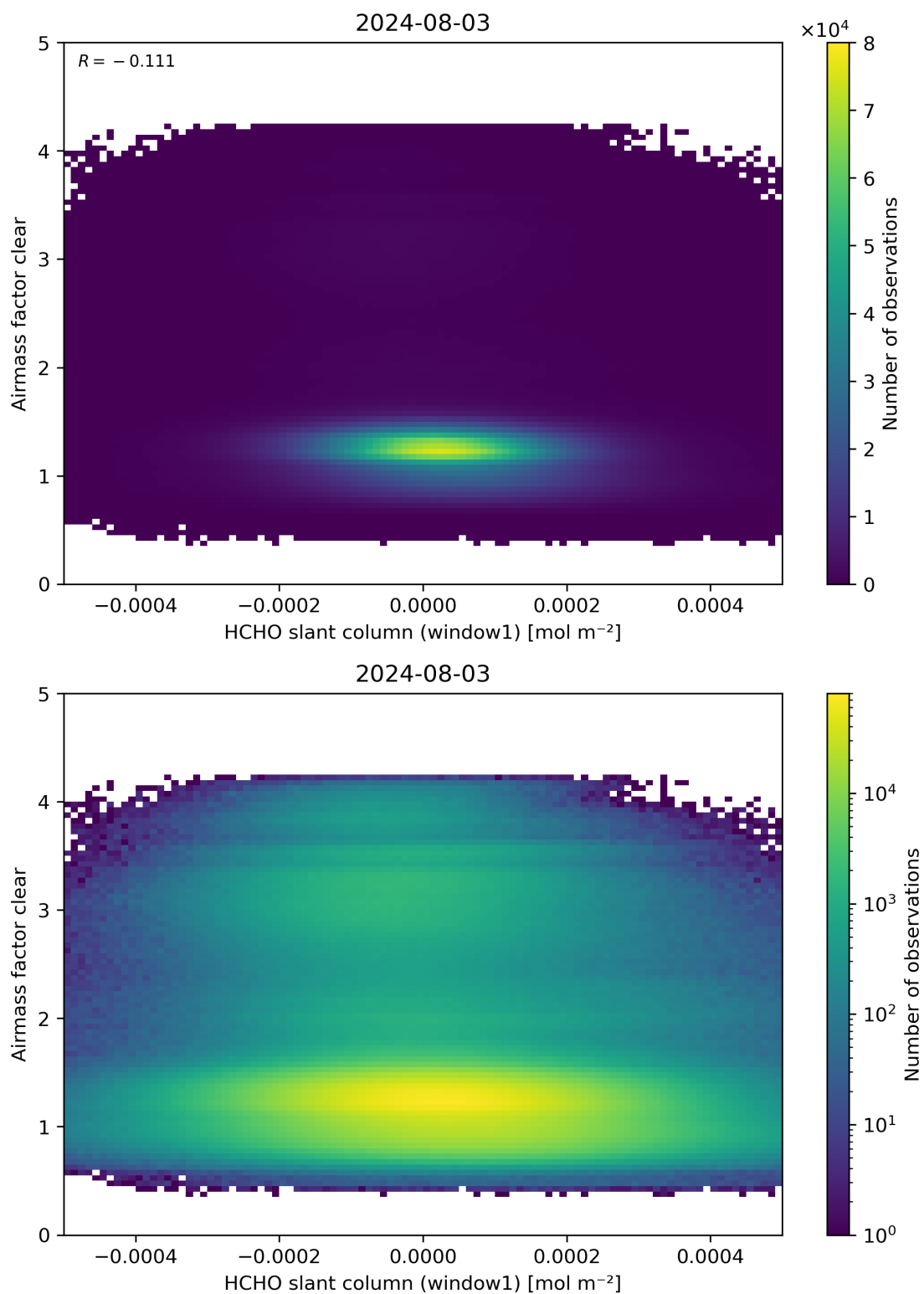
Figure 81: Scatter density plot of “HCHO slant column (window1)” against “Airmass factor clear” for 2024-08-02 to 2024-08-04.
