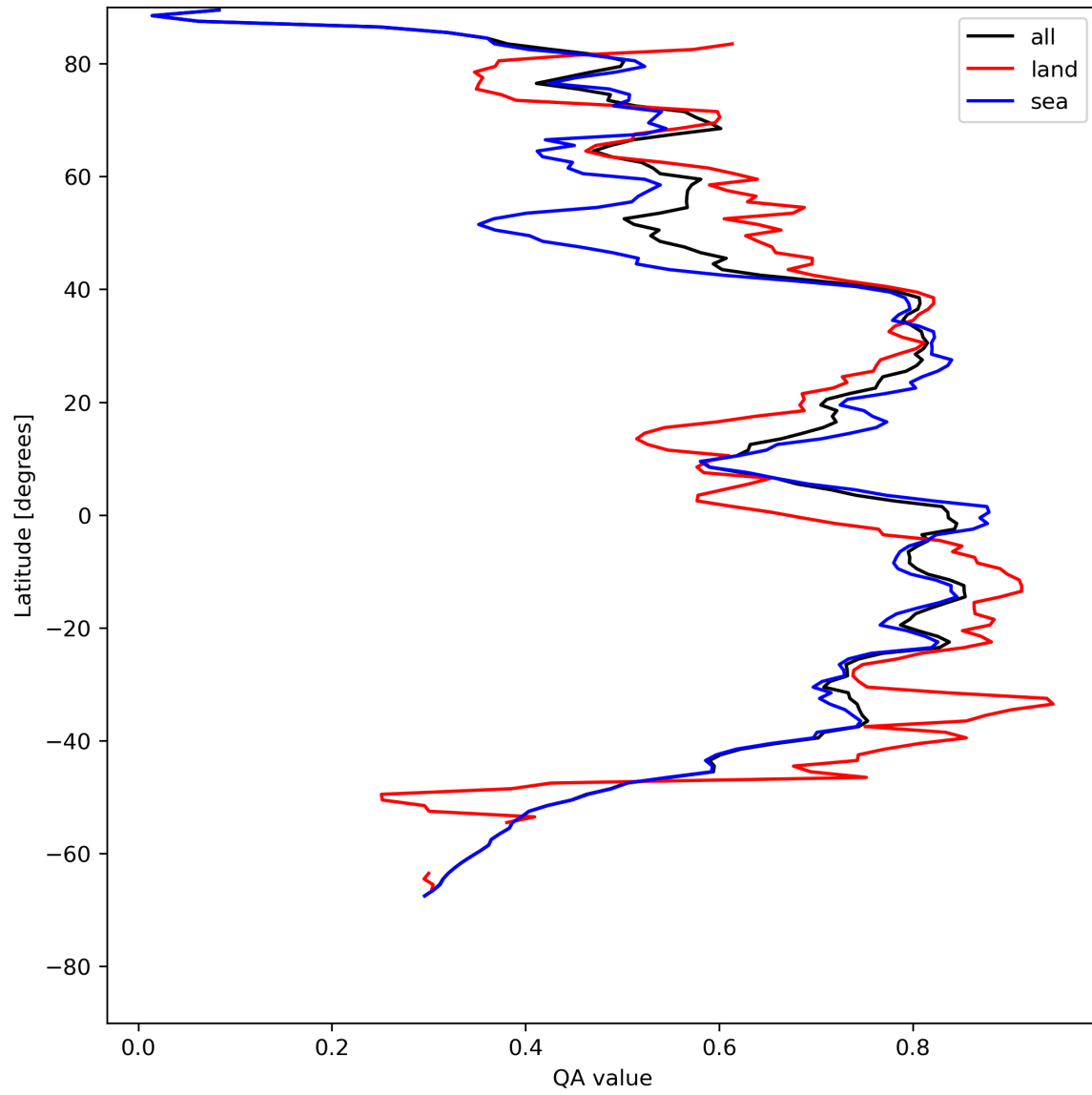
Figure 20: Zonal average of “QA value” for 2024-08-02 to 2024-08-04.
