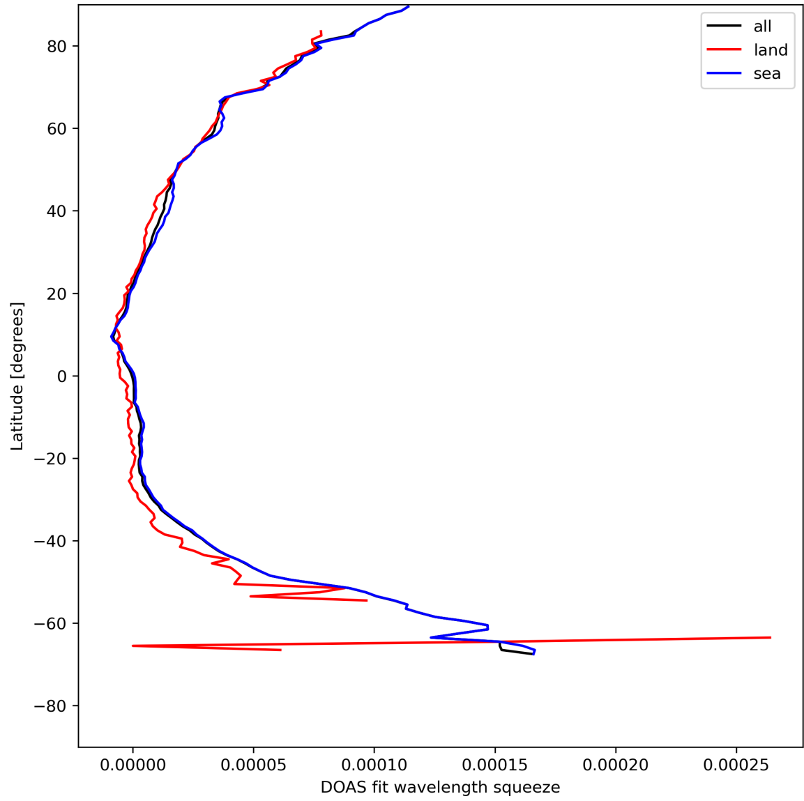
Figure 31: Zonal average of “DOAS fit wavelength squeeze” for 2024-08-02 to 2024-08-04.
