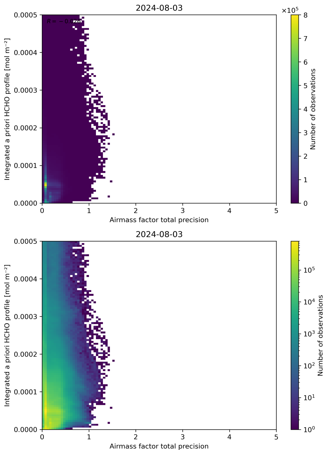
Figure 111: Scatter density plot of “Airmass factor total precision” against “Integrated a priori HCHO profile” for 2024-08-02 to 2024-08-04.
