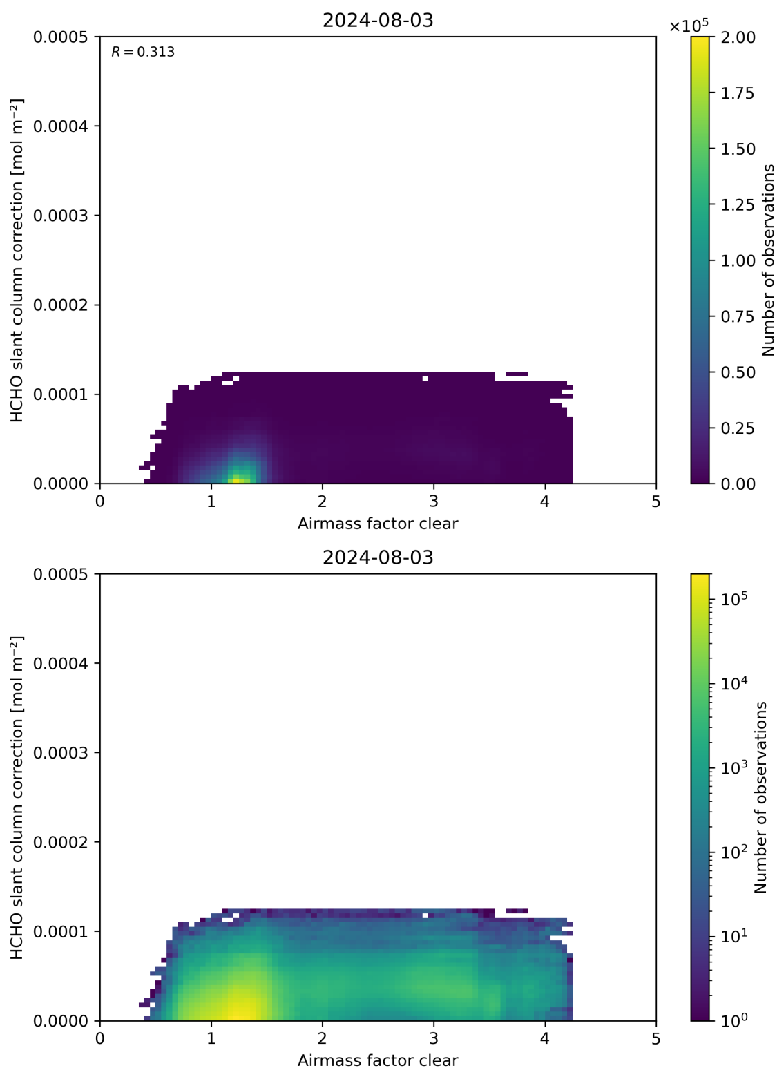
Figure 75: Scatter density plot of “Airmass factor clear” against “HCHO slant column correction” for 2024-08-02 to 2024-08-04.
