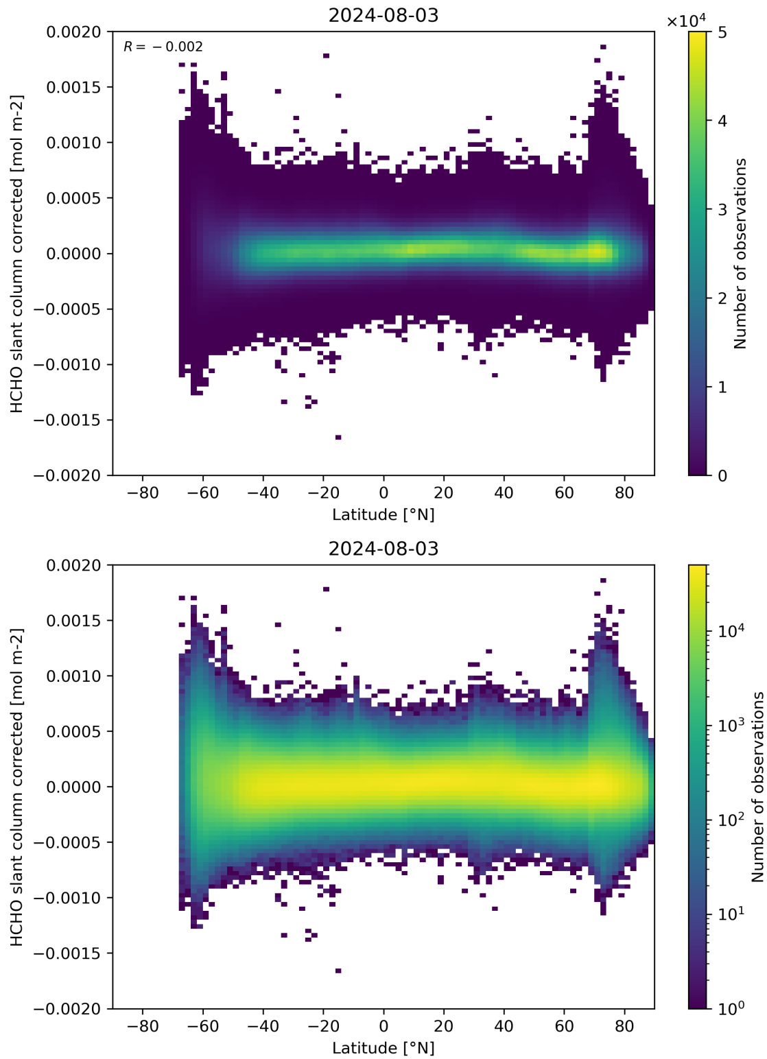
Figure 157: Scatter density plot of “Latitude” against “HCHO slant column corrected” for 2024-08-02 to 2024-08-04.
