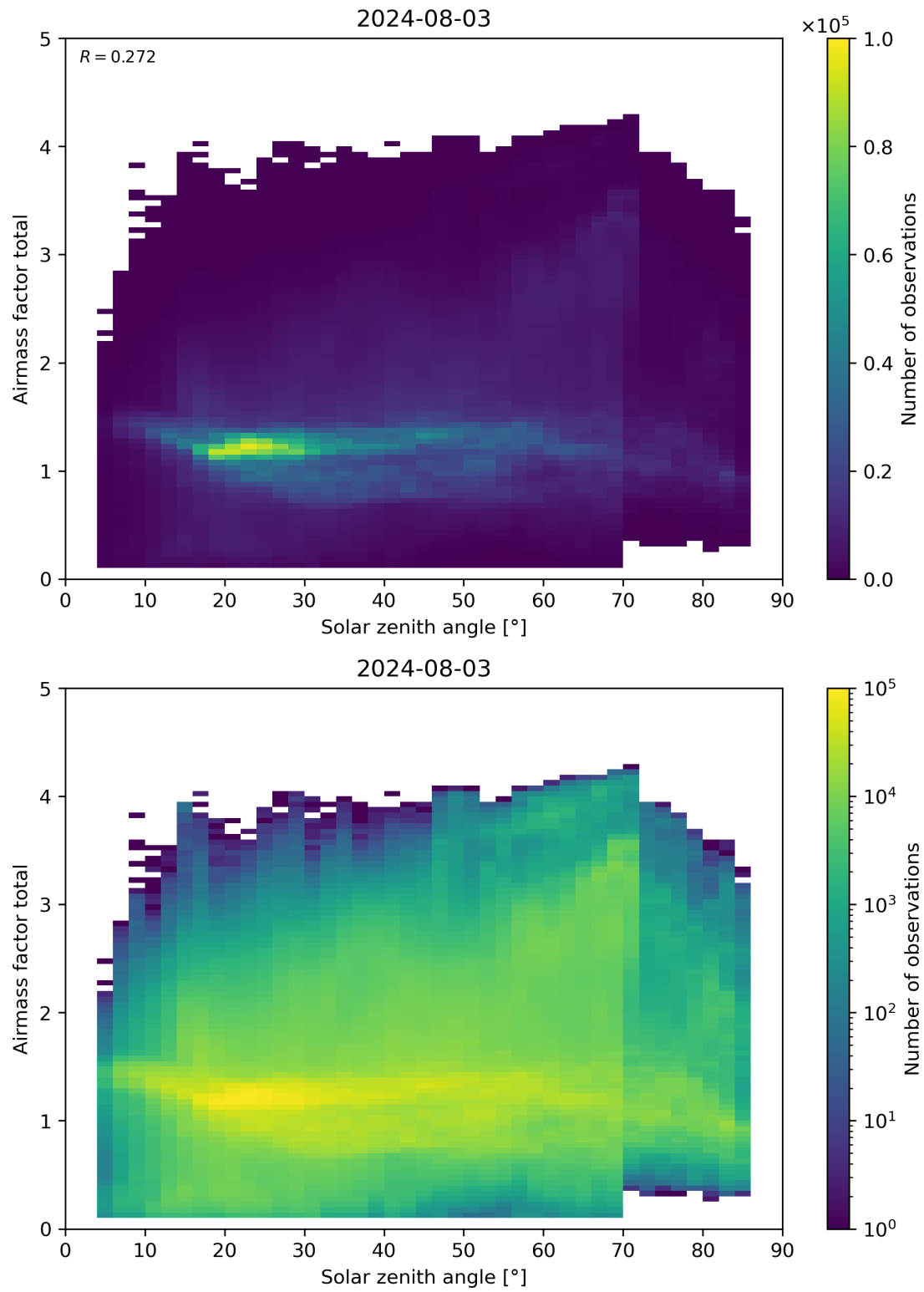
Figure 175: Scatter density plot of “Solar zenith angle” against “Airmass factor total” for 2024-08-02 to 2024-08-04.
