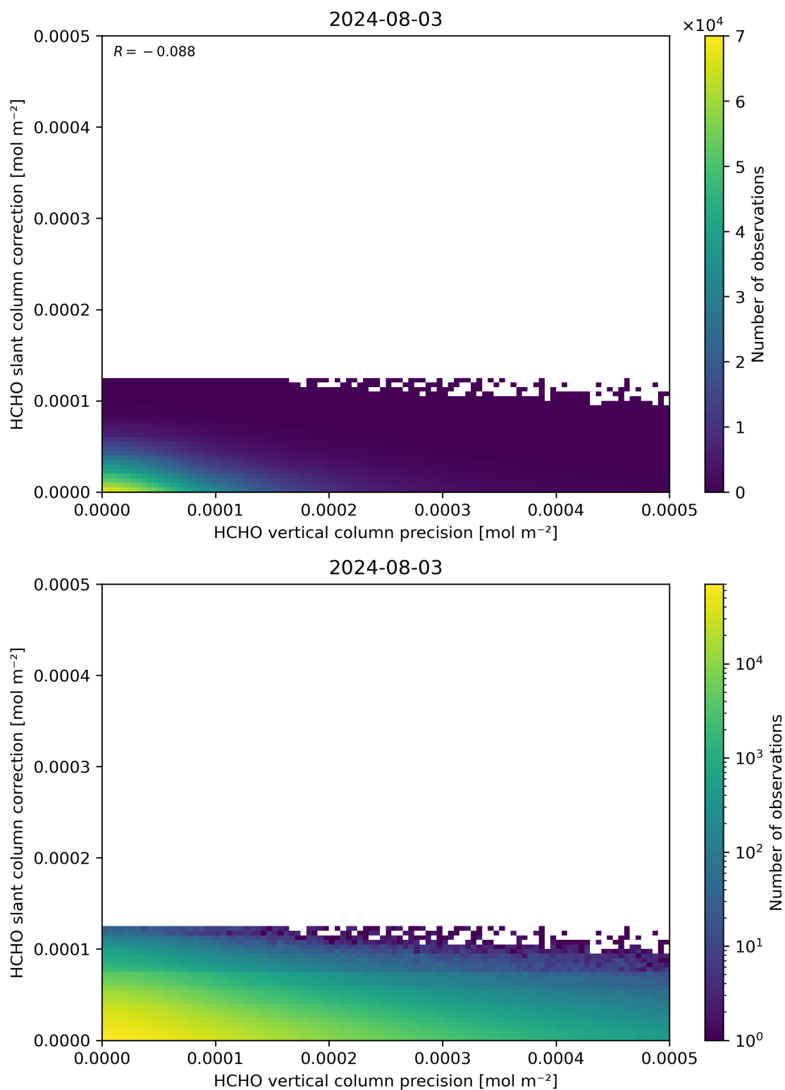
Figure 141: Scatter density plot of “HCHO vertical column precision” against “HCHO slant column correction” for 2024-08-02 to 2024-08-04.
