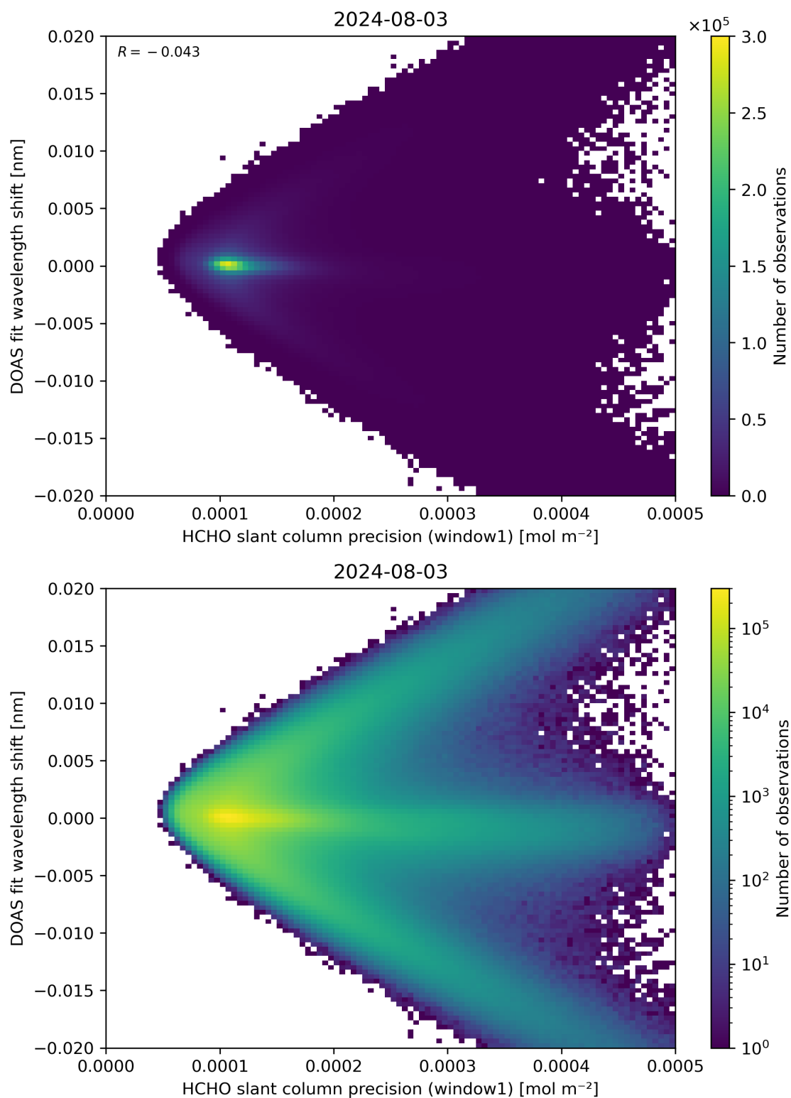
Figure 89: Scatter density plot of “HCHO slant column precision (window1)” against “DOAS fit wavelength shift” for 2024-08-02 to 2024-08-04.
