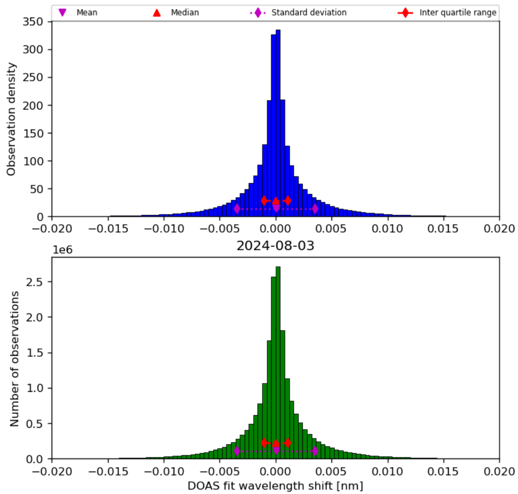
Figure 44: Histogram of “DOAS fit wavelength shift” for 2024-08-02 to 2024-08-04
