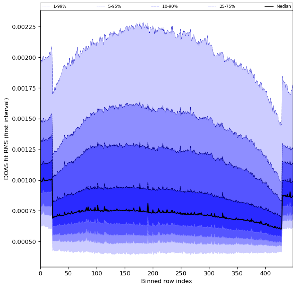
Figure 60: Along track statistics of “DOAS fit RMS (first interval)” for 2024-08-02 to 2024-08-04
