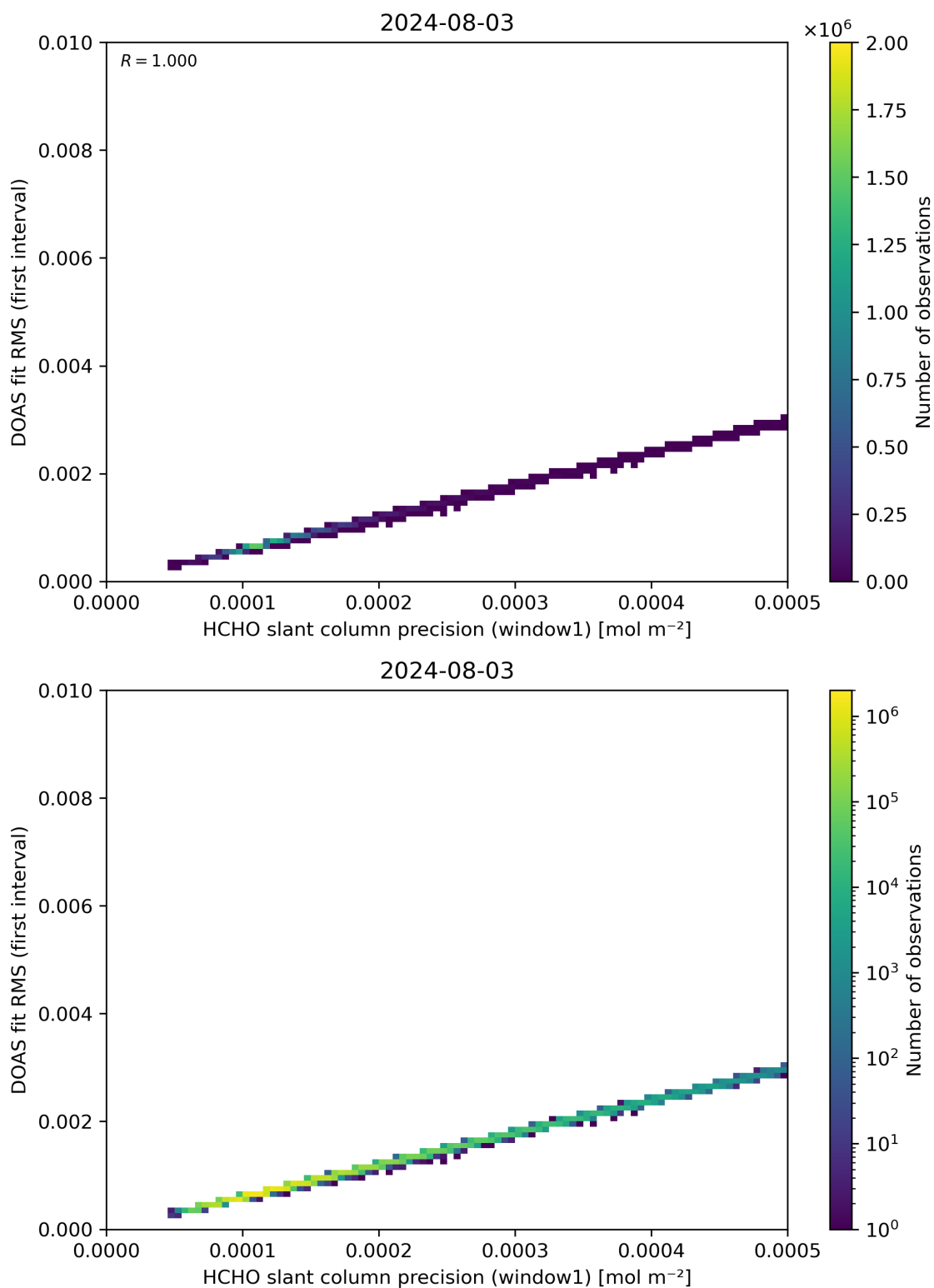
Figure 88: Scatter density plot of “HCHO slant column precision (window1)” against “DOAS fit RMS (first interval)” for 2024-08-02 to 2024-08-04.
