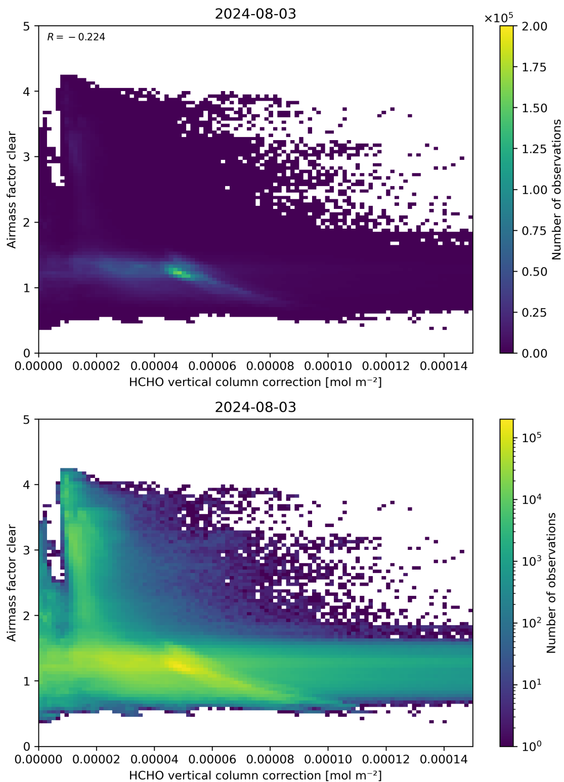
Figure 115: Scatter density plot of “HCHO vertical column correction” against “Airmass factor clear” for 2024-08-02 to 2024-08-04.
