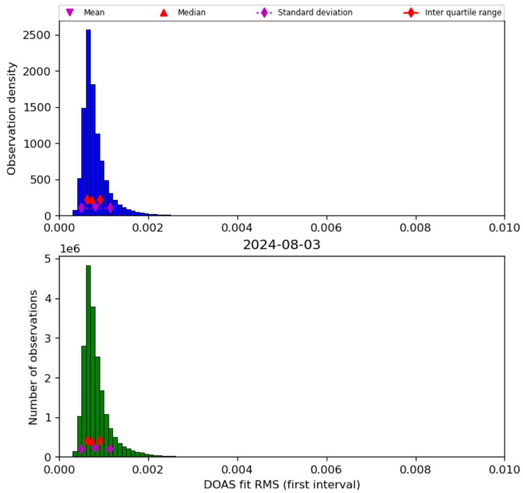
Figure 46: Histogram of “DOAS fit RMS (first interval)” for 2024-08-02 to 2024-08-04
