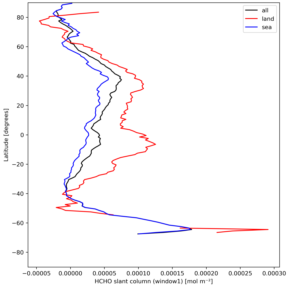
Figure 24: Zonal average of “HCHO slant column (window1)” for 2024-08-02 to 2024-08-04.
