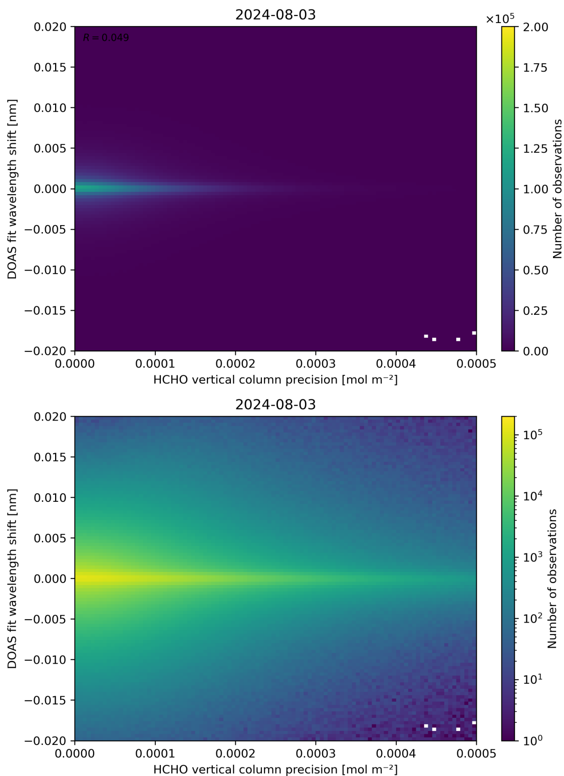
Figure 137: Scatter density plot of “HCHO vertical column precision” against “DOAS fit wavelength shift” for 2024-08-02 to 2024-08-04.
