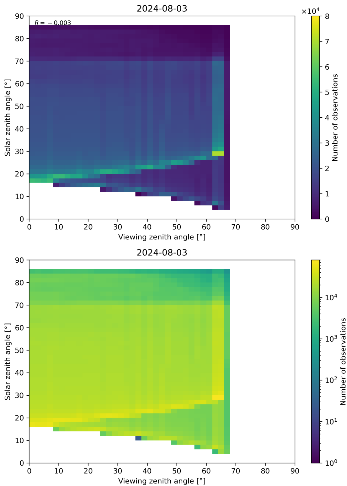
Figure 197: Scatter density plot of “Viewing zenith angle” against “Solar zenith angle” for 2024-08-02 to 2024-08-04.
