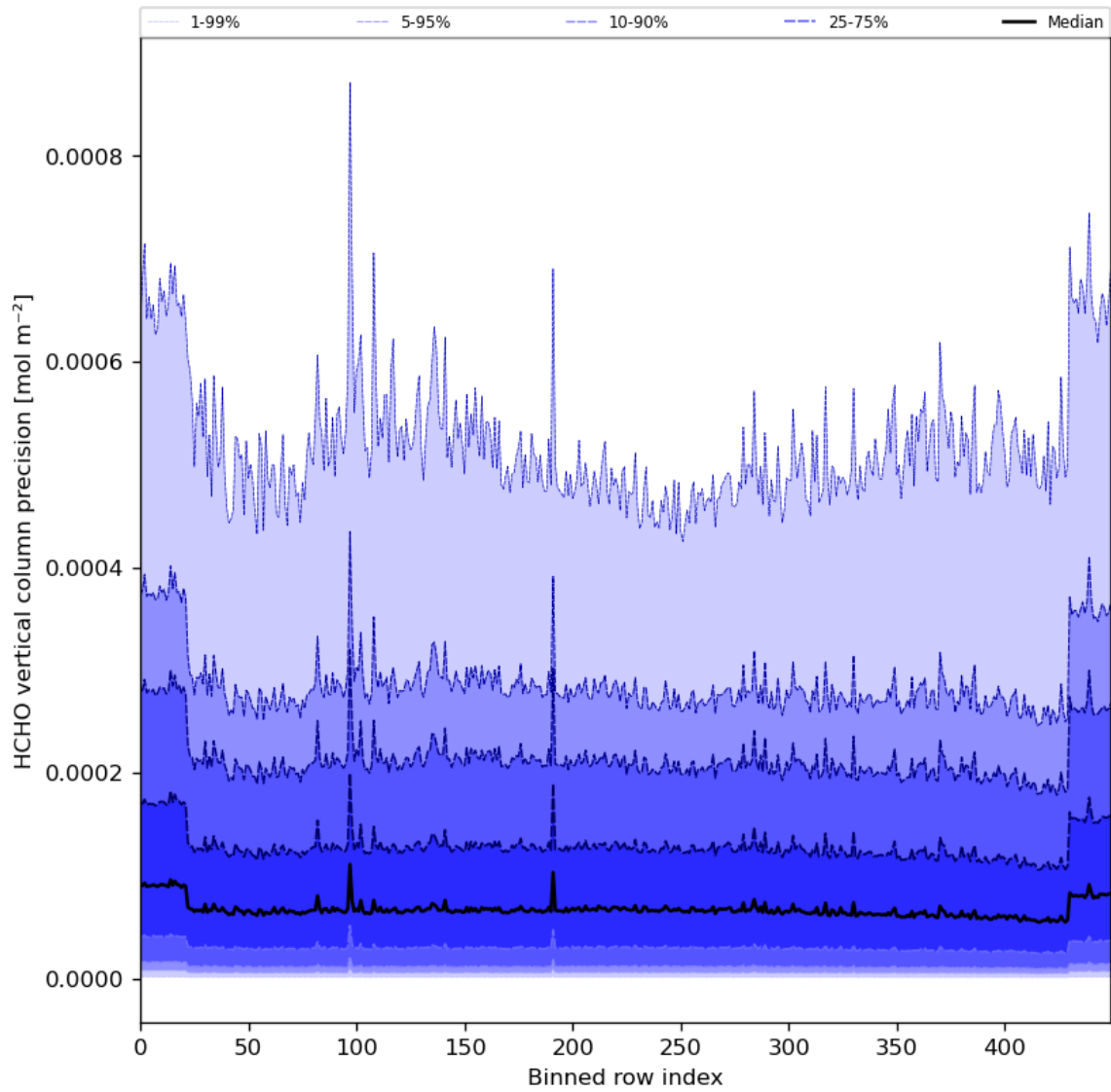
Figure 50: Along track statistics of "HCHO vertical column precision" for 2024-08-02 to 2024-08-04
