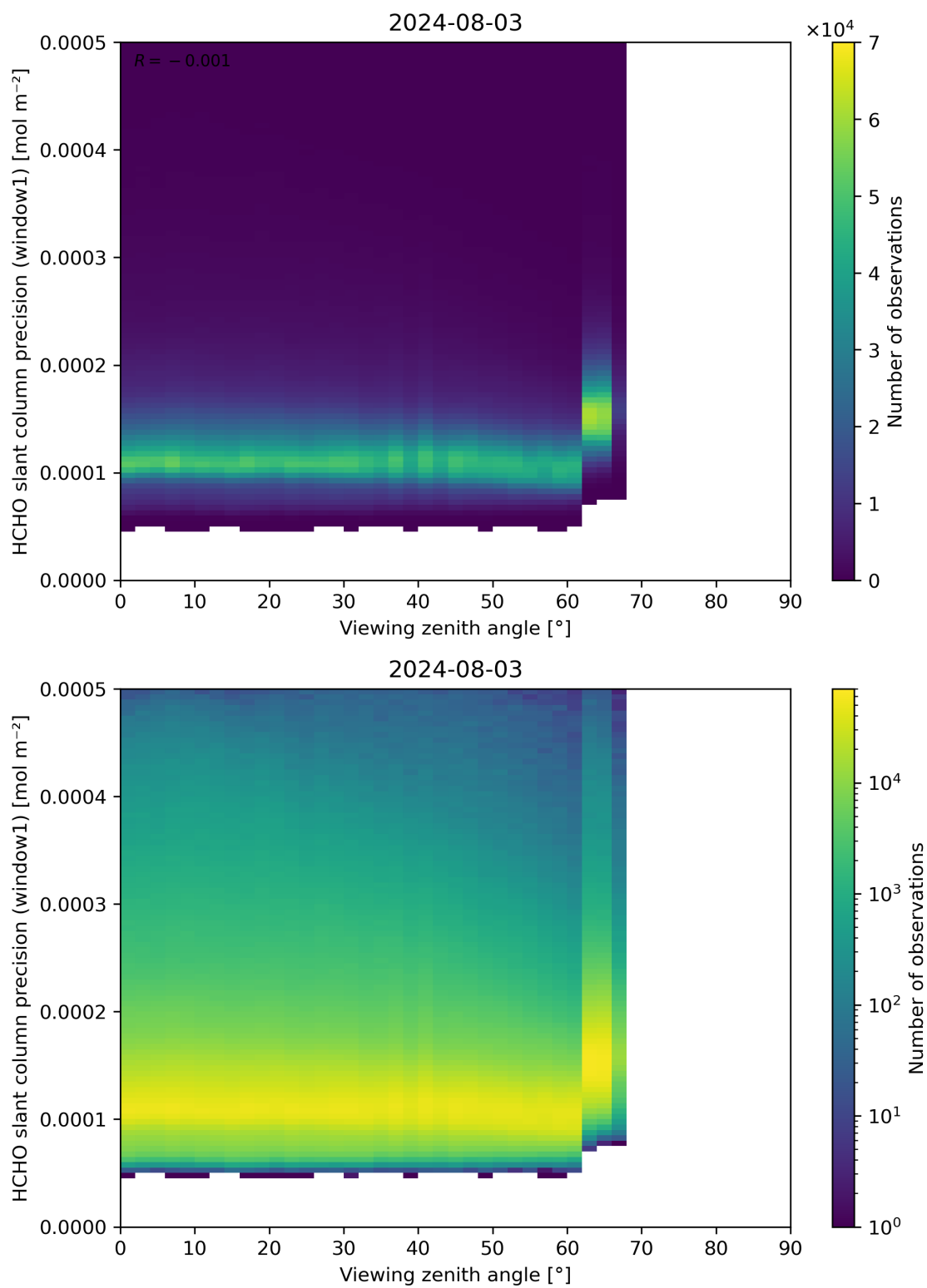
Figure 189: Scatter density plot of “Viewing zenith angle” against “HCHO slant column precision (window1)” for 2024-08-02 to 2024-08-04.
