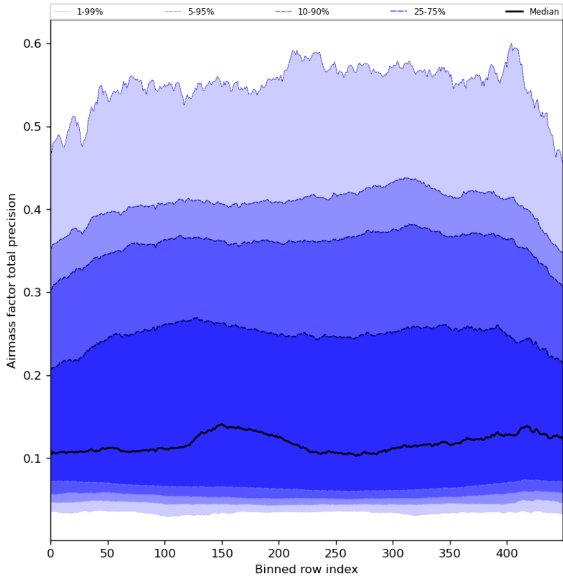
Figure 55: Along track statistics of “Airmass factor total precision” for 2024-08-02 to 2024-08-04
