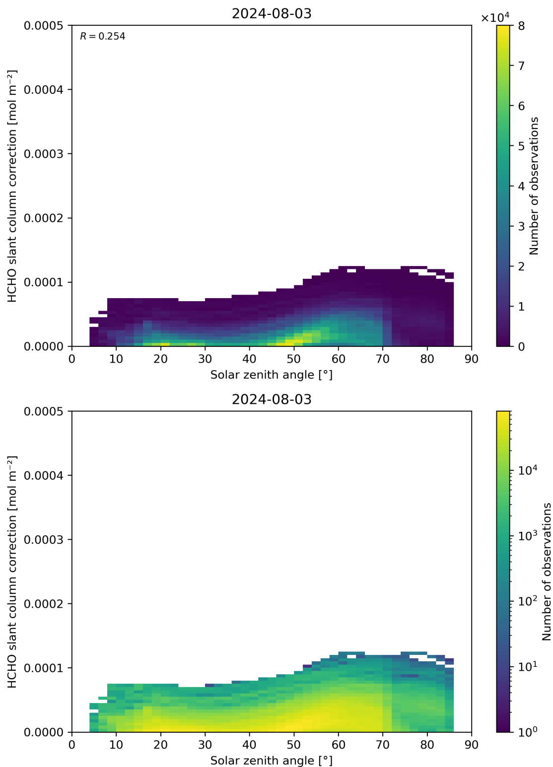
Figure 172: Scatter density plot of “Solar zenith angle” against “HCHO slant column correction” for 2024-08-02 to 2024-08-04.
