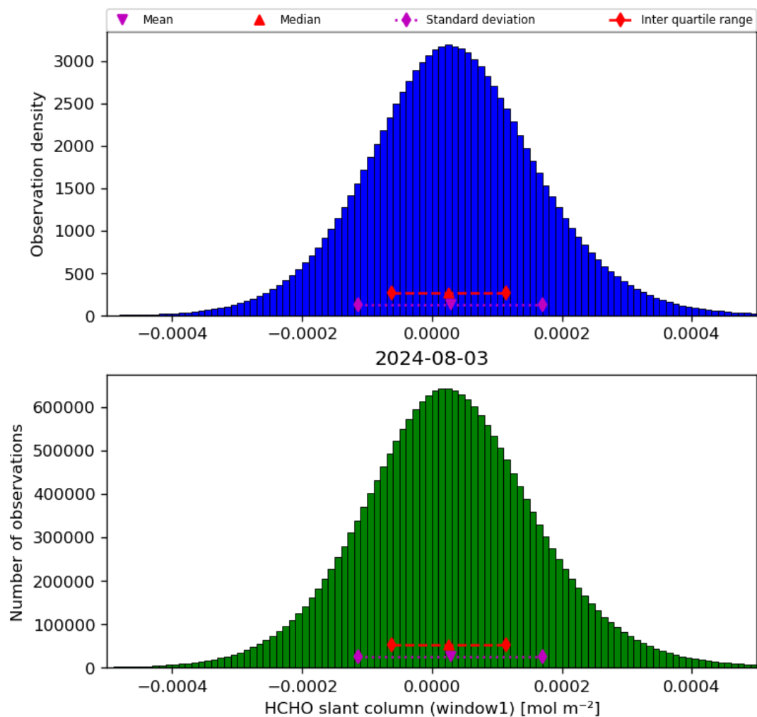
Figure 38: Histogram of “HCHO slant column (window1)” for 2024-08-02 to 2024-08-04
