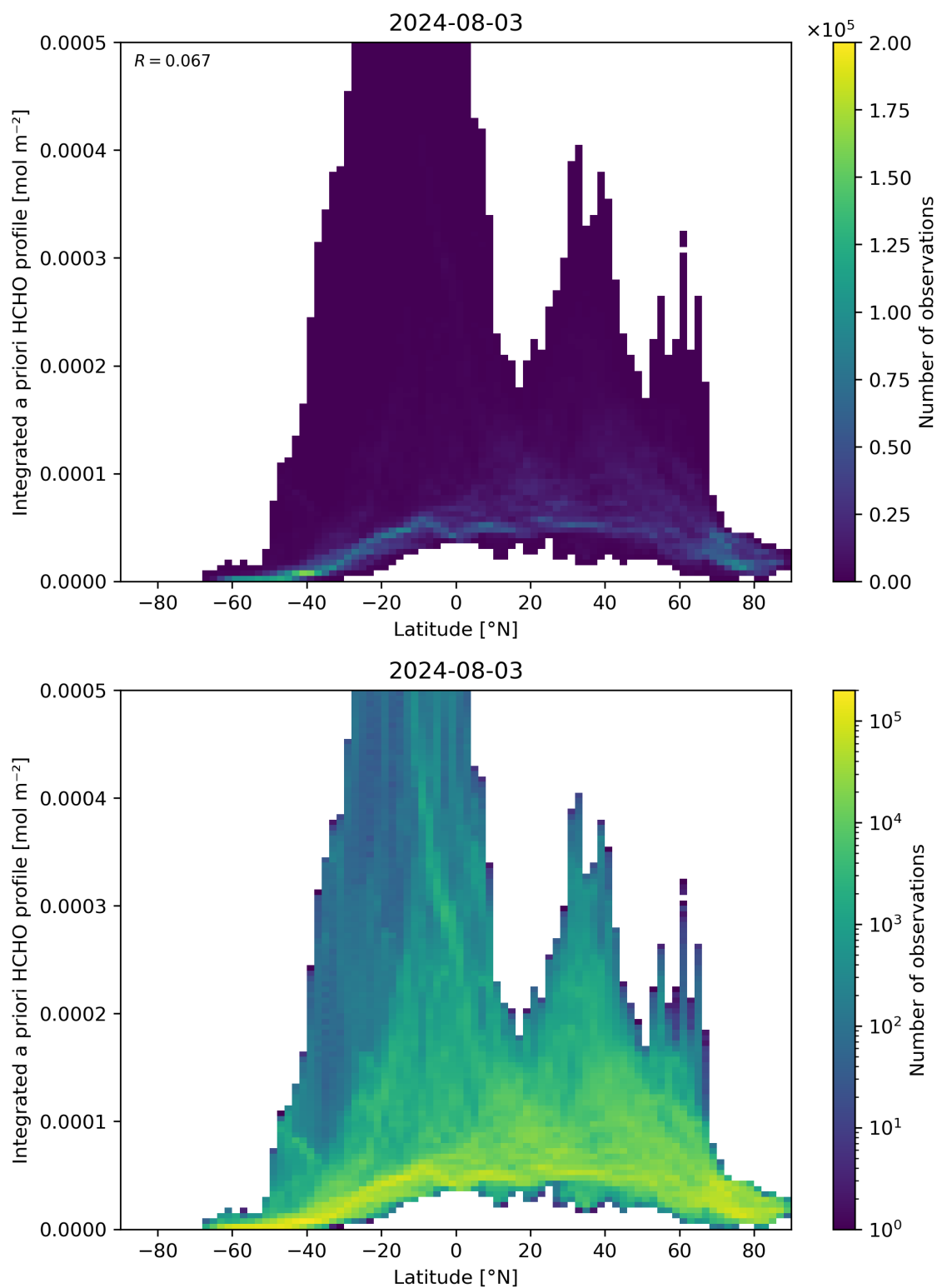
Figure 166: Scatter density plot of “Latitude” against “Integrated a priori HCHO profile” for 2024-08-02 to 2024-08-04.
