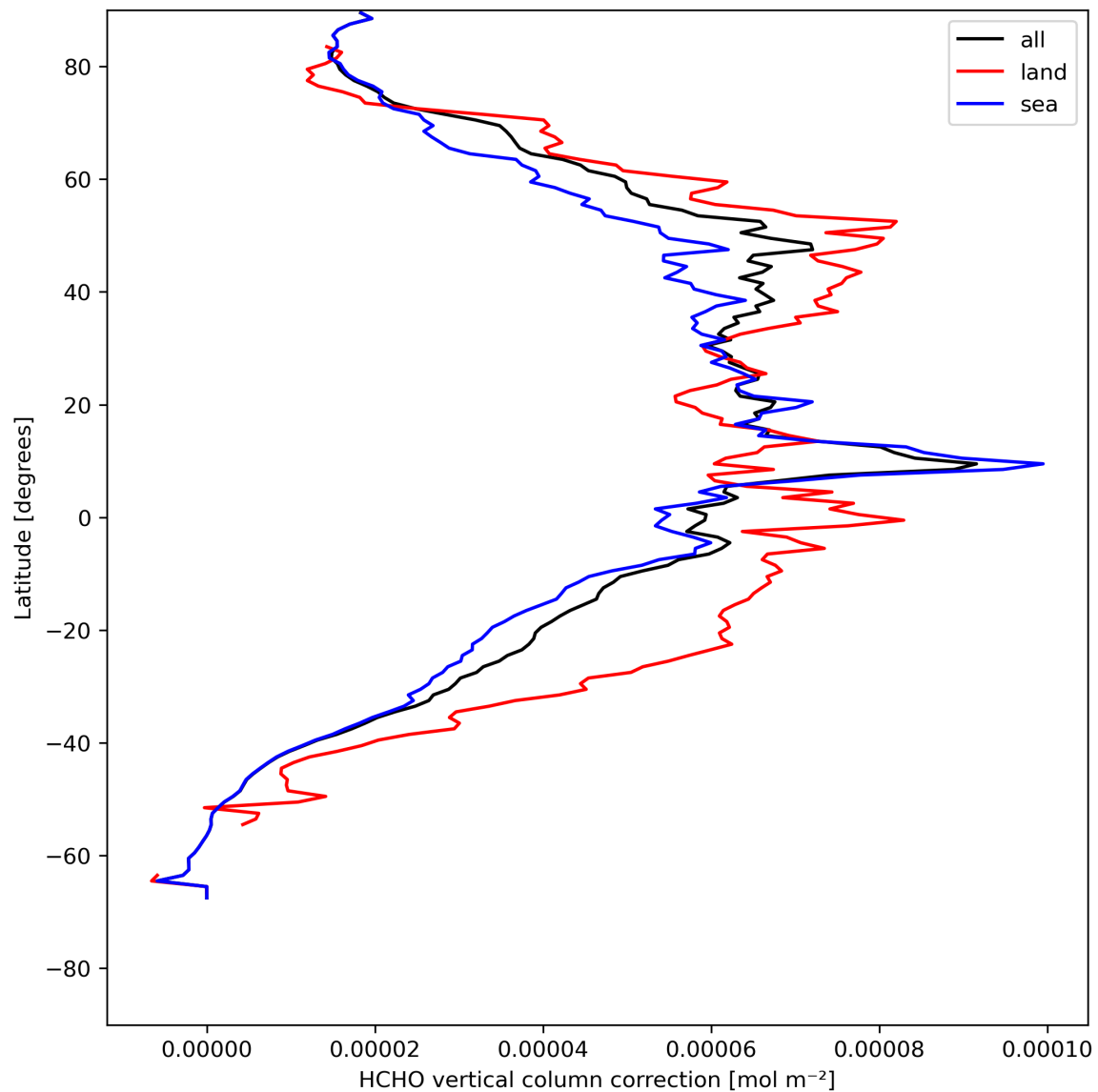
Figure 23: Zonal average of “HCHO vertical column correction” for 2024-08-02 to 2024-08-04.
