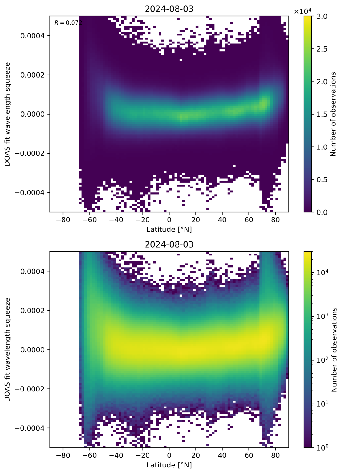
Figure 155: Scatter density plot of “Latitude” against “DOAS fit wavelength squeeze” for 2024-08-02 to 2024-08-04.
