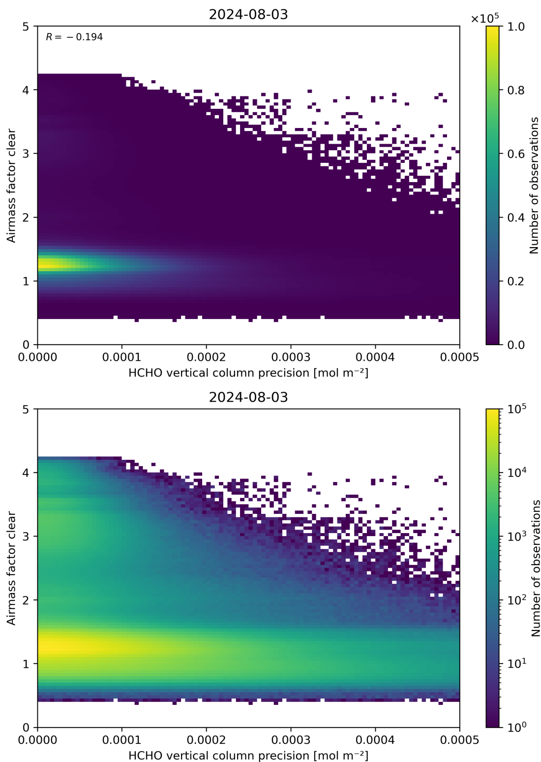
Figure 139: Scatter density plot of “HCHO vertical column precision” against “Airmass factor clear” for 2024-08-02 to 2024-08-04.
