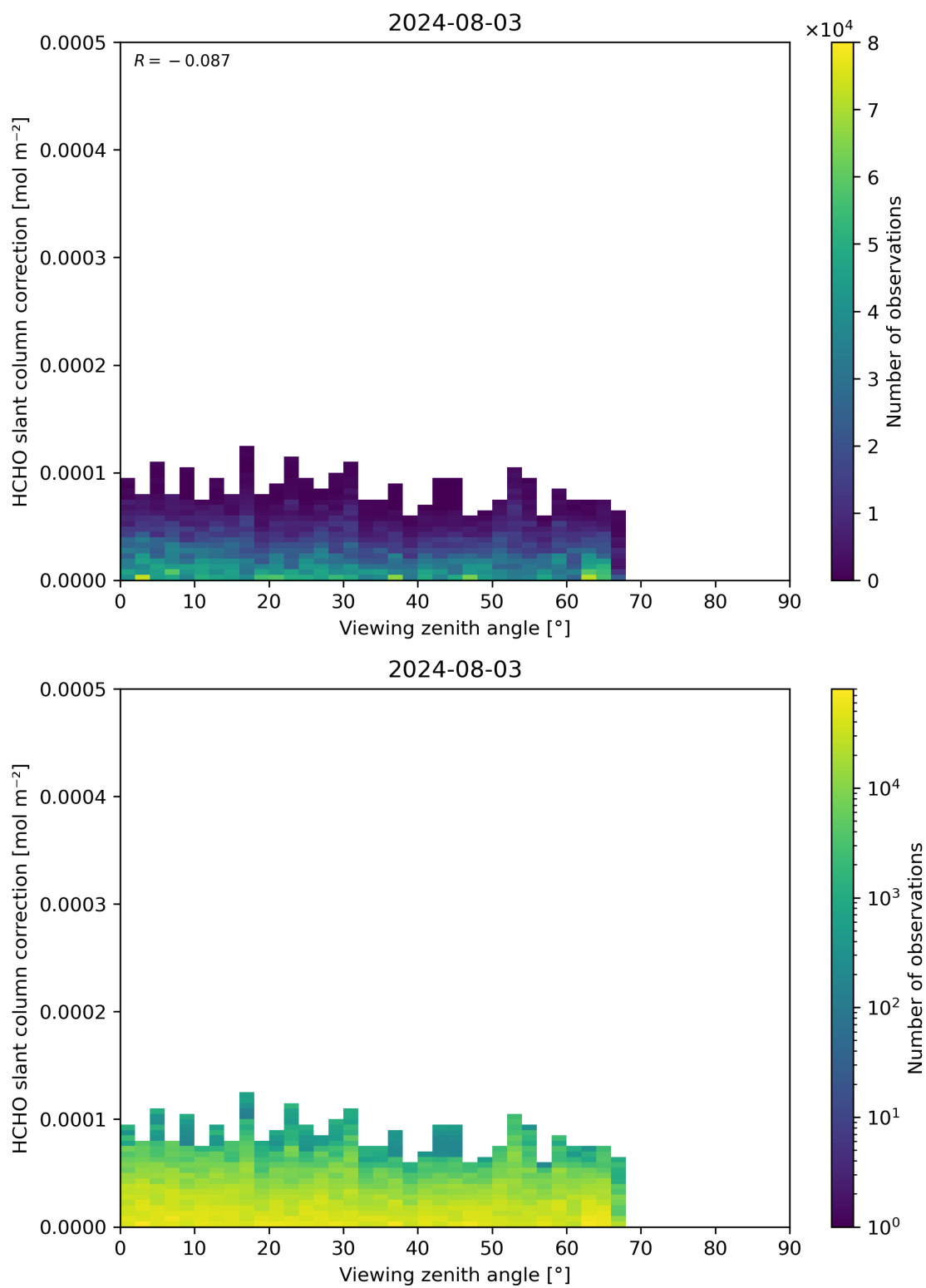
Figure 187: Scatter density plot of “Viewing zenith angle” against “HCHO slant column correction” for 2024-08-02 to 2024-08-04.
