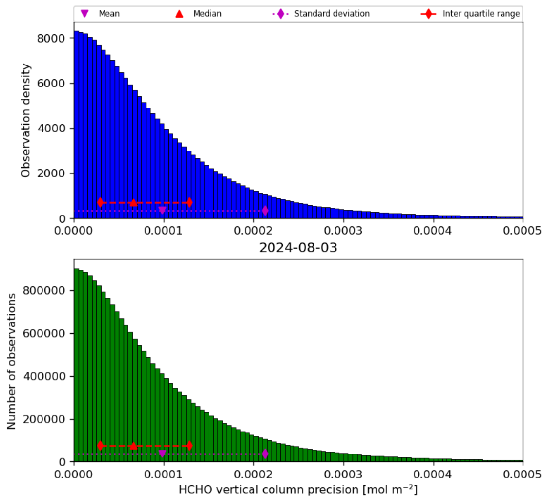
Figure 36: Histogram of “HCHO vertical column precision” for 2024-08-02 to 2024-08-04
