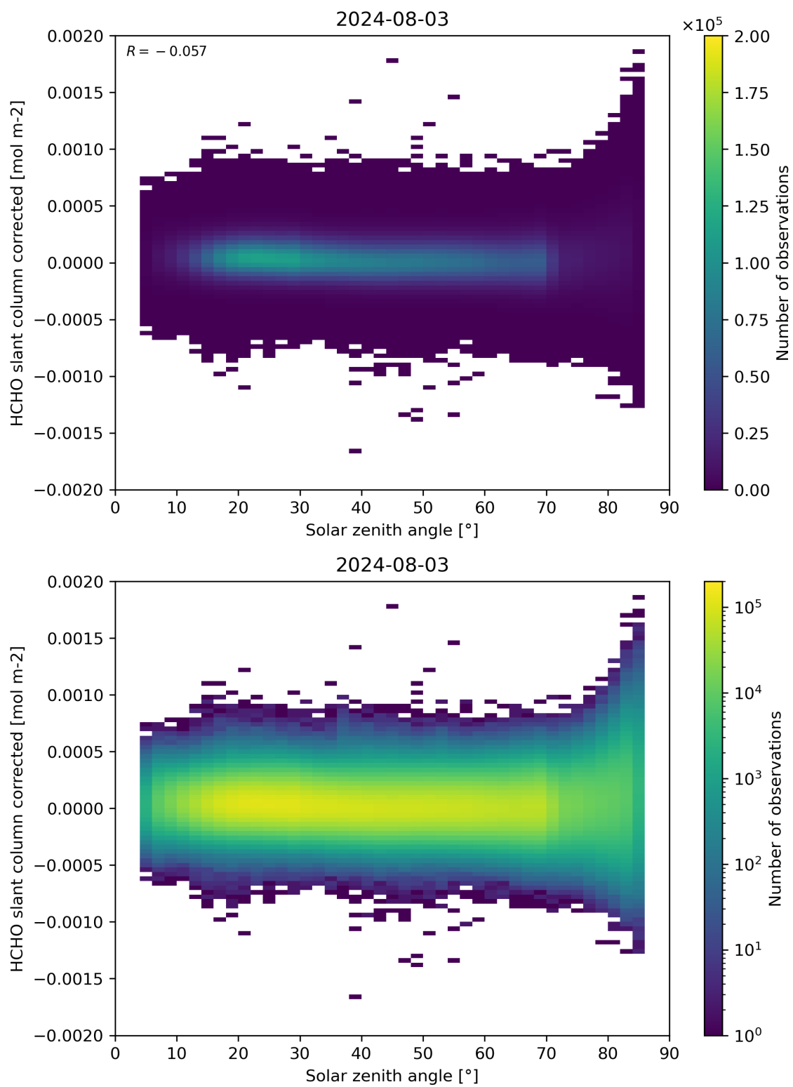
Figure 171: Scatter density plot of “Solar zenith angle” against “HCHO slant column corrected” for 2024-08-02 to 2024-08-04.
