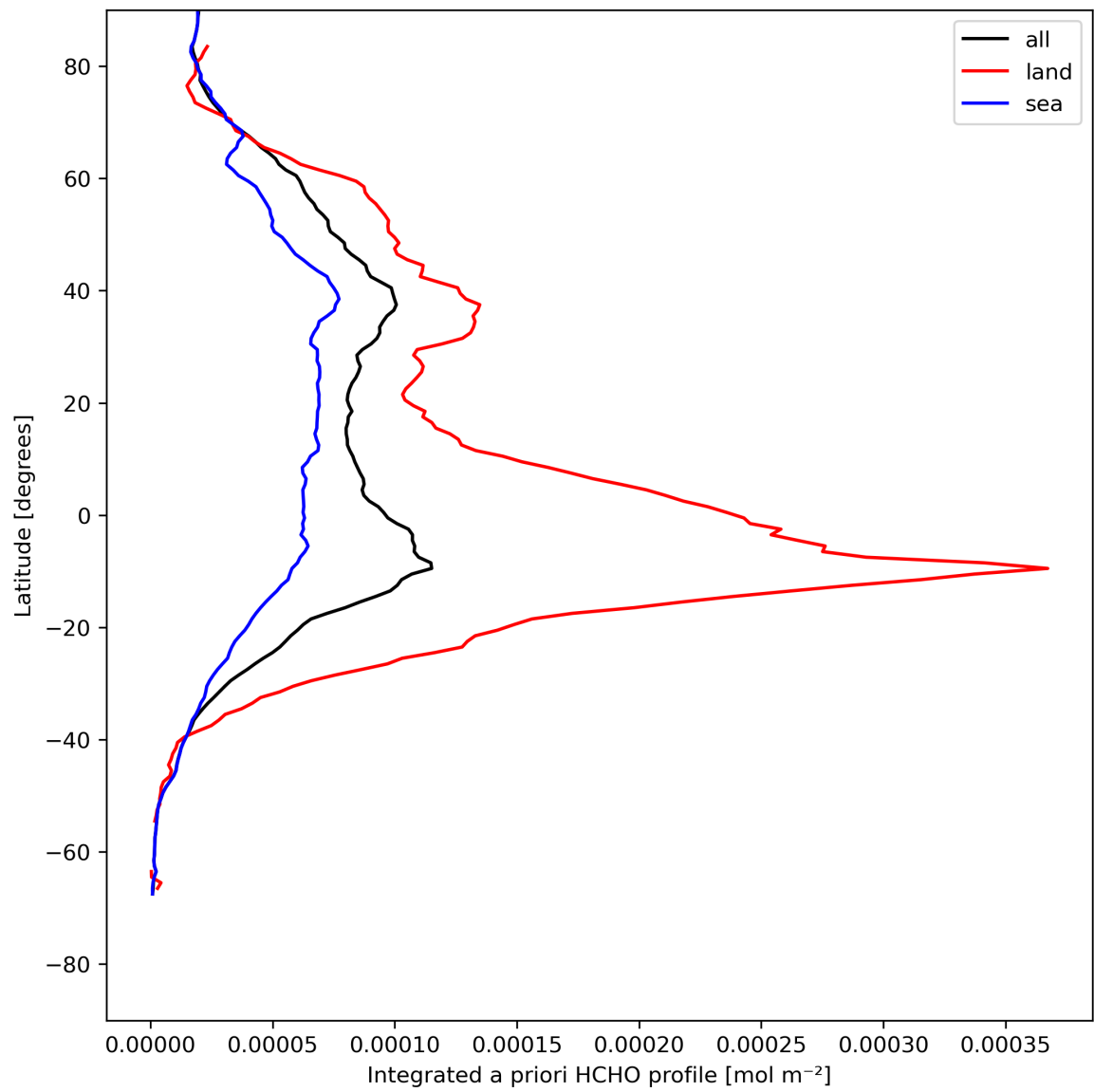
Figure 29: Zonal average of “Integrated a priori HCHO profile” for 2024-08-02 to 2024-08-04.
