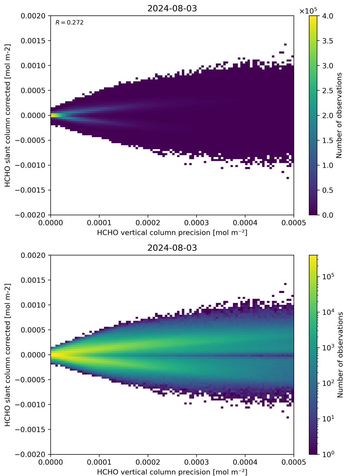
Figure 140: Scatter density plot of “HCHO vertical column precision” against “HCHO slant column corrected” for 2024-08-02 to 2024-08-04.
