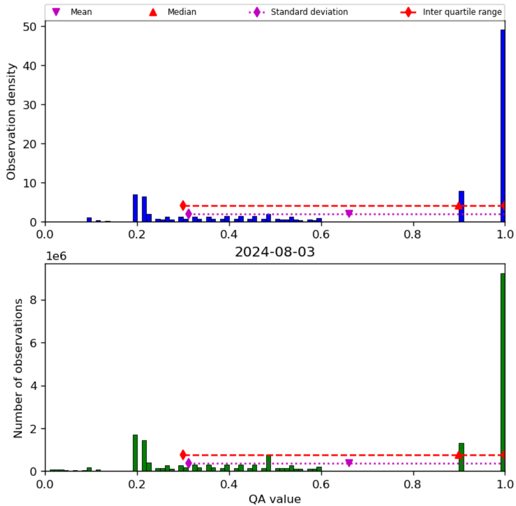
Figure 34: Histogram of “QA value” for 2024-08-02 to 2024-08-04
