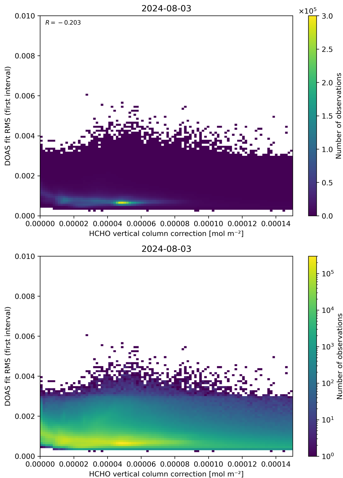
Figure 112: Scatter density plot of “HCHO vertical column correction” against “DOAS fit RMS (first interval)” for 2024-08-02 to 2024-08-04.
