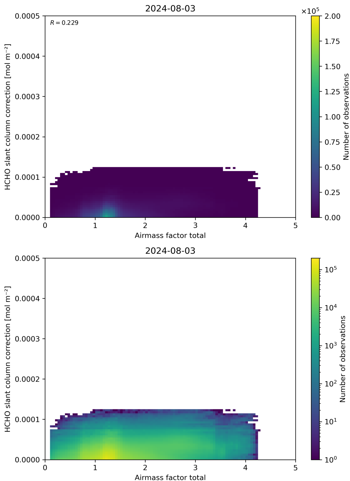
Figure 102: Scatter density plot of “Airmass factor total” against “HCHO slant column correction” for 2024-08-02 to 2024-08-04.
