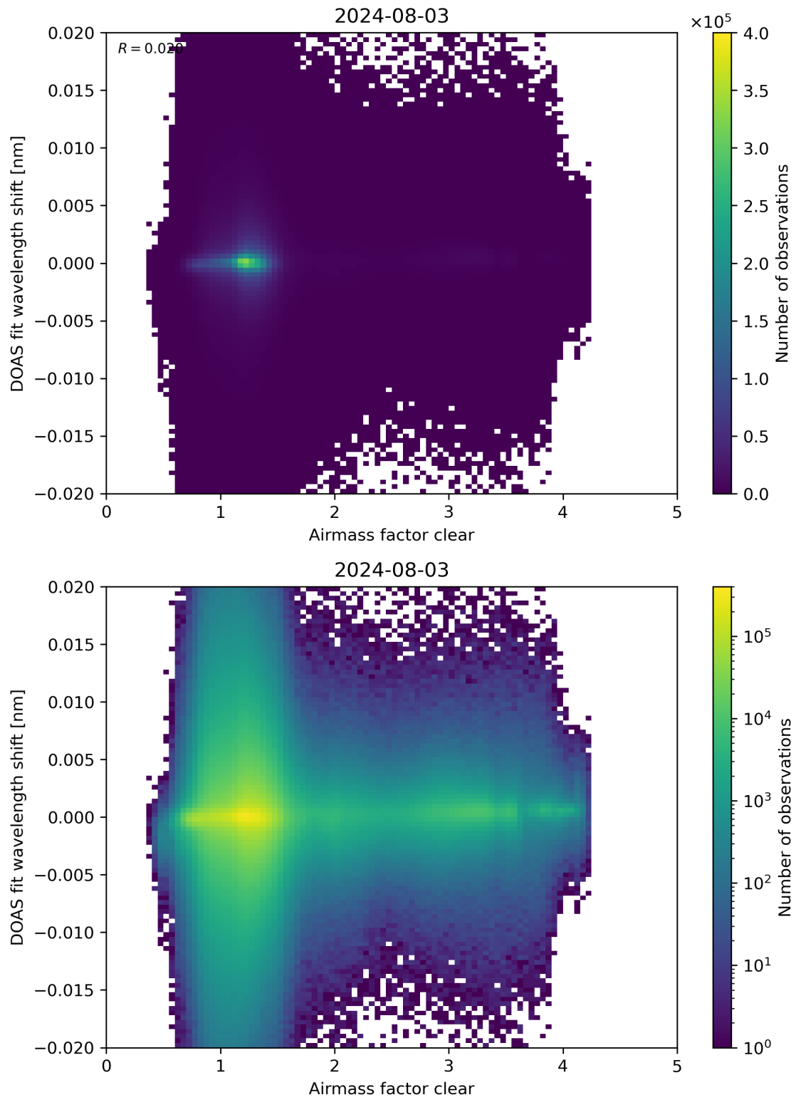
Figure 72: Scatter density plot of “Airmass factor clear” against “DOAS fit wavelength shift” for 2024-08-02 to 2024-08-04.
