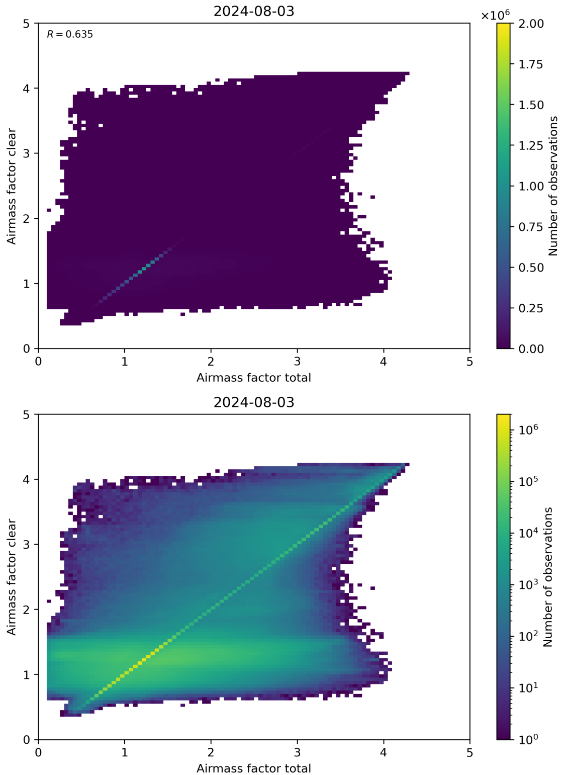
Figure 100: Scatter density plot of “Airmass factor total” against “Airmass factor clear” for 2024-08-02 to 2024-08-04.
