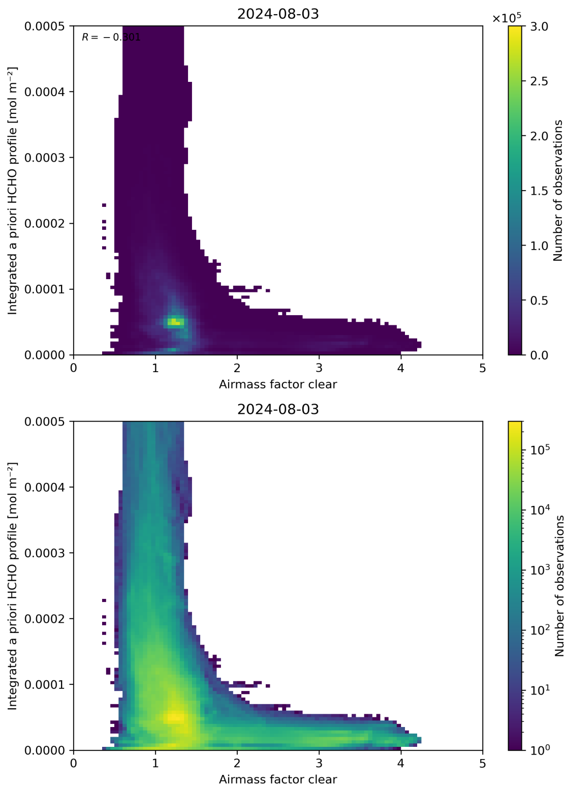
Figure 76: Scatter density plot of “Airmass factor clear” against “Integrated a priori HCHO profile” for 2024-08-02 to 2024-08-04.
