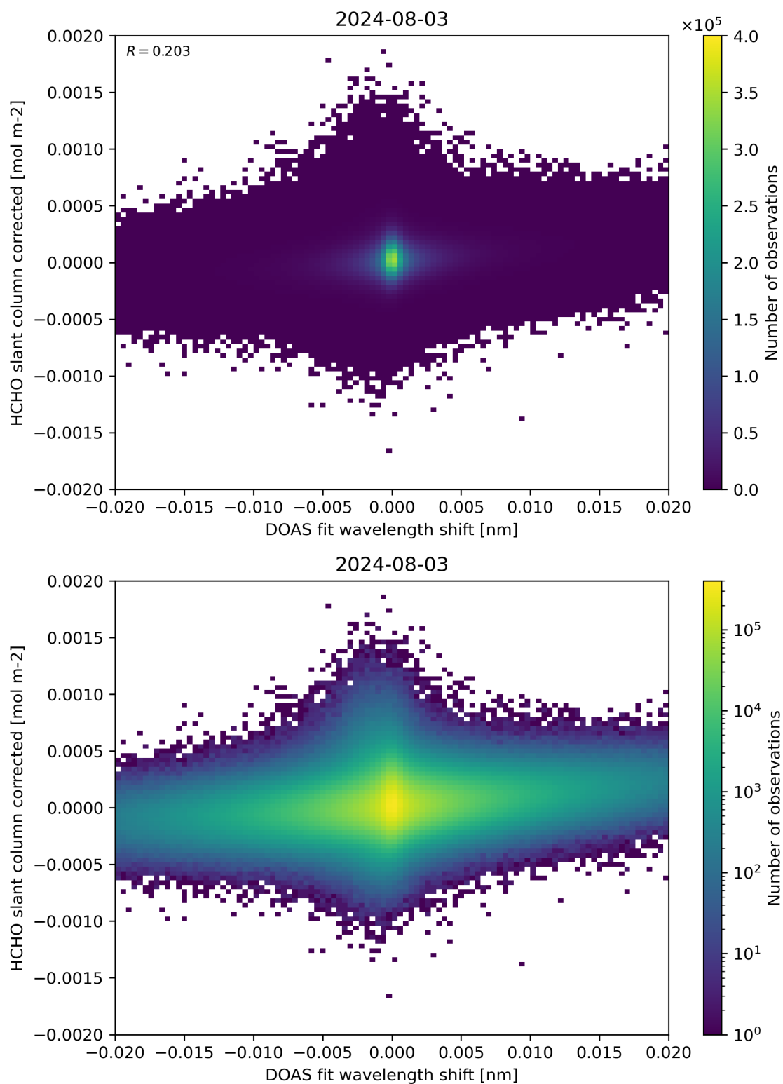
Figure 66: Scatter density plot of “DOAS fit wavelength shift” against “HCHO slant column corrected” for 2024-08-02 to 2024-08-04.
