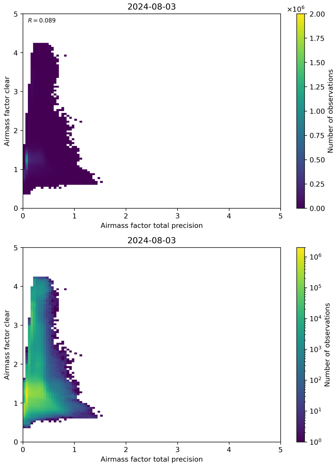
Figure 108: Scatter density plot of “Airmass factor total precision” against “Airmass factor clear” for 2024-08-02 to 2024-08-04.
