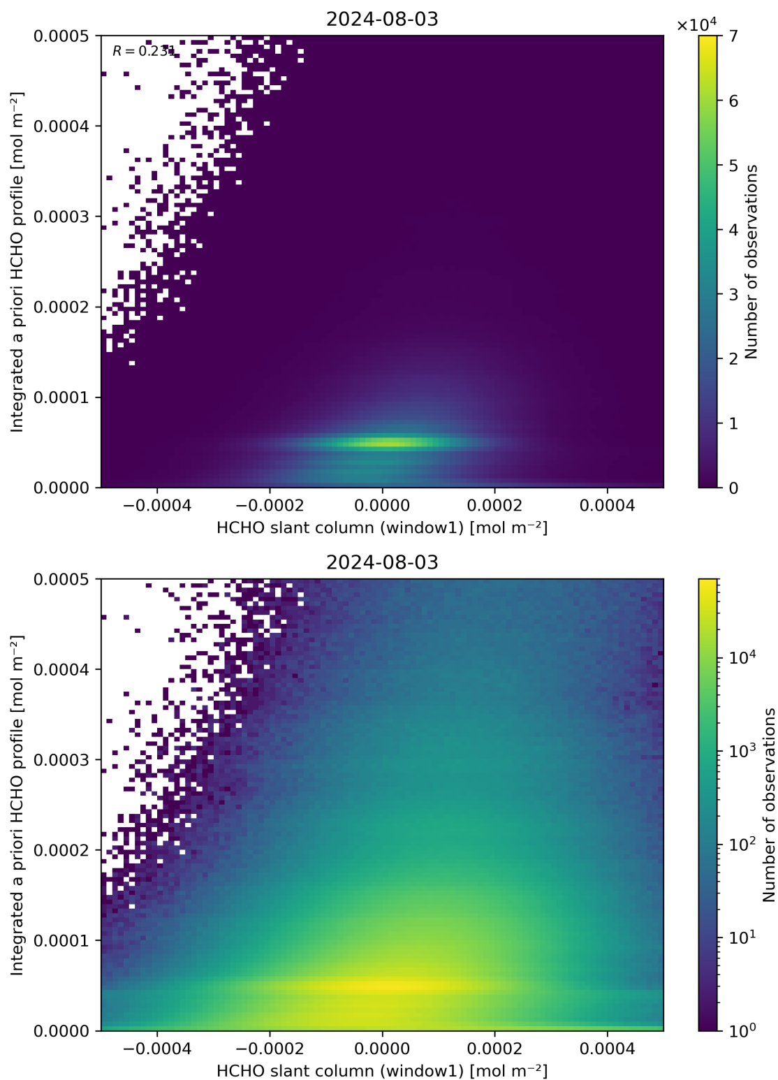
Figure 87: Scatter density plot of “HCHO slant column (window1)” against “Integrated a priori HCHO profile” for 2024-08-02 to 2024-08-04.
