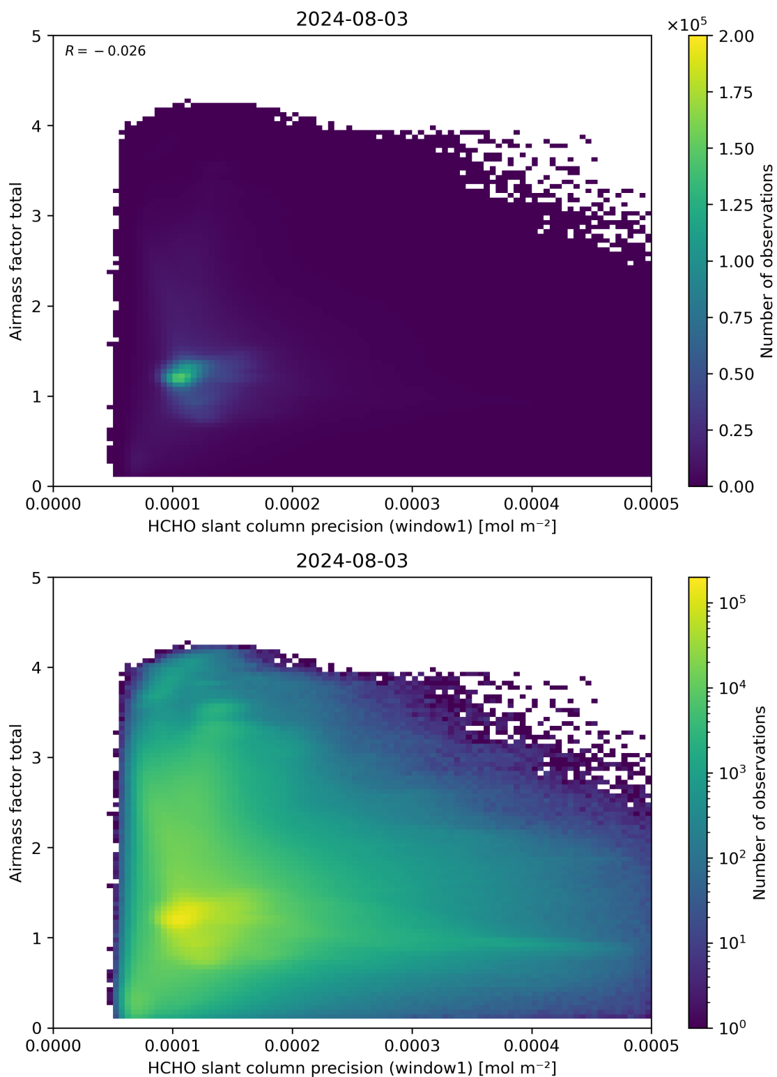
Figure 94: Scatter density plot of “HCHO slant column precision (window1)” against “Airmass factor total” for 2024-08-02 to 2024-08-04.
