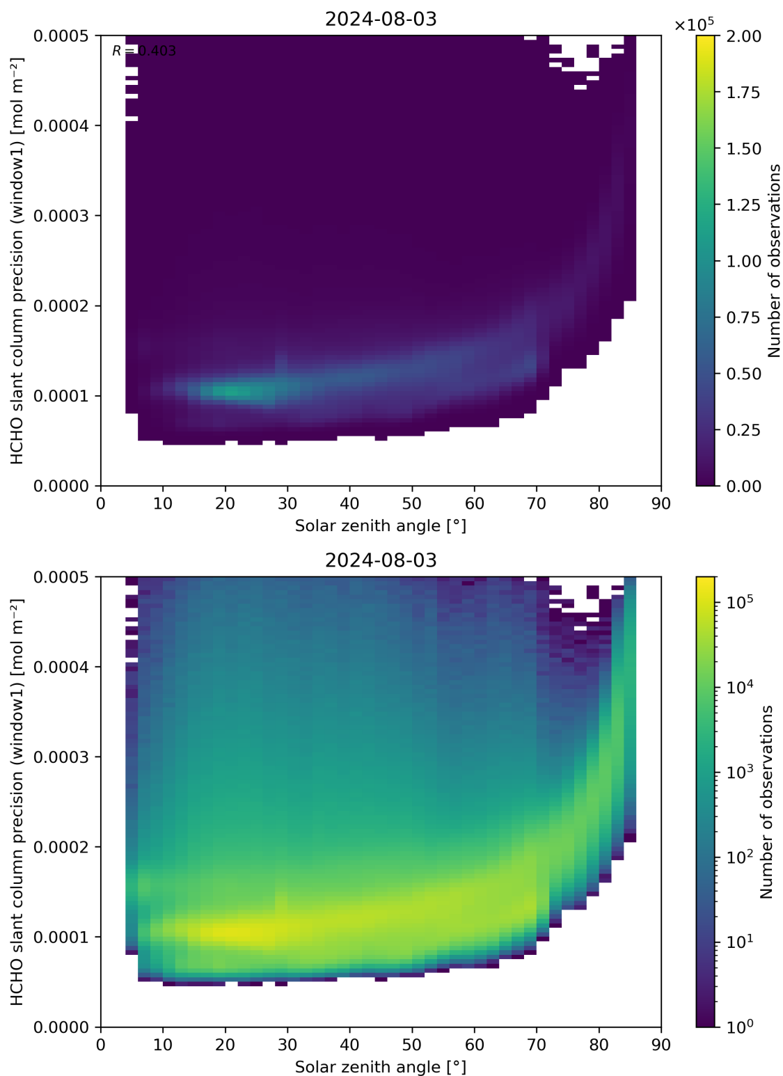
Figure 174: Scatter density plot of “Solar zenith angle” against “HCHO slant column precision (window1)” for 2024-08-02 to 2024-08-04.
