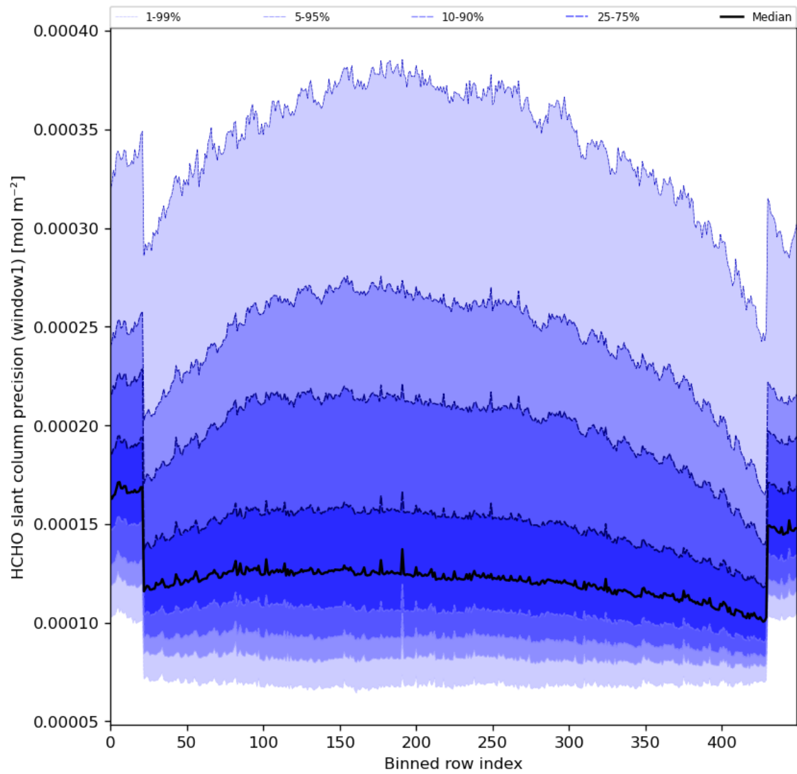
Figure 53: Along track statistics of “HCHO slant column precision (window1)” for 2024-08-02 to 2024-08-04
