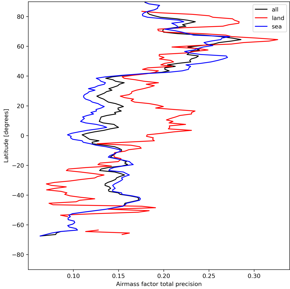
Figure 27: Zonal average of “Airmass factor total precision” for 2024-08-02 to 2024-08-04.
