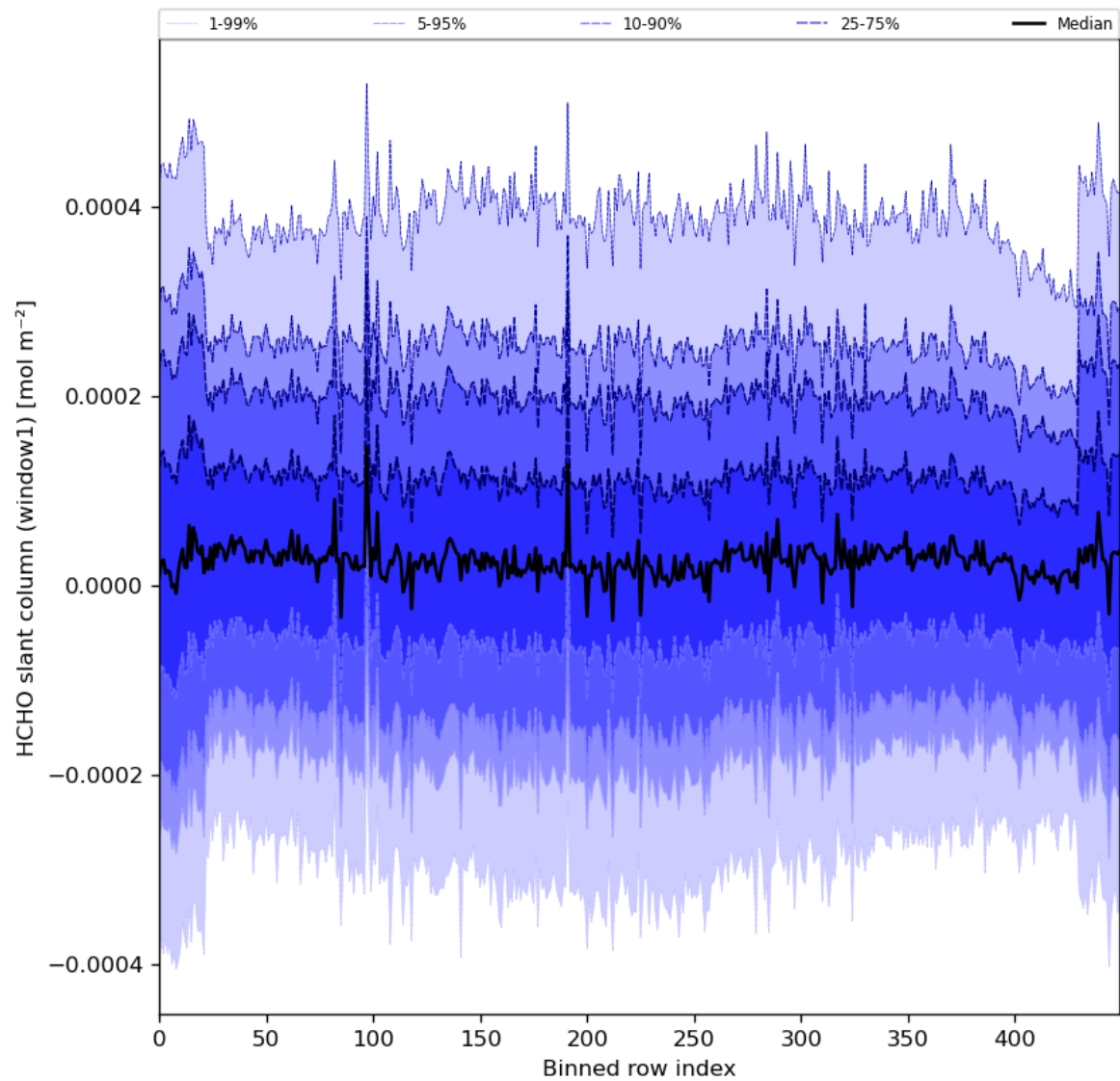
Figure 52: Along track statistics of “HCHO slant column (window1)” for 2024-08-02 to 2024-08-04
