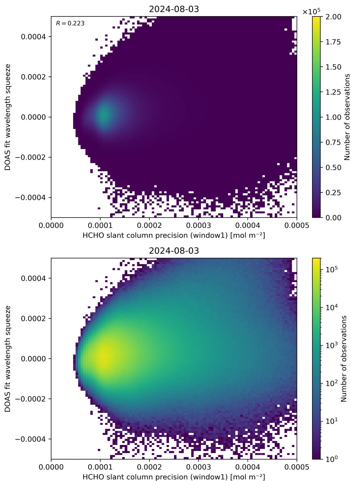
Figure 90: Scatter density plot of “HCHO slant column precision (window1)” against “DOAS fit wavelength squeeze” for 2024-08-02 to 2024-08-04.
