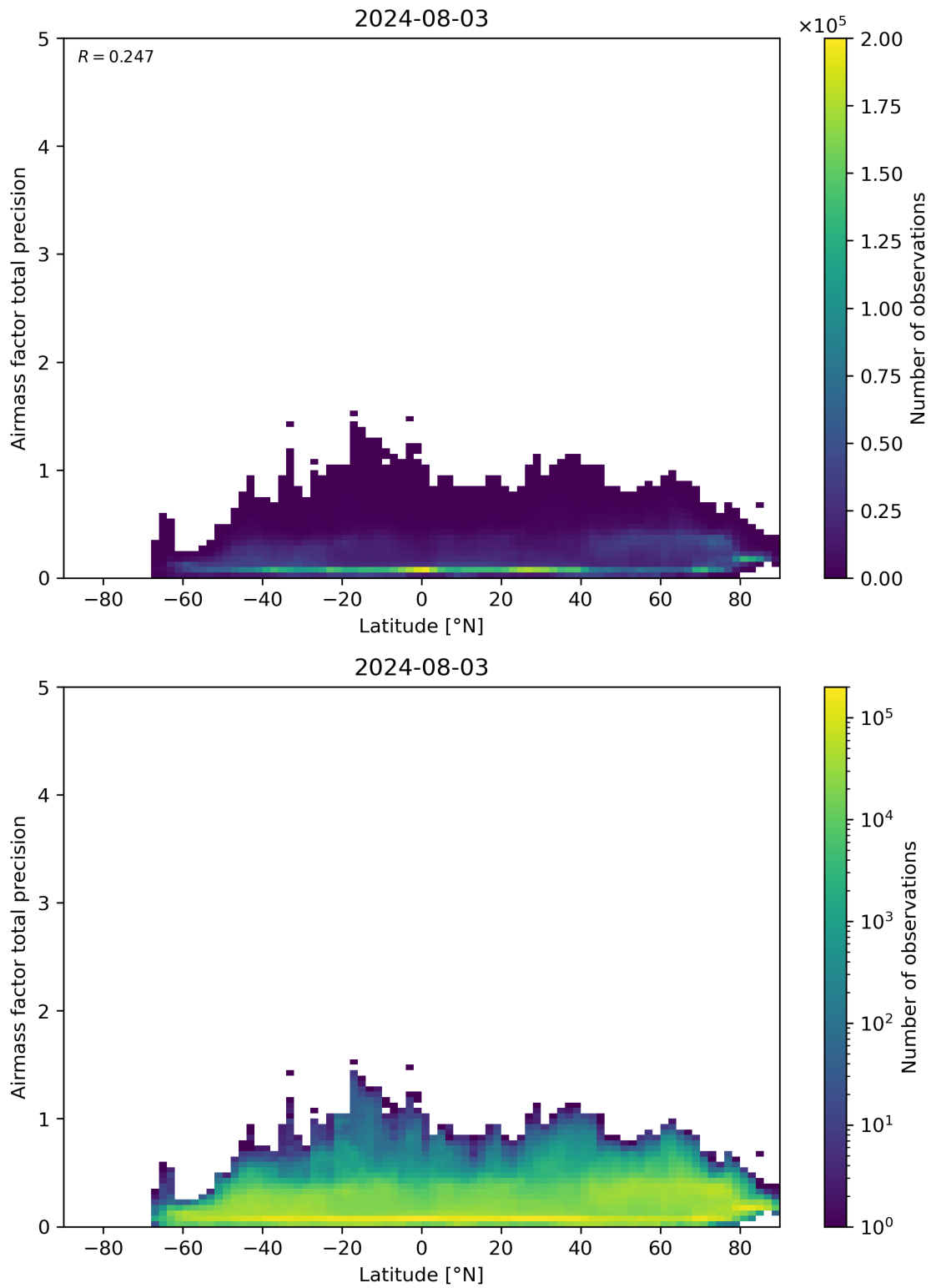
Figure 162: Scatter density plot of “Latitude” against “Airmass factor total precision” for 2024-08-02 to 2024-08-04.
