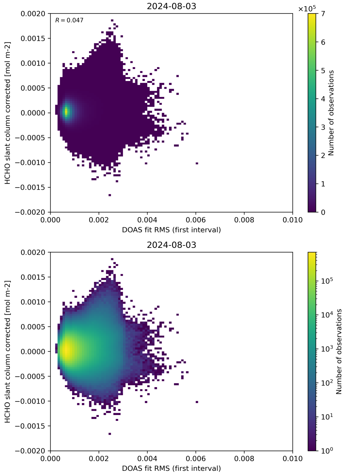
Figure 62: Scatter density plot of “DOAS fit RMS (first interval)” against “HCHO slant column corrected” for 2024-08-02 to 2024-08-04.
