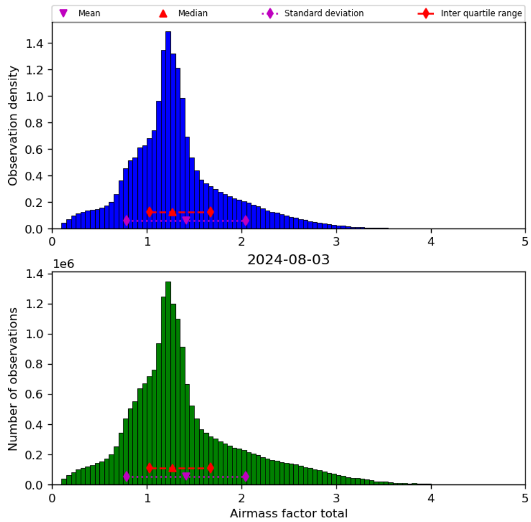
Figure 40: Histogram of “Airmass factor total” for 2024-08-02 to 2024-08-04
