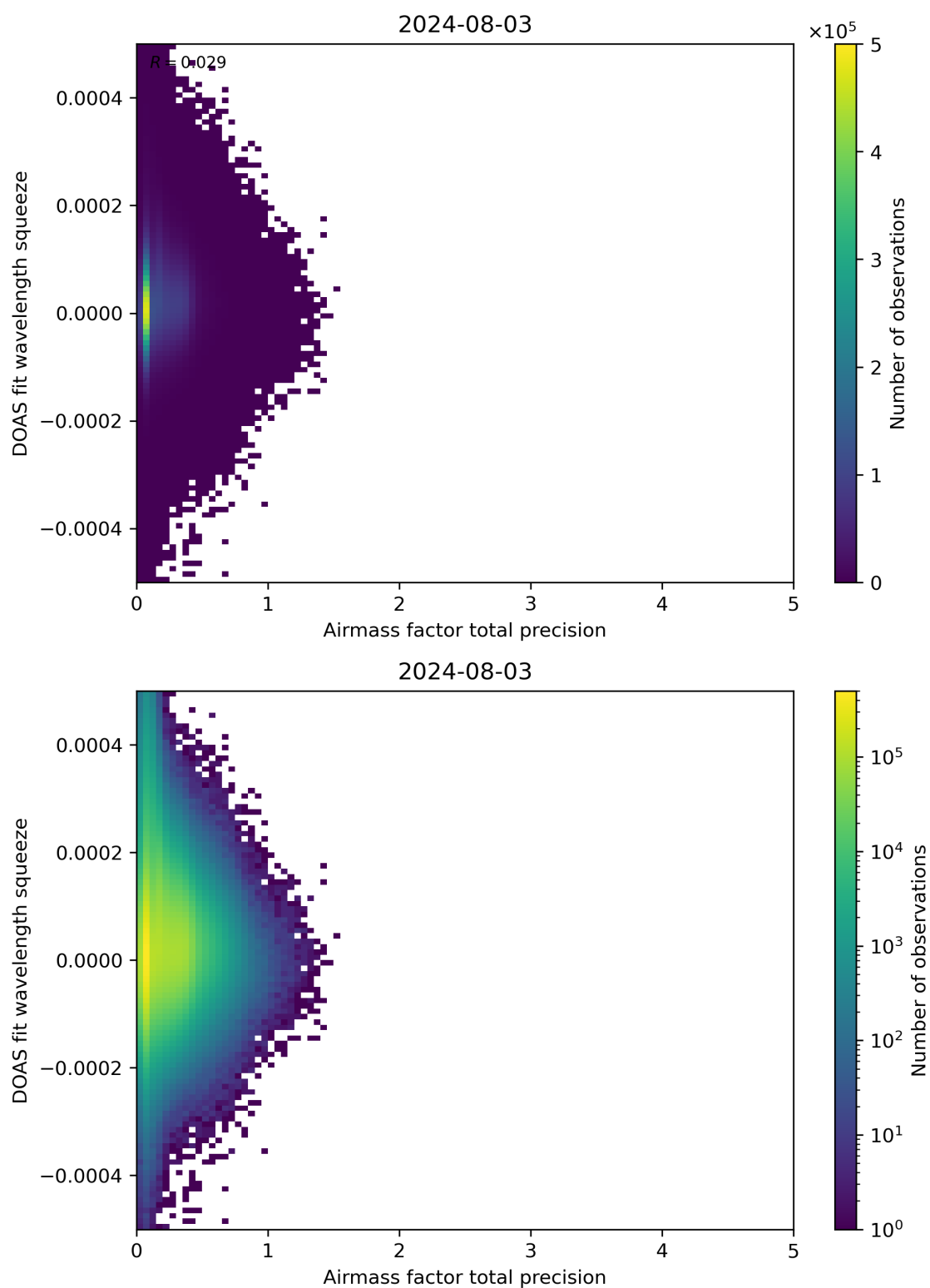
Figure 107: Scatter density plot of “Airmass factor total precision” against “DOAS fit wavelength squeeze” for 2024-08-02 to 2024-08-04.
