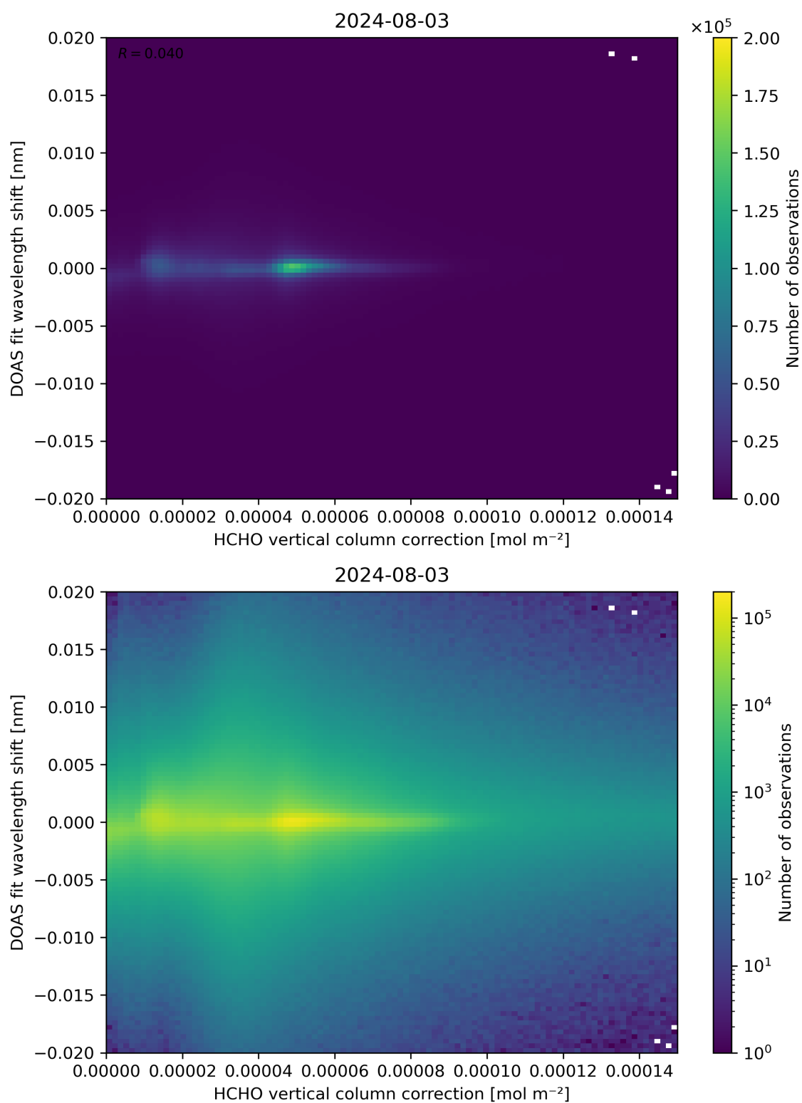
Figure 113: Scatter density plot of “HCHO vertical column correction” against “DOAS fit wavelength shift” for 2024-08-02 to 2024-08-04.
