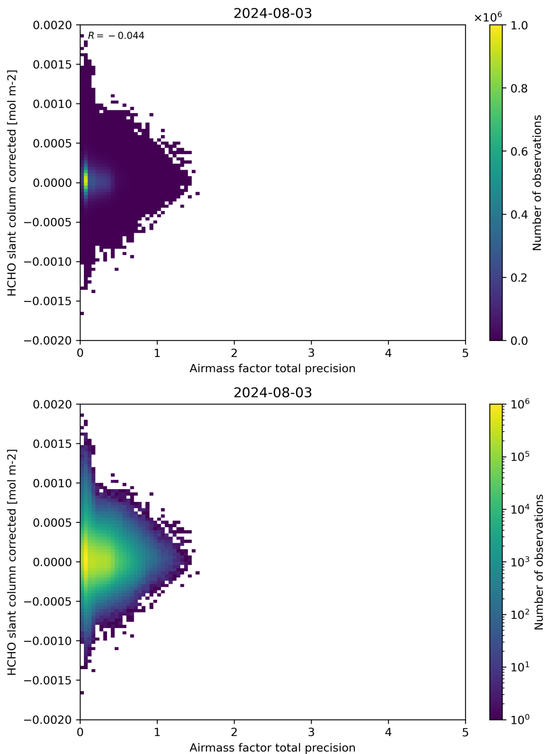
Figure 109: Scatter density plot of “Airmass factor total precision” against “HCHO slant column corrected” for 2024-08-02 to 2024-08-04.
