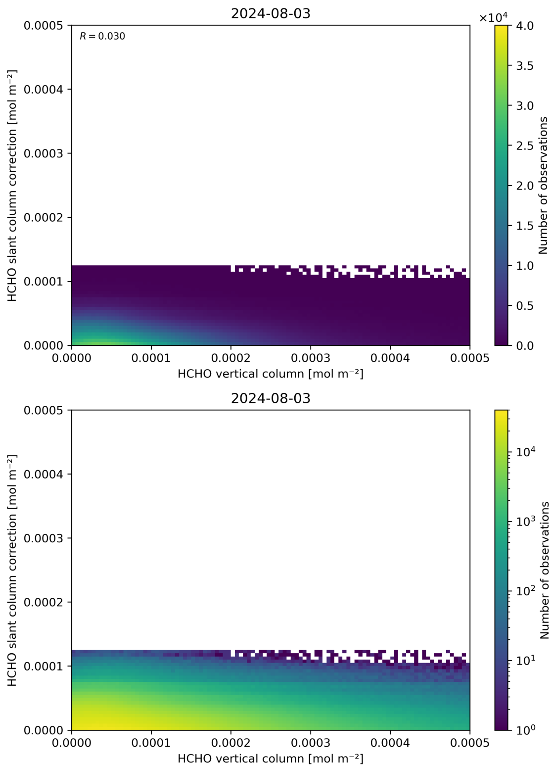
Figure 128: Scatter density plot of “HCHO vertical column” against “HCHO slant column correction” for 2024-08-02 to 2024-08-04.
