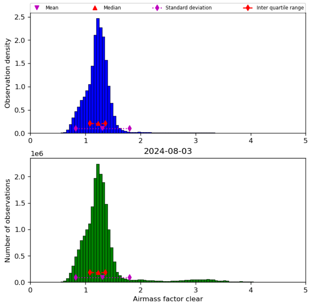
Figure 42: Histogram of “Airmass factor clear” for 2024-08-02 to 2024-08-04
