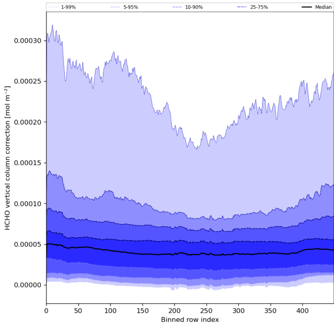
Figure 51: Along track statistics of “HCHO vertical column correction” for 2024-08-02 to 2024-08-04
