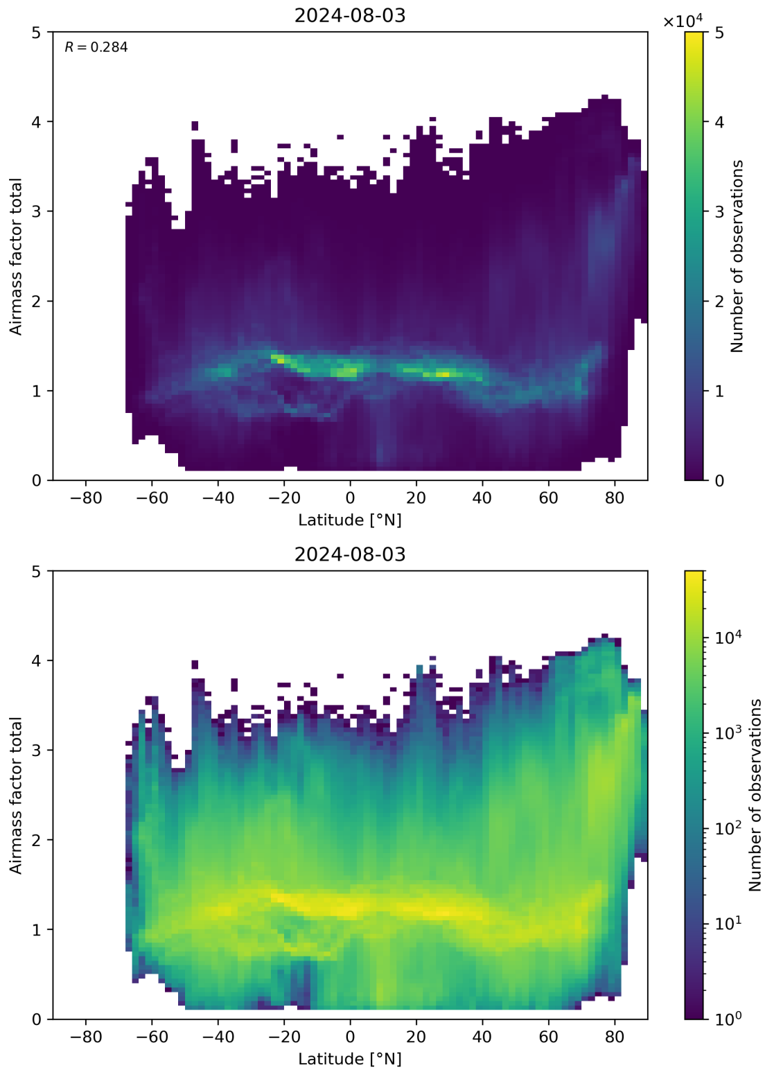
Figure 161: Scatter density plot of “Latitude” against “Airmass factor total” for 2024-08-02 to 2024-08-04.
