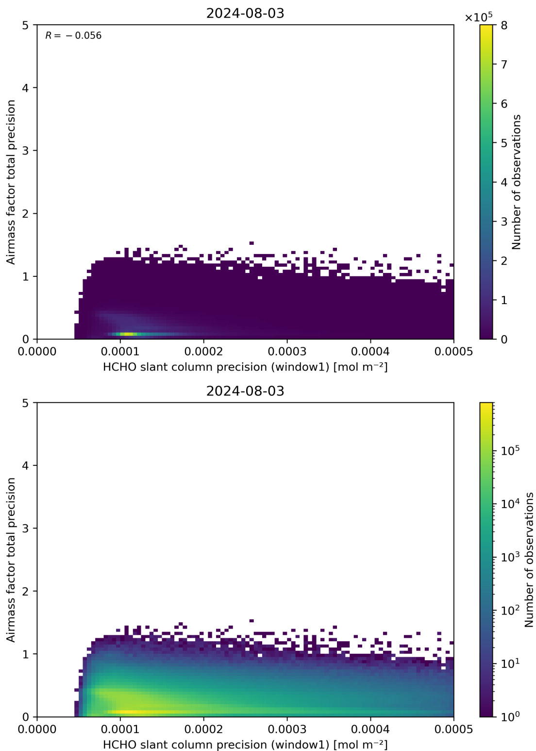
Figure 95: Scatter density plot of “HCHO slant column precision (window1)” against “Airmass factor total precision” for 2024-08-02 to 2024-08-04.
