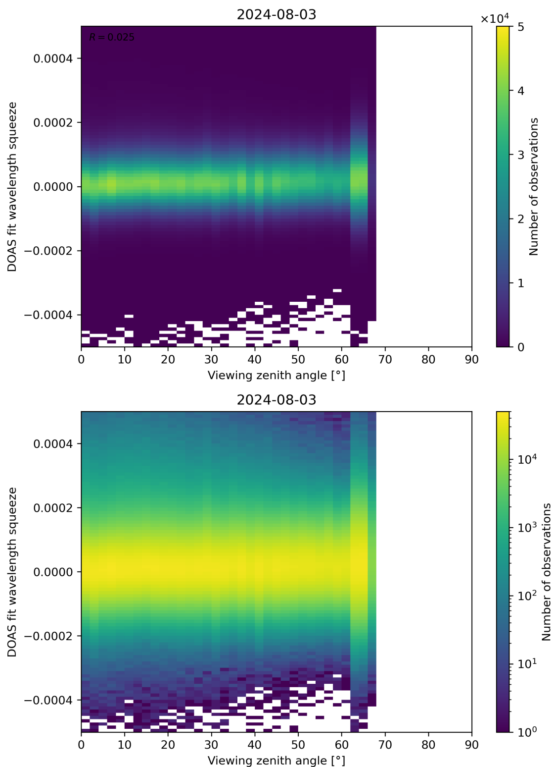
Figure 184: Scatter density plot of “Viewing zenith angle” against “DOAS fit wavelength squeeze” for 2024-08-02 to 2024-08-04.
