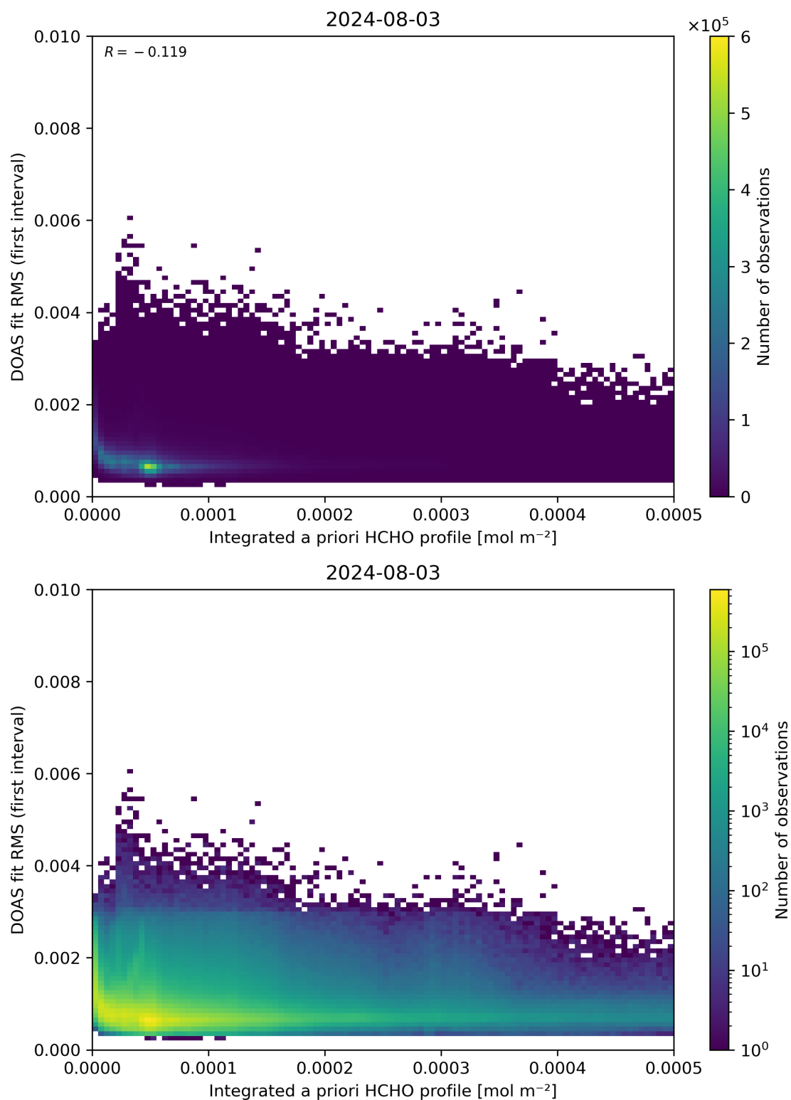
Figure 148: Scatter density plot of “Integrated a priori HCHO profile” against “DOAS fit RMS (first interval)” for 2024-08-02 to 2024-08-04.
