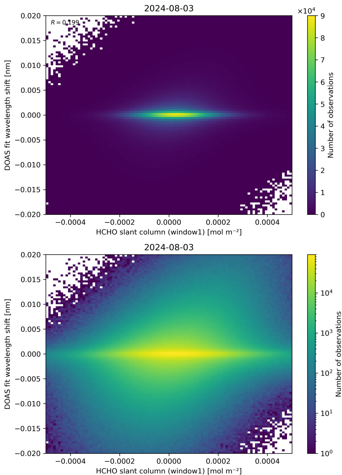
Figure 79: Scatter density plot of “HCHO slant column (window1)” against “DOAS fit wavelength shift” for 2024-08-02 to 2024-08-04.
