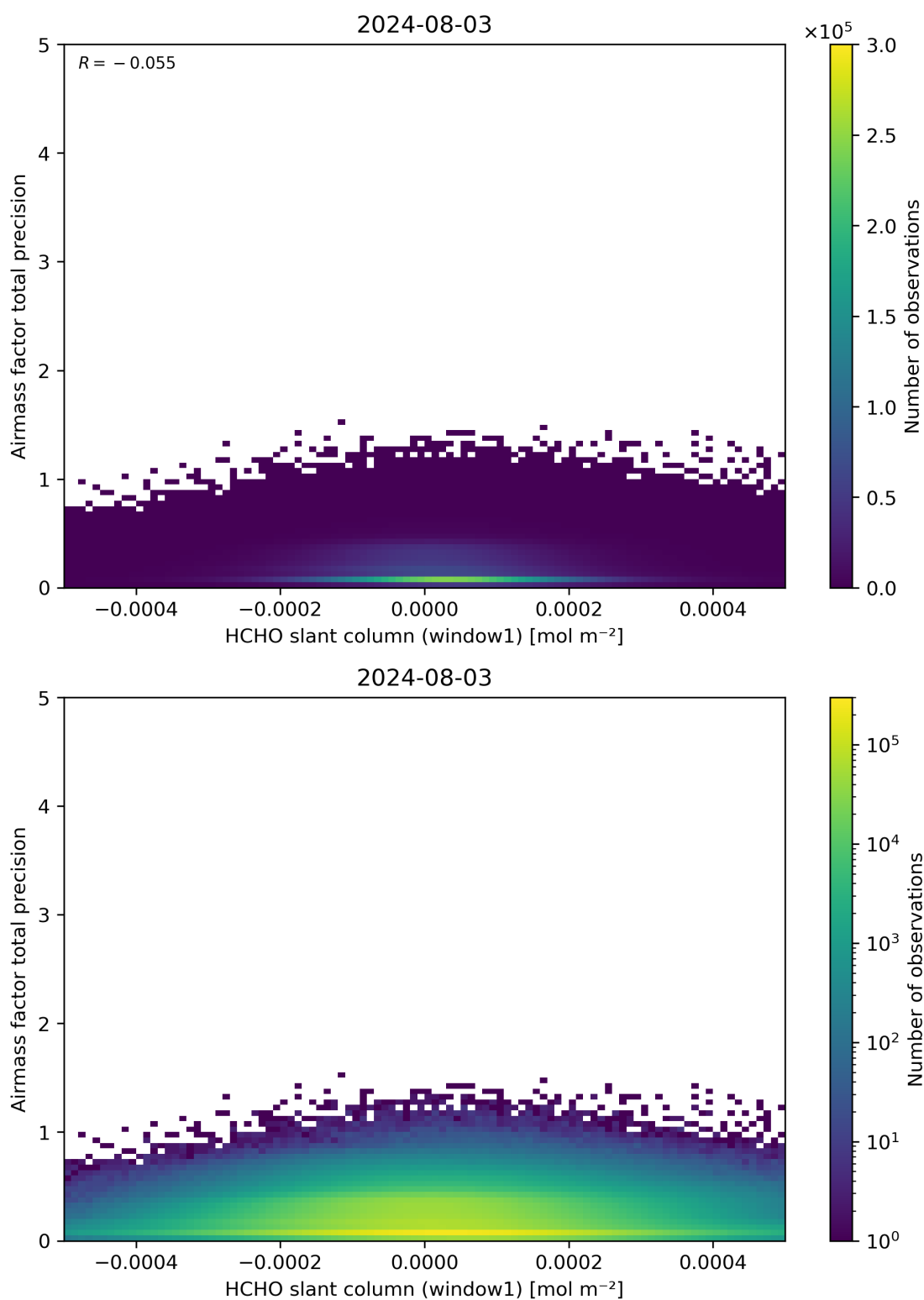
Figure 86: Scatter density plot of “HCHO slant column (window1)” against “Airmass factor total precision” for 2024-08-02 to 2024-08-04.
