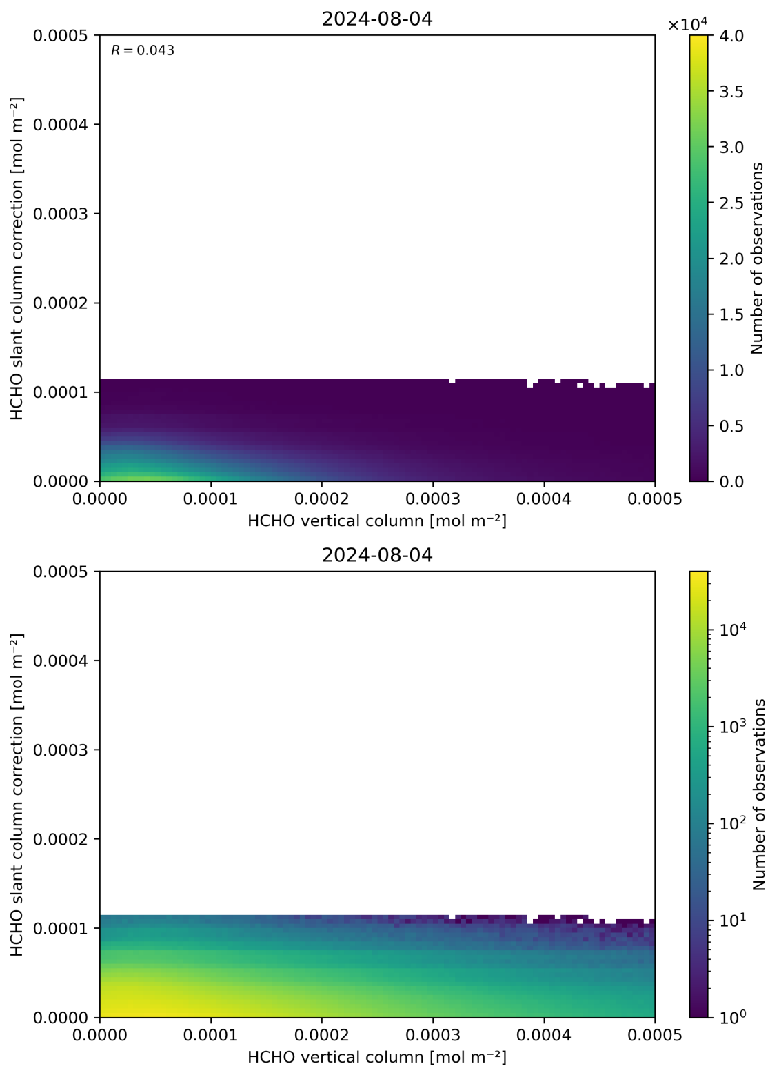
Figure 128: Scatter density plot of “HCHO vertical column” against “HCHO slant column correction” for 2024-08-03 to 2024-08-05.
