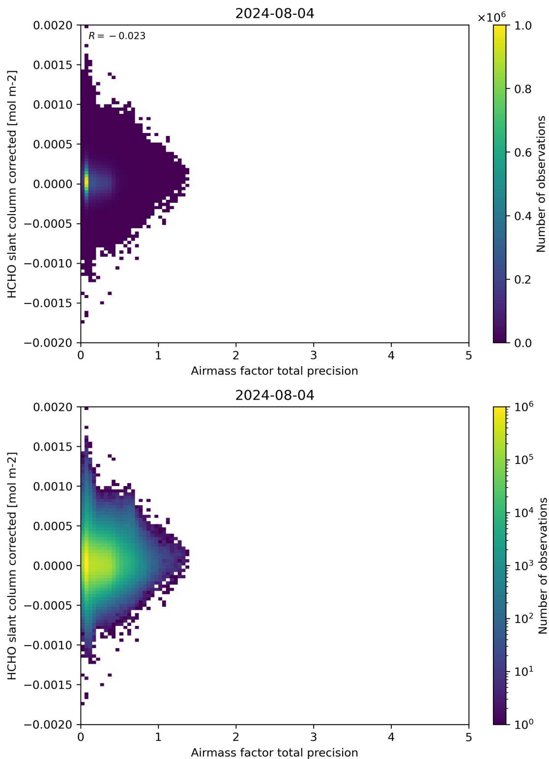
Figure 109: Scatter density plot of “Airmass factor total precision” against “HCHO slant column corrected” for 2024-08-03 to 2024-08-05.
