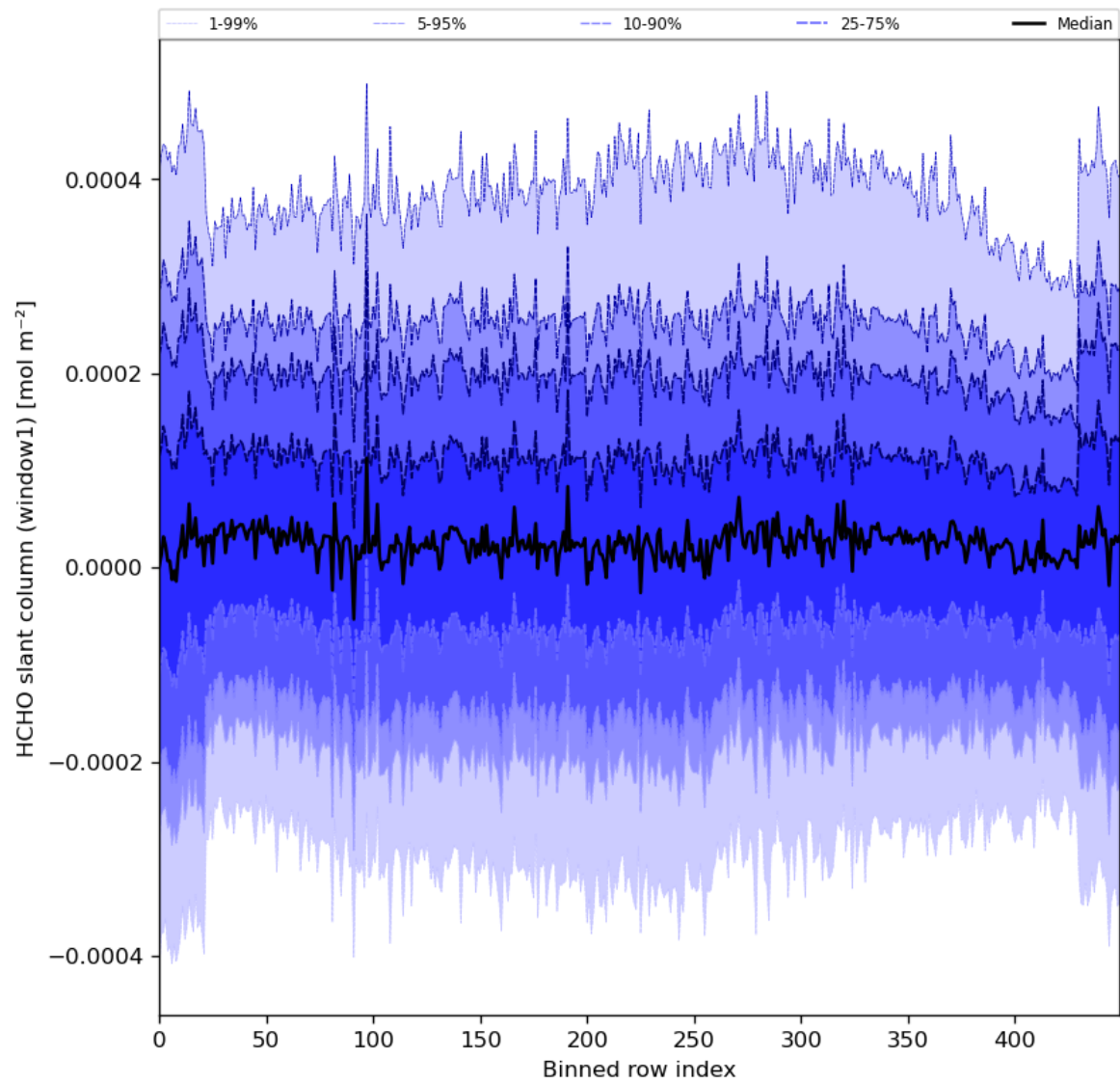
Figure 52: Along track statistics of “HCHO slant column (window1)” for 2024-08-03 to 2024-08-05
