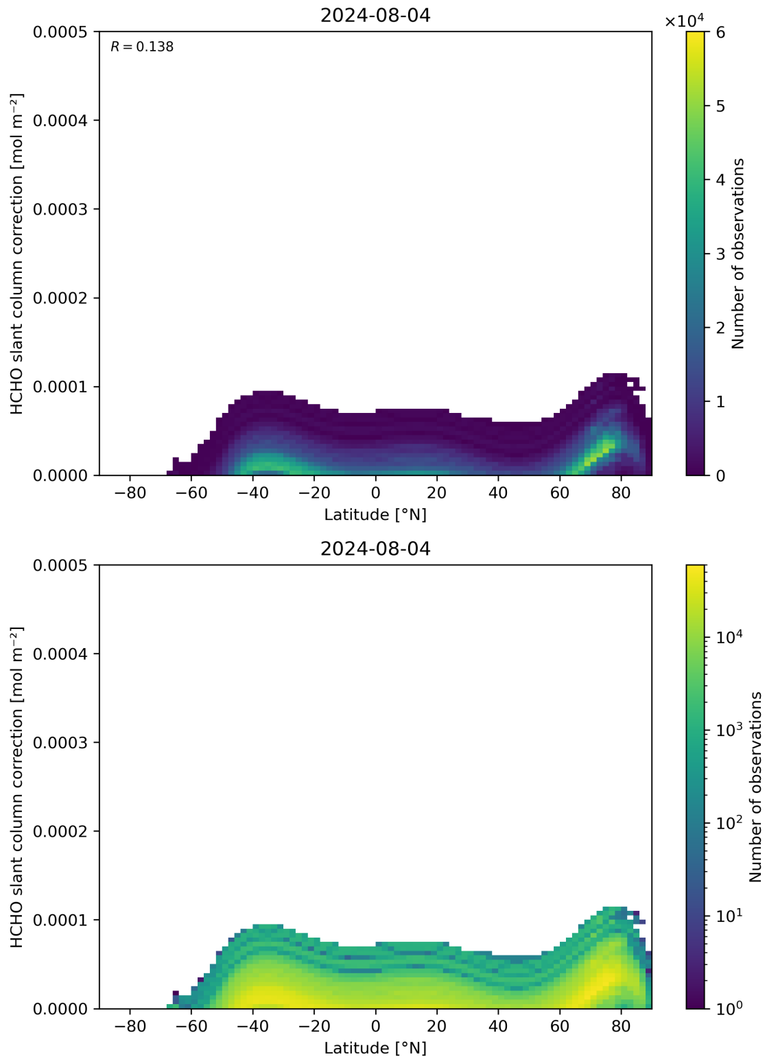
Figure 158: Scatter density plot of “Latitude” against “HCHO slant column correction” for 2024-08-03 to 2024-08-05.
