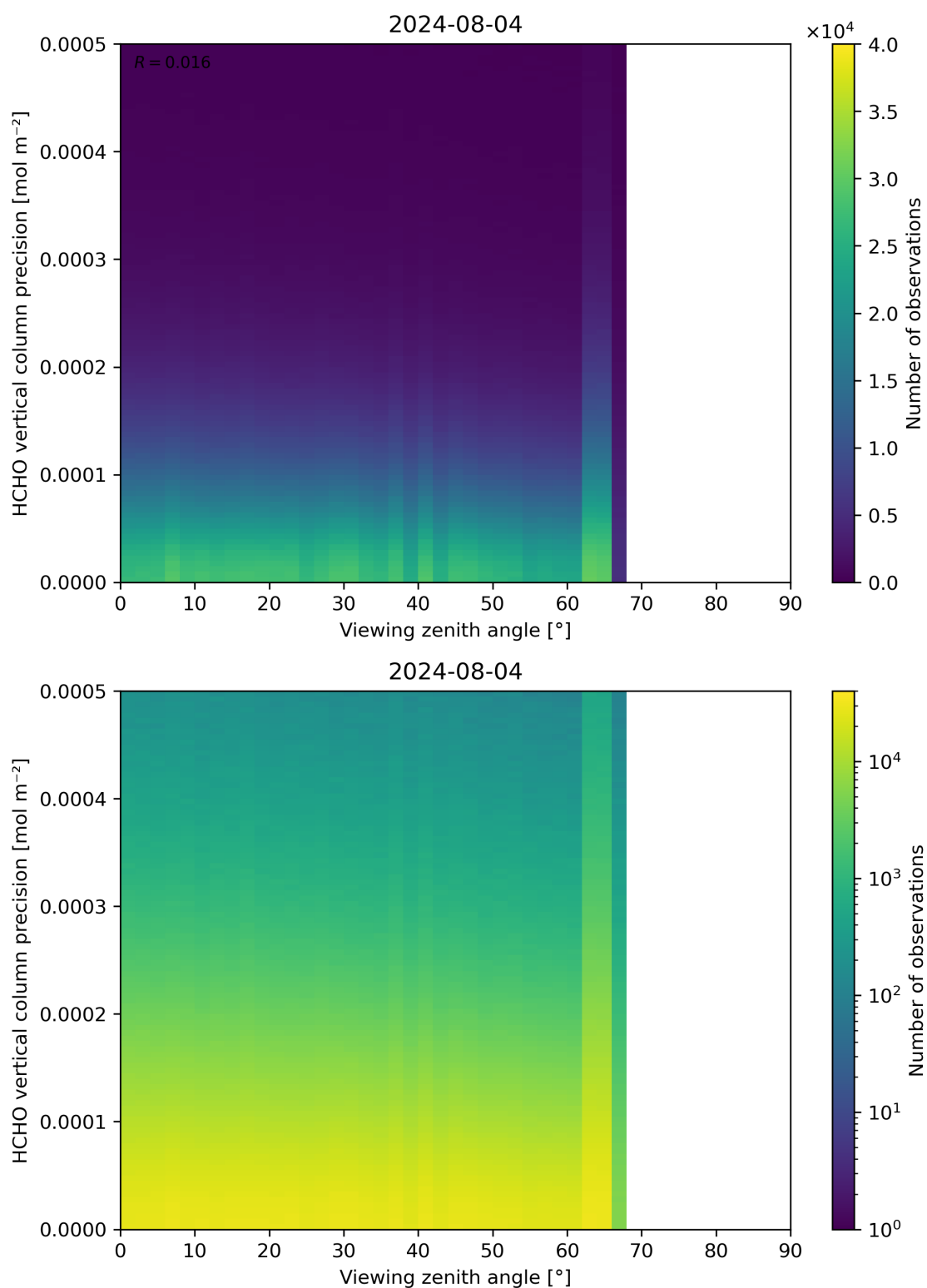
Figure 194: Scatter density plot of “Viewing zenith angle” against “HCHO vertical column precision” for 2024-08-03 to 2024-08-05.
