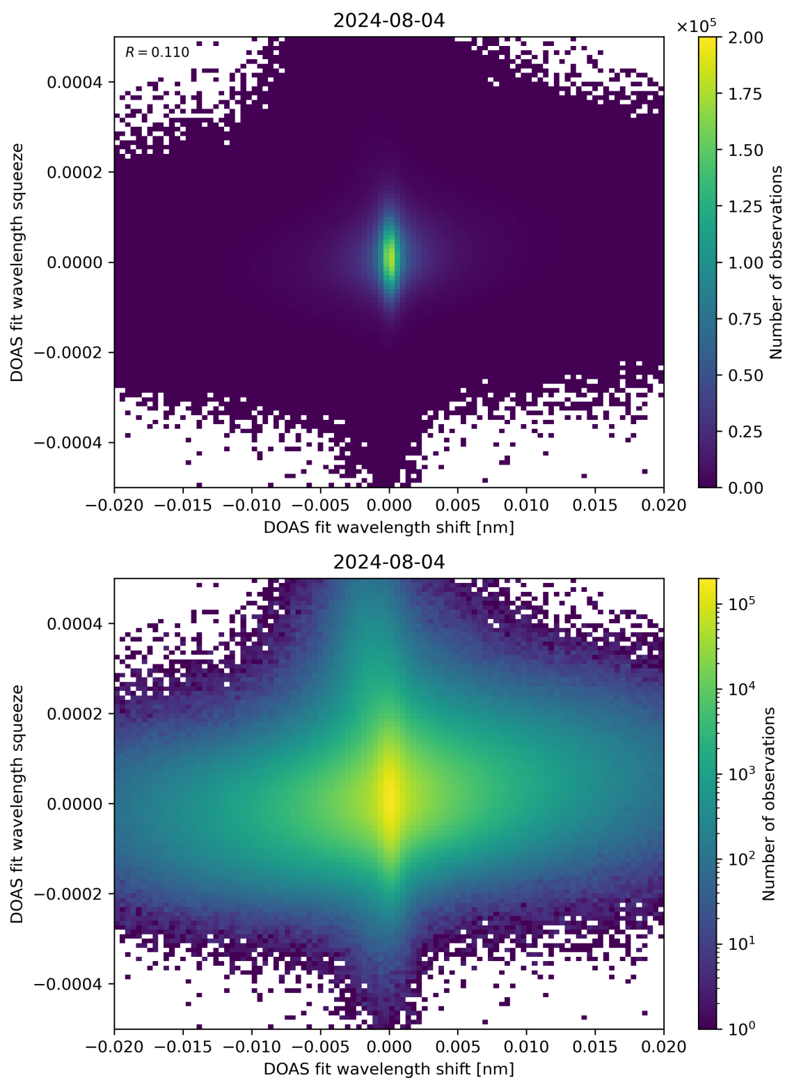
Figure 65: Scatter density plot of “DOAS fit wavelength shift” against “DOAS fit wavelength squeeze” for 2024-08-03 to 2024-08-05.
