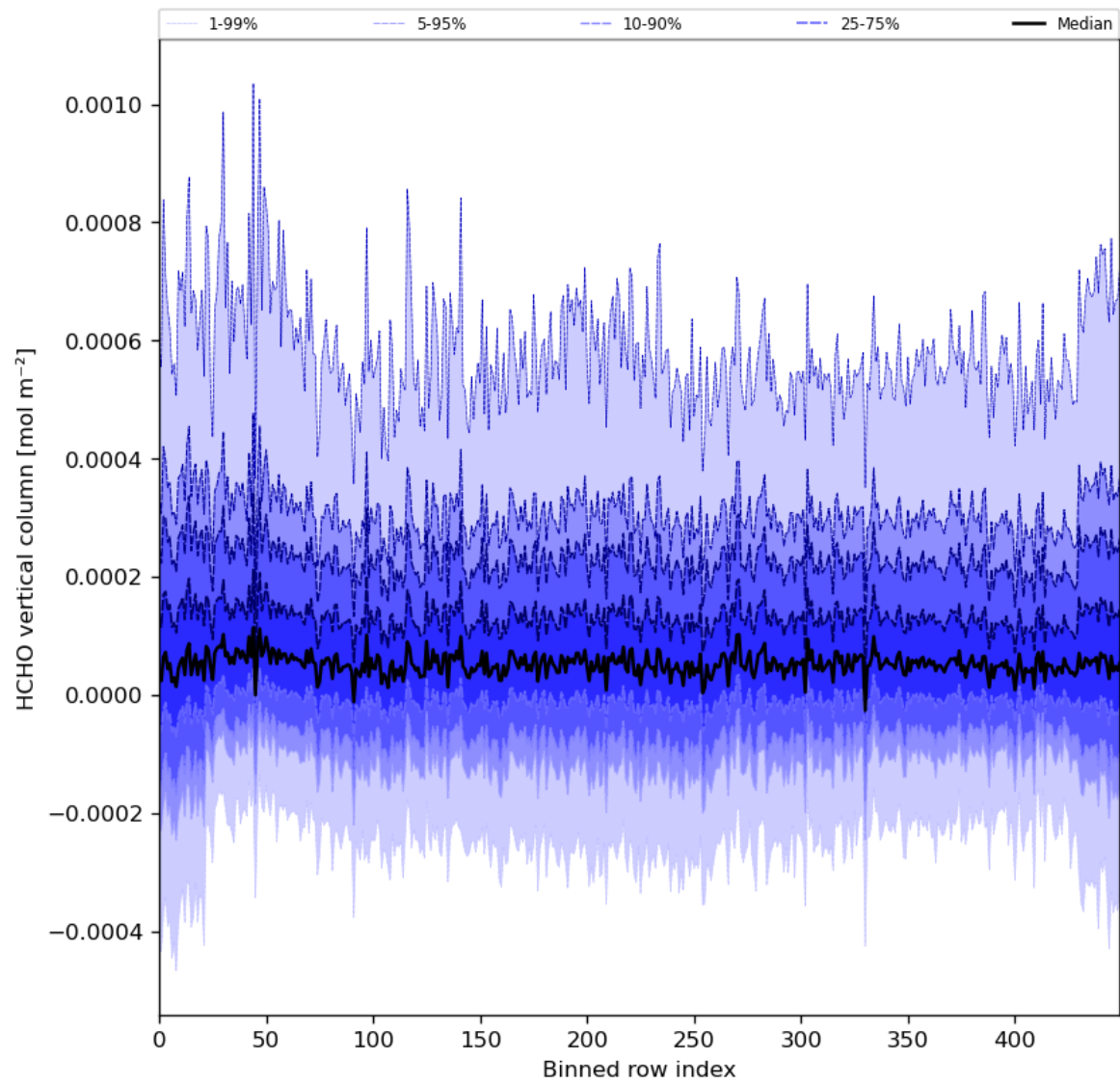
Figure 49: Along track statistics of “HCHO vertical column” for 2024-08-03 to 2024-08-05
