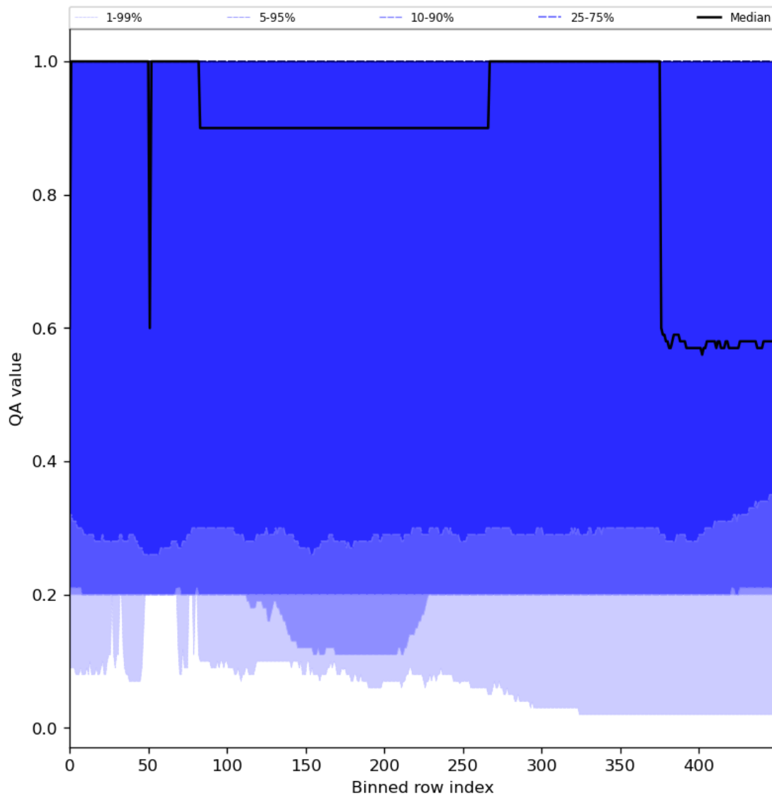
Figure 48: Along track statistics of “QA value” for 2024-08-03 to 2024-08-05
