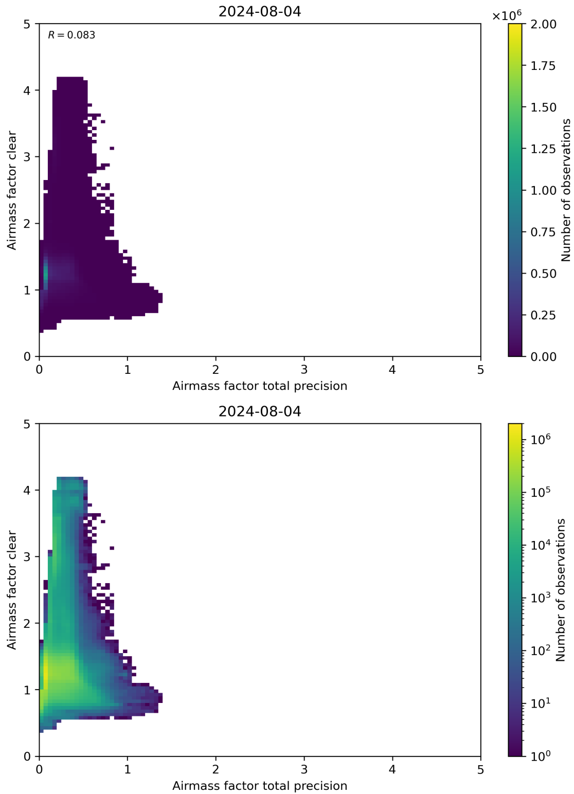
Figure 108: Scatter density plot of “Airmass factor total precision” against “Airmass factor clear” for 2024-08-03 to 2024-08-05.
