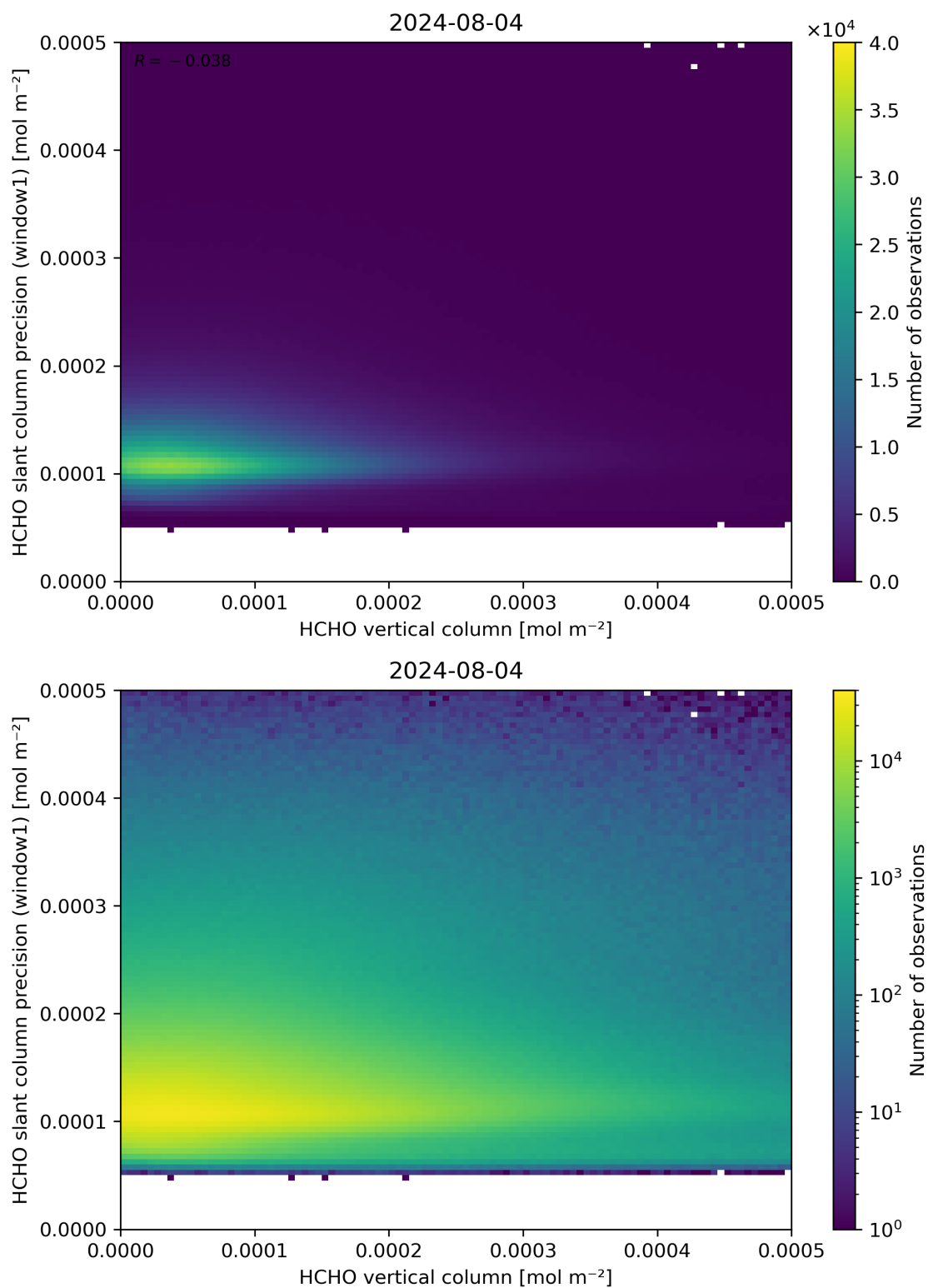
Figure 130: Scatter density plot of “HCHO vertical column” against “HCHO slant column precision (window1)” for 2024-08-03 to 2024-08-05.
