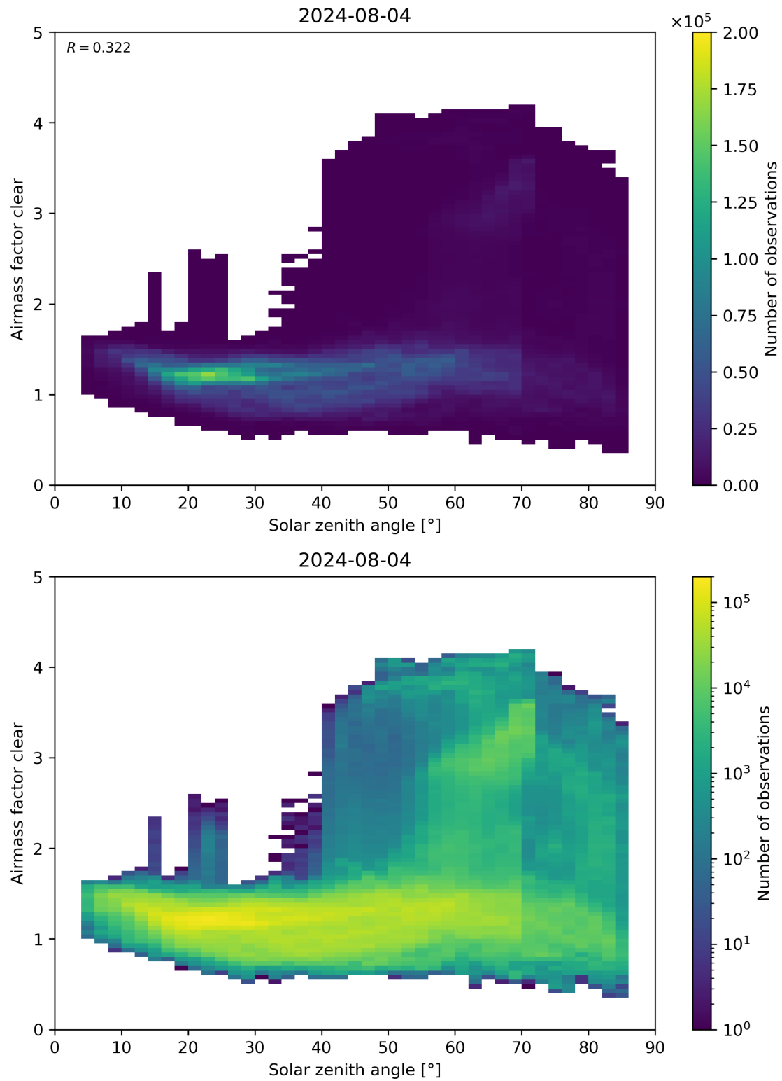
Figure 170: Scatter density plot of “Solar zenith angle” against “Airmass factor clear” for 2024-08-03 to 2024-08-05.
