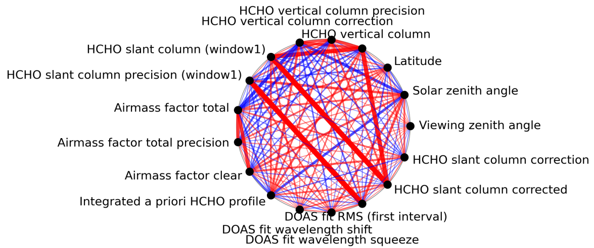
Figure 1: Map of correlation graph for 2024-08-03 to 2024-08-05.
