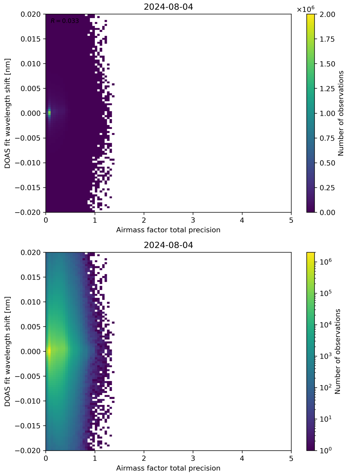
Figure 106: Scatter density plot of “Airmass factor total precision” against “DOAS fit wavelength shift” for 2024-08-03 to 2024-08-05.
