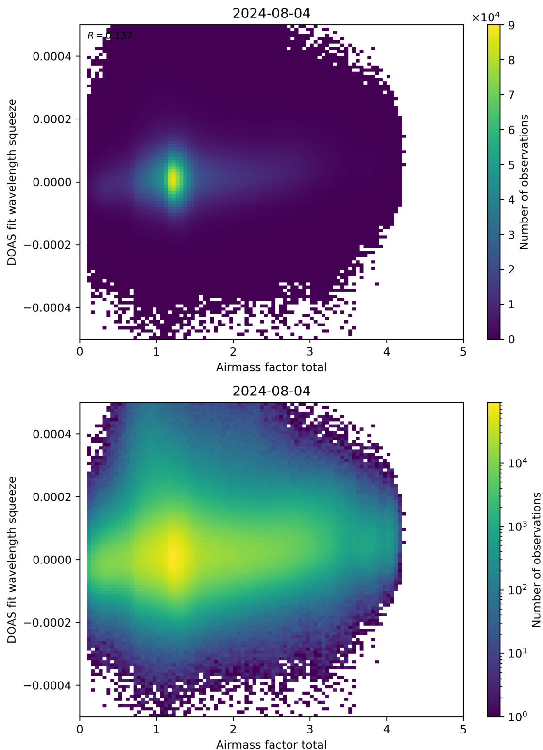
Figure 99: Scatter density plot of “Airmass factor total” against “DOAS fit wavelength squeeze” for 2024-08-03 to 2024-08-05.
