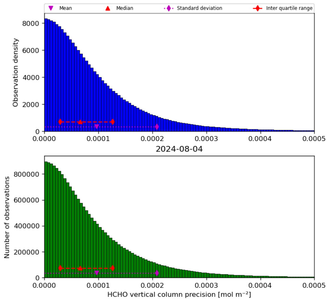
Figure 36: Histogram of “HCHO vertical column precision” for 2024-08-03 to 2024-08-05
