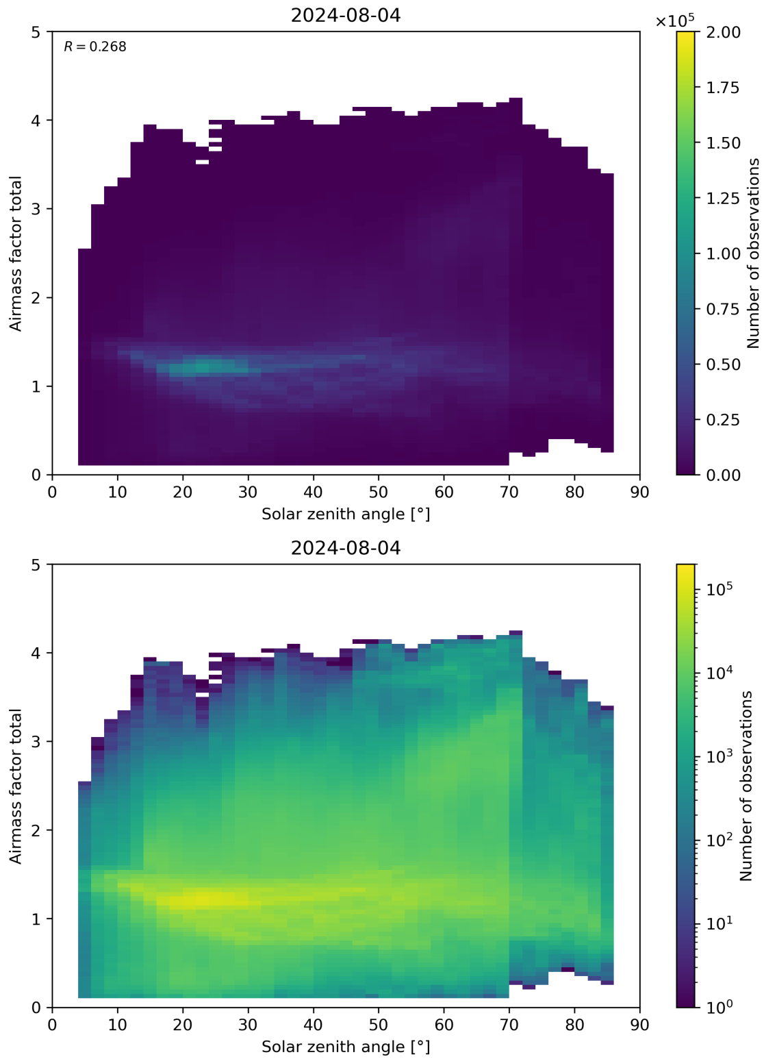
Figure 175: Scatter density plot of “Solar zenith angle” against “Airmass factor total” for 2024-08-03 to 2024-08-05.
