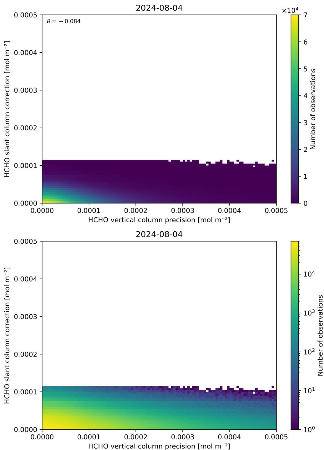
Figure 141: Scatter density plot of “HCHO vertical column precision” against “HCHO slant column correction” for 2024-08-03 to 2024-08-05.
