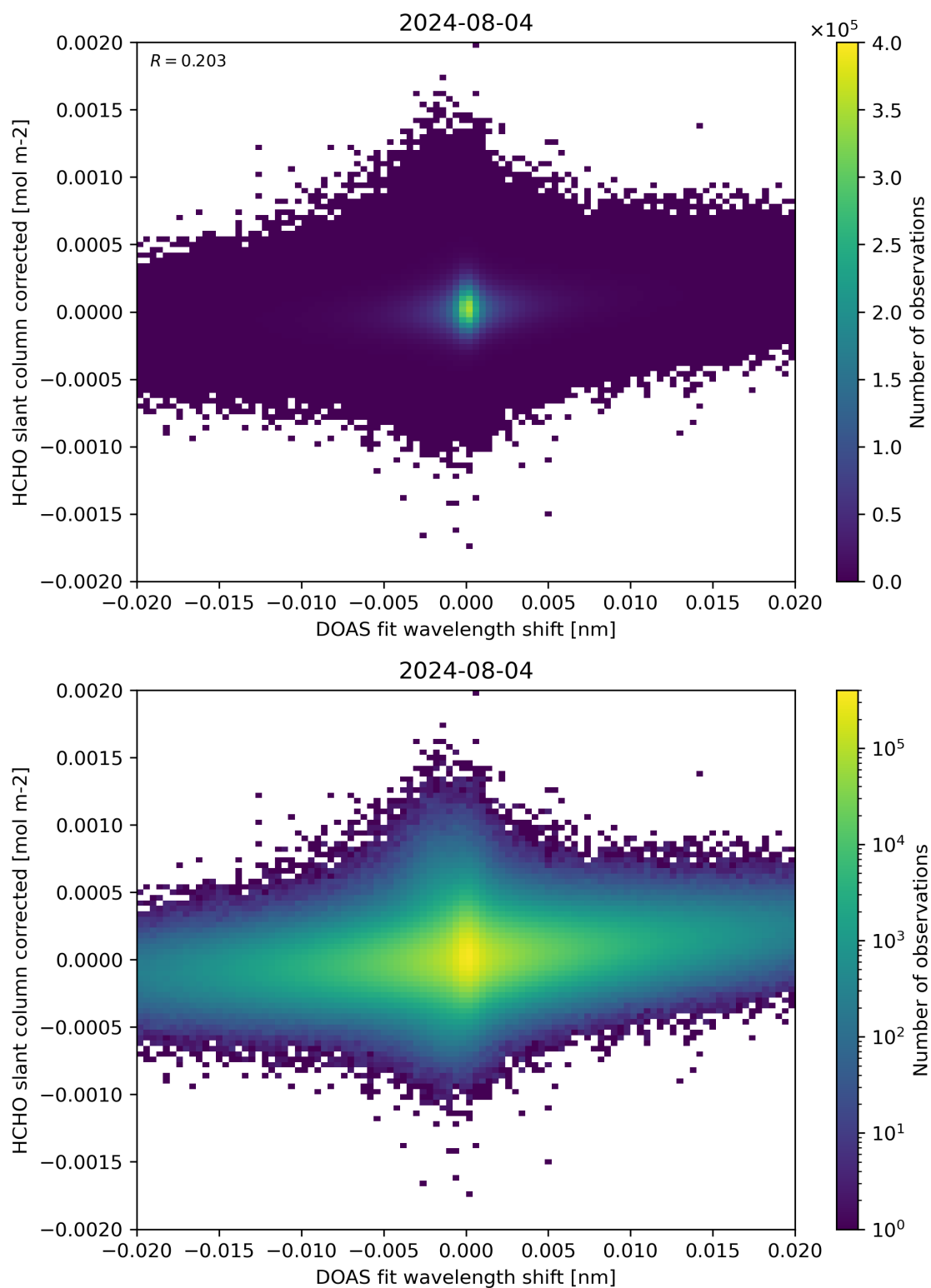
Figure 66: Scatter density plot of “DOAS fit wavelength shift” against “HCHO slant column corrected” for 2024-08-03 to 2024-08-05.
