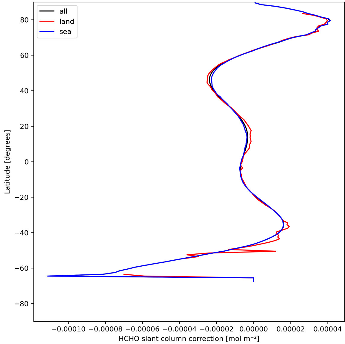
Figure 33: Zonal average of “HCHO slant column correction” for 2024-08-03 to 2024-08-05.
