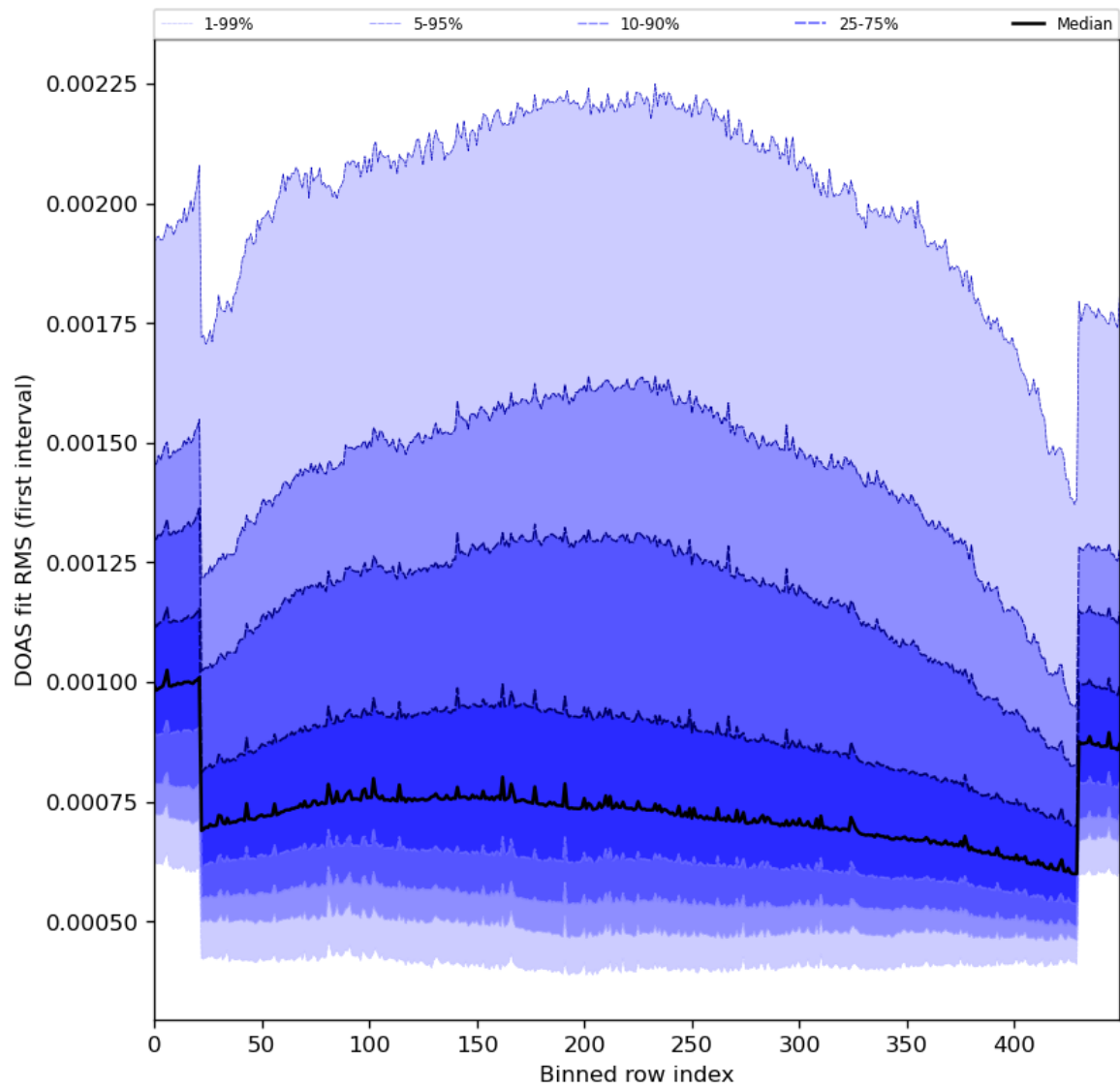
Figure 60: Along track statistics of “DOAS fit RMS (first interval)” for 2024-08-03 to 2024-08-05
