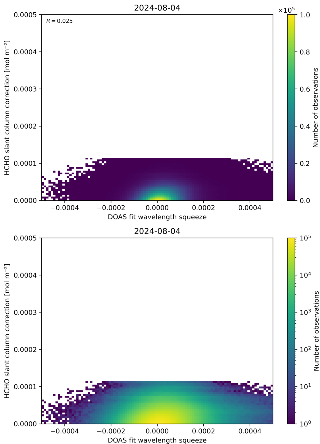
Figure 70: Scatter density plot of “DOAS fit wavelength squeeze” against “HCHO slant column correction” for 2024-08-03 to 2024-08-05.
