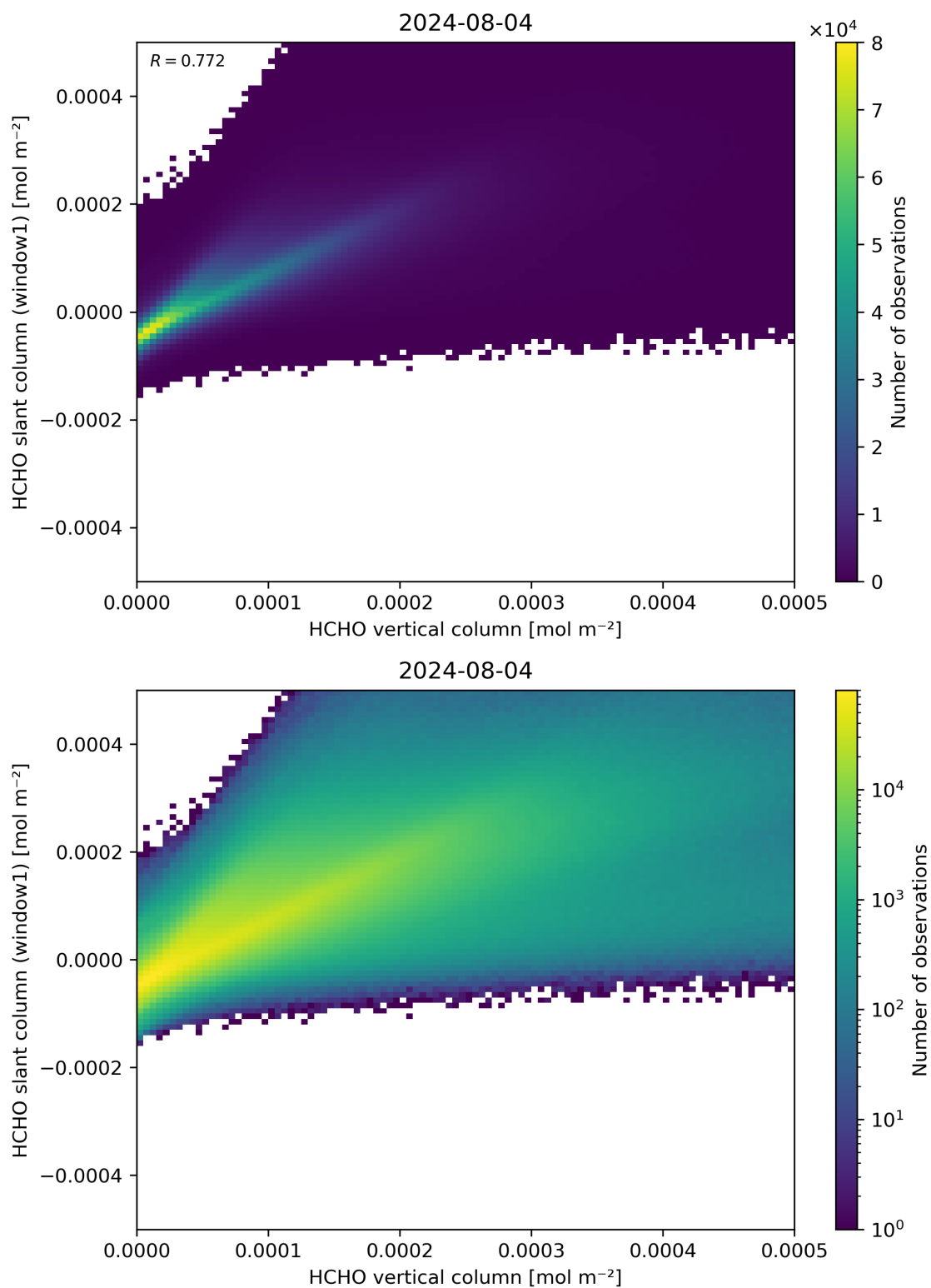
Figure 129: Scatter density plot of “HCHO vertical column” against “HCHO slant column (window1)” for 2024-08-03 to 2024-08-05.
