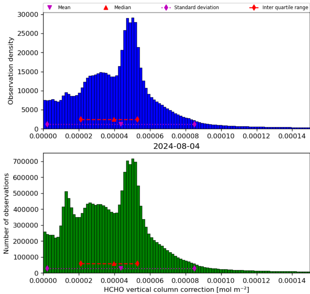
Figure 37: Histogram of “HCHO vertical column correction” for 2024-08-03 to 2024-08-05
