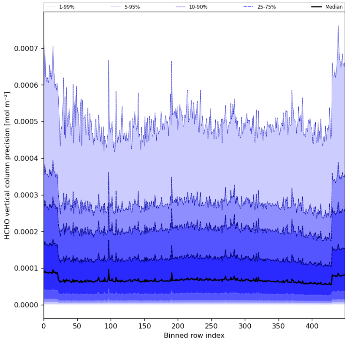
Figure 50: Along track statistics of “HCHO vertical column precision” for 2024-08-03 to 2024-08-05
