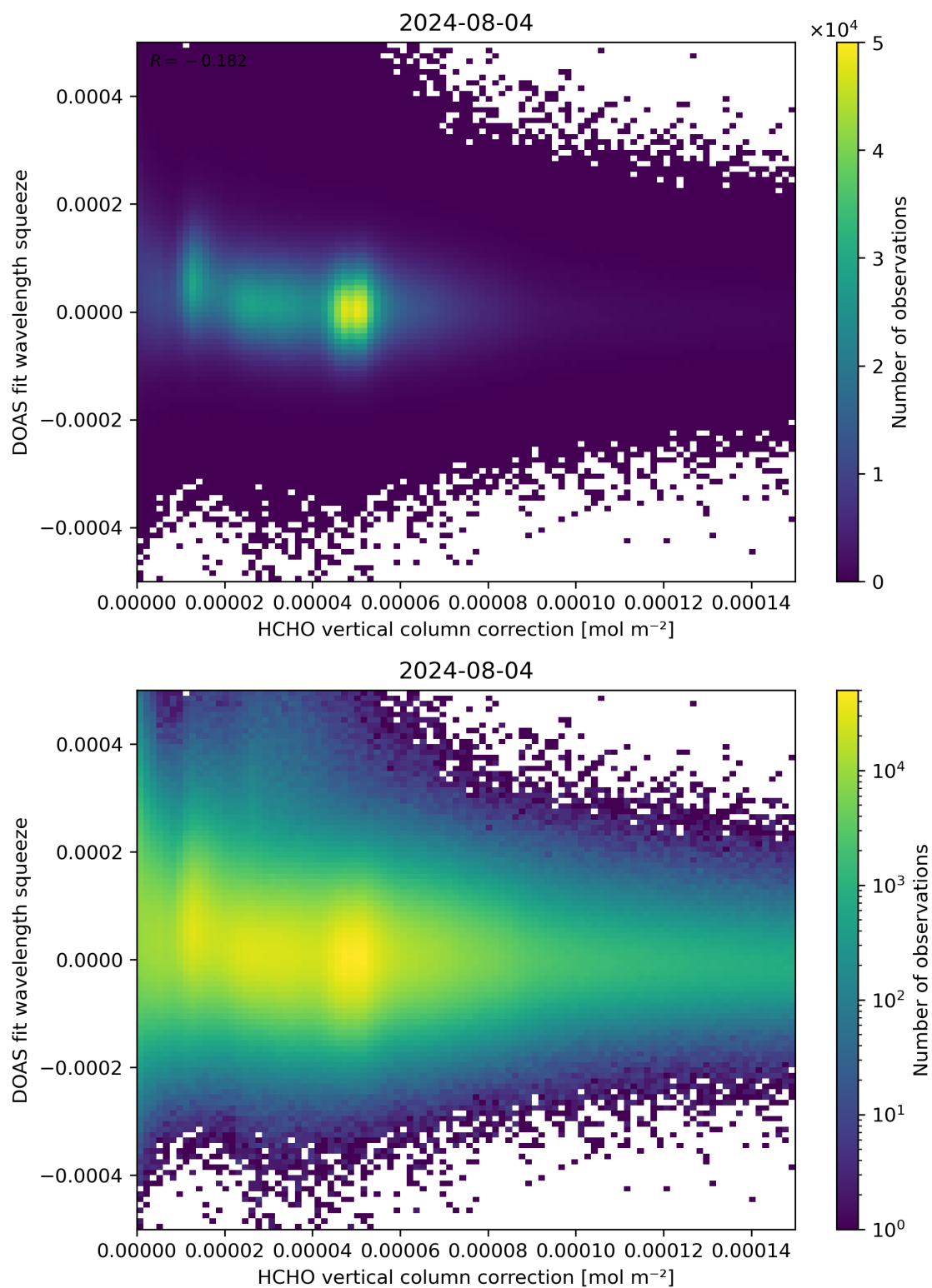
Figure 114: Scatter density plot of “HCHO vertical column correction” against “DOAS fit wavelength squeeze” for 2024-08-03 to 2024-08-05.
