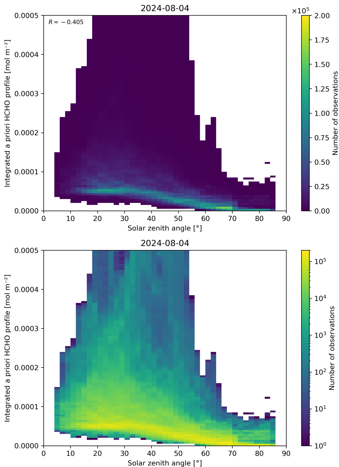
Figure 180: Scatter density plot of “Solar zenith angle” against “Integrated a priori HCHO profile” for 2024-08-03 to 2024-08-05.
