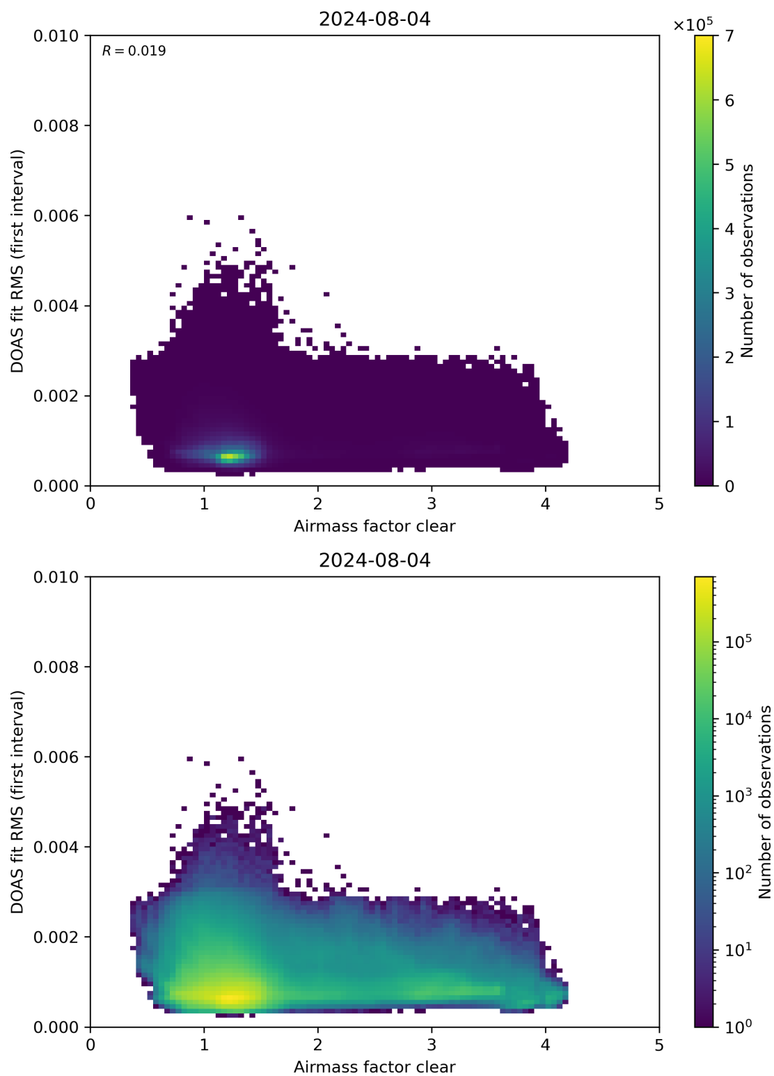
Figure 71: Scatter density plot of “Airmass factor clear” against “DOAS fit RMS (first interval)” for 2024-08-03 to 2024-08-05.
