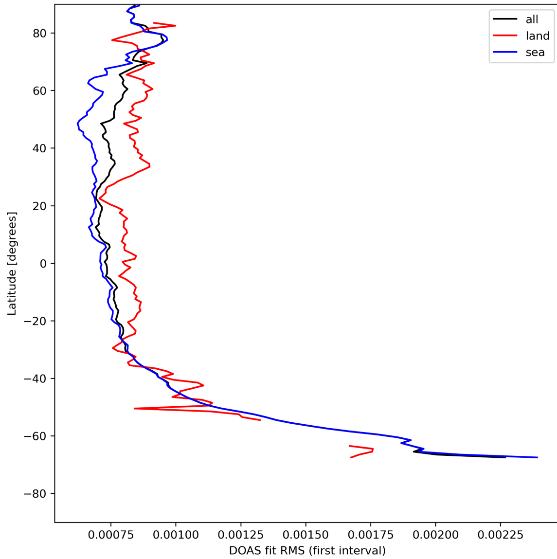
Figure 32: Zonal average of "DOAS fit RMS (first interval)" for 2024-08-03 to 2024-08-05.
