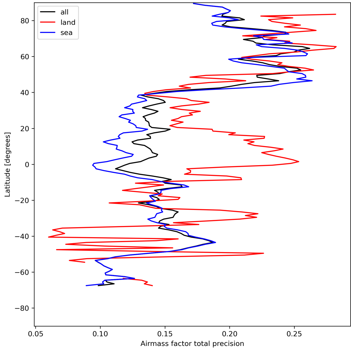
Figure 27: Zonal average of “Airmass factor total precision” for 2024-08-03 to 2024-08-05.
