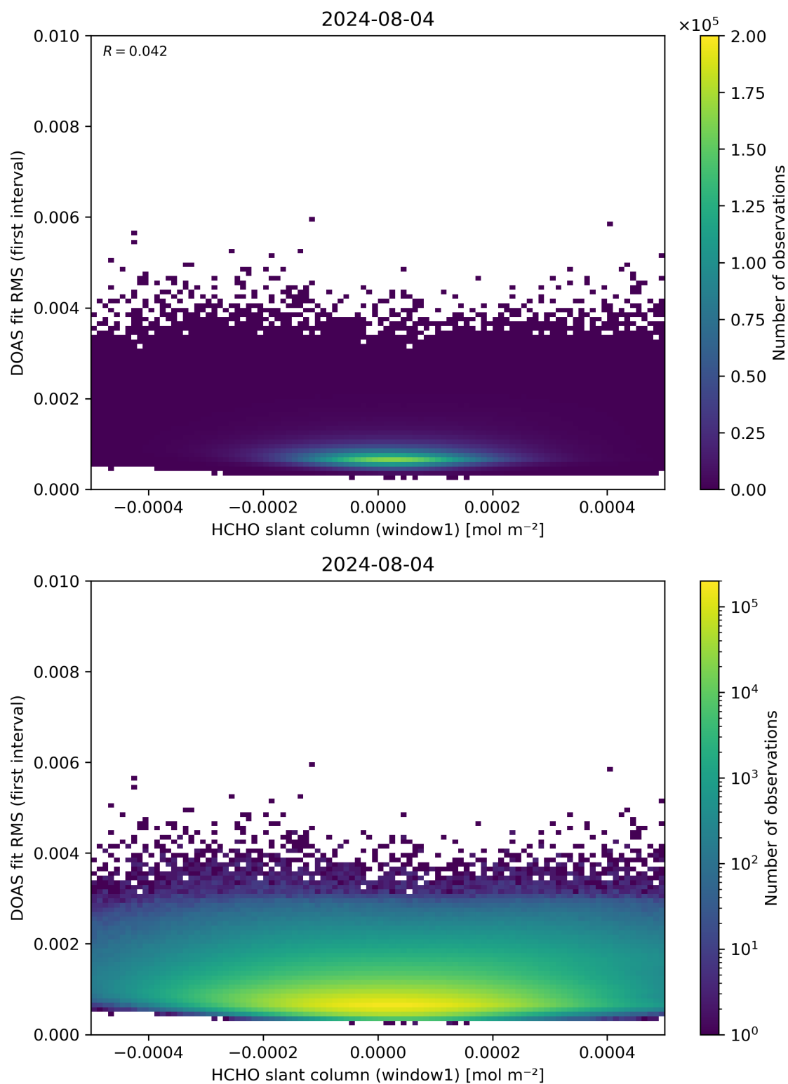
Figure 78: Scatter density plot of “HCHO slant column (window1)” against “DOAS fit RMS (first interval)” for 2024-08-03 to 2024-08-05.
