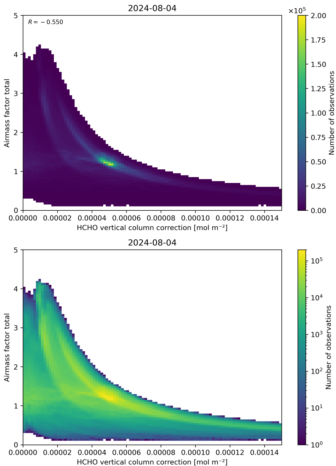
Figure 120: Scatter density plot of “HCHO vertical column correction” against “Airmass factor total” for 2024-08-03 to 2024-08-05.
