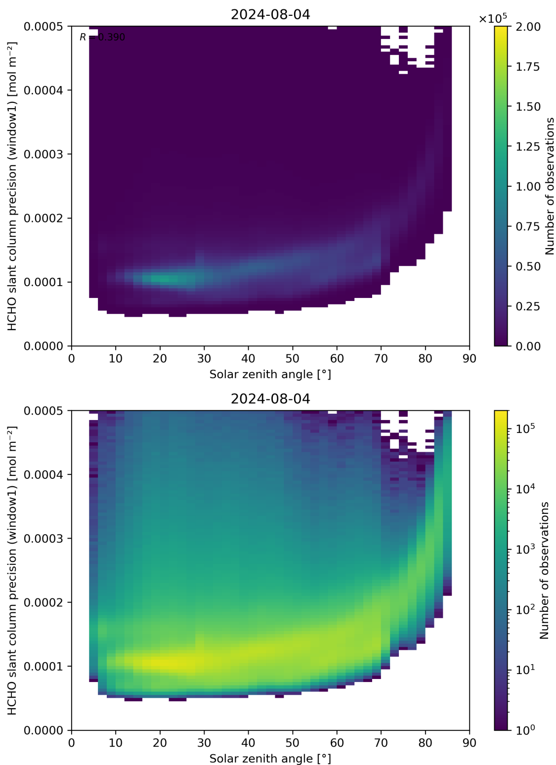
Figure 174: Scatter density plot of “Solar zenith angle” against “HCHO slant column precision (window1)” for 2024-08-03 to 2024-08-05.
