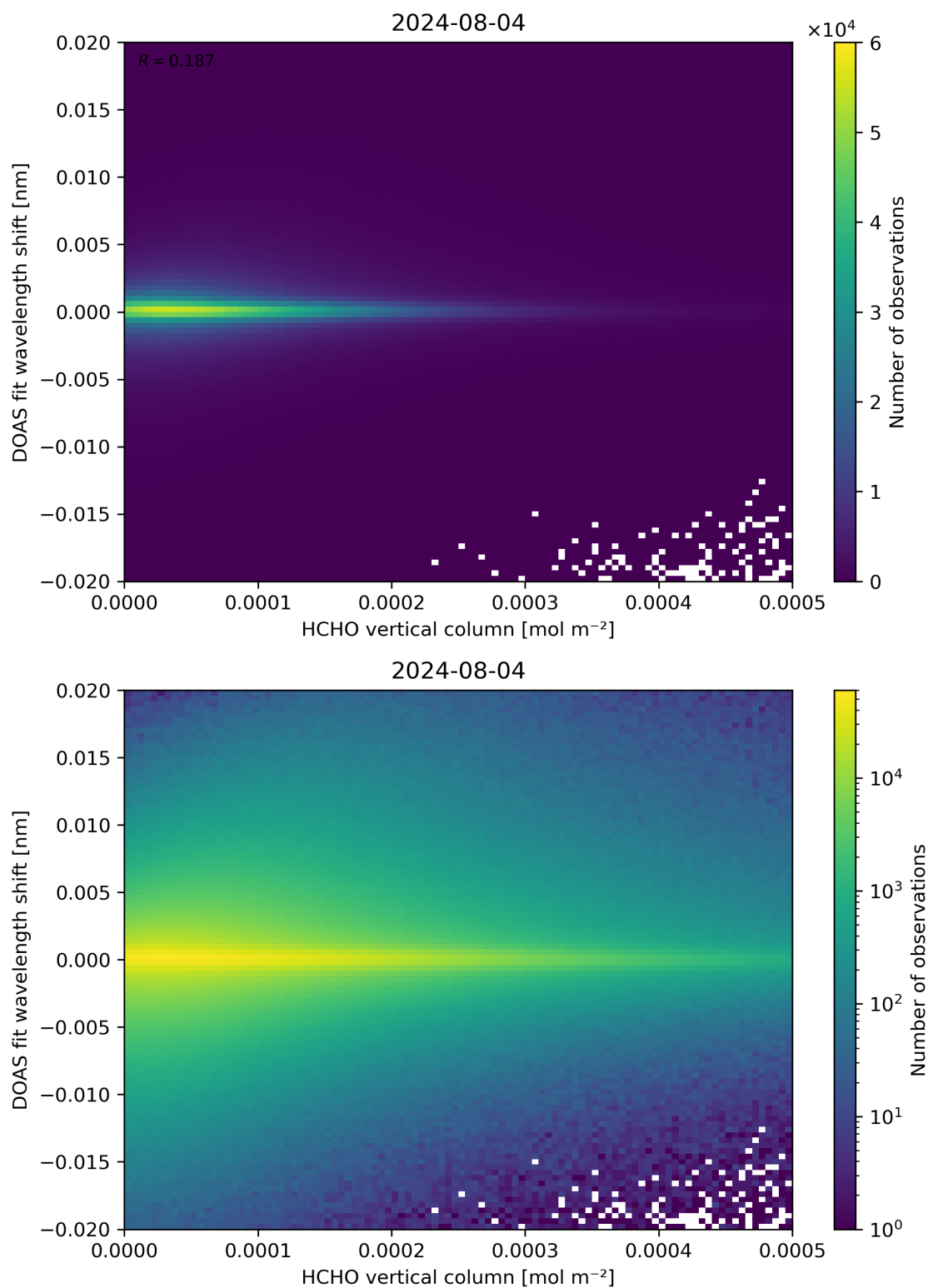
Figure 124: Scatter density plot of “HCHO vertical column” against “DOAS fit wavelength shift” for 2024-08-03 to 2024-08-05.
