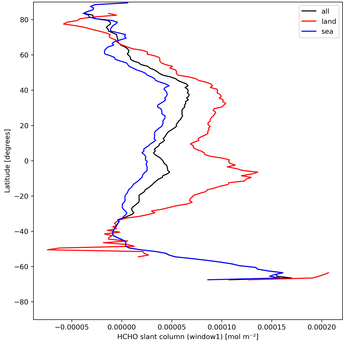
Figure 24: Zonal average of “HCHO slant column (window1)” for 2024-08-03 to 2024-08-05.
