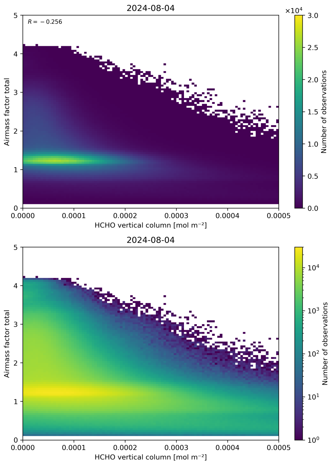
Figure 131: Scatter density plot of “HCHO vertical column” against “Airmass factor total” for 2024-08-03 to 2024-08-05.
