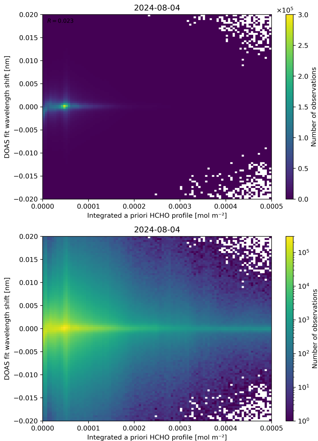
Figure 149: Scatter density plot of “Integrated a priori HCHO profile” against “DOAS fit wavelength shift” for 2024-08-03 to 2024-08-05.
