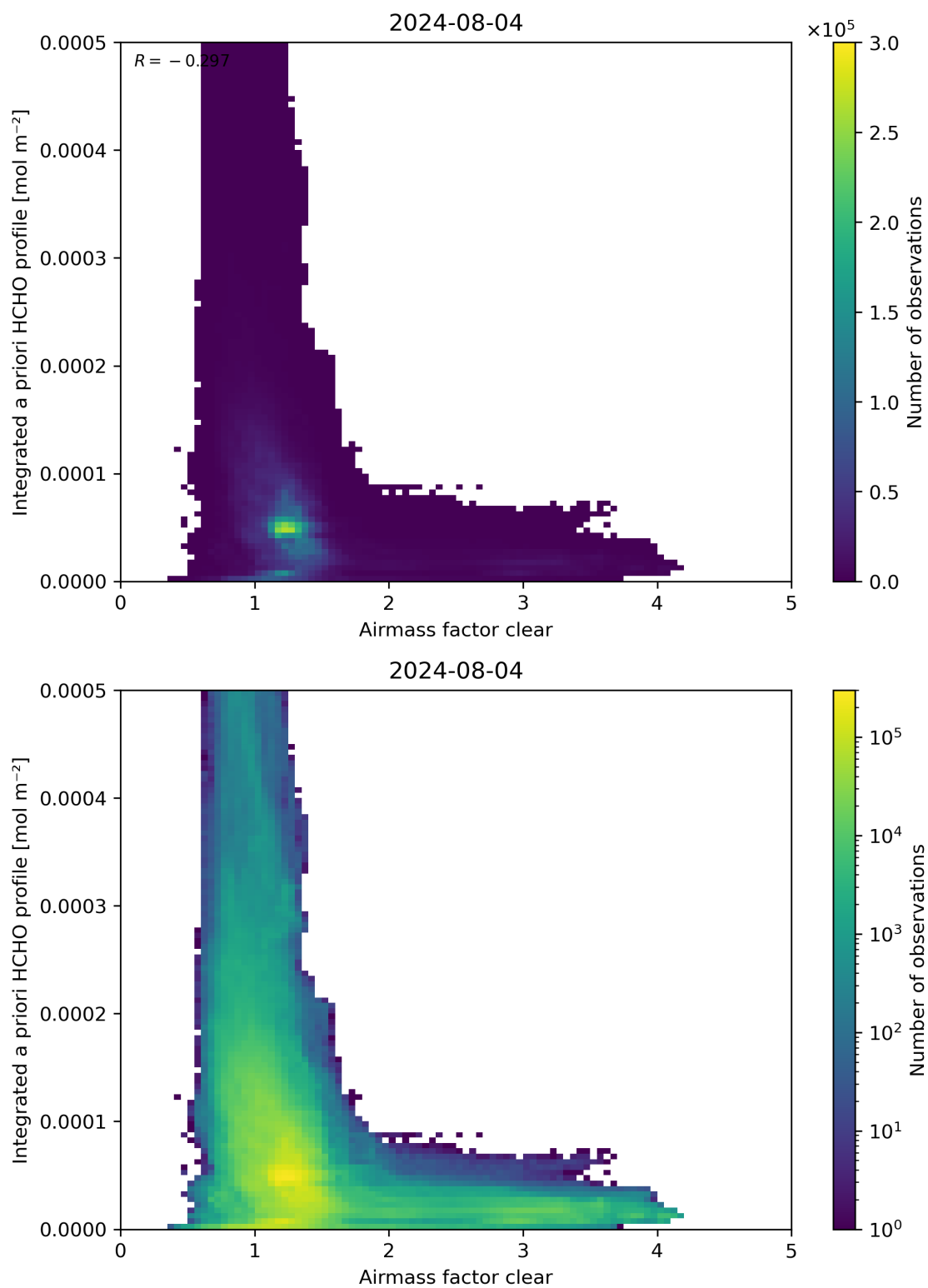
Figure 76: Scatter density plot of “Airmass factor clear” against “Integrated a priori HCHO profile” for 2024-08-03 to 2024-08-05.
