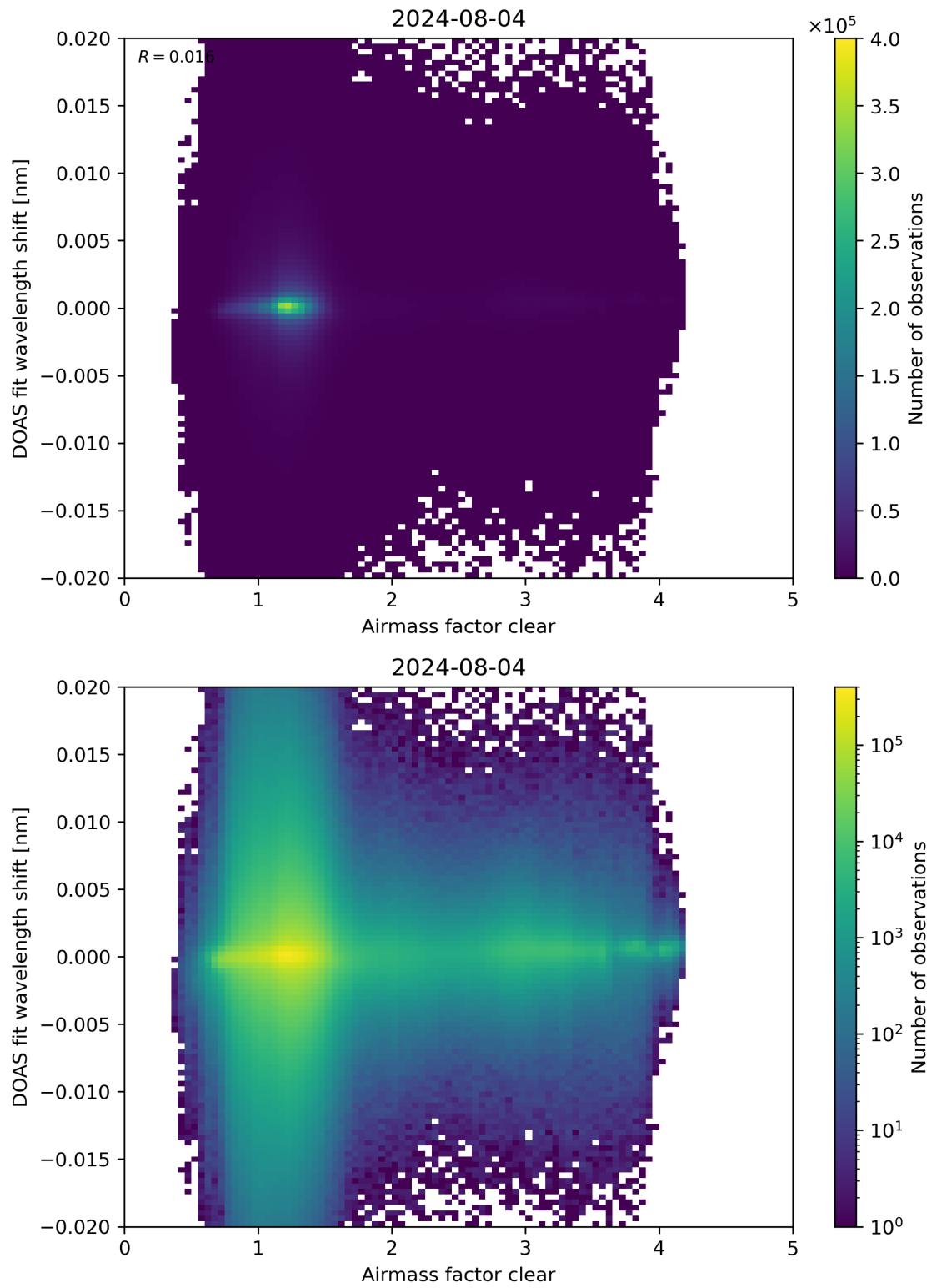
Figure 72: Scatter density plot of “Airmass factor clear” against “DOAS fit wavelength shift” for 2024-08-03 to 2024-08-05.
