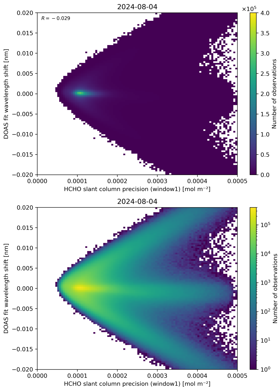
Figure 89: Scatter density plot of “HCHO slant column precision (window1)” against “DOAS fit wavelength shift” for 2024-08-03 to 2024-08-05.
