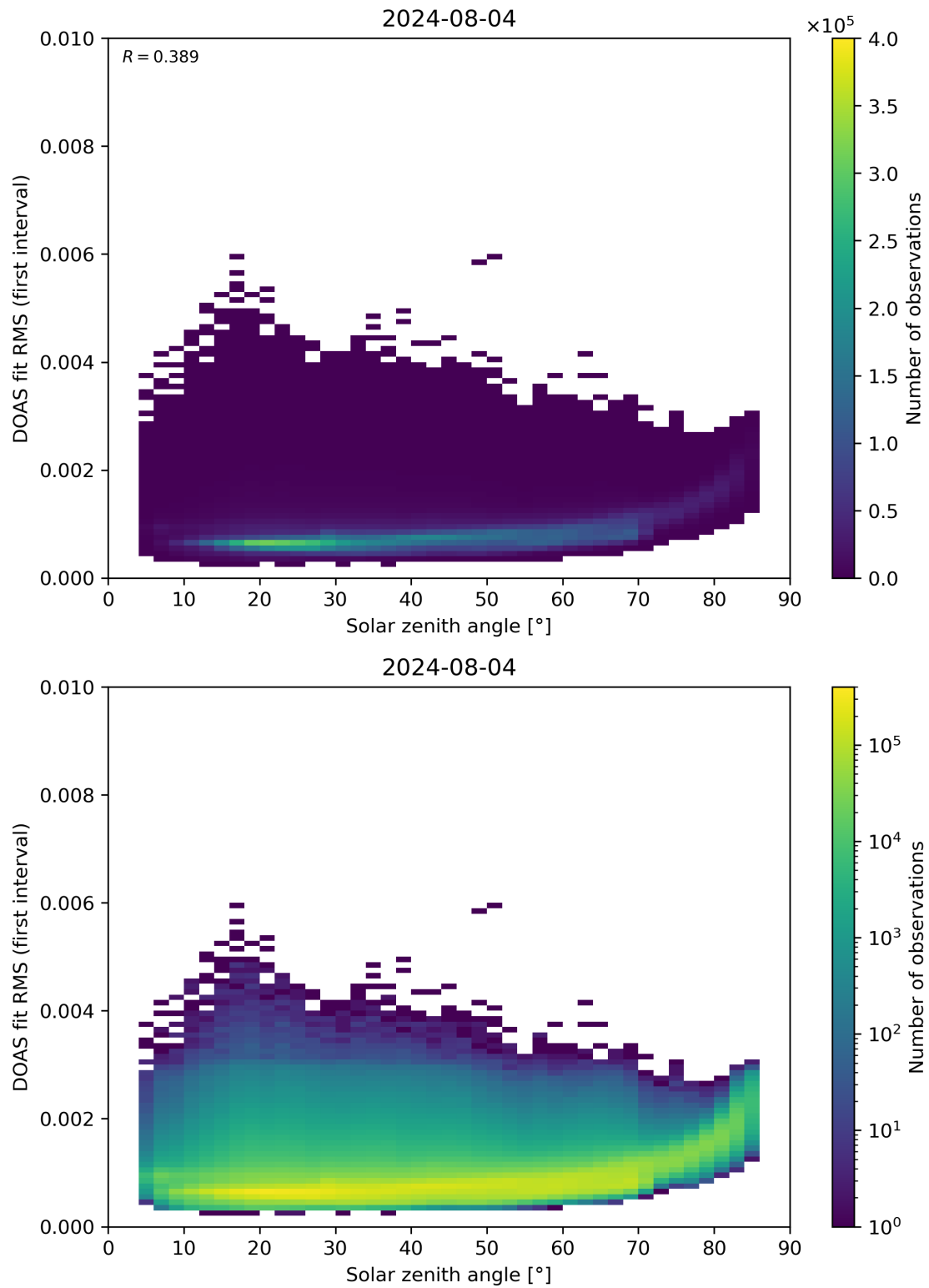
Figure 167: Scatter density plot of “Solar zenith angle” against “DOAS fit RMS (first interval)” for 2024-08-03 to 2024-08-05.
