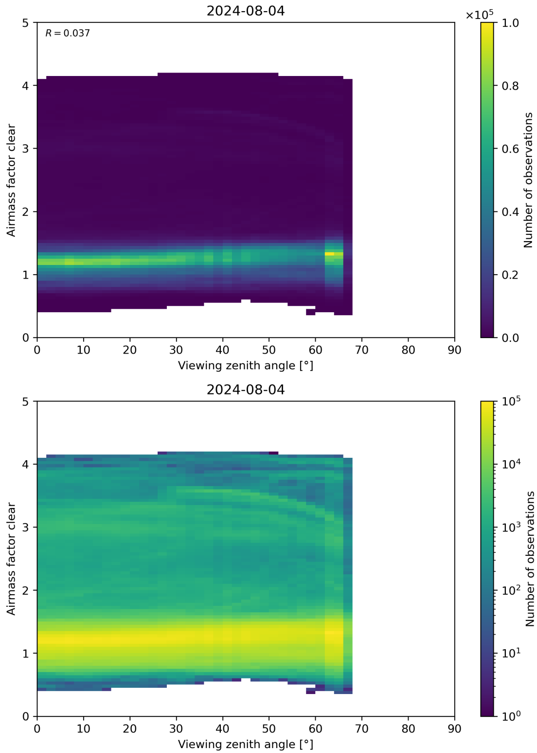
Figure 185: Scatter density plot of “Viewing zenith angle” against “Airmass factor clear” for 2024-08-03 to 2024-08-05.
