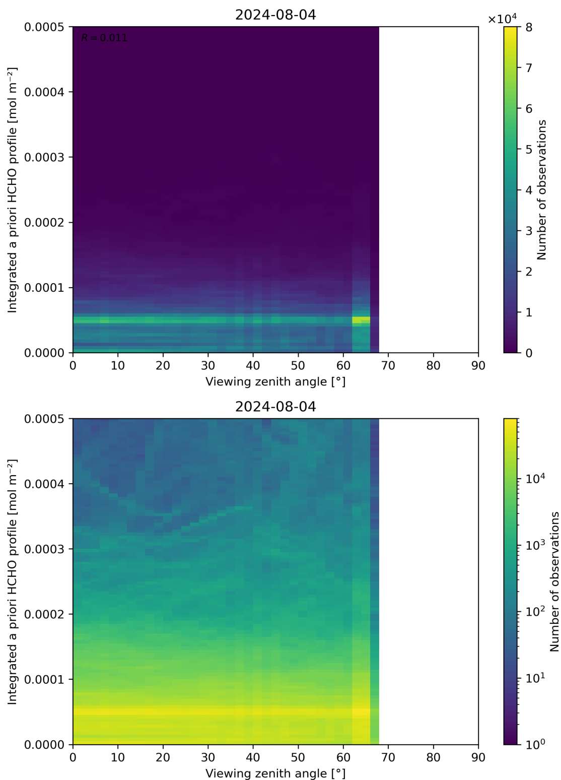
Figure 195: Scatter density plot of “Viewing zenith angle” against “Integrated a priori HCHO profile” for 2024-08-03 to 2024-08-05.
