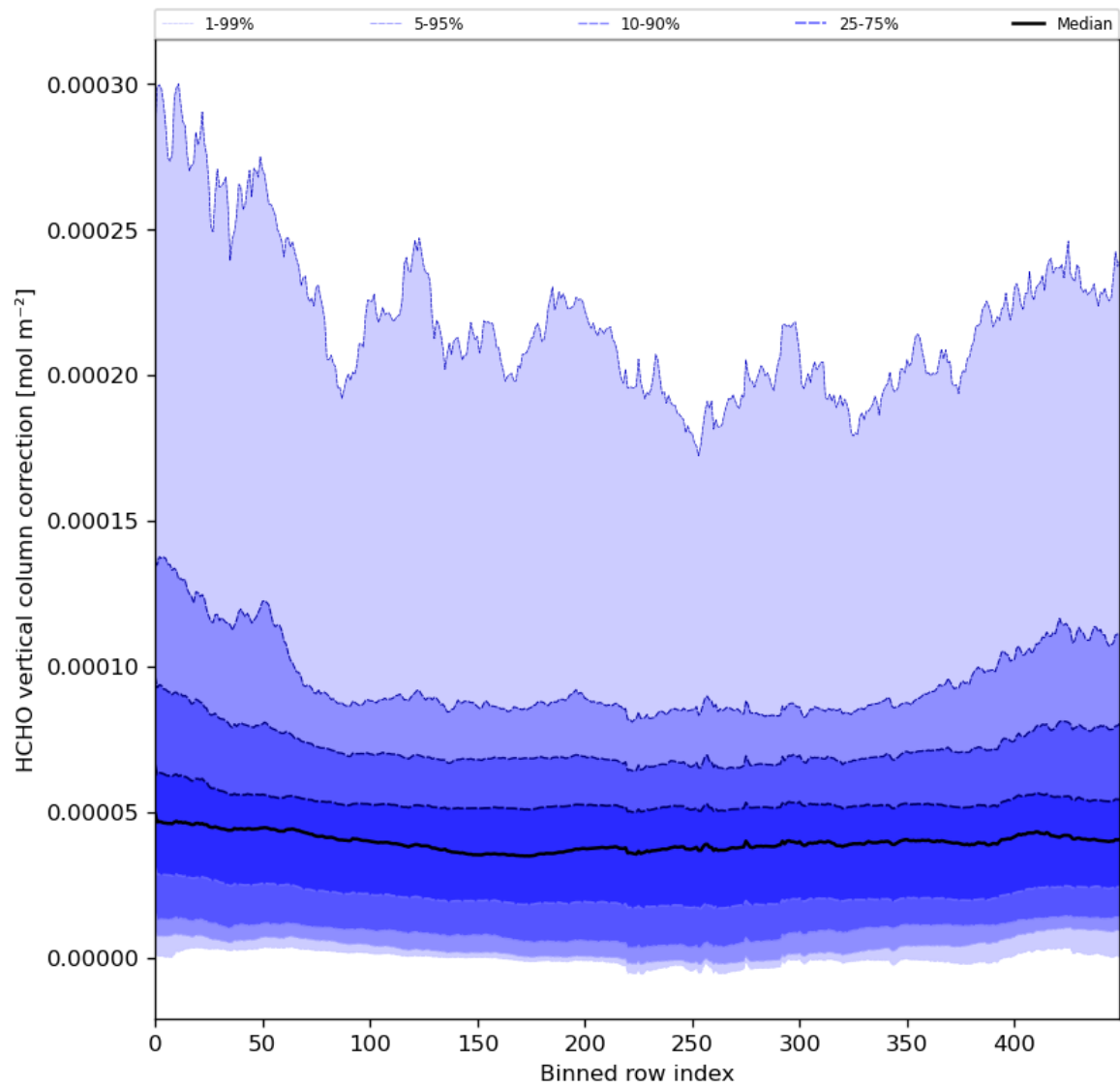
Figure 51: Along track statistics of “HCHO vertical column correction” for 2024-08-03 to 2024-08-05
