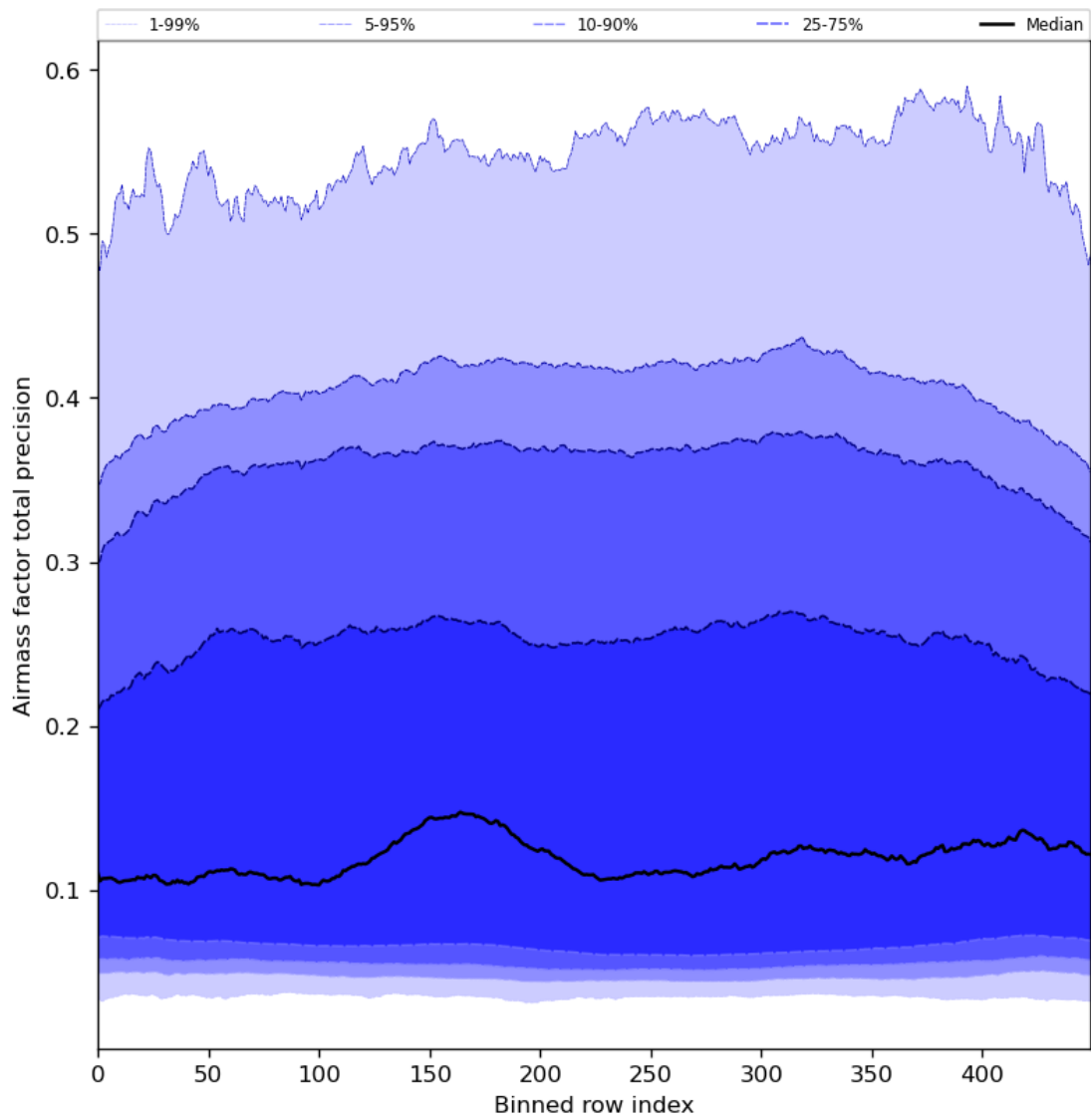
Figure 55: Along track statistics of “Airmass factor total precision” for 2024-08-03 to 2024-08-05
