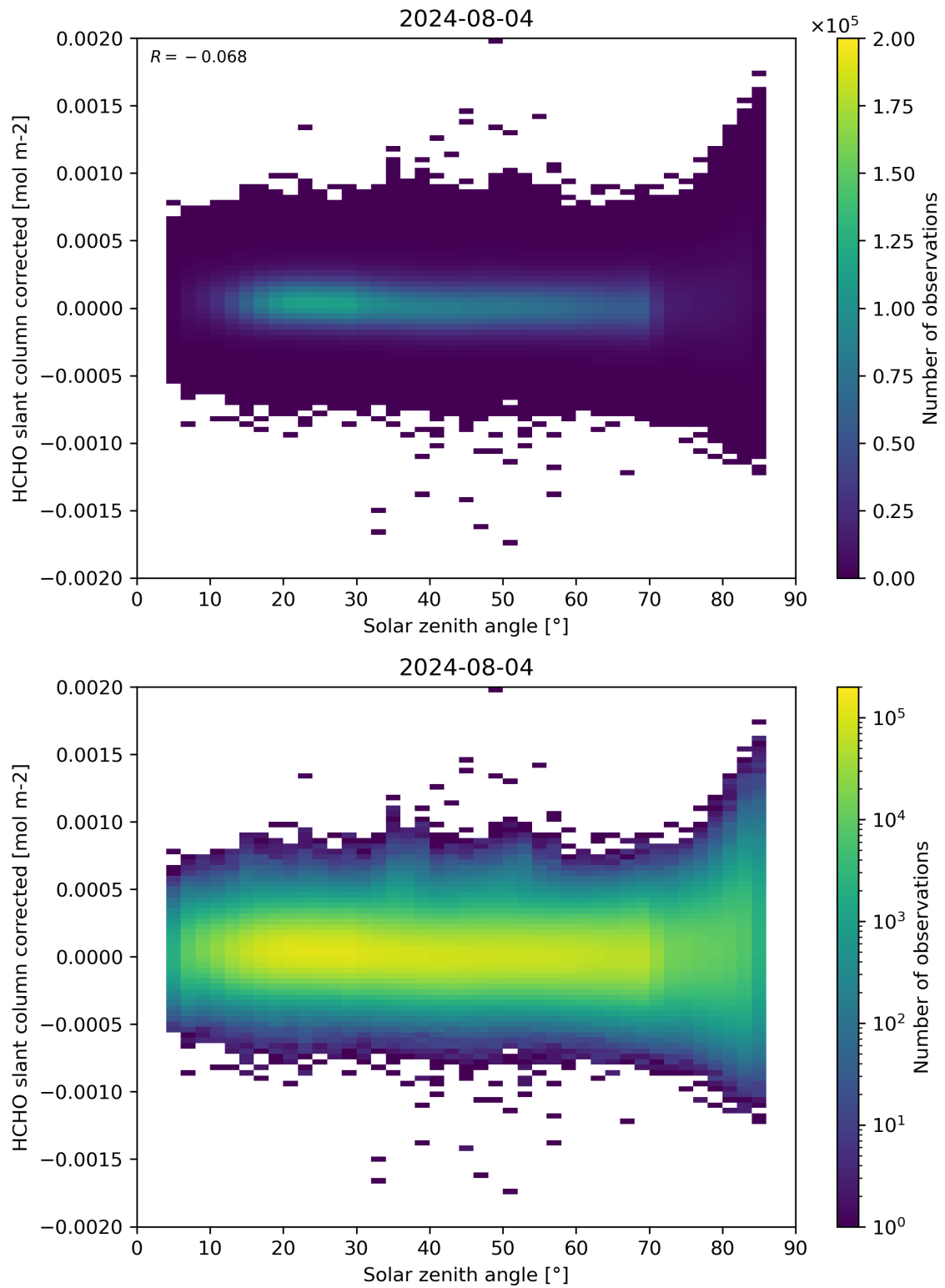
Figure 171: Scatter density plot of “Solar zenith angle” against “HCHO slant column corrected” for 2024-08-03 to 2024-08-05.
