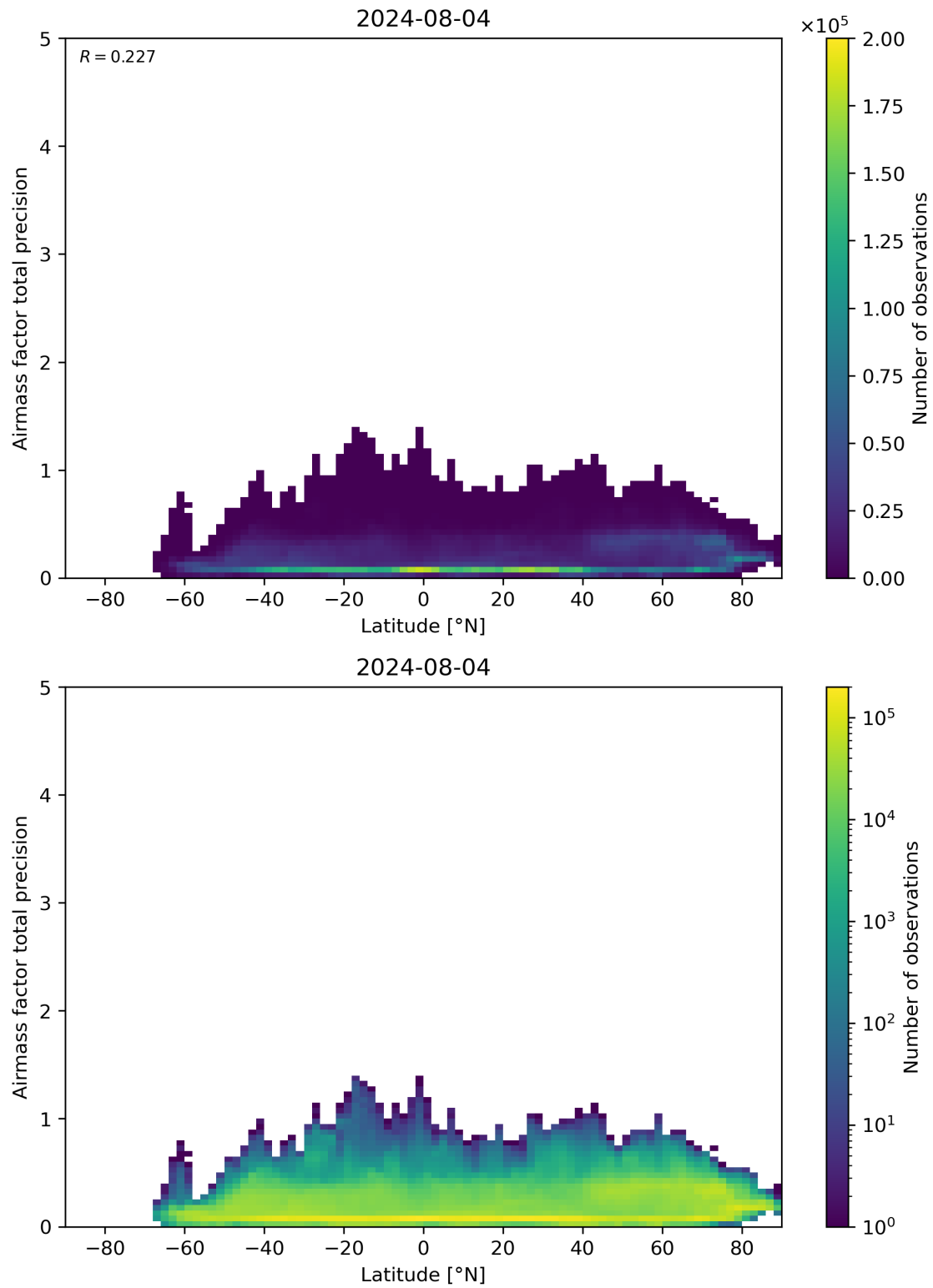
Figure 162: Scatter density plot of “Latitude” against “Airmass factor total precision” for 2024-08-03 to 2024-08-05.
