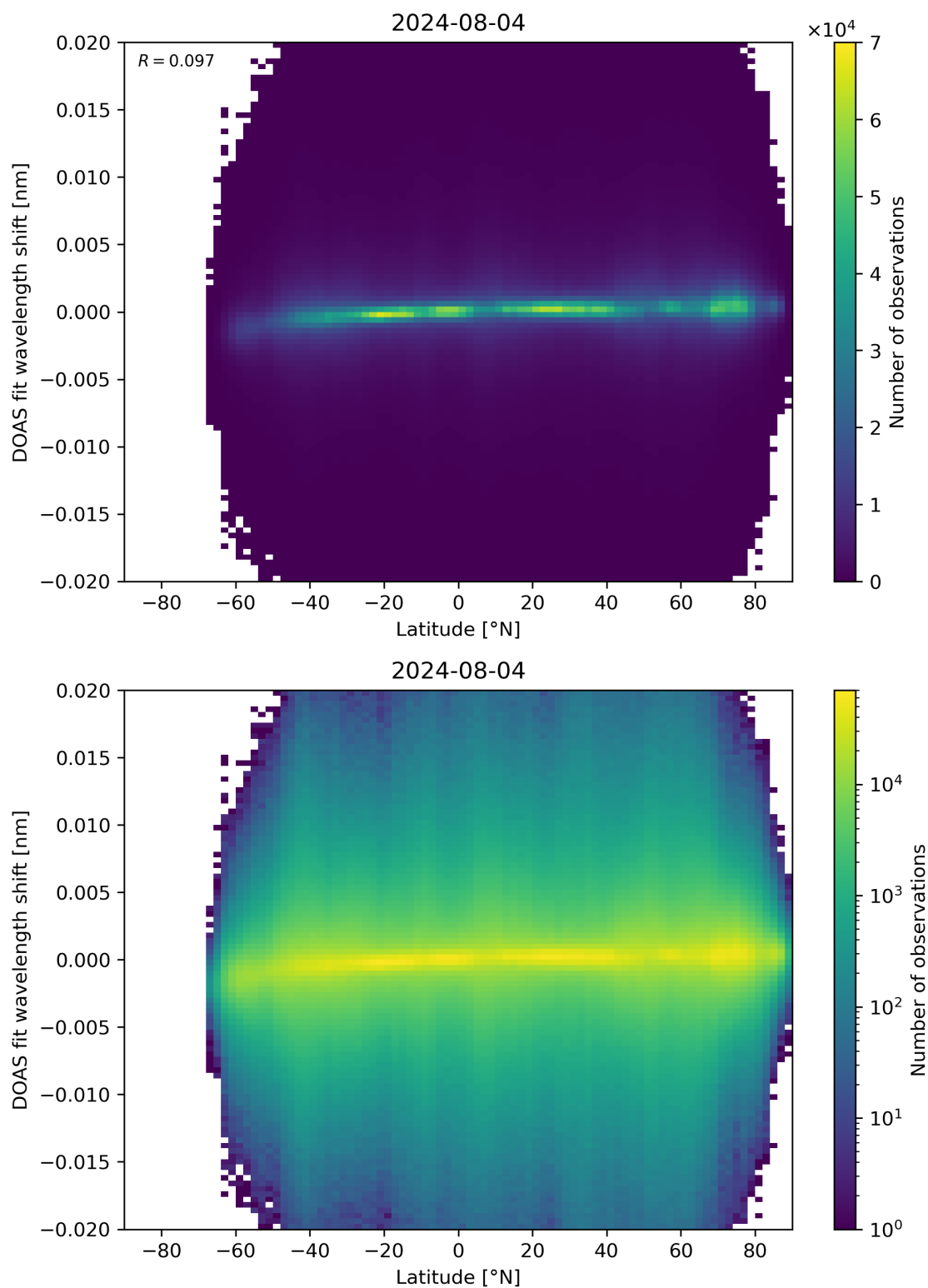
Figure 154: Scatter density plot of “Latitude” against “DOAS fit wavelength shift” for 2024-08-03 to 2024-08-05.
