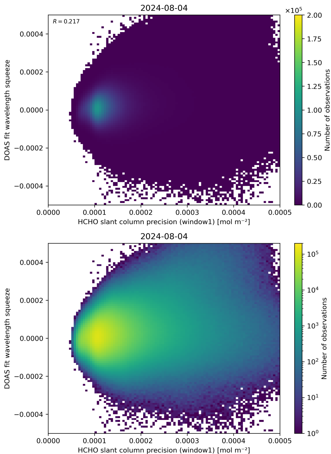
Figure 90: Scatter density plot of “HCHO slant column precision (window1)” against “DOAS fit wavelength squeeze” for 2024-08-03 to 2024-08-05.
