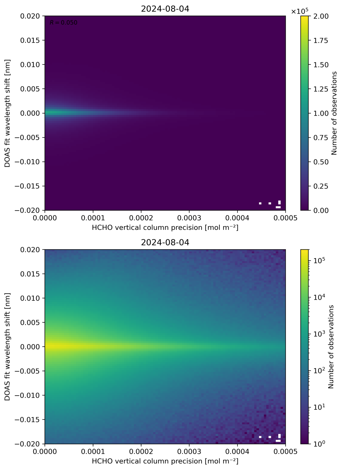
Figure 137: Scatter density plot of “HCHO vertical column precision” against “DOAS fit wavelength shift” for 2024-08-03 to 2024-08-05.
