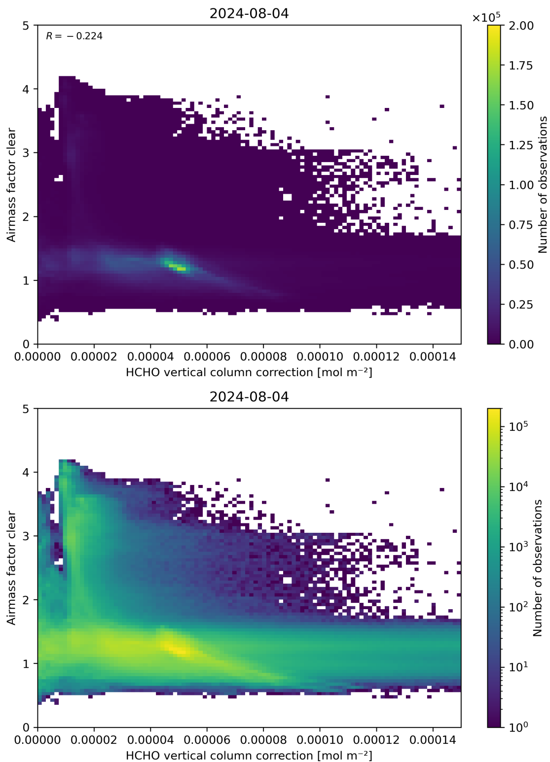
Figure 115: Scatter density plot of “HCHO vertical column correction” against “Airmass factor clear” for 2024-08-03 to 2024-08-05.
