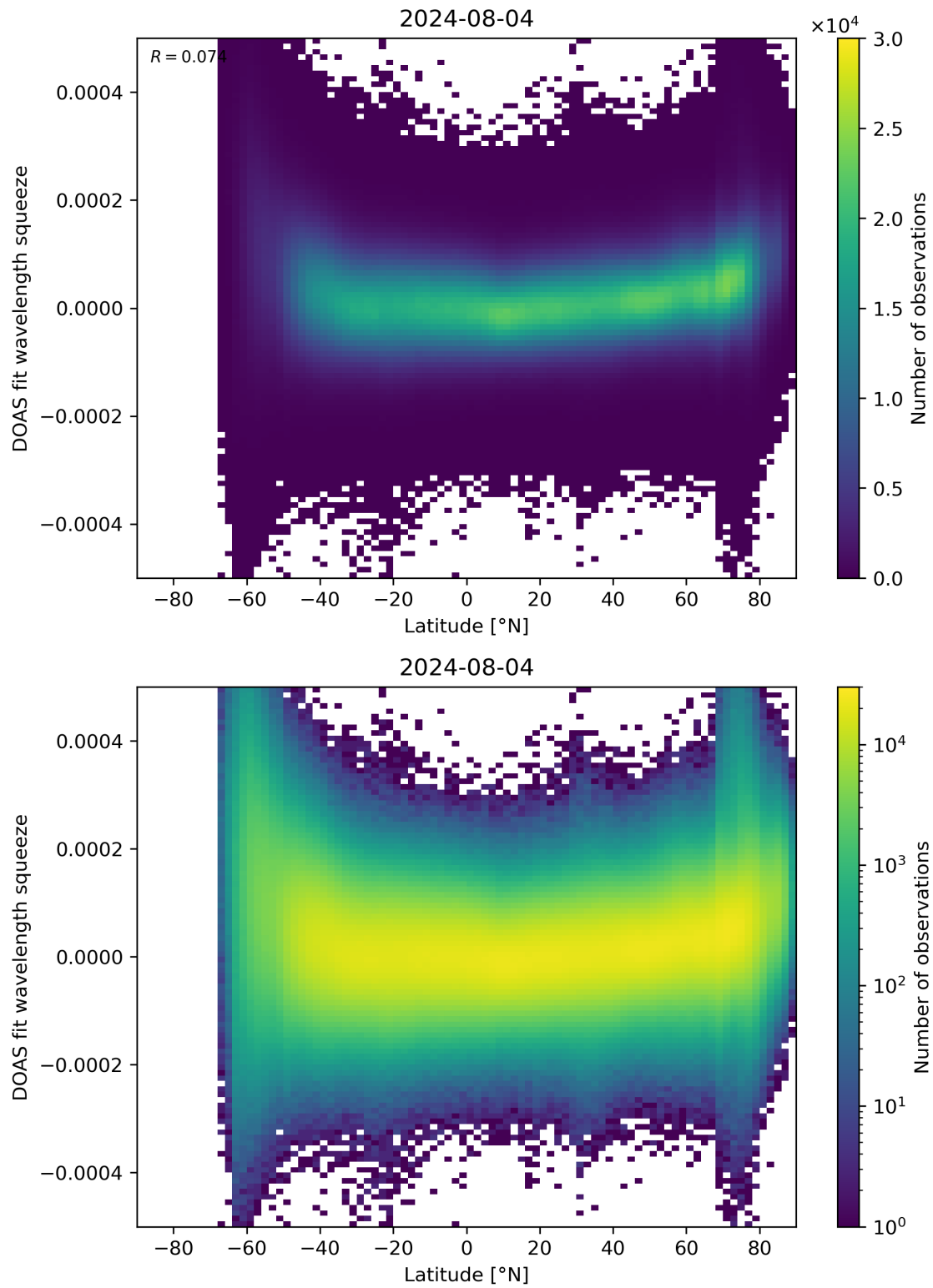
Figure 155: Scatter density plot of “Latitude” against “DOAS fit wavelength squeeze” for 2024-08-03 to 2024-08-05.
