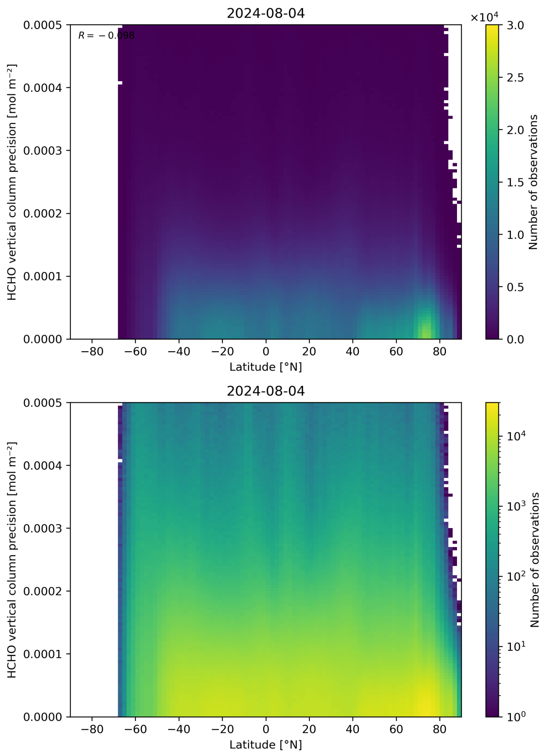
Figure 165: Scatter density plot of “Latitude” against “HCHO vertical column precision” for 2024-08-03 to 2024-08-05.
