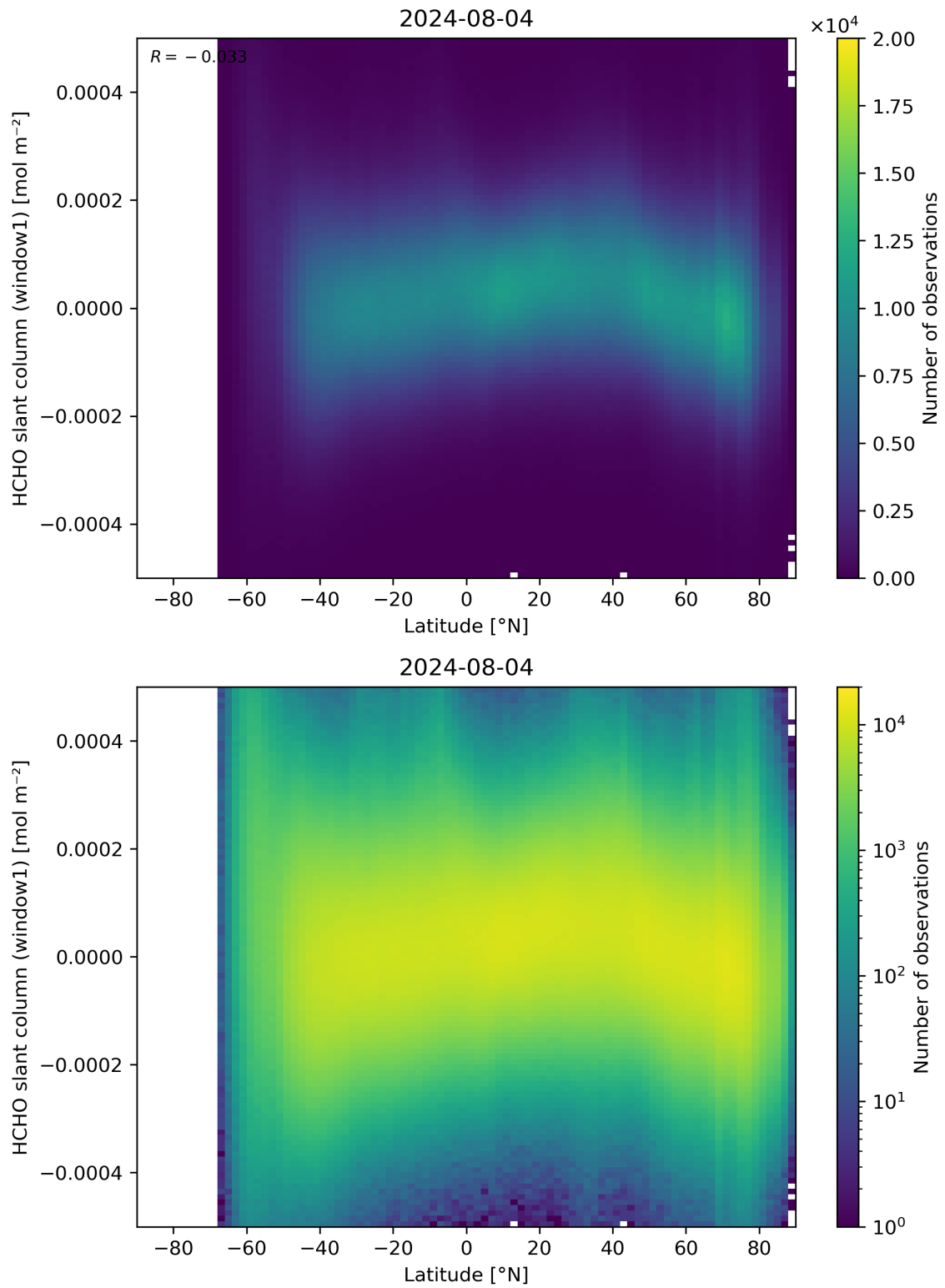
Figure 159: Scatter density plot of “Latitude” against “HCHO slant column (window1)” for 2024-08-03 to 2024-08-05.
