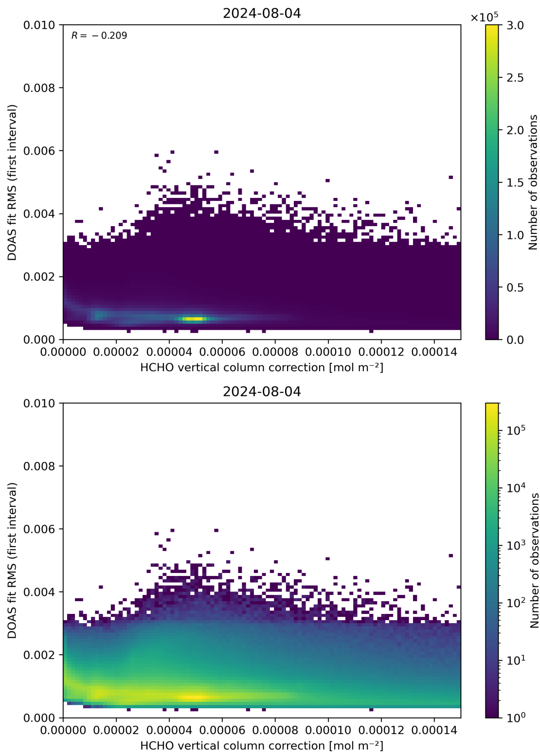
Figure 112: Scatter density plot of “HCHO vertical column correction” against “DOAS fit RMS (first interval)” for 2024-08-03 to 2024-08-05.
