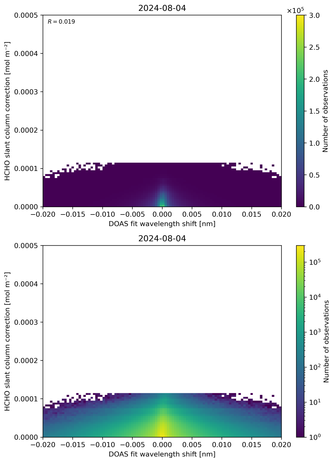
Figure 67: Scatter density plot of “DOAS fit wavelength shift” against “HCHO slant column correction” for 2024-08-03 to 2024-08-05.
