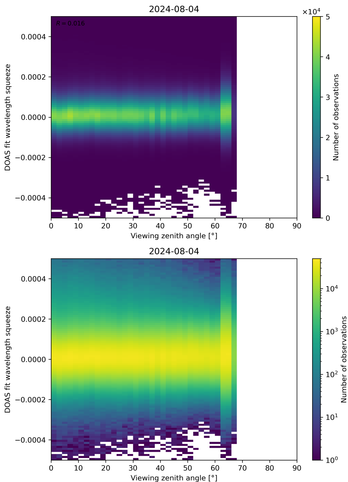
Figure 184: Scatter density plot of “Viewing zenith angle” against “DOAS fit wavelength squeeze” for 2024-08-03 to 2024-08-05.
