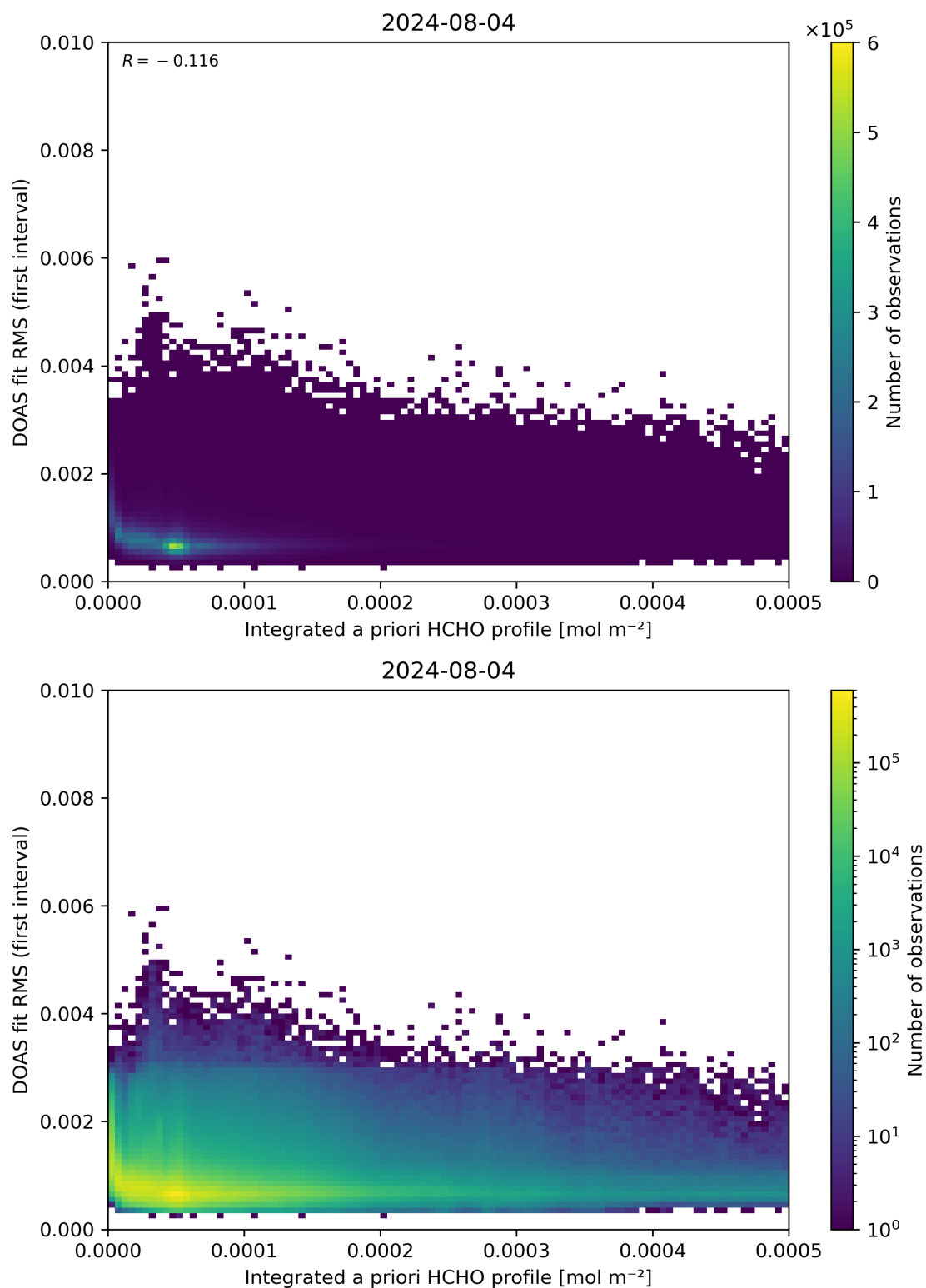
Figure 148: Scatter density plot of “Integrated a priori HCHO profile” against “DOAS fit RMS (first interval)” for 2024-08-03 to 2024-08-05.
