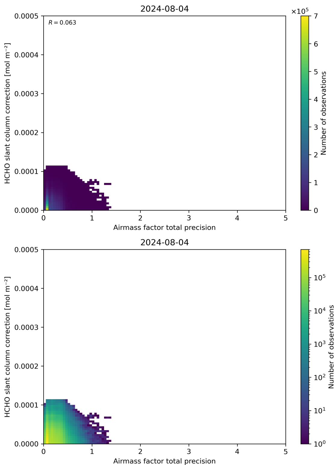
Figure 110: Scatter density plot of “Airmass factor total precision” against “HCHO slant column correction” for 2024-08-03 to 2024-08-05.
