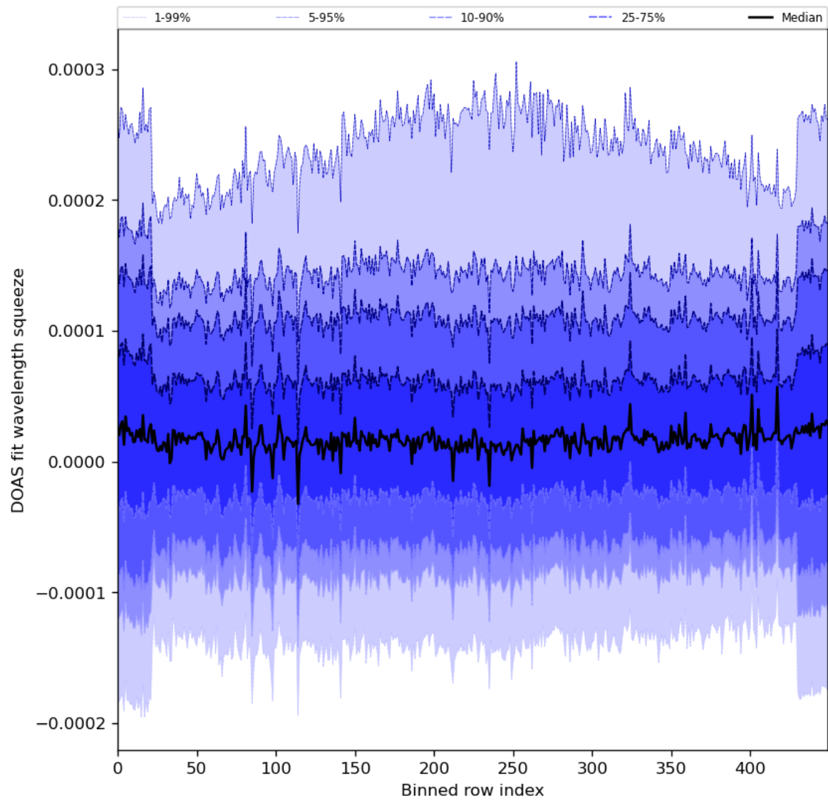
Figure 59: Along track statistics of “DOAS fit wavelength squeeze” for 2024-08-03 to 2024-08-05
