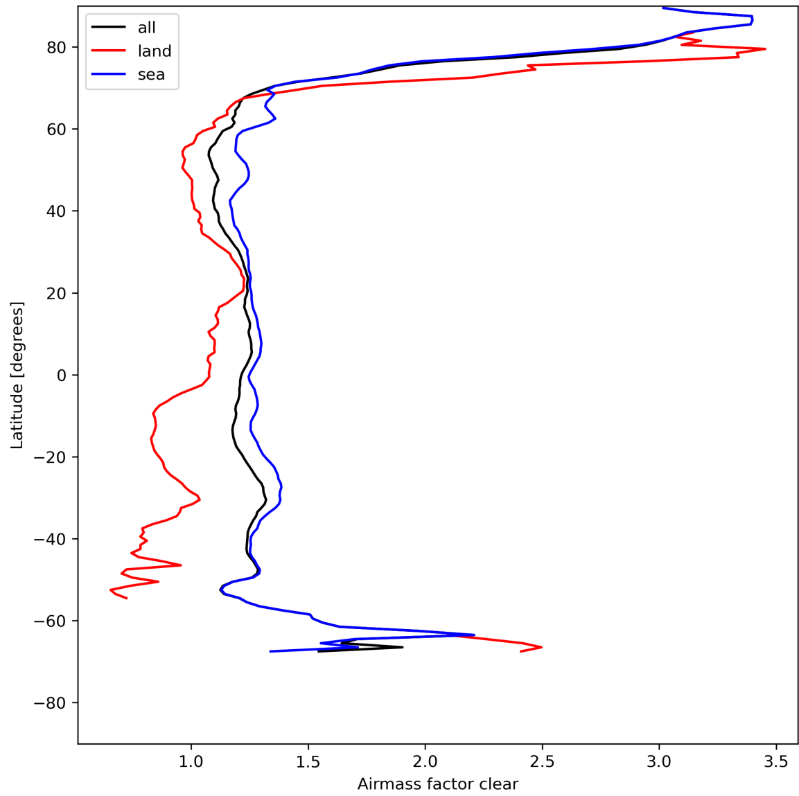
Figure 28: Zonal average of “Airmass factor clear” for 2024-08-03 to 2024-08-05.
