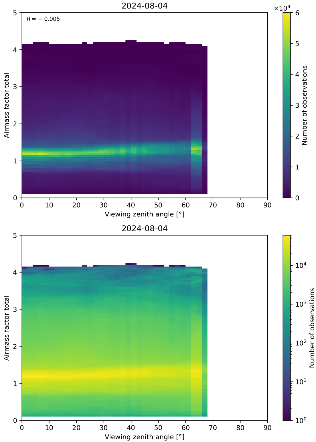
Figure 190: Scatter density plot of “Viewing zenith angle” against “Airmass factor total” for 2024-08-03 to 2024-08-05.
