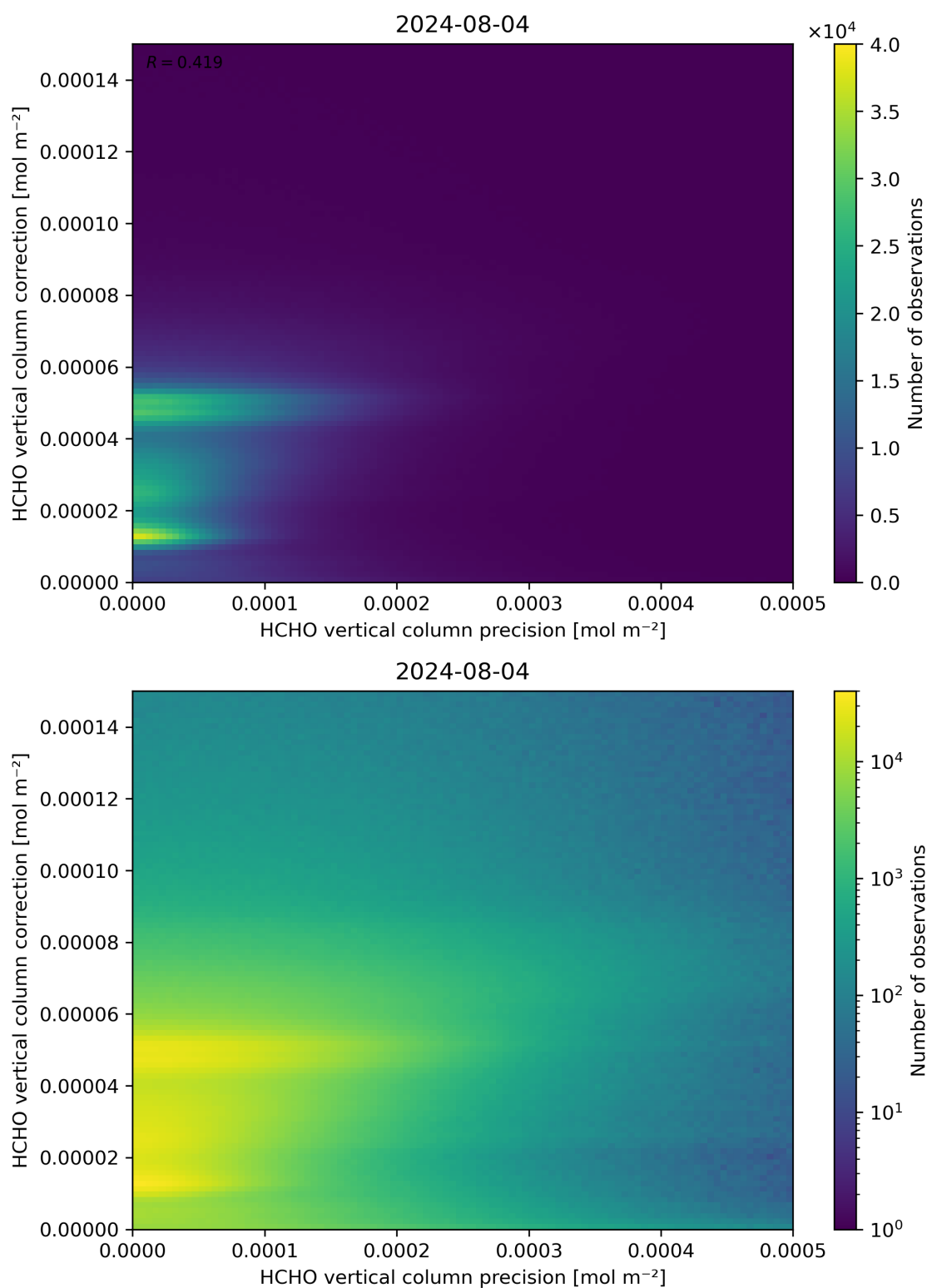
Figure 146: Scatter density plot of “HCHO vertical column precision” against “HCHO vertical column correction” for 2024-08-03 to 2024-08-05.
