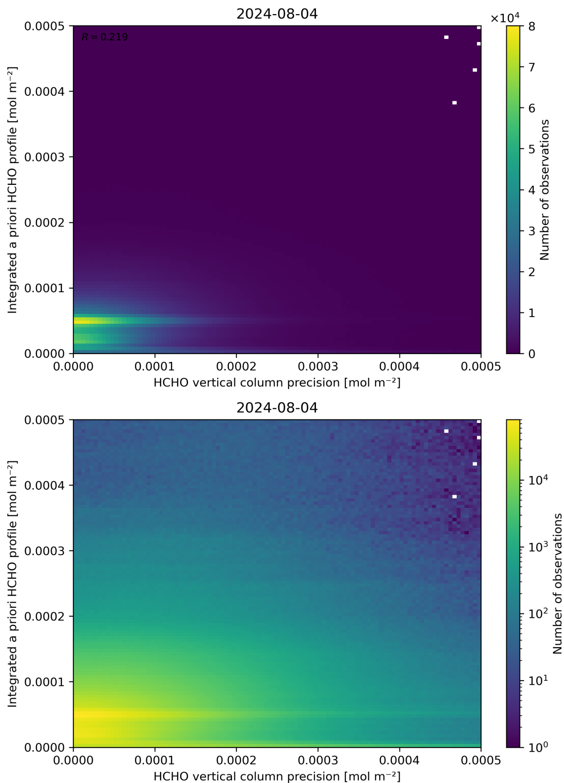
Figure 147: Scatter density plot of “HCHO vertical column precision” against “Integrated a priori HCHO profile” for 2024-08-03 to 2024-08-05.
