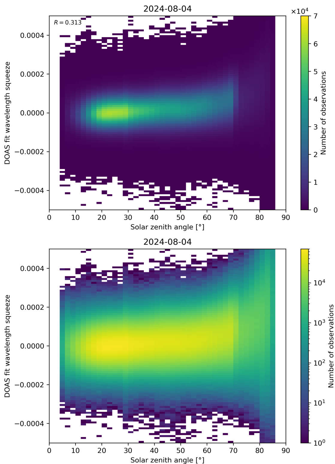
Figure 169: Scatter density plot of “Solar zenith angle” against “DOAS fit wavelength squeeze” for 2024-08-03 to 2024-08-05.
