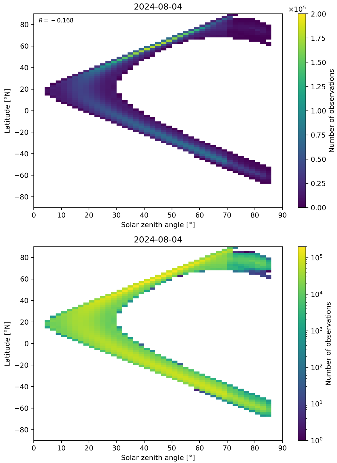
Figure 181: Scatter density plot of “Solar zenith angle” against “Latitude” for 2024-08-03 to 2024-08-05.
