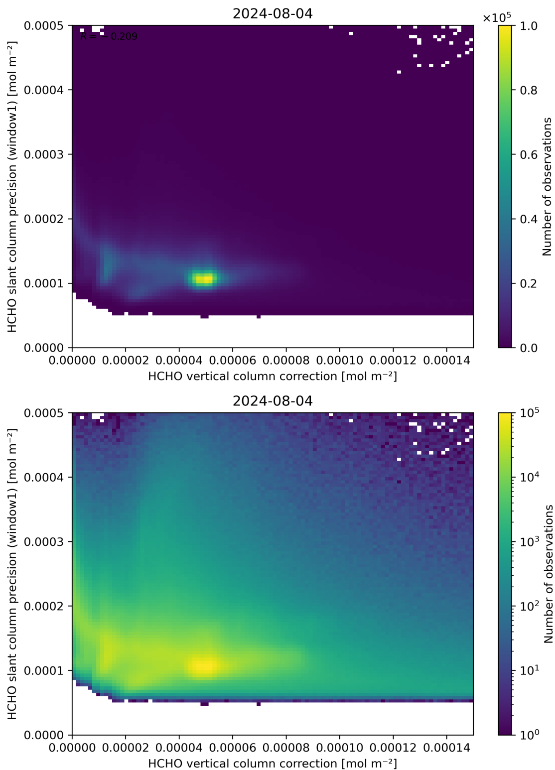
Figure 119: Scatter density plot of “HCHO vertical column correction” against “HCHO slant column precision (window1)” for 2024-08-03 to 2024-08-05.
