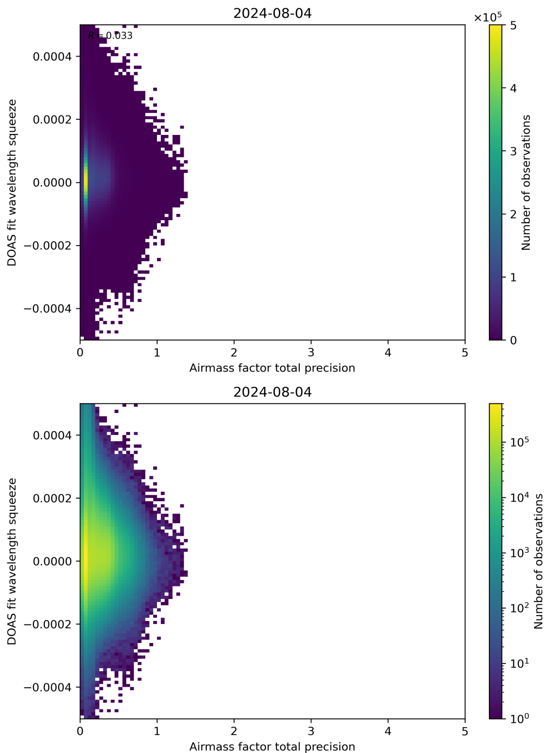
Figure 107: Scatter density plot of “Airmass factor total precision” against “DOAS fit wavelength squeeze” for 2024-08-03 to 2024-08-05.
