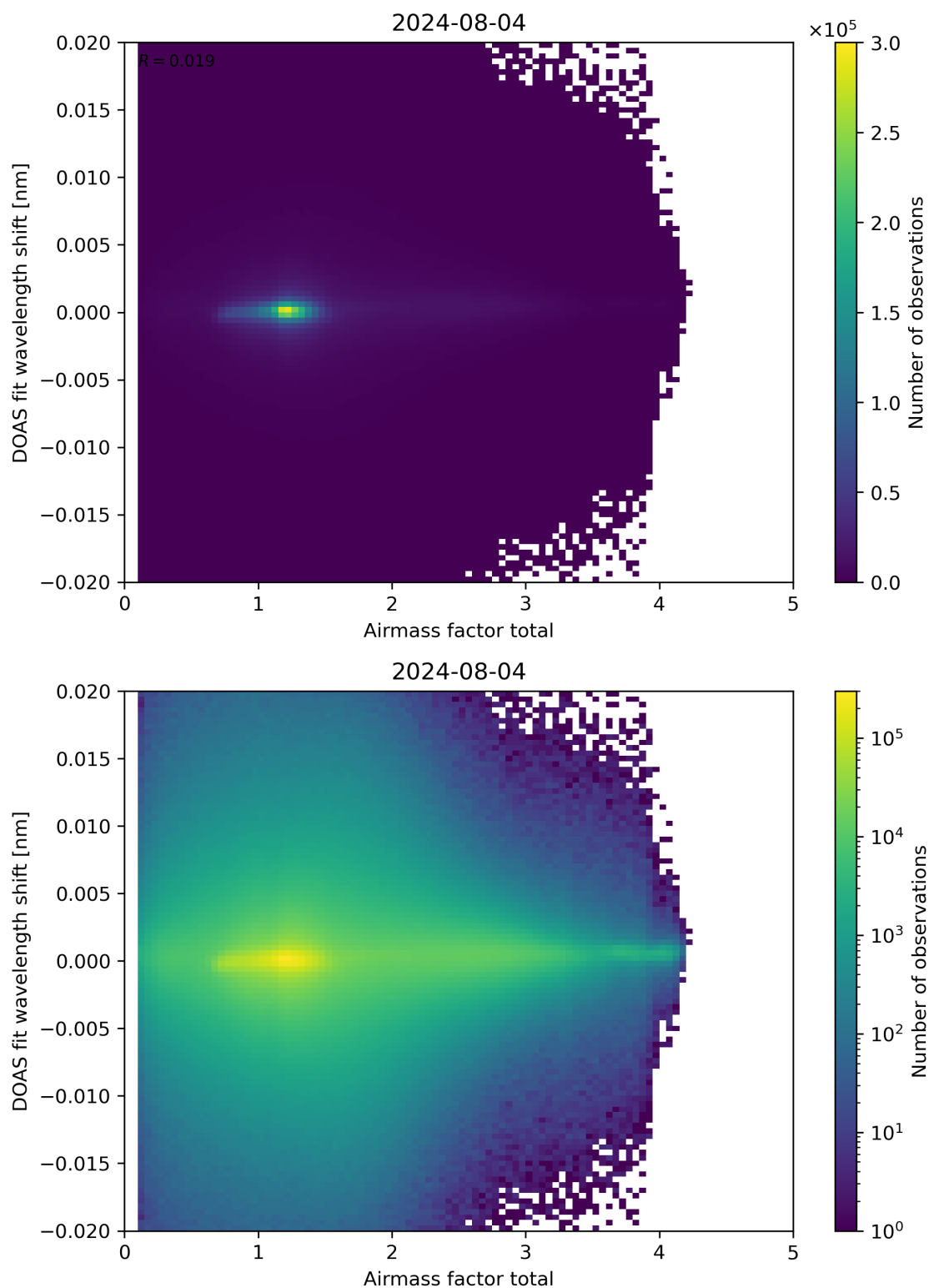
Figure 98: Scatter density plot of “Airmass factor total” against “DOAS fit wavelength shift” for 2024-08-03 to 2024-08-05.
