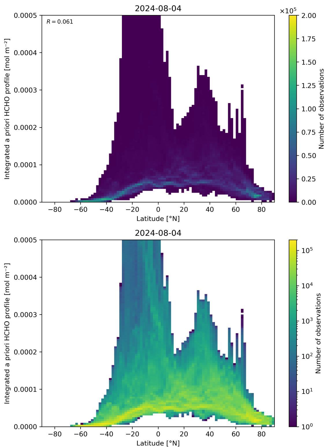
Figure 166: Scatter density plot of “Latitude” against “Integrated a priori HCHO profile” for 2024-08-03 to 2024-08-05.
