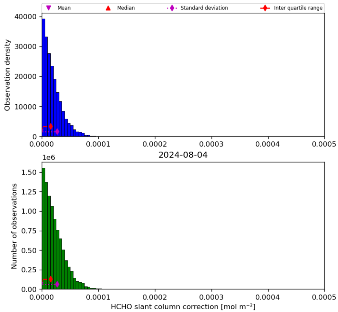
Figure 47: Histogram of “HCHO slant column correction” for 2024-08-03 to 2024-08-05
