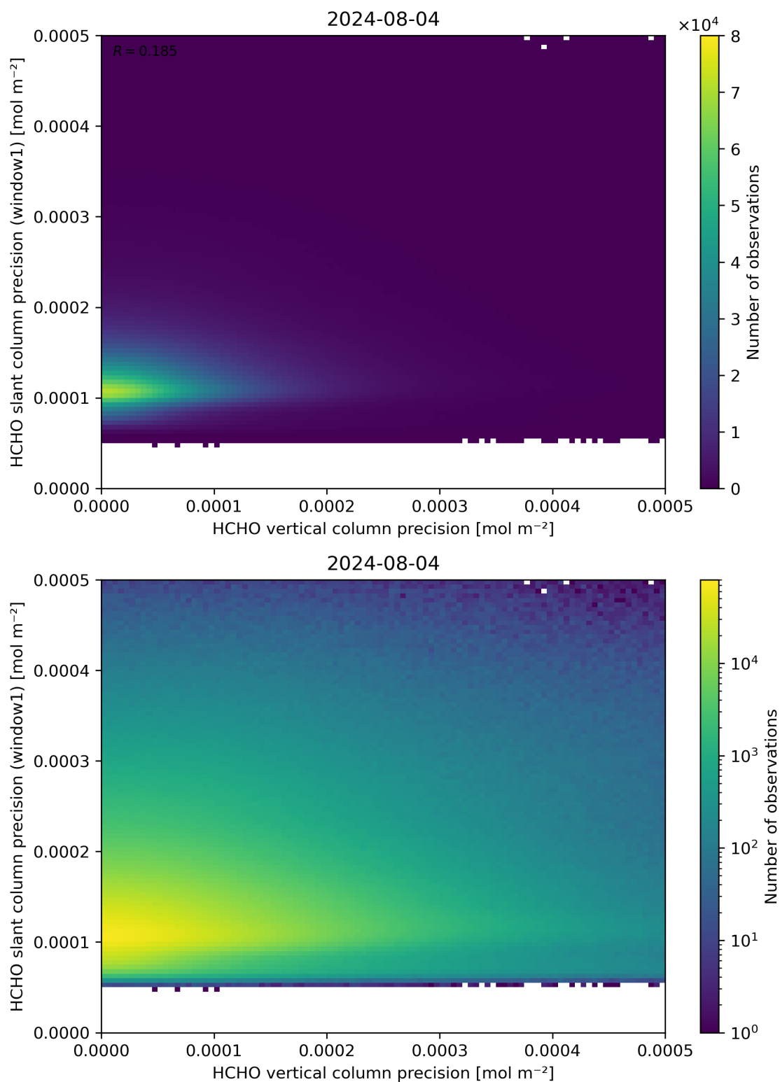
Figure 143: Scatter density plot of “HCHO vertical column precision” against “HCHO slant column precision (window1)” for 2024-08-03 to 2024-08-05.
