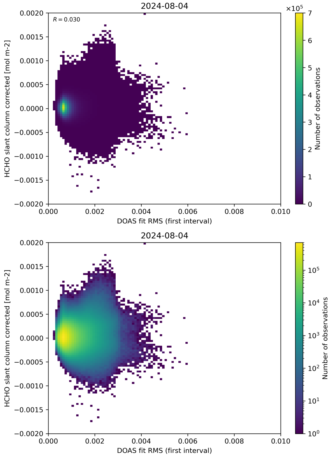
Figure 62: Scatter density plot of “DOAS fit RMS (first interval)” against “HCHO slant column corrected” for 2024-08-03 to 2024-08-05.
