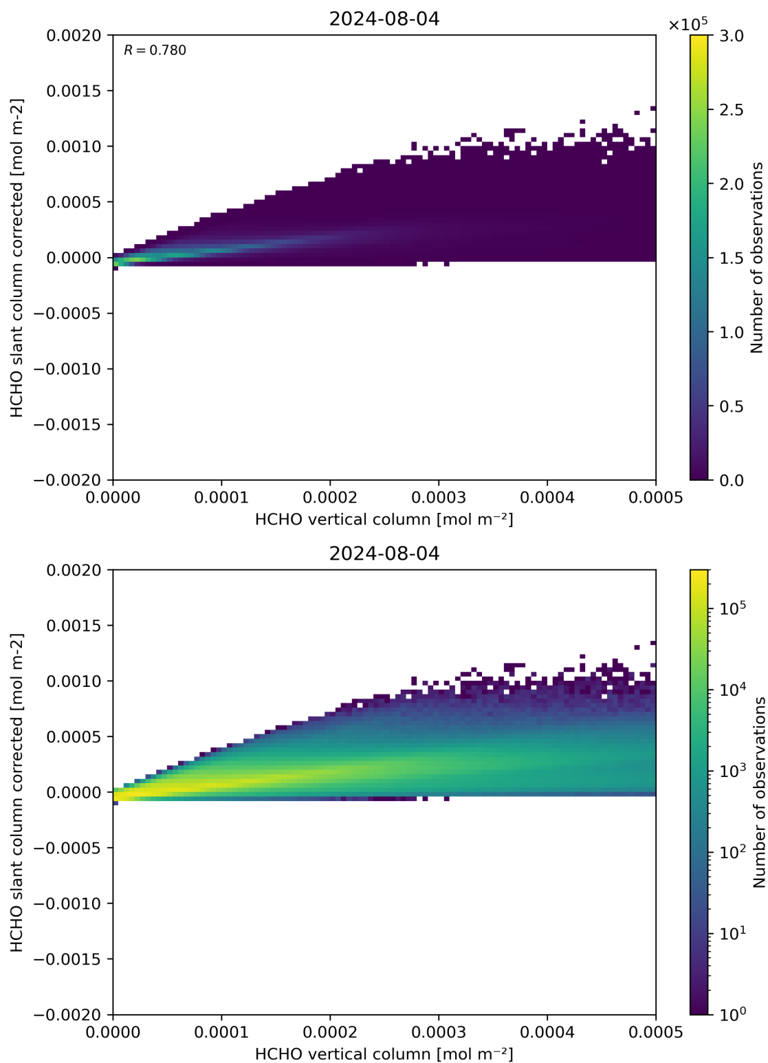
Figure 127: Scatter density plot of “HCHO vertical column” against “HCHO slant column corrected” for 2024-08-03 to 2024-08-05.
