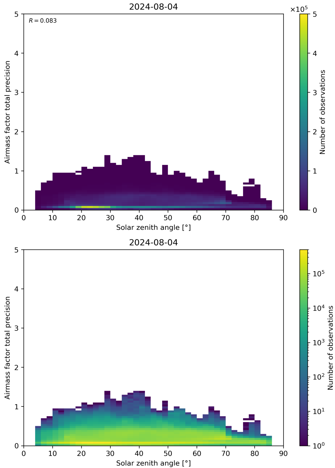
Figure 176: Scatter density plot of “Solar zenith angle” against “Airmass factor total precision” for 2024-08-03 to 2024-08-05.
