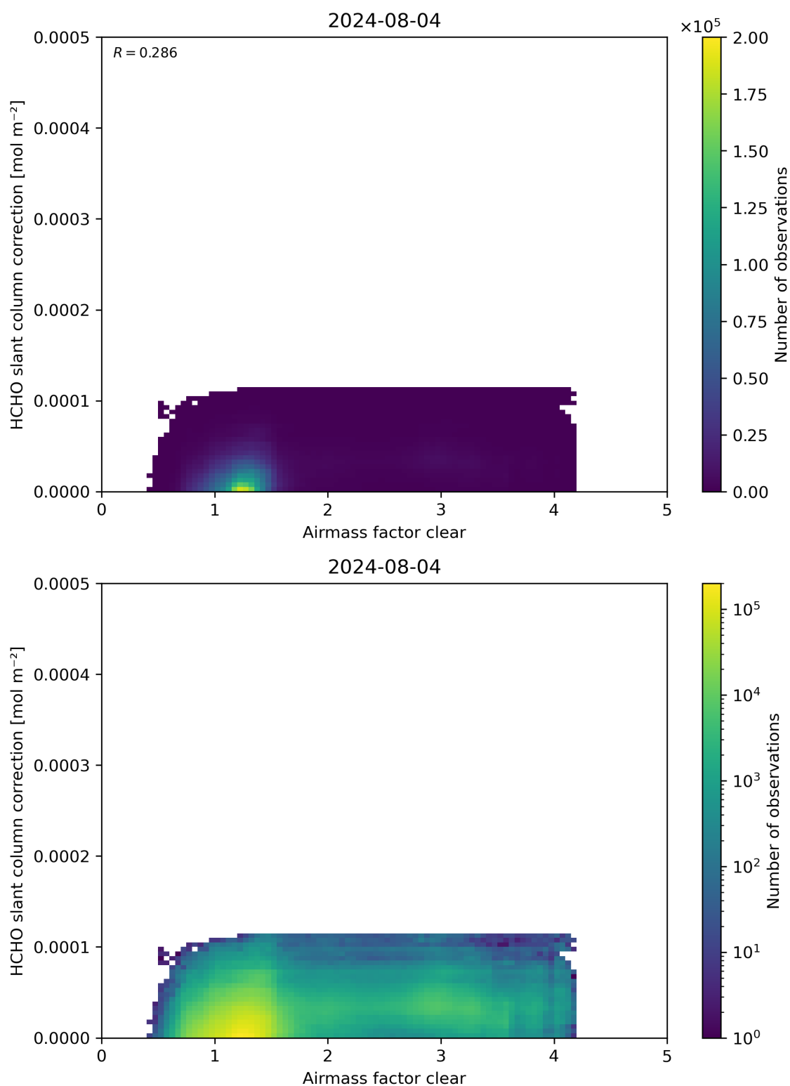
Figure 75: Scatter density plot of “Airmass factor clear” against “HCHO slant column correction” for 2024-08-03 to 2024-08-05.
