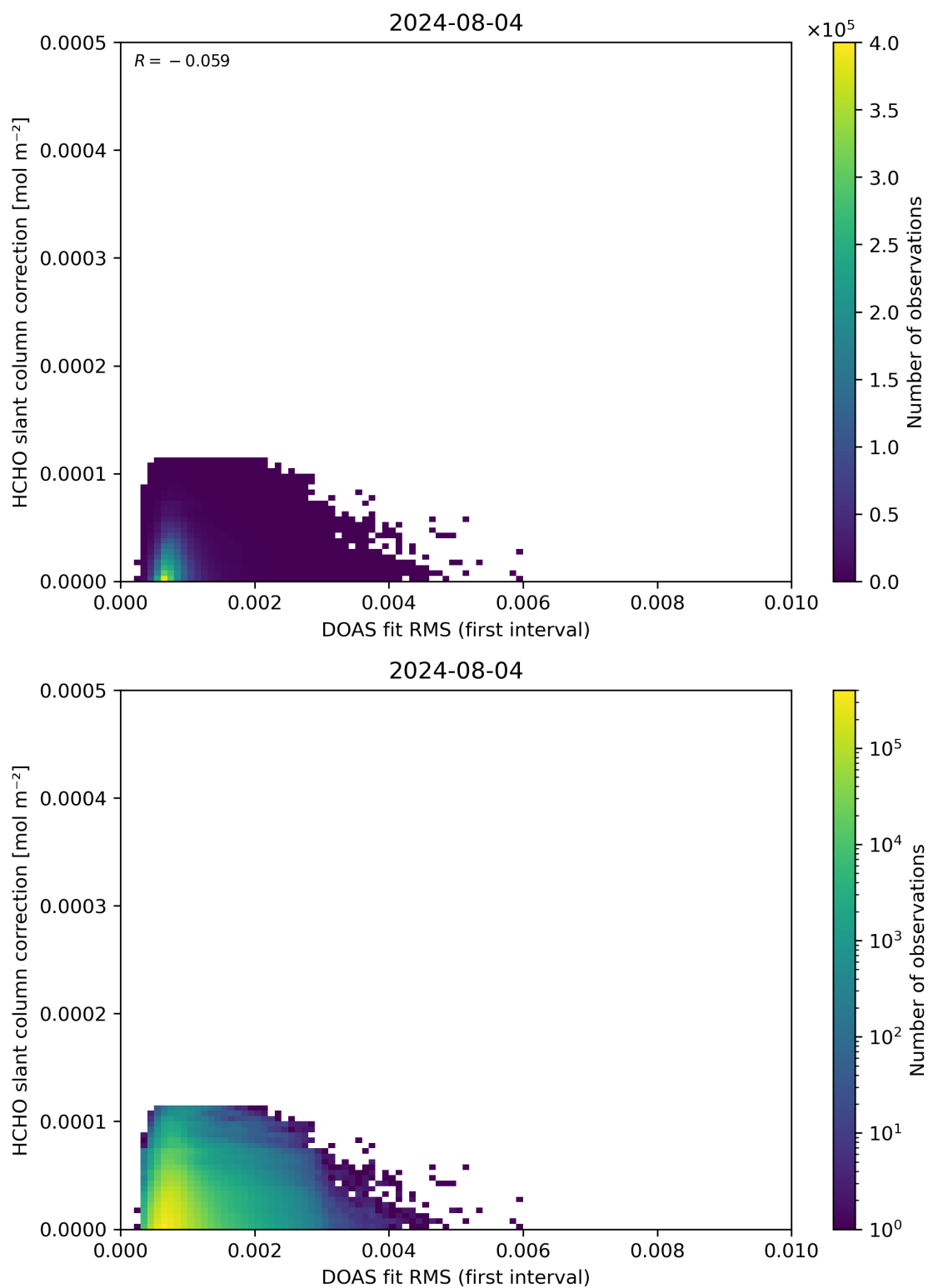
Figure 63: Scatter density plot of “DOAS fit RMS (first interval)” against “HCHO slant column correction” for 2024-08-03 to 2024-08-05.
