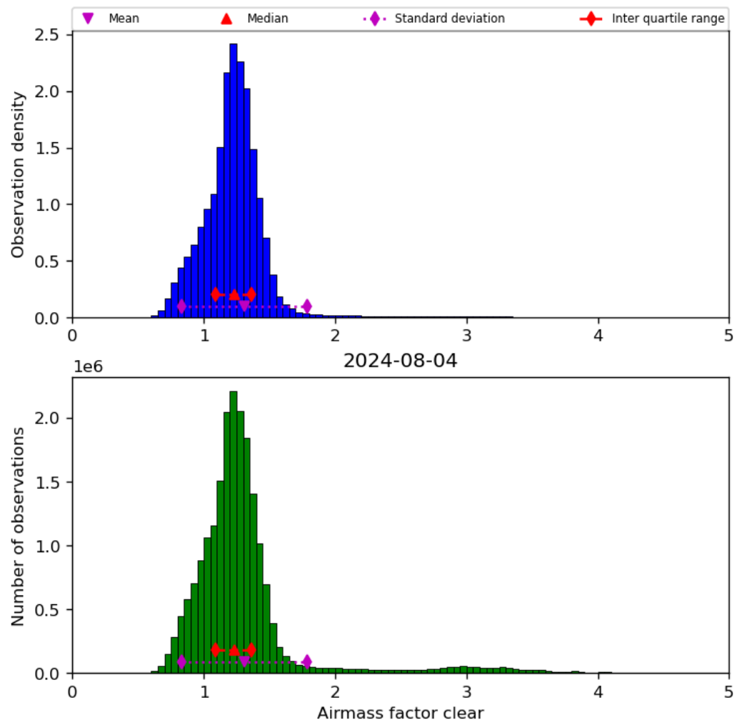
Figure 42: Histogram of “Airmass factor clear” for 2024-08-03 to 2024-08-05
