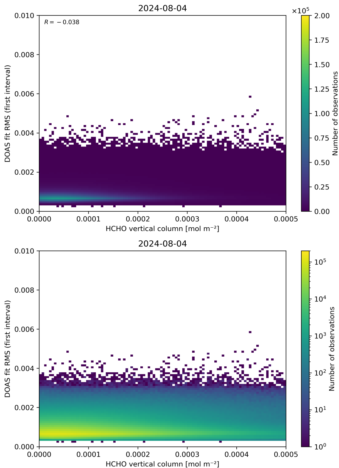
Figure 123: Scatter density plot of “HCHO vertical column” against “DOAS fit RMS (first interval)” for 2024-08-03 to 2024-08-05.
