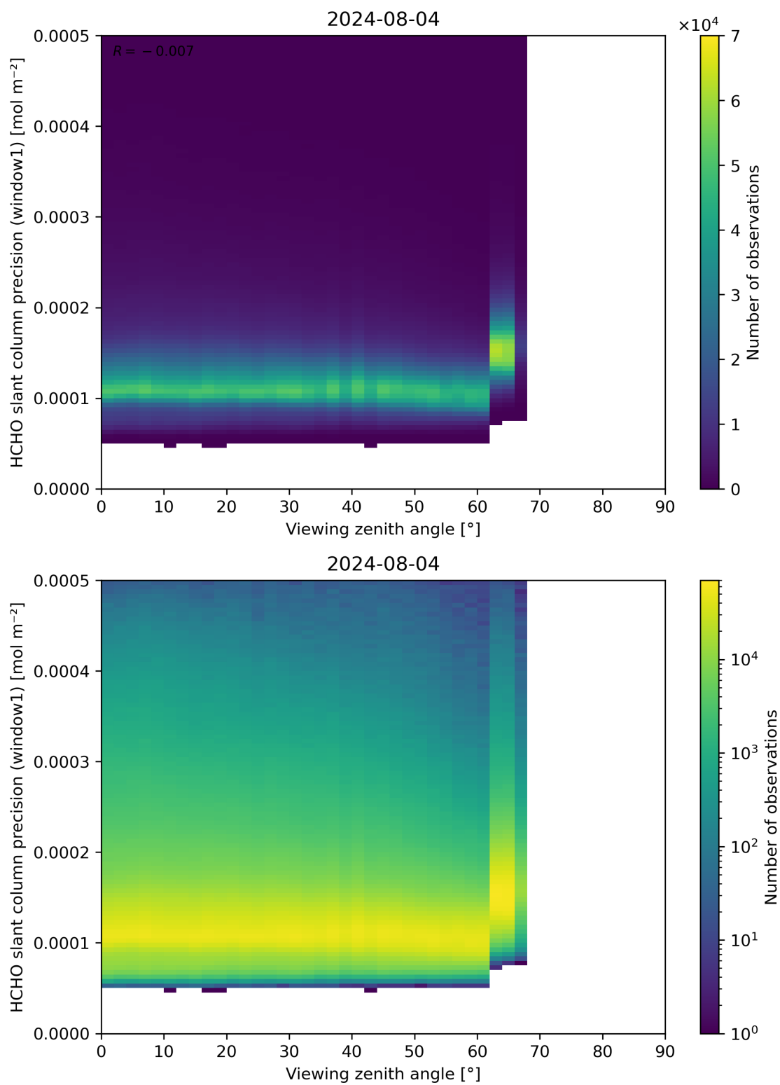
Figure 189: Scatter density plot of “Viewing zenith angle” against “HCHO slant column precision (window1)” for 2024-08-03 to 2024-08-05.
