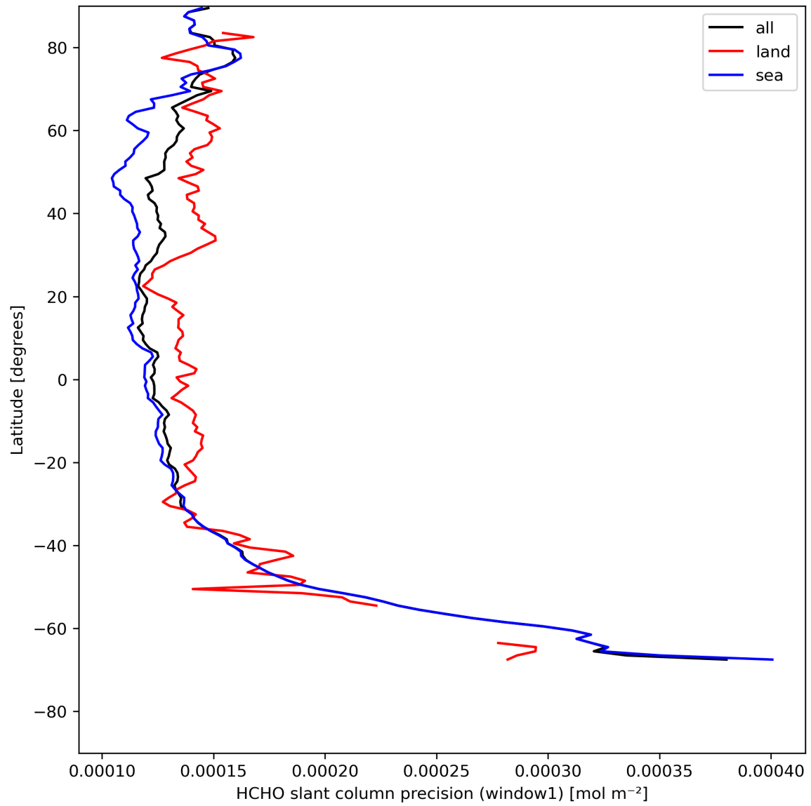
Figure 25: Zonal average of “HCHO slant column precision (window1)” for 2024-08-03 to 2024-08-05.
