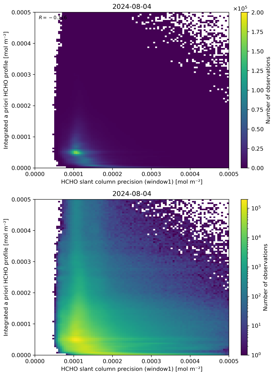
Figure 96: Scatter density plot of “HCHO slant column precision (window1)” against “Integrated a priori HCHO profile” for 2024-08-03 to 2024-08-05.
