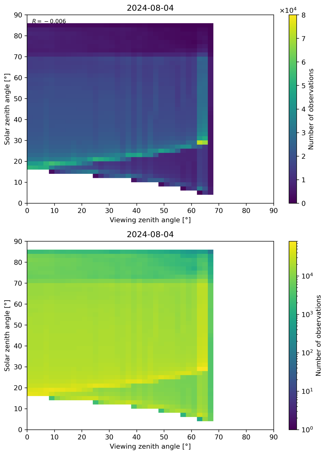
Figure 197: Scatter density plot of “Viewing zenith angle” against “Solar zenith angle” for 2024-08-03 to 2024-08-05.
