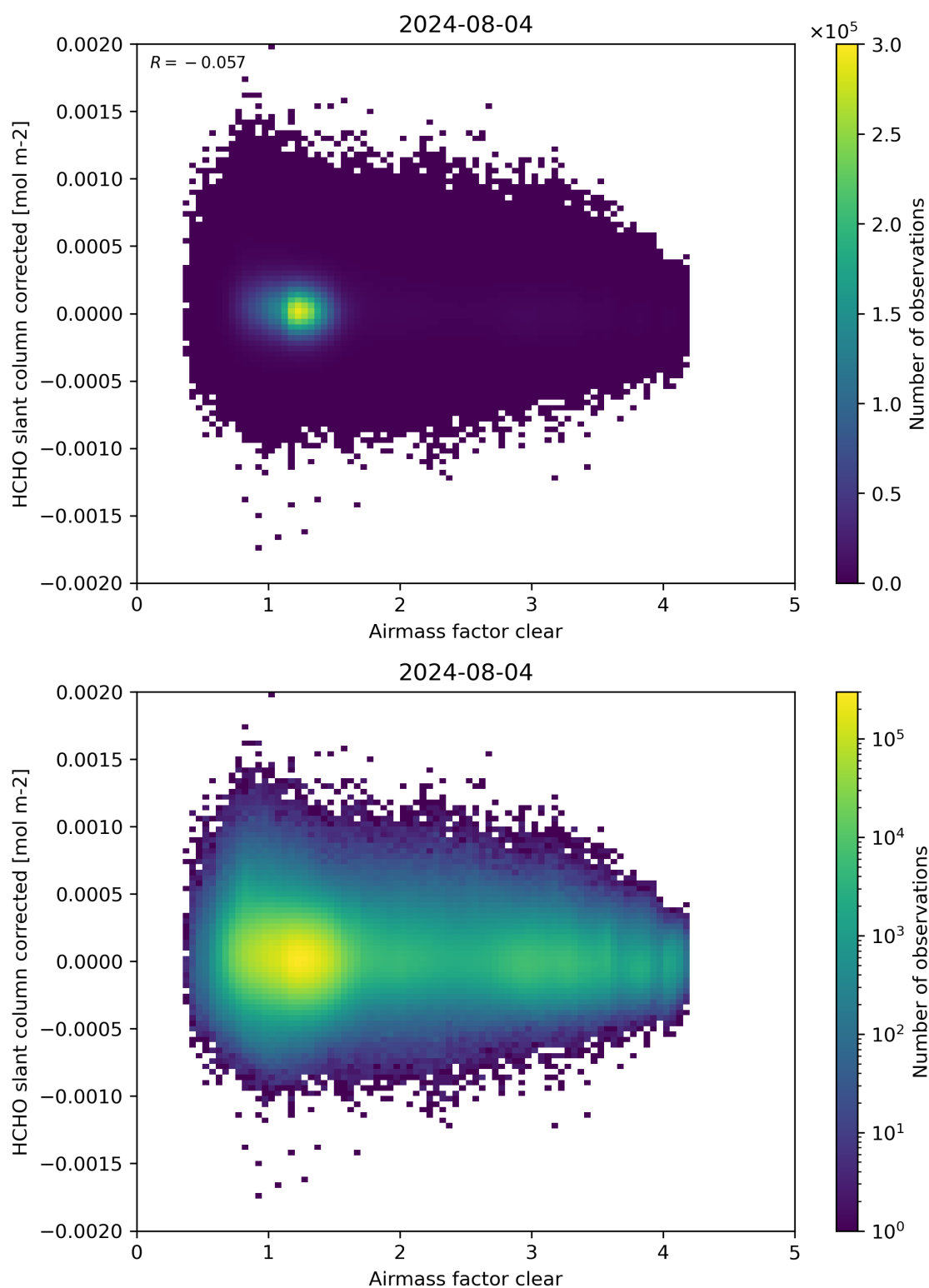
Figure 74: Scatter density plot of “Airmass factor clear” against “HCHO slant column corrected” for 2024-08-03 to 2024-08-05.
