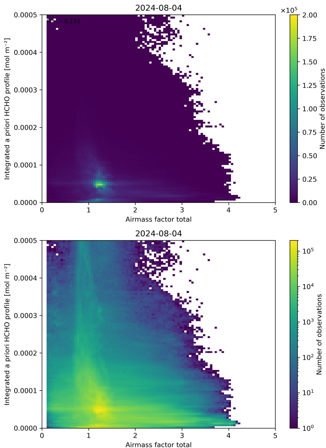
Figure 104: Scatter density plot of “Air mass factor total” against “Integrated a priori HCHO profile” for 2024-08-03 to 2024-08-05.
