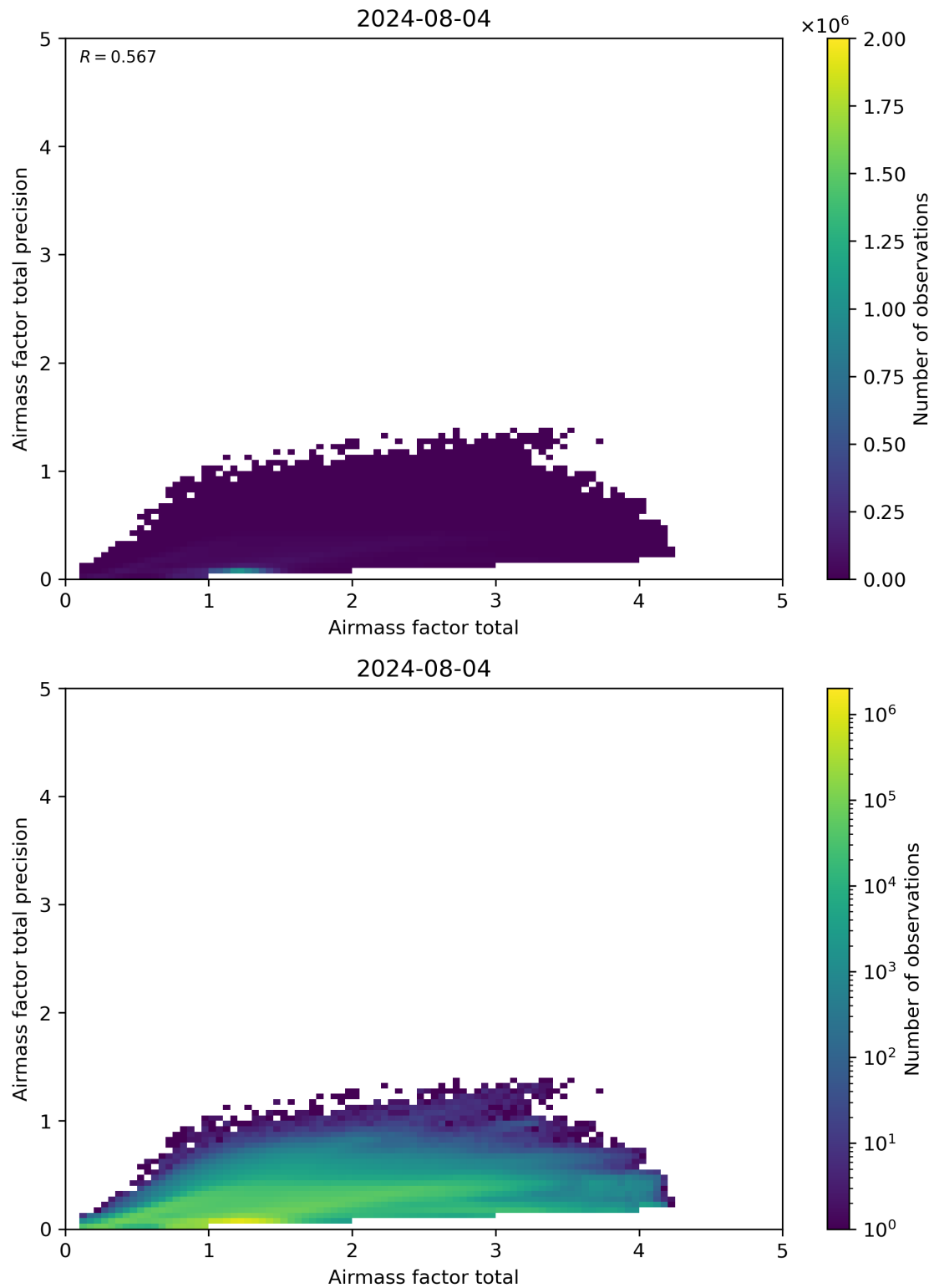
Figure 103: Scatter density plot of “Airmass factor total” against “Airmass factor total precision” for 2024-08-03 to 2024-08-05.
