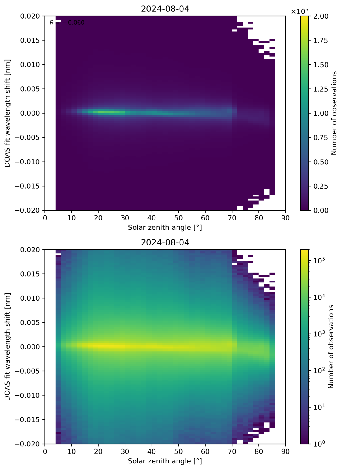
Figure 168: Scatter density plot of “Solar zenith angle” against “DOAS fit wavelength shift” for 2024-08-03 to 2024-08-05.
