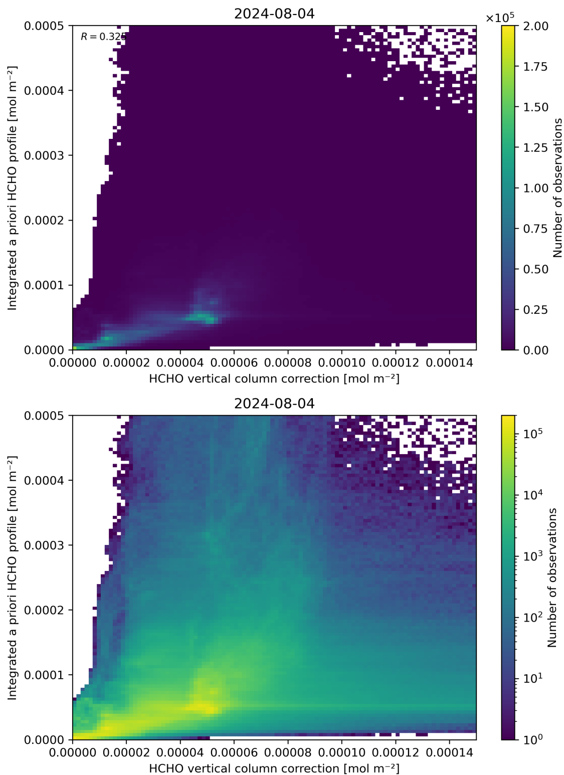
Figure 122: Scatter density plot of “HCHO vertical column correction” against “Integrated a priori HCHO profile” for 2024-08-03 to 2024-08-05.
