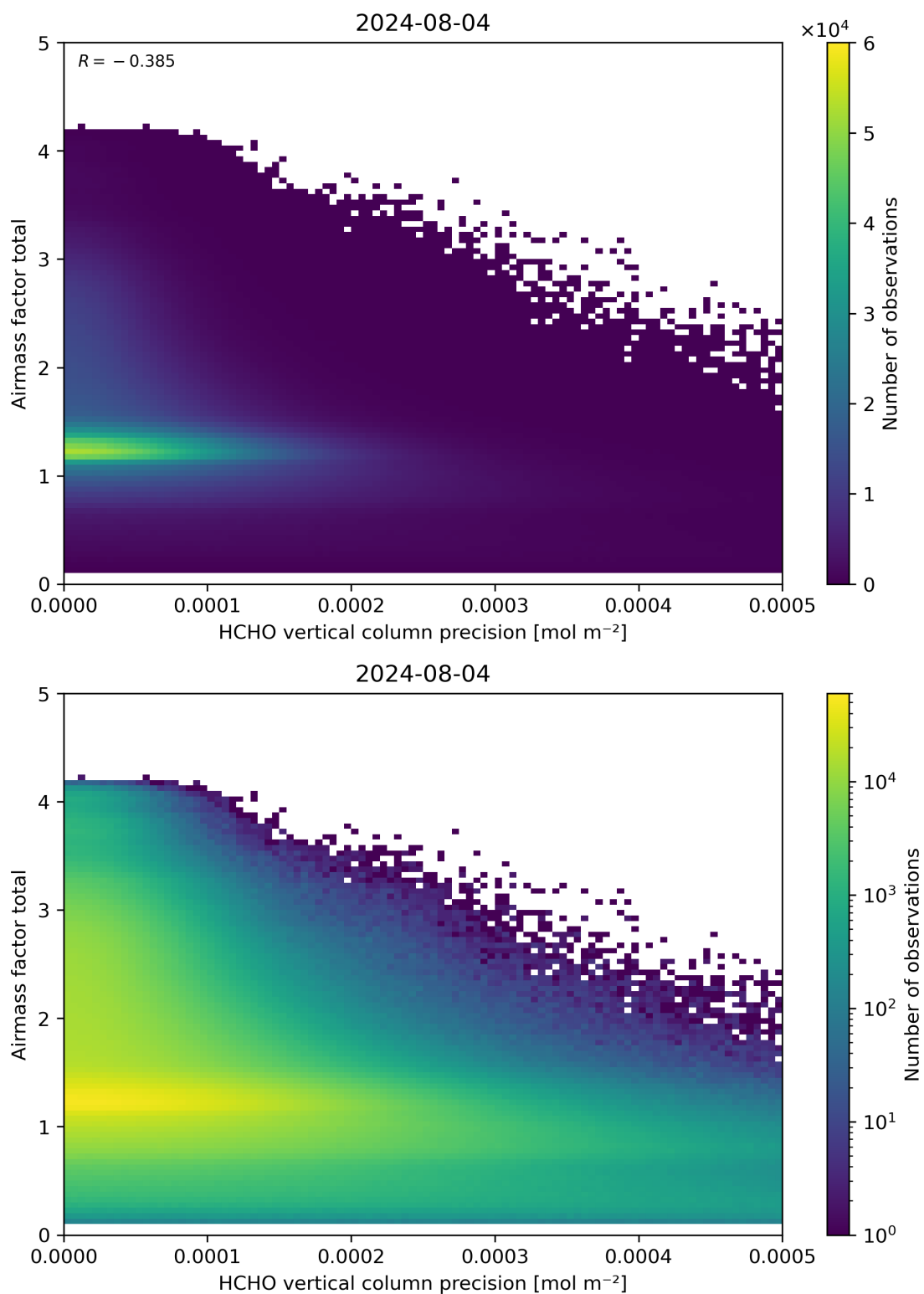
Figure 144: Scatter density plot of “HCHO vertical column precision” against “Airmass factor total” for 2024-08-03 to 2024-08-05.
