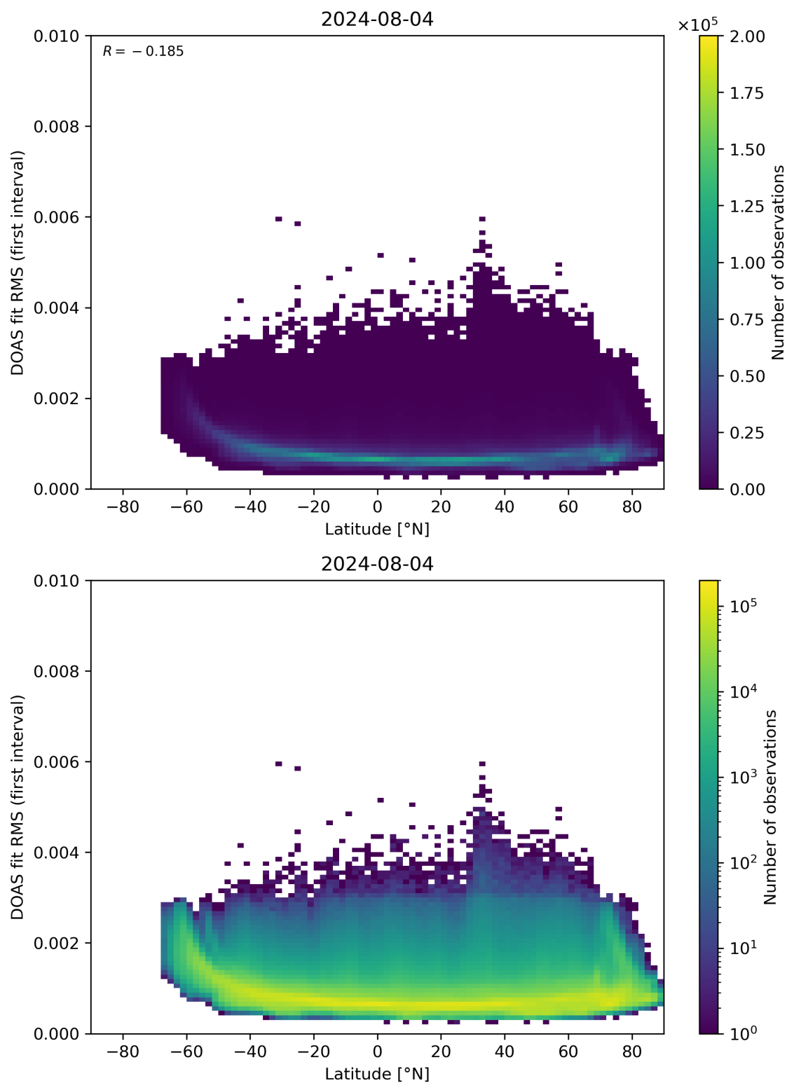
Figure 153: Scatter density plot of “Latitude” against “DOAS fit RMS (first interval)” for 2024-08-03 to 2024-08-05.
