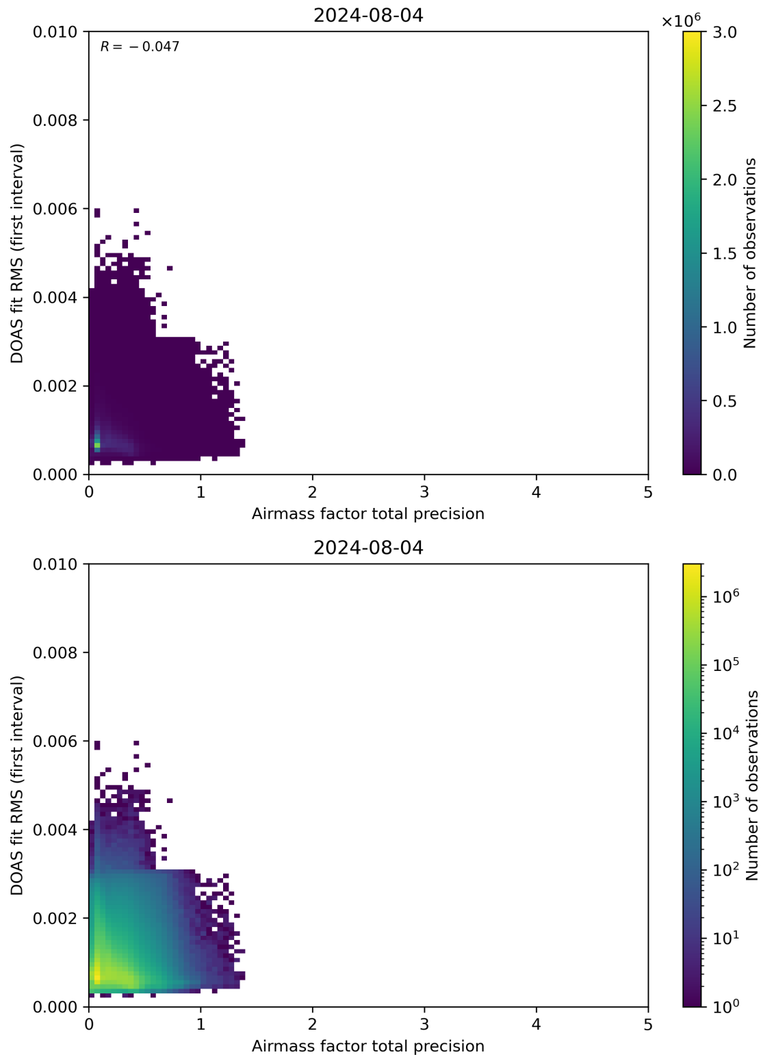
Figure 105: Scatter density plot of “Airmass factor total precision” against “DOAS fit RMS (first interval)” for 2024-08-03 to 2024-08-05.
