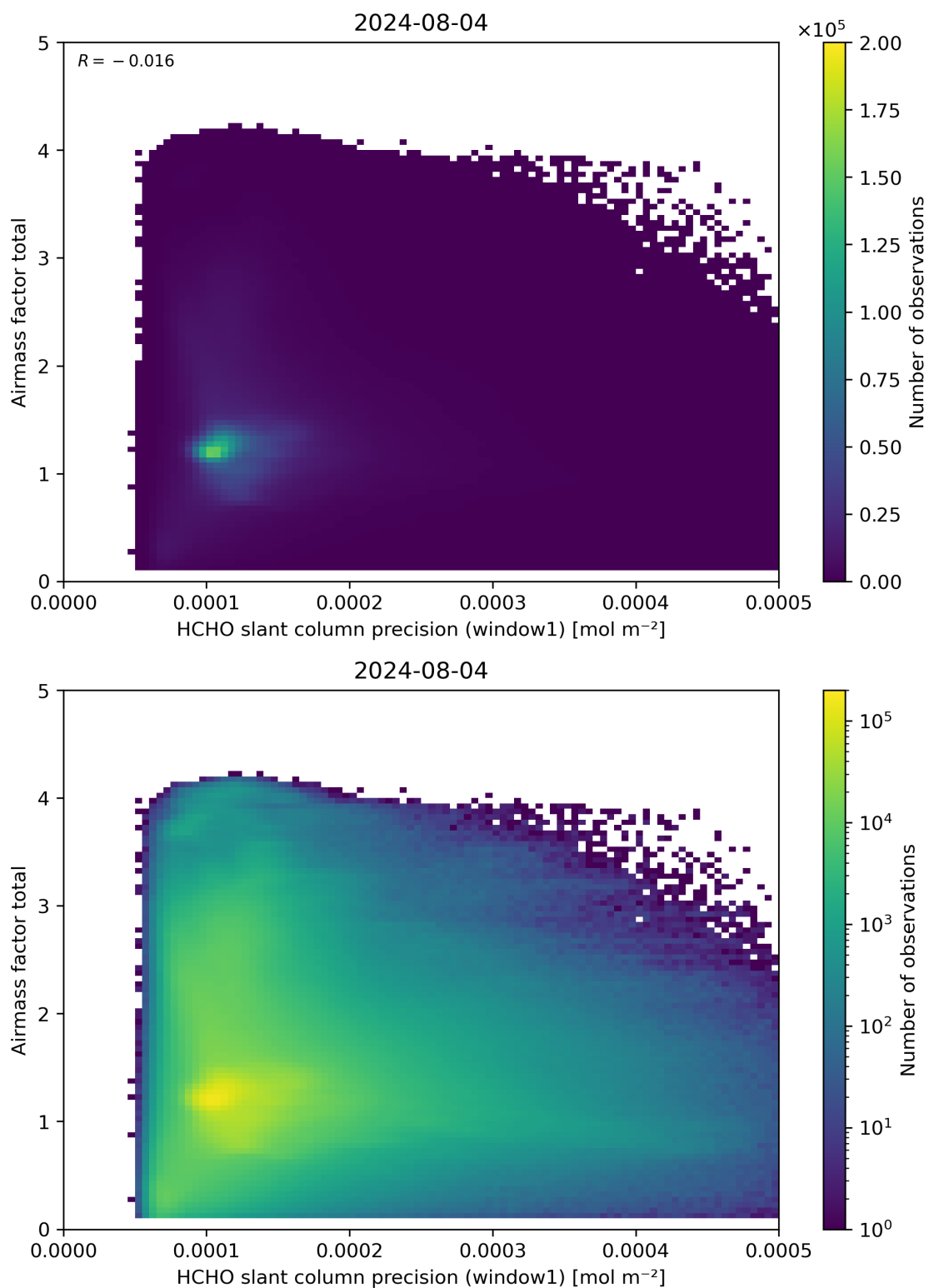
Figure 94: Scatter density plot of “HCHO slant column precision (window1)” against “Airmass factor total” for 2024-08-03 to 2024-08-05.
