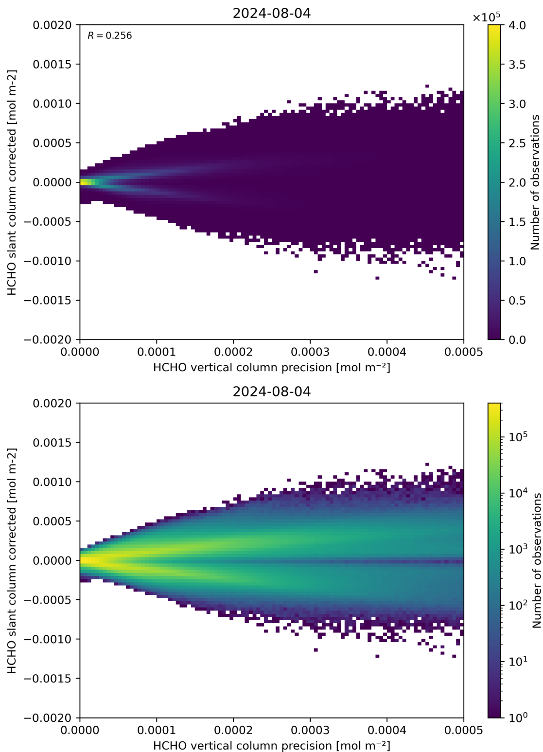
Figure 140: Scatter density plot of “HCHO vertical column precision” against “HCHO slant column corrected” for 2024-08-03 to 2024-08-05.
