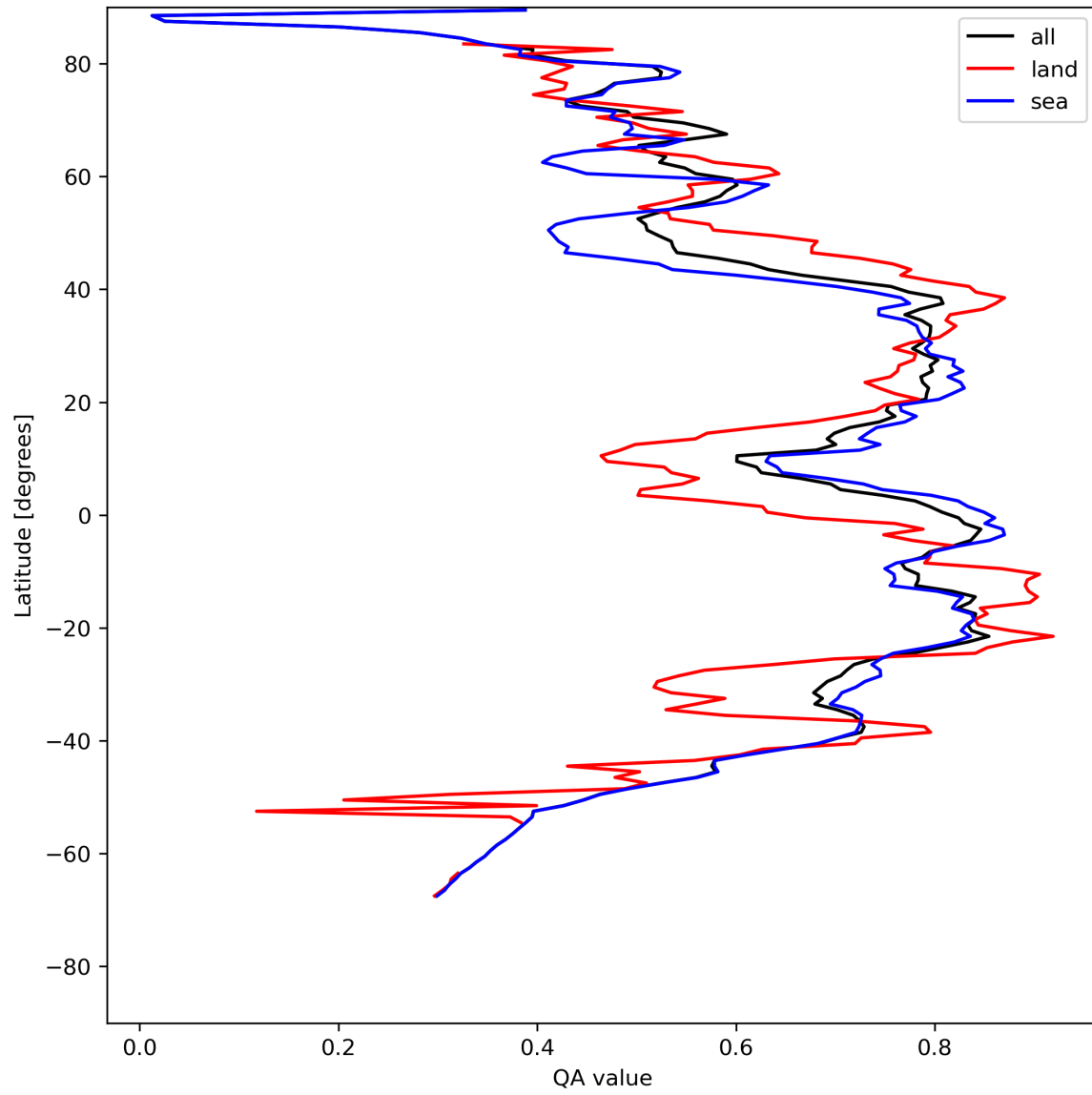
Figure 20: Zonal average of “QA value” for 2024-08-03 to 2024-08-05.
