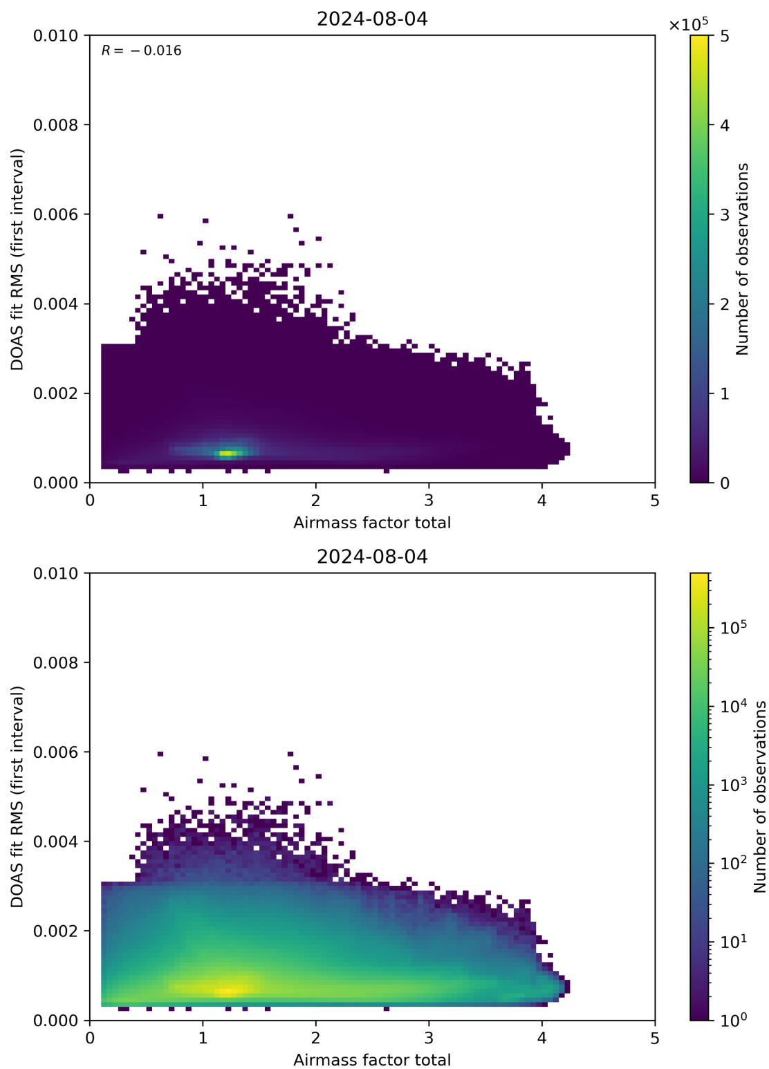
Figure 97: Scatter density plot of “Airmass factor total” against “DOAS fit RMS (first interval)” for 2024-08-03 to 2024-08-05.
