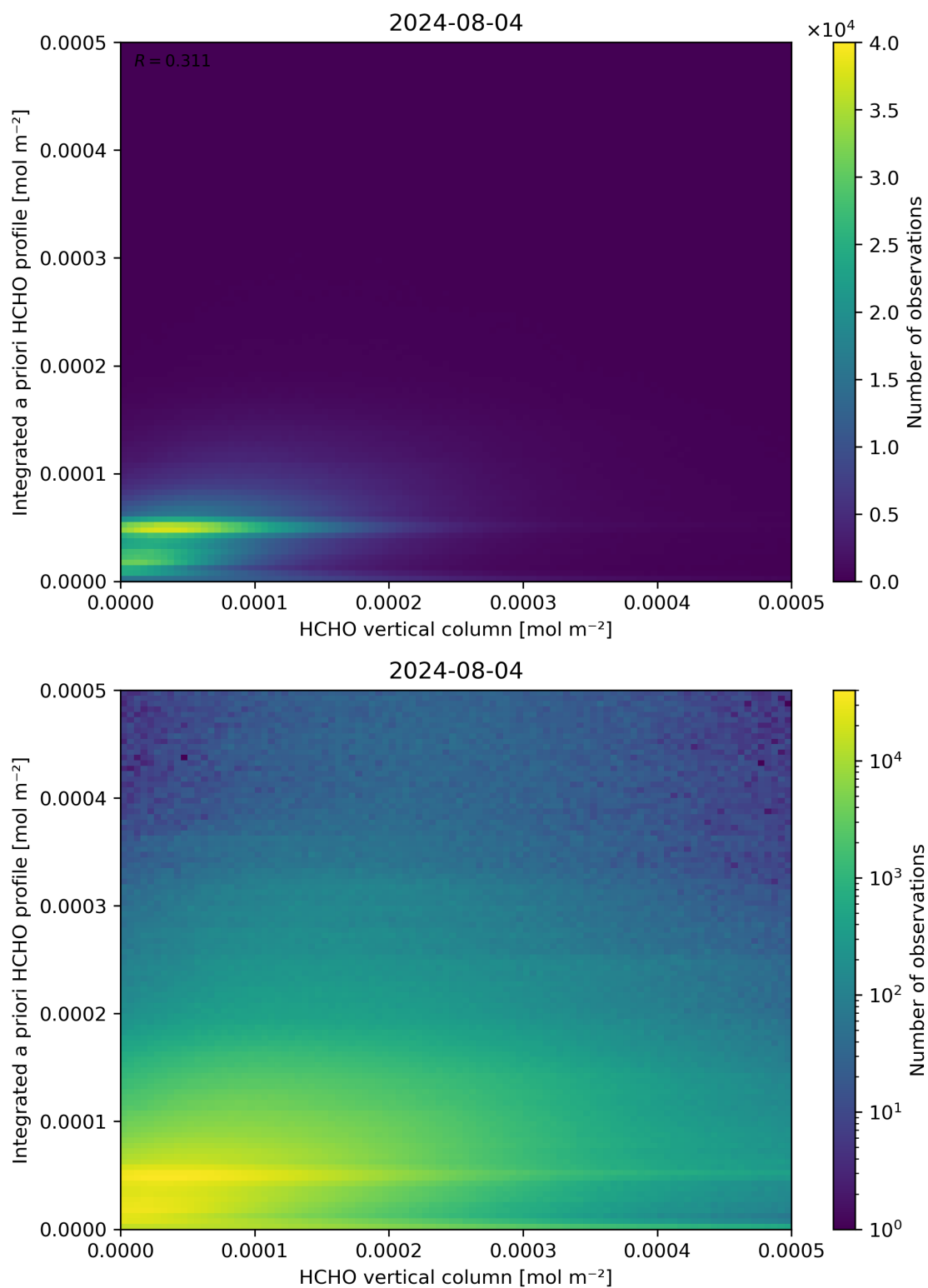
Figure 135: Scatter density plot of “HCHO vertical column” against “Integrated a priori HCHO profile” for 2024-08-03 to 2024-08-05.
