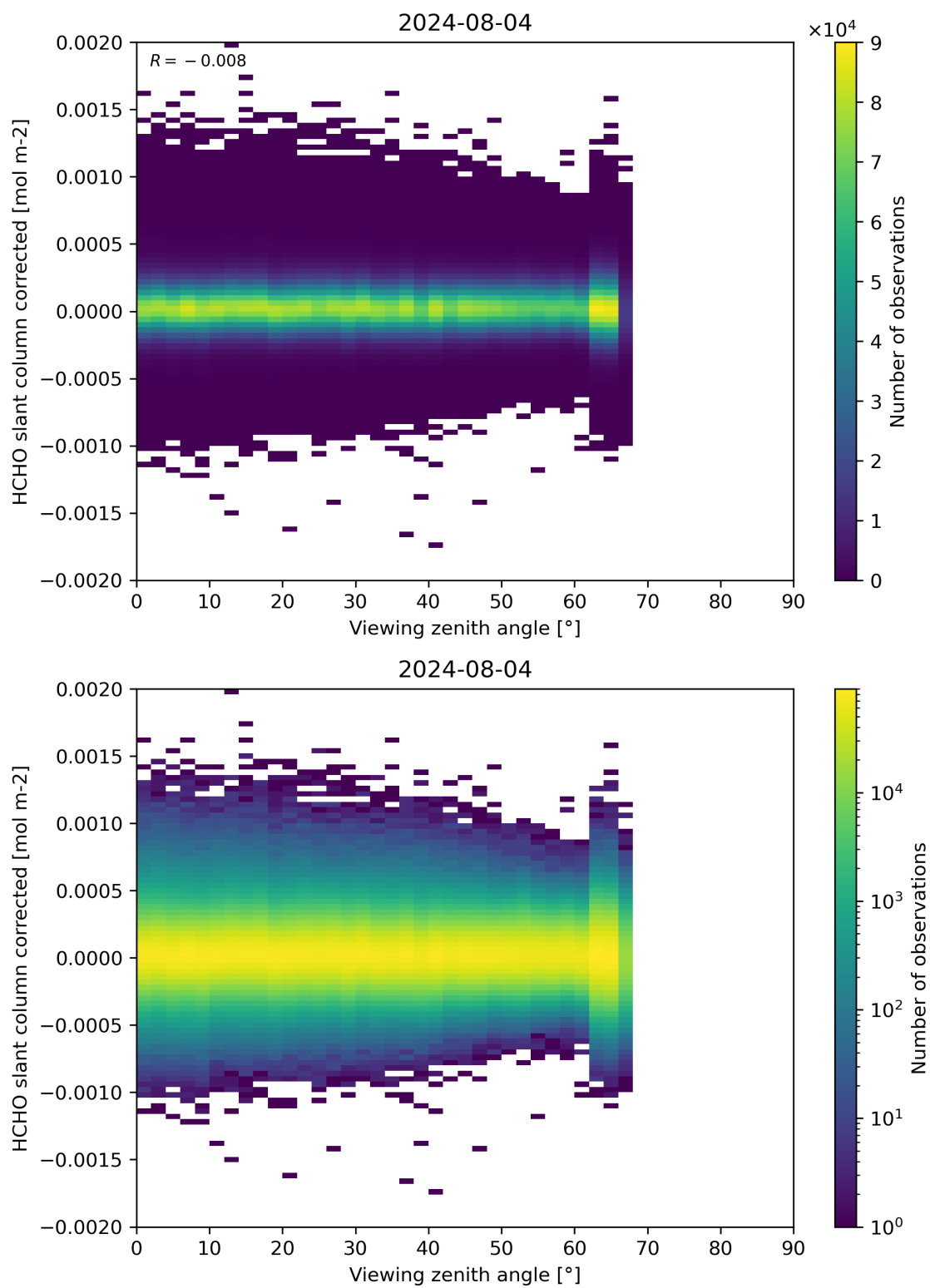
Figure 186: Scatter density plot of “Viewing zenith angle” against “HCHO slant column corrected” for 2024-08-03 to 2024-08-05.
