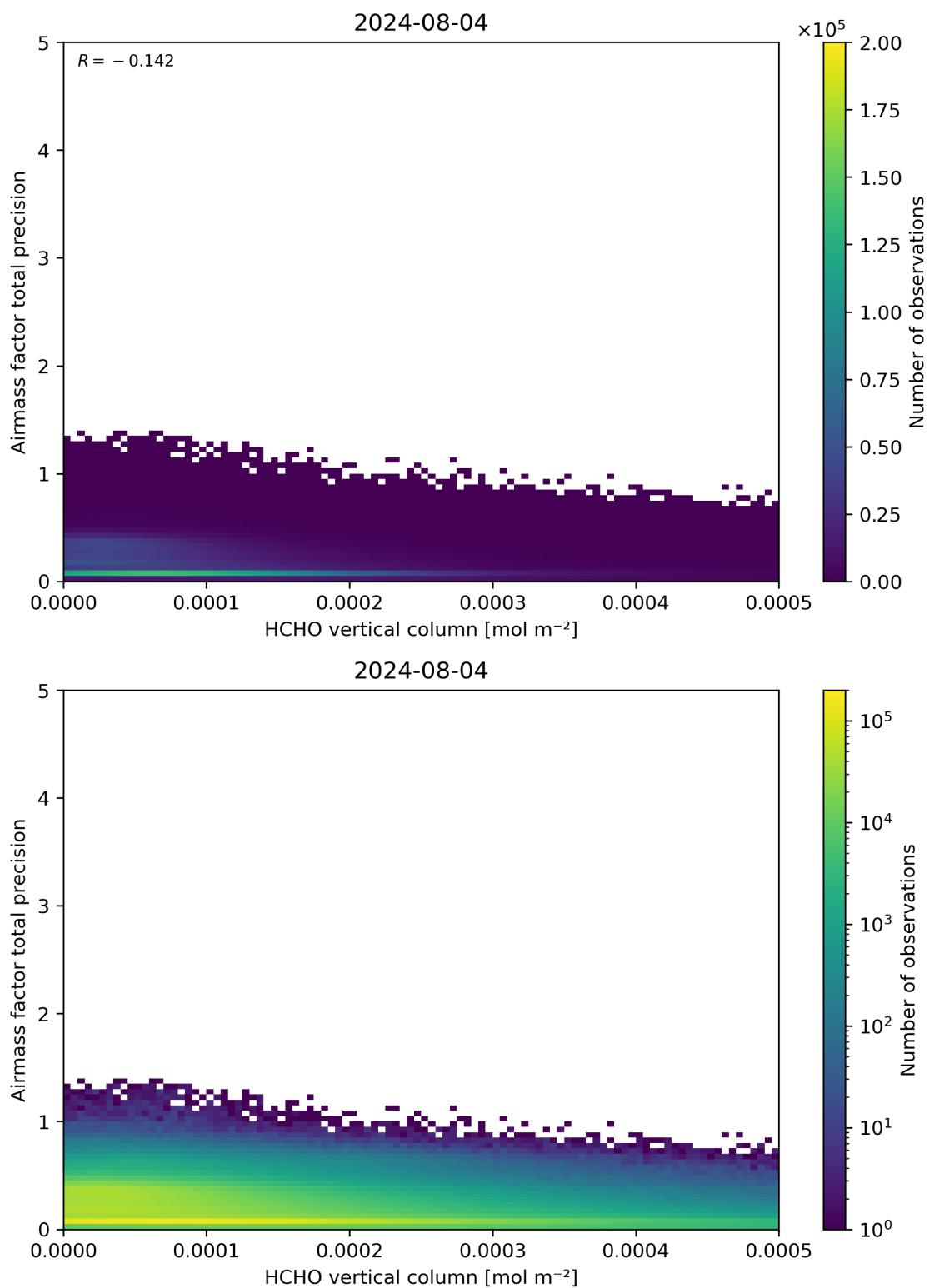
Figure 132: Scatter density plot of “HCHO vertical column” against “Airmass factor total precision” for 2024-08-03 to 2024-08-05.
