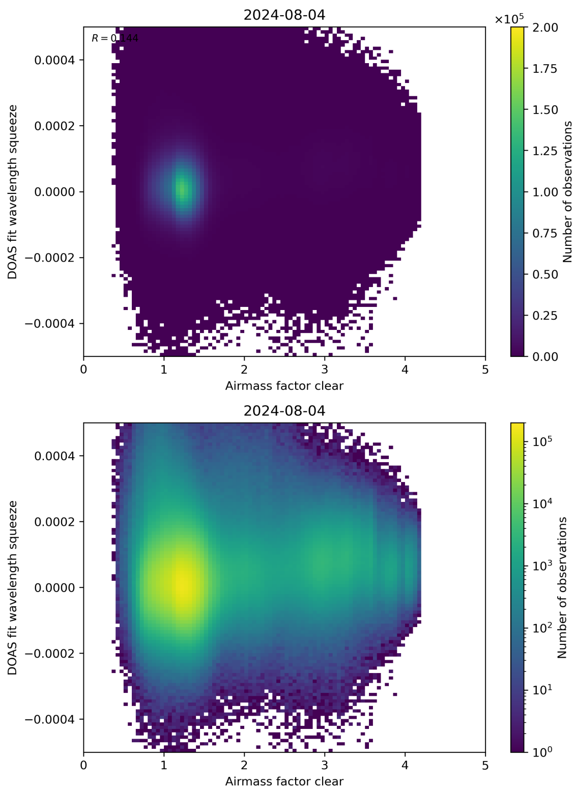
Figure 73: Scatter density plot of “Airmass factor clear” against “DOAS fit wavelength squeeze” for 2024-08-03 to 2024-08-05.
