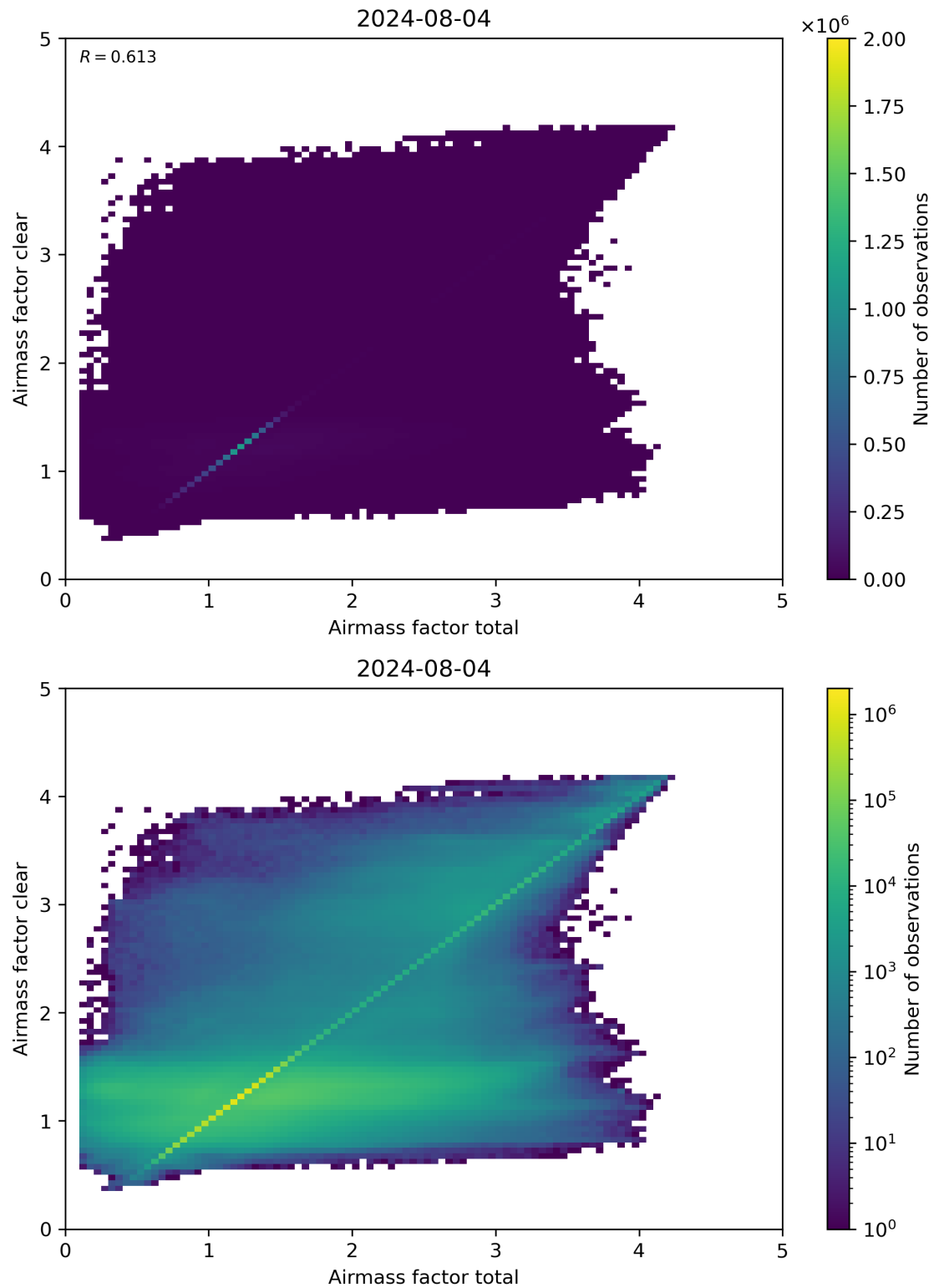
Figure 100: Scatter density plot of “Airmass factor total” against “Airmass factor clear” for 2024-08-03 to 2024-08-05.
