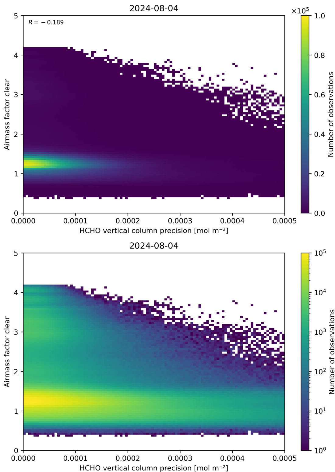
Figure 139: Scatter density plot of “HCHO vertical column precision” against “Airmass factor clear” for 2024-08-03 to 2024-08-05.
