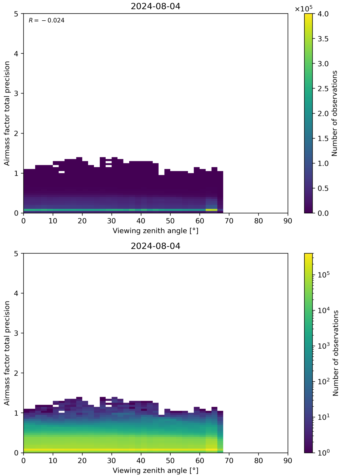
Figure 191: Scatter density plot of “Viewing zenith angle” against “Airmass factor total precision” for 2024-08-03 to 2024-08-05.
