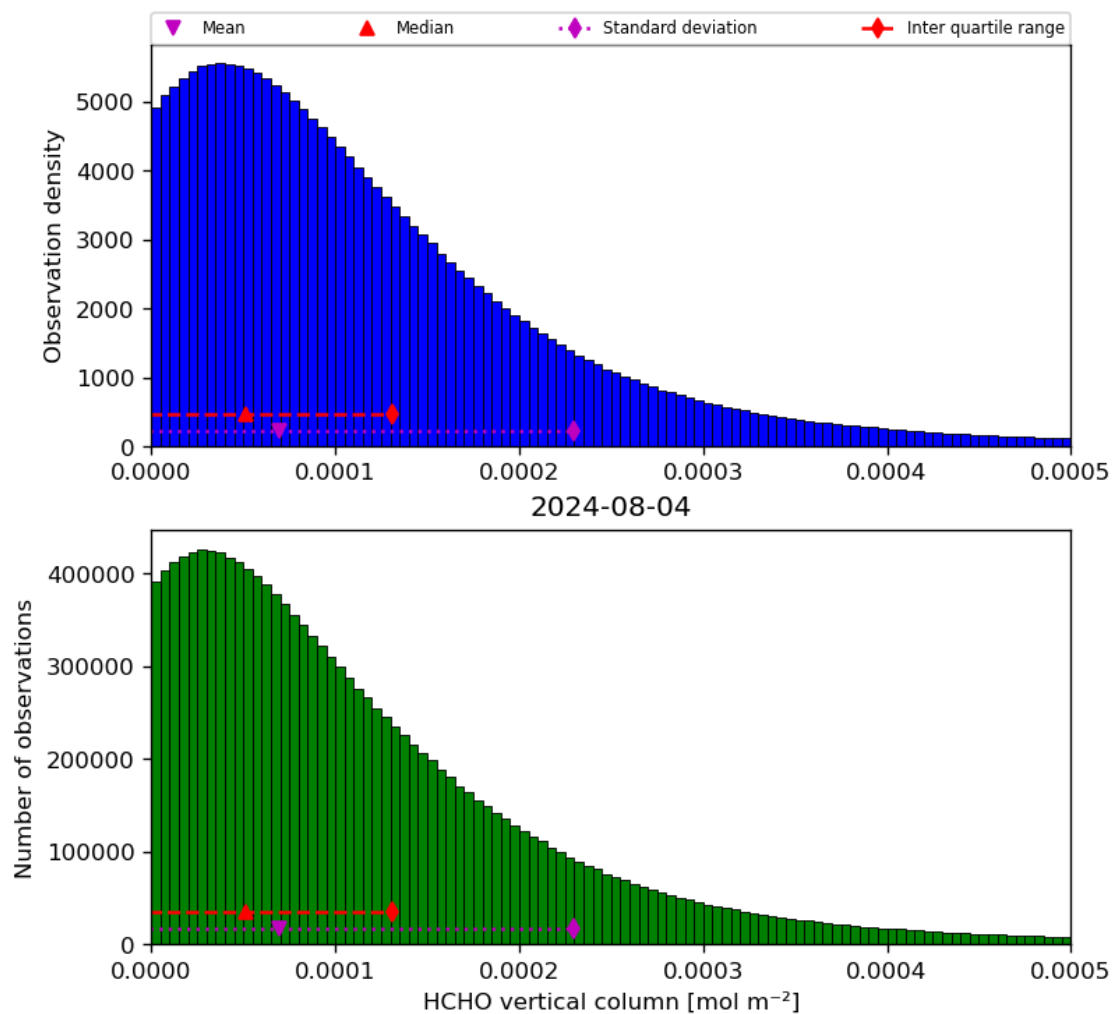
Figure 35: Histogram of “HCHO vertical column” for 2024-08-03 to 2024-08-05
