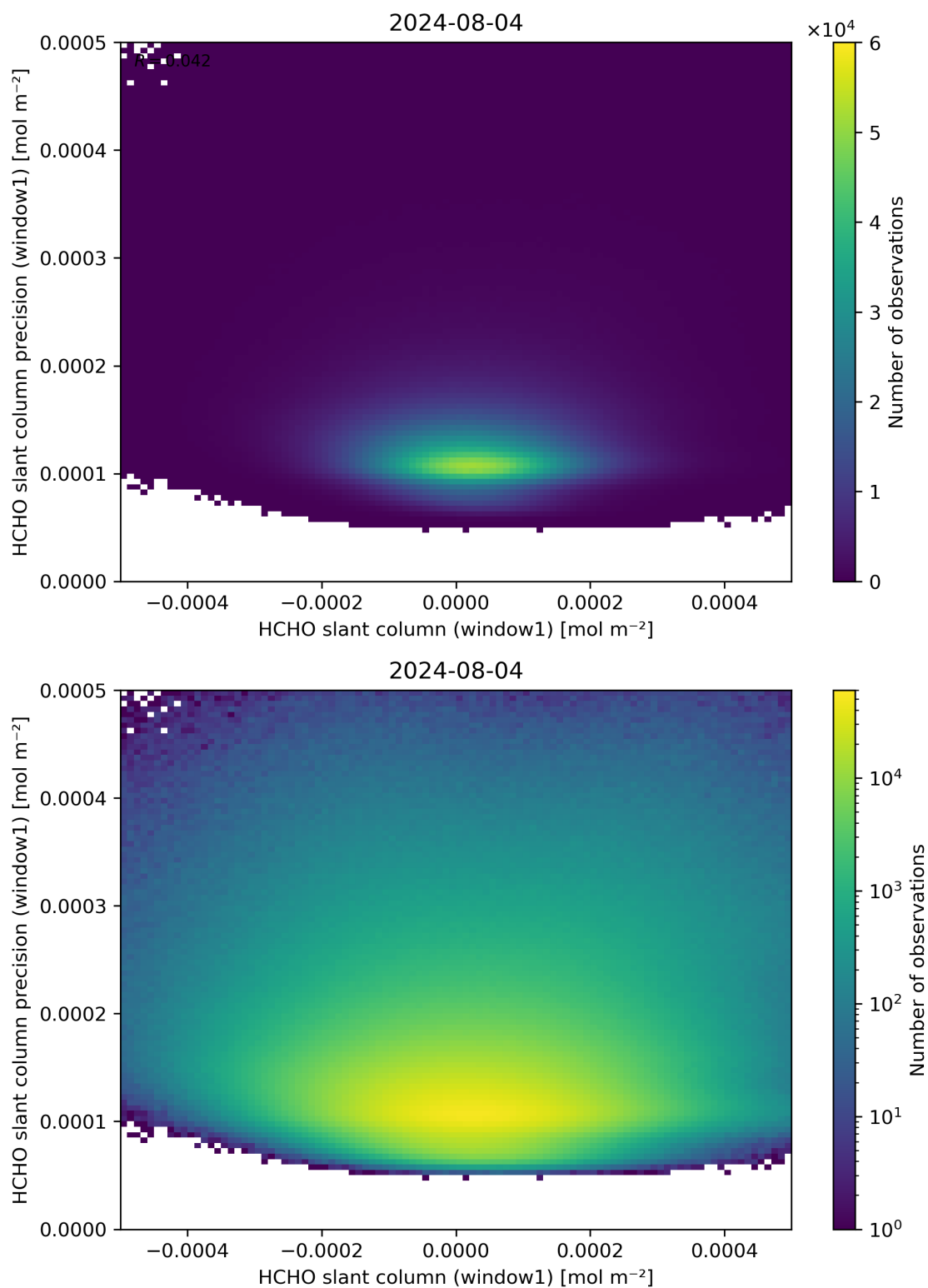
Figure 84: Scatter density plot of “HCHO slant column (window1)” against “HCHO slant column precision (window1)” for 2024-08-03 to 2024-08-05.
