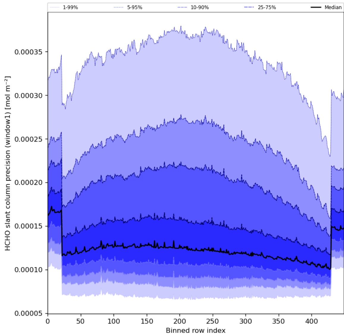
Figure 53: Along track statistics of “HCHO slant column precision (window1)” for 2024-08-03 to 2024-08-05
