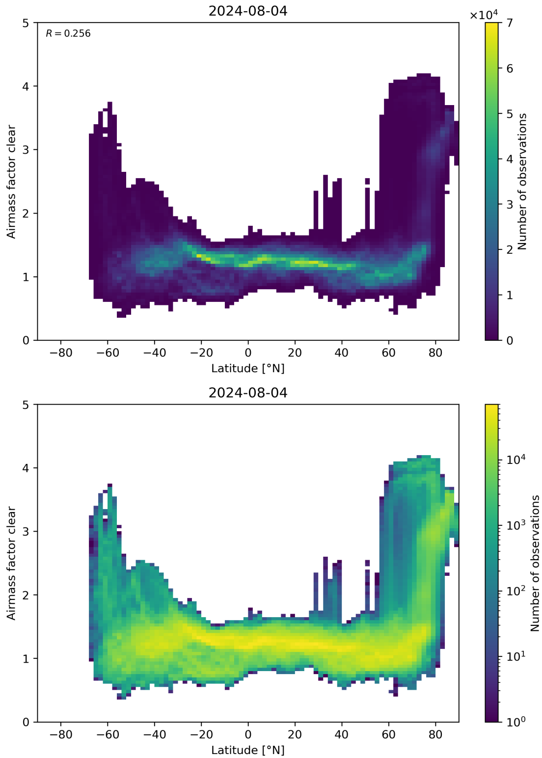
Figure 156: Scatter density plot of “Latitude” against “Airmass factor clear” for 2024-08-03 to 2024-08-05.
