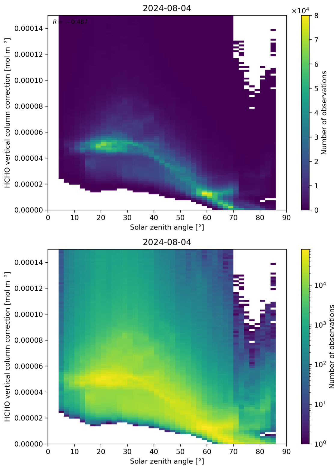
Figure 178: Scatter density plot of “Solar zenith angle” against “HCHO vertical column correction” for 2024-08-03 to 2024-08-05.
