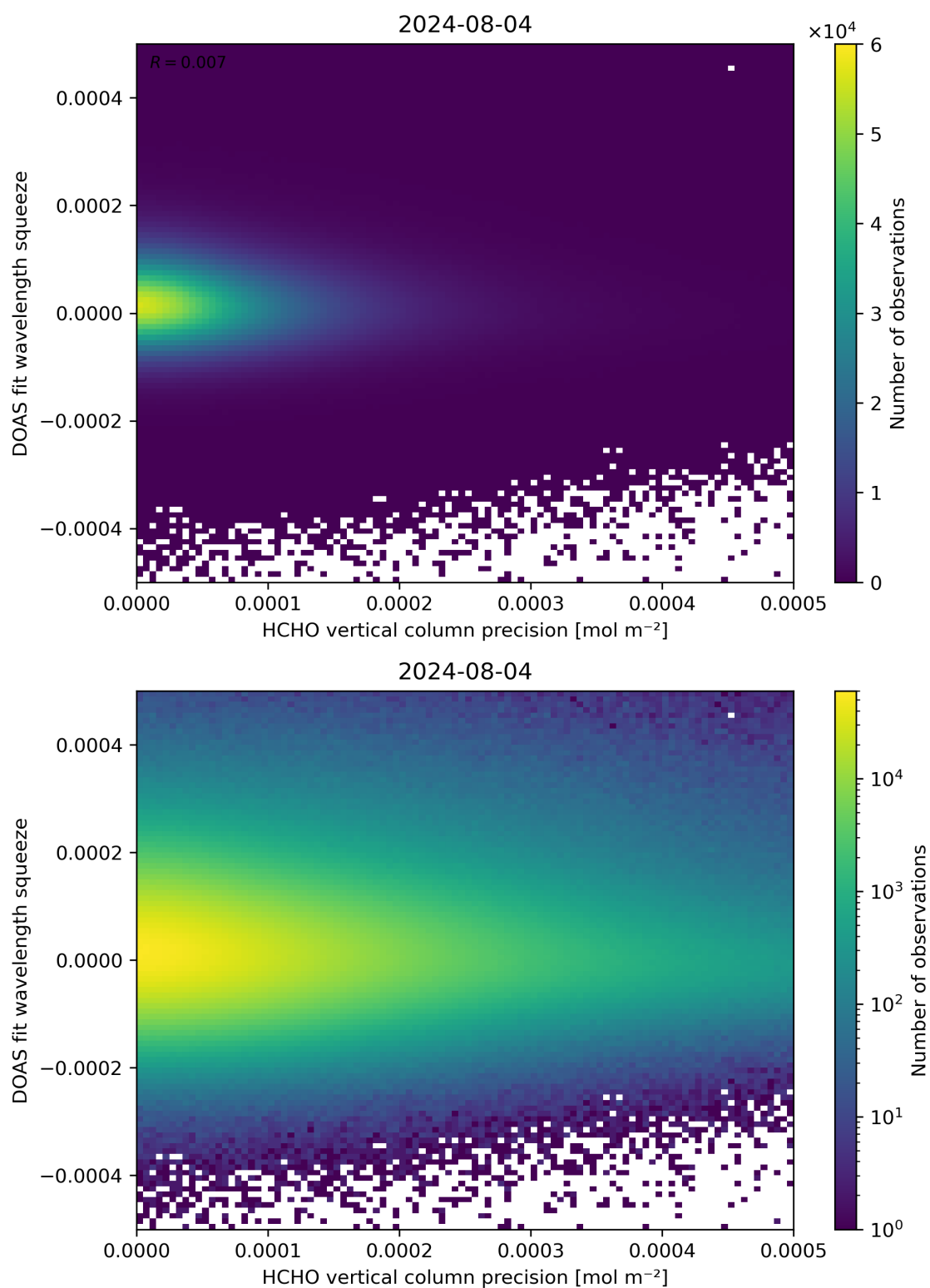
Figure 138: Scatter density plot of “HCHO vertical column precision” against “DOAS fit wavelength squeeze” for 2024-08-03 to 2024-08-05.
