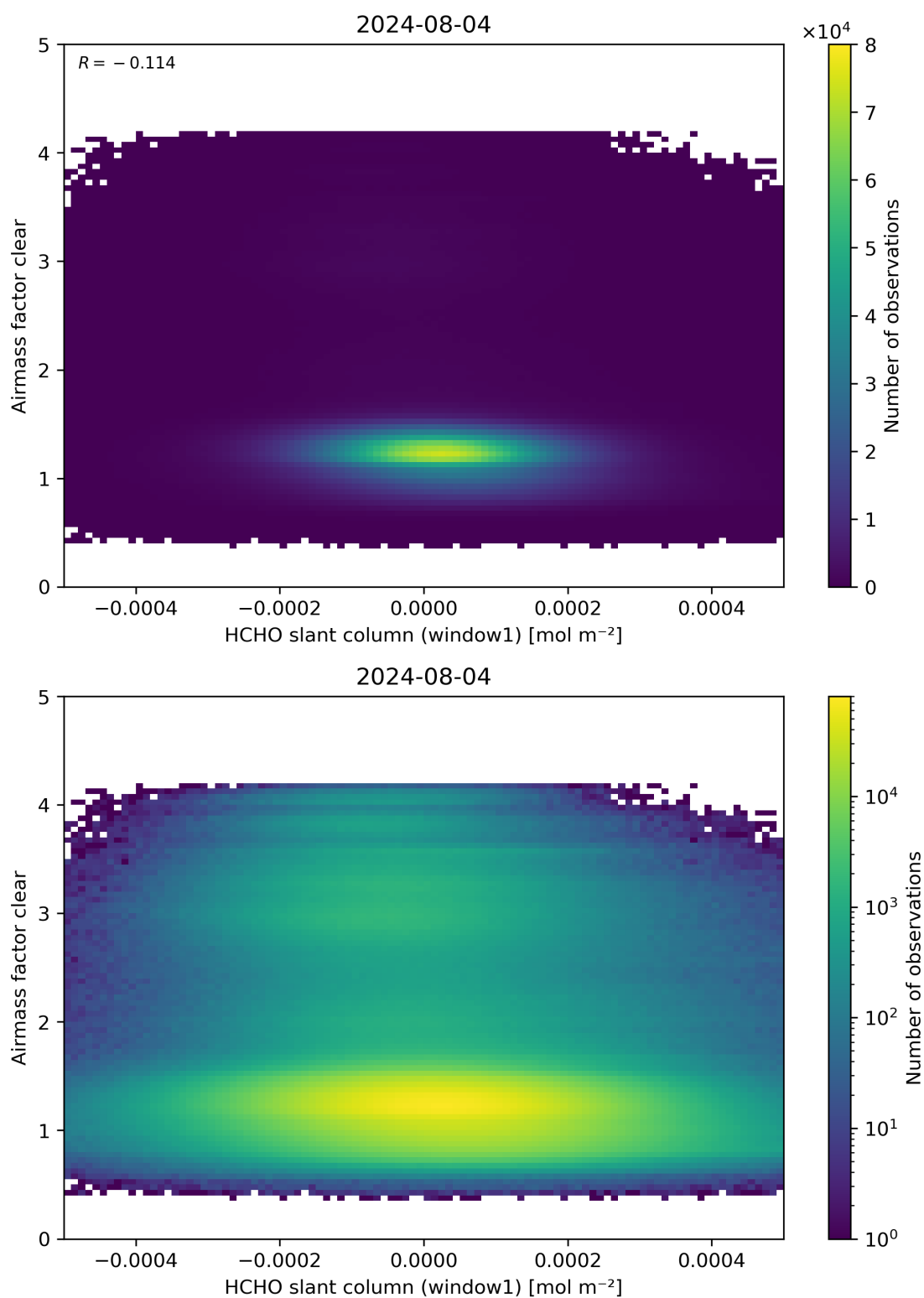
Figure 81: Scatter density plot of “HCHO slant column (window1)” against “Airmass factor clear” for 2024-08-03 to 2024-08-05.
