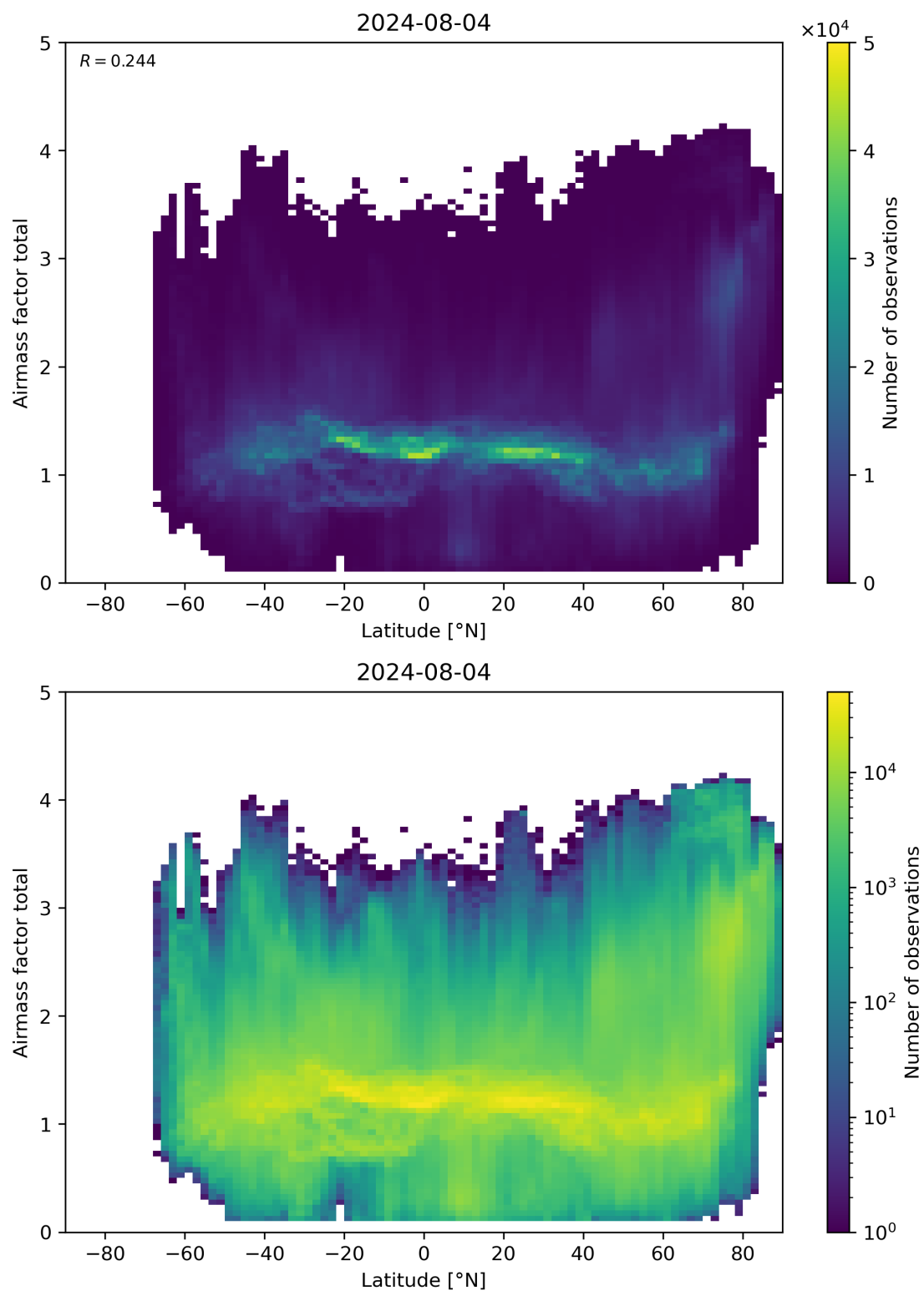
Figure 161: Scatter density plot of “Latitude” against “Airmass factor total” for 2024-08-03 to 2024-08-05.
