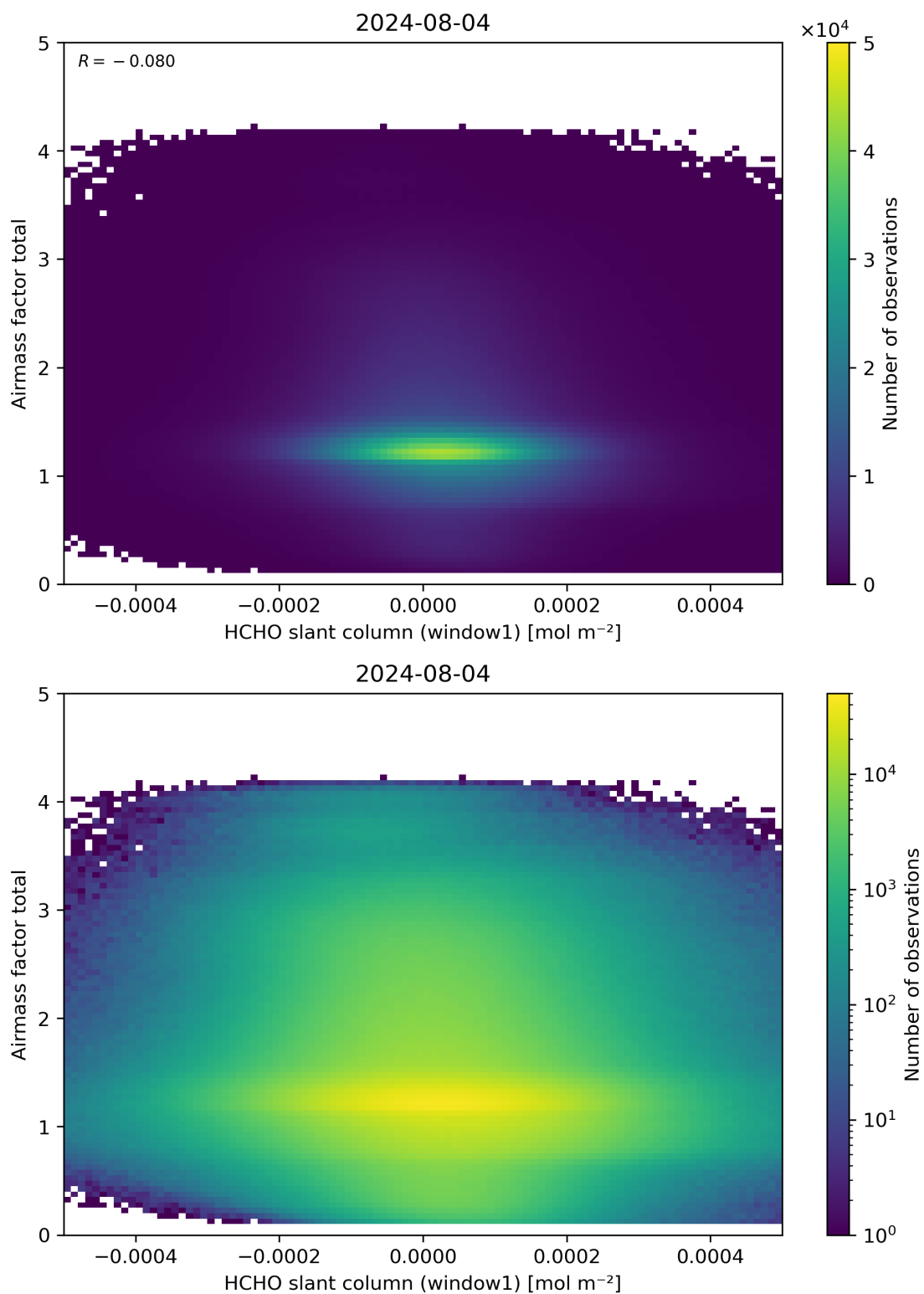
Figure 85: Scatter density plot of “HCHO slant column (window1)” against “Airmass factor total” for 2024-08-03 to 2024-08-05.
