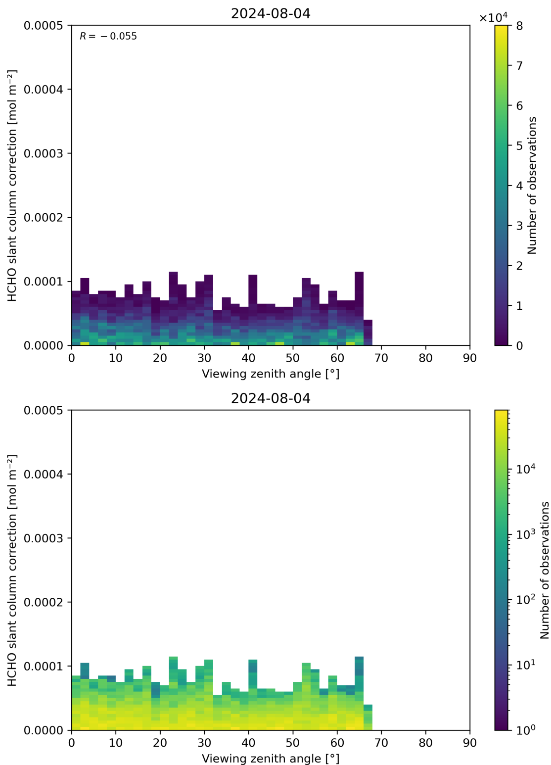
Figure 187: Scatter density plot of “Viewing zenith angle” against “HCHO slant column correction” for 2024-08-03 to 2024-08-05.
