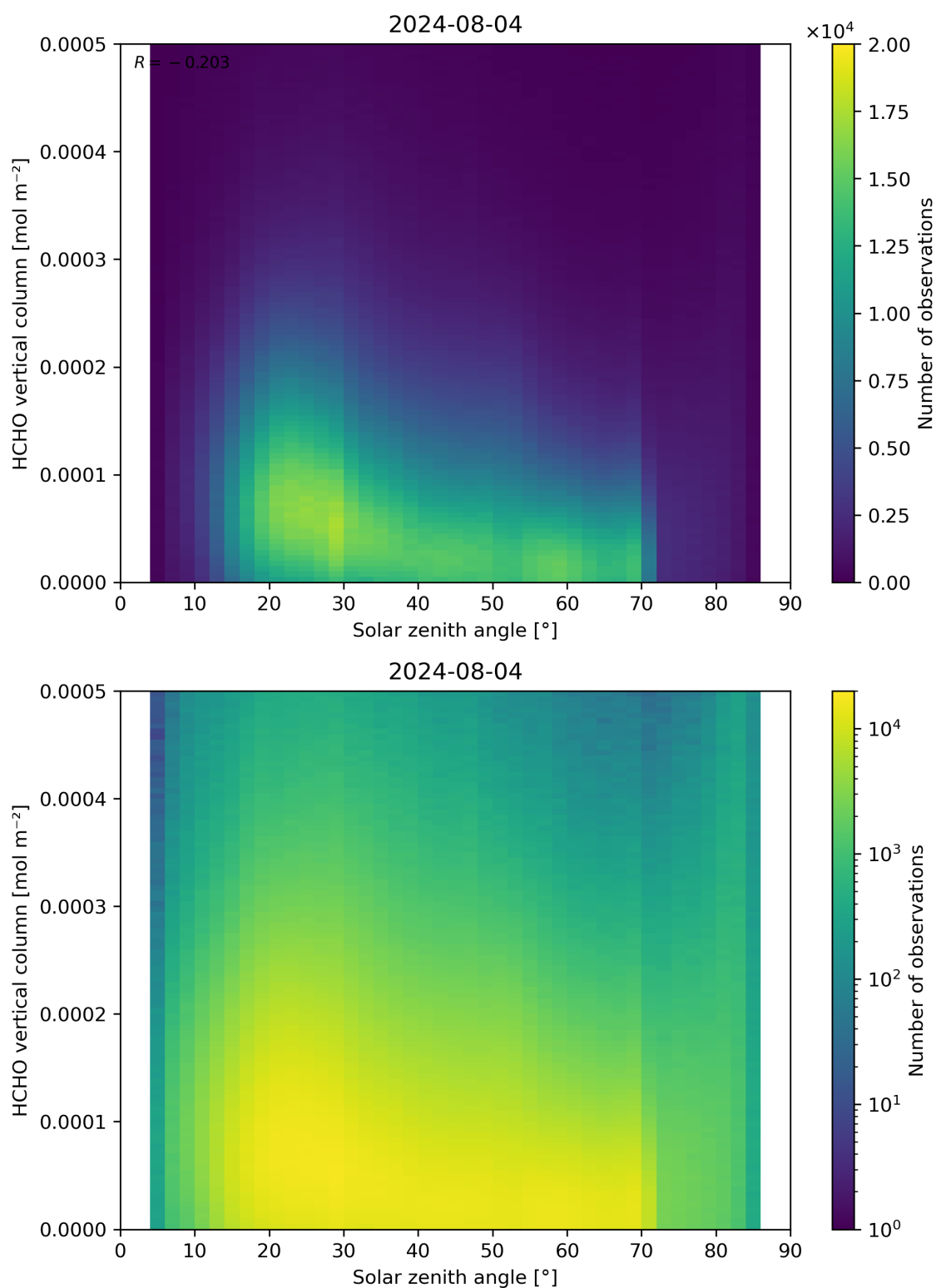
Figure 177: Scatter density plot of “Solar zenith angle” against “HCHO vertical column” for 2024-08-03 to 2024-08-05.
