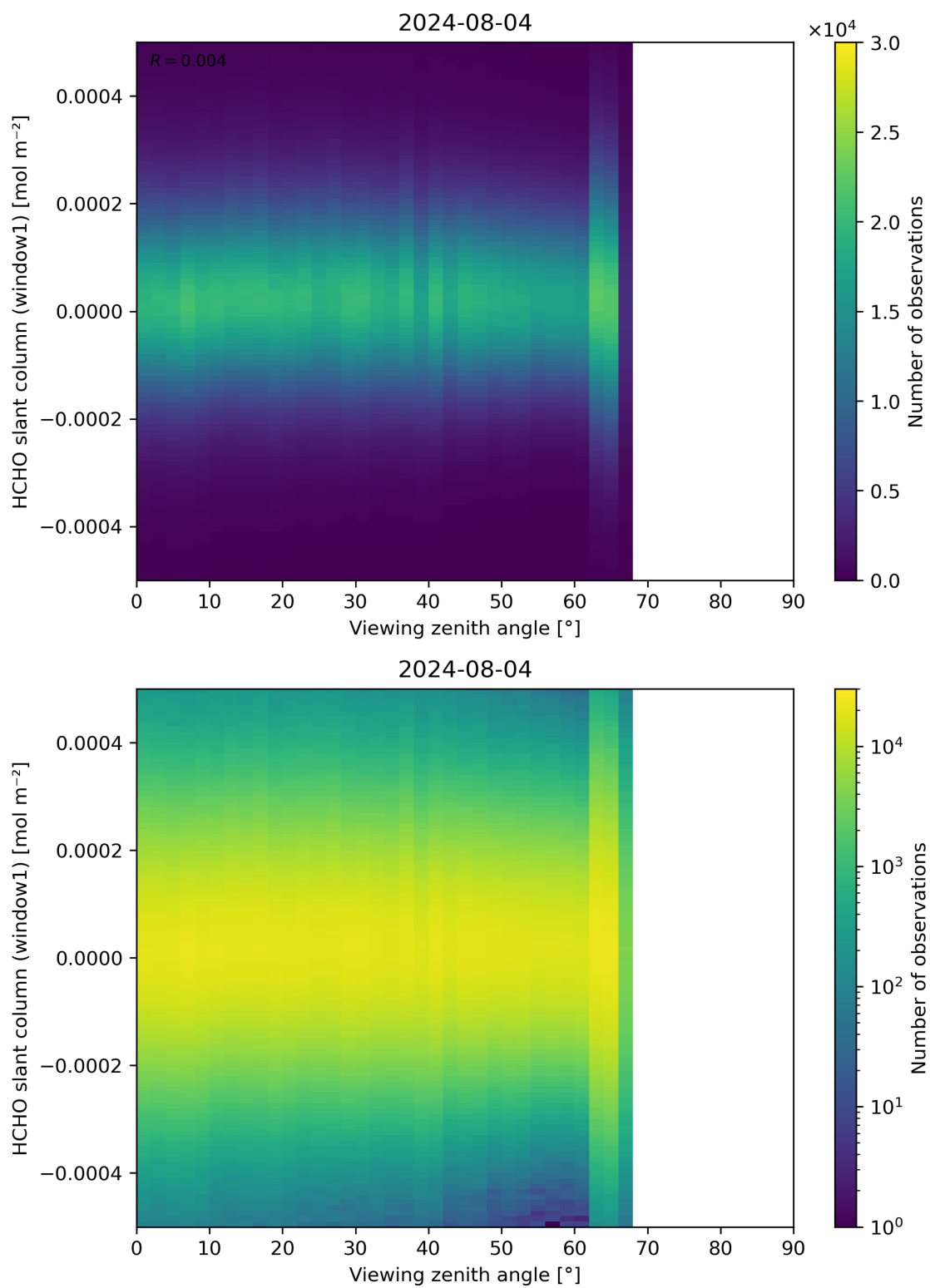
Figure 188: Scatter density plot of “Viewing zenith angle” against “HCHO slant column (window1)” for 2024-08-03 to 2024-08-05.
