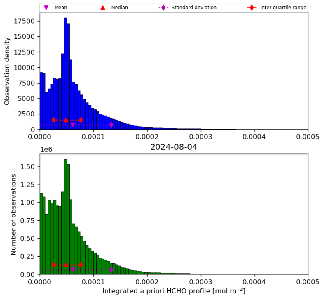
Figure 43: Histogram of “Integrated a priori HCHO profile” for 2024-08-03 to 2024-08-05
