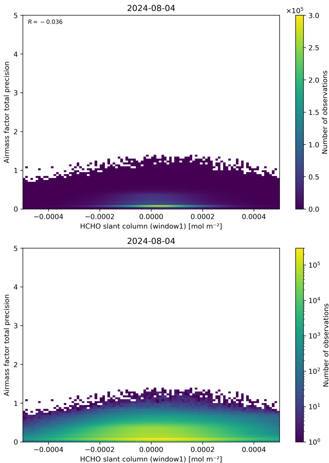
Figure 86: Scatter density plot of “HCHO slant column (window1)” against “Airmass factor total precision” for 2024-08-03 to 2024-08-05.
