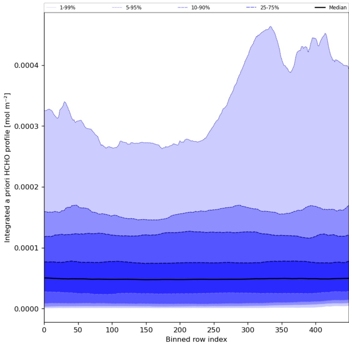
Figure 57: Along track statistics of “Integrated a priori HCHO profile” for 2024-08-03 to 2024-08-05
