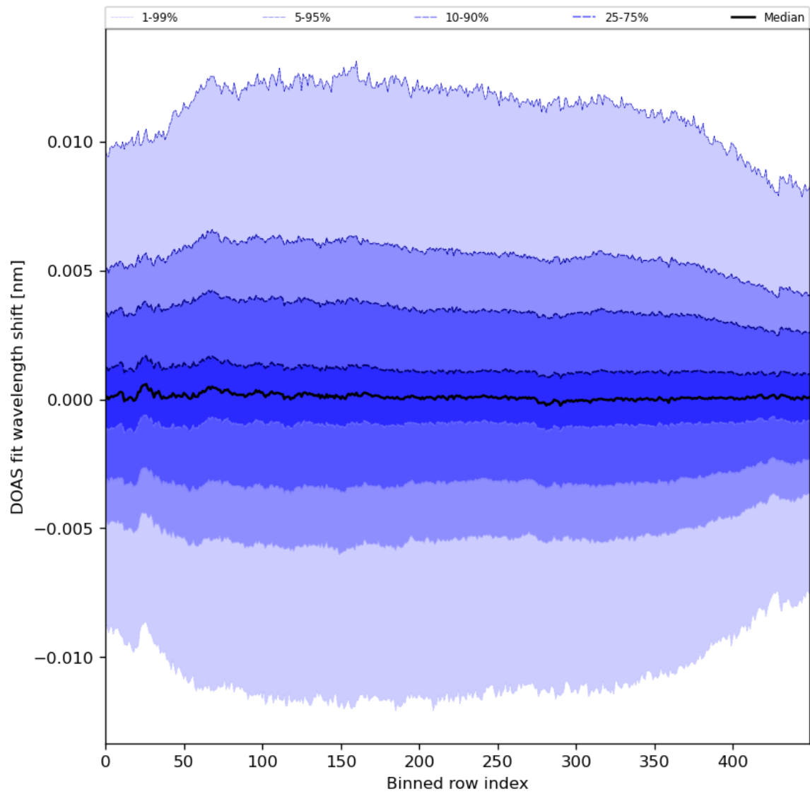
Figure 58: Along track statistics of “DOAS fit wavelength shift” for 2024-08-03 to 2024-08-05
