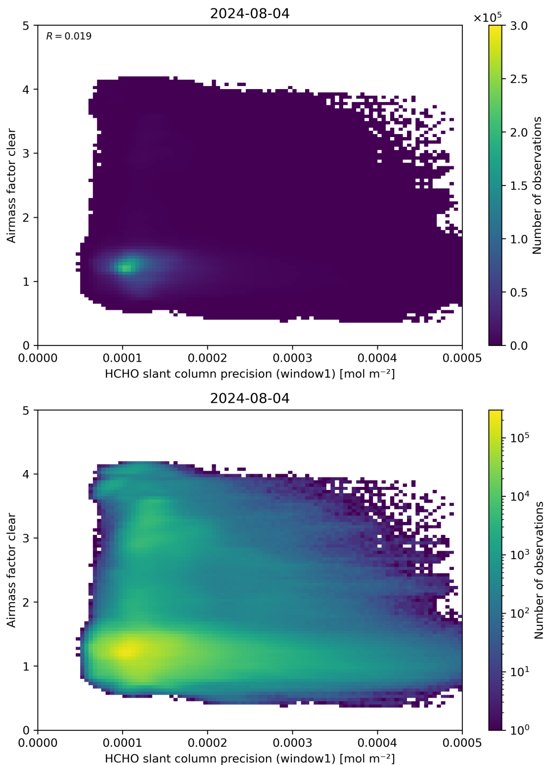
Figure 91: Scatter density plot of “HCHO slant column precision (window1)” against “Airmass factor clear” for 2024-08-03 to 2024-08-05.
