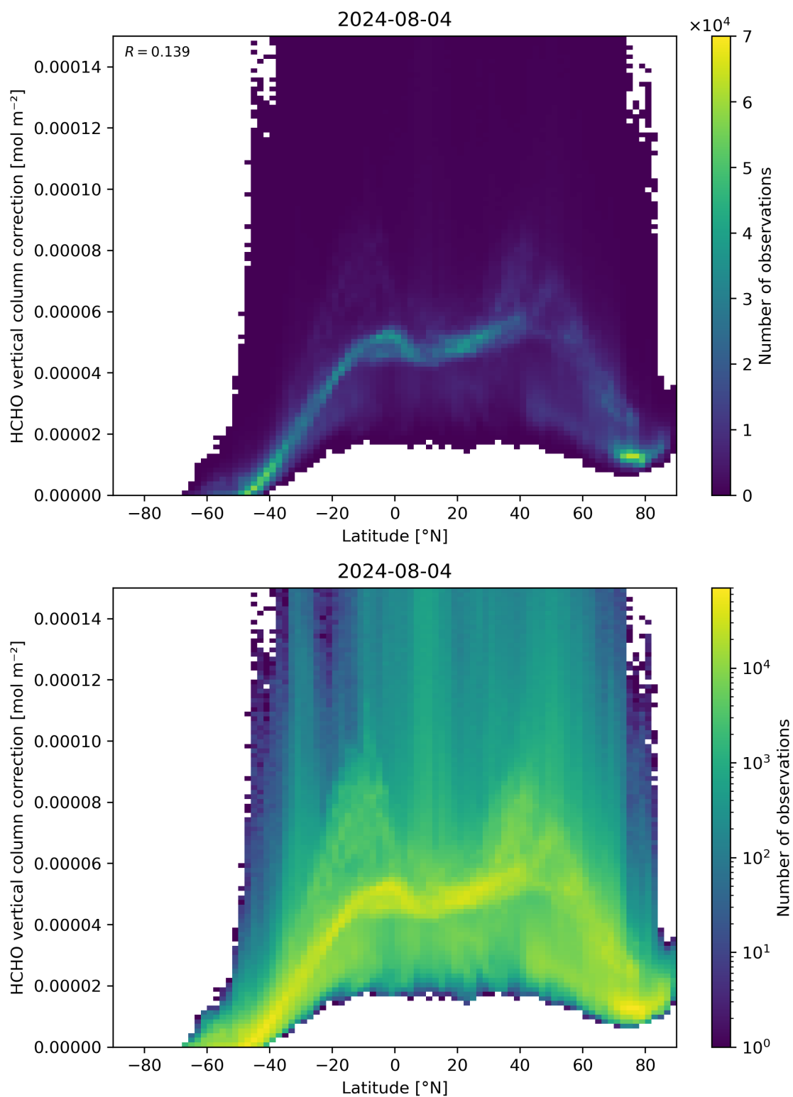
Figure 164: Scatter density plot of “Latitude” against “HCHO vertical column correction” for 2024-08-03 to 2024-08-05.
