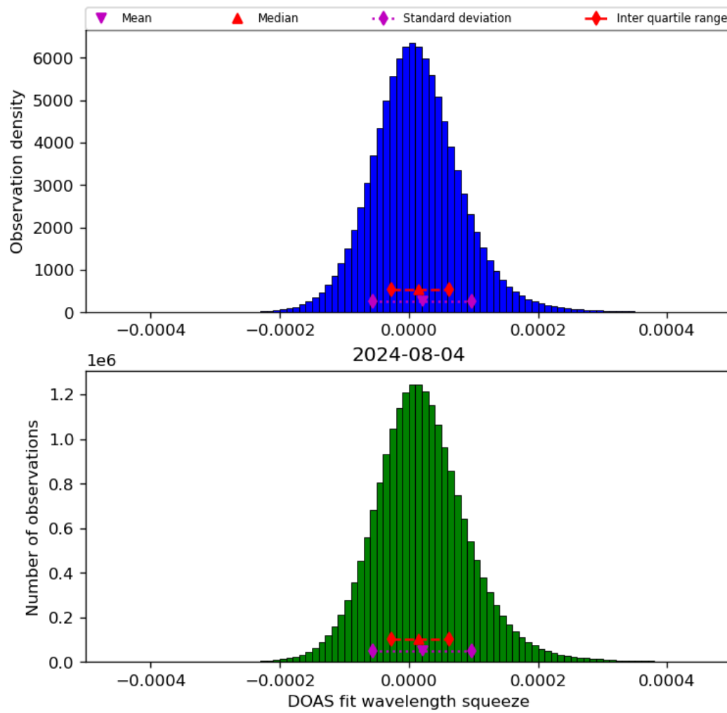
Figure 45: Histogram of “DOAS fit wavelength squeeze” for 2024-08-03 to 2024-08-05
