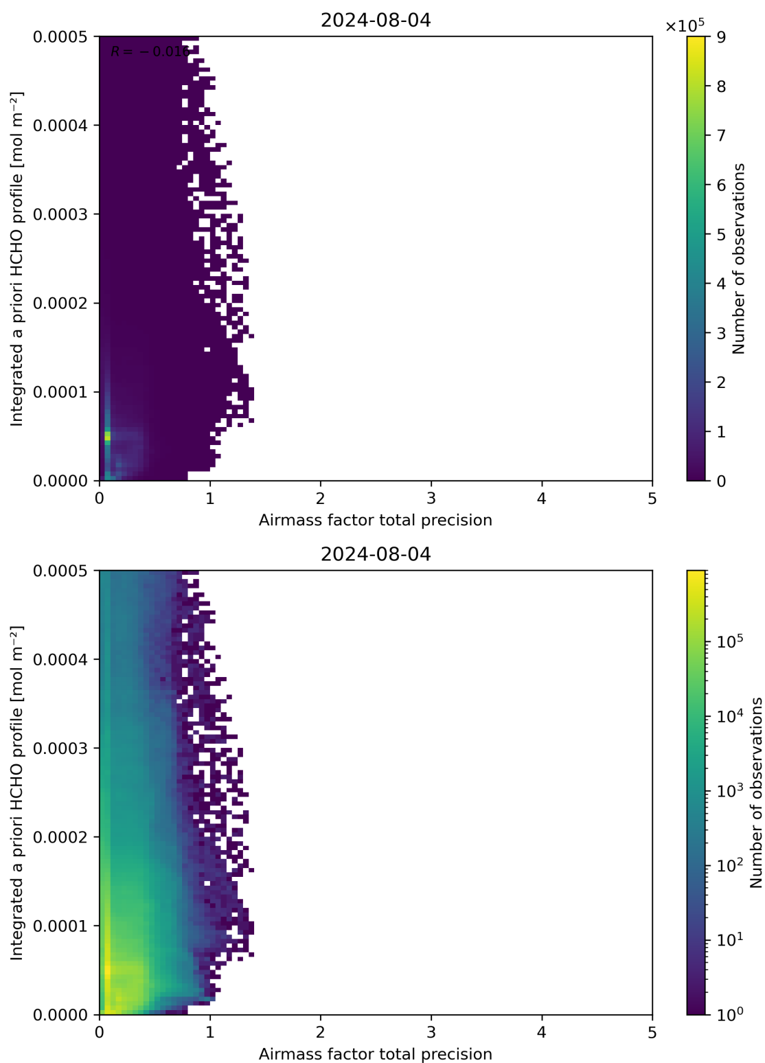
Figure 111: Scatter density plot of “Airmass factor total precision” against “Integrated a priori HCHO profile” for 2024-08-03 to 2024-08-05.
