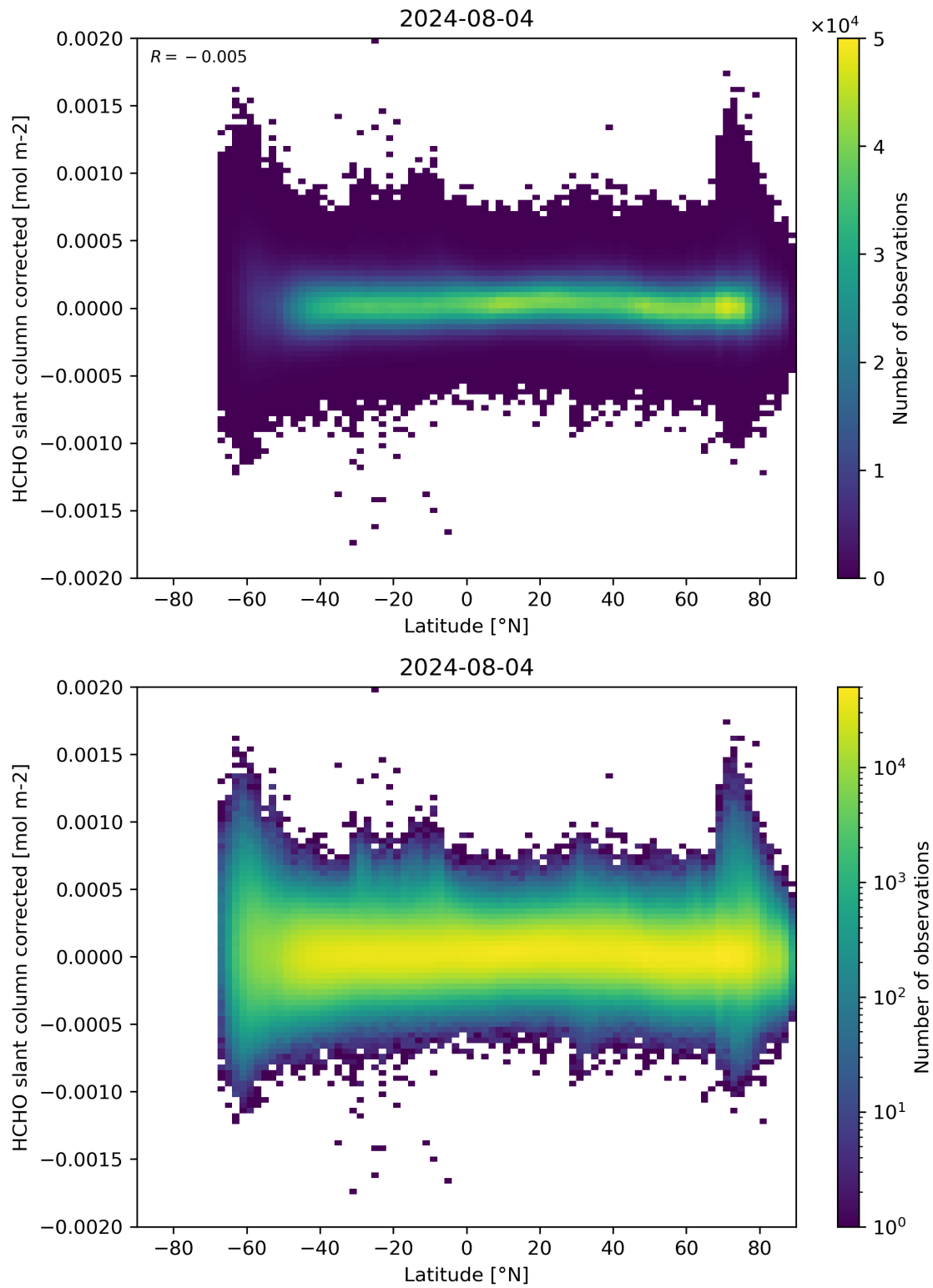
Figure 157: Scatter density plot of “Latitude” against “HCHO slant column corrected” for 2024-08-03 to 2024-08-05.
