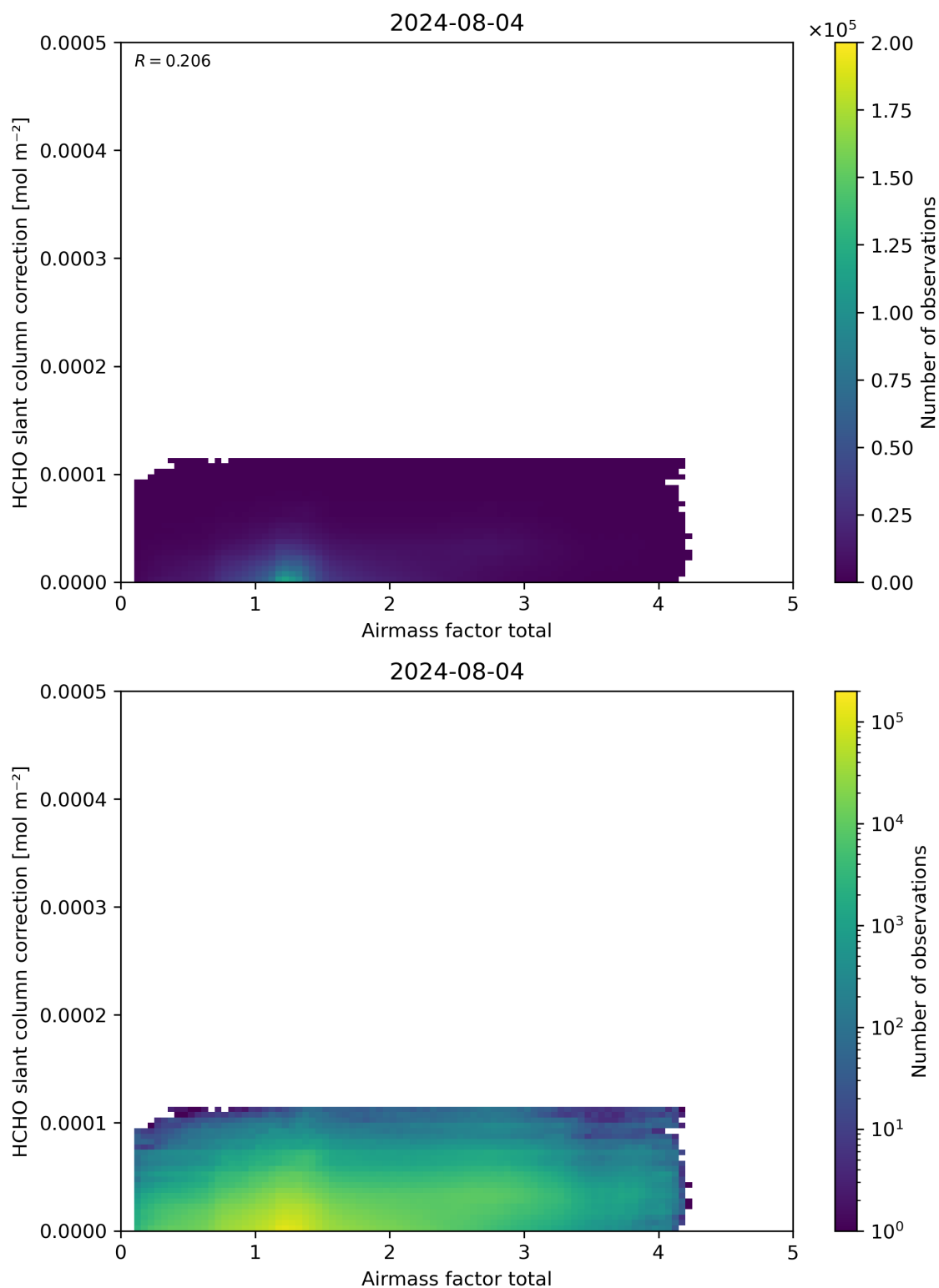
Figure 102: Scatter density plot of “Airmass factor total” against “HCHO slant column correction” for 2024-08-03 to 2024-08-05.
