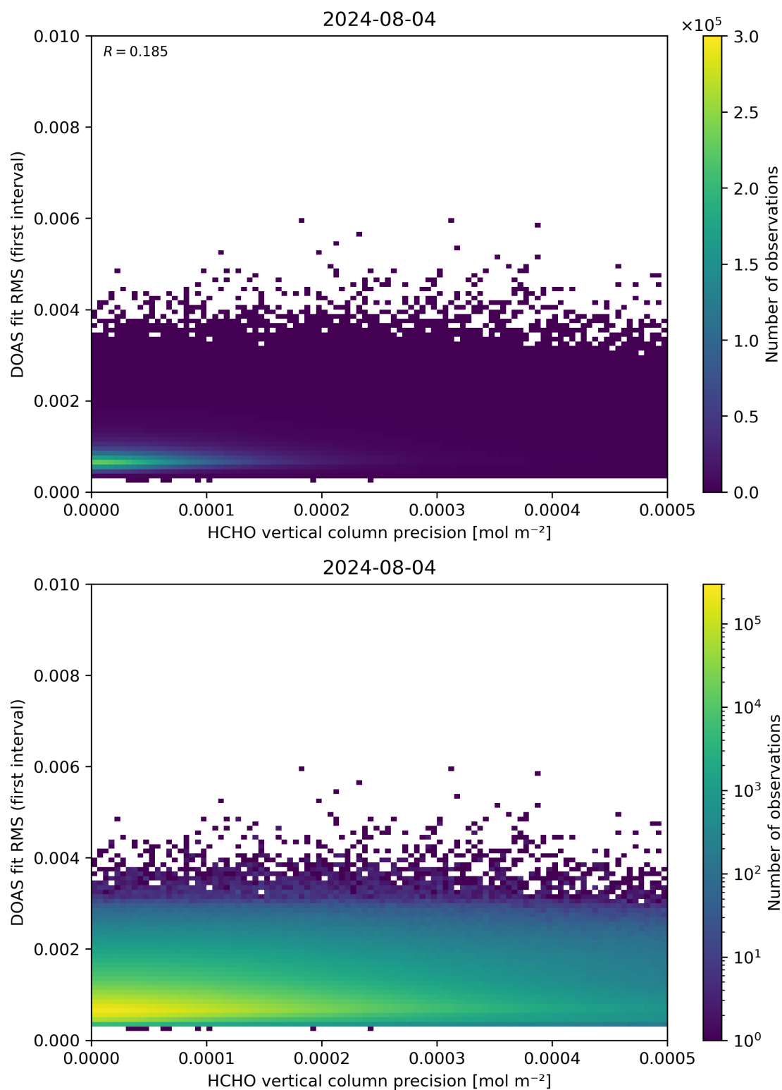
Figure 136: Scatter density plot of “HCHO vertical column precision” against “DOAS fit RMS (first interval)” for 2024-08-03 to 2024-08-05.
