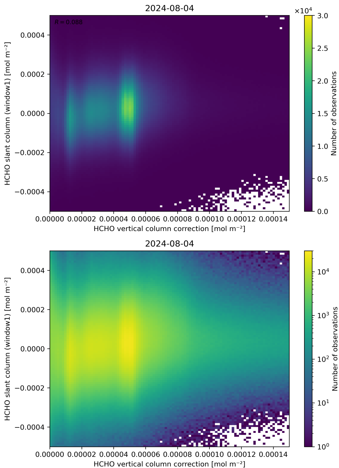
Figure 118: Scatter density plot of “HCHO vertical column correction” against “HCHO slant column (window1)” for 2024-08-03 to 2024-08-05.
