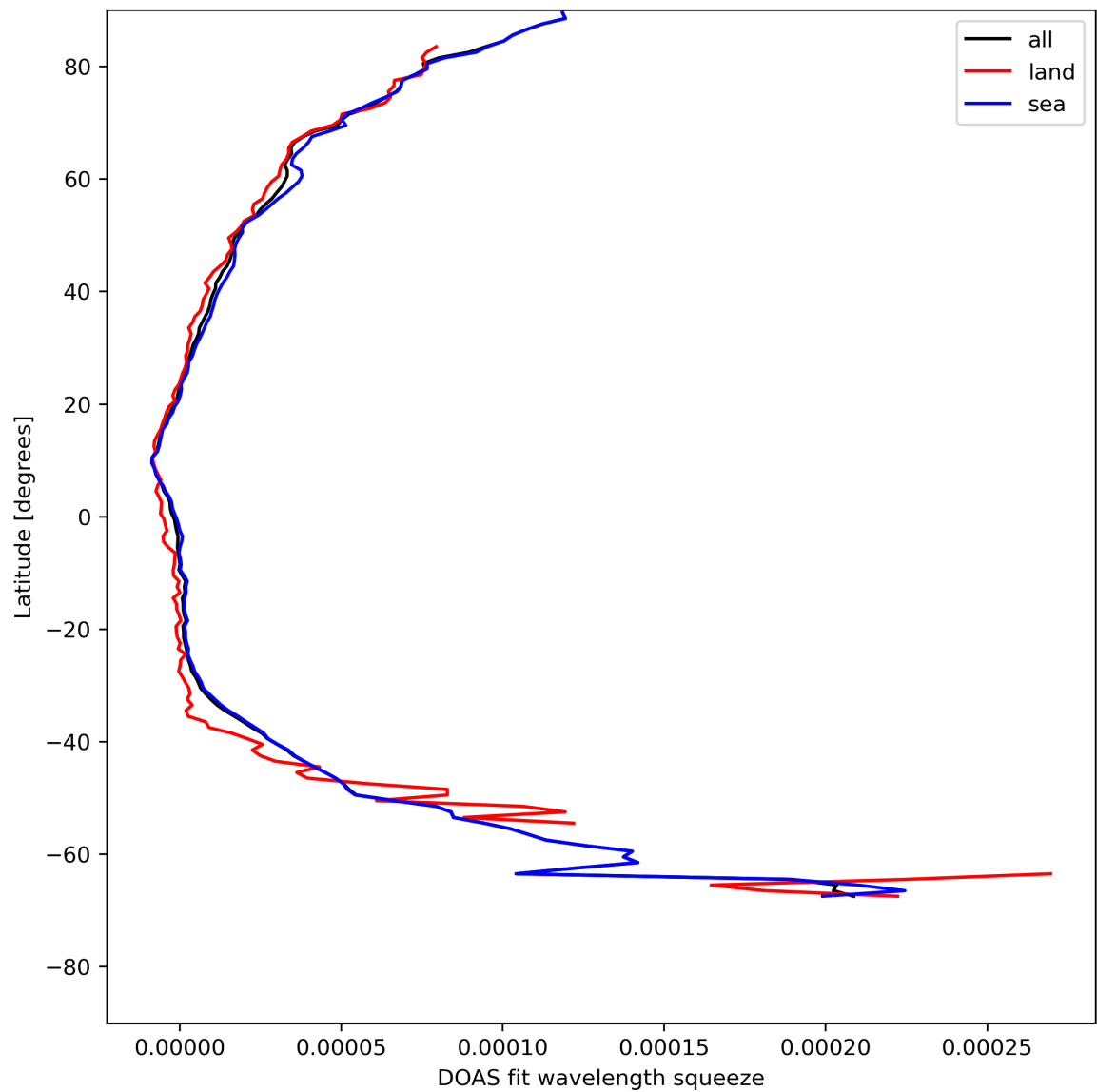
Figure 31: Zonal average of “DOAS fit wavelength squeeze” for 2024-08-03 to 2024-08-05.
