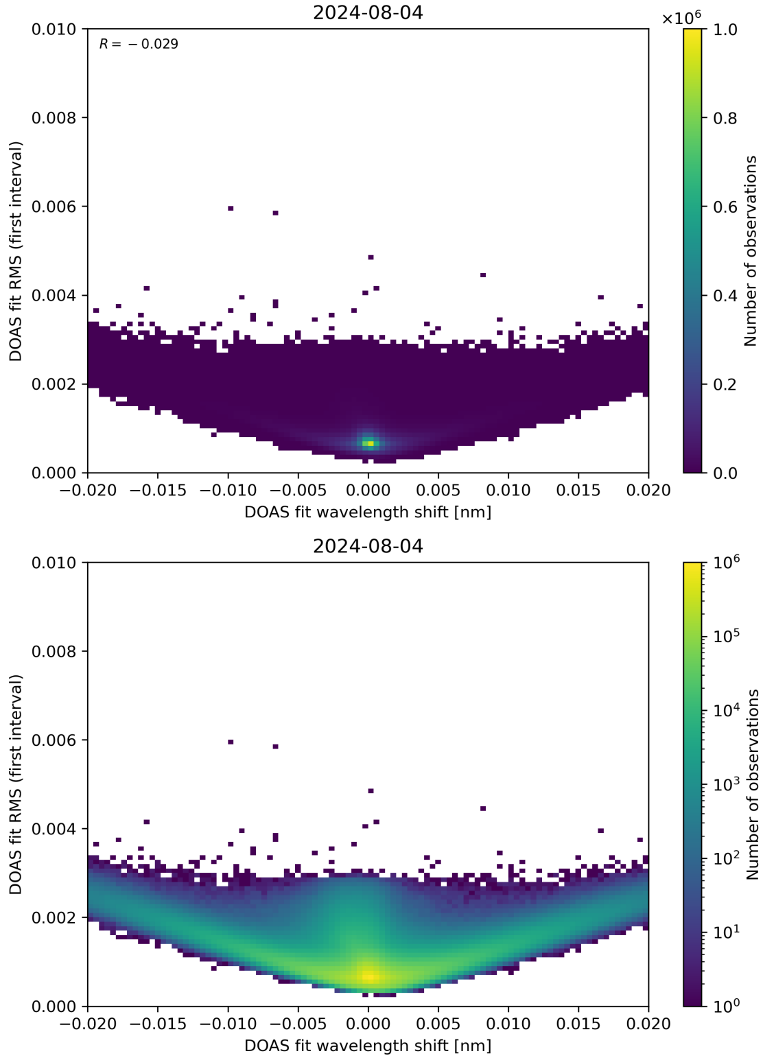
Figure 64: Scatter density plot of “DOAS fit wavelength shift” against “DOAS fit RMS (first interval)” for 2024-08-03 to 2024-08-05.
