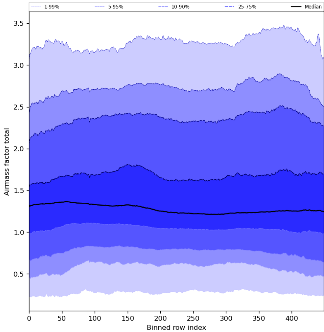
Figure 54: Along track statistics of “Airmass factor total” for 2024-08-03 to 2024-08-05
