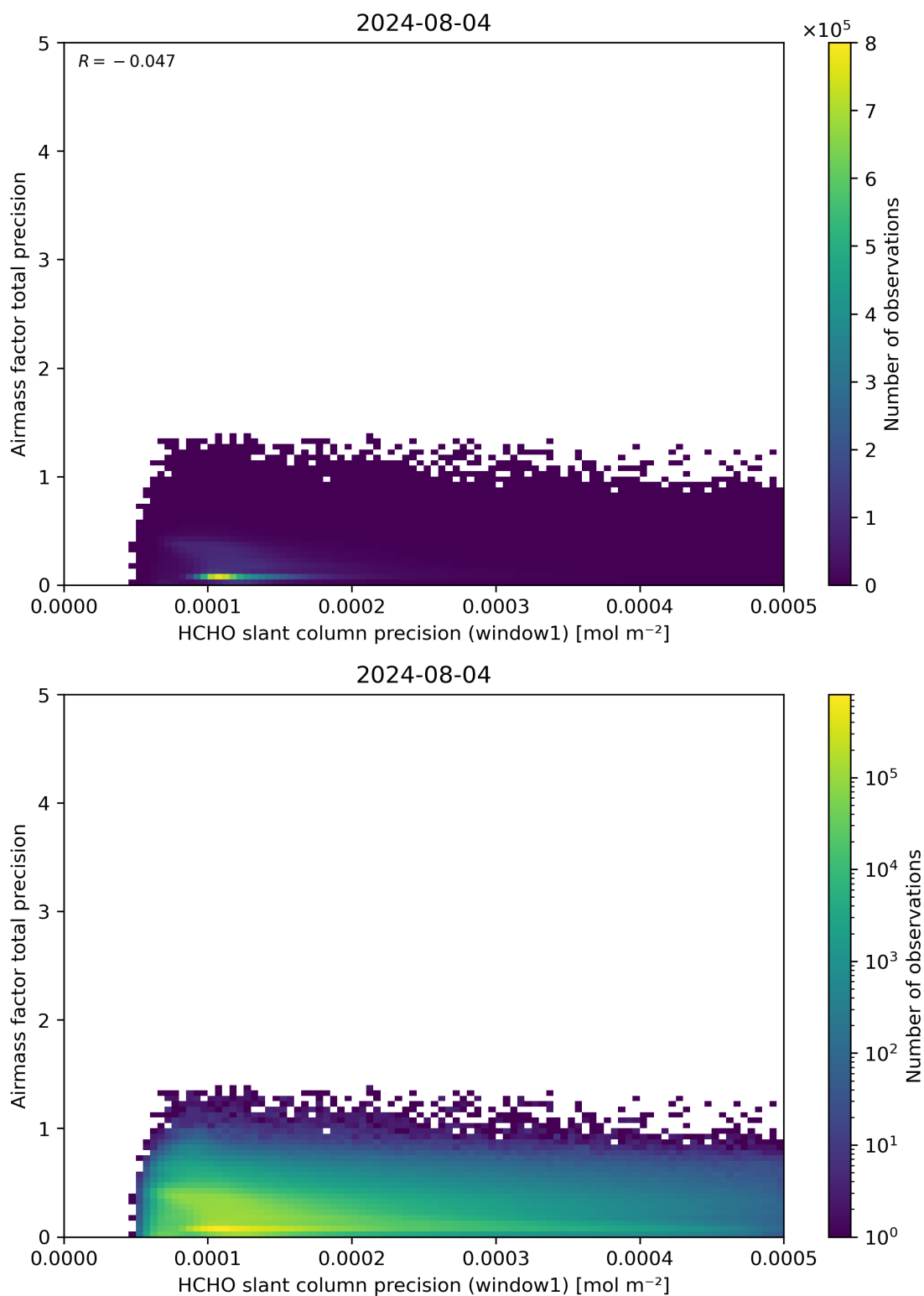
Figure 95: Scatter density plot of “HCHO slant column precision (window1)” against “Airmass factor total precision” for 2024-08-03 to 2024-08-05.
