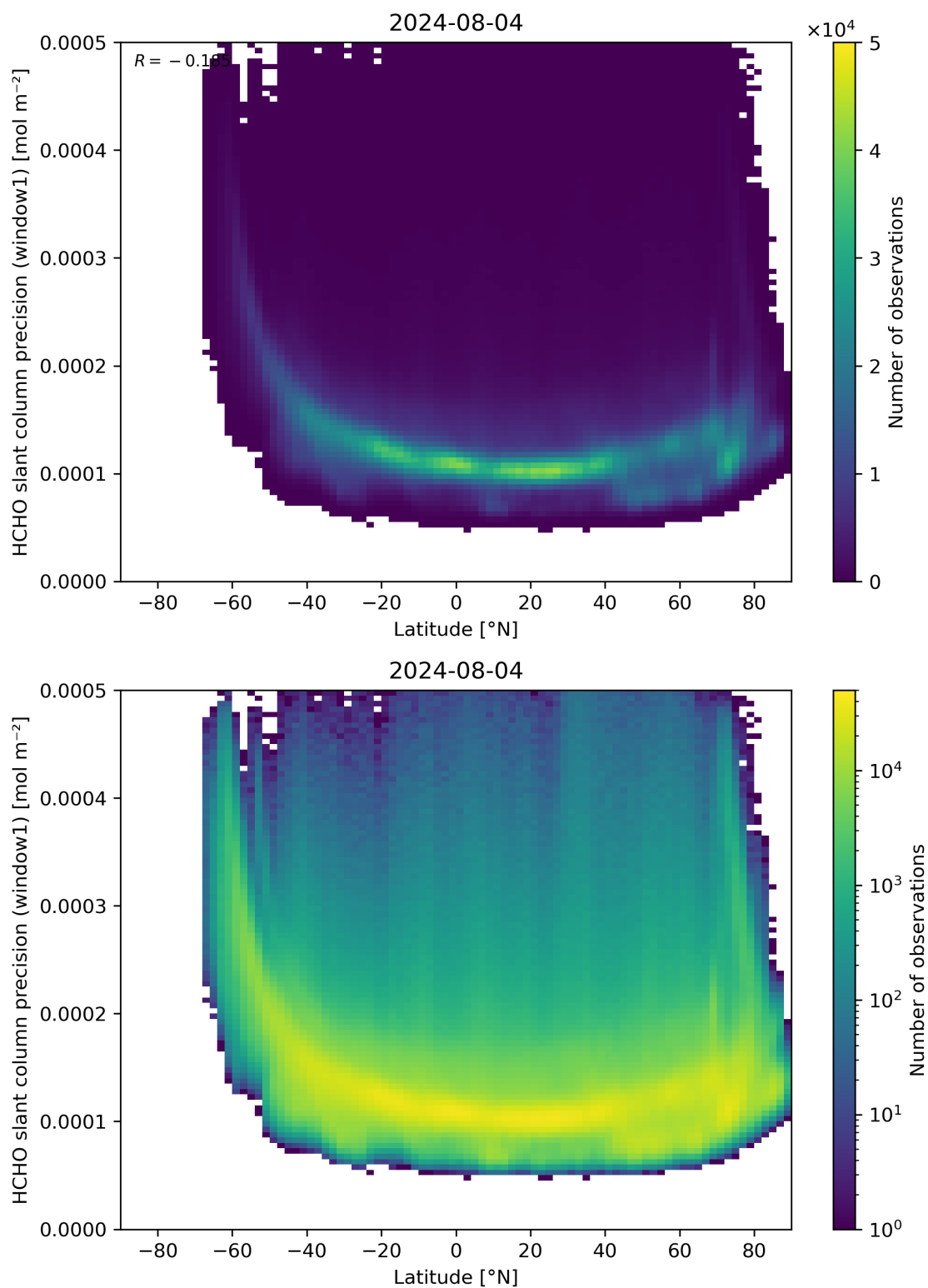
Figure 160: Scatter density plot of “Latitude” against “HCHO slant column precision (window1)” for 2024-08-03 to 2024-08-05.
