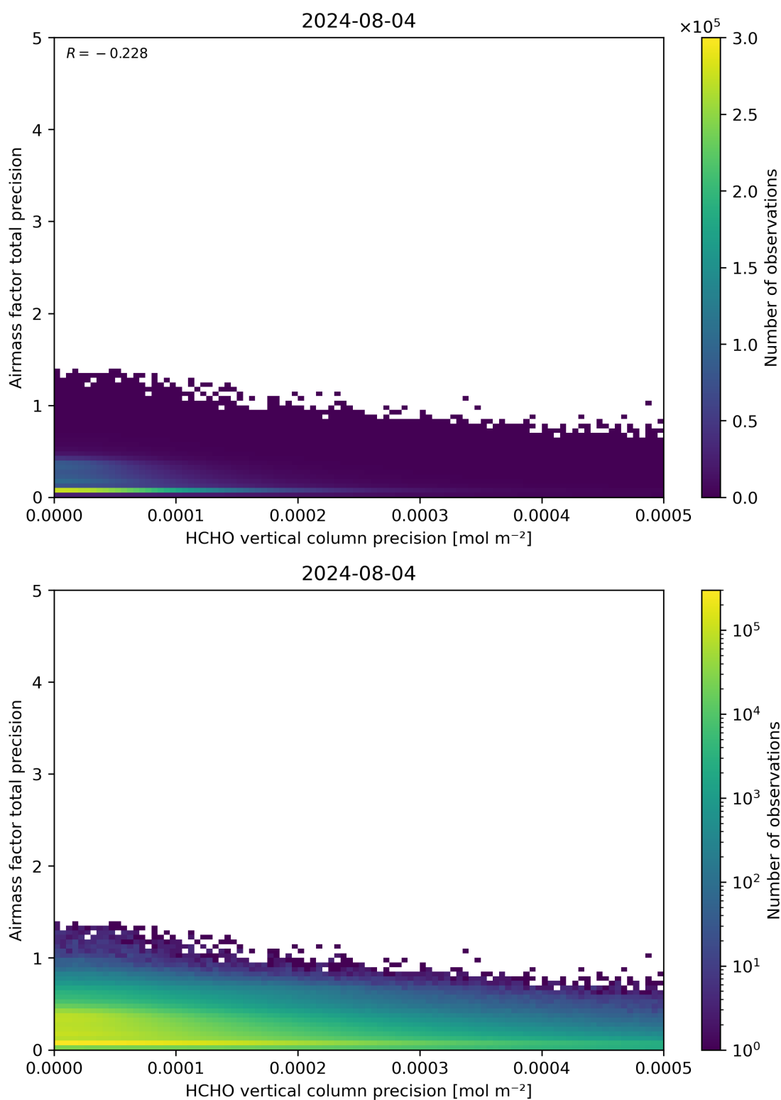
Figure 145: Scatter density plot of “HCHO vertical column precision” against “Airmass factor total precision” for 2024-08-03 to 2024-08-05.
