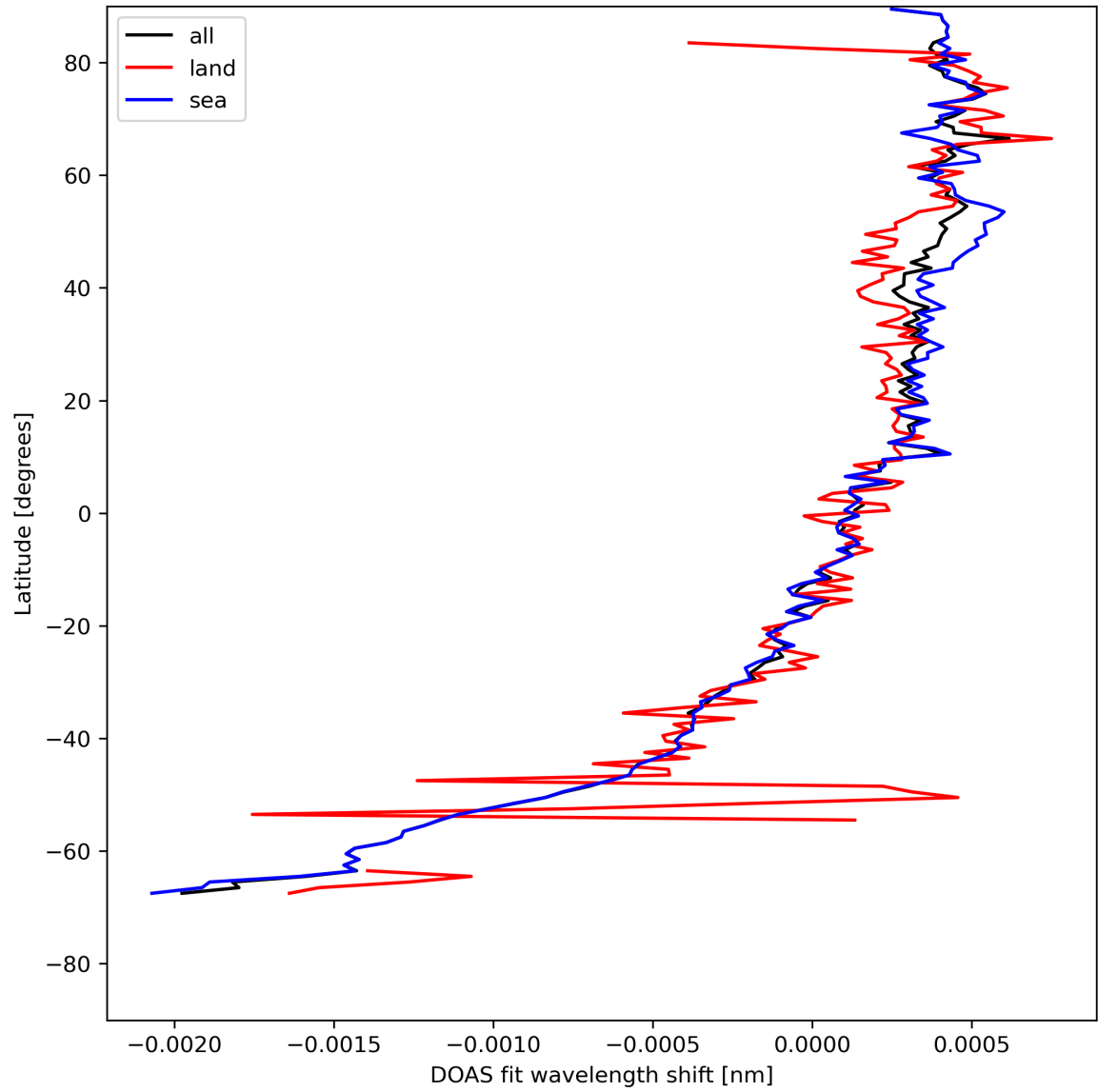
Figure 30: Zonal average of “DOAS fit wavelength shift” for 2024-08-03 to 2024-08-05.
