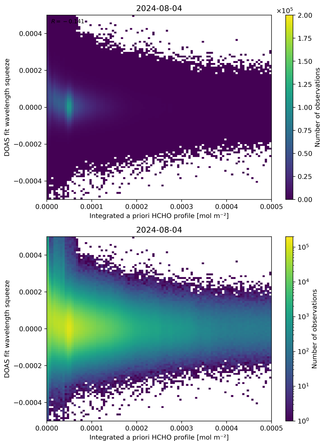
Figure 150: Scatter density plot of “Integrated a priori HCHO profile” against “DOAS fit wavelength squeeze” for 2024-08-03 to 2024-08-05.
