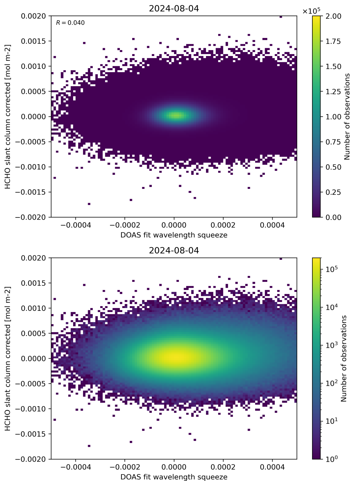
Figure 69: Scatter density plot of “DOAS fit wavelength squeeze” against “HCHO slant column corrected” for 2024-08-03 to 2024-08-05.
