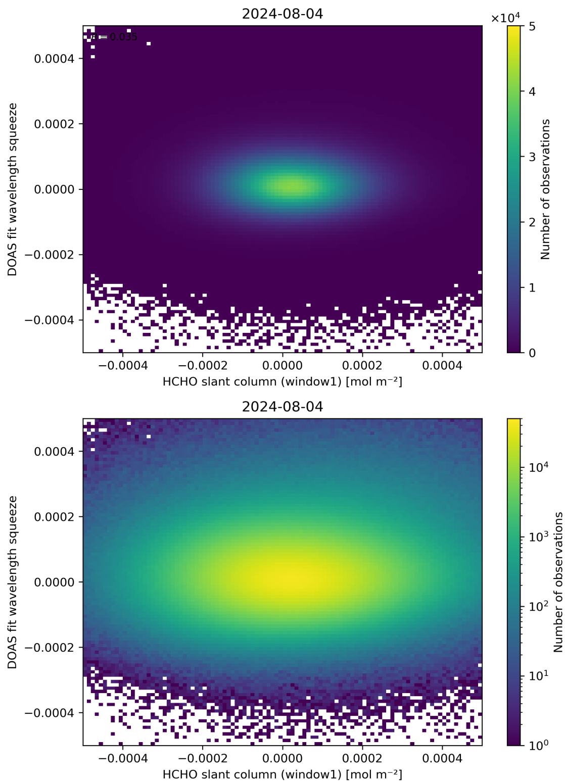
Figure 80: Scatter density plot of “HCHO slant column (window1)” against “DOAS fit wavelength squeeze” for 2024-08-03 to 2024-08-05.
