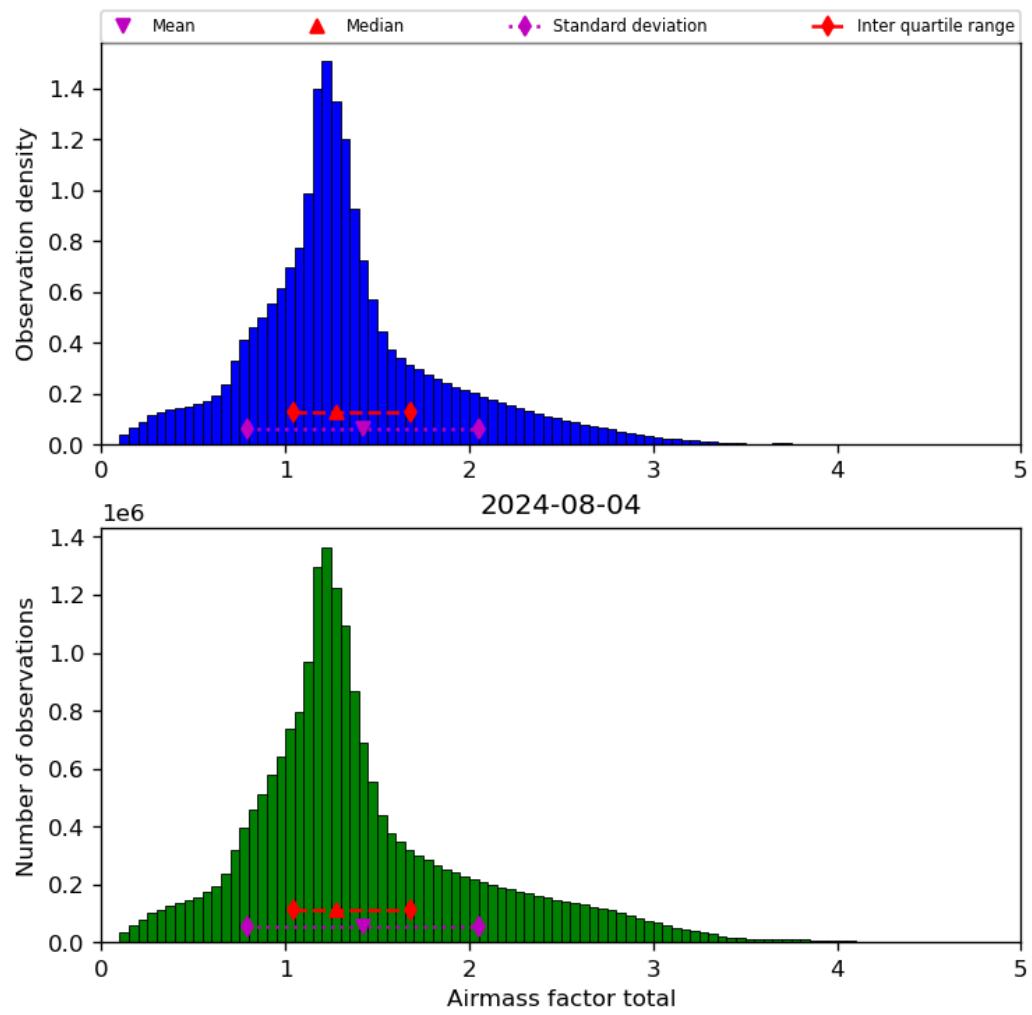
Figure 40: Histogram of “Airmass factor total” for 2024-08-03 to 2024-08-05
