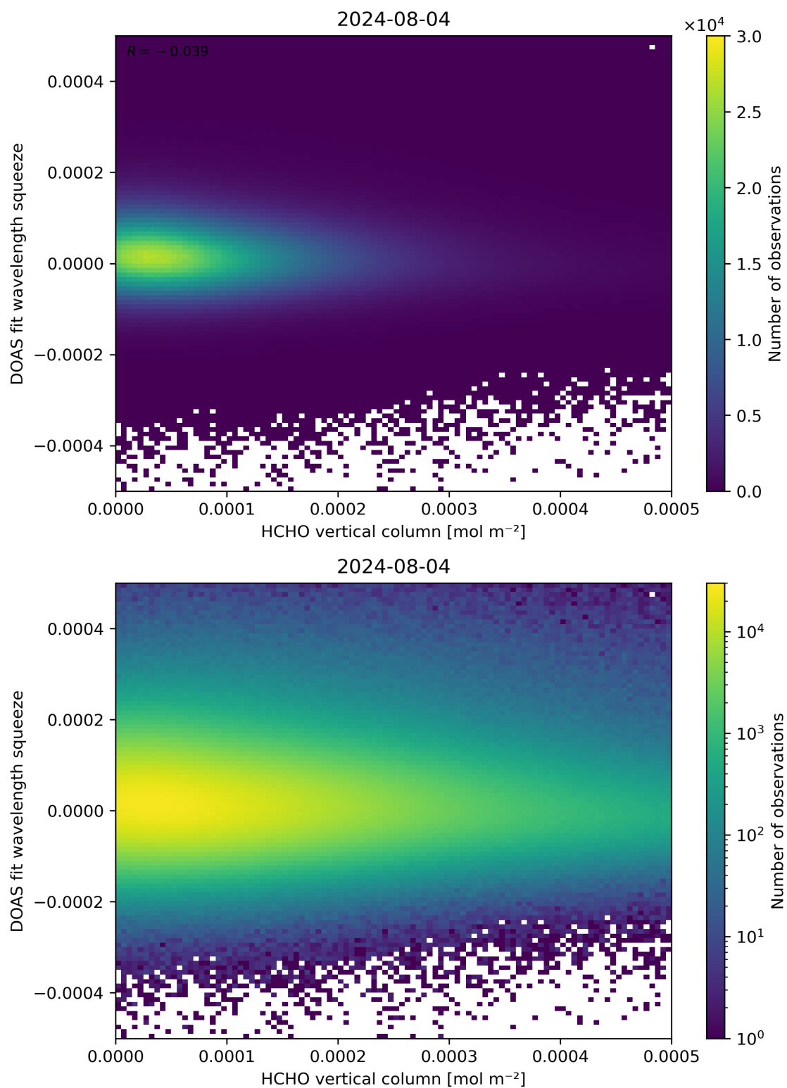
Figure 125: Scatter density plot of “HCHO vertical column” against “DOAS fit wavelength squeeze” for 2024-08-03 to 2024-08-05.
