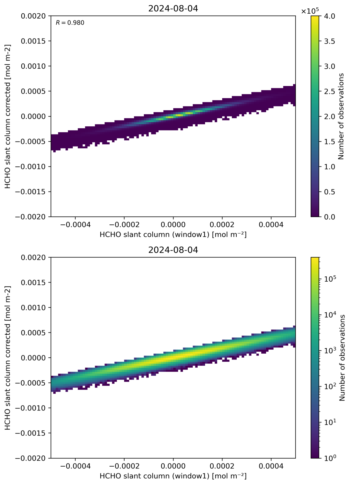
Figure 82: Scatter density plot of “HCHO slant column (window1)” against “HCHO slant column corrected” for 2024-08-03 to 2024-08-05.
