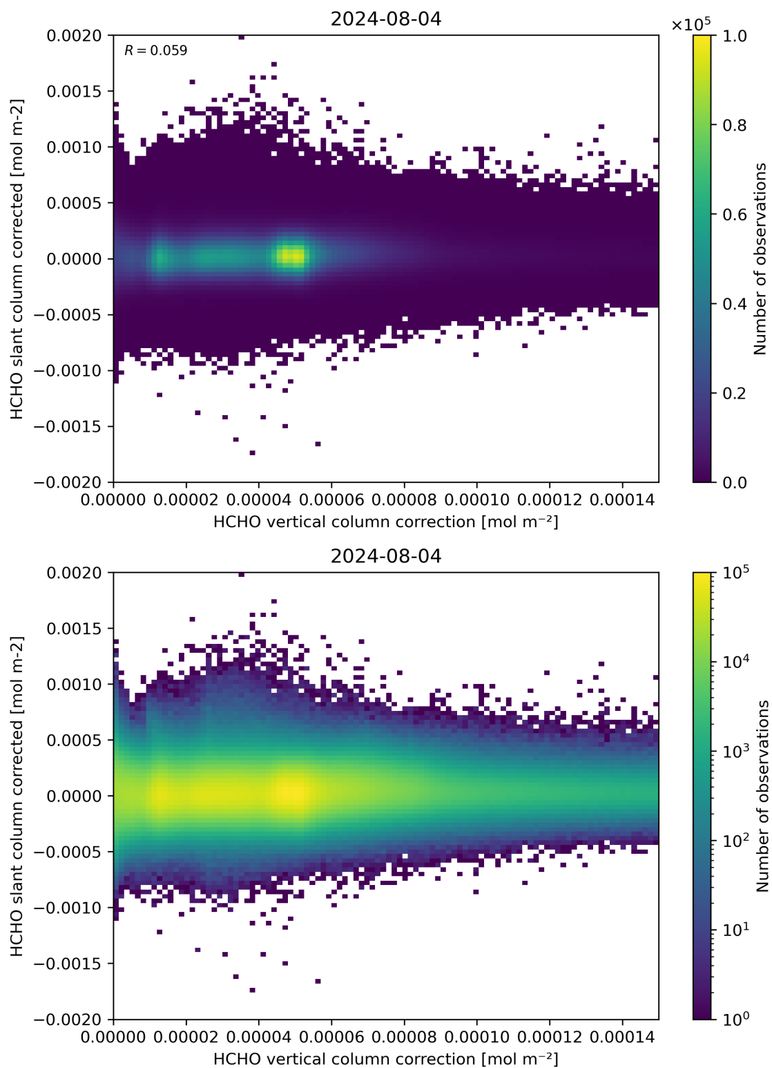
Figure 116: Scatter density plot of “HCHO vertical column correction” against “HCHO slant column corrected” for 2024-08-03 to 2024-08-05.
