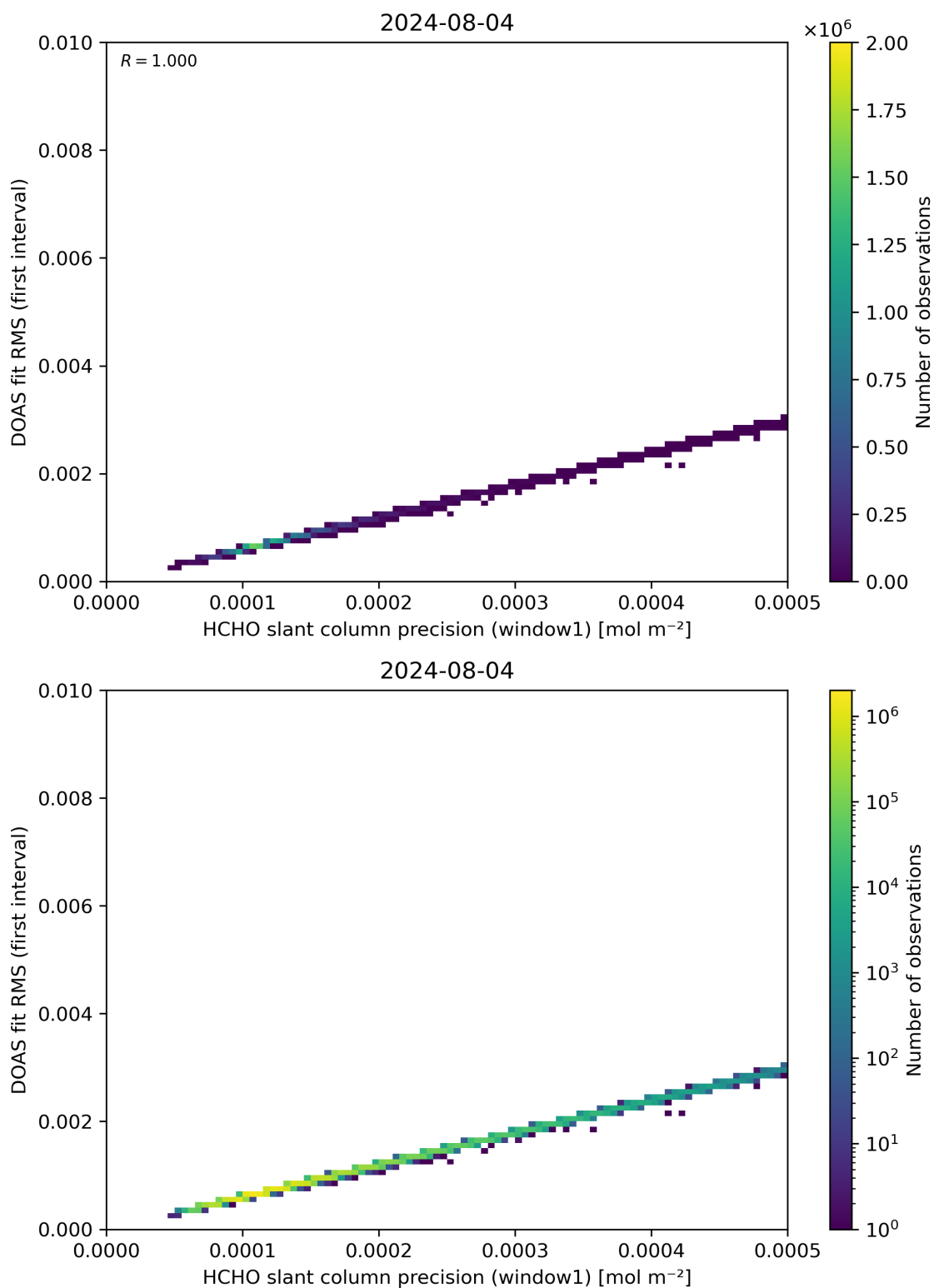
Figure 88: Scatter density plot of “HCHO slant column precision (window1)” against “DOAS fit RMS (first interval)” for 2024-08-03 to 2024-08-05.
