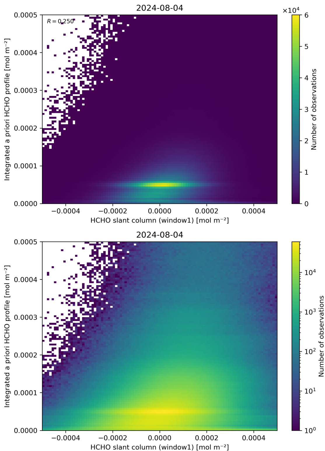
Figure 87: Scatter density plot of “HCHO slant column (window1)” against “Integrated a priori HCHO profile” for 2024-08-03 to 2024-08-05.
