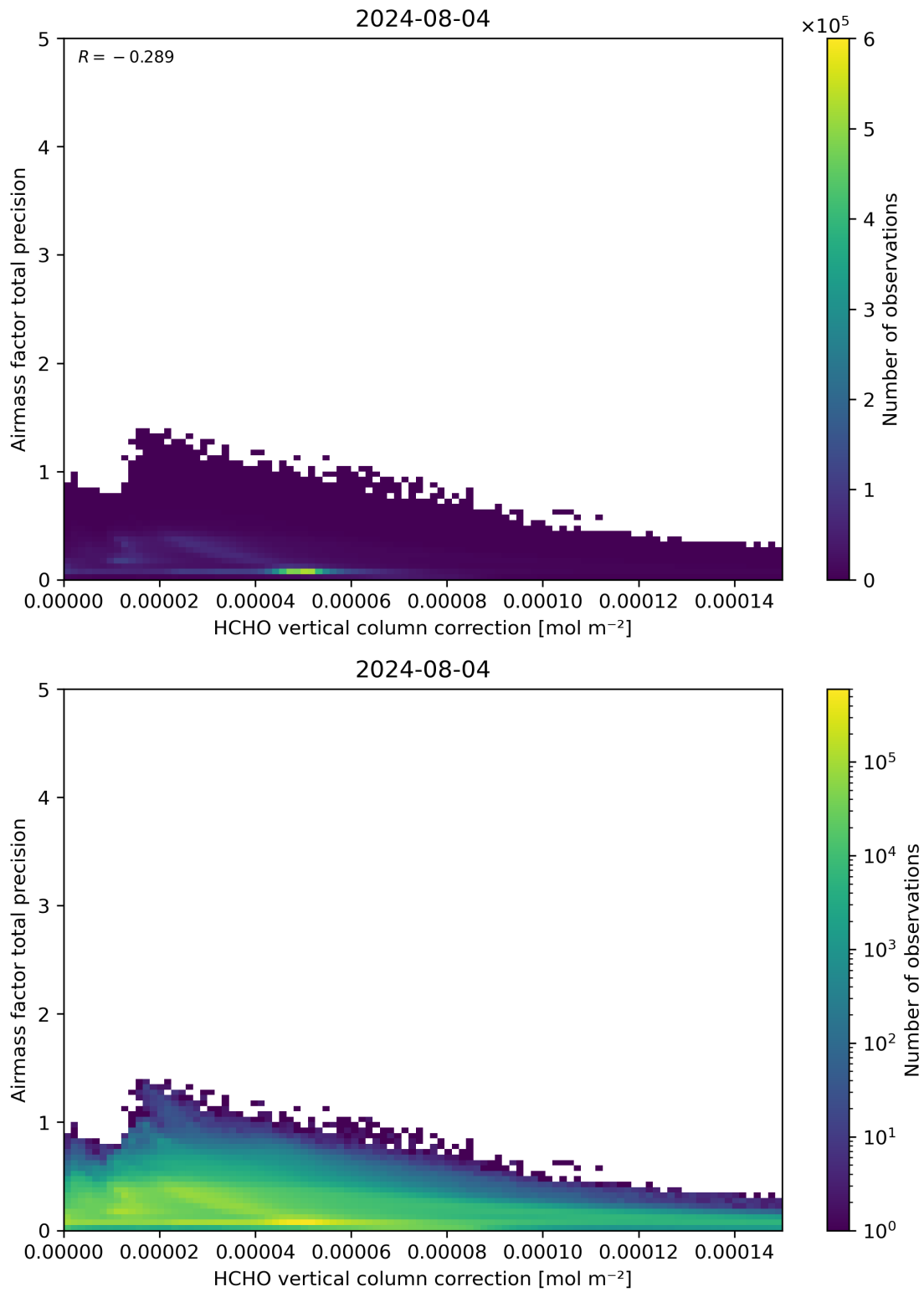
Figure 121: Scatter density plot of “HCHO vertical column correction” against “Airmass factor total precision” for 2024-08-03 to 2024-08-05.
