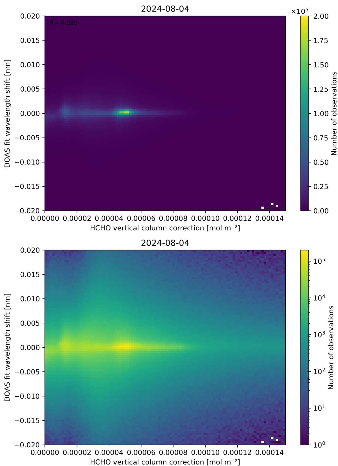
Figure 113: Scatter density plot of “HCHO vertical column correction” against “DOAS fit wavelength shift” for 2024-08-03 to 2024-08-05.
