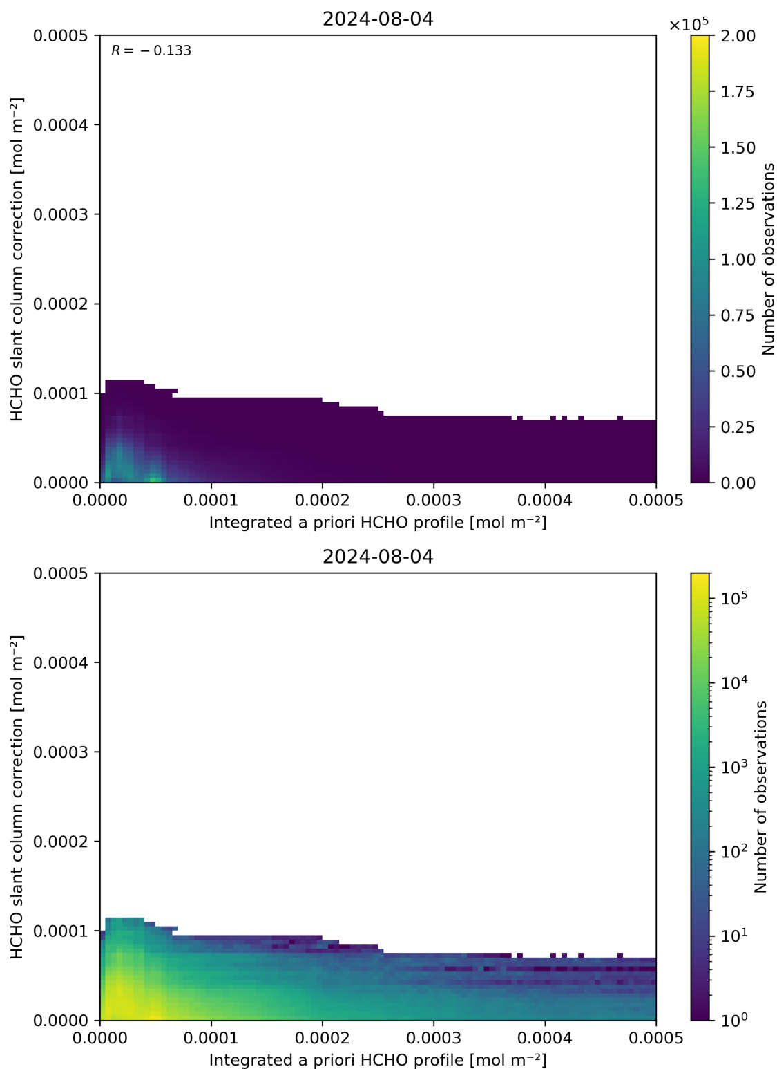
Figure 152: Scatter density plot of “Integrated a priori HCHO profile” against “HCHO slant column correction” for 2024-08-03 to 2024-08-05.
