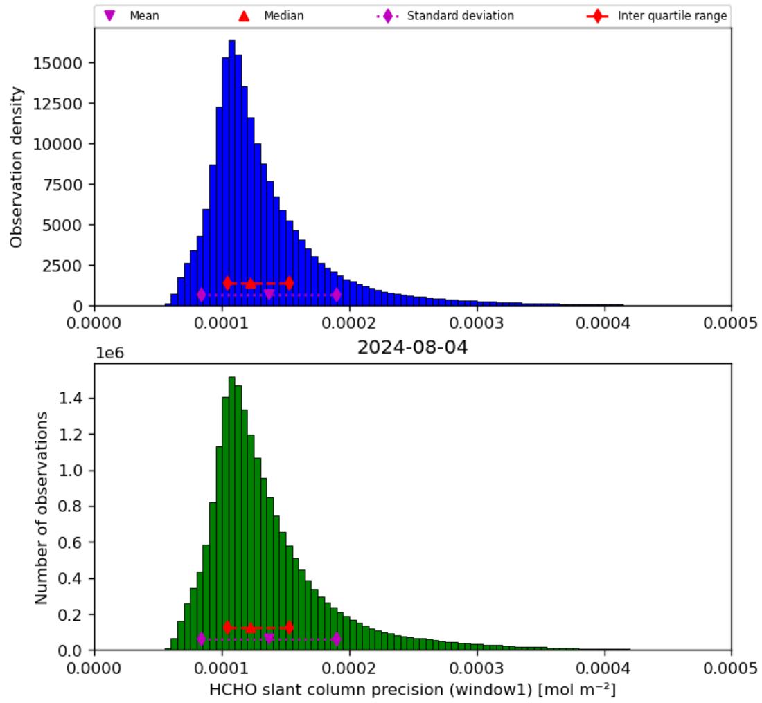
Figure 39: Histogram of “HCHO slant column precision (window1)” for 2024-08-03 to 2024-08-05
