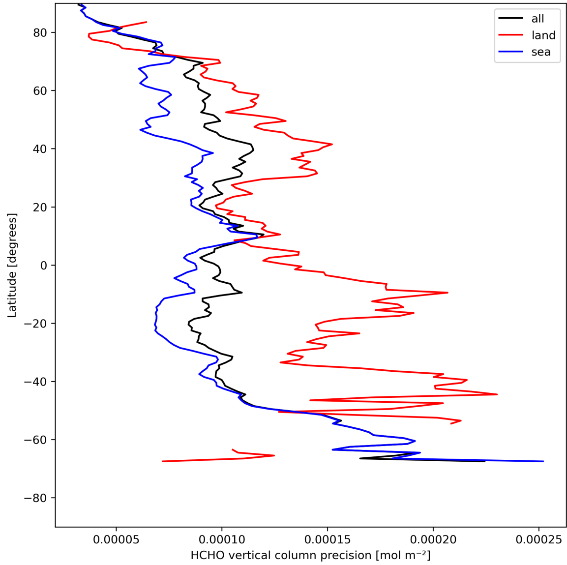
Figure 22: Zonal average of “HCHO vertical column precision” for 2024-08-03 to 2024-08-05.
