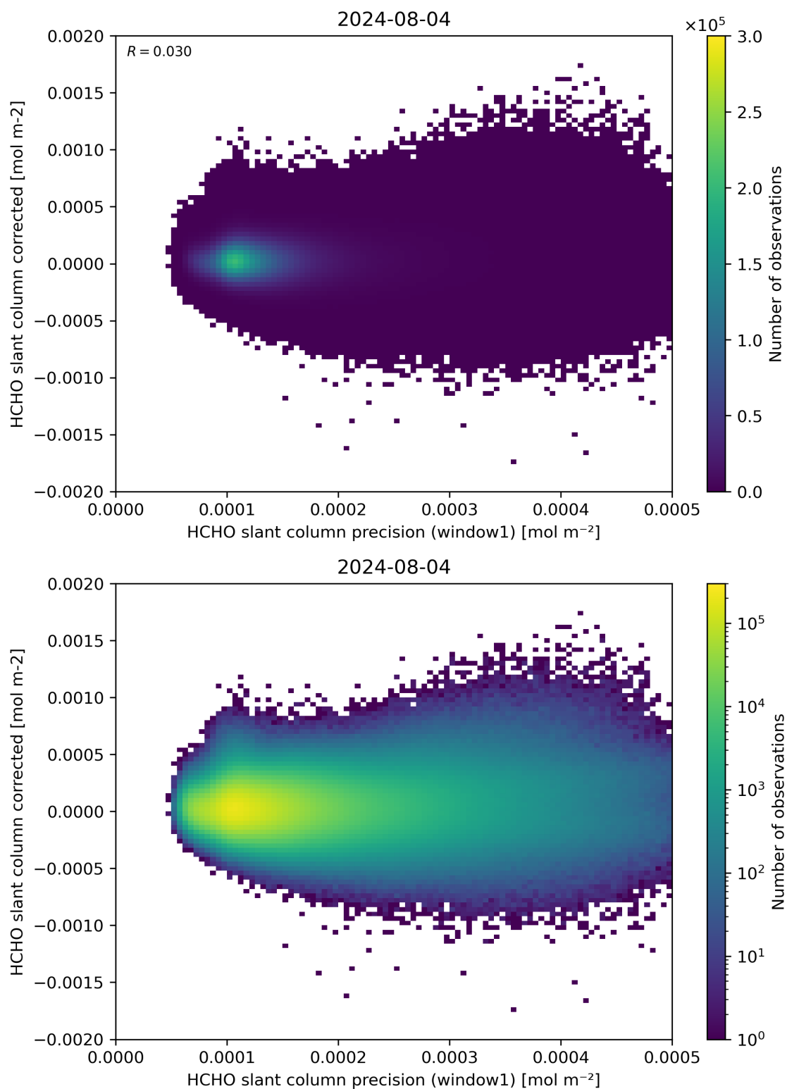
Figure 92: Scatter density plot of “HCHO slant column precision (window1)” against “HCHO slant column corrected” for 2024-08-03 to 2024-08-05.
