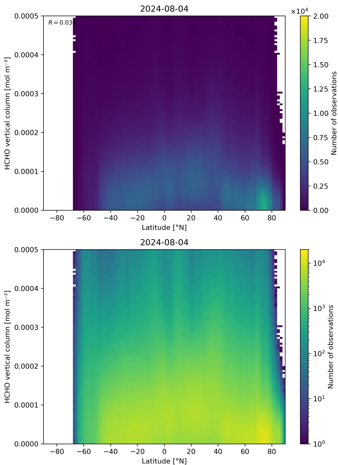
Figure 163: Scatter density plot of “Latitude” against “HCHO vertical column” for 2024-08-03 to 2024-08-05.
