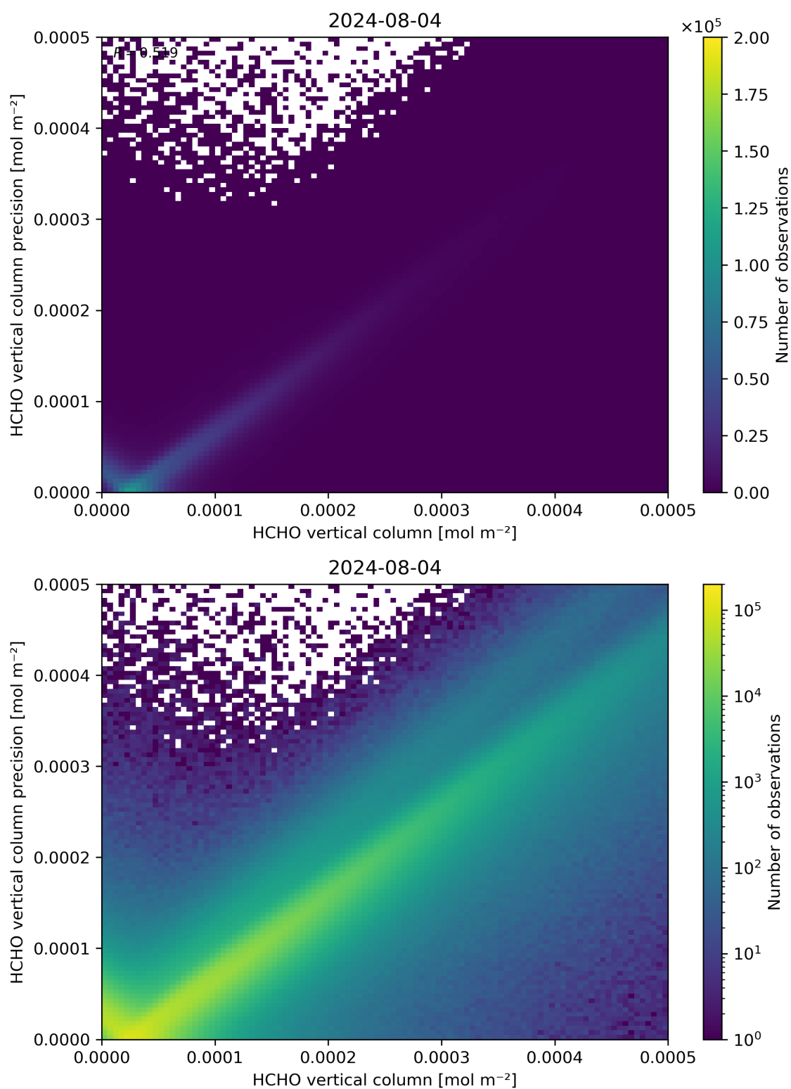
Figure 134: Scatter density plot of “HCHO vertical column” against “HCHO vertical column precision” for 2024-08-03 to 2024-08-05.
