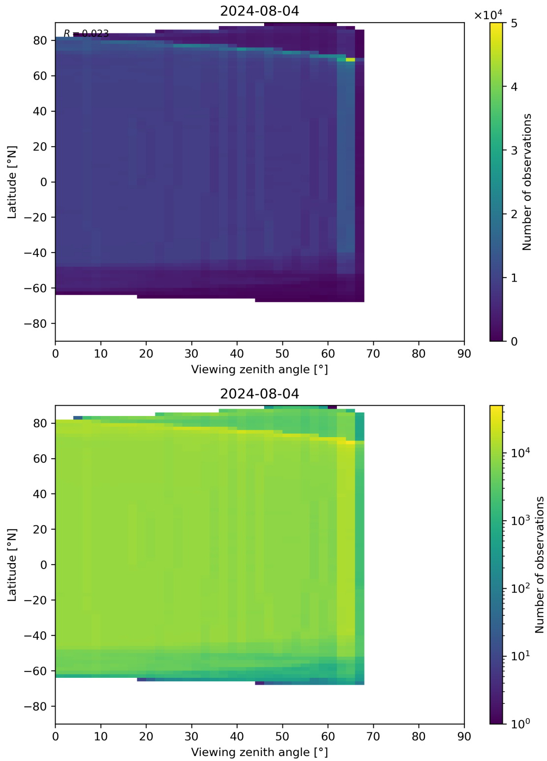
Figure 196: Scatter density plot of “Viewing zenith angle” against “Latitude” for 2024-08-03 to 2024-08-05.
