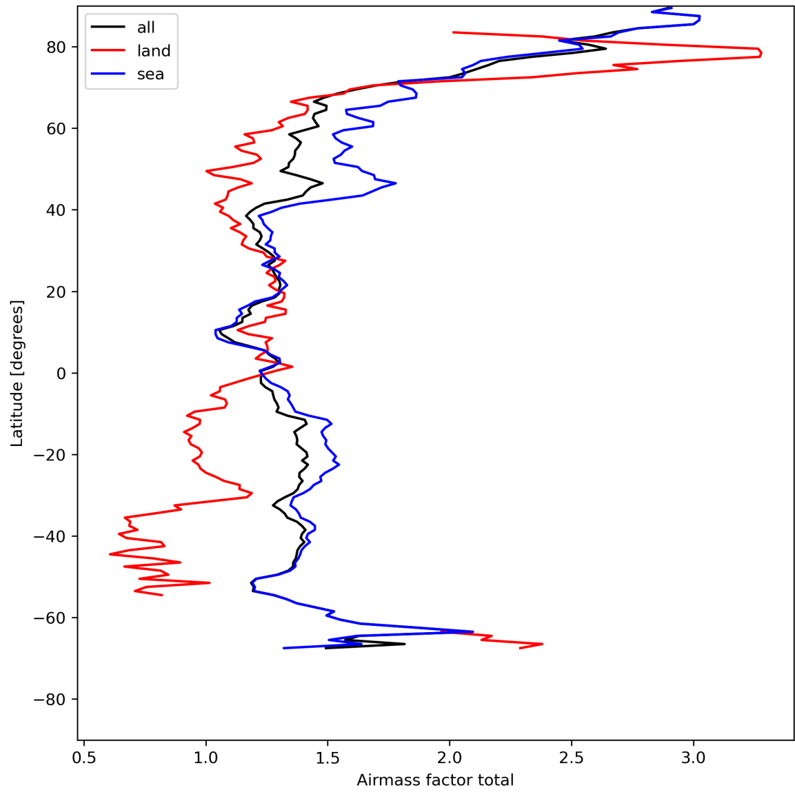
Figure 26: Zonal average of “Airmass factor total” for 2024-08-03 to 2024-08-05.
