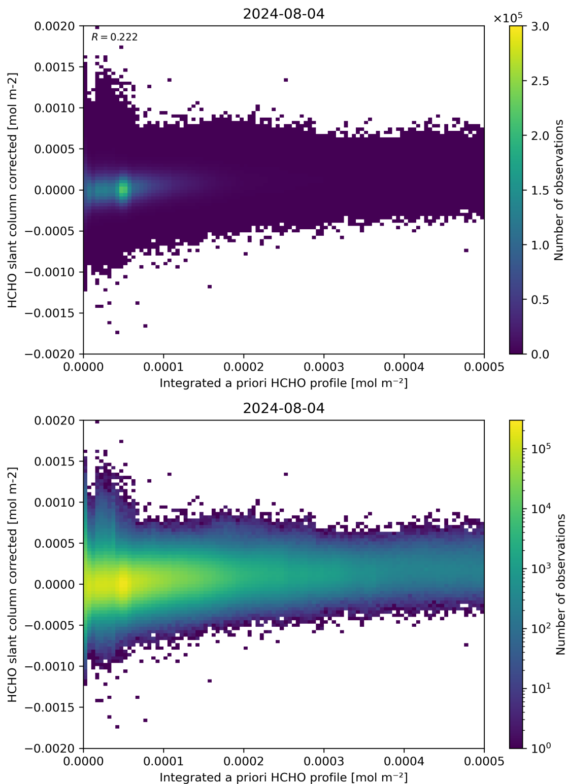
Figure 151: Scatter density plot of “Integrated a priori HCHO profile” against “HCHO slant column corrected” for 2024-08-03 to 2024-08-05.
