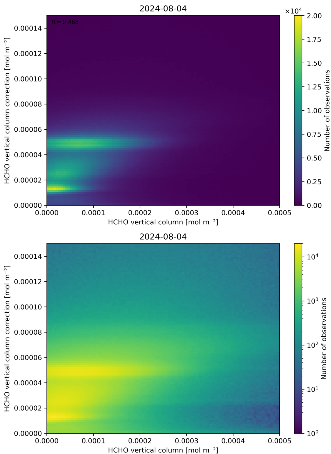
Figure 133: Scatter density plot of “HCHO vertical column” against “HCHO vertical column correction” for 2024-08-03 to 2024-08-05.
