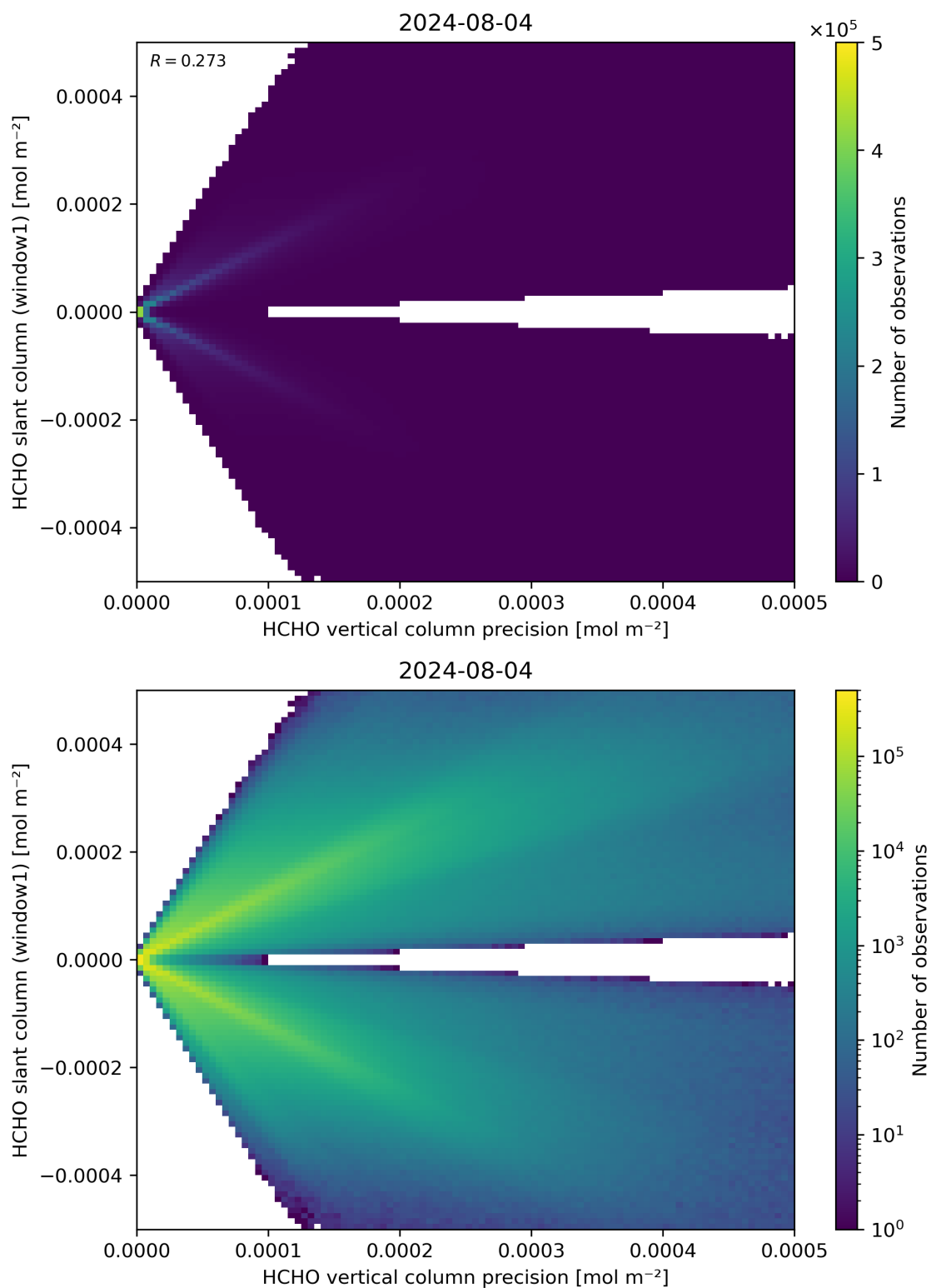
Figure 142: Scatter density plot of “HCHO vertical column precision” against “HCHO slant column (window1)” for 2024-08-03 to 2024-08-05.
