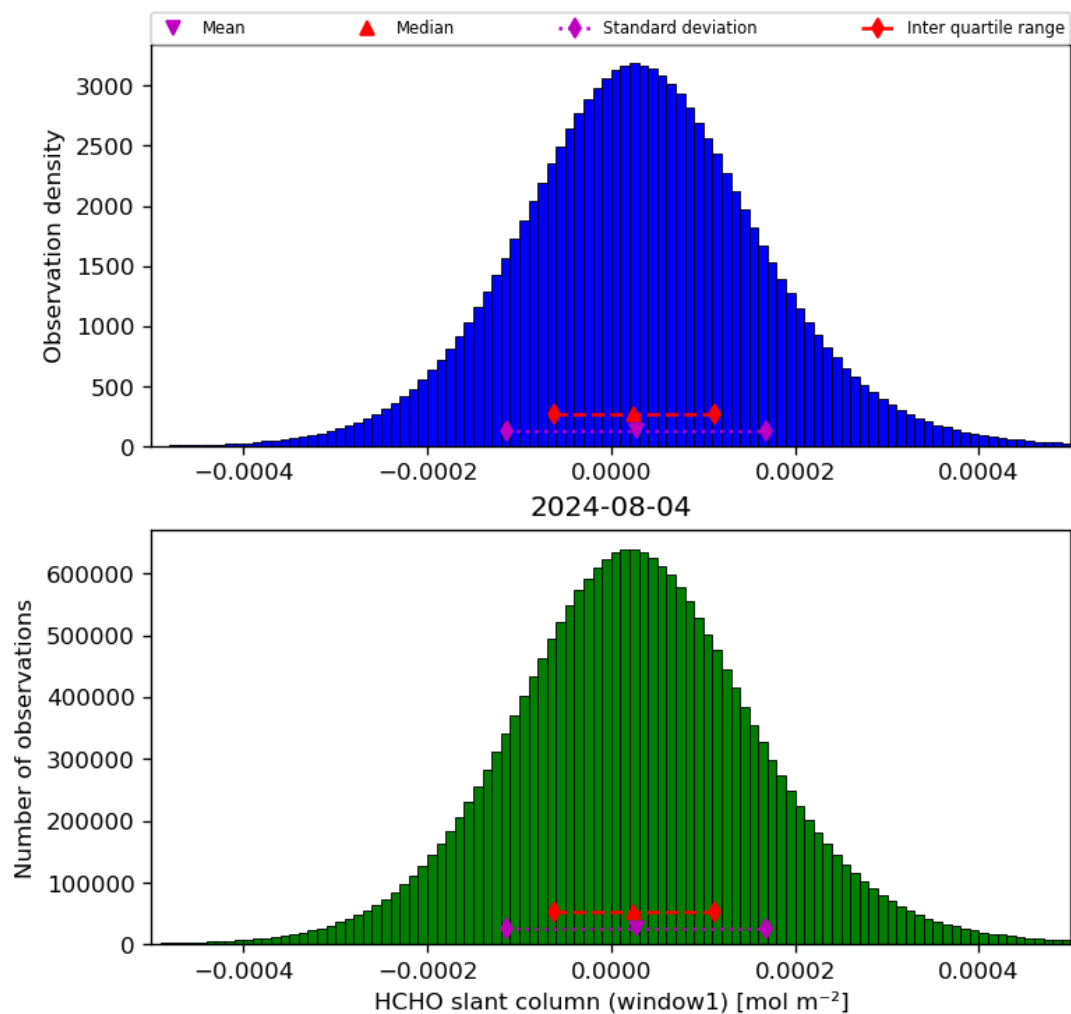
Figure 38: Histogram of “HCHO slant column (window1)” for 2024-08-03 to 2024-08-05
