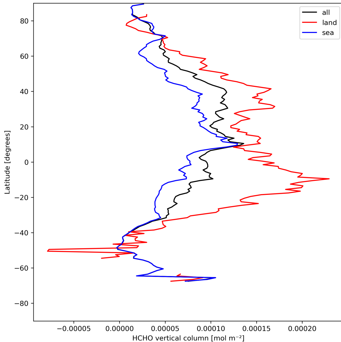
Figure 21: Zonal average of “HCHO vertical column” for 2024-08-03 to 2024-08-05.
