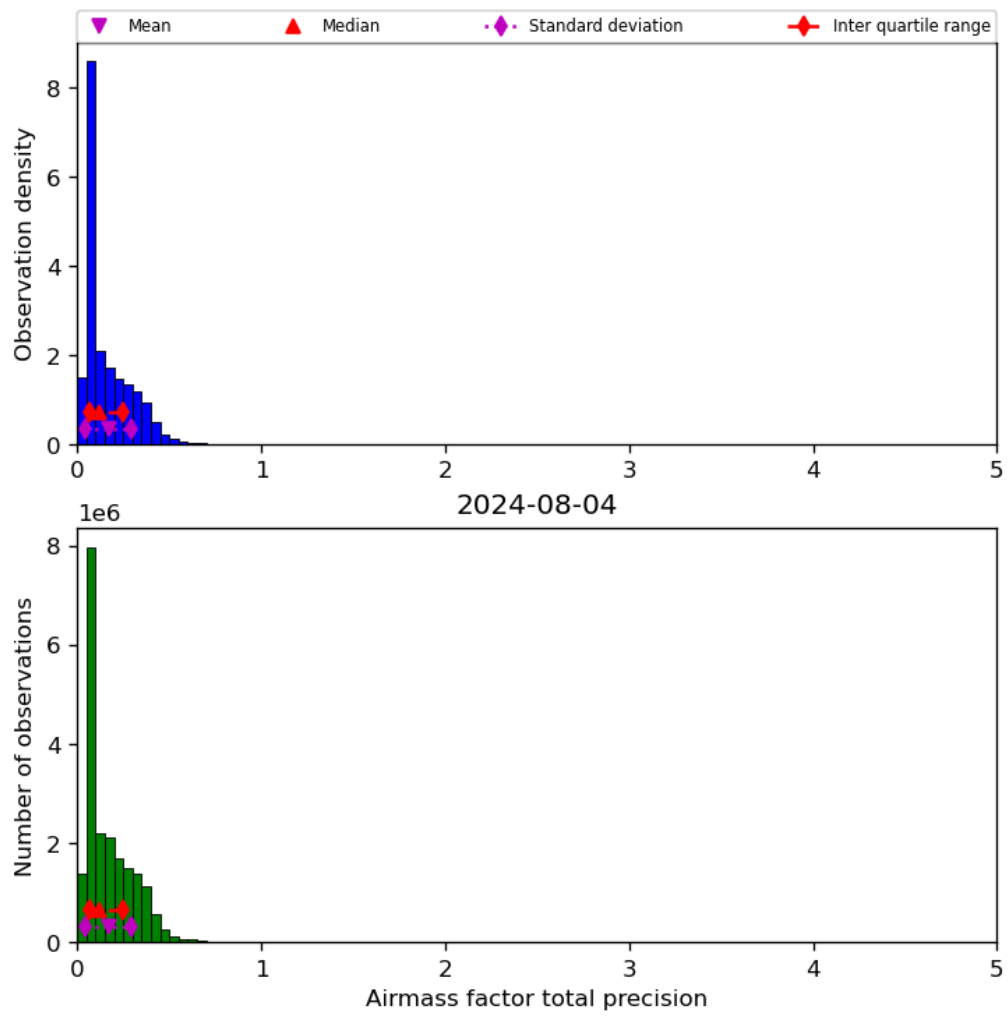
Figure 41: Histogram of "Airmass factor total precision" for 2024-08-03 to 2024-08-05
