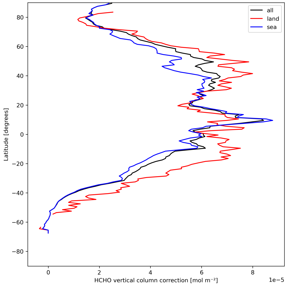
Figure 23: Zonal average of “HCHO vertical column correction” for 2024-08-03 to 2024-08-05.
