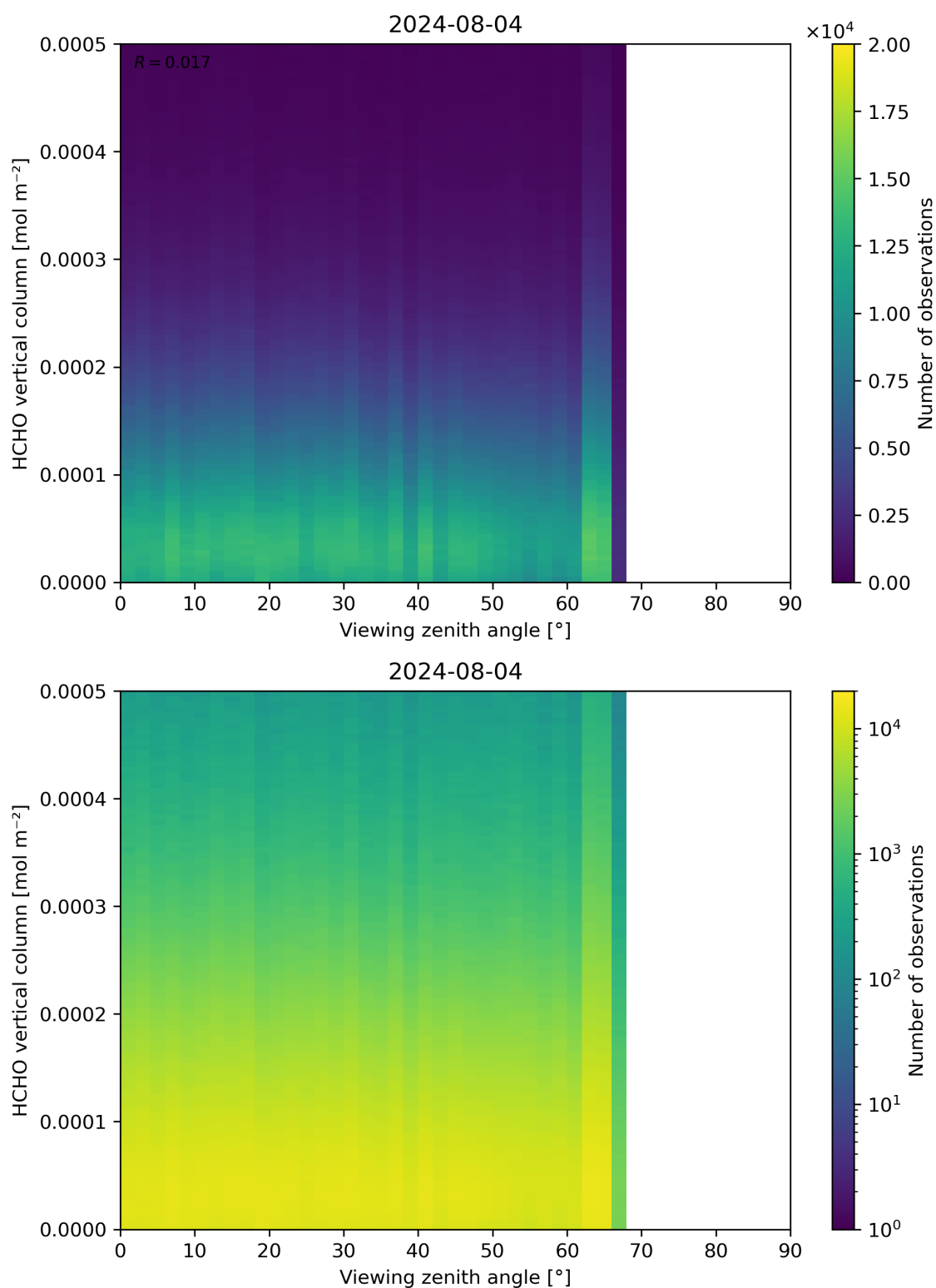
Figure 192: Scatter density plot of “Viewing zenith angle” against “HCHO vertical column” for 2024-08-03 to 2024-08-05.
