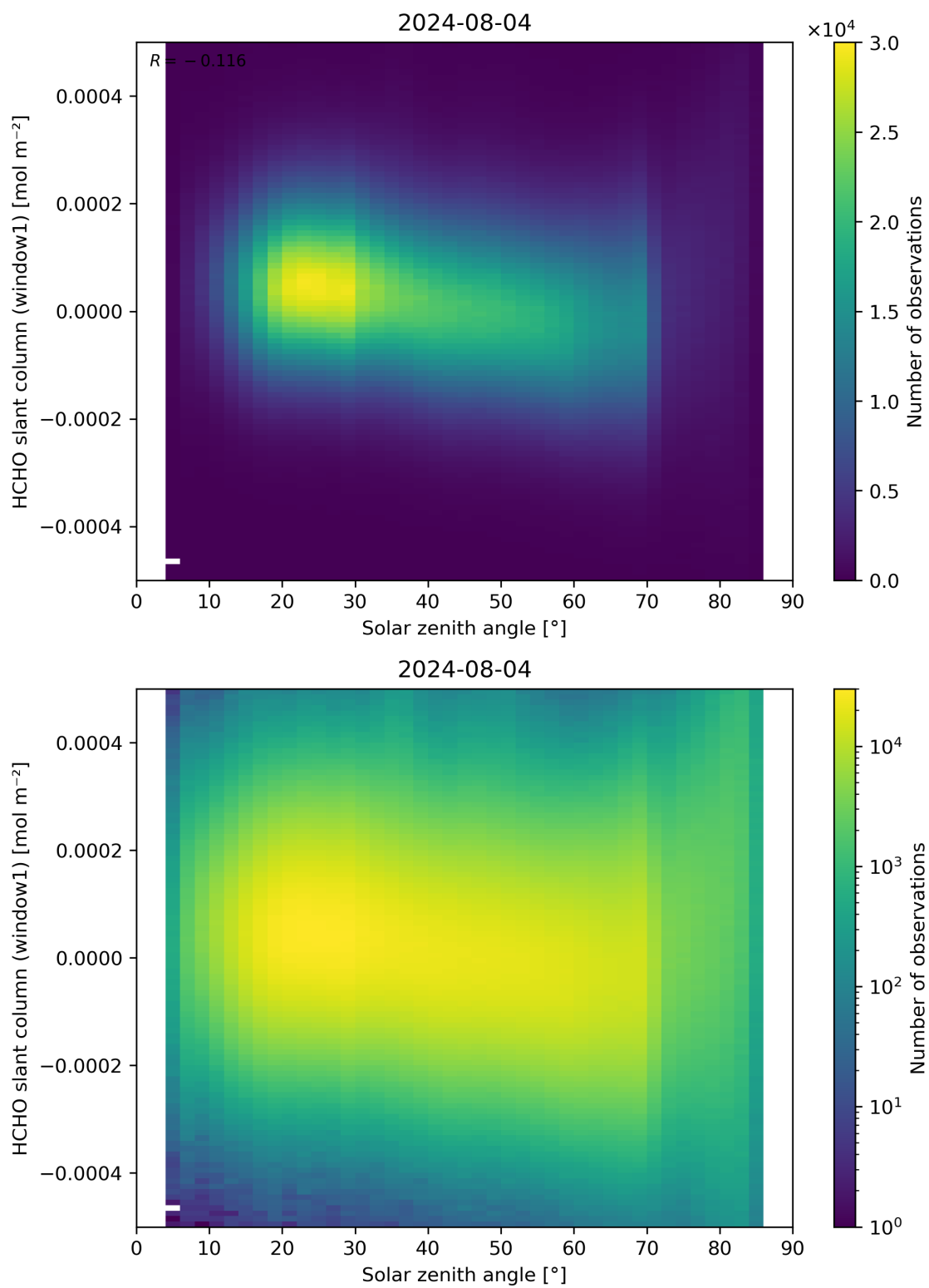
Figure 173: Scatter density plot of “Solar zenith angle” against “HCHO slant column (window1)” for 2024-08-03 to 2024-08-05.
