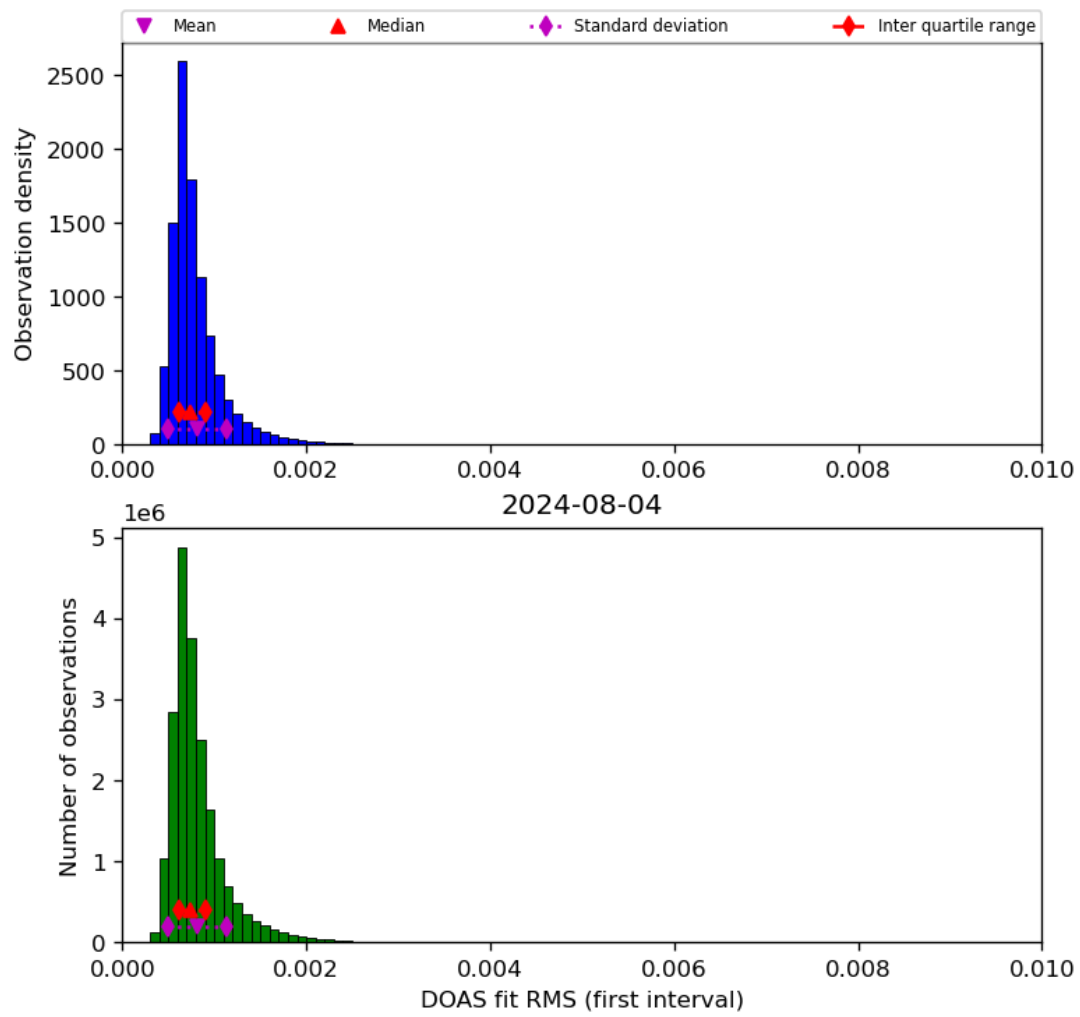
Figure 46: Histogram of “DOAS fit RMS (first interval)” for 2024-08-03 to 2024-08-05
