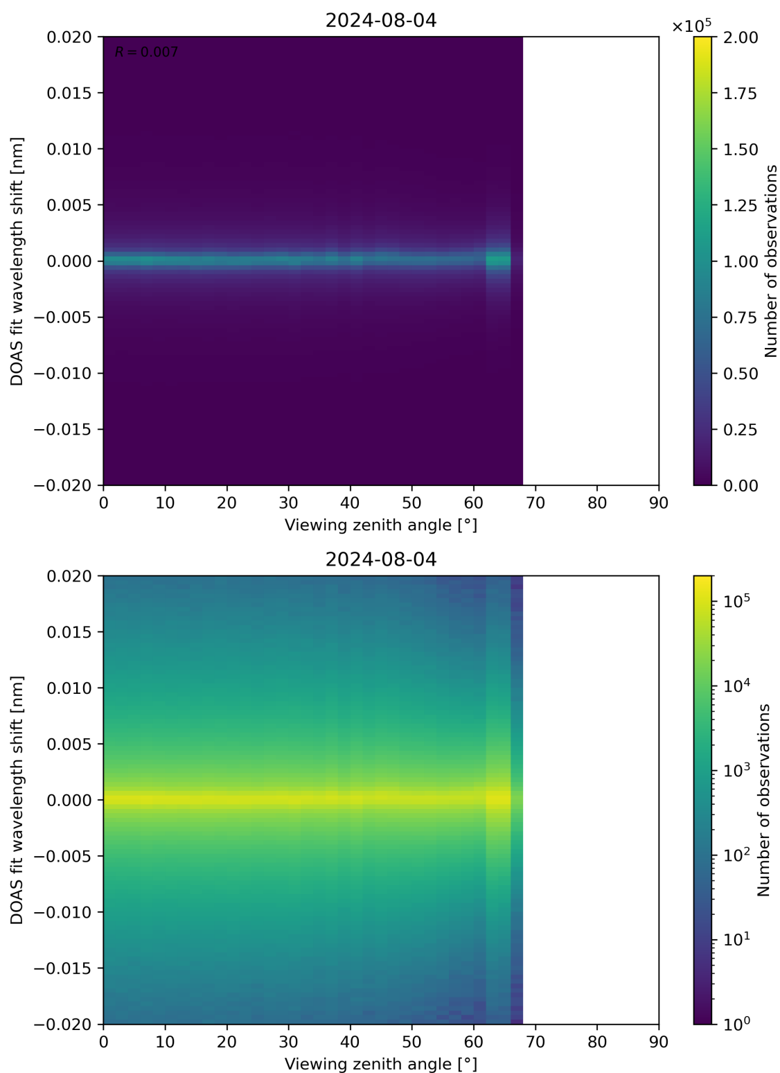
Figure 183: Scatter density plot of “Viewing zenith angle” against “DOAS fit wavelength shift” for 2024-08-03 to 2024-08-05.
