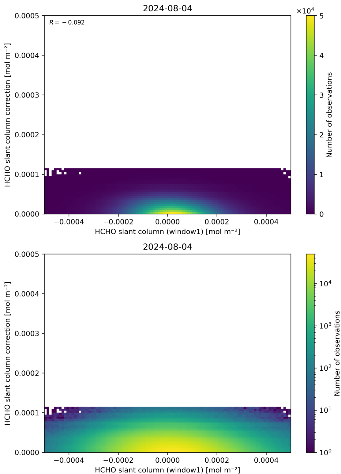
Figure 83: Scatter density plot of “HCHO slant column (window1)” against “HCHO slant column correction” for 2024-08-03 to 2024-08-05.
