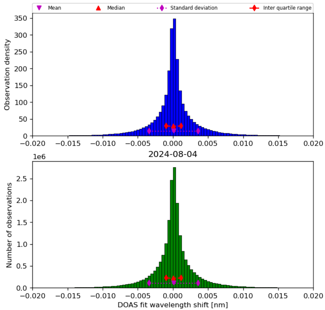
Figure 44: Histogram of “DOAS fit wavelength shift” for 2024-08-03 to 2024-08-05
