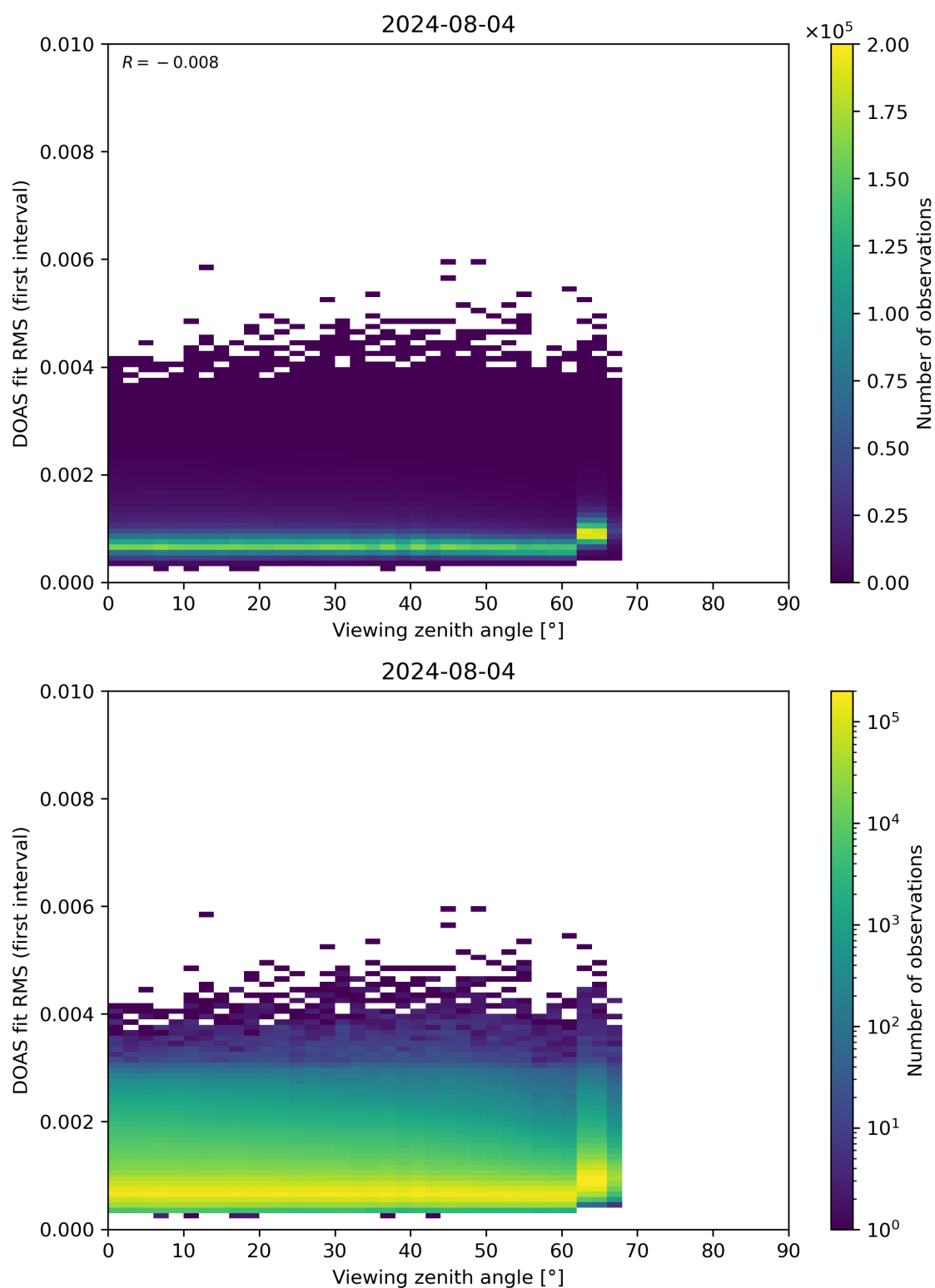
Figure 182: Scatter density plot of “Viewing zenith angle” against “DOAS fit RMS (first interval)” for 2024-08-03 to 2024-08-05.
