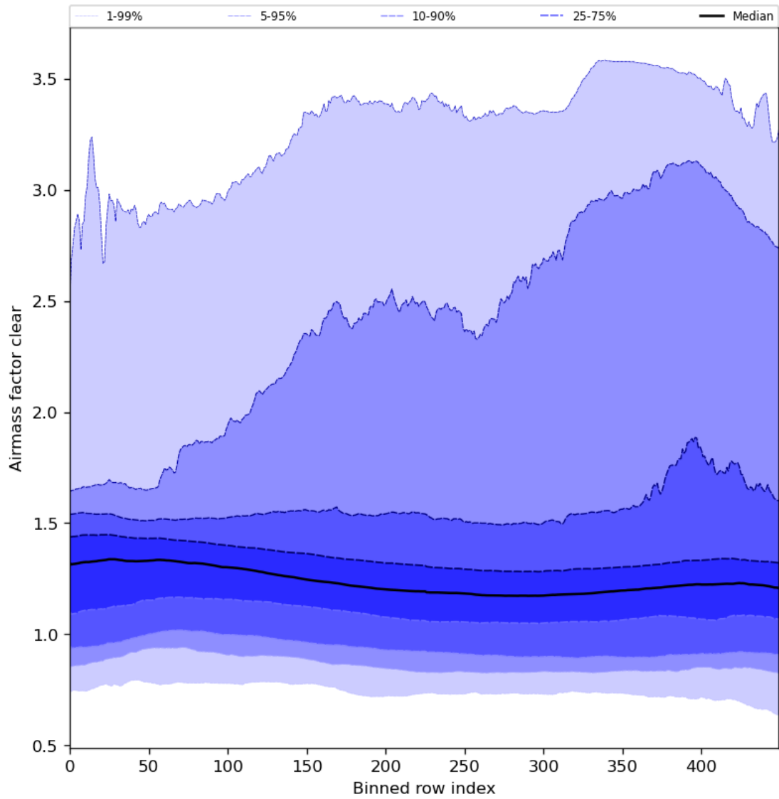
Figure 56: Along track statistics of “Airmass factor clear” for 2024-08-03 to 2024-08-05
