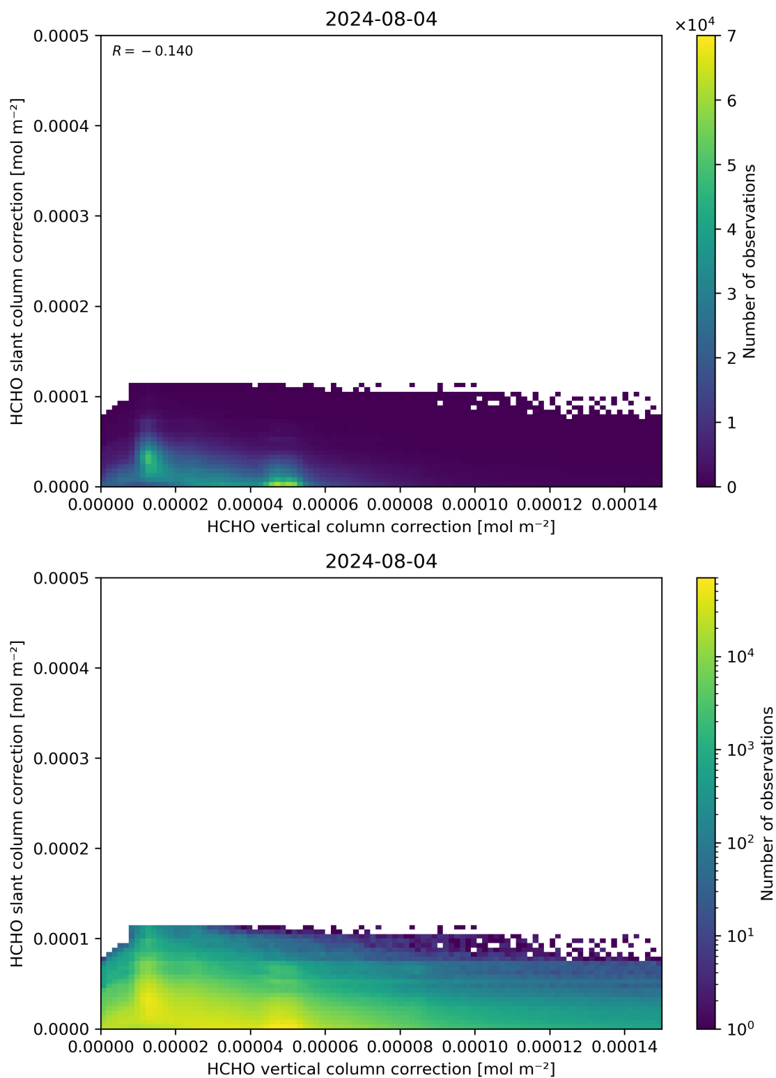
Figure 117: Scatter density plot of “HCHO vertical column correction” against “HCHO slant column correction” for 2024-08-03 to 2024-08-05.
