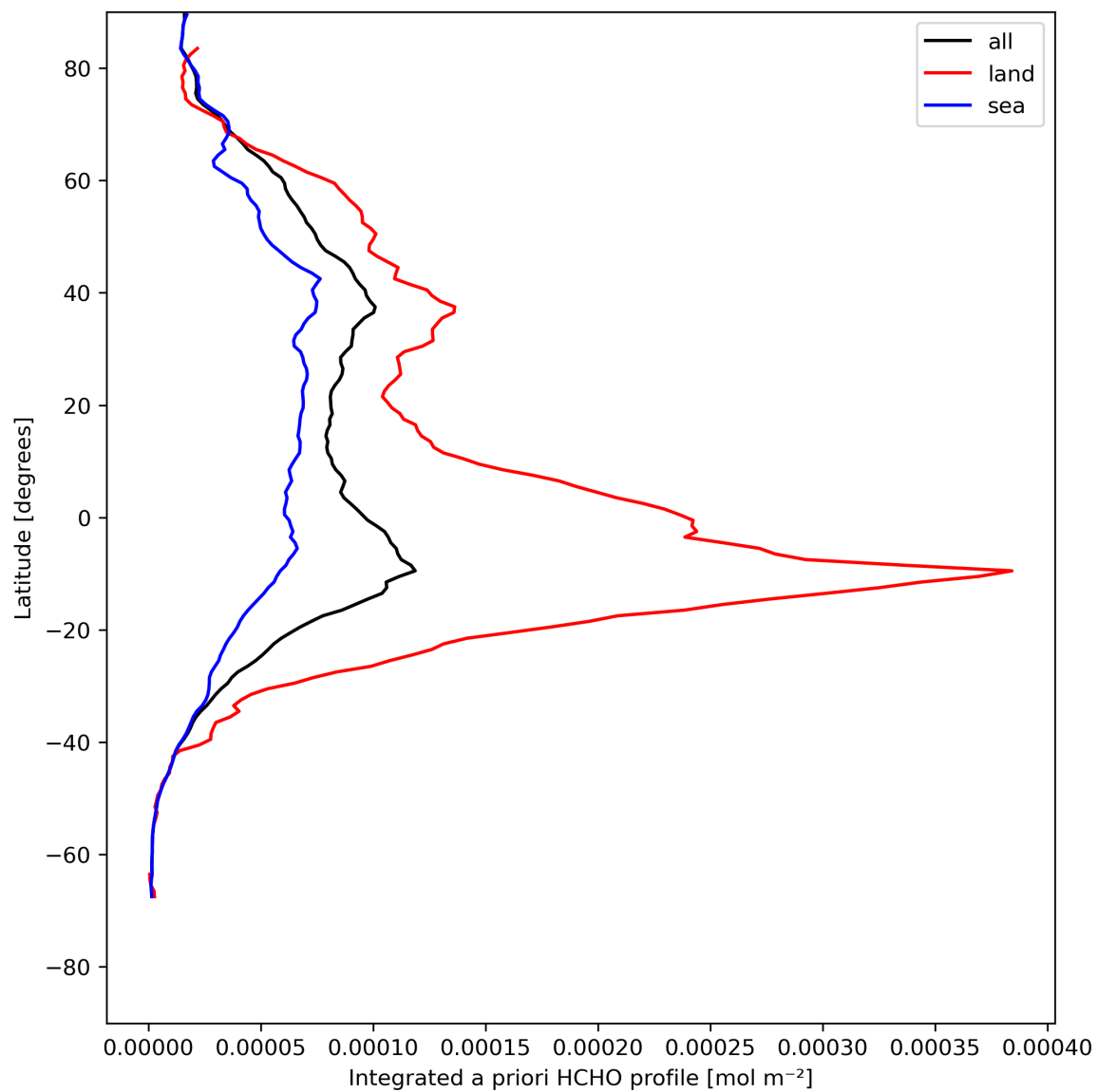
Figure 29: Zonal average of “Integrated a priori HCHO profile” for 2024-08-03 to 2024-08-05.
