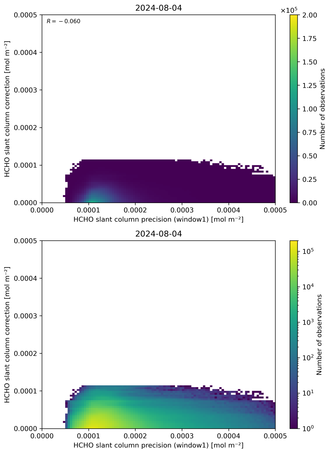
Figure 93: Scatter density plot of “HCHO slant column precision (window1)” against “HCHO slant column correction” for 2024-08-03 to 2024-08-05.
