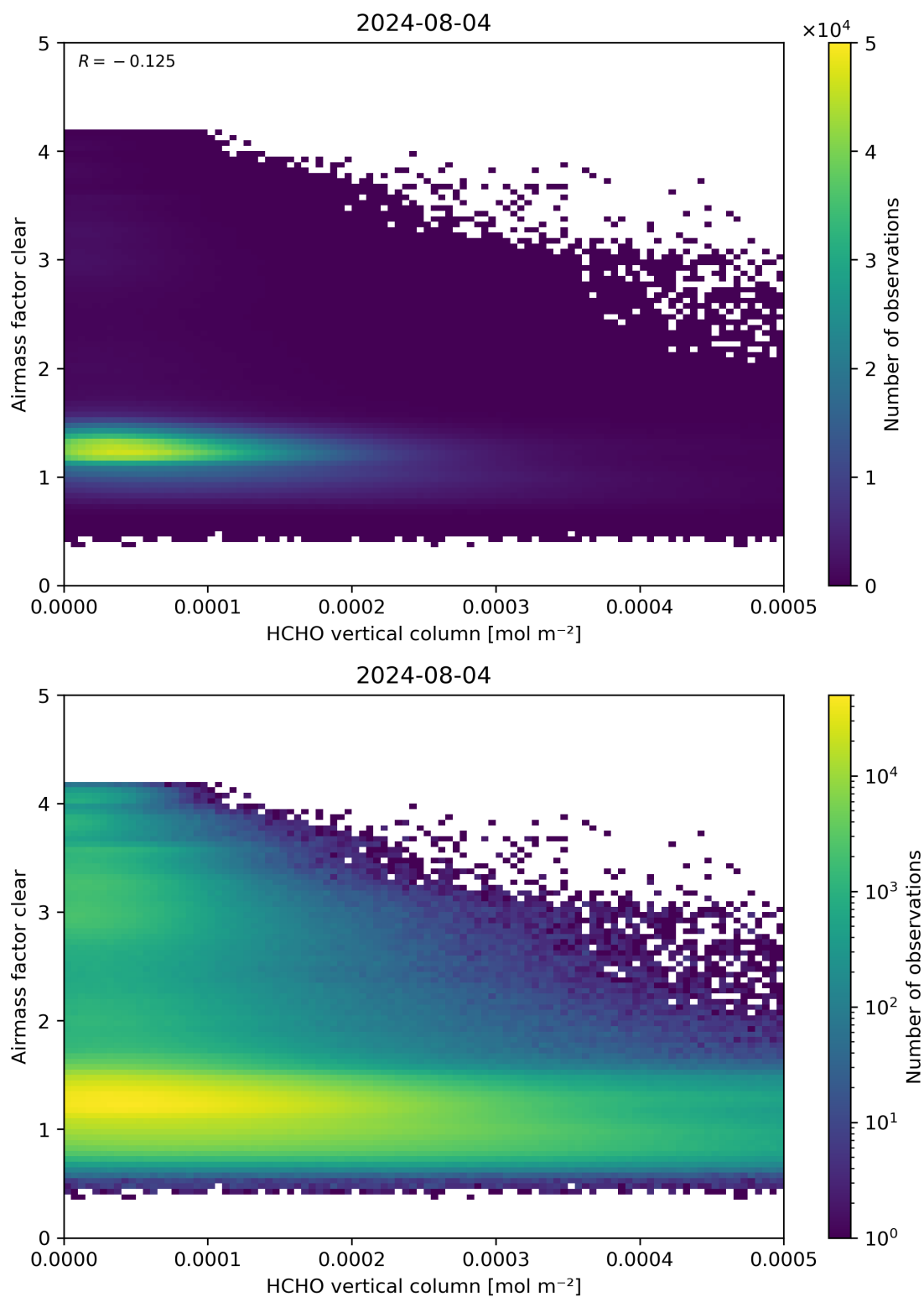
Figure 126: Scatter density plot of “HCHO vertical column” against “Airmass factor clear” for 2024-08-03 to 2024-08-05.
