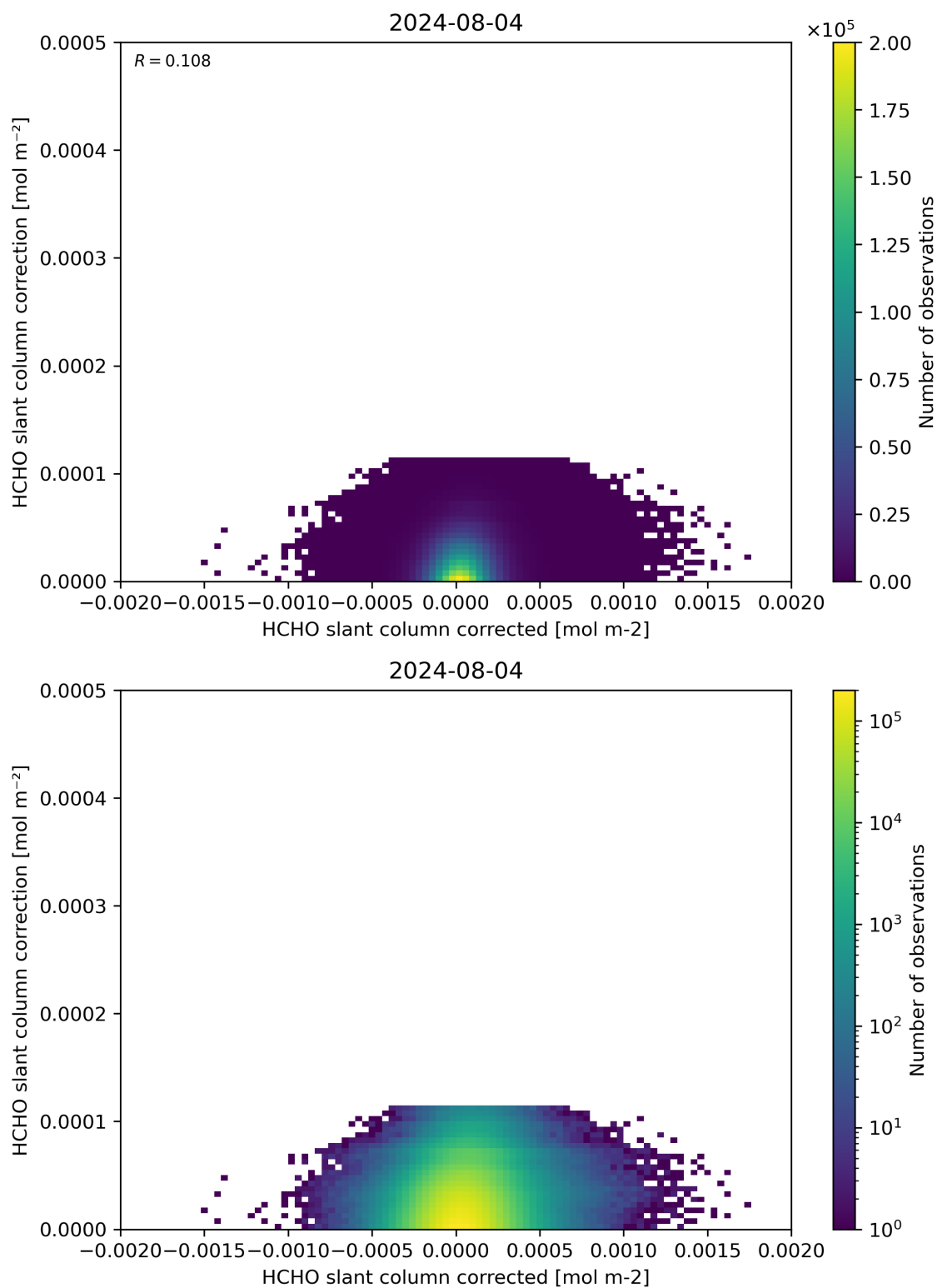
Figure 77: Scatter density plot of “HCHO slant column corrected” against “HCHO slant column correction” for 2024-08-03 to 2024-08-05.
