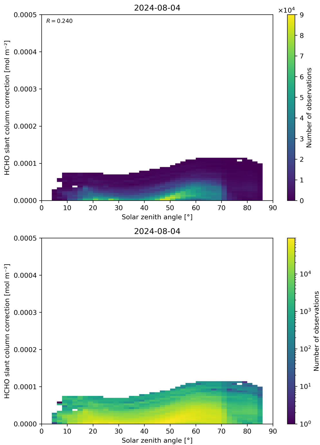
Figure 172: Scatter density plot of “Solar zenith angle” against “HCHO slant column correction” for 2024-08-03 to 2024-08-05.
