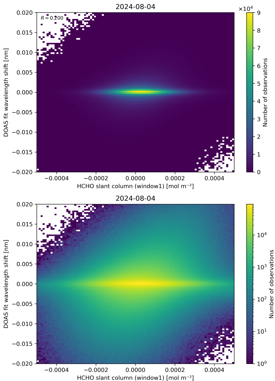
Figure 79: Scatter density plot of “HCHO slant column (window1)” against “DOAS fit wavelength shift” for 2024-08-03 to 2024-08-05.
