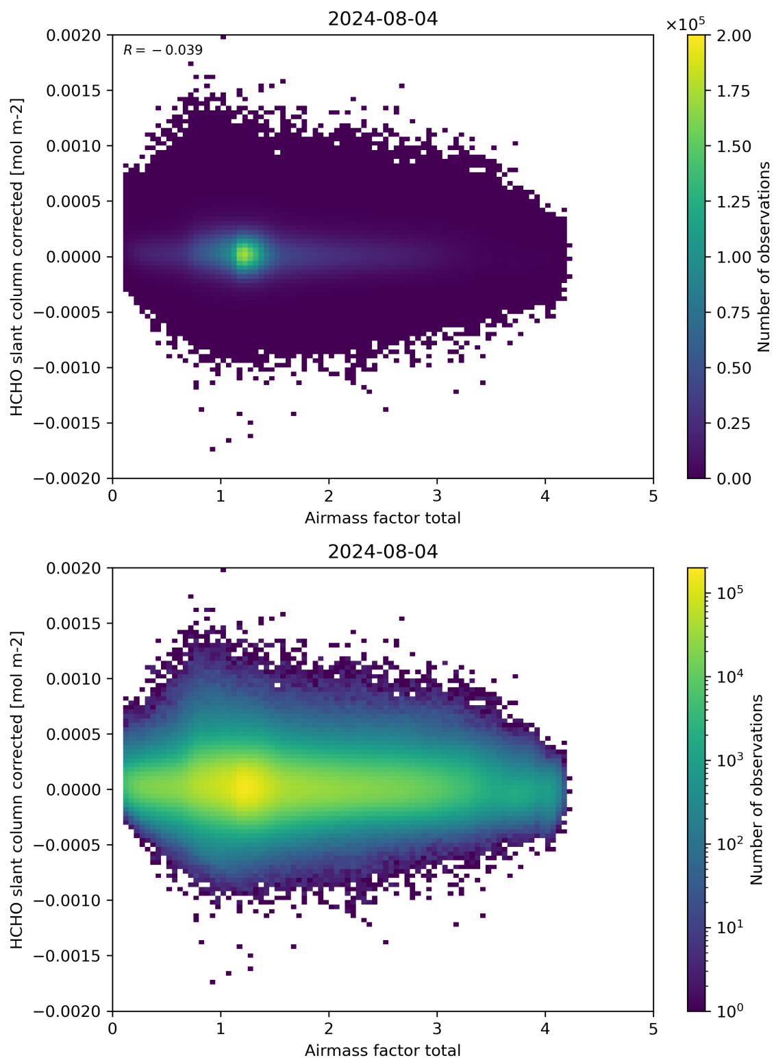
Figure 101: Scatter density plot of “Airmass factor total” against “HCHO slant column corrected” for 2024-08-03 to 2024-08-05.
