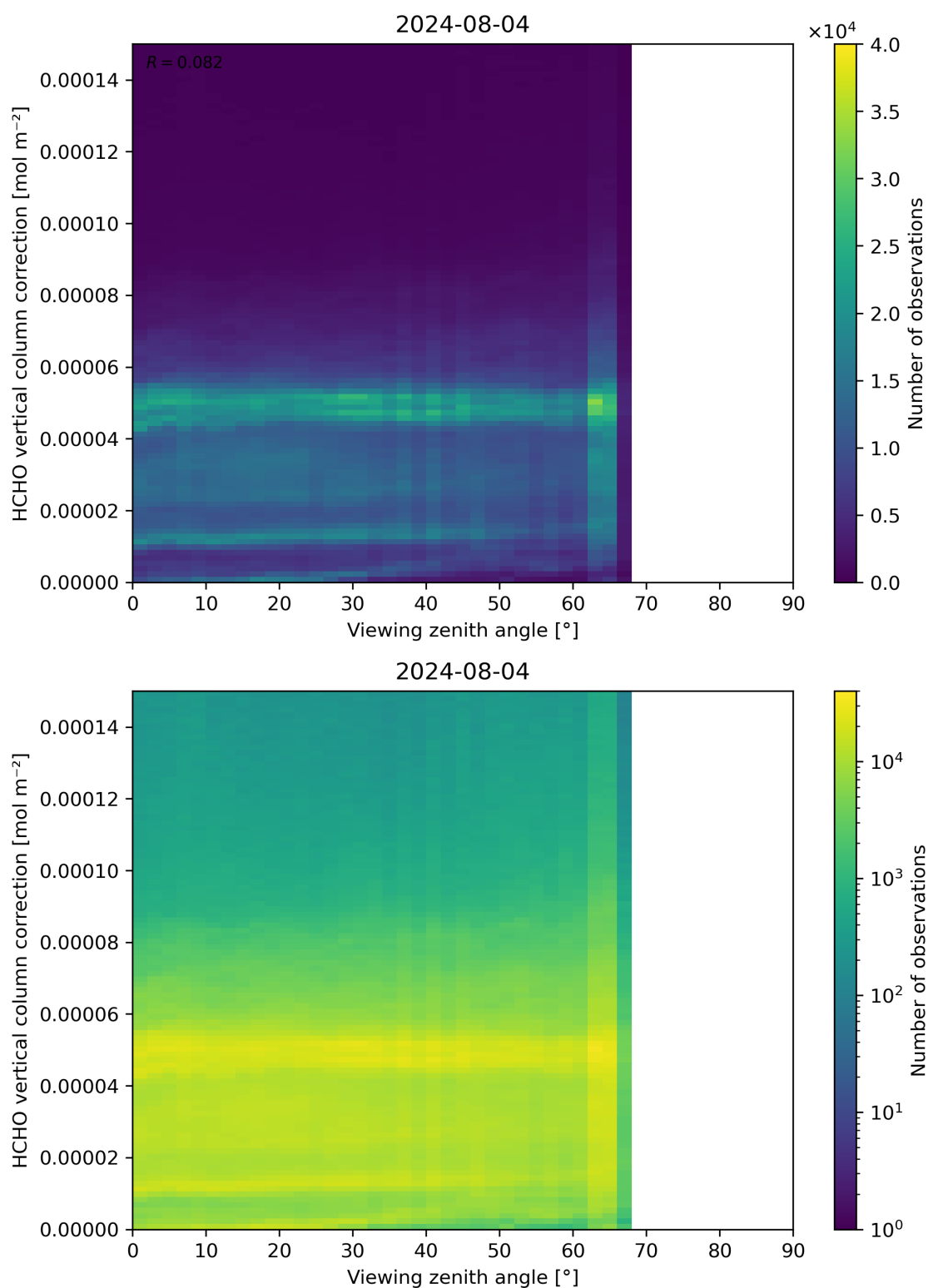
Figure 193: Scatter density plot of “Viewing zenith angle” against “HCHO vertical column correction” for 2024-08-03 to 2024-08-05.
