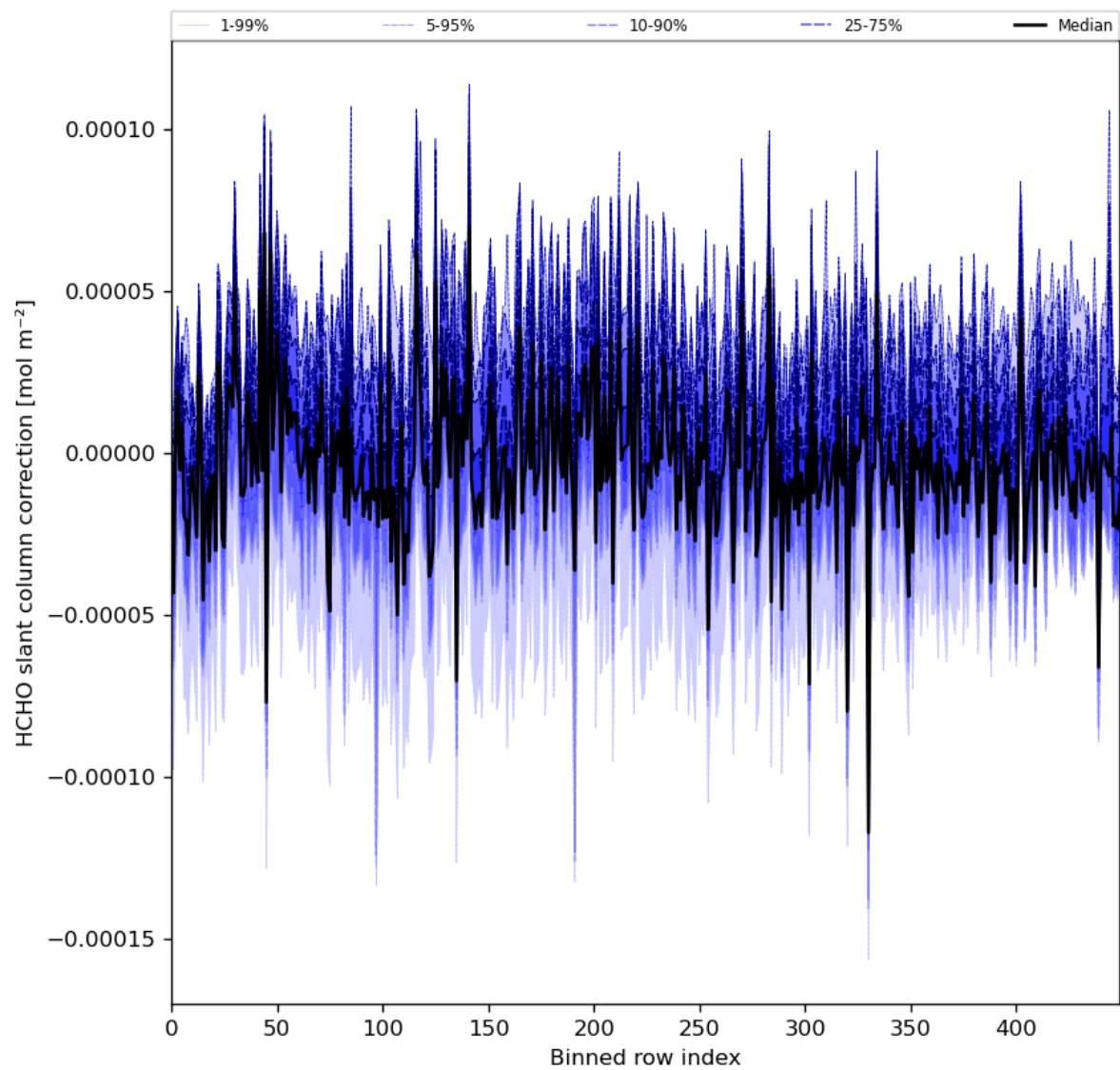
Figure 61: Along track statistics of “HCHO slant column correction” for 2024-08-03 to 2024-08-05
