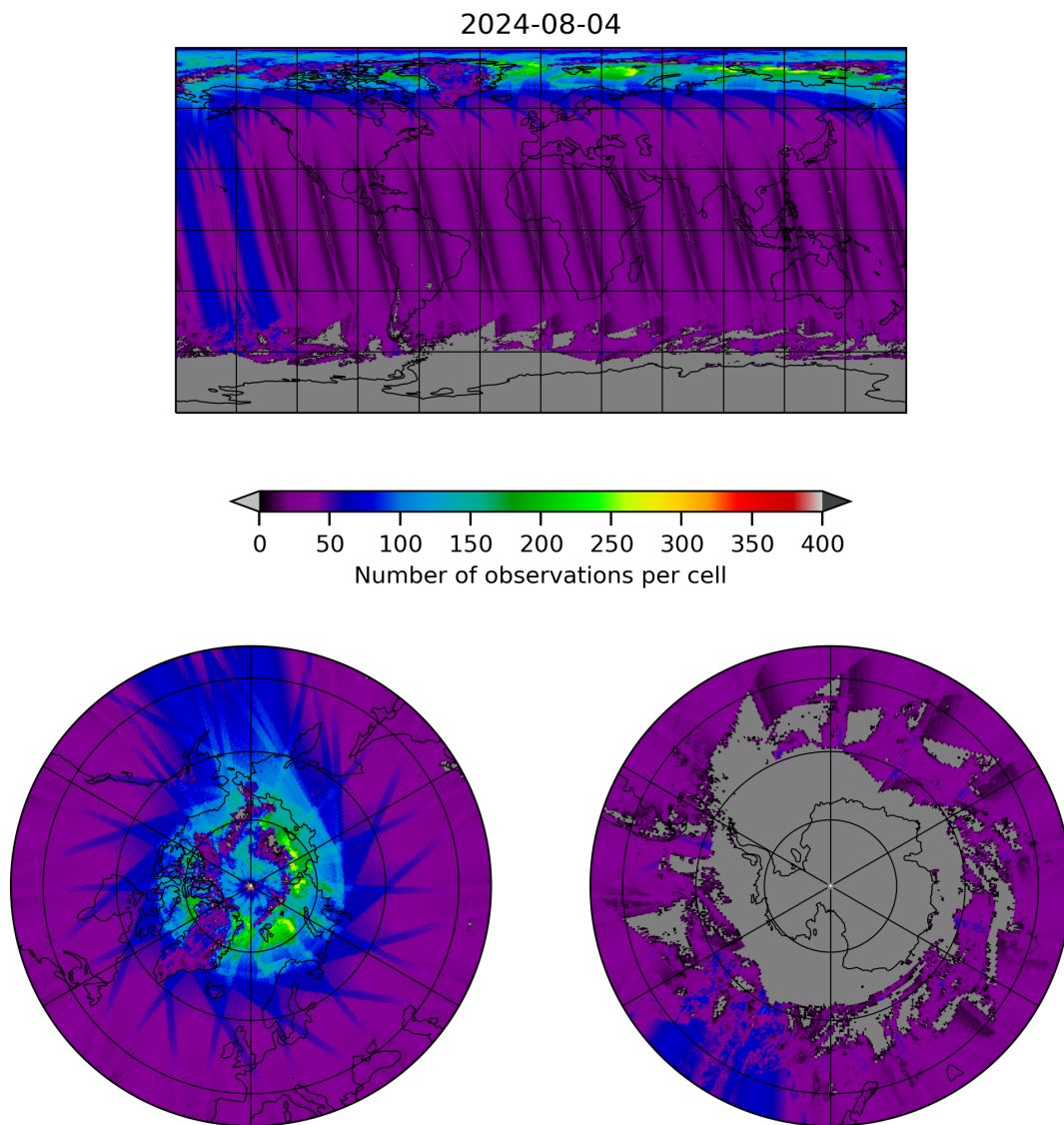
Figure 19: Map of the number of observations for 2024-08-03 to 2024-08-05
