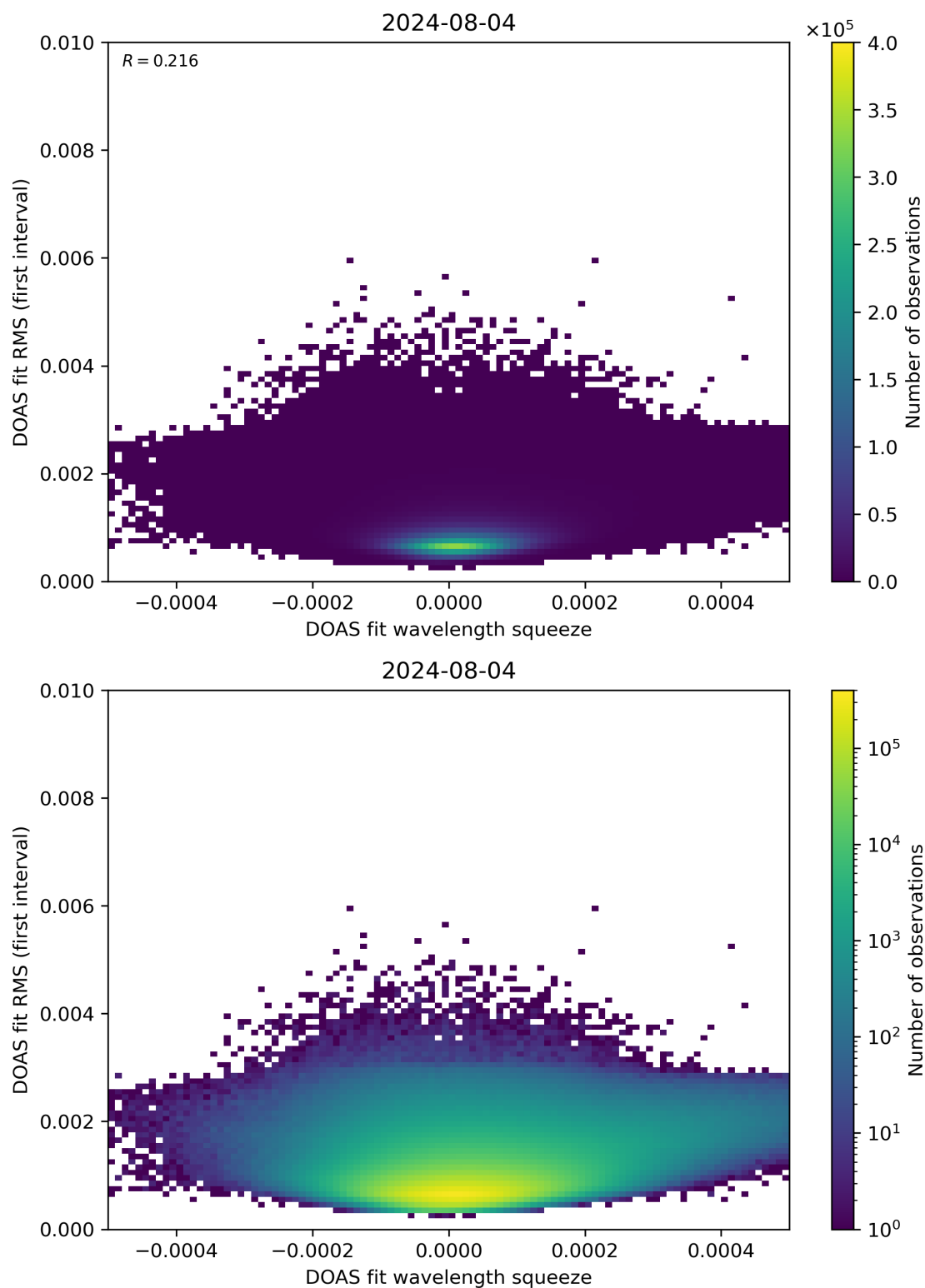
Figure 68: Scatter density plot of “DOAS fit wavelength squeeze” against “DOAS fit RMS (first interval)” for 2024-08-03 to 2024-08-05.
