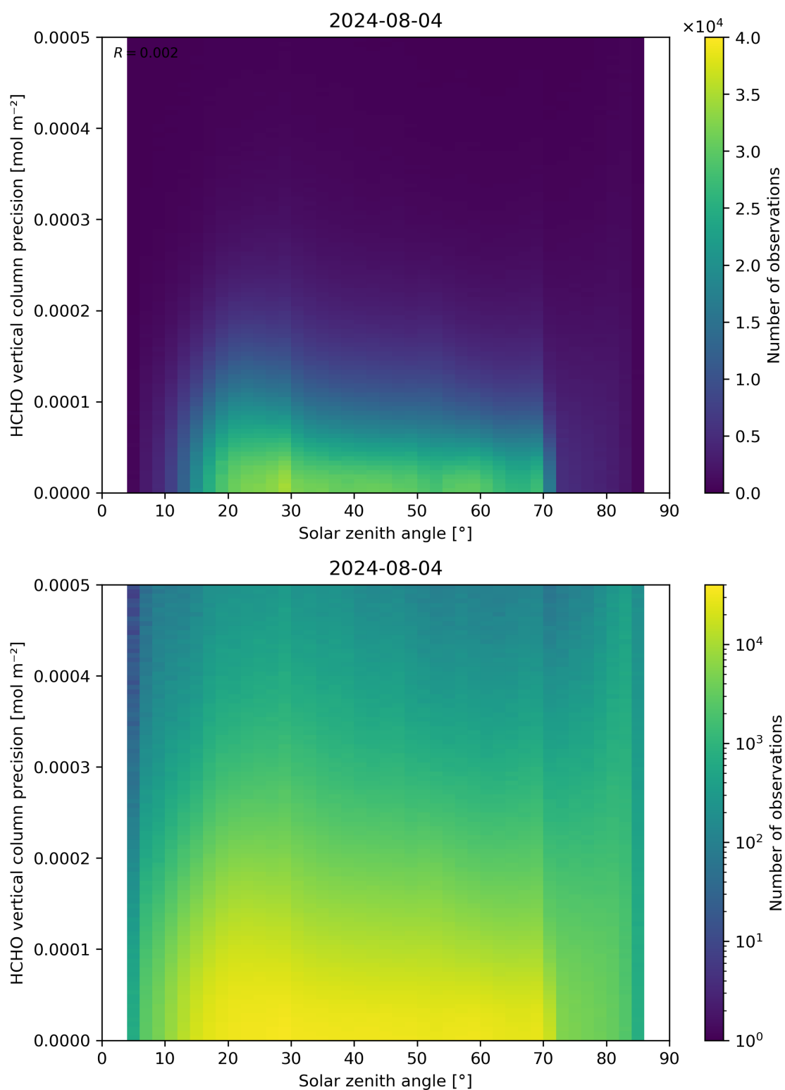
Figure 179: Scatter density plot of “Solar zenith angle” against “HCHO vertical column precision” for 2024-08-03 to 2024-08-05.
