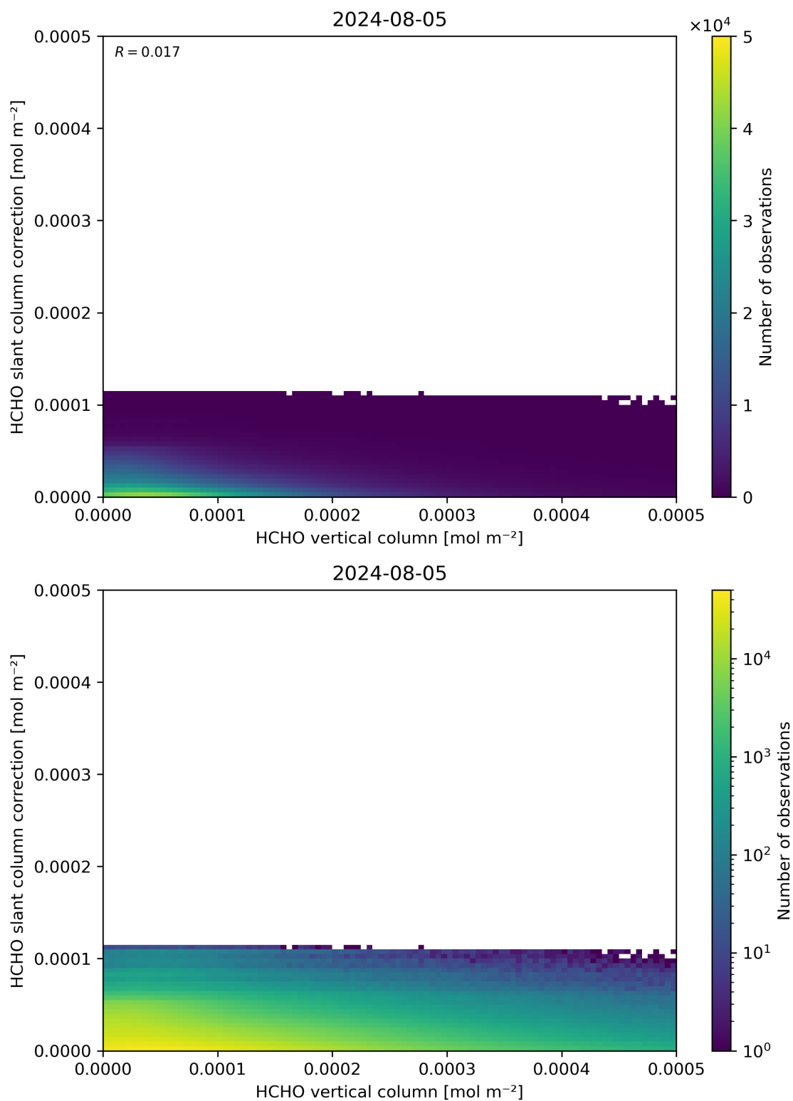
Figure 128: Scatter density plot of “HCHO vertical column” against “HCHO slant column correction” for 2024-08-04 to 2024-08-06.
