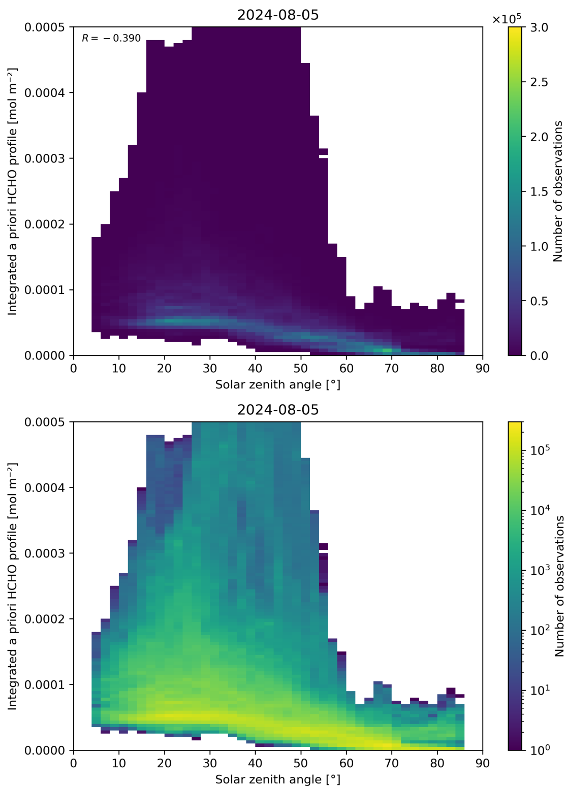
Figure 180: Scatter density plot of “Solar zenith angle” against “Integrated a priori HCHO profile” for 2024-08-04 to 2024-08-06.
