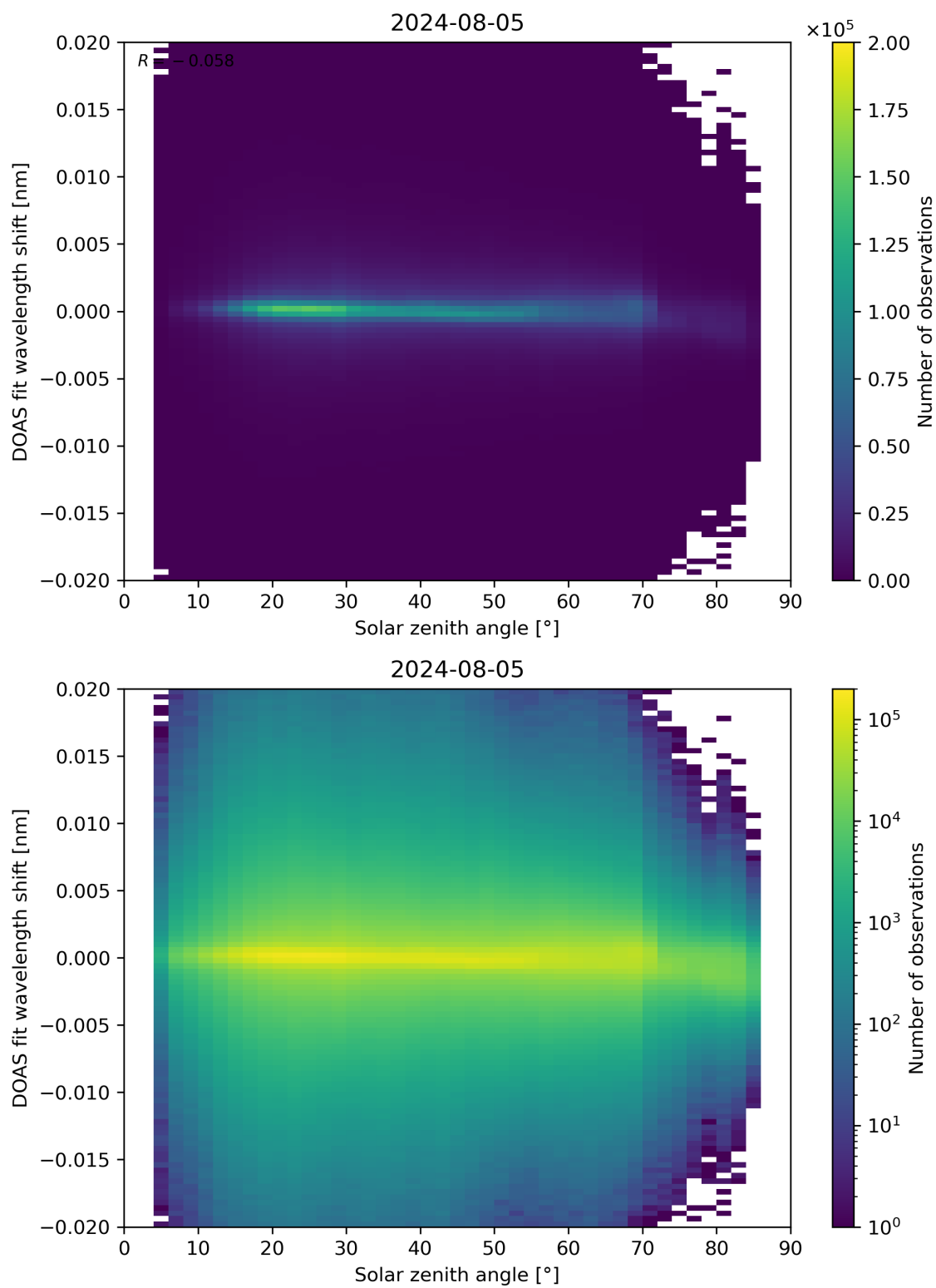
Figure 168: Scatter density plot of “Solar zenith angle” against “DOAS fit wavelength shift” for 2024-08-04 to 2024-08-06.
