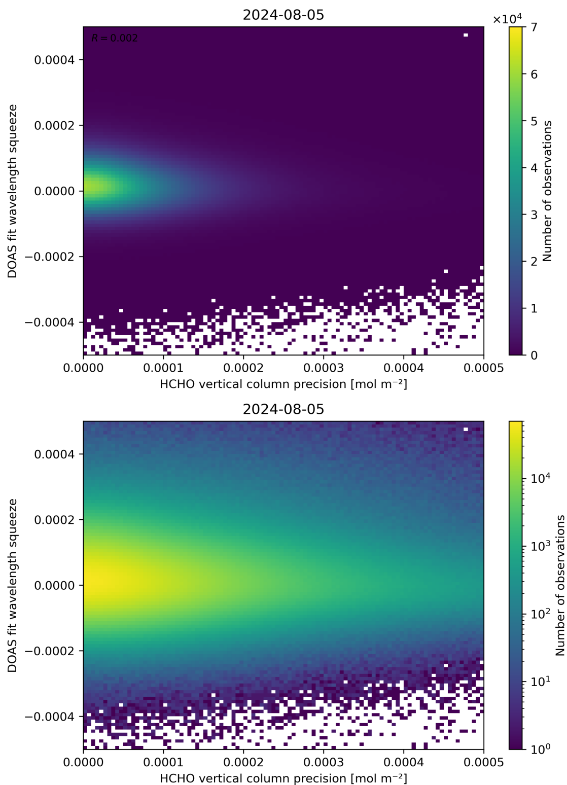
Figure 138: Scatter density plot of “HCHO vertical column precision” against “DOAS fit wavelength squeeze” for 2024-08-04 to 2024-08-06.
