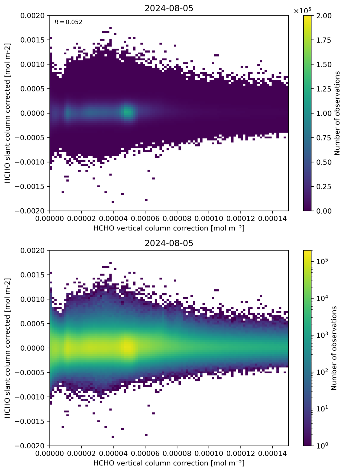
Figure 116: Scatter density plot of “HCHO vertical column correction” against “HCHO slant column corrected” for 2024-08-04 to 2024-08-06.
