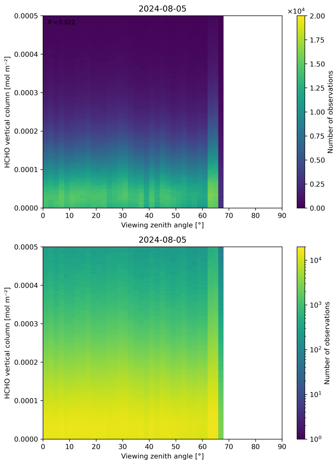
Figure 192: Scatter density plot of “Viewing zenith angle” against “HCHO vertical column” for 2024-08-04 to 2024-08-06.
