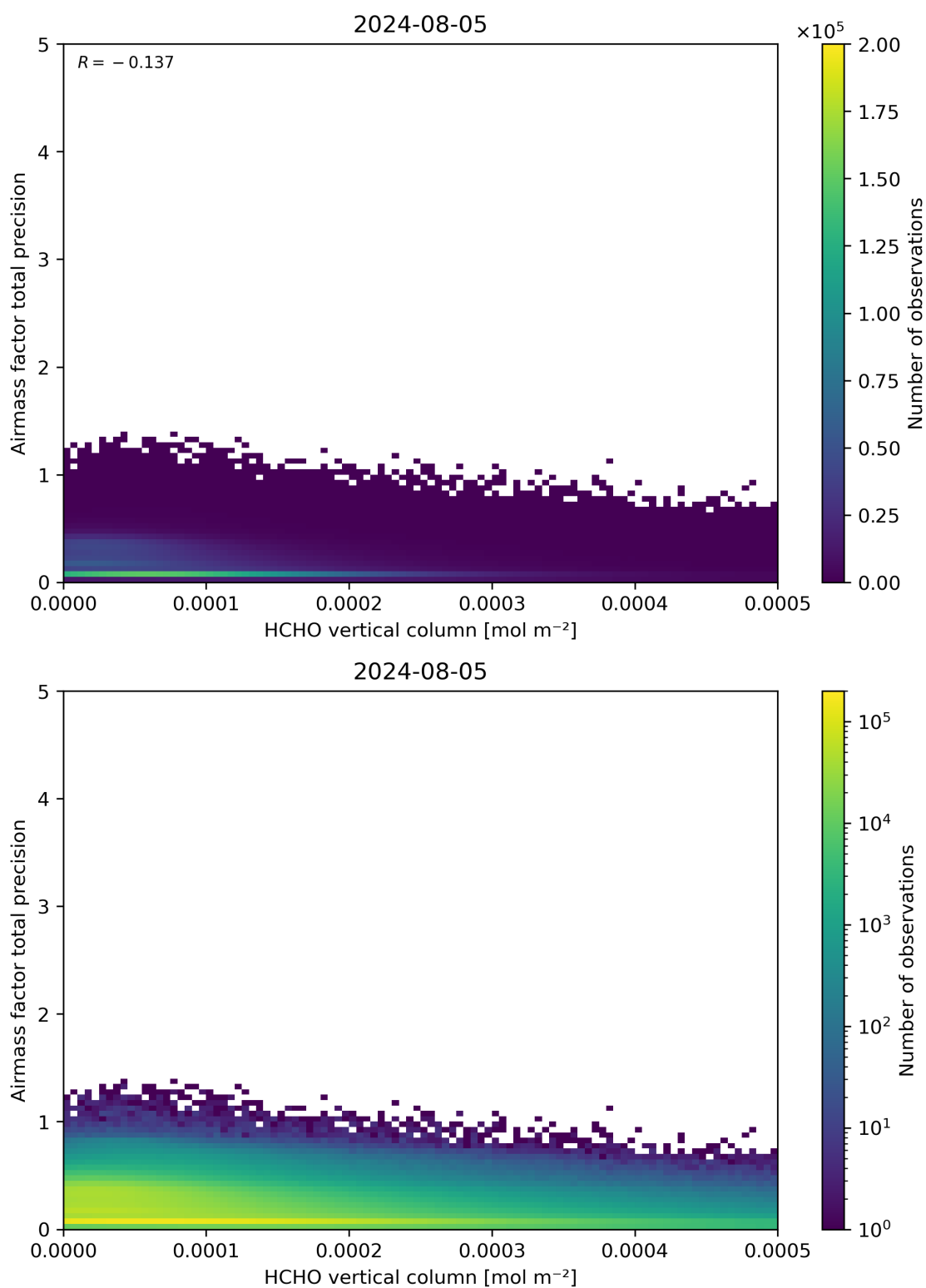
Figure 132: Scatter density plot of “HCHO vertical column” against “Airmass factor total precision” for 2024-08-04 to 2024-08-06.
