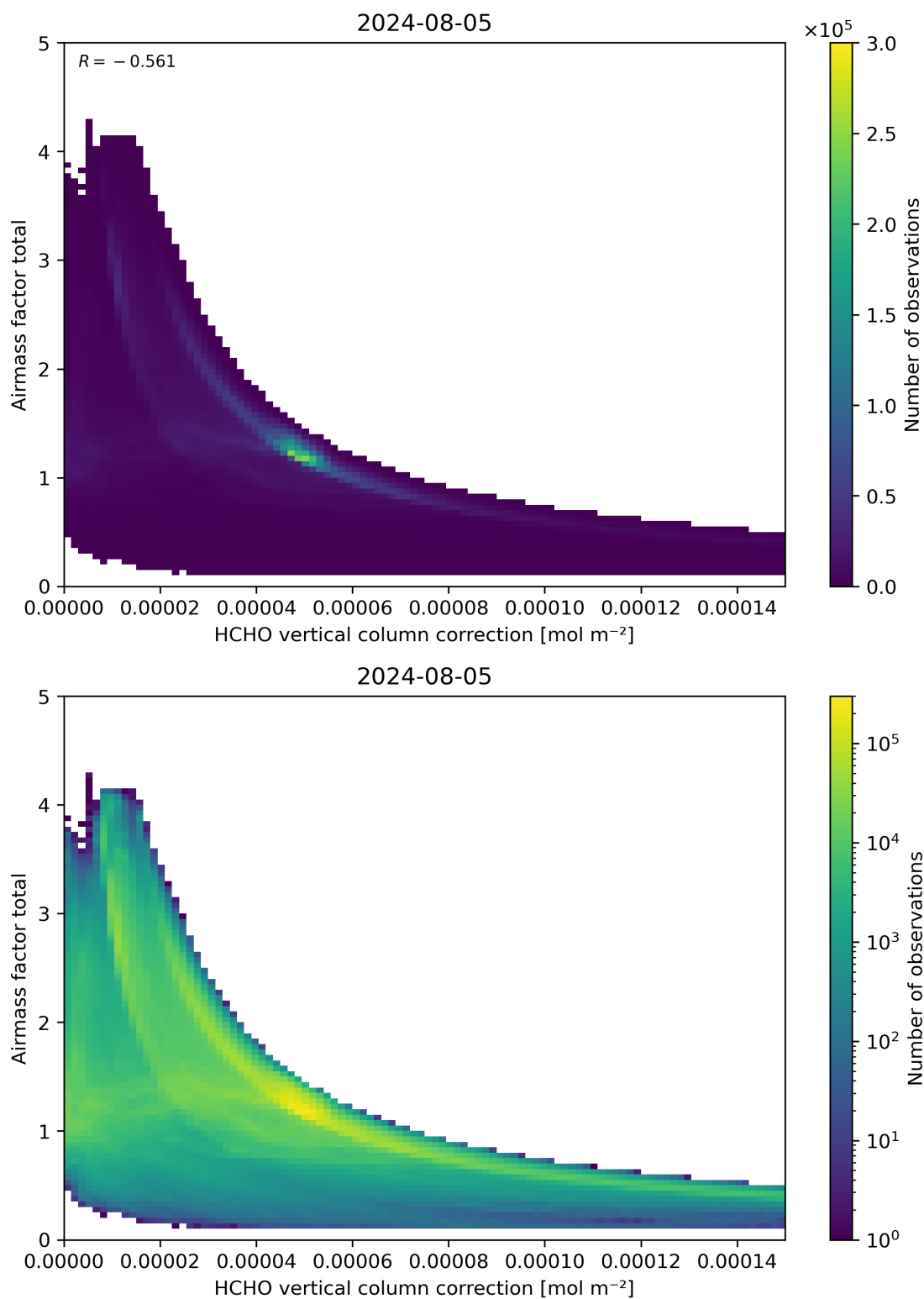
Figure 120: Scatter density plot of “HCHO vertical column correction” against “Airmass factor total” for 2024-08-04 to 2024-08-06.
