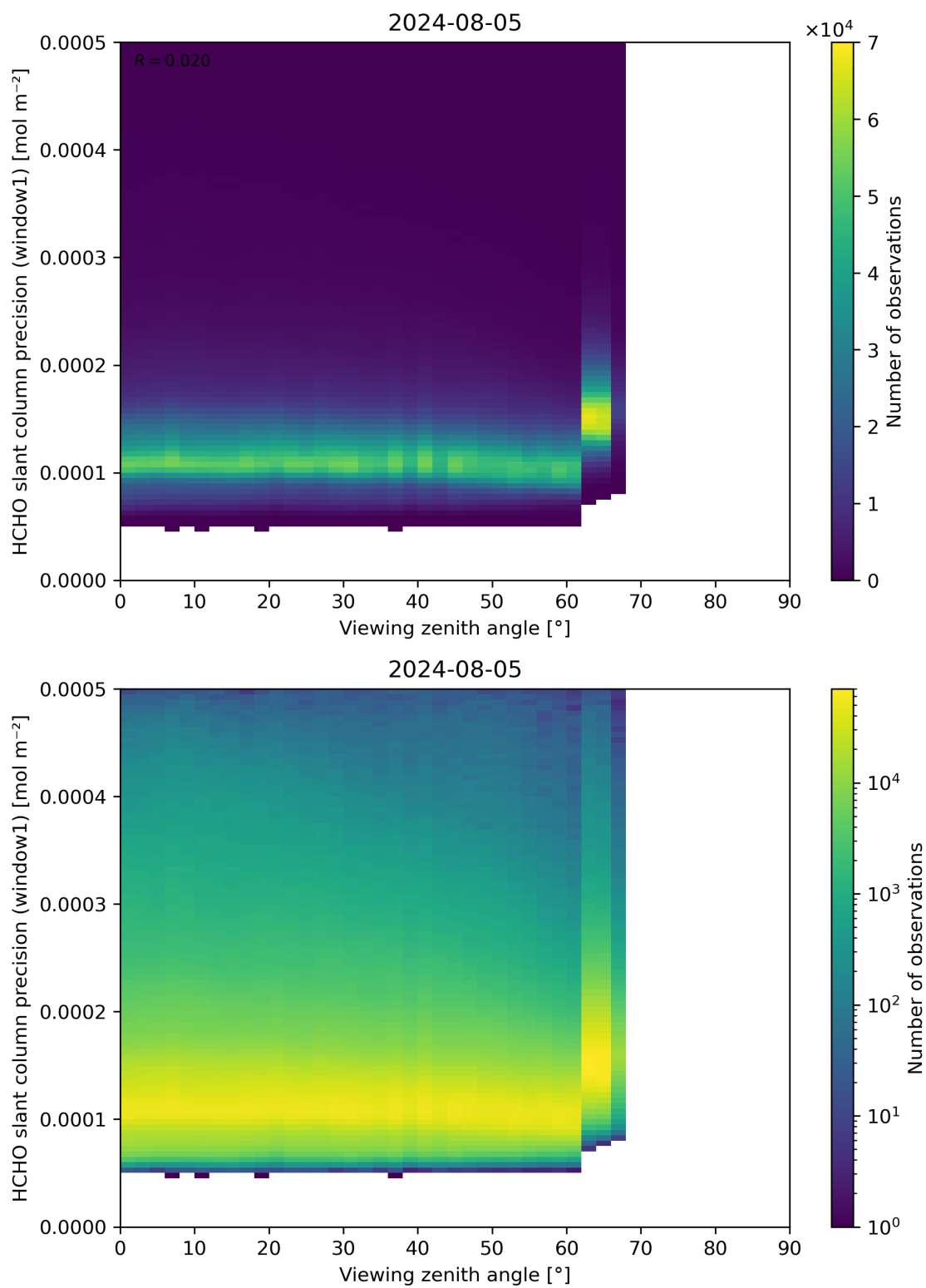
Figure 189: Scatter density plot of “Viewing zenith angle” against “HCHO slant column precision (window1)” for 2024-08-04 to 2024-08-06.
