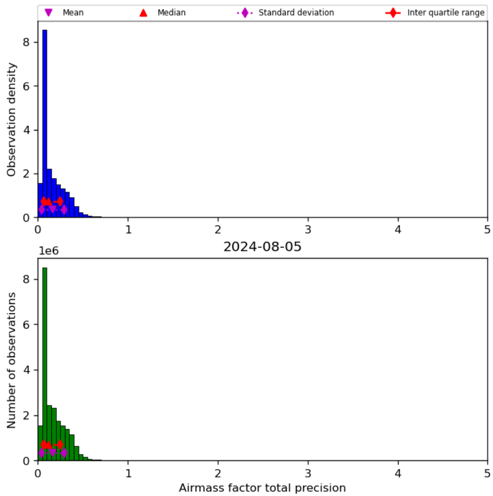
Figure 41: Histogram of “Airmass factor total precision” for 2024-08-04 to 2024-08-06
