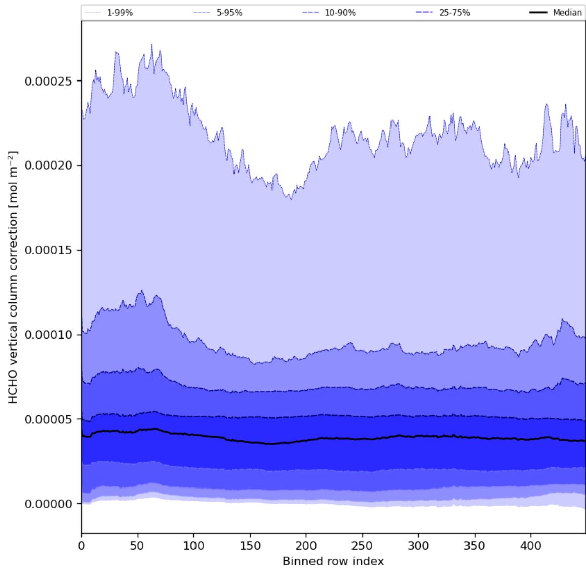
Figure 51: Along track statistics of “HCHO vertical column correction” for 2024-08-04 to 2024-08-06
