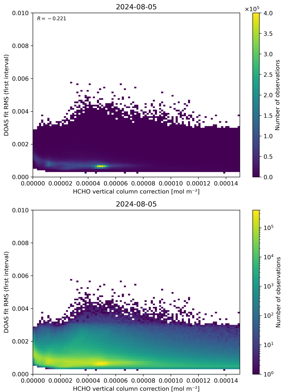
Figure 112: Scatter density plot of “HCHO vertical column correction” against “DOAS fit RMS (first interval)” for 2024-08-04 to 2024-08-06.
