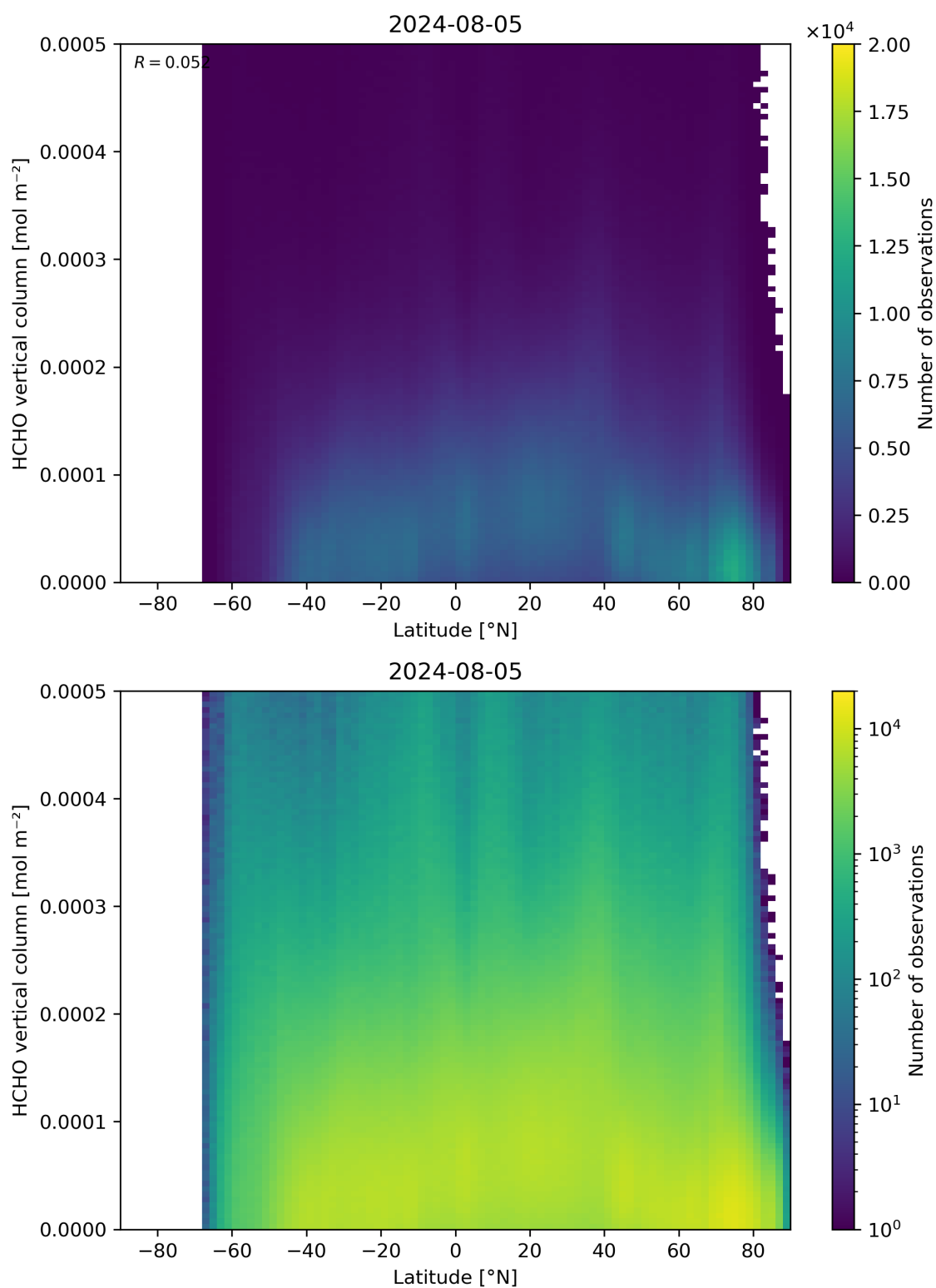
Figure 163: Scatter density plot of “Latitude” against “HCHO vertical column” for 2024-08-04 to 2024-08-06.
