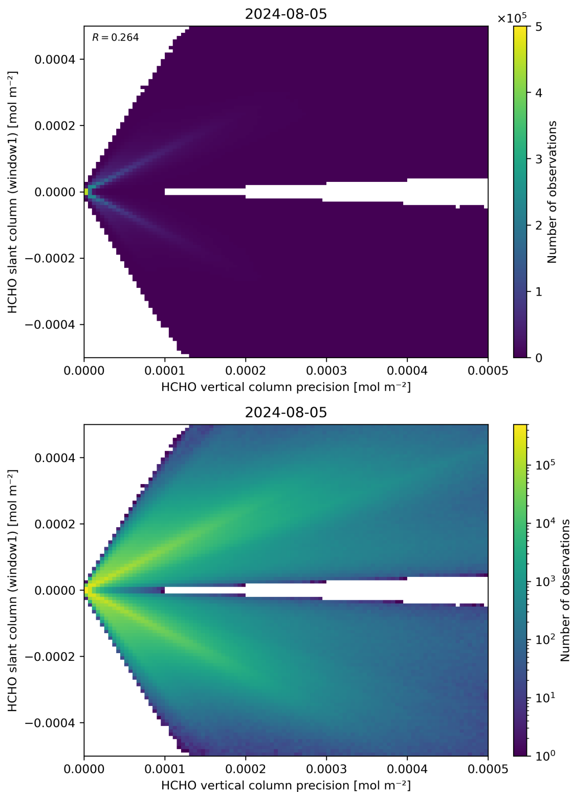
Figure 142: Scatter density plot of “HCHO vertical column precision” against “HCHO slant column (window1)” for 2024-08-04 to 2024-08-06.
