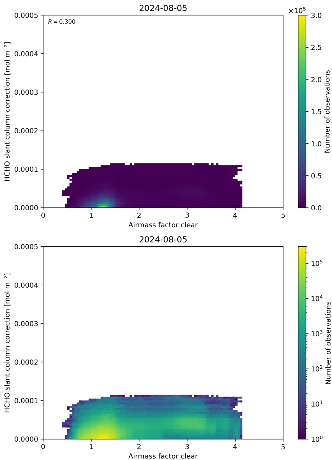
Figure 75: Scatter density plot of “Airmass factor clear” against “HCHO slant column correction” for 2024-08-04 to 2024-08-06.
