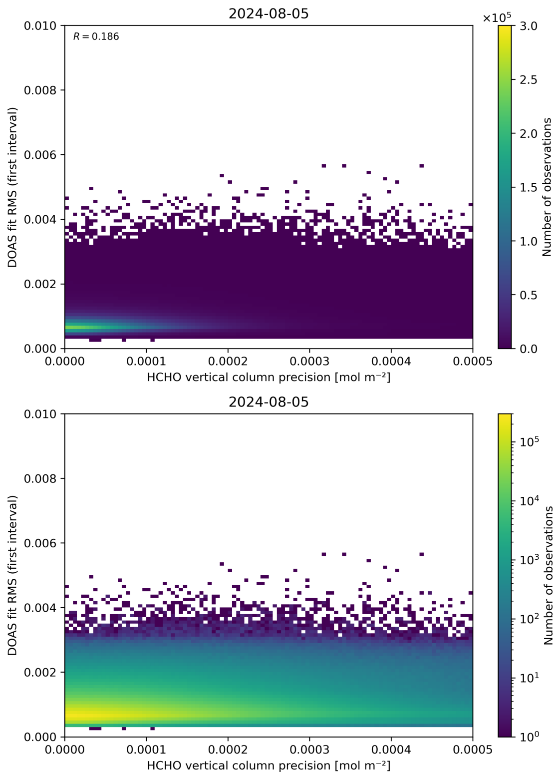
Figure 136: Scatter density plot of “HCHO vertical column precision” against “DOAS fit RMS (first interval)” for 2024-08-04 to 2024-08-06.
