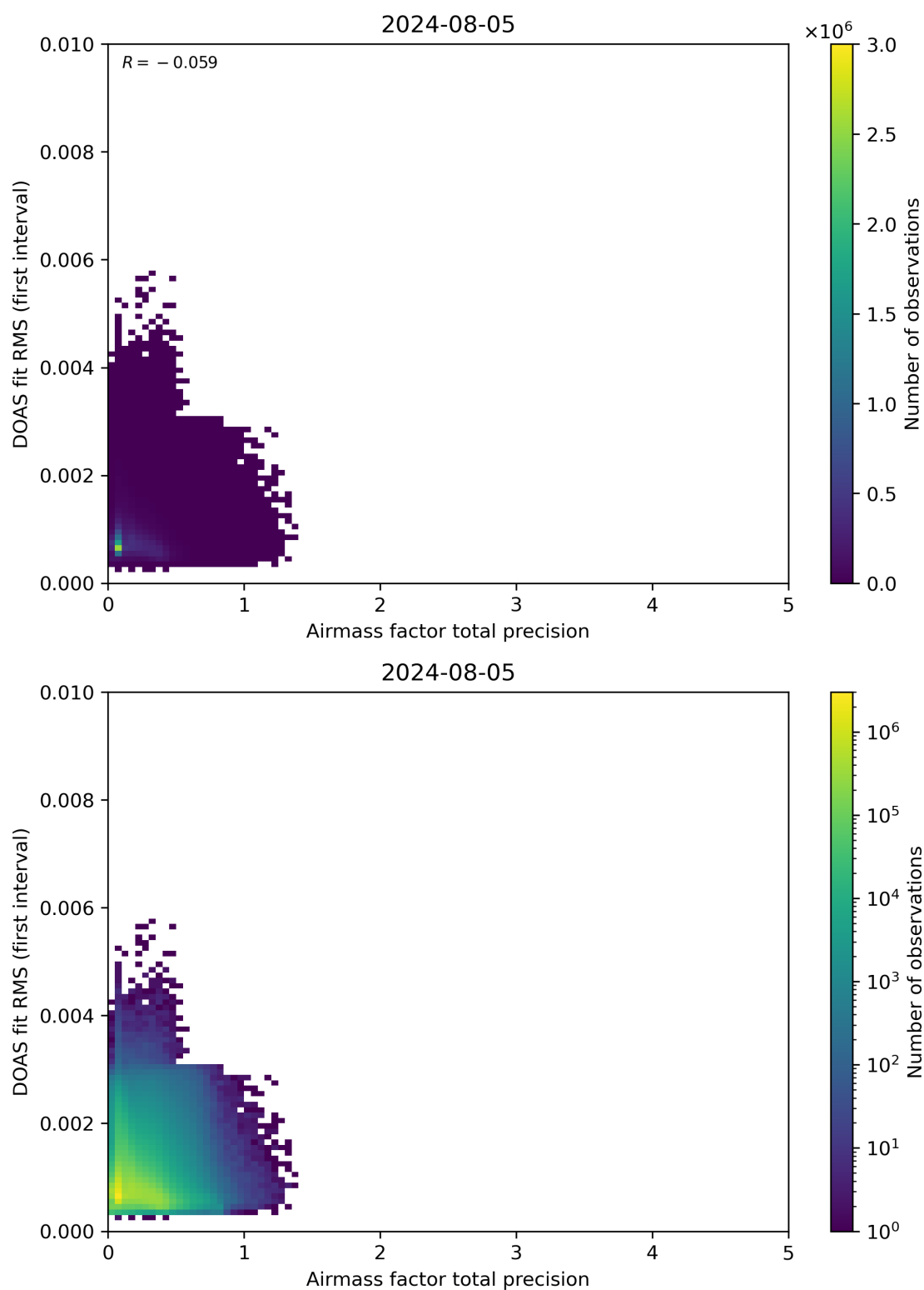
Figure 105: Scatter density plot of “Airmass factor total precision” against “DOAS fit RMS (first interval)” for 2024-08-04 to 2024-08-06.
