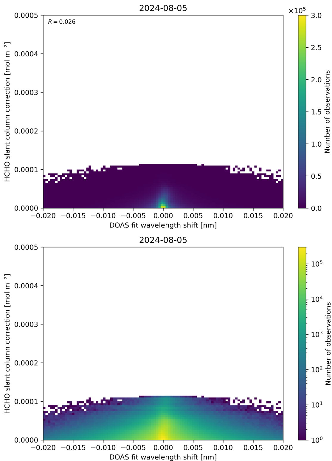
Figure 67: Scatter density plot of “DOAS fit wavelength shift” against “HCHO slant column correction” for 2024-08-04 to 2024-08-06.
