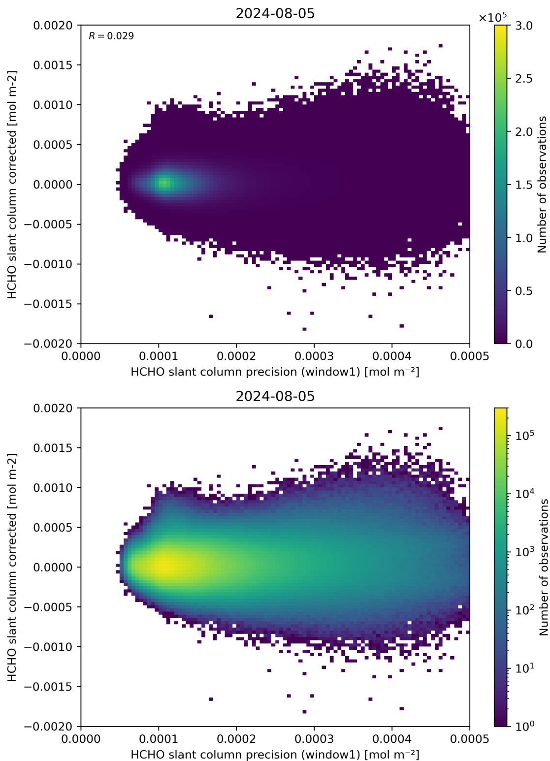
Figure 92: Scatter density plot of “HCHO slant column precision (window1)” against “HCHO slant column corrected” for 2024-08-04 to 2024-08-06.
