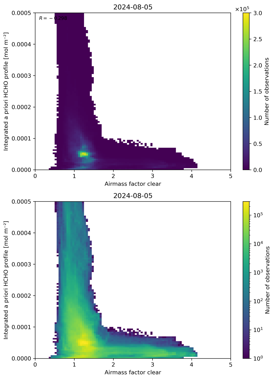
Figure 76: Scatter density plot of “Airmass factor clear” against “Integrated a priori HCHO profile” for 2024-08-04 to 2024-08-06.
