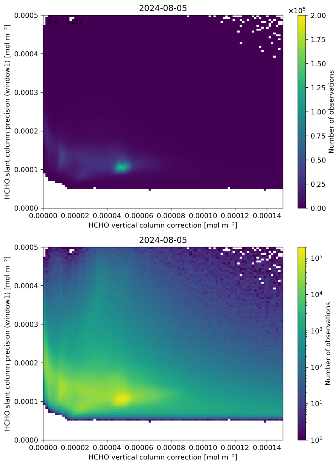
Figure 119: Scatter density plot of “HCHO vertical column correction” against “HCHO slant column precision (window1)” for 2024-08-04 to 2024-08-06.
