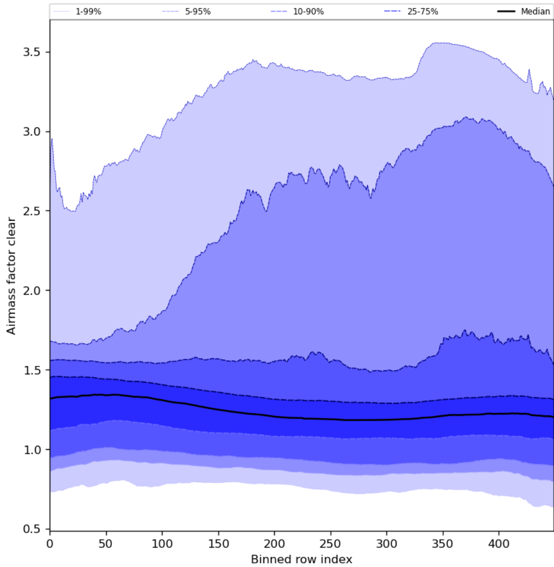
Figure 56: Along track statistics of “Airmass factor clear” for 2024-08-04 to 2024-08-06
