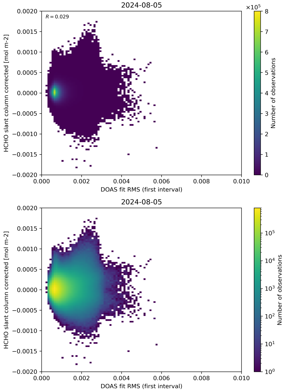
Figure 62: Scatter density plot of “DOAS fit RMS (first interval)” against “HCHO slant column corrected” for 2024-08-04 to 2024-08-06.
