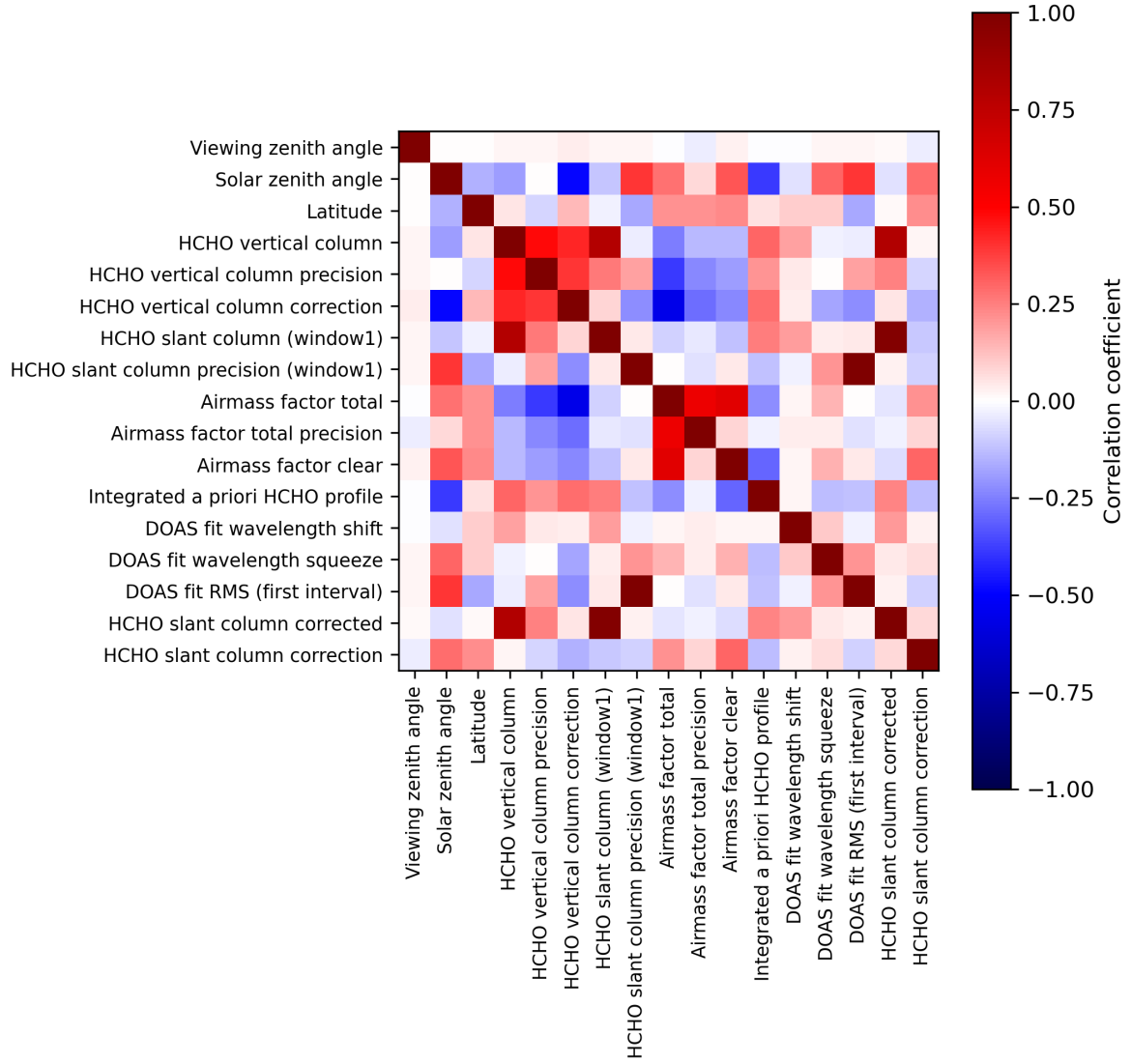
Figure 2: Map of correlation matrix for 2024-08-04 to 2024-08-06.
