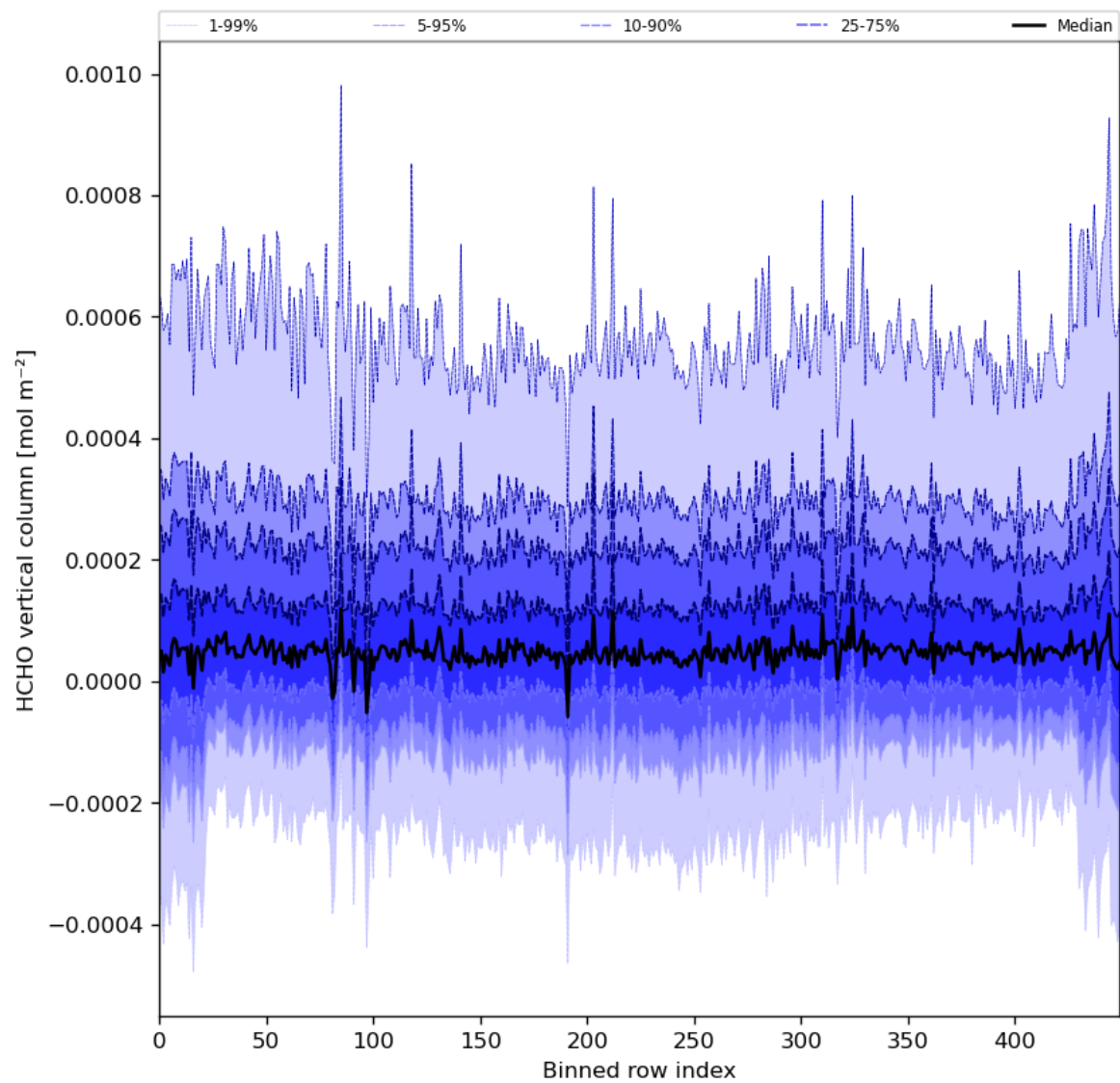
Figure 49: Along track statistics of “HCHO vertical column” for 2024-08-04 to 2024-08-06
