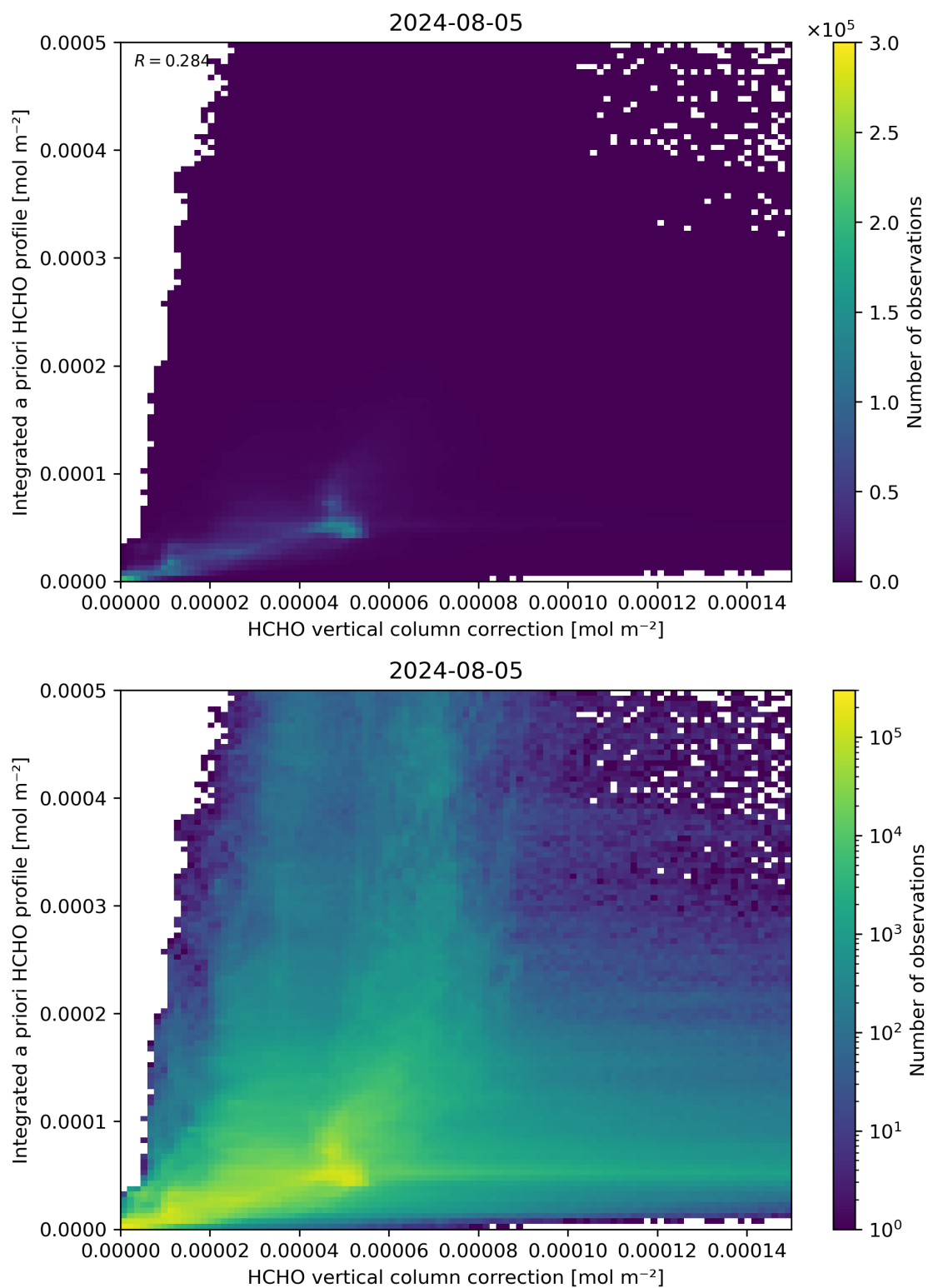
Figure 122: Scatter density plot of “HCHO vertical column correction” against “Integrated a priori HCHO profile” for 2024-08-04 to 2024-08-06.
