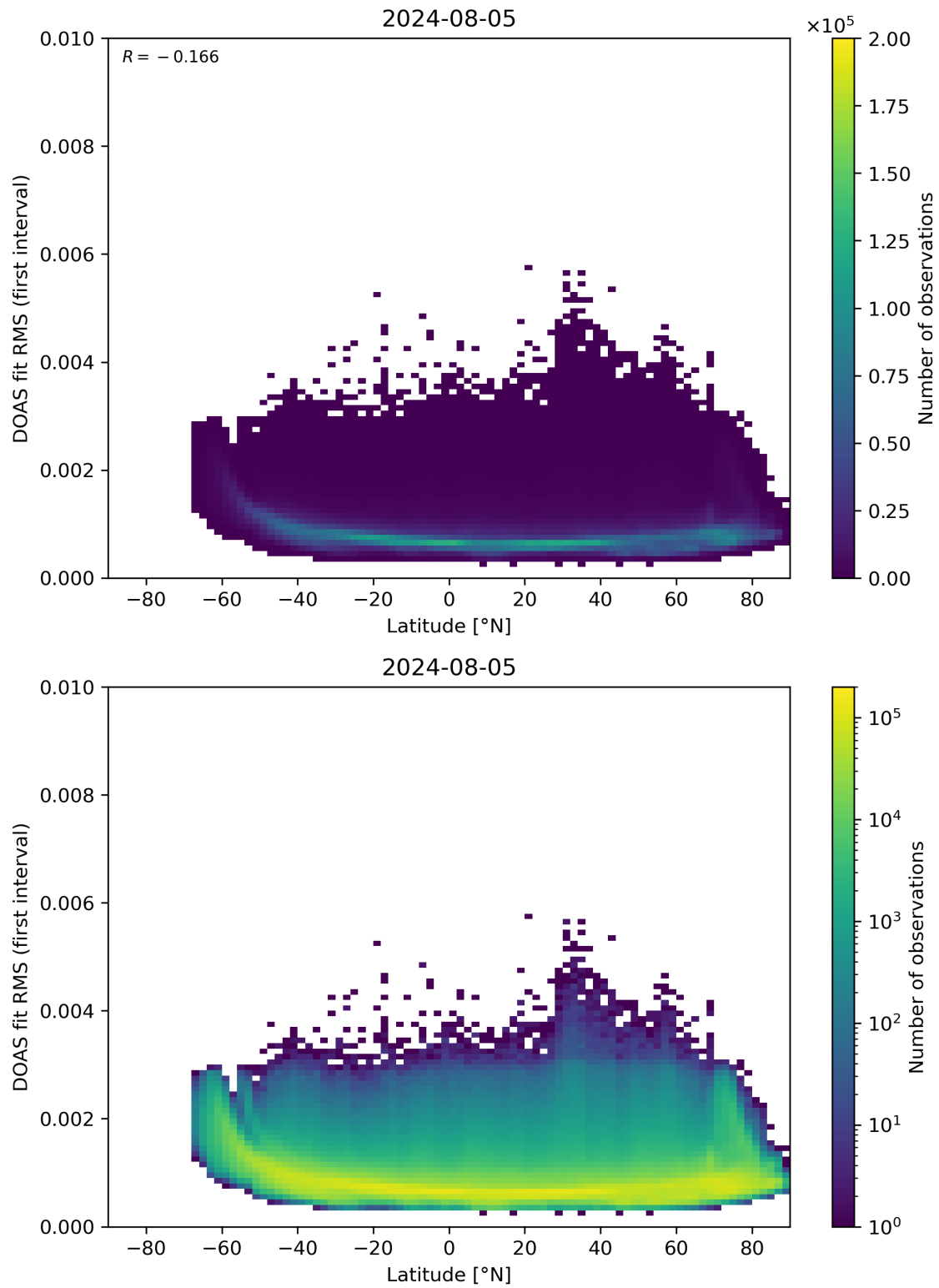
Figure 153: Scatter density plot of “Latitude” against “DOAS fit RMS (first interval)” for 2024-08-04 to 2024-08-06.
