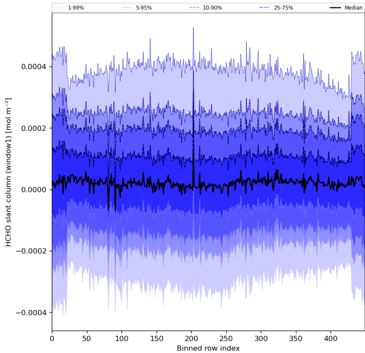
Figure 52: Along track statistics of “HCHO slant column (window1)” for 2024-08-04 to 2024-08-06
