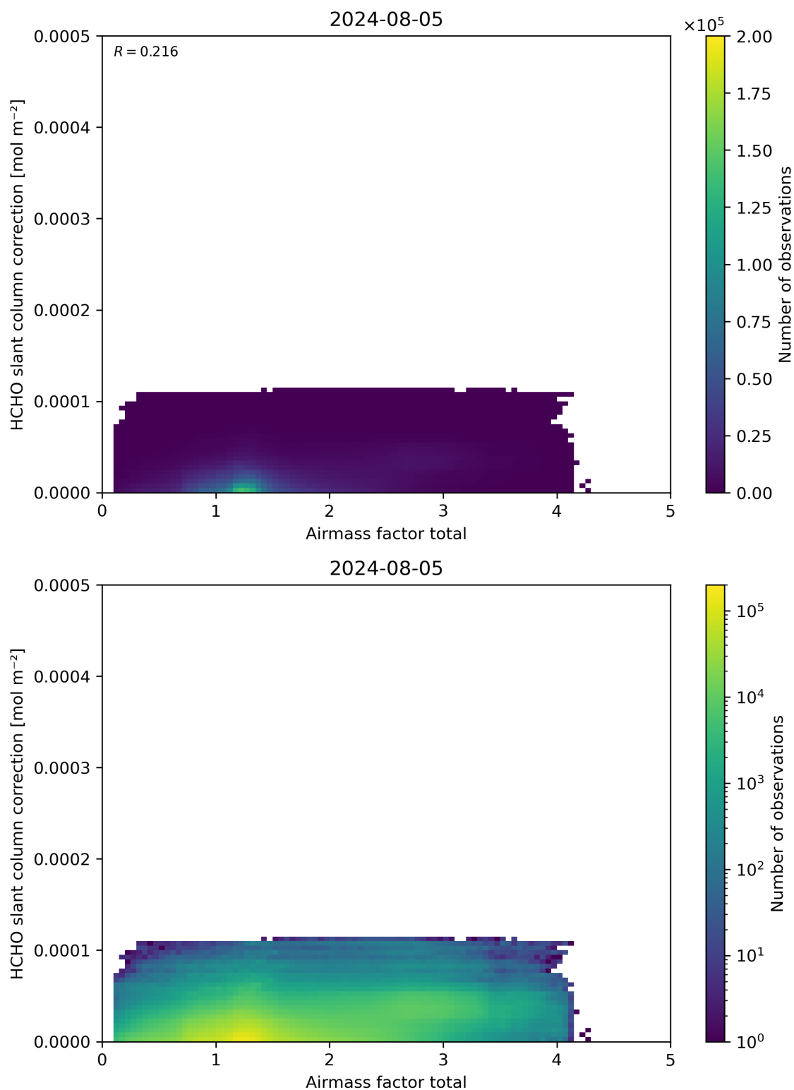
Figure 102: Scatter density plot of “Airmass factor total” against “HCHO slant column correction” for 2024-08-04 to 2024-08-06.
