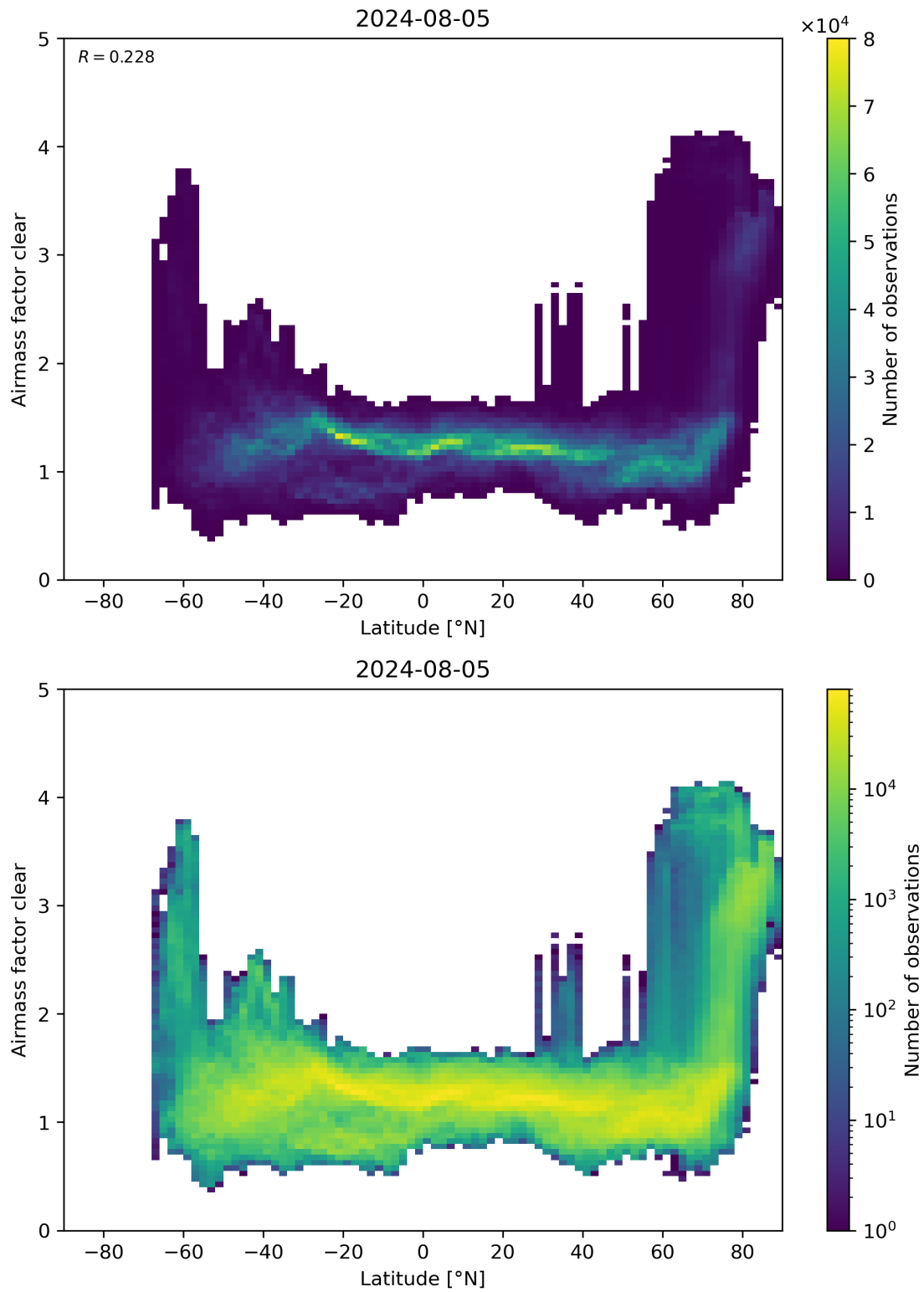
Figure 156: Scatter density plot of “Latitude” against “Airmass factor clear” for 2024-08-04 to 2024-08-06.
