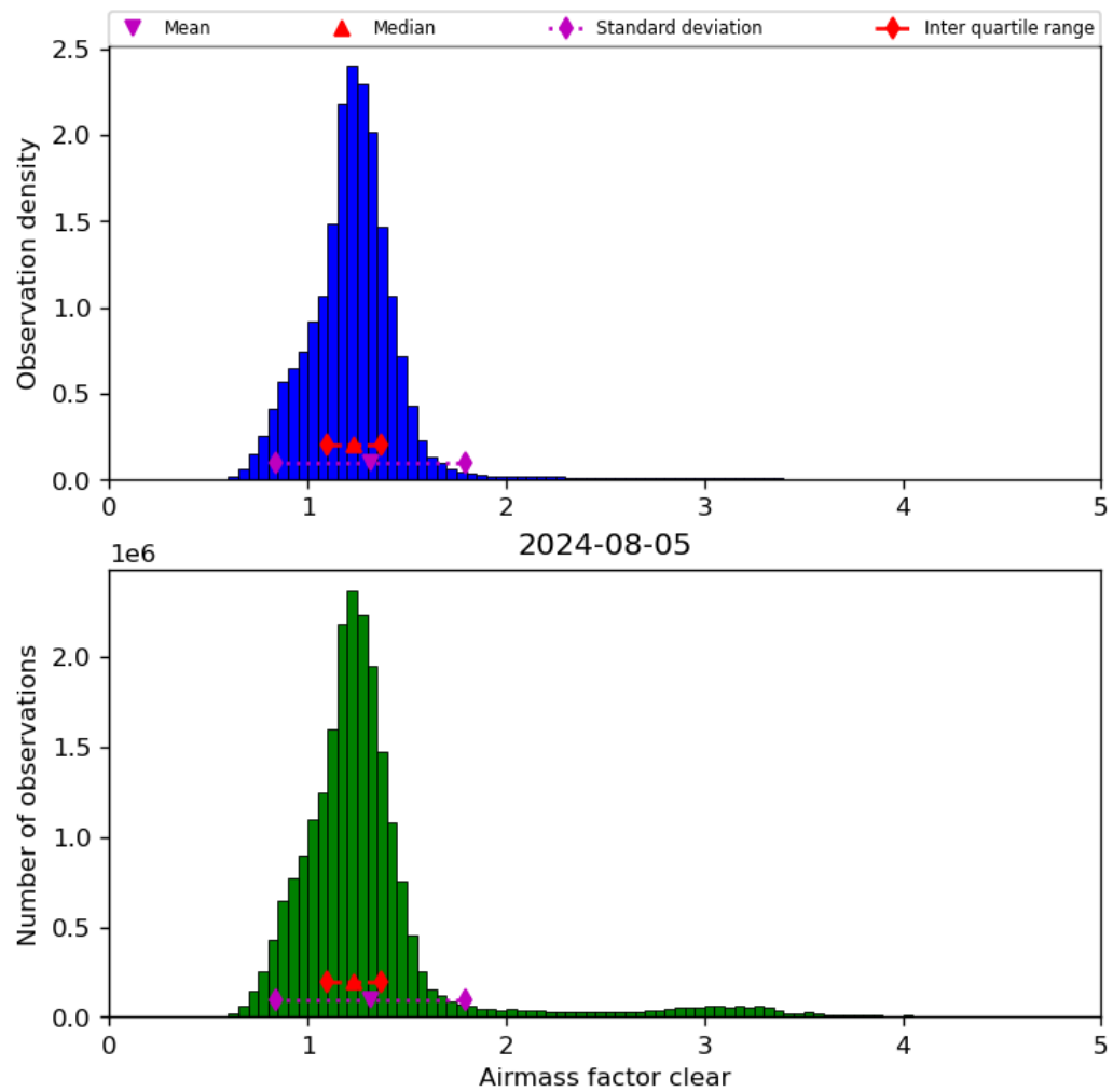
Figure 42: Histogram of “Airmass factor clear” for 2024-08-04 to 2024-08-06
