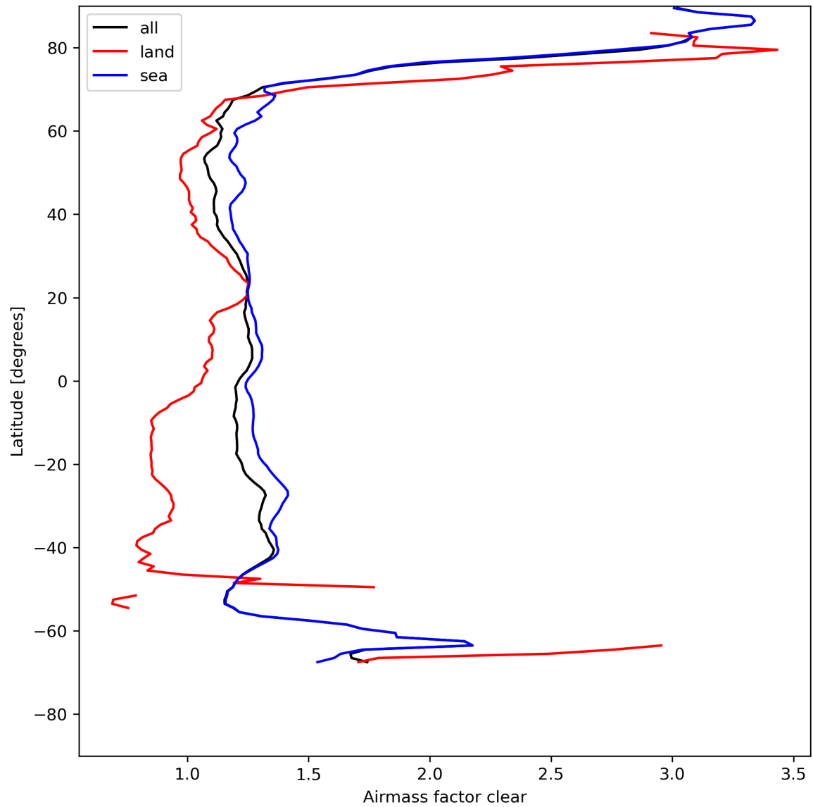
Figure 28: Zonal average of “Airmass factor clear” for 2024-08-04 to 2024-08-06.
