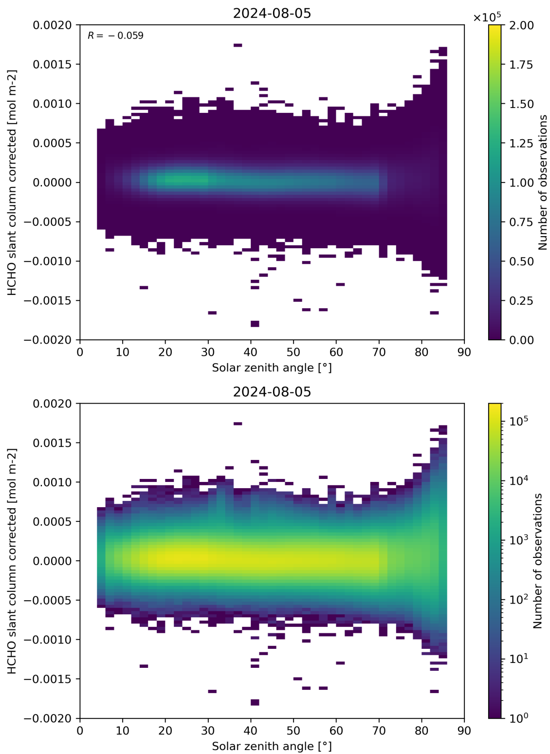
Figure 171: Scatter density plot of “Solar zenith angle” against “HCHO slant column corrected” for 2024-08-04 to 2024-08-06.
