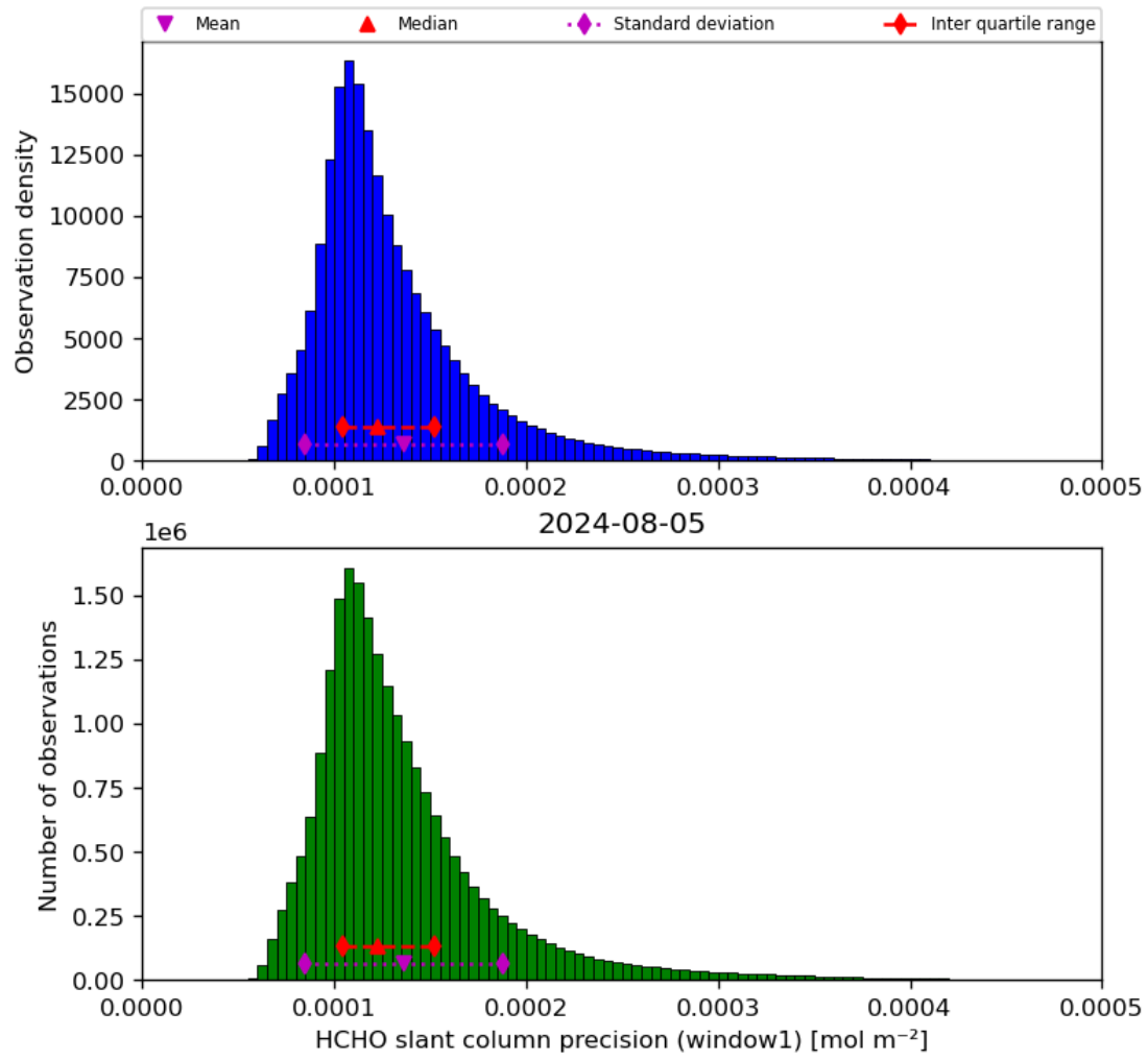
Figure 39: Histogram of “HCHO slant column precision (window1)” for 2024-08-04 to 2024-08-06
