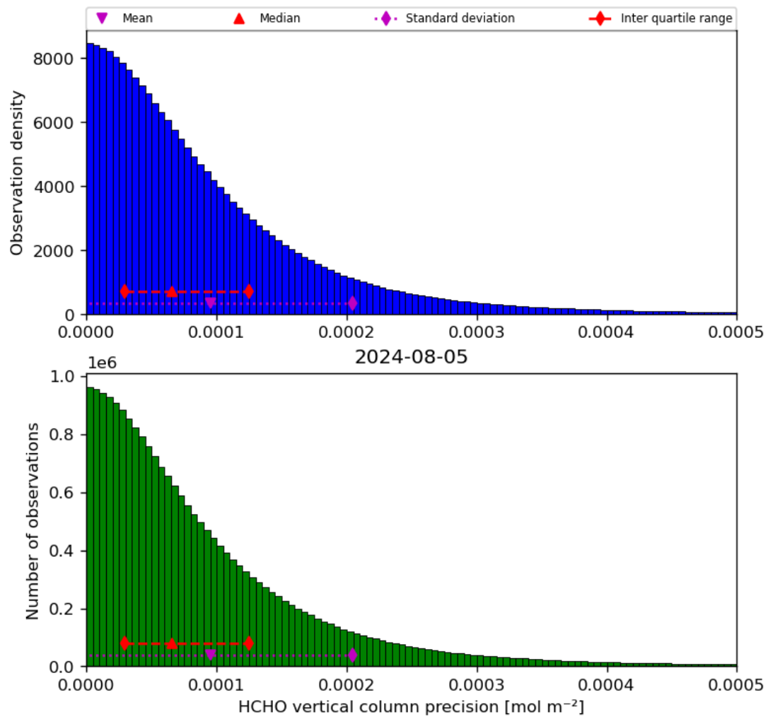
Figure 36: Histogram of “HCHO vertical column precision” for 2024-08-04 to 2024-08-06
