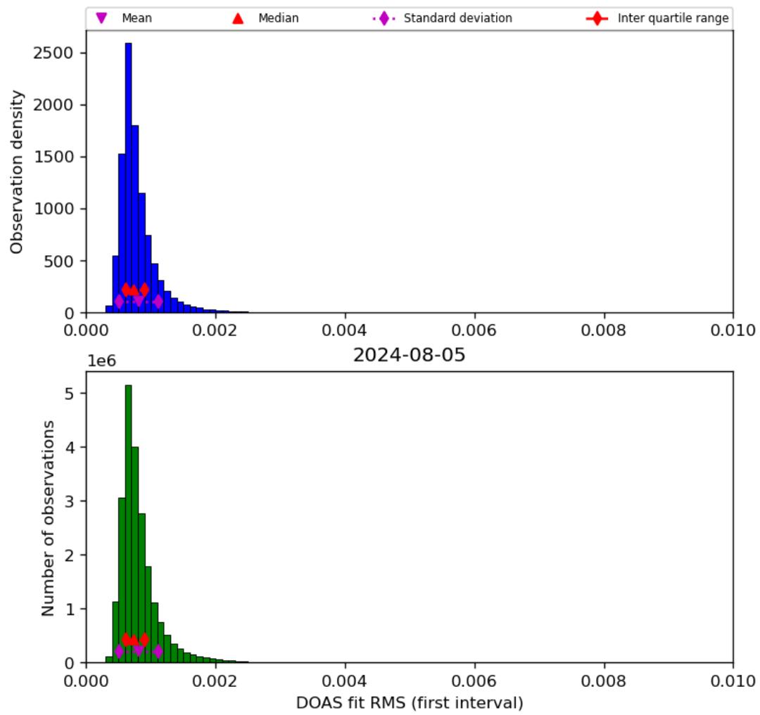
Figure 46: Histogram of “DOAS fit RMS (first interval)” for 2024-08-04 to 2024-08-06
