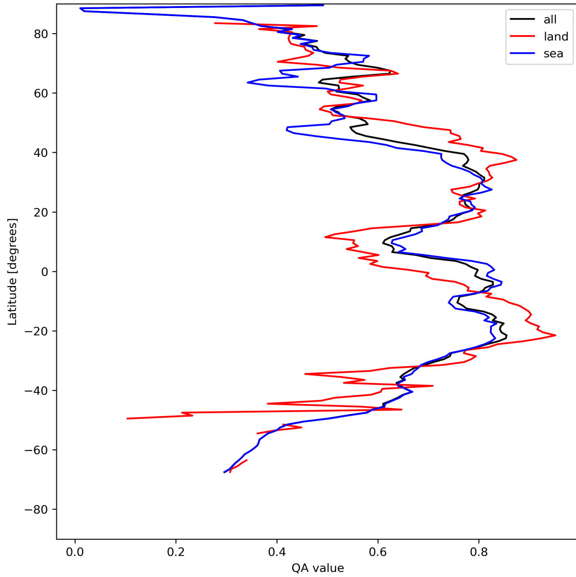
Figure 20: Zonal average of “QA value” for 2024-08-04 to 2024-08-06.
