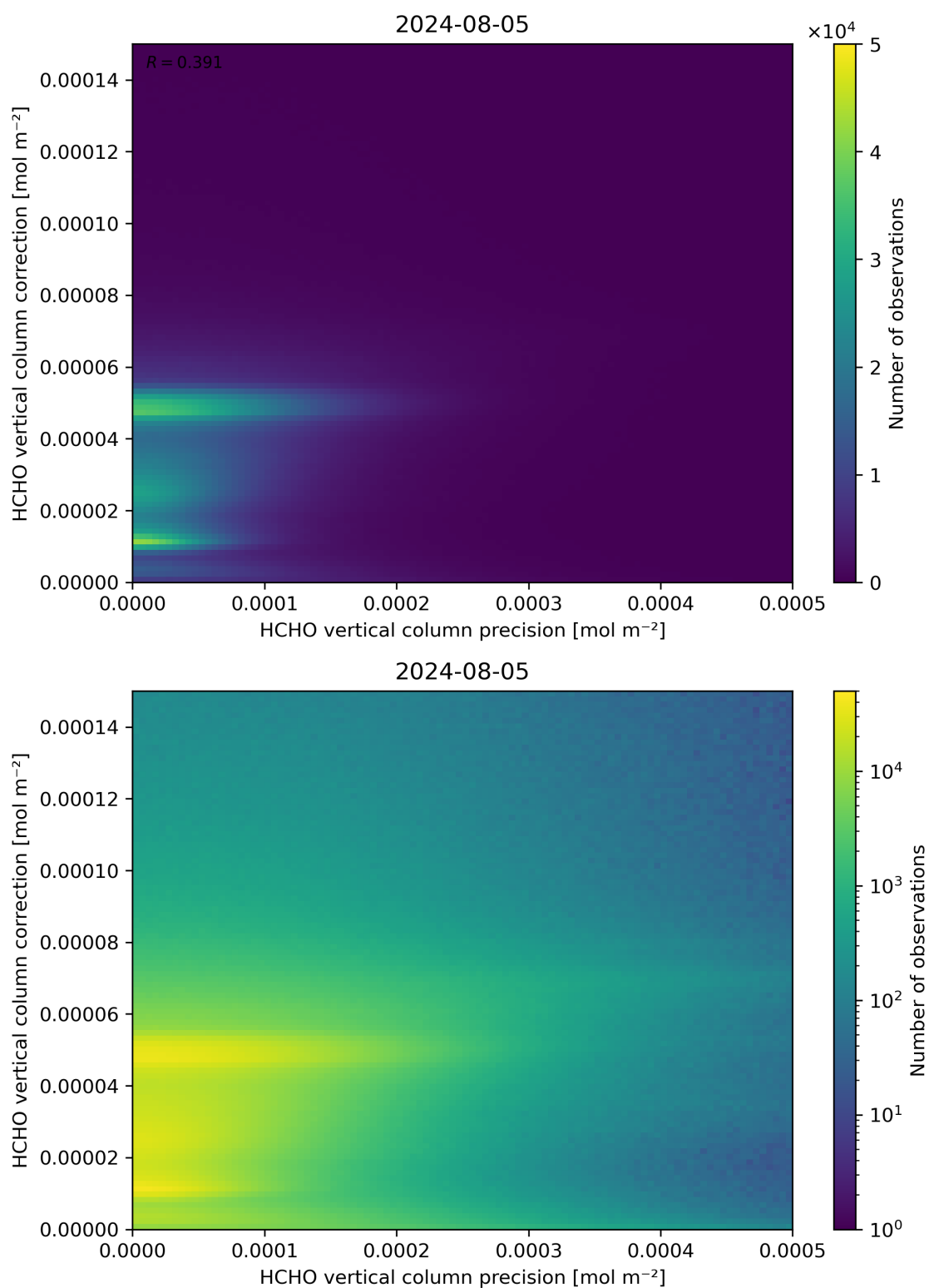
Figure 146: Scatter density plot of “HCHO vertical column precision” against “HCHO vertical column correction” for 2024-08-04 to 2024-08-06.
