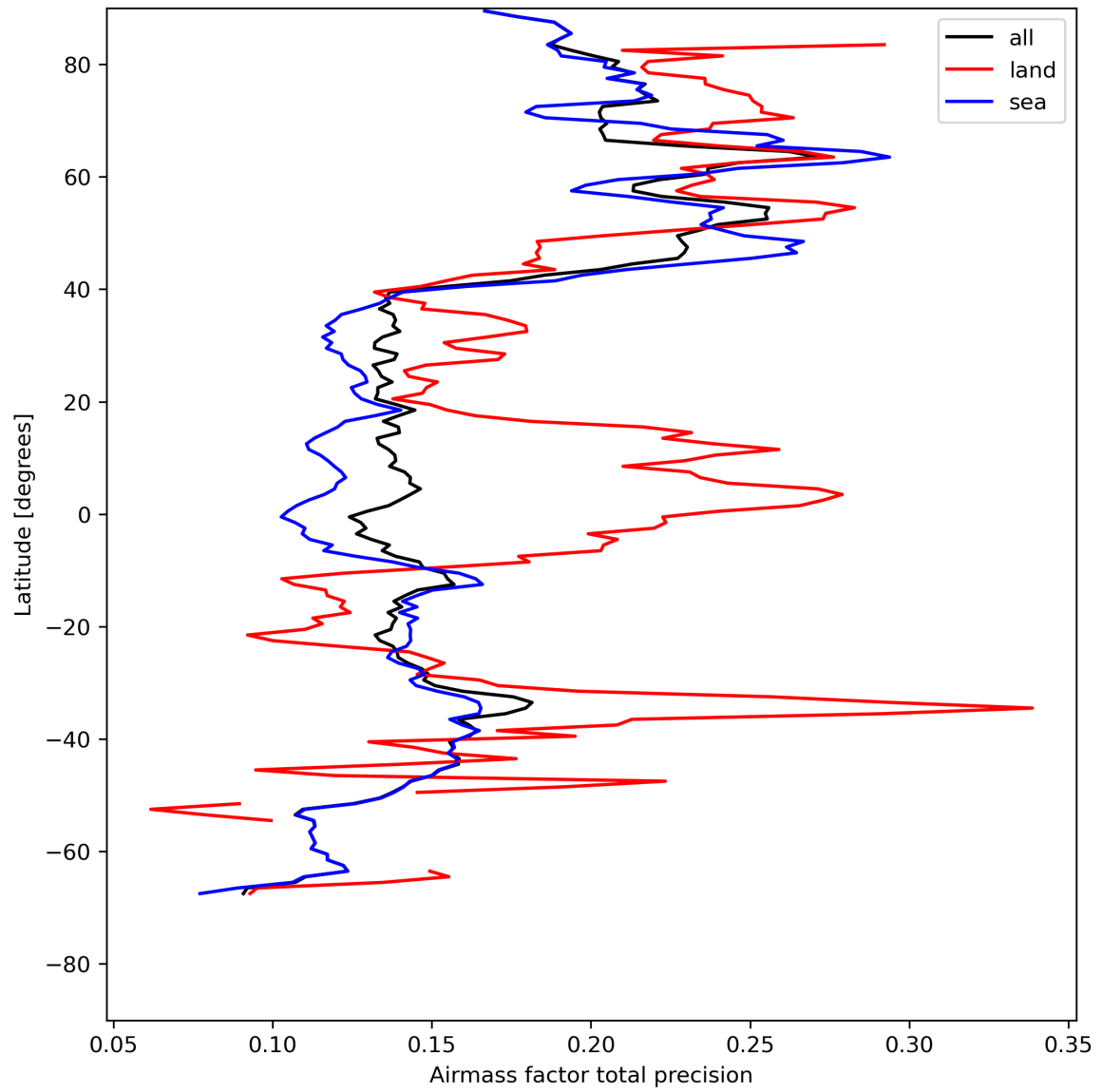
Figure 27: Zonal average of “Airmass factor total precision” for 2024-08-04 to 2024-08-06.
