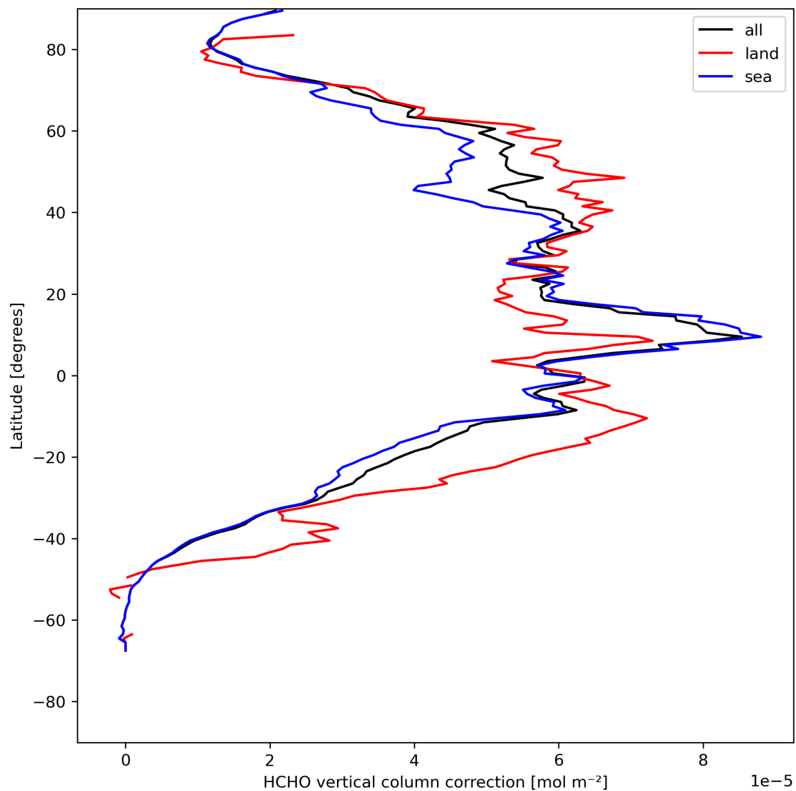
Figure 23: Zonal average of “HCHO vertical column correction” for 2024-08-04 to 2024-08-06.
