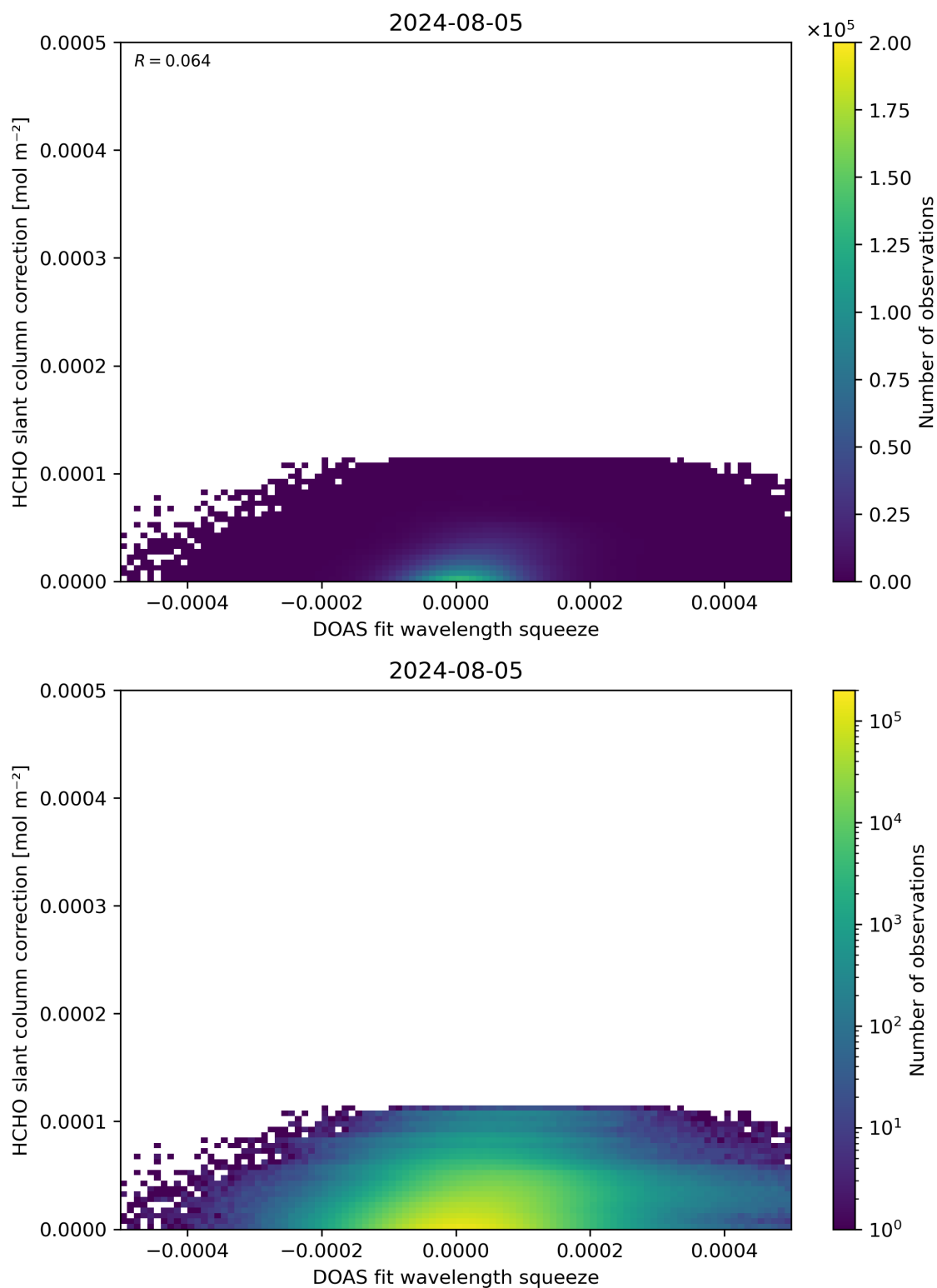
Figure 70: Scatter density plot of “DOAS fit wavelength squeeze” against “HCHO slant column correction” for 2024-08-04 to 2024-08-06.
