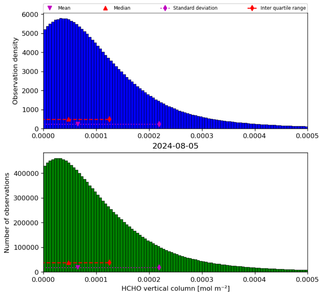
Figure 35: Histogram of “HCHO vertical column” for 2024-08-04 to 2024-08-06
