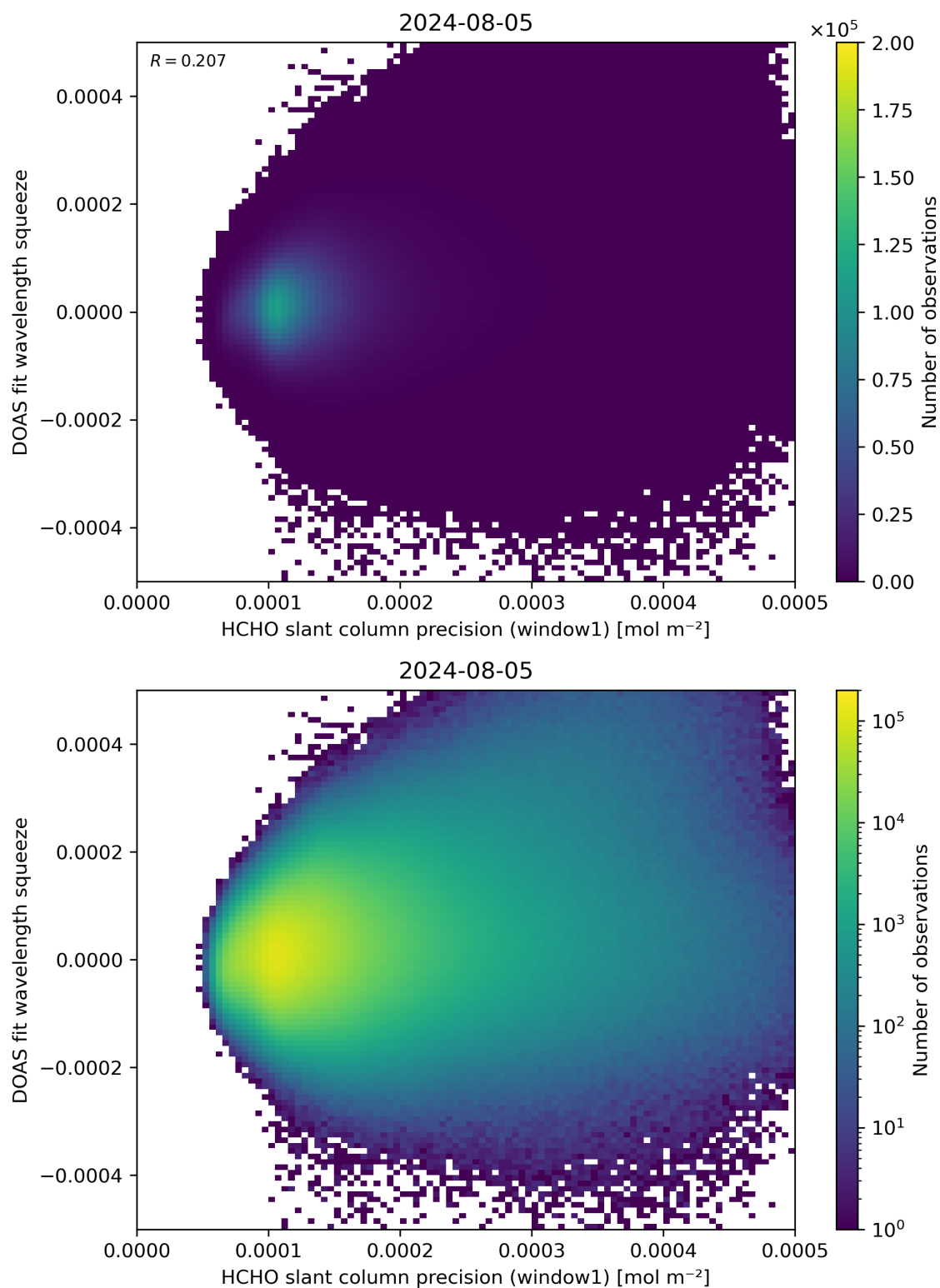
Figure 90: Scatter density plot of “HCHO slant column precision (window1)” against “DOAS fit wavelength squeeze” for 2024-08-04 to 2024-08-06.
