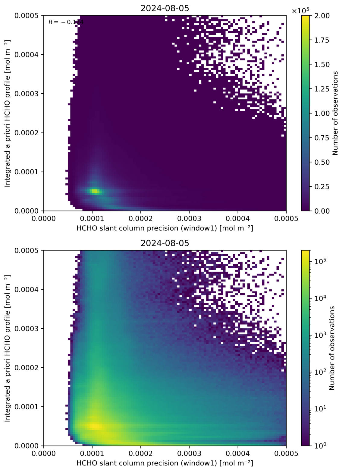
Figure 96: Scatter density plot of “HCHO slant column precision (window1)” against “Integrated a priori HCHO profile” for 2024-08-04 to 2024-08-06.
