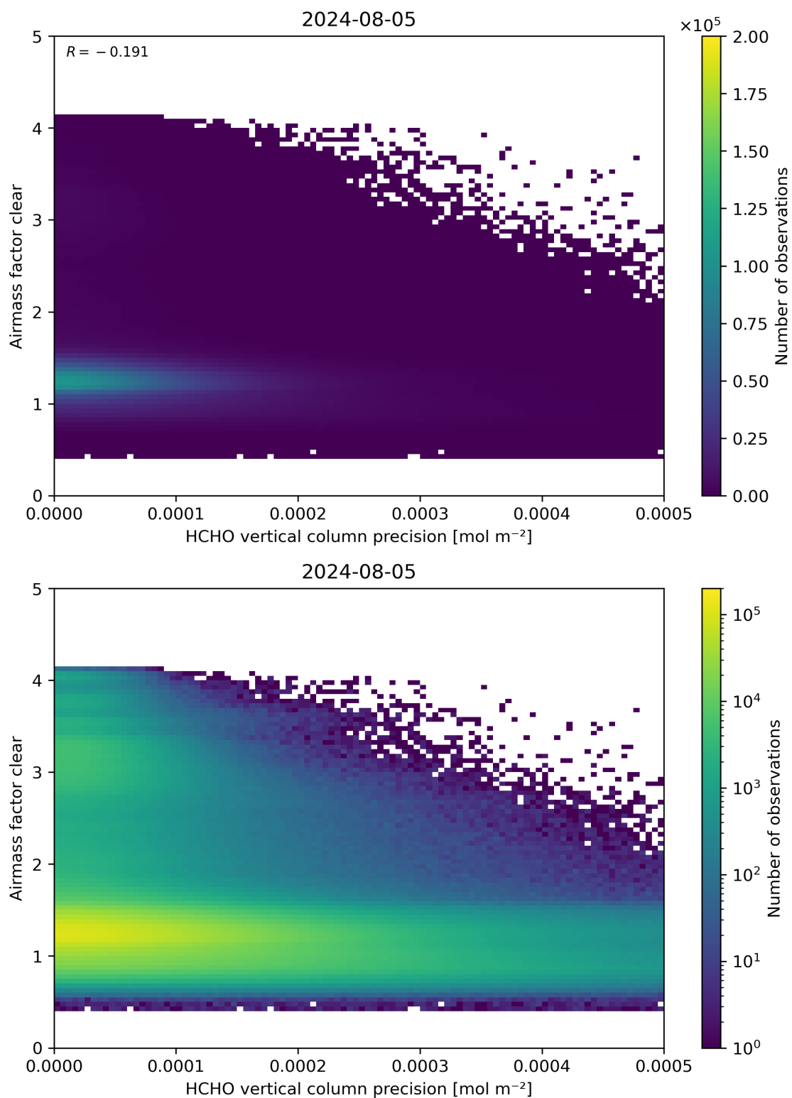
Figure 139: Scatter density plot of “HCHO vertical column precision” against “Airmass factor clear” for 2024-08-04 to 2024-08-06.
