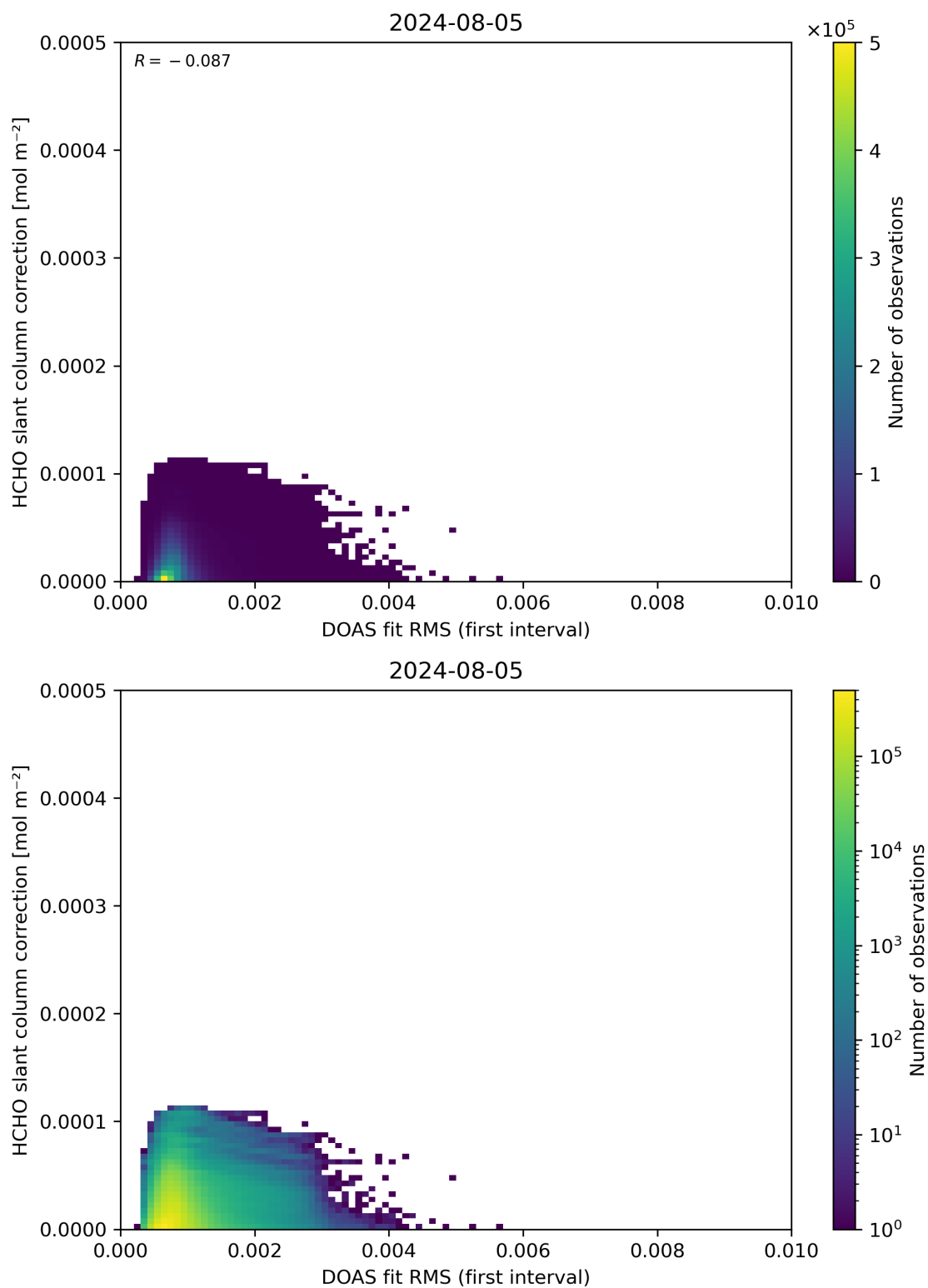
Figure 63: Scatter density plot of “DOAS fit RMS (first interval)” against “HCHO slant column correction” for 2024-08-04 to 2024-08-06.
