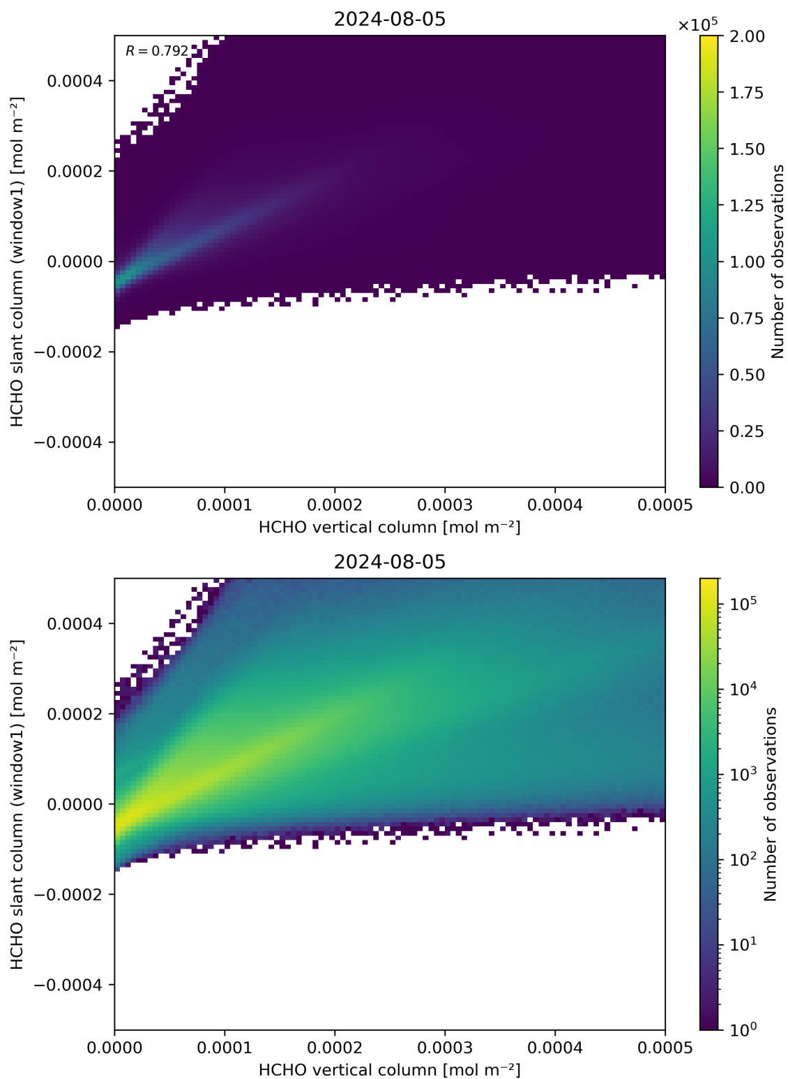
Figure 129: Scatter density plot of “HCHO vertical column” against “HCHO slant column (window1)” for 2024-08-04 to 2024-08-06.
