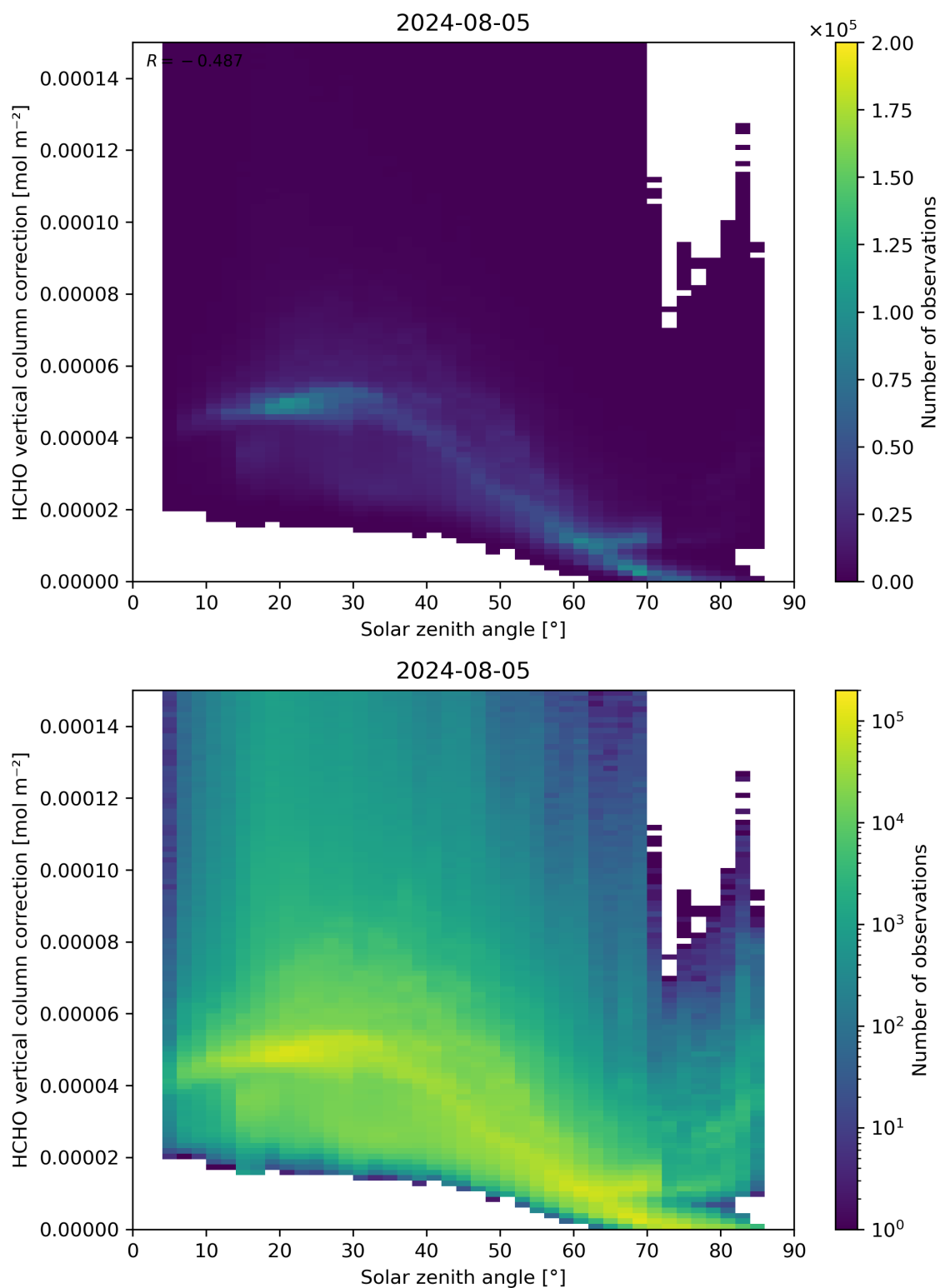
Figure 178: Scatter density plot of “Solar zenith angle” against “HCHO vertical column correction” for 2024-08-04 to 2024-08-06.
