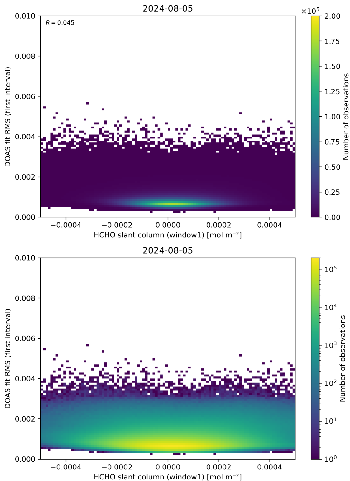
Figure 78: Scatter density plot of “HCHO slant column (window1)” against “DOAS fit RMS (first interval)” for 2024-08-04 to 2024-08-06.
