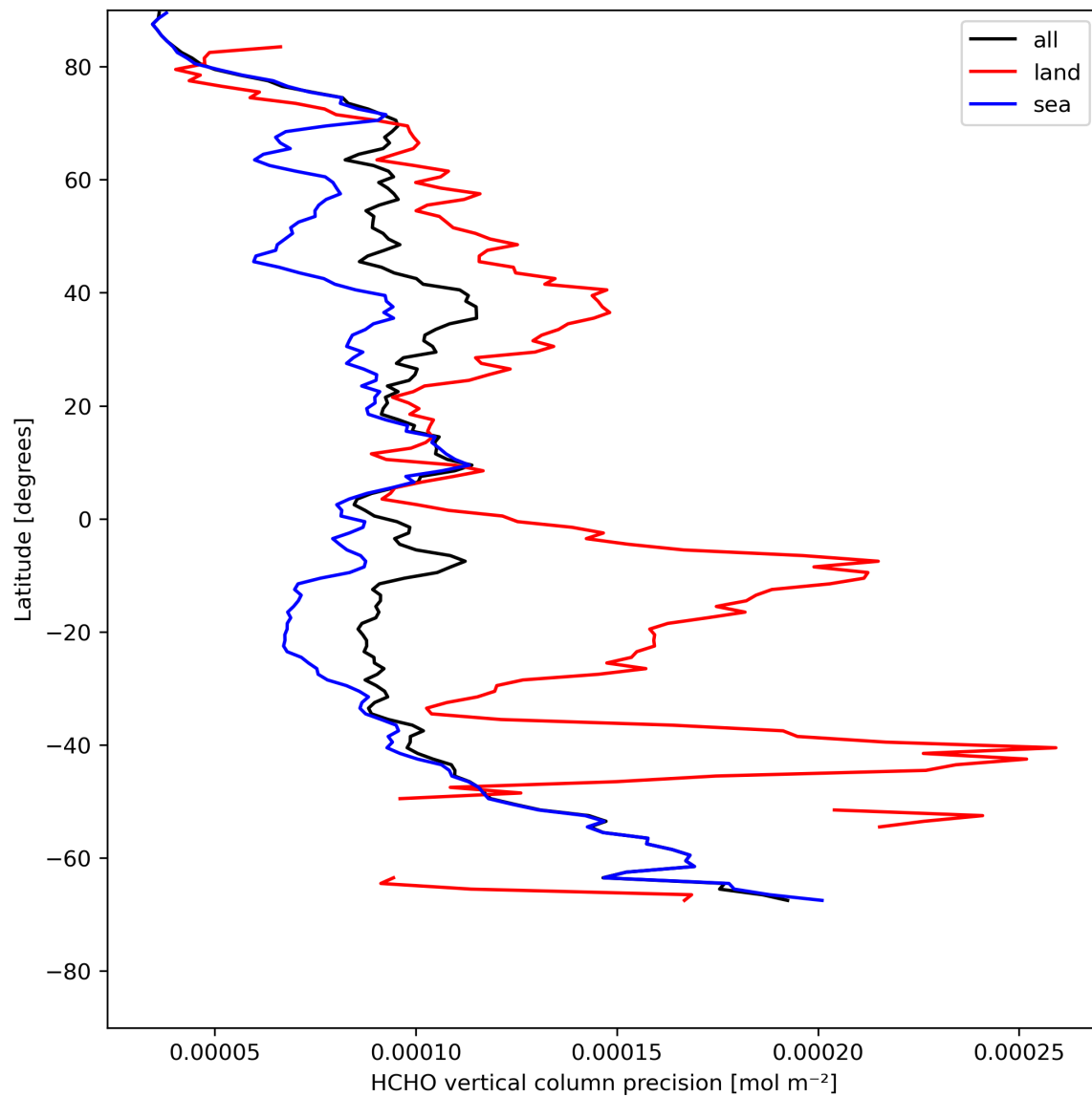
Figure 22: Zonal average of “HCHO vertical column precision” for 2024-08-04 to 2024-08-06.
