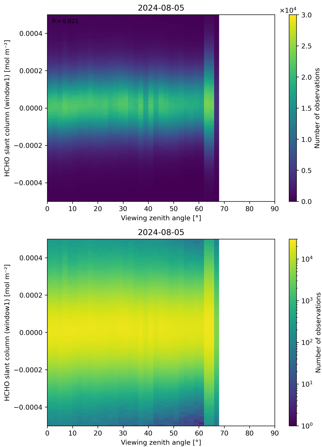
Figure 188: Scatter density plot of “Viewing zenith angle” against “HCHO slant column (window1)” for 2024-08-04 to 2024-08-06.
