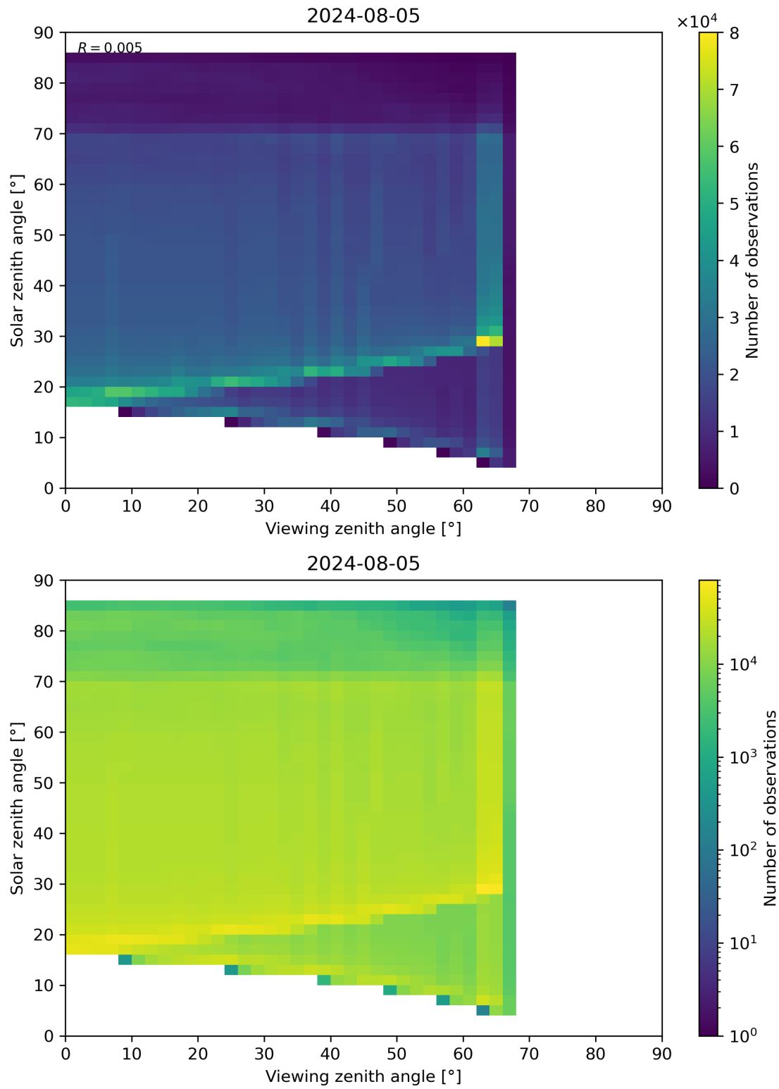
Figure 197: Scatter density plot of “Viewing zenith angle” against “Solar zenith angle” for 2024-08-04 to 2024-08-06.
