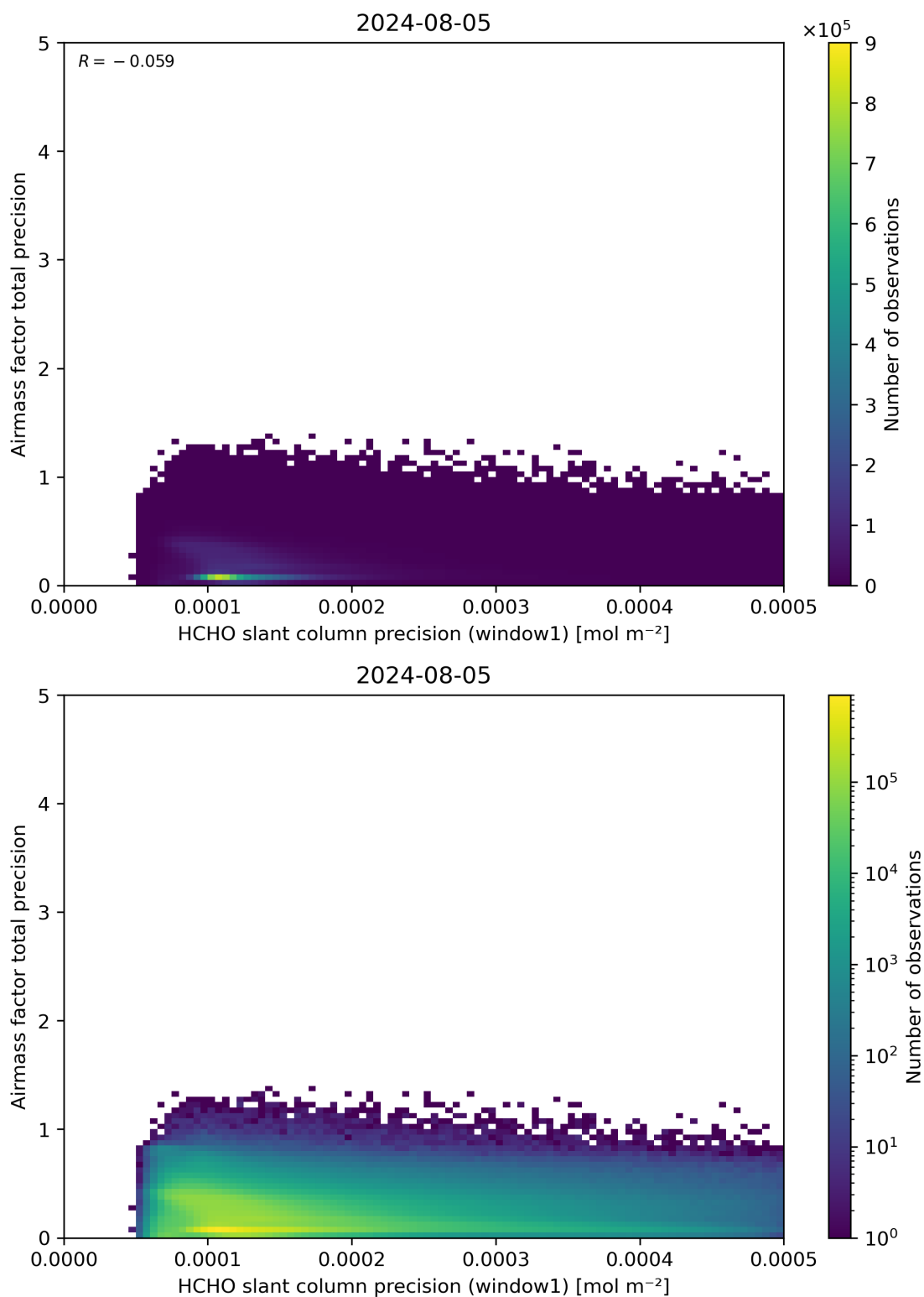
Figure 95: Scatter density plot of “HCHO slant column precision (window1)” against “Airmass factor total precision” for 2024-08-04 to 2024-08-06.
