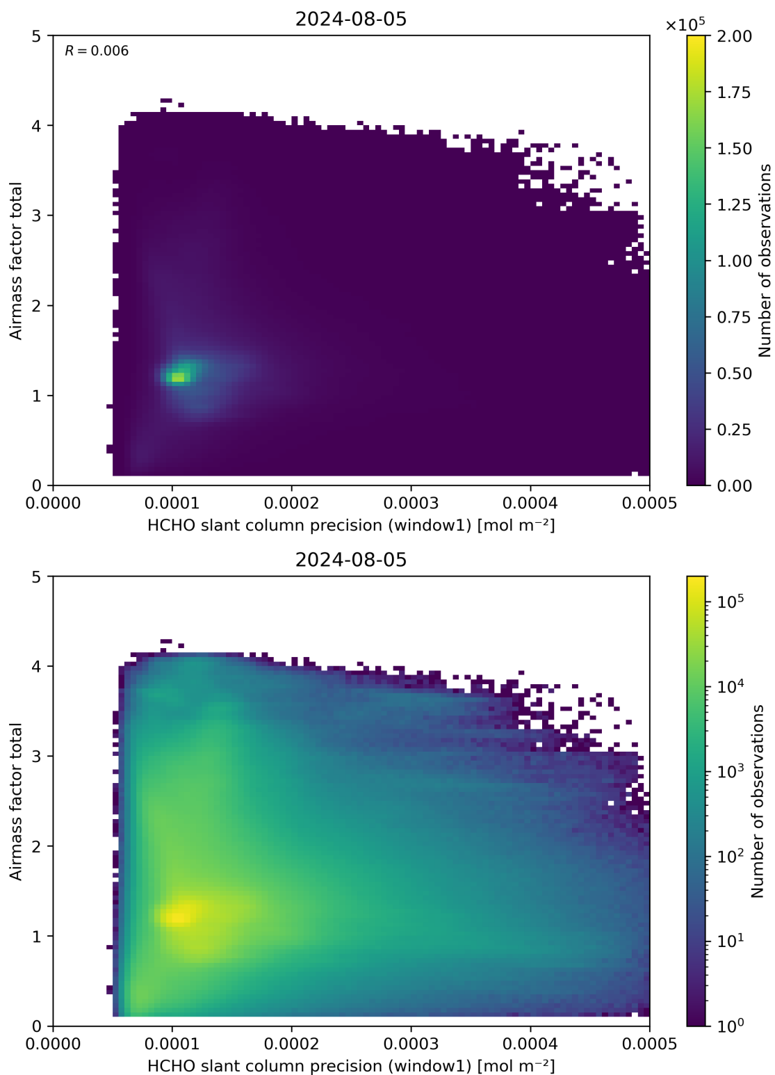
Figure 94: Scatter density plot of “HCHO slant column precision (window1)” against “Airmass factor total” for 2024-08-04 to 2024-08-06.
