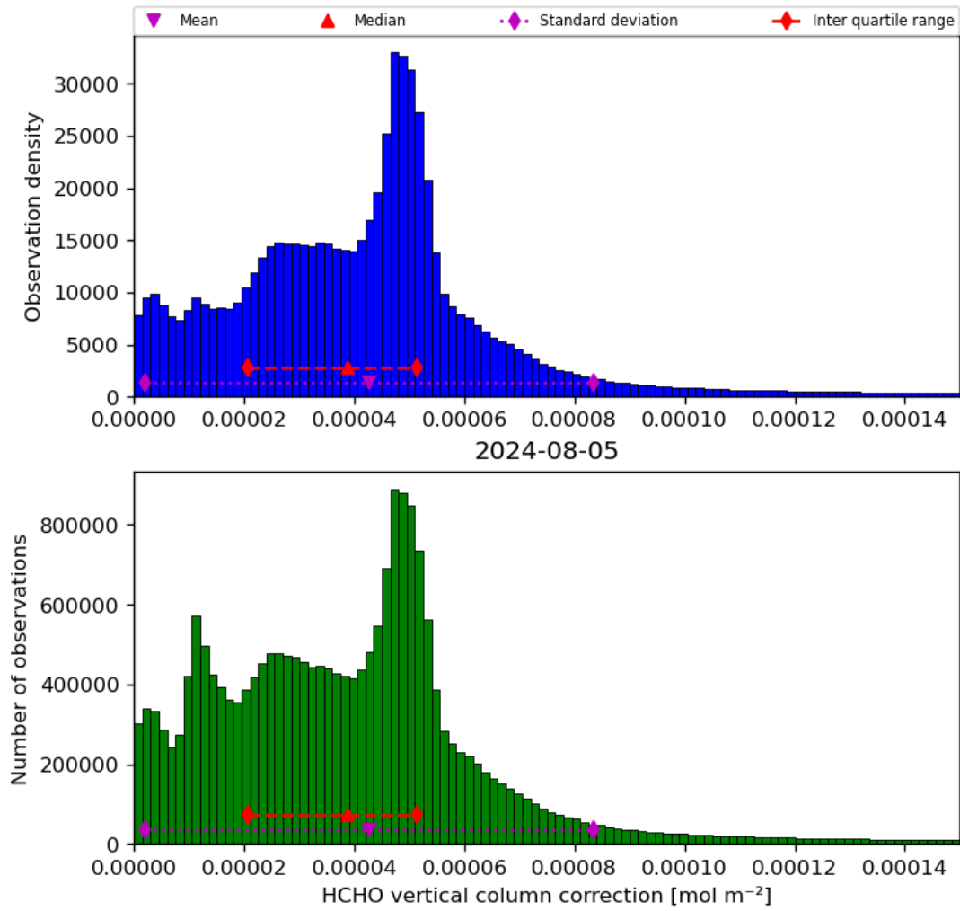
Figure 37: Histogram of “HCHO vertical column correction” for 2024-08-04 to 2024-08-06
