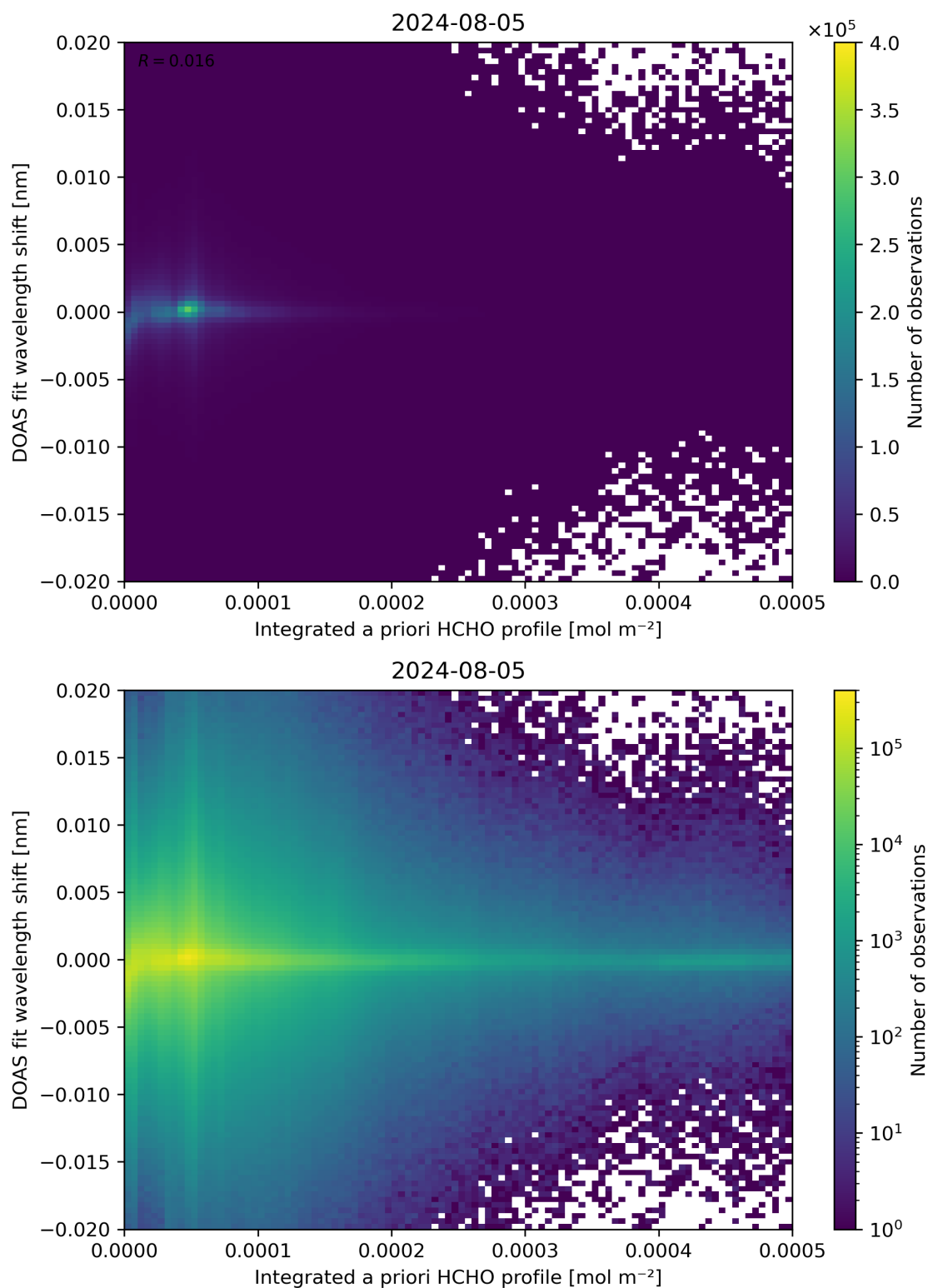
Figure 149: Scatter density plot of “Integrated a priori HCHO profile” against “DOAS fit wavelength shift” for 2024-08-04 to 2024-08-06.
