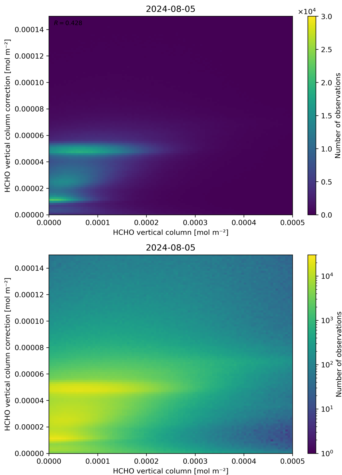
Figure 133: Scatter density plot of “HCHO vertical column” against “HCHO vertical column correction” for 2024-08-04 to 2024-08-06.
