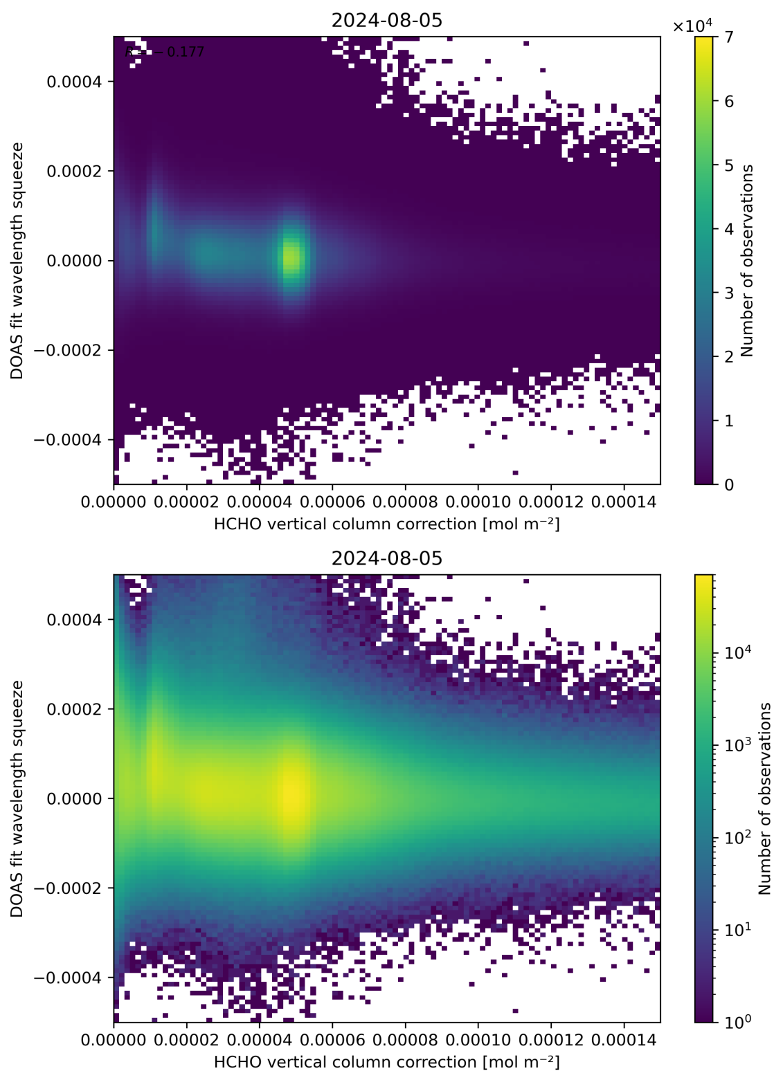
Figure 114: Scatter density plot of “HCHO vertical column correction” against “DOAS fit wavelength squeeze” for 2024-08-04 to 2024-08-06.
