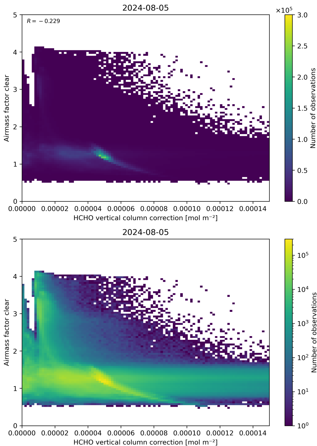
Figure 115: Scatter density plot of “HCHO vertical column correction” against “Airmass factor clear” for 2024-08-04 to 2024-08-06.
