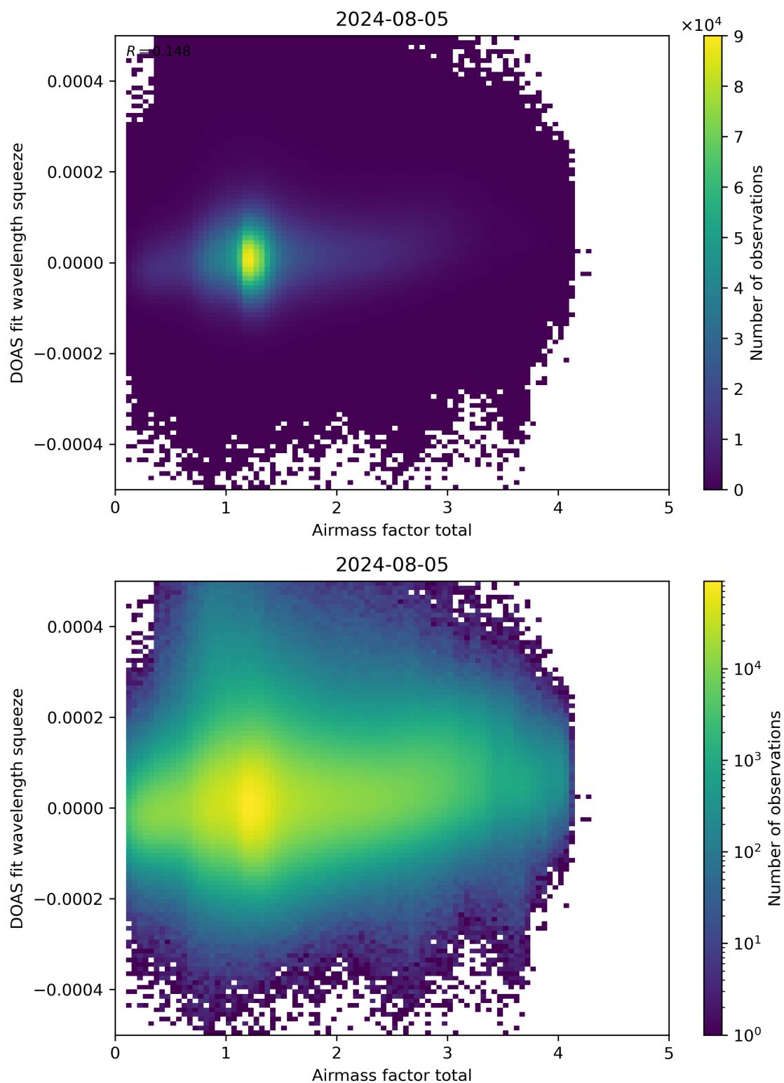
Figure 99: Scatter density plot of “Airmass factor total” against “DOAS fit wavelength squeeze” for 2024-08-04 to 2024-08-06.
