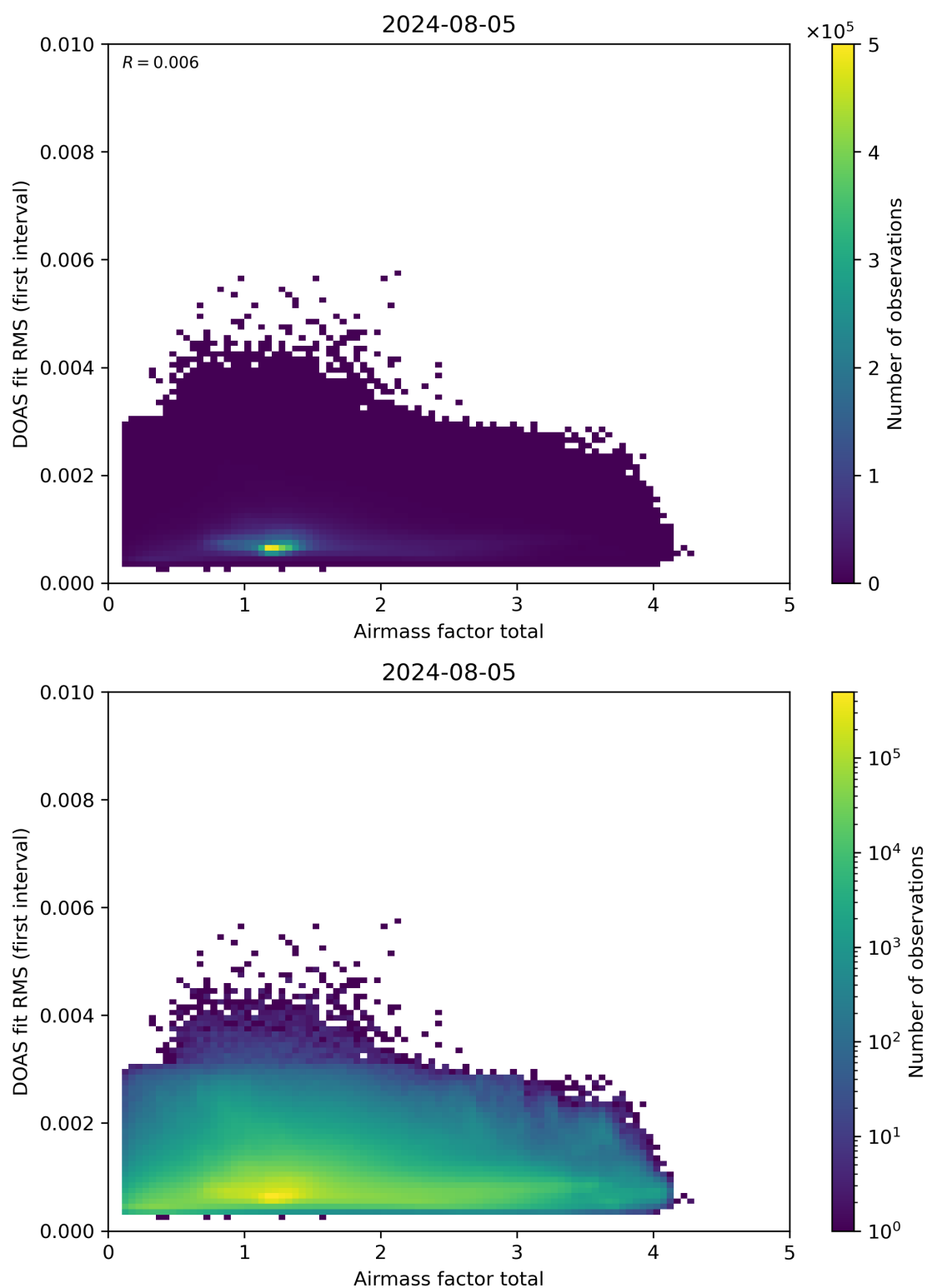
Figure 97: Scatter density plot of “Airmass factor total” against “DOAS fit RMS (first interval)” for 2024-08-04 to 2024-08-06.
