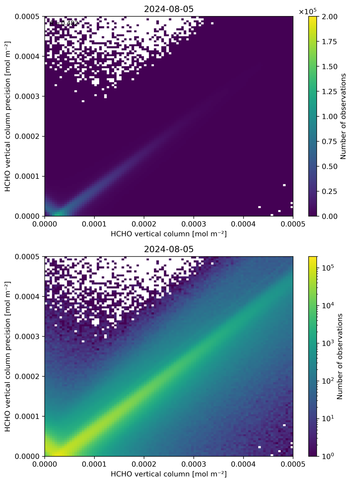
Figure 134: Scatter density plot of “HCHO vertical column” against “HCHO vertical column precision” for 2024-08-04 to 2024-08-06.
