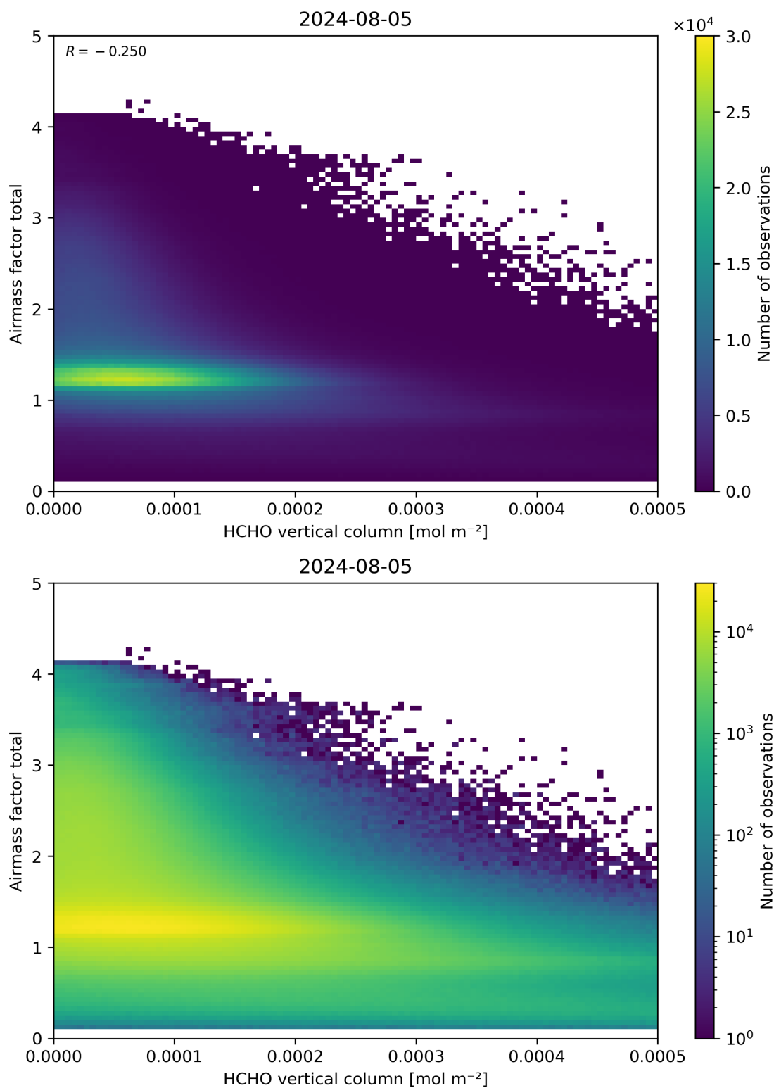
Figure 131: Scatter density plot of “HCHO vertical column” against “Airmass factor total” for 2024-08-04 to 2024-08-06.
