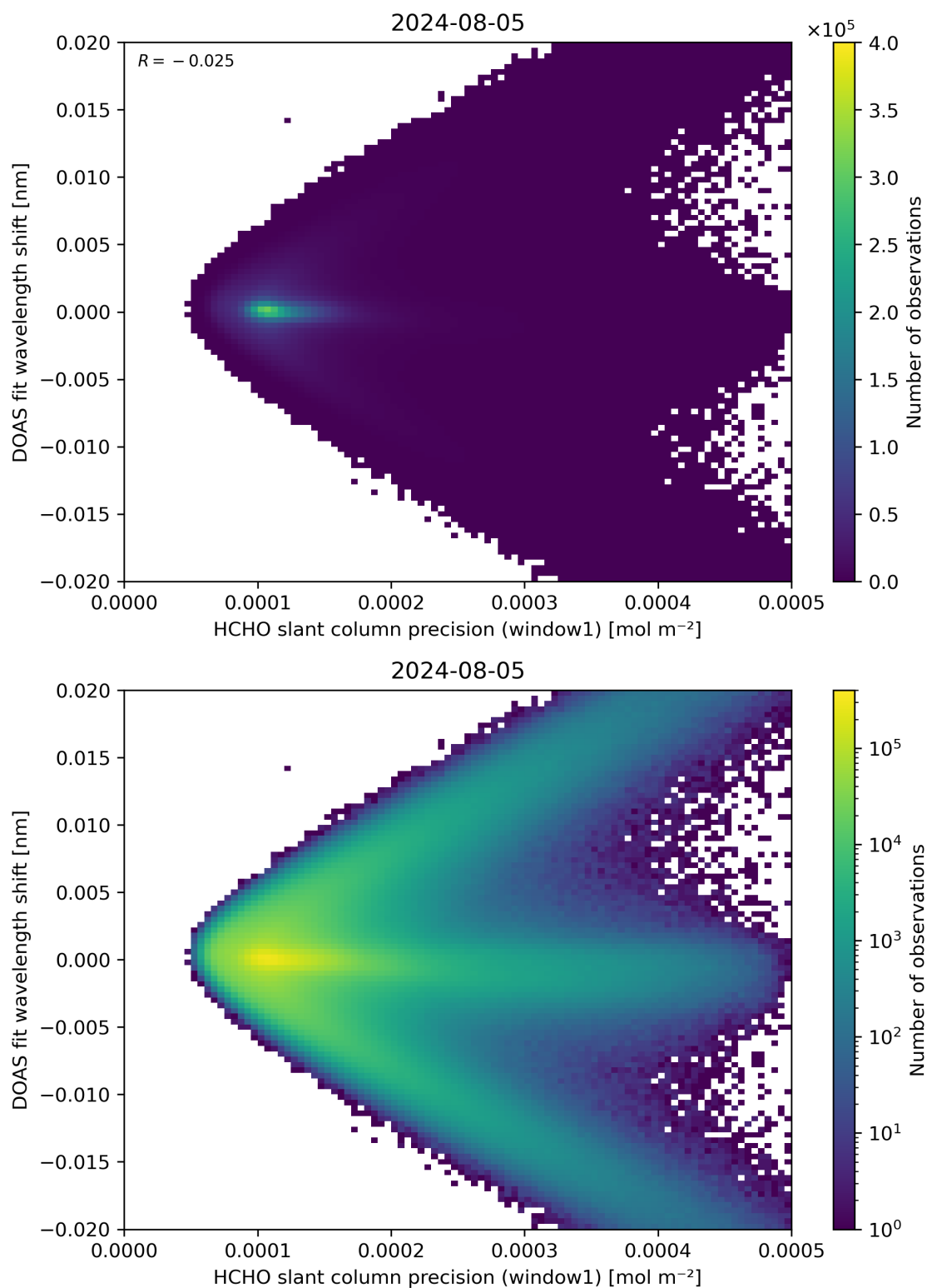
Figure 89: Scatter density plot of “HCHO slant column precision (window1)” against “DOAS fit wavelength shift” for 2024-08-04 to 2024-08-06.
