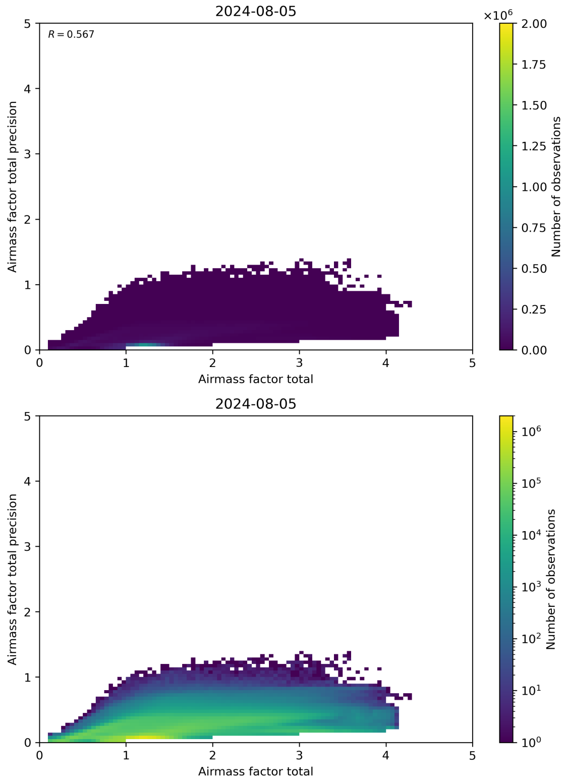
Figure 103: Scatter density plot of “Airmass factor total” against “Airmass factor total precision” for 2024-08-04 to 2024-08-06.
