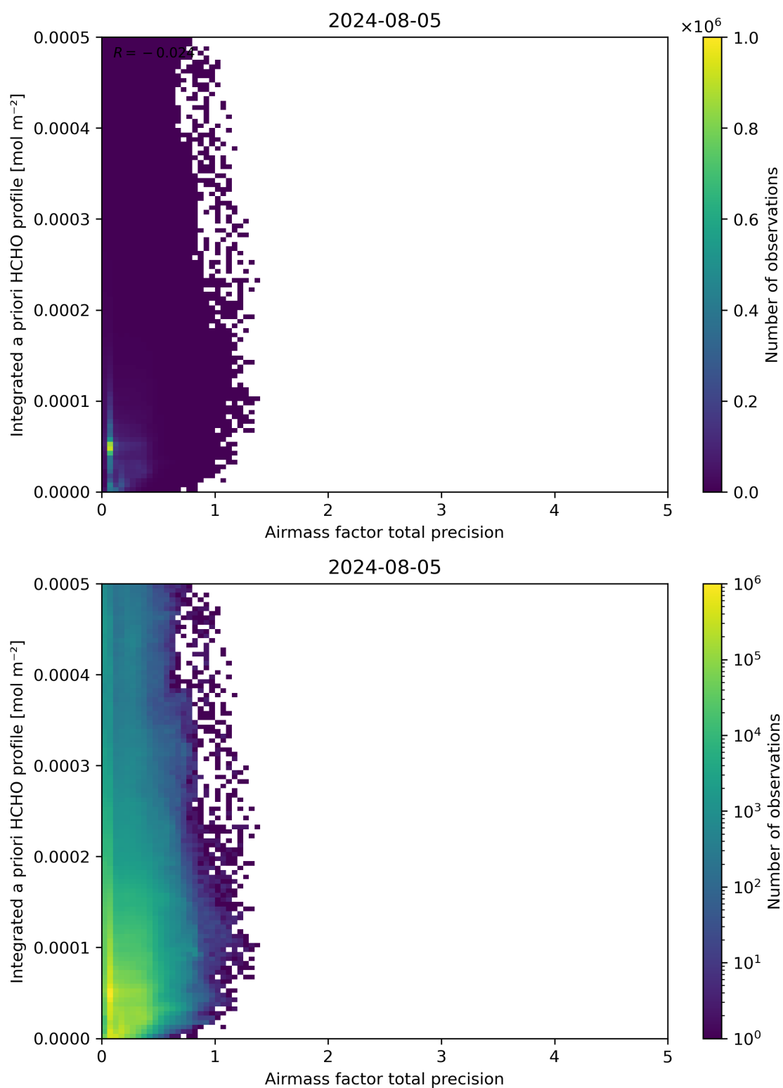
Figure 111: Scatter density plot of “Airmass factor total precision” against “Integrated a priori HCHO profile” for 2024-08-04 to 2024-08-06.
