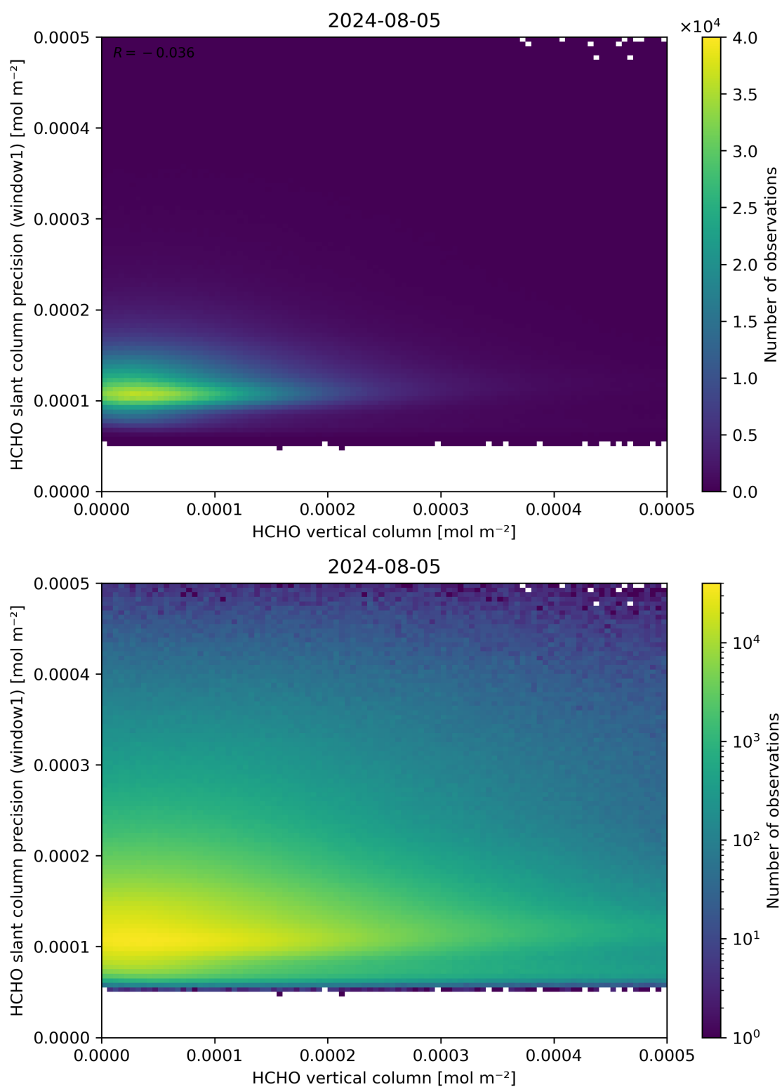
Figure 130: Scatter density plot of “HCHO vertical column” against “HCHO slant column precision (window1)” for 2024-08-04 to 2024-08-06.
