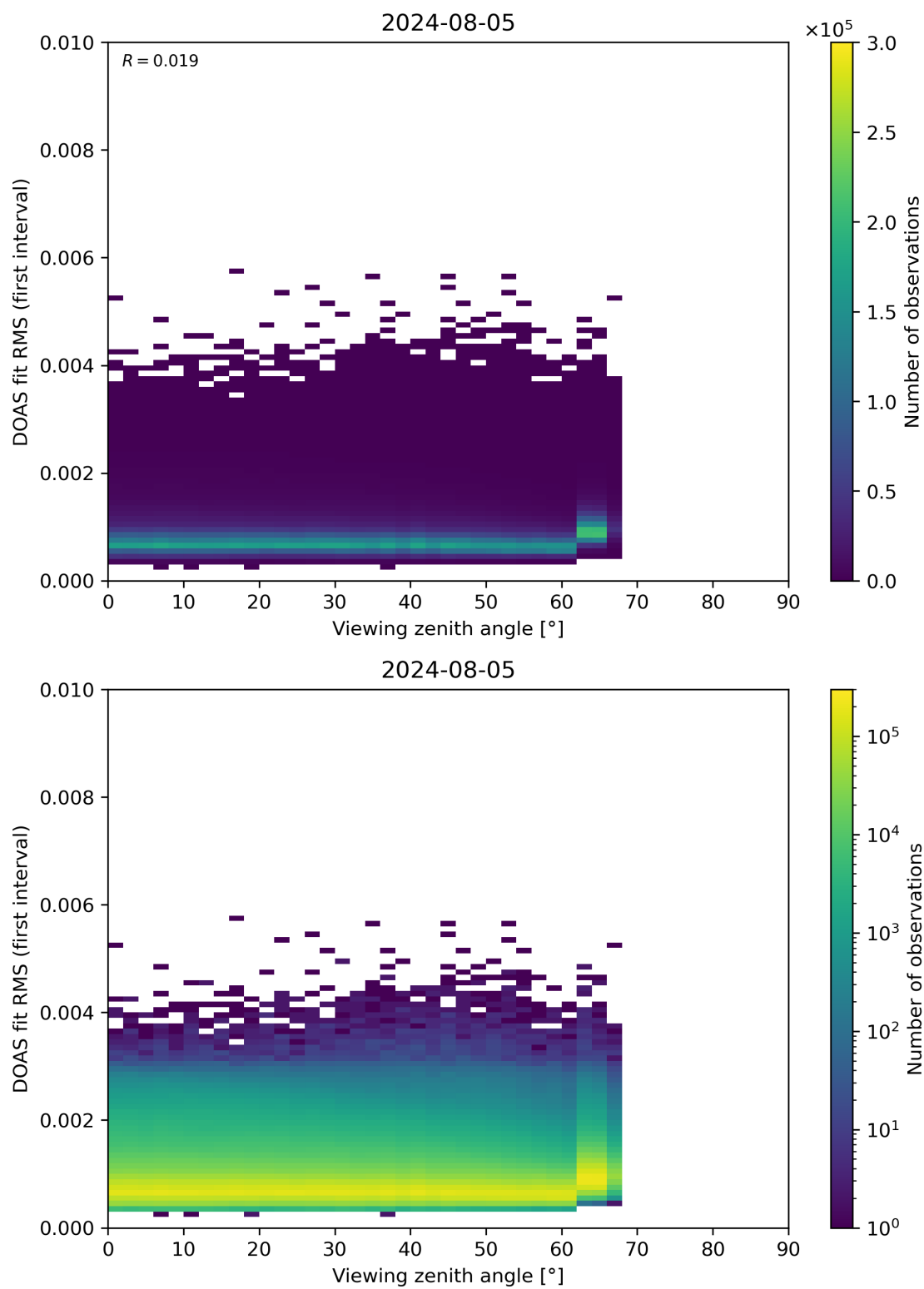
Figure 182: Scatter density plot of “Viewing zenith angle” against “DOAS fit RMS (first interval)” for 2024-08-04 to 2024-08-06.
