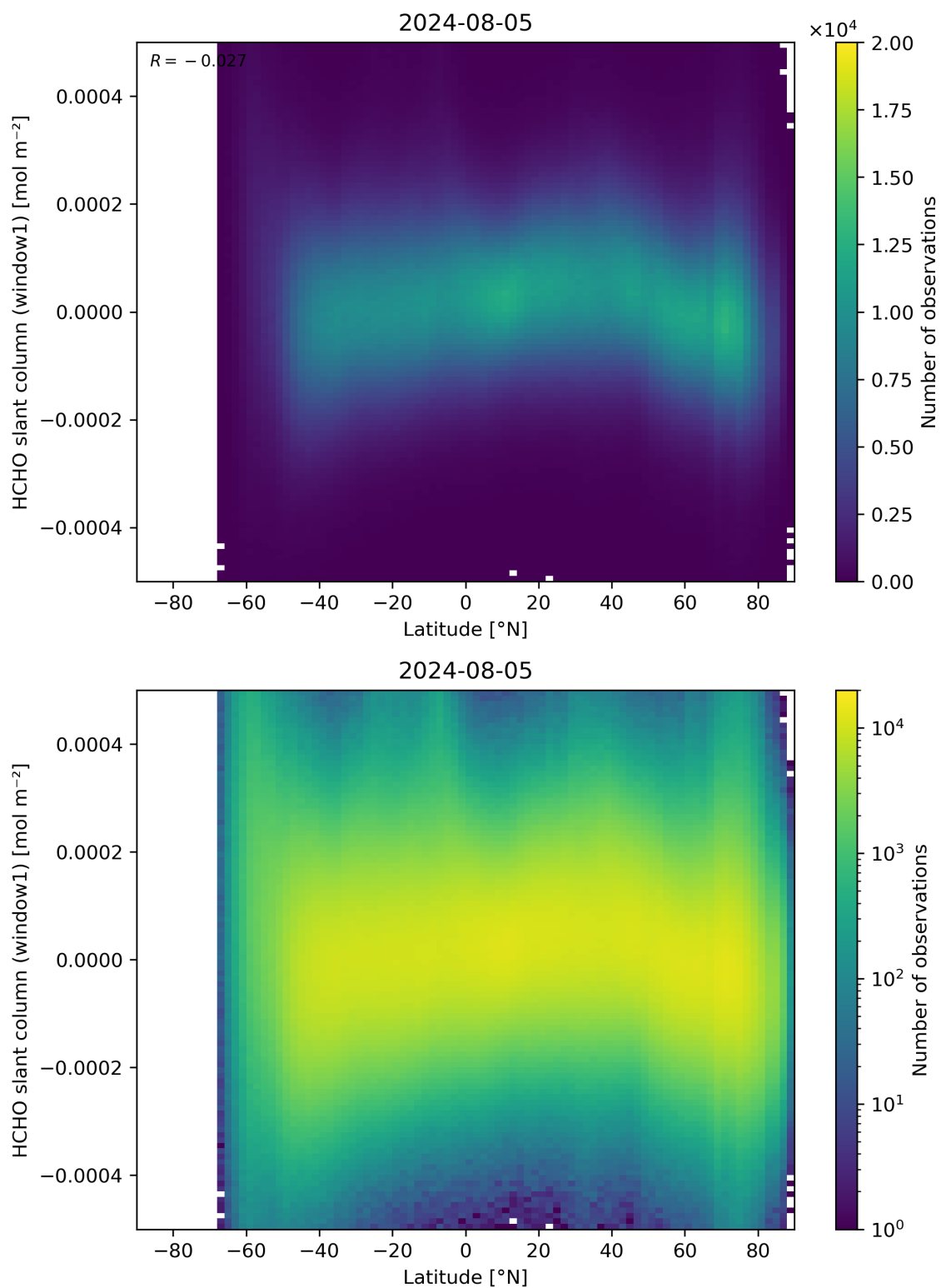
Figure 159: Scatter density plot of “Latitude” against “HCHO slant column (window1)” for 2024-08-04 to 2024-08-06.
