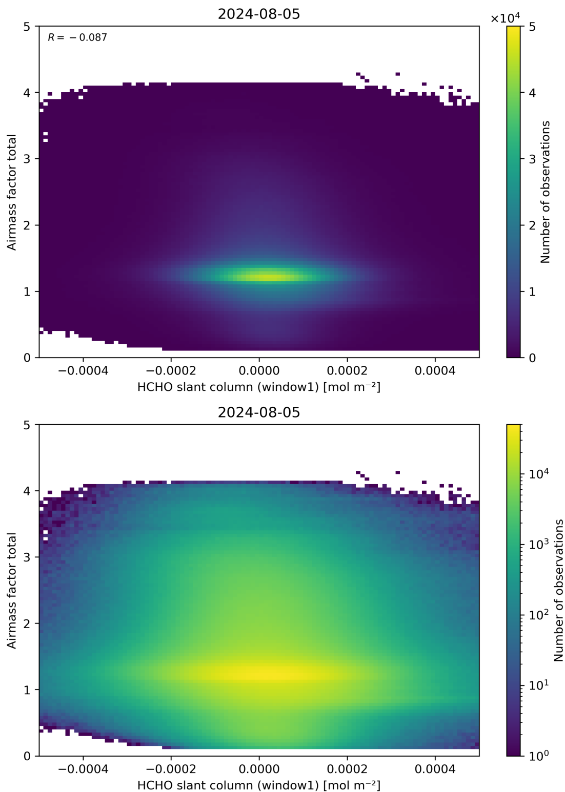
Figure 85: Scatter density plot of “HCHO slant column (window1)” against “Airmass factor total” for 2024-08-04 to 2024-08-06.
