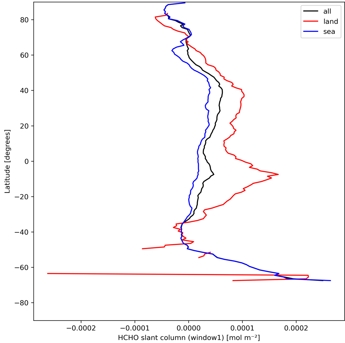
Figure 24: Zonal average of “HCHO slant column (window1)” for 2024-08-04 to 2024-08-06.
