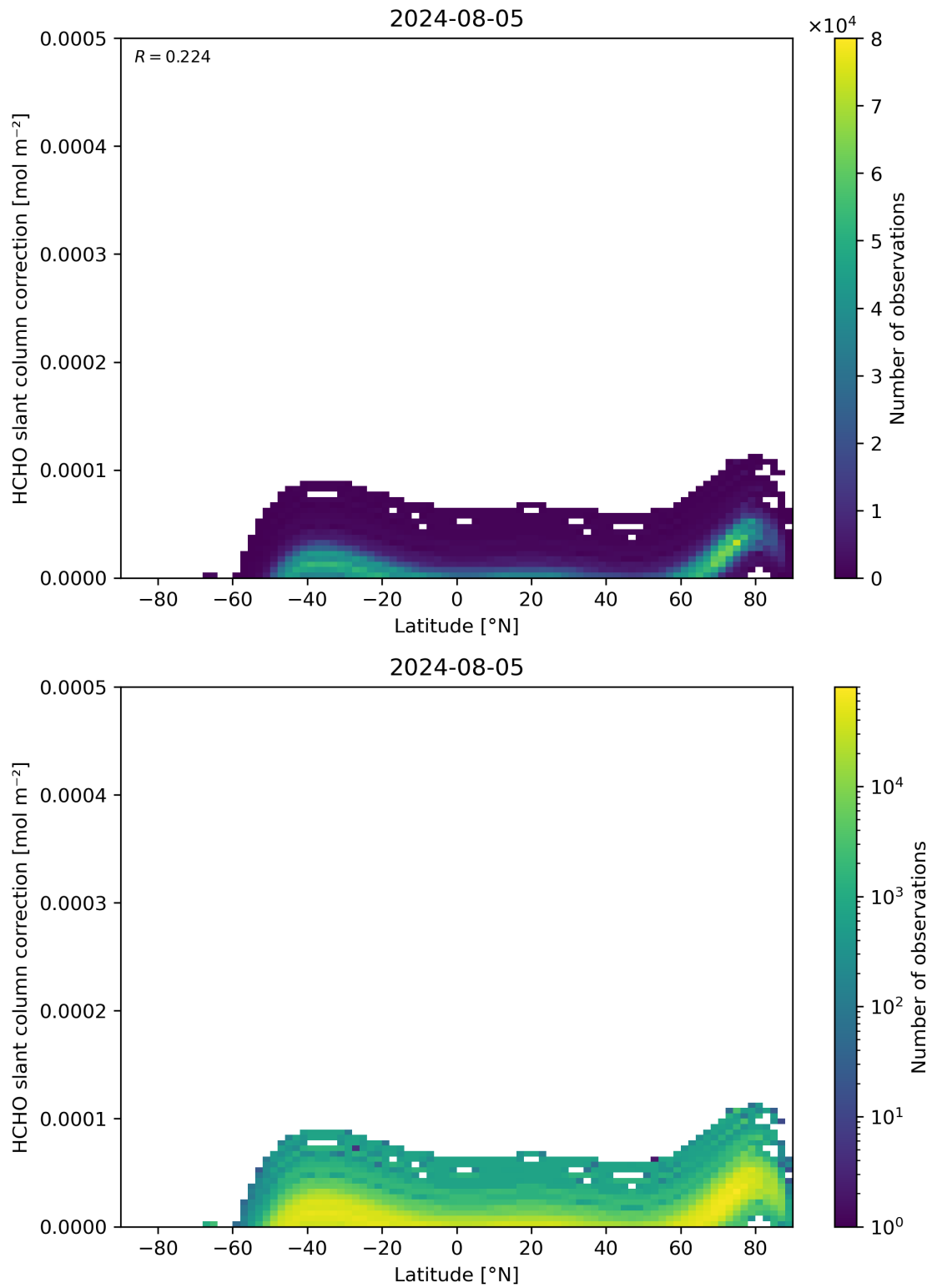
Figure 158: Scatter density plot of “Latitude” against “HCHO slant column correction” for 2024-08-04 to 2024-08-06.
