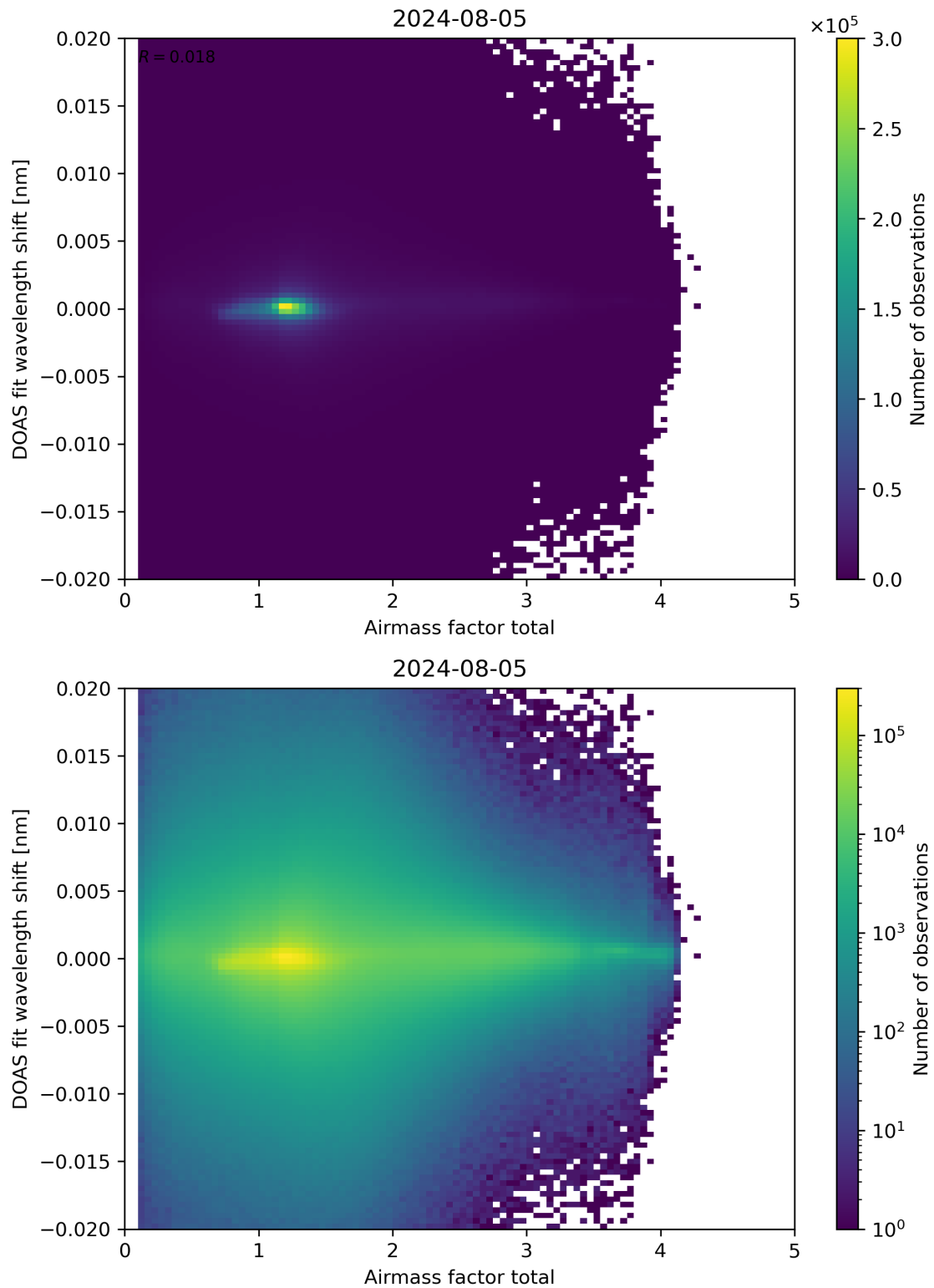
Figure 98: Scatter density plot of “Airmass factor total” against “DOAS fit wavelength shift” for 2024-08-04 to 2024-08-06.
