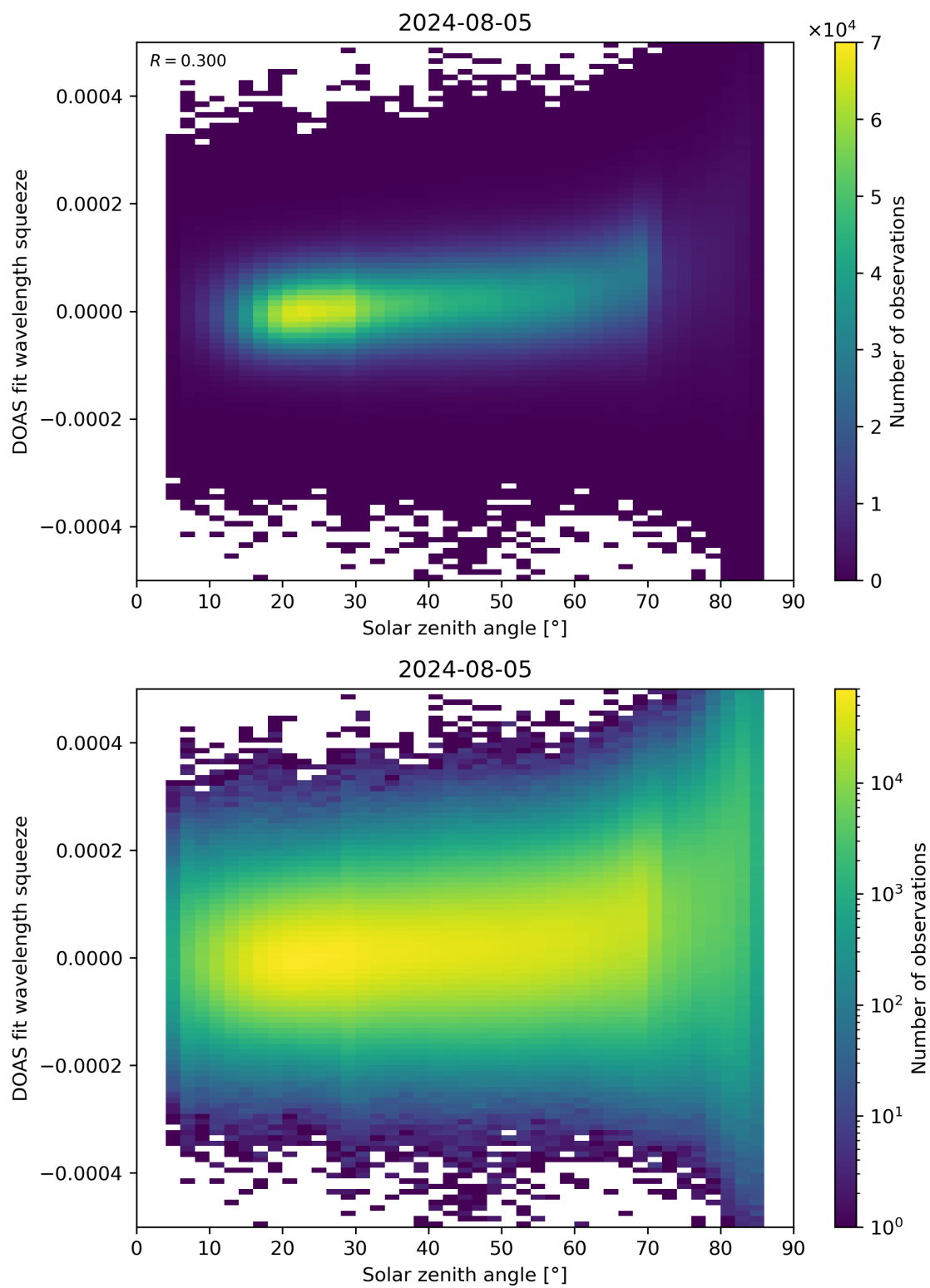
Figure 169: Scatter density plot of “Solar zenith angle” against “DOAS fit wavelength squeeze” for 2024-08-04 to 2024-08-06.
