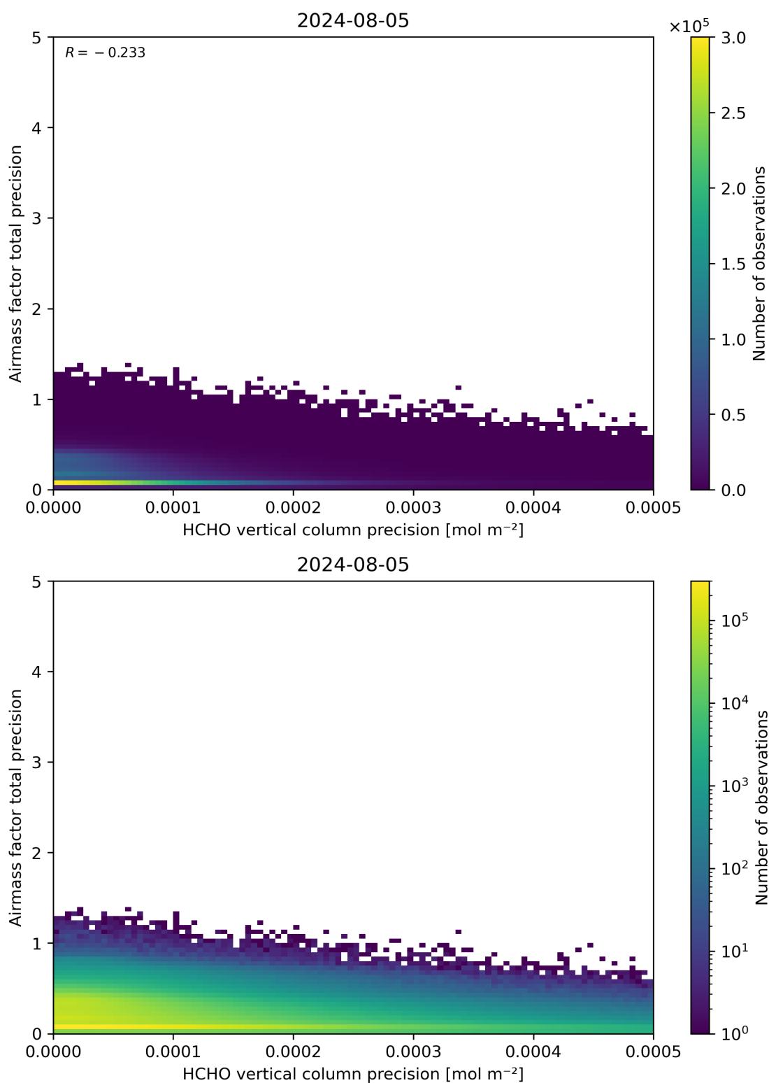
Figure 145: Scatter density plot of “HCHO vertical column precision” against “Airmass factor total precision” for 2024-08-04 to 2024-08-06.
