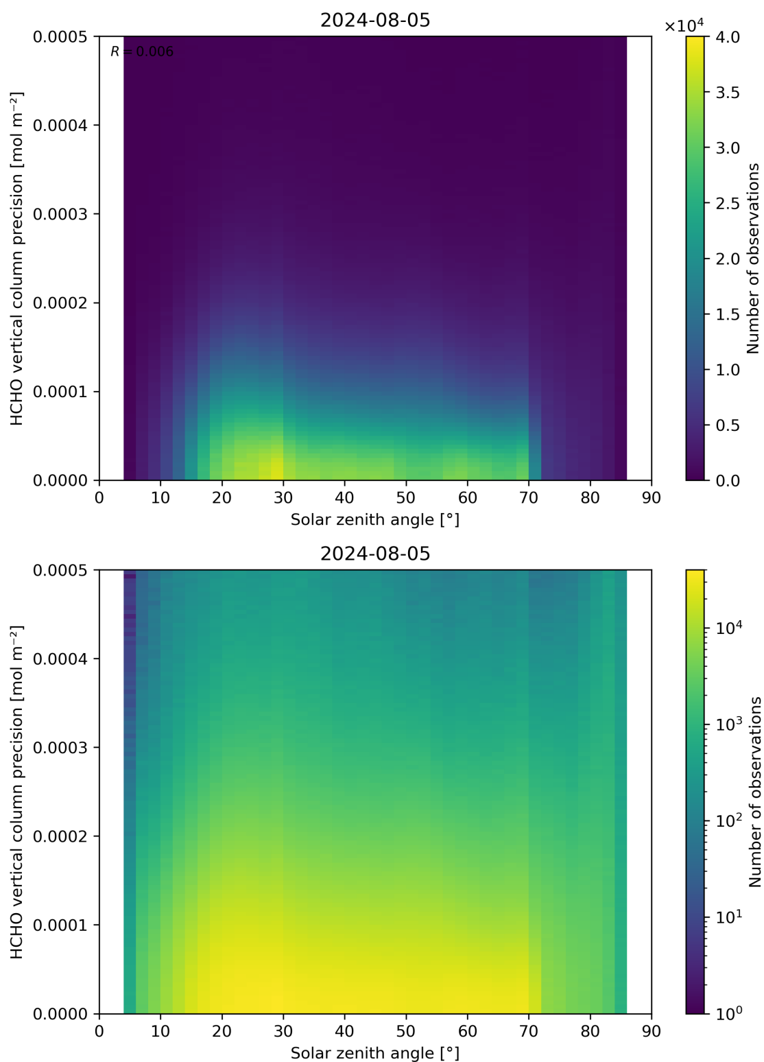
Figure 179: Scatter density plot of “Solar zenith angle” against “HCHO vertical column precision” for 2024-08-04 to 2024-08-06.
