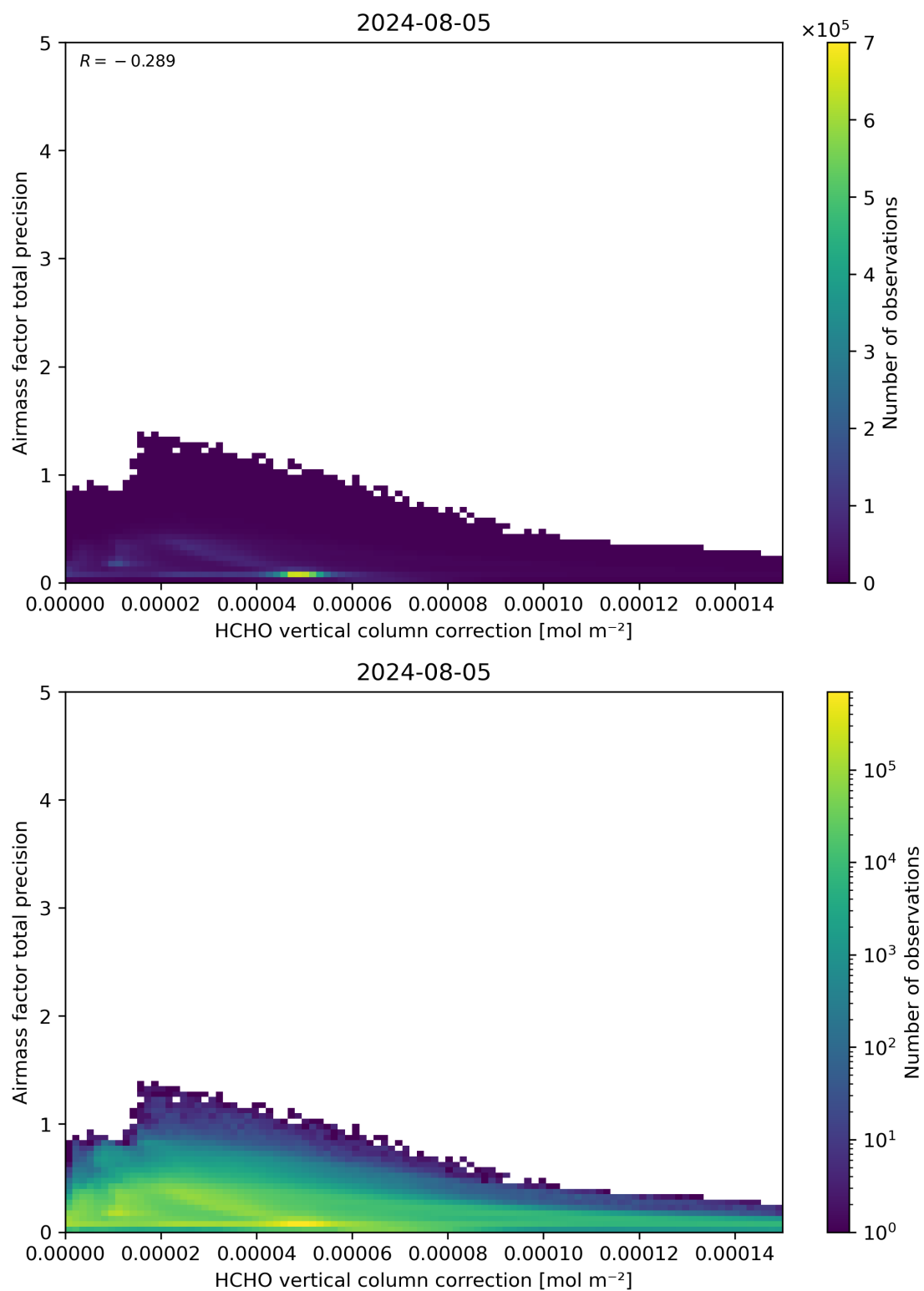
Figure 121: Scatter density plot of “HCHO vertical column correction” against “Airmass factor total precision” for 2024-08-04 to 2024-08-06.
