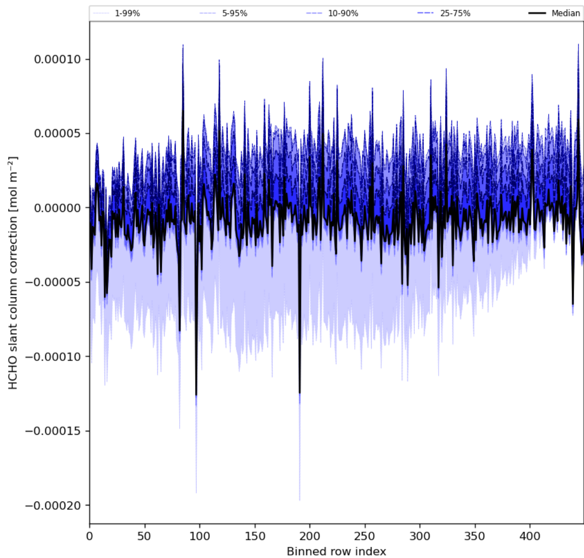
Figure 61: Along track statistics of “HCHO slant column correction” for 2024-08-04 to 2024-08-06
