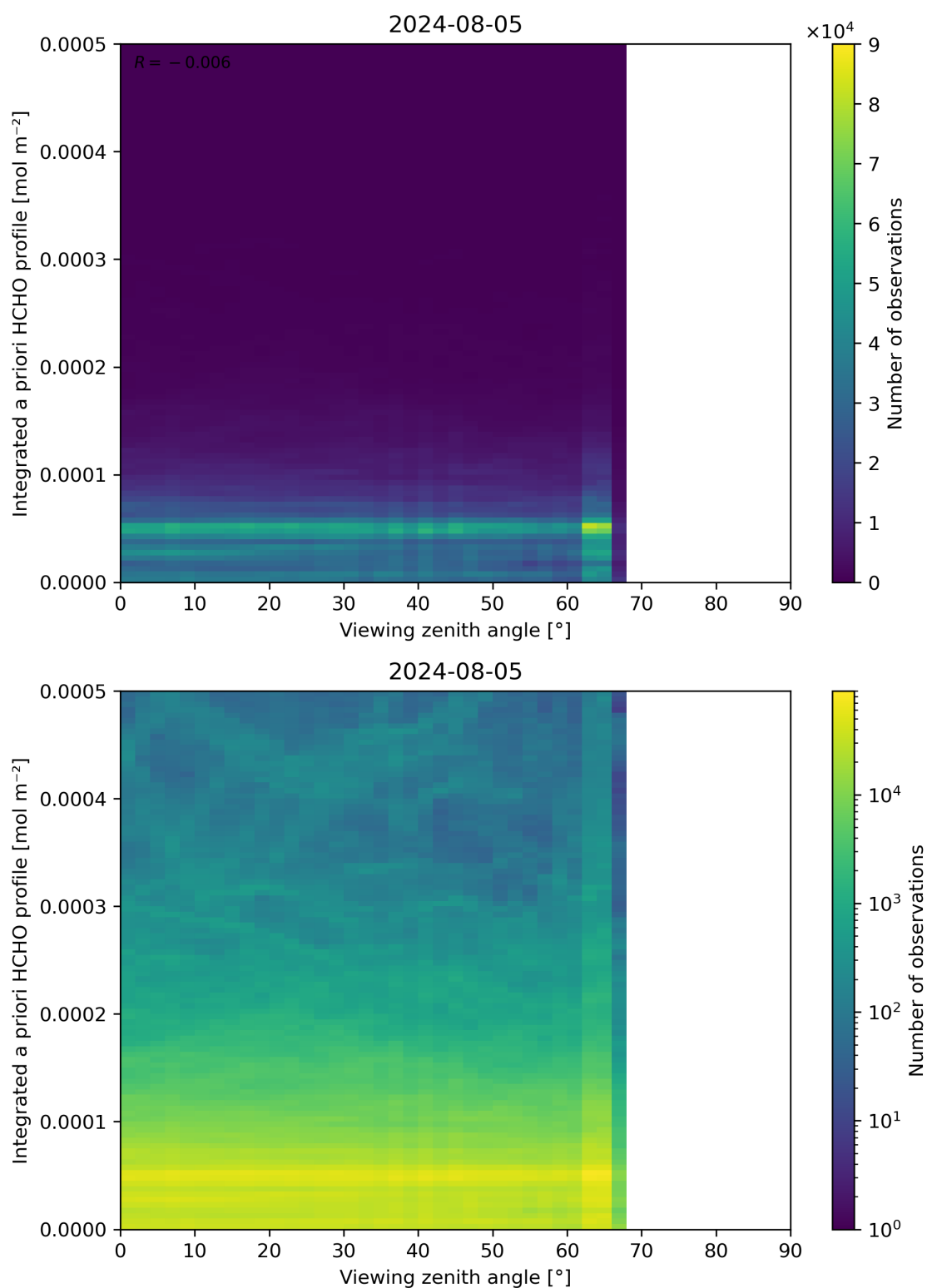
Figure 195: Scatter density plot of “Viewing zenith angle” against “Integrated a priori HCHO profile” for 2024-08-04 to 2024-08-06.
