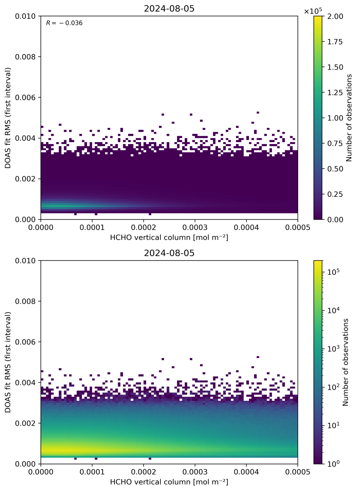
Figure 123: Scatter density plot of “HCHO vertical column” against “DOAS fit RMS (first interval)” for 2024-08-04 to 2024-08-06.
