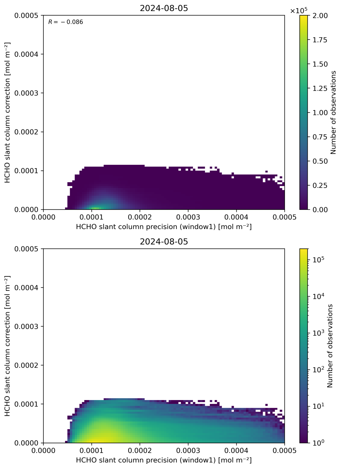
Figure 93: Scatter density plot of “HCHO slant column precision (window1)” against “HCHO slant column correction” for 2024-08-04 to 2024-08-06.
