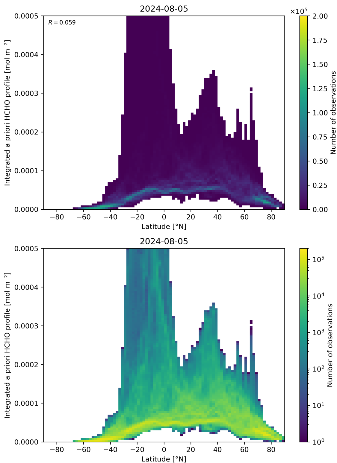
Figure 166: Scatter density plot of “Latitude” against “Integrated a priori HCHO profile” for 2024-08-04 to 2024-08-06.
