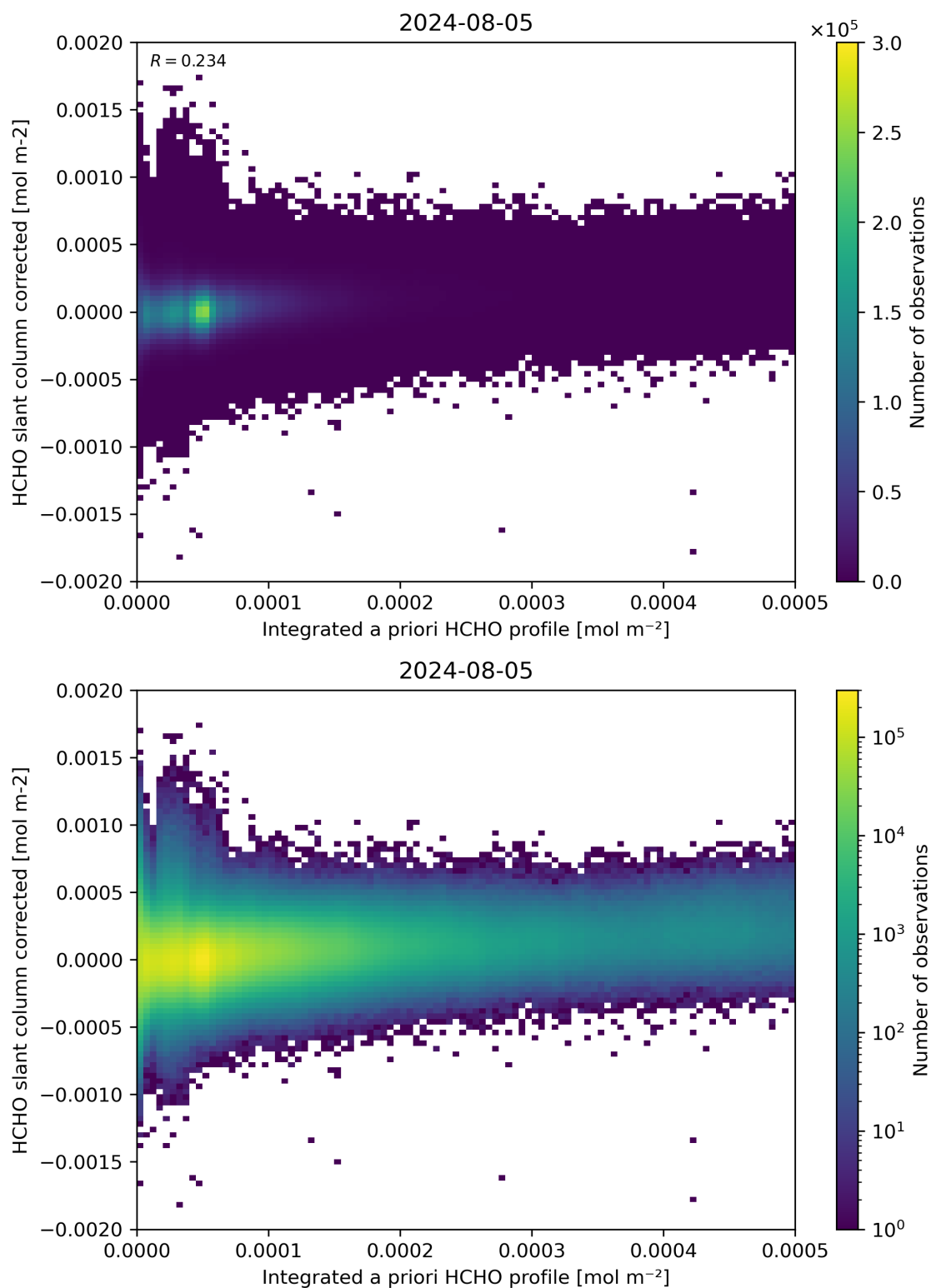
Figure 151: Scatter density plot of “Integrated a priori HCHO profile” against “HCHO slant column corrected” for 2024-08-04 to 2024-08-06.
