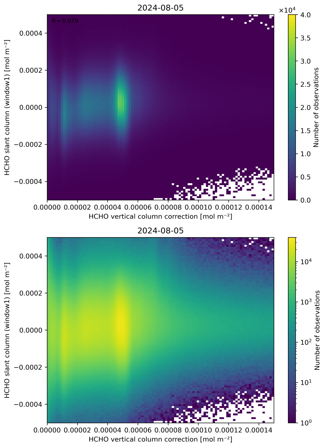
Figure 118: Scatter density plot of “HCHO vertical column correction” against “HCHO slant column (window1)” for 2024-08-04 to 2024-08-06.
