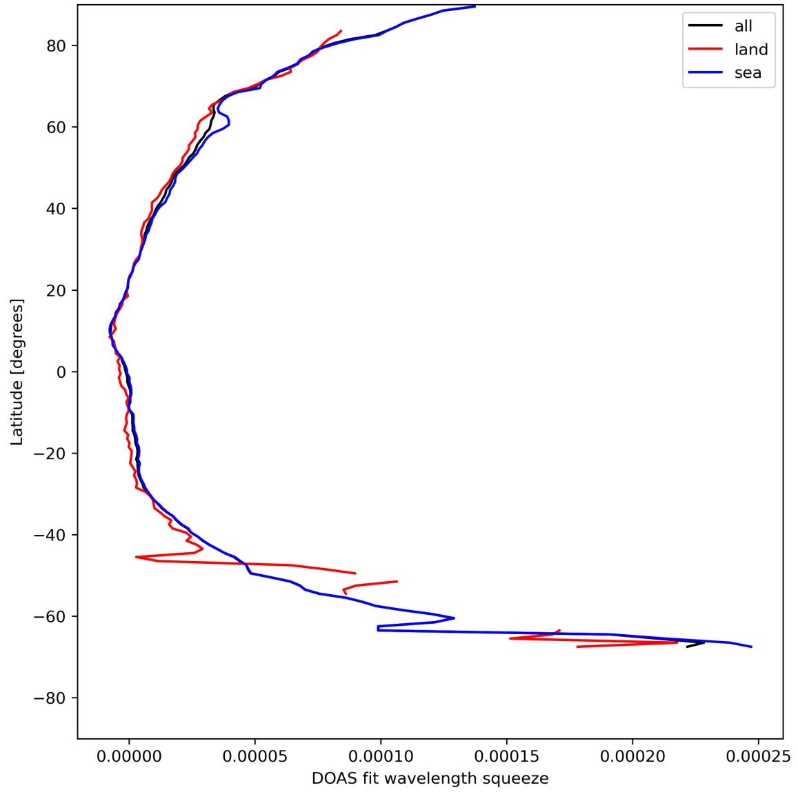
Figure 31: Zonal average of “DOAS fit wavelength squeeze” for 2024-08-04 to 2024-08-06.
