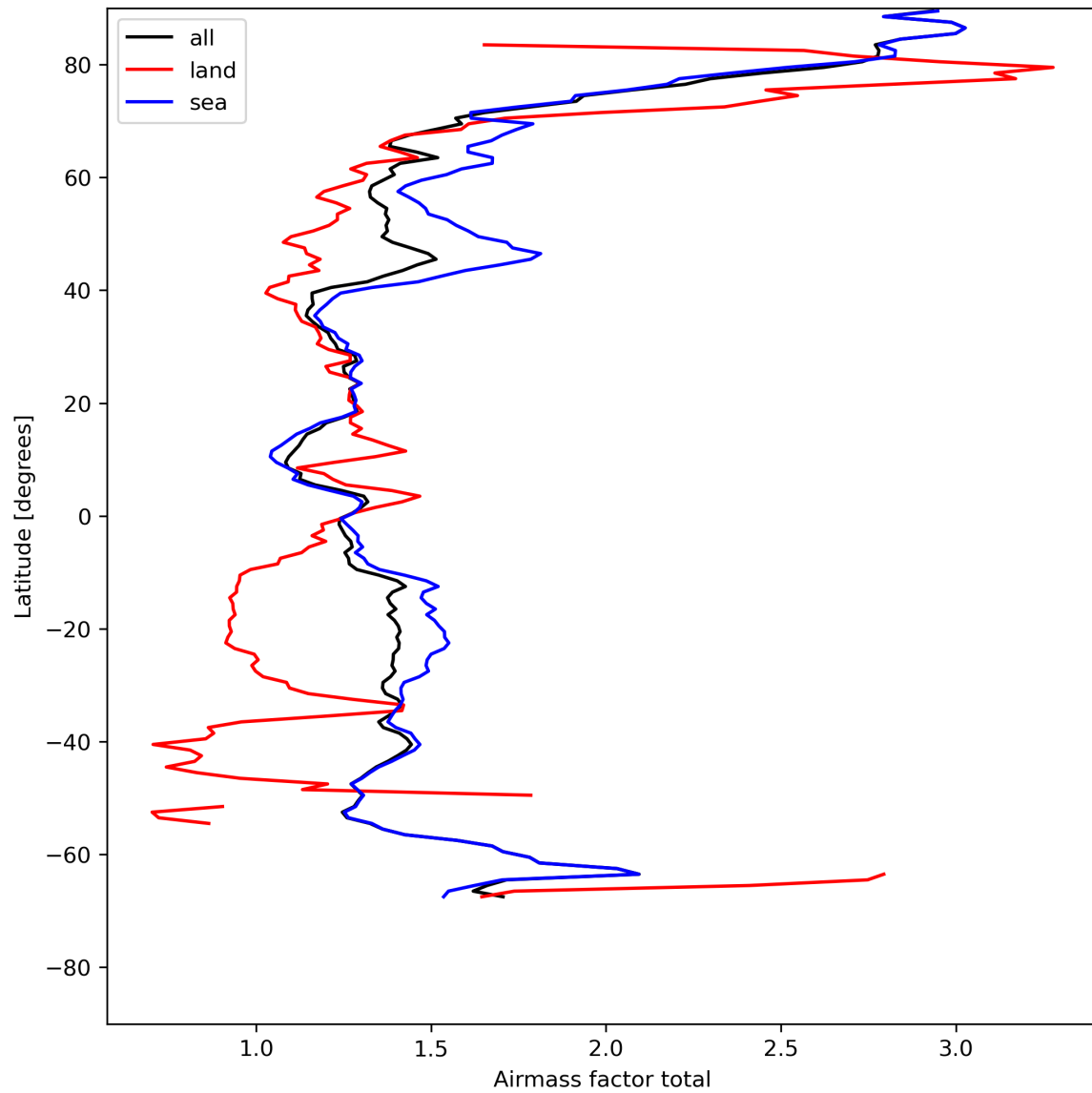
Figure 26: Zonal average of “Airmass factor total” for 2024-08-04 to 2024-08-06.
