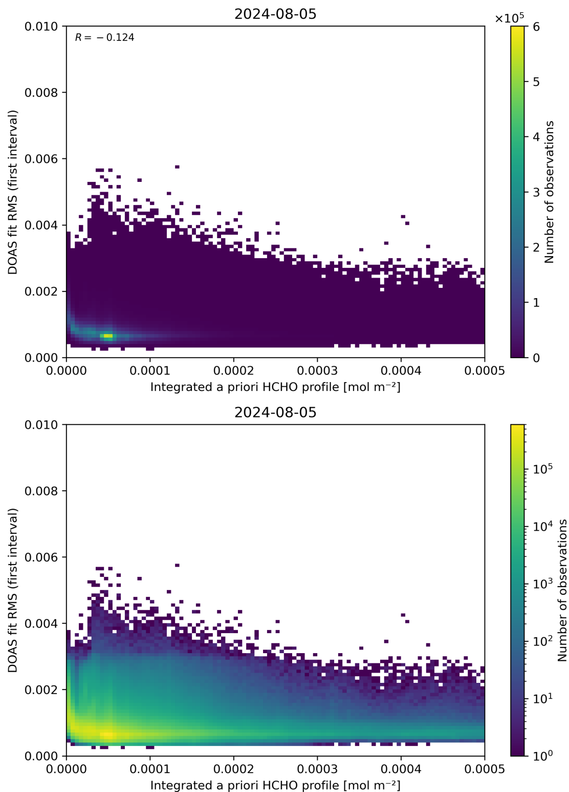
Figure 148: Scatter density plot of “Integrated a priori HCHO profile” against “DOAS fit RMS (first interval)” for 2024-08-04 to 2024-08-06.
