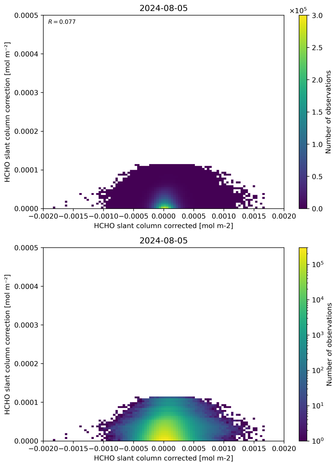
Figure 77: Scatter density plot of “HCHO slant column corrected” against “HCHO slant column correction” for 2024-08-04 to 2024-08-06.
