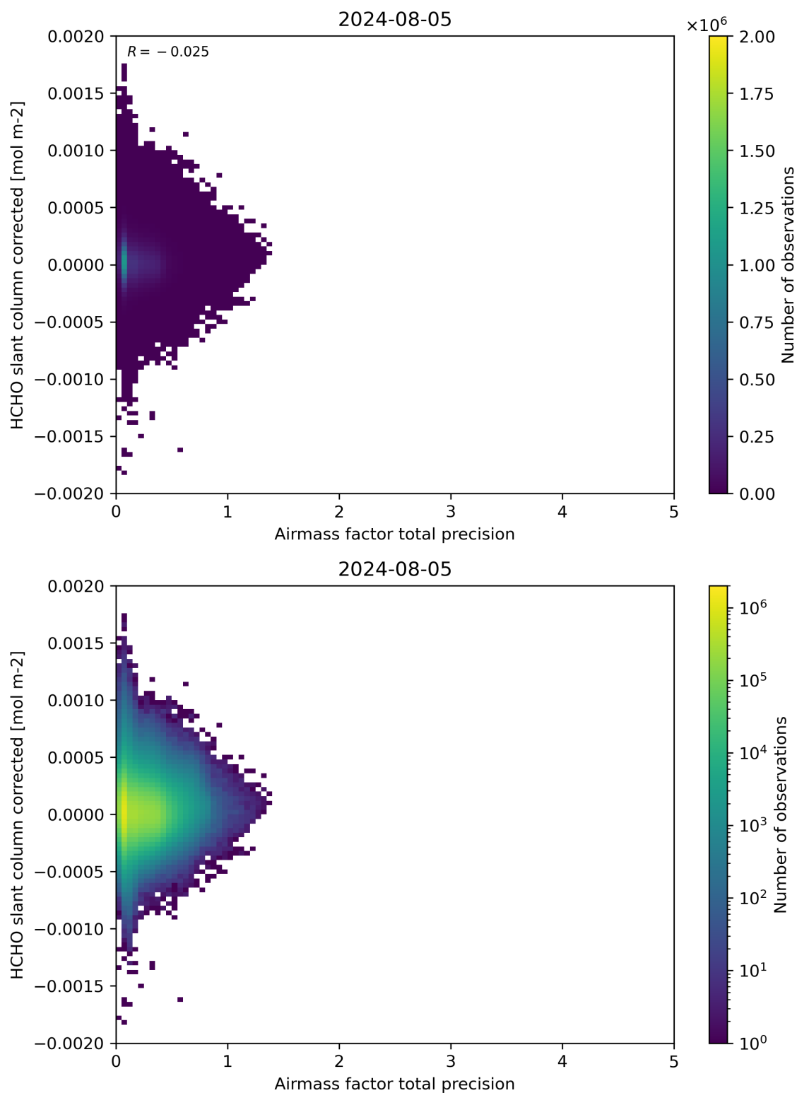
Figure 109: Scatter density plot of “Airmass factor total precision” against “HCHO slant column corrected” for 2024-08-04 to 2024-08-06.
