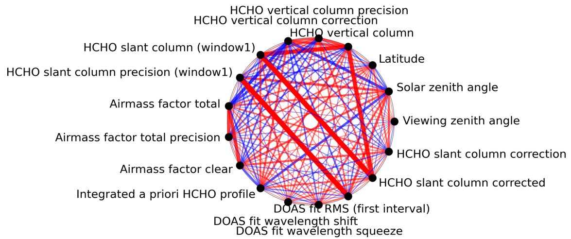
Figure 1: Map of correlation graph for 2024-08-04 to 2024-08-06.
