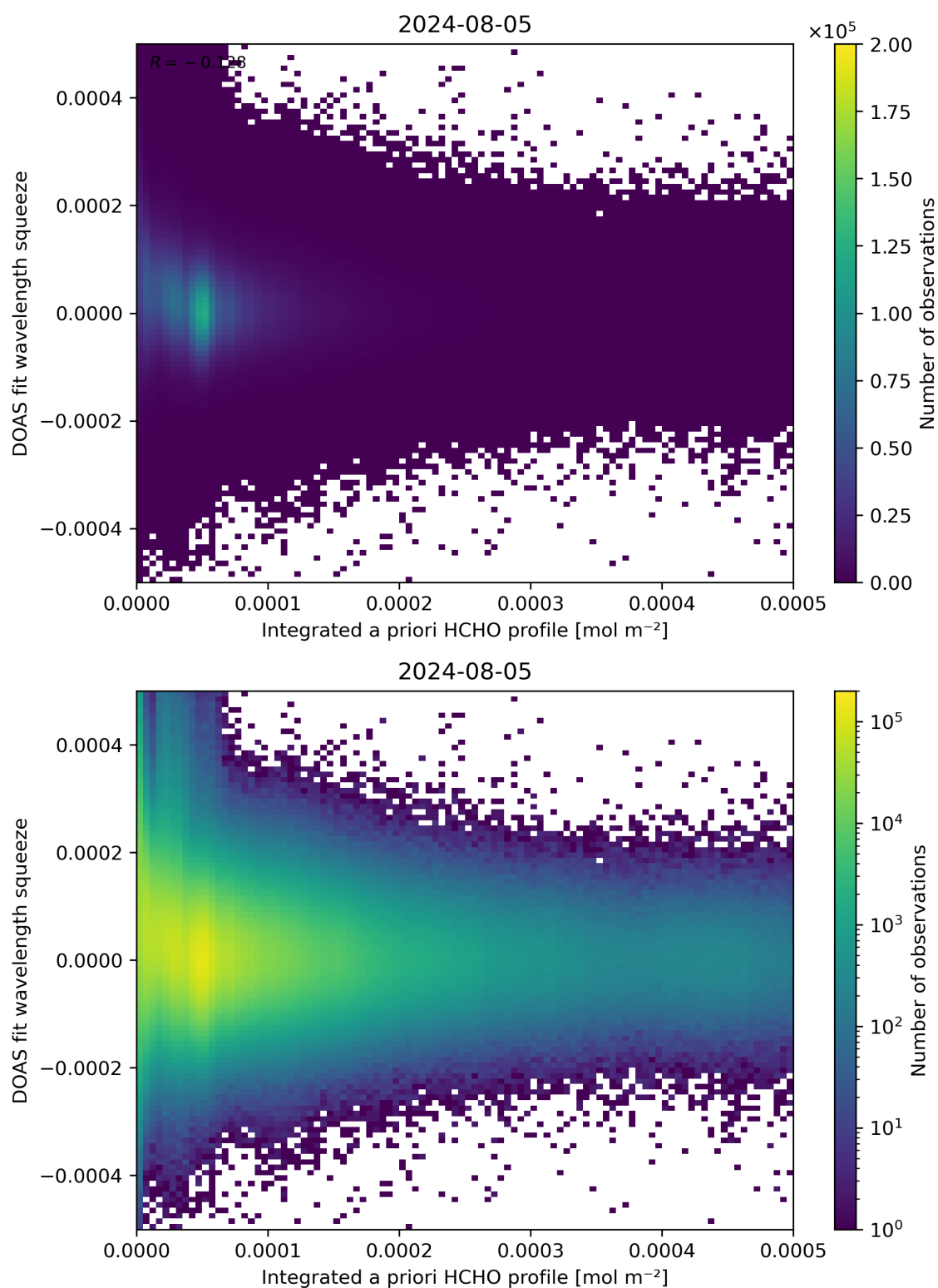
Figure 150: Scatter density plot of “Integrated a priori HCHO profile” against “DOAS fit wavelength squeeze” for 2024-08-04 to 2024-08-06.
