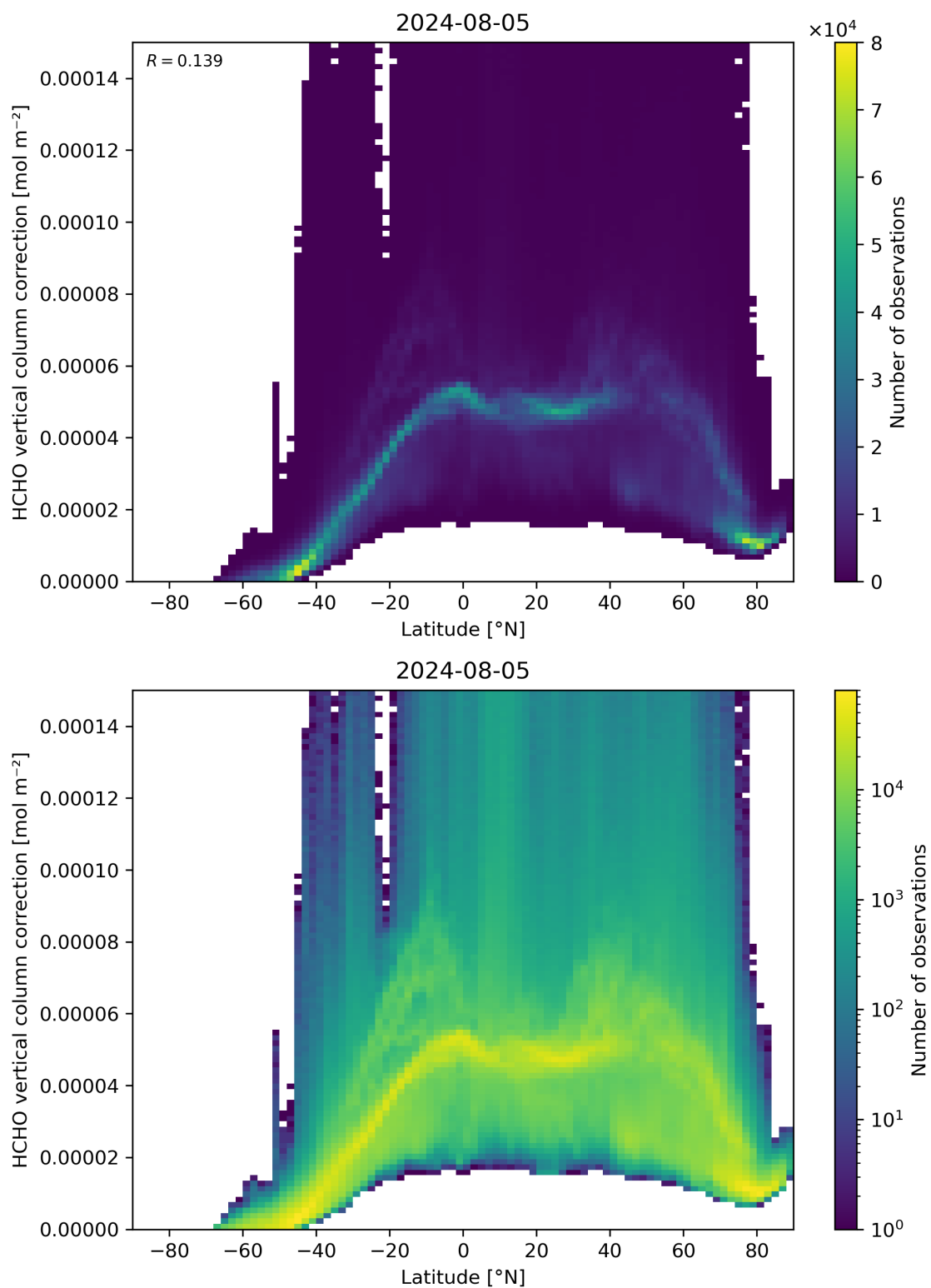
Figure 164: Scatter density plot of “Latitude” against “HCHO vertical column correction” for 2024-08-04 to 2024-08-06.
