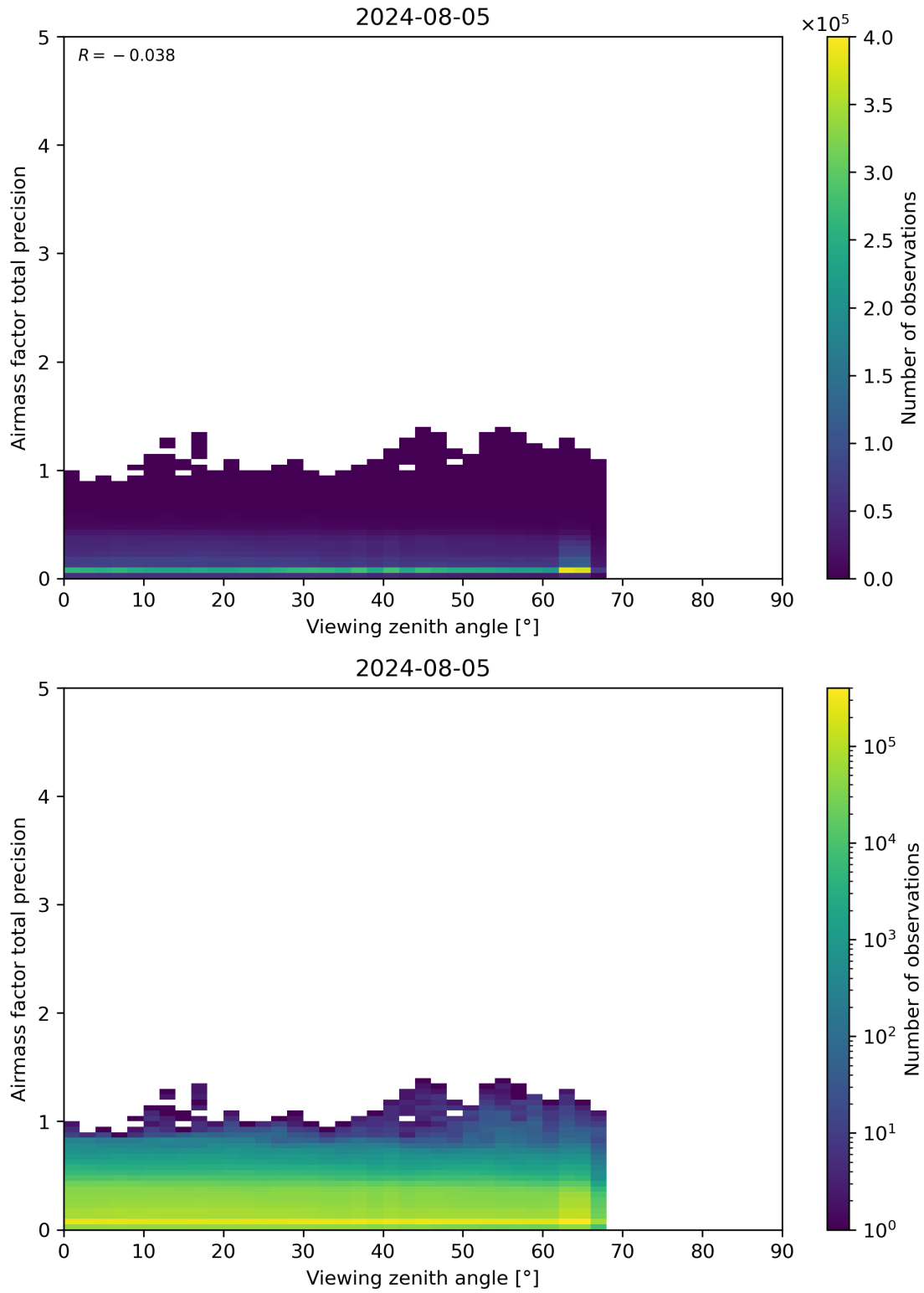
Figure 191: Scatter density plot of “Viewing zenith angle” against “Airmass factor total precision” for 2024-08-04 to 2024-08-06.
