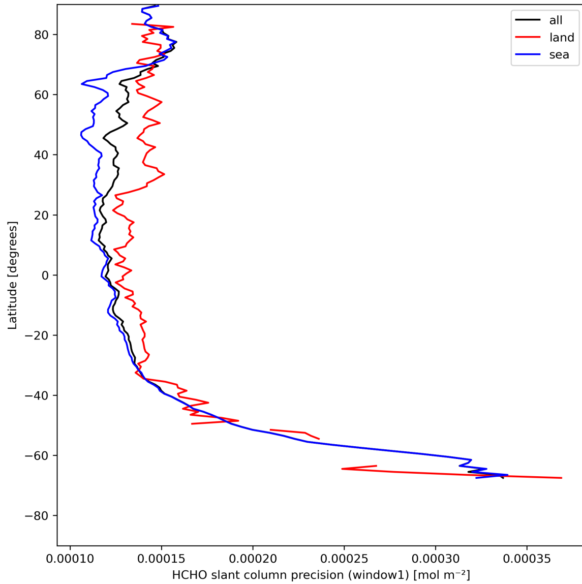
Figure 25: Zonal average of “HCHO slant column precision (window1)” for 2024-08-04 to 2024-08-06.
