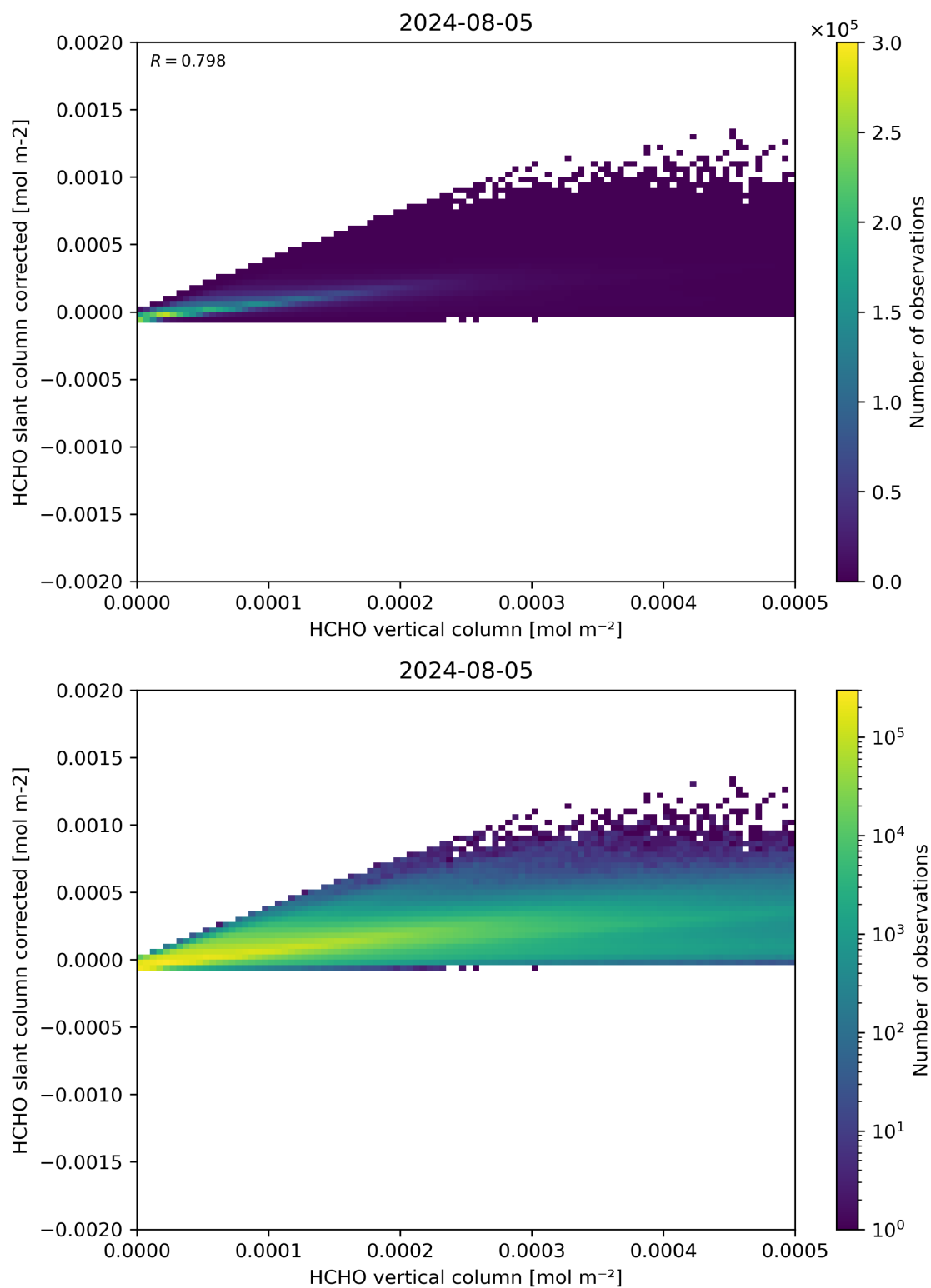
Figure 127: Scatter density plot of “HCHO vertical column” against “HCHO slant column corrected” for 2024-08-04 to 2024-08-06.
