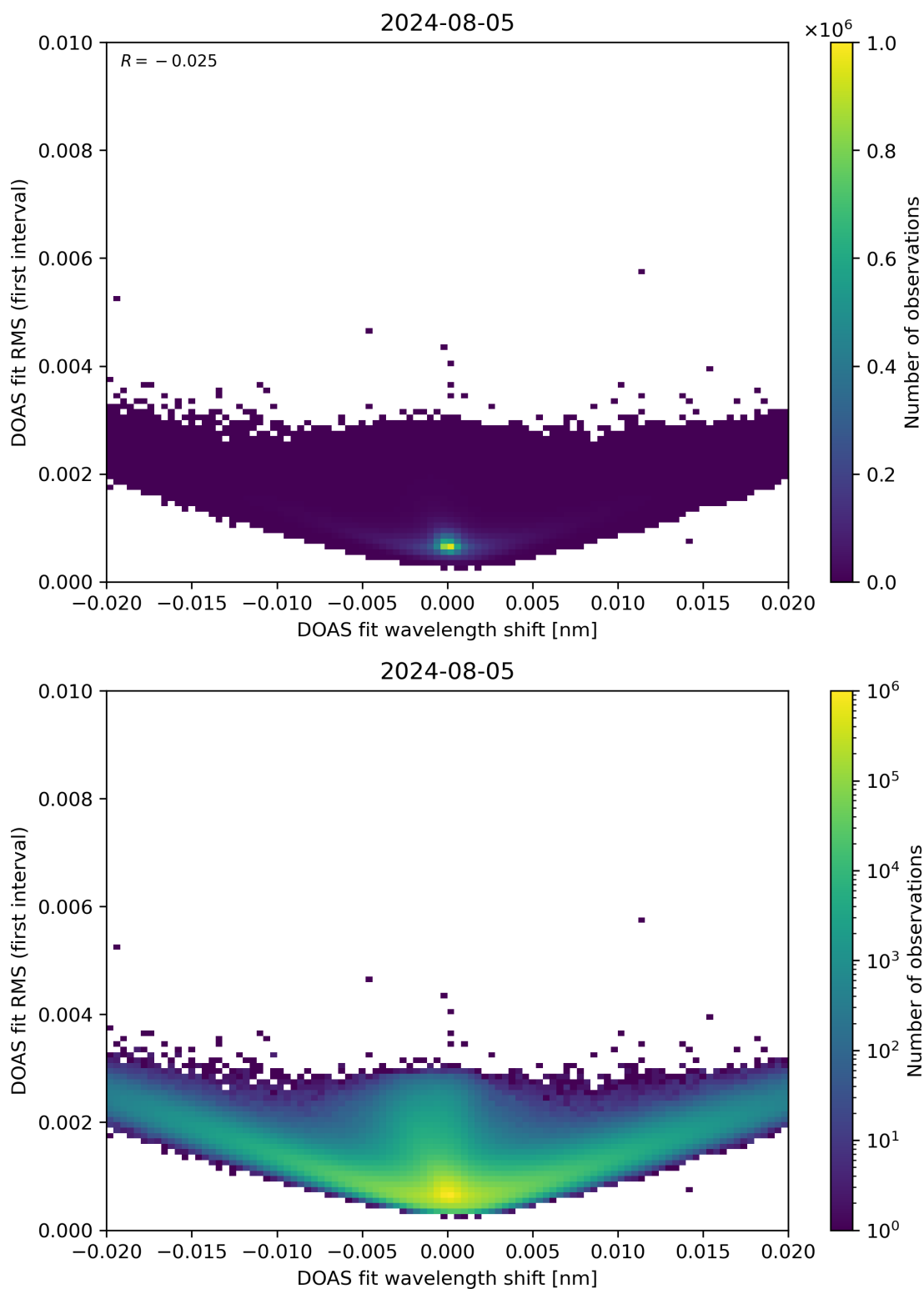
Figure 64: Scatter density plot of “DOAS fit wavelength shift” against “DOAS fit RMS (first interval)” for 2024-08-04 to 2024-08-06.
