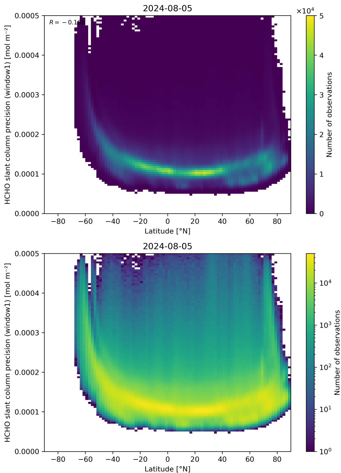
Figure 160: Scatter density plot of “Latitude” against “HCHO slant column precision (window1)” for 2024-08-04 to 2024-08-06.
