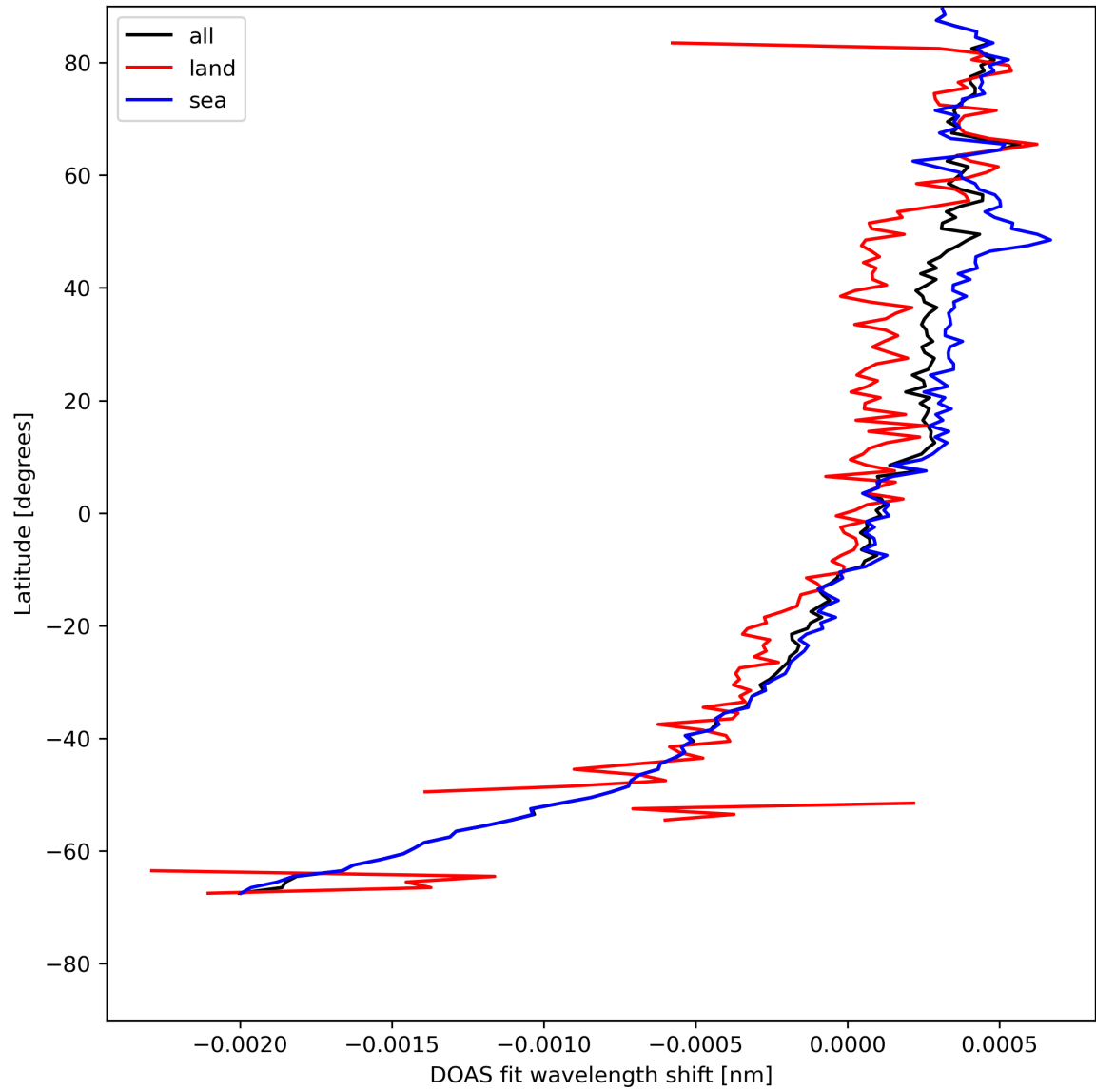
Figure 30: Zonal average of “DOAS fit wavelength shift” for 2024-08-04 to 2024-08-06.
