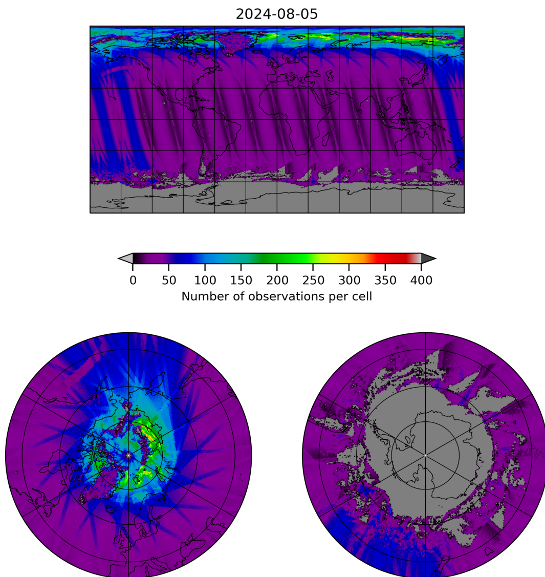
Figure 19: Map of the number of observations for 2024-08-04 to 2024-08-06
