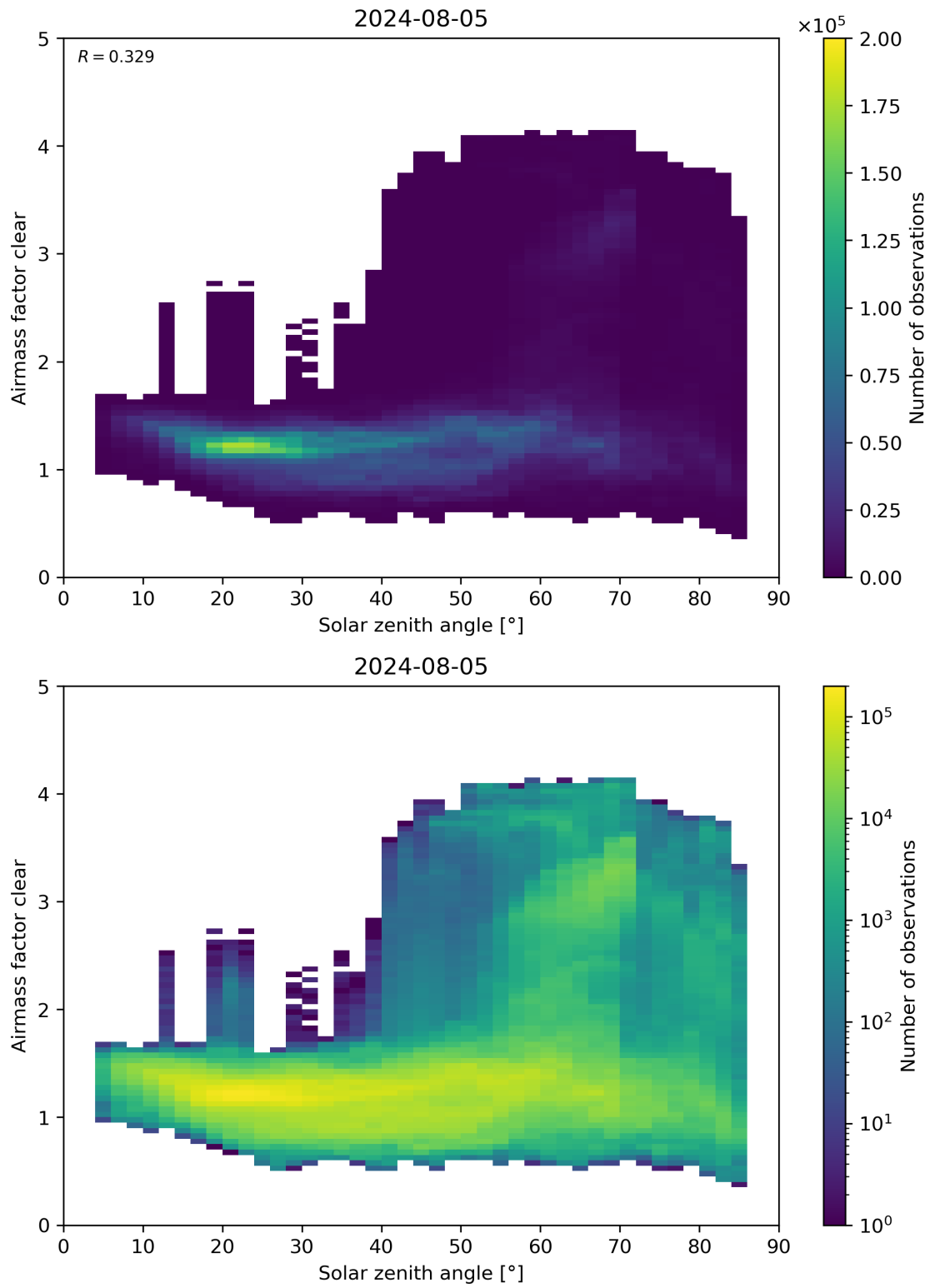
Figure 170: Scatter density plot of “Solar zenith angle” against “Airmass factor clear” for 2024-08-04 to 2024-08-06.
