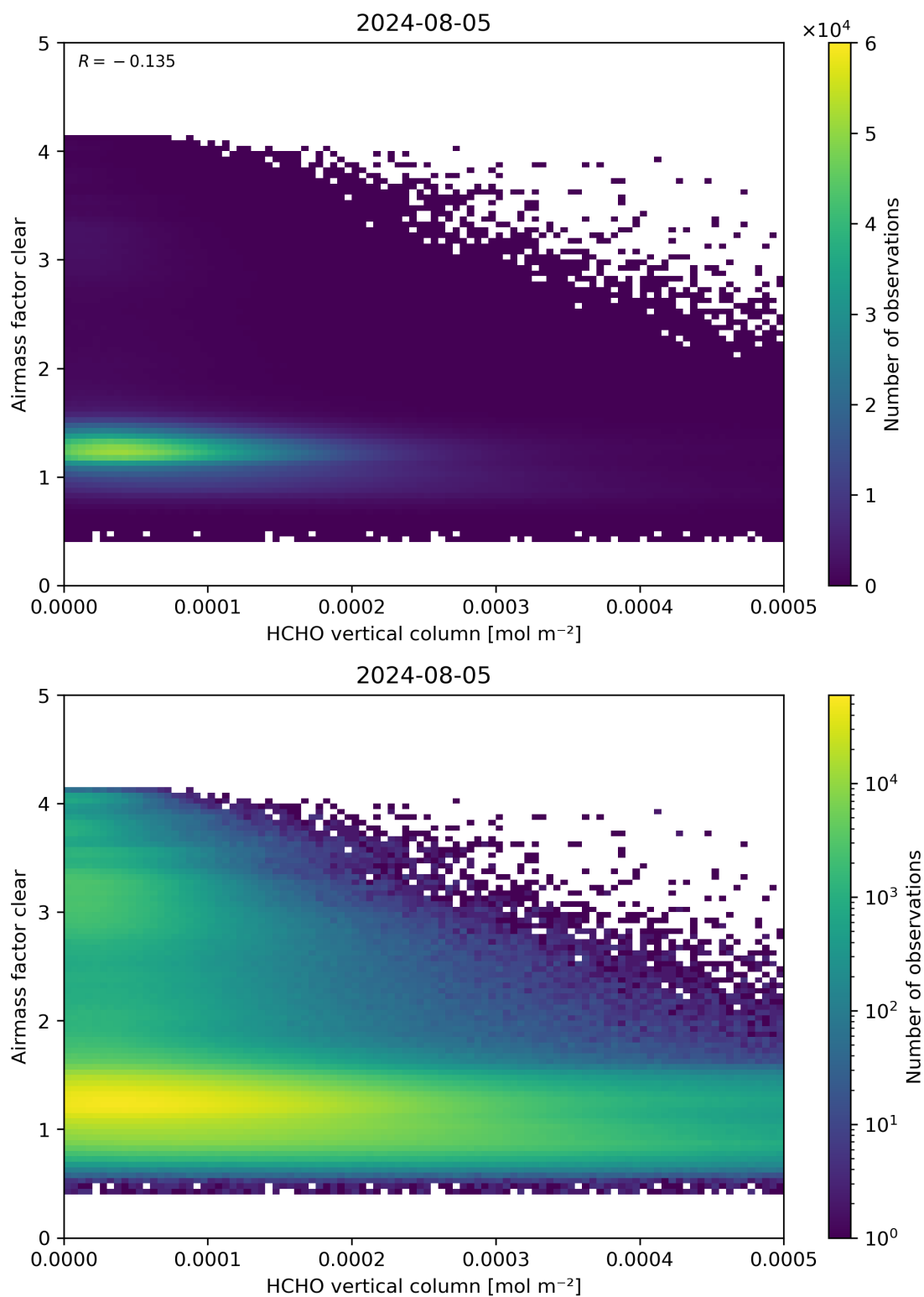
Figure 126: Scatter density plot of “HCHO vertical column” against “Airmass factor clear” for 2024-08-04 to 2024-08-06.
