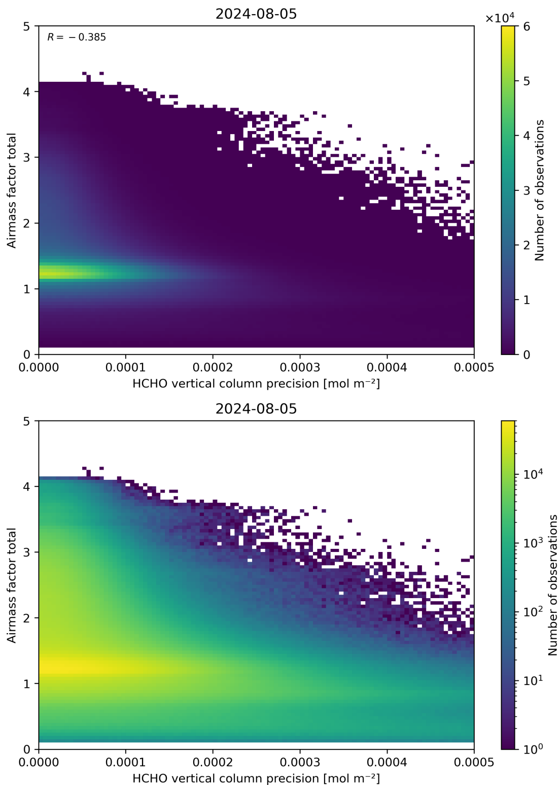
Figure 144: Scatter density plot of “HCHO vertical column precision” against “Airmass factor total” for 2024-08-04 to 2024-08-06.
