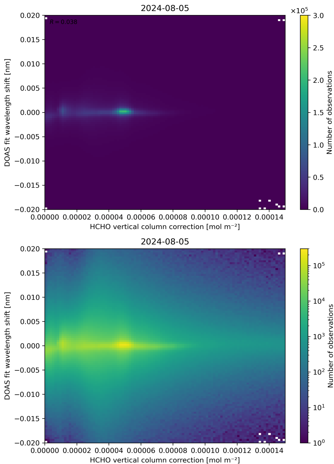
Figure 113: Scatter density plot of “HCHO vertical column correction” against “DOAS fit wavelength shift” for 2024-08-04 to 2024-08-06.
