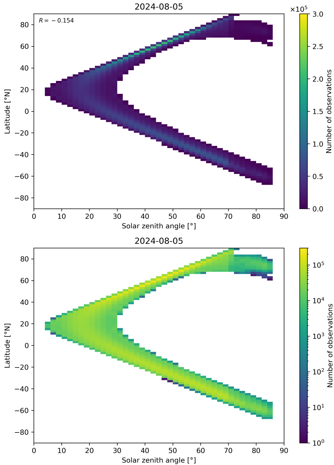
Figure 181: Scatter density plot of “Solar zenith angle” against “Latitude” for 2024-08-04 to 2024-08-06.
