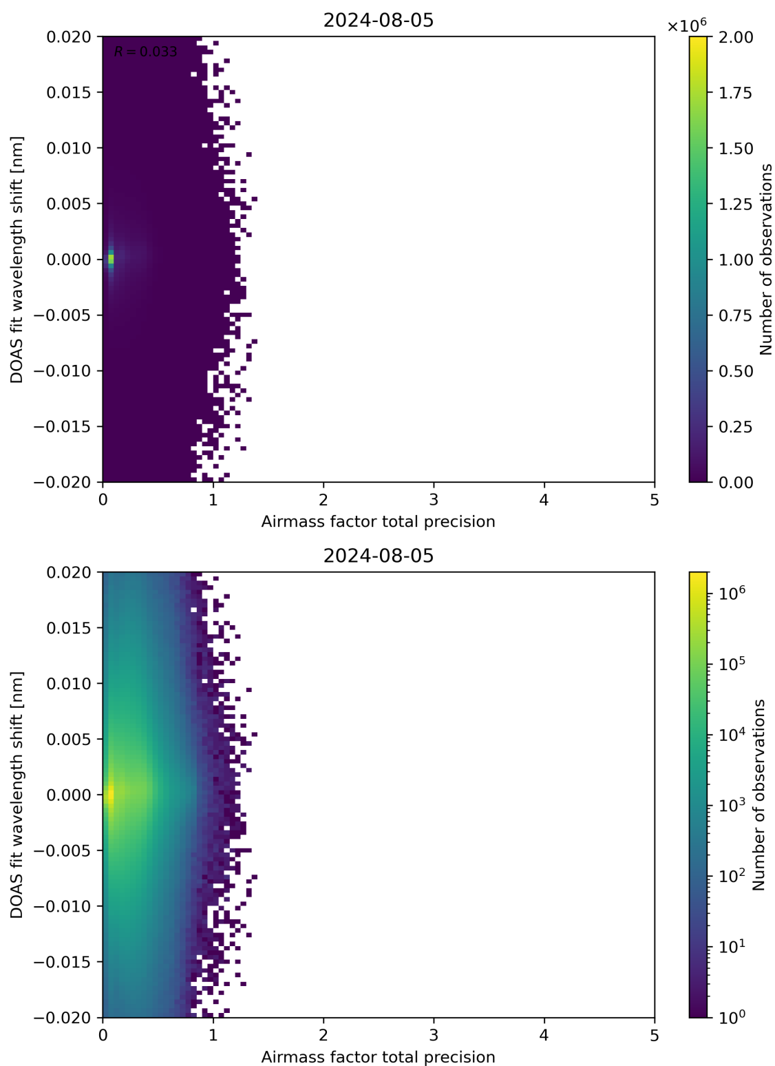
Figure 106: Scatter density plot of “Airmass factor total precision” against “DOAS fit wavelength shift” for 2024-08-04 to 2024-08-06.
