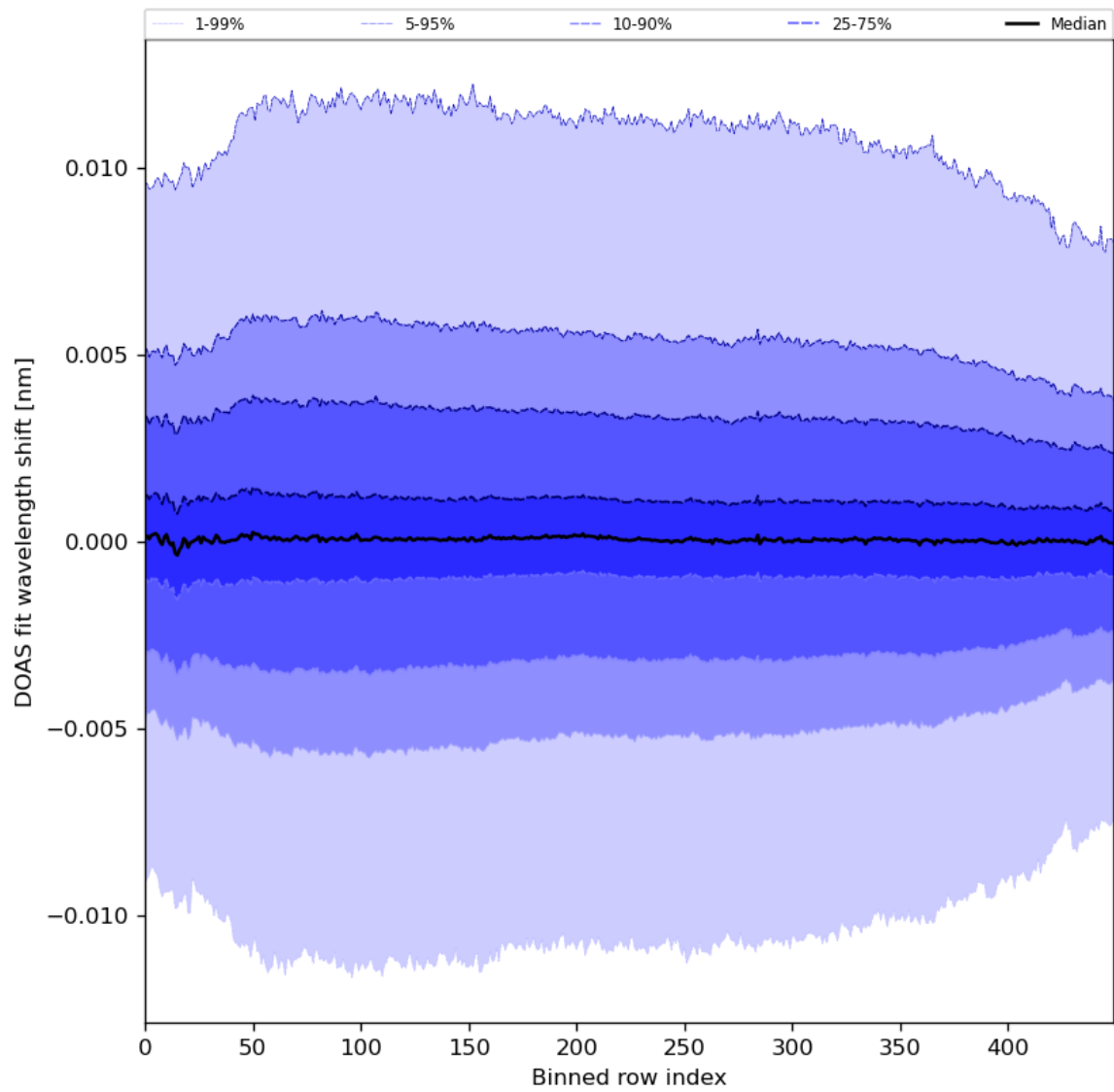
Figure 58: Along track statistics of “DOAS fit wavelength shift” for 2024-08-04 to 2024-08-06
