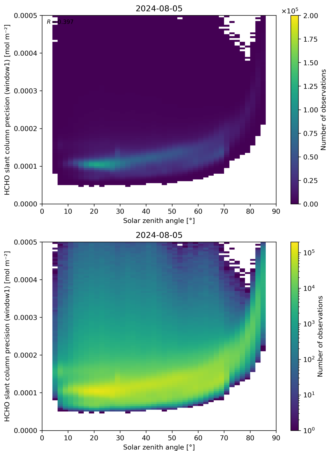
Figure 174: Scatter density plot of “Solar zenith angle” against “HCHO slant column precision (window1)” for 2024-08-04 to 2024-08-06.
