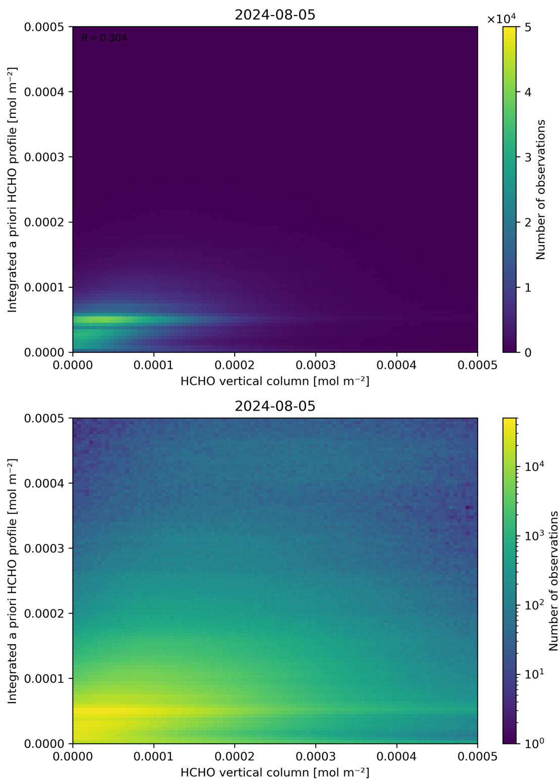
Figure 135: Scatter density plot of “HCHO vertical column” against “Integrated a priori HCHO profile” for 2024-08-04 to 2024-08-06.
