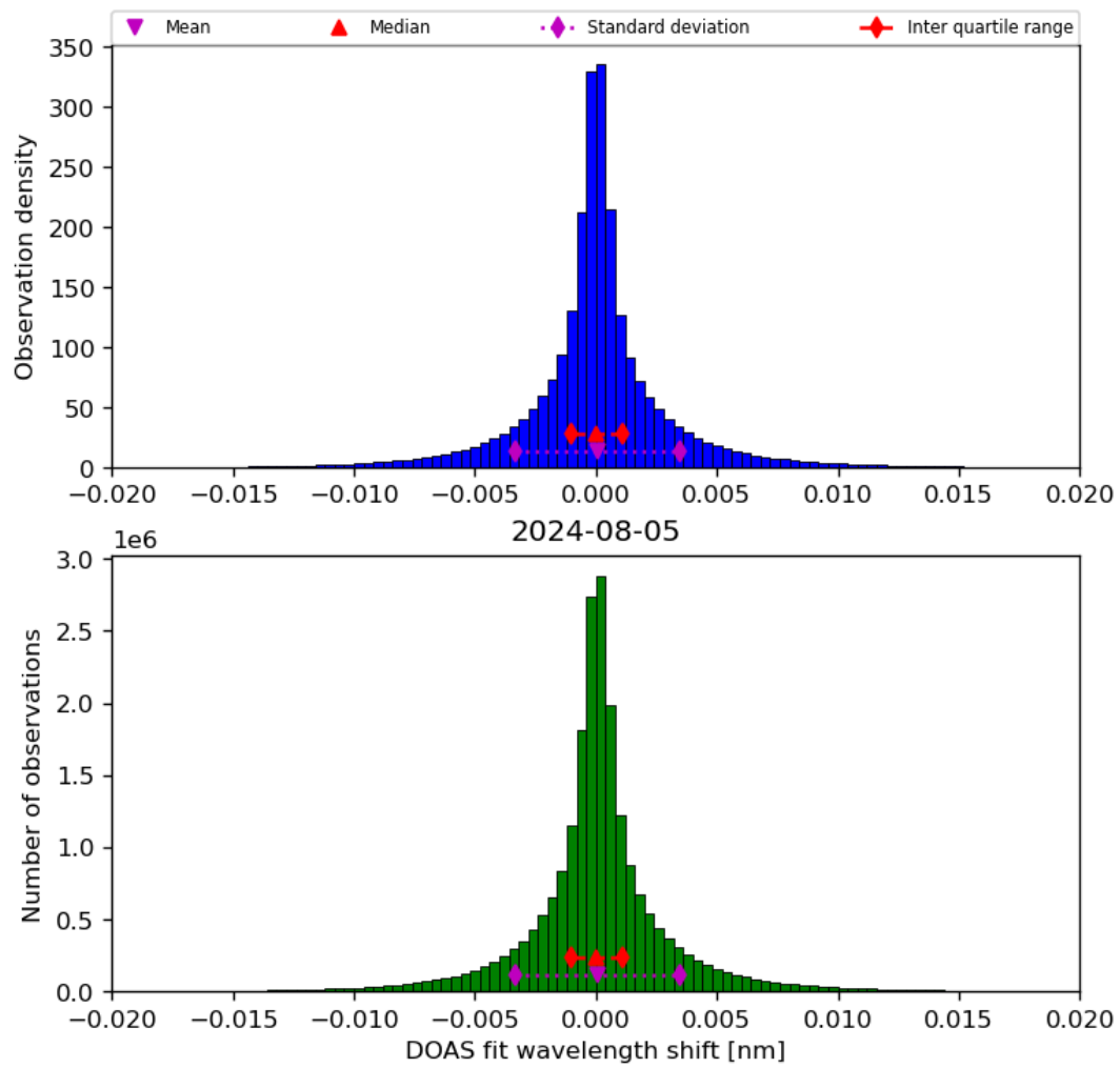
Figure 44: Histogram of “DOAS fit wavelength shift” for 2024-08-04 to 2024-08-06
