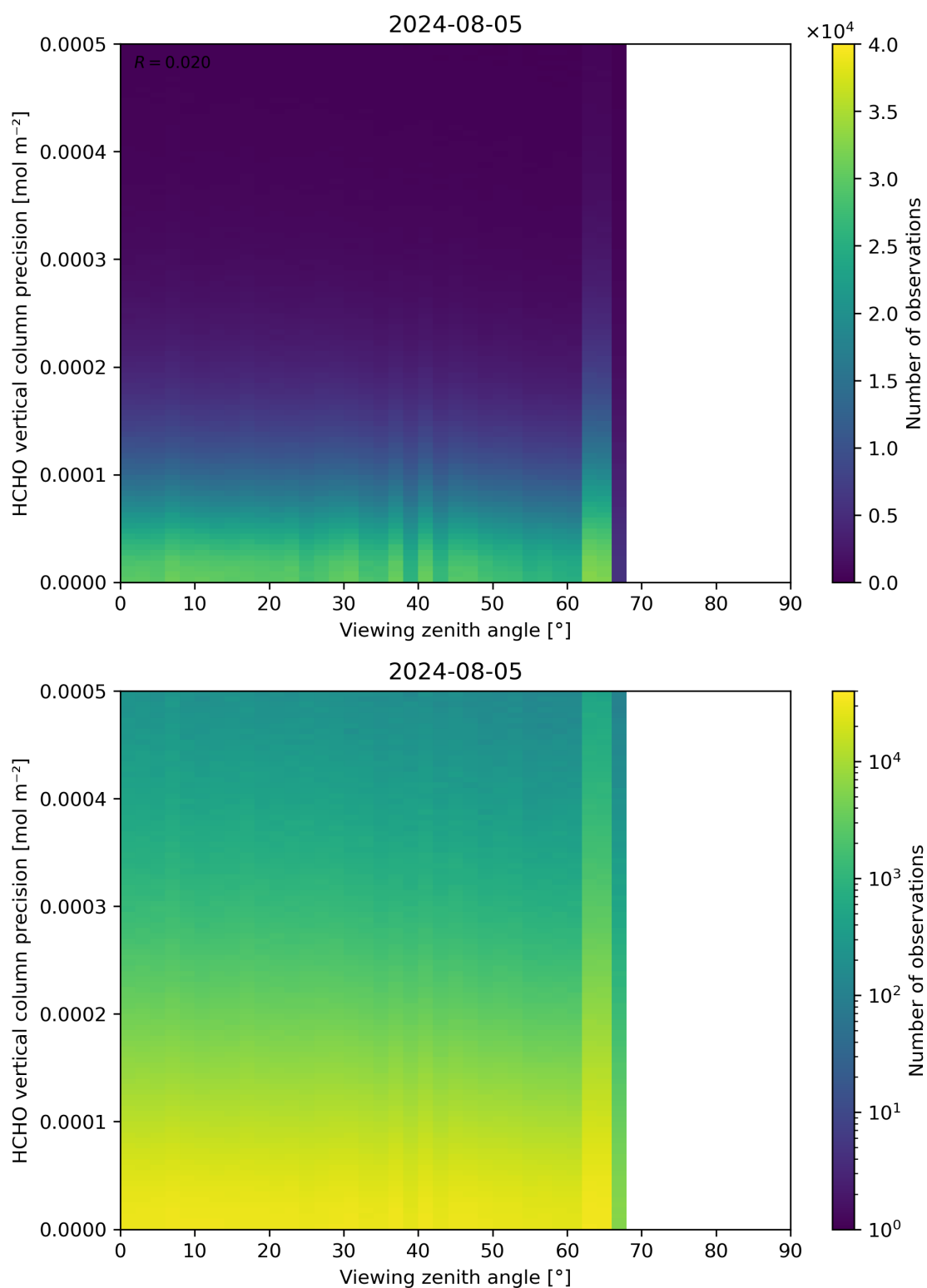
Figure 194: Scatter density plot of “Viewing zenith angle” against “HCHO vertical column precision” for 2024-08-04 to 2024-08-06.
