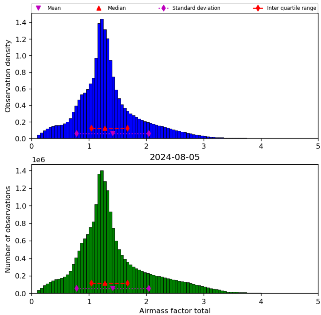
Figure 40: Histogram of “Airmass factor total” for 2024-08-04 to 2024-08-06
