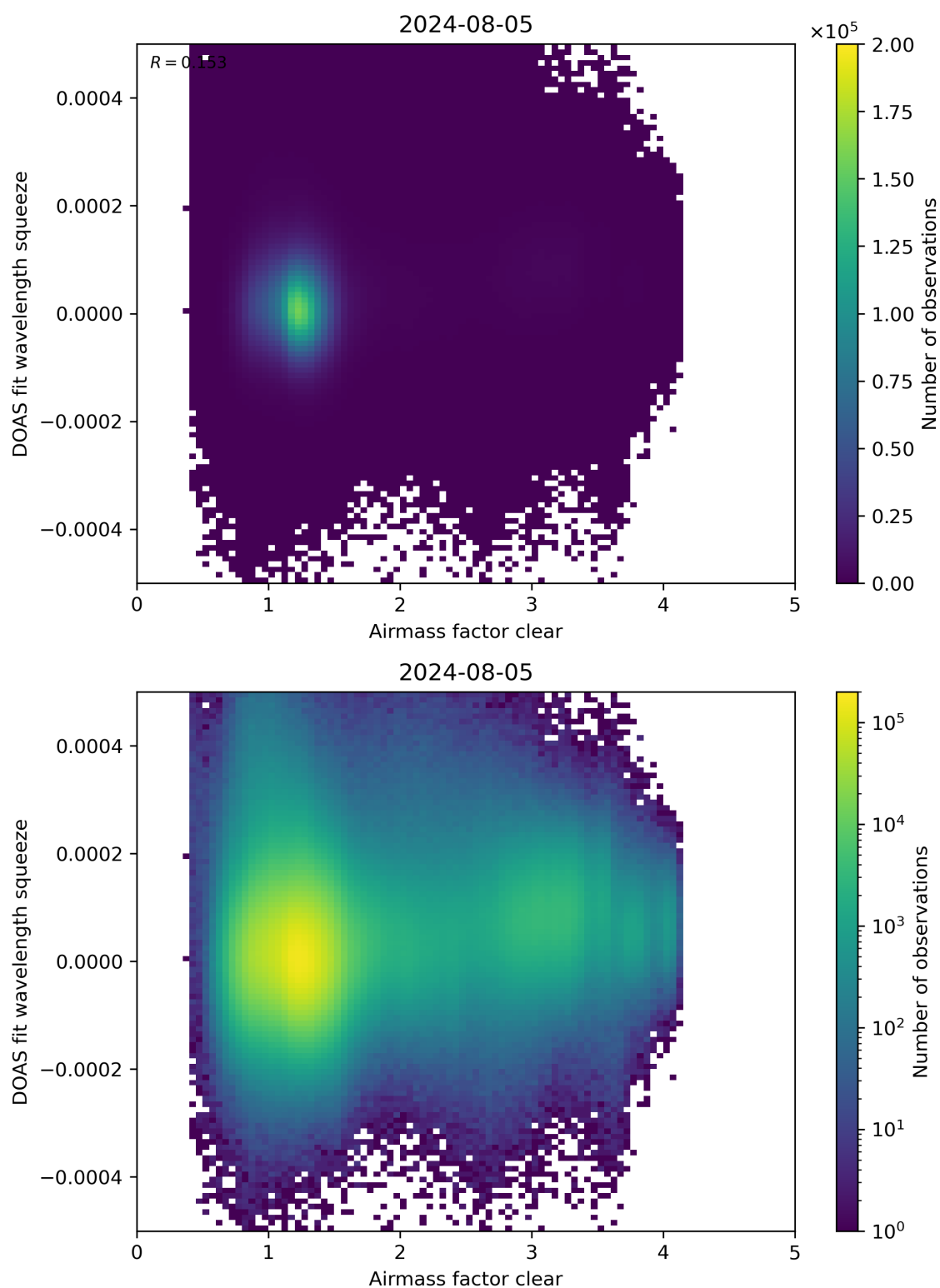
Figure 73: Scatter density plot of “Airmass factor clear” against “DOAS fit wavelength squeeze” for 2024-08-04 to 2024-08-06.
