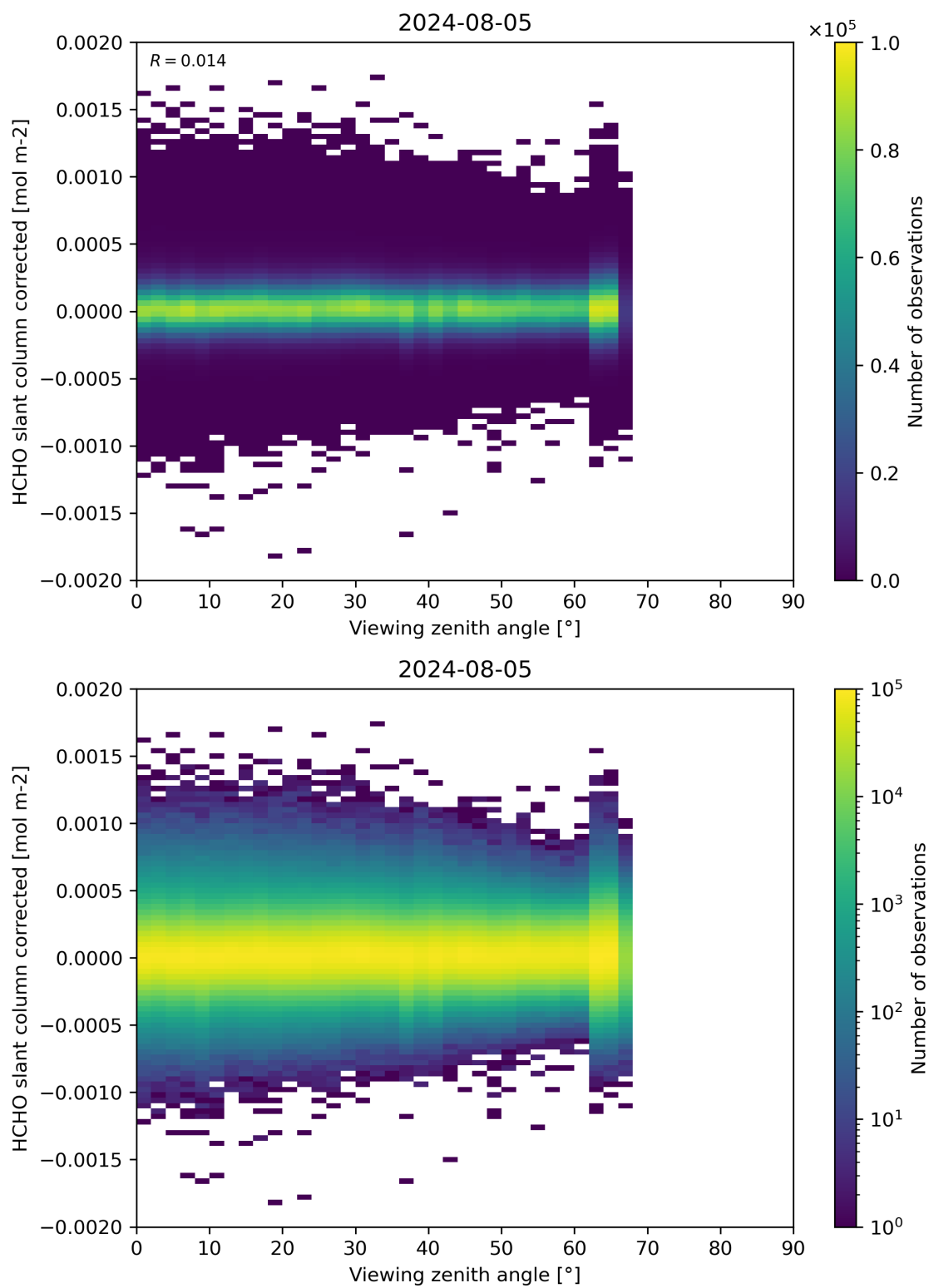
Figure 186: Scatter density plot of “Viewing zenith angle” against “HCHO slant column corrected” for 2024-08-04 to 2024-08-06.
