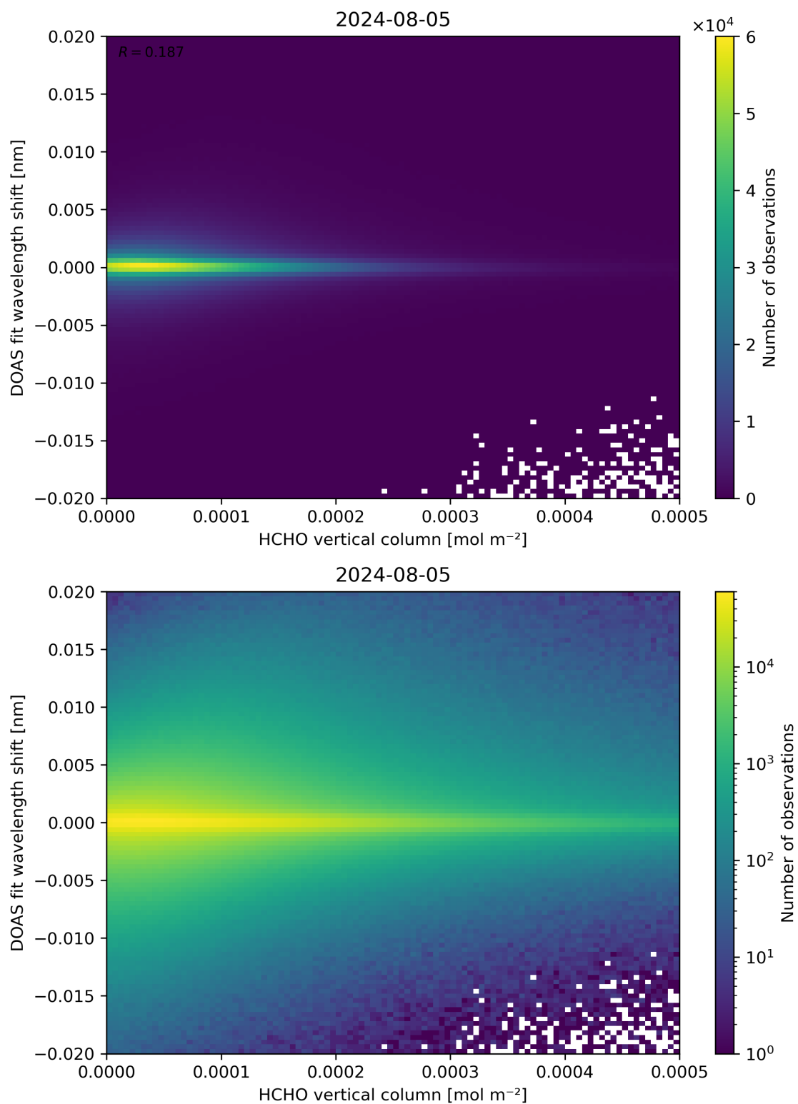
Figure 124: Scatter density plot of “HCHO vertical column” against “DOAS fit wavelength shift” for 2024-08-04 to 2024-08-06.
