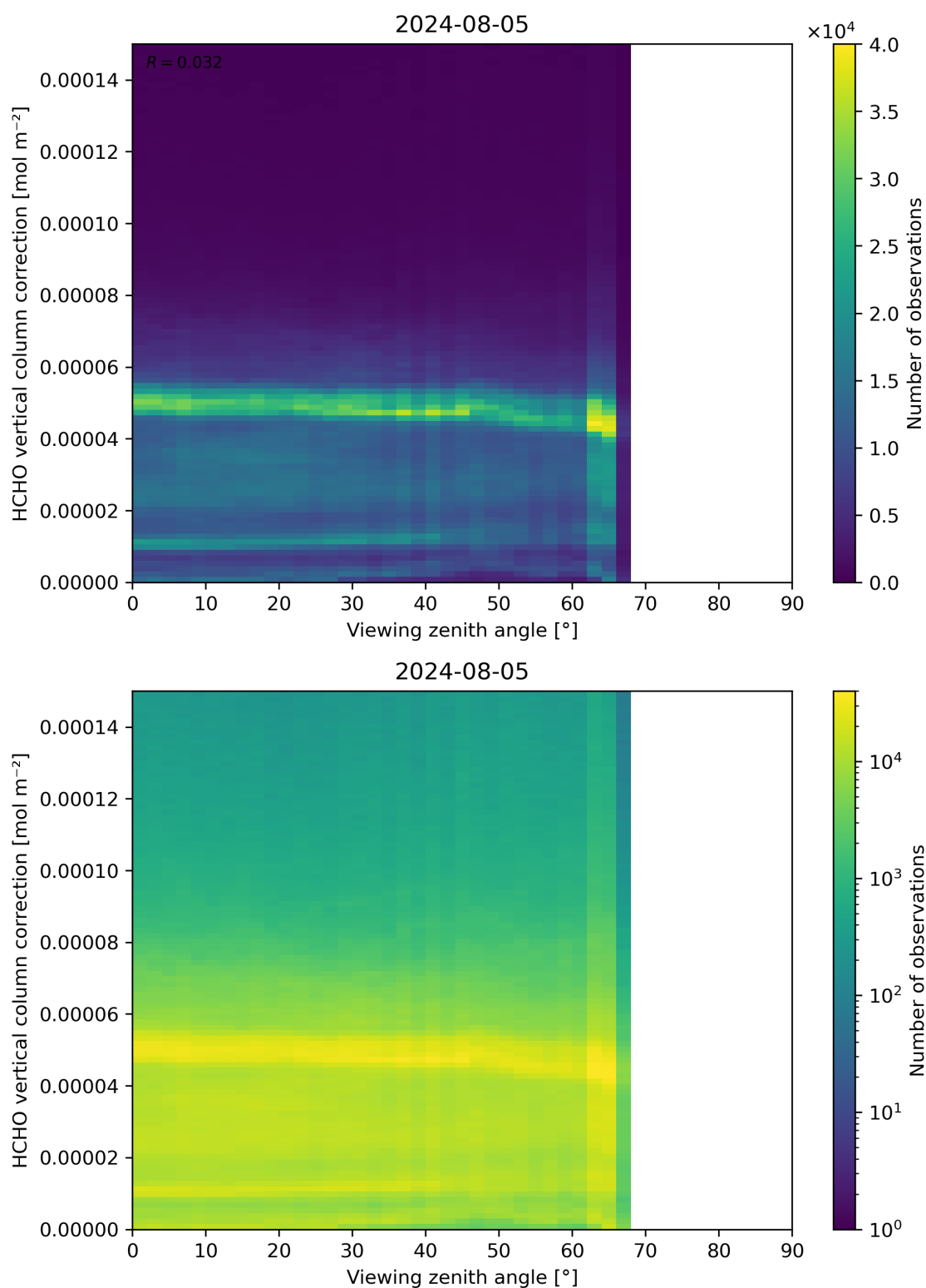
Figure 193: Scatter density plot of “Viewing zenith angle” against “HCHO vertical column correction” for 2024-08-04 to 2024-08-06.
