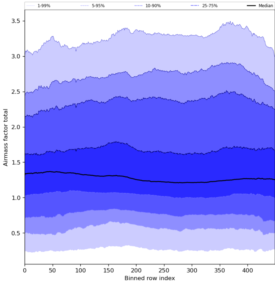
Figure 54: Along track statistics of “Airmass factor total” for 2024-08-04 to 2024-08-06
