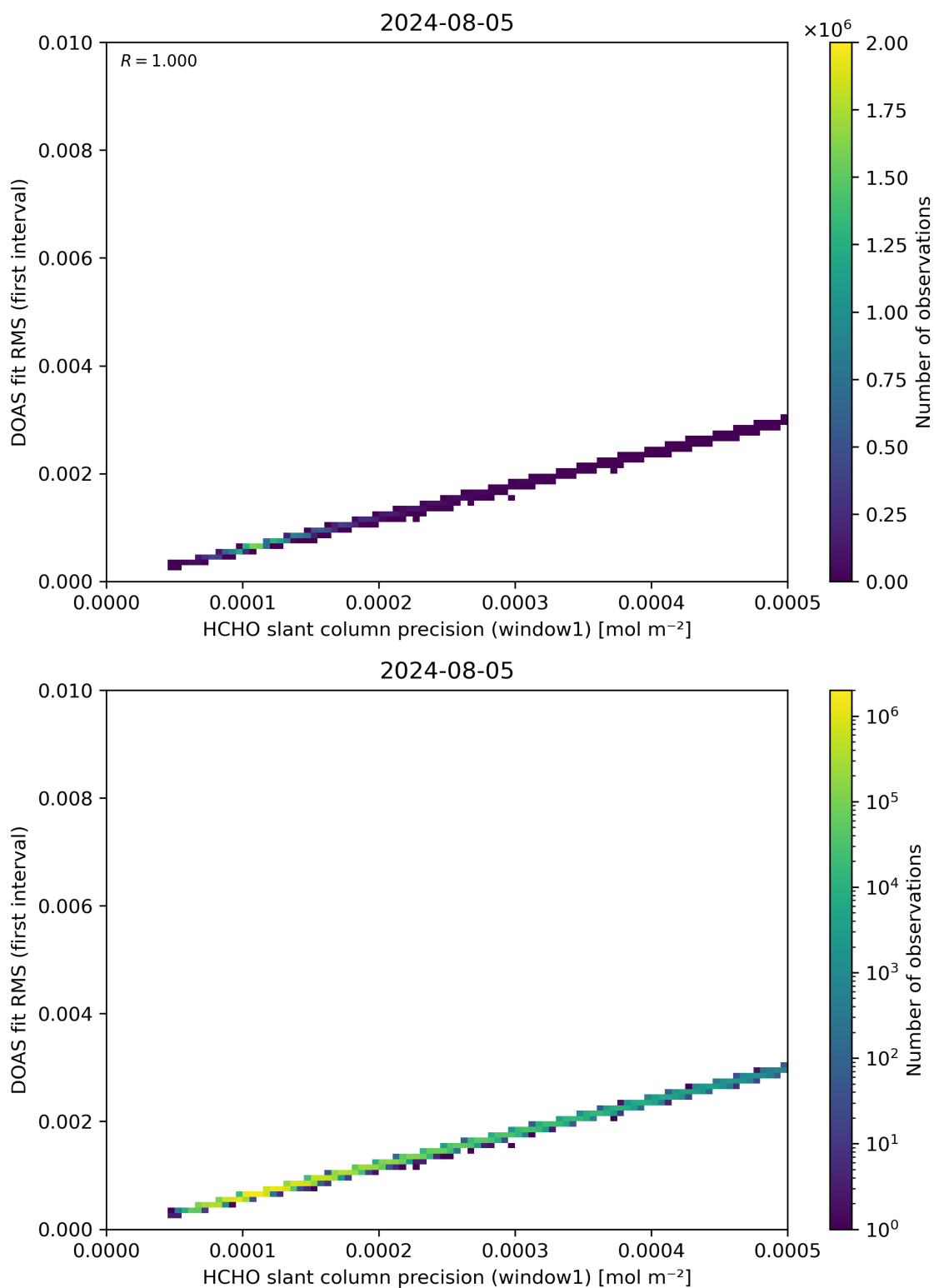
Figure 88: Scatter density plot of “HCHO slant column precision (window1)” against “DOAS fit RMS (first interval)” for 2024-08-04 to 2024-08-06.
