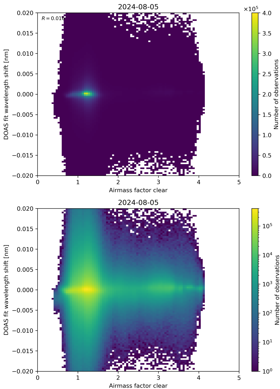
Figure 72: Scatter density plot of “Airmass factor clear” against “DOAS fit wavelength shift” for 2024-08-04 to 2024-08-06.
