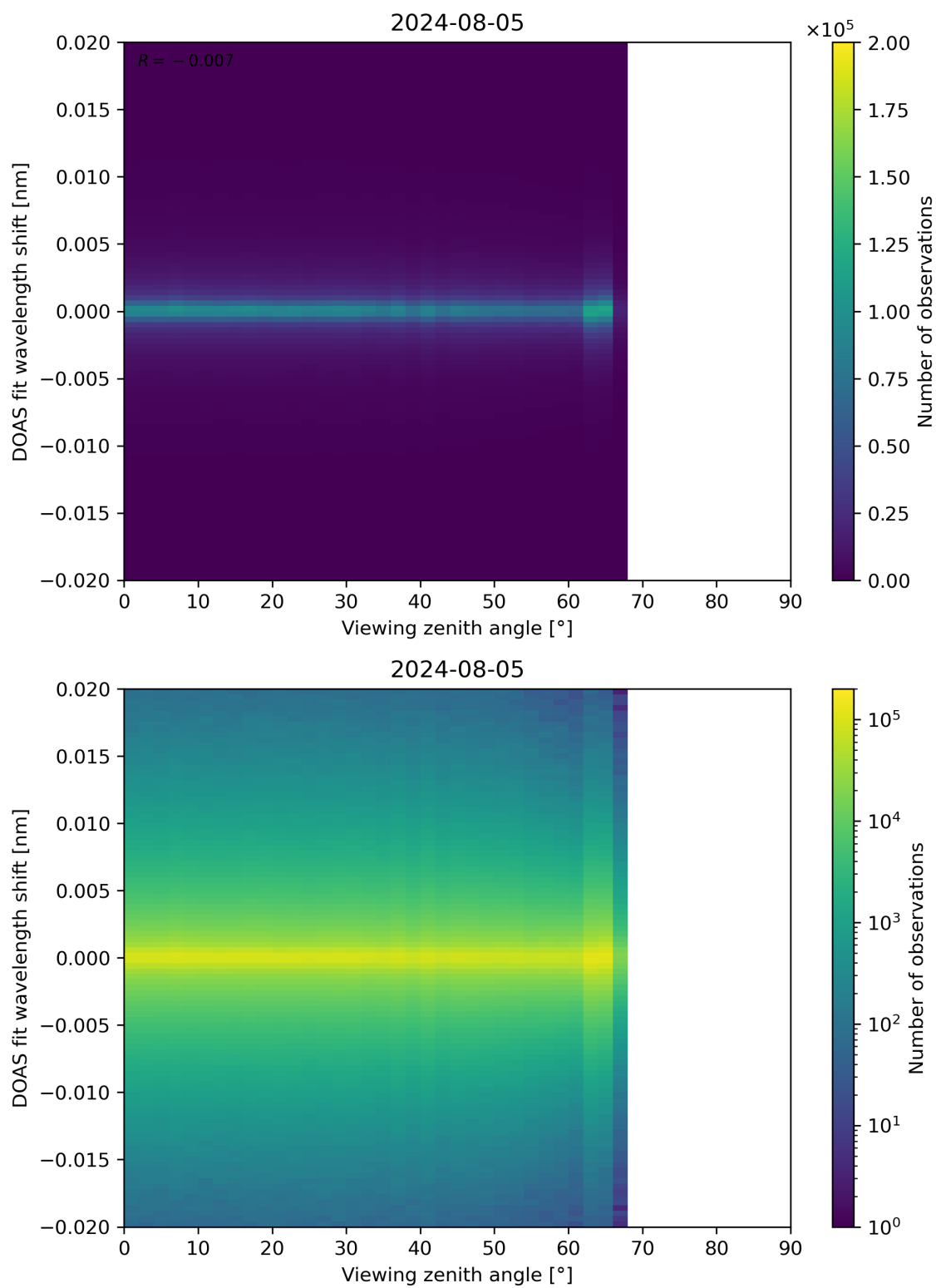
Figure 183: Scatter density plot of “Viewing zenith angle” against “DOAS fit wavelength shift” for 2024-08-04 to 2024-08-06.
