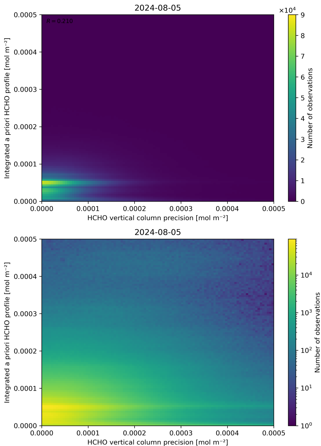
Figure 147: Scatter density plot of “HCHO vertical column precision” against “Integrated a priori HCHO profile” for 2024-08-04 to 2024-08-06.
