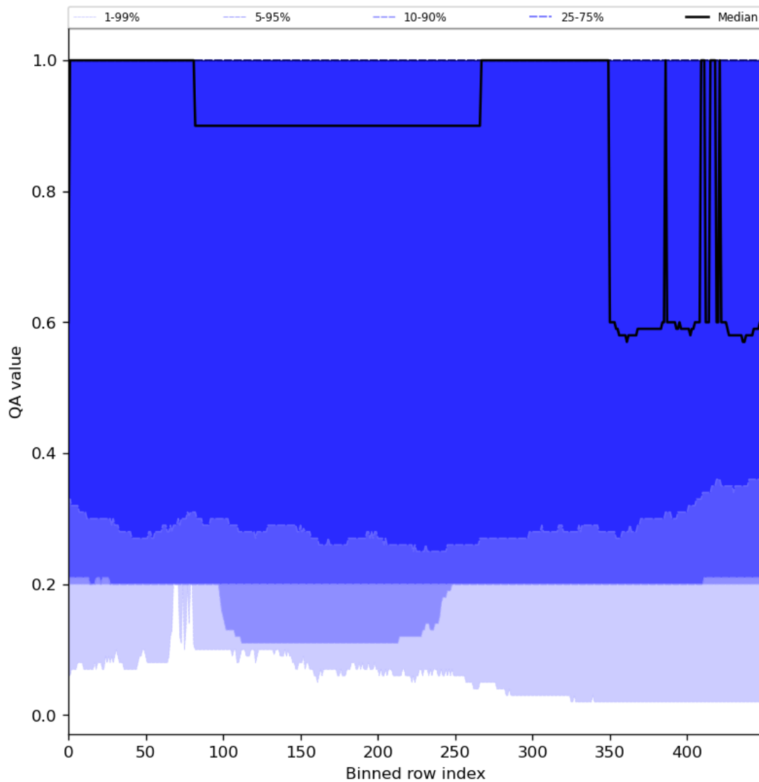
Figure 48: Along track statistics of “QA value” for 2024-08-04 to 2024-08-06
