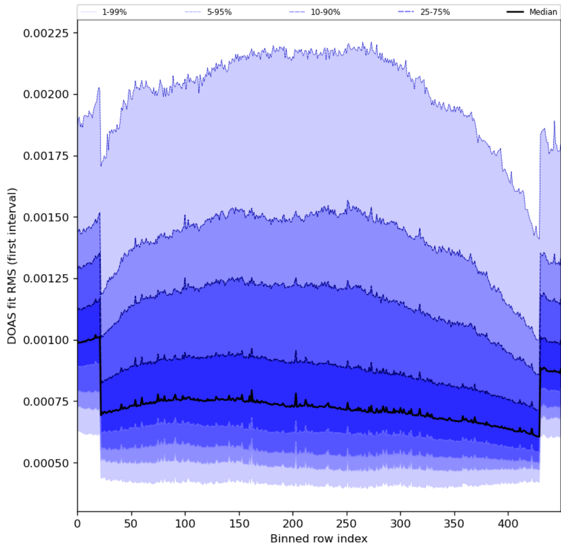
Figure 60: Along track statistics of “DOAS fit RMS (first interval)” for 2024-08-04 to 2024-08-06
