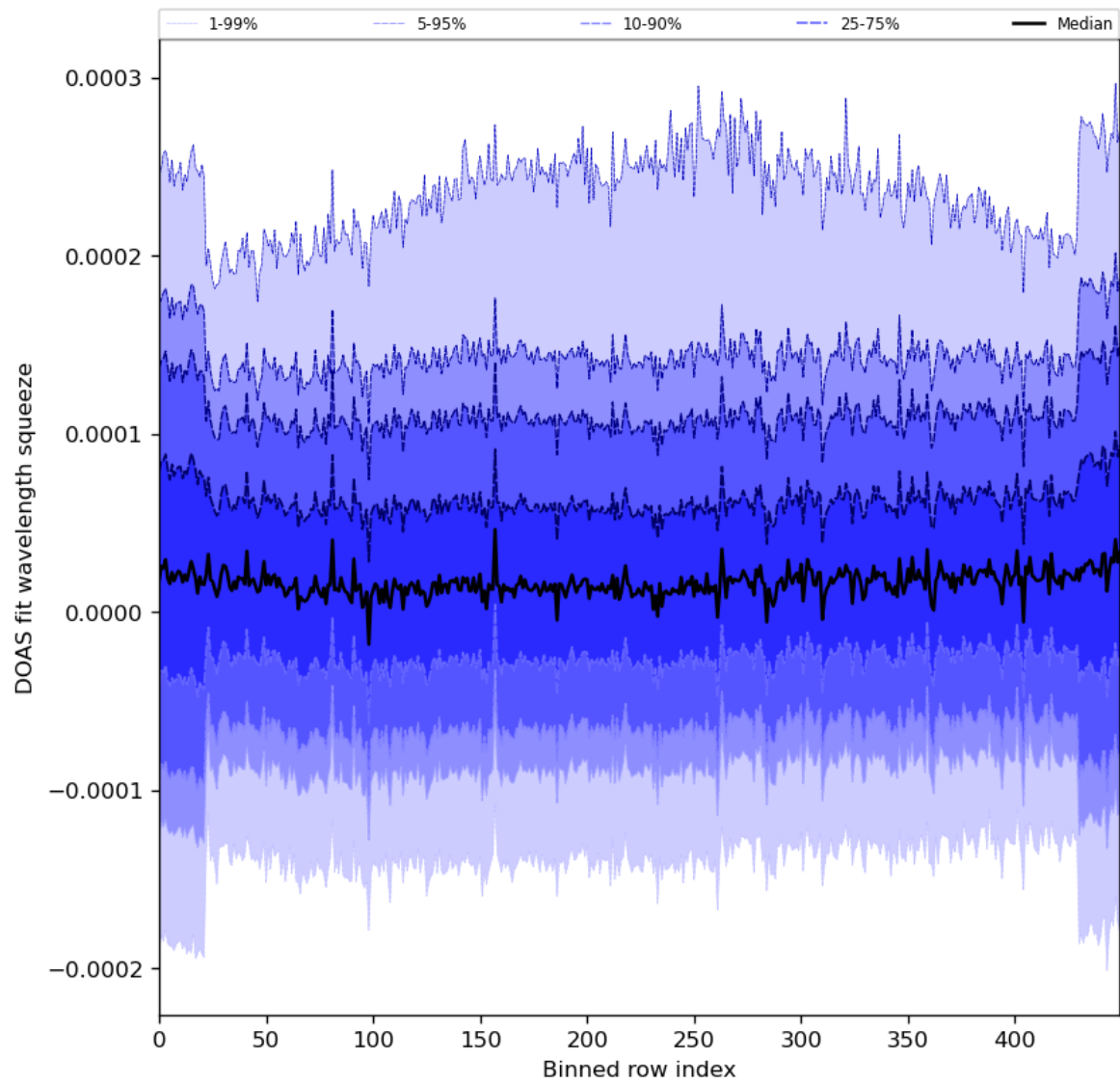
Figure 59: Along track statistics of “DOAS fit wavelength squeeze” for 2024-08-04 to 2024-08-06
