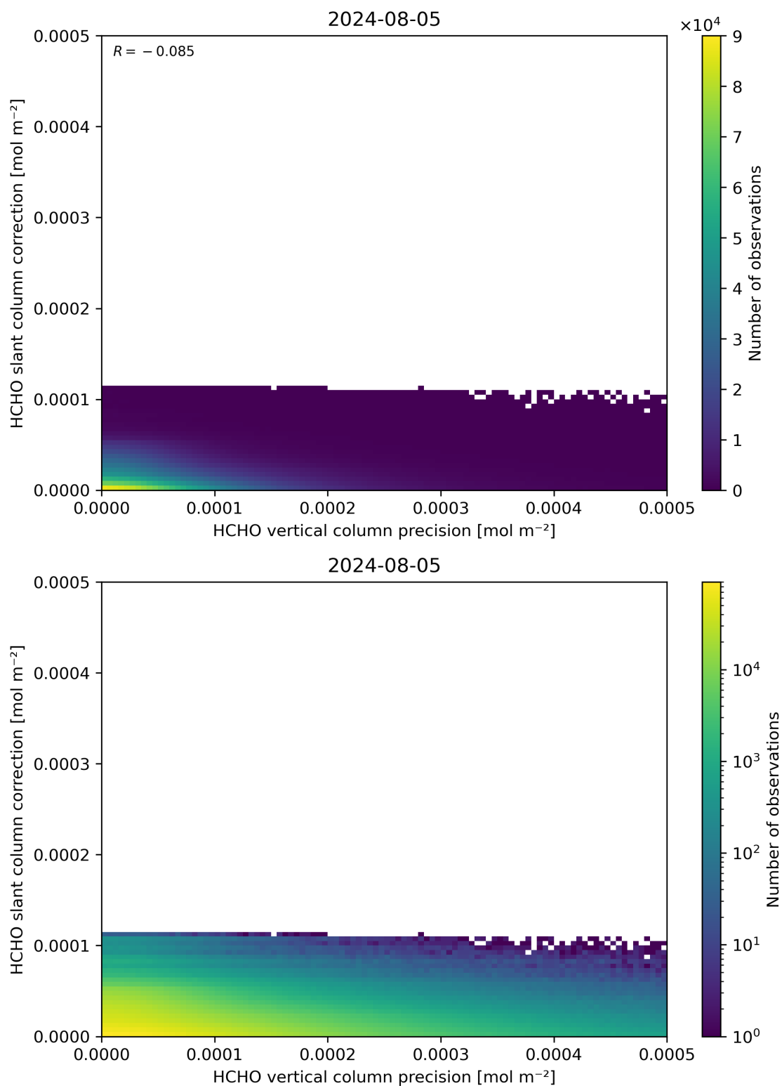
Figure 141: Scatter density plot of “HCHO vertical column precision” against “HCHO slant column correction” for 2024-08-04 to 2024-08-06.
