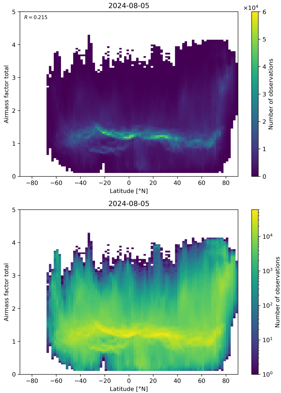
Figure 161: Scatter density plot of “Latitude” against “Airmass factor total” for 2024-08-04 to 2024-08-06.
