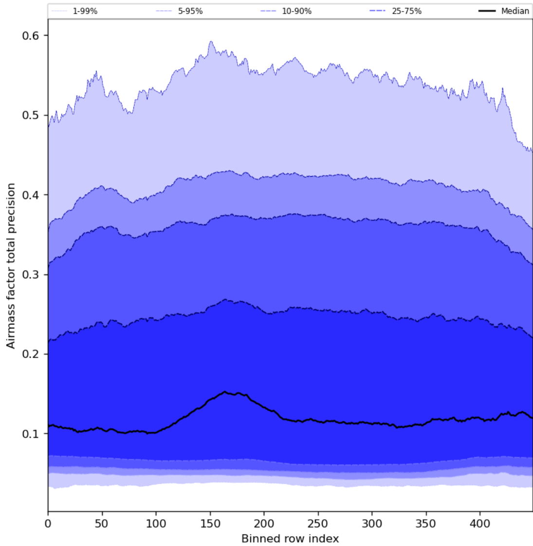
Figure 55: Along track statistics of “Airmass factor total precision” for 2024-08-04 to 2024-08-06
