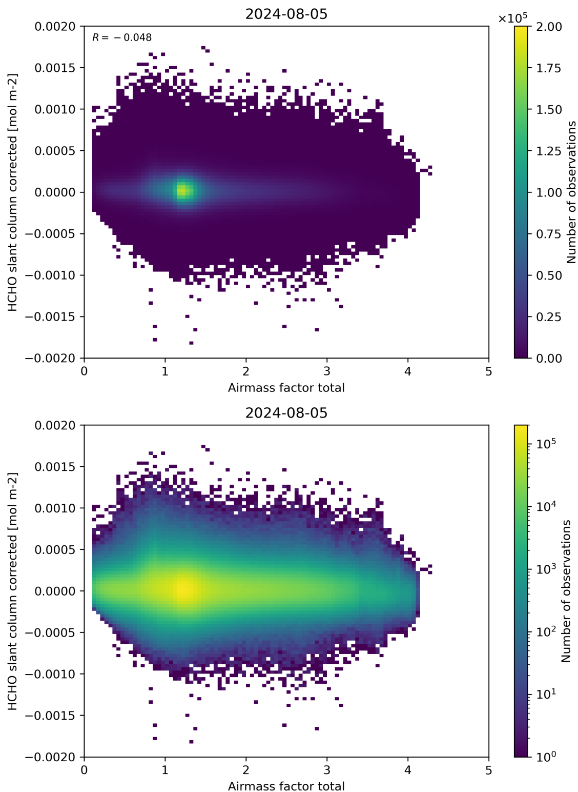
Figure 101: Scatter density plot of “Airmass factor total” against “HCHO slant column corrected” for 2024-08-04 to 2024-08-06.
