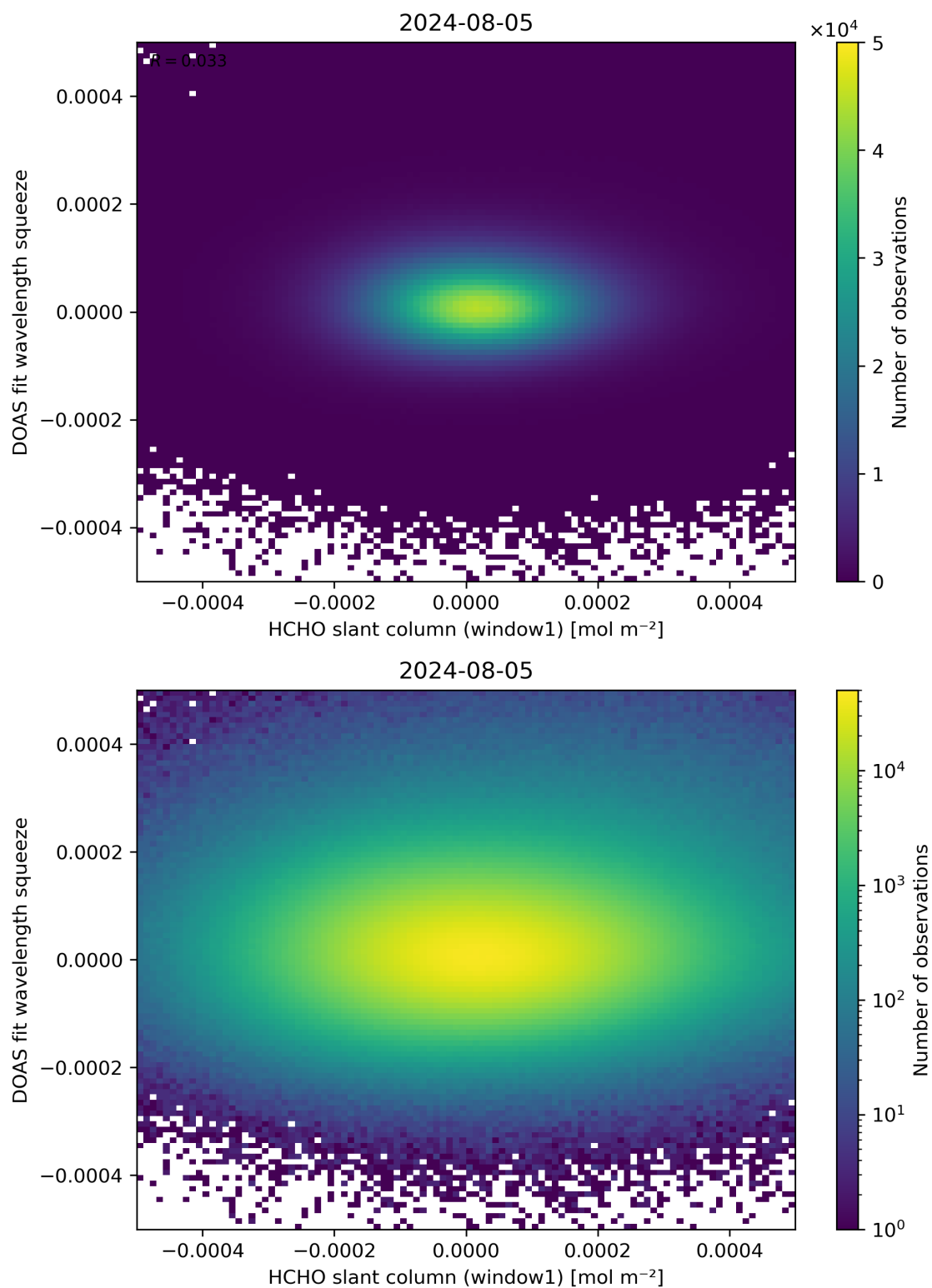
Figure 80: Scatter density plot of “HCHO slant column (window1)” against “DOAS fit wavelength squeeze” for 2024-08-04 to 2024-08-06.
