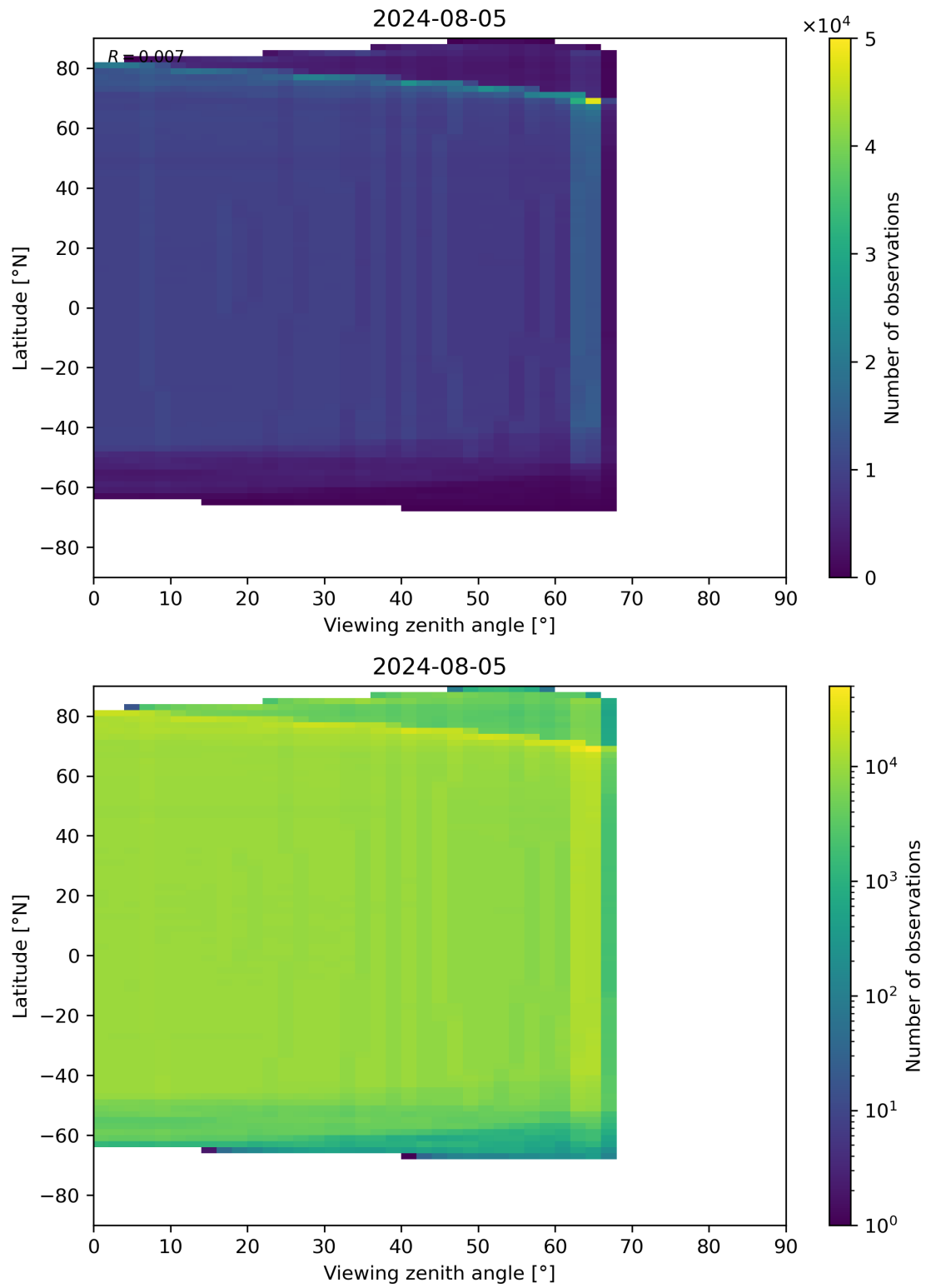
Figure 196: Scatter density plot of “Viewing zenith angle” against “Latitude” for 2024-08-04 to 2024-08-06.
