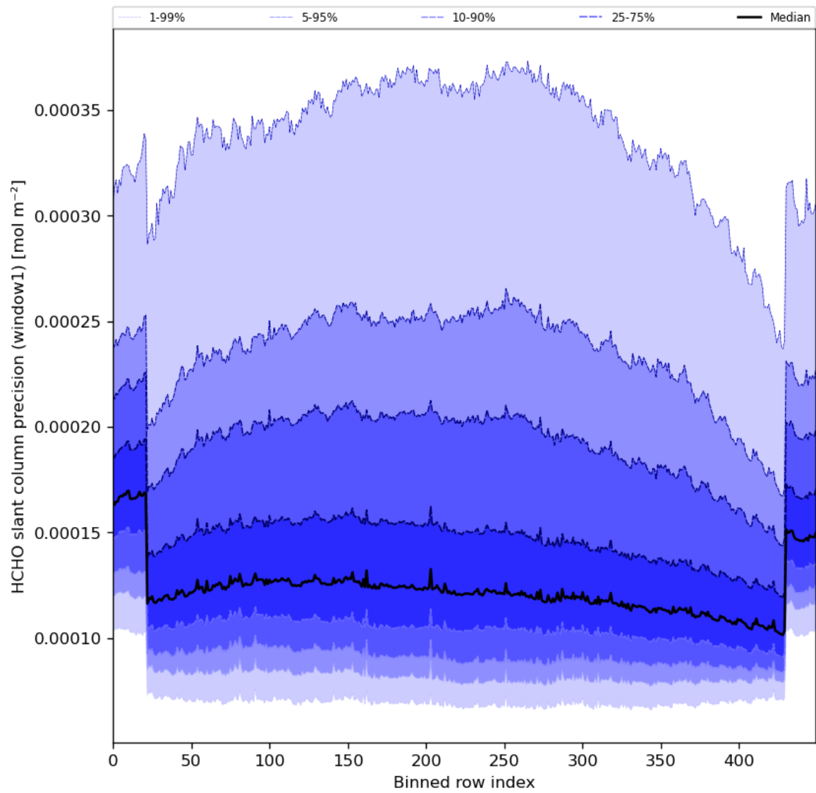
Figure 53: Along track statistics of “HCHO slant column precision (window1)” for 2024-08-04 to 2024-08-06
