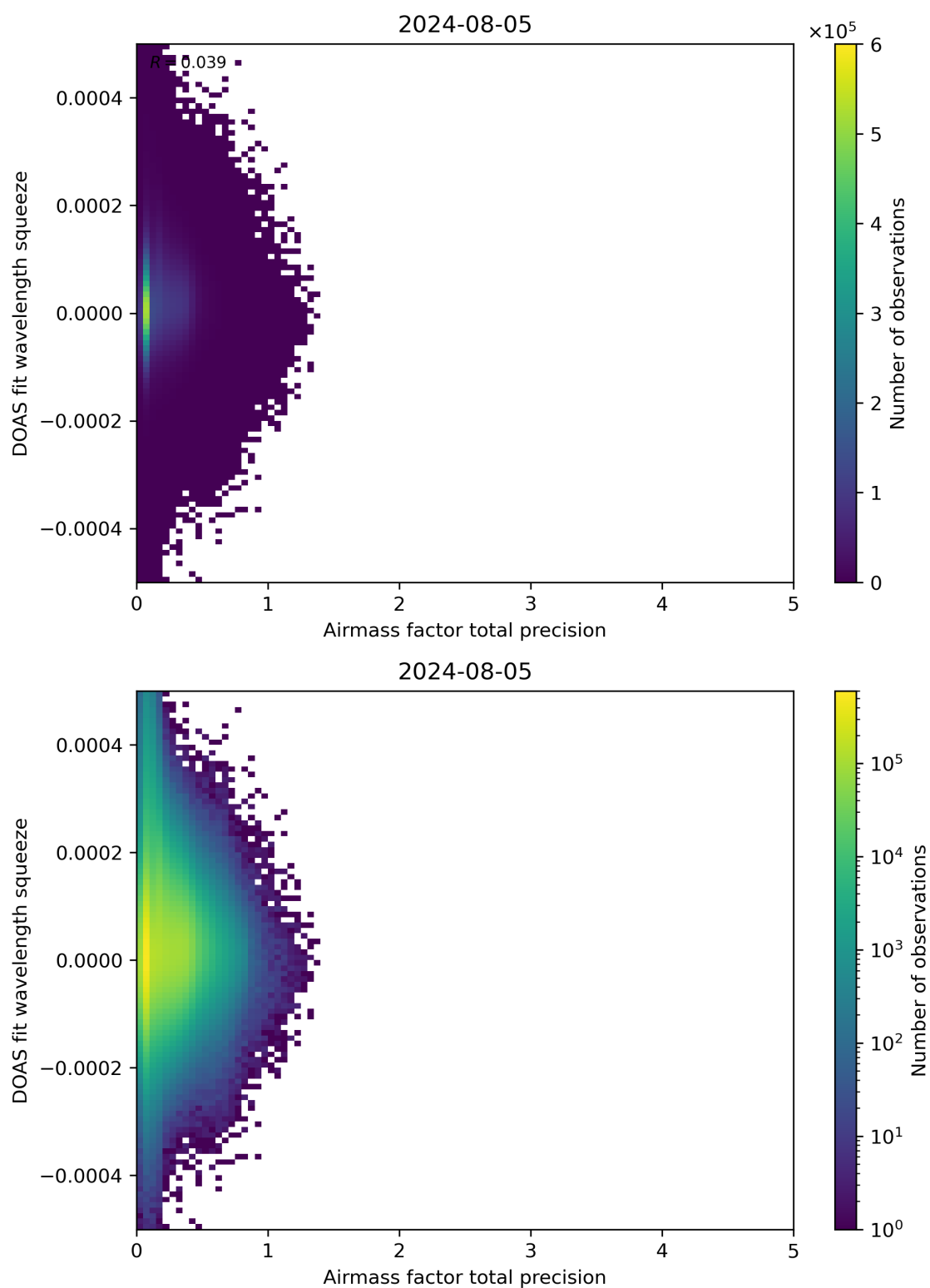
Figure 107: Scatter density plot of “Airmass factor total precision” against “DOAS fit wavelength squeeze” for 2024-08-04 to 2024-08-06.
