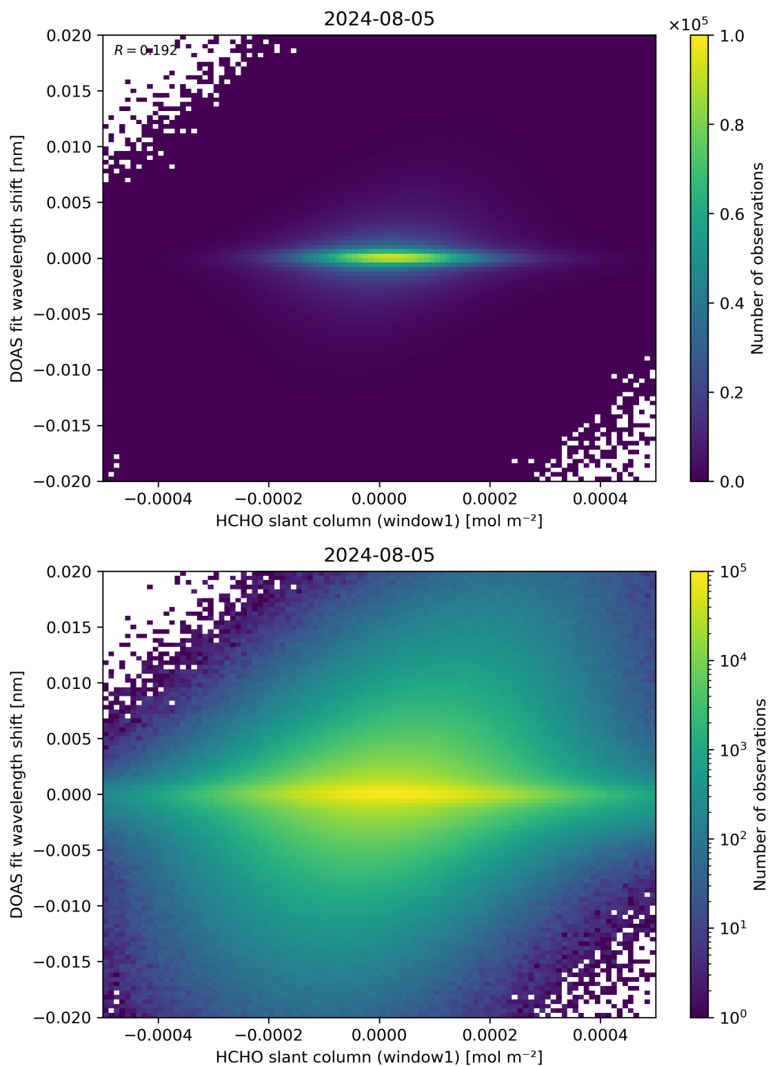
Figure 79: Scatter density plot of “HCHO slant column (window1)” against “DOAS fit wavelength shift” for 2024-08-04 to 2024-08-06.
