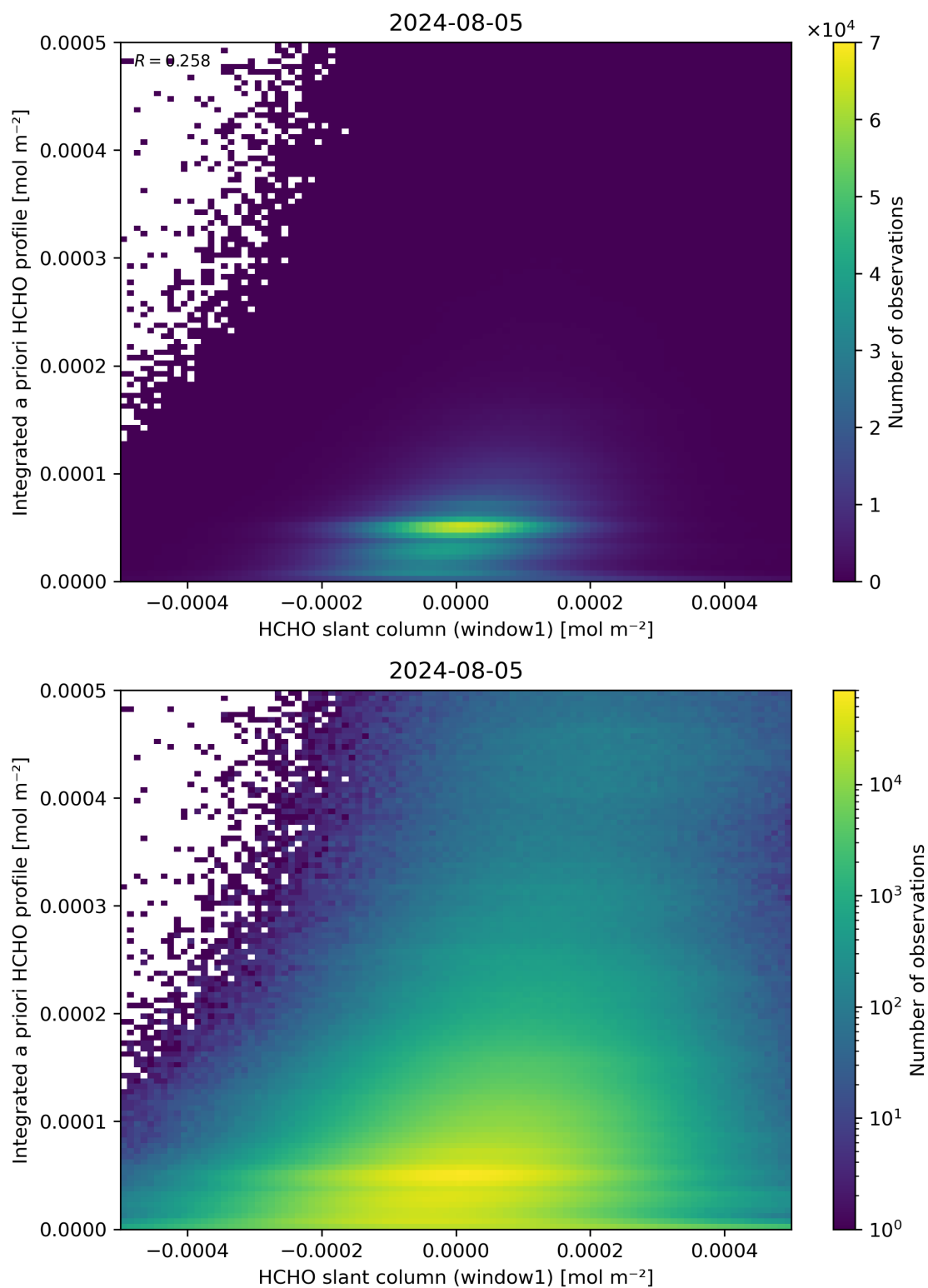
Figure 87: Scatter density plot of “HCHO slant column (window1)” against “Integrated a priori HCHO profile” for 2024-08-04 to 2024-08-06.
