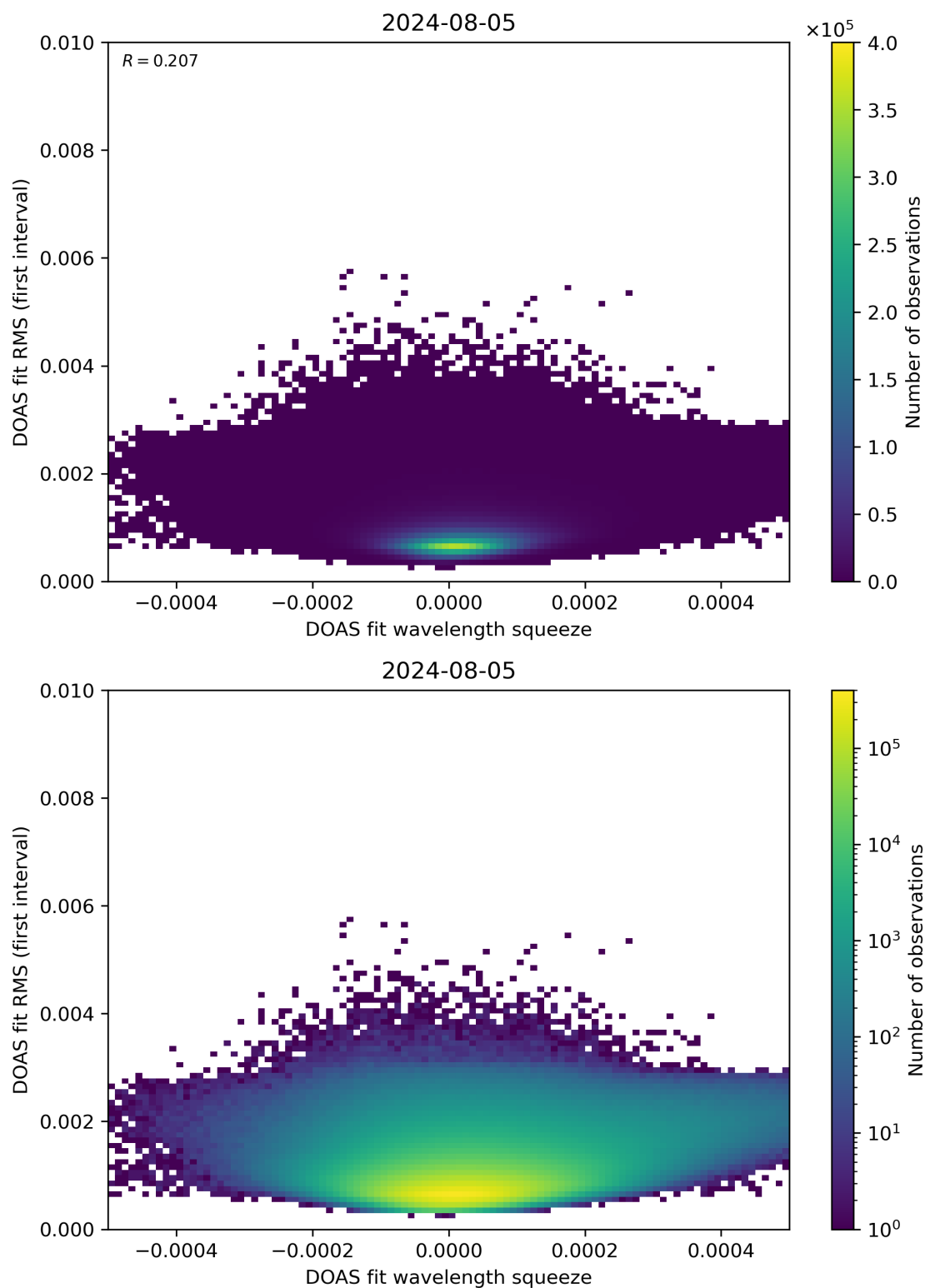
Figure 68: Scatter density plot of “DOAS fit wavelength squeeze” against “DOAS fit RMS (first interval)” for 2024-08-04 to 2024-08-06.
