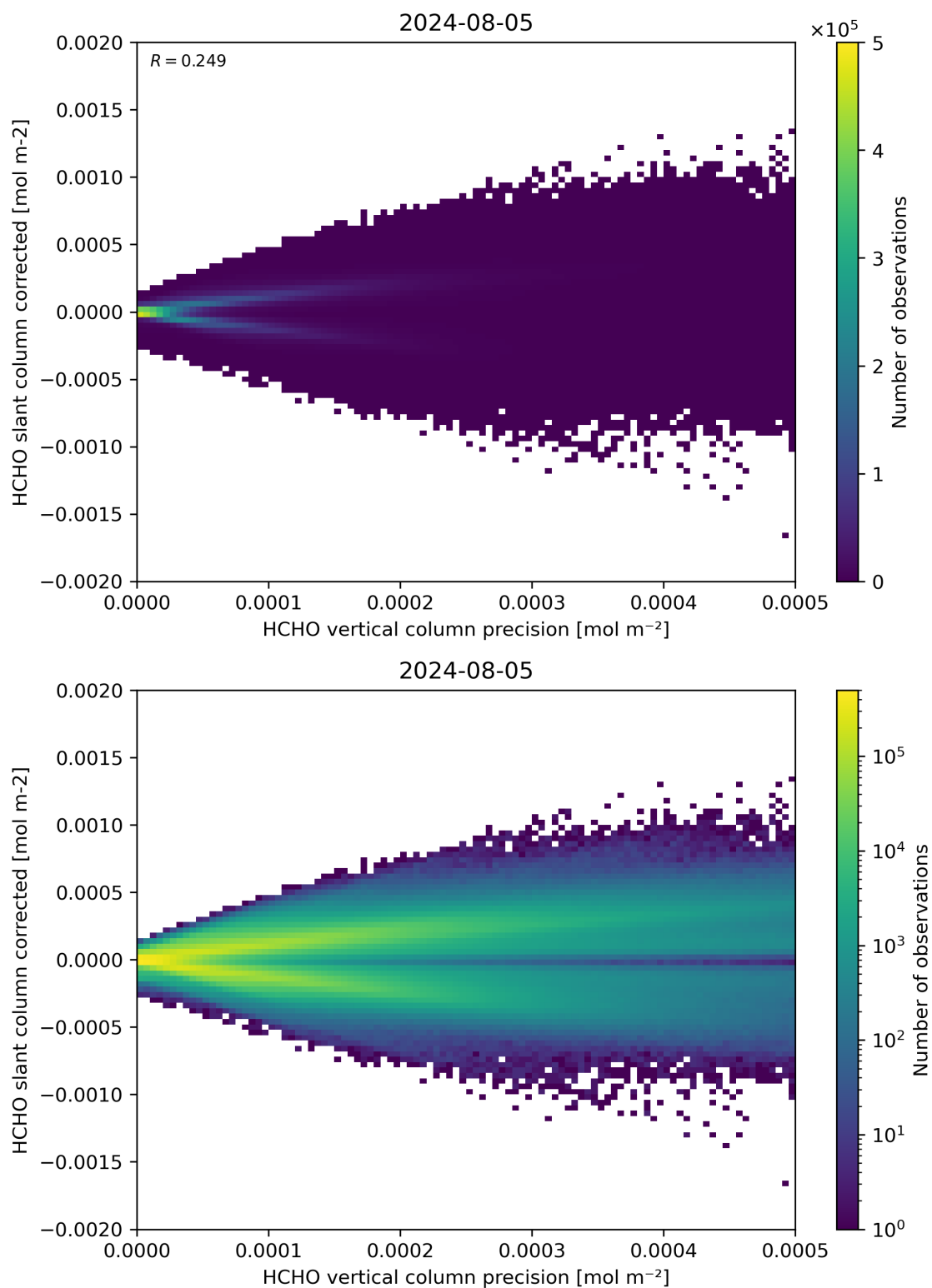
Figure 140: Scatter density plot of “HCHO vertical column precision” against “HCHO slant column corrected” for 2024-08-04 to 2024-08-06.
