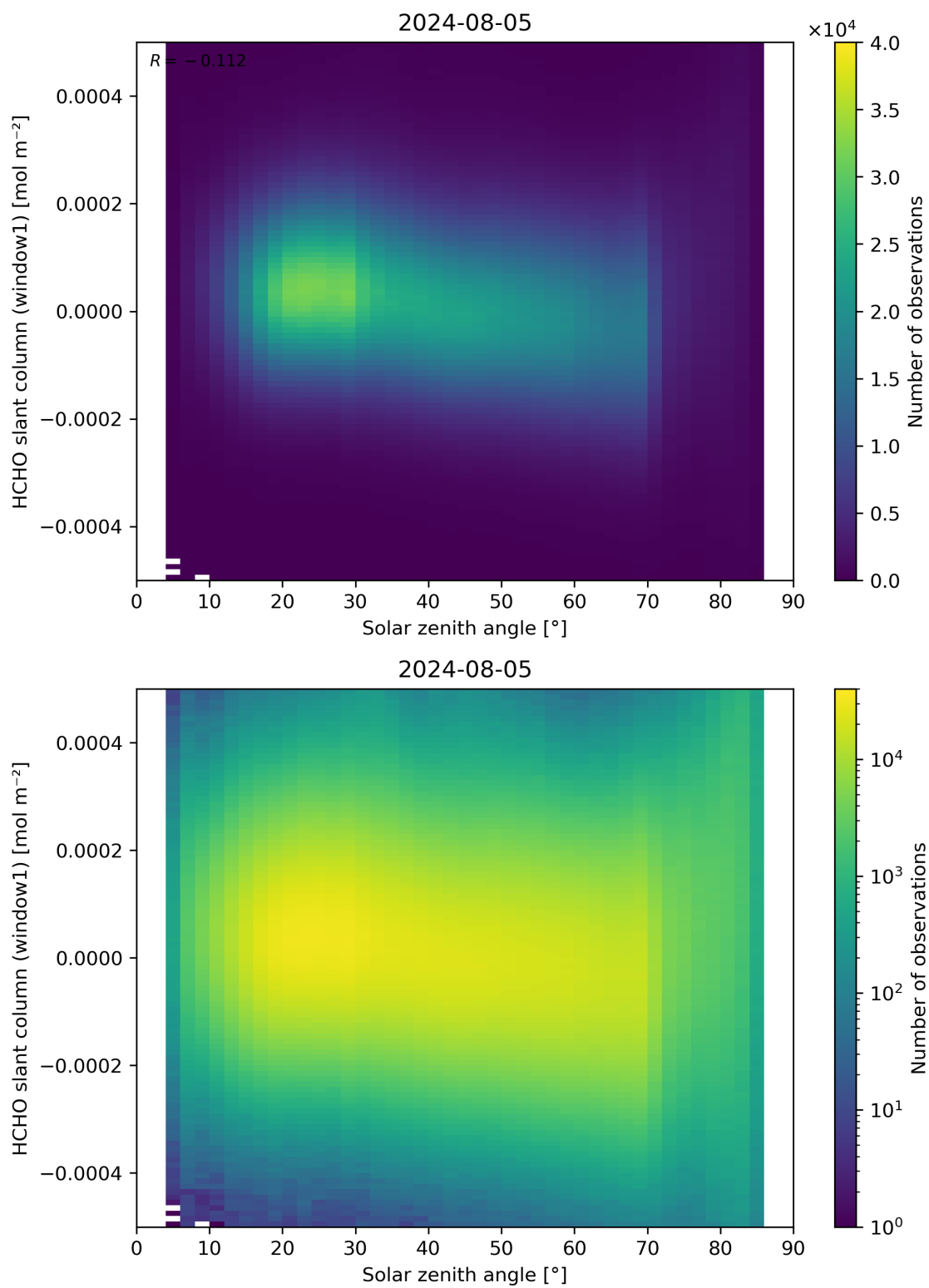
Figure 173: Scatter density plot of “Solar zenith angle” against “HCHO slant column (window1)” for 2024-08-04 to 2024-08-06.
