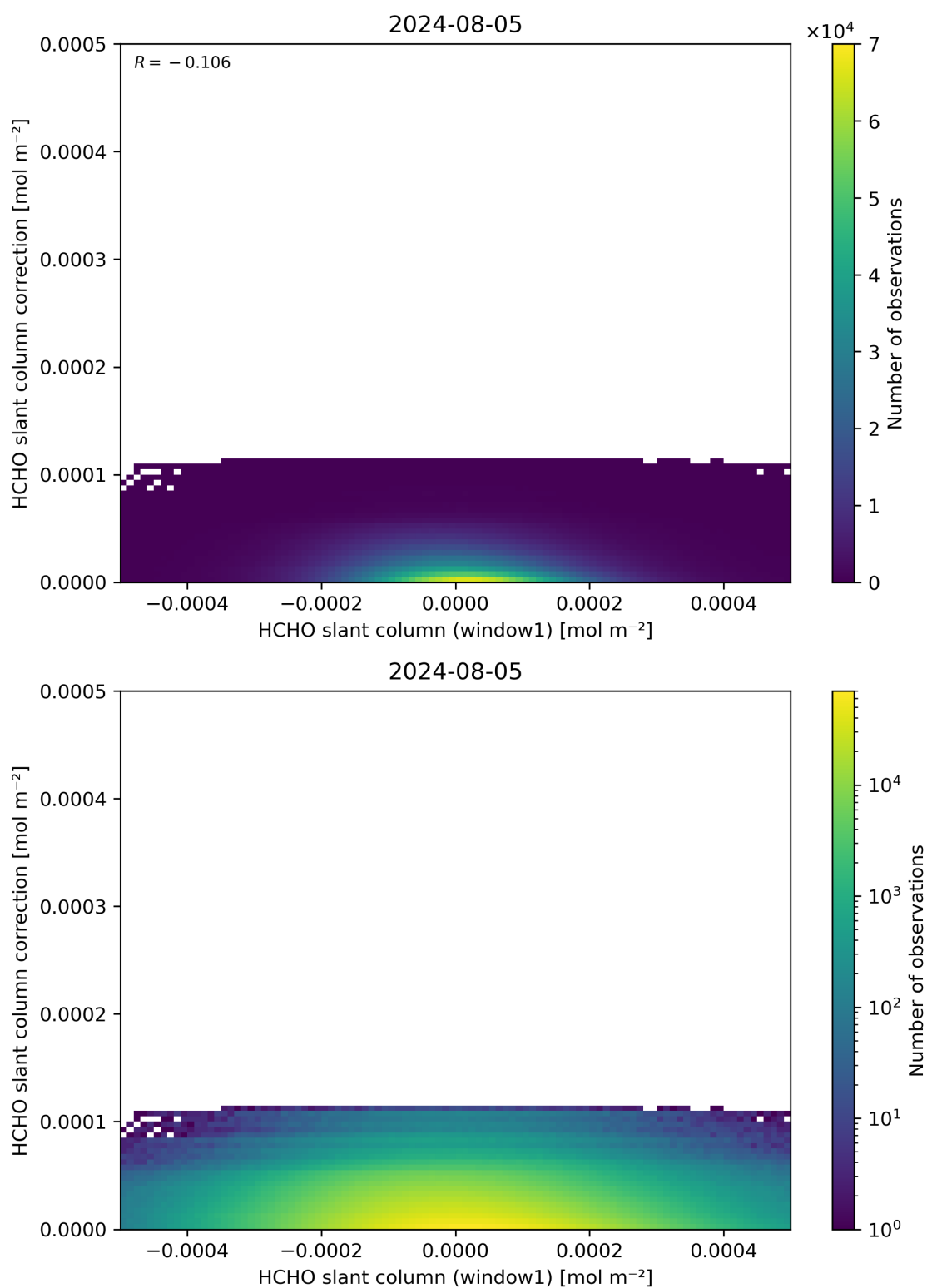
Figure 83: Scatter density plot of “HCHO slant column (window1)” against “HCHO slant column correction” for 2024-08-04 to 2024-08-06.
