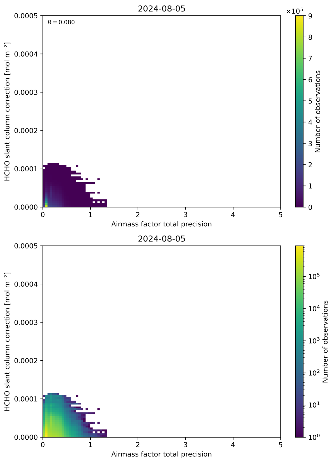
Figure 110: Scatter density plot of “Airmass factor total precision” against “HCHO slant column correction” for 2024-08-04 to 2024-08-06.
