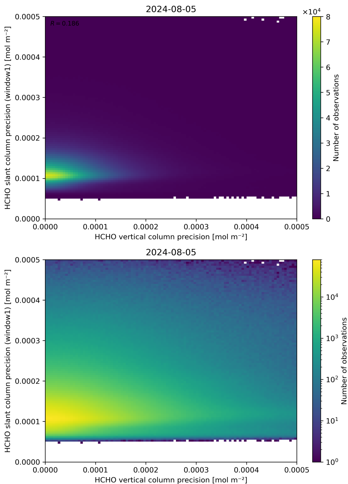
Figure 143: Scatter density plot of “HCHO vertical column precision” against “HCHO slant column precision (window1)” for 2024-08-04 to 2024-08-06.
