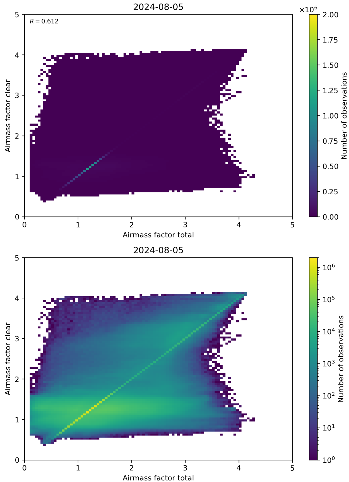
Figure 100: Scatter density plot of “Airmass factor total” against “Airmass factor clear” for 2024-08-04 to 2024-08-06.
