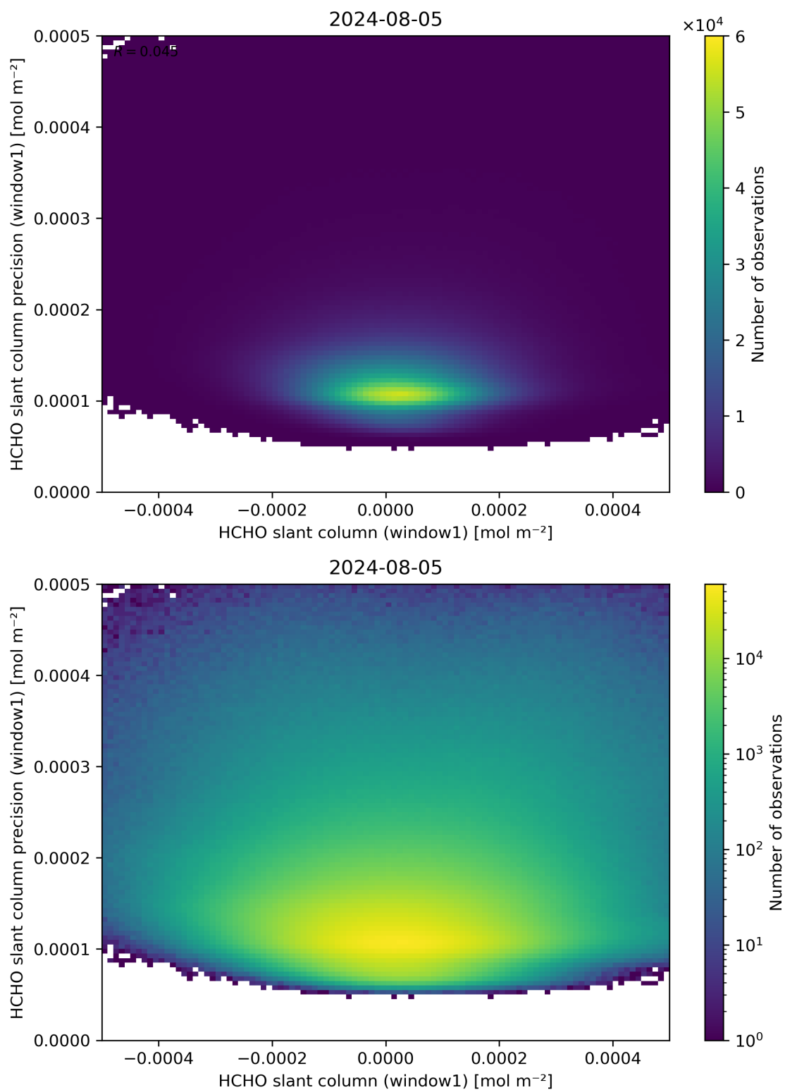
Figure 84: Scatter density plot of “HCHO slant column (window1)” against “HCHO slant column precision (window1)” for 2024-08-04 to 2024-08-06.
