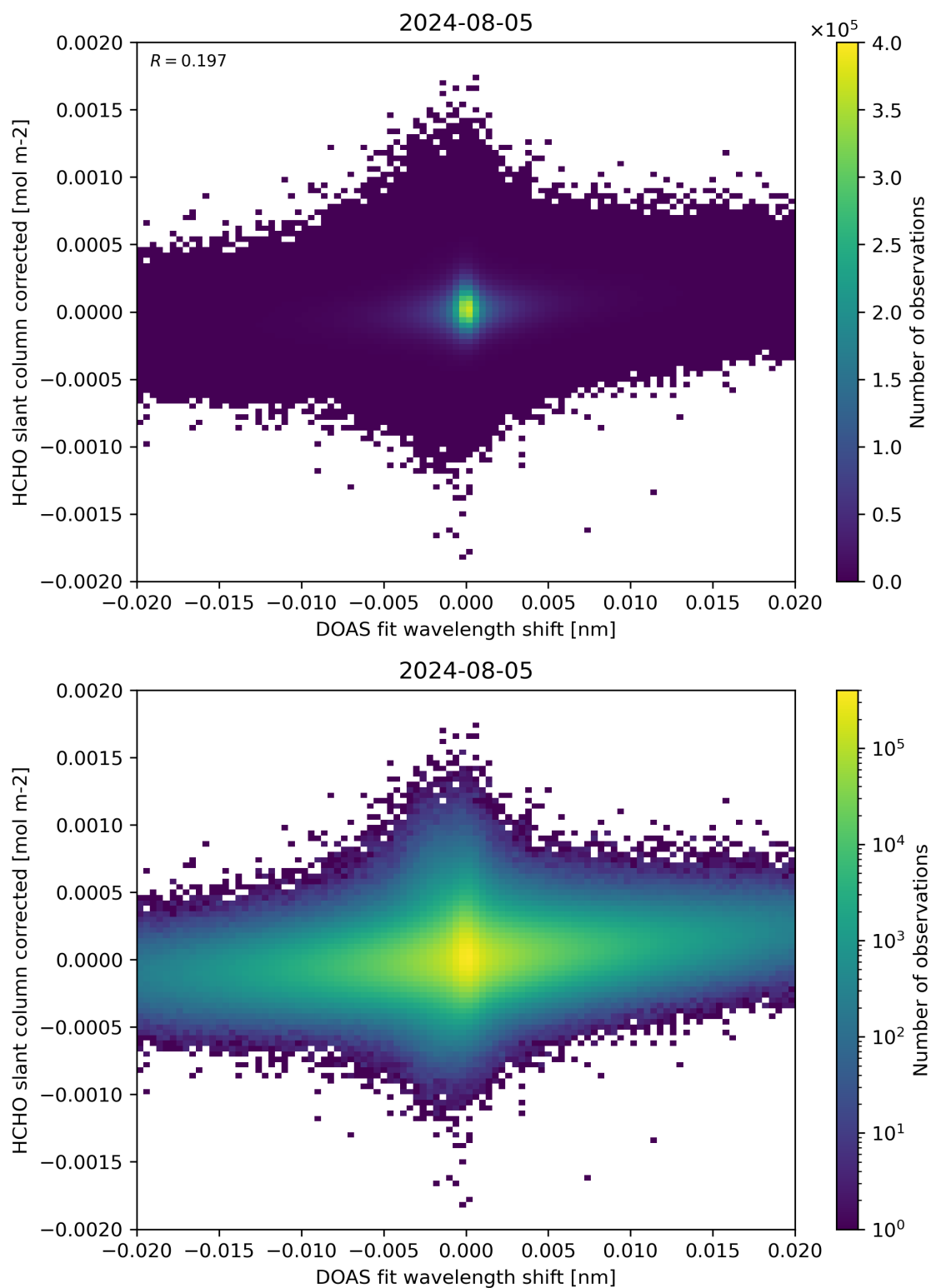
Figure 66: Scatter density plot of “DOAS fit wavelength shift” against “HCHO slant column corrected” for 2024-08-04 to 2024-08-06.
