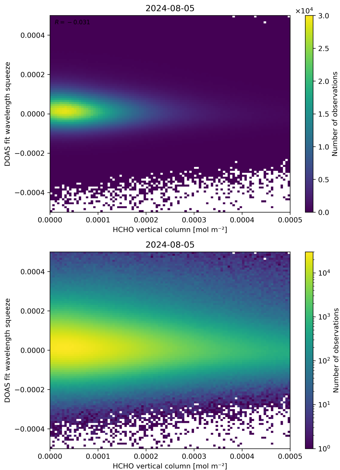
Figure 125: Scatter density plot of “HCHO vertical column” against “DOAS fit wavelength squeeze” for 2024-08-04 to 2024-08-06.
