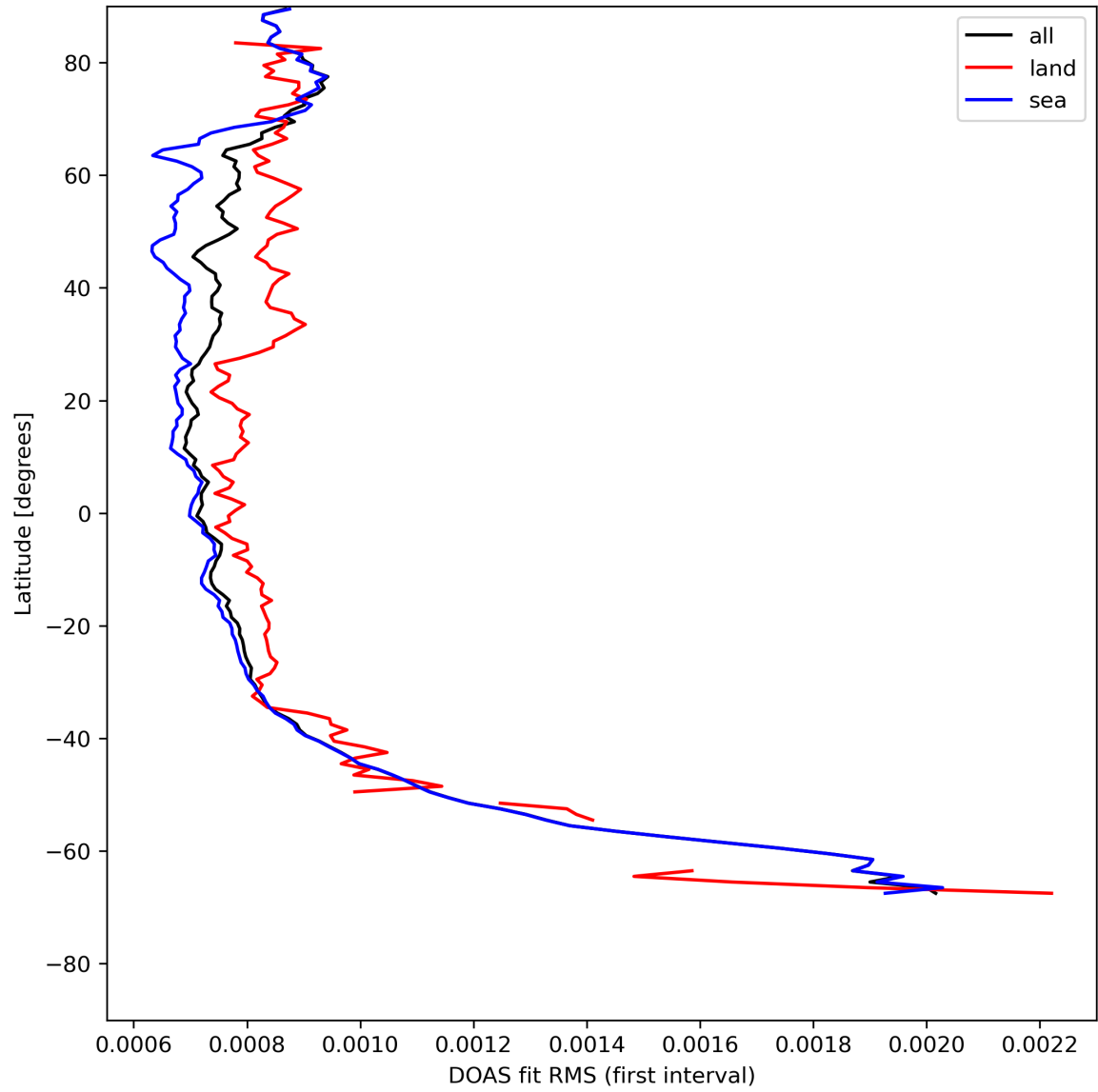
Figure 32: Zonal average of "DOAS fit RMS (first interval)" for 2024-08-04 to 2024-08-06.
