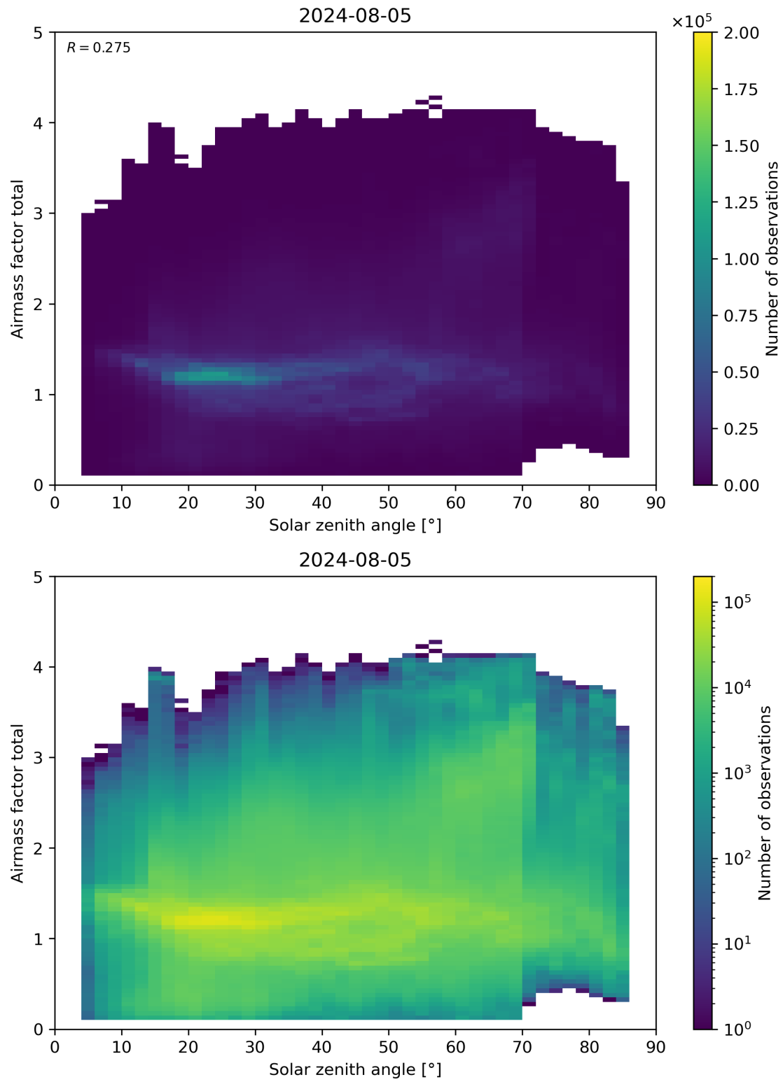
Figure 175: Scatter density plot of “Solar zenith angle” against “Airmass factor total” for 2024-08-04 to 2024-08-06.
