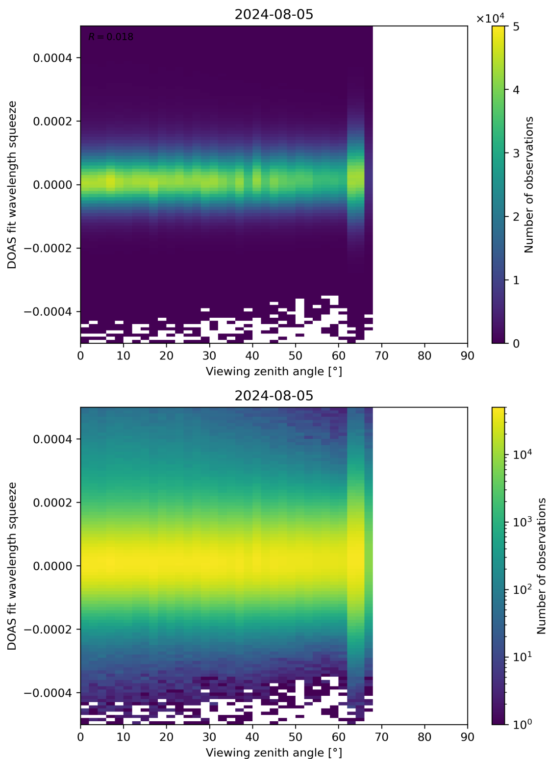
Figure 184: Scatter density plot of “Viewing zenith angle” against “DOAS fit wavelength squeeze” for 2024-08-04 to 2024-08-06.
