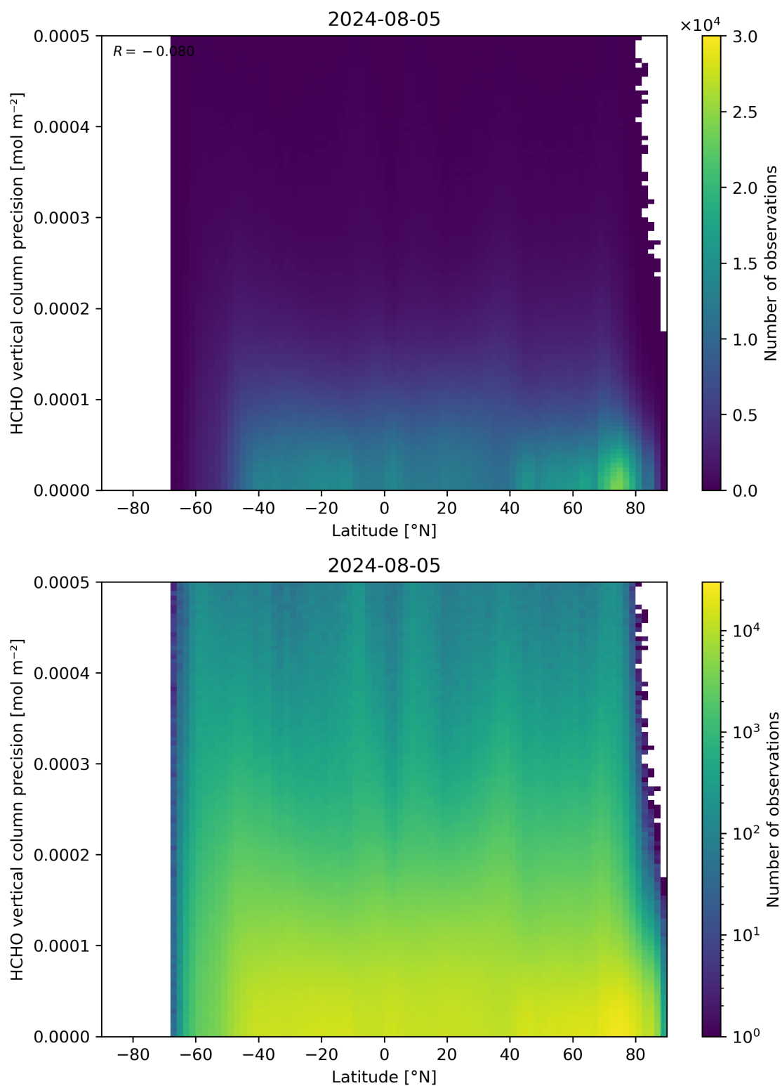
Figure 165: Scatter density plot of “Latitude” against “HCHO vertical column precision” for 2024-08-04 to 2024-08-06.
