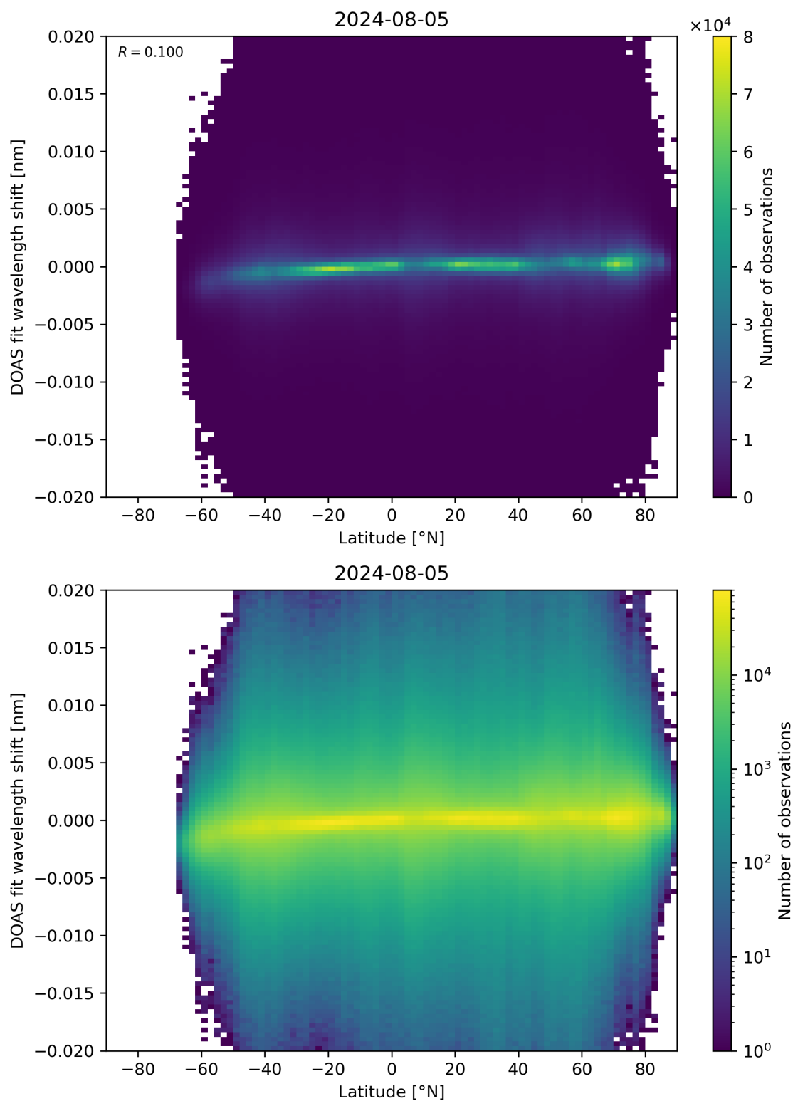
Figure 154: Scatter density plot of “Latitude” against “DOAS fit wavelength shift” for 2024-08-04 to 2024-08-06.
