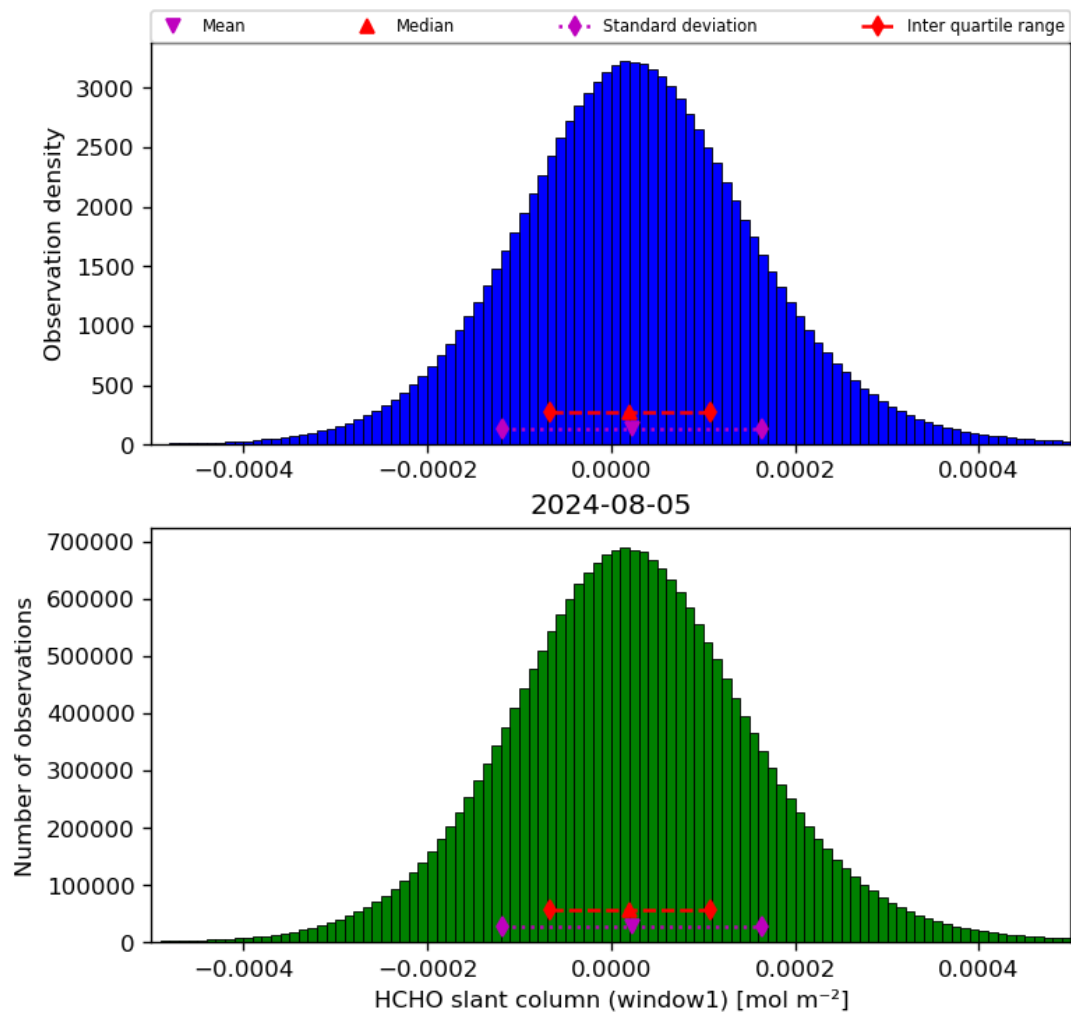
Figure 38: Histogram of “HCHO slant column (window1)” for 2024-08-04 to 2024-08-06
