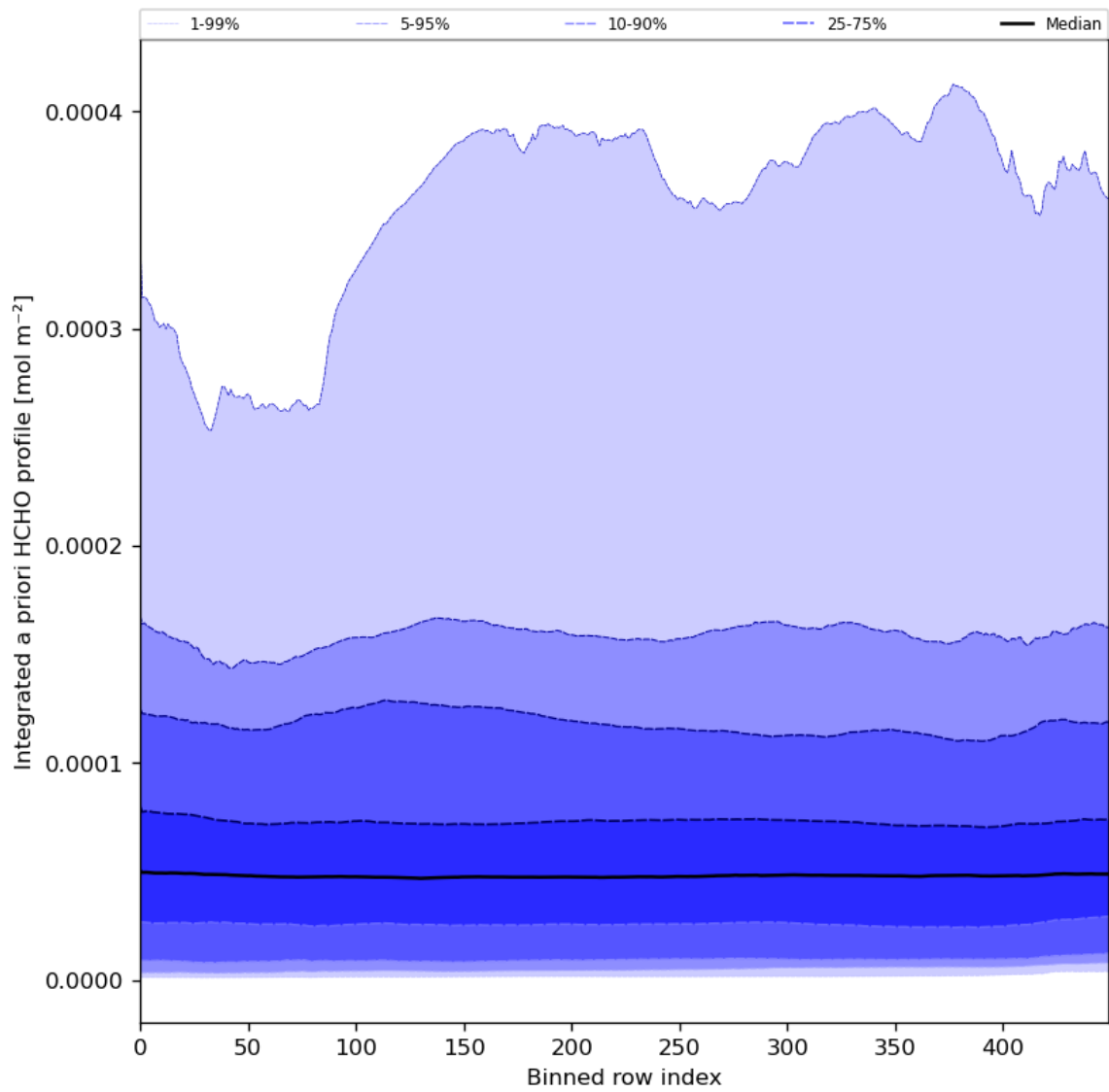
Figure 57: Along track statistics of “Integrated a priori HCHO profile” for 2024-08-04 to 2024-08-06
