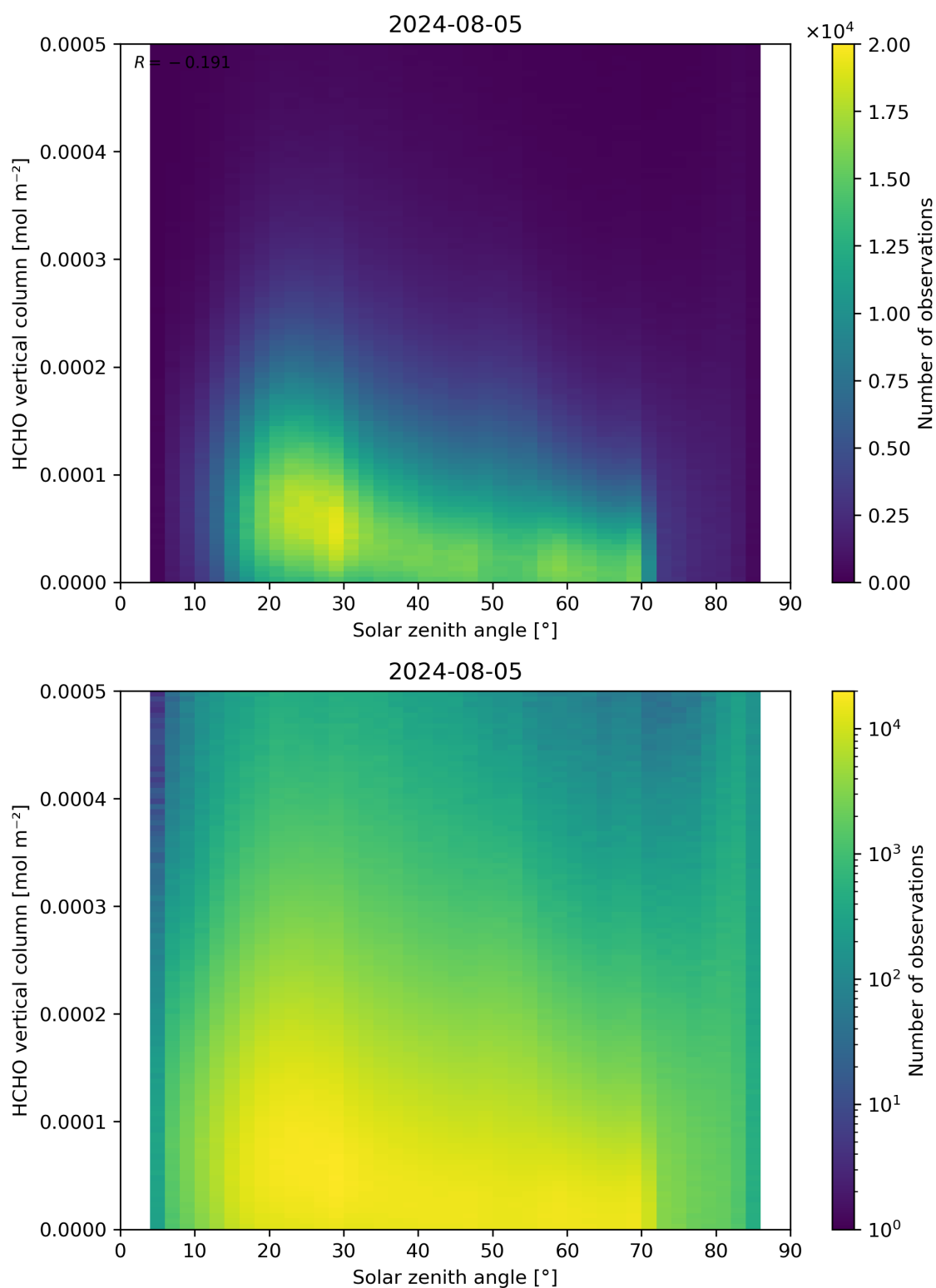
Figure 177: Scatter density plot of “Solar zenith angle” against “HCHO vertical column” for 2024-08-04 to 2024-08-06.
