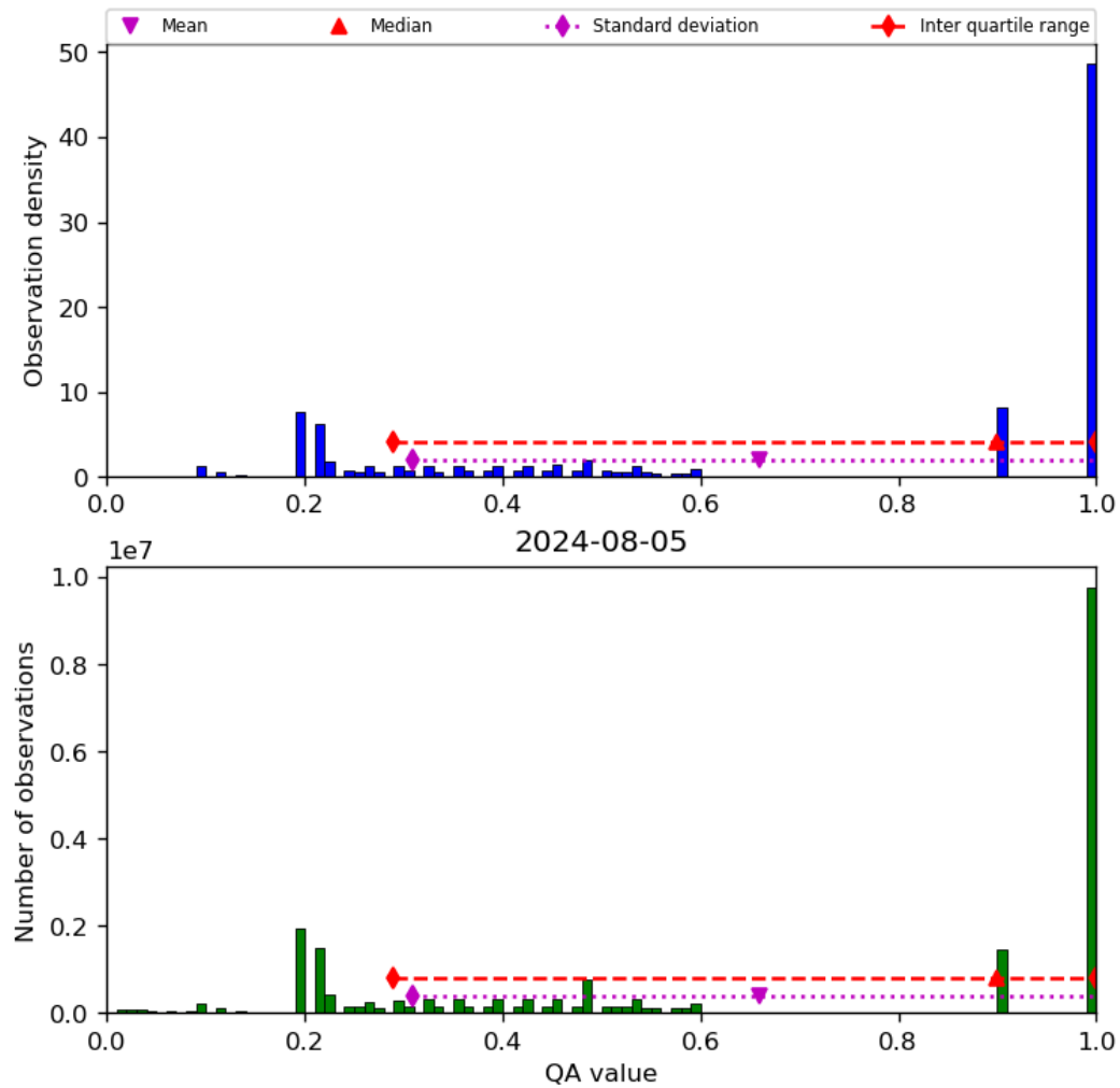
Figure 34: Histogram of “QA value” for 2024-08-04 to 2024-08-06
