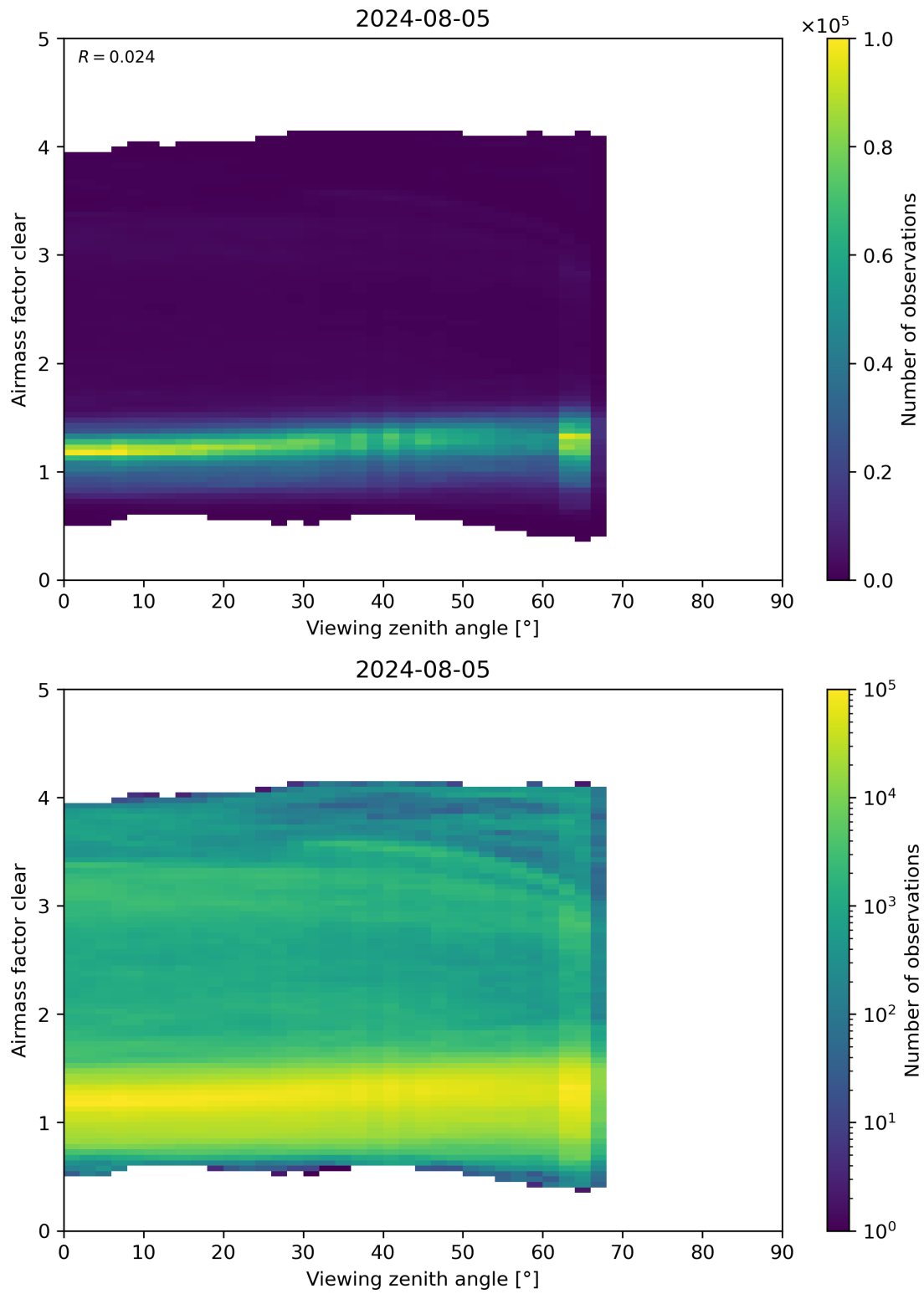
Figure 185: Scatter density plot of “Viewing zenith angle” against “Airmass factor clear” for 2024-08-04 to 2024-08-06.
