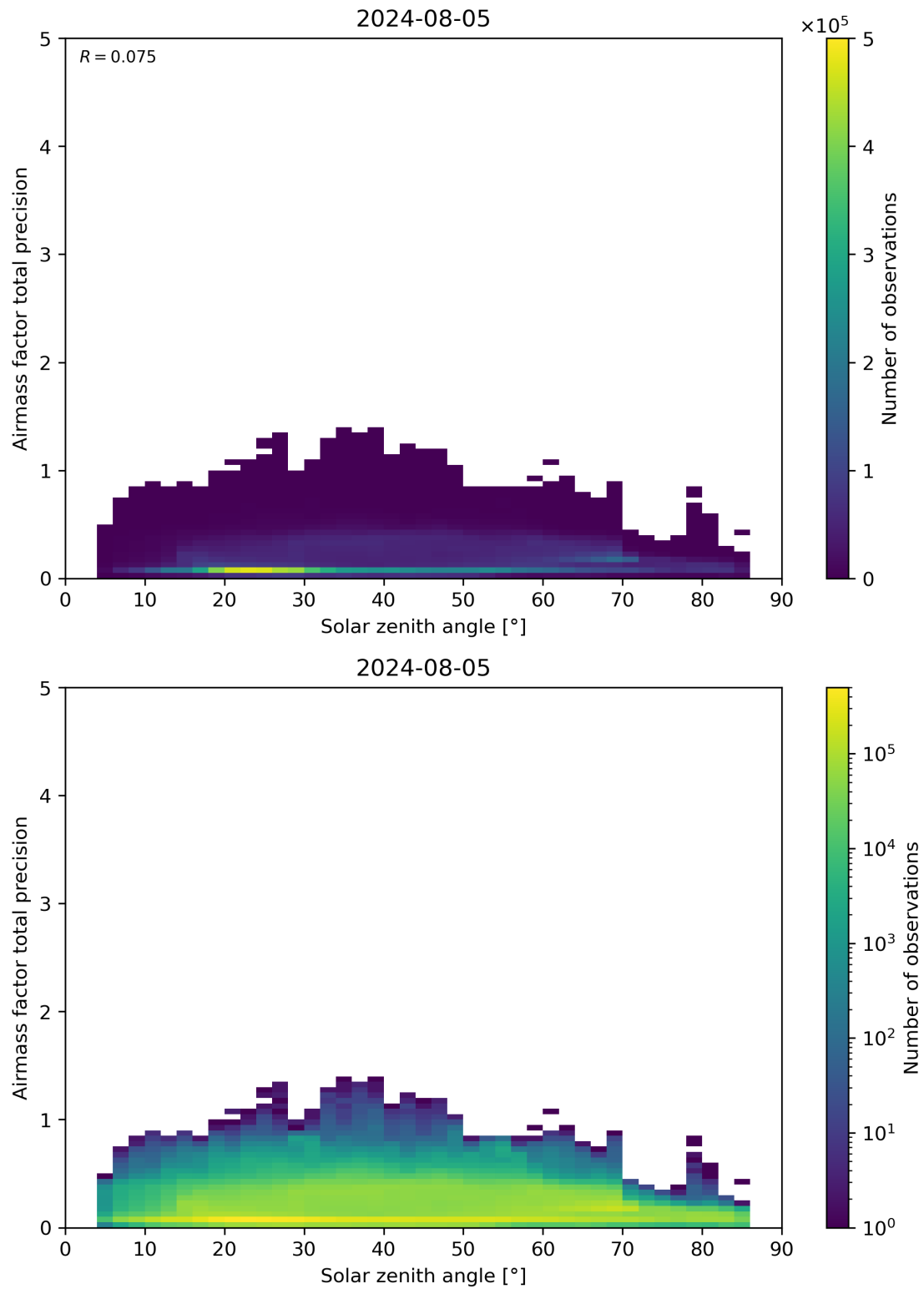
Figure 176: Scatter density plot of “Solar zenith angle” against “Airmass factor total precision” for 2024-08-04 to 2024-08-06.
