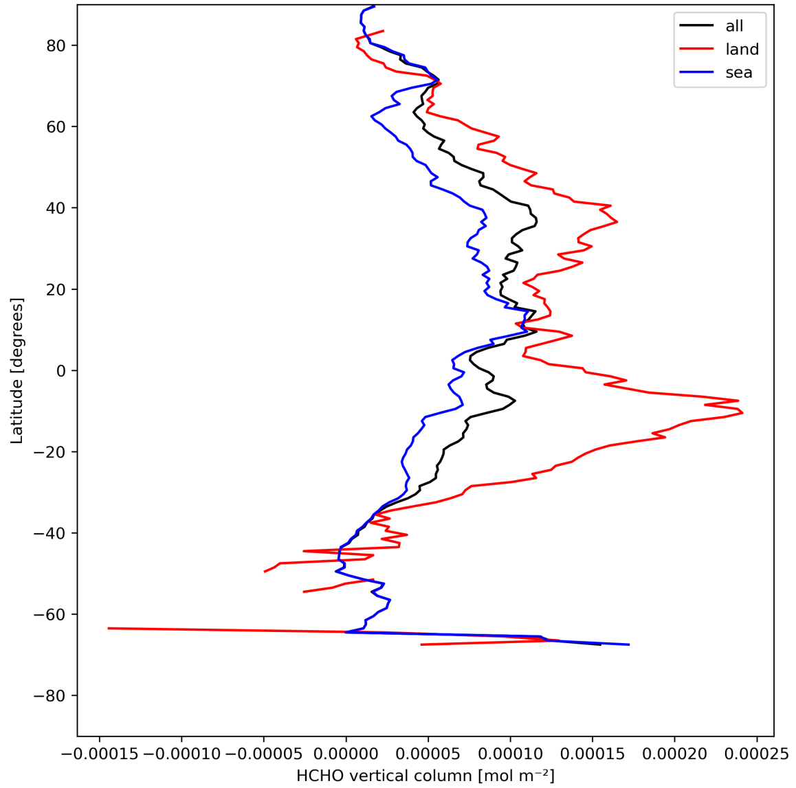
Figure 21: Zonal average of “HCHO vertical column” for 2024-08-04 to 2024-08-06.
