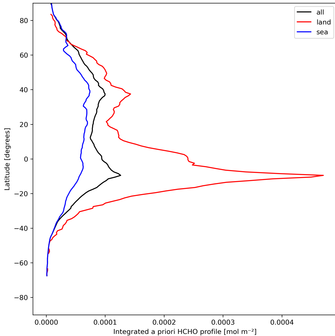
Figure 29: Zonal average of “Integrated a priori HCHO profile” for 2024-08-04 to 2024-08-06.
