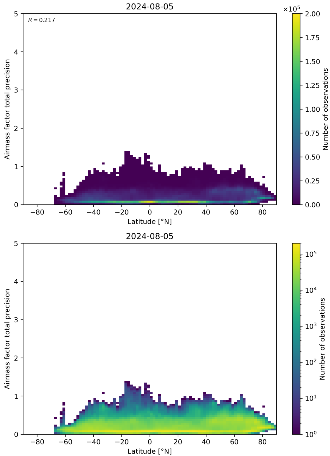
Figure 162: Scatter density plot of “Latitude” against “Airmass factor total precision” for 2024-08-04 to 2024-08-06.
