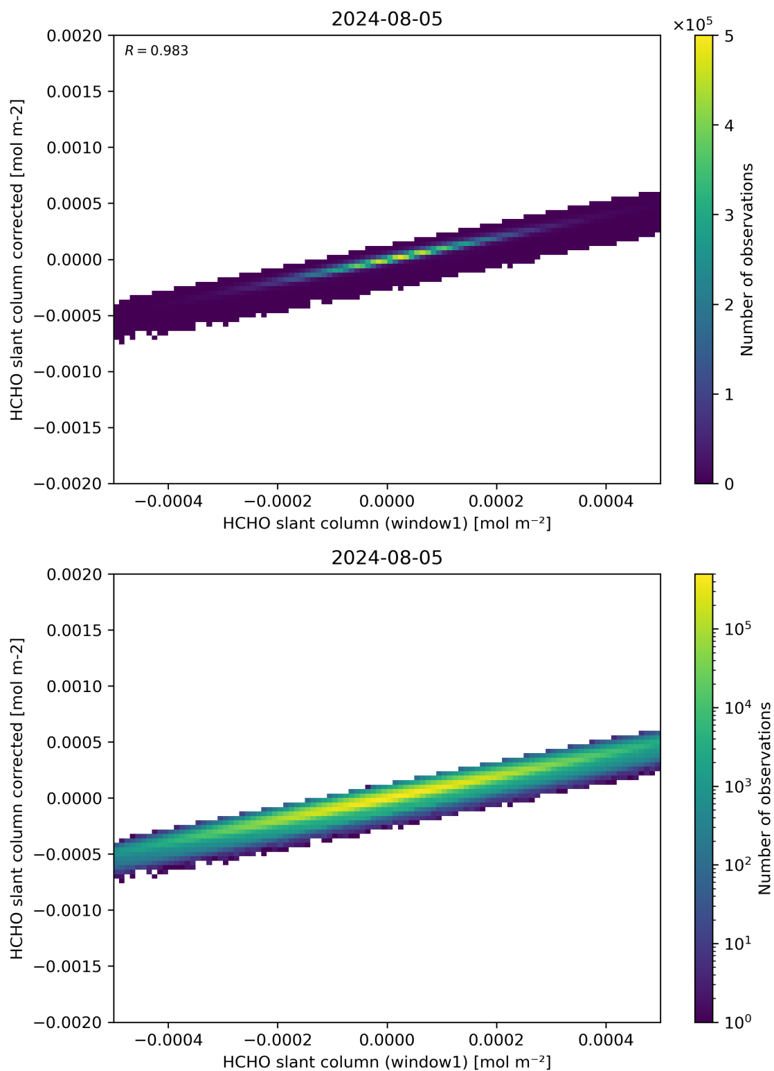
Figure 82: Scatter density plot of “HCHO slant column (window1)” against “HCHO slant column corrected” for 2024-08-04 to 2024-08-06.
