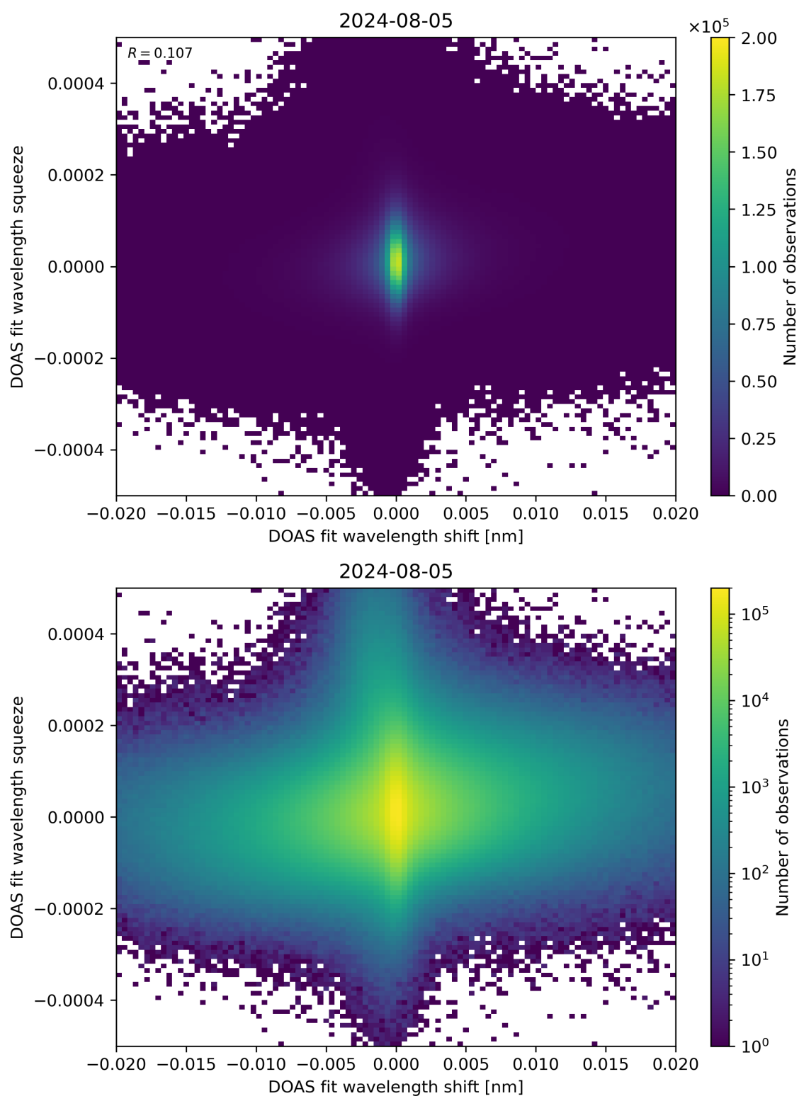
Figure 65: Scatter density plot of “DOAS fit wavelength shift” against “DOAS fit wavelength squeeze” for 2024-08-04 to 2024-08-06.
