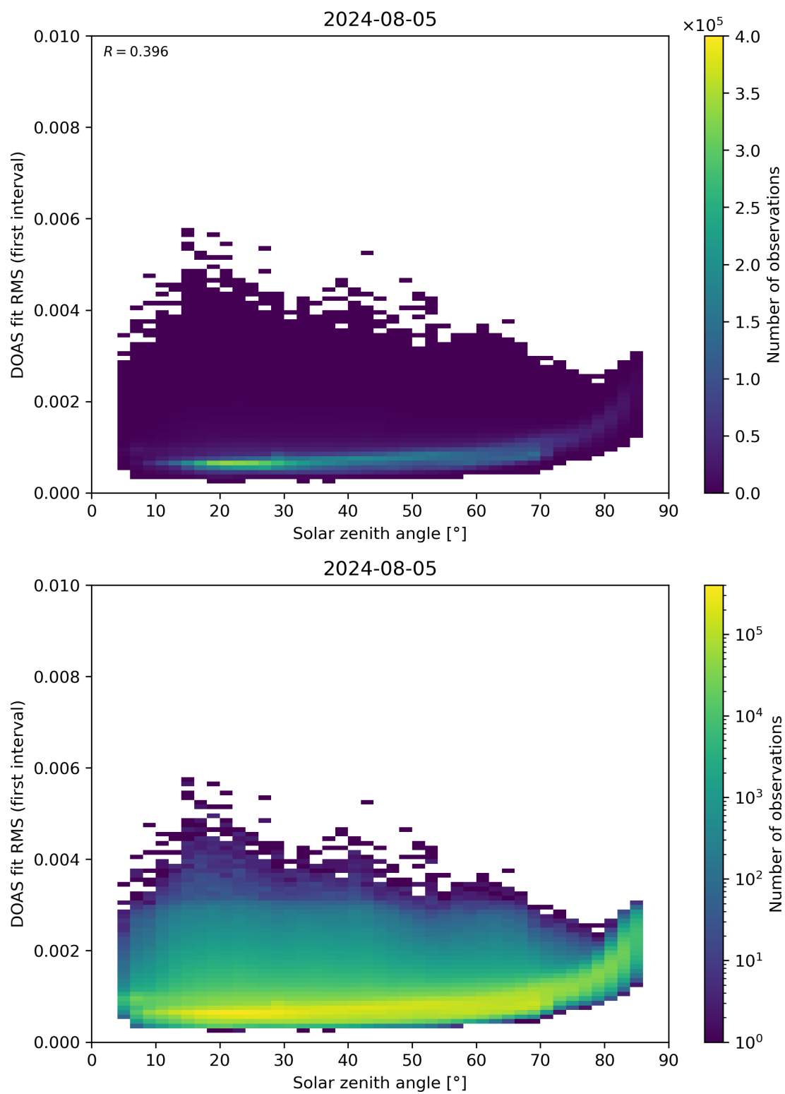
Figure 167: Scatter density plot of “Solar zenith angle” against “DOAS fit RMS (first interval)” for 2024-08-04 to 2024-08-06.
