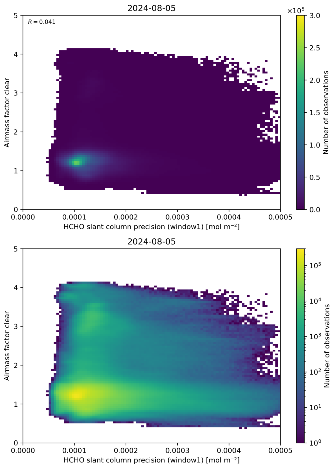
Figure 91: Scatter density plot of “HCHO slant column precision (window1)” against “Airmass factor clear” for 2024-08-04 to 2024-08-06.
