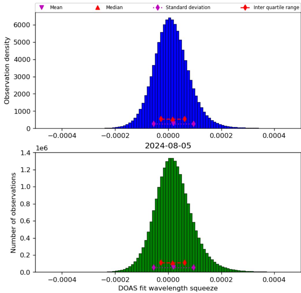
Figure 45: Histogram of “DOAS fit wavelength squeeze” for 2024-08-04 to 2024-08-06
