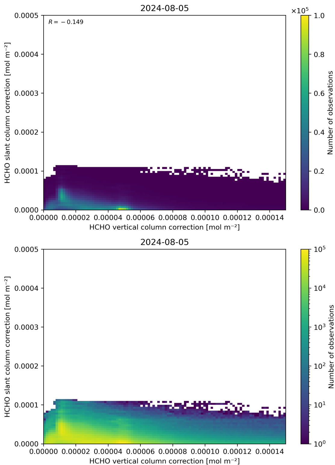
Figure 117: Scatter density plot of “HCHO vertical column correction” against “HCHO slant column correction” for 2024-08-04 to 2024-08-06.
