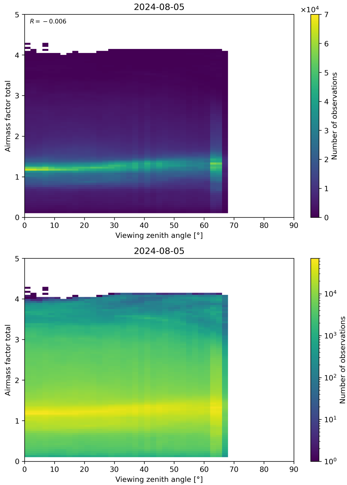
Figure 190: Scatter density plot of “Viewing zenith angle” against “Airmass factor total” for 2024-08-04 to 2024-08-06.
