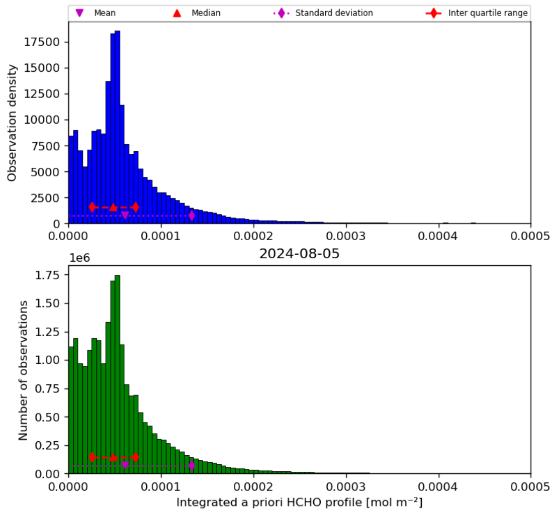
Figure 43: Histogram of “Integrated a priori HCHO profile” for 2024-08-04 to 2024-08-06
