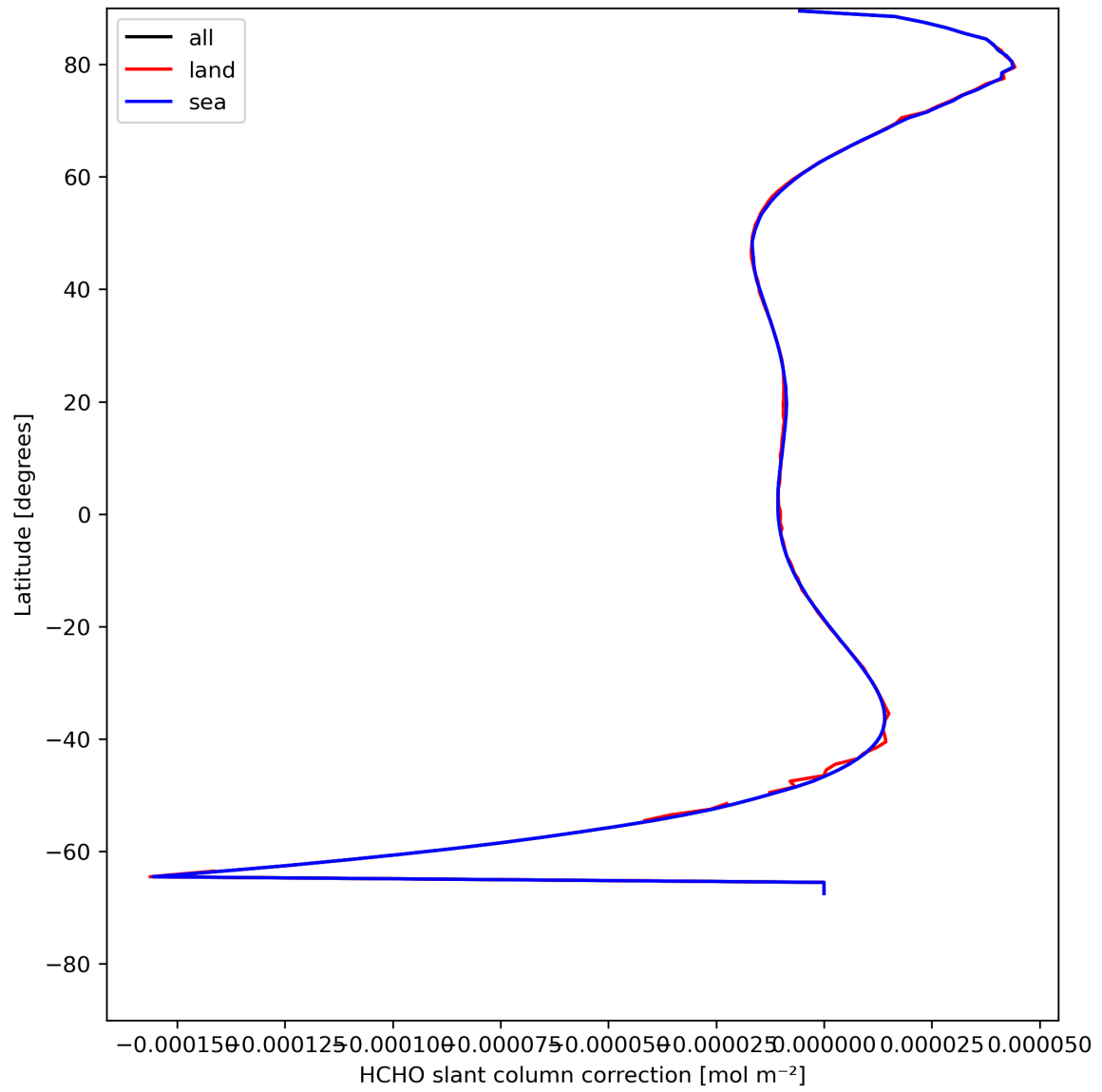
Figure 33: Zonal average of “HCHO slant column correction” for 2024-08-04 to 2024-08-06.
