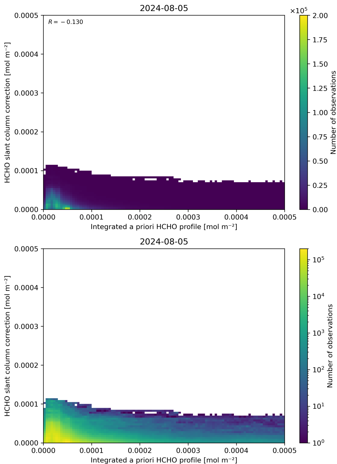
Figure 152: Scatter density plot of “Integrated a priori HCHO profile” against “HCHO slant column correction” for 2024-08-04 to 2024-08-06.
