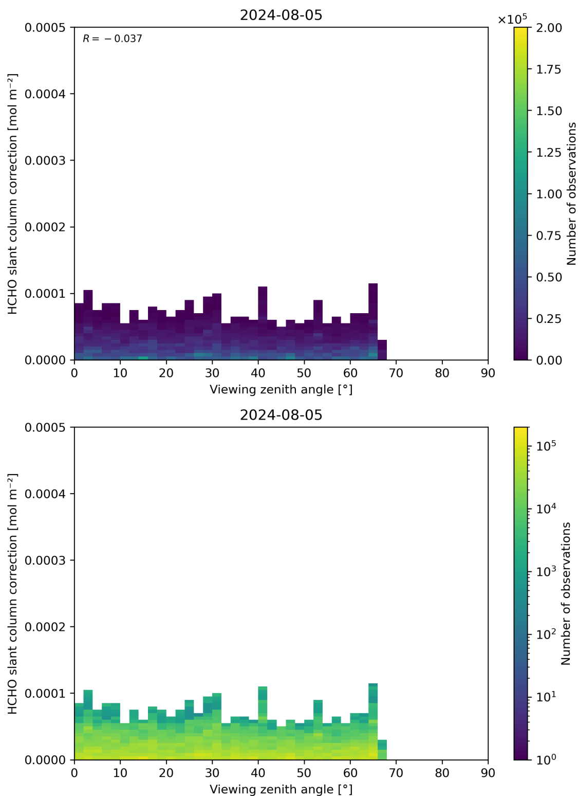
Figure 187: Scatter density plot of “Viewing zenith angle” against “HCHO slant column correction” for 2024-08-04 to 2024-08-06.
