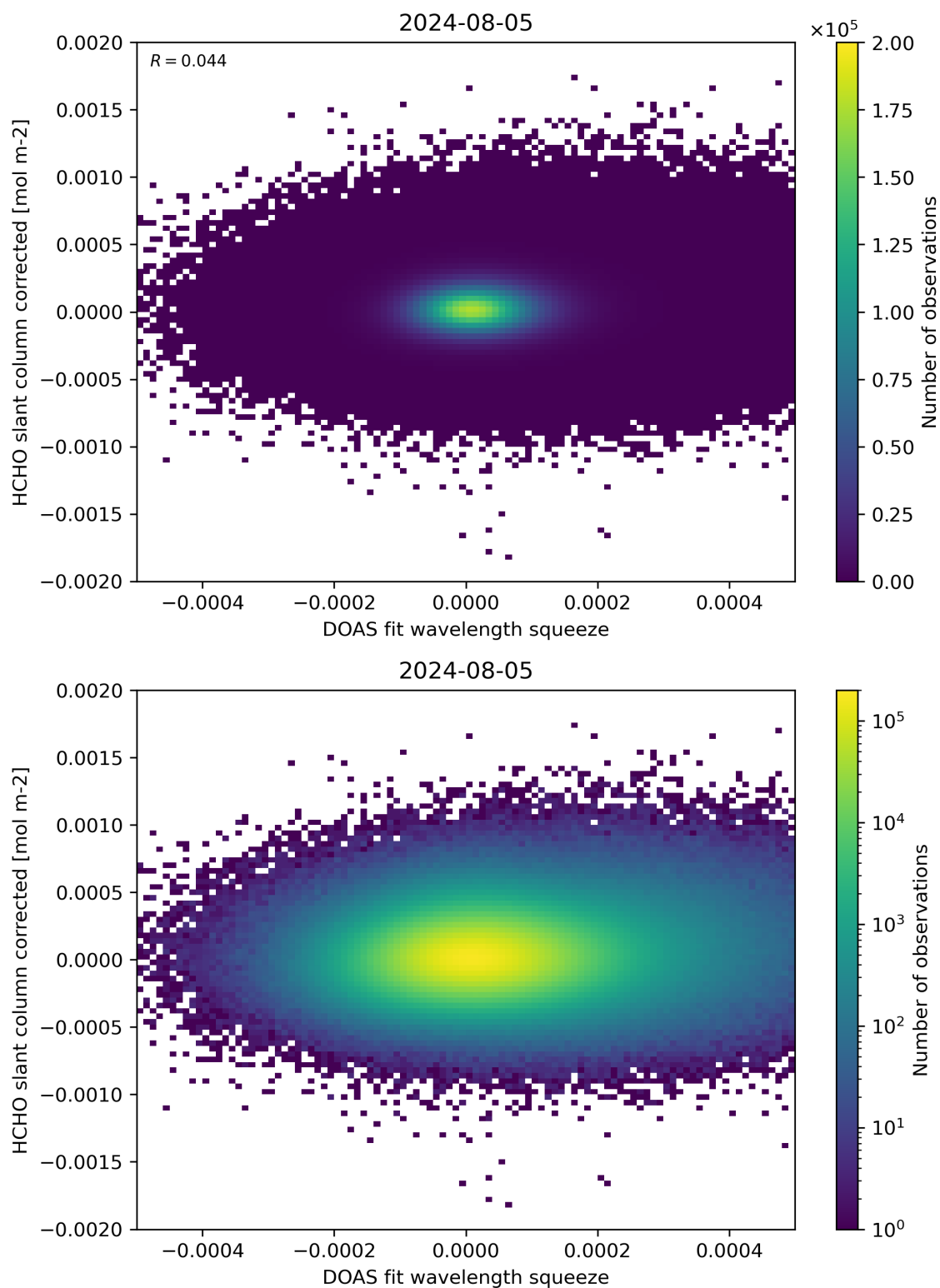
Figure 69: Scatter density plot of “DOAS fit wavelength squeeze” against “HCHO slant column corrected” for 2024-08-04 to 2024-08-06.
