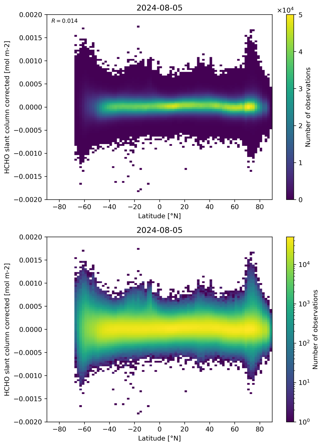
Figure 157: Scatter density plot of “Latitude” against “HCHO slant column corrected” for 2024-08-04 to 2024-08-06.
