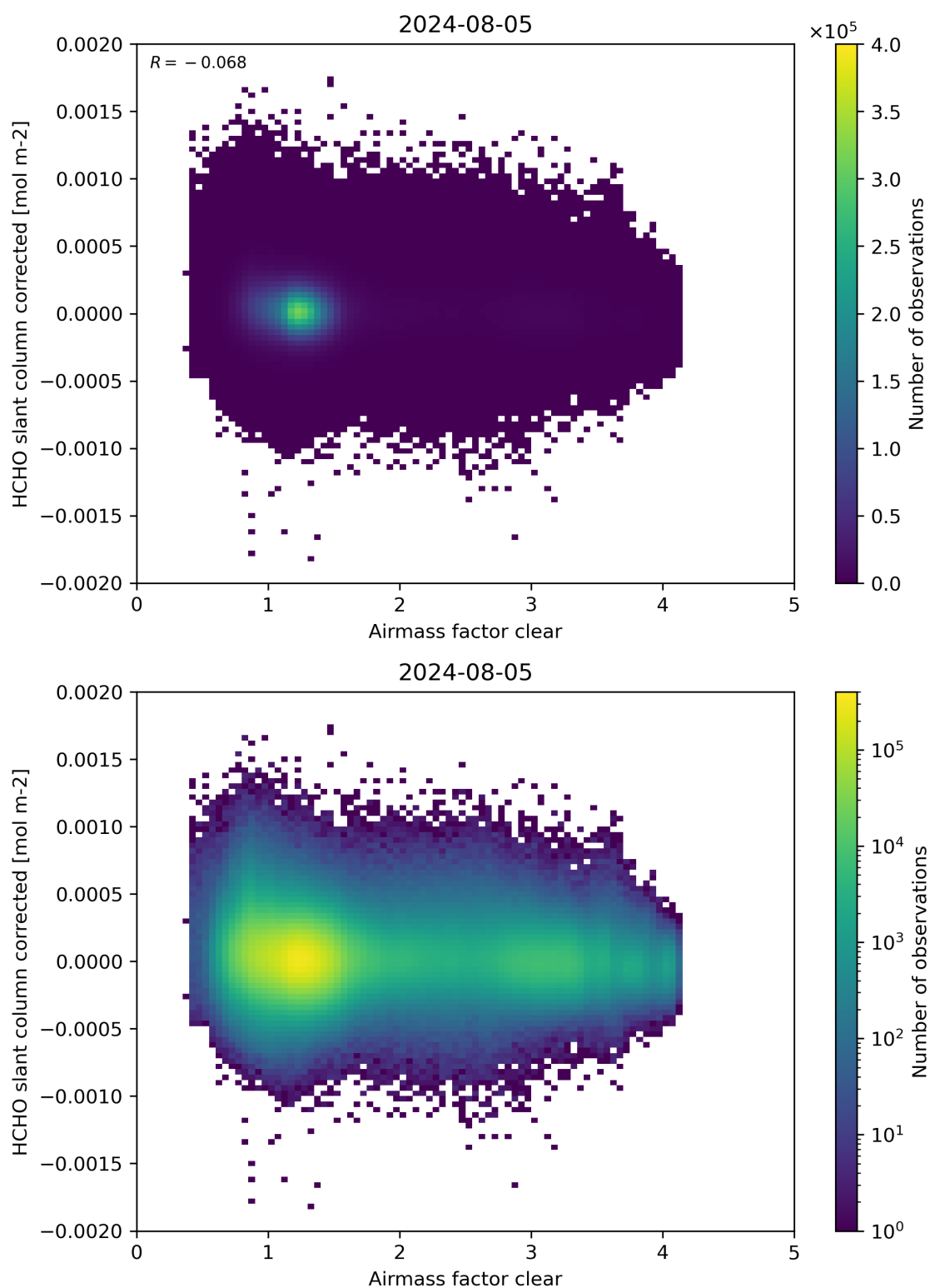
Figure 74: Scatter density plot of “Airmass factor clear” against “HCHO slant column corrected” for 2024-08-04 to 2024-08-06.
