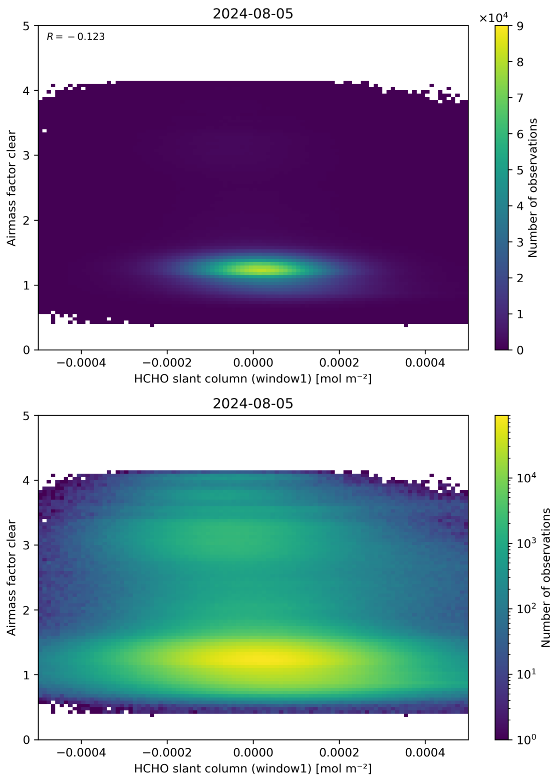
Figure 81: Scatter density plot of “HCHO slant column (window1)” against “Airmass factor clear” for 2024-08-04 to 2024-08-06.
