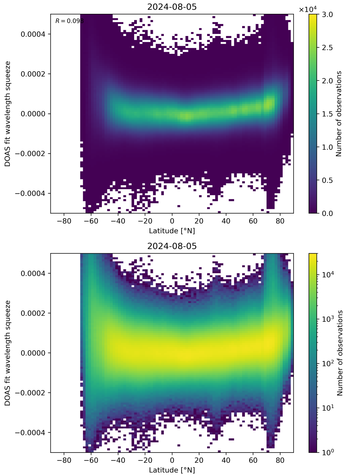
Figure 155: Scatter density plot of “Latitude” against “DOAS fit wavelength squeeze” for 2024-08-04 to 2024-08-06.
