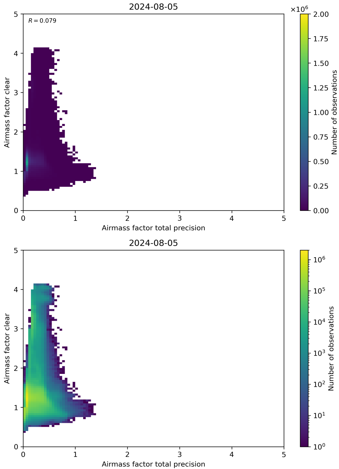
Figure 108: Scatter density plot of “Airmass factor total precision” against “Airmass factor clear” for 2024-08-04 to 2024-08-06.
