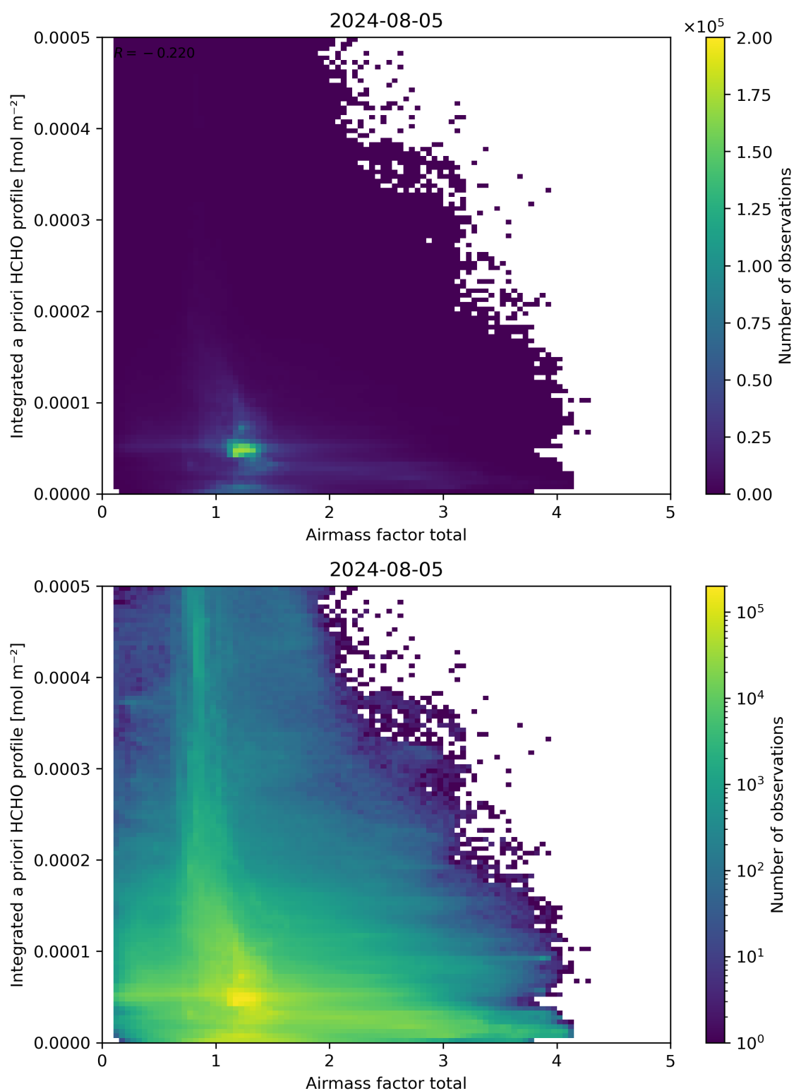
Figure 104: Scatter density plot of “Airmass factor total” against “Integrated a priori HCHO profile” for 2024-08-04 to 2024-08-06.
