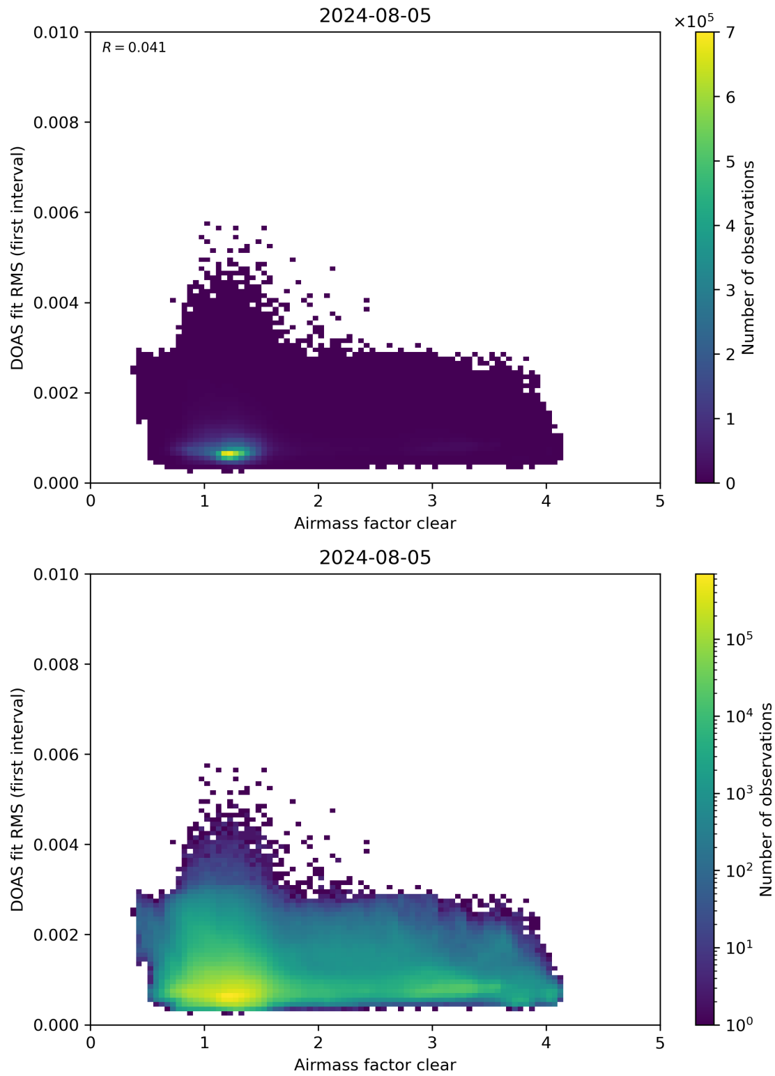
Figure 71: Scatter density plot of “Airmass factor clear” against “DOAS fit RMS (first interval)” for 2024-08-04 to 2024-08-06.
