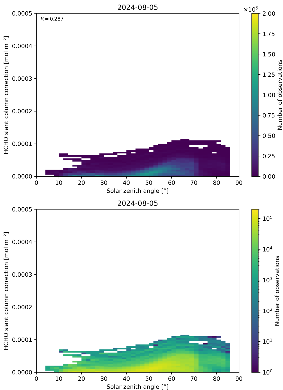
Figure 172: Scatter density plot of “Solar zenith angle” against “HCHO slant column correction” for 2024-08-04 to 2024-08-06.
