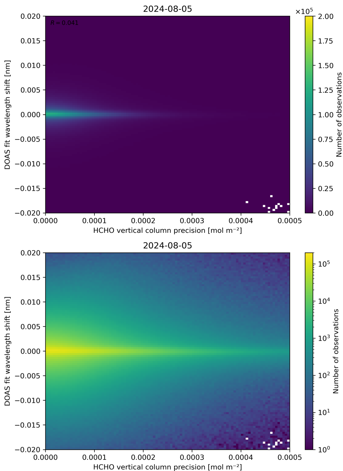
Figure 137: Scatter density plot of “HCHO vertical column precision” against “DOAS fit wavelength shift” for 2024-08-04 to 2024-08-06.
