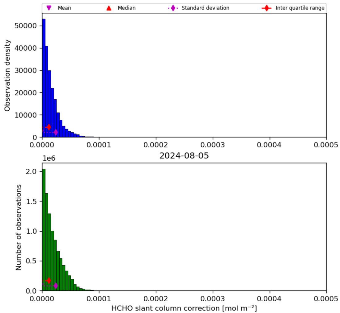
Figure 47: Histogram of “HCHO slant column correction” for 2024-08-04 to 2024-08-06
