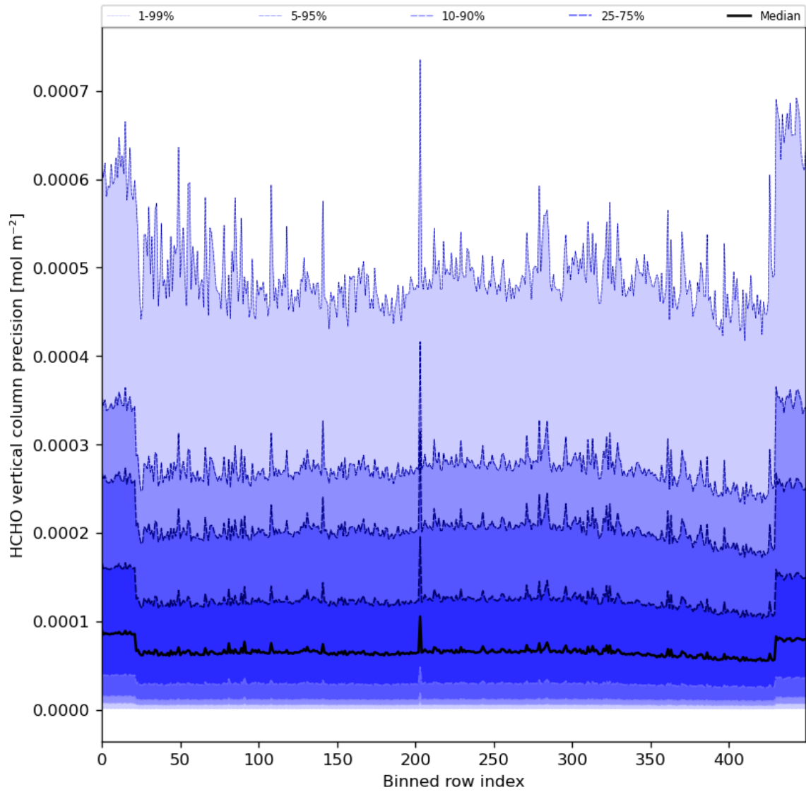
Figure 50: Along track statistics of "HCHO vertical column precision" for 2024-08-04 to 2024-08-06
