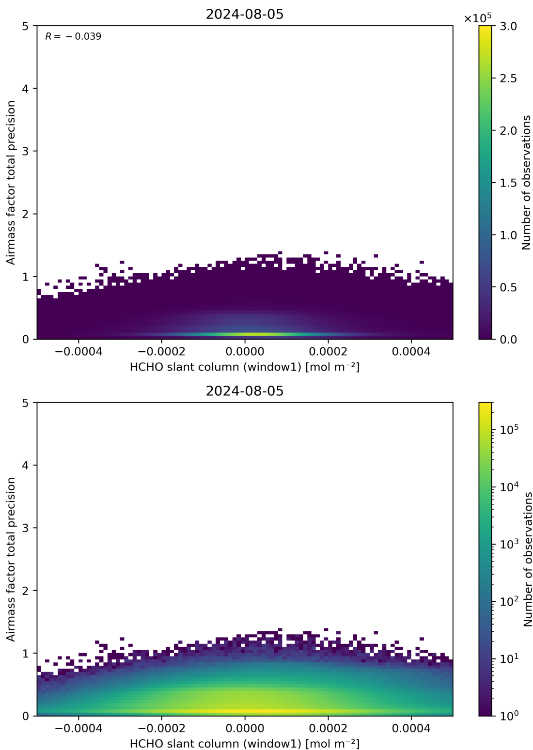
Figure 86: Scatter density plot of “HCHO slant column (window1)” against “Airmass factor total precision” for 2024-08-04 to 2024-08-06.
