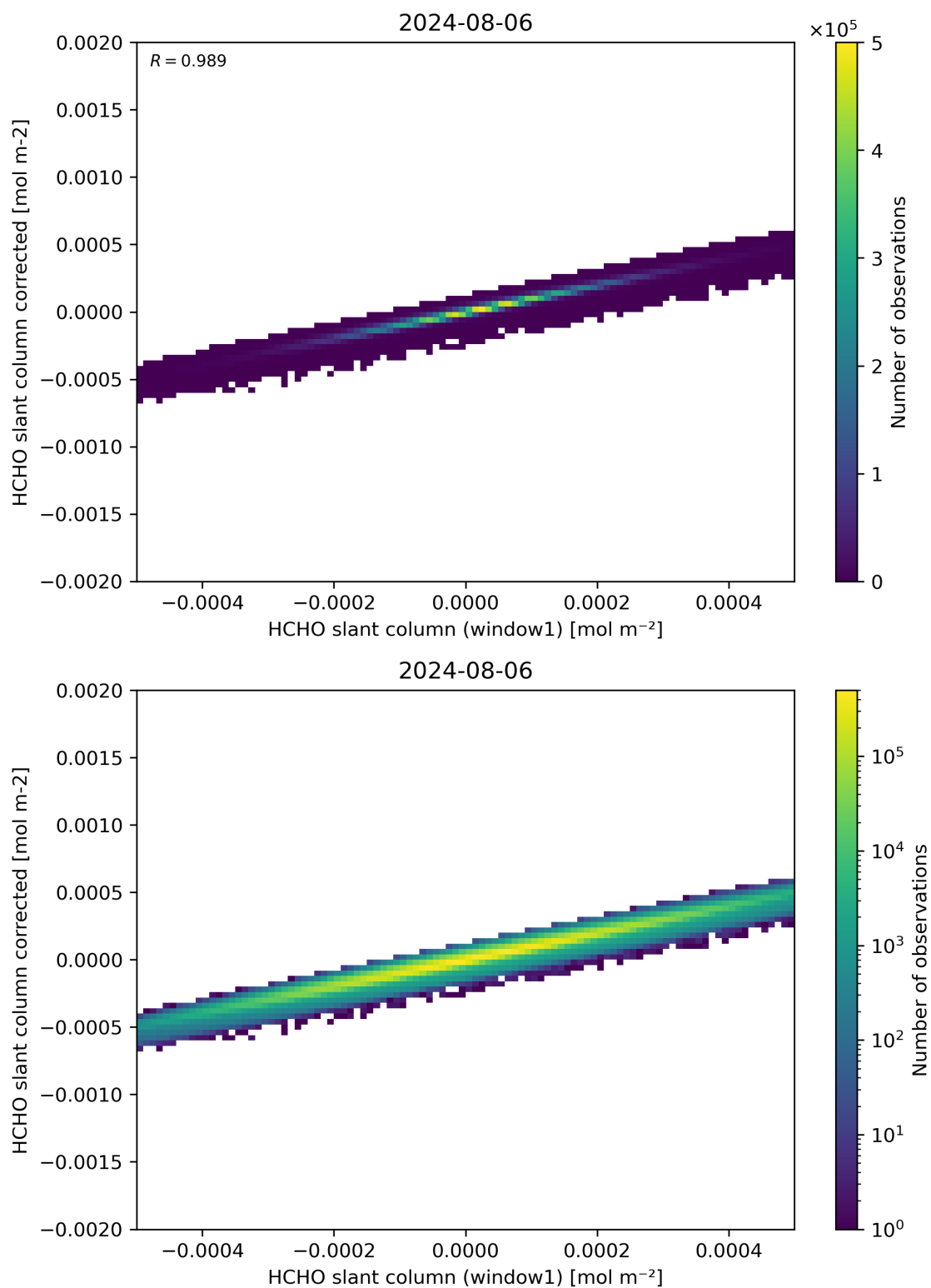
Figure 82: Scatter density plot of “HCHO slant column (window1)” against “HCHO slant column corrected” for 2024-08-06 to 2024-08-07.
