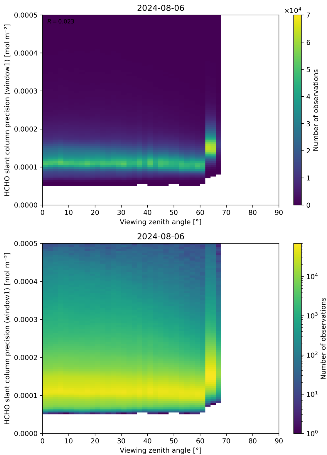
Figure 189: Scatter density plot of “Viewing zenith angle” against “HCHO slant column precision (window1)” for 2024-08-06 to 2024-08-07.
