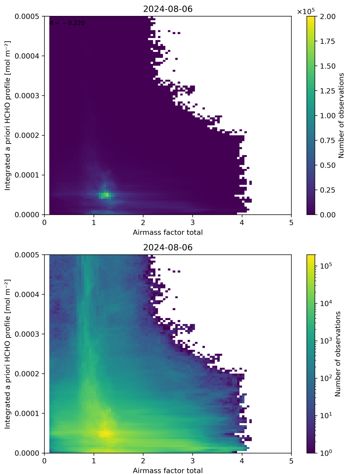
Figure 104: Scatter density plot of “Airmass factor total” against “Integrated a priori HCHO profile” for 2024-08-06 to 2024-08-07.
