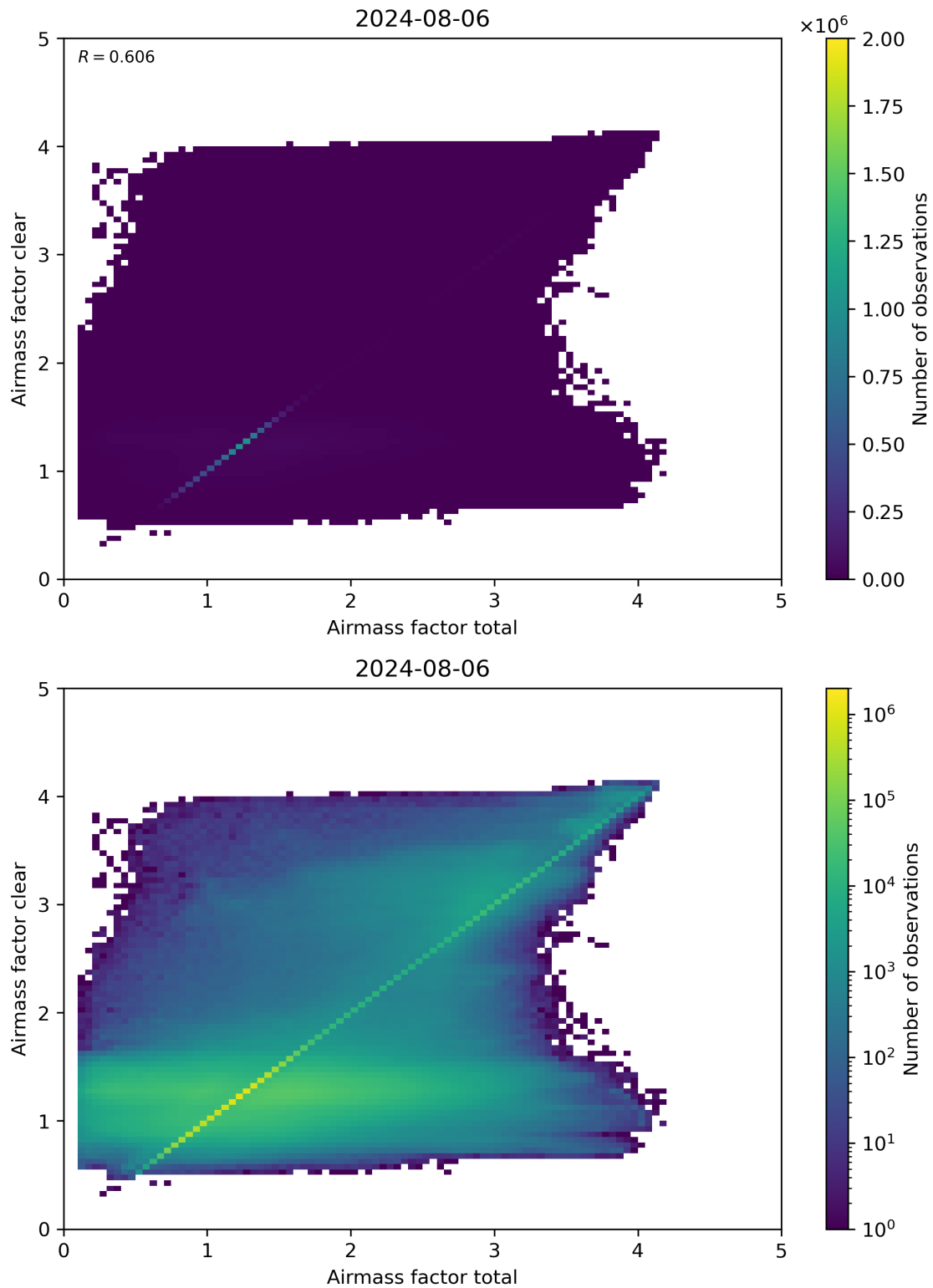
Figure 100: Scatter density plot of “Airmass factor total” against “Airmass factor clear” for 2024-08-06 to 2024-08-07.
