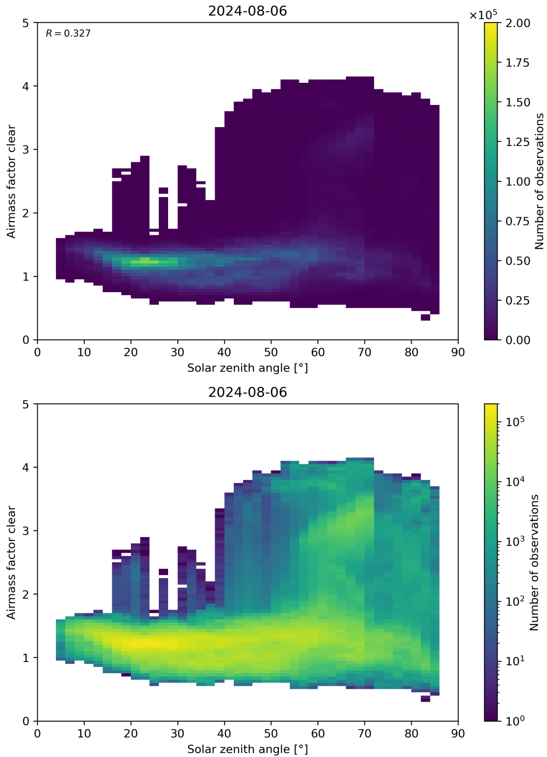
Figure 170: Scatter density plot of “Solar zenith angle” against “Airmass factor clear” for 2024-08-06 to 2024-08-07.
