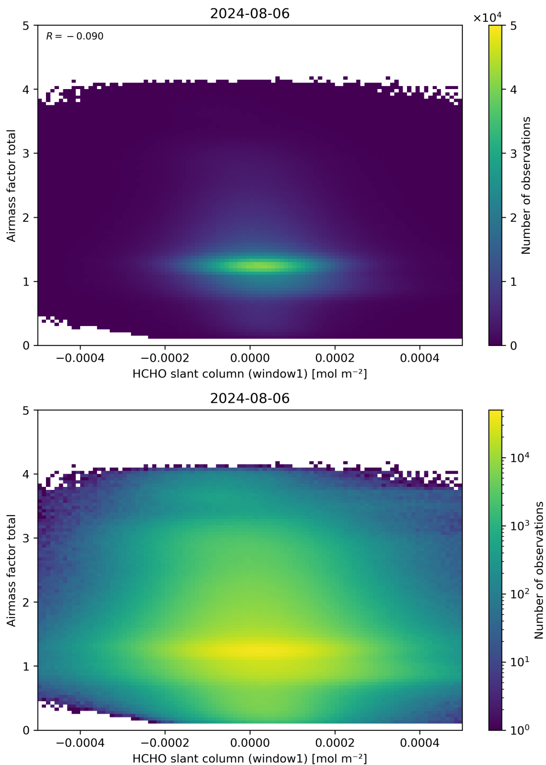
Figure 85: Scatter density plot of “HCHO slant column (window1)” against “Airmass factor total” for 2024-08-06 to 2024-08-07.
