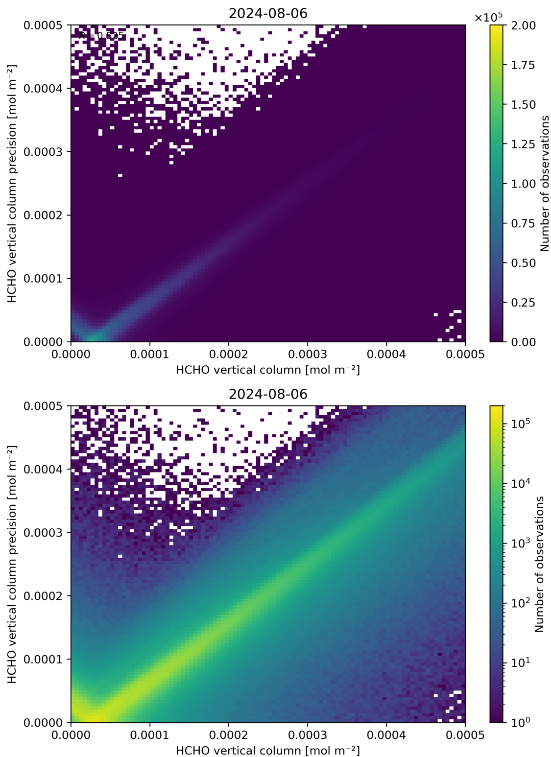
Figure 134: Scatter density plot of “HCHO vertical column” against “HCHO vertical column precision” for 2024-08-06 to 2024-08-07.
