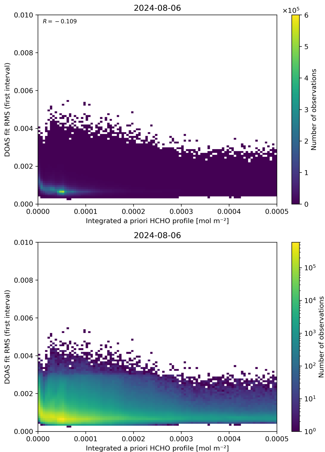
Figure 148: Scatter density plot of “Integrated a priori HCHO profile” against “DOAS fit RMS (first interval)” for 2024-08-06 to 2024-08-07.
