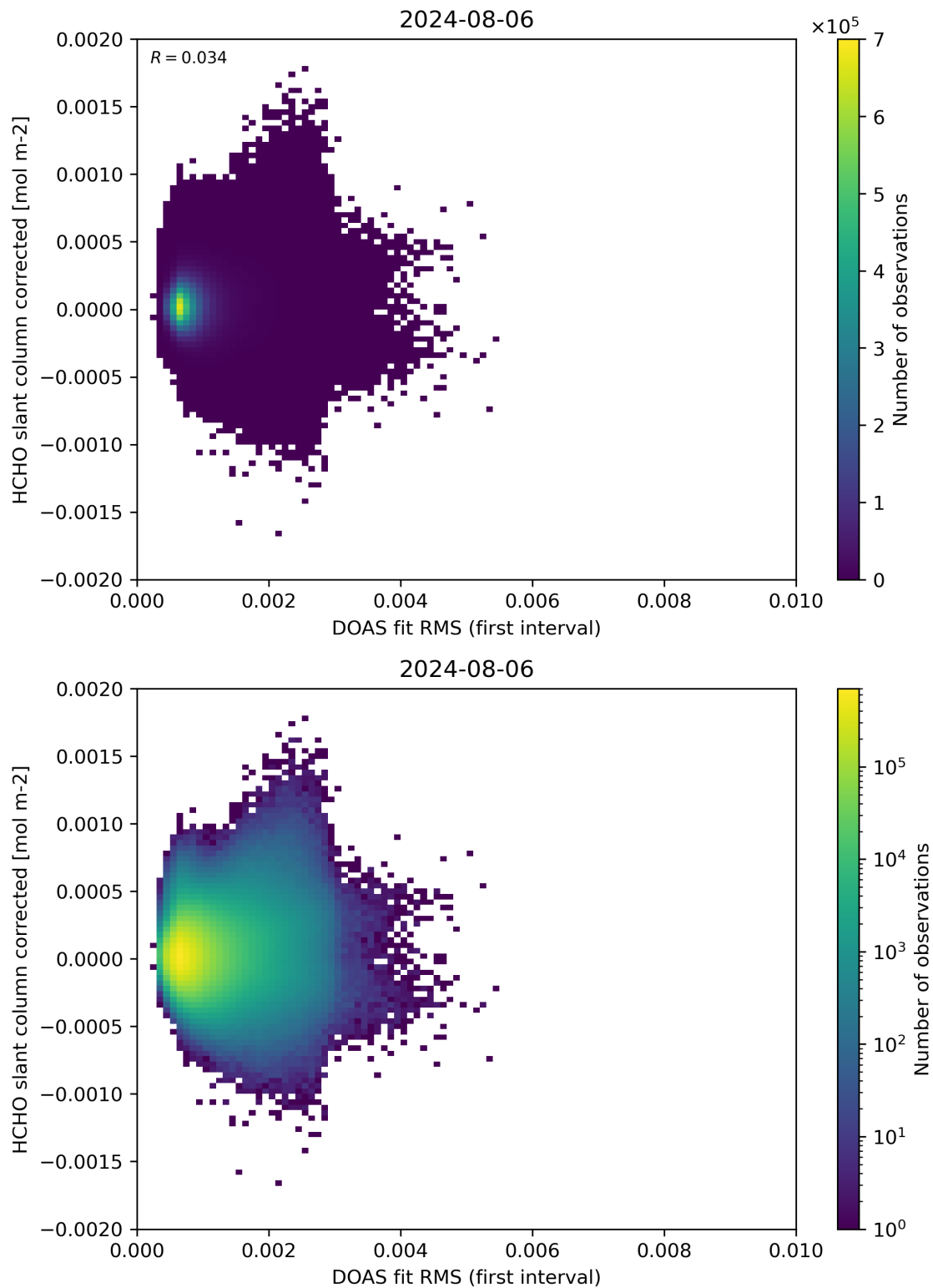
Figure 62: Scatter density plot of “DOAS fit RMS (first interval)” against “HCHO slant column corrected” for 2024-08-06 to 2024-08-07.
