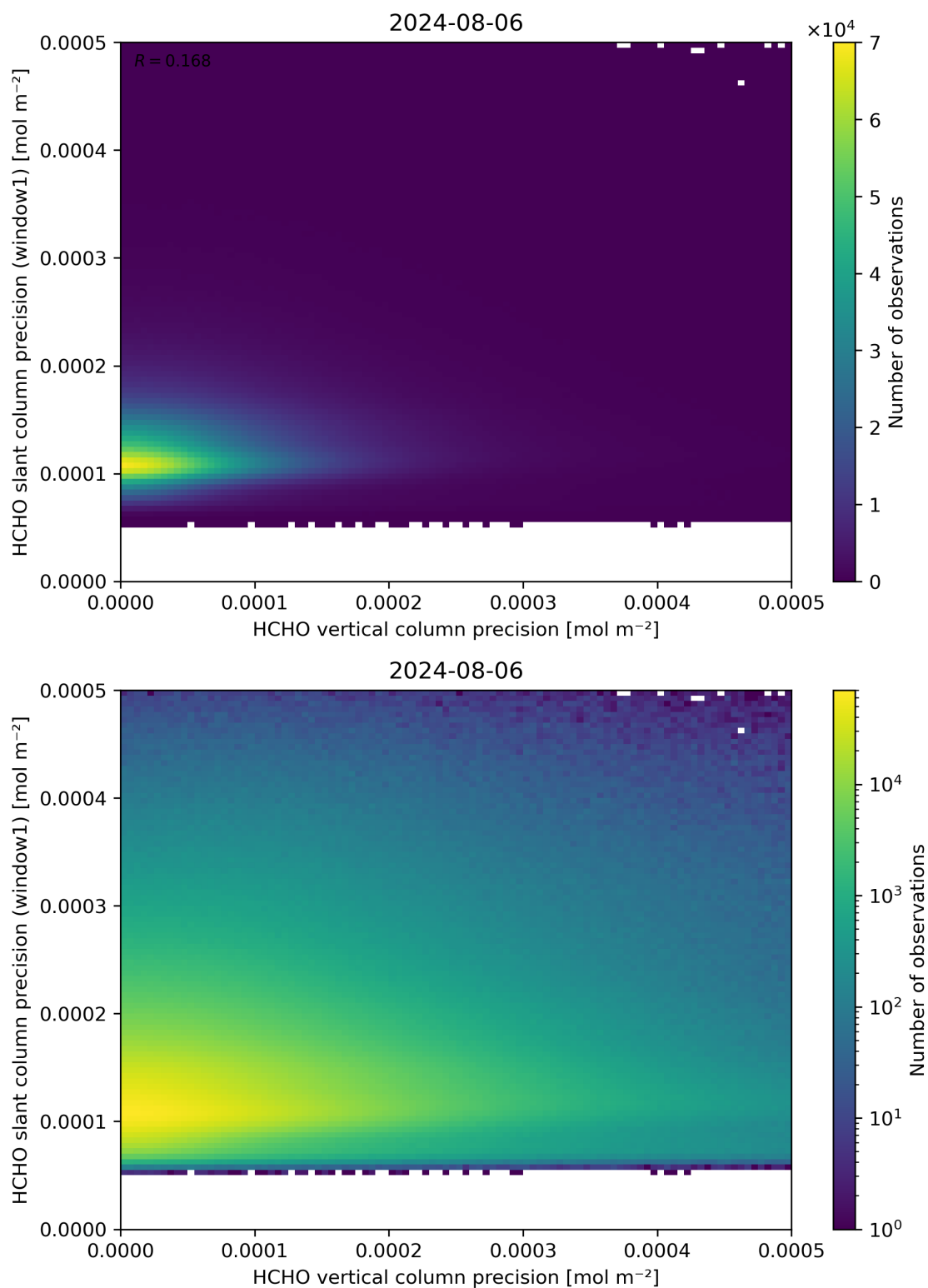
Figure 143: Scatter density plot of “HCHO vertical column precision” against “HCHO slant column precision (window1)” for 2024-08-06 to 2024-08-07.
