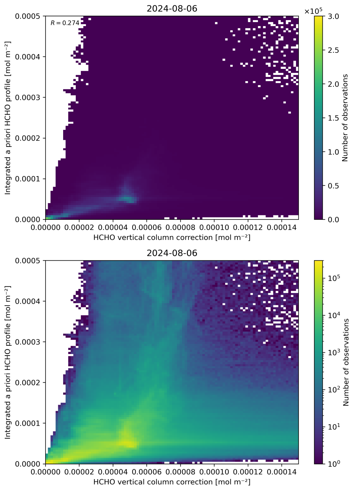
Figure 122: Scatter density plot of “HCHO vertical column correction” against “Integrated a priori HCHO profile” for 2024-08-06 to 2024-08-07.
