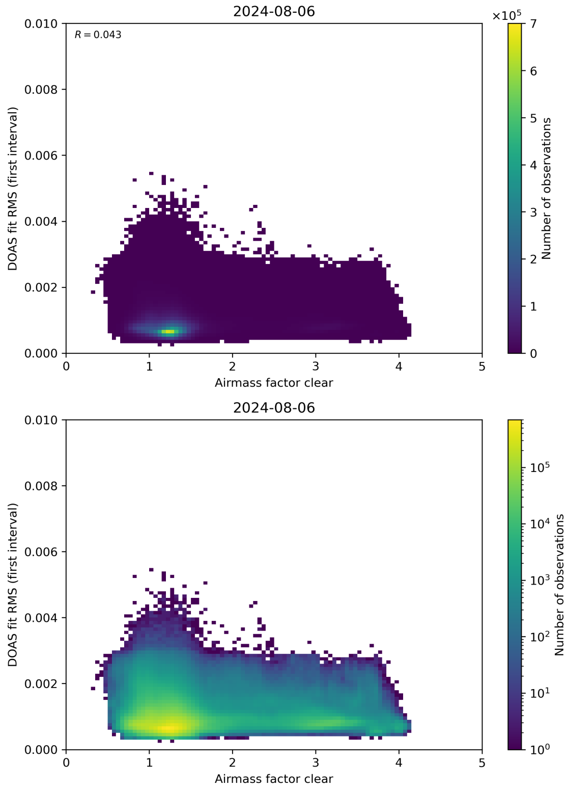
Figure 71: Scatter density plot of “Airmass factor clear” against “DOAS fit RMS (first interval)” for 2024-08-06 to 2024-08-07.
