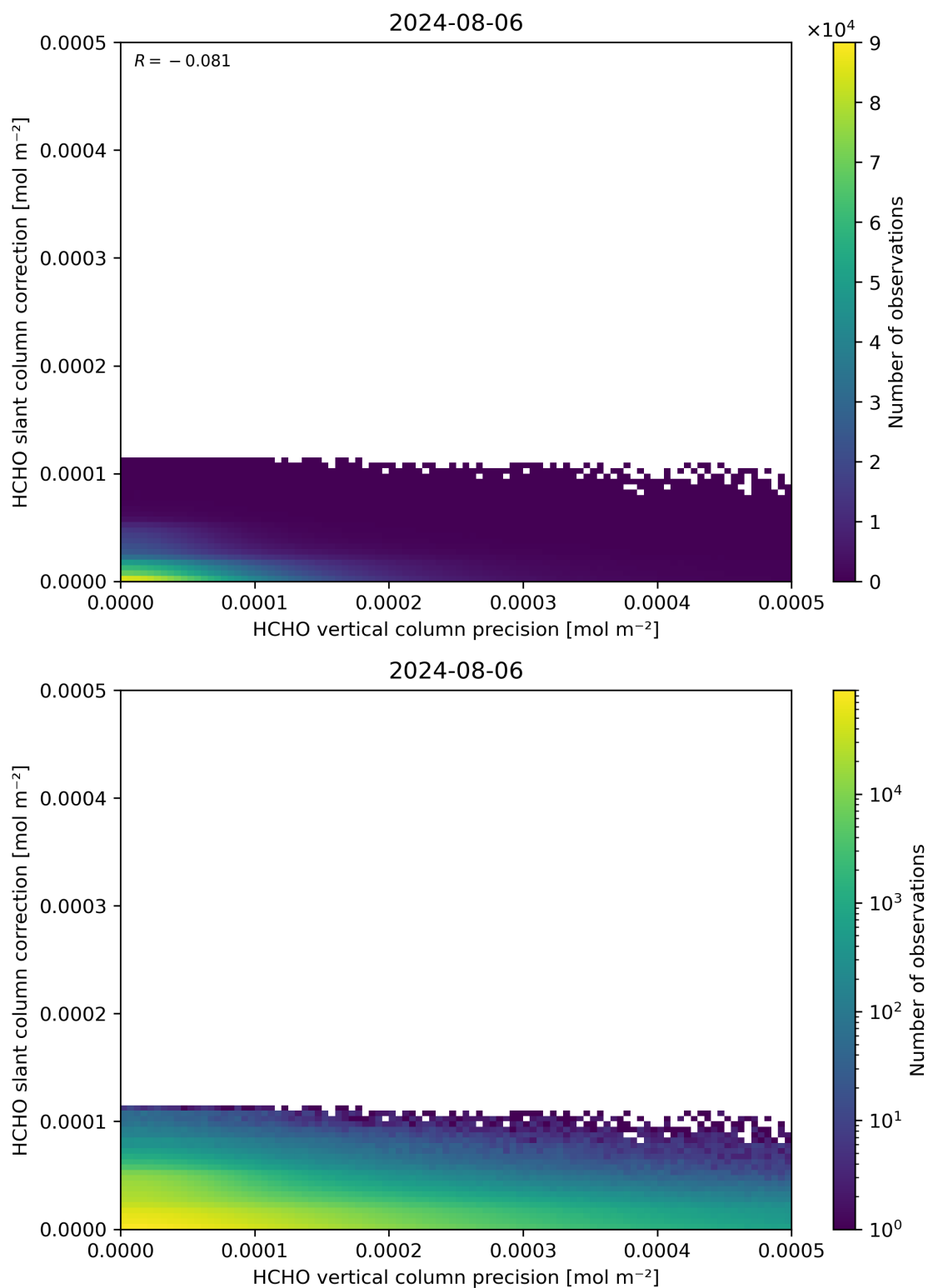
Figure 141: Scatter density plot of “HCHO vertical column precision” against “HCHO slant column correction” for 2024-08-06 to 2024-08-07.
