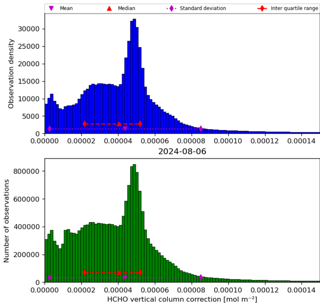
Figure 37: Histogram of “HCHO vertical column correction” for 2024-08-06 to 2024-08-07
