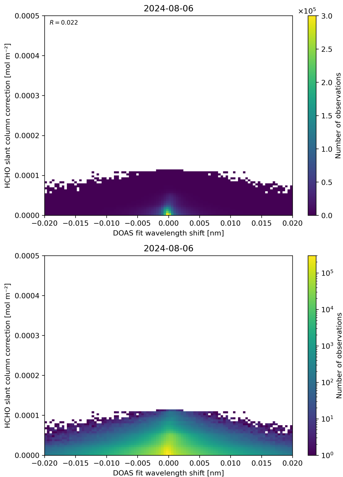
Figure 67: Scatter density plot of “DOAS fit wavelength shift” against “HCHO slant column correction” for 2024-08-06 to 2024-08-07.
