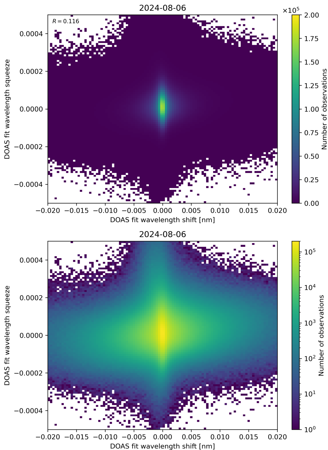
Figure 65: Scatter density plot of “DOAS fit wavelength shift” against “DOAS fit wavelength squeeze” for 2024-08-06 to 2024-08-07.
