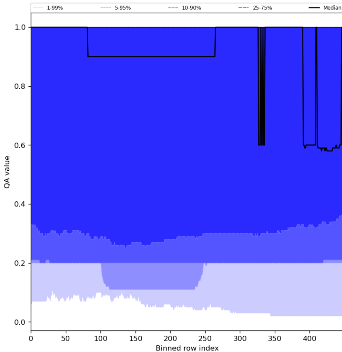
Figure 48: Along track statistics of “QA value” for 2024-08-06 to 2024-08-07
