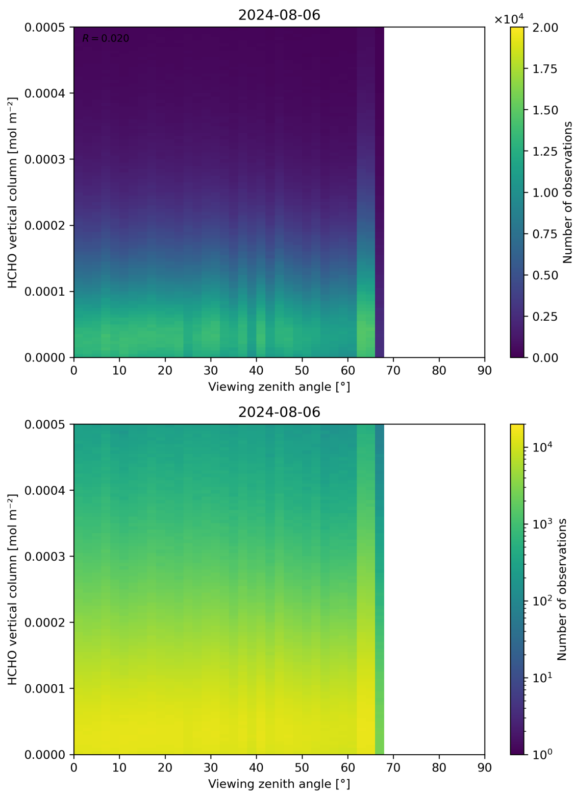
Figure 192: Scatter density plot of “Viewing zenith angle” against “HCHO vertical column” for 2024-08-06 to 2024-08-07.
