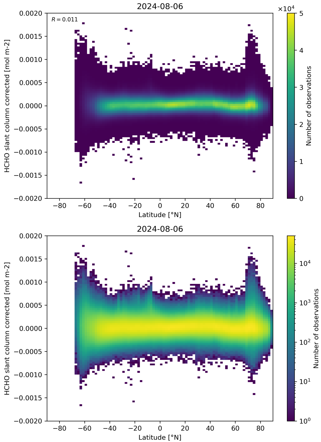
Figure 157: Scatter density plot of “Latitude” against “HCHO slant column corrected” for 2024-08-06 to 2024-08-07.
