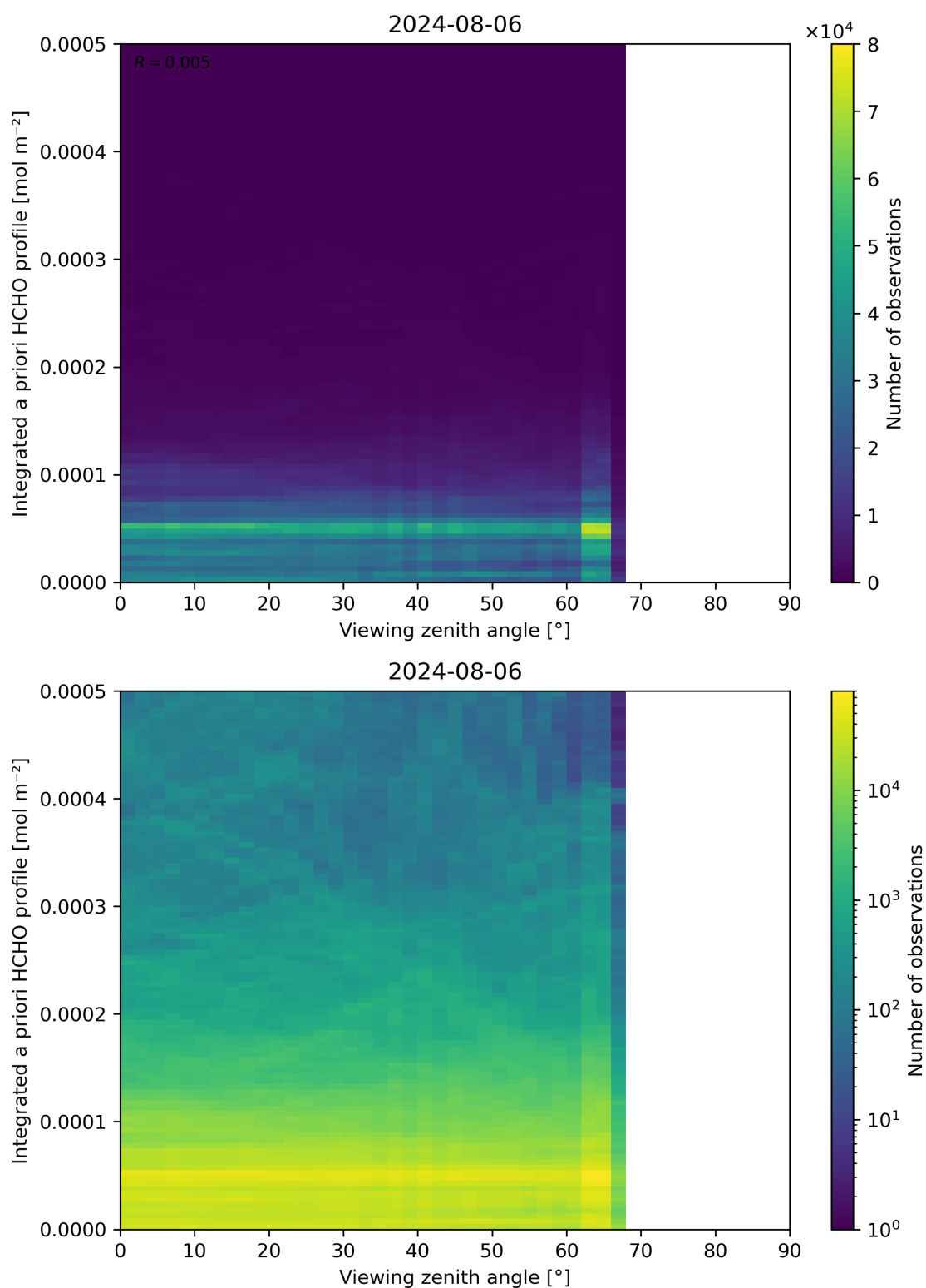
Figure 195: Scatter density plot of “Viewing zenith angle” against “Integrated a priori HCHO profile” for 2024-08-06 to 2024-08-07.
