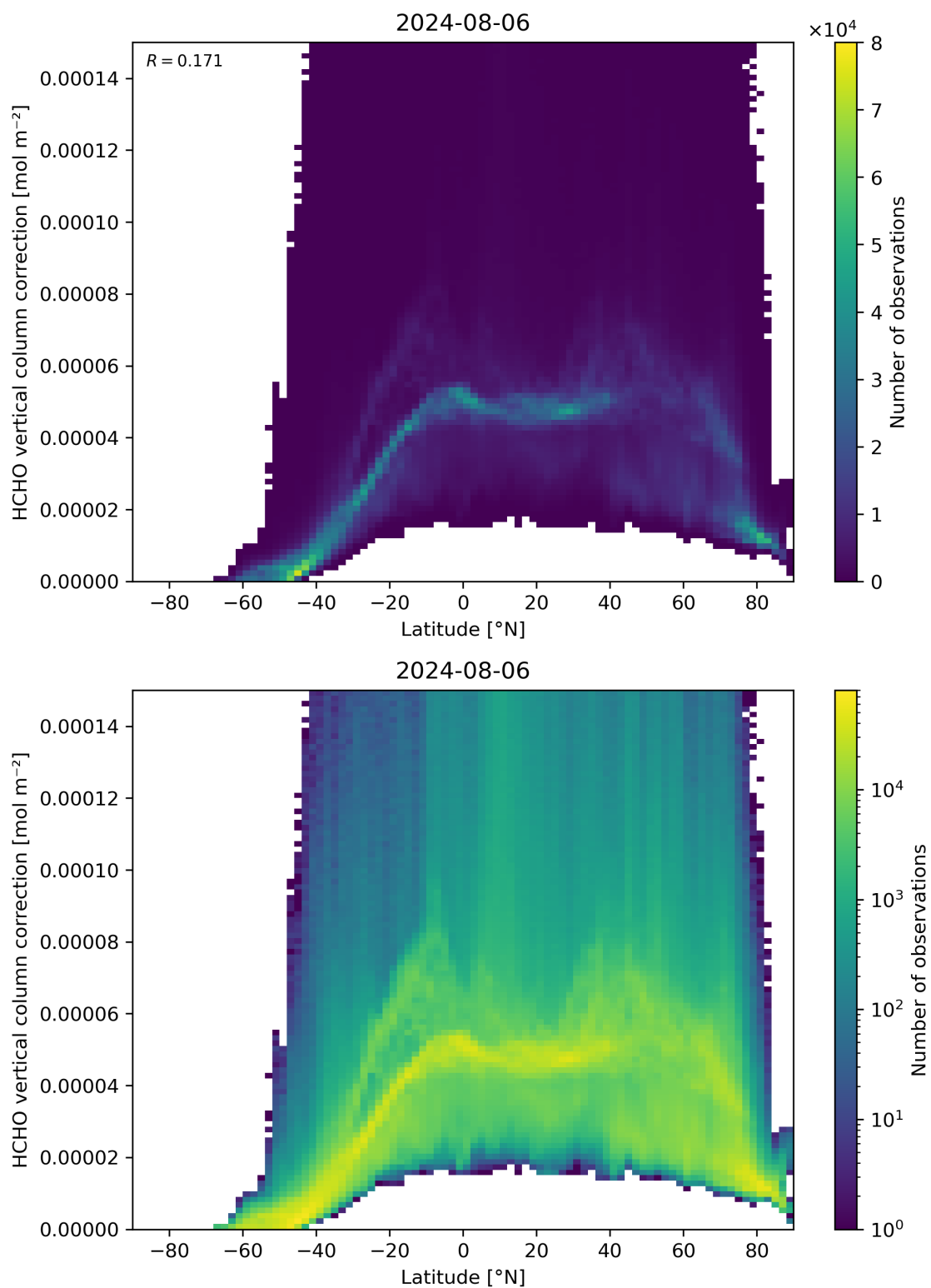
Figure 164: Scatter density plot of “Latitude” against “HCHO vertical column correction” for 2024-08-06 to 2024-08-07.
