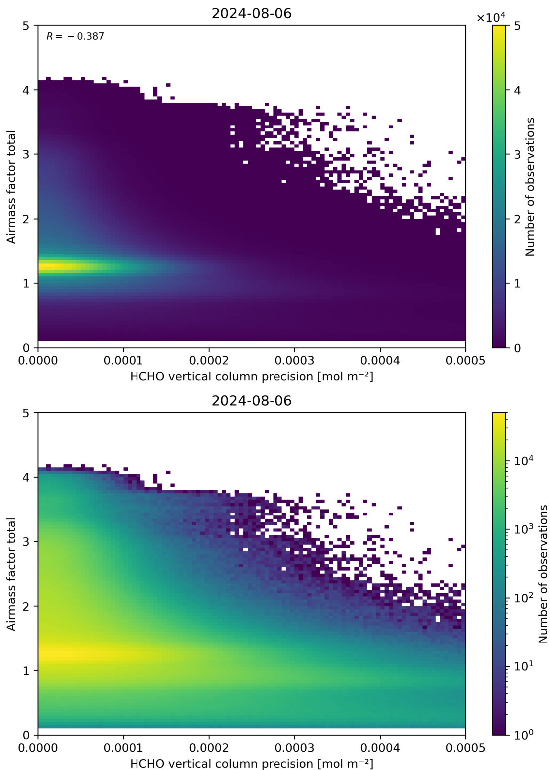
Figure 144: Scatter density plot of “HCHO vertical column precision” against “Airmass factor total” for 2024-08-06 to 2024-08-07.
