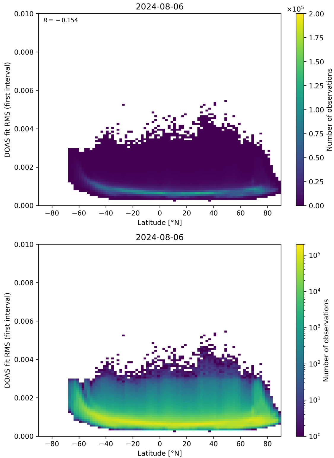
Figure 153: Scatter density plot of “Latitude” against “DOAS fit RMS (first interval)” for 2024-08-06 to 2024-08-07.
