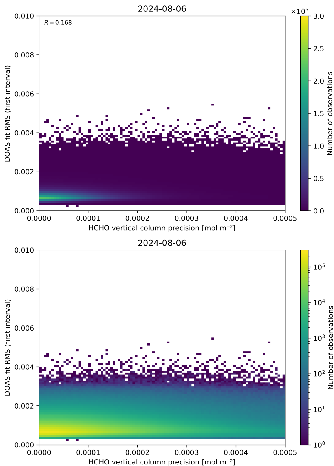
Figure 136: Scatter density plot of “HCHO vertical column precision” against “DOAS fit RMS (first interval)” for 2024-08-06 to 2024-08-07.
