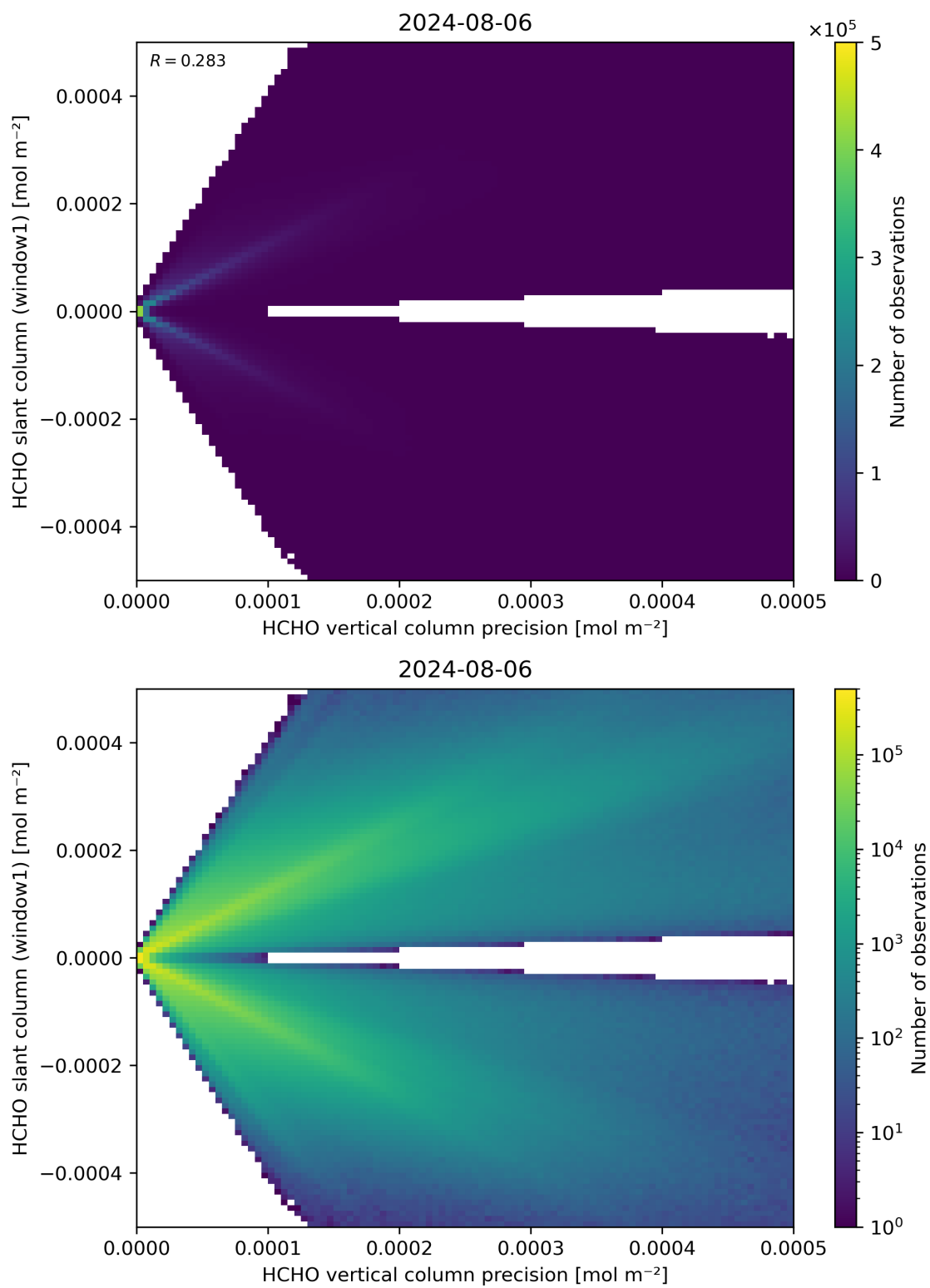
Figure 142: Scatter density plot of “HCHO vertical column precision” against “HCHO slant column (window1)” for 2024-08-06 to 2024-08-07.
