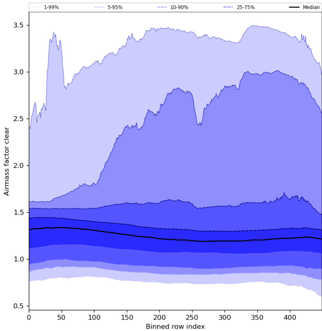
Figure 56: Along track statistics of “Airmass factor clear” for 2024-08-06 to 2024-08-07
