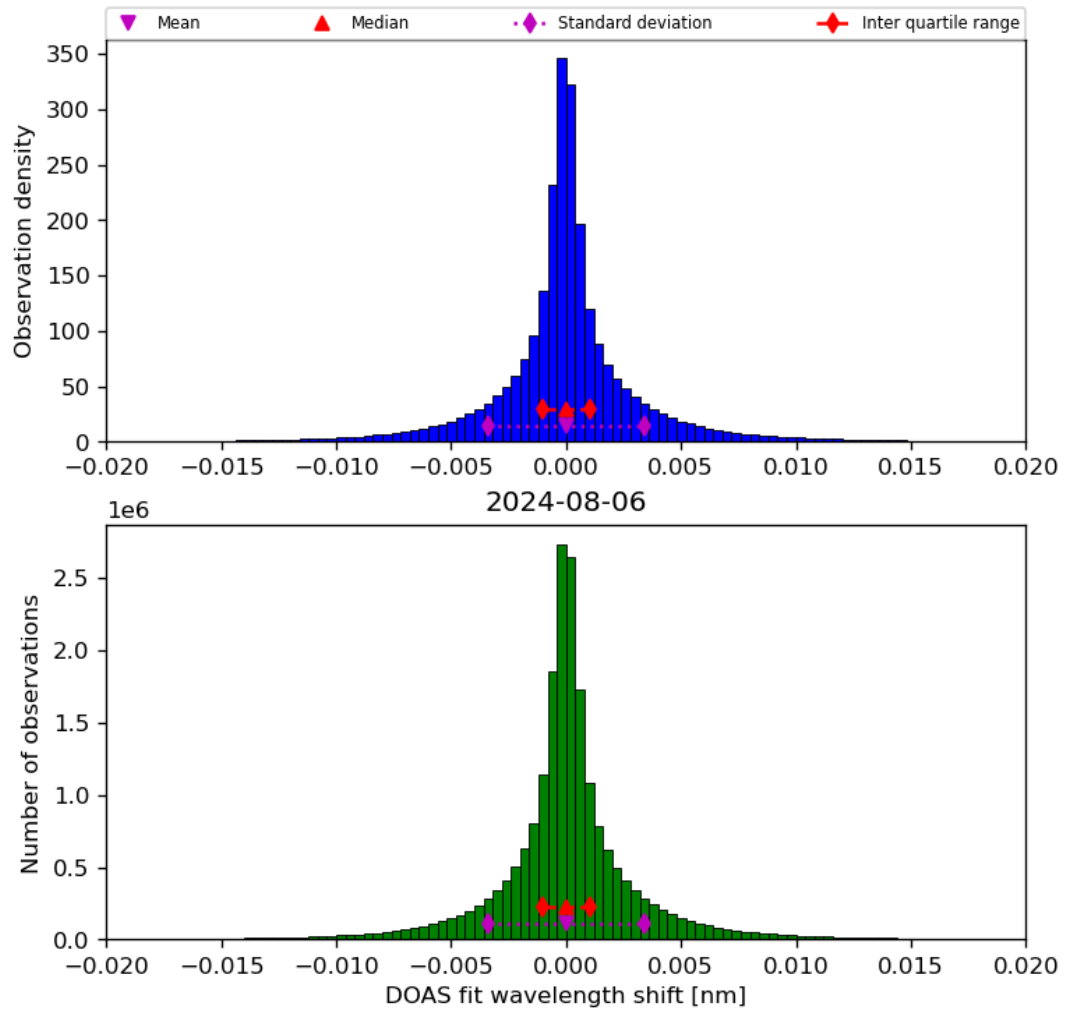
Figure 44: Histogram of “DOAS fit wavelength shift” for 2024-08-06 to 2024-08-07
