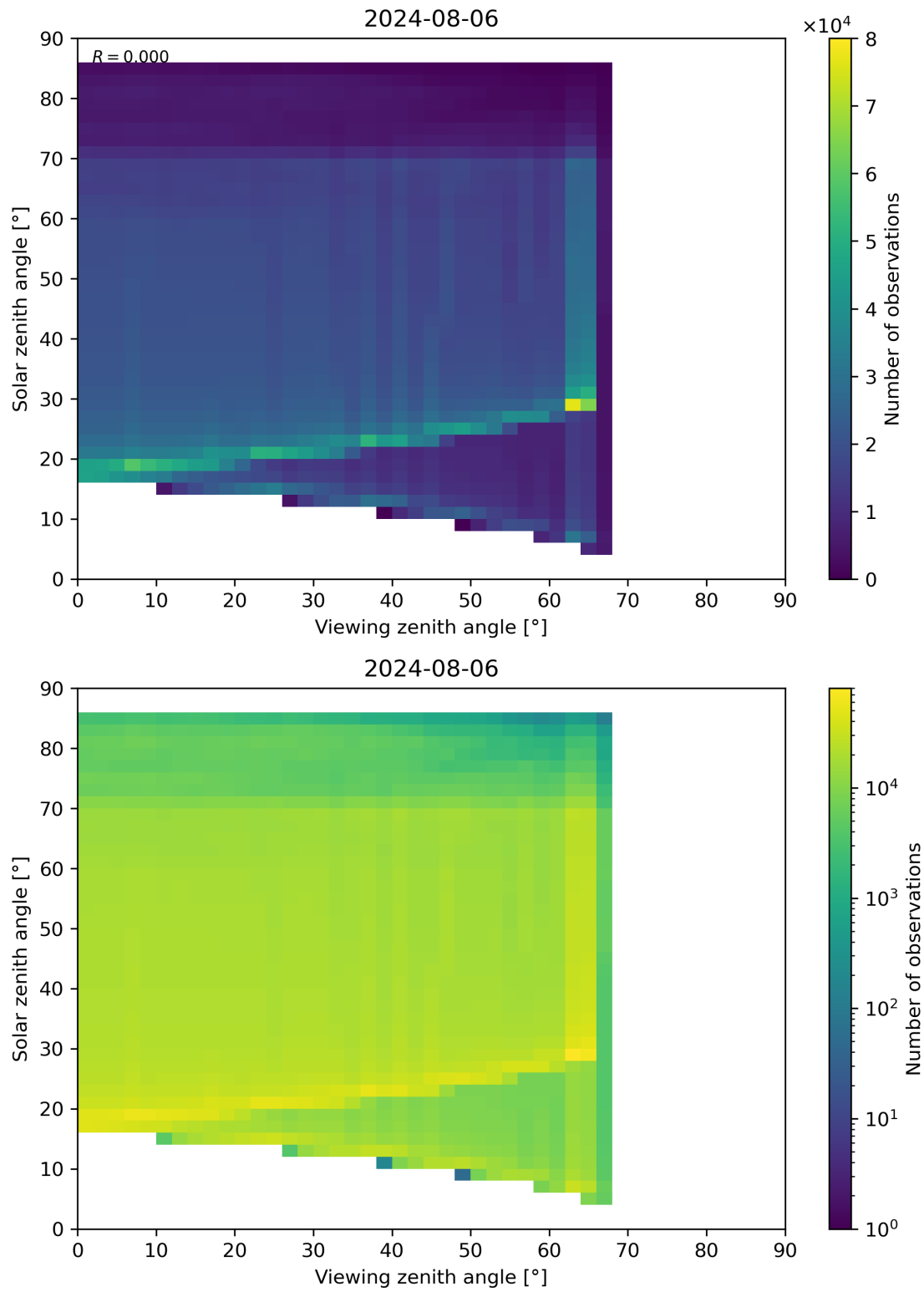
Figure 197: Scatter density plot of “Viewing zenith angle” against “Solar zenith angle” for 2024-08-06 to 2024-08-07.
