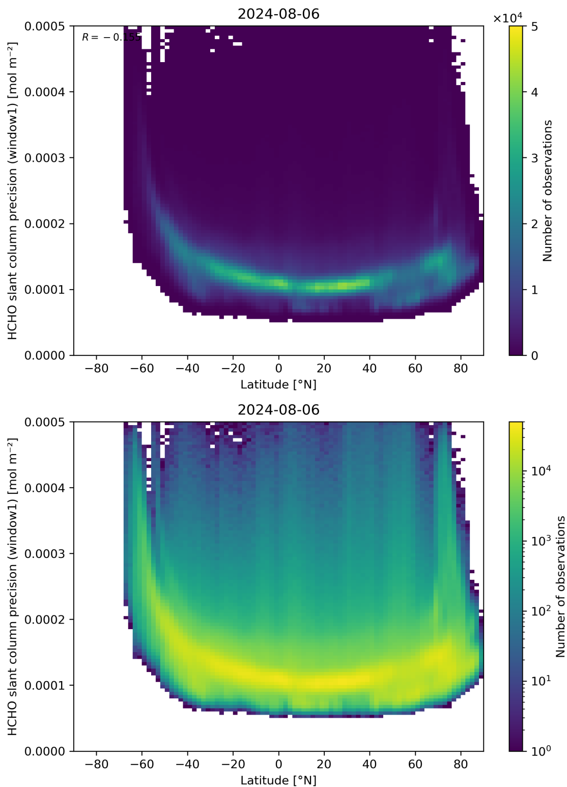
Figure 160: Scatter density plot of “Latitude” against “HCHO slant column precision (window1)” for 2024-08-06 to 2024-08-07.
