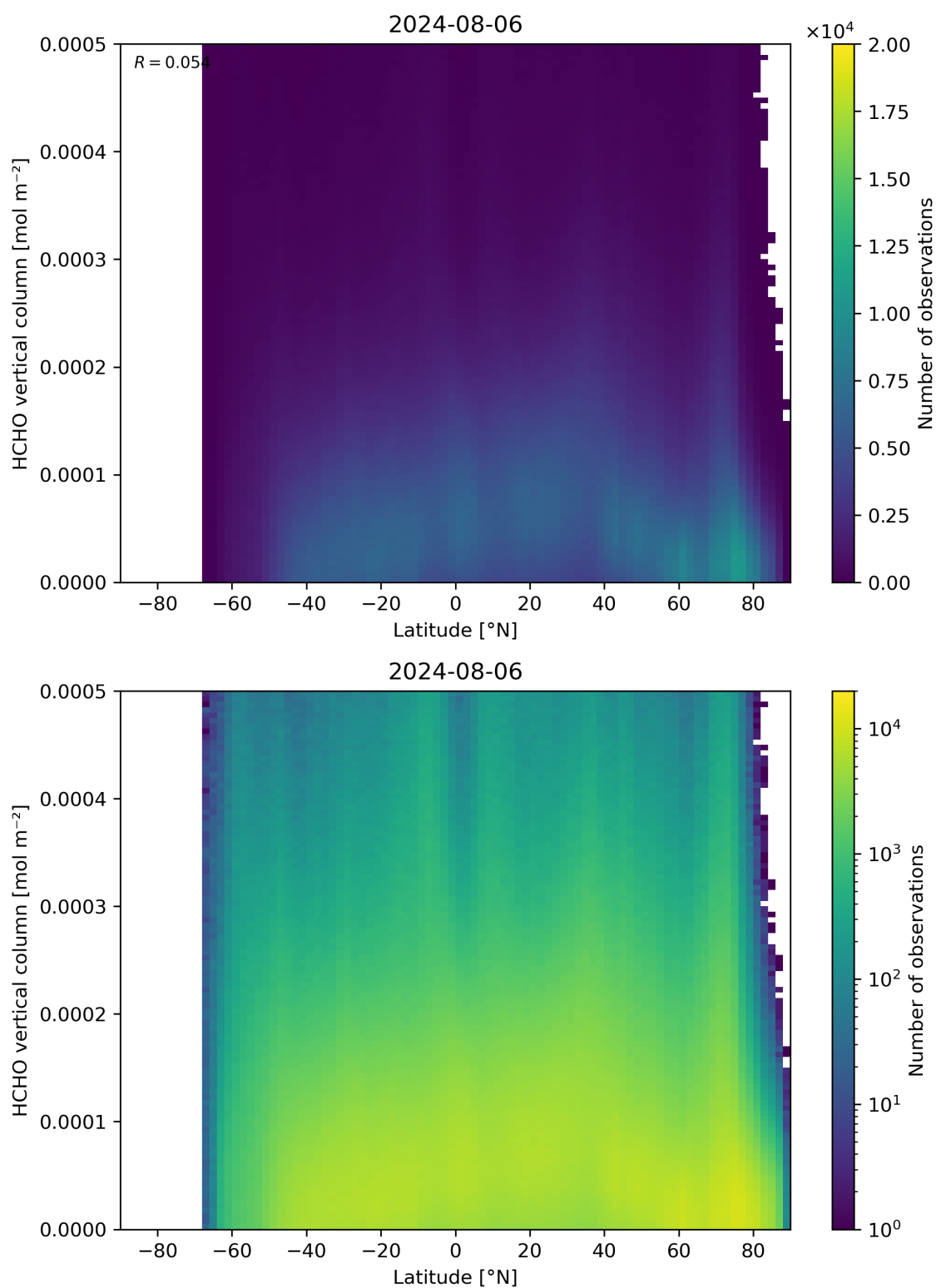
Figure 163: Scatter density plot of “Latitude” against “HCHO vertical column” for 2024-08-06 to 2024-08-07.
