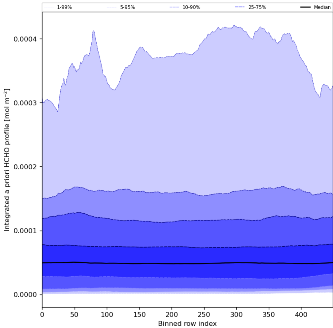
Figure 57: Along track statistics of "Integrated a priori HCHO profile" for 2024-08-06 to 2024-08-07
