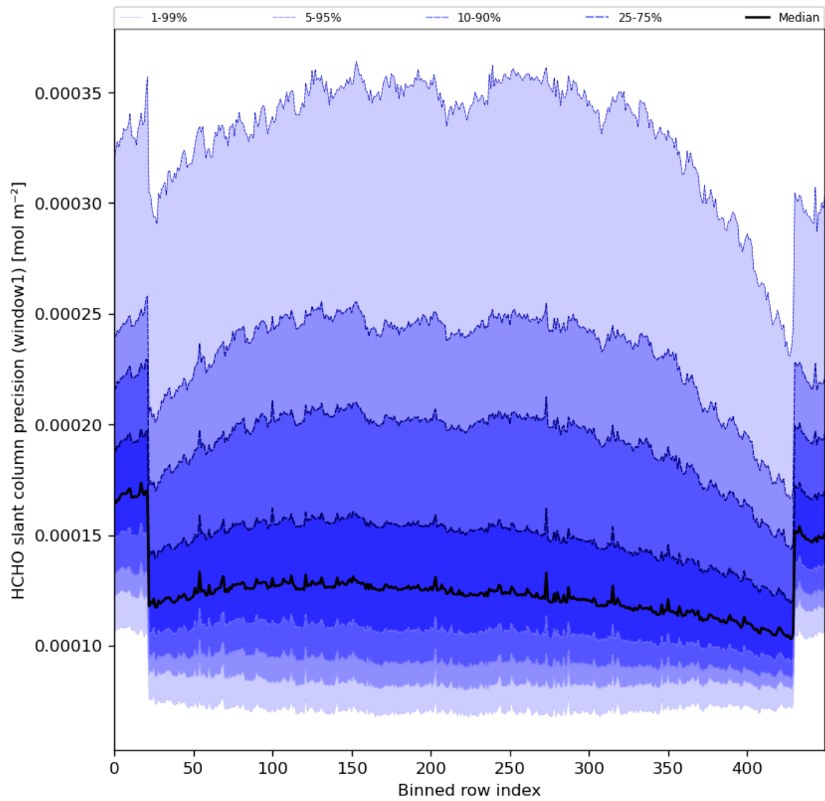
Figure 53: Along track statistics of “HCHO slant column precision (window1)” for 2024-08-06 to 2024-08-07
