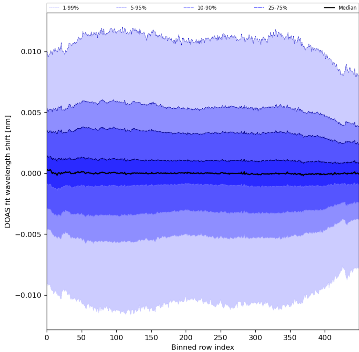
Figure 58: Along track statistics of “DOAS fit wavelength shift” for 2024-08-06 to 2024-08-07
