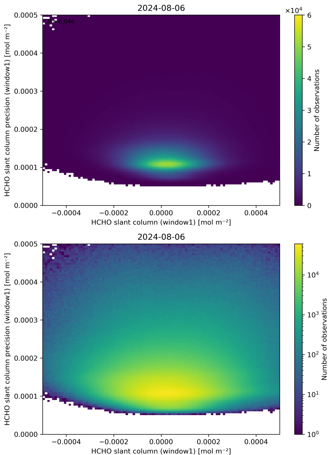
Figure 84: Scatter density plot of “HCHO slant column (window1)” against “HCHO slant column precision (window1)” for 2024-08-06 to 2024-08-07.
