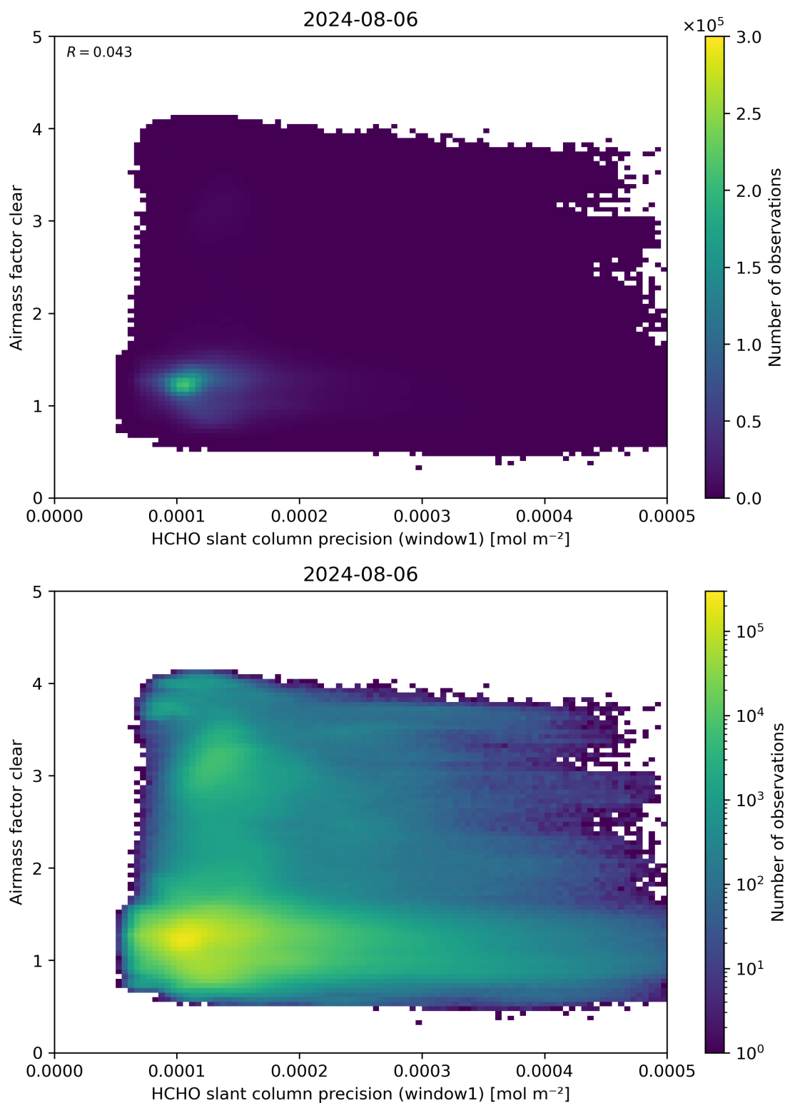
Figure 91: Scatter density plot of “HCHO slant column precision (window1)” against “Airmass factor clear” for 2024-08-06 to 2024-08-07.
