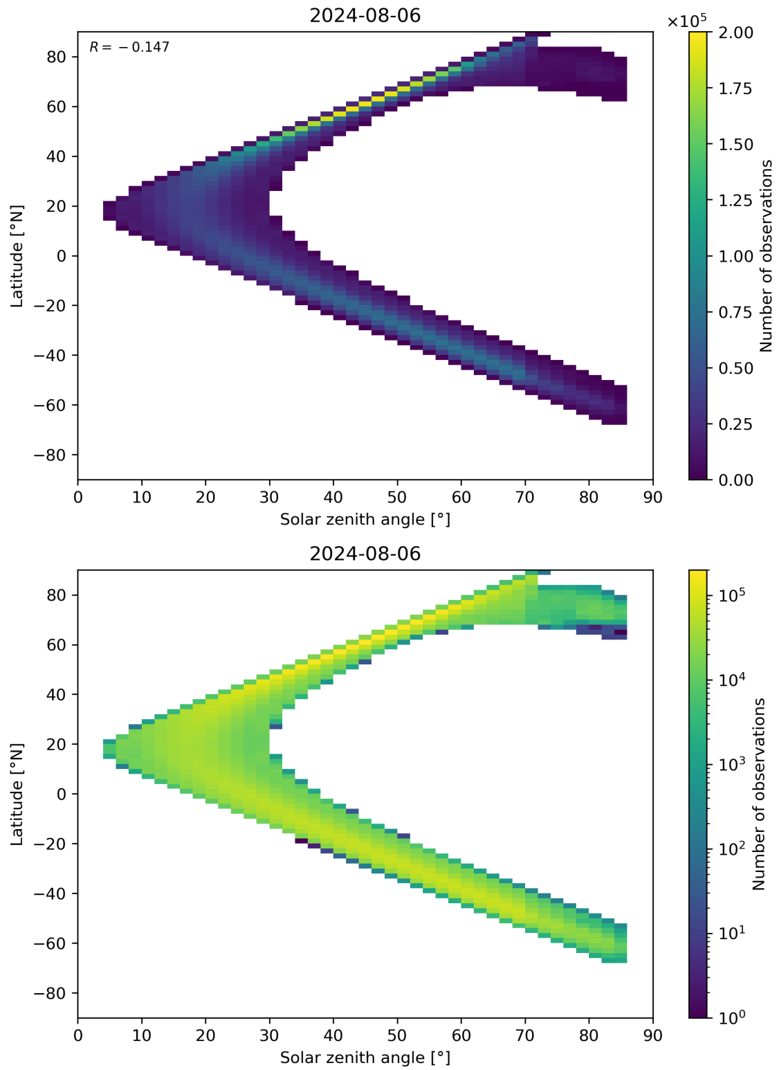
Figure 181: Scatter density plot of “Solar zenith angle” against “Latitude” for 2024-08-06 to 2024-08-07.
