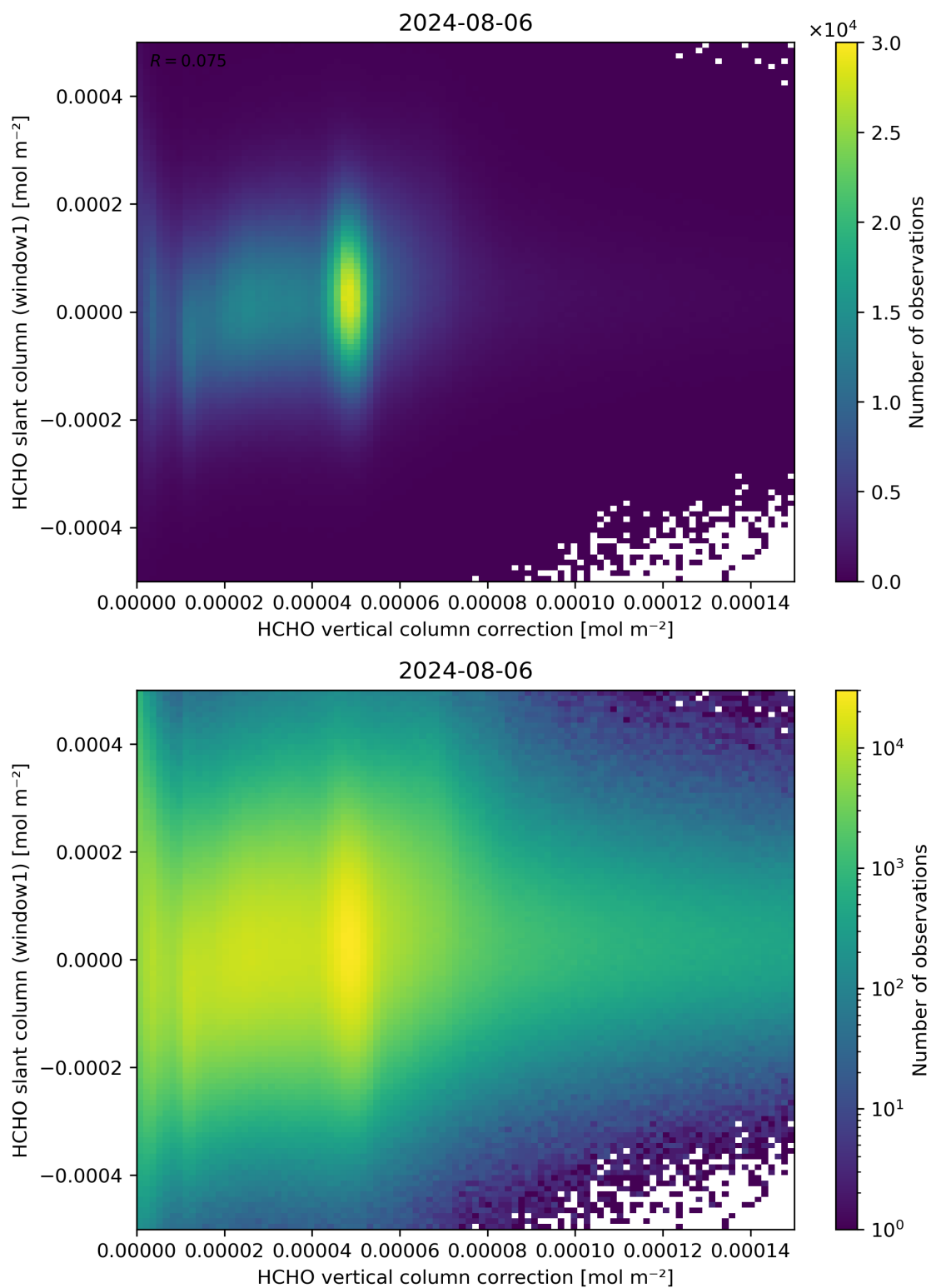
Figure 118: Scatter density plot of “HCHO vertical column correction” against “HCHO slant column (window1)” for 2024-08-06 to 2024-08-07.
