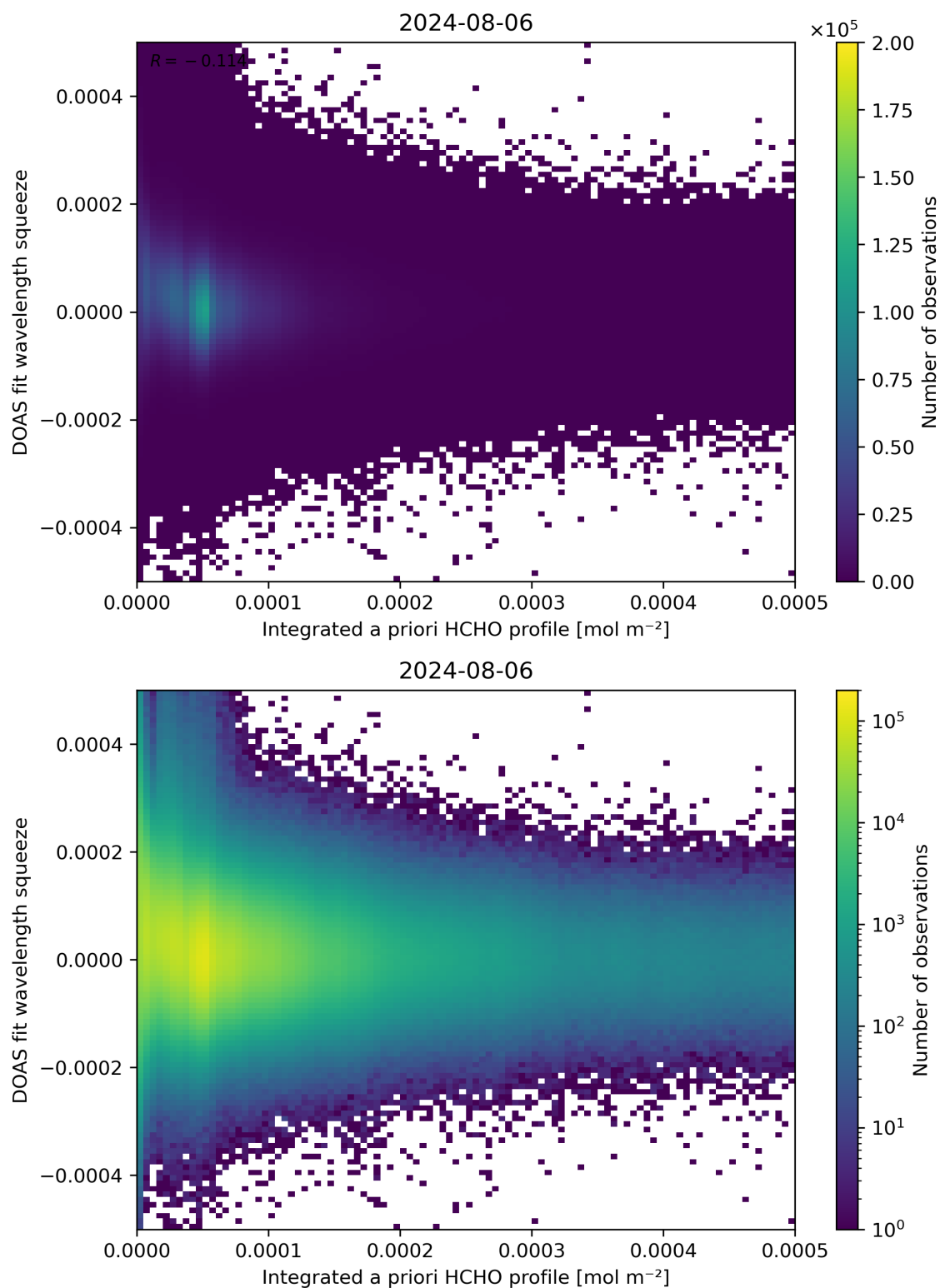
Figure 150: Scatter density plot of “Integrated a priori HCHO profile” against “DOAS fit wavelength squeeze” for 2024-08-06 to 2024-08-07.
