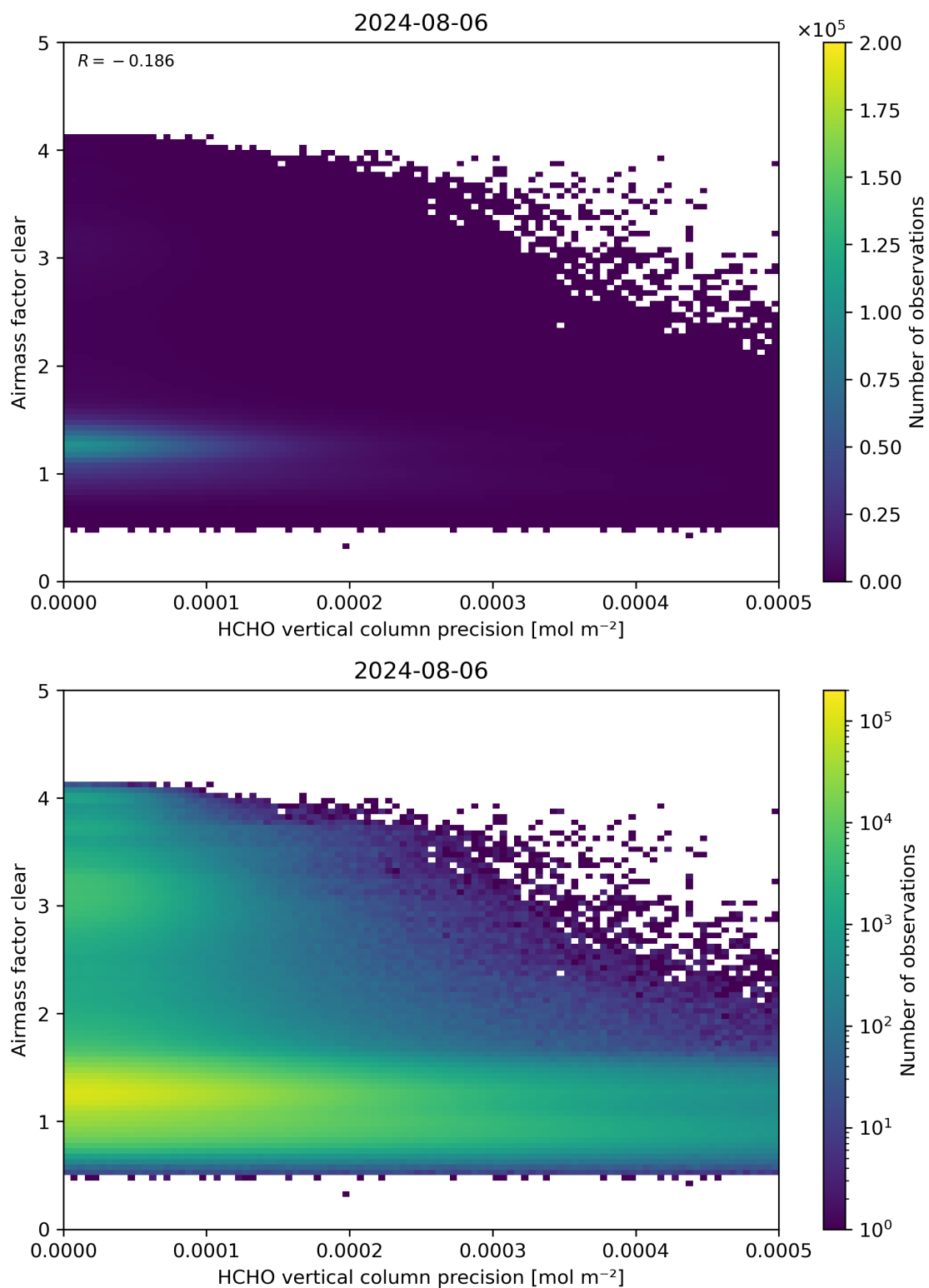
Figure 139: Scatter density plot of “HCHO vertical column precision” against “Airmass factor clear” for 2024-08-06 to 2024-08-07.
