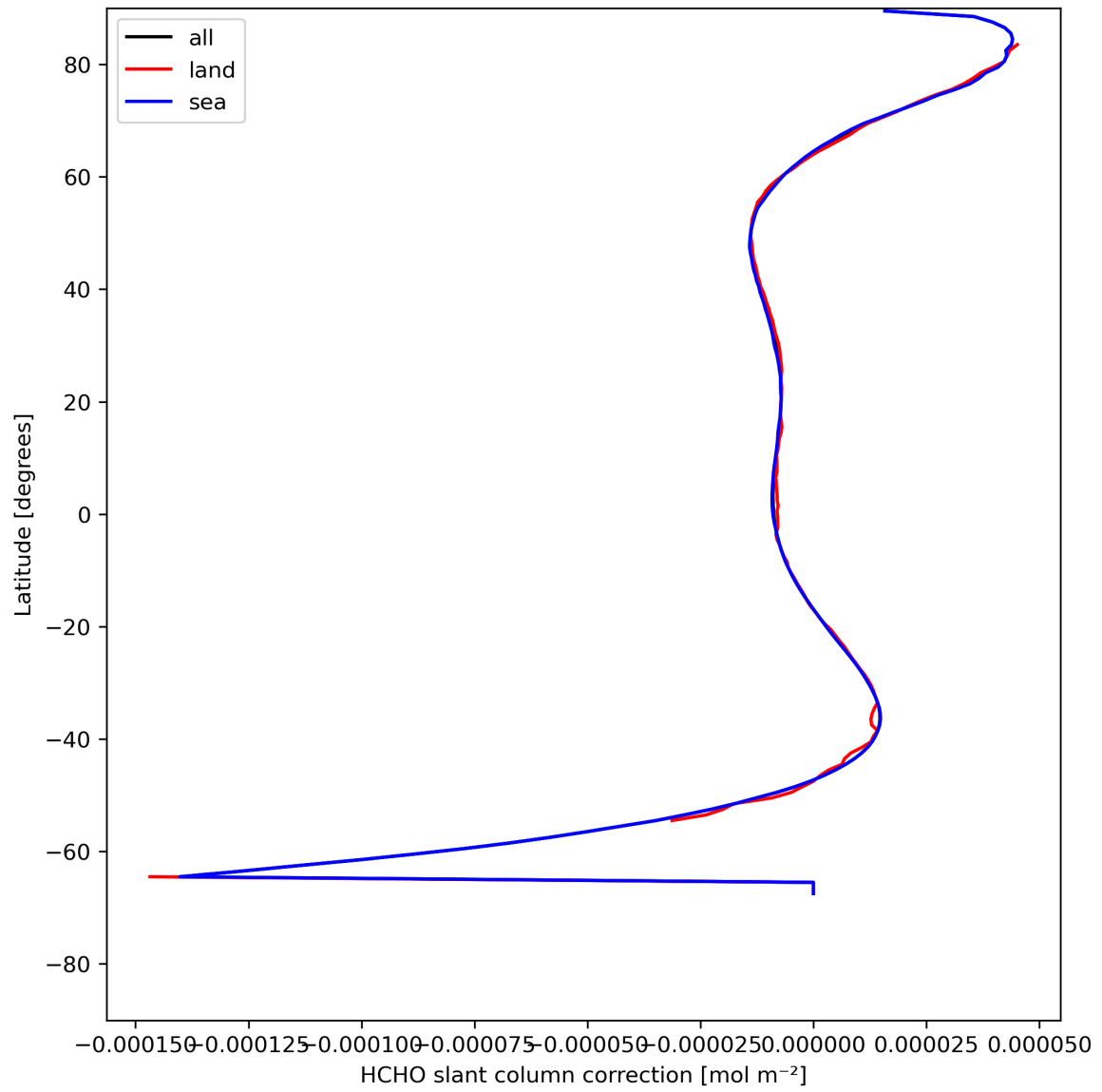
Figure 33: Zonal average of “HCHO slant column correction” for 2024-08-06 to 2024-08-07.
