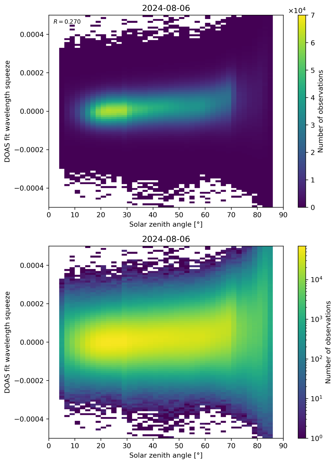
Figure 169: Scatter density plot of “Solar zenith angle” against “DOAS fit wavelength squeeze” for 2024-08-06 to 2024-08-07.
