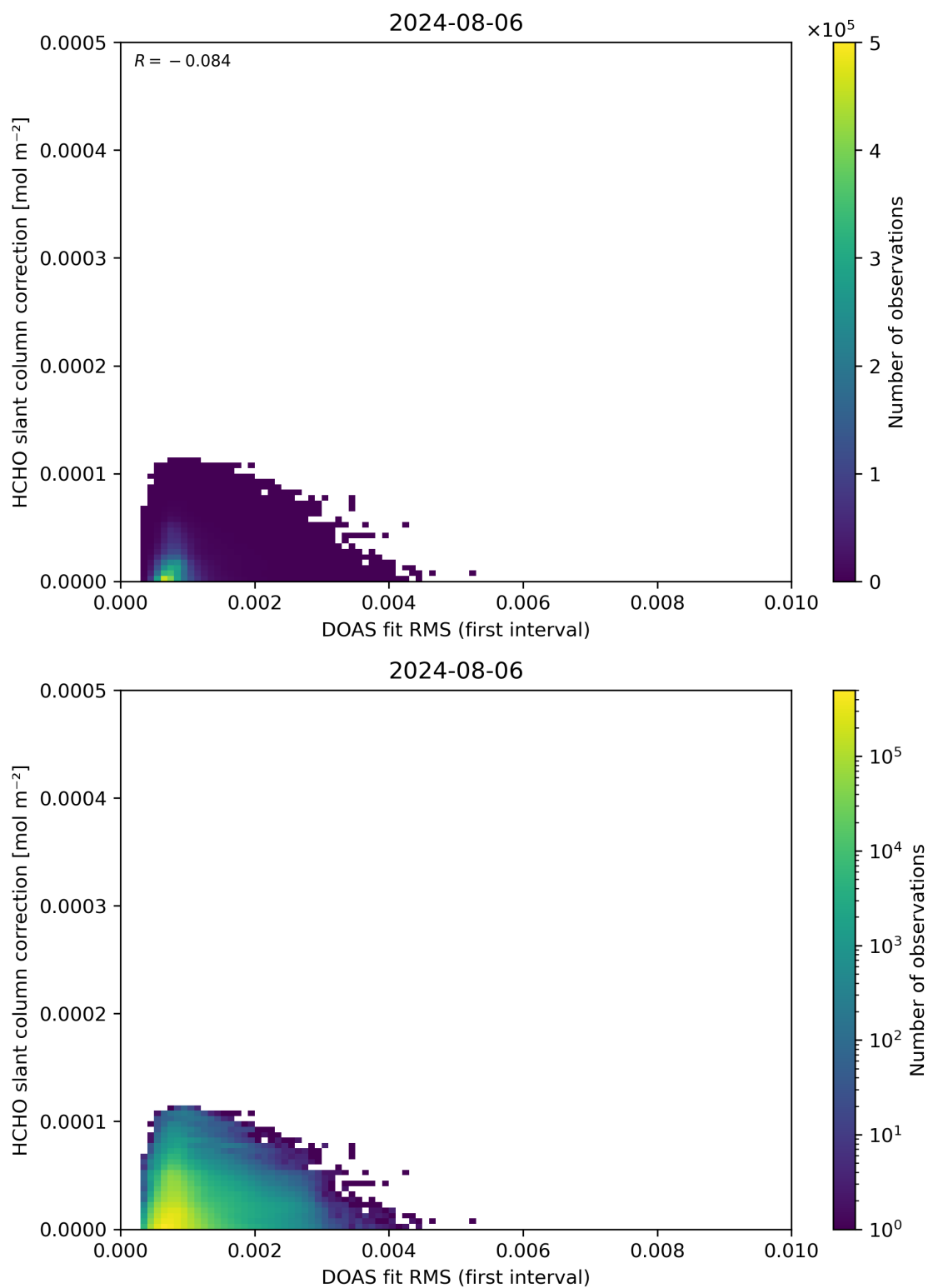
Figure 63: Scatter density plot of “DOAS fit RMS (first interval)” against “HCHO slant column correction” for 2024-08-06 to 2024-08-07.
