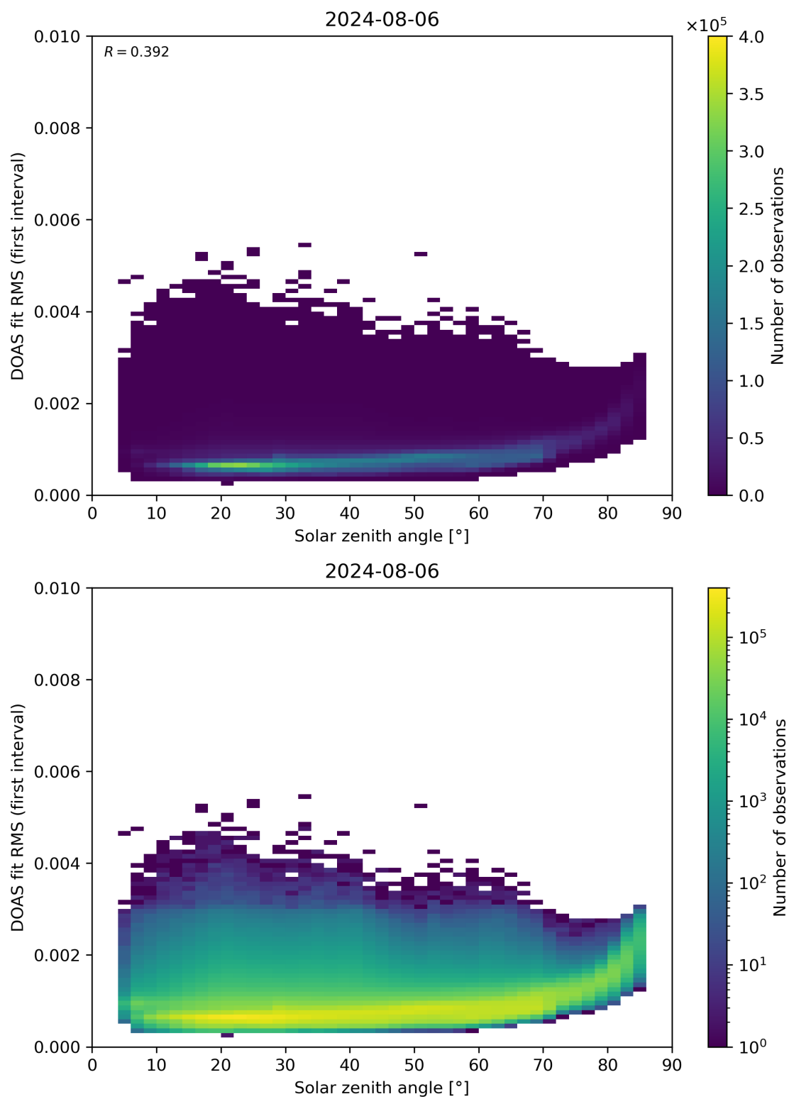
Figure 167: Scatter density plot of “Solar zenith angle” against “DOAS fit RMS (first interval)” for 2024-08-06 to 2024-08-07.
