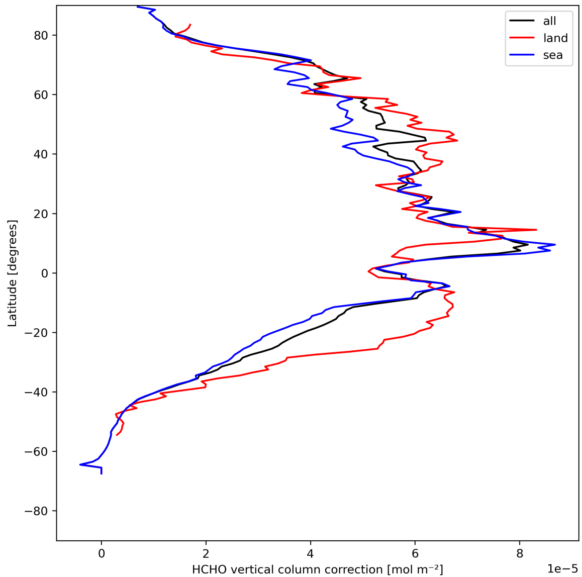
Figure 23: Zonal average of “HCHO vertical column correction” for 2024-08-06 to 2024-08-07.
