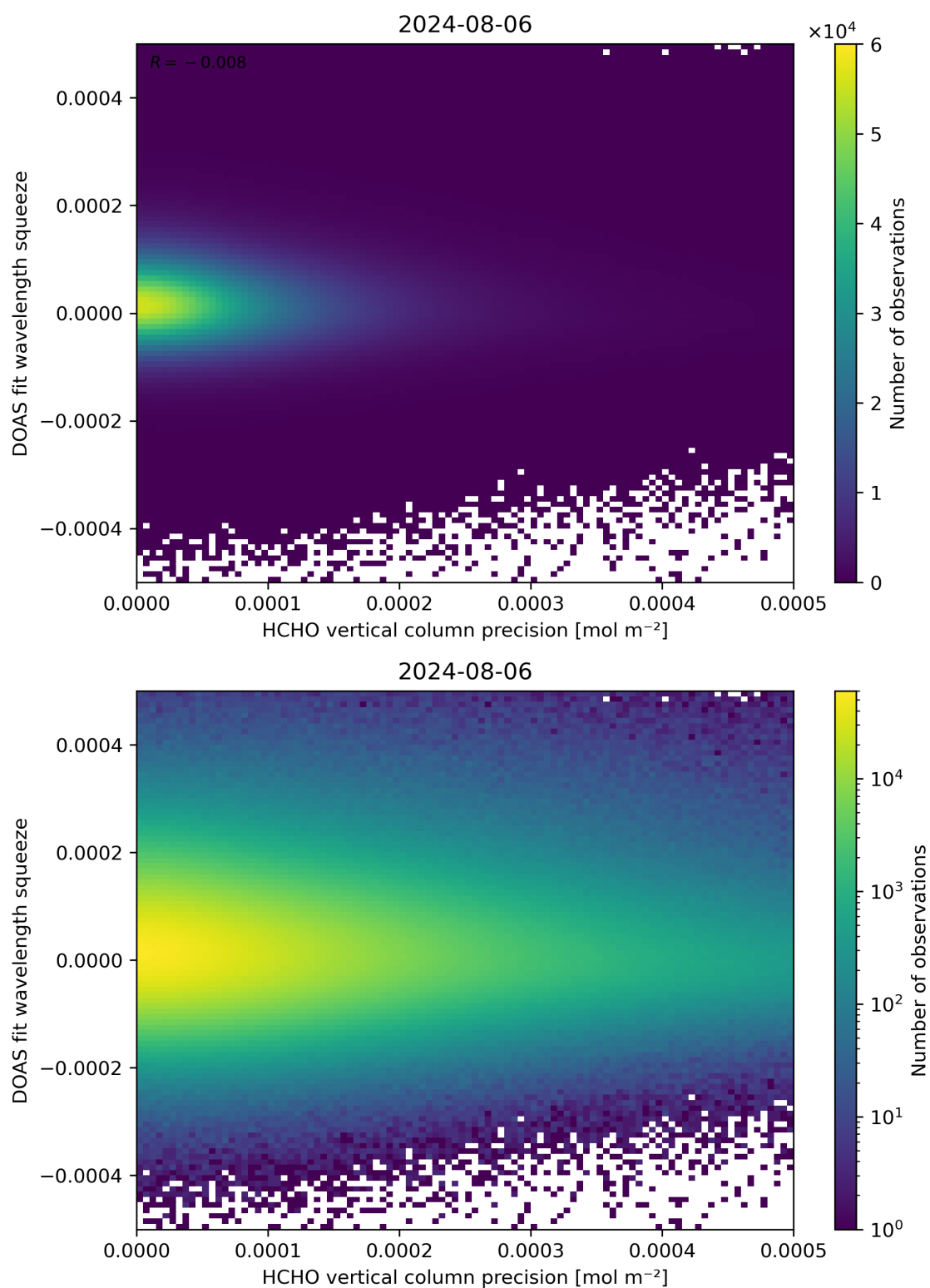
Figure 138: Scatter density plot of “HCHO vertical column precision” against “DOAS fit wavelength squeeze” for 2024-08-06 to 2024-08-07.
