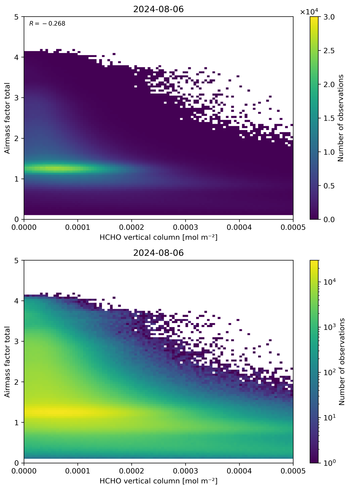
Figure 131: Scatter density plot of “HCHO vertical column” against “Airmass factor total” for 2024-08-06 to 2024-08-07.
