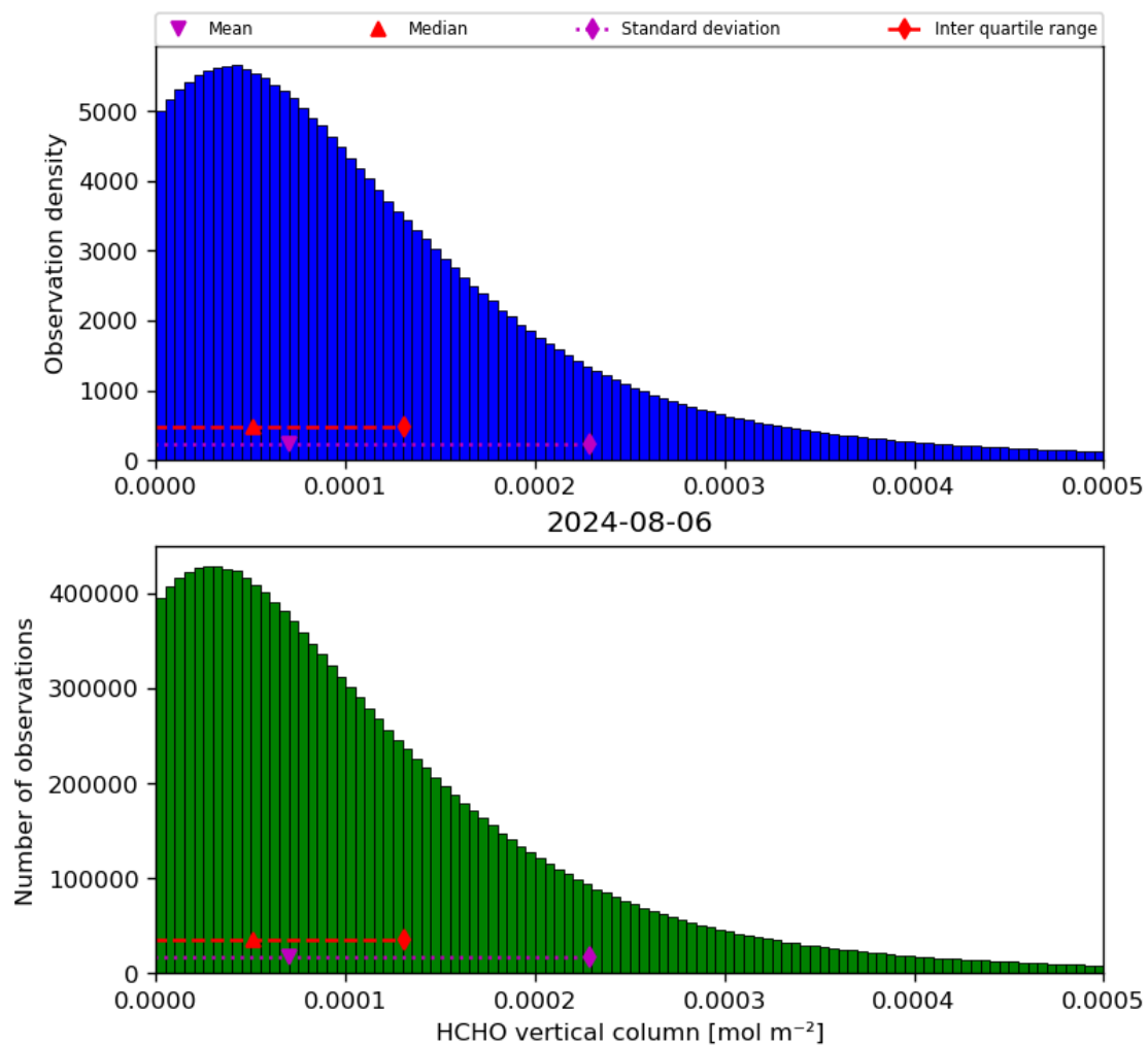
Figure 35: Histogram of “HCHO vertical column” for 2024-08-06 to 2024-08-07
