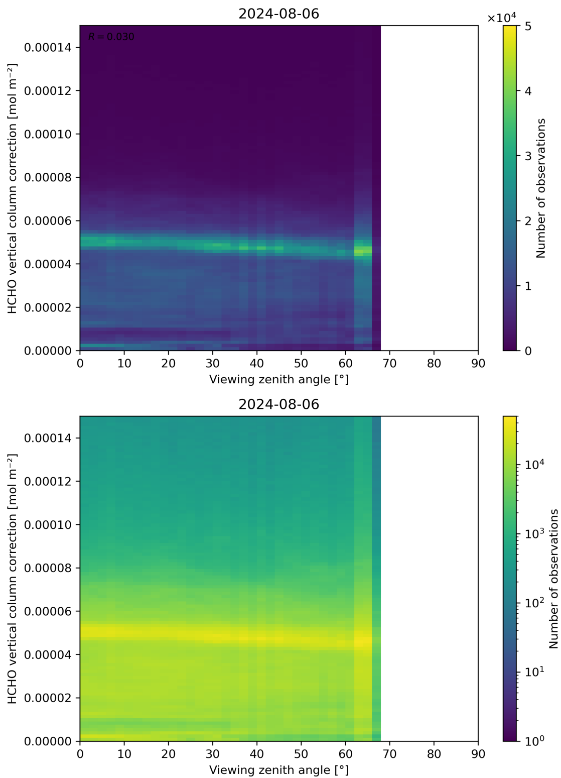
Figure 193: Scatter density plot of “Viewing zenith angle” against “HCHO vertical column correction” for 2024-08-06 to 2024-08-07.
