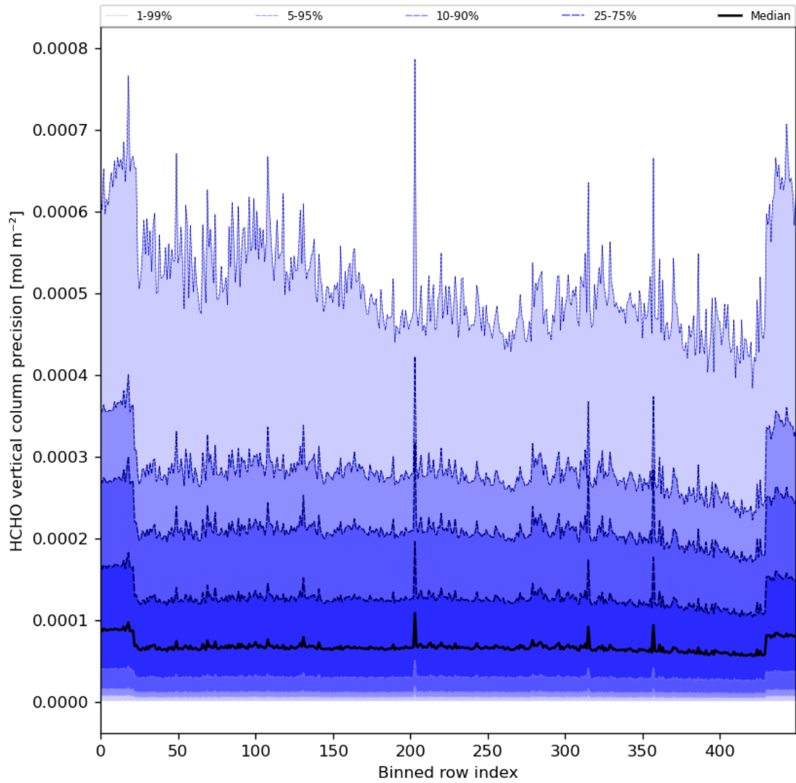
Figure 50: Along track statistics of “HCHO vertical column precision” for 2024-08-06 to 2024-08-07
