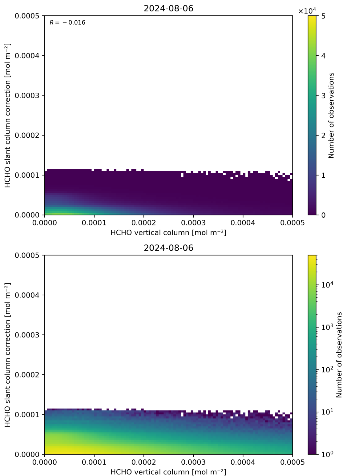
Figure 128: Scatter density plot of “HCHO vertical column” against “HCHO slant column correction” for 2024-08-06 to 2024-08-07.
