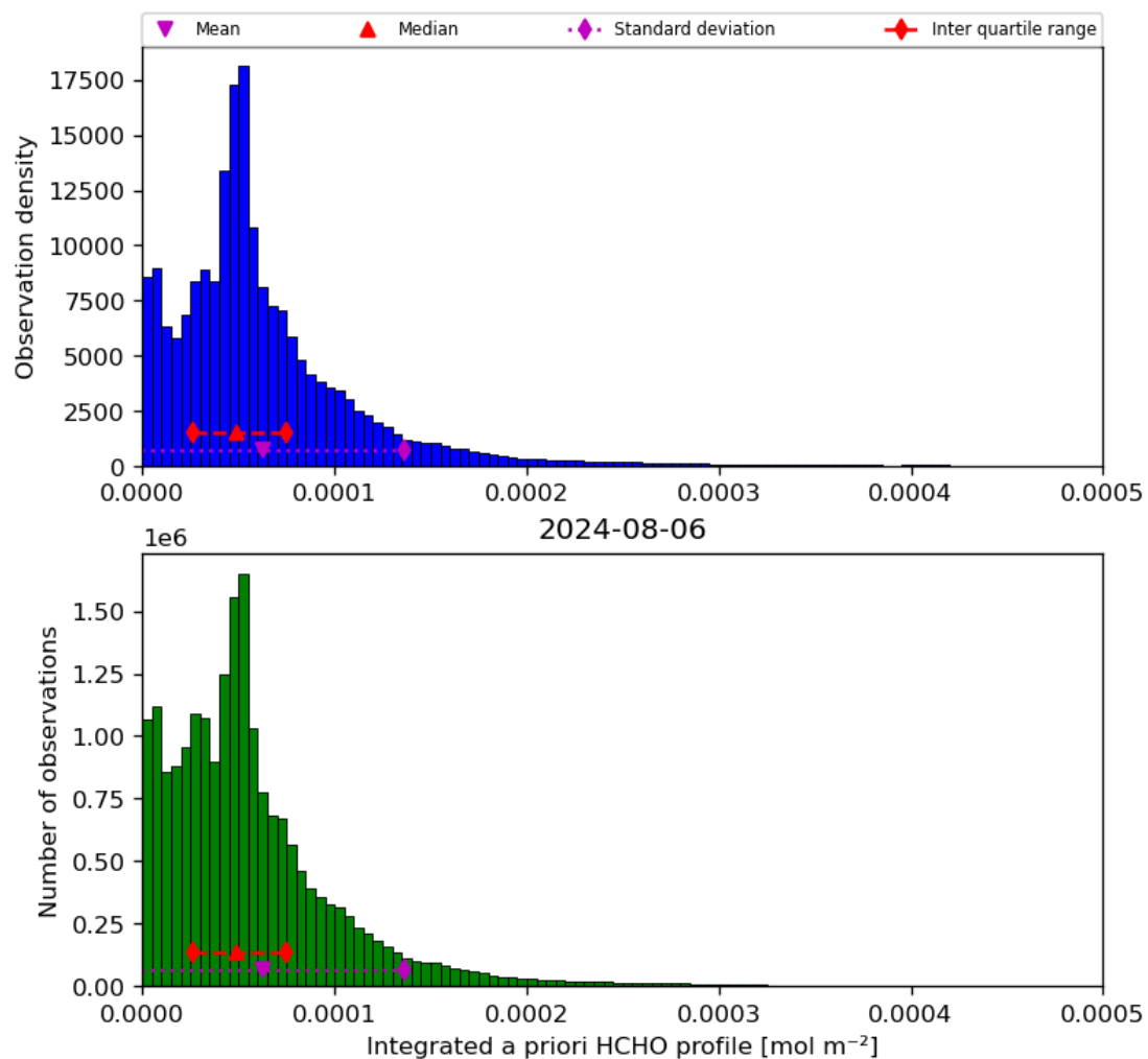
Figure 43: Histogram of “Integrated a priori HCHO profile” for 2024-08-06 to 2024-08-07
