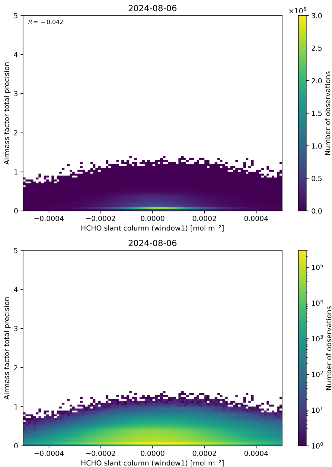
Figure 86: Scatter density plot of “HCHO slant column (window1)” against “Airmass factor total precision” for 2024-08-06 to 2024-08-07.
