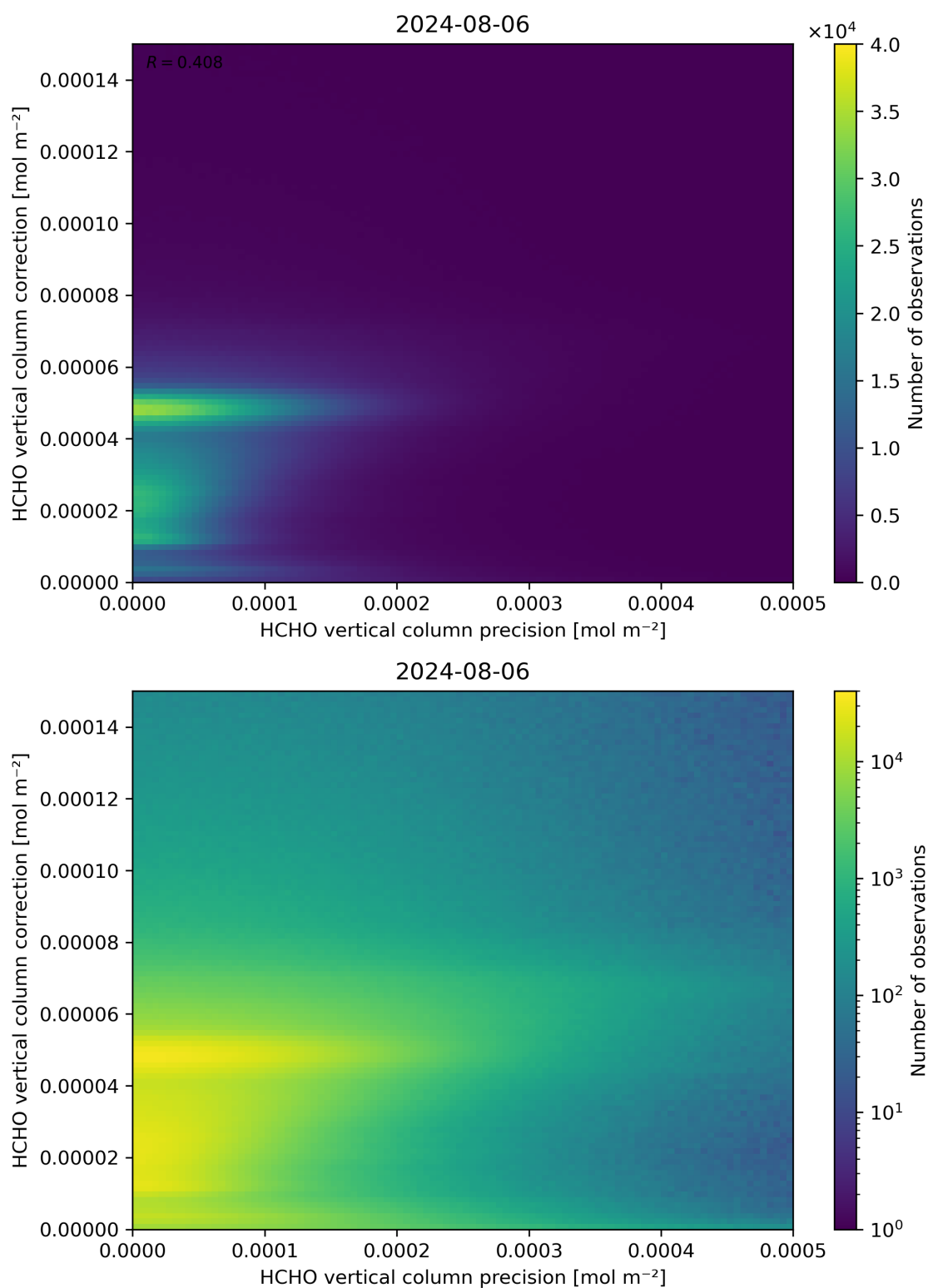
Figure 146: Scatter density plot of “HCHO vertical column precision” against “HCHO vertical column correction” for 2024-08-06 to 2024-08-07.
