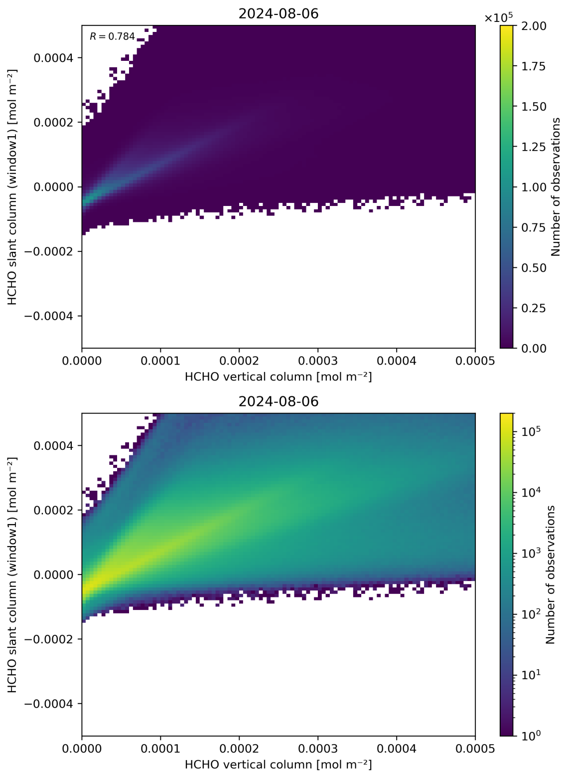
Figure 129: Scatter density plot of “HCHO vertical column” against “HCHO slant column (window1)” for 2024-08-06 to 2024-08-07.
