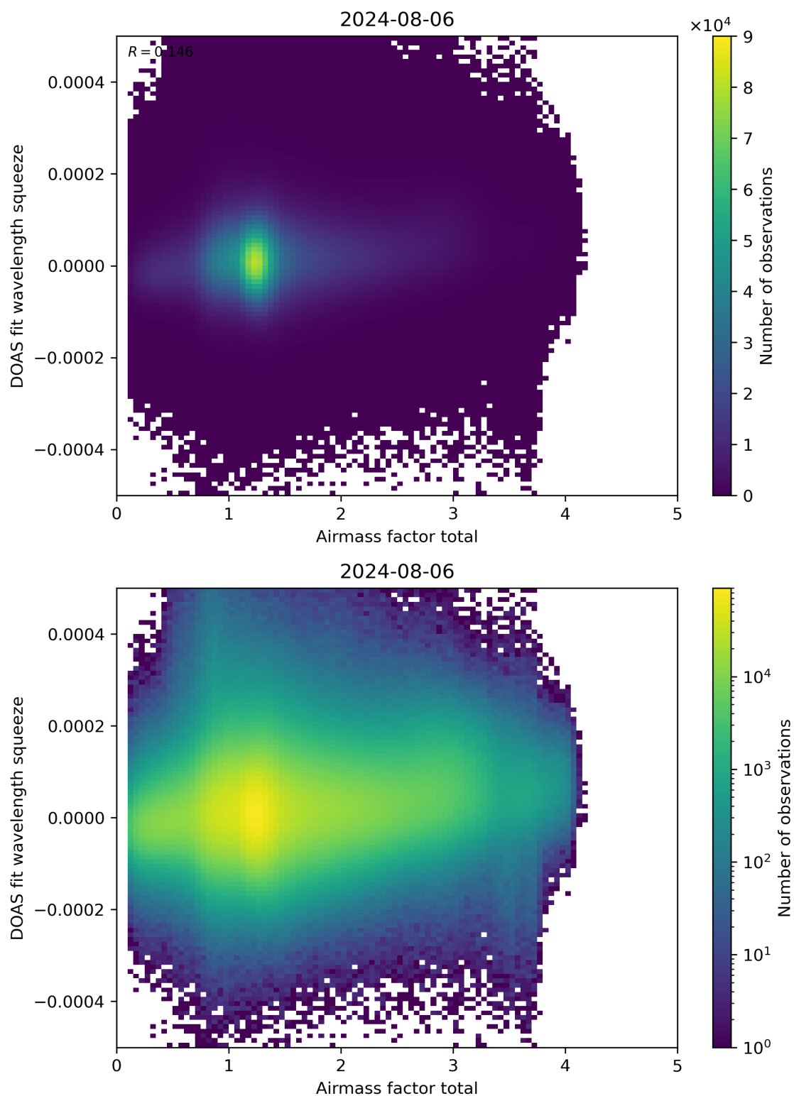
Figure 99: Scatter density plot of “Airmass factor total” against “DOAS fit wavelength squeeze” for 2024-08-06 to 2024-08-07.
