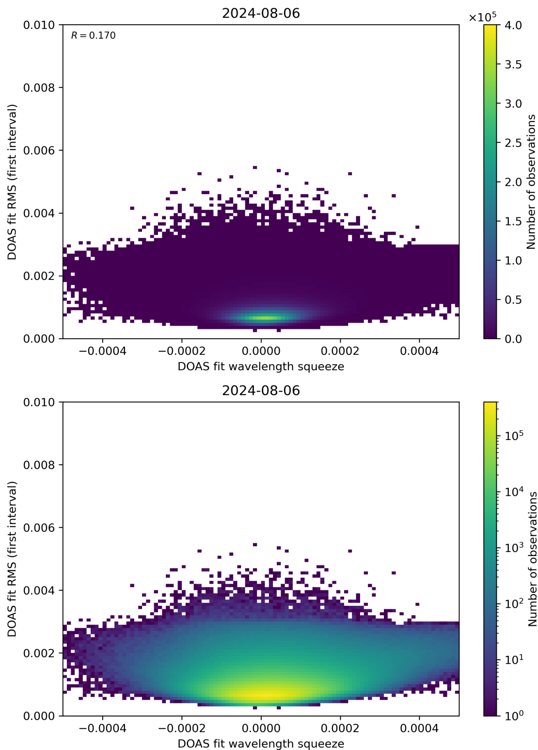
Figure 68: Scatter density plot of “DOAS fit wavelength squeeze” against “DOAS fit RMS (first interval)” for 2024-08-06 to 2024-08-07.
