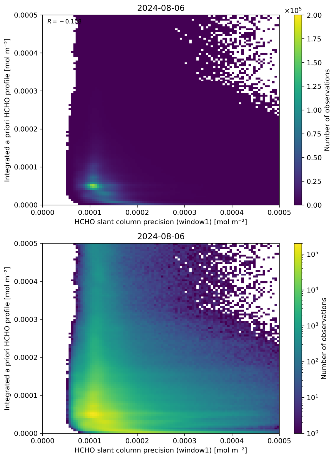
Figure 96: Scatter density plot of “HCHO slant column precision (window1)” against “Integrated a priori HCHO profile” for 2024-08-06 to 2024-08-07.
