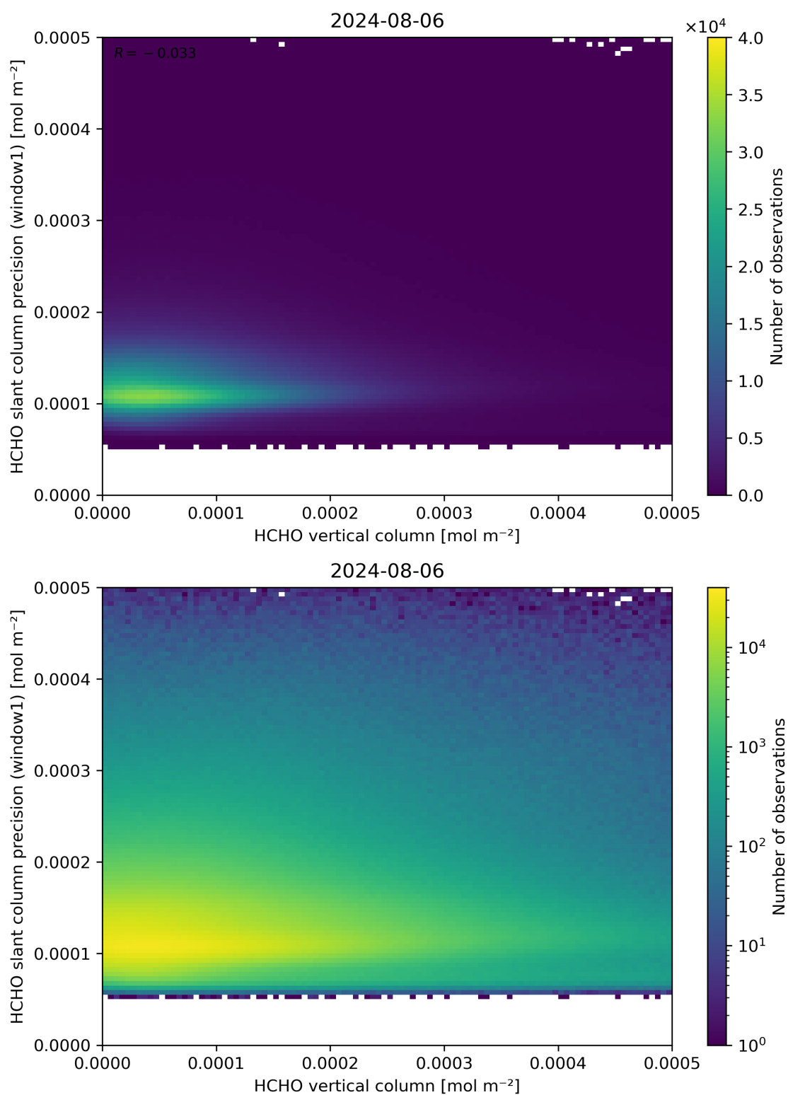
Figure 130: Scatter density plot of “HCHO vertical column” against “HCHO slant column precision (window1)” for 2024-08-06 to 2024-08-07.
