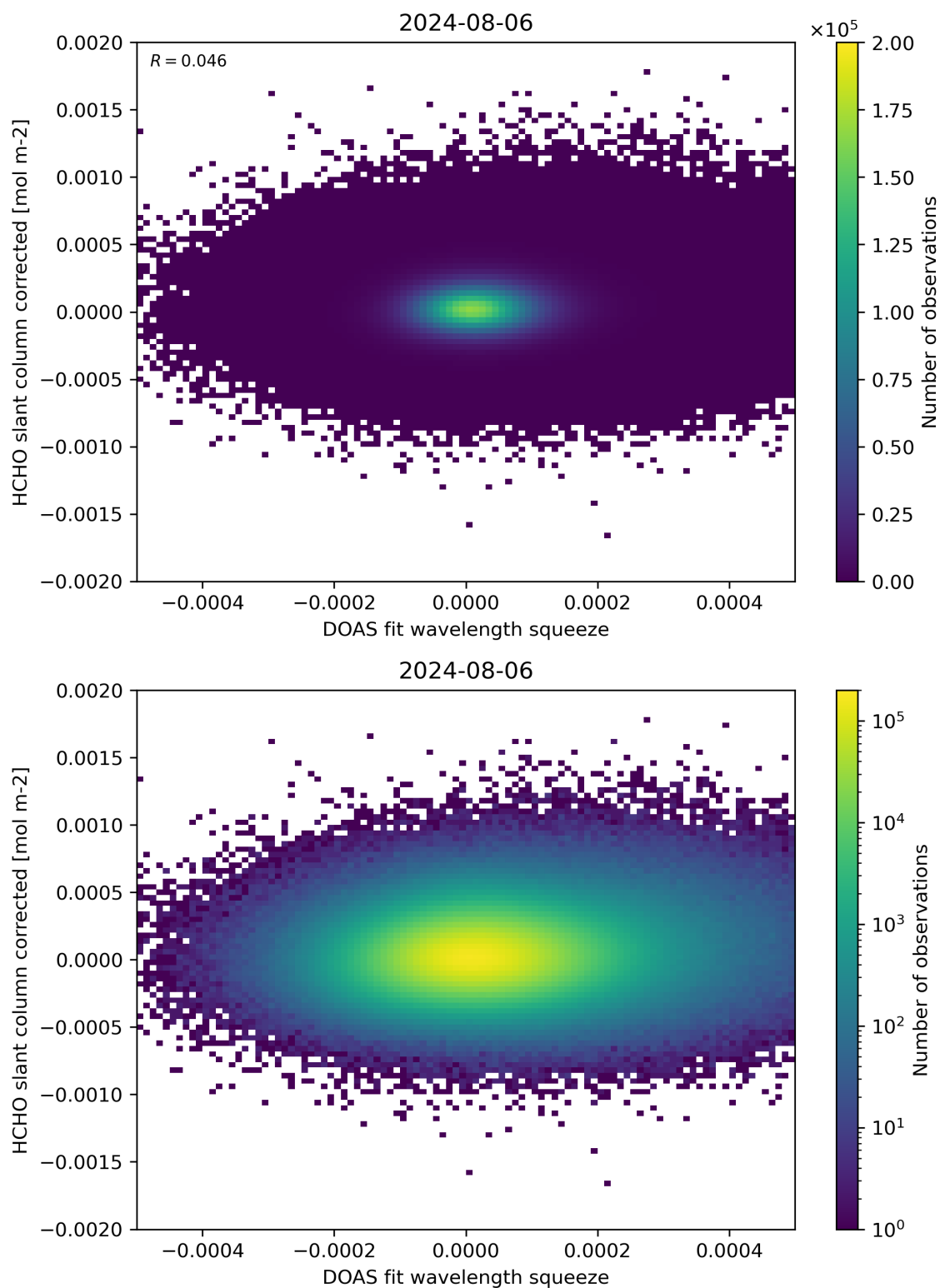
Figure 69: Scatter density plot of “DOAS fit wavelength squeeze” against “HCHO slant column corrected” for 2024-08-06 to 2024-08-07.
