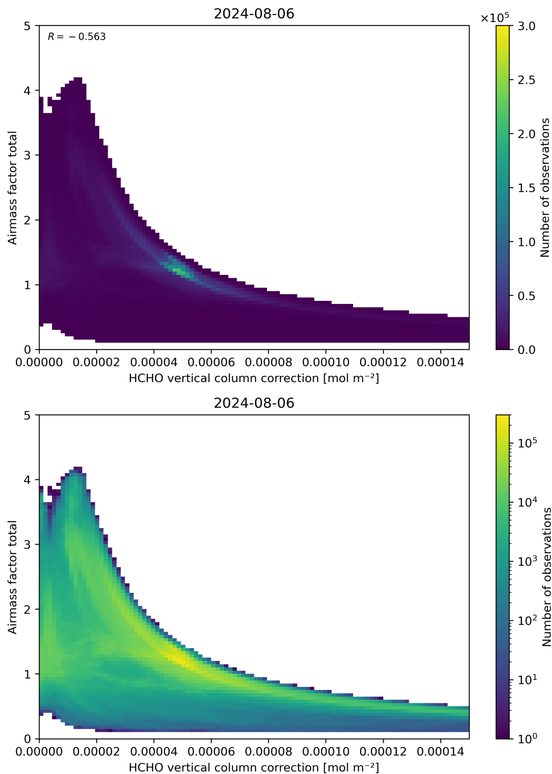
Figure 120: Scatter density plot of “HCHO vertical column correction” against “Airmass factor total” for 2024-08-06 to 2024-08-07.
