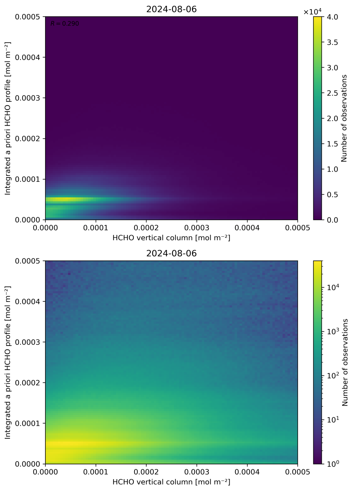
Figure 135: Scatter density plot of “HCHO vertical column” against “Integrated a priori HCHO profile” for 2024-08-06 to 2024-08-07.
