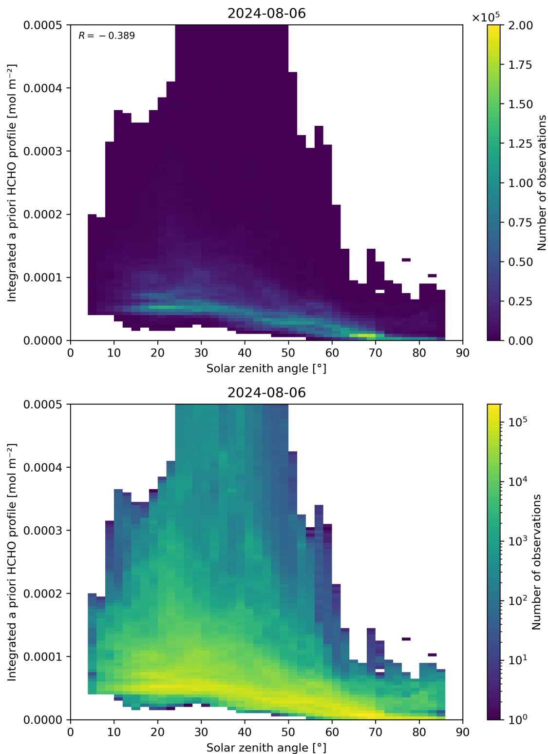
Figure 180: Scatter density plot of “Solar zenith angle” against “Integrated a priori HCHO profile” for 2024-08-06 to 2024-08-07.
