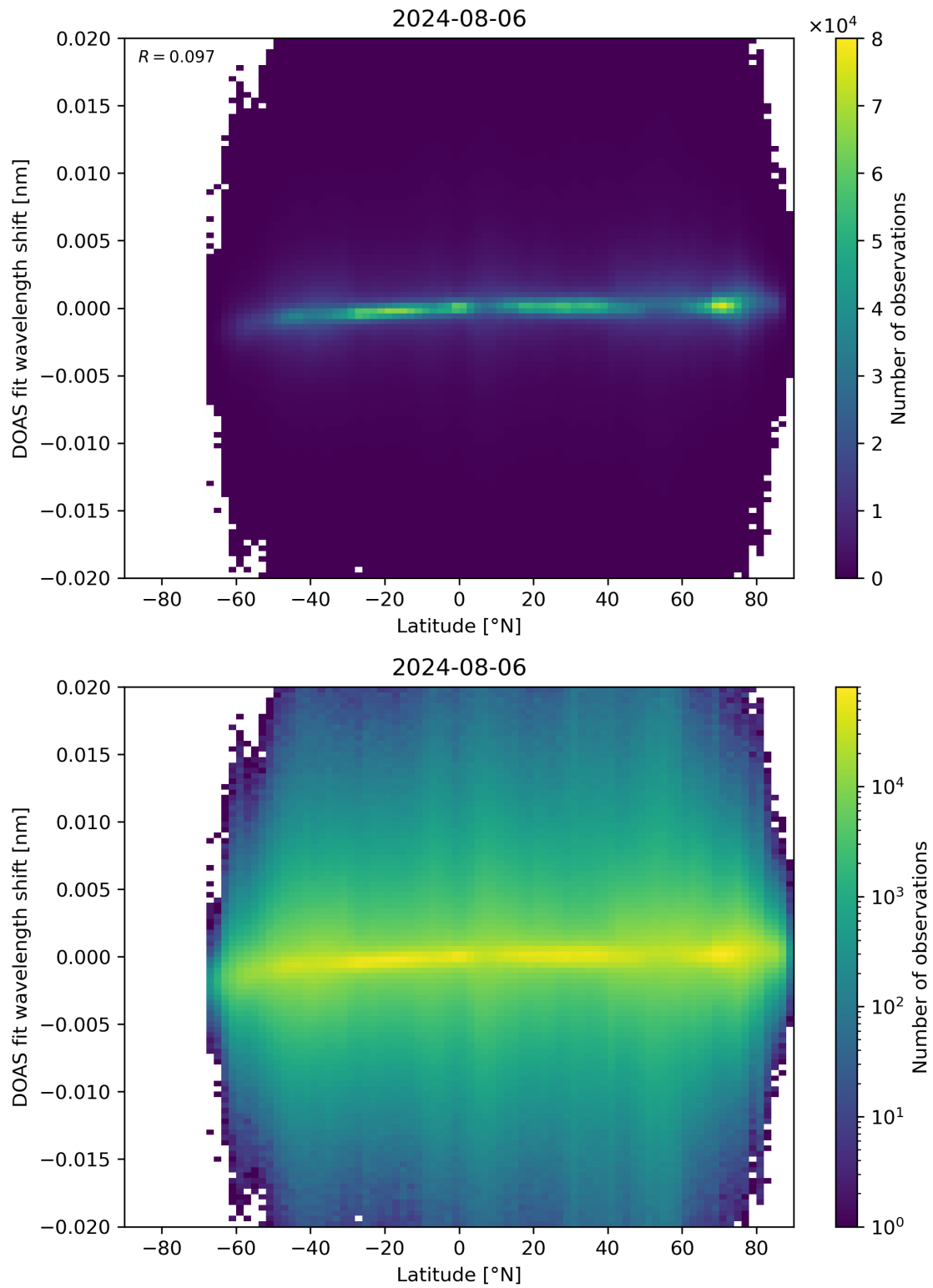
Figure 154: Scatter density plot of “Latitude” against “DOAS fit wavelength shift” for 2024-08-06 to 2024-08-07.
