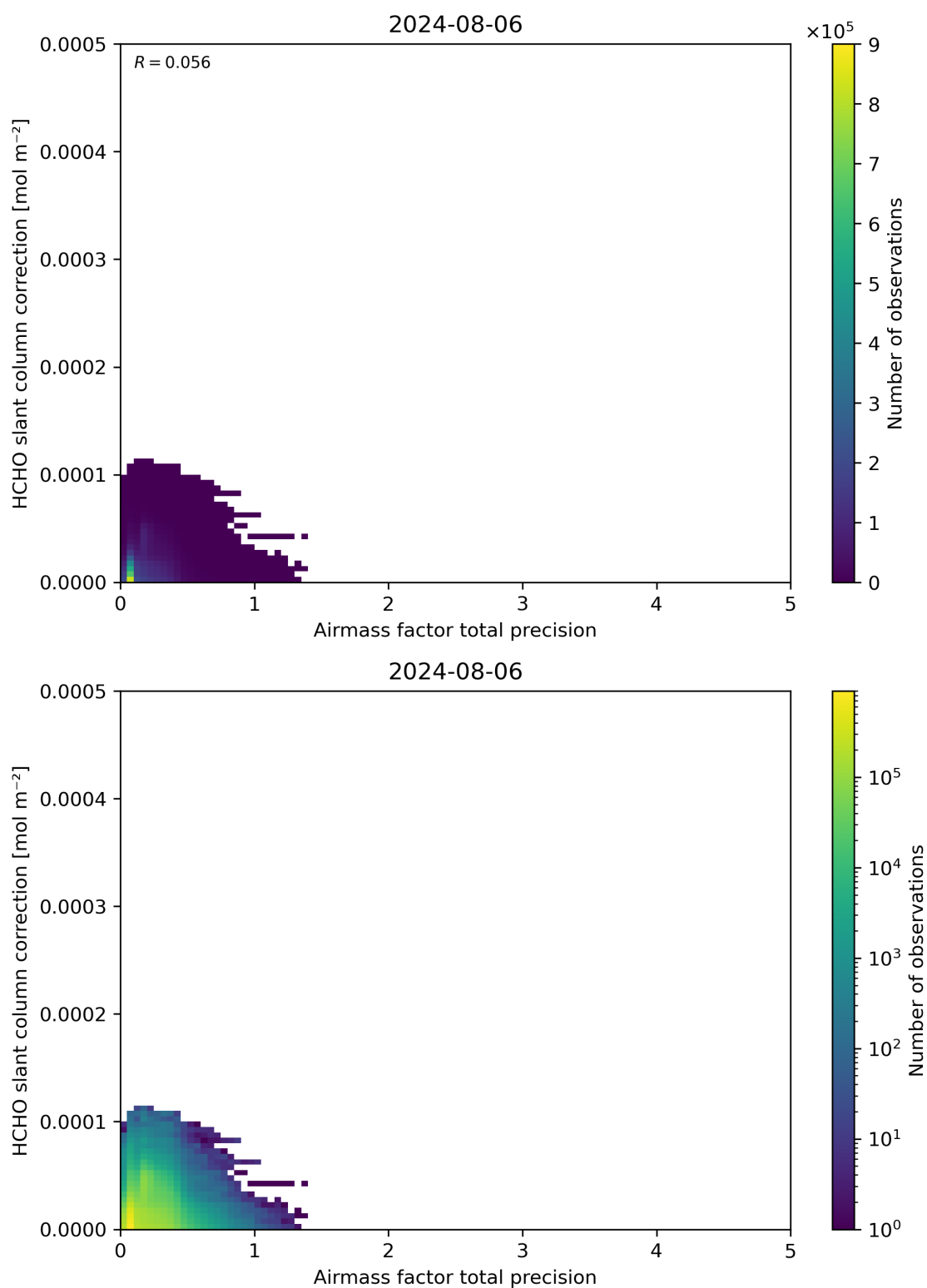
Figure 110: Scatter density plot of “Airmass factor total precision” against “HCHO slant column correction” for 2024-08-06 to 2024-08-07.
