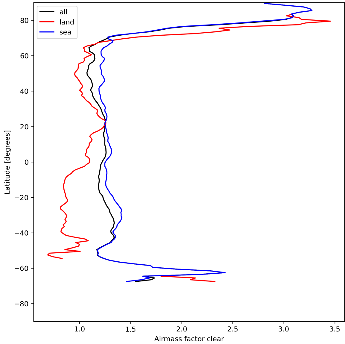
Figure 28: Zonal average of “Airmass factor clear” for 2024-08-06 to 2024-08-07.
