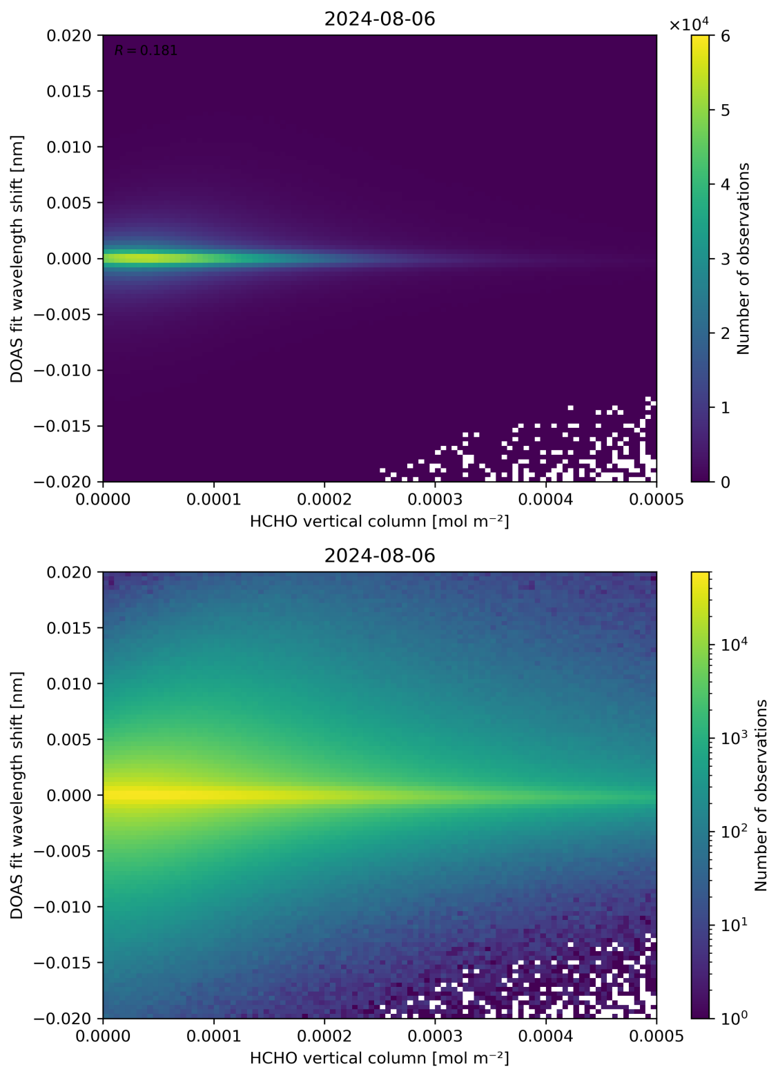
Figure 124: Scatter density plot of “HCHO vertical column” against “DOAS fit wavelength shift” for 2024-08-06 to 2024-08-07.
