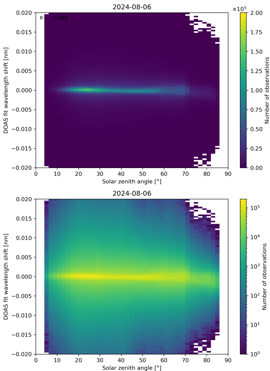
Figure 168: Scatter density plot of “Solar zenith angle” against “DOAS fit wavelength shift” for 2024-08-06 to 2024-08-07.
