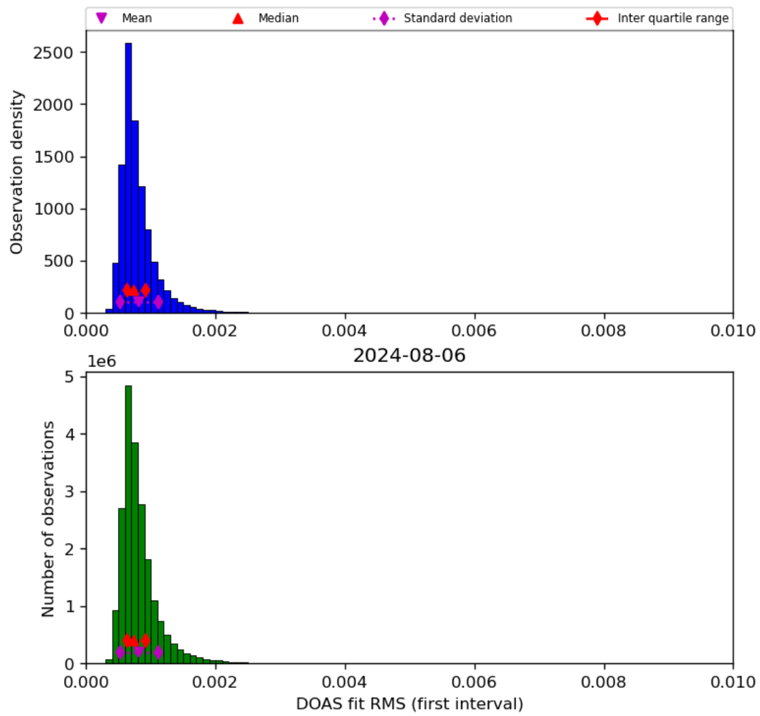
Figure 46: Histogram of “DOAS fit RMS (first interval)” for 2024-08-06 to 2024-08-07
