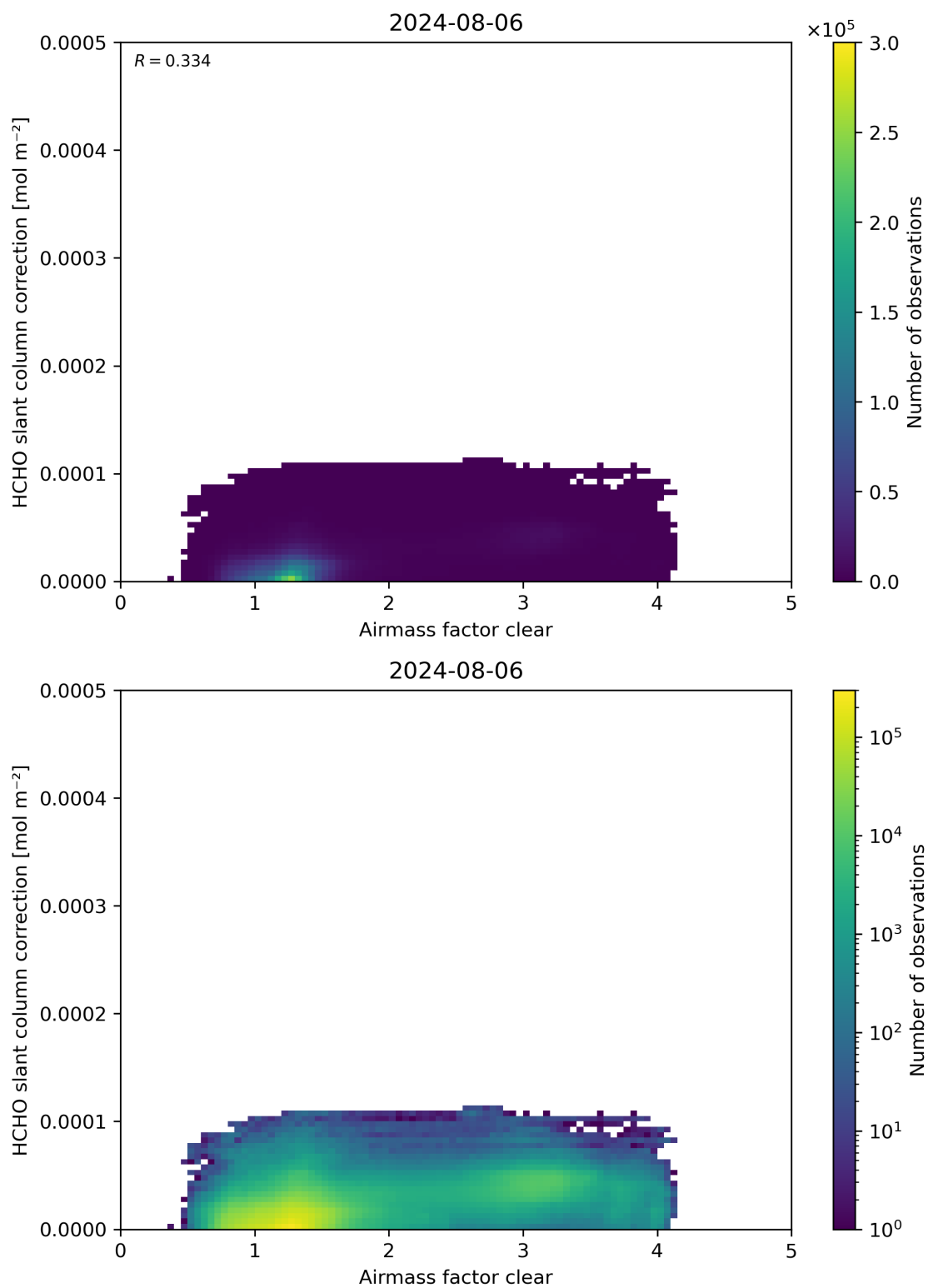
Figure 75: Scatter density plot of “Airmass factor clear” against “HCHO slant column correction” for 2024-08-06 to 2024-08-07.
