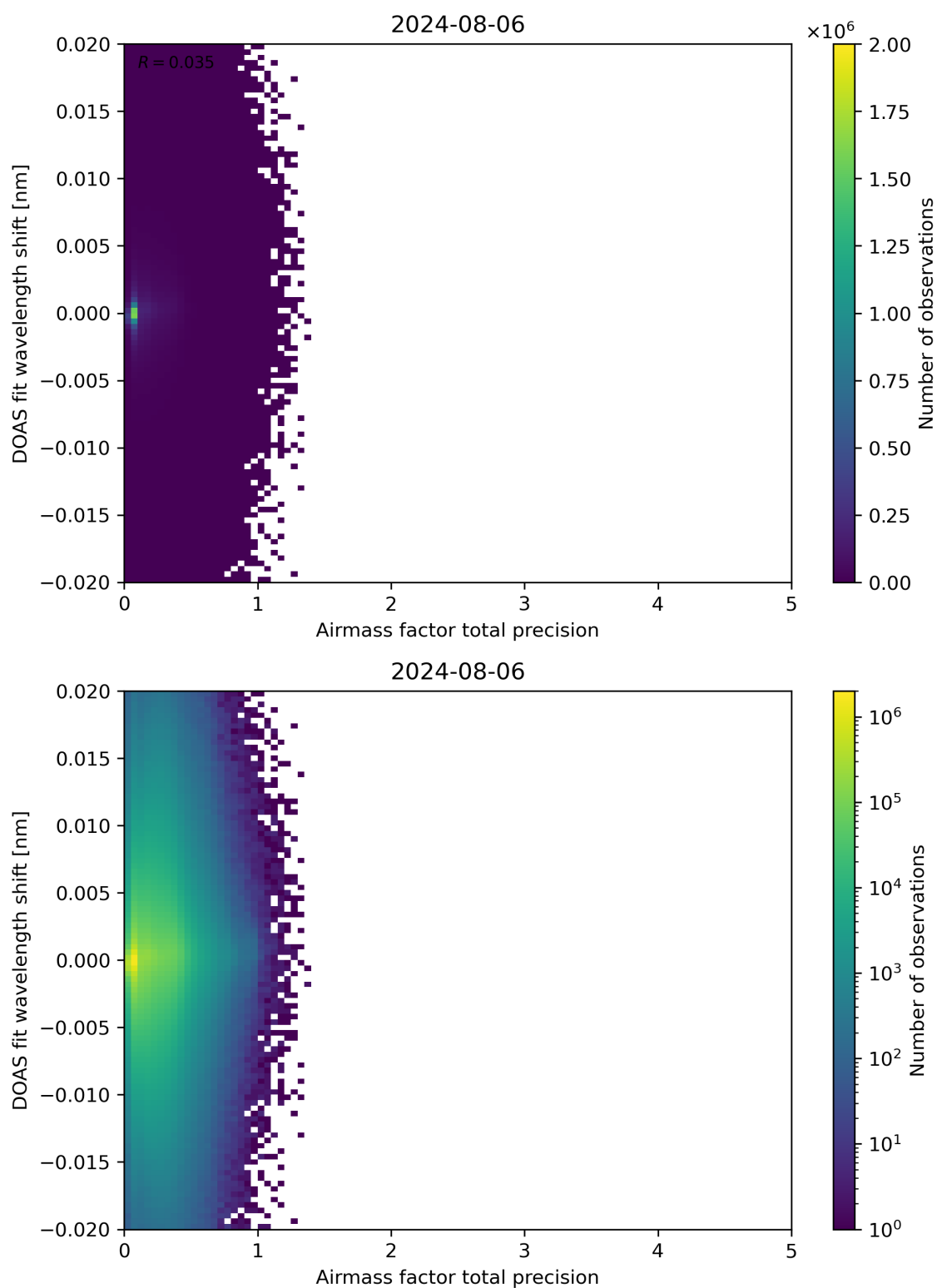
Figure 106: Scatter density plot of “Airmass factor total precision” against “DOAS fit wavelength shift” for 2024-08-06 to 2024-08-07.
