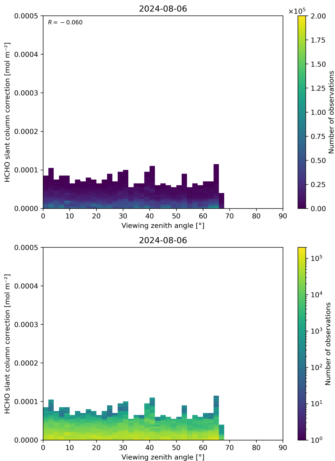
Figure 187: Scatter density plot of “Viewing zenith angle” against “HCHO slant column correction” for 2024-08-06 to 2024-08-07.
