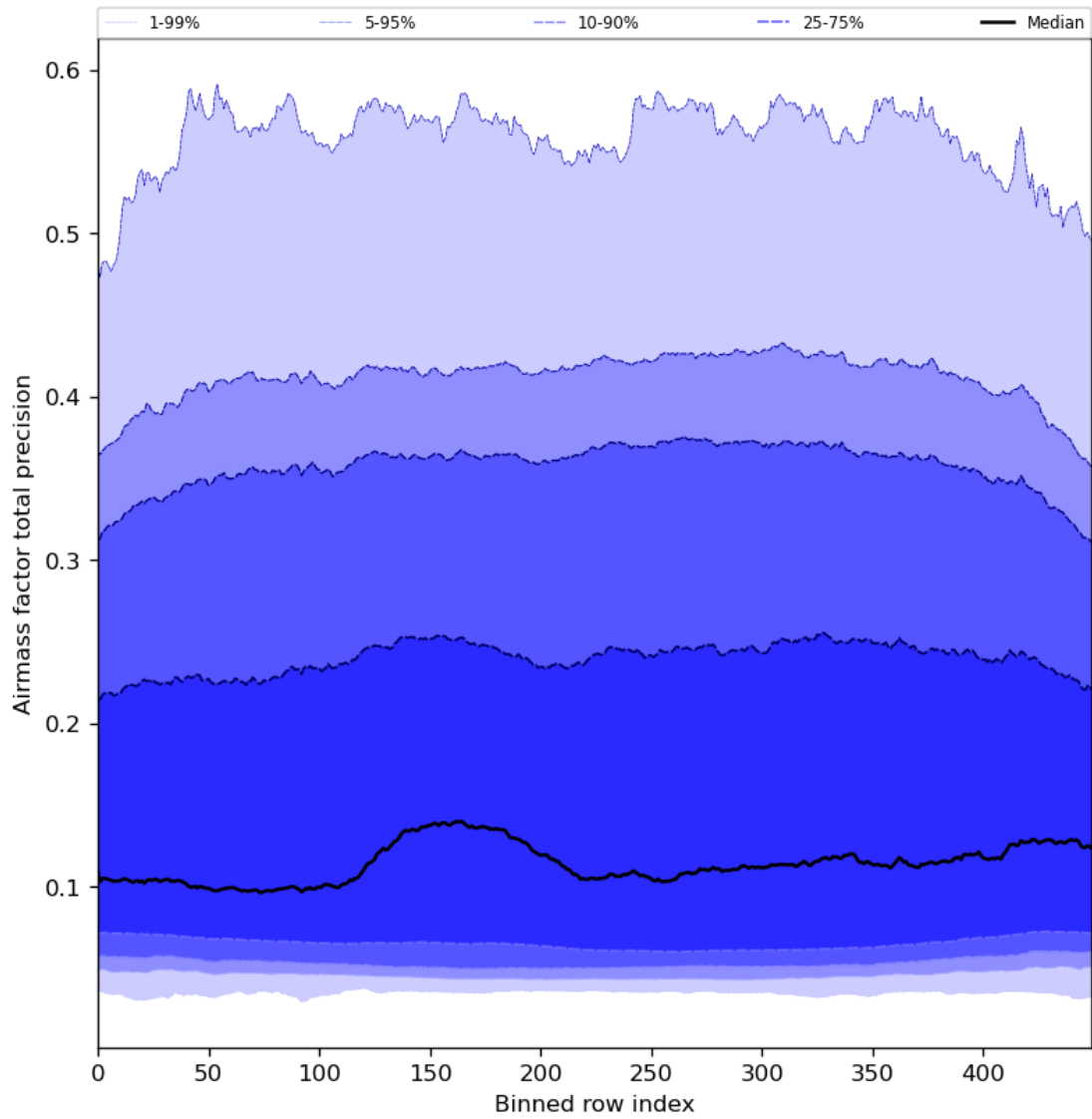
Figure 55: Along track statistics of “Airmass factor total precision” for 2024-08-06 to 2024-08-07
