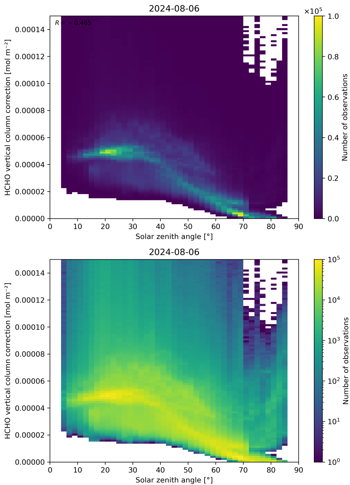
Figure 178: Scatter density plot of “Solar zenith angle” against “HCHO vertical column correction” for 2024-08-06 to 2024-08-07.
