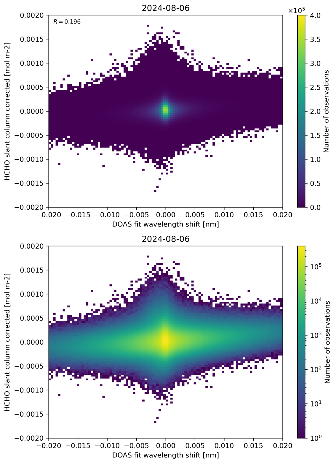
Figure 66: Scatter density plot of “DOAS fit wavelength shift” against “HCHO slant column corrected” for 2024-08-06 to 2024-08-07.
