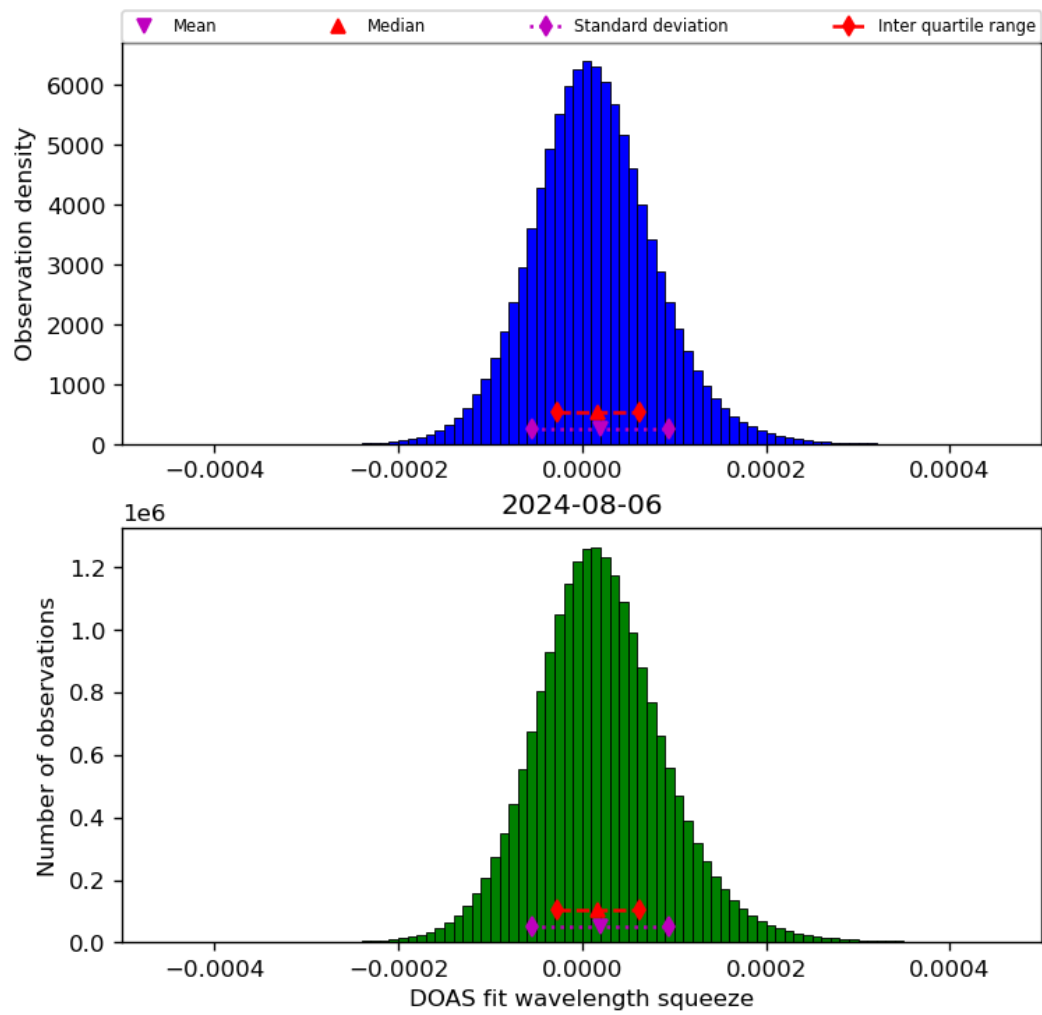
Figure 45: Histogram of “DOAS fit wavelength squeeze” for 2024-08-06 to 2024-08-07
