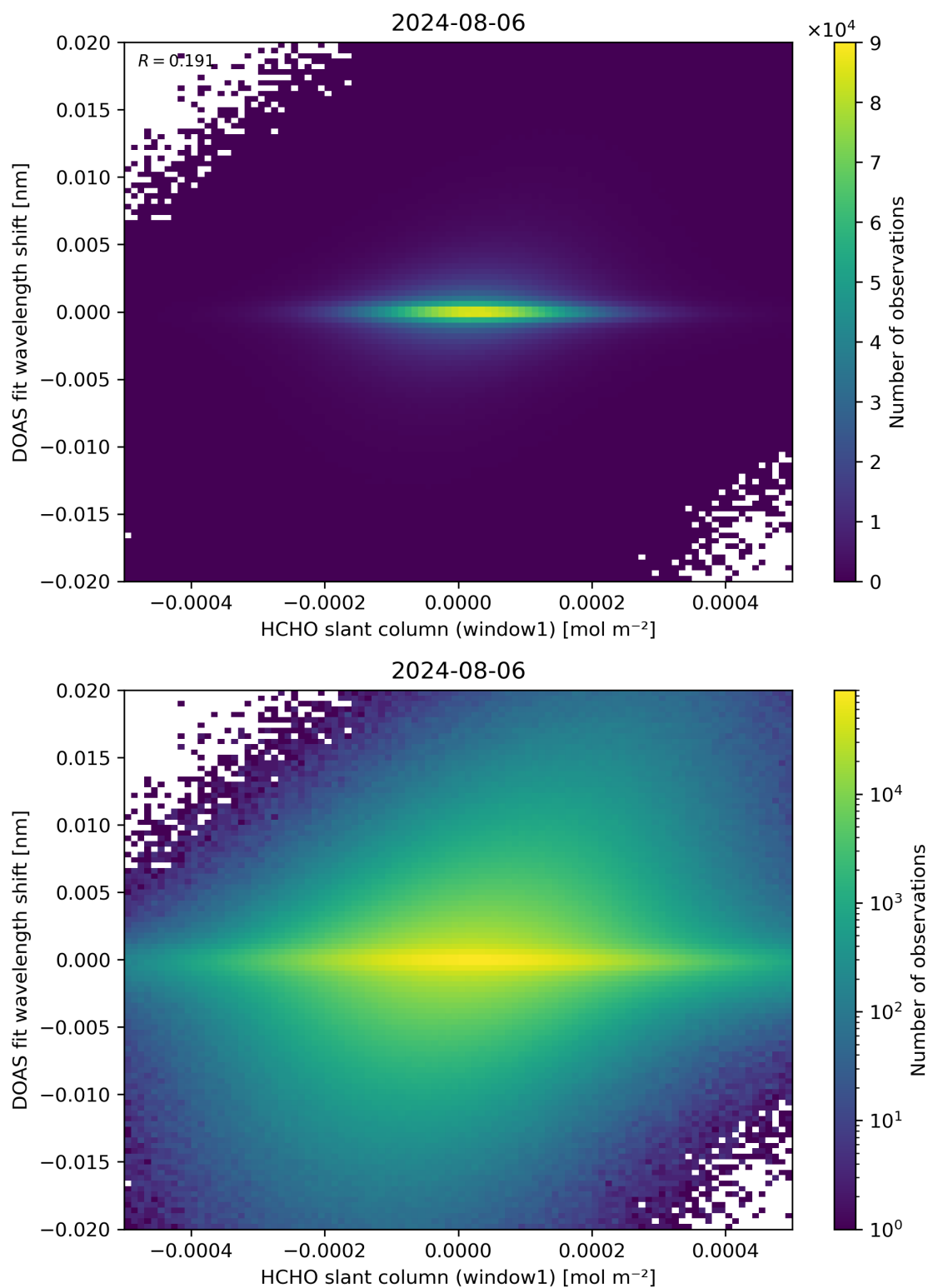
Figure 79: Scatter density plot of “HCHO slant column (window1)” against “DOAS fit wavelength shift” for 2024-08-06 to 2024-08-07.
