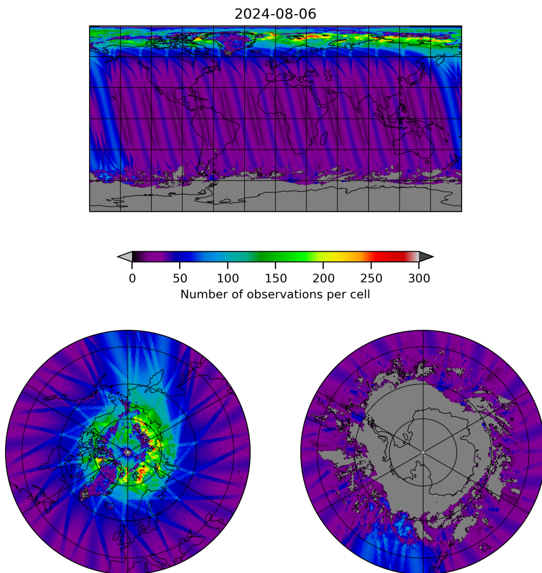
Figure 19: Map of the number of observations for 2024-08-06 to 2024-08-07
