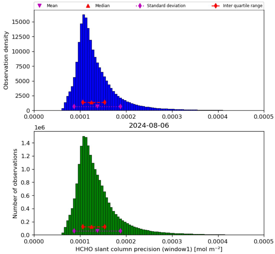
Figure 39: Histogram of “HCHO slant column precision (window1)” for 2024-08-06 to 2024-08-07
