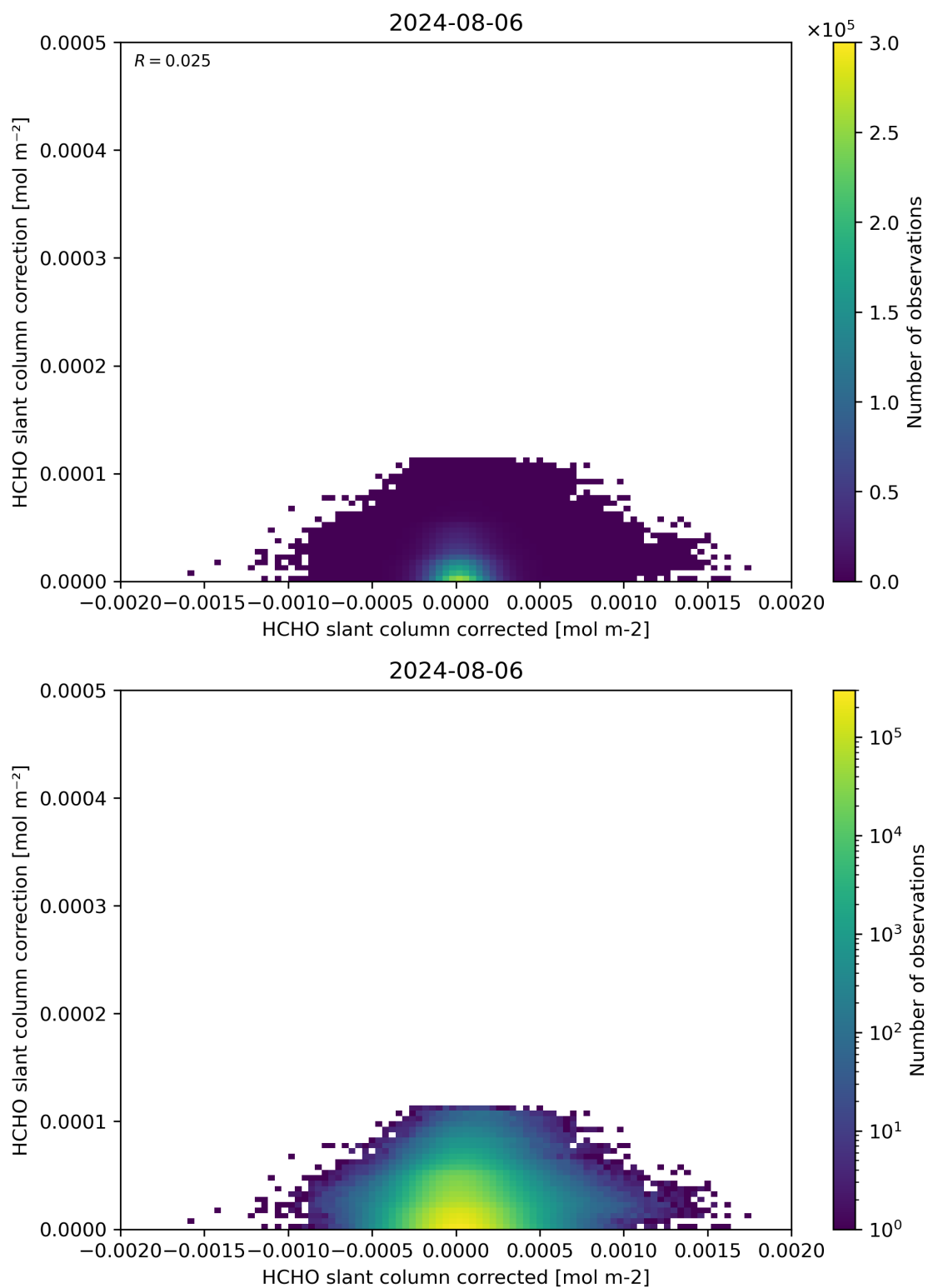
Figure 77: Scatter density plot of “HCHO slant column corrected” against “HCHO slant column correction” for 2024-08-06 to 2024-08-07.
