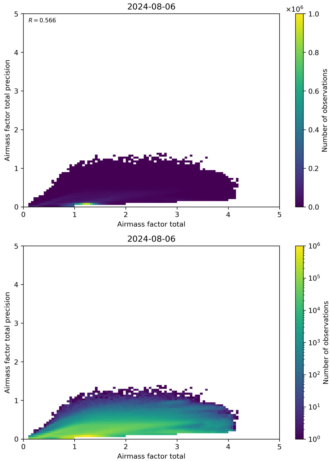
Figure 103: Scatter density plot of “Airmass factor total” against “Airmass factor total precision” for 2024-08-06 to 2024-08-07.
