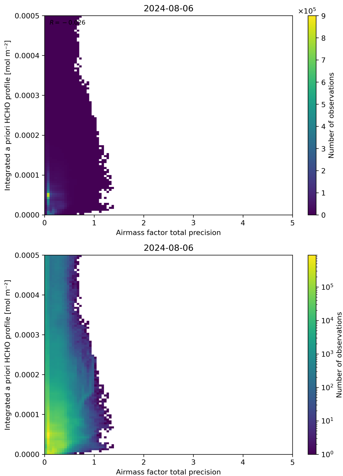
Figure 111: Scatter density plot of “Airmass factor total precision” against “Integrated a priori HCHO profile” for 2024-08-06 to 2024-08-07.
