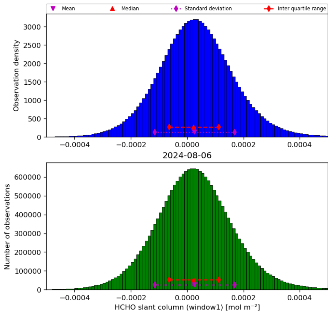
Figure 38: Histogram of “HCHO slant column (window1)” for 2024-08-06 to 2024-08-07
