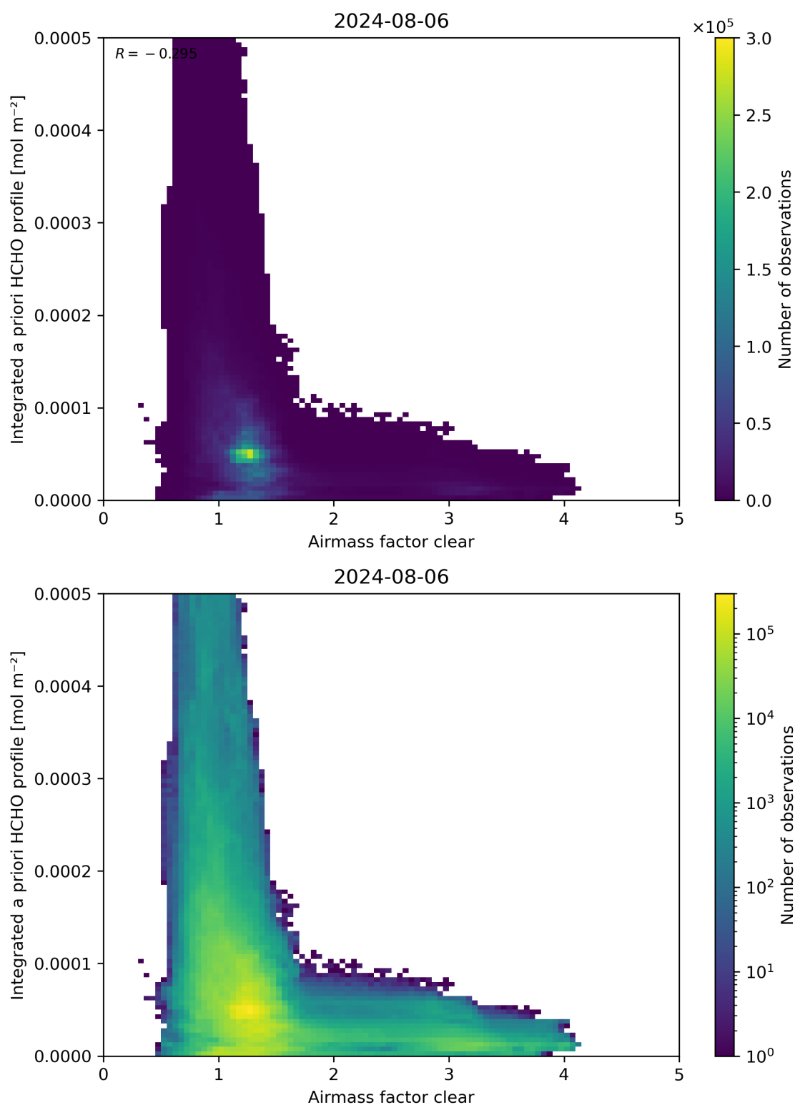
Figure 76: Scatter density plot of “Airmass factor clear” against “Integrated a priori HCHO profile” for 2024-08-06 to 2024-08-07.
