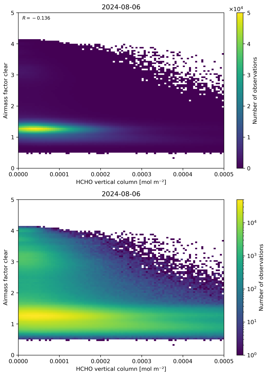
Figure 126: Scatter density plot of “HCHO vertical column” against “Airmass factor clear” for 2024-08-06 to 2024-08-07.
