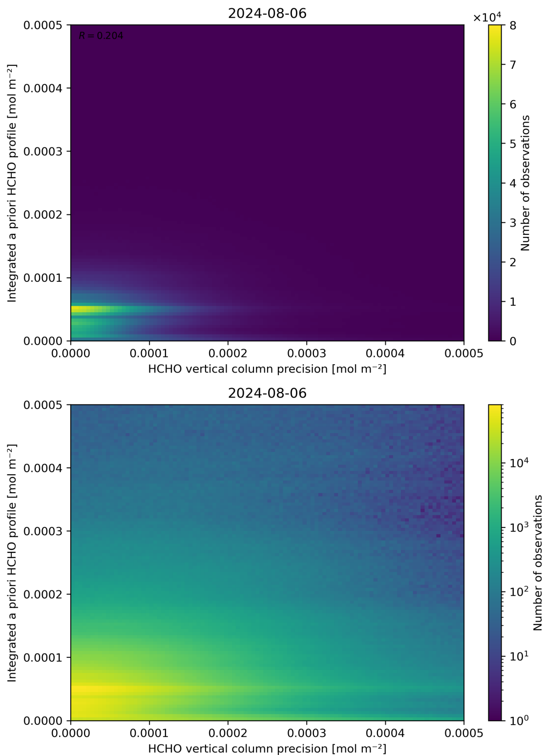
Figure 147: Scatter density plot of “HCHO vertical column precision” against “Integrated a priori HCHO profile” for 2024-08-06 to 2024-08-07.
