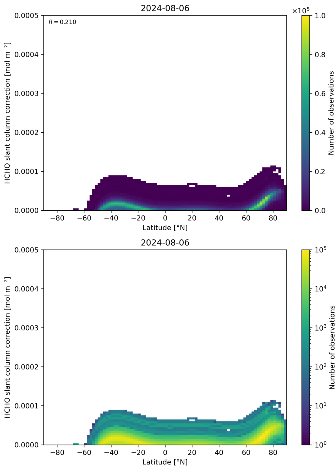
Figure 158: Scatter density plot of “Latitude” against “HCHO slant column correction” for 2024-08-06 to 2024-08-07.
