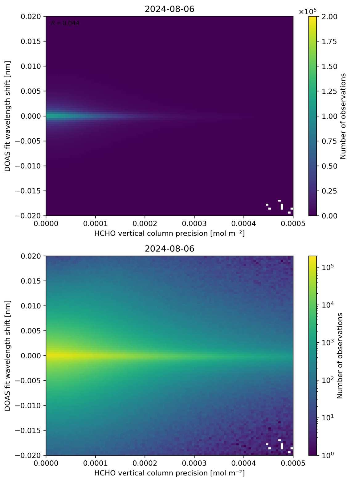
Figure 137: Scatter density plot of “HCHO vertical column precision” against “DOAS fit wavelength shift” for 2024-08-06 to 2024-08-07.
