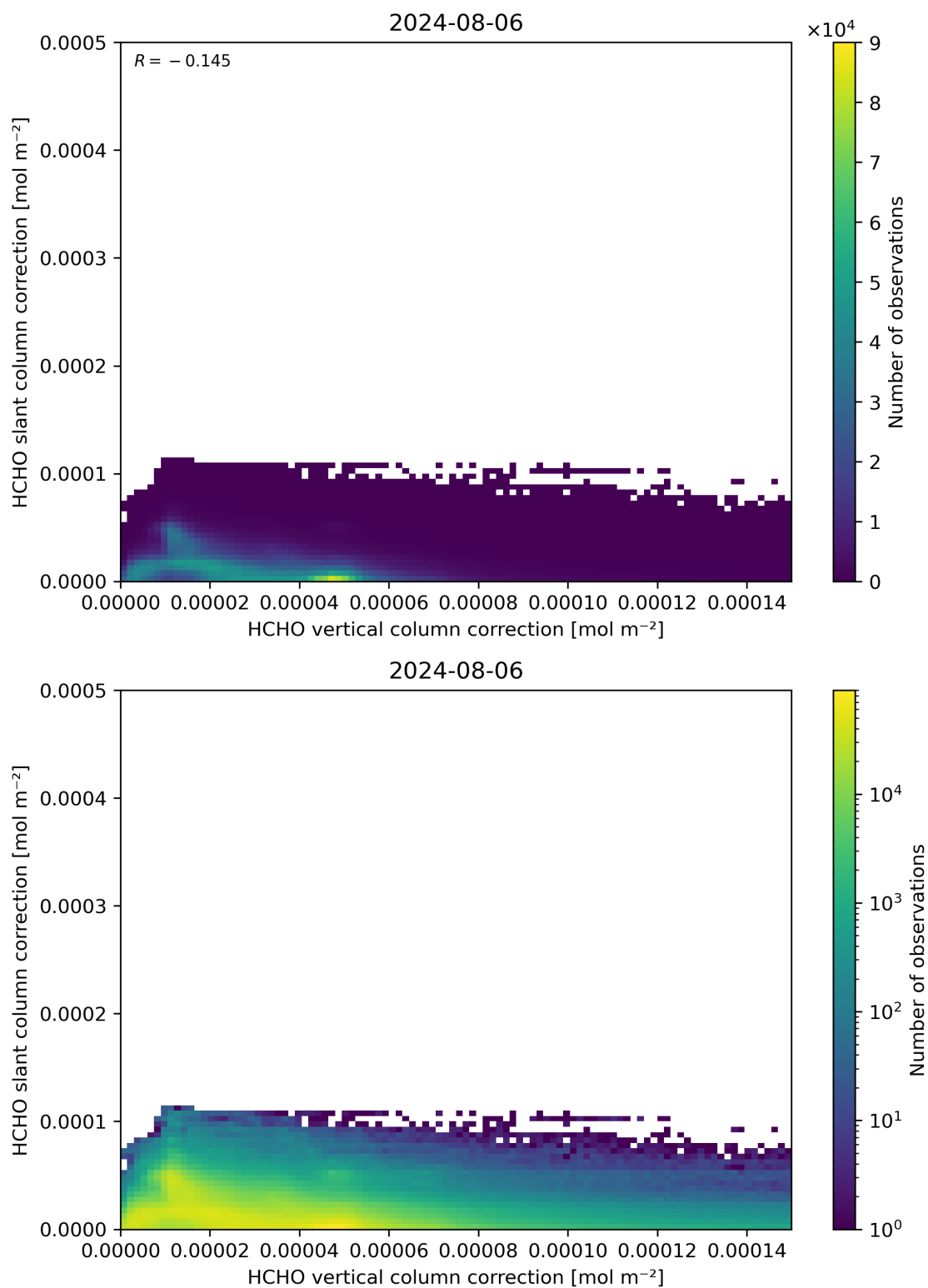
Figure 117: Scatter density plot of “HCHO vertical column correction” against “HCHO slant column correction” for 2024-08-06 to 2024-08-07.
