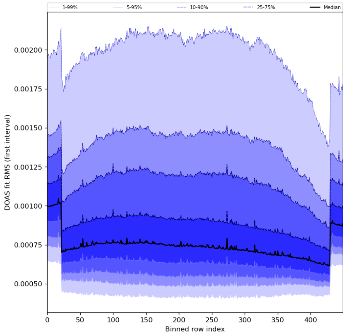
Figure 60: Along track statistics of “DOAS fit RMS (first interval)” for 2024-08-06 to 2024-08-07
