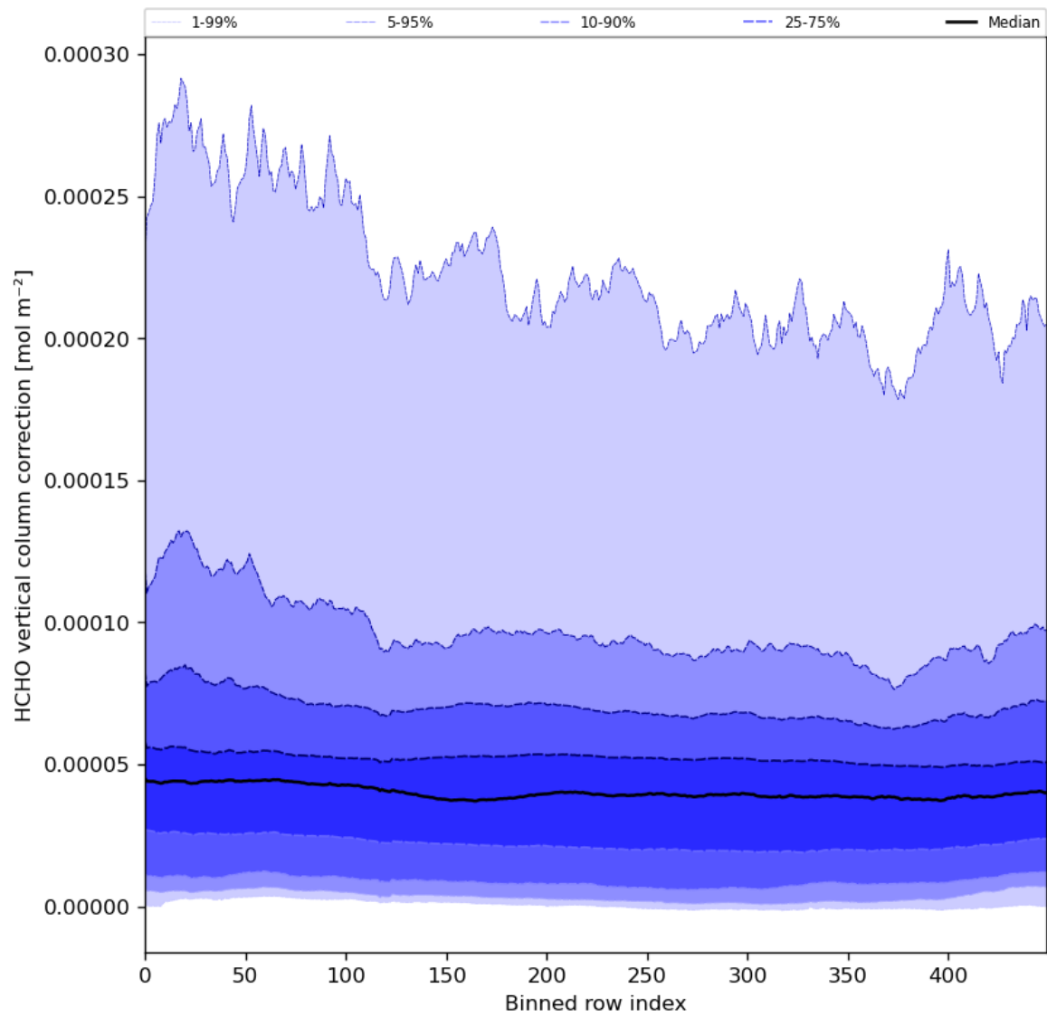
Figure 51: Along track statistics of “HCHO vertical column correction” for 2024-08-06 to 2024-08-07
