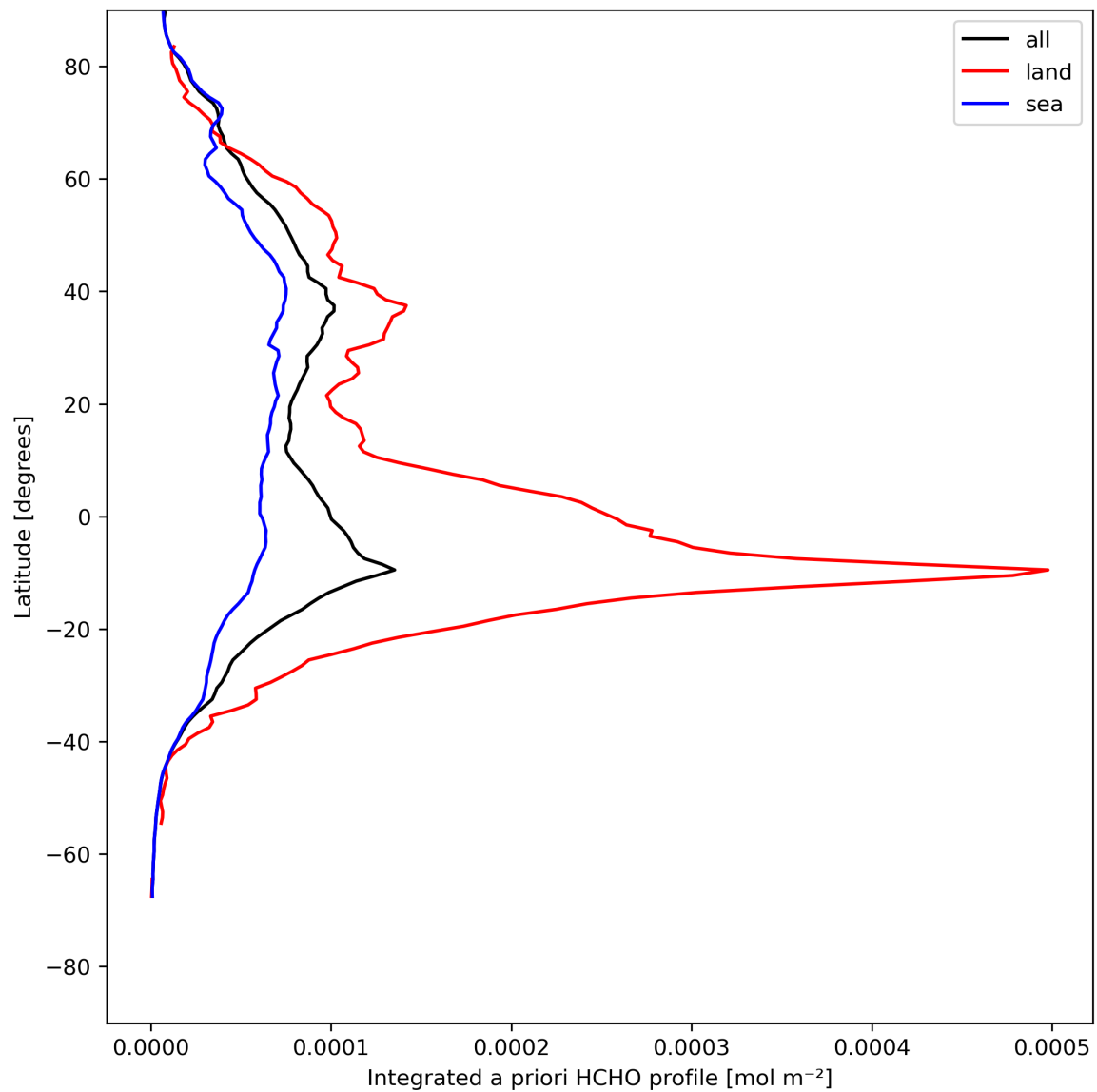
Figure 29: Zonal average of “Integrated a priori HCHO profile” for 2024-08-06 to 2024-08-07.
