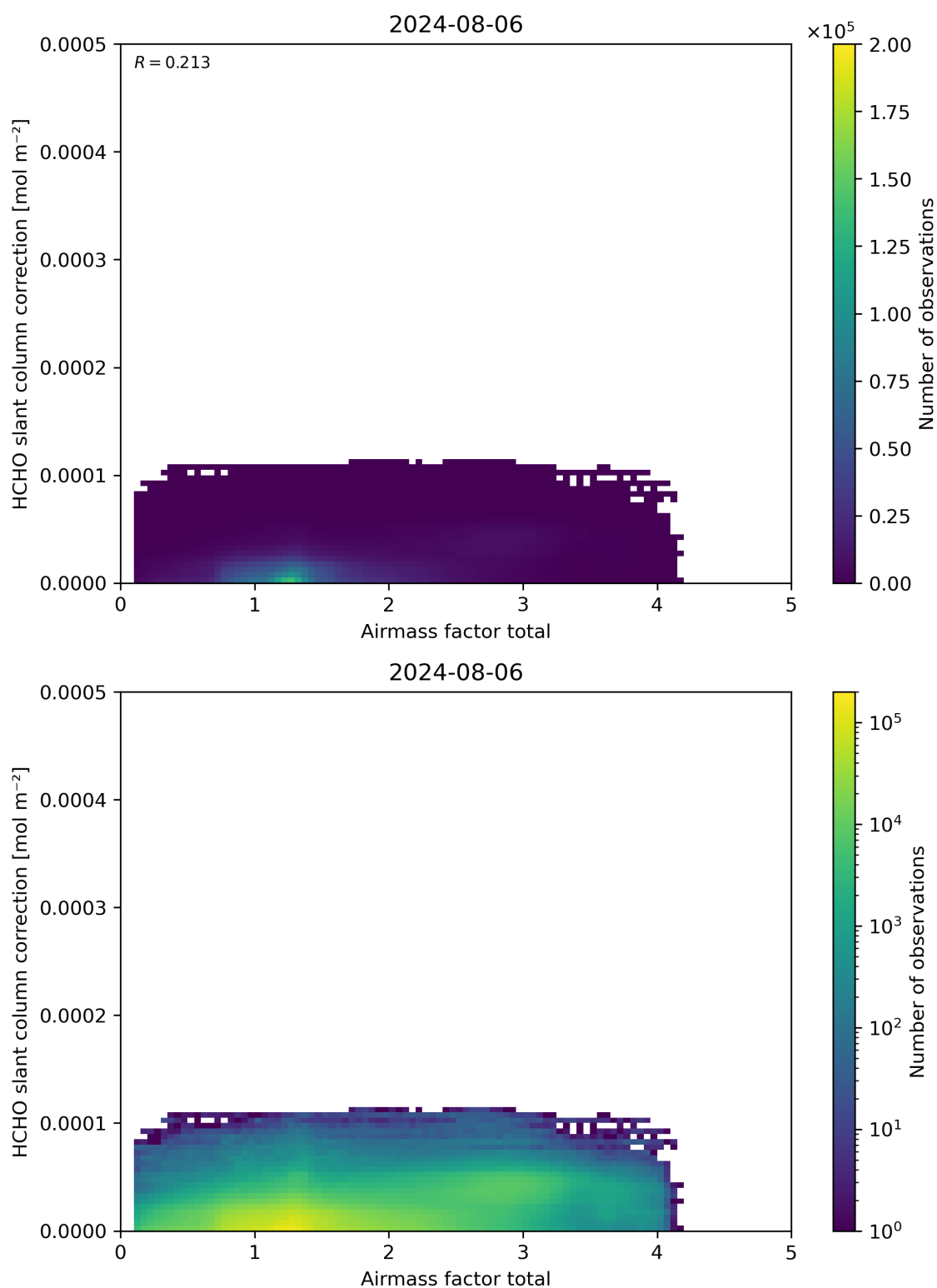
Figure 102: Scatter density plot of “Airmass factor total” against “HCHO slant column correction” for 2024-08-06 to 2024-08-07.
