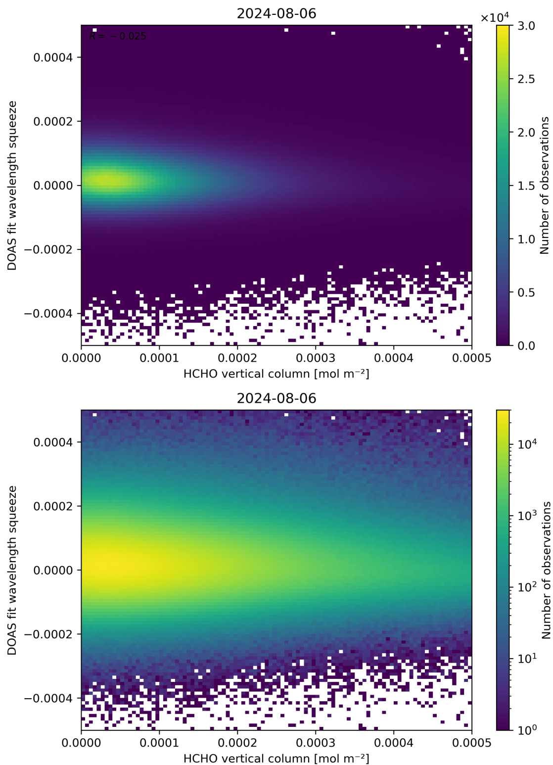
Figure 125: Scatter density plot of “HCHO vertical column” against “DOAS fit wavelength squeeze” for 2024-08-06 to 2024-08-07.
