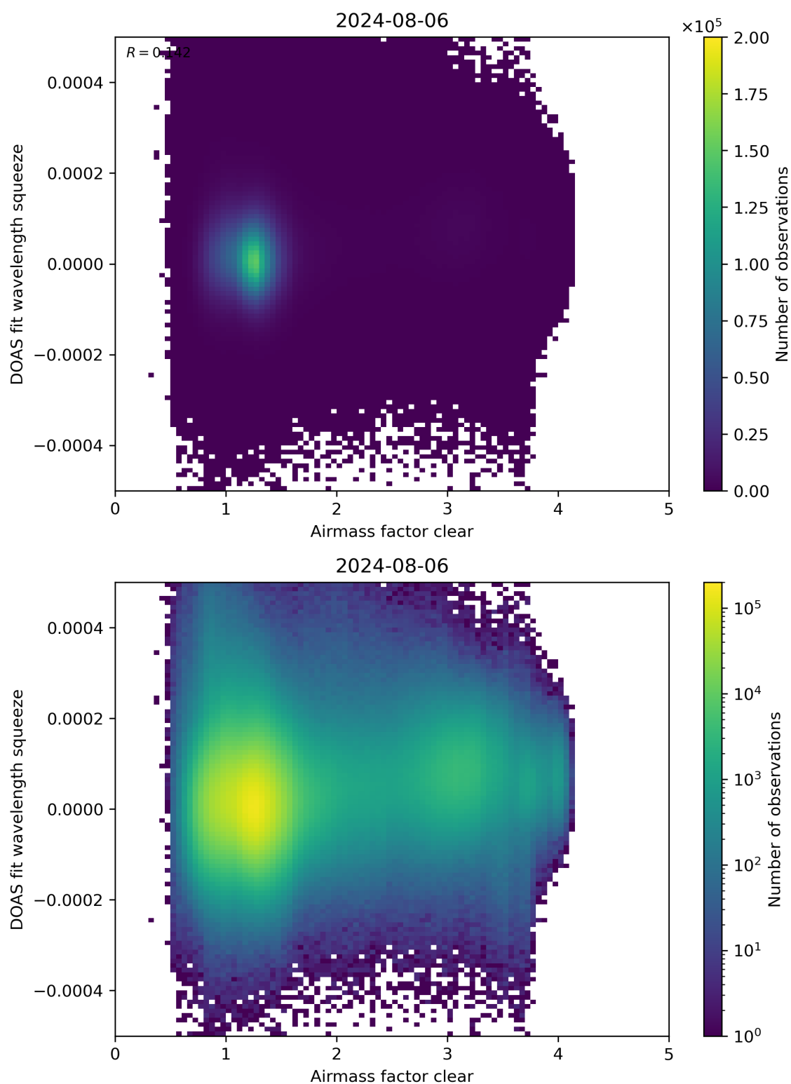
Figure 73: Scatter density plot of “Airmass factor clear” against “DOAS fit wavelength squeeze” for 2024-08-06 to 2024-08-07.
