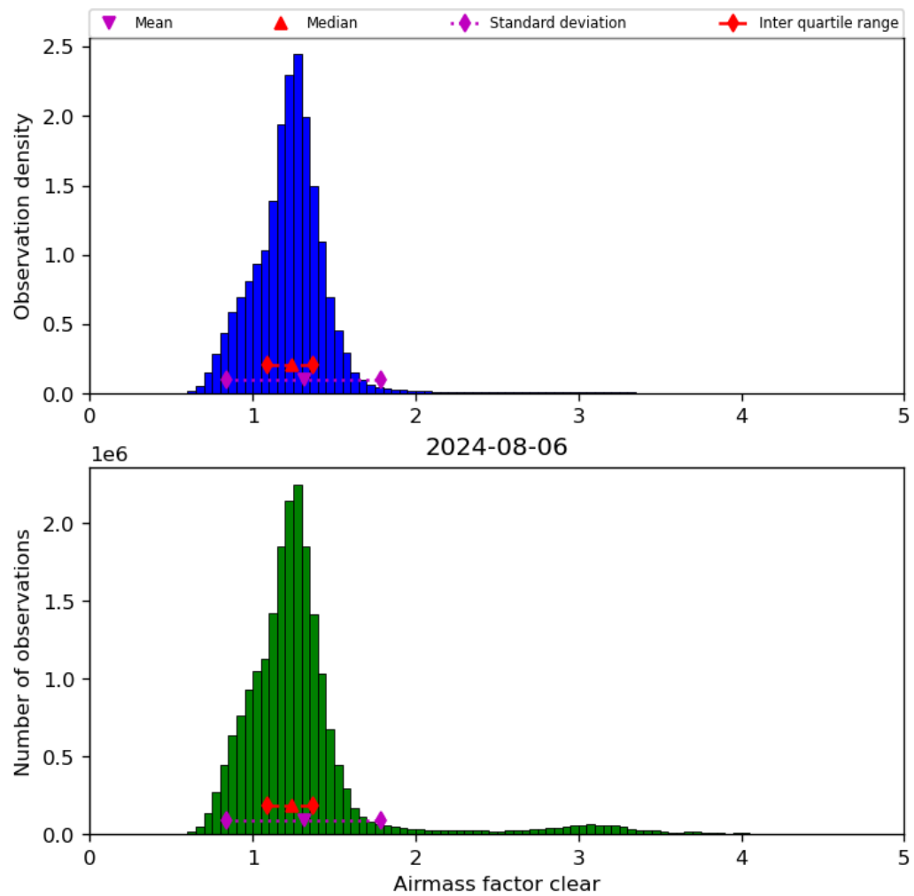
Figure 42: Histogram of “Airmass factor clear” for 2024-08-06 to 2024-08-07
