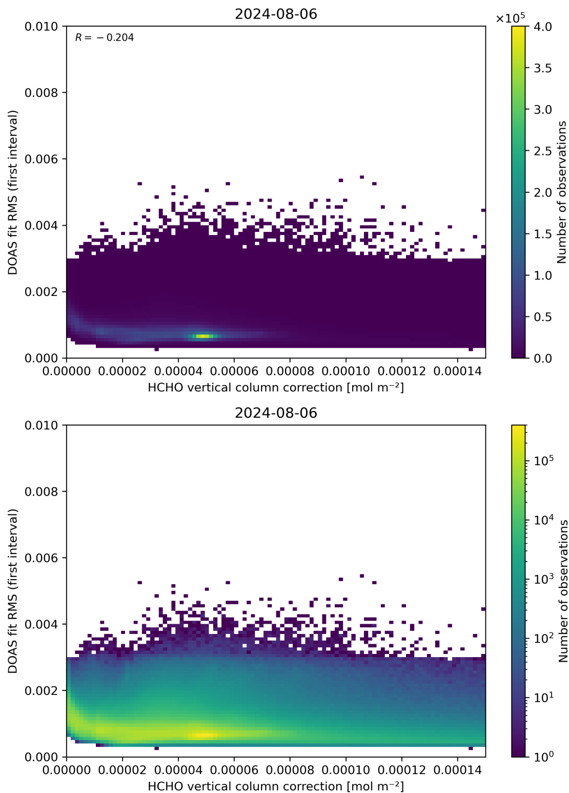
Figure 112: Scatter density plot of “HCHO vertical column correction” against “DOAS fit RMS (first interval)” for 2024-08-06 to 2024-08-07.
