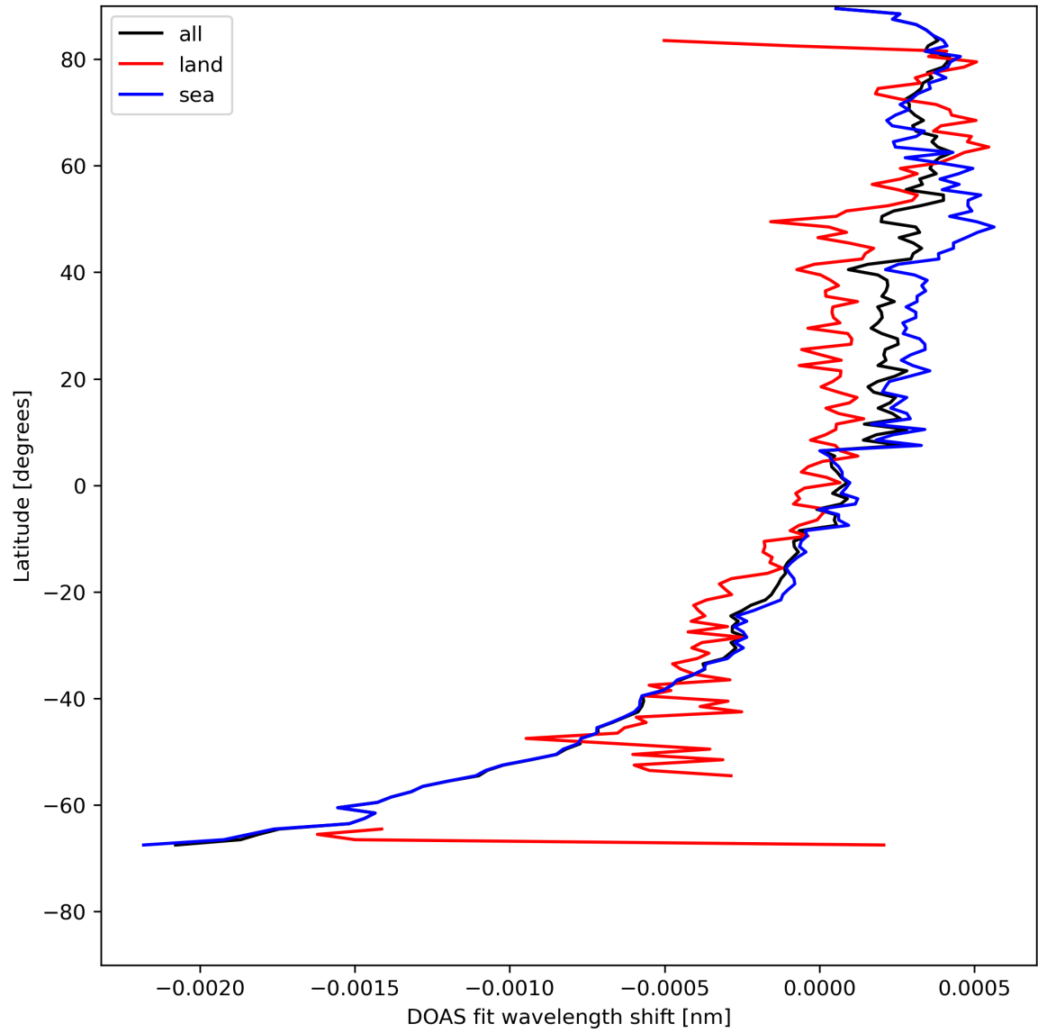
Figure 30: Zonal average of "DOAS fit wavelength shift" for 2024-08-06 to 2024-08-07.
