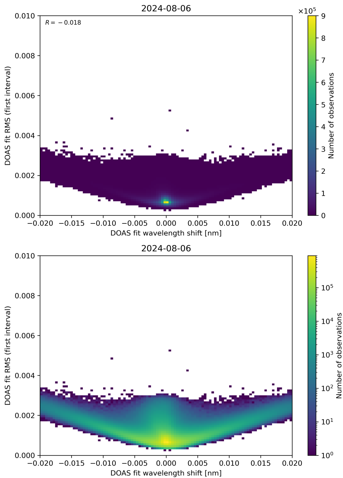
Figure 64: Scatter density plot of “DOAS fit wavelength shift” against “DOAS fit RMS (first interval)” for 2024-08-06 to 2024-08-07.
