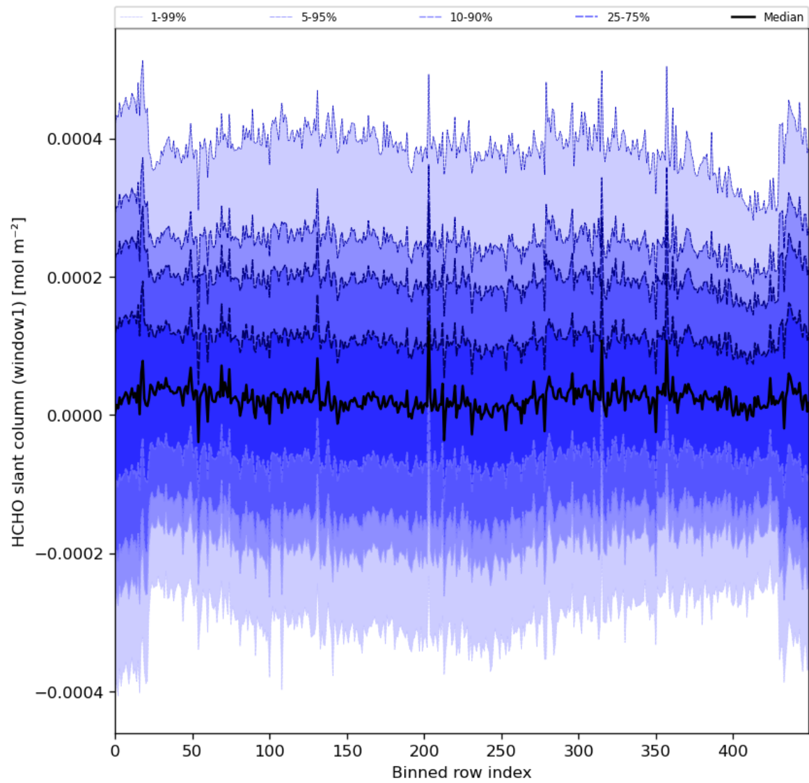
Figure 52: Along track statistics of “HCHO slant column (window1)” for 2024-08-06 to 2024-08-07
