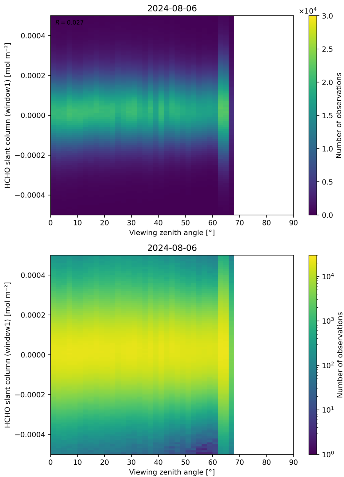
Figure 188: Scatter density plot of “Viewing zenith angle” against “HCHO slant column (window1)” for 2024-08-06 to 2024-08-07.
