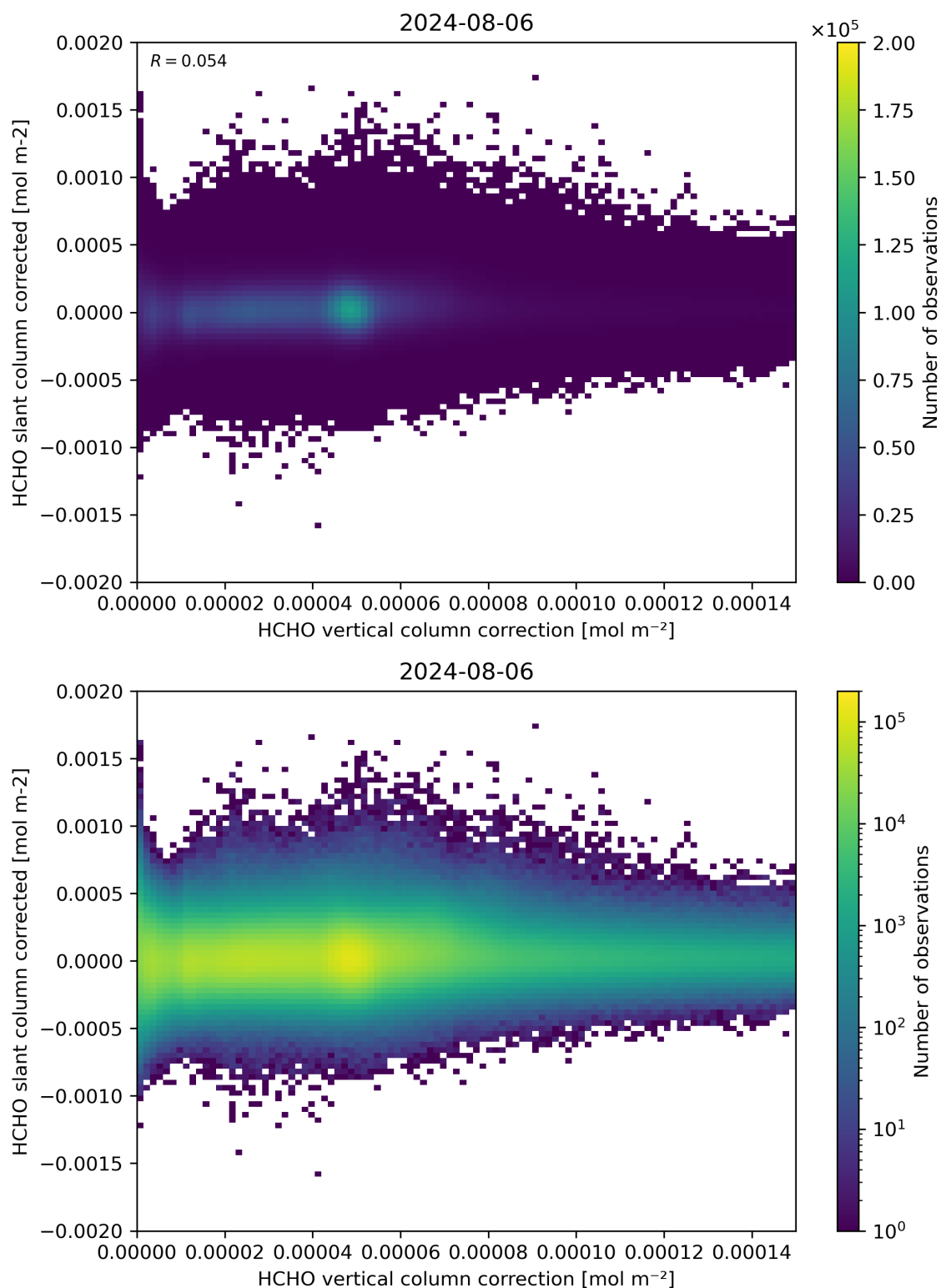
Figure 116: Scatter density plot of “HCHO vertical column correction” against “HCHO slant column corrected” for 2024-08-06 to 2024-08-07.
