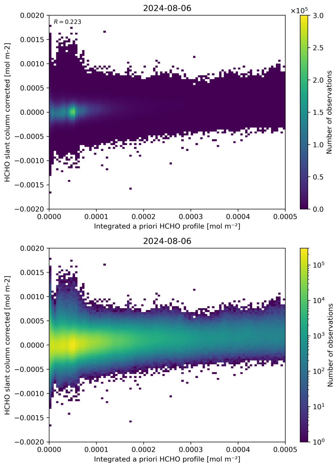
Figure 151: Scatter density plot of “Integrated a priori HCHO profile” against “HCHO slant column corrected” for 2024-08-06 to 2024-08-07.
