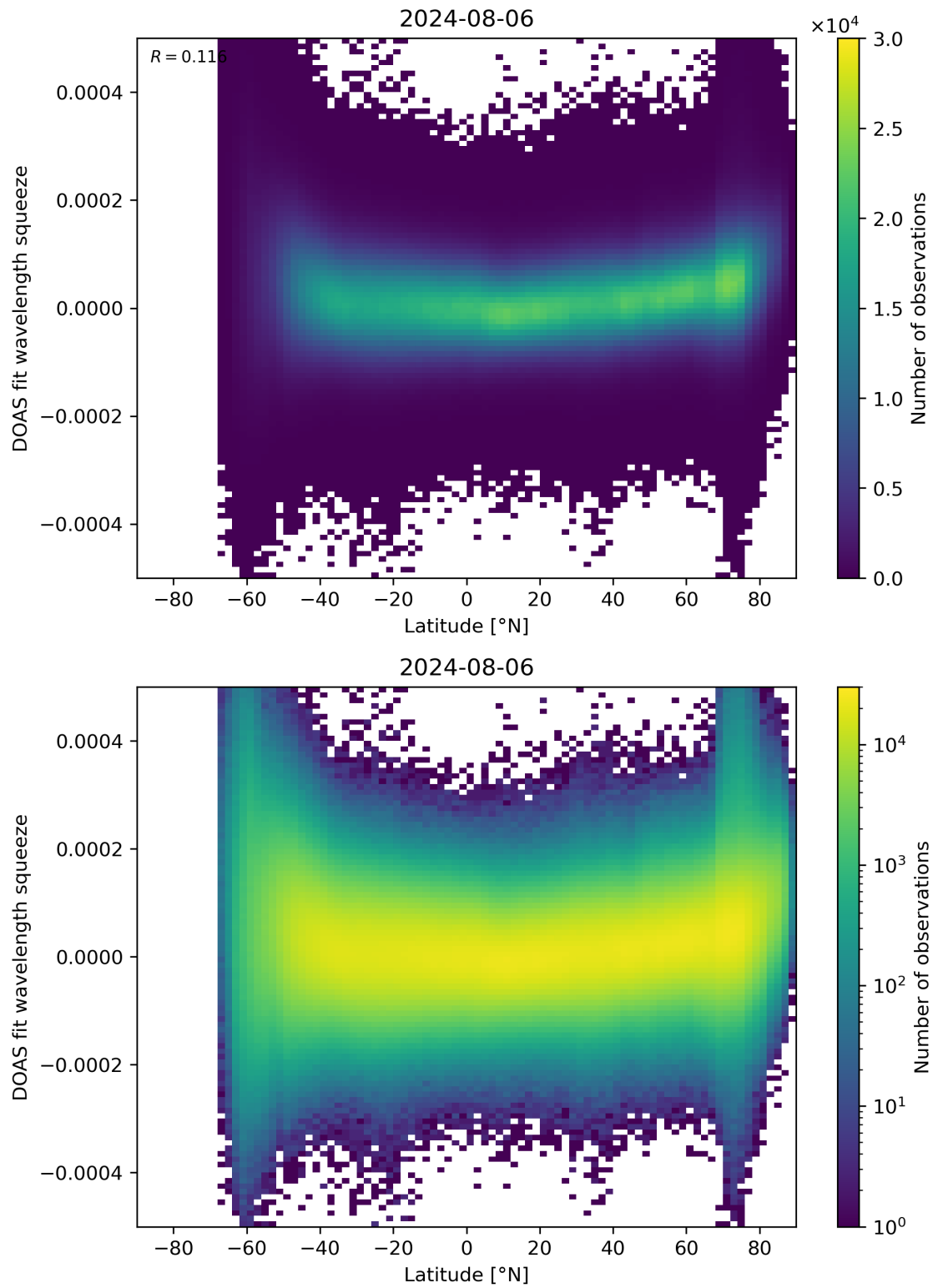
Figure 155: Scatter density plot of “Latitude” against “DOAS fit wavelength squeeze” for 2024-08-06 to 2024-08-07.
