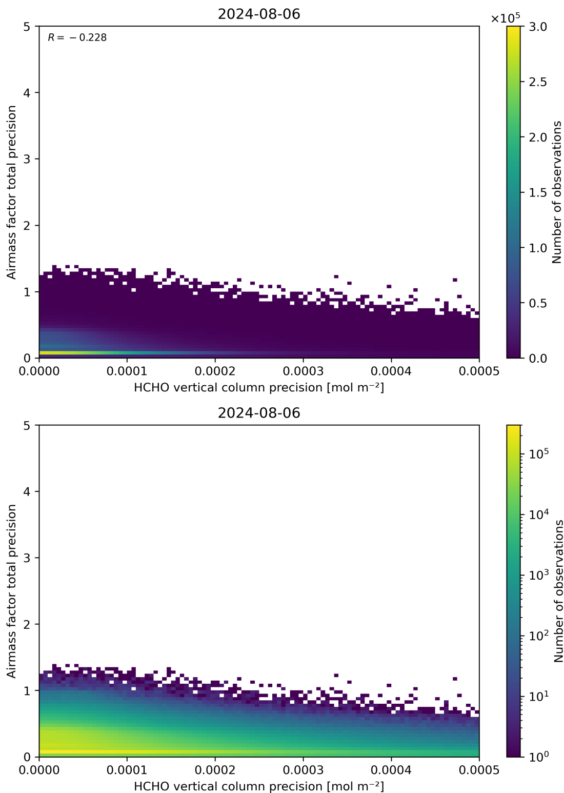
Figure 145: Scatter density plot of “HCHO vertical column precision” against “Airmass factor total precision” for 2024-08-06 to 2024-08-07.
