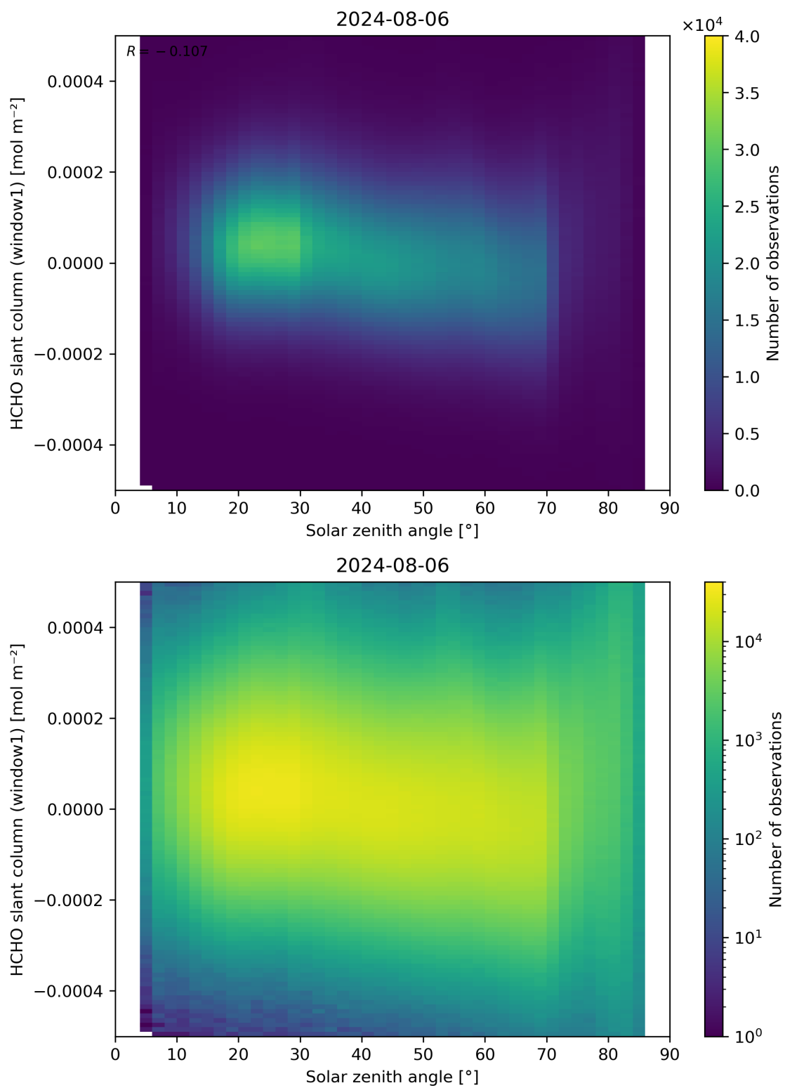
Figure 173: Scatter density plot of “Solar zenith angle” against “HCHO slant column (window1)” for 2024-08-06 to 2024-08-07.
