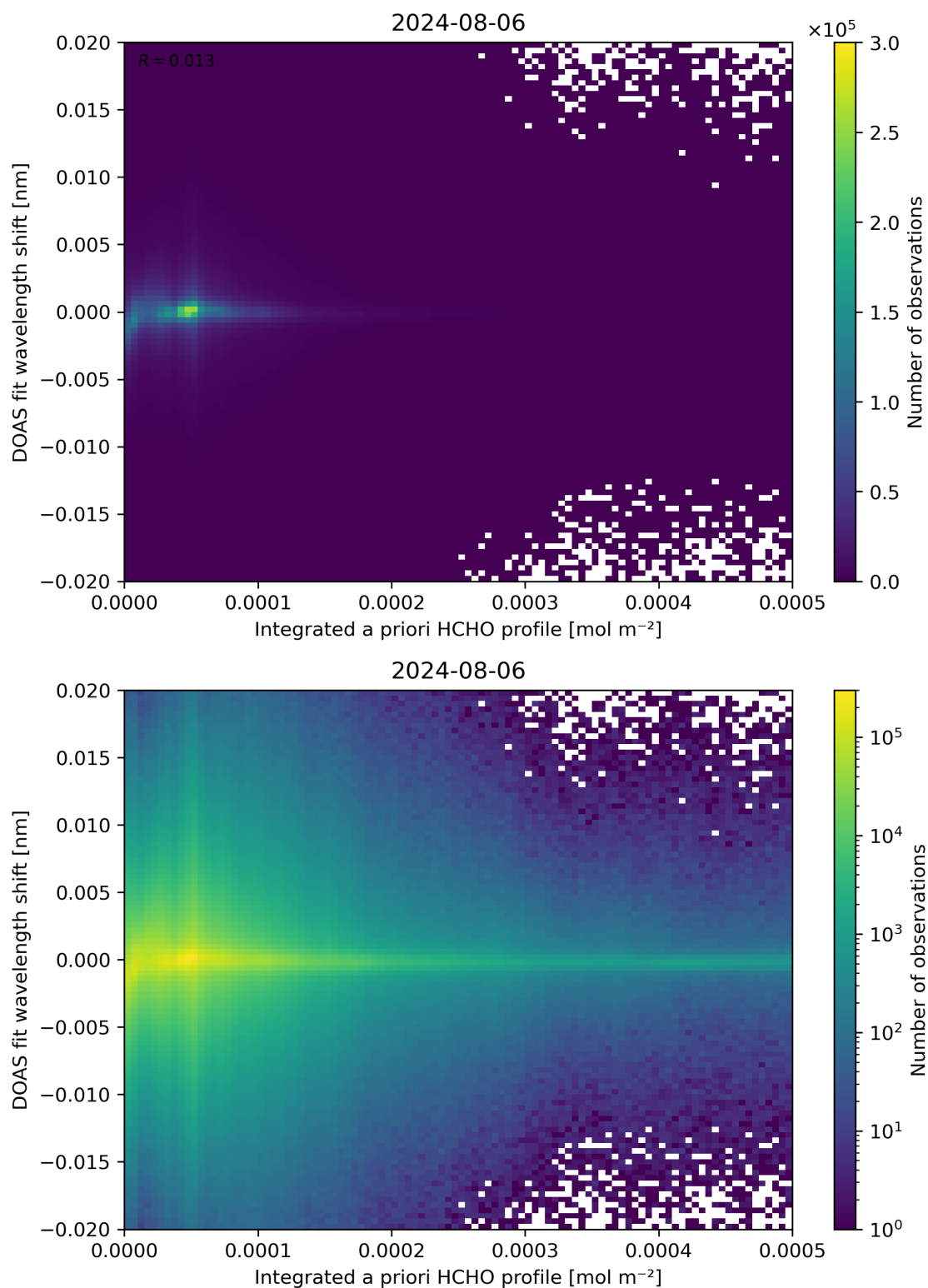
Figure 149: Scatter density plot of “Integrated a priori HCHO profile” against “DOAS fit wavelength shift” for 2024-08-06 to 2024-08-07.
