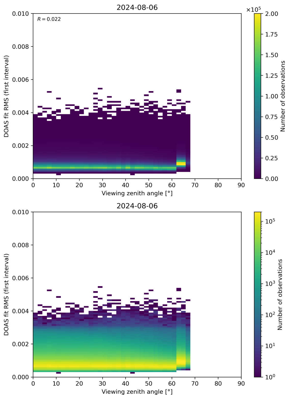
Figure 182: Scatter density plot of “Viewing zenith angle” against “DOAS fit RMS (first interval)” for 2024-08-06 to 2024-08-07.
