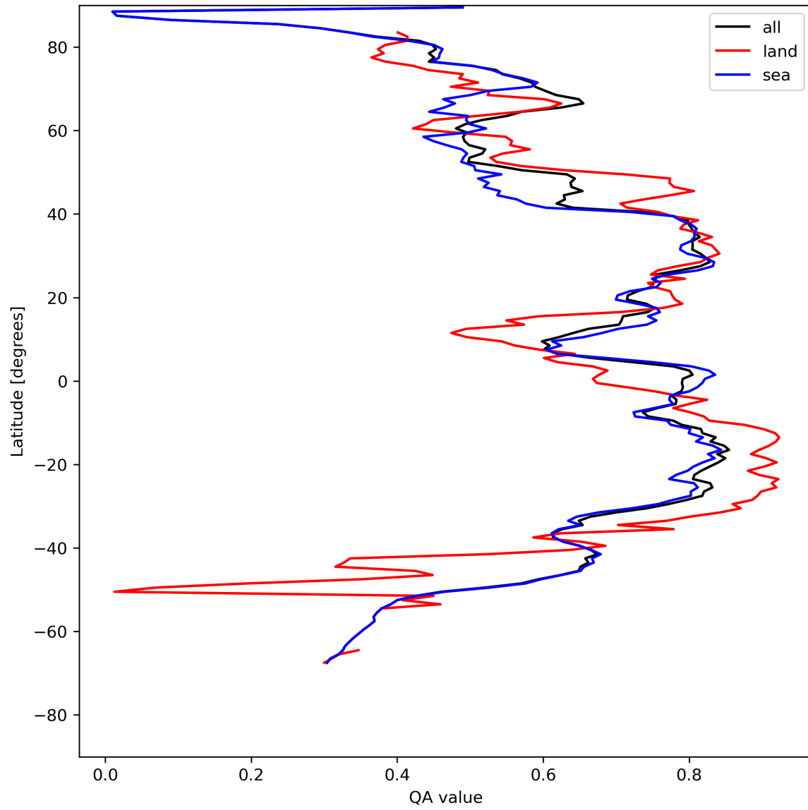
Figure 20: Zonal average of “QA value” for 2024-08-06 to 2024-08-07.
