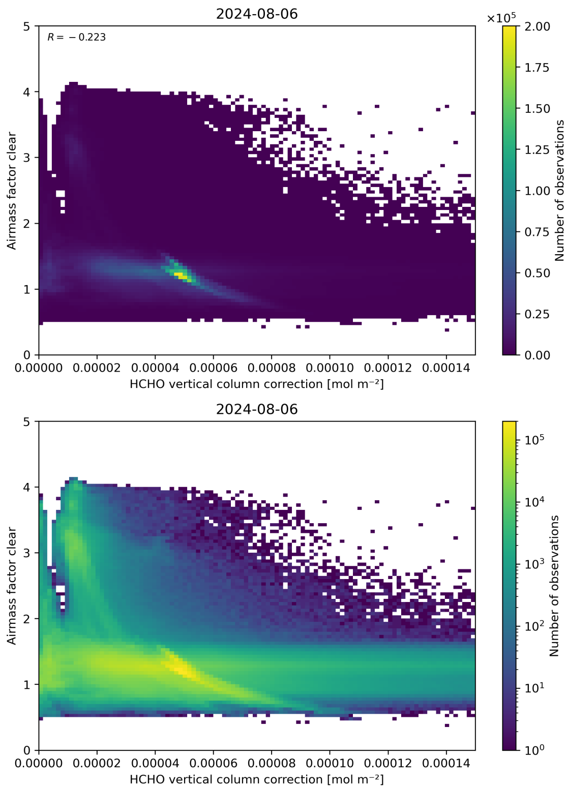
Figure 115: Scatter density plot of “HCHO vertical column correction” against “Airmass factor clear” for 2024-08-06 to 2024-08-07.
