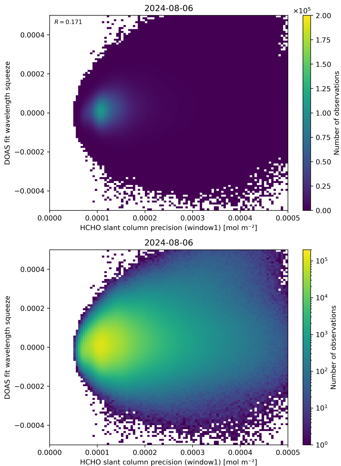
Figure 90: Scatter density plot of “HCHO slant column precision (window1)” against “DOAS fit wavelength squeeze” for 2024-08-06 to 2024-08-07.
