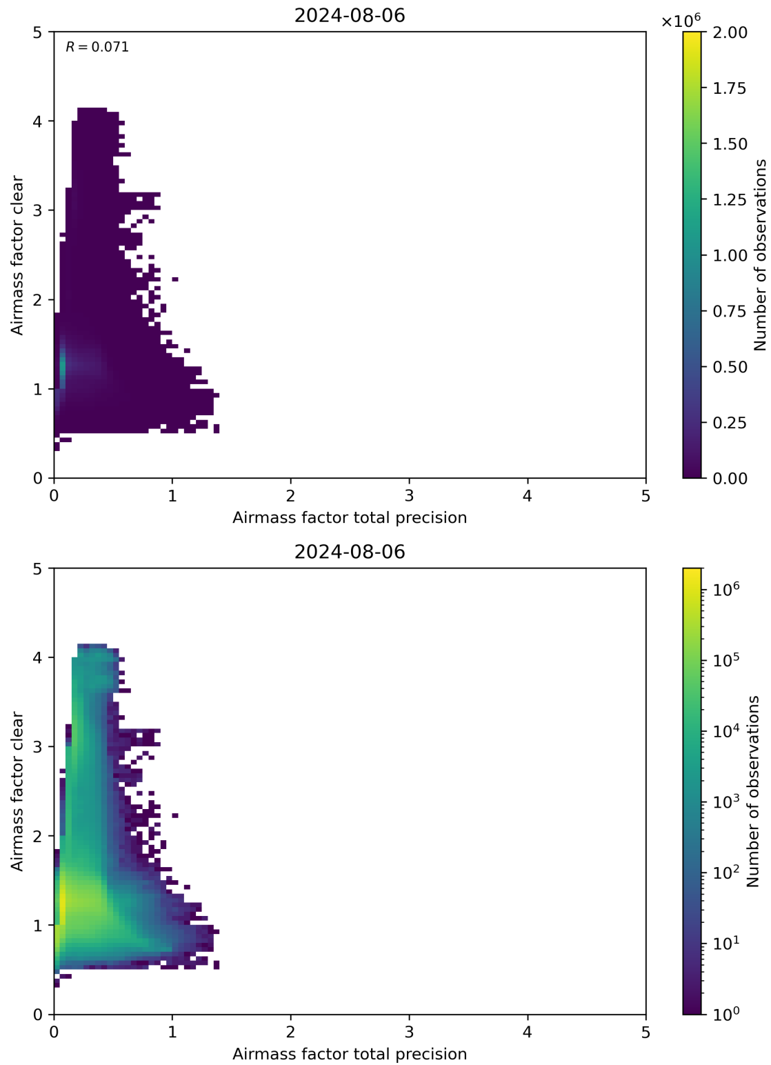
Figure 108: Scatter density plot of “Airmass factor total precision” against “Airmass factor clear” for 2024-08-06 to 2024-08-07.
