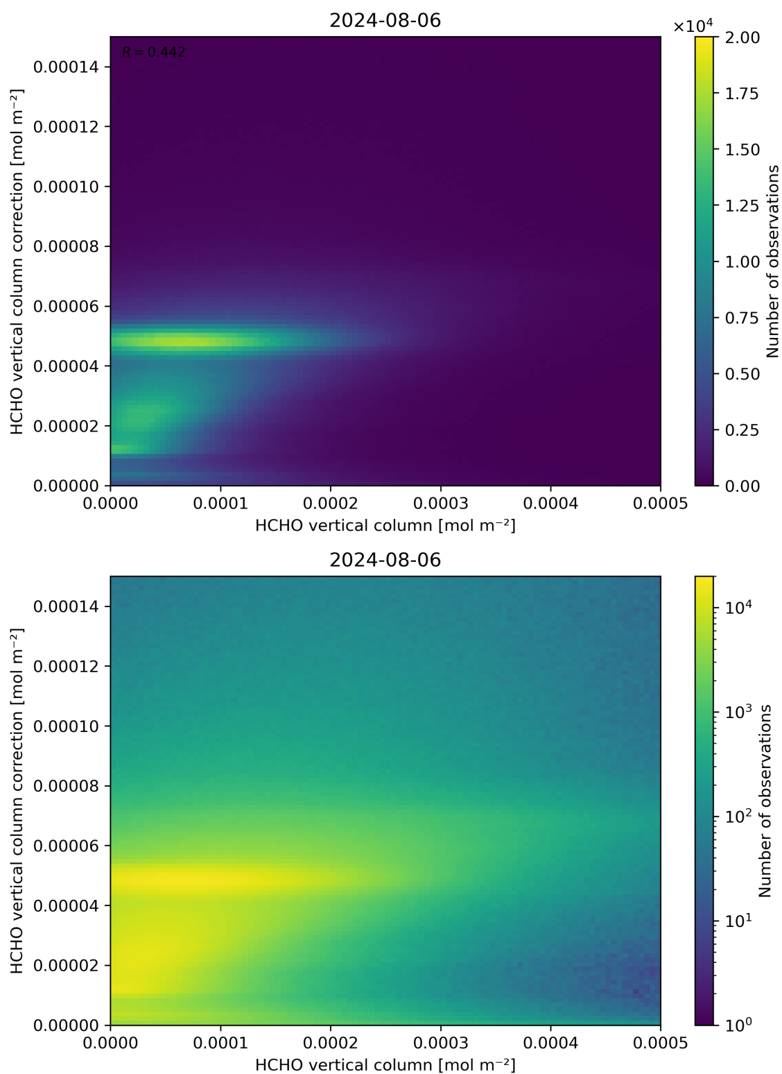
Figure 133: Scatter density plot of “HCHO vertical column” against “HCHO vertical column correction” for 2024-08-06 to 2024-08-07.
