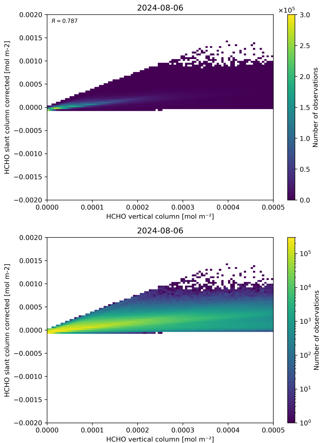
Figure 127: Scatter density plot of “HCHO vertical column” against “HCHO slant column corrected” for 2024-08-06 to 2024-08-07.
