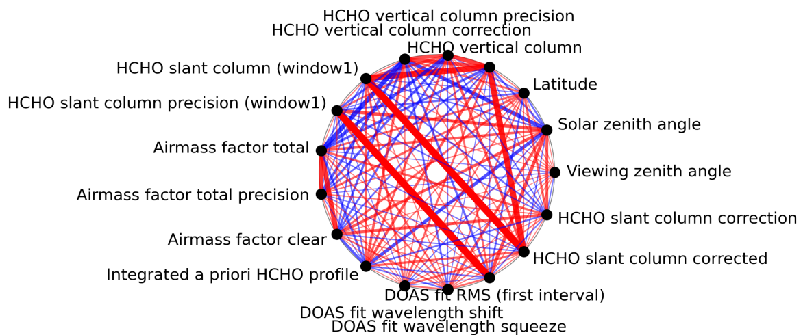
Figure 1: Map of correlation graph for 2024-08-06 to 2024-08-07.
