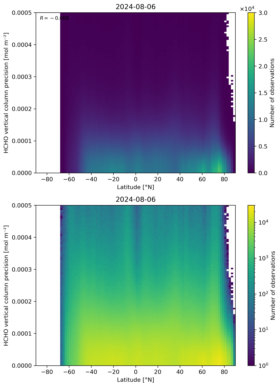
Figure 165: Scatter density plot of “Latitude” against “HCHO vertical column precision” for 2024-08-06 to 2024-08-07.
