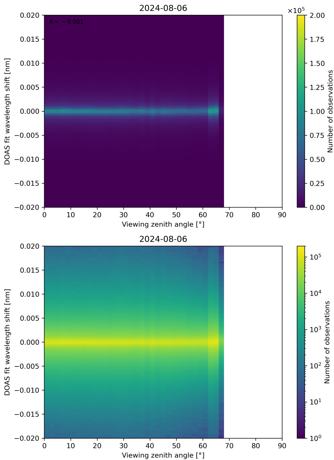
Figure 183: Scatter density plot of “Viewing zenith angle” against “DOAS fit wavelength shift” for 2024-08-06 to 2024-08-07.
