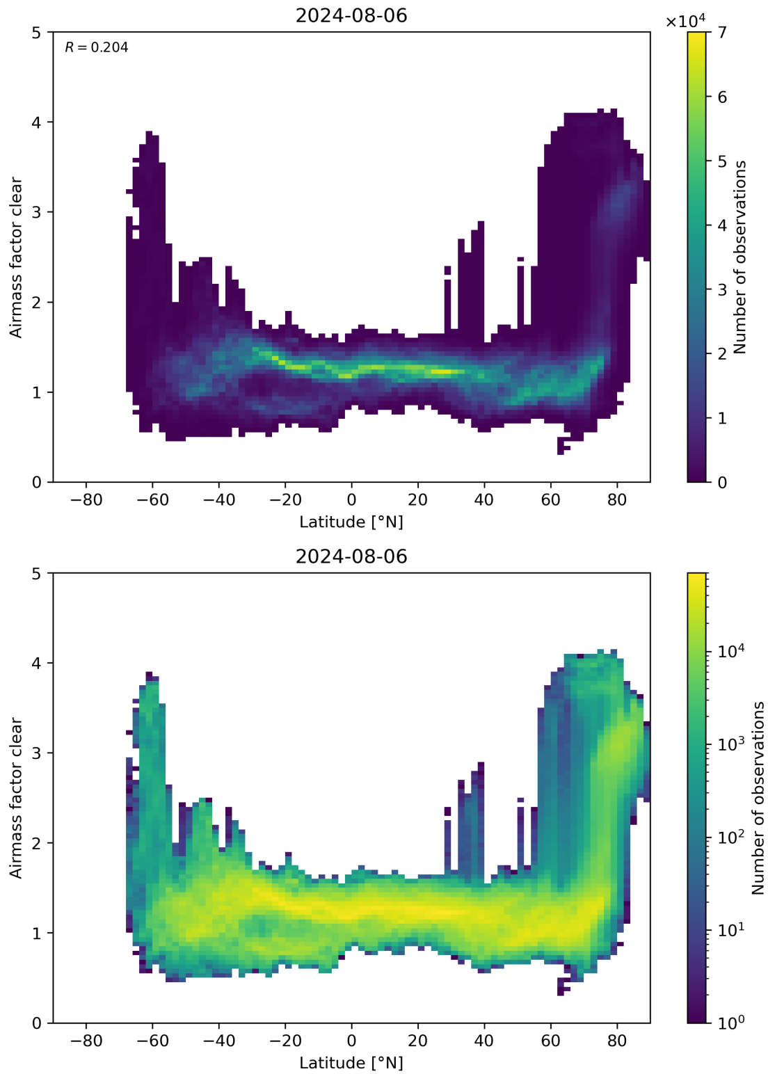
Figure 156: Scatter density plot of “Latitude” against “Airmass factor clear” for 2024-08-06 to 2024-08-07.
