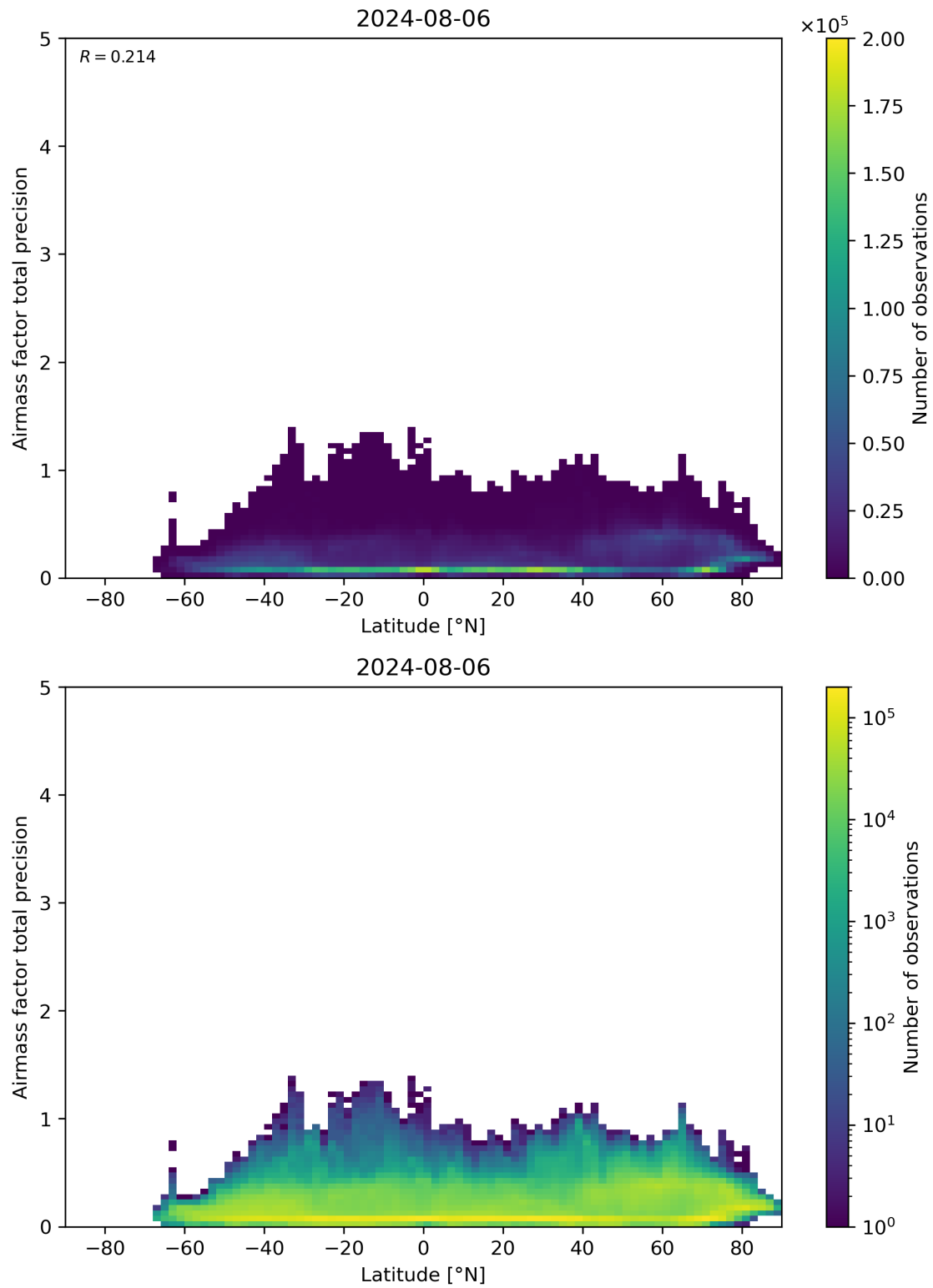
Figure 162: Scatter density plot of “Latitude” against “Airmass factor total precision” for 2024-08-06 to 2024-08-07.
