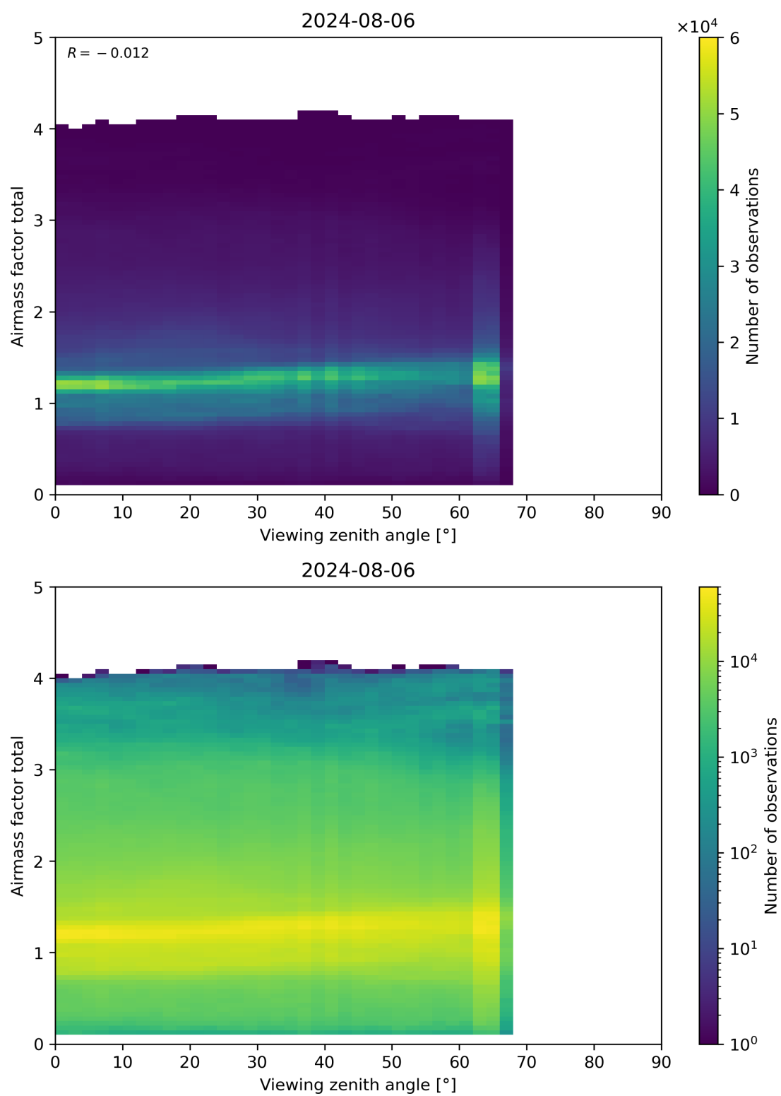
Figure 190: Scatter density plot of “Viewing zenith angle” against “Airmass factor total” for 2024-08-06 to 2024-08-07.
