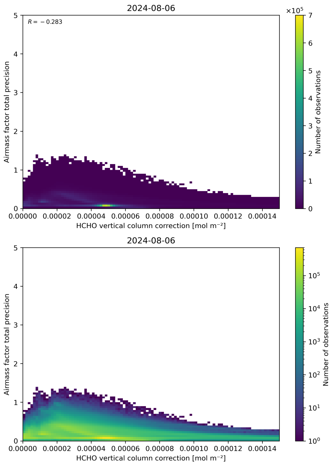
Figure 121: Scatter density plot of “HCHO vertical column correction” against “Airmass factor total precision” for 2024-08-06 to 2024-08-07.
