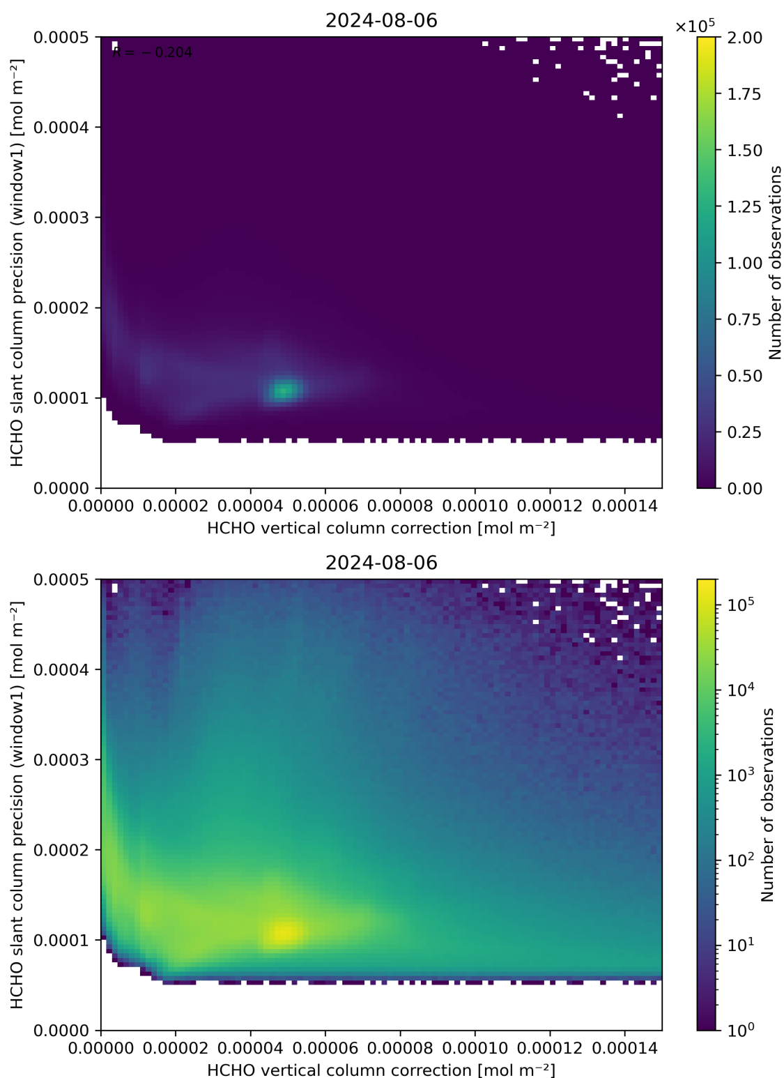
Figure 119: Scatter density plot of “HCHO vertical column correction” against “HCHO slant column precision (window1)” for 2024-08-06 to 2024-08-07.
