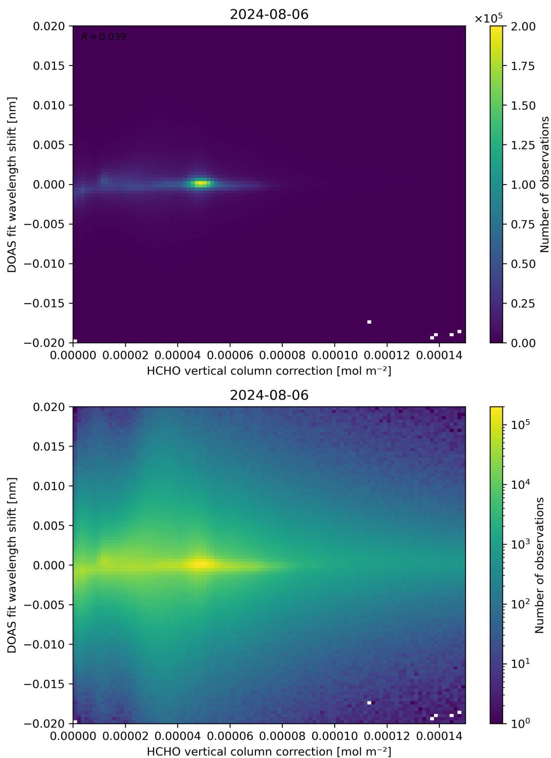
Figure 113: Scatter density plot of “HCHO vertical column correction” against “DOAS fit wavelength shift” for 2024-08-06 to 2024-08-07.
