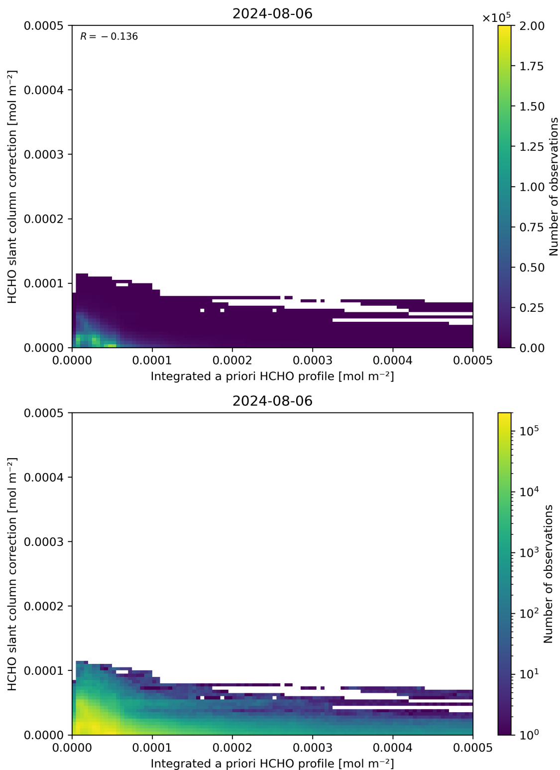
Figure 152: Scatter density plot of “Integrated a priori HCHO profile” against “HCHO slant column correction” for 2024-08-06 to 2024-08-07.
