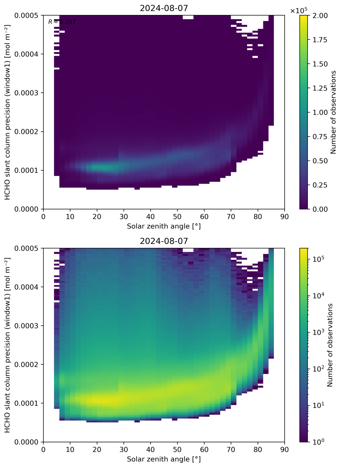
Figure 174: Scatter density plot of “Solar zenith angle” against “HCHO slant column precision (window1)” for 2024-08-06 to 2024-08-08.
