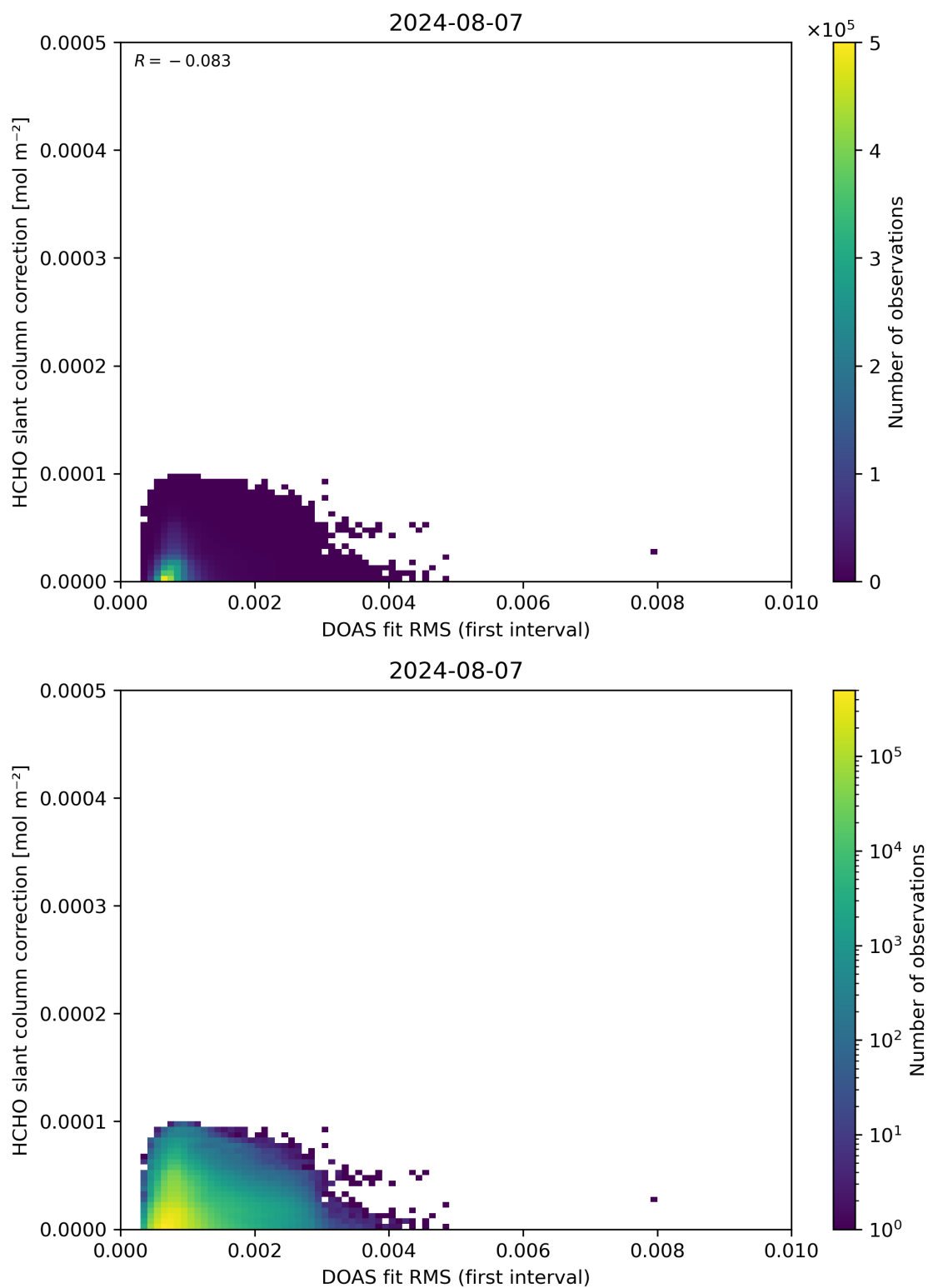
Figure 63: Scatter density plot of “DOAS fit RMS (first interval)” against “HCHO slant column correction” for 2024-08-06 to 2024-08-08.
