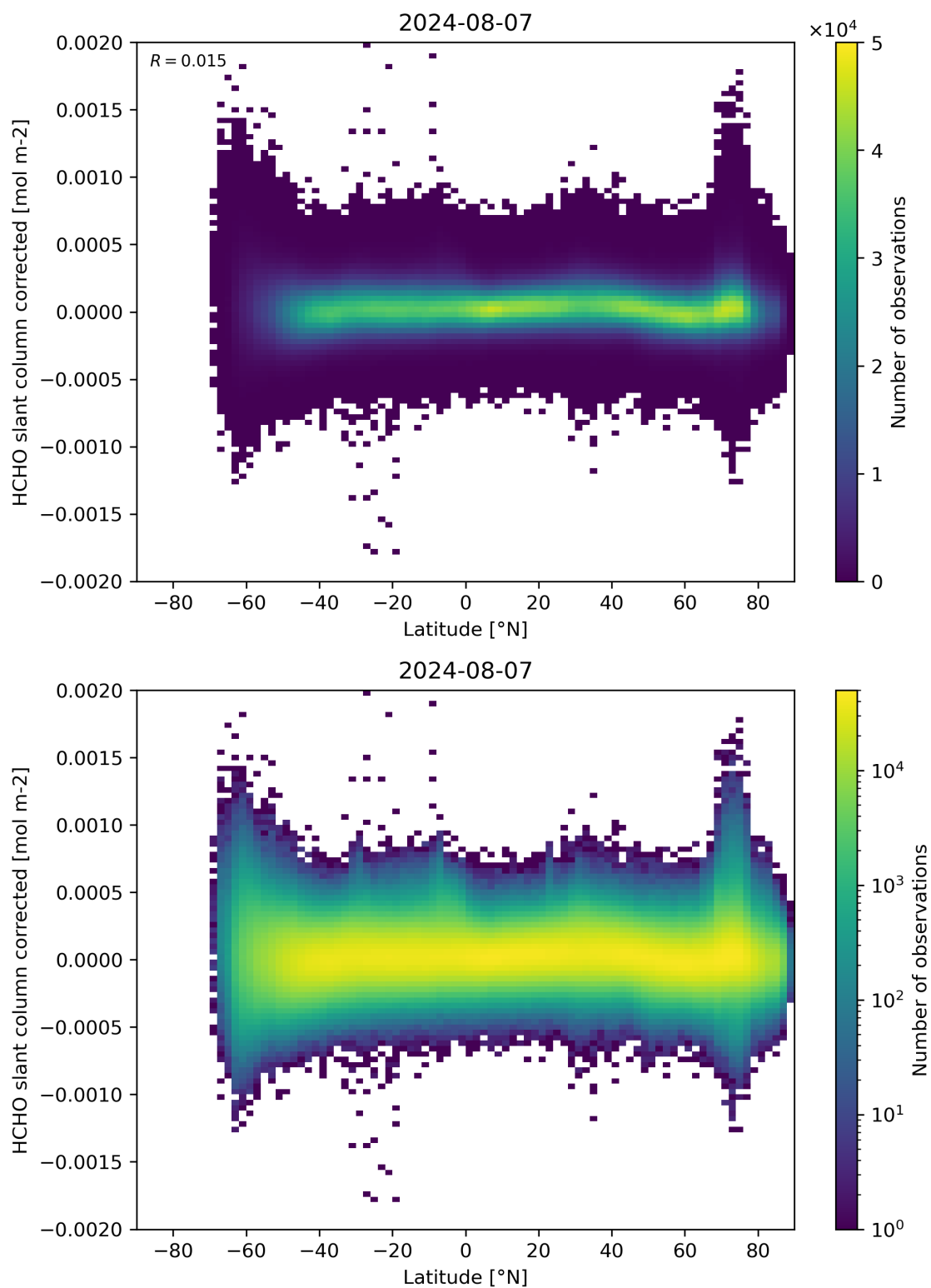
Figure 157: Scatter density plot of “Latitude” against “HCHO slant column corrected” for 2024-08-06 to 2024-08-08.
