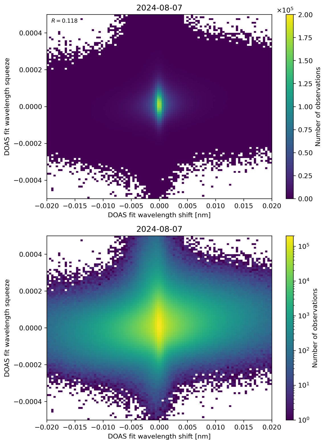
Figure 65: Scatter density plot of “DOAS fit wavelength shift” against “DOAS fit wavelength squeeze” for 2024-08-06 to 2024-08-08.
