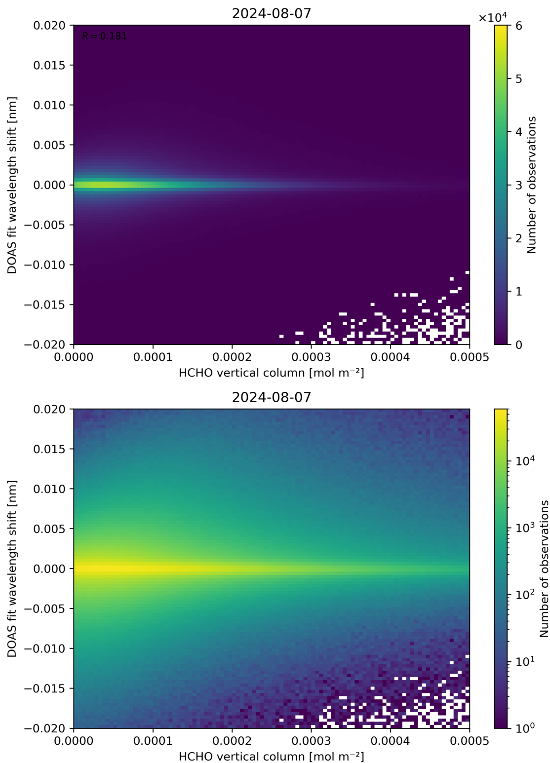
Figure 124: Scatter density plot of “HCHO vertical column” against “DOAS fit wavelength shift” for 2024-08-06 to 2024-08-08.
