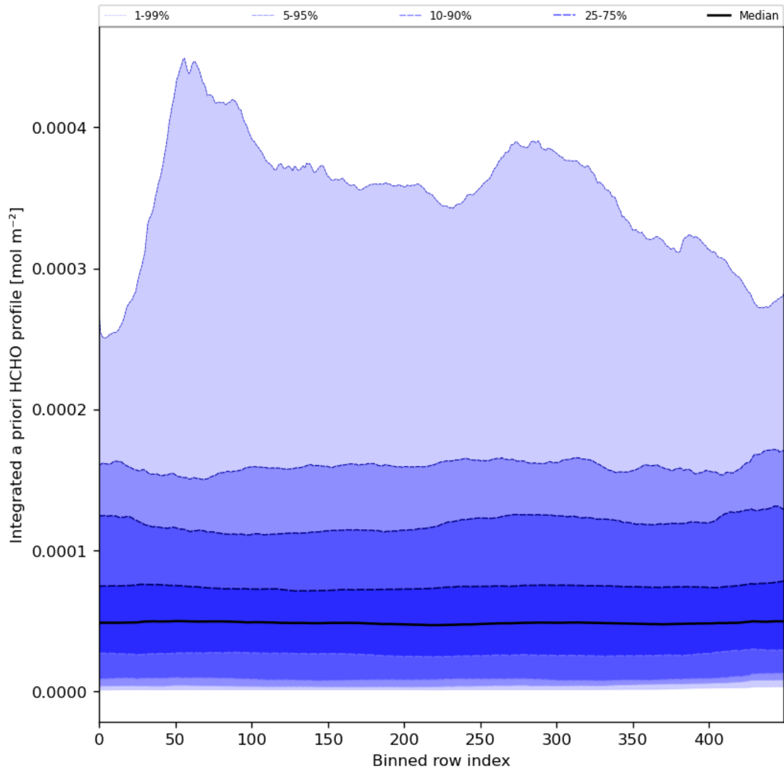
Figure 57: Along track statistics of “Integrated a priori HCHO profile” for 2024-08-06 to 2024-08-08
