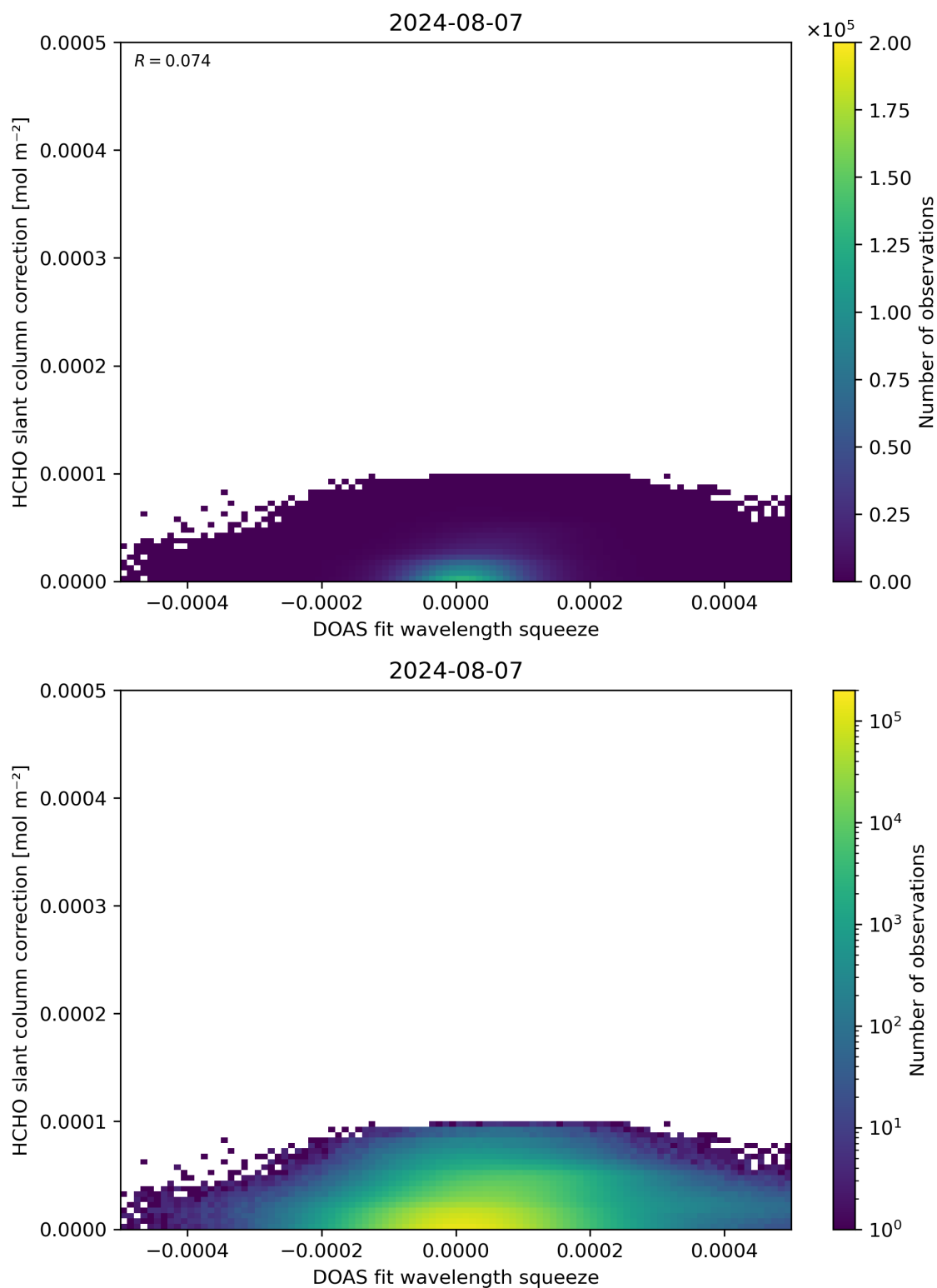
Figure 70: Scatter density plot of “DOAS fit wavelength squeeze” against “HCHO slant column correction” for 2024-08-06 to 2024-08-08.
