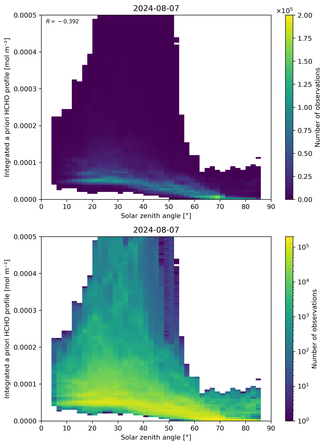
Figure 180: Scatter density plot of “Solar zenith angle” against “Integrated a priori HCHO profile” for 2024-08-06 to 2024-08-08.
