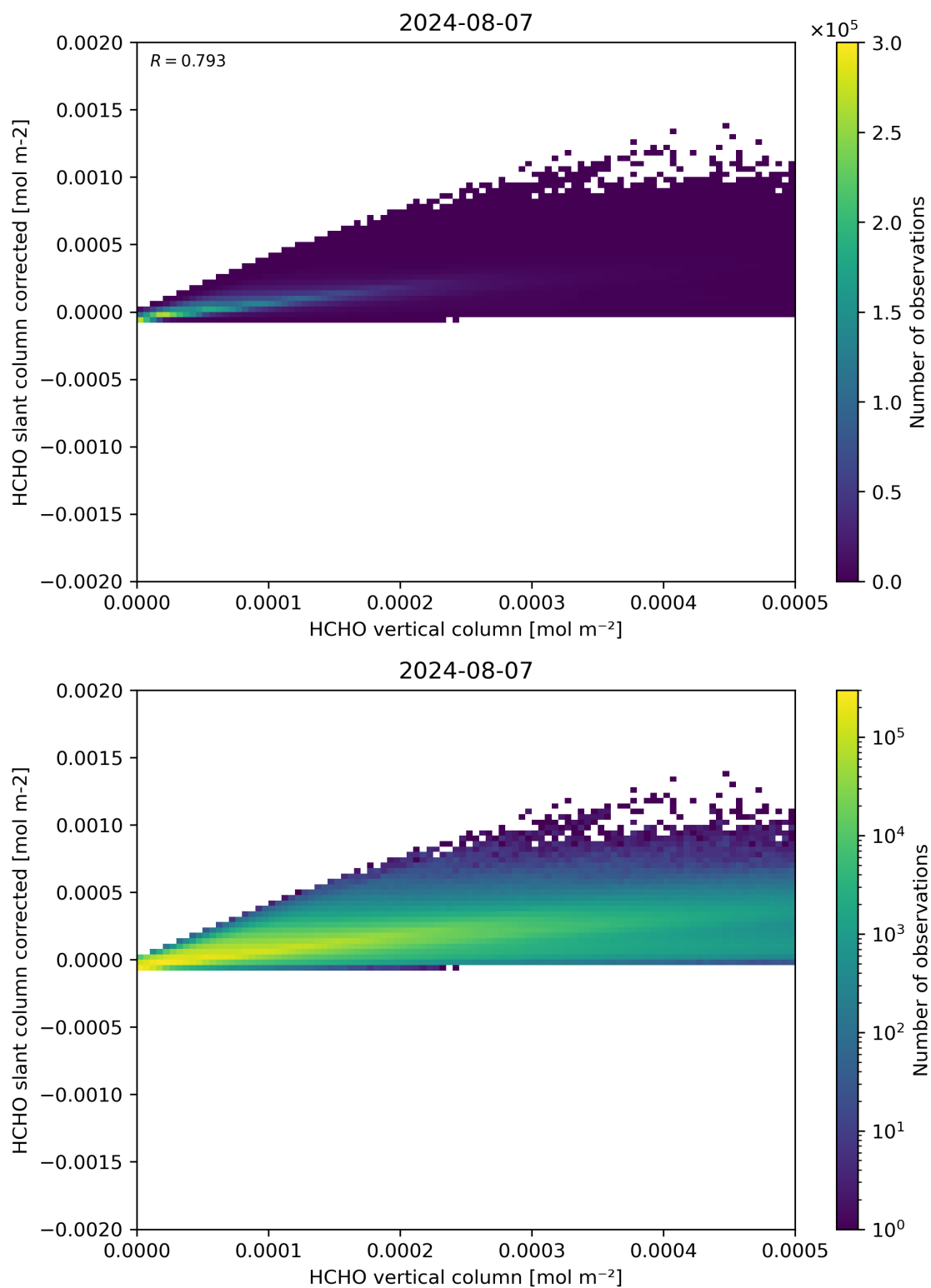
Figure 127: Scatter density plot of “HCHO vertical column” against “HCHO slant column corrected” for 2024-08-06 to 2024-08-08.
