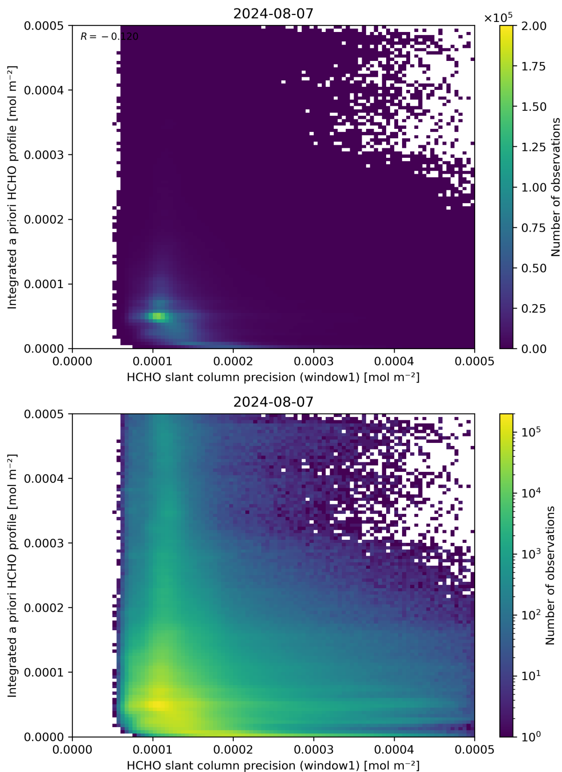
Figure 96: Scatter density plot of “HCHO slant column precision (window1)” against “Integrated a priori HCHO profile” for 2024-08-06 to 2024-08-08.
