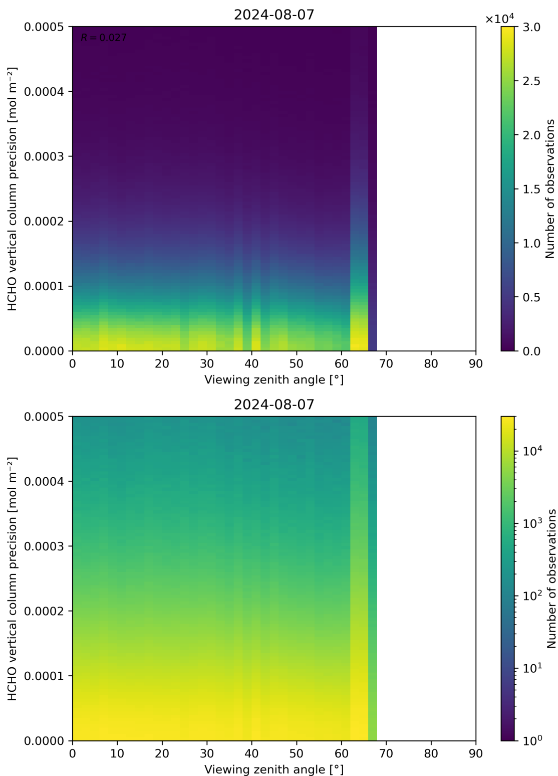
Figure 194: Scatter density plot of “Viewing zenith angle” against “HCHO vertical column precision” for 2024-08-06 to 2024-08-08.
