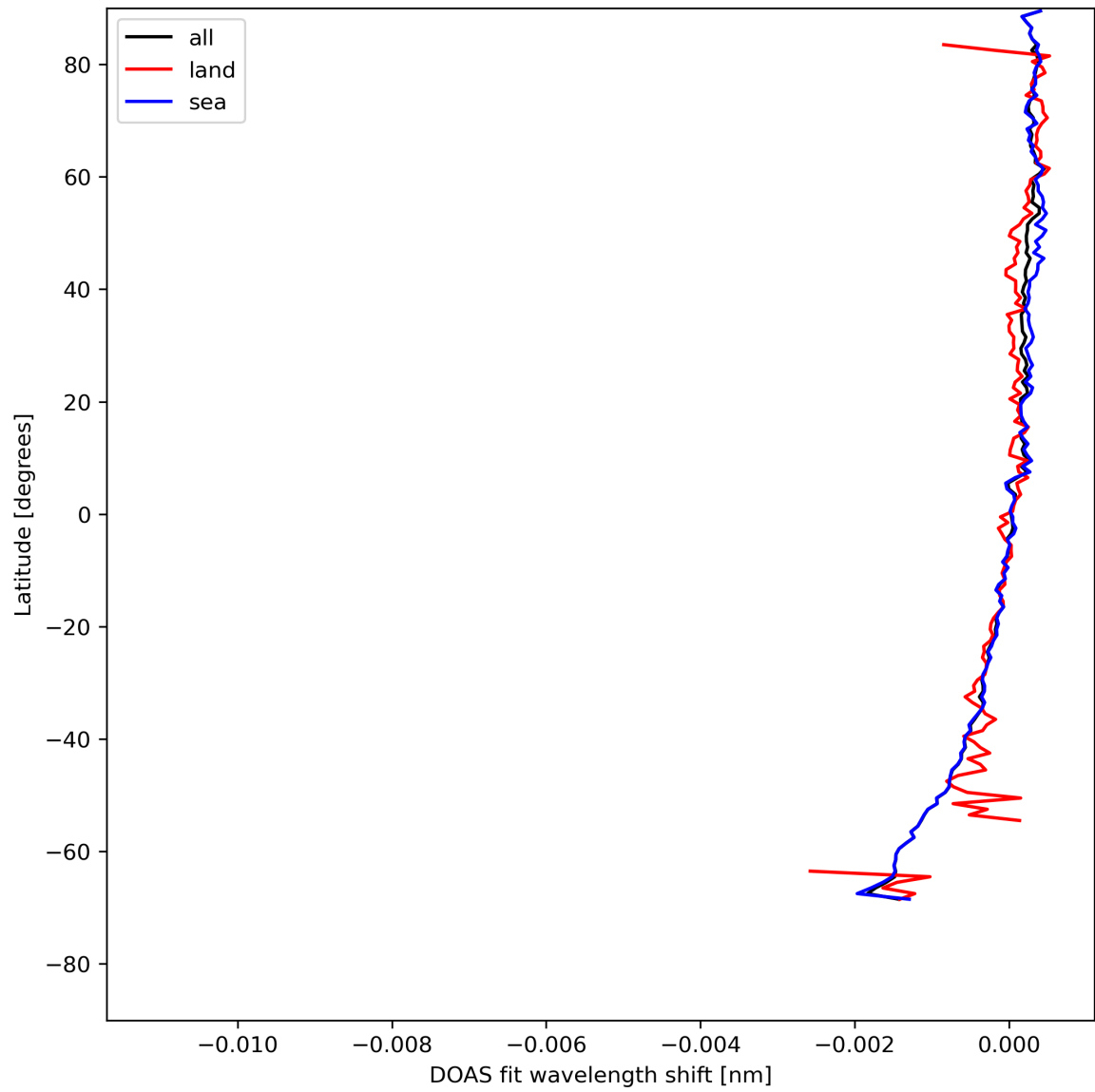
Figure 30: Zonal average of "DOAS fit wavelength shift" for 2024-08-06 to 2024-08-08.
