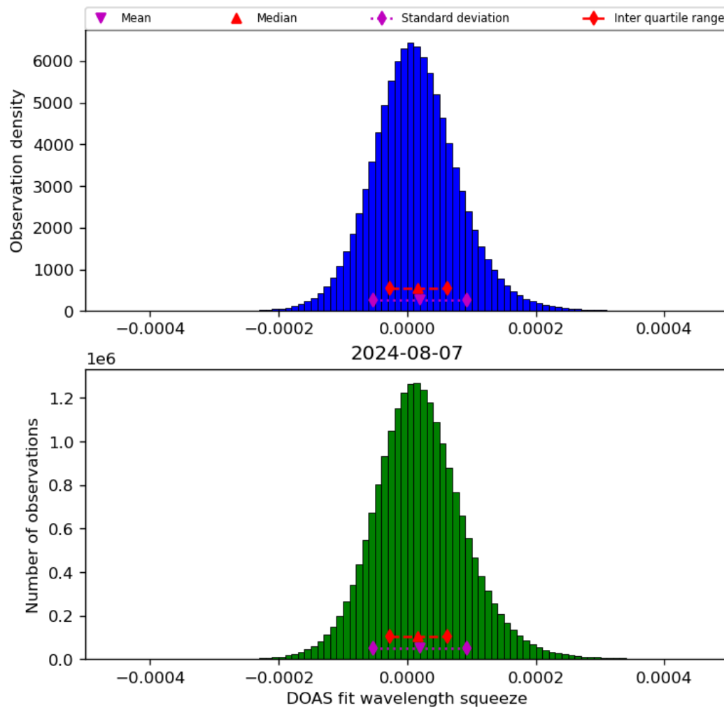
Figure 45: Histogram of “DOAS fit wavelength squeeze” for 2024-08-06 to 2024-08-08
