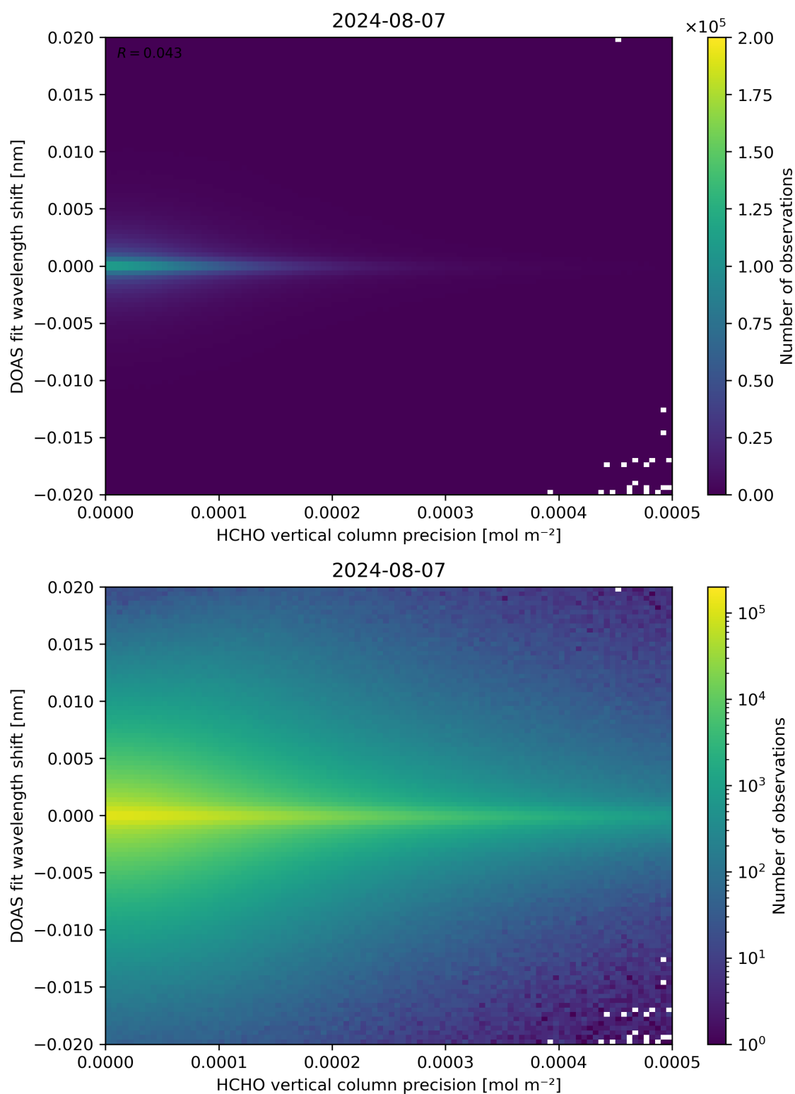
Figure 137: Scatter density plot of “HCHO vertical column precision” against “DOAS fit wavelength shift” for 2024-08-06 to 2024-08-08.
