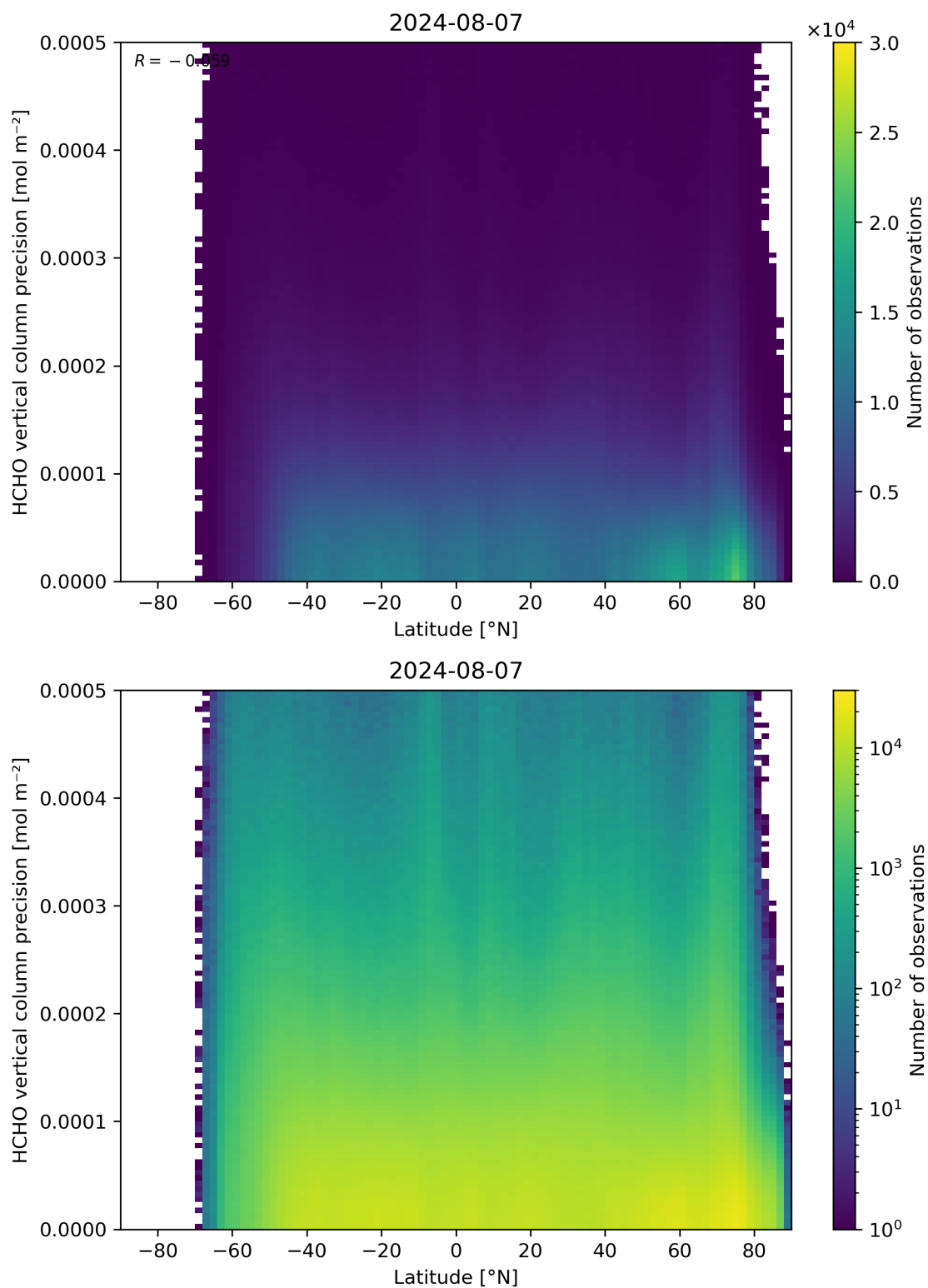
Figure 165: Scatter density plot of “Latitude” against “HCHO vertical column precision” for 2024-08-06 to 2024-08-08.
