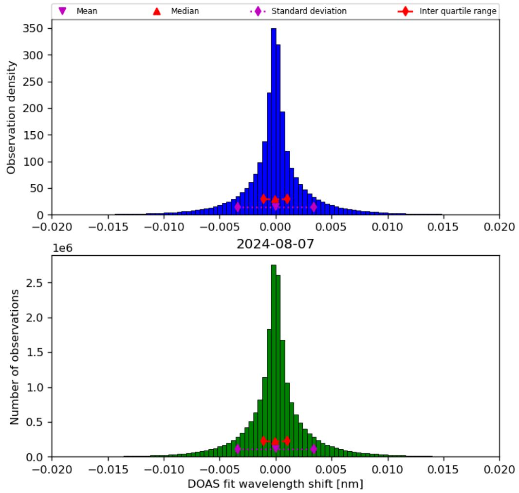
Figure 44: Histogram of “DOAS fit wavelength shift” for 2024-08-06 to 2024-08-08
