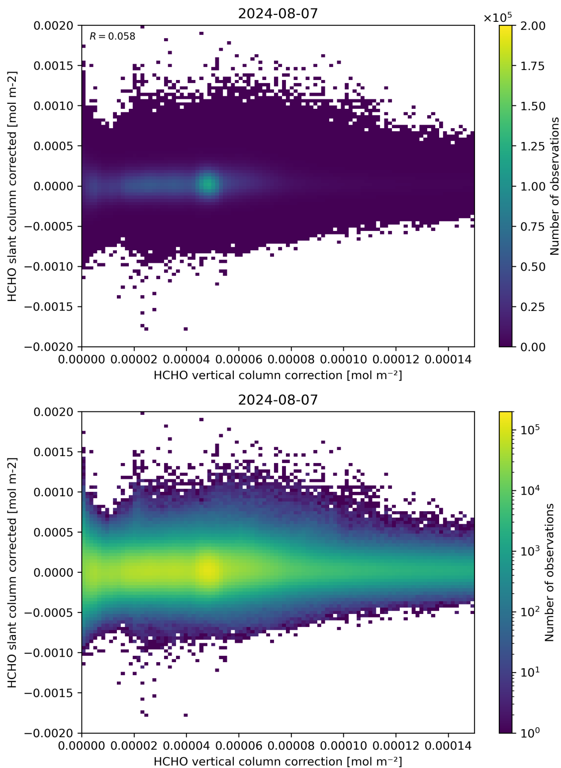
Figure 116: Scatter density plot of “HCHO vertical column correction” against “HCHO slant column corrected” for 2024-08-06 to 2024-08-08.
