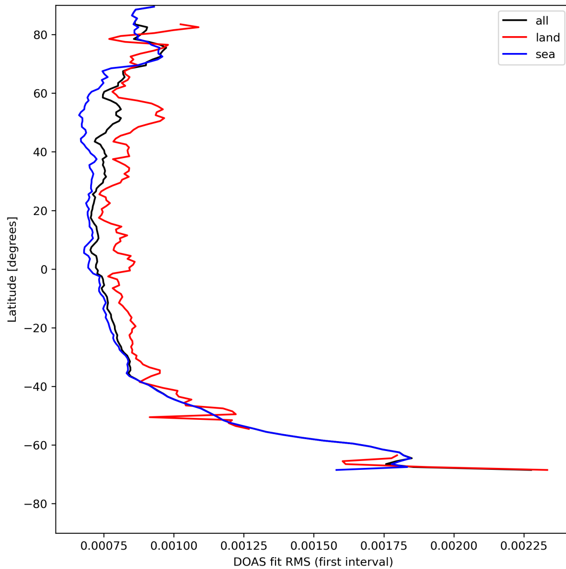
Figure 32: Zonal average of “DOAS fit RMS (first interval)” for 2024-08-06 to 2024-08-08.
