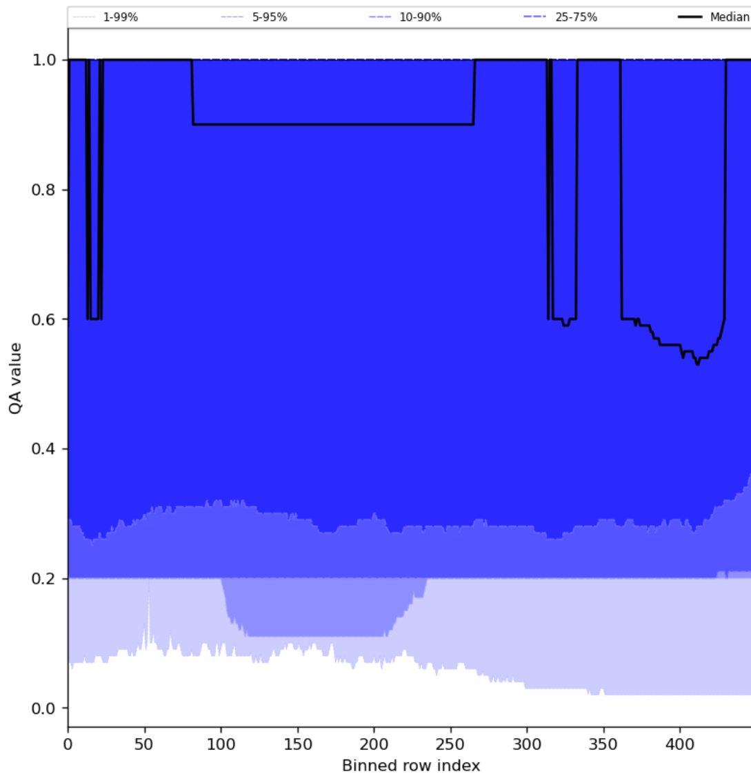
Figure 48: Along track statistics of “QA value” for 2024-08-06 to 2024-08-08
