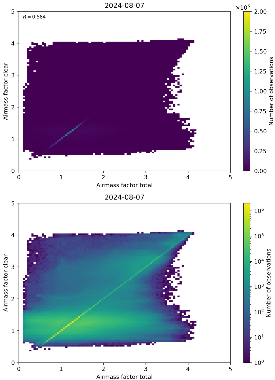
Figure 100: Scatter density plot of “Airmass factor total” against “Airmass factor clear” for 2024-08-06 to 2024-08-08.
