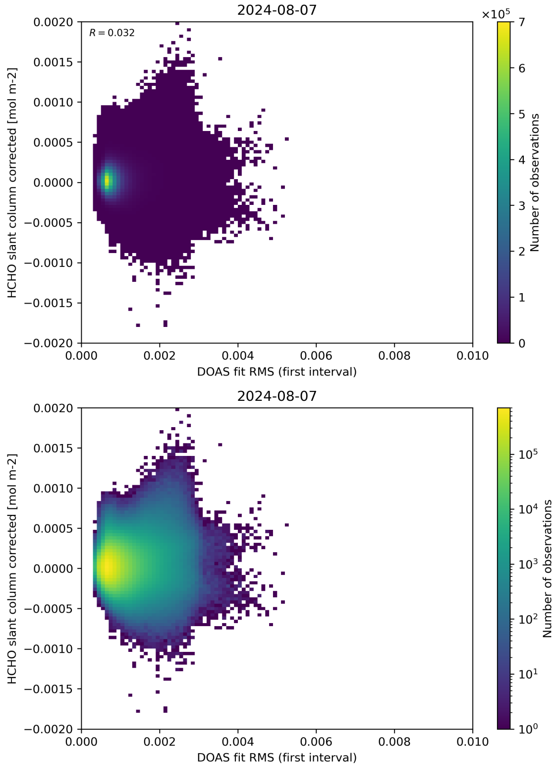
Figure 62: Scatter density plot of “DOAS fit RMS (first interval)” against “HCHO slant column corrected” for 2024-08-06 to 2024-08-08.
