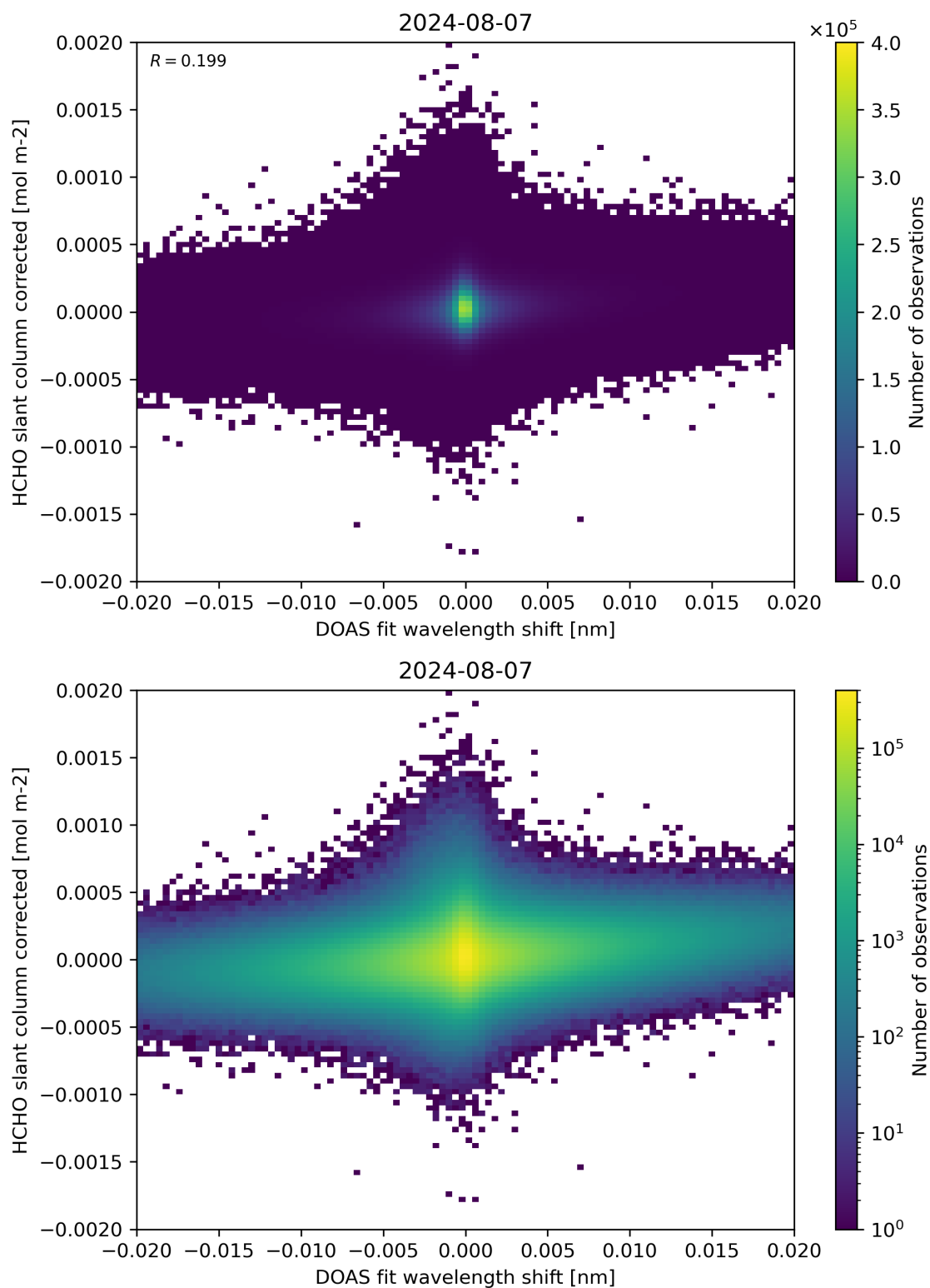
Figure 66: Scatter density plot of “DOAS fit wavelength shift” against “HCHO slant column corrected” for 2024-08-06 to 2024-08-08.
