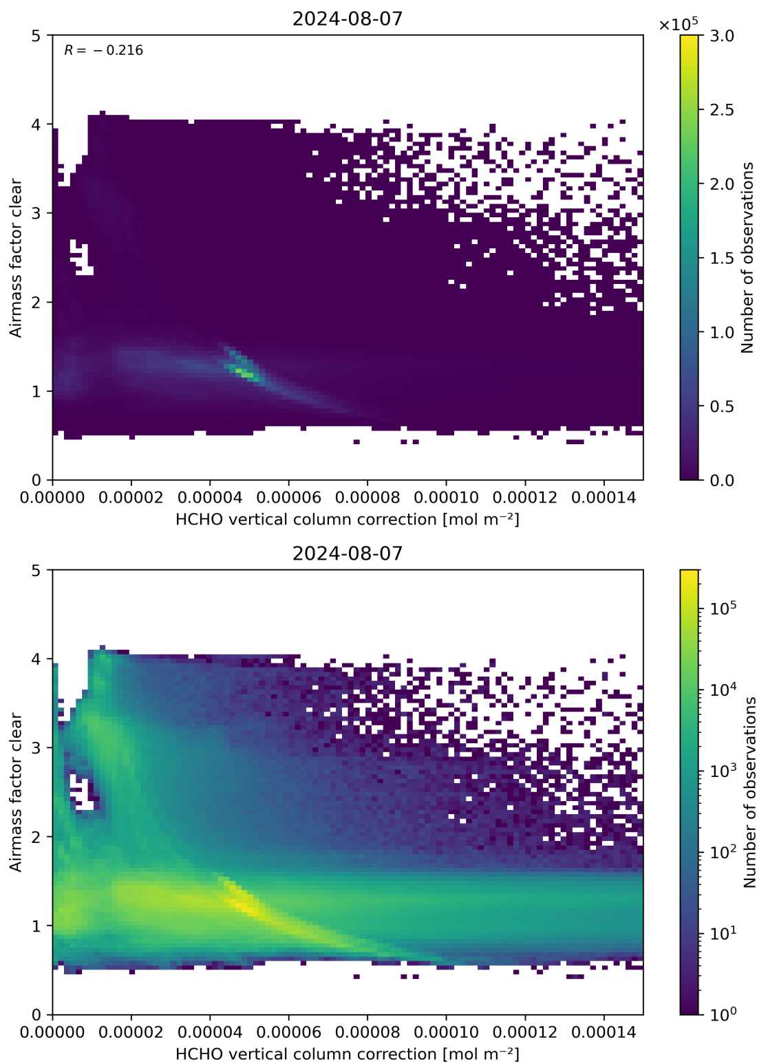
Figure 115: Scatter density plot of “HCHO vertical column correction” against “Airmass factor clear” for 2024-08-06 to 2024-08-08.
