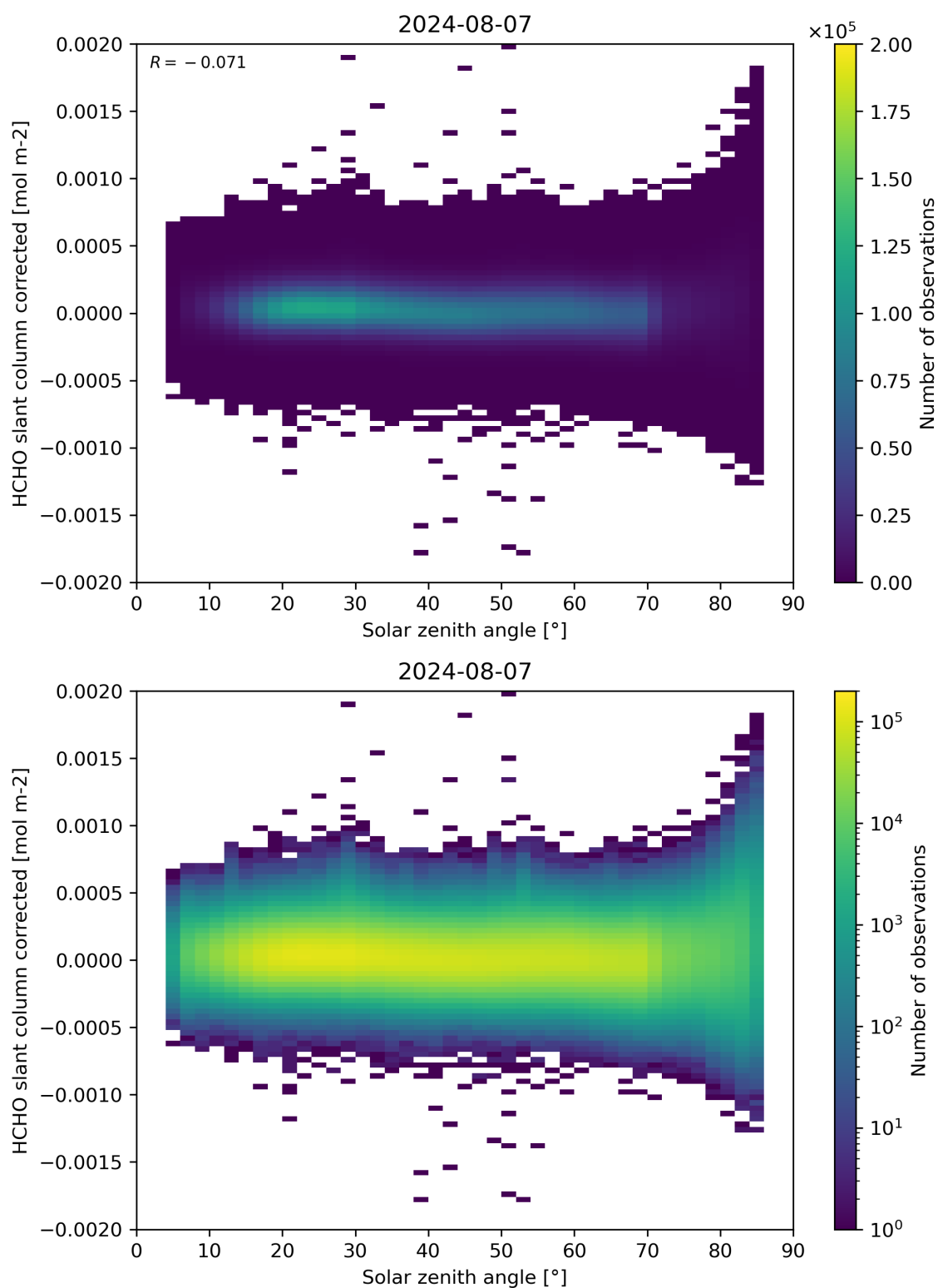
Figure 171: Scatter density plot of “Solar zenith angle” against “HCHO slant column corrected” for 2024-08-06 to 2024-08-08.
