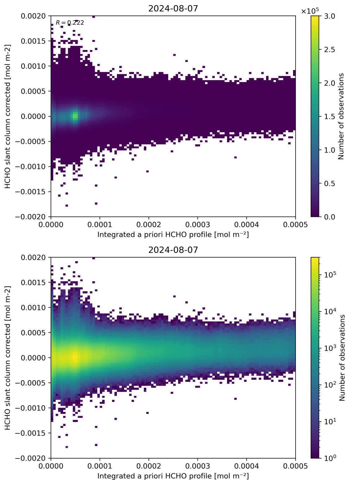
Figure 151: Scatter density plot of “Integrated a priori HCHO profile” against “HCHO slant column corrected” for 2024-08-06 to 2024-08-08.
