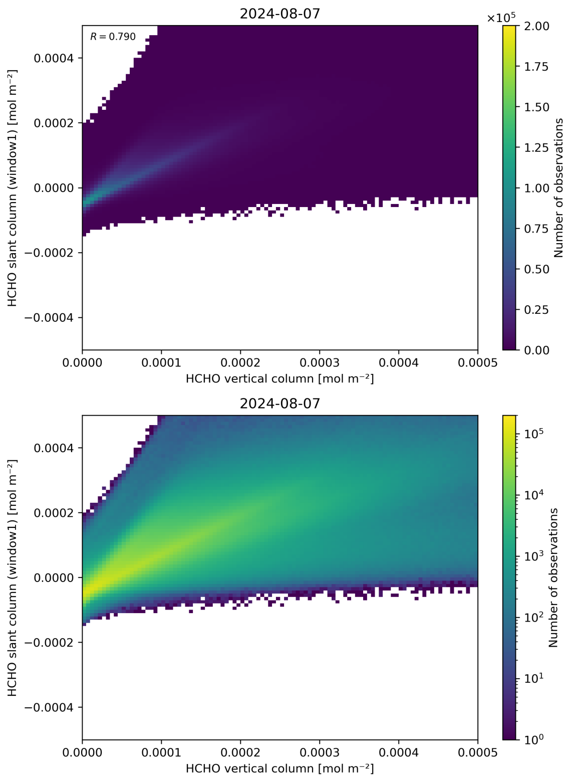
Figure 129: Scatter density plot of “HCHO vertical column” against “HCHO slant column (window1)” for 2024-08-06 to 2024-08-08.
