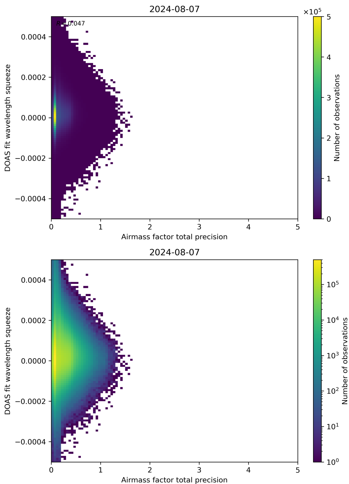
Figure 107: Scatter density plot of “Airmass factor total precision” against “DOAS fit wavelength squeeze” for 2024-08-06 to 2024-08-08.
