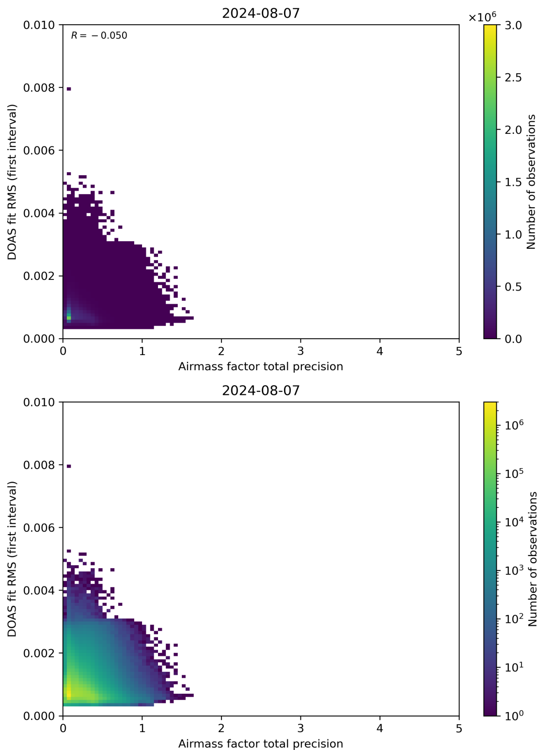
Figure 105: Scatter density plot of “Airmass factor total precision” against “DOAS fit RMS (first interval)” for 2024-08-06 to 2024-08-08.
