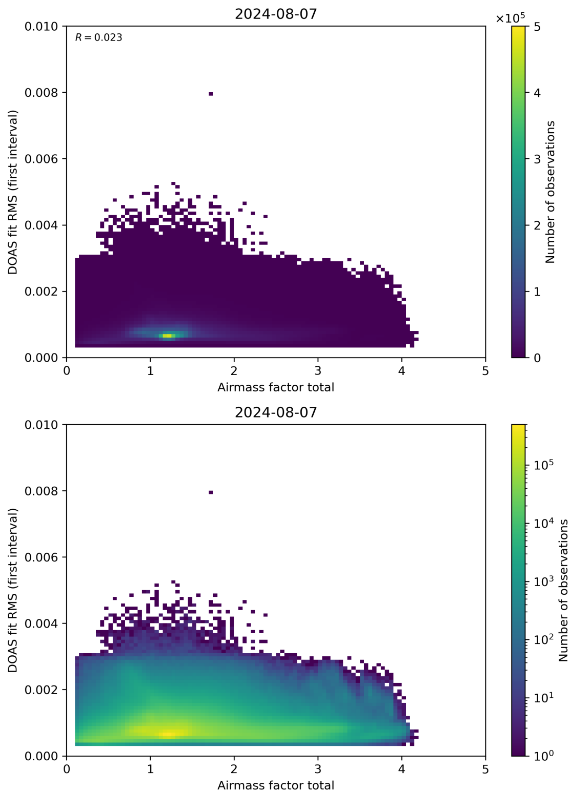
Figure 97: Scatter density plot of “Airmass factor total” against “DOAS fit RMS (first interval)” for 2024-08-06 to 2024-08-08.
