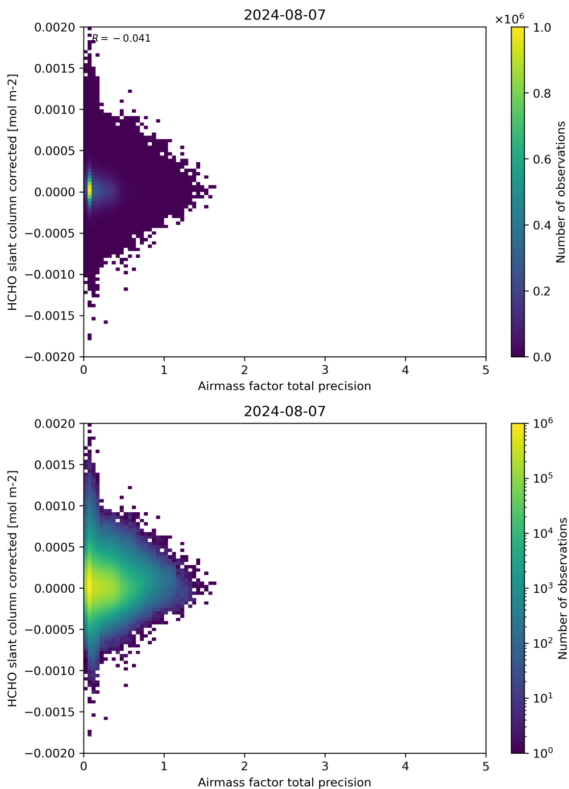
Figure 109: Scatter density plot of “Airmass factor total precision” against “HCHO slant column corrected” for 2024-08-06 to 2024-08-08.
