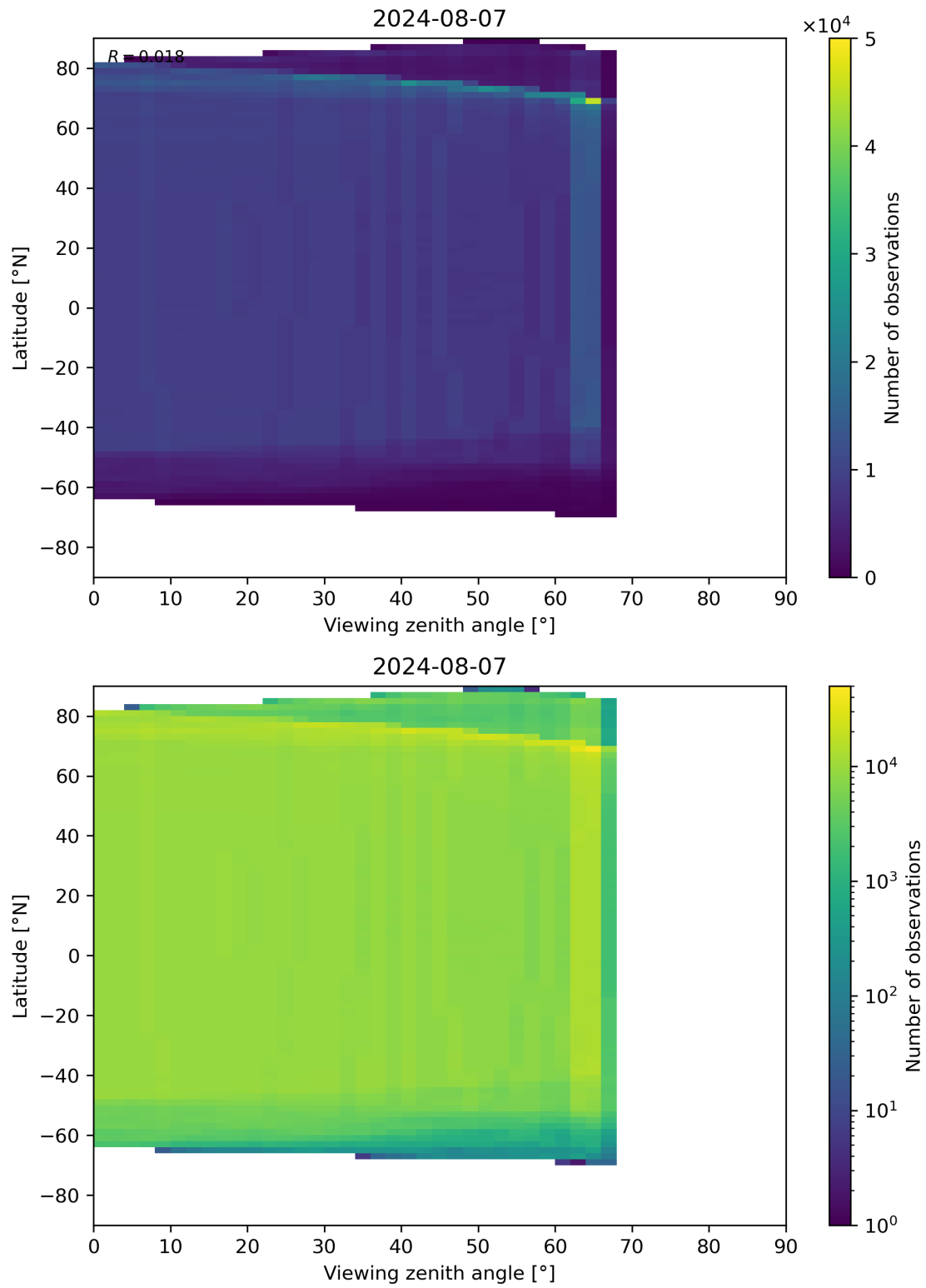
Figure 196: Scatter density plot of “Viewing zenith angle” against “Latitude” for 2024-08-06 to 2024-08-08.
