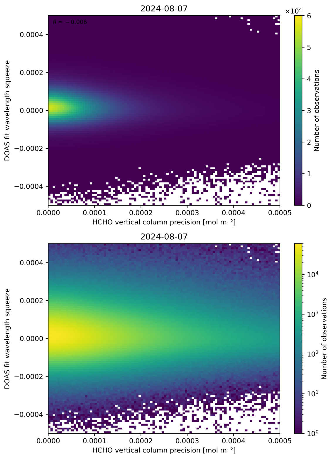
Figure 138: Scatter density plot of “HCHO vertical column precision” against “DOAS fit wavelength squeeze” for 2024-08-06 to 2024-08-08.
