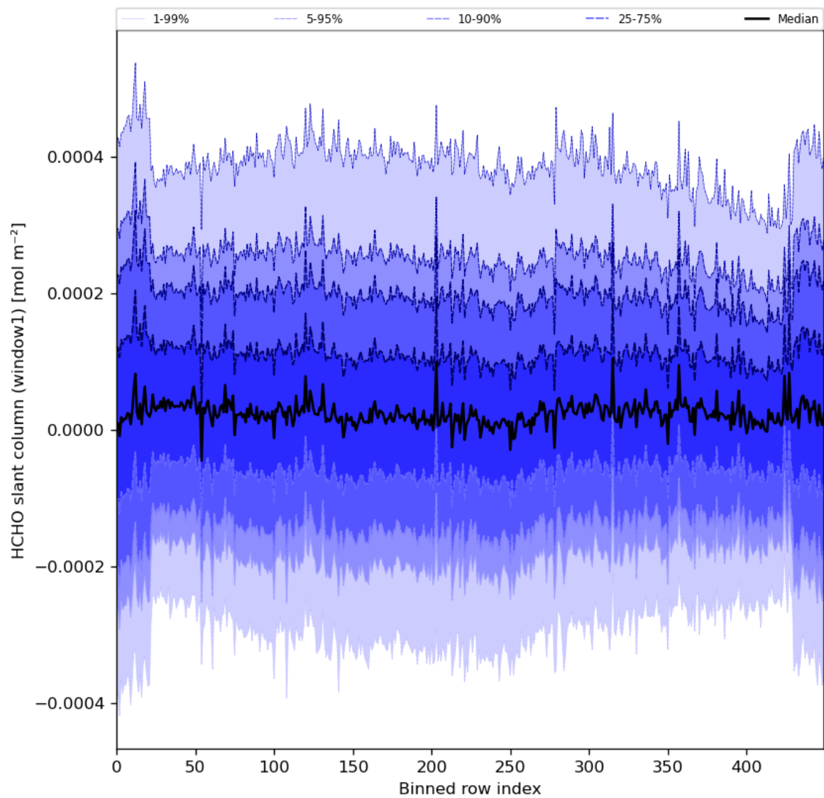
Figure 52: Along track statistics of “HCHO slant column (window1)” for 2024-08-06 to 2024-08-08
