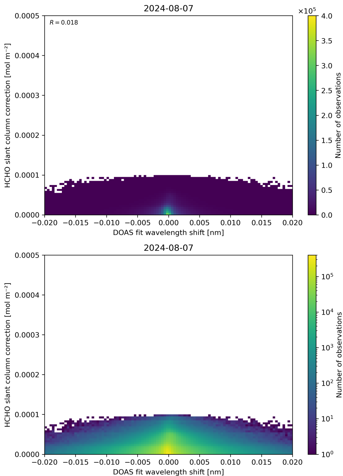
Figure 67: Scatter density plot of “DOAS fit wavelength shift” against “HCHO slant column correction” for 2024-08-06 to 2024-08-08.
