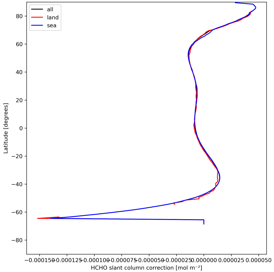
Figure 33: Zonal average of “HCHO slant column correction” for 2024-08-06 to 2024-08-08.
