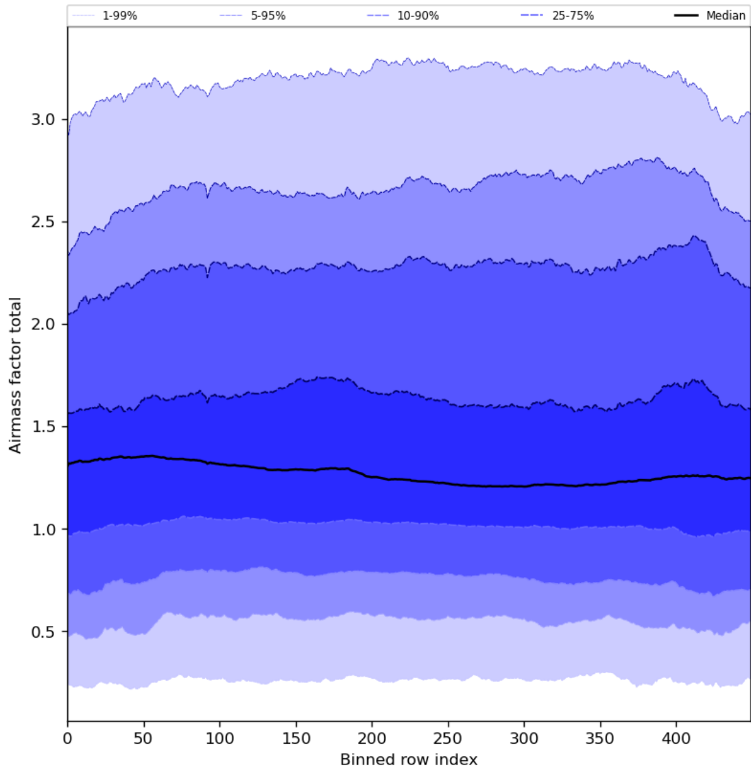
Figure 54: Along track statistics of “Airmass factor total” for 2024-08-06 to 2024-08-08
