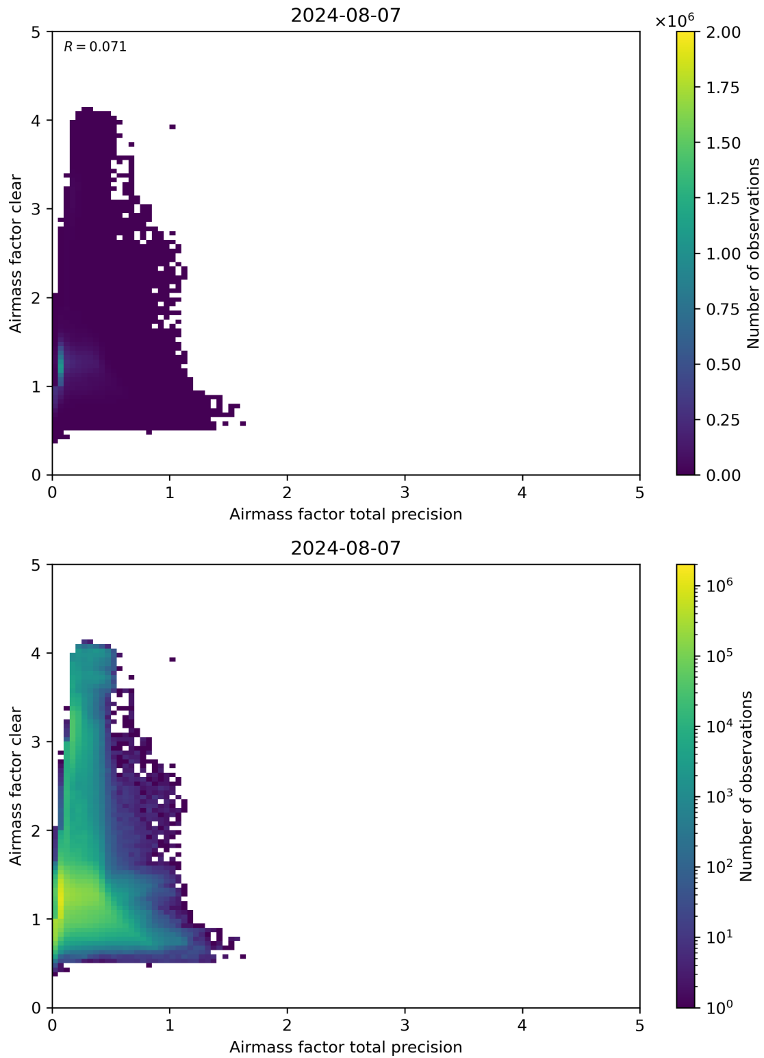
Figure 108: Scatter density plot of “Airmass factor total precision” against “Airmass factor clear” for 2024-08-06 to 2024-08-08.
