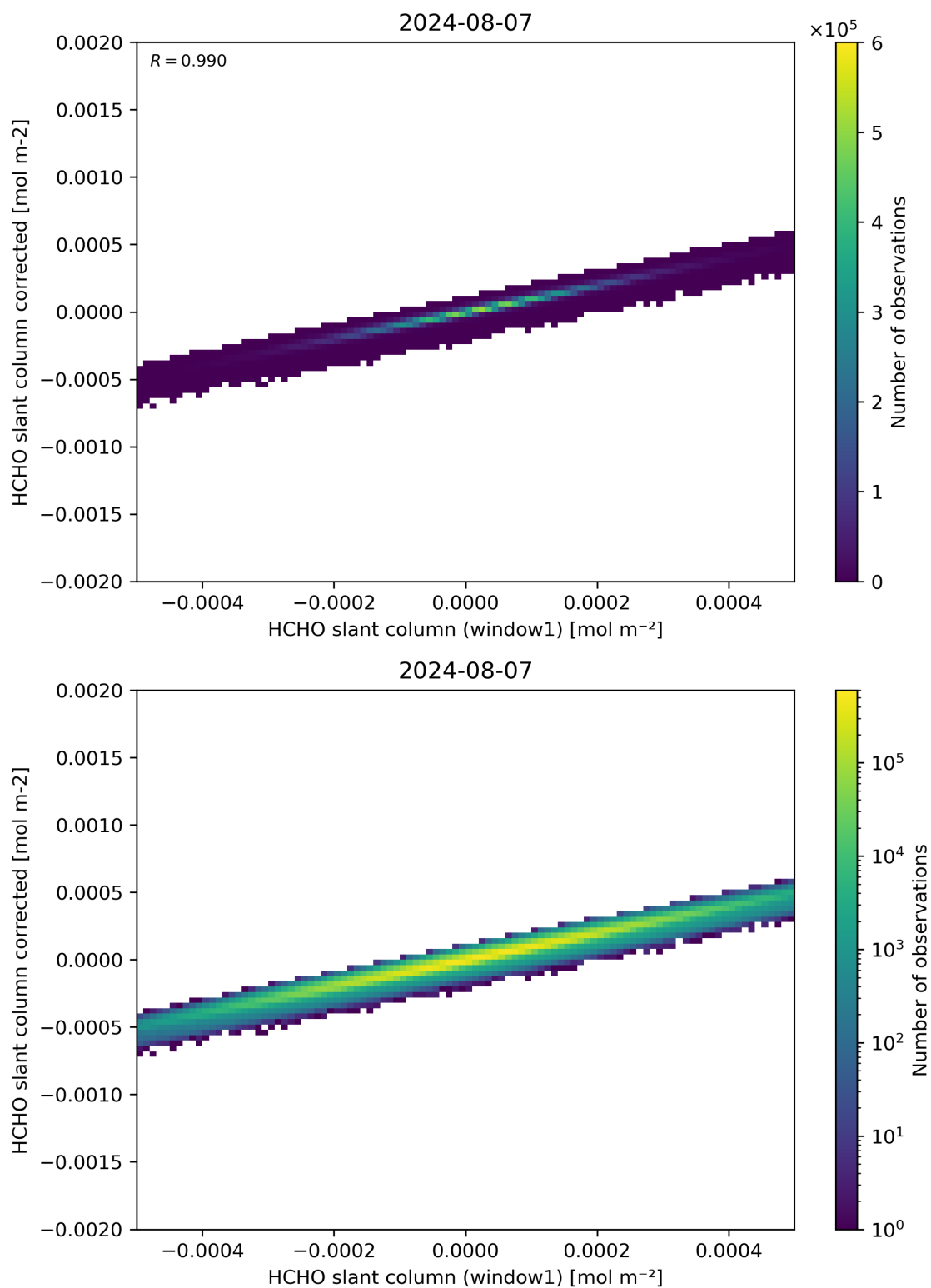
Figure 82: Scatter density plot of “HCHO slant column (window1)” against “HCHO slant column corrected” for 2024-08-06 to 2024-08-08.
