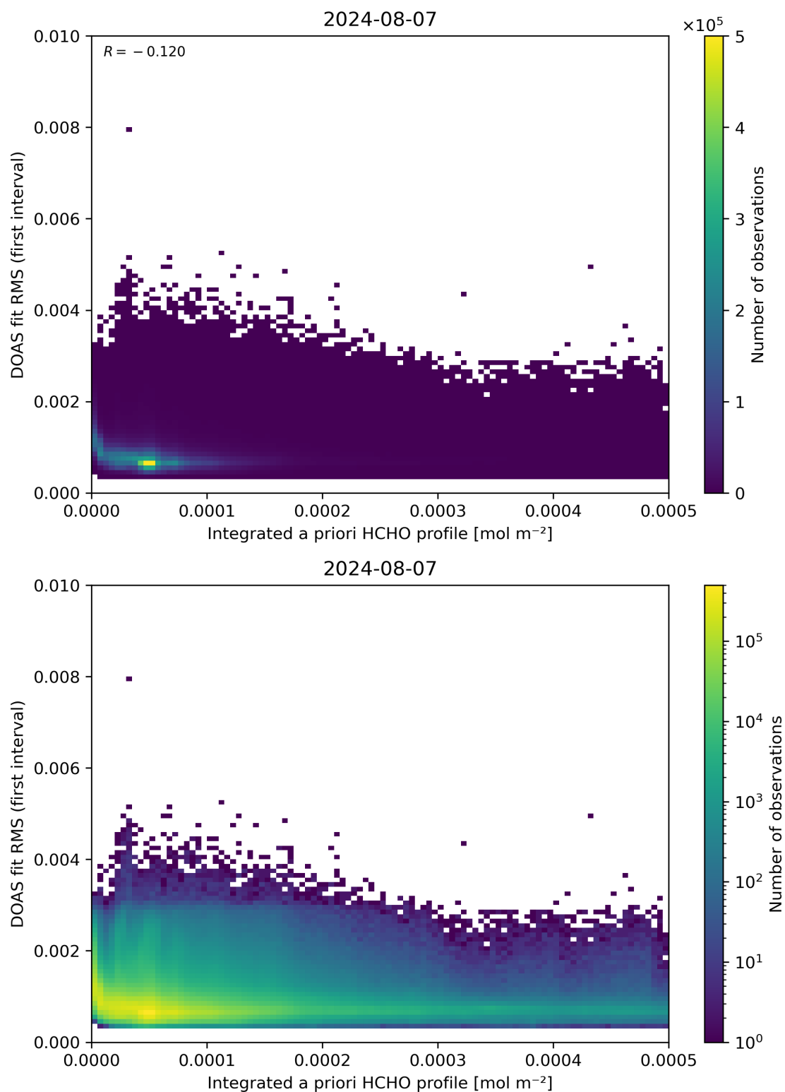
Figure 148: Scatter density plot of “Integrated a priori HCHO profile” against “DOAS fit RMS (first interval)” for 2024-08-06 to 2024-08-08.
