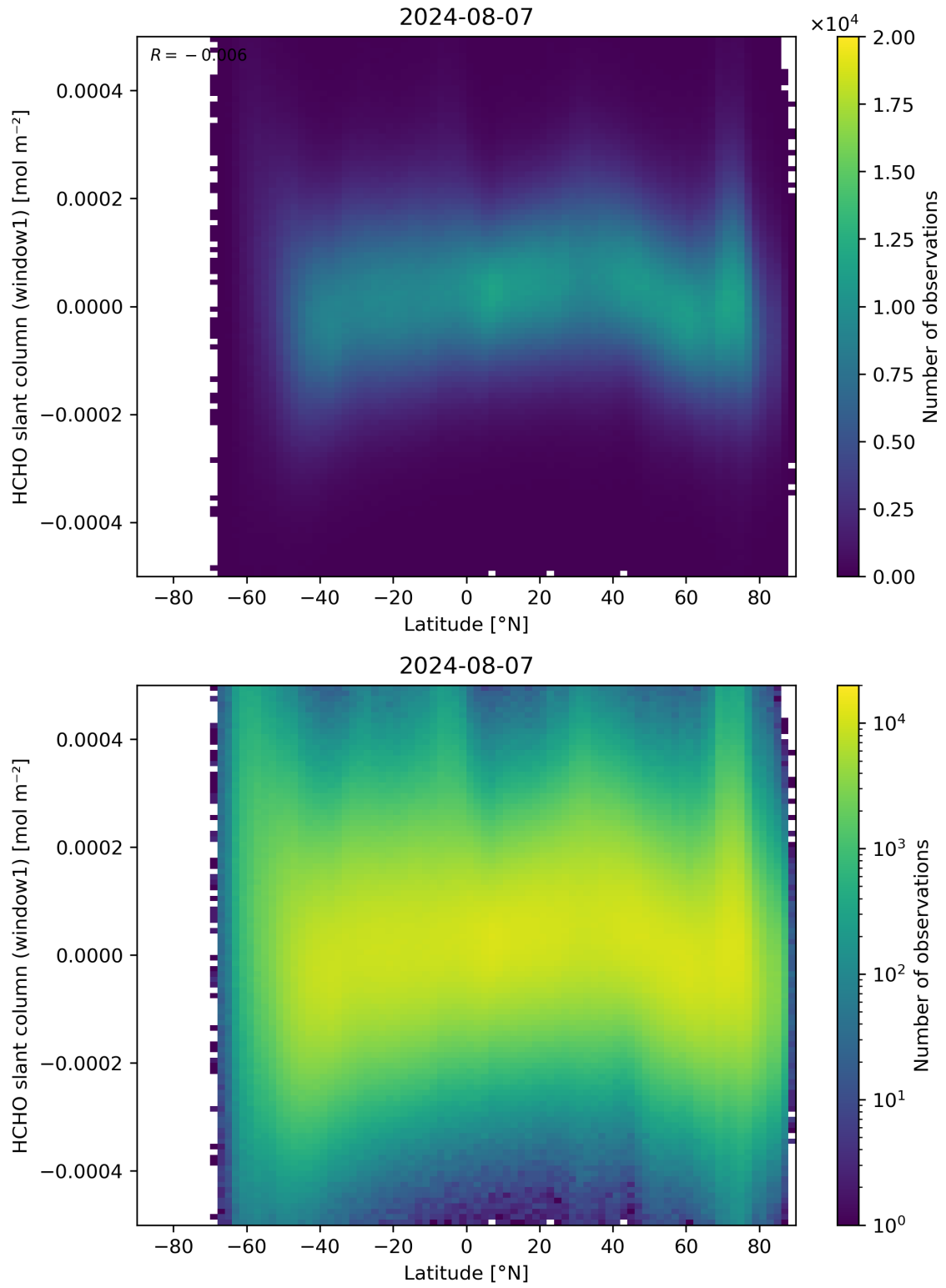
Figure 159: Scatter density plot of “Latitude” against “HCHO slant column (window1)” for 2024-08-06 to 2024-08-08.
