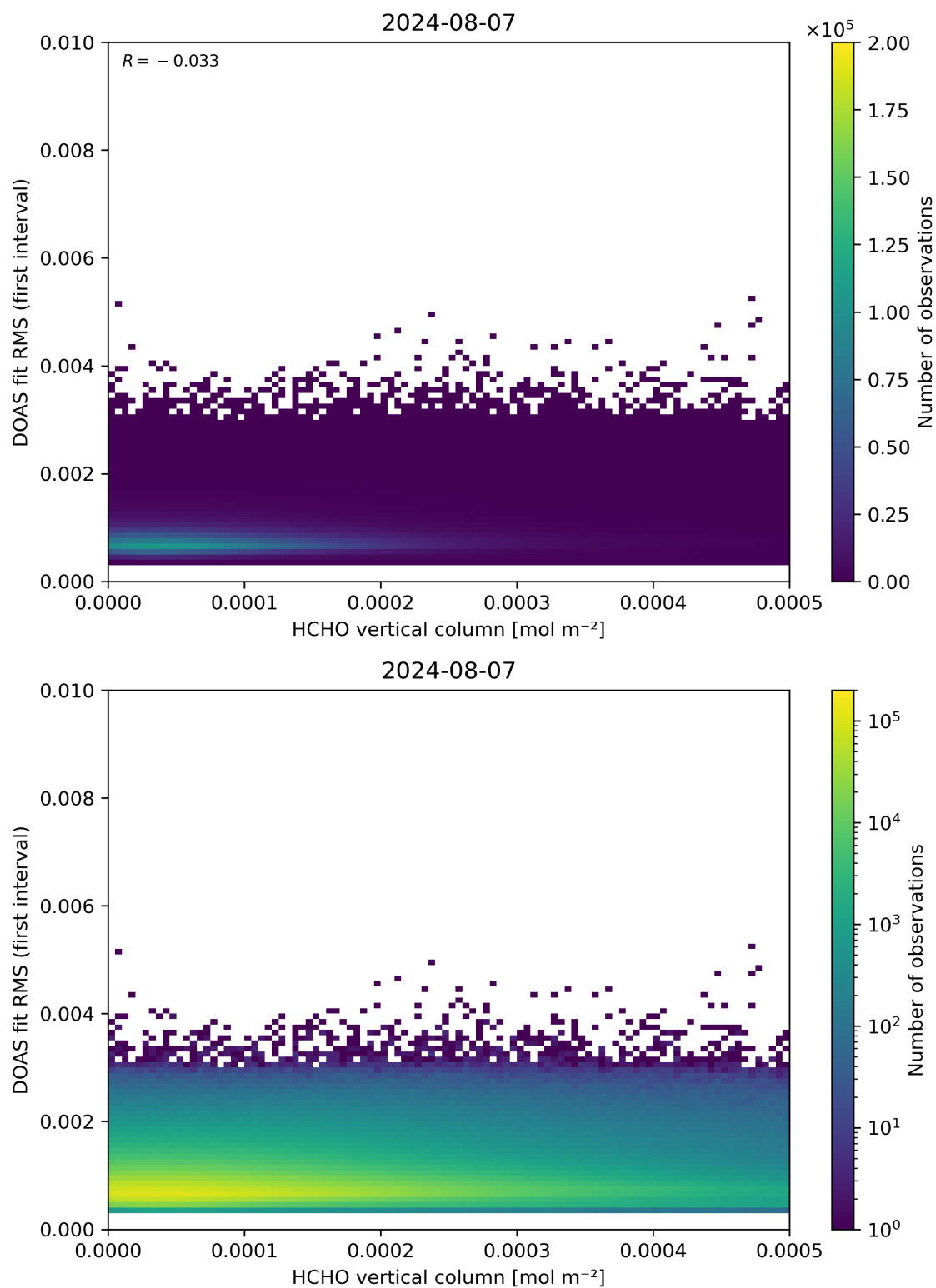
Figure 123: Scatter density plot of “HCHO vertical column” against “DOAS fit RMS (first interval)” for 2024-08-06 to 2024-08-08.
