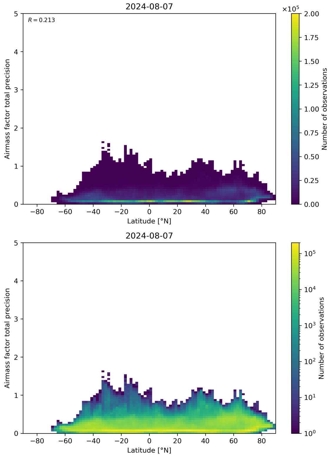
Figure 162: Scatter density plot of “Latitude” against “Airmass factor total precision” for 2024-08-06 to 2024-08-08.
