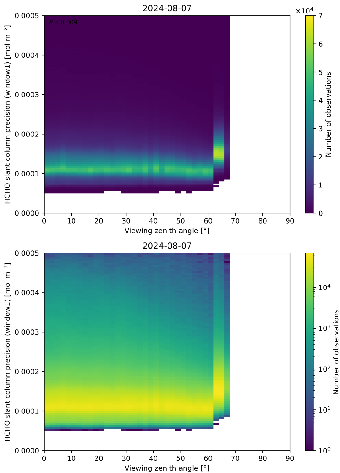
Figure 189: Scatter density plot of “Viewing zenith angle” against “HCHO slant column precision (window1)” for 2024-08-06 to 2024-08-08.
