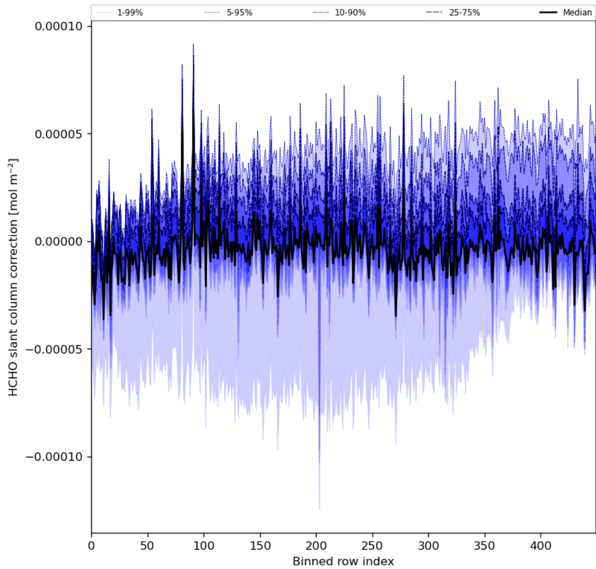
Figure 61: Along track statistics of “HCHO slant column correction” for 2024-08-06 to 2024-08-08
