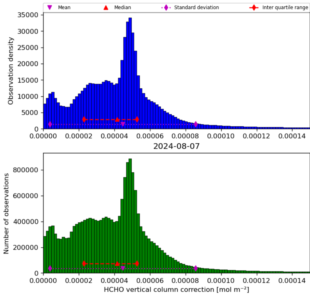
Figure 37: Histogram of “HCHO vertical column correction” for 2024-08-06 to 2024-08-08
