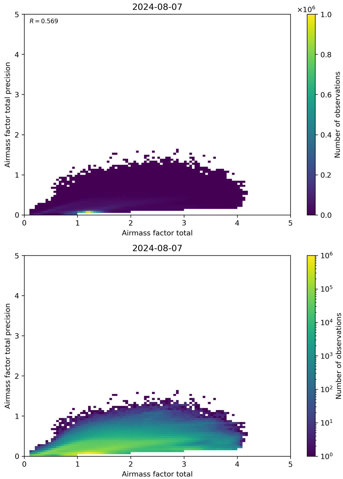
Figure 103: Scatter density plot of “Airmass factor total” against “Airmass factor total precision” for 2024-08-06 to 2024-08-08.
