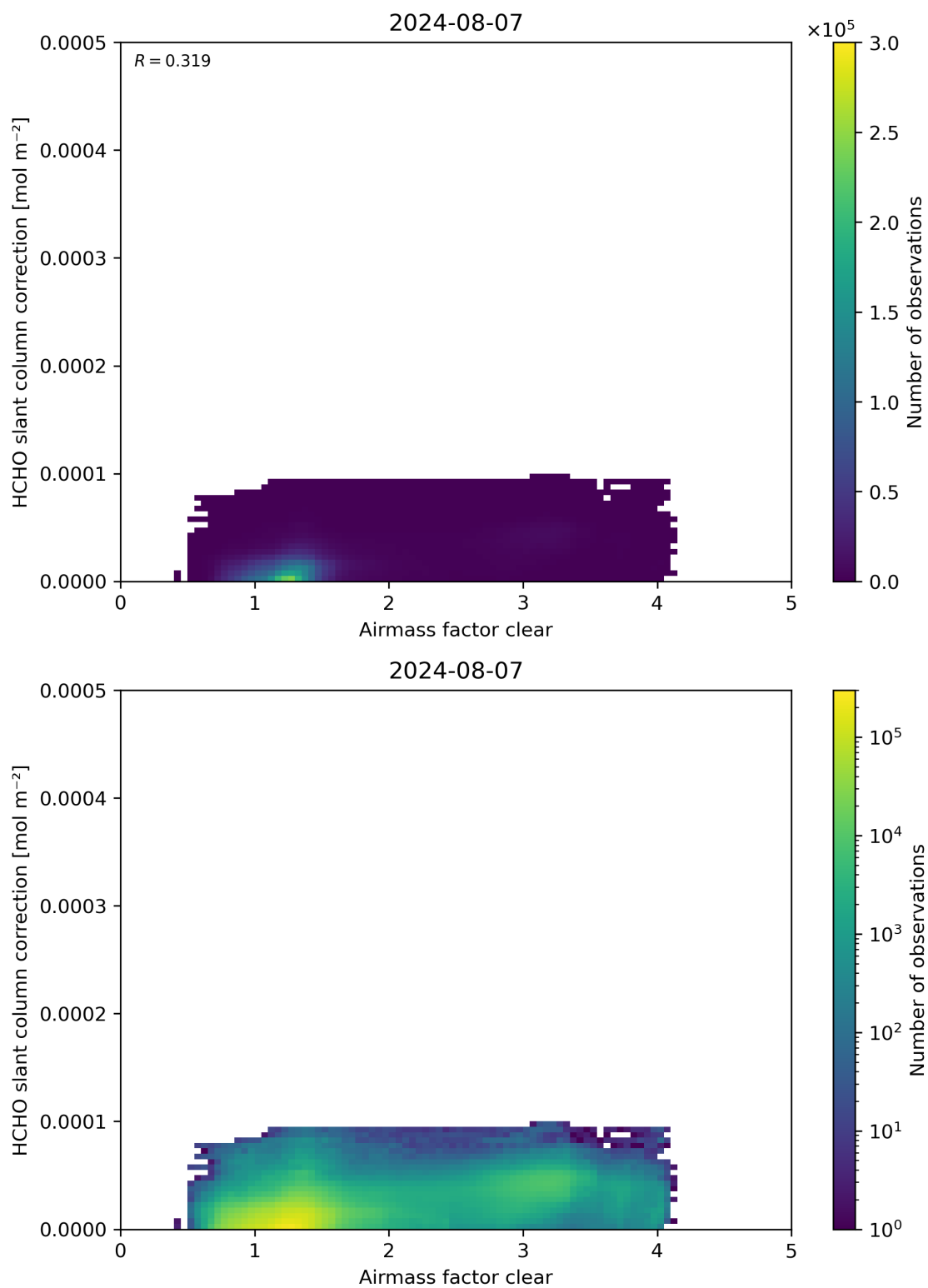
Figure 75: Scatter density plot of “Airmass factor clear” against “HCHO slant column correction” for 2024-08-06 to 2024-08-08.
