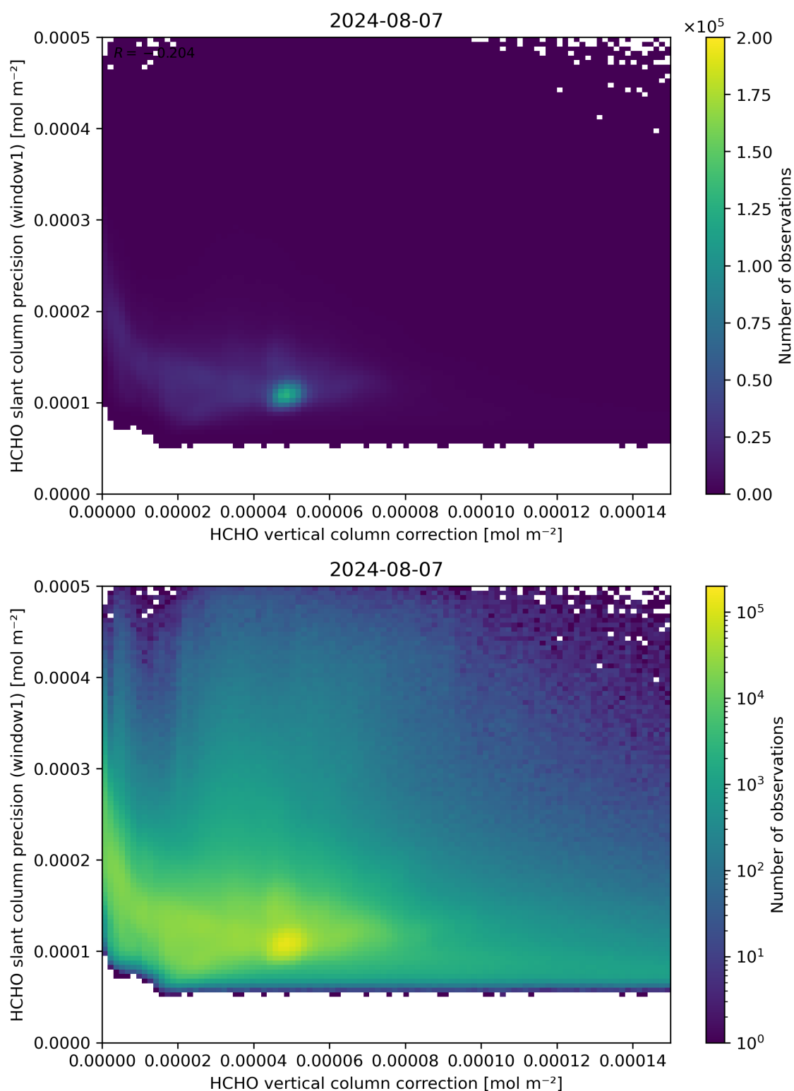
Figure 119: Scatter density plot of “HCHO vertical column correction” against “HCHO slant column precision (window1)” for 2024-08-06 to 2024-08-08.
