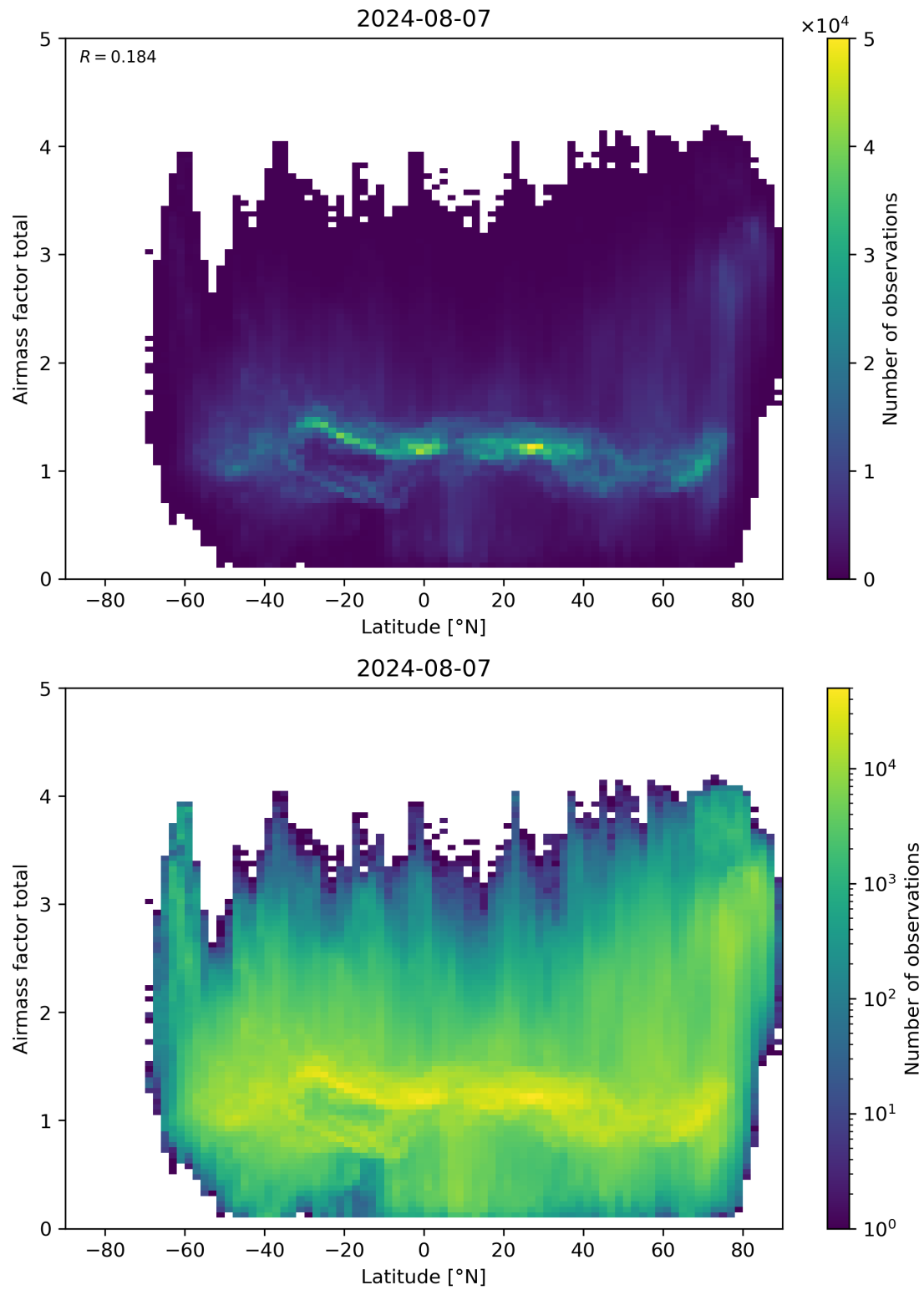
Figure 161: Scatter density plot of “Latitude” against “Airmass factor total” for 2024-08-06 to 2024-08-08.
