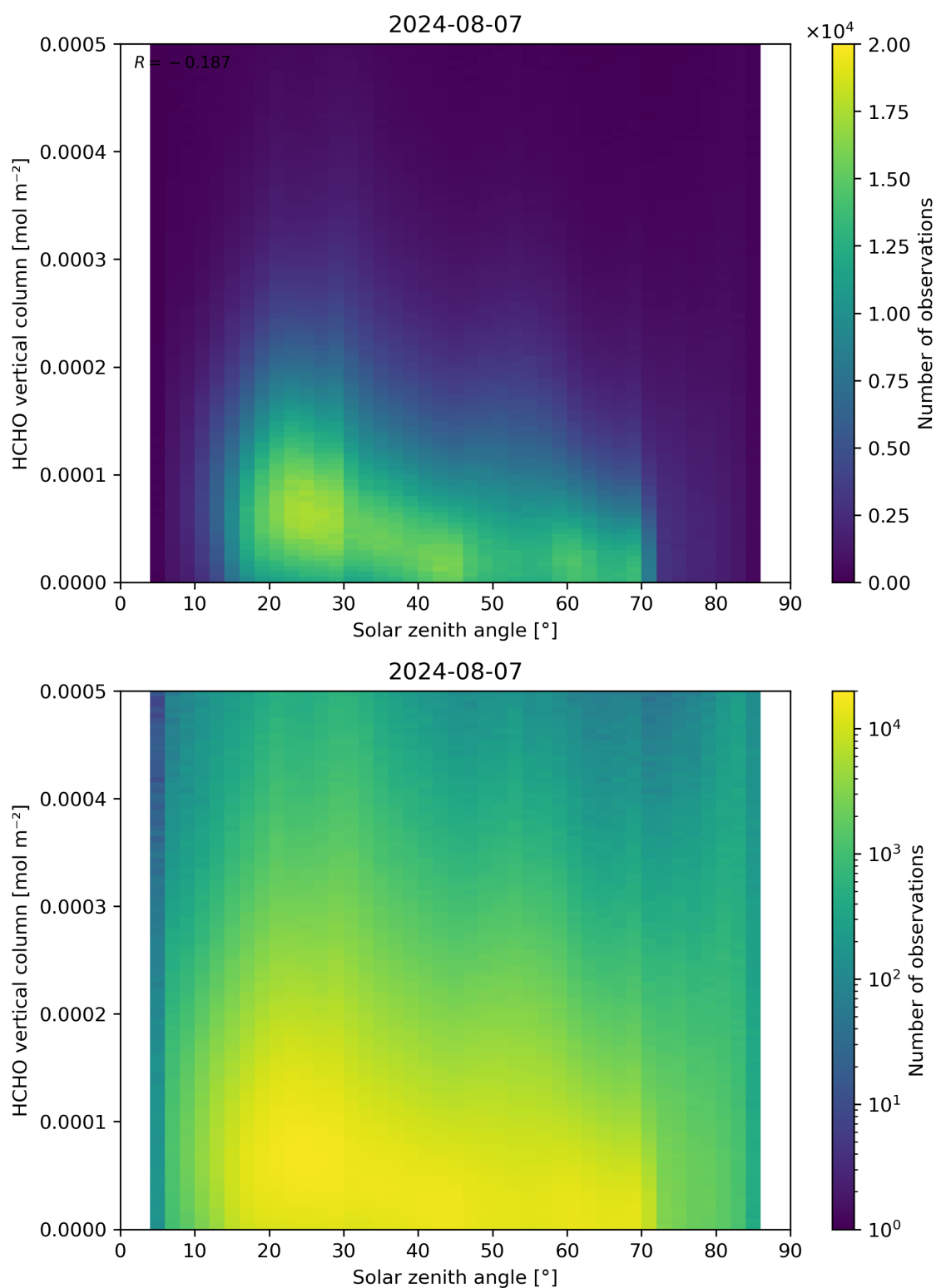
Figure 177: Scatter density plot of “Solar zenith angle” against “HCHO vertical column” for 2024-08-06 to 2024-08-08.
