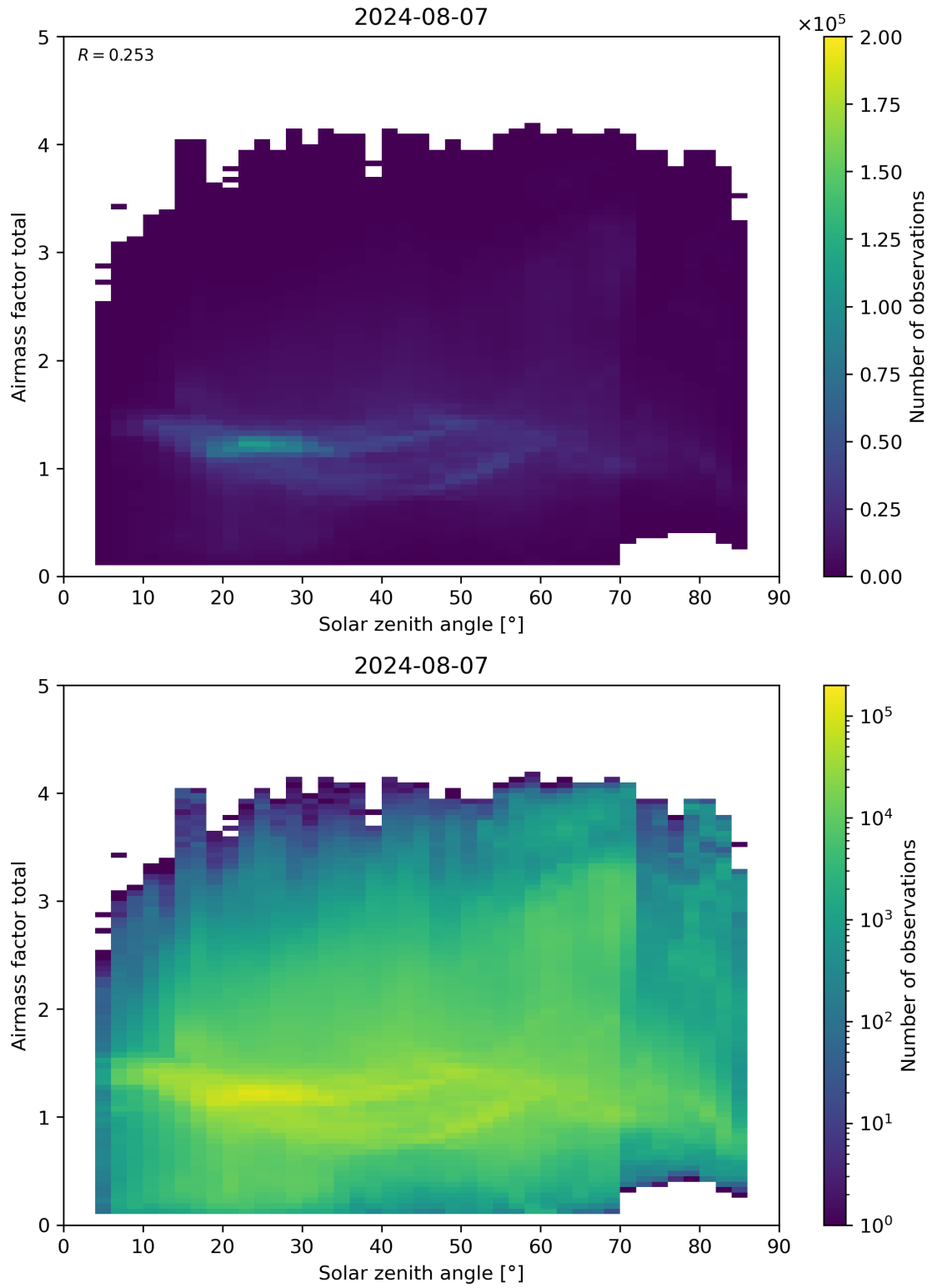
Figure 175: Scatter density plot of “Solar zenith angle” against “Airmass factor total” for 2024-08-06 to 2024-08-08.
