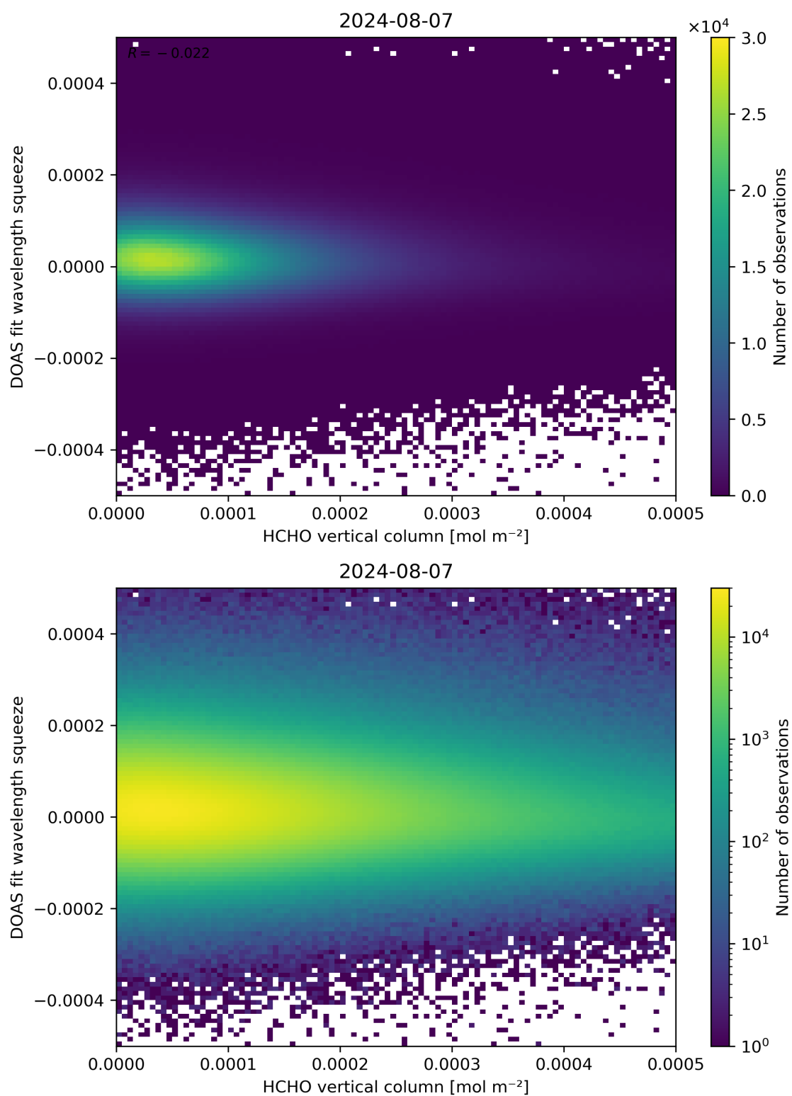
Figure 125: Scatter density plot of “HCHO vertical column” against “DOAS fit wavelength squeeze” for 2024-08-06 to 2024-08-08.
