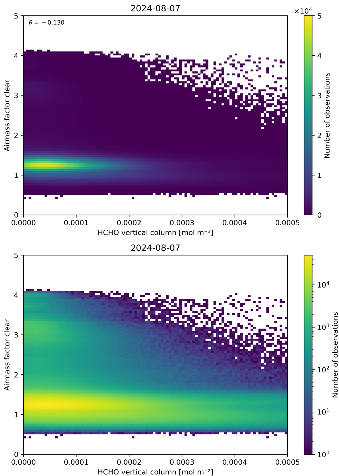
Figure 126: Scatter density plot of “HCHO vertical column” against “Airmass factor clear” for 2024-08-06 to 2024-08-08.
