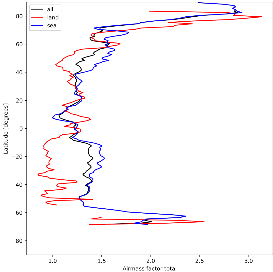
Figure 26: Zonal average of “Airmass factor total” for 2024-08-06 to 2024-08-08.
