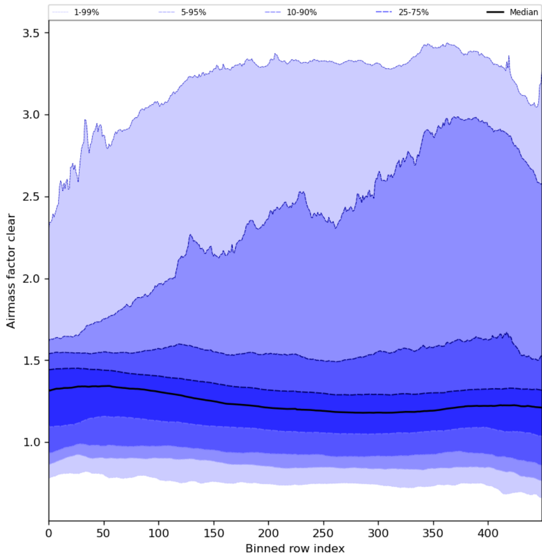
Figure 56: Along track statistics of “Airmass factor clear” for 2024-08-06 to 2024-08-08
