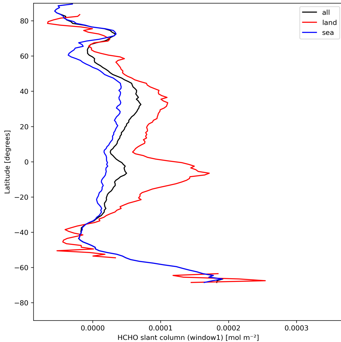
Figure 24: Zonal average of “HCHO slant column (window1)” for 2024-08-06 to 2024-08-08.
