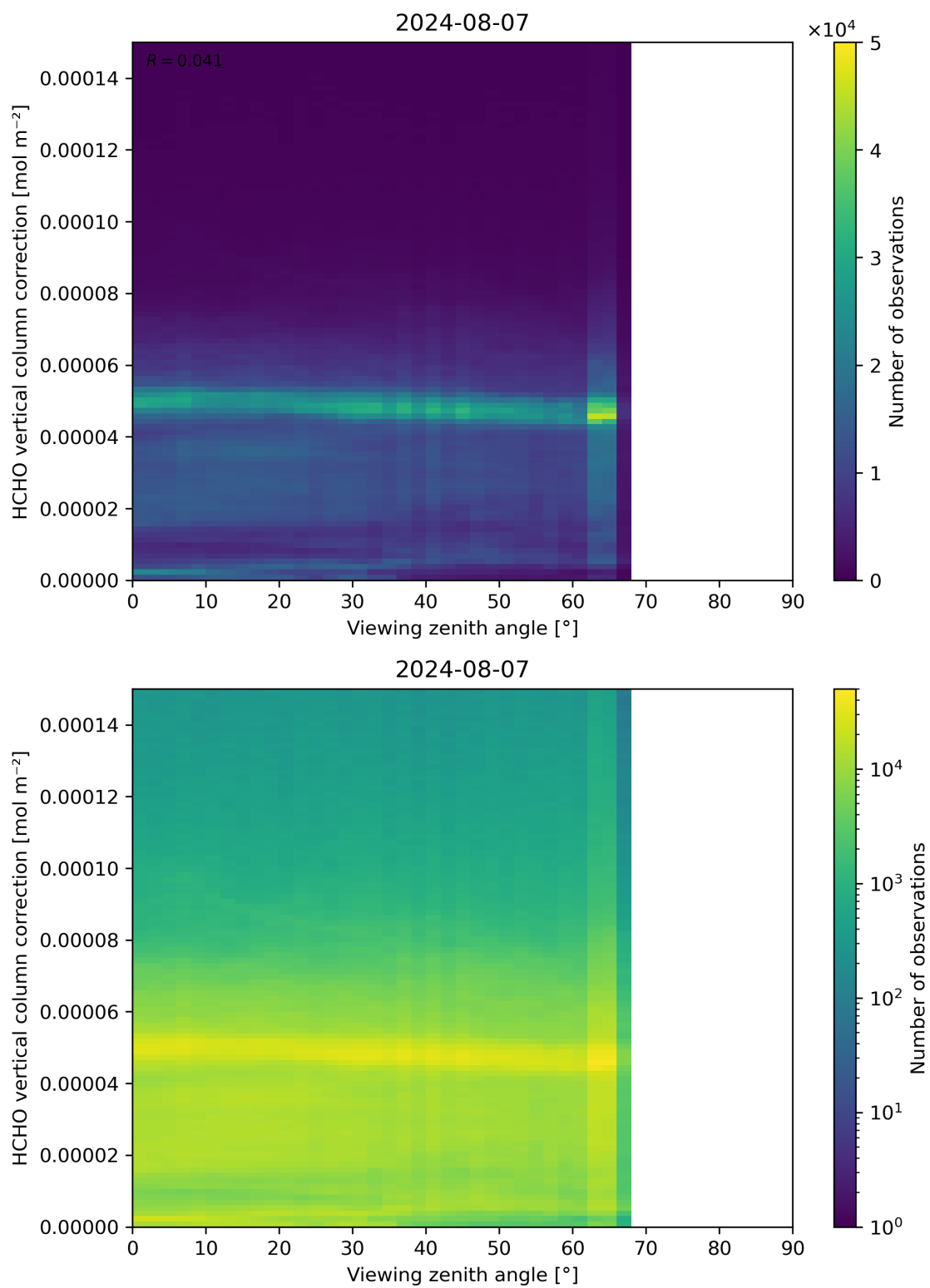
Figure 193: Scatter density plot of “Viewing zenith angle” against “HCHO vertical column correction” for 2024-08-06 to 2024-08-08.
