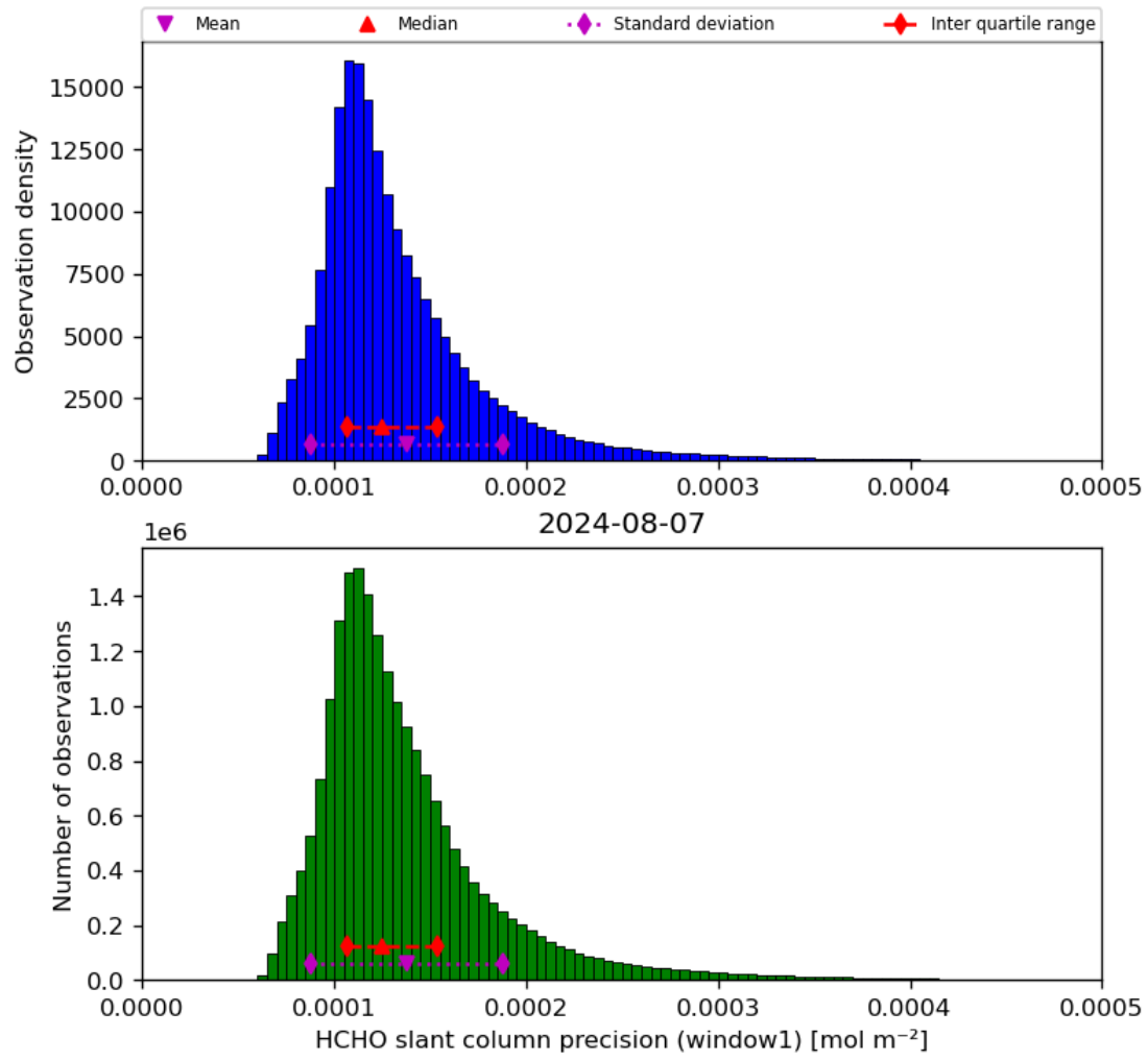
Figure 39: Histogram of “HCHO slant column precision (window1)” for 2024-08-06 to 2024-08-08
