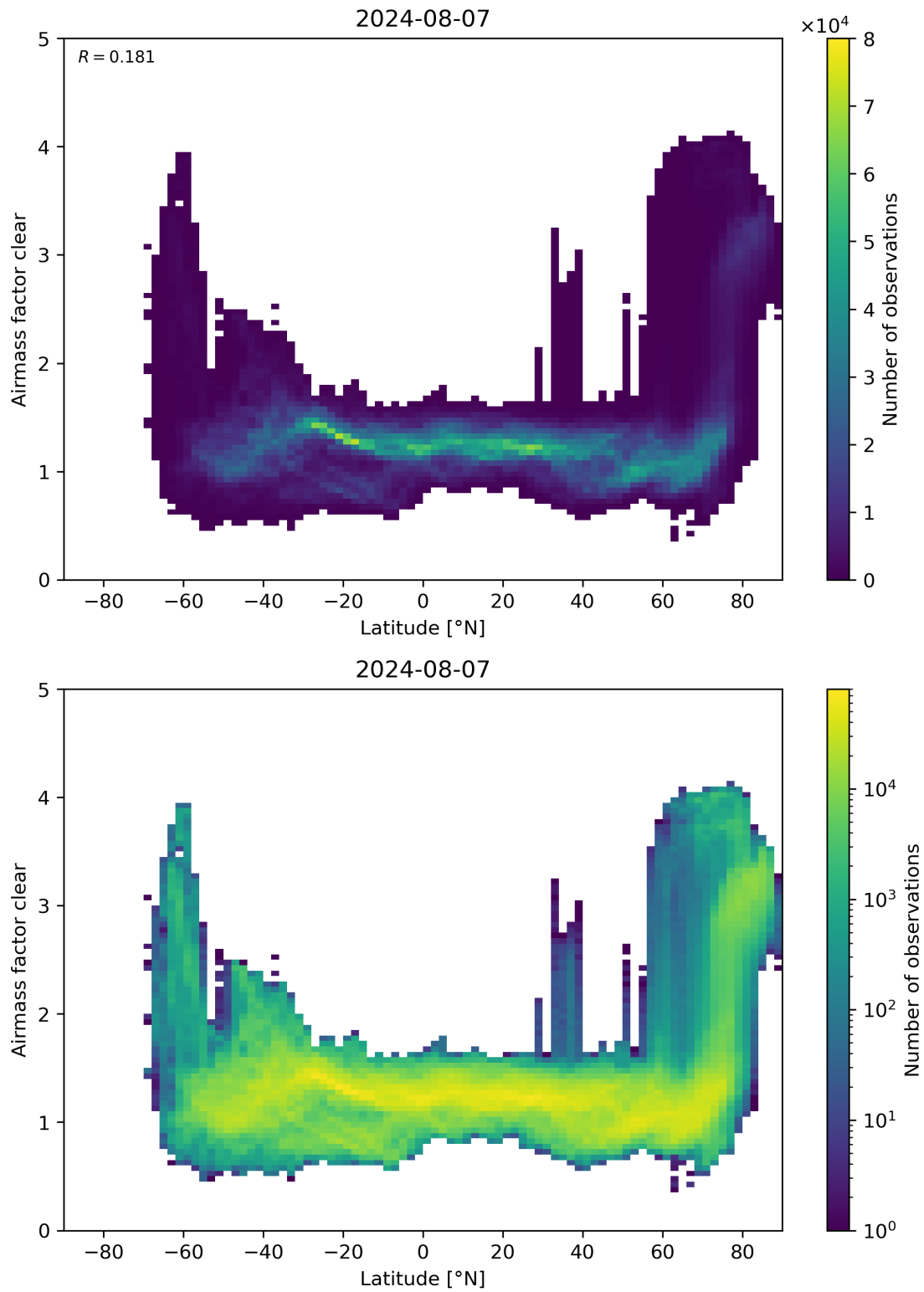
Figure 156: Scatter density plot of “Latitude” against “Airmass factor clear” for 2024-08-06 to 2024-08-08.
