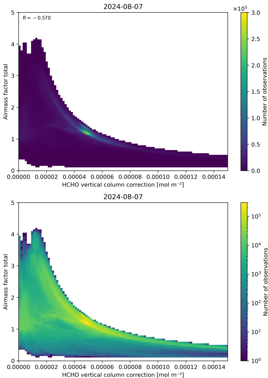
Figure 120: Scatter density plot of “HCHO vertical column correction” against “Airmass factor total” for 2024-08-06 to 2024-08-08.
