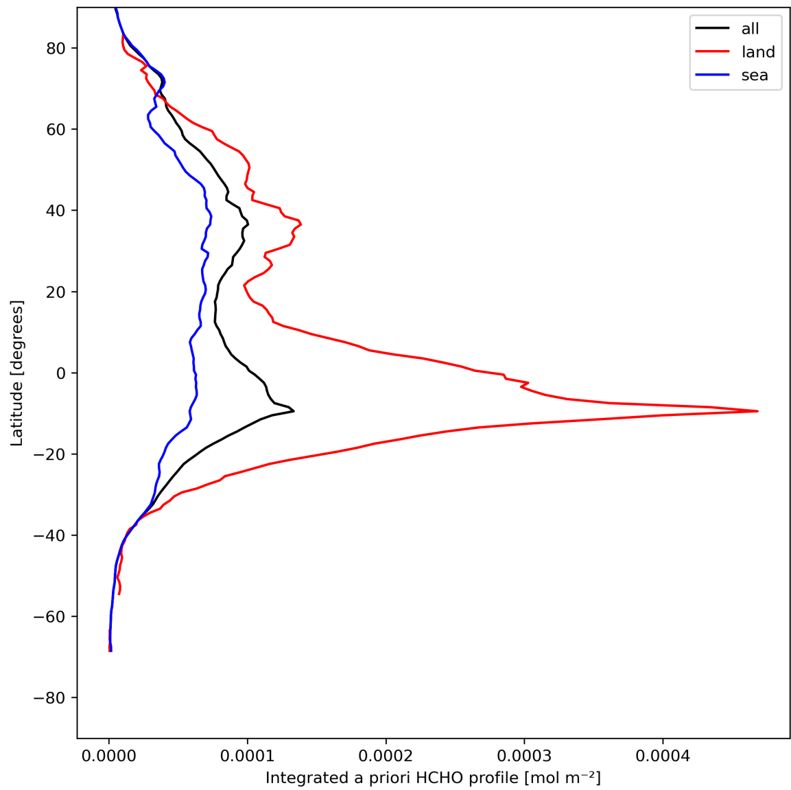
Figure 29: Zonal average of “Integrated a priori HCHO profile” for 2024-08-06 to 2024-08-08.
