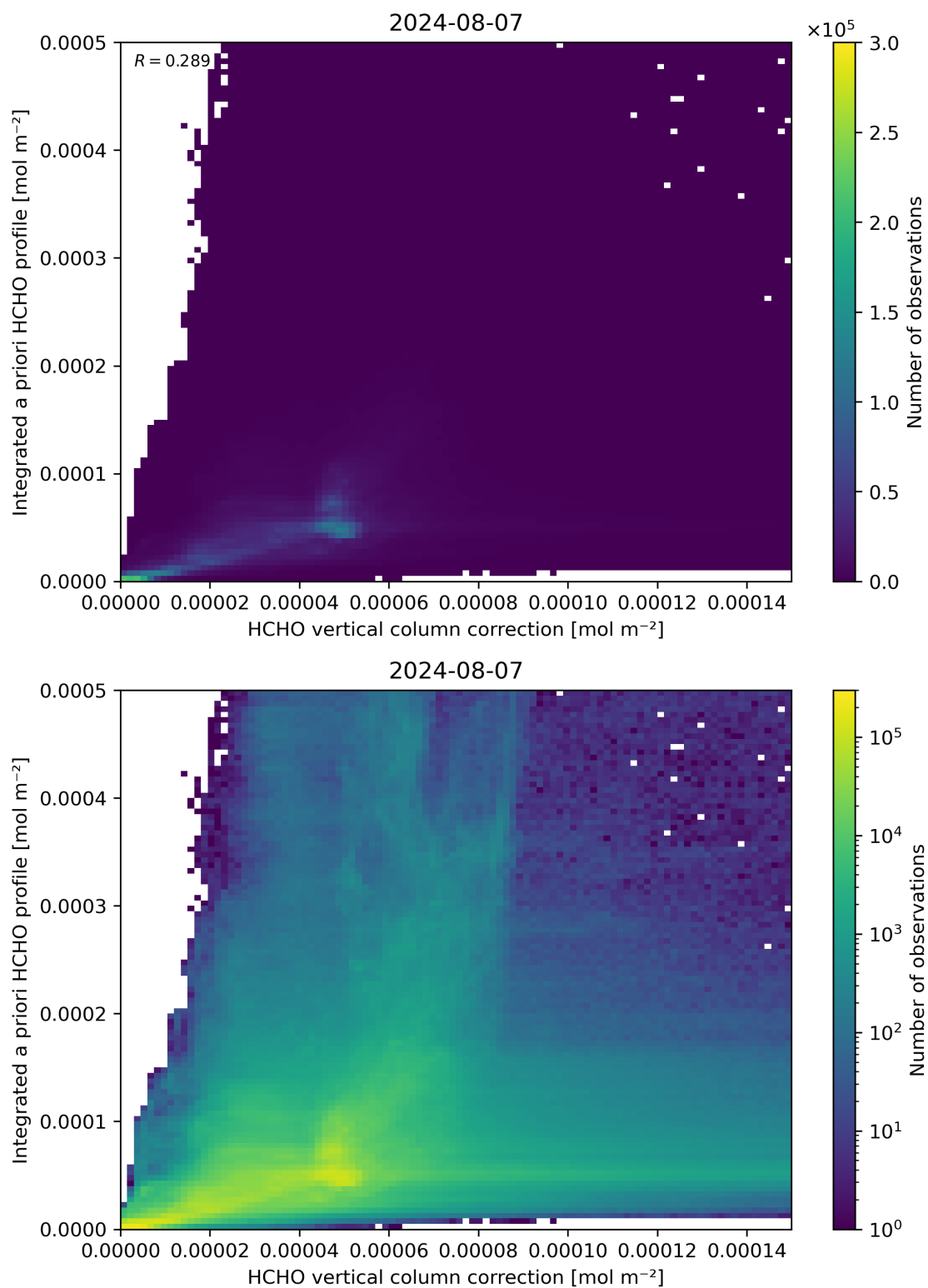
Figure 122: Scatter density plot of “HCHO vertical column correction” against “Integrated a priori HCHO profile” for 2024-08-06 to 2024-08-08.
