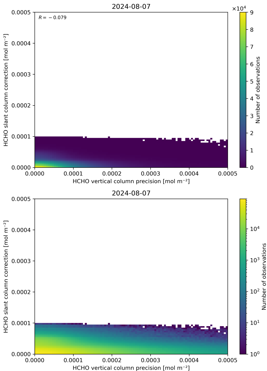
Figure 141: Scatter density plot of “HCHO vertical column precision” against “HCHO slant column correction” for 2024-08-06 to 2024-08-08.
