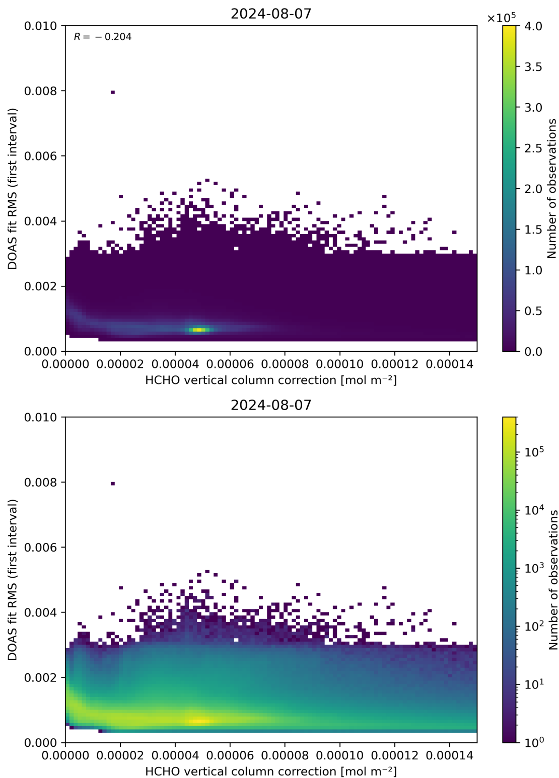
Figure 112: Scatter density plot of “HCHO vertical column correction” against “DOAS fit RMS (first interval)” for 2024-08-06 to 2024-08-08.
