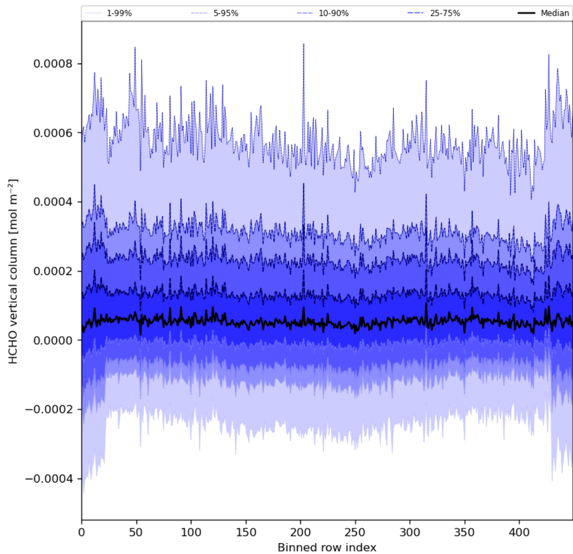
Figure 49: Along track statistics of “HCHO vertical column” for 2024-08-06 to 2024-08-08
