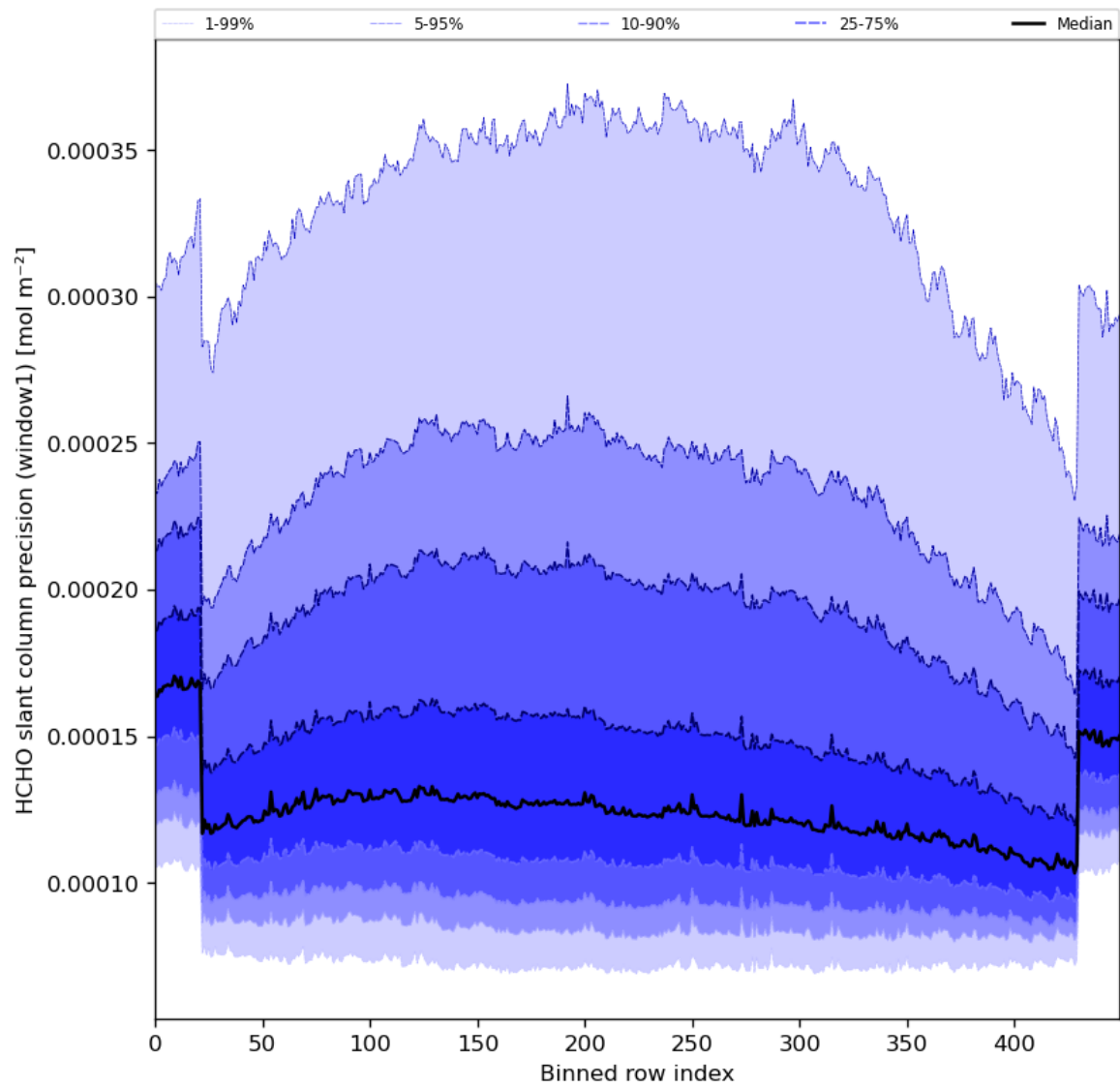
Figure 53: Along track statistics of “HCHO slant column precision (window1)” for 2024-08-06 to 2024-08-08
