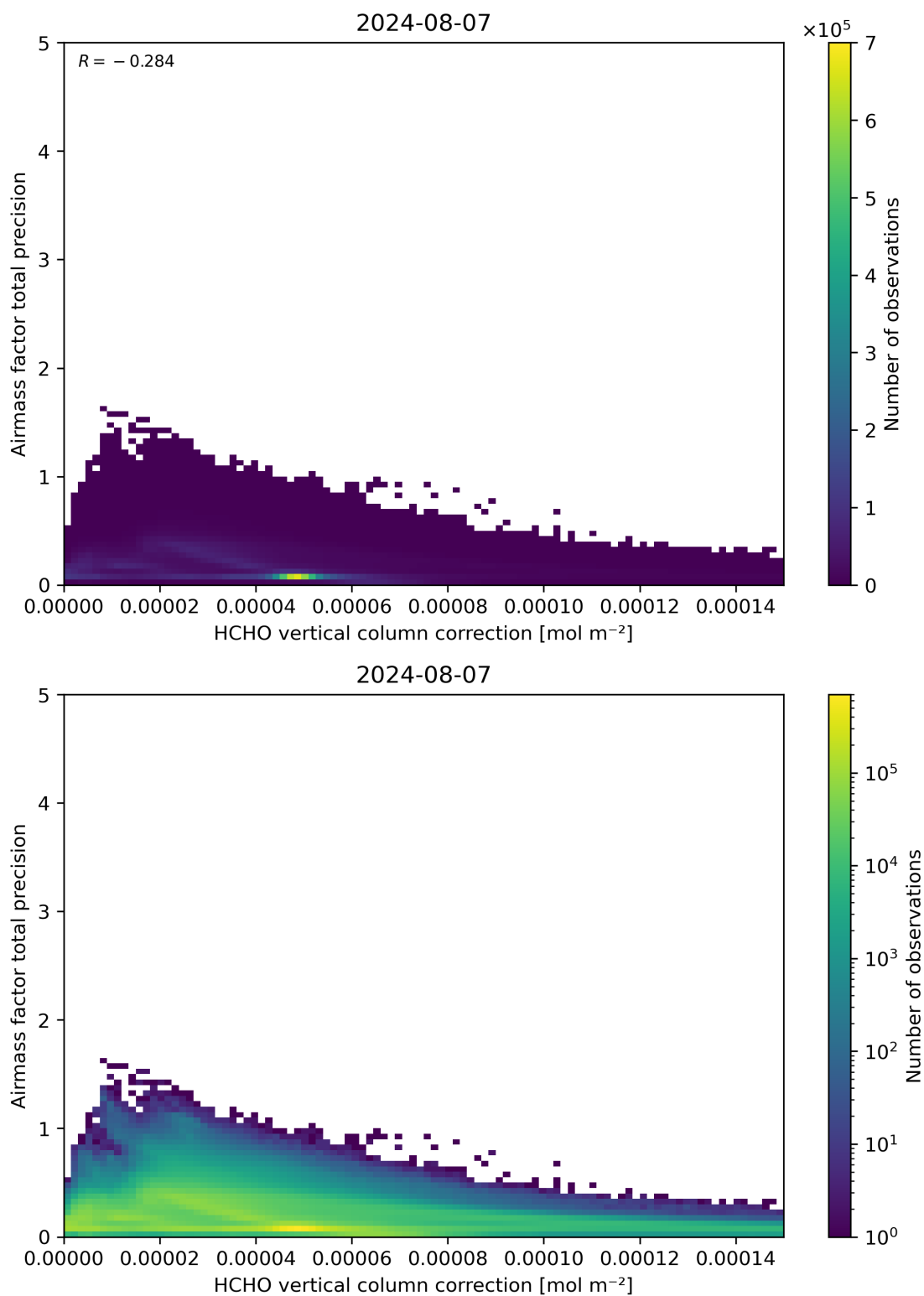
Figure 121: Scatter density plot of “HCHO vertical column correction” against “Airmass factor total precision” for 2024-08-06 to 2024-08-08.
