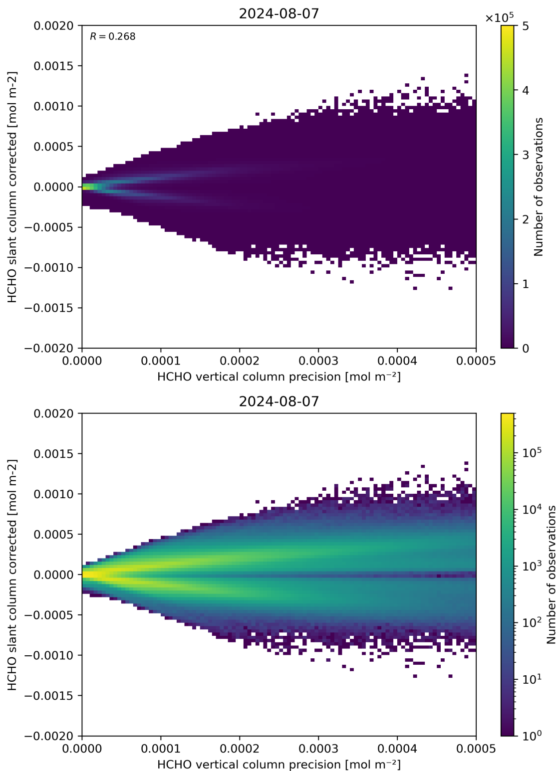
Figure 140: Scatter density plot of “HCHO vertical column precision” against “HCHO slant column corrected” for 2024-08-06 to 2024-08-08.
