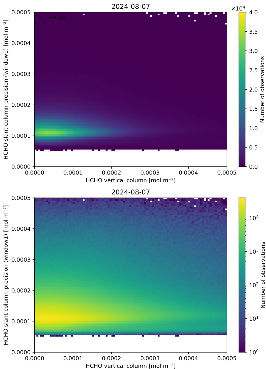
Figure 130: Scatter density plot of “HCHO vertical column” against “HCHO slant column precision (window1)” for 2024-08-06 to 2024-08-08.
