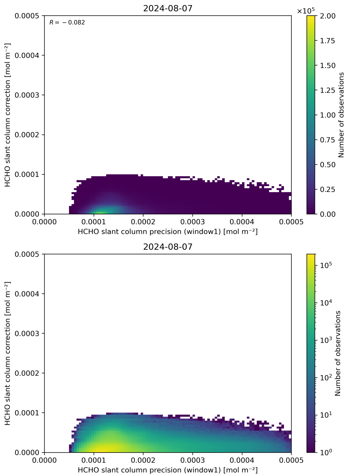
Figure 93: Scatter density plot of “HCHO slant column precision (window1)” against “HCHO slant column correction” for 2024-08-06 to 2024-08-08.
