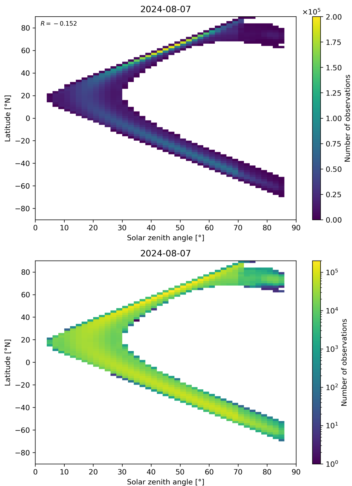
Figure 181: Scatter density plot of “Solar zenith angle” against “Latitude” for 2024-08-06 to 2024-08-08.
