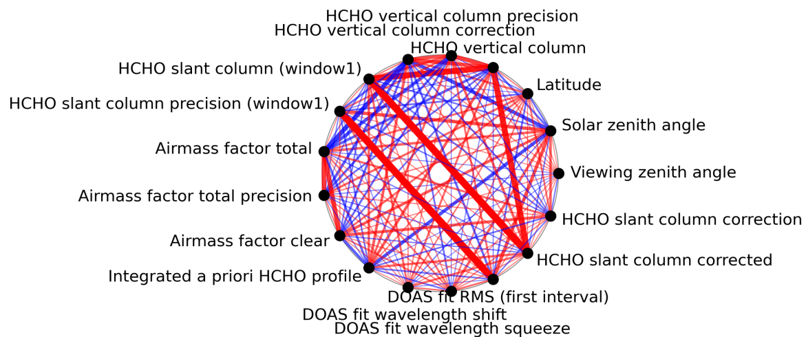
Figure 1: Map of correlation graph for 2024-08-06 to 2024-08-08.
