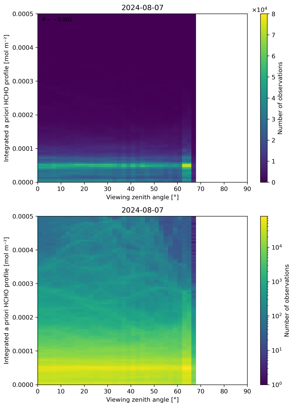
Figure 195: Scatter density plot of “Viewing zenith angle” against “Integrated a priori HCHO profile” for 2024-08-06 to 2024-08-08.
