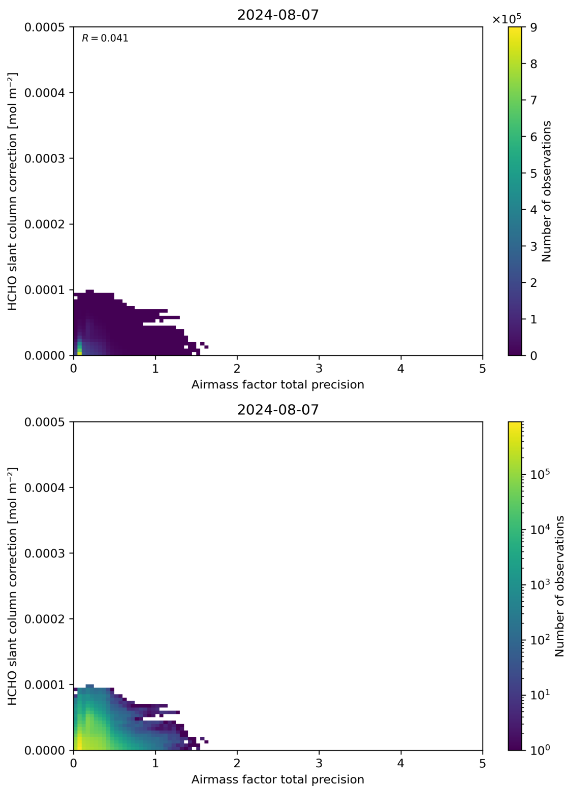
Figure 110: Scatter density plot of “Airmass factor total precision” against “HCHO slant column correction” for 2024-08-06 to 2024-08-08.
