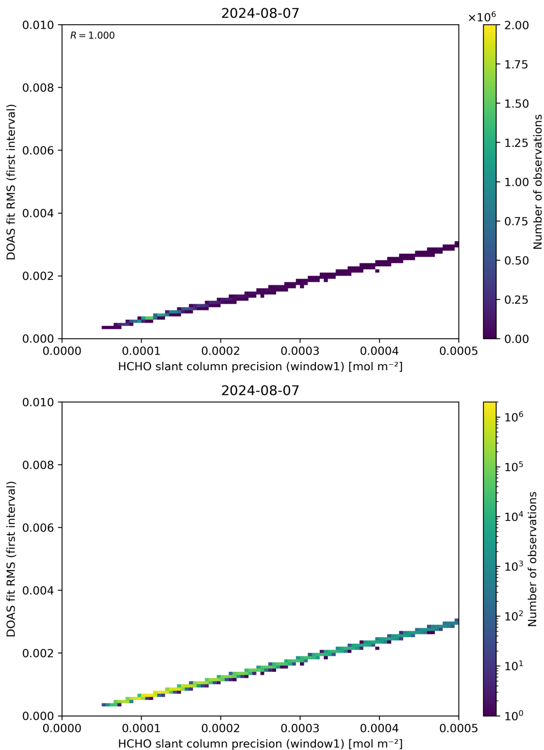
Figure 88: Scatter density plot of “HCHO slant column precision (window1)” against “DOAS fit RMS (first interval)” for 2024-08-06 to 2024-08-08.
