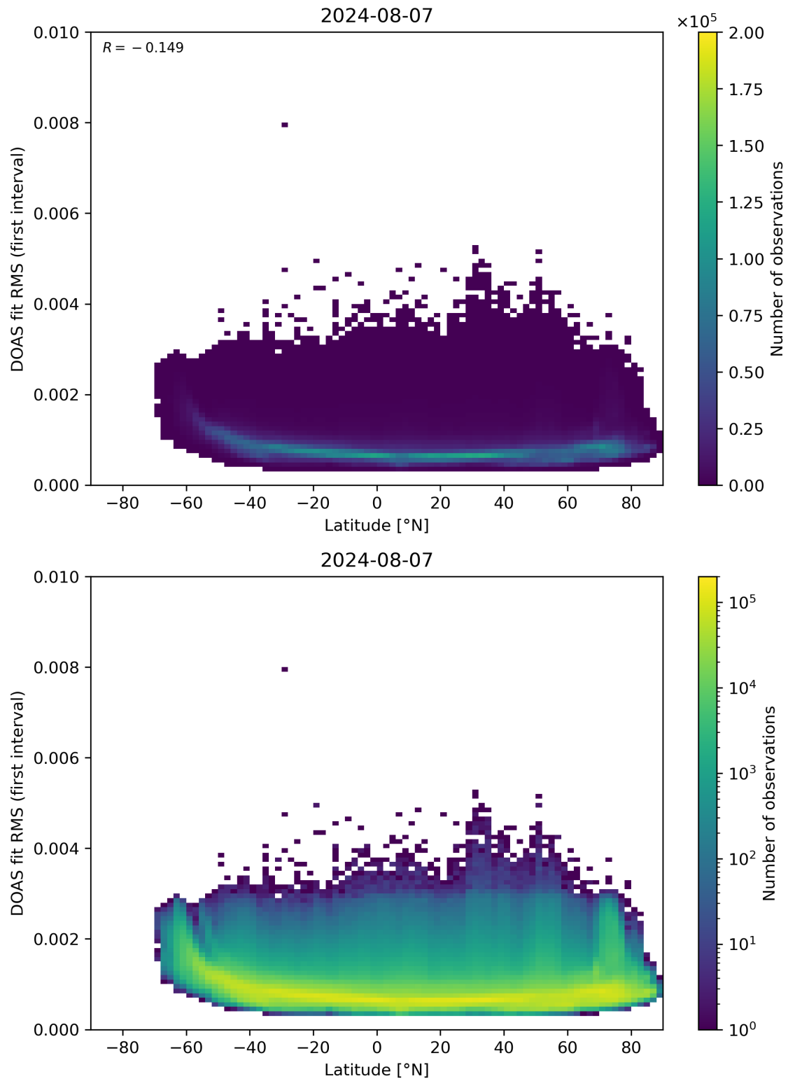
Figure 153: Scatter density plot of “Latitude” against “DOAS fit RMS (first interval)” for 2024-08-06 to 2024-08-08.
