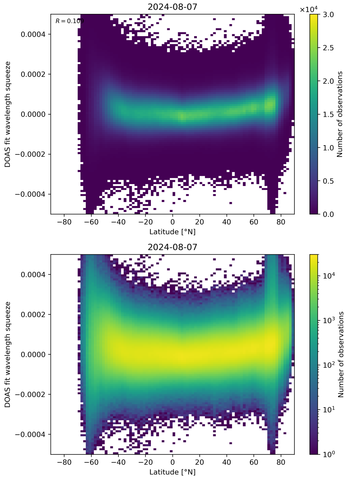
Figure 155: Scatter density plot of “Latitude” against “DOAS fit wavelength squeeze” for 2024-08-06 to 2024-08-08.
