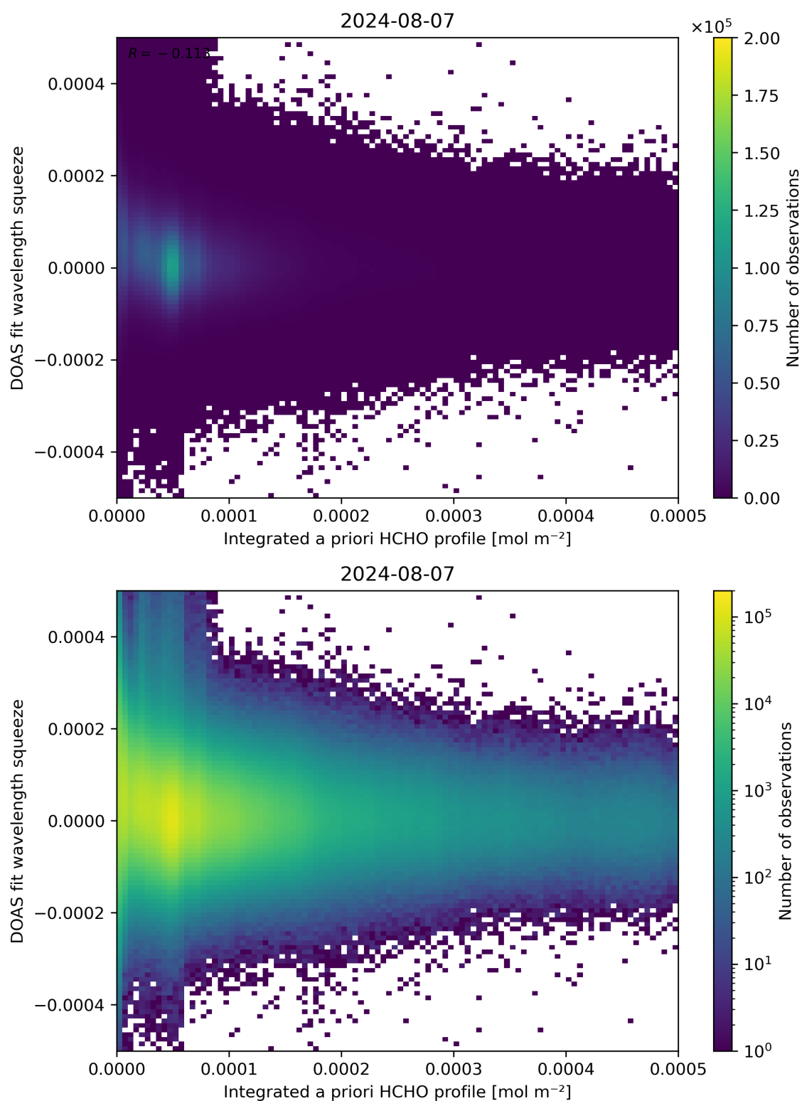
Figure 150: Scatter density plot of “Integrated a priori HCHO profile” against “DOAS fit wavelength squeeze” for 2024-08-06 to 2024-08-08.
