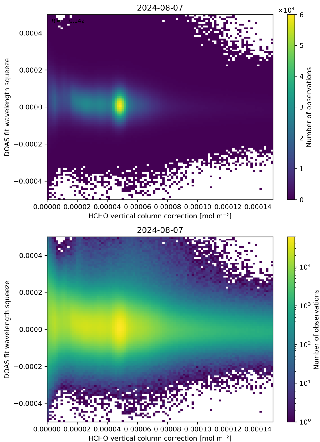
Figure 114: Scatter density plot of “HCHO vertical column correction” against “DOAS fit wavelength squeeze” for 2024-08-06 to 2024-08-08.
