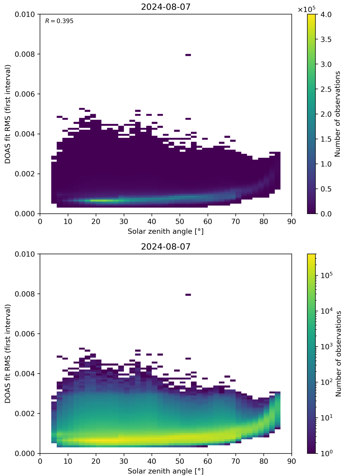
Figure 167: Scatter density plot of “Solar zenith angle” against “DOAS fit RMS (first interval)” for 2024-08-06 to 2024-08-08.
