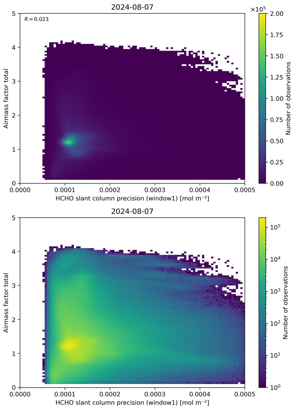
Figure 94: Scatter density plot of “HCHO slant column precision (window1)” against “Airmass factor total” for 2024-08-06 to 2024-08-08.
