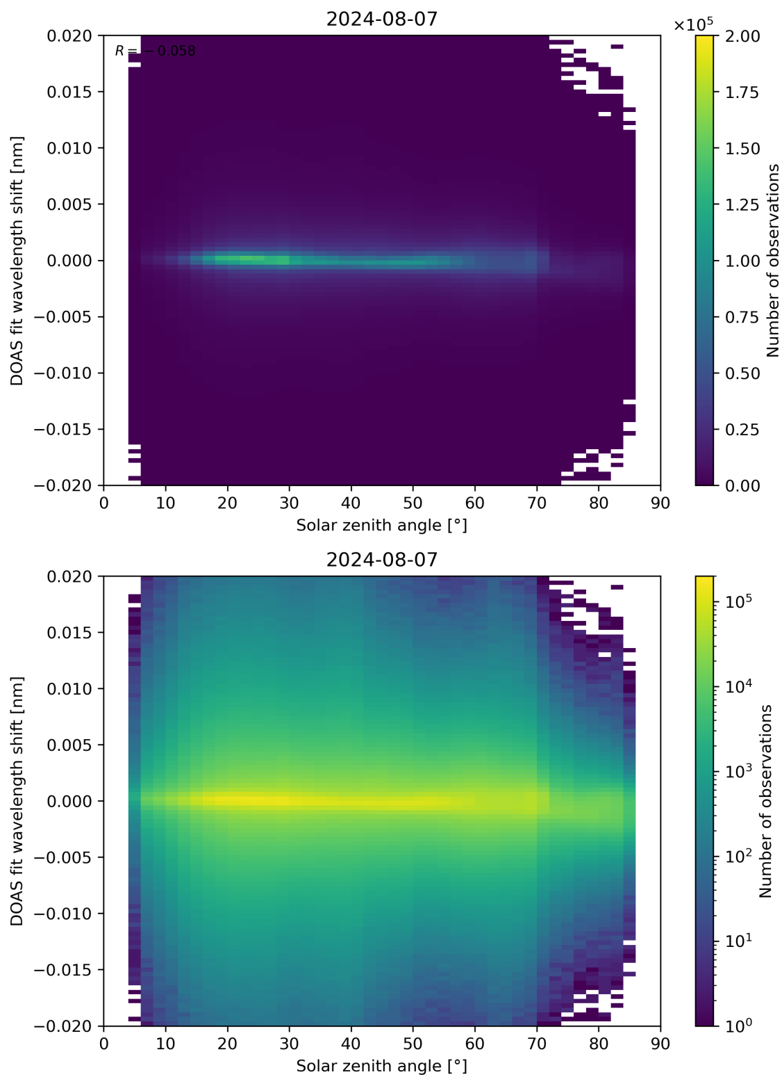
Figure 168: Scatter density plot of “Solar zenith angle” against “DOAS fit wavelength shift” for 2024-08-06 to 2024-08-08.
