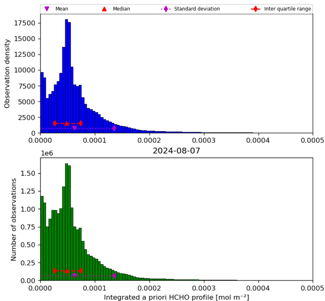
Figure 43: Histogram of “Integrated a priori HCHO profile” for 2024-08-06 to 2024-08-08
