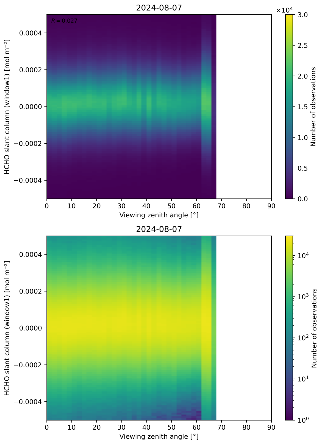
Figure 188: Scatter density plot of “Viewing zenith angle” against “HCHO slant column (window1)” for 2024-08-06 to 2024-08-08.
