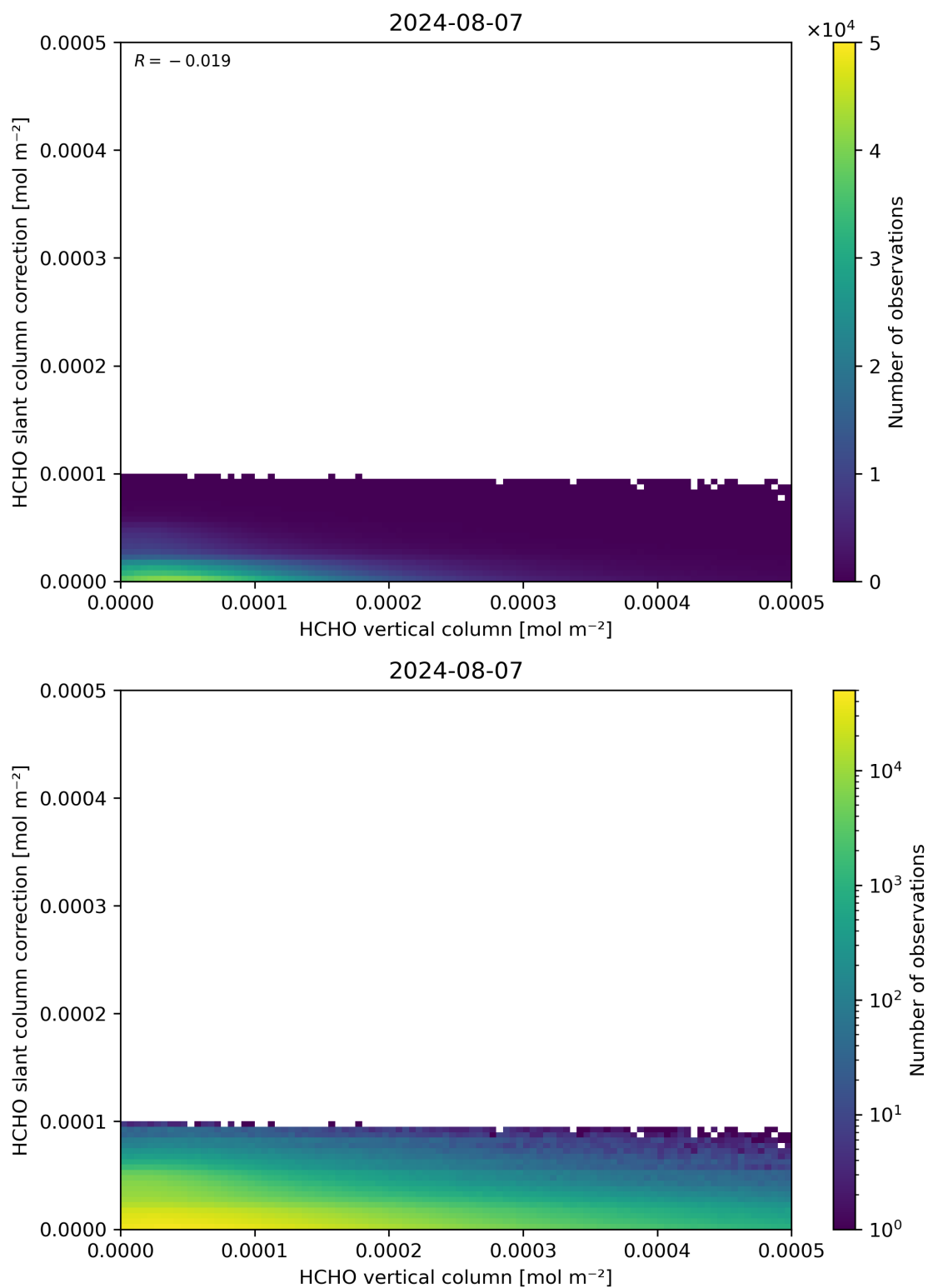
Figure 128: Scatter density plot of “HCHO vertical column” against “HCHO slant column correction” for 2024-08-06 to 2024-08-08.
