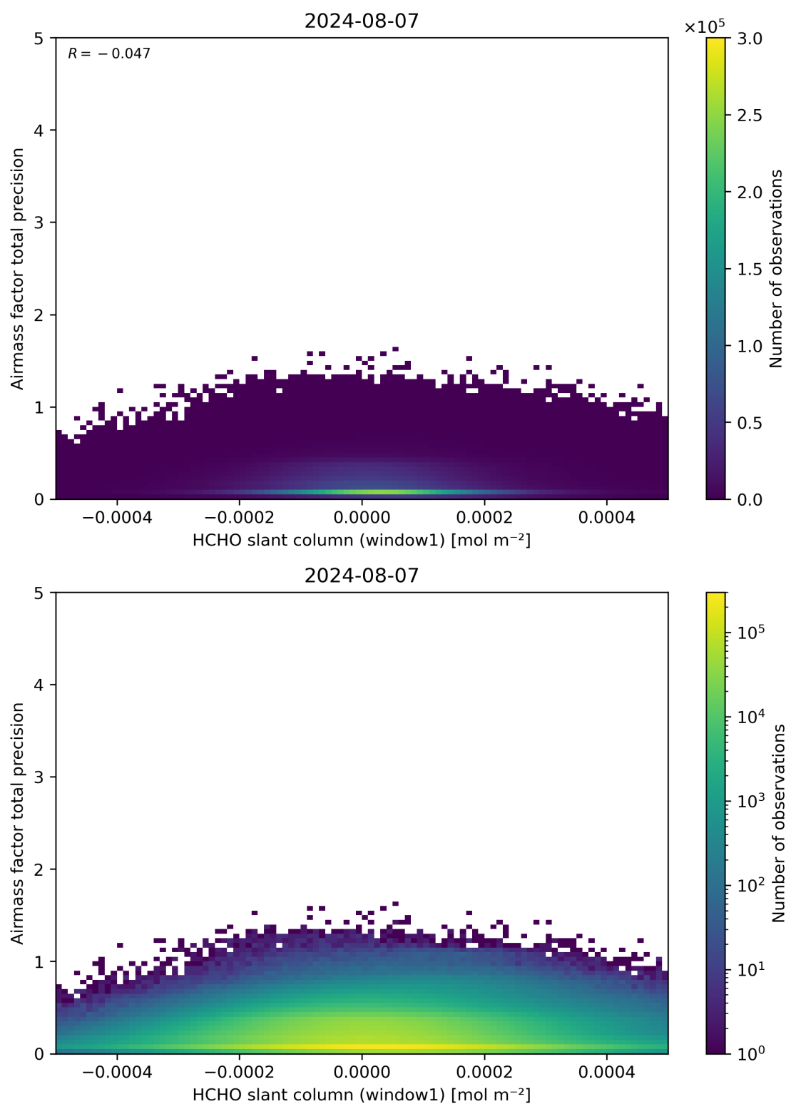
Figure 86: Scatter density plot of “HCHO slant column (window1)” against “Airmass factor total precision” for 2024-08-06 to 2024-08-08.
