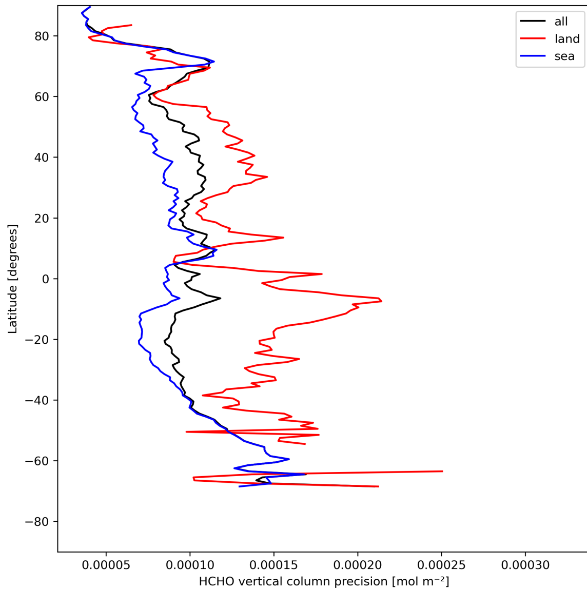
Figure 22: Zonal average of “HCHO vertical column precision” for 2024-08-06 to 2024-08-08.
