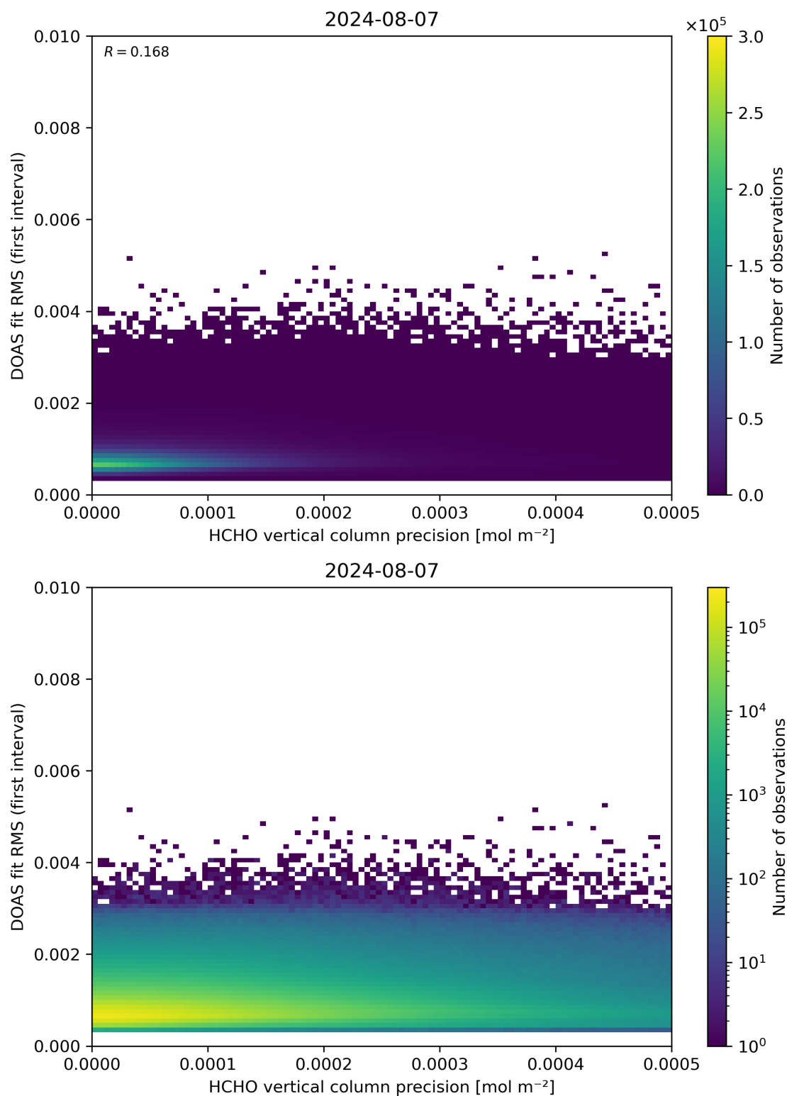
Figure 136: Scatter density plot of “HCHO vertical column precision” against “DOAS fit RMS (first interval)” for 2024-08-06 to 2024-08-08.
