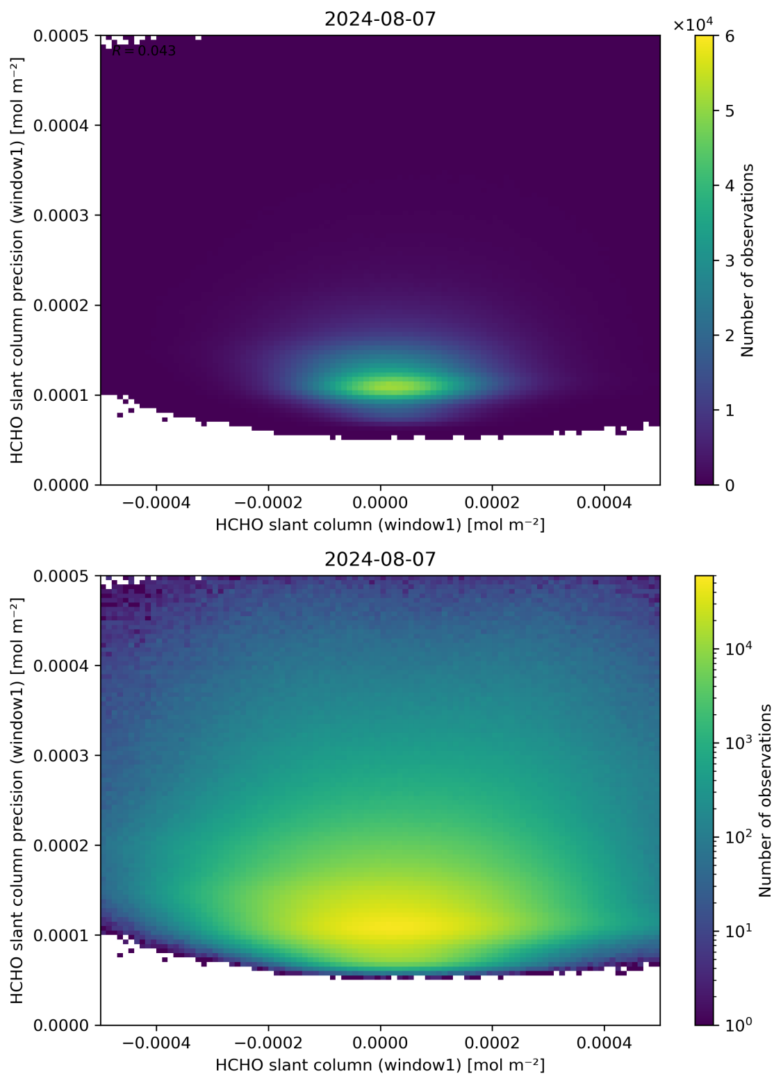
Figure 84: Scatter density plot of “HCHO slant column (window1)” against “HCHO slant column precision (window1)” for 2024-08-06 to 2024-08-08.
