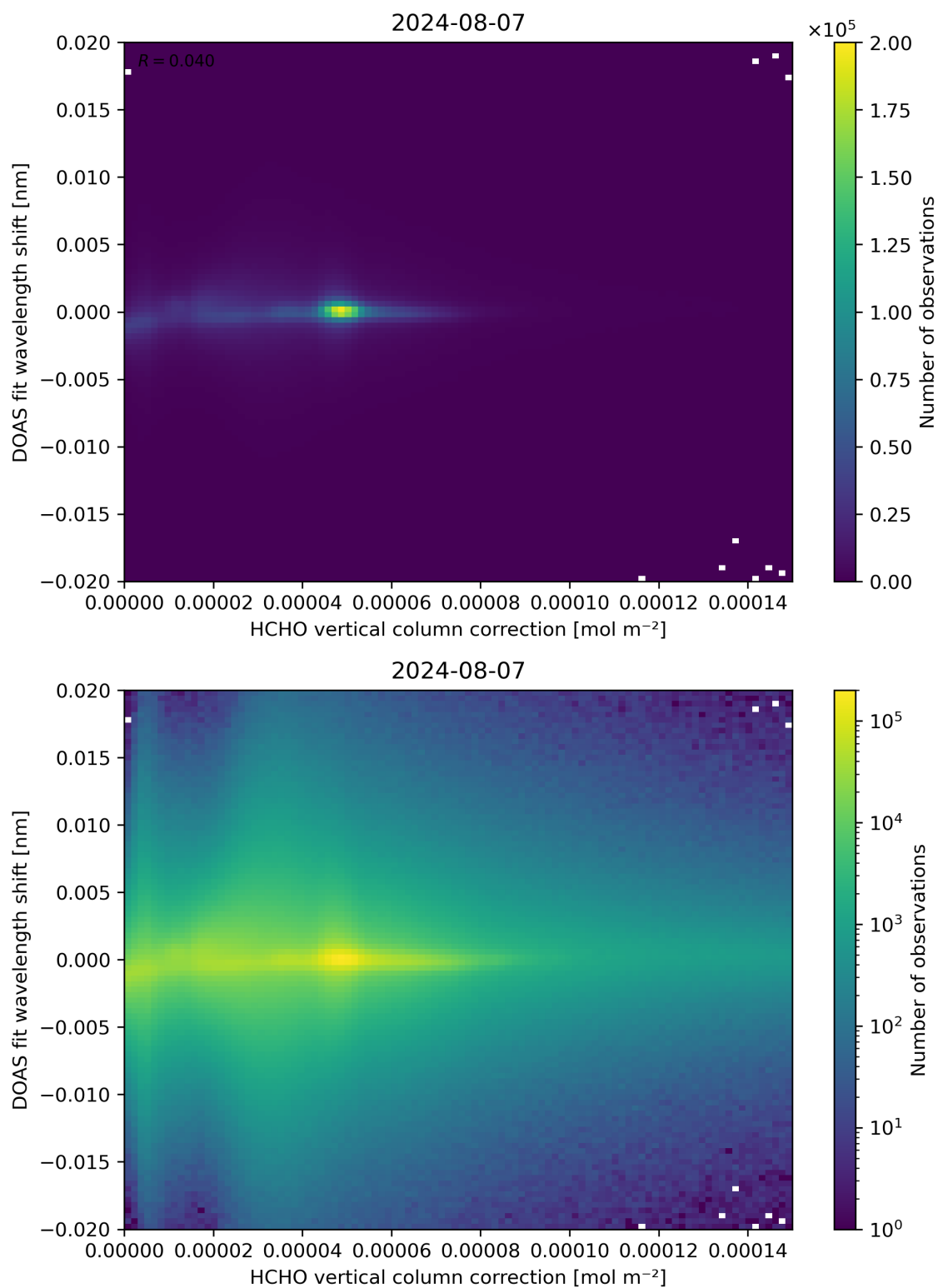
Figure 113: Scatter density plot of “HCHO vertical column correction” against “DOAS fit wavelength shift” for 2024-08-06 to 2024-08-08.
