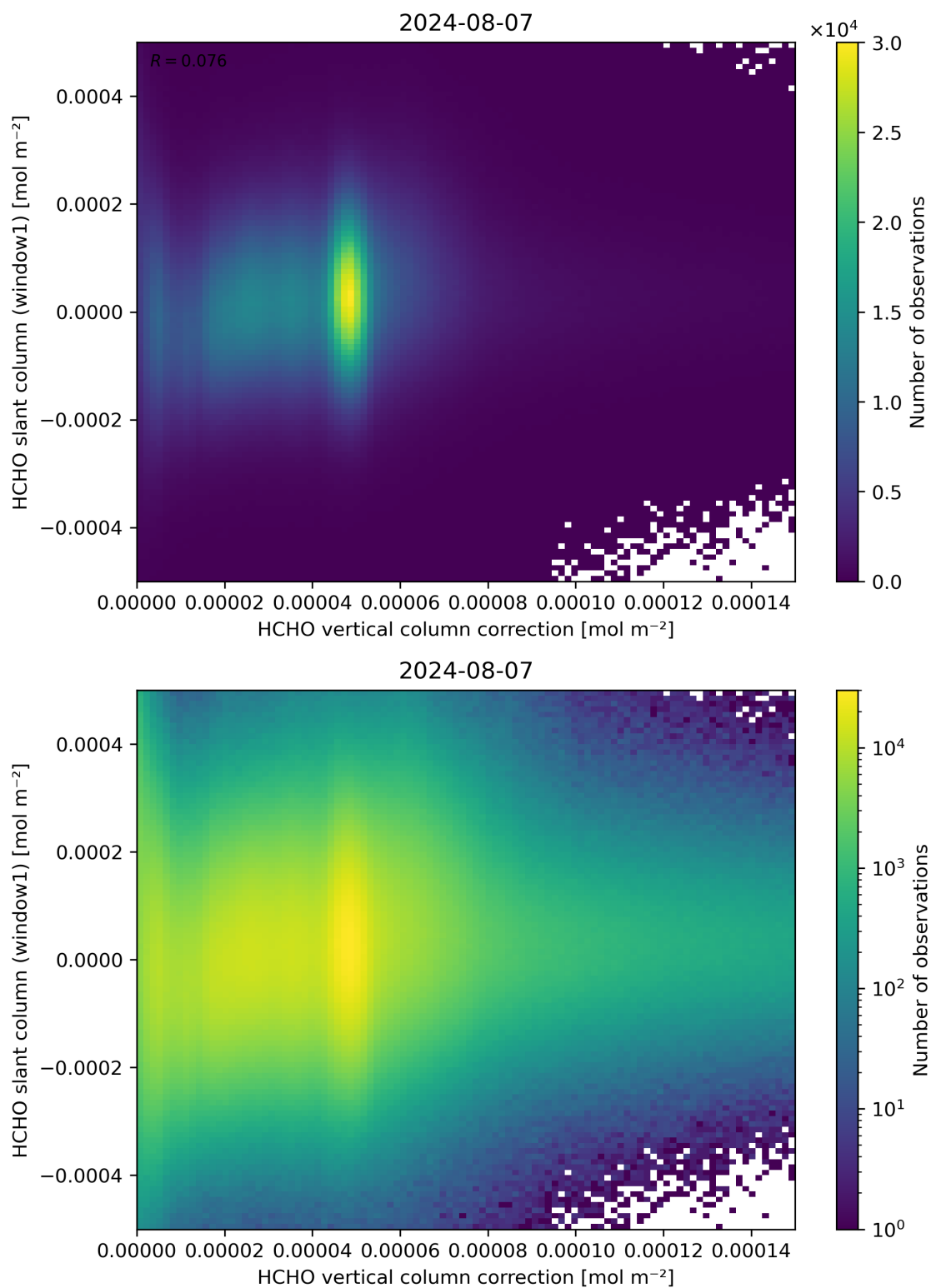
Figure 118: Scatter density plot of “HCHO vertical column correction” against “HCHO slant column (window1)” for 2024-08-06 to 2024-08-08.
