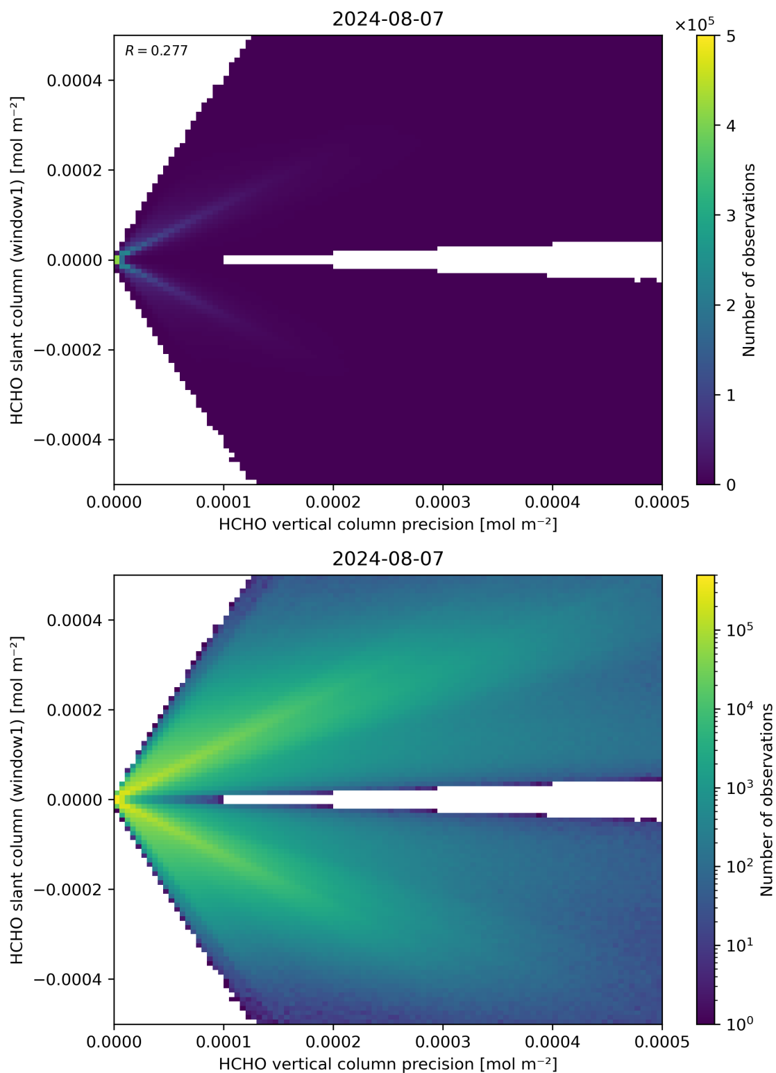
Figure 142: Scatter density plot of “HCHO vertical column precision” against “HCHO slant column (window1)” for 2024-08-06 to 2024-08-08.
