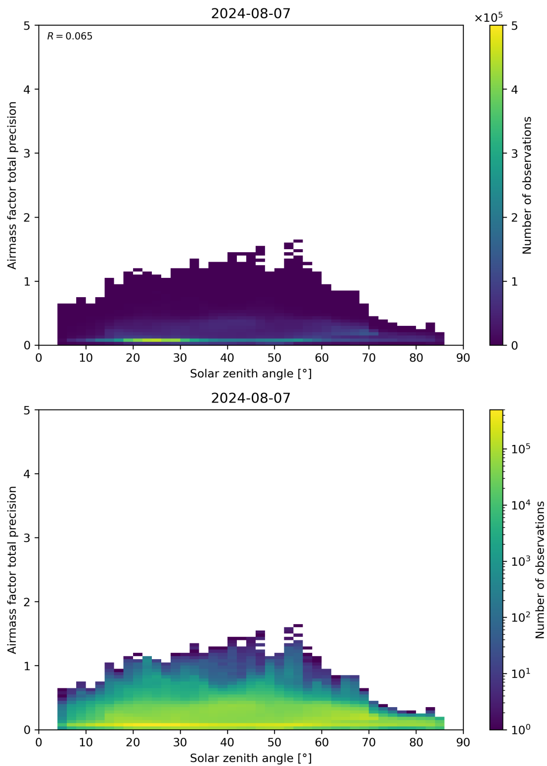
Figure 176: Scatter density plot of “Solar zenith angle” against “Airmass factor total precision” for 2024-08-06 to 2024-08-08.
