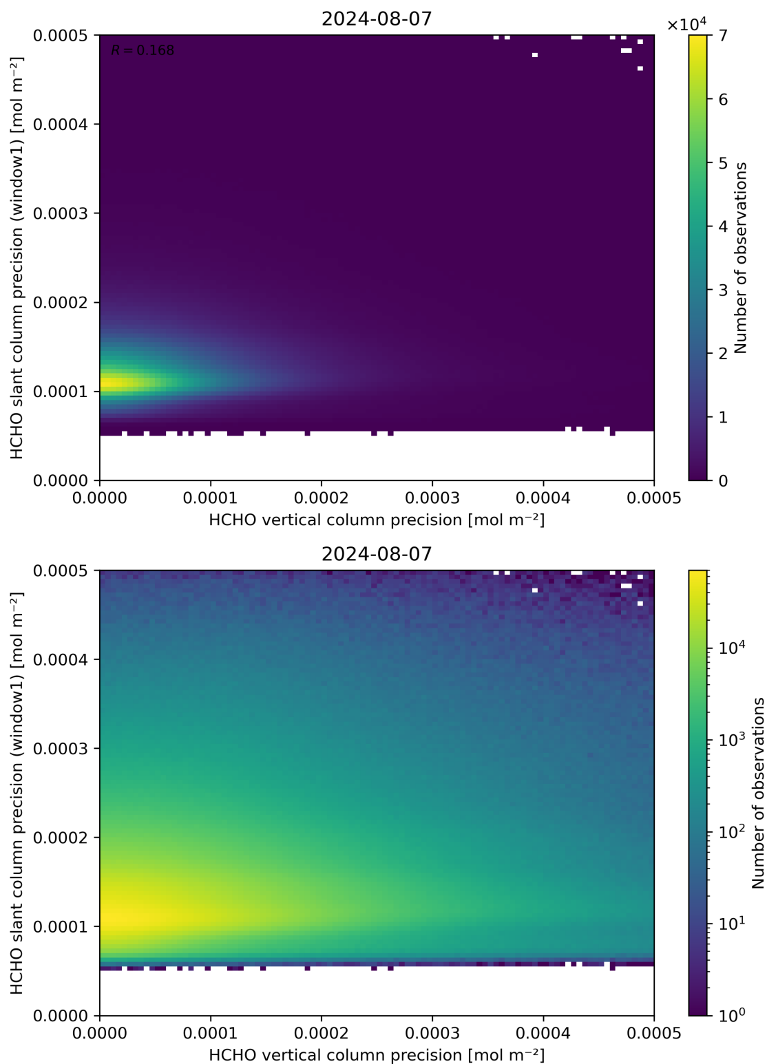
Figure 143: Scatter density plot of “HCHO vertical column precision” against “HCHO slant column precision (window1)” for 2024-08-06 to 2024-08-08.
