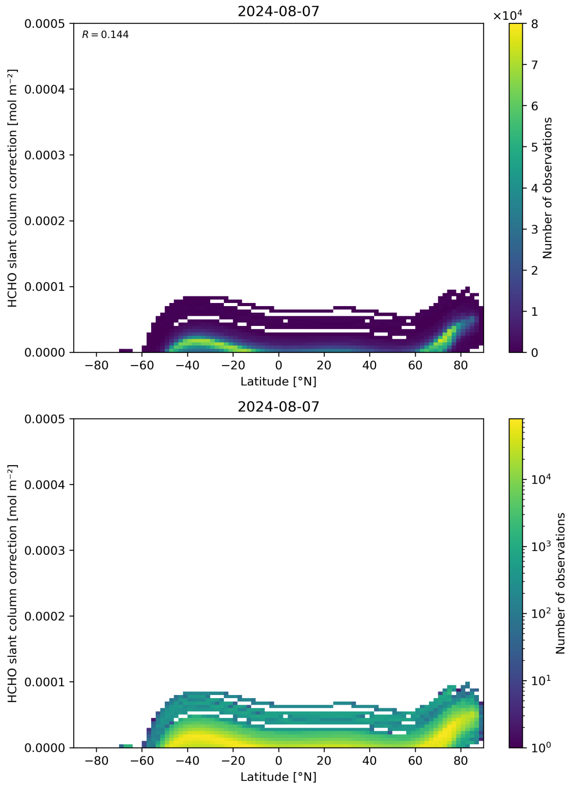
Figure 158: Scatter density plot of “Latitude” against “HCHO slant column correction” for 2024-08-06 to 2024-08-08.
