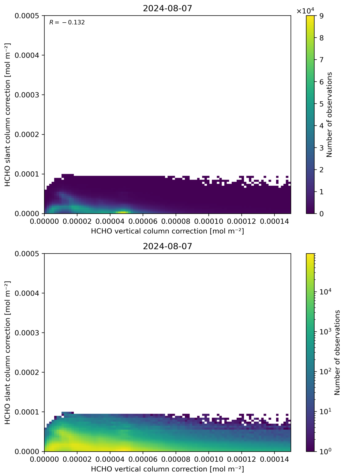
Figure 117: Scatter density plot of “HCHO vertical column correction” against “HCHO slant column correction” for 2024-08-06 to 2024-08-08.
