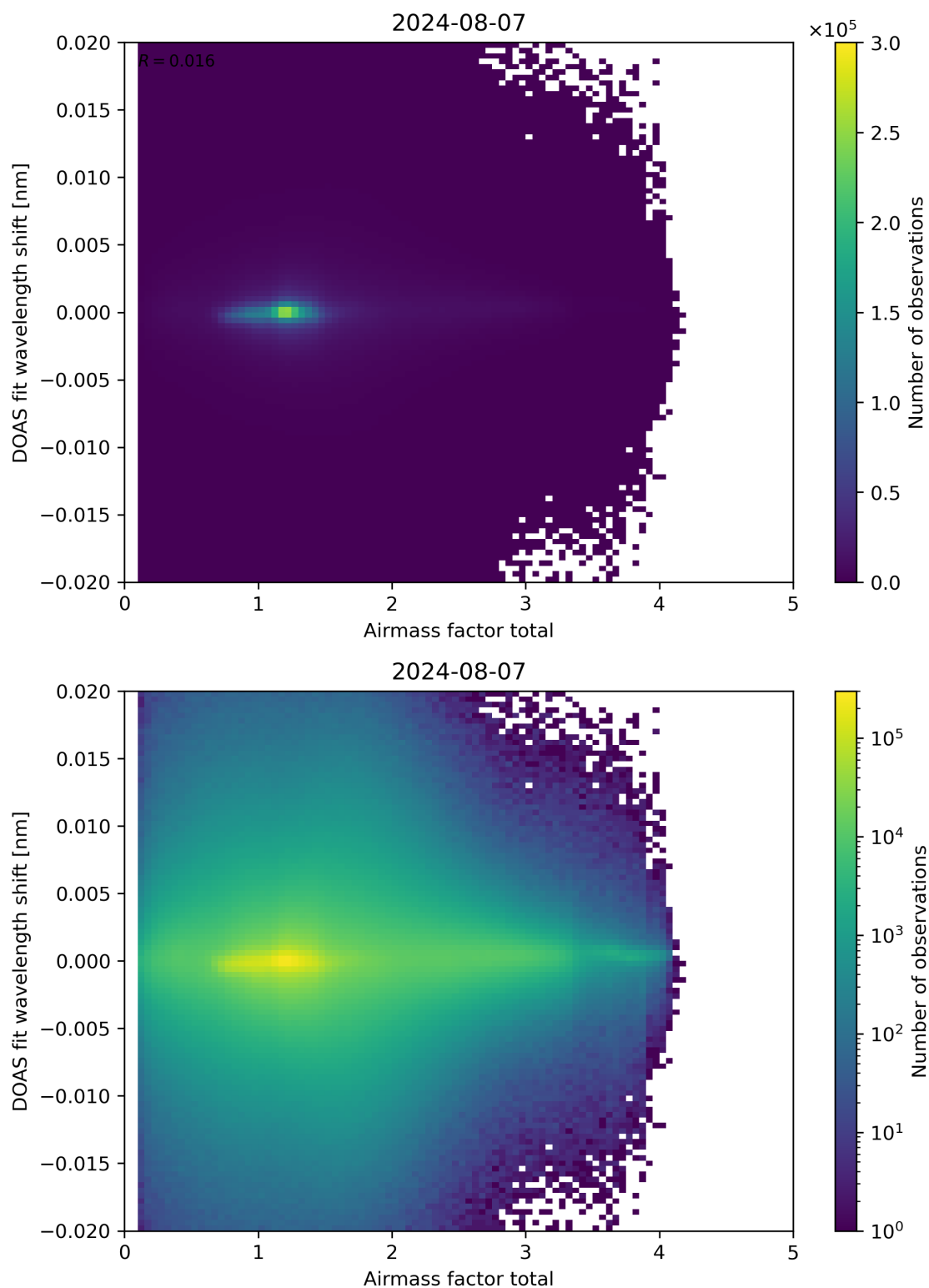
Figure 98: Scatter density plot of “Airmass factor total” against “DOAS fit wavelength shift” for 2024-08-06 to 2024-08-08.
