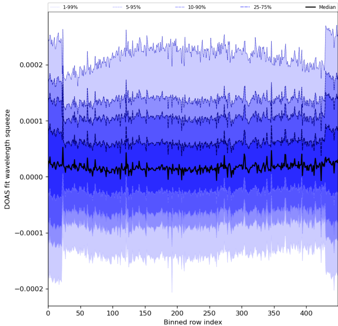
Figure 59: Along track statistics of “DOAS fit wavelength squeeze” for 2024-08-06 to 2024-08-08
