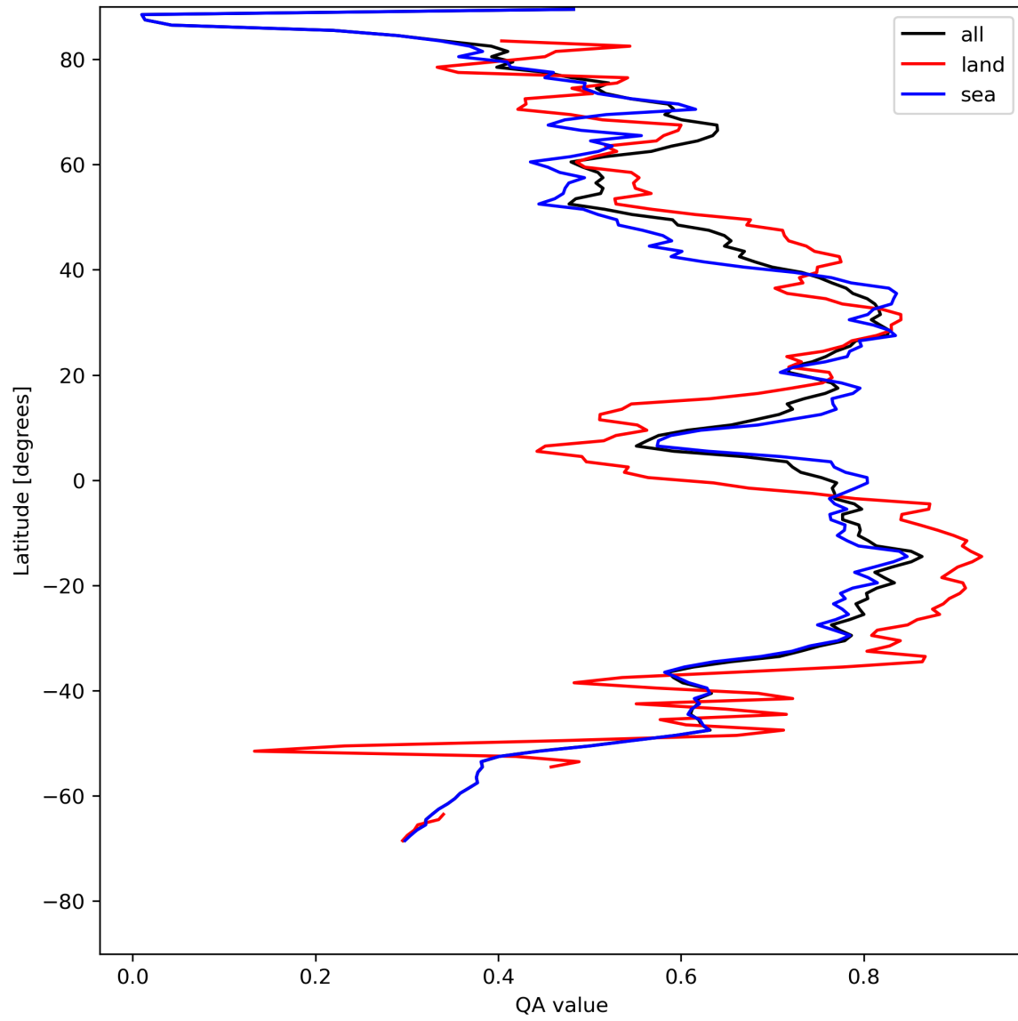
Figure 20: Zonal average of “QA value” for 2024-08-06 to 2024-08-08.
