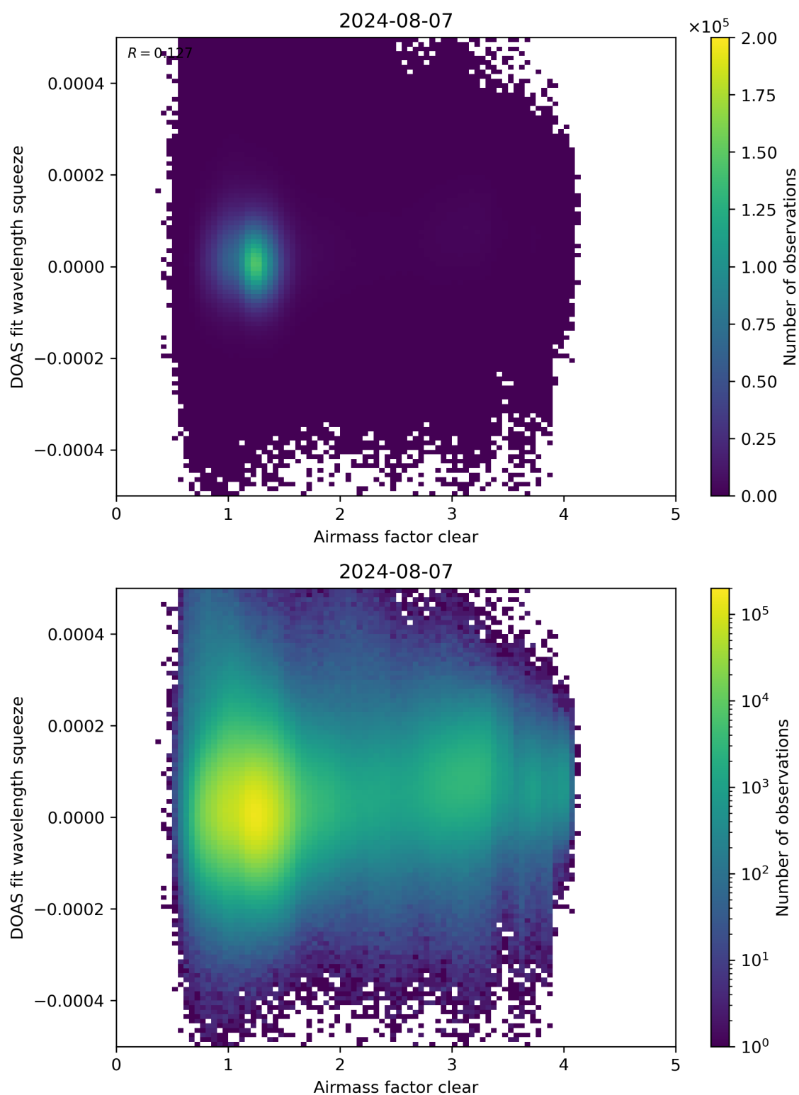
Figure 73: Scatter density plot of “Airmass factor clear” against “DOAS fit wavelength squeeze” for 2024-08-06 to 2024-08-08.
