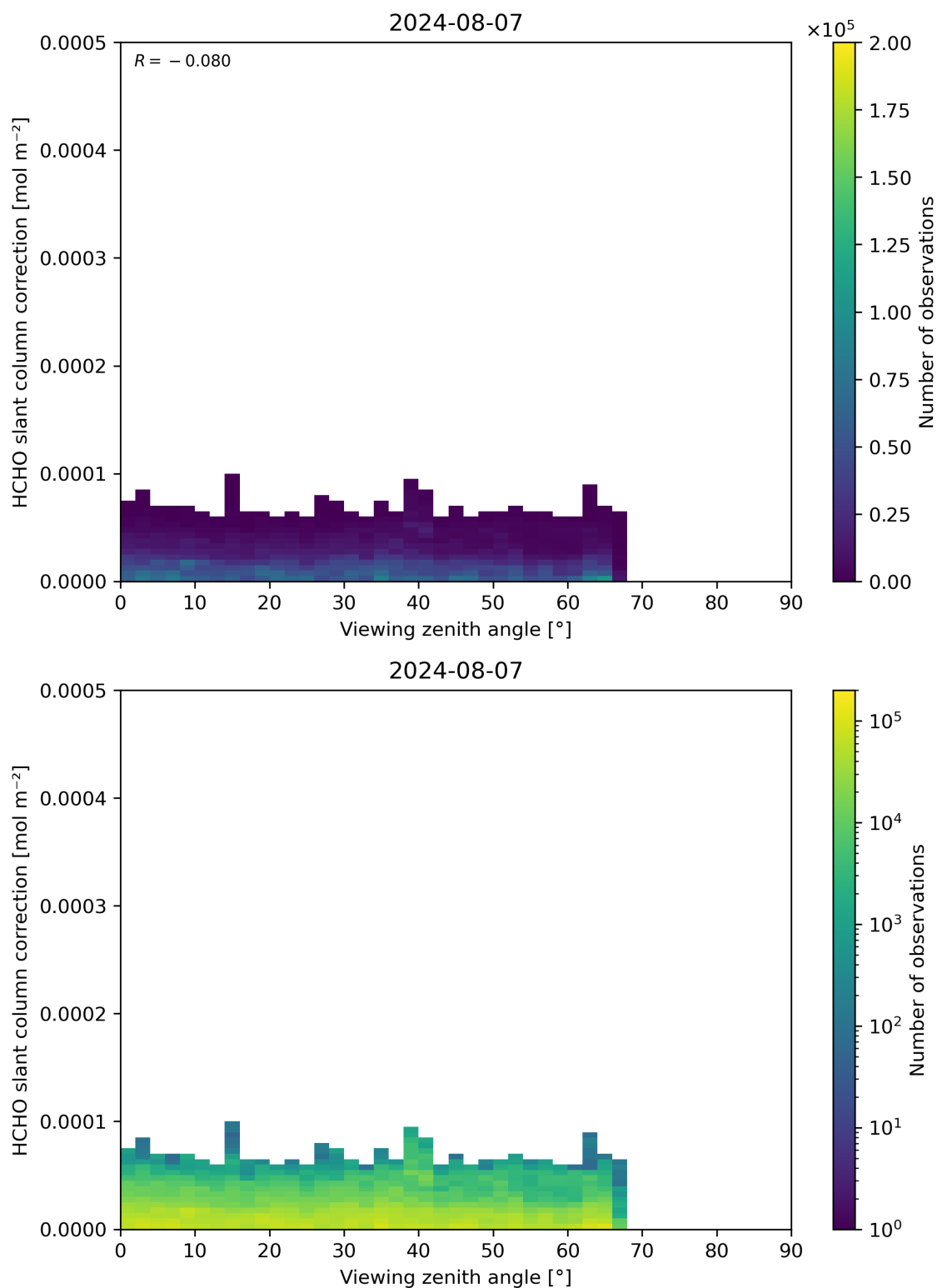
Figure 187: Scatter density plot of “Viewing zenith angle” against “HCHO slant column correction” for 2024-08-06 to 2024-08-08.
