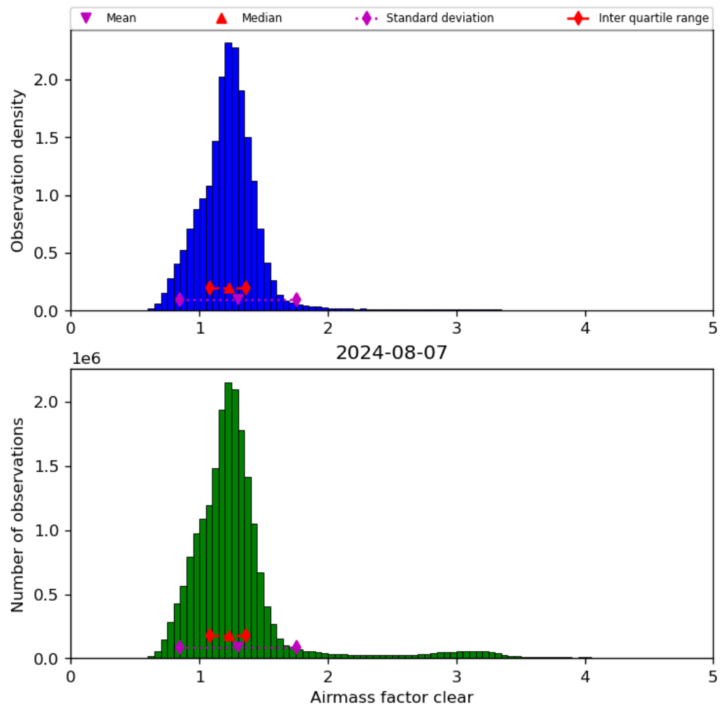
Figure 42: Histogram of “Airmass factor clear” for 2024-08-06 to 2024-08-08
