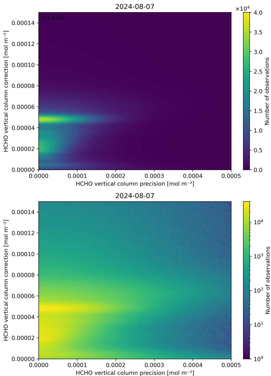
Figure 146: Scatter density plot of “HCHO vertical column precision” against “HCHO vertical column correction” for 2024-08-06 to 2024-08-08.
