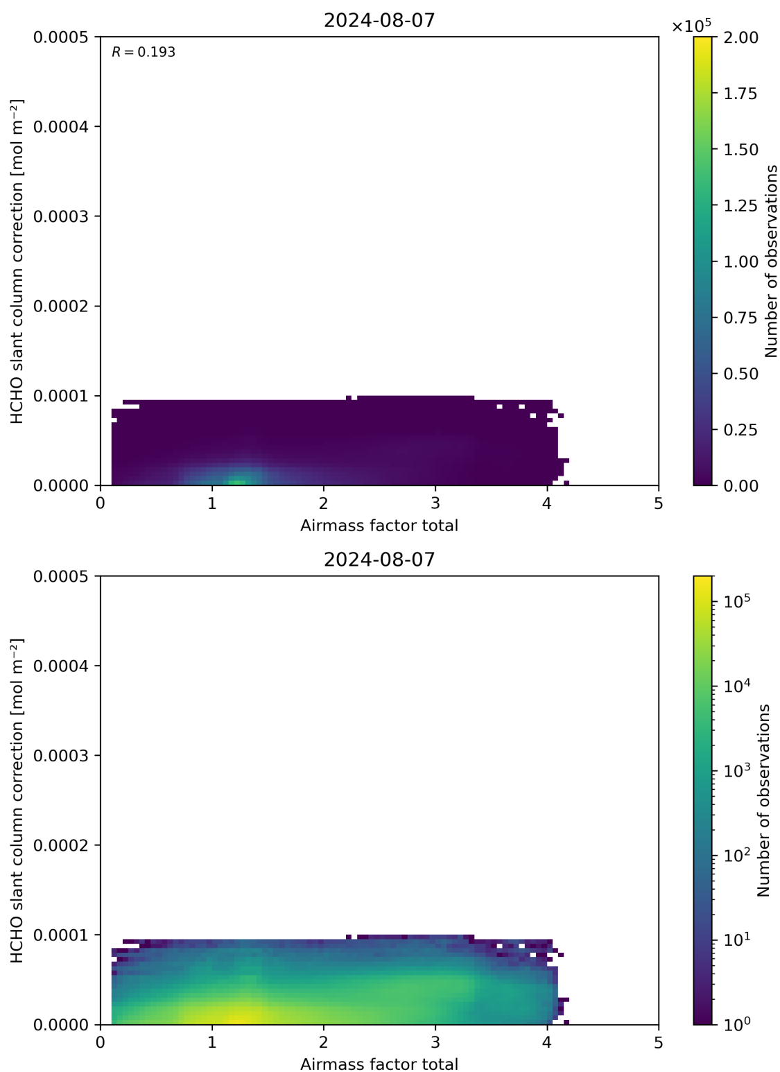
Figure 102: Scatter density plot of “Airmass factor total” against “HCHO slant column correction” for 2024-08-06 to 2024-08-08.
