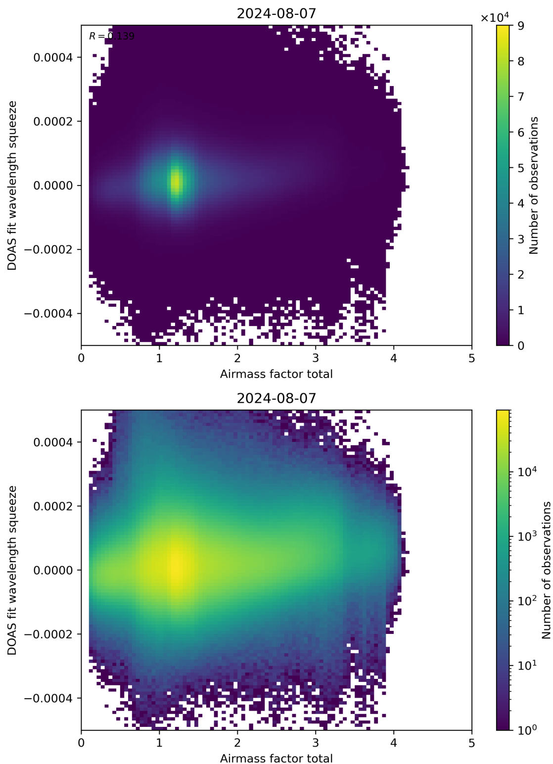
Figure 99: Scatter density plot of “Airmass factor total” against “DOAS fit wavelength squeeze” for 2024-08-06 to 2024-08-08.
