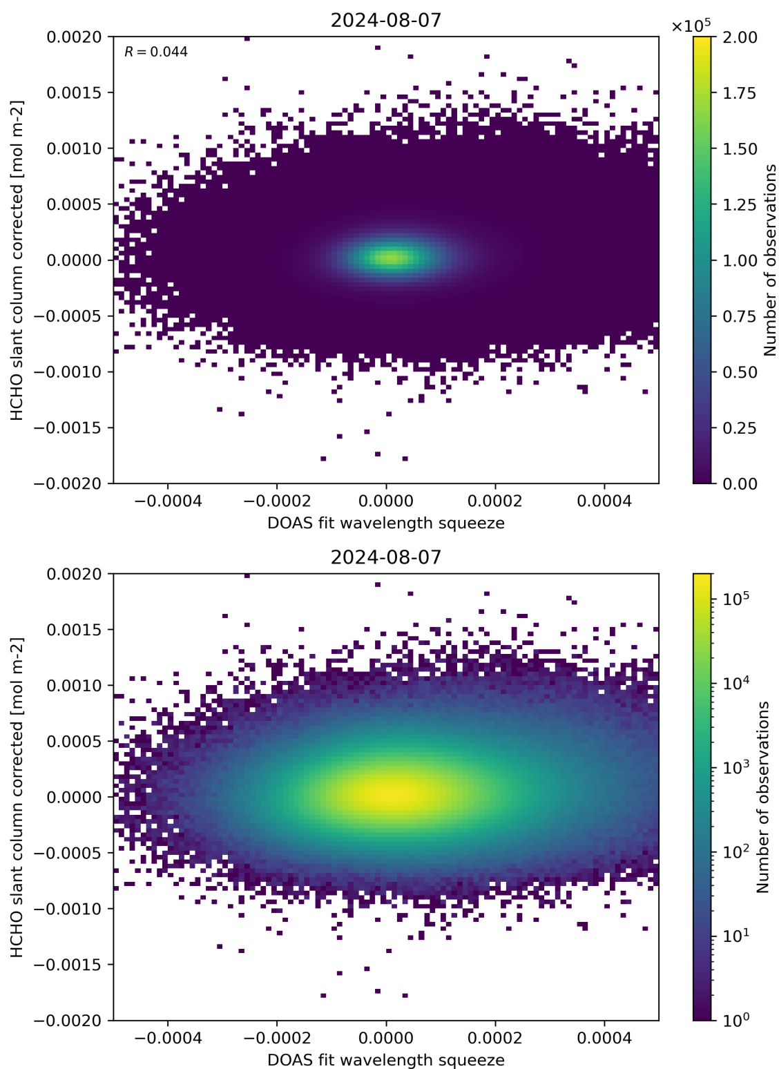
Figure 69: Scatter density plot of “DOAS fit wavelength squeeze” against “HCHO slant column corrected” for 2024-08-06 to 2024-08-08.
