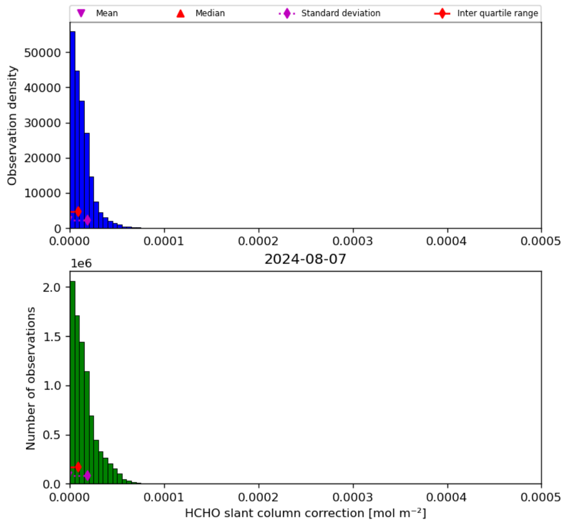
Figure 47: Histogram of “HCHO slant column correction” for 2024-08-06 to 2024-08-08
