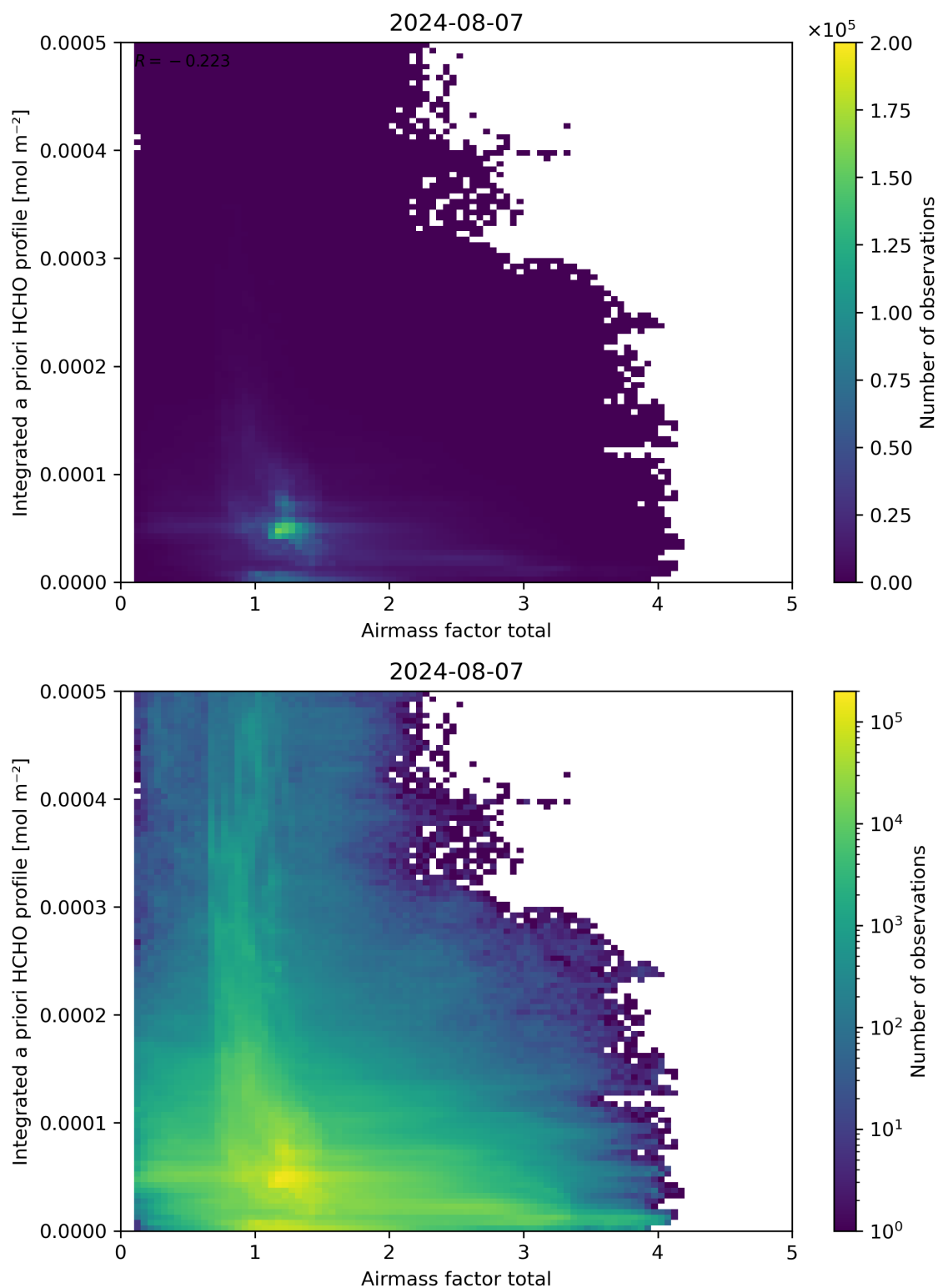
Figure 104: Scatter density plot of “Airmass factor total” against “Integrated a priori HCHO profile” for 2024-08-06 to 2024-08-08.
