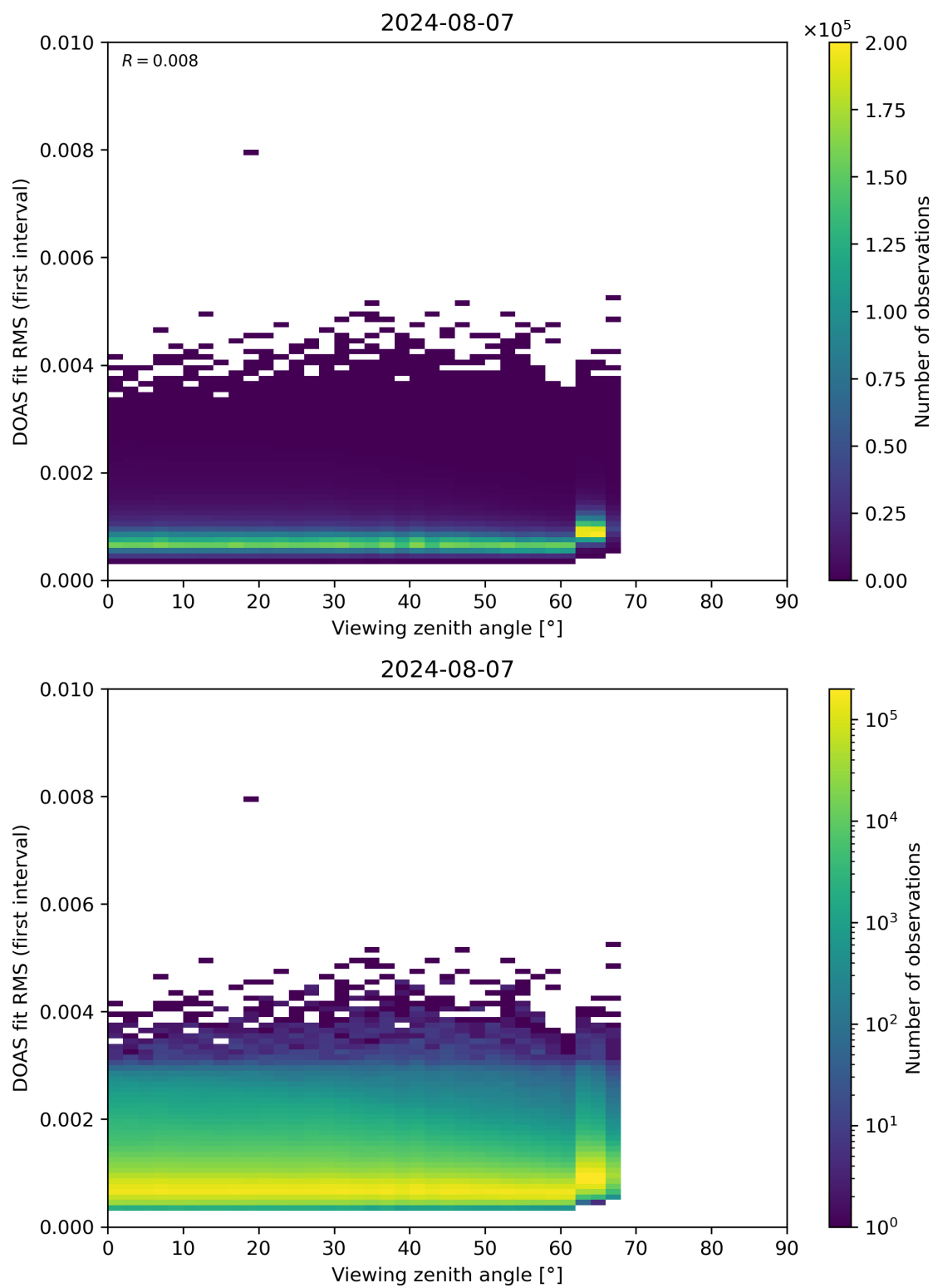
Figure 182: Scatter density plot of “Viewing zenith angle” against “DOAS fit RMS (first interval)” for 2024-08-06 to 2024-08-08.
