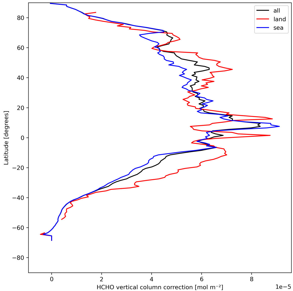
Figure 23: Zonal average of “HCHO vertical column correction” for 2024-08-06 to 2024-08-08.
