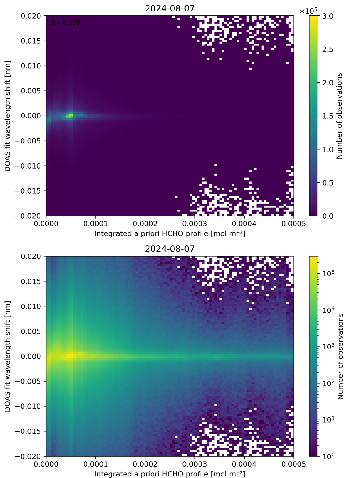
Figure 149: Scatter density plot of “Integrated a priori HCHO profile” against “DOAS fit wavelength shift” for 2024-08-06 to 2024-08-08.
