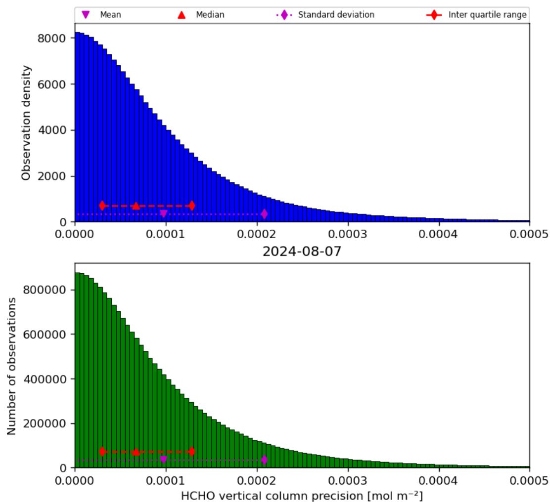
Figure 36: Histogram of “HCHO vertical column precision” for 2024-08-06 to 2024-08-08
