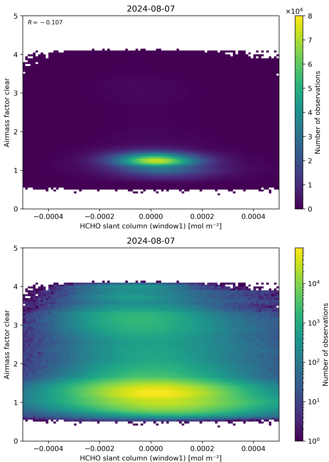
Figure 81: Scatter density plot of “HCHO slant column (window1)” against “Airmass factor clear” for 2024-08-06 to 2024-08-08.
