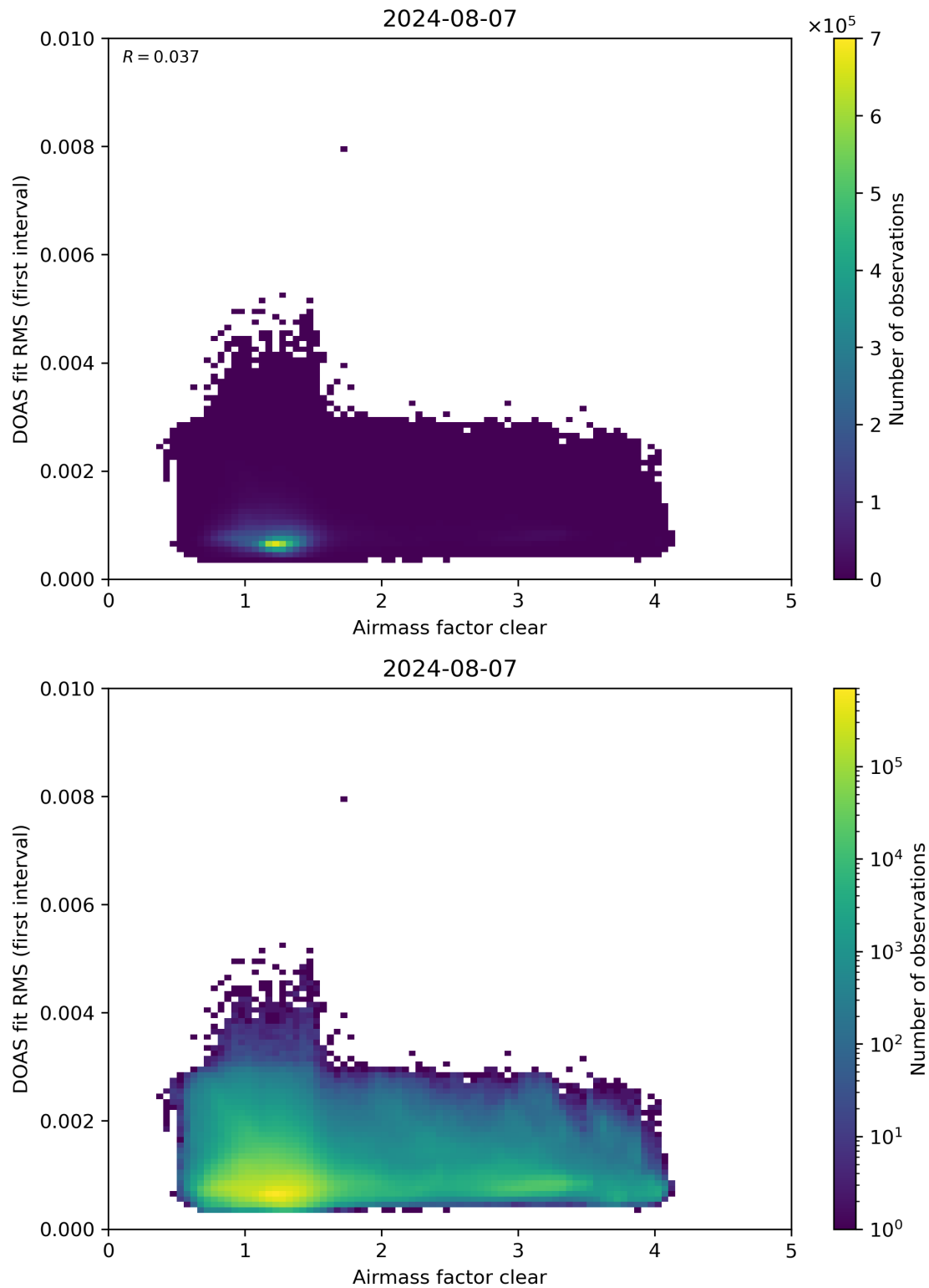
Figure 71: Scatter density plot of “Airmass factor clear” against “DOAS fit RMS (first interval)” for 2024-08-06 to 2024-08-08.
