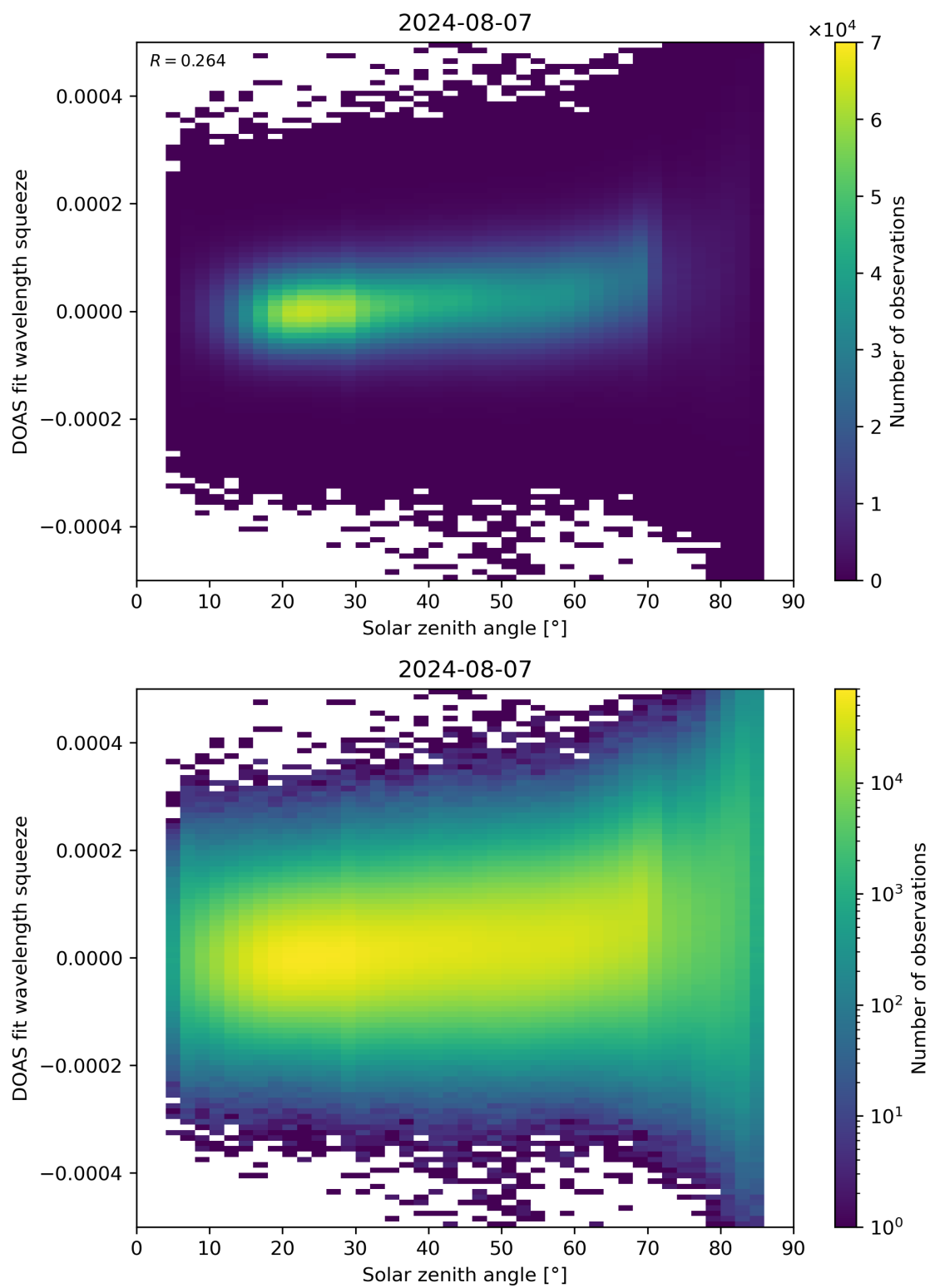
Figure 169: Scatter density plot of “Solar zenith angle” against “DOAS fit wavelength squeeze” for 2024-08-06 to 2024-08-08.
