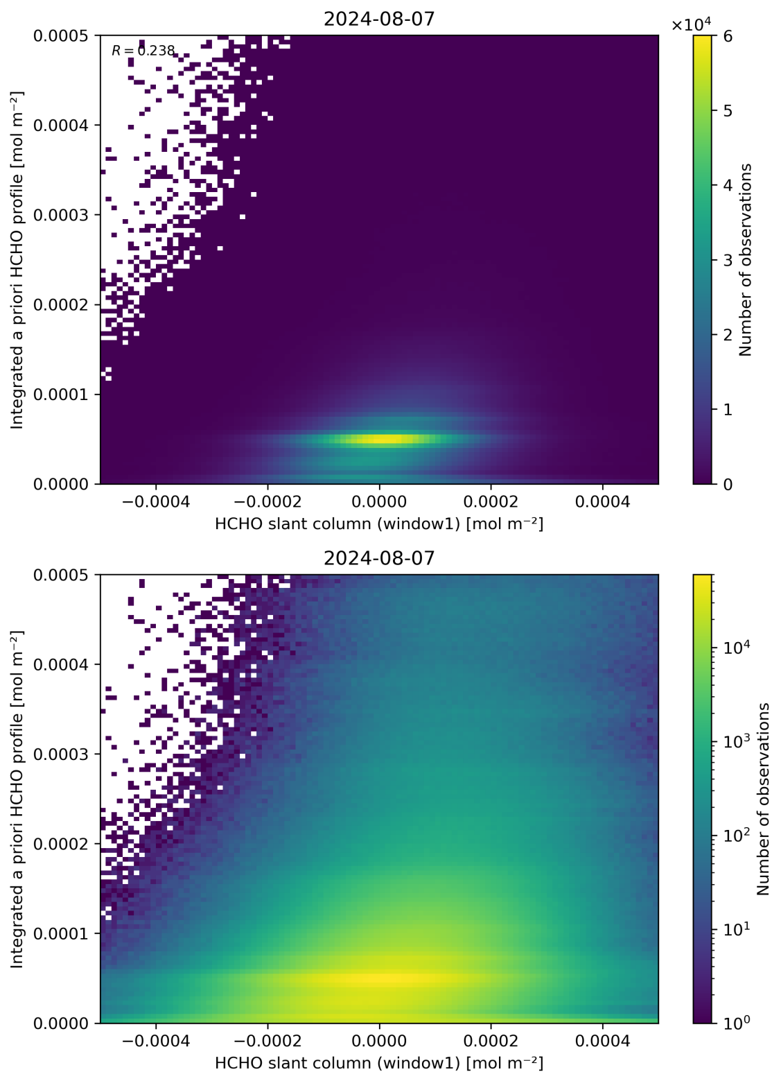
Figure 87: Scatter density plot of “HCHO slant column (window1)” against “Integrated a priori HCHO profile” for 2024-08-06 to 2024-08-08.
