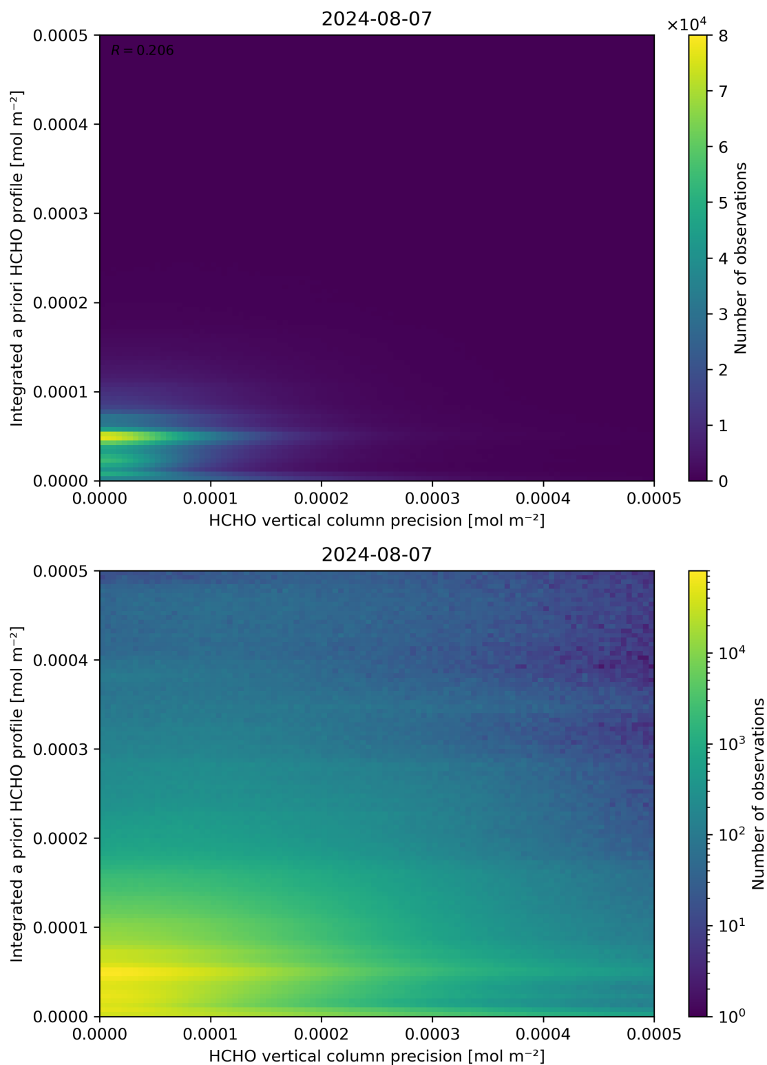
Figure 147: Scatter density plot of “HCHO vertical column precision” against “Integrated a priori HCHO profile” for 2024-08-06 to 2024-08-08.
