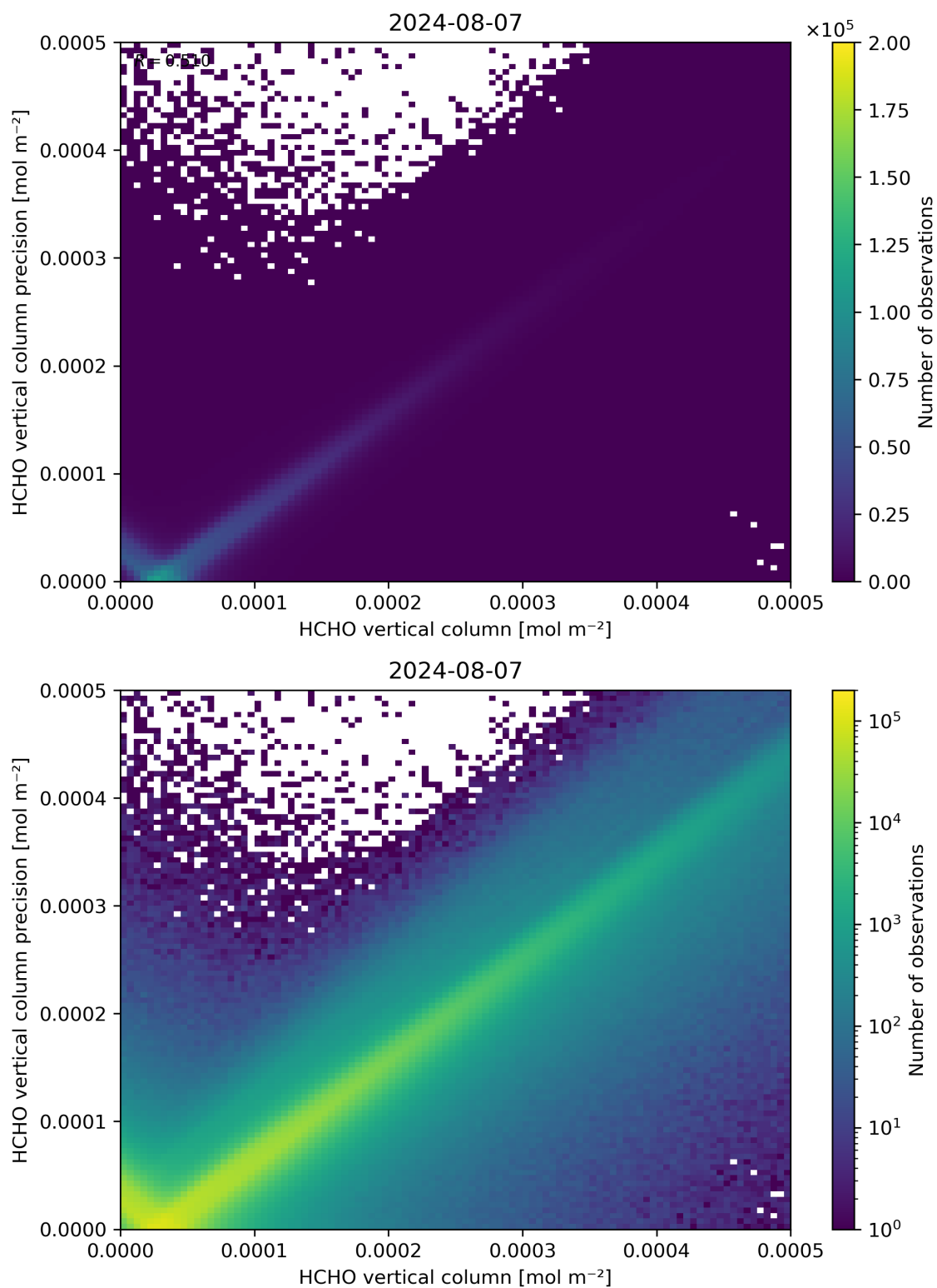
Figure 134: Scatter density plot of “HCHO vertical column” against “HCHO vertical column precision” for 2024-08-06 to 2024-08-08.
