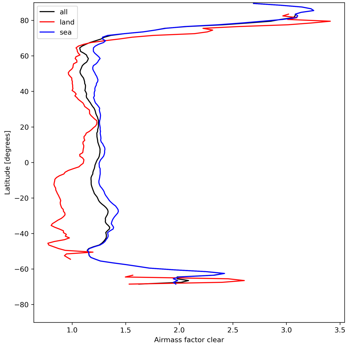
Figure 28: Zonal average of “Airmass factor clear” for 2024-08-06 to 2024-08-08.
