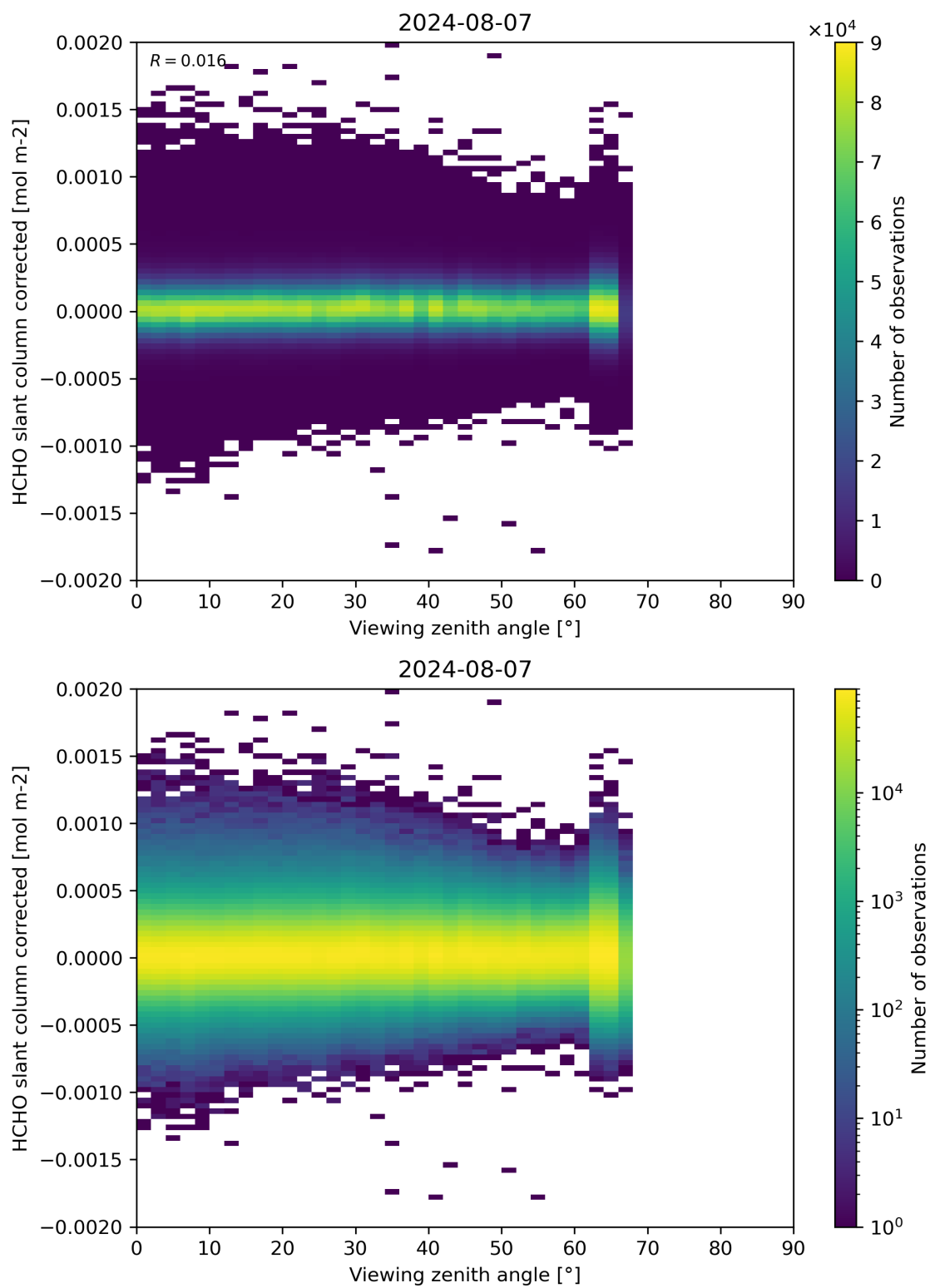
Figure 186: Scatter density plot of “Viewing zenith angle” against “HCHO slant column corrected” for 2024-08-06 to 2024-08-08.
