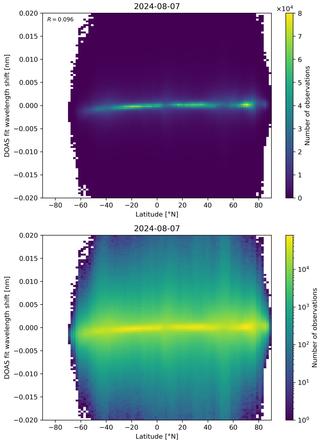
Figure 154: Scatter density plot of “Latitude” against “DOAS fit wavelength shift” for 2024-08-06 to 2024-08-08.
