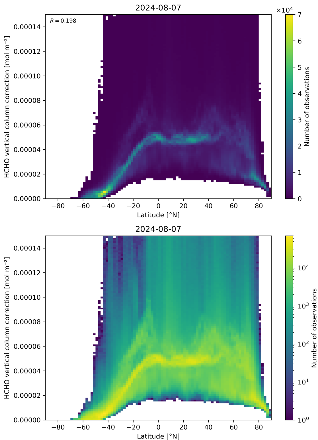
Figure 164: Scatter density plot of “Latitude” against “HCHO vertical column correction” for 2024-08-06 to 2024-08-08.
