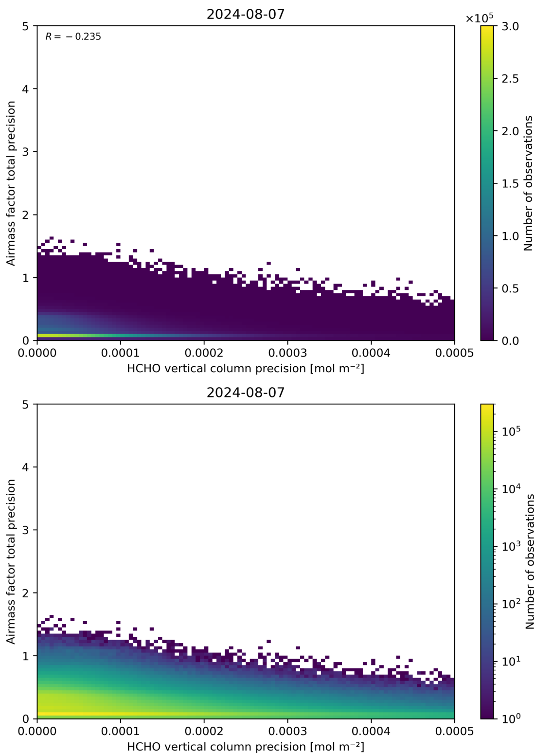
Figure 145: Scatter density plot of “HCHO vertical column precision” against “Airmass factor total precision” for 2024-08-06 to 2024-08-08.
