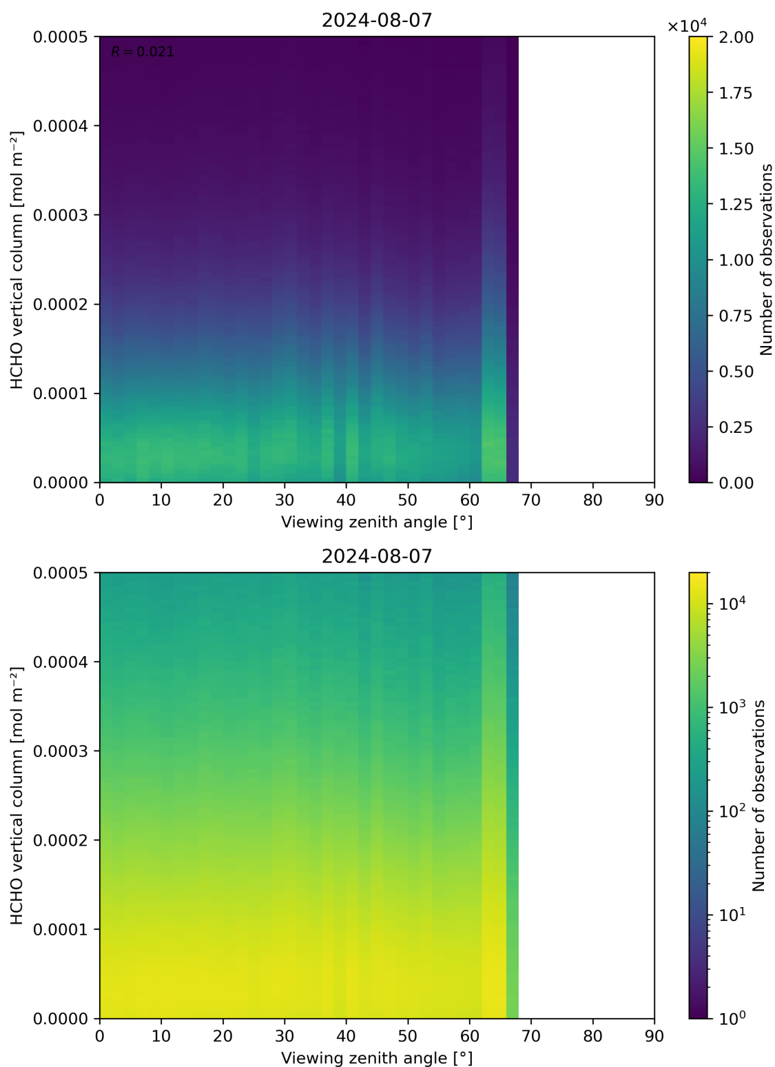
Figure 192: Scatter density plot of “Viewing zenith angle” against “HCHO vertical column” for 2024-08-06 to 2024-08-08.
