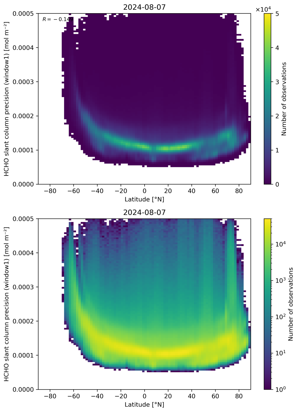
Figure 160: Scatter density plot of “Latitude” against “HCHO slant column precision (window1)” for 2024-08-06 to 2024-08-08.
