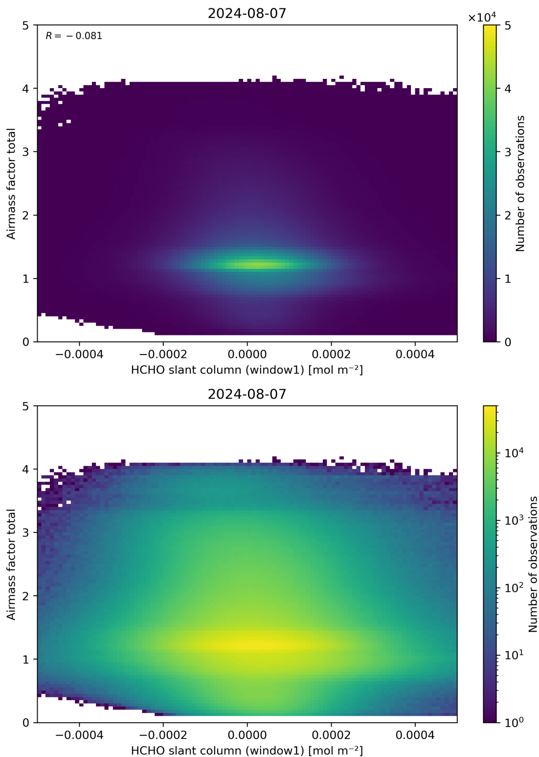
Figure 85: Scatter density plot of “HCHO slant column (window1)” against “Airmass factor total” for 2024-08-06 to 2024-08-08.
