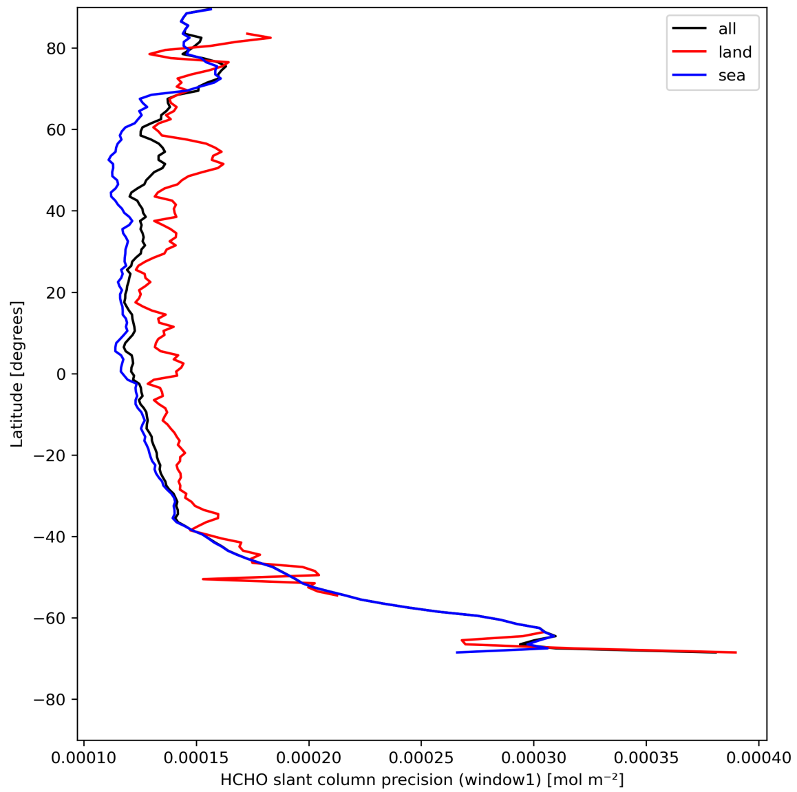
Figure 25: Zonal average of “HCHO slant column precision (window1)” for 2024-08-06 to 2024-08-08.
