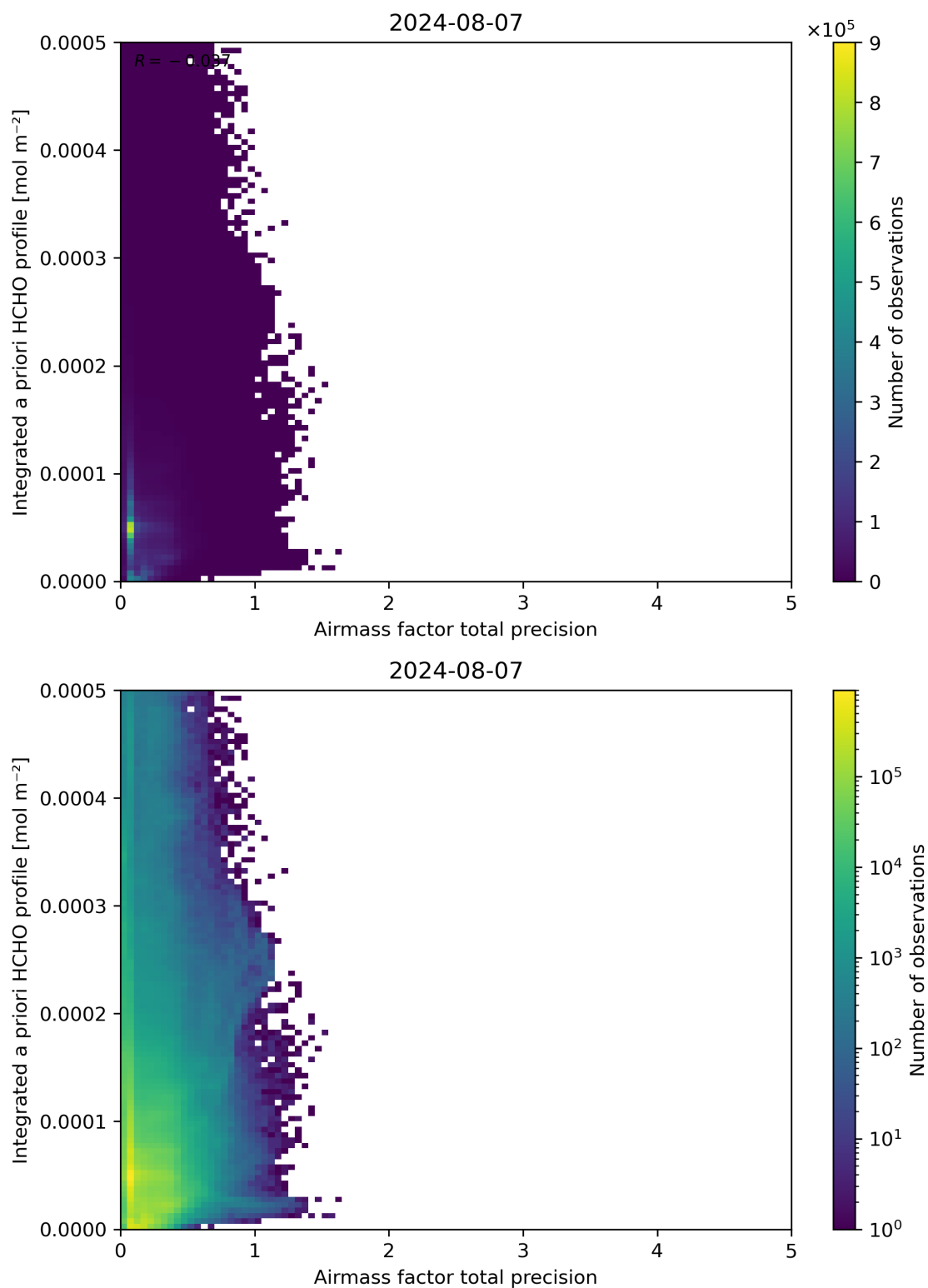
Figure 111: Scatter density plot of “Airmass factor total precision” against “Integrated a priori HCHO profile” for 2024-08-06 to 2024-08-08.
