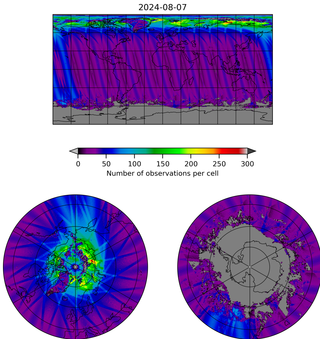
Figure 19: Map of the number of observations for 2024-08-06 to 2024-08-08
