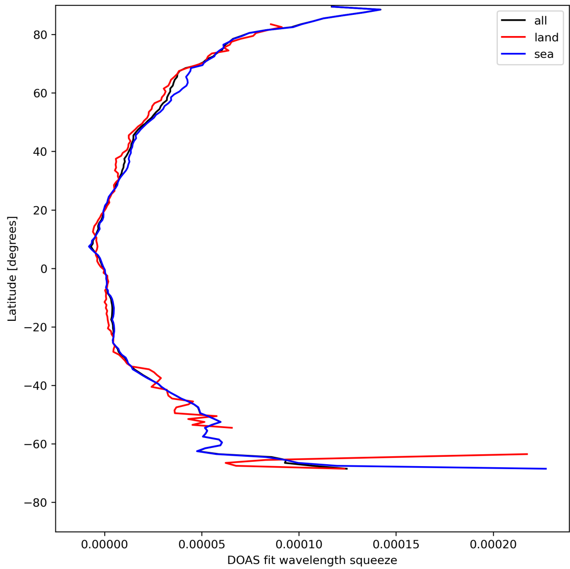
Figure 31: Zonal average of “DOAS fit wavelength squeeze” for 2024-08-06 to 2024-08-08.
