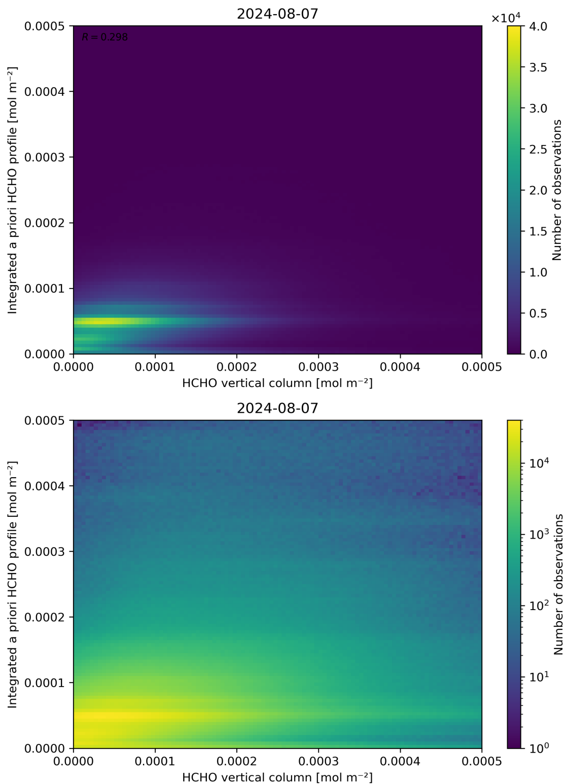
Figure 135: Scatter density plot of “HCHO vertical column” against “Integrated a priori HCHO profile” for 2024-08-06 to 2024-08-08.
