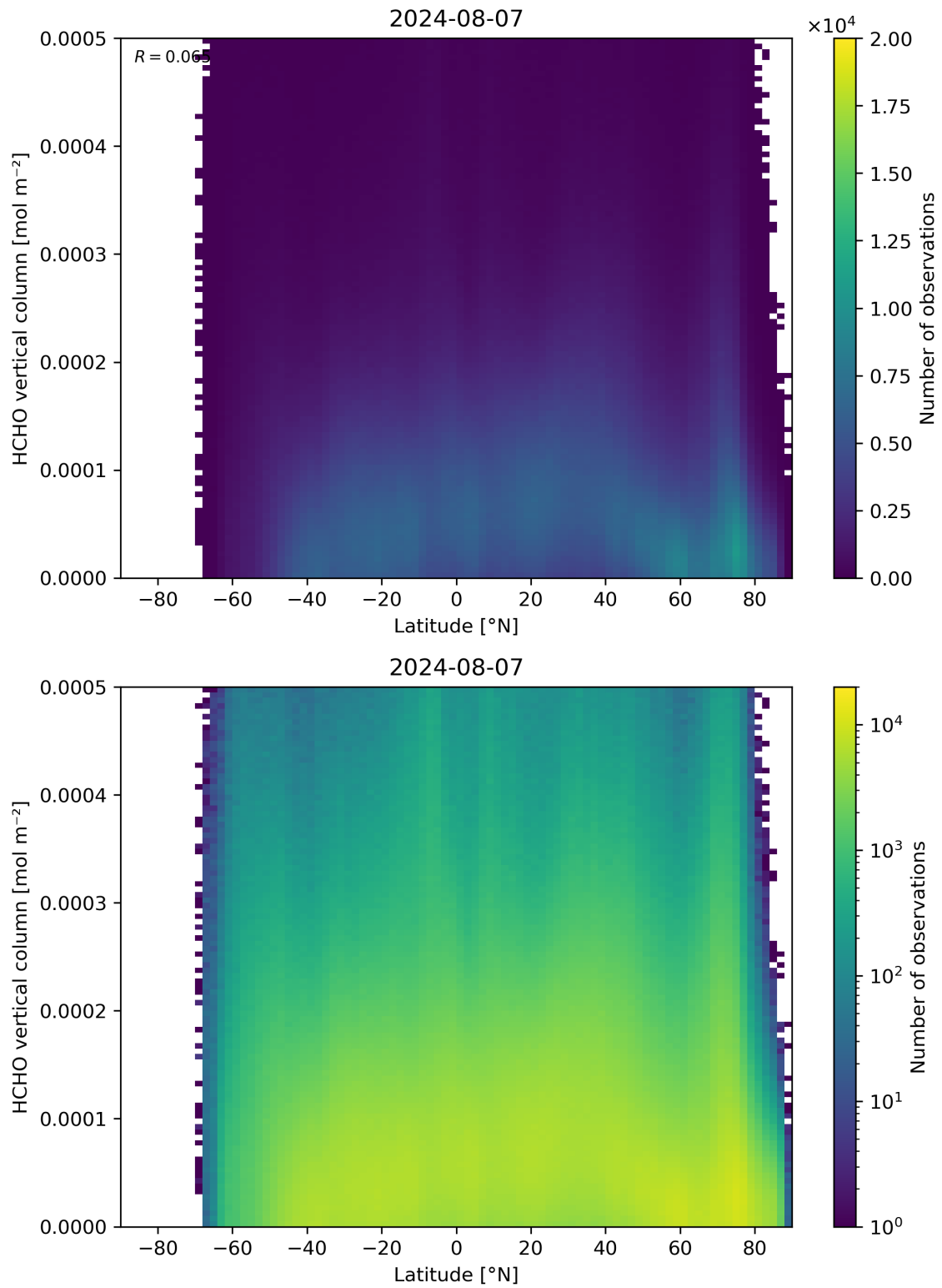
Figure 163: Scatter density plot of “Latitude” against “HCHO vertical column” for 2024-08-06 to 2024-08-08.
