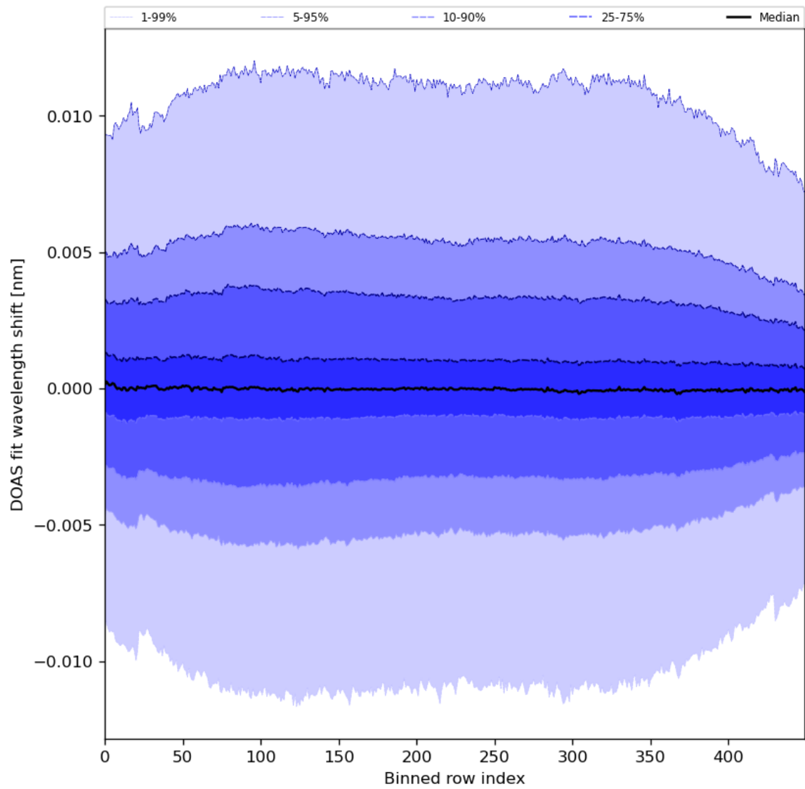
Figure 58: Along track statistics of “DOAS fit wavelength shift” for 2024-08-06 to 2024-08-08
