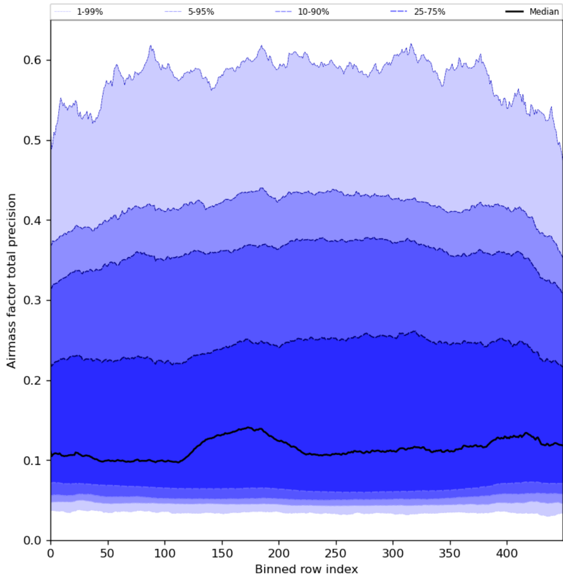
Figure 55: Along track statistics of “Airmass factor total precision” for 2024-08-06 to 2024-08-08
