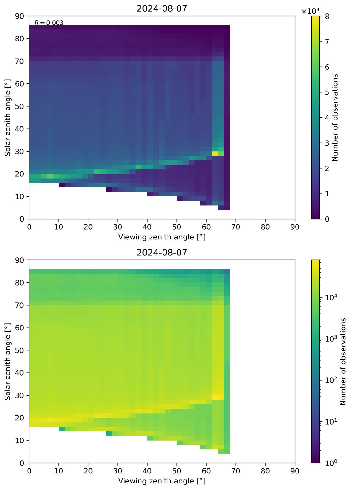
Figure 197: Scatter density plot of “Viewing zenith angle” against “Solar zenith angle” for 2024-08-06 to 2024-08-08.
