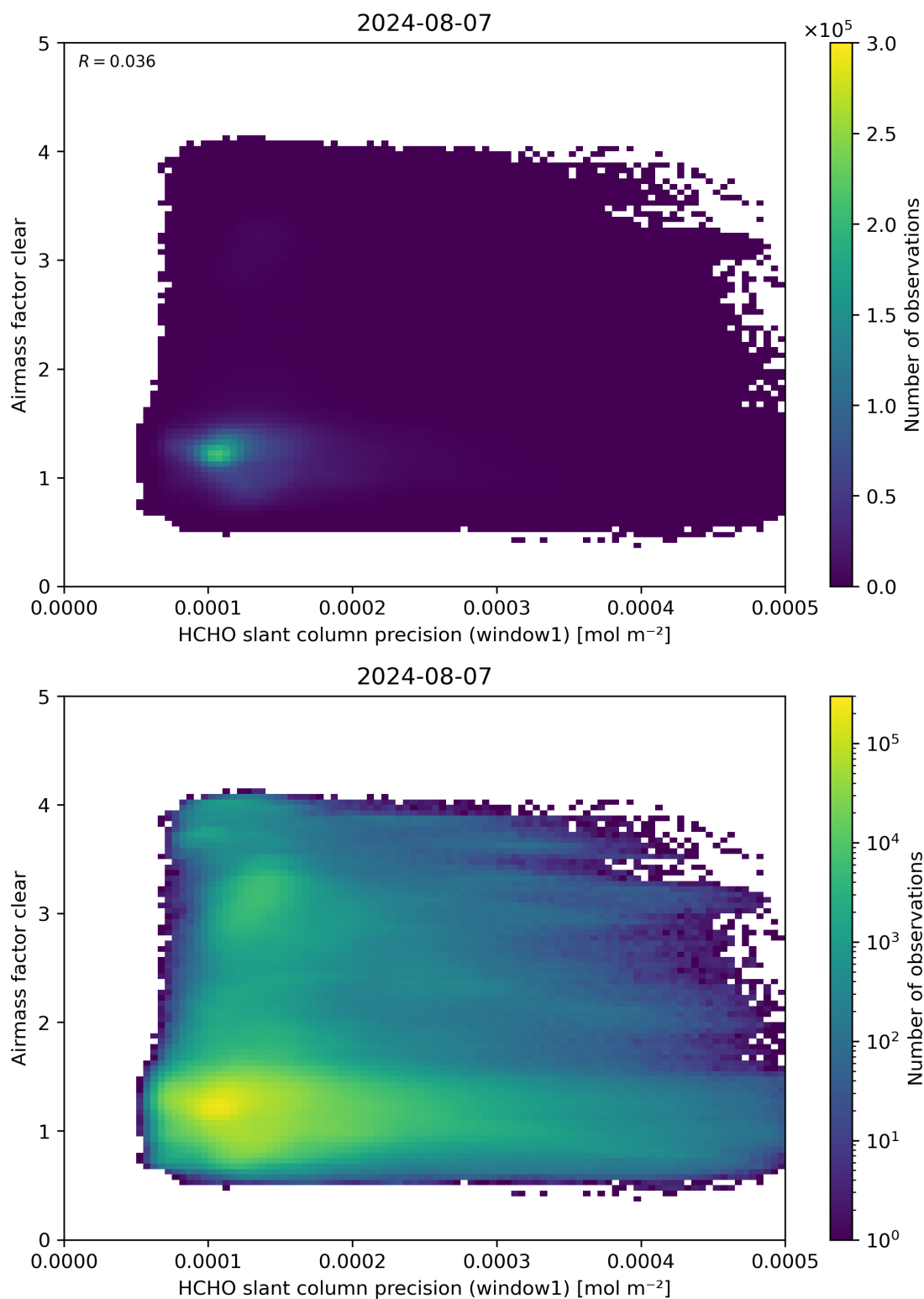
Figure 91: Scatter density plot of “HCHO slant column precision (window1)” against “Airmass factor clear” for 2024-08-06 to 2024-08-08.
