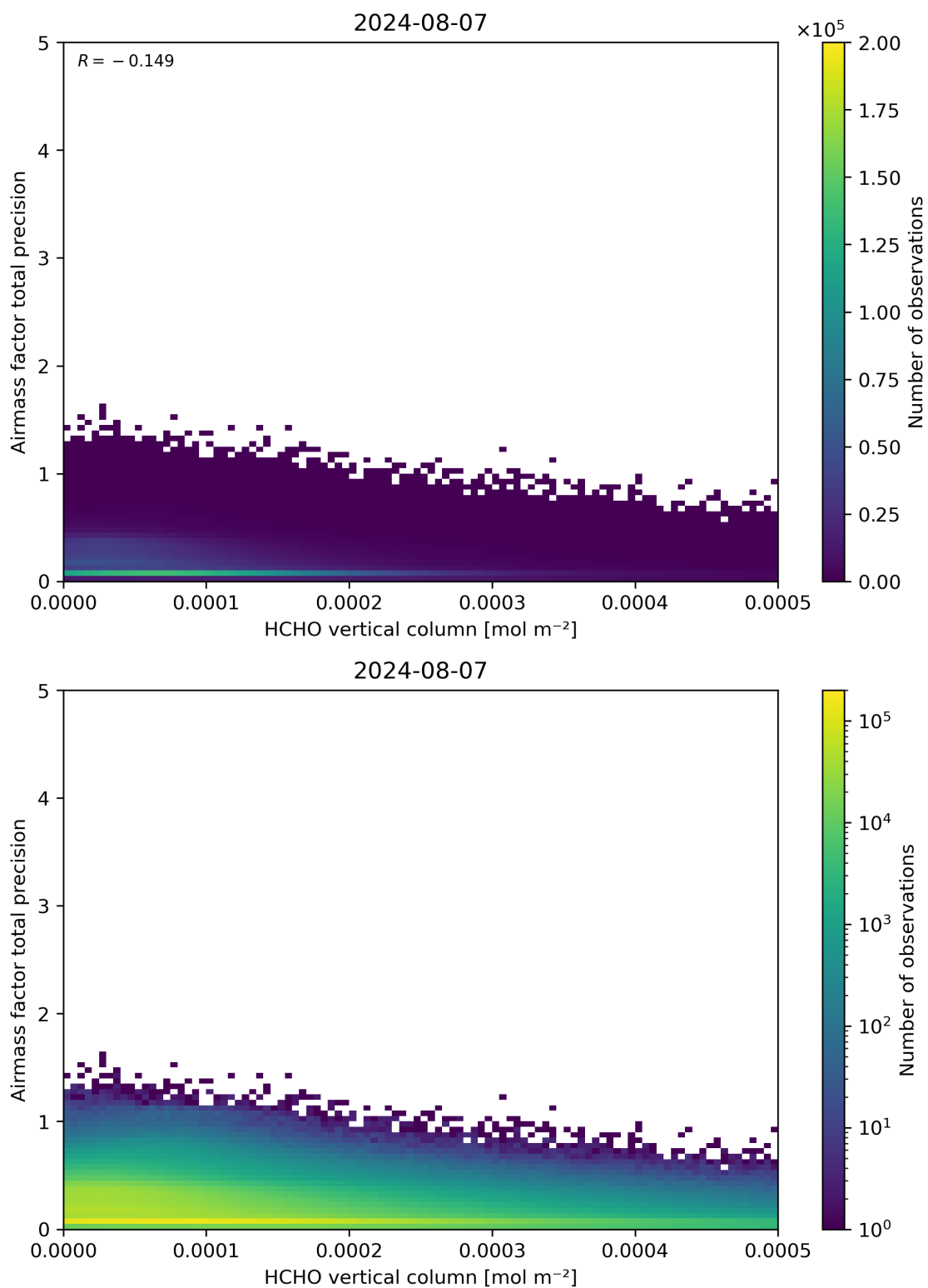
Figure 132: Scatter density plot of “HCHO vertical column” against “Airmass factor total precision” for 2024-08-06 to 2024-08-08.
