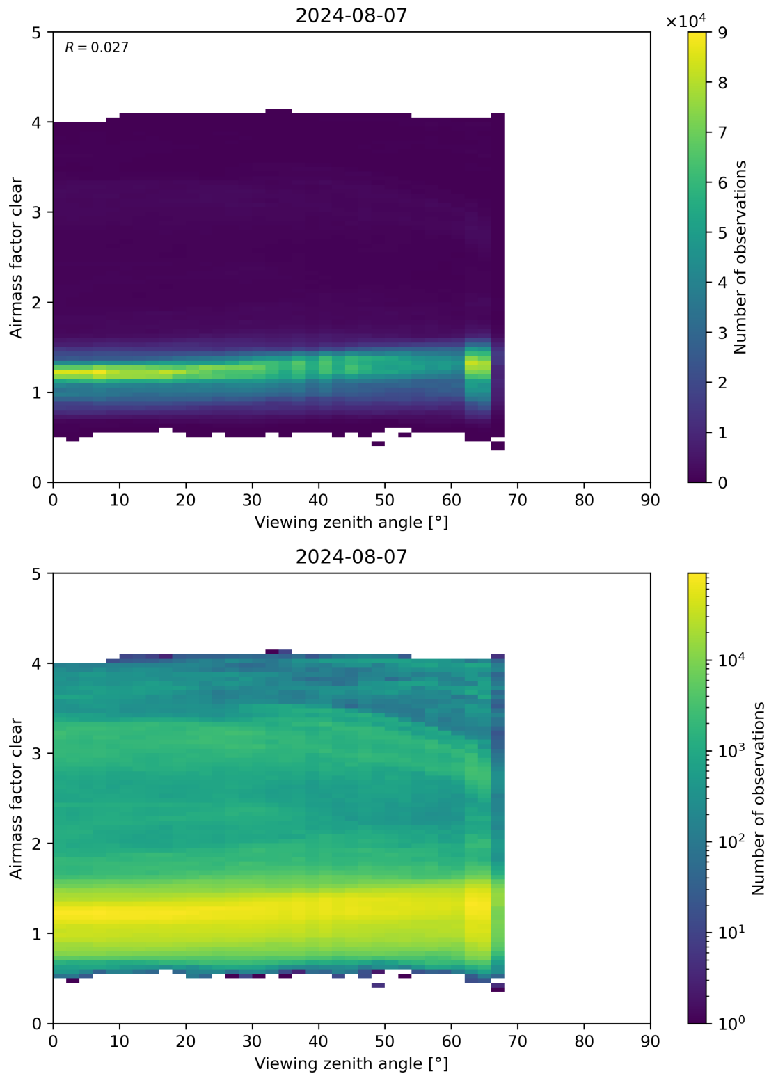
Figure 185: Scatter density plot of “Viewing zenith angle” against “Airmass factor clear” for 2024-08-06 to 2024-08-08.
