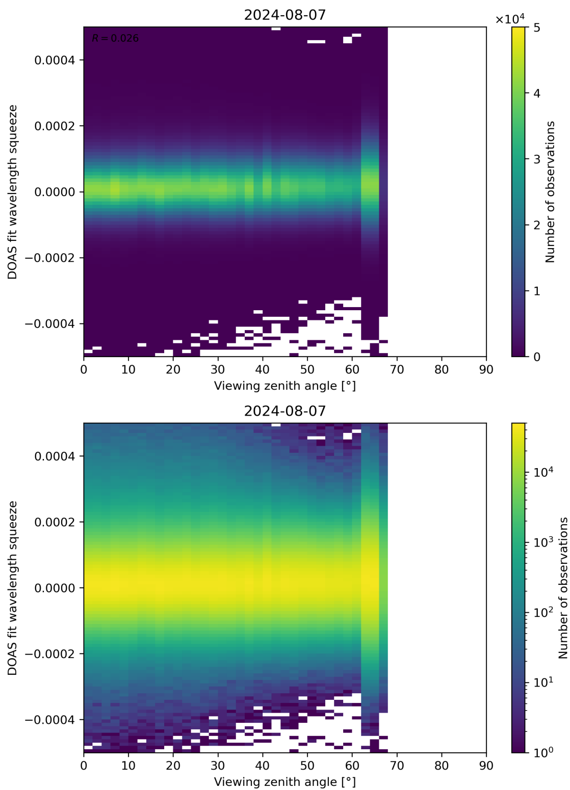
Figure 184: Scatter density plot of “Viewing zenith angle” against “DOAS fit wavelength squeeze” for 2024-08-06 to 2024-08-08.
