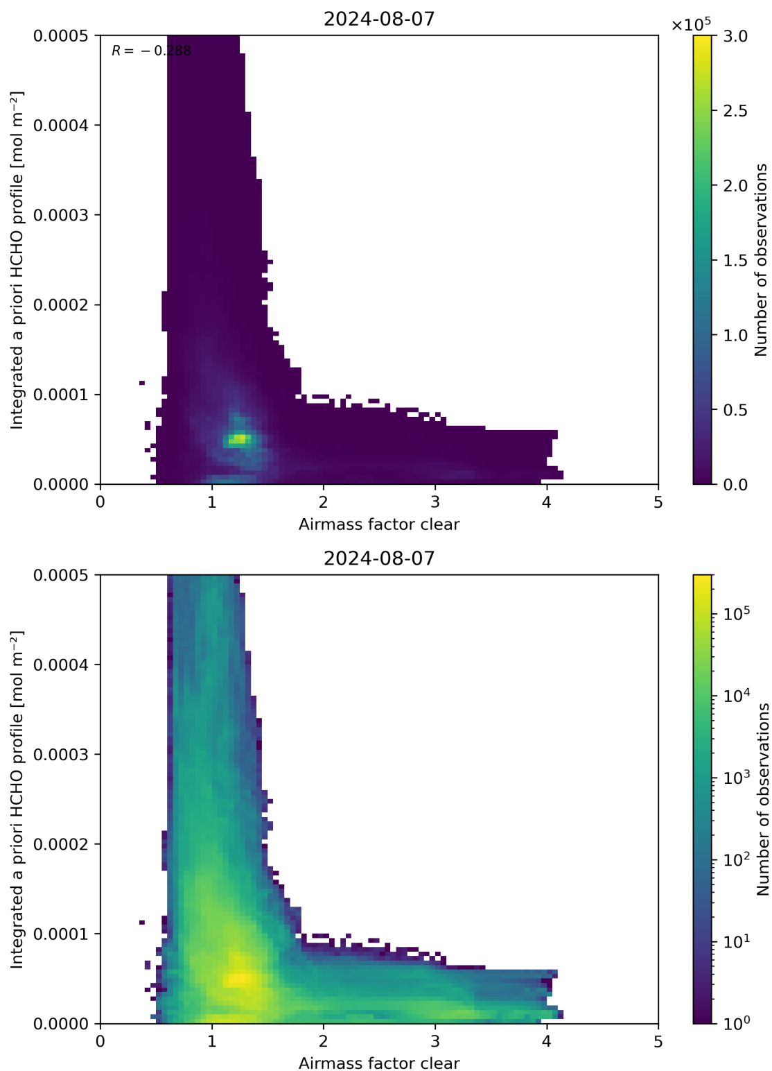
Figure 76: Scatter density plot of “Airmass factor clear” against “Integrated a priori HCHO profile” for 2024-08-06 to 2024-08-08.
