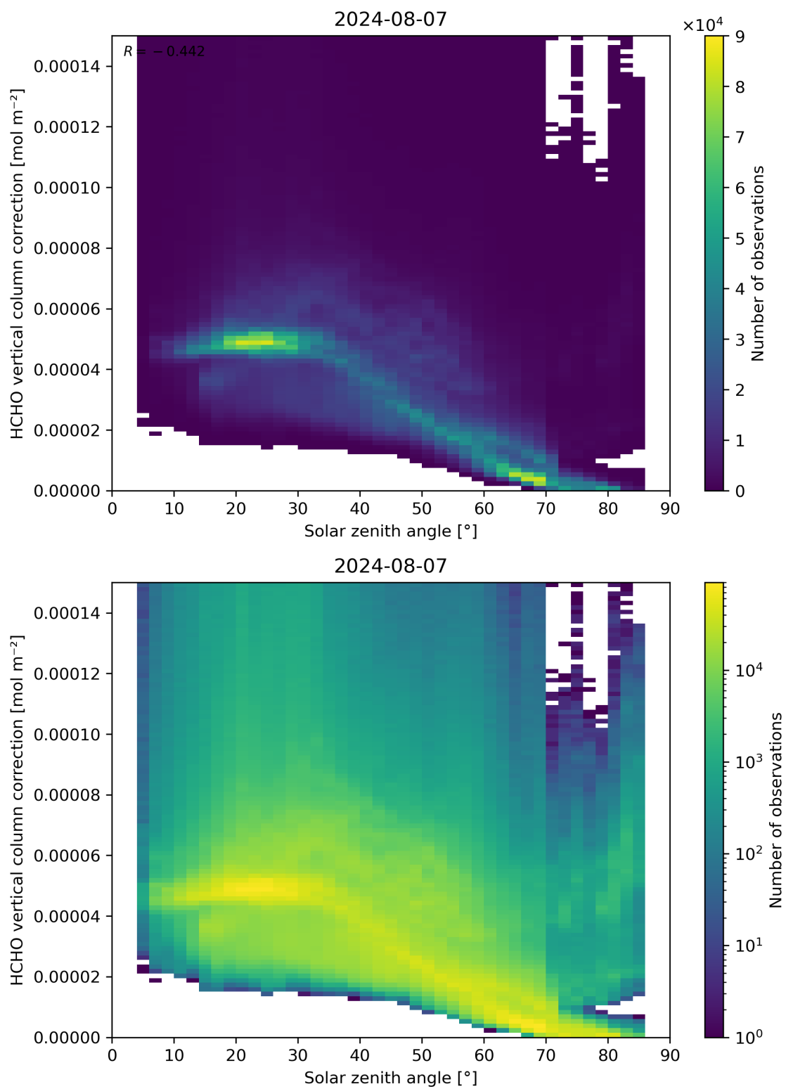
Figure 178: Scatter density plot of “Solar zenith angle” against “HCHO vertical column correction” for 2024-08-06 to 2024-08-08.
