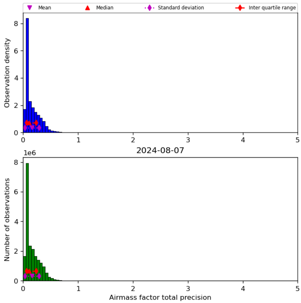
Figure 41: Histogram of “Airmass factor total precision” for 2024-08-06 to 2024-08-08
