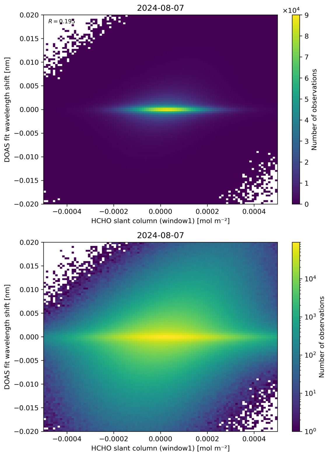
Figure 79: Scatter density plot of “HCHO slant column (window1)” against “DOAS fit wavelength shift” for 2024-08-06 to 2024-08-08.
