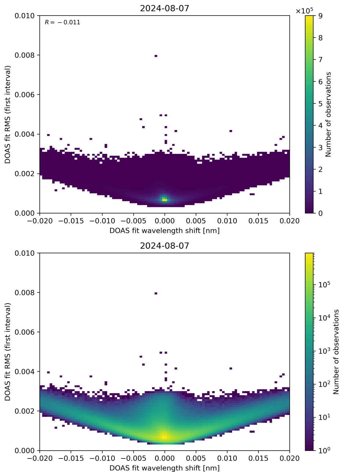
Figure 64: Scatter density plot of “DOAS fit wavelength shift” against “DOAS fit RMS (first interval)” for 2024-08-06 to 2024-08-08.
