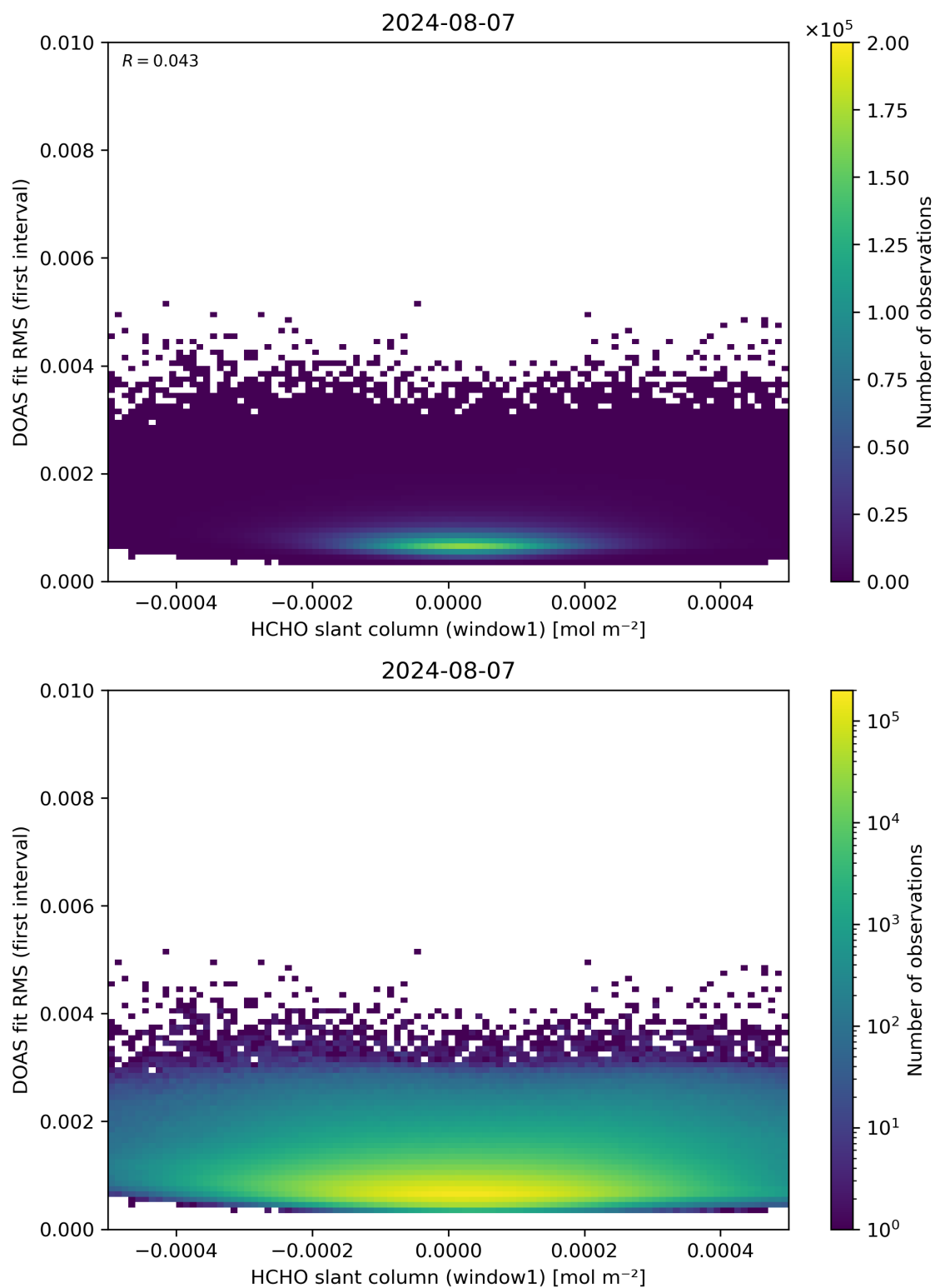
Figure 78: Scatter density plot of “HCHO slant column (window1)” against “DOAS fit RMS (first interval)” for 2024-08-06 to 2024-08-08.
