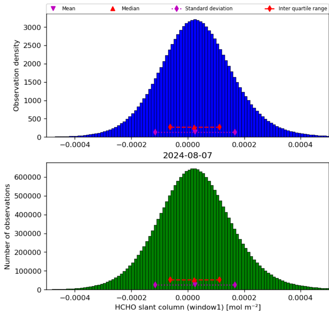
Figure 38: Histogram of “HCHO slant column (window1)” for 2024-08-06 to 2024-08-08
