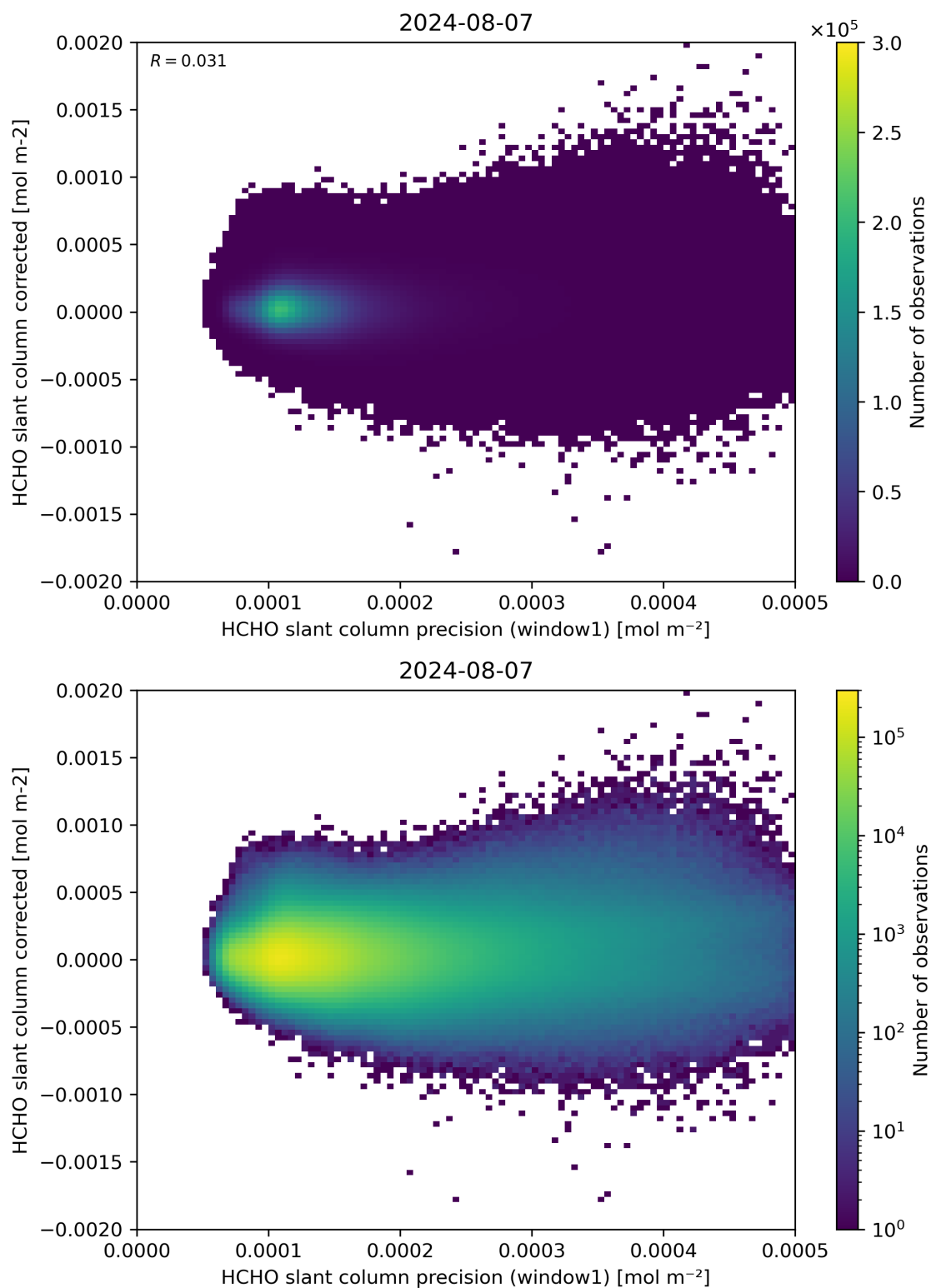
Figure 92: Scatter density plot of “HCHO slant column precision (window1)” against “HCHO slant column corrected” for 2024-08-06 to 2024-08-08.
