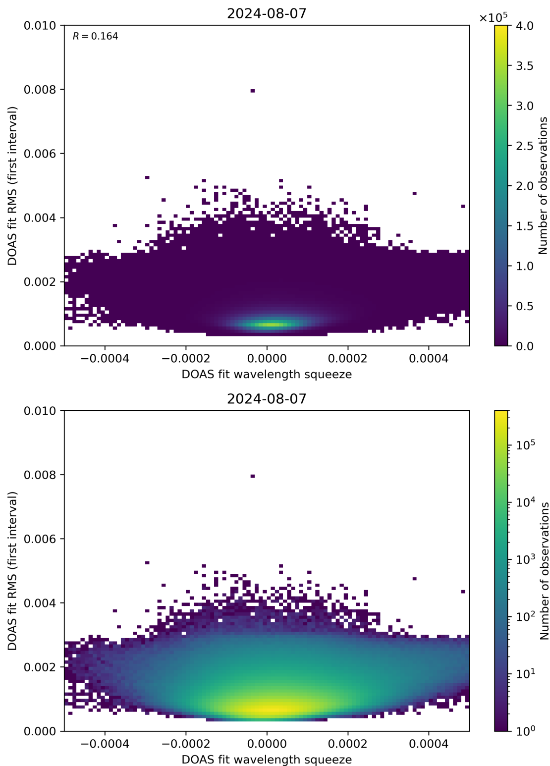
Figure 68: Scatter density plot of “DOAS fit wavelength squeeze” against “DOAS fit RMS (first interval)” for 2024-08-06 to 2024-08-08.
