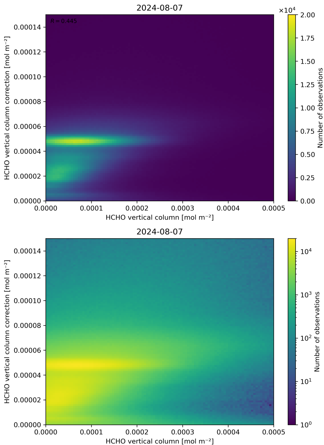
Figure 133: Scatter density plot of “HCHO vertical column” against “HCHO vertical column correction” for 2024-08-06 to 2024-08-08.
