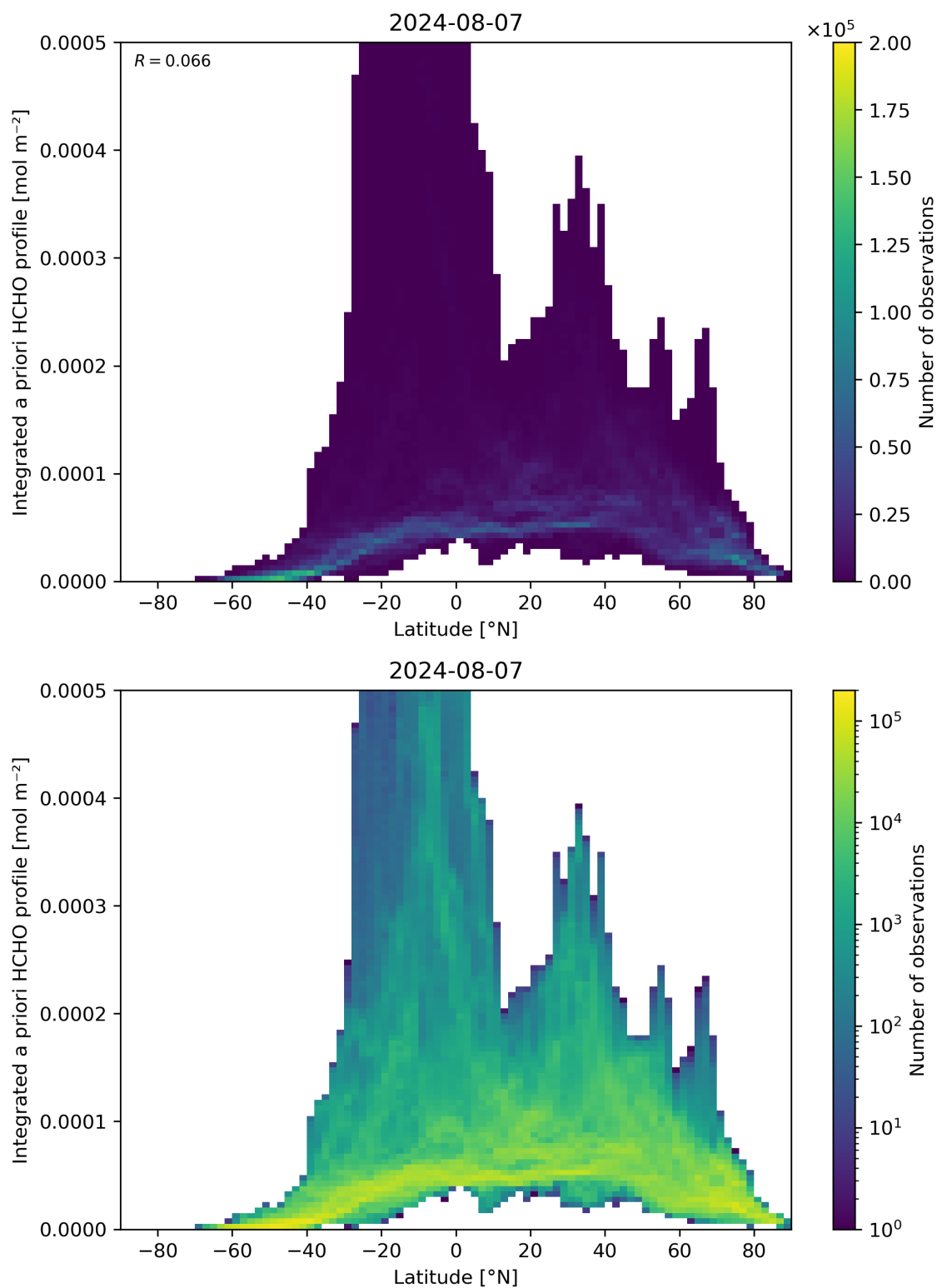
Figure 166: Scatter density plot of “Latitude” against “Integrated a priori HCHO profile” for 2024-08-06 to 2024-08-08.
