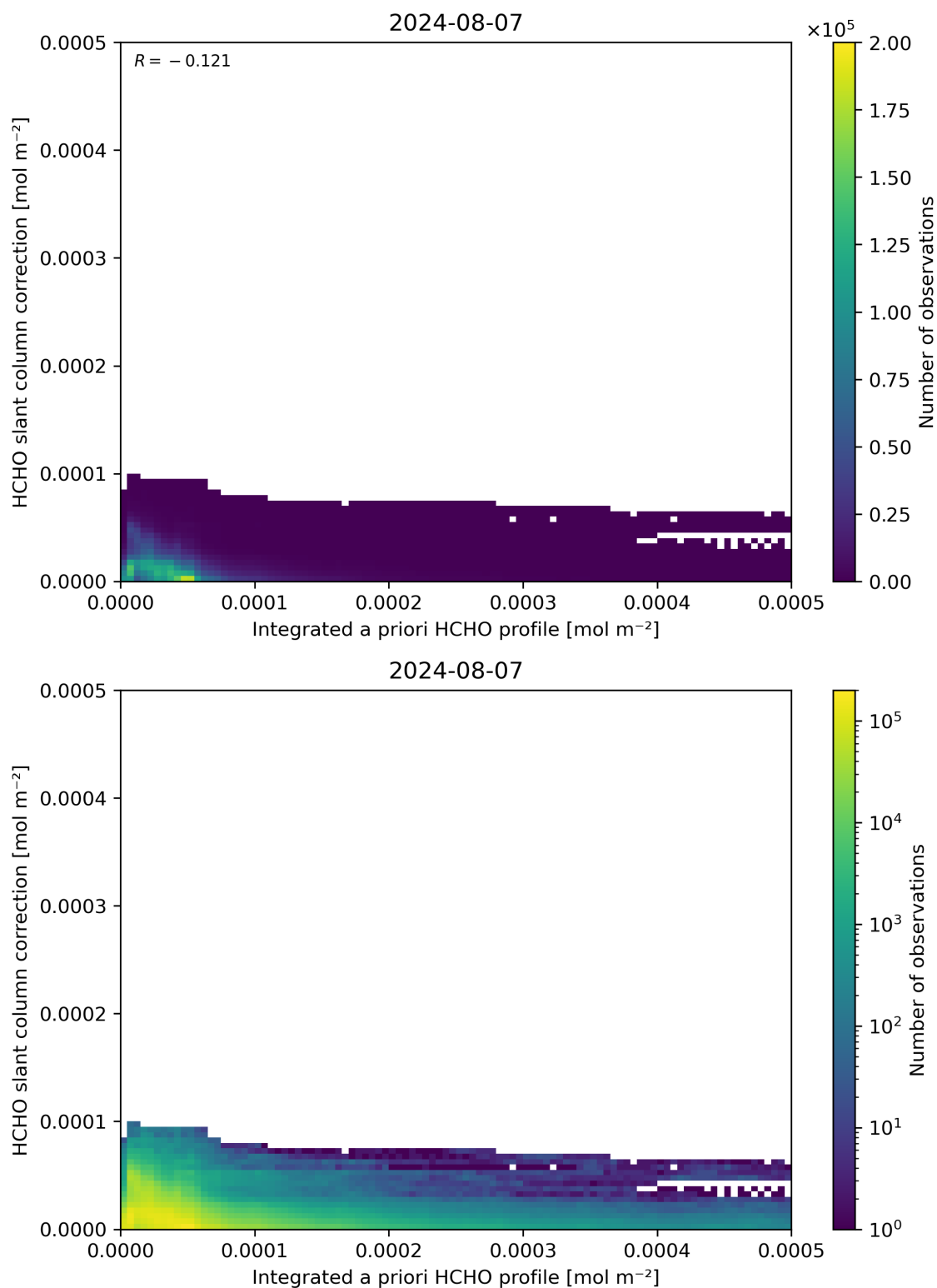
Figure 152: Scatter density plot of “Integrated a priori HCHO profile” against “HCHO slant column correction” for 2024-08-06 to 2024-08-08.
