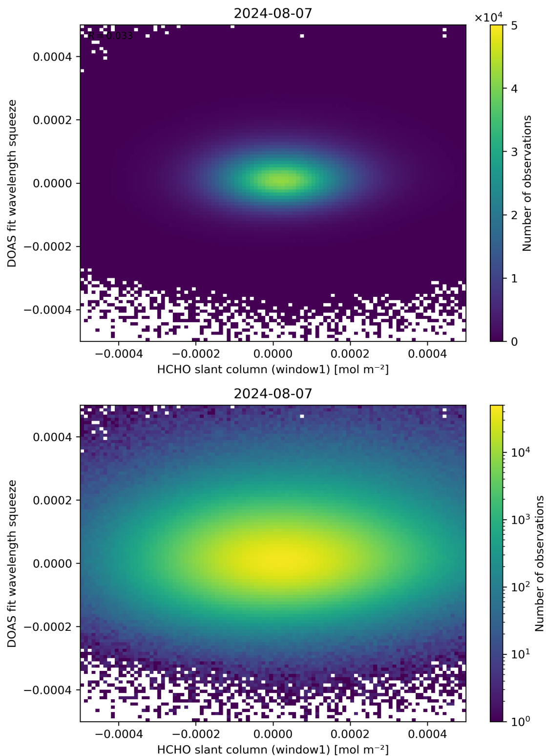
Figure 80: Scatter density plot of “HCHO slant column (window1)” against “DOAS fit wavelength squeeze” for 2024-08-06 to 2024-08-08.
