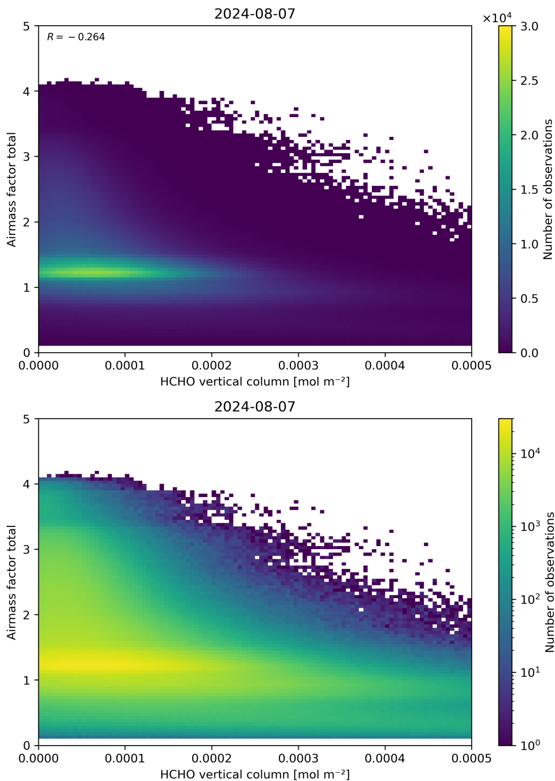
Figure 131: Scatter density plot of “HCHO vertical column” against “Airmass factor total” for 2024-08-06 to 2024-08-08.
