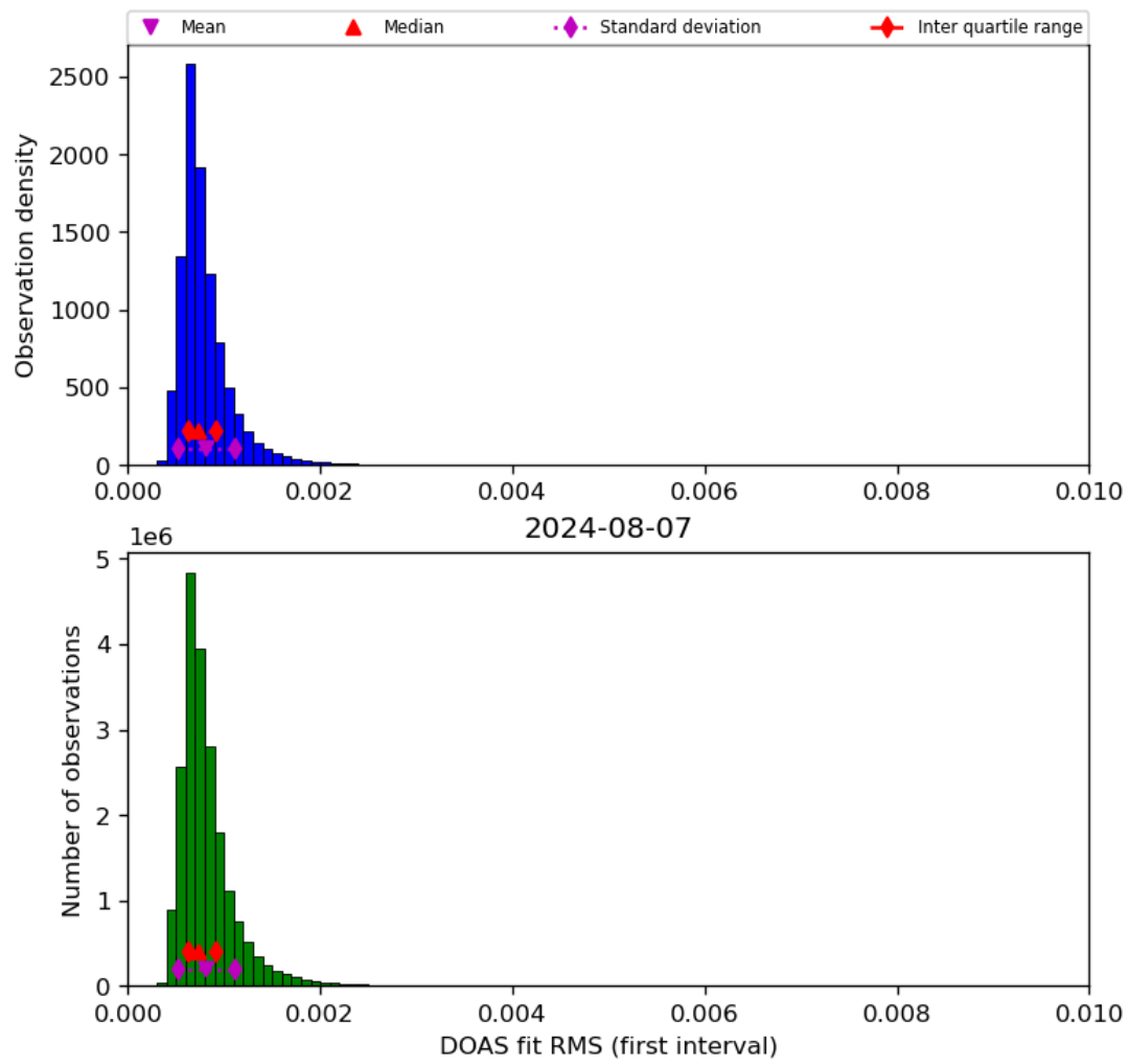
Figure 46: Histogram of “DOAS fit RMS (first interval)” for 2024-08-06 to 2024-08-08
