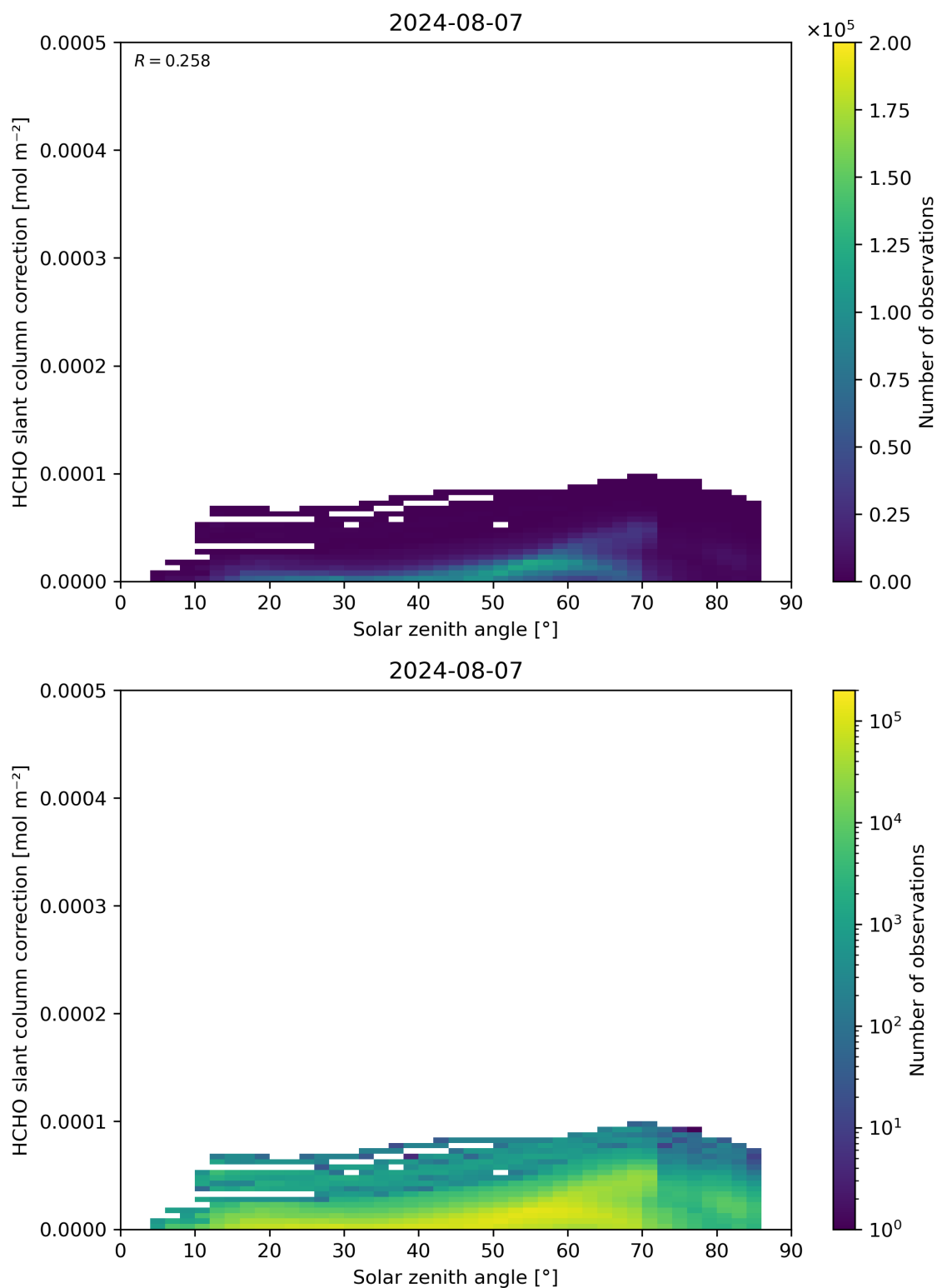
Figure 172: Scatter density plot of “Solar zenith angle” against “HCHO slant column correction” for 2024-08-06 to 2024-08-08.
