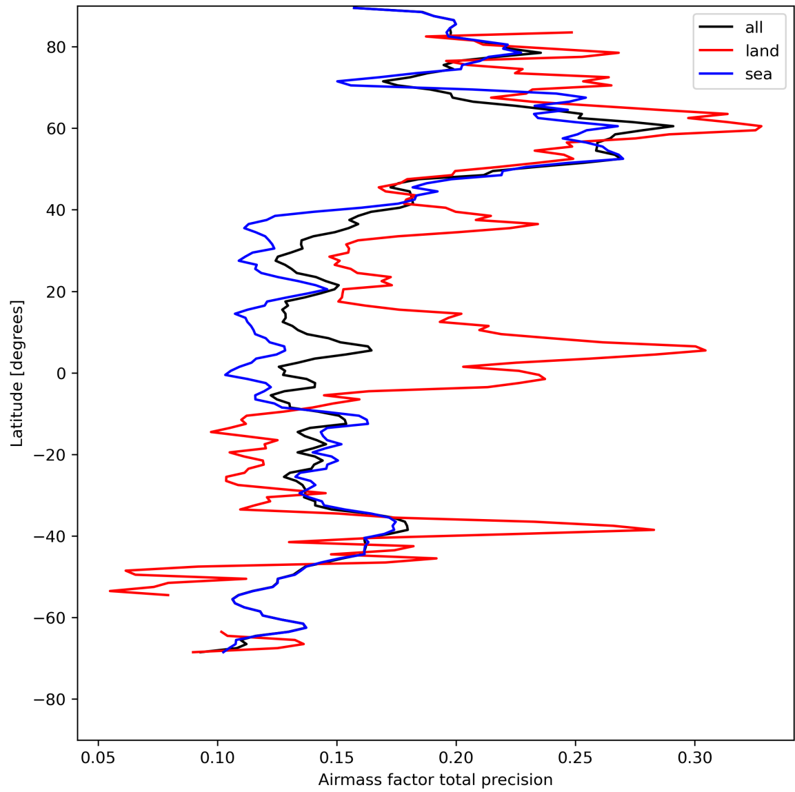
Figure 27: Zonal average of “Airmass factor total precision” for 2024-08-06 to 2024-08-08.
