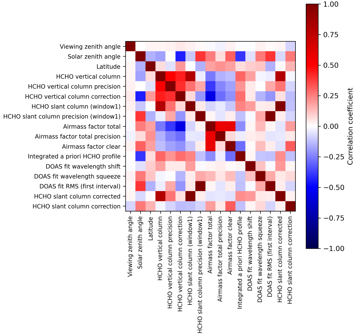
Figure 2: Map of correlation matrix for 2024-08-06 to 2024-08-08.
