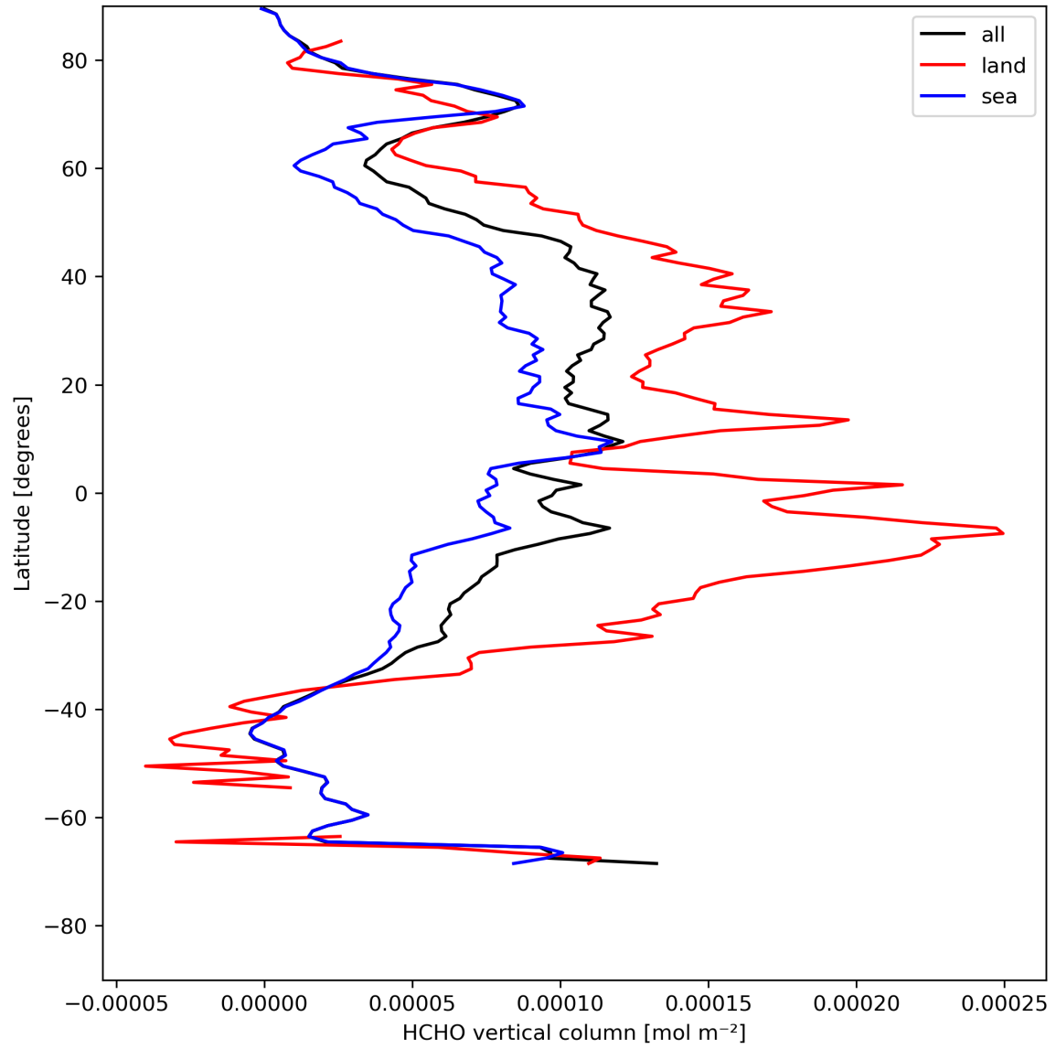
Figure 21: Zonal average of “HCHO vertical column” for 2024-08-06 to 2024-08-08.
