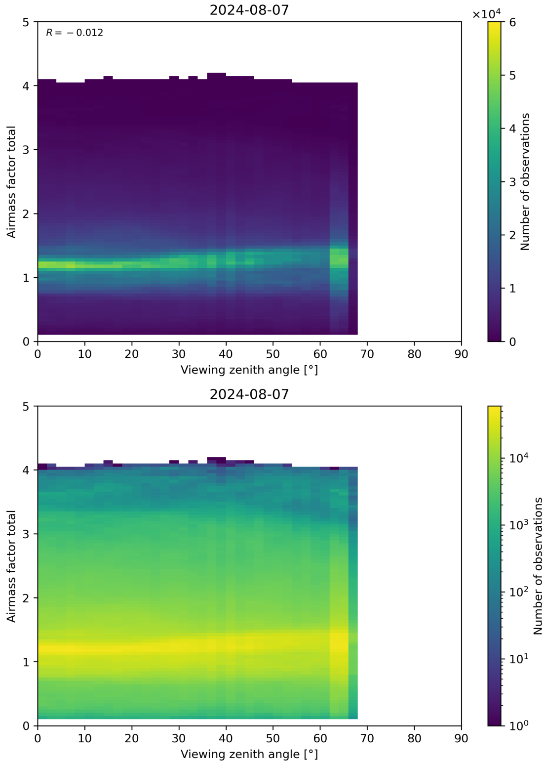
Figure 190: Scatter density plot of “Viewing zenith angle” against “Airmass factor total” for 2024-08-06 to 2024-08-08.
