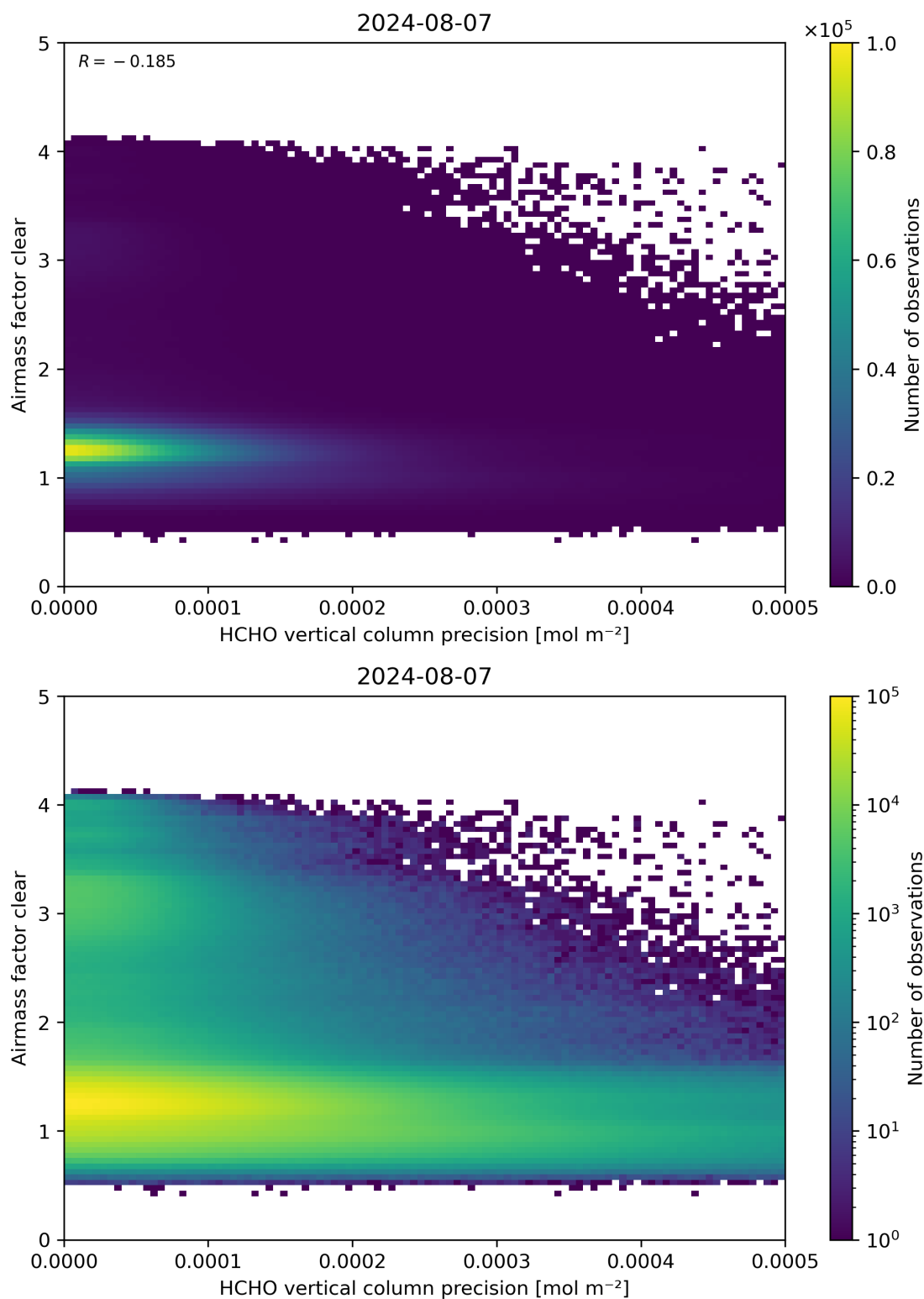
Figure 139: Scatter density plot of “HCHO vertical column precision” against “Airmass factor clear” for 2024-08-06 to 2024-08-08.
