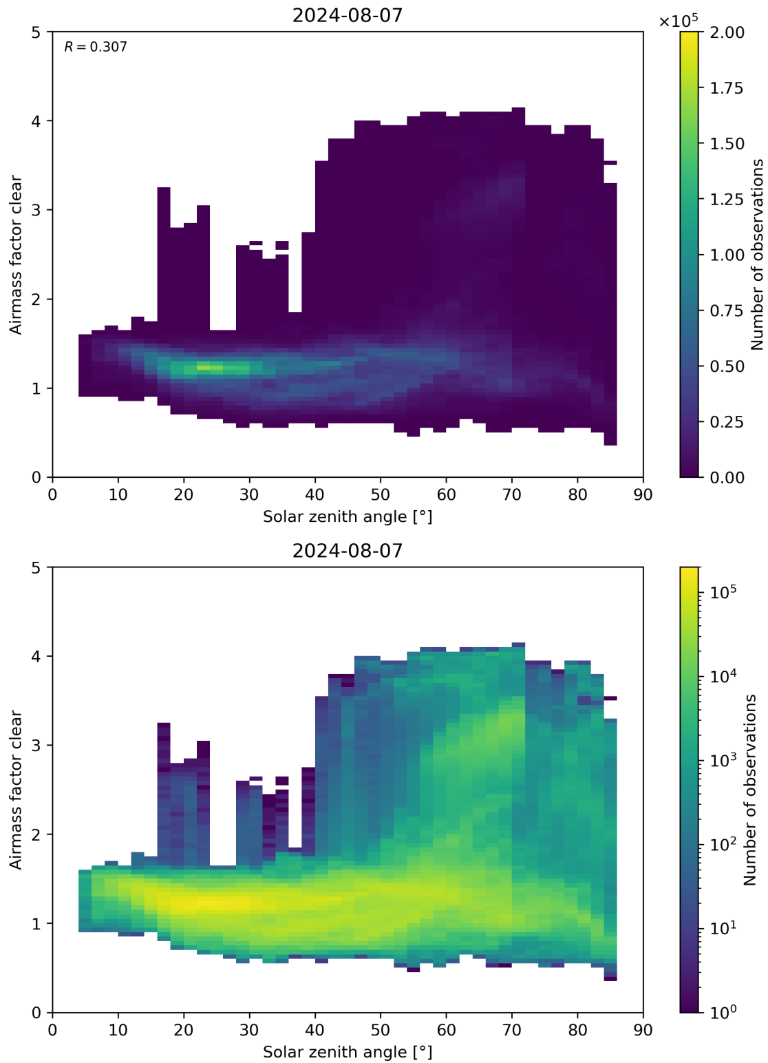
Figure 170: Scatter density plot of “Solar zenith angle” against “Airmass factor clear” for 2024-08-06 to 2024-08-08.
