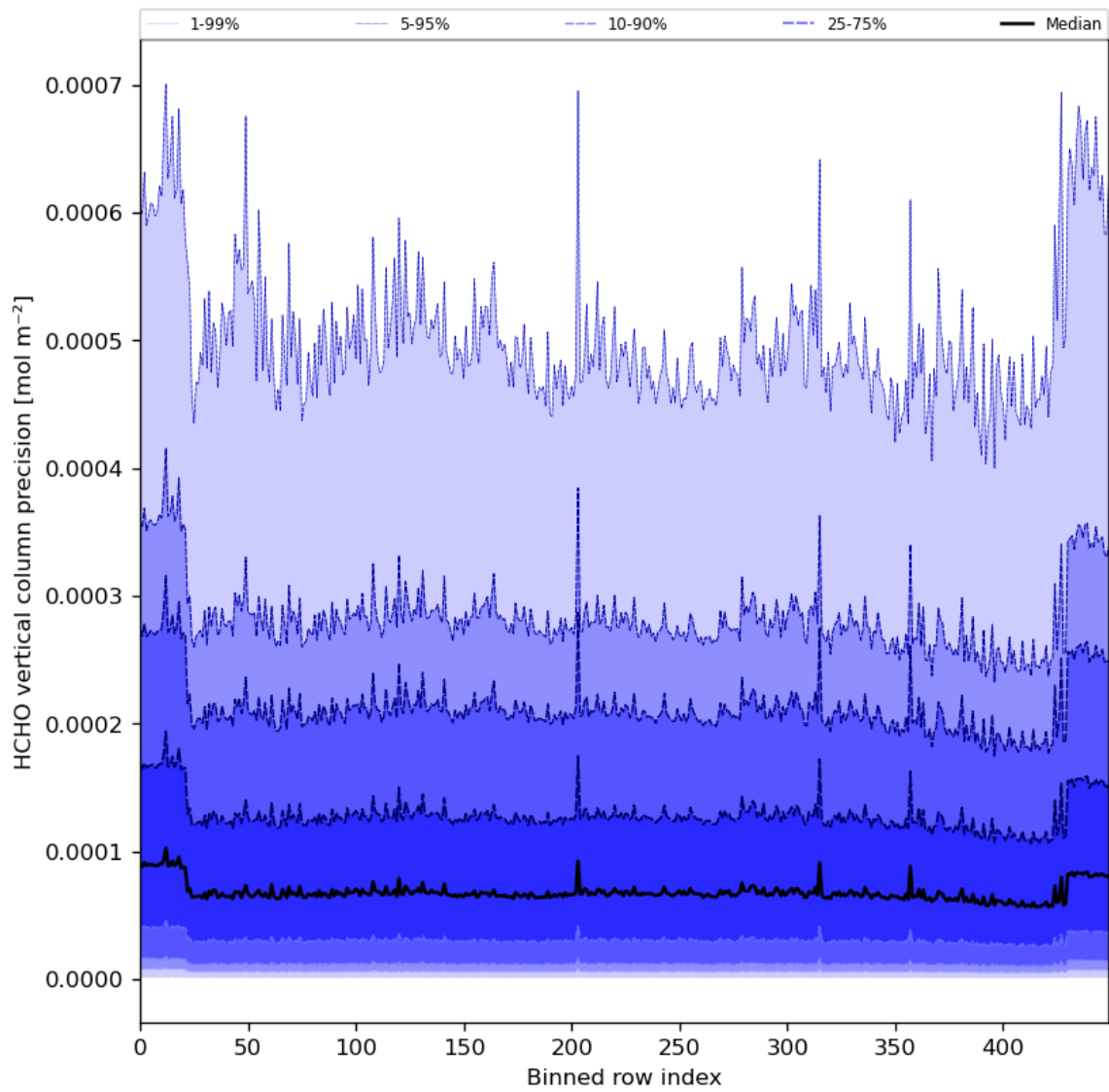
Figure 50: Along track statistics of “HCHO vertical column precision” for 2024-08-06 to 2024-08-08
