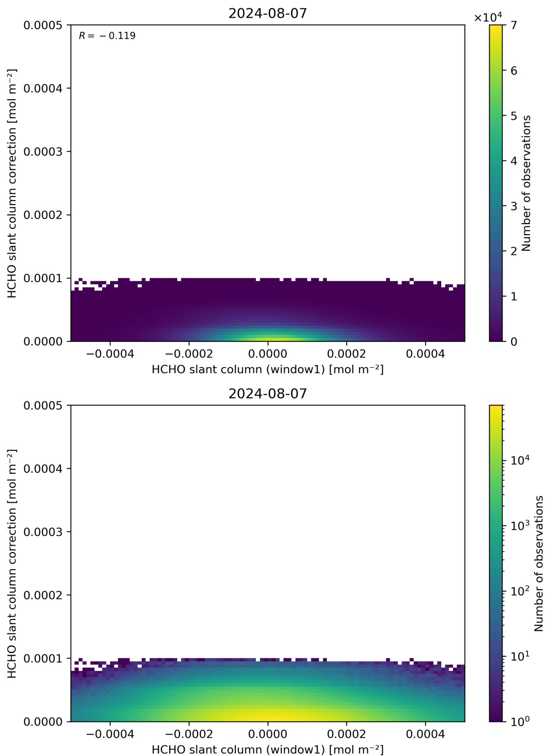
Figure 83: Scatter density plot of “HCHO slant column (window1)” against “HCHO slant column correction” for 2024-08-06 to 2024-08-08.
