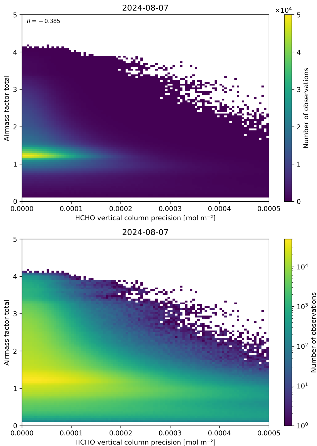
Figure 144: Scatter density plot of “HCHO vertical column precision” against “Airmass factor total” for 2024-08-06 to 2024-08-08.
