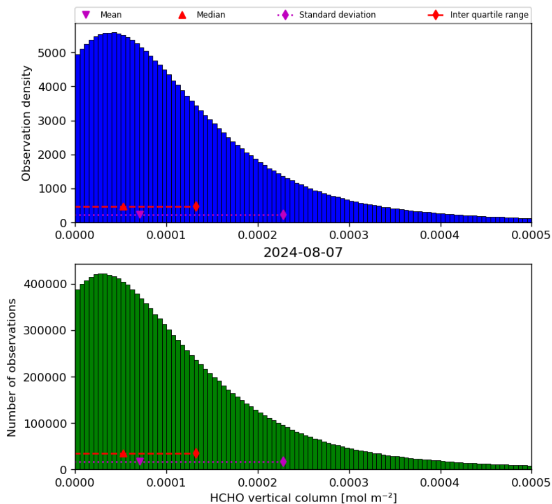
Figure 35: Histogram of “HCHO vertical column” for 2024-08-06 to 2024-08-08
