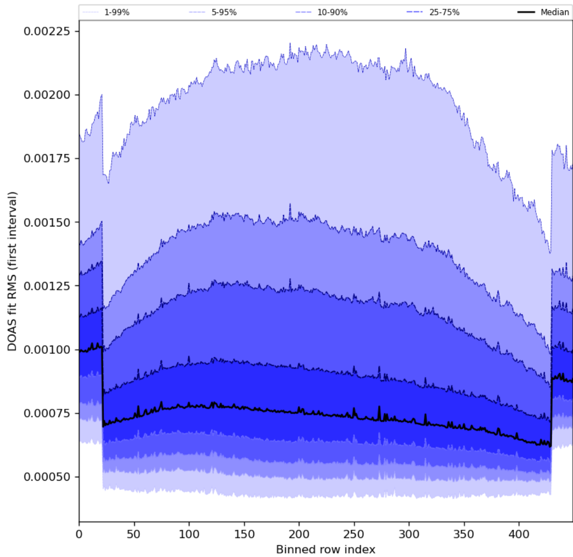
Figure 60: Along track statistics of “DOAS fit RMS (first interval)” for 2024-08-06 to 2024-08-08
