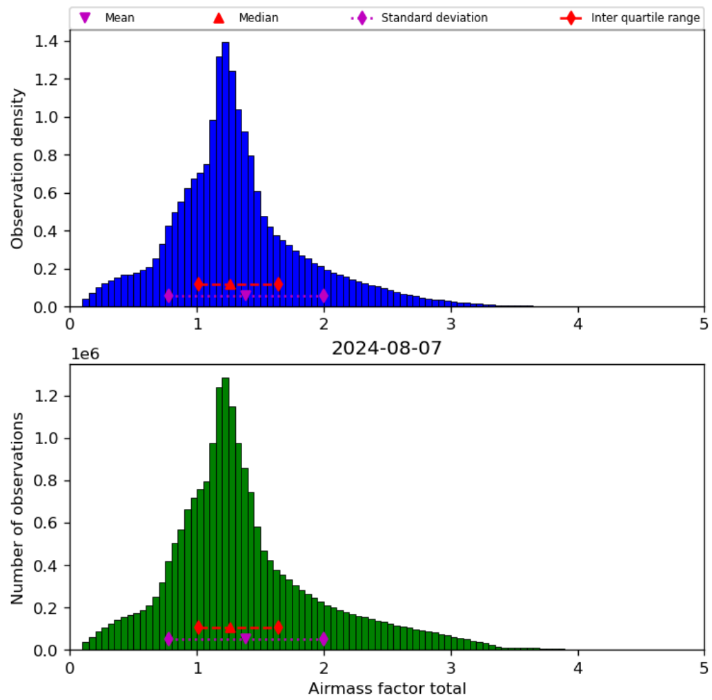
Figure 40: Histogram of “Airmass factor total” for 2024-08-06 to 2024-08-08
