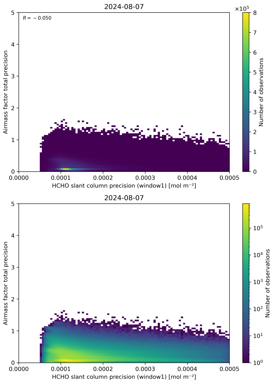
Figure 95: Scatter density plot of “HCHO slant column precision (window1)” against “Airmass factor total precision” for 2024-08-06 to 2024-08-08.
