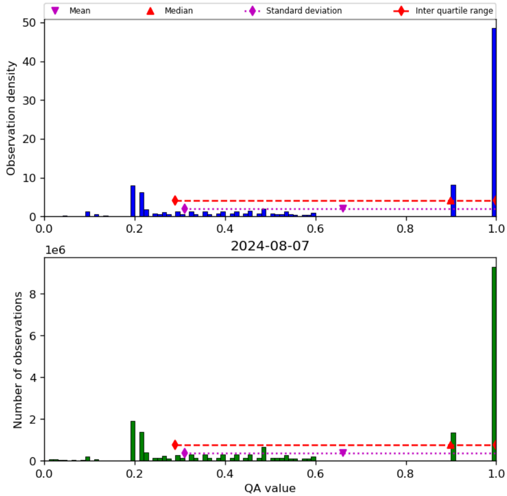
Figure 34: Histogram of “QA value” for 2024-08-06 to 2024-08-08
