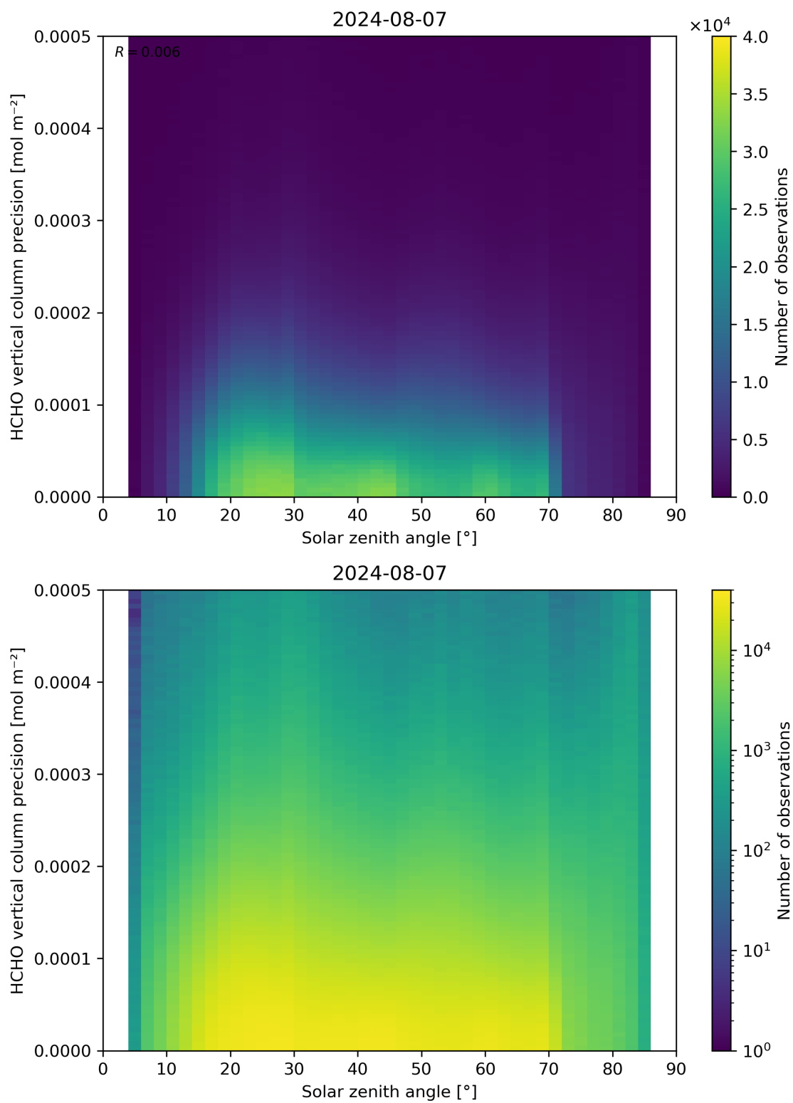
Figure 179: Scatter density plot of “Solar zenith angle” against “HCHO vertical column precision” for 2024-08-06 to 2024-08-08.
