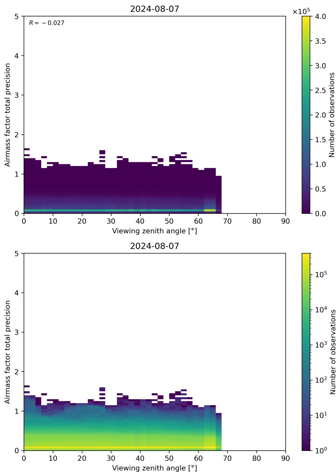
Figure 191: Scatter density plot of “Viewing zenith angle” against “Airmass factor total precision” for 2024-08-06 to 2024-08-08.
