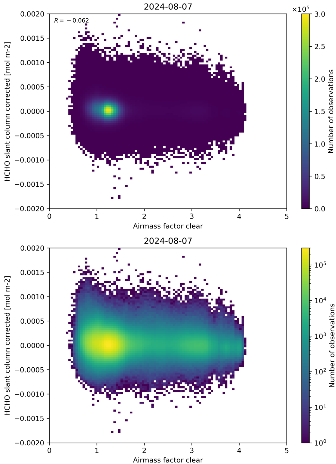
Figure 74: Scatter density plot of “Airmass factor clear” against “HCHO slant column corrected” for 2024-08-06 to 2024-08-08.
