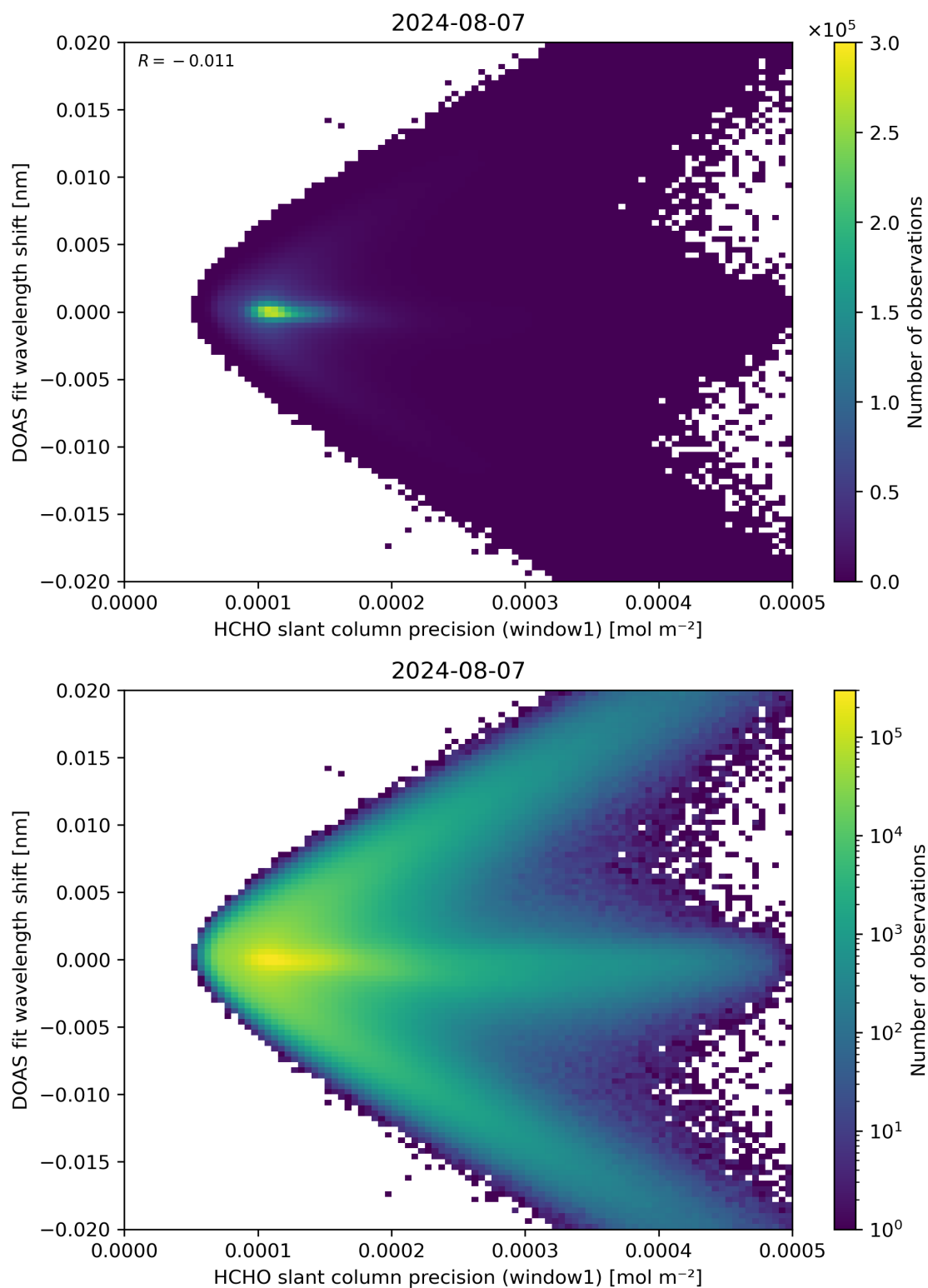
Figure 89: Scatter density plot of “HCHO slant column precision (window1)” against “DOAS fit wavelength shift” for 2024-08-06 to 2024-08-08.
