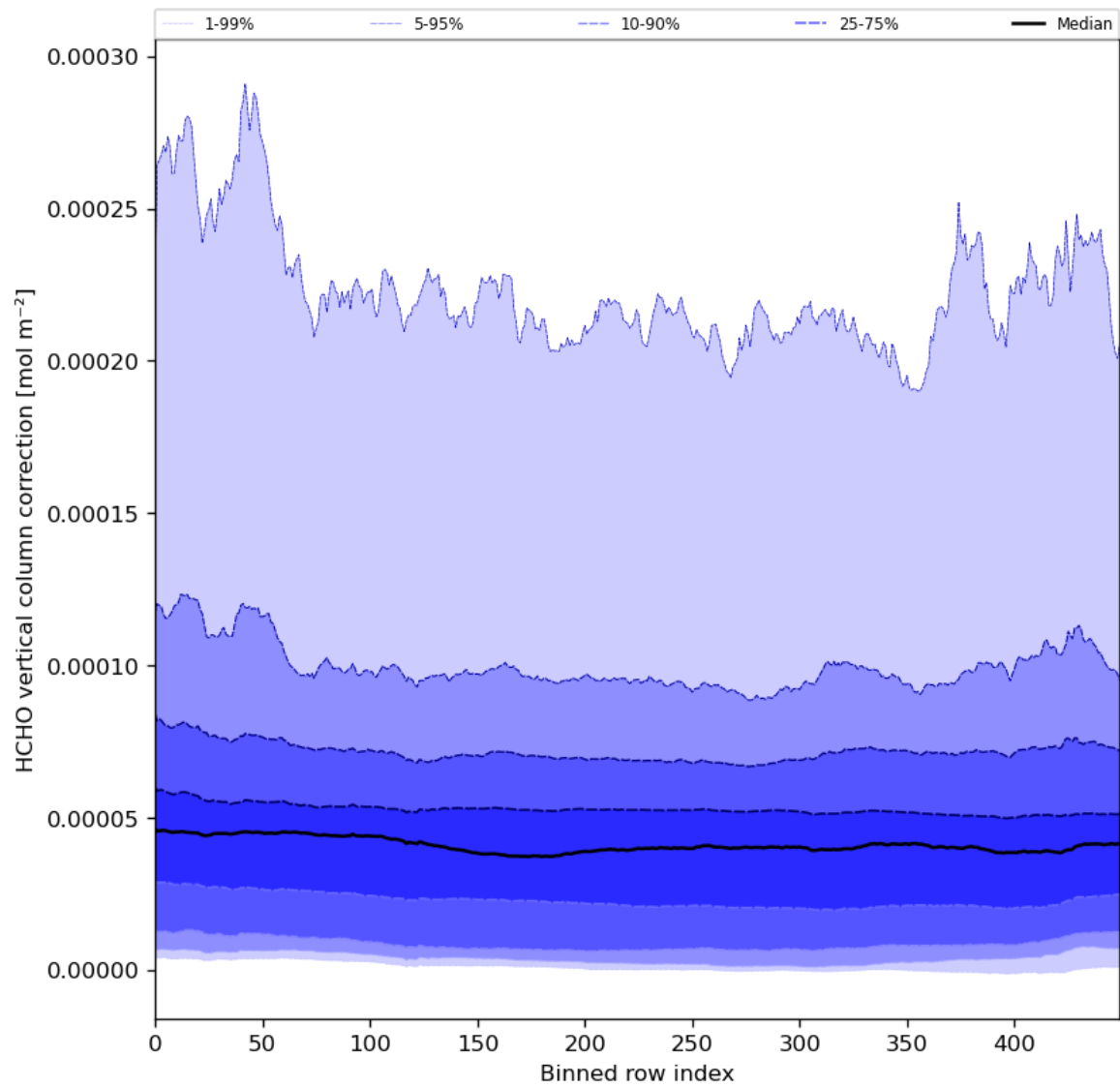
Figure 51: Along track statistics of "HCHO vertical column correction" for 2024-08-06 to 2024-08-08
