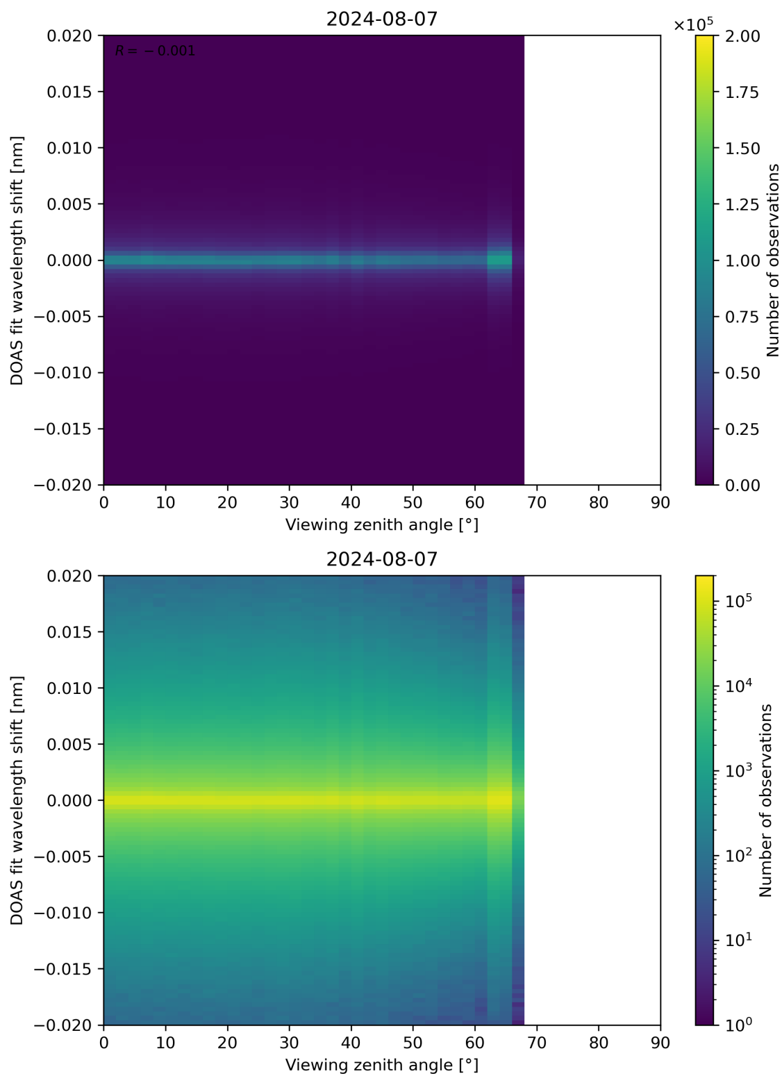
Figure 183: Scatter density plot of “Viewing zenith angle” against “DOAS fit wavelength shift” for 2024-08-06 to 2024-08-08.
