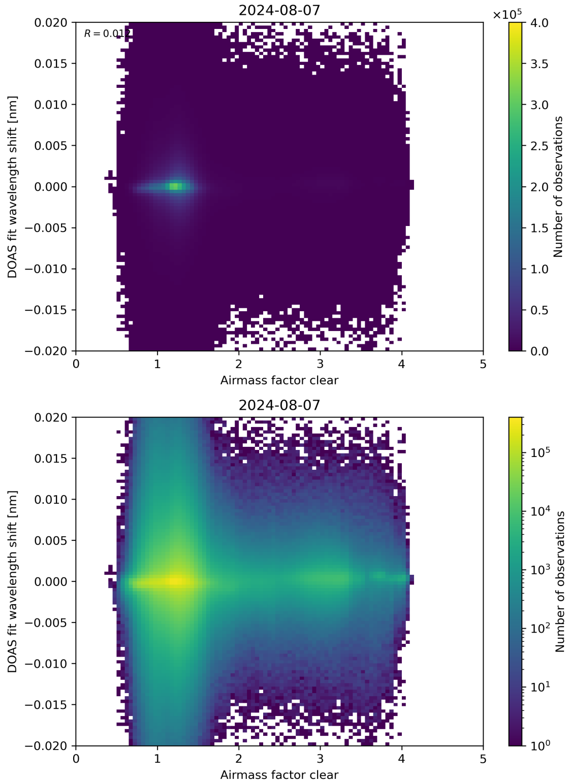
Figure 72: Scatter density plot of “Airmass factor clear” against “DOAS fit wavelength shift” for 2024-08-06 to 2024-08-08.
