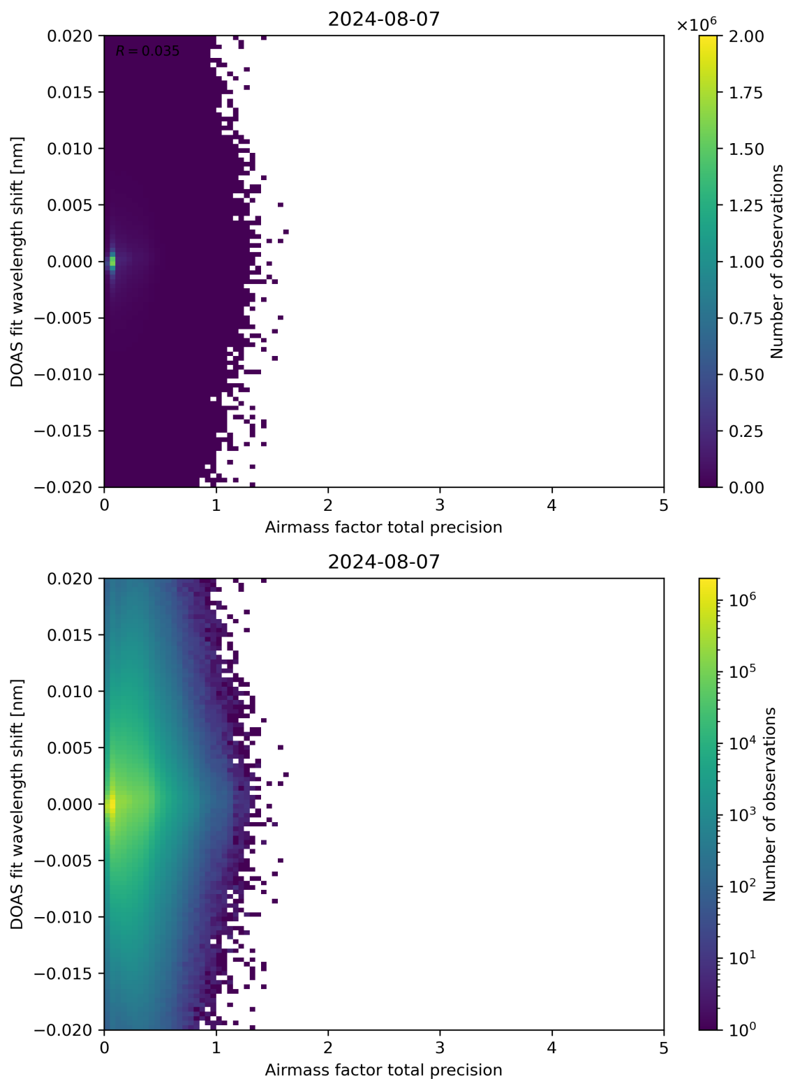
Figure 106: Scatter density plot of “Airmass factor total precision” against “DOAS fit wavelength shift” for 2024-08-06 to 2024-08-08.
