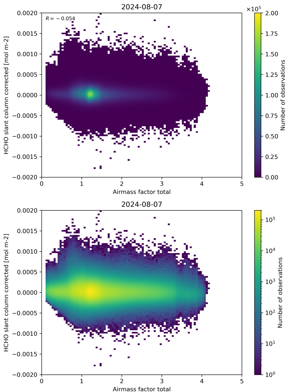
Figure 101: Scatter density plot of “Airmass factor total” against “HCHO slant column corrected” for 2024-08-06 to 2024-08-08.
