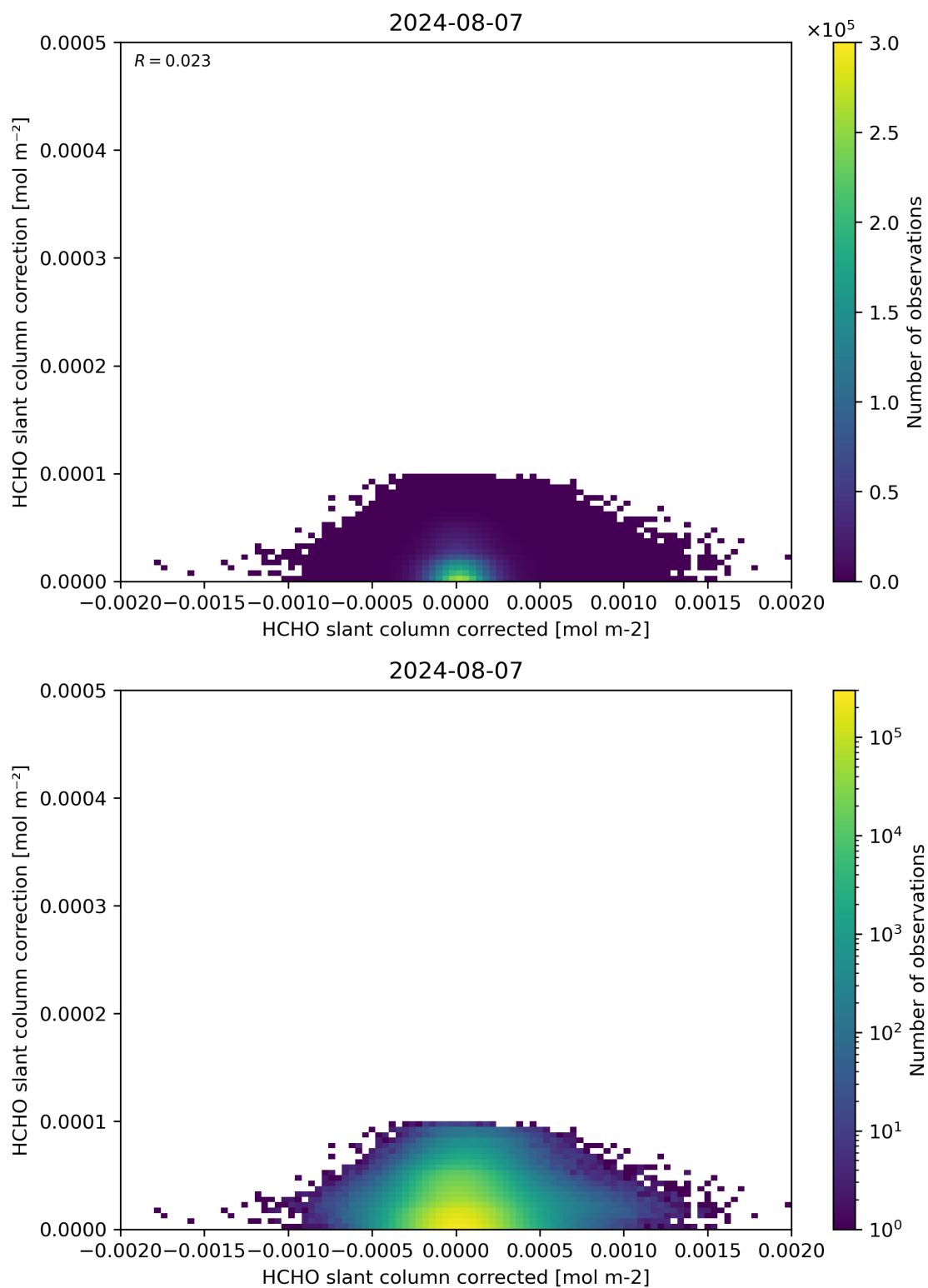
Figure 77: Scatter density plot of “HCHO slant column corrected” against “HCHO slant column correction” for 2024-08-06 to 2024-08-08.
