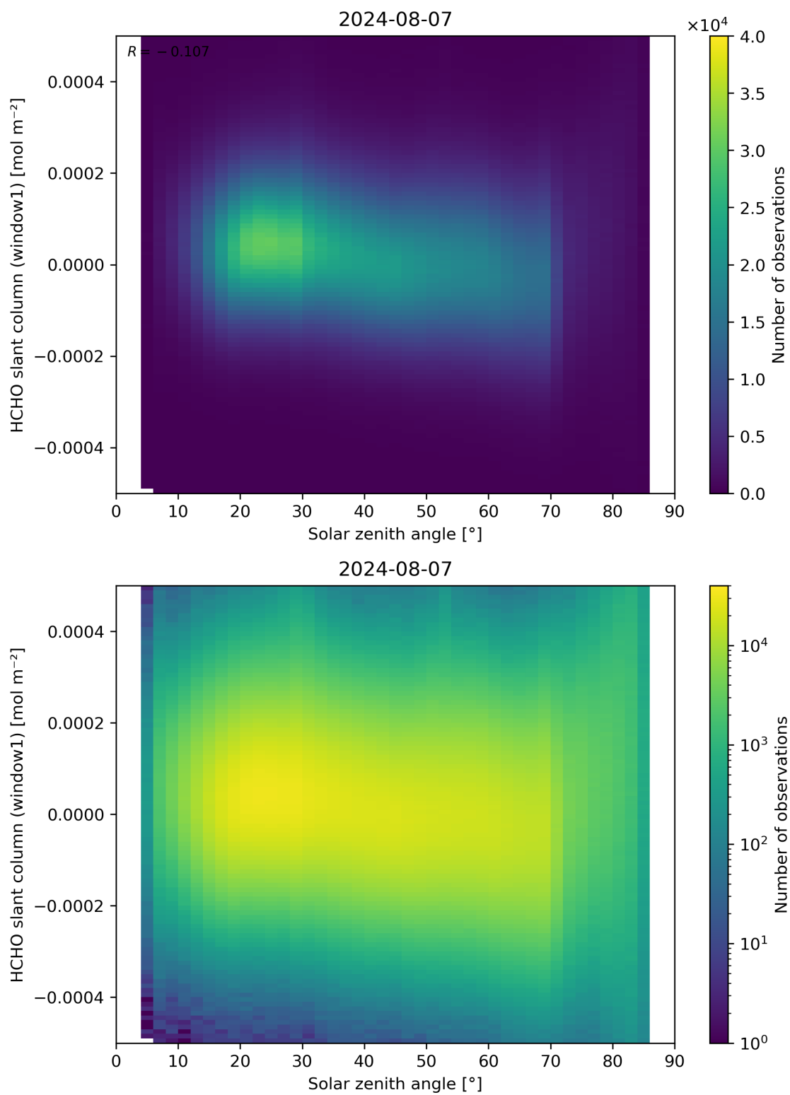
Figure 173: Scatter density plot of “Solar zenith angle” against “HCHO slant column (window1)” for 2024-08-06 to 2024-08-08.
