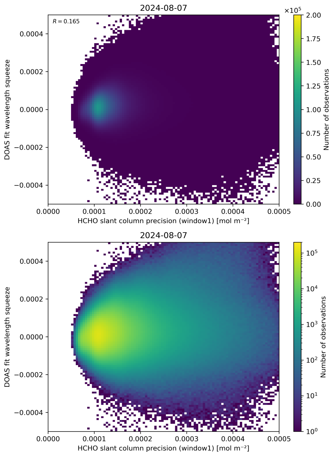
Figure 90: Scatter density plot of “HCHO slant column precision (window1)” against “DOAS fit wavelength squeeze” for 2024-08-06 to 2024-08-08.
