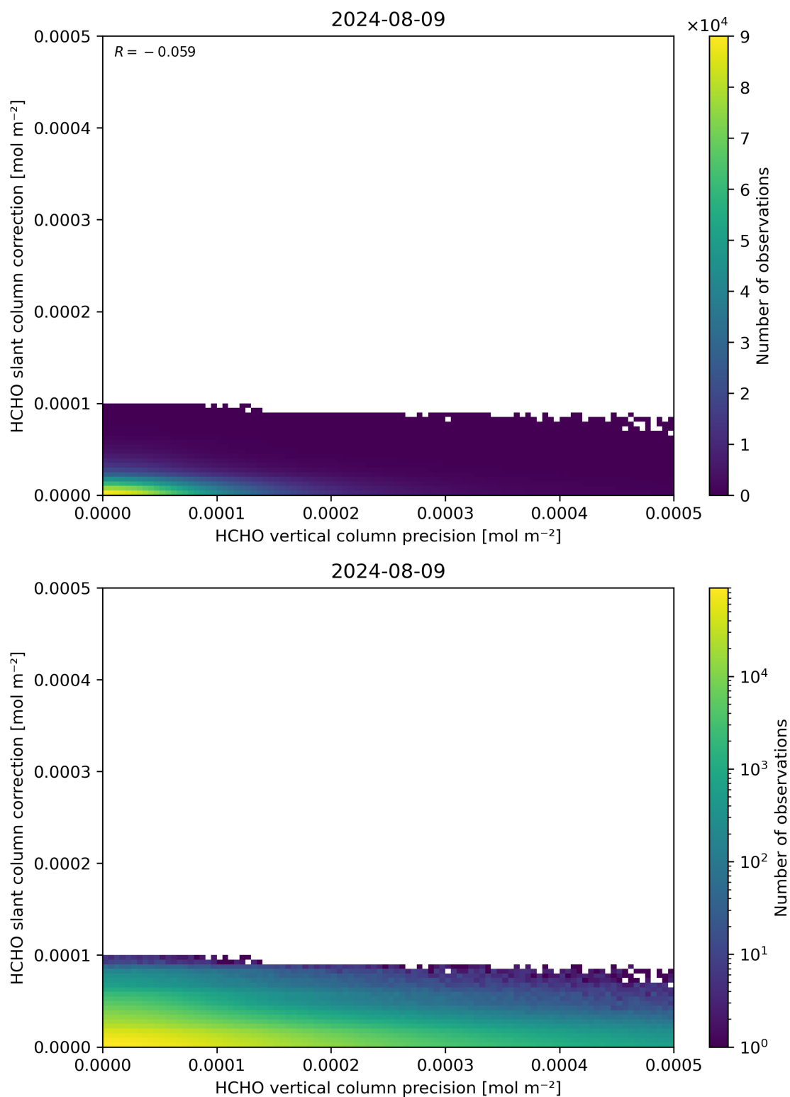
Figure 141: Scatter density plot of “HCHO vertical column precision” against “HCHO slant column correction” for 2024-08-08 to 2024-08-10.
