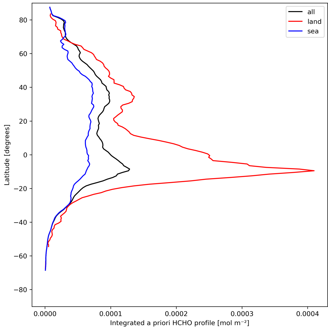
Figure 29: Zonal average of “Integrated a priori HCHO profile” for 2024-08-08 to 2024-08-10.
