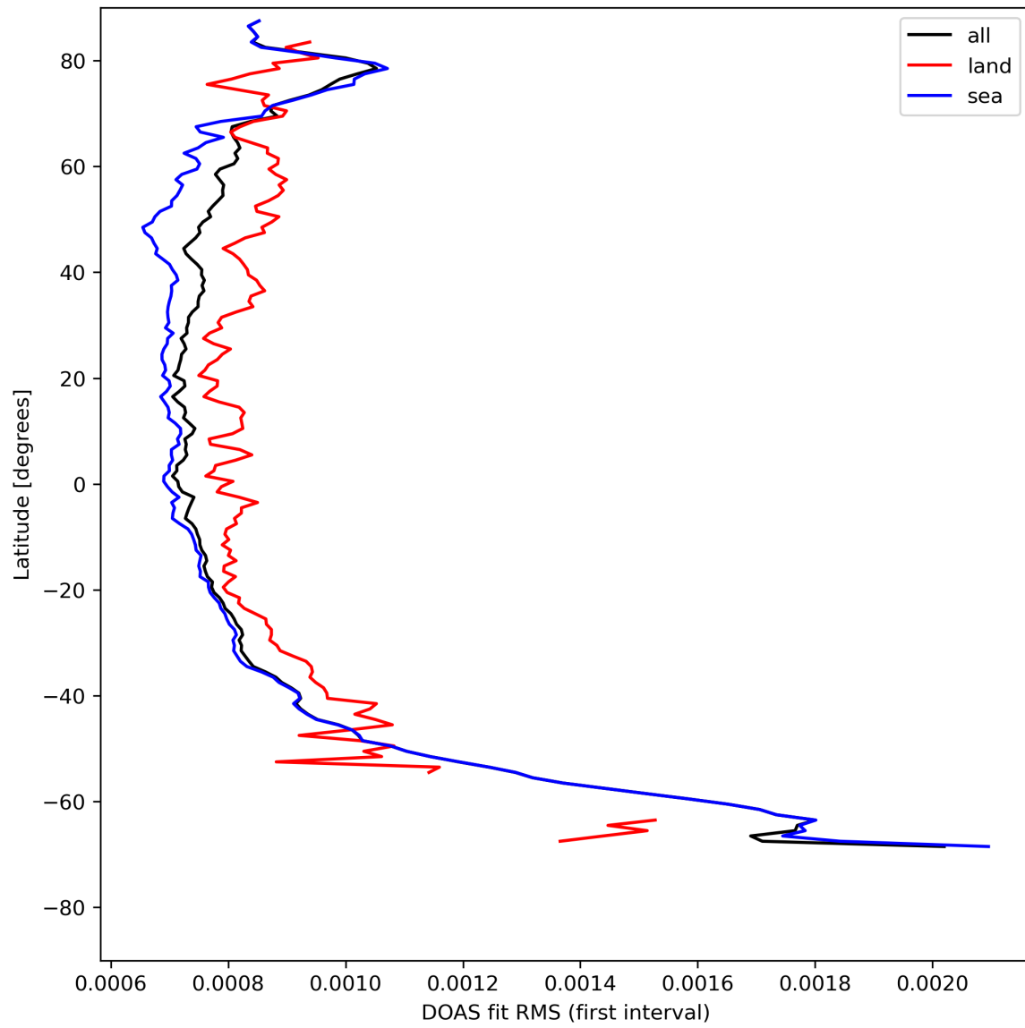
Figure 32: Zonal average of "DOAS fit RMS (first interval)" for 2024-08-08 to 2024-08-10.
