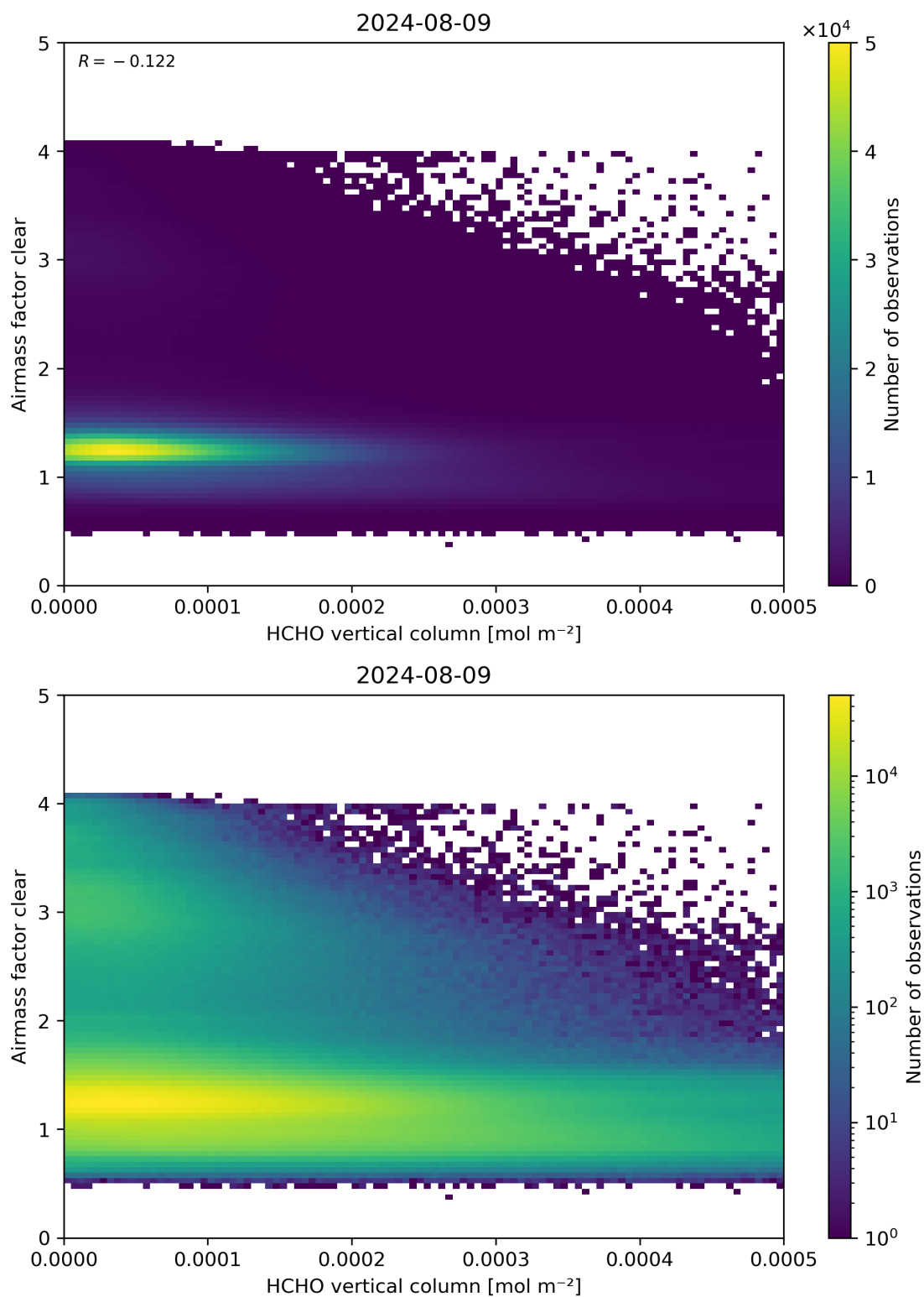
Figure 126: Scatter density plot of “HCHO vertical column” against “Airmass factor clear” for 2024-08-08 to 2024-08-10.
