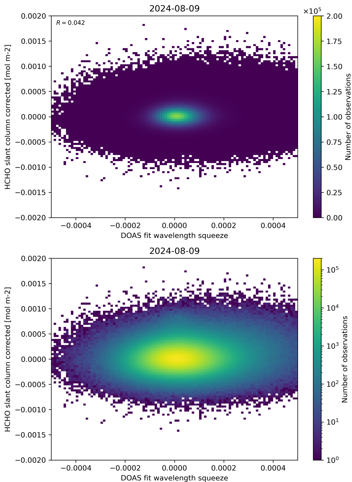
Figure 69: Scatter density plot of “DOAS fit wavelength squeeze” against “HCHO slant column corrected” for 2024-08-08 to 2024-08-10.
