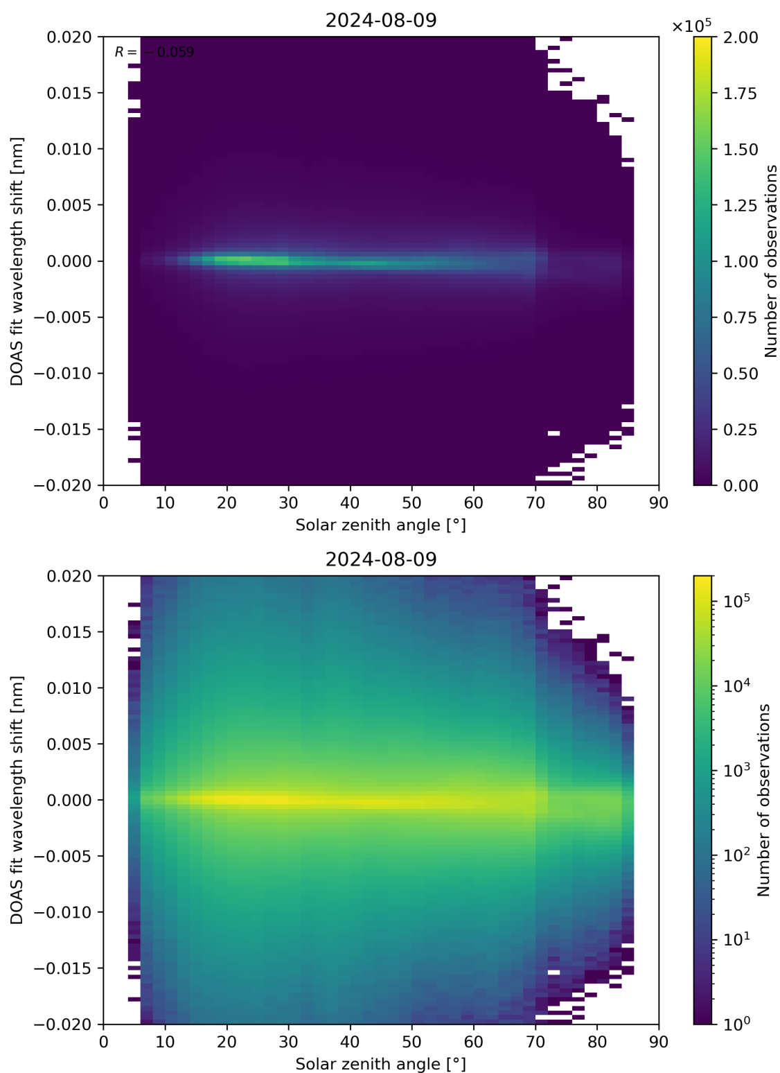
Figure 168: Scatter density plot of “Solar zenith angle” against “DOAS fit wavelength shift” for 2024-08-08 to 2024-08-10.
