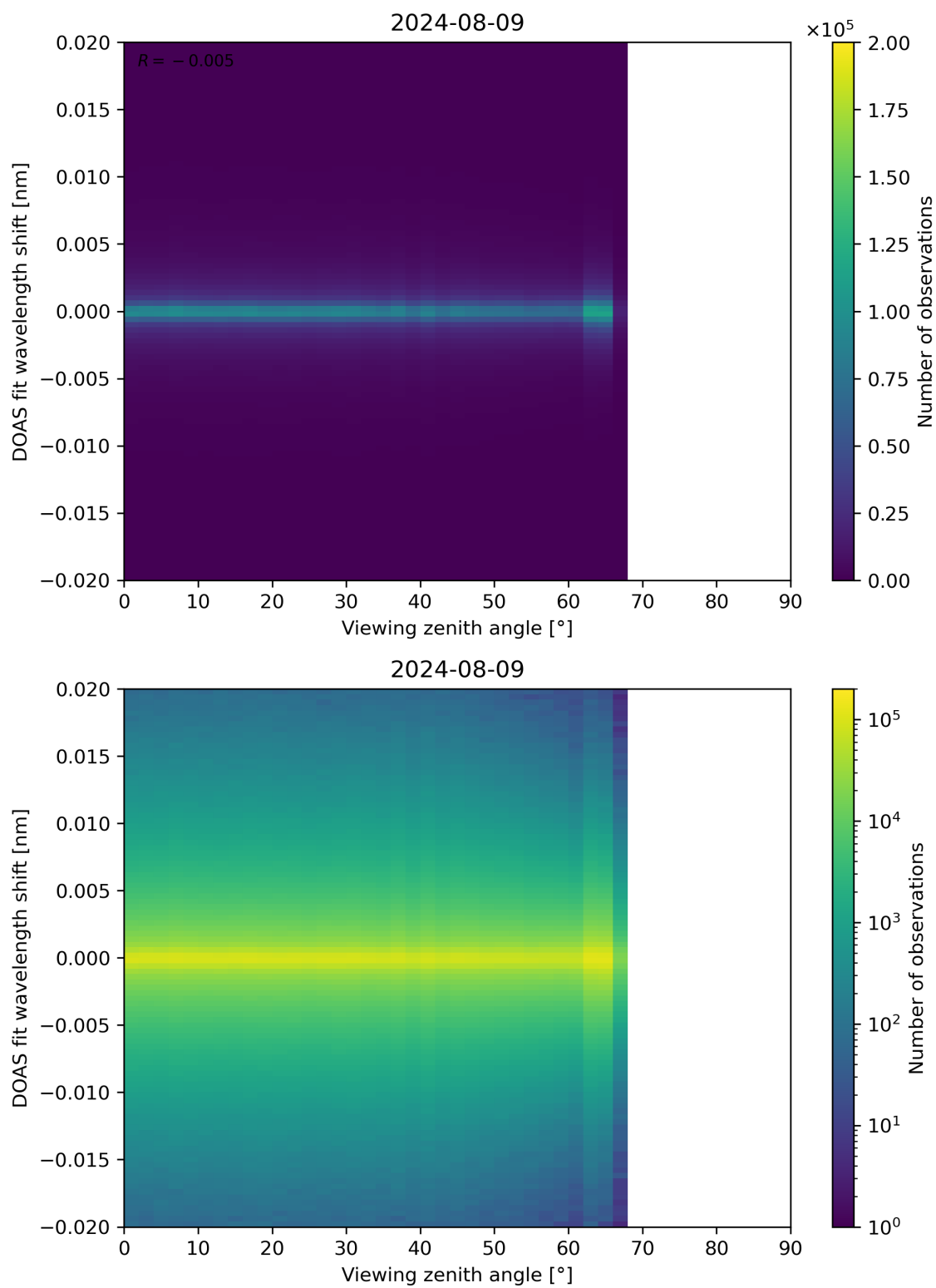
Figure 183: Scatter density plot of “Viewing zenith angle” against “DOAS fit wavelength shift” for 2024-08-08 to 2024-08-10.
