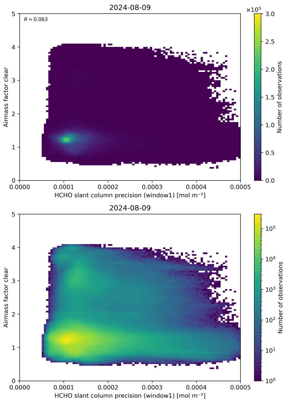
Figure 91: Scatter density plot of “HCHO slant column precision (window1)” against “Airmass factor clear” for 2024-08-08 to 2024-08-10.
