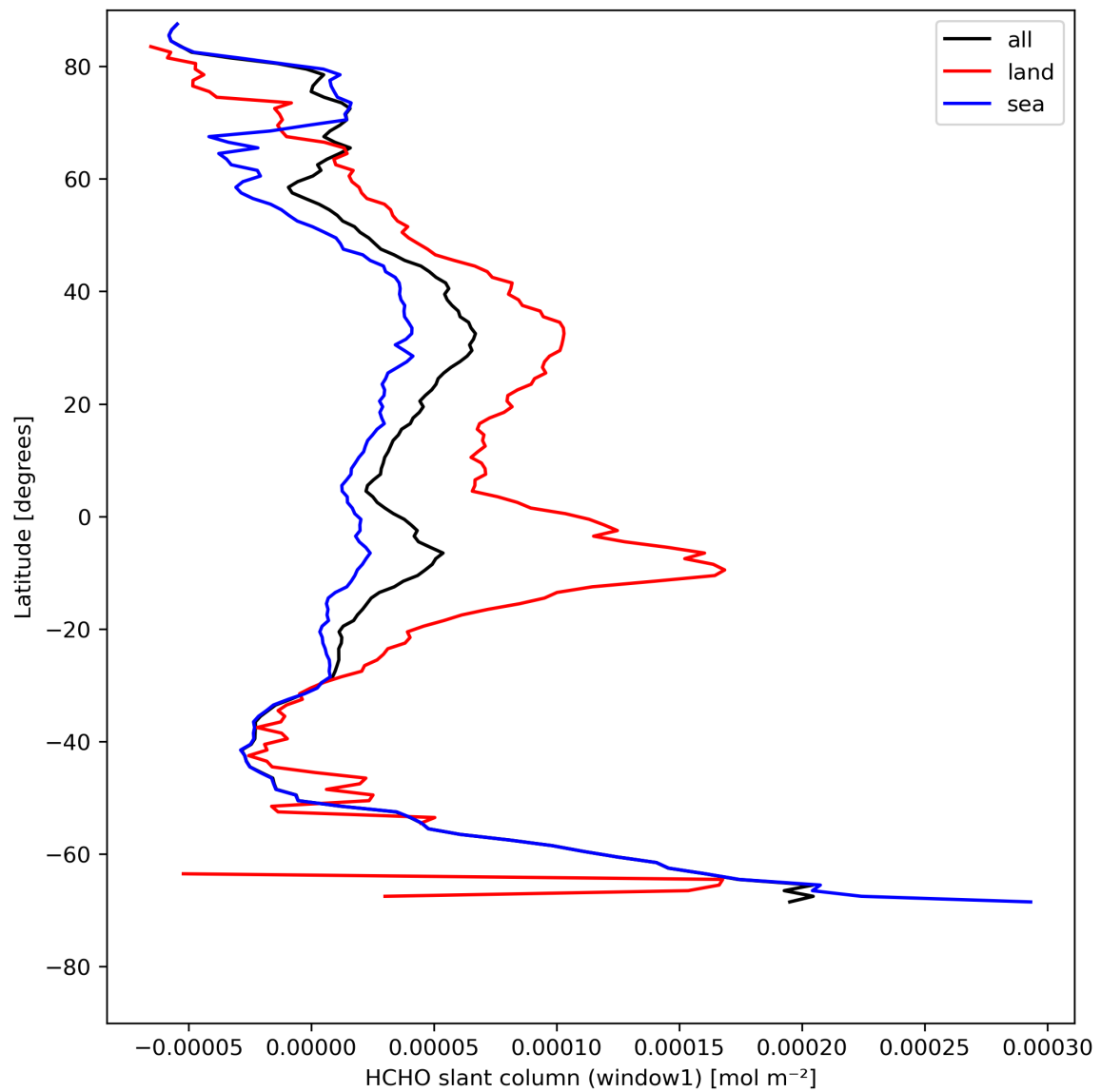
Figure 24: Zonal average of “HCHO slant column (window1)” for 2024-08-08 to 2024-08-10.
