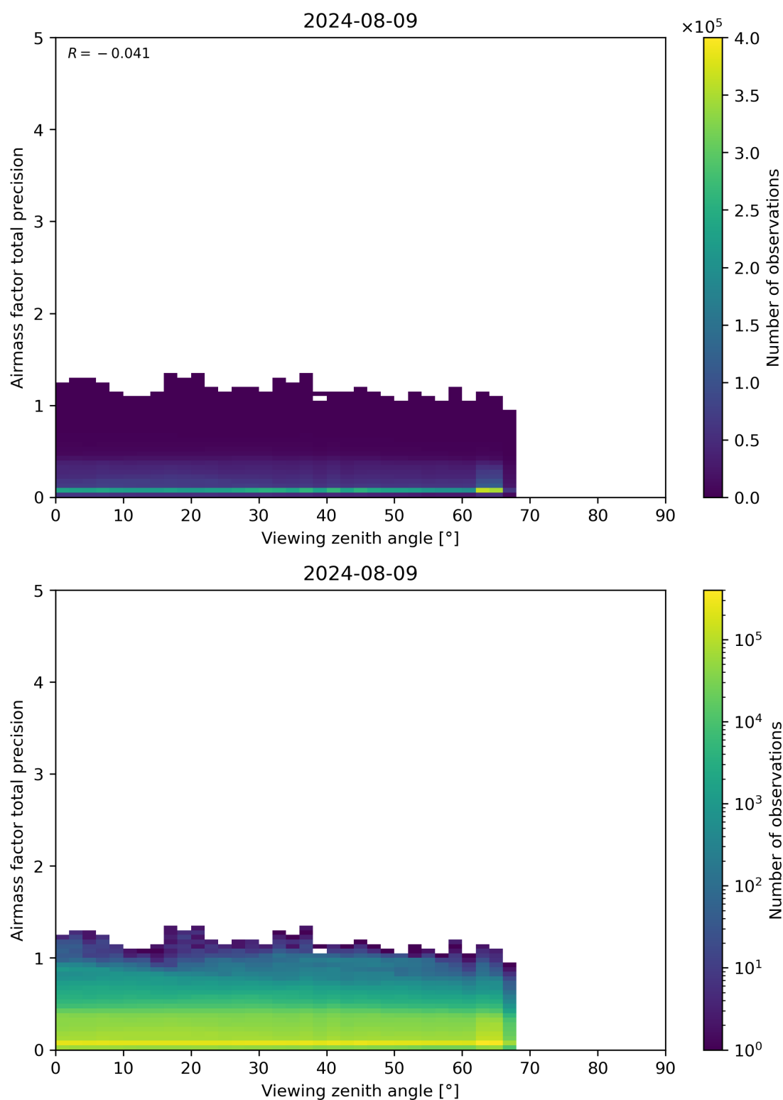
Figure 191: Scatter density plot of “Viewing zenith angle” against “Airmass factor total precision” for 2024-08-08 to 2024-08-10.
