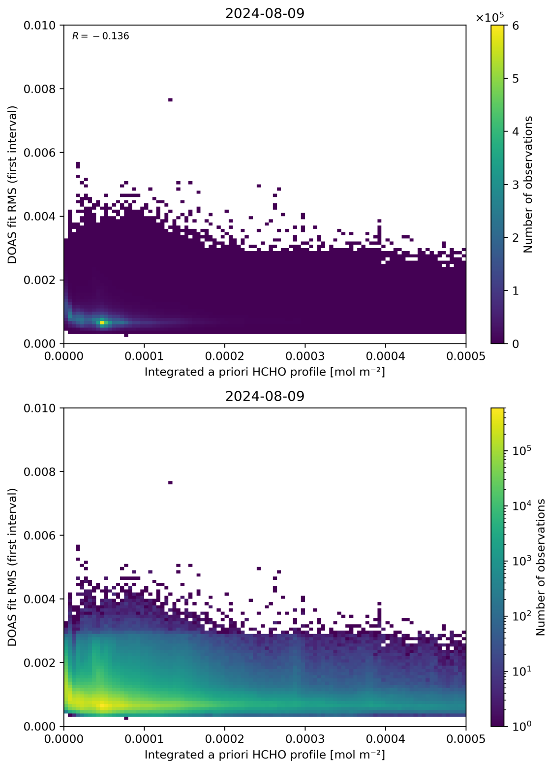
Figure 148: Scatter density plot of “Integrated a priori HCHO profile” against “DOAS fit RMS (first interval)” for 2024-08-08 to 2024-08-10.
