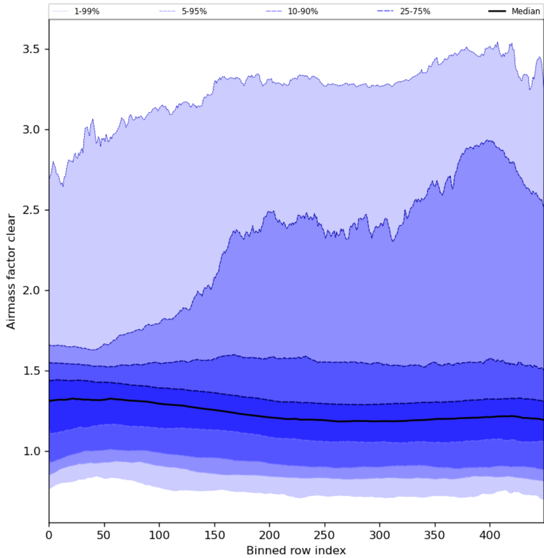
Figure 56: Along track statistics of “Airmass factor clear” for 2024-08-08 to 2024-08-10
