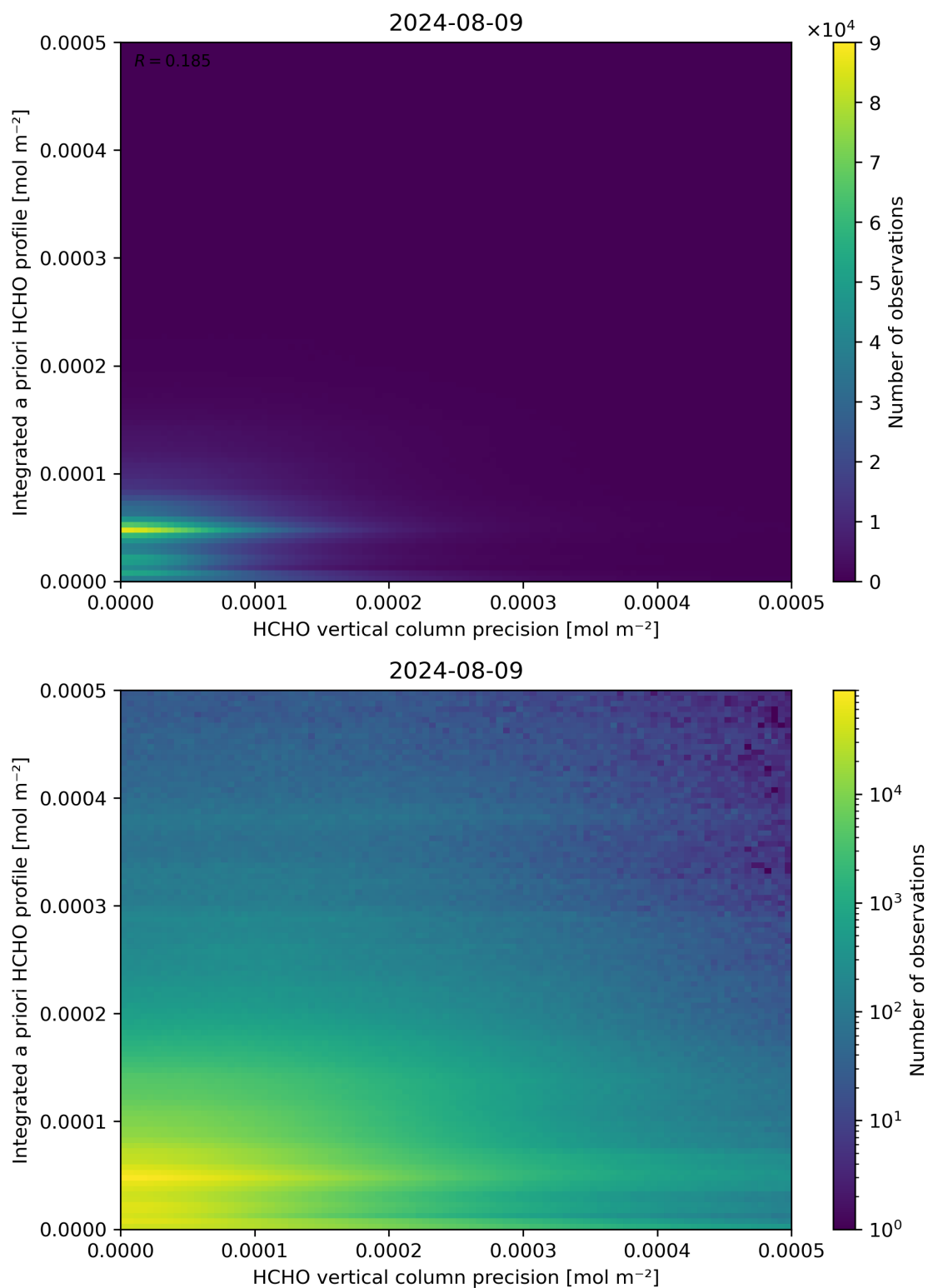
Figure 147: Scatter density plot of “HCHO vertical column precision” against “Integrated a priori HCHO profile” for 2024-08-08 to 2024-08-10.
