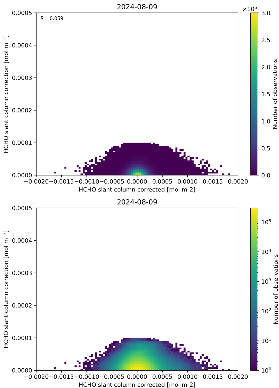
Figure 77: Scatter density plot of “HCHO slant column corrected” against “HCHO slant column correction” for 2024-08-08 to 2024-08-10.
