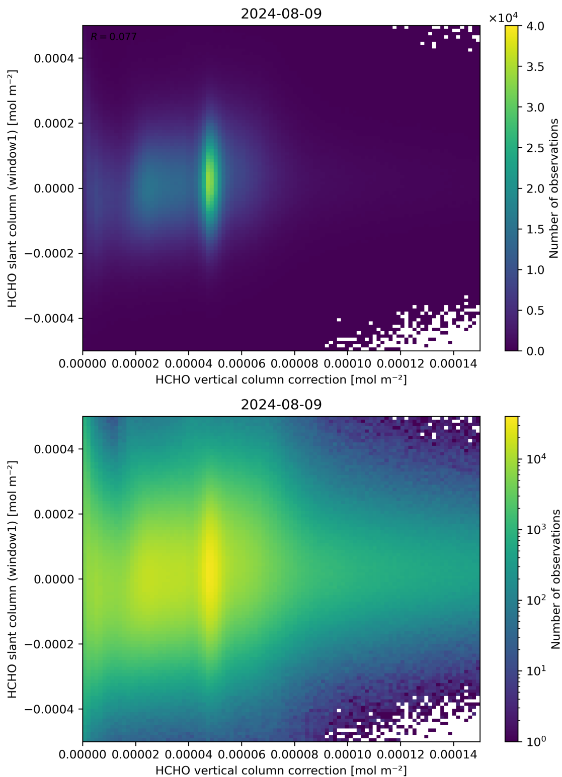
Figure 118: Scatter density plot of “HCHO vertical column correction” against “HCHO slant column (window1)” for 2024-08-08 to 2024-08-10.
