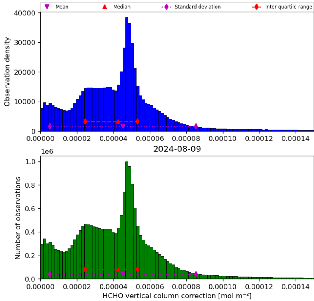
Figure 37: Histogram of “HCHO vertical column correction” for 2024-08-08 to 2024-08-10
