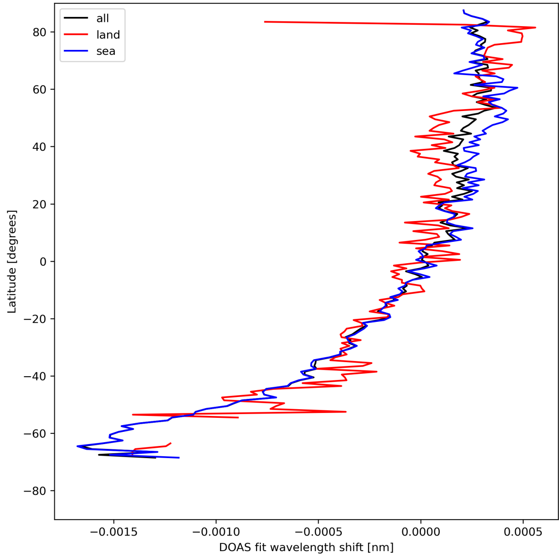
Figure 30: Zonal average of “DOAS fit wavelength shift” for 2024-08-08 to 2024-08-10.
