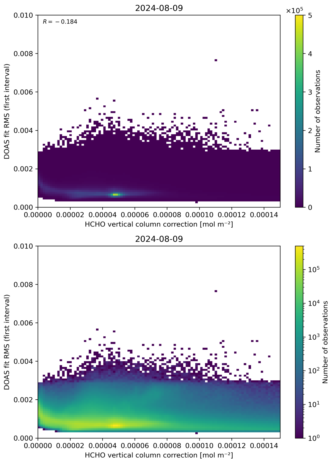
Figure 112: Scatter density plot of “HCHO vertical column correction” against “DOAS fit RMS (first interval)” for 2024-08-08 to 2024-08-10.
