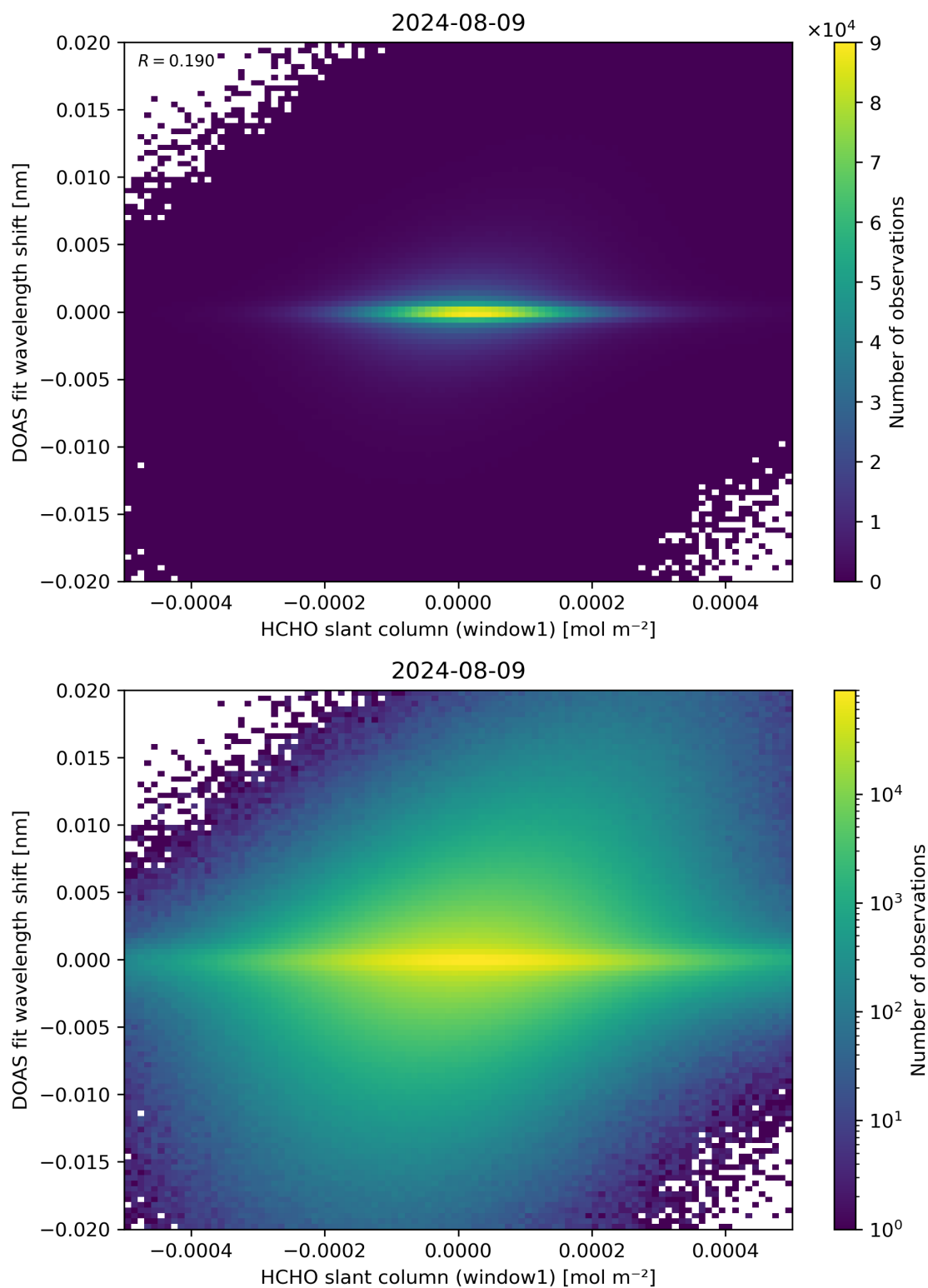
Figure 79: Scatter density plot of “HCHO slant column (window1)” against “DOAS fit wavelength shift” for 2024-08-08 to 2024-08-10.
