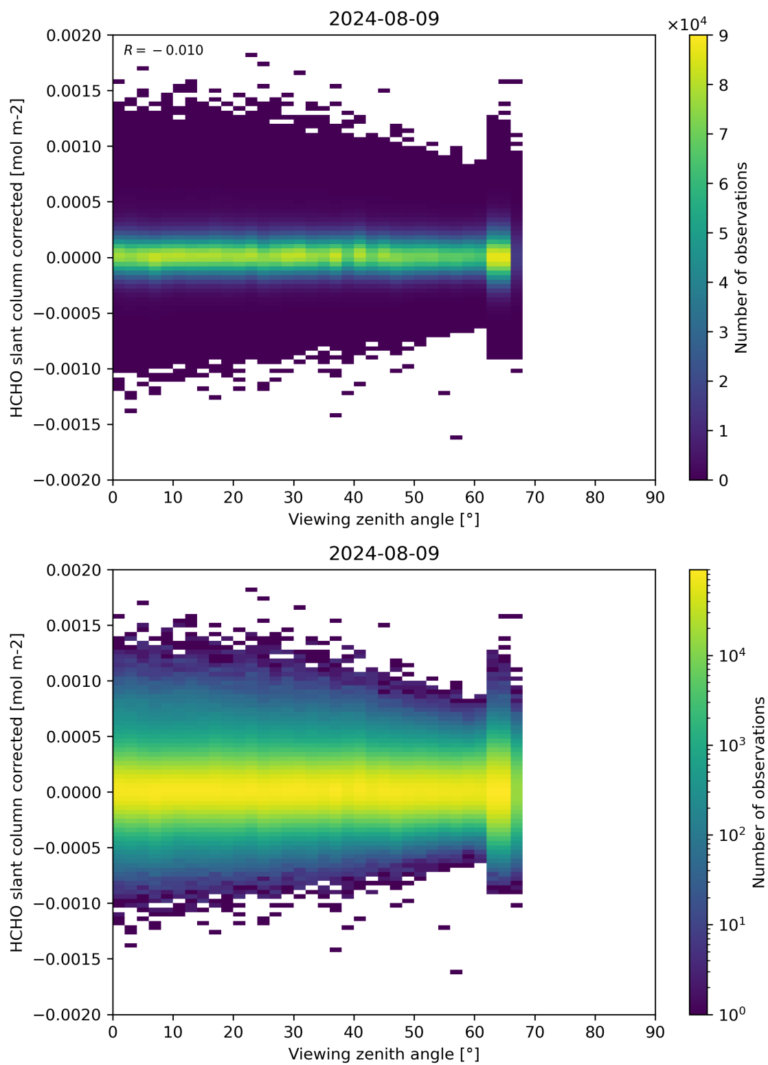
Figure 186: Scatter density plot of “Viewing zenith angle” against “HCHO slant column corrected” for 2024-08-08 to 2024-08-10.
