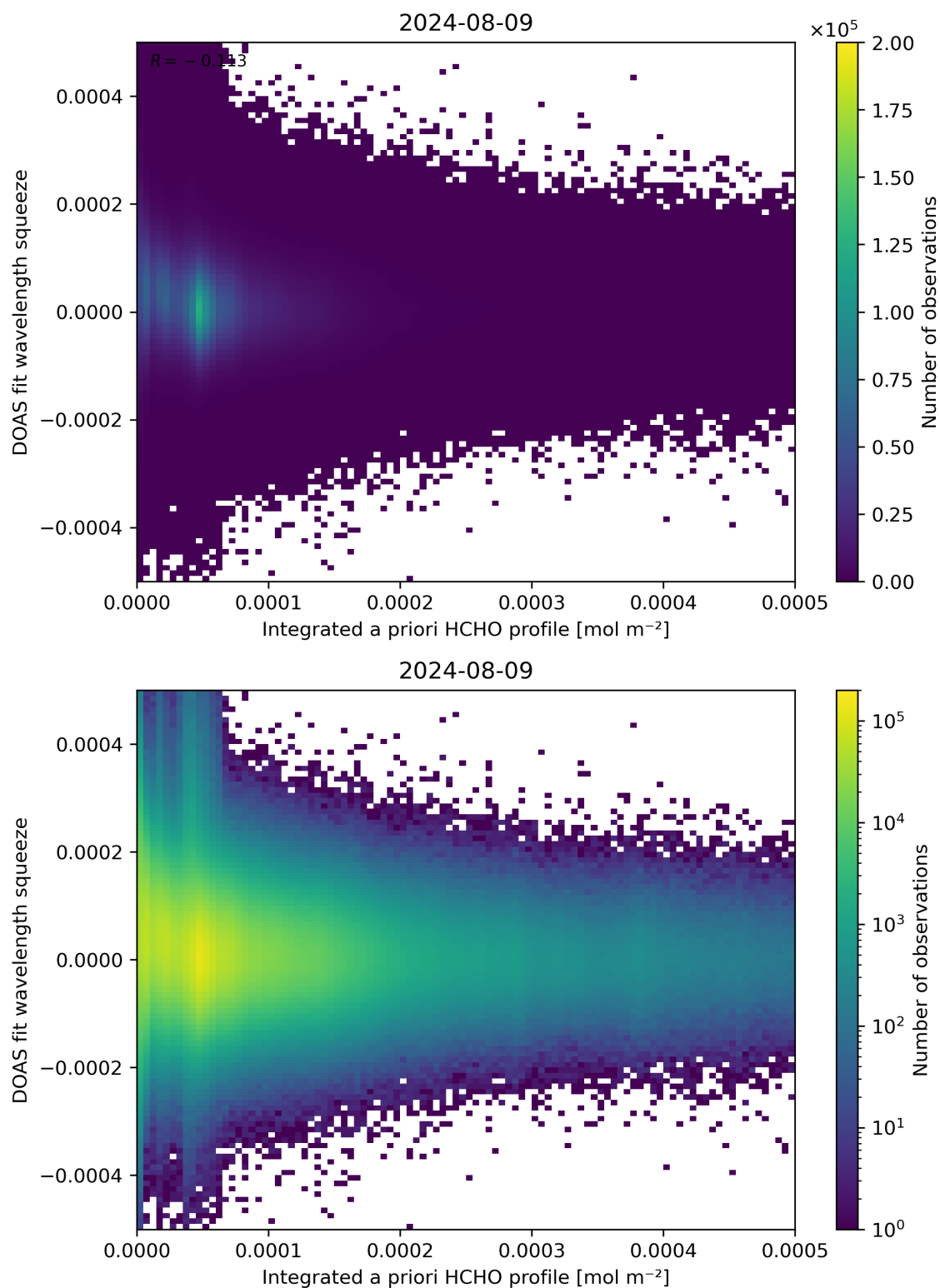
Figure 150: Scatter density plot of “Integrated a priori HCHO profile” against “DOAS fit wavelength squeeze” for 2024-08-08 to 2024-08-10.
