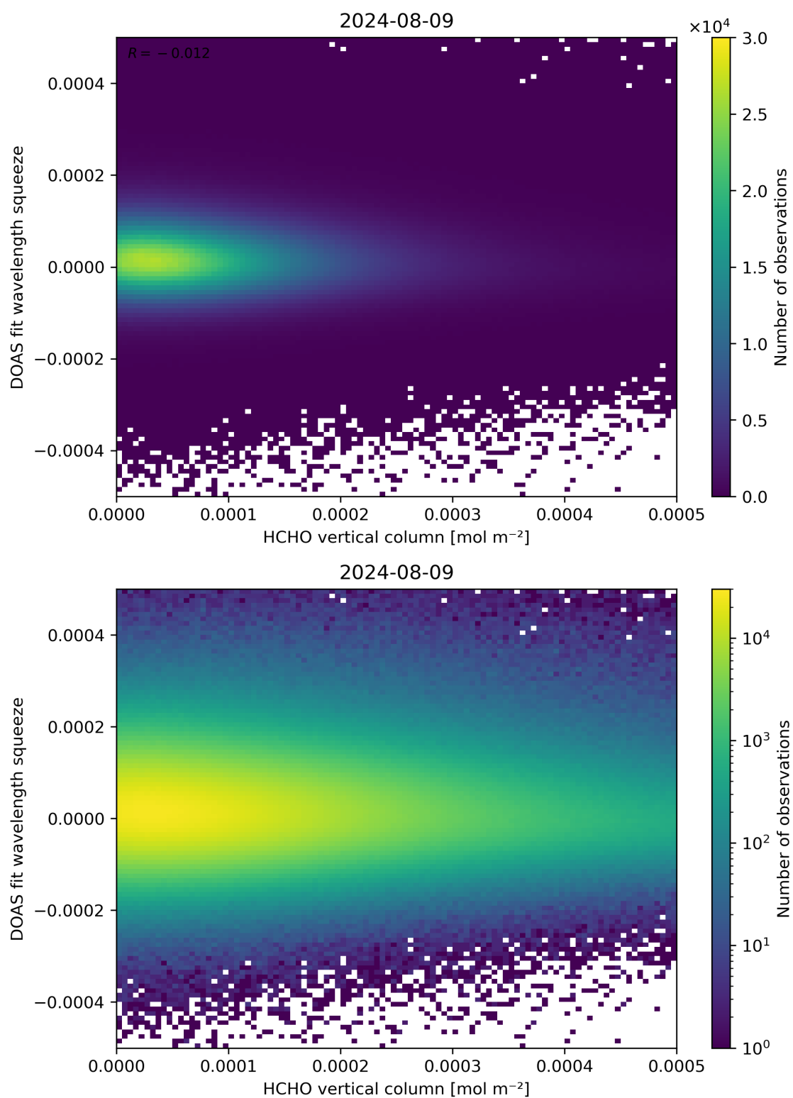
Figure 125: Scatter density plot of “HCHO vertical column” against “DOAS fit wavelength squeeze” for 2024-08-08 to 2024-08-10.
