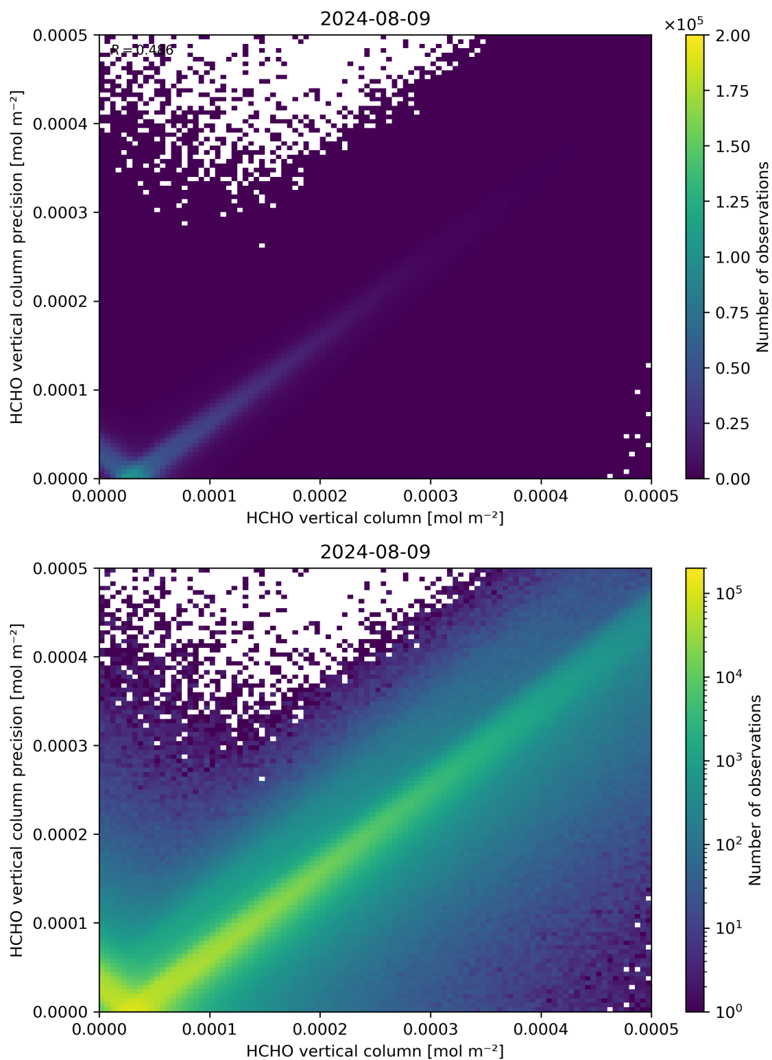
Figure 134: Scatter density plot of “HCHO vertical column” against “HCHO vertical column precision” for 2024-08-08 to 2024-08-10.
