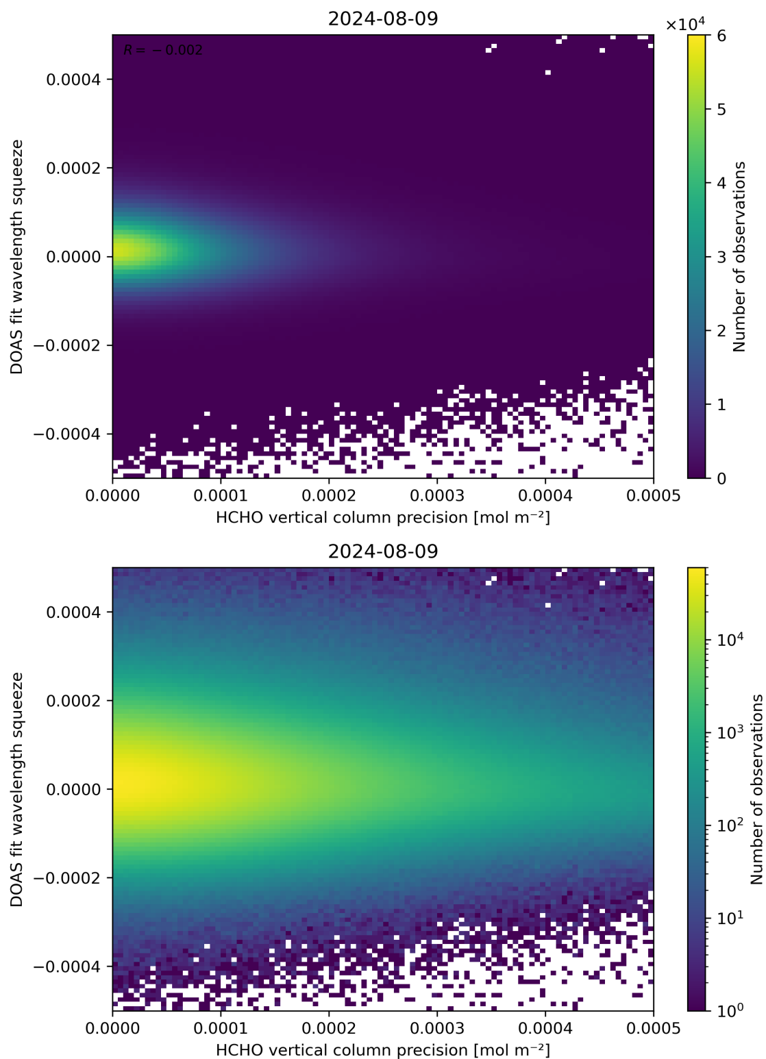
Figure 138: Scatter density plot of “HCHO vertical column precision” against “DOAS fit wavelength squeeze” for 2024-08-08 to 2024-08-10.
