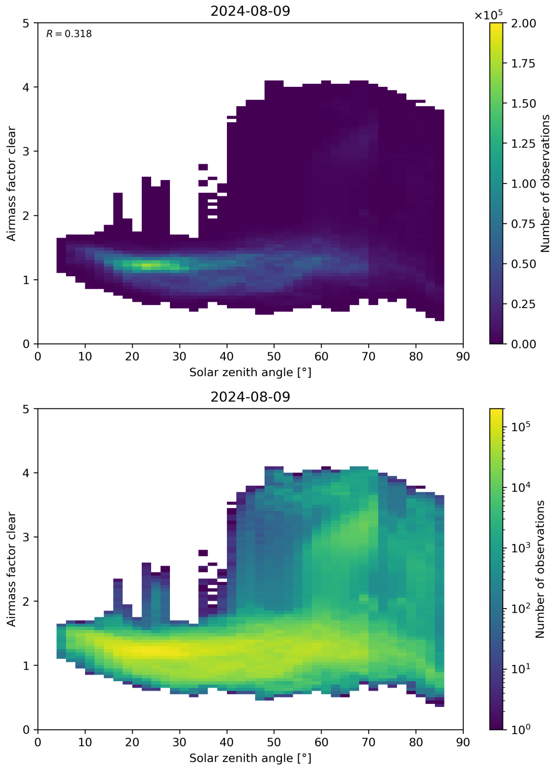
Figure 170: Scatter density plot of “Solar zenith angle” against “Airmass factor clear” for 2024-08-08 to 2024-08-10.
