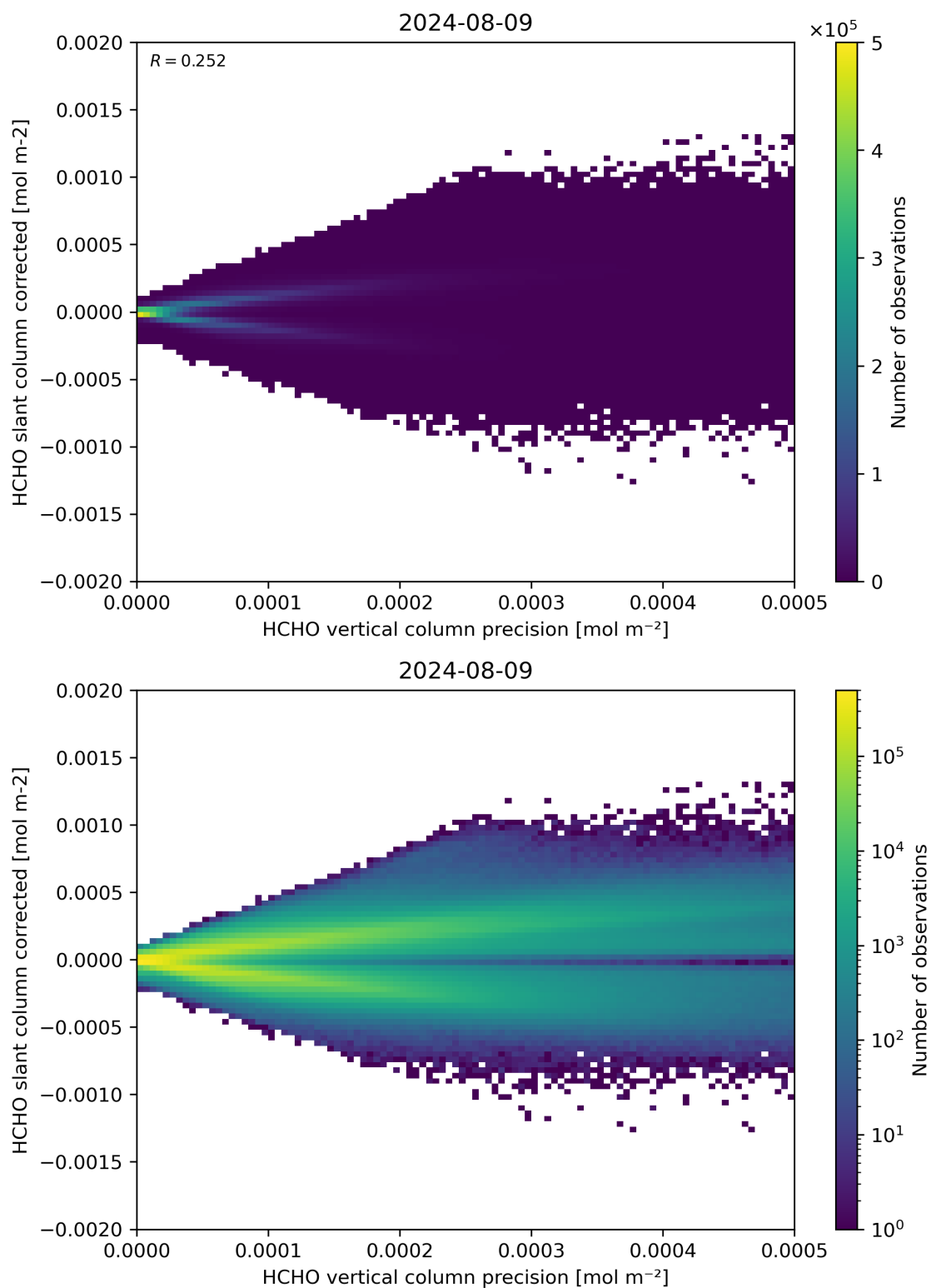
Figure 140: Scatter density plot of “HCHO vertical column precision” against “HCHO slant column corrected” for 2024-08-08 to 2024-08-10.
