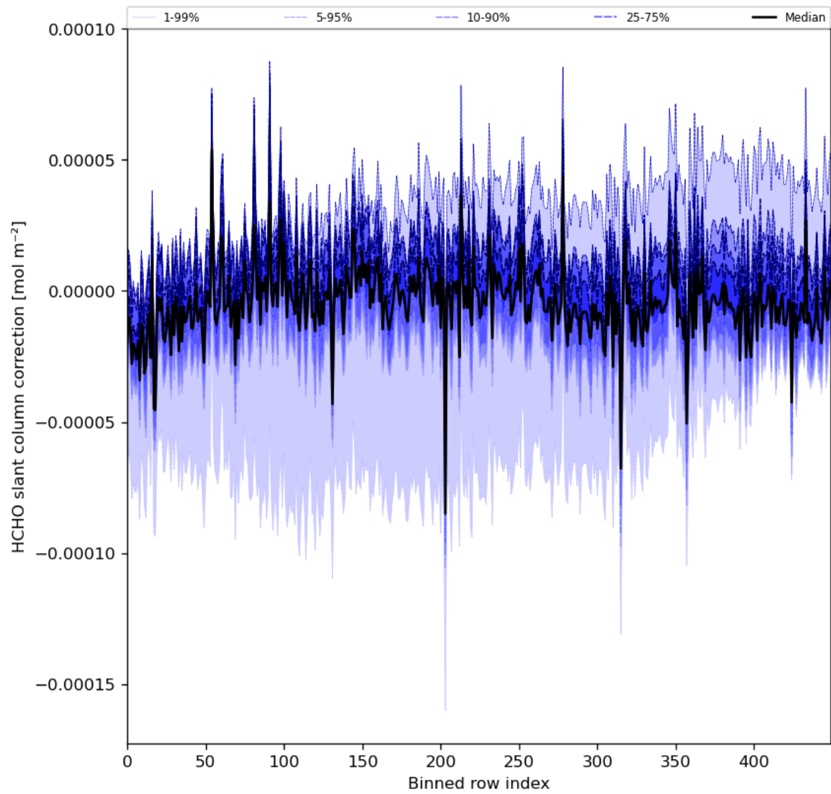
Figure 61: Along track statistics of “HCHO slant column correction” for 2024-08-08 to 2024-08-10
