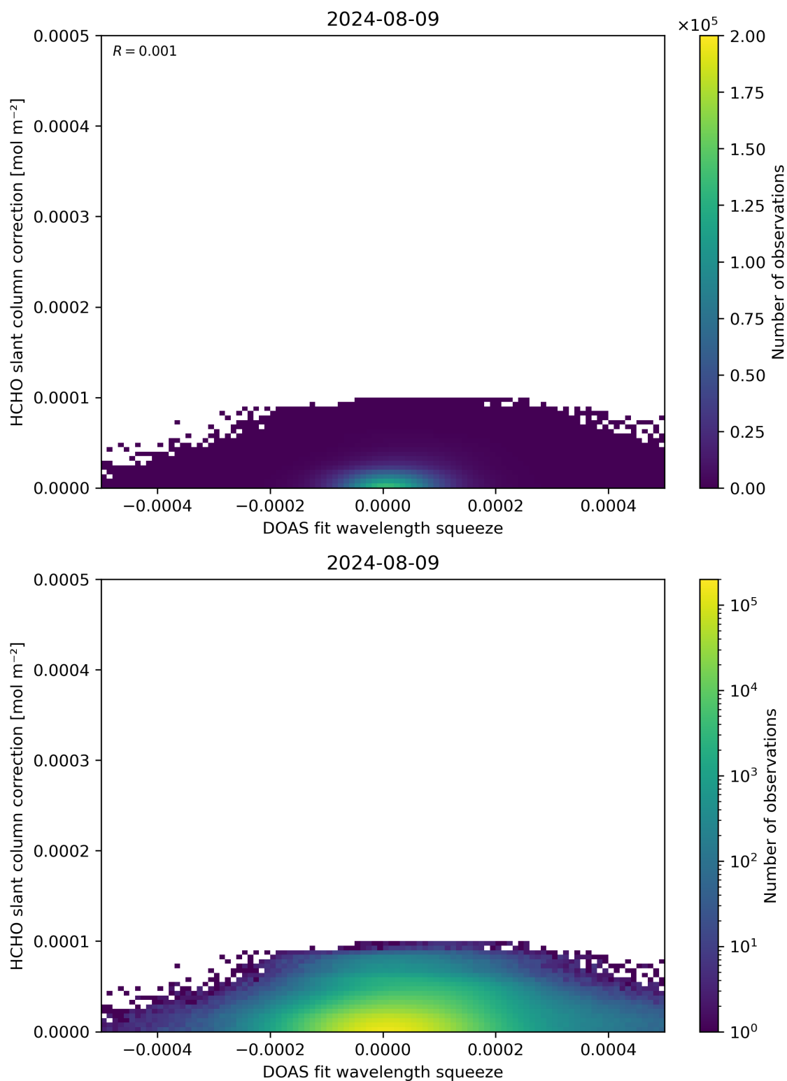
Figure 70: Scatter density plot of “DOAS fit wavelength squeeze” against “HCHO slant column correction” for 2024-08-08 to 2024-08-10.
