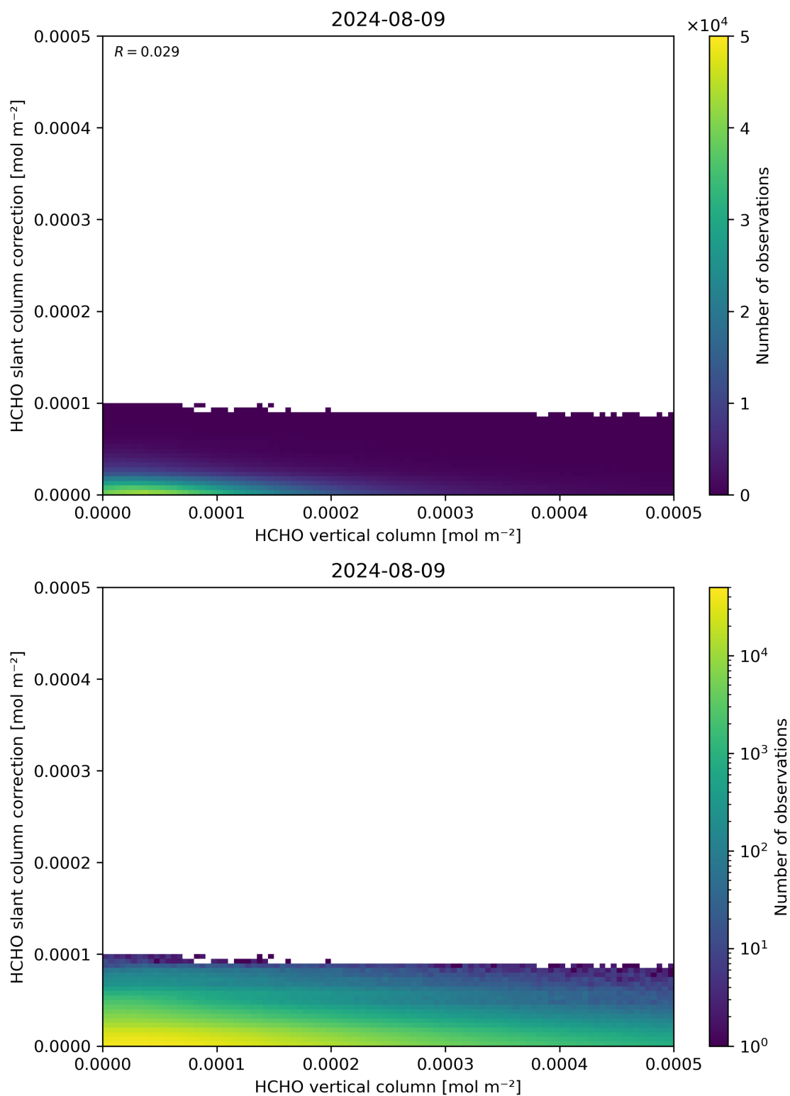
Figure 128: Scatter density plot of “HCHO vertical column” against “HCHO slant column correction” for 2024-08-08 to 2024-08-10.
