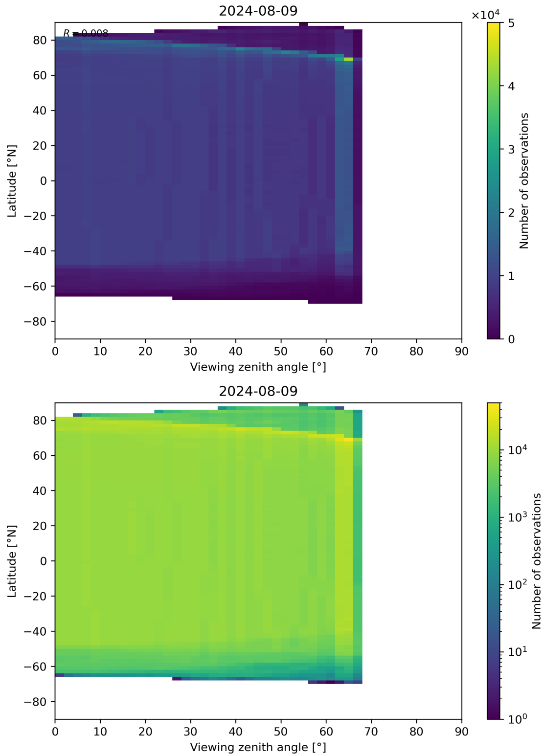
Figure 196: Scatter density plot of “Viewing zenith angle” against “Latitude” for 2024-08-08 to 2024-08-10.
