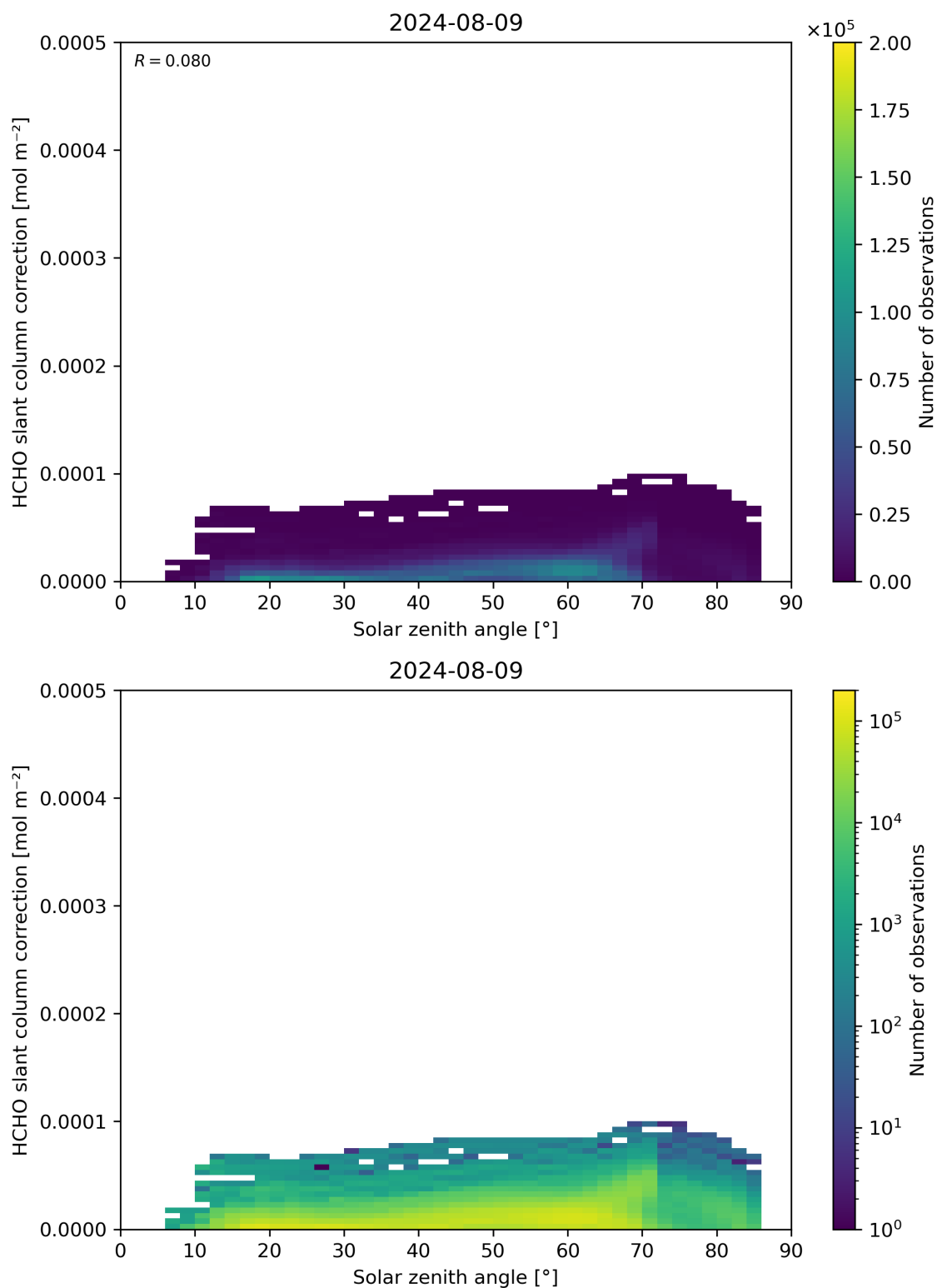
Figure 172: Scatter density plot of “Solar zenith angle” against “HCHO slant column correction” for 2024-08-08 to 2024-08-10.
