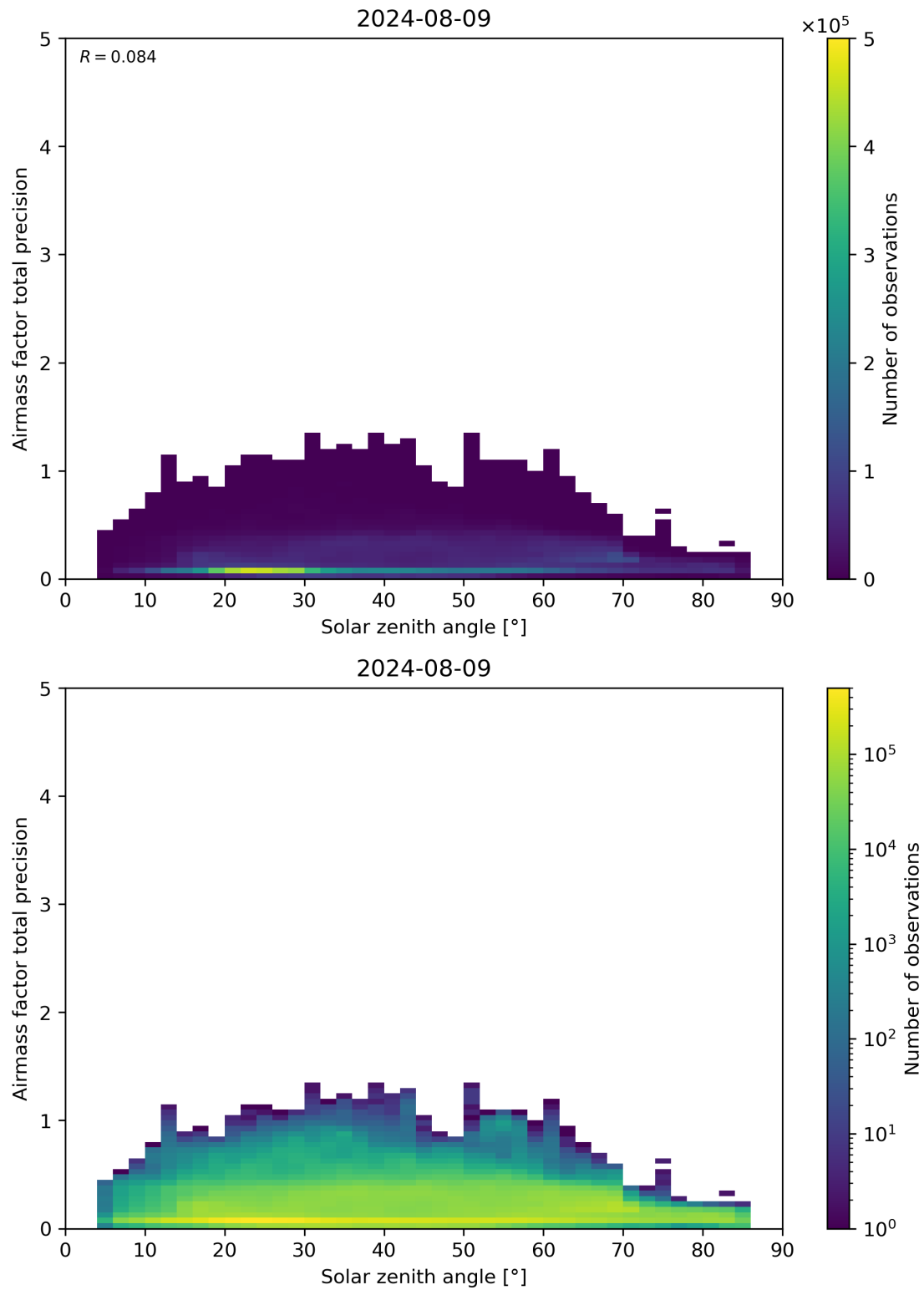
Figure 176: Scatter density plot of “Solar zenith angle” against “Airmass factor total precision” for 2024-08-08 to 2024-08-10.
