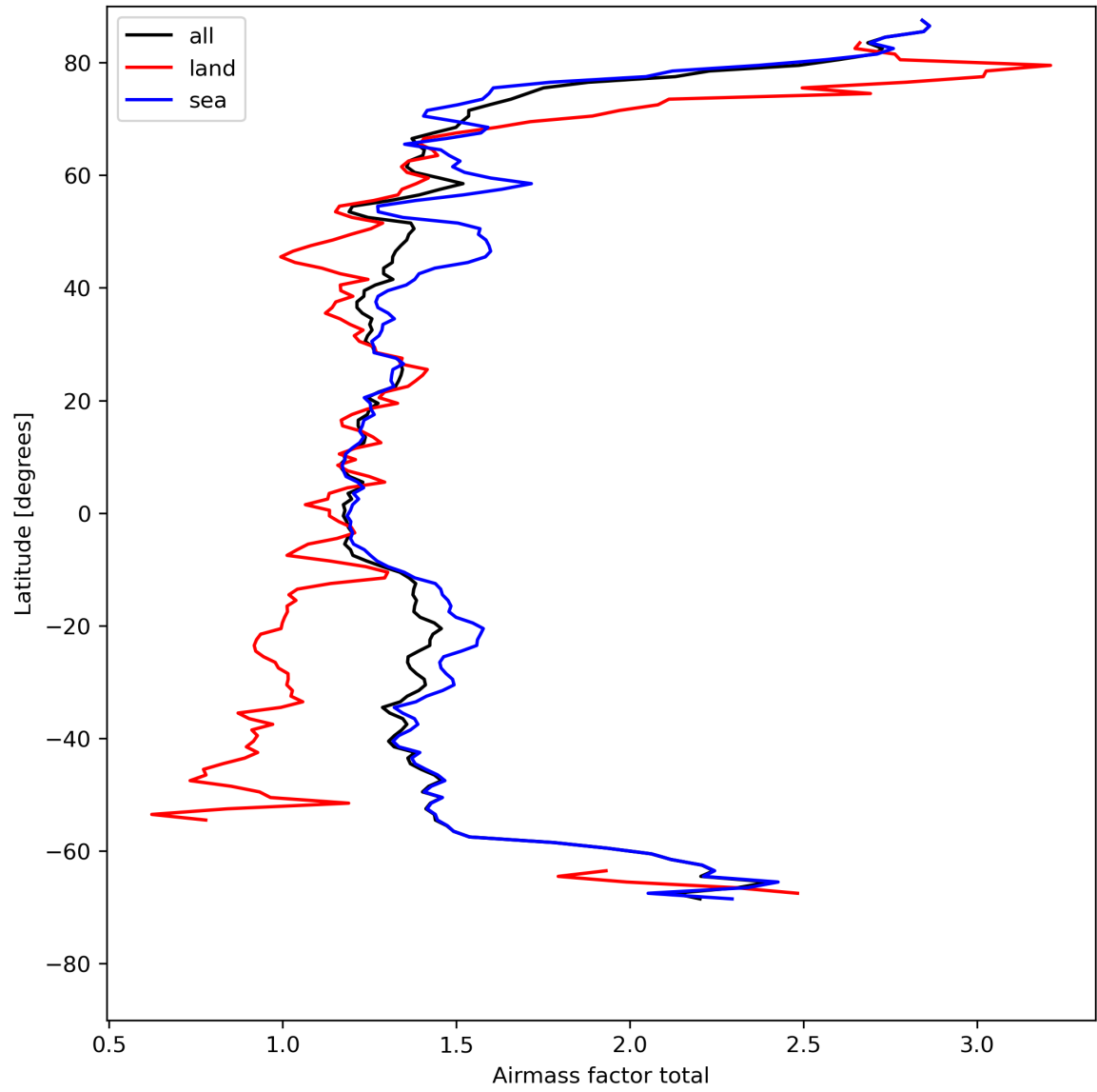
Figure 26: Zonal average of “Airmass factor total” for 2024-08-08 to 2024-08-10.
