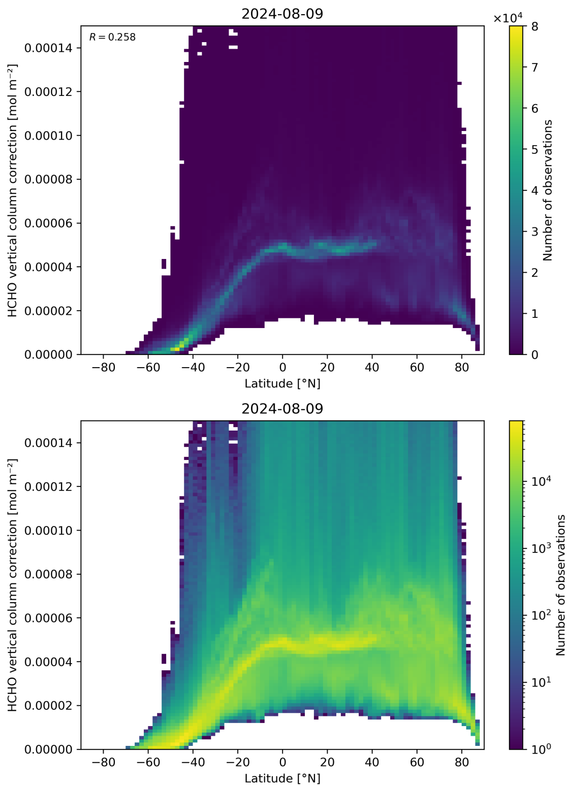
Figure 164: Scatter density plot of “Latitude” against “HCHO vertical column correction” for 2024-08-08 to 2024-08-10.
