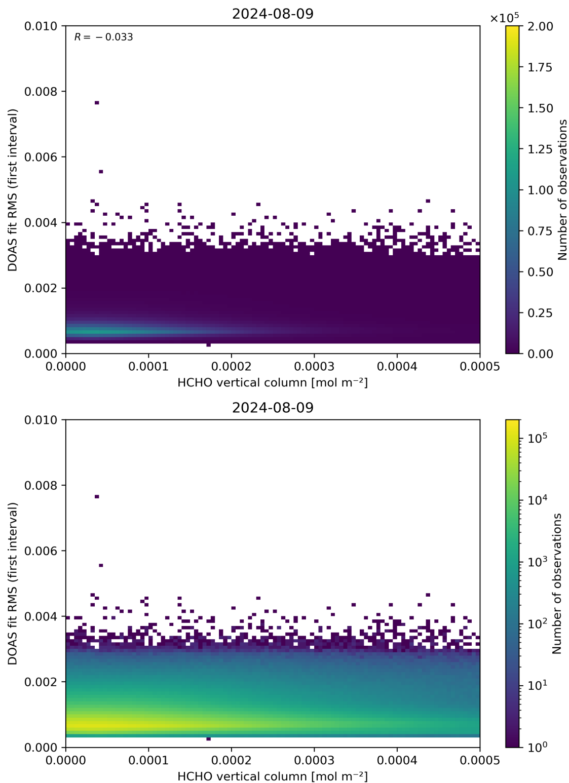
Figure 123: Scatter density plot of “HCHO vertical column” against “DOAS fit RMS (first interval)” for 2024-08-08 to 2024-08-10.
