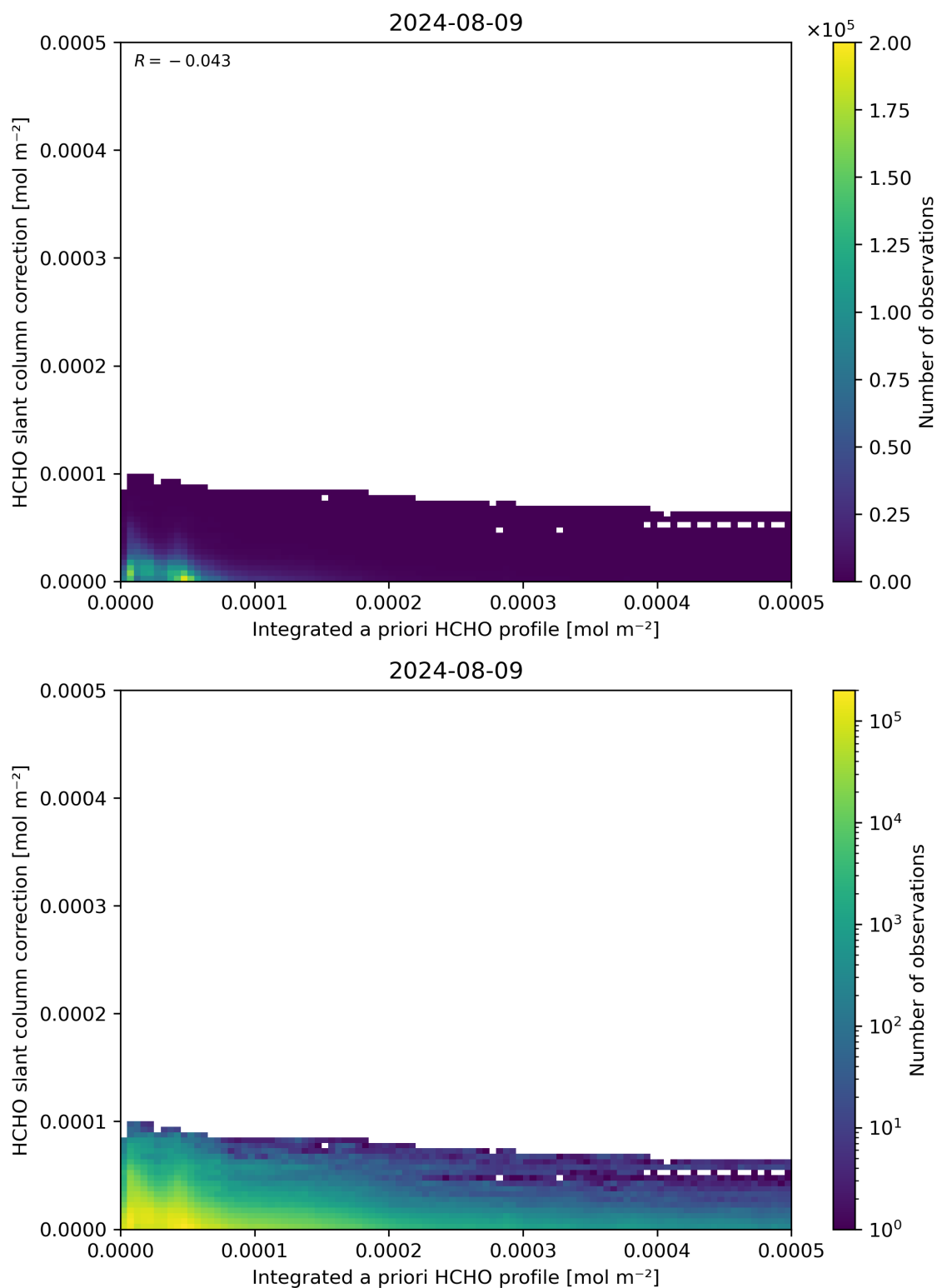
Figure 152: Scatter density plot of “Integrated a priori HCHO profile” against “HCHO slant column correction” for 2024-08-08 to 2024-08-10.
