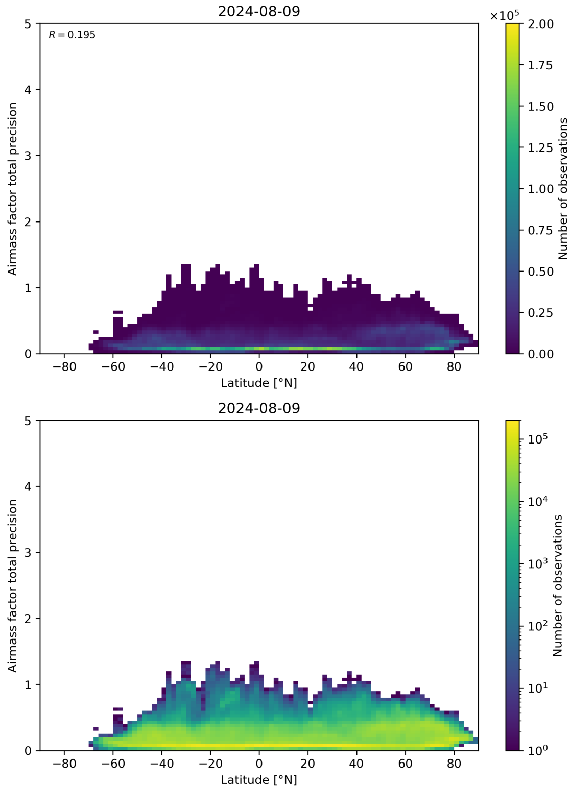
Figure 162: Scatter density plot of “Latitude” against “Airmass factor total precision” for 2024-08-08 to 2024-08-10.
