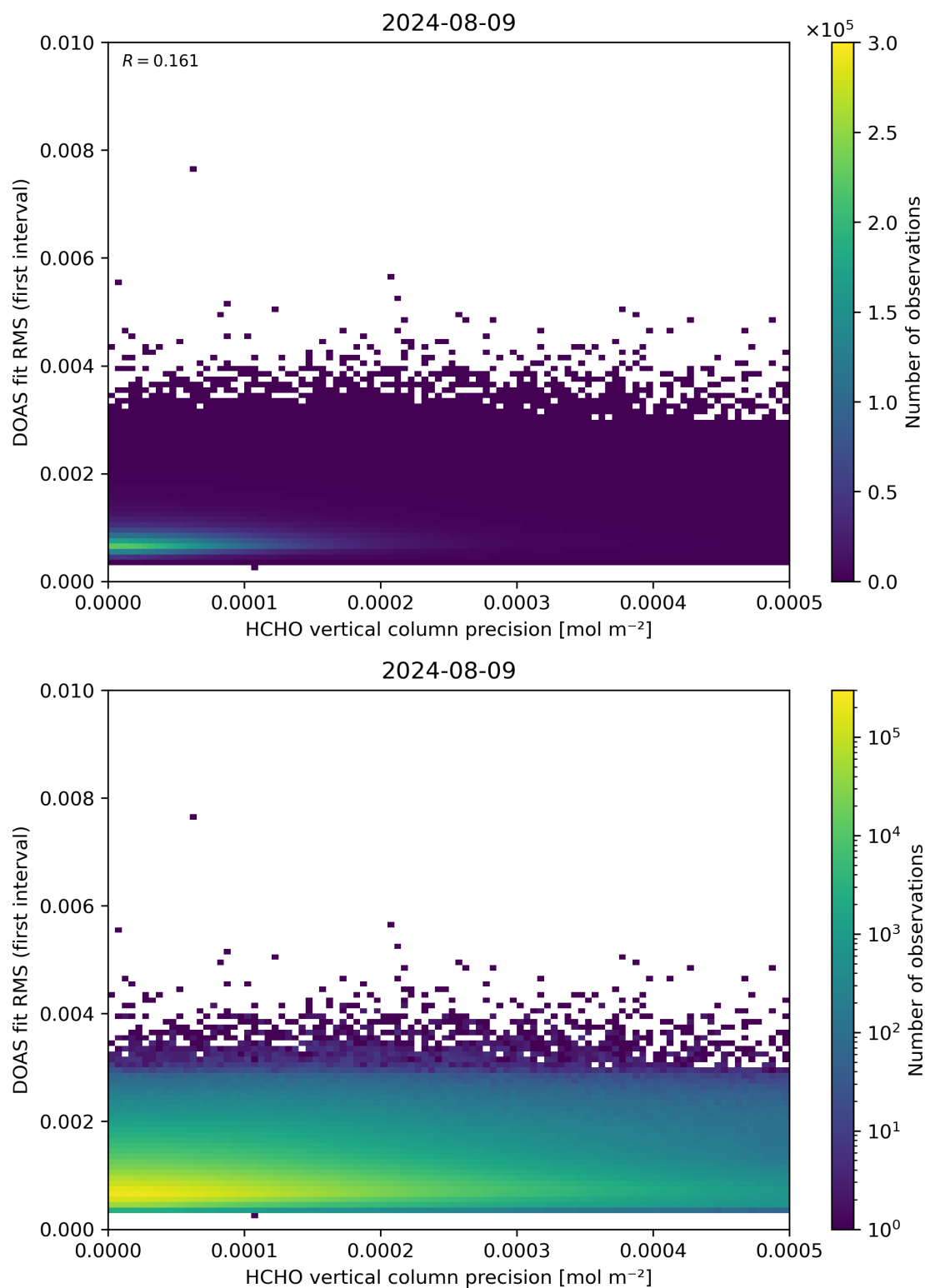
Figure 136: Scatter density plot of “HCHO vertical column precision” against “DOAS fit RMS (first interval)” for 2024-08-08 to 2024-08-10.
