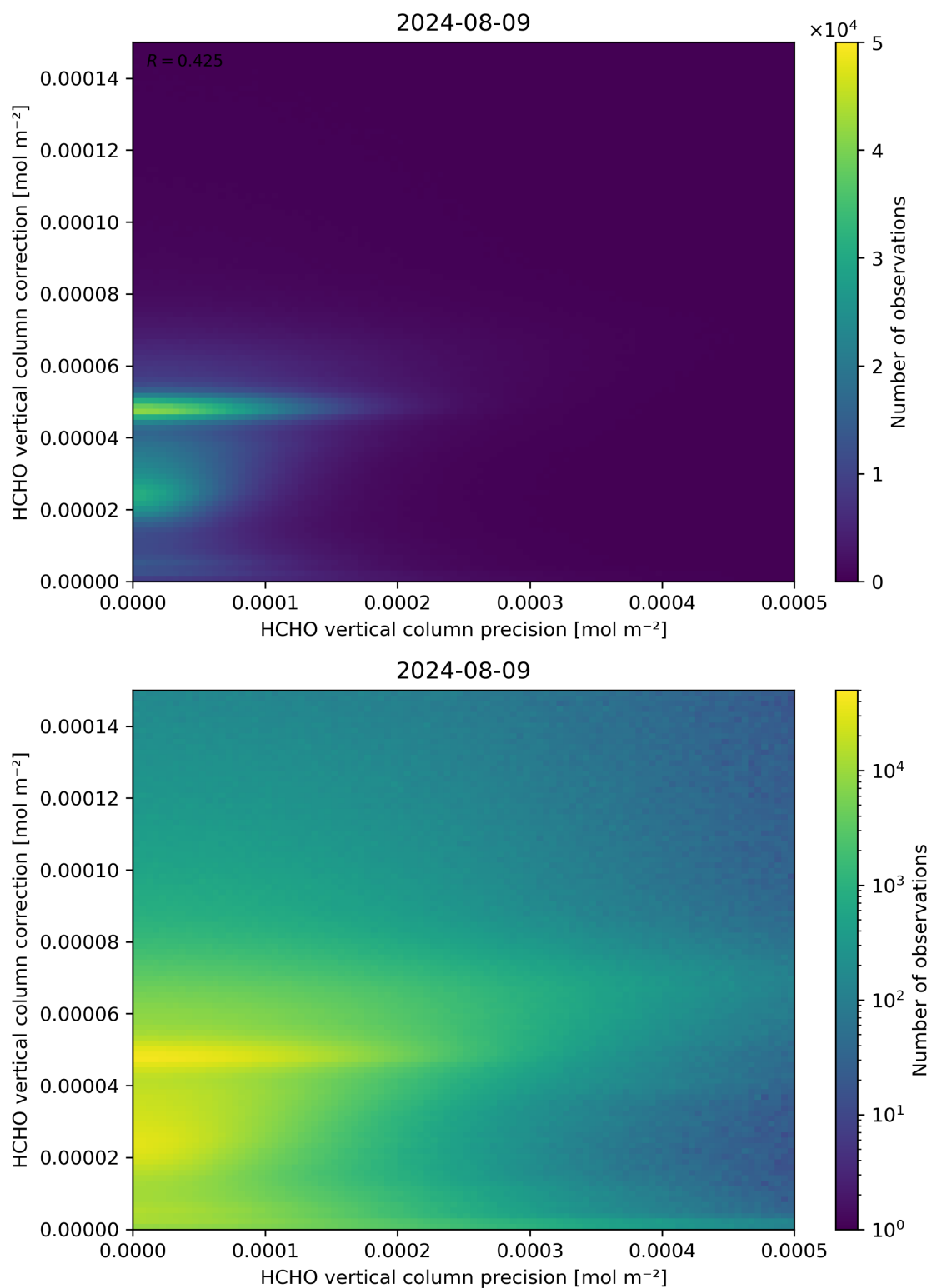
Figure 146: Scatter density plot of “HCHO vertical column precision” against “HCHO vertical column correction” for 2024-08-08 to 2024-08-10.
