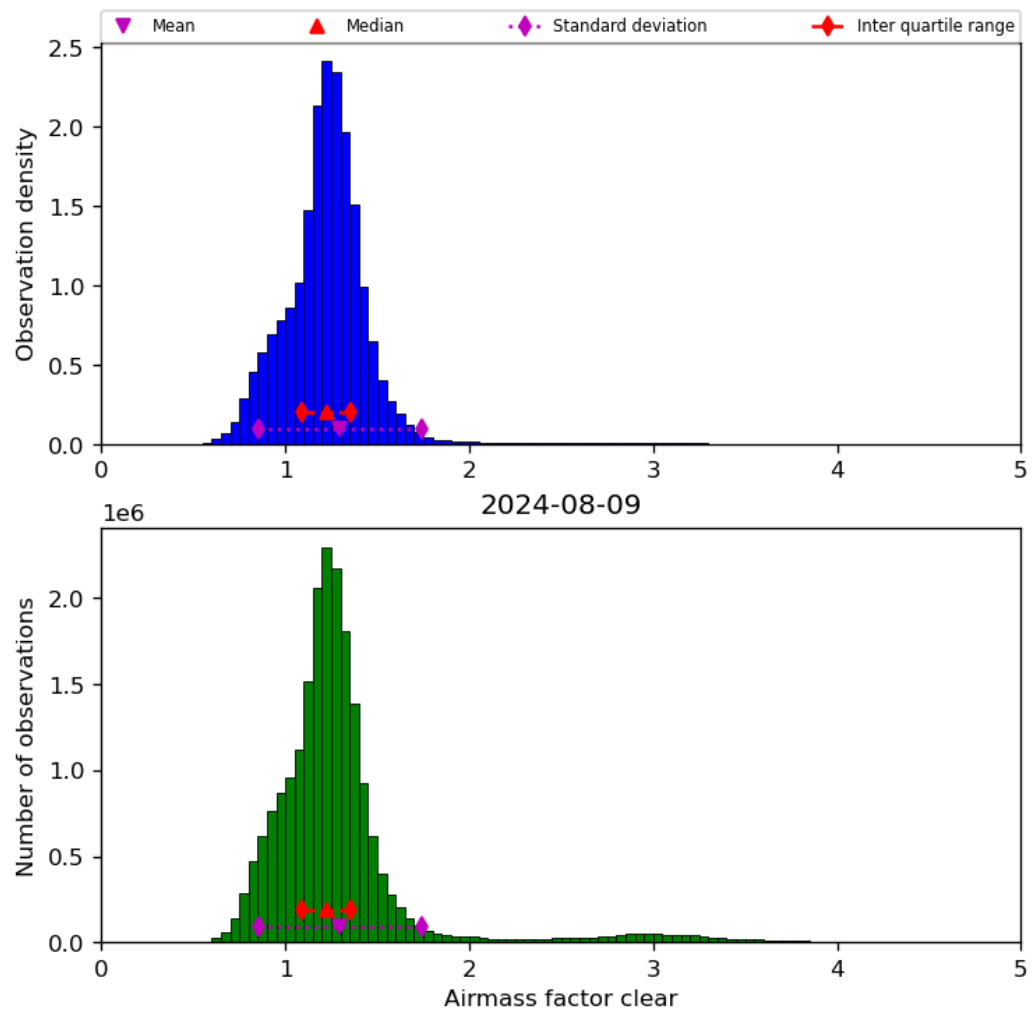
Figure 42: Histogram of “Airmass factor clear” for 2024-08-08 to 2024-08-10
