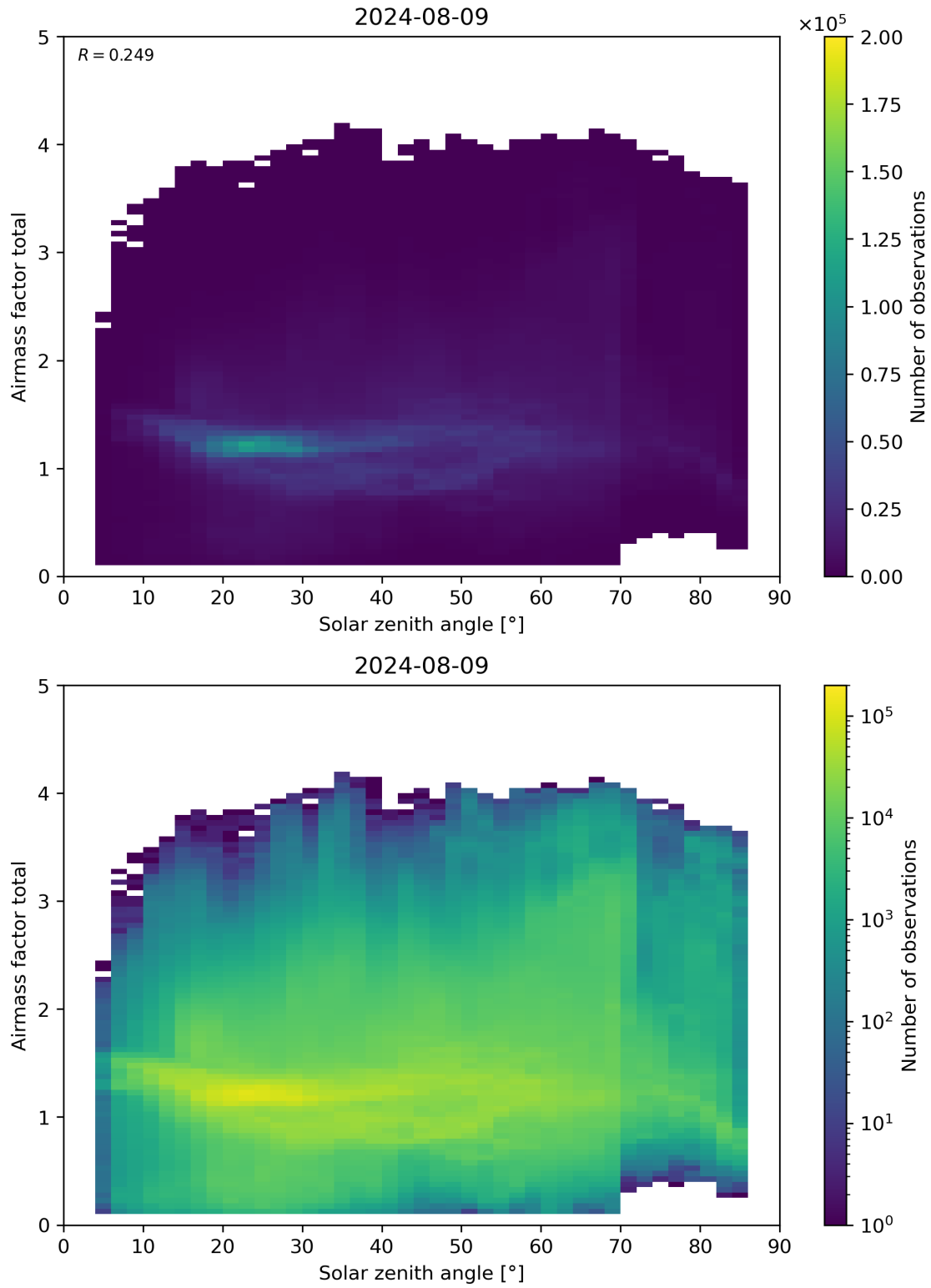
Figure 175: Scatter density plot of “Solar zenith angle” against “Airmass factor total” for 2024-08-08 to 2024-08-10.
