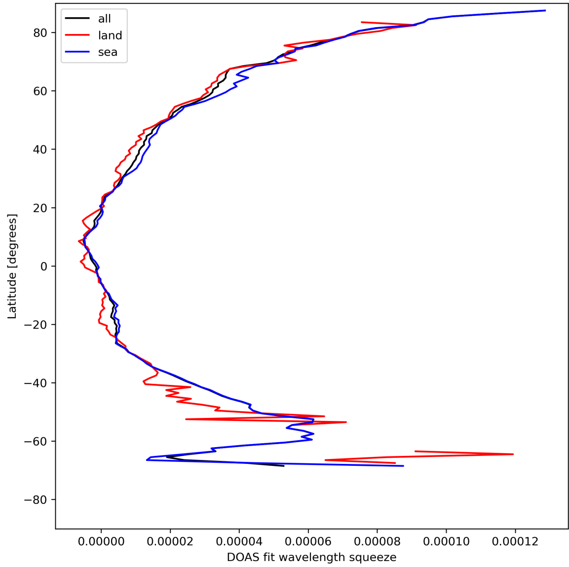
Figure 31: Zonal average of “DOAS fit wavelength squeeze” for 2024-08-08 to 2024-08-10.
