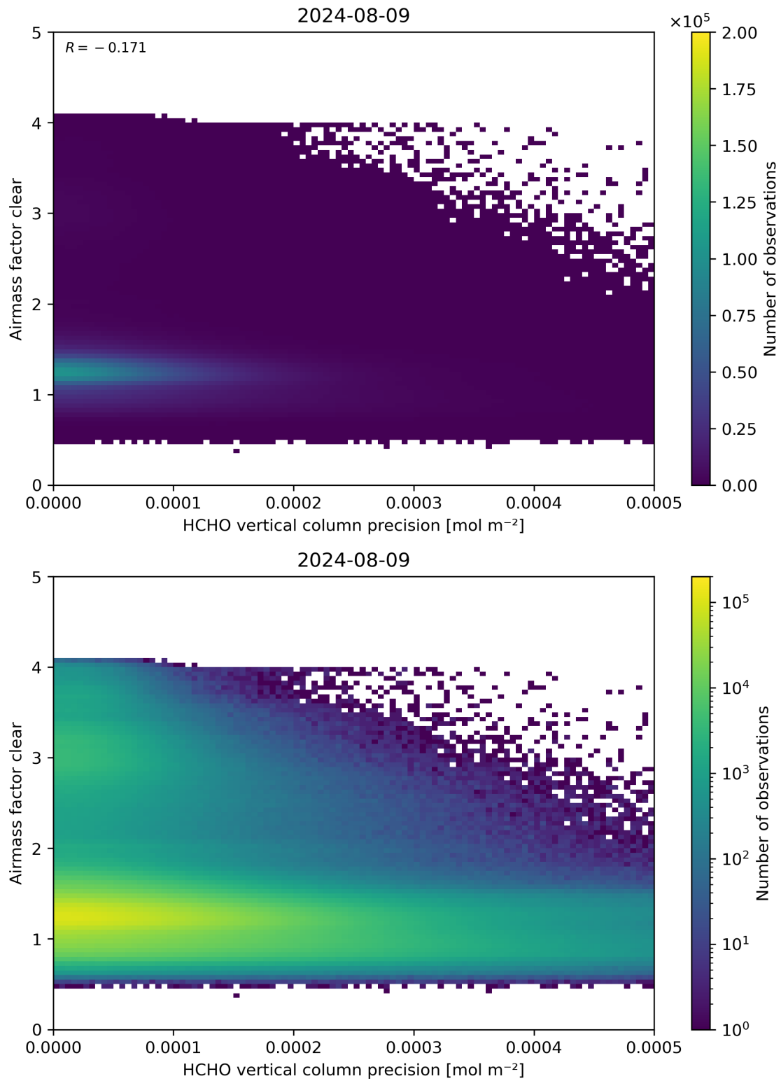
Figure 139: Scatter density plot of “HCHO vertical column precision” against “Airmass factor clear” for 2024-08-08 to 2024-08-10.
