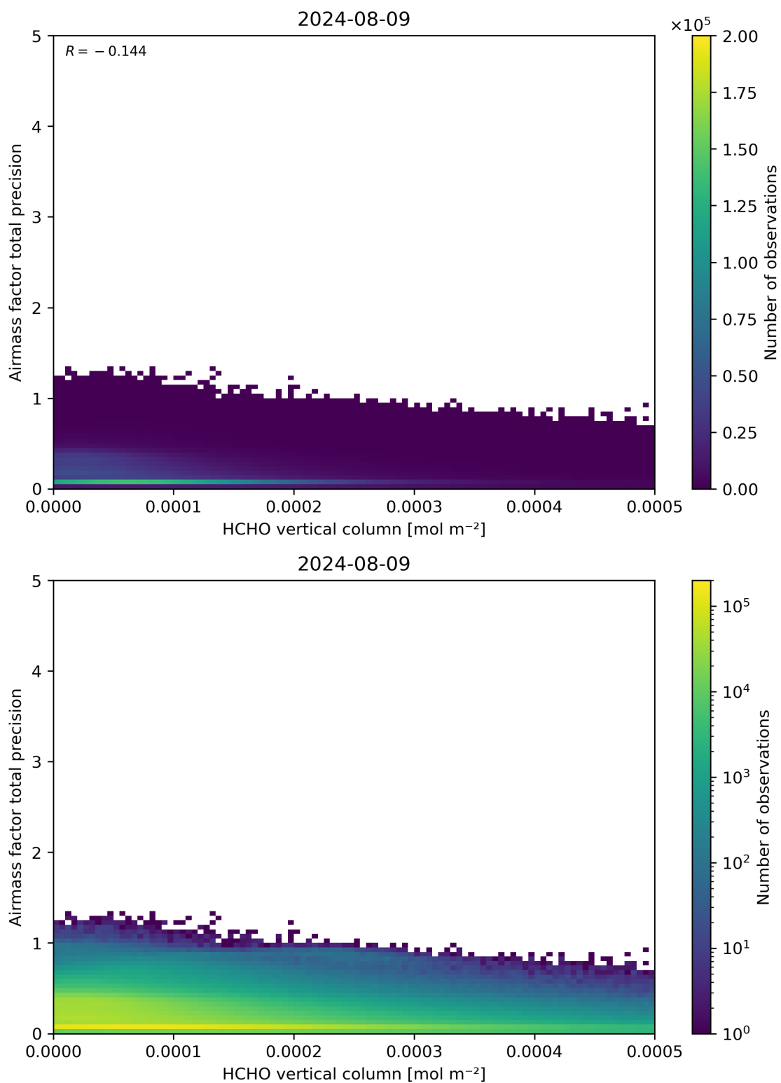
Figure 132: Scatter density plot of “HCHO vertical column” against “Airmass factor total precision” for 2024-08-08 to 2024-08-10.
