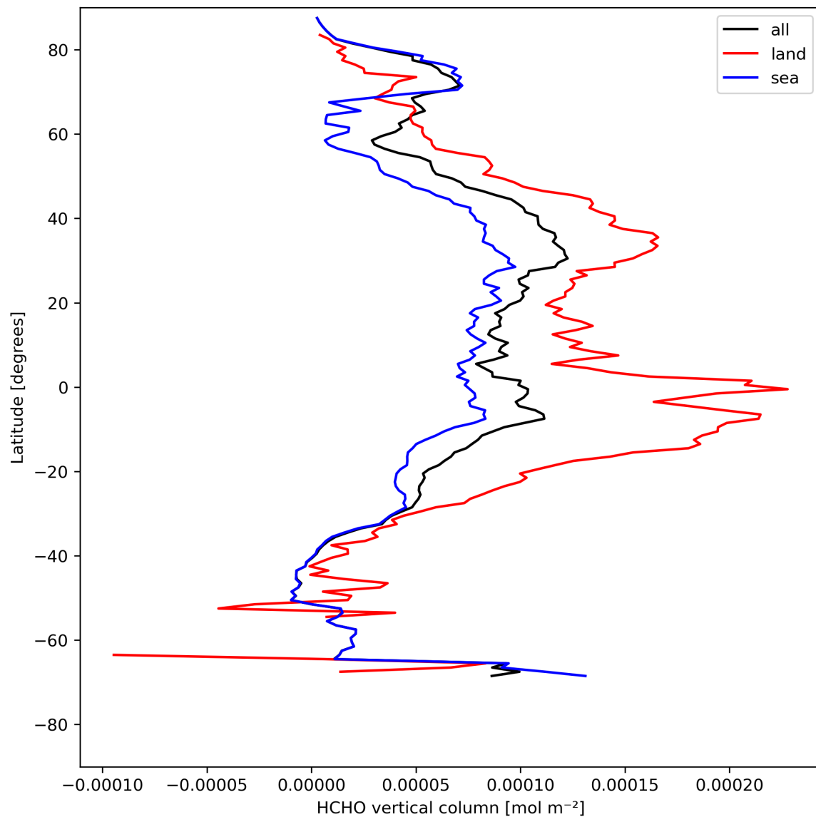
Figure 21: Zonal average of “HCHO vertical column” for 2024-08-08 to 2024-08-10.
