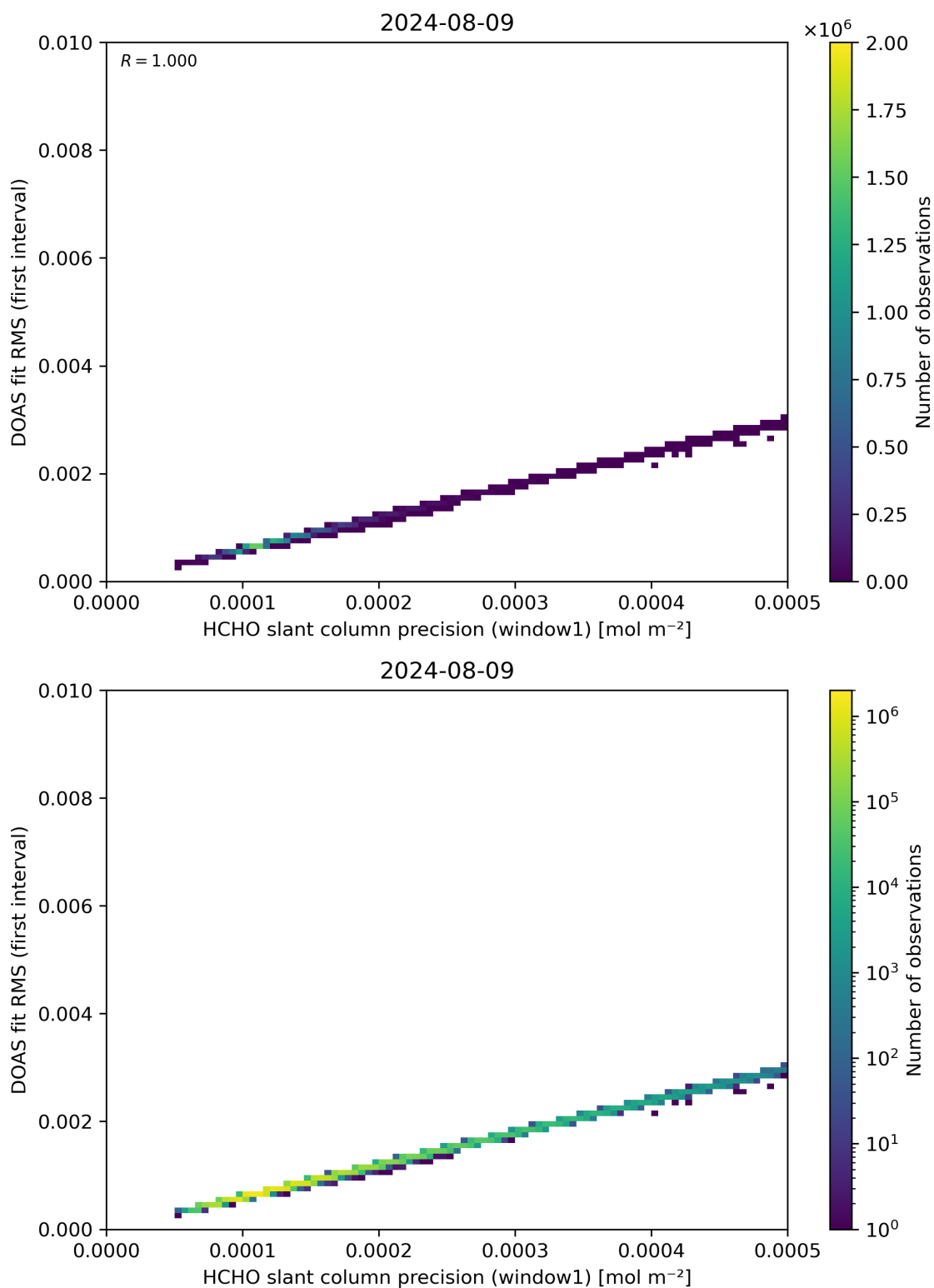
Figure 88: Scatter density plot of “HCHO slant column precision (window1)” against “DOAS fit RMS (first interval)” for 2024-08-08 to 2024-08-10.
