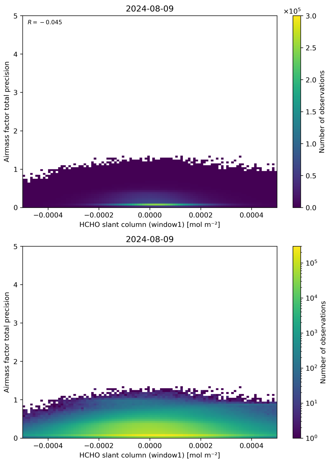
Figure 86: Scatter density plot of “HCHO slant column (window1)” against “Airmass factor total precision” for 2024-08-08 to 2024-08-10.
