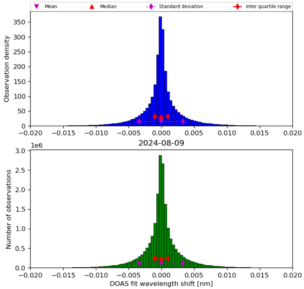
Figure 44: Histogram of “DOAS fit wavelength shift” for 2024-08-08 to 2024-08-10
