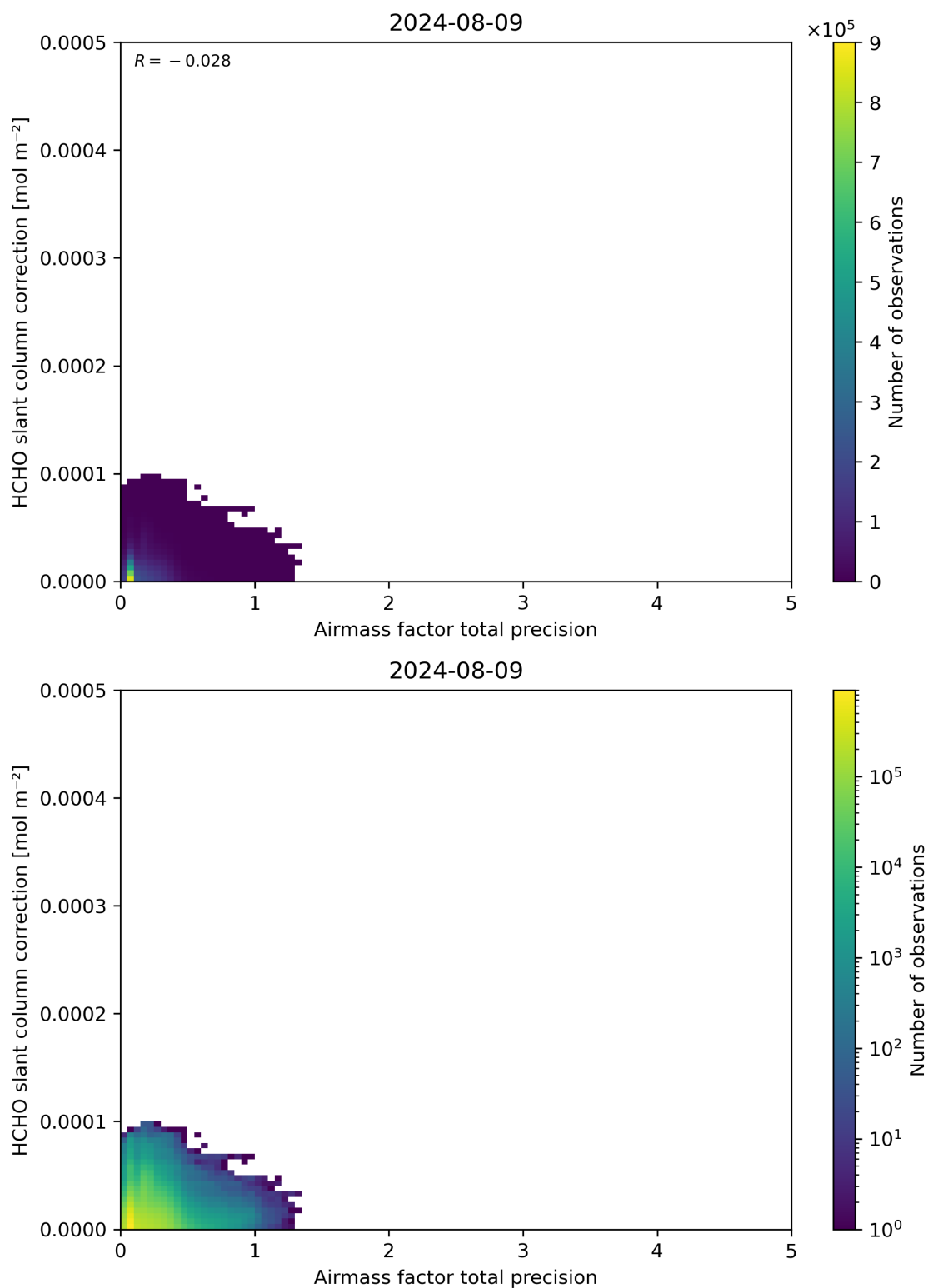
Figure 110: Scatter density plot of “Airmass factor total precision” against “HCHO slant column correction” for 2024-08-08 to 2024-08-10.
