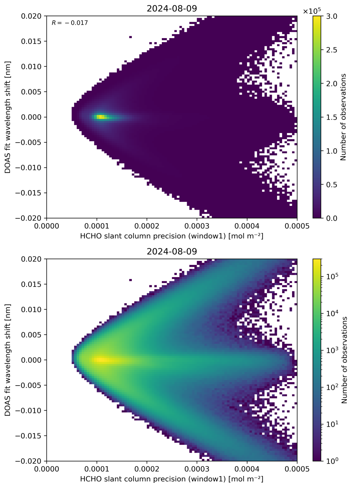
Figure 89: Scatter density plot of “HCHO slant column precision (window1)” against “DOAS fit wavelength shift” for 2024-08-08 to 2024-08-10.
