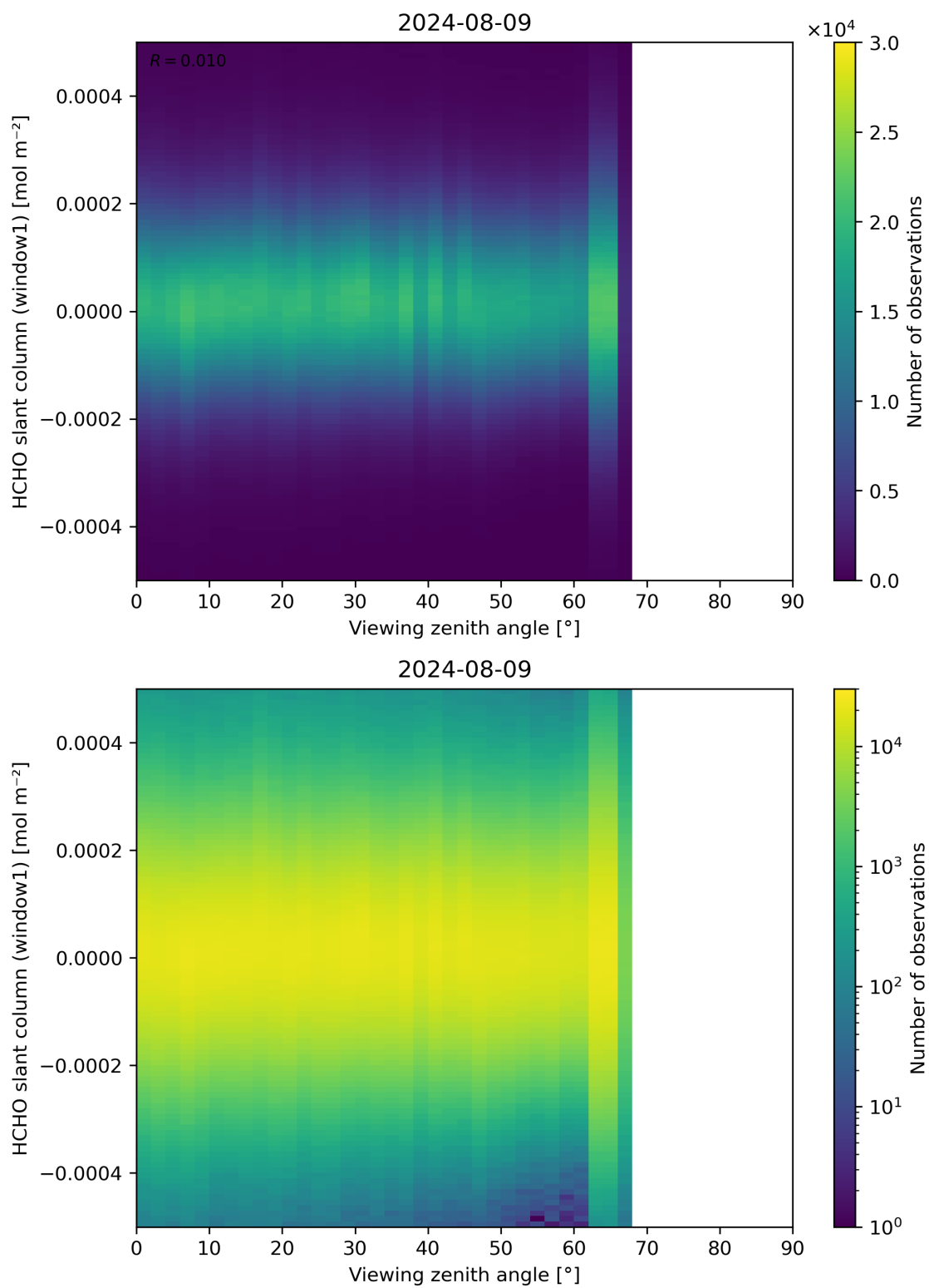
Figure 188: Scatter density plot of “Viewing zenith angle” against “HCHO slant column (window1)” for 2024-08-08 to 2024-08-10.
