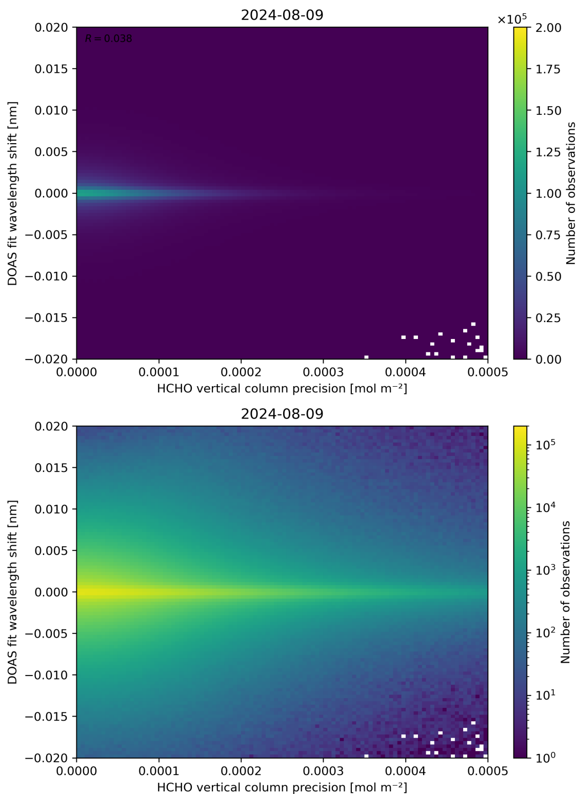
Figure 137: Scatter density plot of “HCHO vertical column precision” against “DOAS fit wavelength shift” for 2024-08-08 to 2024-08-10.
