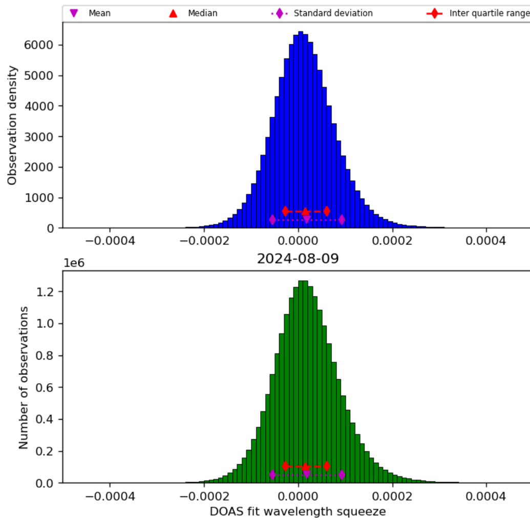
Figure 45: Histogram of “DOAS fit wavelength squeeze” for 2024-08-08 to 2024-08-10
