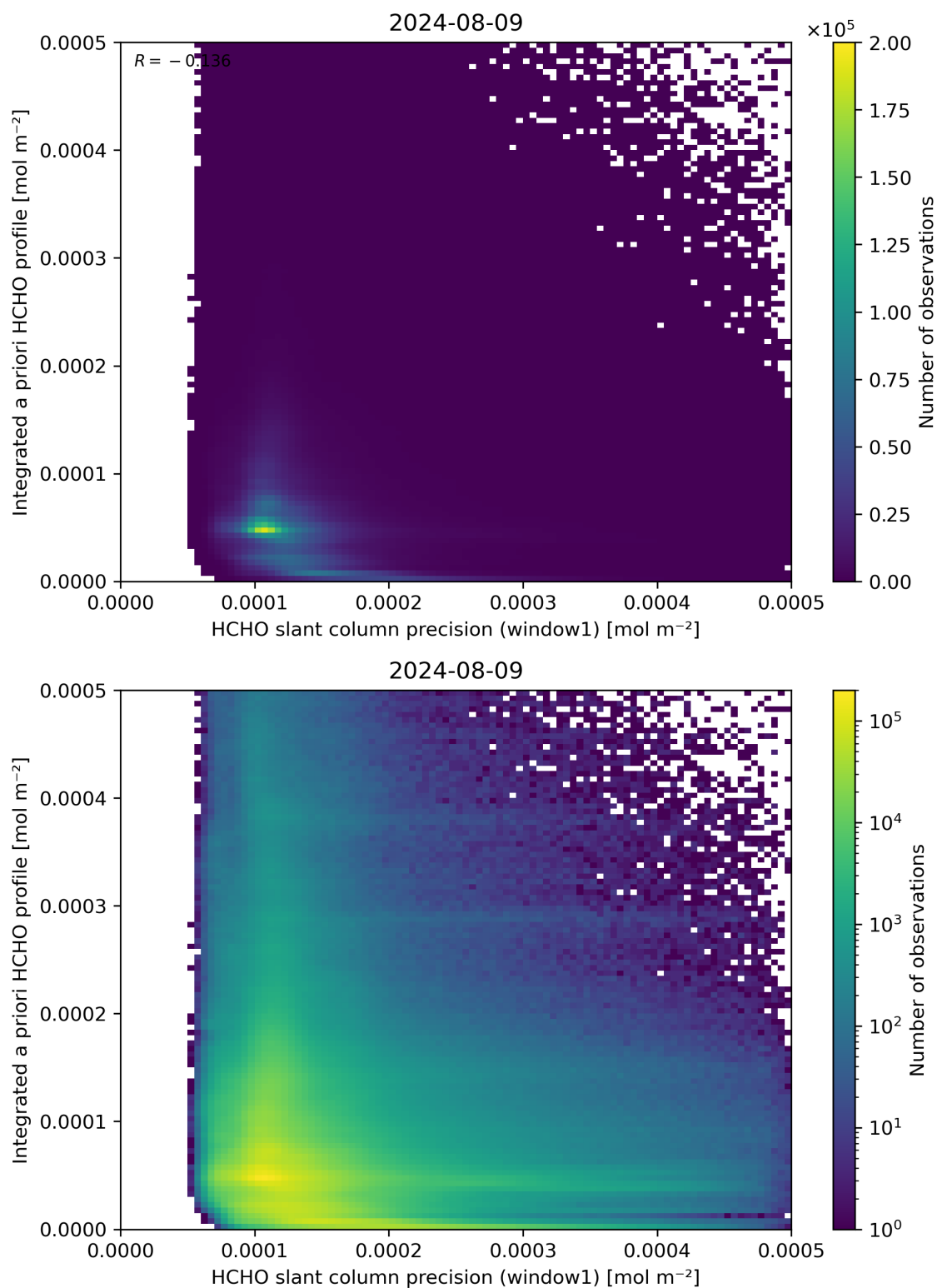
Figure 96: Scatter density plot of “HCHO slant column precision (window1)” against “Integrated a priori HCHO profile” for 2024-08-08 to 2024-08-10.
