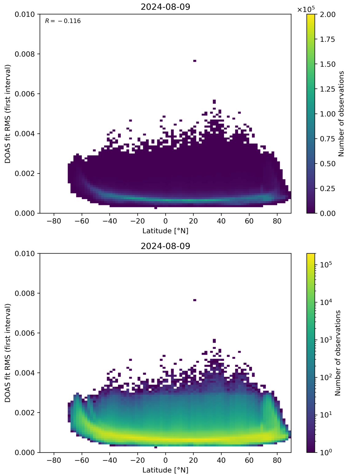
Figure 153: Scatter density plot of “Latitude” against “DOAS fit RMS (first interval)” for 2024-08-08 to 2024-08-10.
