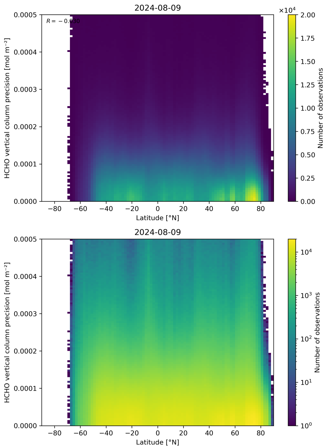
Figure 165: Scatter density plot of “Latitude” against “HCHO vertical column precision” for 2024-08-08 to 2024-08-10.
