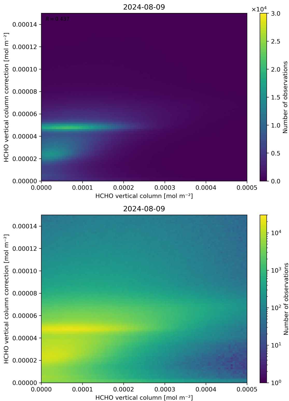
Figure 133: Scatter density plot of “HCHO vertical column” against “HCHO vertical column correction” for 2024-08-08 to 2024-08-10.
