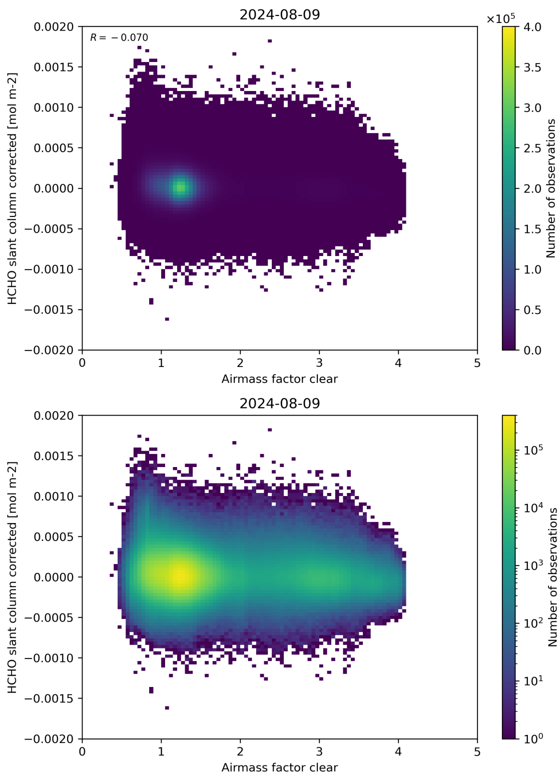
Figure 74: Scatter density plot of “Airmass factor clear” against “HCHO slant column corrected” for 2024-08-08 to 2024-08-10.
