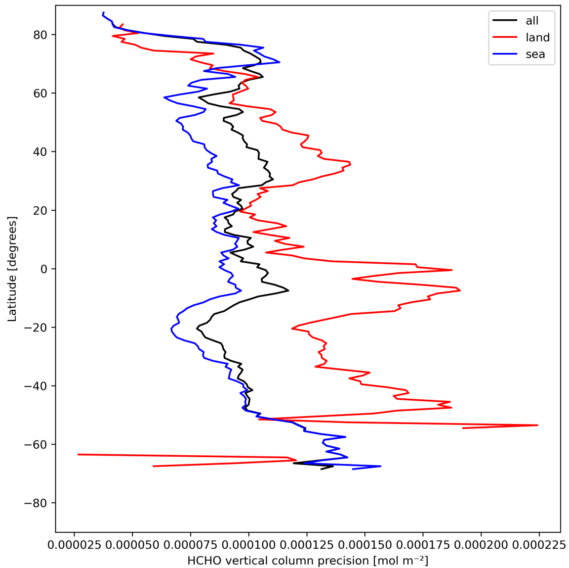
Figure 22: Zonal average of “HCHO vertical column precision” for 2024-08-08 to 2024-08-10.
