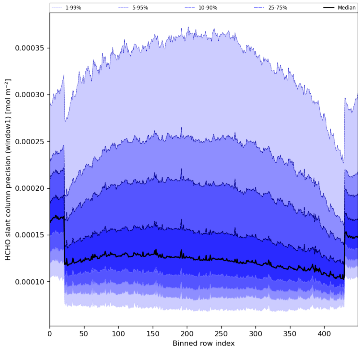
Figure 53: Along track statistics of “HCHO slant column precision (window1)” for 2024-08-08 to 2024-08-10
