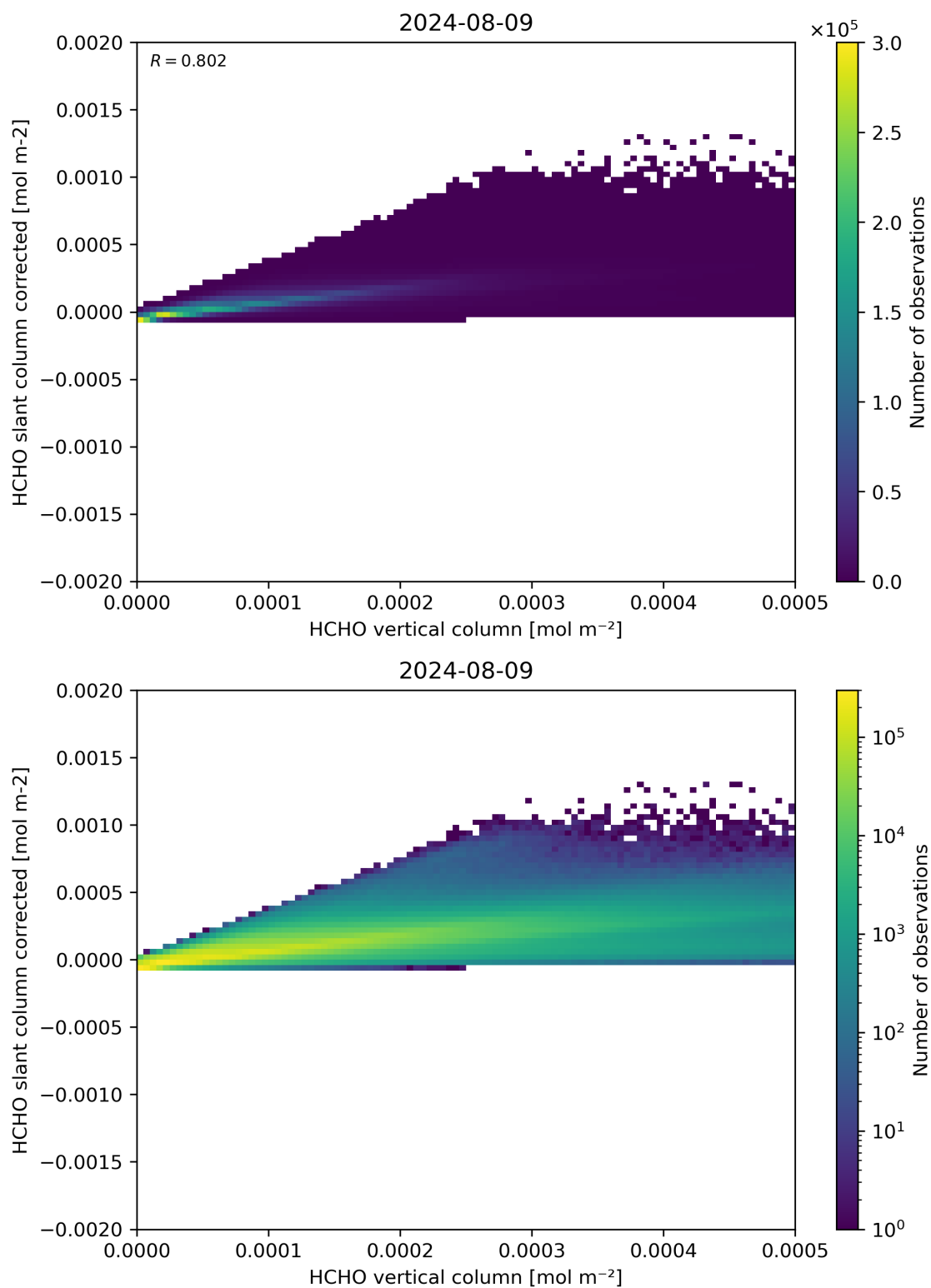
Figure 127: Scatter density plot of “HCHO vertical column” against “HCHO slant column corrected” for 2024-08-08 to 2024-08-10.
