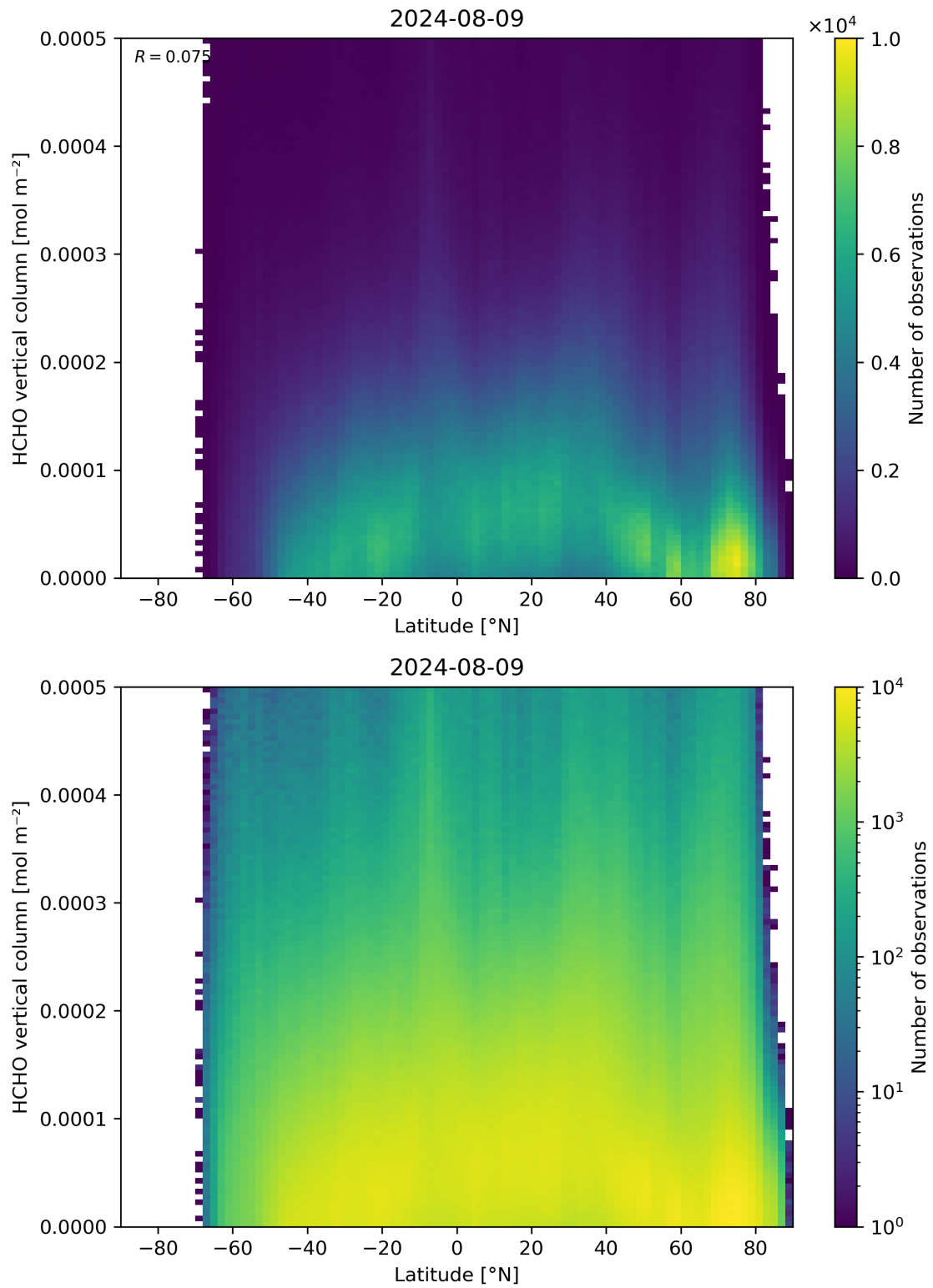
Figure 163: Scatter density plot of “Latitude” against “HCHO vertical column” for 2024-08-08 to 2024-08-10.
