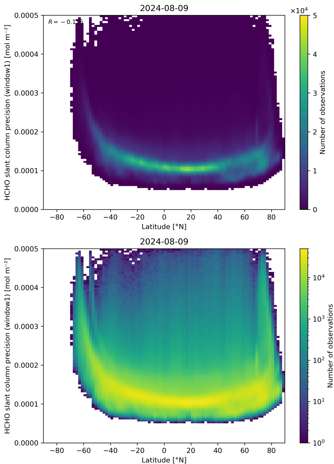
Figure 160: Scatter density plot of “Latitude” against “HCHO slant column precision (window1)” for 2024-08-08 to 2024-08-10.
