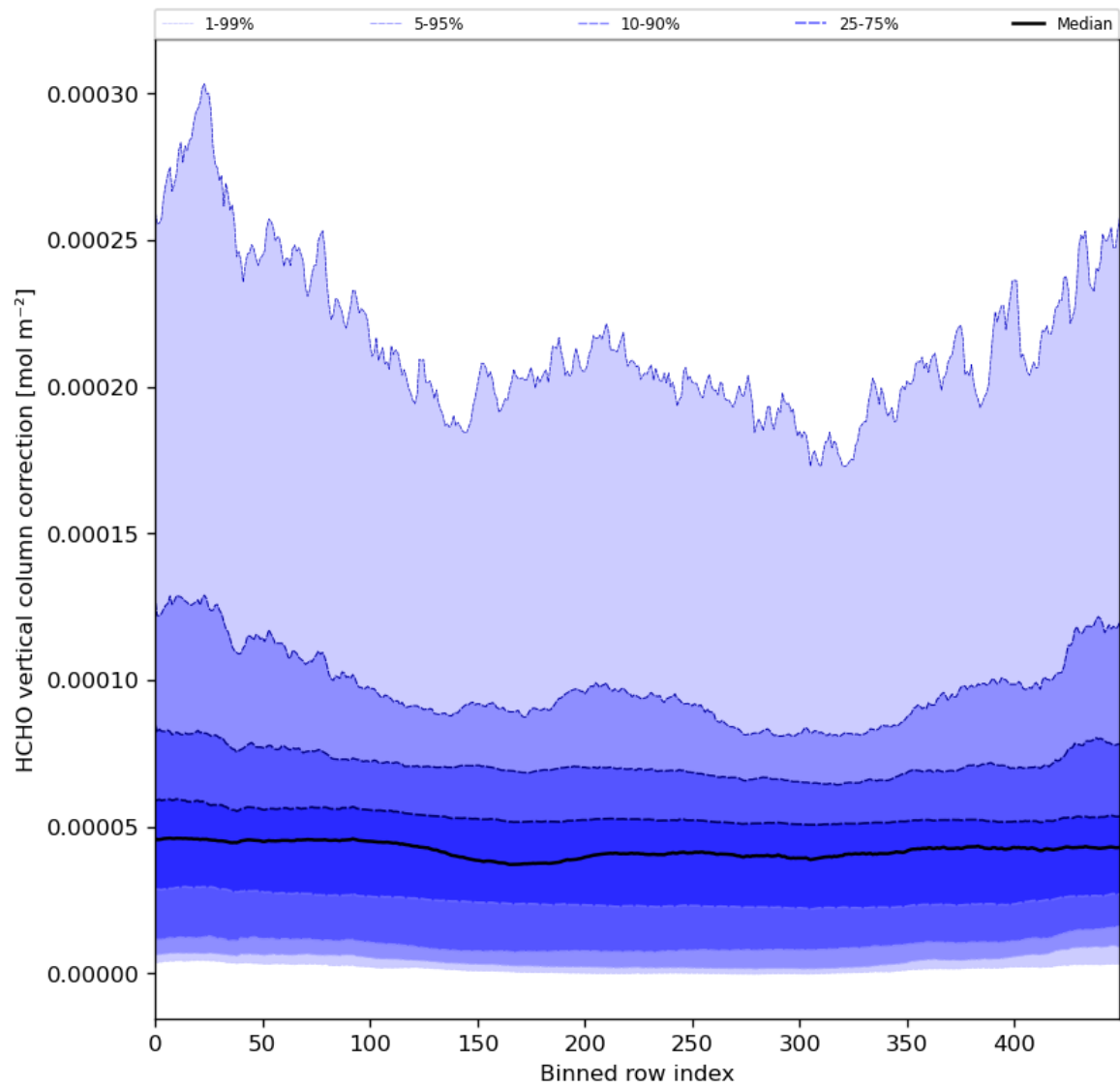
Figure 51: Along track statistics of “HCHO vertical column correction” for 2024-08-08 to 2024-08-10
