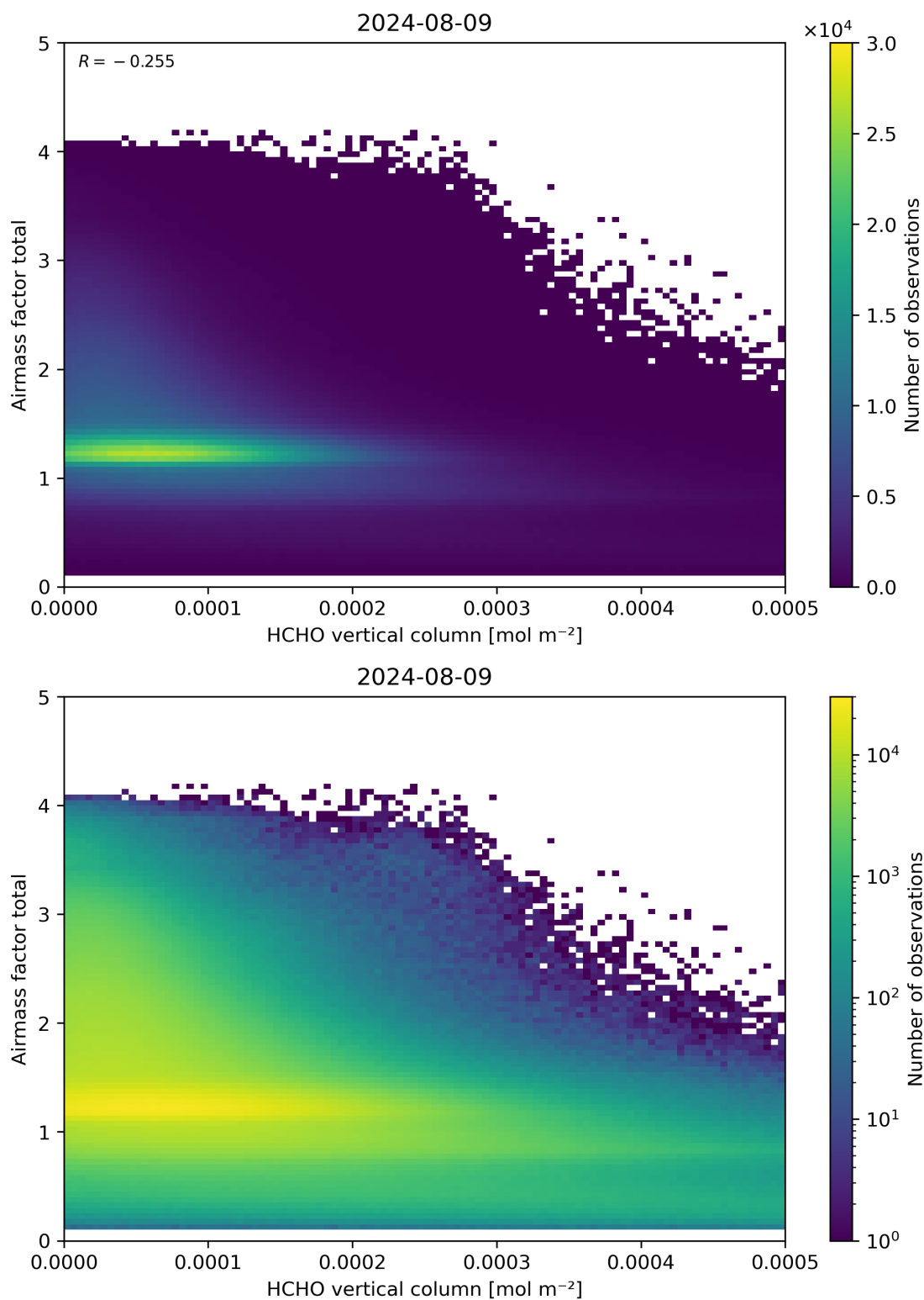
Figure 131: Scatter density plot of “HCHO vertical column” against “Airmass factor total” for 2024-08-08 to 2024-08-10.
