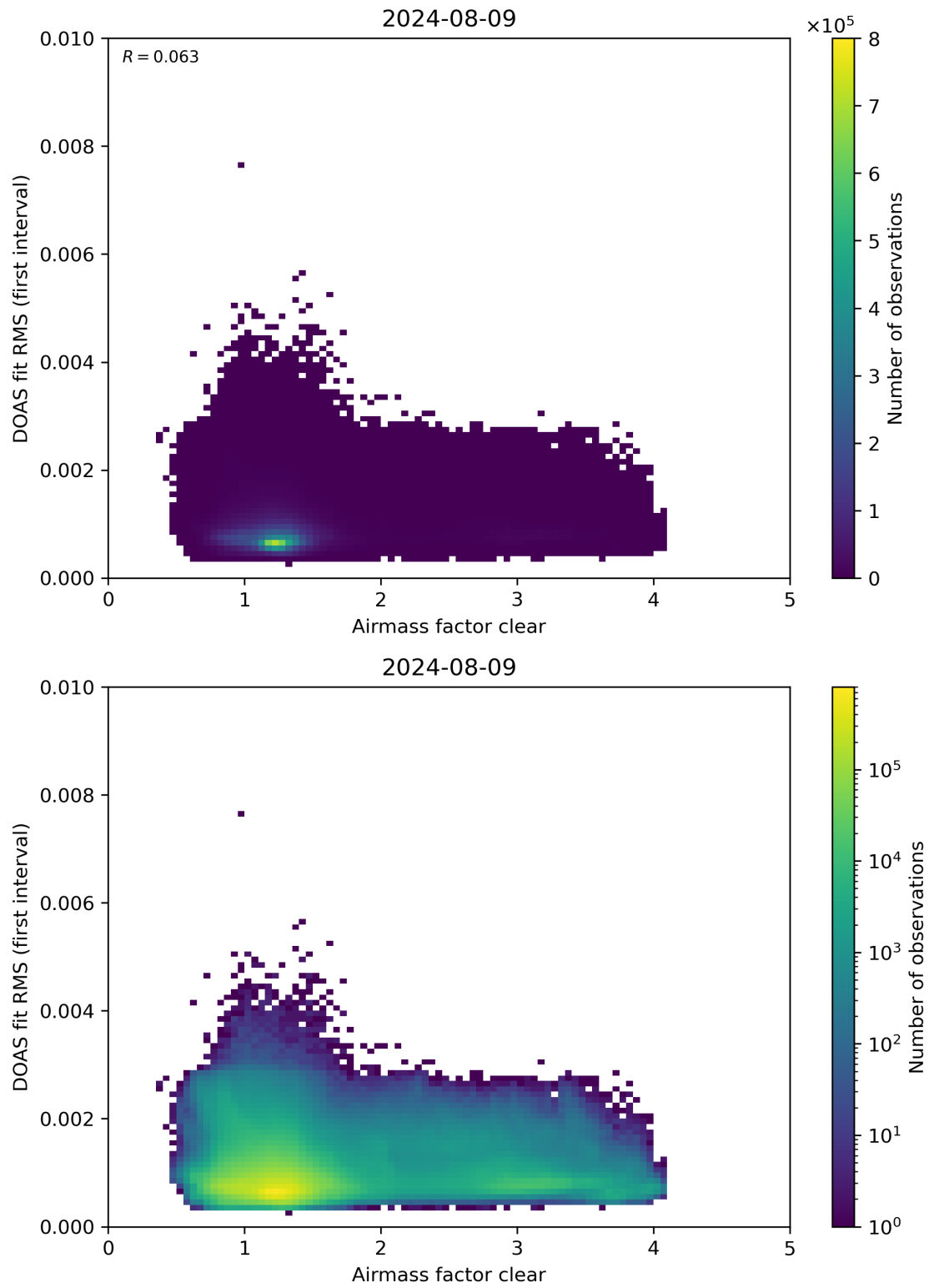
Figure 71: Scatter density plot of “Airmass factor clear” against “DOAS fit RMS (first interval)” for 2024-08-08 to 2024-08-10.
