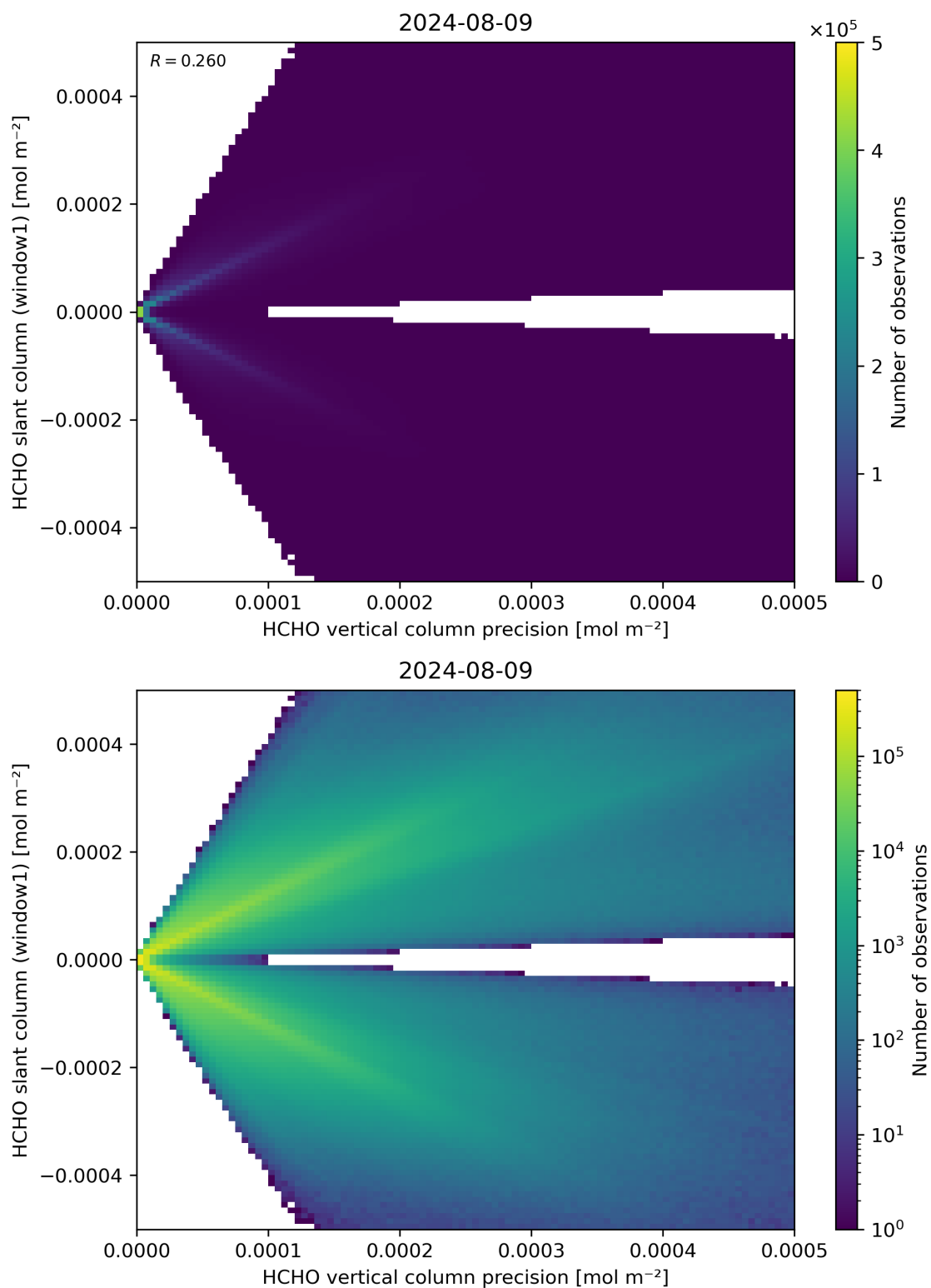
Figure 142: Scatter density plot of “HCHO vertical column precision” against “HCHO slant column (window1)” for 2024-08-08 to 2024-08-10.
