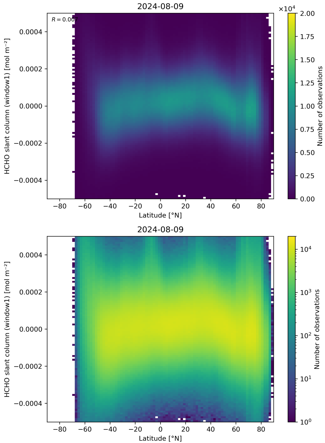
Figure 159: Scatter density plot of “Latitude” against “HCHO slant column (window1)” for 2024-08-08 to 2024-08-10.
