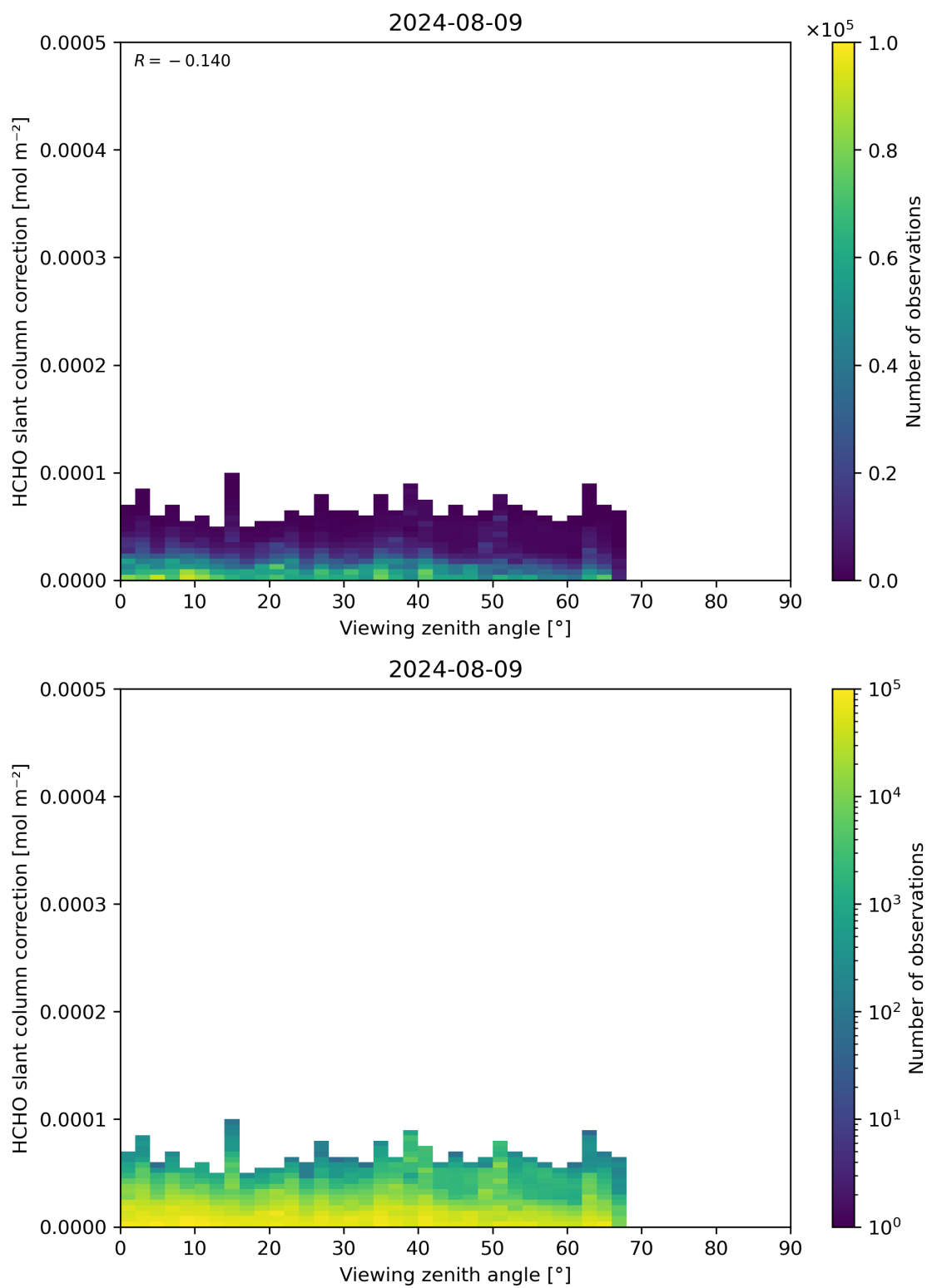
Figure 187: Scatter density plot of “Viewing zenith angle” against “HCHO slant column correction” for 2024-08-08 to 2024-08-10.
