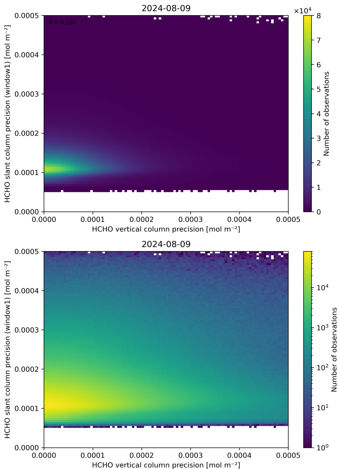
Figure 143: Scatter density plot of “HCHO vertical column precision” against “HCHO slant column precision (window1)” for 2024-08-08 to 2024-08-10.
