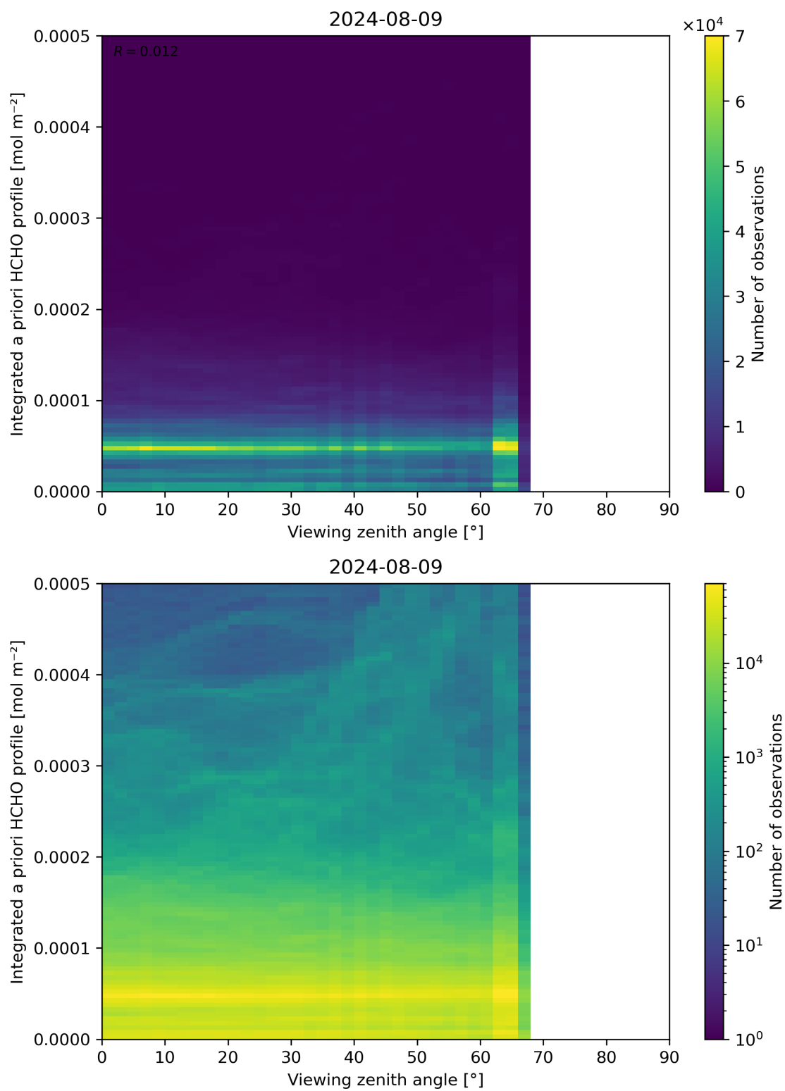
Figure 195: Scatter density plot of “Viewing zenith angle” against “Integrated a priori HCHO profile” for 2024-08-08 to 2024-08-10.
