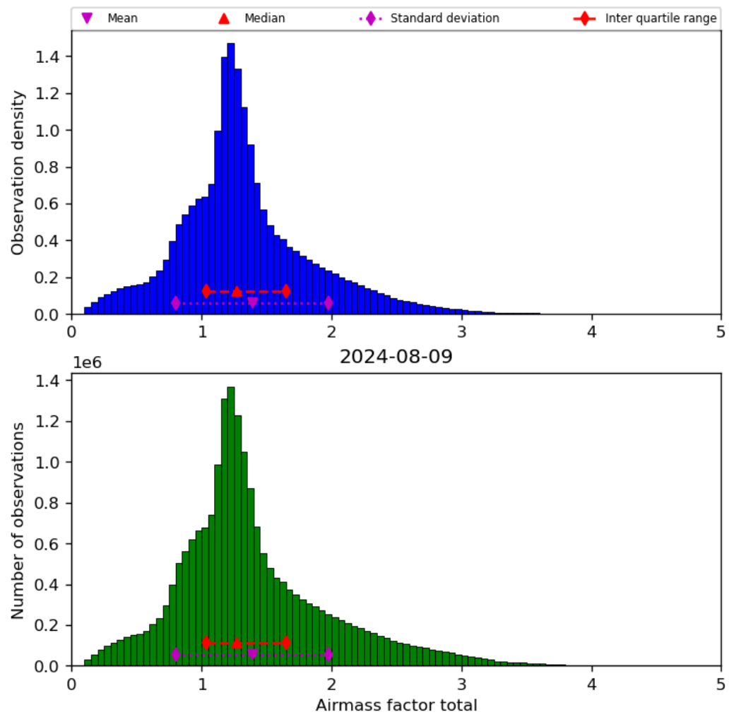
Figure 40: Histogram of “Airmass factor total” for 2024-08-08 to 2024-08-10
