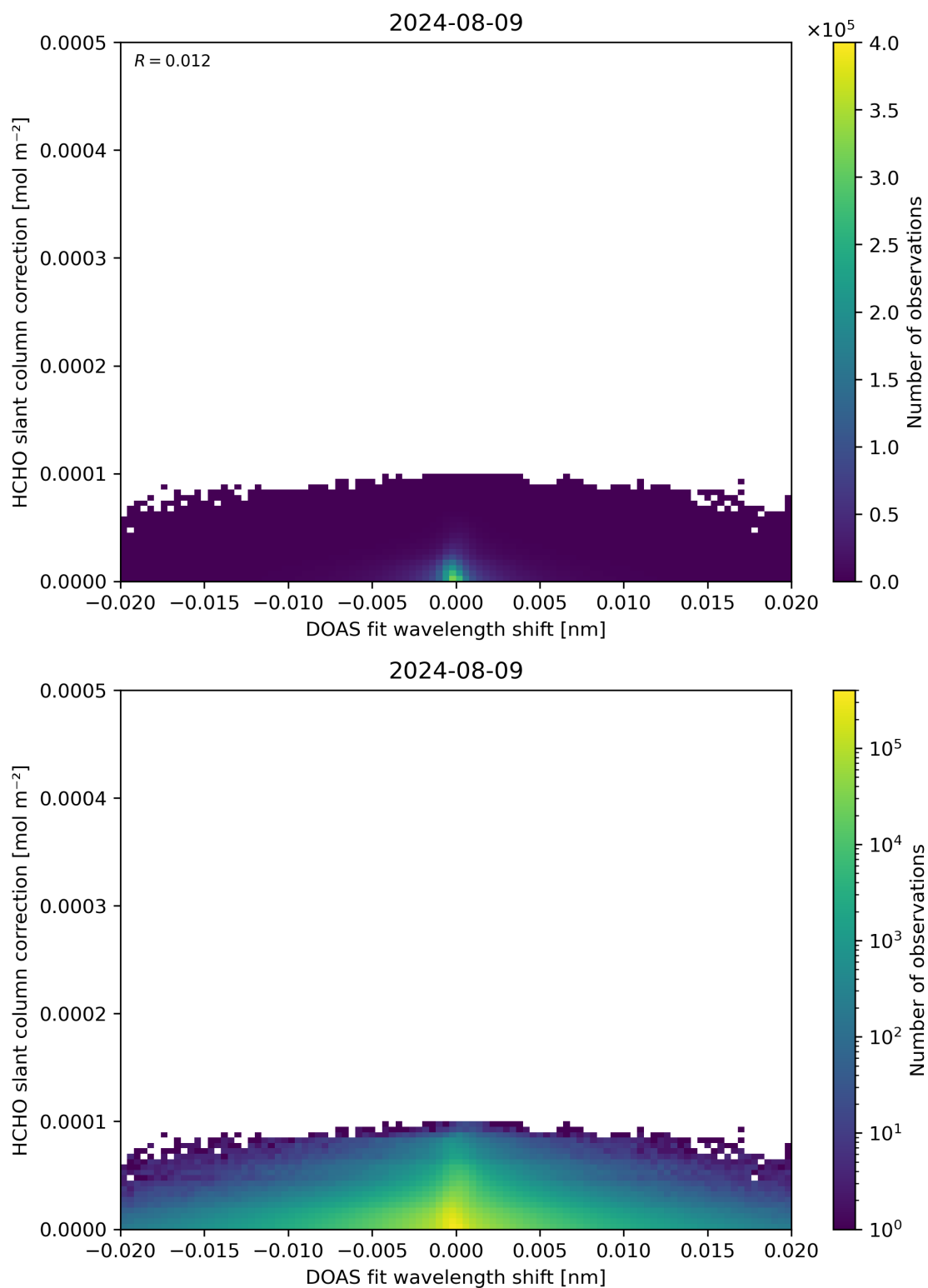
Figure 67: Scatter density plot of “DOAS fit wavelength shift” against “HCHO slant column correction” for 2024-08-08 to 2024-08-10.
