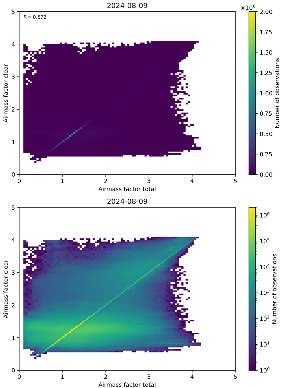
Figure 100: Scatter density plot of “Airmass factor total” against “Airmass factor clear” for 2024-08-08 to 2024-08-10.
