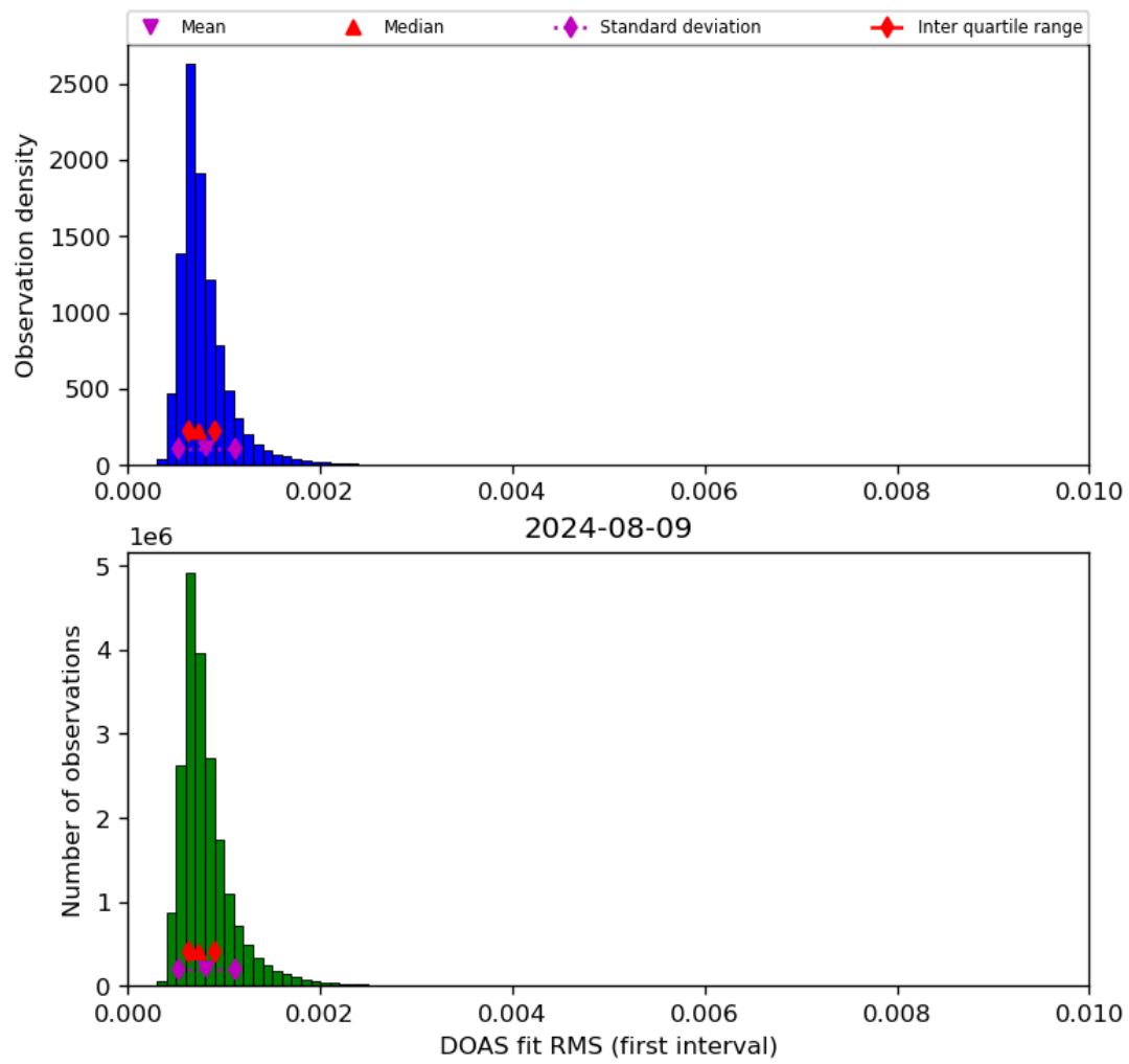
Figure 46: Histogram of “DOAS fit RMS (first interval)” for 2024-08-08 to 2024-08-10
