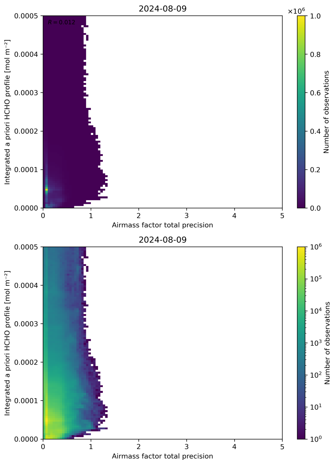
Figure 111: Scatter density plot of “Airmass factor total precision” against “Integrated a priori HCHO profile” for 2024-08-08 to 2024-08-10.
