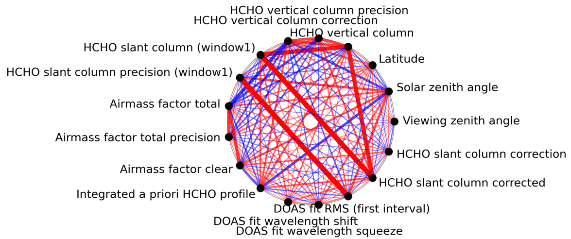
Figure 1: Map of correlation graph for 2024-08-08 to 2024-08-10.
