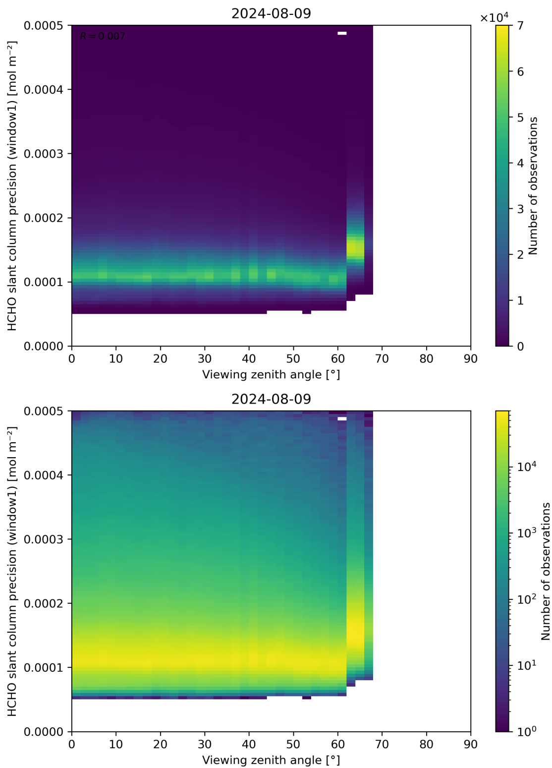
Figure 189: Scatter density plot of “Viewing zenith angle” against “HCHO slant column precision (window1)” for 2024-08-08 to 2024-08-10.
