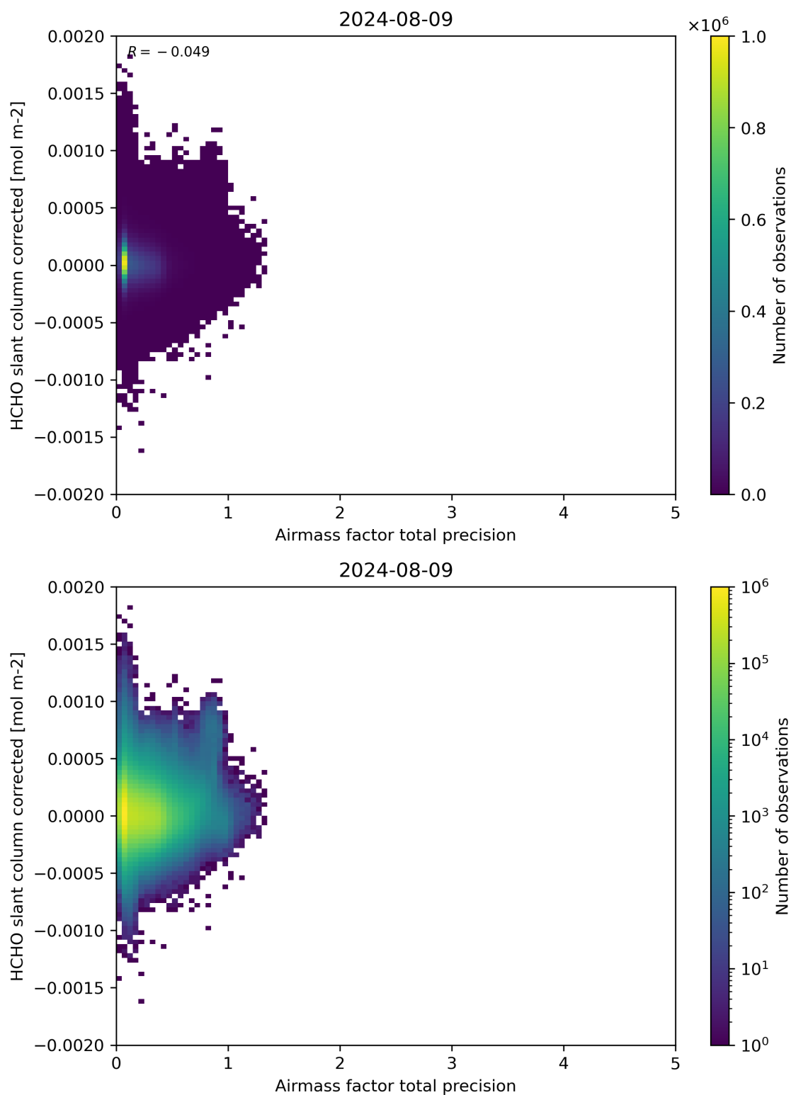
Figure 109: Scatter density plot of “Airmass factor total precision” against “HCHO slant column corrected” for 2024-08-08 to 2024-08-10.
