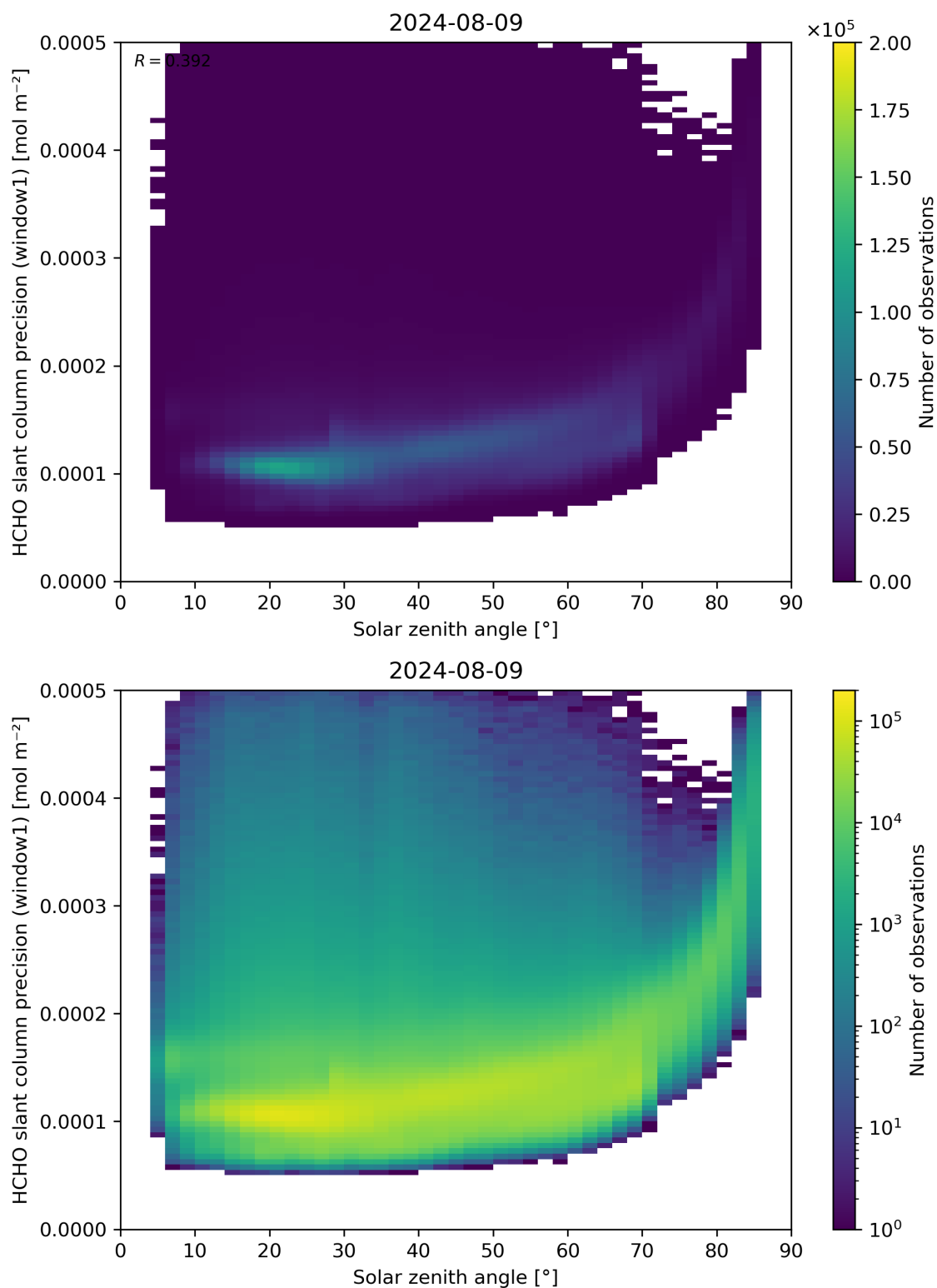
Figure 174: Scatter density plot of “Solar zenith angle” against “HCHO slant column precision (window1)” for 2024-08-08 to 2024-08-10.
