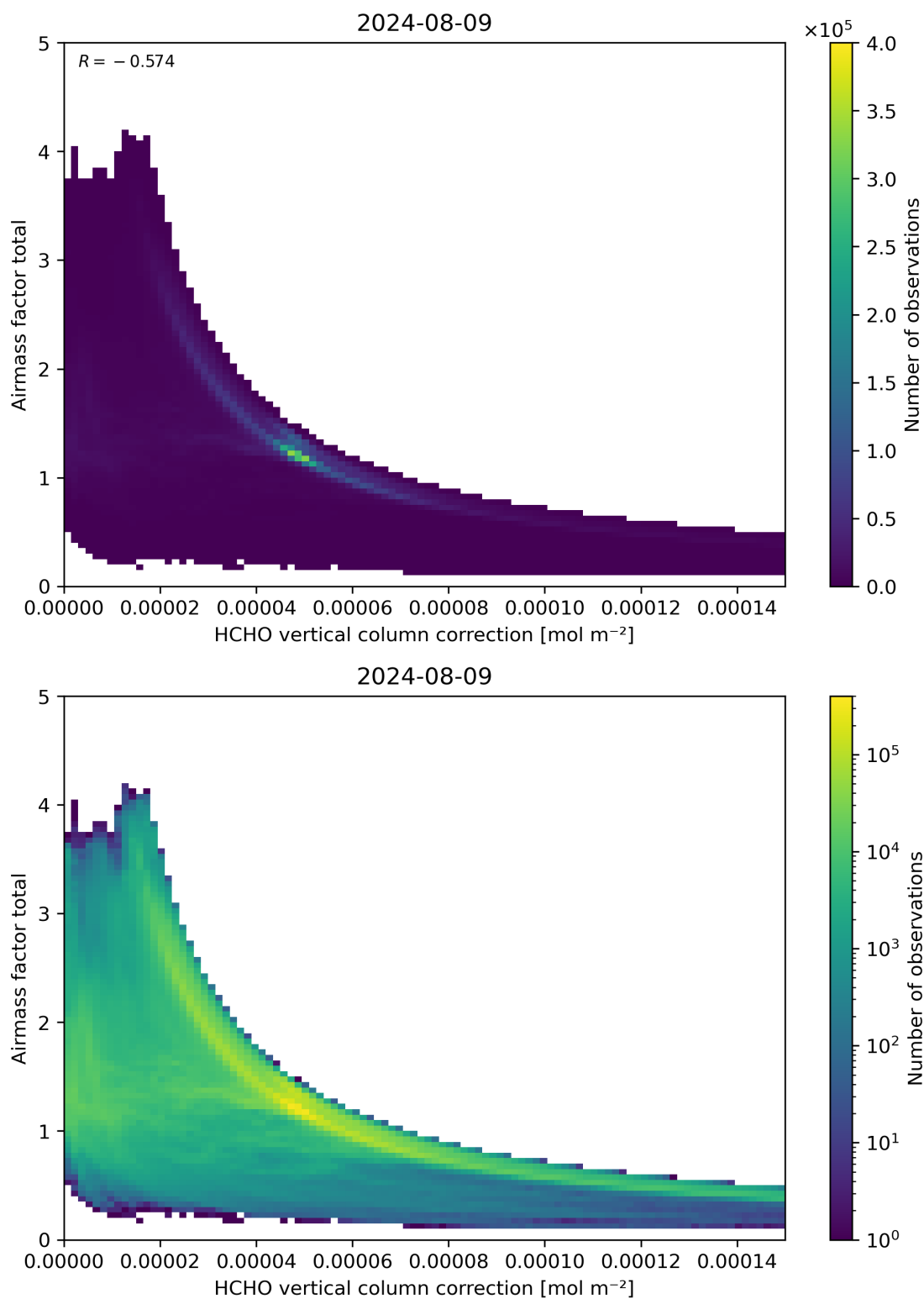
Figure 120: Scatter density plot of “HCHO vertical column correction” against “Airmass factor total” for 2024-08-08 to 2024-08-10.
