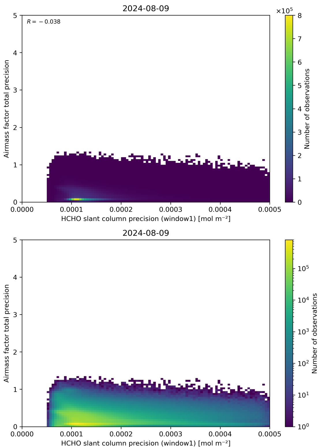
Figure 95: Scatter density plot of “HCHO slant column precision (window1)” against “Airmass factor total precision” for 2024-08-08 to 2024-08-10.
