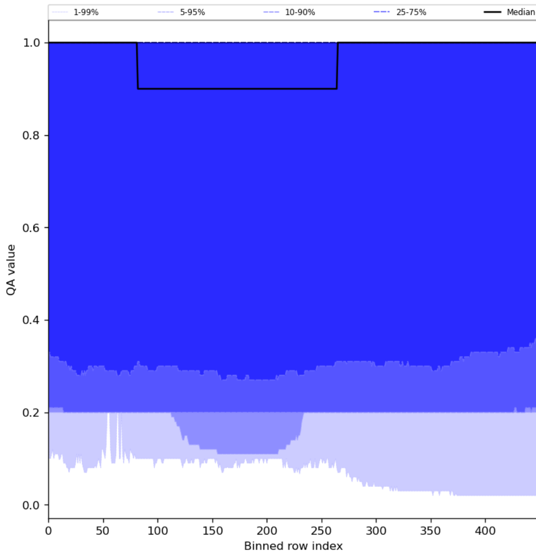
Figure 48: Along track statistics of “QA value” for 2024-08-08 to 2024-08-10
