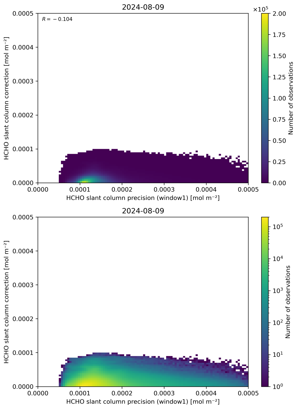
Figure 93: Scatter density plot of “HCHO slant column precision (window1)” against “HCHO slant column correction” for 2024-08-08 to 2024-08-10.
