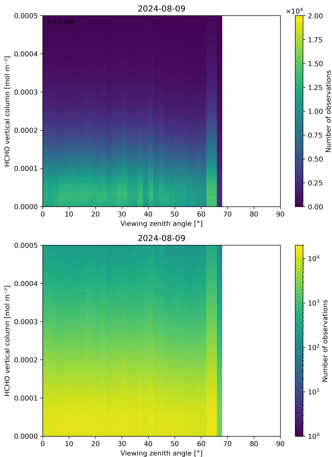
Figure 192: Scatter density plot of “Viewing zenith angle” against “HCHO vertical column” for 2024-08-08 to 2024-08-10.
