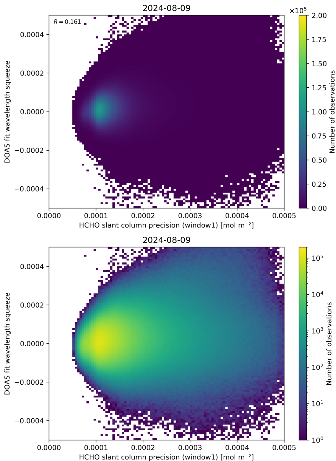
Figure 90: Scatter density plot of “HCHO slant column precision (window1)” against “DOAS fit wavelength squeeze” for 2024-08-08 to 2024-08-10.
