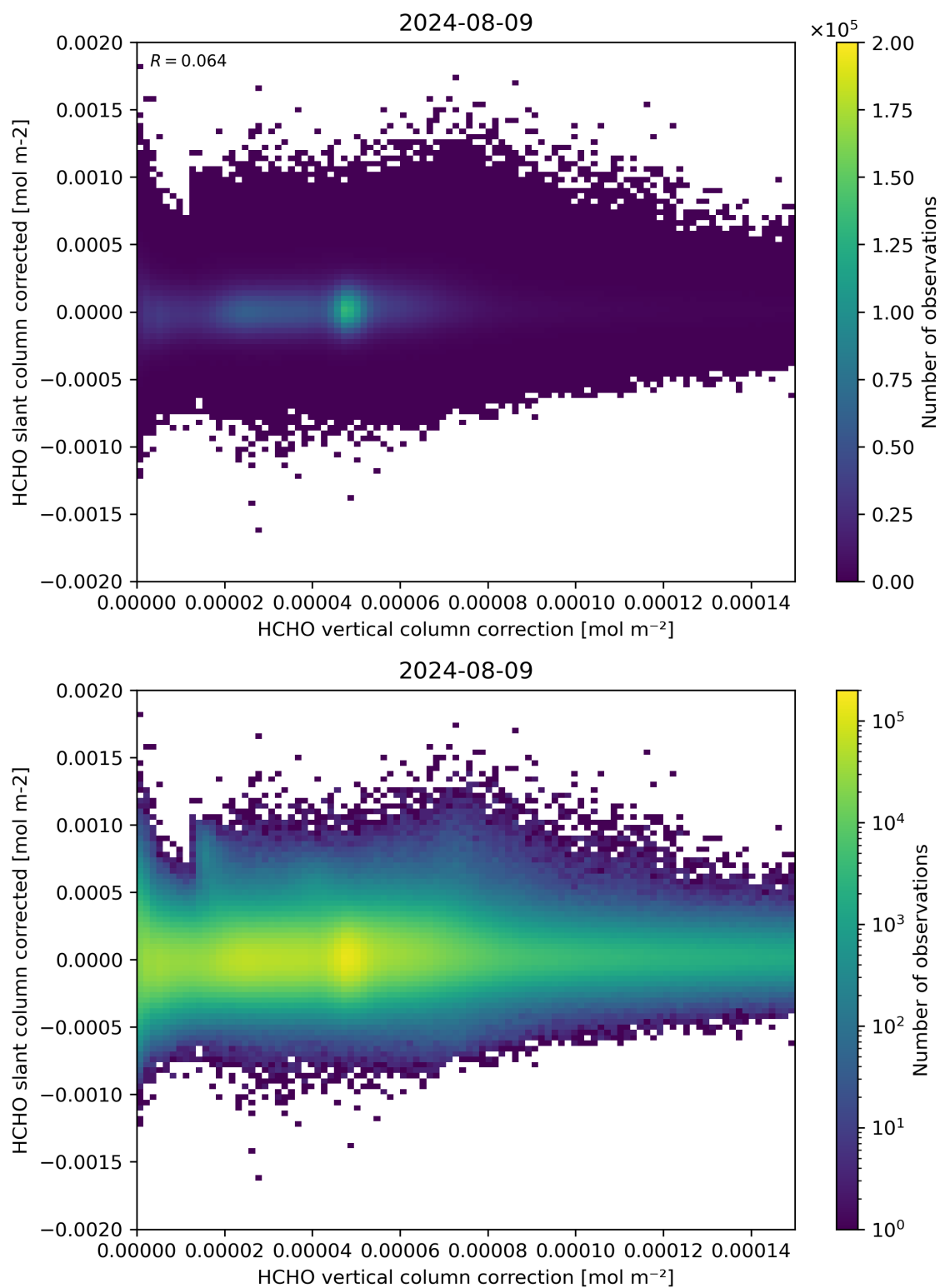
Figure 116: Scatter density plot of “HCHO vertical column correction” against “HCHO slant column corrected” for 2024-08-08 to 2024-08-10.
