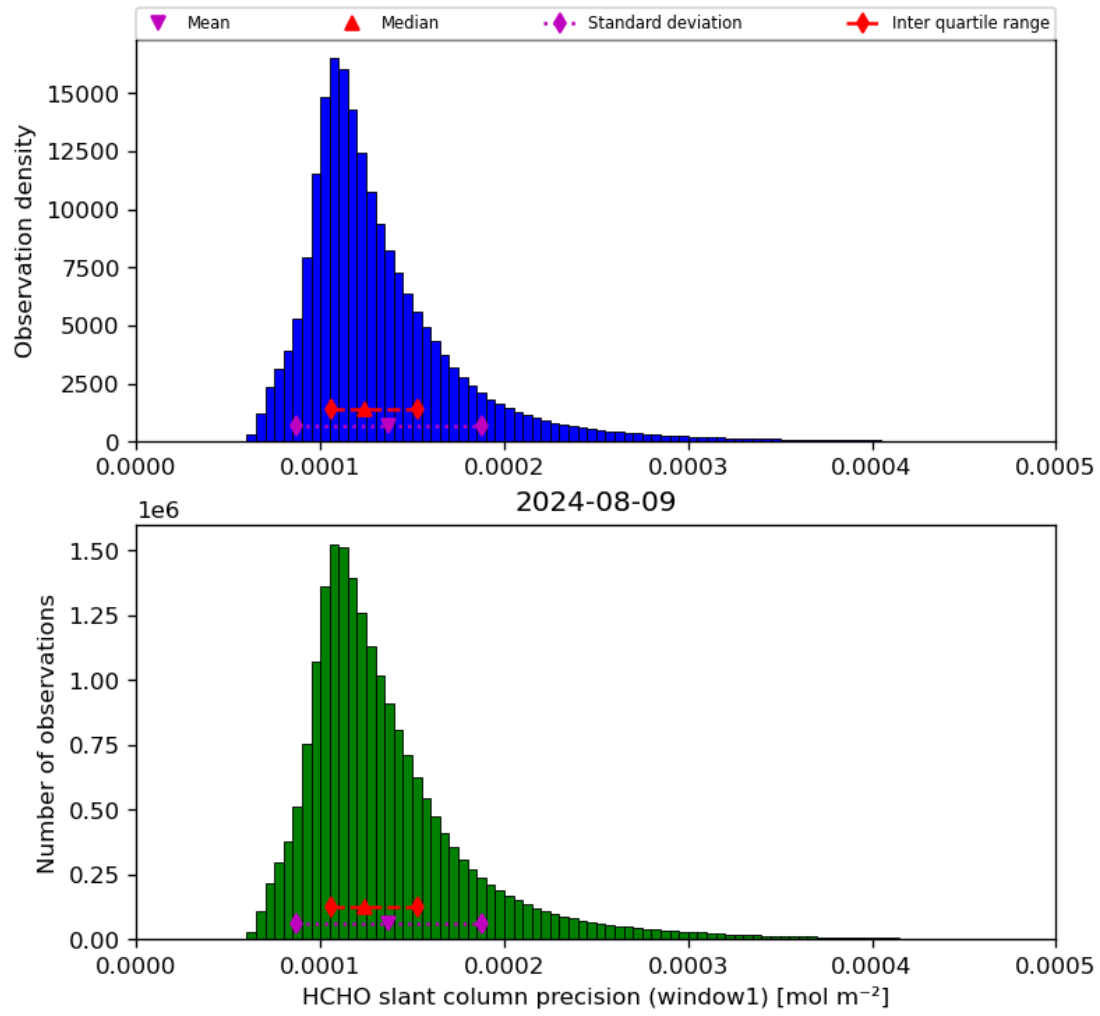
Figure 39: Histogram of “HCHO slant column precision (window1)” for 2024-08-08 to 2024-08-10
