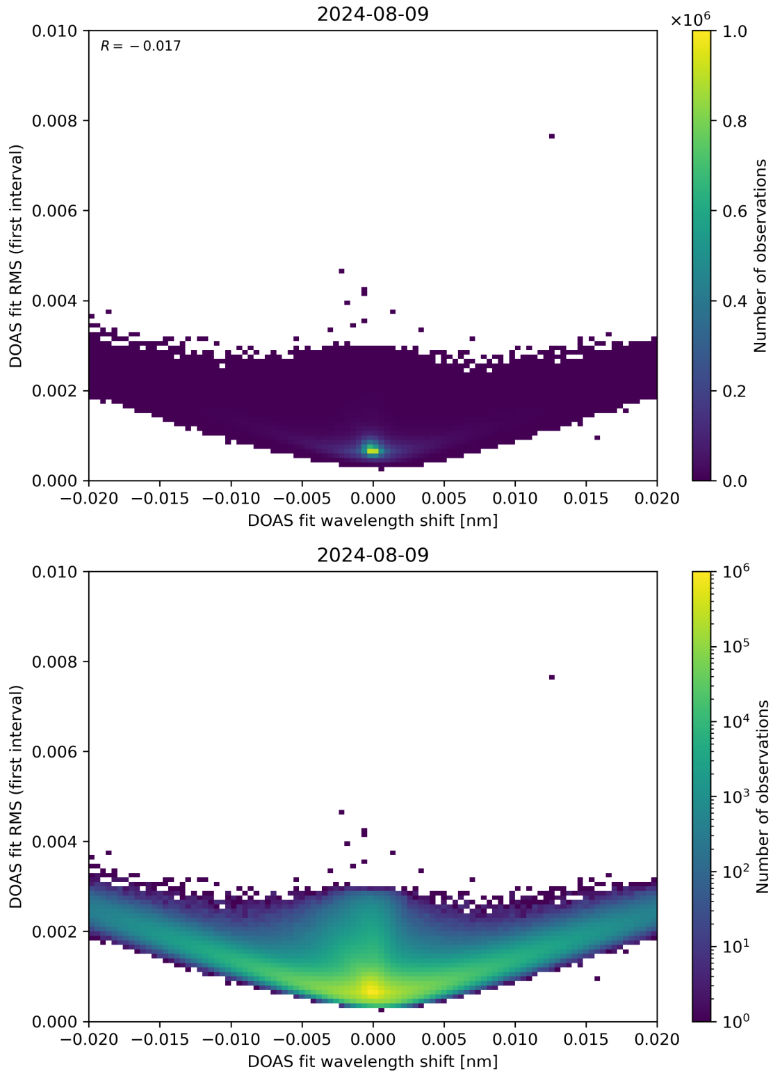
Figure 64: Scatter density plot of “DOAS fit wavelength shift” against “DOAS fit RMS (first interval)” for 2024-08-08 to 2024-08-10.
