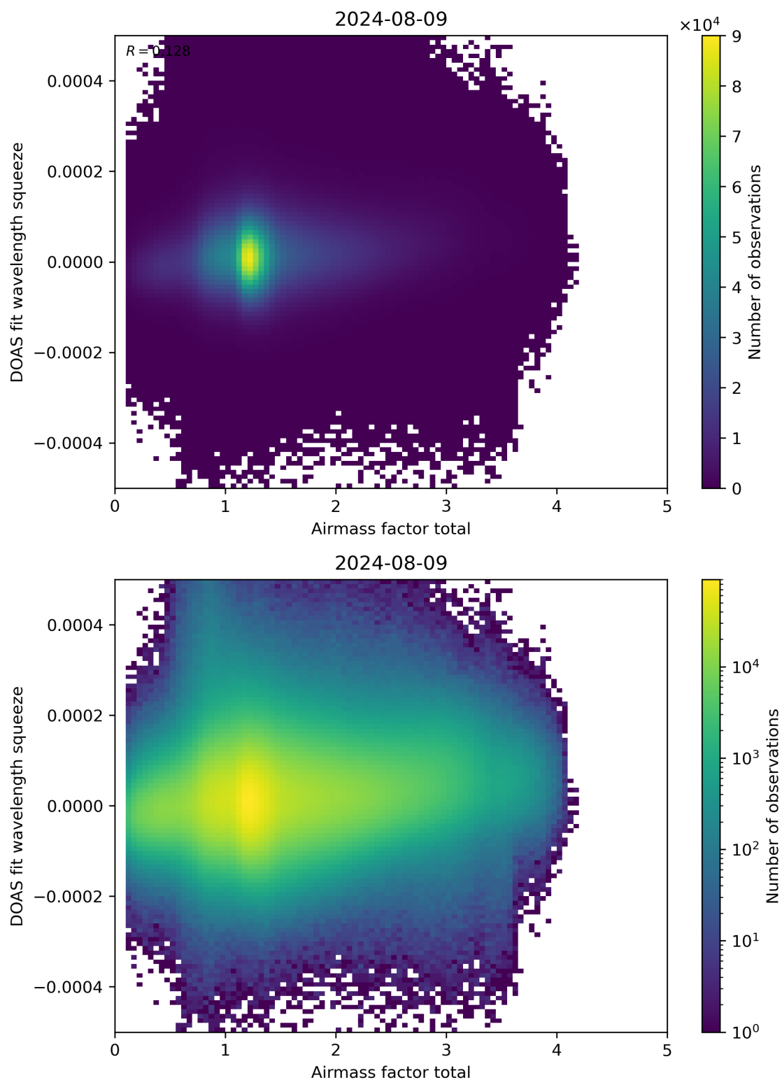
Figure 99: Scatter density plot of “Airmass factor total” against “DOAS fit wavelength squeeze” for 2024-08-08 to 2024-08-10.
