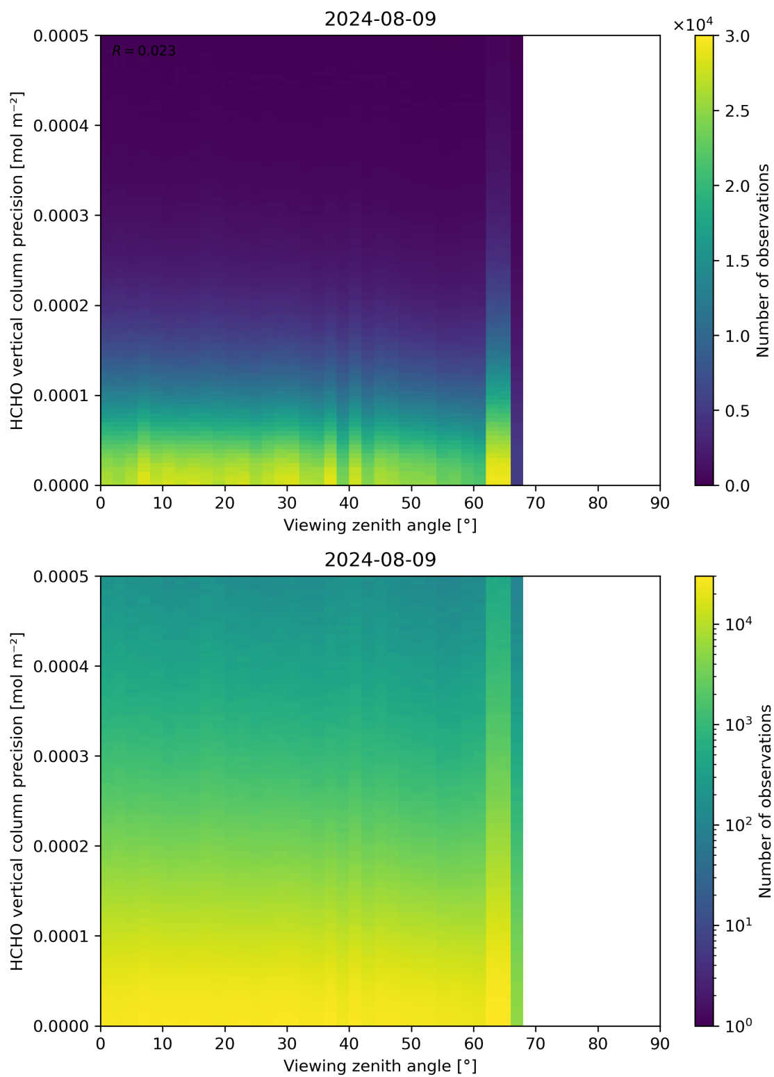
Figure 194: Scatter density plot of “Viewing zenith angle” against “HCHO vertical column precision” for 2024-08-08 to 2024-08-10.
