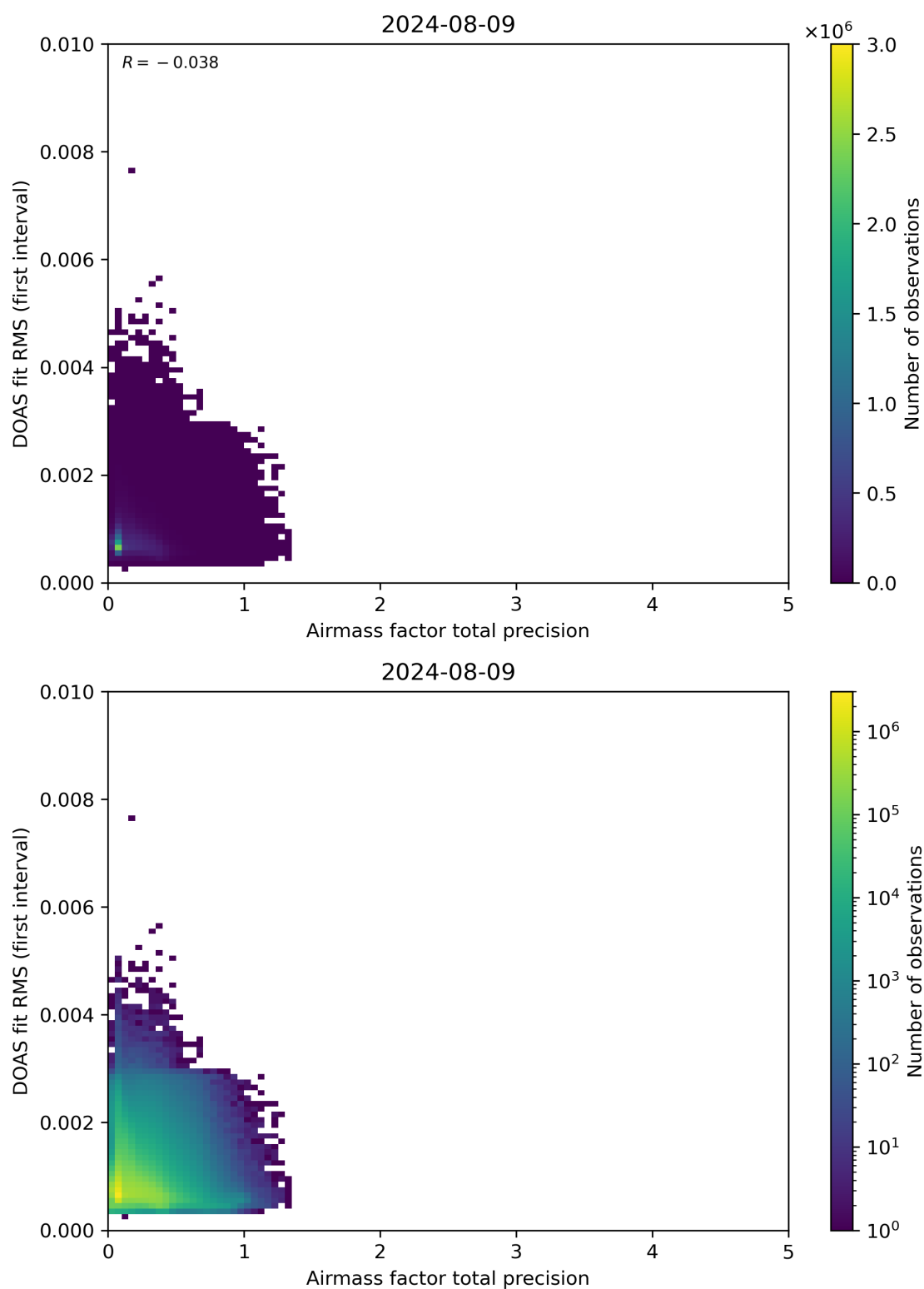
Figure 105: Scatter density plot of “Airmass factor total precision” against “DOAS fit RMS (first interval)” for 2024-08-08 to 2024-08-10.
