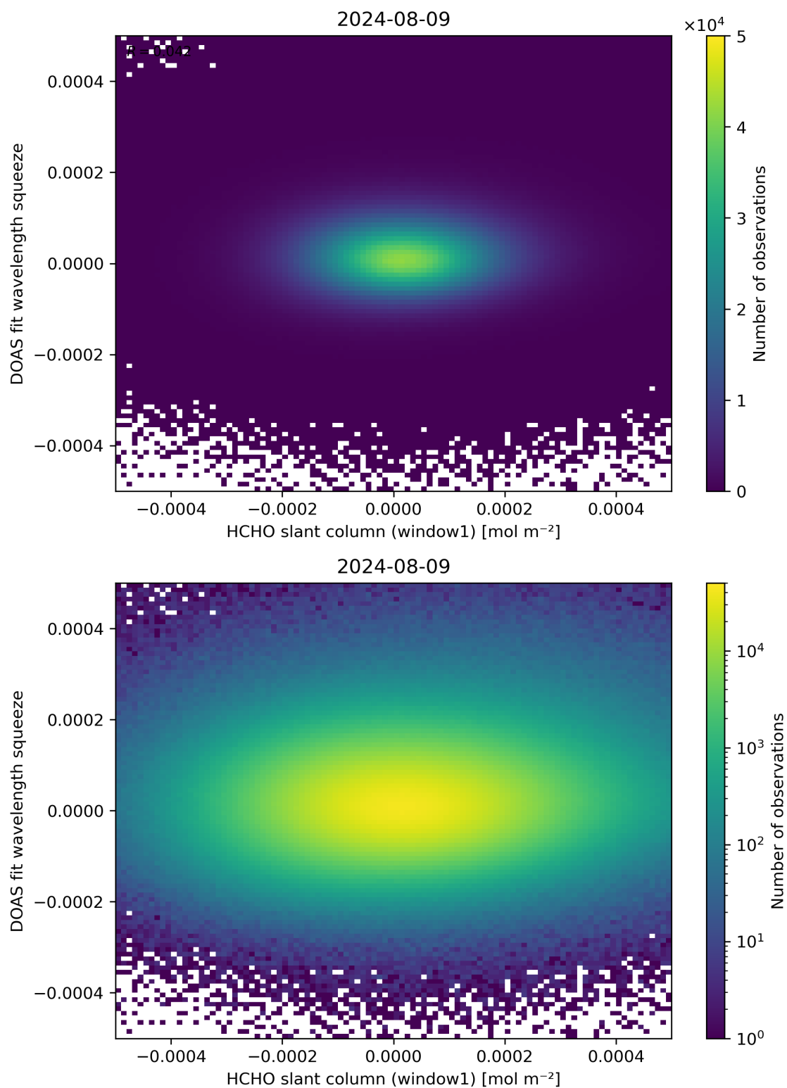
Figure 80: Scatter density plot of “HCHO slant column (window1)” against “DOAS fit wavelength squeeze” for 2024-08-08 to 2024-08-10.
