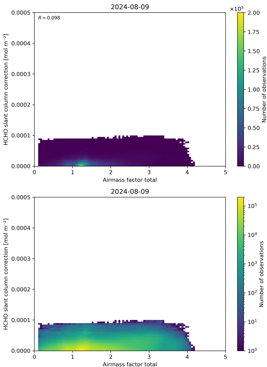
Figure 102: Scatter density plot of “Airmass factor total” against “HCHO slant column correction” for 2024-08-08 to 2024-08-10.
