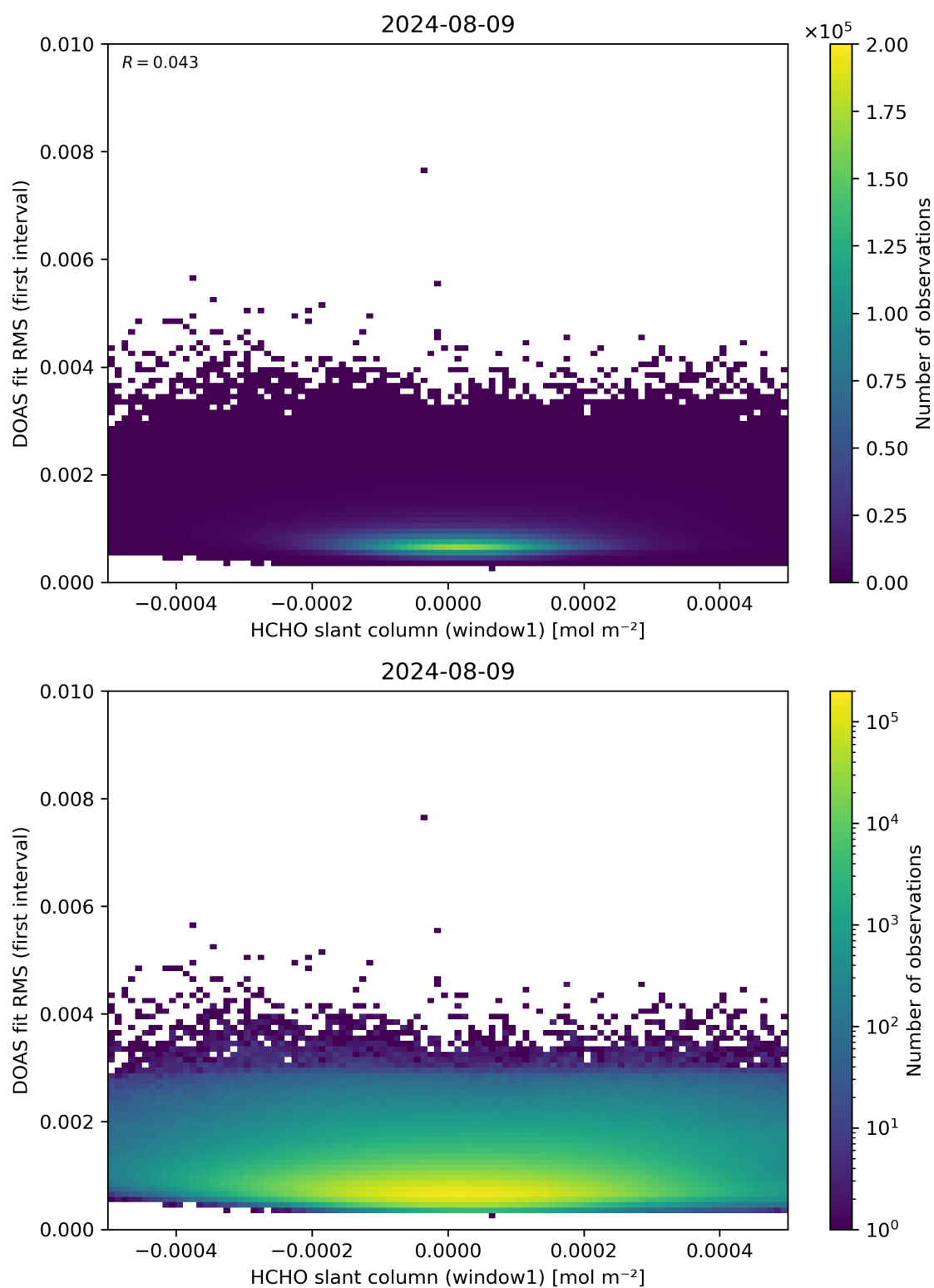
Figure 78: Scatter density plot of “HCHO slant column (window1)” against “DOAS fit RMS (first interval)” for 2024-08-08 to 2024-08-10.
