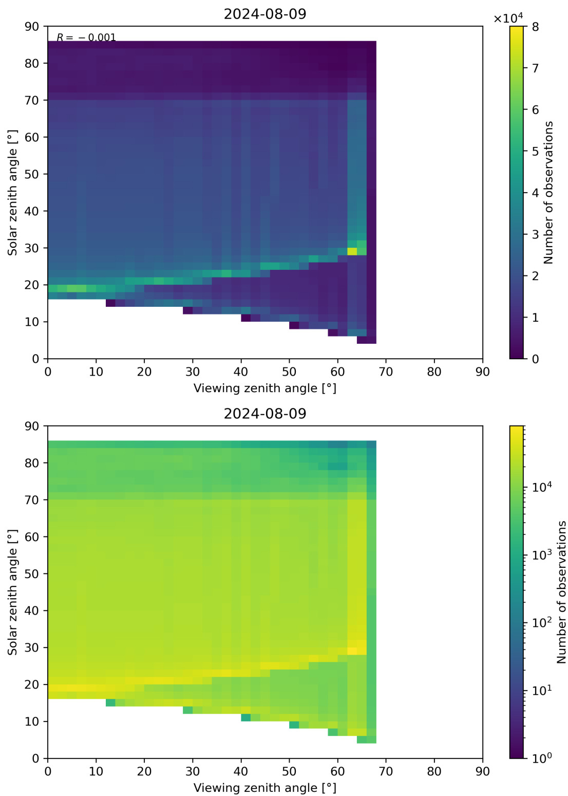
Figure 197: Scatter density plot of “Viewing zenith angle” against “Solar zenith angle” for 2024-08-08 to 2024-08-10.
