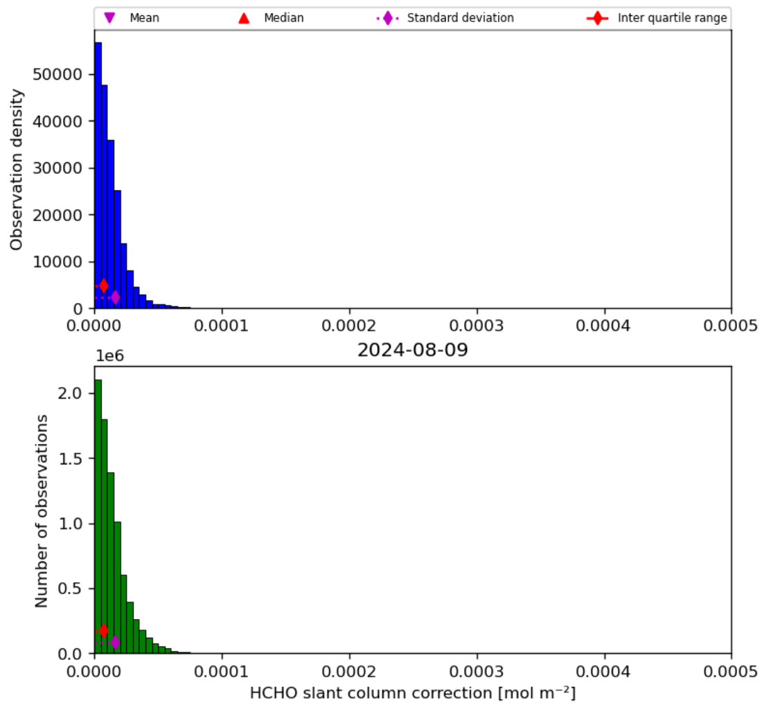
Figure 47: Histogram of “HCHO slant column correction” for 2024-08-08 to 2024-08-10
