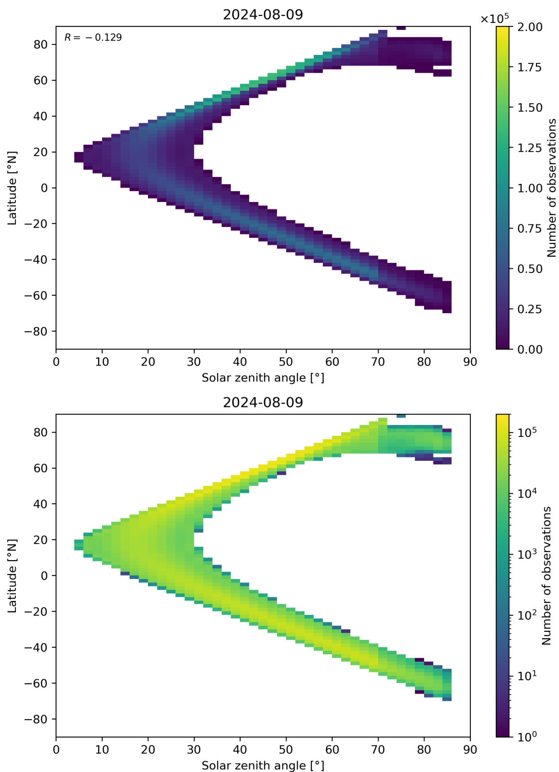
Figure 181: Scatter density plot of “Solar zenith angle” against “Latitude” for 2024-08-08 to 2024-08-10.
