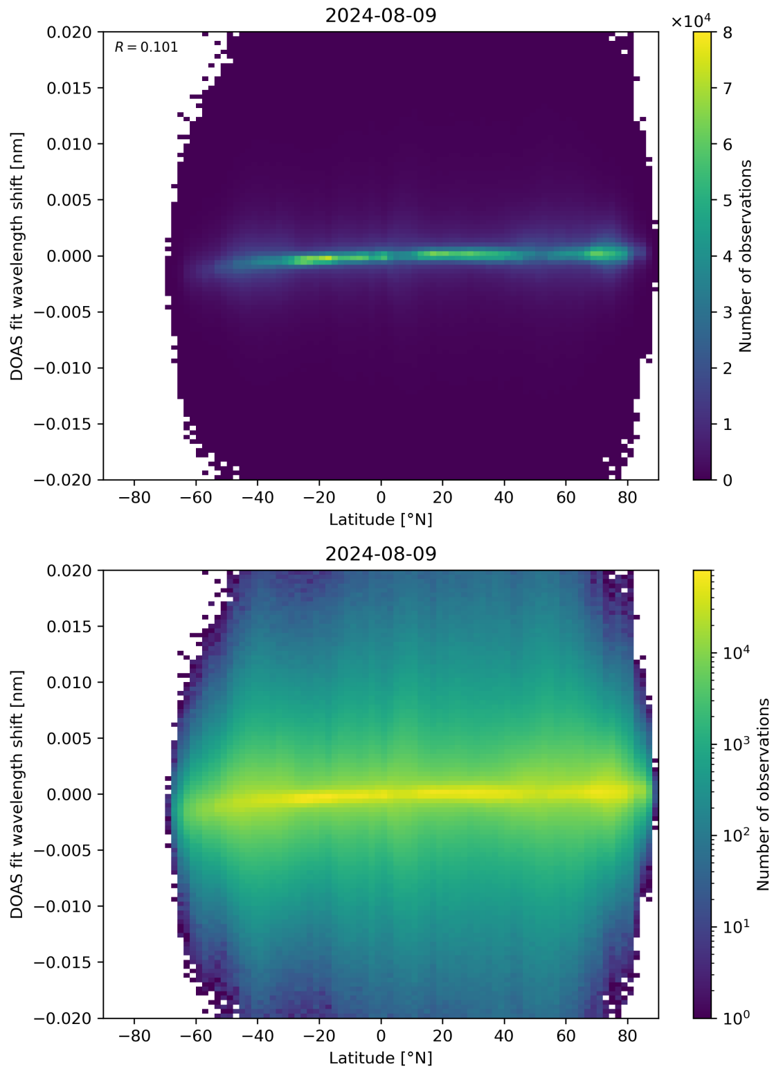
Figure 154: Scatter density plot of “Latitude” against “DOAS fit wavelength shift” for 2024-08-08 to 2024-08-10.
