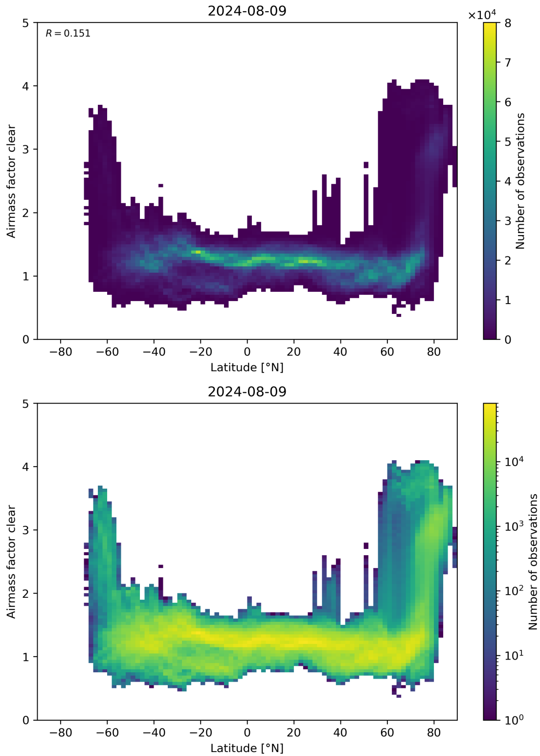
Figure 156: Scatter density plot of “Latitude” against “Airmass factor clear” for 2024-08-08 to 2024-08-10.
