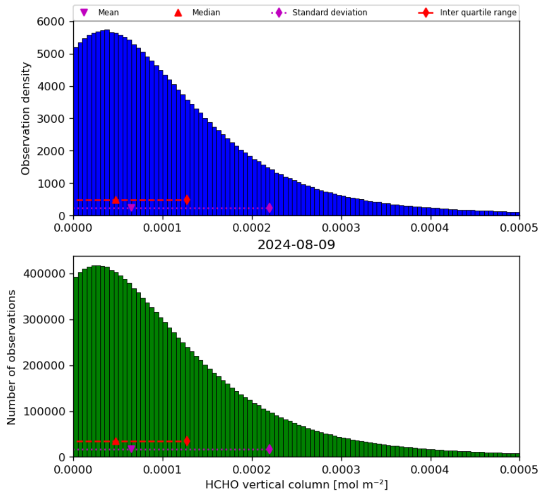
Figure 35: Histogram of “HCHO vertical column” for 2024-08-08 to 2024-08-10
