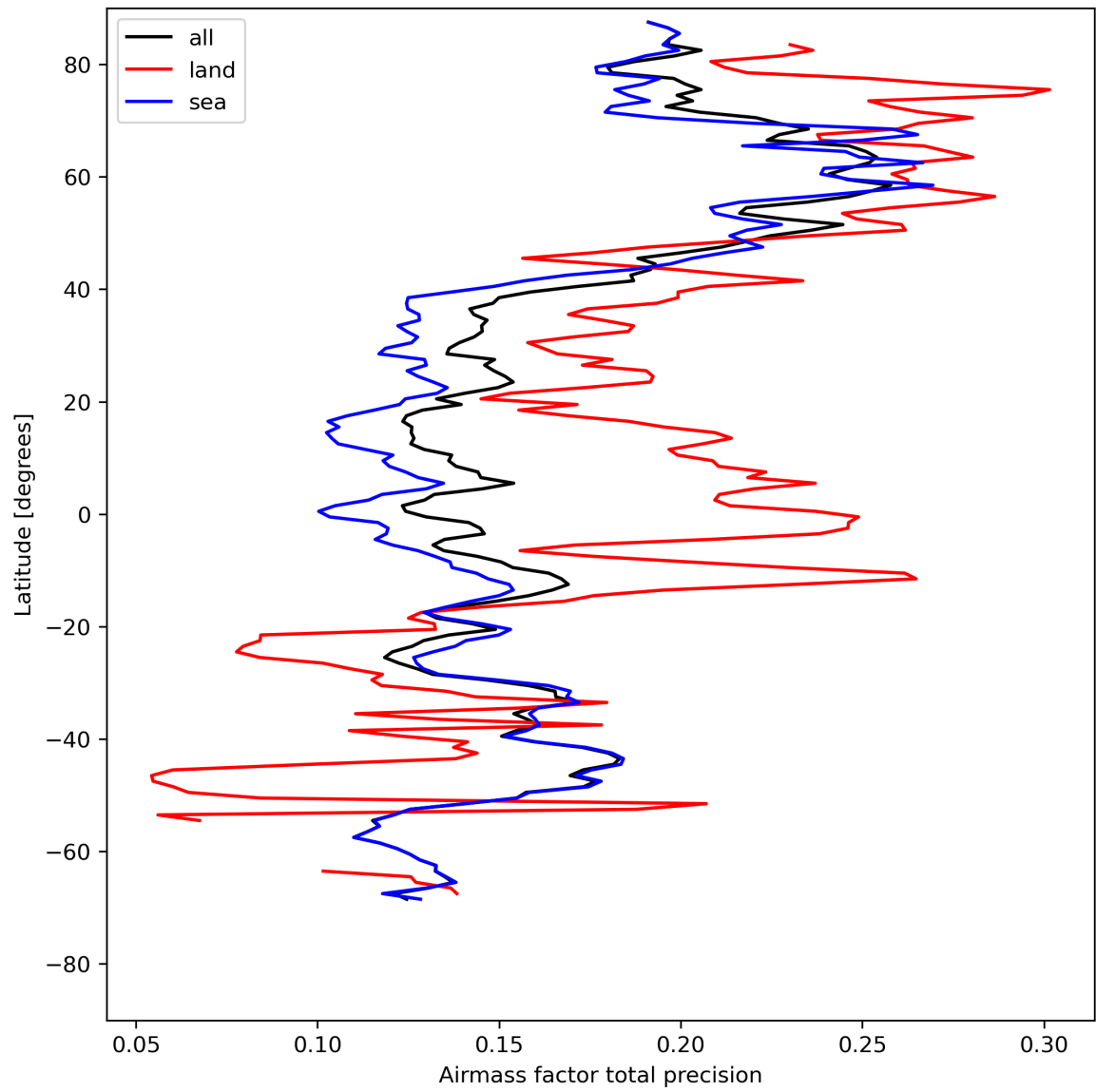
Figure 27: Zonal average of “Airmass factor total precision” for 2024-08-08 to 2024-08-10.
