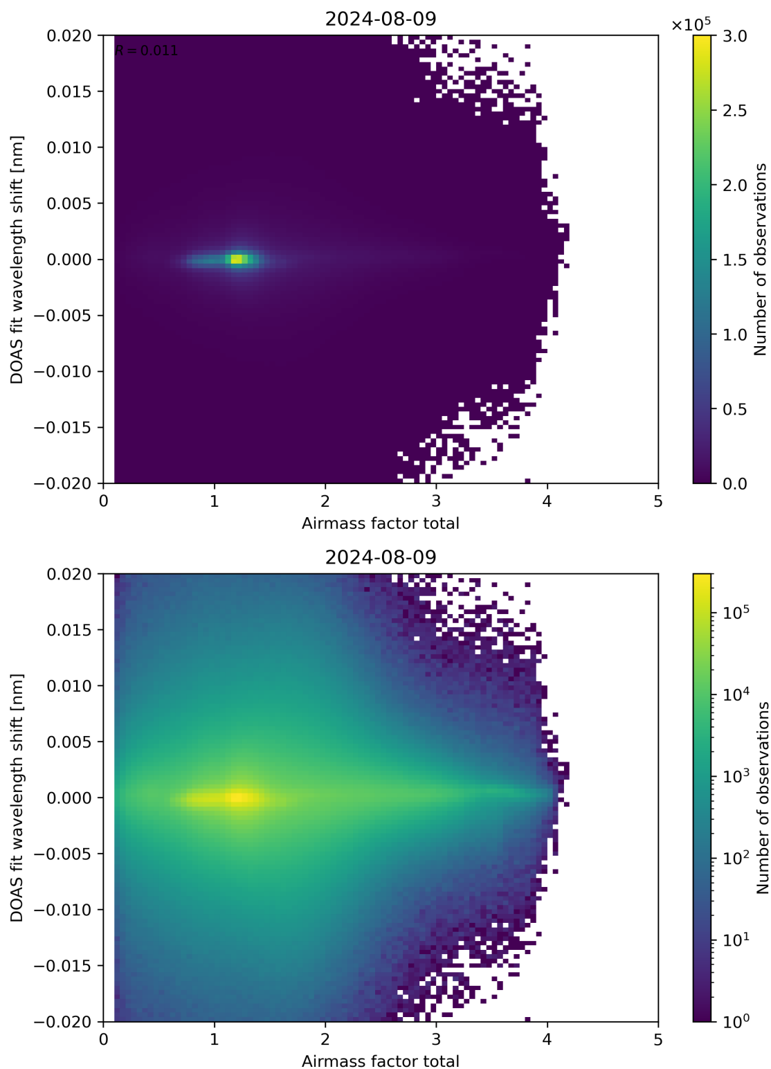
Figure 98: Scatter density plot of “Airmass factor total” against “DOAS fit wavelength shift” for 2024-08-08 to 2024-08-10.
