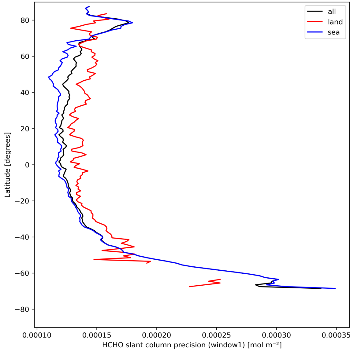
Figure 25: Zonal average of “HCHO slant column precision (window1)” for 2024-08-08 to 2024-08-10.
