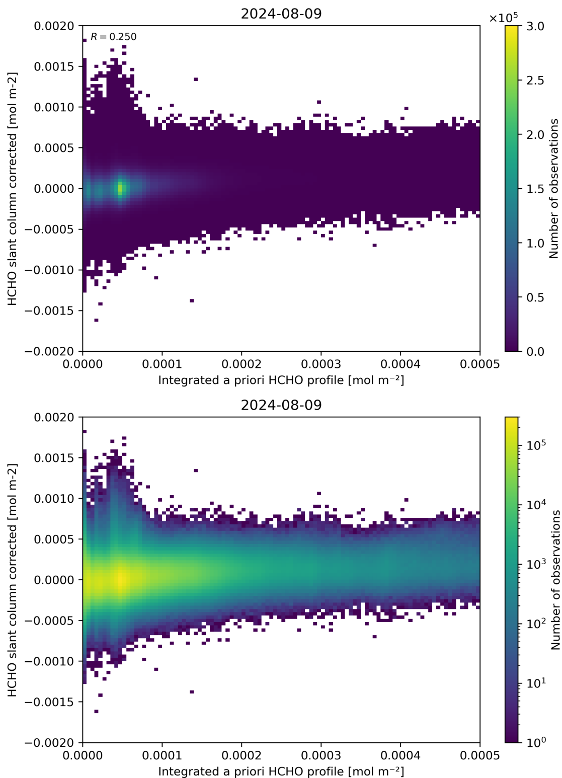
Figure 151: Scatter density plot of “Integrated a priori HCHO profile” against “HCHO slant column corrected” for 2024-08-08 to 2024-08-10.
