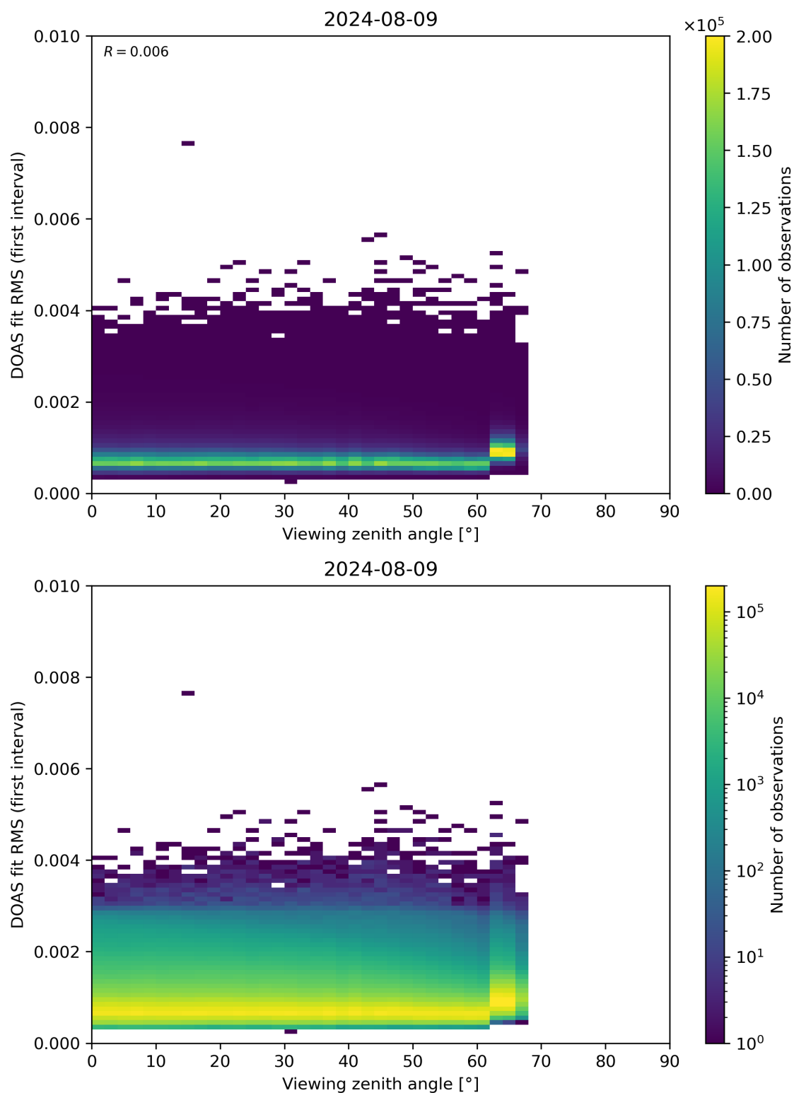
Figure 182: Scatter density plot of “Viewing zenith angle” against “DOAS fit RMS (first interval)” for 2024-08-08 to 2024-08-10.
