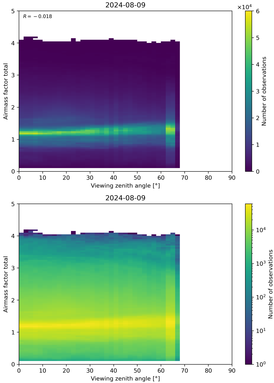
Figure 190: Scatter density plot of “Viewing zenith angle” against “Airmass factor total” for 2024-08-08 to 2024-08-10.
