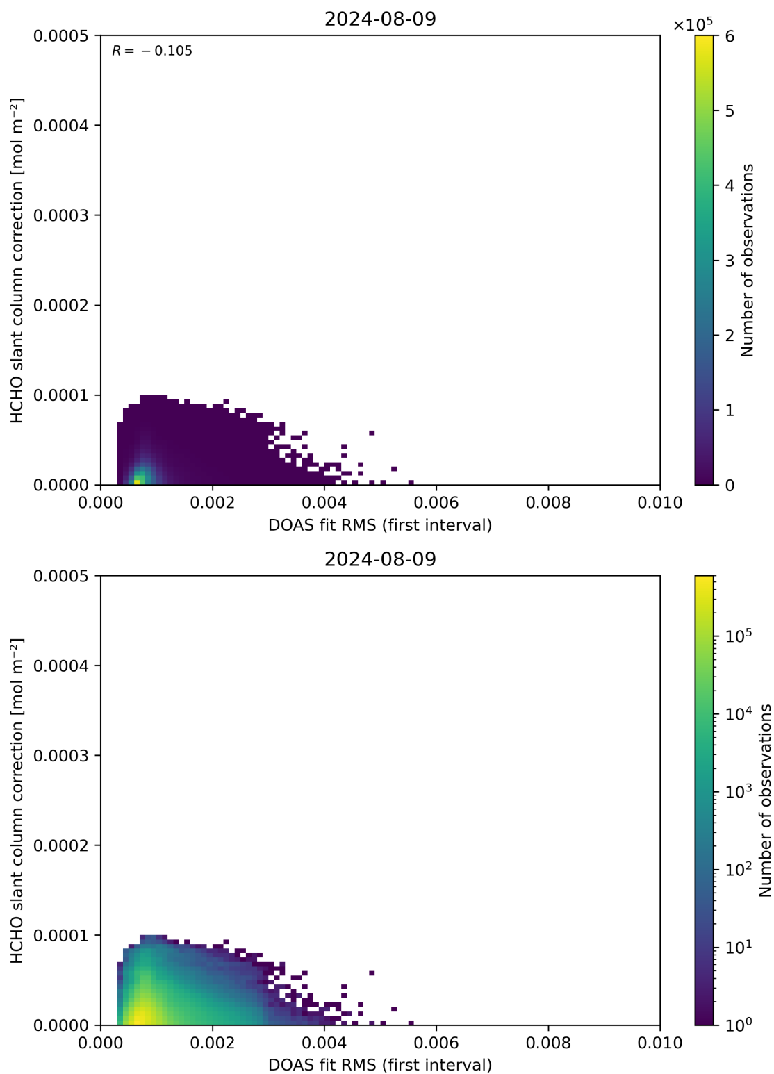
Figure 63: Scatter density plot of “DOAS fit RMS (first interval)” against “HCHO slant column correction” for 2024-08-08 to 2024-08-10.
