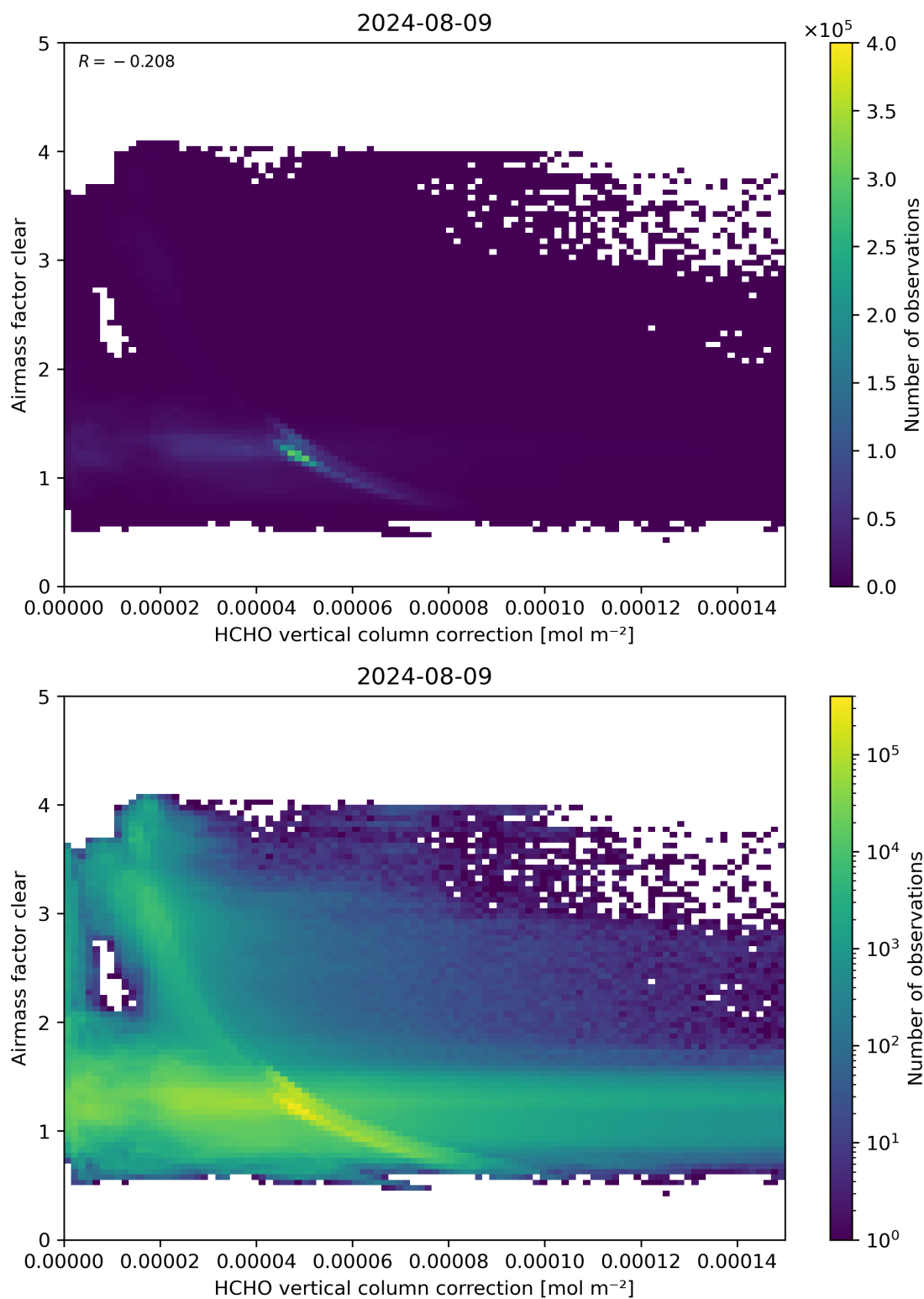
Figure 115: Scatter density plot of “HCHO vertical column correction” against “Airmass factor clear” for 2024-08-08 to 2024-08-10.
