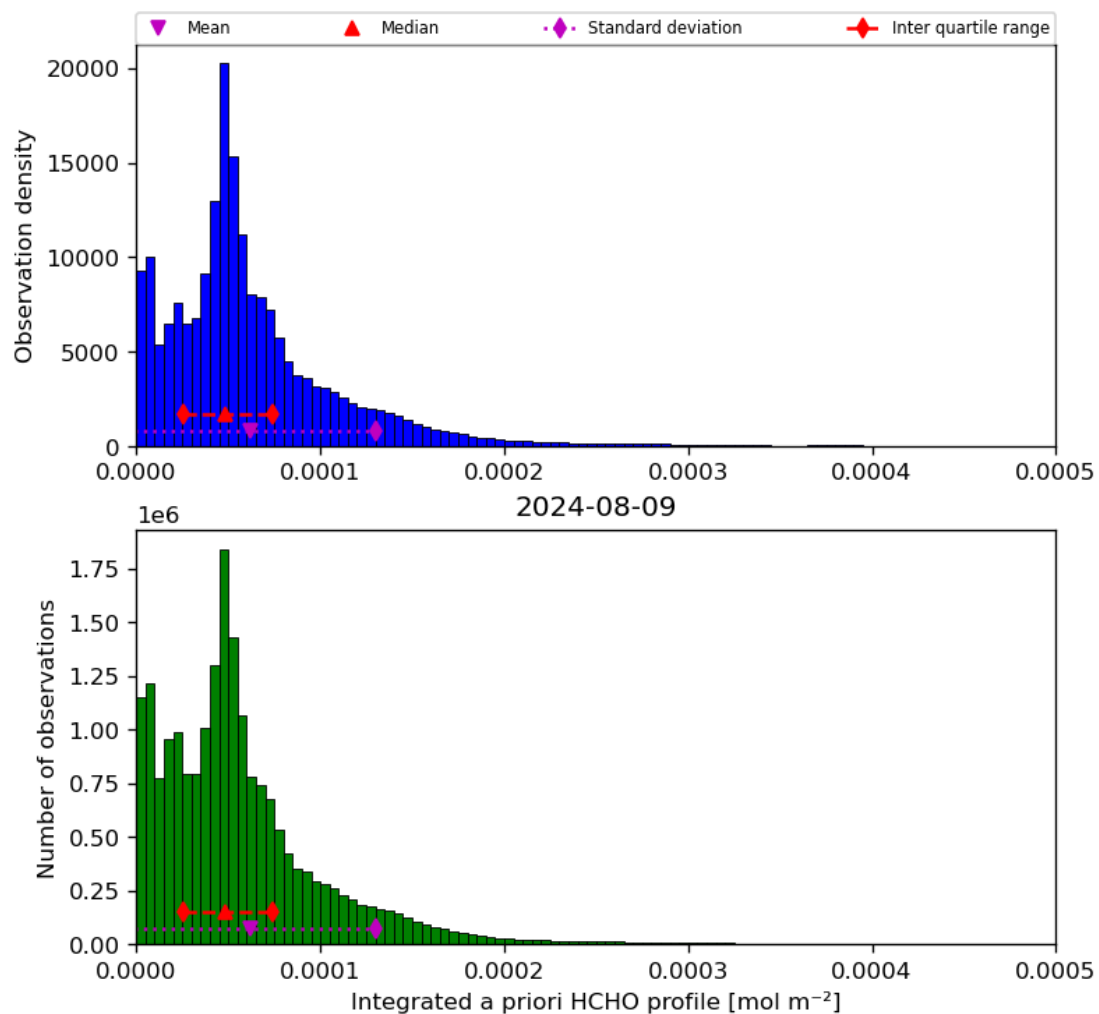
Figure 43: Histogram of “Integrated a priori HCHO profile” for 2024-08-08 to 2024-08-10
