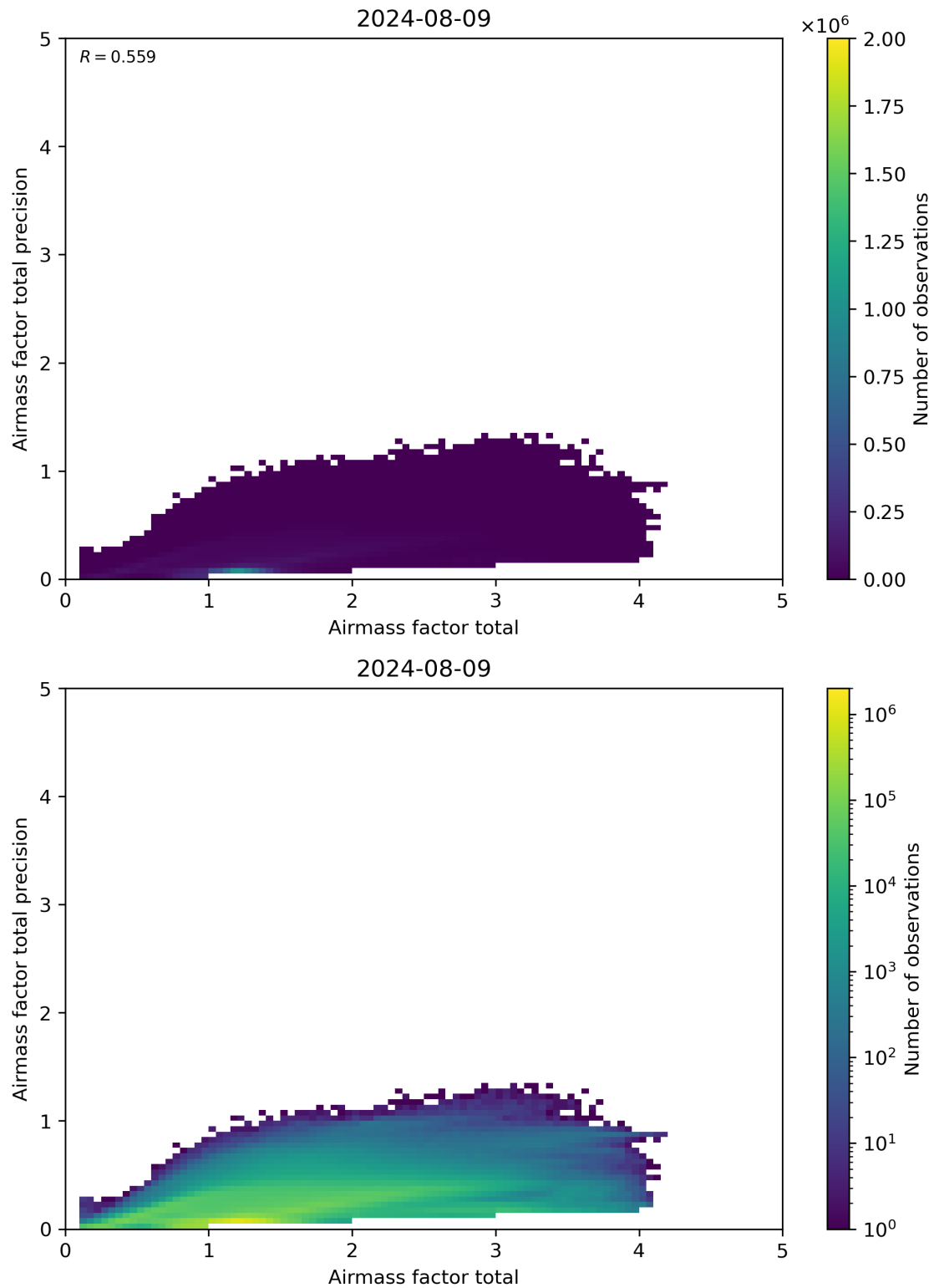
Figure 103: Scatter density plot of “Airmass factor total” against “Airmass factor total precision” for 2024-08-08 to 2024-08-10.
