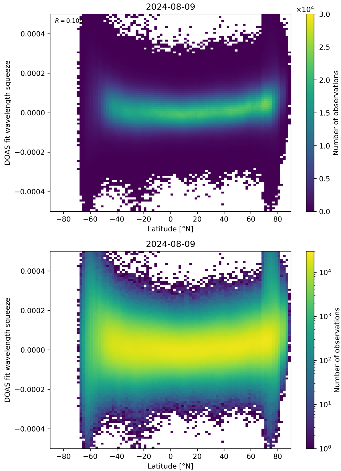
Figure 155: Scatter density plot of “Latitude” against “DOAS fit wavelength squeeze” for 2024-08-08 to 2024-08-10.
