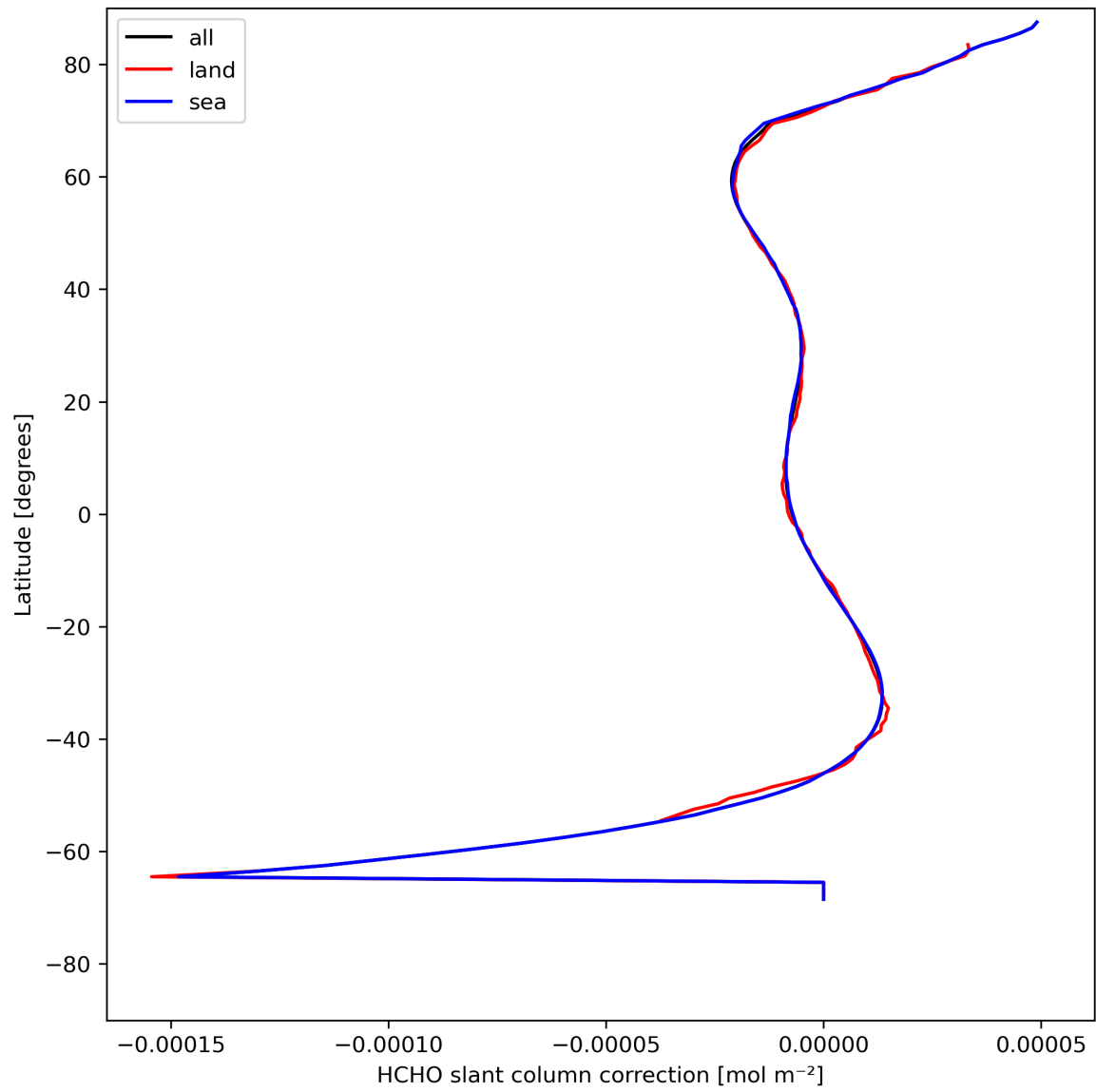
Figure 33: Zonal average of “HCHO slant column correction” for 2024-08-08 to 2024-08-10.
