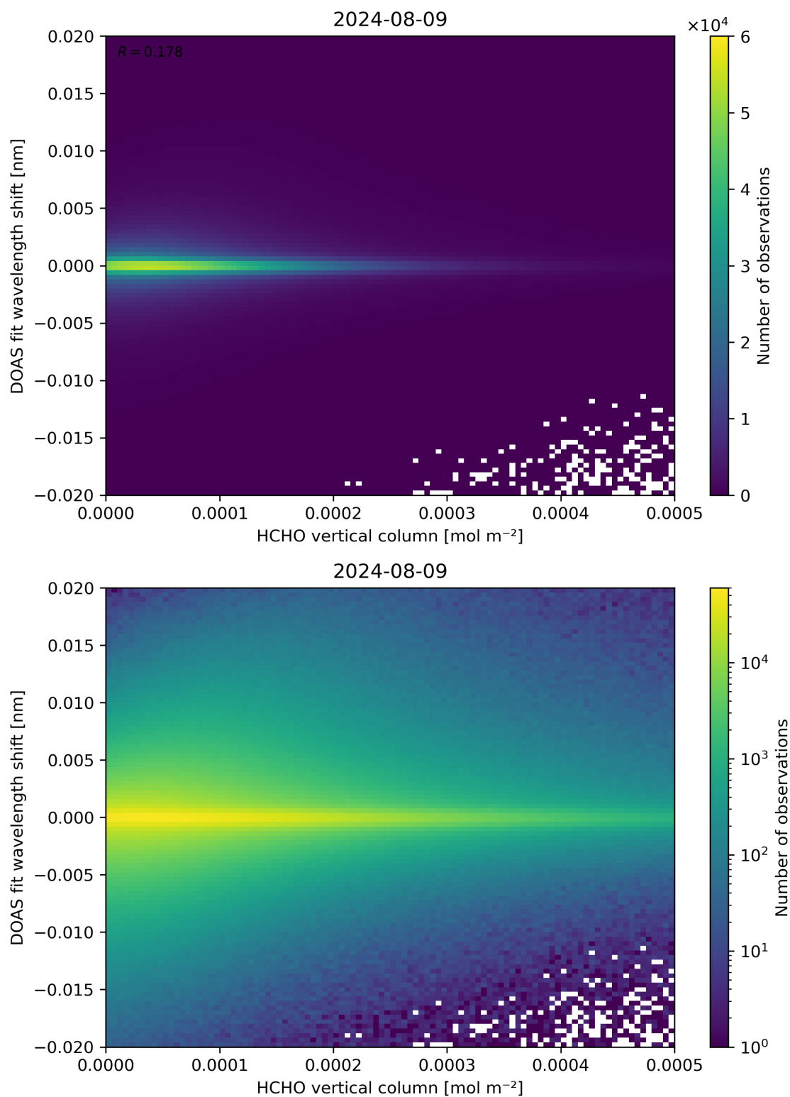
Figure 124: Scatter density plot of “HCHO vertical column” against “DOAS fit wavelength shift” for 2024-08-08 to 2024-08-10.
