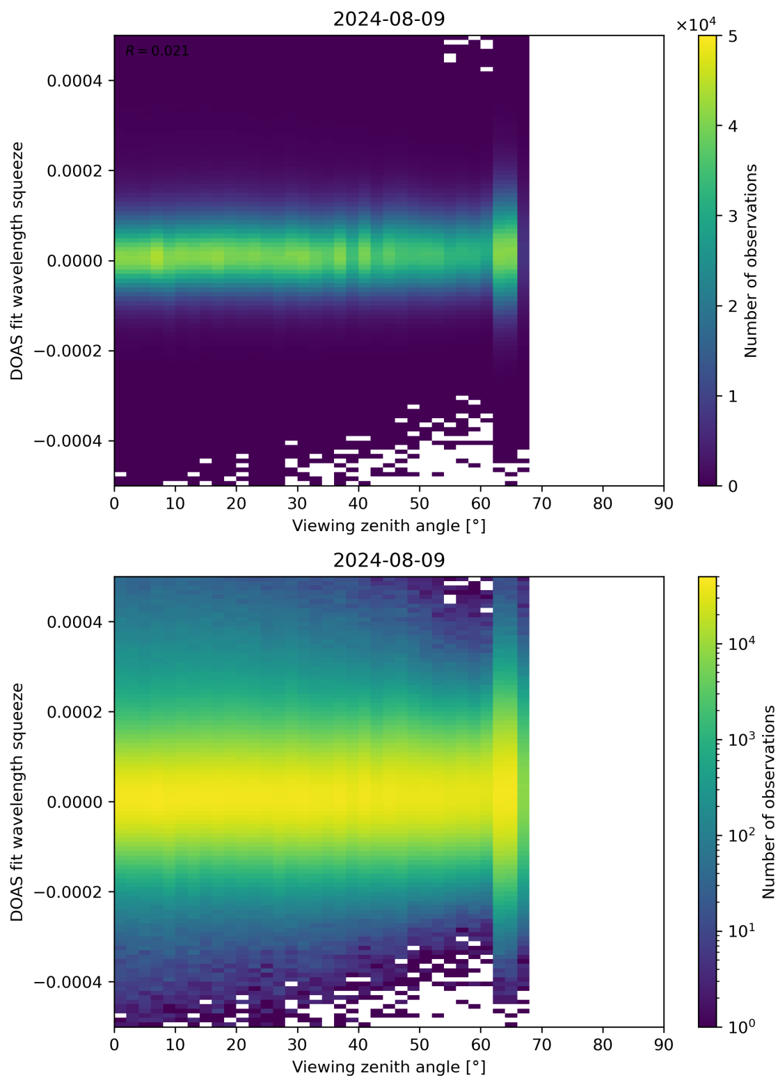
Figure 184: Scatter density plot of “Viewing zenith angle” against “DOAS fit wavelength squeeze” for 2024-08-08 to 2024-08-10.
