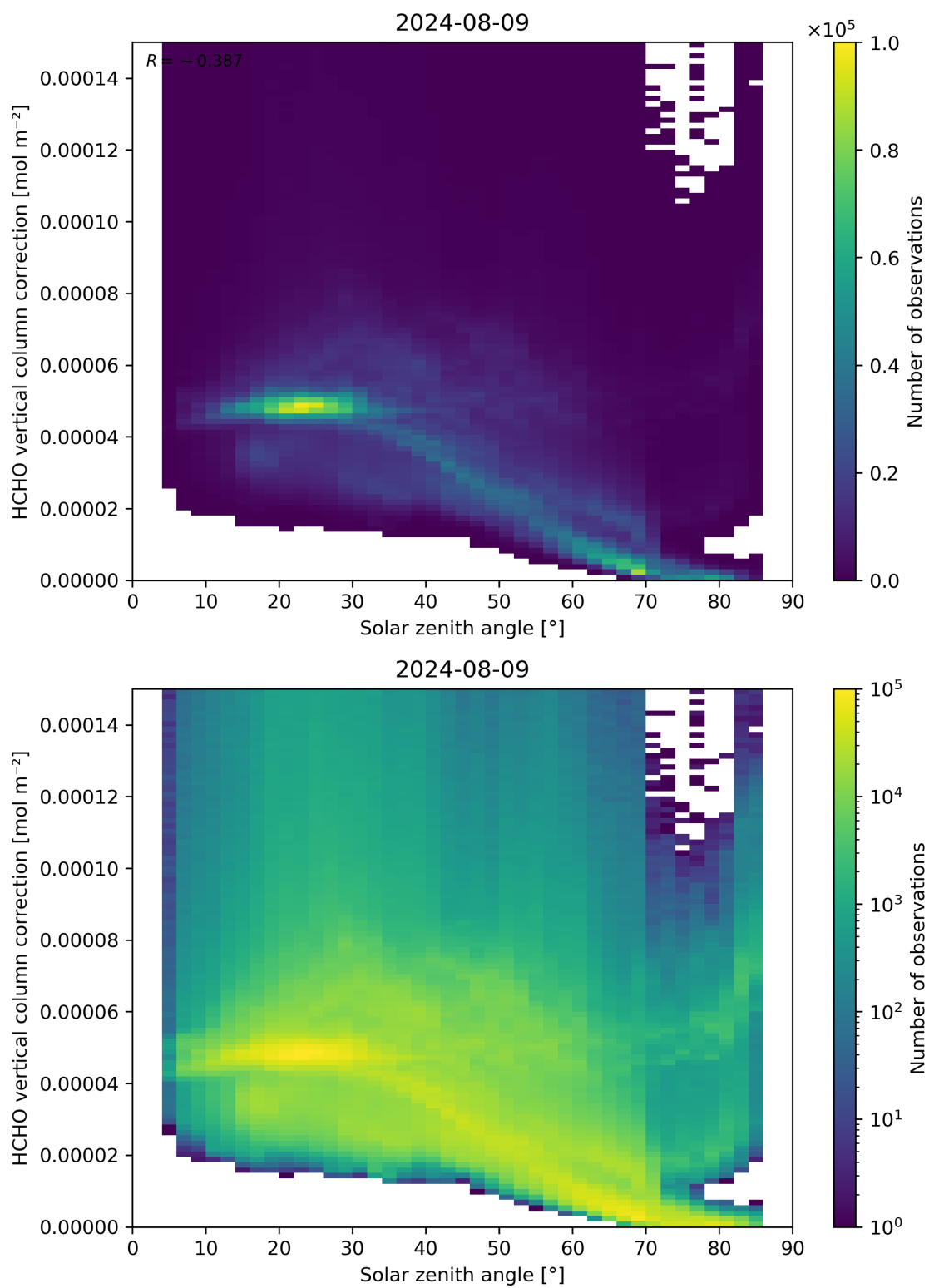
Figure 178: Scatter density plot of “Solar zenith angle” against “HCHO vertical column correction” for 2024-08-08 to 2024-08-10.
