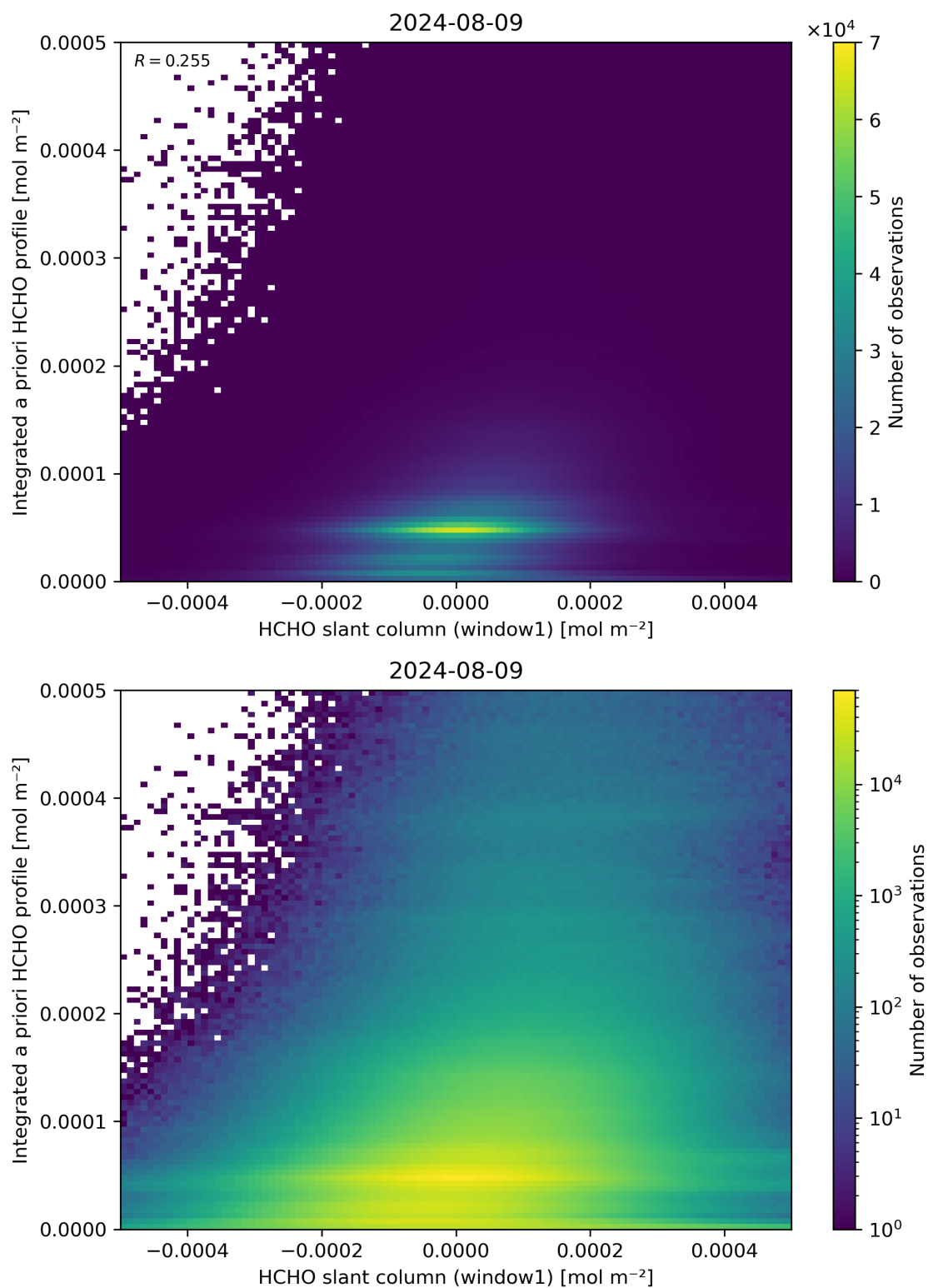
Figure 87: Scatter density plot of “HCHO slant column (window1)” against “Integrated a priori HCHO profile” for 2024-08-08 to 2024-08-10.
