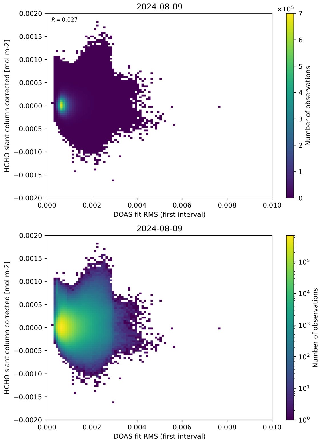
Figure 62: Scatter density plot of “DOAS fit RMS (first interval)” against “HCHO slant column corrected” for 2024-08-08 to 2024-08-10.
