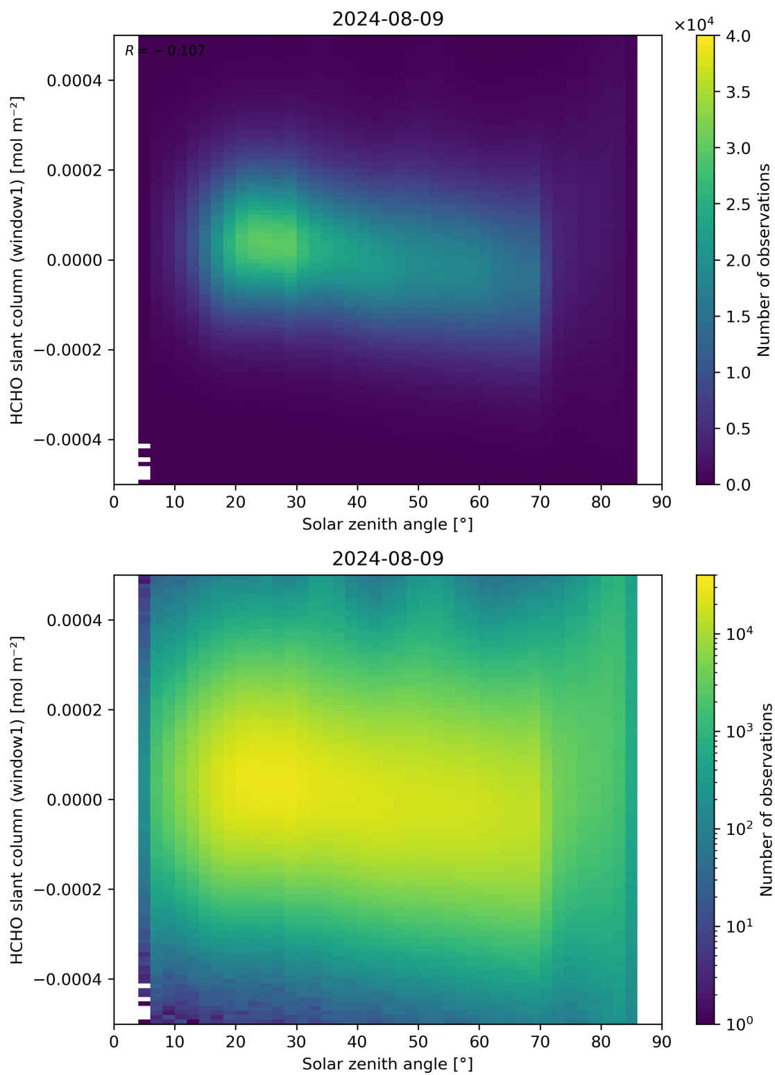
Figure 173: Scatter density plot of “Solar zenith angle” against “HCHO slant column (window1)” for 2024-08-08 to 2024-08-10.
