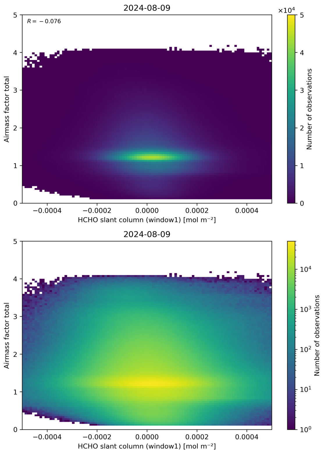
Figure 85: Scatter density plot of “HCHO slant column (window1)” against “Airmass factor total” for 2024-08-08 to 2024-08-10.
