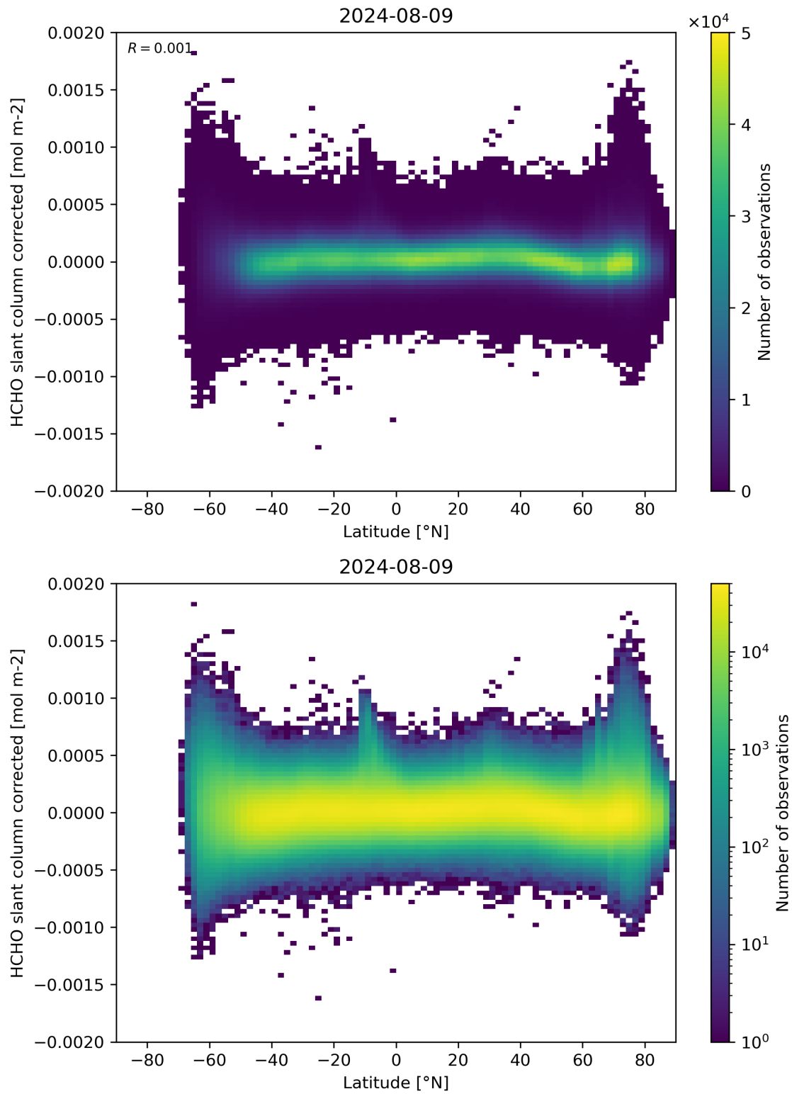
Figure 157: Scatter density plot of “Latitude” against “HCHO slant column corrected” for 2024-08-08 to 2024-08-10.
