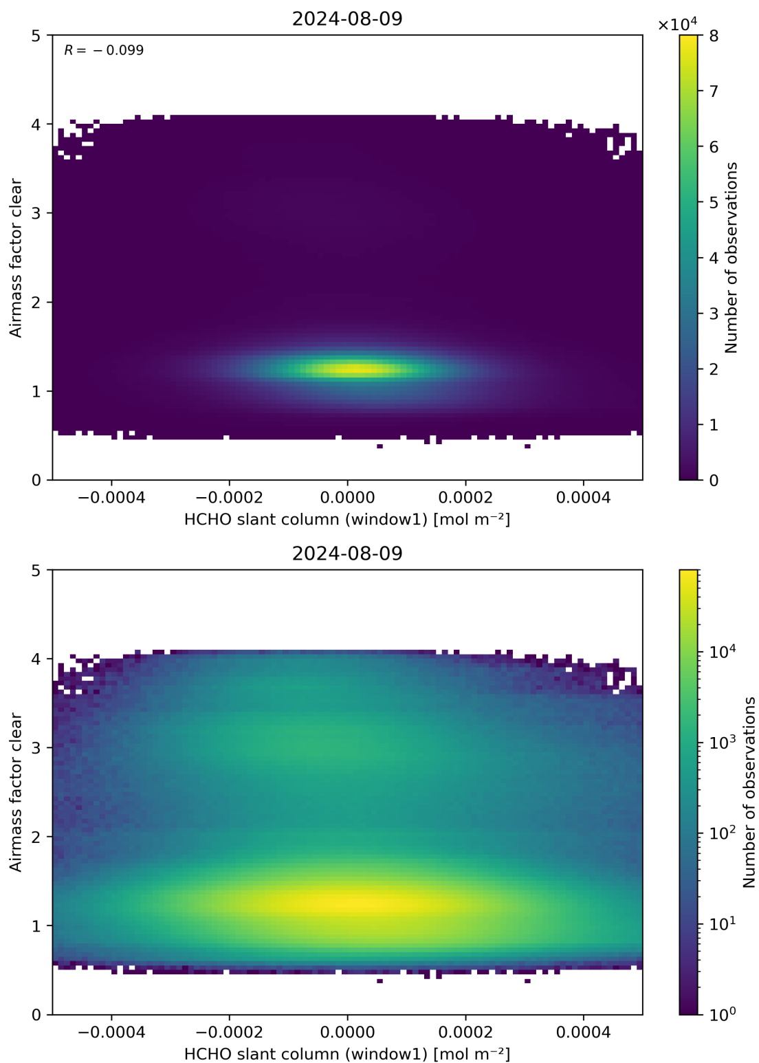
Figure 81: Scatter density plot of “HCHO slant column (window1)” against “Airmass factor clear” for 2024-08-08 to 2024-08-10.
