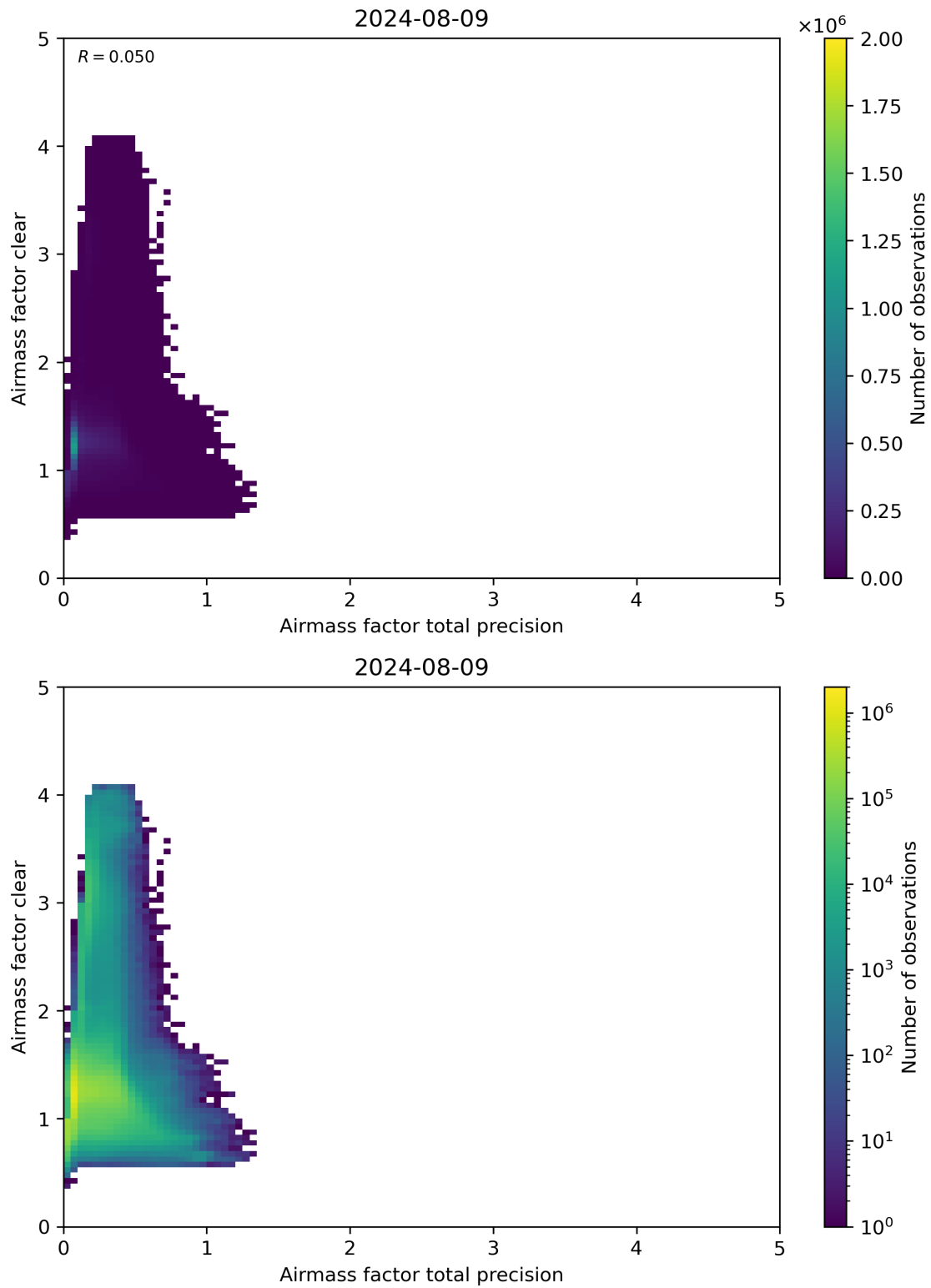
Figure 108: Scatter density plot of “Airmass factor total precision” against “Airmass factor clear” for 2024-08-08 to 2024-08-10.
