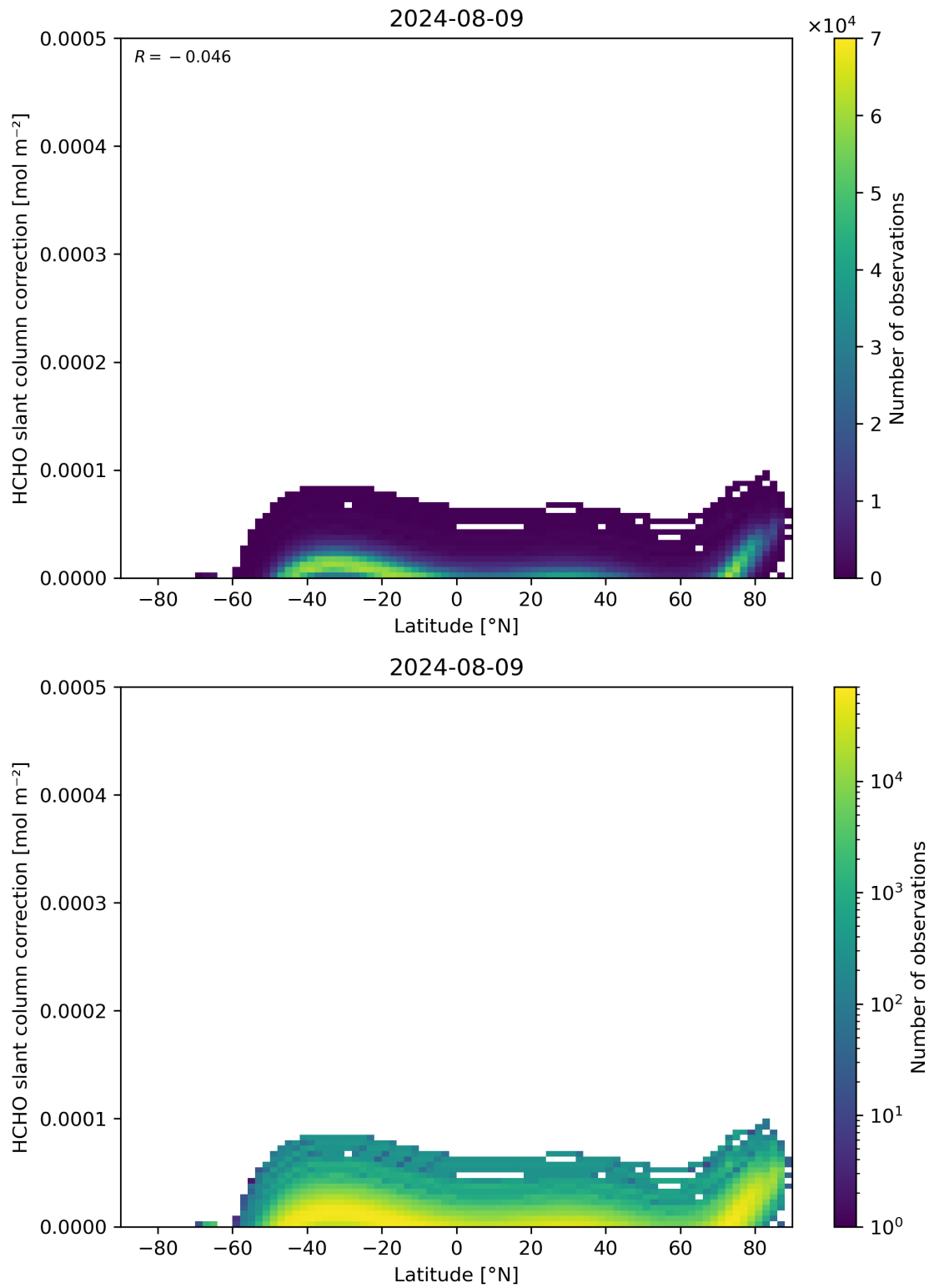
Figure 158: Scatter density plot of “Latitude” against “HCHO slant column correction” for 2024-08-08 to 2024-08-10.
