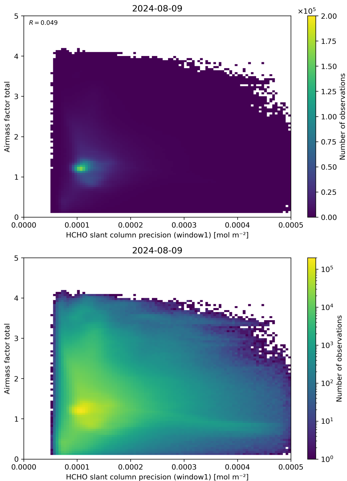
Figure 94: Scatter density plot of “HCHO slant column precision (window1)” against “Airmass factor total” for 2024-08-08 to 2024-08-10.
