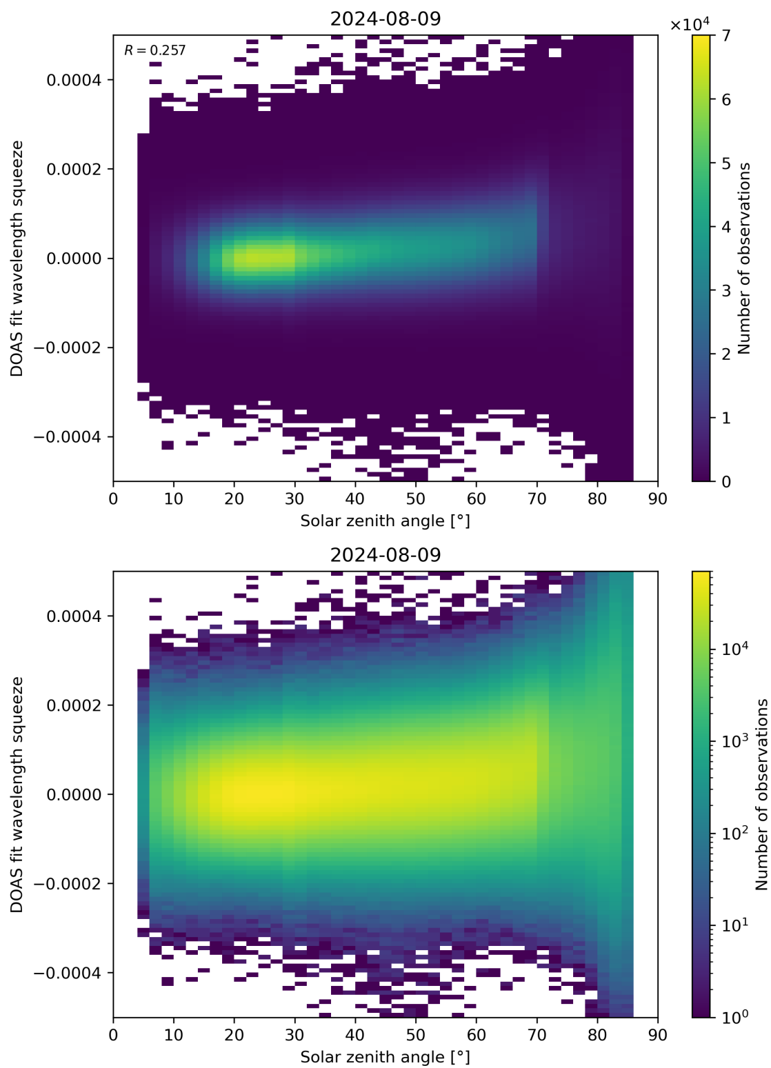
Figure 169: Scatter density plot of “Solar zenith angle” against “DOAS fit wavelength squeeze” for 2024-08-08 to 2024-08-10.
