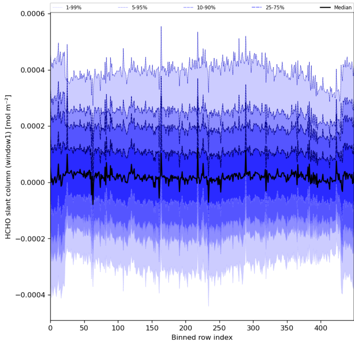
Figure 52: Along track statistics of "HCHO slant column (window1)" for 2024-08-08 to 2024-08-10
