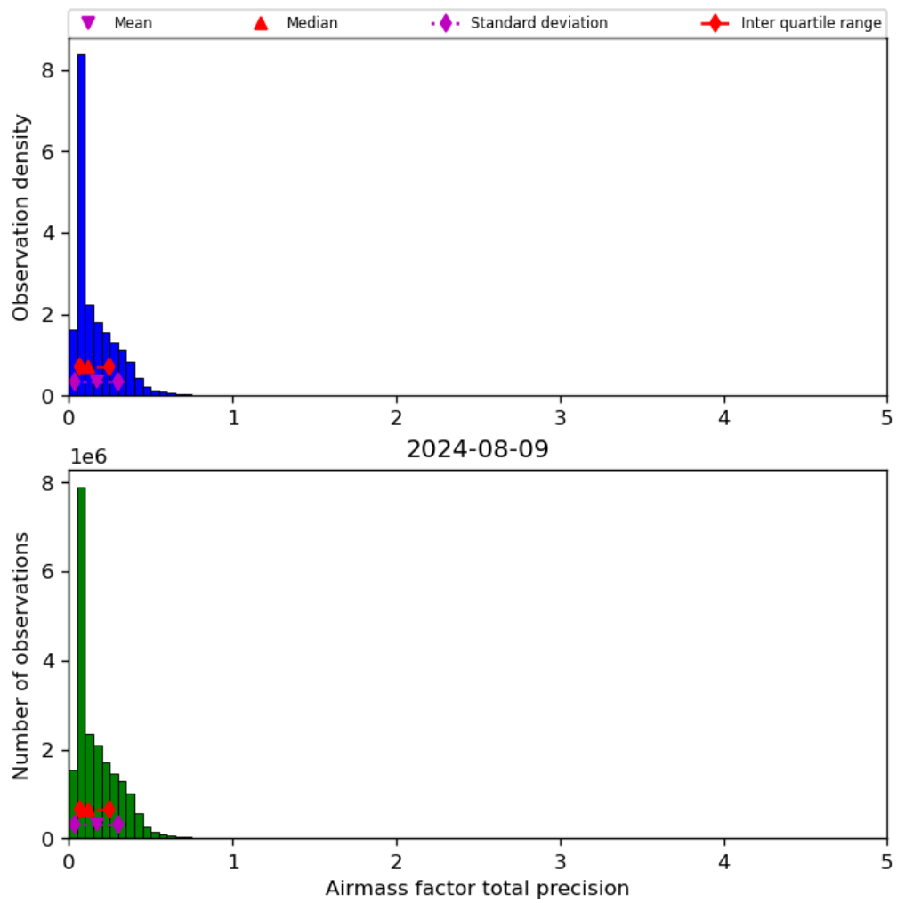
Figure 41: Histogram of “Airmass factor total precision” for 2024-08-08 to 2024-08-10
