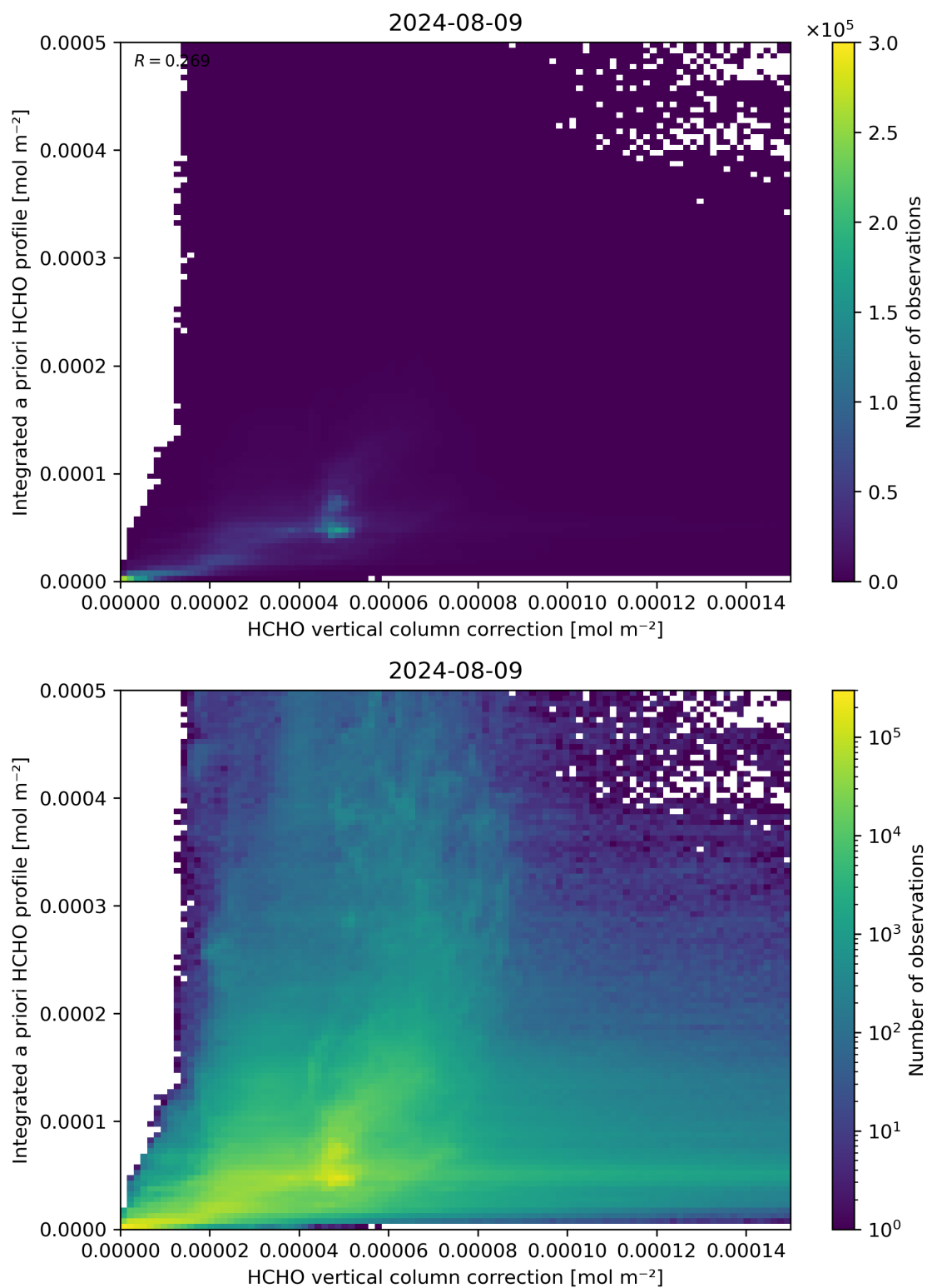
Figure 122: Scatter density plot of “HCHO vertical column correction” against “Integrated a priori HCHO profile” for 2024-08-08 to 2024-08-10.
