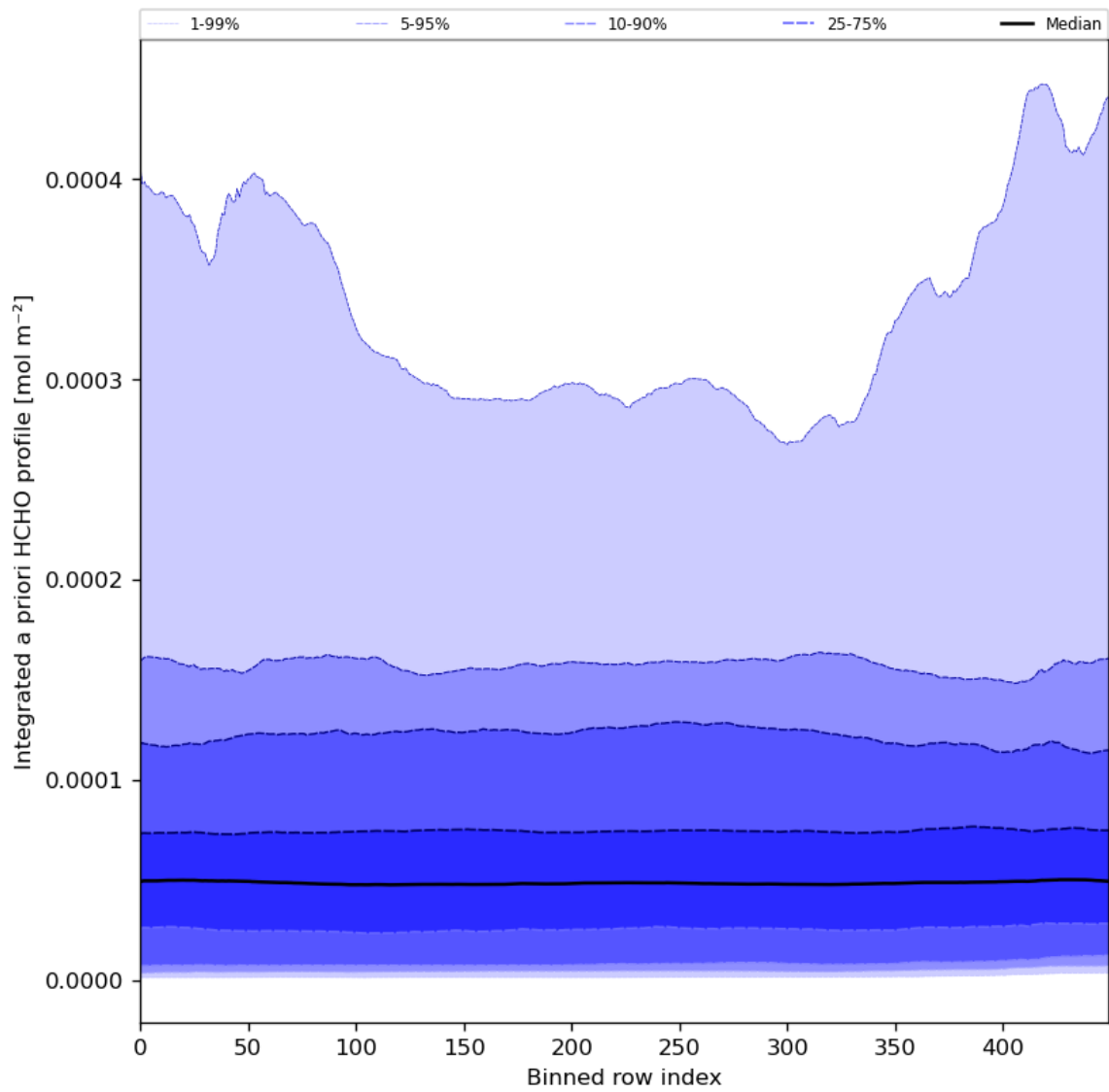
Figure 57: Along track statistics of “Integrated a priori HCHO profile” for 2024-08-08 to 2024-08-10
