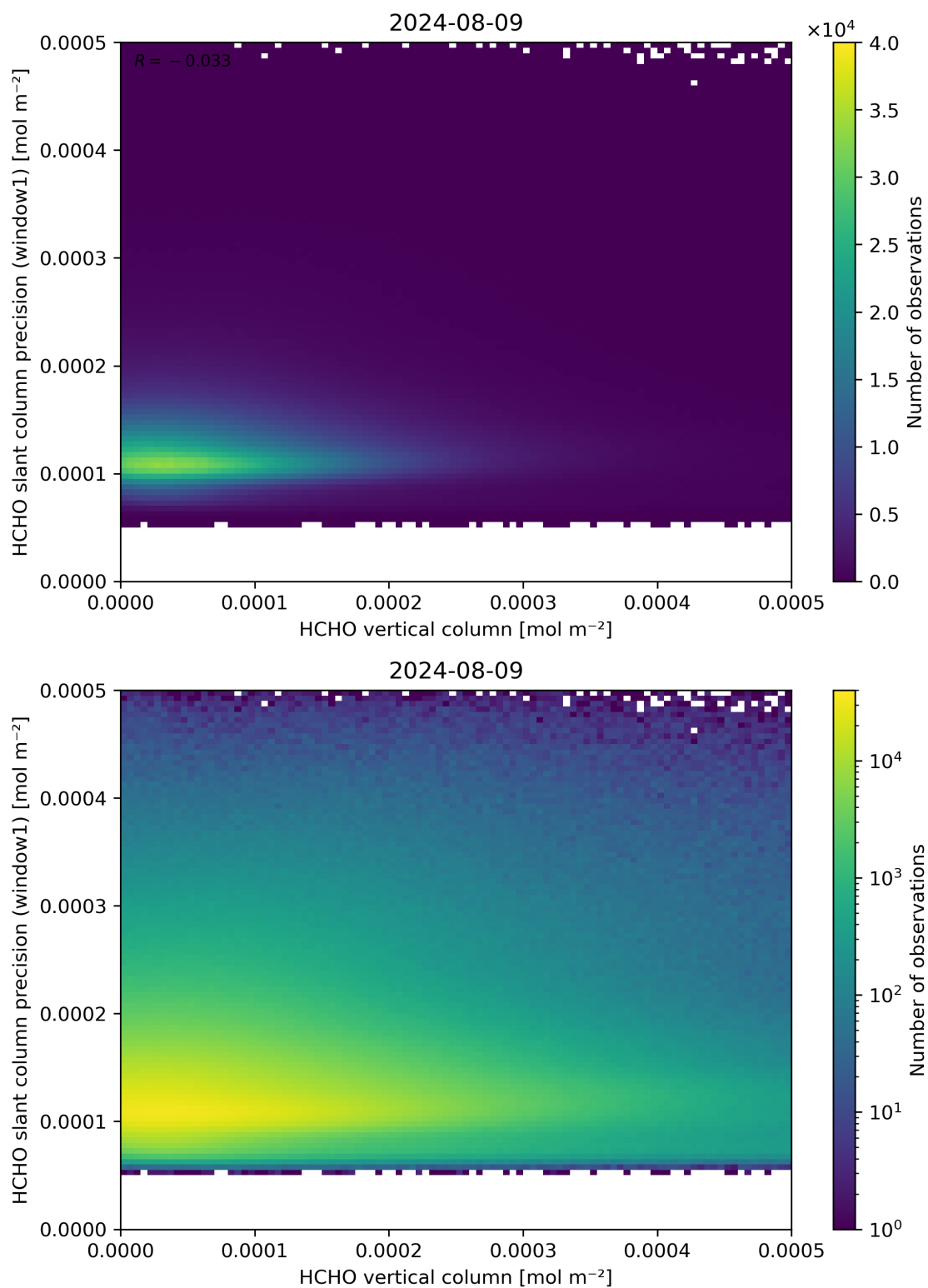
Figure 130: Scatter density plot of “HCHO vertical column” against “HCHO slant column precision (window1)” for 2024-08-08 to 2024-08-10.
