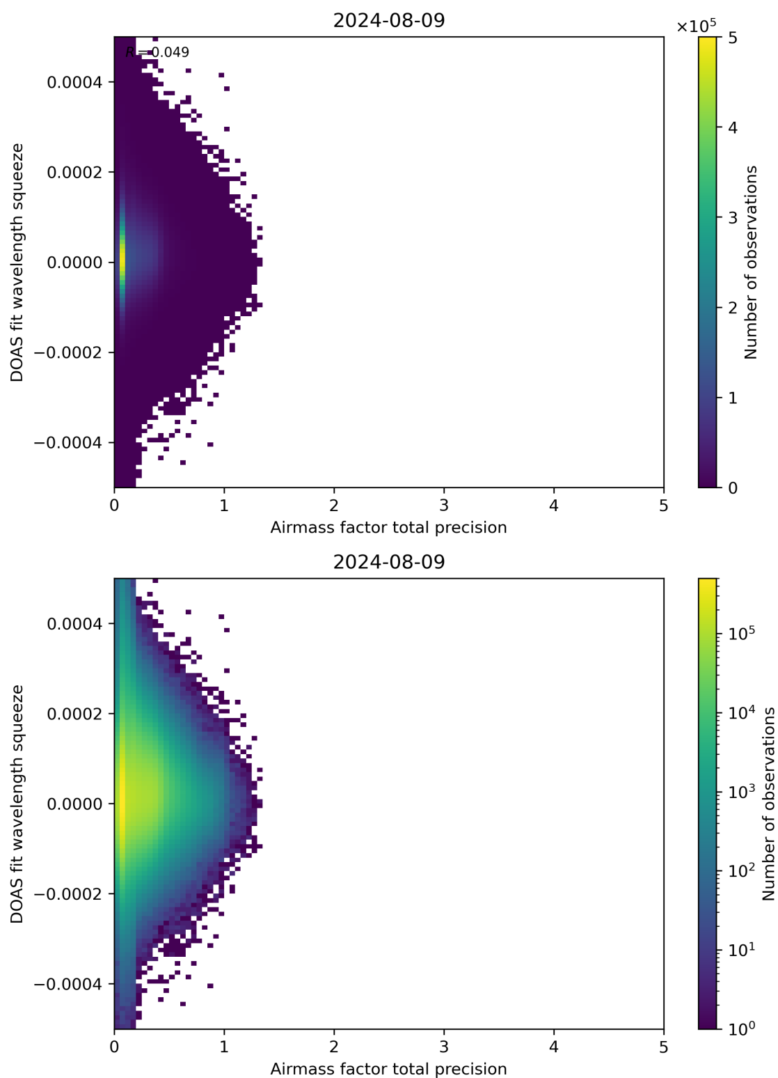
Figure 107: Scatter density plot of “Airmass factor total precision” against “DOAS fit wavelength squeeze” for 2024-08-08 to 2024-08-10.
