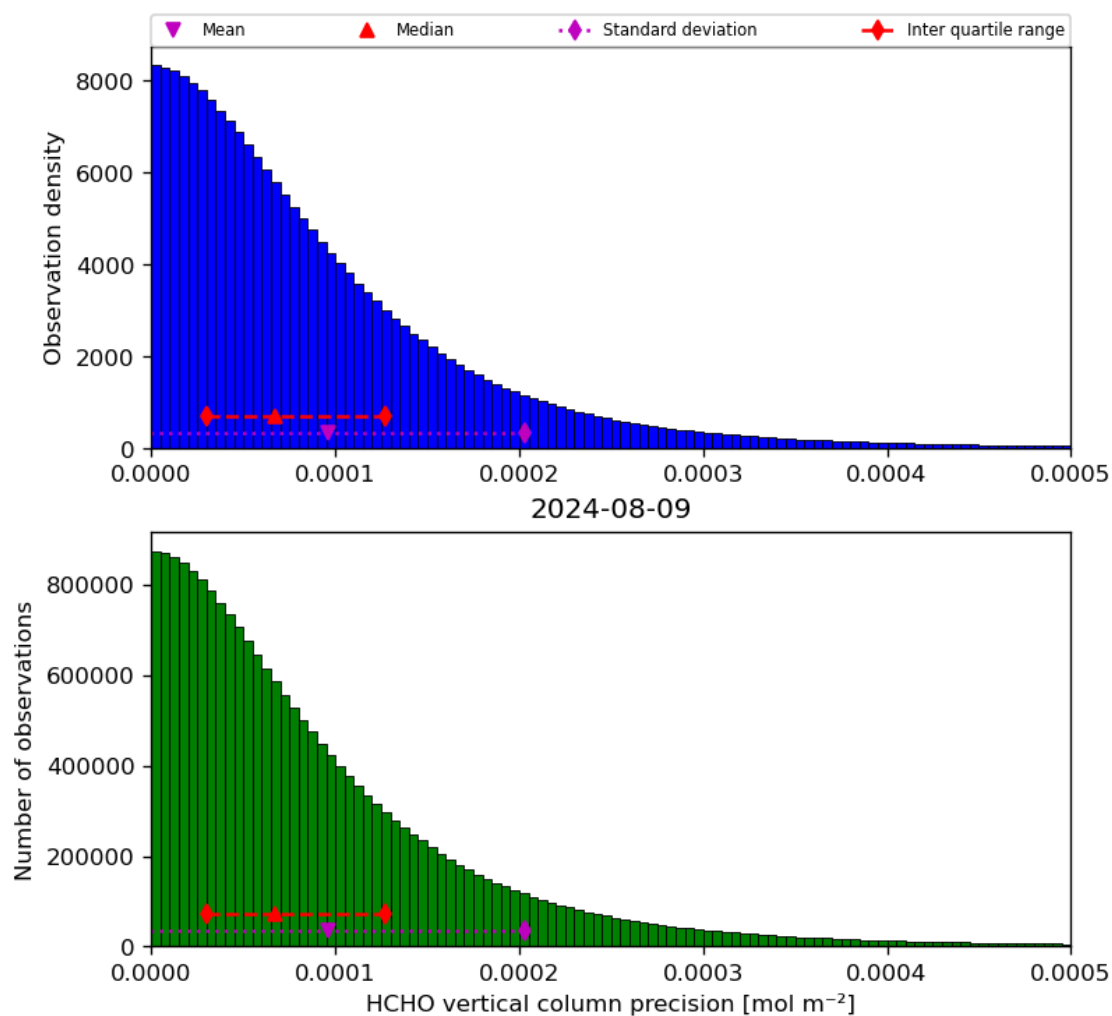
Figure 36: Histogram of “HCHO vertical column precision” for 2024-08-08 to 2024-08-10
