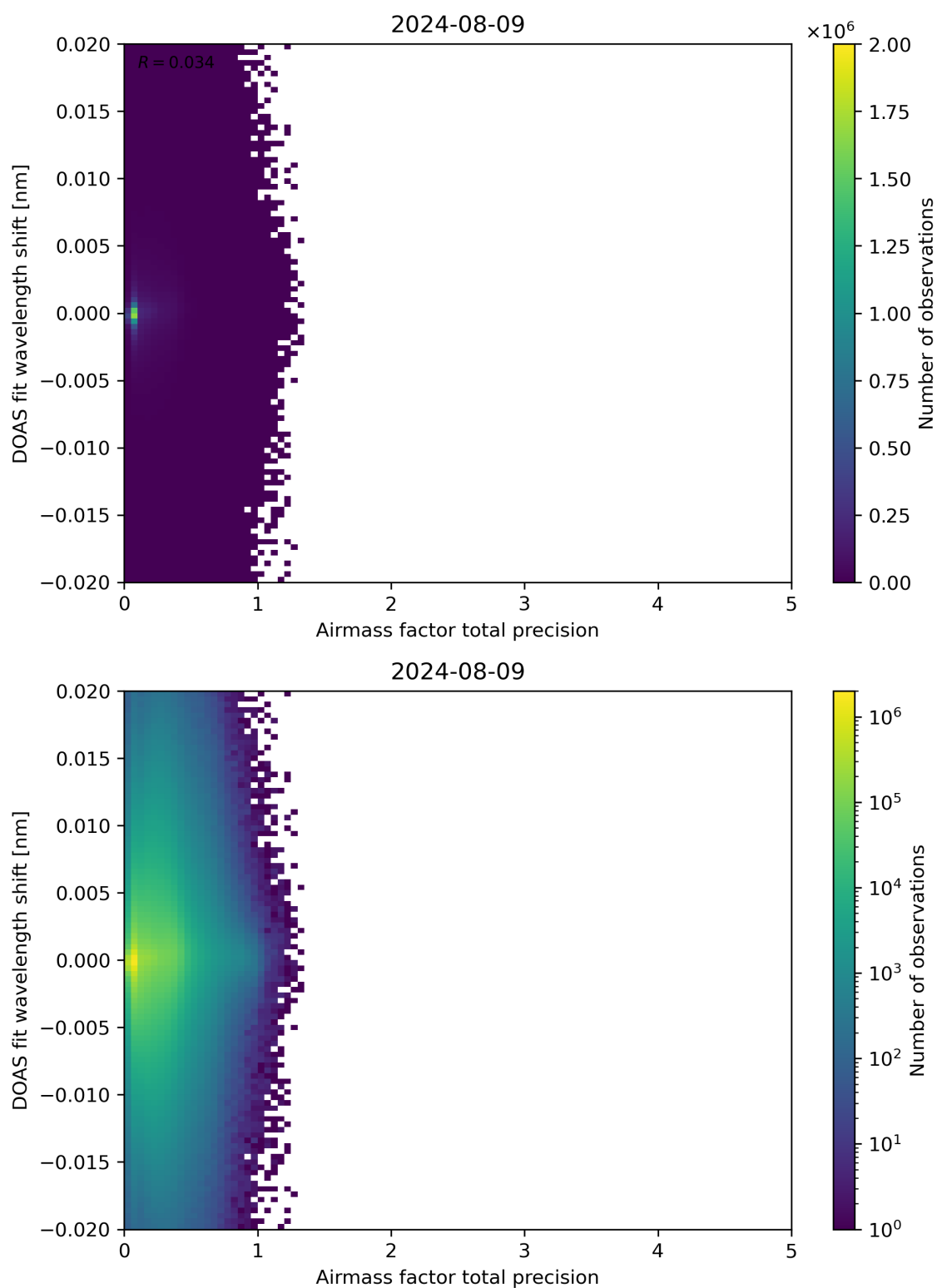
Figure 106: Scatter density plot of “Airmass factor total precision” against “DOAS fit wavelength shift” for 2024-08-08 to 2024-08-10.
