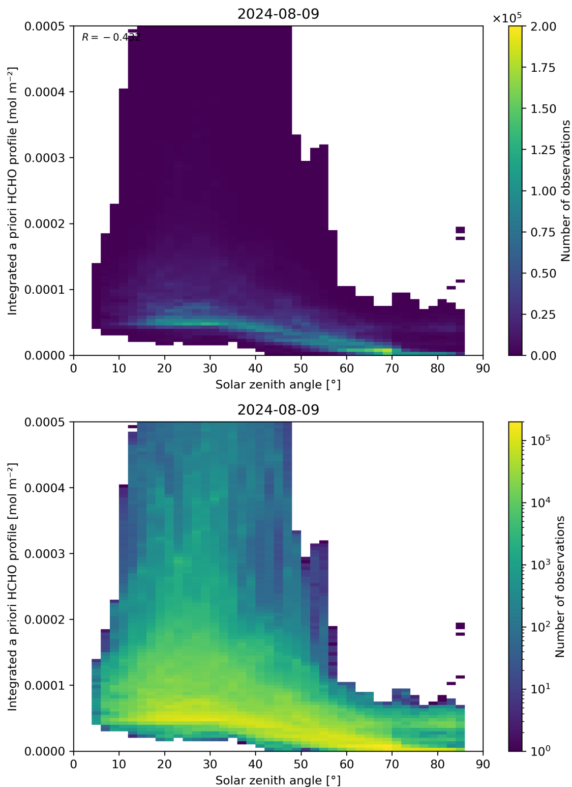
Figure 180: Scatter density plot of “Solar zenith angle” against “Integrated a priori HCHO profile” for 2024-08-08 to 2024-08-10.
