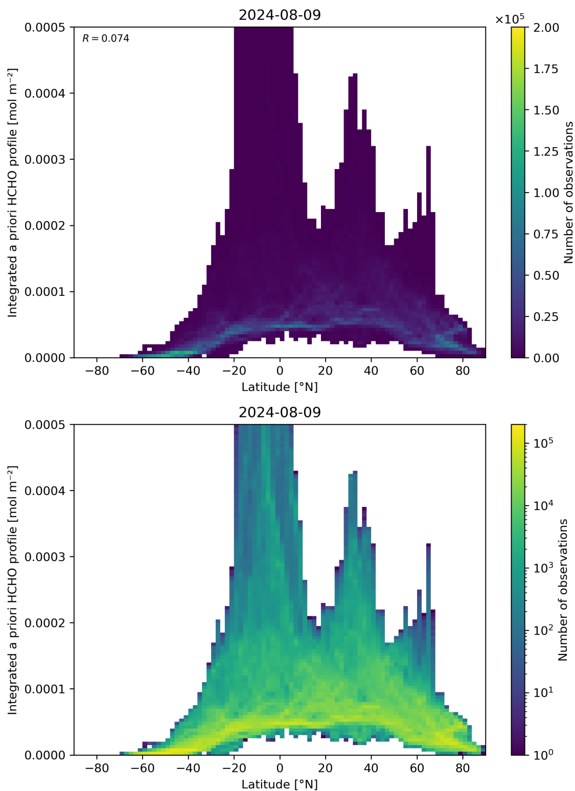
Figure 166: Scatter density plot of “Latitude” against “Integrated a priori HCHO profile” for 2024-08-08 to 2024-08-10.
