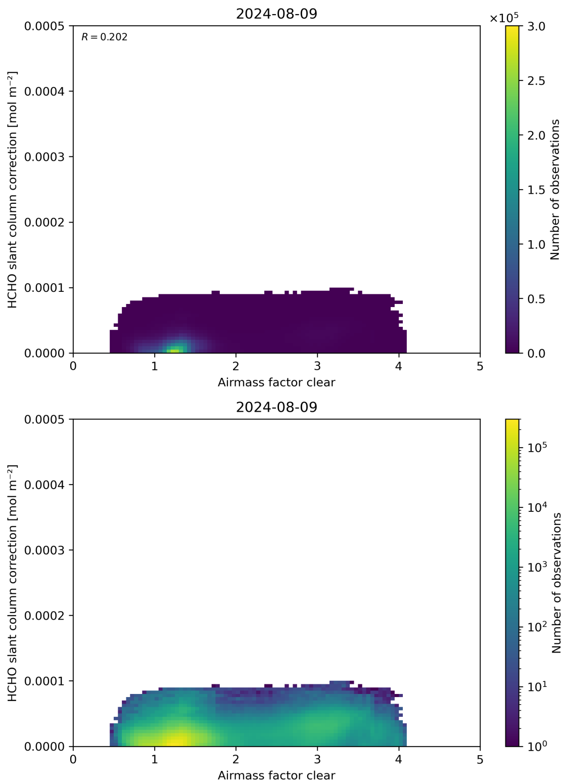
Figure 75: Scatter density plot of “Airmass factor clear” against “HCHO slant column correction” for 2024-08-08 to 2024-08-10.
