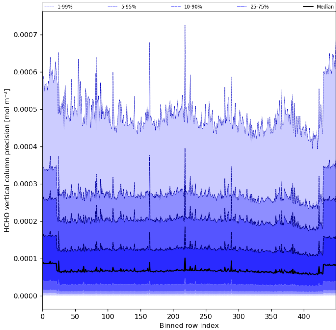
Figure 50: Along track statistics of “HCHO vertical column precision” for 2024-08-08 to 2024-08-10
