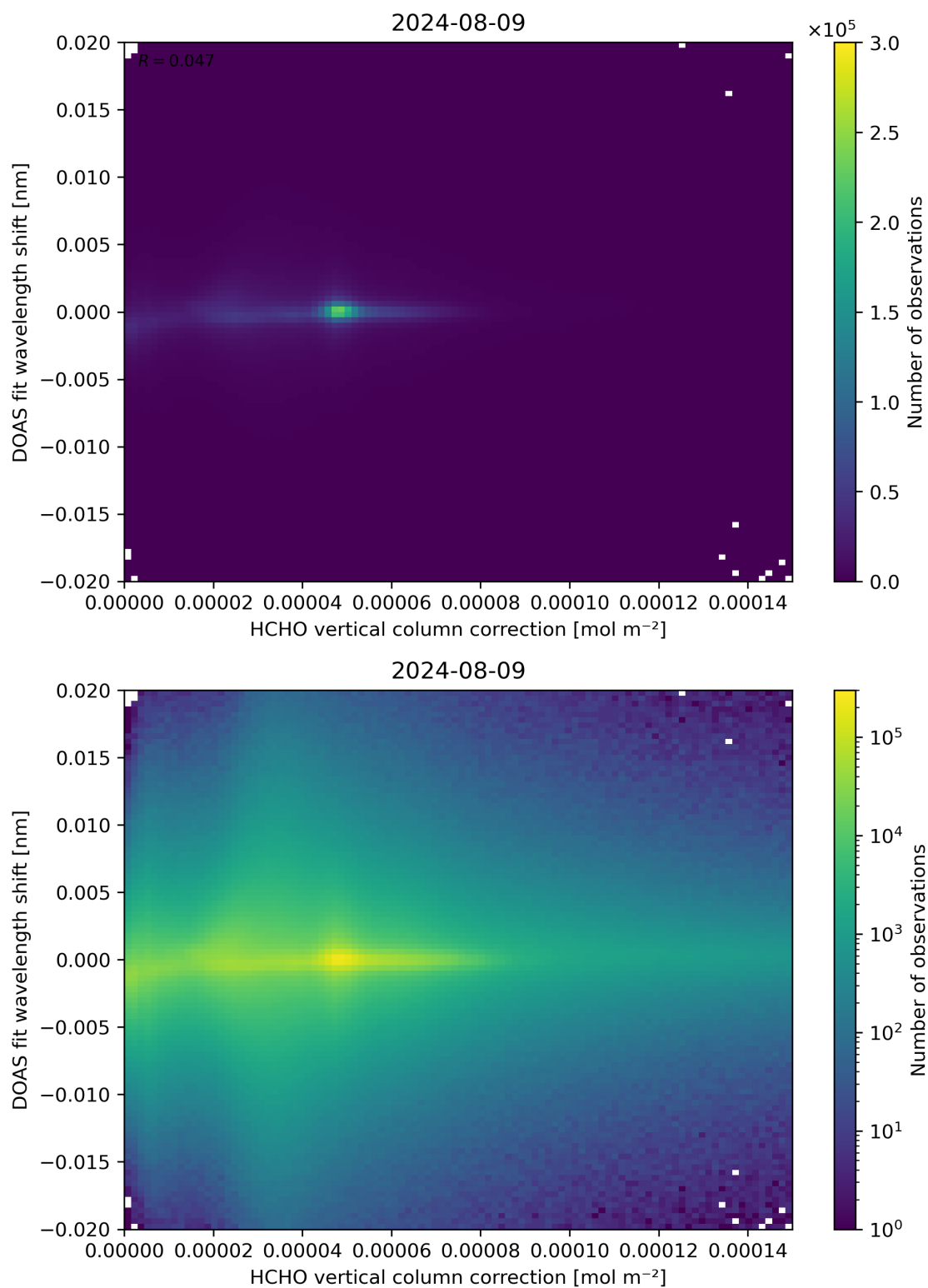
Figure 113: Scatter density plot of “HCHO vertical column correction” against “DOAS fit wavelength shift” for 2024-08-08 to 2024-08-10.
