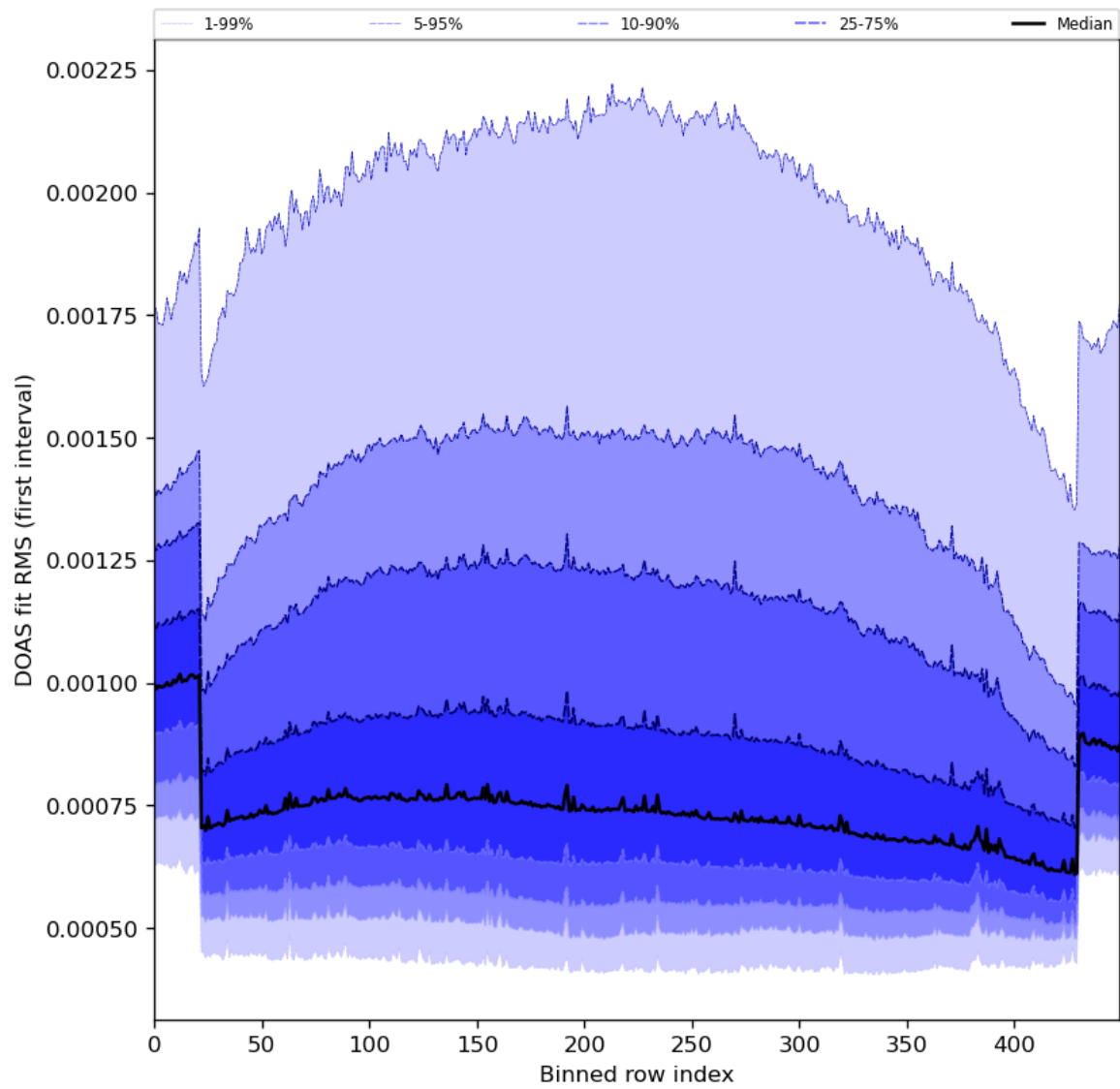
Figure 60: Along track statistics of “DOAS fit RMS (first interval)” for 2024-08-08 to 2024-08-10
