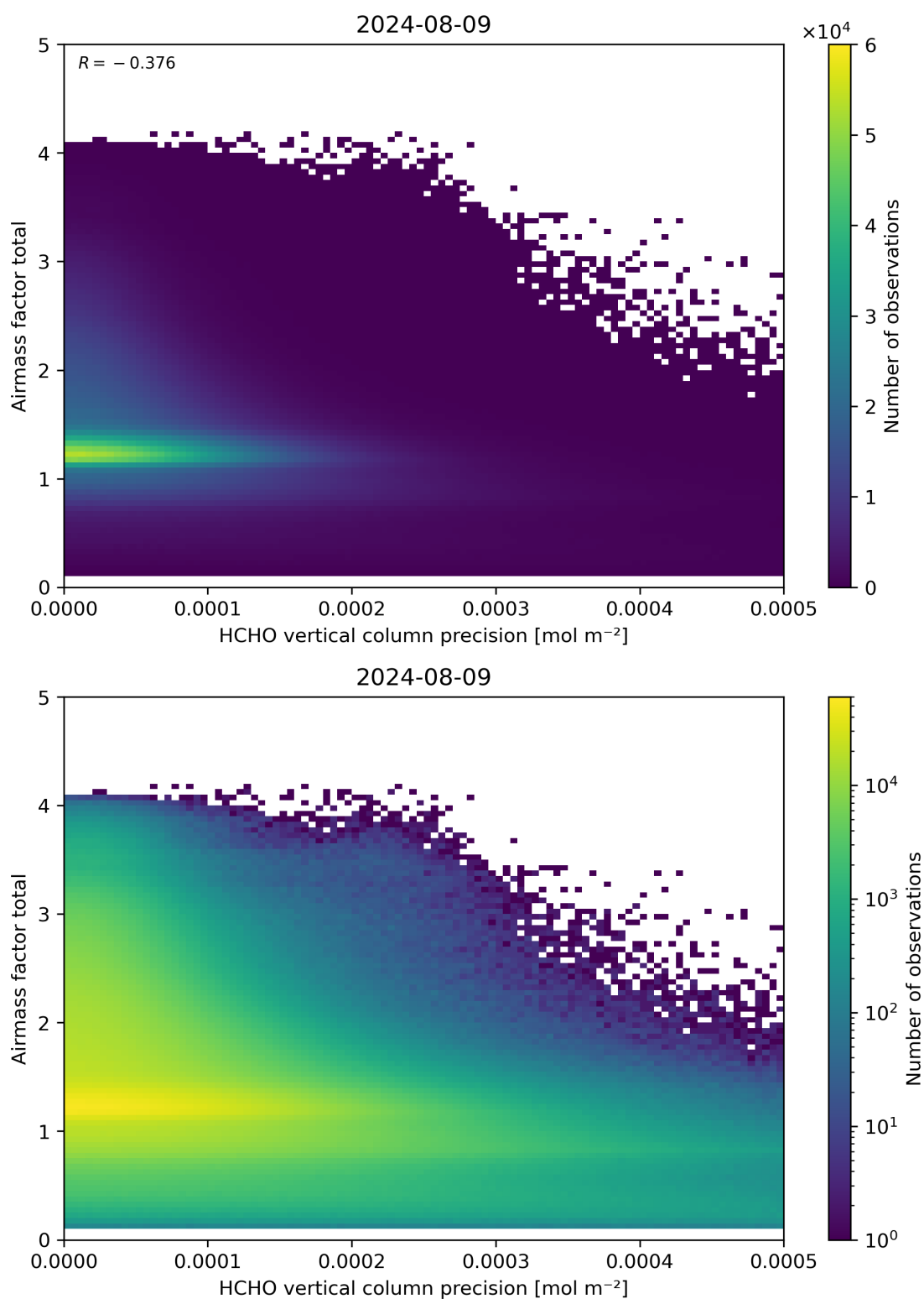
Figure 144: Scatter density plot of “HCHO vertical column precision” against “Airmass factor total” for 2024-08-08 to 2024-08-10.
