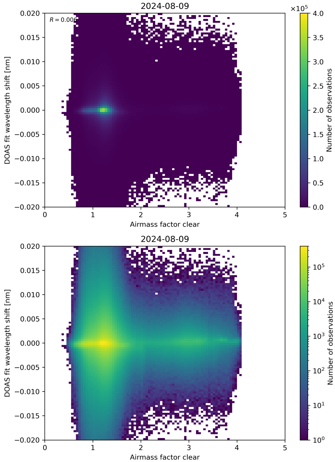
Figure 72: Scatter density plot of “Airmass factor clear” against “DOAS fit wavelength shift” for 2024-08-08 to 2024-08-10.
