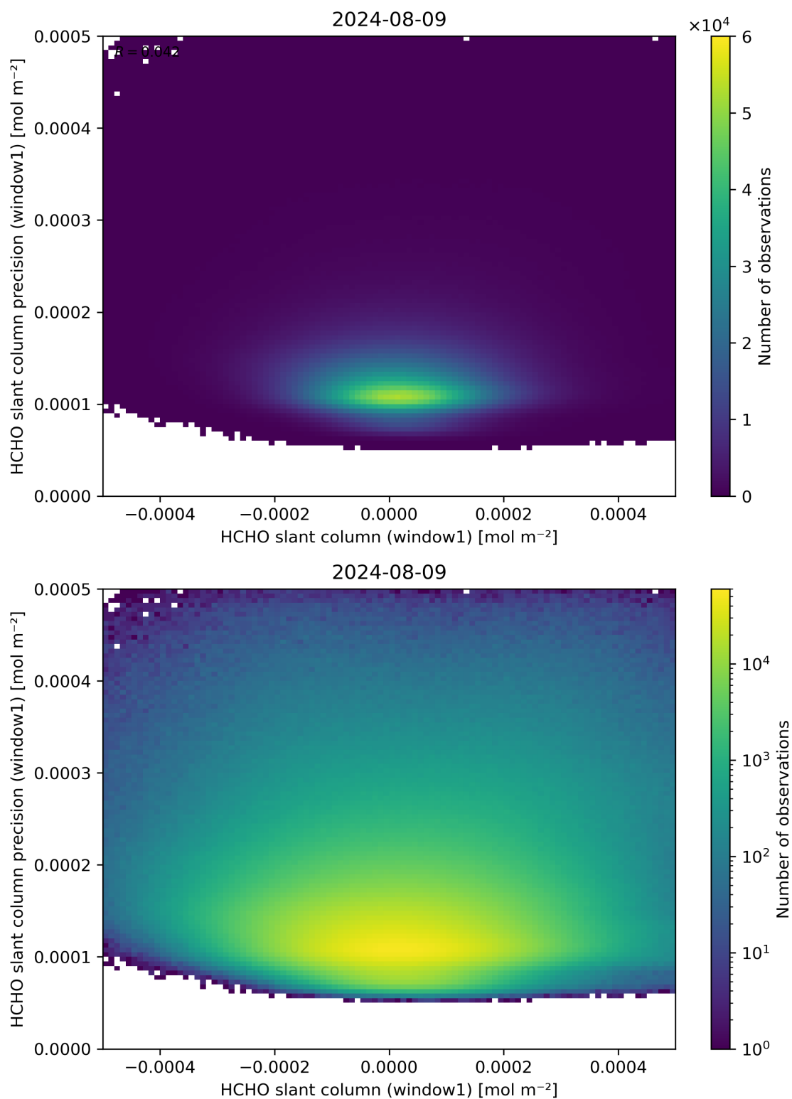
Figure 84: Scatter density plot of “HCHO slant column (window1)” against “HCHO slant column precision (window1)” for 2024-08-08 to 2024-08-10.
