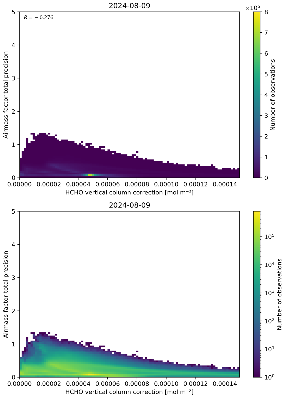
Figure 121: Scatter density plot of “HCHO vertical column correction” against “Airmass factor total precision” for 2024-08-08 to 2024-08-10.
