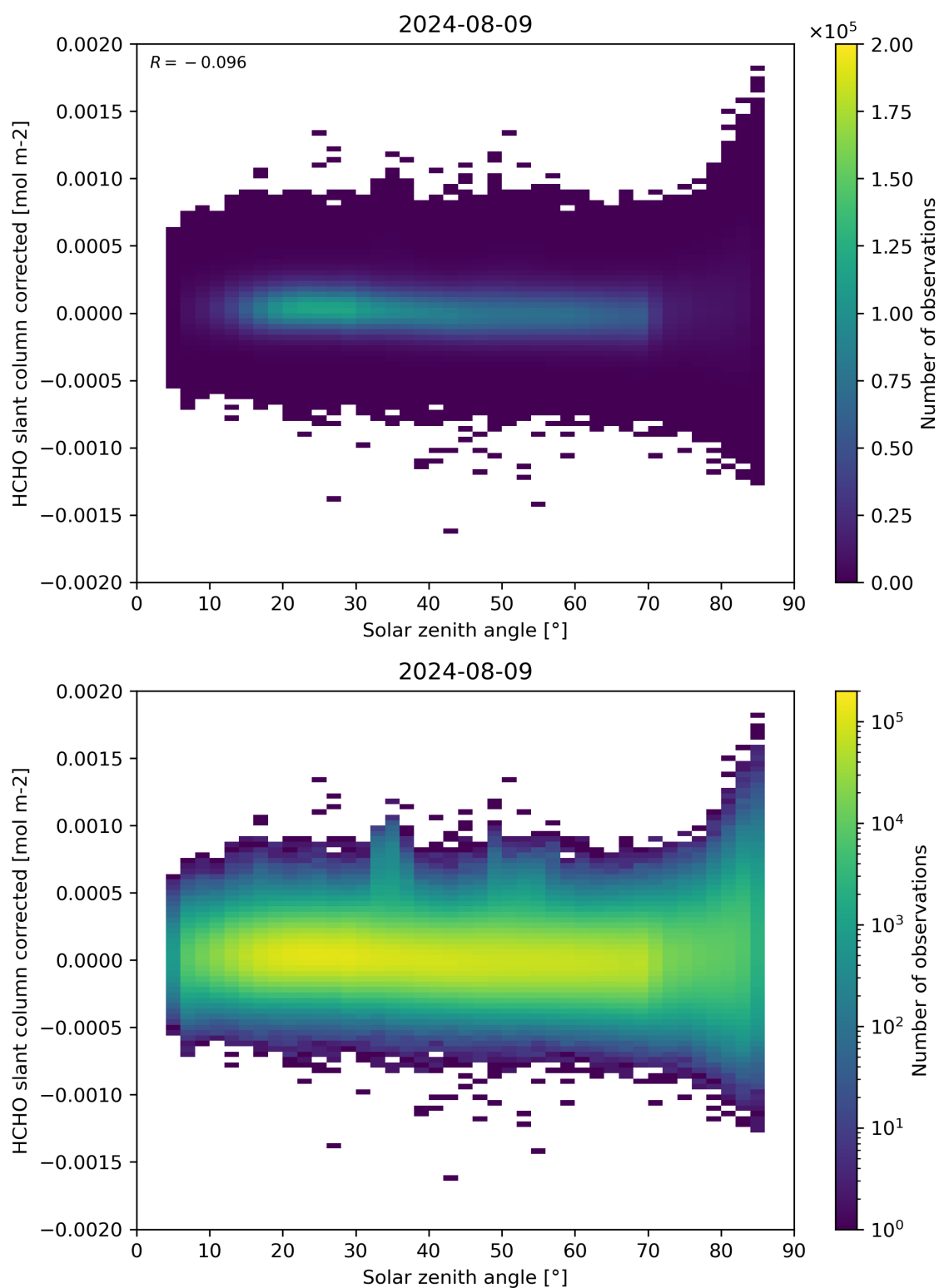
Figure 171: Scatter density plot of “Solar zenith angle” against “HCHO slant column corrected” for 2024-08-08 to 2024-08-10.
