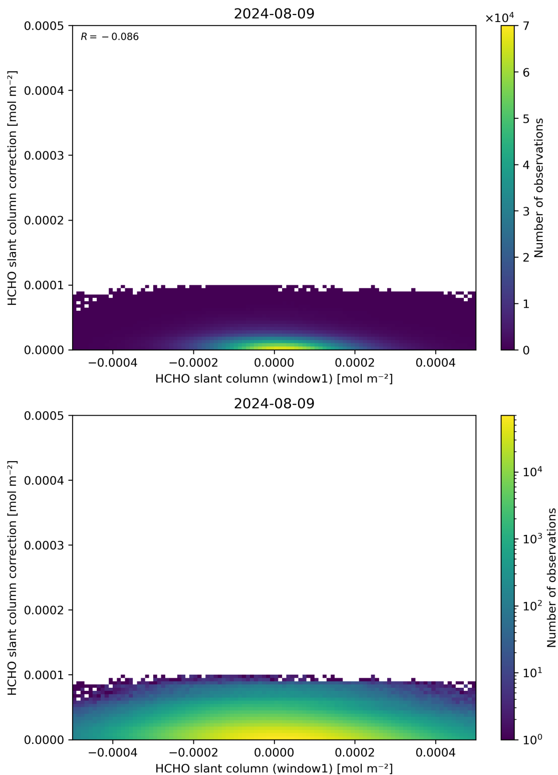
Figure 83: Scatter density plot of “HCHO slant column (window1)” against “HCHO slant column correction” for 2024-08-08 to 2024-08-10.
