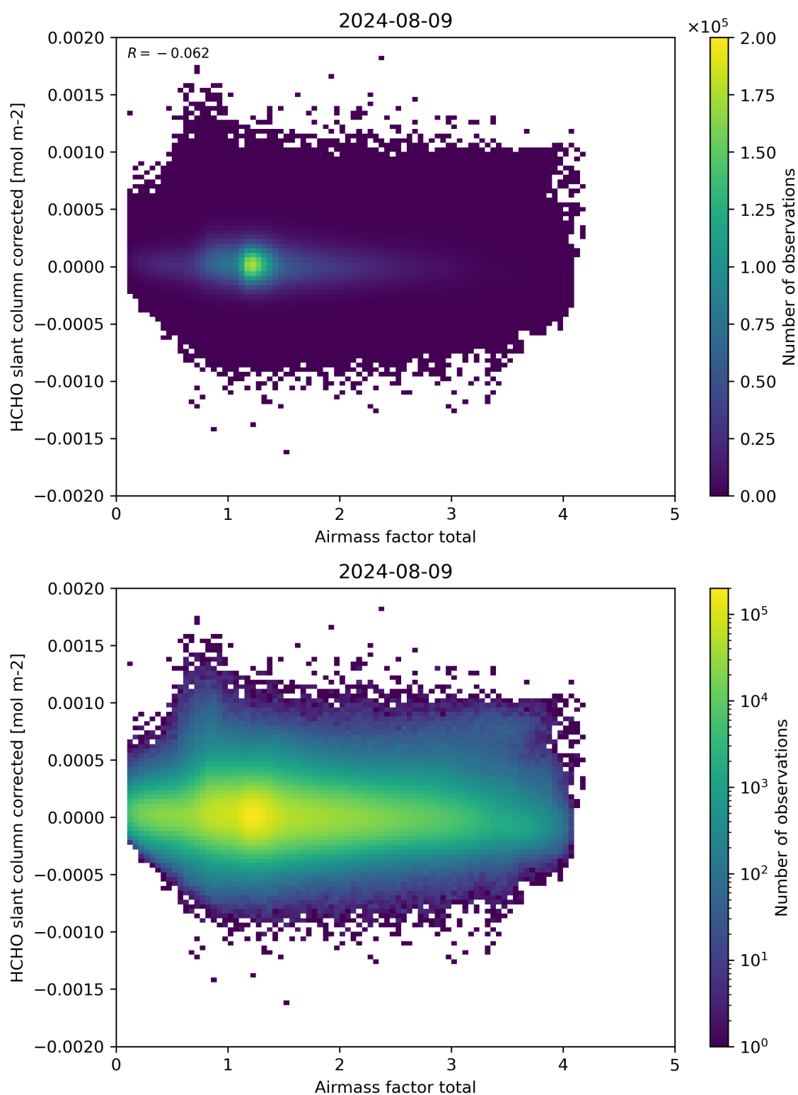
Figure 101: Scatter density plot of “Airmass factor total” against “HCHO slant column corrected” for 2024-08-08 to 2024-08-10.
