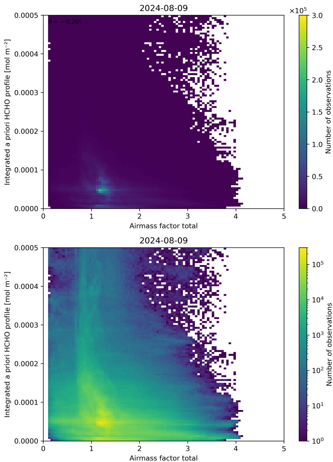
Figure 104: Scatter density plot of “Airmass factor total” against “Integrated a priori HCHO profile” for 2024-08-08 to 2024-08-10.
