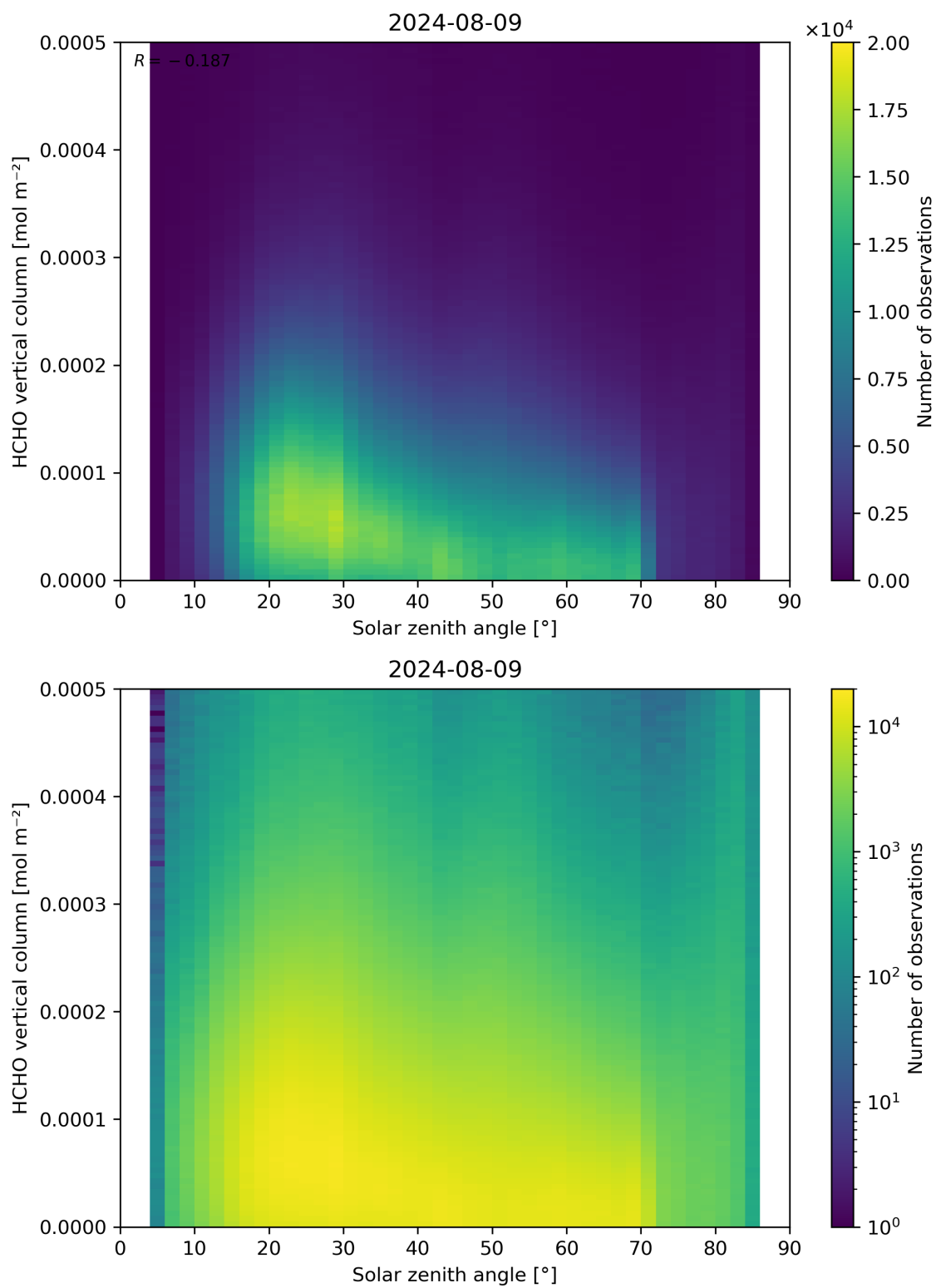
Figure 177: Scatter density plot of “Solar zenith angle” against “HCHO vertical column” for 2024-08-08 to 2024-08-10.
