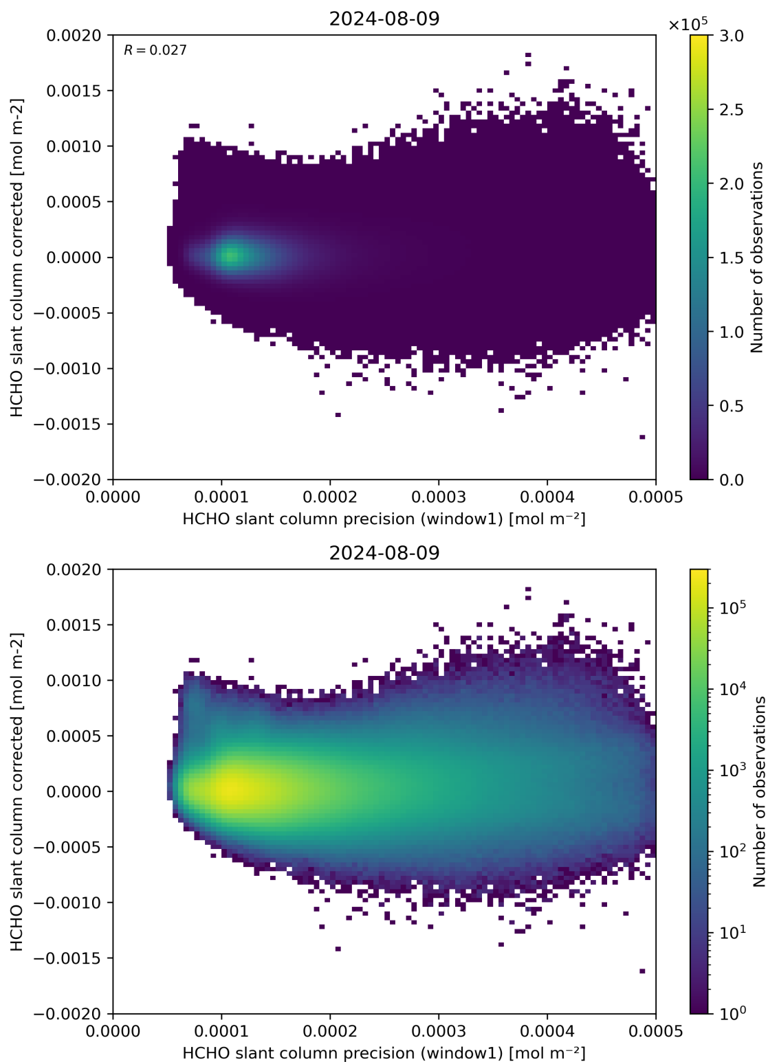
Figure 92: Scatter density plot of “HCHO slant column precision (window1)” against “HCHO slant column corrected” for 2024-08-08 to 2024-08-10.
