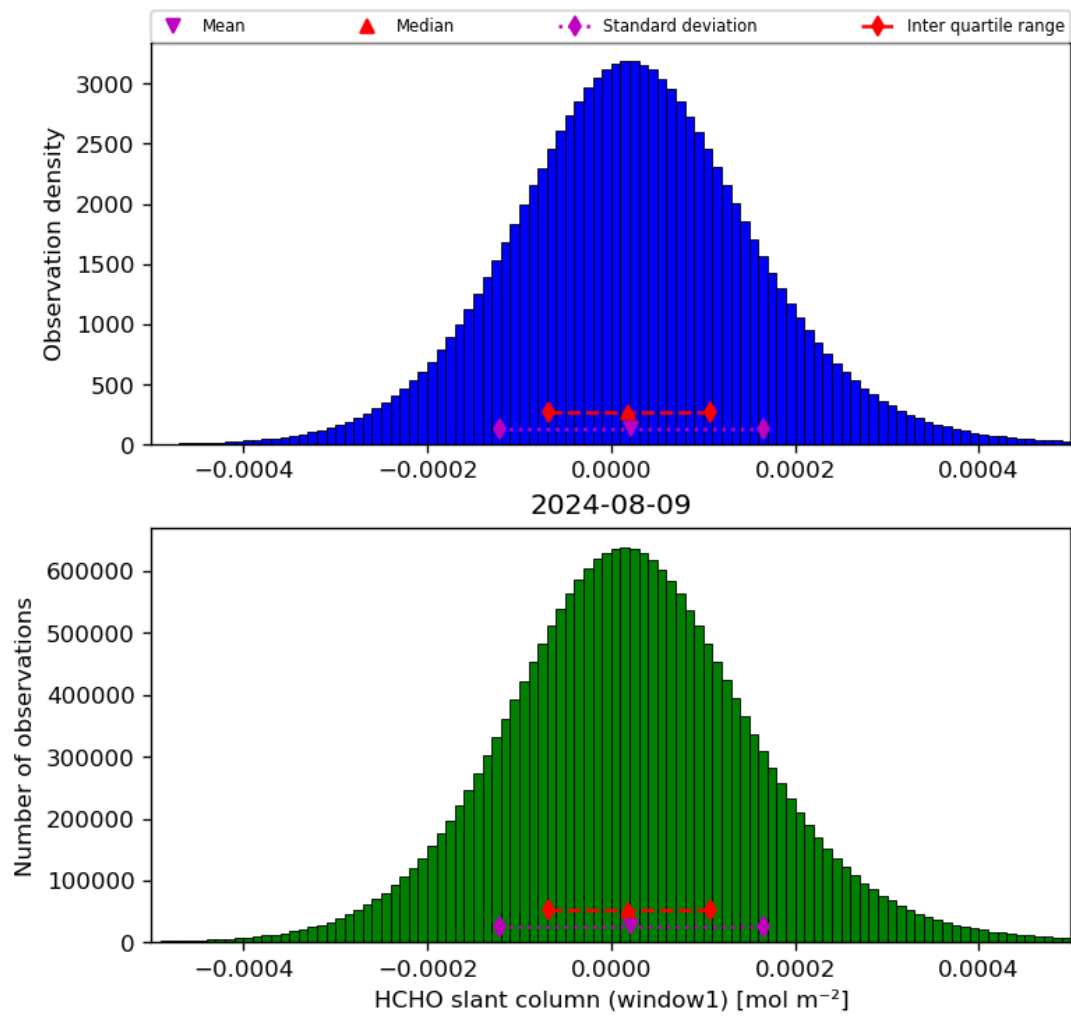
Figure 38: Histogram of “HCHO slant column (window1)” for 2024-08-08 to 2024-08-10
