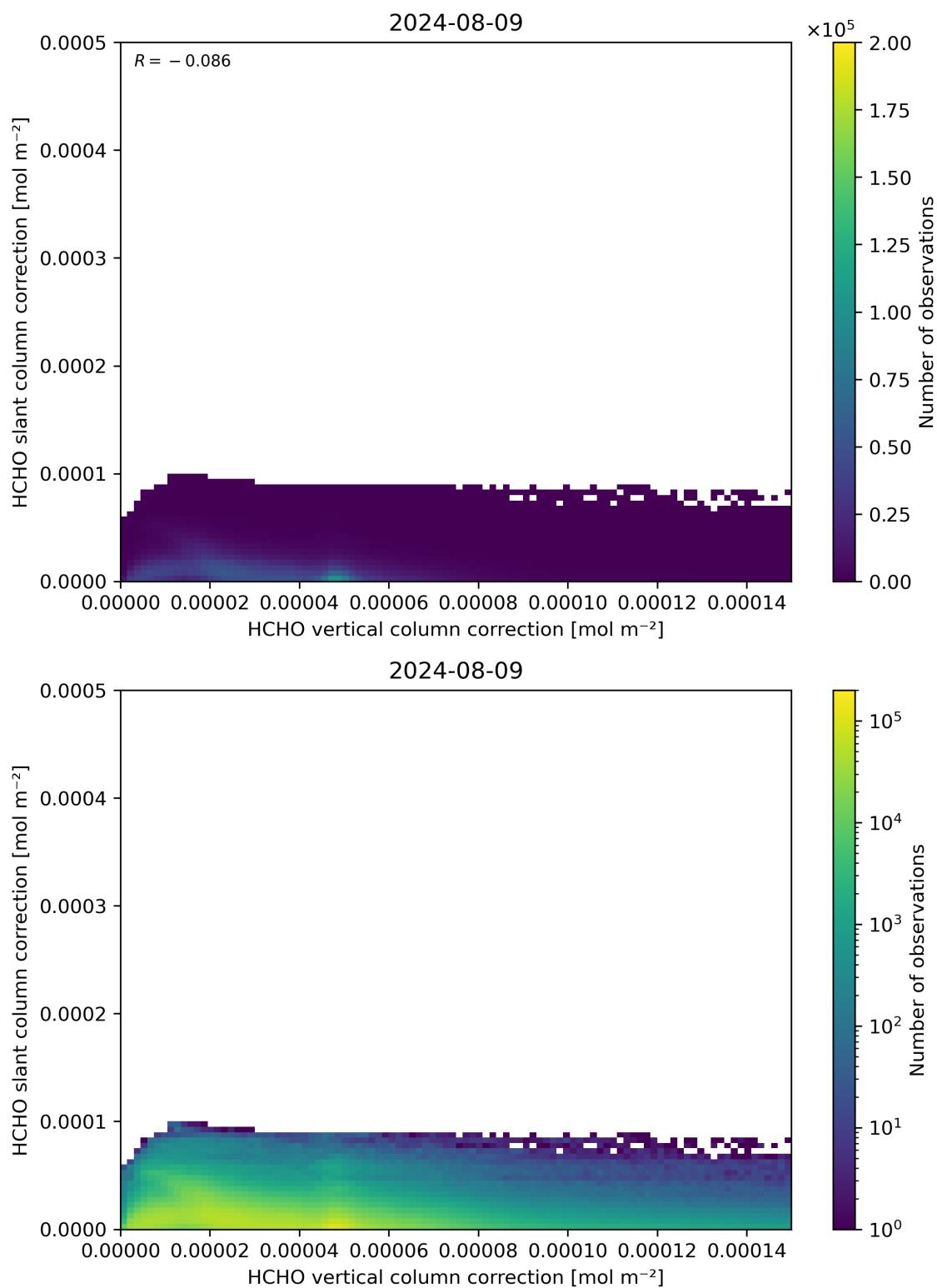
Figure 117: Scatter density plot of “HCHO vertical column correction” against “HCHO slant column correction” for 2024-08-08 to 2024-08-10.
