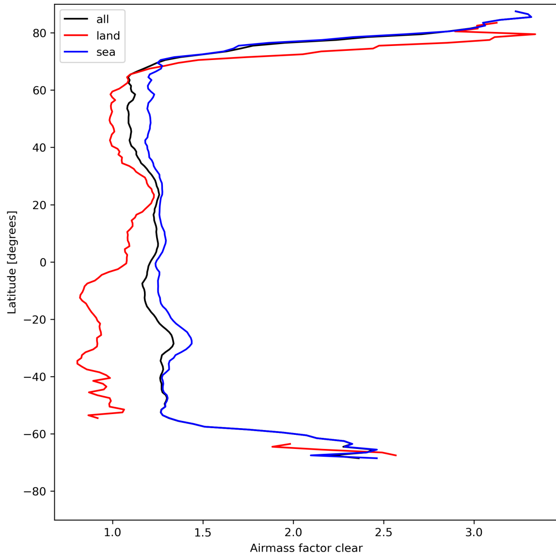
Figure 28: Zonal average of “Airmass factor clear” for 2024-08-08 to 2024-08-10.
