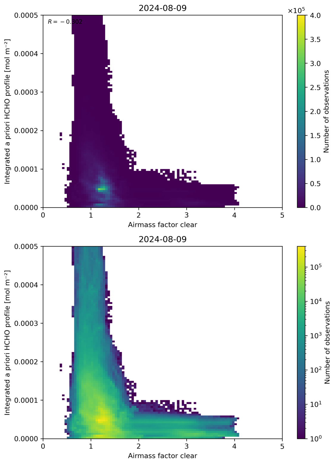
Figure 76: Scatter density plot of “Airmass factor clear” against “Integrated a priori HCHO profile” for 2024-08-08 to 2024-08-10.
