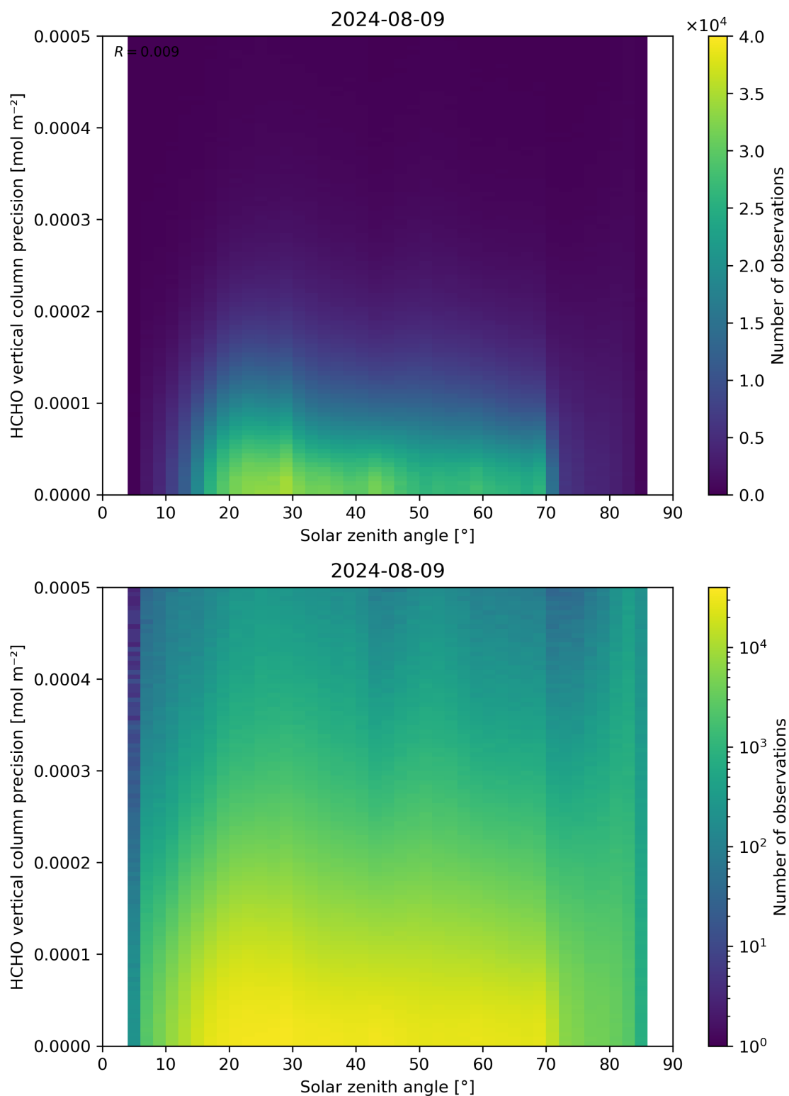
Figure 179: Scatter density plot of “Solar zenith angle” against “HCHO vertical column precision” for 2024-08-08 to 2024-08-10.
