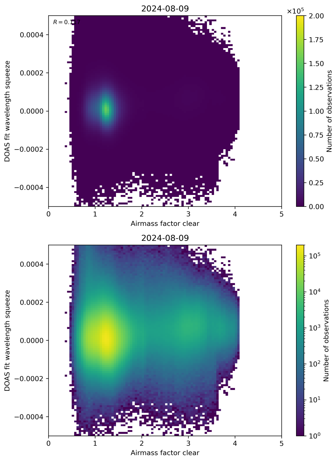
Figure 73: Scatter density plot of “Airmass factor clear” against “DOAS fit wavelength squeeze” for 2024-08-08 to 2024-08-10.
