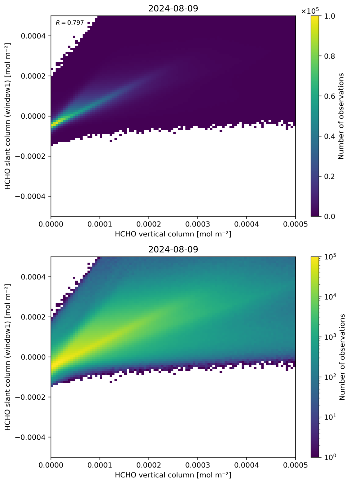
Figure 129: Scatter density plot of “HCHO vertical column” against “HCHO slant column (window1)” for 2024-08-08 to 2024-08-10.
