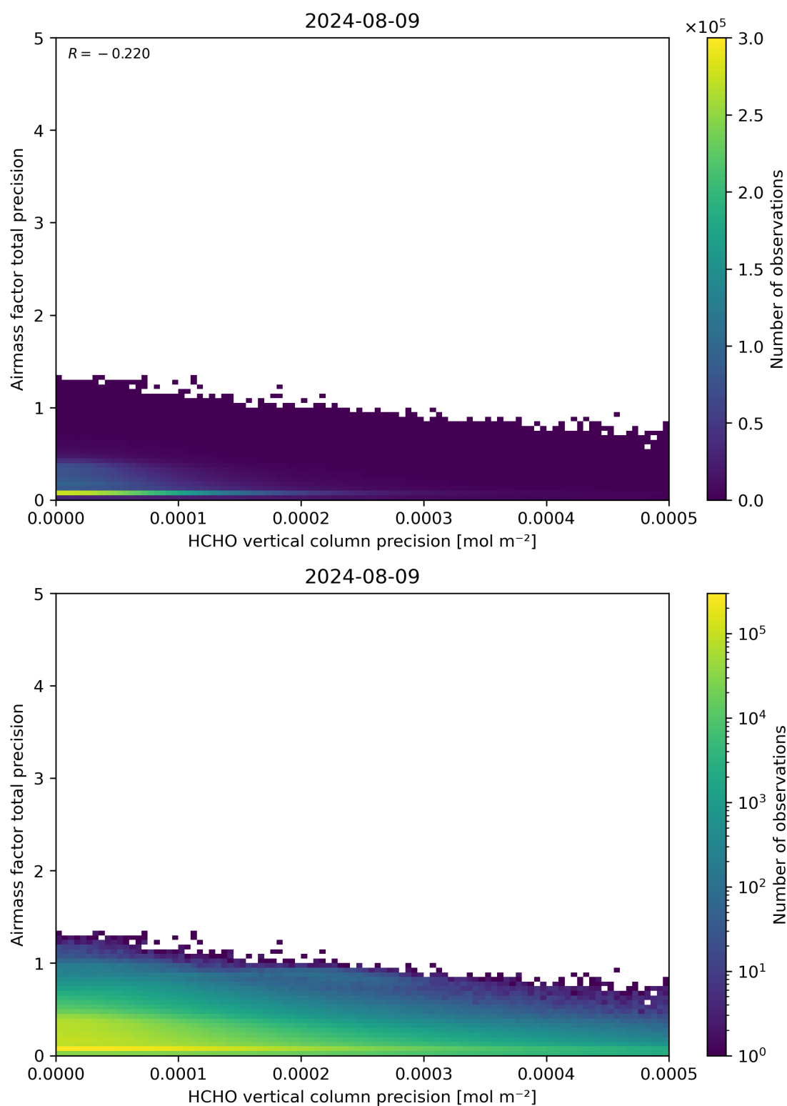
Figure 145: Scatter density plot of “HCHO vertical column precision” against “Airmass factor total precision” for 2024-08-08 to 2024-08-10.
