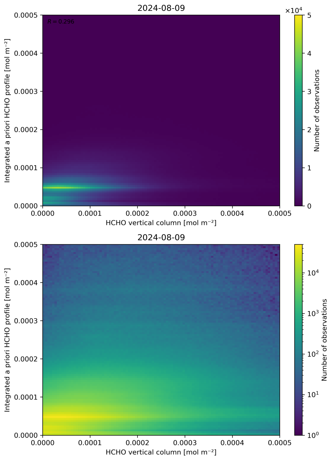
Figure 135: Scatter density plot of “HCHO vertical column” against “Integrated a priori HCHO profile” for 2024-08-08 to 2024-08-10.
