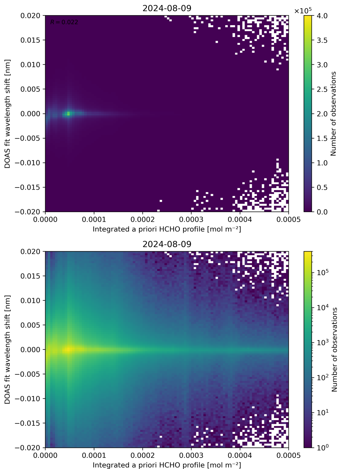
Figure 149: Scatter density plot of “Integrated a priori HCHO profile” against “DOAS fit wavelength shift” for 2024-08-08 to 2024-08-10.
