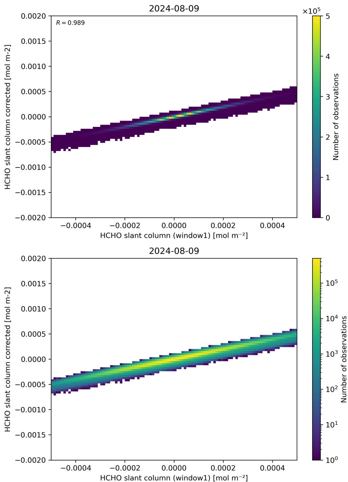
Figure 82: Scatter density plot of “HCHO slant column (window1)” against “HCHO slant column corrected” for 2024-08-08 to 2024-08-10.
