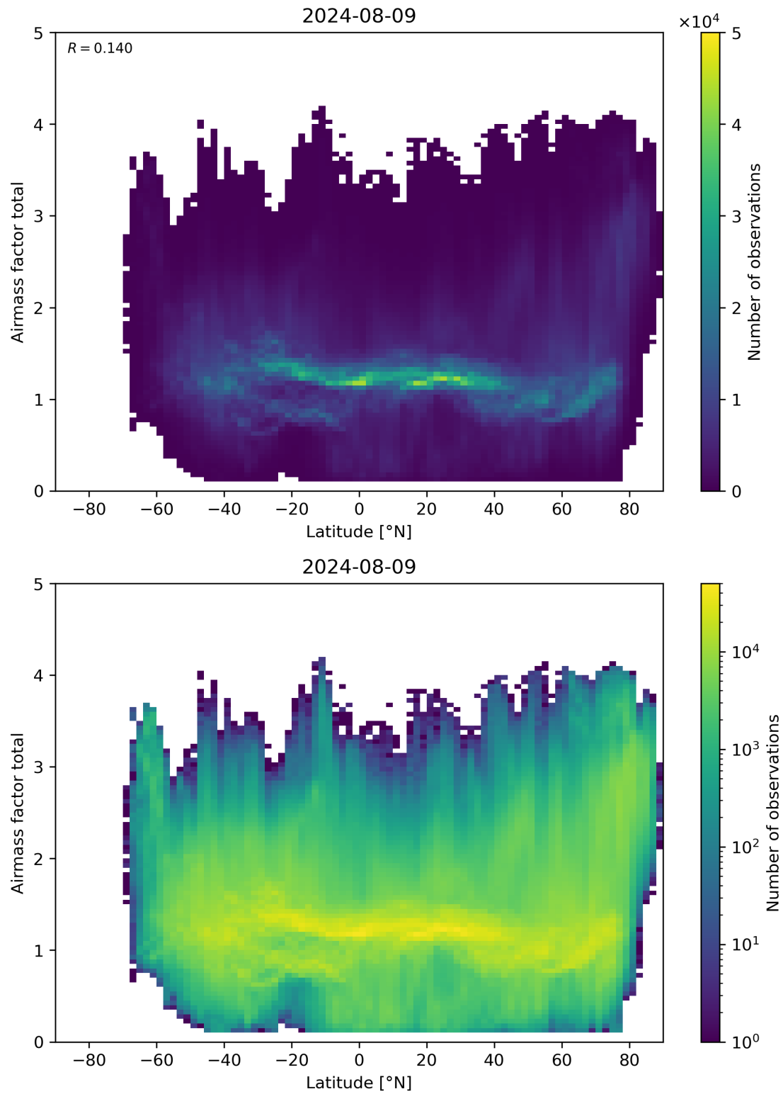
Figure 161: Scatter density plot of “Latitude” against “Airmass factor total” for 2024-08-08 to 2024-08-10.
