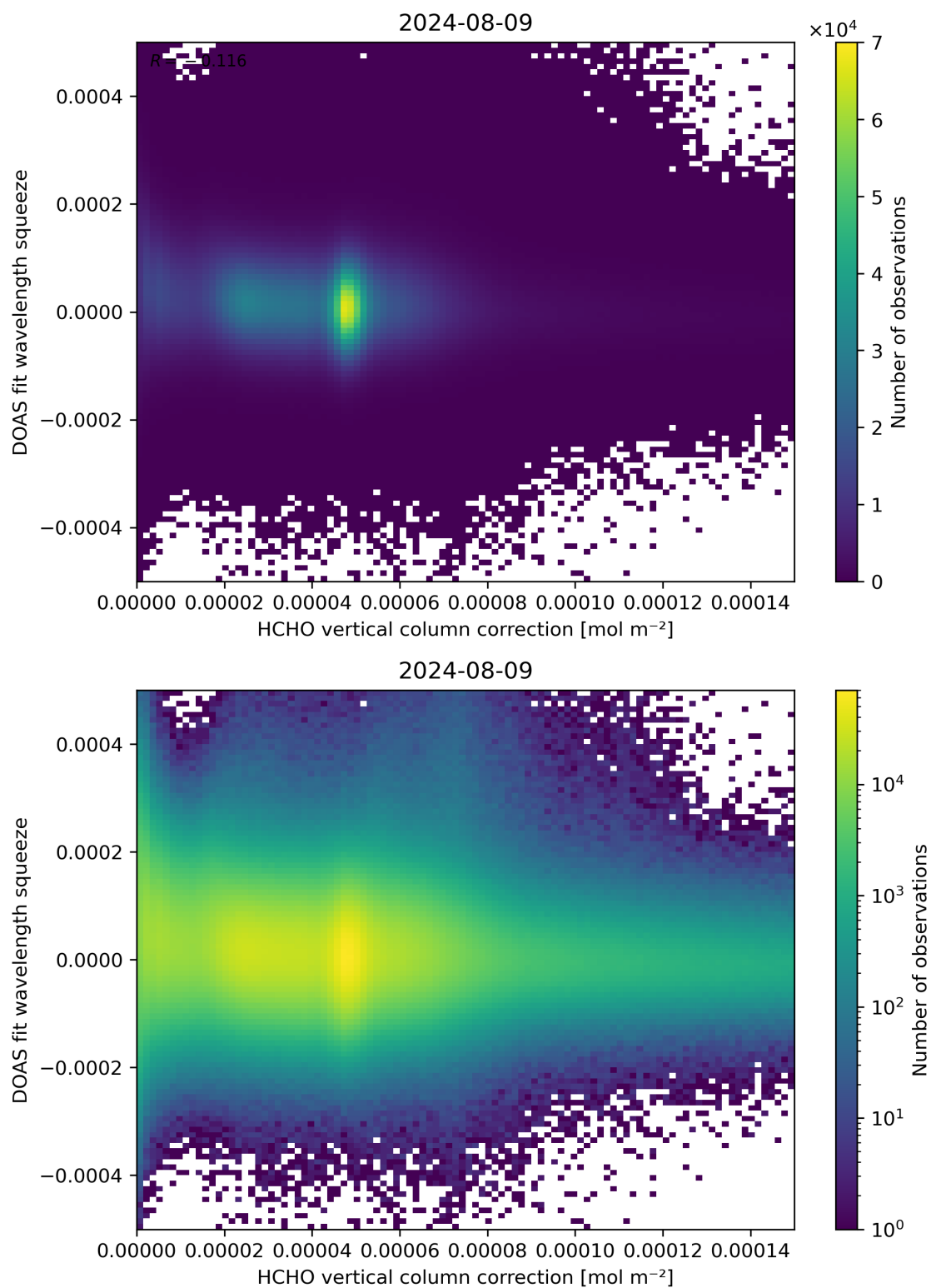
Figure 114: Scatter density plot of “HCHO vertical column correction” against “DOAS fit wavelength squeeze” for 2024-08-08 to 2024-08-10.
