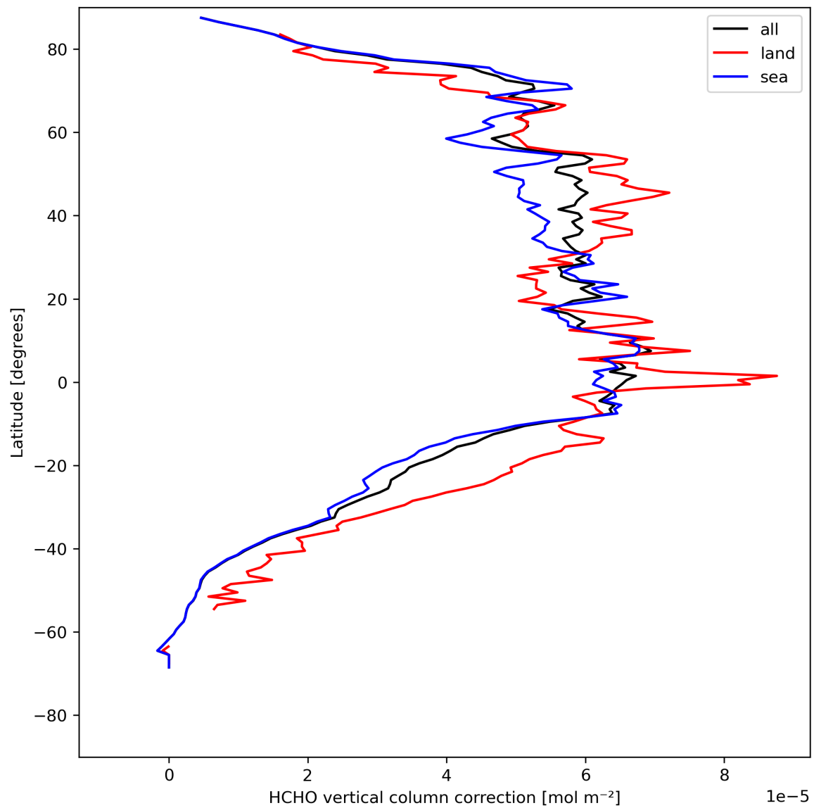
Figure 23: Zonal average of “HCHO vertical column correction” for 2024-08-08 to 2024-08-10.
