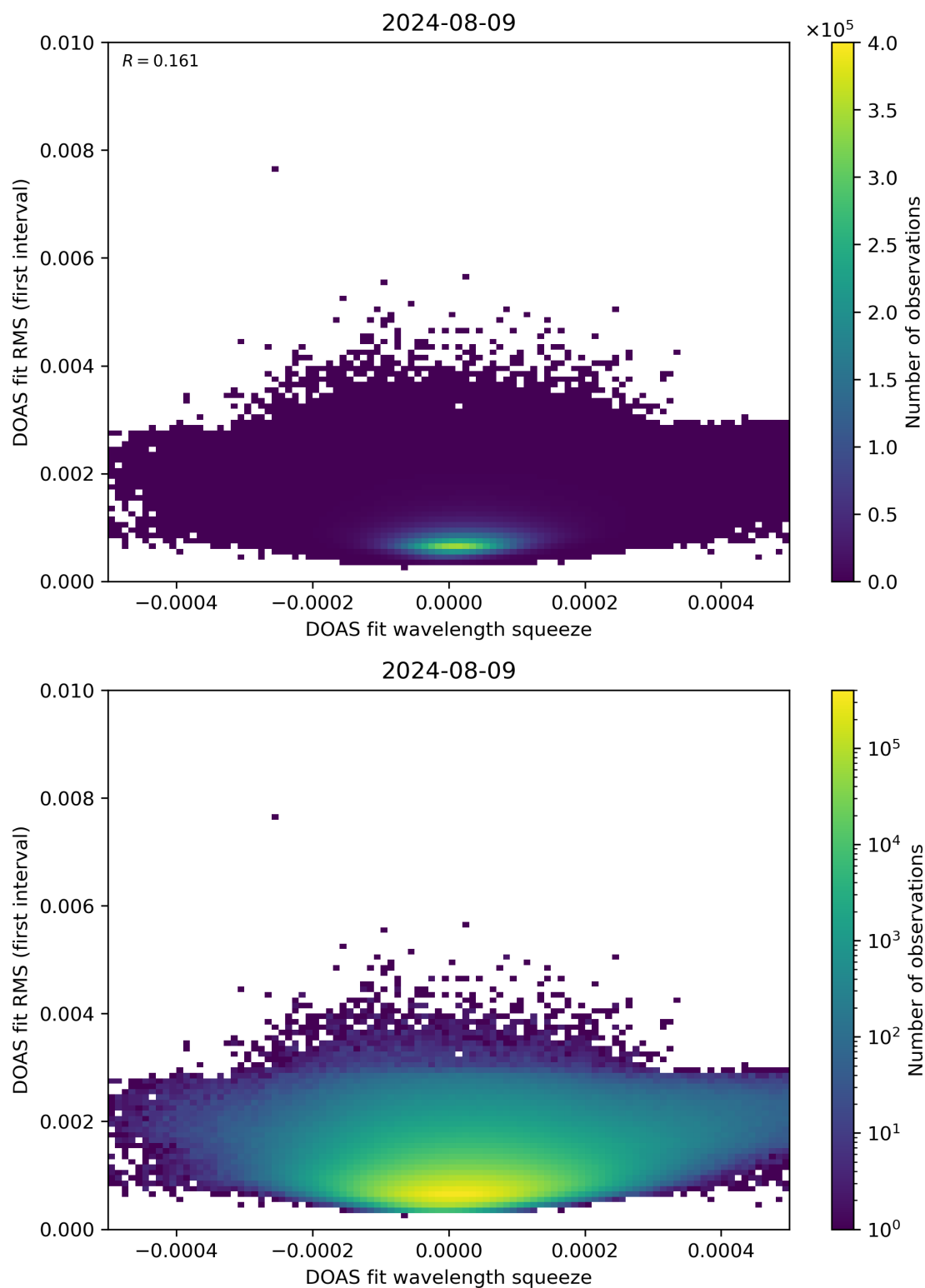
Figure 68: Scatter density plot of “DOAS fit wavelength squeeze” against “DOAS fit RMS (first interval)” for 2024-08-08 to 2024-08-10.
