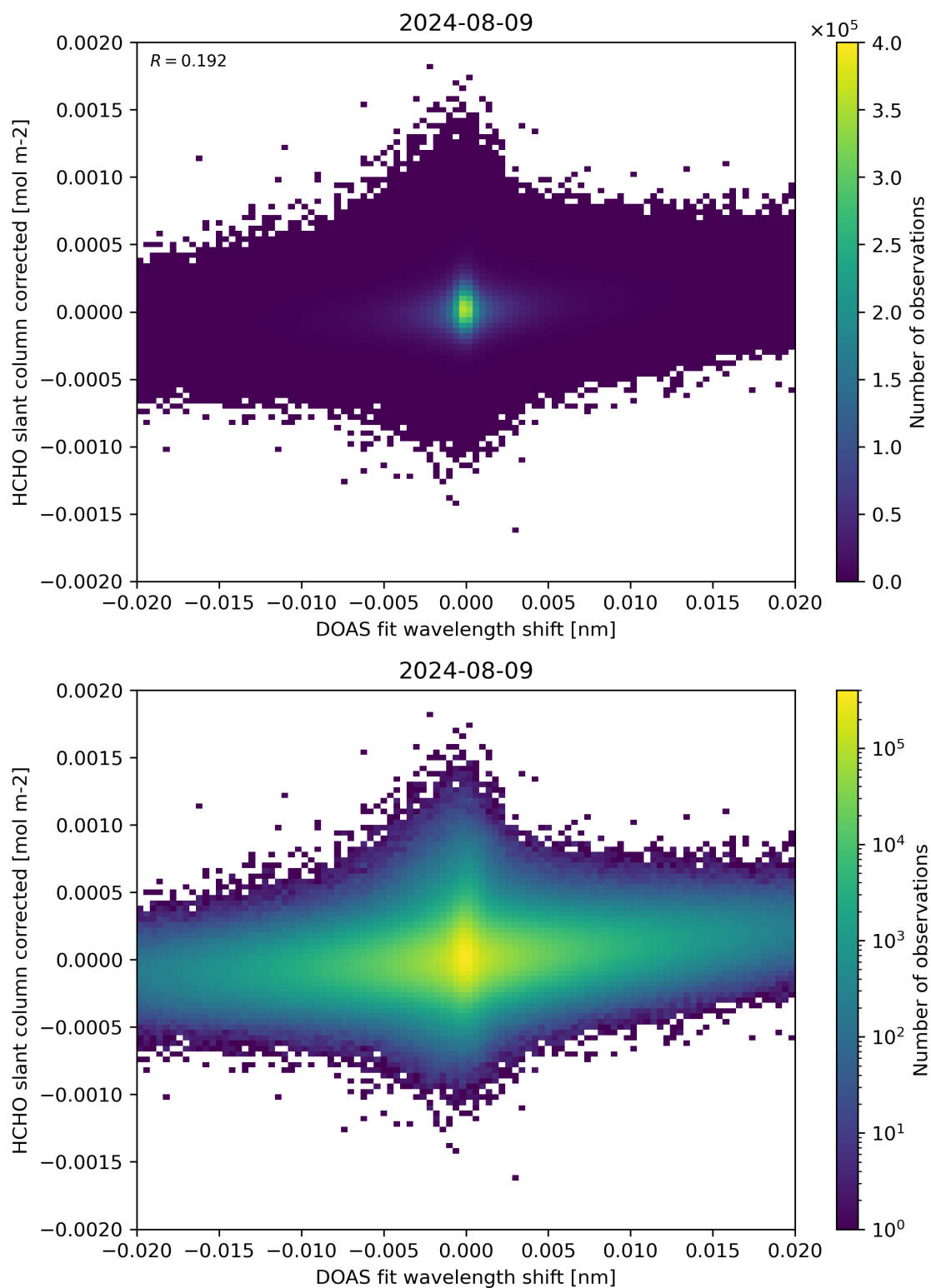
Figure 66: Scatter density plot of “DOAS fit wavelength shift” against “HCHO slant column corrected” for 2024-08-08 to 2024-08-10.
