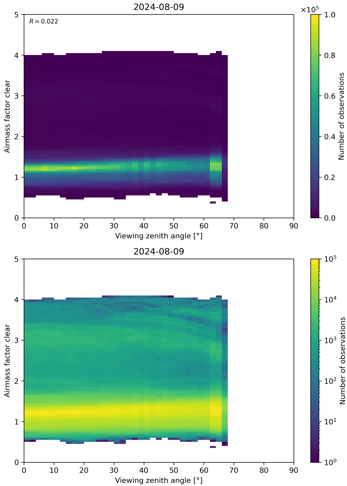
Figure 185: Scatter density plot of “Viewing zenith angle” against “Airmass factor clear” for 2024-08-08 to 2024-08-10.
