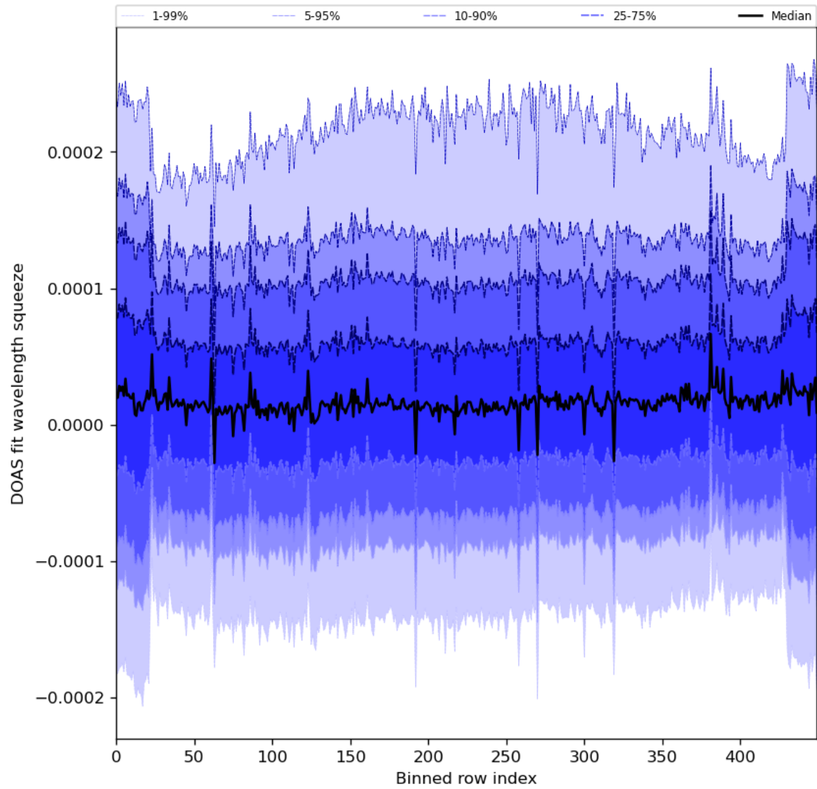
Figure 59: Along track statistics of “DOAS fit wavelength squeeze” for 2024-08-08 to 2024-08-10
