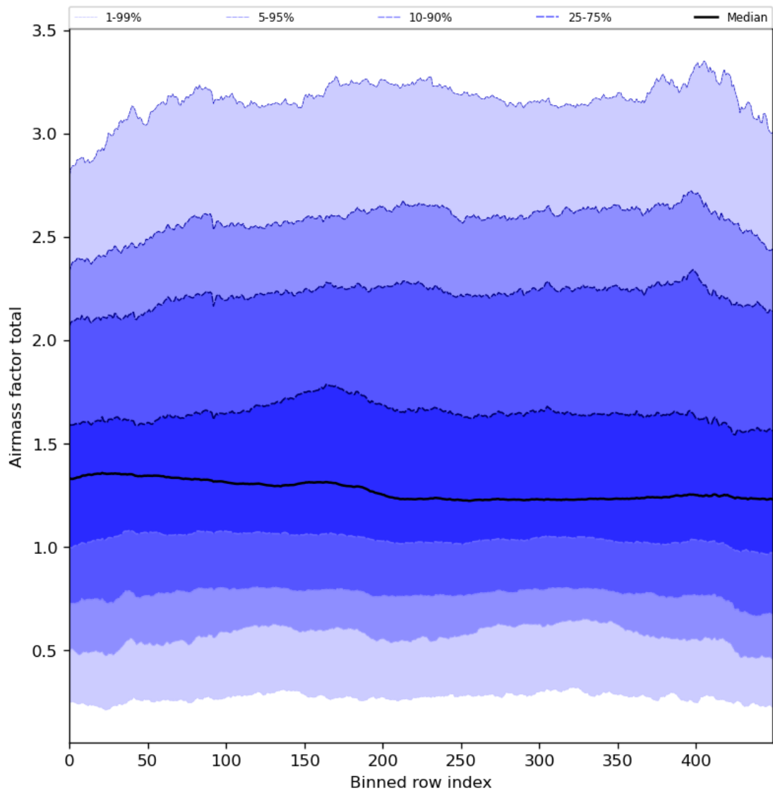
Figure 54: Along track statistics of “Airmass factor total” for 2024-08-08 to 2024-08-10
