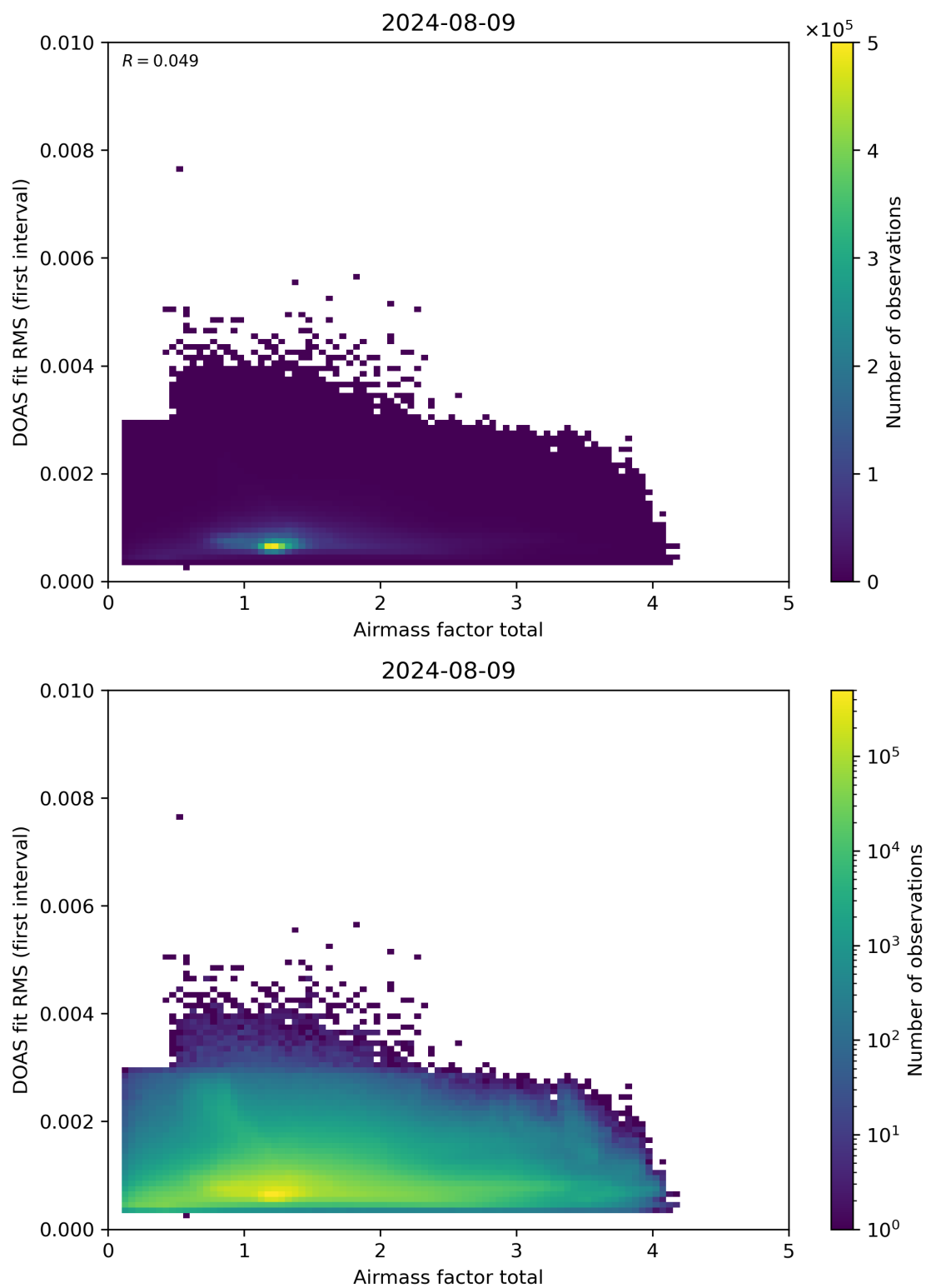
Figure 97: Scatter density plot of “Airmass factor total” against “DOAS fit RMS (first interval)” for 2024-08-08 to 2024-08-10.
