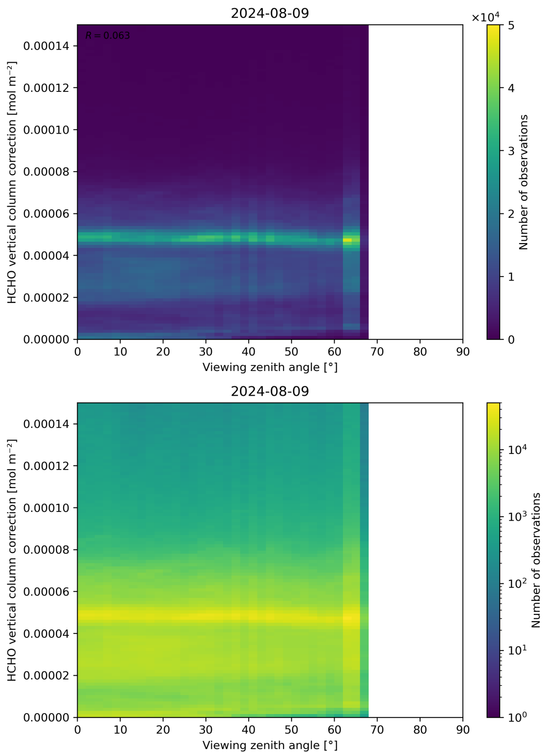
Figure 193: Scatter density plot of “Viewing zenith angle” against “HCHO vertical column correction” for 2024-08-08 to 2024-08-10.
