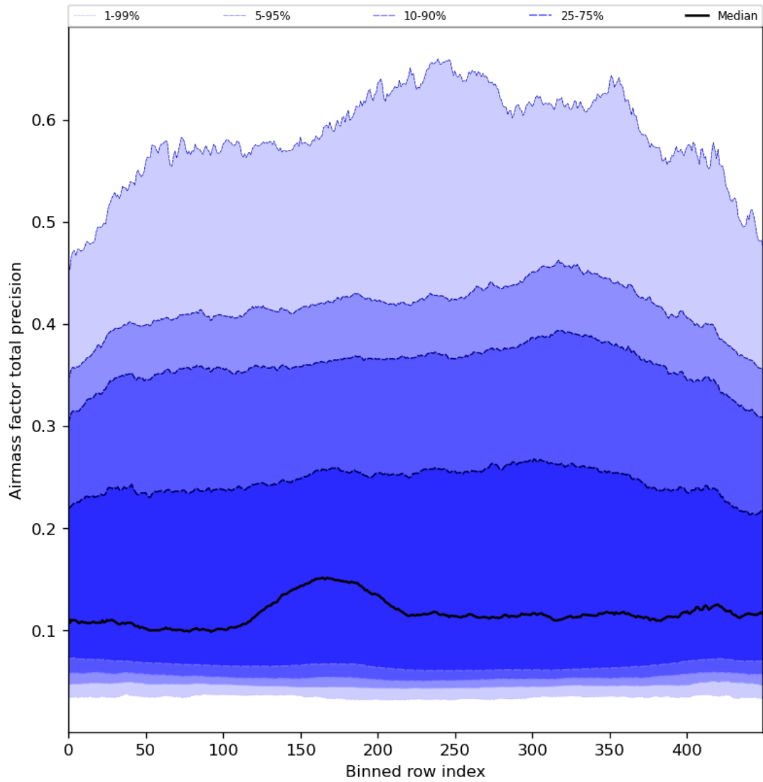
Figure 55: Along track statistics of “Airmass factor total precision” for 2024-08-08 to 2024-08-10
