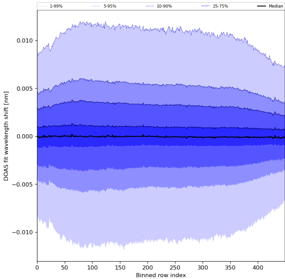
Figure 58: Along track statistics of “DOAS fit wavelength shift” for 2024-08-08 to 2024-08-10
