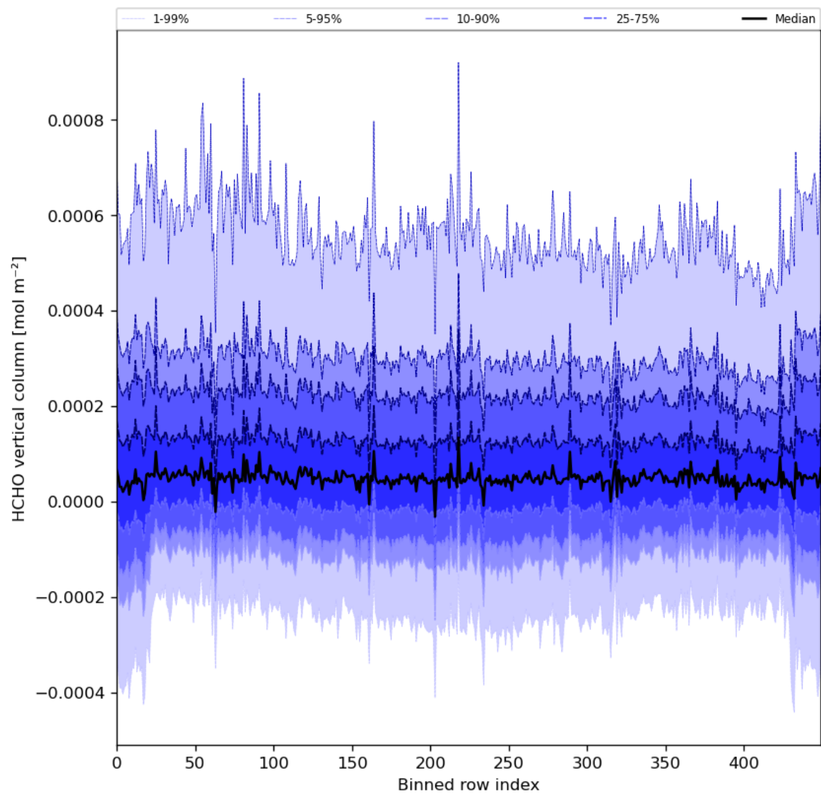
Figure 49: Along track statistics of “HCHO vertical column” for 2024-08-08 to 2024-08-10
