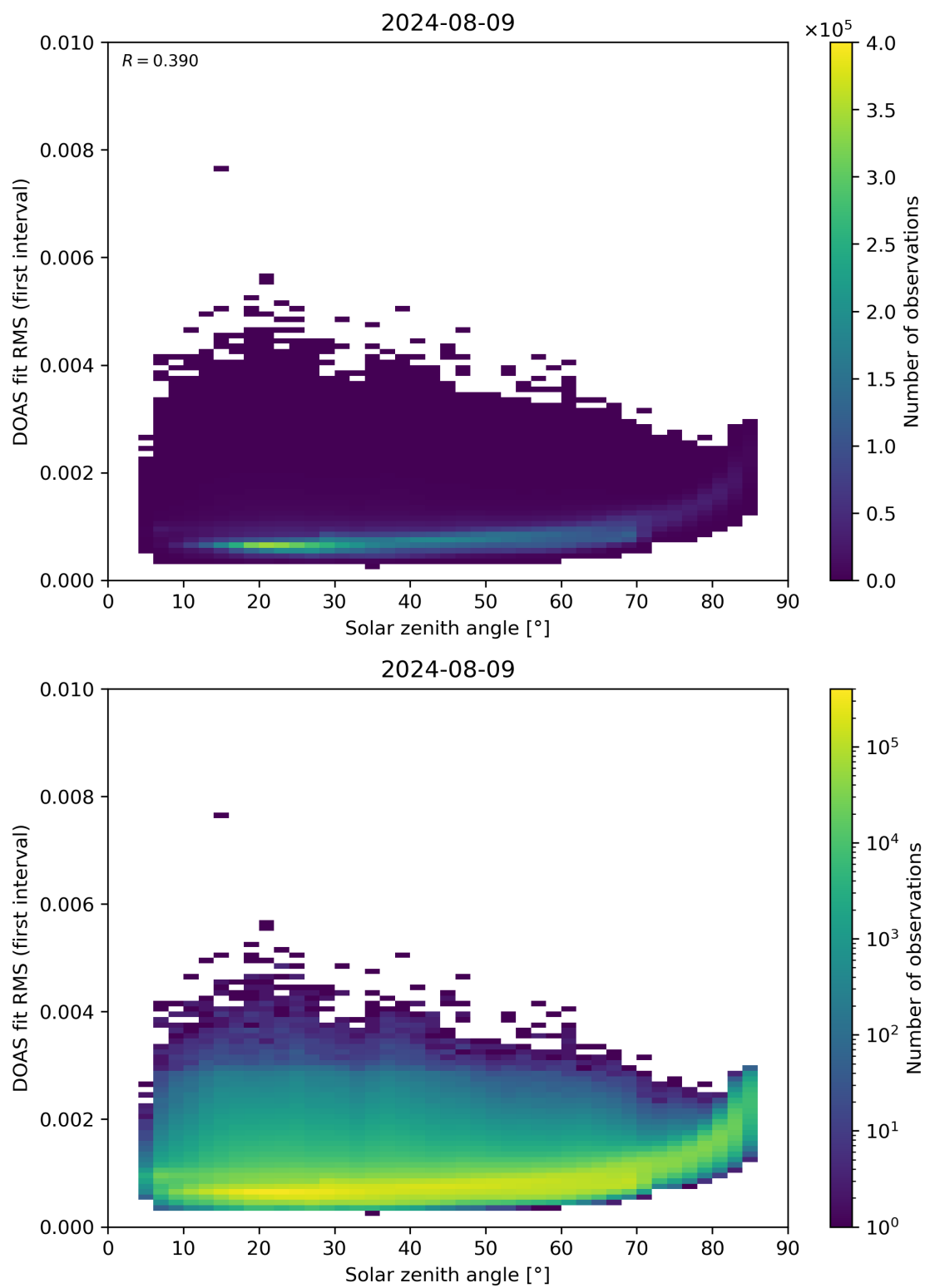
Figure 167: Scatter density plot of “Solar zenith angle” against “DOAS fit RMS (first interval)” for 2024-08-08 to 2024-08-10.
