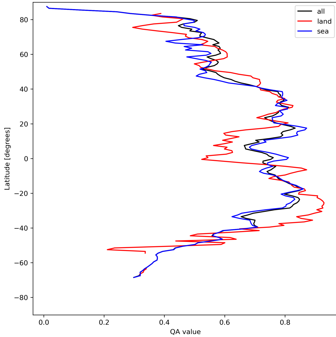
Figure 20: Zonal average of “QA value” for 2024-08-08 to 2024-08-10.
