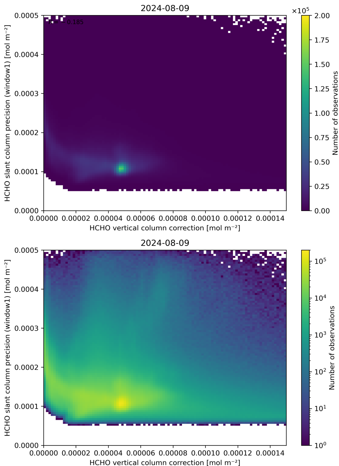
Figure 119: Scatter density plot of “HCHO vertical column correction” against “HCHO slant column precision (window1)” for 2024-08-08 to 2024-08-10.
