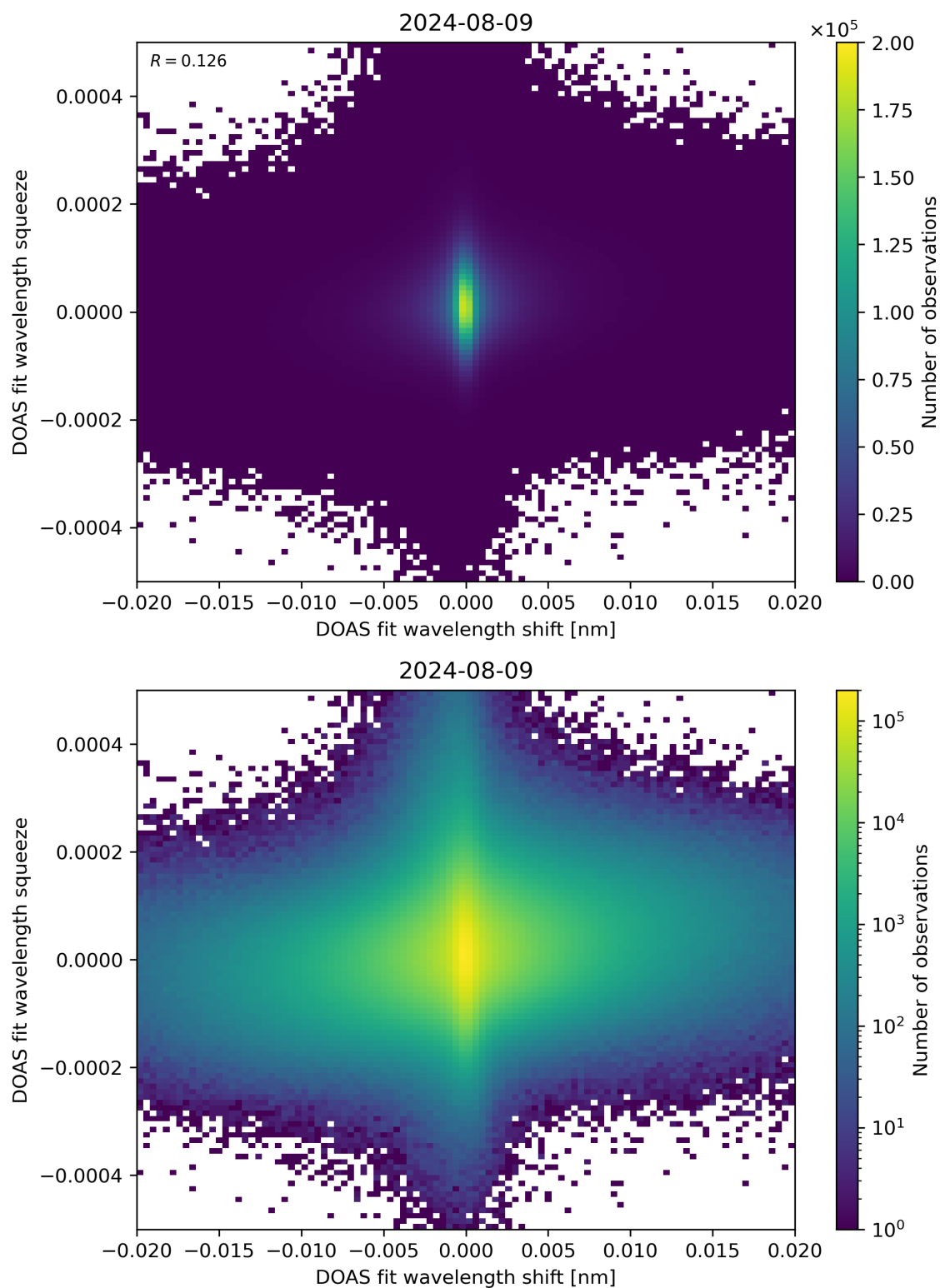
Figure 65: Scatter density plot of “DOAS fit wavelength shift” against “DOAS fit wavelength squeeze” for 2024-08-08 to 2024-08-10.
