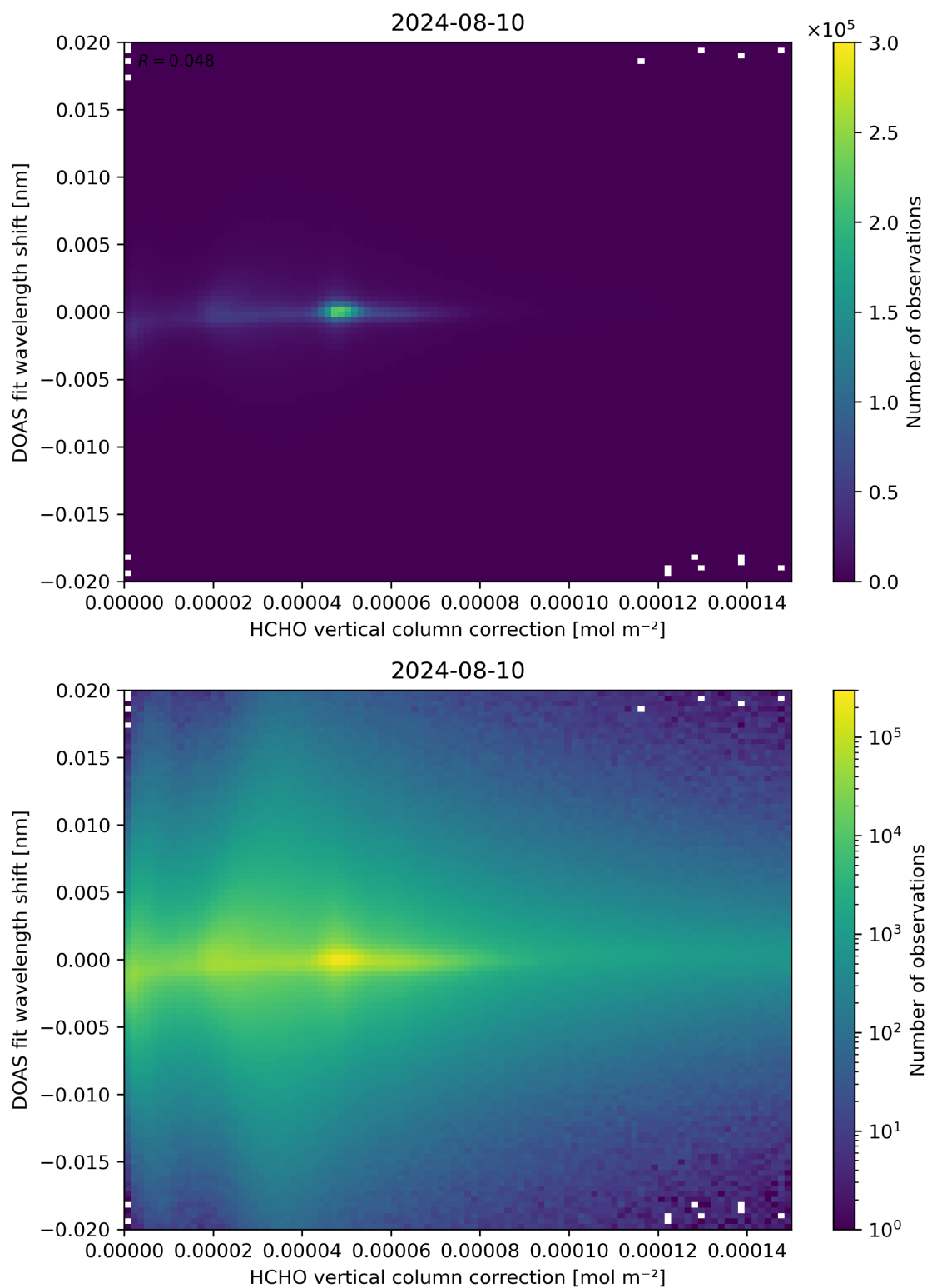
Figure 113: Scatter density plot of “HCHO vertical column correction” against “DOAS fit wavelength shift” for 2024-08-09 to 2024-08-11.
