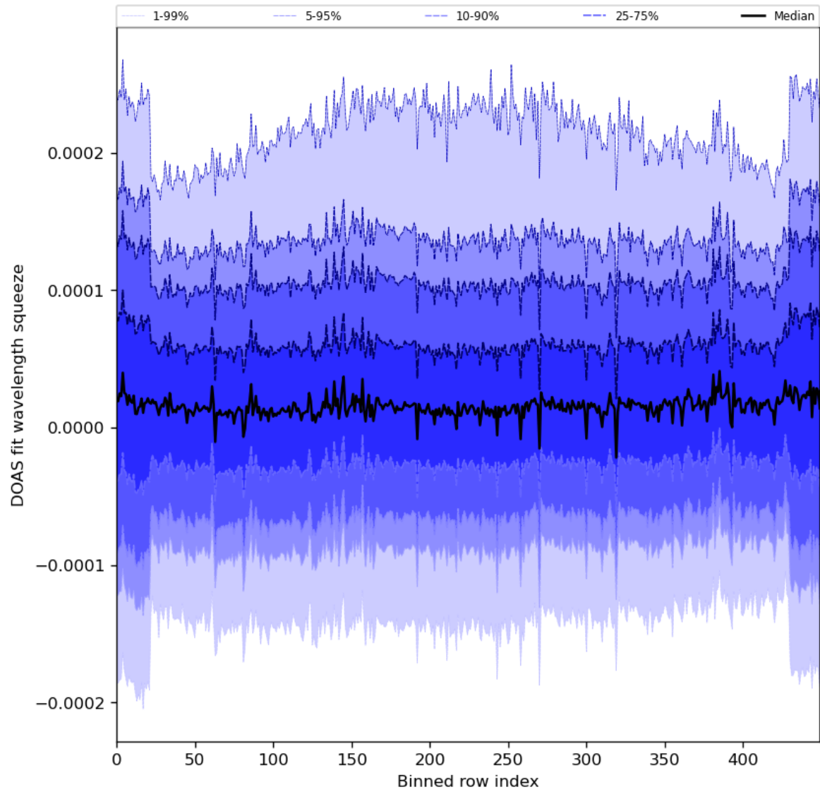
Figure 59: Along track statistics of “DOAS fit wavelength squeeze” for 2024-08-09 to 2024-08-11
