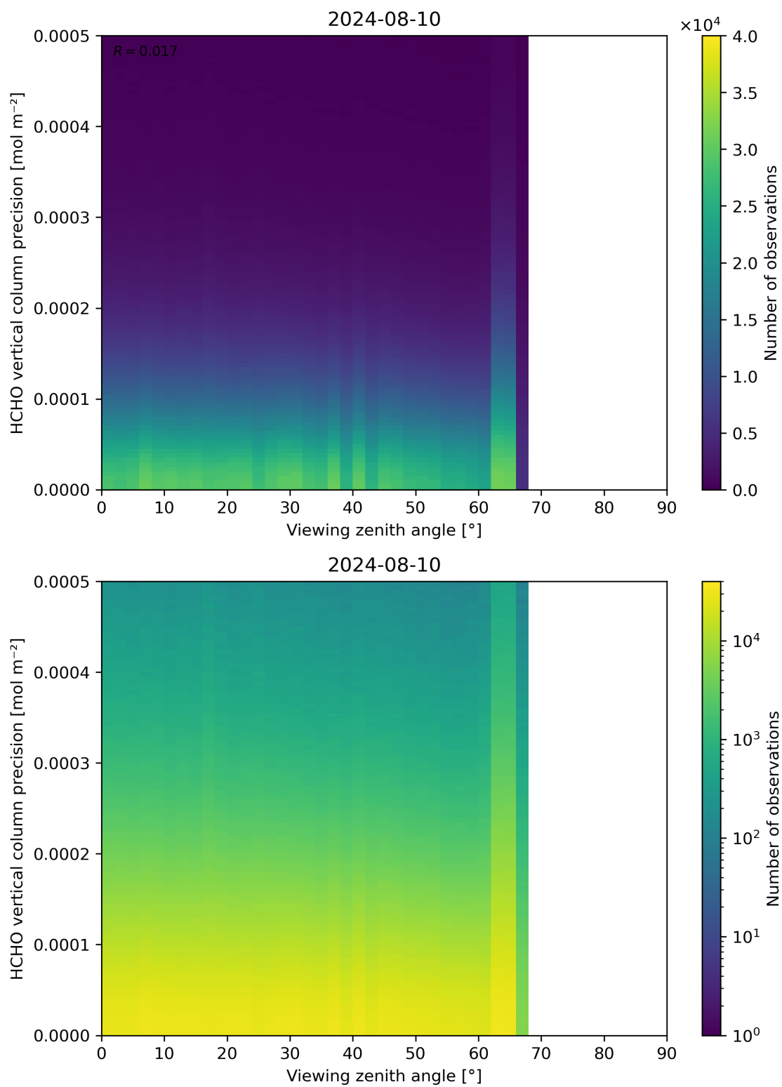
Figure 194: Scatter density plot of “Viewing zenith angle” against “HCHO vertical column precision” for 2024-08-09 to 2024-08-11.
