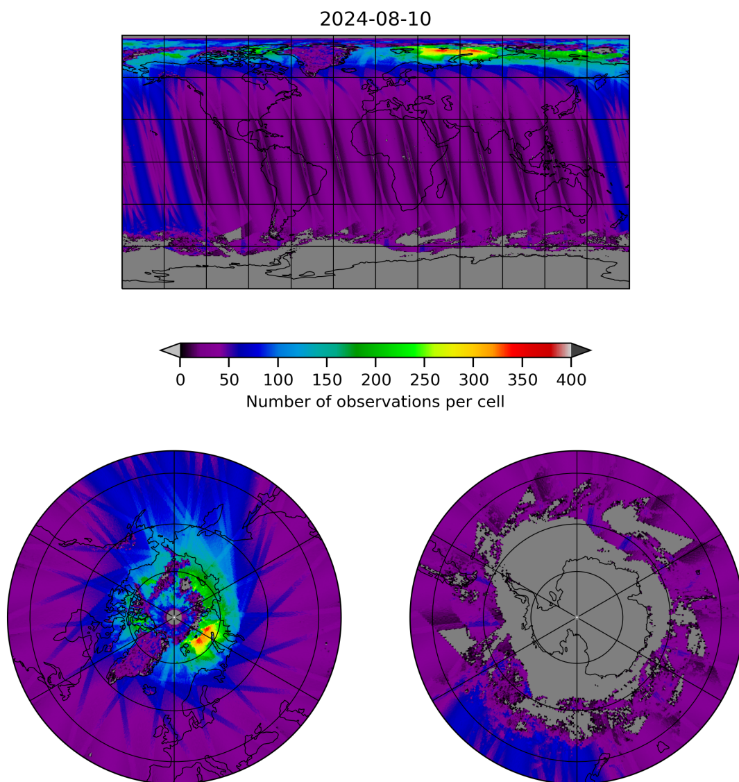
Figure 19: Map of the number of observations for 2024-08-09 to 2024-08-11
