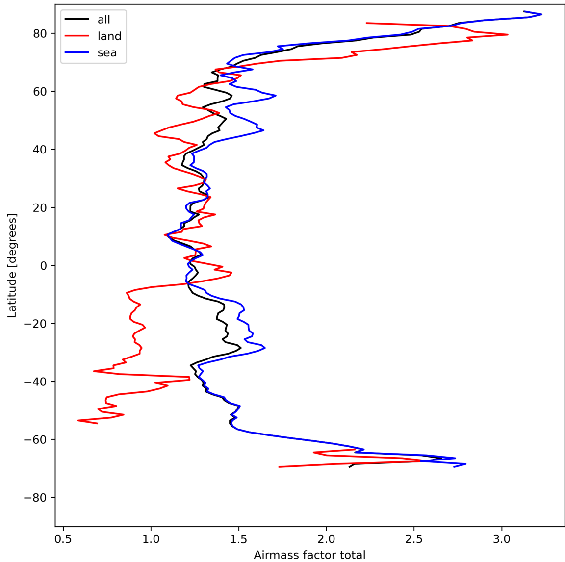
Figure 26: Zonal average of “Airmass factor total” for 2024-08-09 to 2024-08-11.
