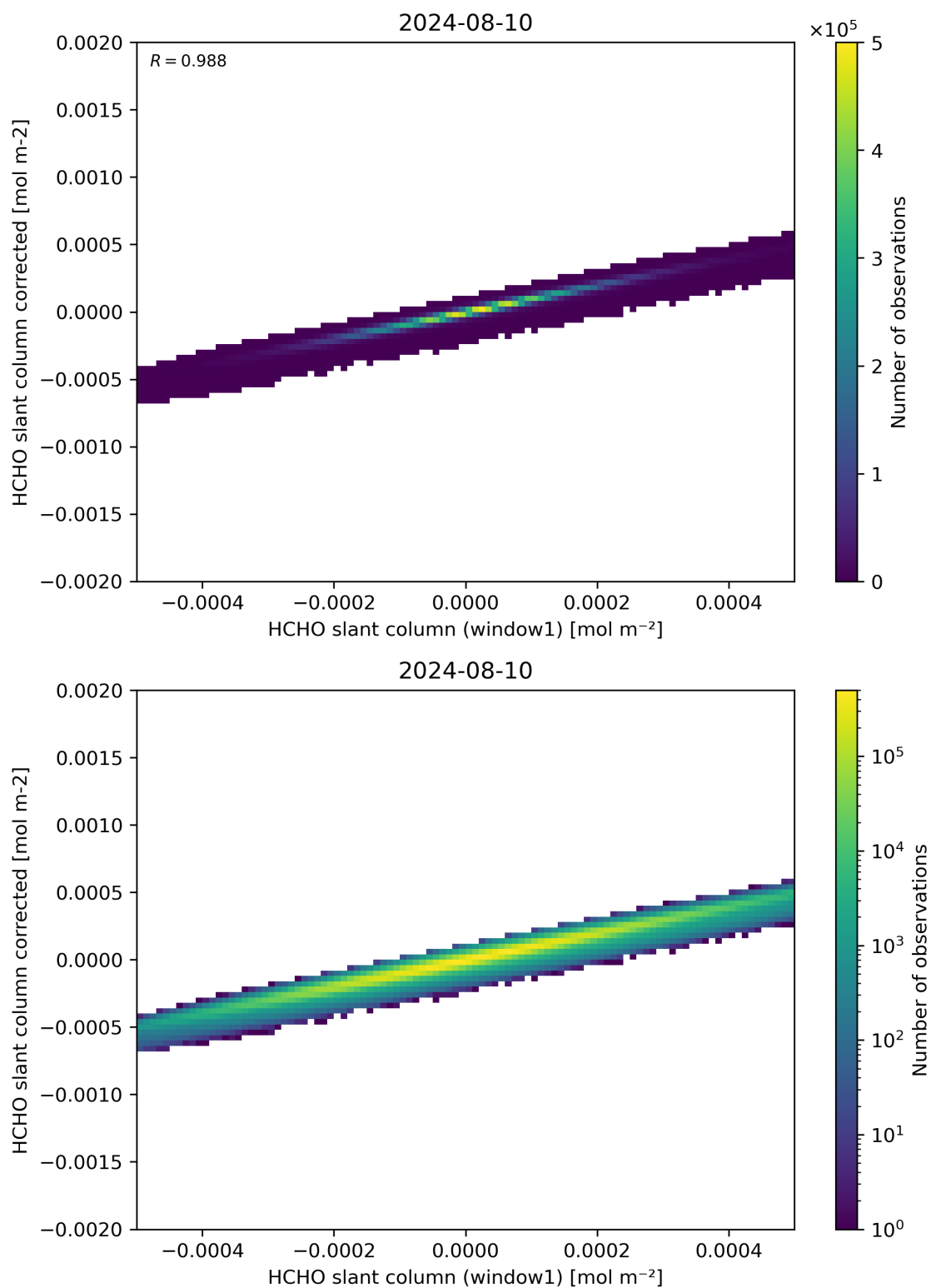
Figure 82: Scatter density plot of “HCHO slant column (window1)” against “HCHO slant column corrected” for 2024-08-09 to 2024-08-11.
