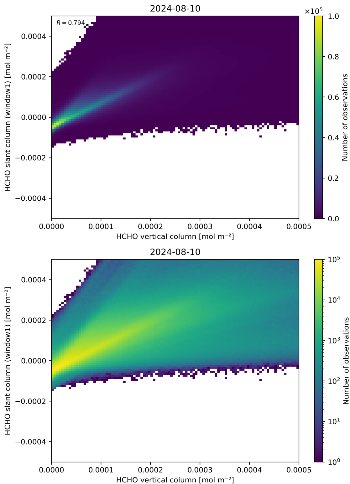
Figure 129: Scatter density plot of “HCHO vertical column” against “HCHO slant column (window1)” for 2024-08-09 to 2024-08-11.
