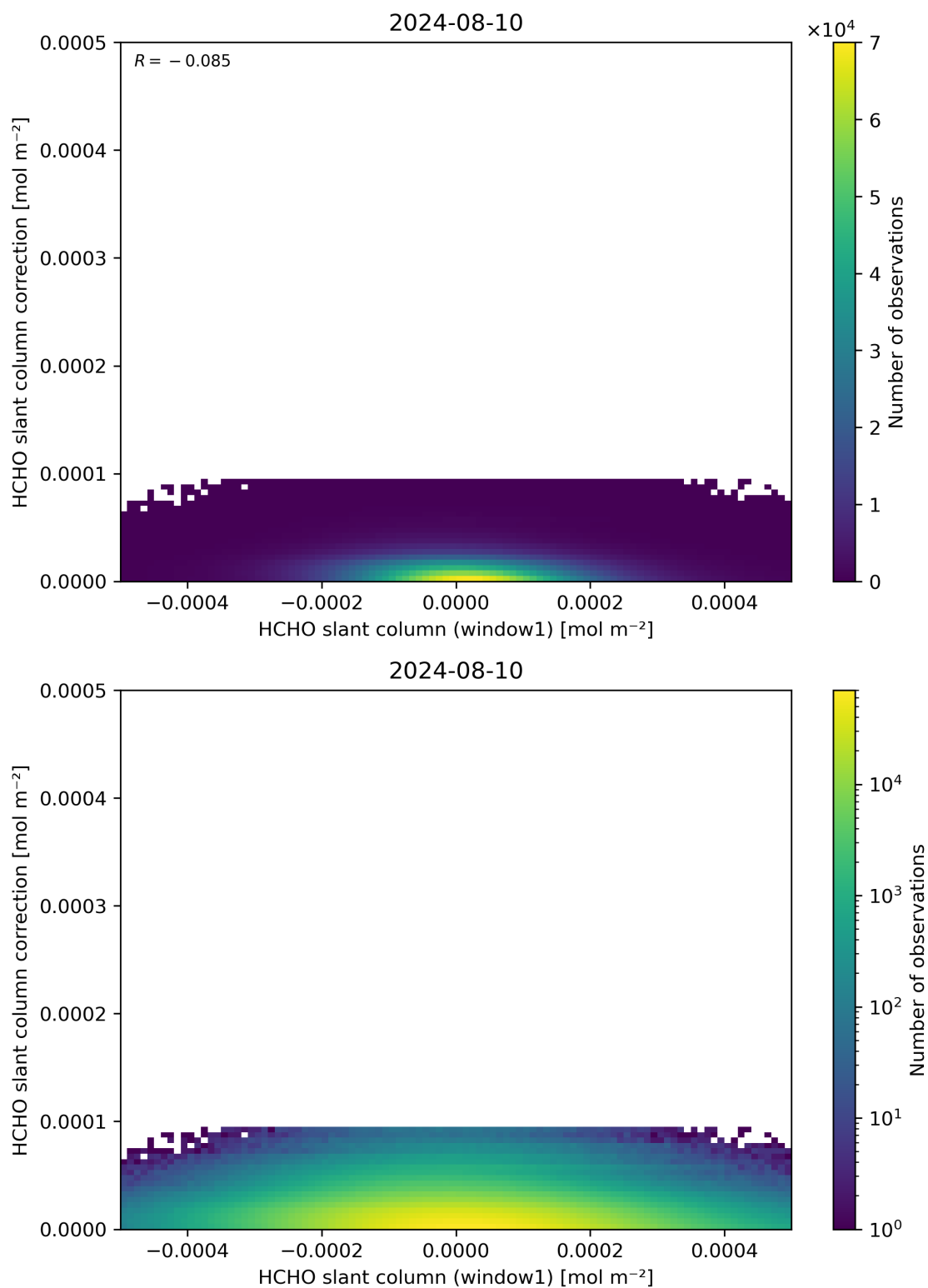
Figure 83: Scatter density plot of “HCHO slant column (window1)” against “HCHO slant column correction” for 2024-08-09 to 2024-08-11.
