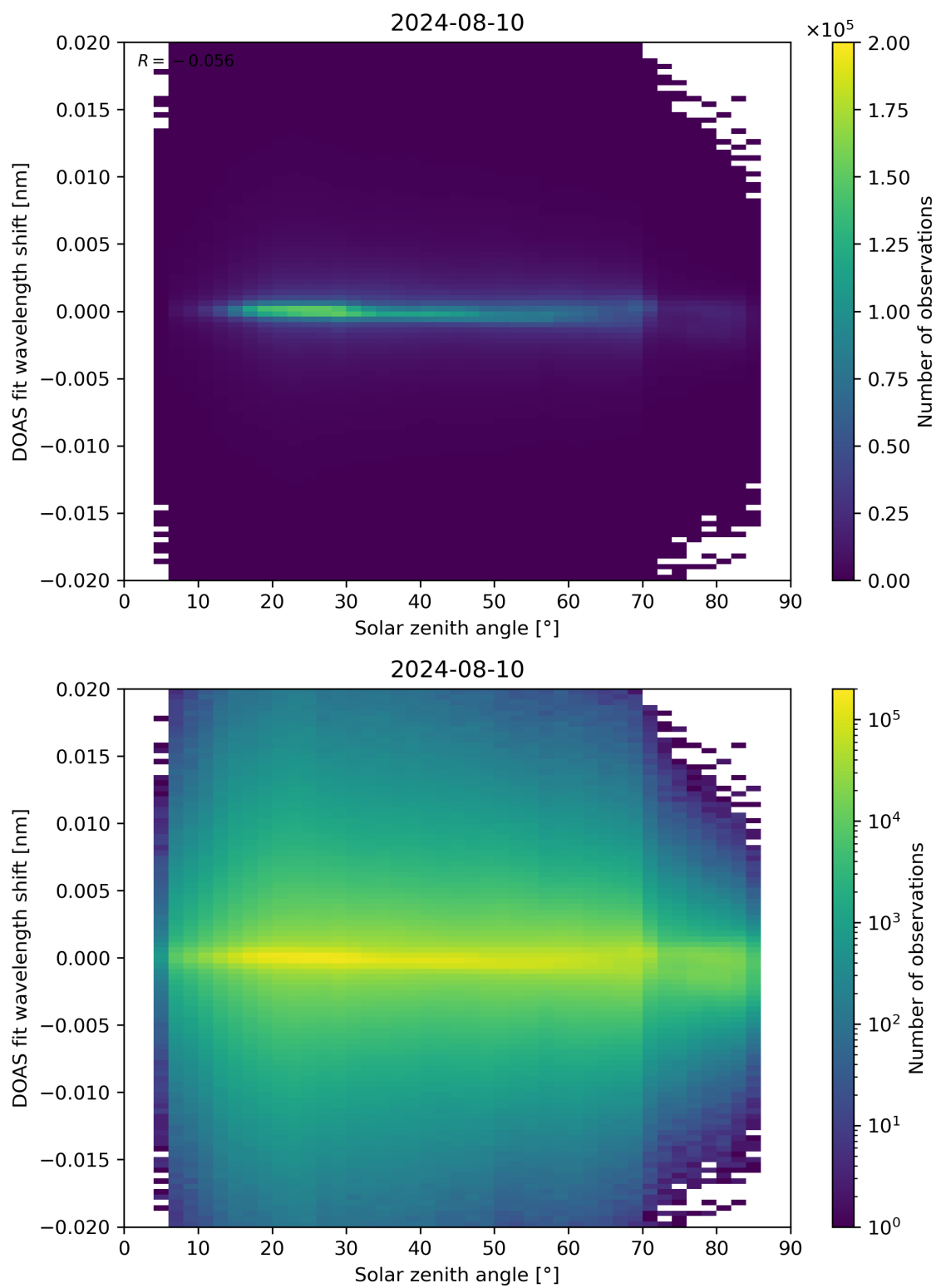
Figure 168: Scatter density plot of “Solar zenith angle” against “DOAS fit wavelength shift” for 2024-08-09 to 2024-08-11.
