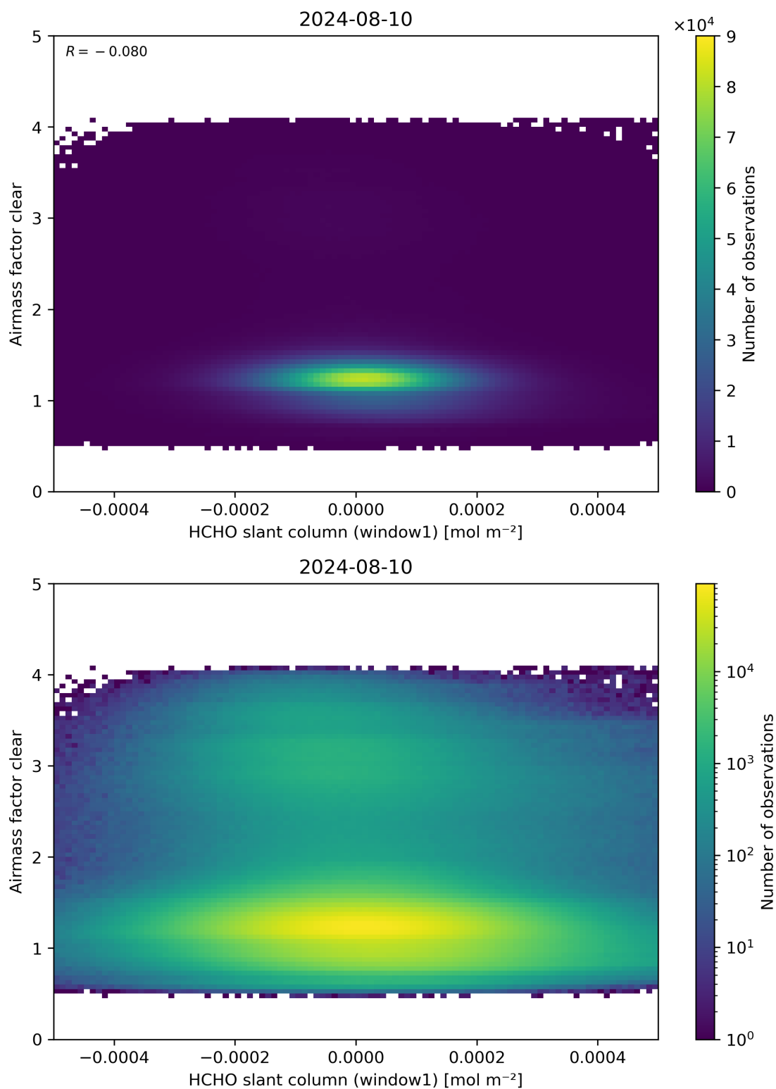
Figure 81: Scatter density plot of “HCHO slant column (window1)” against “Airmass factor clear” for 2024-08-09 to 2024-08-11.
