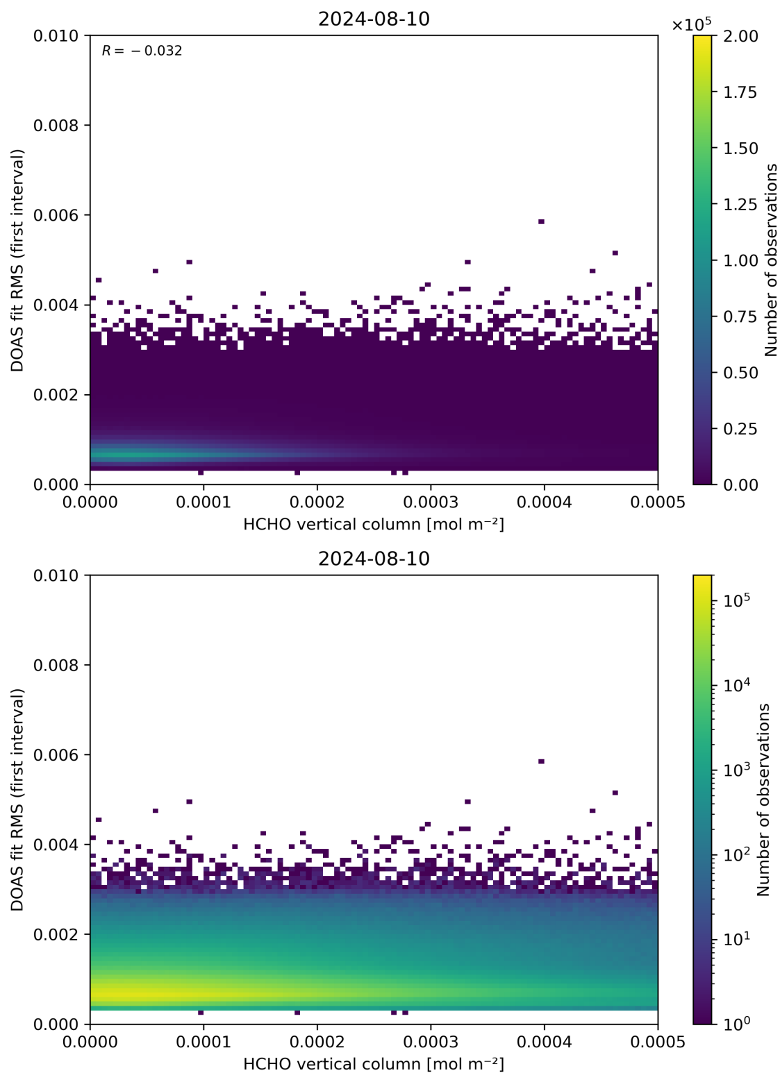
Figure 123: Scatter density plot of “HCHO vertical column” against “DOAS fit RMS (first interval)” for 2024-08-09 to 2024-08-11.
