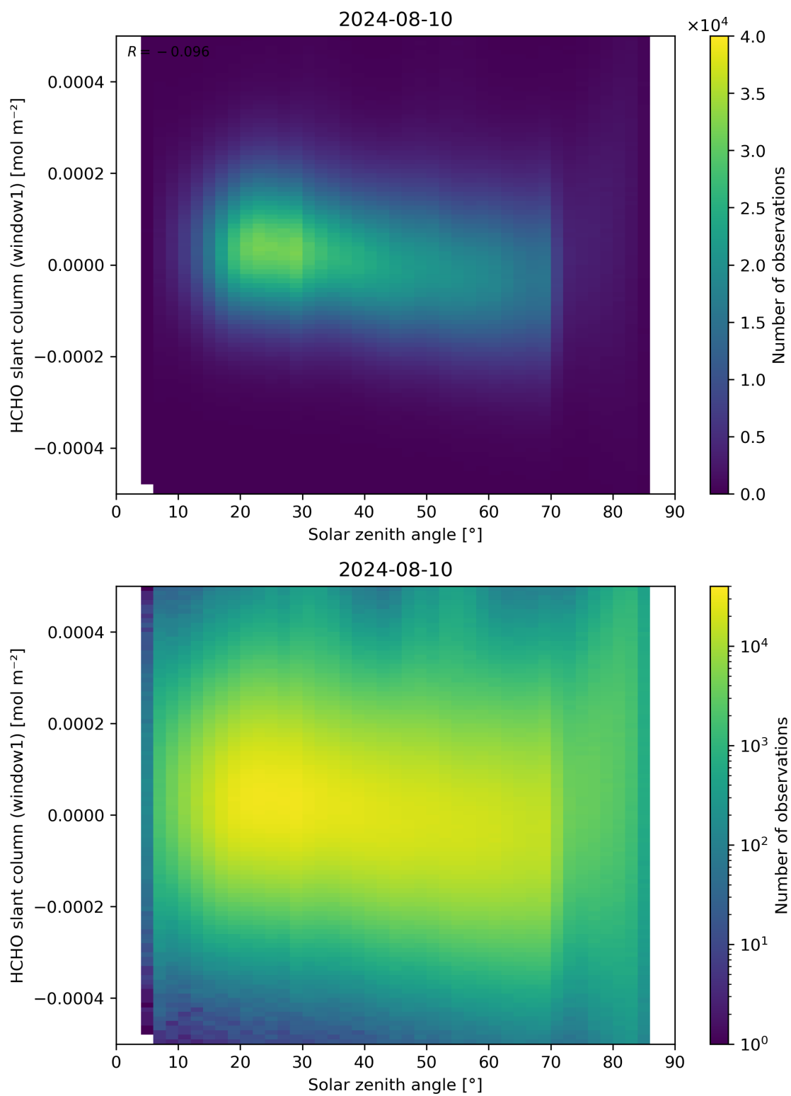
Figure 173: Scatter density plot of “Solar zenith angle” against “HCHO slant column (window1)” for 2024-08-09 to 2024-08-11.
