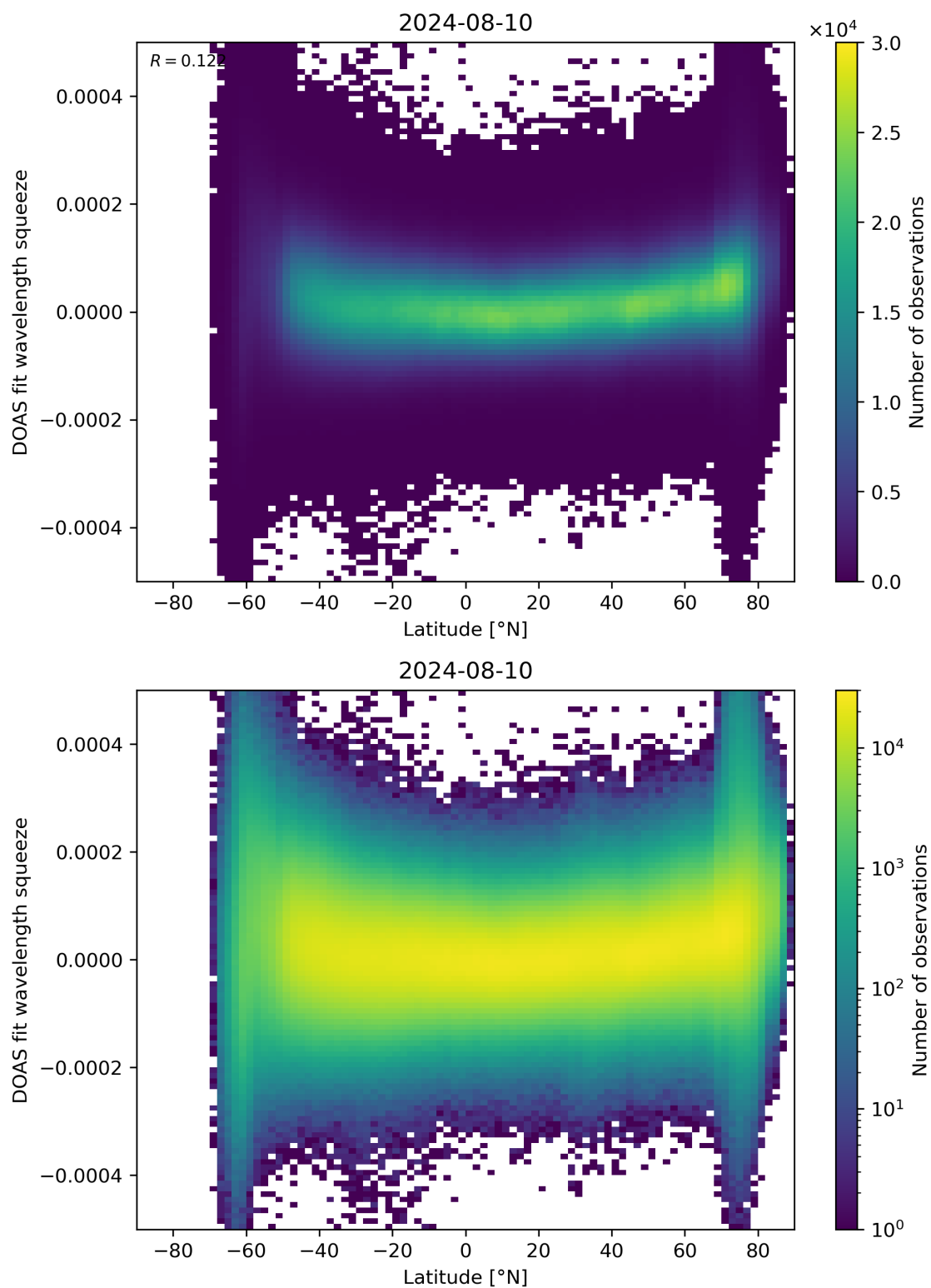
Figure 155: Scatter density plot of “Latitude” against “DOAS fit wavelength squeeze” for 2024-08-09 to 2024-08-11.
