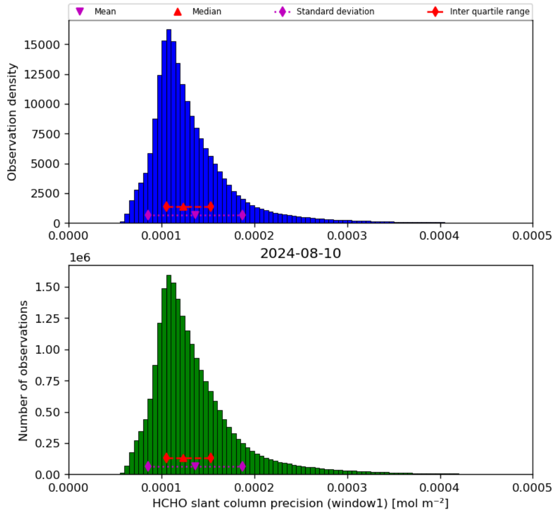
Figure 39: Histogram of “HCHO slant column precision (window1)” for 2024-08-09 to 2024-08-11
