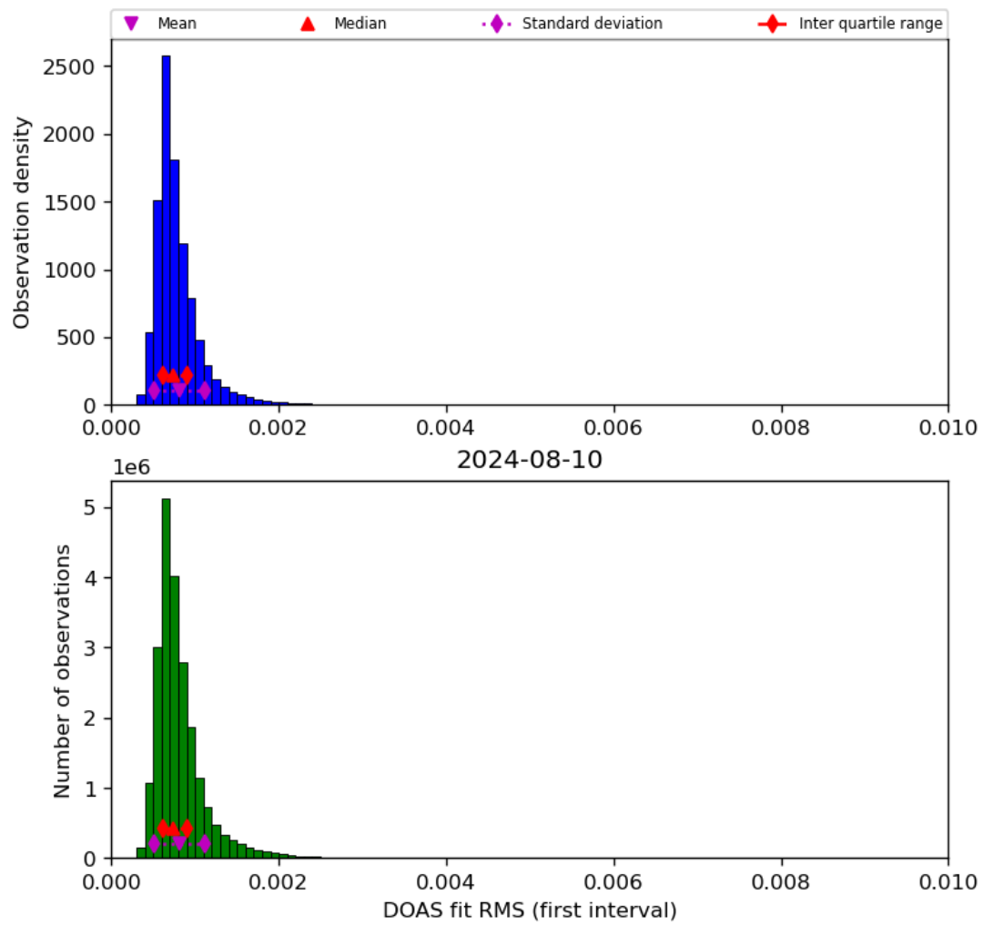
Figure 46: Histogram of “DOAS fit RMS (first interval)” for 2024-08-09 to 2024-08-11
