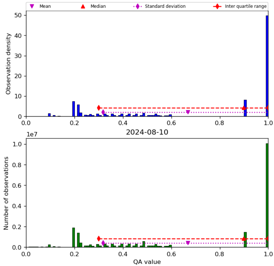
Figure 34: Histogram of “QA value” for 2024-08-09 to 2024-08-11
