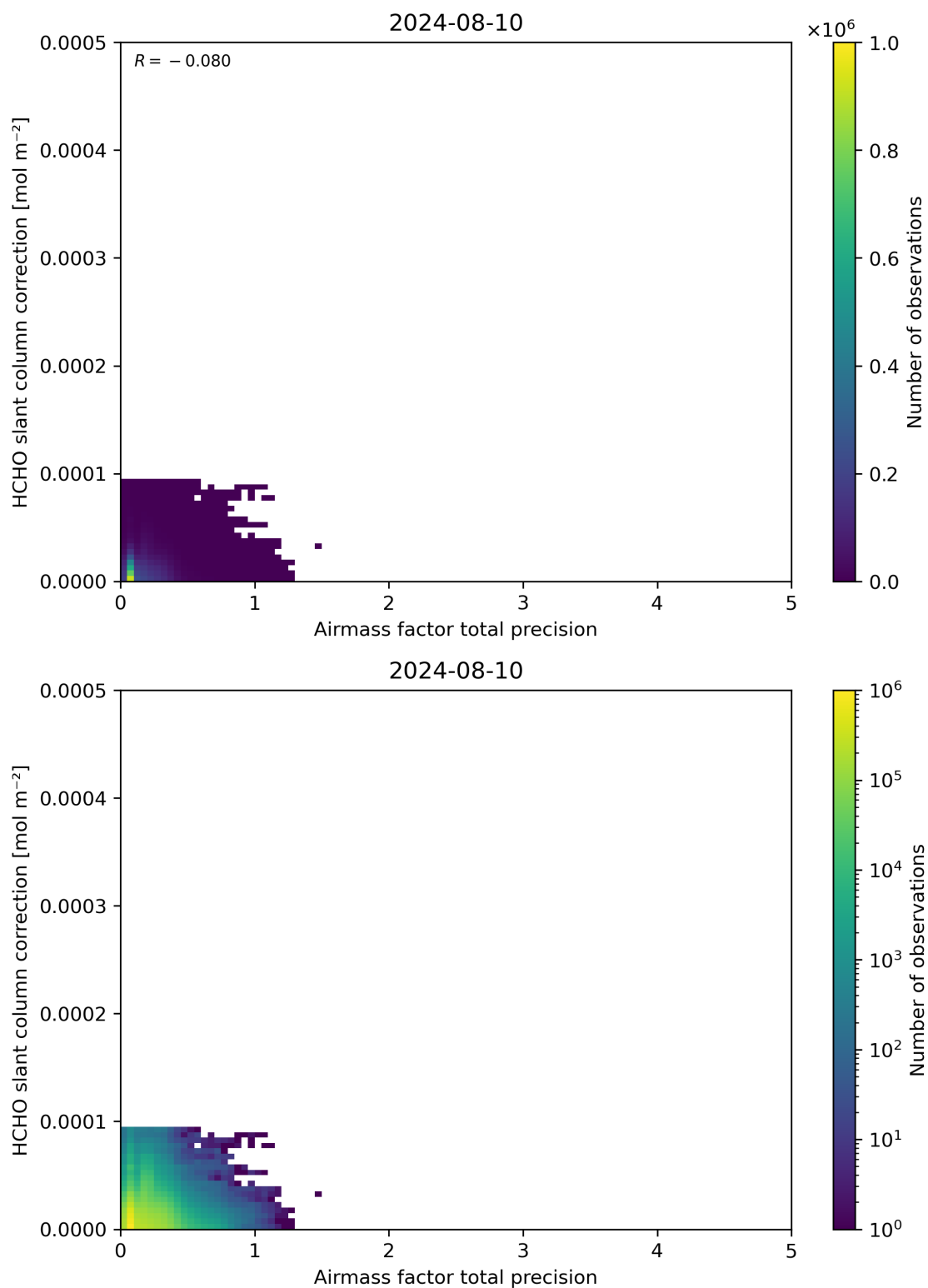
Figure 110: Scatter density plot of “Airmass factor total precision” against “HCHO slant column correction” for 2024-08-09 to 2024-08-11.
