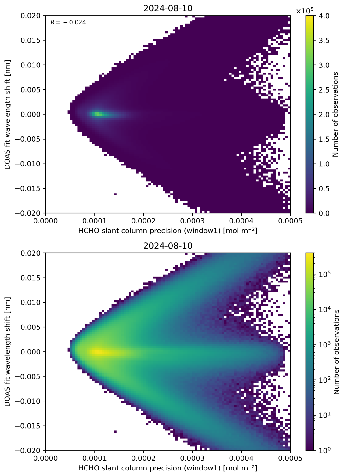
Figure 89: Scatter density plot of “HCHO slant column precision (window1)” against “DOAS fit wavelength shift” for 2024-08-09 to 2024-08-11.
