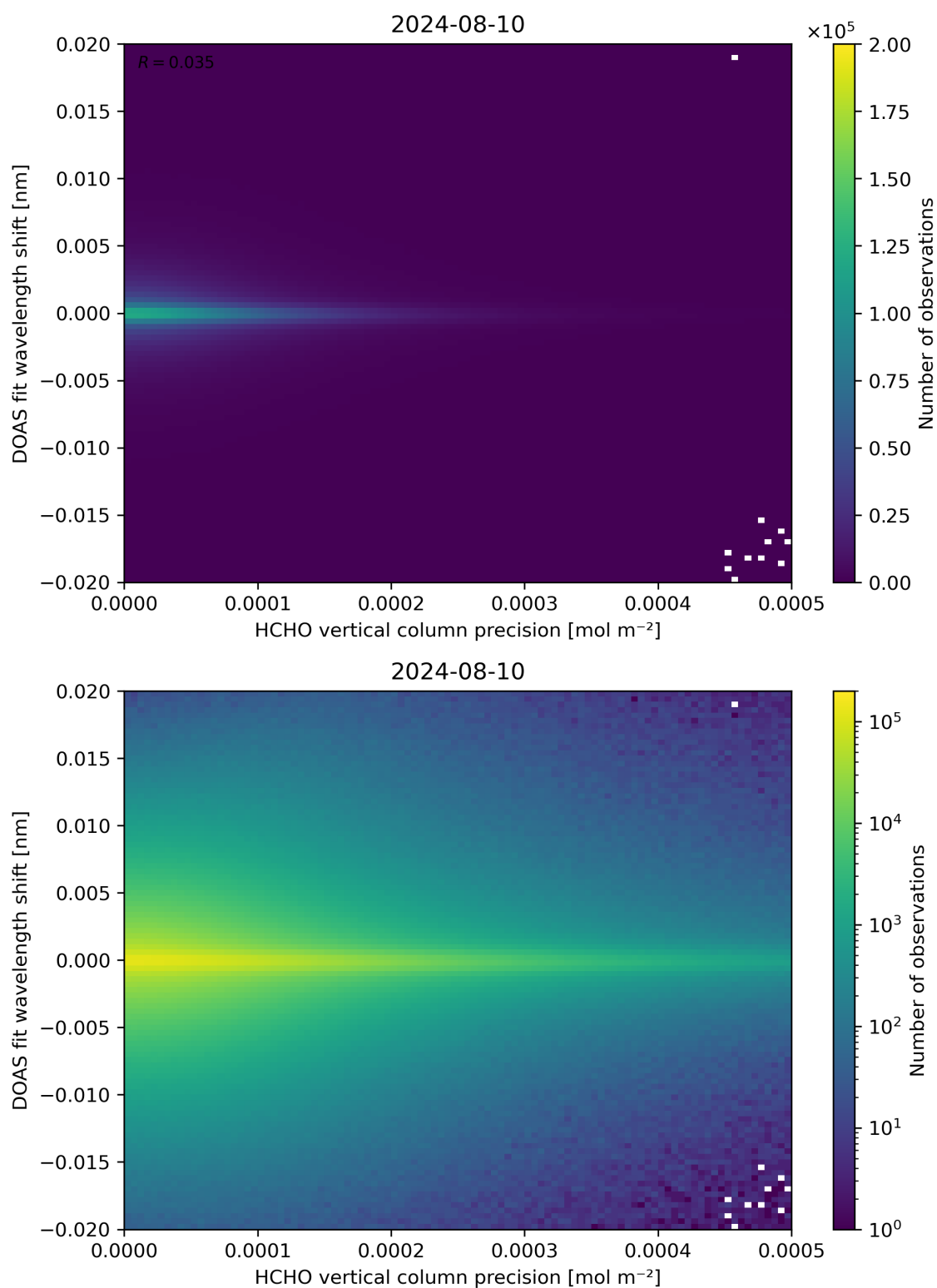
Figure 137: Scatter density plot of “HCHO vertical column precision” against “DOAS fit wavelength shift” for 2024-08-09 to 2024-08-11.
