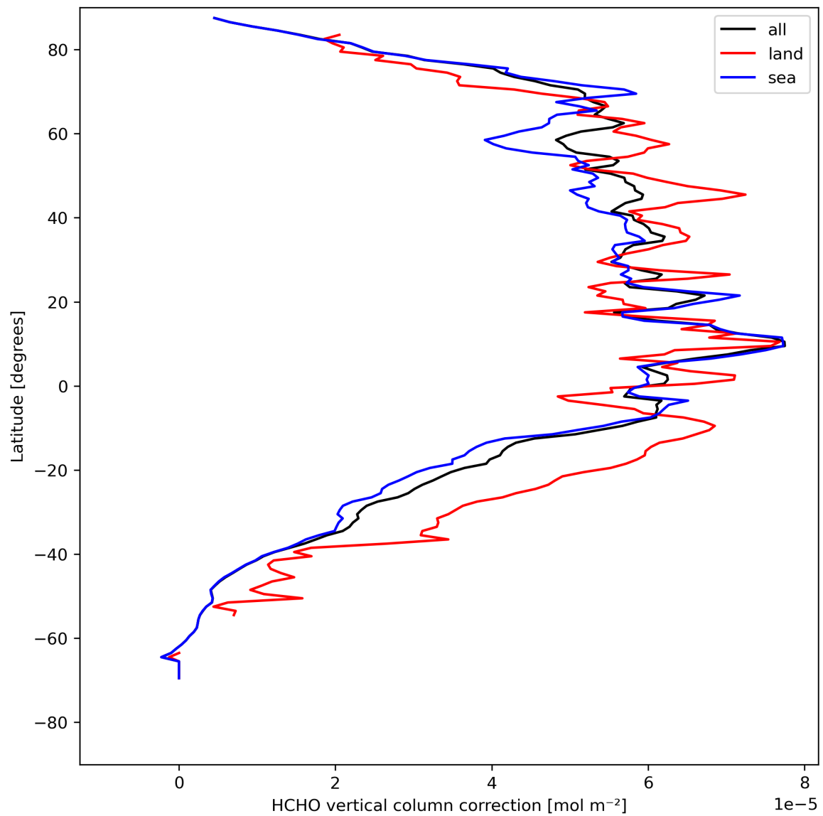
Figure 23: Zonal average of "HCHO vertical column correction" for 2024-08-09 to 2024-08-11.
