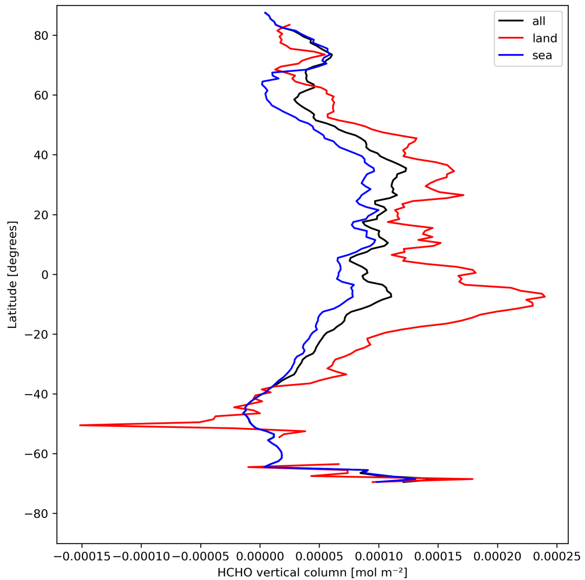
Figure 21: Zonal average of “HCHO vertical column” for 2024-08-09 to 2024-08-11.
