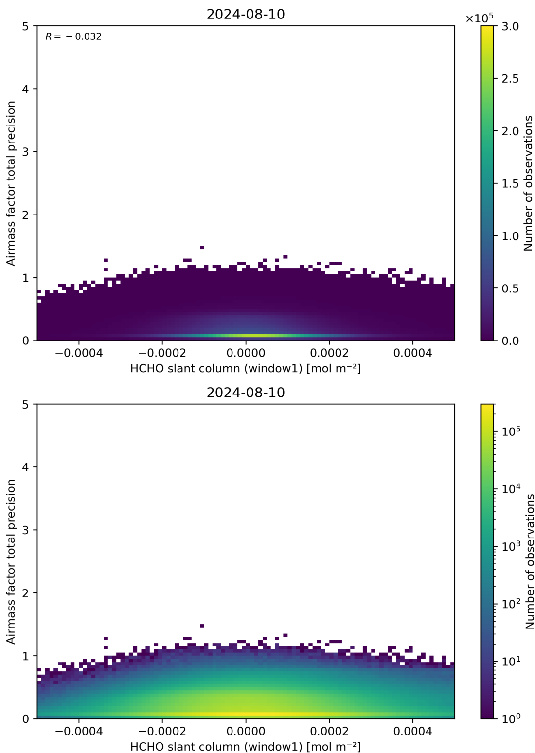
Figure 86: Scatter density plot of “HCHO slant column (window1)” against “Airmass factor total precision” for 2024-08-09 to 2024-08-11.
