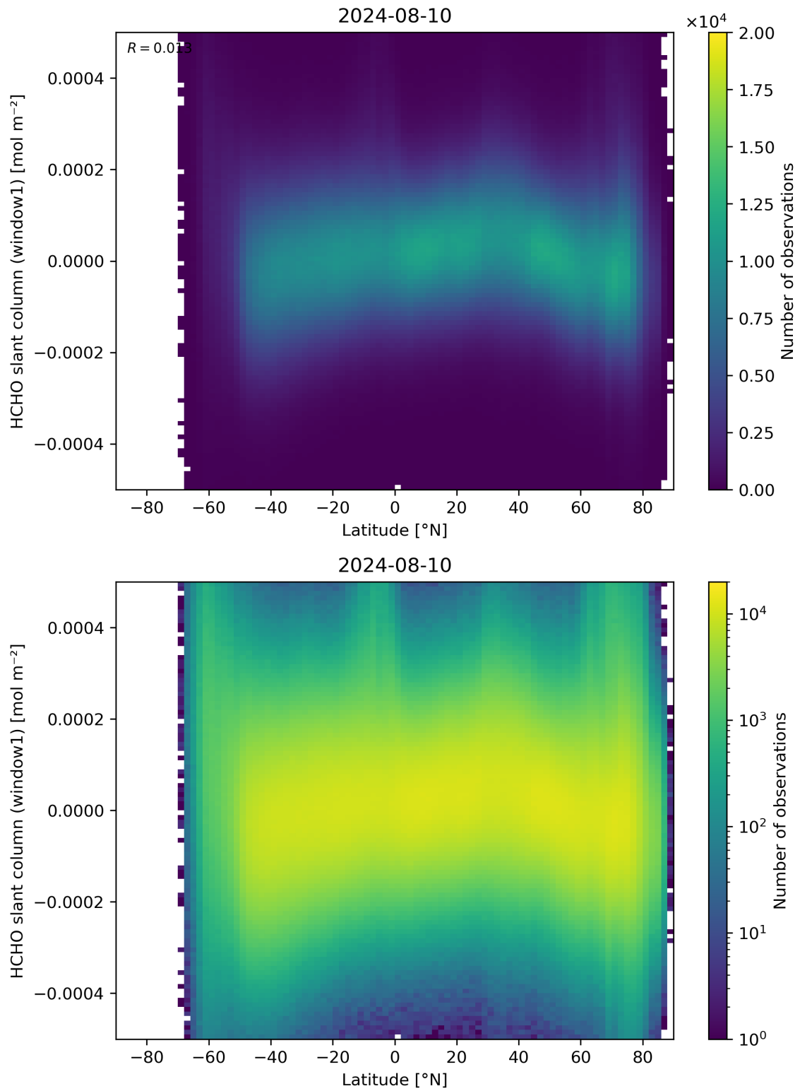
Figure 159: Scatter density plot of “Latitude” against “HCHO slant column (window1)” for 2024-08-09 to 2024-08-11.
