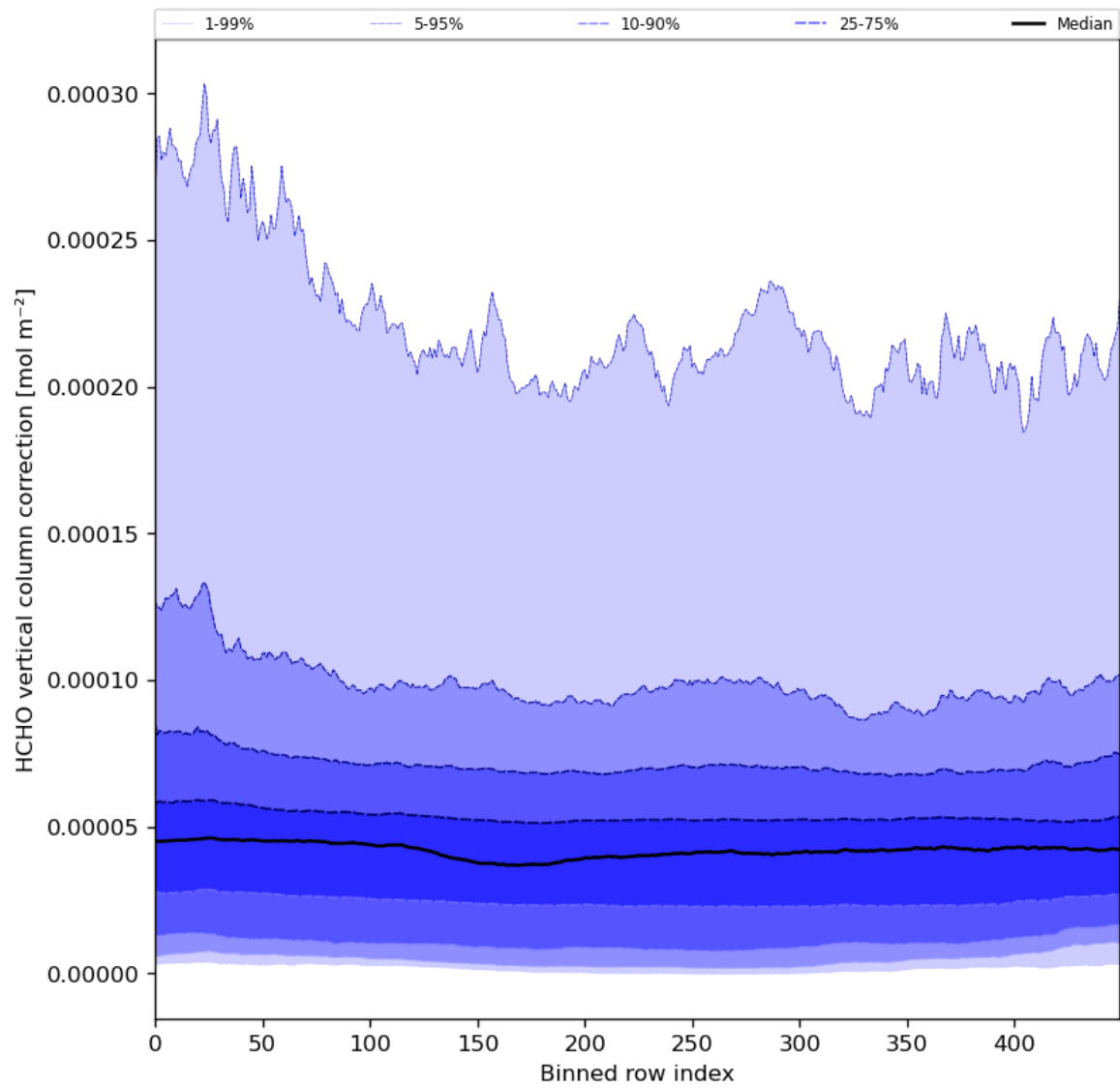
Figure 51: Along track statistics of “HCHO vertical column correction” for 2024-08-09 to 2024-08-11
