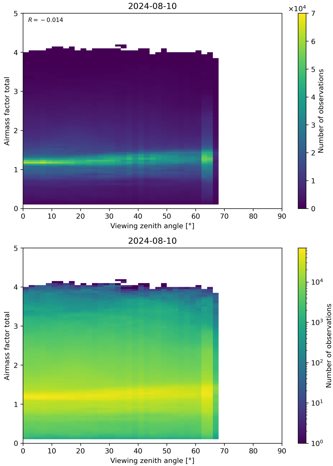
Figure 190: Scatter density plot of “Viewing zenith angle” against “Airmass factor total” for 2024-08-09 to 2024-08-11.
