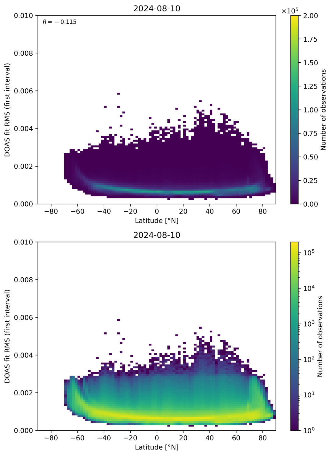
Figure 153: Scatter density plot of “Latitude” against “DOAS fit RMS (first interval)” for 2024-08-09 to 2024-08-11.
