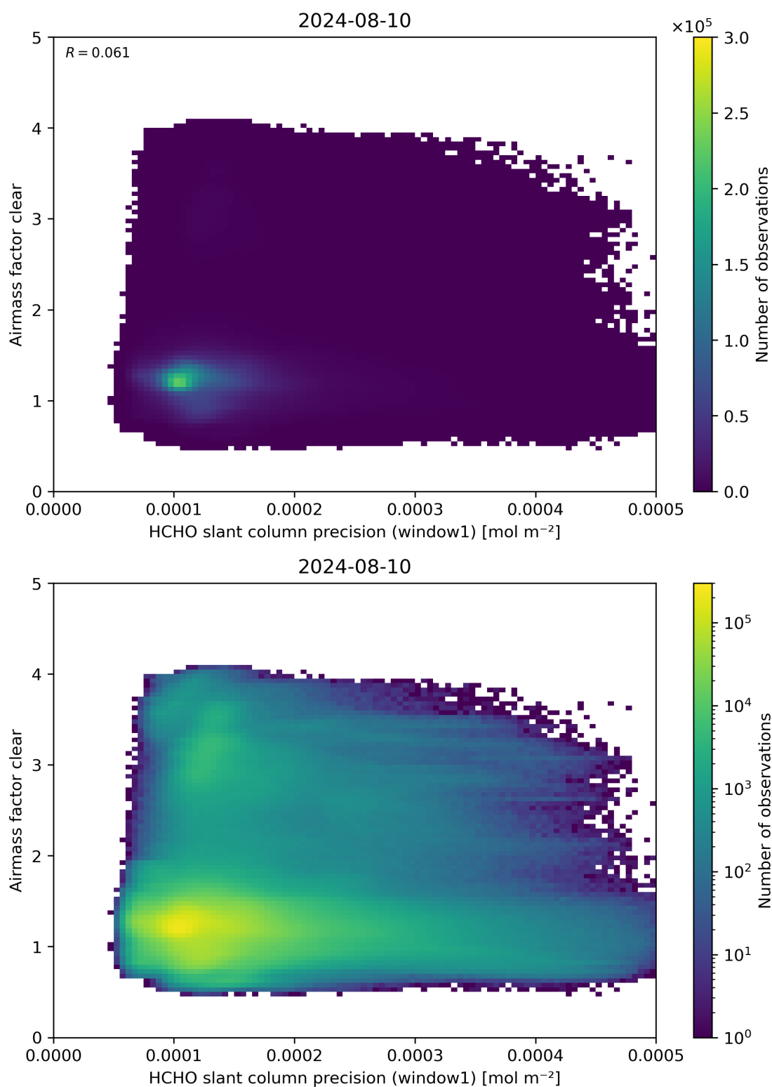
Figure 91: Scatter density plot of “HCHO slant column precision (window1)” against “Airmass factor clear” for 2024-08-09 to 2024-08-11.
