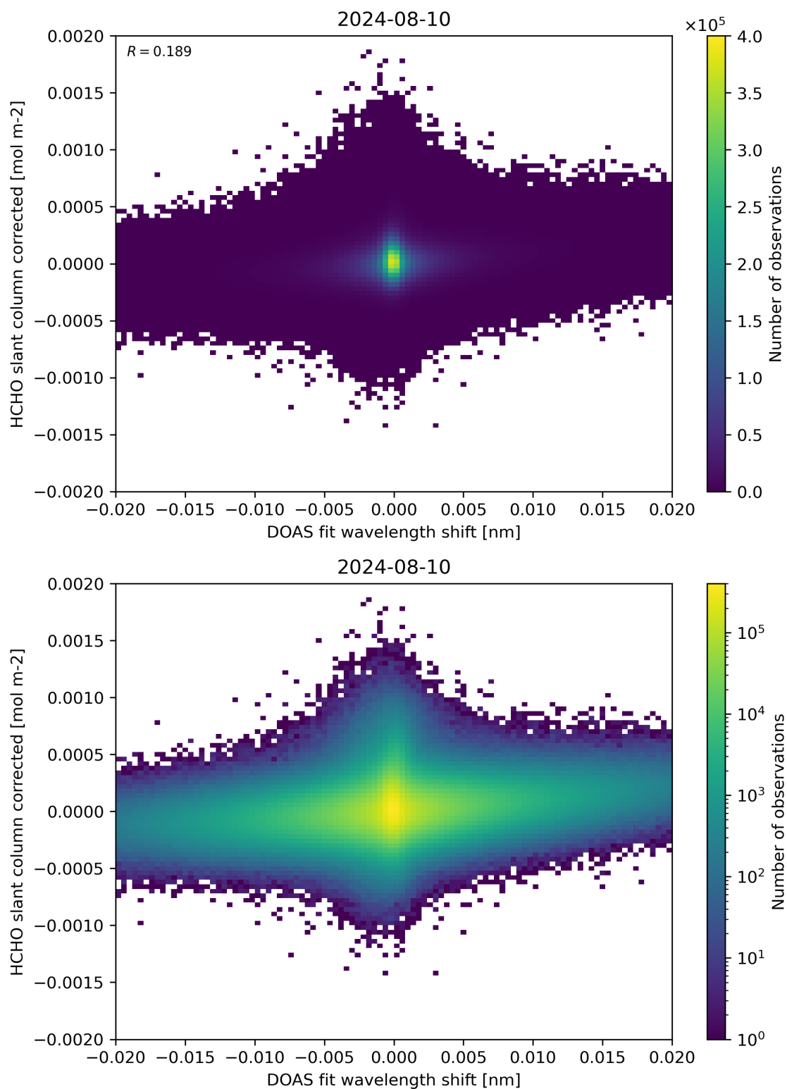
Figure 66: Scatter density plot of “DOAS fit wavelength shift” against “HCHO slant column corrected” for 2024-08-09 to 2024-08-11.
