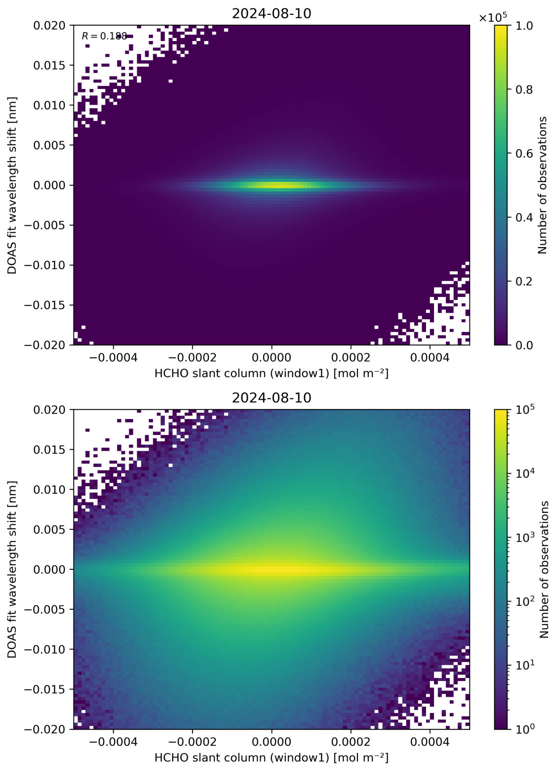
Figure 79: Scatter density plot of “HCHO slant column (window1)” against “DOAS fit wavelength shift” for 2024-08-09 to 2024-08-11.
