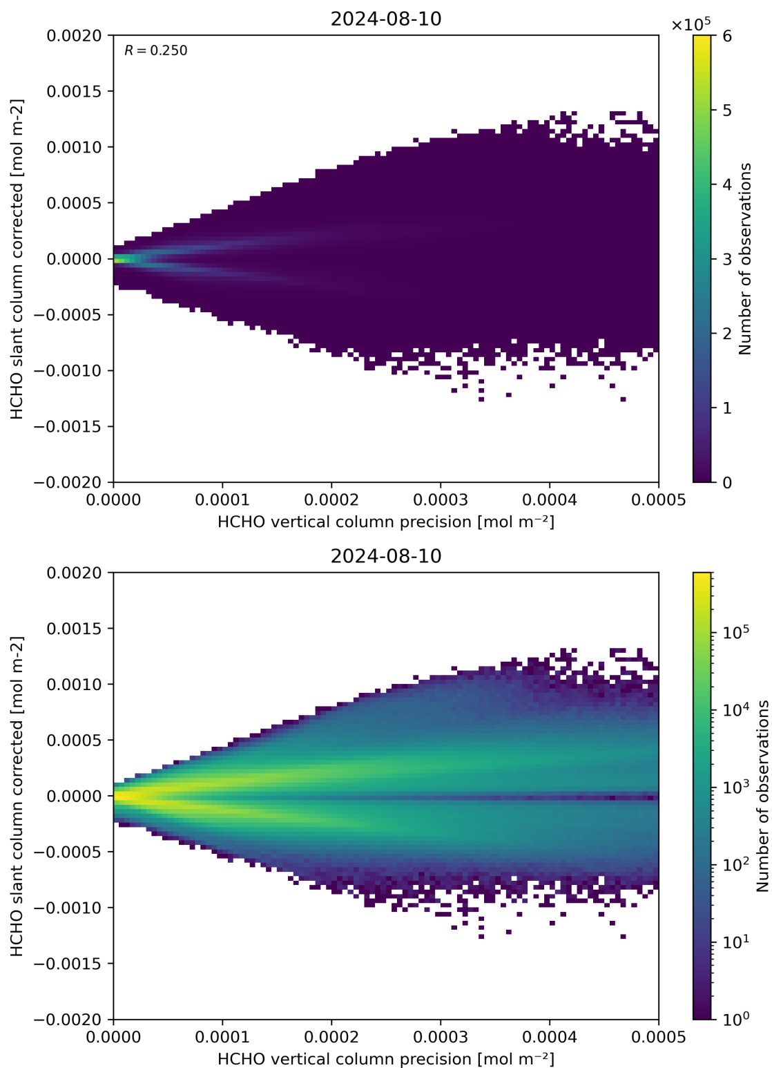
Figure 140: Scatter density plot of “HCHO vertical column precision” against “HCHO slant column corrected” for 2024-08-09 to 2024-08-11.
