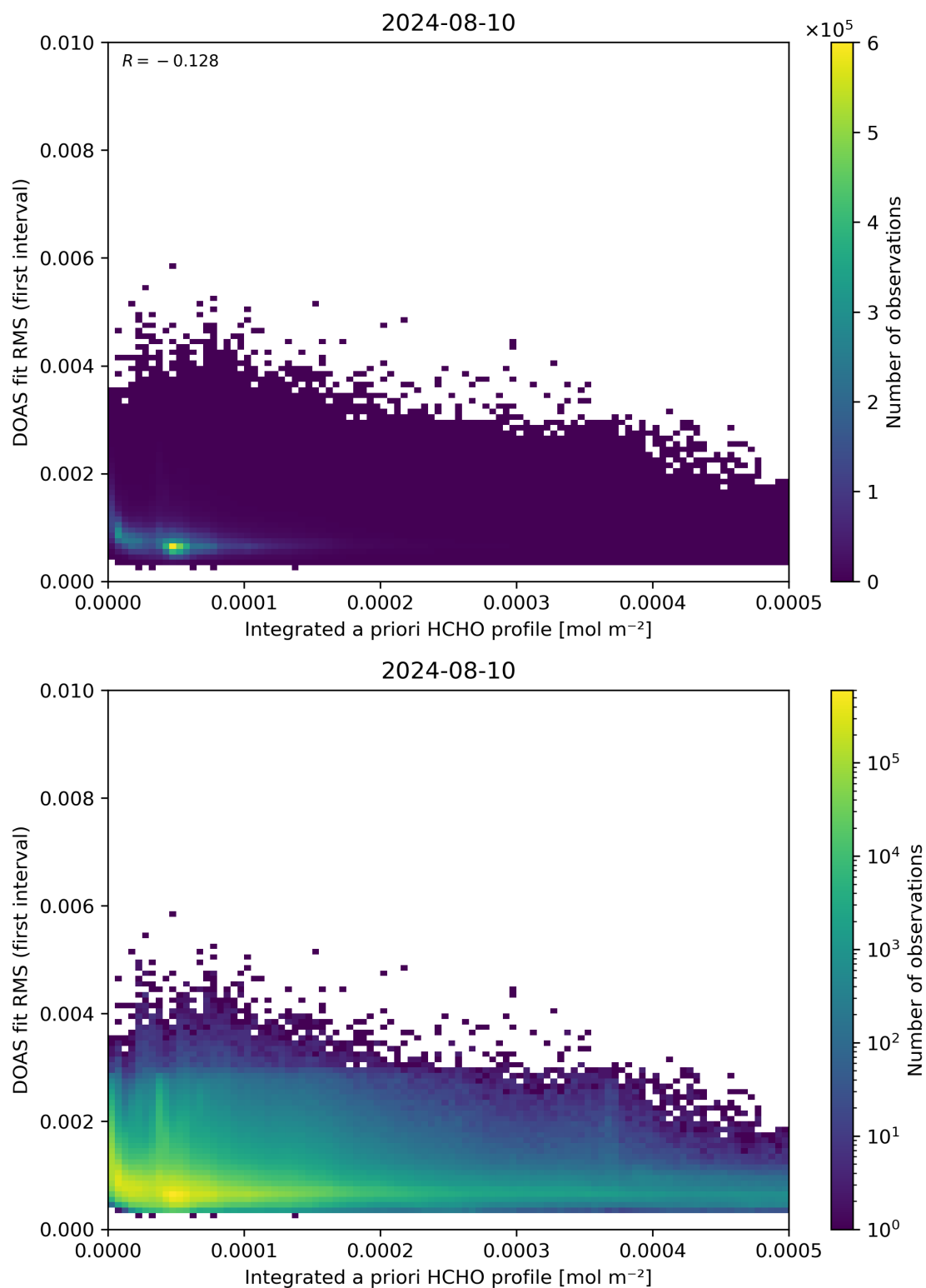
Figure 148: Scatter density plot of “Integrated a priori HCHO profile” against “DOAS fit RMS (first interval)” for 2024-08-09 to 2024-08-11.
