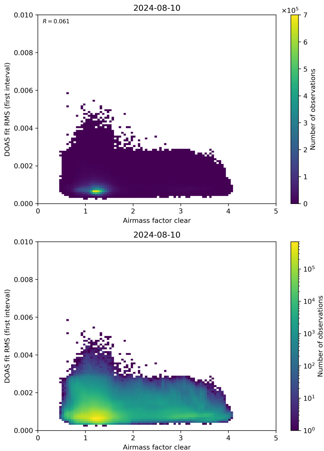
Figure 71: Scatter density plot of “Airmass factor clear” against “DOAS fit RMS (first interval)” for 2024-08-09 to 2024-08-11.
