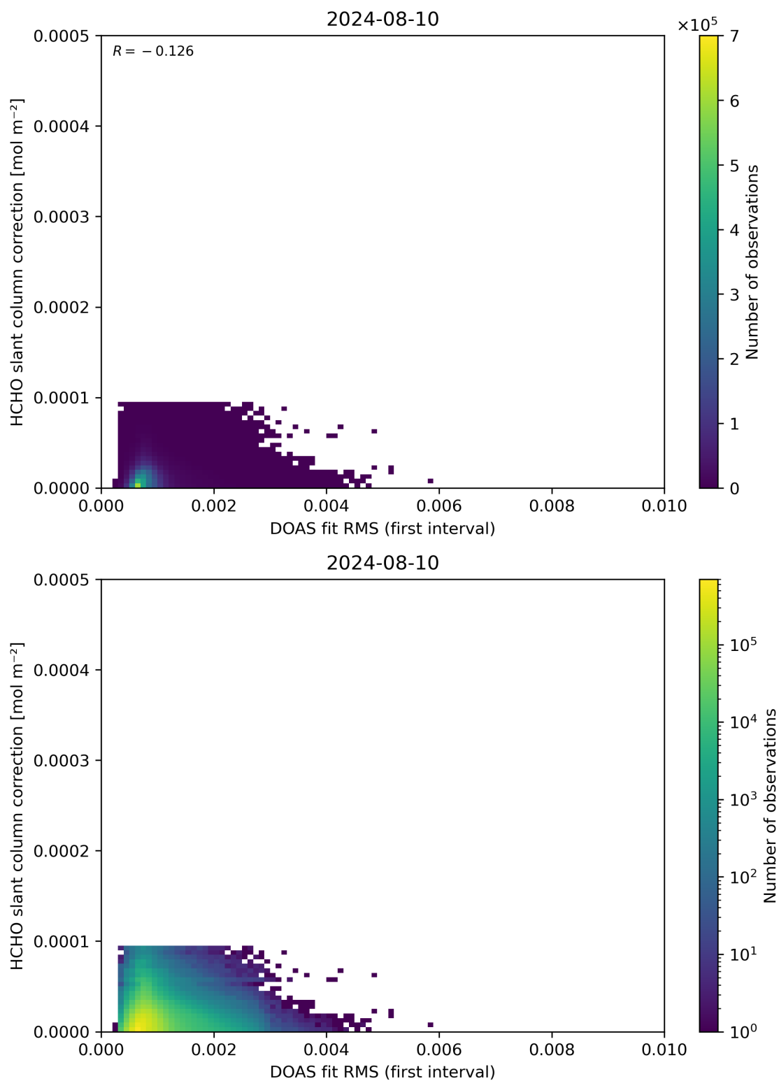
Figure 63: Scatter density plot of “DOAS fit RMS (first interval)” against “HCHO slant column correction” for 2024-08-09 to 2024-08-11.
