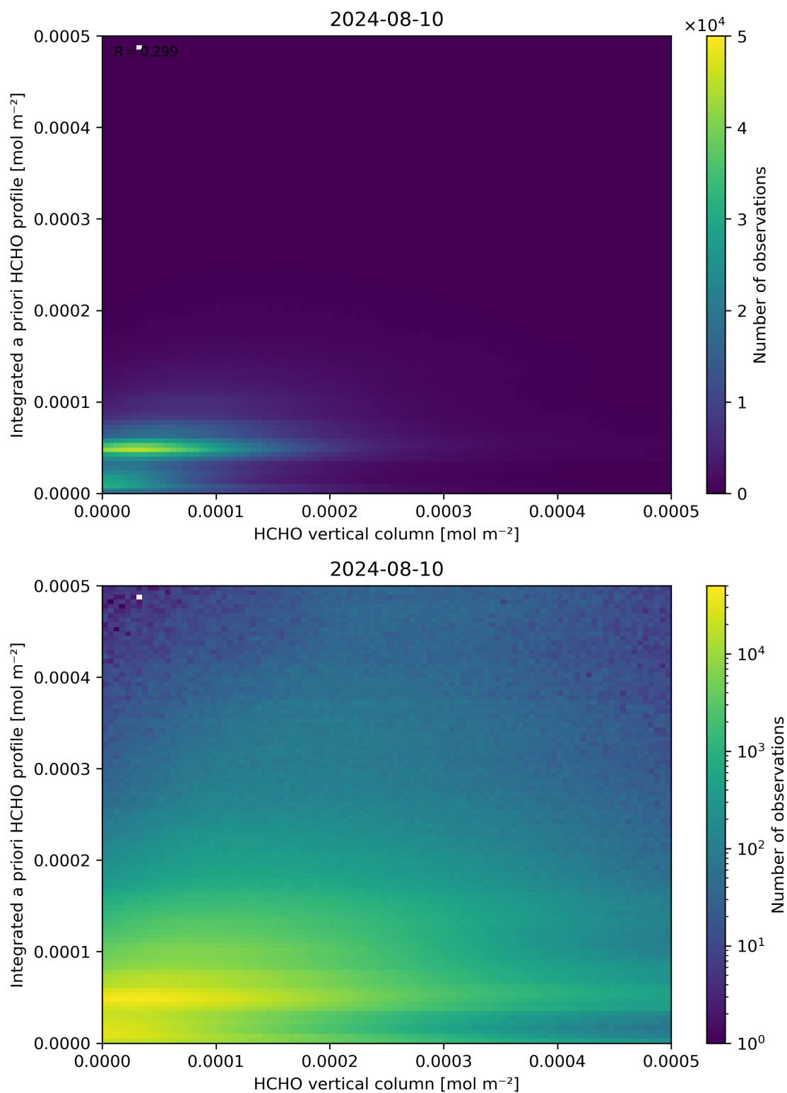
Figure 135: Scatter density plot of “HCHO vertical column” against “Integrated a priori HCHO profile” for 2024-08-09 to 2024-08-11.
