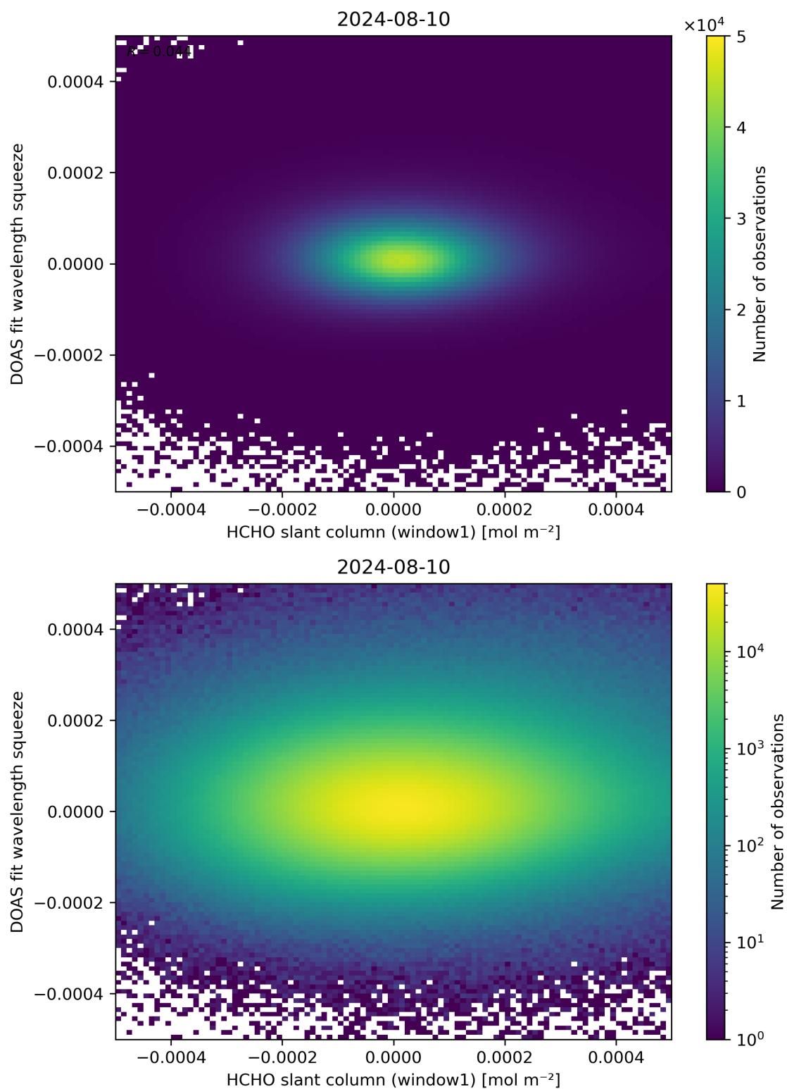
Figure 80: Scatter density plot of “HCHO slant column (window1)” against “DOAS fit wavelength squeeze” for 2024-08-09 to 2024-08-11.
