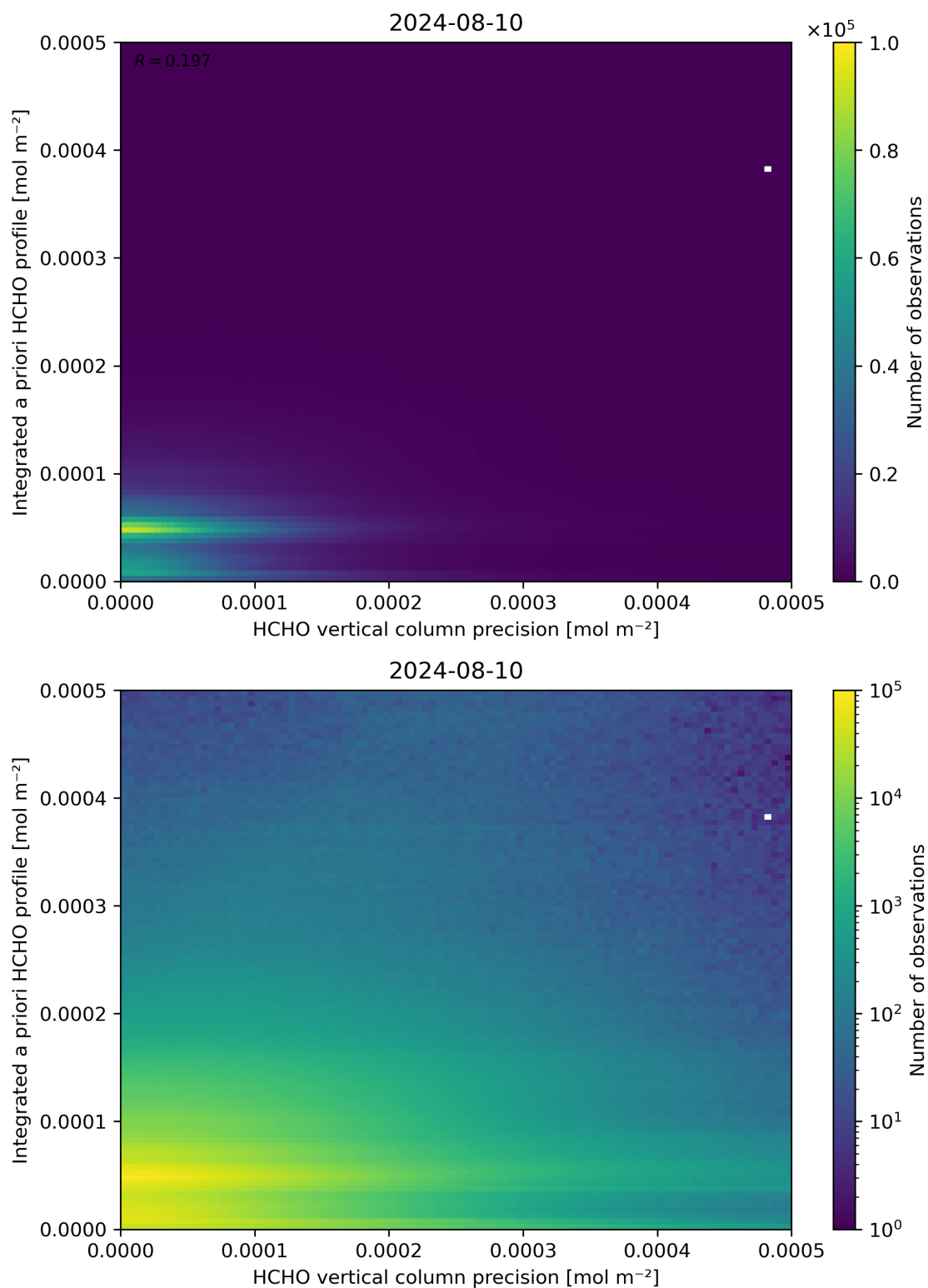
Figure 147: Scatter density plot of “HCHO vertical column precision” against “Integrated a priori HCHO profile” for 2024-08-09 to 2024-08-11.
