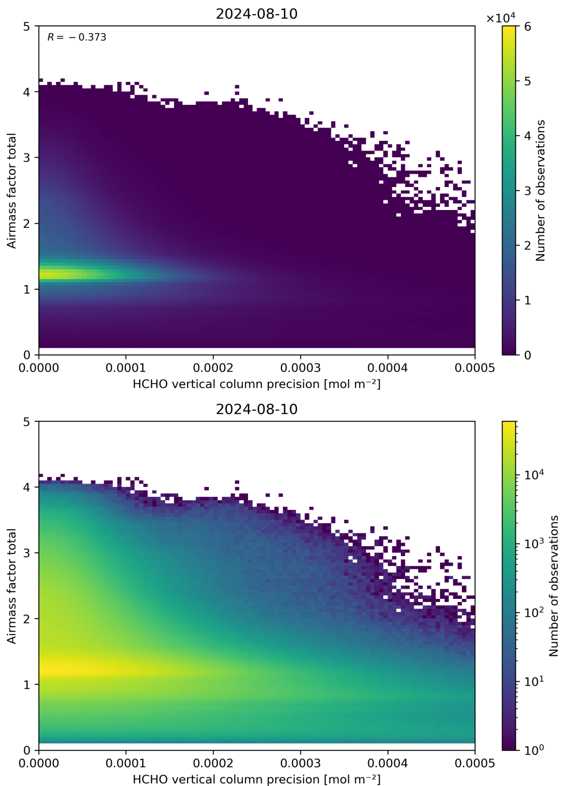
Figure 144: Scatter density plot of “HCHO vertical column precision” against “Airmass factor total” for 2024-08-09 to 2024-08-11.
