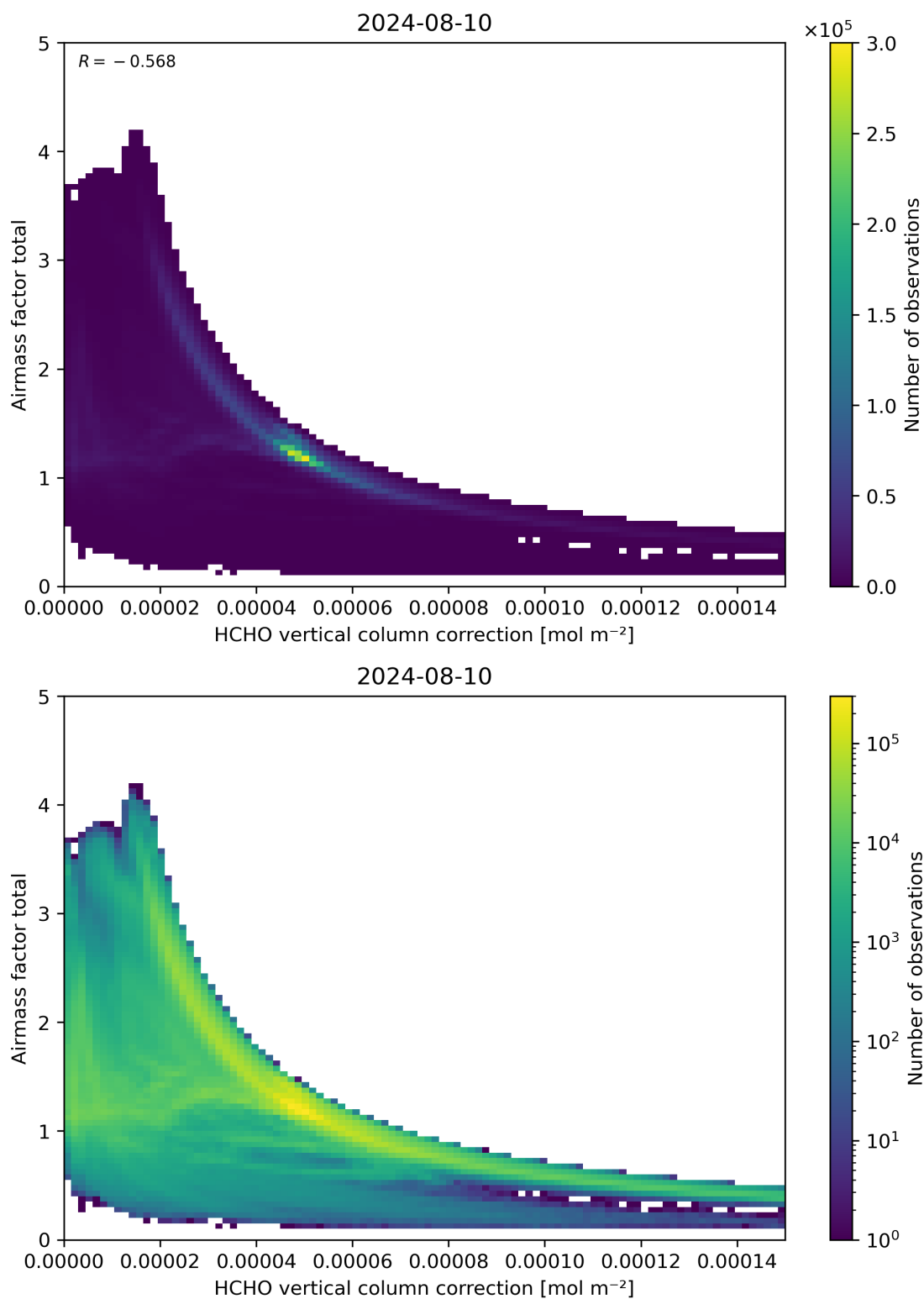
Figure 120: Scatter density plot of “HCHO vertical column correction” against “Airmass factor total” for 2024-08-09 to 2024-08-11.
