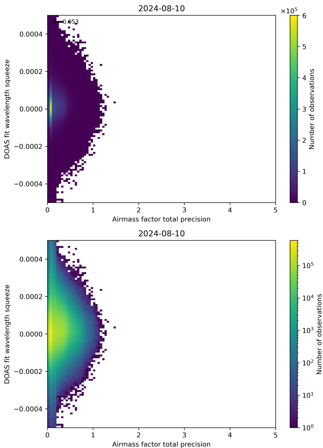
Figure 107: Scatter density plot of “Airmass factor total precision” against “DOAS fit wavelength squeeze” for 2024-08-09 to 2024-08-11.
