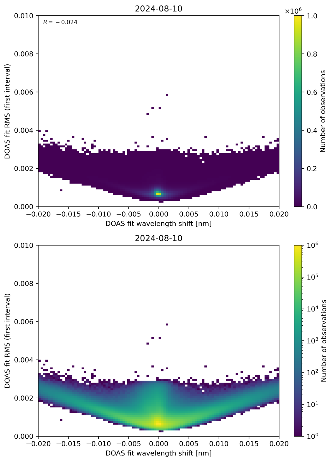
Figure 64: Scatter density plot of “DOAS fit wavelength shift” against “DOAS fit RMS (first interval)” for 2024-08-09 to 2024-08-11.
