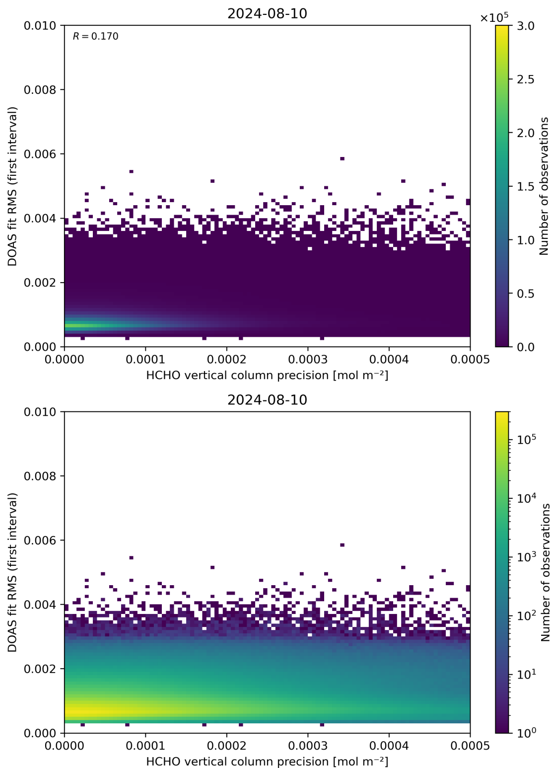
Figure 136: Scatter density plot of “HCHO vertical column precision” against “DOAS fit RMS (first interval)” for 2024-08-09 to 2024-08-11.
