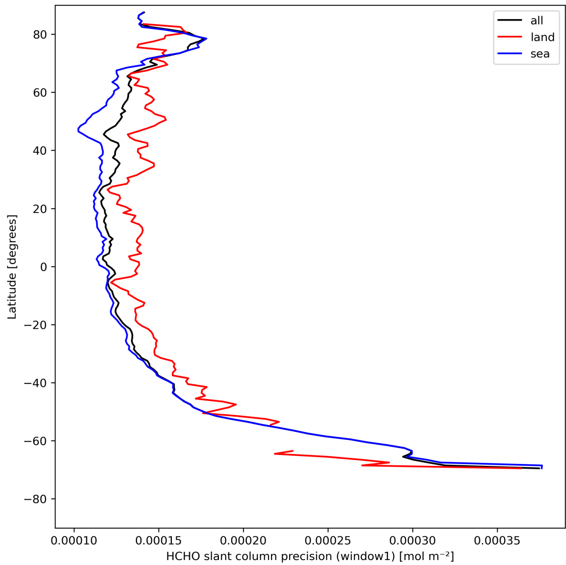
Figure 25: Zonal average of “HCHO slant column precision (window1)” for 2024-08-09 to 2024-08-11.
