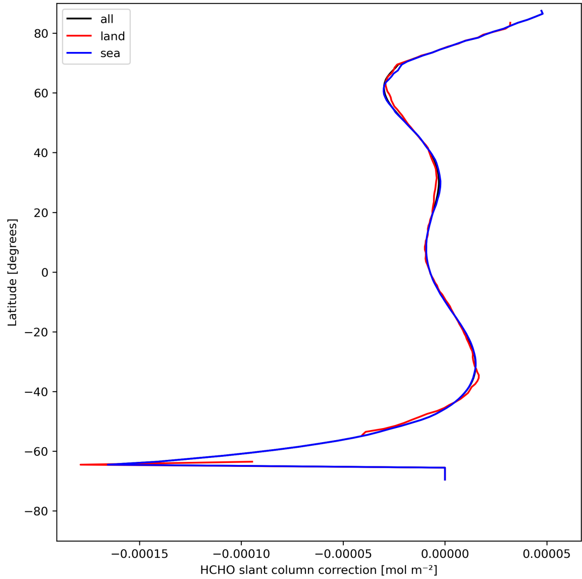
Figure 33: Zonal average of “HCHO slant column correction” for 2024-08-09 to 2024-08-11.
