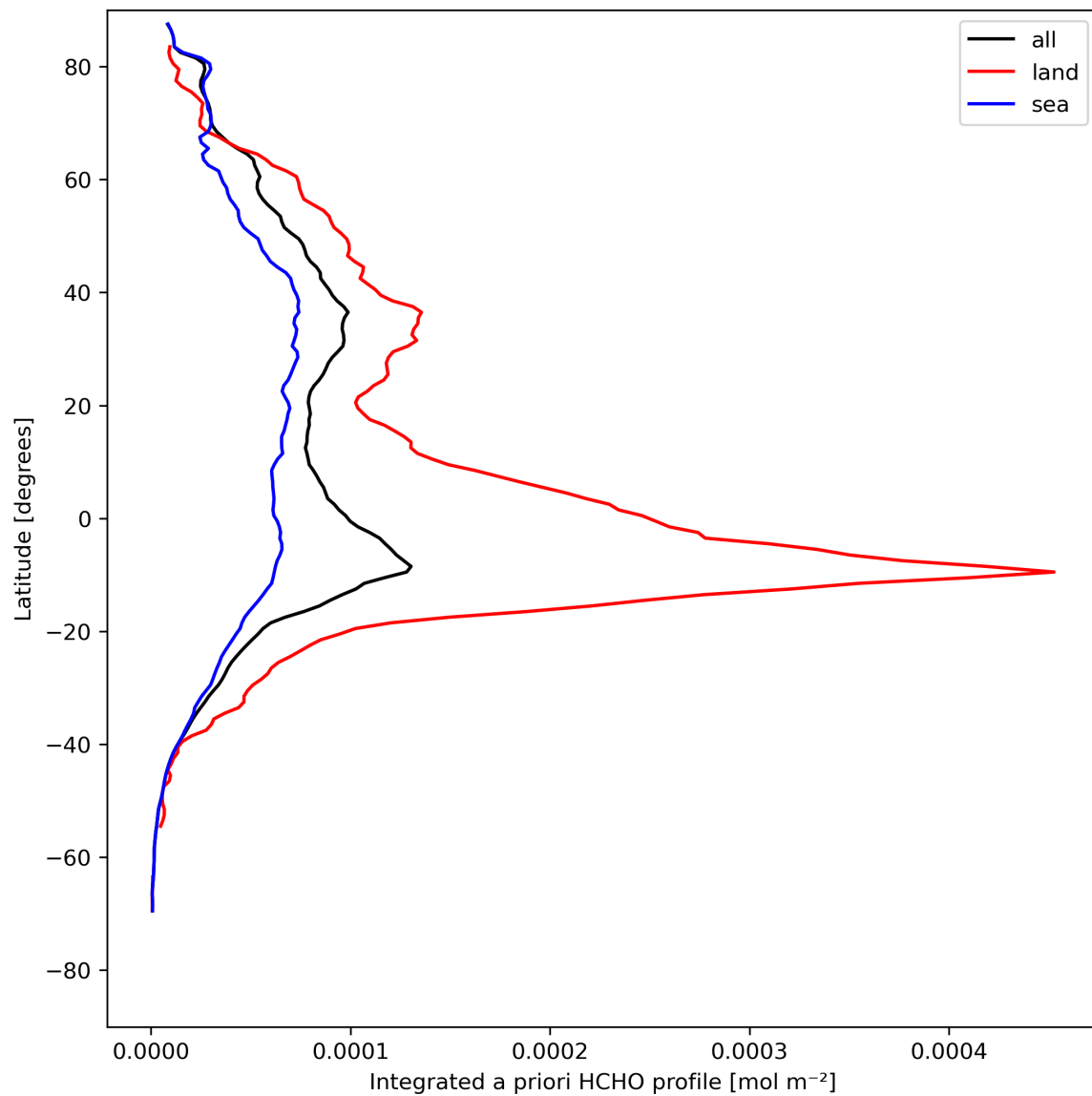
Figure 29: Zonal average of “Integrated a priori HCHO profile” for 2024-08-09 to 2024-08-11.
