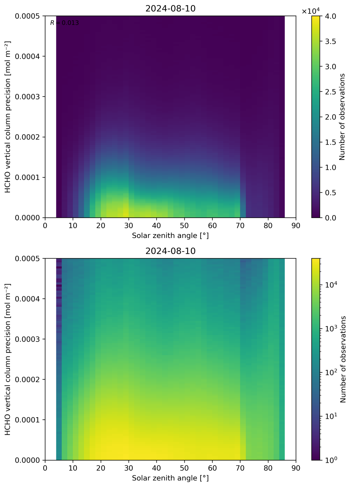
Figure 179: Scatter density plot of “Solar zenith angle” against “HCHO vertical column precision” for 2024-08-09 to 2024-08-11.
