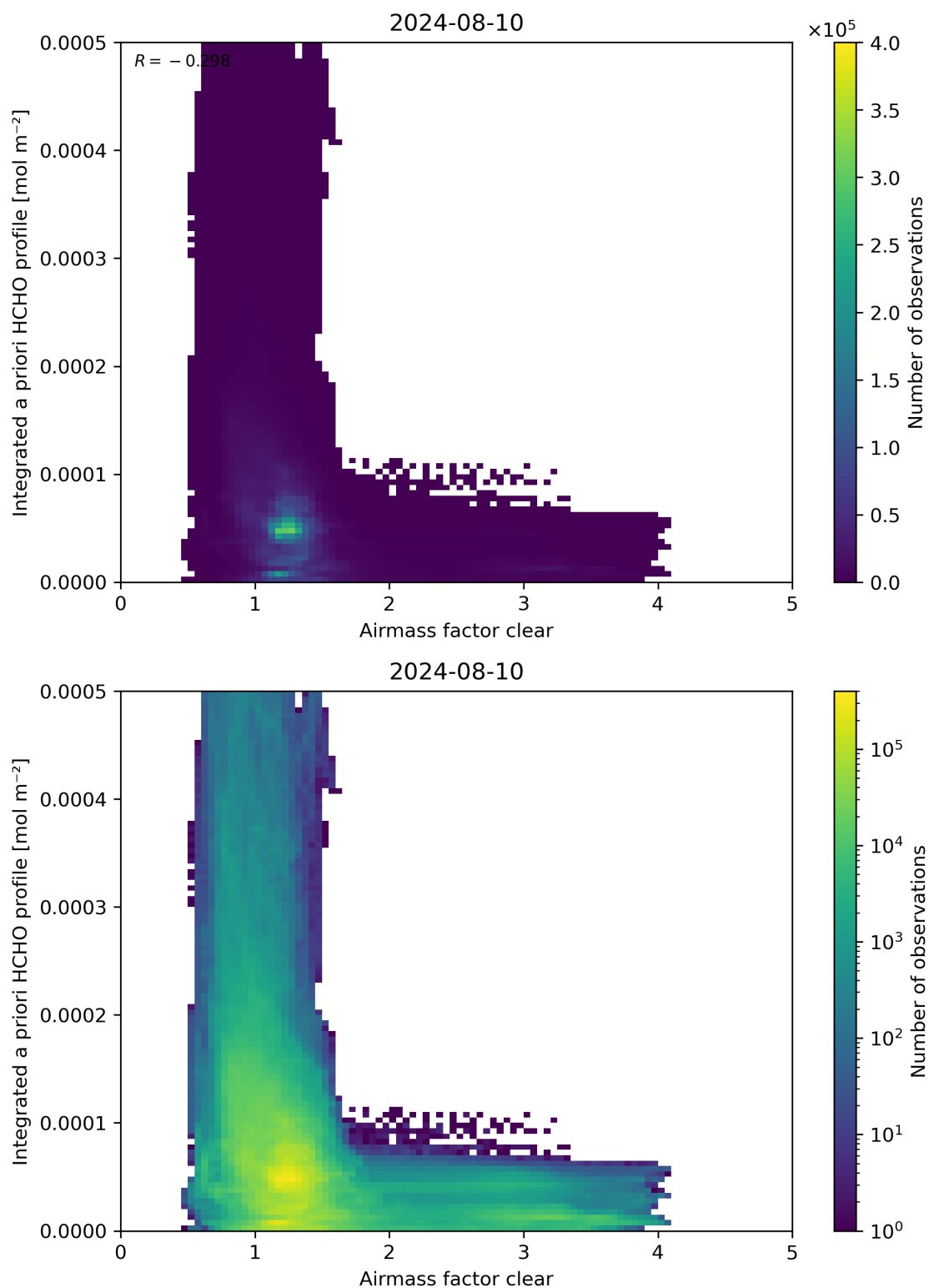
Figure 76: Scatter density plot of “Airmass factor clear” against “Integrated a priori HCHO profile” for 2024-08-09 to 2024-08-11.
