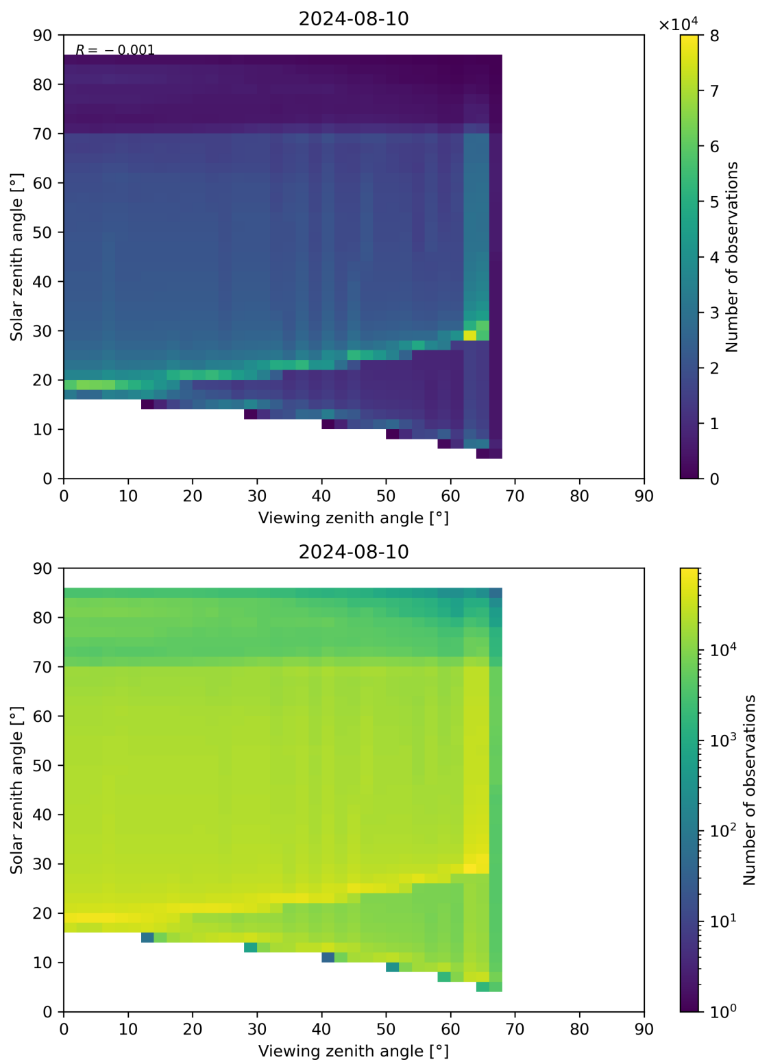
Figure 197: Scatter density plot of “Viewing zenith angle” against “Solar zenith angle” for 2024-08-09 to 2024-08-11.
