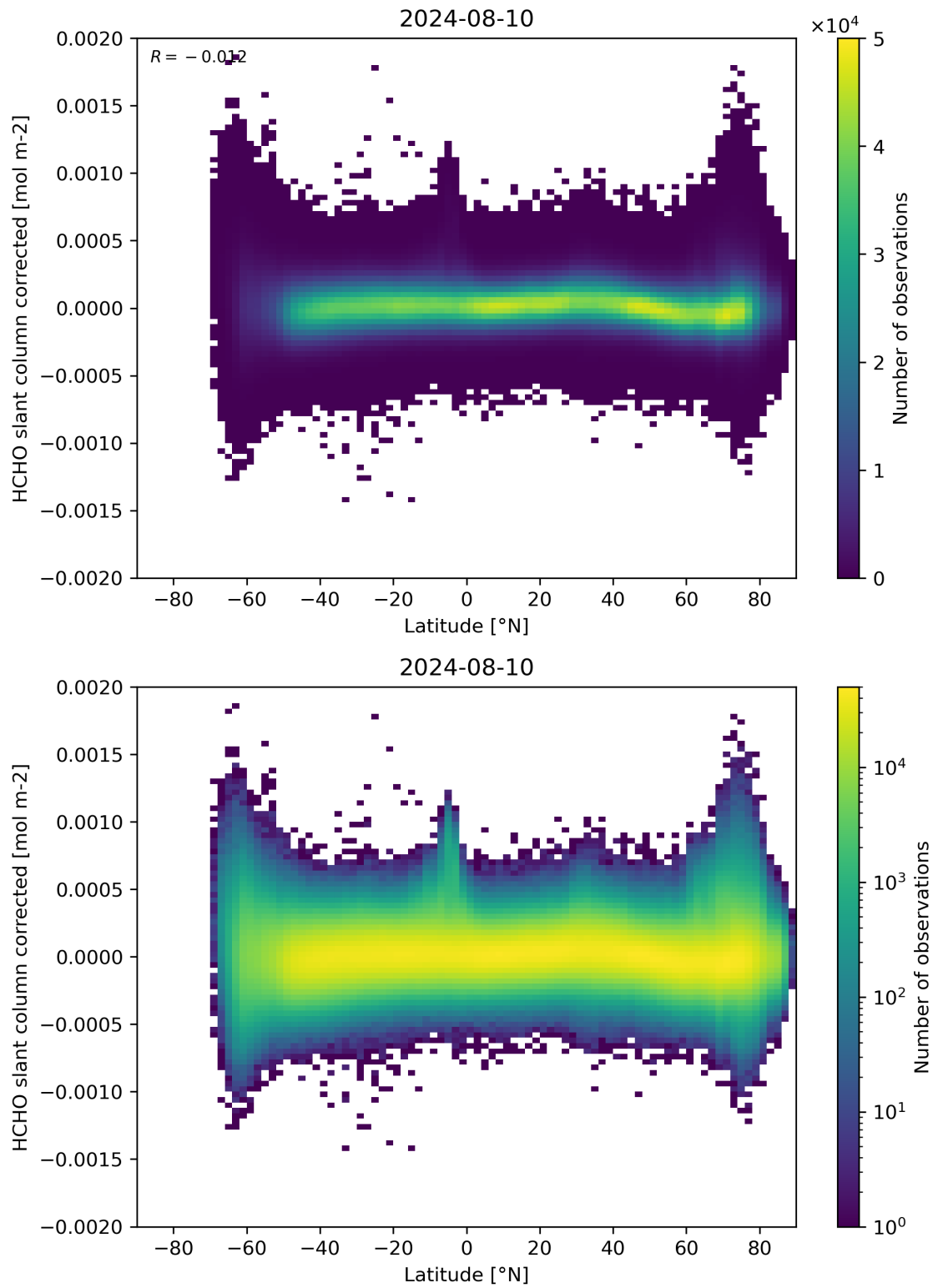
Figure 157: Scatter density plot of “Latitude” against “HCHO slant column corrected” for 2024-08-09 to 2024-08-11.
