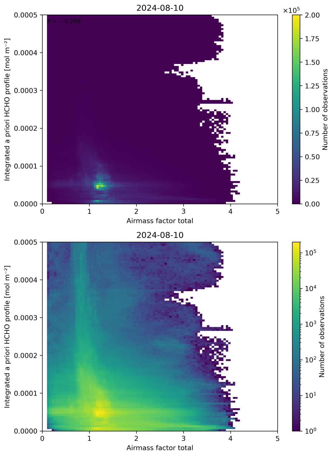
Figure 104: Scatter density plot of “Airmass factor total” against “Integrated a priori HCHO profile” for 2024-08-09 to 2024-08-11.
