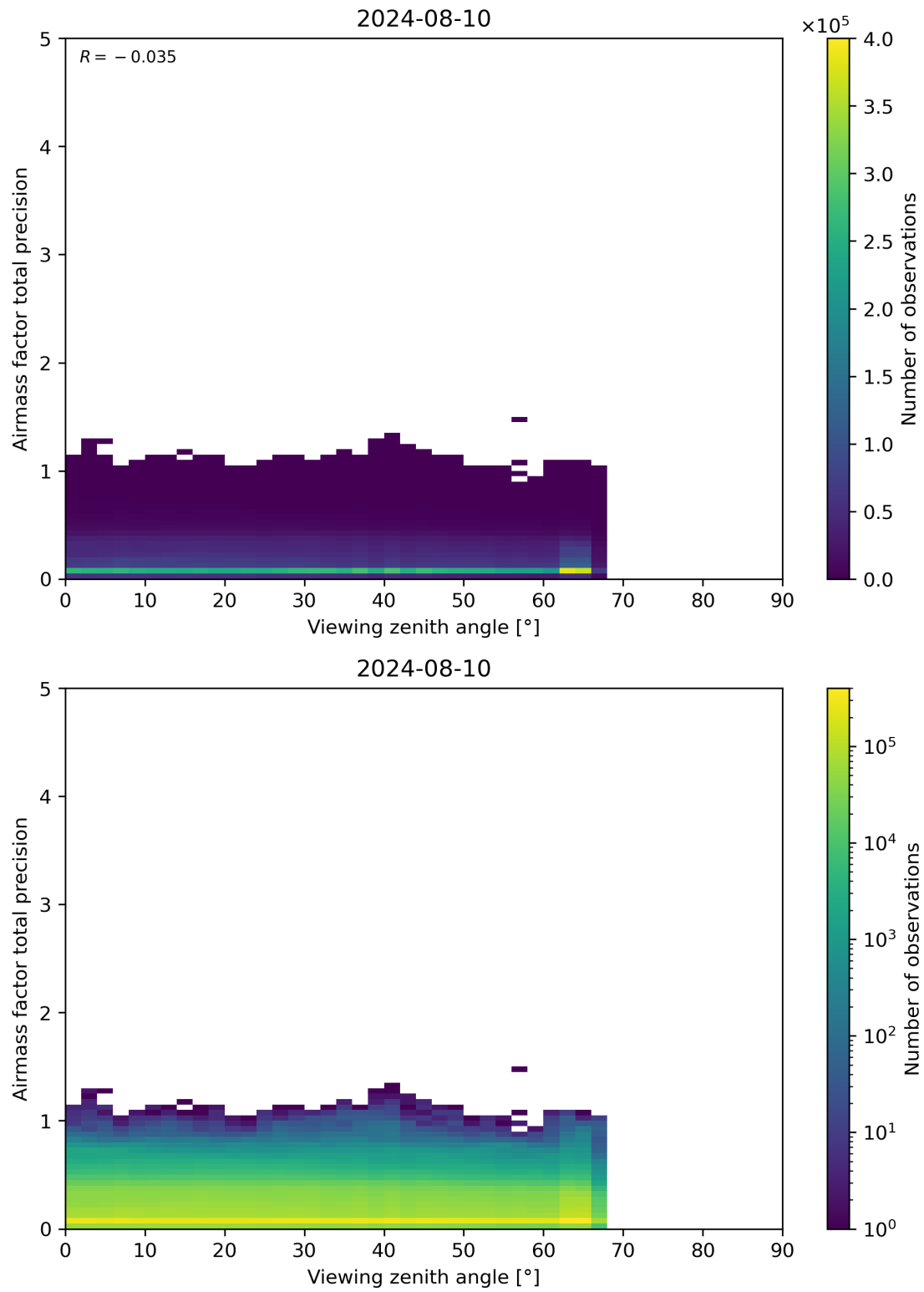
Figure 191: Scatter density plot of “Viewing zenith angle” against “Airmass factor total precision” for 2024-08-09 to 2024-08-11.
