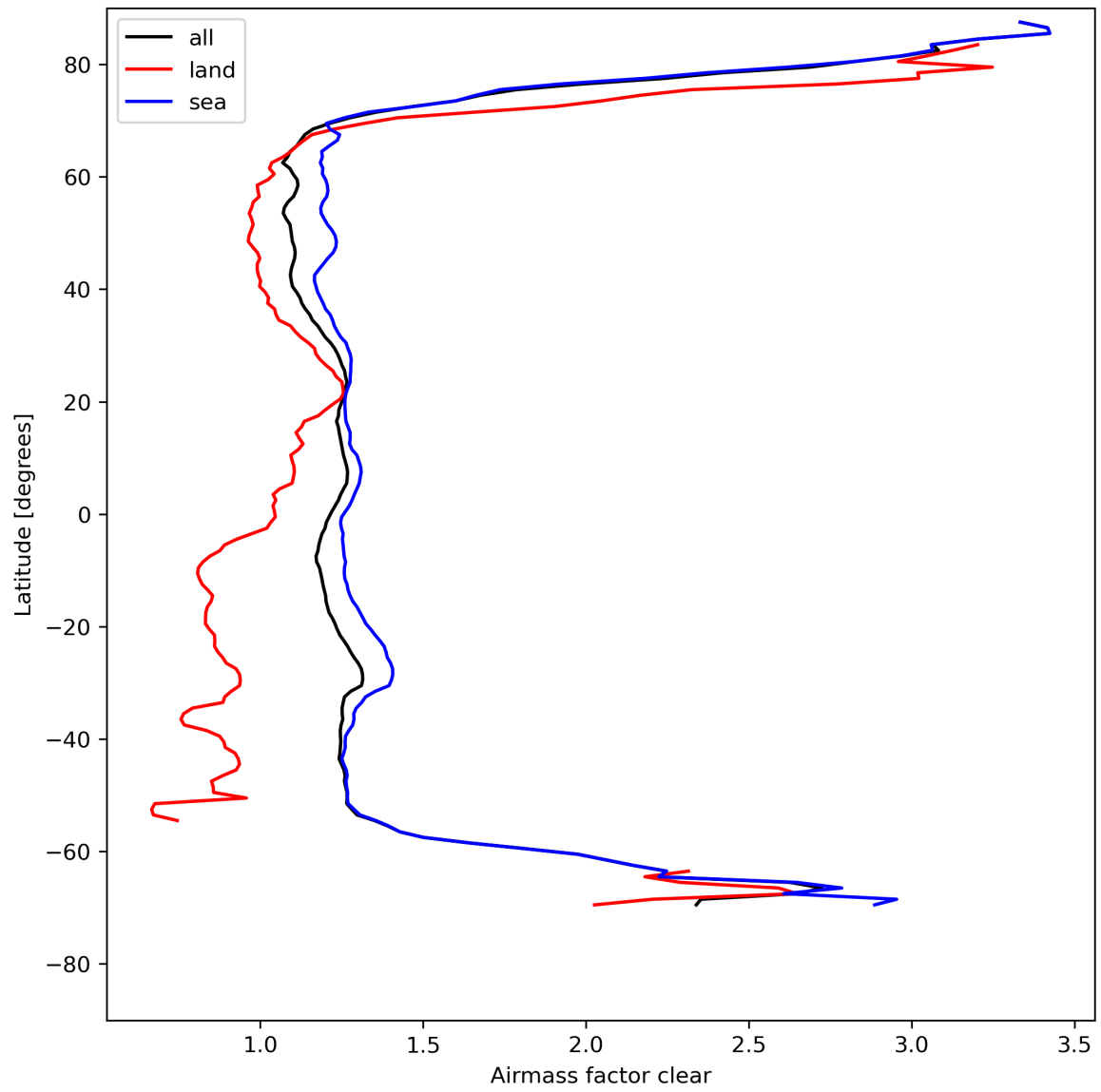
Figure 28: Zonal average of “Airmass factor clear” for 2024-08-09 to 2024-08-11.
