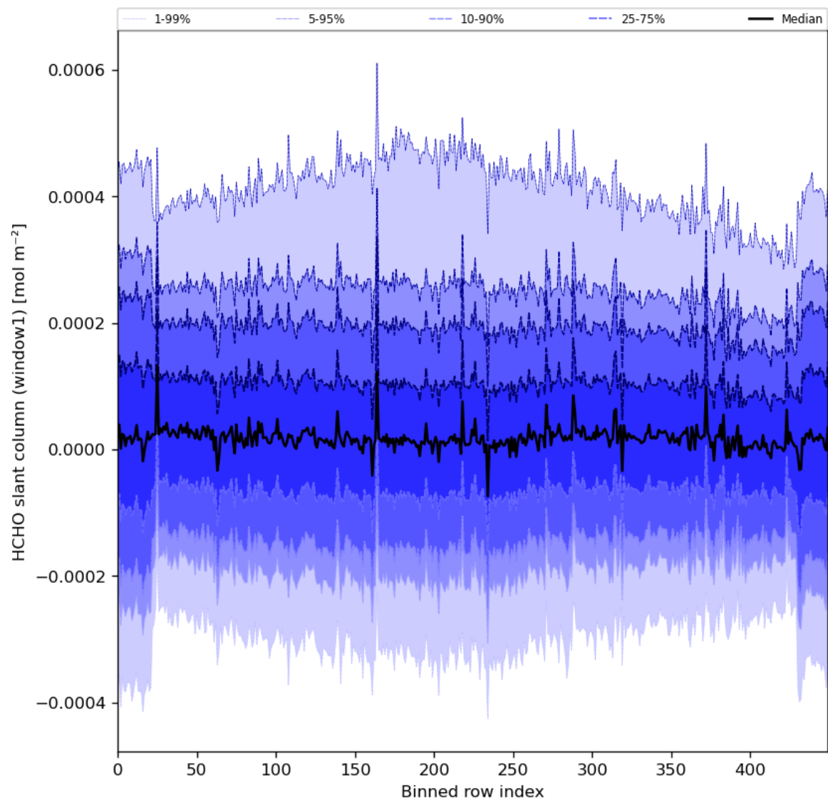
Figure 52: Along track statistics of “HCHO slant column (window1)” for 2024-08-09 to 2024-08-11
