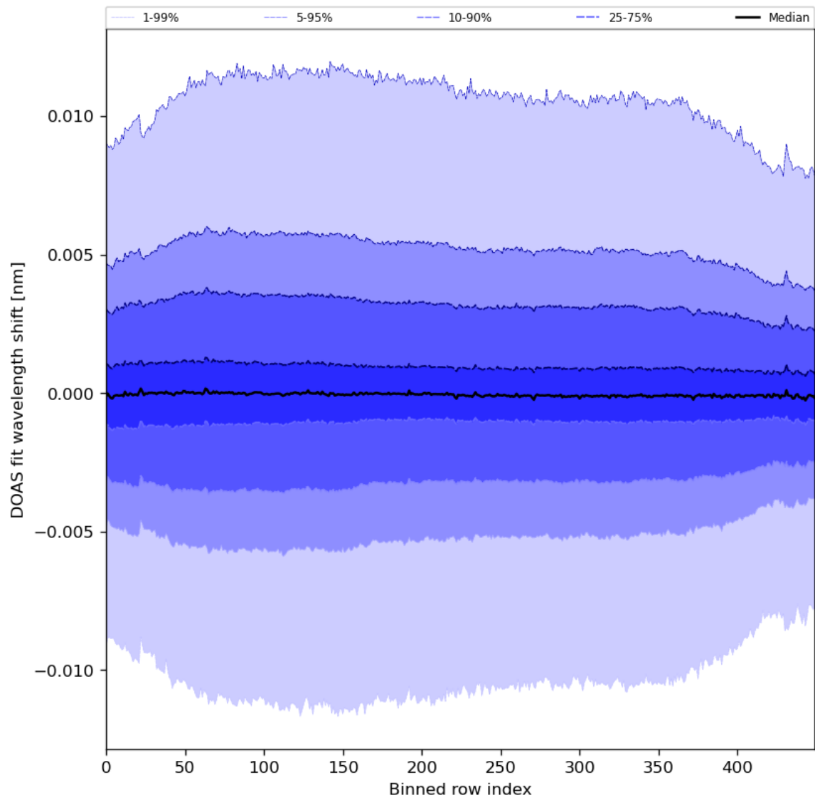
Figure 58: Along track statistics of “DOAS fit wavelength shift” for 2024-08-09 to 2024-08-11
