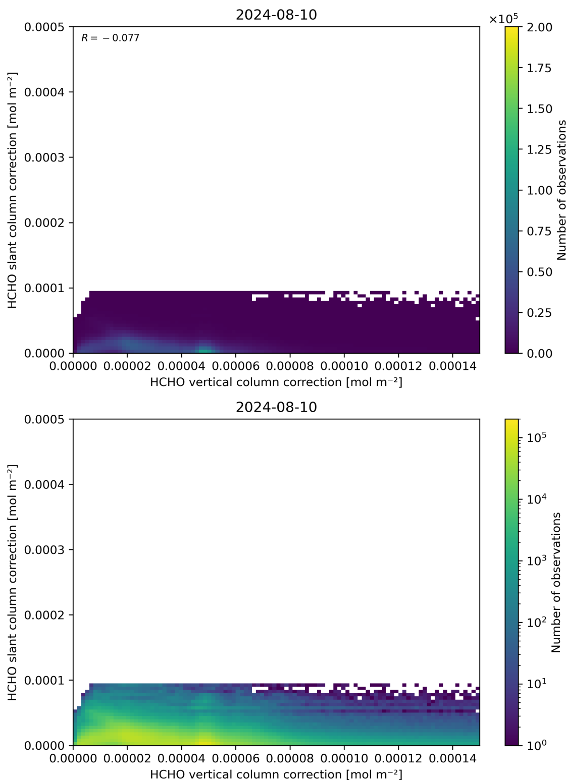
Figure 117: Scatter density plot of “HCHO vertical column correction” against “HCHO slant column correction” for 2024-08-09 to 2024-08-11.
