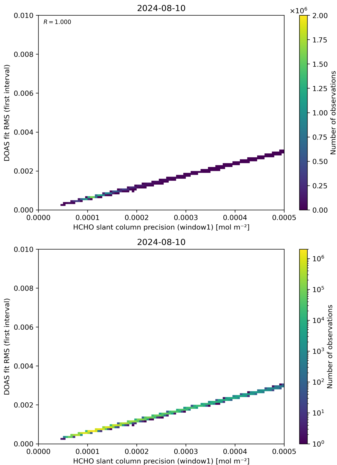
Figure 88: Scatter density plot of “HCHO slant column precision (window1)” against “DOAS fit RMS (first interval)” for 2024-08-09 to 2024-08-11.
