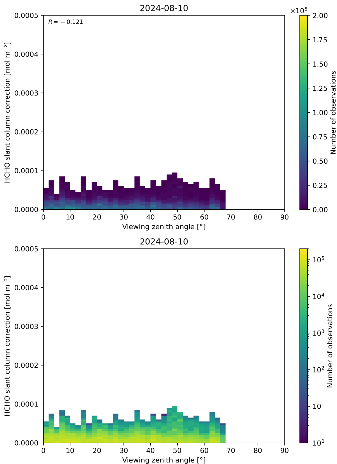
Figure 187: Scatter density plot of “Viewing zenith angle” against “HCHO slant column correction” for 2024-08-09 to 2024-08-11.
