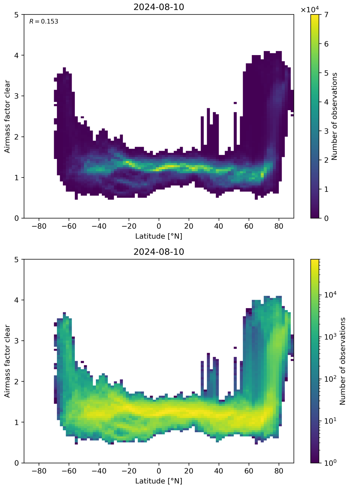
Figure 156: Scatter density plot of “Latitude” against “Airmass factor clear” for 2024-08-09 to 2024-08-11.
