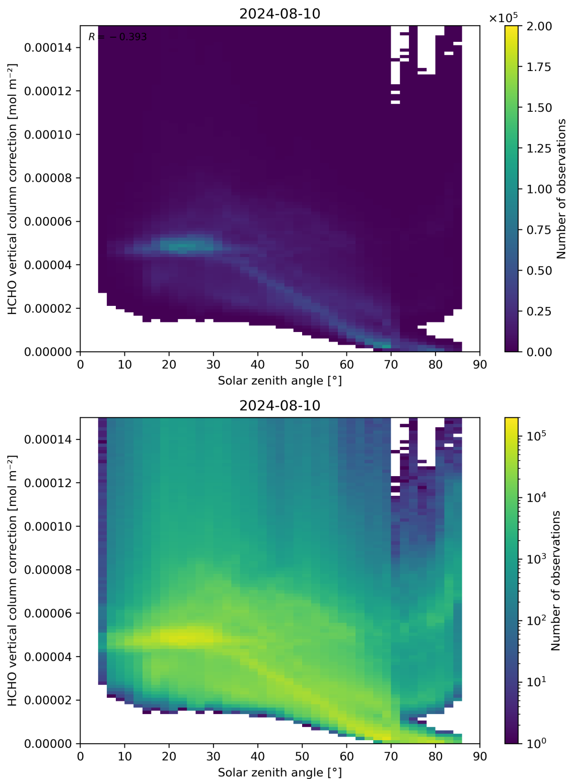
Figure 178: Scatter density plot of “Solar zenith angle” against “HCHO vertical column correction” for 2024-08-09 to 2024-08-11.
