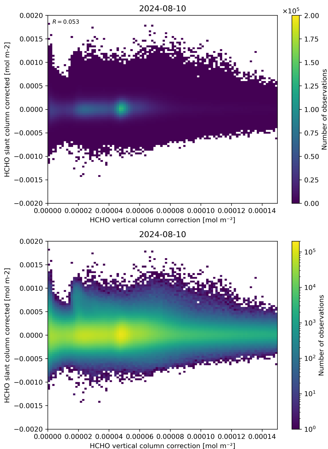
Figure 116: Scatter density plot of “HCHO vertical column correction” against “HCHO slant column corrected” for 2024-08-09 to 2024-08-11.
