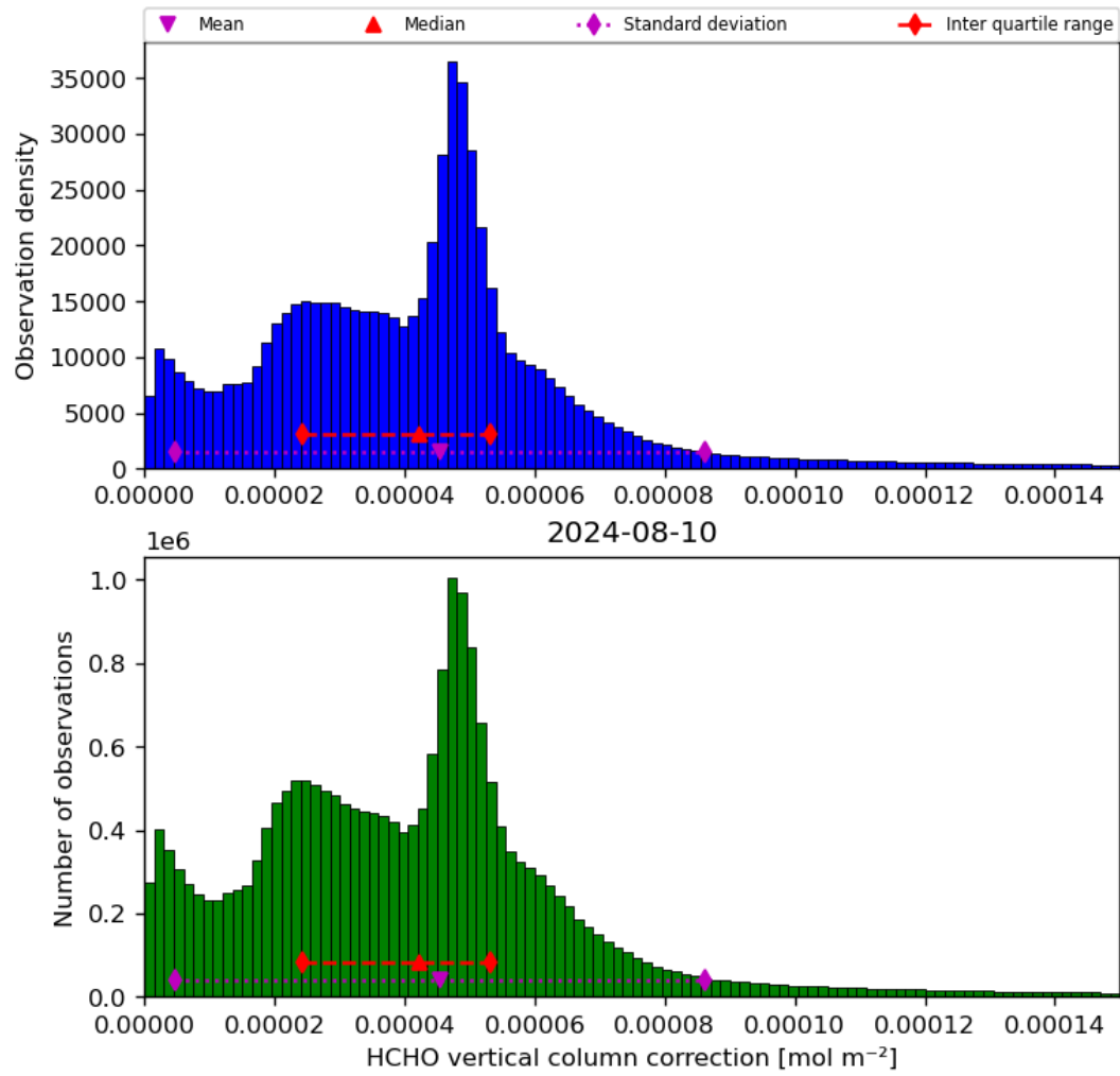
Figure 37: Histogram of “HCHO vertical column correction” for 2024-08-09 to 2024-08-11
