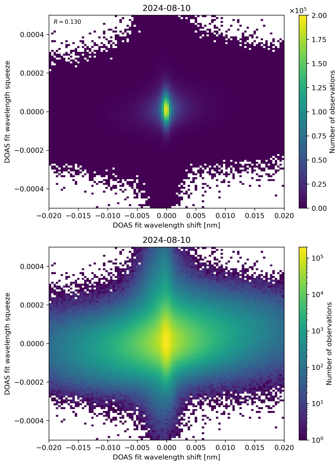
Figure 65: Scatter density plot of “DOAS fit wavelength shift” against “DOAS fit wavelength squeeze” for 2024-08-09 to 2024-08-11.
