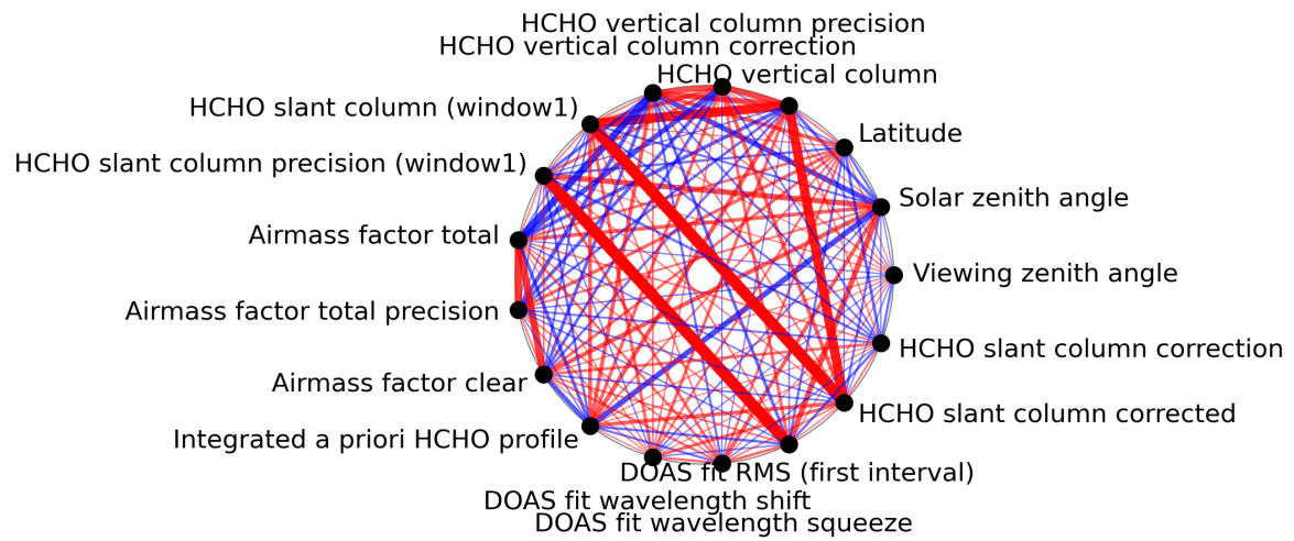
Figure 1: Map of correlation graph for 2024-08-09 to 2024-08-11.
