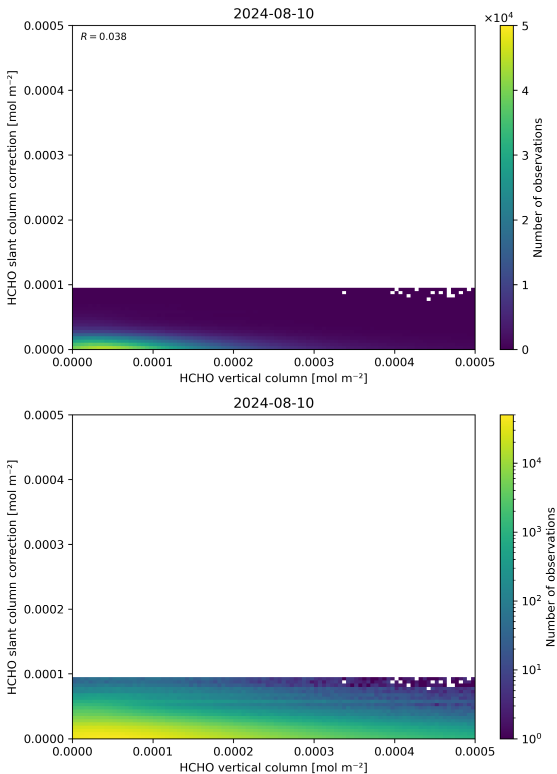
Figure 128: Scatter density plot of “HCHO vertical column” against “HCHO slant column correction” for 2024-08-09 to 2024-08-11.
