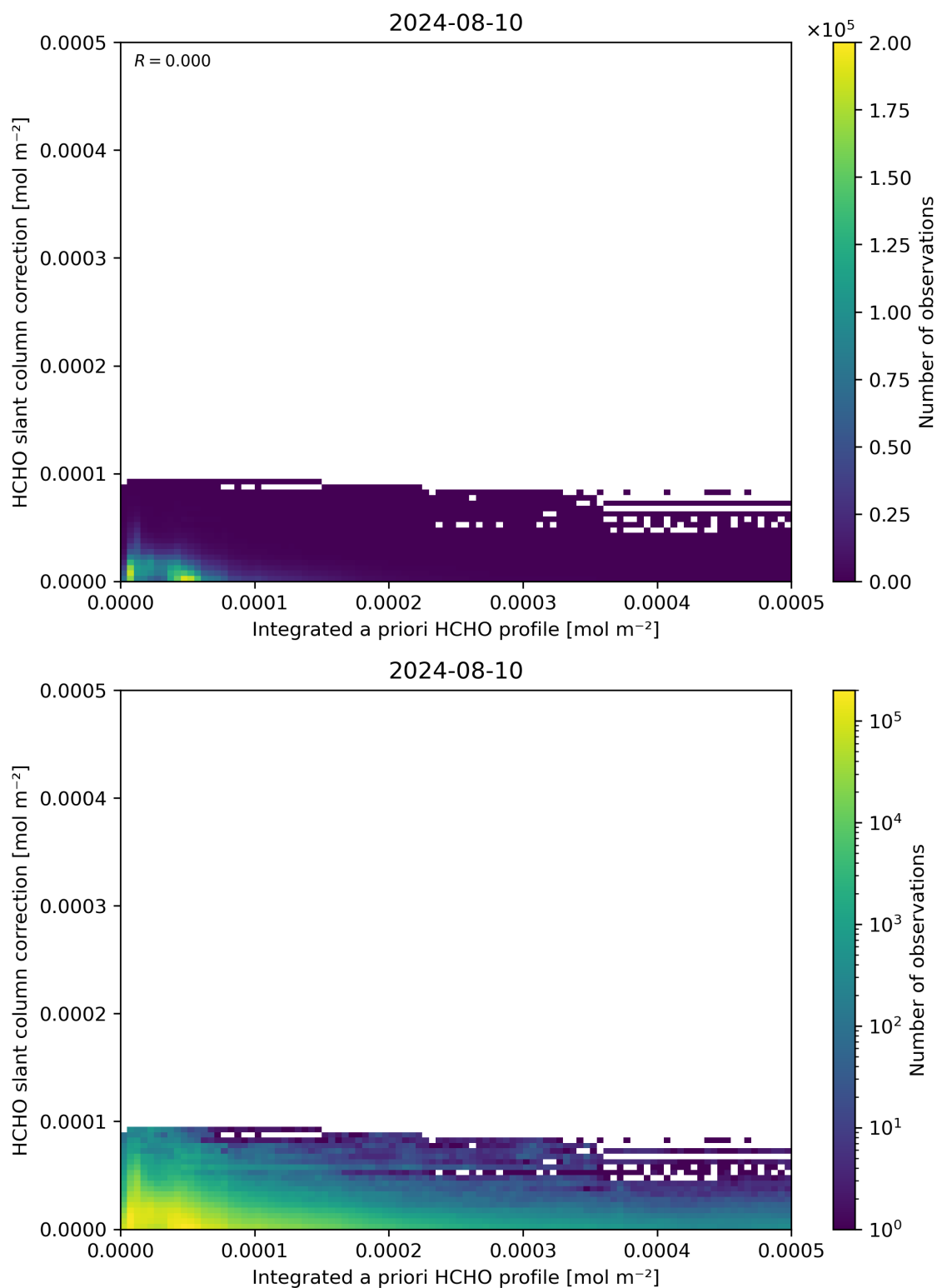
Figure 152: Scatter density plot of “Integrated a priori HCHO profile” against “HCHO slant column correction” for 2024-08-09 to 2024-08-11.
