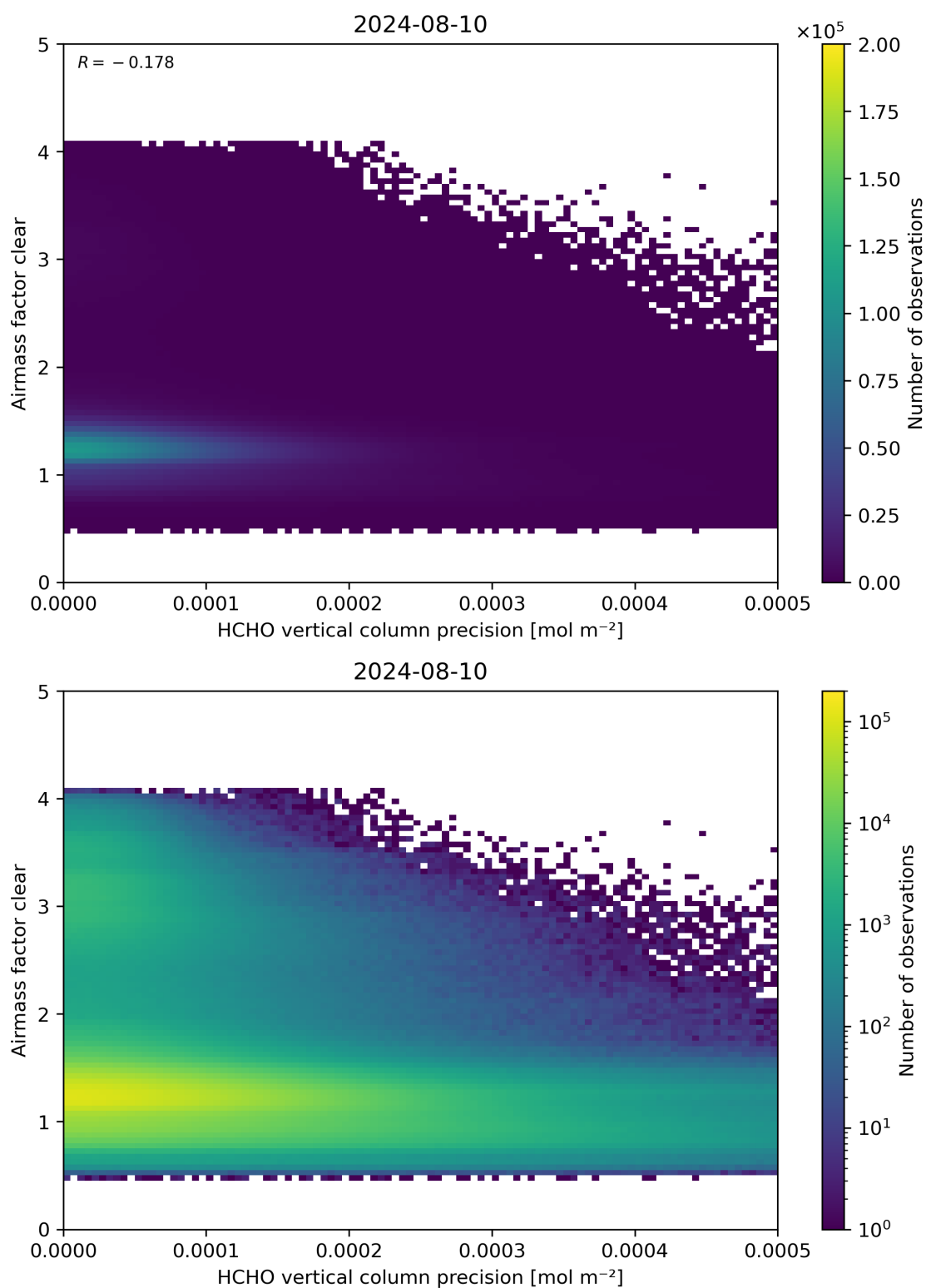
Figure 139: Scatter density plot of “HCHO vertical column precision” against “Airmass factor clear” for 2024-08-09 to 2024-08-11.
