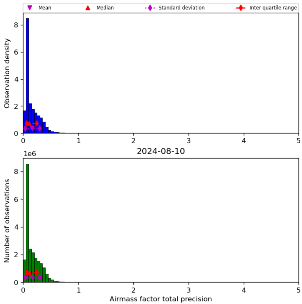
Figure 41: Histogram of “Airmass factor total precision” for 2024-08-09 to 2024-08-11
