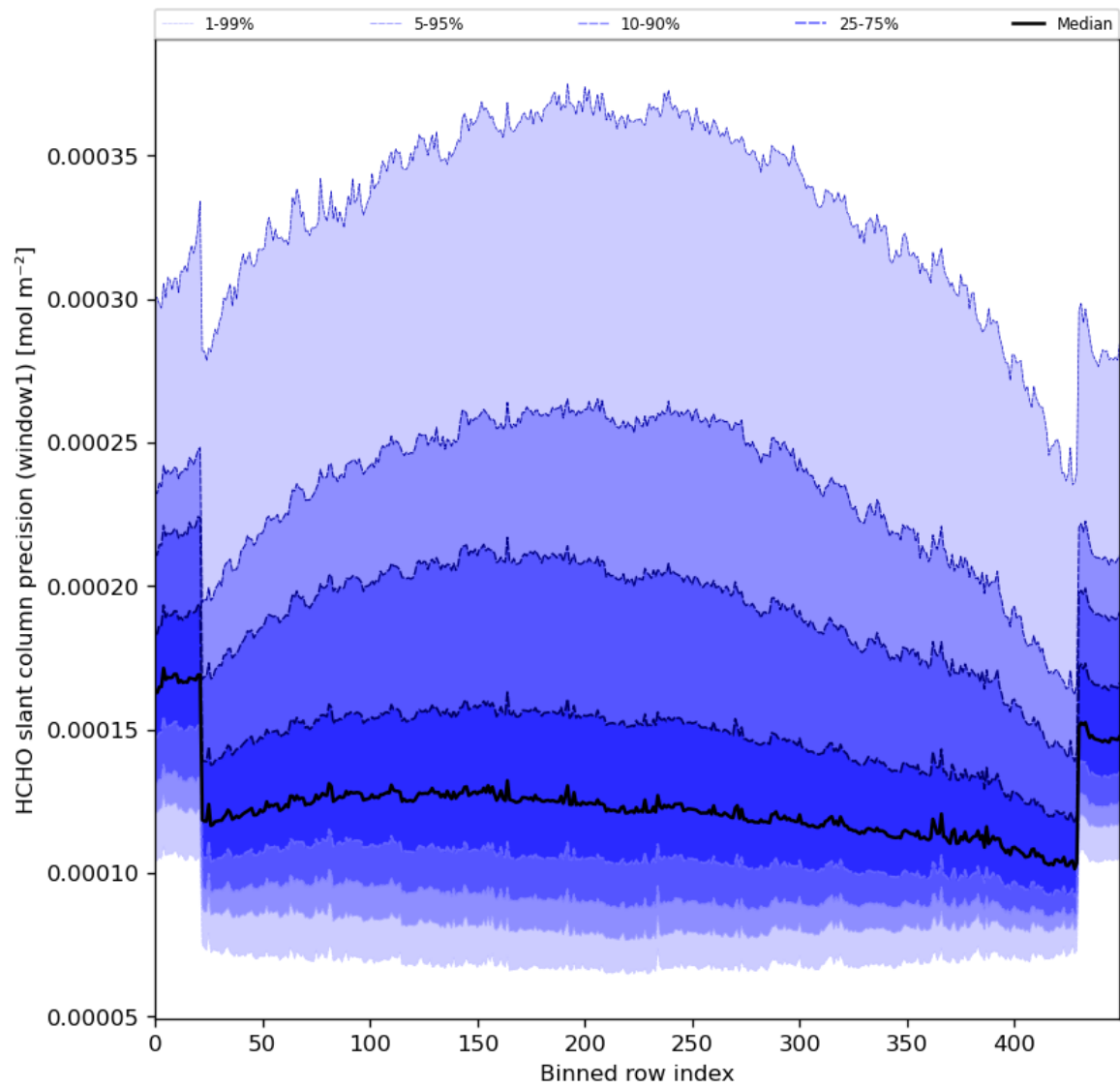
Figure 53: Along track statistics of “HCHO slant column precision (window1)” for 2024-08-09 to 2024-08-11
