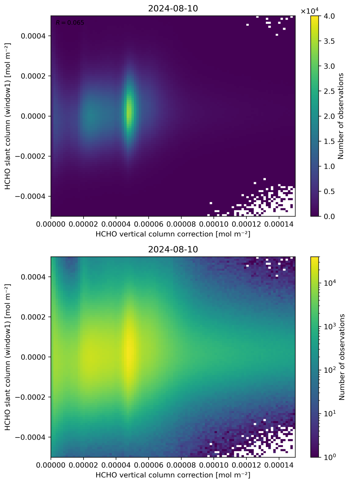
Figure 118: Scatter density plot of “HCHO vertical column correction” against “HCHO slant column (window1)” for 2024-08-09 to 2024-08-11.
