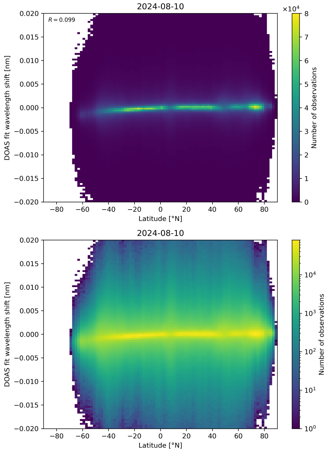
Figure 154: Scatter density plot of “Latitude” against “DOAS fit wavelength shift” for 2024-08-09 to 2024-08-11.
