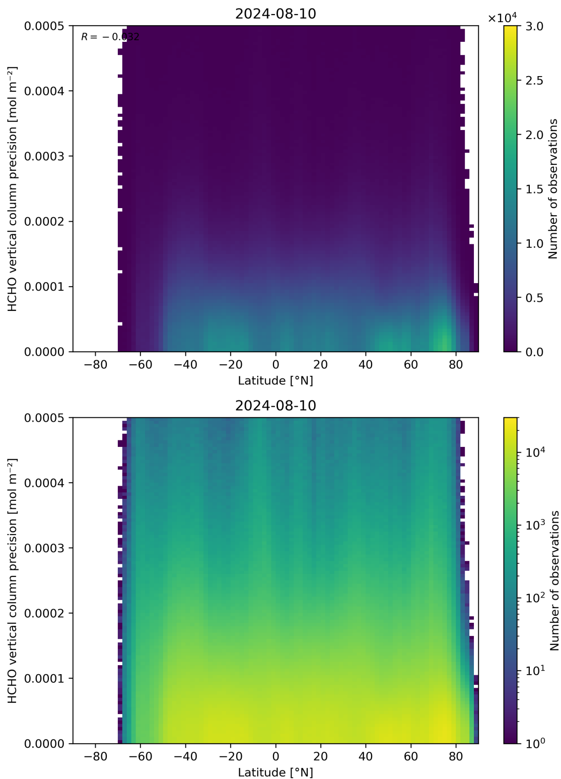
Figure 165: Scatter density plot of “Latitude” against “HCHO vertical column precision” for 2024-08-09 to 2024-08-11.
