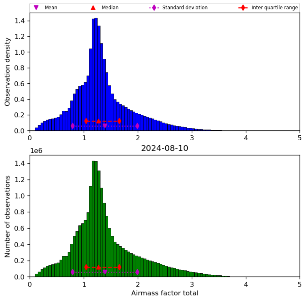
Figure 40: Histogram of “Airmass factor total” for 2024-08-09 to 2024-08-11
