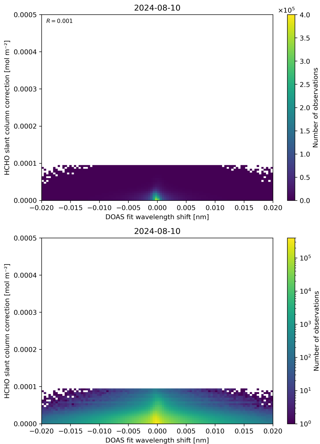
Figure 67: Scatter density plot of “DOAS fit wavelength shift” against “HCHO slant column correction” for 2024-08-09 to 2024-08-11.
