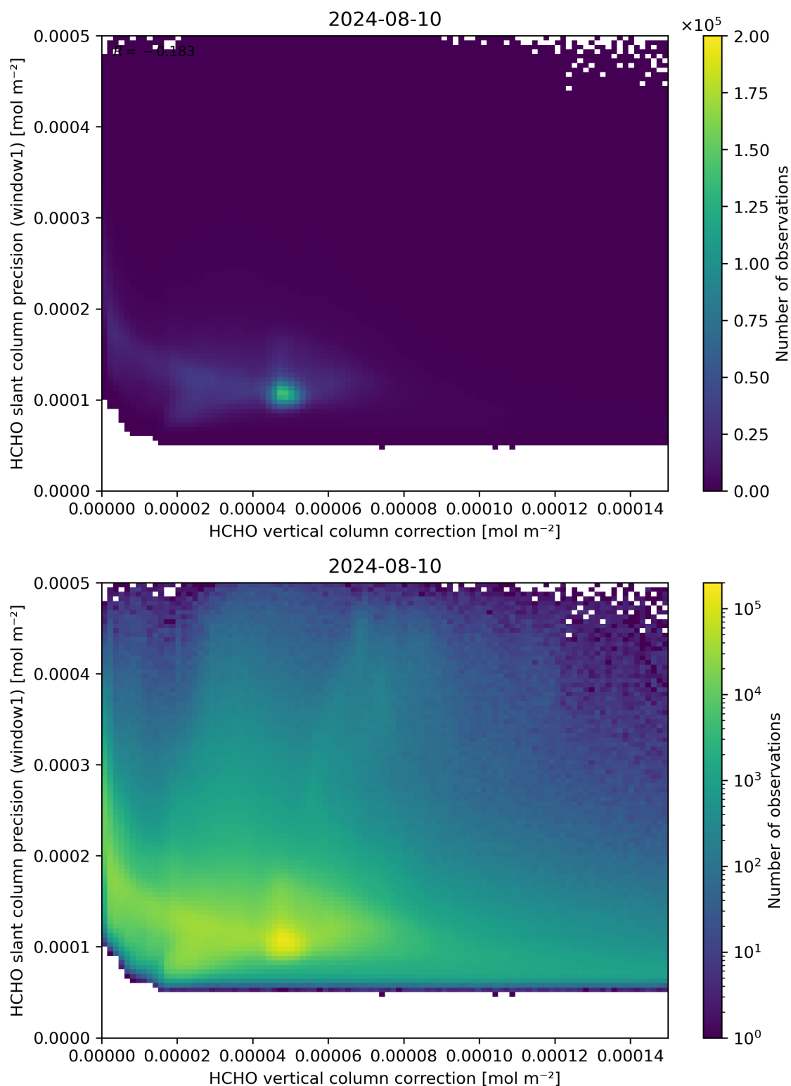
Figure 119: Scatter density plot of “HCHO vertical column correction” against “HCHO slant column precision (window1)” for 2024-08-09 to 2024-08-11.
