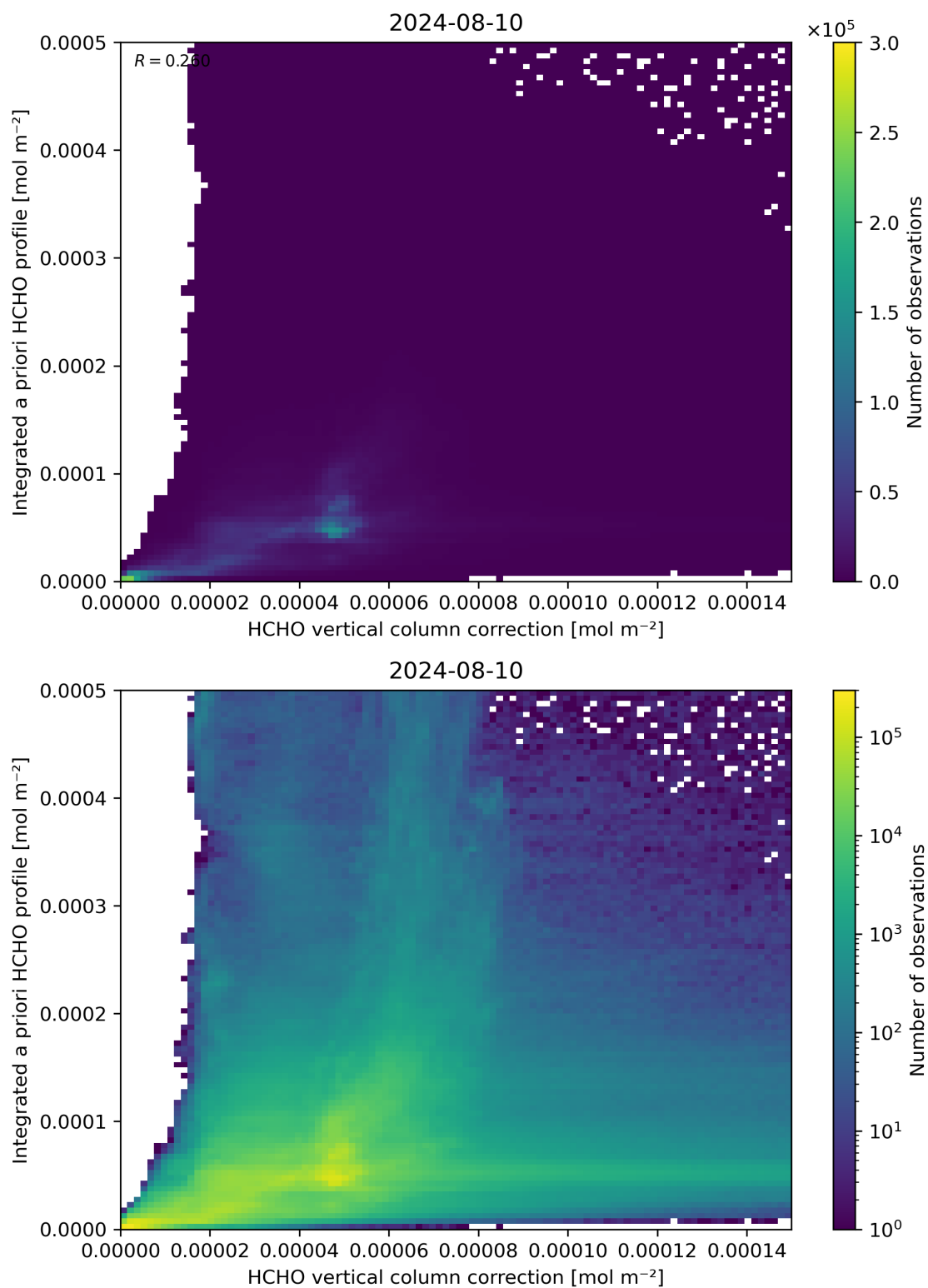
Figure 122: Scatter density plot of “HCHO vertical column correction” against “Integrated a priori HCHO profile” for 2024-08-09 to 2024-08-11.
