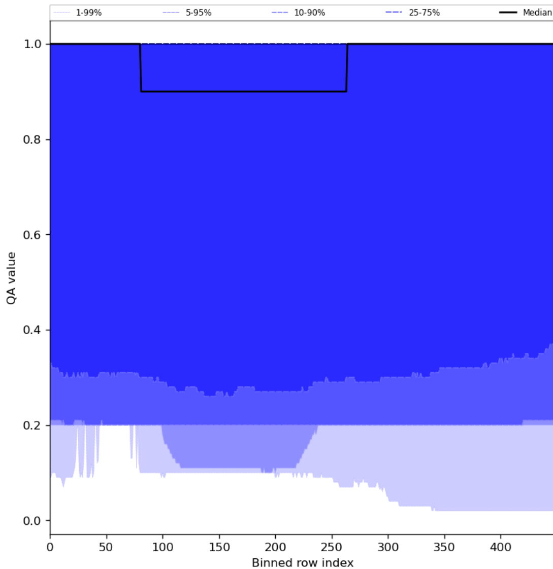
Figure 48: Along track statistics of “QA value” for 2024-08-09 to 2024-08-11
