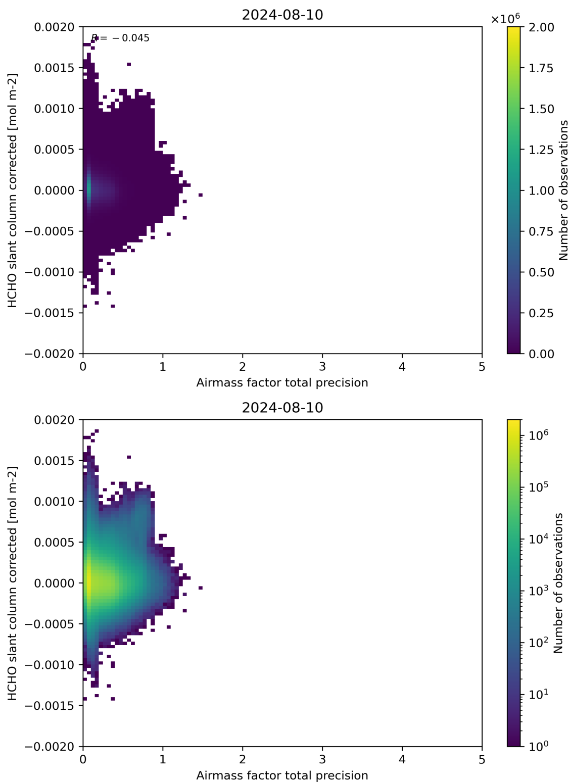
Figure 109: Scatter density plot of “Airmass factor total precision” against “HCHO slant column corrected” for 2024-08-09 to 2024-08-11.
