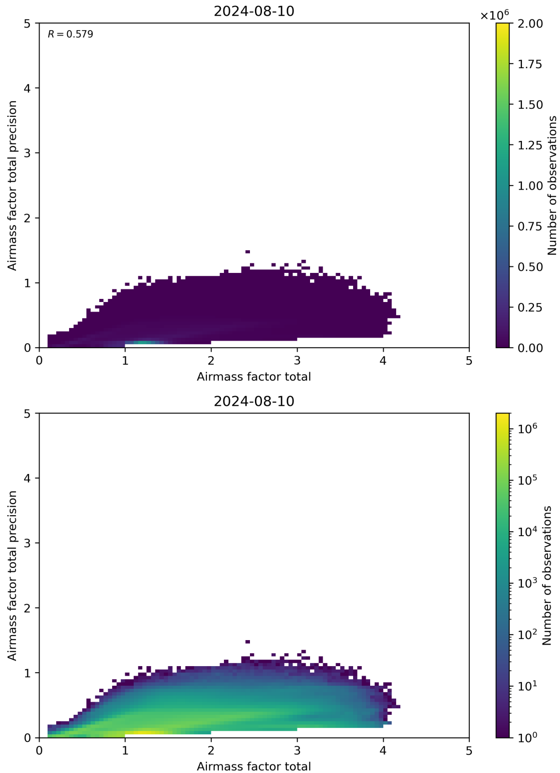
Figure 103: Scatter density plot of “Airmass factor total” against “Airmass factor total precision” for 2024-08-09 to 2024-08-11.
