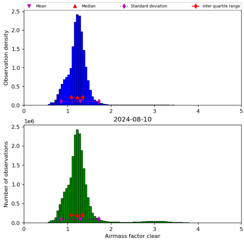
Figure 42: Histogram of “Airmass factor clear” for 2024-08-09 to 2024-08-11
