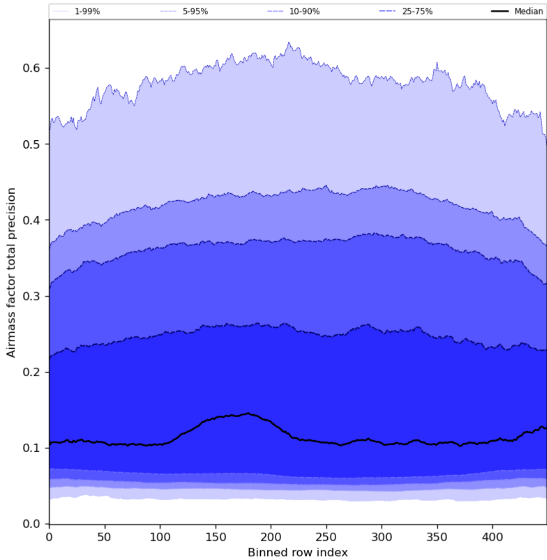
Figure 55: Along track statistics of “Airmass factor total precision” for 2024-08-09 to 2024-08-11
