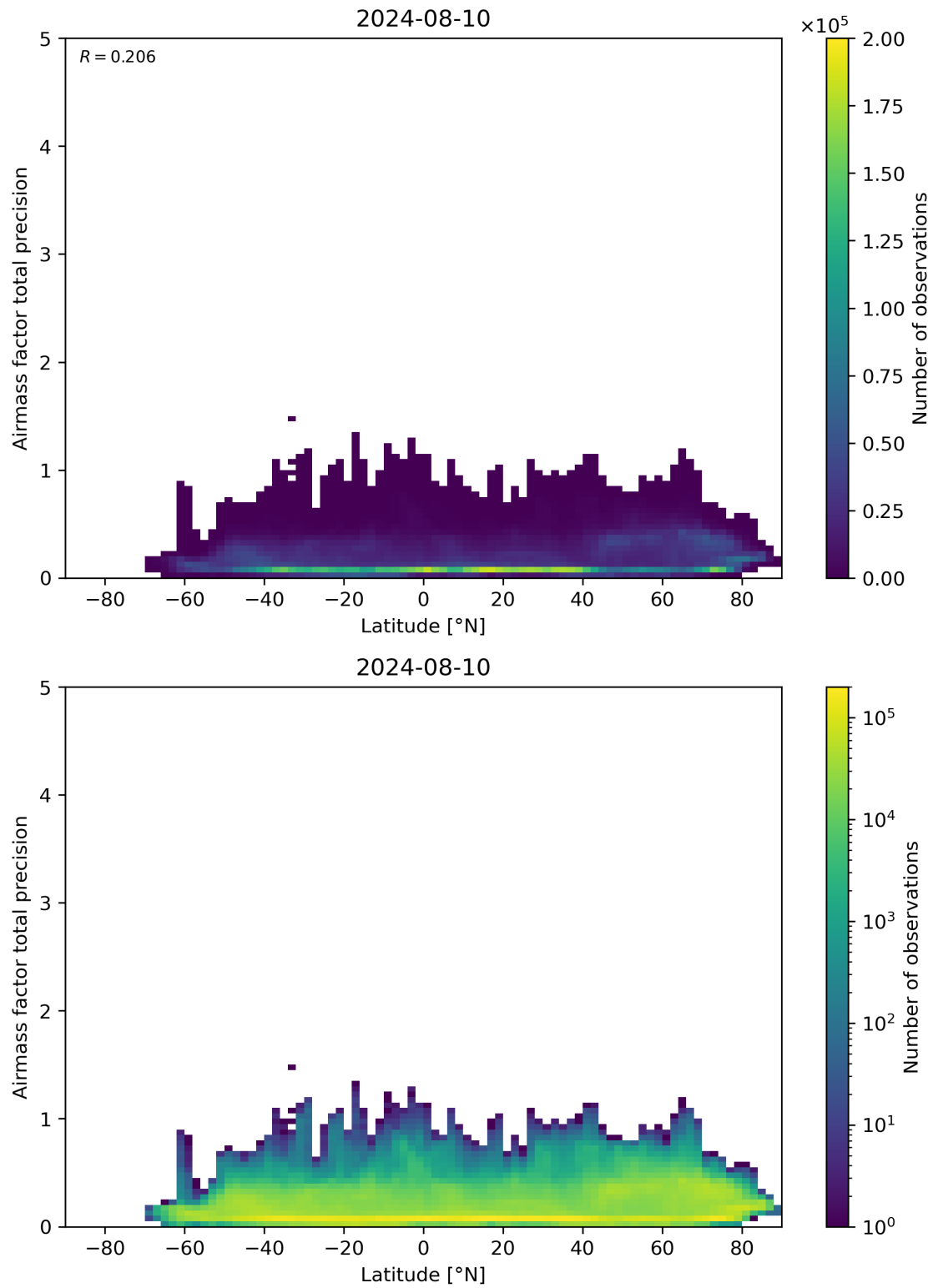
Figure 162: Scatter density plot of “Latitude” against “Airmass factor total precision” for 2024-08-09 to 2024-08-11.
