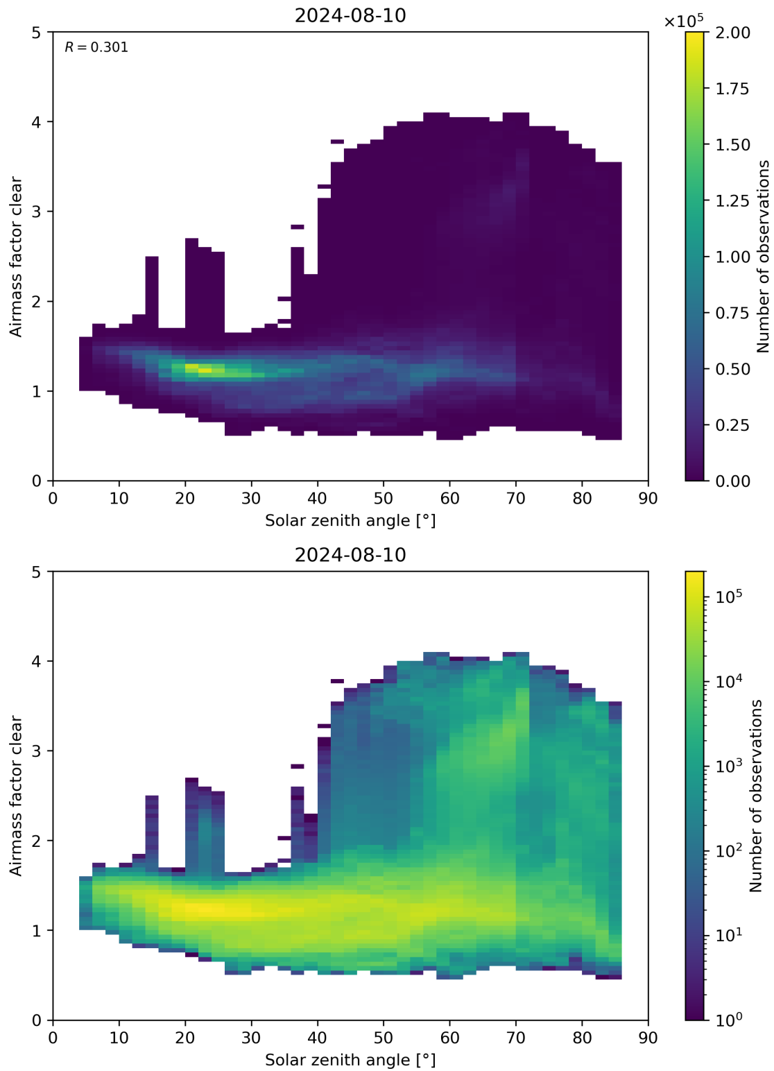
Figure 170: Scatter density plot of “Solar zenith angle” against “Airmass factor clear” for 2024-08-09 to 2024-08-11.
