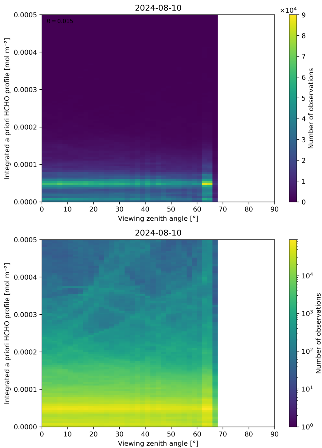
Figure 195: Scatter density plot of “Viewing zenith angle” against “Integrated a priori HCHO profile” for 2024-08-09 to 2024-08-11.
