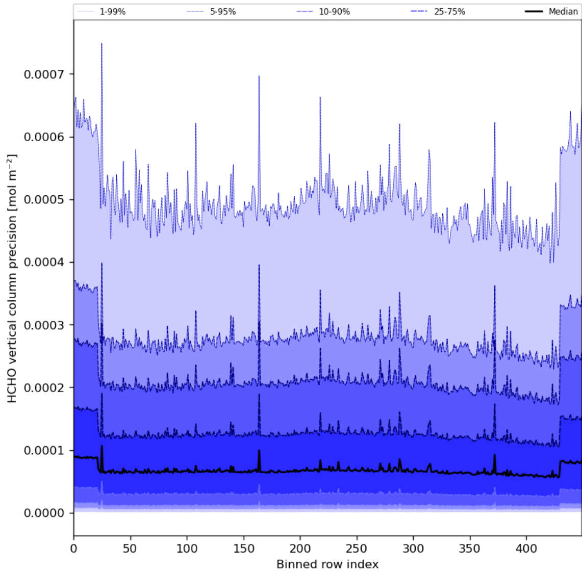
Figure 50: Along track statistics of “HCHO vertical column precision” for 2024-08-09 to 2024-08-11
