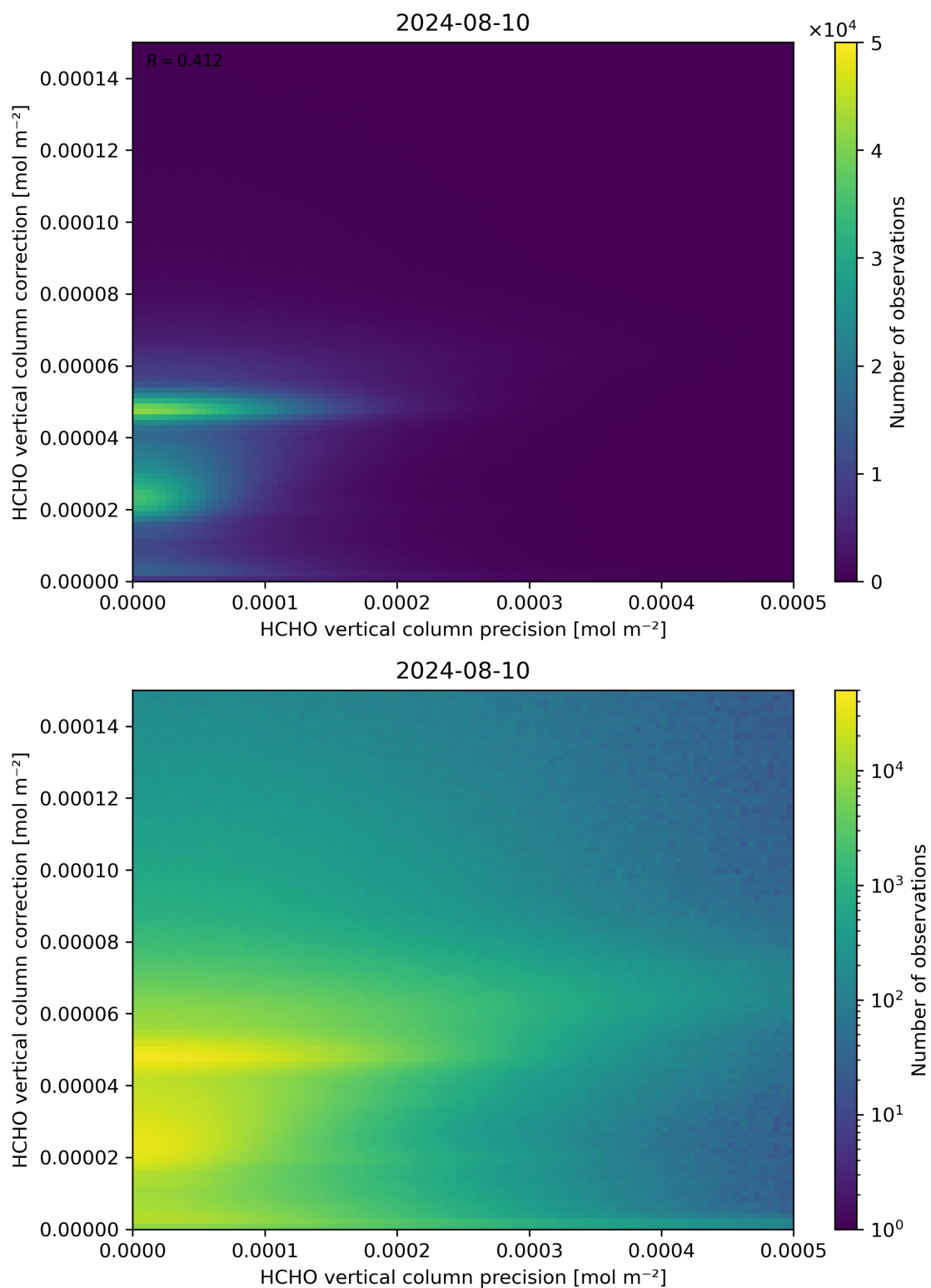
Figure 146: Scatter density plot of “HCHO vertical column precision” against “HCHO vertical column correction” for 2024-08-09 to 2024-08-11.
