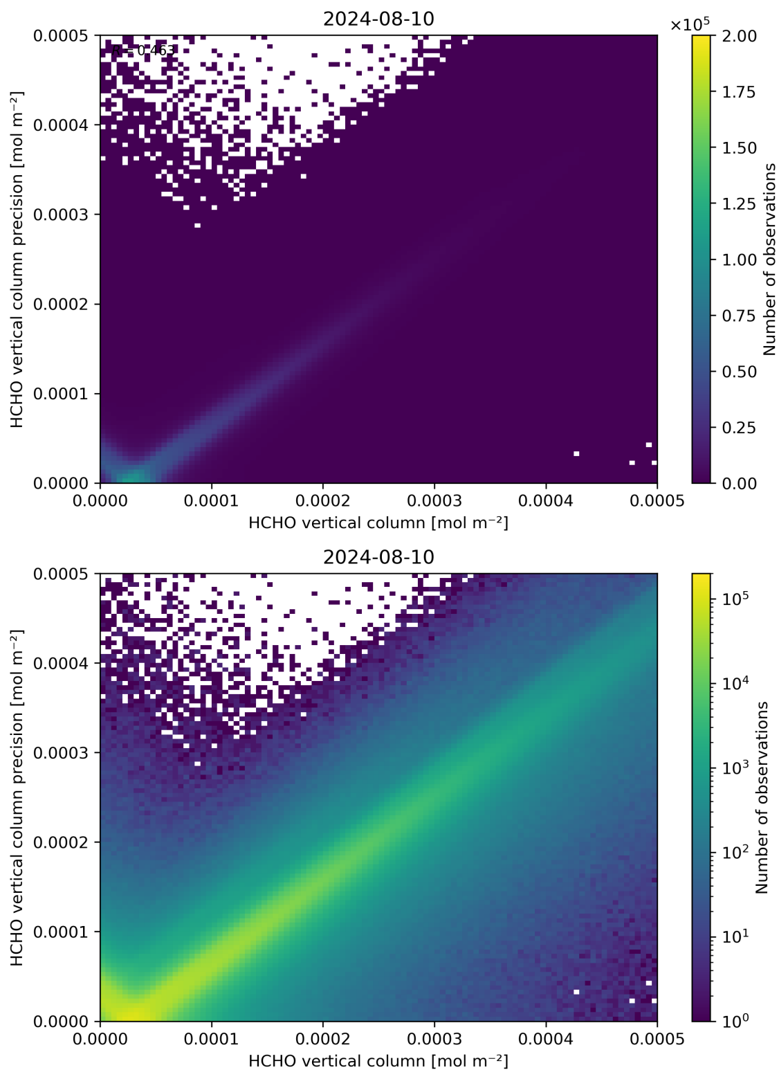
Figure 134: Scatter density plot of “HCHO vertical column” against “HCHO vertical column precision” for 2024-08-09 to 2024-08-11.
