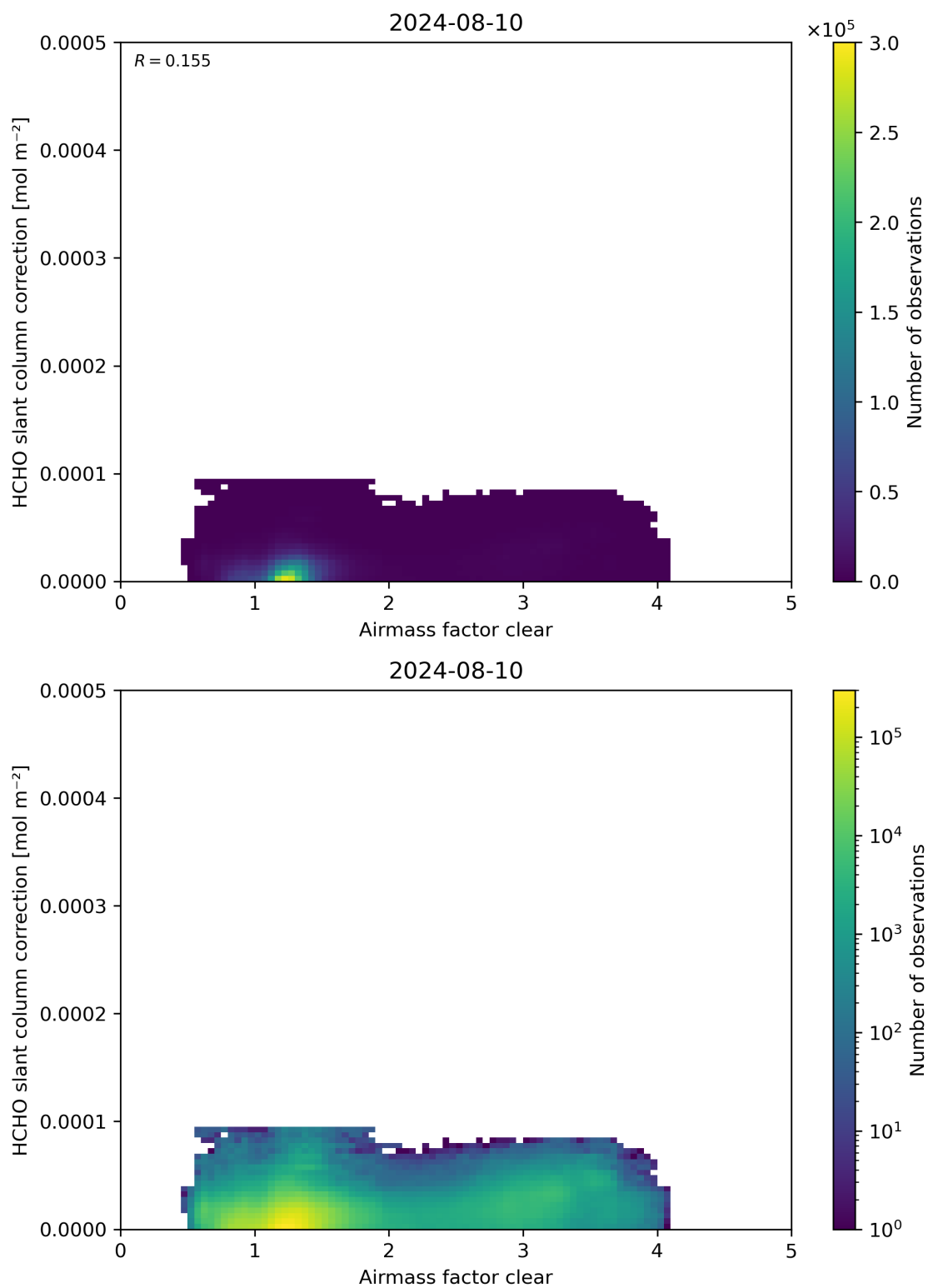
Figure 75: Scatter density plot of “Airmass factor clear” against “HCHO slant column correction” for 2024-08-09 to 2024-08-11.
