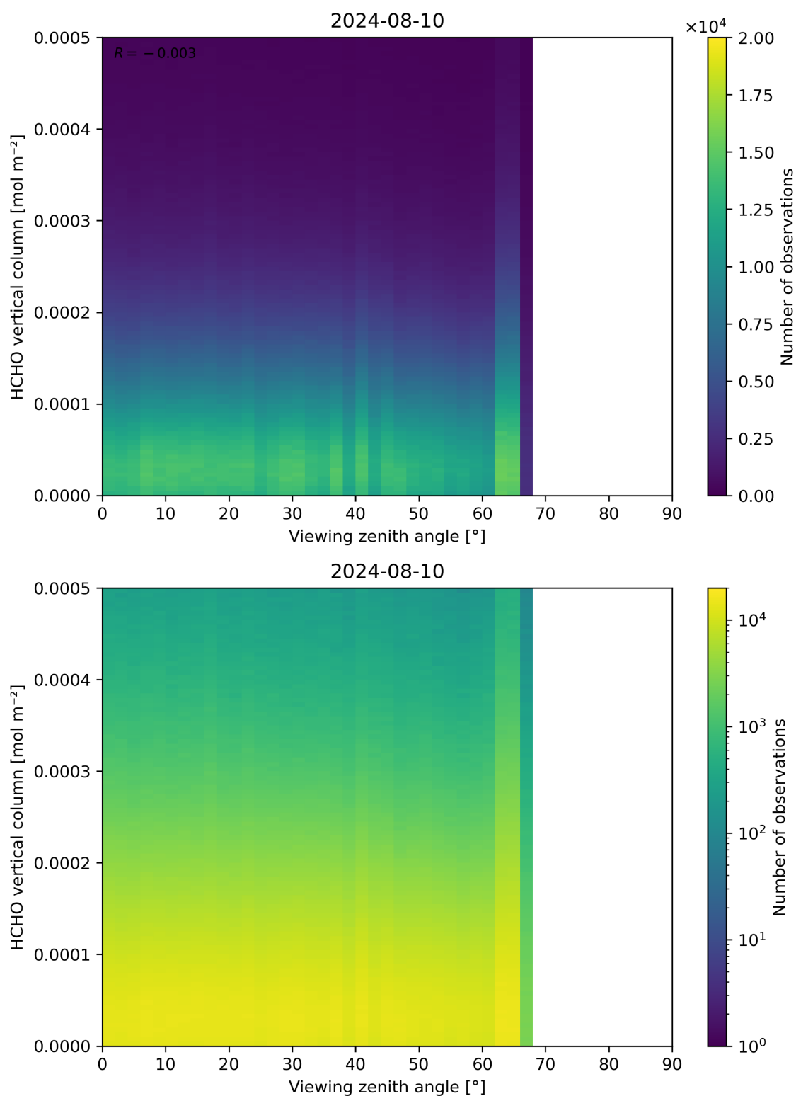
Figure 192: Scatter density plot of “Viewing zenith angle” against “HCHO vertical column” for 2024-08-09 to 2024-08-11.
