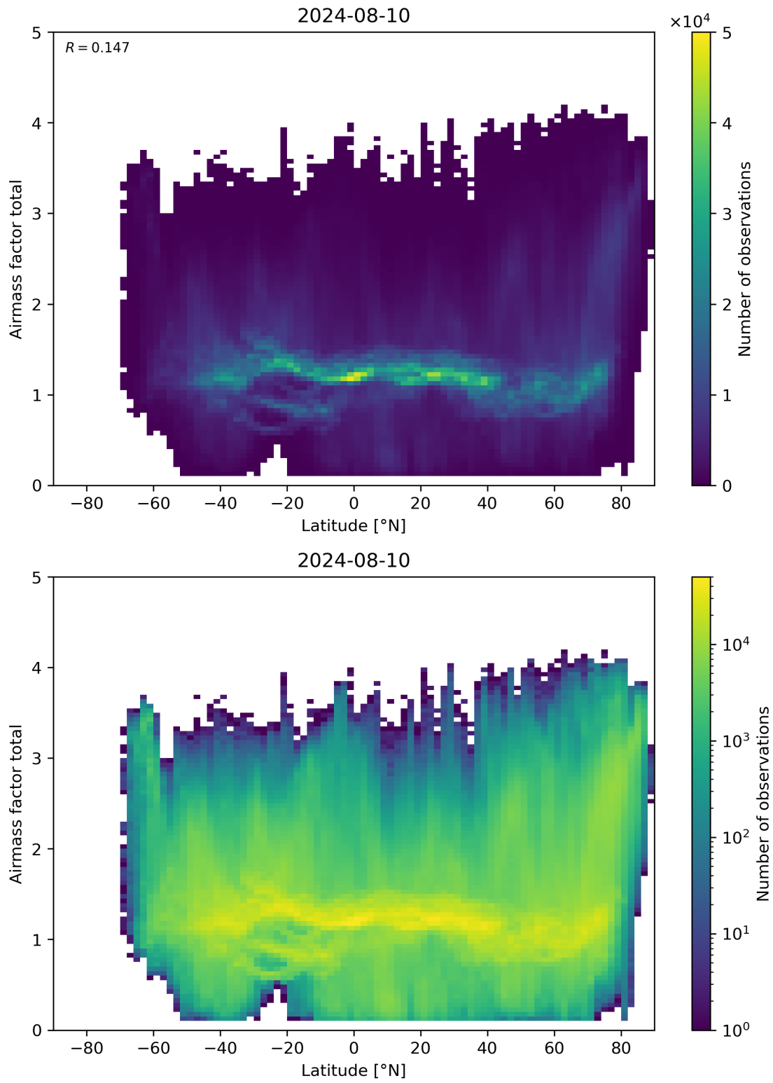
Figure 161: Scatter density plot of “Latitude” against “Airmass factor total” for 2024-08-09 to 2024-08-11.
