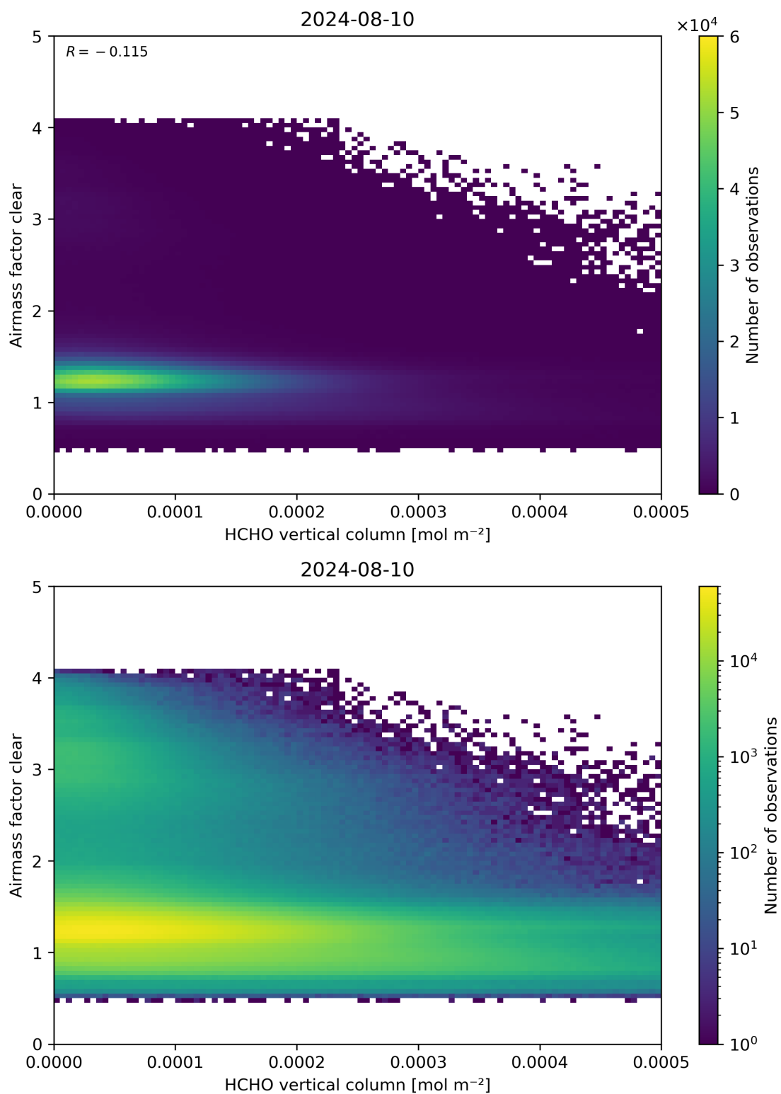
Figure 126: Scatter density plot of “HCHO vertical column” against “Airmass factor clear” for 2024-08-09 to 2024-08-11.
