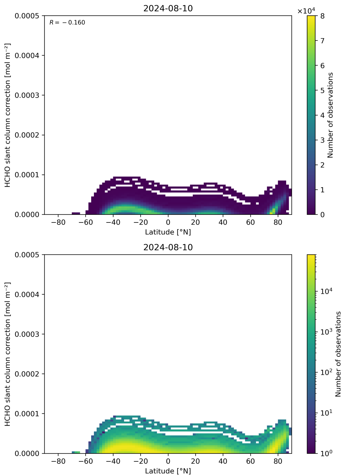
Figure 158: Scatter density plot of “Latitude” against “HCHO slant column correction” for 2024-08-09 to 2024-08-11.
