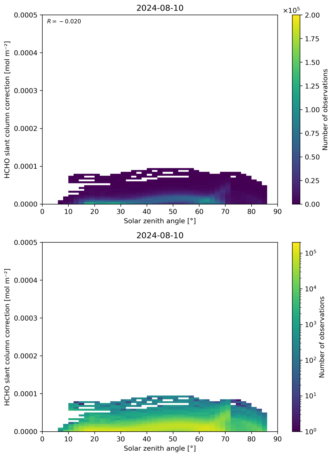
Figure 172: Scatter density plot of “Solar zenith angle” against “HCHO slant column correction” for 2024-08-09 to 2024-08-11.
