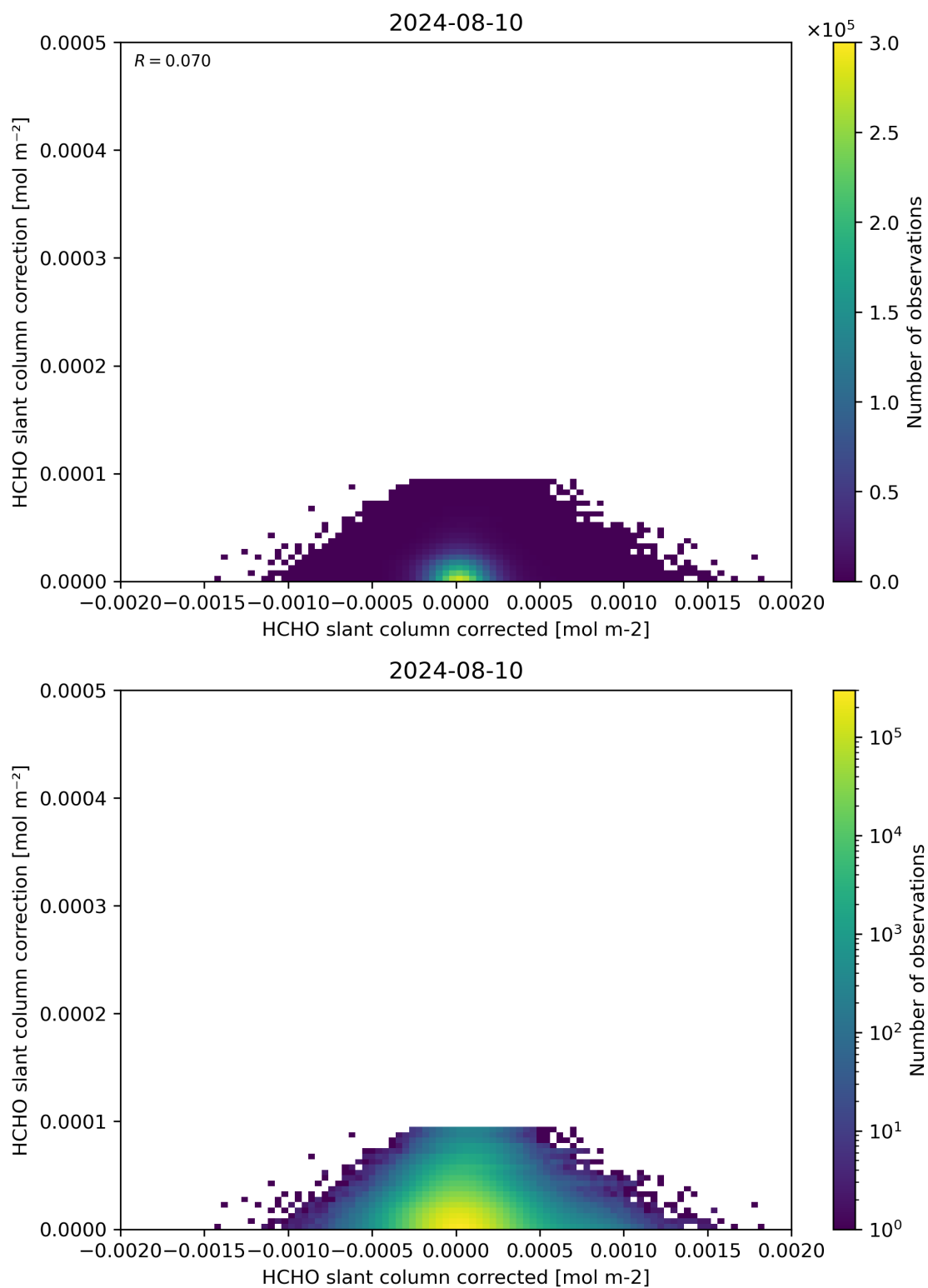
Figure 77: Scatter density plot of “HCHO slant column corrected” against “HCHO slant column correction” for 2024-08-09 to 2024-08-11.
