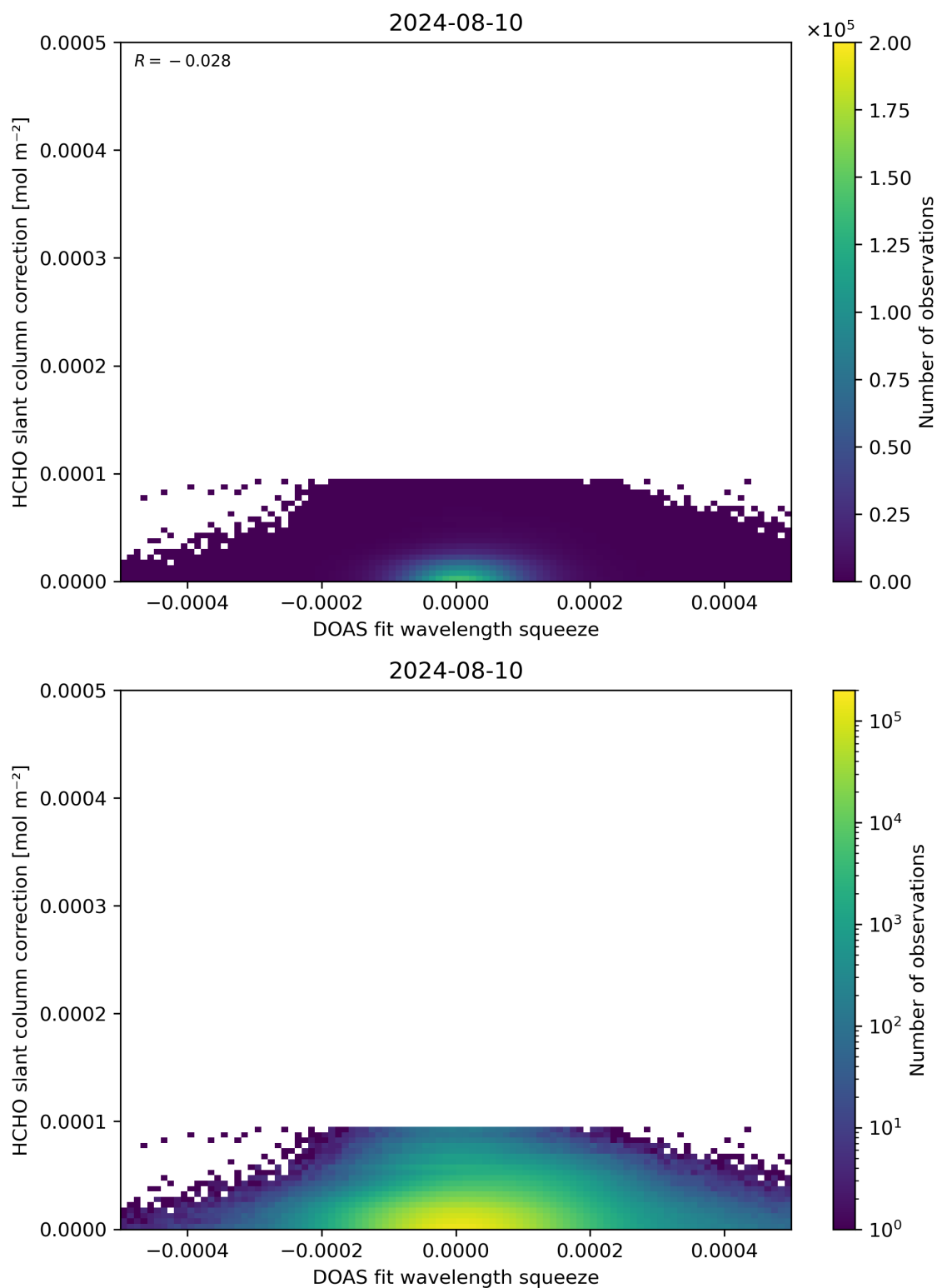
Figure 70: Scatter density plot of “DOAS fit wavelength squeeze” against “HCHO slant column correction” for 2024-08-09 to 2024-08-11.
