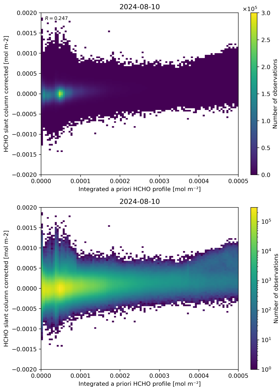
Figure 151: Scatter density plot of “Integrated a priori HCHO profile” against “HCHO slant column corrected” for 2024-08-09 to 2024-08-11.
