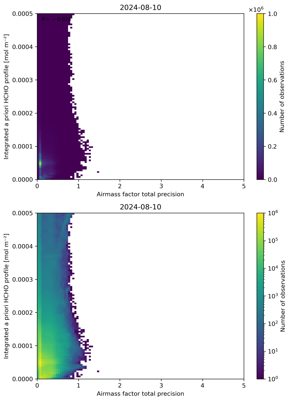
Figure 111: Scatter density plot of “Airmass factor total precision” against “Integrated a priori HCHO profile” for 2024-08-09 to 2024-08-11.
