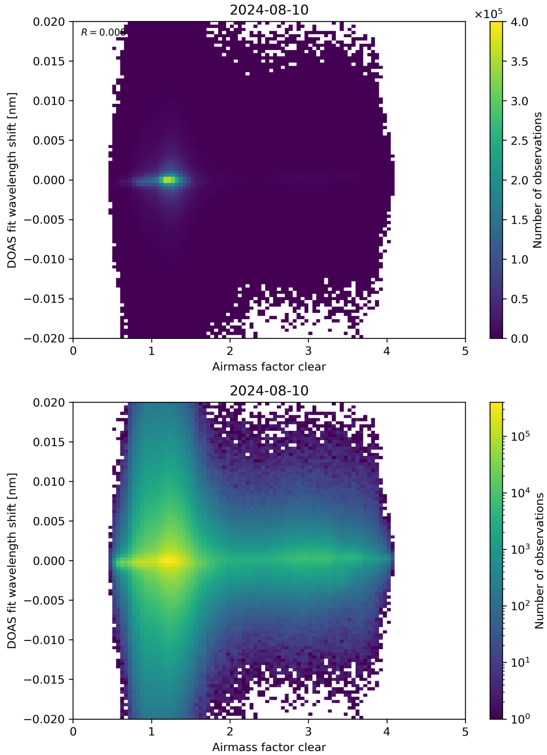
Figure 72: Scatter density plot of “Airmass factor clear” against “DOAS fit wavelength shift” for 2024-08-09 to 2024-08-11.
