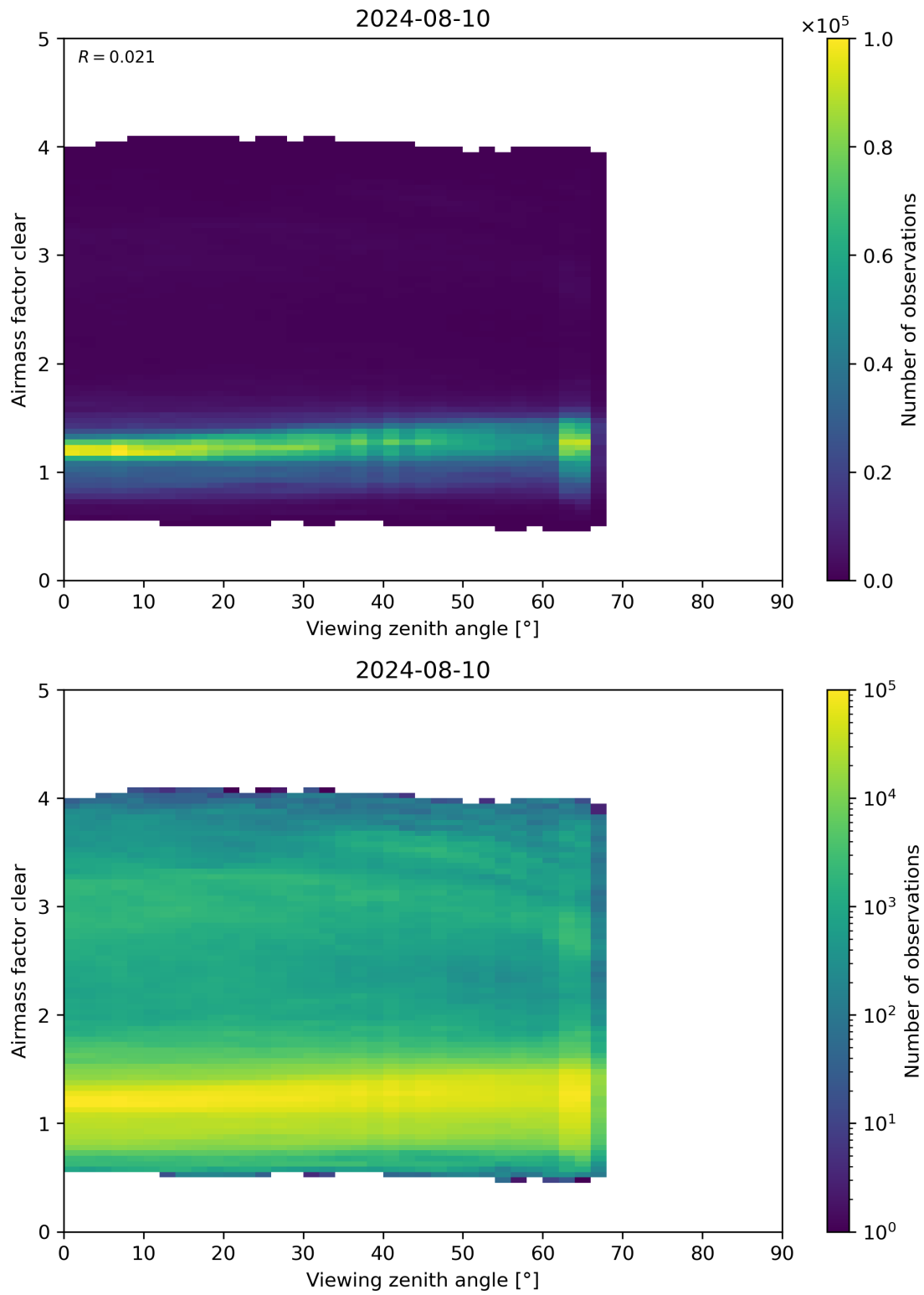
Figure 185: Scatter density plot of “Viewing zenith angle” against “Airmass factor clear” for 2024-08-09 to 2024-08-11.
