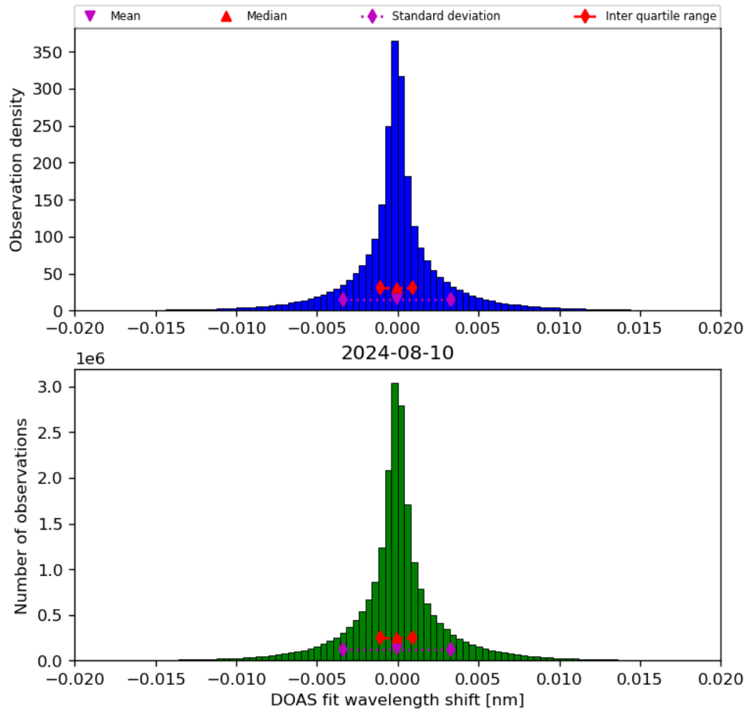
Figure 44: Histogram of “DOAS fit wavelength shift” for 2024-08-09 to 2024-08-11
