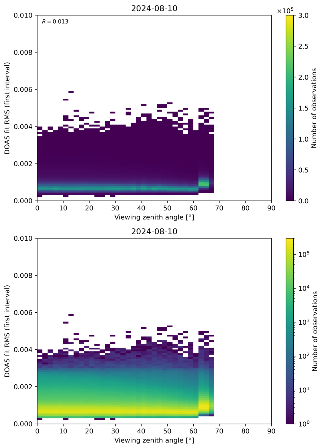
Figure 182: Scatter density plot of “Viewing zenith angle” against “DOAS fit RMS (first interval)” for 2024-08-09 to 2024-08-11.
