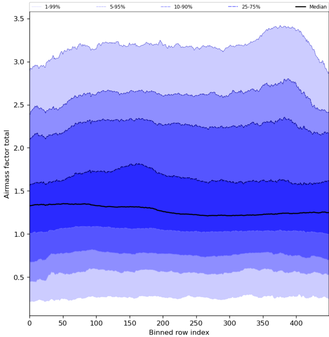
Figure 54: Along track statistics of “Airmass factor total” for 2024-08-09 to 2024-08-11
