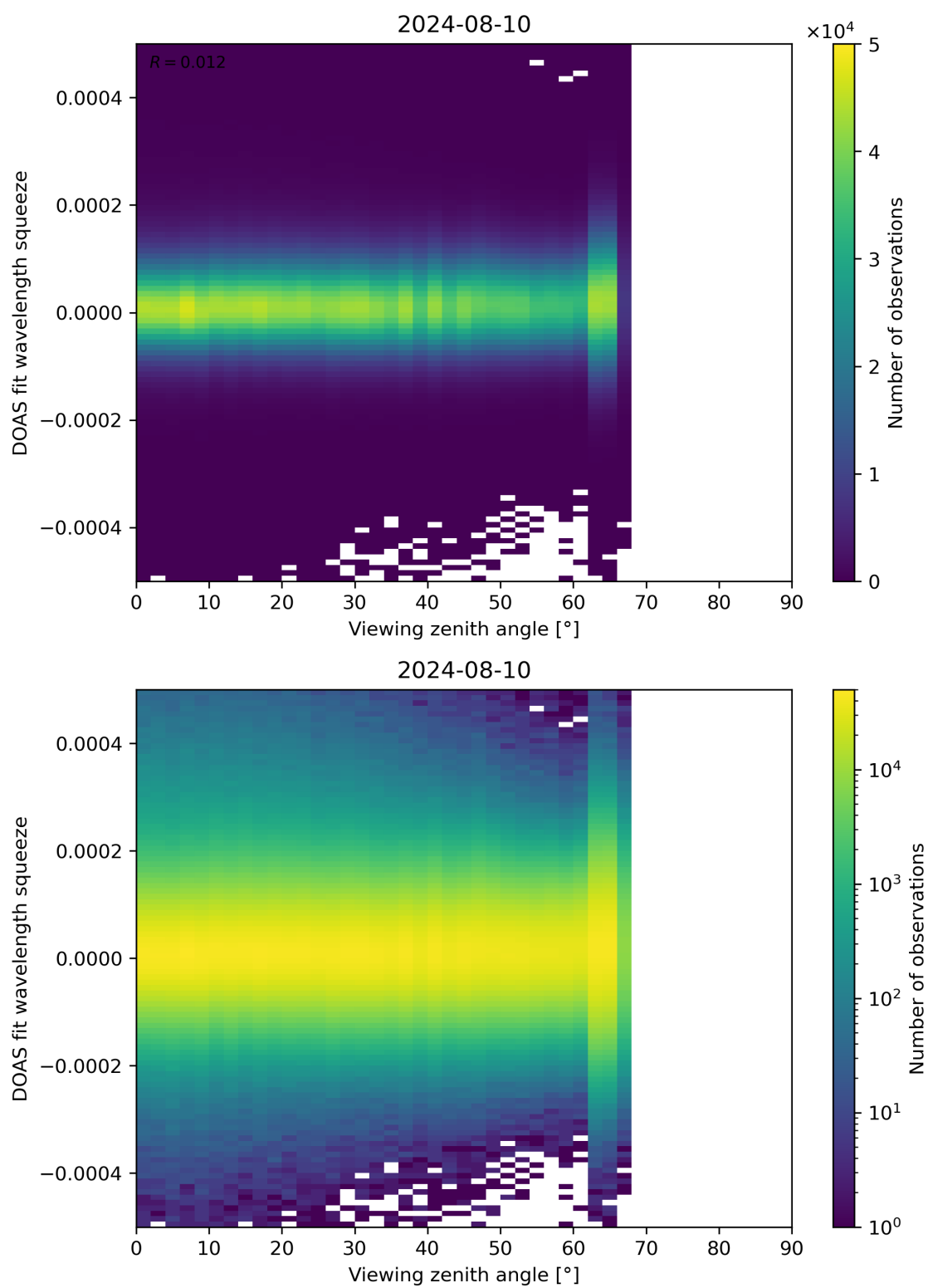
Figure 184: Scatter density plot of “Viewing zenith angle” against “DOAS fit wavelength squeeze” for 2024-08-09 to 2024-08-11.
