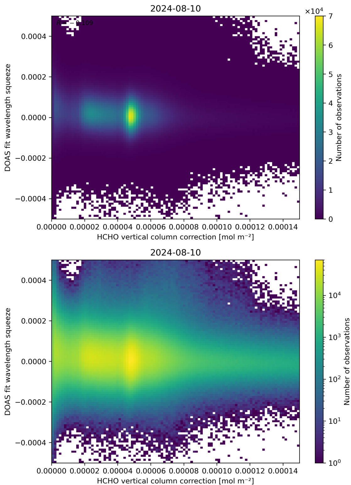
Figure 114: Scatter density plot of “HCHO vertical column correction” against “DOAS fit wavelength squeeze” for 2024-08-09 to 2024-08-11.
