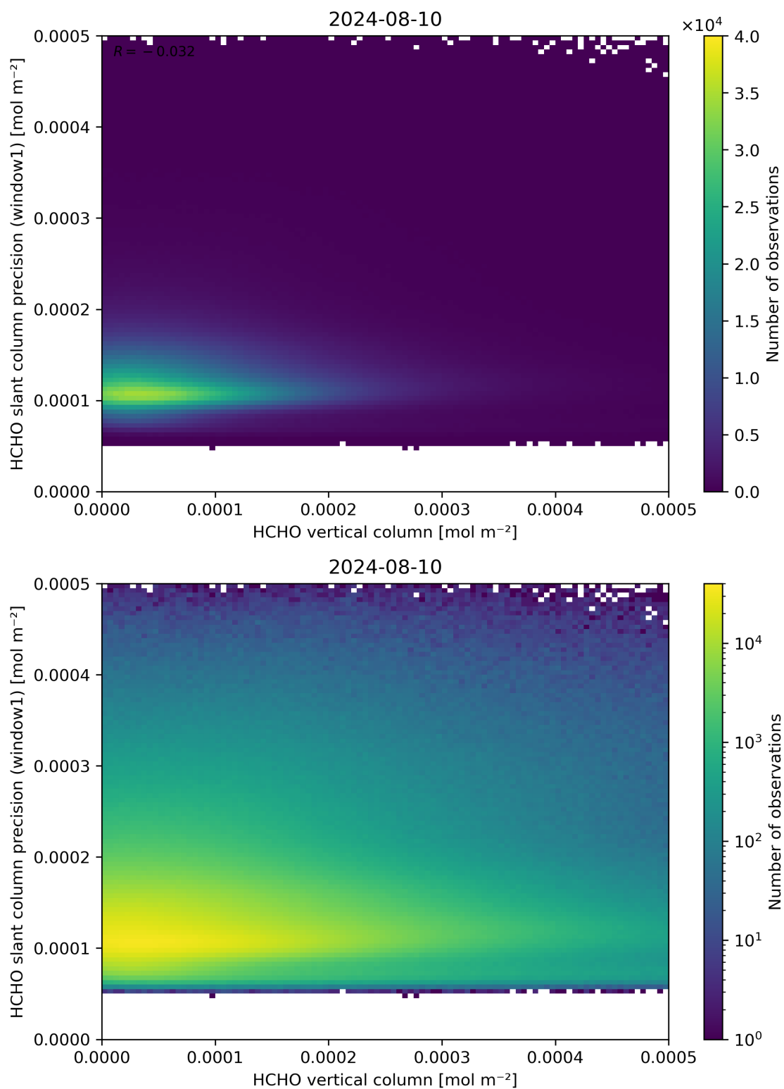
Figure 130: Scatter density plot of “HCHO vertical column” against “HCHO slant column precision (window1)” for 2024-08-09 to 2024-08-11.
