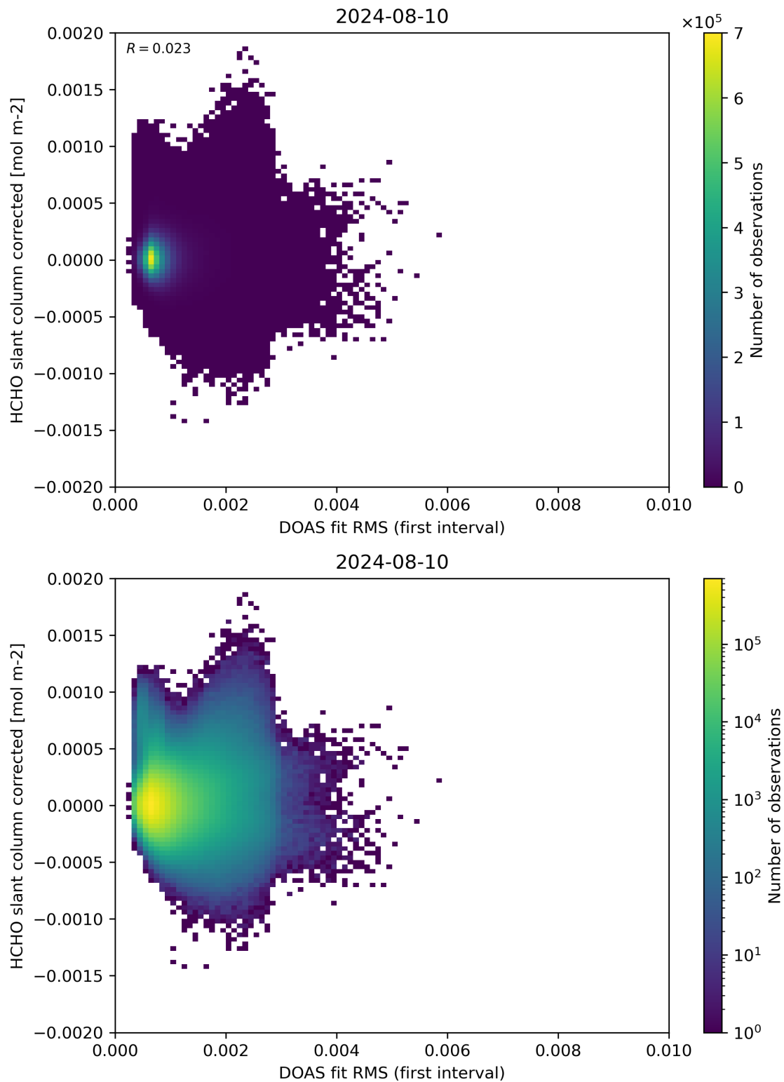
Figure 62: Scatter density plot of “DOAS fit RMS (first interval)” against “HCHO slant column corrected” for 2024-08-09 to 2024-08-11.
