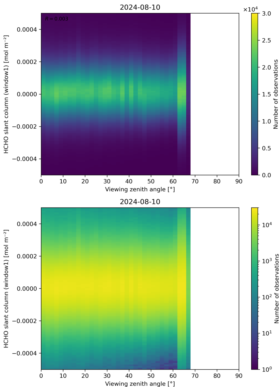
Figure 188: Scatter density plot of “Viewing zenith angle” against “HCHO slant column (window1)” for 2024-08-09 to 2024-08-11.
