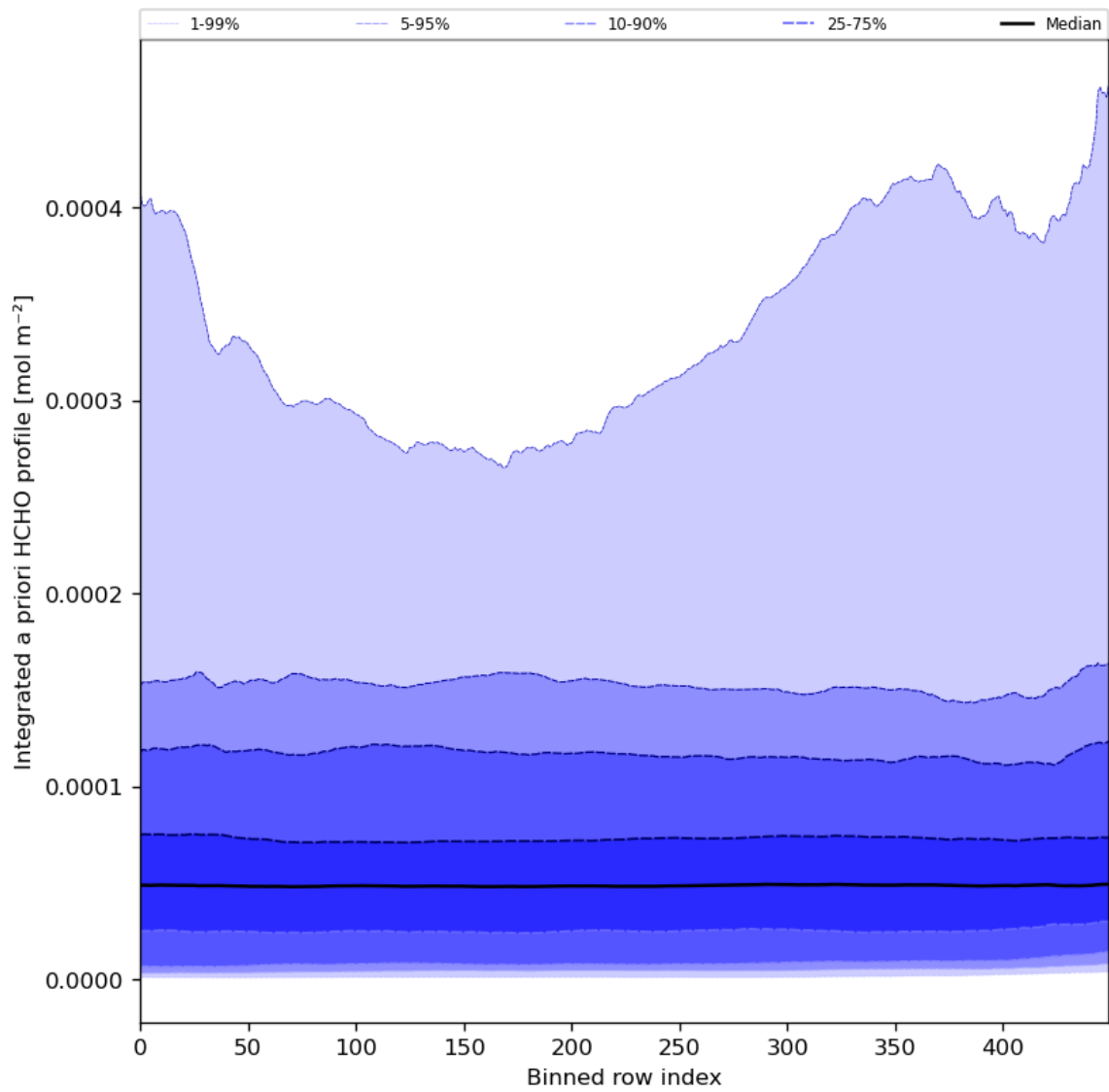
Figure 57: Along track statistics of “Integrated a priori HCHO profile” for 2024-08-09 to 2024-08-11
