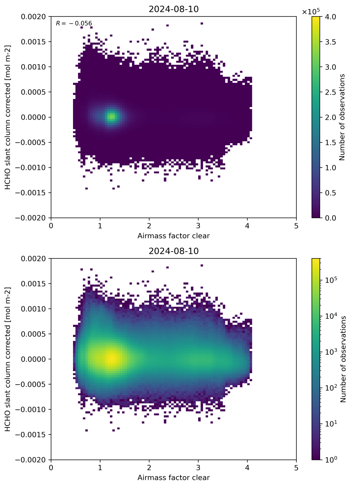
Figure 74: Scatter density plot of “Airmass factor clear” against “HCHO slant column corrected” for 2024-08-09 to 2024-08-11.
