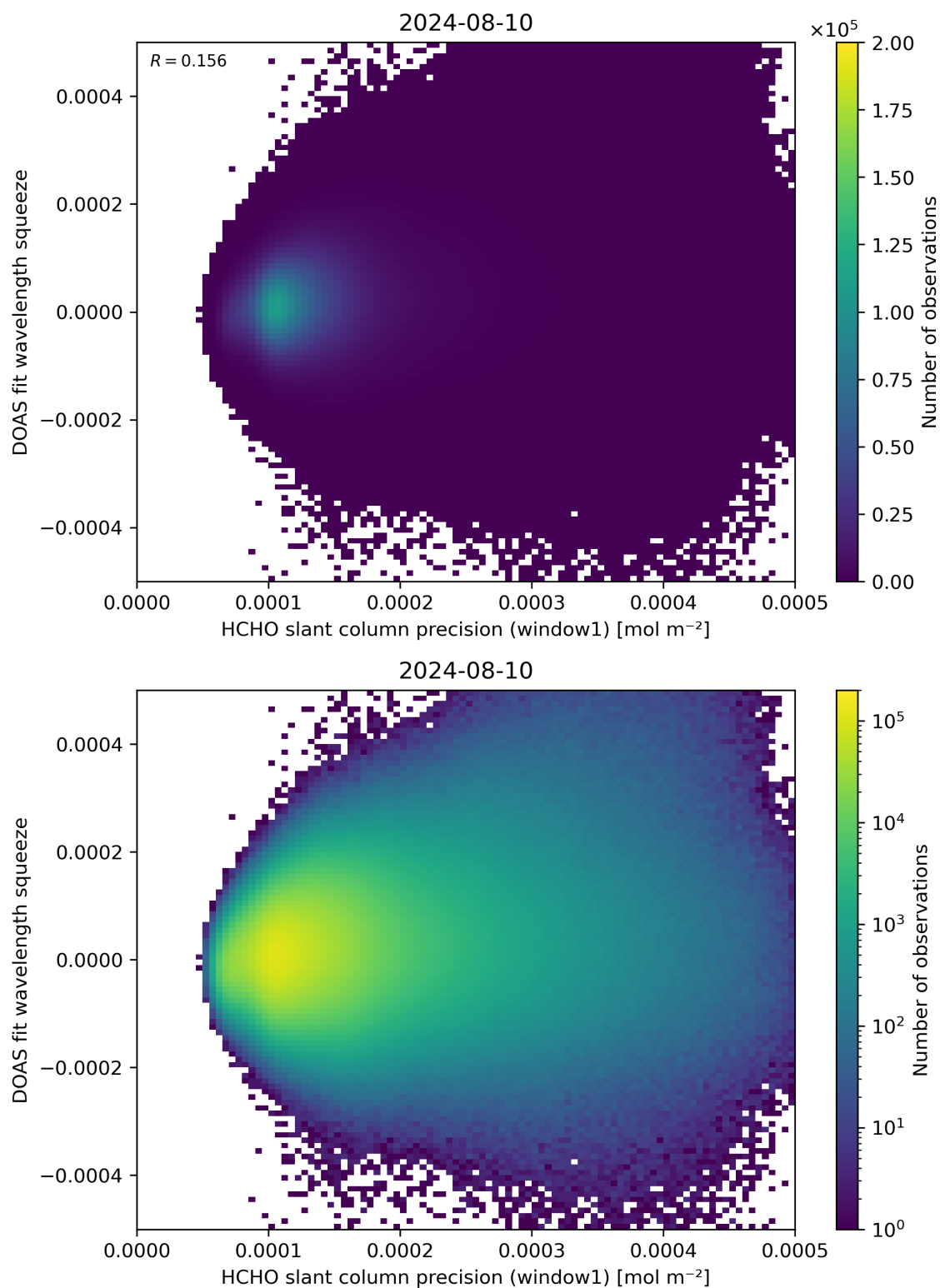
Figure 90: Scatter density plot of “HCHO slant column precision (window1)” against “DOAS fit wavelength squeeze” for 2024-08-09 to 2024-08-11.
