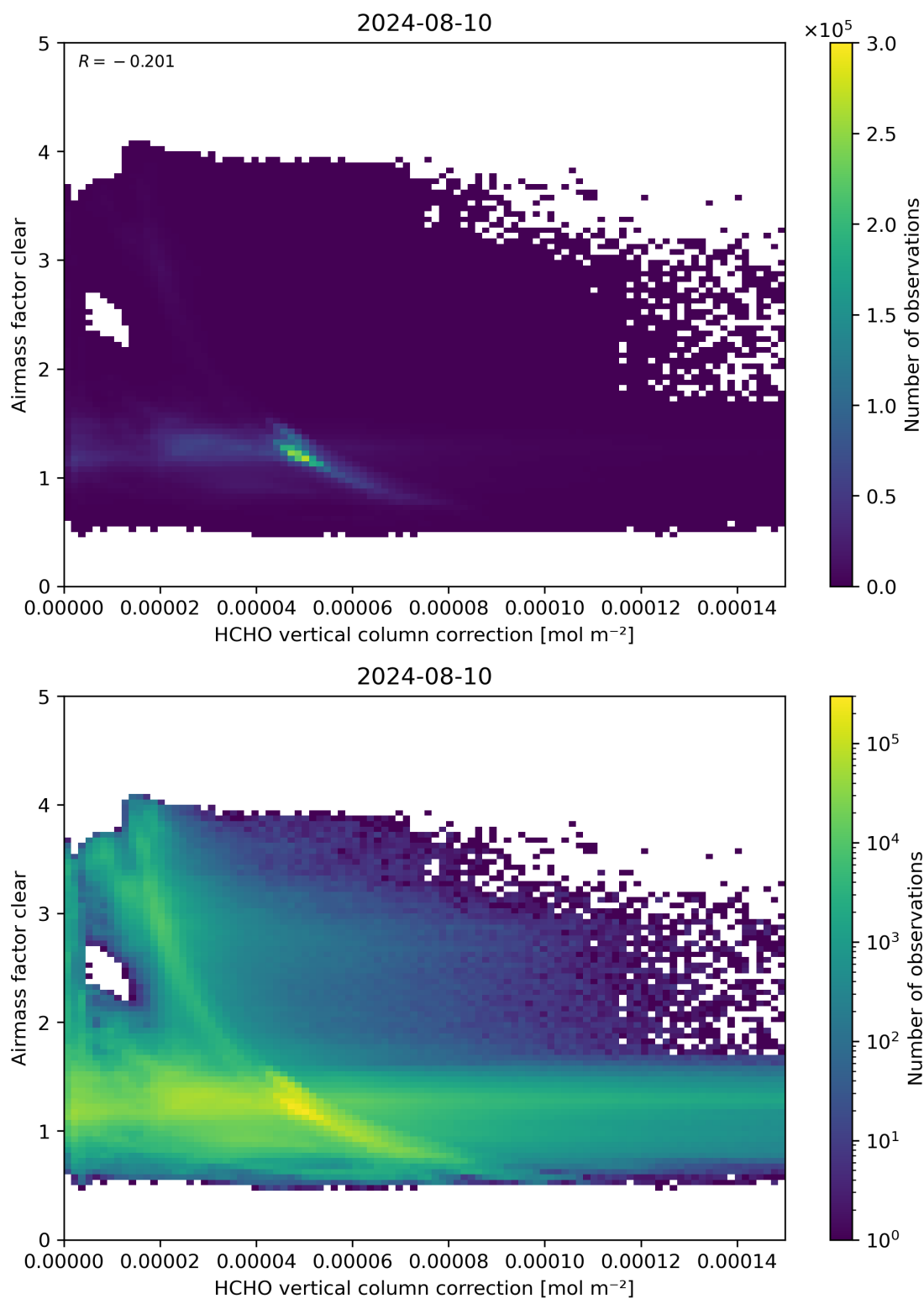
Figure 115: Scatter density plot of “HCHO vertical column correction” against “Airmass factor clear” for 2024-08-09 to 2024-08-11.
