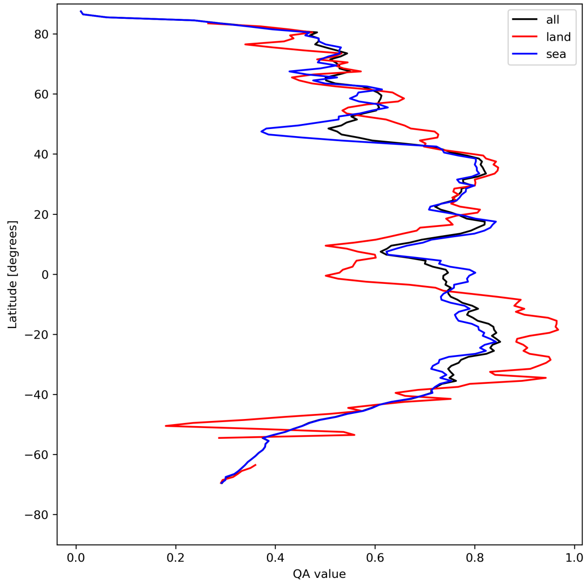
Figure 20: Zonal average of “QA value” for 2024-08-09 to 2024-08-11.
