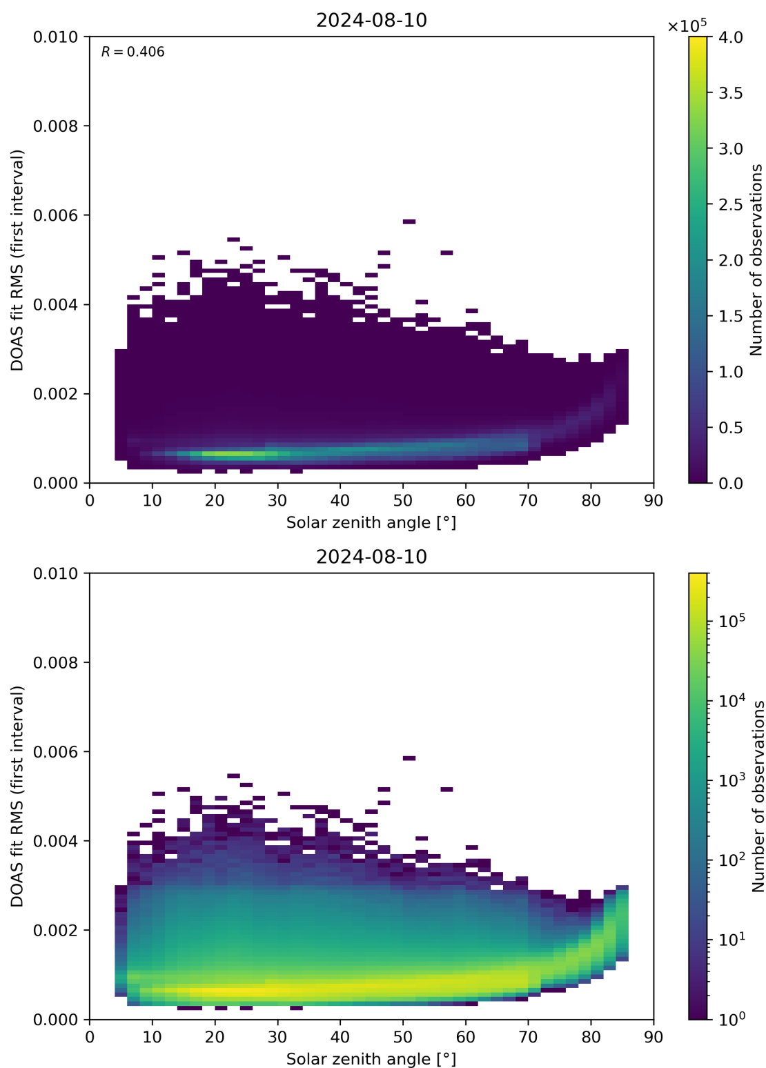
Figure 167: Scatter density plot of “Solar zenith angle” against “DOAS fit RMS (first interval)” for 2024-08-09 to 2024-08-11.
