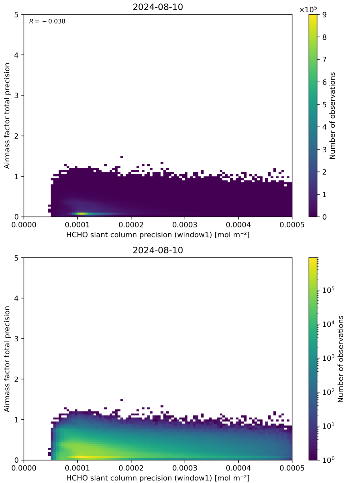
Figure 95: Scatter density plot of “HCHO slant column precision (window1)” against “Airmass factor total precision” for 2024-08-09 to 2024-08-11.
