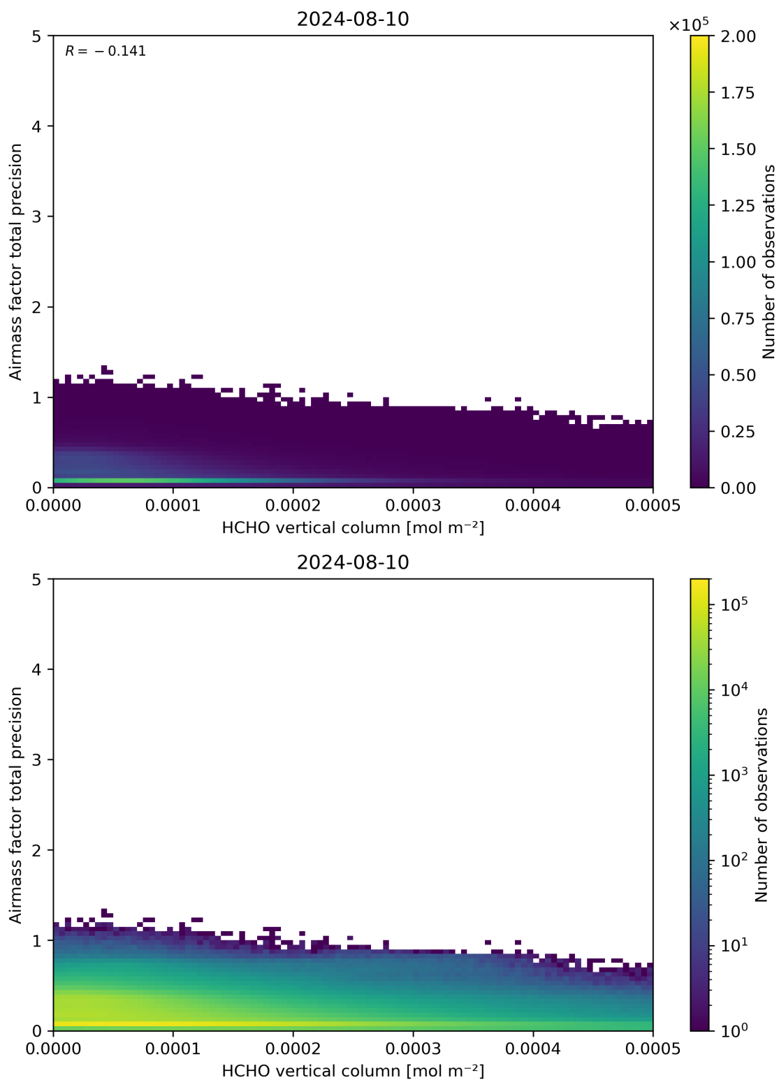
Figure 132: Scatter density plot of “HCHO vertical column” against “Airmass factor total precision” for 2024-08-09 to 2024-08-11.
