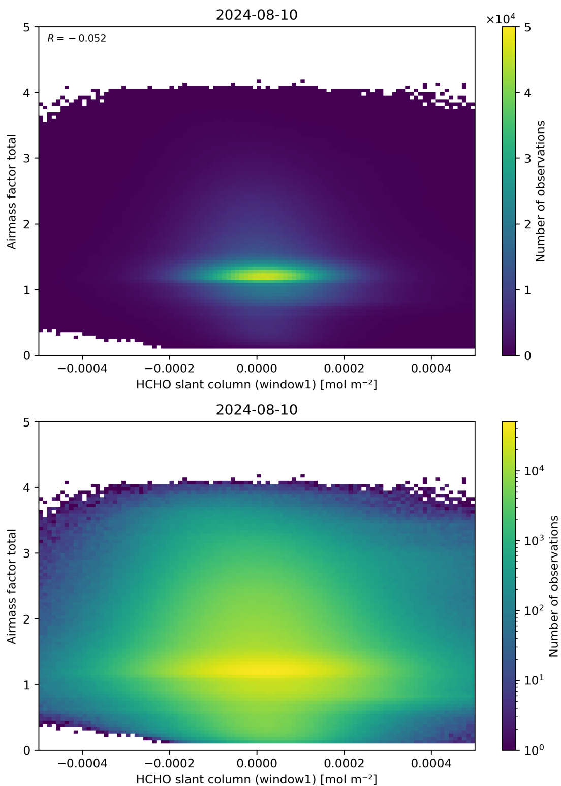
Figure 85: Scatter density plot of “HCHO slant column (window1)” against “Airmass factor total” for 2024-08-09 to 2024-08-11.
