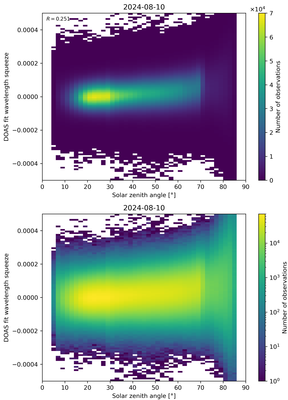
Figure 169: Scatter density plot of “Solar zenith angle” against “DOAS fit wavelength squeeze” for 2024-08-09 to 2024-08-11.
