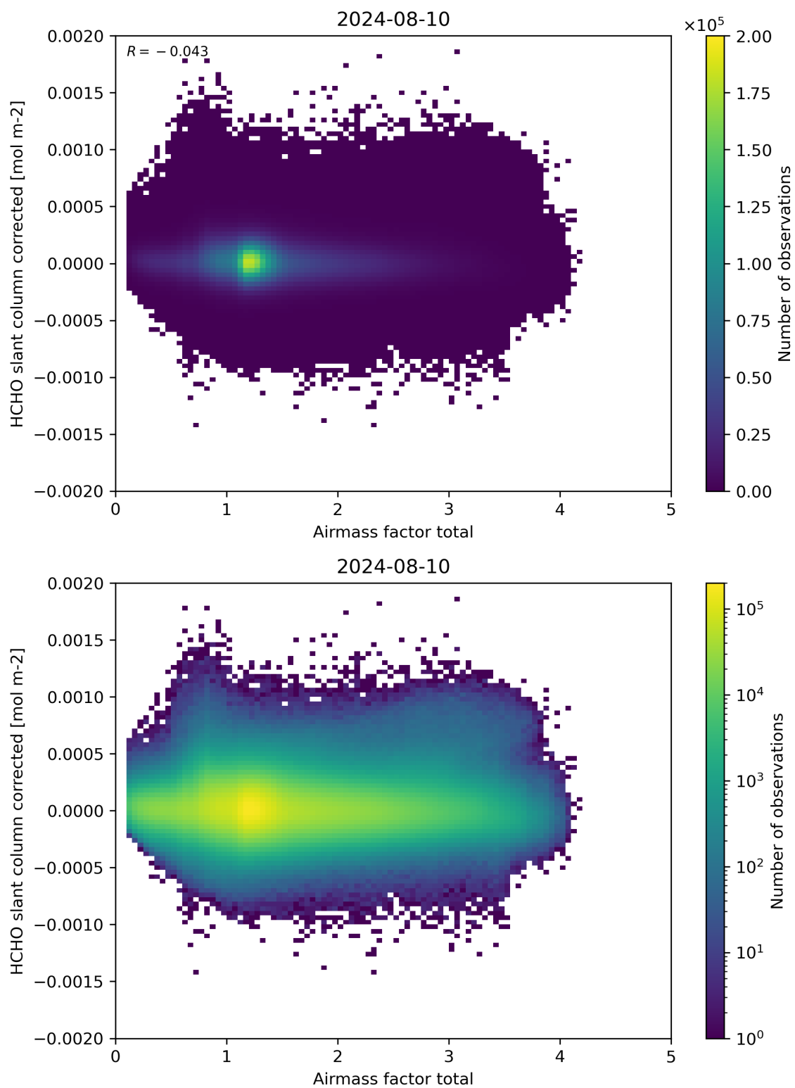
Figure 101: Scatter density plot of “Airmass factor total” against “HCHO slant column corrected” for 2024-08-09 to 2024-08-11.
