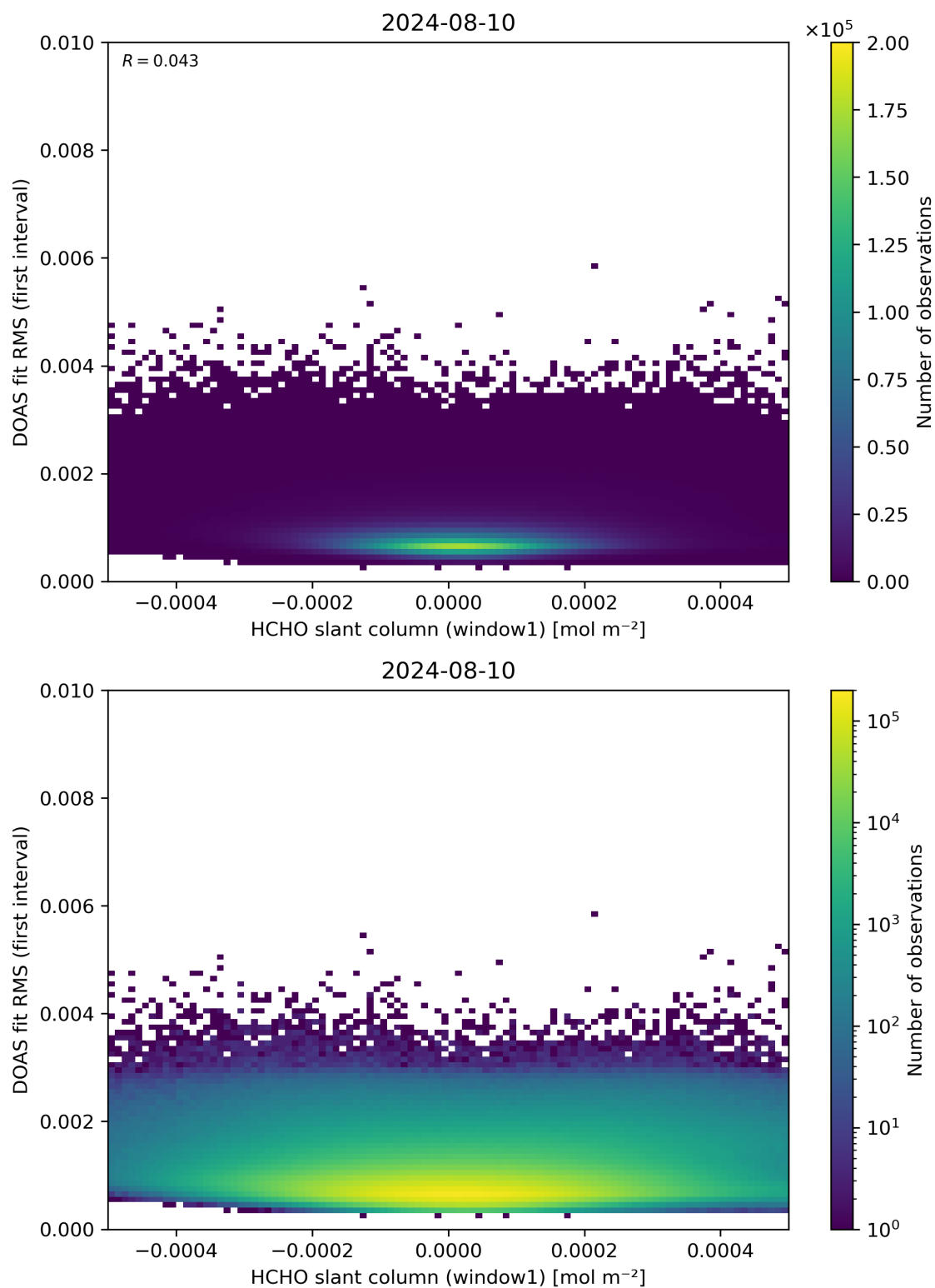
Figure 78: Scatter density plot of “HCHO slant column (window1)” against “DOAS fit RMS (first interval)” for 2024-08-09 to 2024-08-11.
