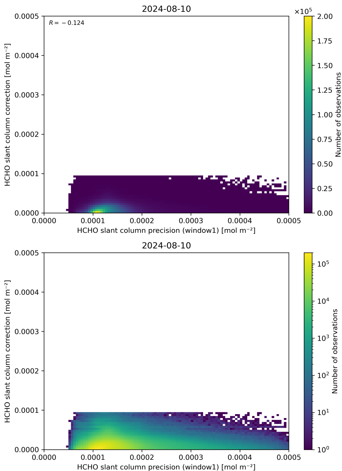
Figure 93: Scatter density plot of “HCHO slant column precision (window1)” against “HCHO slant column correction” for 2024-08-09 to 2024-08-11.
