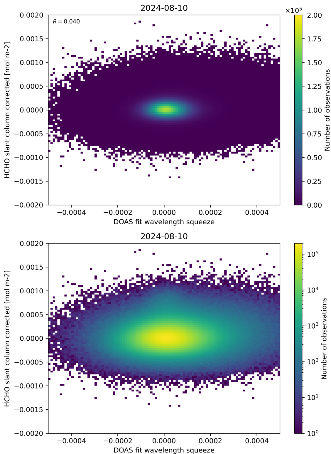
Figure 69: Scatter density plot of “DOAS fit wavelength squeeze” against “HCHO slant column corrected” for 2024-08-09 to 2024-08-11.
