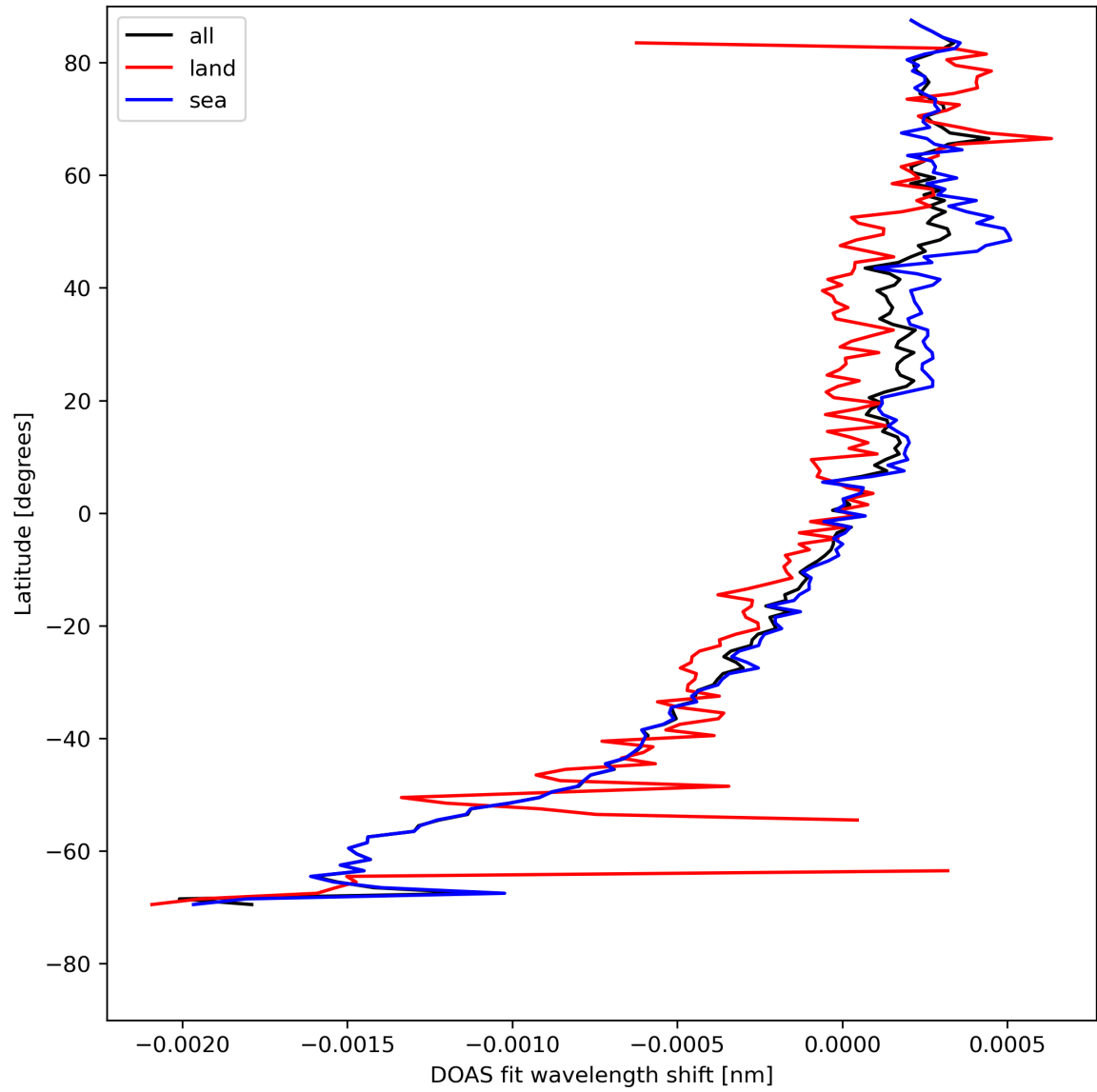
Figure 30: Zonal average of “DOAS fit wavelength shift” for 2024-08-09 to 2024-08-11.
