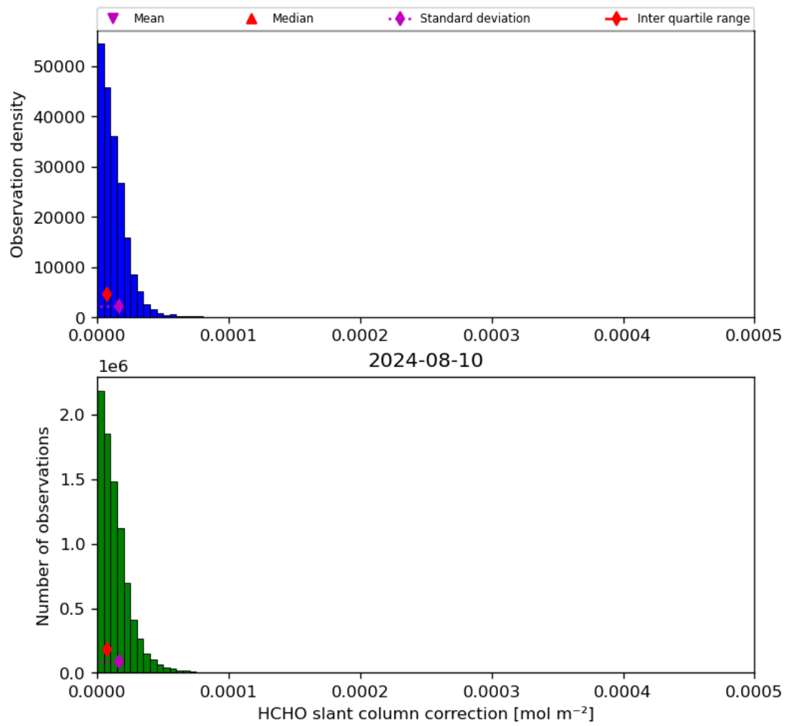
Figure 47: Histogram of "HCHO slant column correction" for 2024-08-09 to 2024-08-11
