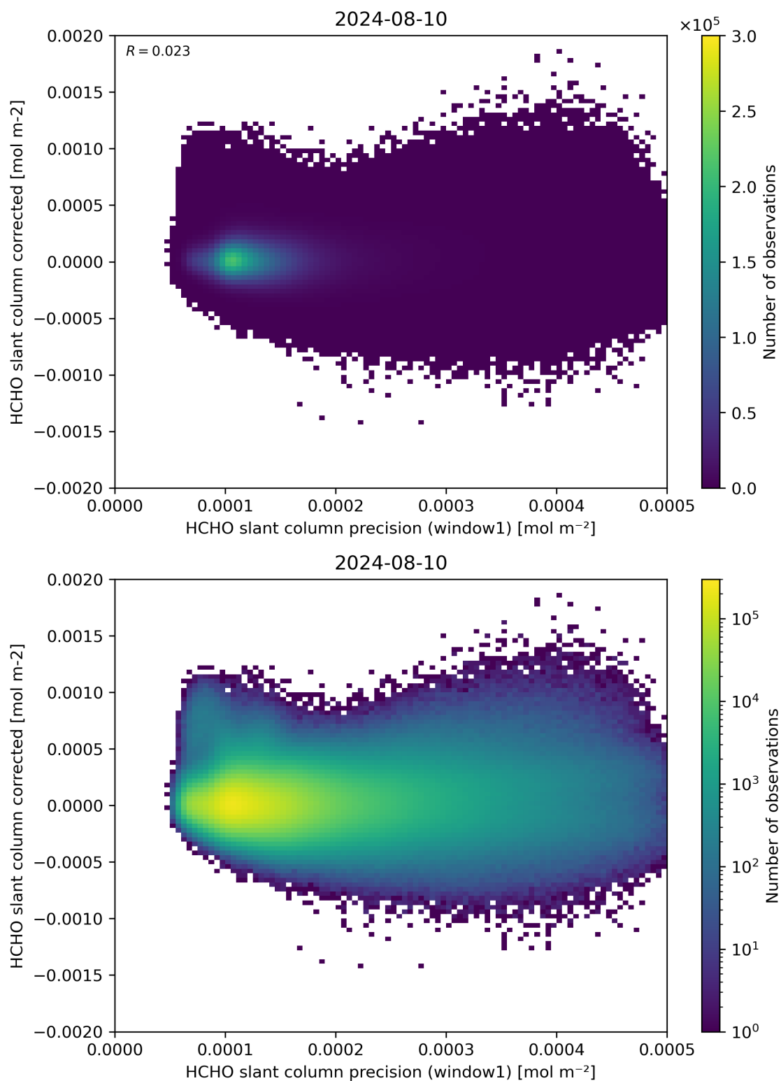
Figure 92: Scatter density plot of “HCHO slant column precision (window1)” against “HCHO slant column corrected” for 2024-08-09 to 2024-08-11.
