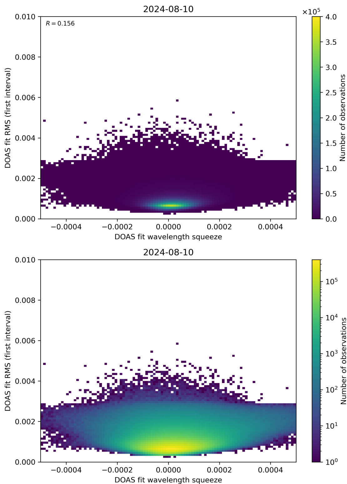
Figure 68: Scatter density plot of “DOAS fit wavelength squeeze” against “DOAS fit RMS (first interval)” for 2024-08-09 to 2024-08-11.
