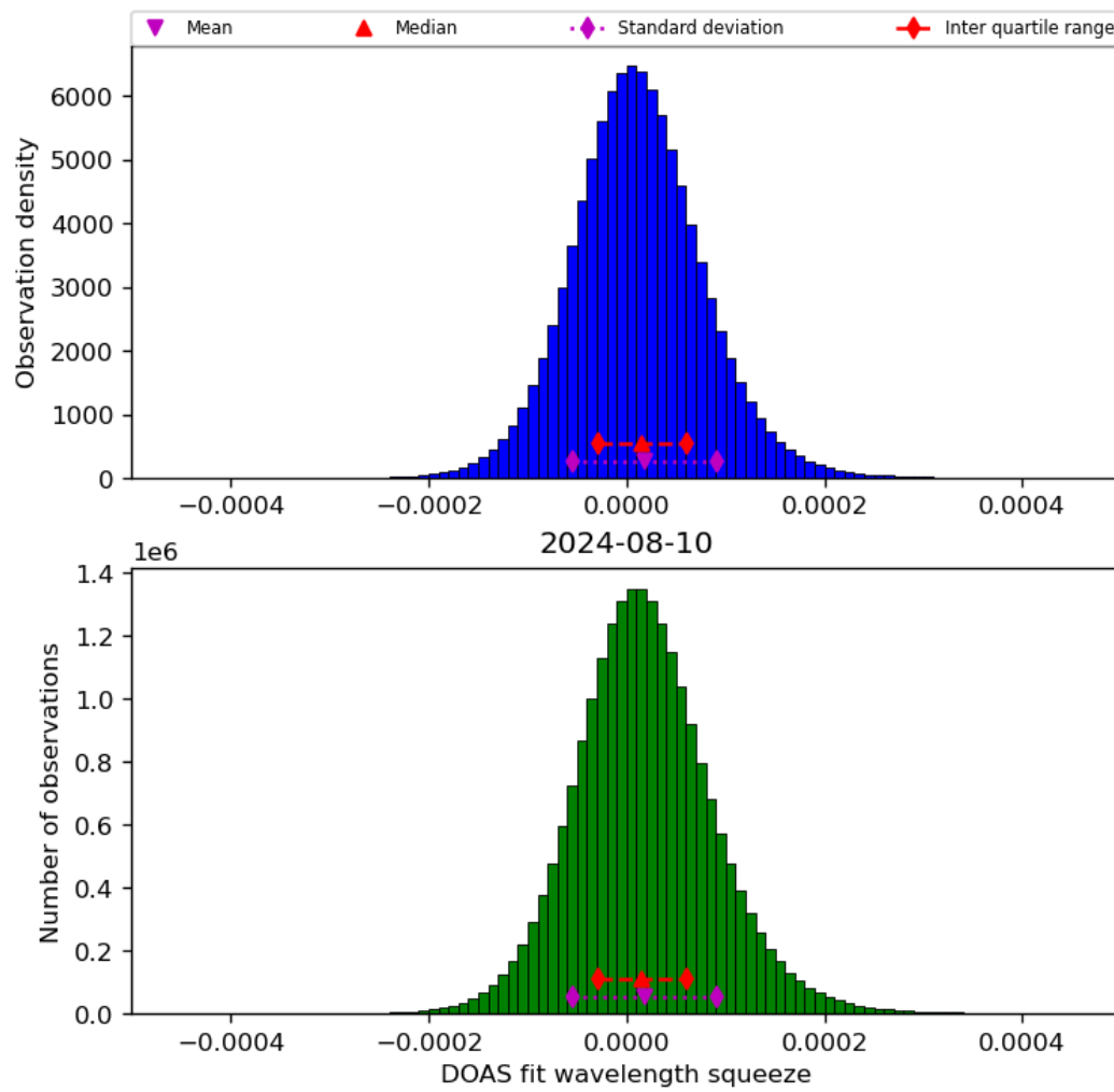
Figure 45: Histogram of “DOAS fit wavelength squeeze” for 2024-08-09 to 2024-08-11
