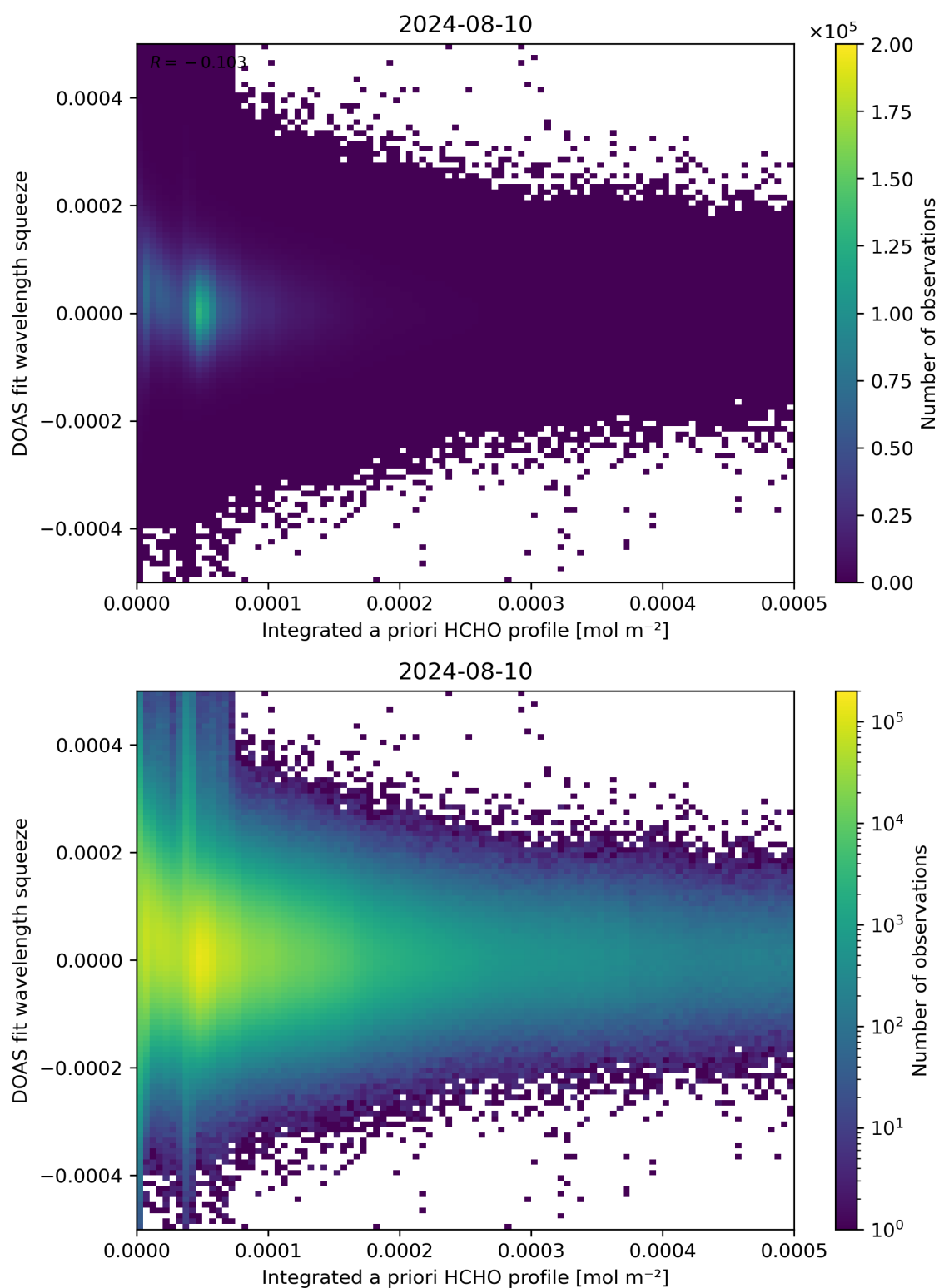
Figure 150: Scatter density plot of “Integrated a priori HCHO profile” against “DOAS fit wavelength squeeze” for 2024-08-09 to 2024-08-11.
