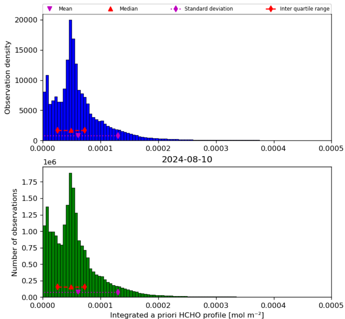
Figure 43: Histogram of “Integrated a priori HCHO profile” for 2024-08-09 to 2024-08-11
