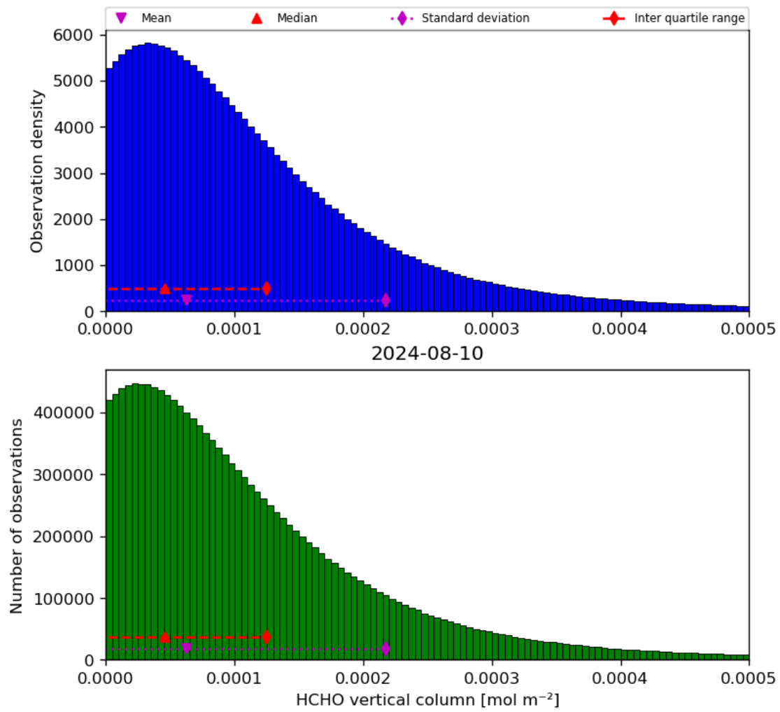
Figure 35: Histogram of “HCHO vertical column” for 2024-08-09 to 2024-08-11
