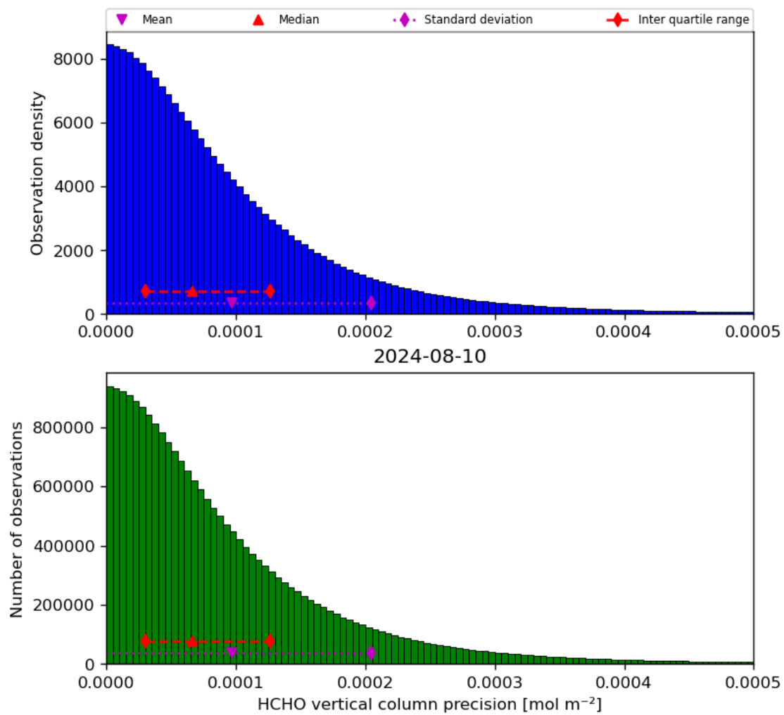
Figure 36: Histogram of “HCHO vertical column precision” for 2024-08-09 to 2024-08-11
