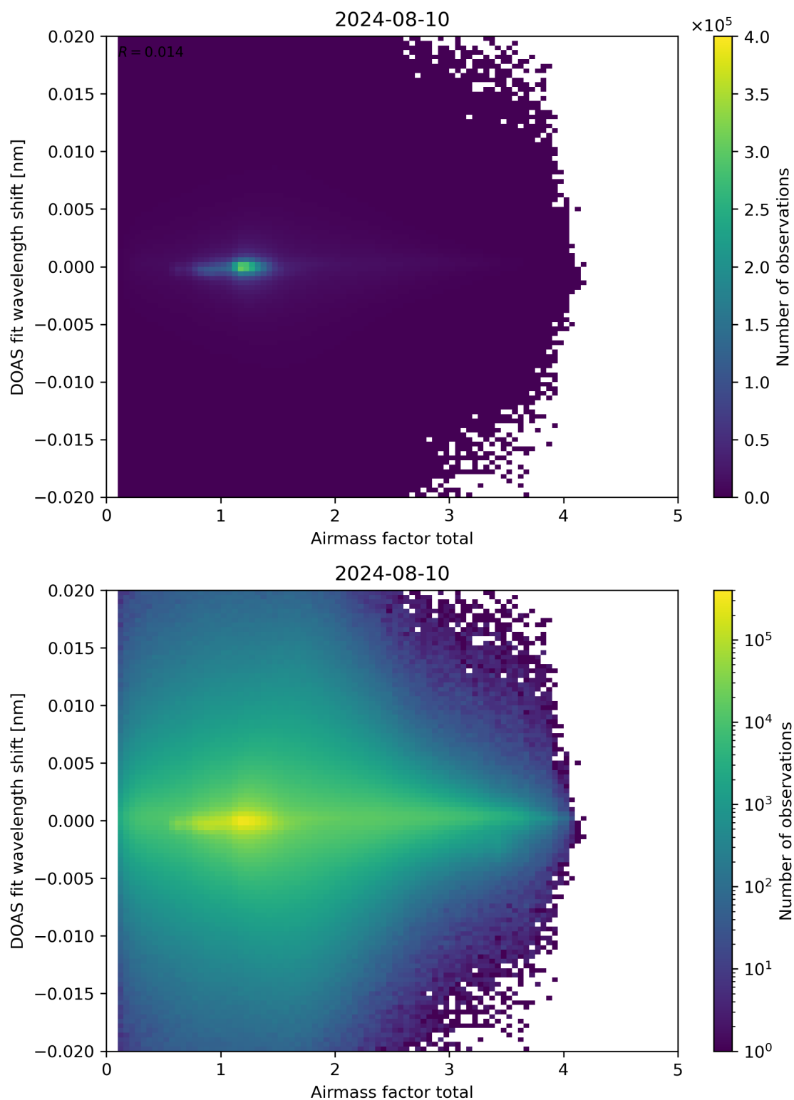
Figure 98: Scatter density plot of “Airmass factor total” against “DOAS fit wavelength shift” for 2024-08-09 to 2024-08-11.
