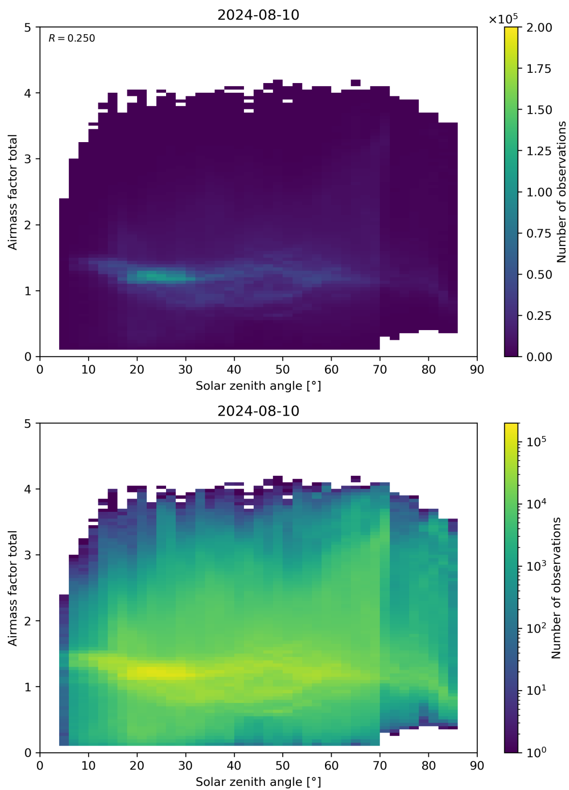
Figure 175: Scatter density plot of “Solar zenith angle” against “Airmass factor total” for 2024-08-09 to 2024-08-11.
