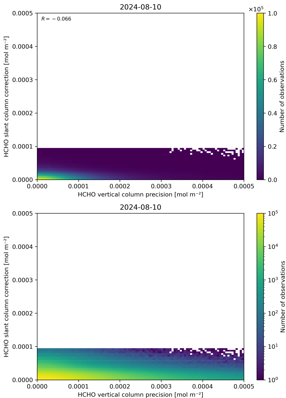
Figure 141: Scatter density plot of “HCHO vertical column precision” against “HCHO slant column correction” for 2024-08-09 to 2024-08-11.
