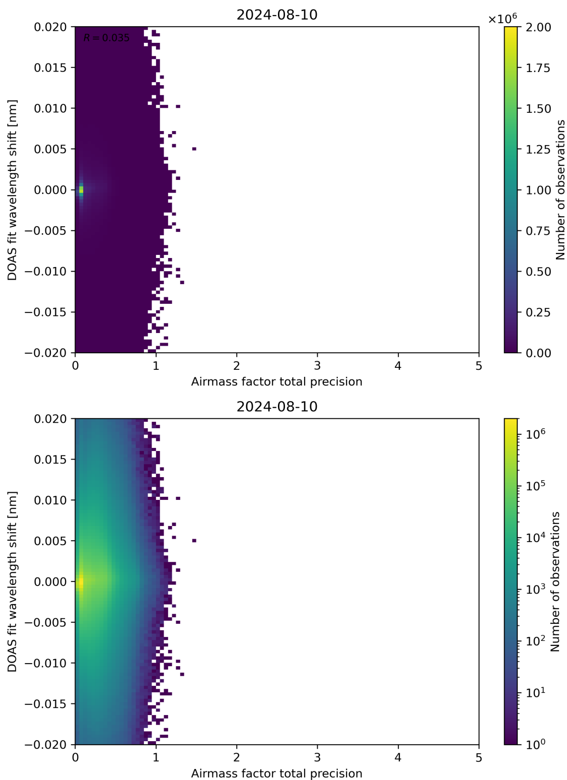
Figure 106: Scatter density plot of “Airmass factor total precision” against “DOAS fit wavelength shift” for 2024-08-09 to 2024-08-11.
