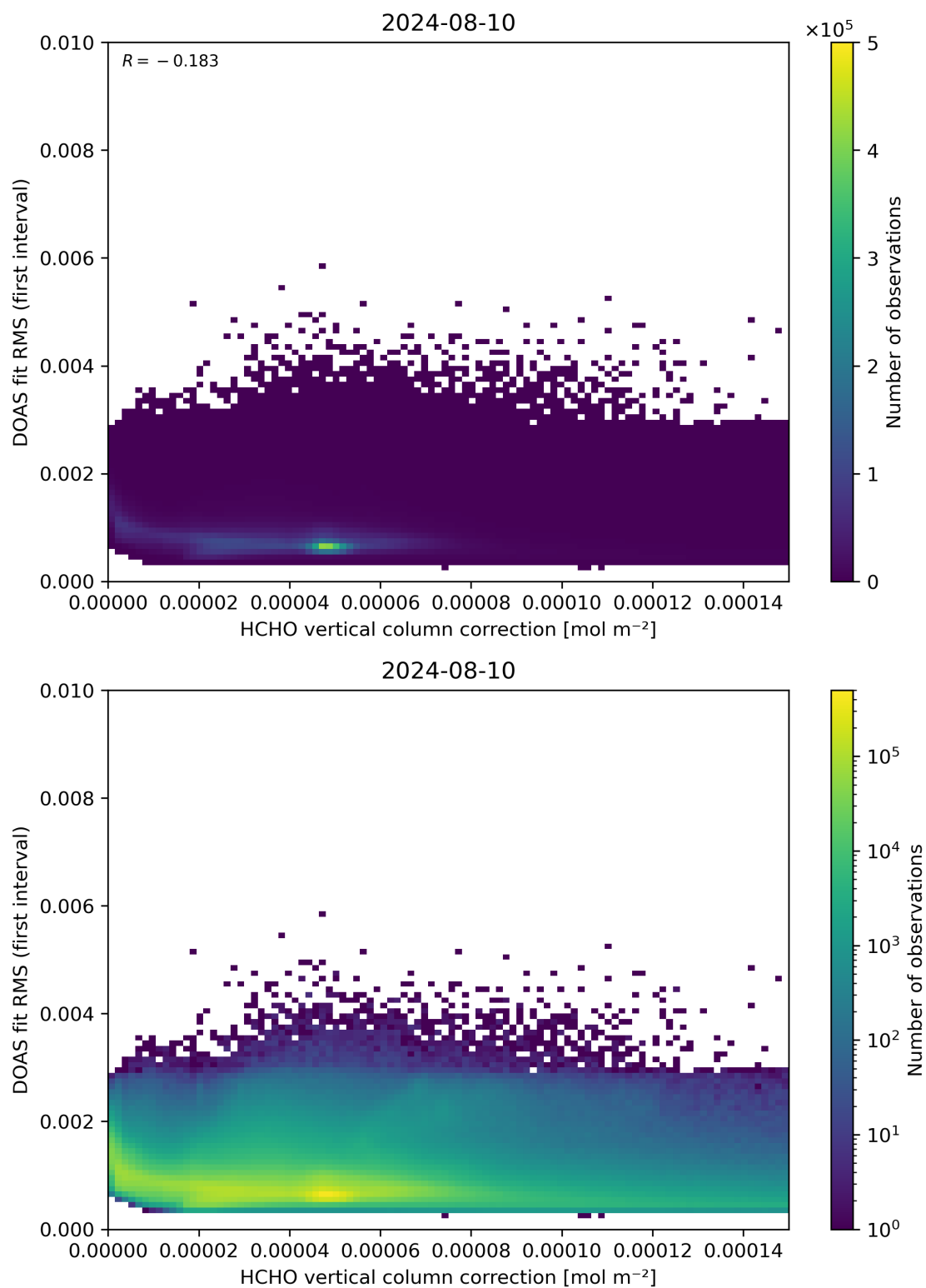
Figure 112: Scatter density plot of “HCHO vertical column correction” against “DOAS fit RMS (first interval)” for 2024-08-09 to 2024-08-11.
