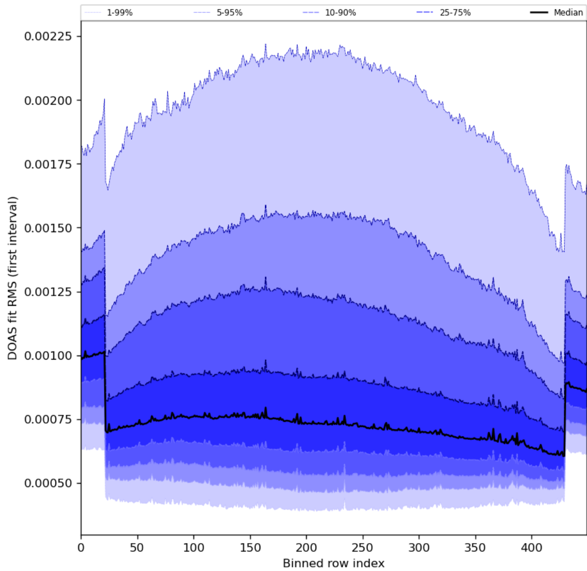
Figure 60: Along track statistics of “DOAS fit RMS (first interval)” for 2024-08-09 to 2024-08-11
