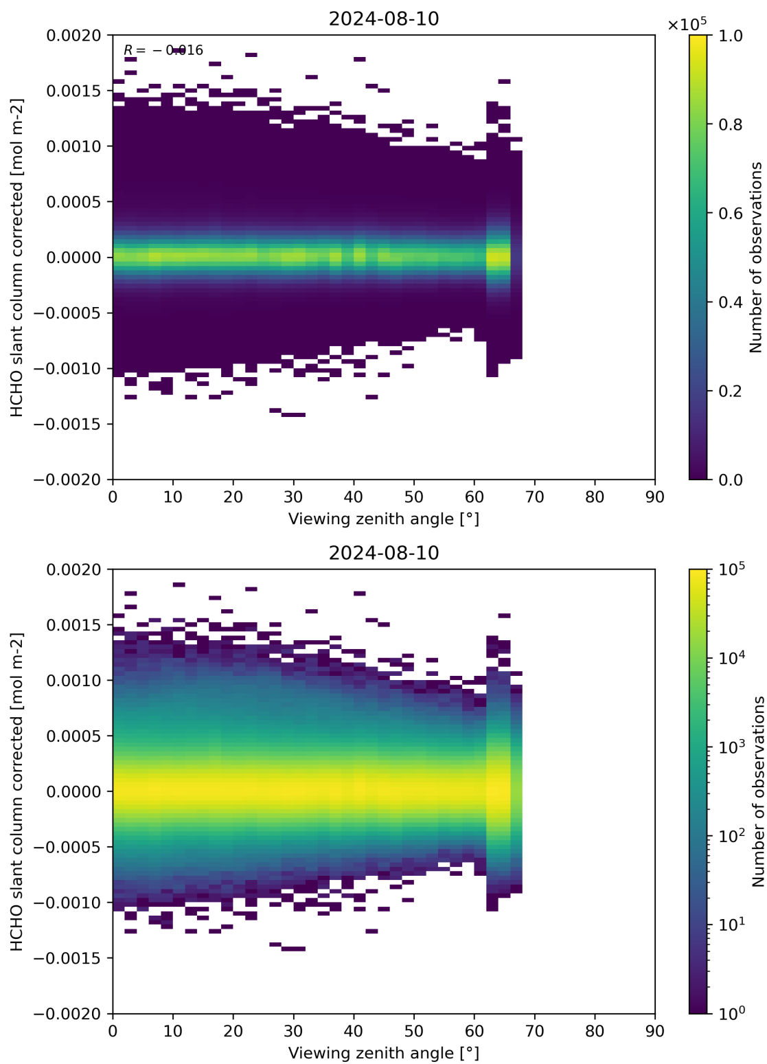
Figure 186: Scatter density plot of “Viewing zenith angle” against “HCHO slant column corrected” for 2024-08-09 to 2024-08-11.
