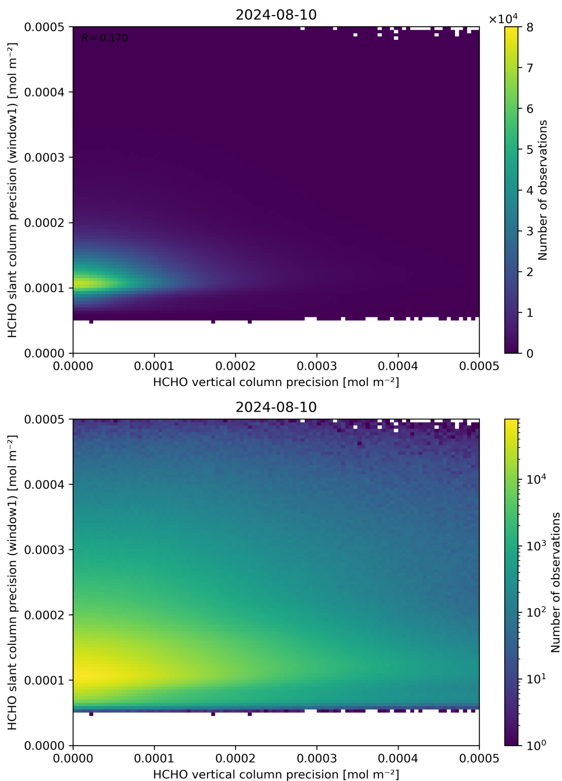
Figure 143: Scatter density plot of “HCHO vertical column precision” against “HCHO slant column precision (window1)” for 2024-08-09 to 2024-08-11.
