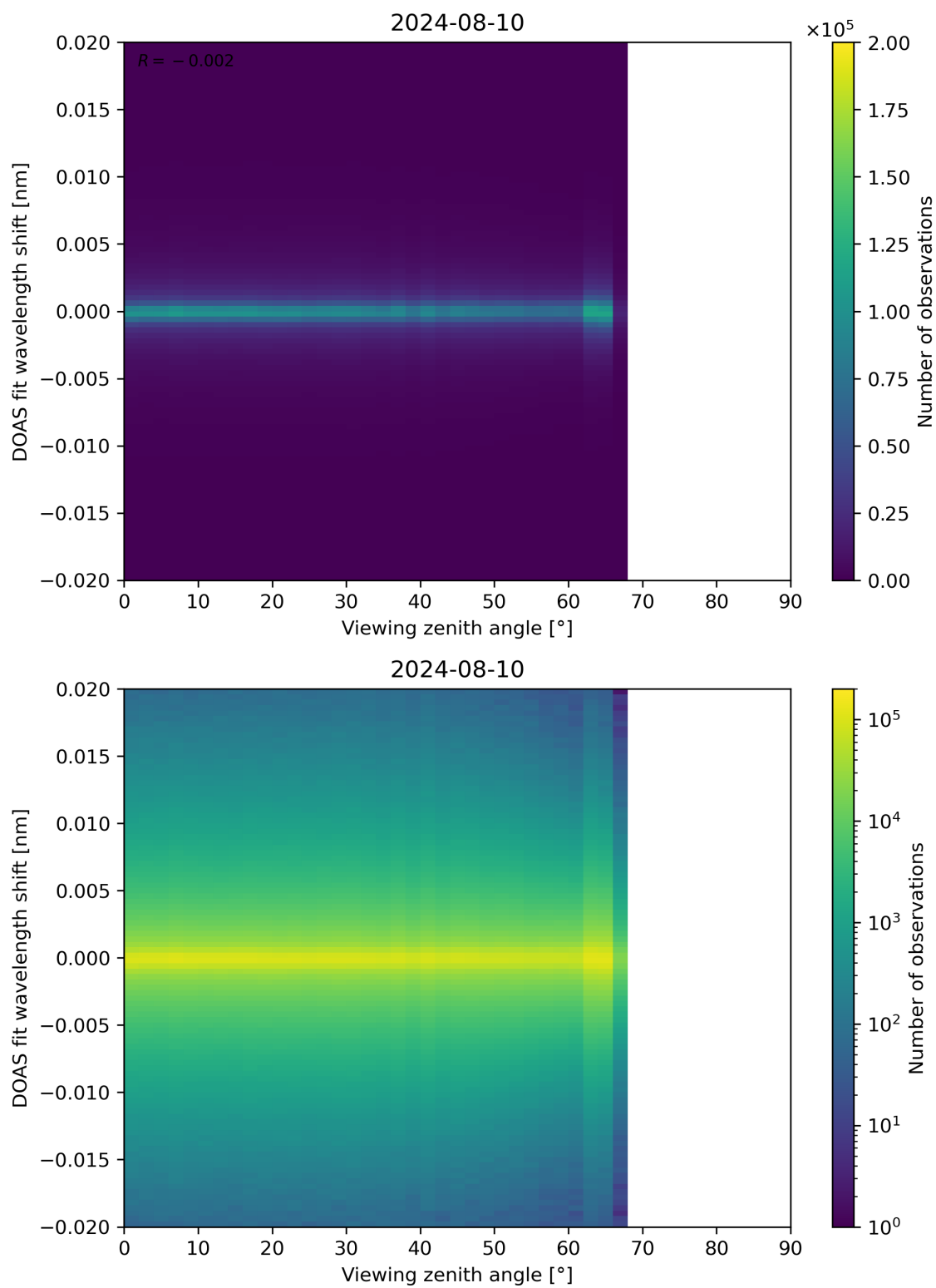
Figure 183: Scatter density plot of “Viewing zenith angle” against “DOAS fit wavelength shift” for 2024-08-09 to 2024-08-11.
