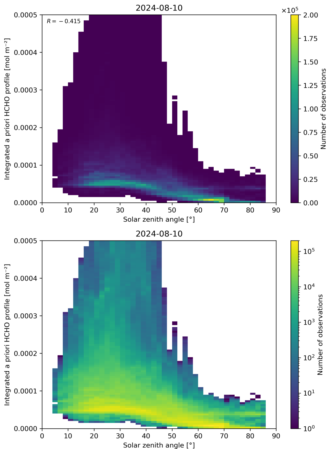
Figure 180: Scatter density plot of “Solar zenith angle” against “Integrated a priori HCHO profile” for 2024-08-09 to 2024-08-11.
