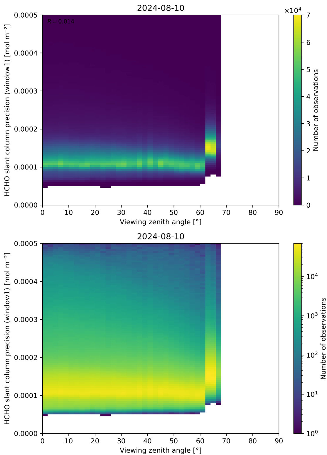
Figure 189: Scatter density plot of “Viewing zenith angle” against “HCHO slant column precision (window1)” for 2024-08-09 to 2024-08-11.
