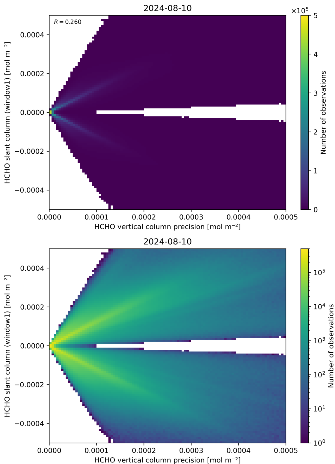
Figure 142: Scatter density plot of “HCHO vertical column precision” against “HCHO slant column (window1)” for 2024-08-09 to 2024-08-11.
