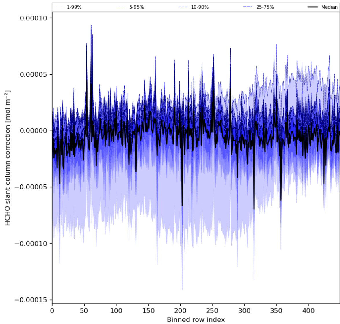
Figure 61: Along track statistics of “HCHO slant column correction” for 2024-08-09 to 2024-08-11
