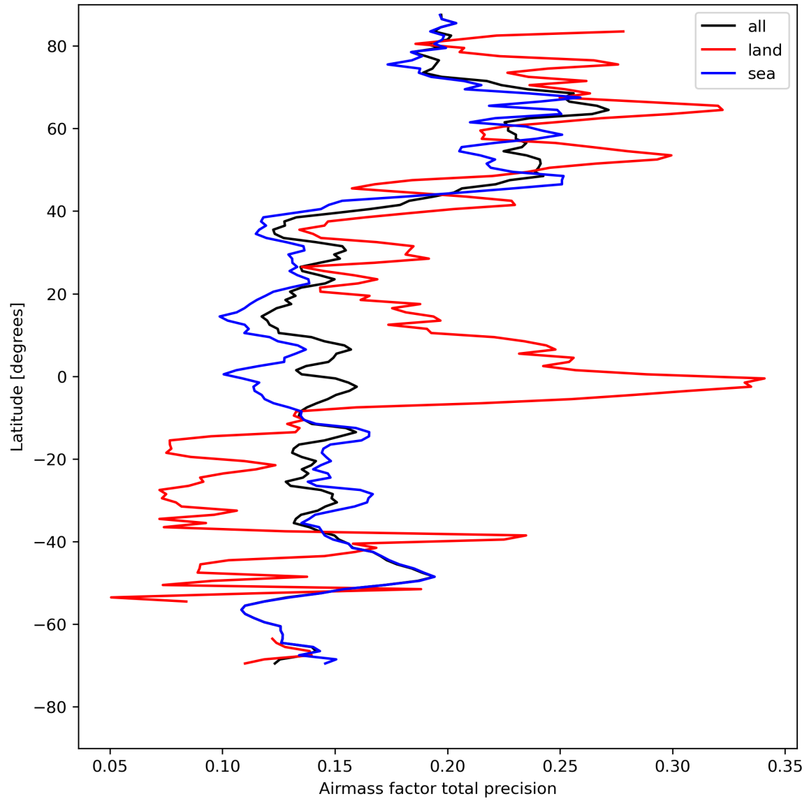
Figure 27: Zonal average of “Airmass factor total precision” for 2024-08-09 to 2024-08-11.
