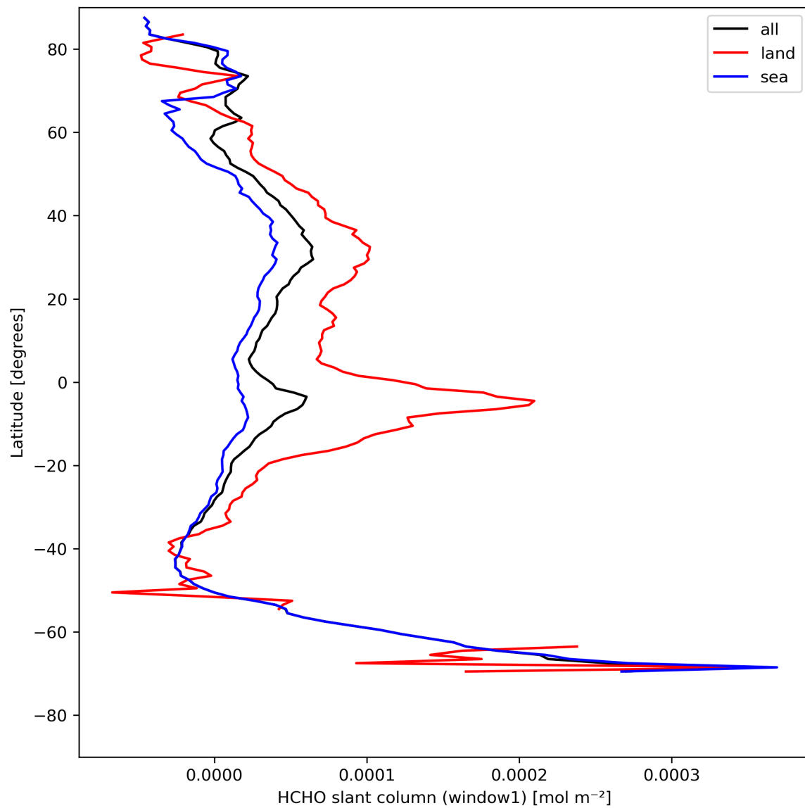
Figure 24: Zonal average of “HCHO slant column (window1)” for 2024-08-09 to 2024-08-11.
