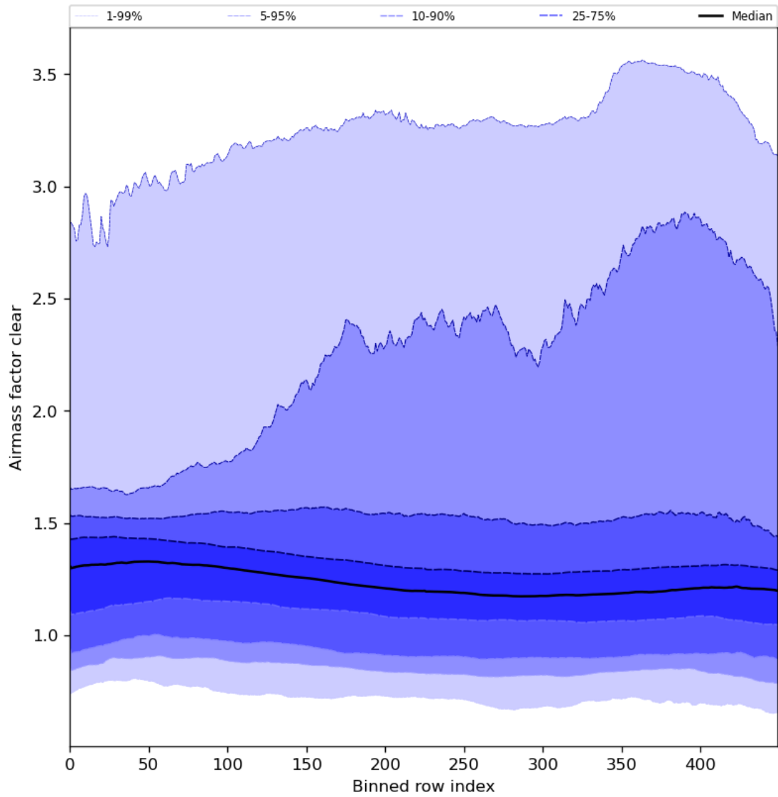
Figure 56: Along track statistics of “Airmass factor clear” for 2024-08-09 to 2024-08-11
