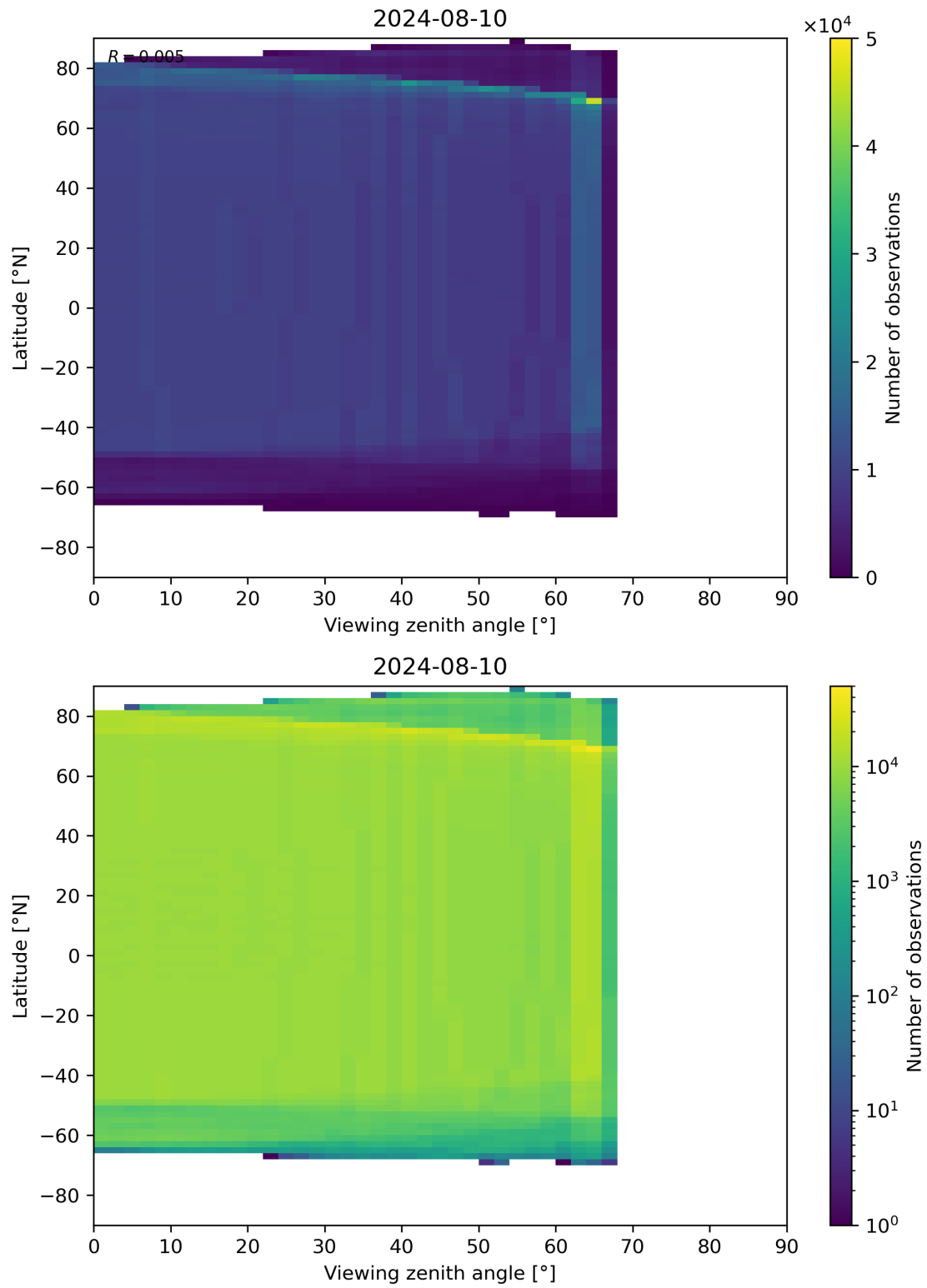
Figure 196: Scatter density plot of “Viewing zenith angle” against “Latitude” for 2024-08-09 to 2024-08-11.
