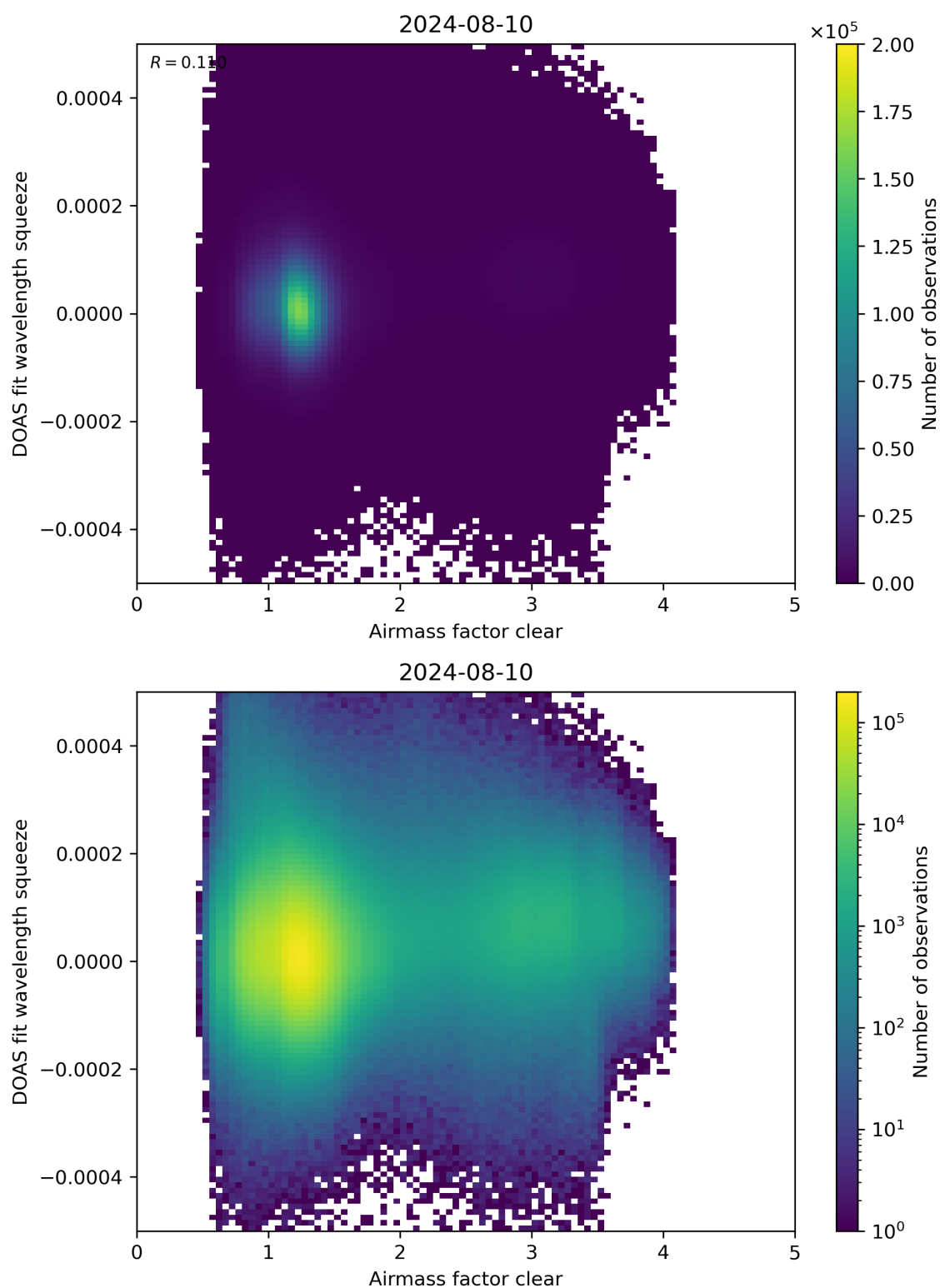
Figure 73: Scatter density plot of “Airmass factor clear” against “DOAS fit wavelength squeeze” for 2024-08-09 to 2024-08-11.
