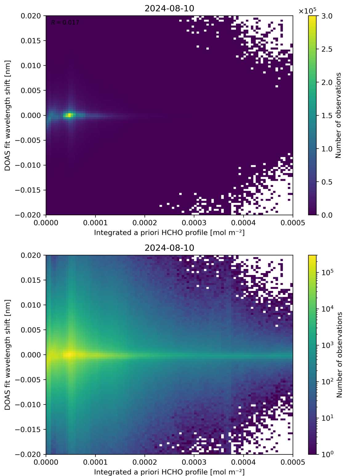
Figure 149: Scatter density plot of “Integrated a priori HCHO profile” against “DOAS fit wavelength shift” for 2024-08-09 to 2024-08-11.
