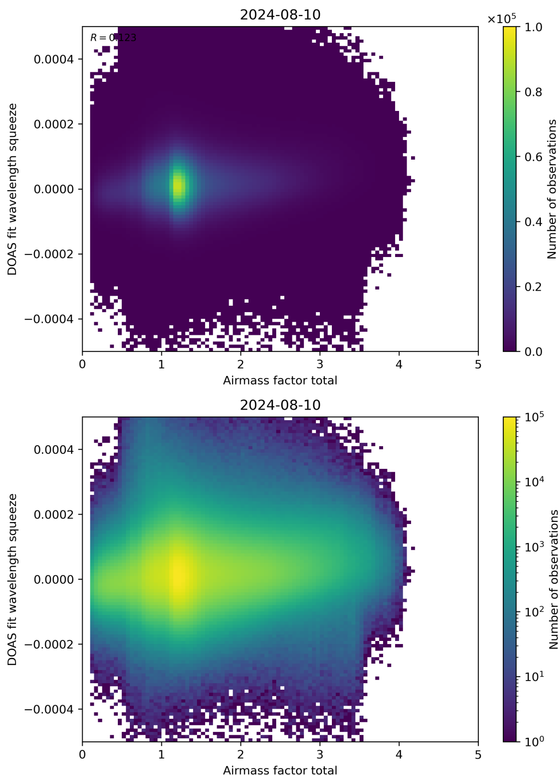
Figure 99: Scatter density plot of “Airmass factor total” against “DOAS fit wavelength squeeze” for 2024-08-09 to 2024-08-11.
