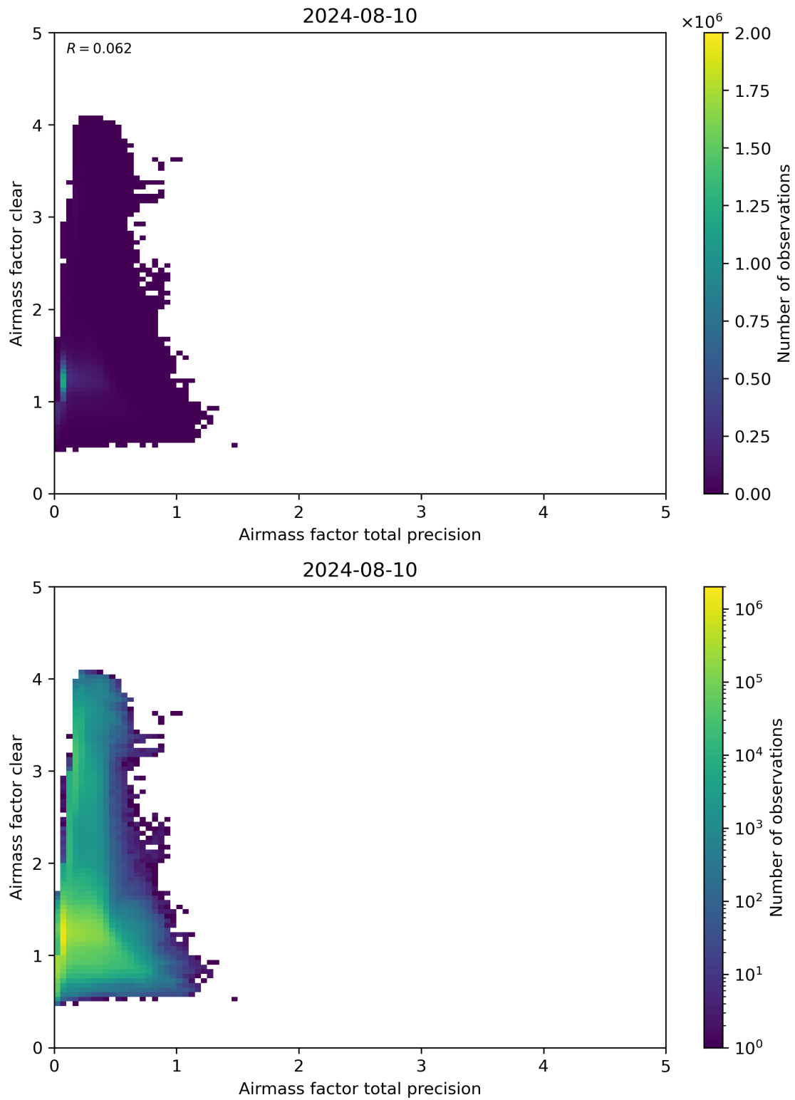
Figure 108: Scatter density plot of “Airmass factor total precision” against “Airmass factor clear” for 2024-08-09 to 2024-08-11.
