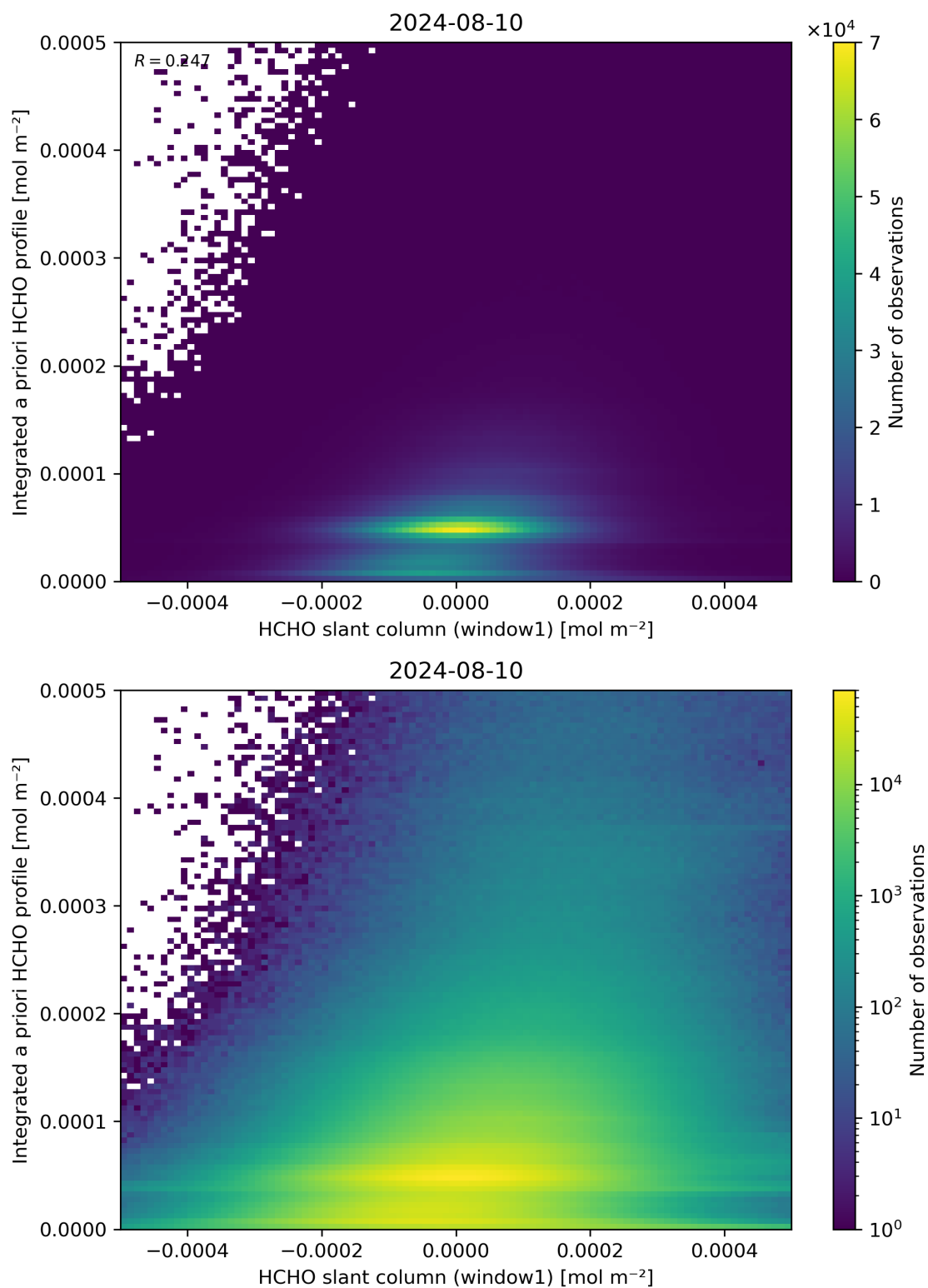
Figure 87: Scatter density plot of “HCHO slant column (window1)” against “Integrated a priori HCHO profile” for 2024-08-09 to 2024-08-11.
