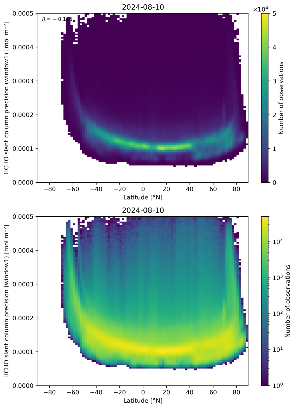
Figure 160: Scatter density plot of “Latitude” against “HCHO slant column precision (window1)” for 2024-08-09 to 2024-08-11.
