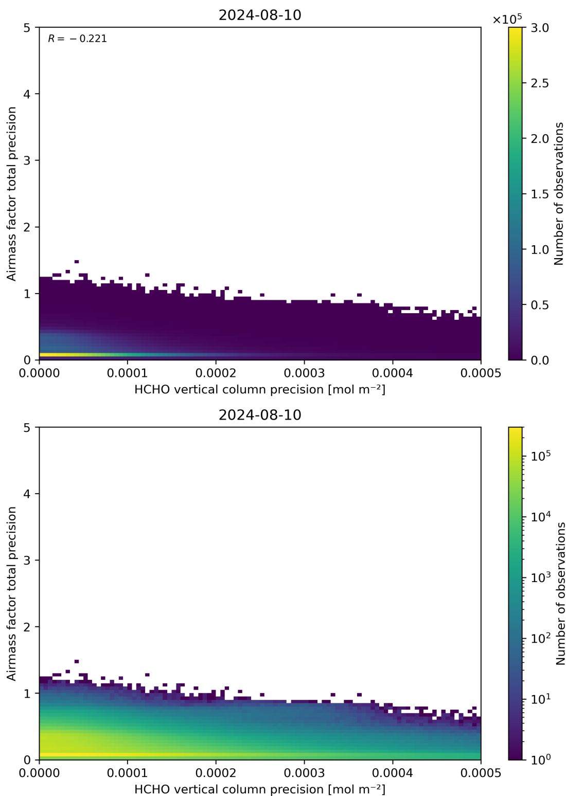
Figure 145: Scatter density plot of “HCHO vertical column precision” against “Airmass factor total precision” for 2024-08-09 to 2024-08-11.
