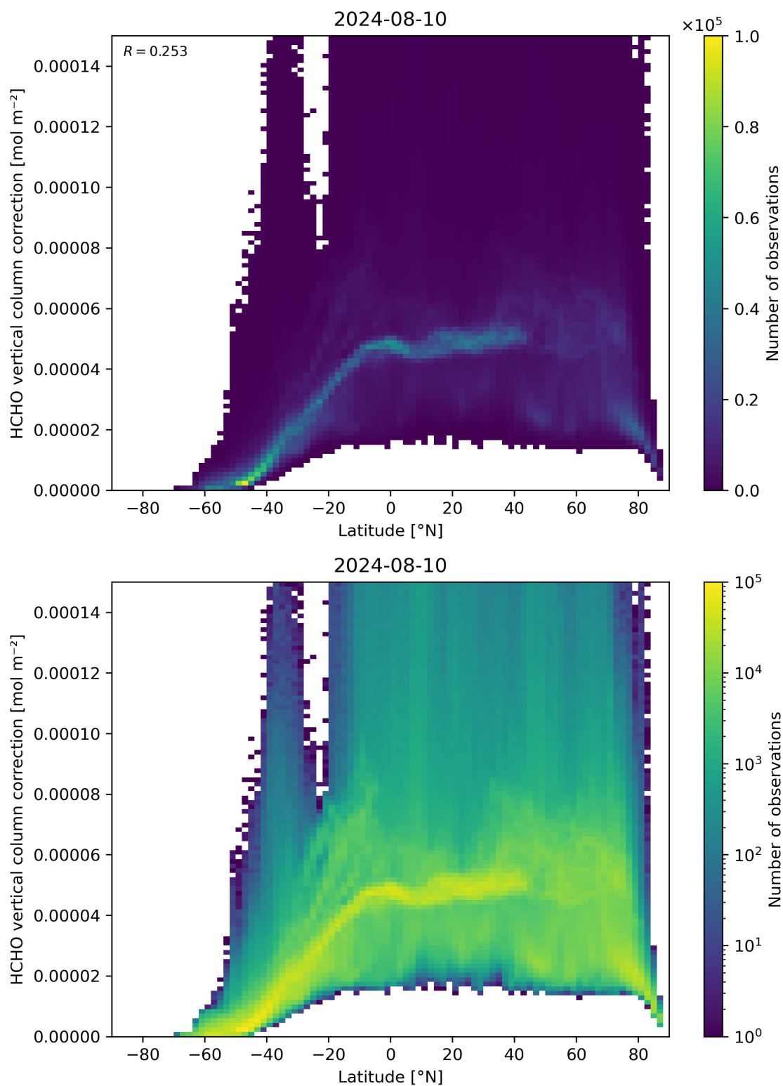
Figure 164: Scatter density plot of “Latitude” against “HCHO vertical column correction” for 2024-08-09 to 2024-08-11.
