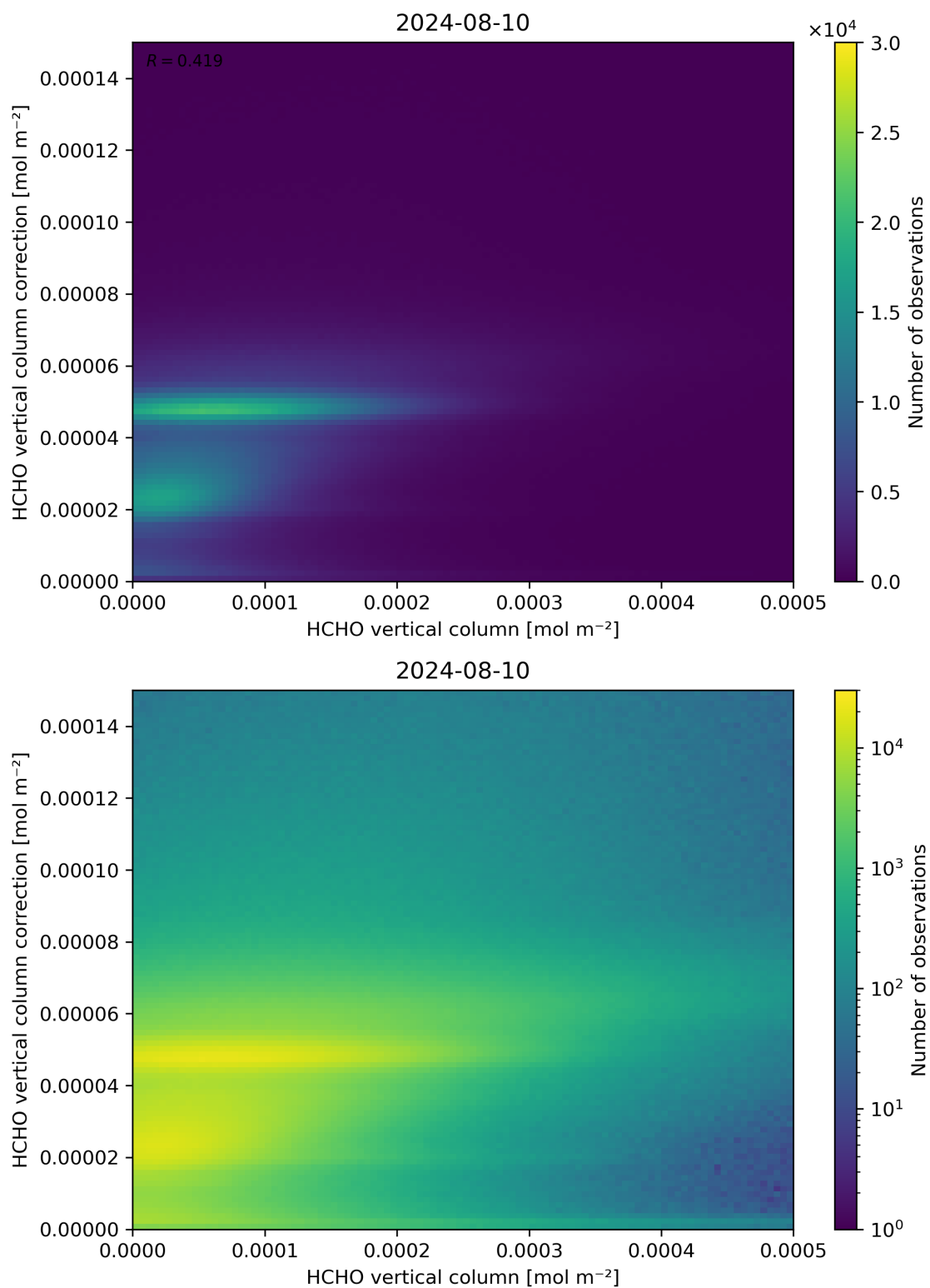
Figure 133: Scatter density plot of “HCHO vertical column” against “HCHO vertical column correction” for 2024-08-09 to 2024-08-11.
