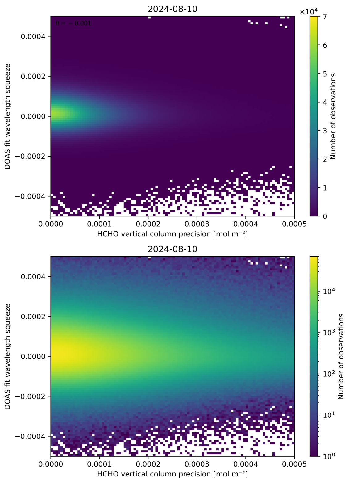
Figure 138: Scatter density plot of “HCHO vertical column precision” against “DOAS fit wavelength squeeze” for 2024-08-09 to 2024-08-11.
