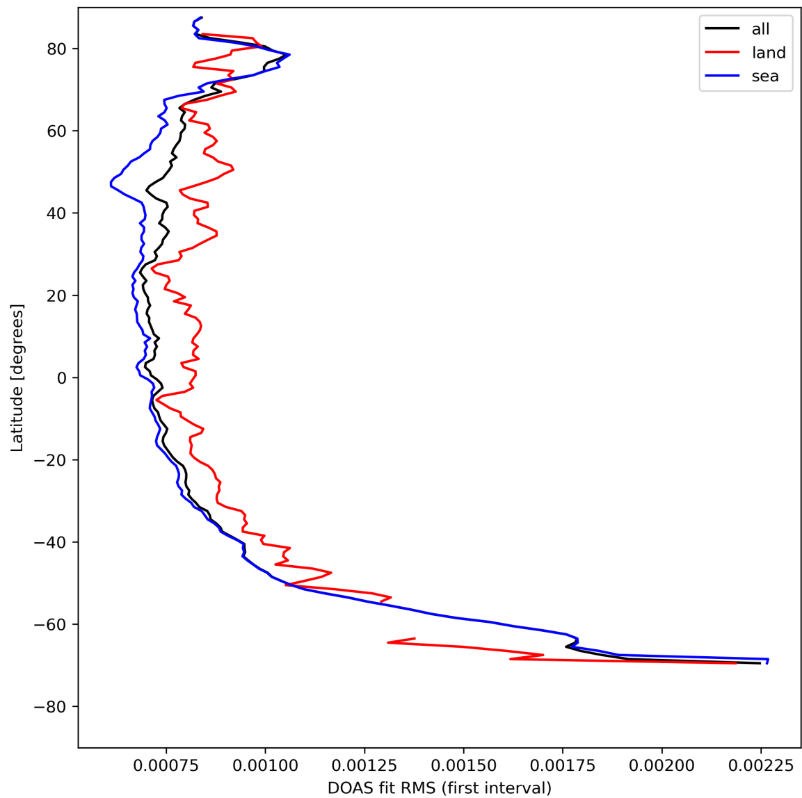
Figure 32: Zonal average of “DOAS fit RMS (first interval)” for 2024-08-09 to 2024-08-11.
