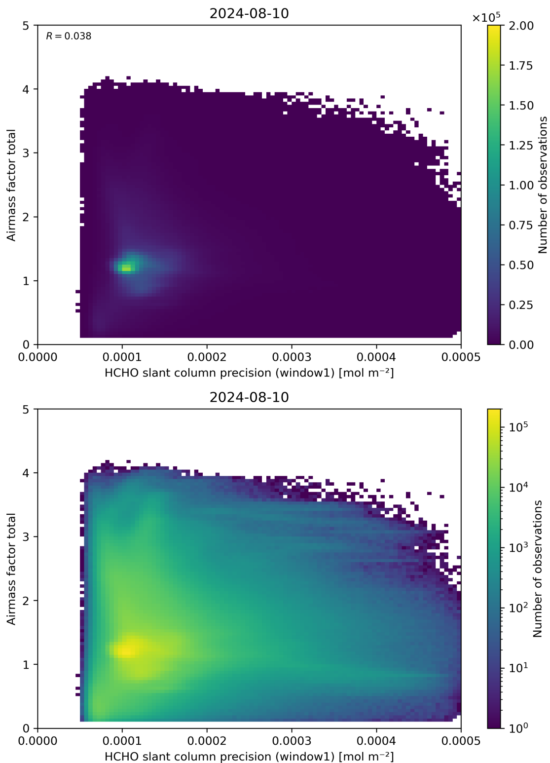
Figure 94: Scatter density plot of “HCHO slant column precision (window1)” against “Airmass factor total” for 2024-08-09 to 2024-08-11.
