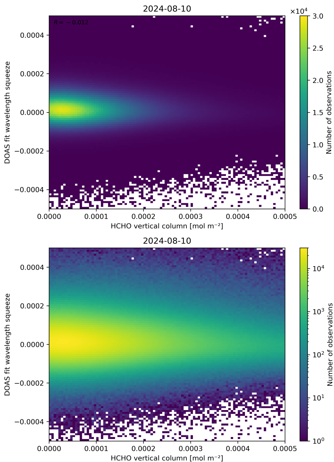
Figure 125: Scatter density plot of “HCHO vertical column” against “DOAS fit wavelength squeeze” for 2024-08-09 to 2024-08-11.
