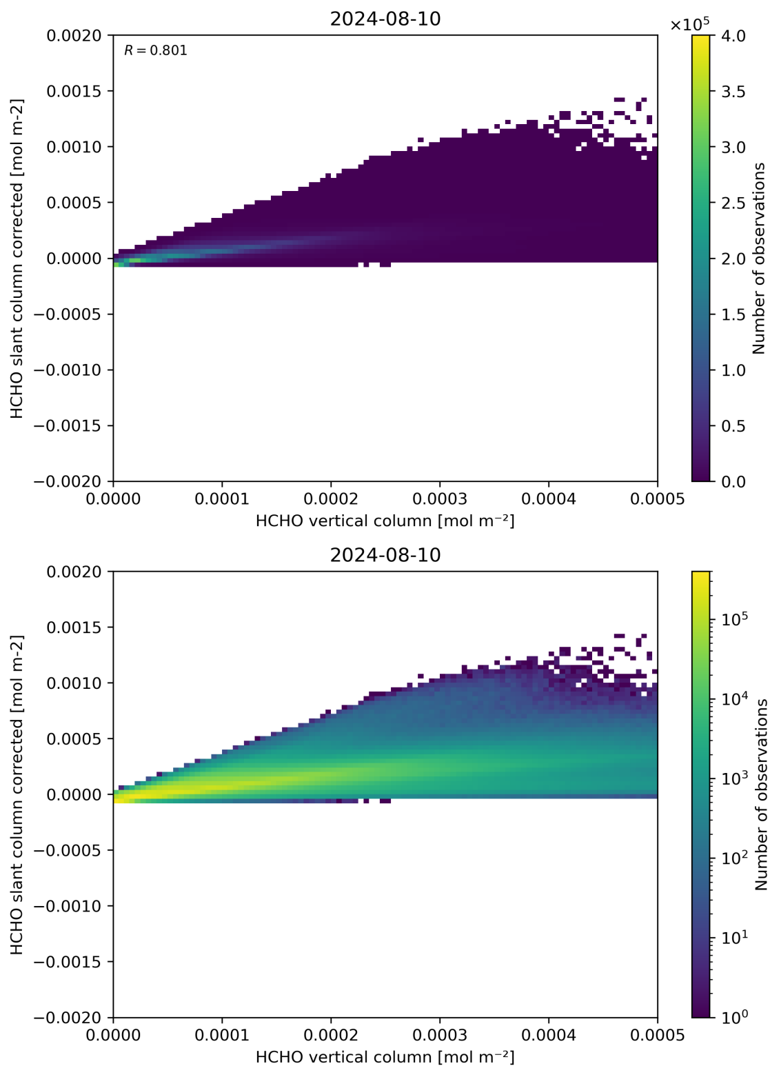
Figure 127: Scatter density plot of “HCHO vertical column” against “HCHO slant column corrected” for 2024-08-09 to 2024-08-11.
