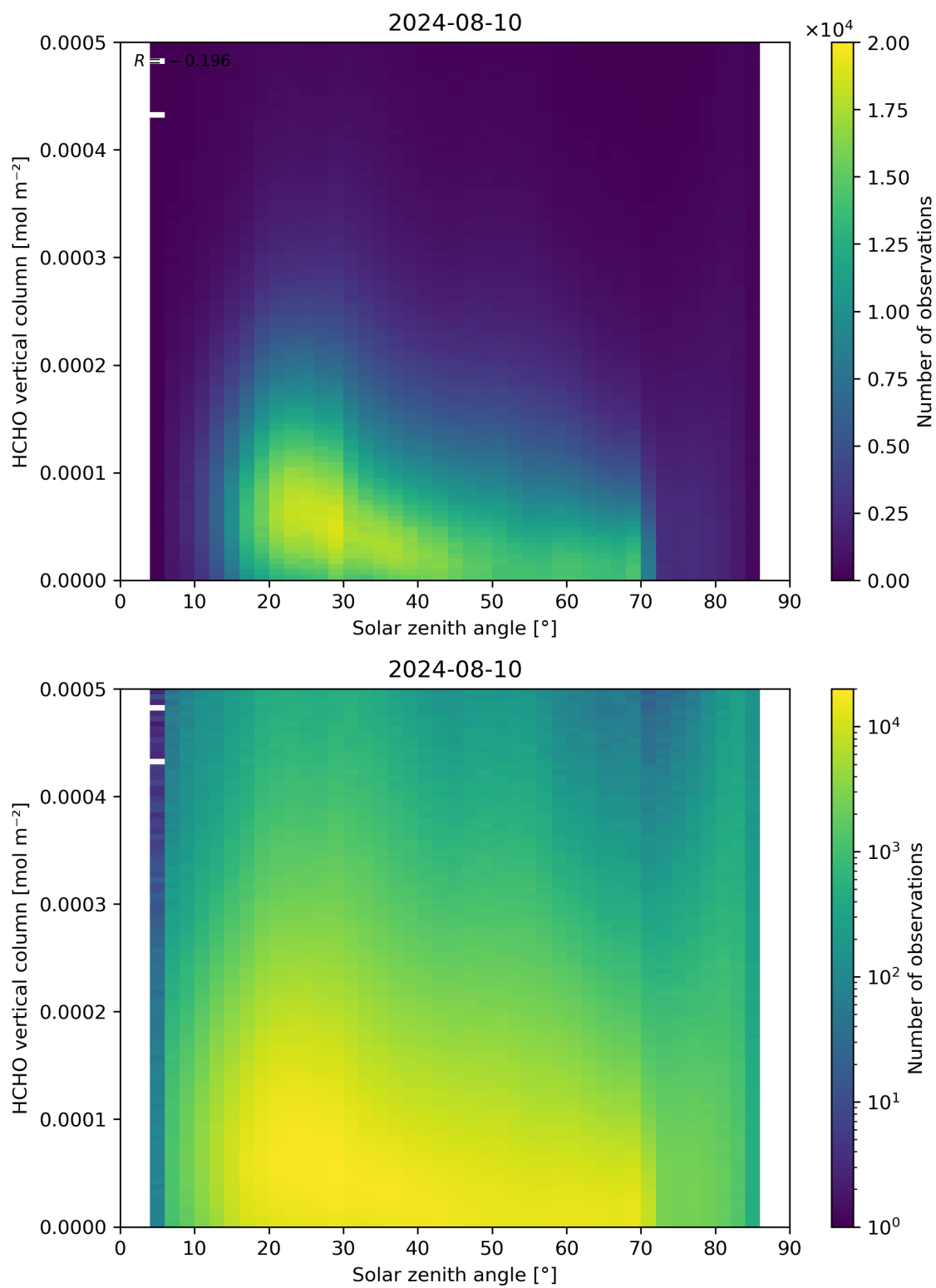
Figure 177: Scatter density plot of “Solar zenith angle” against “HCHO vertical column” for 2024-08-09 to 2024-08-11.
