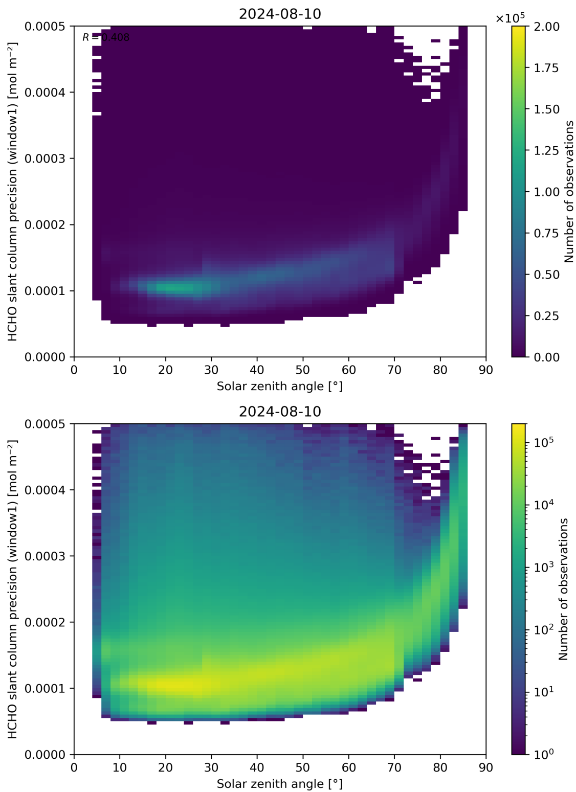
Figure 174: Scatter density plot of “Solar zenith angle” against “HCHO slant column precision (window1)” for 2024-08-09 to 2024-08-11.
