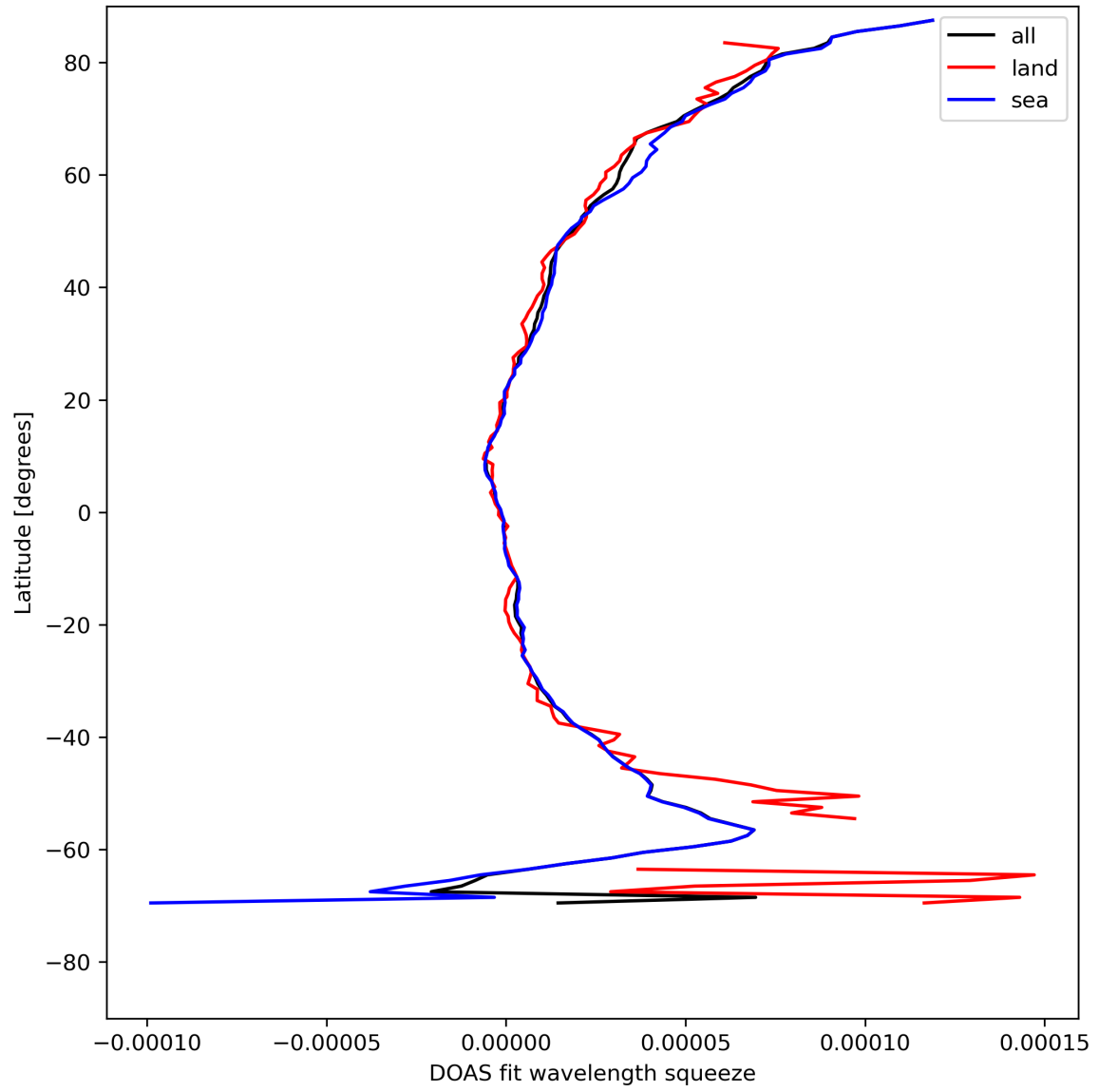
Figure 31: Zonal average of “DOAS fit wavelength squeeze” for 2024-08-09 to 2024-08-11.
