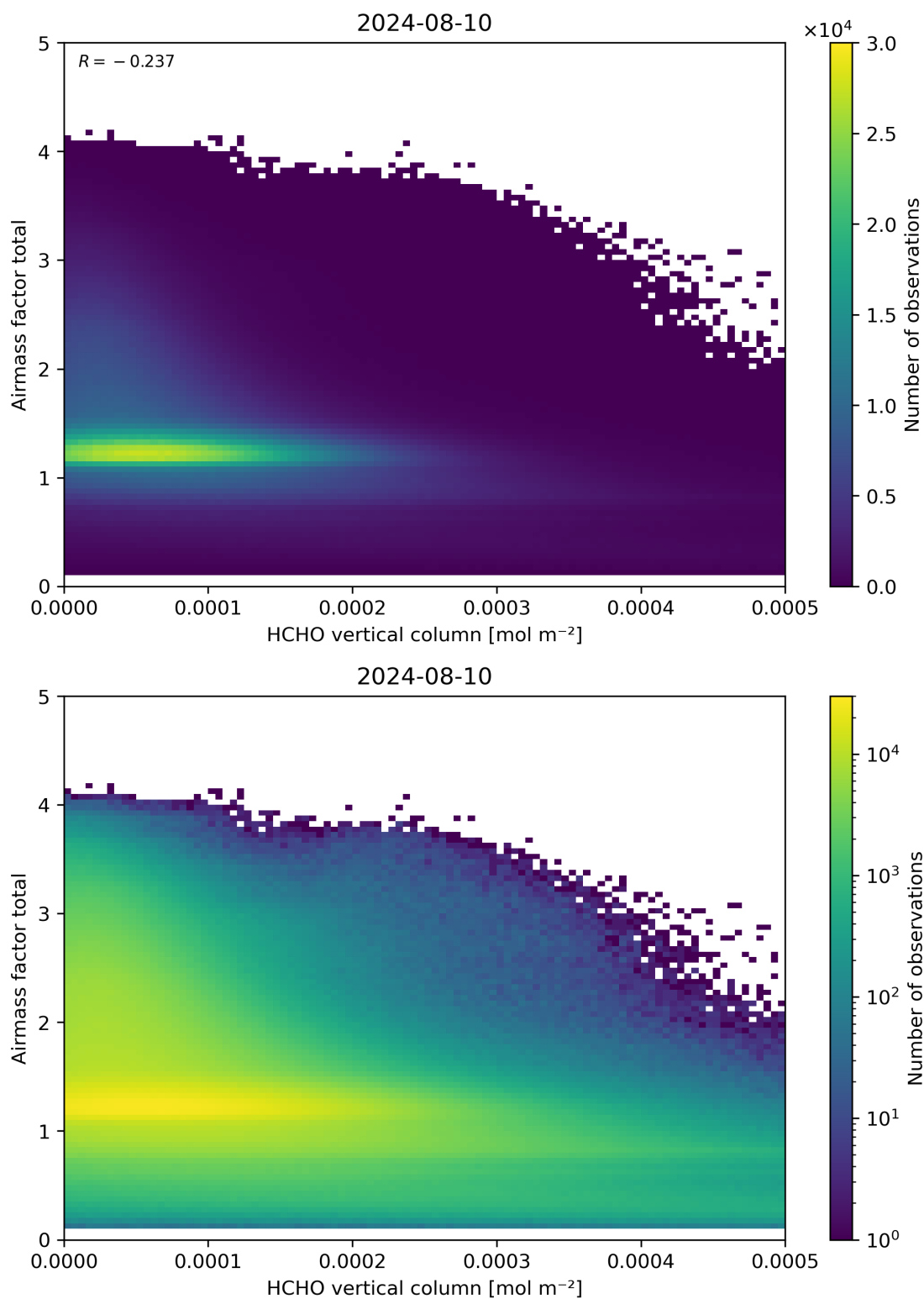
Figure 131: Scatter density plot of “HCHO vertical column” against “Airmass factor total” for 2024-08-09 to 2024-08-11.
