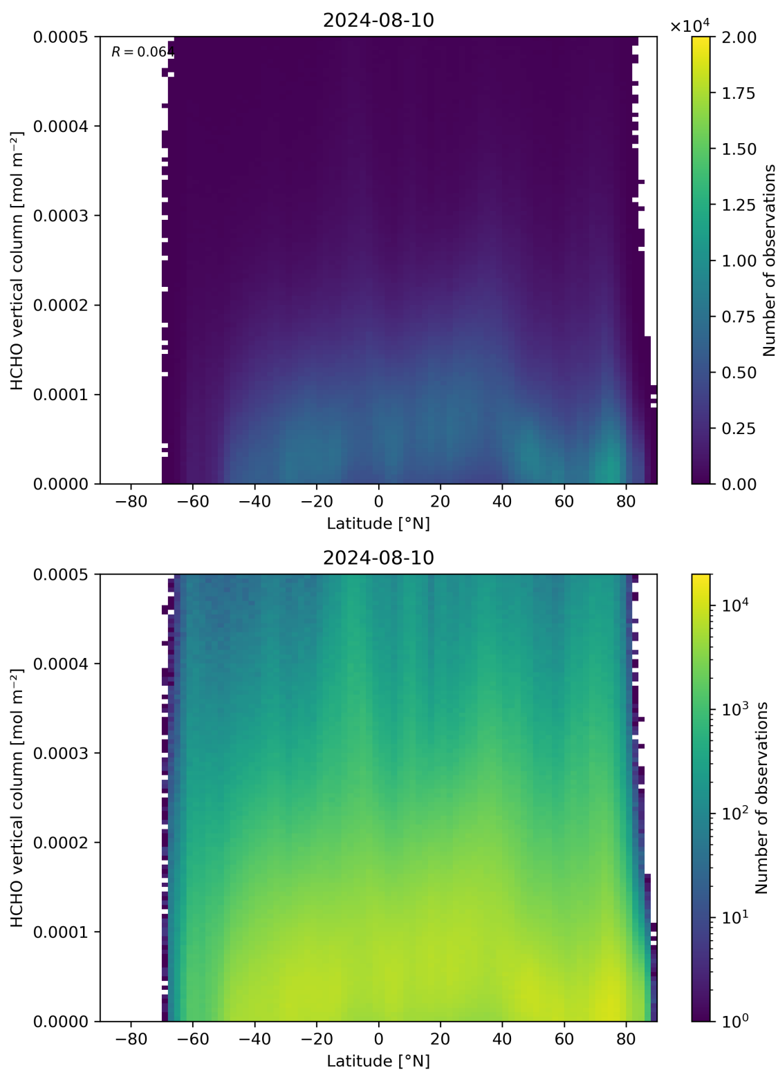
Figure 163: Scatter density plot of “Latitude” against “HCHO vertical column” for 2024-08-09 to 2024-08-11.
