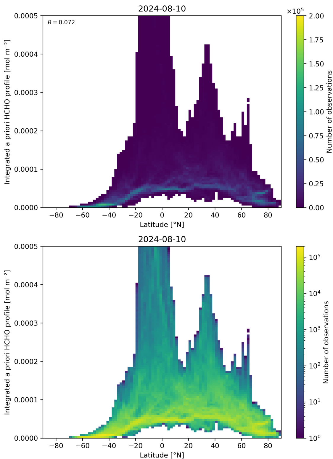
Figure 166: Scatter density plot of “Latitude” against “Integrated a priori HCHO profile” for 2024-08-09 to 2024-08-11.
