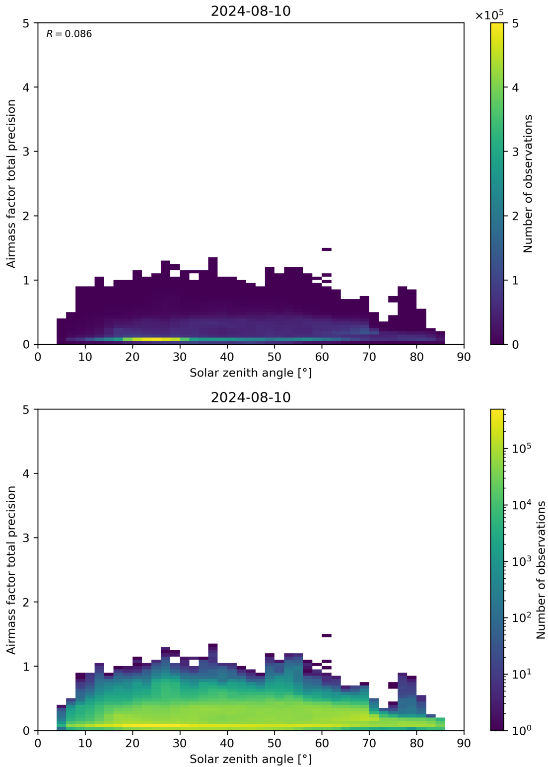
Figure 176: Scatter density plot of “Solar zenith angle” against “Airmass factor total precision” for 2024-08-09 to 2024-08-11.
