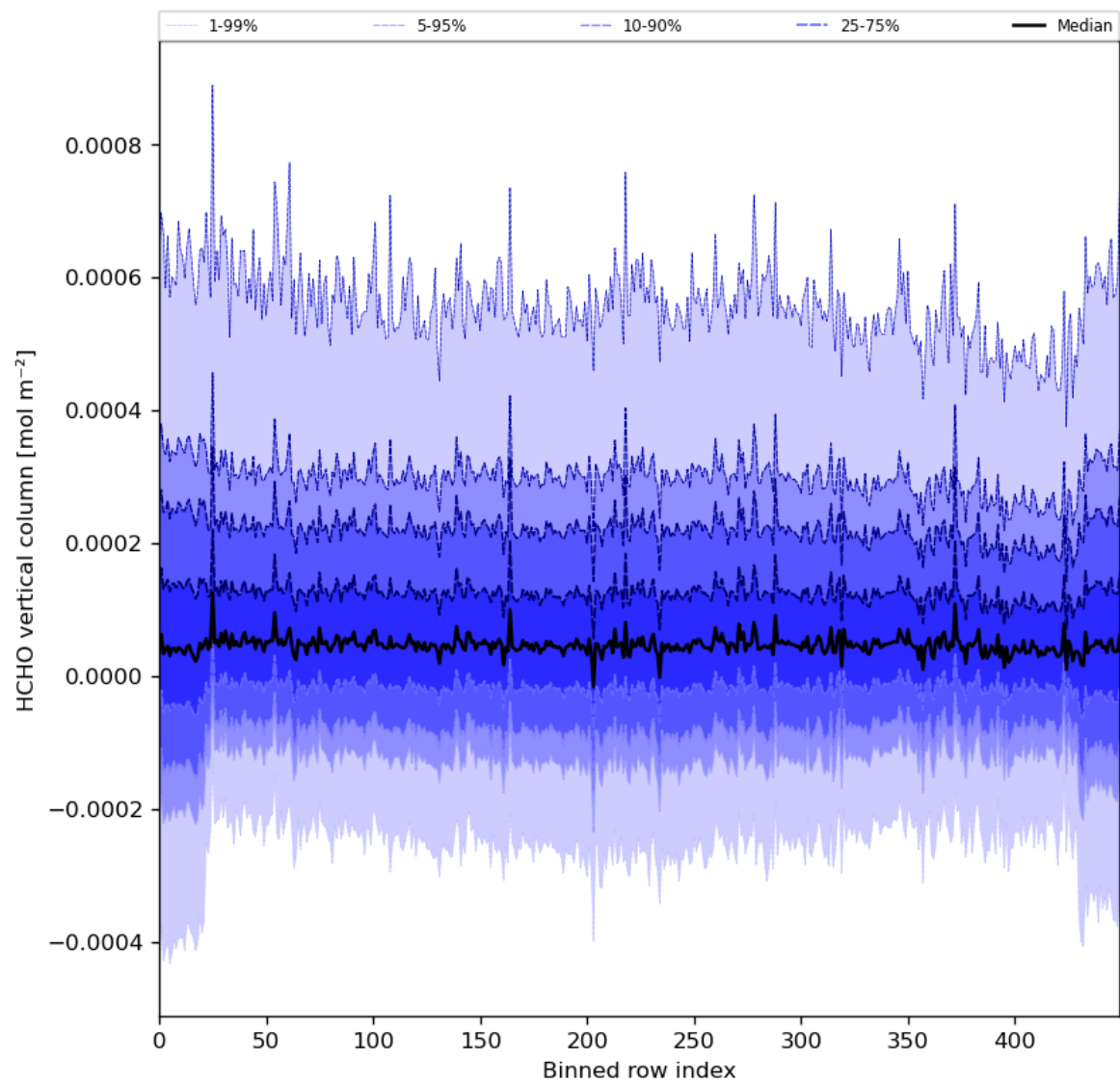
Figure 49: Along track statistics of “HCHO vertical column” for 2024-08-09 to 2024-08-11
