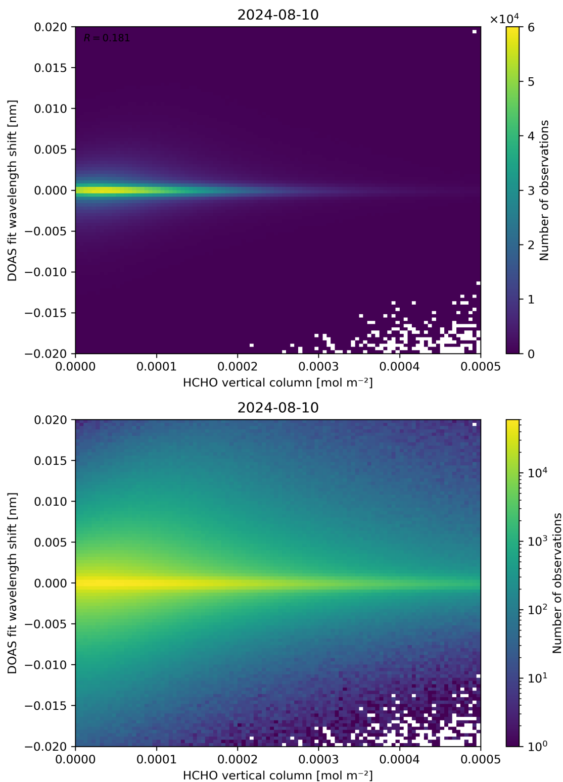
Figure 124: Scatter density plot of “HCHO vertical column” against “DOAS fit wavelength shift” for 2024-08-09 to 2024-08-11.
