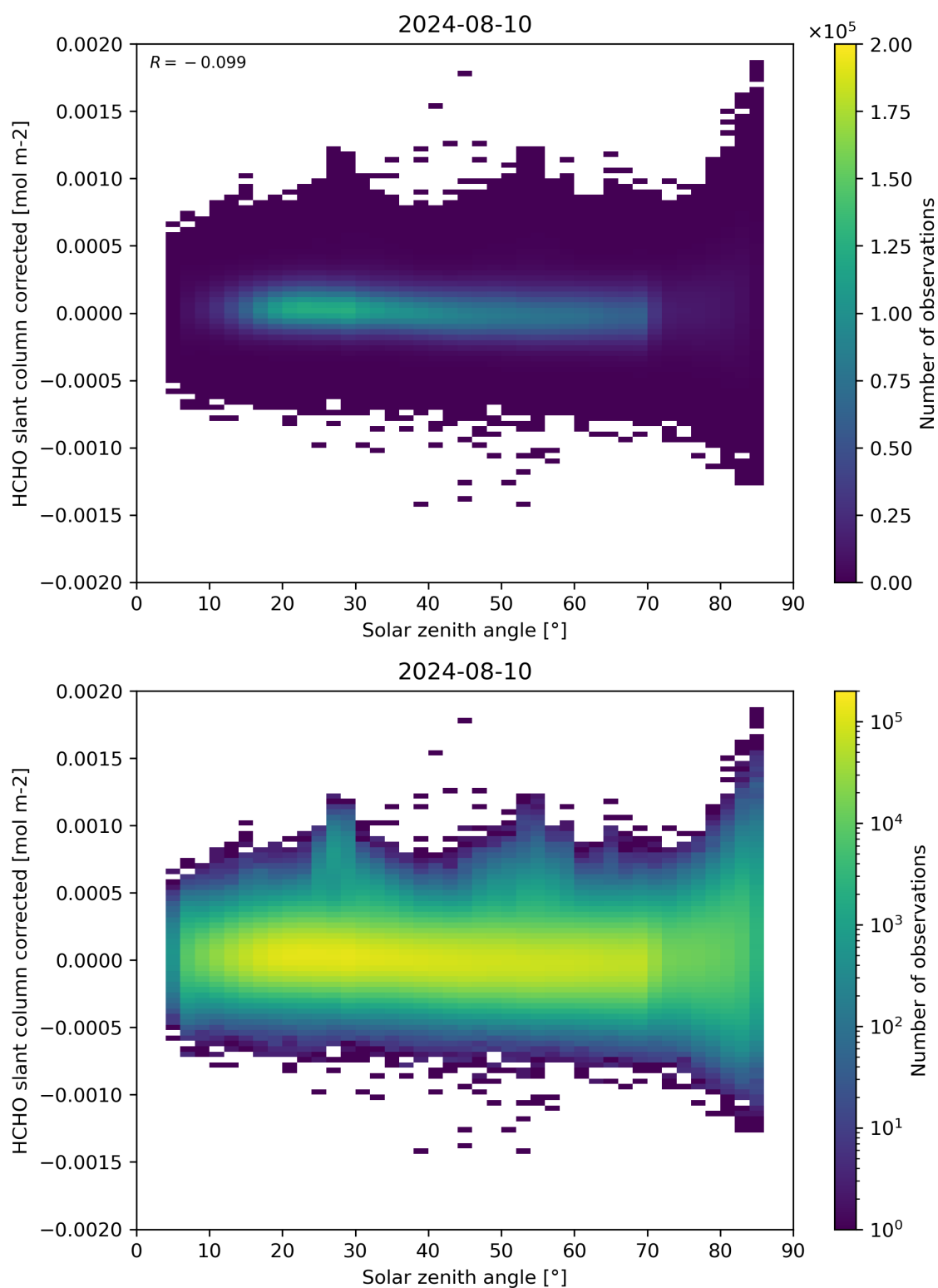
Figure 171: Scatter density plot of “Solar zenith angle” against “HCHO slant column corrected” for 2024-08-09 to 2024-08-11.
