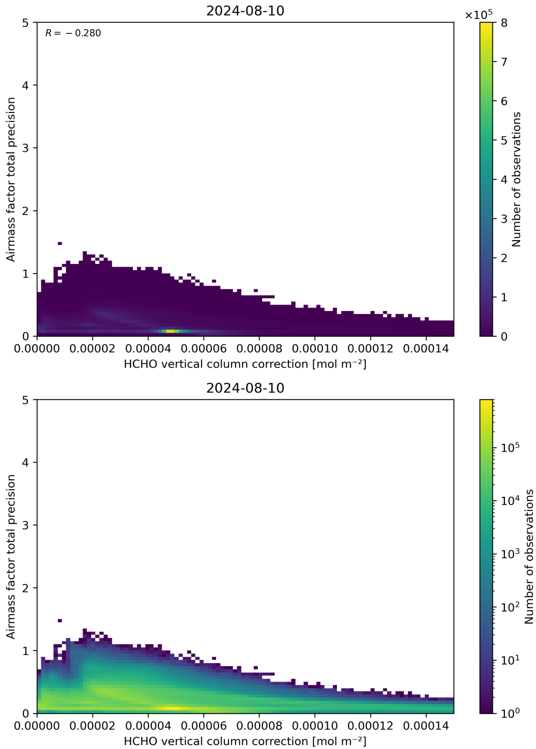
Figure 121: Scatter density plot of “HCHO vertical column correction” against “Airmass factor total precision” for 2024-08-09 to 2024-08-11.
