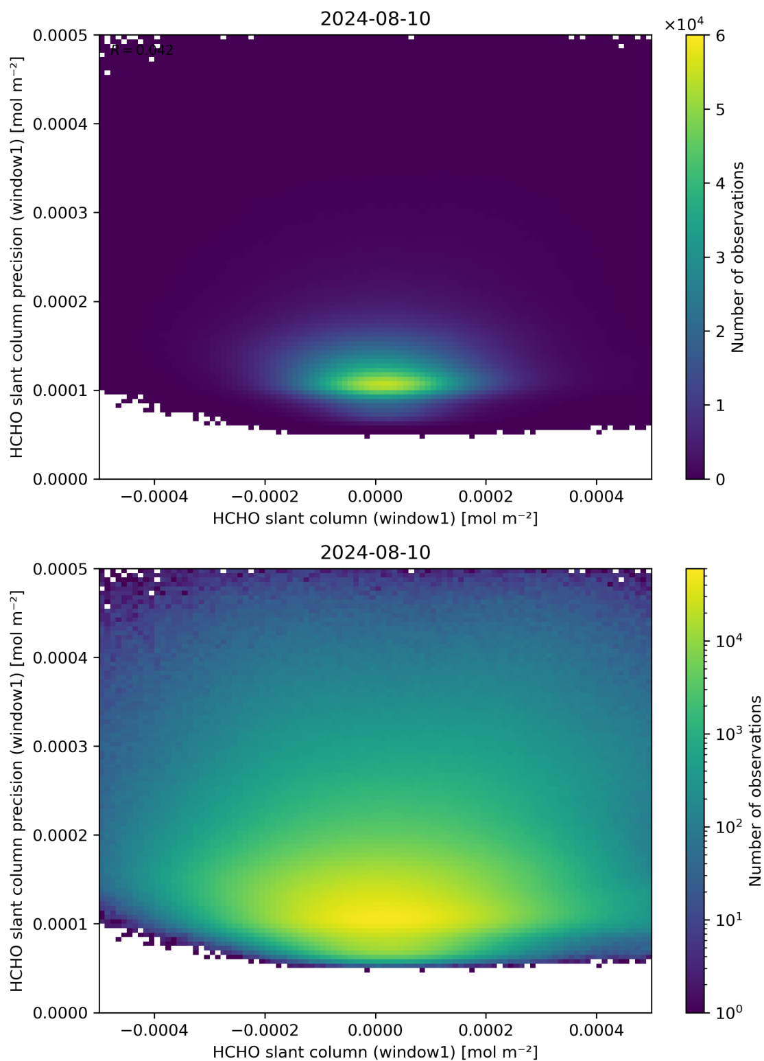
Figure 84: Scatter density plot of “HCHO slant column (window1)” against “HCHO slant column precision (window1)” for 2024-08-09 to 2024-08-11.
