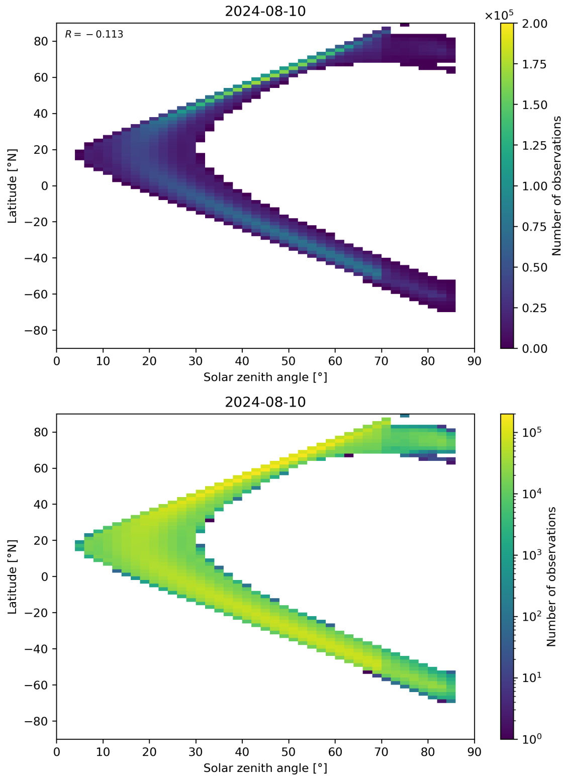
Figure 181: Scatter density plot of “Solar zenith angle” against “Latitude” for 2024-08-09 to 2024-08-11.
