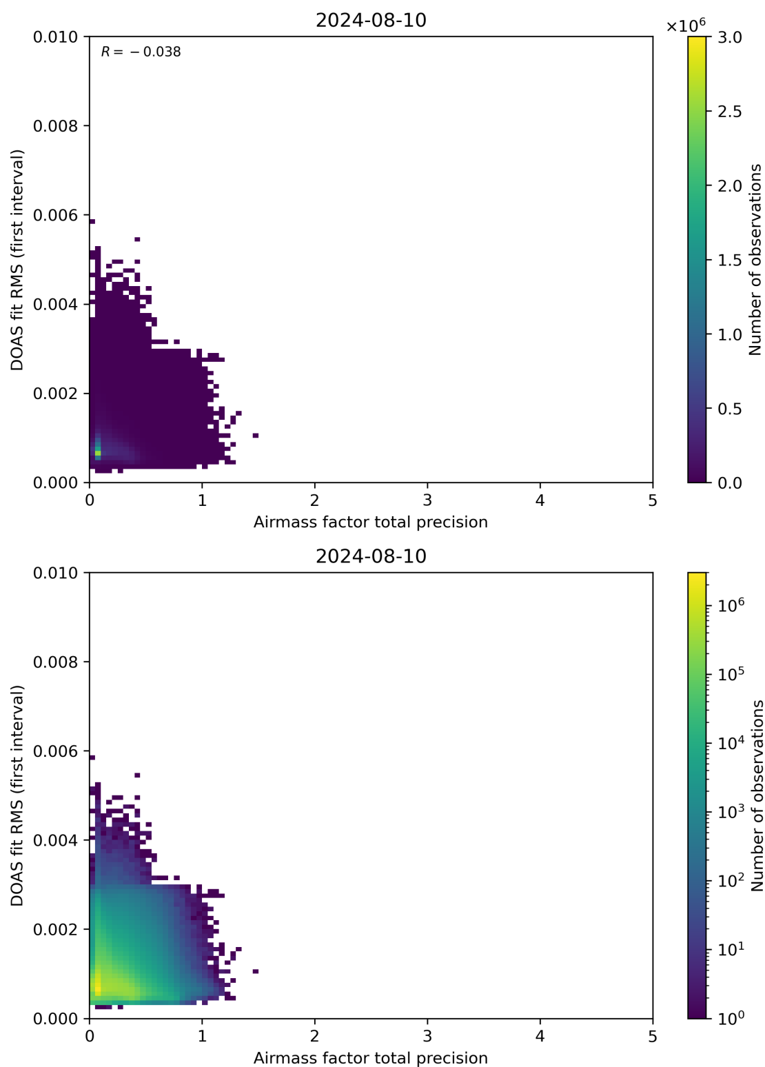
Figure 105: Scatter density plot of “Airmass factor total precision” against “DOAS fit RMS (first interval)” for 2024-08-09 to 2024-08-11.
