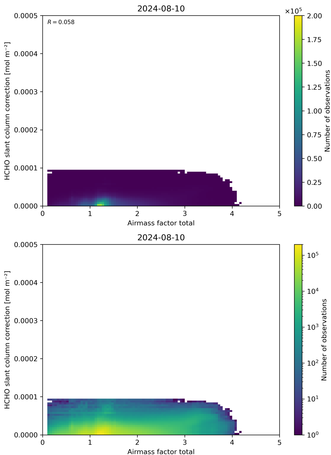
Figure 102: Scatter density plot of “Airmass factor total” against “HCHO slant column correction” for 2024-08-09 to 2024-08-11.
