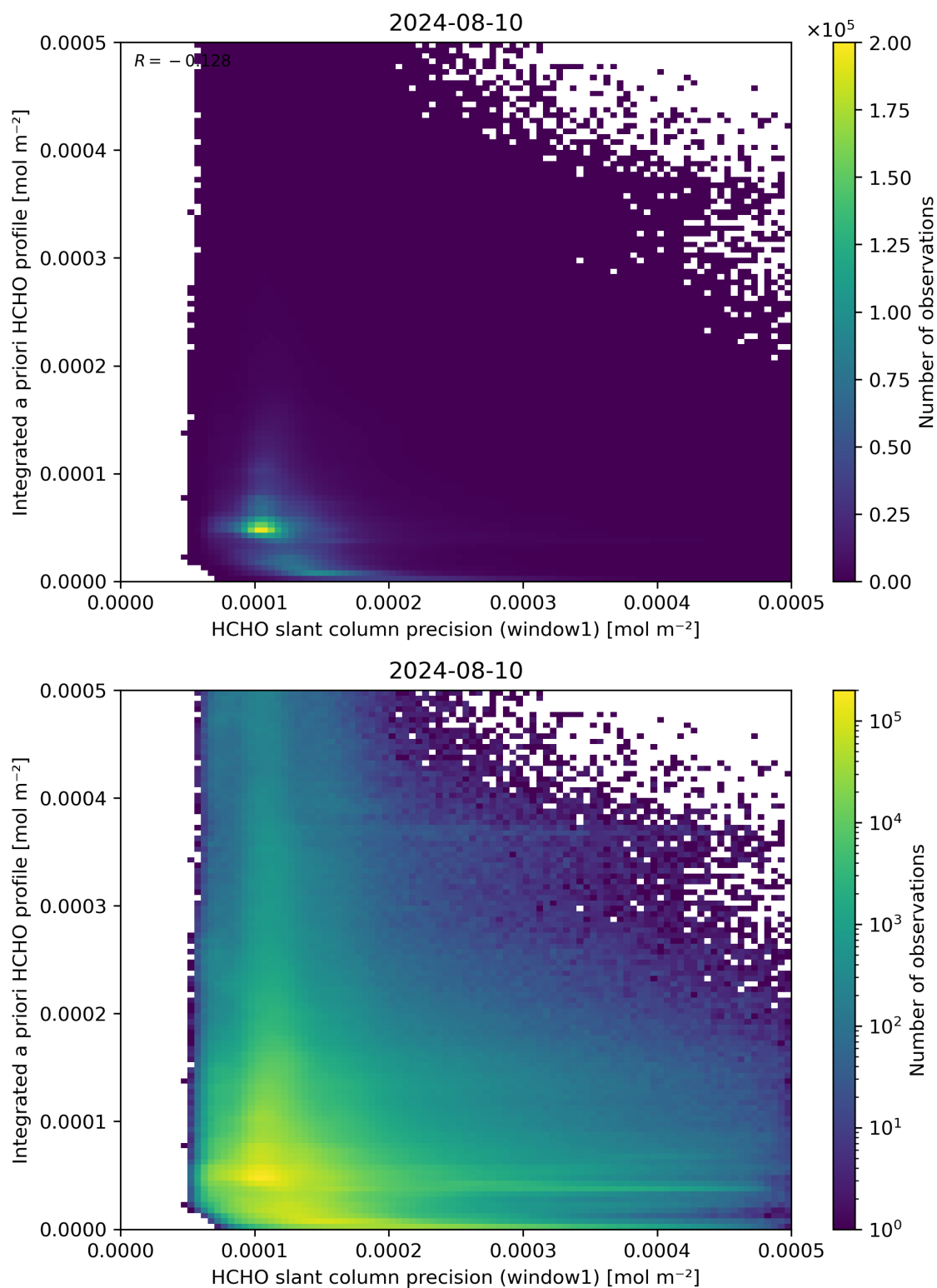
Figure 96: Scatter density plot of “HCHO slant column precision (window1)” against “Integrated a priori HCHO profile” for 2024-08-09 to 2024-08-11.
