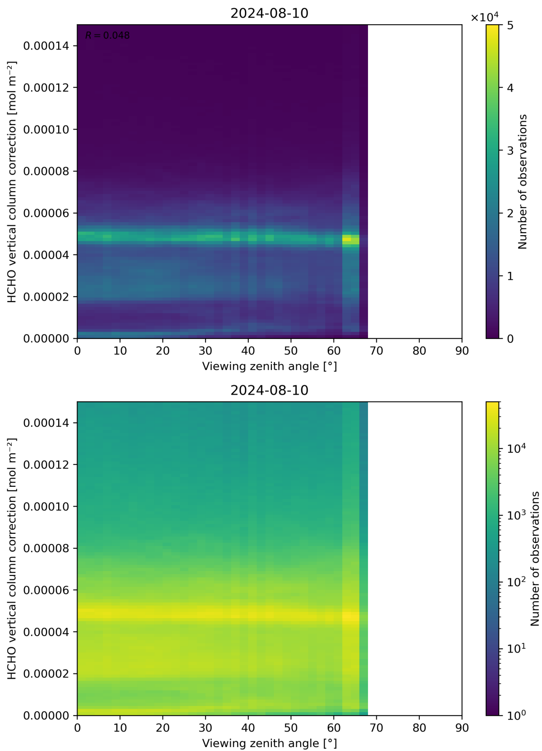
Figure 193: Scatter density plot of “Viewing zenith angle” against “HCHO vertical column correction” for 2024-08-09 to 2024-08-11.
