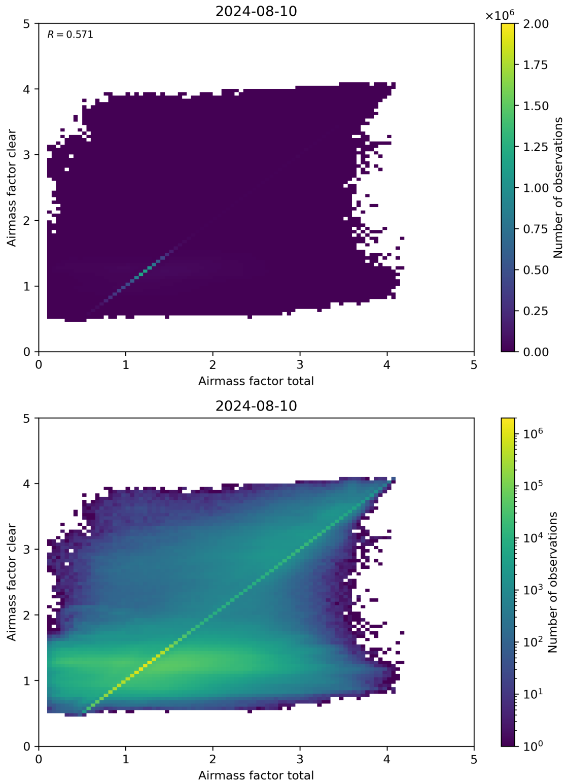
Figure 100: Scatter density plot of “Airmass factor total” against “Airmass factor clear” for 2024-08-09 to 2024-08-11.
