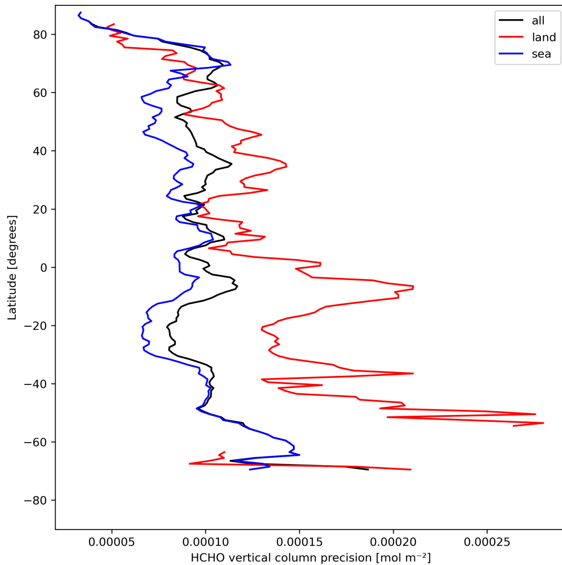
Figure 22: Zonal average of “HCHO vertical column precision” for 2024-08-09 to 2024-08-11.
