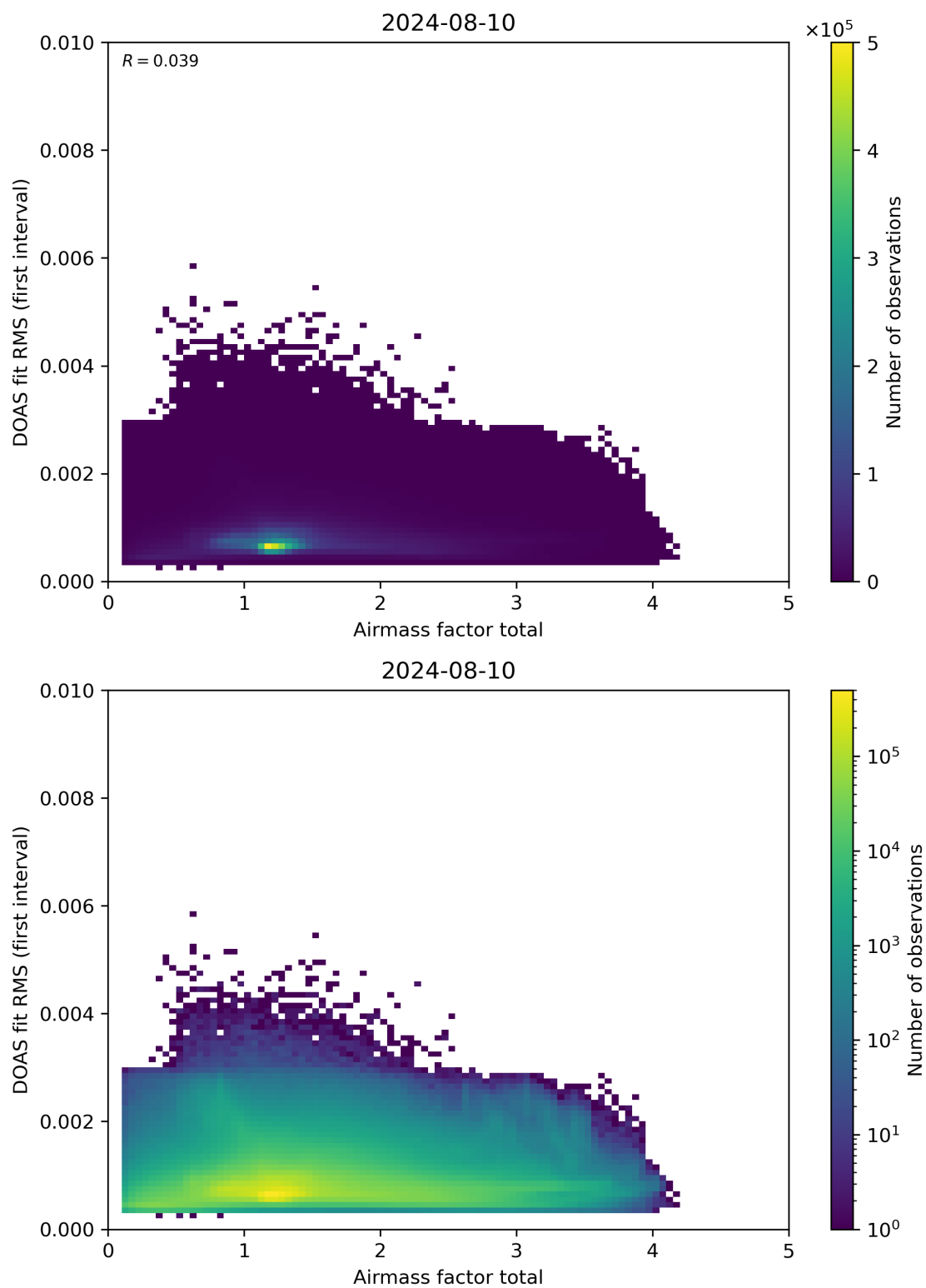
Figure 97: Scatter density plot of “Airmass factor total” against “DOAS fit RMS (first interval)” for 2024-08-09 to 2024-08-11.
