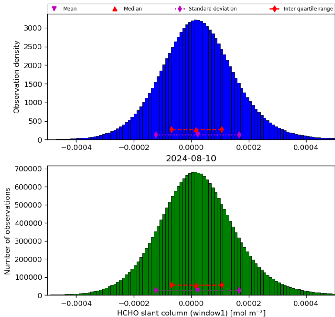
Figure 38: Histogram of “HCHO slant column (window1)” for 2024-08-09 to 2024-08-11
