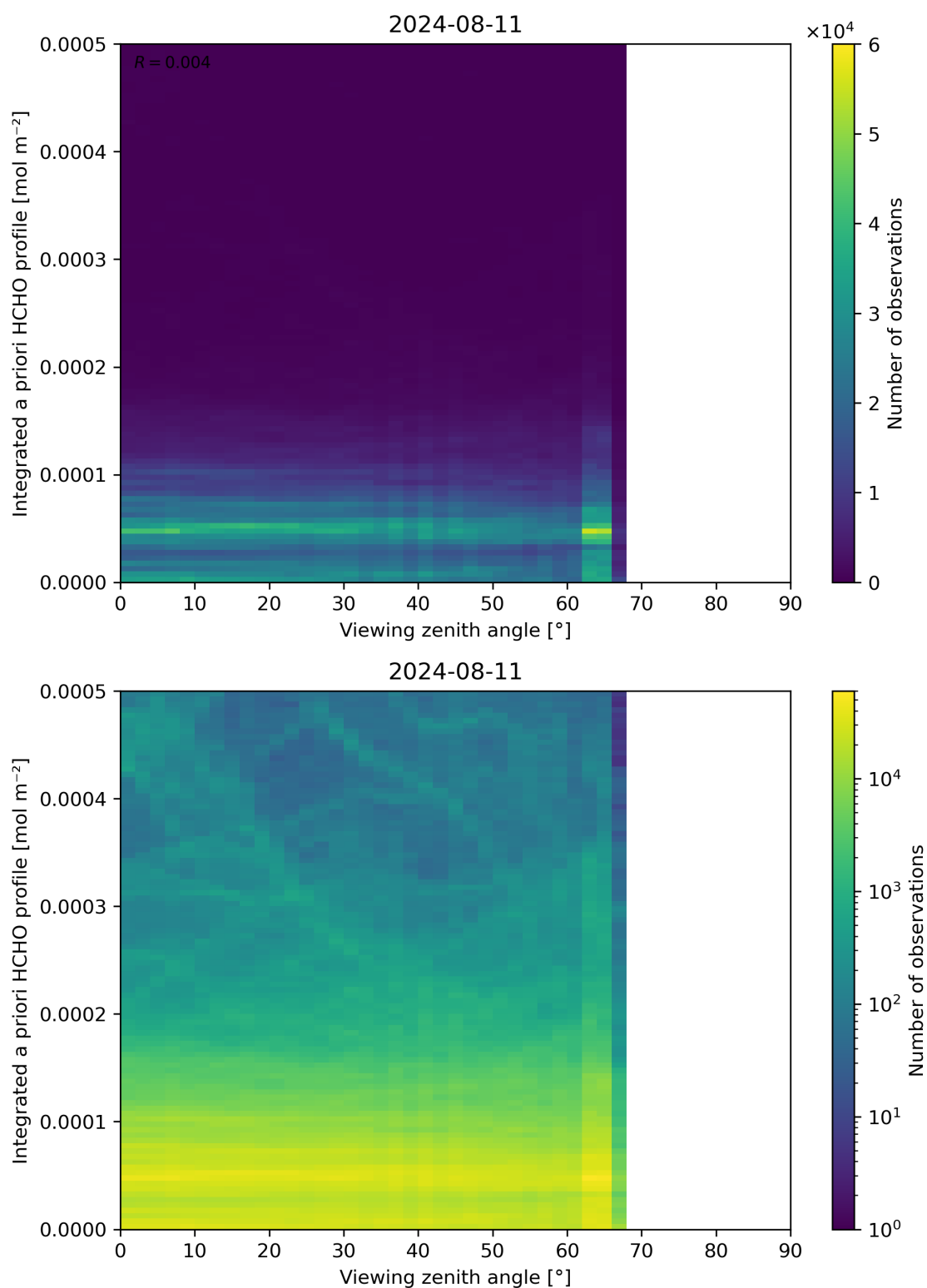
Figure 195: Scatter density plot of “Viewing zenith angle” against “Integrated a priori HCHO profile” for 2024-08-11 to 2024-08-11.
