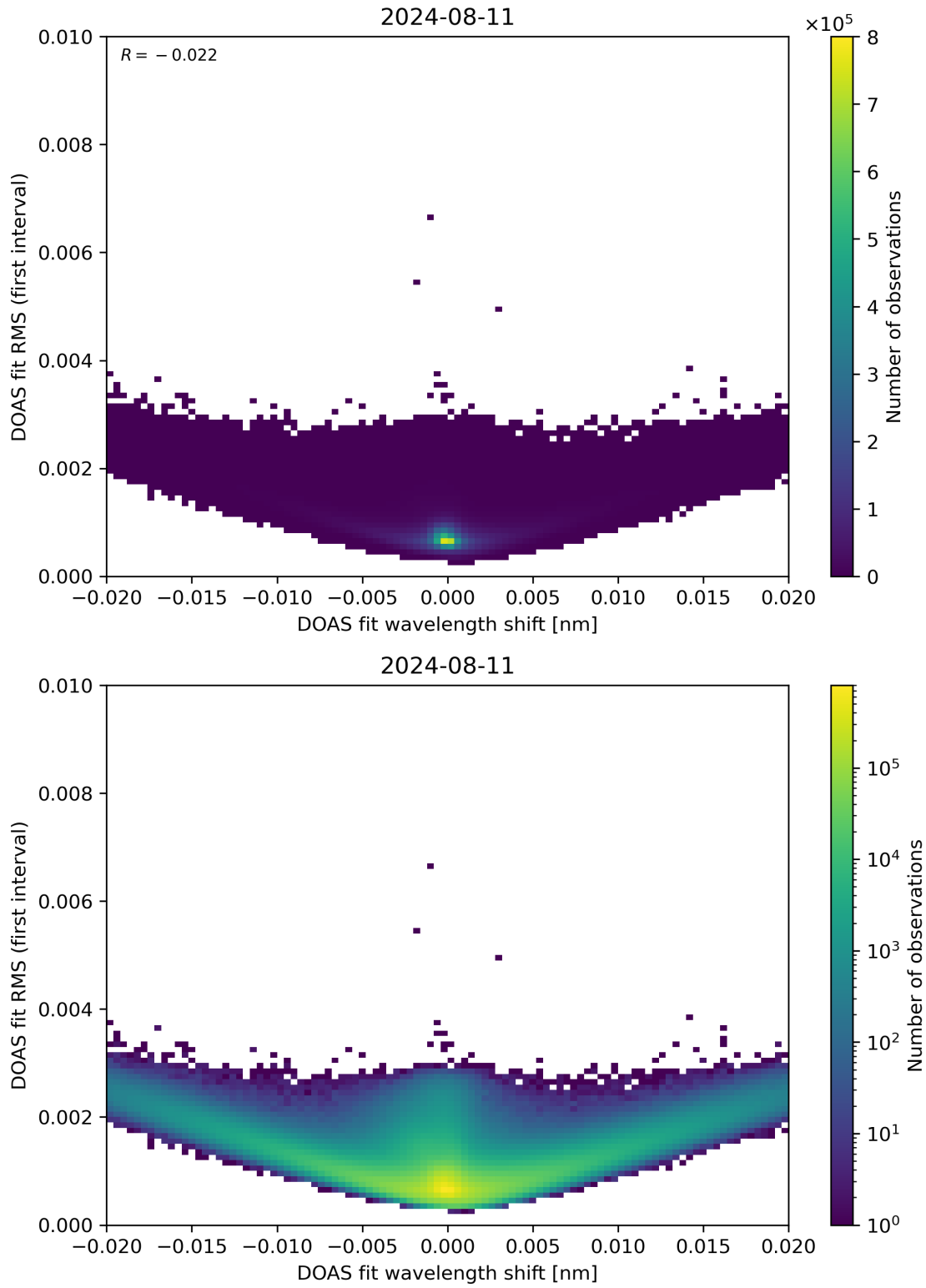
Figure 64: Scatter density plot of “DOAS fit wavelength shift” against “DOAS fit RMS (first interval)” for 2024-08-11 to 2024-08-11.
