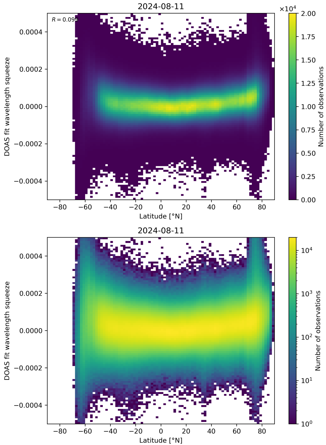
Figure 155: Scatter density plot of “Latitude” against “DOAS fit wavelength squeeze” for 2024-08-11 to 2024-08-11.
