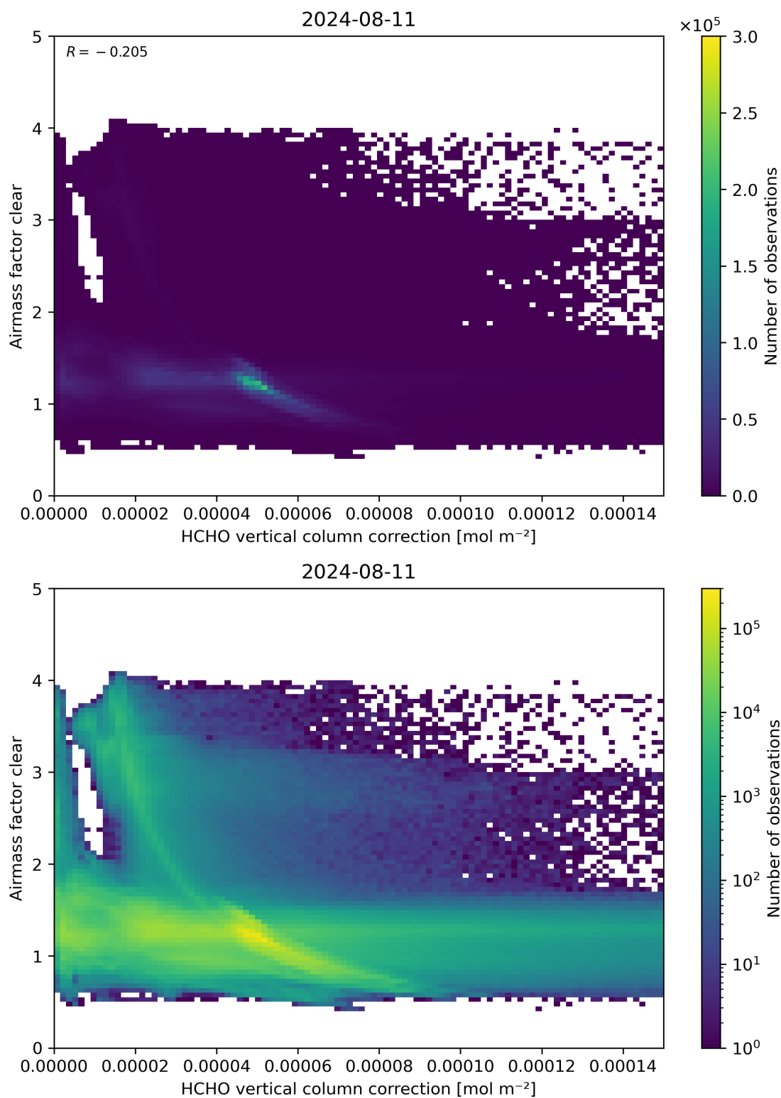
Figure 115: Scatter density plot of “HCHO vertical column correction” against “Airmass factor clear” for 2024-08-11 to 2024-08-11.
