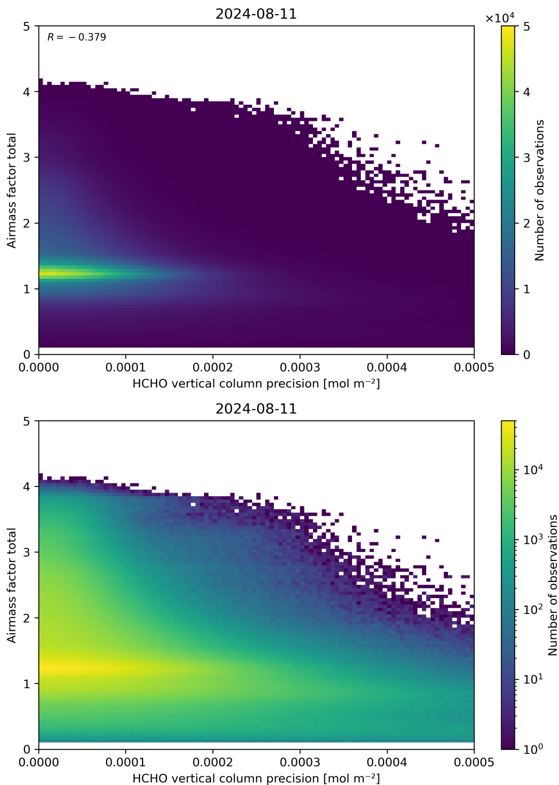
Figure 144: Scatter density plot of “HCHO vertical column precision” against “Airmass factor total” for 2024-08-11 to 2024-08-11.
