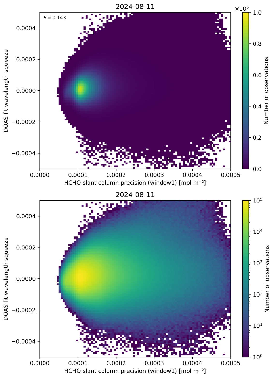
Figure 90: Scatter density plot of “HCHO slant column precision (window1)” against “DOAS fit wavelength squeeze” for 2024-08-11 to 2024-08-11.
