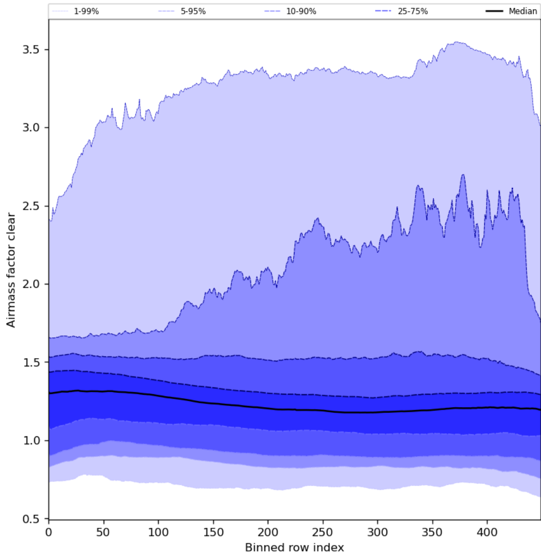
Figure 56: Along track statistics of “Airmass factor clear” for 2024-08-11 to 2024-08-11
