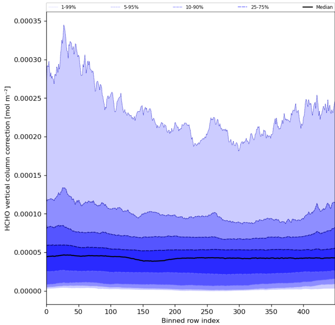
Figure 51: Along track statistics of “HCHO vertical column correction” for 2024-08-11 to 2024-08-11
