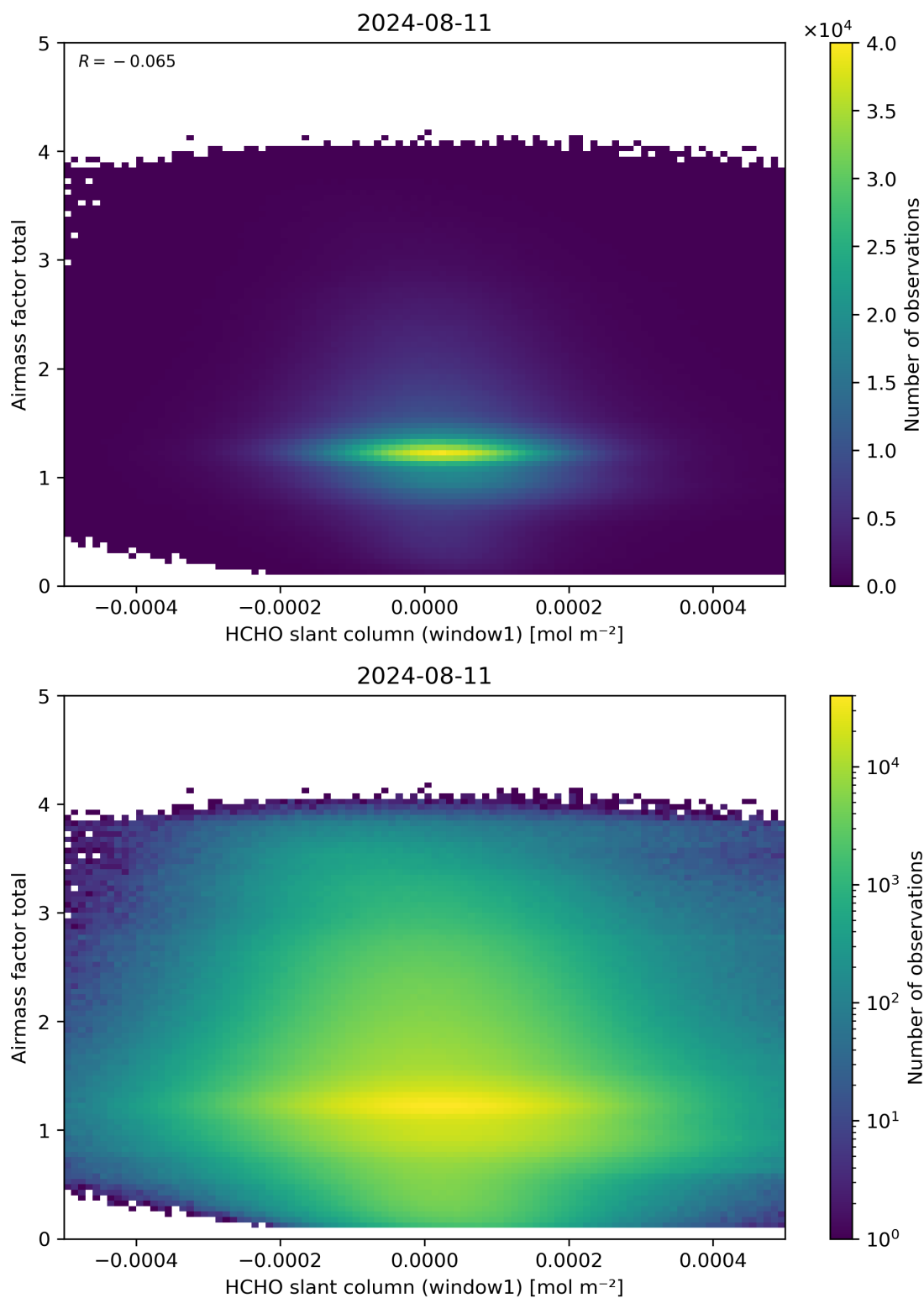
Figure 85: Scatter density plot of “HCHO slant column (window1)” against “Airmass factor total” for 2024-08-11 to 2024-08-11.
