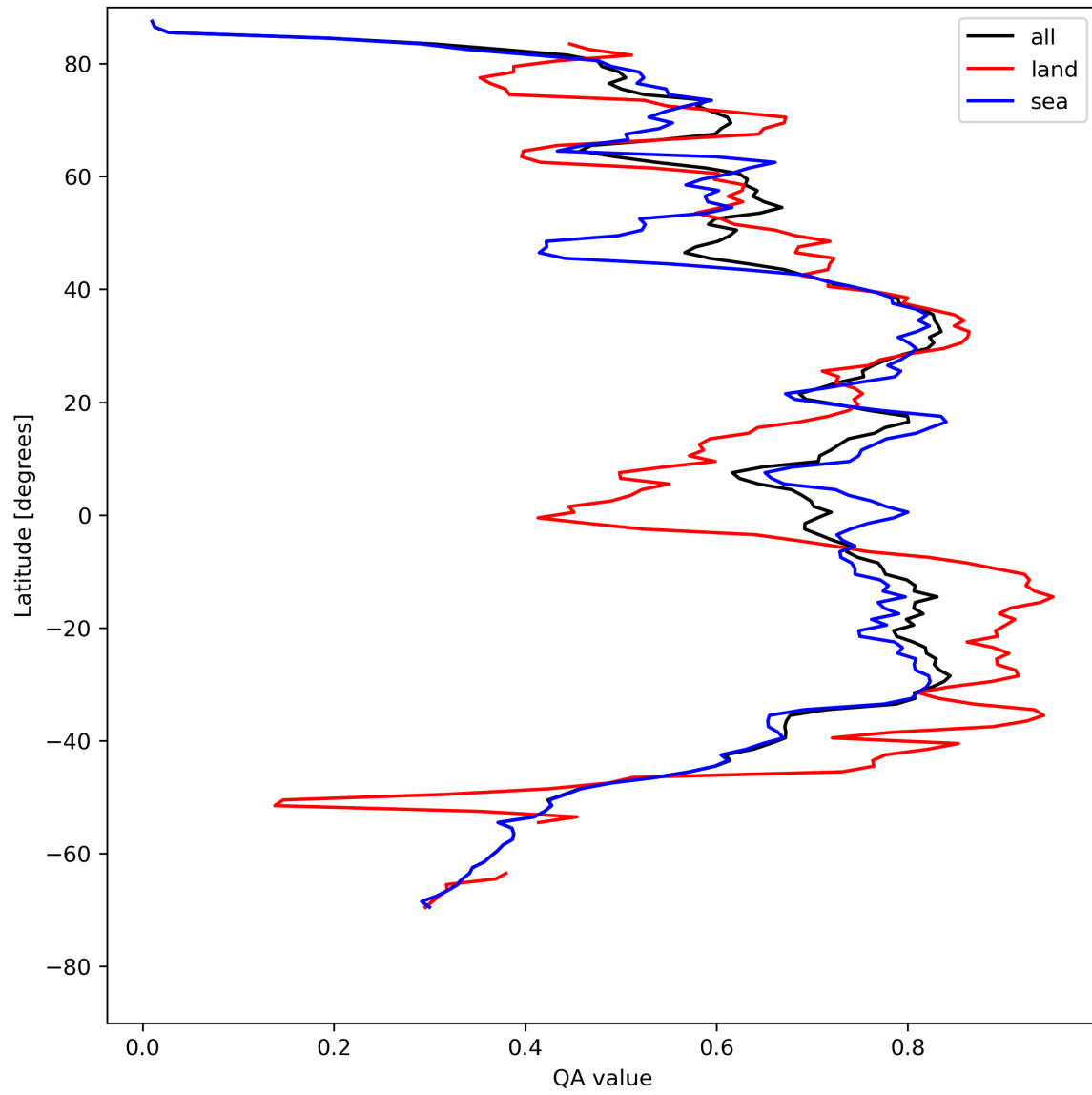
Figure 20: Zonal average of “QA value” for 2024-08-11 to 2024-08-11.
