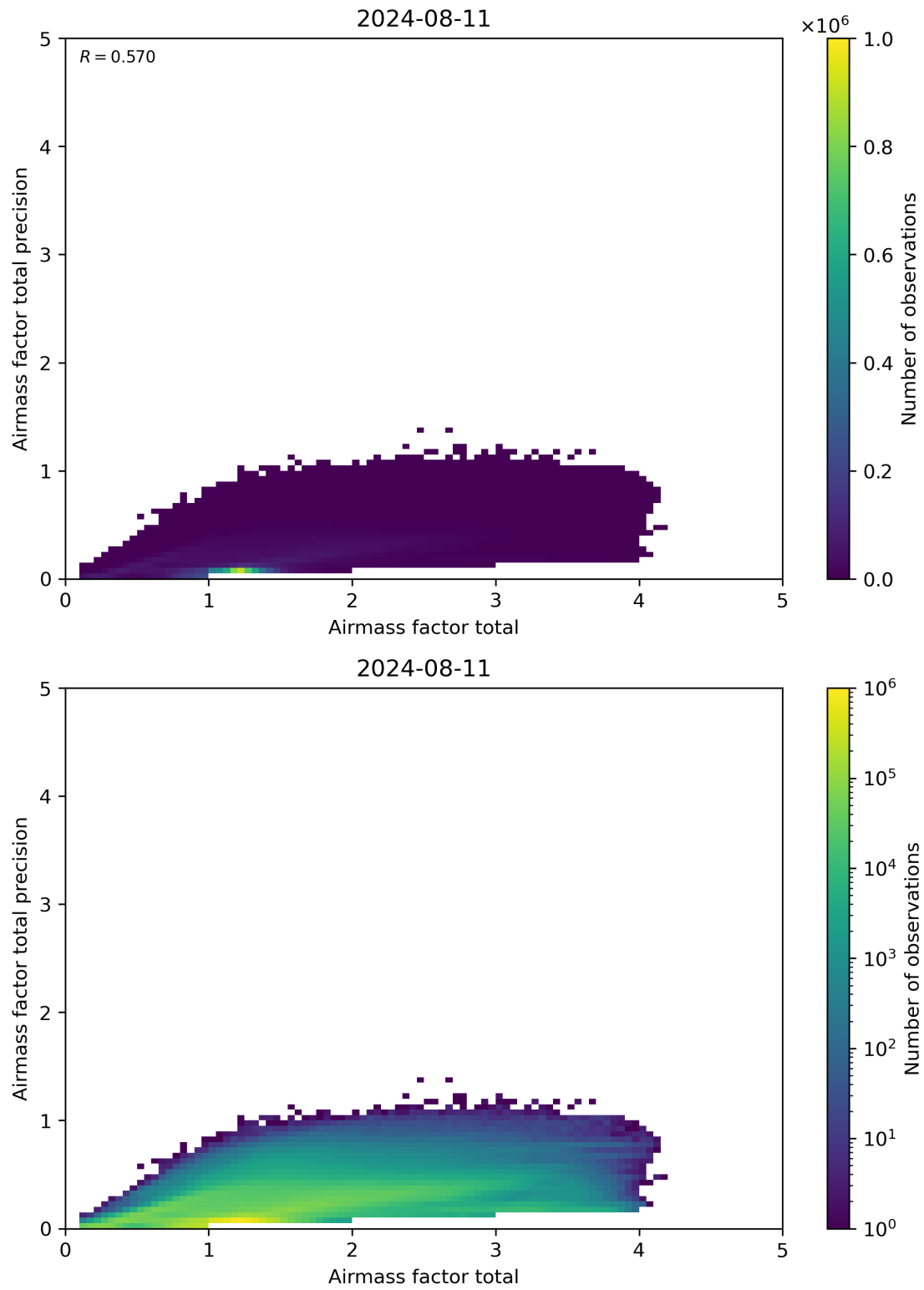
Figure 103: Scatter density plot of “Airmass factor total” against “Airmass factor total precision” for 2024-08-11 to 2024-08-11.
