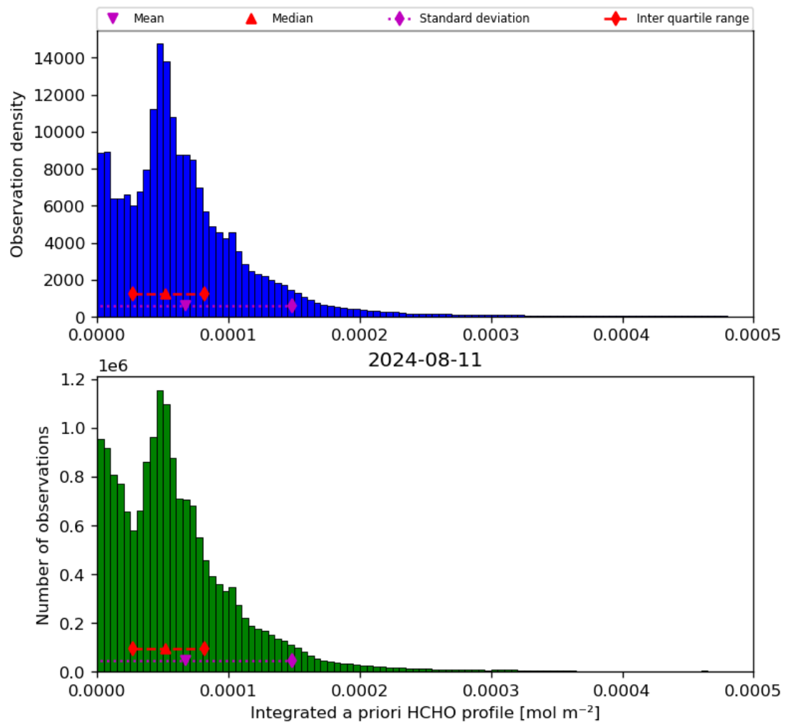
Figure 43: Histogram of “Integrated a priori HCHO profile” for 2024-08-11 to 2024-08-11
