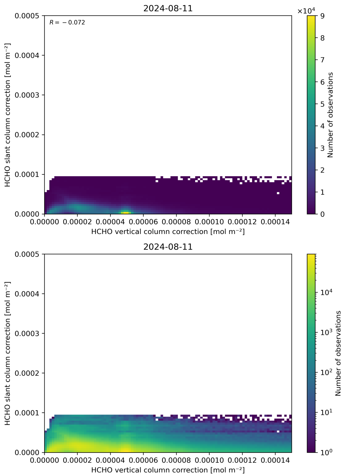
Figure 117: Scatter density plot of “HCHO vertical column correction” against “HCHO slant column correction” for 2024-08-11 to 2024-08-11.
