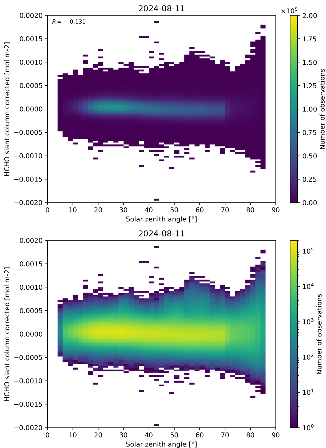
Figure 171: Scatter density plot of “Solar zenith angle” against “HCHO slant column corrected” for 2024-08-11 to 2024-08-11.
