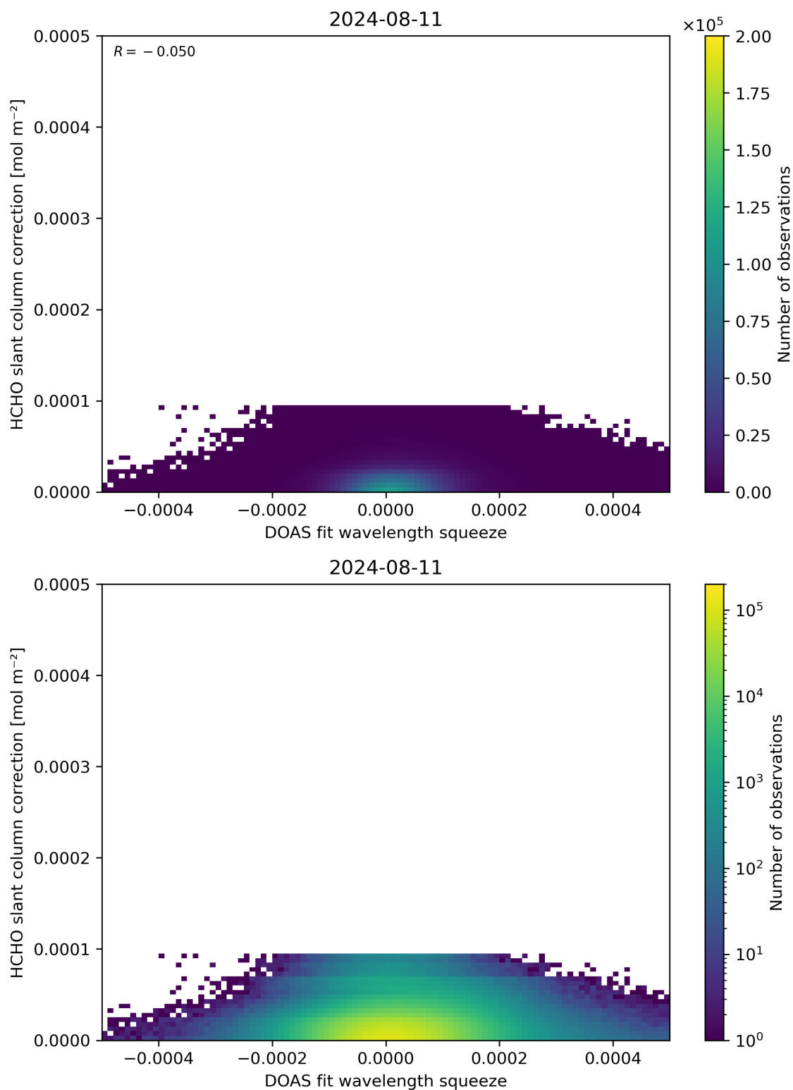
Figure 70: Scatter density plot of “DOAS fit wavelength squeeze” against “HCHO slant column correction” for 2024-08-11 to 2024-08-11.
