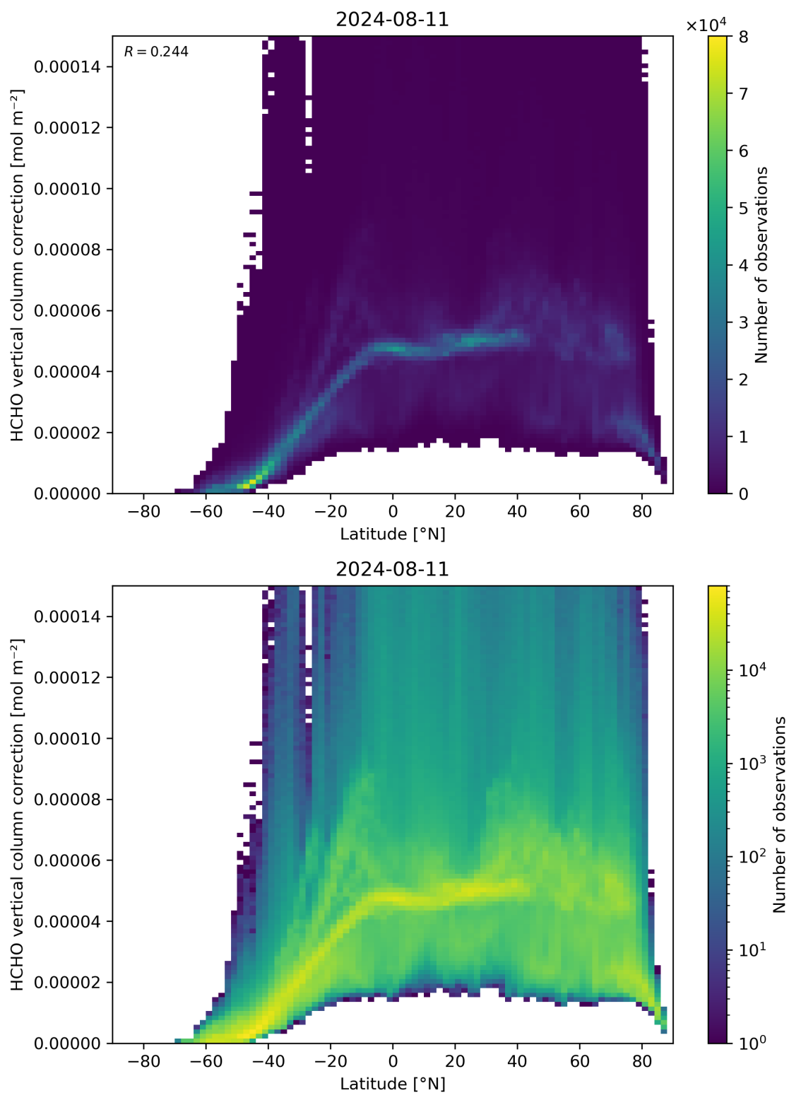
Figure 164: Scatter density plot of “Latitude” against “HCHO vertical column correction” for 2024-08-11 to 2024-08-11.
