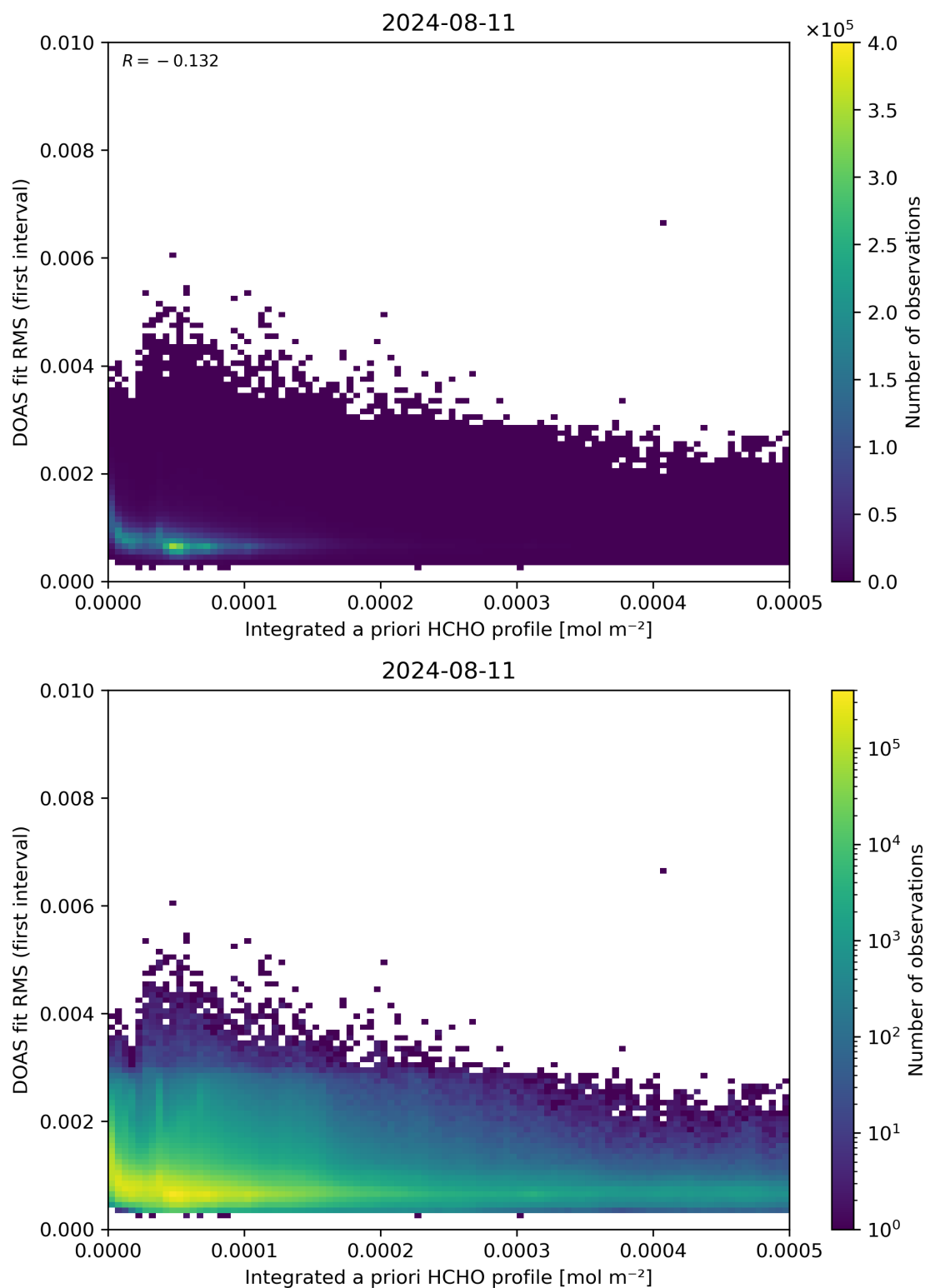
Figure 148: Scatter density plot of “Integrated a priori HCHO profile” against “DOAS fit RMS (first interval)” for 2024-08-11 to 2024-08-11.
