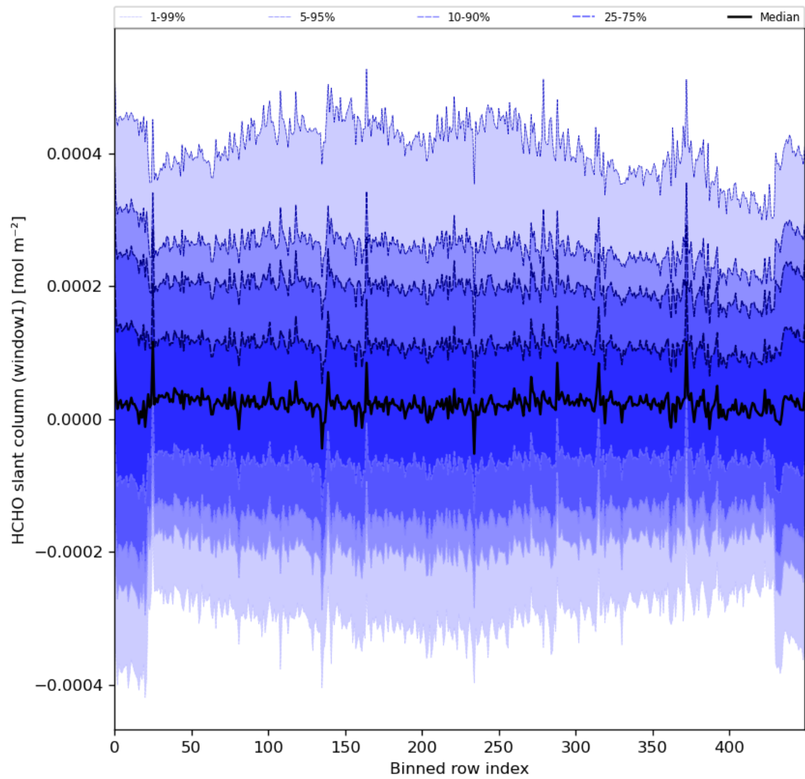
Figure 52: Along track statistics of “HCHO slant column (window1)” for 2024-08-11 to 2024-08-11
