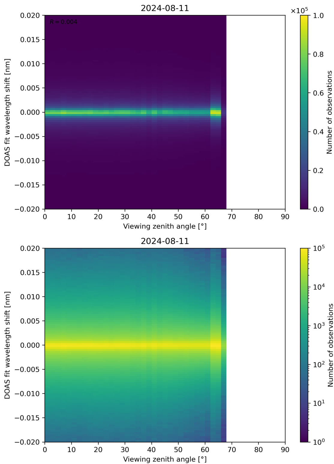
Figure 183: Scatter density plot of “Viewing zenith angle” against “DOAS fit wavelength shift” for 2024-08-11 to 2024-08-11.
