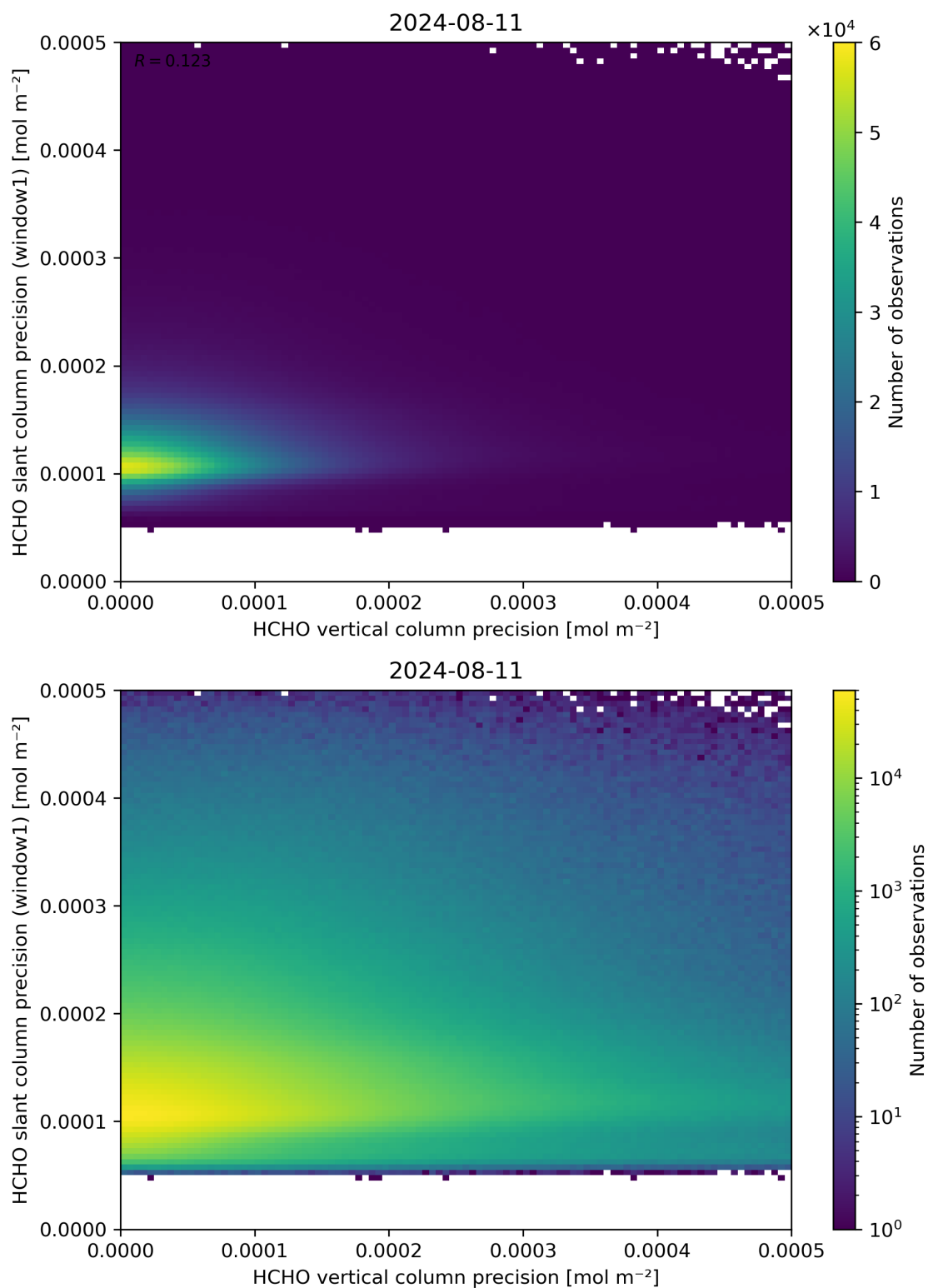
Figure 143: Scatter density plot of “HCHO vertical column precision” against “HCHO slant column precision (window1)” for 2024-08-11 to 2024-08-11.
