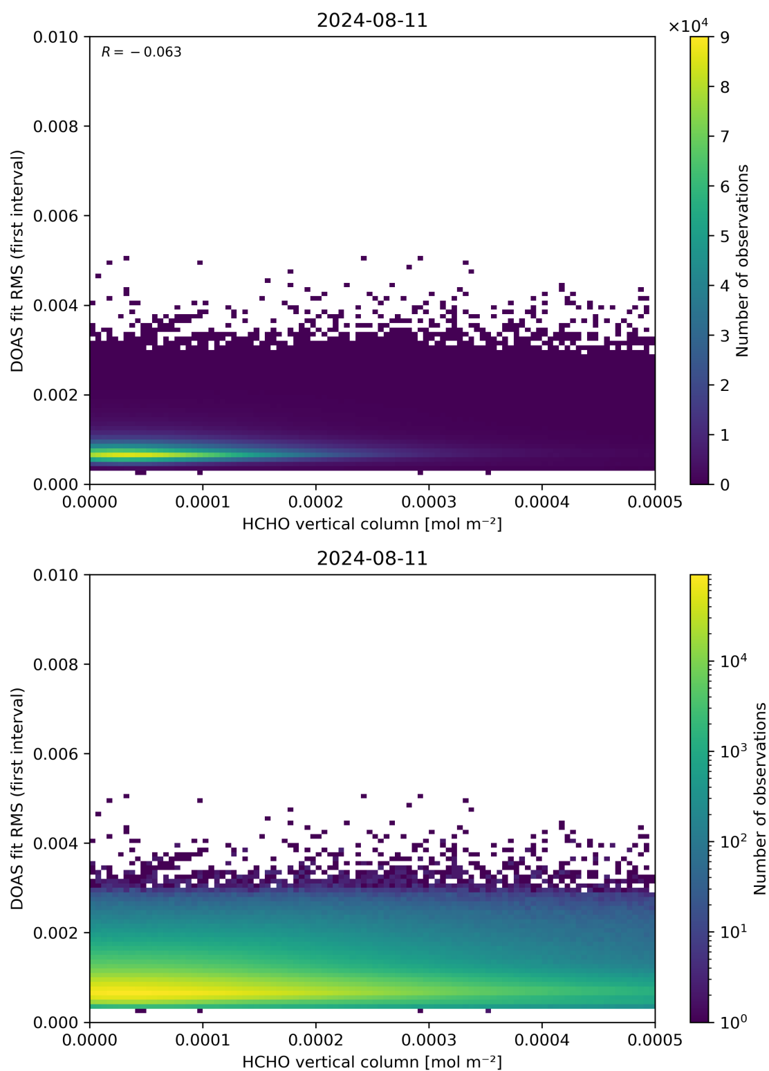
Figure 123: Scatter density plot of “HCHO vertical column” against “DOAS fit RMS (first interval)” for 2024-08-11 to 2024-08-11.
