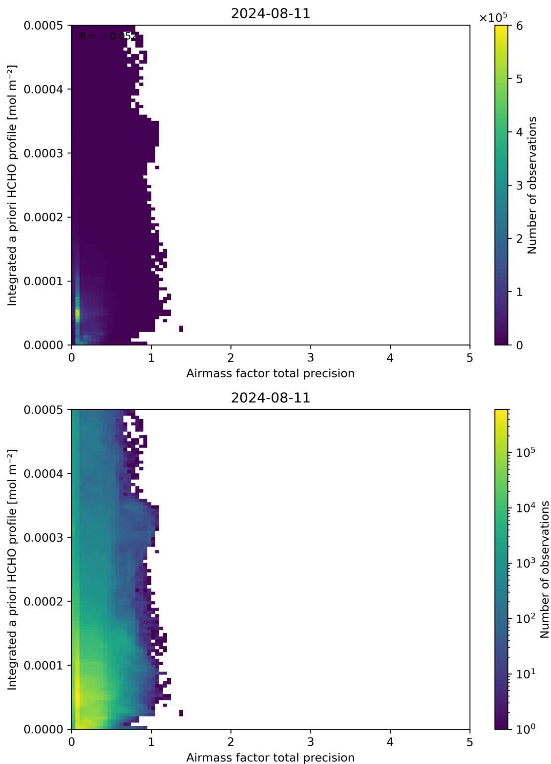
Figure 111: Scatter density plot of “Airmass factor total precision” against “Integrated a priori HCHO profile” for 2024-08-11 to 2024-08-11.
