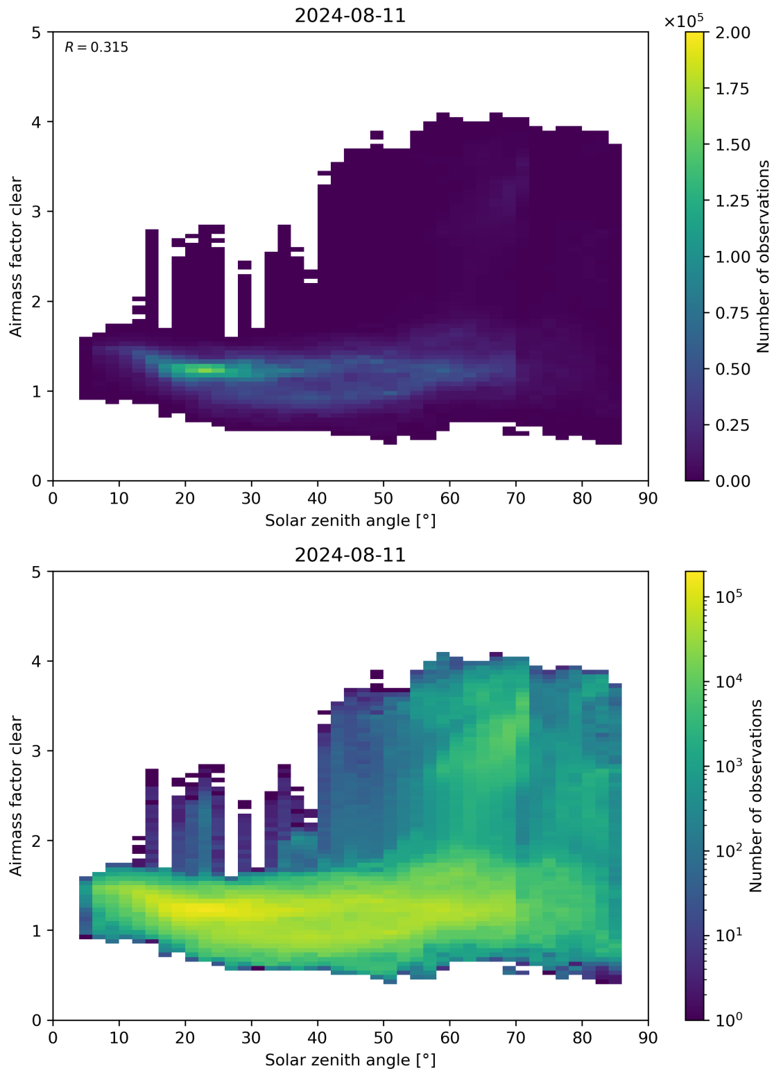
Figure 170: Scatter density plot of “Solar zenith angle” against “Airmass factor clear” for 2024-08-11 to 2024-08-11.
