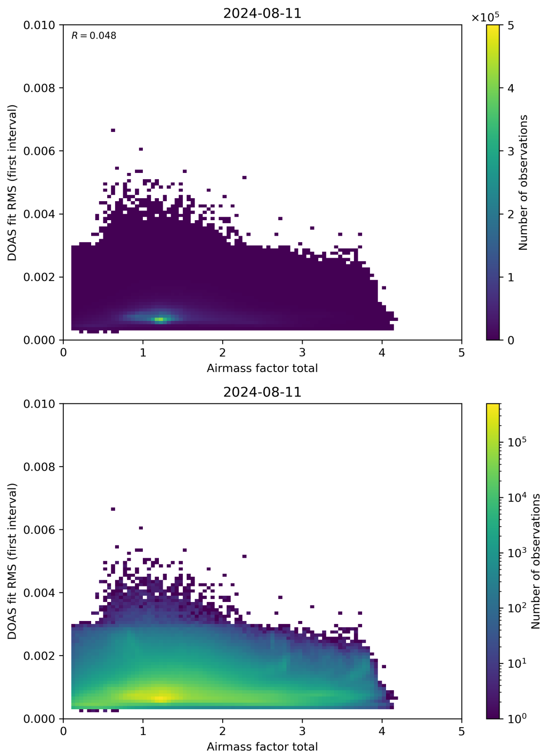
Figure 97: Scatter density plot of “Airmass factor total” against “DOAS fit RMS (first interval)” for 2024-08-11 to 2024-08-11.
