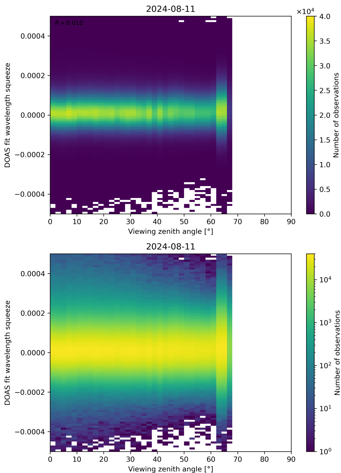
Figure 184: Scatter density plot of “Viewing zenith angle” against “DOAS fit wavelength squeeze” for 2024-08-11 to 2024-08-11.
