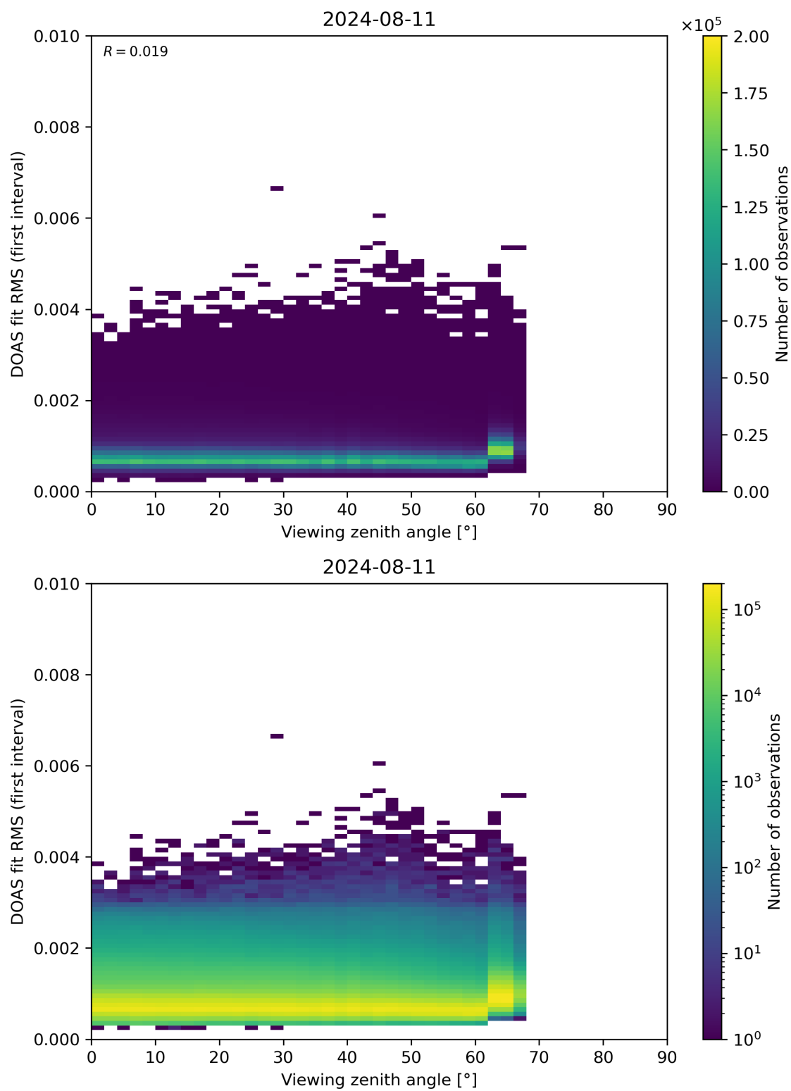
Figure 182: Scatter density plot of “Viewing zenith angle” against “DOAS fit RMS (first interval)” for 2024-08-11 to 2024-08-11.
