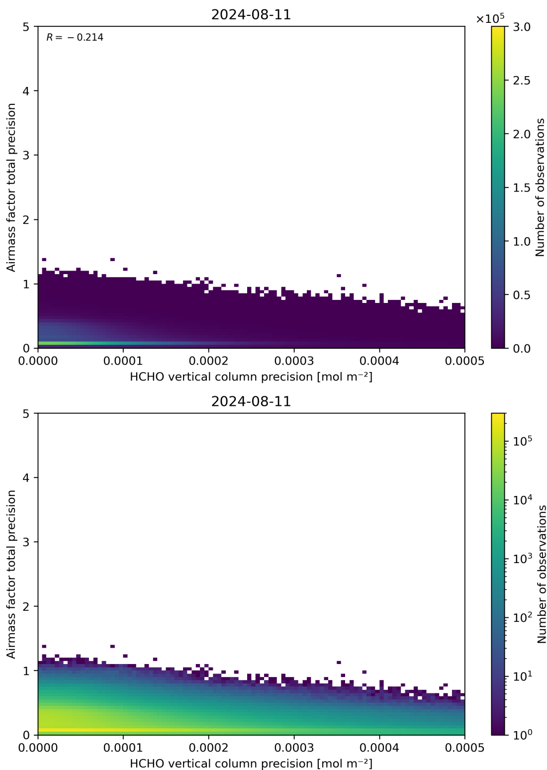
Figure 145: Scatter density plot of “HCHO vertical column precision” against “Airmass factor total precision” for 2024-08-11 to 2024-08-11.
