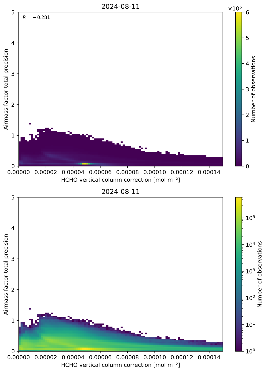
Figure 121: Scatter density plot of “HCHO vertical column correction” against “Airmass factor total precision” for 2024-08-11 to 2024-08-11.
