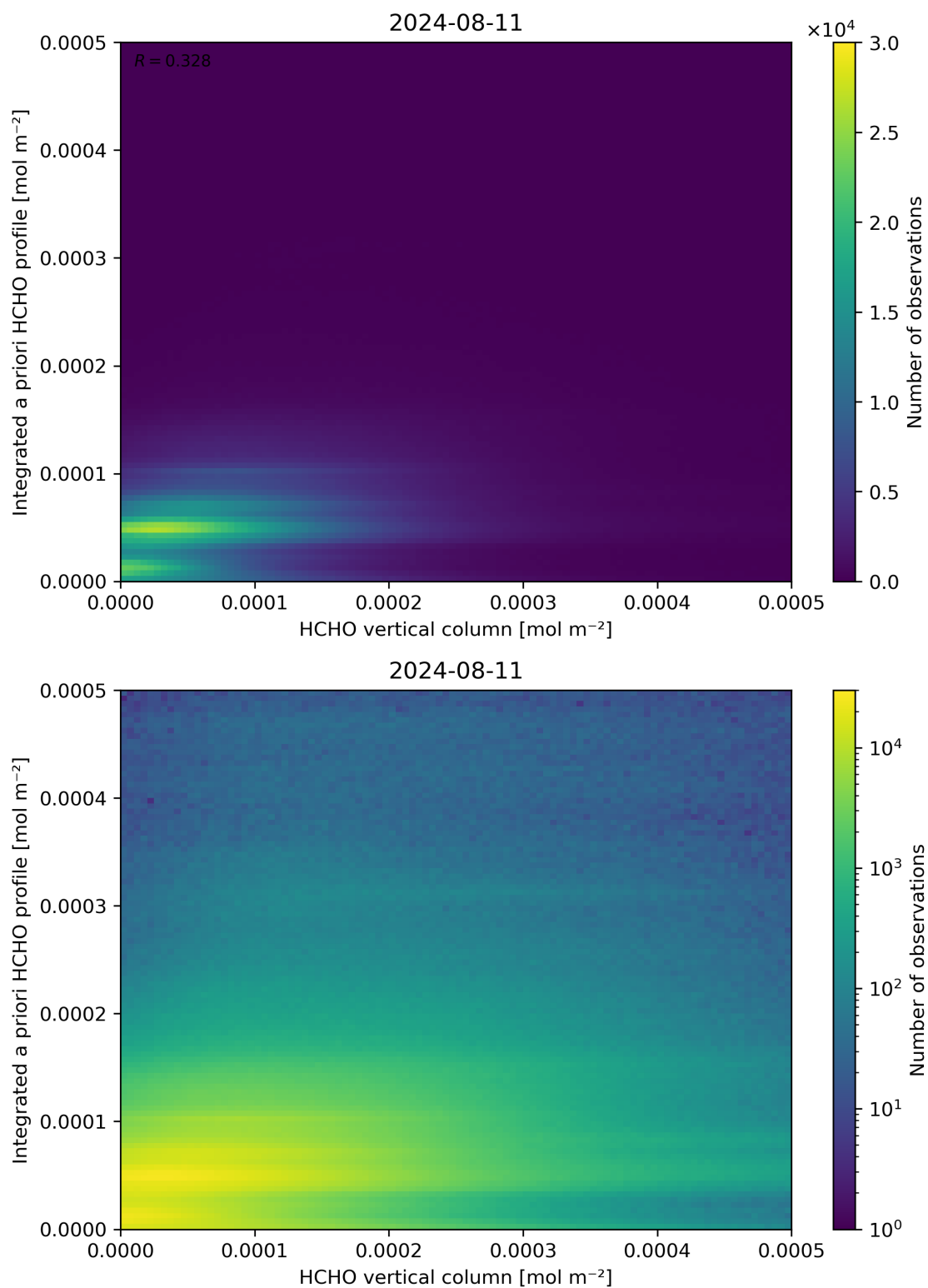
Figure 135: Scatter density plot of “HCHO vertical column” against “Integrated a priori HCHO profile” for 2024-08-11 to 2024-08-11.
