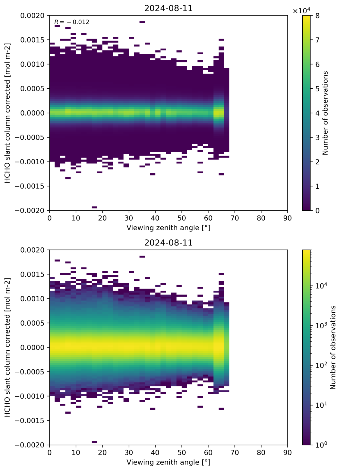
Figure 186: Scatter density plot of “Viewing zenith angle” against “HCHO slant column corrected” for 2024-08-11 to 2024-08-11.
