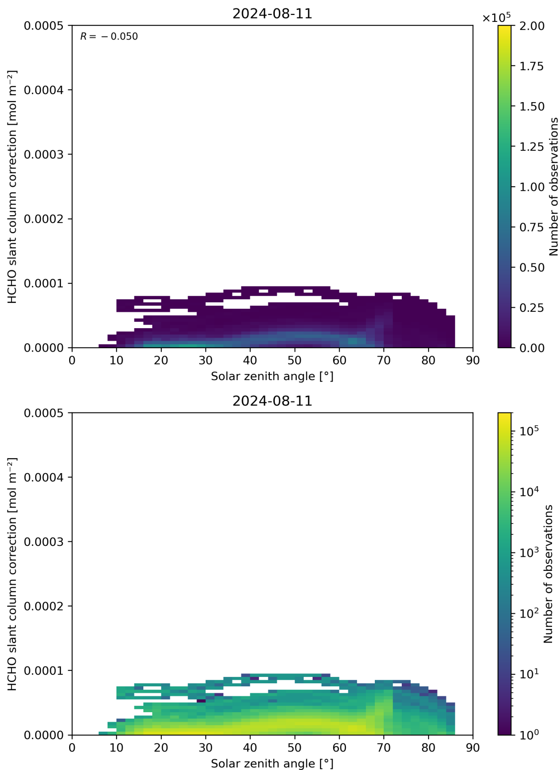
Figure 172: Scatter density plot of “Solar zenith angle” against “HCHO slant column correction” for 2024-08-11 to 2024-08-11.
