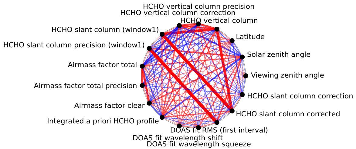
Figure 1: Map of correlation graph for 2024-08-11 to 2024-08-11.
