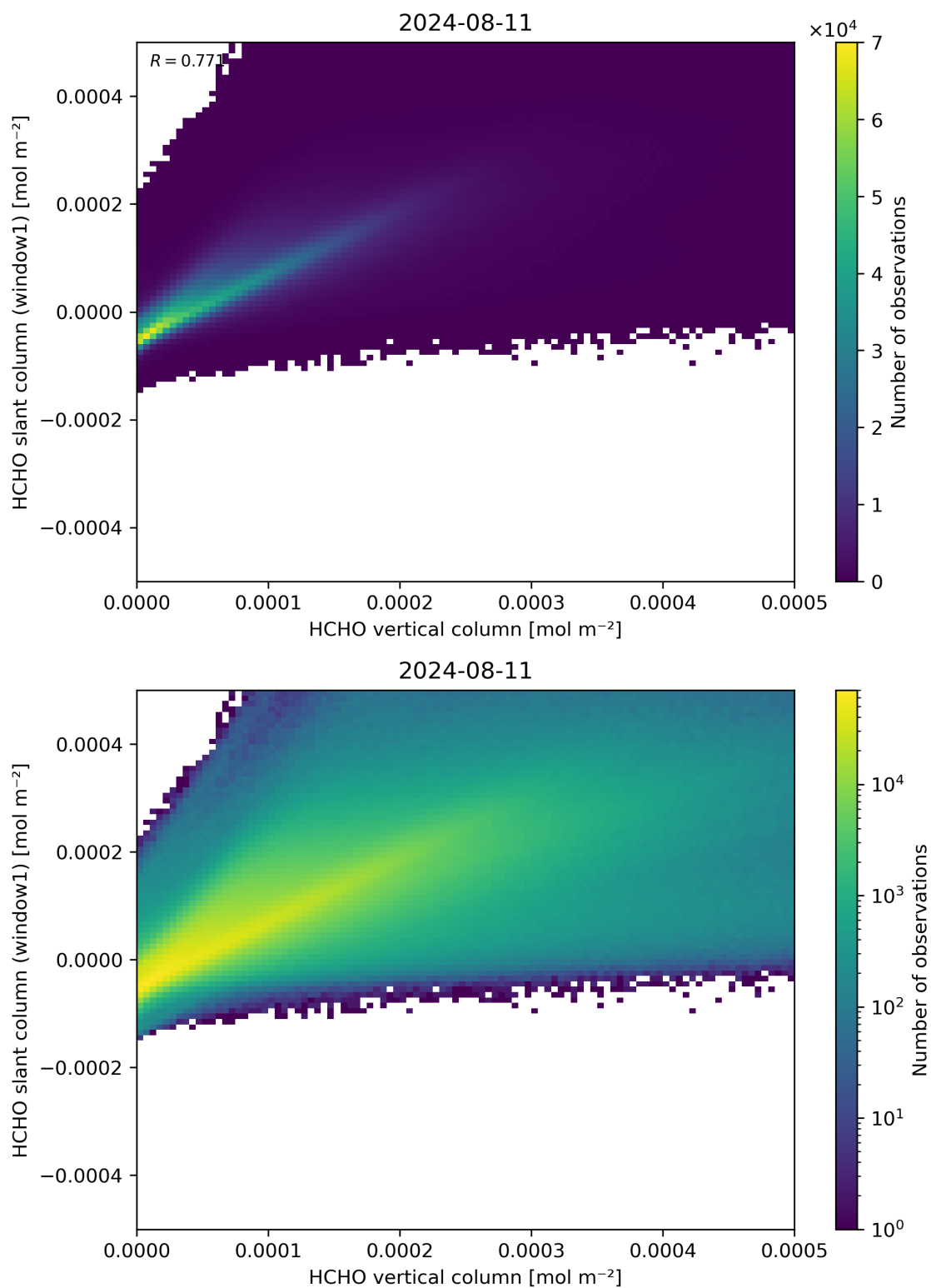
Figure 129: Scatter density plot of “HCHO vertical column” against “HCHO slant column (window1)” for 2024-08-11 to 2024-08-11.
