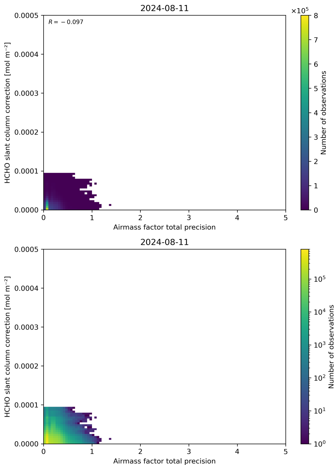
Figure 110: Scatter density plot of “Airmass factor total precision” against “HCHO slant column correction” for 2024-08-11 to 2024-08-11.
