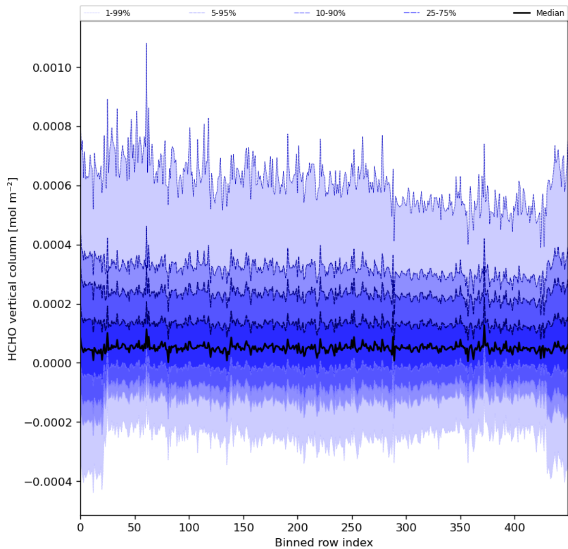
Figure 49: Along track statistics of “HCHO vertical column” for 2024-08-11 to 2024-08-11
