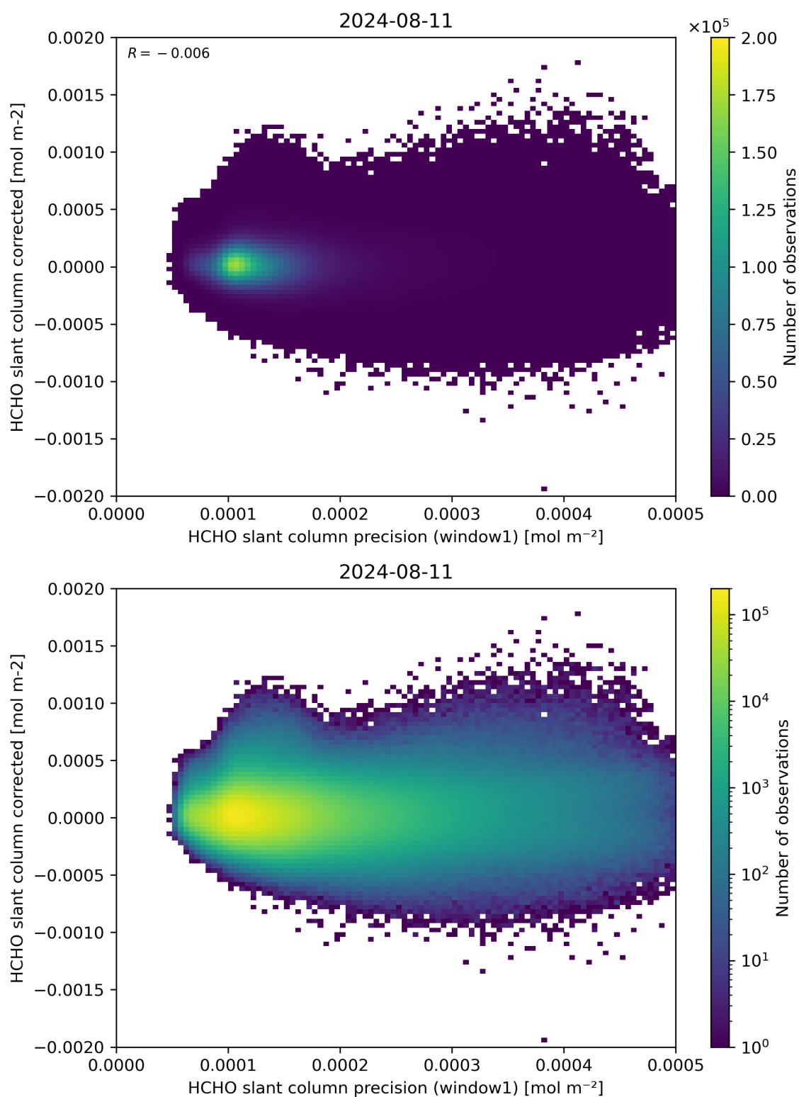
Figure 92: Scatter density plot of “HCHO slant column precision (window1)” against “HCHO slant column corrected” for 2024-08-11 to 2024-08-11.
