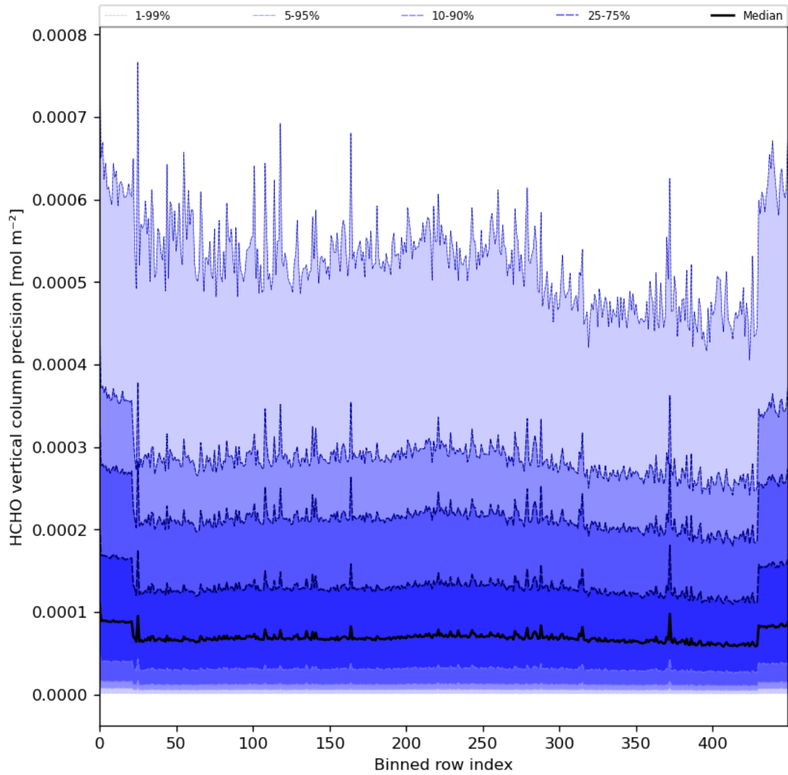
Figure 50: Along track statistics of “HCHO vertical column precision” for 2024-08-11 to 2024-08-11
