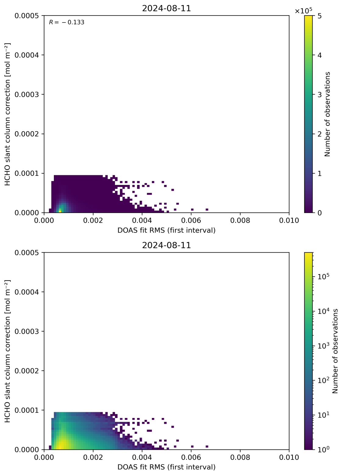
Figure 63: Scatter density plot of “DOAS fit RMS (first interval)” against “HCHO slant column correction” for 2024-08-11 to 2024-08-11.
