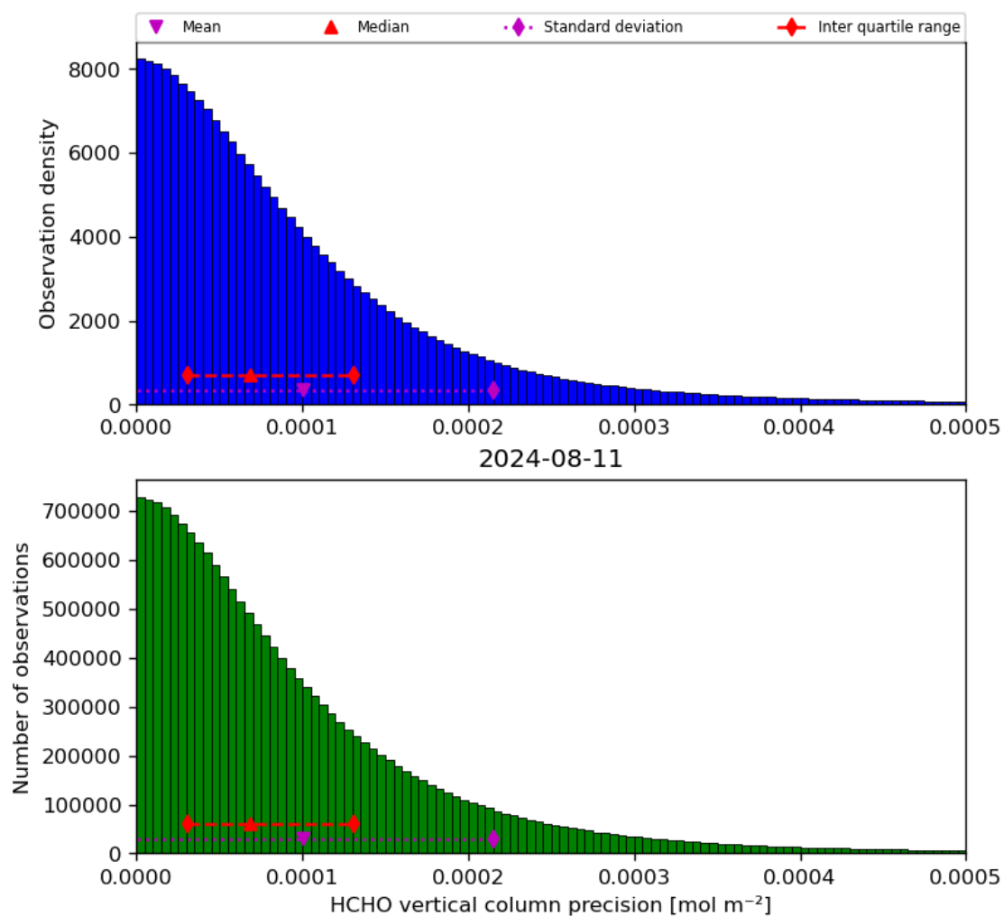
Figure 36: Histogram of “HCHO vertical column precision” for 2024-08-11 to 2024-08-11
