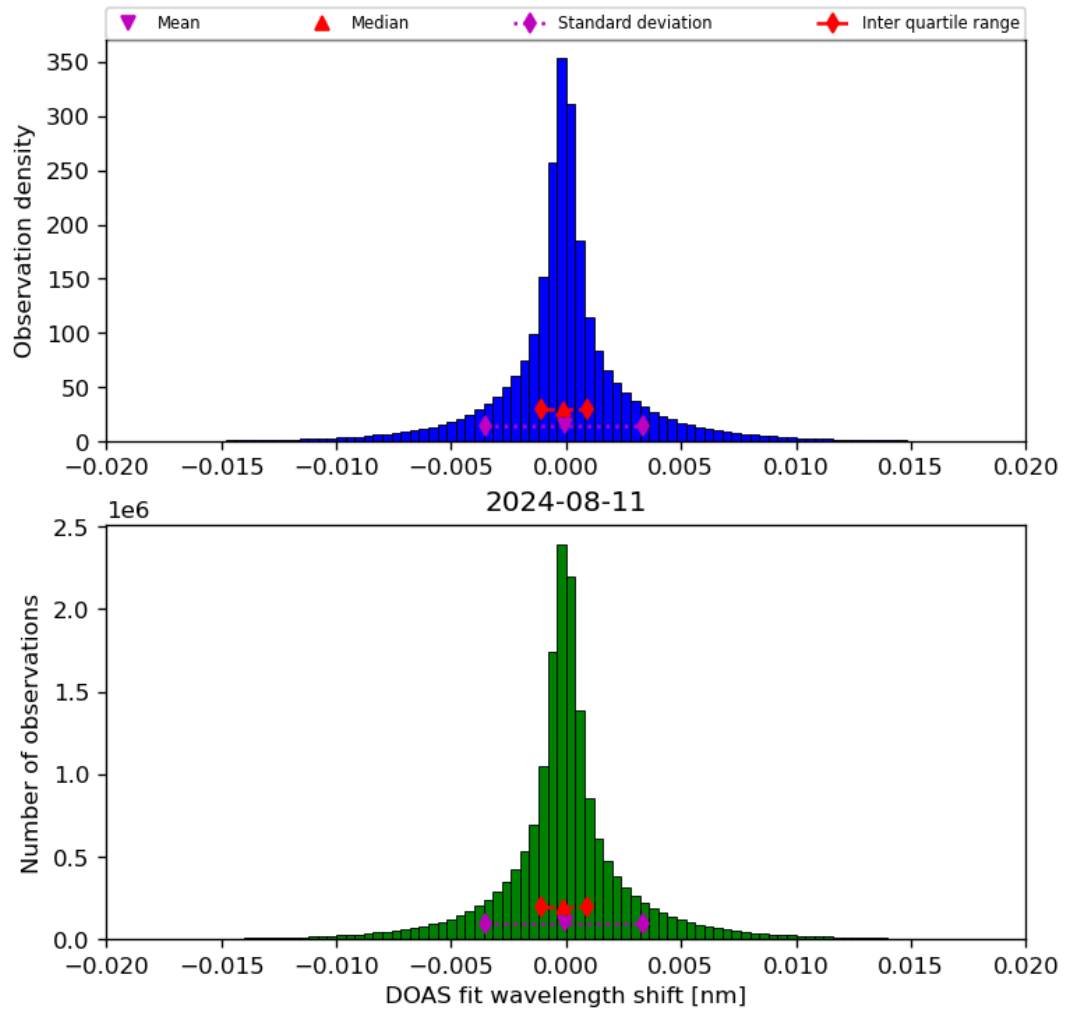
Figure 44: Histogram of “DOAS fit wavelength shift” for 2024-08-11 to 2024-08-11
