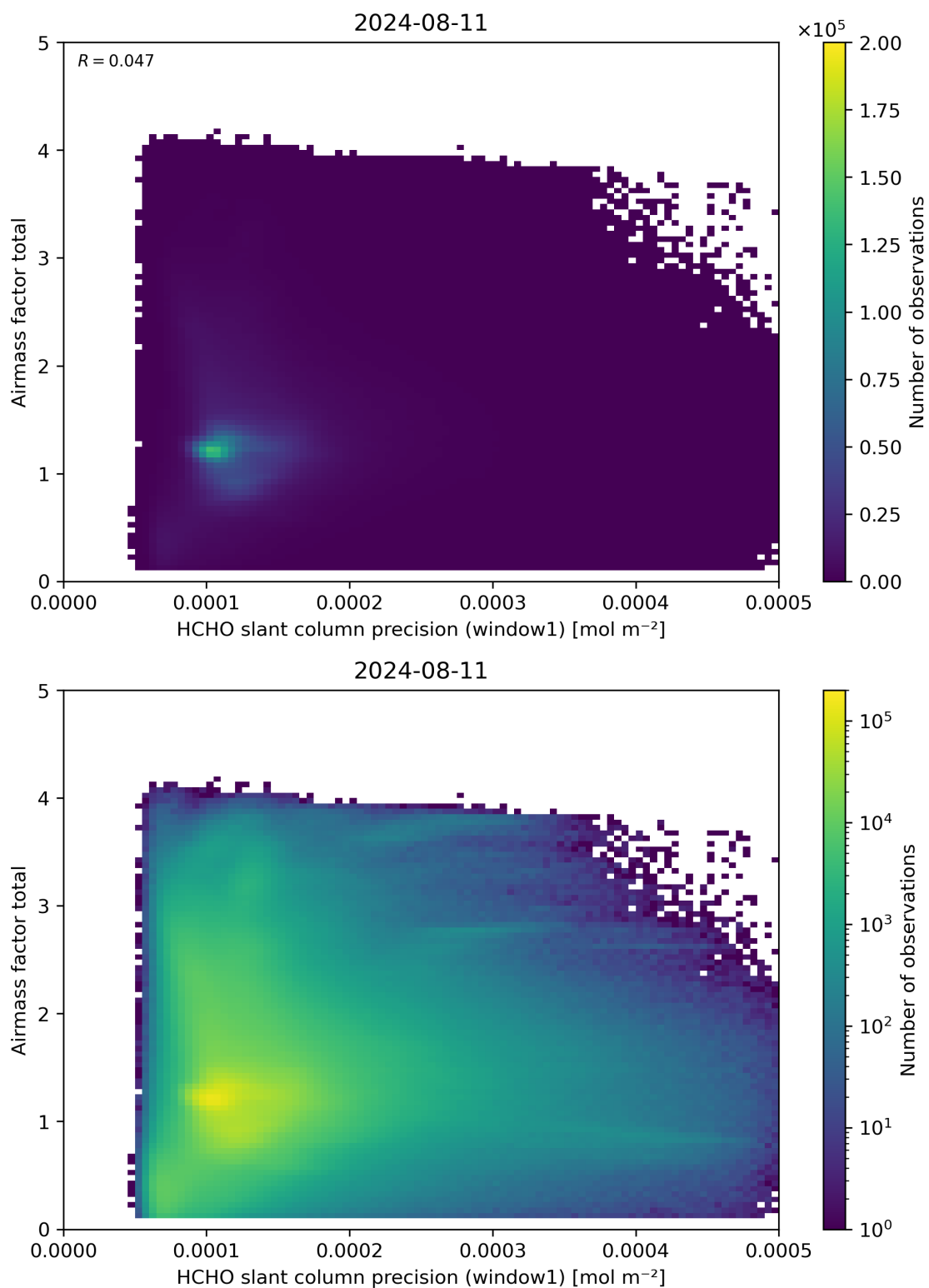
Figure 94: Scatter density plot of “HCHO slant column precision (window1)” against “Airmass factor total” for 2024-08-11 to 2024-08-11.
