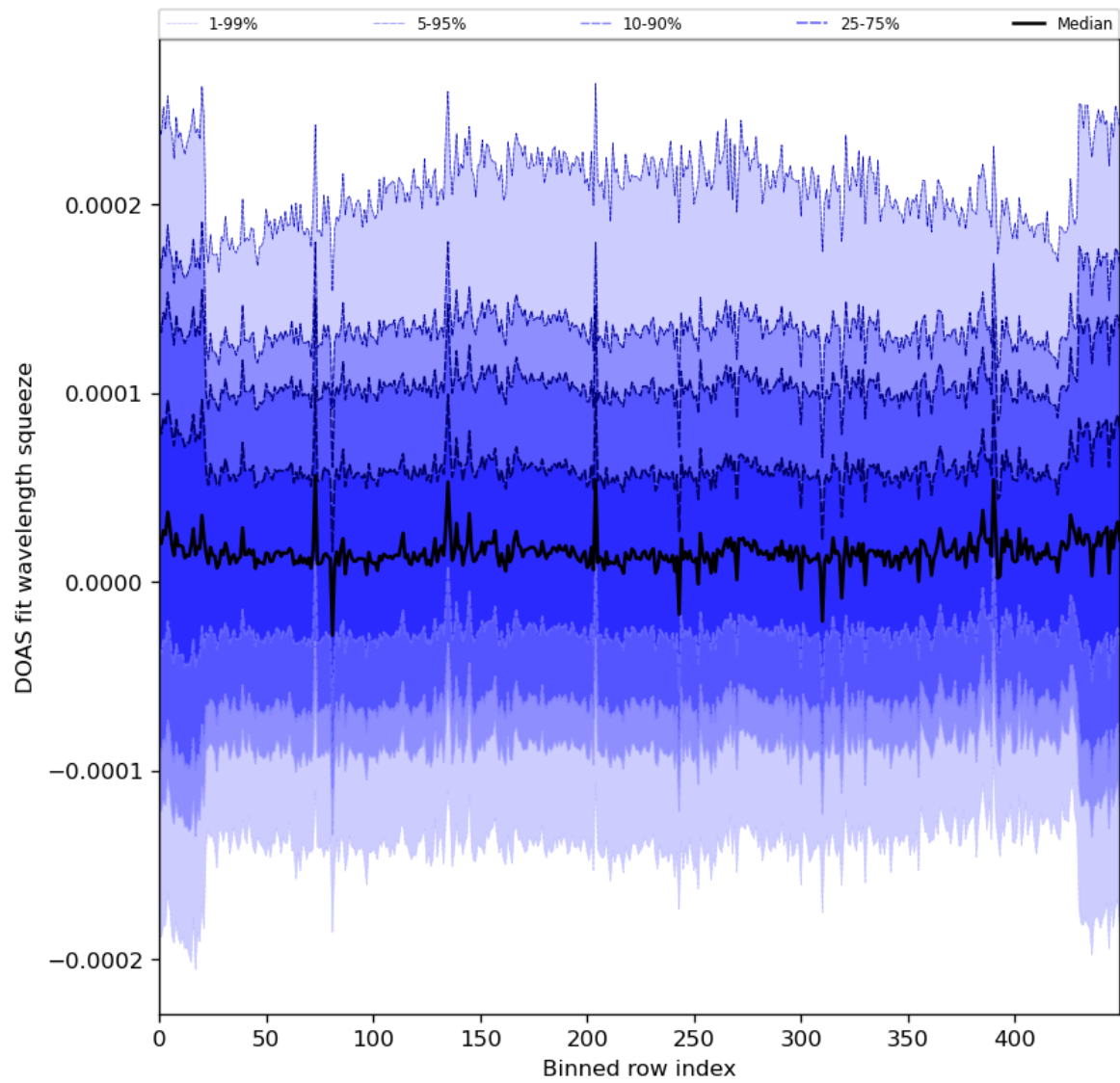
Figure 59: Along track statistics of “DOAS fit wavelength squeeze” for 2024-08-11 to 2024-08-11
