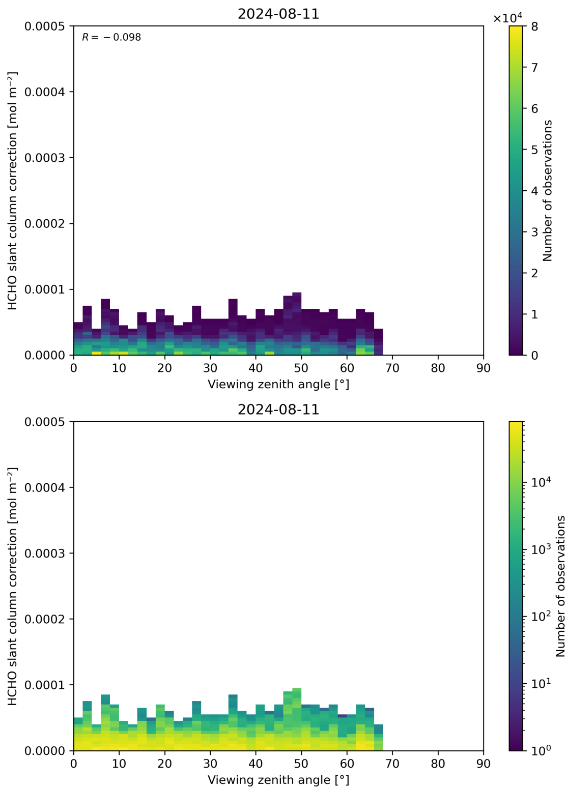
Figure 187: Scatter density plot of “Viewing zenith angle” against “HCHO slant column correction” for 2024-08-11 to 2024-08-11.
