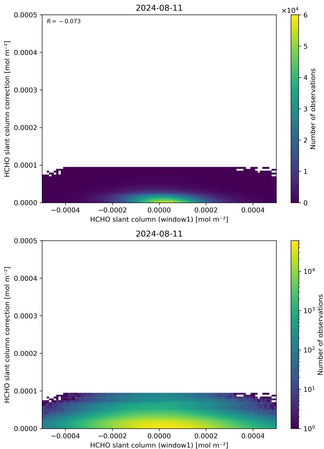
Figure 83: Scatter density plot of “HCHO slant column (window1)” against “HCHO slant column correction” for 2024-08-11 to 2024-08-11.
