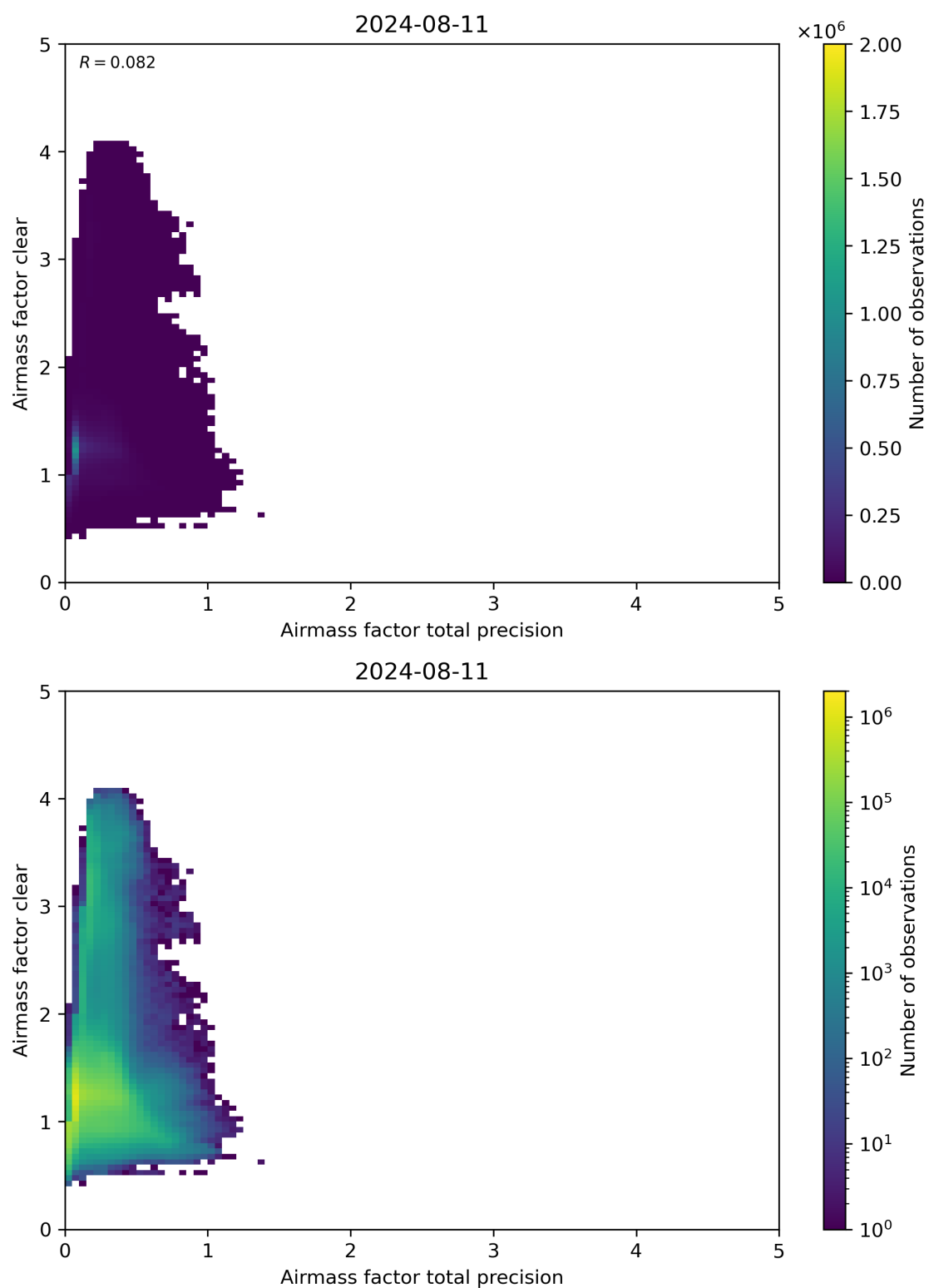
Figure 108: Scatter density plot of “Airmass factor total precision” against “Airmass factor clear” for 2024-08-11 to 2024-08-11.
