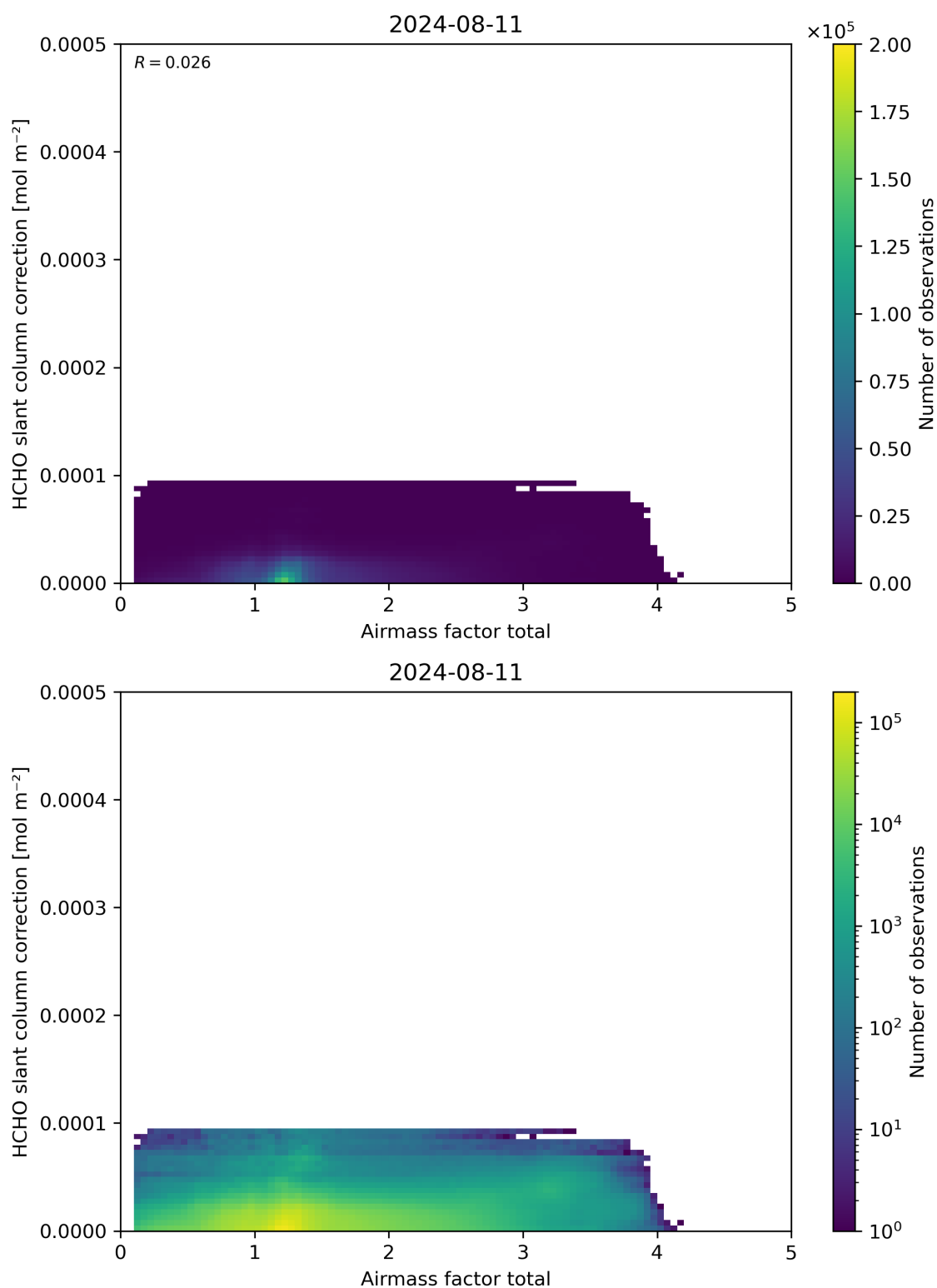
Figure 102: Scatter density plot of “Airmass factor total” against “HCHO slant column correction” for 2024-08-11 to 2024-08-11.
