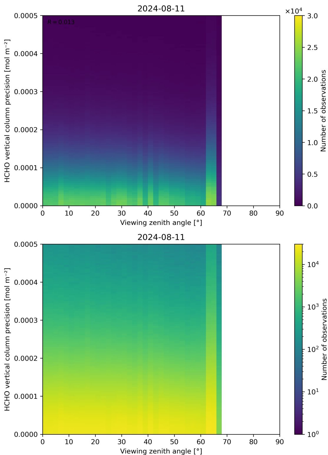
Figure 194: Scatter density plot of “Viewing zenith angle” against “HCHO vertical column precision” for 2024-08-11 to 2024-08-11.
