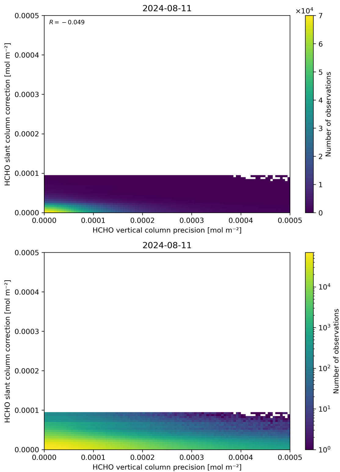
Figure 141: Scatter density plot of “HCHO vertical column precision” against “HCHO slant column correction” for 2024-08-11 to 2024-08-11.
