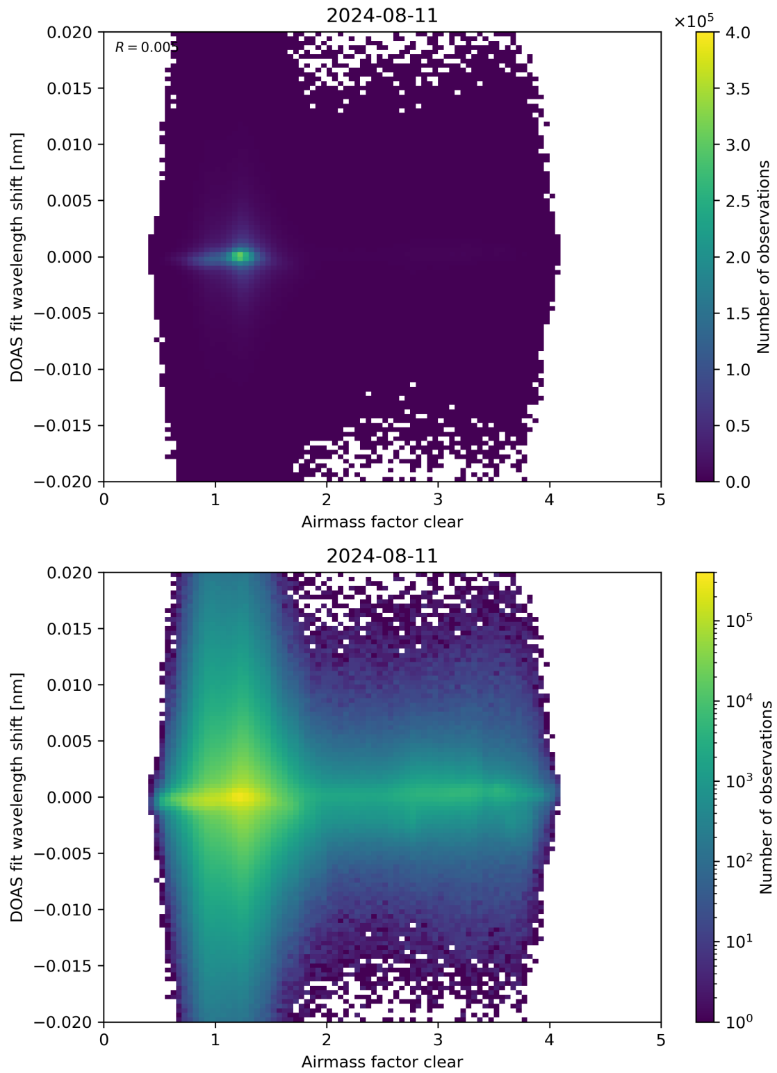
Figure 72: Scatter density plot of “Airmass factor clear” against “DOAS fit wavelength shift” for 2024-08-11 to 2024-08-11.
