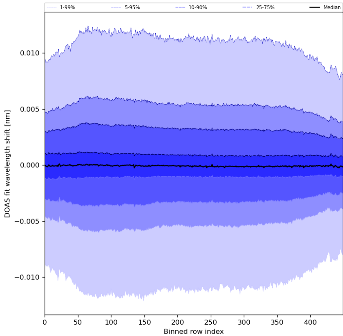
Figure 58: Along track statistics of “DOAS fit wavelength shift” for 2024-08-11 to 2024-08-11
