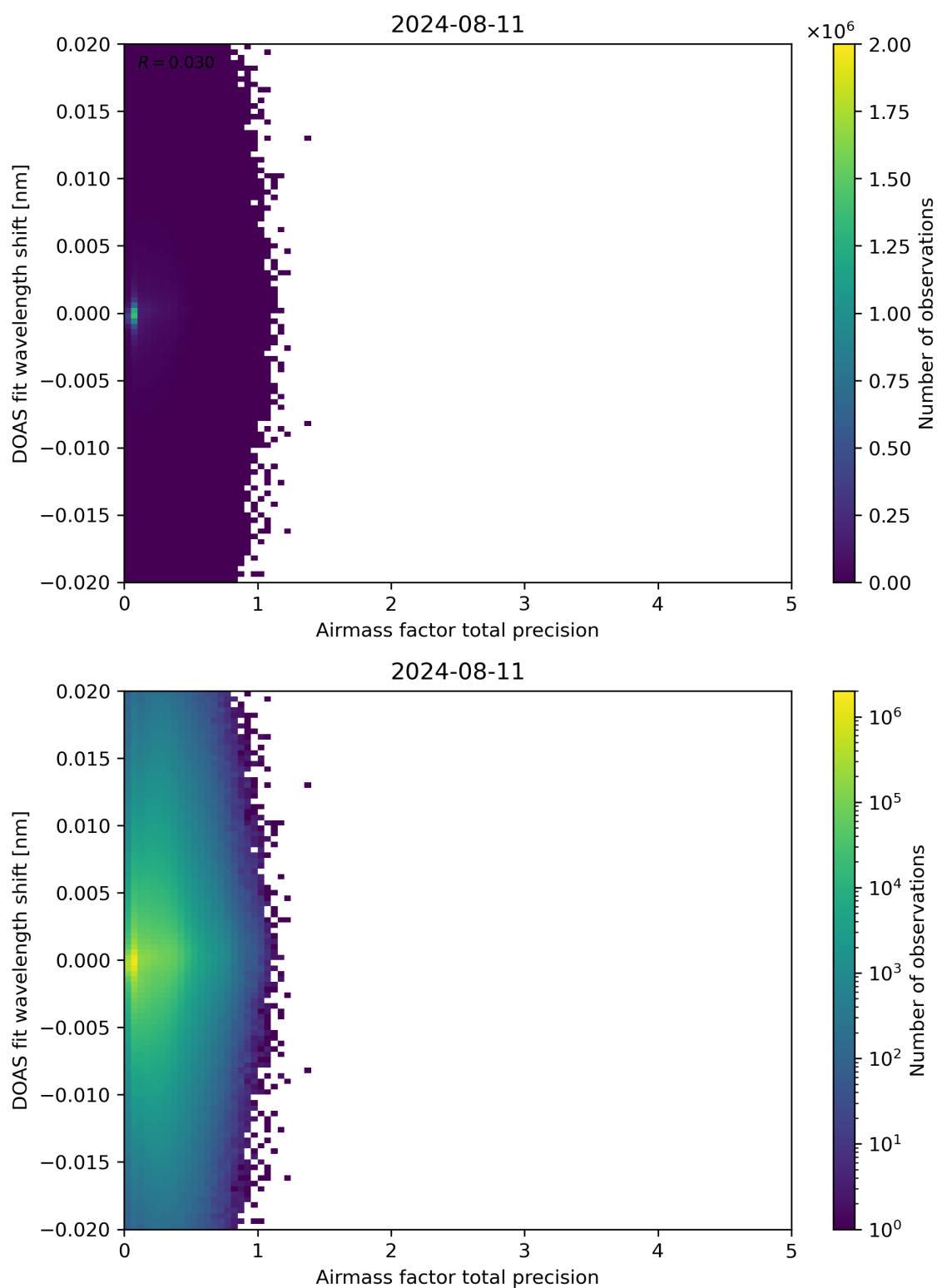
Figure 106: Scatter density plot of “Airmass factor total precision” against “DOAS fit wavelength shift” for 2024-08-11 to 2024-08-11.
