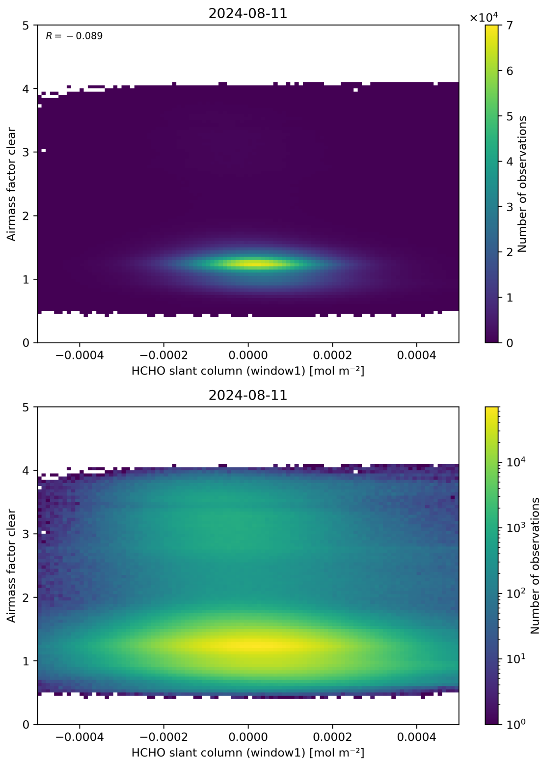
Figure 81: Scatter density plot of “HCHO slant column (window1)” against “Airmass factor clear” for 2024-08-11 to 2024-08-11.
