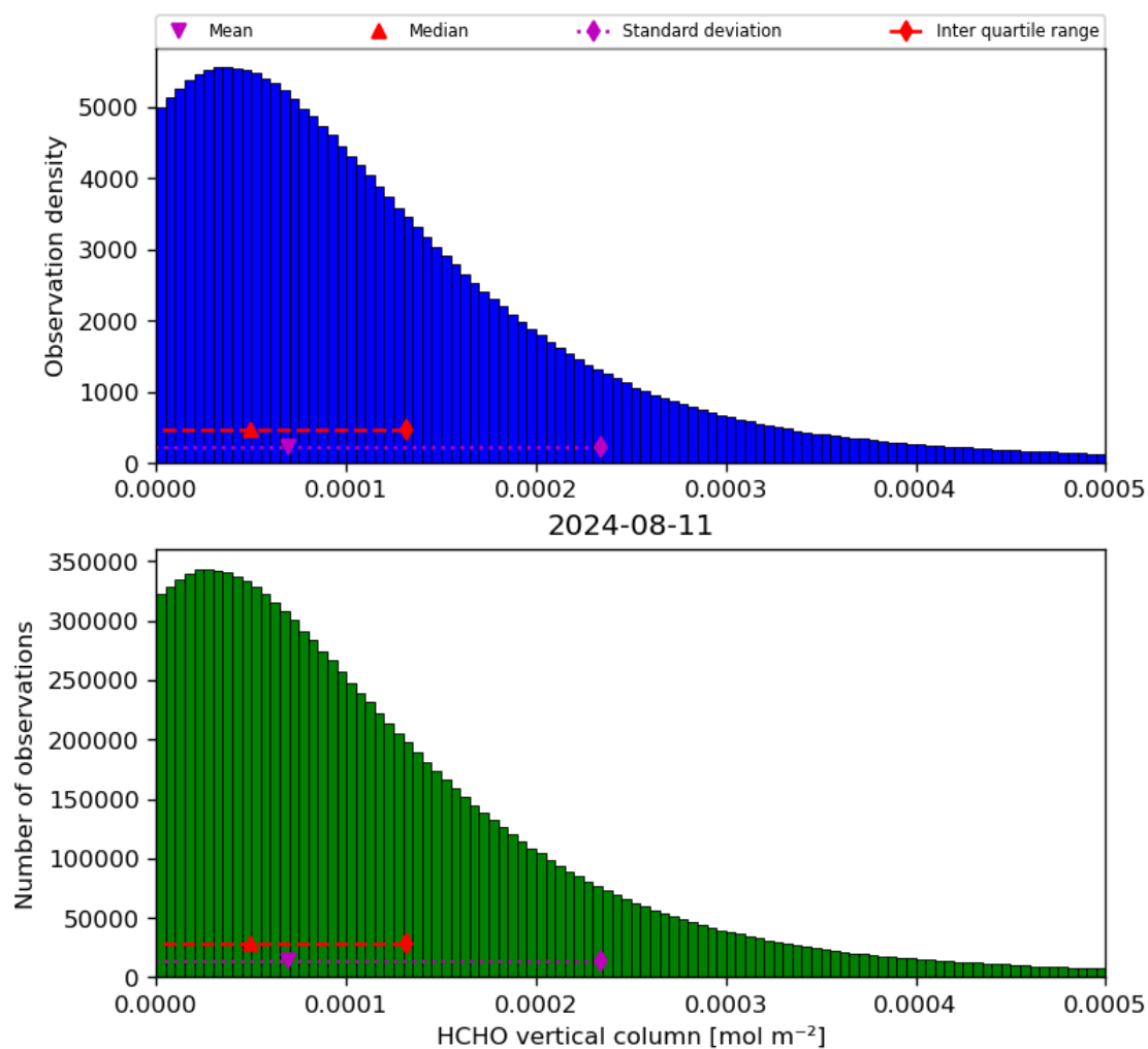
Figure 35: Histogram of “HCHO vertical column” for 2024-08-11 to 2024-08-11
