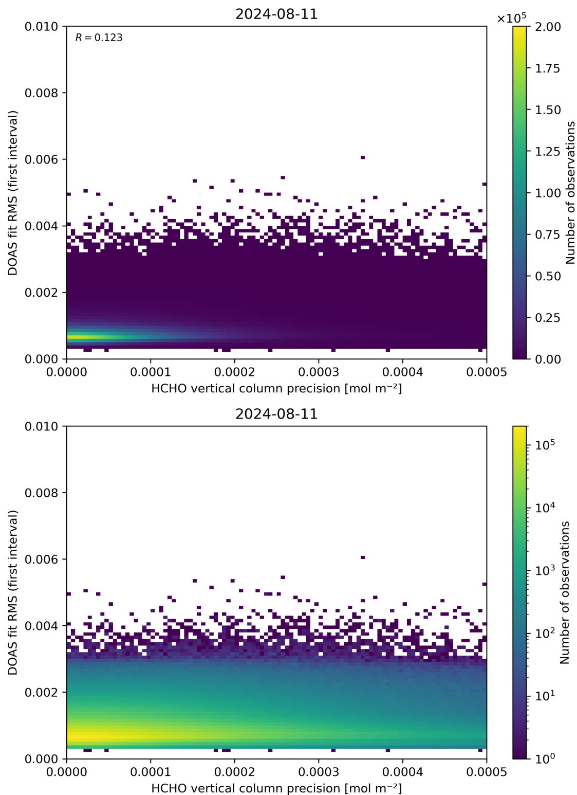
Figure 136: Scatter density plot of “HCHO vertical column precision” against “DOAS fit RMS (first interval)” for 2024-08-11 to 2024-08-11.
