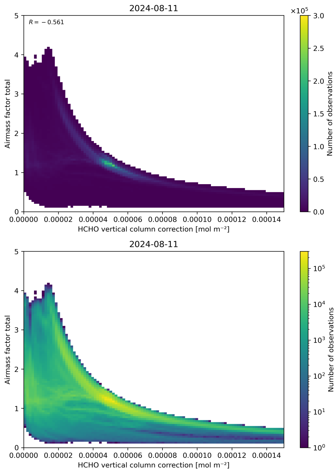
Figure 120: Scatter density plot of “HCHO vertical column correction” against “Airmass factor total” for 2024-08-11 to 2024-08-11.
