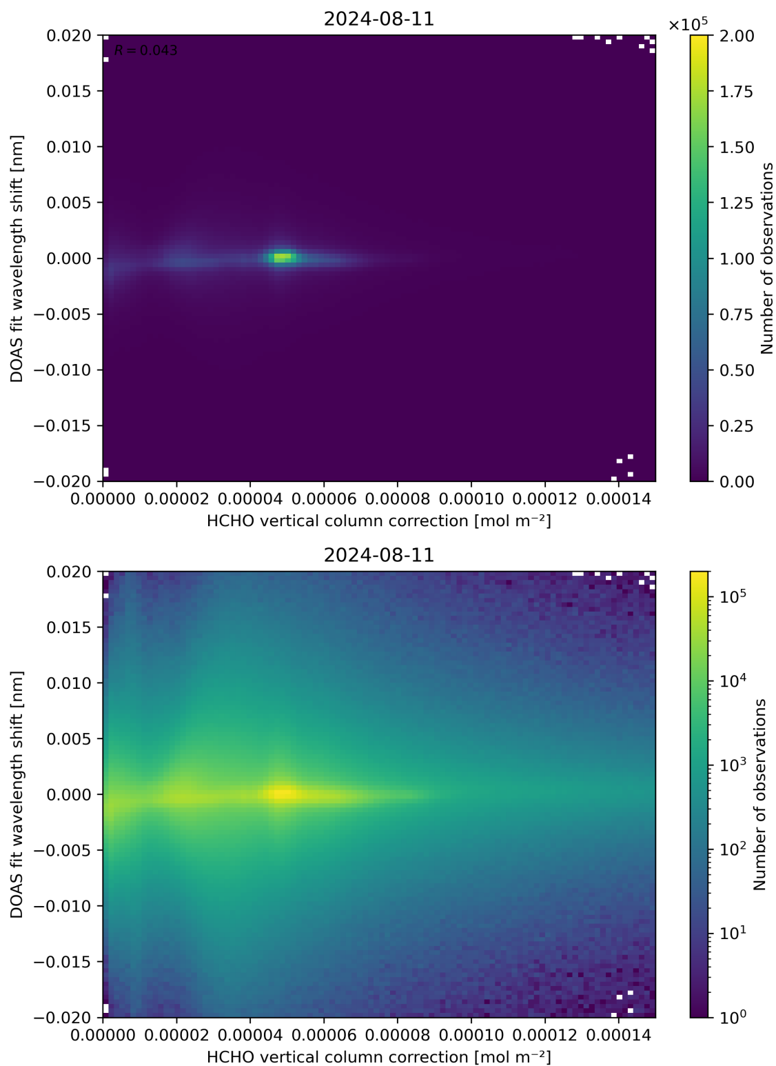
Figure 113: Scatter density plot of “HCHO vertical column correction” against “DOAS fit wavelength shift” for 2024-08-11 to 2024-08-11.
