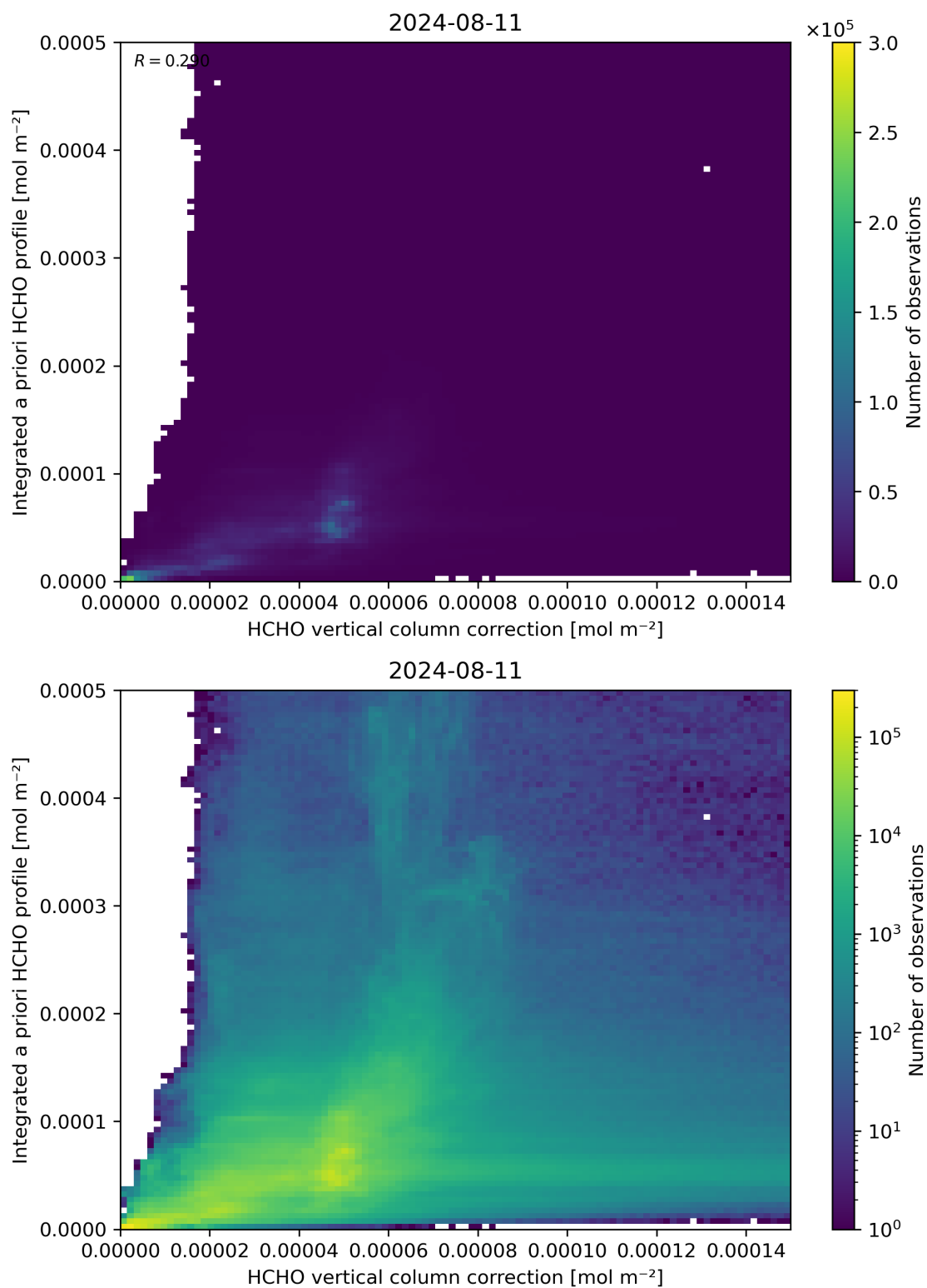
Figure 122: Scatter density plot of “HCHO vertical column correction” against “Integrated a priori HCHO profile” for 2024-08-11 to 2024-08-11.
