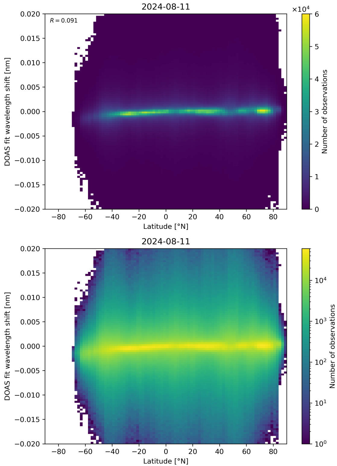
Figure 154: Scatter density plot of “Latitude” against “DOAS fit wavelength shift” for 2024-08-11 to 2024-08-11.
