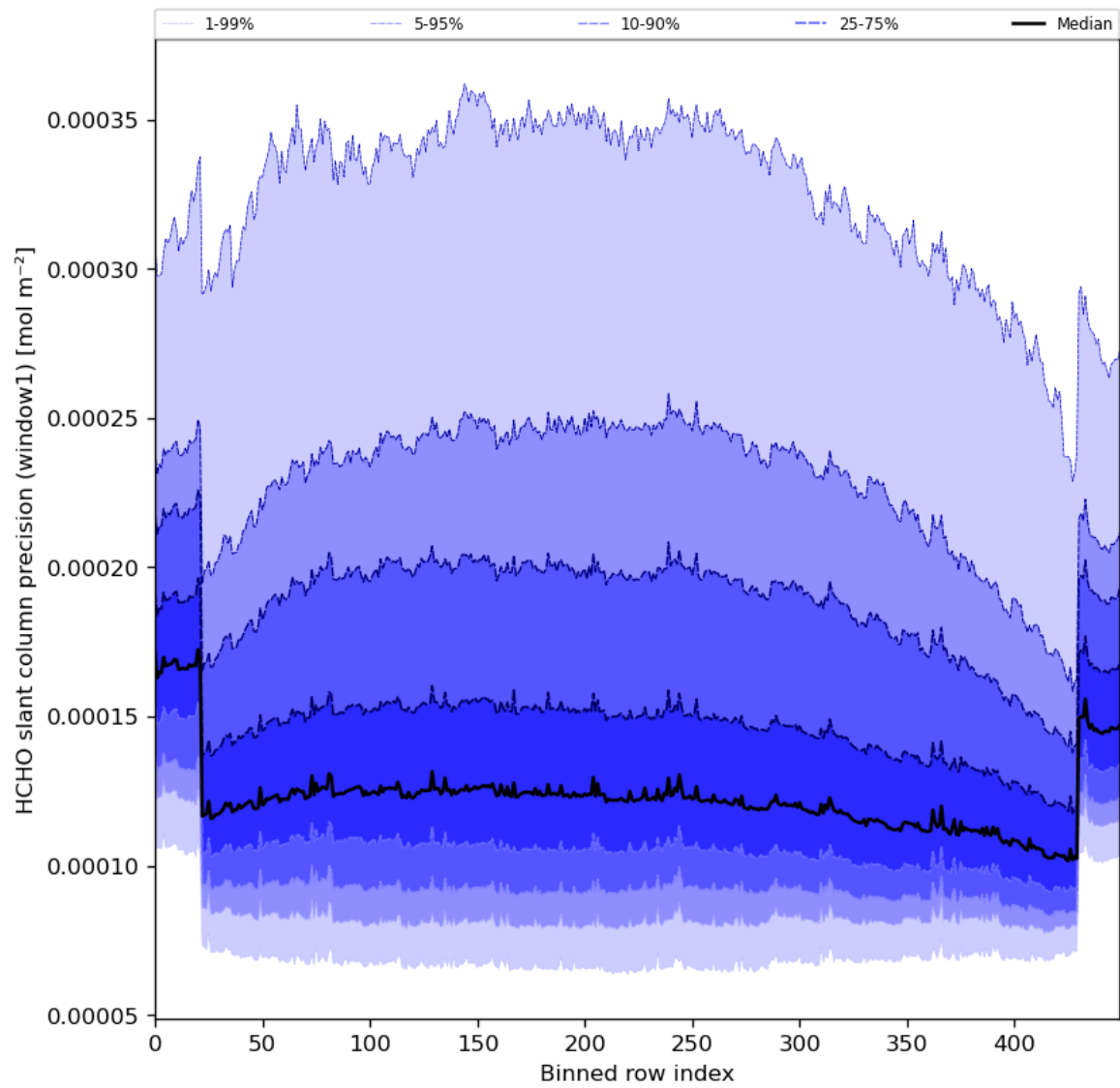
Figure 53: Along track statistics of “HCHO slant column precision (window1)” for 2024-08-11 to 2024-08-11
