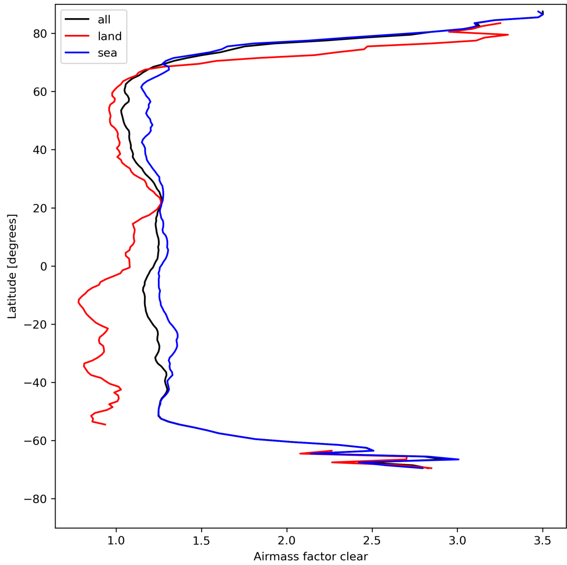
Figure 28: Zonal average of “Airmass factor clear” for 2024-08-11 to 2024-08-11.
