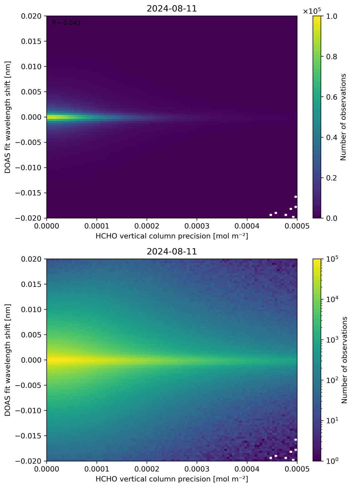
Figure 137: Scatter density plot of “HCHO vertical column precision” against “DOAS fit wavelength shift” for 2024-08-11 to 2024-08-11.
