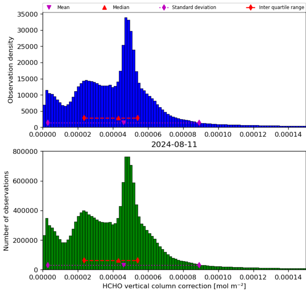
Figure 37: Histogram of “HCHO vertical column correction” for 2024-08-11 to 2024-08-11
