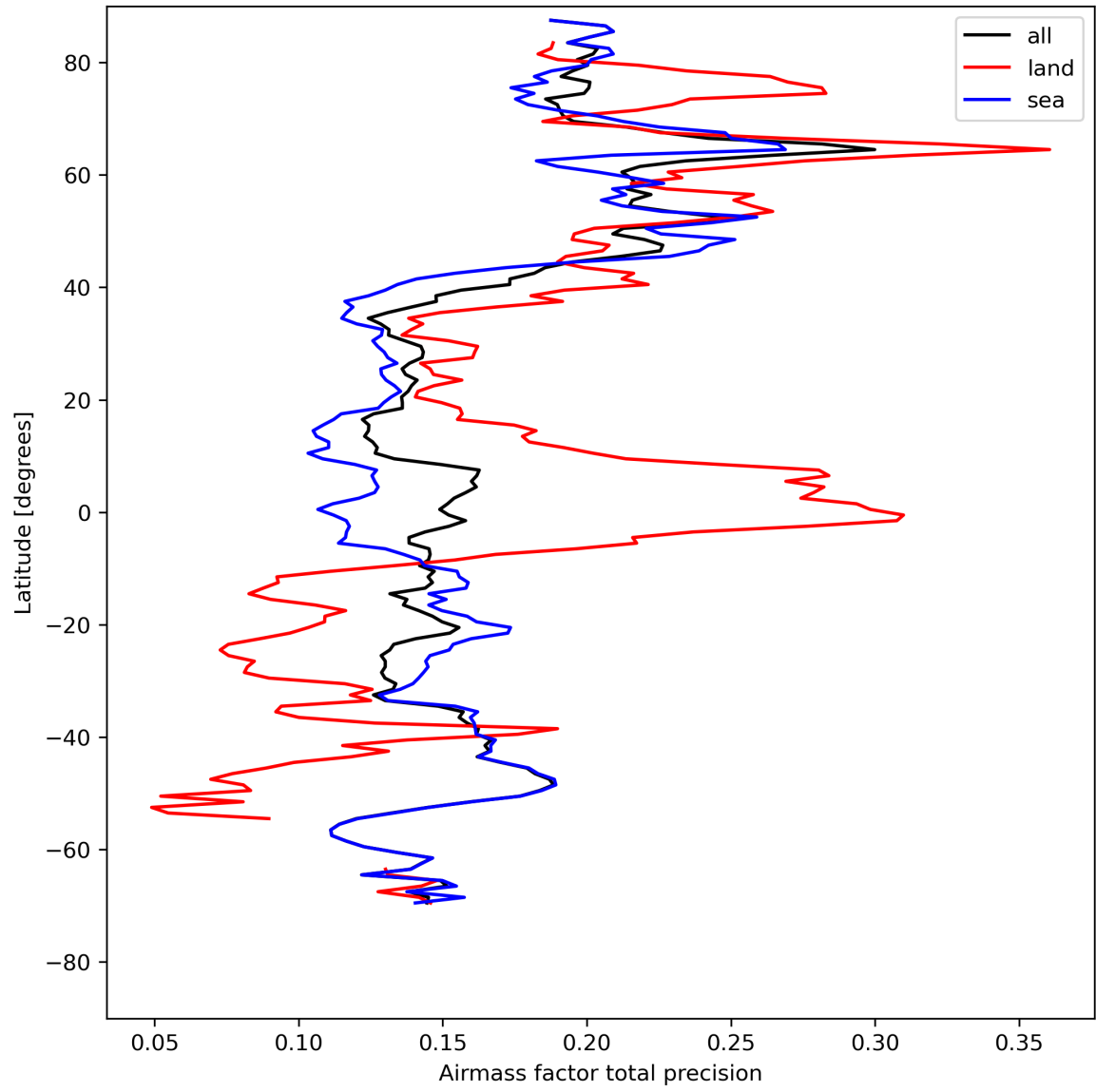
Figure 27: Zonal average of “Airmass factor total precision” for 2024-08-11 to 2024-08-11.
