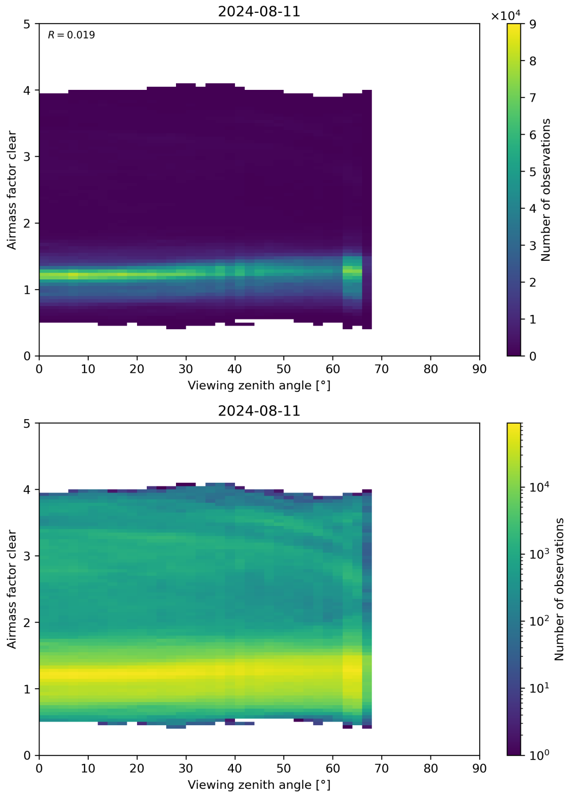
Figure 185: Scatter density plot of “Viewing zenith angle” against “Airmass factor clear” for 2024-08-11 to 2024-08-11.
