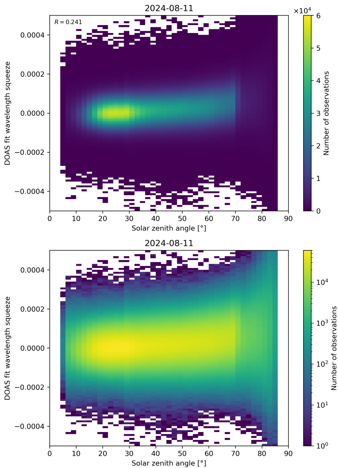
Figure 169: Scatter density plot of “Solar zenith angle” against “DOAS fit wavelength squeeze” for 2024-08-11 to 2024-08-11.
