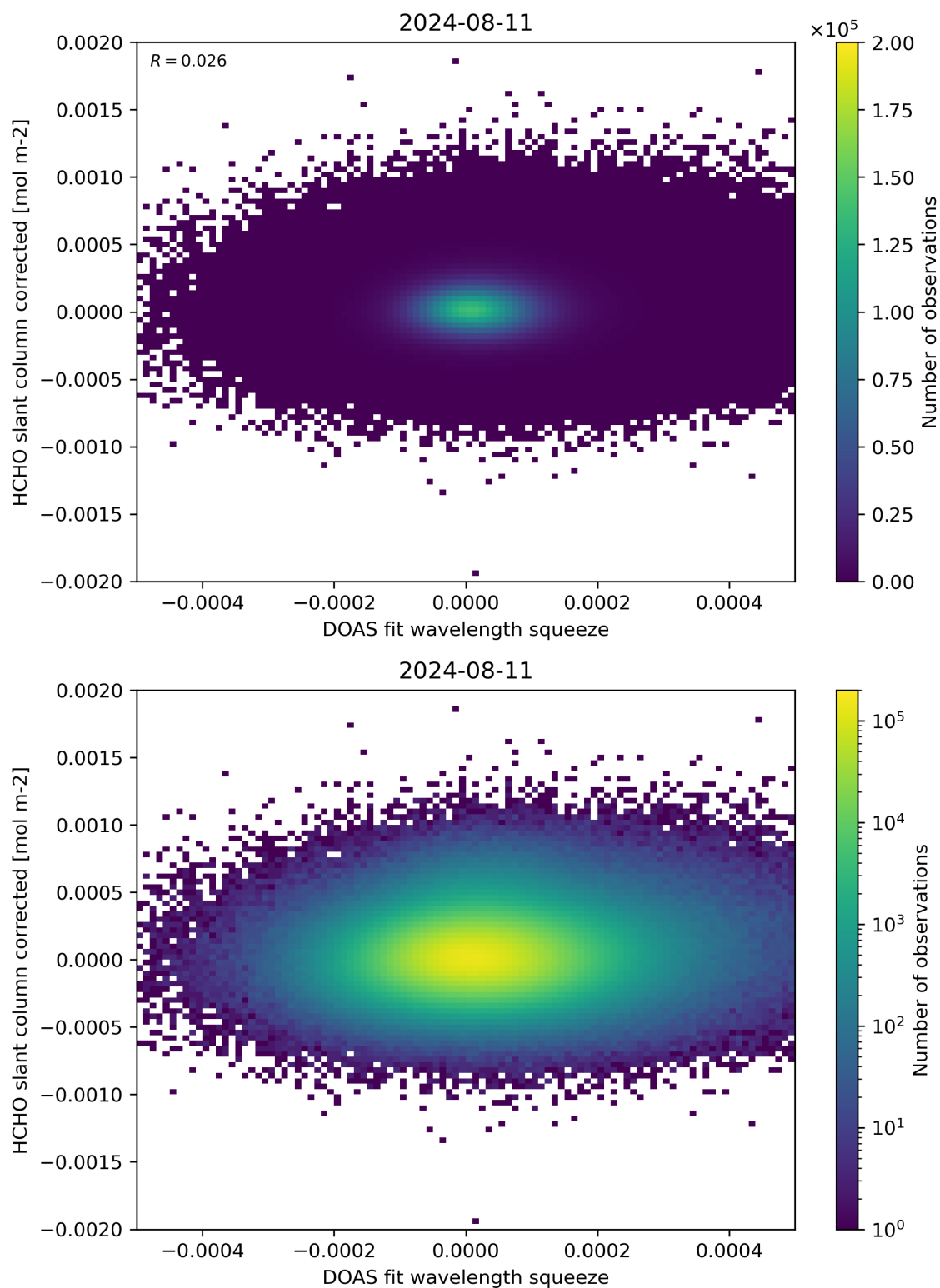
Figure 69: Scatter density plot of “DOAS fit wavelength squeeze” against “HCHO slant column corrected” for 2024-08-11 to 2024-08-11.
