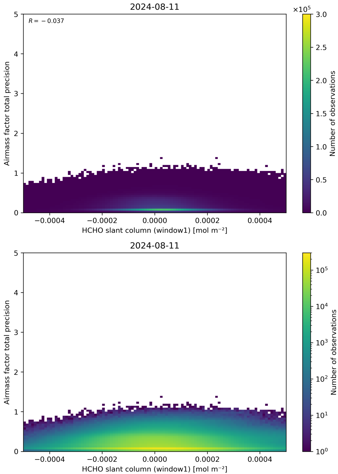
Figure 86: Scatter density plot of “HCHO slant column (window1)” against “Airmass factor total precision” for 2024-08-11 to 2024-08-11.
