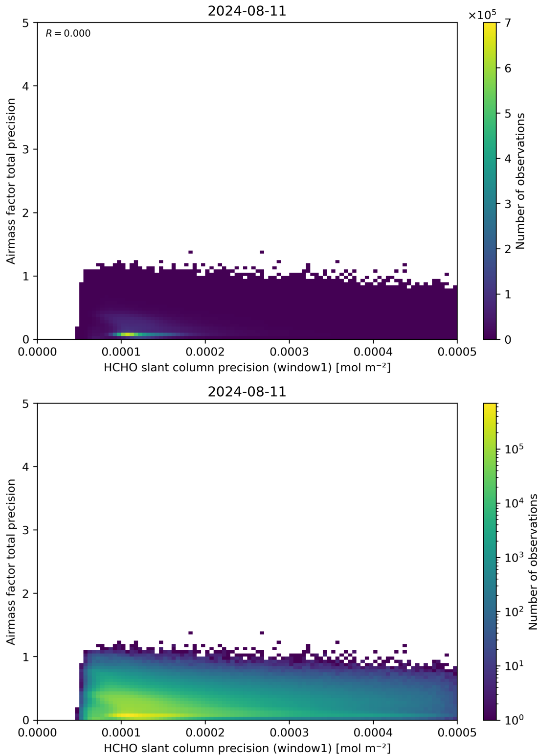
Figure 95: Scatter density plot of “HCHO slant column precision (window1)” against “Airmass factor total precision” for 2024-08-11 to 2024-08-11.
