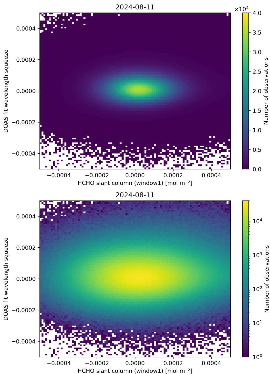
Figure 80: Scatter density plot of “HCHO slant column (window1)” against “DOAS fit wavelength squeeze” for 2024-08-11 to 2024-08-11.
