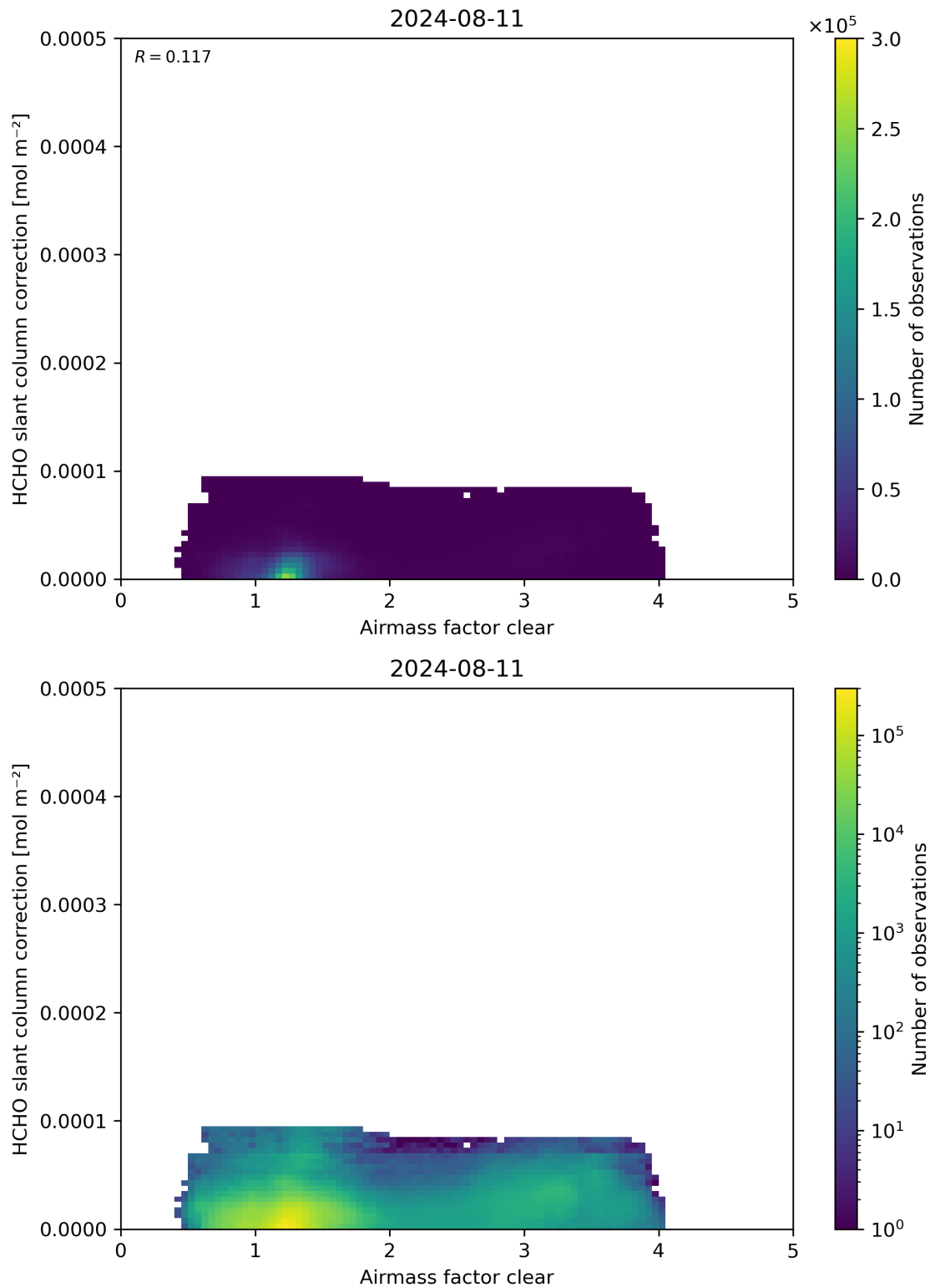
Figure 75: Scatter density plot of “Airmass factor clear” against “HCHO slant column correction” for 2024-08-11 to 2024-08-11.
