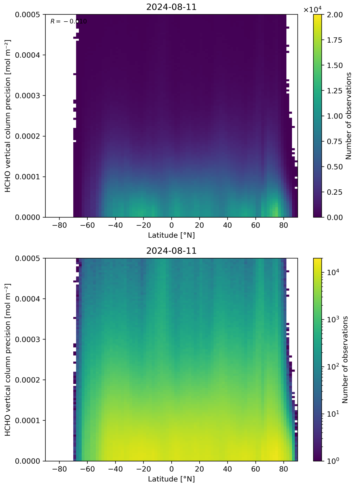
Figure 165: Scatter density plot of “Latitude” against “HCHO vertical column precision” for 2024-08-11 to 2024-08-11.
