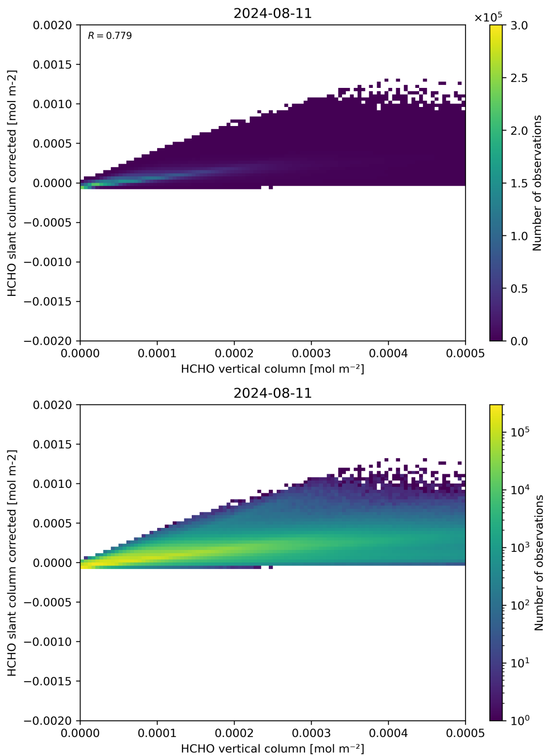
Figure 127: Scatter density plot of “HCHO vertical column” against “HCHO slant column corrected” for 2024-08-11 to 2024-08-11.
