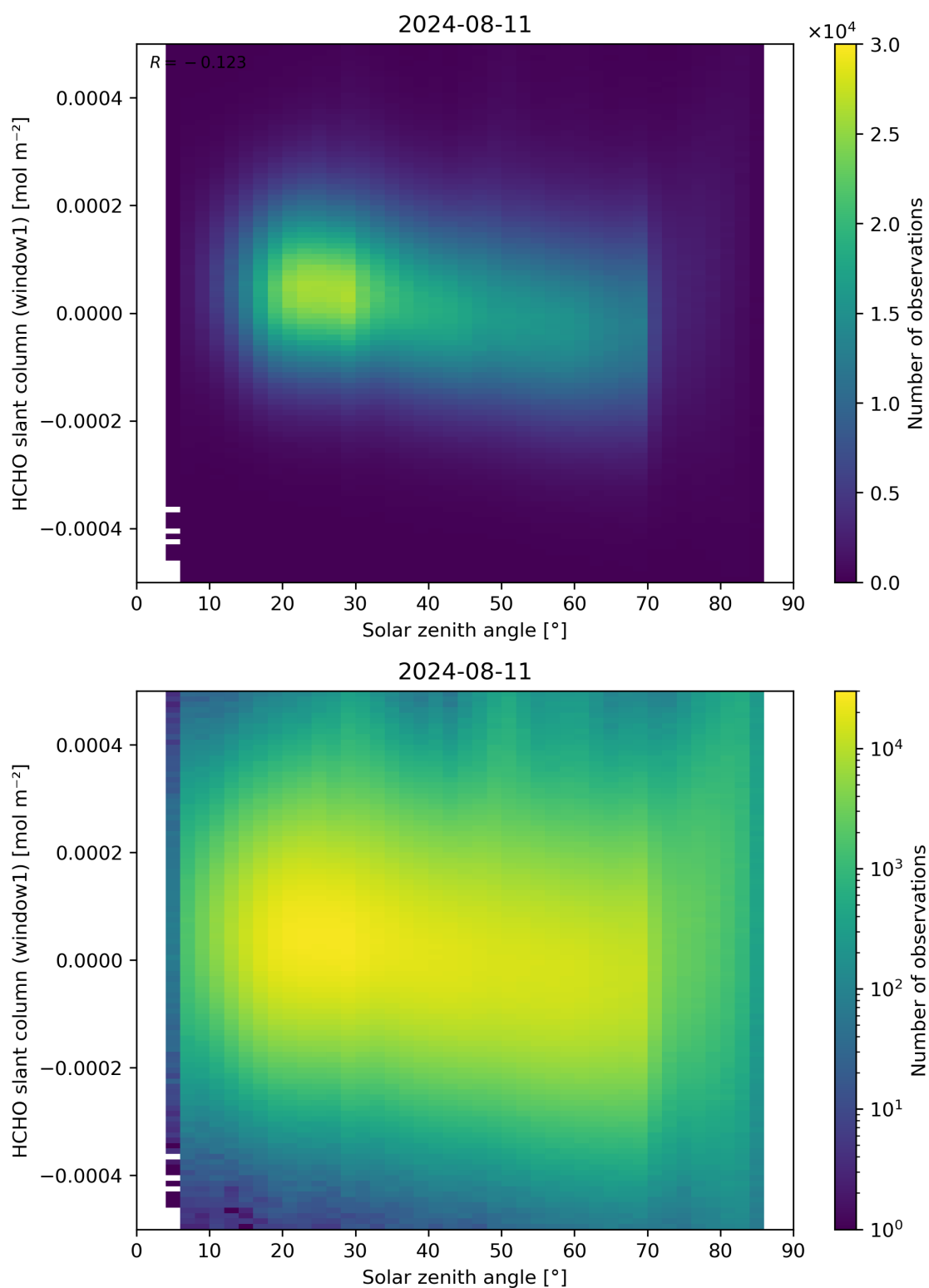
Figure 173: Scatter density plot of “Solar zenith angle” against “HCHO slant column (window1)” for 2024-08-11 to 2024-08-11.
