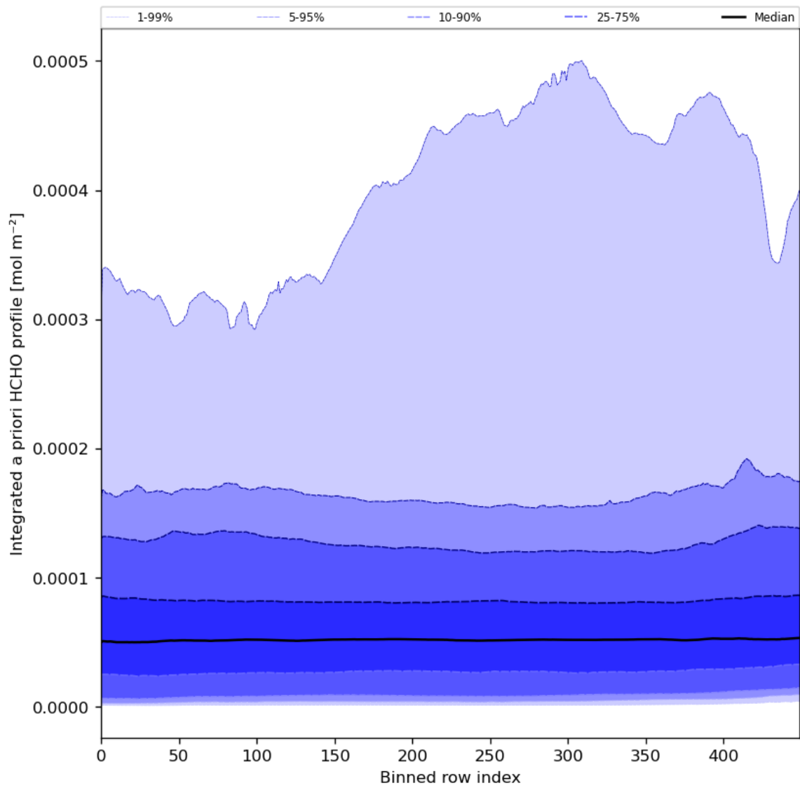
Figure 57: Along track statistics of “Integrated a priori HCHO profile” for 2024-08-11 to 2024-08-11
