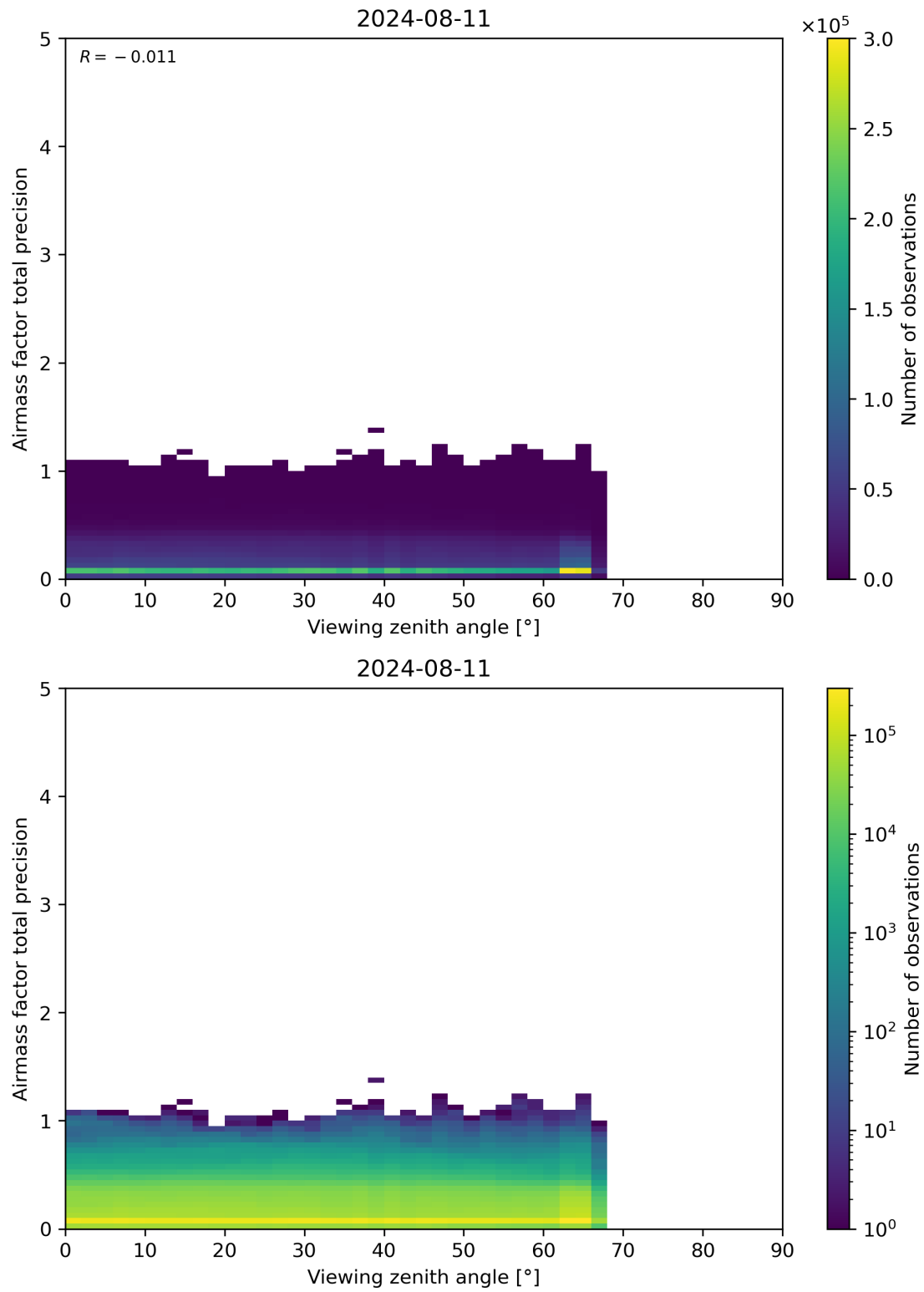
Figure 191: Scatter density plot of “Viewing zenith angle” against “Airmass factor total precision” for 2024-08-11 to 2024-08-11.
