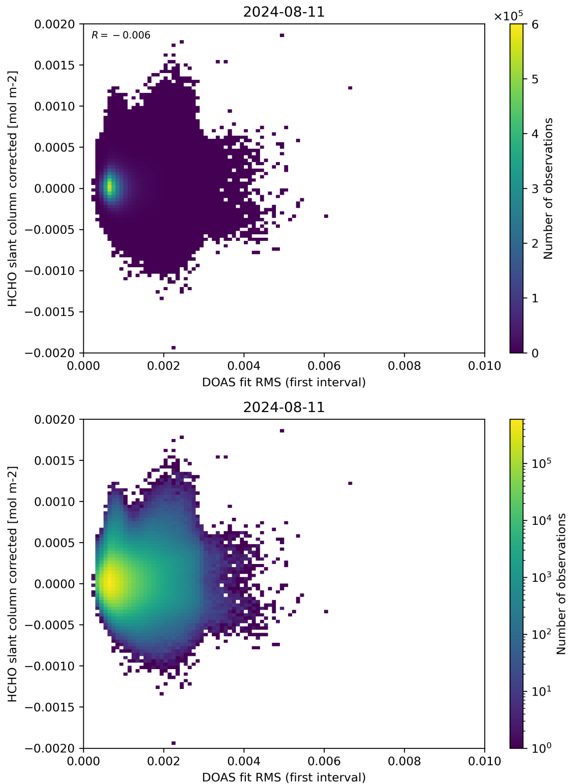
Figure 62: Scatter density plot of “DOAS fit RMS (first interval)” against “HCHO slant column corrected” for 2024-08-11 to 2024-08-11.
