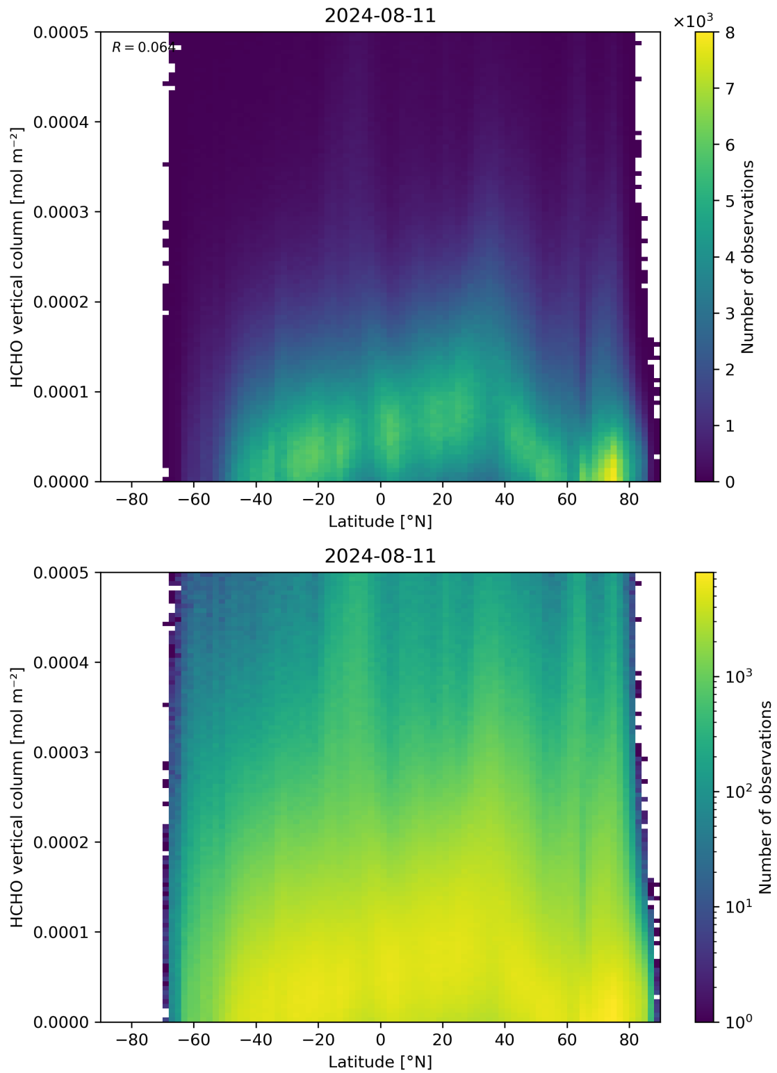
Figure 163: Scatter density plot of “Latitude” against “HCHO vertical column” for 2024-08-11 to 2024-08-11.
