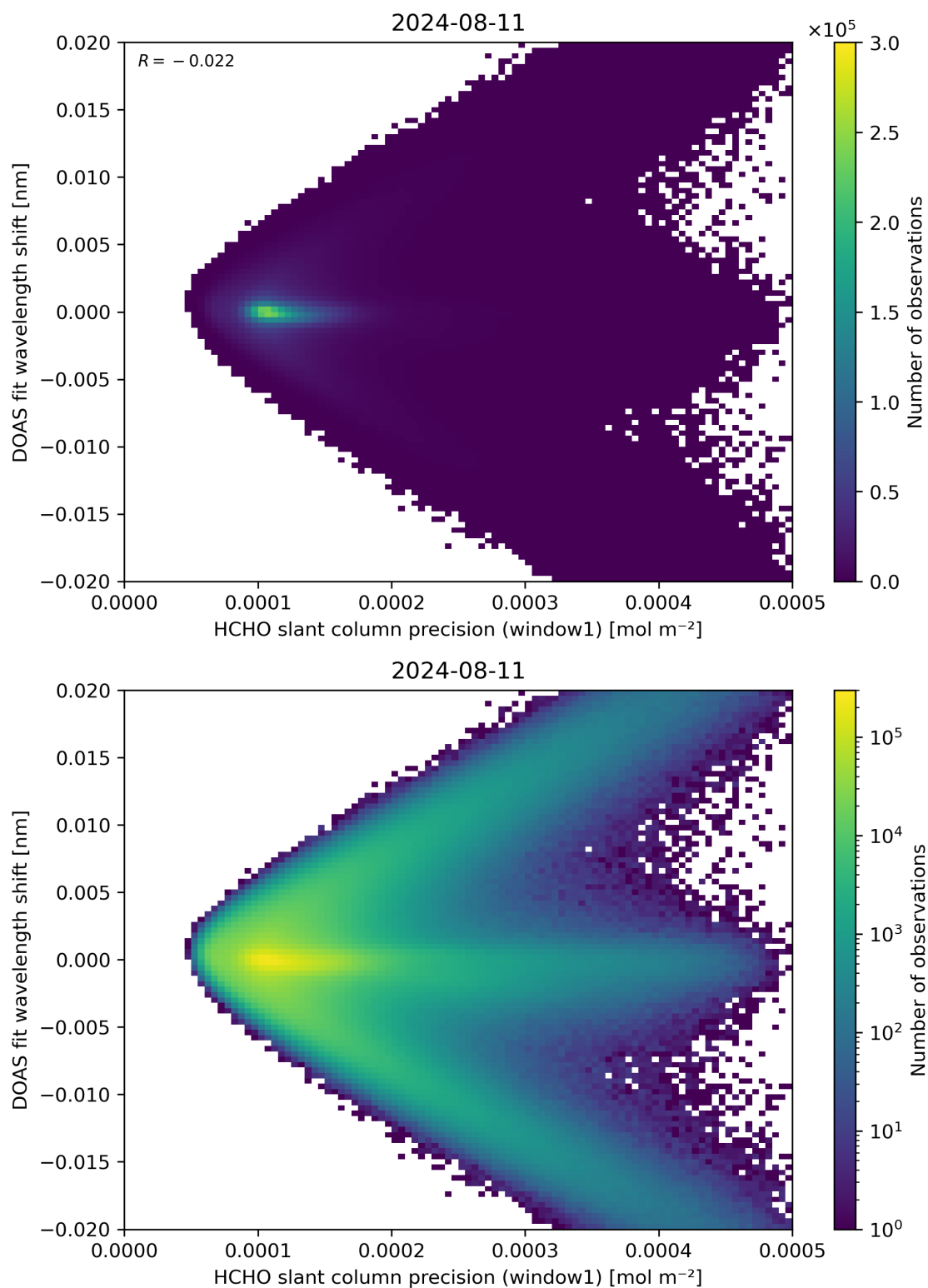
Figure 89: Scatter density plot of “HCHO slant column precision (window1)” against “DOAS fit wavelength shift” for 2024-08-11 to 2024-08-11.
