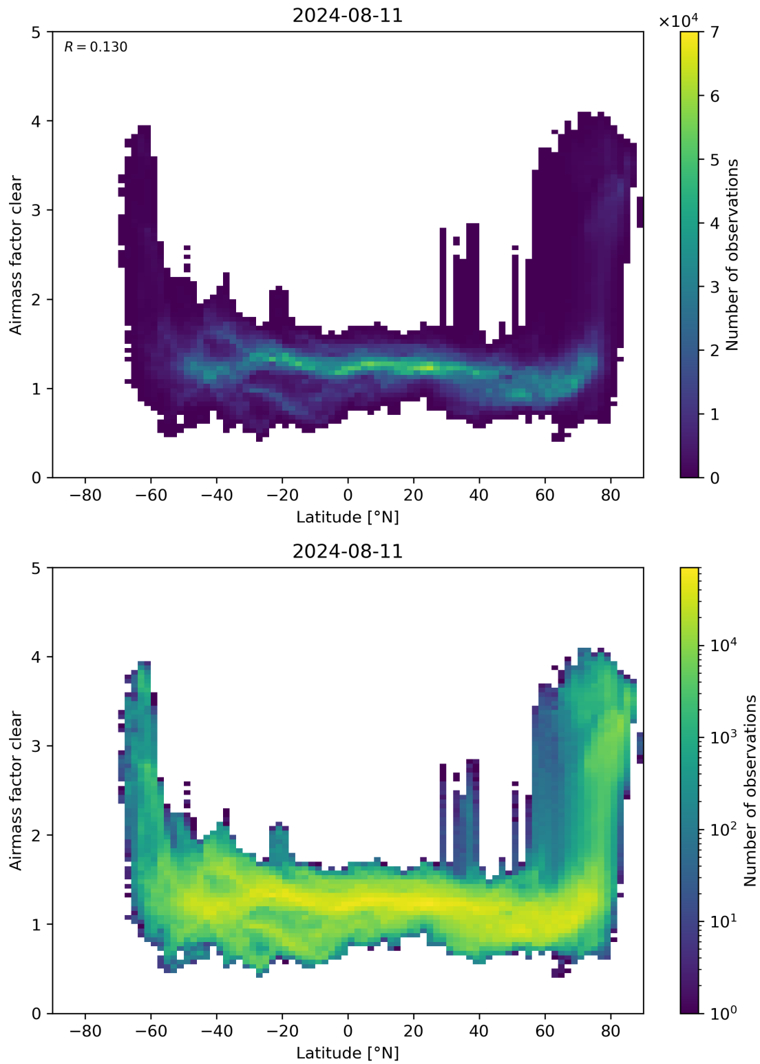
Figure 156: Scatter density plot of “Latitude” against “Airmass factor clear” for 2024-08-11 to 2024-08-11.
