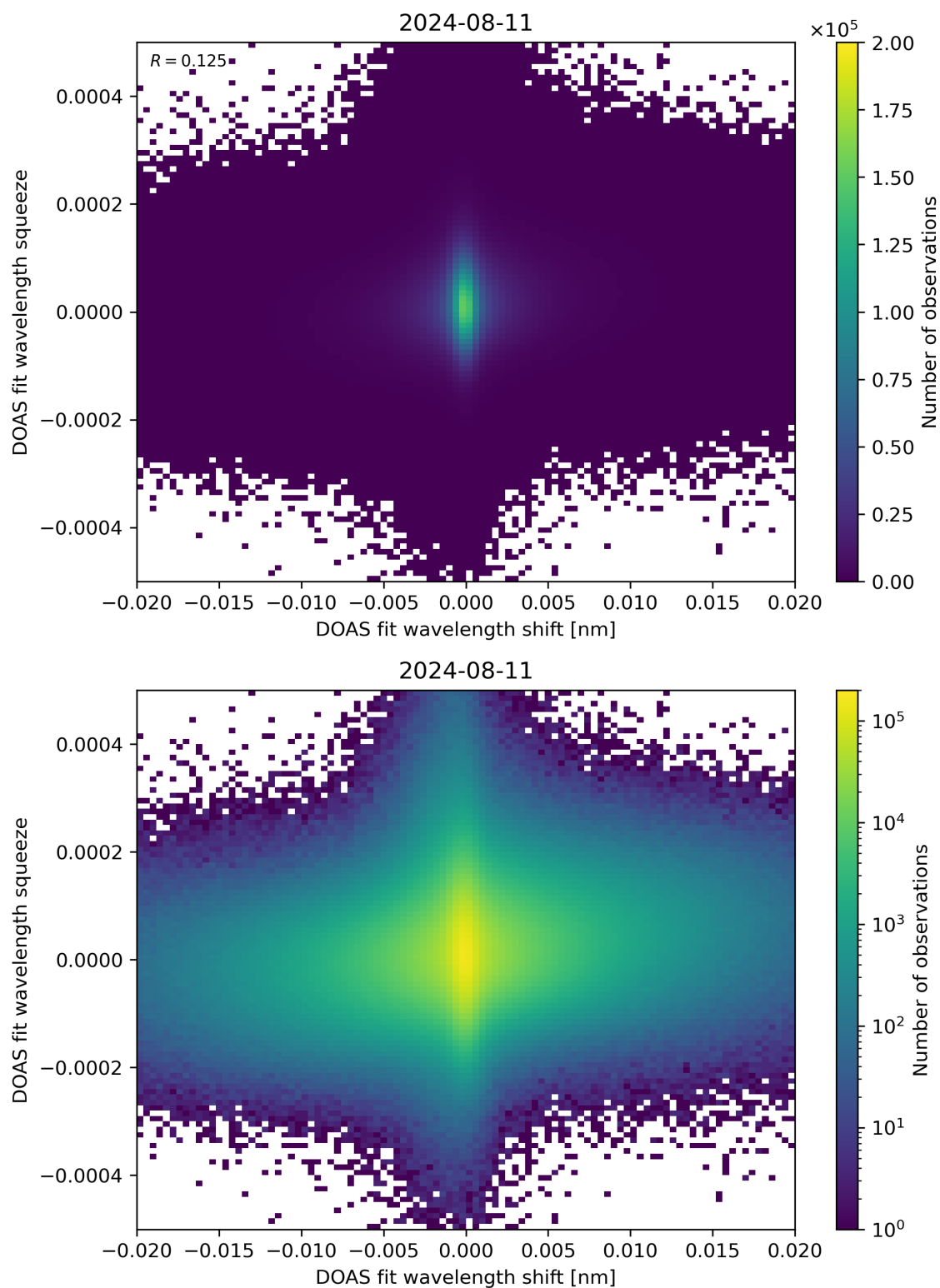
Figure 65: Scatter density plot of “DOAS fit wavelength shift” against “DOAS fit wavelength squeeze” for 2024-08-11 to 2024-08-11.
