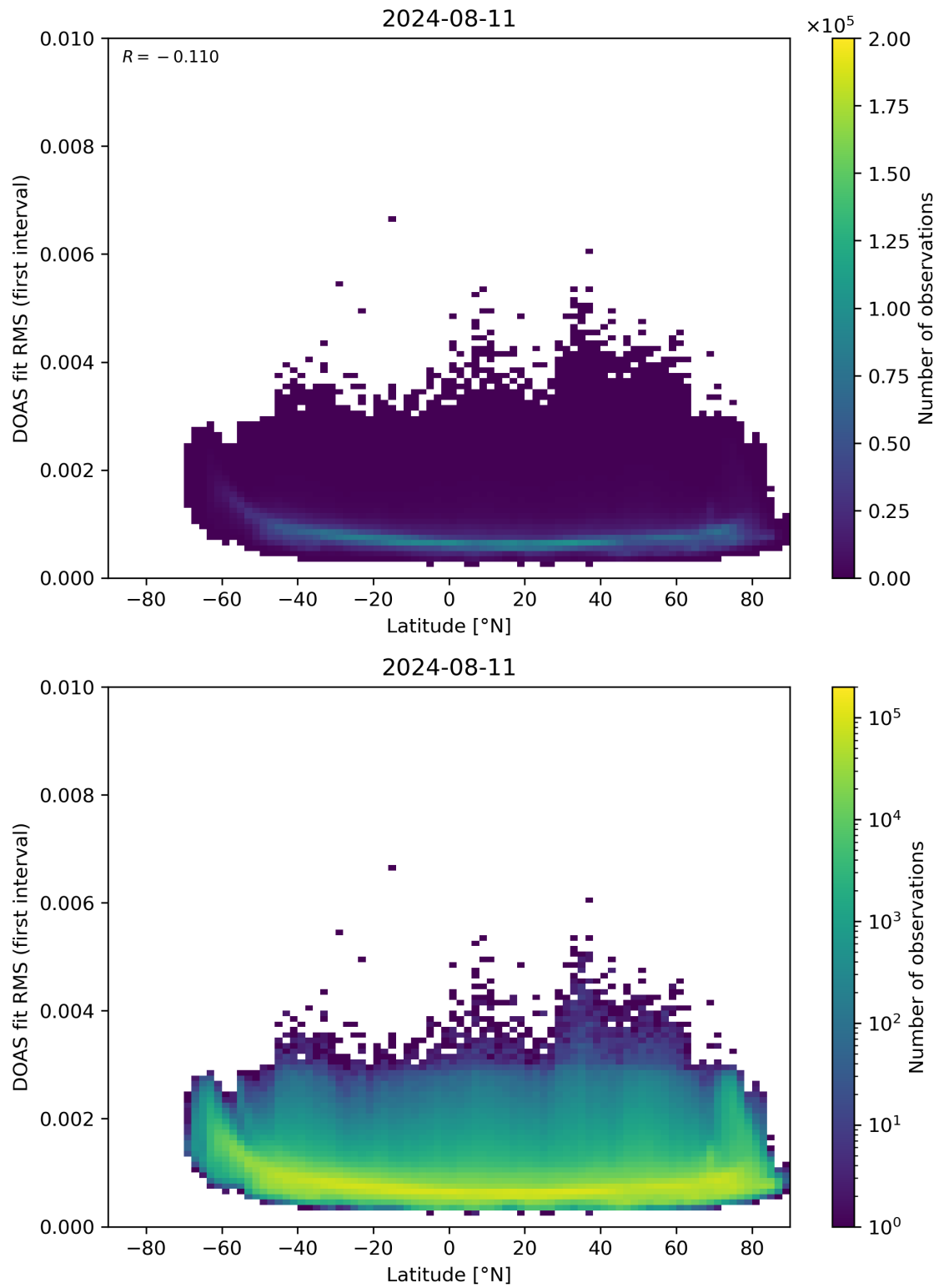
Figure 153: Scatter density plot of “Latitude” against “DOAS fit RMS (first interval)” for 2024-08-11 to 2024-08-11.
