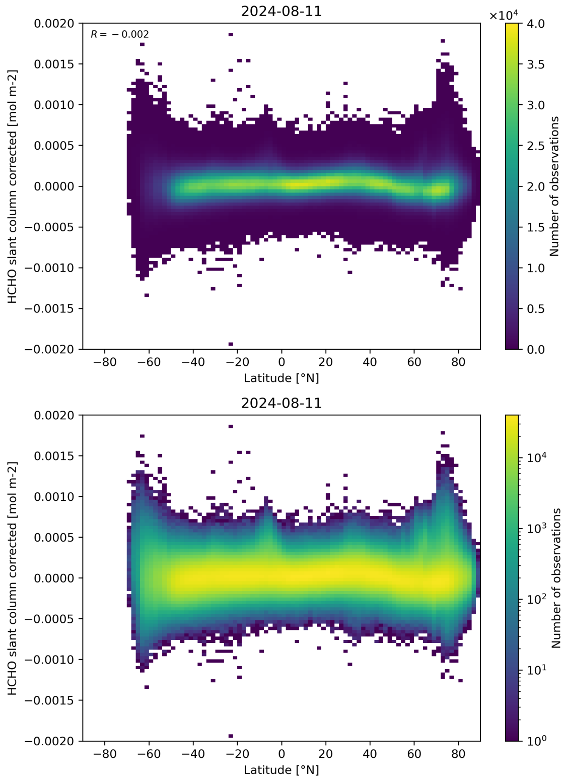
Figure 157: Scatter density plot of “Latitude” against “HCHO slant column corrected” for 2024-08-11 to 2024-08-11.
