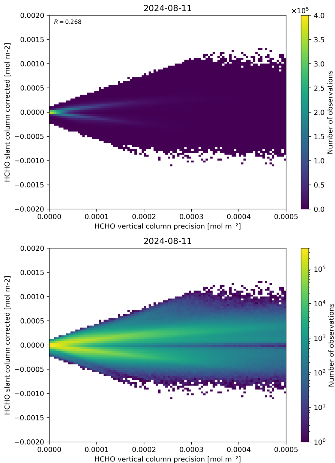
Figure 140: Scatter density plot of “HCHO vertical column precision” against “HCHO slant column corrected” for 2024-08-11 to 2024-08-11.
