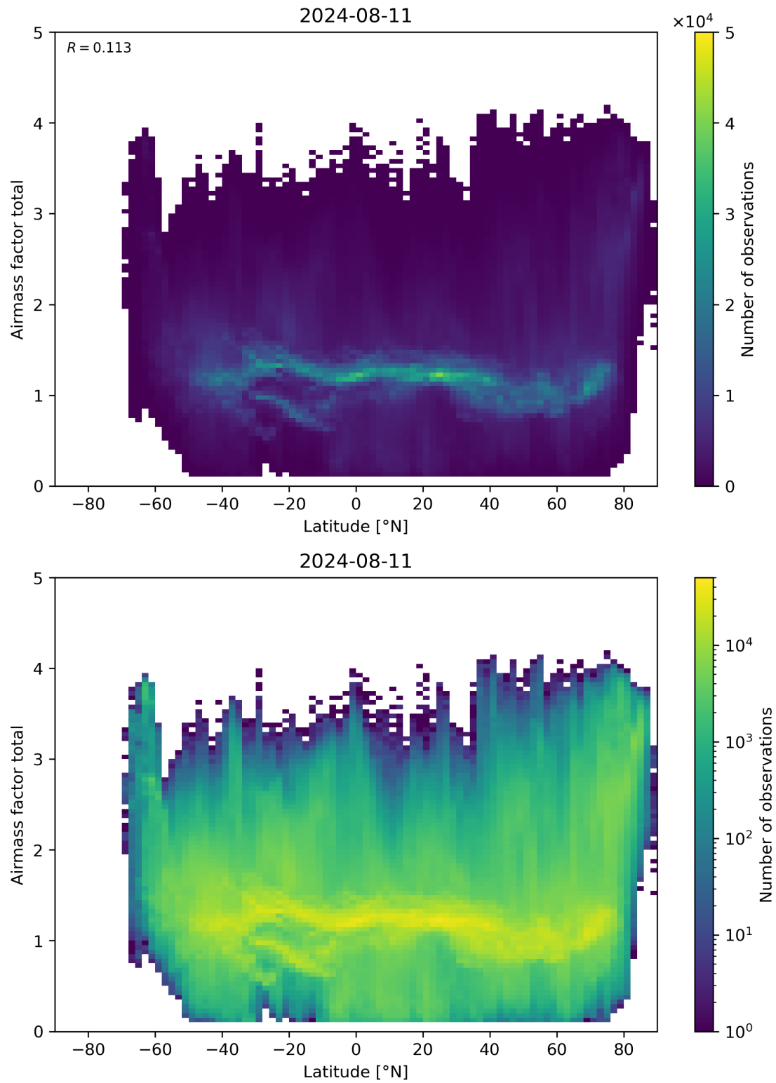
Figure 161: Scatter density plot of “Latitude” against “Airmass factor total” for 2024-08-11 to 2024-08-11.
