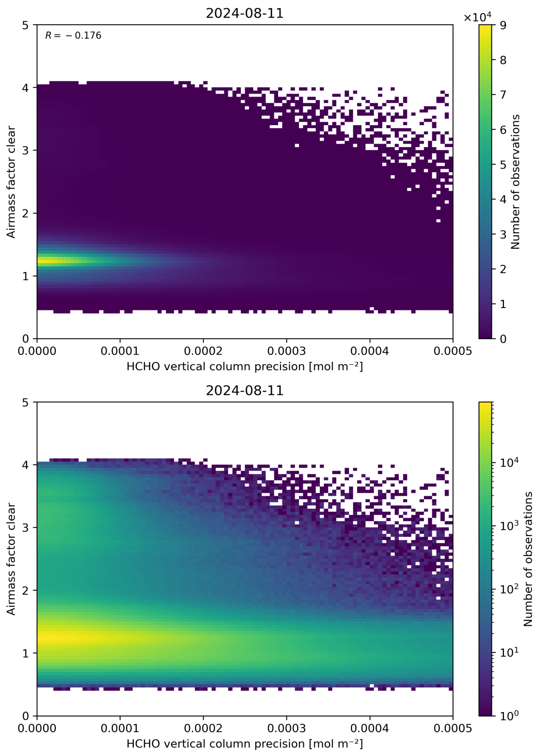
Figure 139: Scatter density plot of “HCHO vertical column precision” against “Airmass factor clear” for 2024-08-11 to 2024-08-11.
