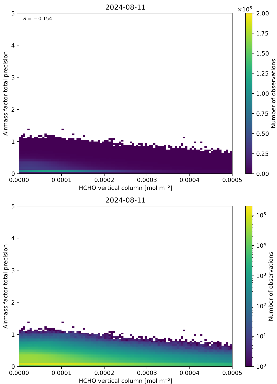
Figure 132: Scatter density plot of “HCHO vertical column” against “Airmass factor total precision” for 2024-08-11 to 2024-08-11.
