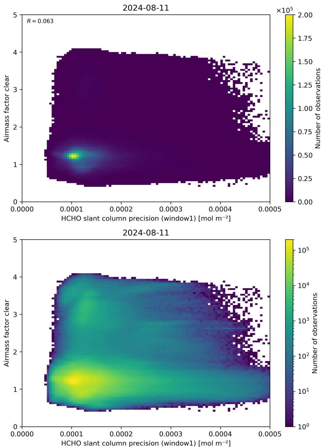
Figure 91: Scatter density plot of “HCHO slant column precision (window1)” against “Airmass factor clear” for 2024-08-11 to 2024-08-11.
