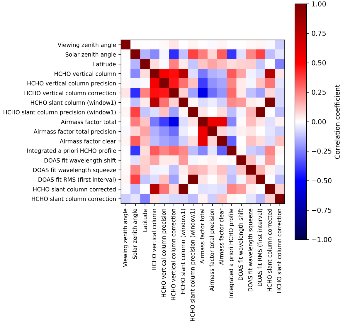
Figure 2: Map of correlation matrix for 2024-08-11 to 2024-08-11.
