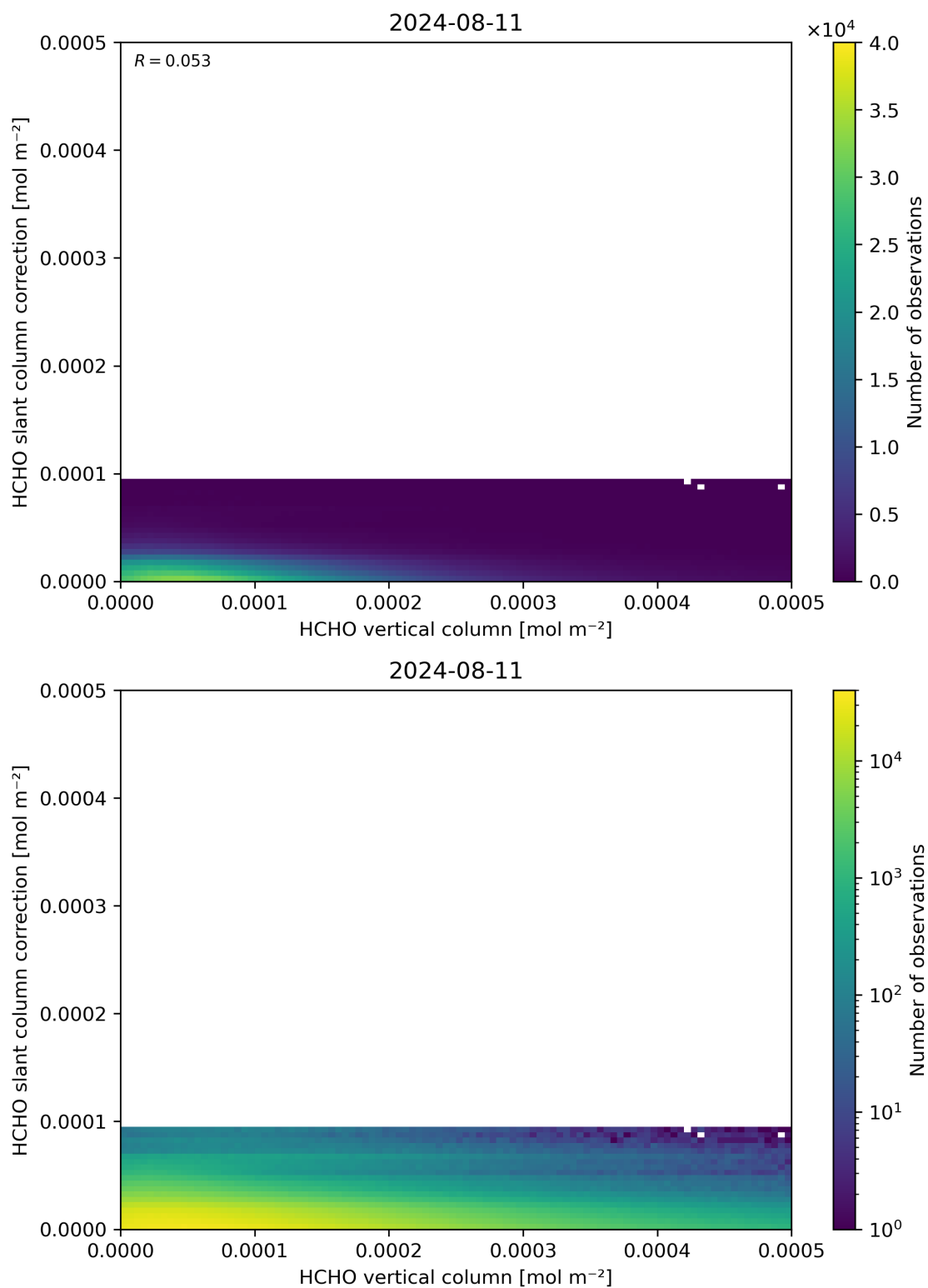
Figure 128: Scatter density plot of “HCHO vertical column” against “HCHO slant column correction” for 2024-08-11 to 2024-08-11.
