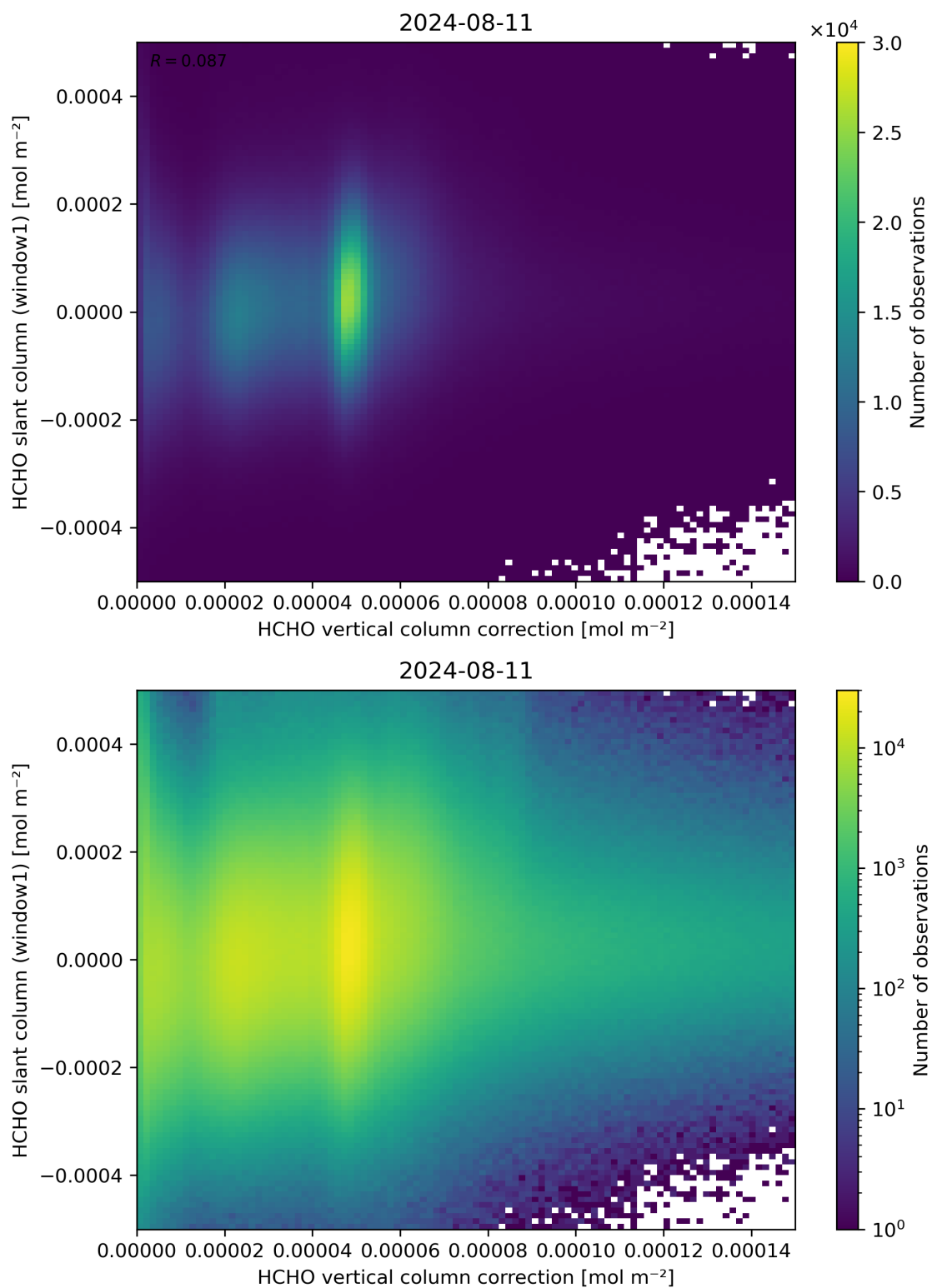
Figure 118: Scatter density plot of “HCHO vertical column correction” against “HCHO slant column (window1)” for 2024-08-11 to 2024-08-11.
