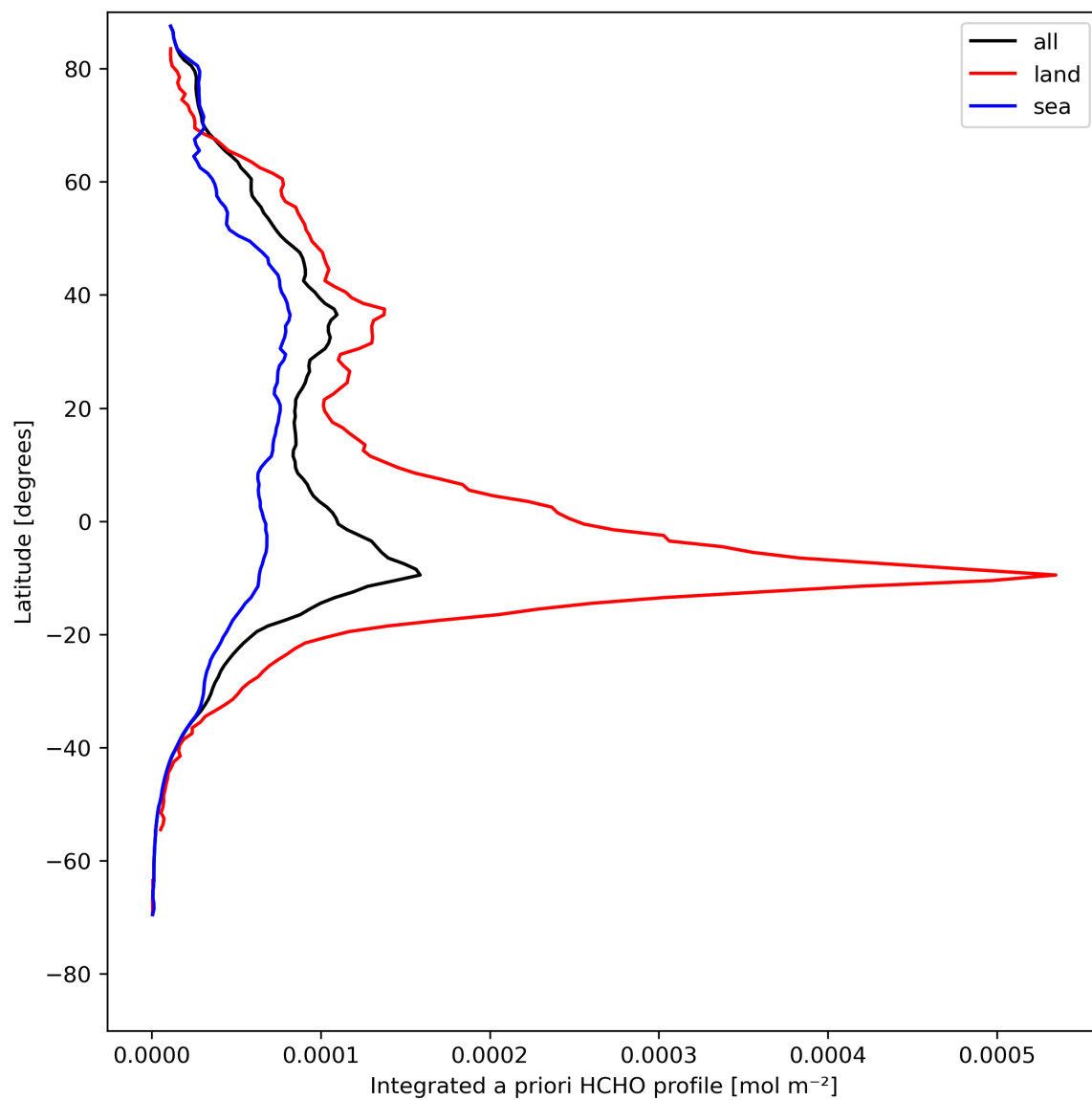
Figure 29: Zonal average of “Integrated a priori HCHO profile” for 2024-08-11 to 2024-08-11.
