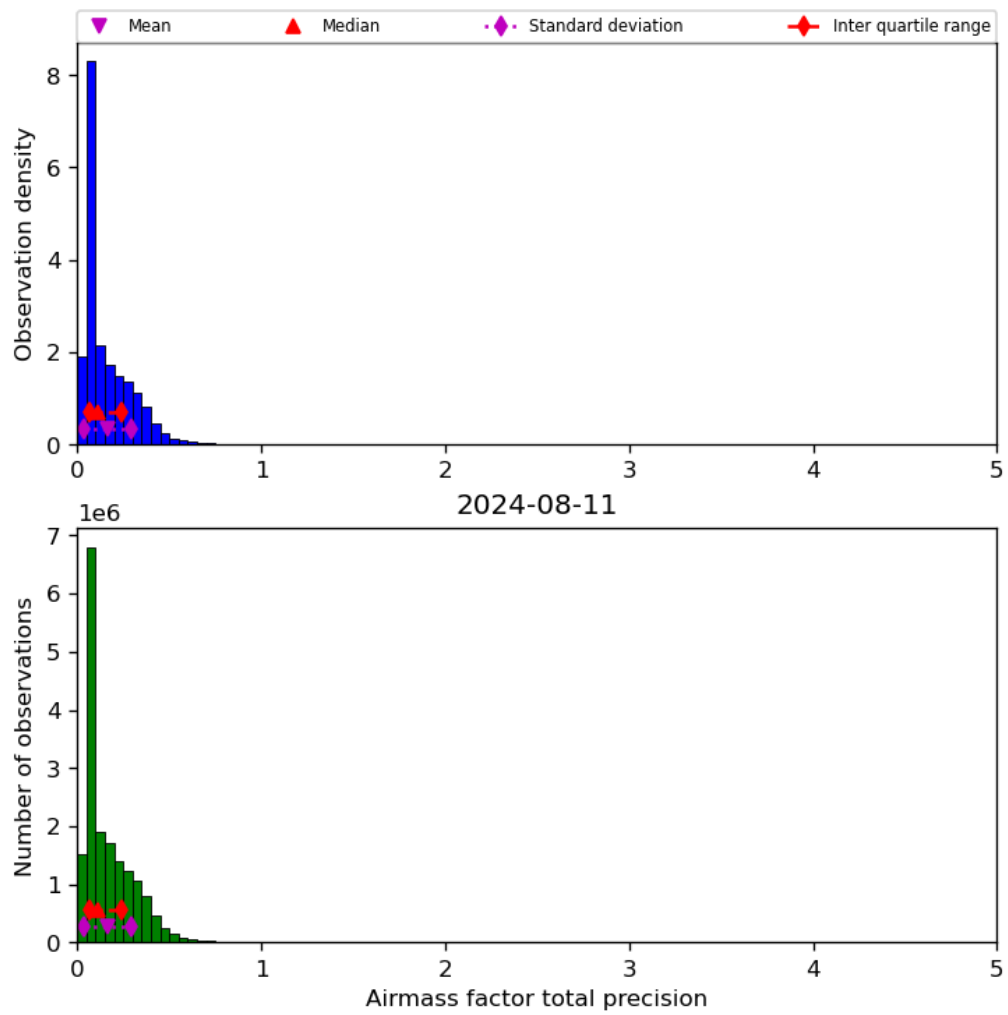
Figure 41: Histogram of “Airmass factor total precision” for 2024-08-11 to 2024-08-11
