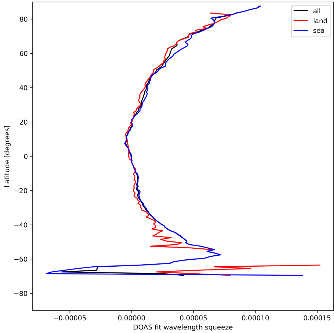
Figure 31: Zonal average of “DOAS fit wavelength squeeze” for 2024-08-11 to 2024-08-11.
