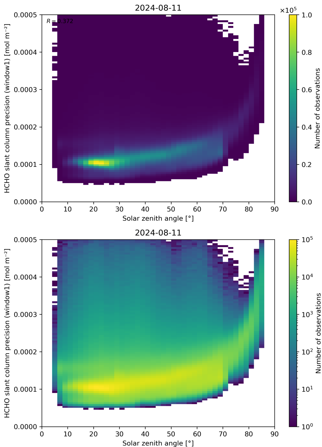
Figure 174: Scatter density plot of “Solar zenith angle” against “HCHO slant column precision (window1)” for 2024-08-11 to 2024-08-11.
