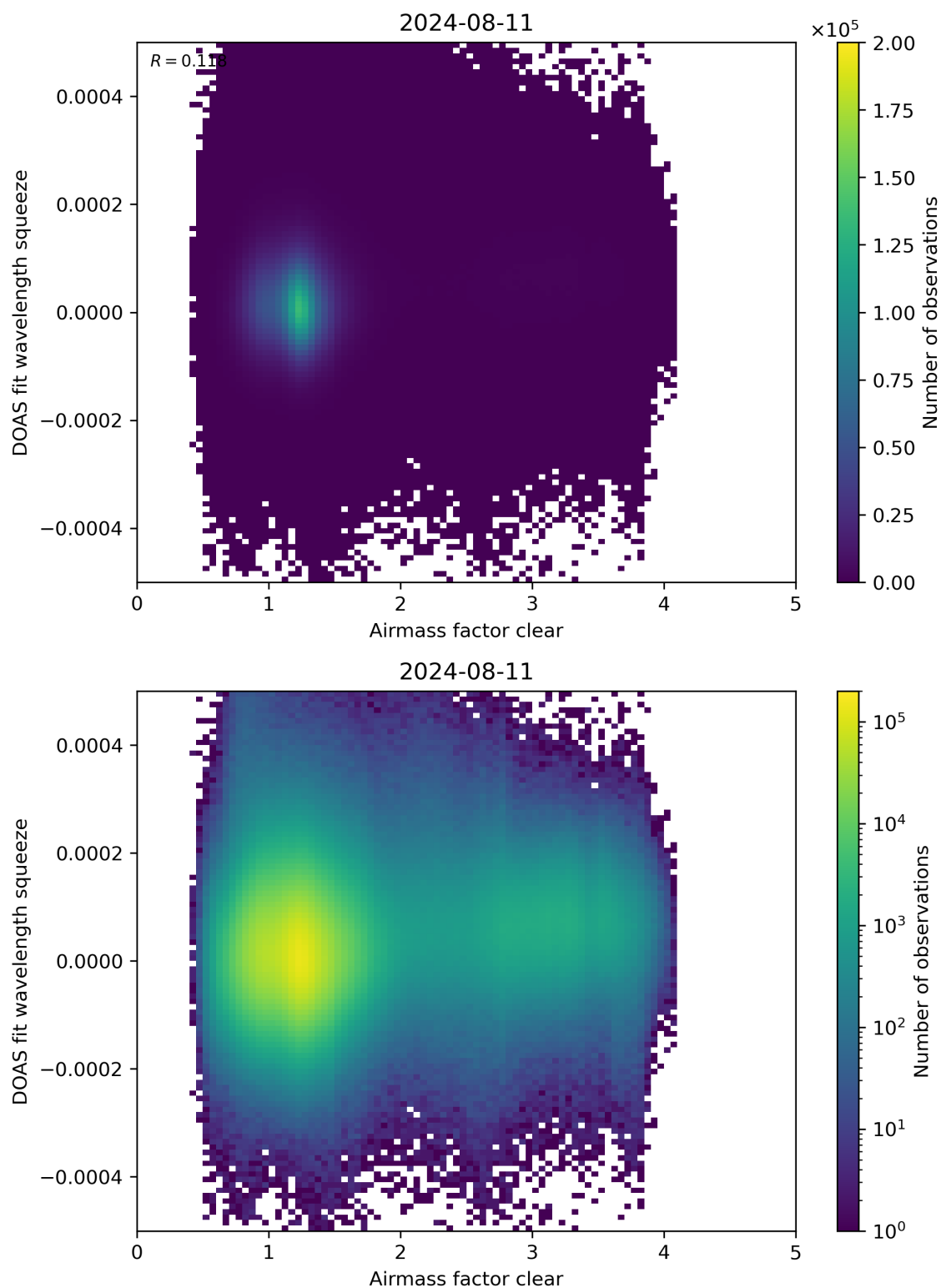
Figure 73: Scatter density plot of “Airmass factor clear” against “DOAS fit wavelength squeeze” for 2024-08-11 to 2024-08-11.
