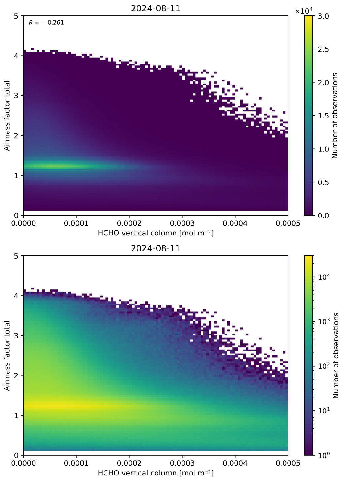
Figure 131: Scatter density plot of “HCHO vertical column” against “Airmass factor total” for 2024-08-11 to 2024-08-11.
