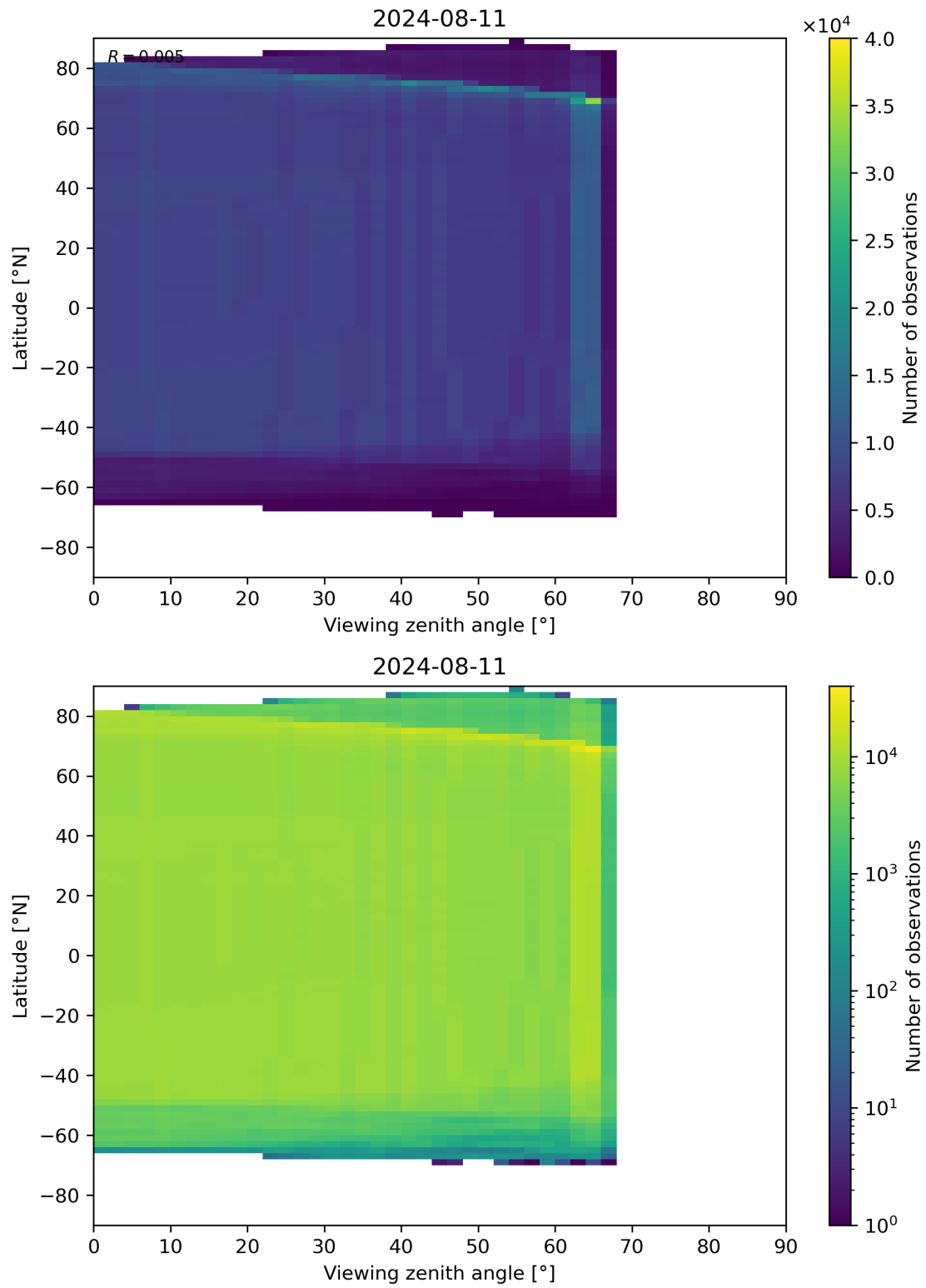
Figure 196: Scatter density plot of “Viewing zenith angle” against “Latitude” for 2024-08-11 to 2024-08-11.
