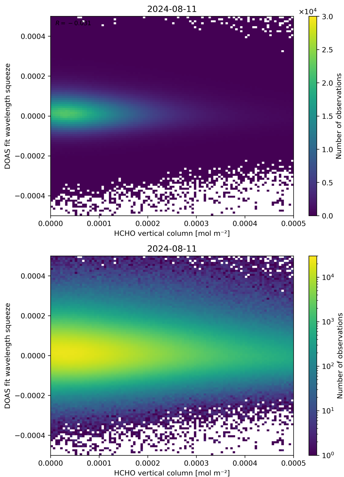
Figure 125: Scatter density plot of “HCHO vertical column” against “DOAS fit wavelength squeeze” for 2024-08-11 to 2024-08-11.
