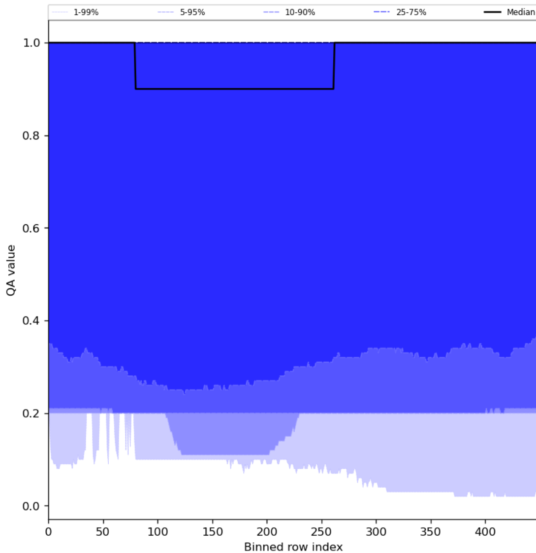
Figure 48: Along track statistics of “QA value” for 2024-08-11 to 2024-08-11
