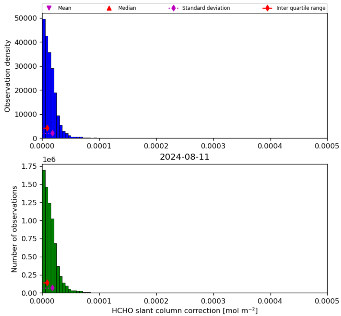
Figure 47: Histogram of “HCHO slant column correction” for 2024-08-11 to 2024-08-11
