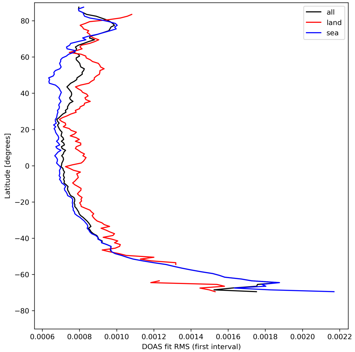
Figure 32: Zonal average of "DOAS fit RMS (first interval)" for 2024-08-11 to 2024-08-11.
