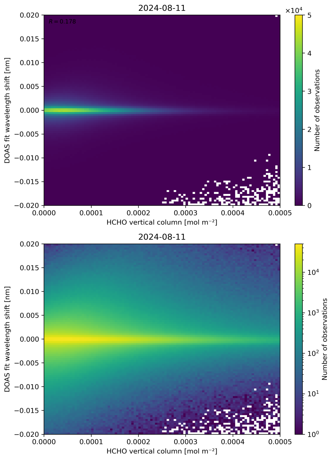
Figure 124: Scatter density plot of “HCHO vertical column” against “DOAS fit wavelength shift” for 2024-08-11 to 2024-08-11.
