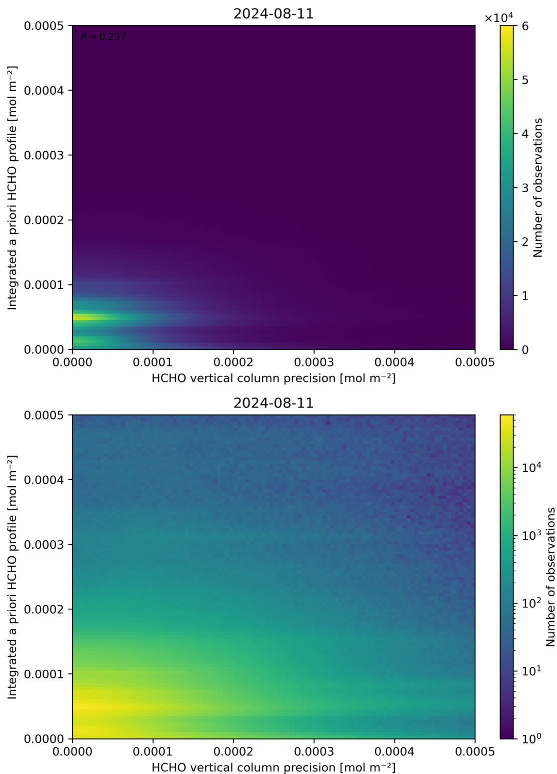
Figure 147: Scatter density plot of “HCHO vertical column precision” against “Integrated a priori HCHO profile” for 2024-08-11 to 2024-08-11.
