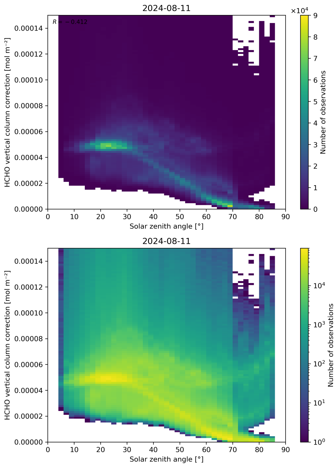
Figure 178: Scatter density plot of “Solar zenith angle” against “HCHO vertical column correction” for 2024-08-11 to 2024-08-11.
