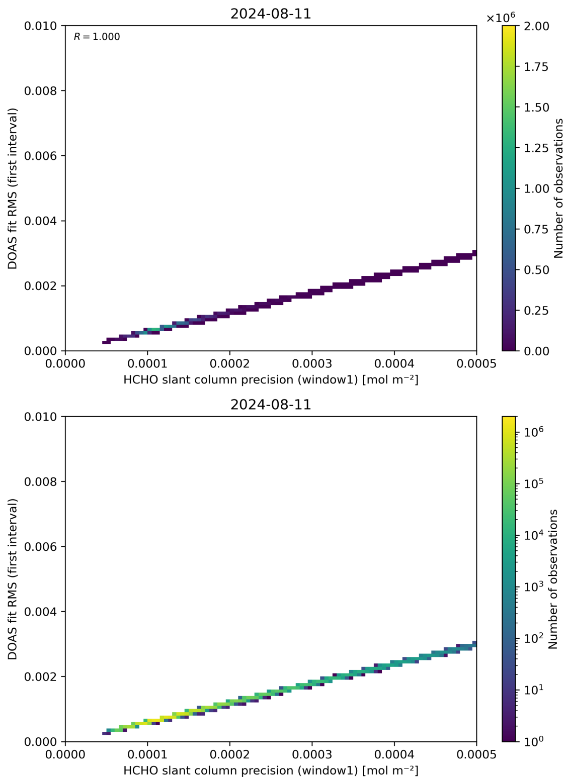
Figure 88: Scatter density plot of “HCHO slant column precision (window1)” against “DOAS fit RMS (first interval)” for 2024-08-11 to 2024-08-11.
