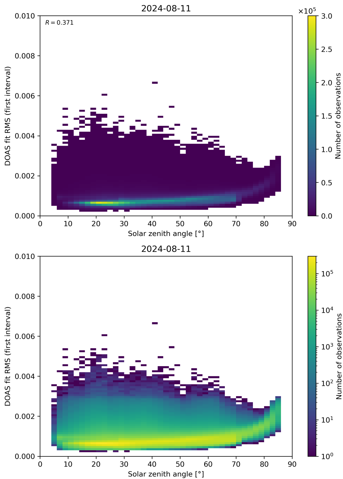
Figure 167: Scatter density plot of “Solar zenith angle” against “DOAS fit RMS (first interval)” for 2024-08-11 to 2024-08-11.
