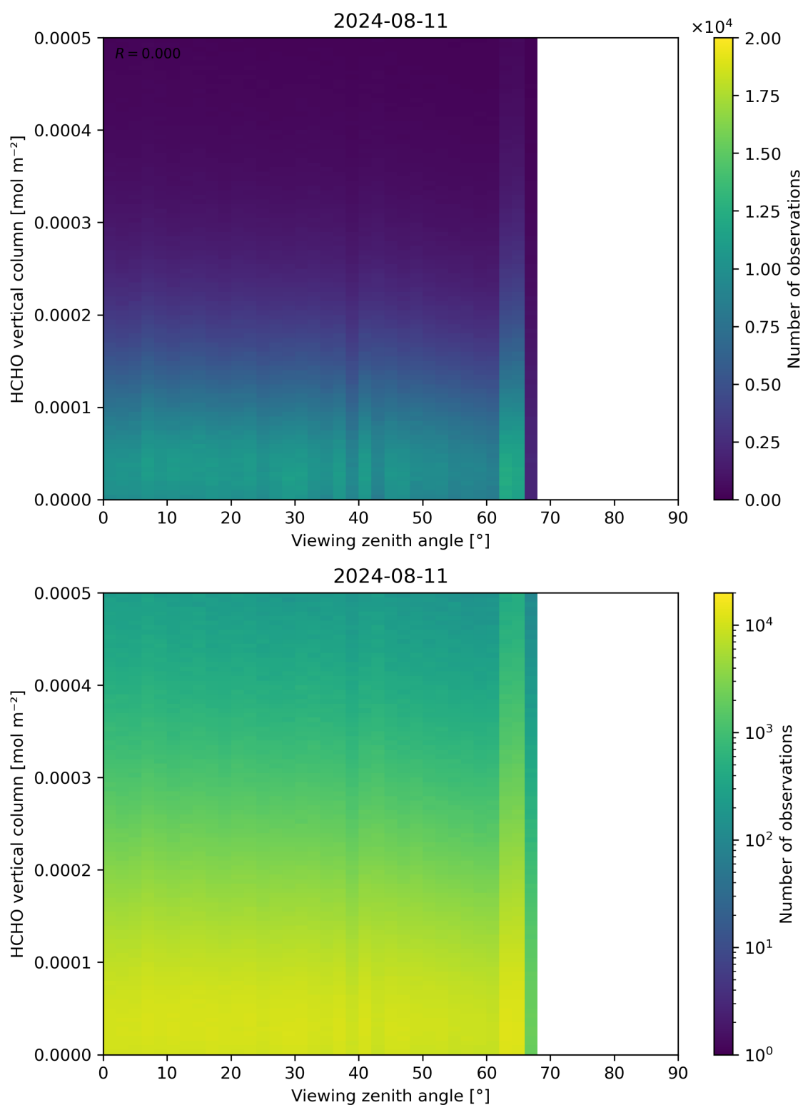
Figure 192: Scatter density plot of “Viewing zenith angle” against “HCHO vertical column” for 2024-08-11 to 2024-08-11.
