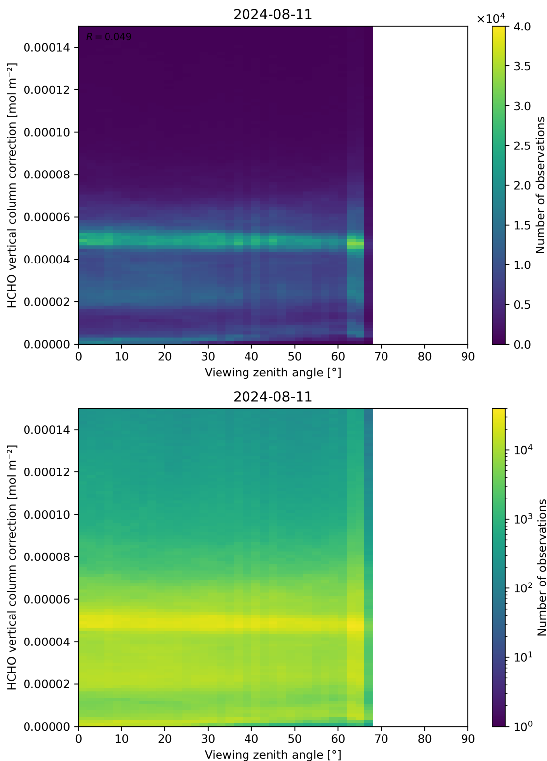
Figure 193: Scatter density plot of “Viewing zenith angle” against “HCHO vertical column correction” for 2024-08-11 to 2024-08-11.
