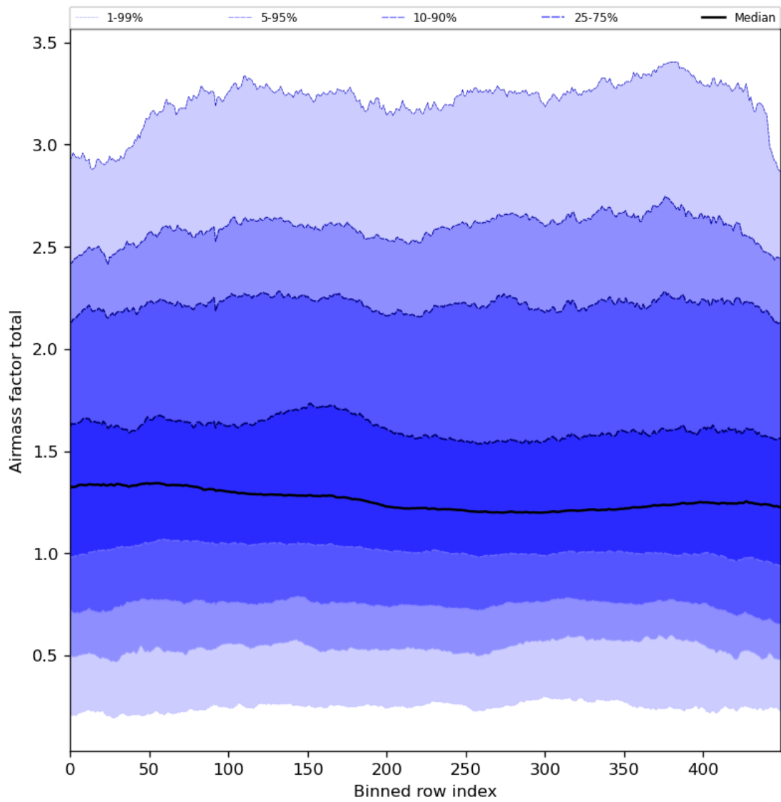
Figure 54: Along track statistics of “Airmass factor total” for 2024-08-11 to 2024-08-11
