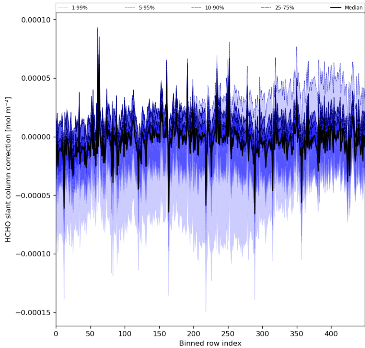
Figure 61: Along track statistics of “HCHO slant column correction” for 2024-08-11 to 2024-08-11
