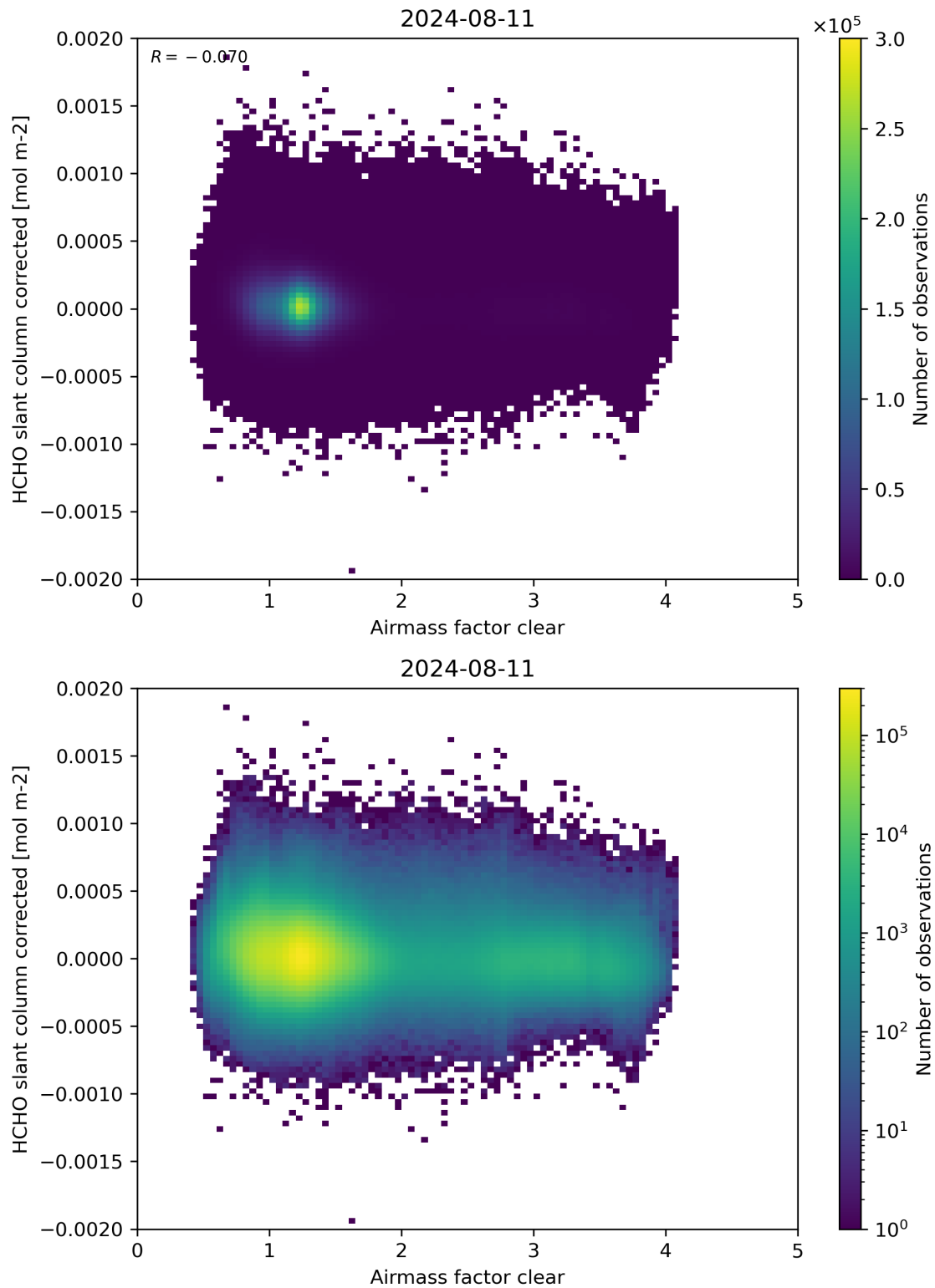
Figure 74: Scatter density plot of “Airmass factor clear” against “HCHO slant column corrected” for 2024-08-11 to 2024-08-11.
