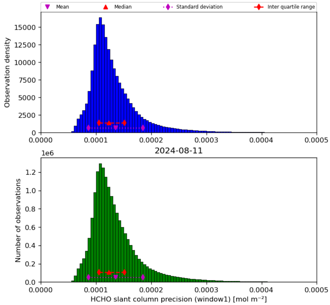
Figure 39: Histogram of “HCHO slant column precision (window1)” for 2024-08-11 to 2024-08-11
