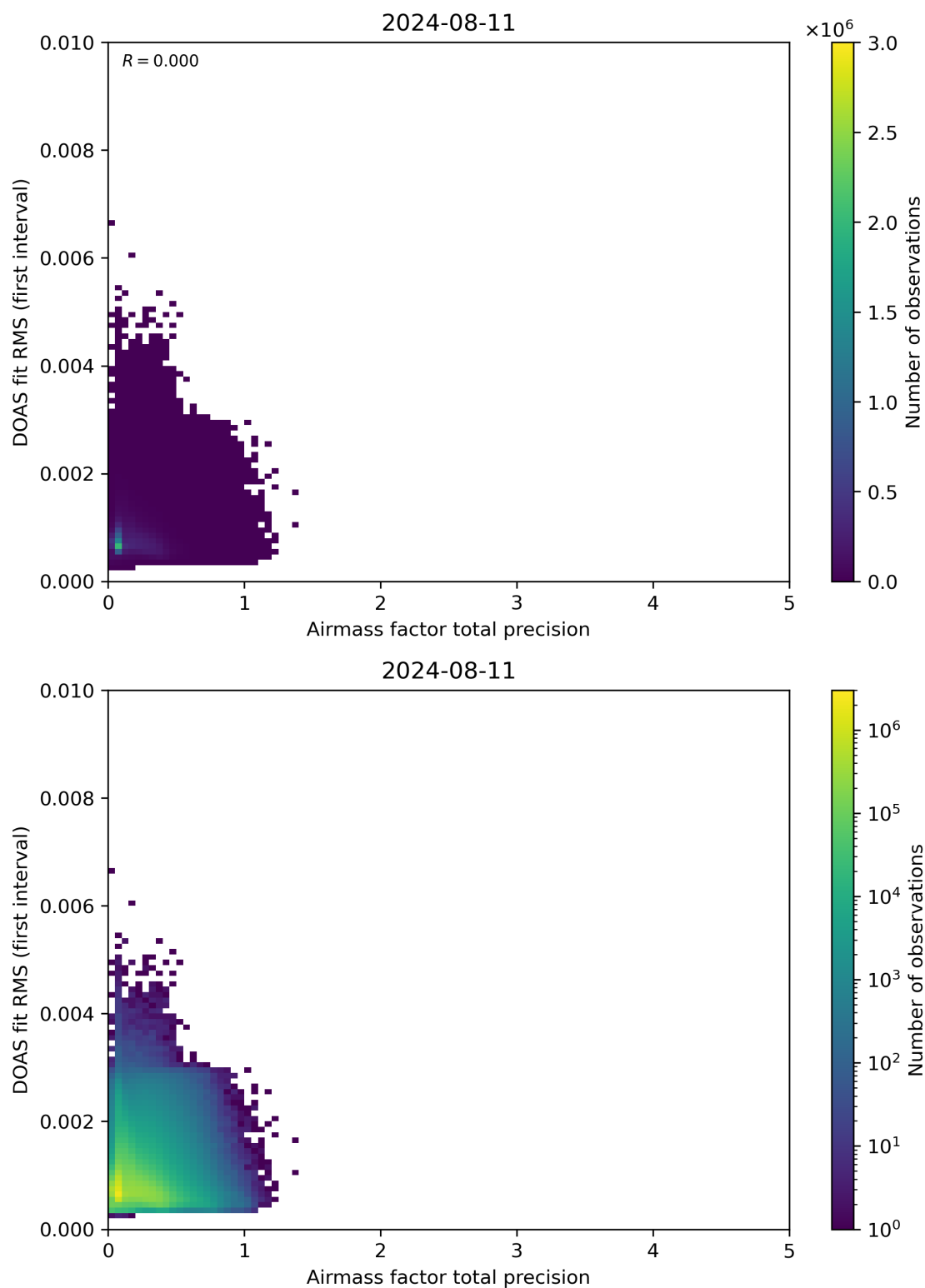
Figure 105: Scatter density plot of “Airmass factor total precision” against “DOAS fit RMS (first interval)” for 2024-08-11 to 2024-08-11.
