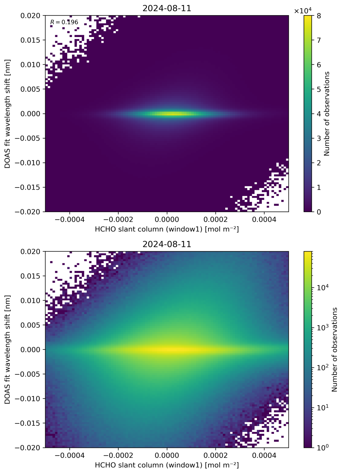
Figure 79: Scatter density plot of “HCHO slant column (window1)” against “DOAS fit wavelength shift” for 2024-08-11 to 2024-08-11.
