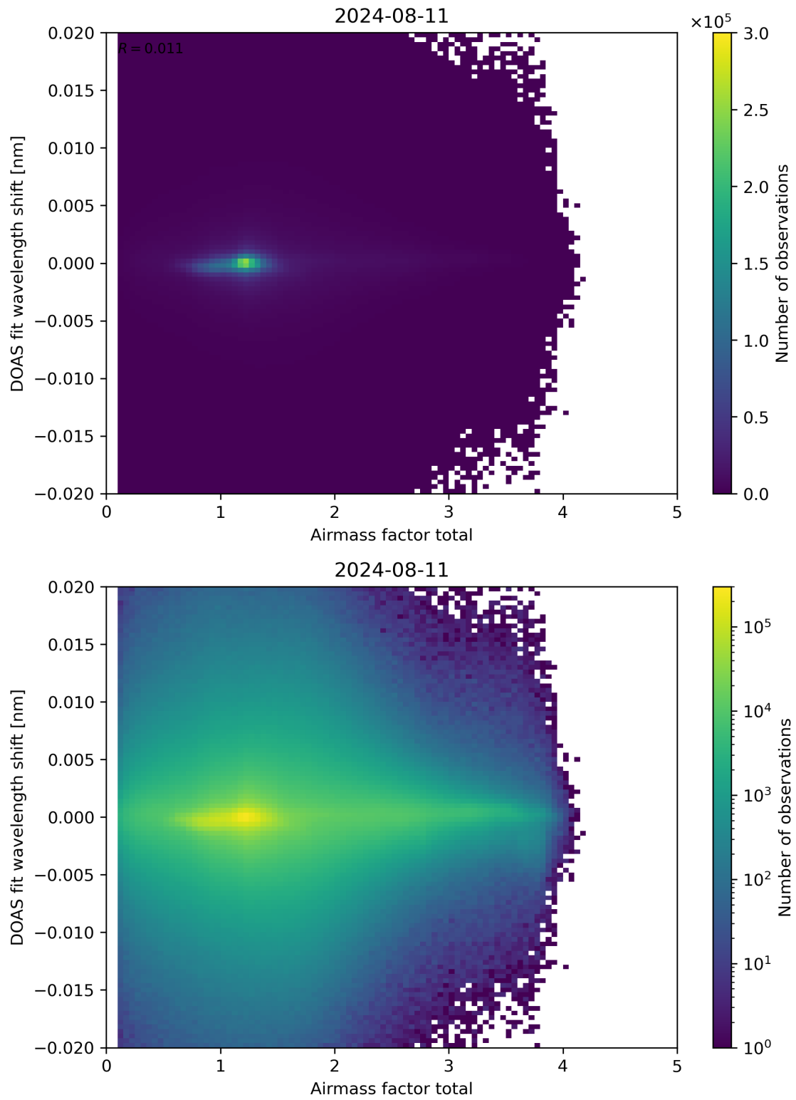
Figure 98: Scatter density plot of “Airmass factor total” against “DOAS fit wavelength shift” for 2024-08-11 to 2024-08-11.
