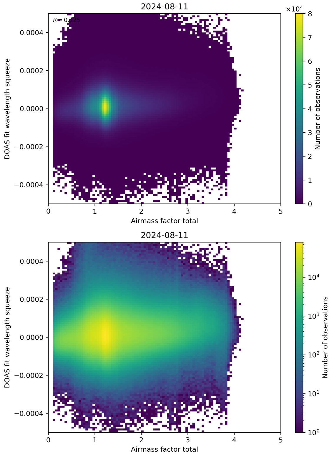
Figure 99: Scatter density plot of “Airmass factor total” against “DOAS fit wavelength squeeze” for 2024-08-11 to 2024-08-11.
