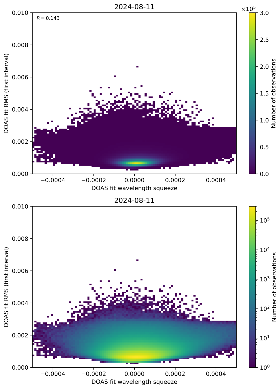
Figure 68: Scatter density plot of “DOAS fit wavelength squeeze” against “DOAS fit RMS (first interval)” for 2024-08-11 to 2024-08-11.
