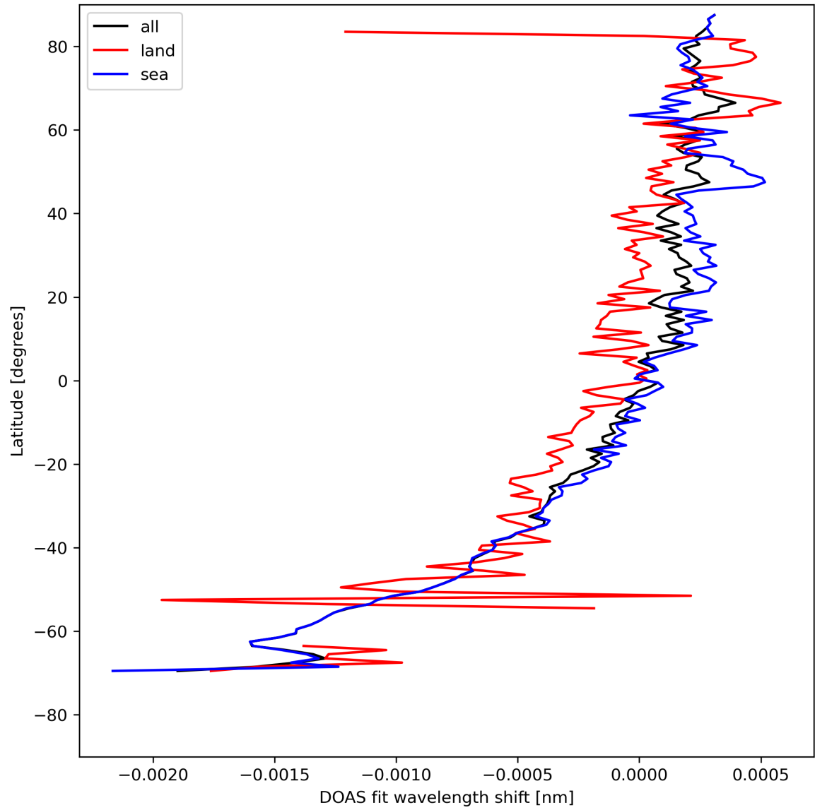
Figure 30: Zonal average of “DOAS fit wavelength shift” for 2024-08-11 to 2024-08-11.
