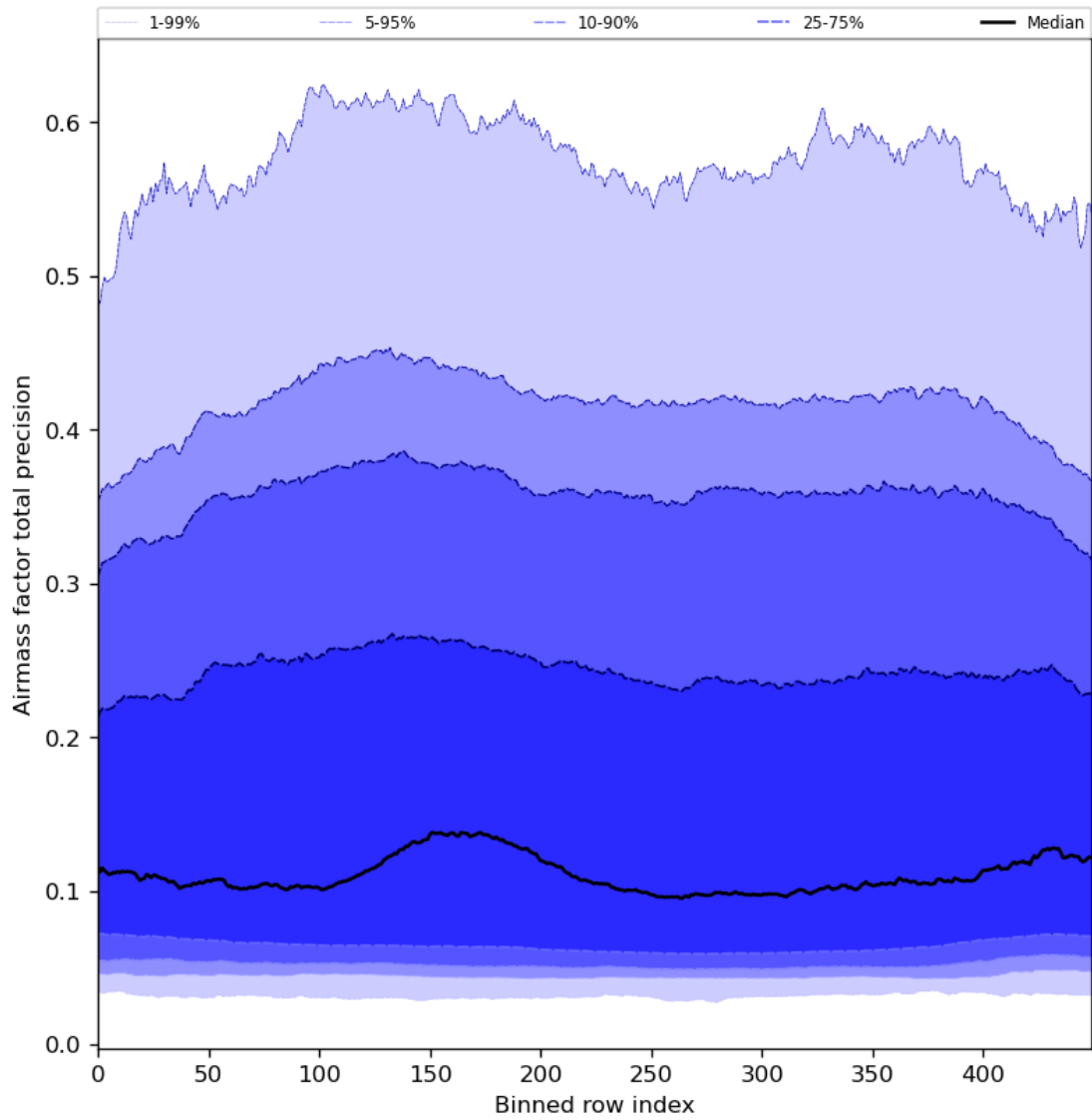
Figure 55: Along track statistics of “Airmass factor total precision” for 2024-08-11 to 2024-08-11
