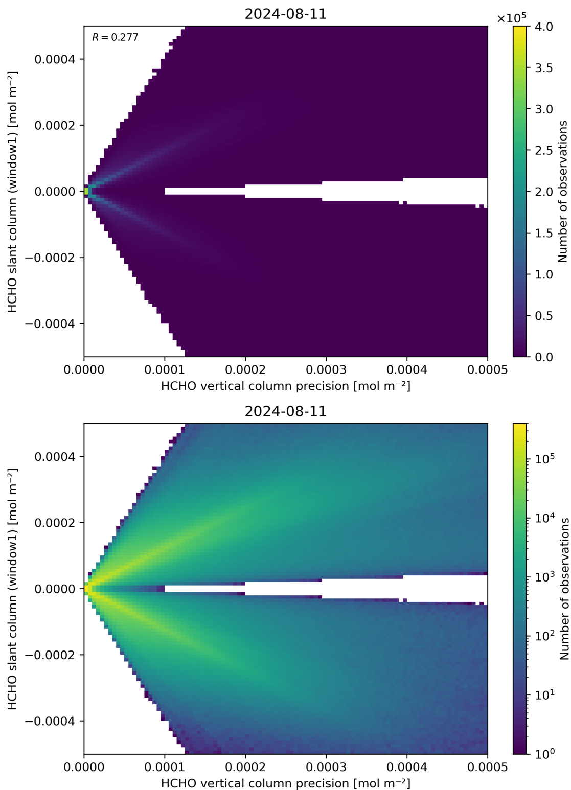
Figure 142: Scatter density plot of “HCHO vertical column precision” against “HCHO slant column (window1)” for 2024-08-11 to 2024-08-11.
