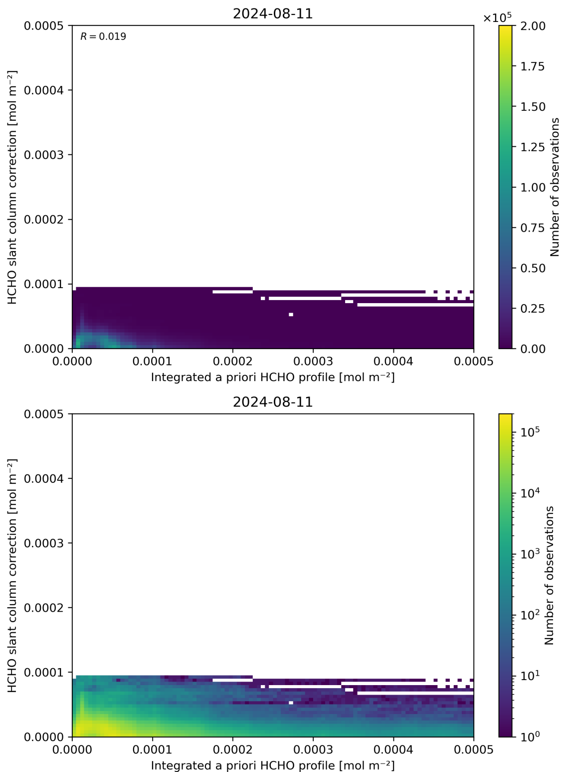
Figure 152: Scatter density plot of “Integrated a priori HCHO profile” against “HCHO slant column correction” for 2024-08-11 to 2024-08-11.
