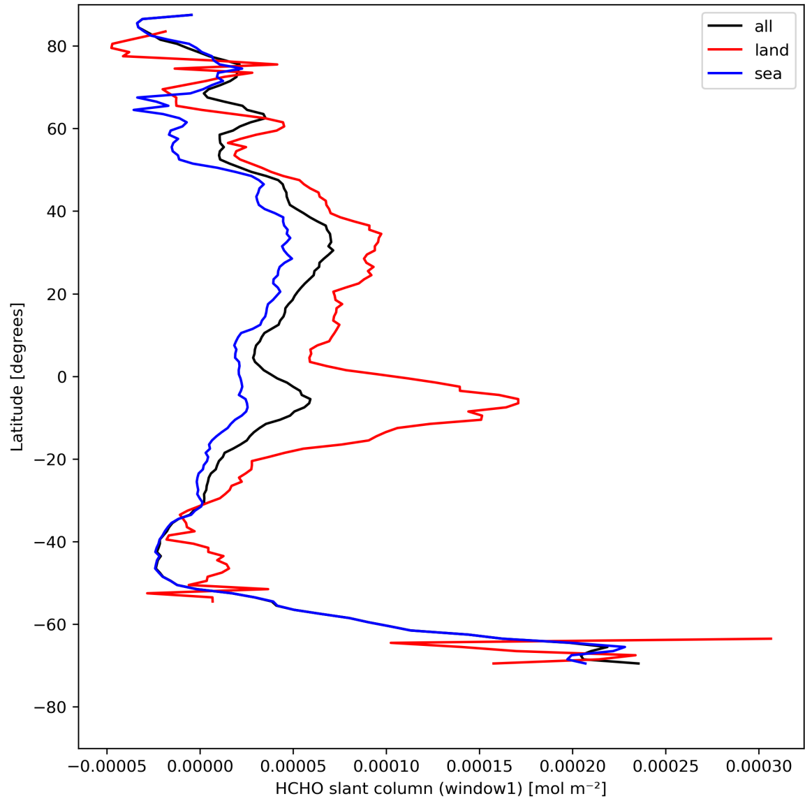
Figure 24: Zonal average of “HCHO slant column (window1)” for 2024-08-11 to 2024-08-11.
