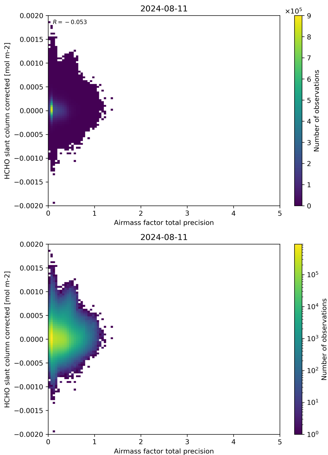
Figure 109: Scatter density plot of “Airmass factor total precision” against “HCHO slant column corrected” for 2024-08-11 to 2024-08-11.
