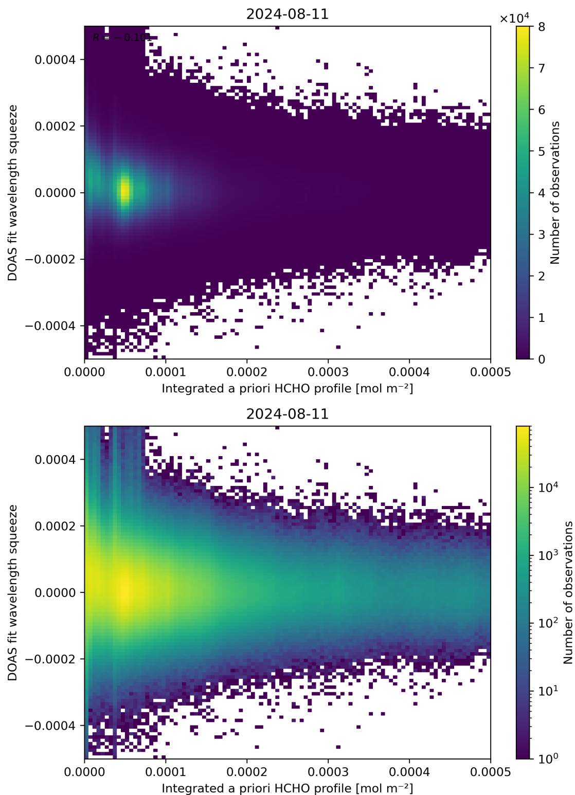
Figure 150: Scatter density plot of “Integrated a priori HCHO profile” against “DOAS fit wavelength squeeze” for 2024-08-11 to 2024-08-11.
