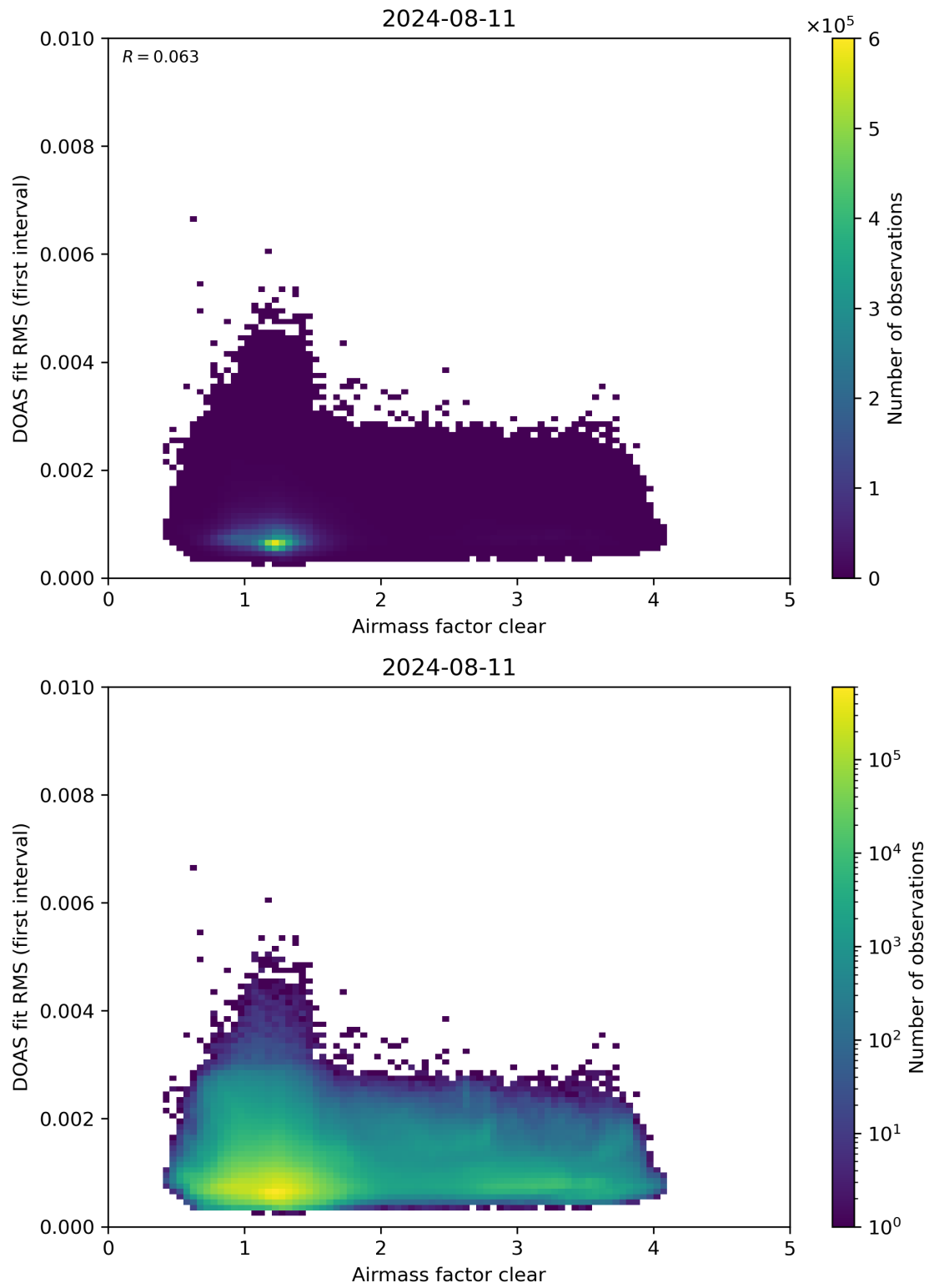
Figure 71: Scatter density plot of “Airmass factor clear” against “DOAS fit RMS (first interval)” for 2024-08-11 to 2024-08-11.
