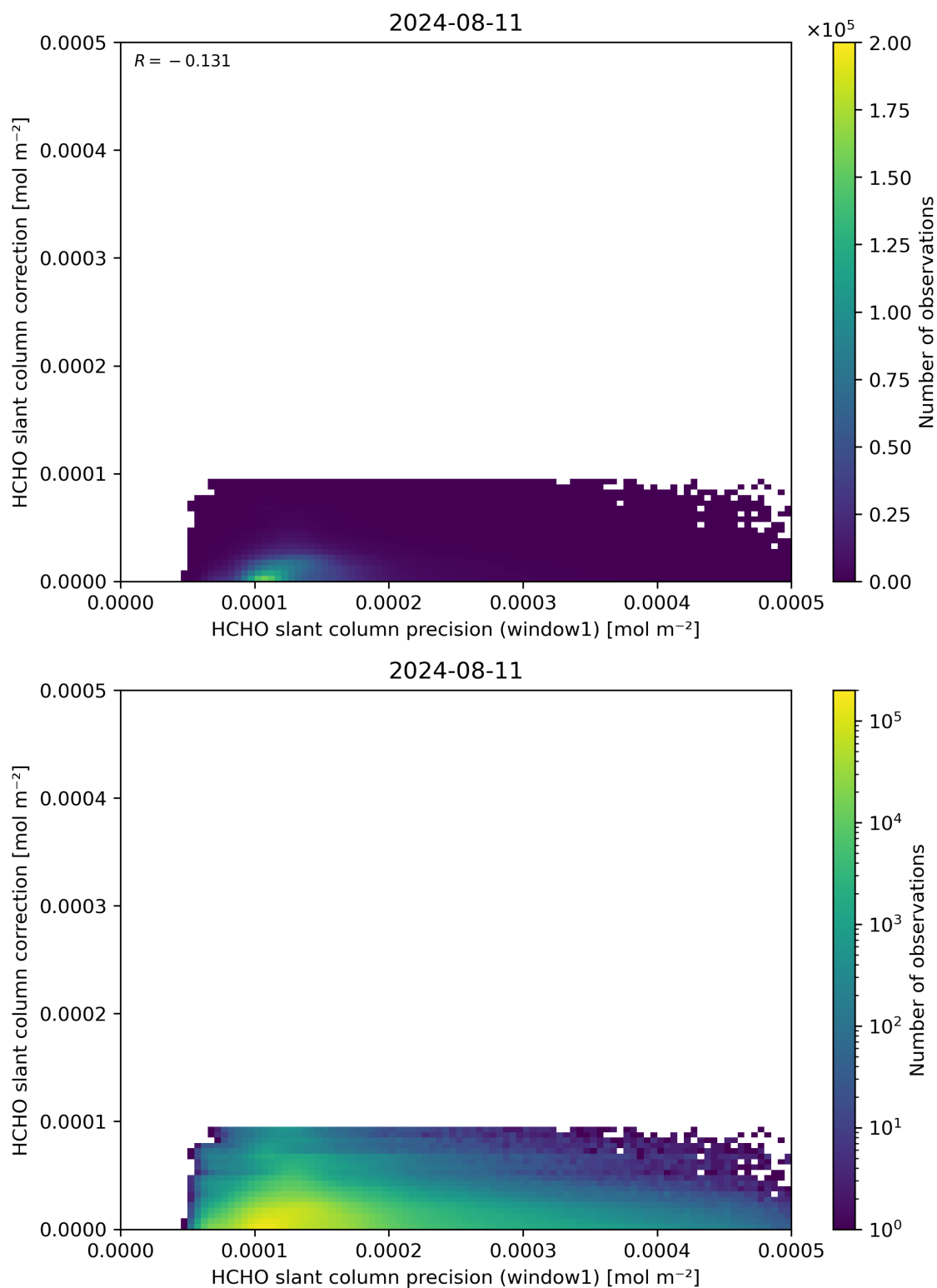
Figure 93: Scatter density plot of “HCHO slant column precision (window1)” against “HCHO slant column correction” for 2024-08-11 to 2024-08-11.
