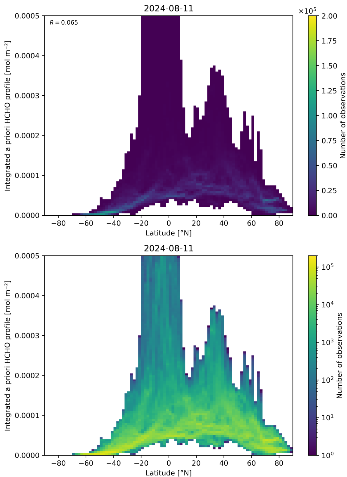
Figure 166: Scatter density plot of “Latitude” against “Integrated a priori HCHO profile” for 2024-08-11 to 2024-08-11.
