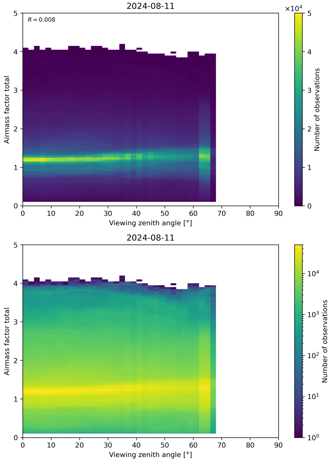
Figure 190: Scatter density plot of “Viewing zenith angle” against “Airmass factor total” for 2024-08-11 to 2024-08-11.
