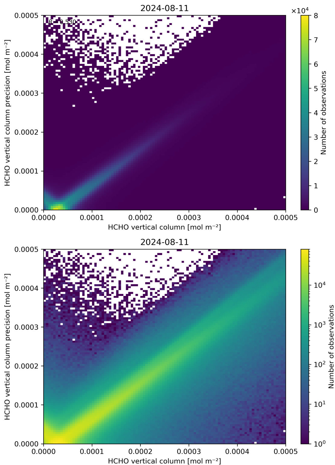
Figure 134: Scatter density plot of “HCHO vertical column” against “HCHO vertical column precision” for 2024-08-11 to 2024-08-11.
