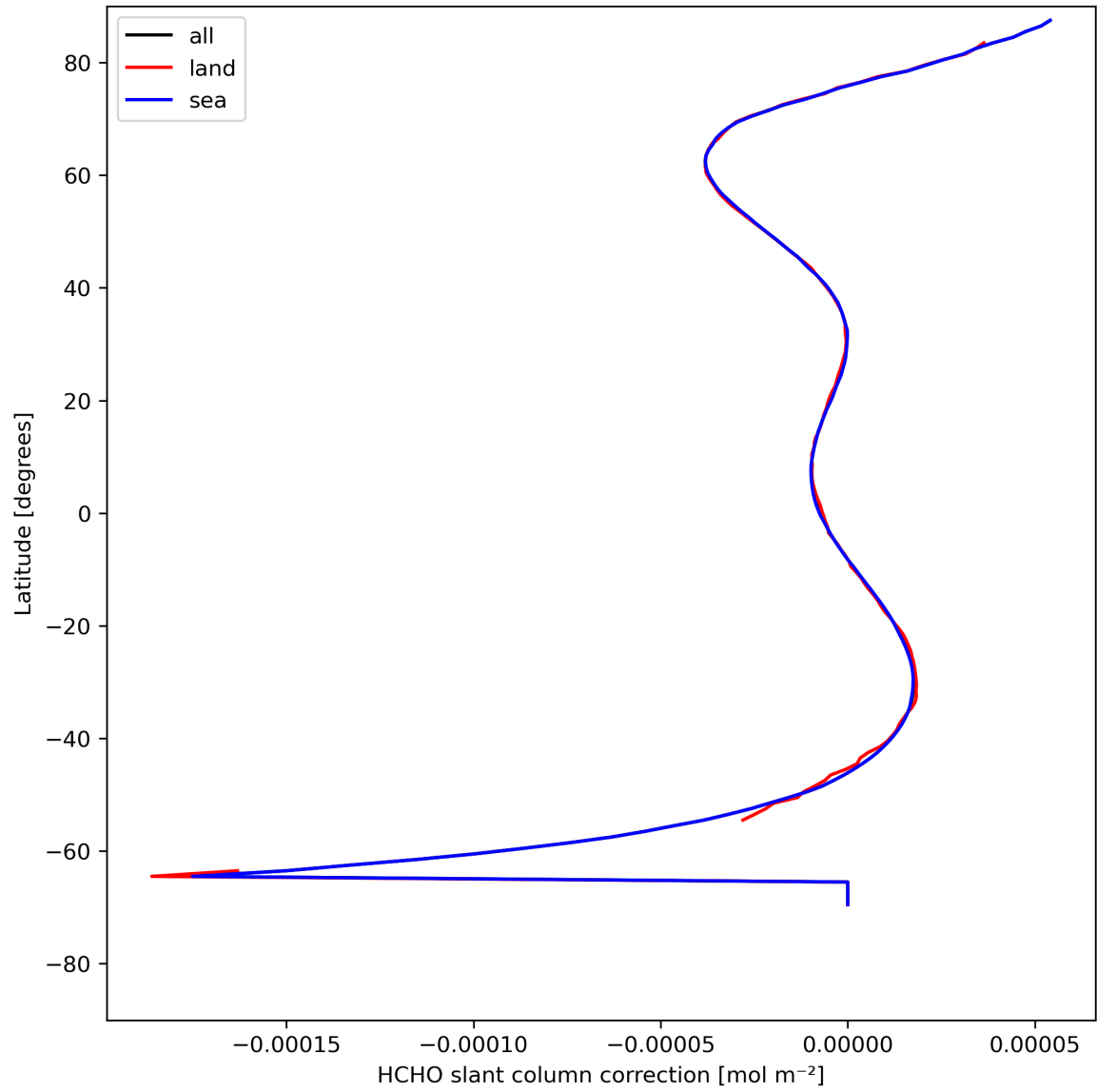
Figure 33: Zonal average of “HCHO slant column correction” for 2024-08-11 to 2024-08-11.
