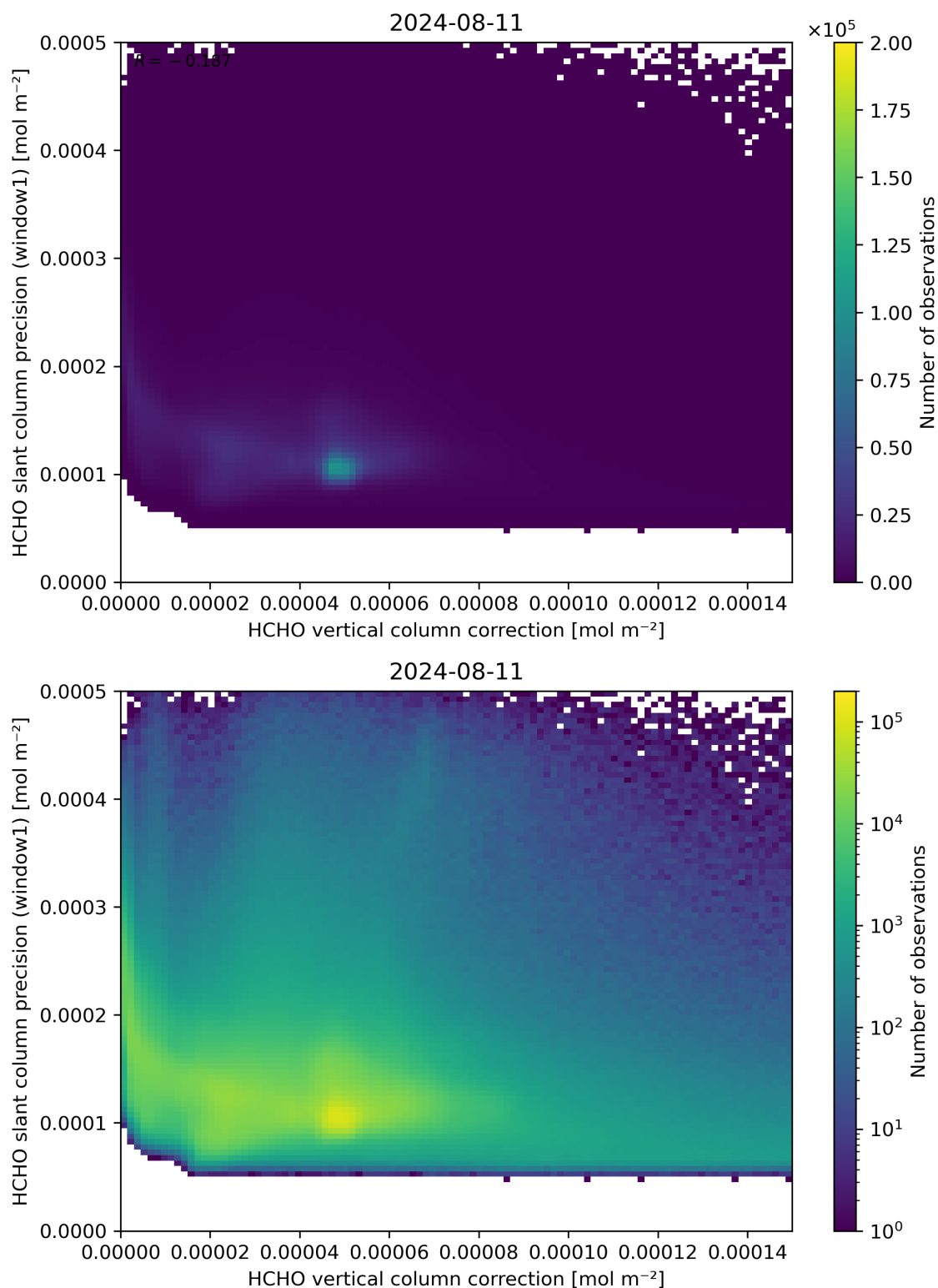
Figure 119: Scatter density plot of “HCHO vertical column correction” against “HCHO slant column precision (window1)” for 2024-08-11 to 2024-08-11.
