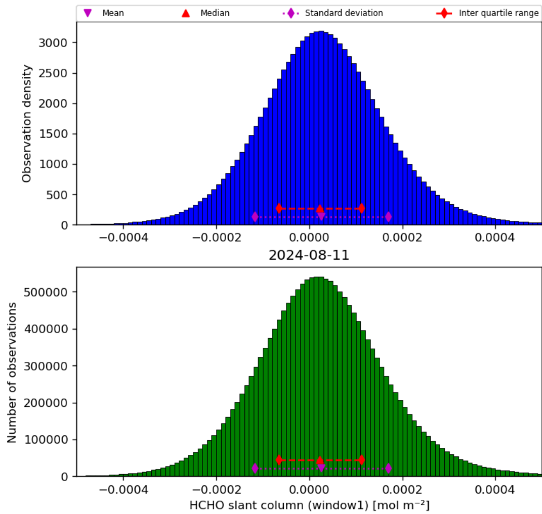
Figure 38: Histogram of “HCHO slant column (window1)” for 2024-08-11 to 2024-08-11
