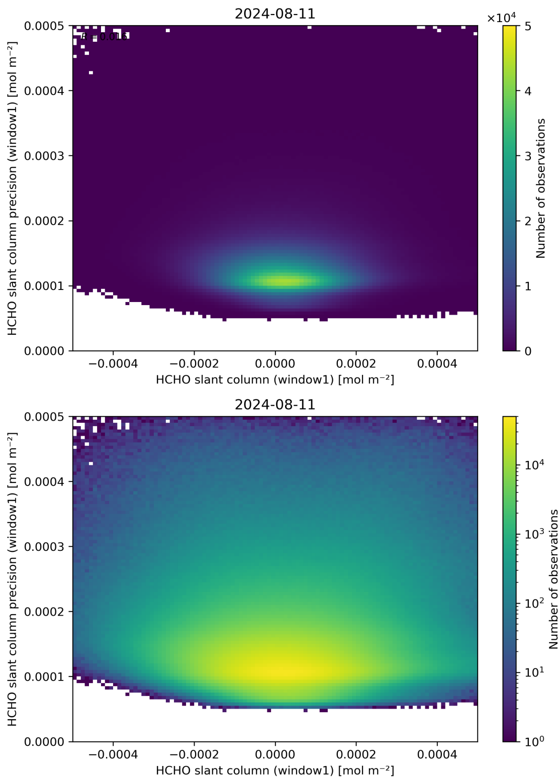
Figure 84: Scatter density plot of “HCHO slant column (window1)” against “HCHO slant column precision (window1)” for 2024-08-11 to 2024-08-11.
