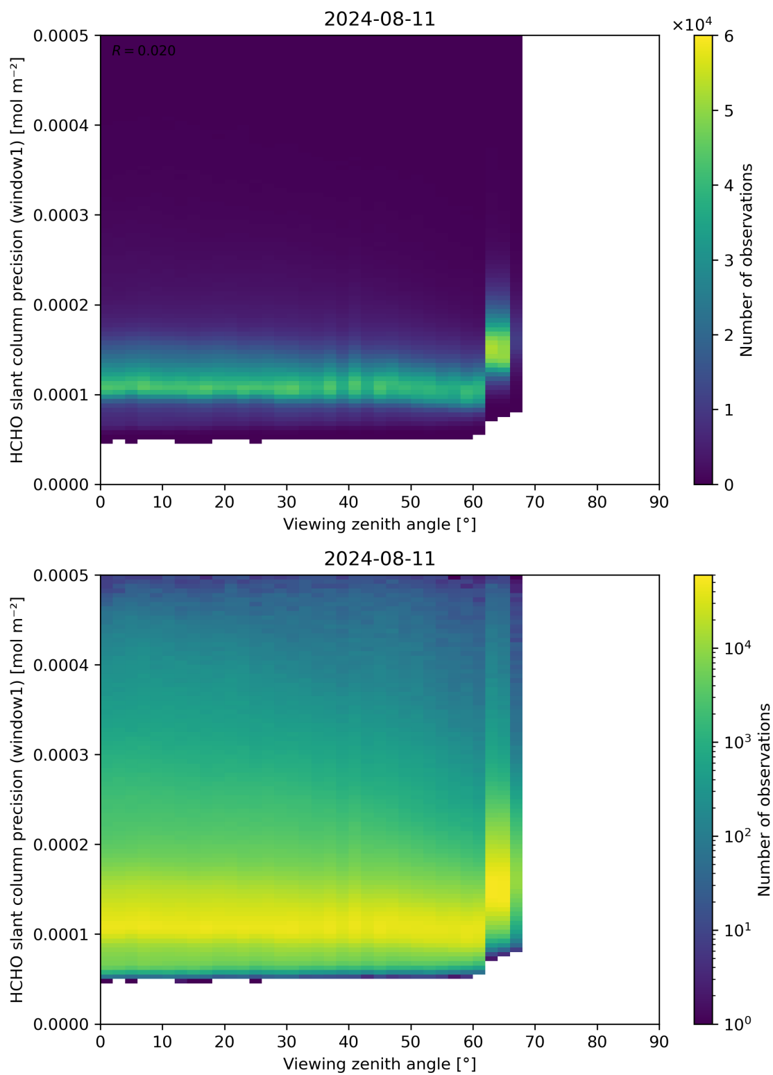
Figure 189: Scatter density plot of “Viewing zenith angle” against “HCHO slant column precision (window1)” for 2024-08-11 to 2024-08-11.
