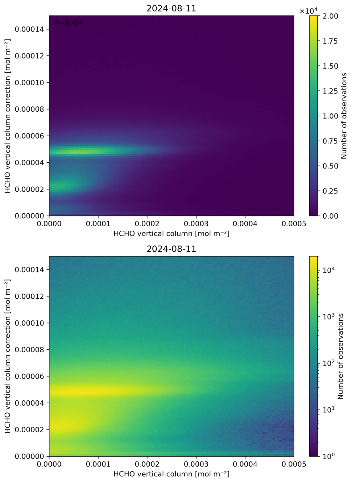
Figure 133: Scatter density plot of “HCHO vertical column” against “HCHO vertical column correction” for 2024-08-11 to 2024-08-11.
