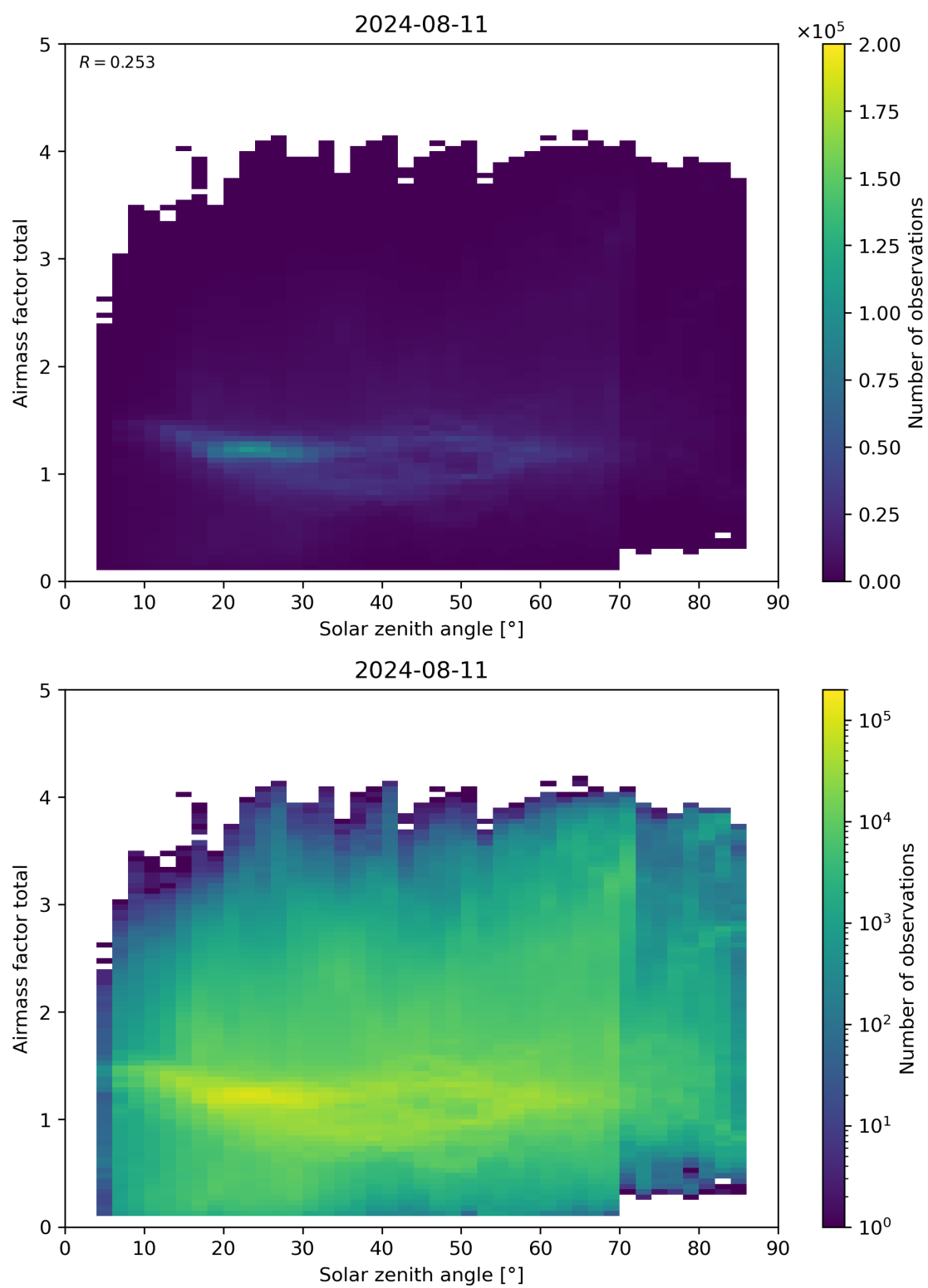
Figure 175: Scatter density plot of “Solar zenith angle” against “Airmass factor total” for 2024-08-11 to 2024-08-11.
