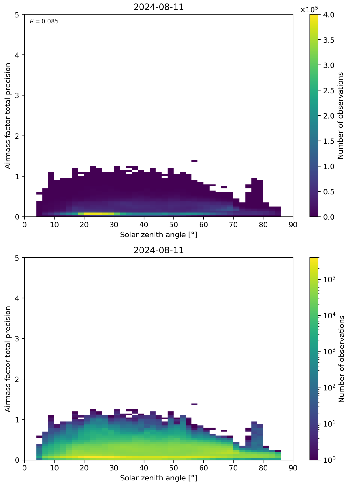
Figure 176: Scatter density plot of “Solar zenith angle” against “Airmass factor total precision” for 2024-08-11 to 2024-08-11.
