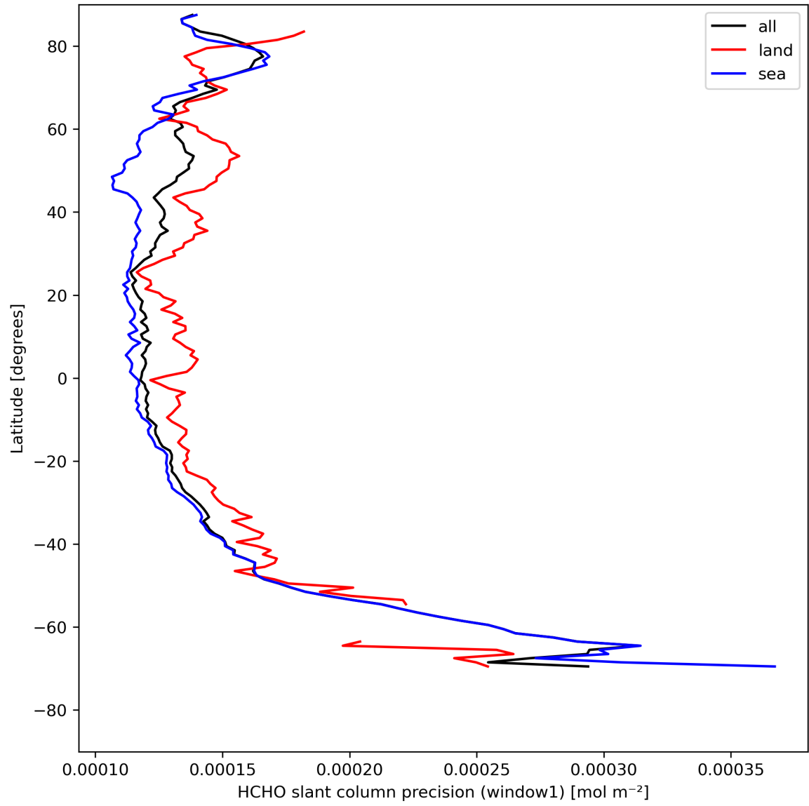
Figure 25: Zonal average of “HCHO slant column precision (window1)” for 2024-08-11 to 2024-08-11.
