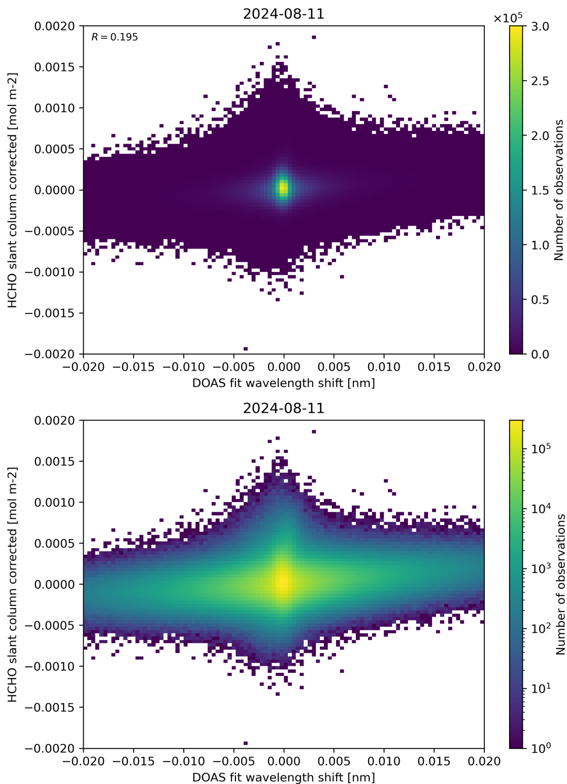
Figure 66: Scatter density plot of “DOAS fit wavelength shift” against “HCHO slant column corrected” for 2024-08-11 to 2024-08-11.
