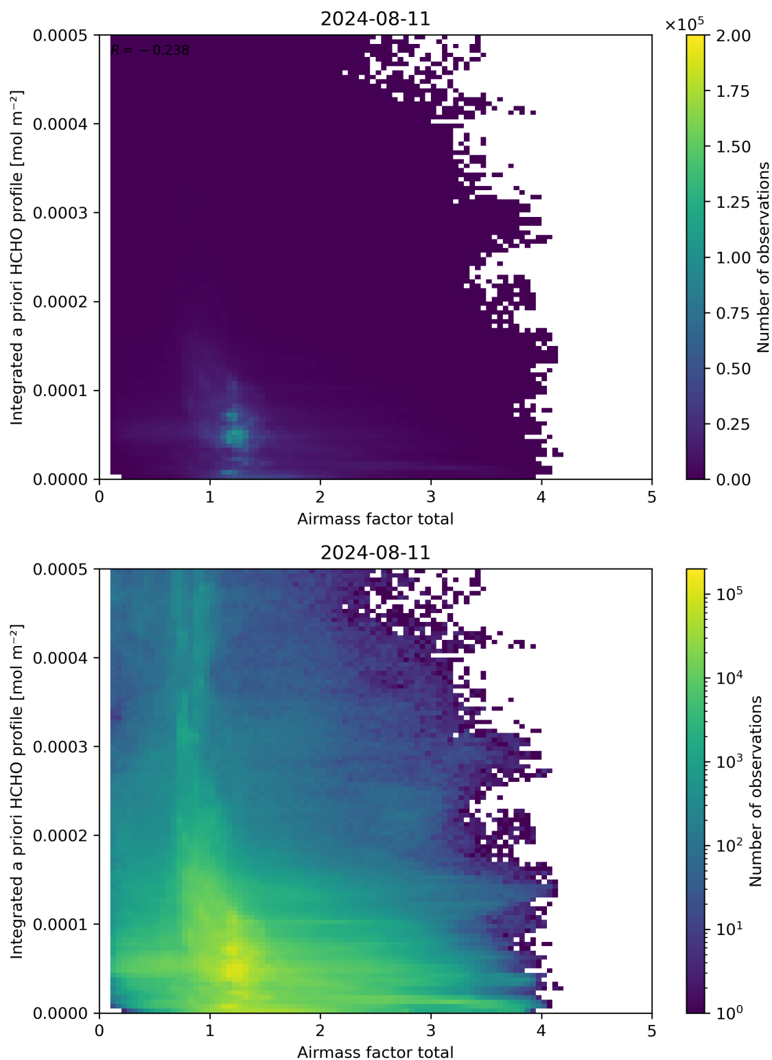
Figure 104: Scatter density plot of “Airmass factor total” against “Integrated a priori HCHO profile” for 2024-08-11 to 2024-08-11.
