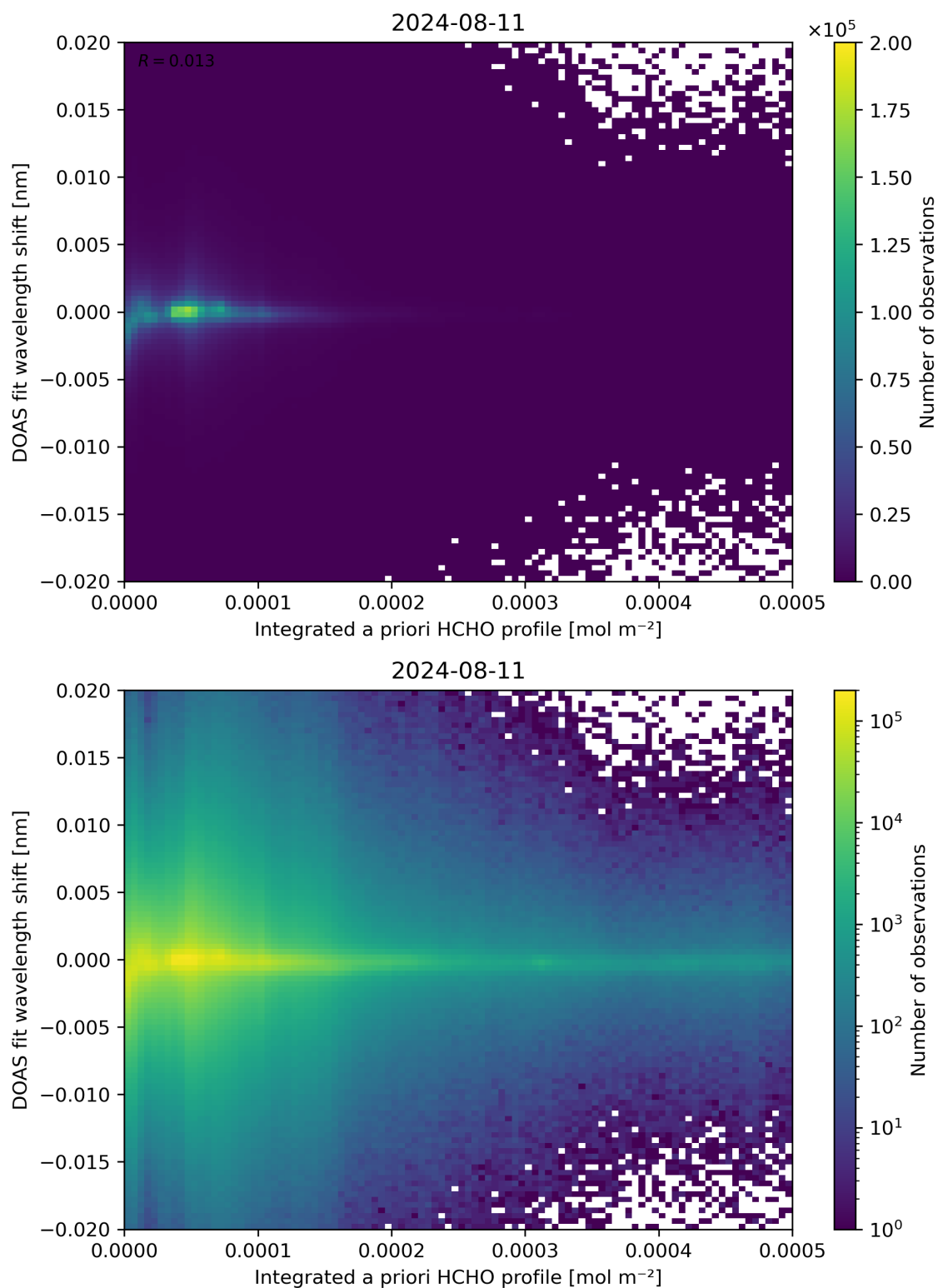
Figure 149: Scatter density plot of “Integrated a priori HCHO profile” against “DOAS fit wavelength shift” for 2024-08-11 to 2024-08-11.
