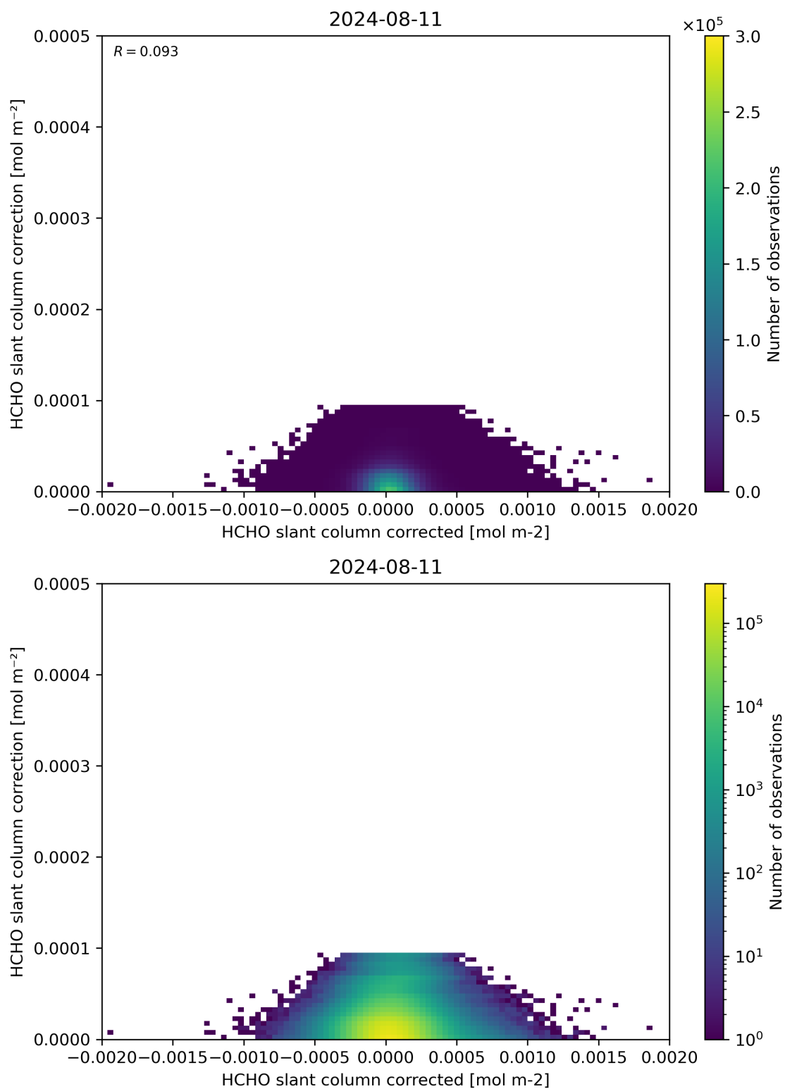
Figure 77: Scatter density plot of “HCHO slant column corrected” against “HCHO slant column correction” for 2024-08-11 to 2024-08-11.
