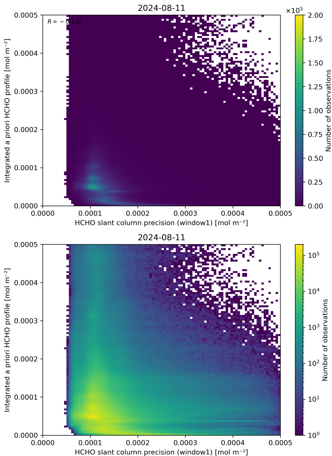
Figure 96: Scatter density plot of “HCHO slant column precision (window1)” against “Integrated a priori HCHO profile” for 2024-08-11 to 2024-08-11.
