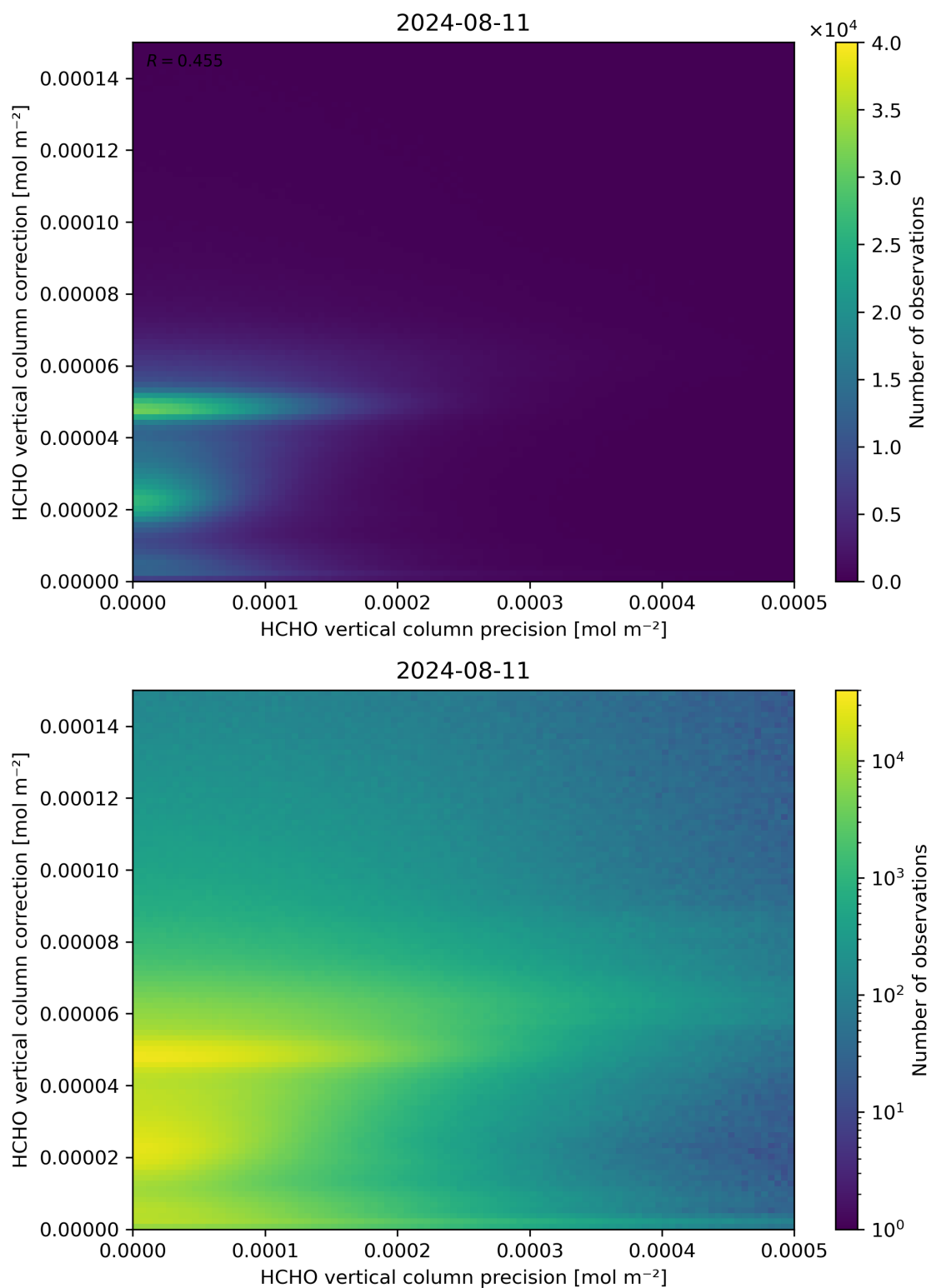
Figure 146: Scatter density plot of “HCHO vertical column precision” against “HCHO vertical column correction” for 2024-08-11 to 2024-08-11.
