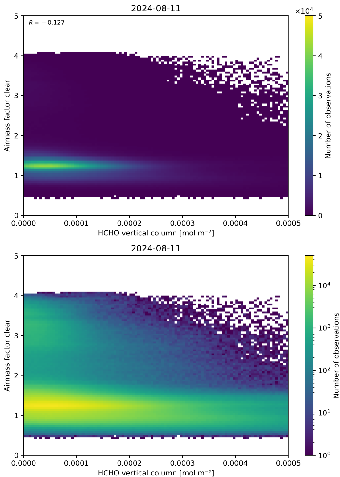
Figure 126: Scatter density plot of “HCHO vertical column” against “Airmass factor clear” for 2024-08-11 to 2024-08-11.
