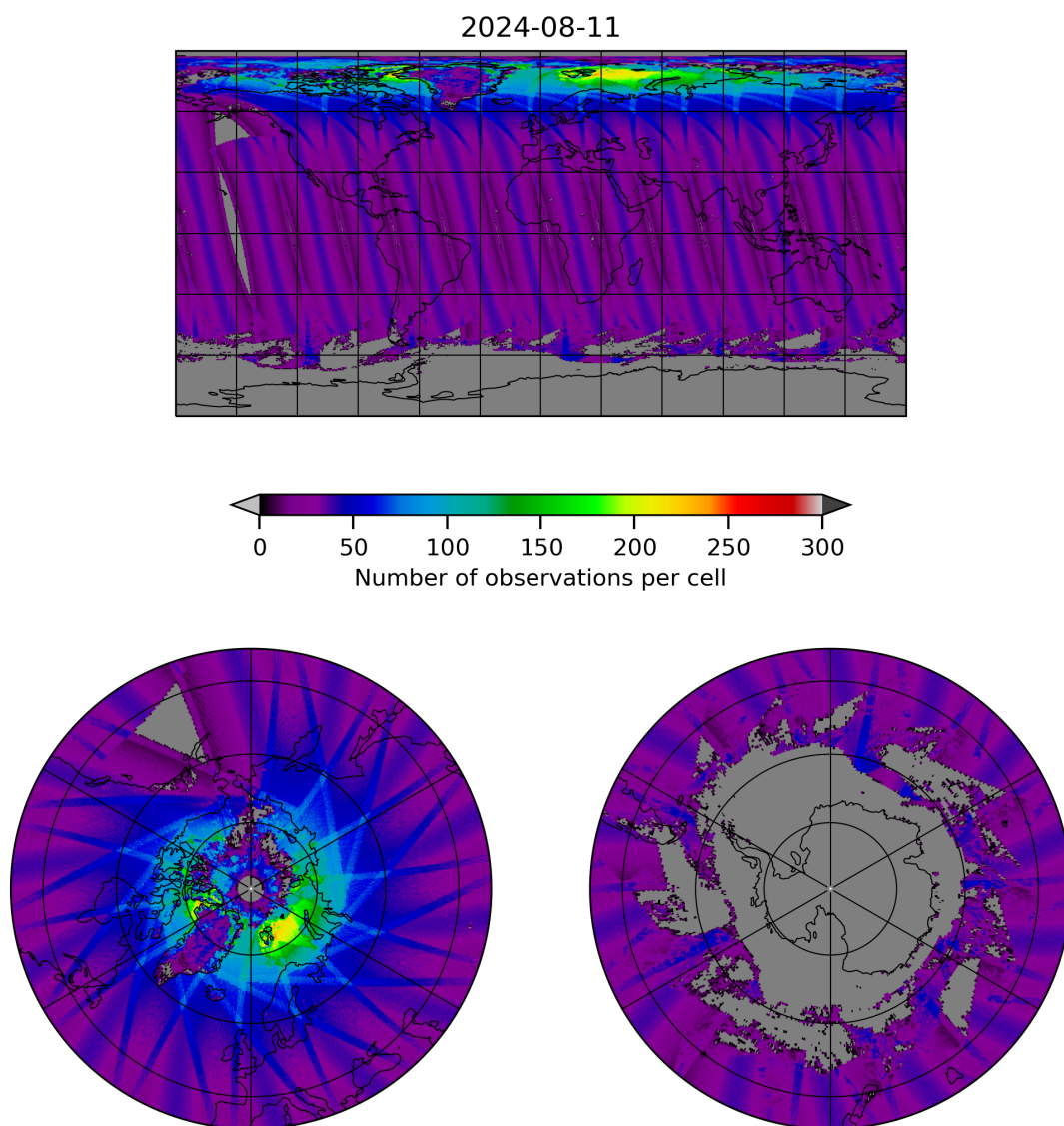
Figure 19: Map of the number of observations for 2024-08-11 to 2024-08-11
