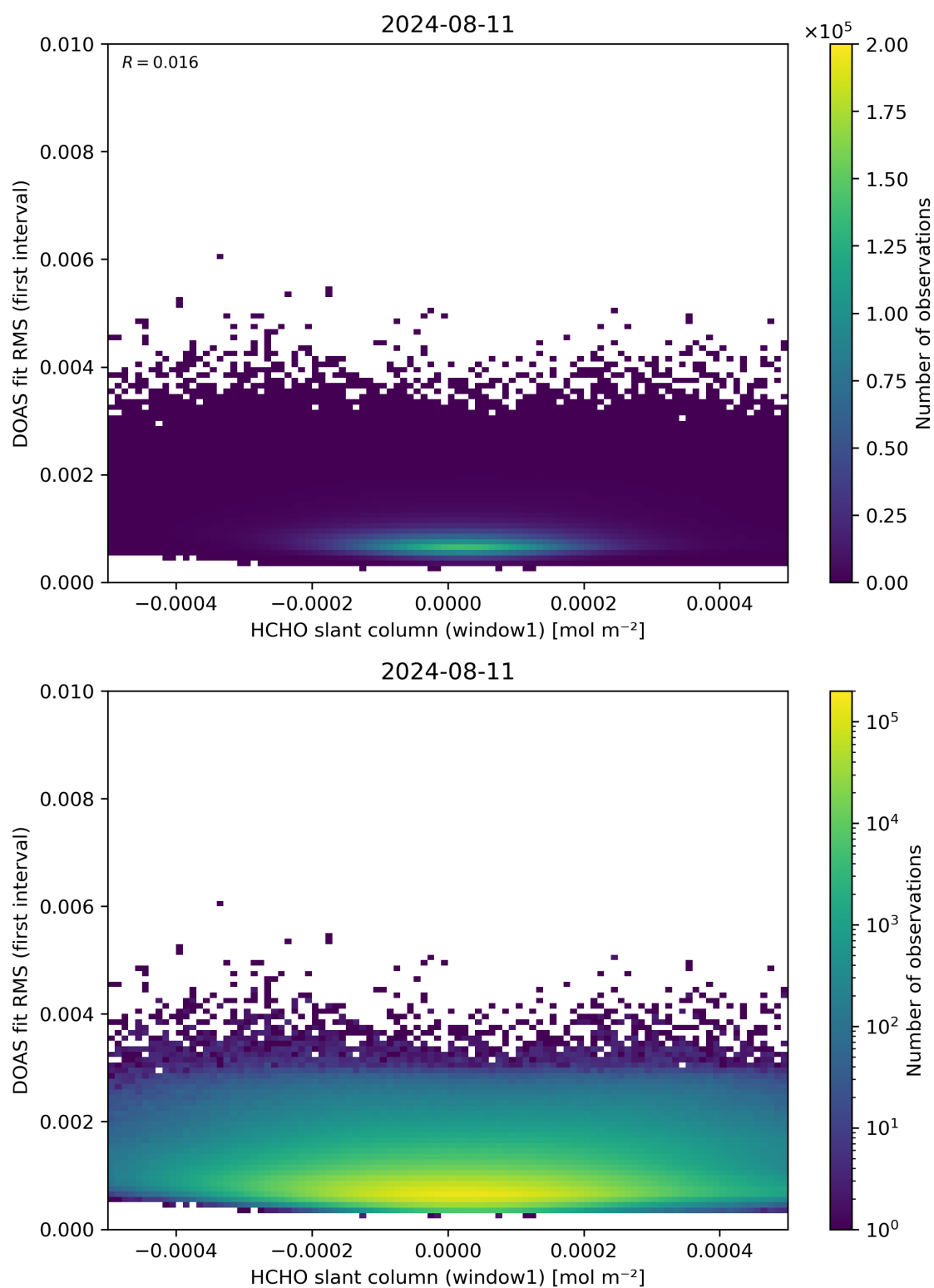
Figure 78: Scatter density plot of “HCHO slant column (window1)” against “DOAS fit RMS (first interval)” for 2024-08-11 to 2024-08-11.
