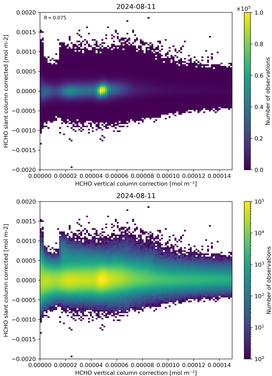
Figure 116: Scatter density plot of “HCHO vertical column correction” against “HCHO slant column corrected” for 2024-08-11 to 2024-08-11.
