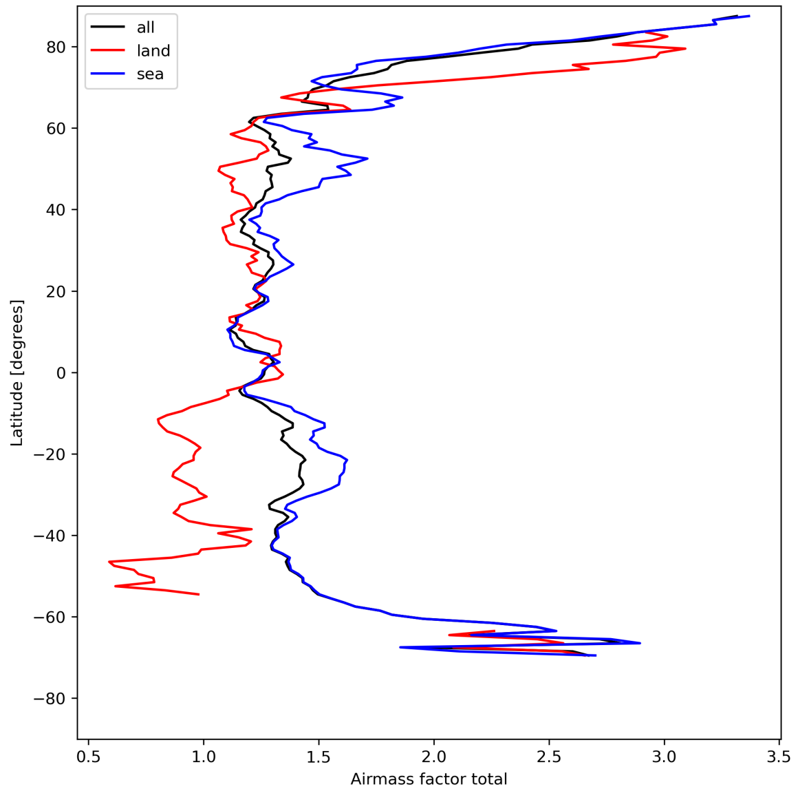
Figure 26: Zonal average of “Airmass factor total” for 2024-08-11 to 2024-08-11.
