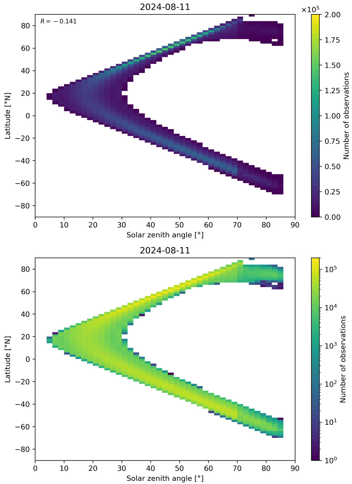
Figure 181: Scatter density plot of “Solar zenith angle” against “Latitude” for 2024-08-11 to 2024-08-11.
