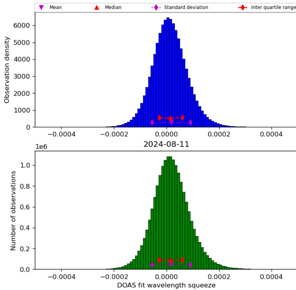
Figure 45: Histogram of “DOAS fit wavelength squeeze” for 2024-08-11 to 2024-08-11
