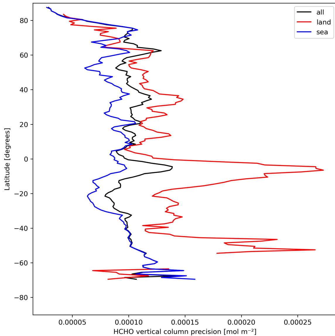
Figure 22: Zonal average of “HCHO vertical column precision” for 2024-08-11 to 2024-08-11.
