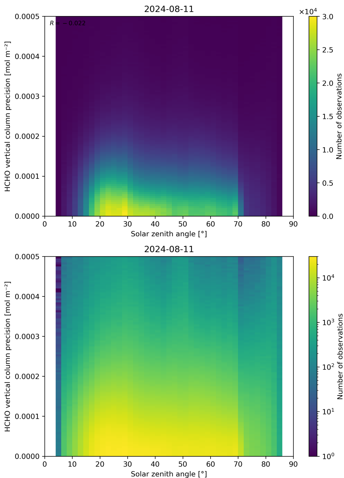
Figure 179: Scatter density plot of “Solar zenith angle” against “HCHO vertical column precision” for 2024-08-11 to 2024-08-11.
