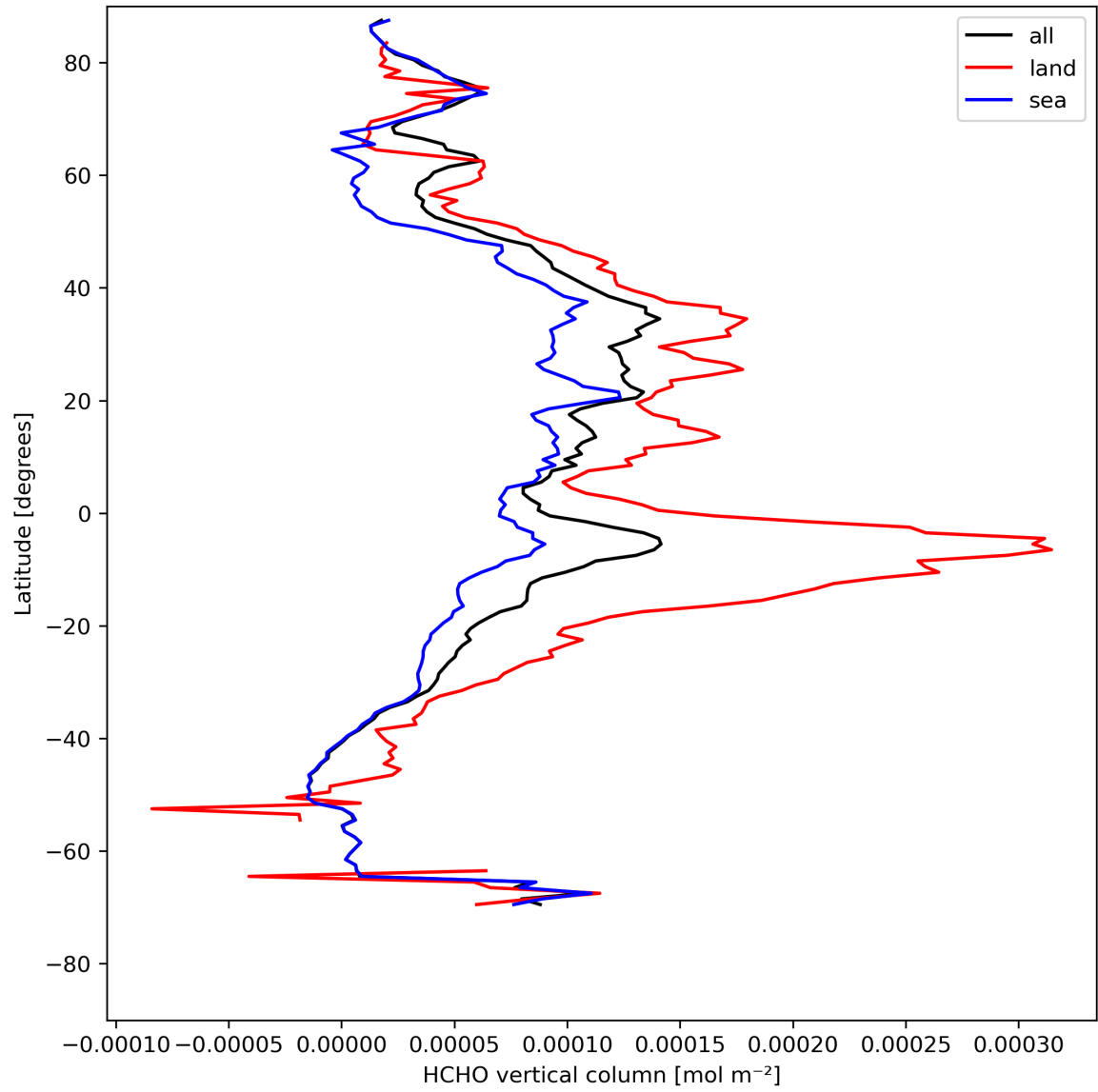
Figure 21: Zonal average of “HCHO vertical column” for 2024-08-11 to 2024-08-11.
