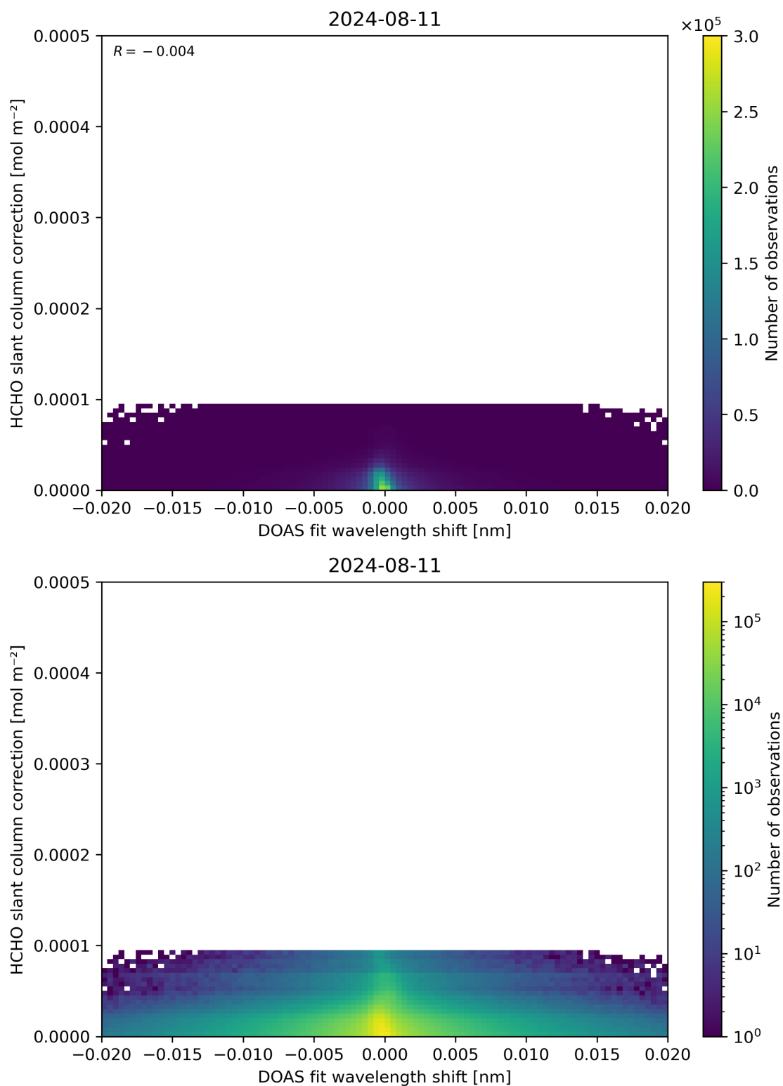
Figure 67: Scatter density plot of “DOAS fit wavelength shift” against “HCHO slant column correction” for 2024-08-11 to 2024-08-11.
