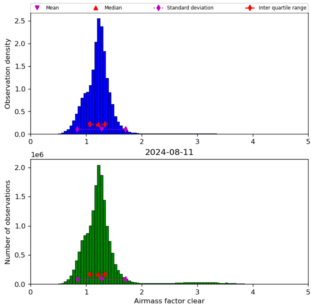
Figure 42: Histogram of “Airmass factor clear” for 2024-08-11 to 2024-08-11
