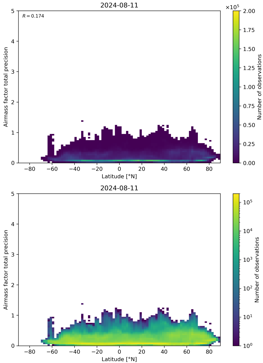
Figure 162: Scatter density plot of “Latitude” against “Airmass factor total precision” for 2024-08-11 to 2024-08-11.
