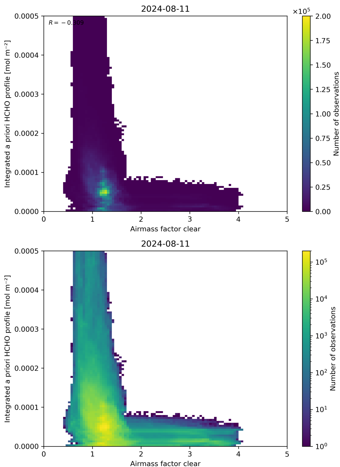
Figure 76: Scatter density plot of “Airmass factor clear” against “Integrated a priori HCHO profile” for 2024-08-11 to 2024-08-11.
