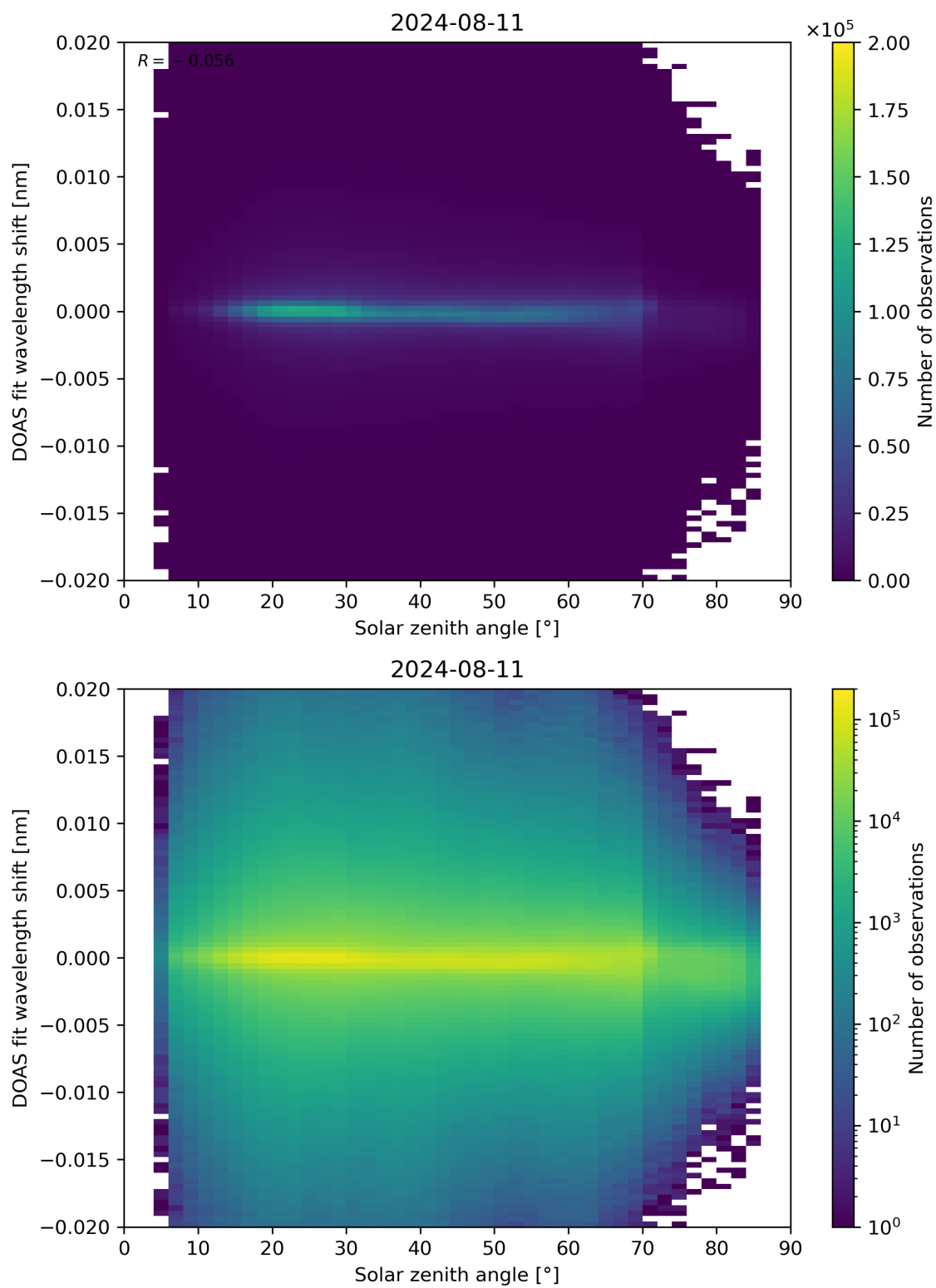
Figure 168: Scatter density plot of “Solar zenith angle” against “DOAS fit wavelength shift” for 2024-08-11 to 2024-08-11.
