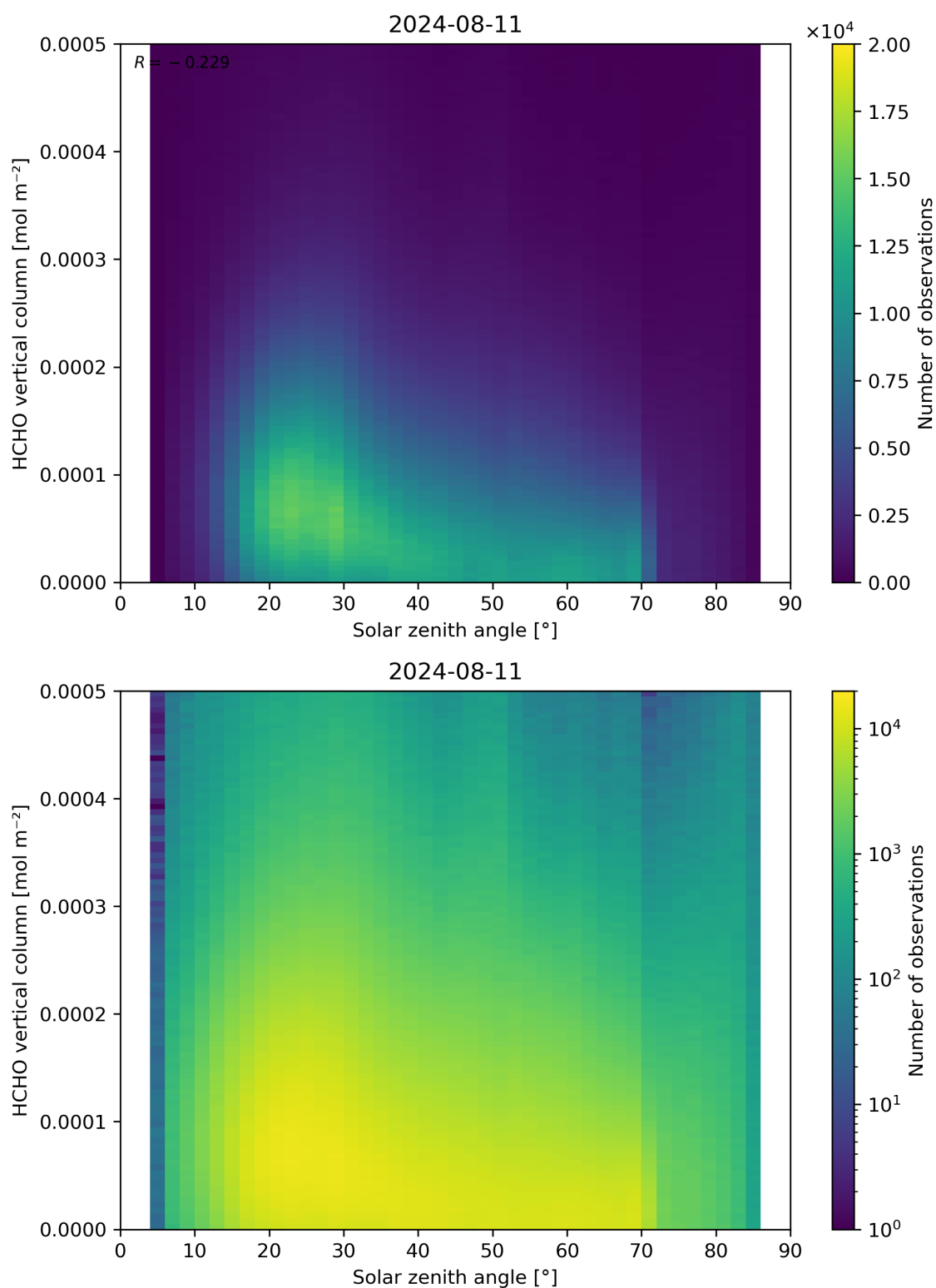
Figure 177: Scatter density plot of “Solar zenith angle” against “HCHO vertical column” for 2024-08-11 to 2024-08-11.
