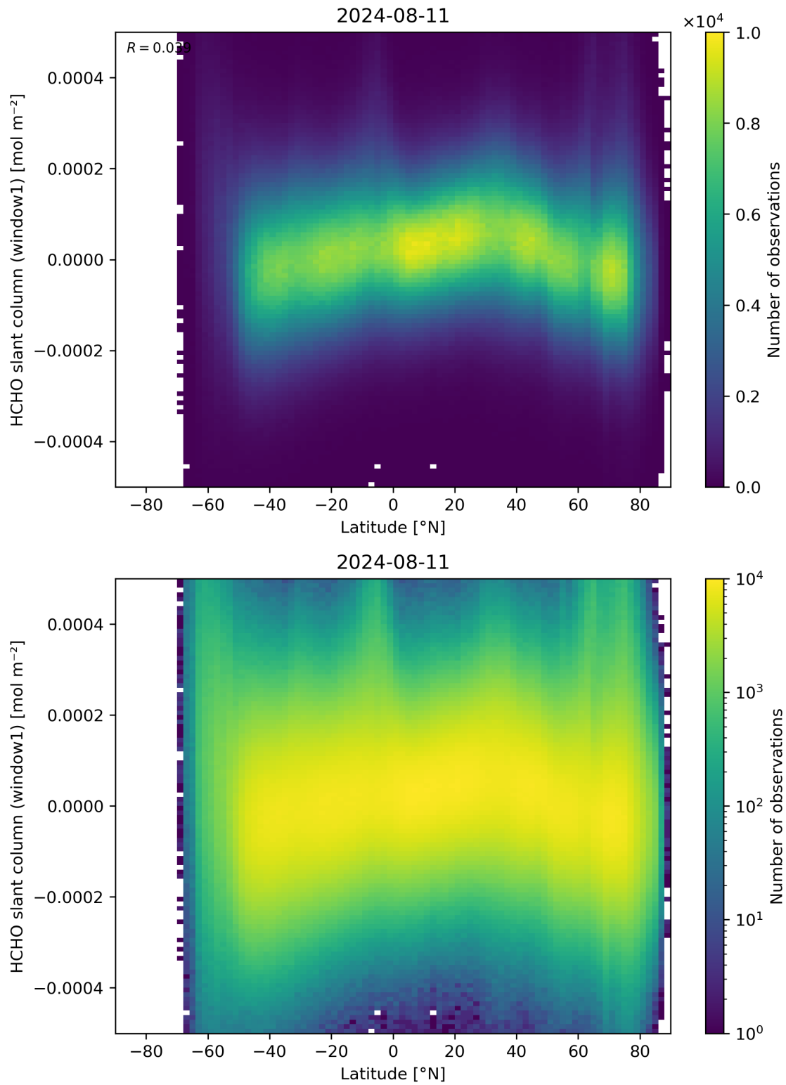
Figure 159: Scatter density plot of “Latitude” against “HCHO slant column (window1)” for 2024-08-11 to 2024-08-11.
