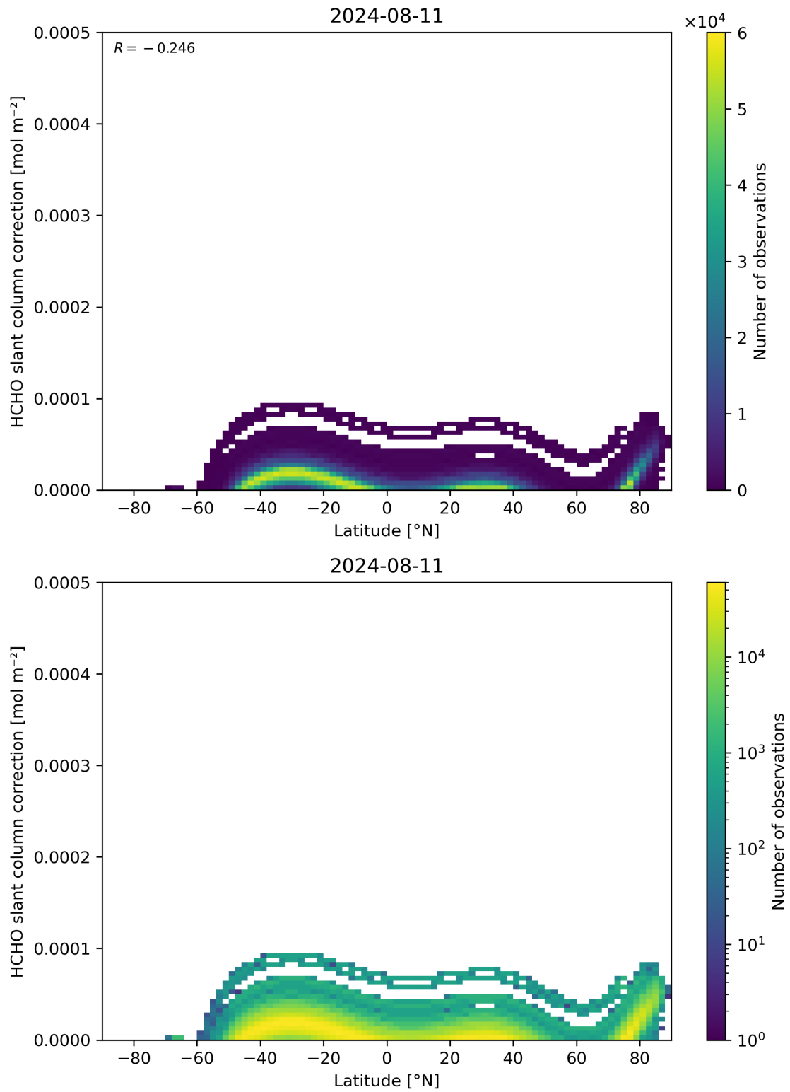
Figure 158: Scatter density plot of “Latitude” against “HCHO slant column correction” for 2024-08-11 to 2024-08-11.
