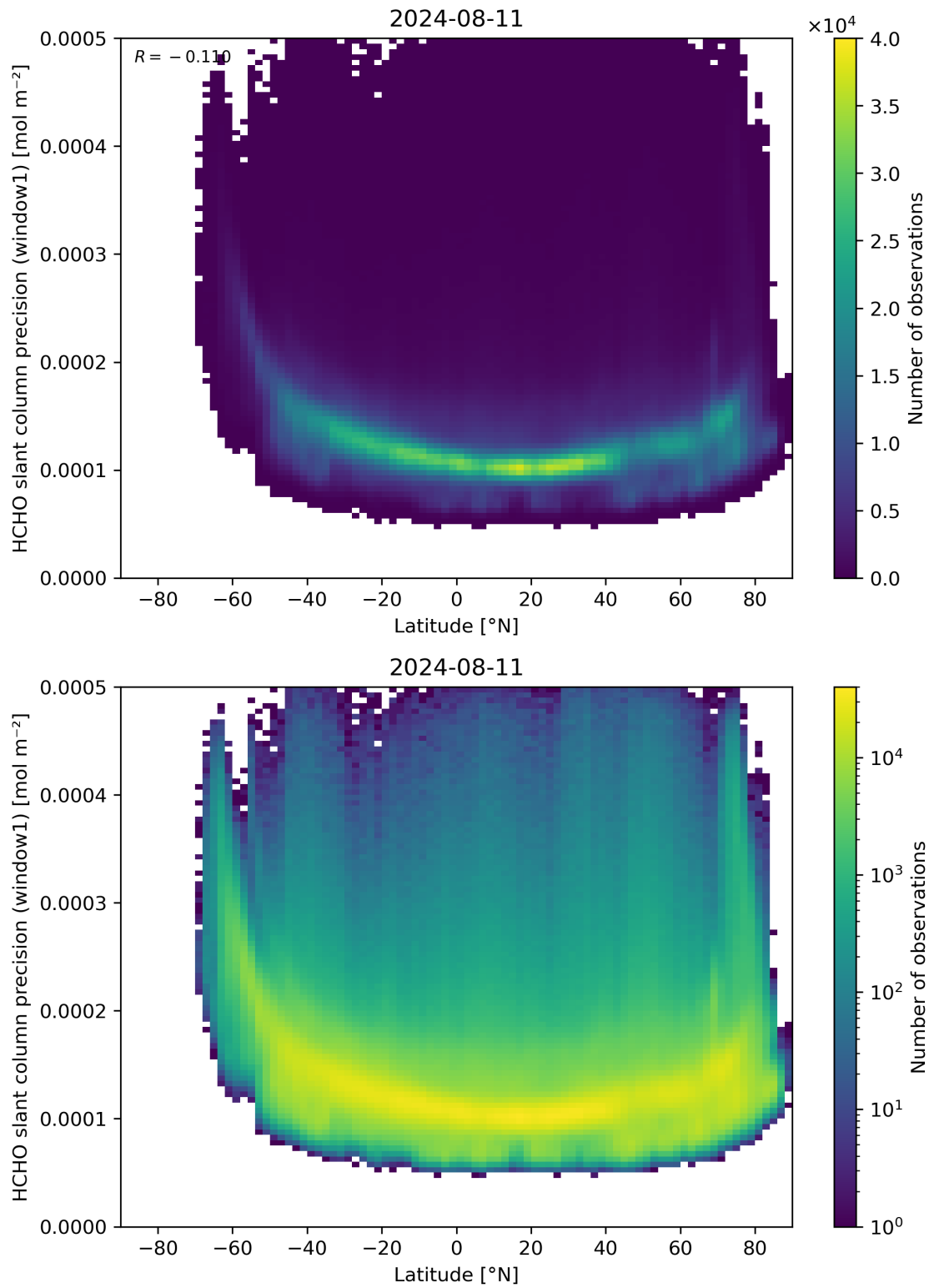
Figure 160: Scatter density plot of “Latitude” against “HCHO slant column precision (window1)” for 2024-08-11 to 2024-08-11.
