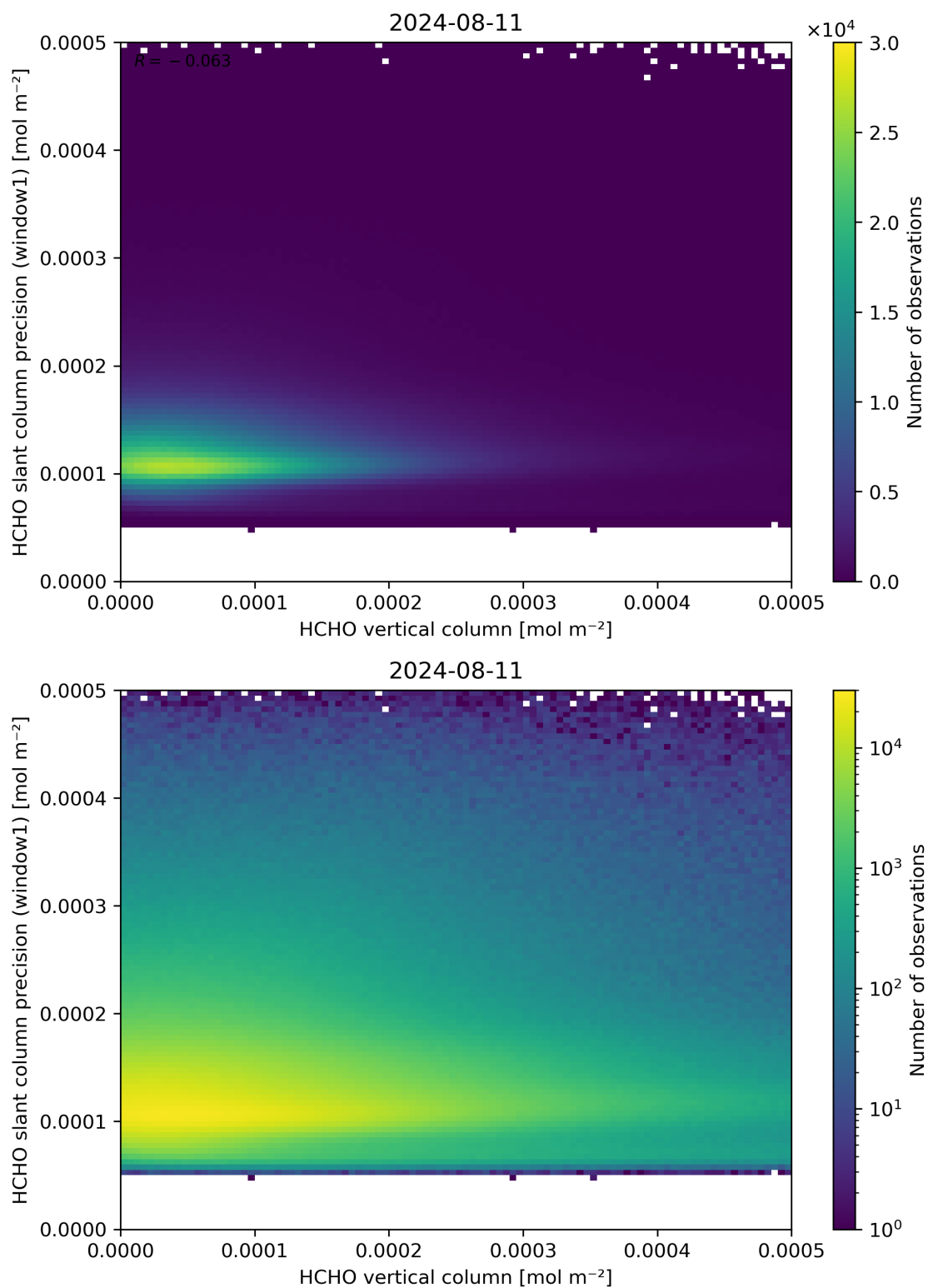
Figure 130: Scatter density plot of “HCHO vertical column” against “HCHO slant column precision (window1)” for 2024-08-11 to 2024-08-11.
