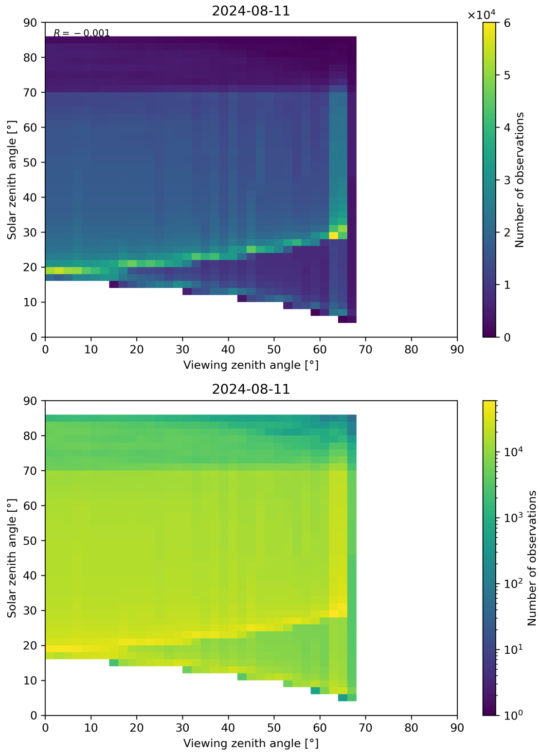
Figure 197: Scatter density plot of “Viewing zenith angle” against “Solar zenith angle” for 2024-08-11 to 2024-08-11.
