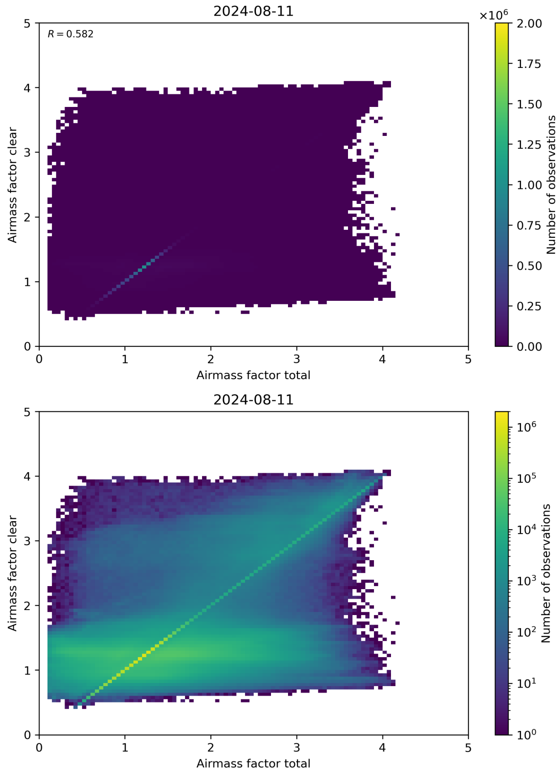
Figure 100: Scatter density plot of “Airmass factor total” against “Airmass factor clear” for 2024-08-11 to 2024-08-11.
