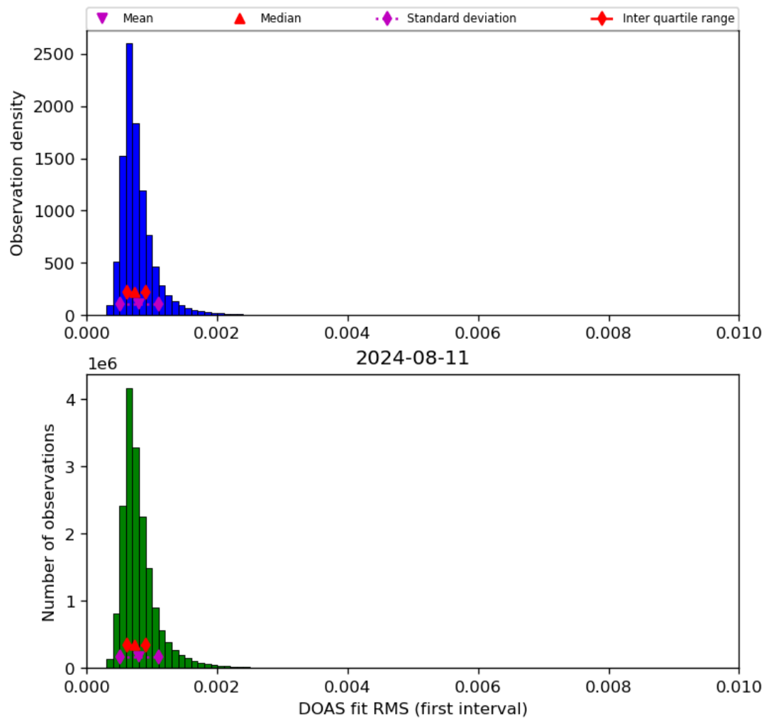
Figure 46: Histogram of “DOAS fit RMS (first interval)” for 2024-08-11 to 2024-08-11
