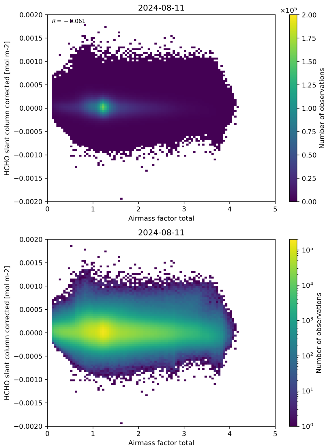
Figure 101: Scatter density plot of “Airmass factor total” against “HCHO slant column corrected” for 2024-08-11 to 2024-08-11.
