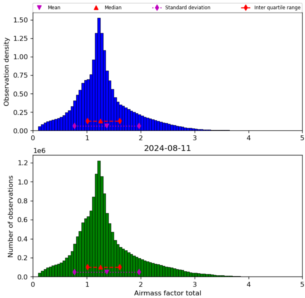
Figure 40: Histogram of “Airmass factor total” for 2024-08-11 to 2024-08-11
