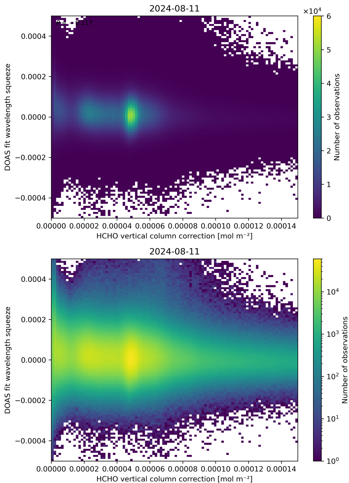
Figure 114: Scatter density plot of “HCHO vertical column correction” against “DOAS fit wavelength squeeze” for 2024-08-11 to 2024-08-11.
