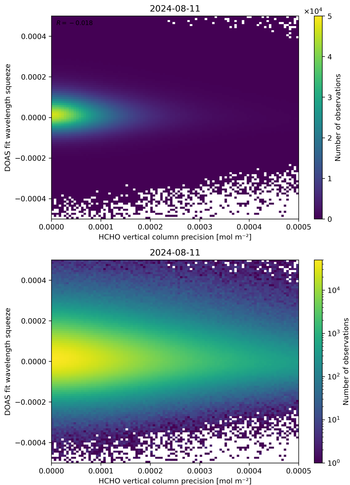
Figure 138: Scatter density plot of “HCHO vertical column precision” against “DOAS fit wavelength squeeze” for 2024-08-11 to 2024-08-11.
