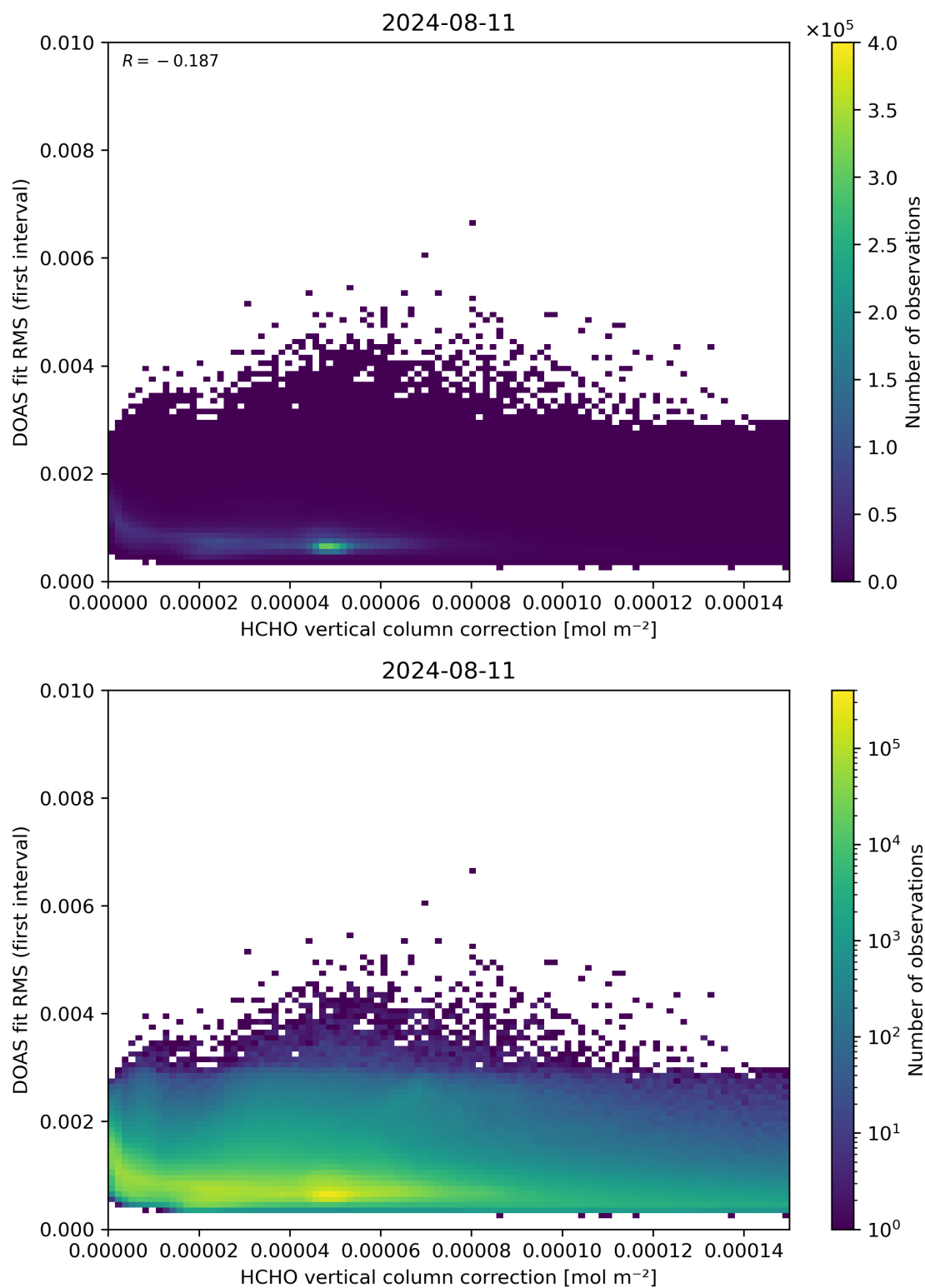
Figure 112: Scatter density plot of “HCHO vertical column correction” against “DOAS fit RMS (first interval)” for 2024-08-11 to 2024-08-11.
