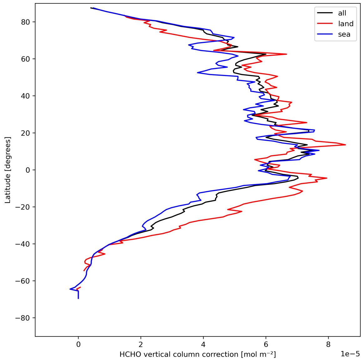
Figure 23: Zonal average of “HCHO vertical column correction” for 2024-08-11 to 2024-08-11.
