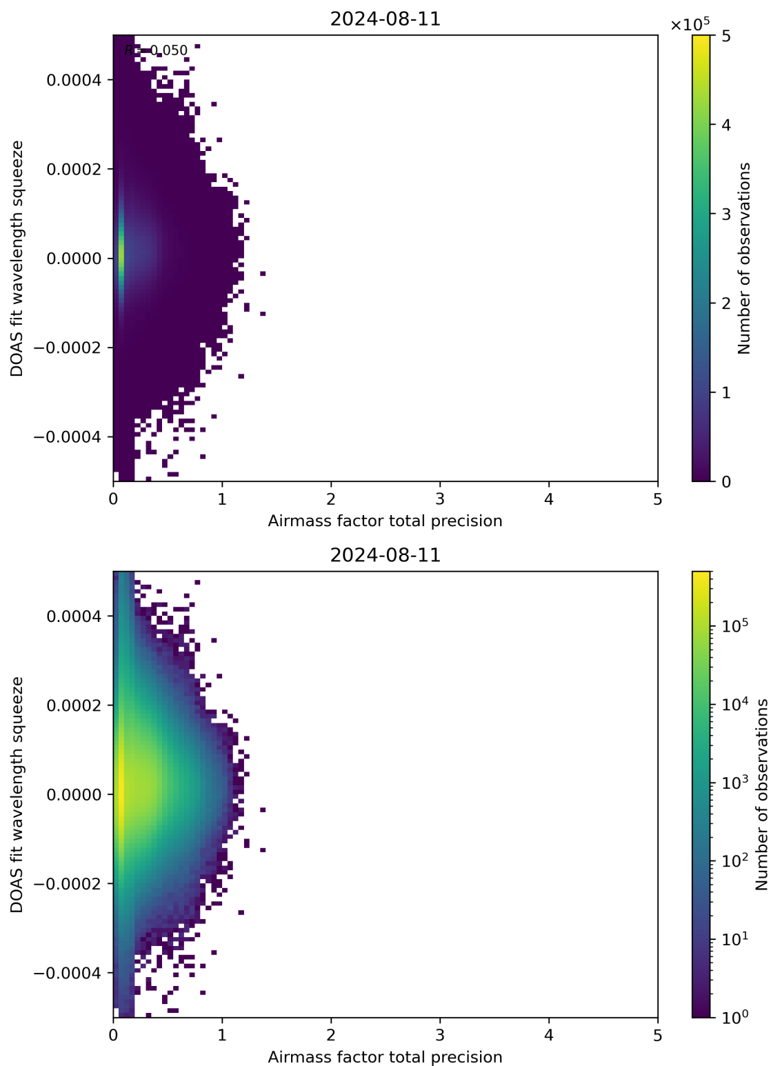
Figure 107: Scatter density plot of “Airmass factor total precision” against “DOAS fit wavelength squeeze” for 2024-08-11 to 2024-08-11.
