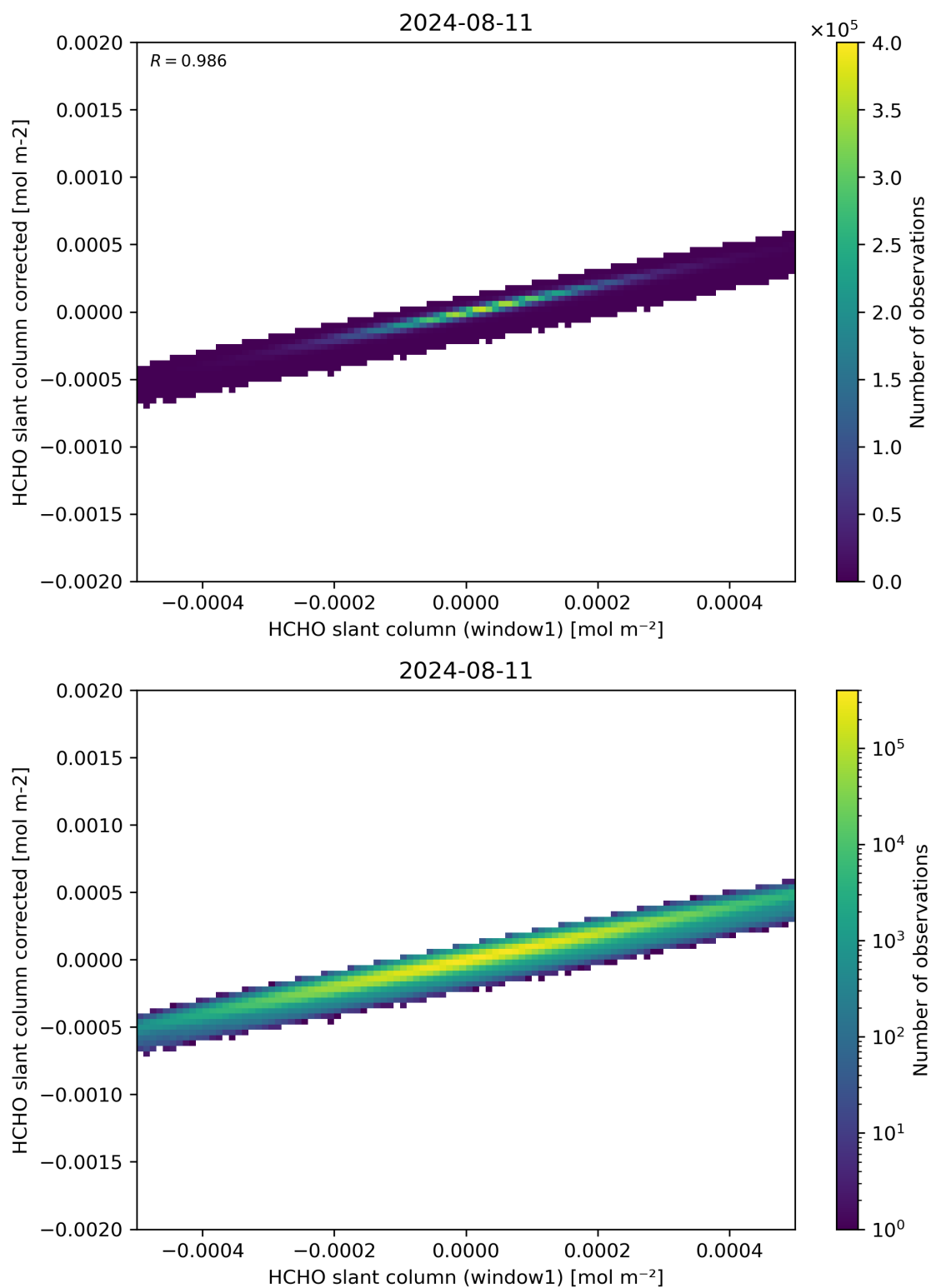
Figure 82: Scatter density plot of “HCHO slant column (window1)” against “HCHO slant column corrected” for 2024-08-11 to 2024-08-11.
