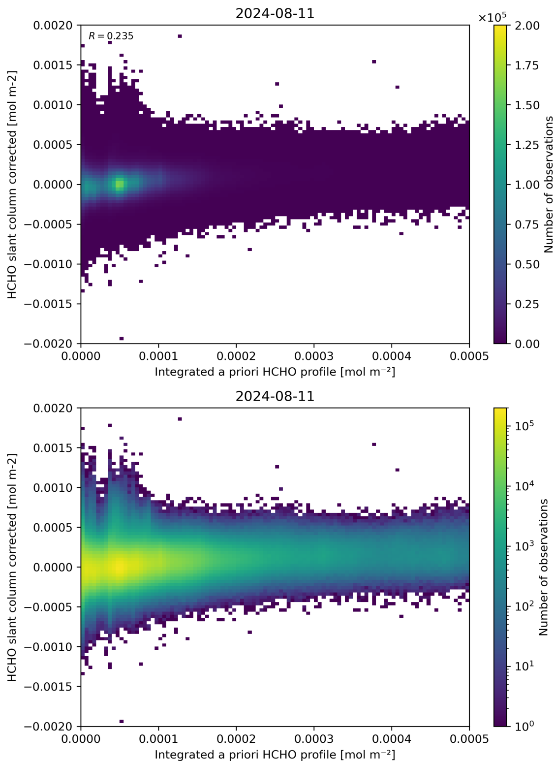
Figure 151: Scatter density plot of “Integrated a priori HCHO profile” against “HCHO slant column corrected” for 2024-08-11 to 2024-08-11.
