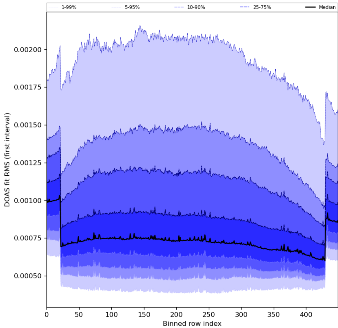
Figure 60: Along track statistics of “DOAS fit RMS (first interval)” for 2024-08-11 to 2024-08-11
