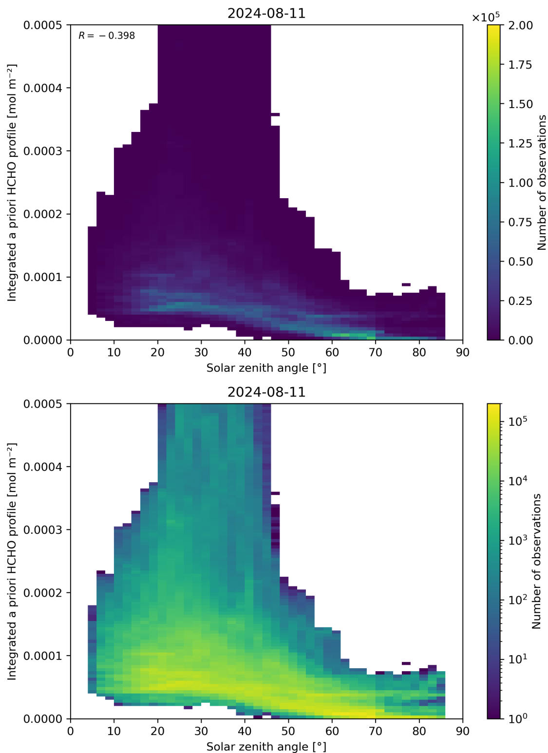
Figure 180: Scatter density plot of “Solar zenith angle” against “Integrated a priori HCHO profile” for 2024-08-11 to 2024-08-11.
