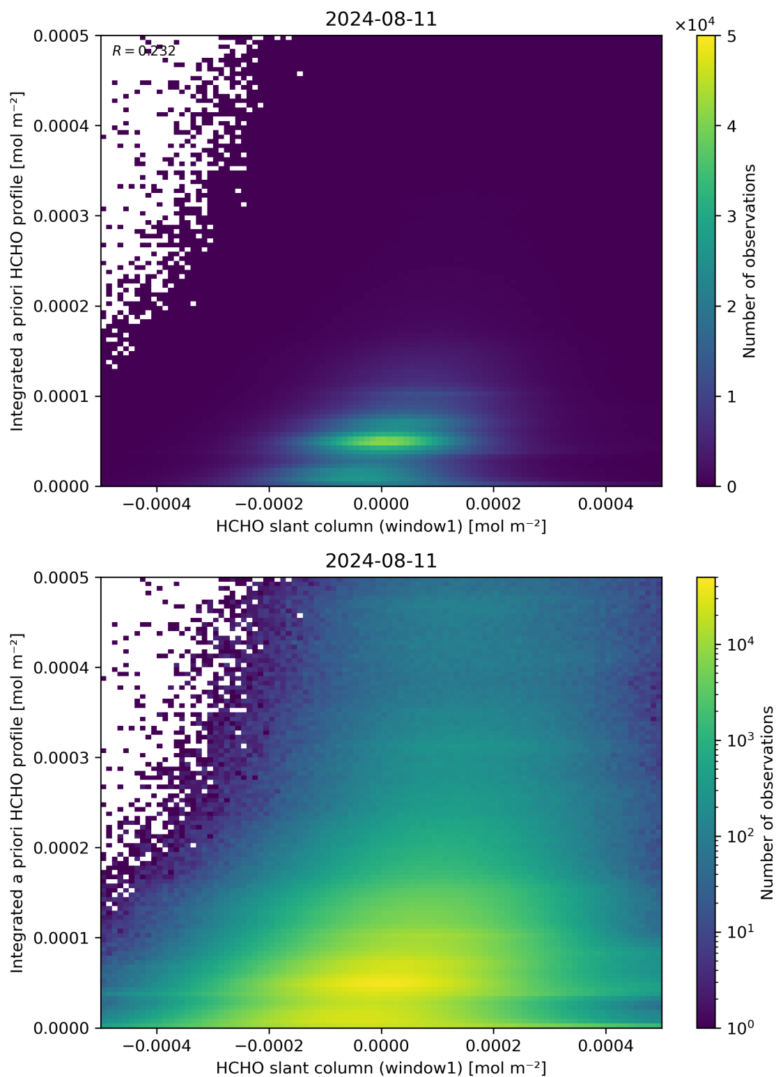
Figure 87: Scatter density plot of “HCHO slant column (window1)” against “Integrated a priori HCHO profile” for 2024-08-11 to 2024-08-11.
