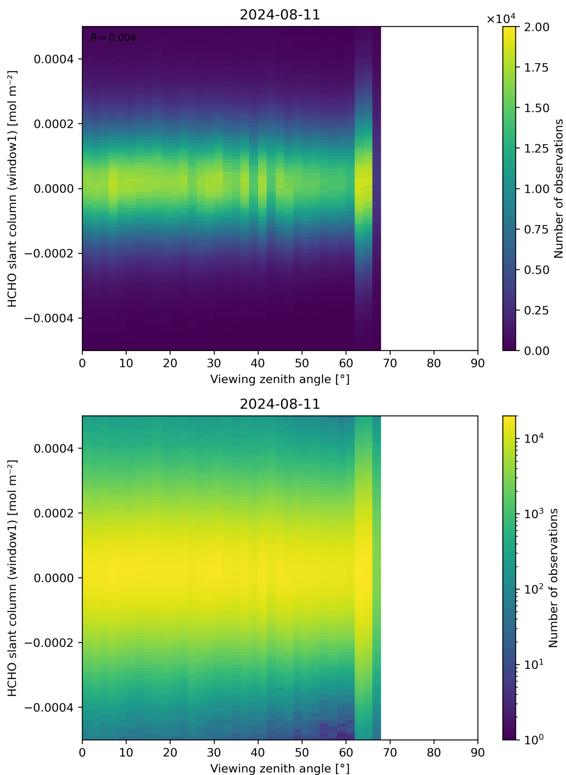
Figure 188: Scatter density plot of “Viewing zenith angle” against “HCHO slant column (window1)” for 2024-08-11 to 2024-08-11.
