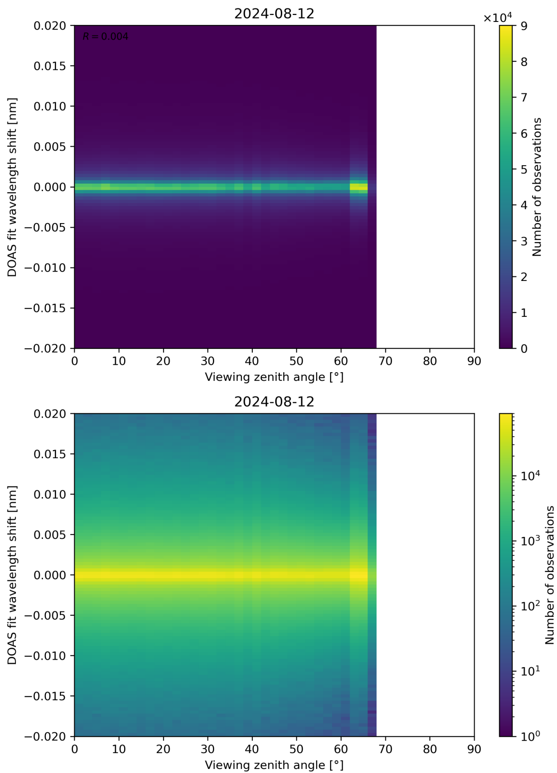
Figure 183: Scatter density plot of “Viewing zenith angle” against “DOAS fit wavelength shift” for 2024-08-12 to 2024-08-13.
