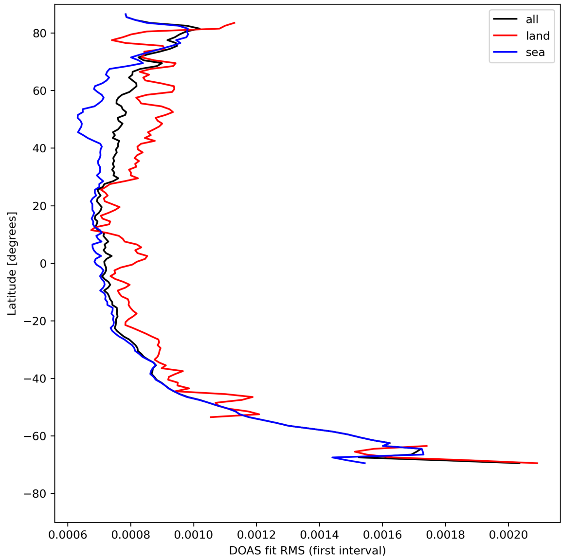
Figure 32: Zonal average of “DOAS fit RMS (first interval)” for 2024-08-12 to 2024-08-13.
