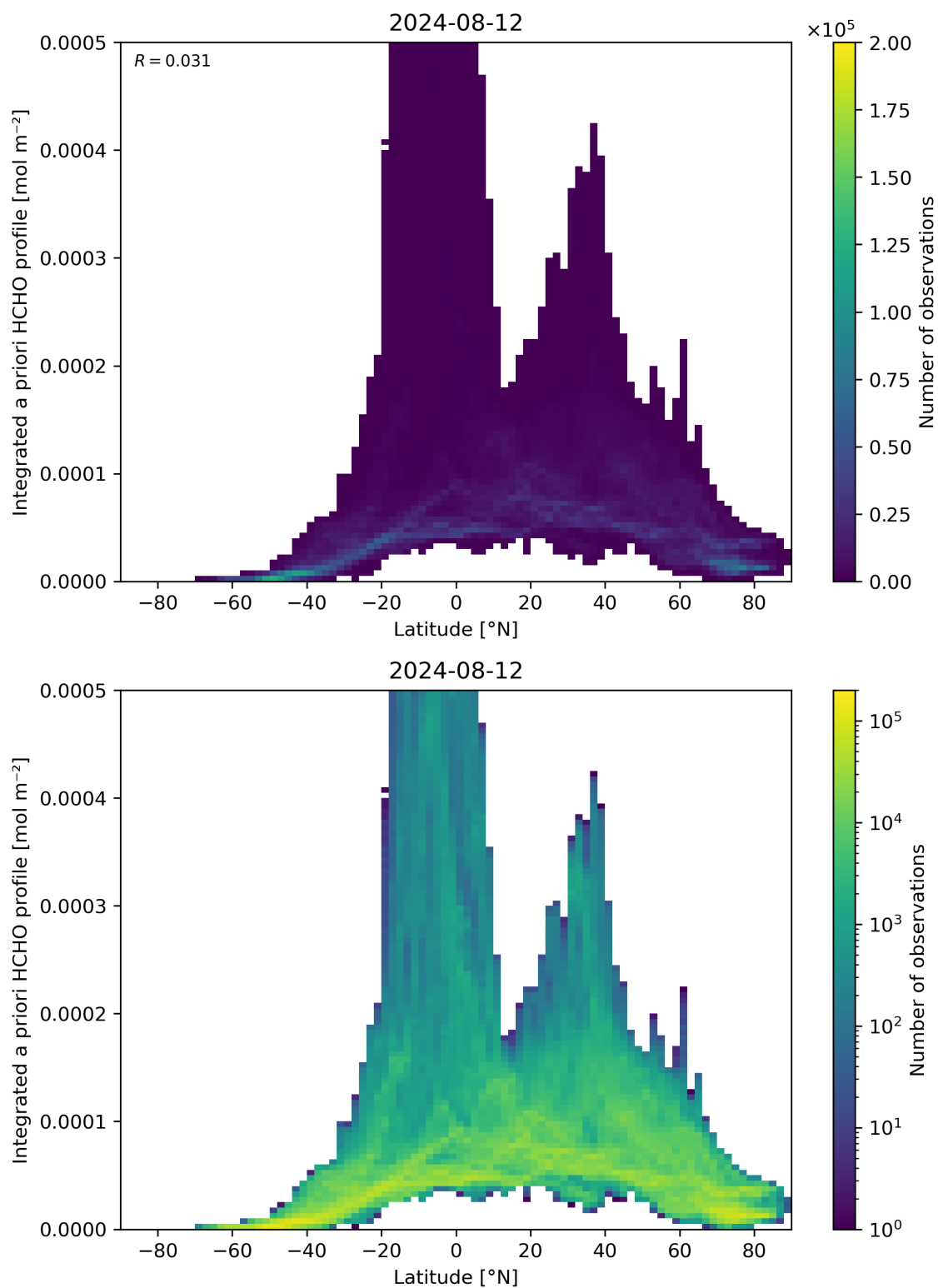
Figure 166: Scatter density plot of “Latitude” against “Integrated a priori HCHO profile” for 2024-08-12 to 2024-08-13.
