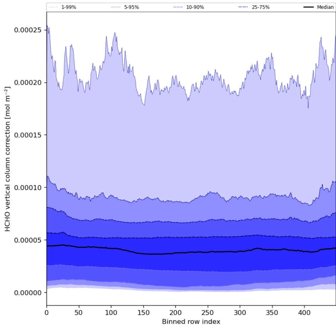
Figure 51: Along track statistics of “HCHO vertical column correction” for 2024-08-12 to 2024-08-13
