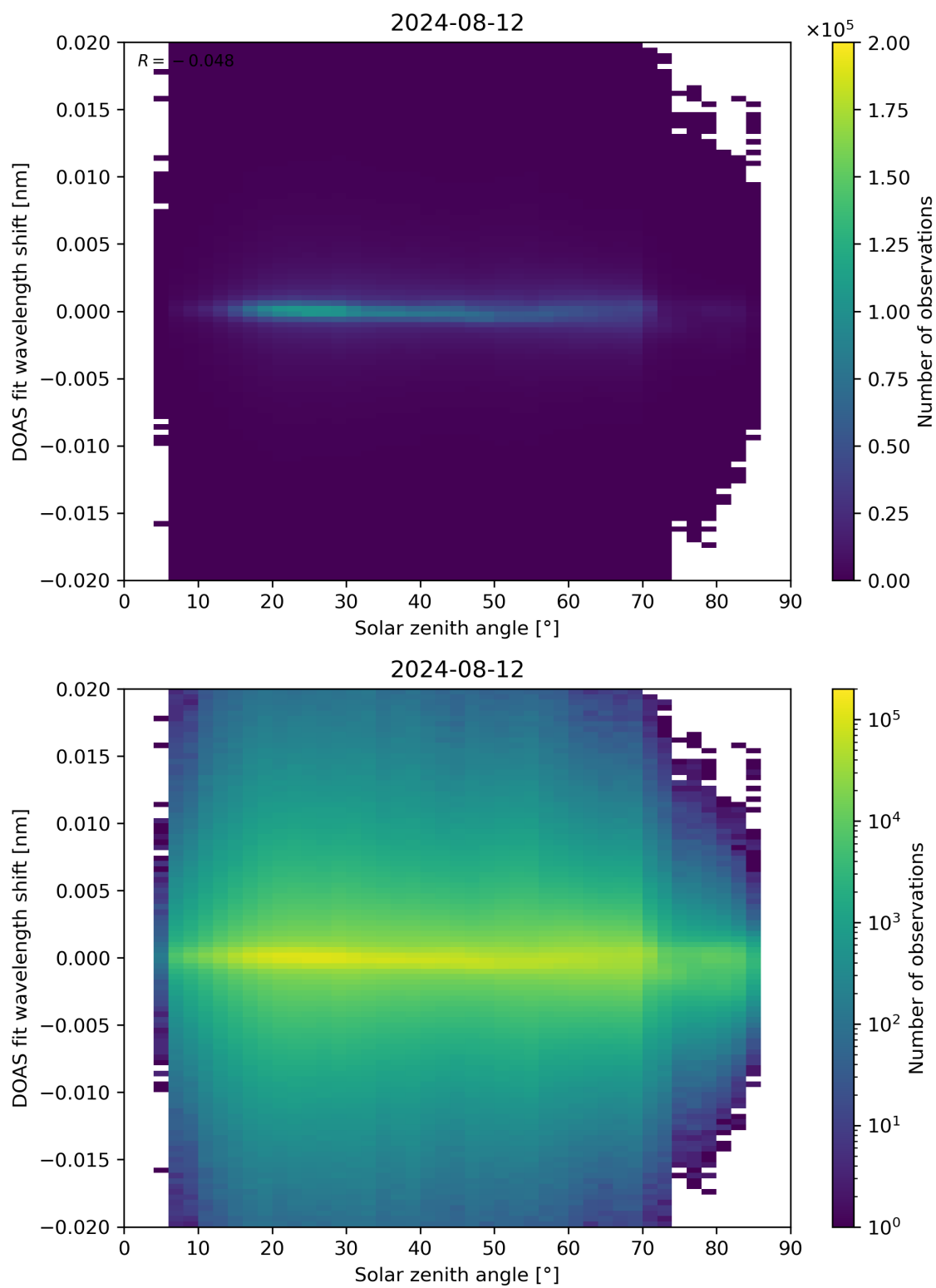
Figure 168: Scatter density plot of “Solar zenith angle” against “DOAS fit wavelength shift” for 2024-08-12 to 2024-08-13.
