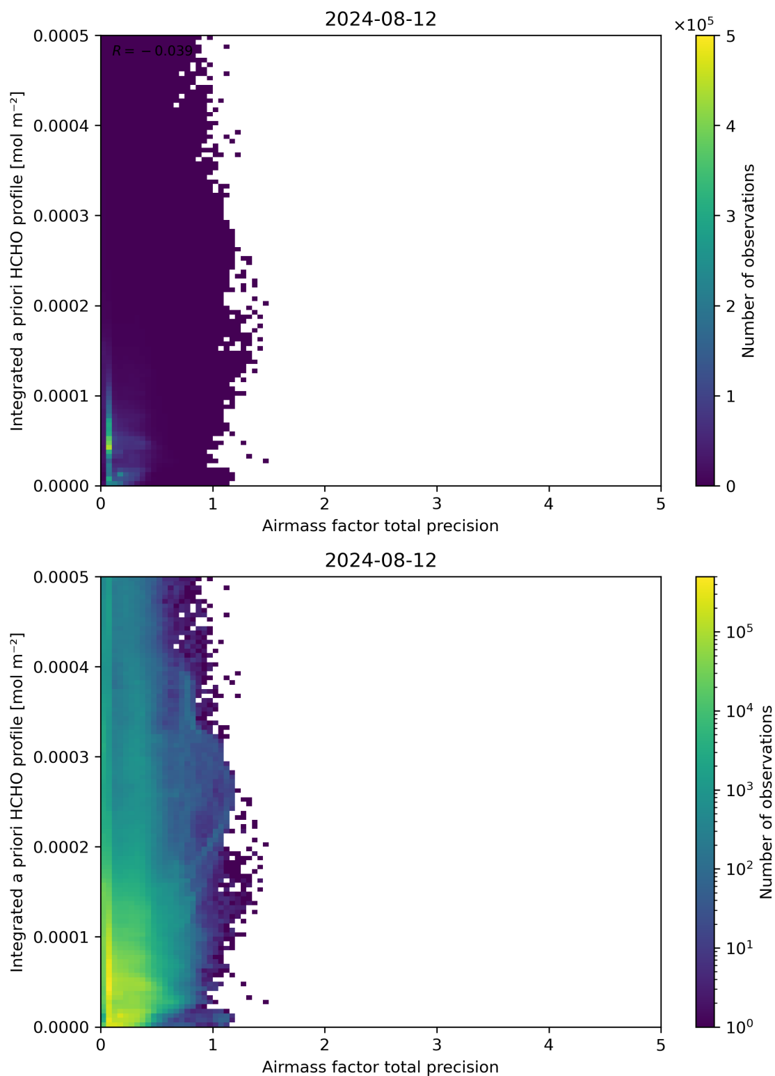
Figure 111: Scatter density plot of “Airmass factor total precision” against “Integrated a priori HCHO profile” for 2024-08-12 to 2024-08-13.
