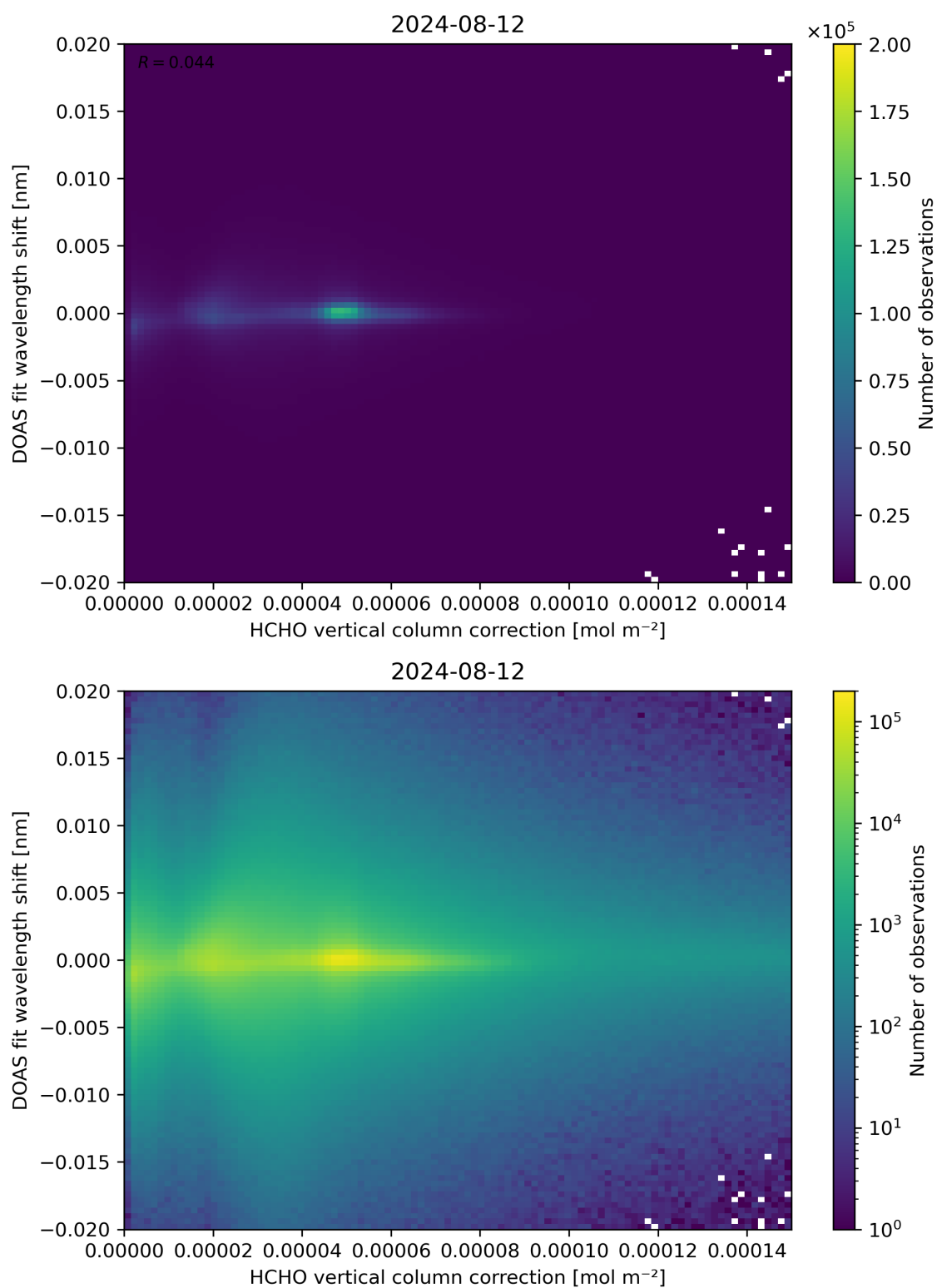
Figure 113: Scatter density plot of “HCHO vertical column correction” against “DOAS fit wavelength shift” for 2024-08-12 to 2024-08-13.
