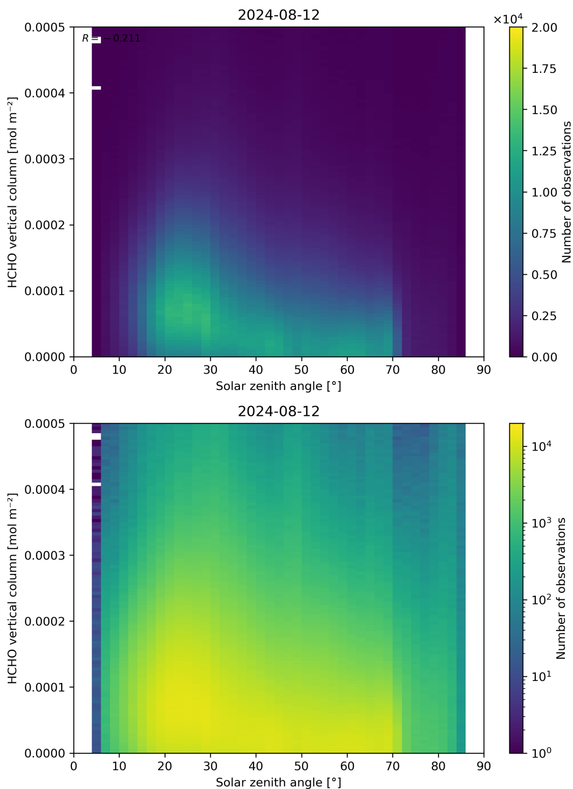
Figure 177: Scatter density plot of “Solar zenith angle” against “HCHO vertical column” for 2024-08-12 to 2024-08-13.
