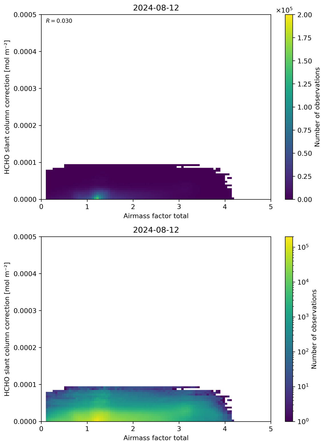
Figure 102: Scatter density plot of “Airmass factor total” against “HCHO slant column correction” for 2024-08-12 to 2024-08-13.
