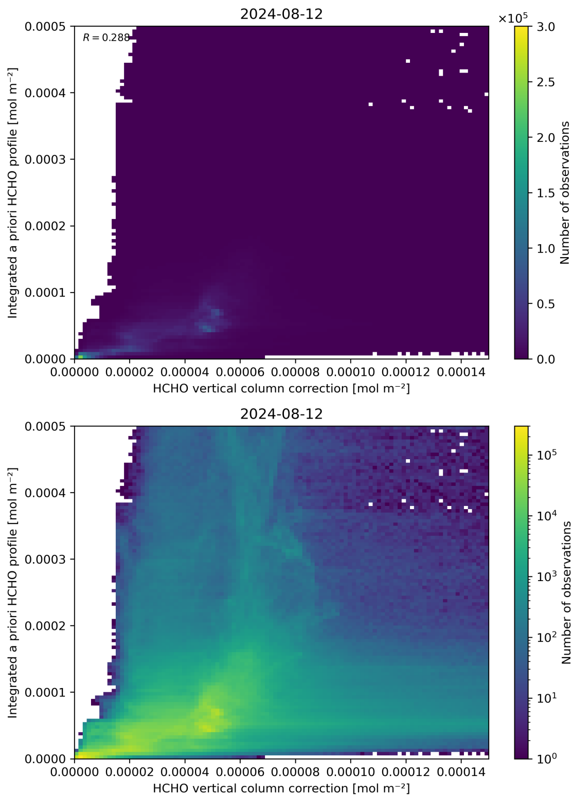
Figure 122: Scatter density plot of “HCHO vertical column correction” against “Integrated a priori HCHO profile” for 2024-08-12 to 2024-08-13.
