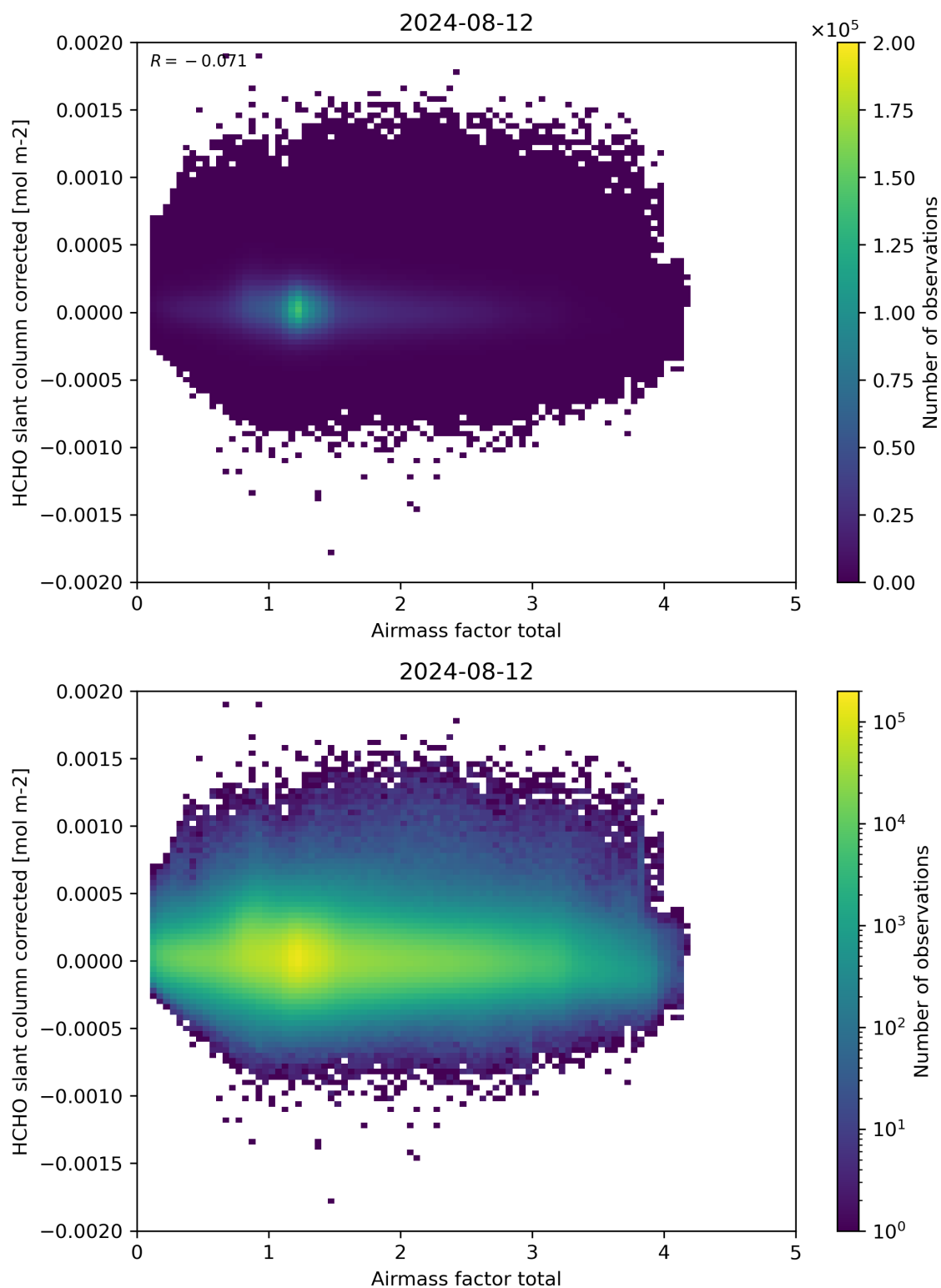
Figure 101: Scatter density plot of “Airmass factor total” against “HCHO slant column corrected” for 2024-08-12 to 2024-08-13.
