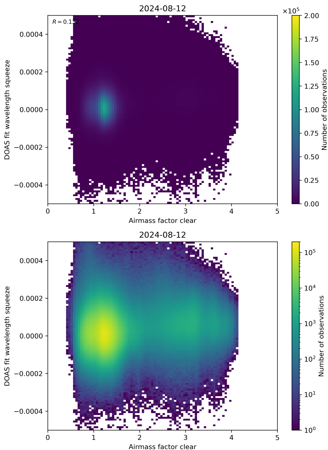
Figure 73: Scatter density plot of “Airmass factor clear” against “DOAS fit wavelength squeeze” for 2024-08-12 to 2024-08-13.
