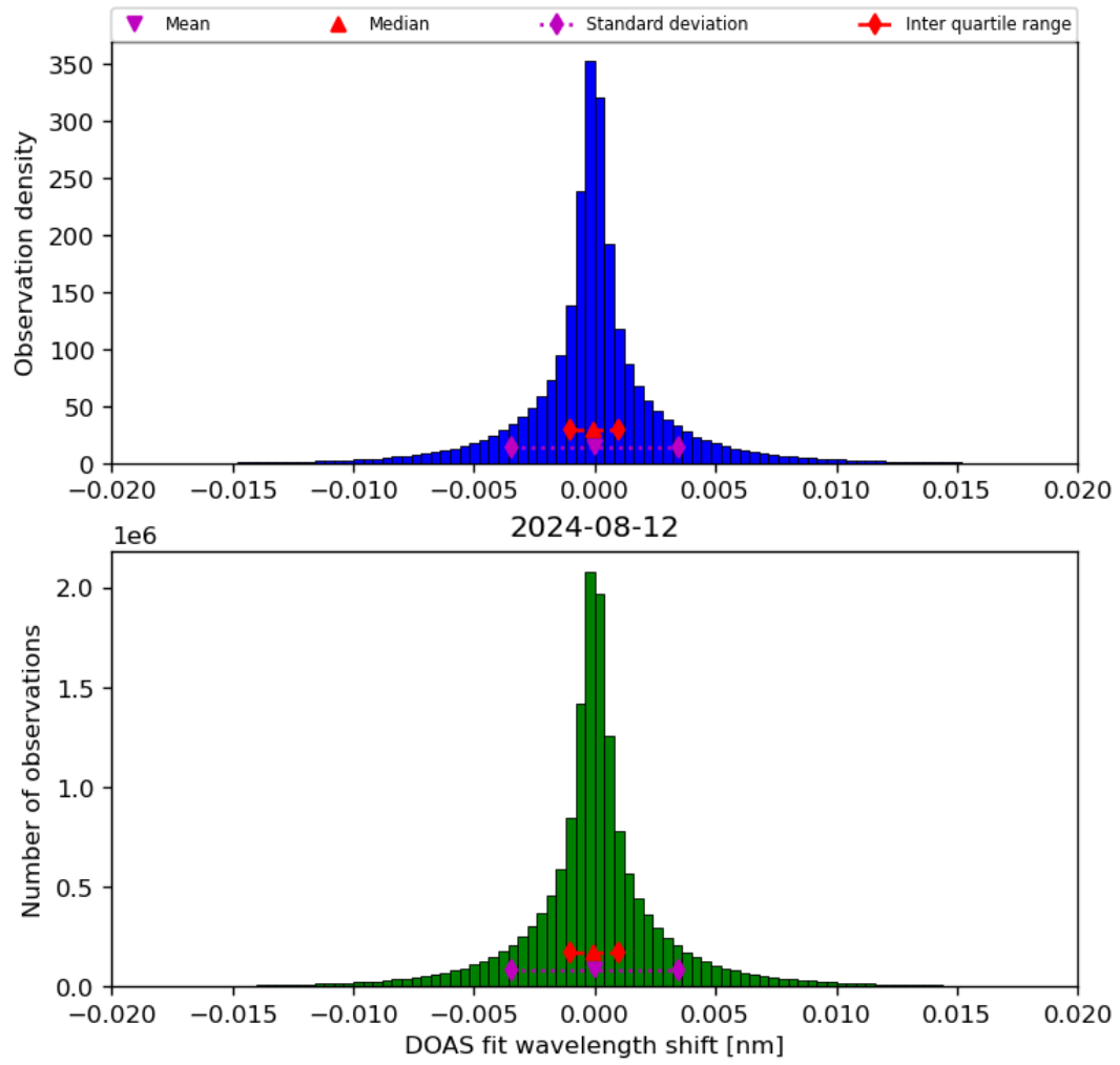
Figure 44: Histogram of “DOAS fit wavelength shift” for 2024-08-12 to 2024-08-13
