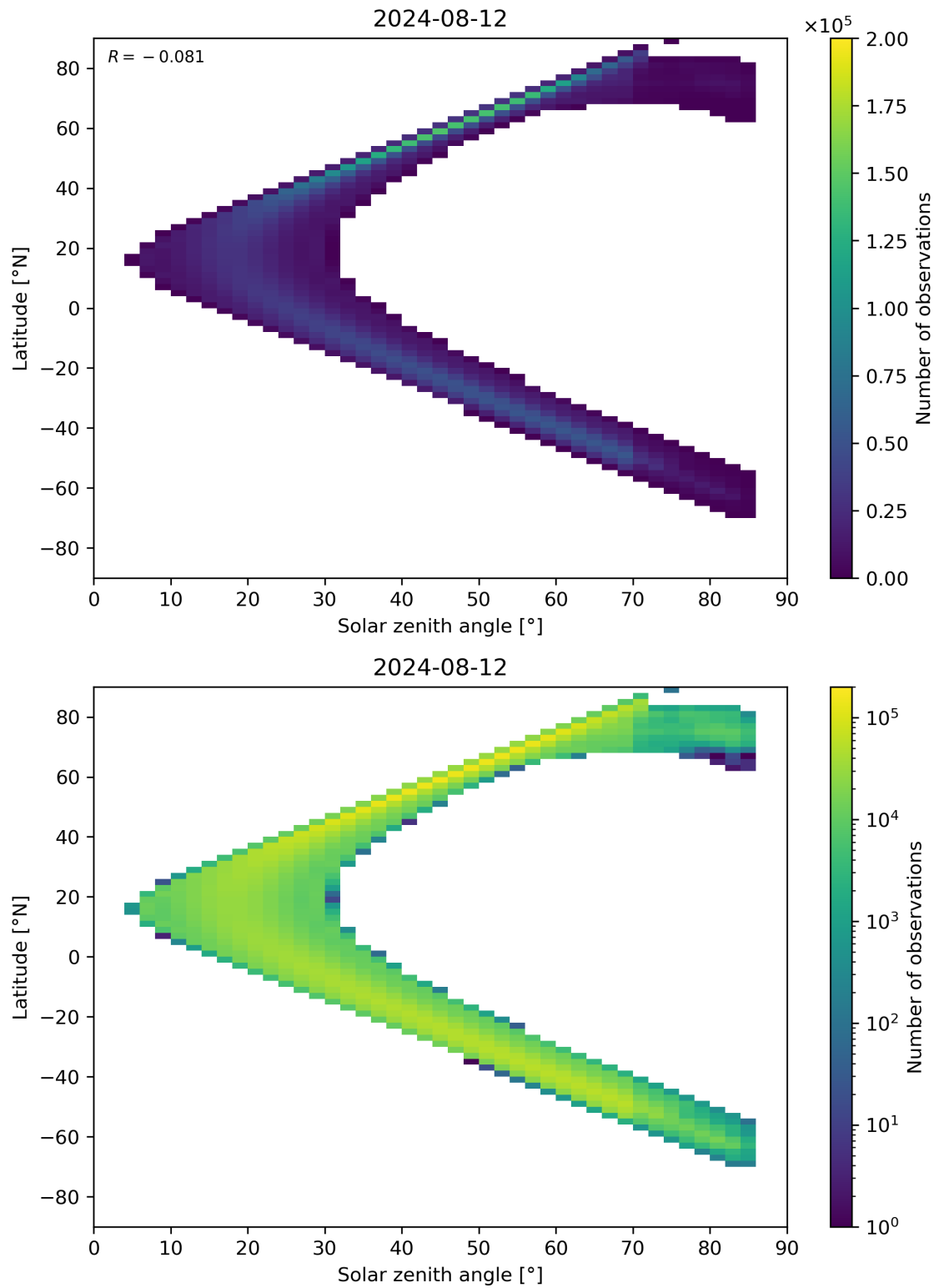
Figure 181: Scatter density plot of “Solar zenith angle” against “Latitude” for 2024-08-12 to 2024-08-13.
