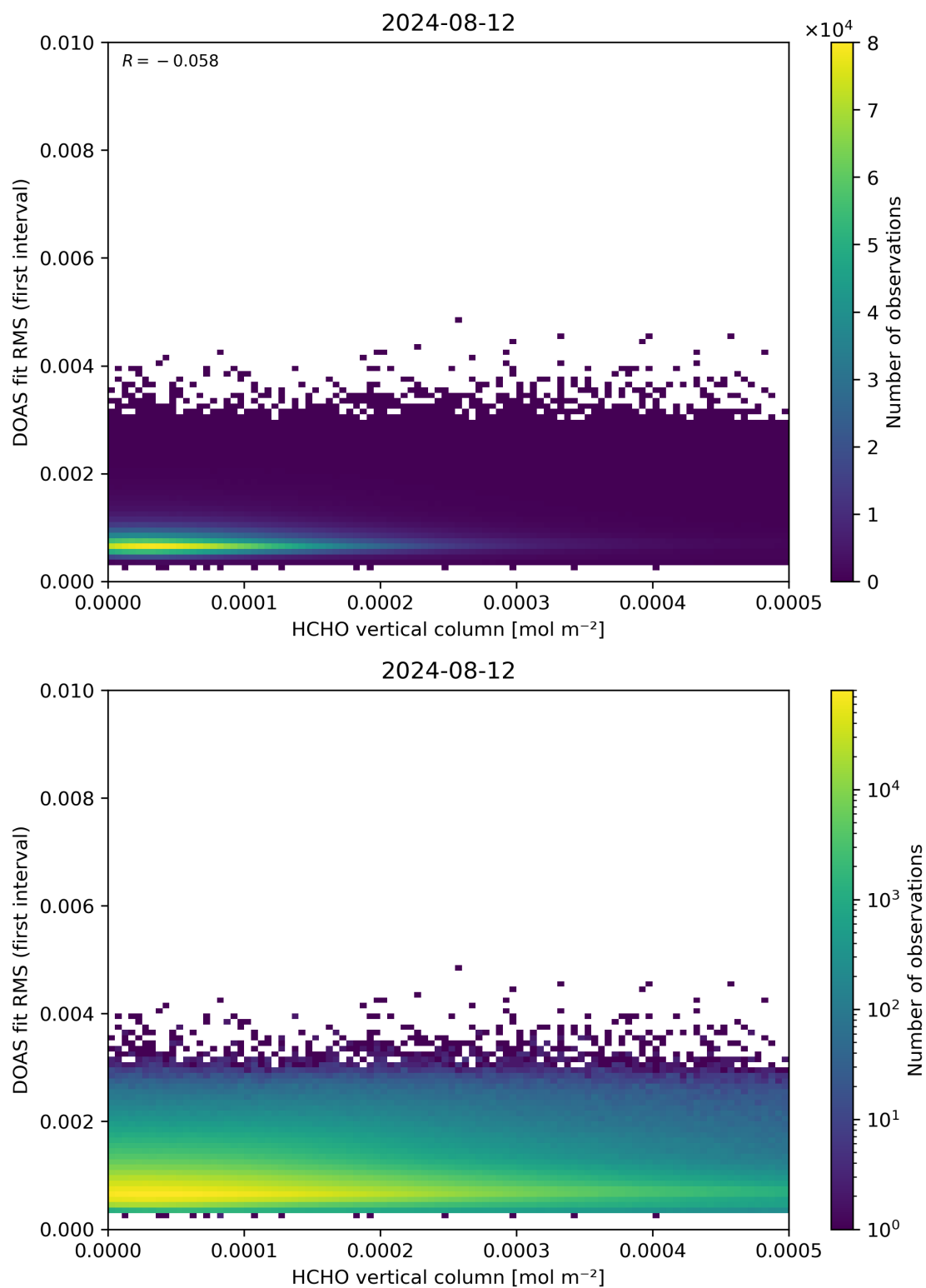
Figure 123: Scatter density plot of “HCHO vertical column” against “DOAS fit RMS (first interval)” for 2024-08-12 to 2024-08-13.
