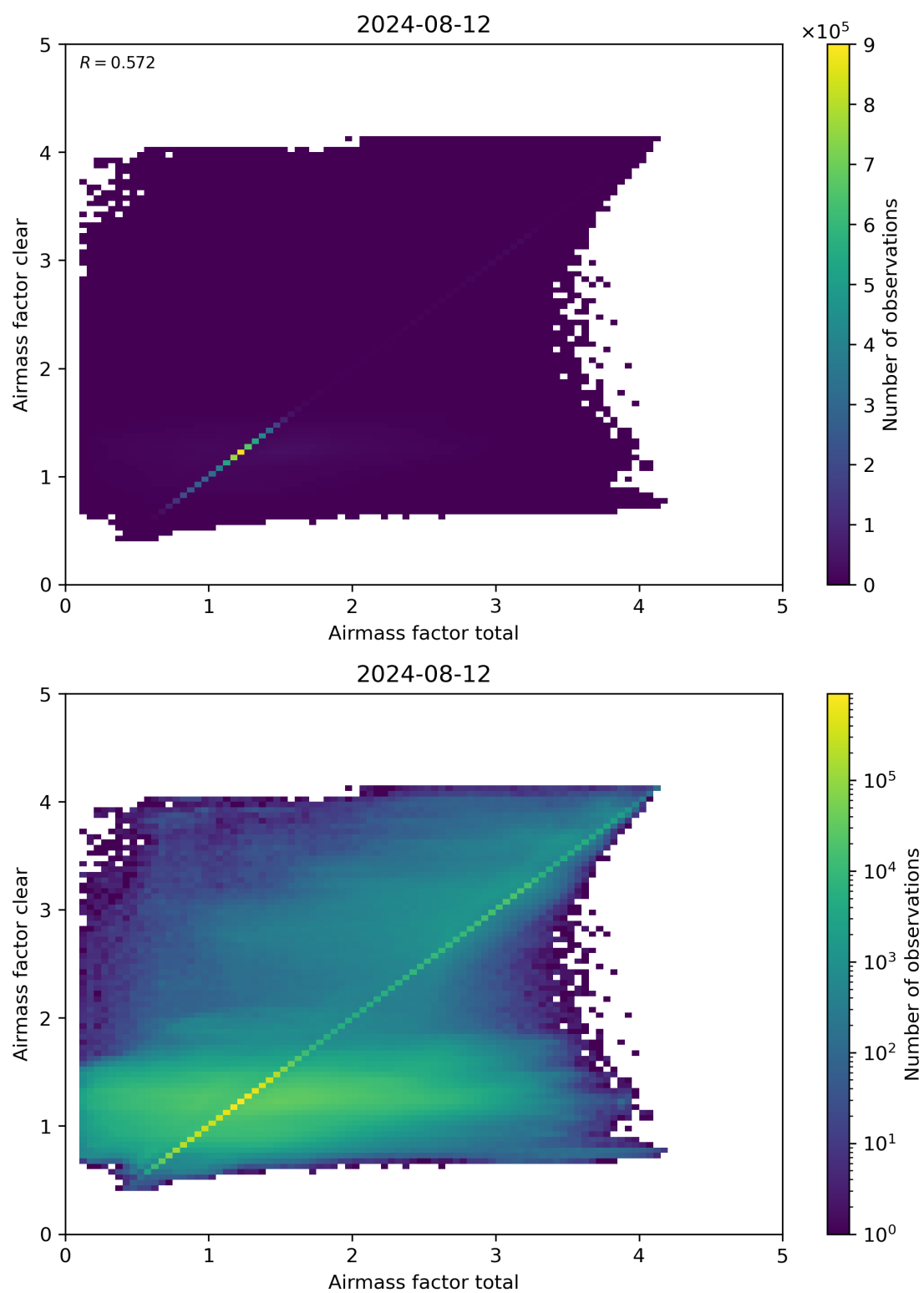
Figure 100: Scatter density plot of “Airmass factor total” against “Airmass factor clear” for 2024-08-12 to 2024-08-13.
