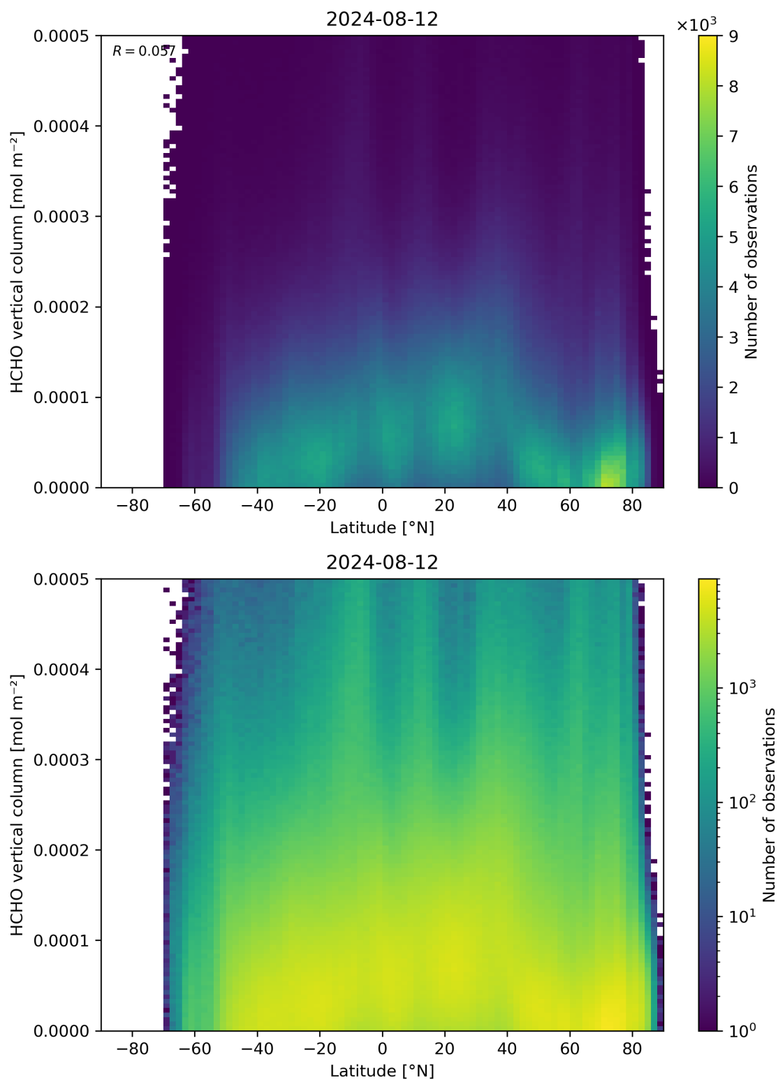
Figure 163: Scatter density plot of “Latitude” against “HCHO vertical column” for 2024-08-12 to 2024-08-13.
