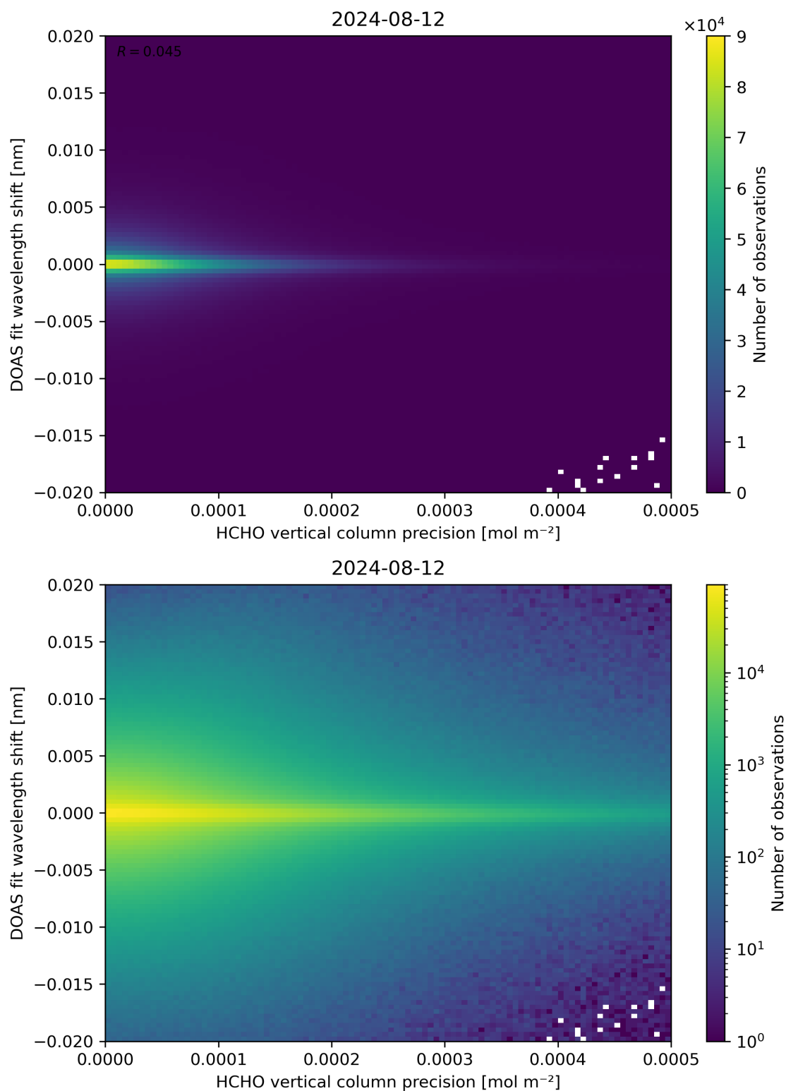
Figure 137: Scatter density plot of “HCHO vertical column precision” against “DOAS fit wavelength shift” for 2024-08-12 to 2024-08-13.
