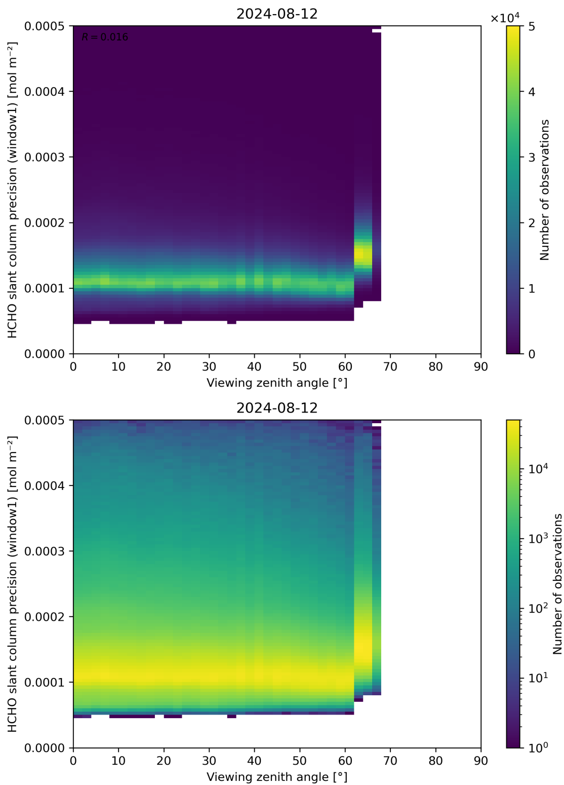
Figure 189: Scatter density plot of “Viewing zenith angle” against “HCHO slant column precision (window1)” for 2024-08-12 to 2024-08-13.
