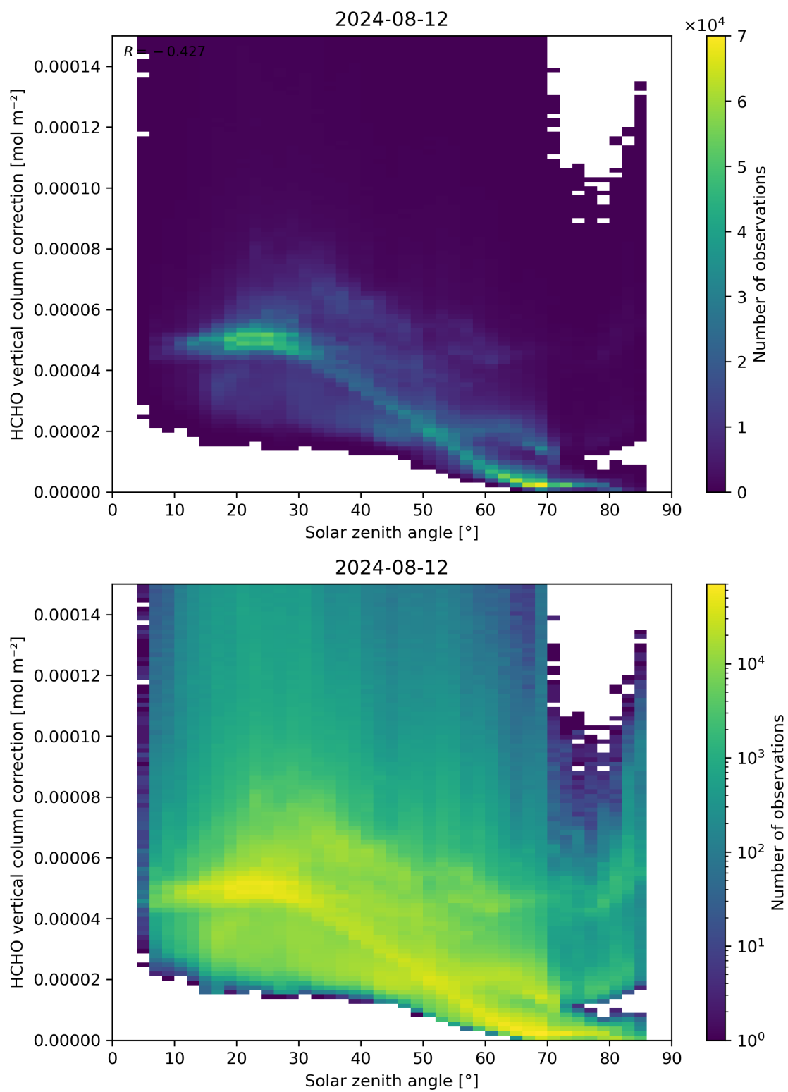
Figure 178: Scatter density plot of “Solar zenith angle” against “HCHO vertical column correction” for 2024-08-12 to 2024-08-13.
