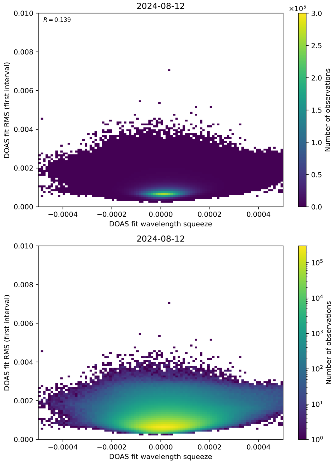
Figure 68: Scatter density plot of “DOAS fit wavelength squeeze” against “DOAS fit RMS (first interval)” for 2024-08-12 to 2024-08-13.
