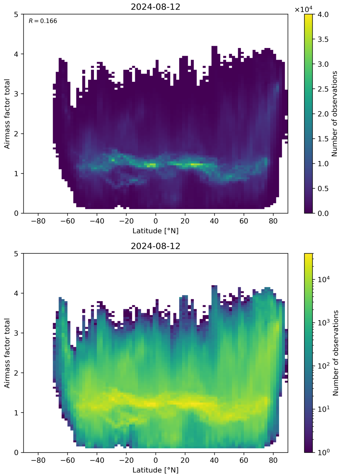
Figure 161: Scatter density plot of “Latitude” against “Airmass factor total” for 2024-08-12 to 2024-08-13.
