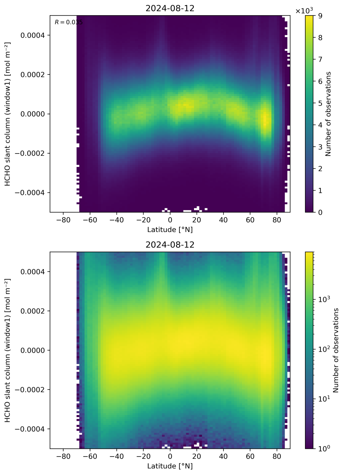
Figure 159: Scatter density plot of “Latitude” against “HCHO slant column (window1)” for 2024-08-12 to 2024-08-13.
