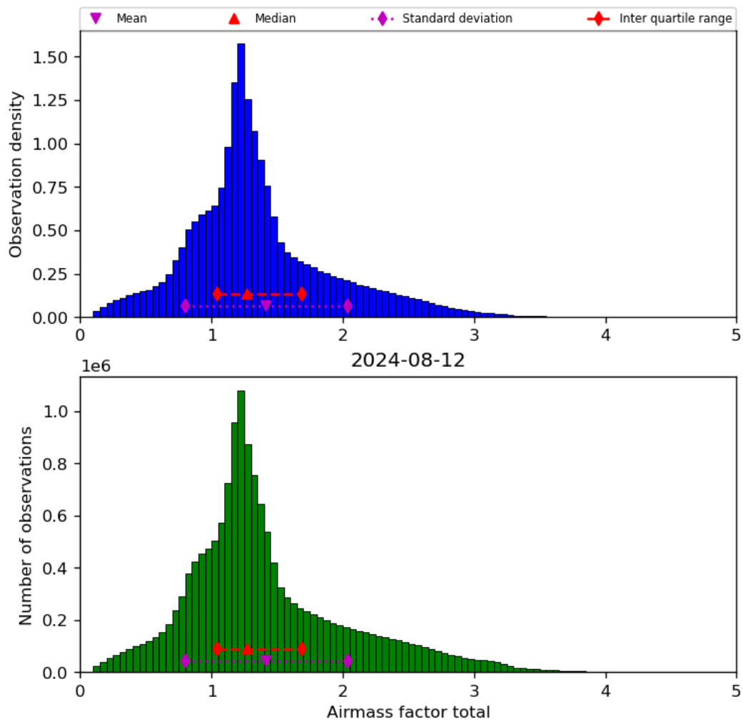
Figure 40: Histogram of “Airmass factor total” for 2024-08-12 to 2024-08-13
