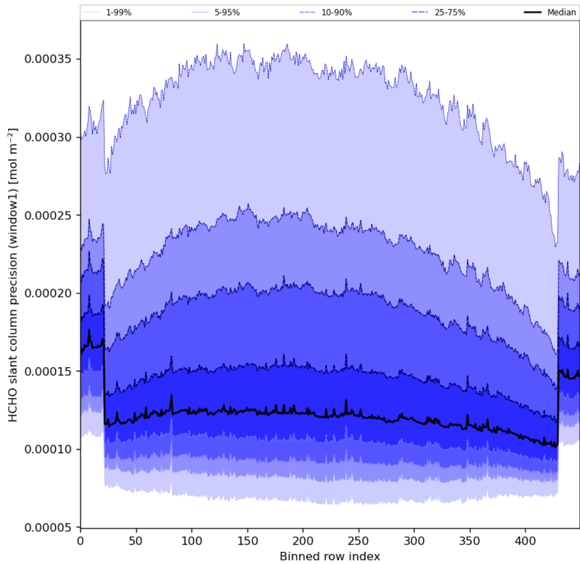
Figure 53: Along track statistics of “HCHO slant column precision (window1)” for 2024-08-12 to 2024-08-13
