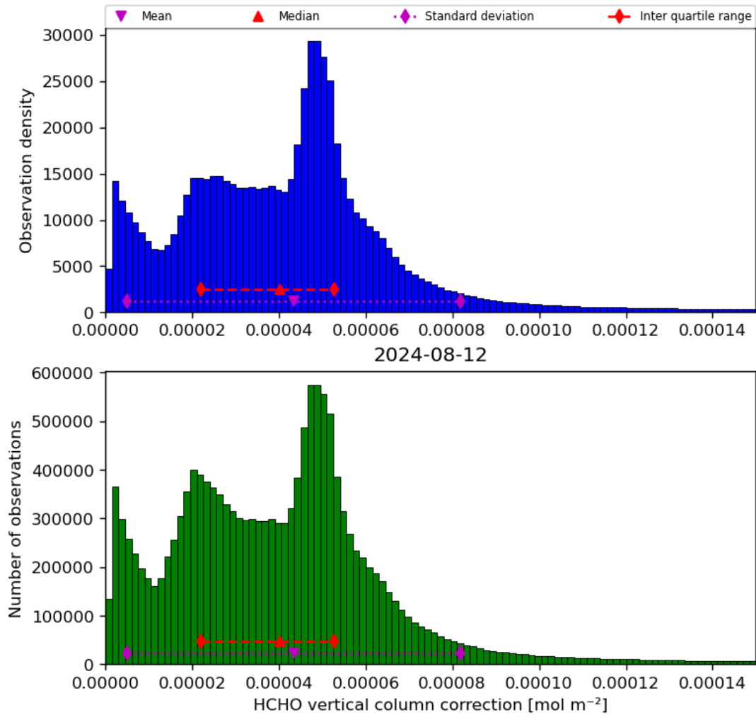
Figure 37: Histogram of “HCHO vertical column correction” for 2024-08-12 to 2024-08-13
