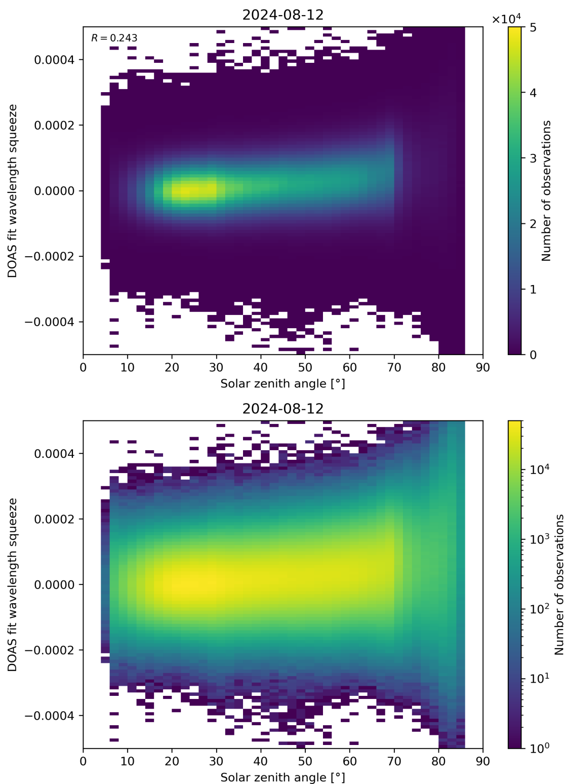
Figure 169: Scatter density plot of “Solar zenith angle” against “DOAS fit wavelength squeeze” for 2024-08-12 to 2024-08-13.
