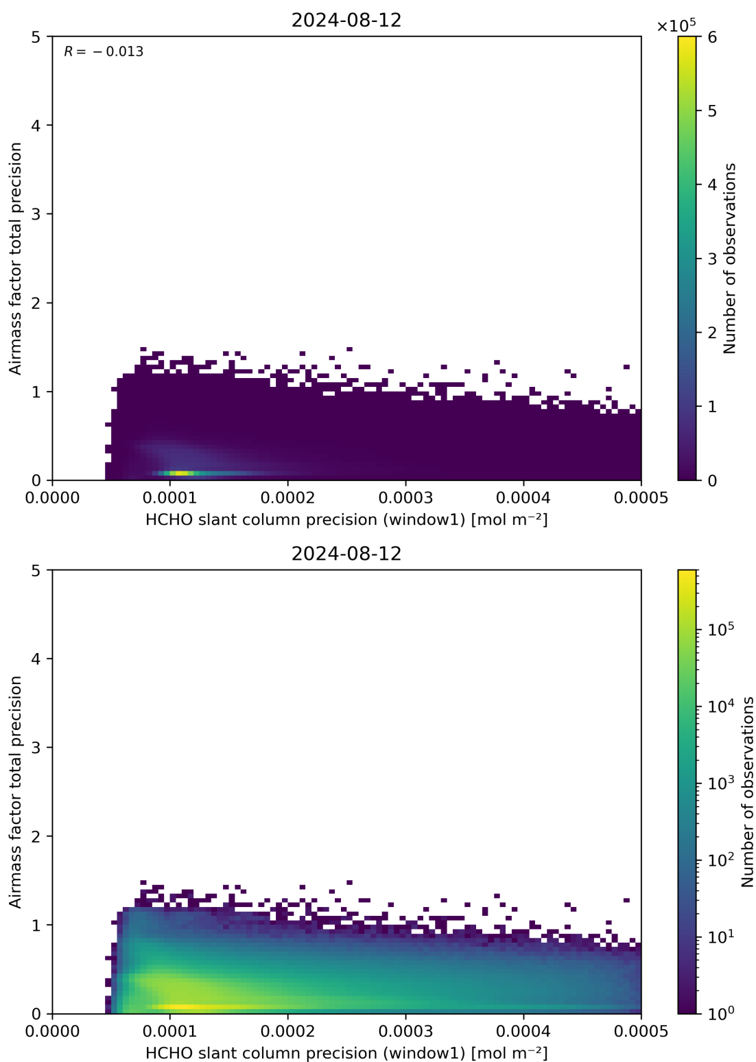
Figure 95: Scatter density plot of “HCHO slant column precision (window1)” against “Airmass factor total precision” for 2024-08-12 to 2024-08-13.
