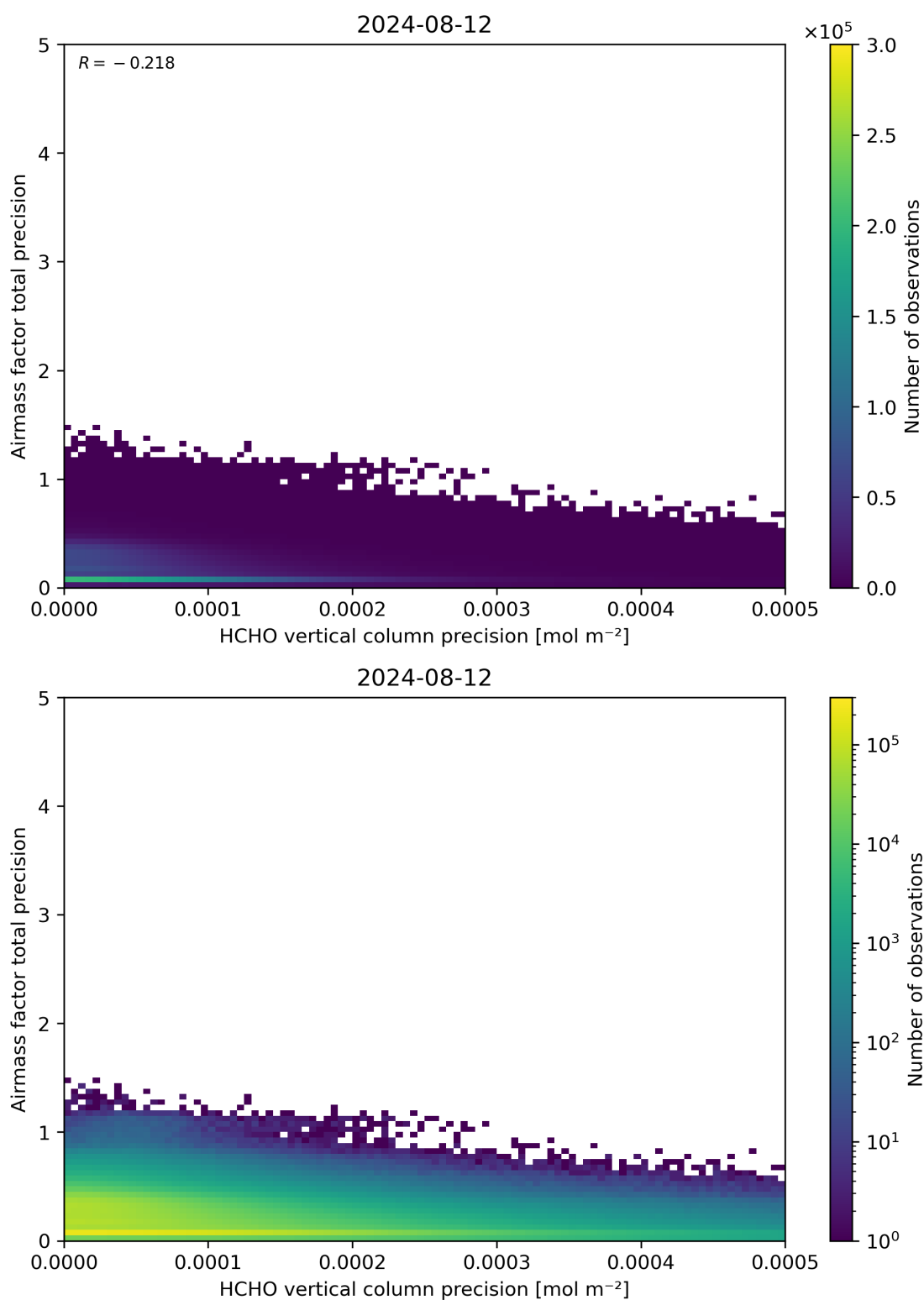
Figure 145: Scatter density plot of “HCHO vertical column precision” against “Airmass factor total precision” for 2024-08-12 to 2024-08-13.
