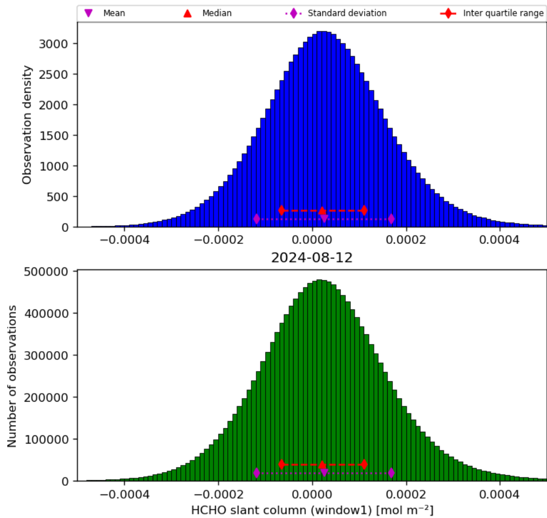
Figure 38: Histogram of “HCHO slant column (window1)” for 2024-08-12 to 2024-08-13
