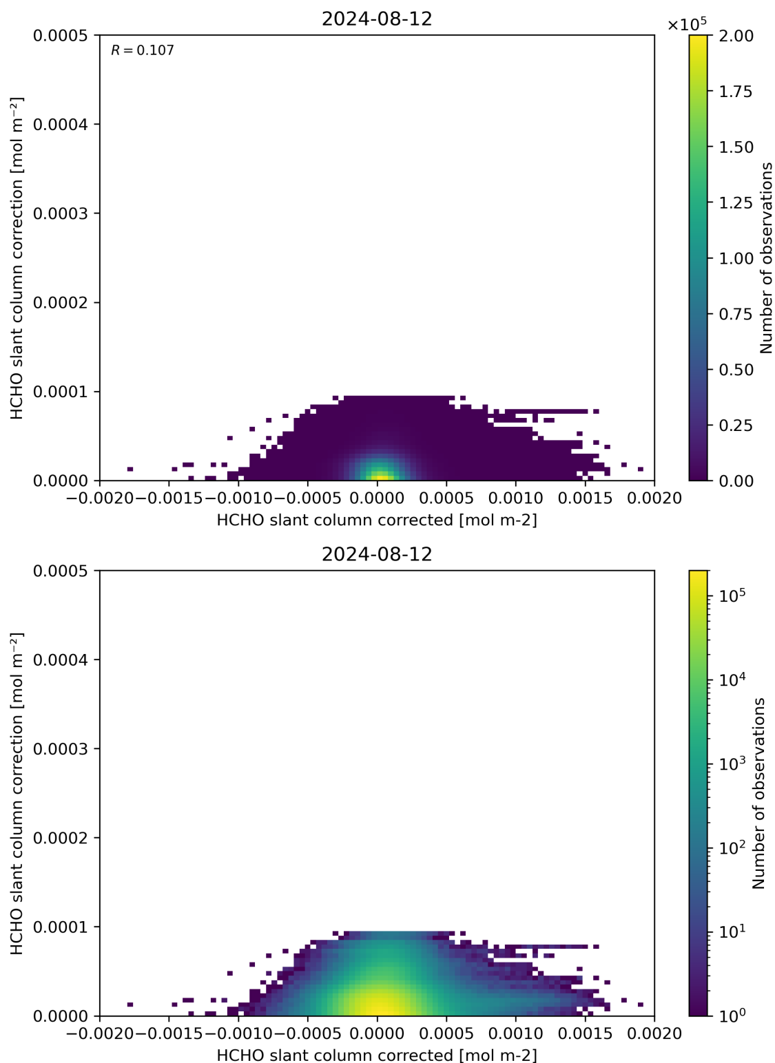
Figure 77: Scatter density plot of “HCHO slant column corrected” against “HCHO slant column correction” for 2024-08-12 to 2024-08-13.
