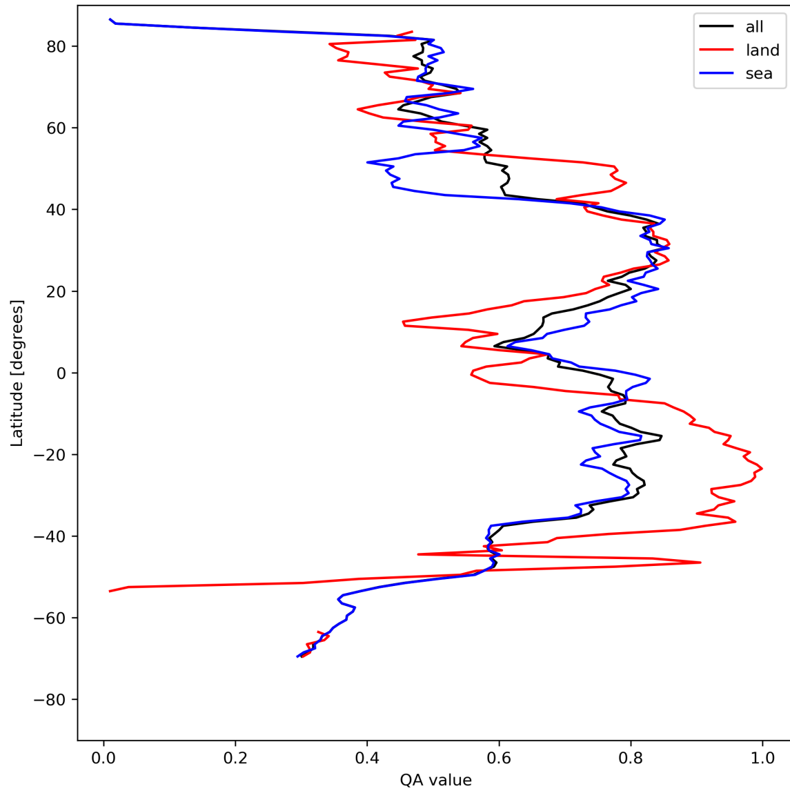
Figure 20: Zonal average of “QA value” for 2024-08-12 to 2024-08-13.
