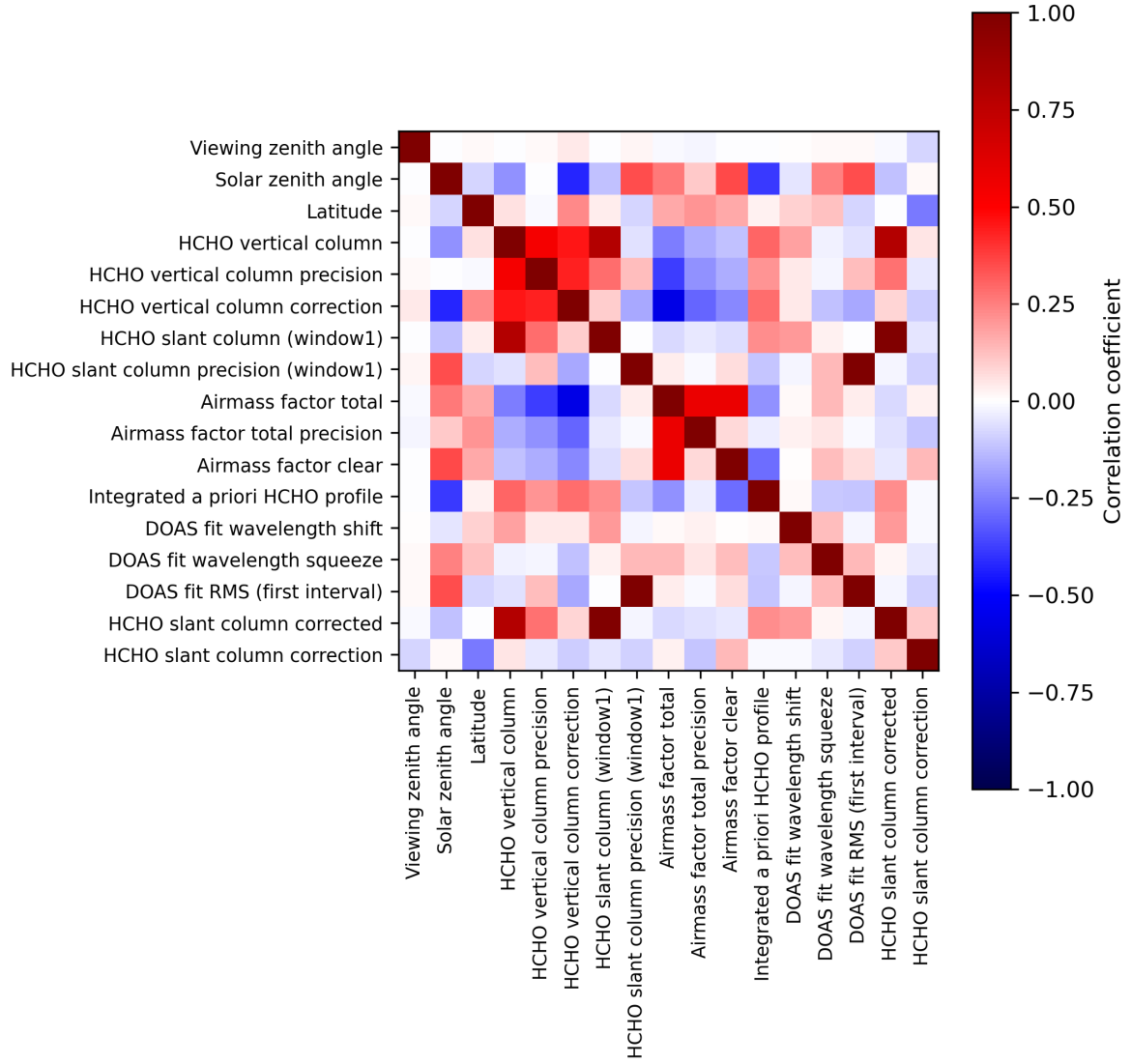
Figure 2: Map of correlation matrix for 2024-08-12 to 2024-08-13.
