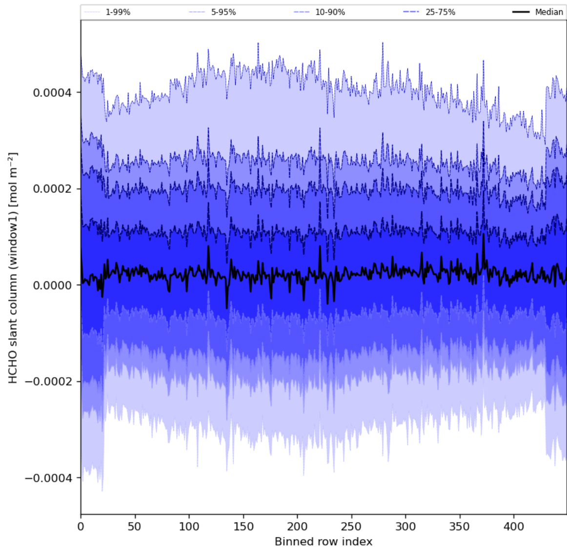
Figure 52: Along track statistics of “HCHO slant column (window1)” for 2024-08-12 to 2024-08-13
