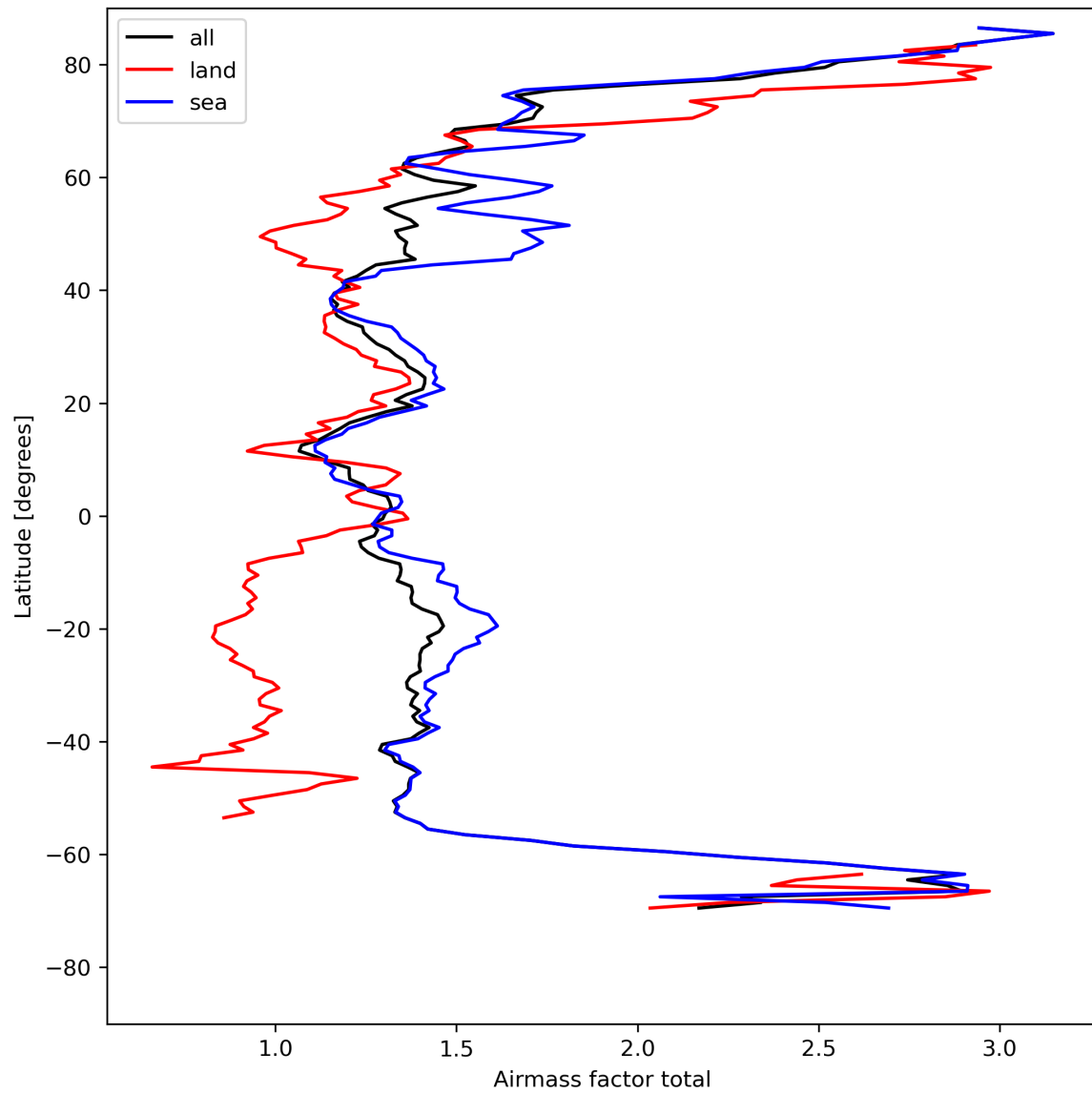
Figure 26: Zonal average of “Airmass factor total” for 2024-08-12 to 2024-08-13.
