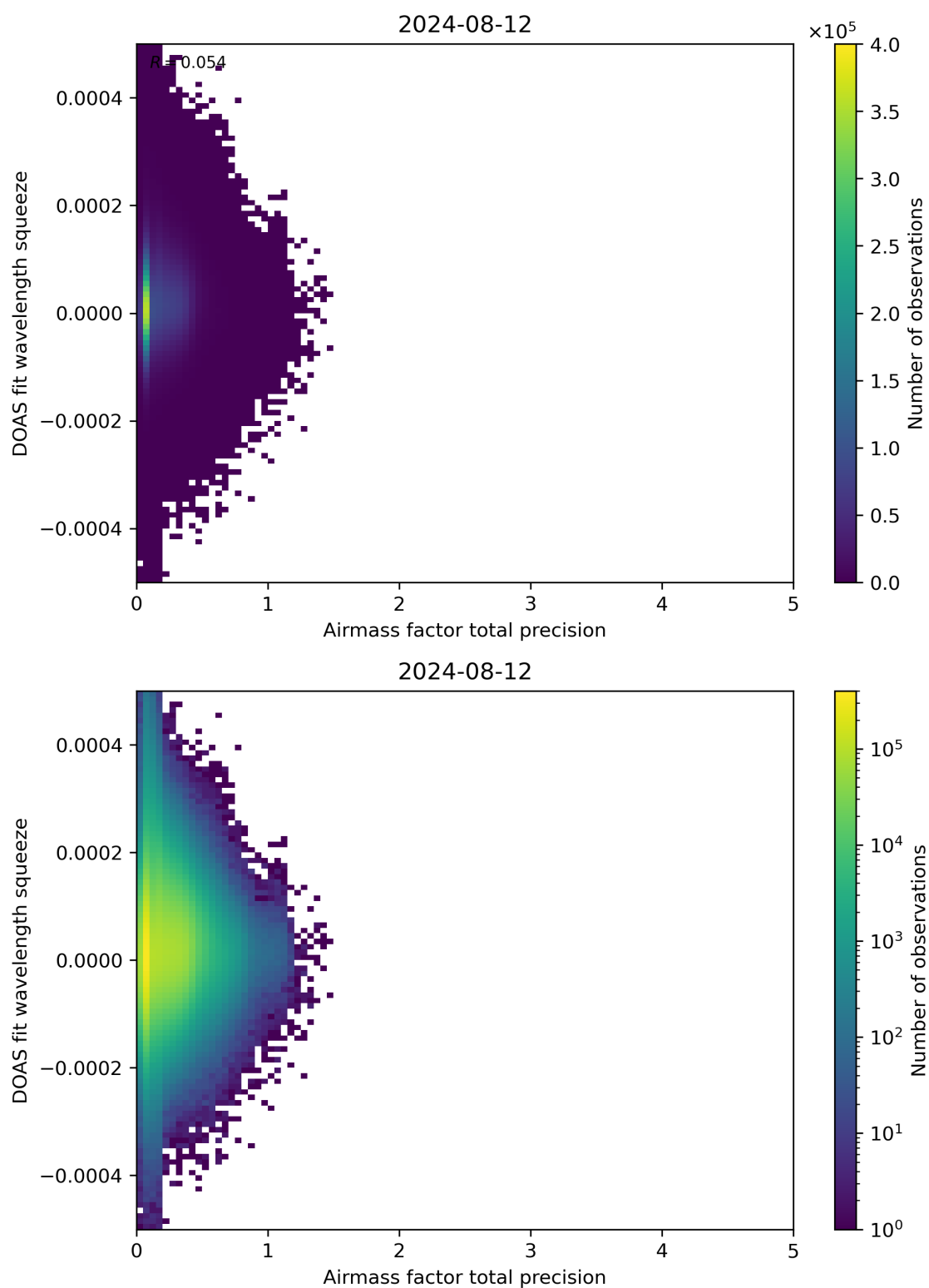
Figure 107: Scatter density plot of “Airmass factor total precision” against “DOAS fit wavelength squeeze” for 2024-08-12 to 2024-08-13.
