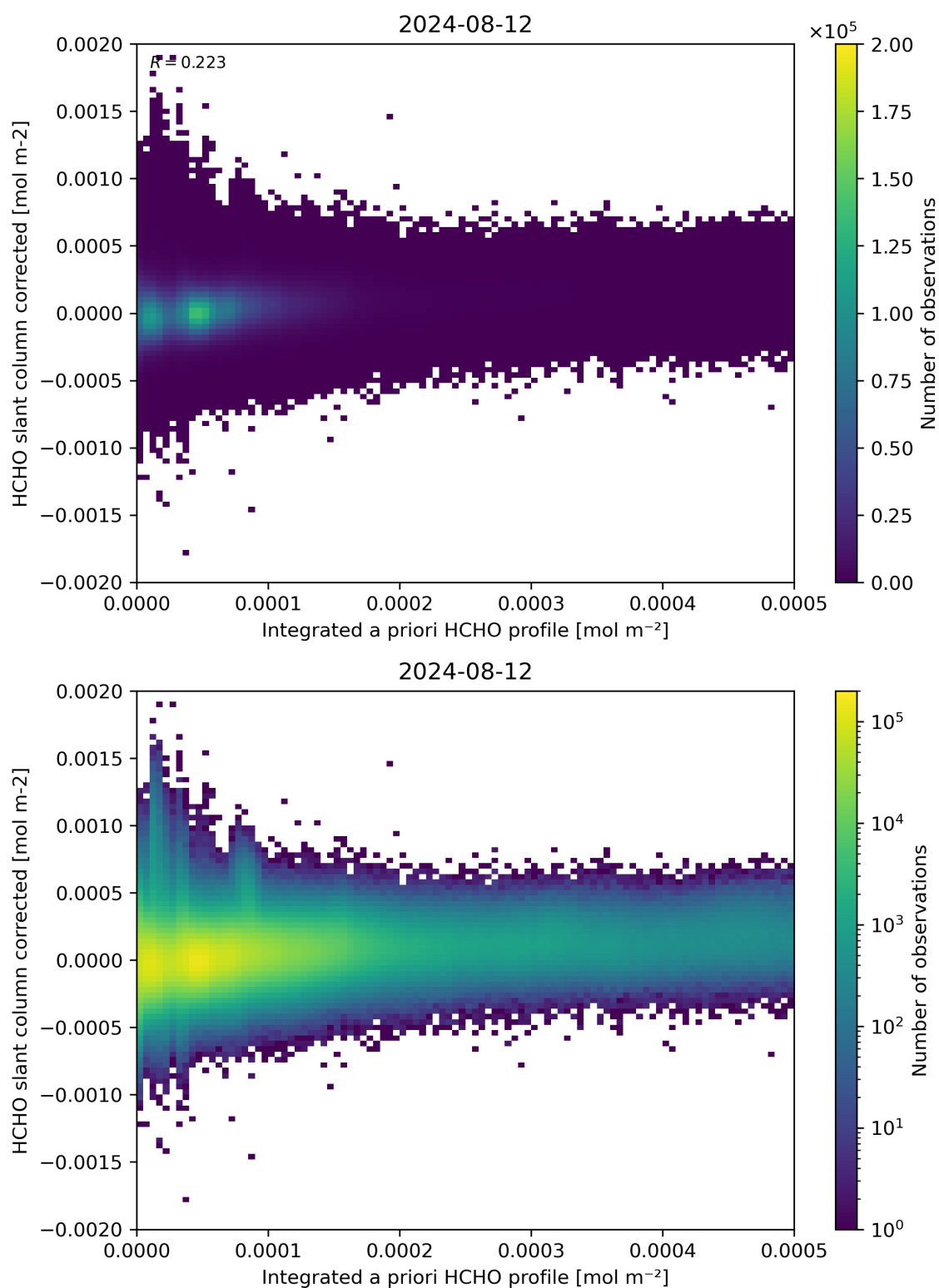
Figure 151: Scatter density plot of “Integrated a priori HCHO profile” against “HCHO slant column corrected” for 2024-08-12 to 2024-08-13.
