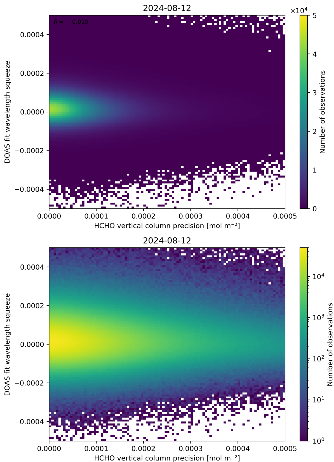
Figure 138: Scatter density plot of “HCHO vertical column precision” against “DOAS fit wavelength squeeze” for 2024-08-12 to 2024-08-13.
