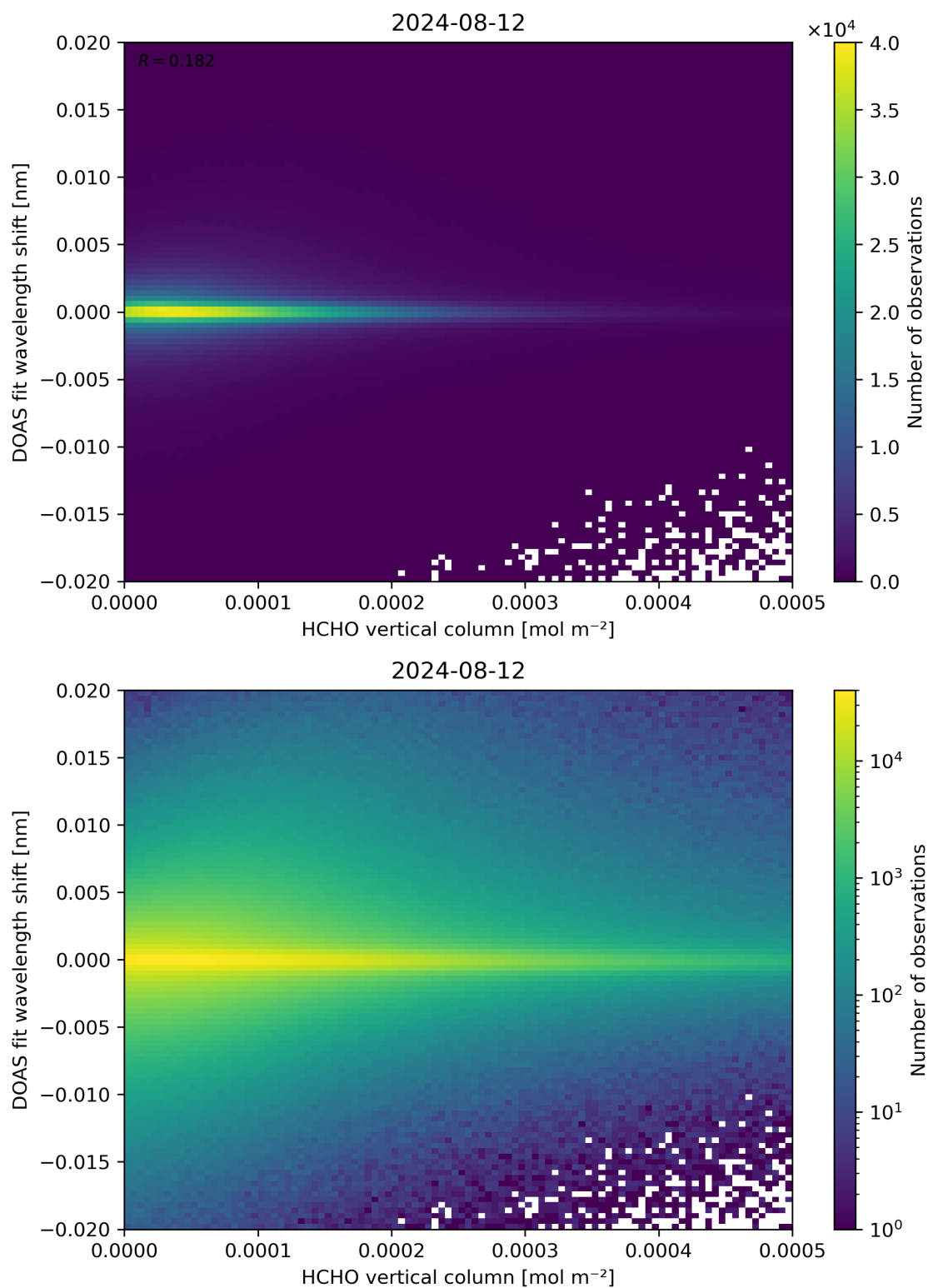
Figure 124: Scatter density plot of “HCHO vertical column” against “DOAS fit wavelength shift” for 2024-08-12 to 2024-08-13.
