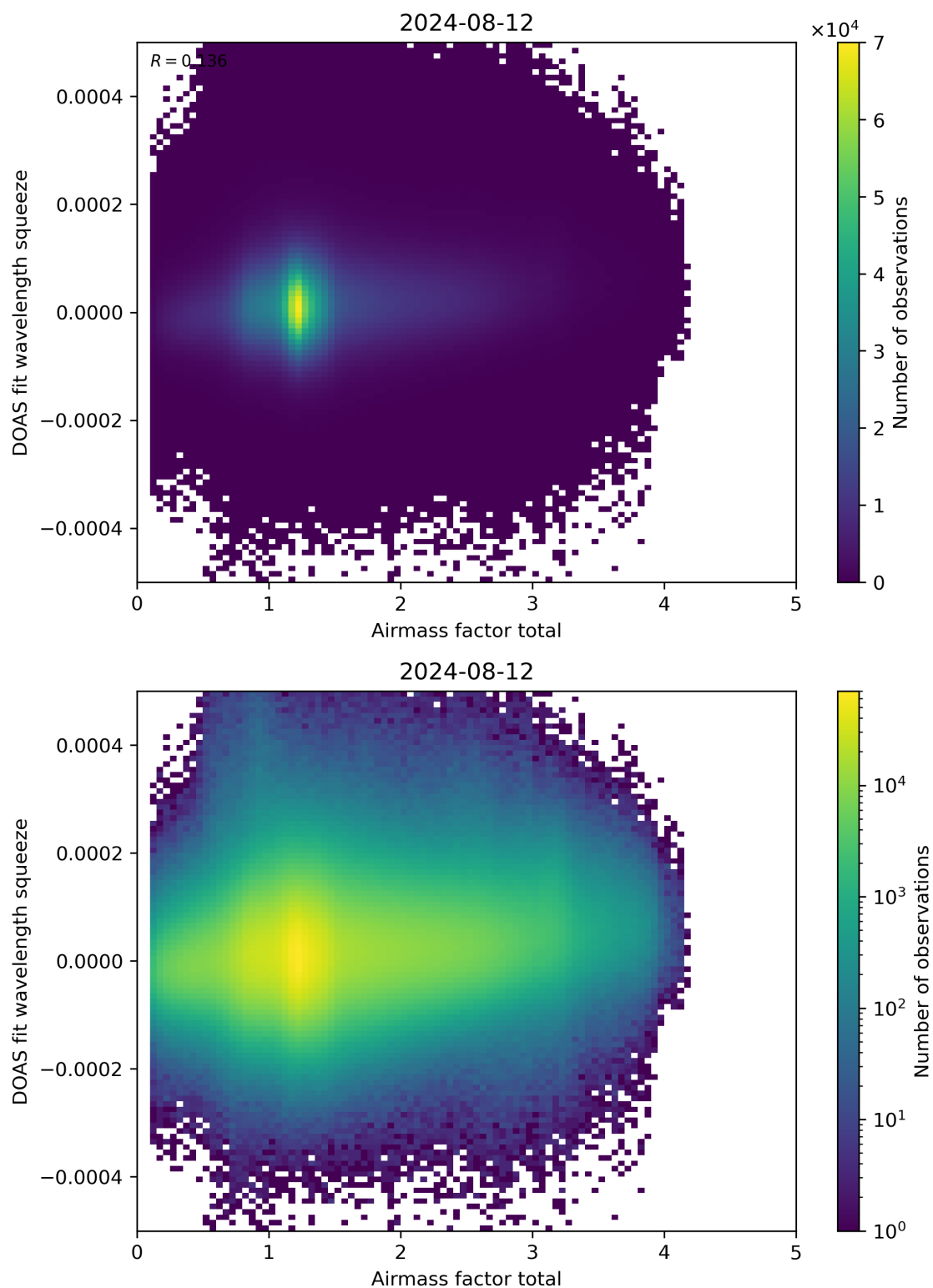
Figure 99: Scatter density plot of “Airmass factor total” against “DOAS fit wavelength squeeze” for 2024-08-12 to 2024-08-13.
