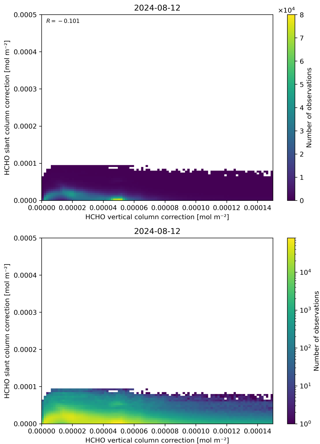
Figure 117: Scatter density plot of “HCHO vertical column correction” against “HCHO slant column correction” for 2024-08-12 to 2024-08-13.
