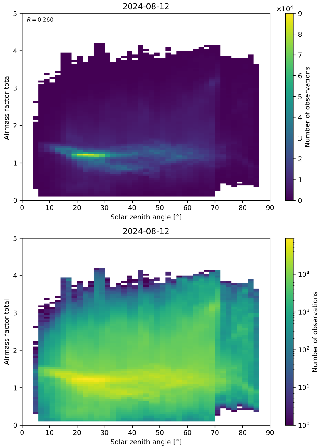
Figure 175: Scatter density plot of “Solar zenith angle” against “Airmass factor total” for 2024-08-12 to 2024-08-13.
