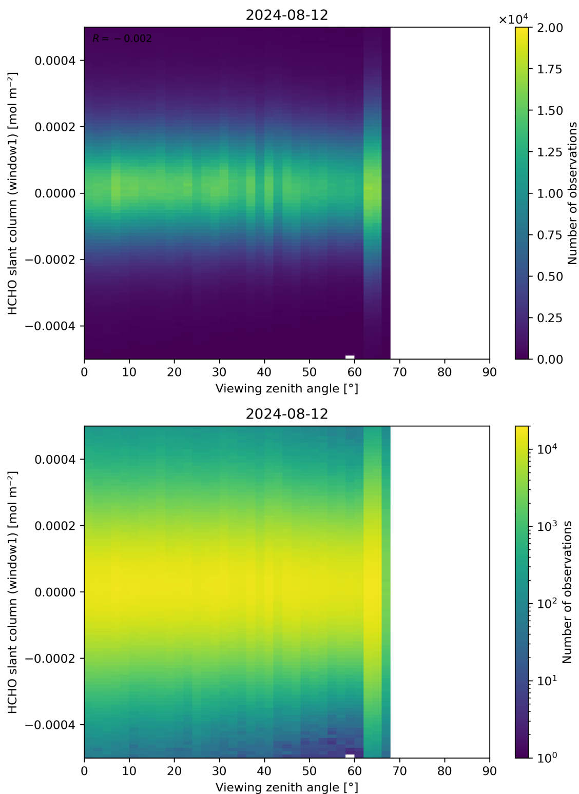
Figure 188: Scatter density plot of “Viewing zenith angle” against “HCHO slant column (window1)” for 2024-08-12 to 2024-08-13.
