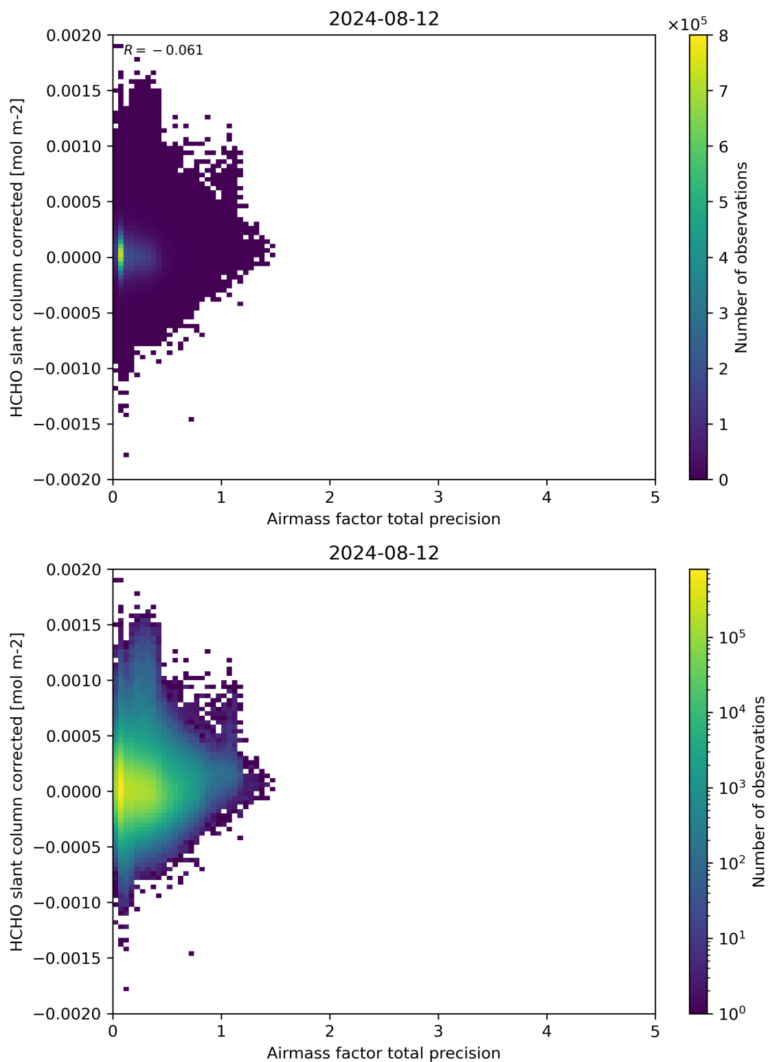
Figure 109: Scatter density plot of “Airmass factor total precision” against “HCHO slant column corrected” for 2024-08-12 to 2024-08-13.
