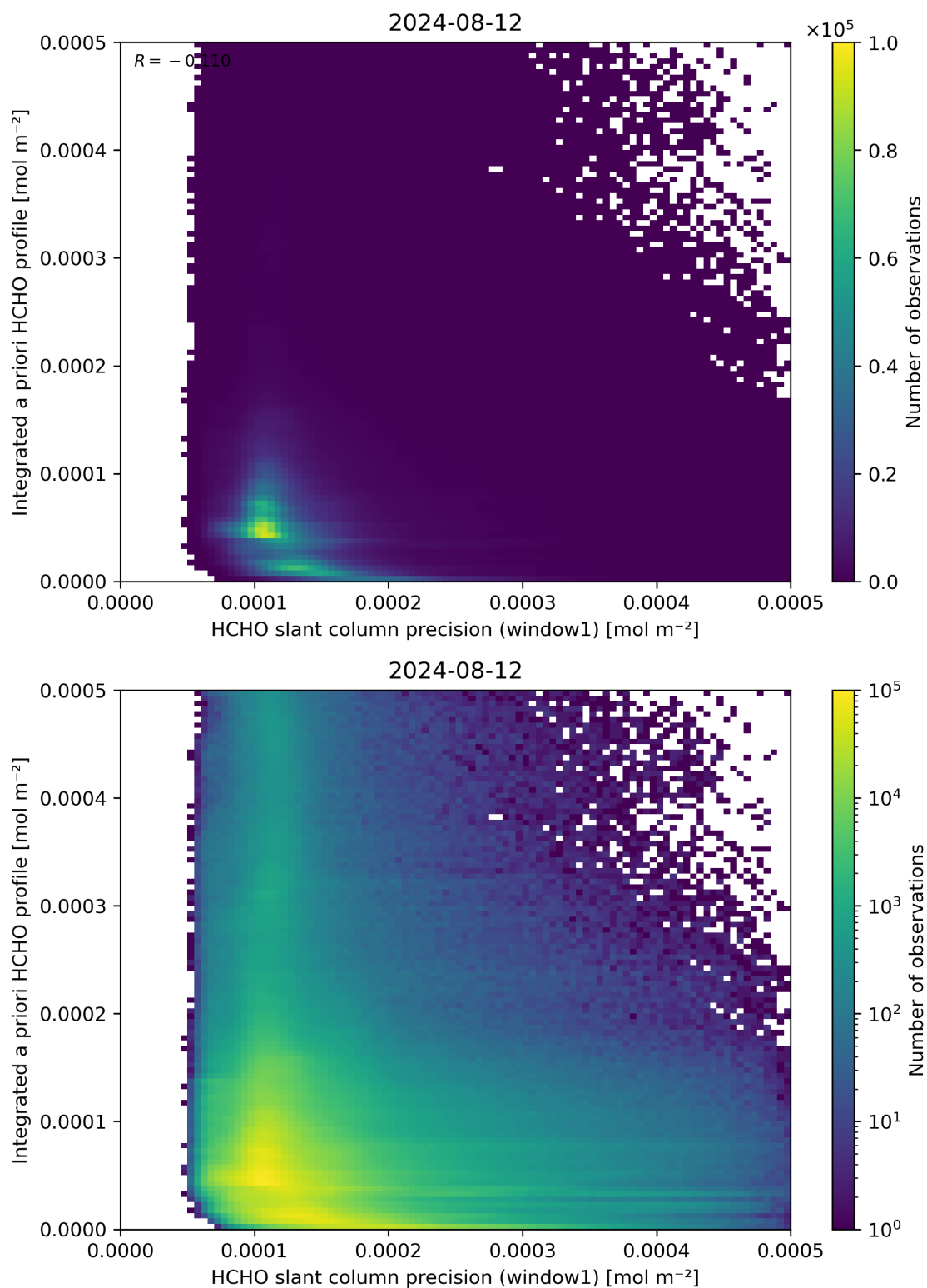
Figure 96: Scatter density plot of “HCHO slant column precision (window1)” against “Integrated a priori HCHO profile” for 2024-08-12 to 2024-08-13.
