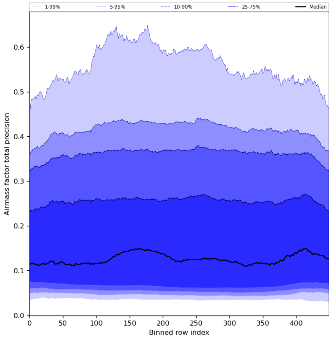
Figure 55: Along track statistics of “Airmass factor total precision” for 2024-08-12 to 2024-08-13
