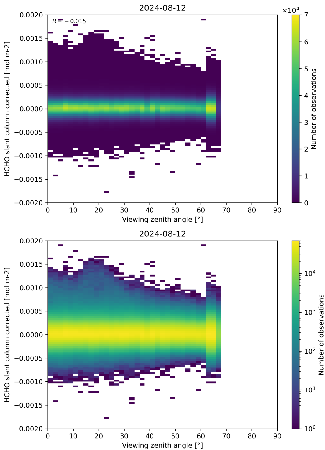
Figure 186: Scatter density plot of “Viewing zenith angle” against “HCHO slant column corrected” for 2024-08-12 to 2024-08-13.
