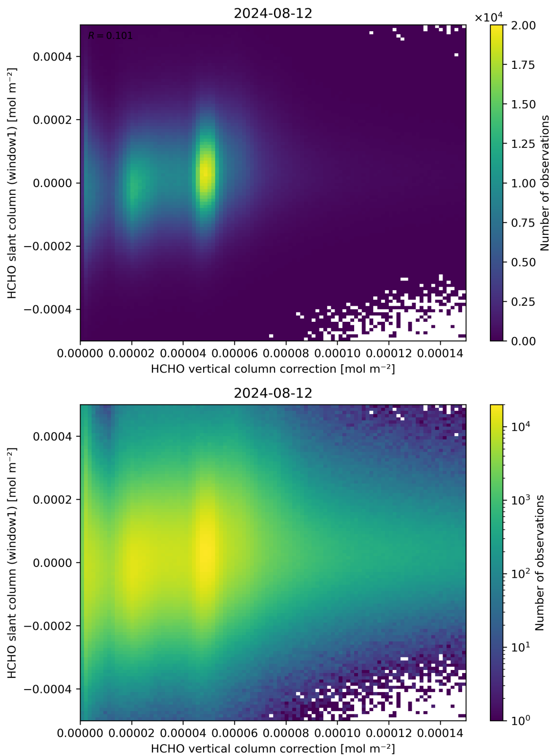
Figure 118: Scatter density plot of “HCHO vertical column correction” against “HCHO slant column (window1)” for 2024-08-12 to 2024-08-13.
