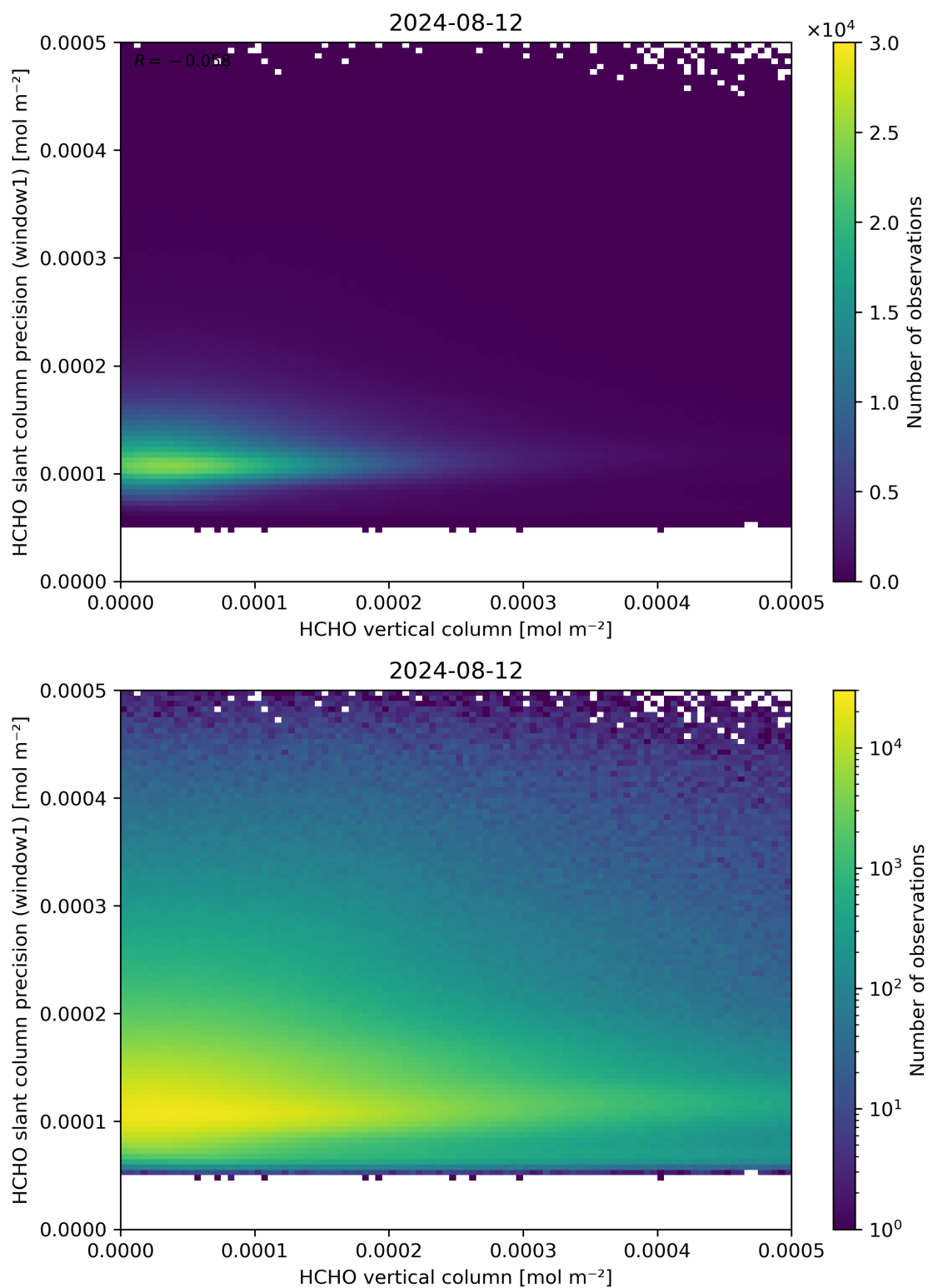
Figure 130: Scatter density plot of “HCHO vertical column” against “HCHO slant column precision (window1)” for 2024-08-12 to 2024-08-13.
