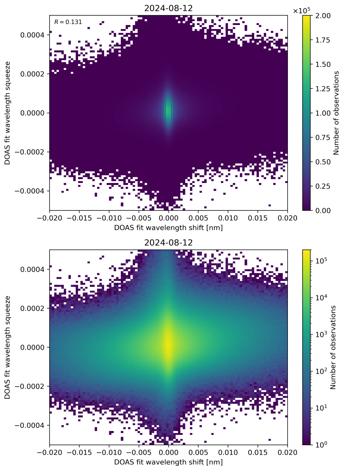
Figure 65: Scatter density plot of “DOAS fit wavelength shift” against “DOAS fit wavelength squeeze” for 2024-08-12 to 2024-08-13.
