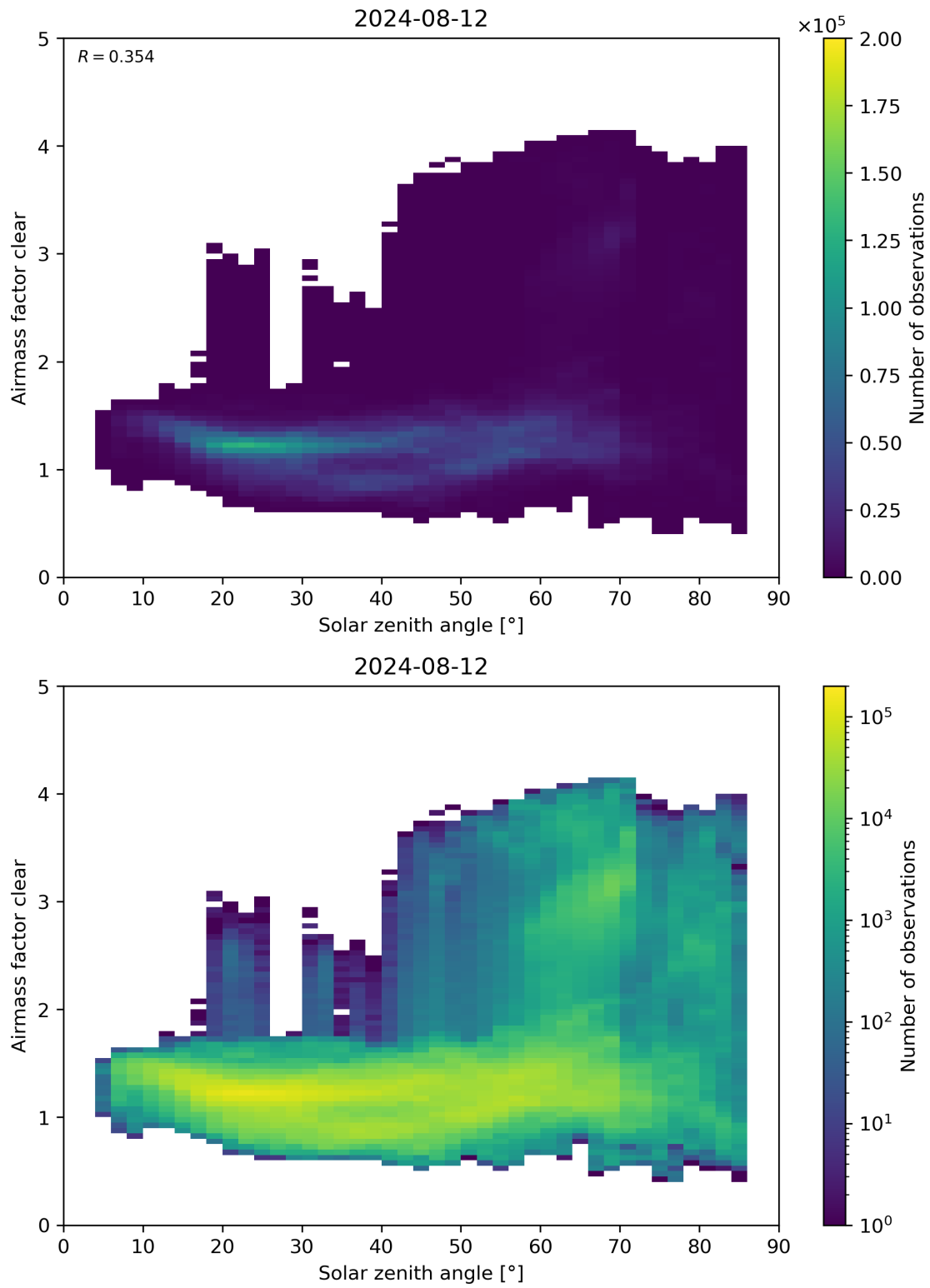
Figure 170: Scatter density plot of “Solar zenith angle” against “Airmass factor clear” for 2024-08-12 to 2024-08-13.
