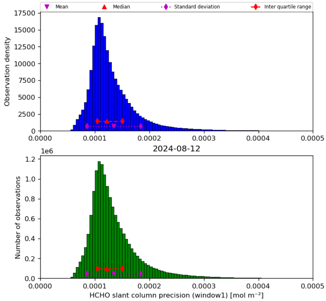
Figure 39: Histogram of “HCHO slant column precision (window1)” for 2024-08-12 to 2024-08-13
