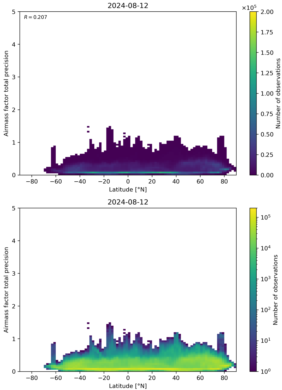
Figure 162: Scatter density plot of “Latitude” against “Airmass factor total precision” for 2024-08-12 to 2024-08-13.
