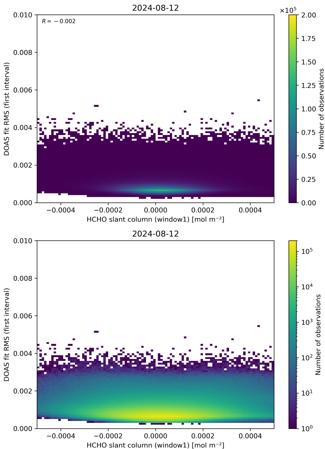
Figure 78: Scatter density plot of “HCHO slant column (window1)” against “DOAS fit RMS (first interval)” for 2024-08-12 to 2024-08-13.
