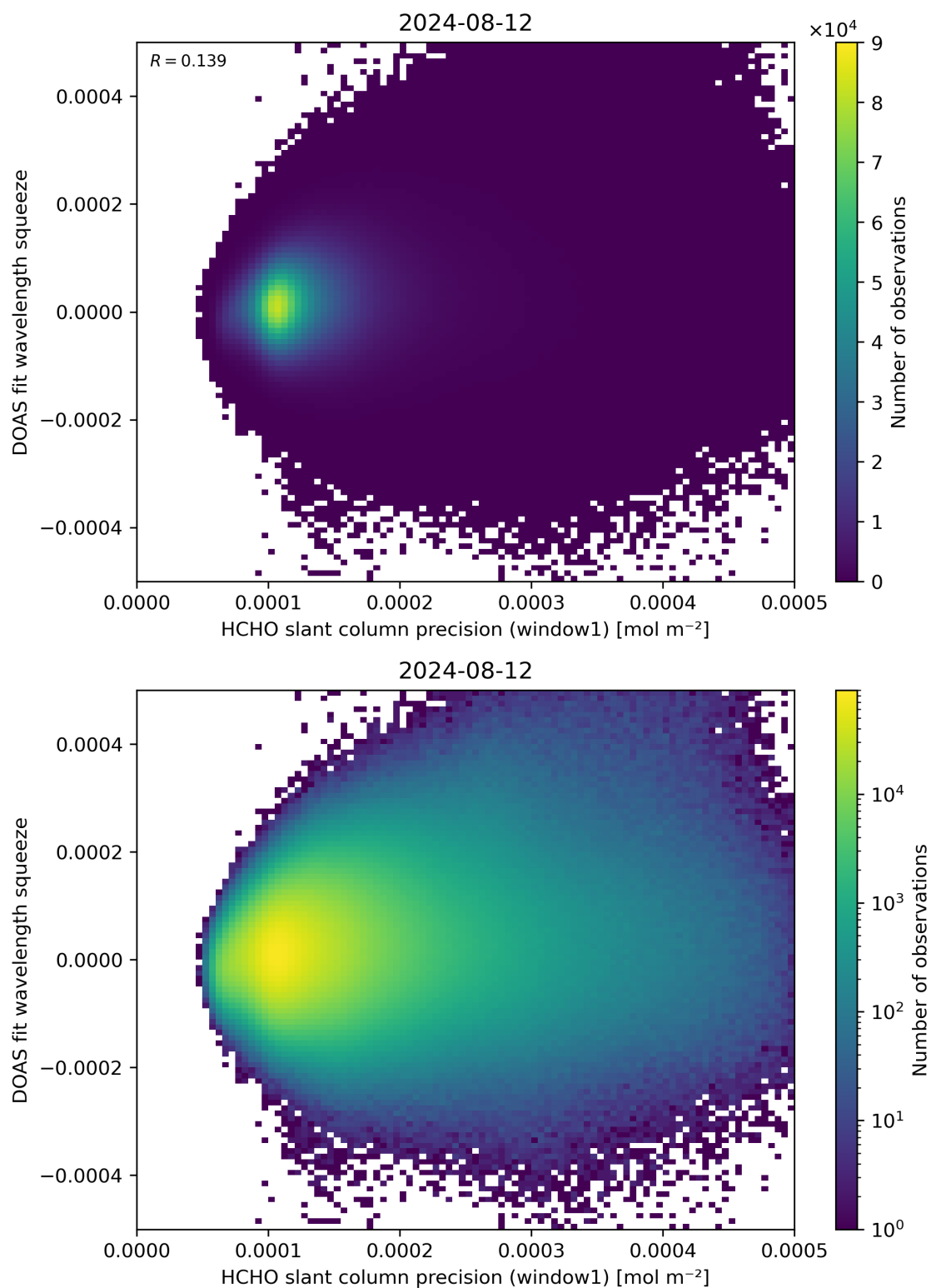
Figure 90: Scatter density plot of “HCHO slant column precision (window1)” against “DOAS fit wavelength squeeze” for 2024-08-12 to 2024-08-13.
