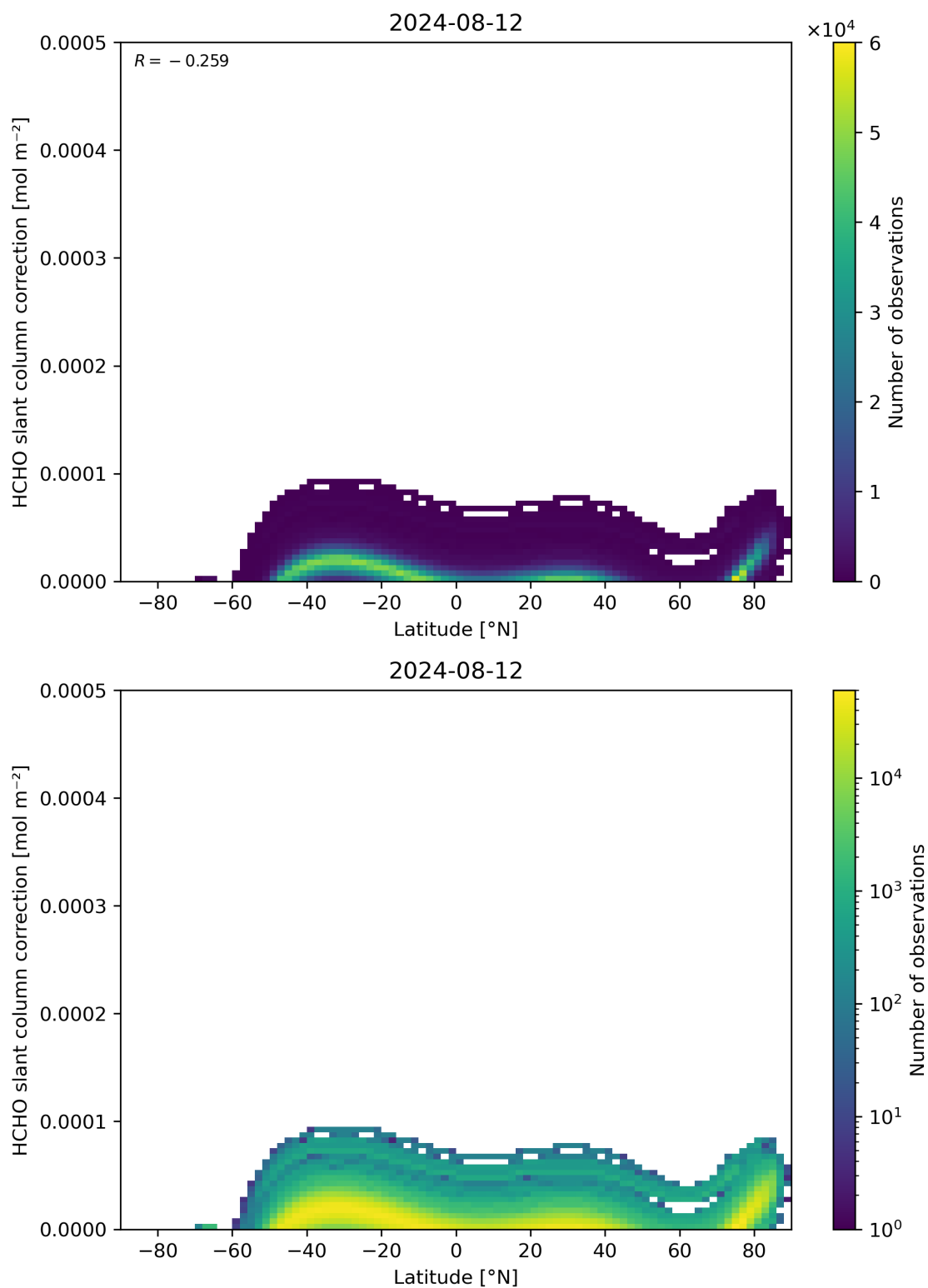
Figure 158: Scatter density plot of “Latitude” against “HCHO slant column correction” for 2024-08-12 to 2024-08-13.
