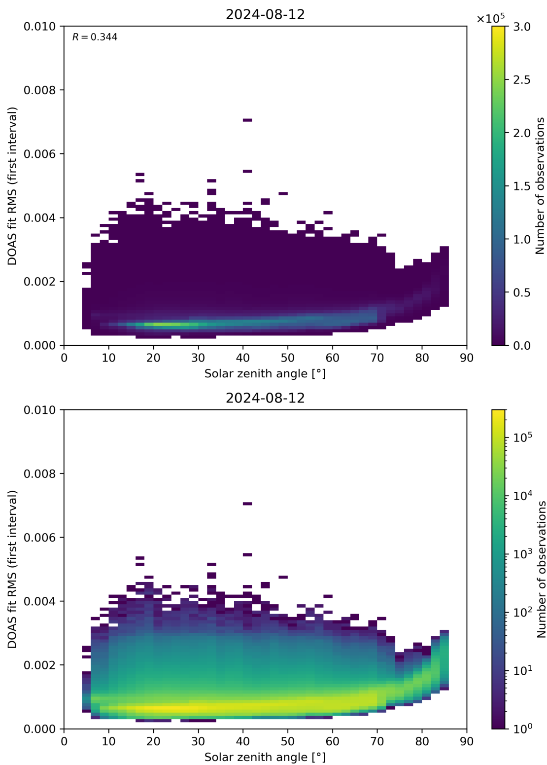
Figure 167: Scatter density plot of “Solar zenith angle” against “DOAS fit RMS (first interval)” for 2024-08-12 to 2024-08-13.
