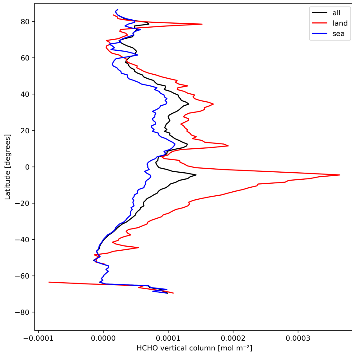
Figure 21: Zonal average of “HCHO vertical column” for 2024-08-12 to 2024-08-13.
