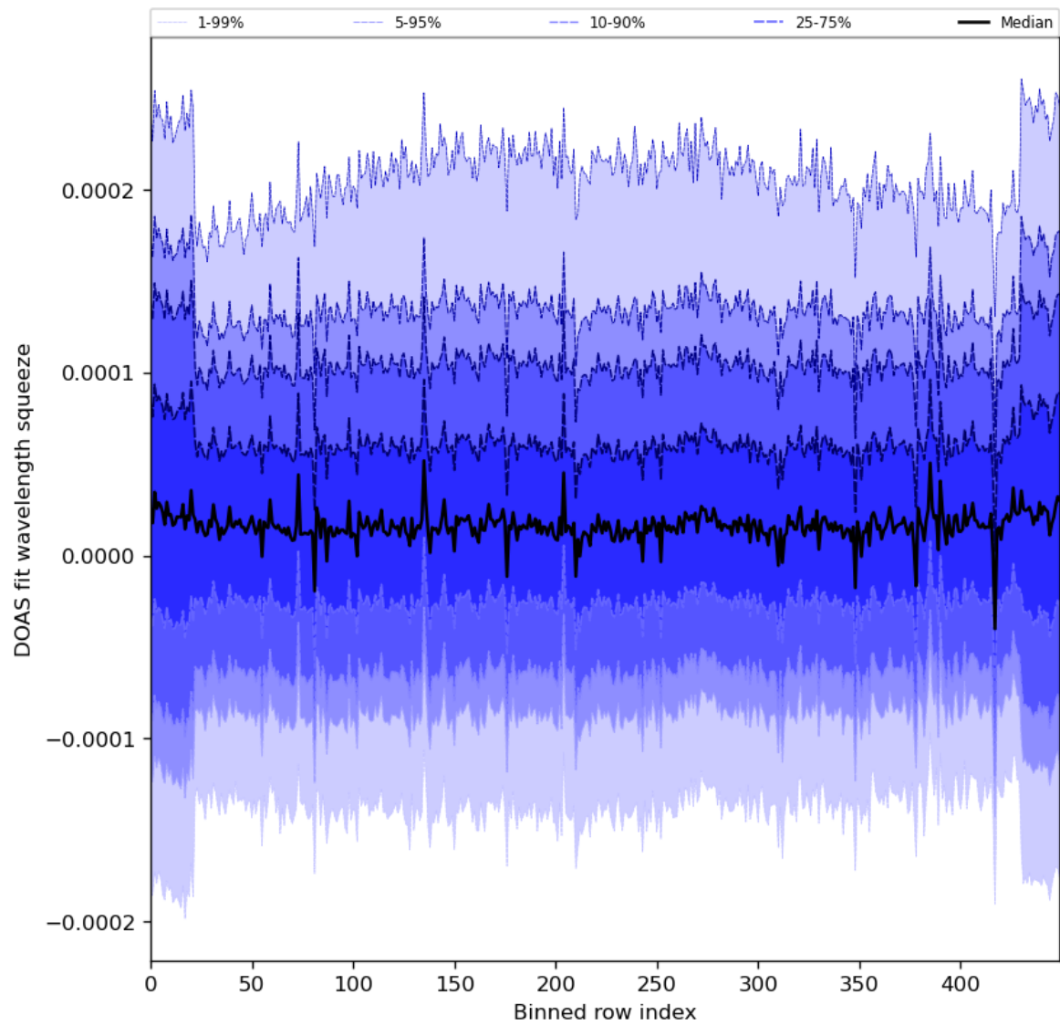
Figure 59: Along track statistics of “DOAS fit wavelength squeeze” for 2024-08-12 to 2024-08-13
