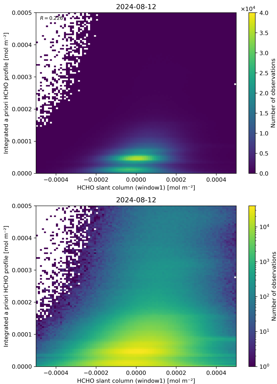
Figure 87: Scatter density plot of “HCHO slant column (window1)” against “Integrated a priori HCHO profile” for 2024-08-12 to 2024-08-13.
