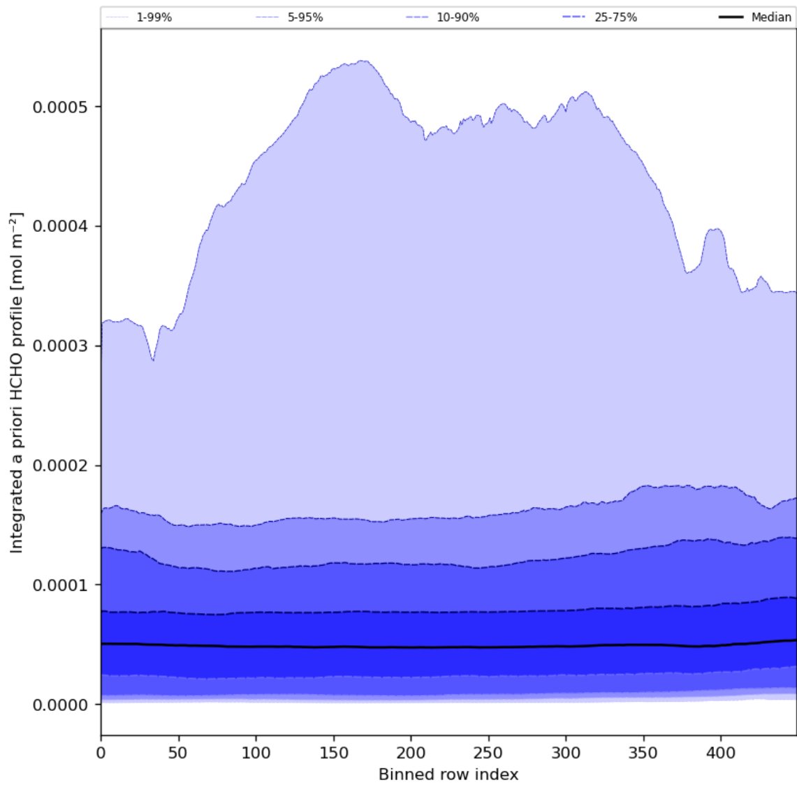
Figure 57: Along track statistics of “Integrated a priori HCHO profile” for 2024-08-12 to 2024-08-13
