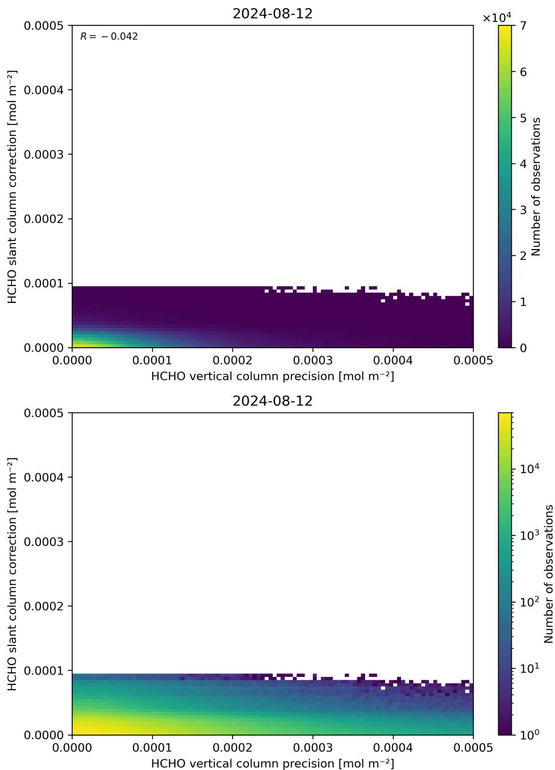
Figure 141: Scatter density plot of “HCHO vertical column precision” against “HCHO slant column correction” for 2024-08-12 to 2024-08-13.
