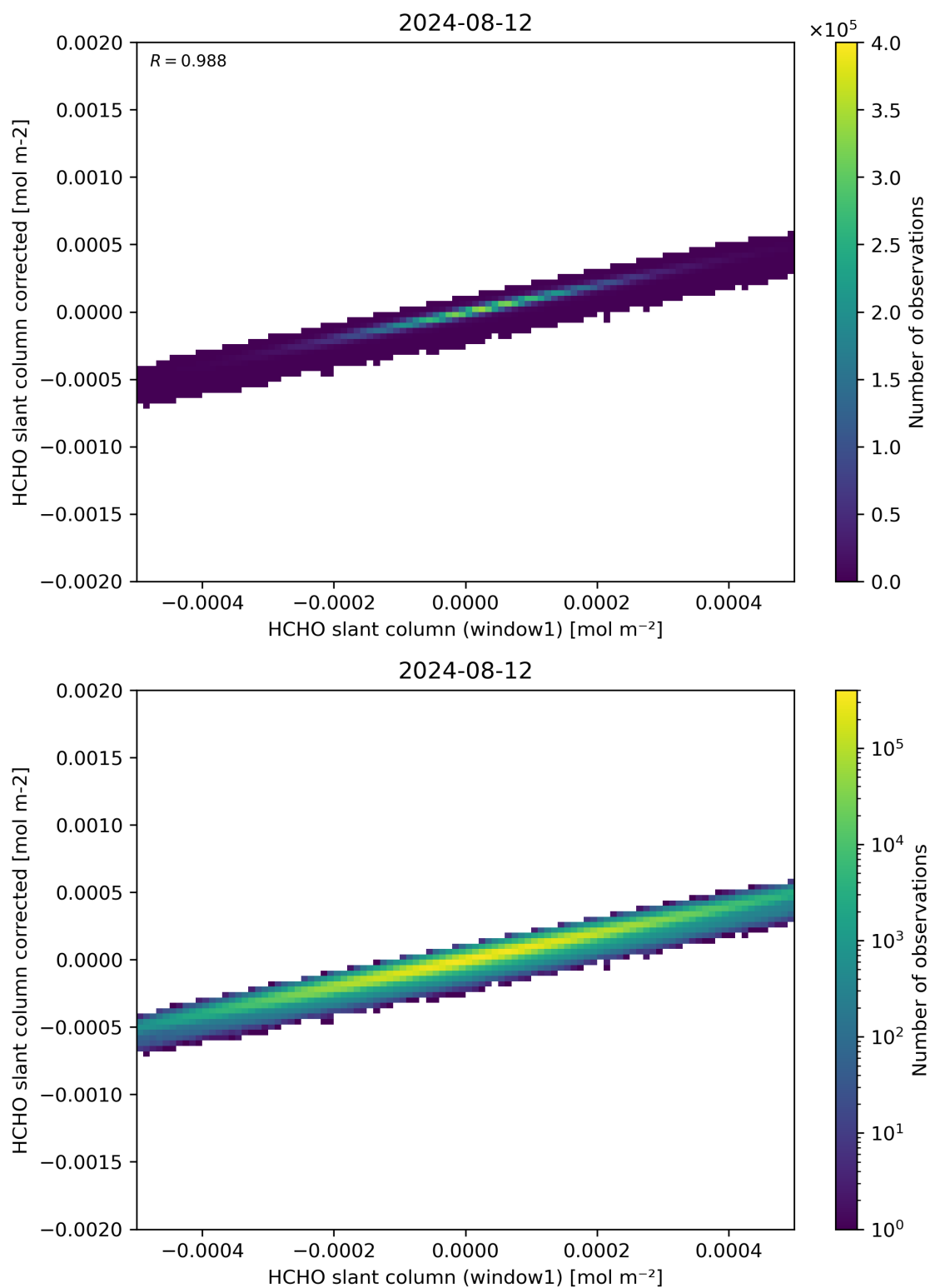
Figure 82: Scatter density plot of “HCHO slant column (window1)” against “HCHO slant column corrected” for 2024-08-12 to 2024-08-13.
