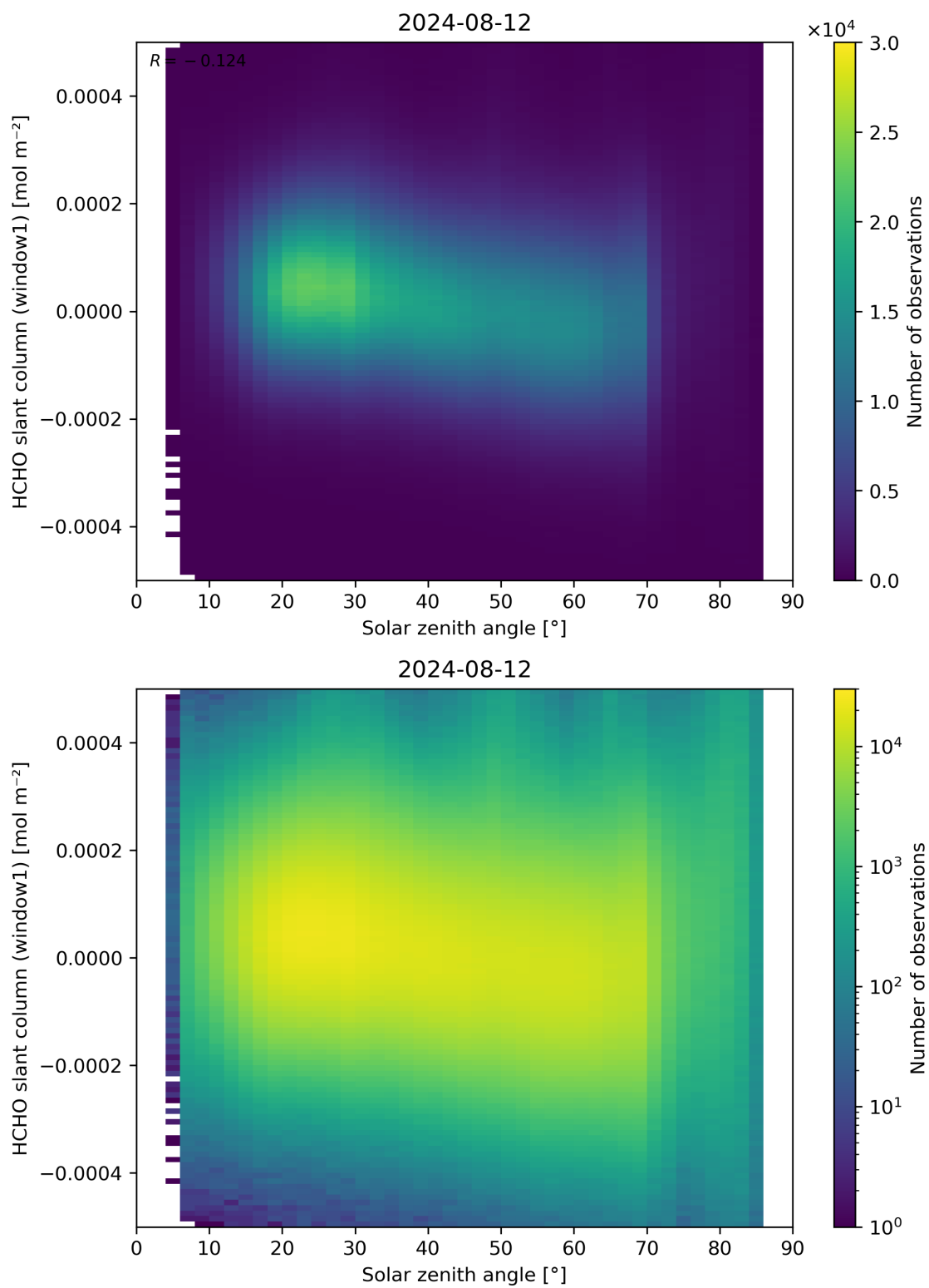
Figure 173: Scatter density plot of “Solar zenith angle” against “HCHO slant column (window1)” for 2024-08-12 to 2024-08-13.
