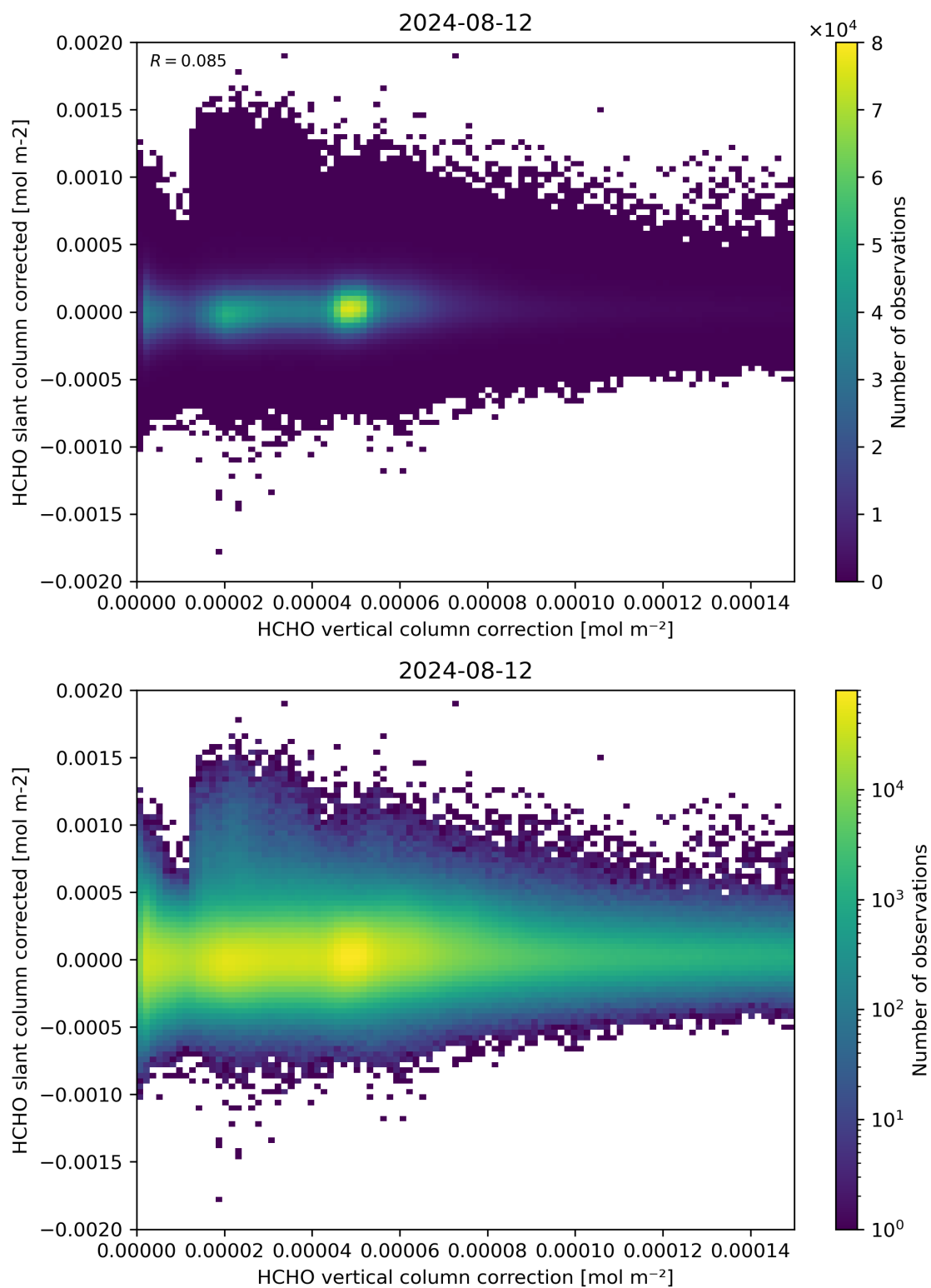
Figure 116: Scatter density plot of “HCHO vertical column correction” against “HCHO slant column corrected” for 2024-08-12 to 2024-08-13.
