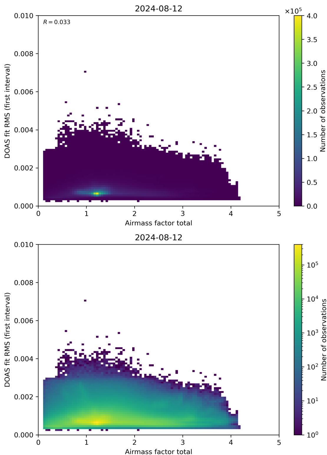
Figure 97: Scatter density plot of “Airmass factor total” against “DOAS fit RMS (first interval)” for 2024-08-12 to 2024-08-13.
