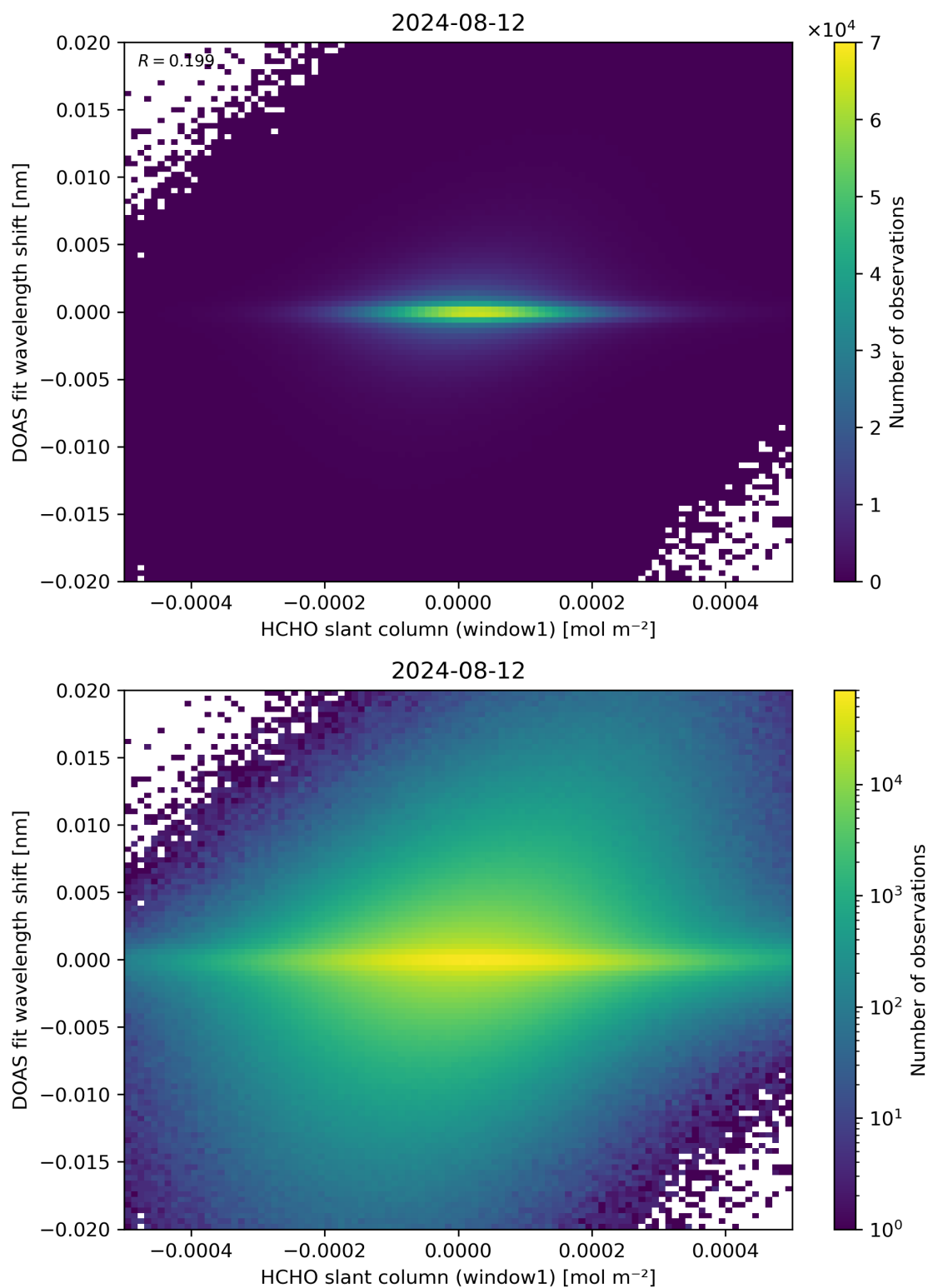
Figure 79: Scatter density plot of “HCHO slant column (window1)” against “DOAS fit wavelength shift” for 2024-08-12 to 2024-08-13.
