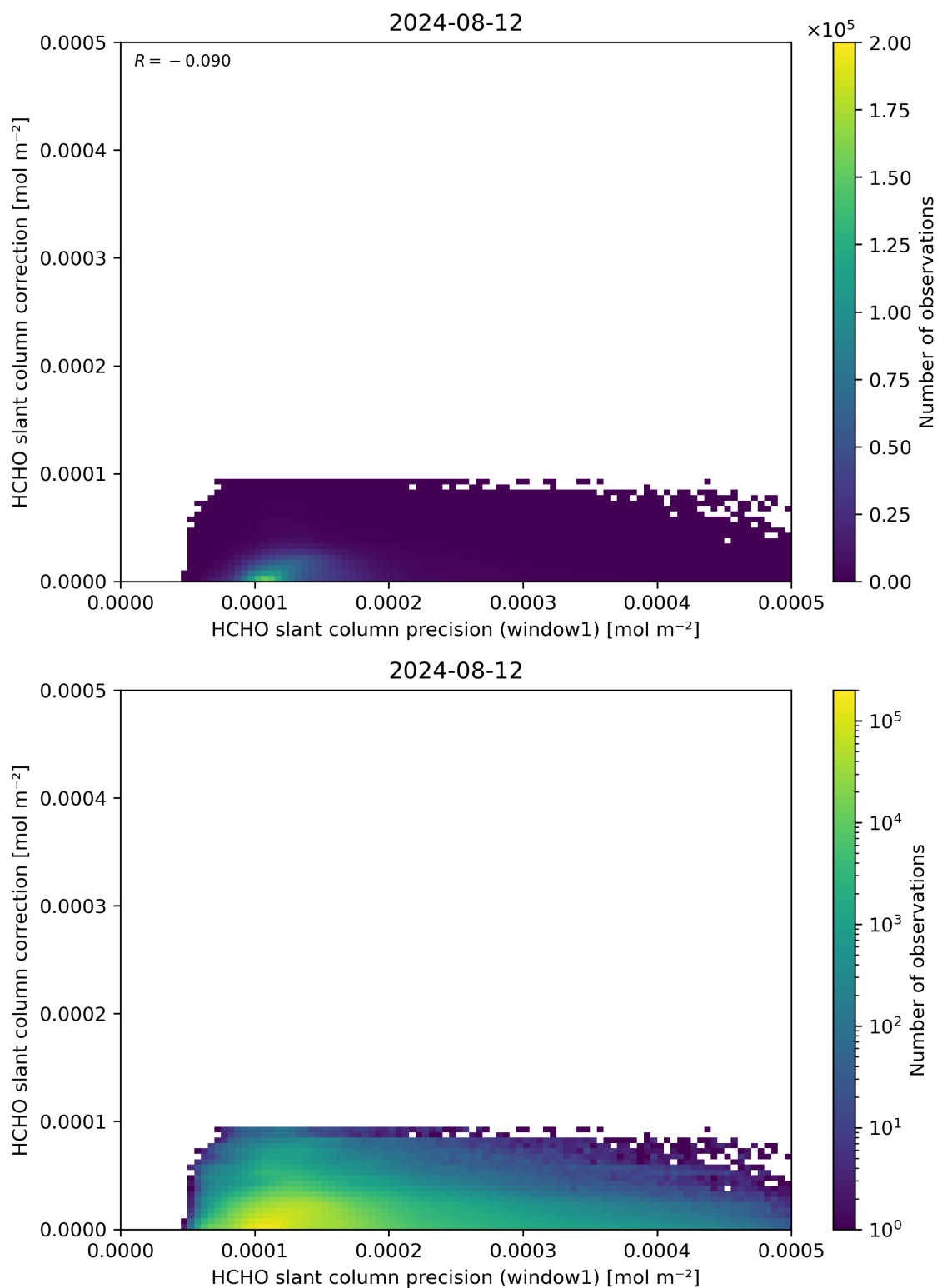
Figure 93: Scatter density plot of “HCHO slant column precision (window1)” against “HCHO slant column correction” for 2024-08-12 to 2024-08-13.
