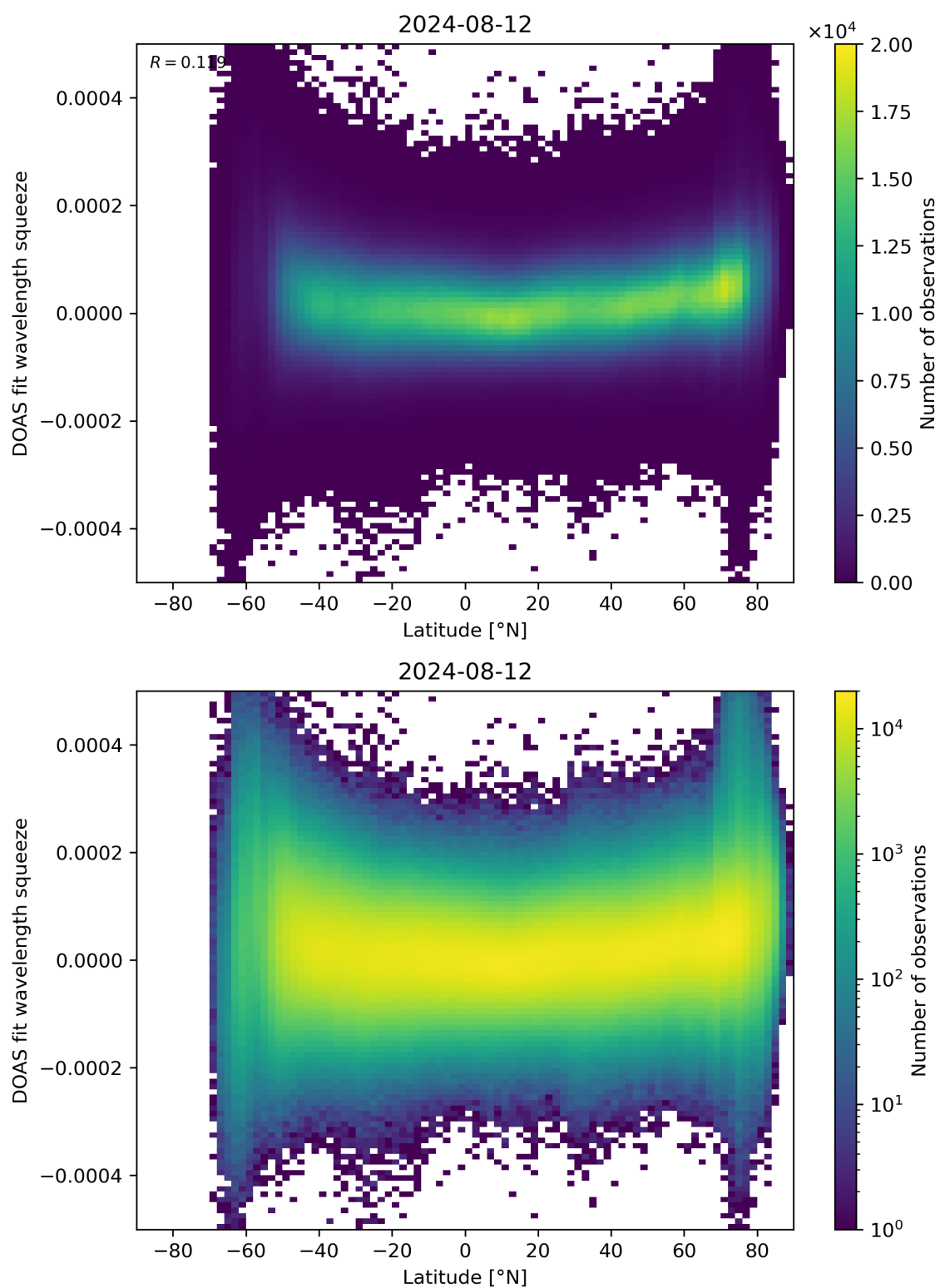
Figure 155: Scatter density plot of “Latitude” against “DOAS fit wavelength squeeze” for 2024-08-12 to 2024-08-13.
