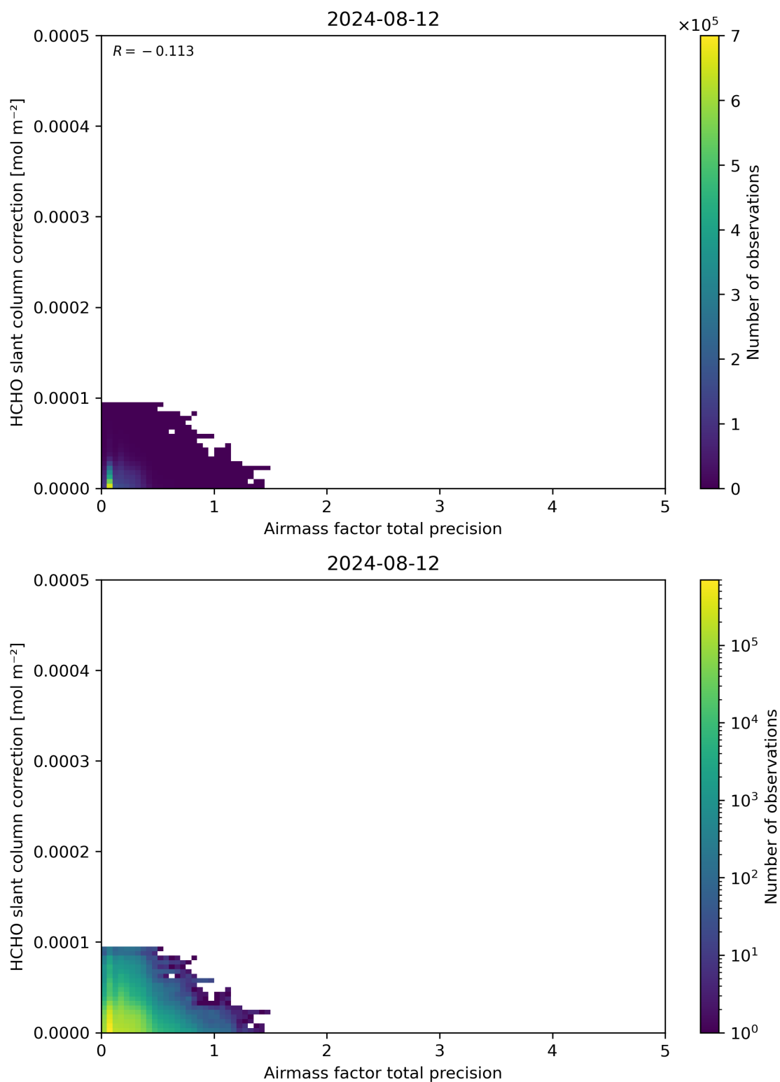
Figure 110: Scatter density plot of “Airmass factor total precision” against “HCHO slant column correction” for 2024-08-12 to 2024-08-13.
