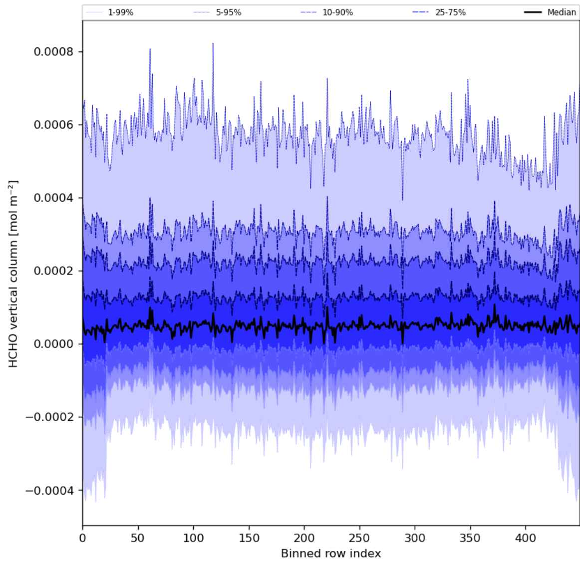
Figure 49: Along track statistics of “HCHO vertical column” for 2024-08-12 to 2024-08-13
