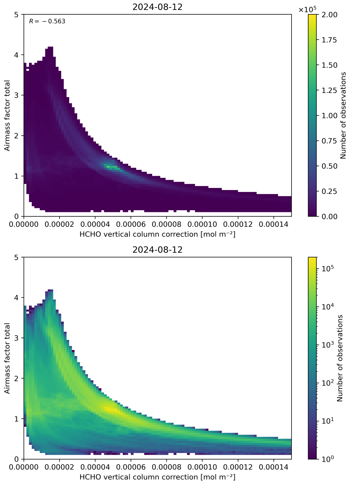
Figure 120: Scatter density plot of “HCHO vertical column correction” against “Airmass factor total” for 2024-08-12 to 2024-08-13.
