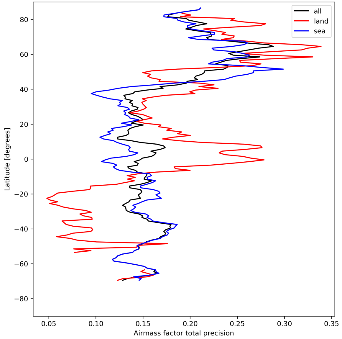
Figure 27: Zonal average of “Airmass factor total precision” for 2024-08-12 to 2024-08-13.
