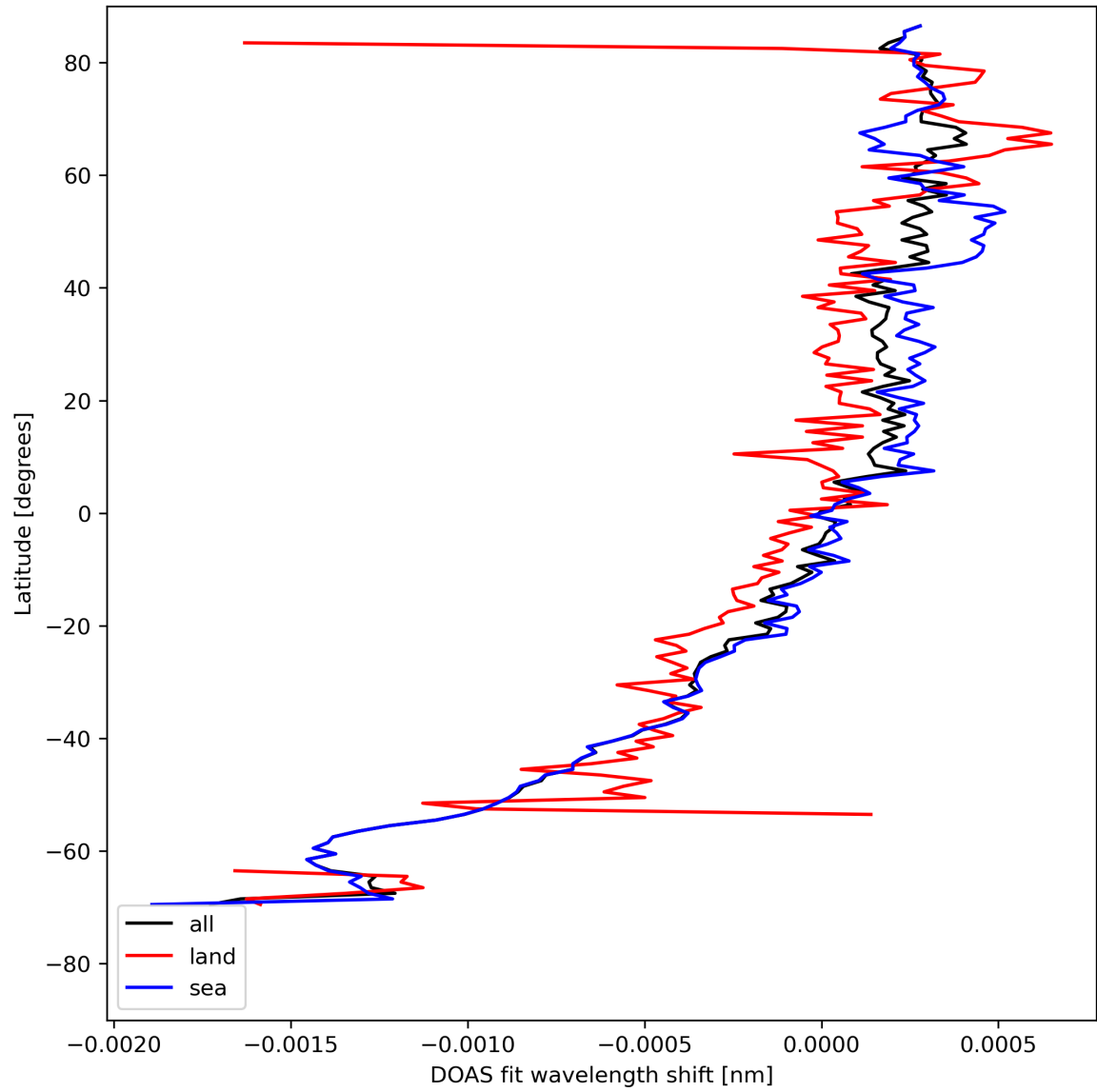
Figure 30: Zonal average of “DOAS fit wavelength shift” for 2024-08-12 to 2024-08-13.
