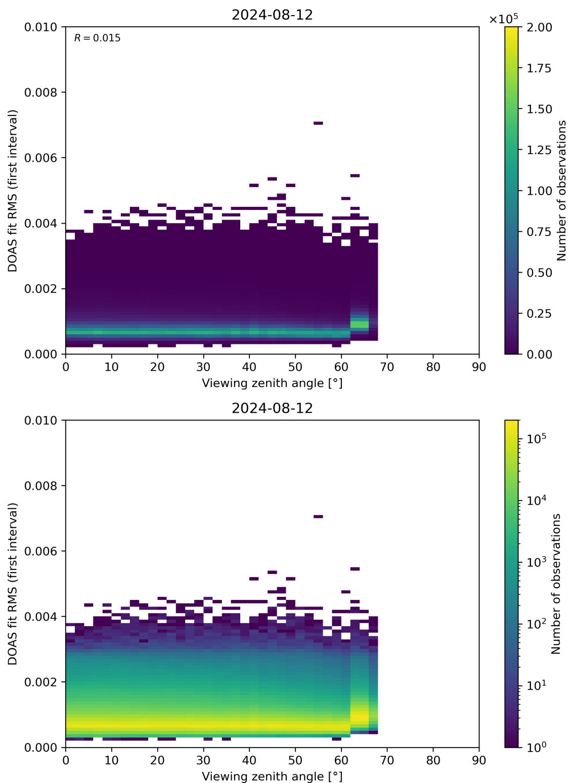
Figure 182: Scatter density plot of “Viewing zenith angle” against “DOAS fit RMS (first interval)” for 2024-08-12 to 2024-08-13.
