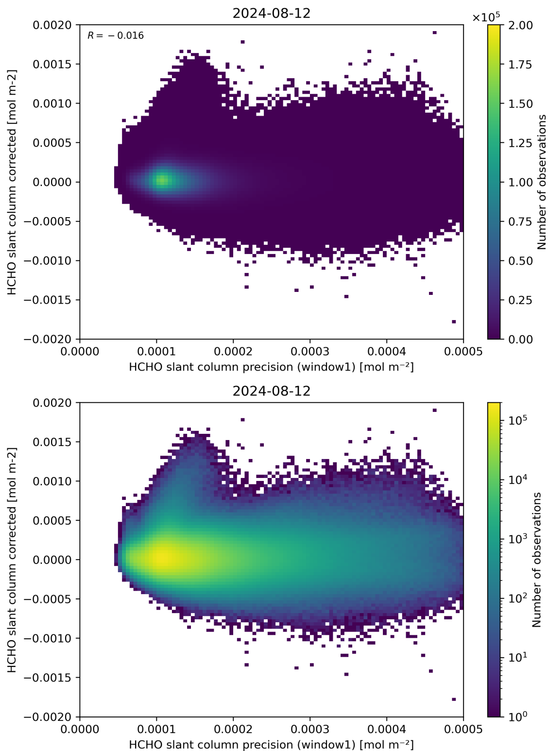
Figure 92: Scatter density plot of “HCHO slant column precision (window1)” against “HCHO slant column corrected” for 2024-08-12 to 2024-08-13.
