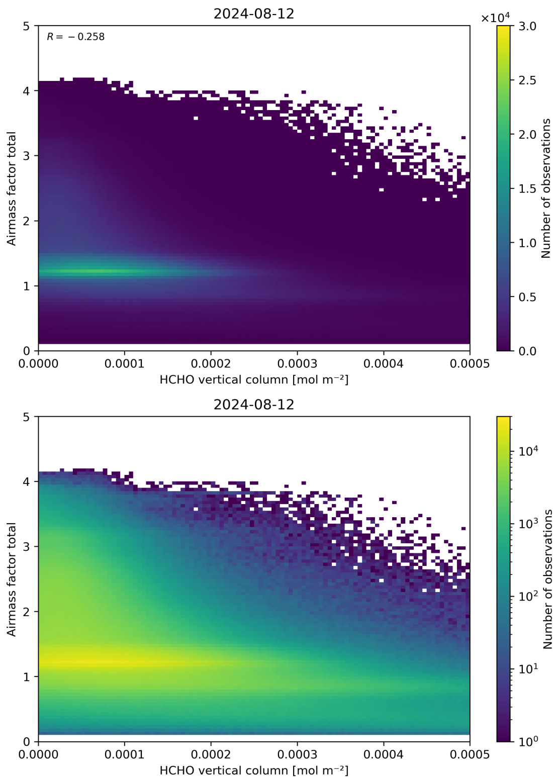
Figure 131: Scatter density plot of “HCHO vertical column” against “Airmass factor total” for 2024-08-12 to 2024-08-13.
