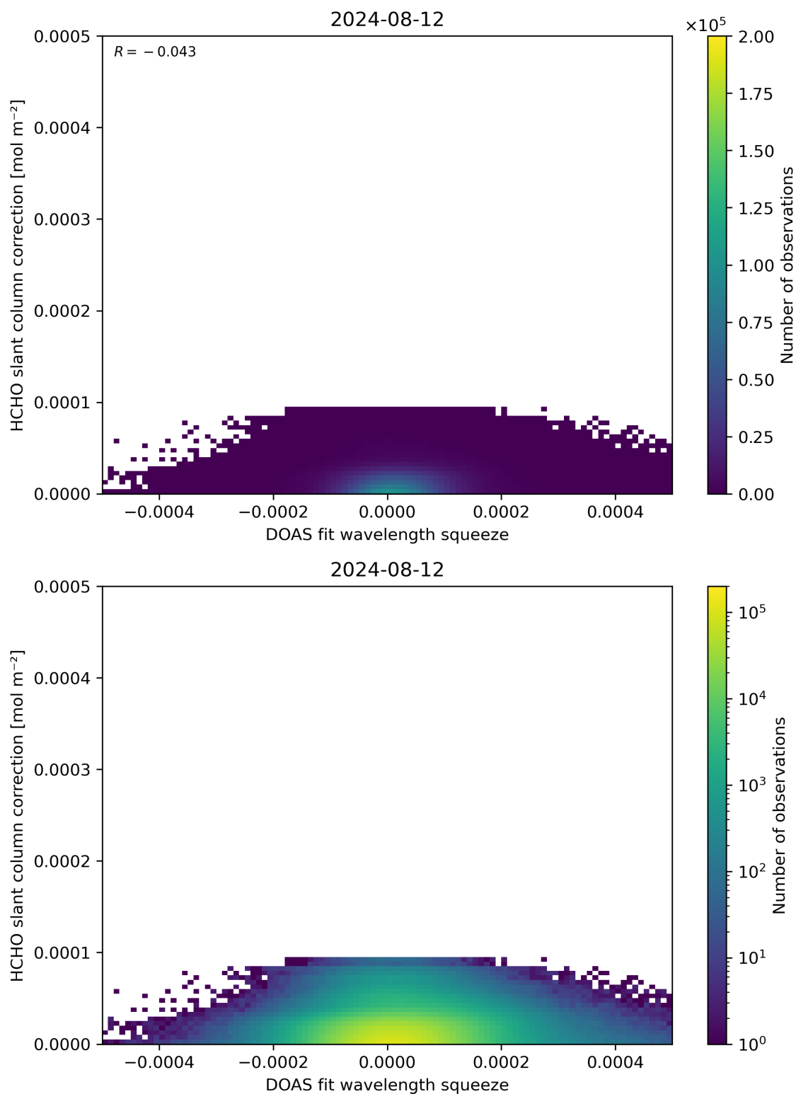
Figure 70: Scatter density plot of “DOAS fit wavelength squeeze” against “HCHO slant column correction” for 2024-08-12 to 2024-08-13.
