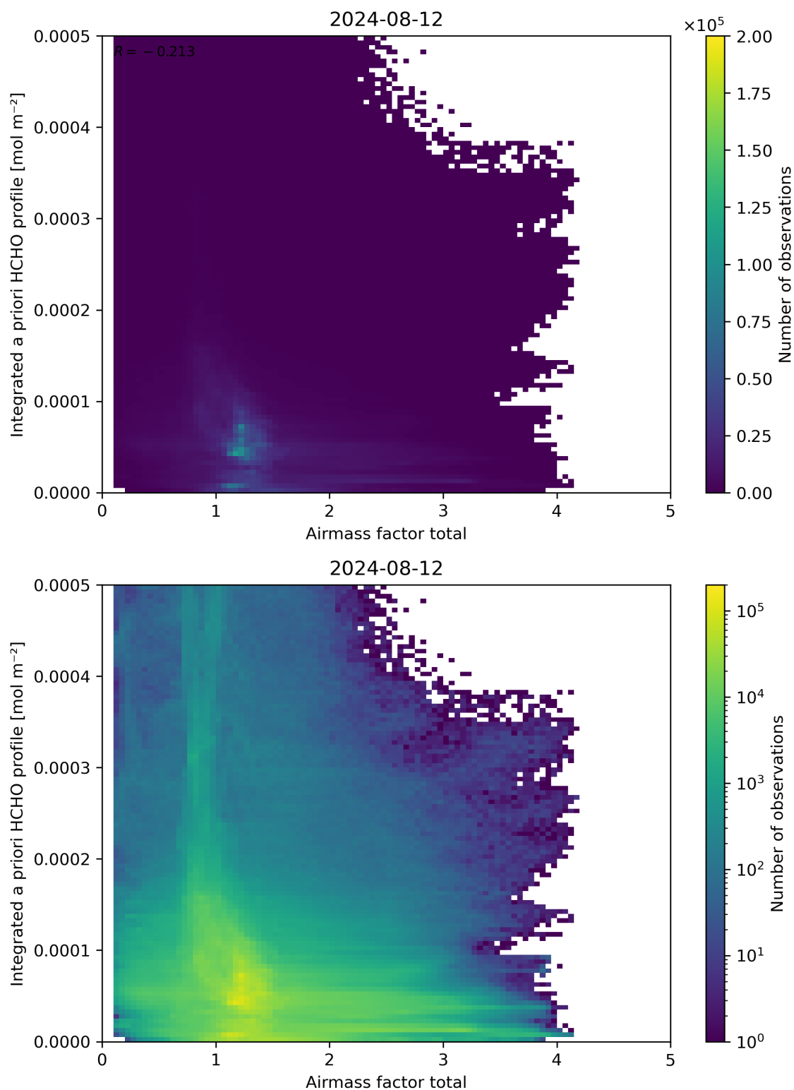
Figure 104: Scatter density plot of “Airmass factor total” against “Integrated a priori HCHO profile” for 2024-08-12 to 2024-08-13.
