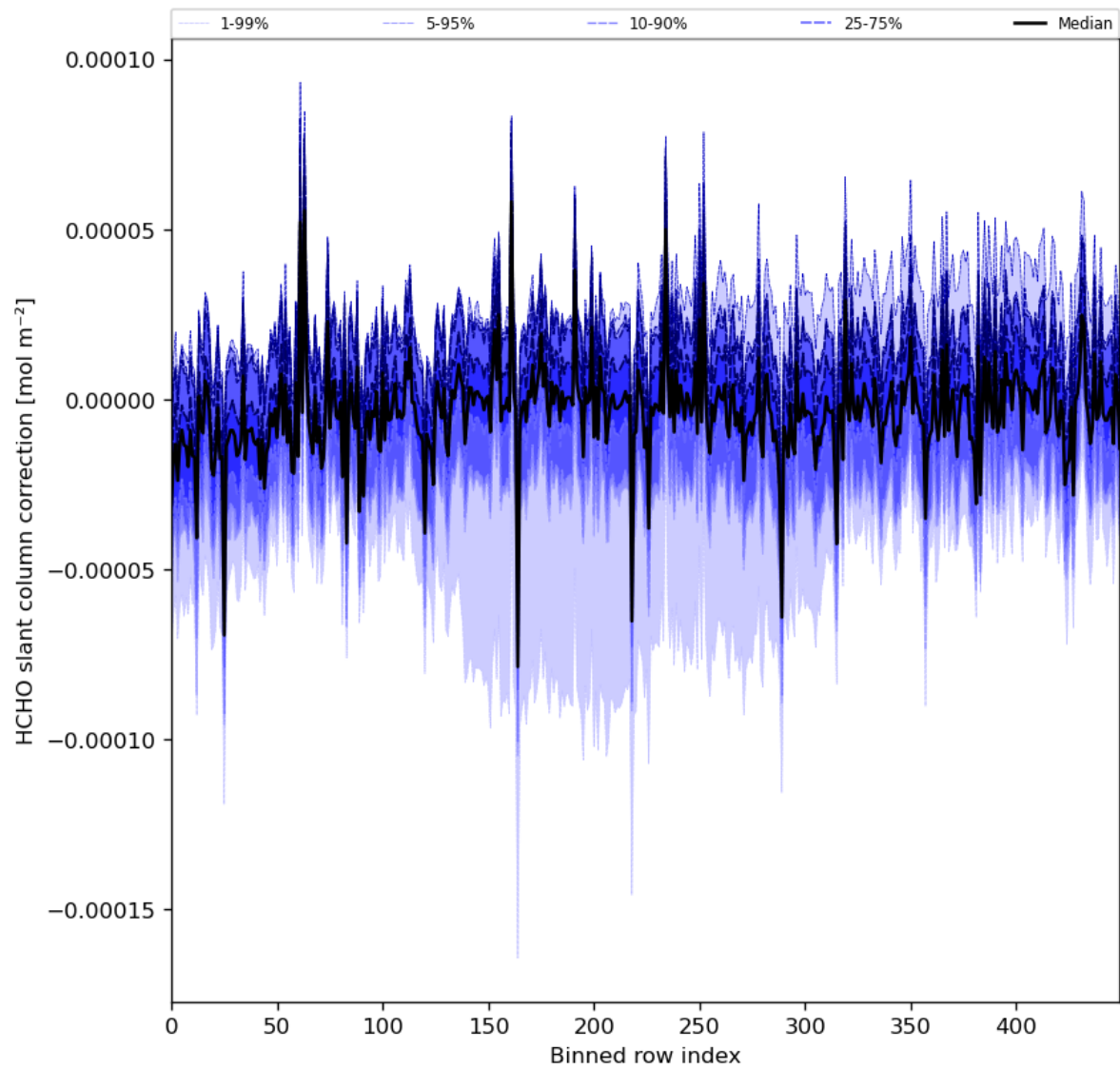
Figure 61: Along track statistics of “HCHO slant column correction” for 2024-08-12 to 2024-08-13
