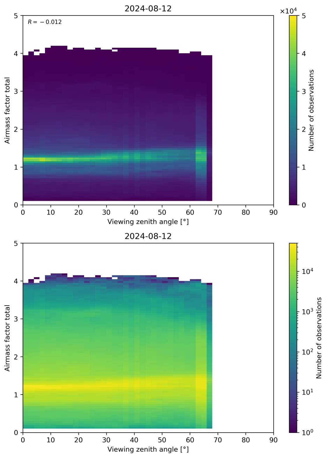
Figure 190: Scatter density plot of “Viewing zenith angle” against “Airmass factor total” for 2024-08-12 to 2024-08-13.
