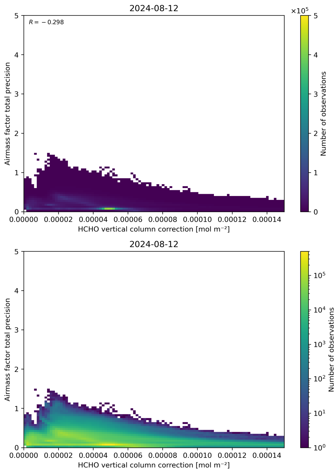
Figure 121: Scatter density plot of “HCHO vertical column correction” against “Airmass factor total precision” for 2024-08-12 to 2024-08-13.
