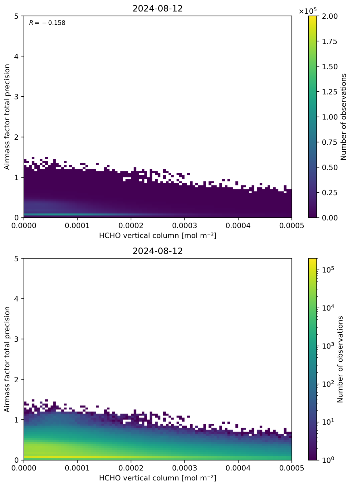
Figure 132: Scatter density plot of “HCHO vertical column” against “Airmass factor total precision” for 2024-08-12 to 2024-08-13.
