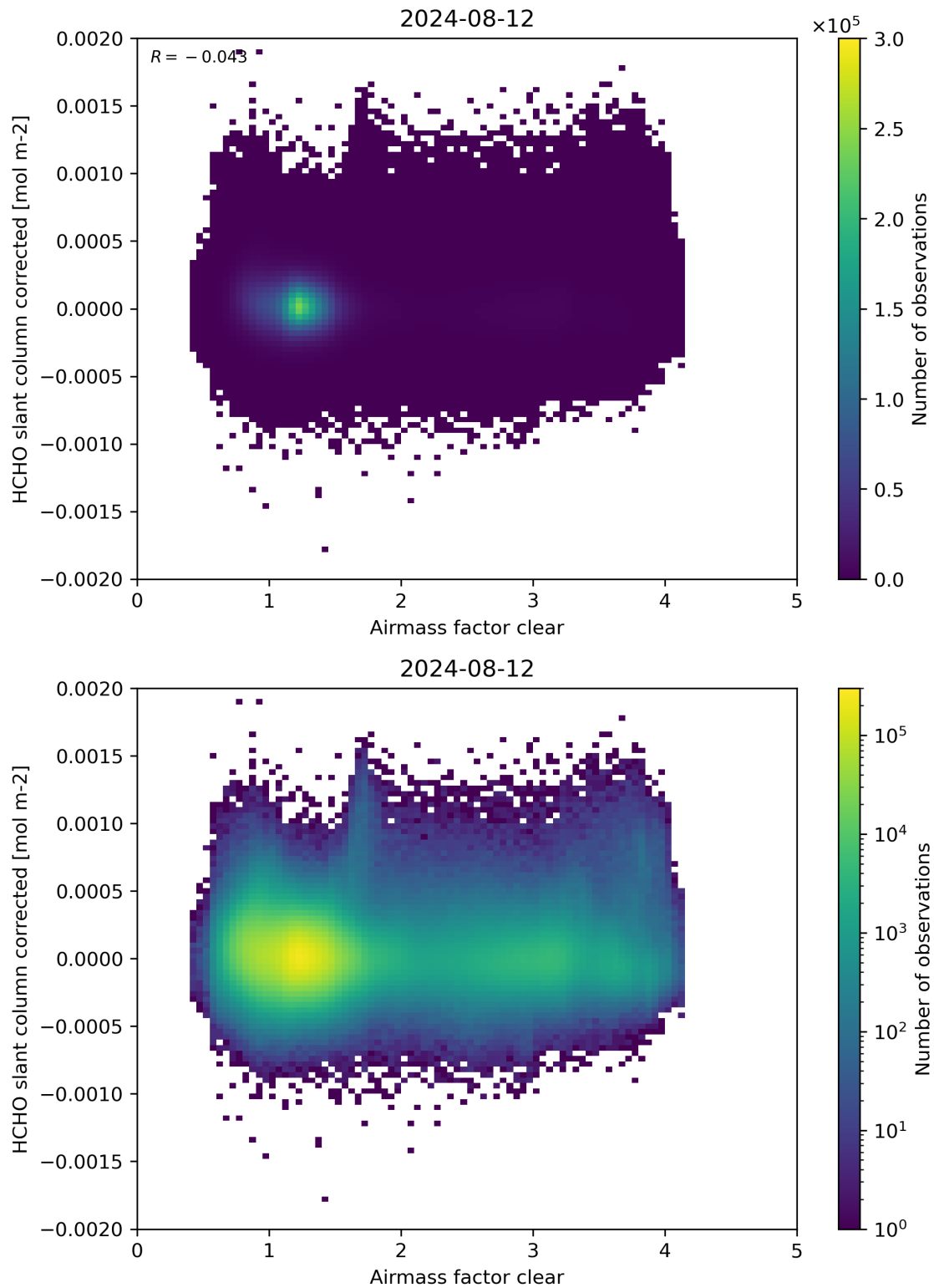
Figure 74: Scatter density plot of “Airmass factor clear” against “HCHO slant column corrected” for 2024-08-12 to 2024-08-13.
