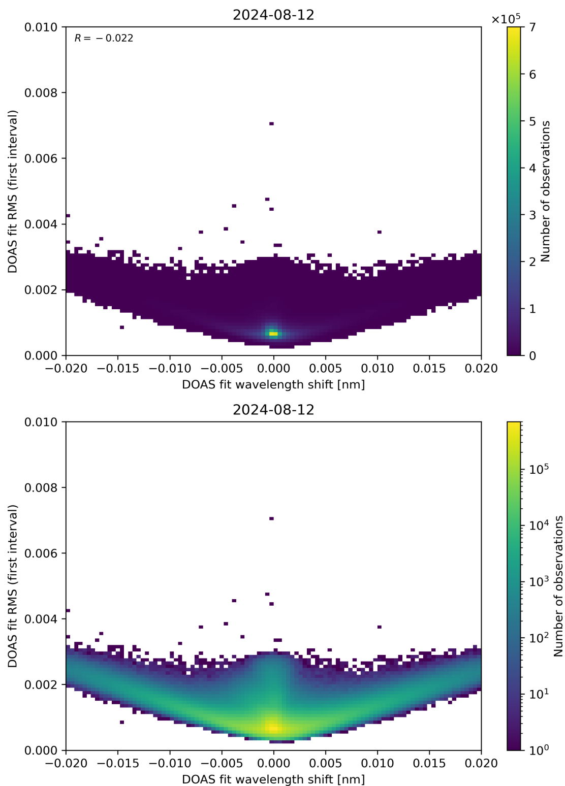
Figure 64: Scatter density plot of “DOAS fit wavelength shift” against “DOAS fit RMS (first interval)” for 2024-08-12 to 2024-08-13.
