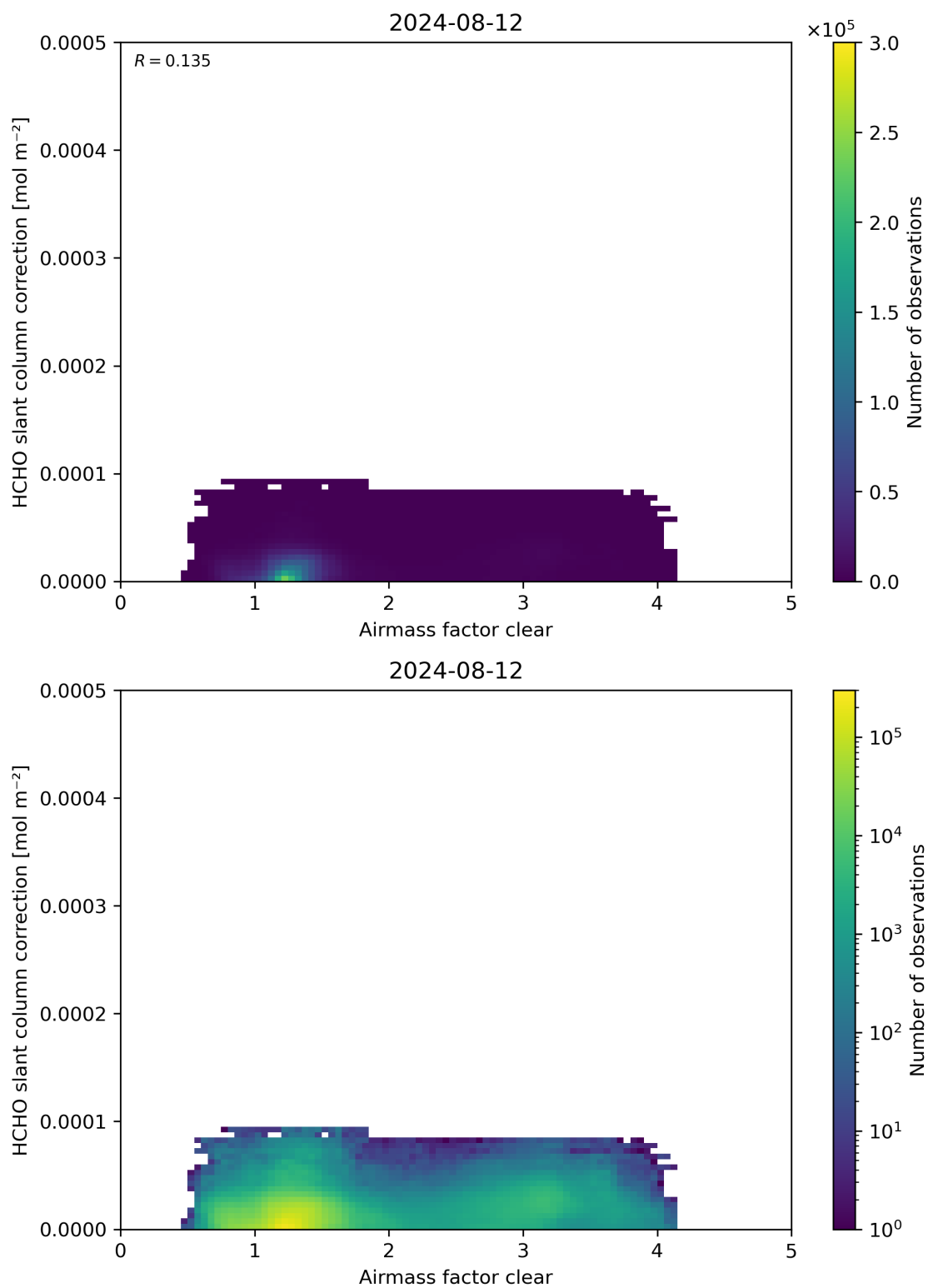
Figure 75: Scatter density plot of “Airmass factor clear” against “HCHO slant column correction” for 2024-08-12 to 2024-08-13.
