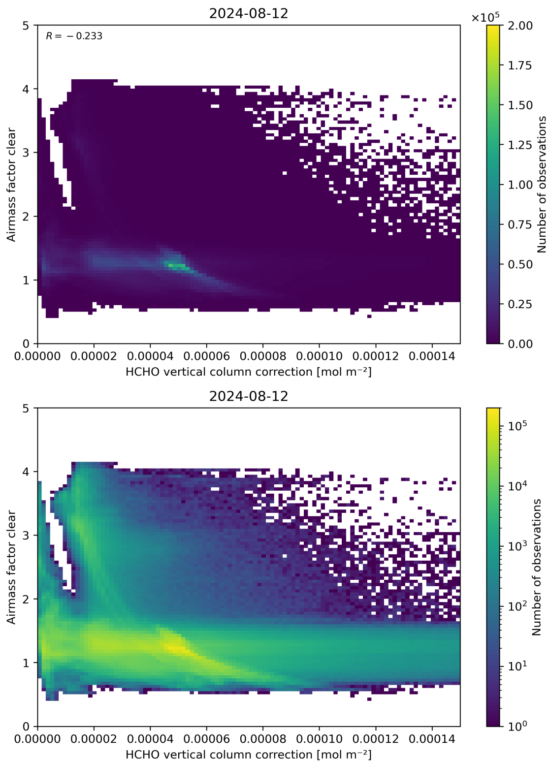
Figure 115: Scatter density plot of “HCHO vertical column correction” against “Airmass factor clear” for 2024-08-12 to 2024-08-13.
