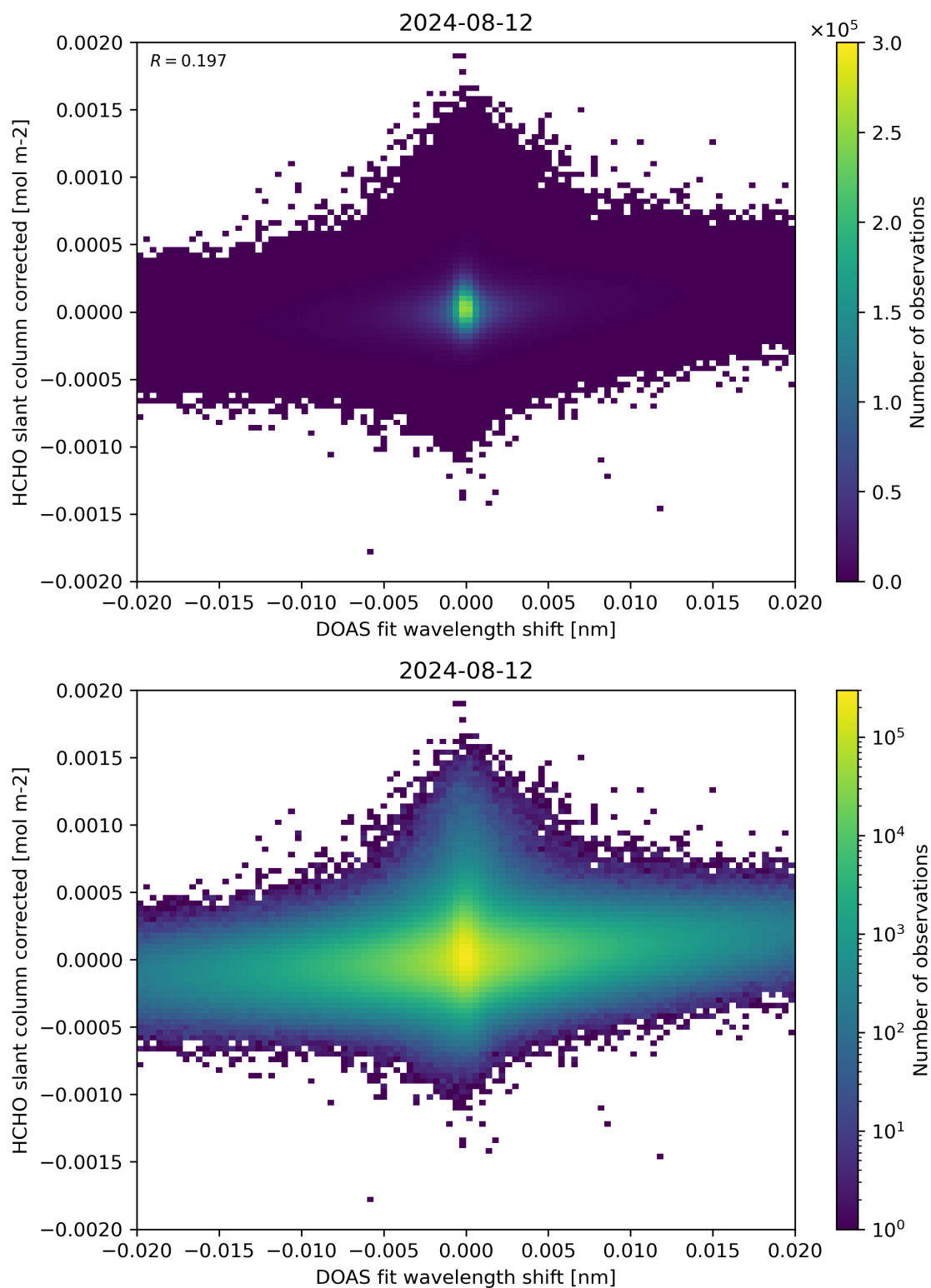
Figure 66: Scatter density plot of “DOAS fit wavelength shift” against “HCHO slant column corrected” for 2024-08-12 to 2024-08-13.
