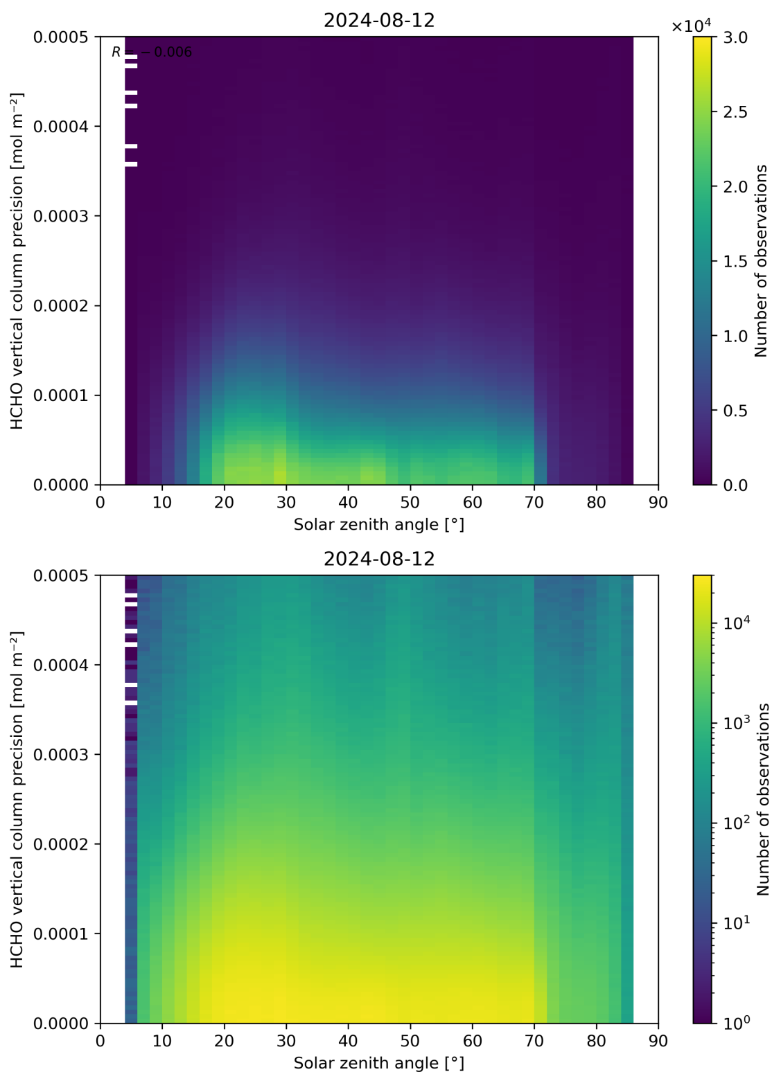
Figure 179: Scatter density plot of “Solar zenith angle” against “HCHO vertical column precision” for 2024-08-12 to 2024-08-13.
