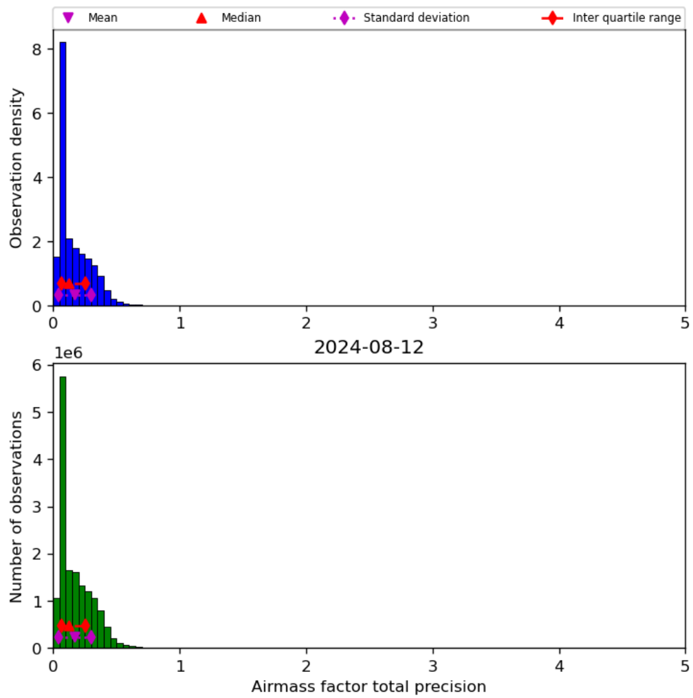
Figure 41: Histogram of “Airmass factor total precision” for 2024-08-12 to 2024-08-13
