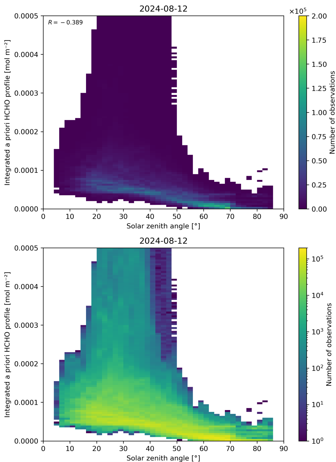
Figure 180: Scatter density plot of “Solar zenith angle” against “Integrated a priori HCHO profile” for 2024-08-12 to 2024-08-13.
