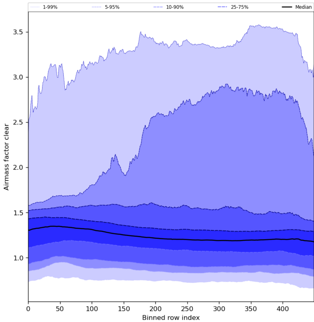
Figure 56: Along track statistics of “Airmass factor clear” for 2024-08-12 to 2024-08-13
