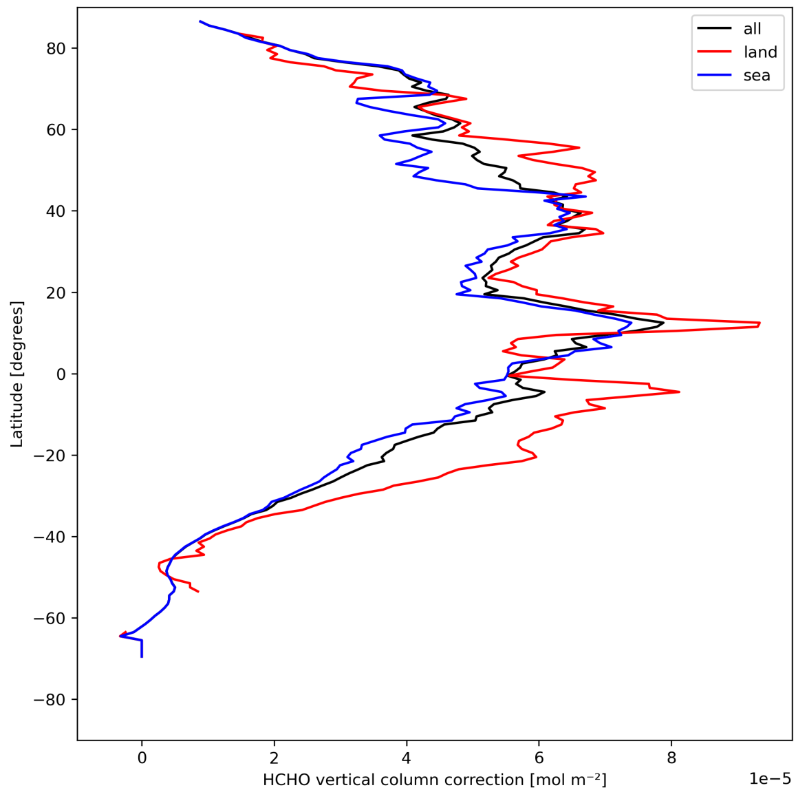
Figure 23: Zonal average of “HCHO vertical column correction” for 2024-08-12 to 2024-08-13.
