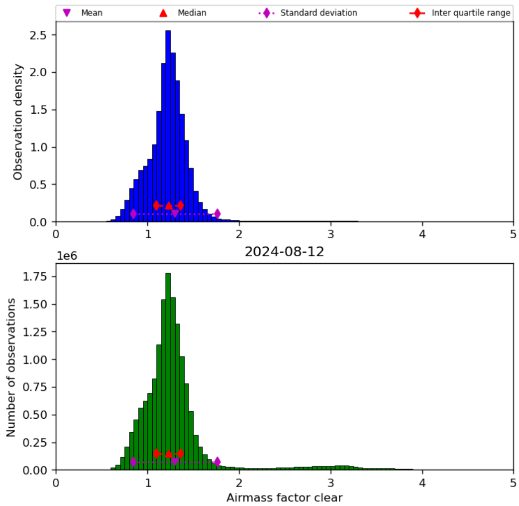
Figure 42: Histogram of “Airmass factor clear” for 2024-08-12 to 2024-08-13
