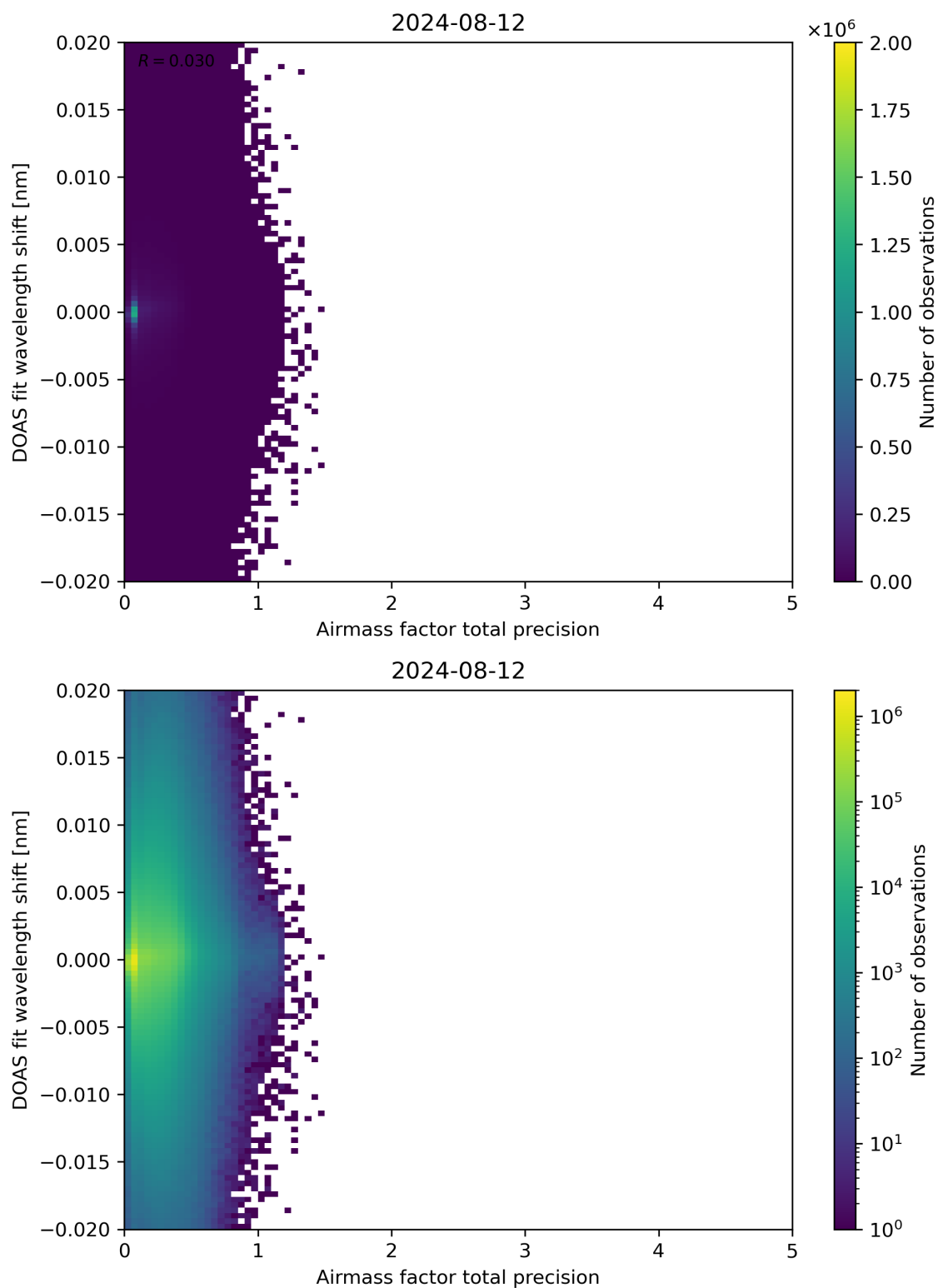
Figure 106: Scatter density plot of “Airmass factor total precision” against “DOAS fit wavelength shift” for 2024-08-12 to 2024-08-13.
