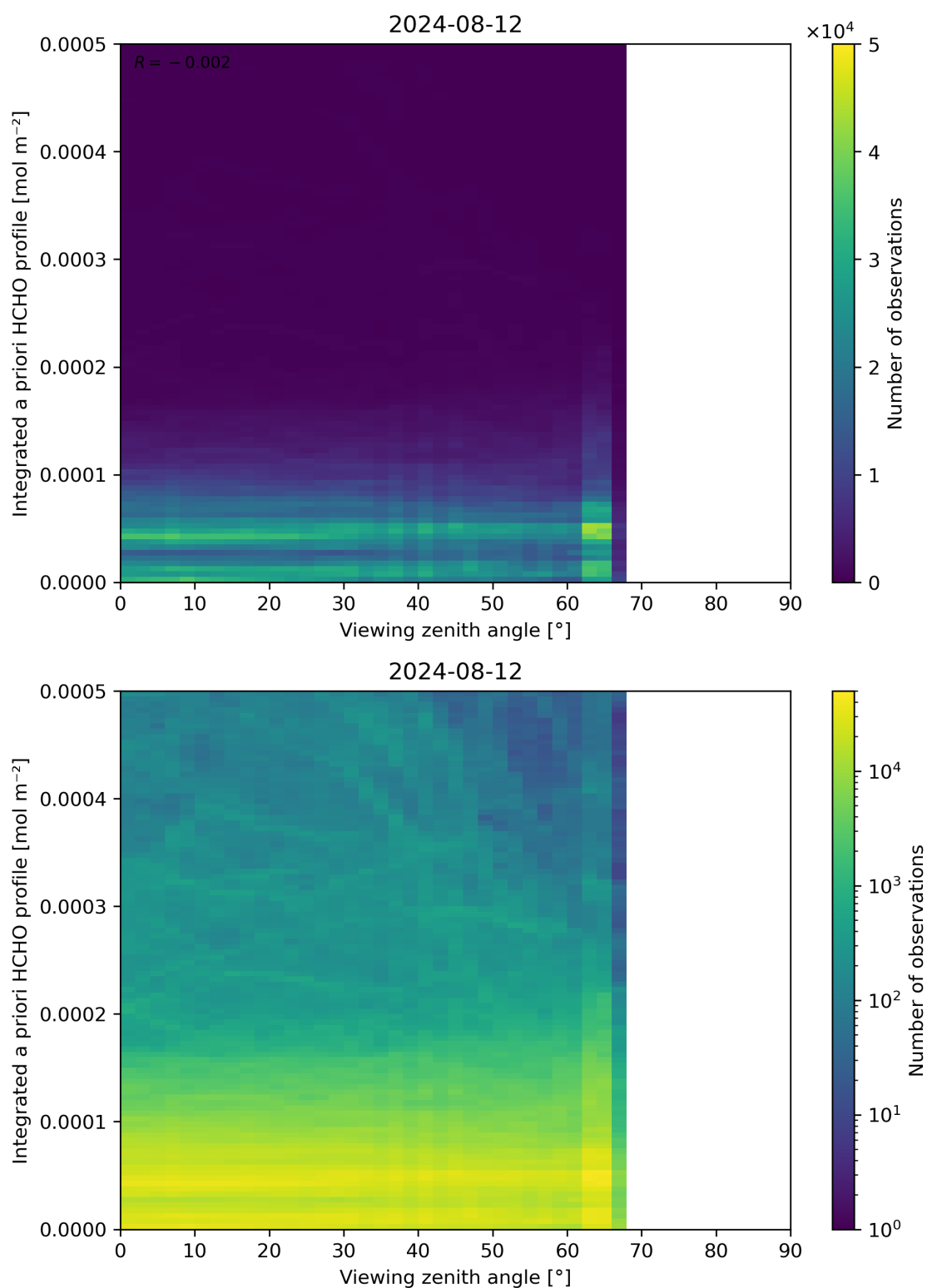
Figure 195: Scatter density plot of “Viewing zenith angle” against “Integrated a priori HCHO profile” for 2024-08-12 to 2024-08-13.
