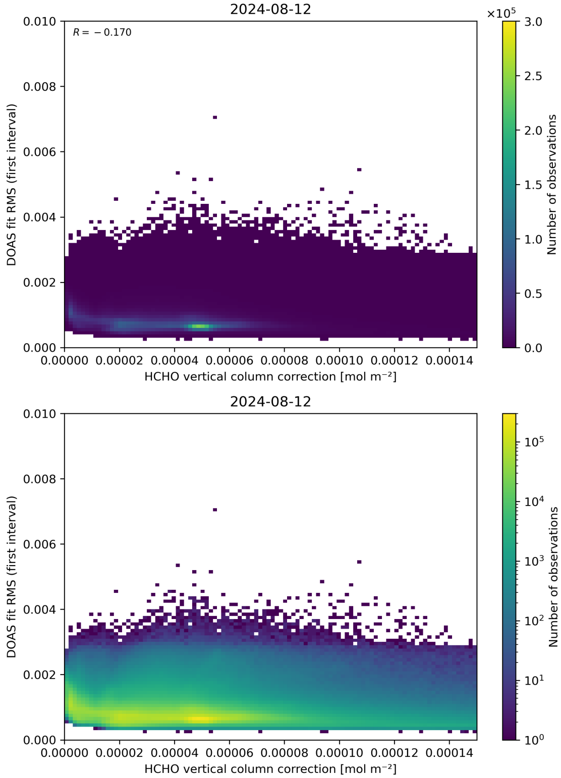
Figure 112: Scatter density plot of “HCHO vertical column correction” against “DOAS fit RMS (first interval)” for 2024-08-12 to 2024-08-13.
