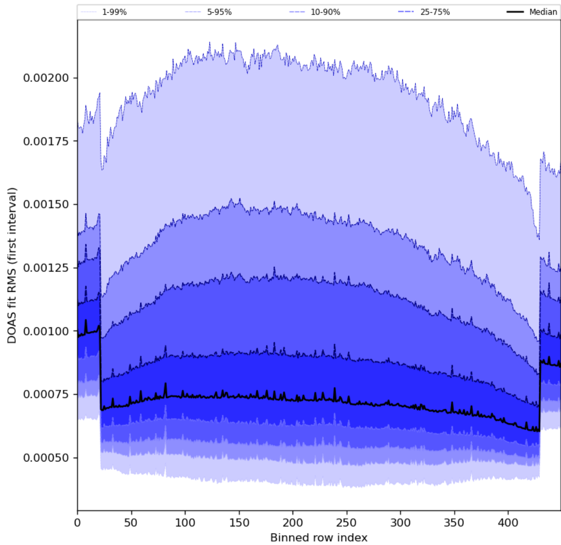
Figure 60: Along track statistics of “DOAS fit RMS (first interval)” for 2024-08-12 to 2024-08-13
