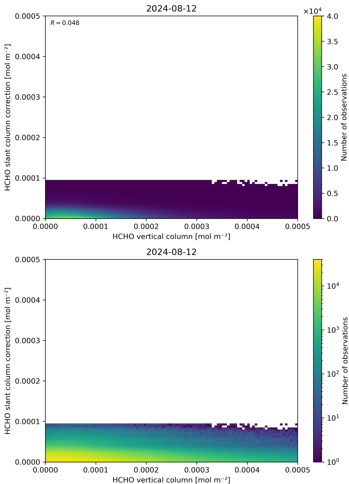
Figure 128: Scatter density plot of “HCHO vertical column” against “HCHO slant column correction” for 2024-08-12 to 2024-08-13.
