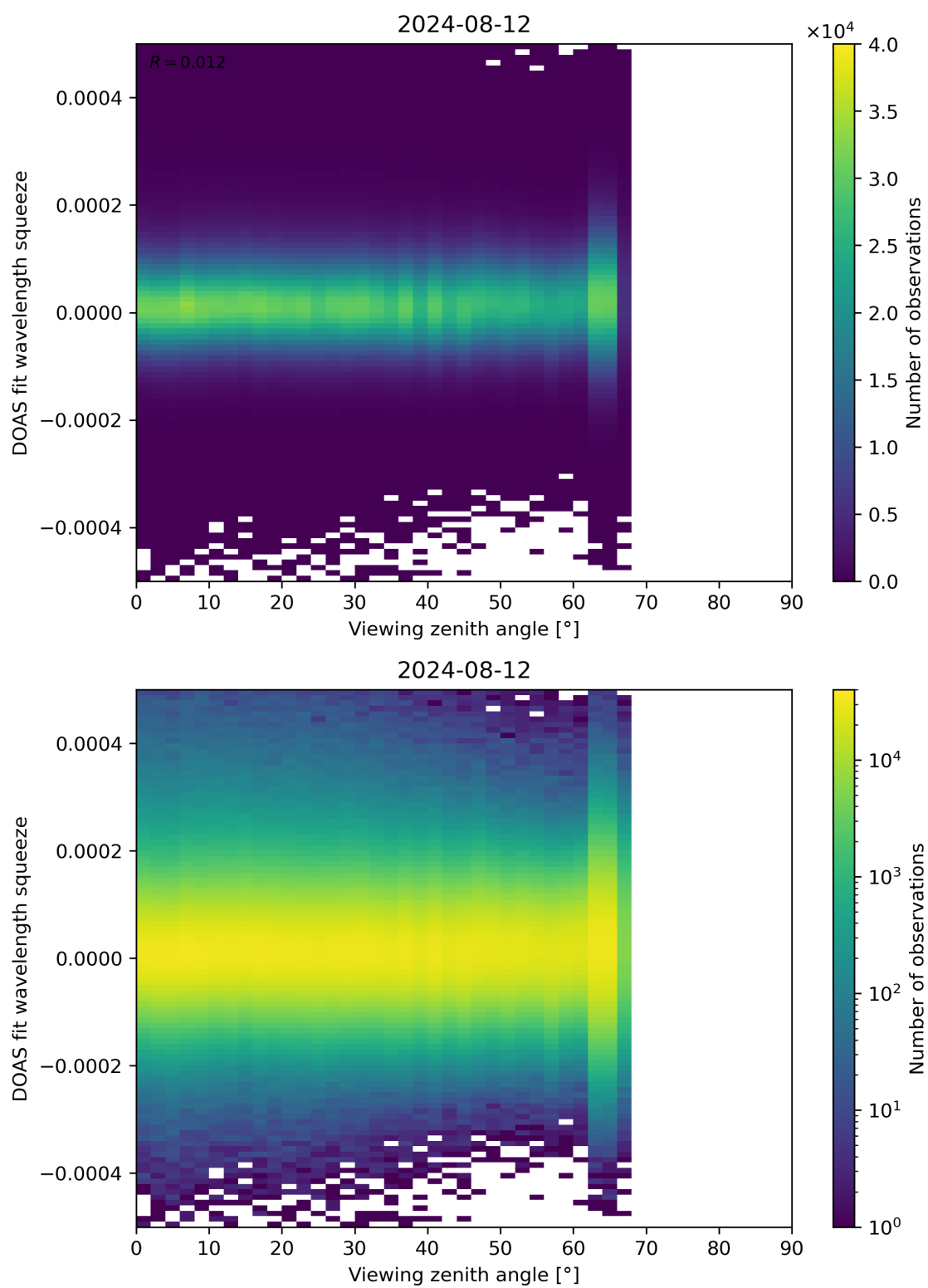
Figure 184: Scatter density plot of “Viewing zenith angle” against “DOAS fit wavelength squeeze” for 2024-08-12 to 2024-08-13.
