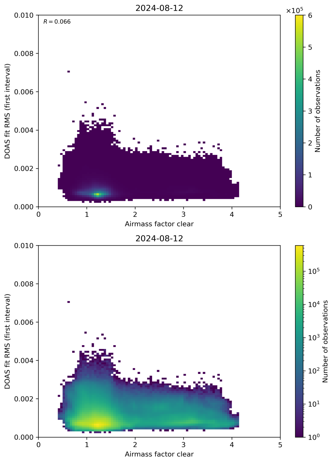
Figure 71: Scatter density plot of “Airmass factor clear” against “DOAS fit RMS (first interval)” for 2024-08-12 to 2024-08-13.
