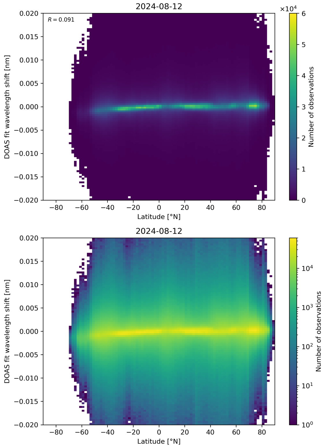
Figure 154: Scatter density plot of “Latitude” against “DOAS fit wavelength shift” for 2024-08-12 to 2024-08-13.
