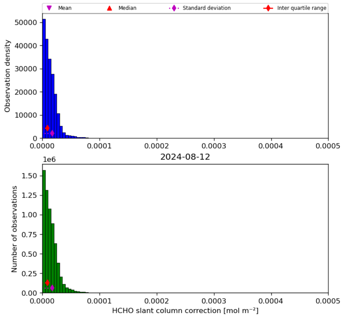
Figure 47: Histogram of “HCHO slant column correction” for 2024-08-12 to 2024-08-13
