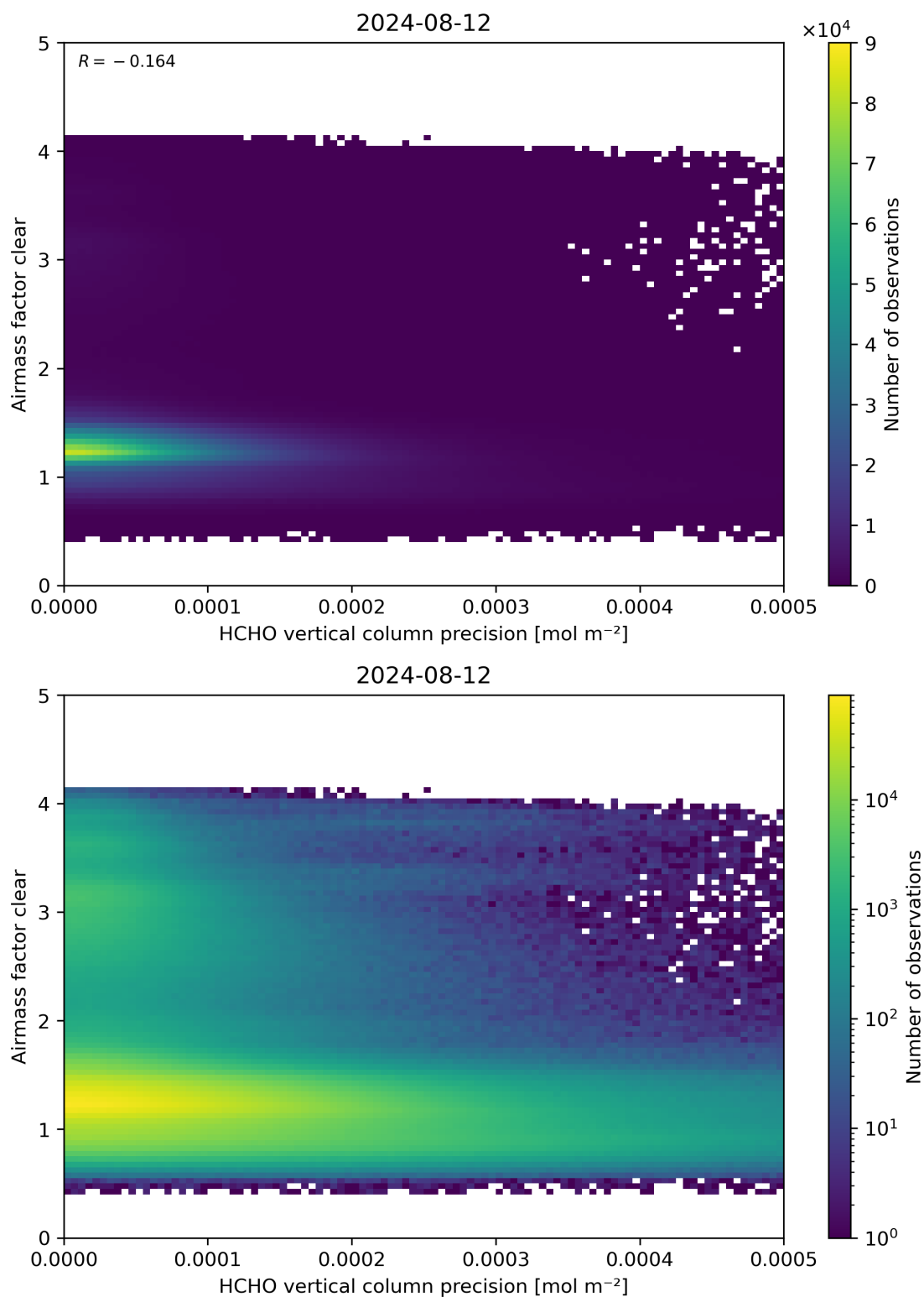
Figure 139: Scatter density plot of “HCHO vertical column precision” against “Airmass factor clear” for 2024-08-12 to 2024-08-13.
