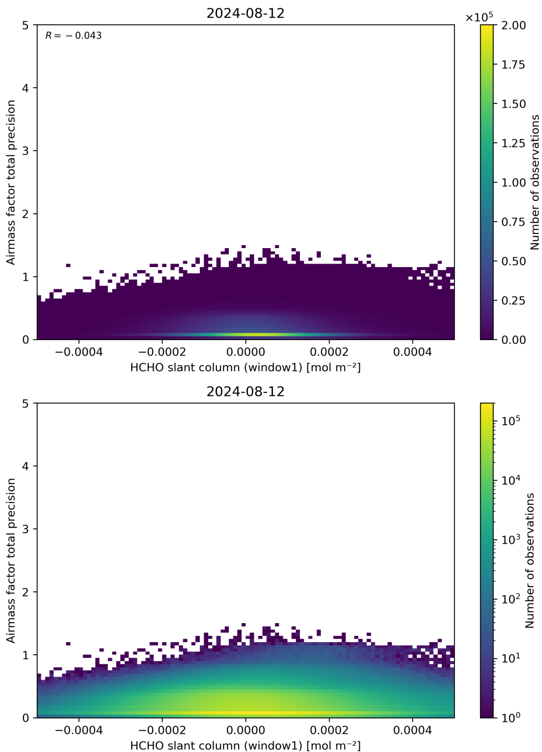
Figure 86: Scatter density plot of “HCHO slant column (window1)” against “Airmass factor total precision” for 2024-08-12 to 2024-08-13.
