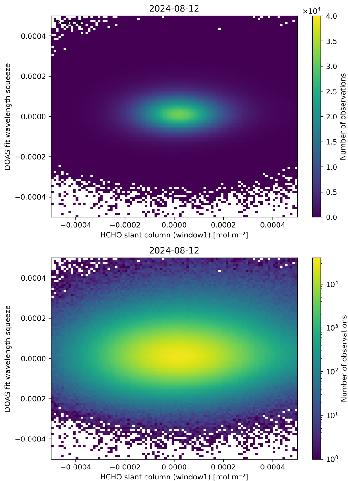
Figure 80: Scatter density plot of “HCHO slant column (window1)” against “DOAS fit wavelength squeeze” for 2024-08-12 to 2024-08-13.
