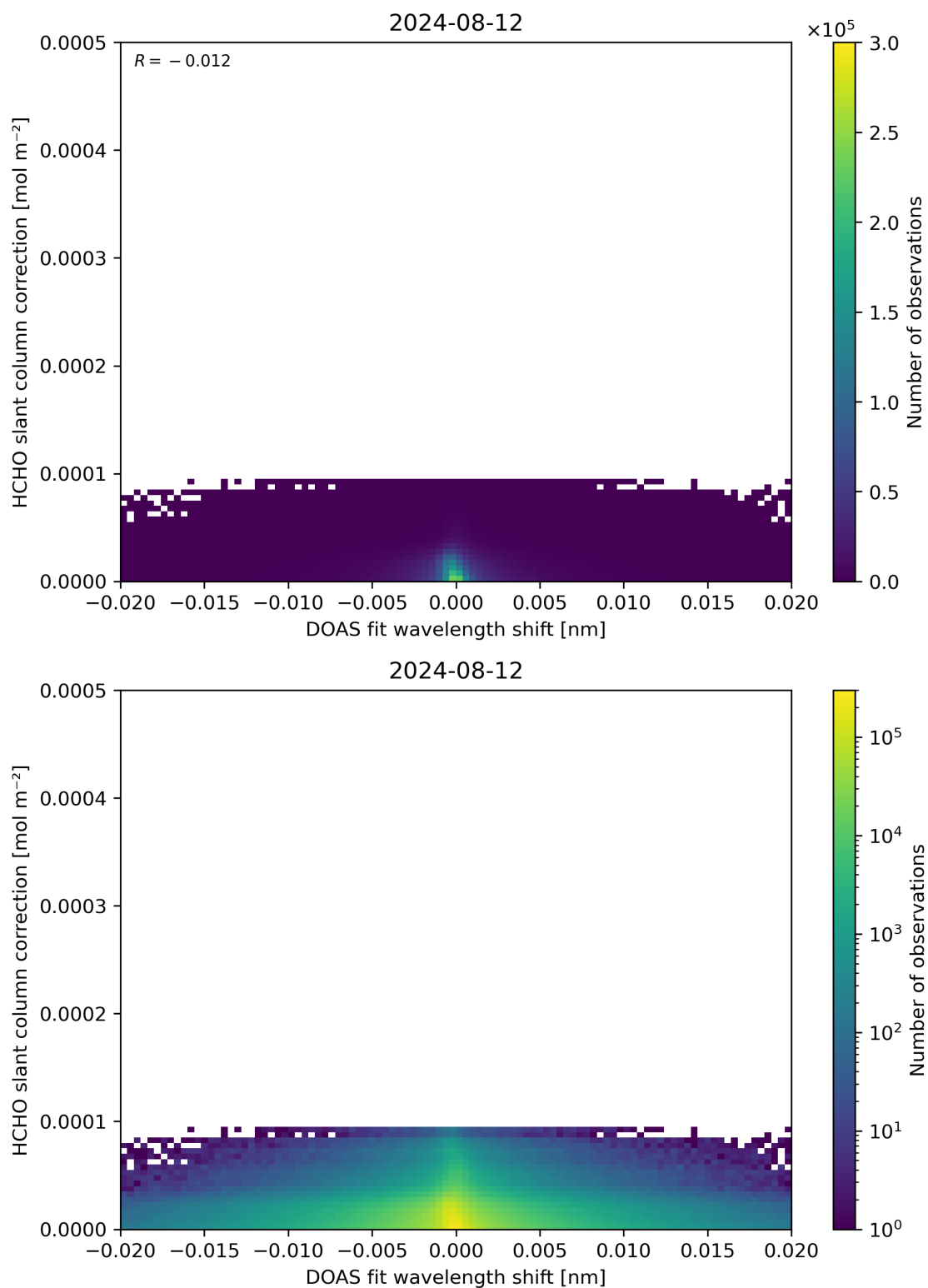
Figure 67: Scatter density plot of “DOAS fit wavelength shift” against “HCHO slant column correction” for 2024-08-12 to 2024-08-13.
