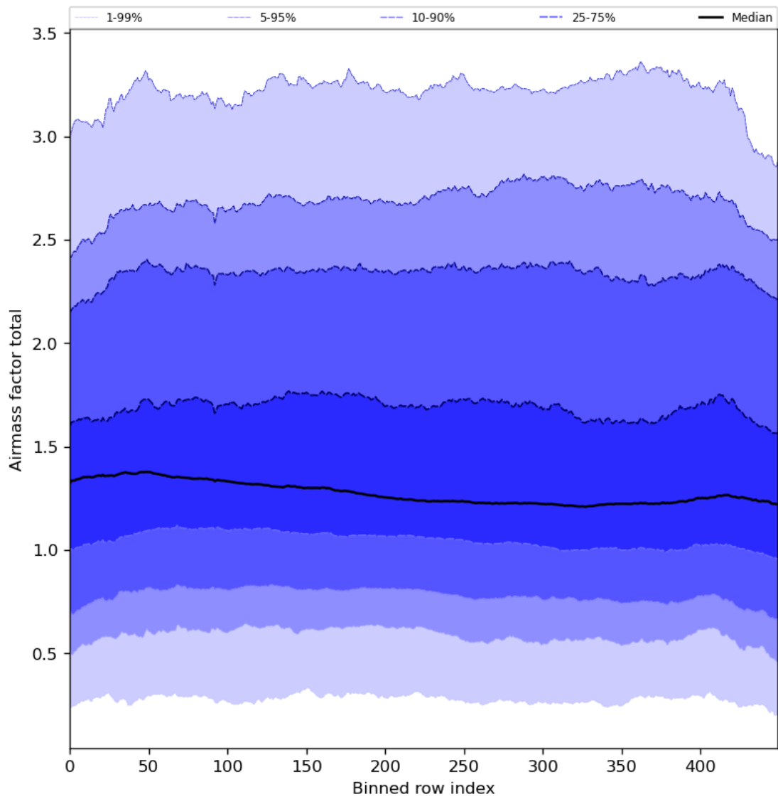
Figure 54: Along track statistics of “Airmass factor total” for 2024-08-12 to 2024-08-13
