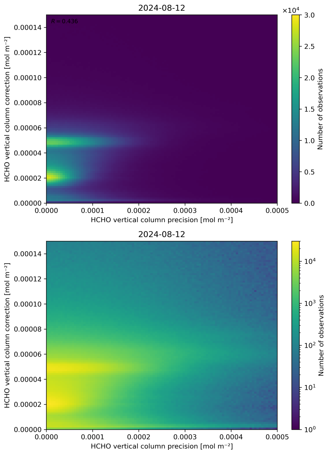
Figure 146: Scatter density plot of “HCHO vertical column precision” against “HCHO vertical column correction” for 2024-08-12 to 2024-08-13.
