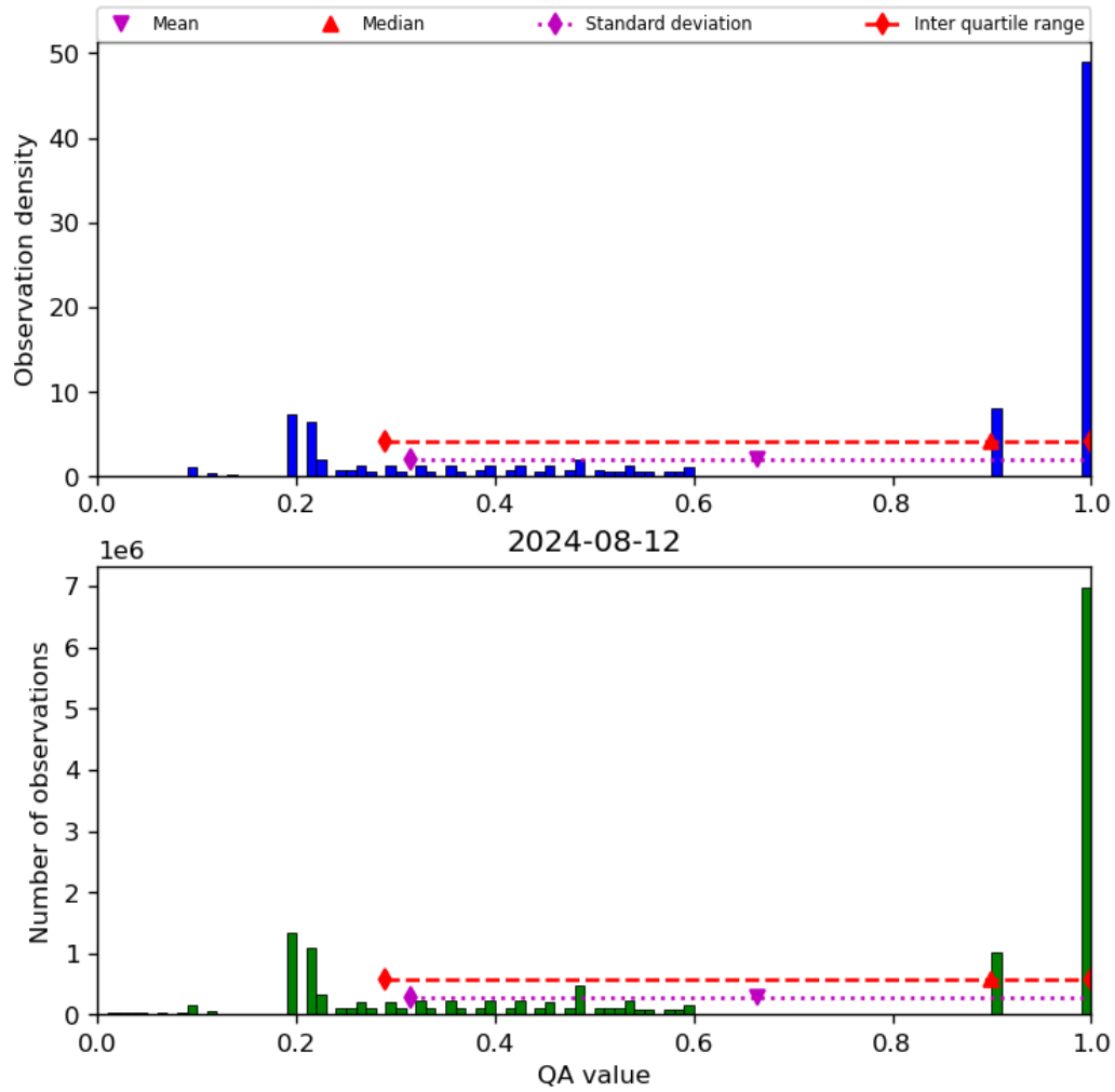
Figure 34: Histogram of “QA value” for 2024-08-12 to 2024-08-13
