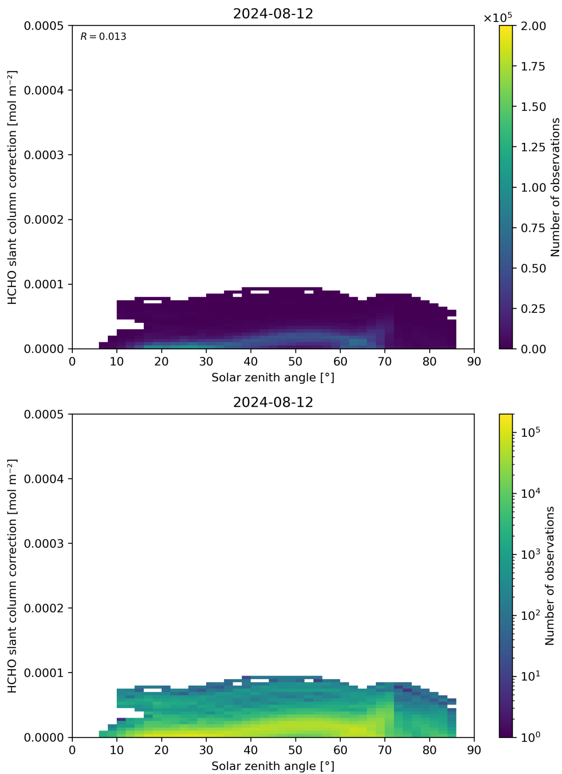
Figure 172: Scatter density plot of “Solar zenith angle” against “HCHO slant column correction” for 2024-08-12 to 2024-08-13.
