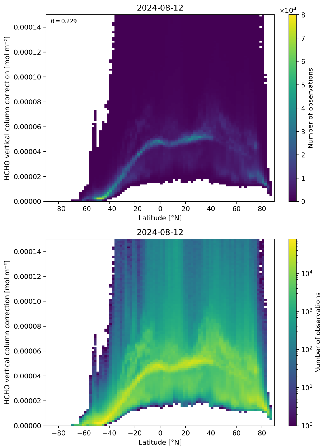
Figure 164: Scatter density plot of “Latitude” against “HCHO vertical column correction” for 2024-08-12 to 2024-08-13.
