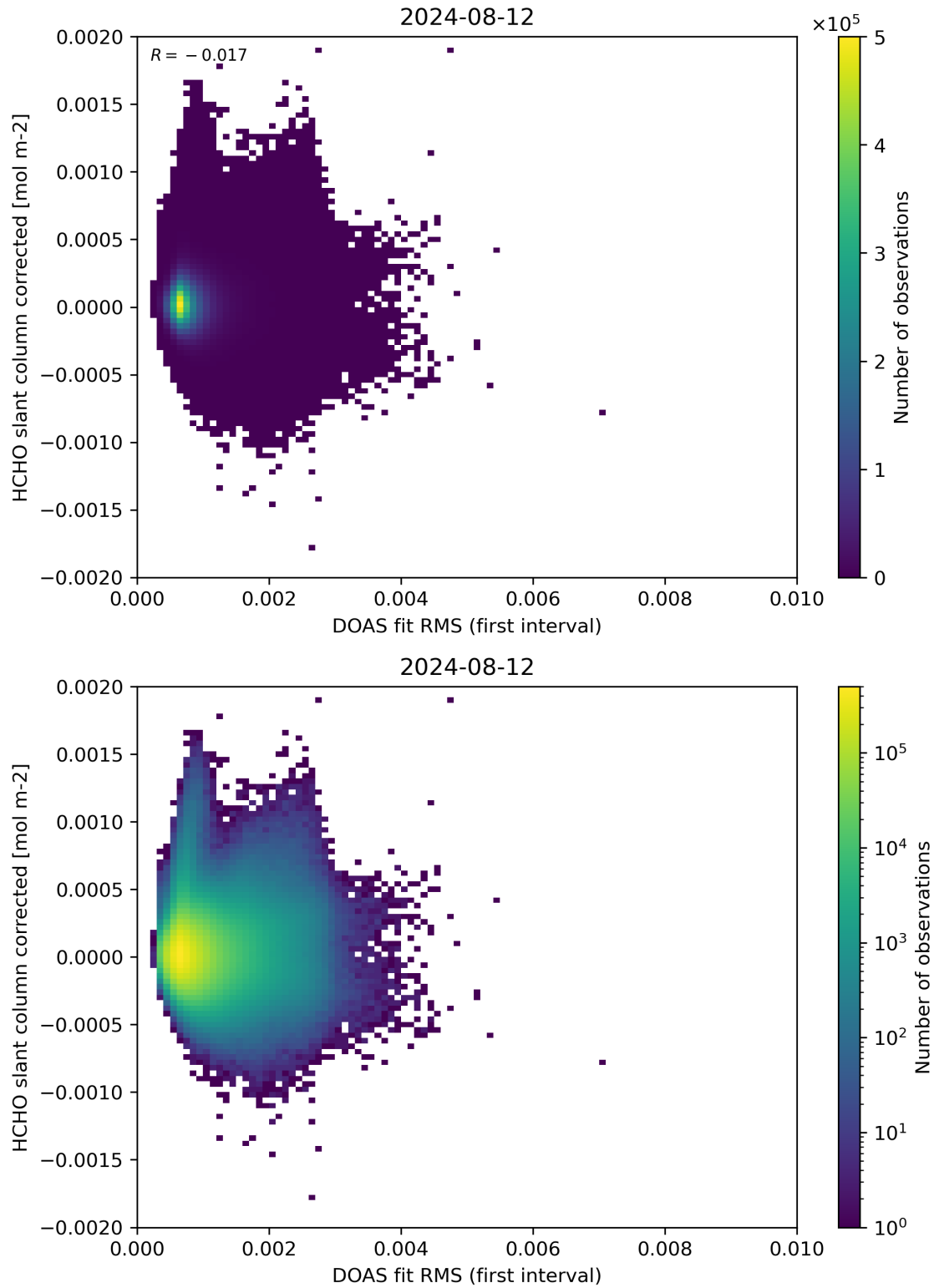
Figure 62: Scatter density plot of “DOAS fit RMS (first interval)” against “HCHO slant column corrected” for 2024-08-12 to 2024-08-13.
