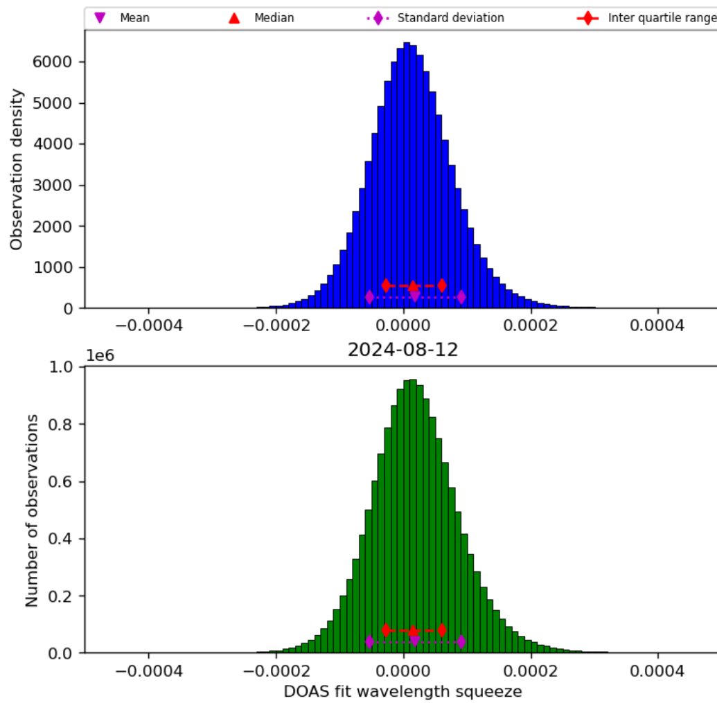
Figure 45: Histogram of “DOAS fit wavelength squeeze” for 2024-08-12 to 2024-08-13
