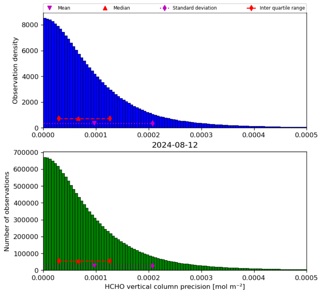
Figure 36: Histogram of “HCHO vertical column precision” for 2024-08-12 to 2024-08-13
