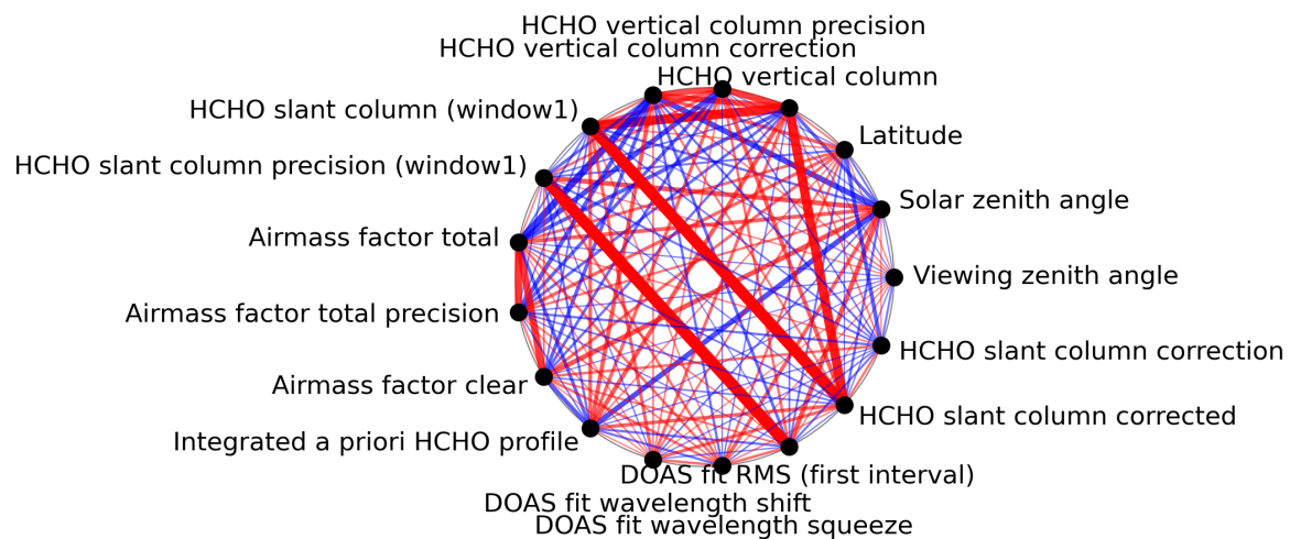
Figure 1: Map of correlation graph for 2024-08-12 to 2024-08-13.
