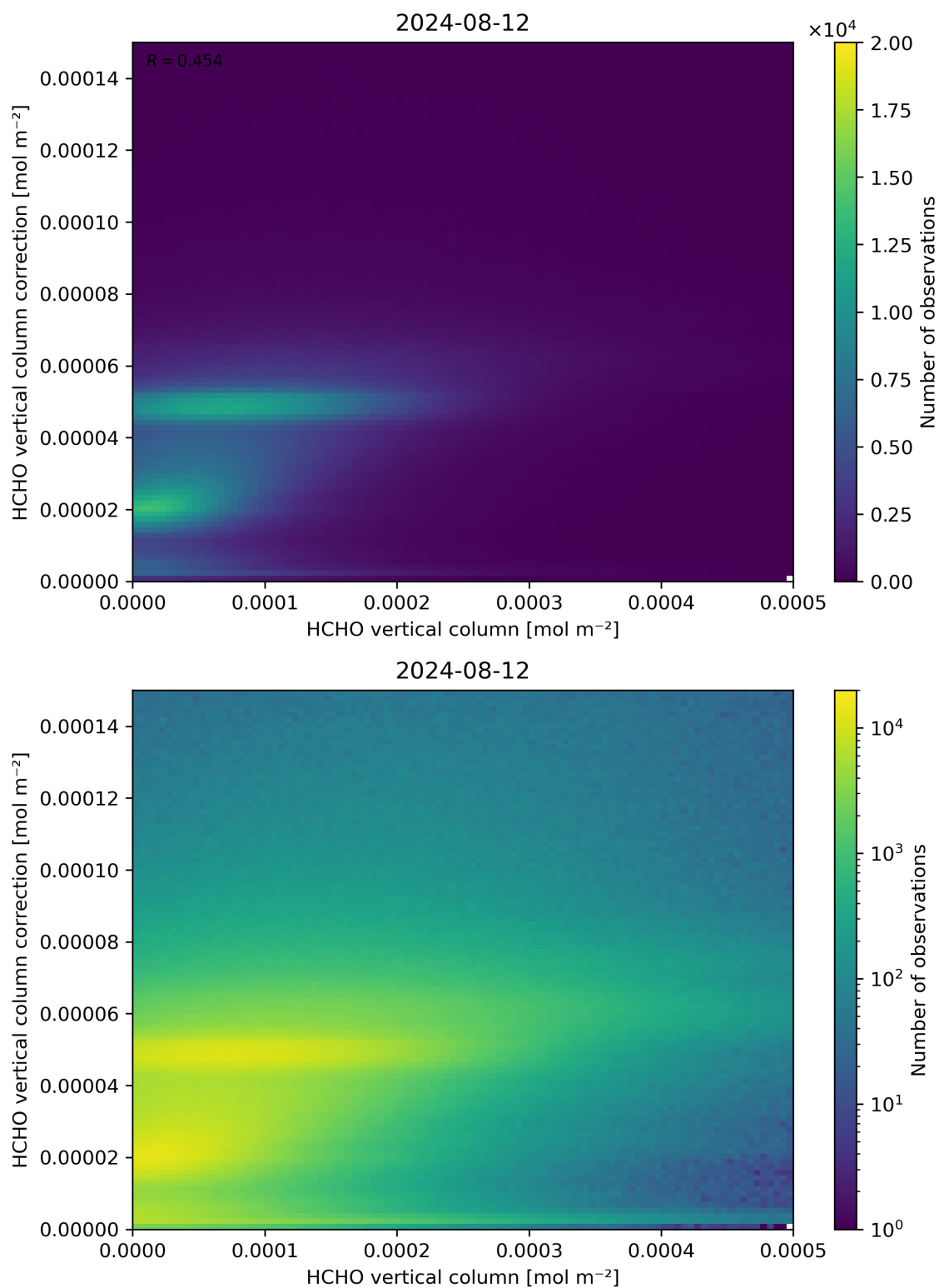
Figure 133: Scatter density plot of “HCHO vertical column” against “HCHO vertical column correction” for 2024-08-12 to 2024-08-13.
