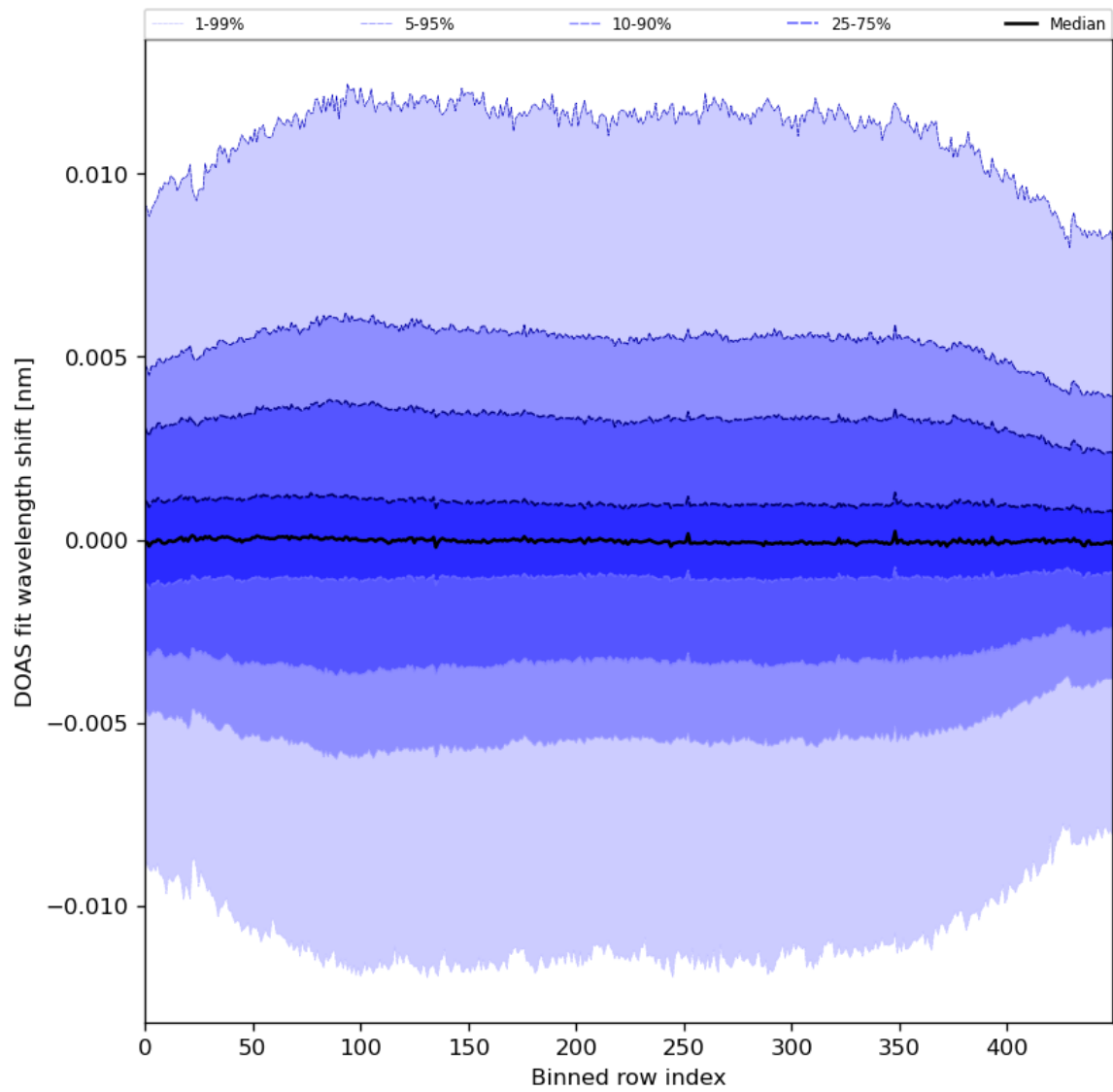
Figure 58: Along track statistics of “DOAS fit wavelength shift” for 2024-08-12 to 2024-08-13
