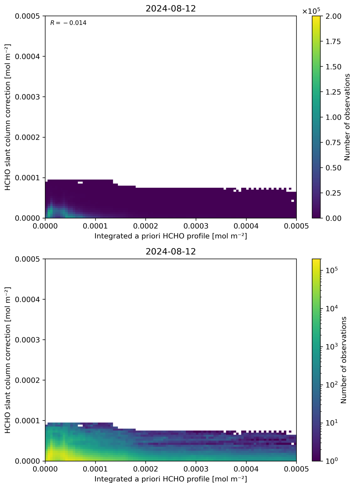
Figure 152: Scatter density plot of “Integrated a priori HCHO profile” against “HCHO slant column correction” for 2024-08-12 to 2024-08-13.
