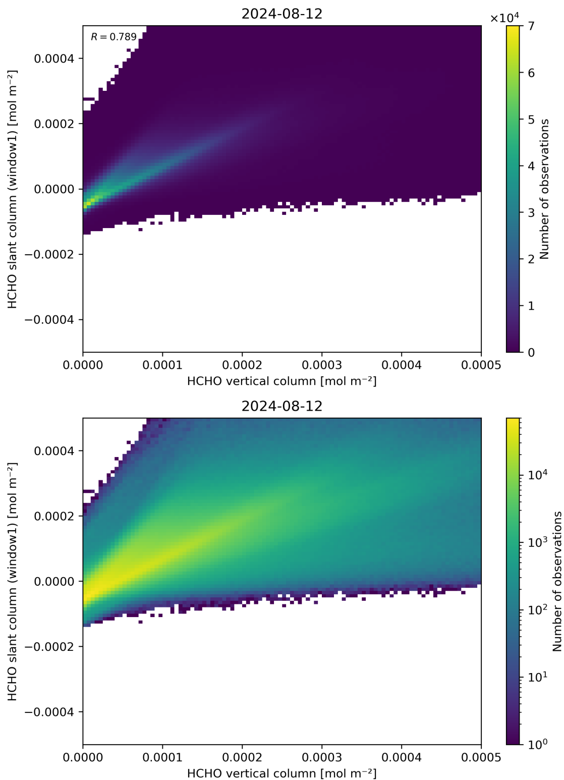
Figure 129: Scatter density plot of “HCHO vertical column” against “HCHO slant column (window1)” for 2024-08-12 to 2024-08-13.
