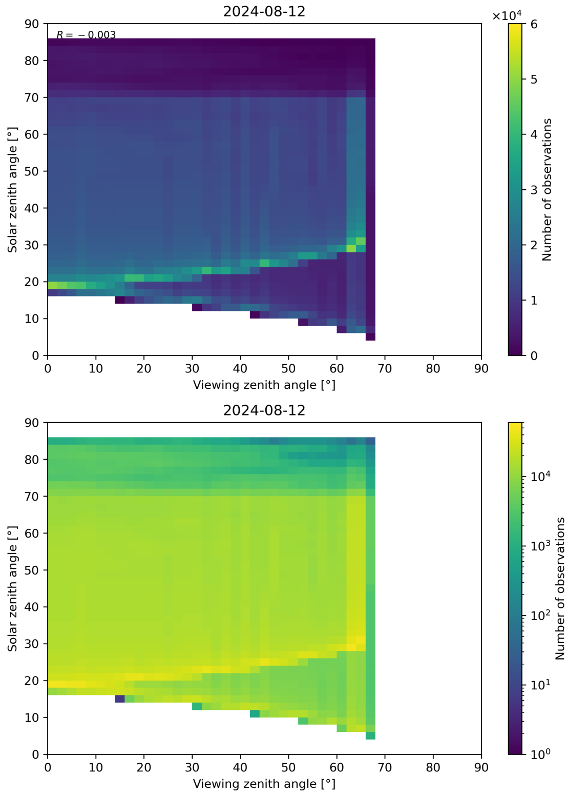
Figure 197: Scatter density plot of “Viewing zenith angle” against “Solar zenith angle” for 2024-08-12 to 2024-08-13.
