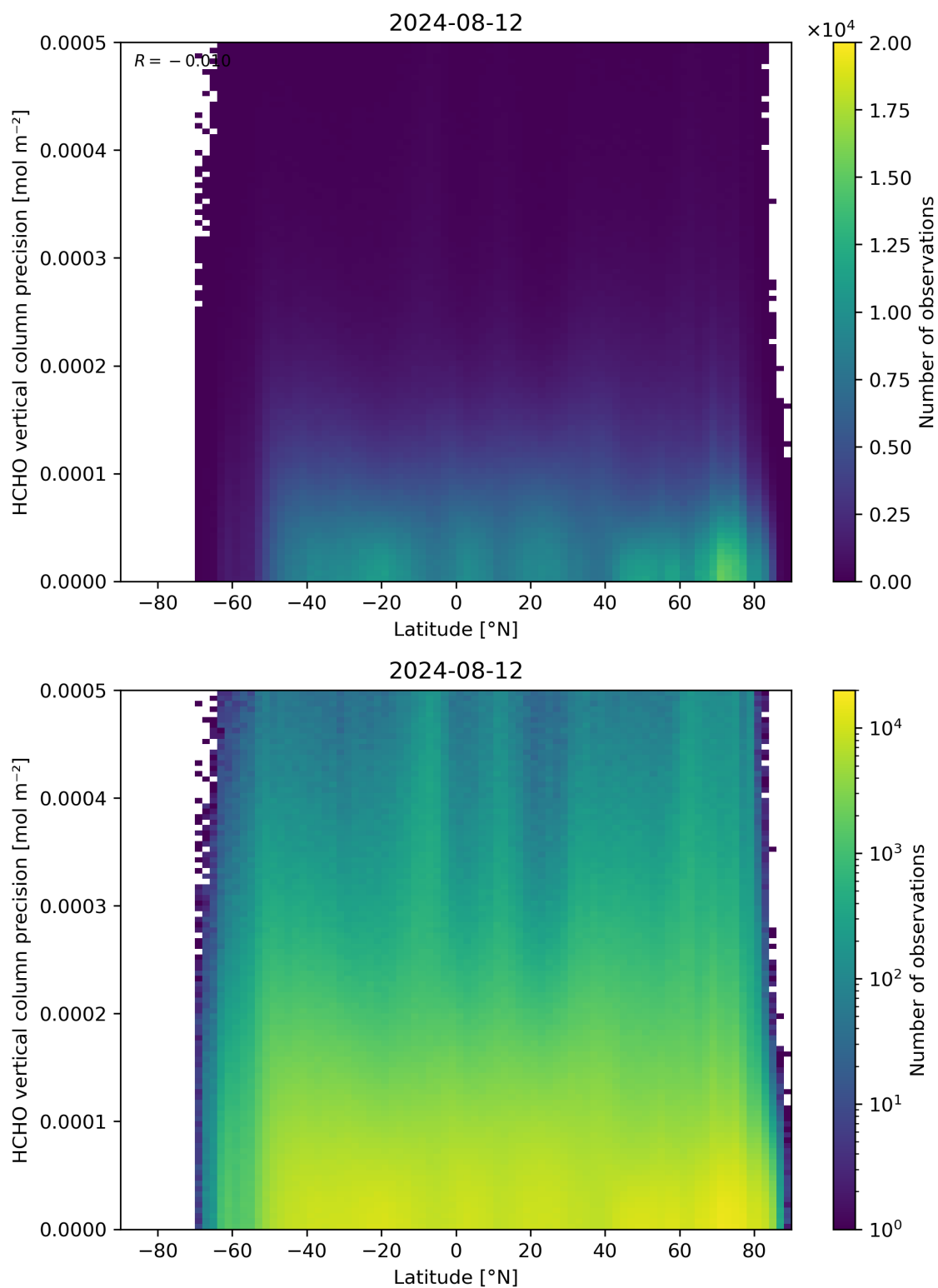
Figure 165: Scatter density plot of “Latitude” against “HCHO vertical column precision” for 2024-08-12 to 2024-08-13.
