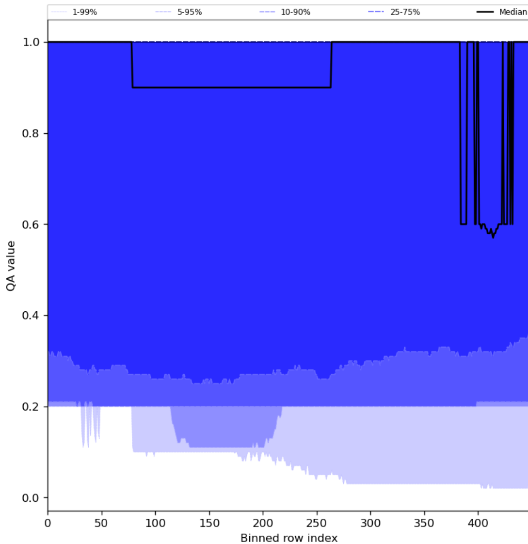
Figure 48: Along track statistics of “QA value” for 2024-08-12 to 2024-08-13
