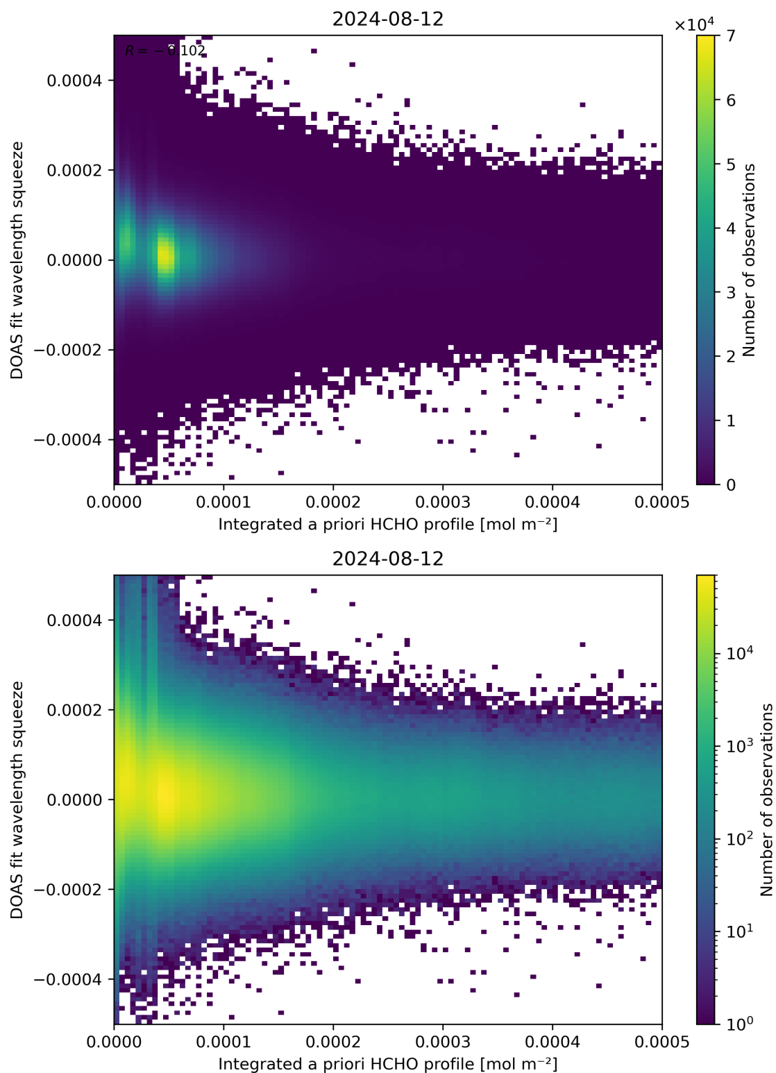
Figure 150: Scatter density plot of “Integrated a priori HCHO profile” against “DOAS fit wavelength squeeze” for 2024-08-12 to 2024-08-13.
