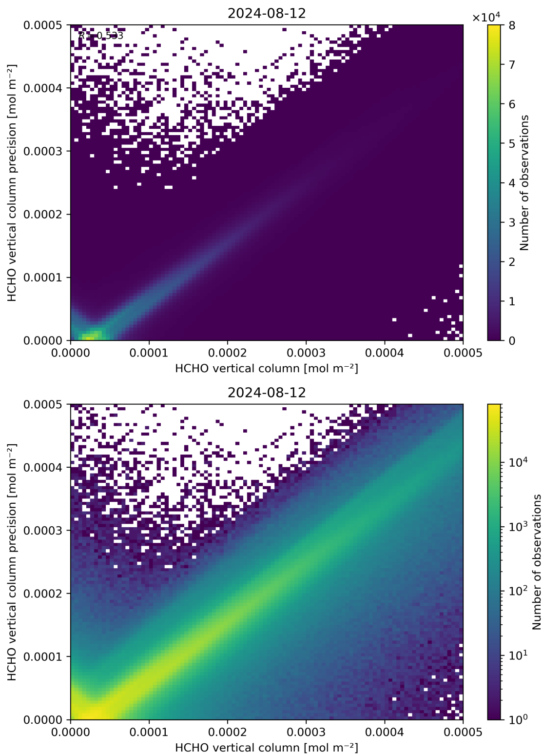
Figure 134: Scatter density plot of “HCHO vertical column” against “HCHO vertical column precision” for 2024-08-12 to 2024-08-13.
