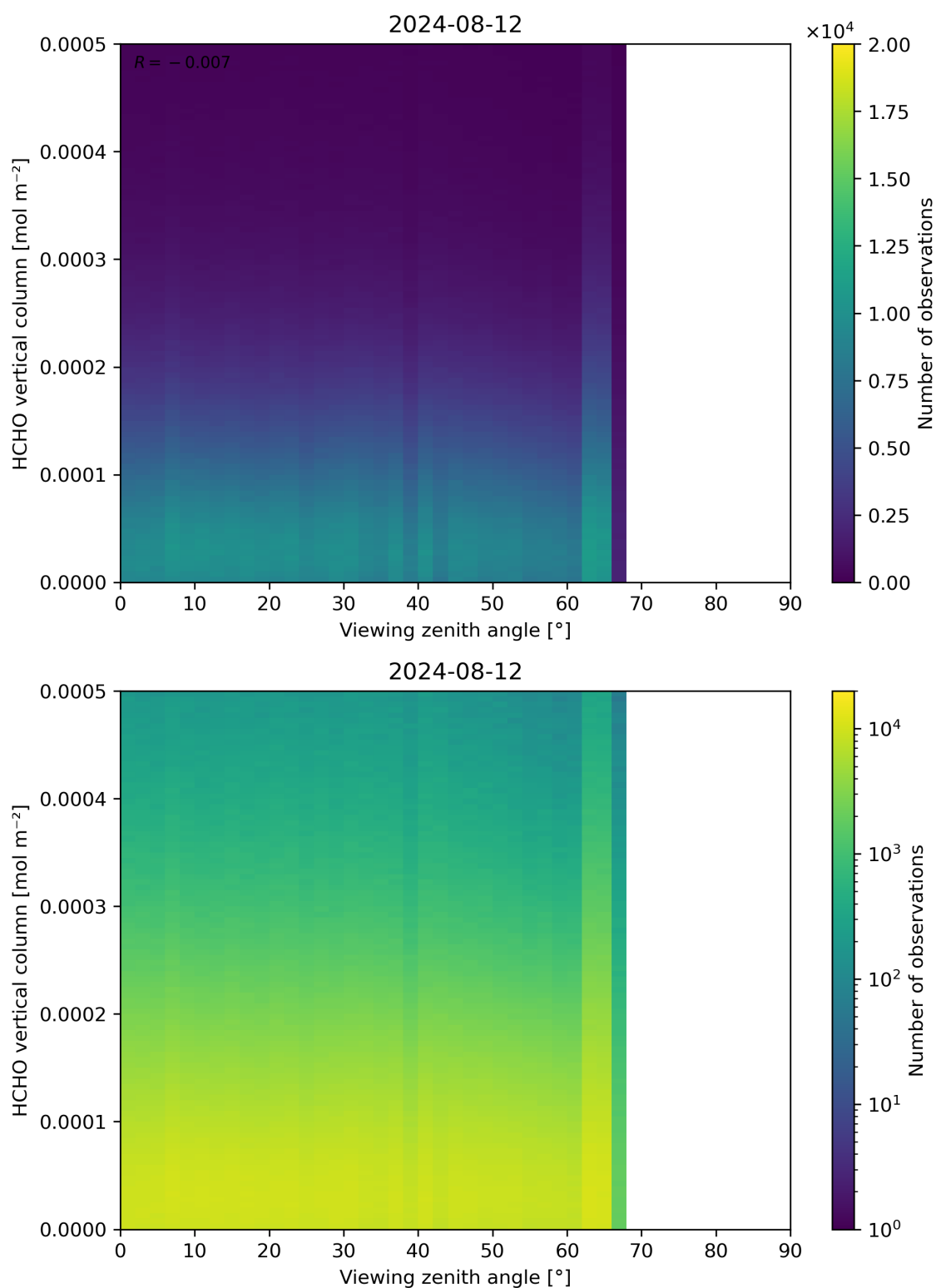
Figure 192: Scatter density plot of “Viewing zenith angle” against “HCHO vertical column” for 2024-08-12 to 2024-08-13.
