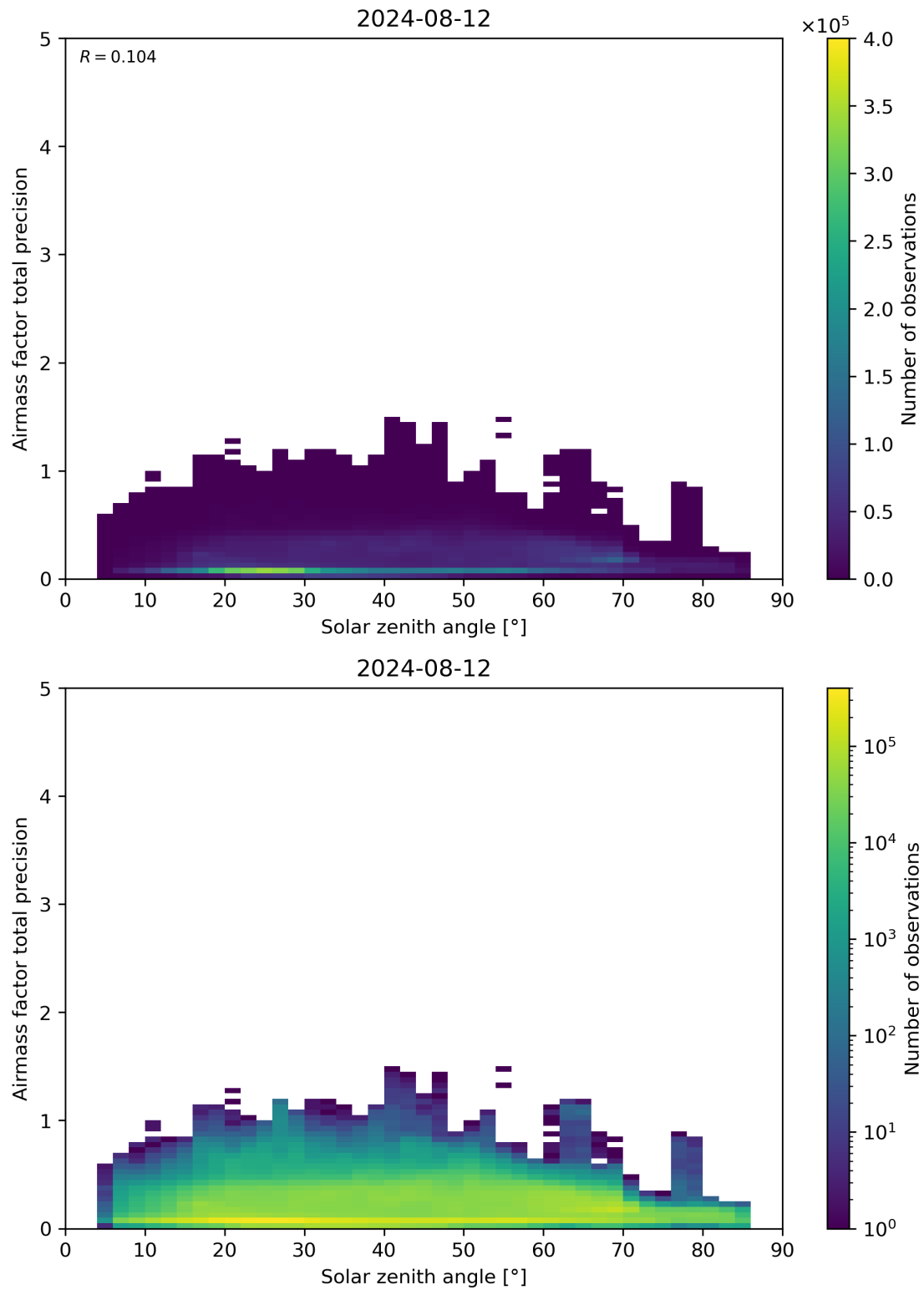
Figure 176: Scatter density plot of “Solar zenith angle” against “Airmass factor total precision” for 2024-08-12 to 2024-08-13.
