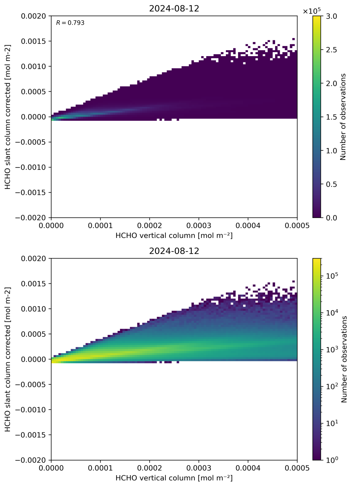
Figure 127: Scatter density plot of “HCHO vertical column” against “HCHO slant column corrected” for 2024-08-12 to 2024-08-13.
