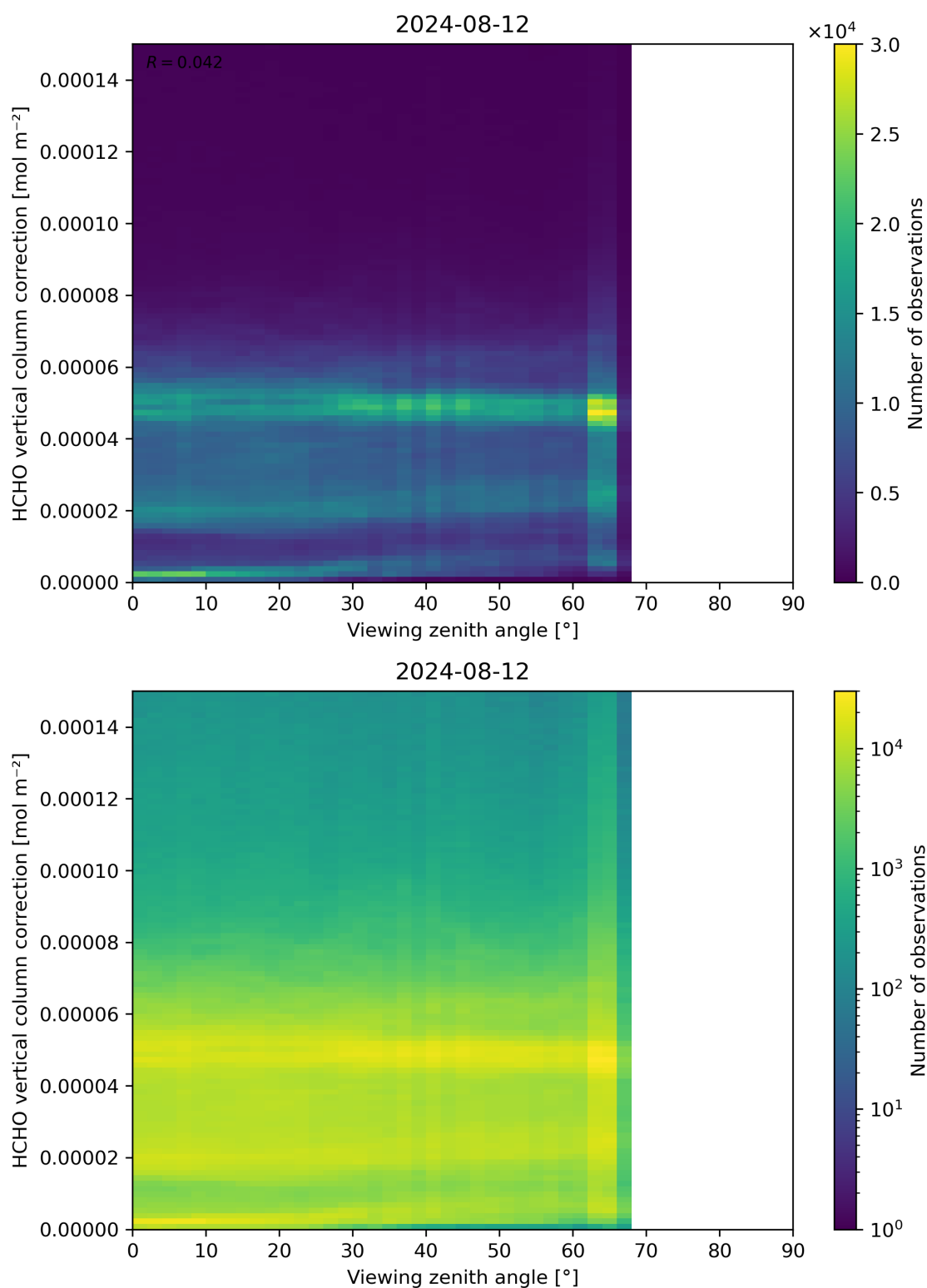
Figure 193: Scatter density plot of “Viewing zenith angle” against “HCHO vertical column correction” for 2024-08-12 to 2024-08-13.
