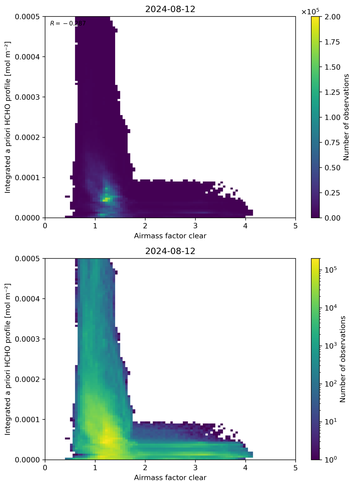
Figure 76: Scatter density plot of “Airmass factor clear” against “Integrated a priori HCHO profile” for 2024-08-12 to 2024-08-13.
