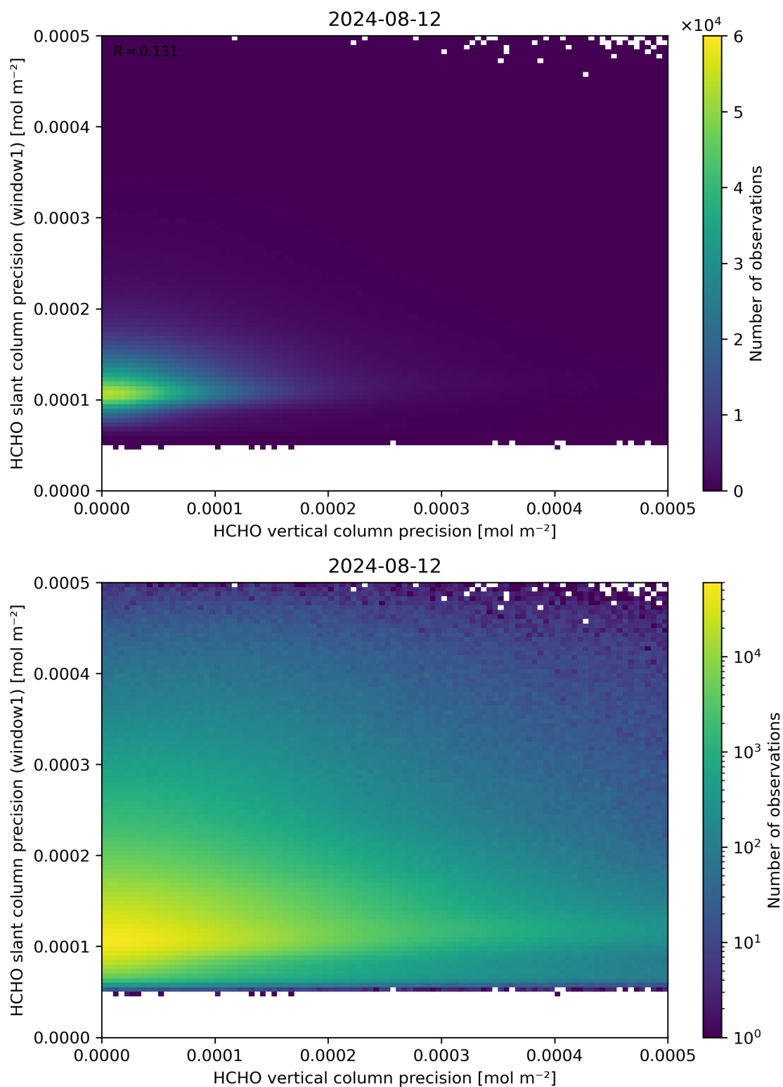
Figure 143: Scatter density plot of “HCHO vertical column precision” against “HCHO slant column precision (window1)” for 2024-08-12 to 2024-08-13.
