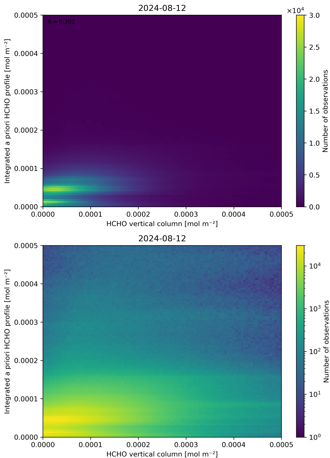
Figure 135: Scatter density plot of “HCHO vertical column” against “Integrated a priori HCHO profile” for 2024-08-12 to 2024-08-13.
