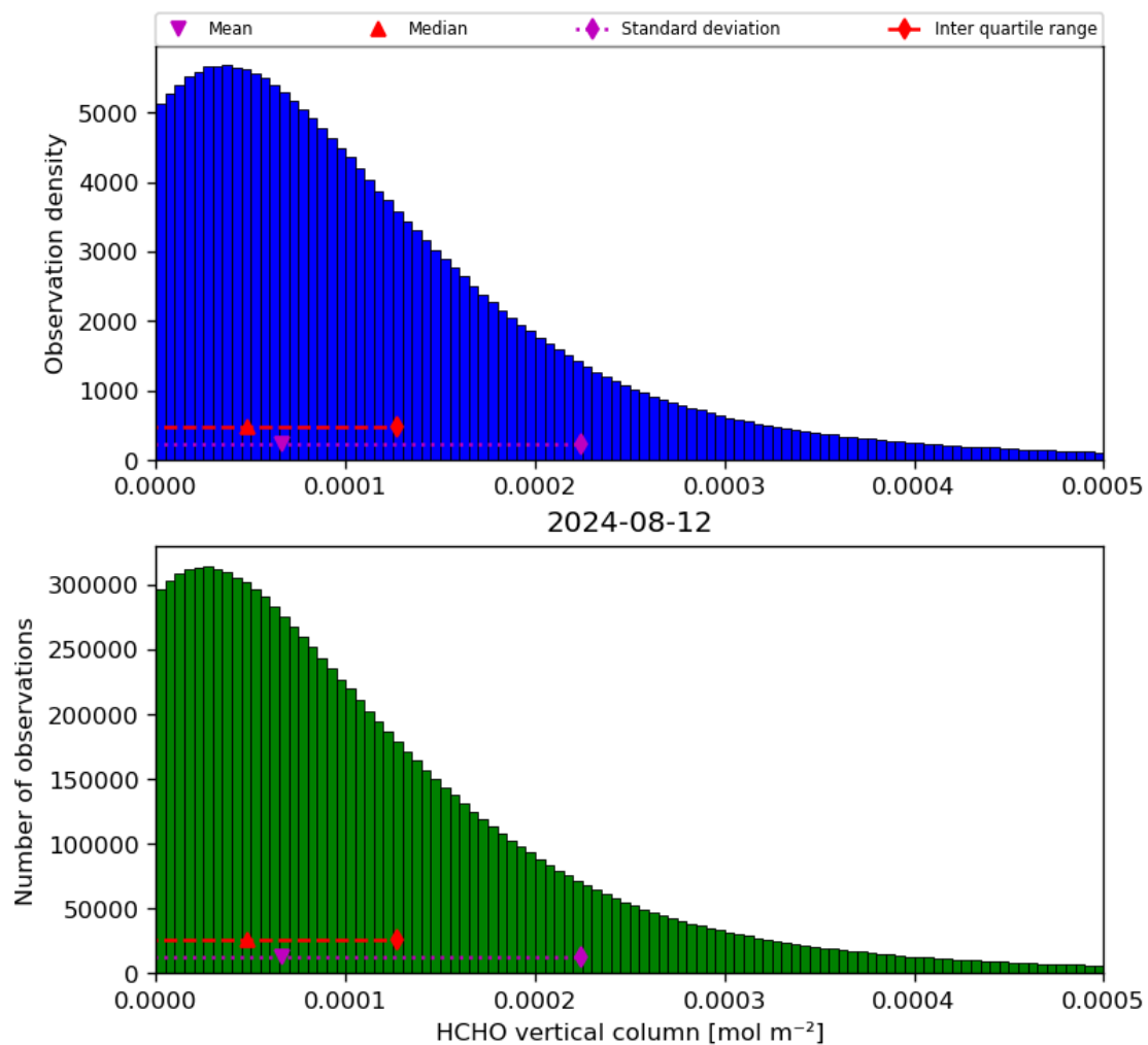
Figure 35: Histogram of “HCHO vertical column” for 2024-08-12 to 2024-08-13
