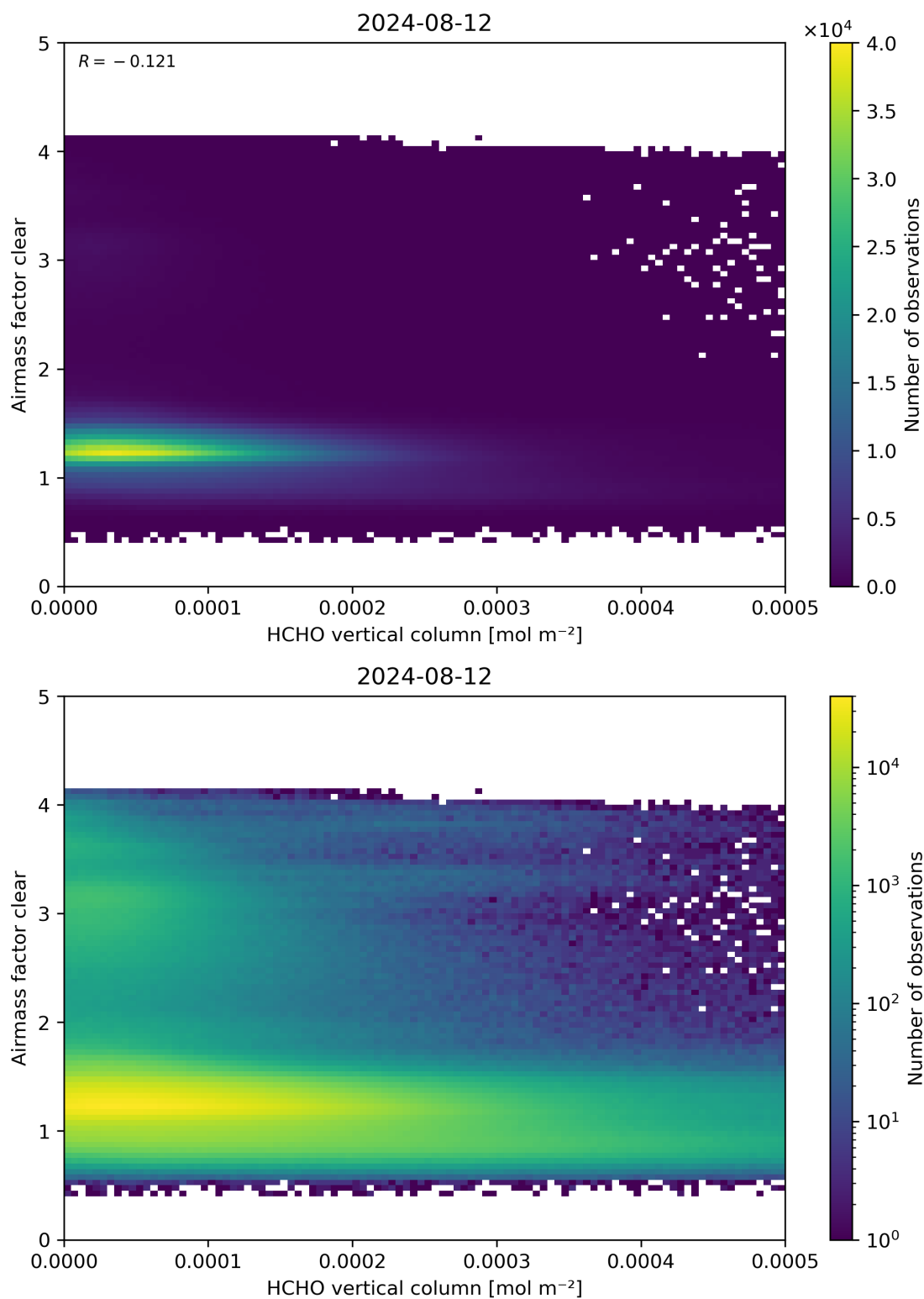
Figure 126: Scatter density plot of “HCHO vertical column” against “Airmass factor clear” for 2024-08-12 to 2024-08-13.
