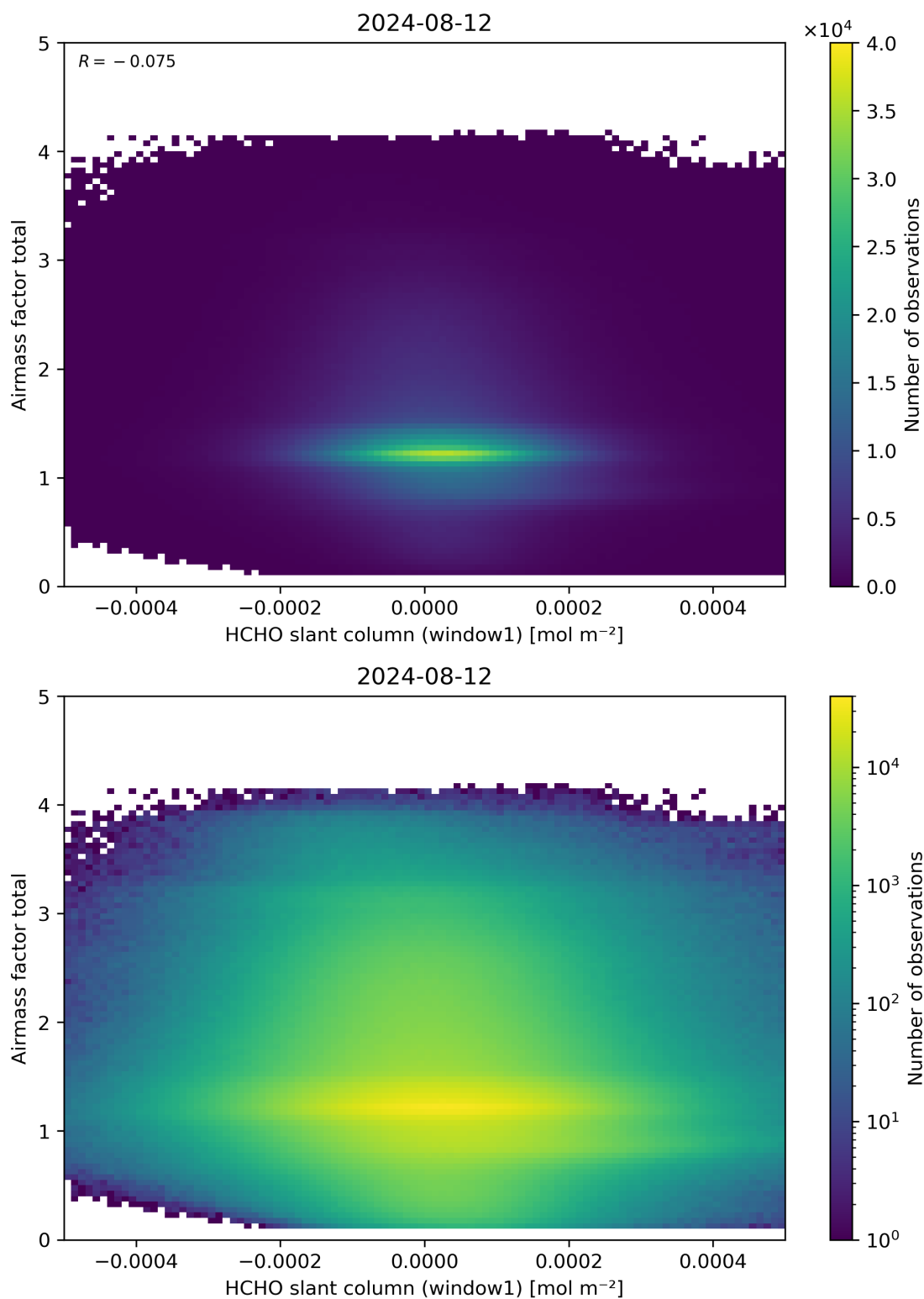
Figure 85: Scatter density plot of “HCHO slant column (window1)” against “Airmass factor total” for 2024-08-12 to 2024-08-13.
