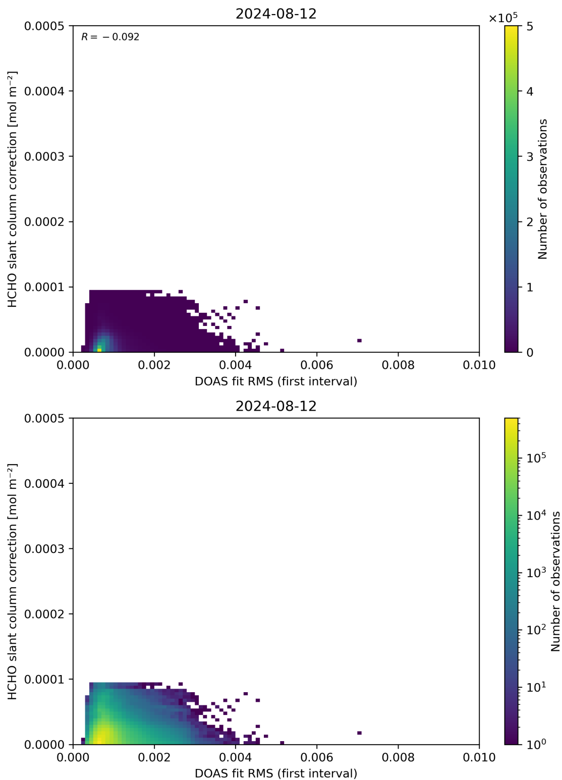
Figure 63: Scatter density plot of “DOAS fit RMS (first interval)” against “HCHO slant column correction” for 2024-08-12 to 2024-08-13.
