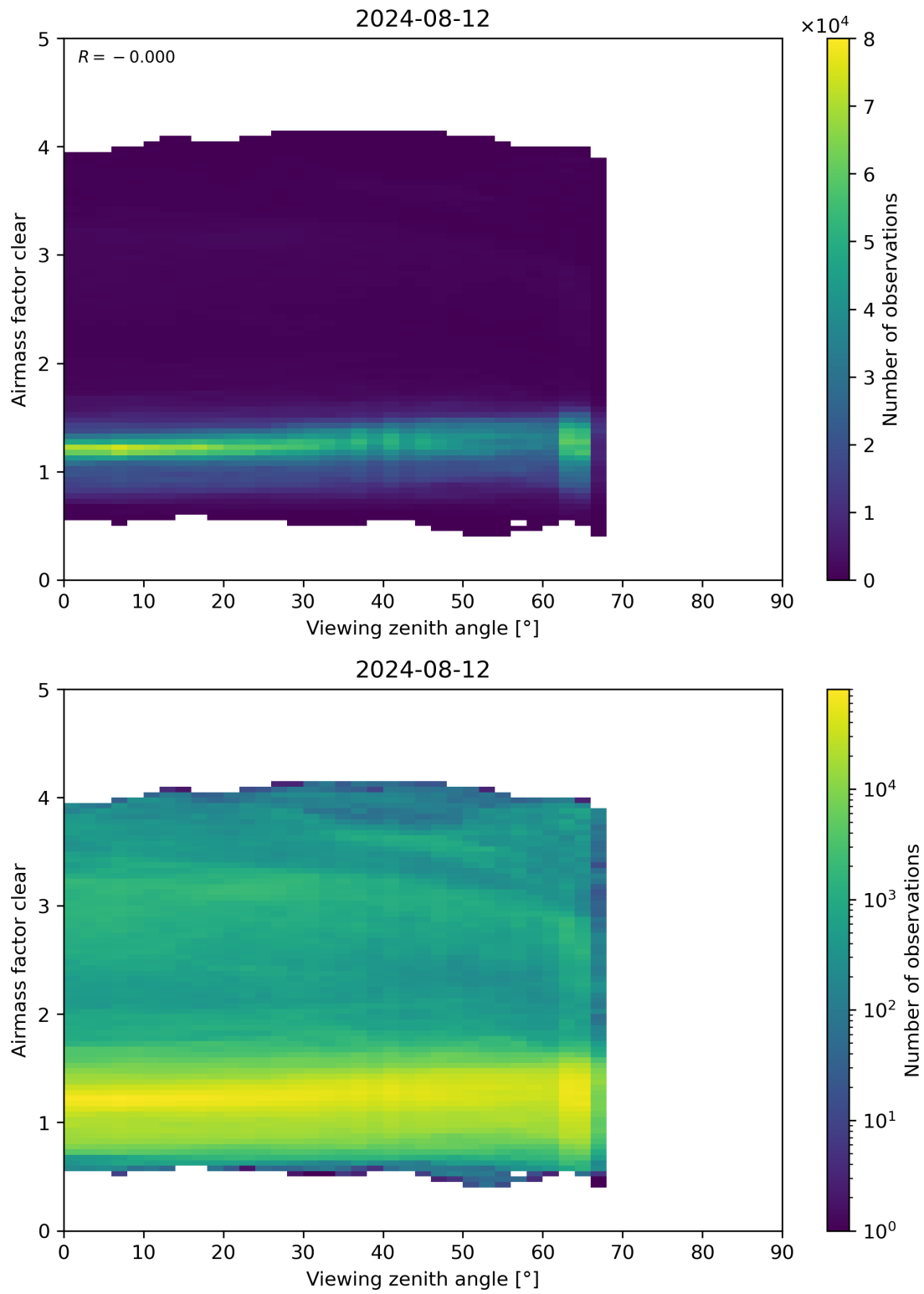
Figure 185: Scatter density plot of “Viewing zenith angle” against “Airmass factor clear” for 2024-08-12 to 2024-08-13.
