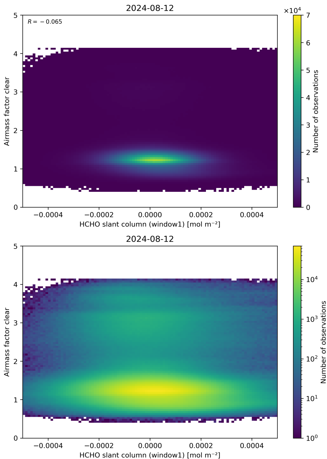
Figure 81: Scatter density plot of “HCHO slant column (window1)” against “Airmass factor clear” for 2024-08-12 to 2024-08-13.
