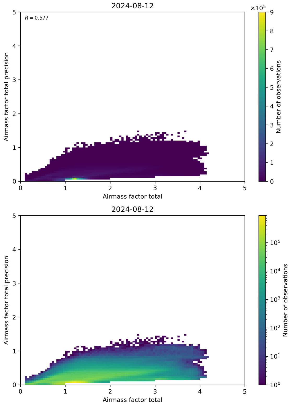
Figure 103: Scatter density plot of “Airmass factor total” against “Airmass factor total precision” for 2024-08-12 to 2024-08-13.
