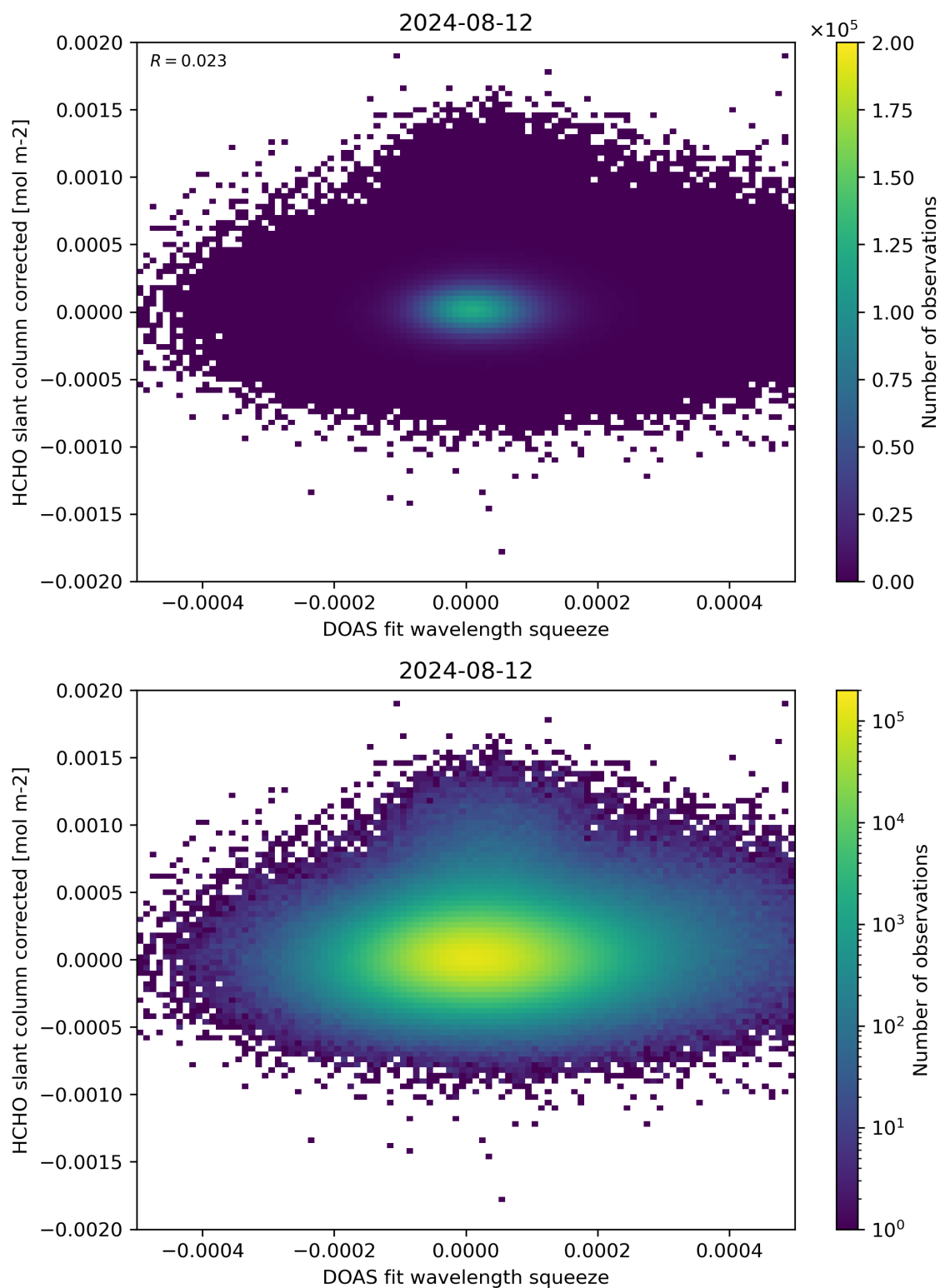
Figure 69: Scatter density plot of “DOAS fit wavelength squeeze” against “HCHO slant column corrected” for 2024-08-12 to 2024-08-13.
