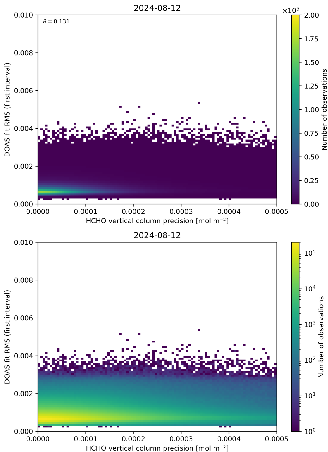
Figure 136: Scatter density plot of “HCHO vertical column precision” against “DOAS fit RMS (first interval)” for 2024-08-12 to 2024-08-13.
