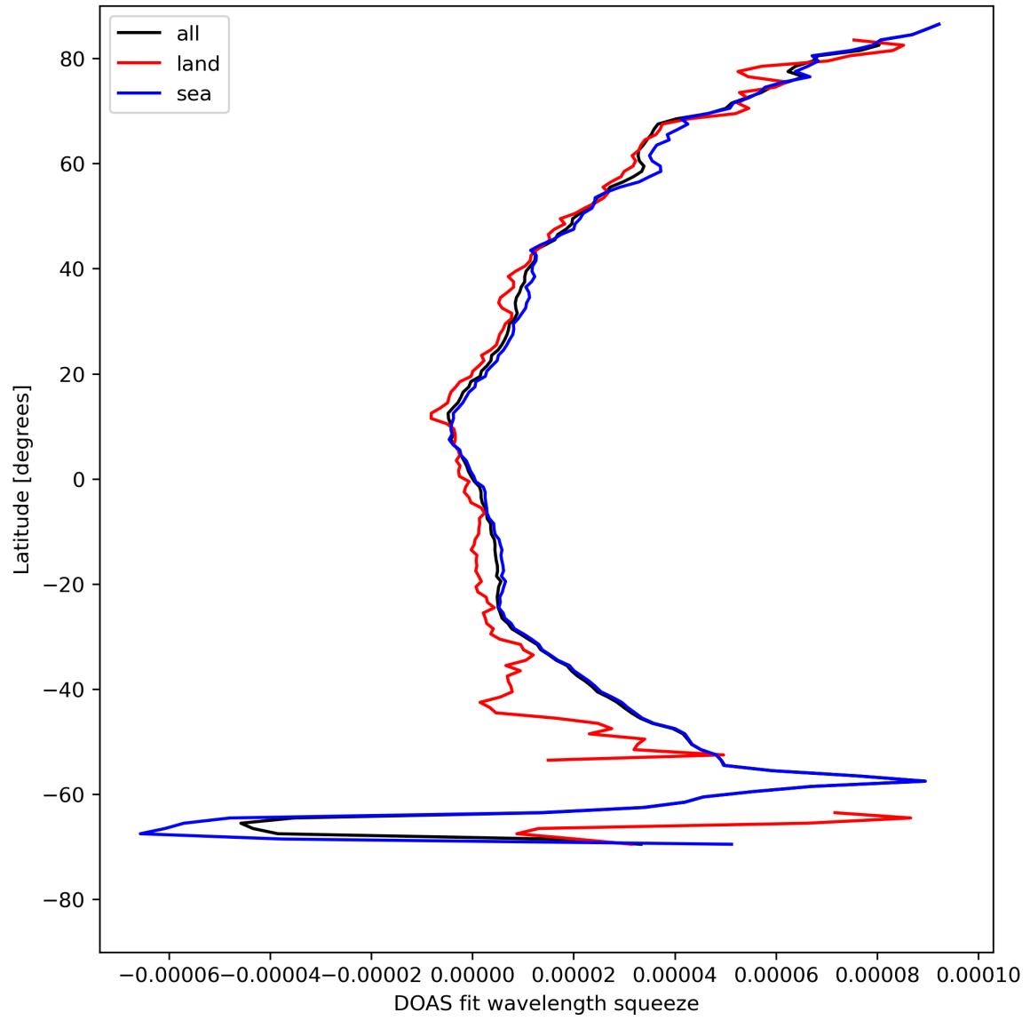
Figure 31: Zonal average of “DOAS fit wavelength squeeze” for 2024-08-12 to 2024-08-13.
