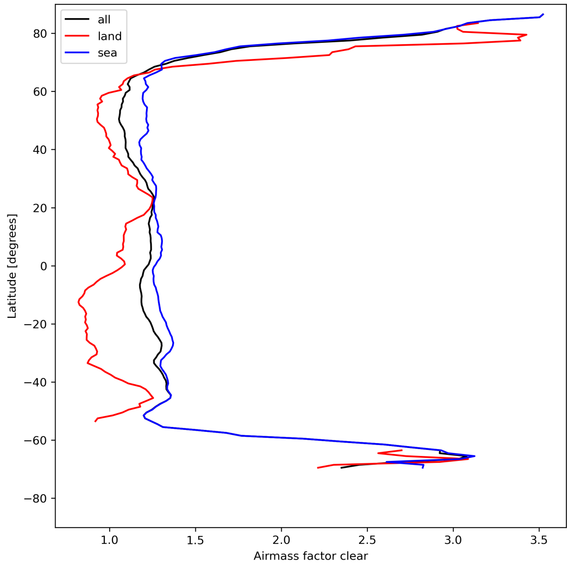
Figure 28: Zonal average of “Airmass factor clear” for 2024-08-12 to 2024-08-13.
