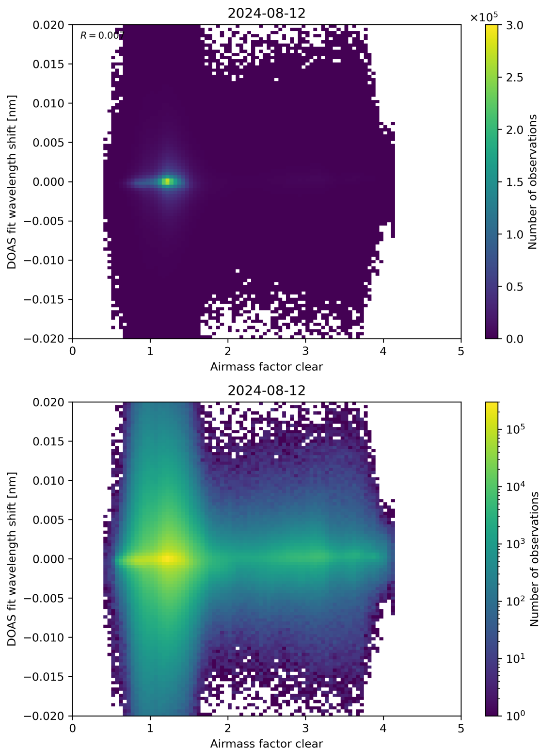
Figure 72: Scatter density plot of “Airmass factor clear” against “DOAS fit wavelength shift” for 2024-08-12 to 2024-08-13.
