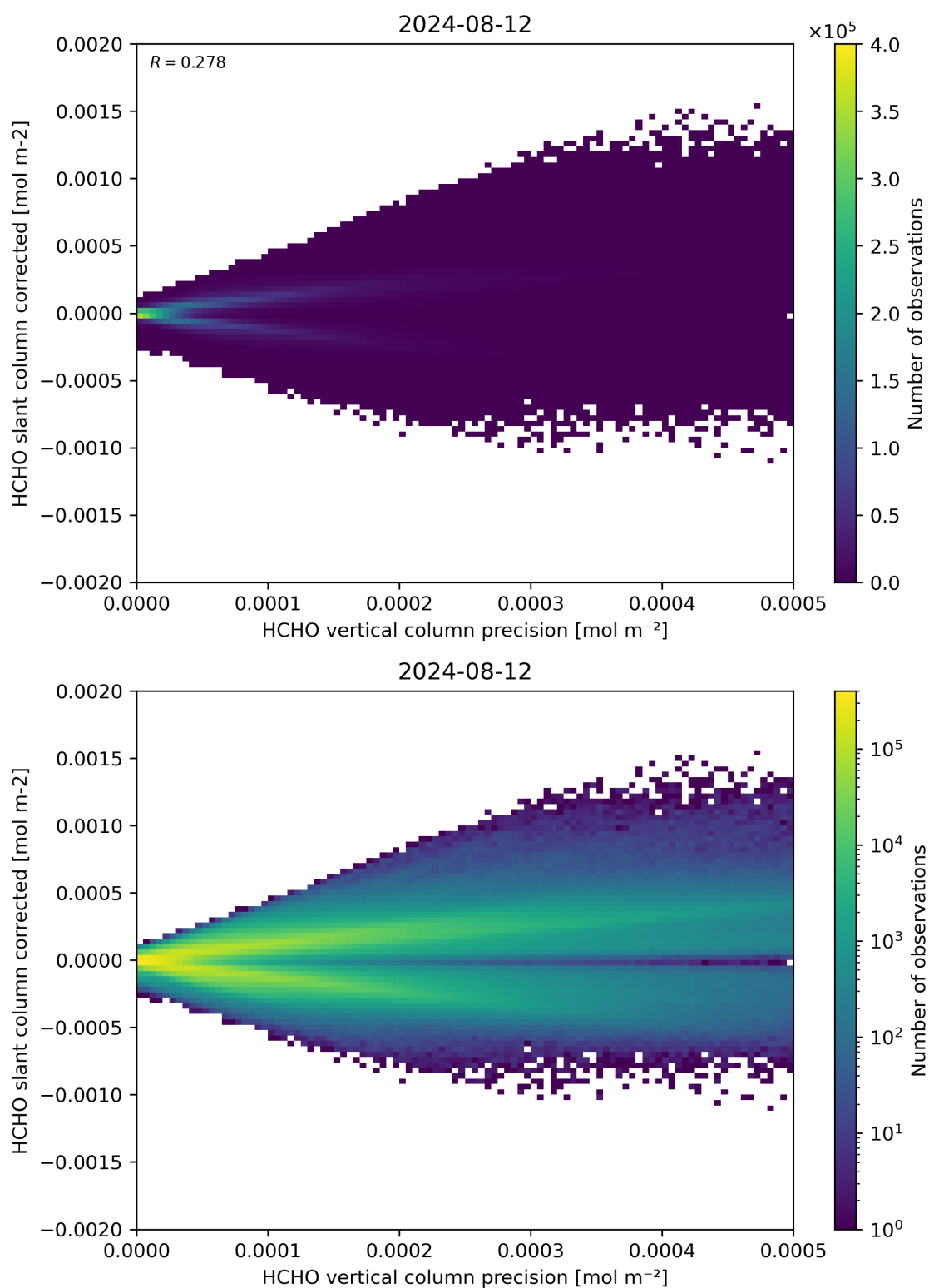
Figure 140: Scatter density plot of “HCHO vertical column precision” against “HCHO slant column corrected” for 2024-08-12 to 2024-08-13.
