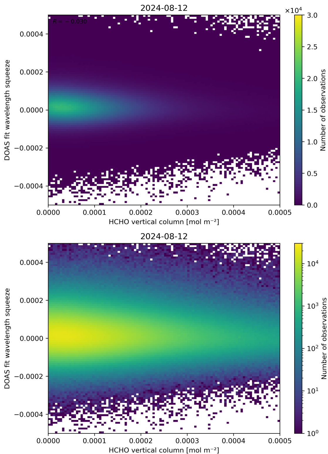
Figure 125: Scatter density plot of “HCHO vertical column” against “DOAS fit wavelength squeeze” for 2024-08-12 to 2024-08-13.
