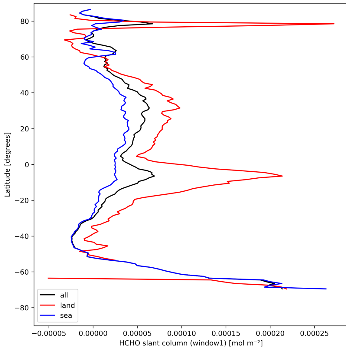
Figure 24: Zonal average of “HCHO slant column (window1)” for 2024-08-12 to 2024-08-13.
