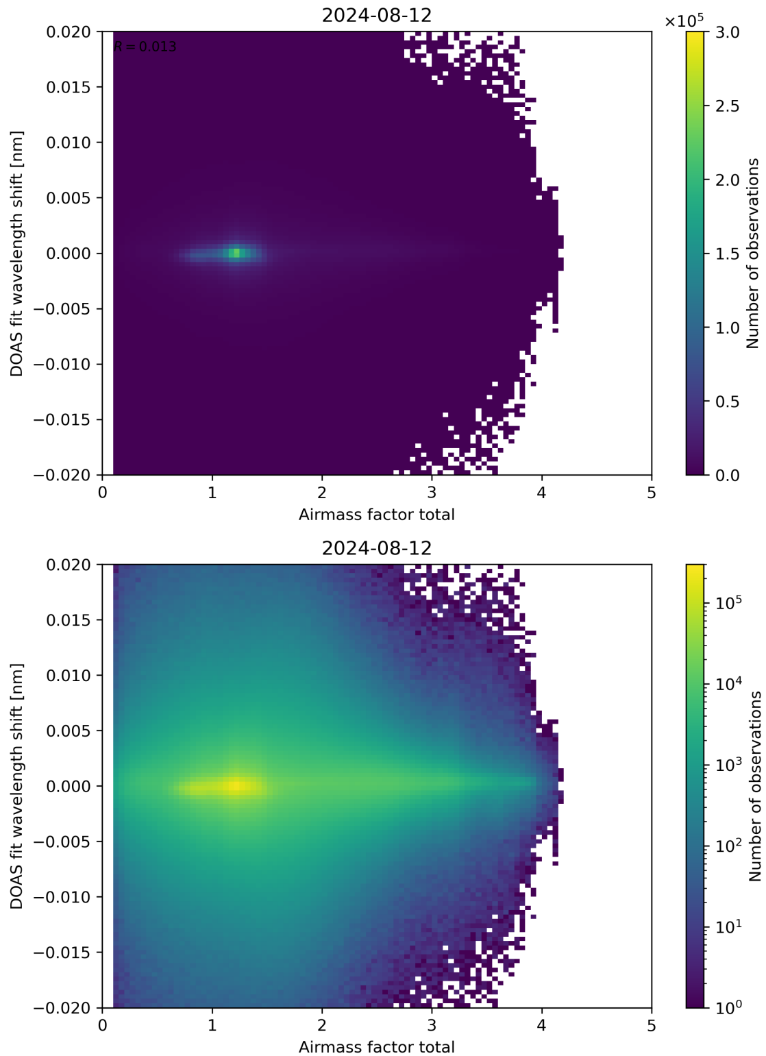
Figure 98: Scatter density plot of “Airmass factor total” against “DOAS fit wavelength shift” for 2024-08-12 to 2024-08-13.
