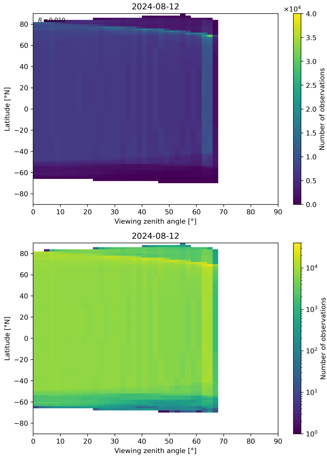
Figure 196: Scatter density plot of “Viewing zenith angle” against “Latitude” for 2024-08-12 to 2024-08-13.
