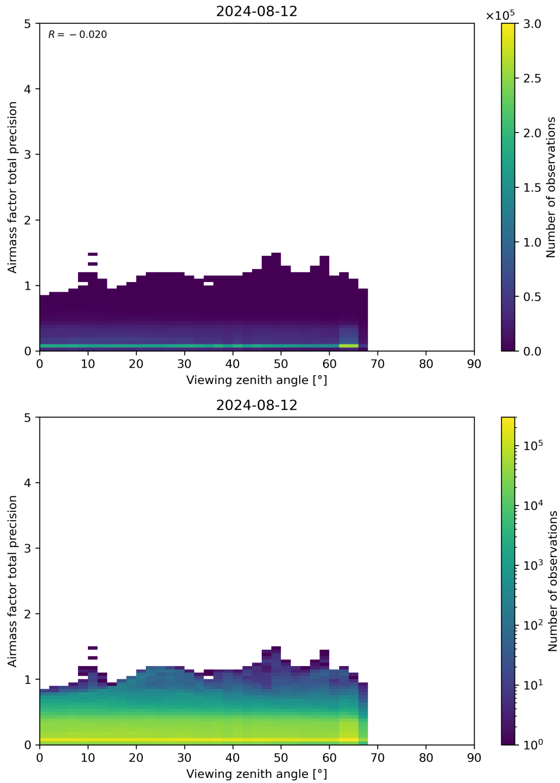
Figure 191: Scatter density plot of “Viewing zenith angle” against “Airmass factor total precision” for 2024-08-12 to 2024-08-13.
