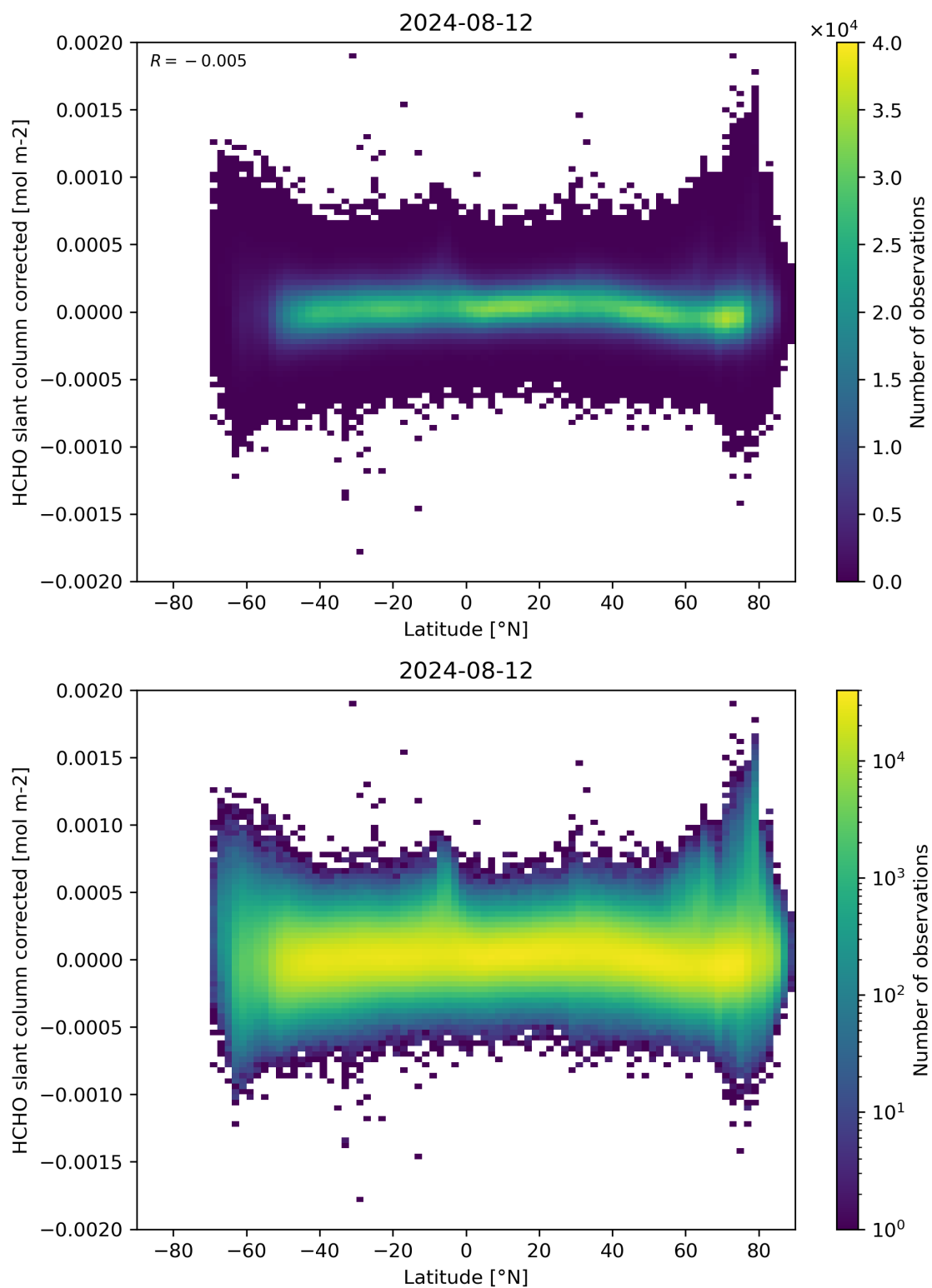
Figure 157: Scatter density plot of “Latitude” against “HCHO slant column corrected” for 2024-08-12 to 2024-08-13.
