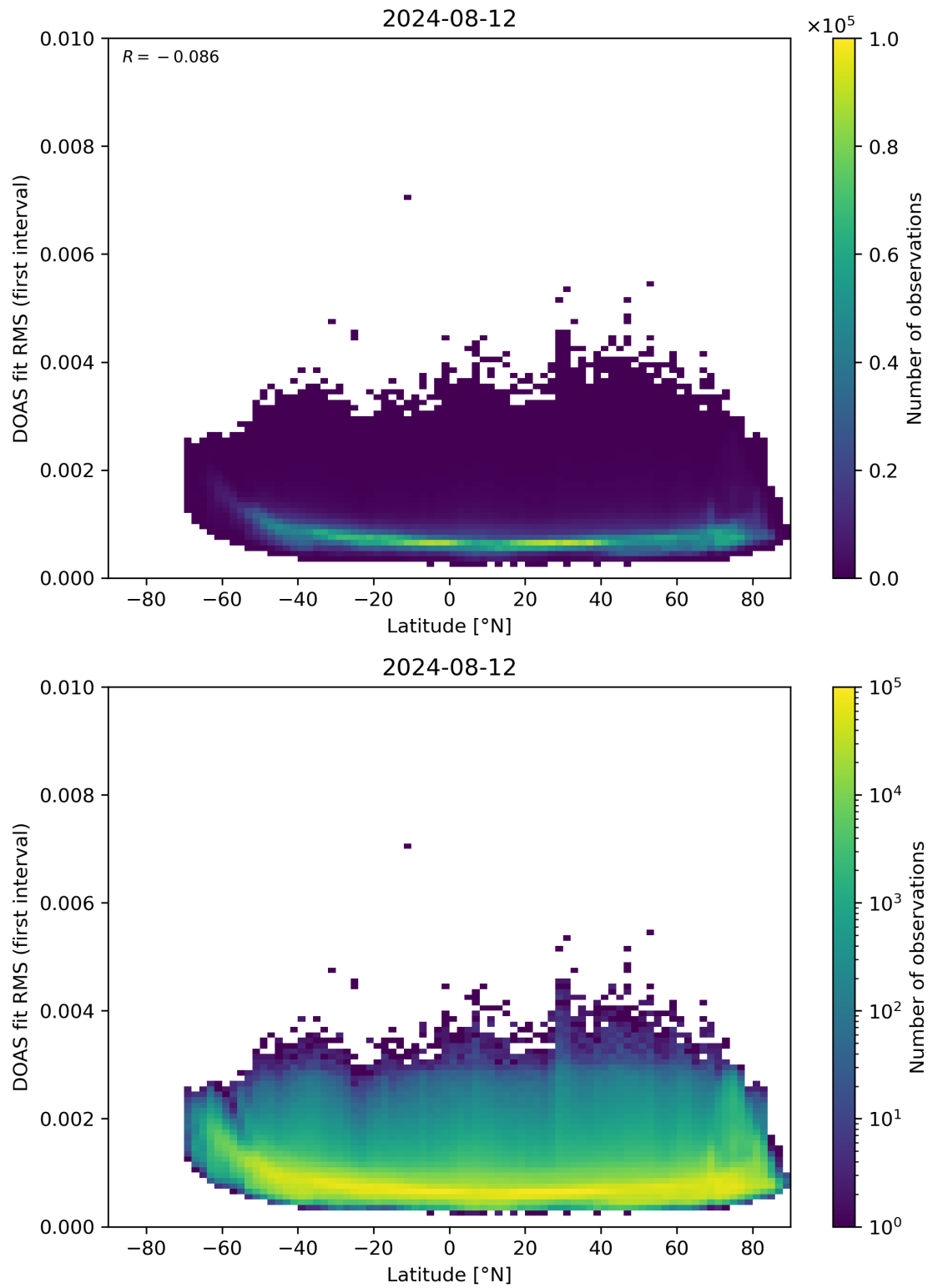
Figure 153: Scatter density plot of “Latitude” against “DOAS fit RMS (first interval)” for 2024-08-12 to 2024-08-13.
