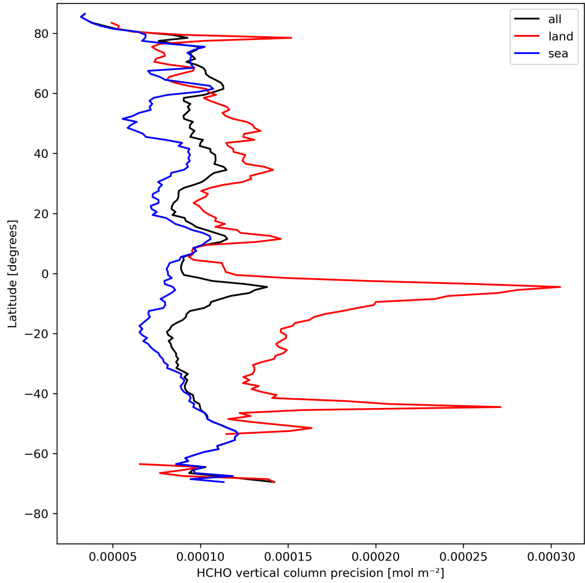
Figure 22: Zonal average of “HCHO vertical column precision” for 2024-08-12 to 2024-08-13.
