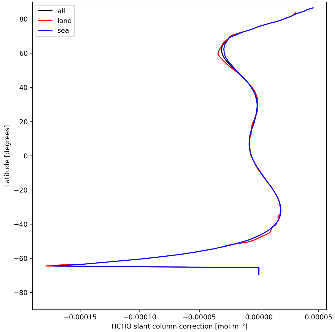
Figure 33: Zonal average of “HCHO slant column correction” for 2024-08-12 to 2024-08-13.
