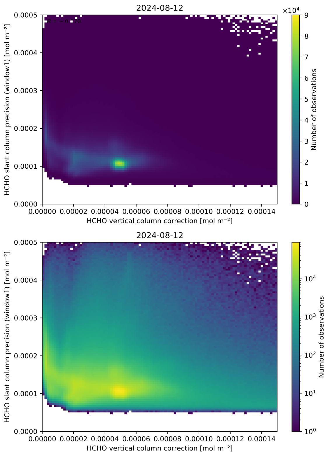
Figure 119: Scatter density plot of “HCHO vertical column correction” against “HCHO slant column precision (window1)” for 2024-08-12 to 2024-08-13.
