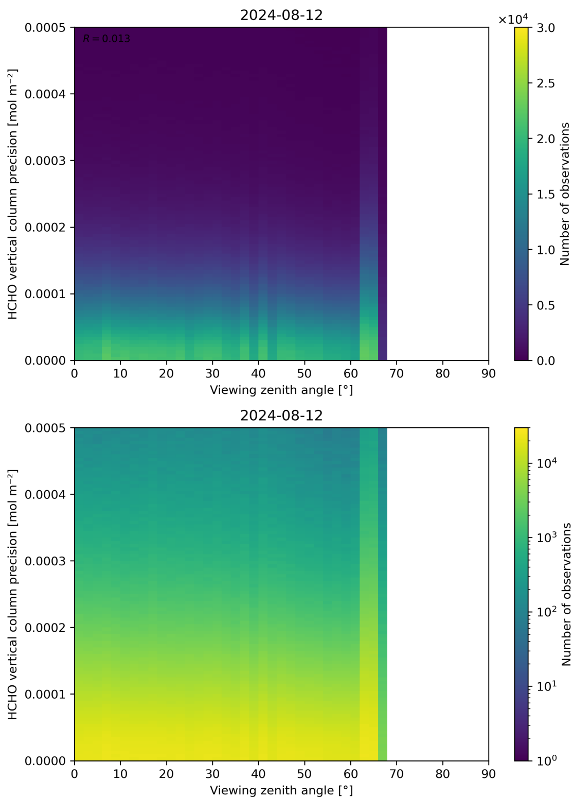
Figure 194: Scatter density plot of “Viewing zenith angle” against “HCHO vertical column precision” for 2024-08-12 to 2024-08-13.
