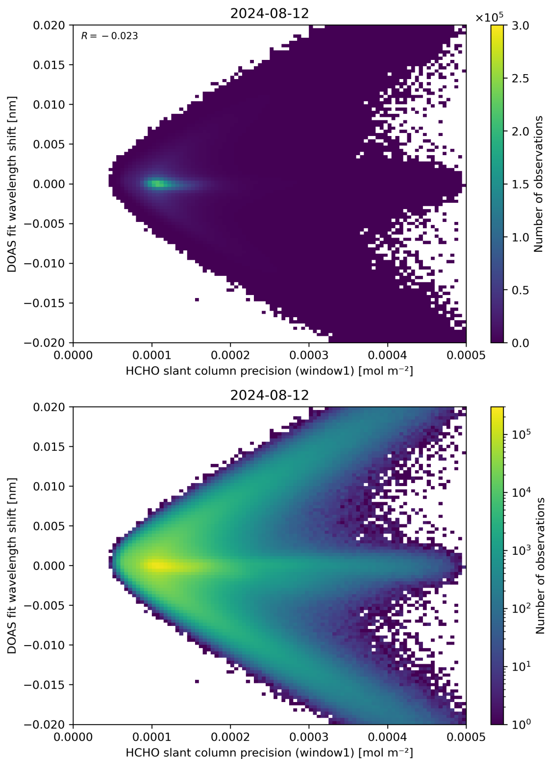
Figure 89: Scatter density plot of “HCHO slant column precision (window1)” against “DOAS fit wavelength shift” for 2024-08-12 to 2024-08-13.
