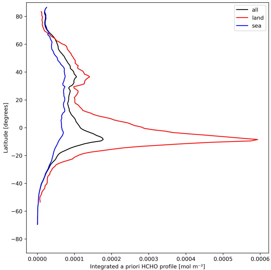
Figure 29: Zonal average of “Integrated a priori HCHO profile” for 2024-08-12 to 2024-08-13.
