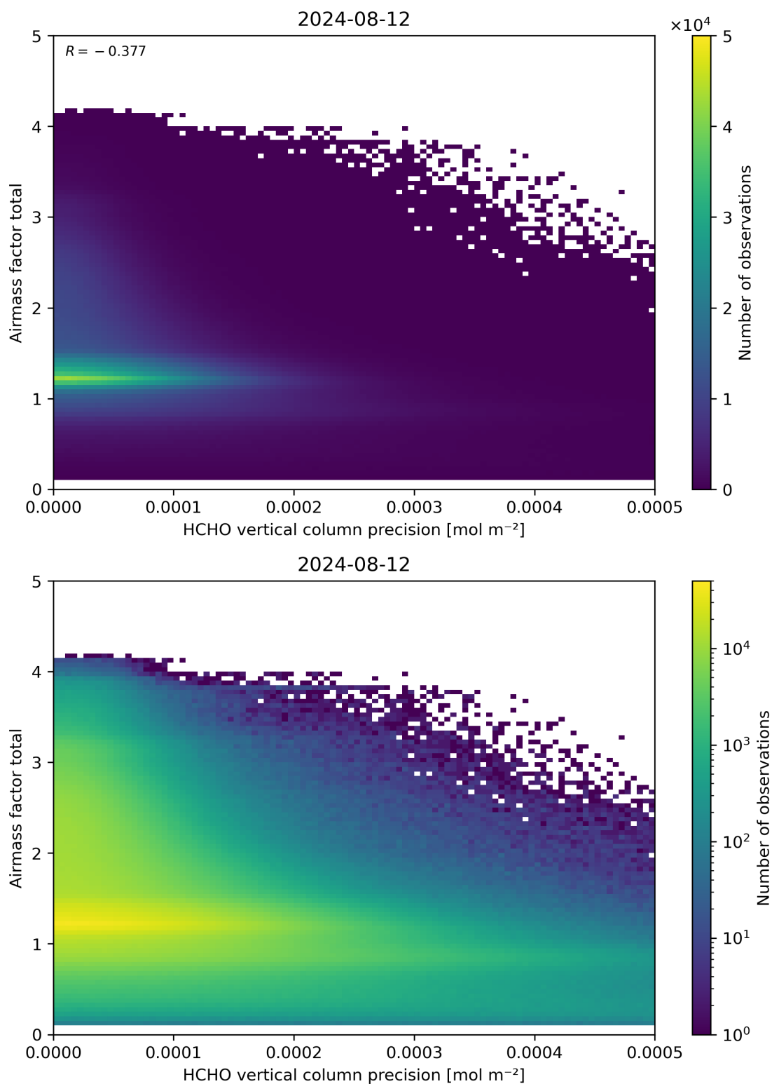
Figure 144: Scatter density plot of “HCHO vertical column precision” against “Airmass factor total” for 2024-08-12 to 2024-08-13.
