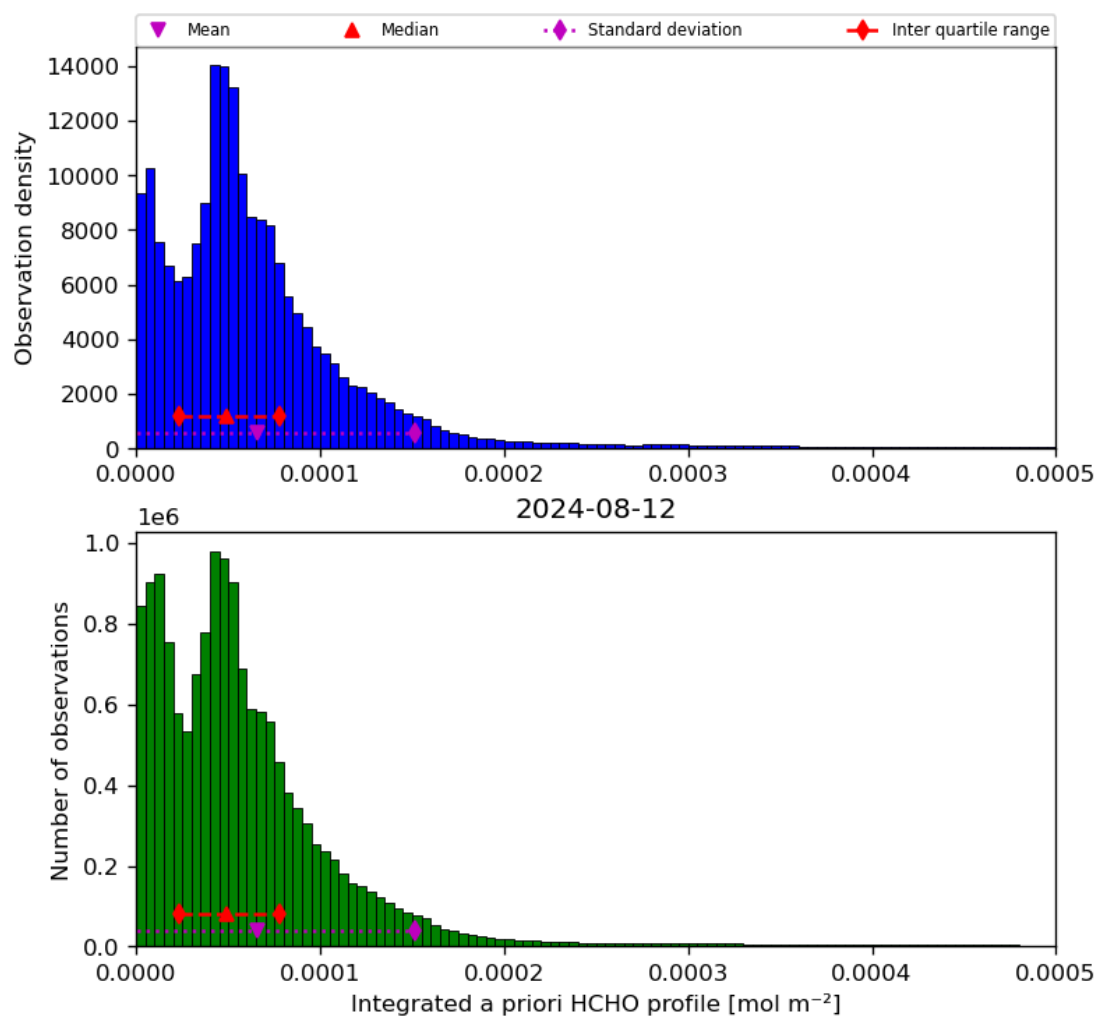
Figure 43: Histogram of “Integrated a priori HCHO profile” for 2024-08-12 to 2024-08-13
