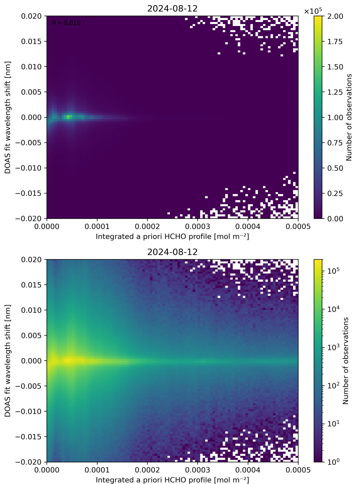
Figure 149: Scatter density plot of “Integrated a priori HCHO profile” against “DOAS fit wavelength shift” for 2024-08-12 to 2024-08-13.
