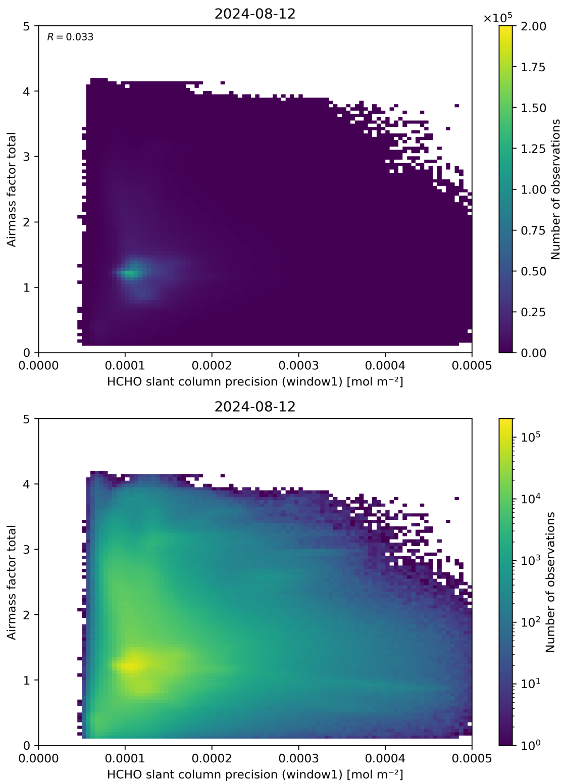
Figure 94: Scatter density plot of “HCHO slant column precision (window1)” against “Airmass factor total” for 2024-08-12 to 2024-08-13.
