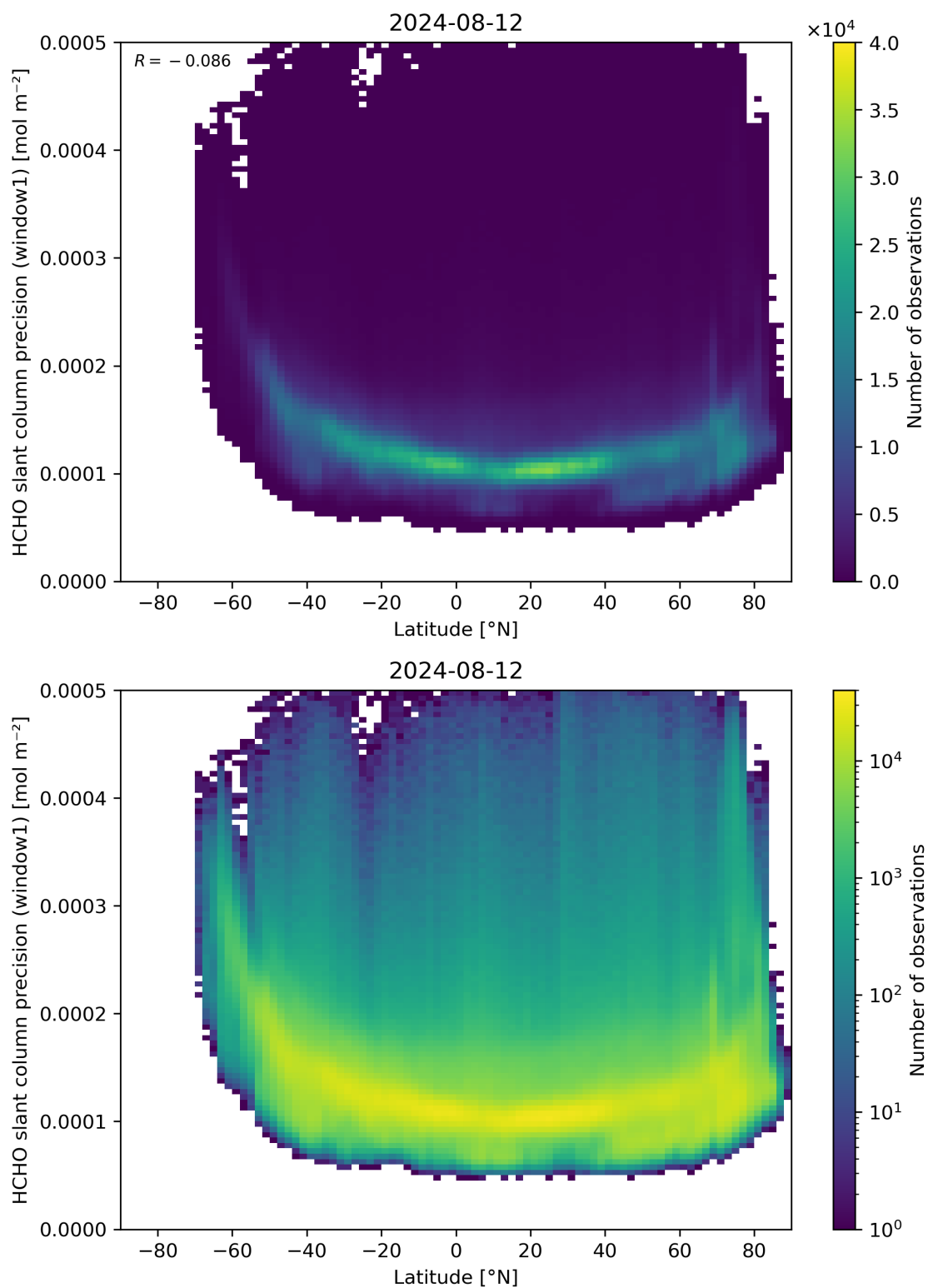
Figure 160: Scatter density plot of “Latitude” against “HCHO slant column precision (window1)” for 2024-08-12 to 2024-08-13.
