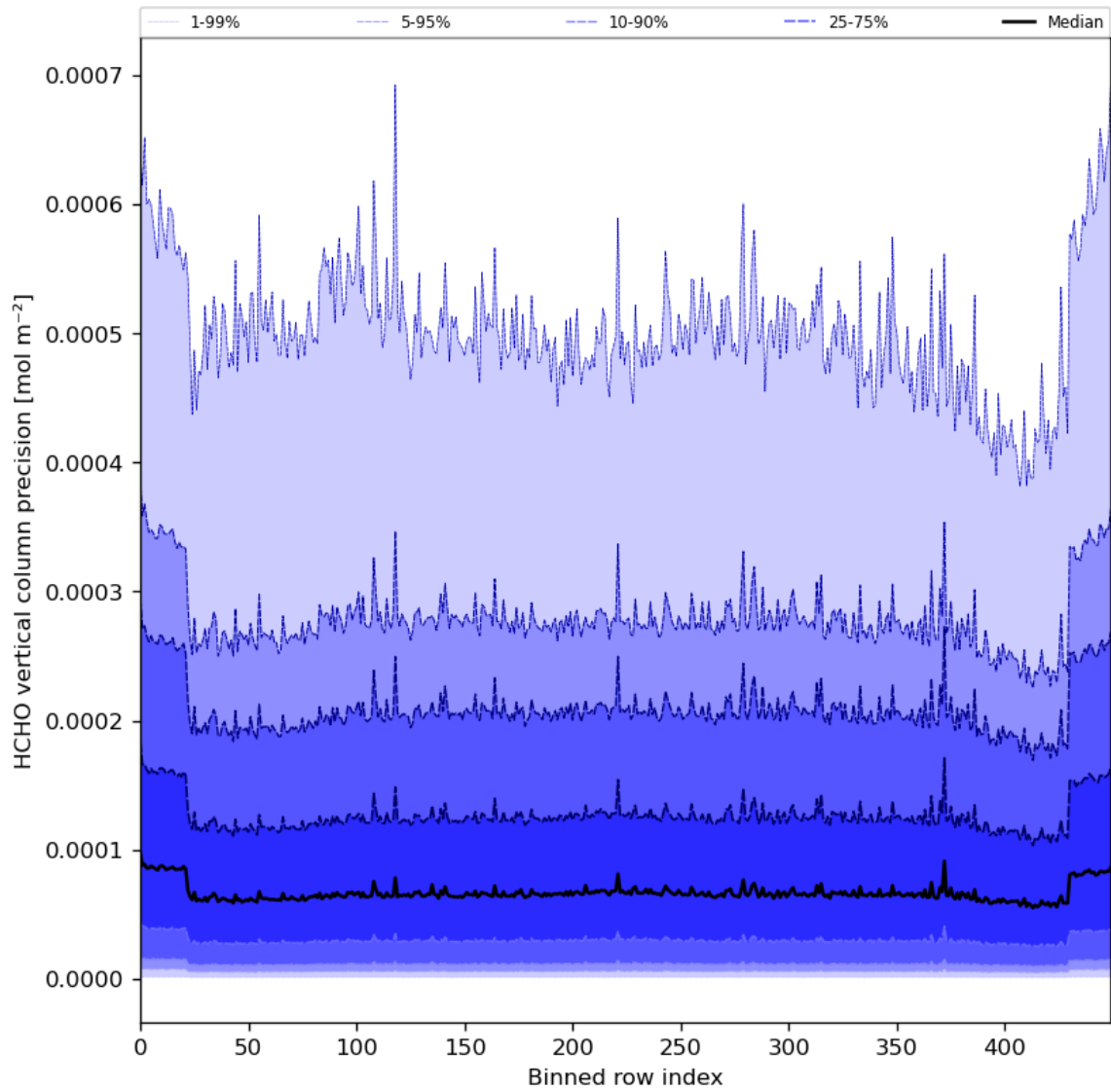
Figure 50: Along track statistics of “HCHO vertical column precision” for 2024-08-12 to 2024-08-13
