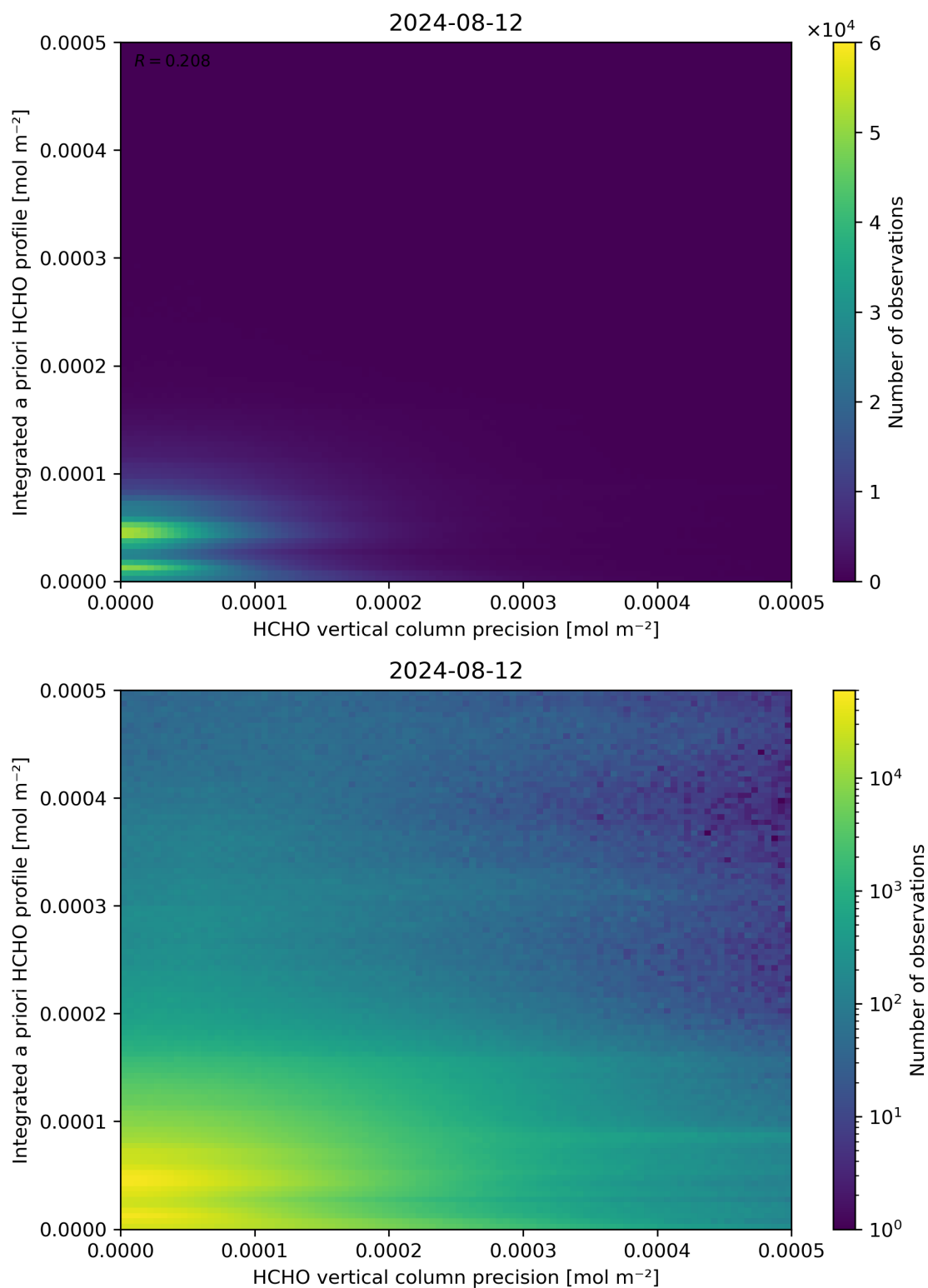
Figure 147: Scatter density plot of “HCHO vertical column precision” against “Integrated a priori HCHO profile” for 2024-08-12 to 2024-08-13.
