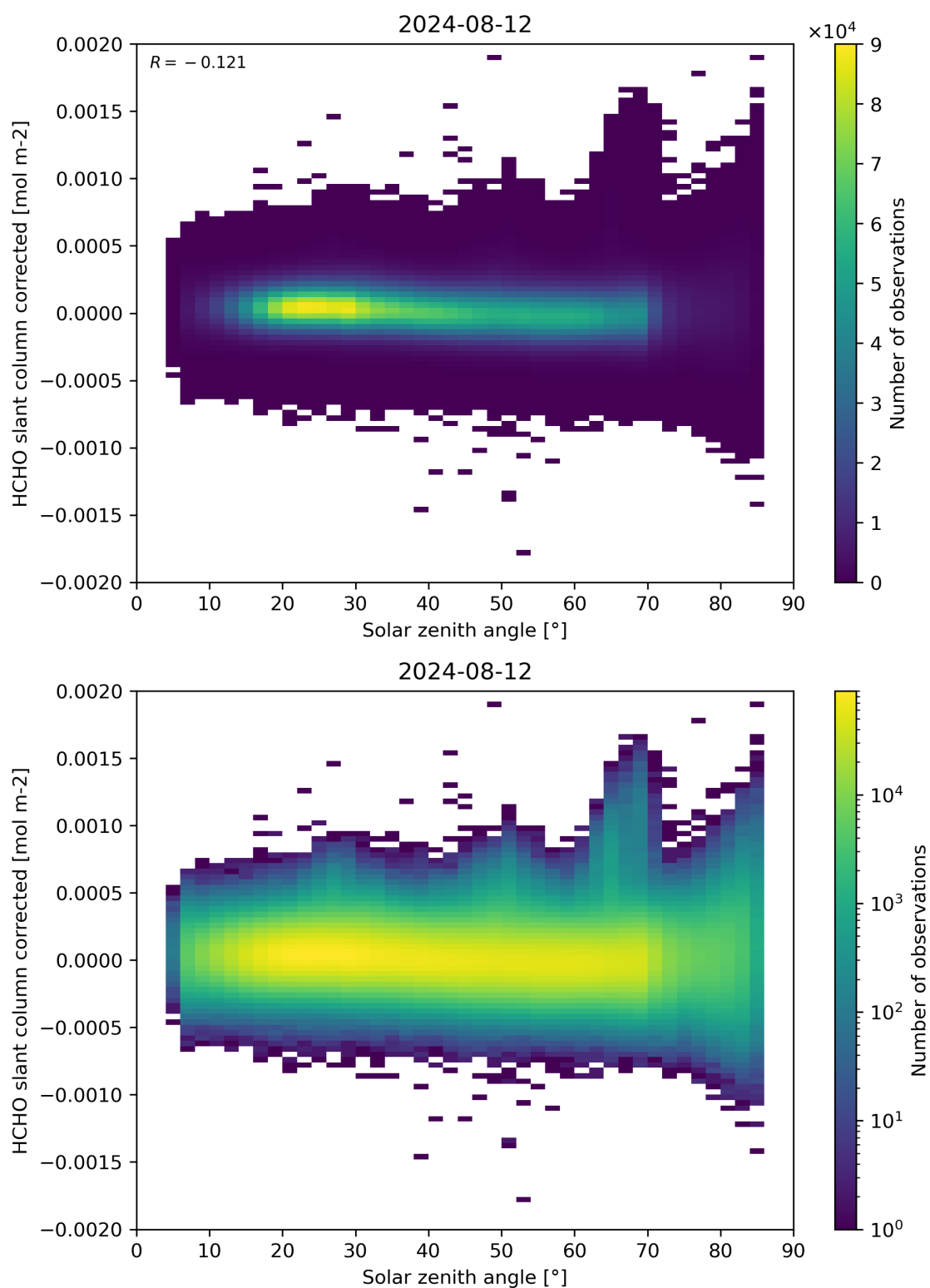
Figure 171: Scatter density plot of “Solar zenith angle” against “HCHO slant column corrected” for 2024-08-12 to 2024-08-13.
