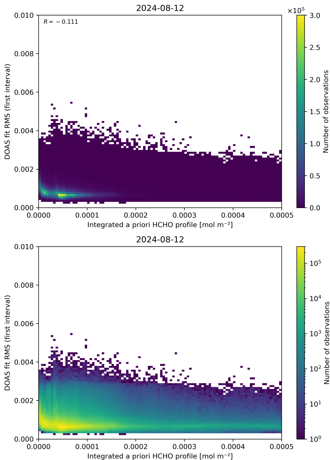
Figure 148: Scatter density plot of “Integrated a priori HCHO profile” against “DOAS fit RMS (first interval)” for 2024-08-12 to 2024-08-13.
