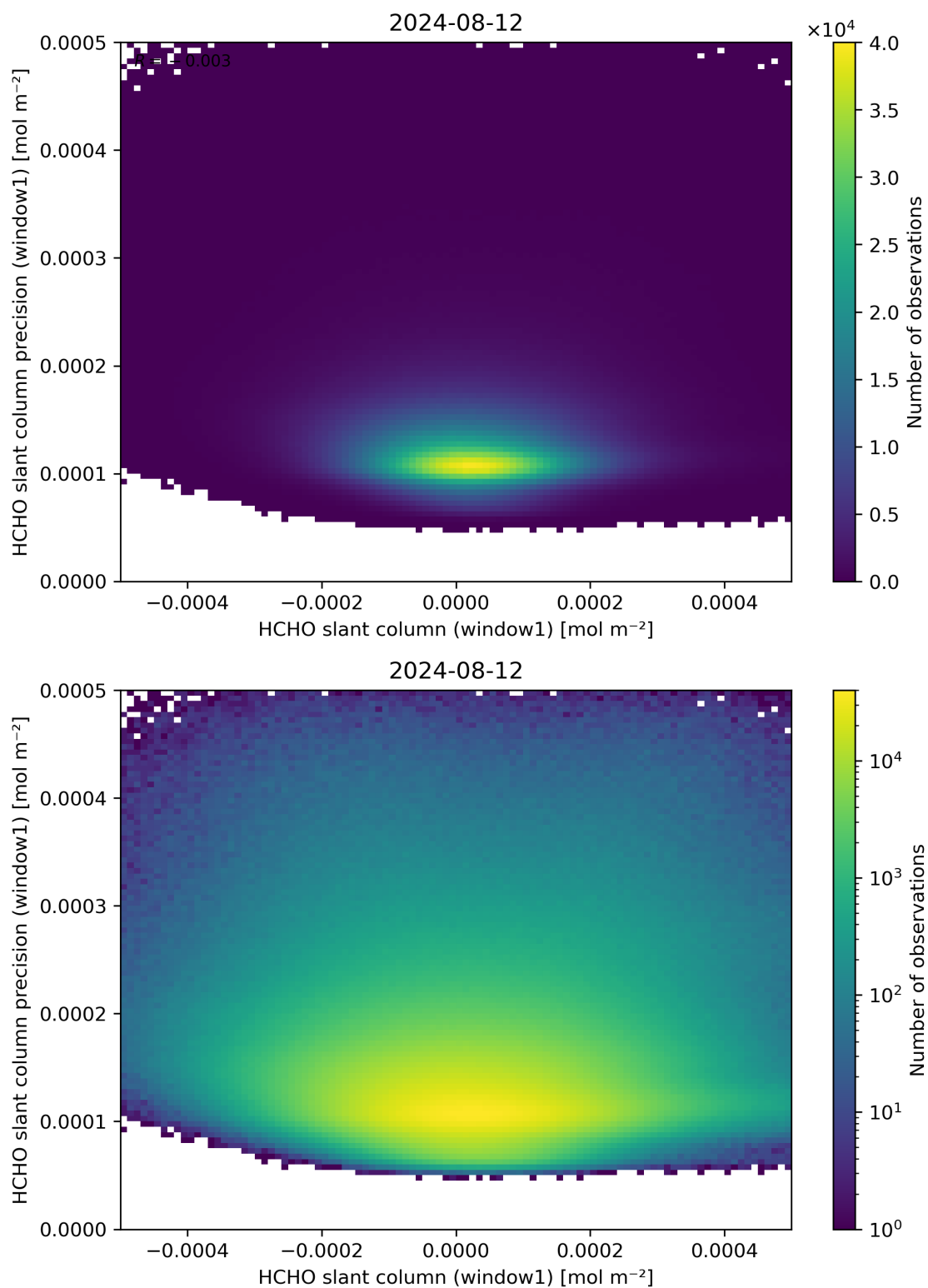
Figure 84: Scatter density plot of “HCHO slant column (window1)” against “HCHO slant column precision (window1)” for 2024-08-12 to 2024-08-13.
