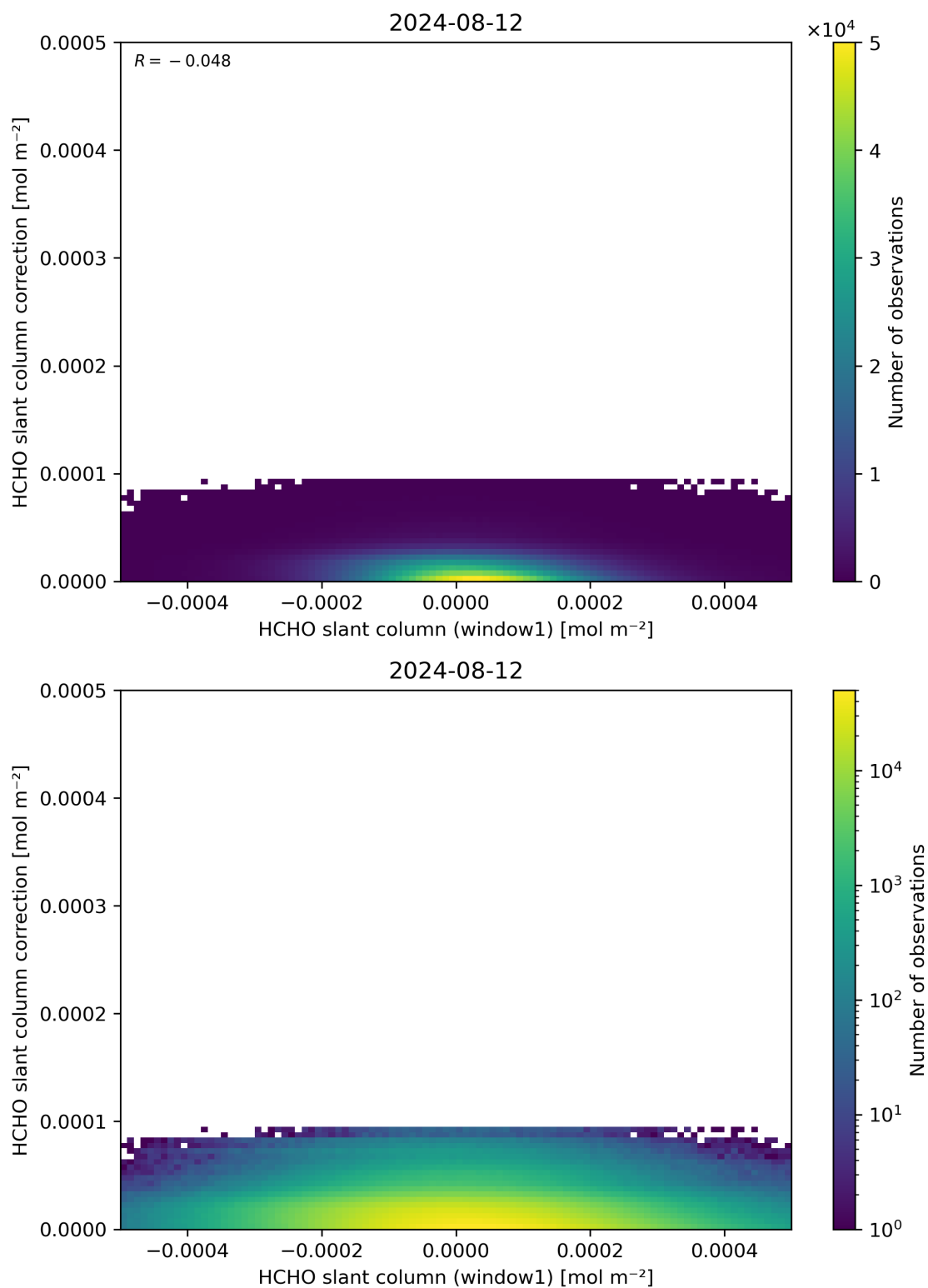
Figure 83: Scatter density plot of “HCHO slant column (window1)” against “HCHO slant column correction” for 2024-08-12 to 2024-08-13.
