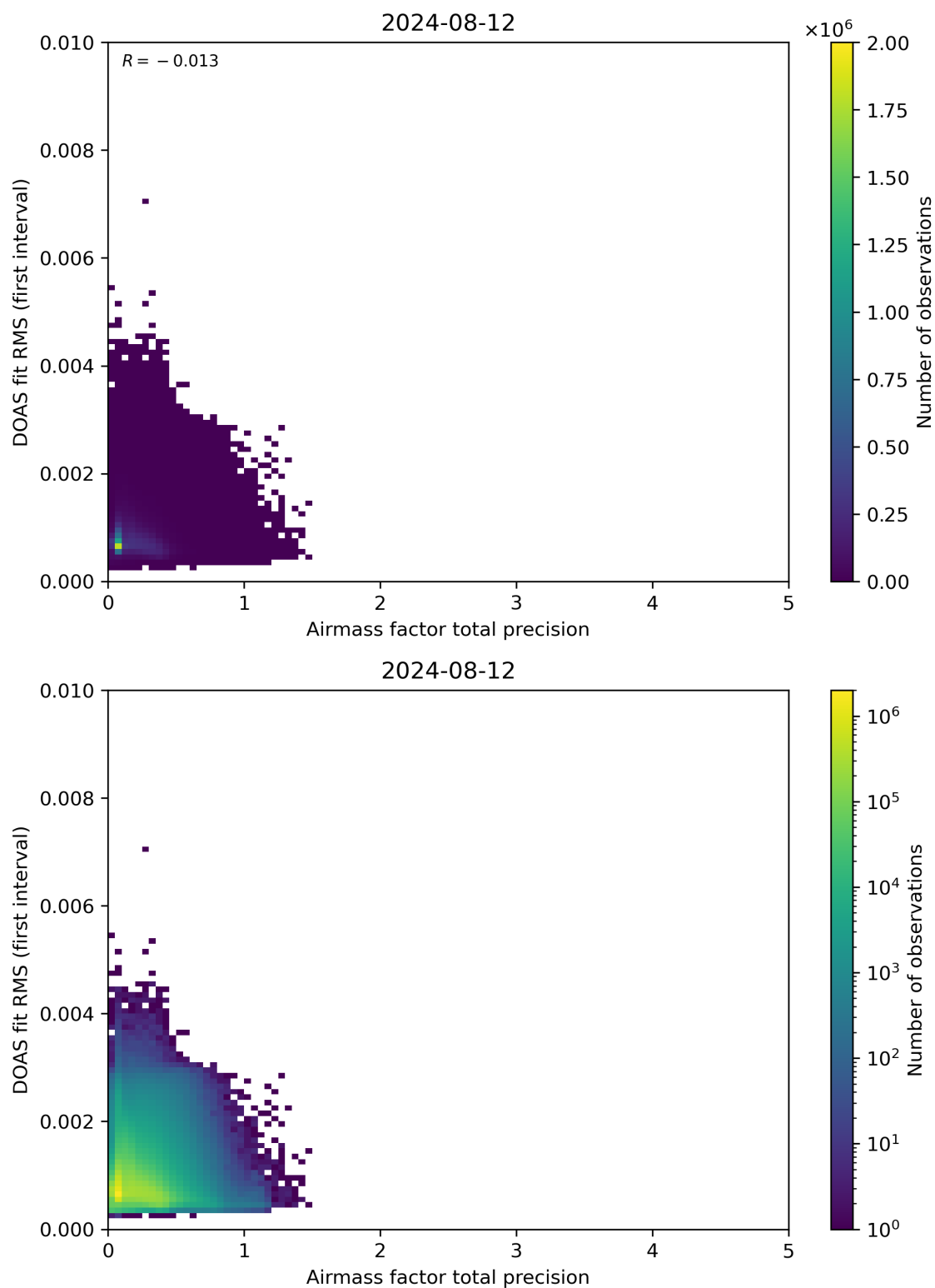
Figure 105: Scatter density plot of “Airmass factor total precision” against “DOAS fit RMS (first interval)” for 2024-08-12 to 2024-08-13.
