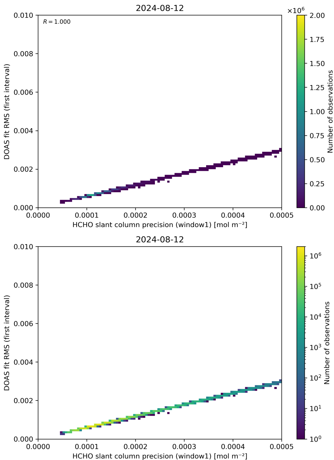
Figure 88: Scatter density plot of “HCHO slant column precision (window1)” against “DOAS fit RMS (first interval)” for 2024-08-12 to 2024-08-13.
