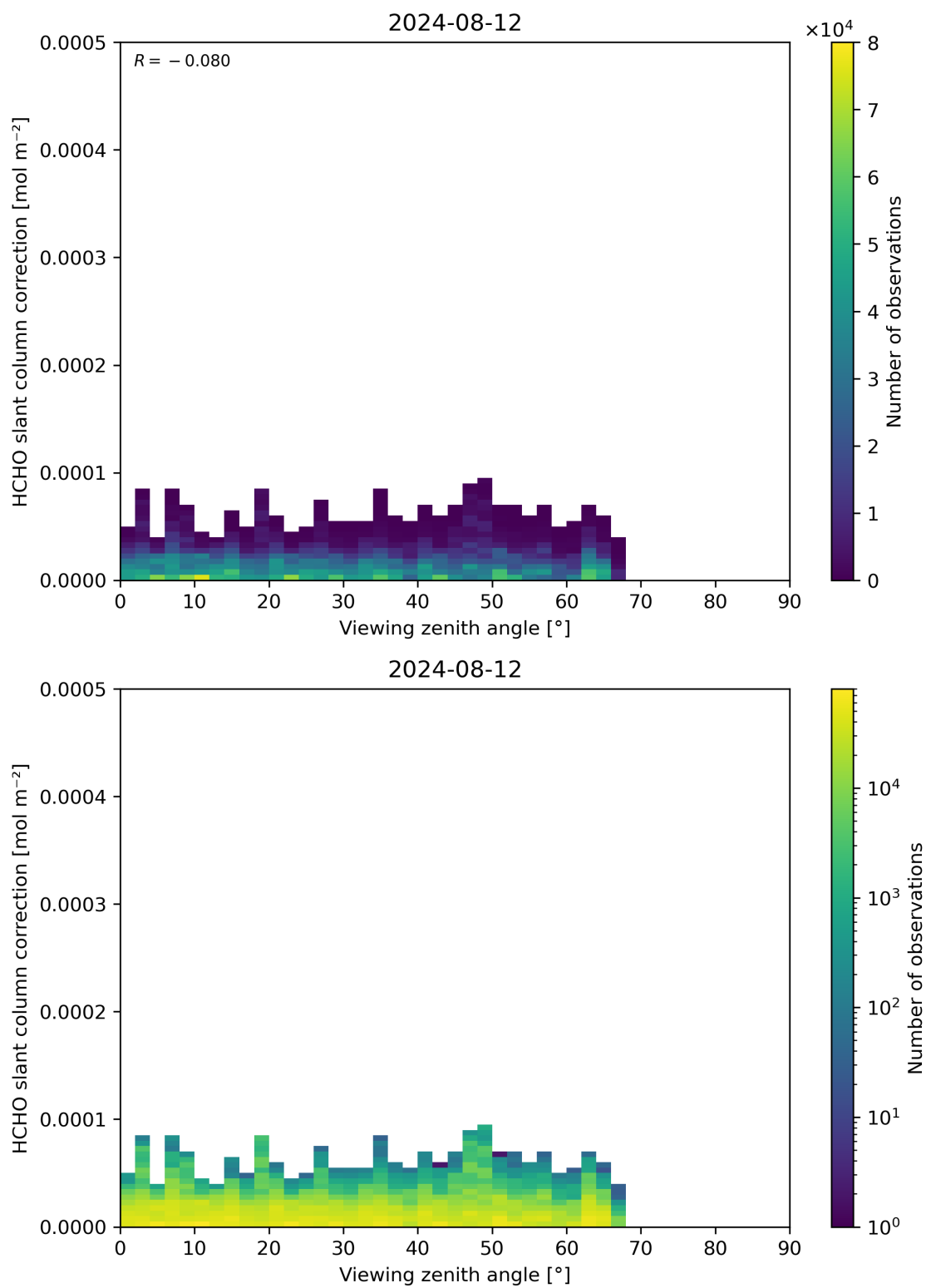
Figure 187: Scatter density plot of “Viewing zenith angle” against “HCHO slant column correction” for 2024-08-12 to 2024-08-13.
