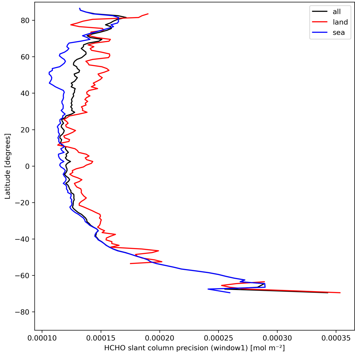
Figure 25: Zonal average of “HCHO slant column precision (window1)” for 2024-08-12 to 2024-08-13.
