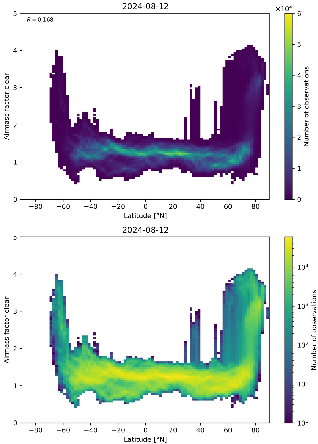
Figure 156: Scatter density plot of “Latitude” against “Airmass factor clear” for 2024-08-12 to 2024-08-13.
