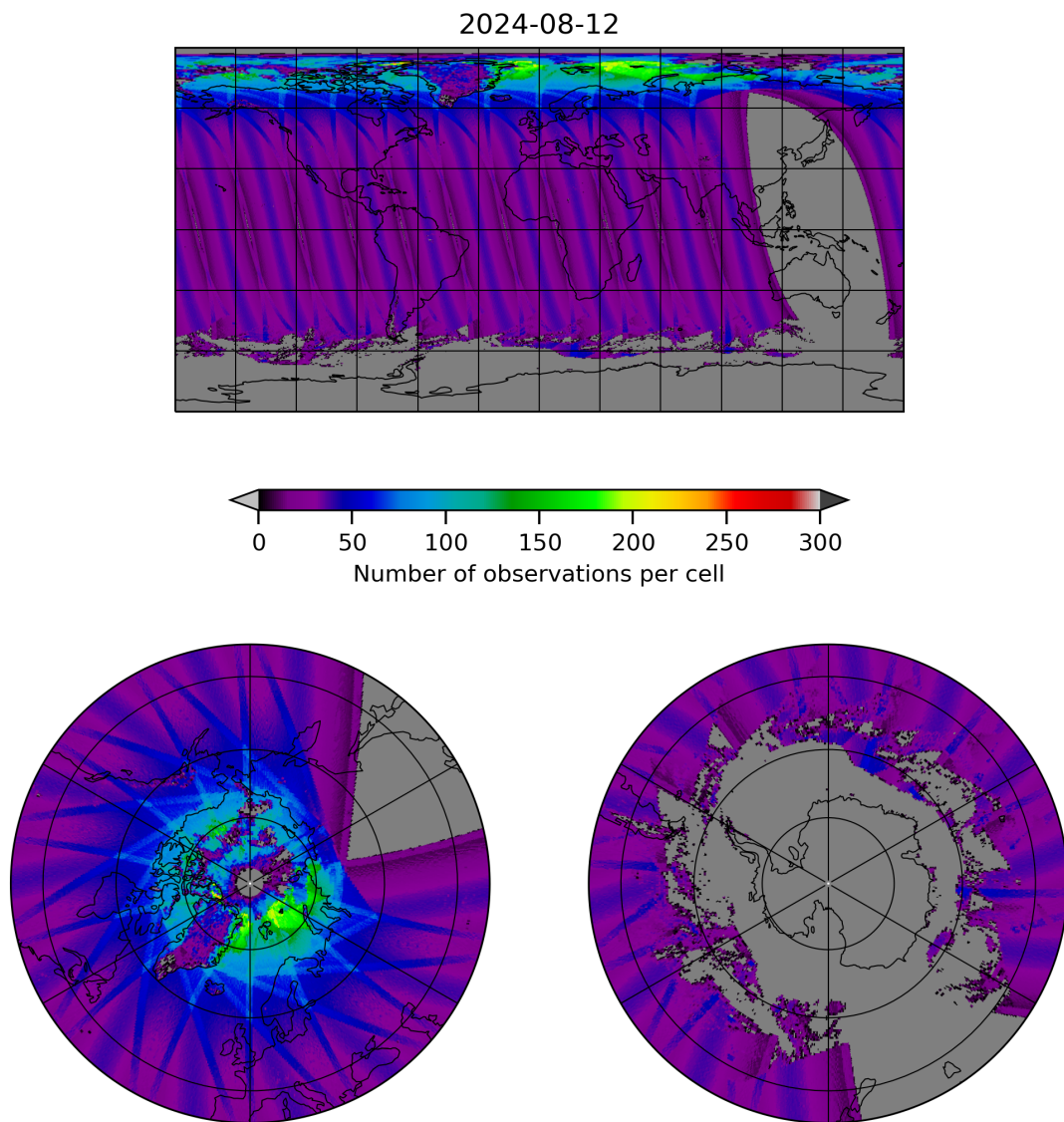
Figure 19: Map of the number of observations for 2024-08-12 to 2024-08-13
