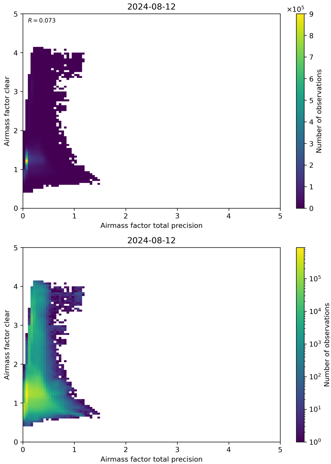
Figure 108: Scatter density plot of “Airmass factor total precision” against “Airmass factor clear” for 2024-08-12 to 2024-08-13.
