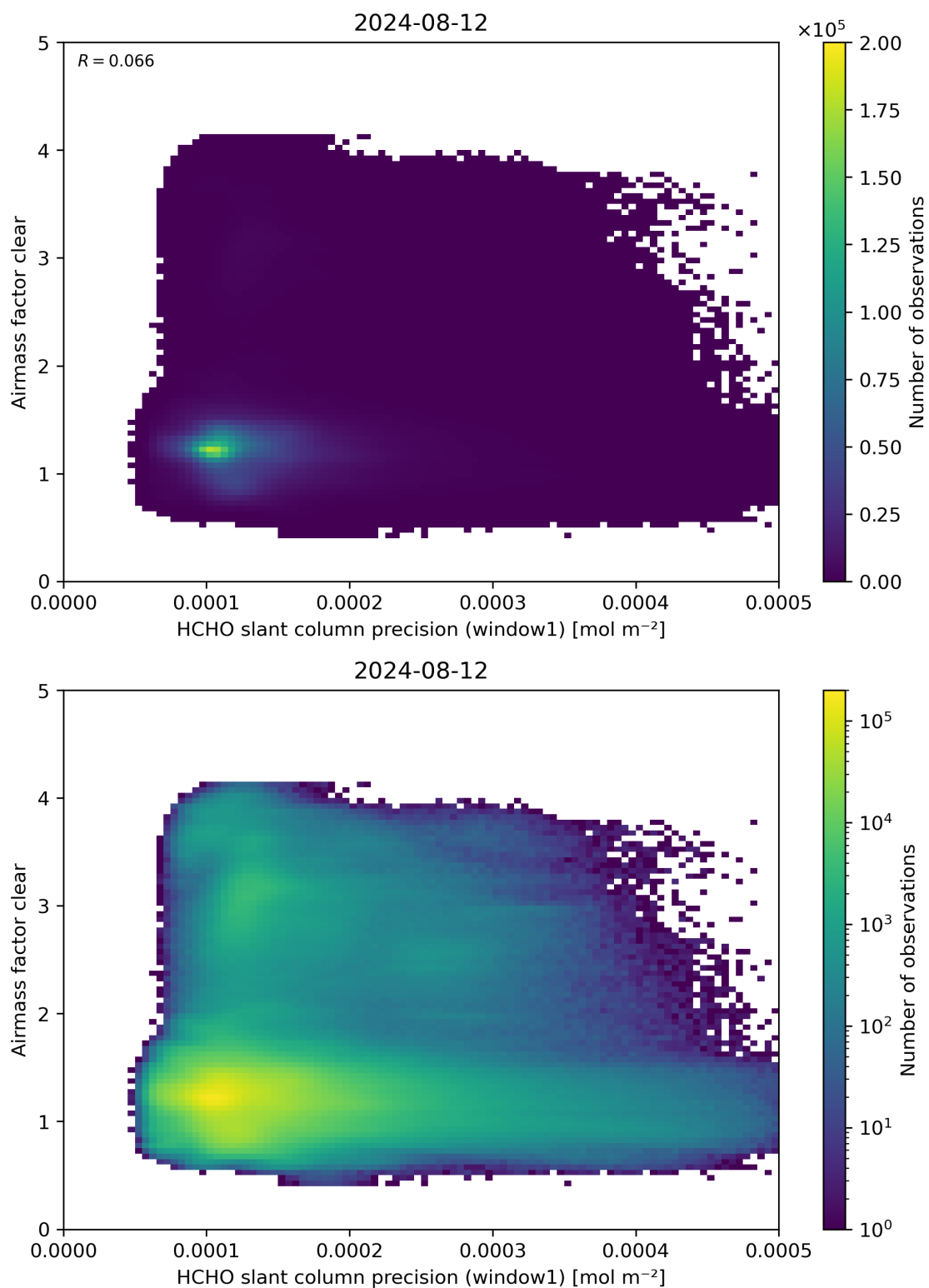
Figure 91: Scatter density plot of “HCHO slant column precision (window1)” against “Airmass factor clear” for 2024-08-12 to 2024-08-13.
