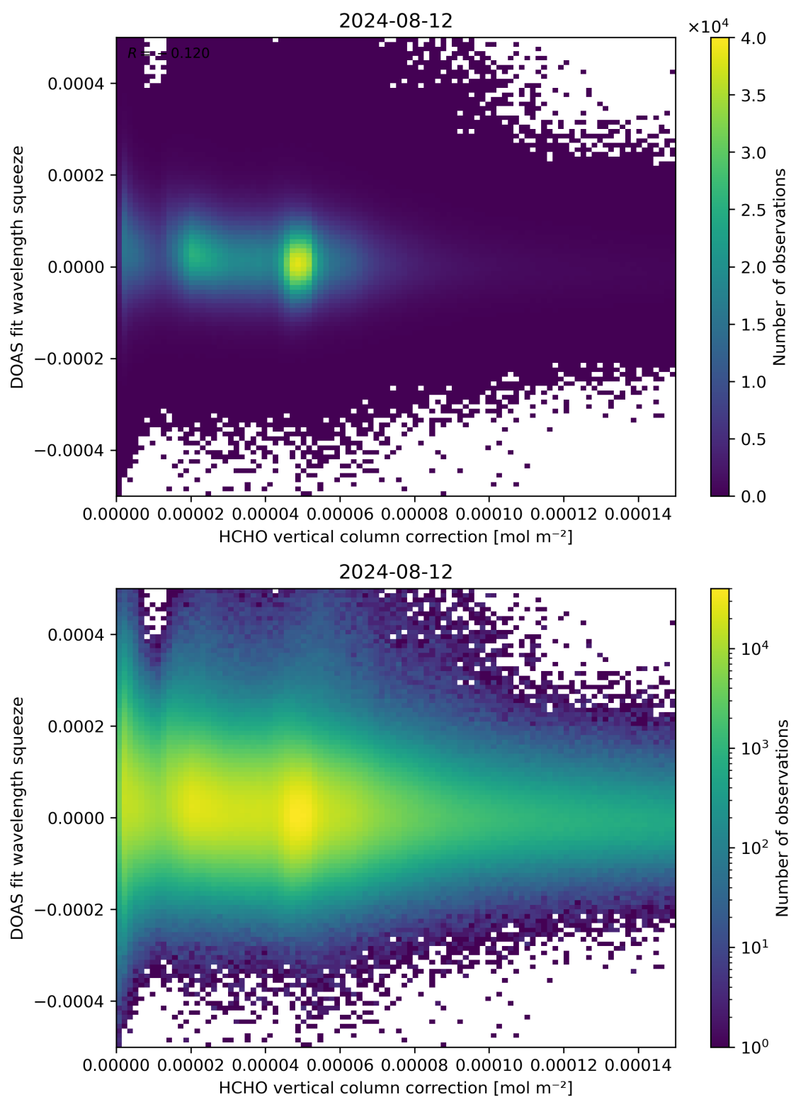
Figure 114: Scatter density plot of “HCHO vertical column correction” against “DOAS fit wavelength squeeze” for 2024-08-12 to 2024-08-13.
