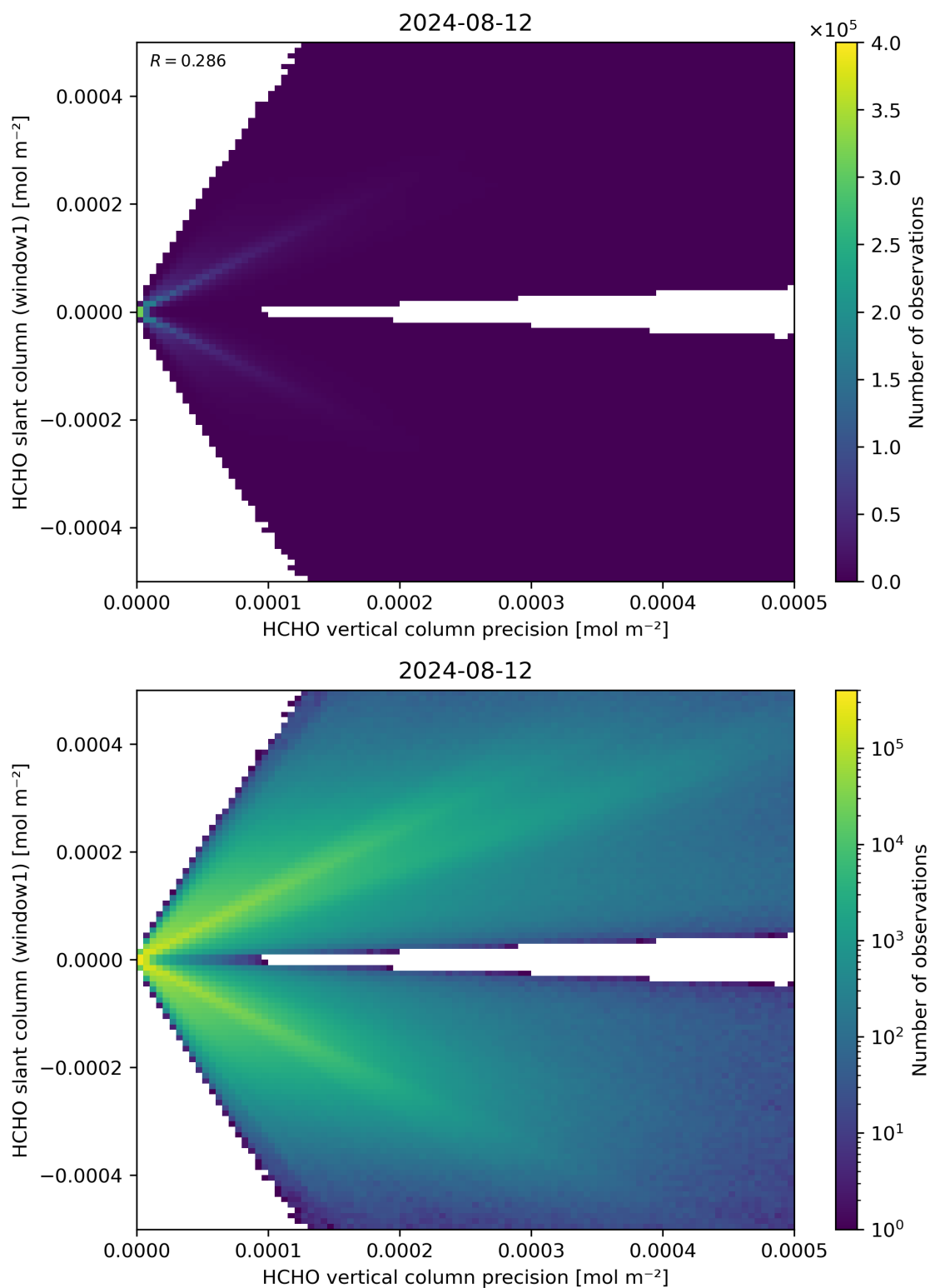
Figure 142: Scatter density plot of “HCHO vertical column precision” against “HCHO slant column (window1)” for 2024-08-12 to 2024-08-13.
