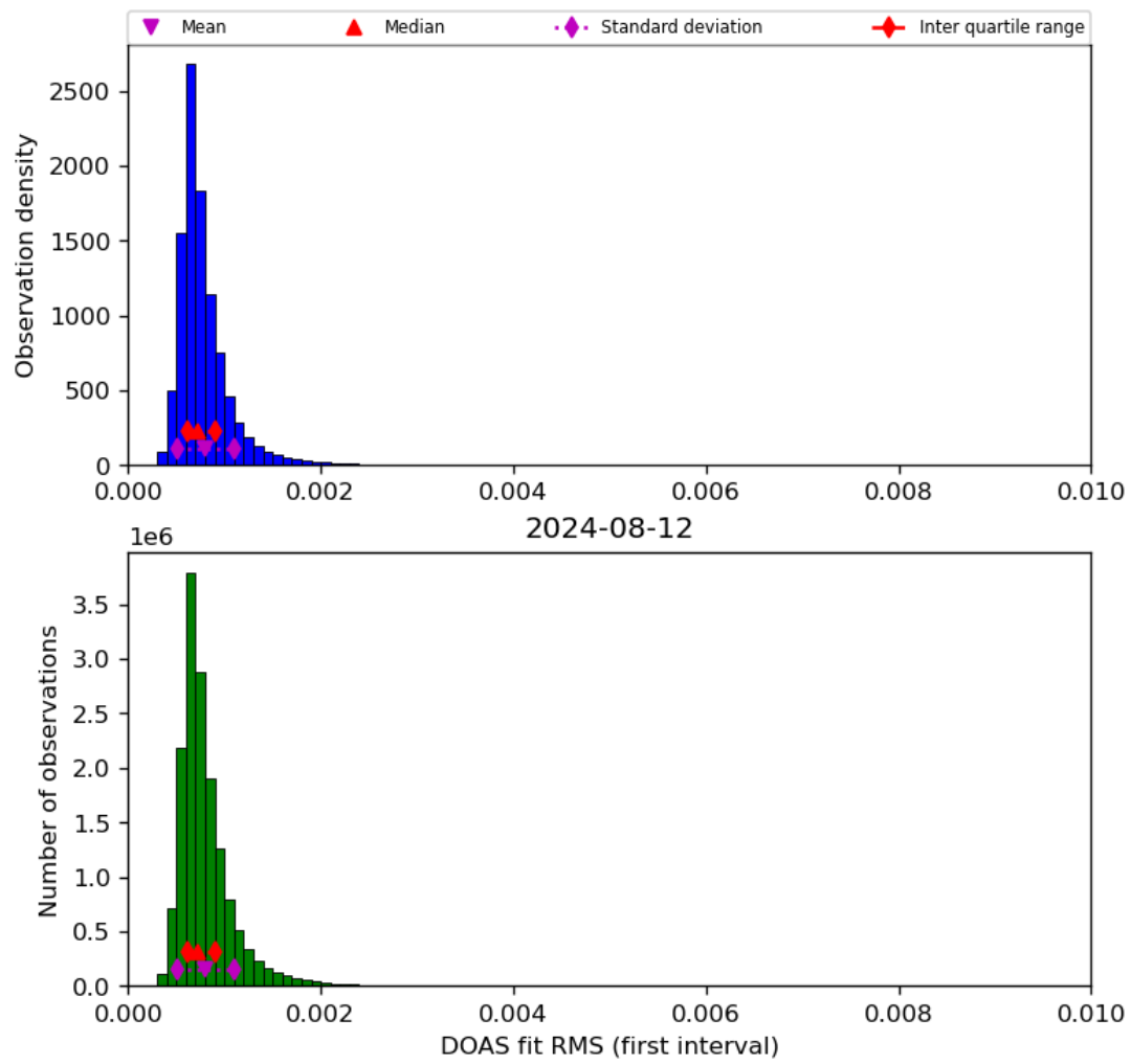
Figure 46: Histogram of “DOAS fit RMS (first interval)” for 2024-08-12 to 2024-08-13
