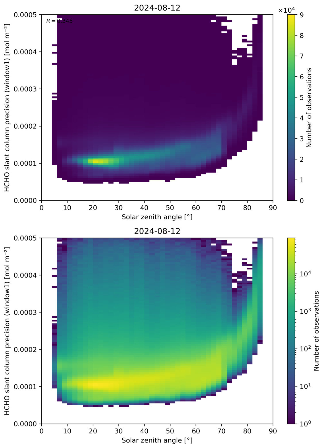
Figure 174: Scatter density plot of “Solar zenith angle” against “HCHO slant column precision (window1)” for 2024-08-12 to 2024-08-13.
