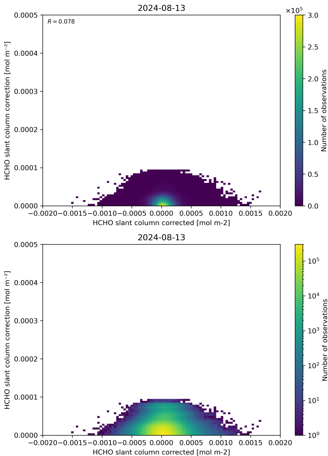
Figure 77: Scatter density plot of “HCHO slant column corrected” against “HCHO slant column correction” for 2024-08-12 to 2024-08-14.
