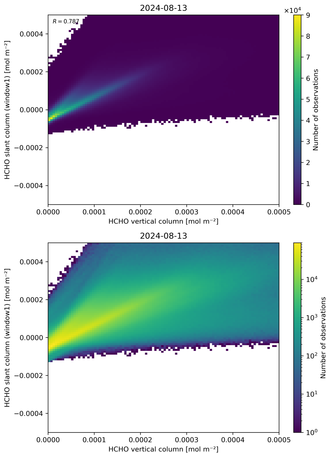
Figure 129: Scatter density plot of “HCHO vertical column” against “HCHO slant column (window1)” for 2024-08-12 to 2024-08-14.
