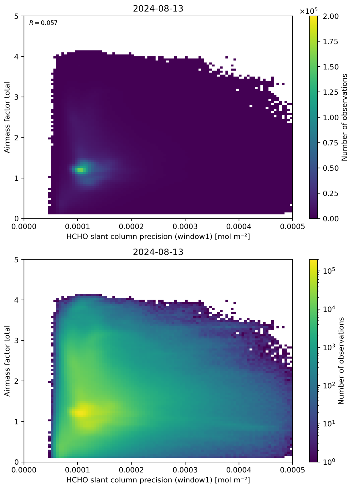
Figure 94: Scatter density plot of “HCHO slant column precision (window1)” against “Airmass factor total” for 2024-08-12 to 2024-08-14.
