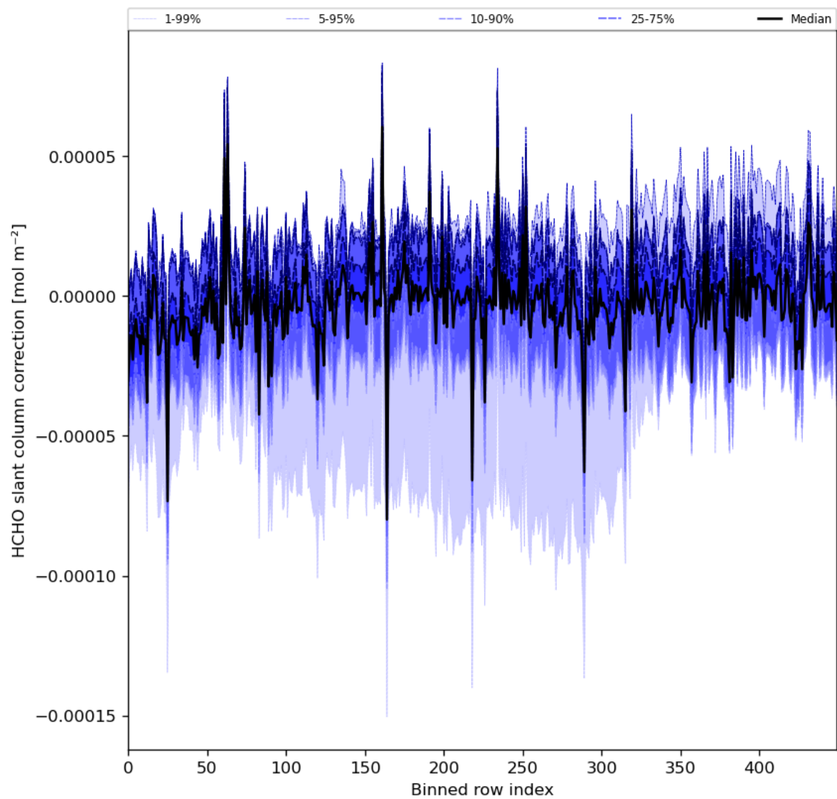
Figure 61: Along track statistics of “HCHO slant column correction” for 2024-08-12 to 2024-08-14
