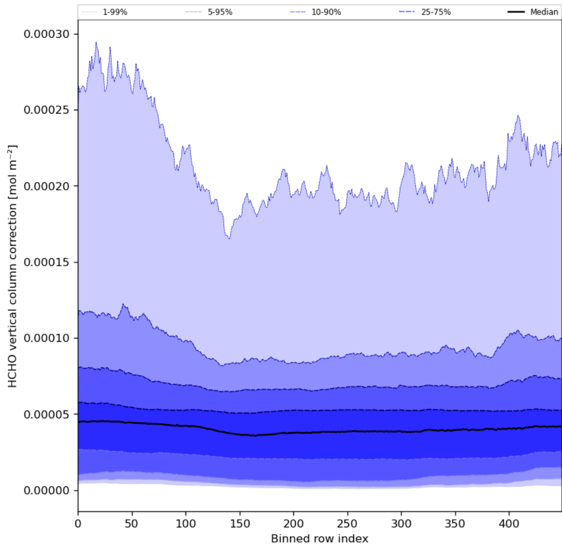
Figure 51: Along track statistics of “HCHO vertical column correction” for 2024-08-12 to 2024-08-14
