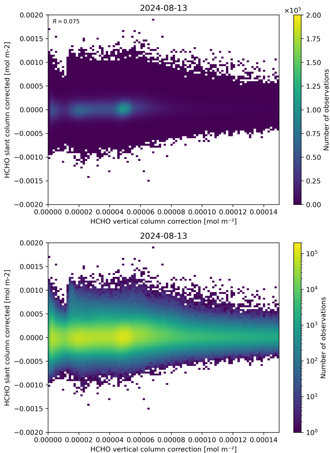
Figure 116: Scatter density plot of “HCHO vertical column correction” against “HCHO slant column corrected” for 2024-08-12 to 2024-08-14.
