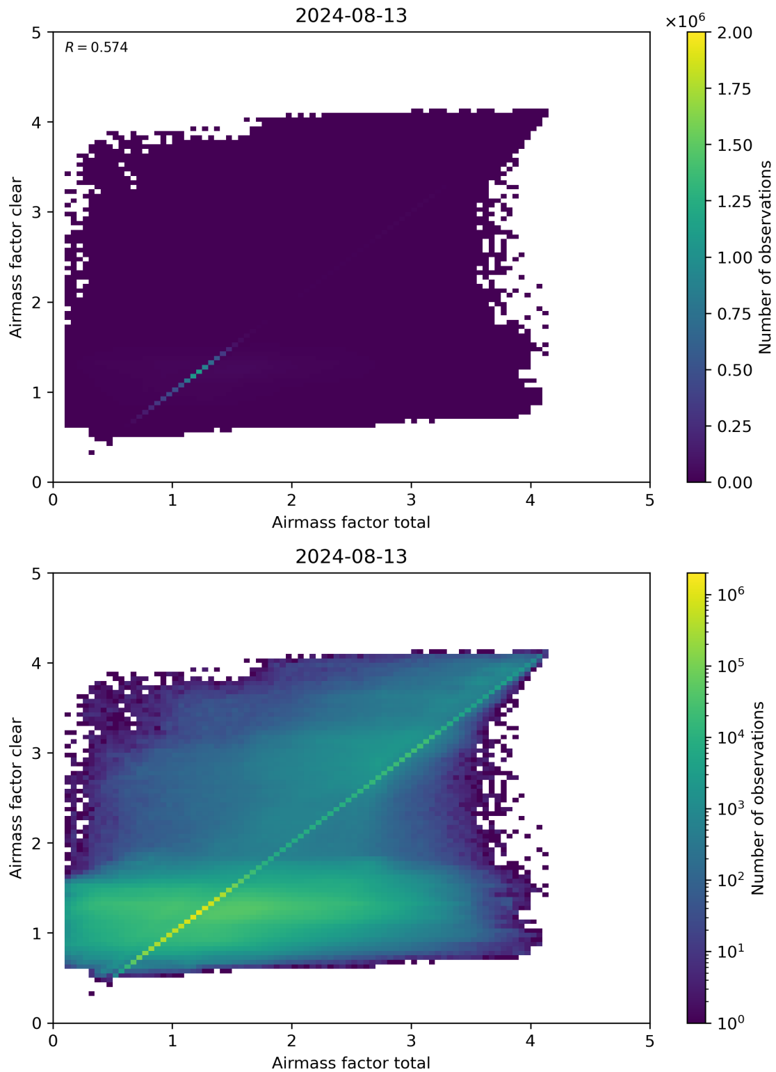
Figure 100: Scatter density plot of “Airmass factor total” against “Airmass factor clear” for 2024-08-12 to 2024-08-14.
