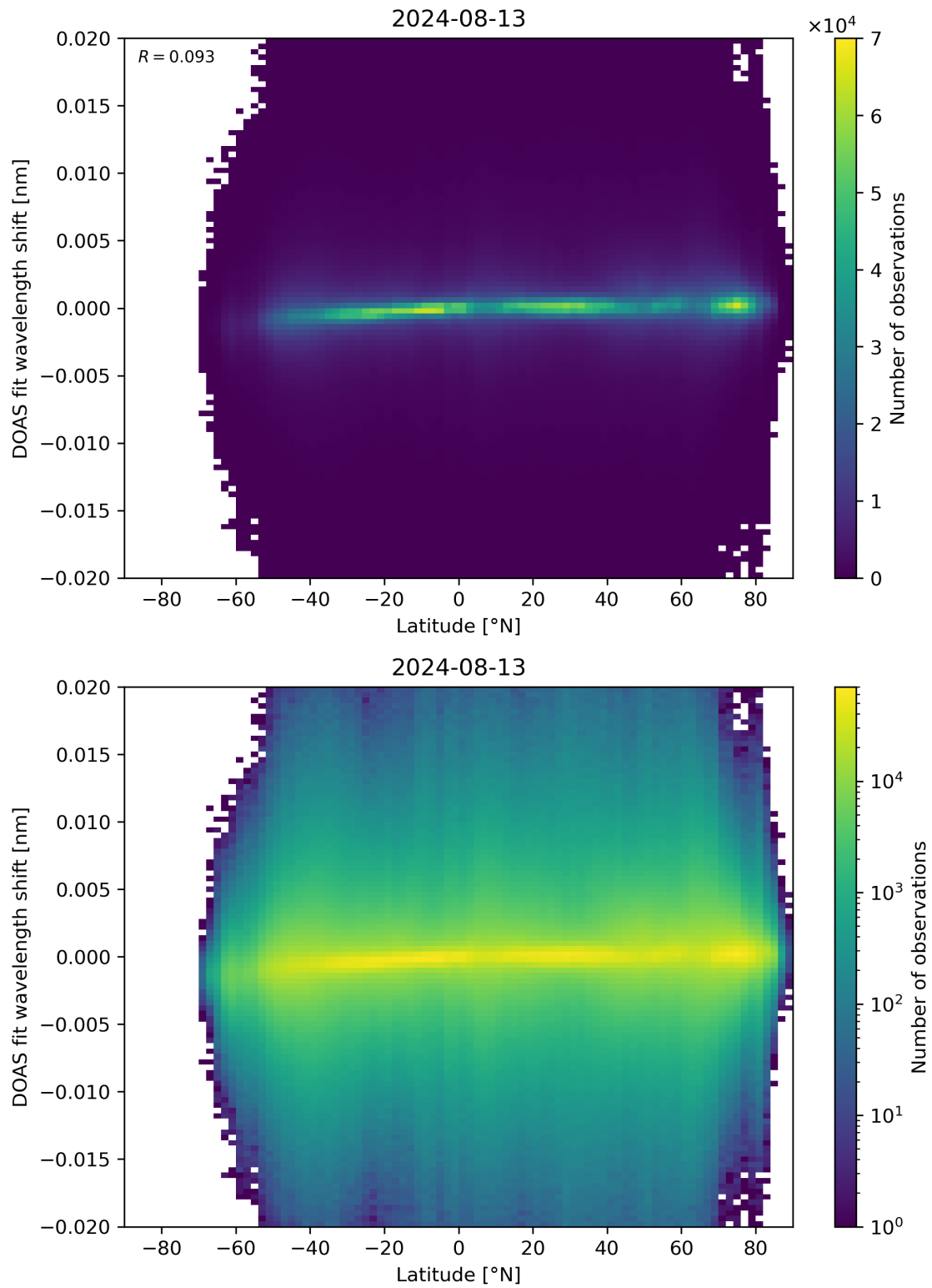
Figure 154: Scatter density plot of “Latitude” against “DOAS fit wavelength shift” for 2024-08-12 to 2024-08-14.
