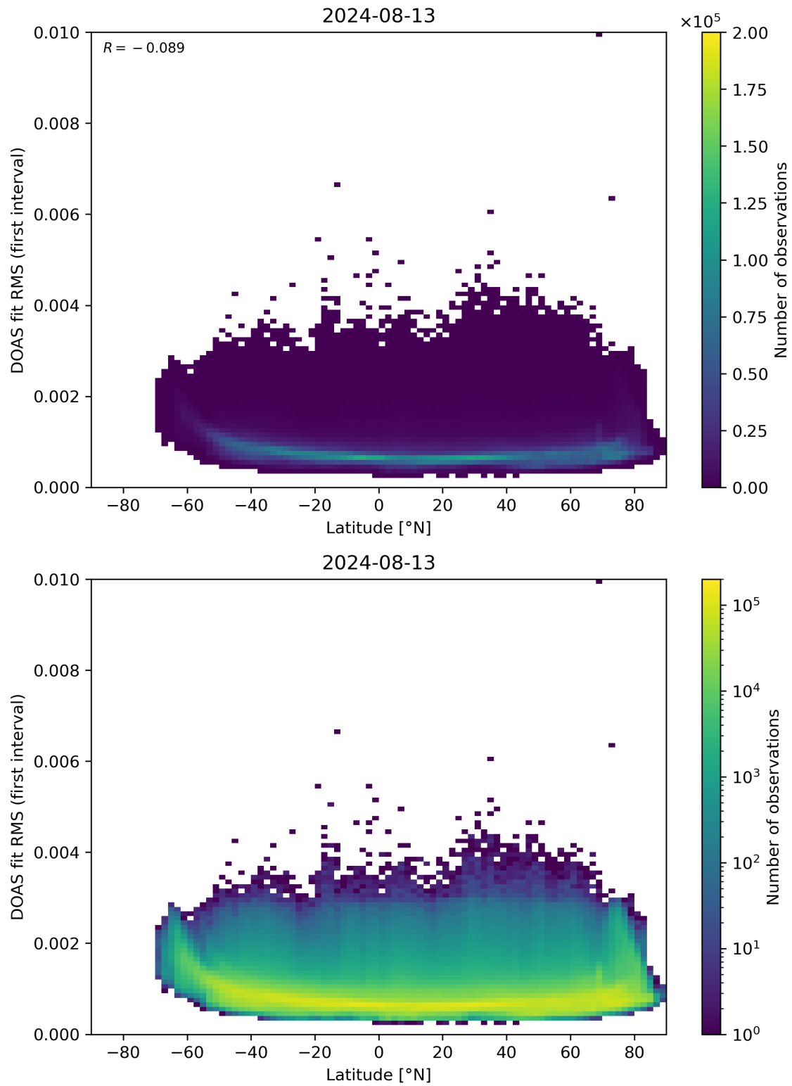
Figure 153: Scatter density plot of “Latitude” against “DOAS fit RMS (first interval)” for 2024-08-12 to 2024-08-14.
