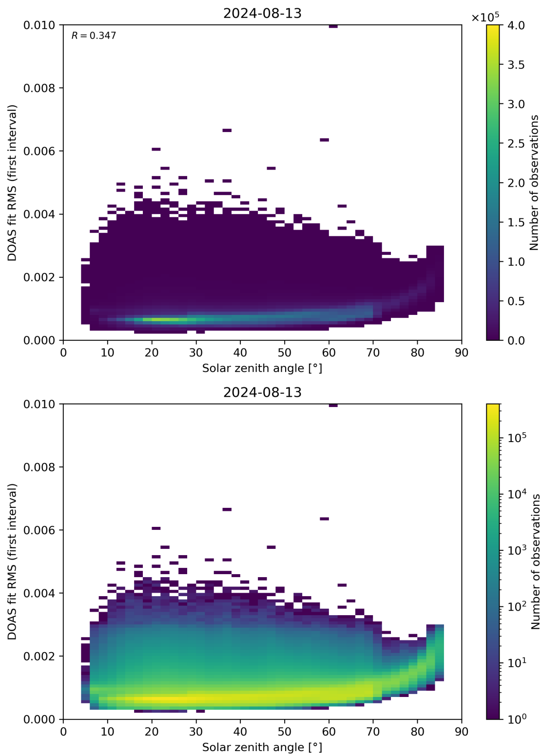
Figure 167: Scatter density plot of “Solar zenith angle” against “DOAS fit RMS (first interval)” for 2024-08-12 to 2024-08-14.
