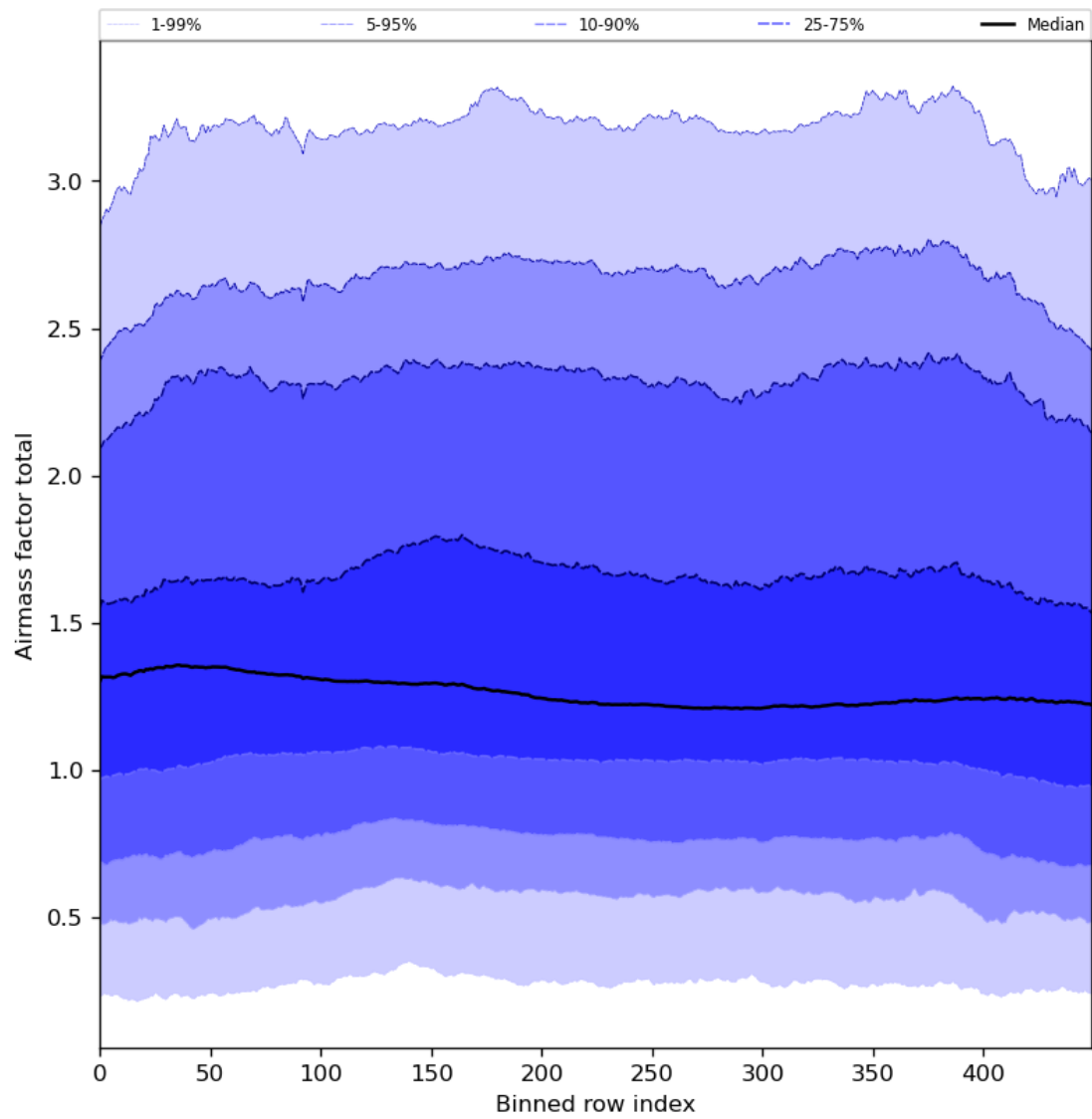
Figure 54: Along track statistics of “Airmass factor total” for 2024-08-12 to 2024-08-14
