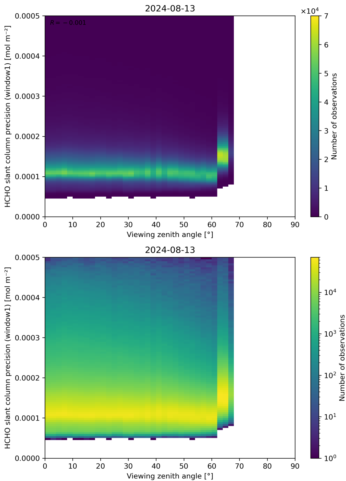
Figure 189: Scatter density plot of “Viewing zenith angle” against “HCHO slant column precision (window1)” for 2024-08-12 to 2024-08-14.
