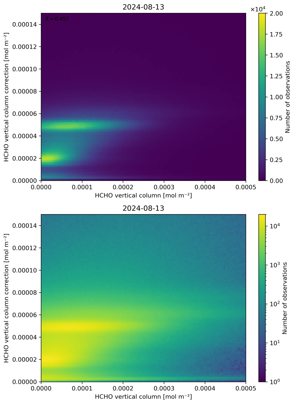
Figure 133: Scatter density plot of “HCHO vertical column” against “HCHO vertical column correction” for 2024-08-12 to 2024-08-14.
