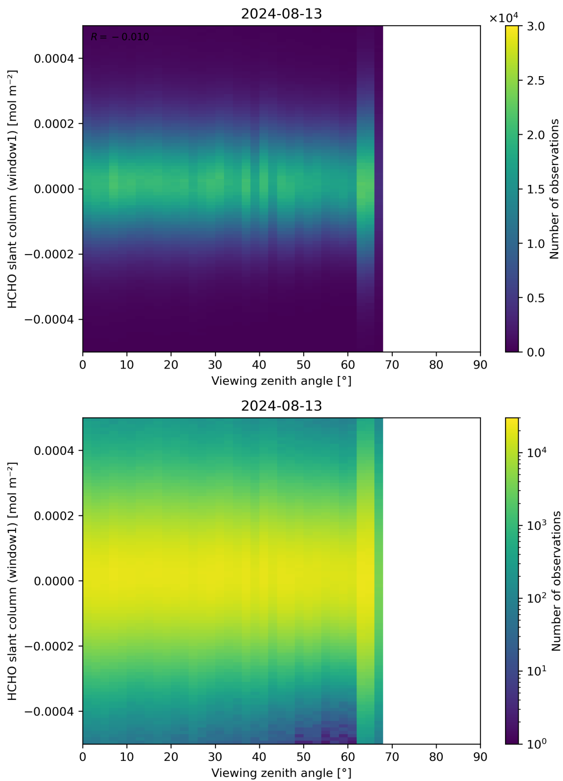
Figure 188: Scatter density plot of “Viewing zenith angle” against “HCHO slant column (window1)” for 2024-08-12 to 2024-08-14.
