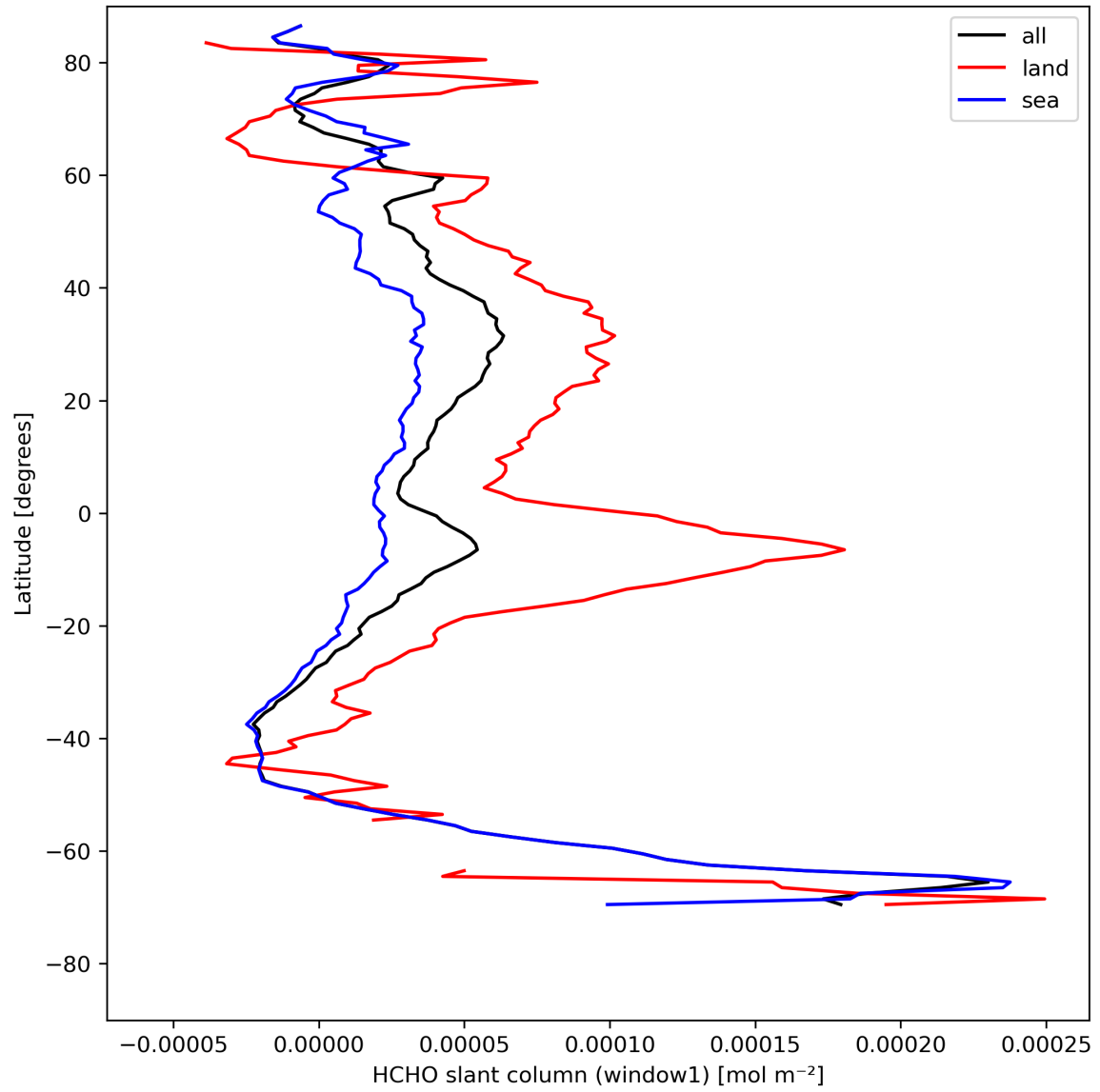
Figure 24: Zonal average of “HCHO slant column (window1)” for 2024-08-12 to 2024-08-14.
