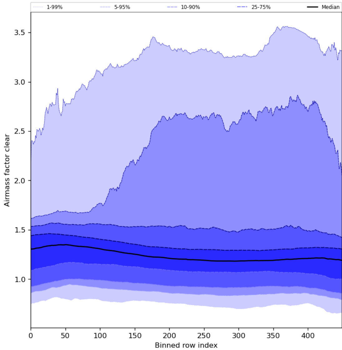
Figure 56: Along track statistics of “Airmass factor clear” for 2024-08-12 to 2024-08-14
