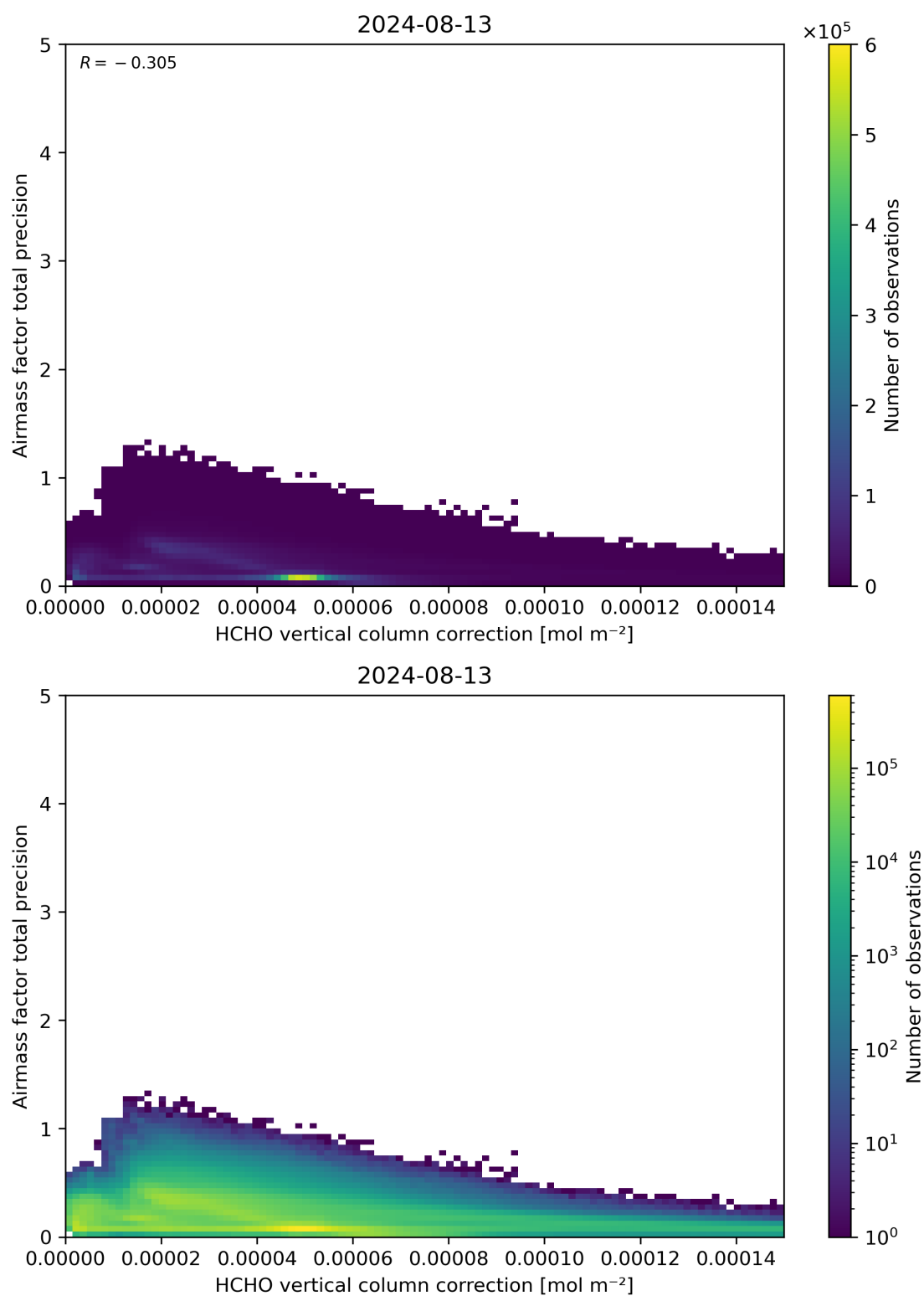
Figure 121: Scatter density plot of “HCHO vertical column correction” against “Airmass factor total precision” for 2024-08-12 to 2024-08-14.
