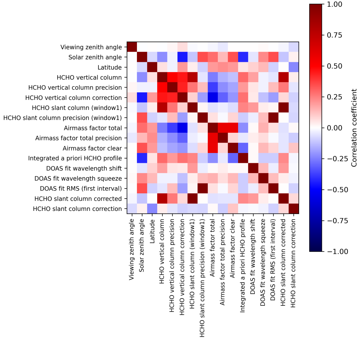
Figure 2: Map of correlation matrix for 2024-08-12 to 2024-08-14.
