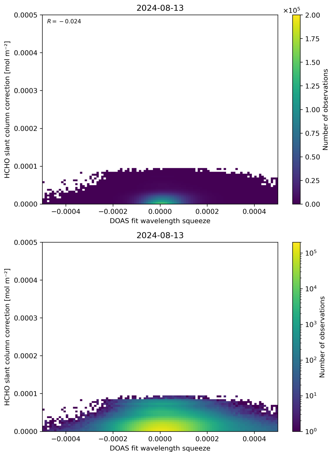
Figure 70: Scatter density plot of “DOAS fit wavelength squeeze” against “HCHO slant column correction” for 2024-08-12 to 2024-08-14.
