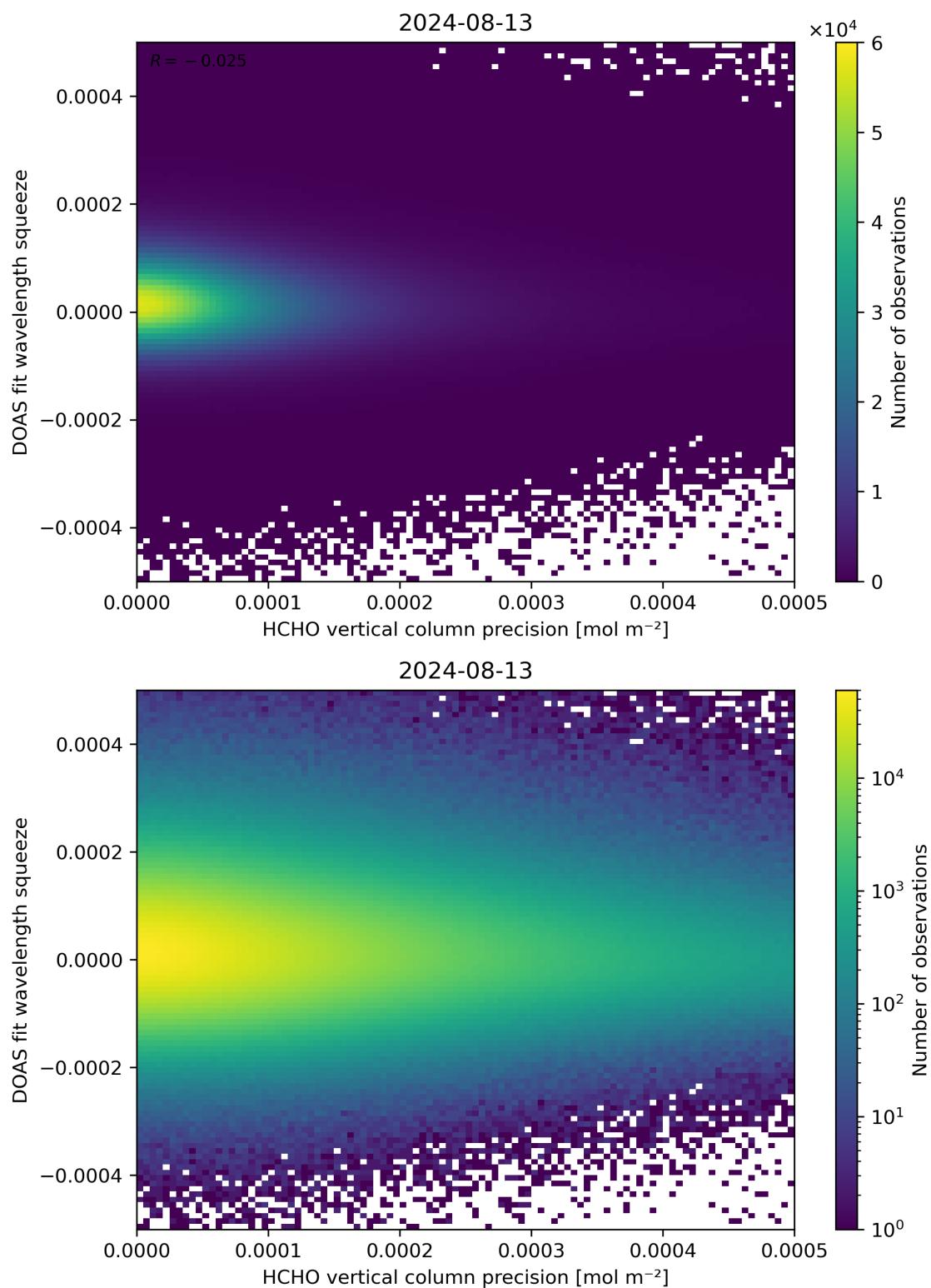
Figure 138: Scatter density plot of “HCHO vertical column precision” against “DOAS fit wavelength squeeze” for 2024-08-12 to 2024-08-14.
