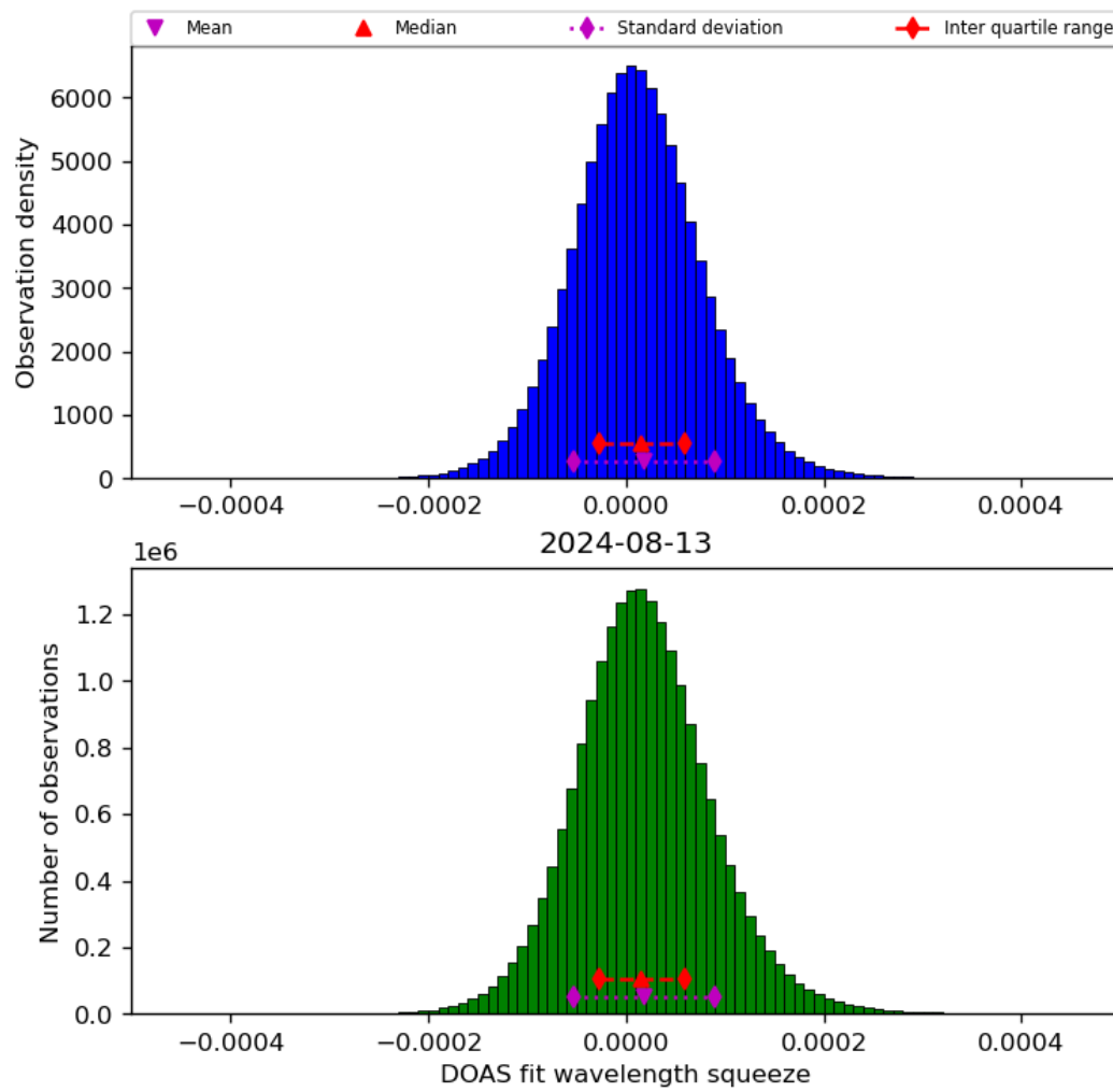
Figure 45: Histogram of “DOAS fit wavelength squeeze” for 2024-08-12 to 2024-08-14
