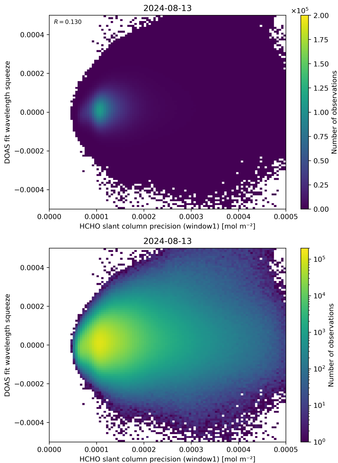
Figure 90: Scatter density plot of “HCHO slant column precision (window1)” against “DOAS fit wavelength squeeze” for 2024-08-12 to 2024-08-14.
