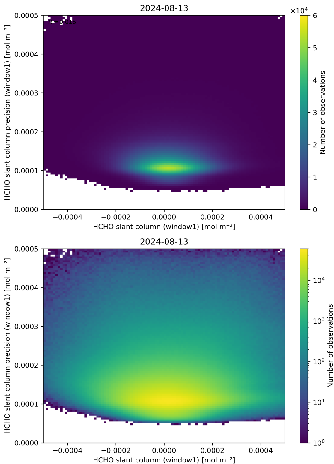
Figure 84: Scatter density plot of “HCHO slant column (window1)” against “HCHO slant column precision (window1)” for 2024-08-12 to 2024-08-14.
