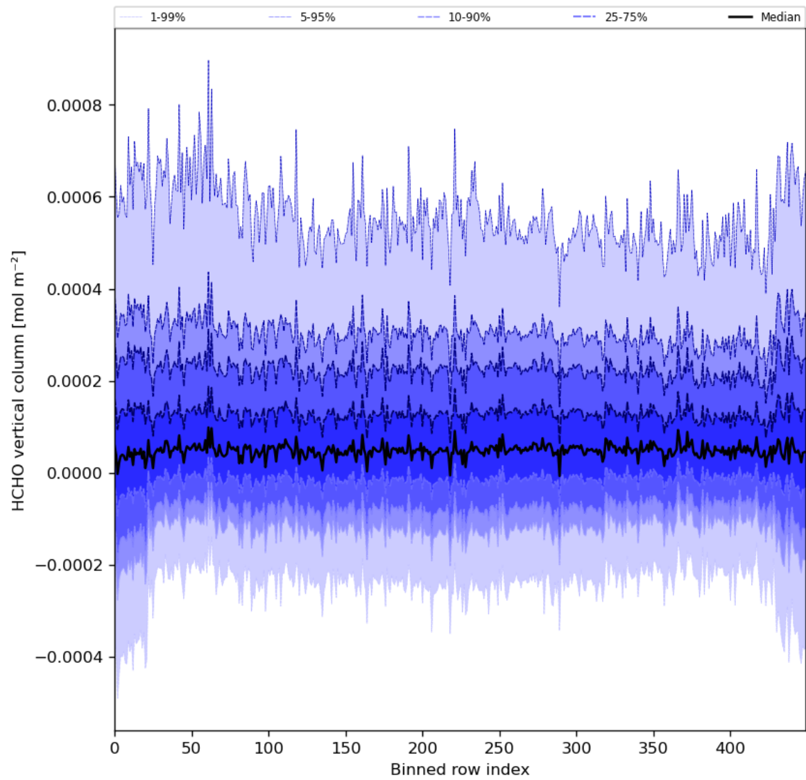
Figure 49: Along track statistics of “HCHO vertical column” for 2024-08-12 to 2024-08-14
