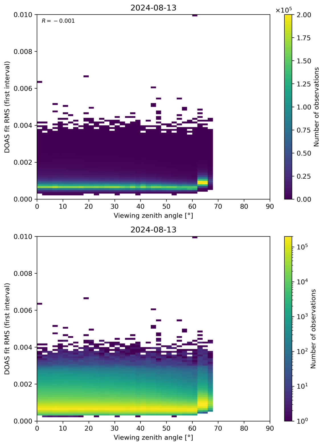
Figure 182: Scatter density plot of “Viewing zenith angle” against “DOAS fit RMS (first interval)” for 2024-08-12 to 2024-08-14.
