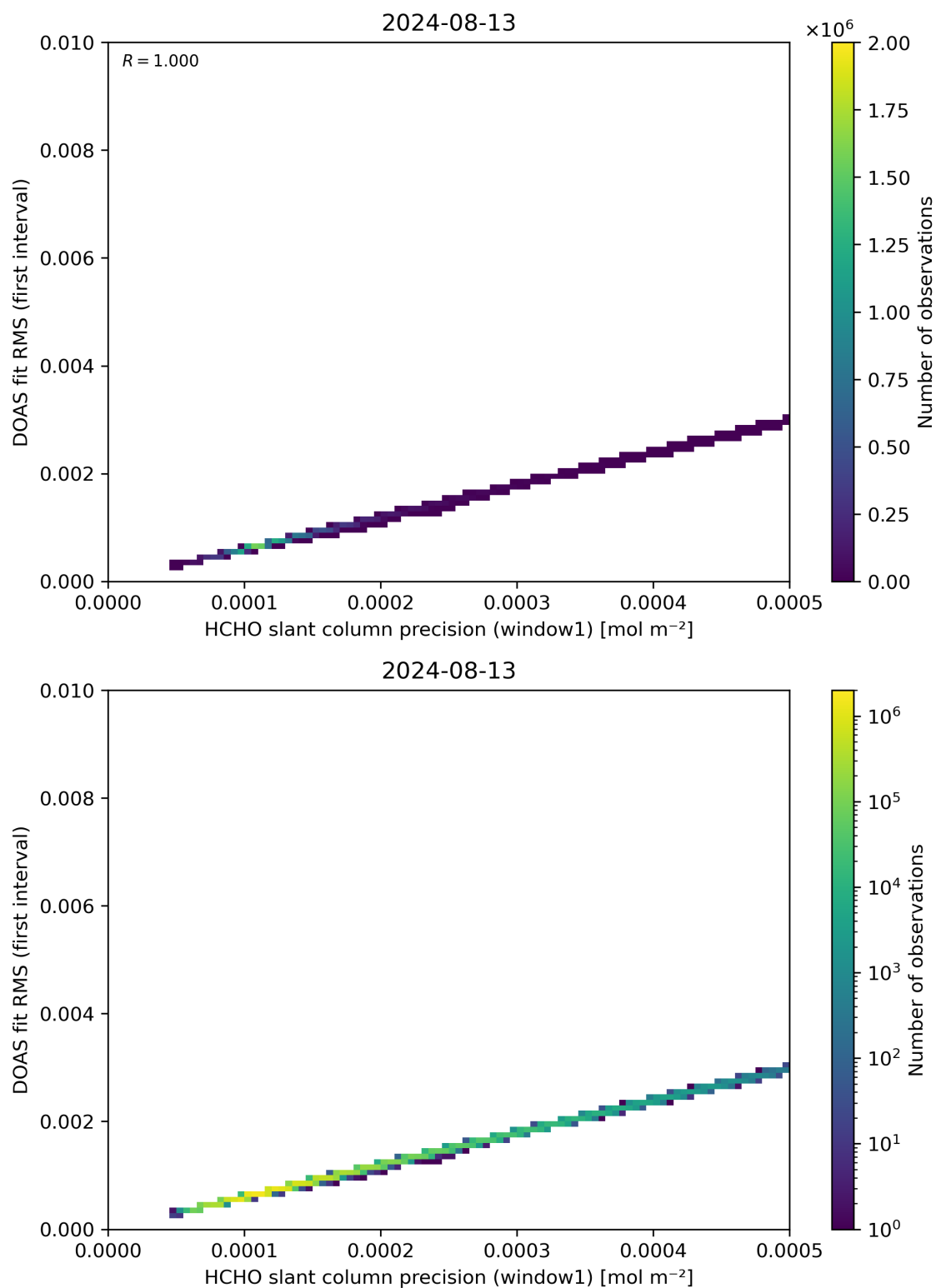
Figure 88: Scatter density plot of “HCHO slant column precision (window1)” against “DOAS fit RMS (first interval)” for 2024-08-12 to 2024-08-14.
