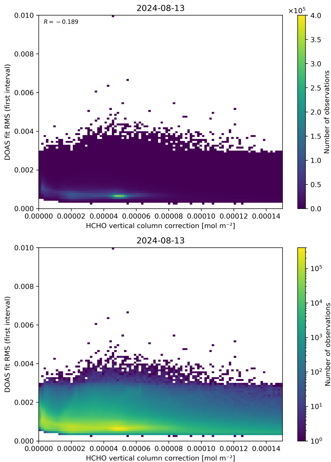
Figure 112: Scatter density plot of “HCHO vertical column correction” against “DOAS fit RMS (first interval)” for 2024-08-12 to 2024-08-14.
