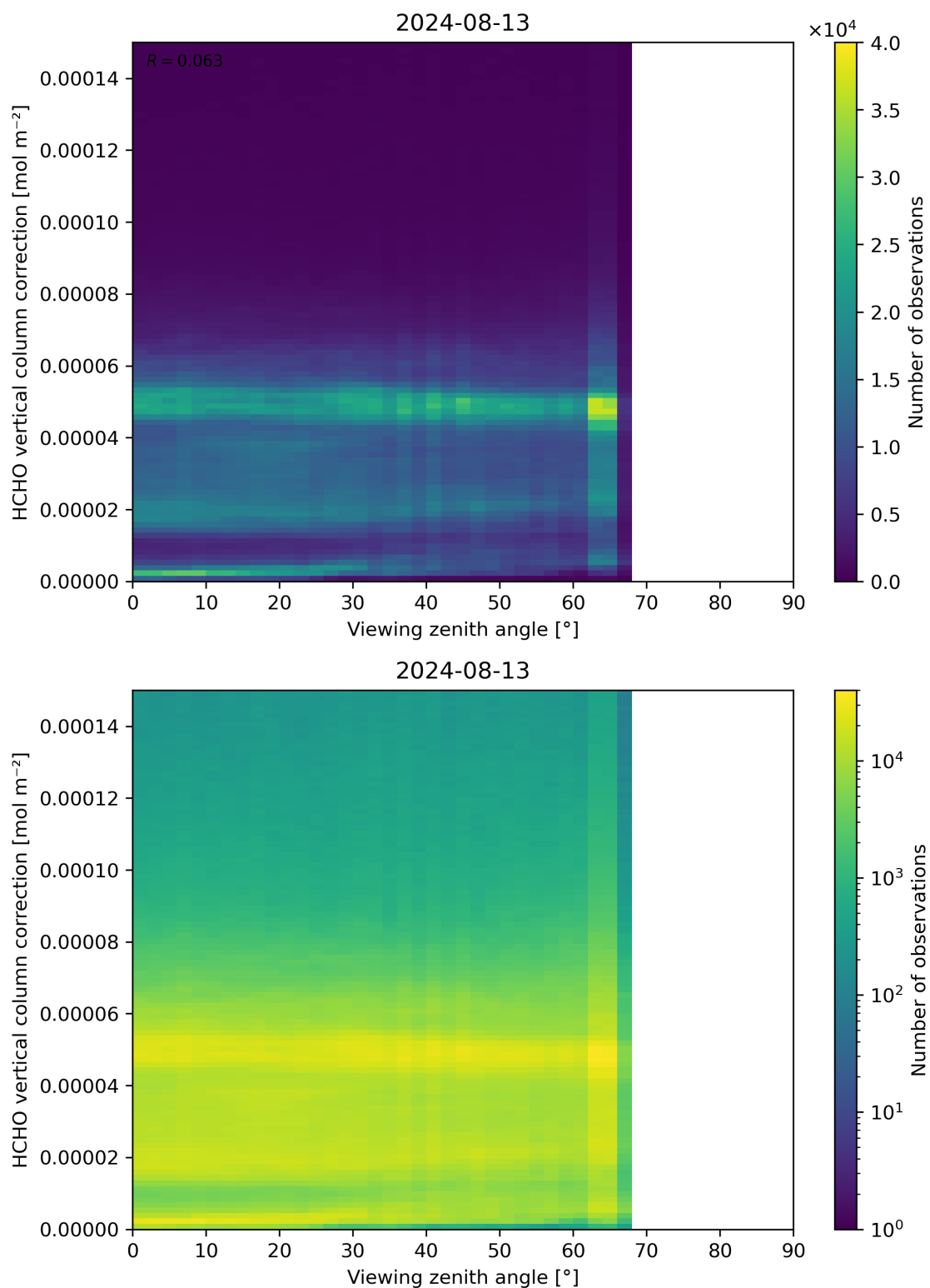
Figure 193: Scatter density plot of “Viewing zenith angle” against “HCHO vertical column correction” for 2024-08-12 to 2024-08-14.
