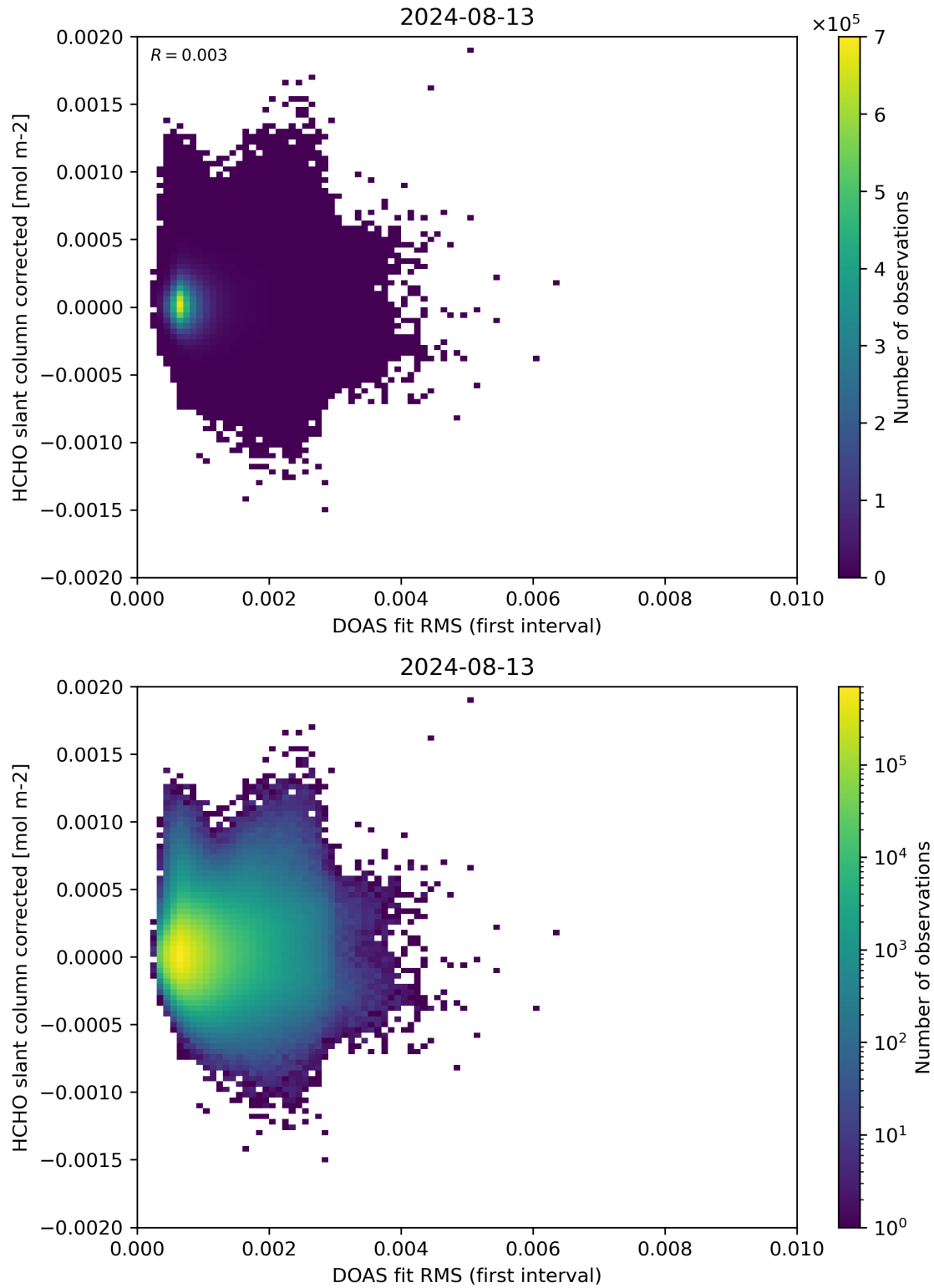
Figure 62: Scatter density plot of “DOAS fit RMS (first interval)” against “HCHO slant column corrected” for 2024-08-12 to 2024-08-14.
