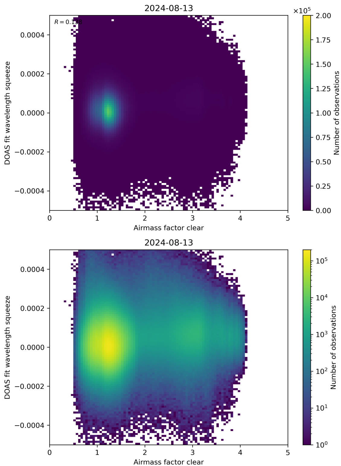
Figure 73: Scatter density plot of “Airmass factor clear” against “DOAS fit wavelength squeeze” for 2024-08-12 to 2024-08-14.
