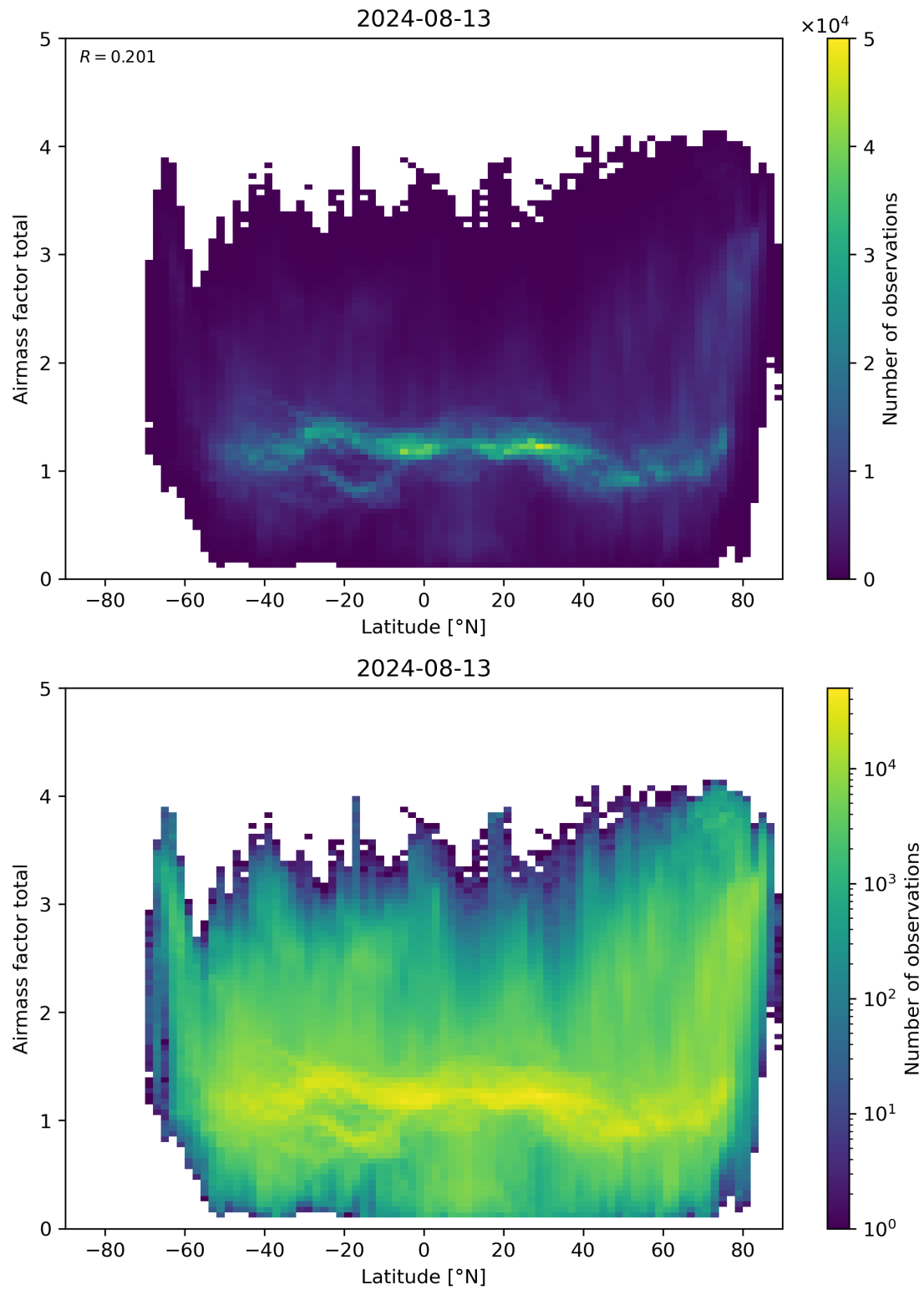
Figure 161: Scatter density plot of “Latitude” against “Airmass factor total” for 2024-08-12 to 2024-08-14.
