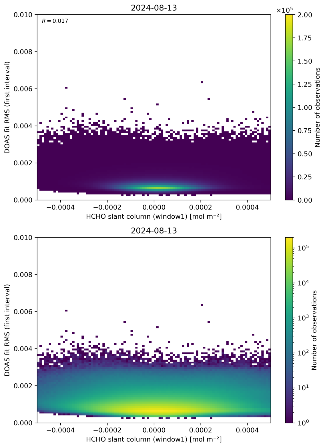
Figure 78: Scatter density plot of “HCHO slant column (window1)” against “DOAS fit RMS (first interval)” for 2024-08-12 to 2024-08-14.
