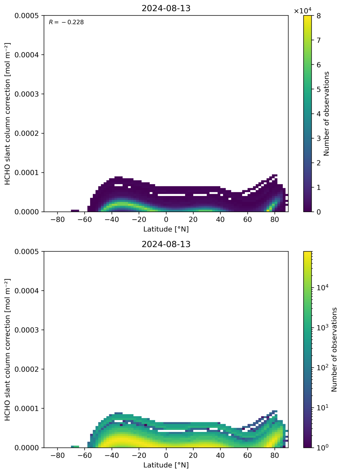
Figure 158: Scatter density plot of “Latitude” against “HCHO slant column correction” for 2024-08-12 to 2024-08-14.
