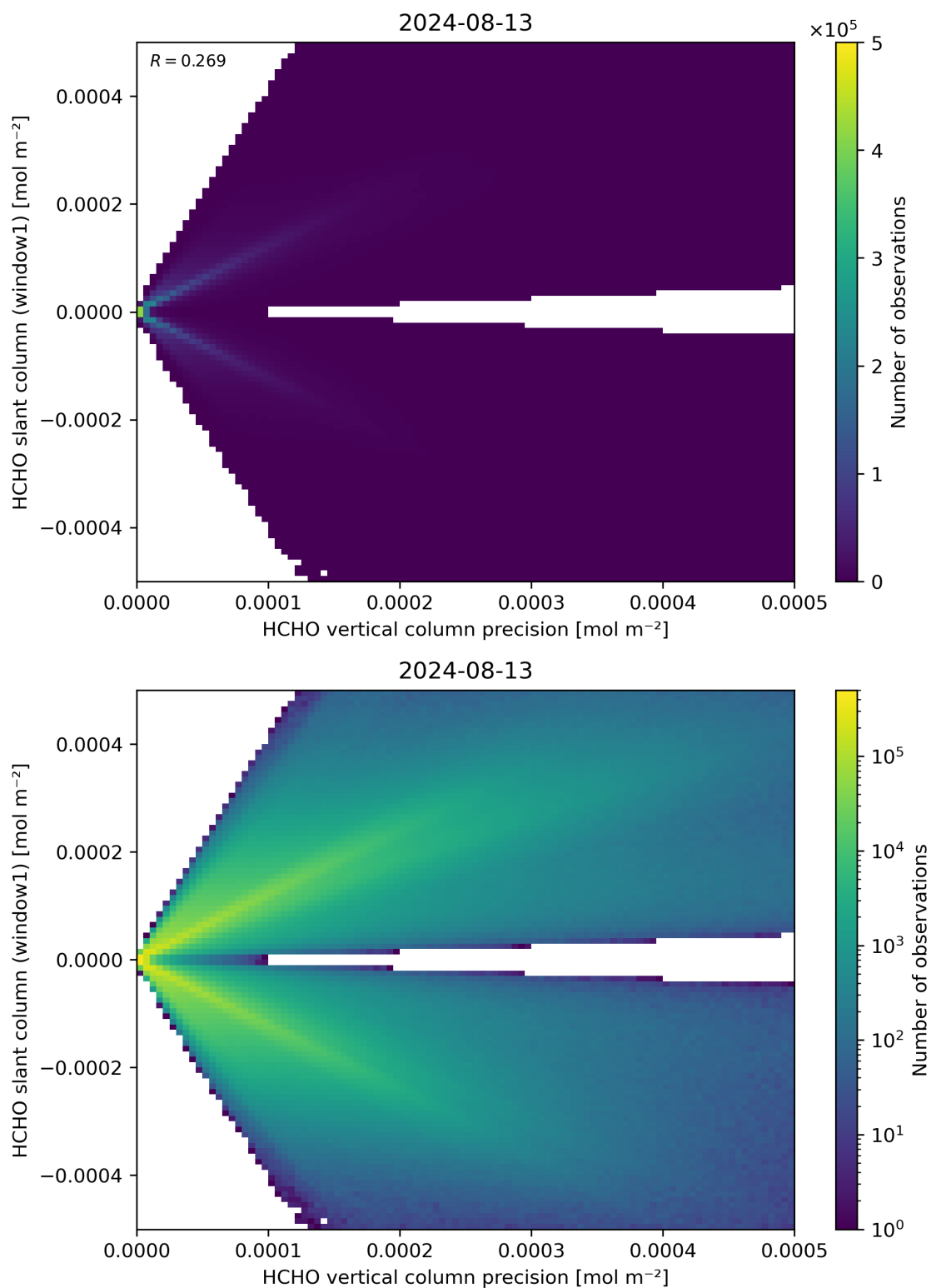
Figure 142: Scatter density plot of “HCHO vertical column precision” against “HCHO slant column (window1)” for 2024-08-12 to 2024-08-14.
