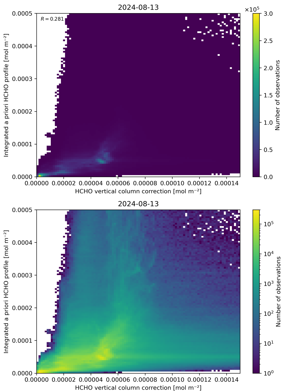
Figure 122: Scatter density plot of “HCHO vertical column correction” against “Integrated a priori HCHO profile” for 2024-08-12 to 2024-08-14.
