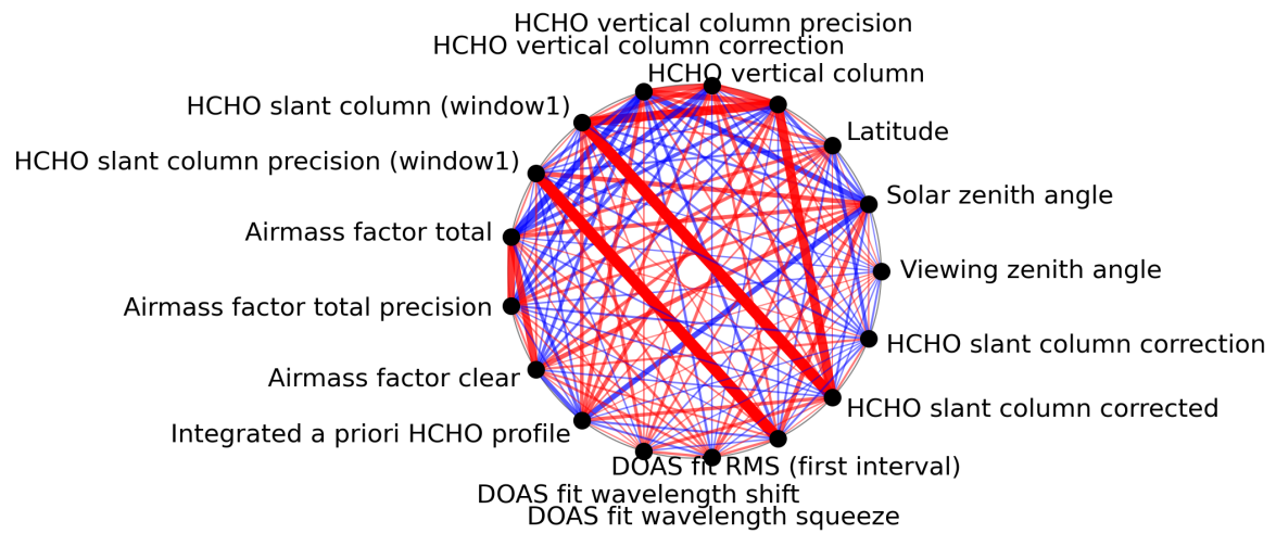
Figure 1: Map of correlation graph for 2024-08-12 to 2024-08-14.
