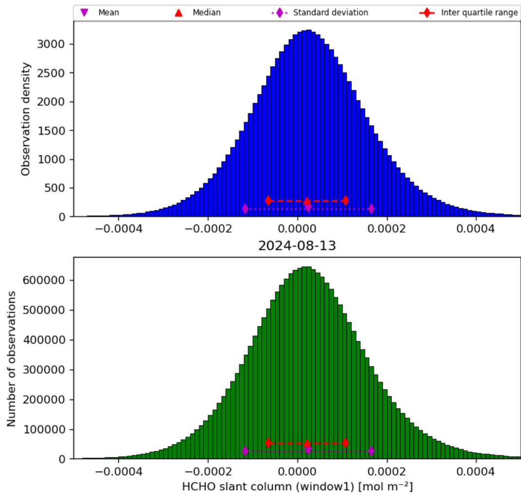
Figure 38: Histogram of “HCHO slant column (window1)” for 2024-08-12 to 2024-08-14
