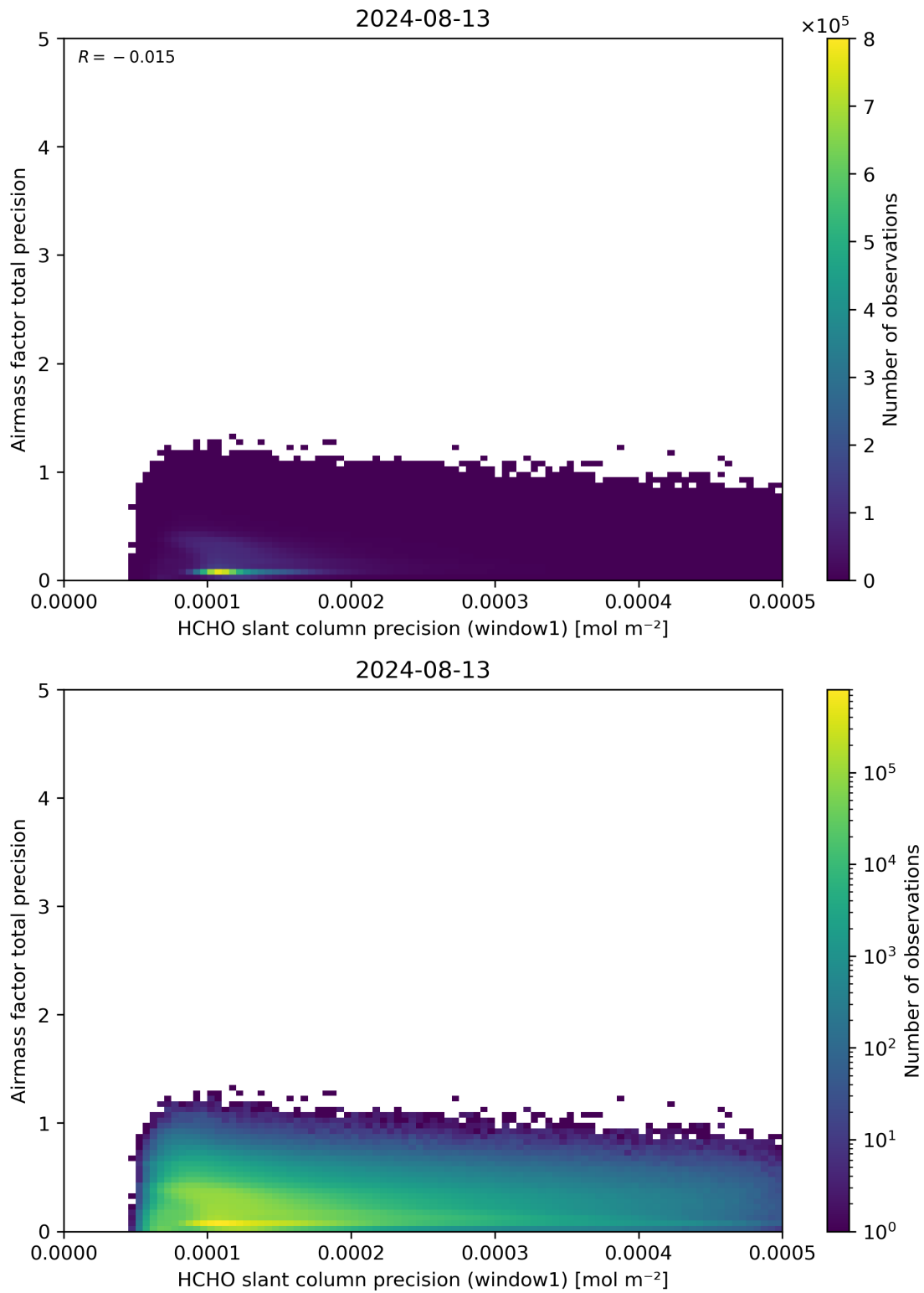
Figure 95: Scatter density plot of “HCHO slant column precision (window1)” against “Airmass factor total precision” for 2024-08-12 to 2024-08-14.
