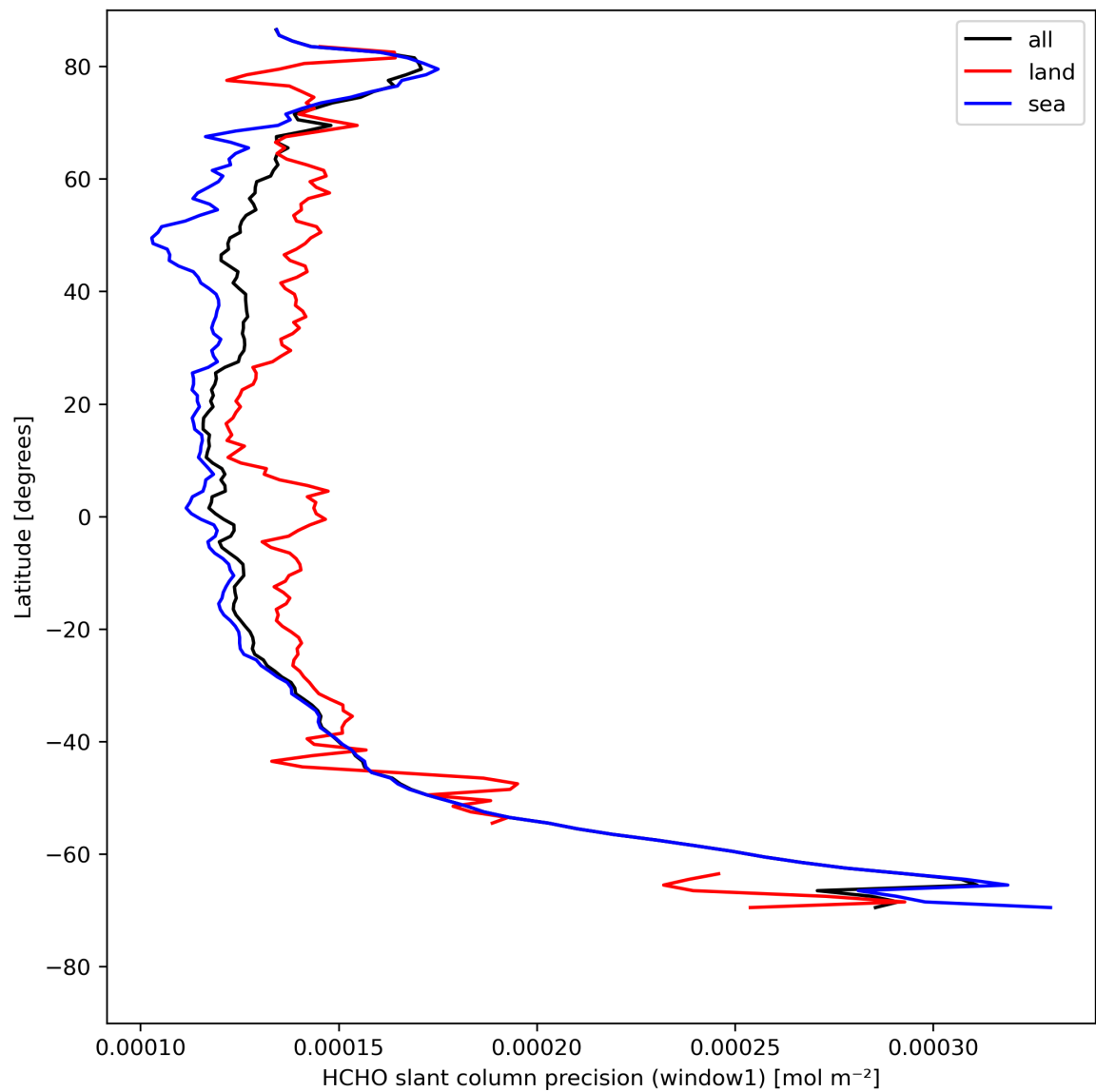
Figure 25: Zonal average of “HCHO slant column precision (window1)” for 2024-08-12 to 2024-08-14.
