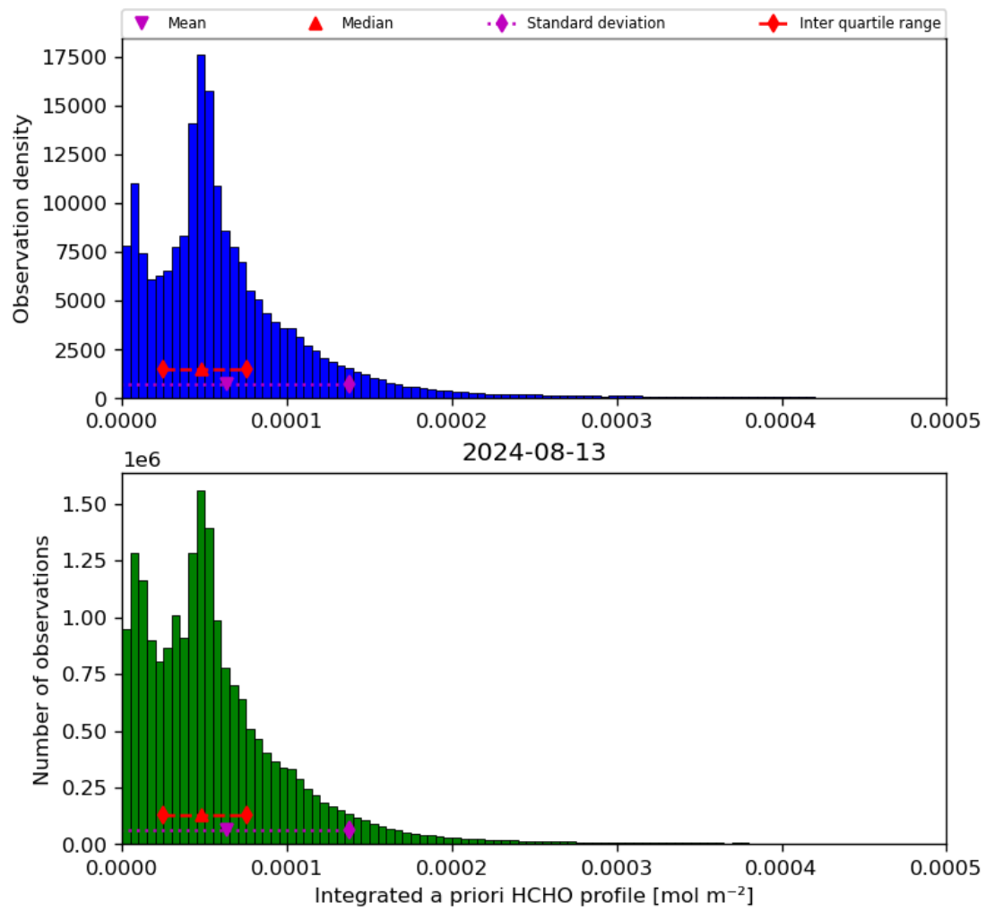
Figure 43: Histogram of “Integrated a priori HCHO profile” for 2024-08-12 to 2024-08-14
