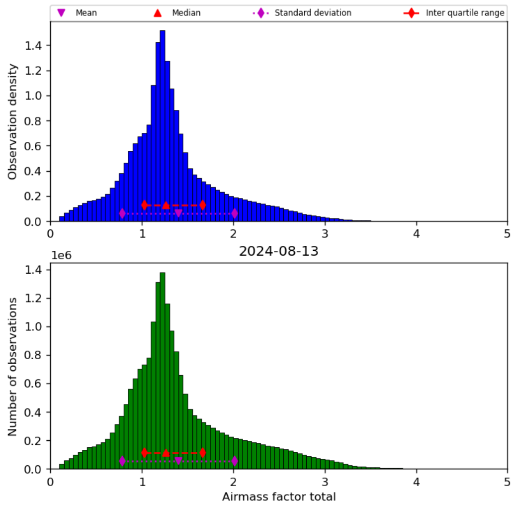
Figure 40: Histogram of “Airmass factor total” for 2024-08-12 to 2024-08-14
