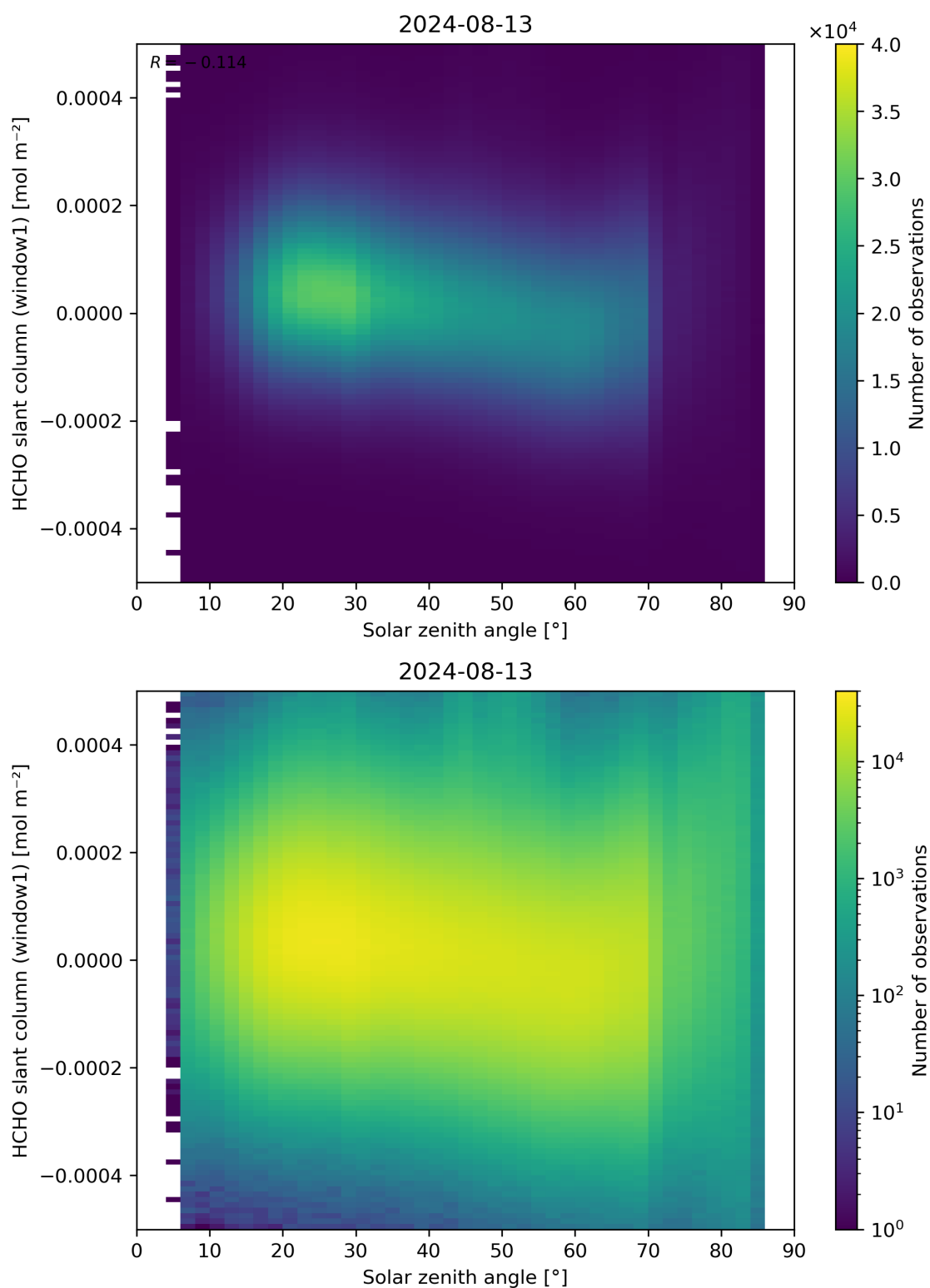
Figure 173: Scatter density plot of “Solar zenith angle” against “HCHO slant column (window1)” for 2024-08-12 to 2024-08-14.
