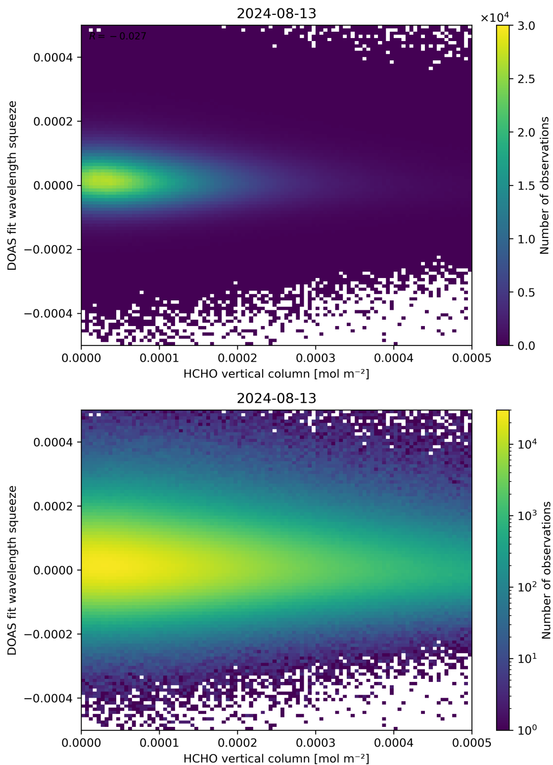
Figure 125: Scatter density plot of “HCHO vertical column” against “DOAS fit wavelength squeeze” for 2024-08-12 to 2024-08-14.
