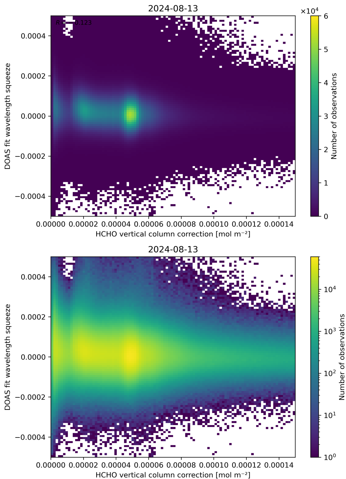
Figure 114: Scatter density plot of “HCHO vertical column correction” against “DOAS fit wavelength squeeze” for 2024-08-12 to 2024-08-14.
