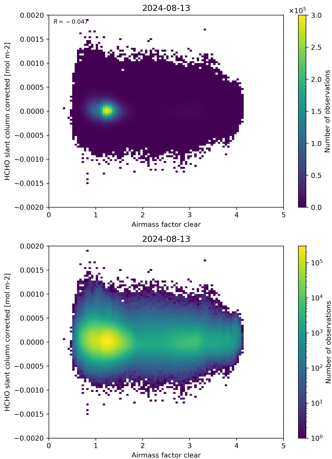
Figure 74: Scatter density plot of “Airmass factor clear” against “HCHO slant column corrected” for 2024-08-12 to 2024-08-14.
