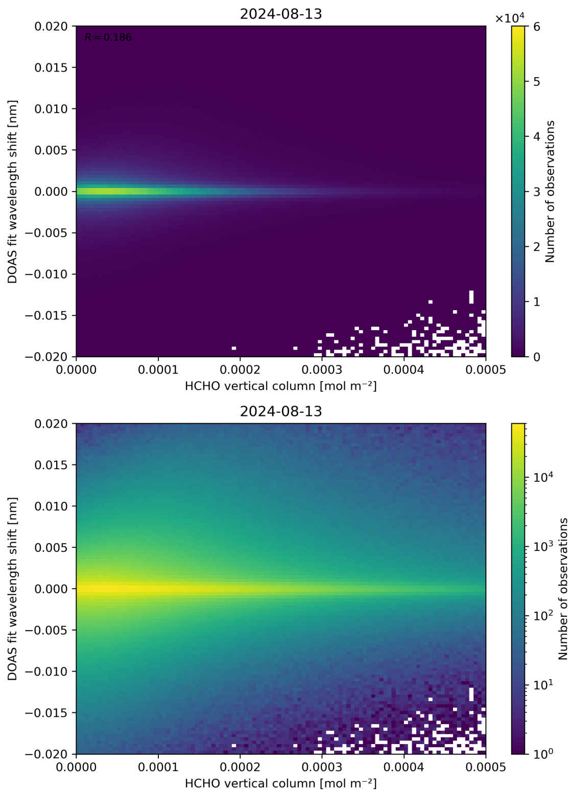
Figure 124: Scatter density plot of “HCHO vertical column” against “DOAS fit wavelength shift” for 2024-08-12 to 2024-08-14.
