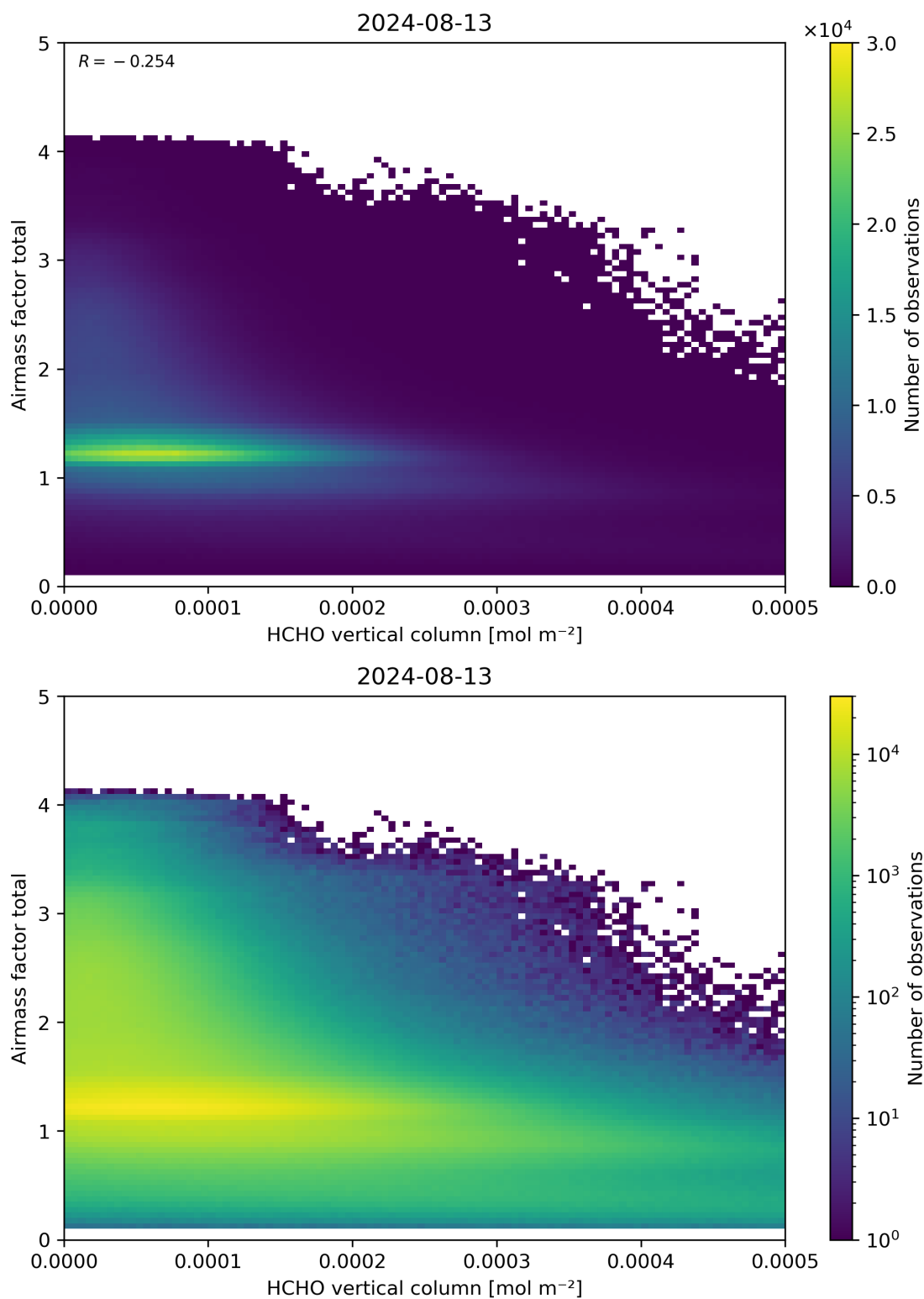
Figure 131: Scatter density plot of “HCHO vertical column” against “Airmass factor total” for 2024-08-12 to 2024-08-14.
