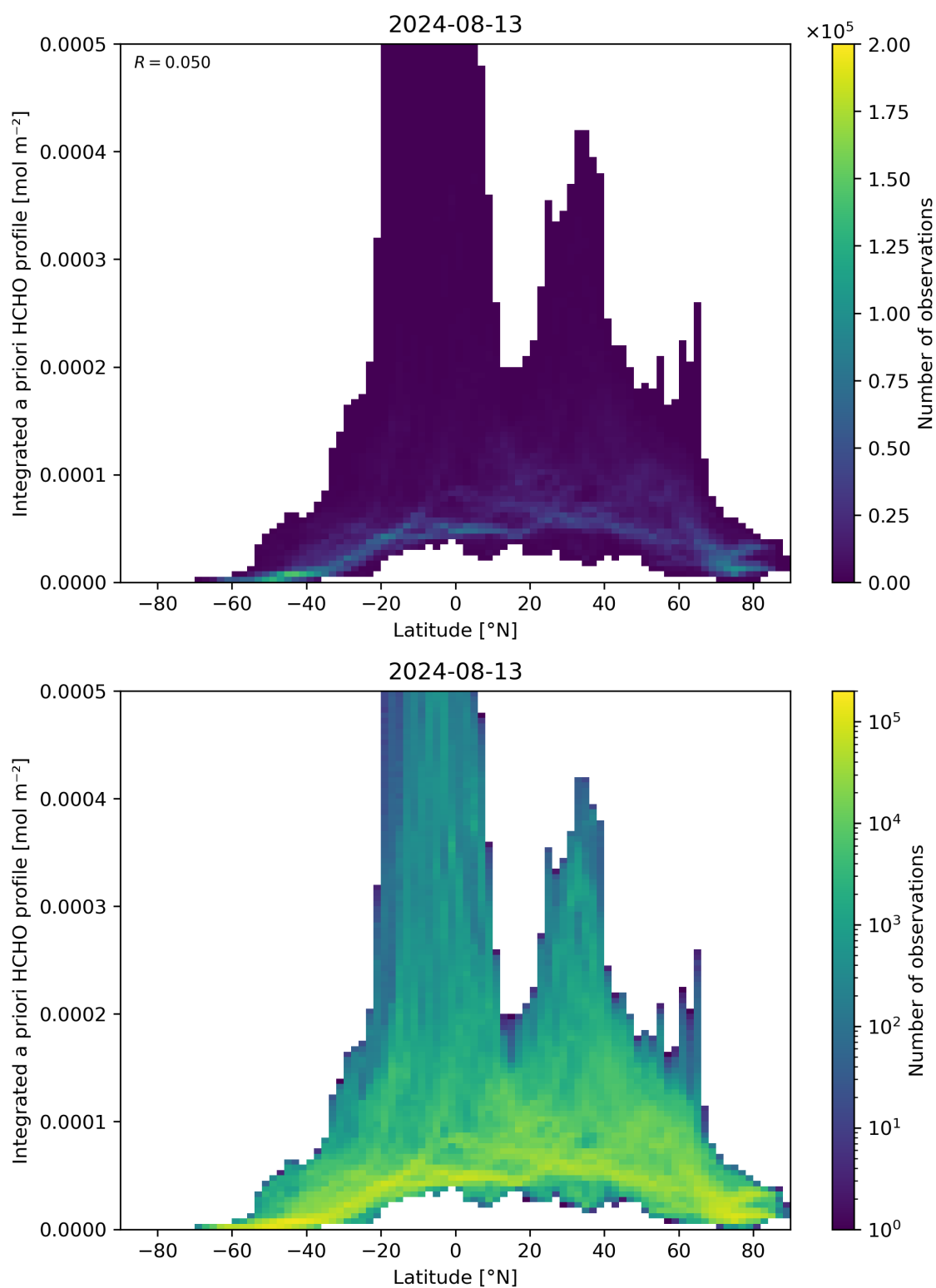
Figure 166: Scatter density plot of “Latitude” against “Integrated a priori HCHO profile” for 2024-08-12 to 2024-08-14.
