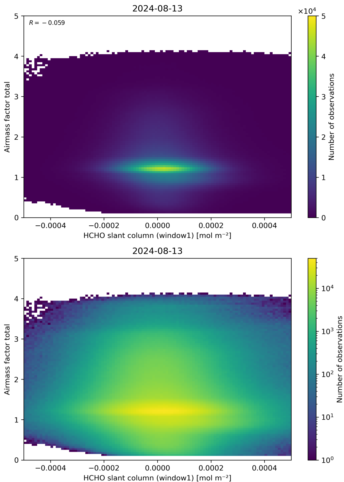
Figure 85: Scatter density plot of “HCHO slant column (window1)” against “Airmass factor total” for 2024-08-12 to 2024-08-14.
