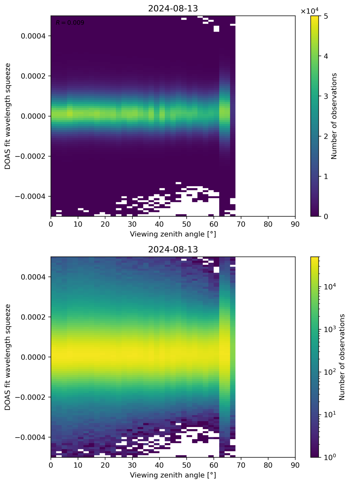
Figure 184: Scatter density plot of “Viewing zenith angle” against “DOAS fit wavelength squeeze” for 2024-08-12 to 2024-08-14.
