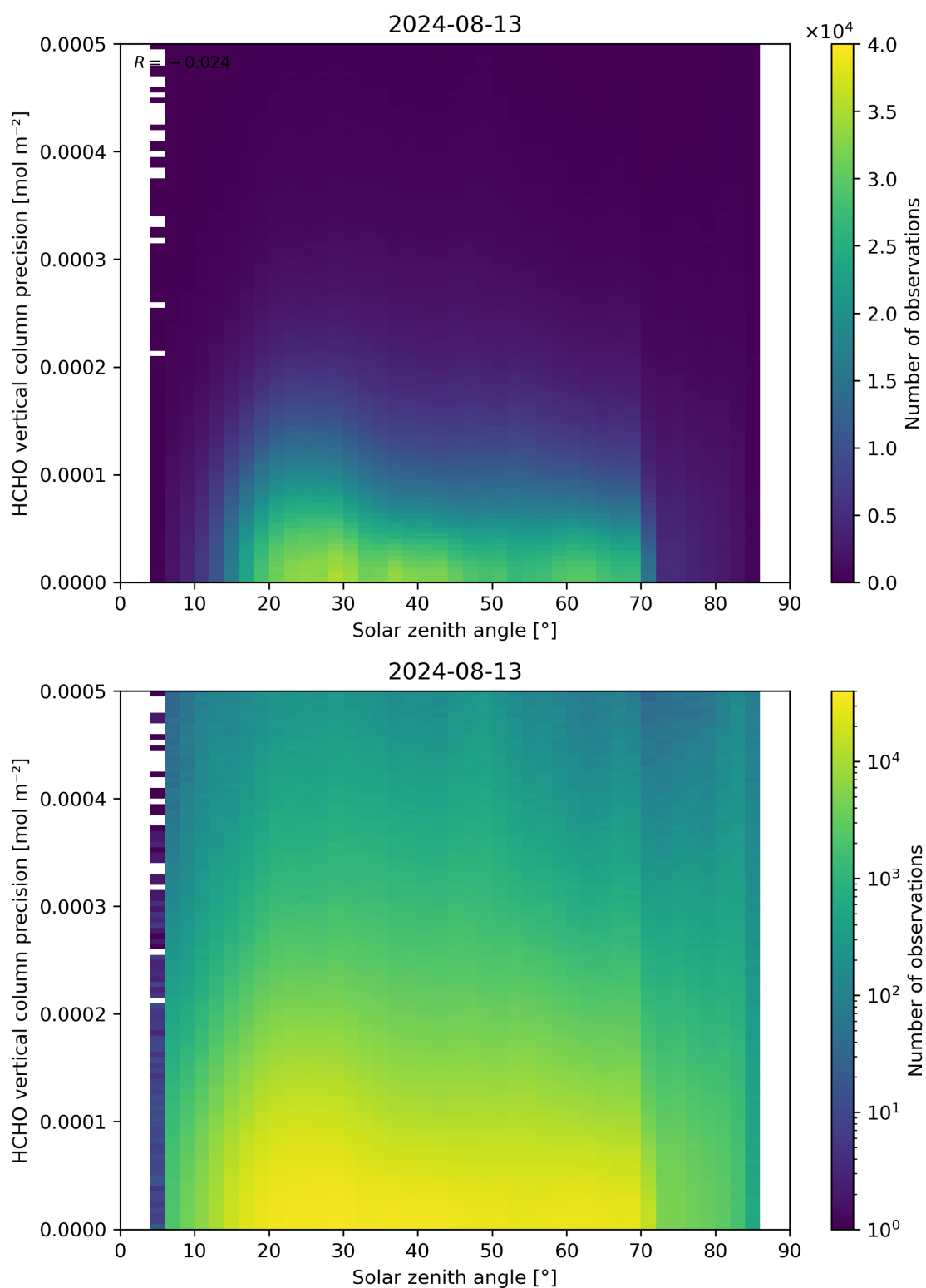
Figure 179: Scatter density plot of “Solar zenith angle” against “HCHO vertical column precision” for 2024-08-12 to 2024-08-14.
