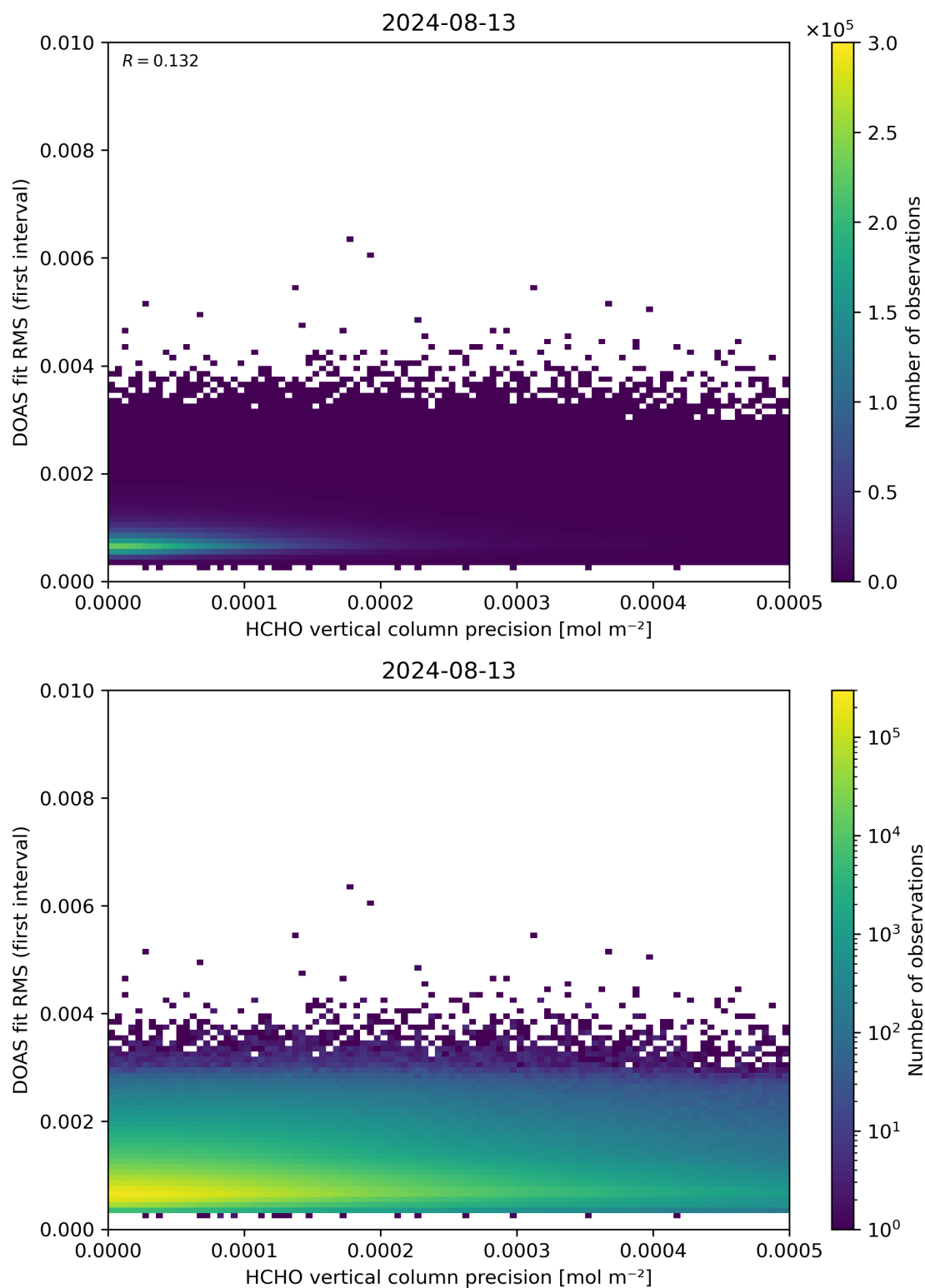
Figure 136: Scatter density plot of “HCHO vertical column precision” against “DOAS fit RMS (first interval)” for 2024-08-12 to 2024-08-14.
