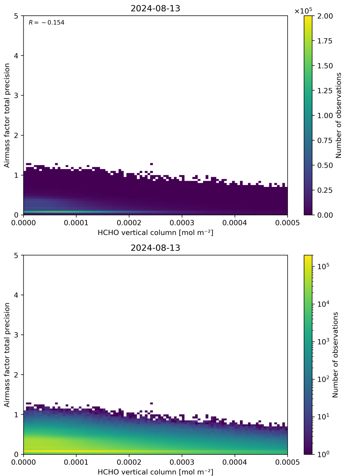
Figure 132: Scatter density plot of “HCHO vertical column” against “Airmass factor total precision” for 2024-08-12 to 2024-08-14.
