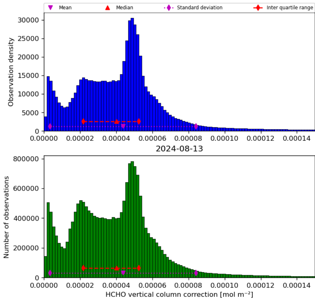
Figure 37: Histogram of “HCHO vertical column correction” for 2024-08-12 to 2024-08-14
