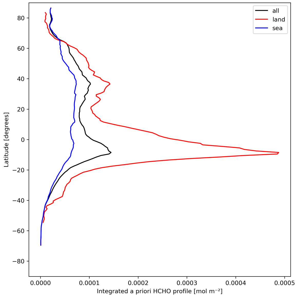
Figure 29: Zonal average of “Integrated a priori HCHO profile” for 2024-08-12 to 2024-08-14.
