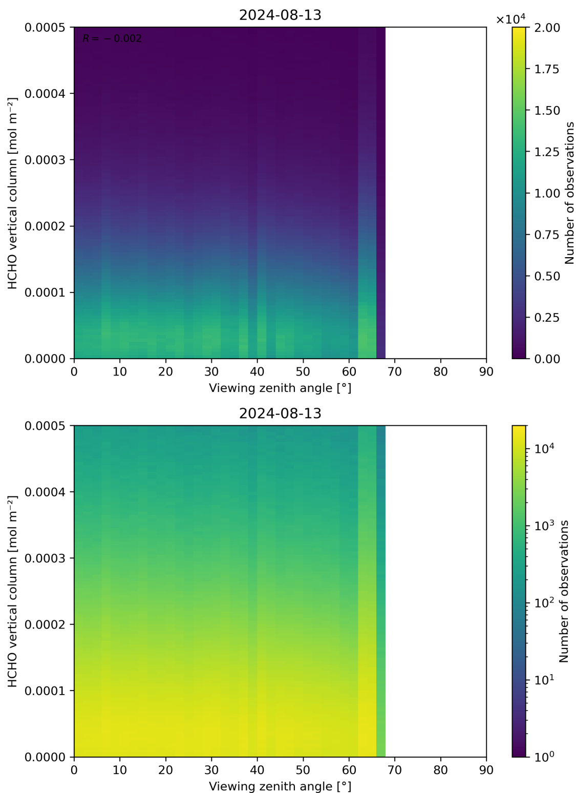
Figure 192: Scatter density plot of “Viewing zenith angle” against “HCHO vertical column” for 2024-08-12 to 2024-08-14.
