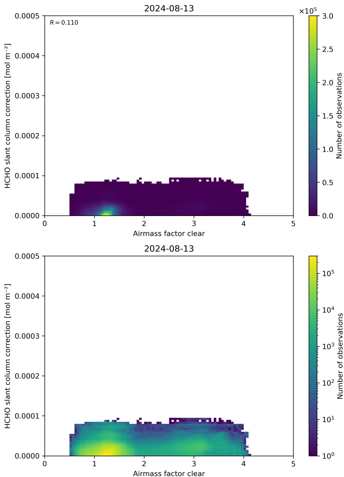
Figure 75: Scatter density plot of “Airmass factor clear” against “HCHO slant column correction” for 2024-08-12 to 2024-08-14.
