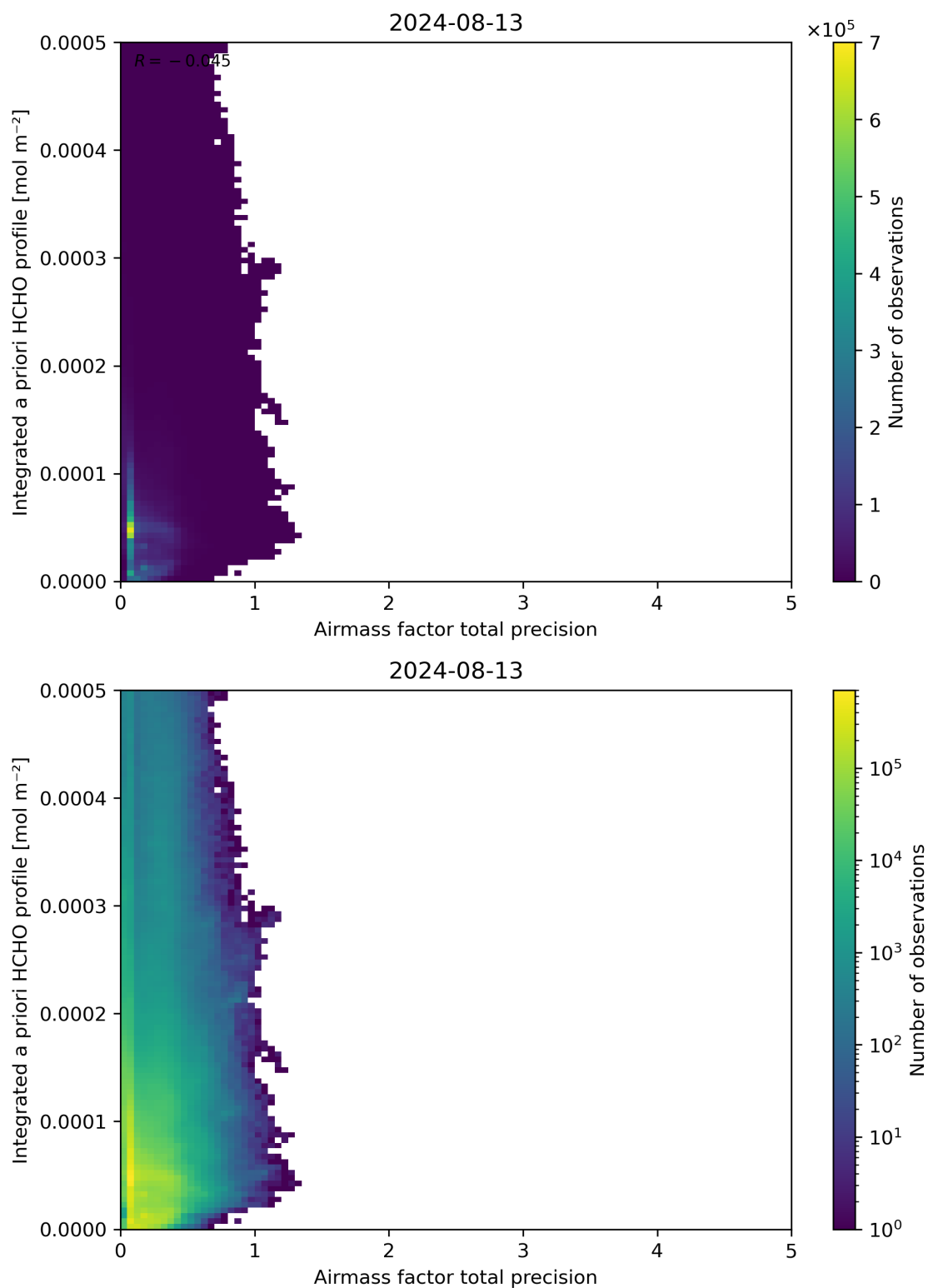
Figure 111: Scatter density plot of “Airmass factor total precision” against “Integrated a priori HCHO profile” for 2024-08-12 to 2024-08-14.
