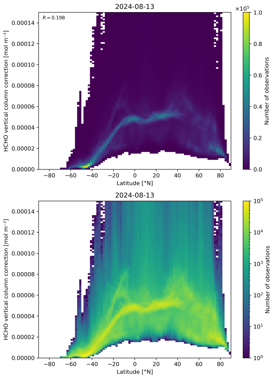
Figure 164: Scatter density plot of “Latitude” against “HCHO vertical column correction” for 2024-08-12 to 2024-08-14.
