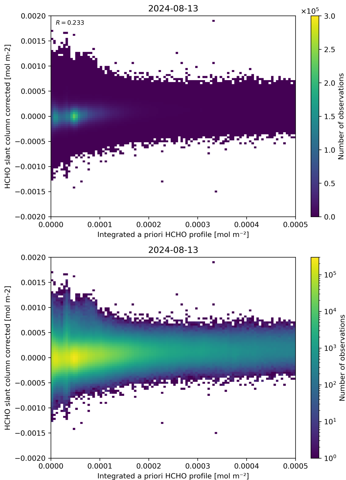
Figure 151: Scatter density plot of “Integrated a priori HCHO profile” against “HCHO slant column corrected” for 2024-08-12 to 2024-08-14.
