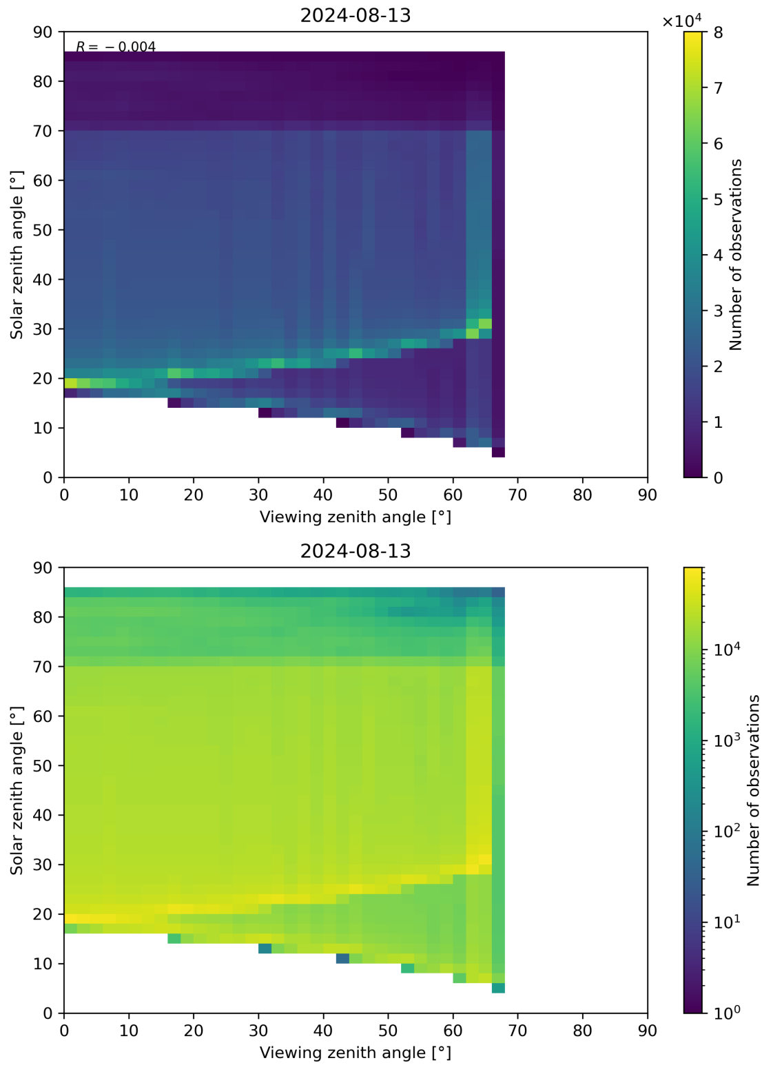
Figure 197: Scatter density plot of “Viewing zenith angle” against “Solar zenith angle” for 2024-08-12 to 2024-08-14.
