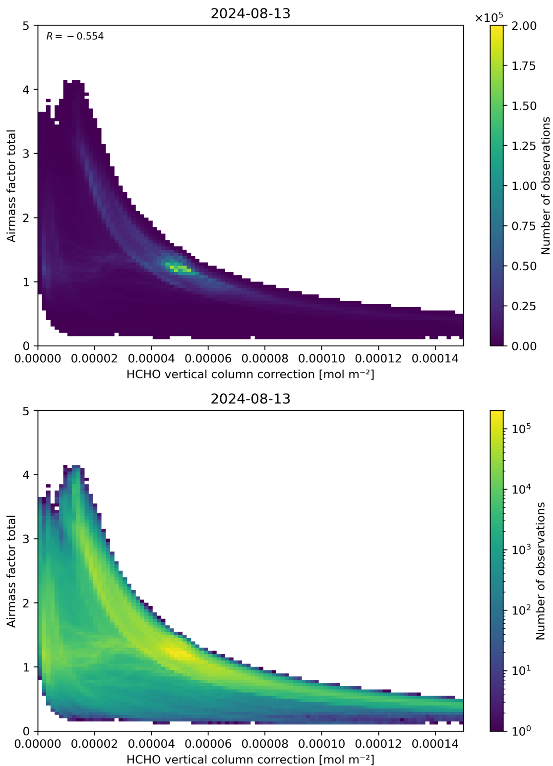
Figure 120: Scatter density plot of “HCHO vertical column correction” against “Airmass factor total” for 2024-08-12 to 2024-08-14.
