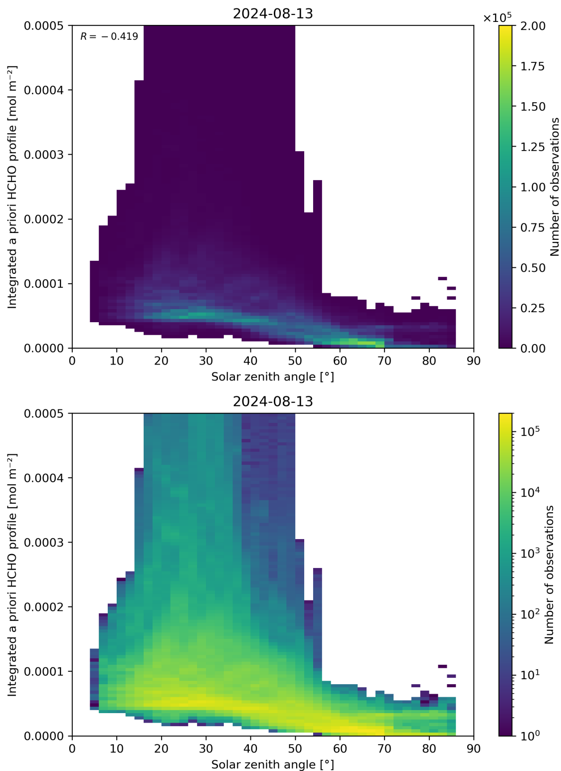
Figure 180: Scatter density plot of “Solar zenith angle” against “Integrated a priori HCHO profile” for 2024-08-12 to 2024-08-14.
