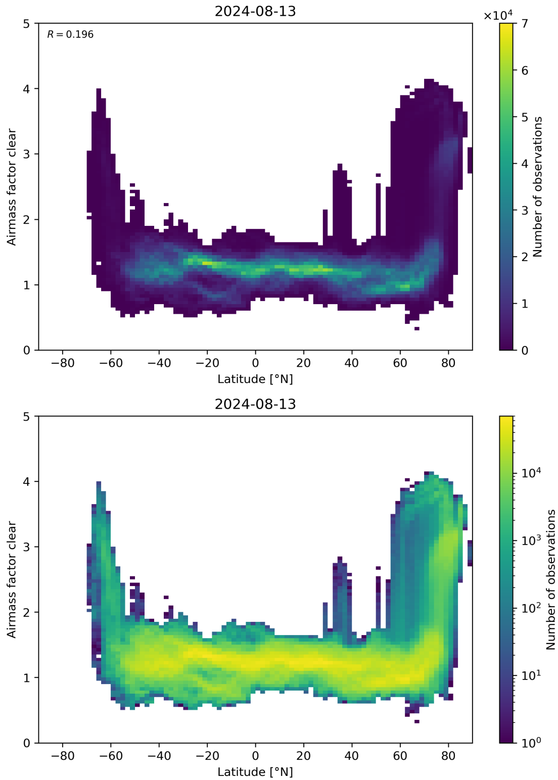
Figure 156: Scatter density plot of “Latitude” against “Airmass factor clear” for 2024-08-12 to 2024-08-14.
