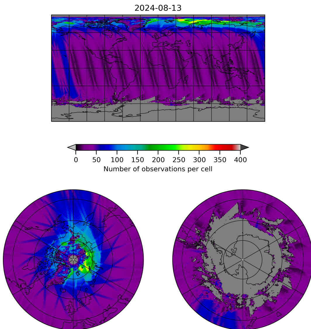
Figure 19: Map of the number of observations for 2024-08-12 to 2024-08-14
