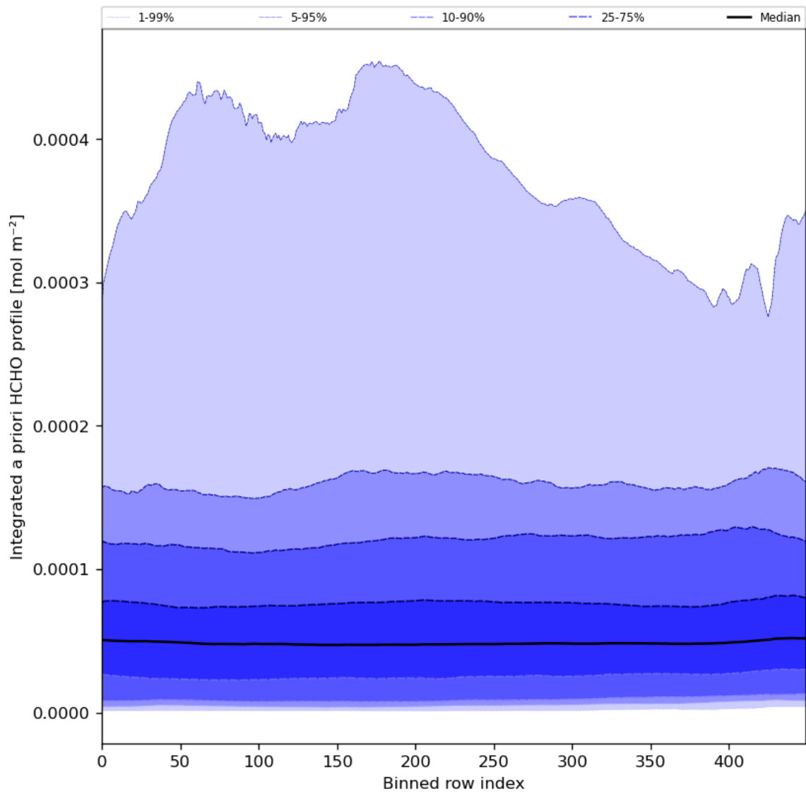
Figure 57: Along track statistics of “Integrated a priori HCHO profile” for 2024-08-12 to 2024-08-14
