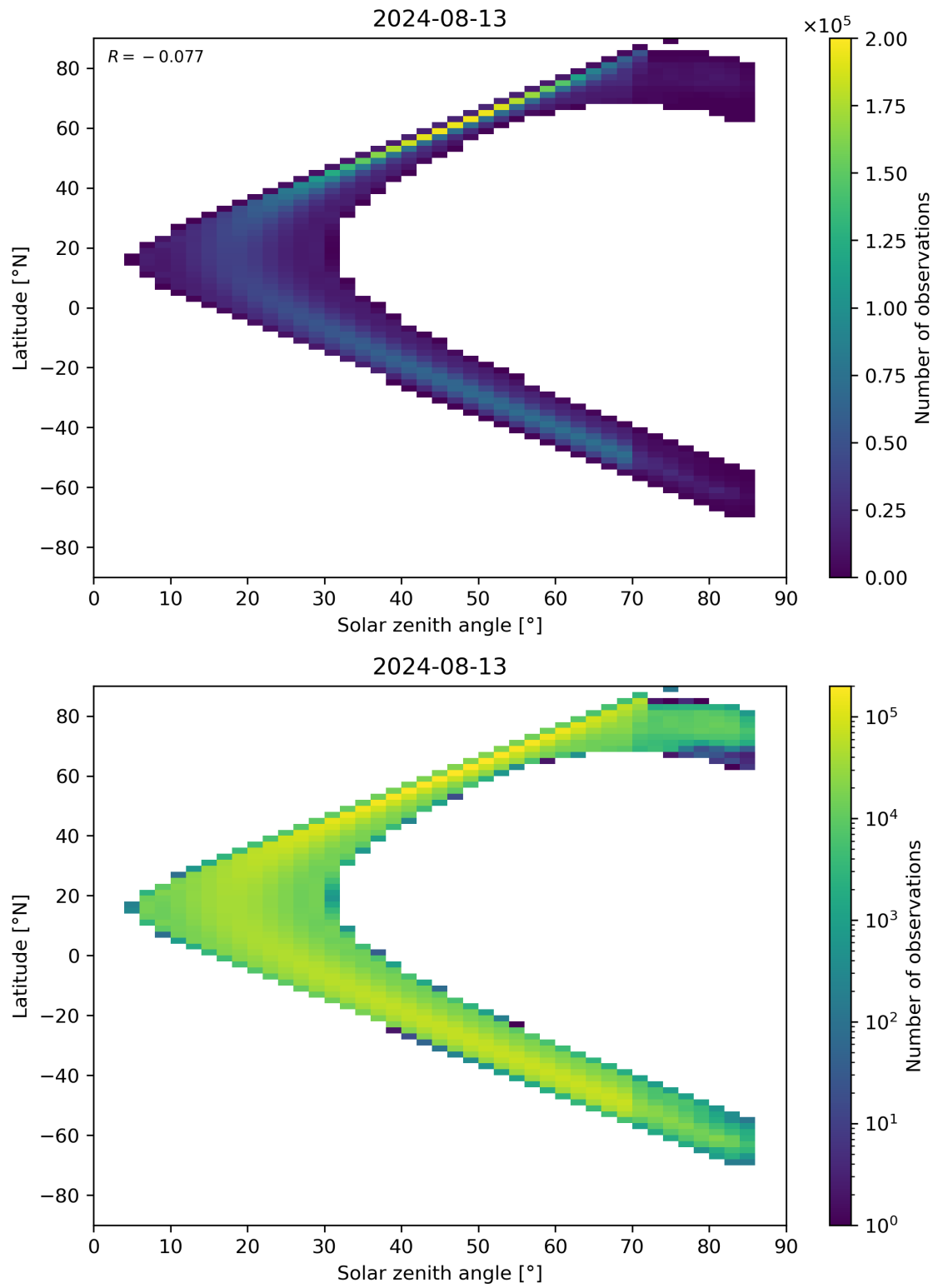
Figure 181: Scatter density plot of “Solar zenith angle” against “Latitude” for 2024-08-12 to 2024-08-14.
