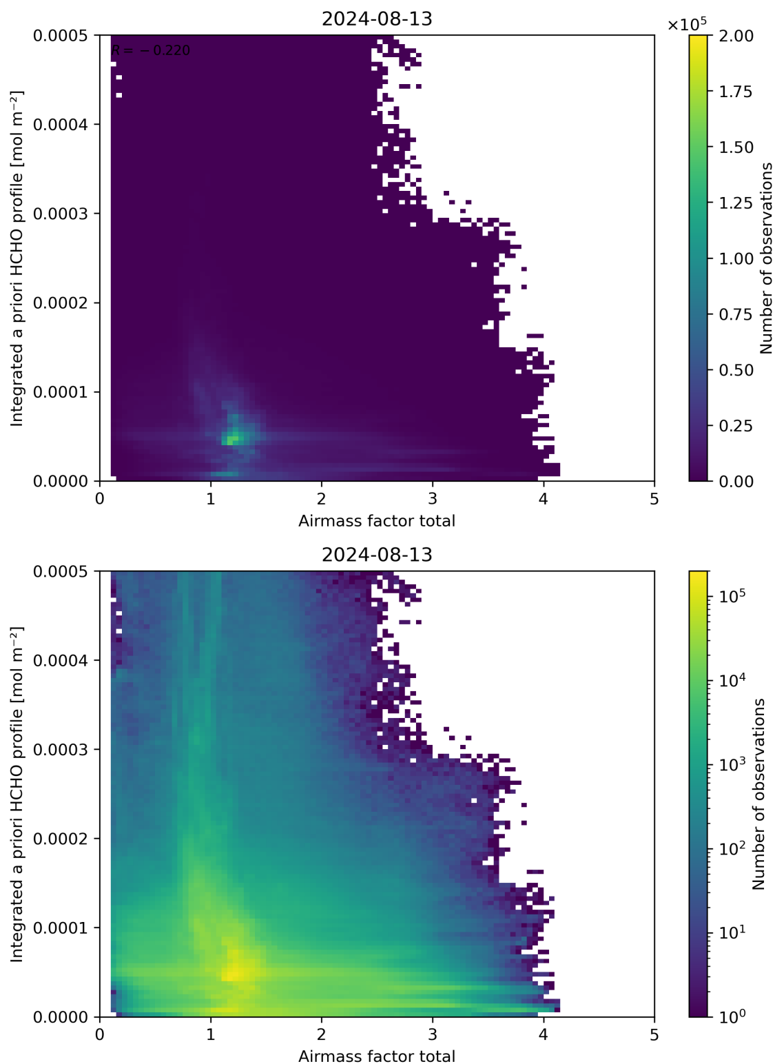
Figure 104: Scatter density plot of “Airmass factor total” against “Integrated a priori HCHO profile” for 2024-08-12 to 2024-08-14.
