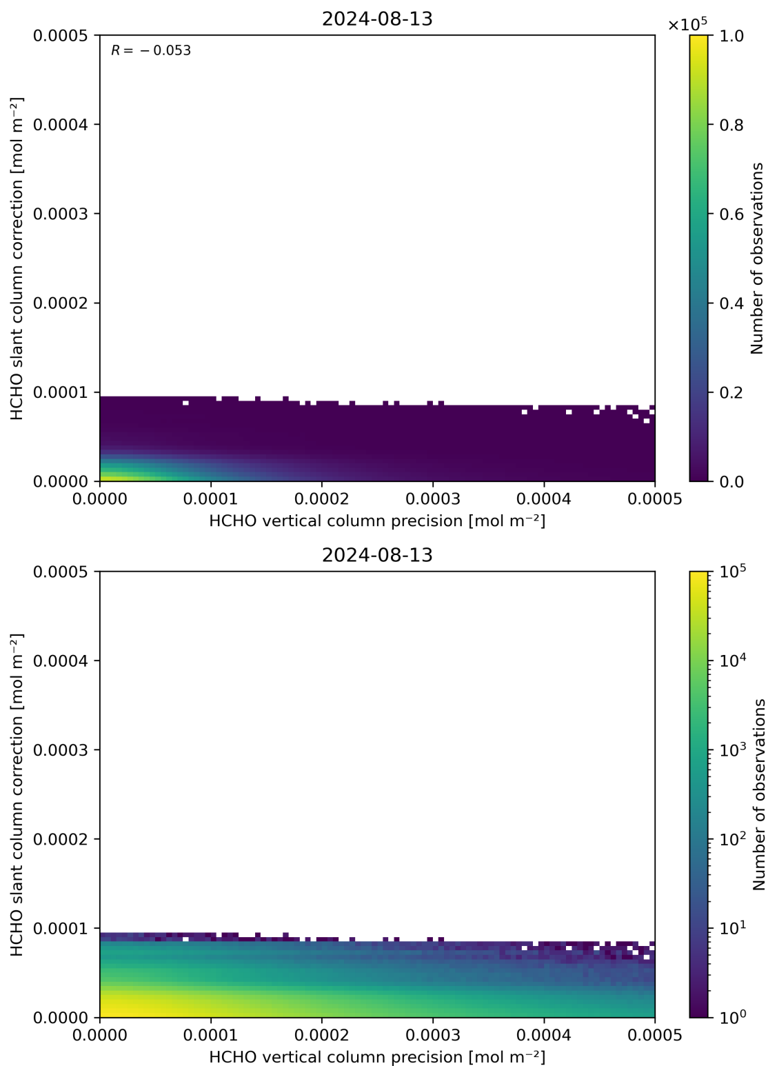
Figure 141: Scatter density plot of “HCHO vertical column precision” against “HCHO slant column correction” for 2024-08-12 to 2024-08-14.
