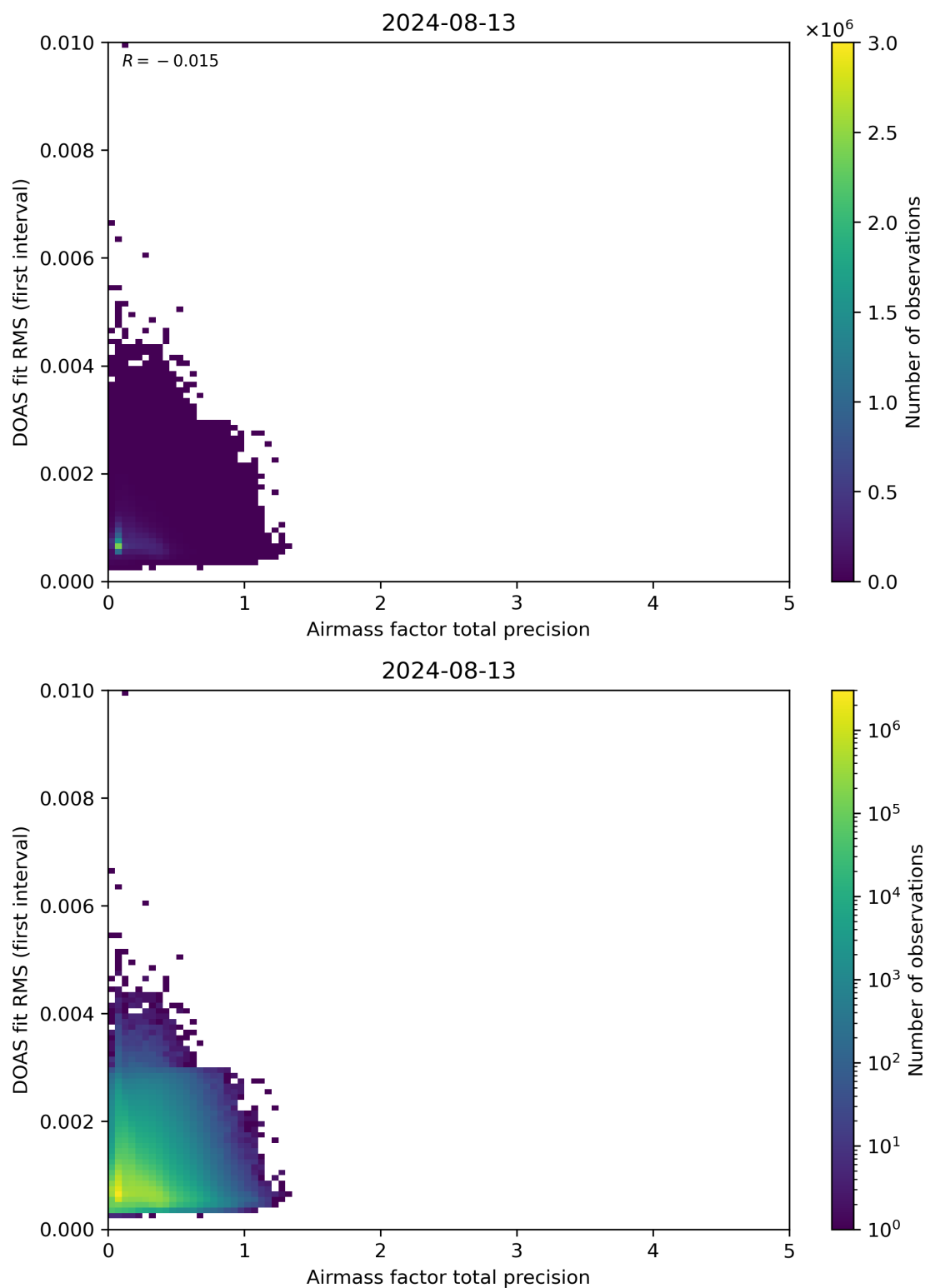
Figure 105: Scatter density plot of “Airmass factor total precision” against “DOAS fit RMS (first interval)” for 2024-08-12 to 2024-08-14.
