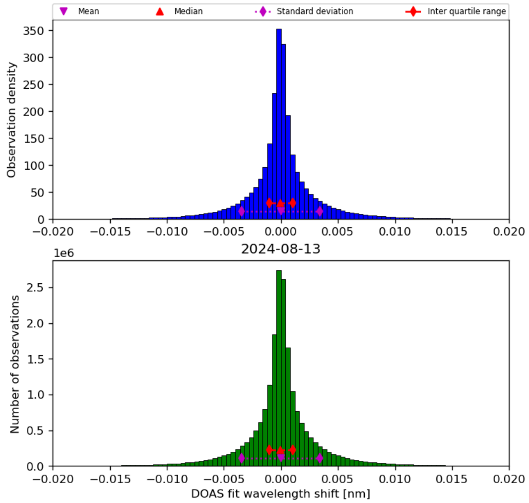
Figure 44: Histogram of “DOAS fit wavelength shift” for 2024-08-12 to 2024-08-14
