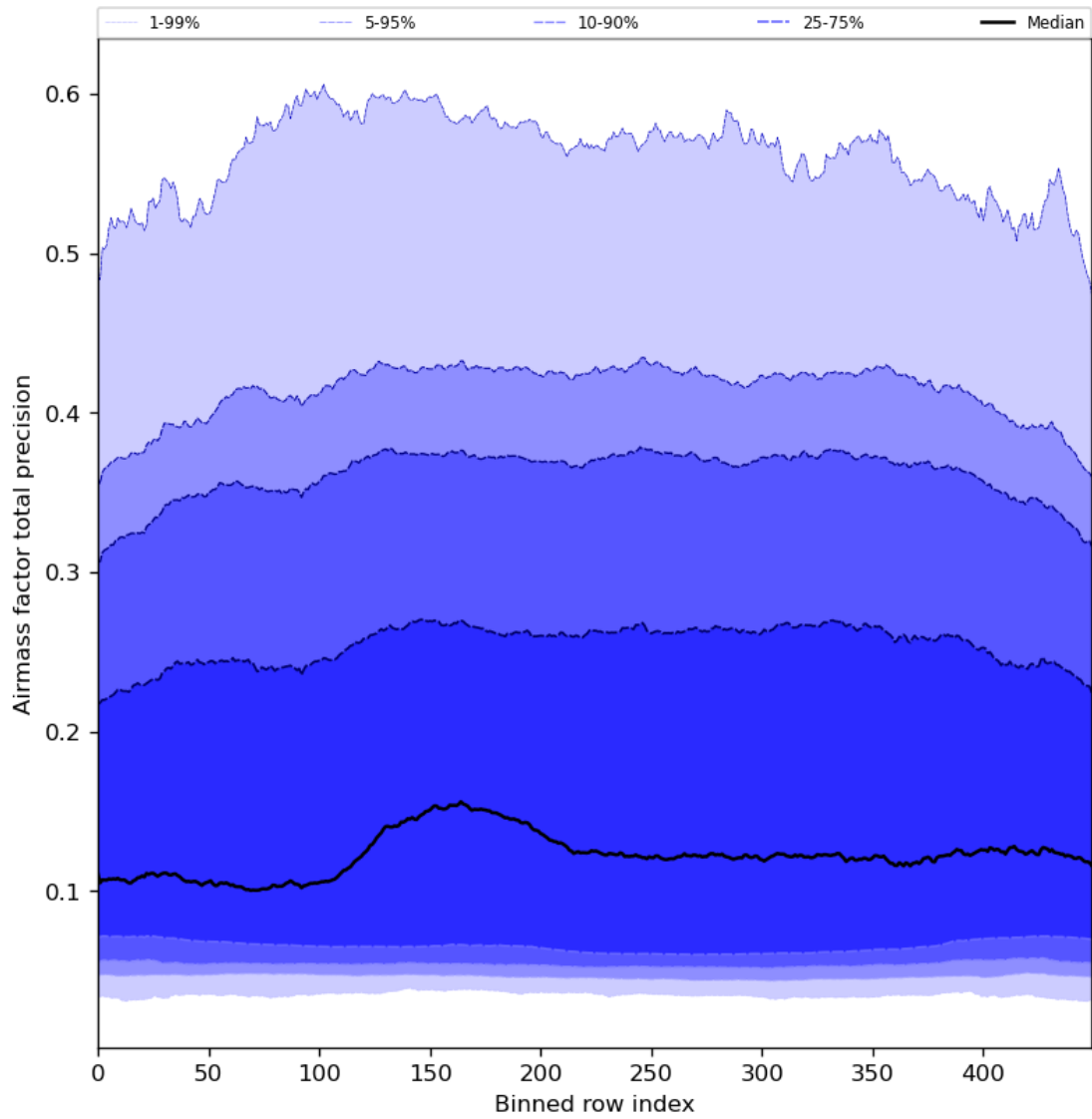
Figure 55: Along track statistics of “Airmass factor total precision” for 2024-08-12 to 2024-08-14
