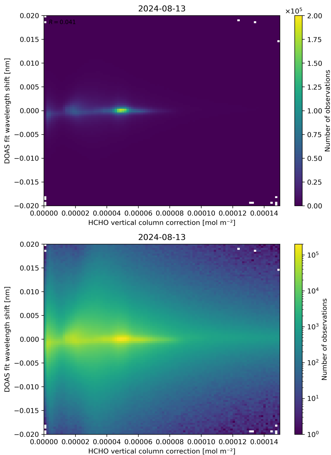
Figure 113: Scatter density plot of “HCHO vertical column correction” against “DOAS fit wavelength shift” for 2024-08-12 to 2024-08-14.
