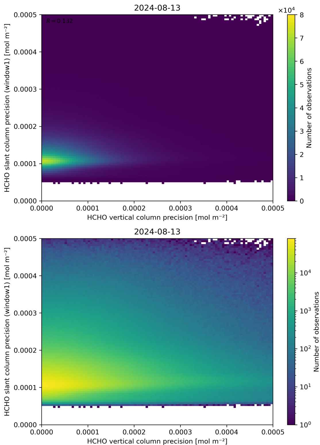
Figure 143: Scatter density plot of “HCHO vertical column precision” against “HCHO slant column precision (window1)” for 2024-08-12 to 2024-08-14.
