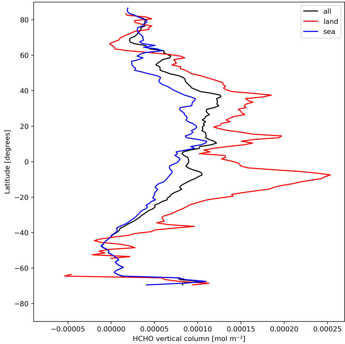
Figure 21: Zonal average of “HCHO vertical column” for 2024-08-12 to 2024-08-14.
