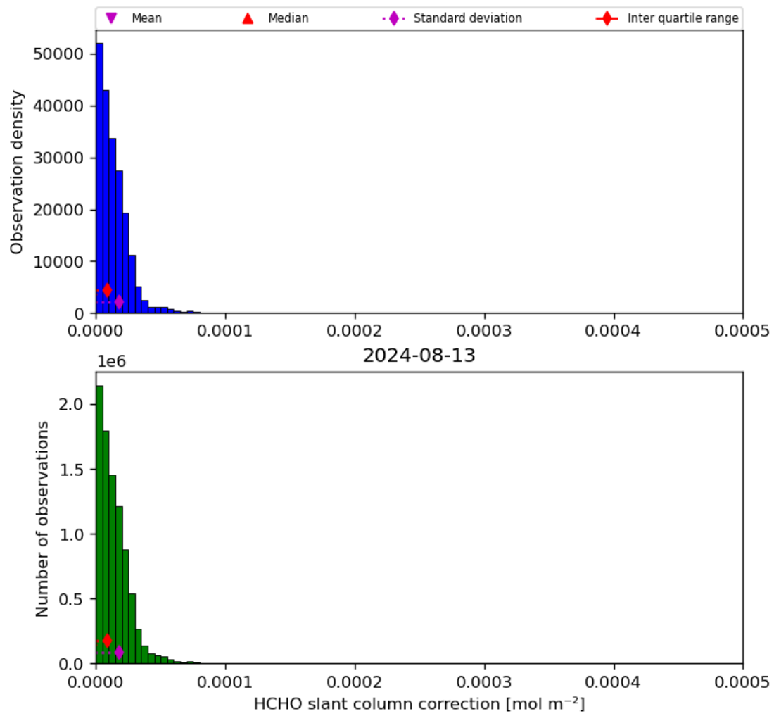
Figure 47: Histogram of “HCHO slant column correction” for 2024-08-12 to 2024-08-14
