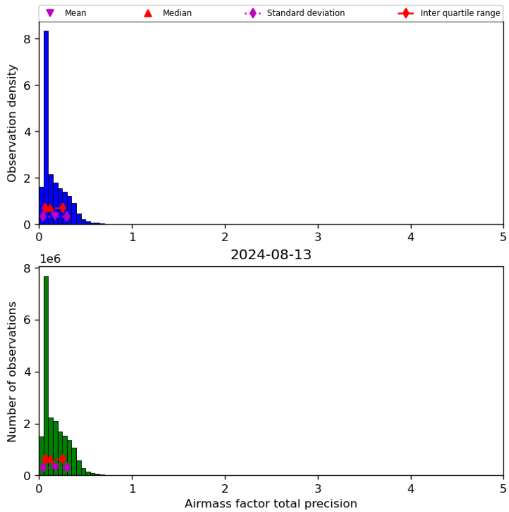
Figure 41: Histogram of “Airmass factor total precision” for 2024-08-12 to 2024-08-14
