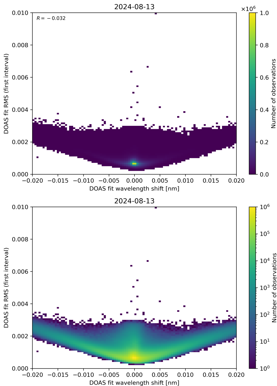
Figure 64: Scatter density plot of “DOAS fit wavelength shift” against “DOAS fit RMS (first interval)” for 2024-08-12 to 2024-08-14.
