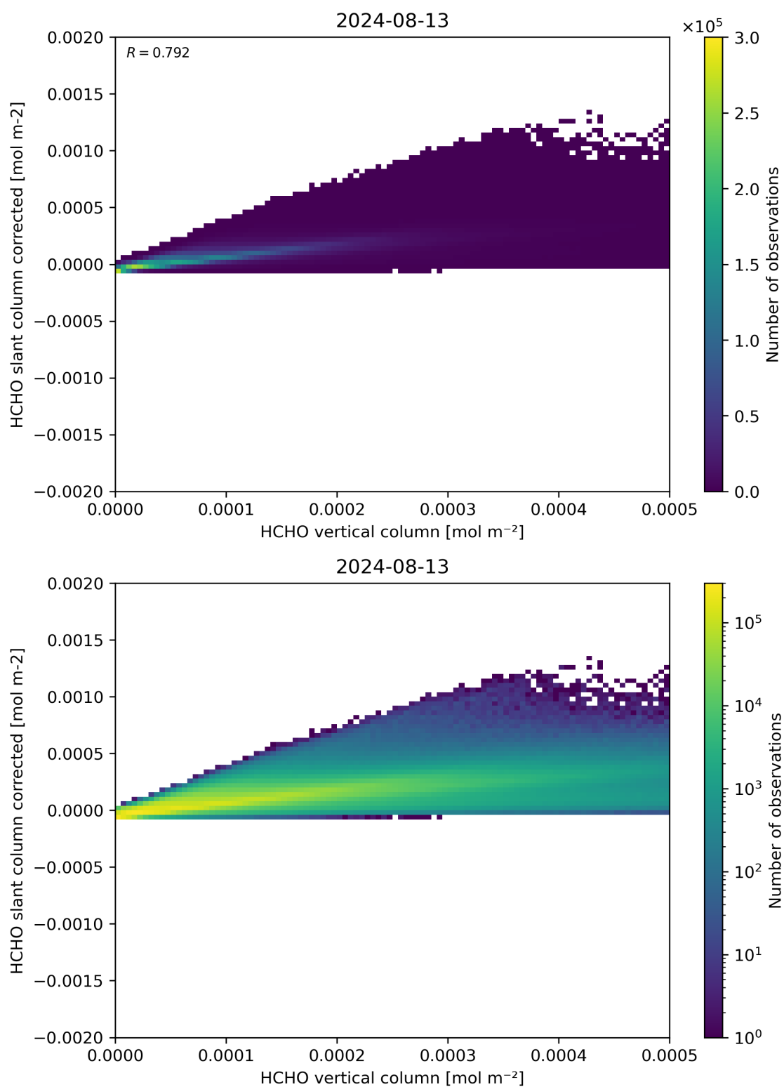
Figure 127: Scatter density plot of “HCHO vertical column” against “HCHO slant column corrected” for 2024-08-12 to 2024-08-14.
