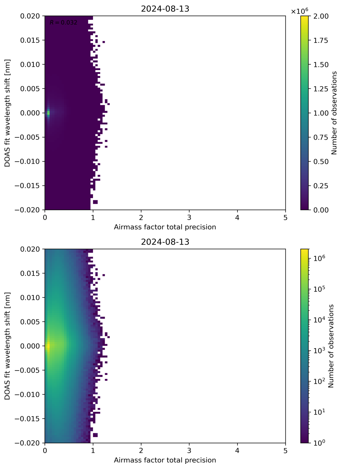
Figure 106: Scatter density plot of “Airmass factor total precision” against “DOAS fit wavelength shift” for 2024-08-12 to 2024-08-14.
