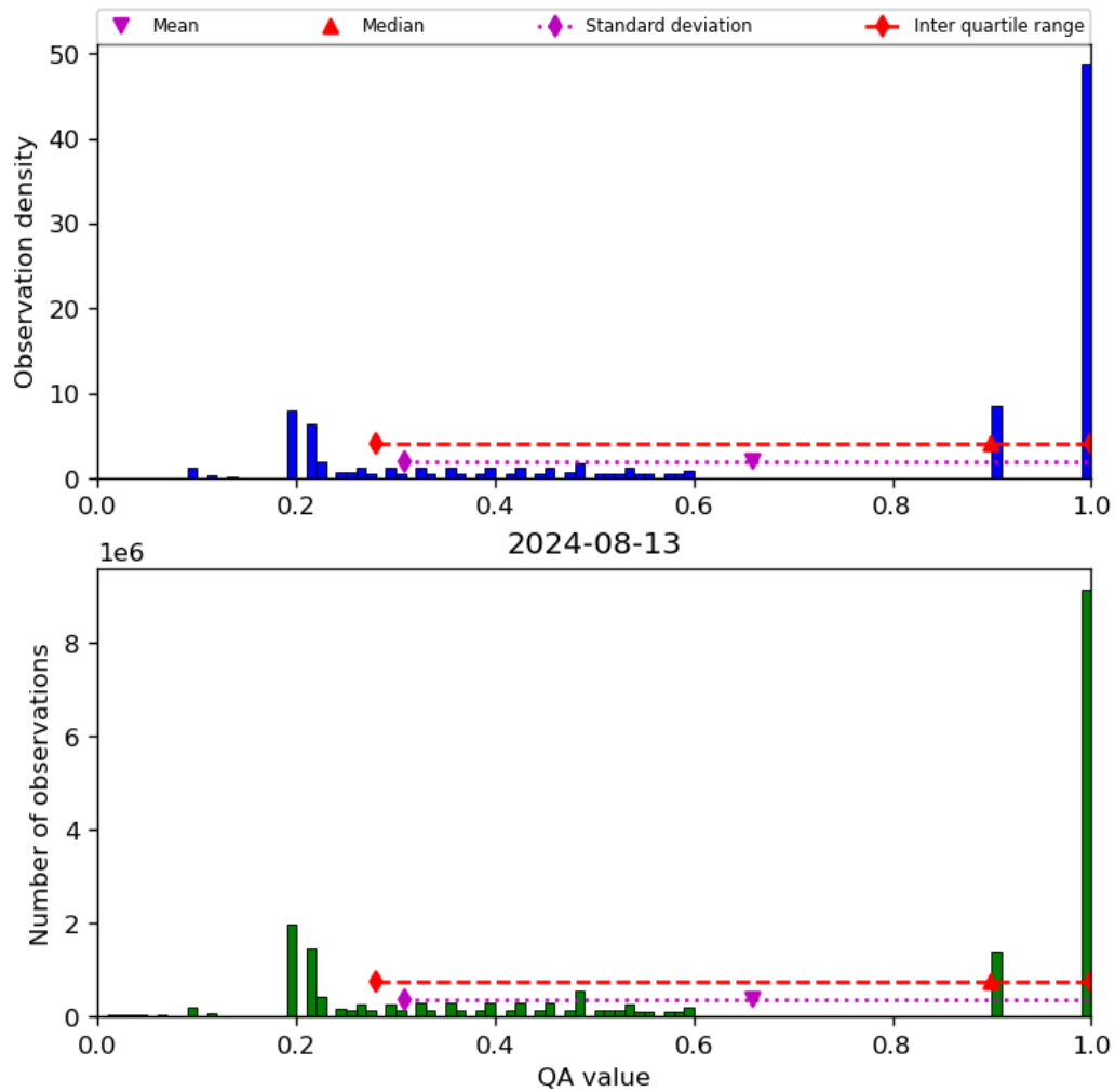
Figure 34: Histogram of “QA value” for 2024-08-12 to 2024-08-14
