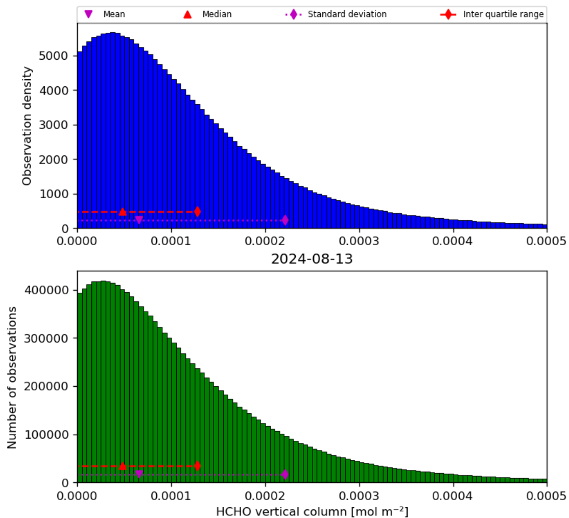
Figure 35: Histogram of “HCHO vertical column” for 2024-08-12 to 2024-08-14
