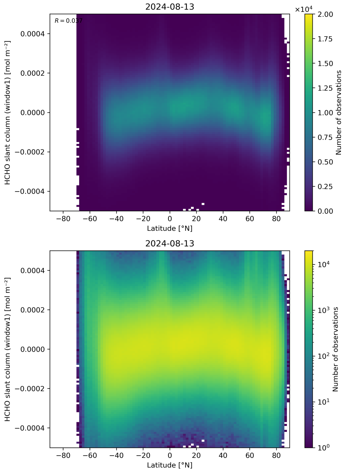
Figure 159: Scatter density plot of “Latitude” against “HCHO slant column (window1)” for 2024-08-12 to 2024-08-14.
