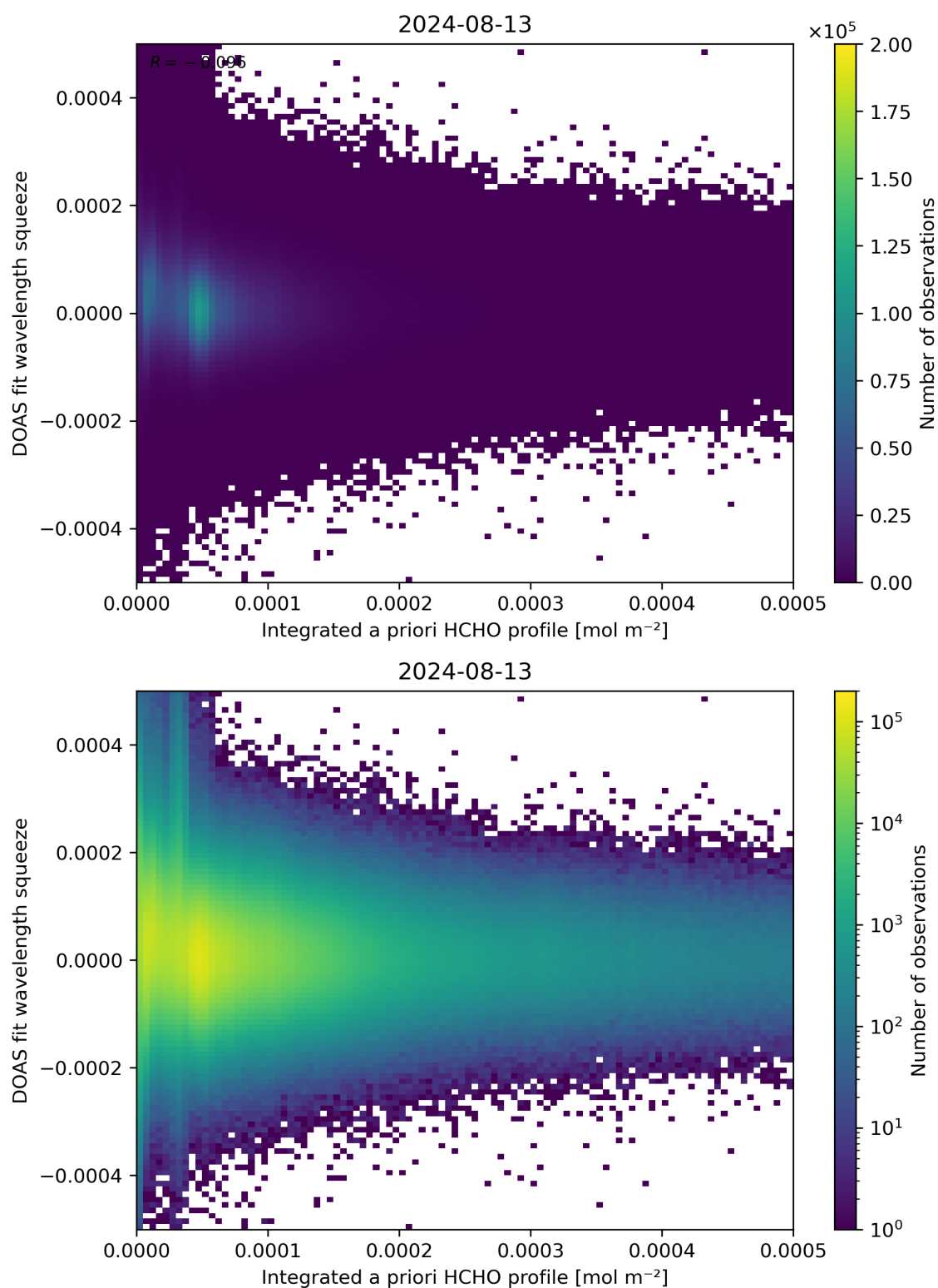
Figure 150: Scatter density plot of “Integrated a priori HCHO profile” against “DOAS fit wavelength squeeze” for 2024-08-12 to 2024-08-14.
