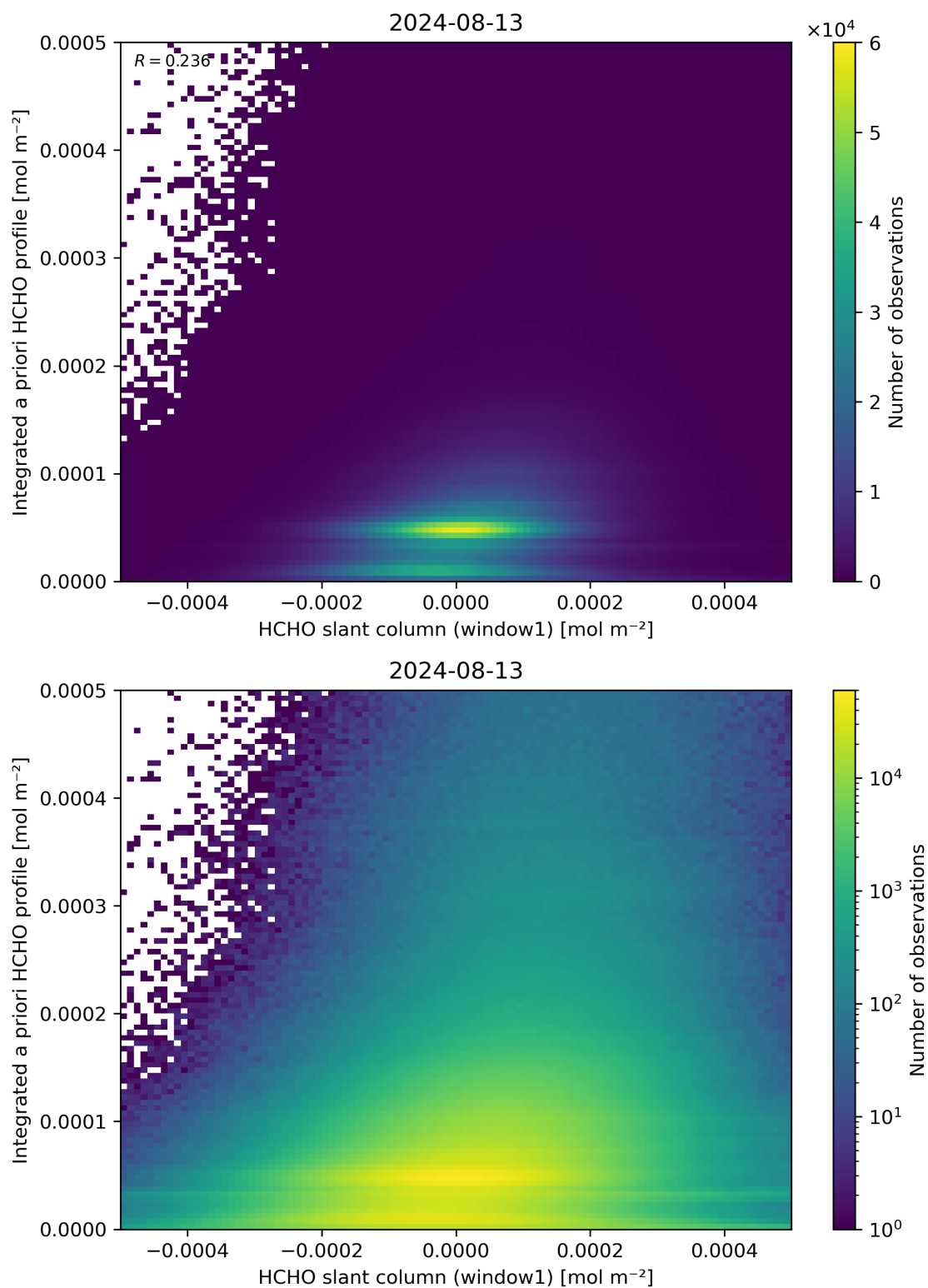
Figure 87: Scatter density plot of “HCHO slant column (window1)” against “Integrated a priori HCHO profile” for 2024-08-12 to 2024-08-14.
