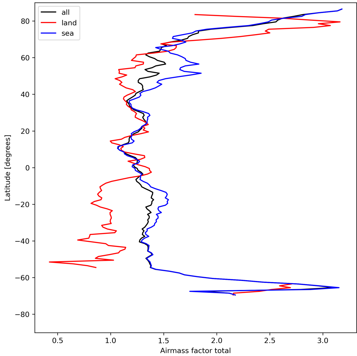
Figure 26: Zonal average of “Airmass factor total” for 2024-08-12 to 2024-08-14.
