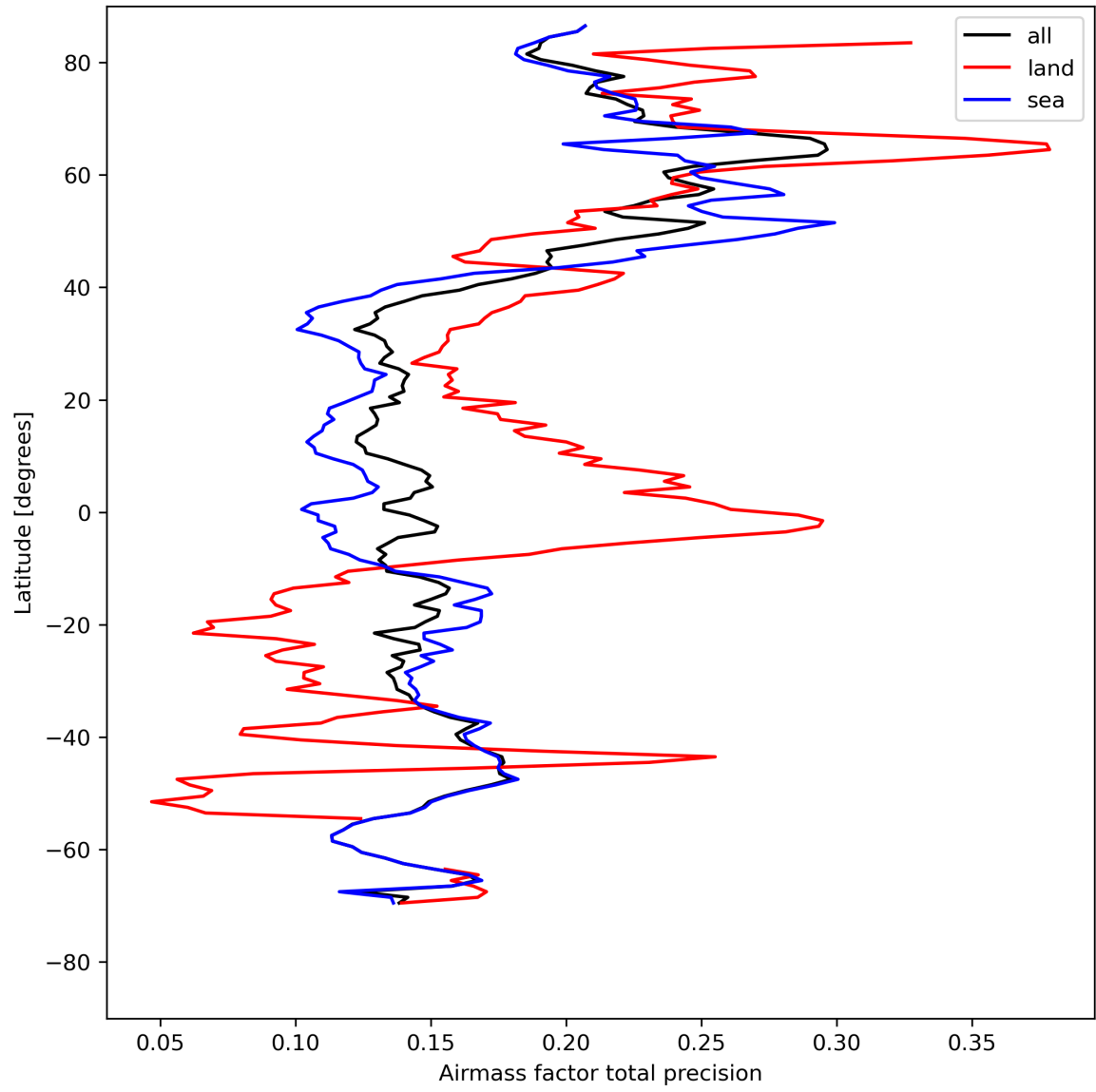
Figure 27: Zonal average of “Airmass factor total precision” for 2024-08-12 to 2024-08-14.
