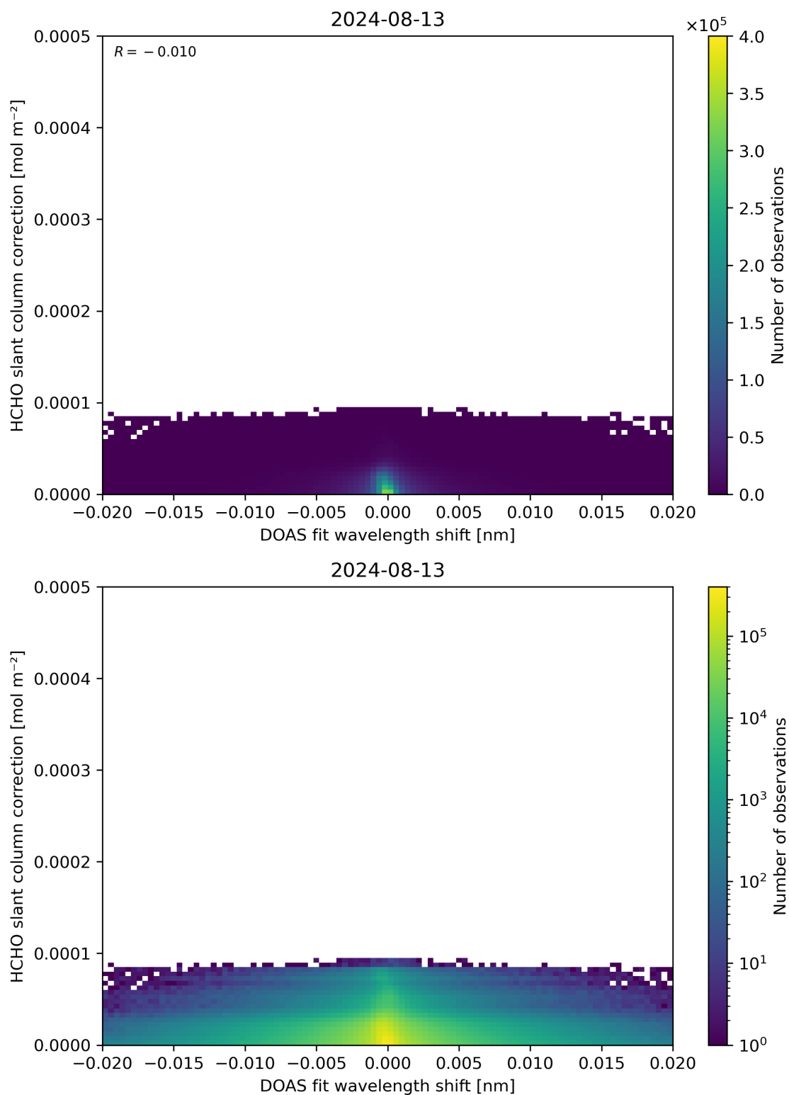
Figure 67: Scatter density plot of “DOAS fit wavelength shift” against “HCHO slant column correction” for 2024-08-12 to 2024-08-14.
