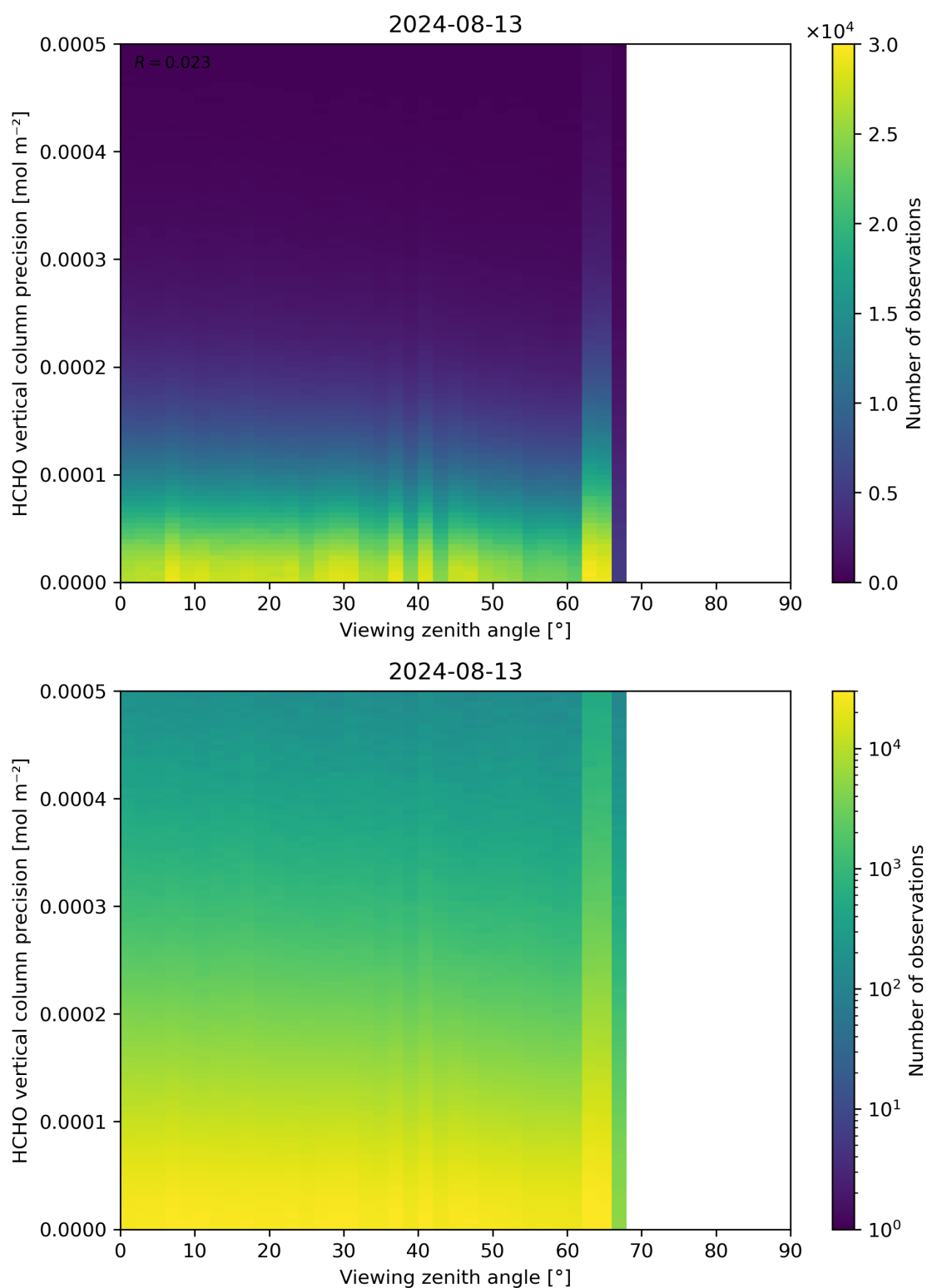
Figure 194: Scatter density plot of “Viewing zenith angle” against “HCHO vertical column precision” for 2024-08-12 to 2024-08-14.
