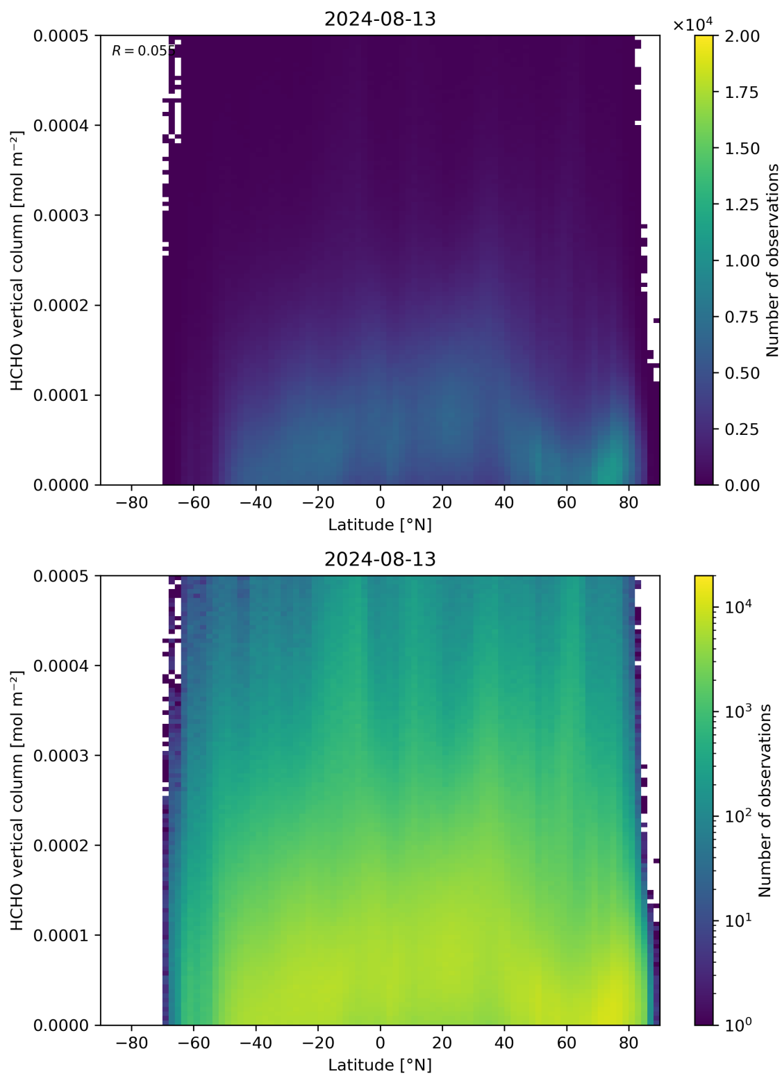
Figure 163: Scatter density plot of “Latitude” against “HCHO vertical column” for 2024-08-12 to 2024-08-14.
