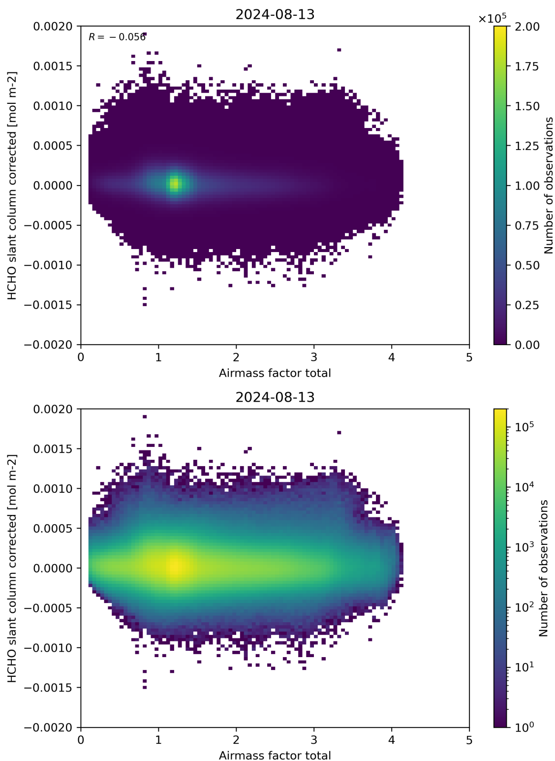
Figure 101: Scatter density plot of “Airmass factor total” against “HCHO slant column corrected” for 2024-08-12 to 2024-08-14.
