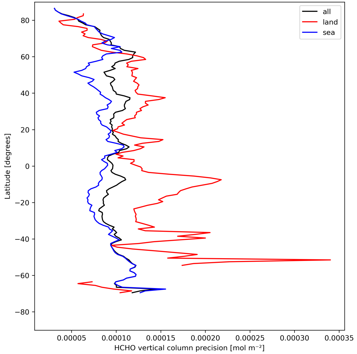
Figure 22: Zonal average of “HCHO vertical column precision” for 2024-08-12 to 2024-08-14.
