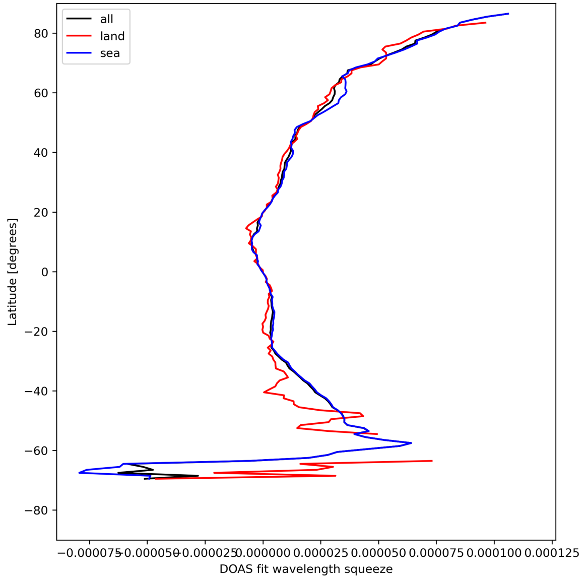
Figure 31: Zonal average of “DOAS fit wavelength squeeze” for 2024-08-12 to 2024-08-14.
