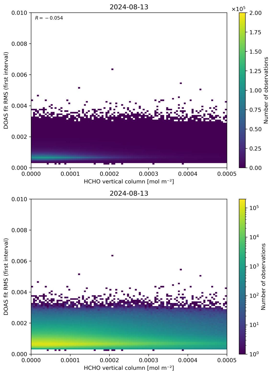
Figure 123: Scatter density plot of “HCHO vertical column” against “DOAS fit RMS (first interval)” for 2024-08-12 to 2024-08-14.
