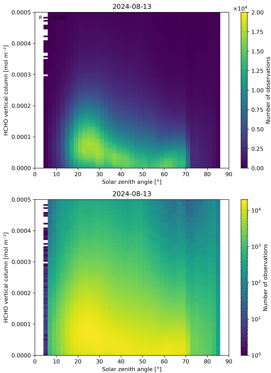
Figure 177: Scatter density plot of “Solar zenith angle” against “HCHO vertical column” for 2024-08-12 to 2024-08-14.
