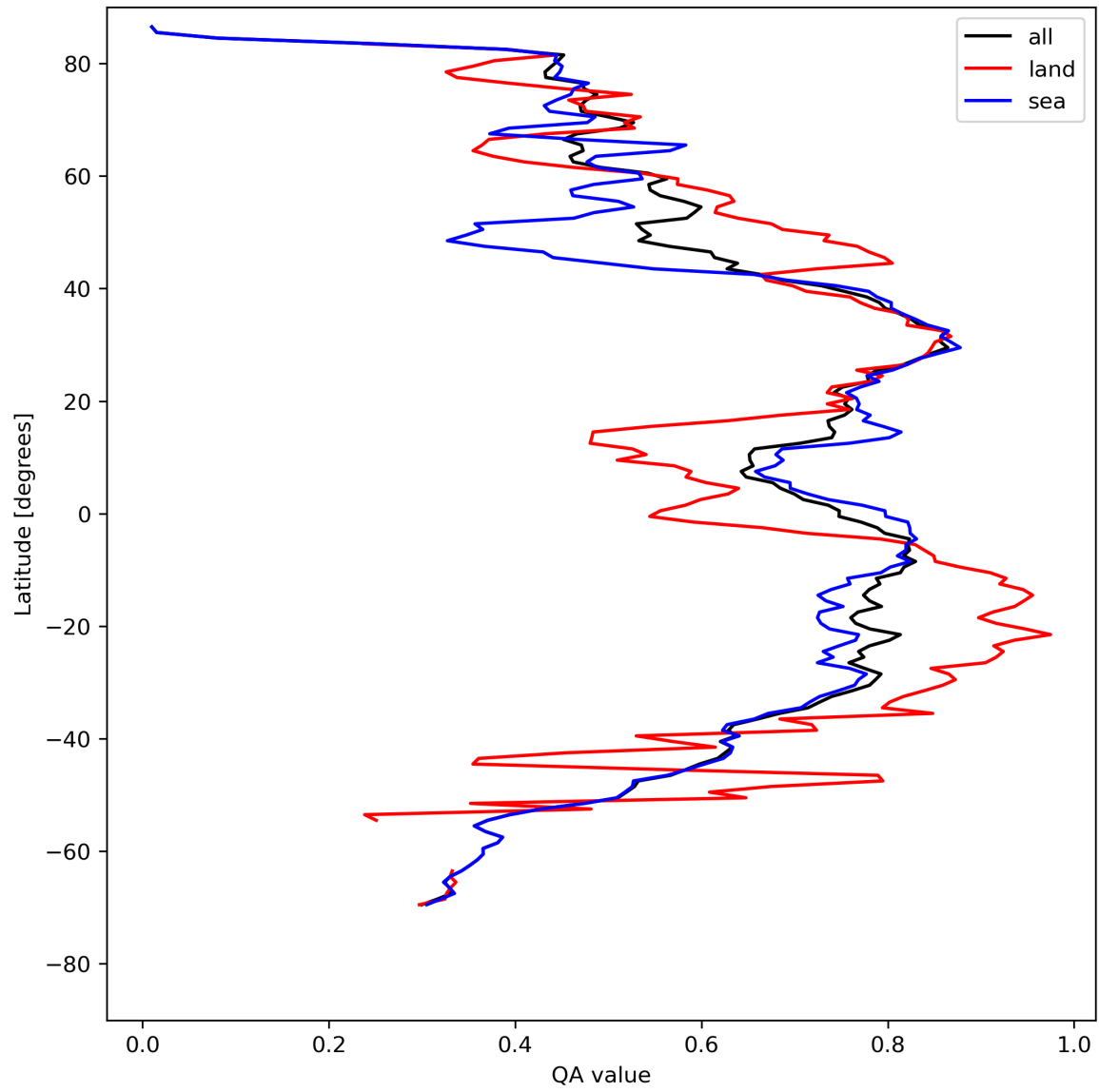
Figure 20: Zonal average of “QA value” for 2024-08-12 to 2024-08-14.
