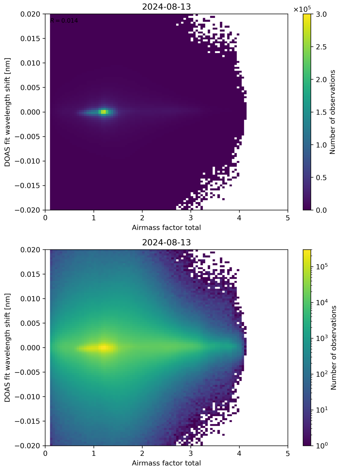
Figure 98: Scatter density plot of “Airmass factor total” against “DOAS fit wavelength shift” for 2024-08-12 to 2024-08-14.
