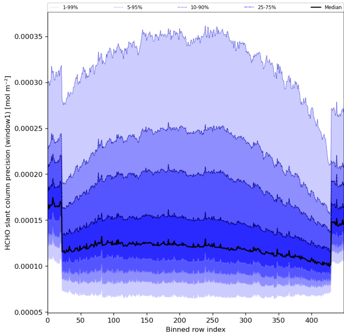
Figure 53: Along track statistics of “HCHO slant column precision (window1)” for 2024-08-12 to 2024-08-14
