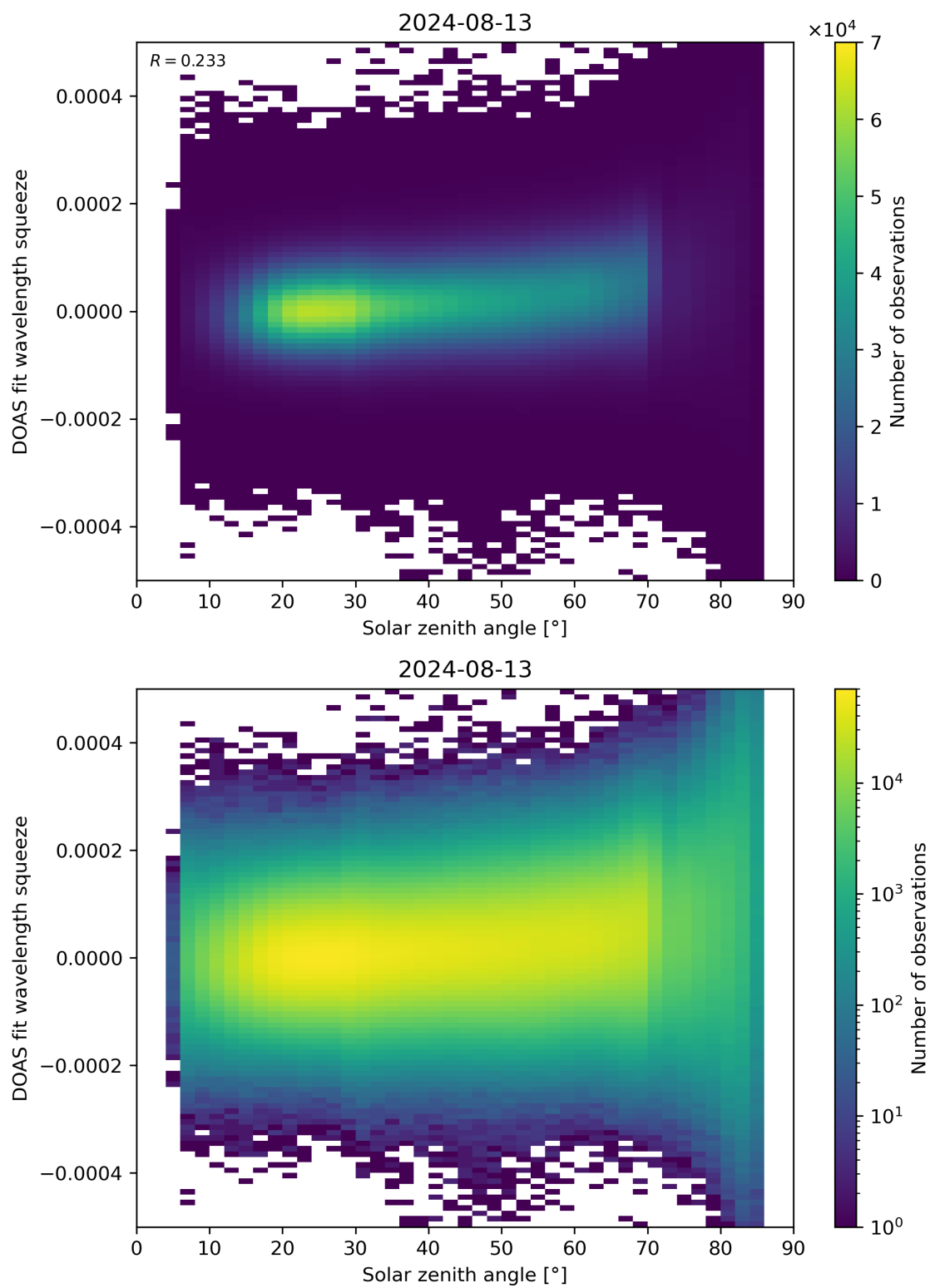
Figure 169: Scatter density plot of “Solar zenith angle” against “DOAS fit wavelength squeeze” for 2024-08-12 to 2024-08-14.
