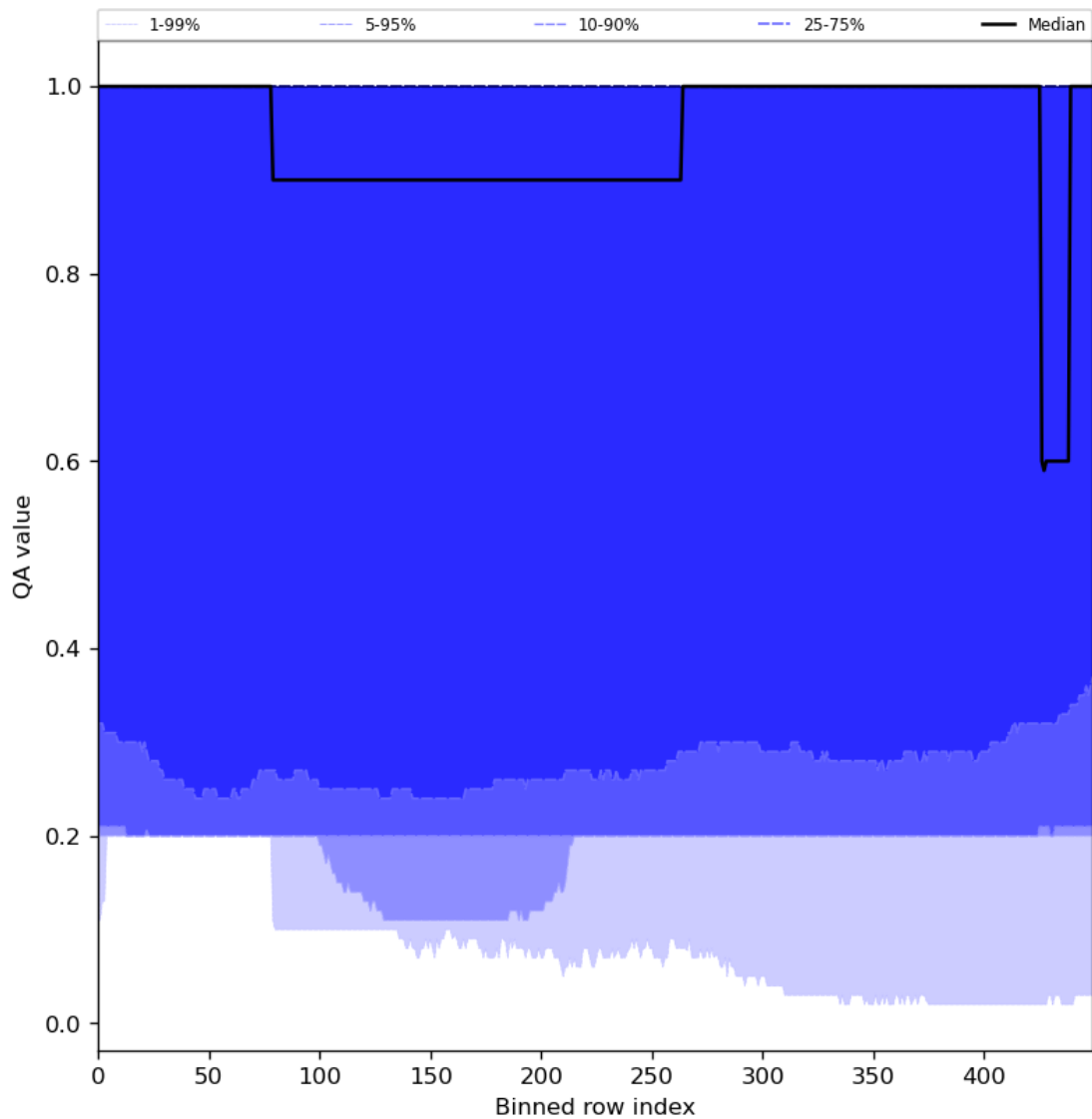
Figure 48: Along track statistics of “QA value” for 2024-08-12 to 2024-08-14
