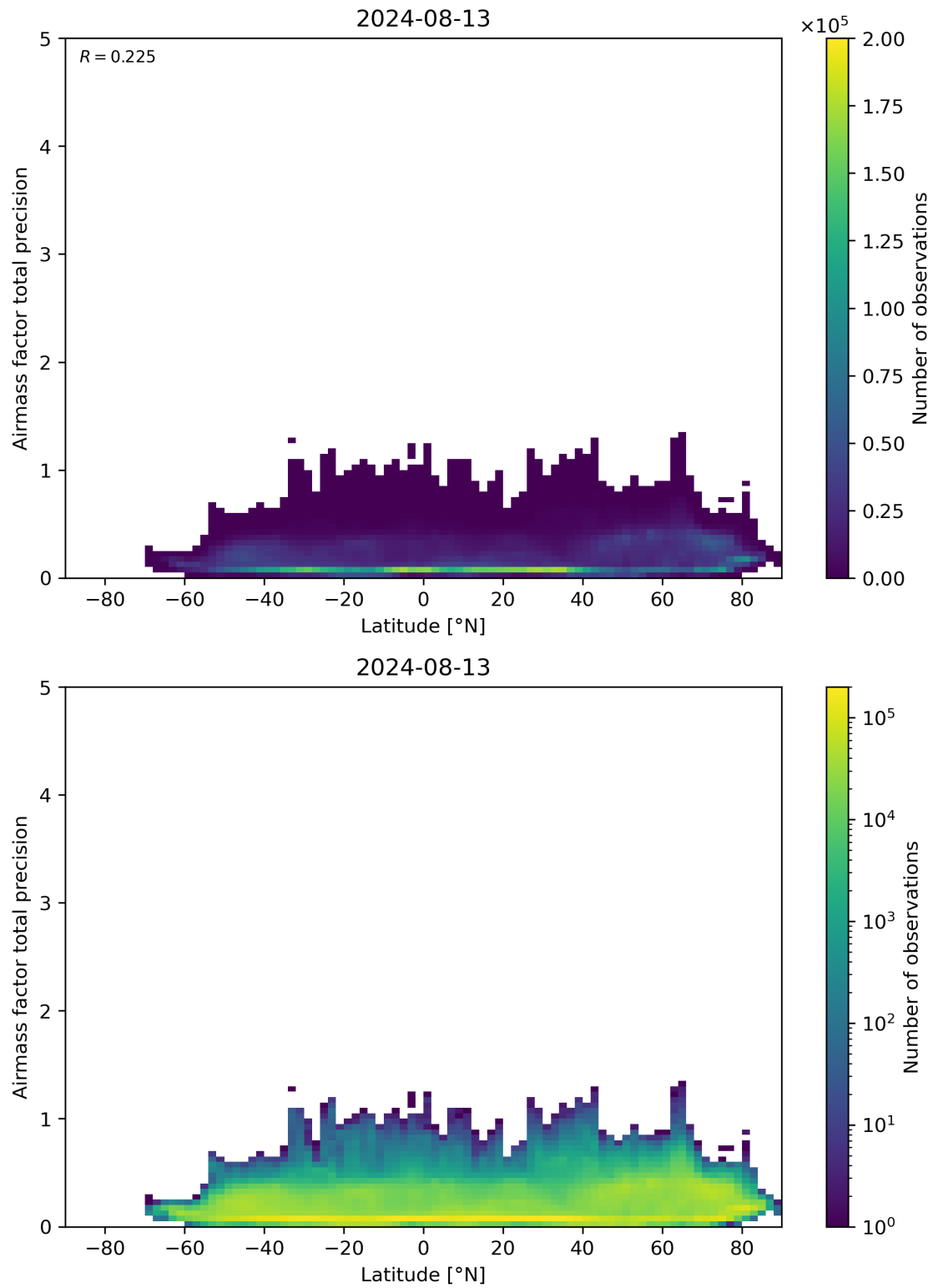
Figure 162: Scatter density plot of “Latitude” against “Airmass factor total precision” for 2024-08-12 to 2024-08-14.
