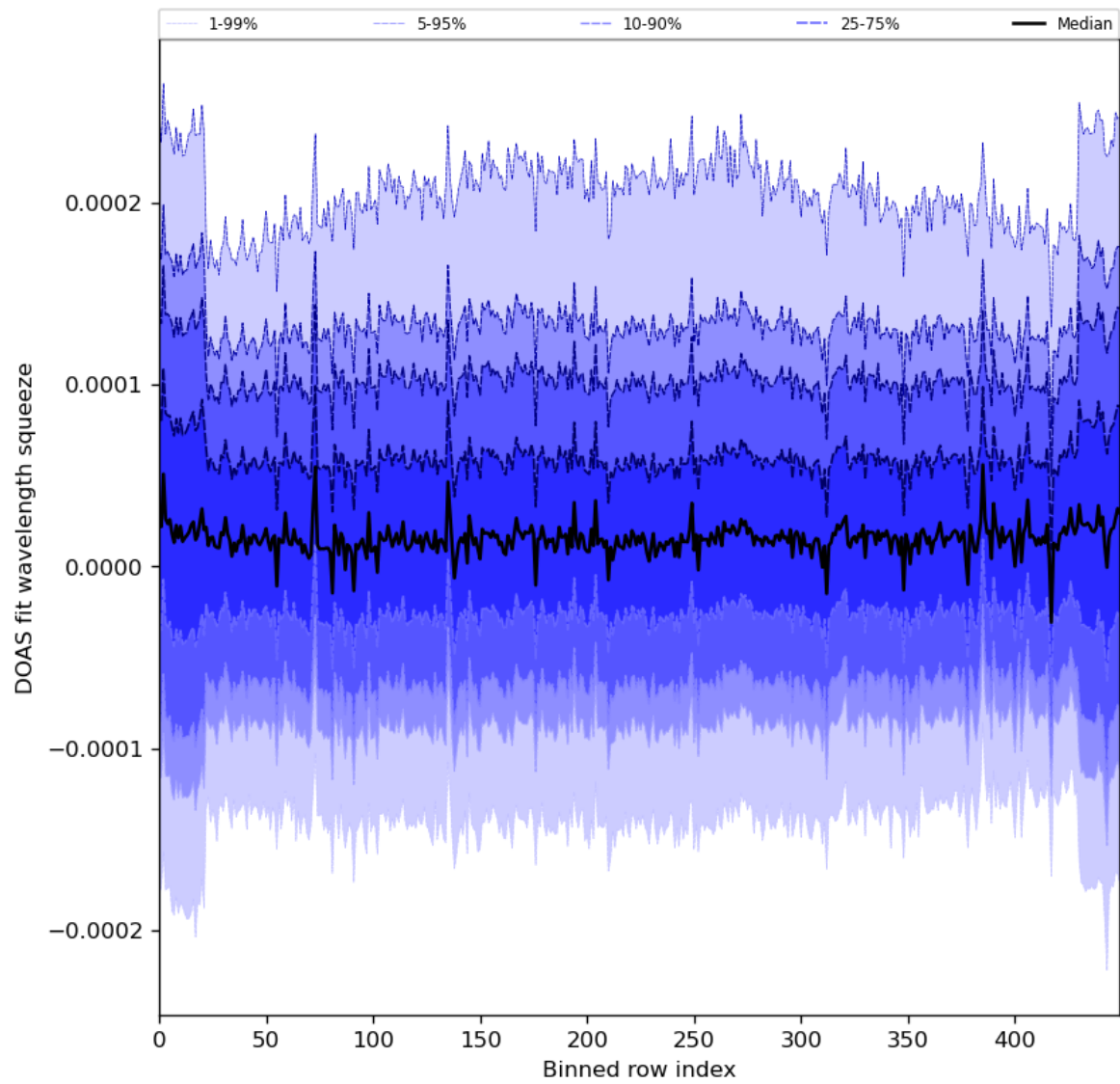
Figure 59: Along track statistics of “DOAS fit wavelength squeeze” for 2024-08-12 to 2024-08-14
