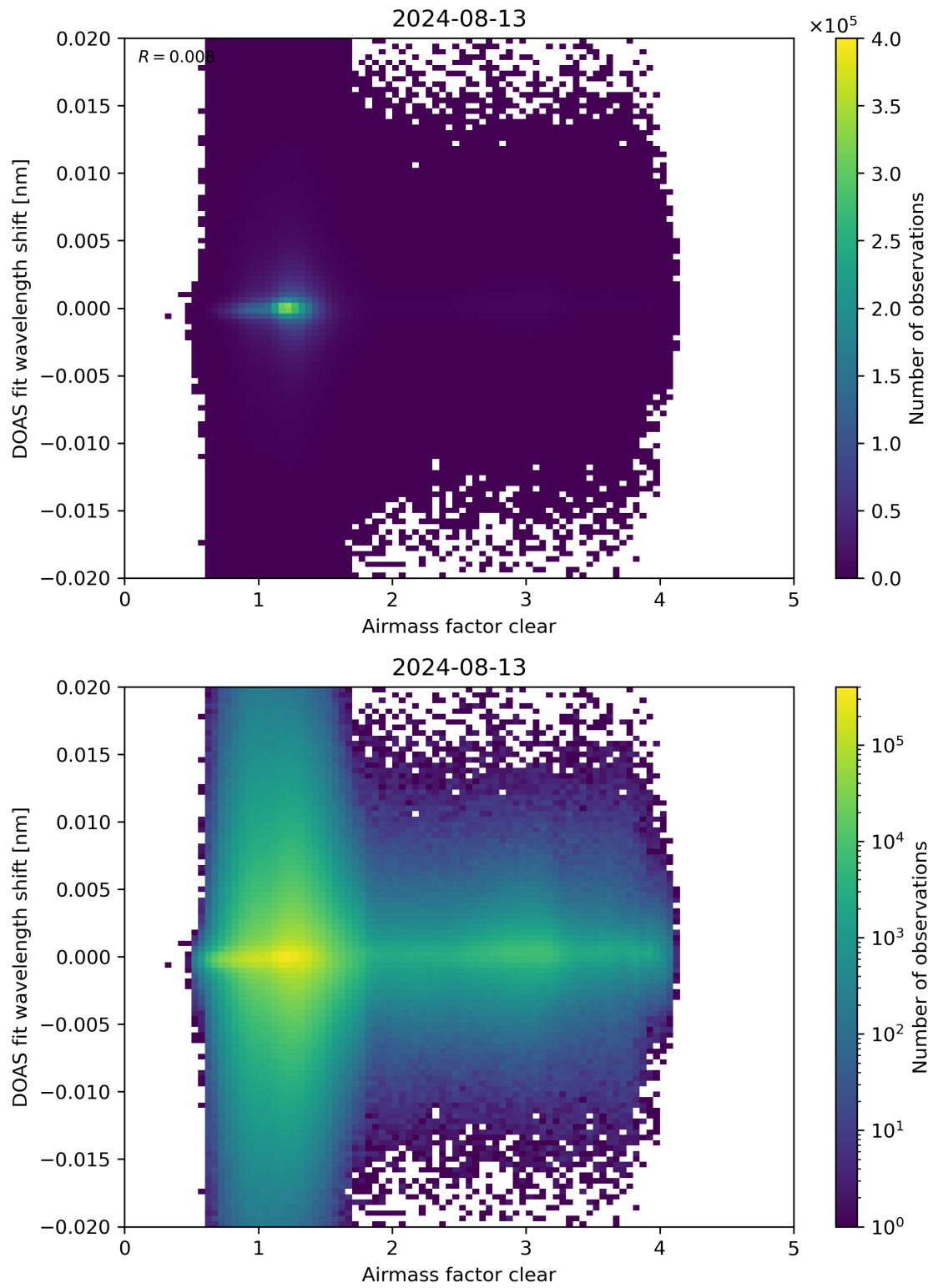
Figure 72: Scatter density plot of “Airmass factor clear” against “DOAS fit wavelength shift” for 2024-08-12 to 2024-08-14.
