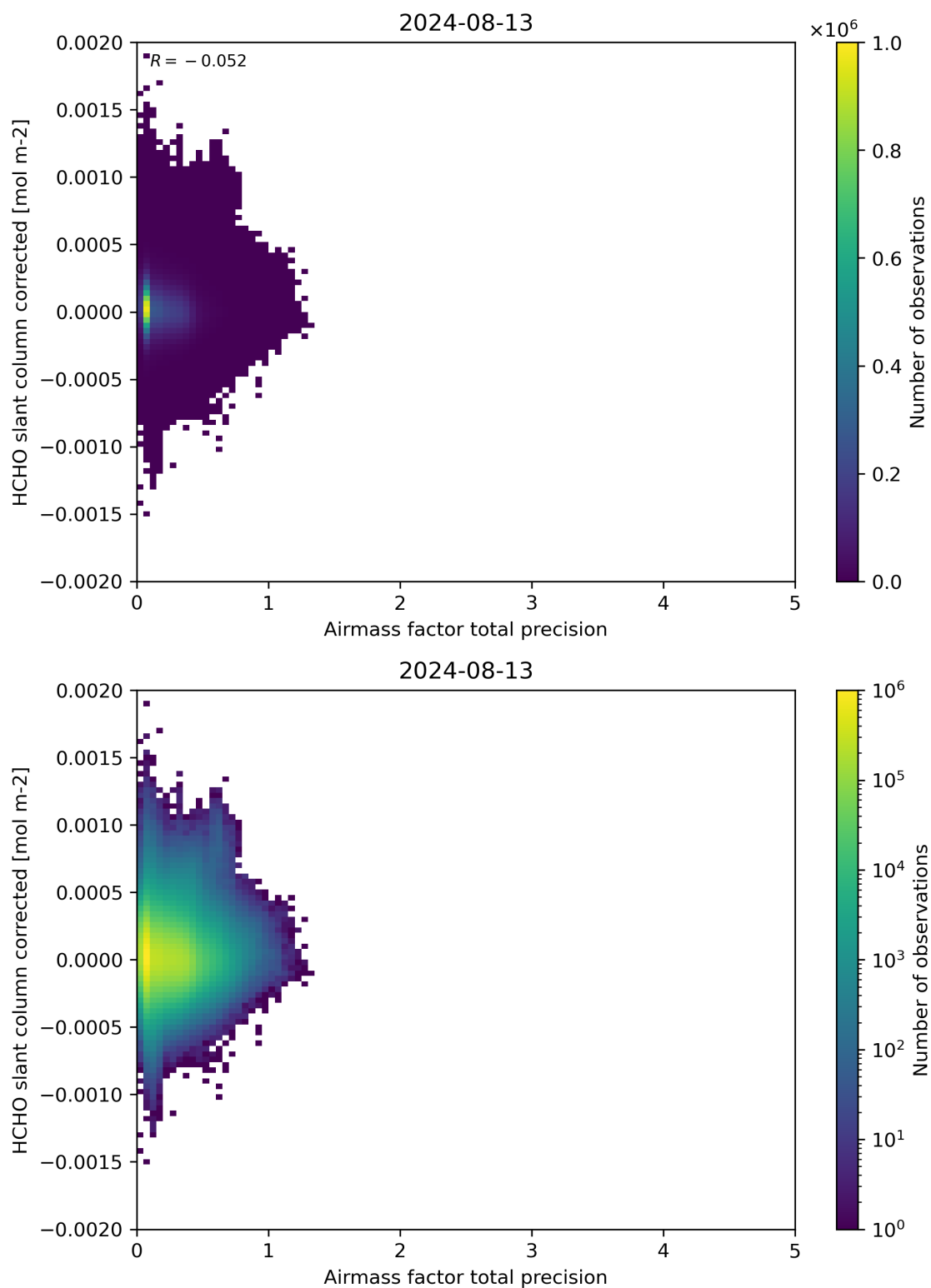
Figure 109: Scatter density plot of “Airmass factor total precision” against “HCHO slant column corrected” for 2024-08-12 to 2024-08-14.
