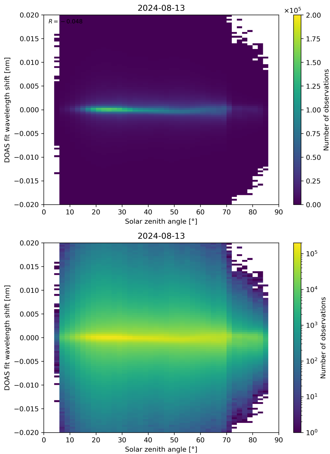
Figure 168: Scatter density plot of “Solar zenith angle” against “DOAS fit wavelength shift” for 2024-08-12 to 2024-08-14.
