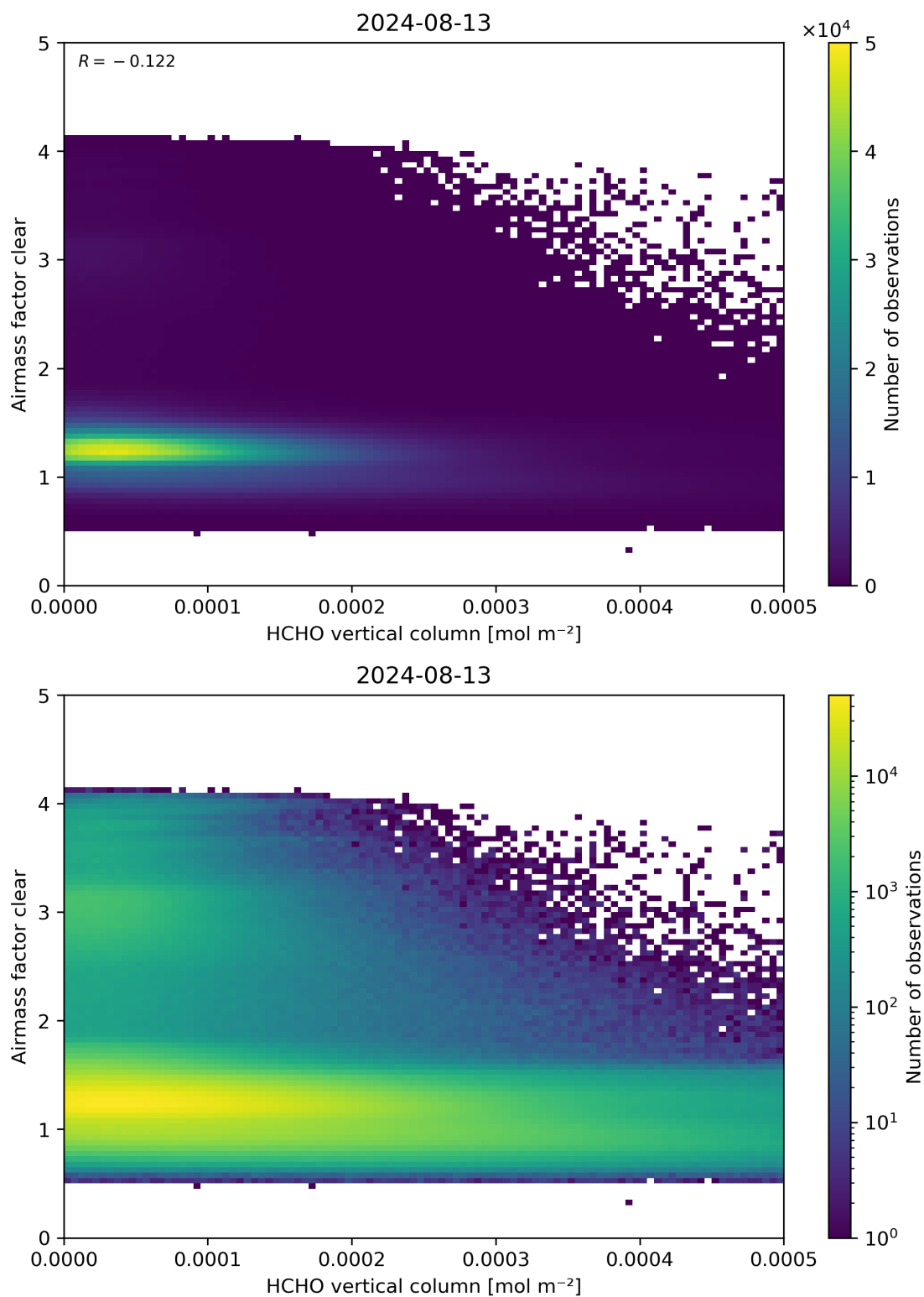
Figure 126: Scatter density plot of “HCHO vertical column” against “Airmass factor clear” for 2024-08-12 to 2024-08-14.
