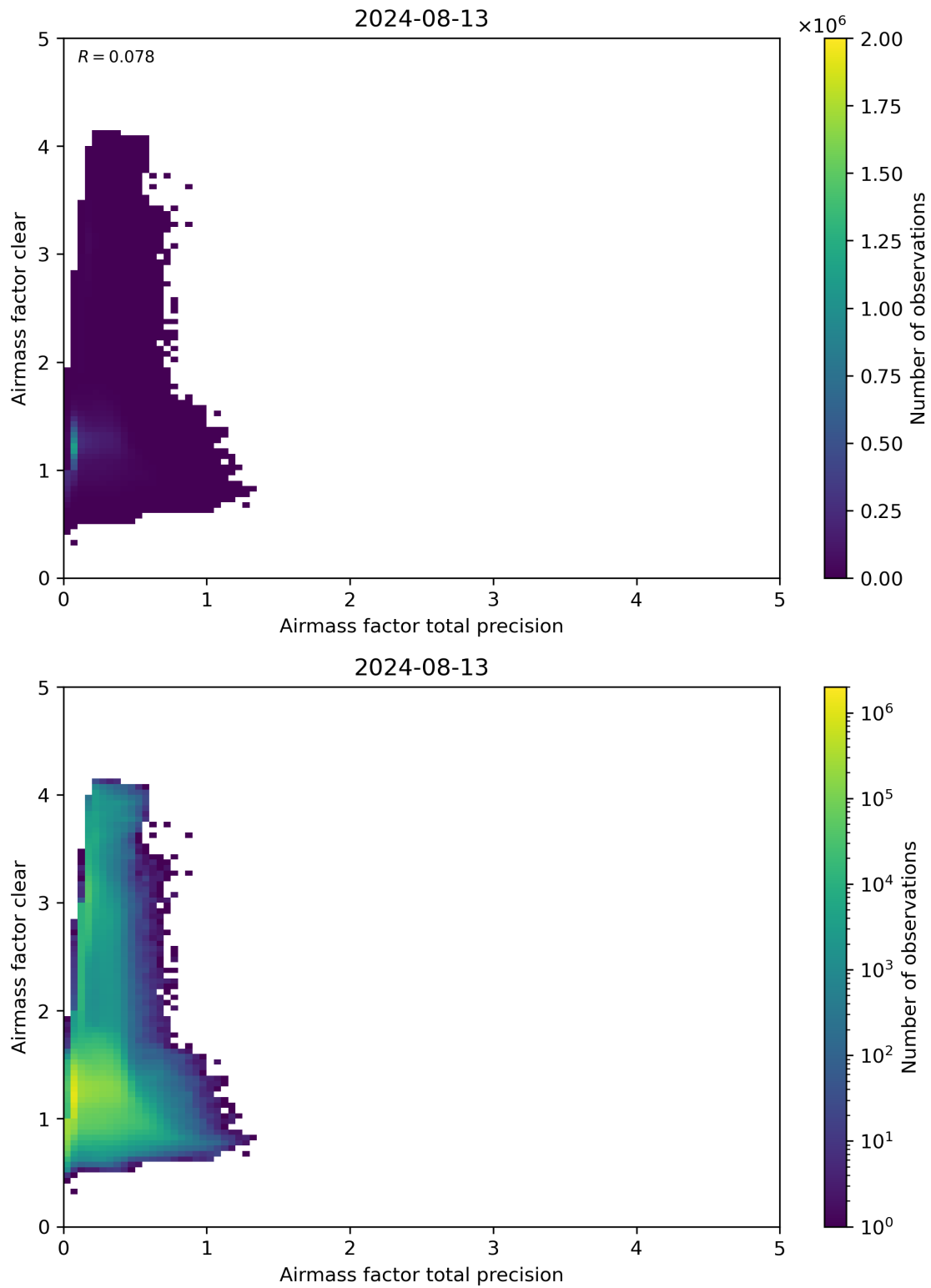
Figure 108: Scatter density plot of “Airmass factor total precision” against “Airmass factor clear” for 2024-08-12 to 2024-08-14.
