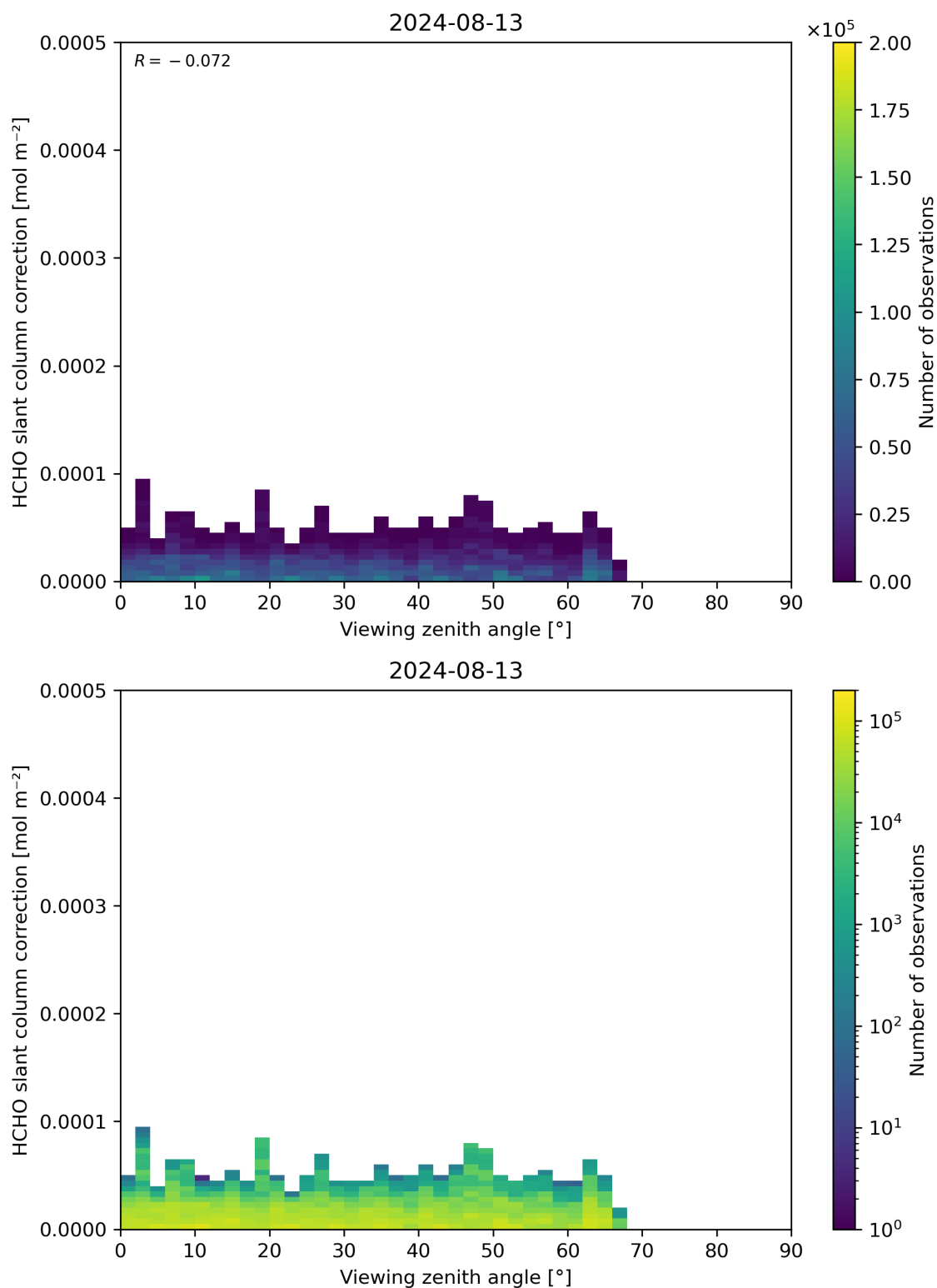
Figure 187: Scatter density plot of “Viewing zenith angle” against “HCHO slant column correction” for 2024-08-12 to 2024-08-14.
