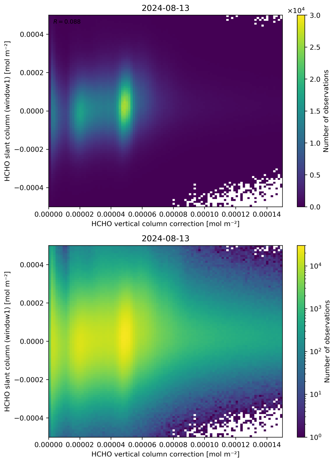
Figure 118: Scatter density plot of “HCHO vertical column correction” against “HCHO slant column (window1)” for 2024-08-12 to 2024-08-14.
