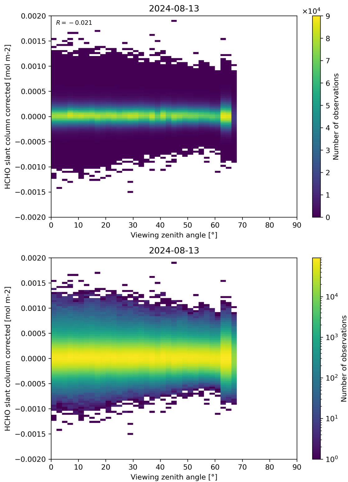
Figure 186: Scatter density plot of “Viewing zenith angle” against “HCHO slant column corrected” for 2024-08-12 to 2024-08-14.
