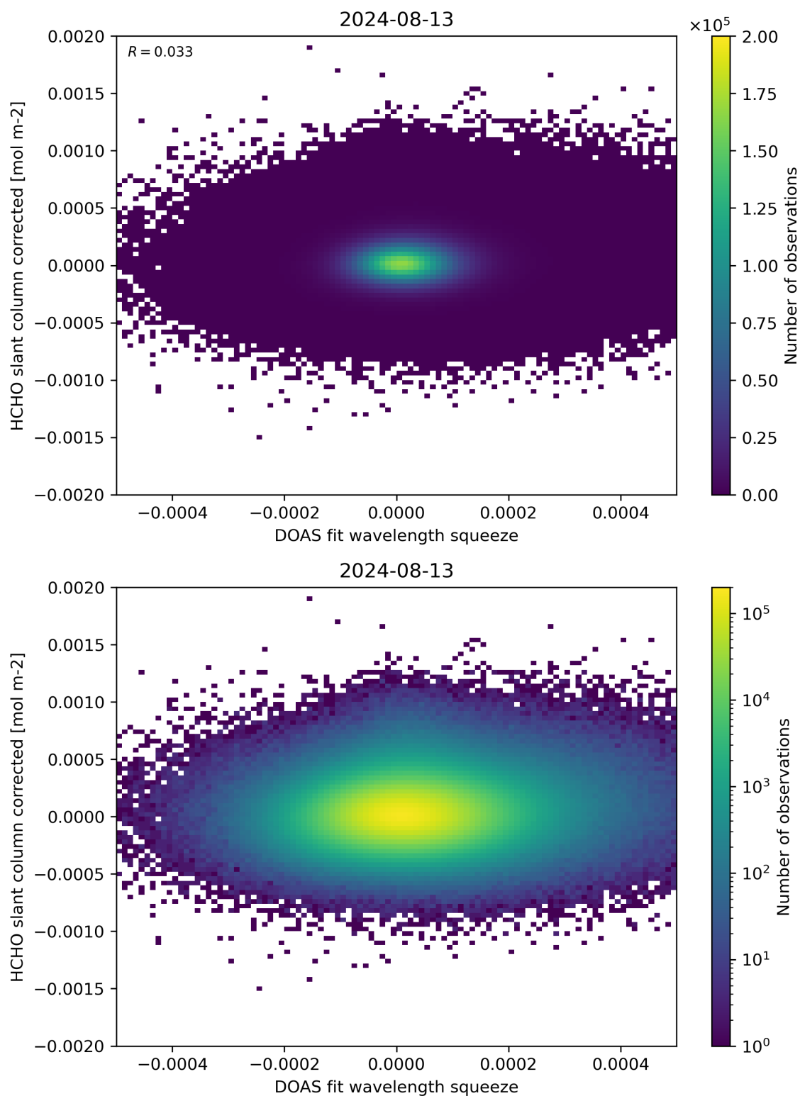
Figure 69: Scatter density plot of “DOAS fit wavelength squeeze” against “HCHO slant column corrected” for 2024-08-12 to 2024-08-14.
