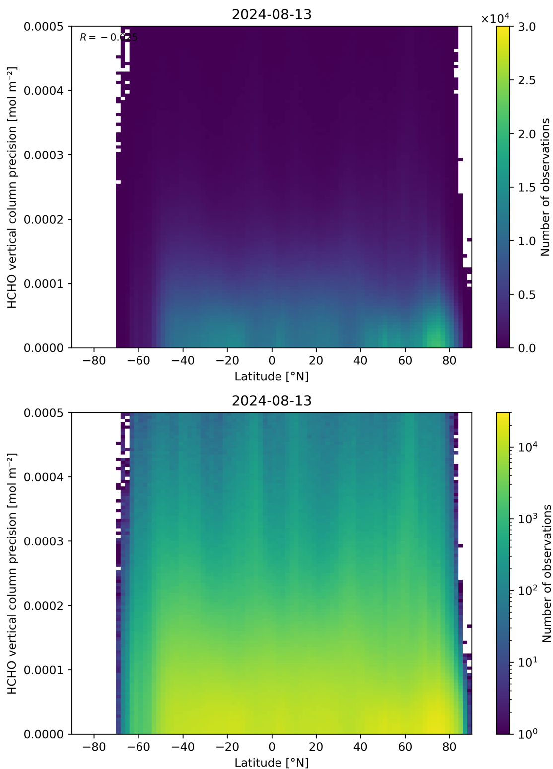
Figure 165: Scatter density plot of “Latitude” against “HCHO vertical column precision” for 2024-08-12 to 2024-08-14.
