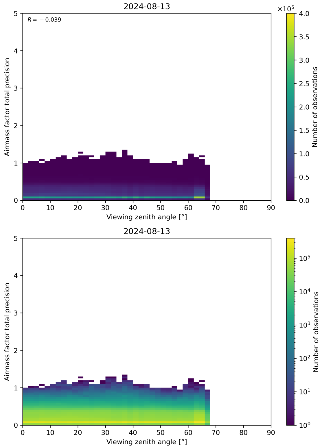
Figure 191: Scatter density plot of “Viewing zenith angle” against “Airmass factor total precision” for 2024-08-12 to 2024-08-14.
