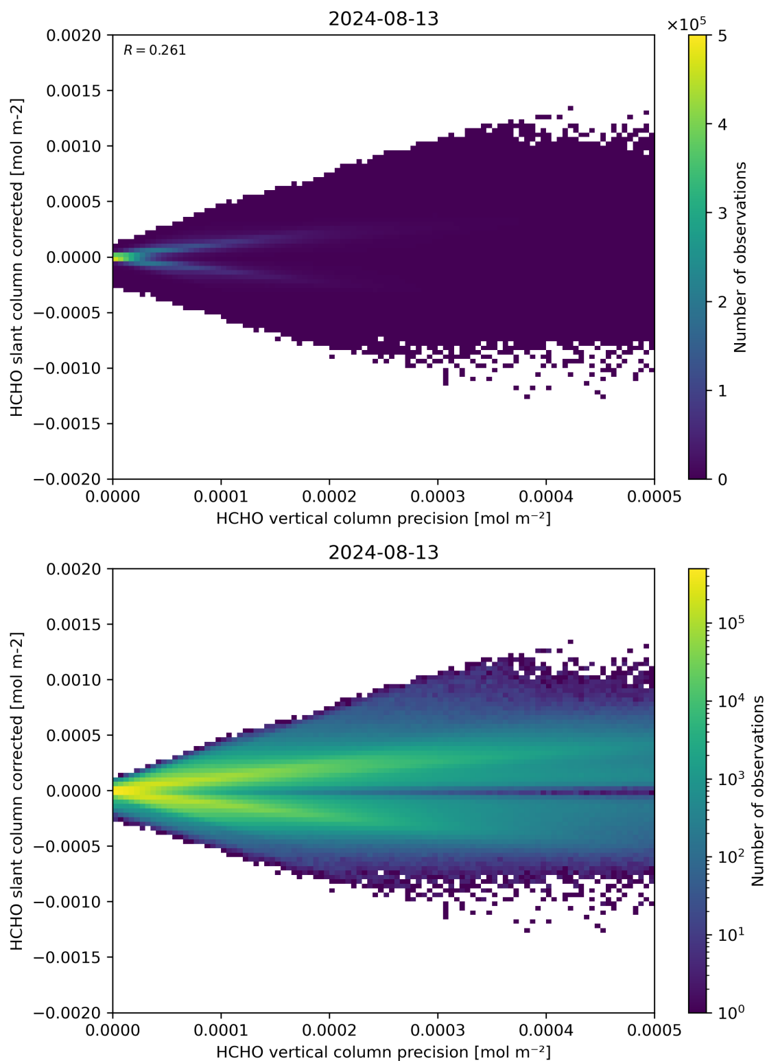
Figure 140: Scatter density plot of “HCHO vertical column precision” against “HCHO slant column corrected” for 2024-08-12 to 2024-08-14.
