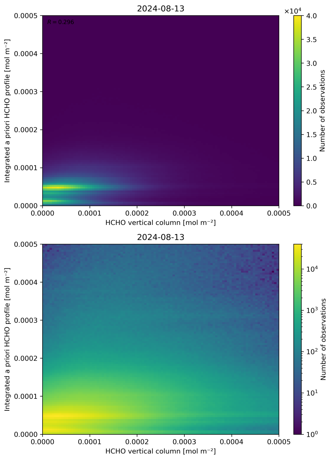
Figure 135: Scatter density plot of “HCHO vertical column” against “Integrated a priori HCHO profile” for 2024-08-12 to 2024-08-14.
