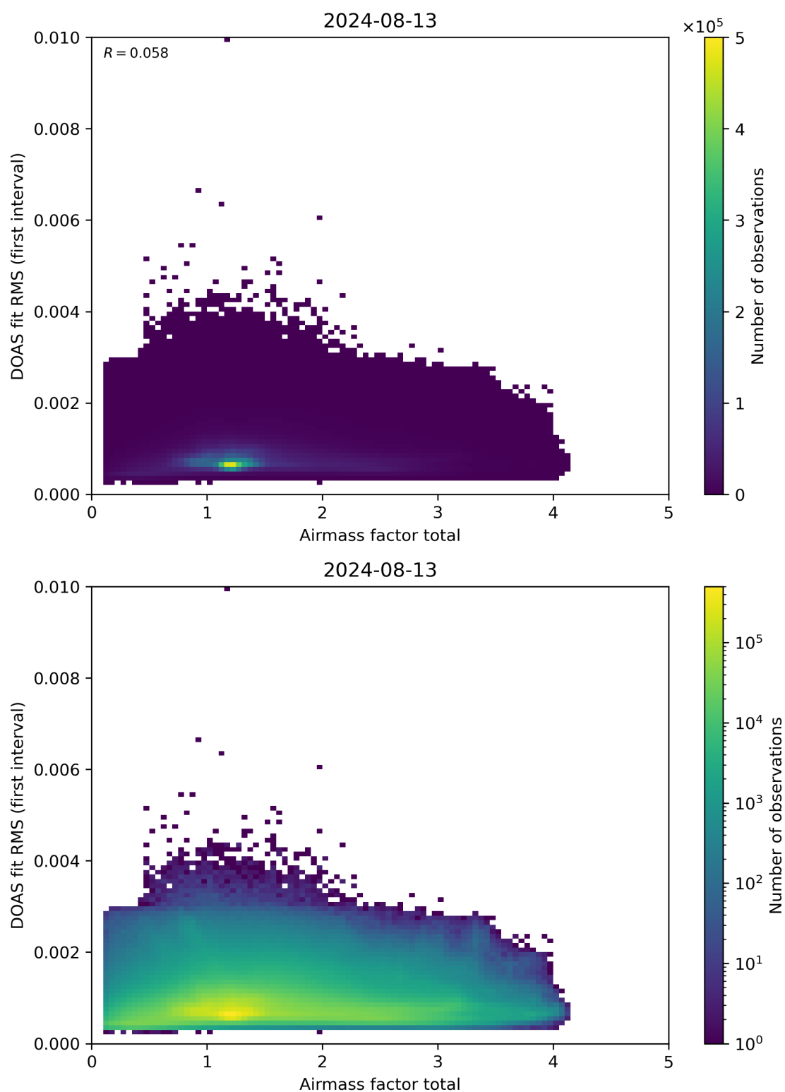
Figure 97: Scatter density plot of “Airmass factor total” against “DOAS fit RMS (first interval)” for 2024-08-12 to 2024-08-14.
