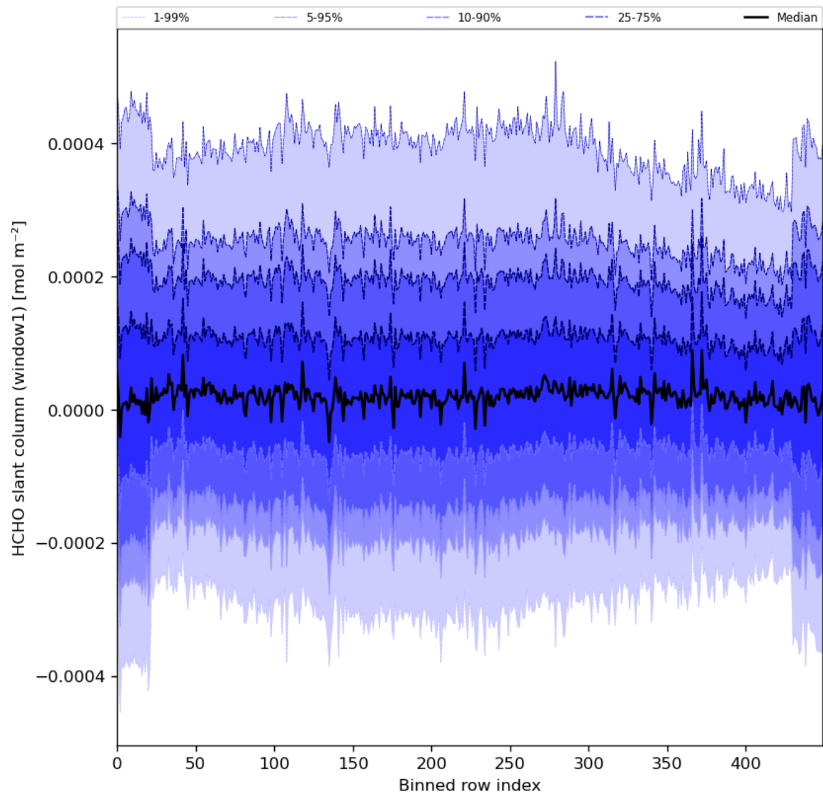
Figure 52: Along track statistics of “HCHO slant column (window1)” for 2024-08-12 to 2024-08-14
