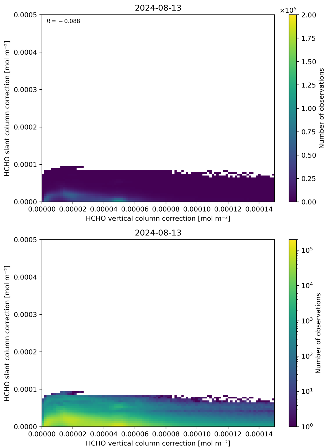
Figure 117: Scatter density plot of “HCHO vertical column correction” against “HCHO slant column correction” for 2024-08-12 to 2024-08-14.
