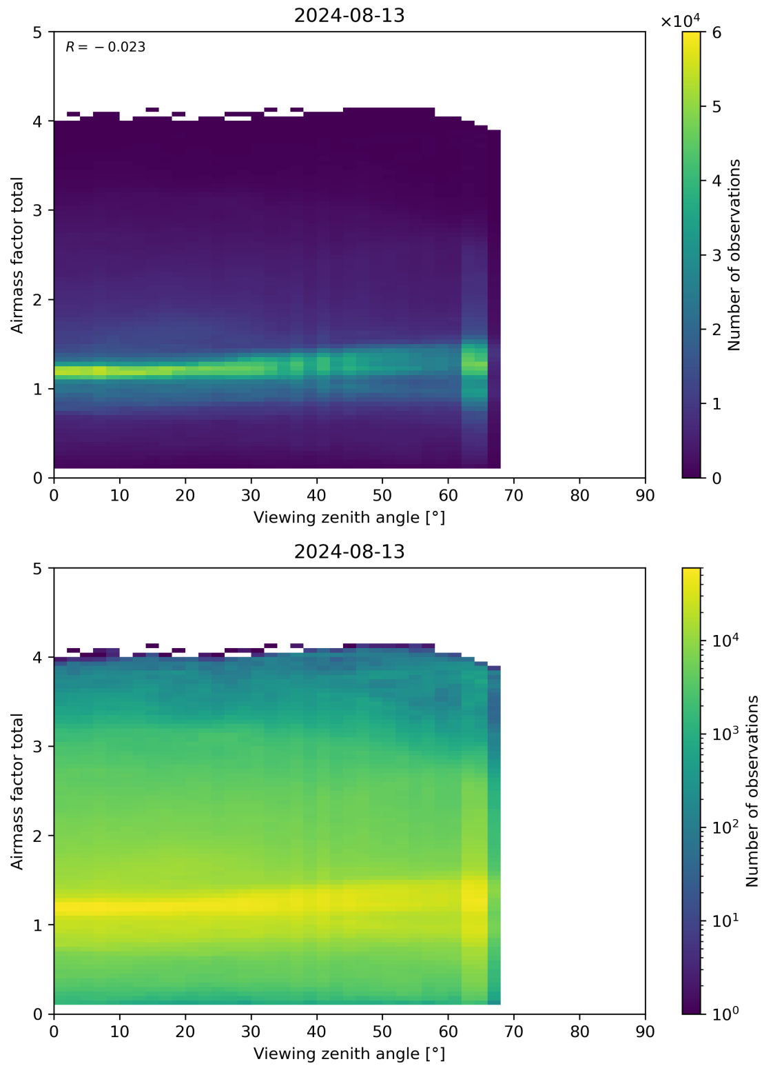
Figure 190: Scatter density plot of “Viewing zenith angle” against “Airmass factor total” for 2024-08-12 to 2024-08-14.
