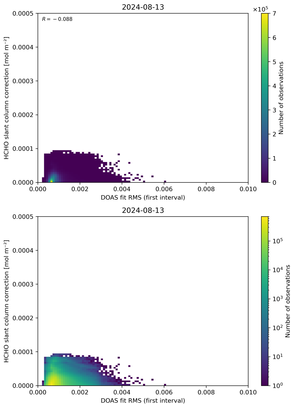
Figure 63: Scatter density plot of “DOAS fit RMS (first interval)” against “HCHO slant column correction” for 2024-08-12 to 2024-08-14.
