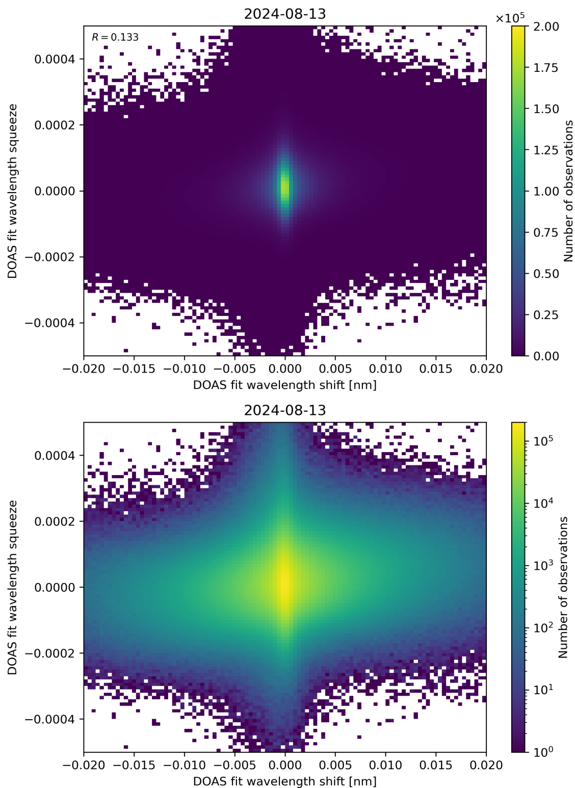
Figure 65: Scatter density plot of “DOAS fit wavelength shift” against “DOAS fit wavelength squeeze” for 2024-08-12 to 2024-08-14.
