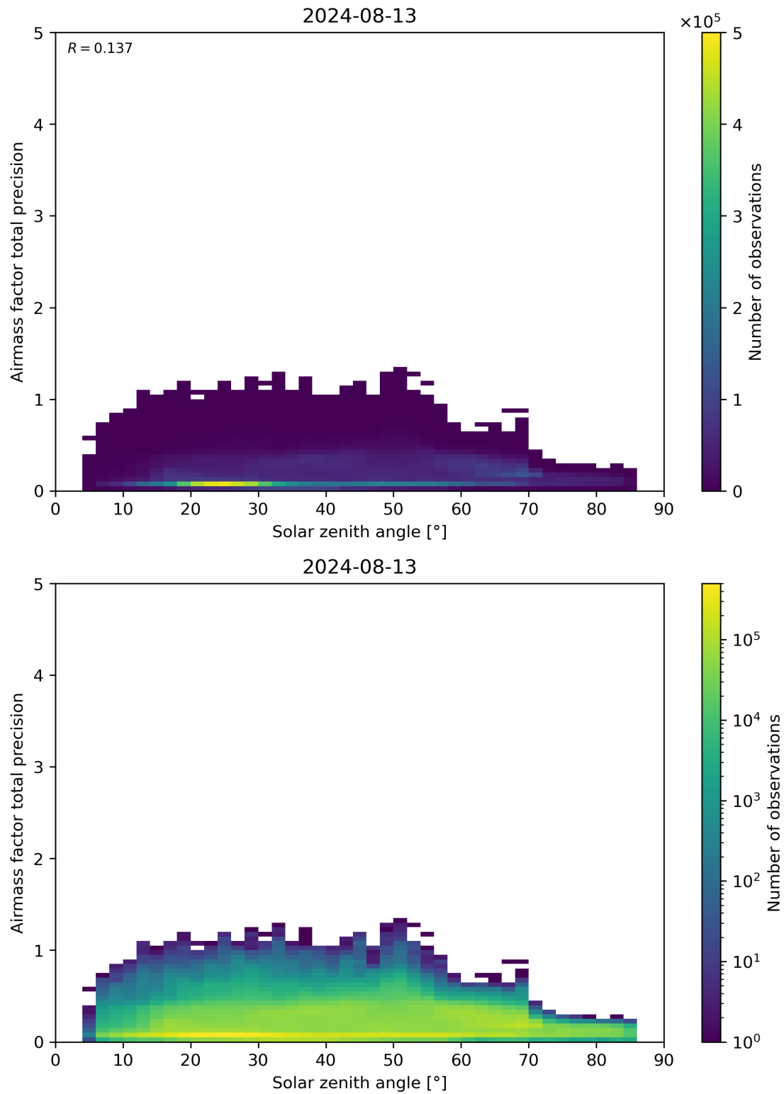
Figure 176: Scatter density plot of “Solar zenith angle” against “Airmass factor total precision” for 2024-08-12 to 2024-08-14.
