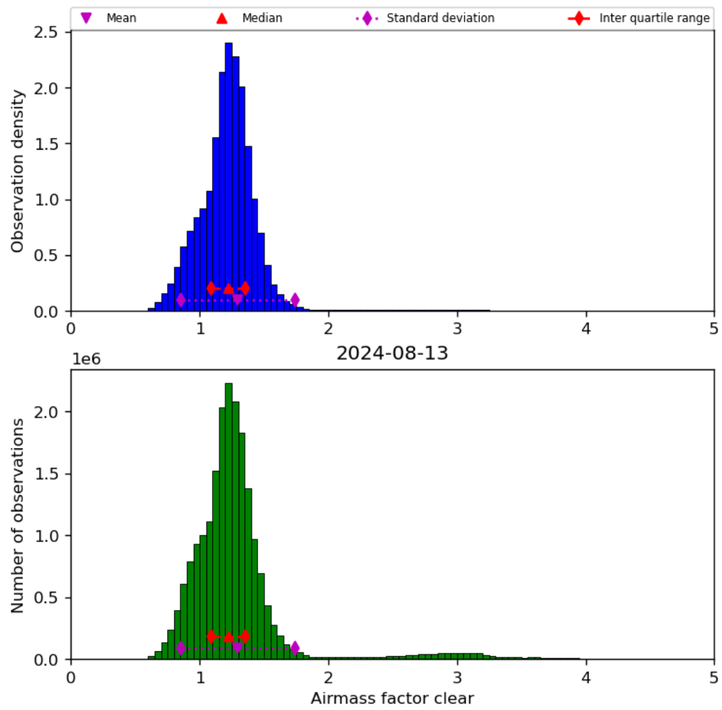
Figure 42: Histogram of “Airmass factor clear” for 2024-08-12 to 2024-08-14
