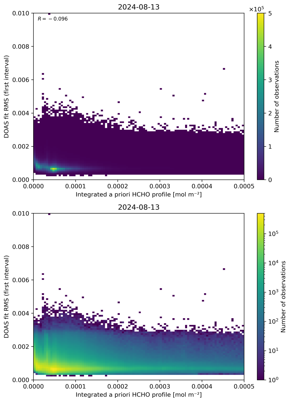
Figure 148: Scatter density plot of “Integrated a priori HCHO profile” against “DOAS fit RMS (first interval)” for 2024-08-12 to 2024-08-14.
