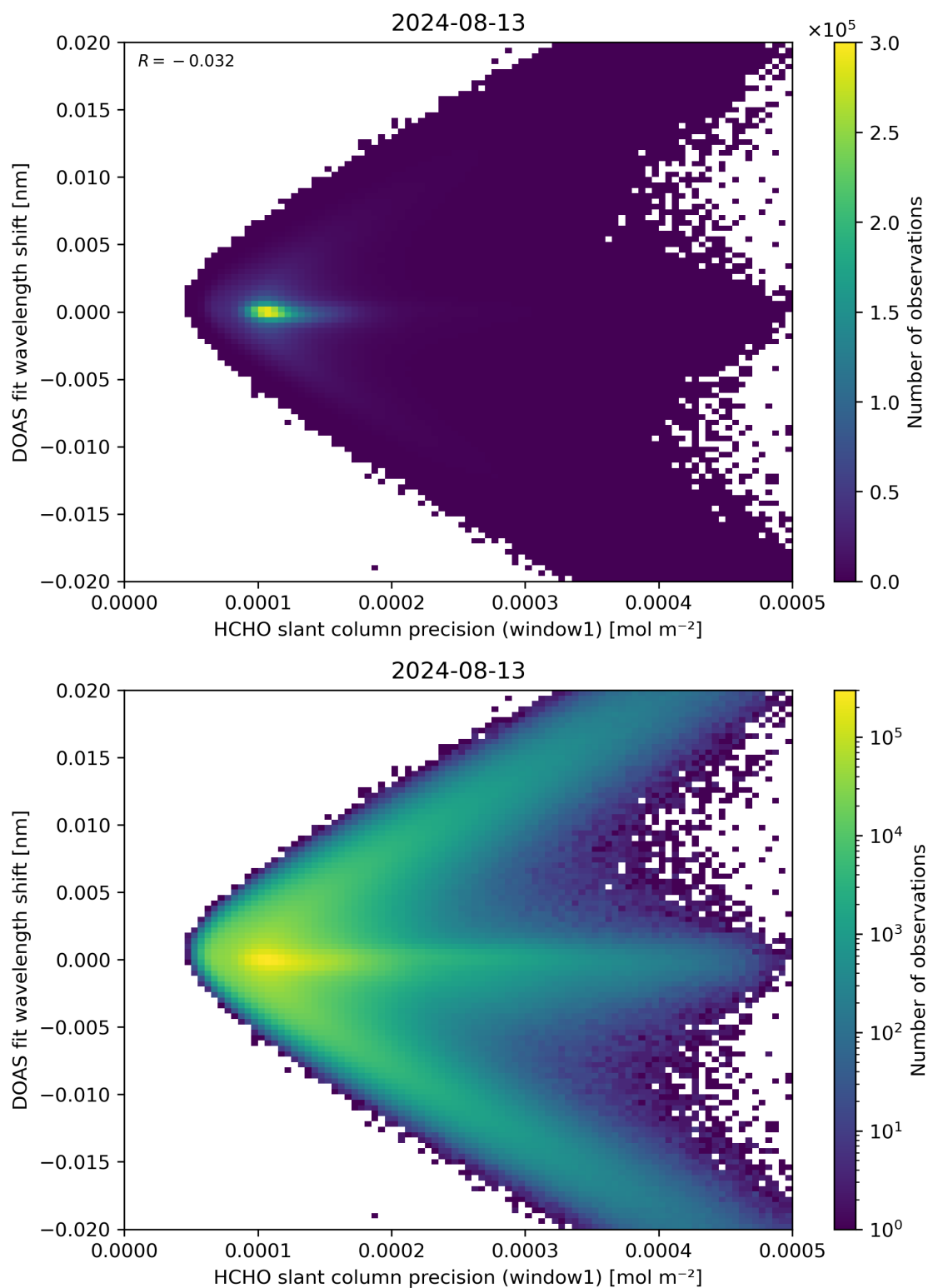
Figure 89: Scatter density plot of “HCHO slant column precision (window1)” against “DOAS fit wavelength shift” for 2024-08-12 to 2024-08-14.
