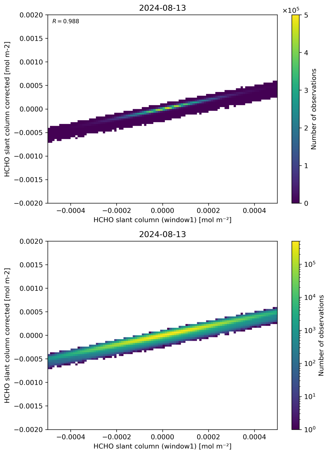
Figure 82: Scatter density plot of “HCHO slant column (window1)” against “HCHO slant column corrected” for 2024-08-12 to 2024-08-14.
