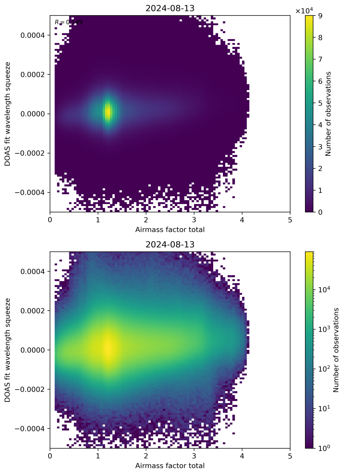
Figure 99: Scatter density plot of “Airmass factor total” against “DOAS fit wavelength squeeze” for 2024-08-12 to 2024-08-14.
