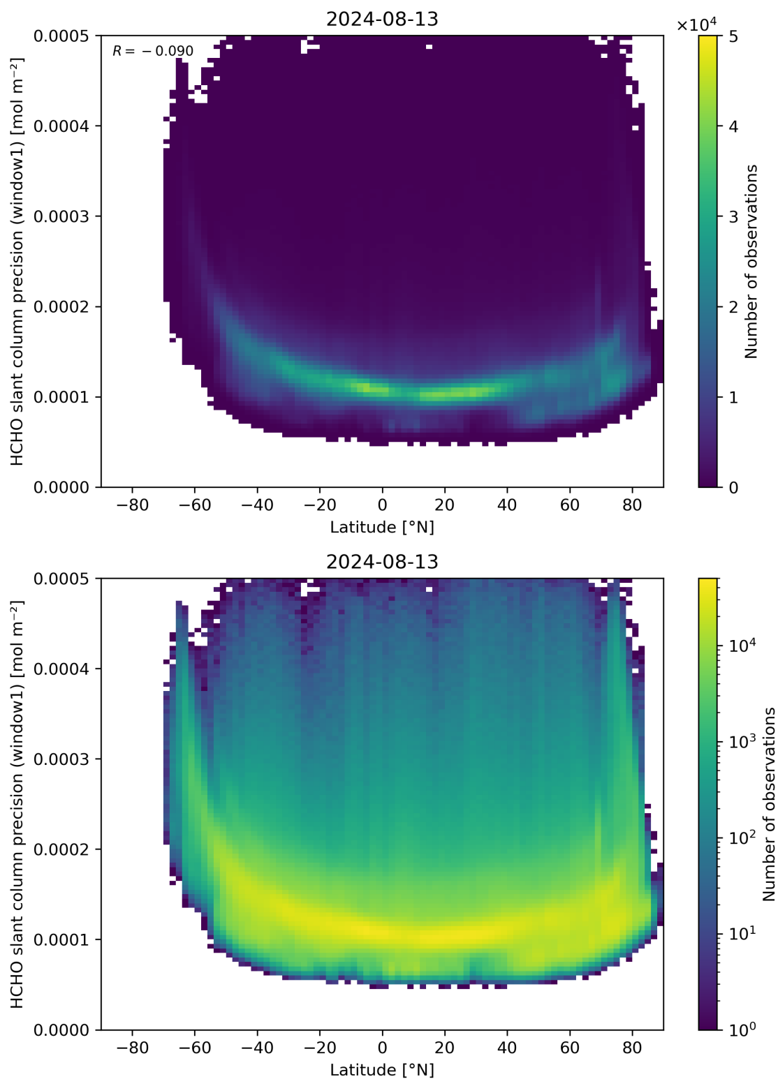
Figure 160: Scatter density plot of “Latitude” against “HCHO slant column precision (window1)” for 2024-08-12 to 2024-08-14.
