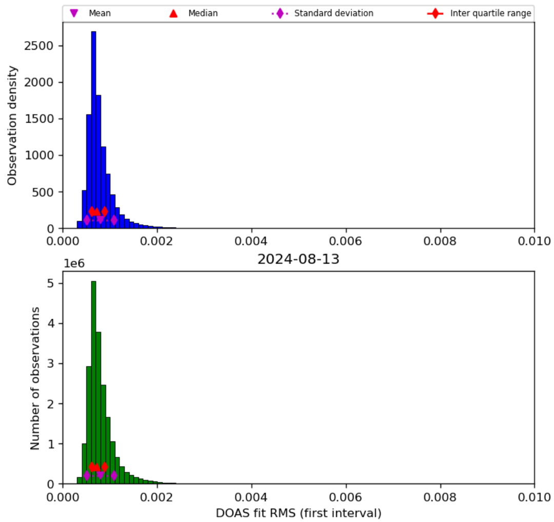
Figure 46: Histogram of “DOAS fit RMS (first interval)” for 2024-08-12 to 2024-08-14
