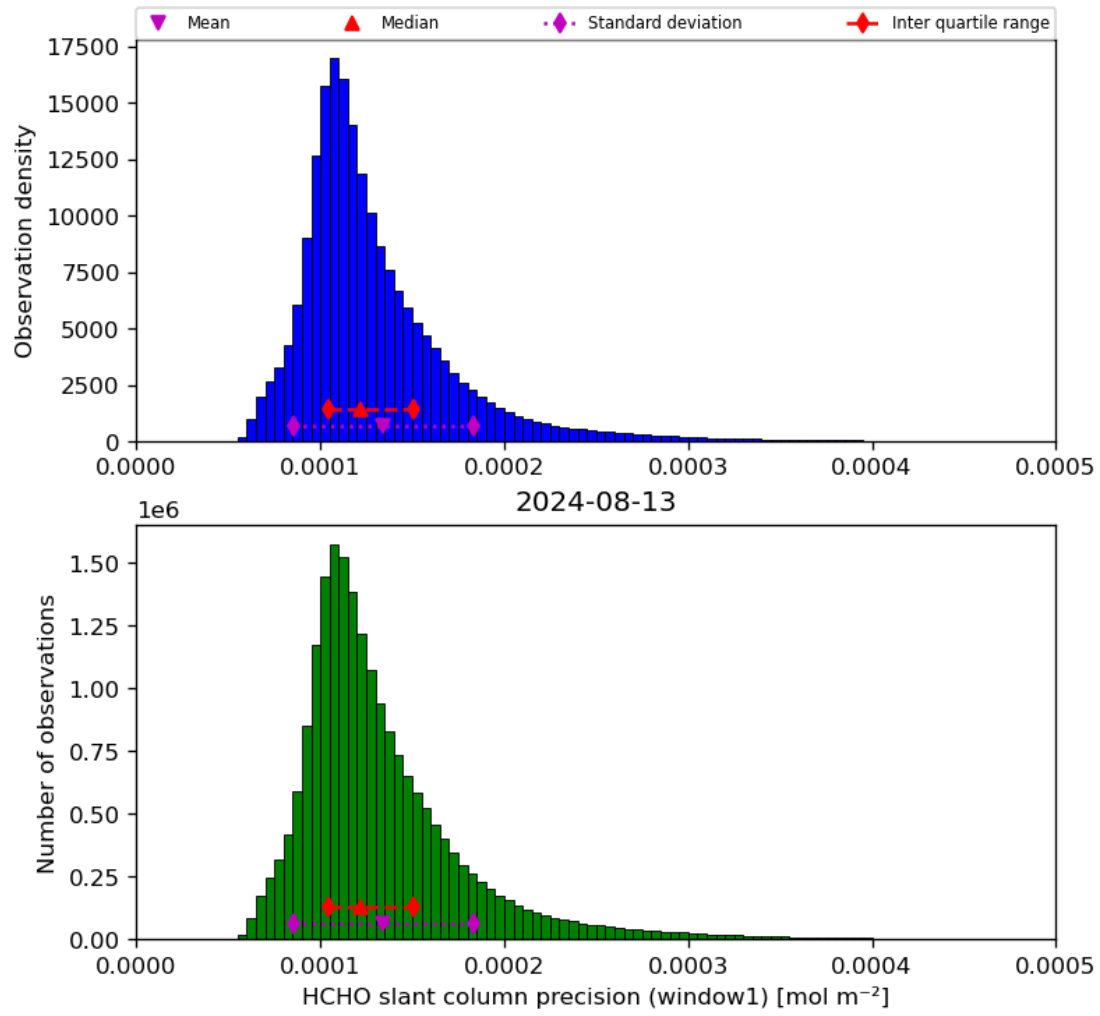
Figure 39: Histogram of “HCHO slant column precision (window1)” for 2024-08-12 to 2024-08-14
