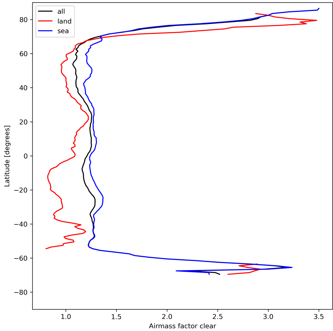
Figure 28: Zonal average of “Airmass factor clear” for 2024-08-12 to 2024-08-14.
