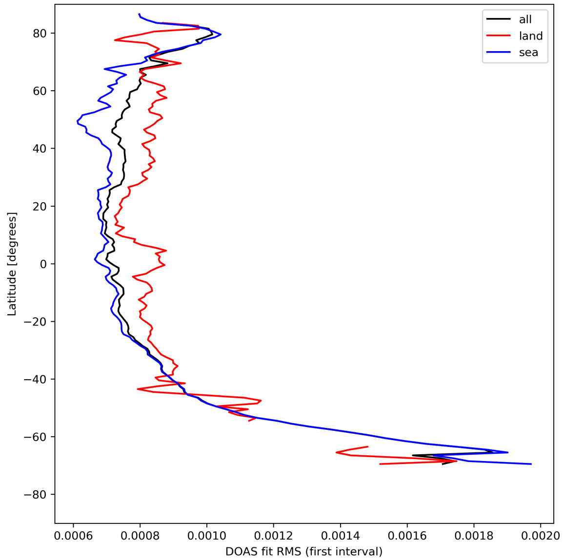
Figure 32: Zonal average of “DOAS fit RMS (first interval)” for 2024-08-12 to 2024-08-14.
