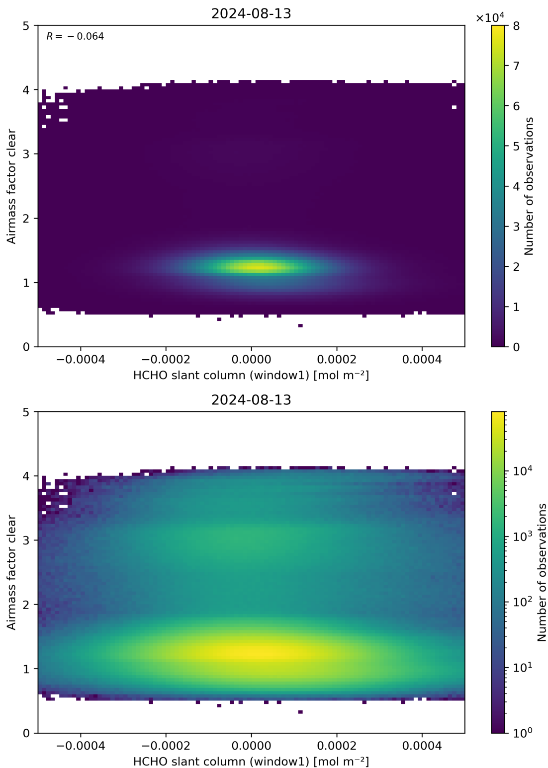
Figure 81: Scatter density plot of “HCHO slant column (window1)” against “Airmass factor clear” for 2024-08-12 to 2024-08-14.
