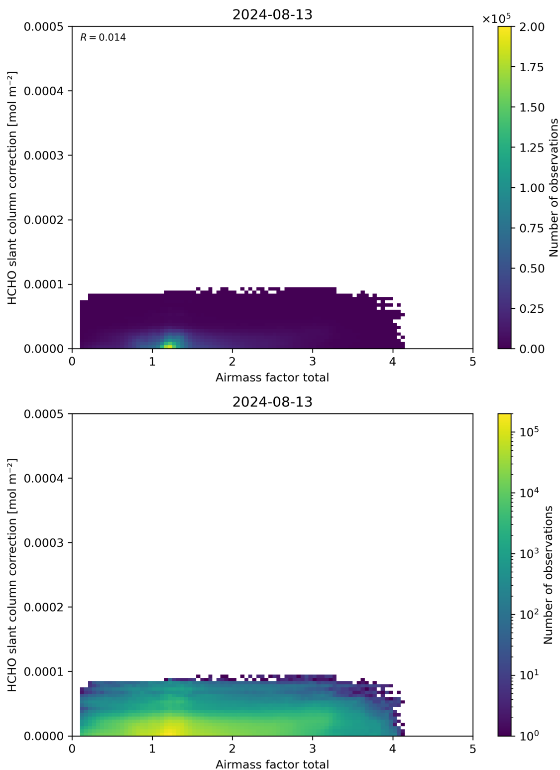
Figure 102: Scatter density plot of “Airmass factor total” against “HCHO slant column correction” for 2024-08-12 to 2024-08-14.
