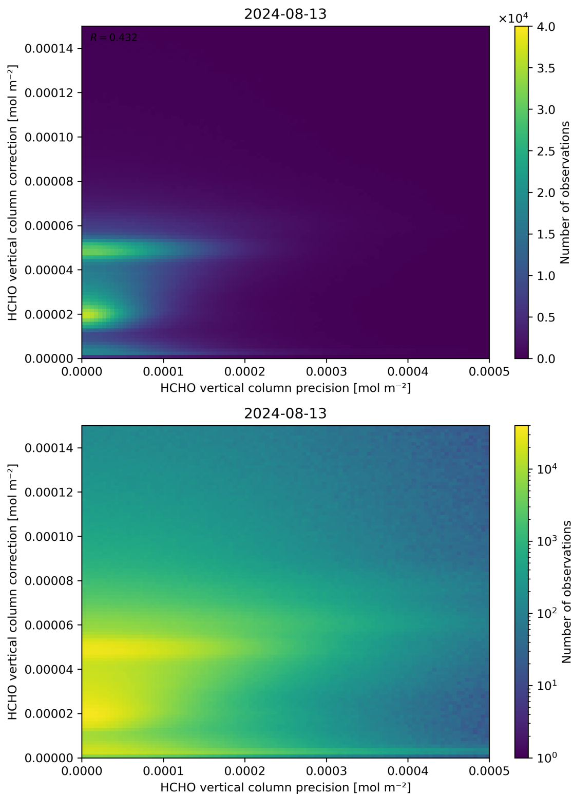
Figure 146: Scatter density plot of “HCHO vertical column precision” against “HCHO vertical column correction” for 2024-08-12 to 2024-08-14.
