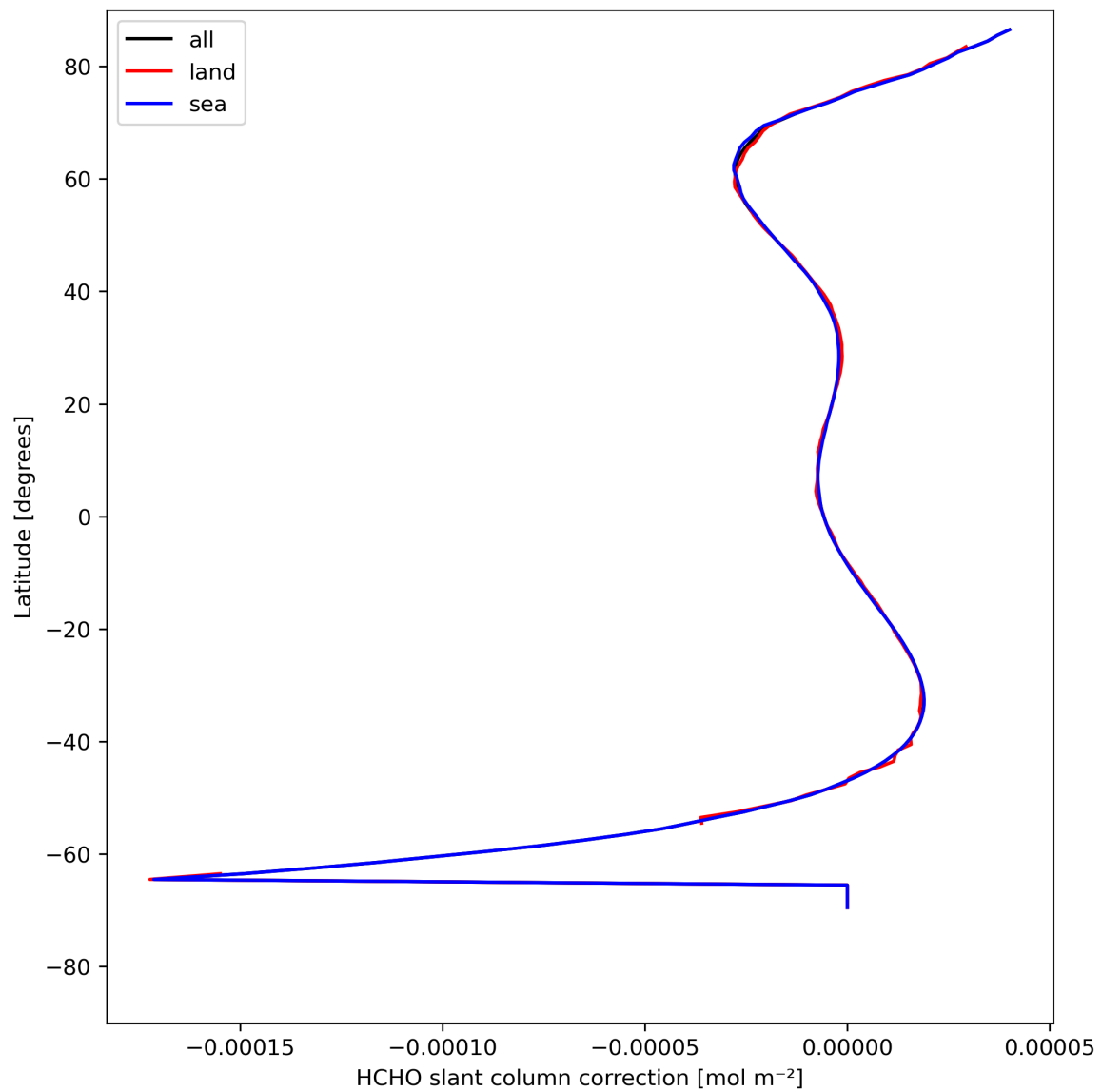
Figure 33: Zonal average of “HCHO slant column correction” for 2024-08-12 to 2024-08-14.
