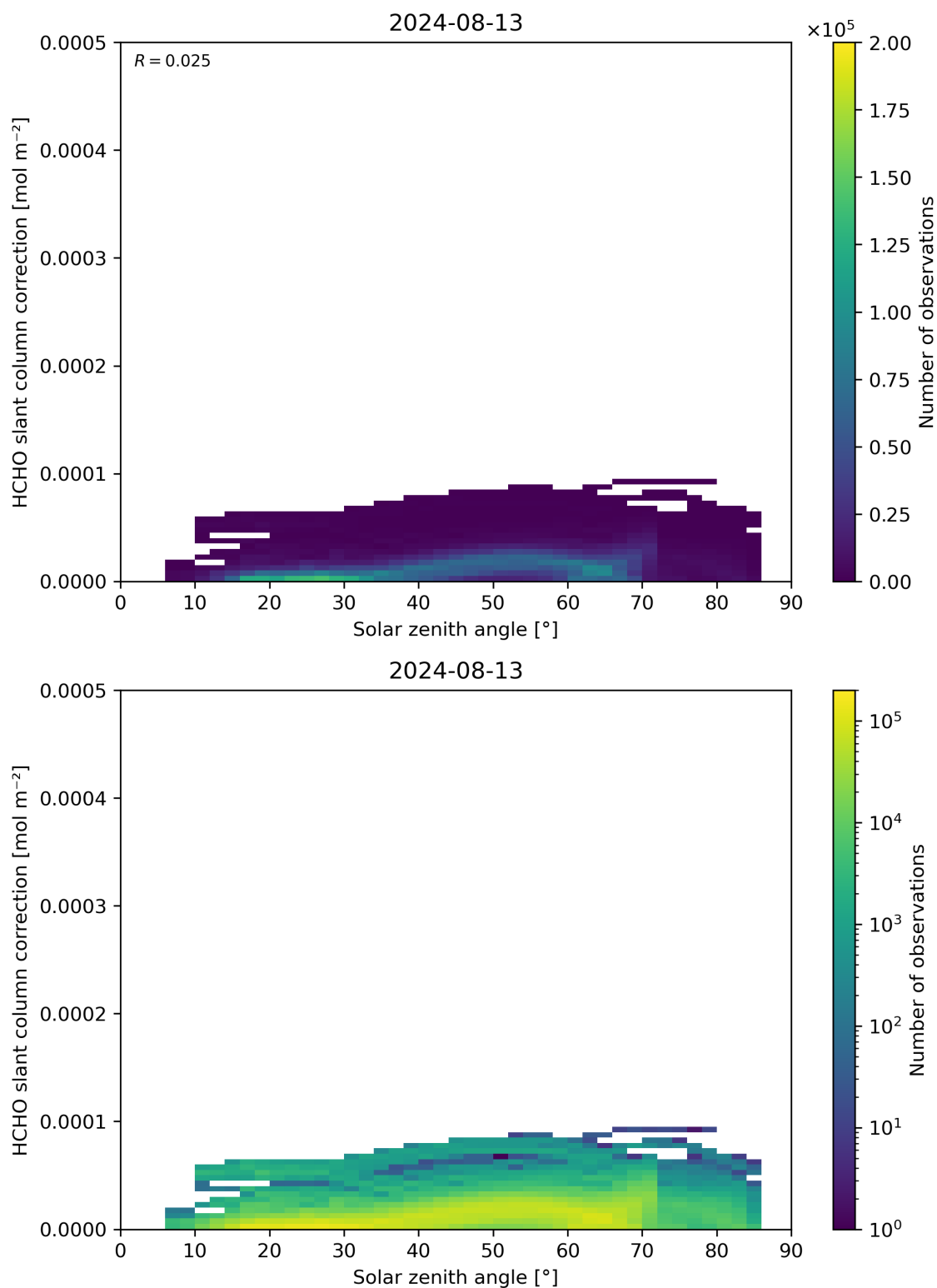
Figure 172: Scatter density plot of “Solar zenith angle” against “HCHO slant column correction” for 2024-08-12 to 2024-08-14.
