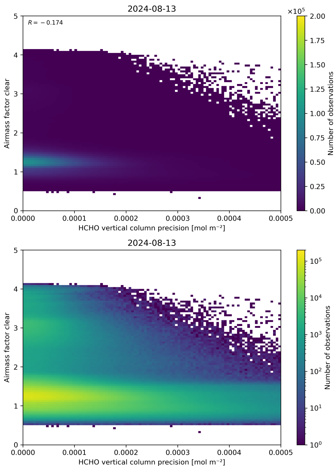
Figure 139: Scatter density plot of “HCHO vertical column precision” against “Airmass factor clear” for 2024-08-12 to 2024-08-14.
