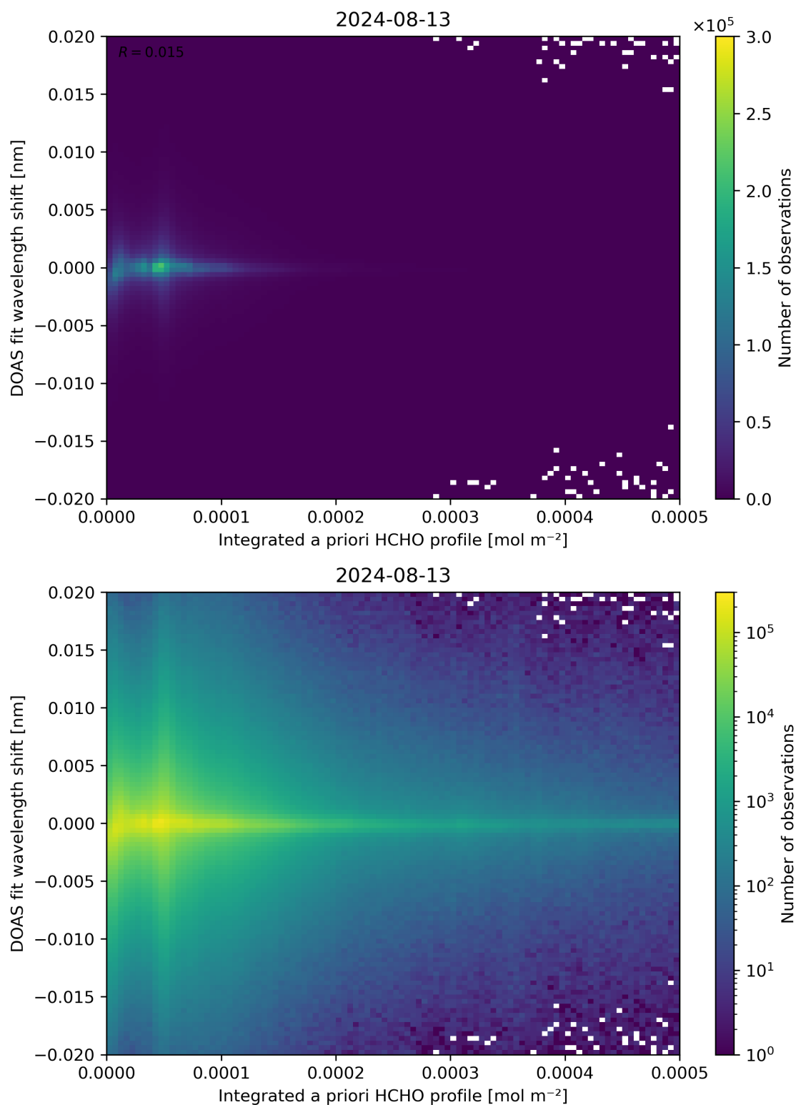
Figure 149: Scatter density plot of “Integrated a priori HCHO profile” against “DOAS fit wavelength shift” for 2024-08-12 to 2024-08-14.
