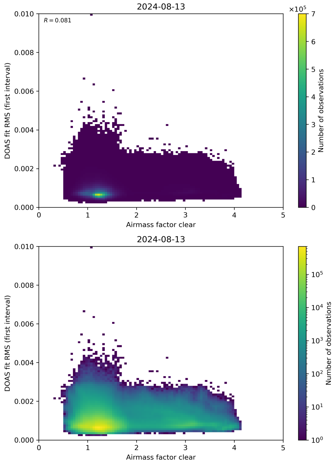
Figure 71: Scatter density plot of “Airmass factor clear” against “DOAS fit RMS (first interval)” for 2024-08-12 to 2024-08-14.
