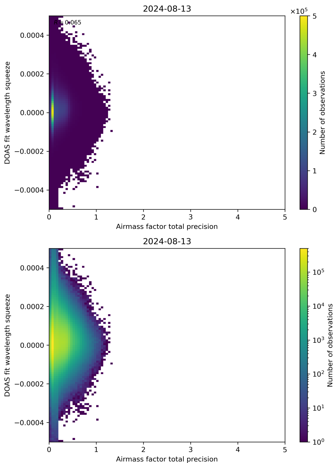
Figure 107: Scatter density plot of “Airmass factor total precision” against “DOAS fit wavelength squeeze” for 2024-08-12 to 2024-08-14.
