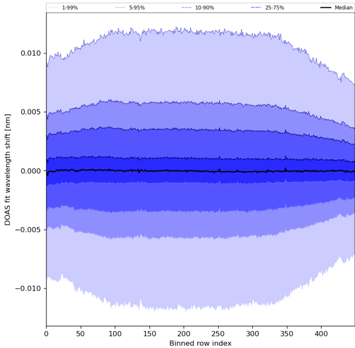
Figure 58: Along track statistics of “DOAS fit wavelength shift” for 2024-08-12 to 2024-08-14
