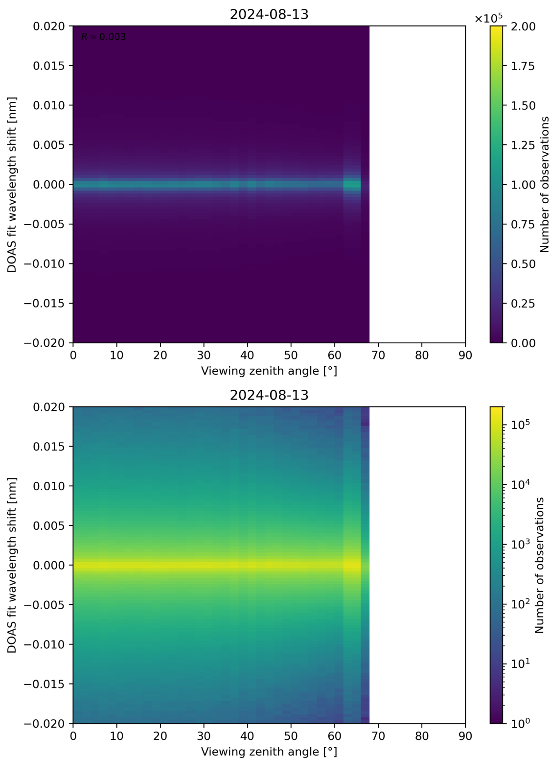
Figure 183: Scatter density plot of “Viewing zenith angle” against “DOAS fit wavelength shift” for 2024-08-12 to 2024-08-14.
