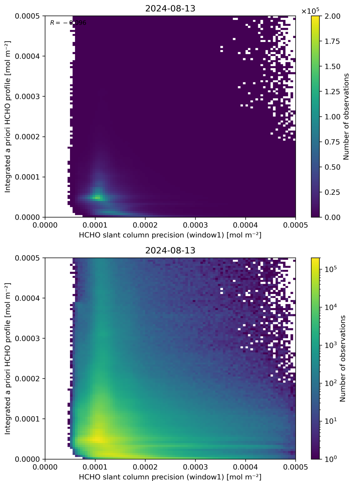
Figure 96: Scatter density plot of “HCHO slant column precision (window1)” against “Integrated a priori HCHO profile” for 2024-08-12 to 2024-08-14.
