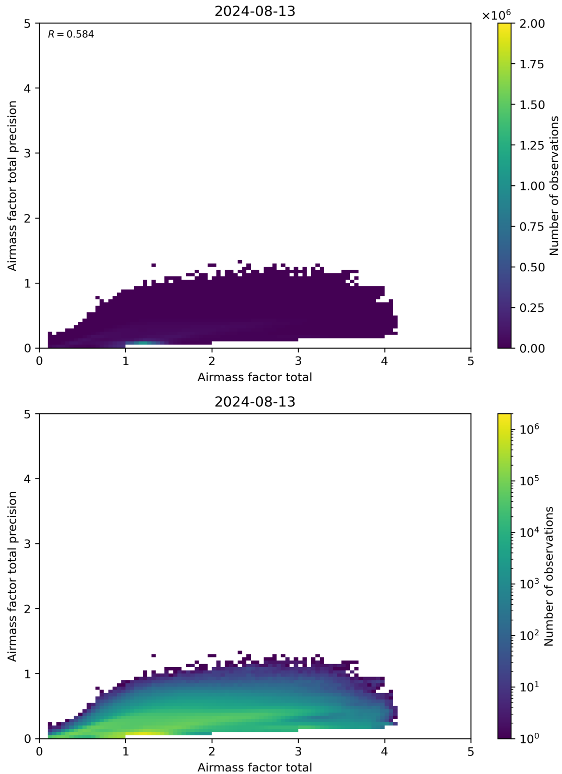
Figure 103: Scatter density plot of “Airmass factor total” against “Airmass factor total precision” for 2024-08-12 to 2024-08-14.
