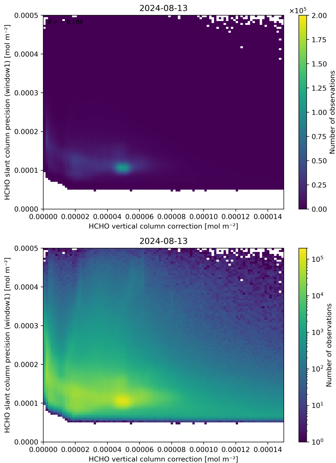
Figure 119: Scatter density plot of “HCHO vertical column correction” against “HCHO slant column precision (window1)” for 2024-08-12 to 2024-08-14.
