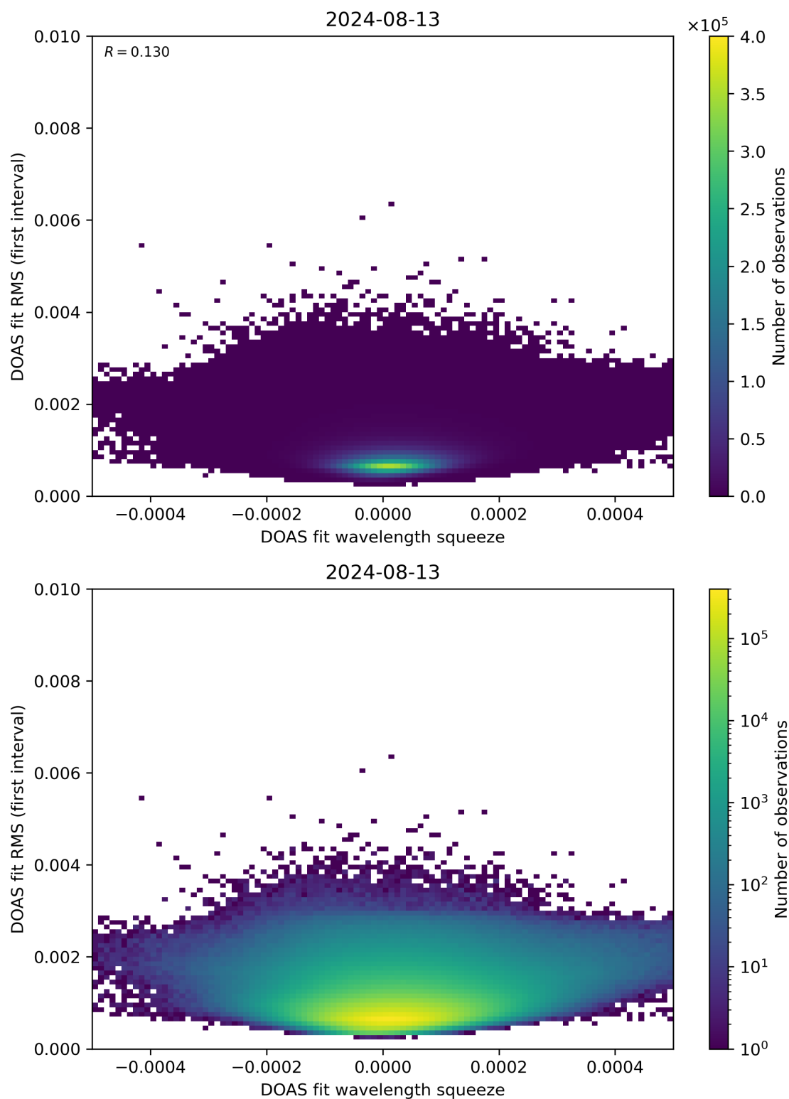
Figure 68: Scatter density plot of “DOAS fit wavelength squeeze” against “DOAS fit RMS (first interval)” for 2024-08-12 to 2024-08-14.
