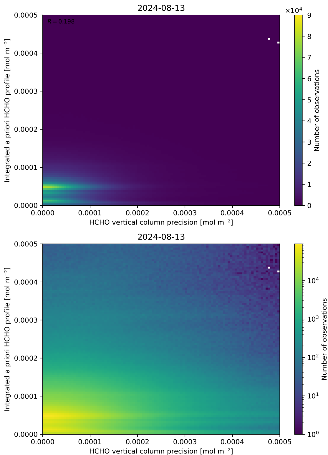
Figure 147: Scatter density plot of “HCHO vertical column precision” against “Integrated a priori HCHO profile” for 2024-08-12 to 2024-08-14.
