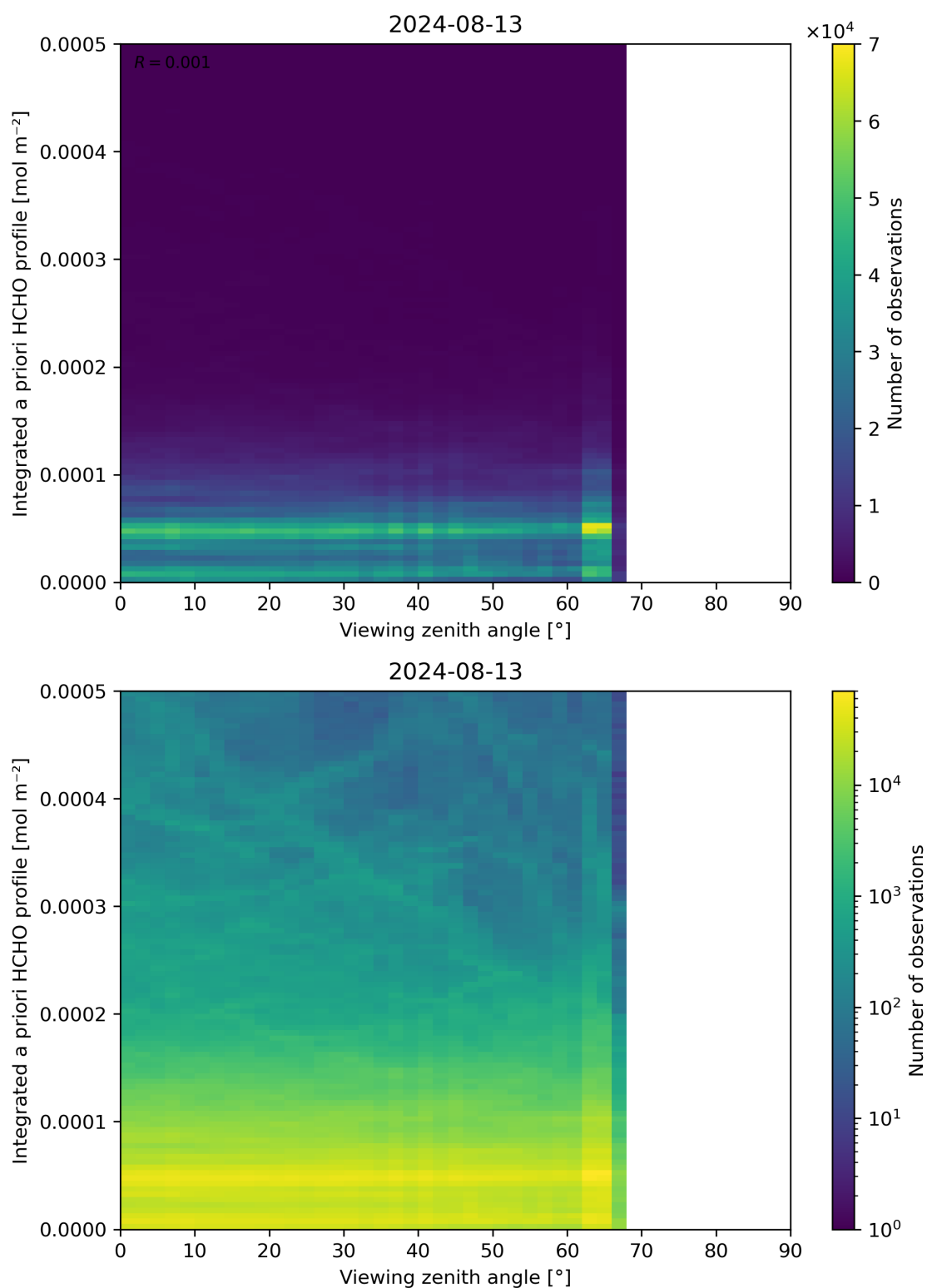
Figure 195: Scatter density plot of “Viewing zenith angle” against “Integrated a priori HCHO profile” for 2024-08-12 to 2024-08-14.
