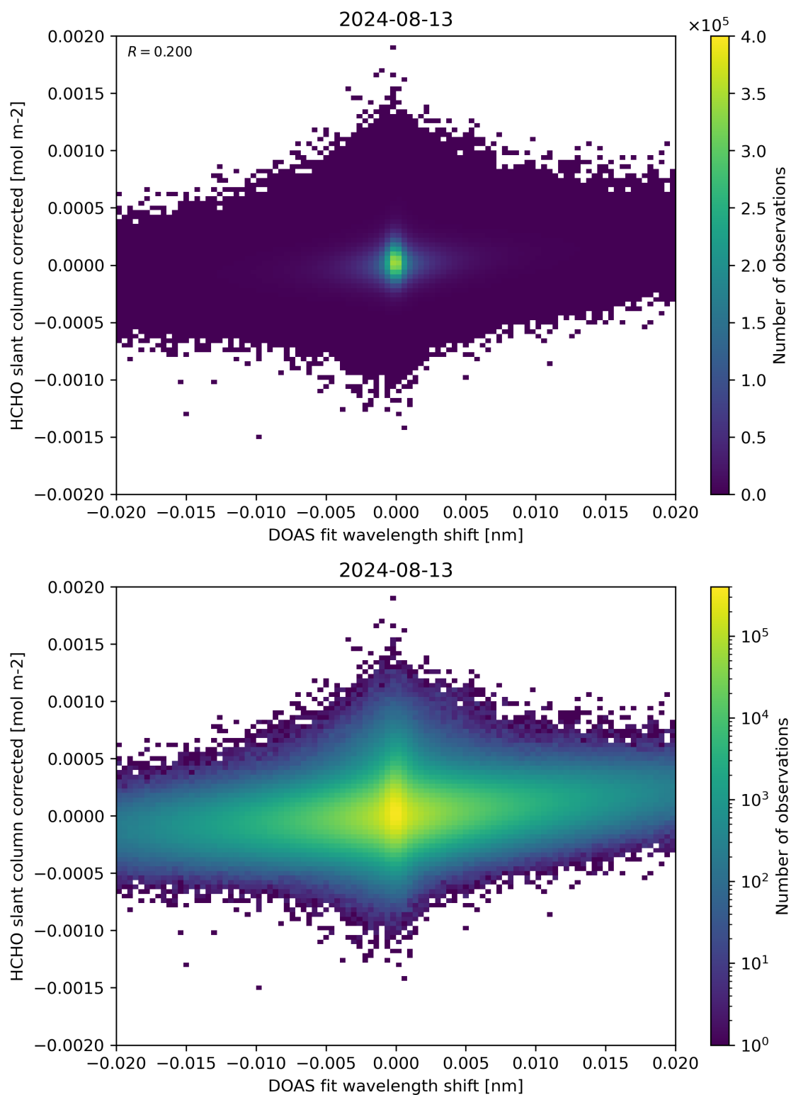
Figure 66: Scatter density plot of “DOAS fit wavelength shift” against “HCHO slant column corrected” for 2024-08-12 to 2024-08-14.
