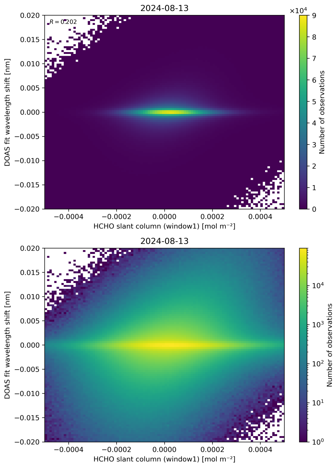
Figure 79: Scatter density plot of “HCHO slant column (window1)” against “DOAS fit wavelength shift” for 2024-08-12 to 2024-08-14.
