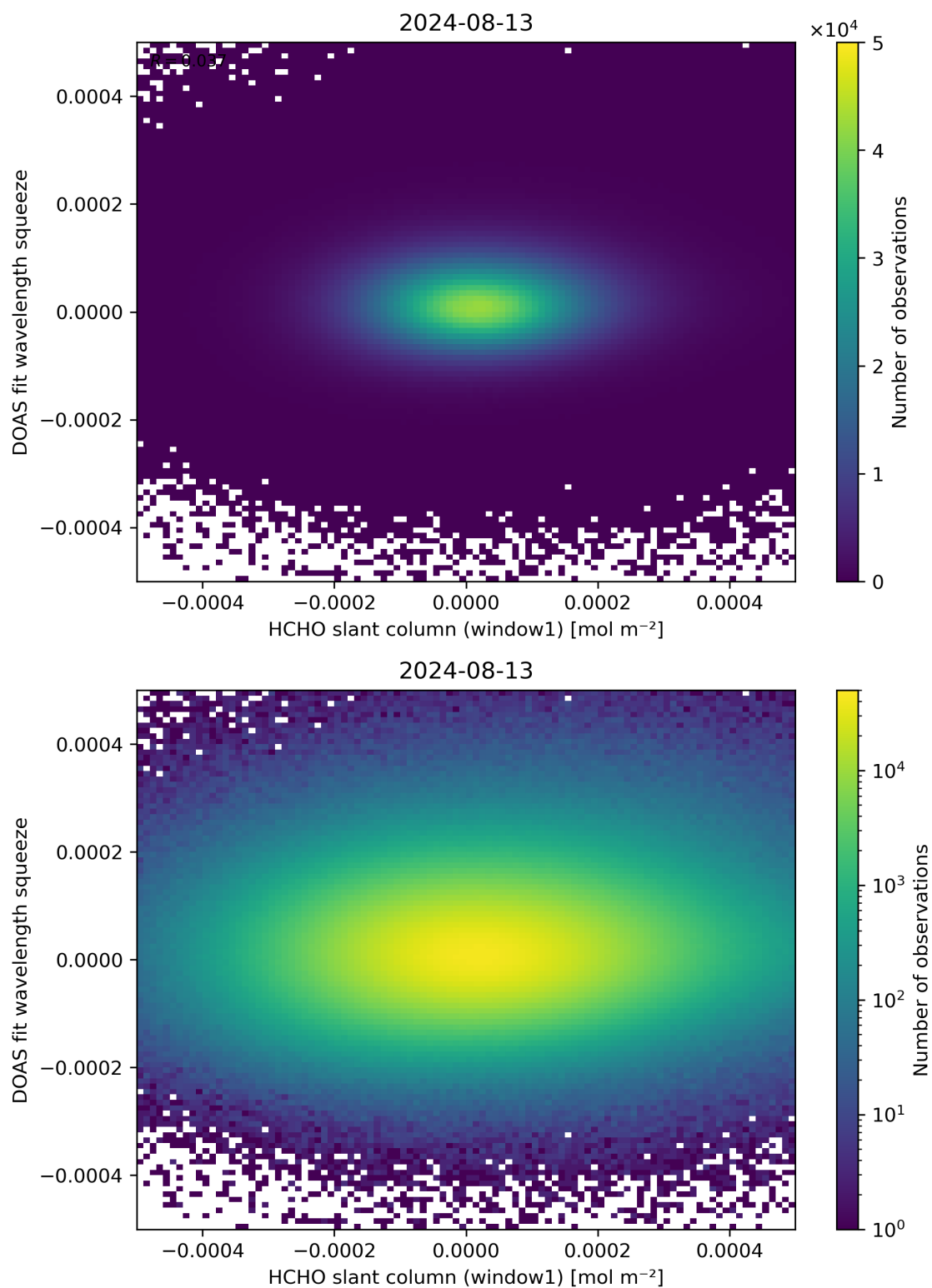
Figure 80: Scatter density plot of “HCHO slant column (window1)” against “DOAS fit wavelength squeeze” for 2024-08-12 to 2024-08-14.
