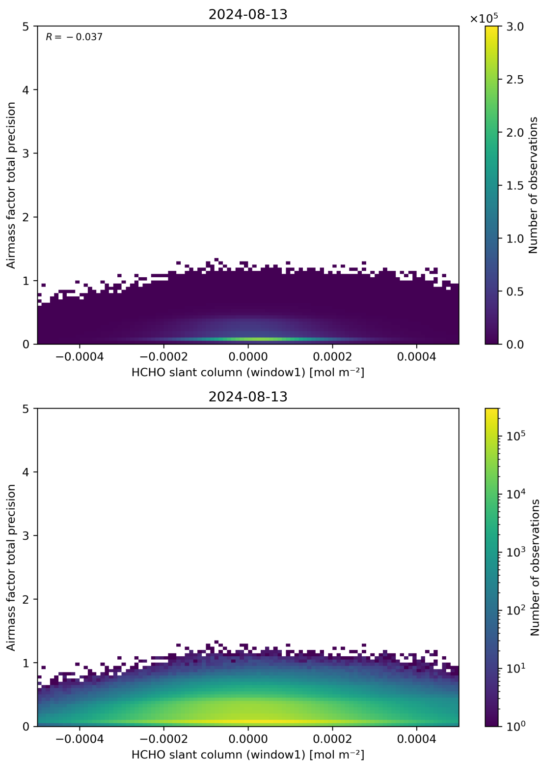
Figure 86: Scatter density plot of “HCHO slant column (window1)” against “Airmass factor total precision” for 2024-08-12 to 2024-08-14.
