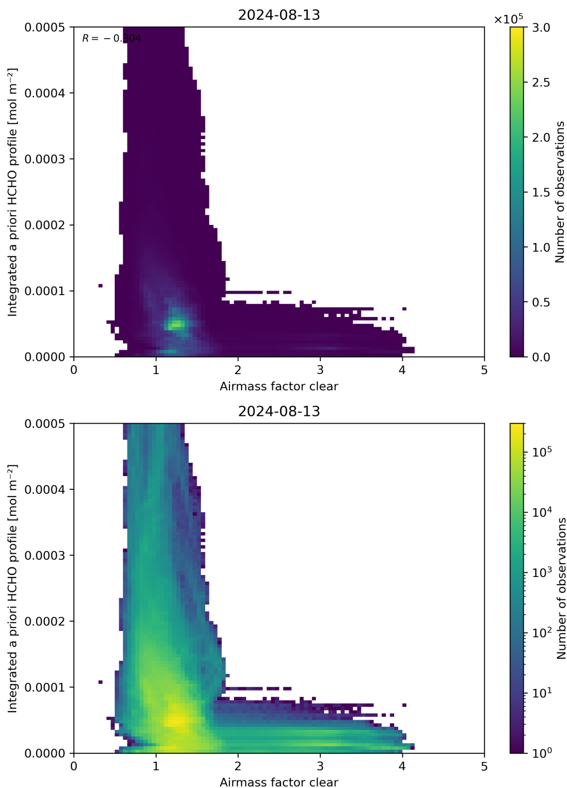
Figure 76: Scatter density plot of “Airmass factor clear” against “Integrated a priori HCHO profile” for 2024-08-12 to 2024-08-14.
