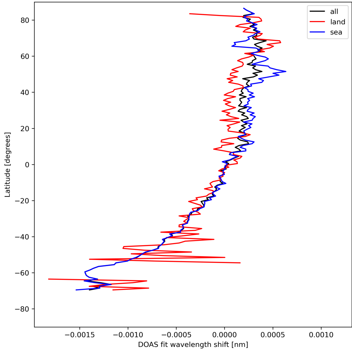
Figure 30: Zonal average of “DOAS fit wavelength shift” for 2024-08-12 to 2024-08-14.
