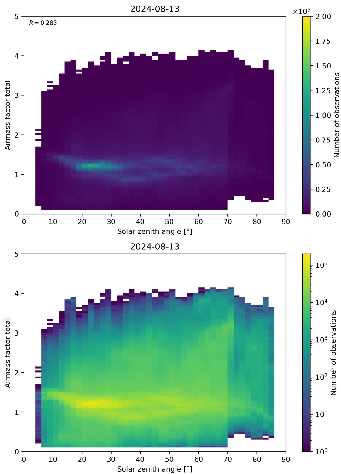
Figure 175: Scatter density plot of “Solar zenith angle” against “Airmass factor total” for 2024-08-12 to 2024-08-14.
