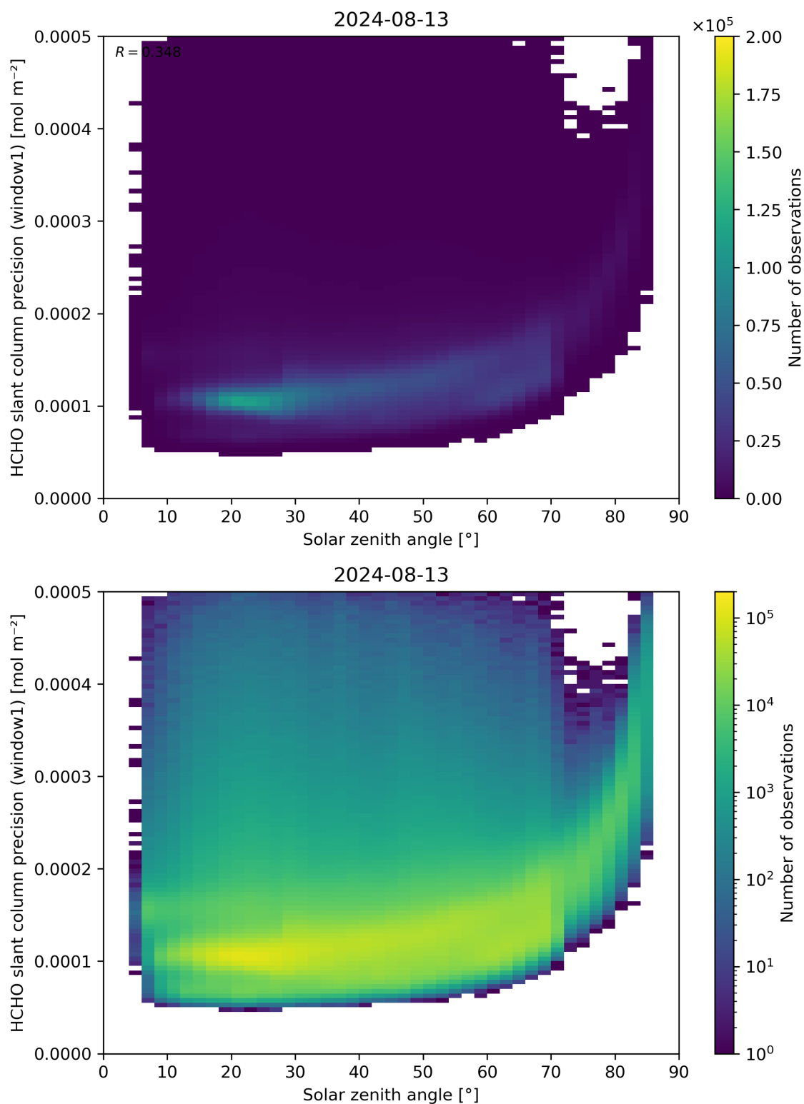
Figure 174: Scatter density plot of “Solar zenith angle” against “HCHO slant column precision (window1)” for 2024-08-12 to 2024-08-14.
