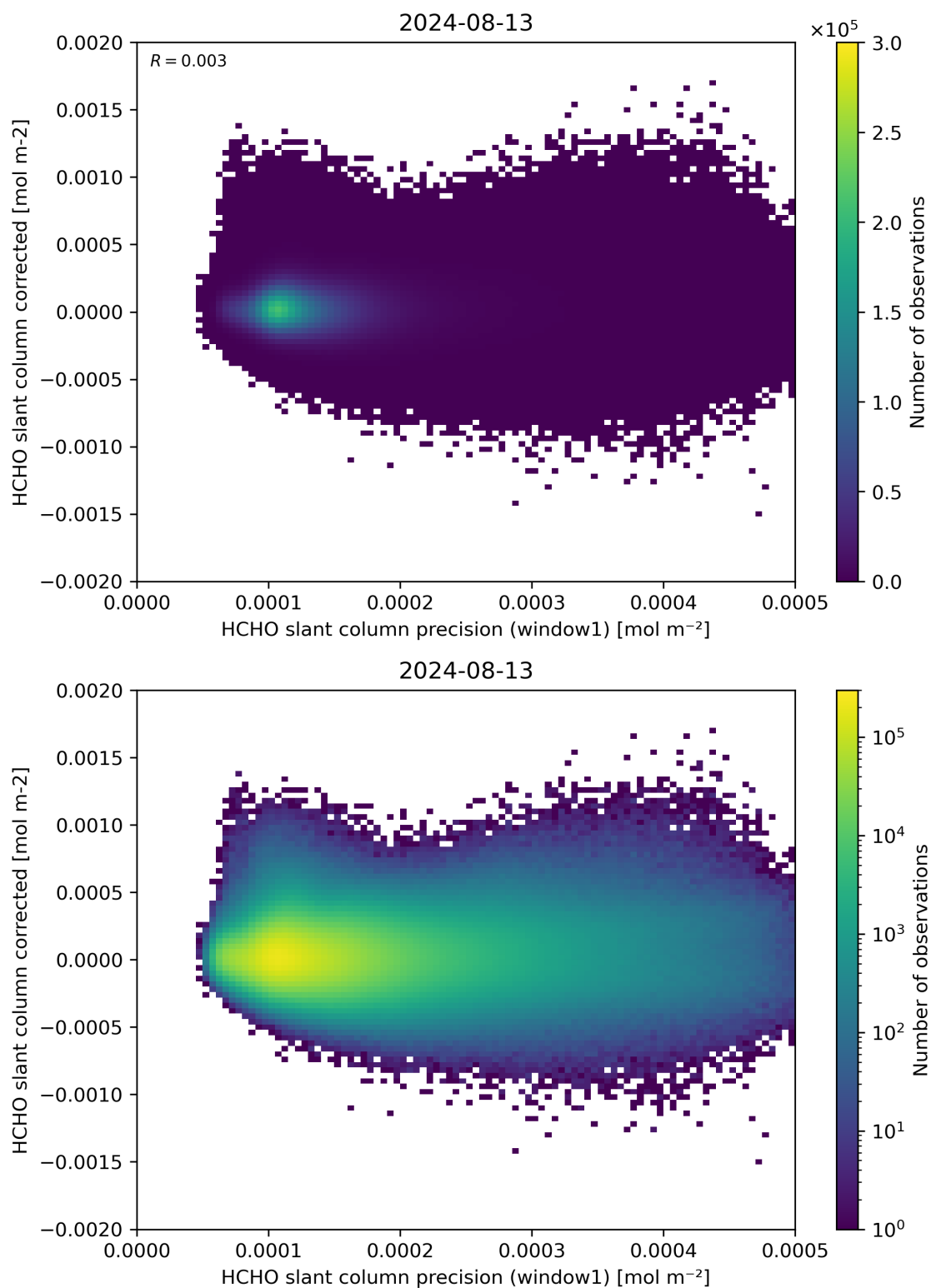
Figure 92: Scatter density plot of “HCHO slant column precision (window1)” against “HCHO slant column corrected” for 2024-08-12 to 2024-08-14.
