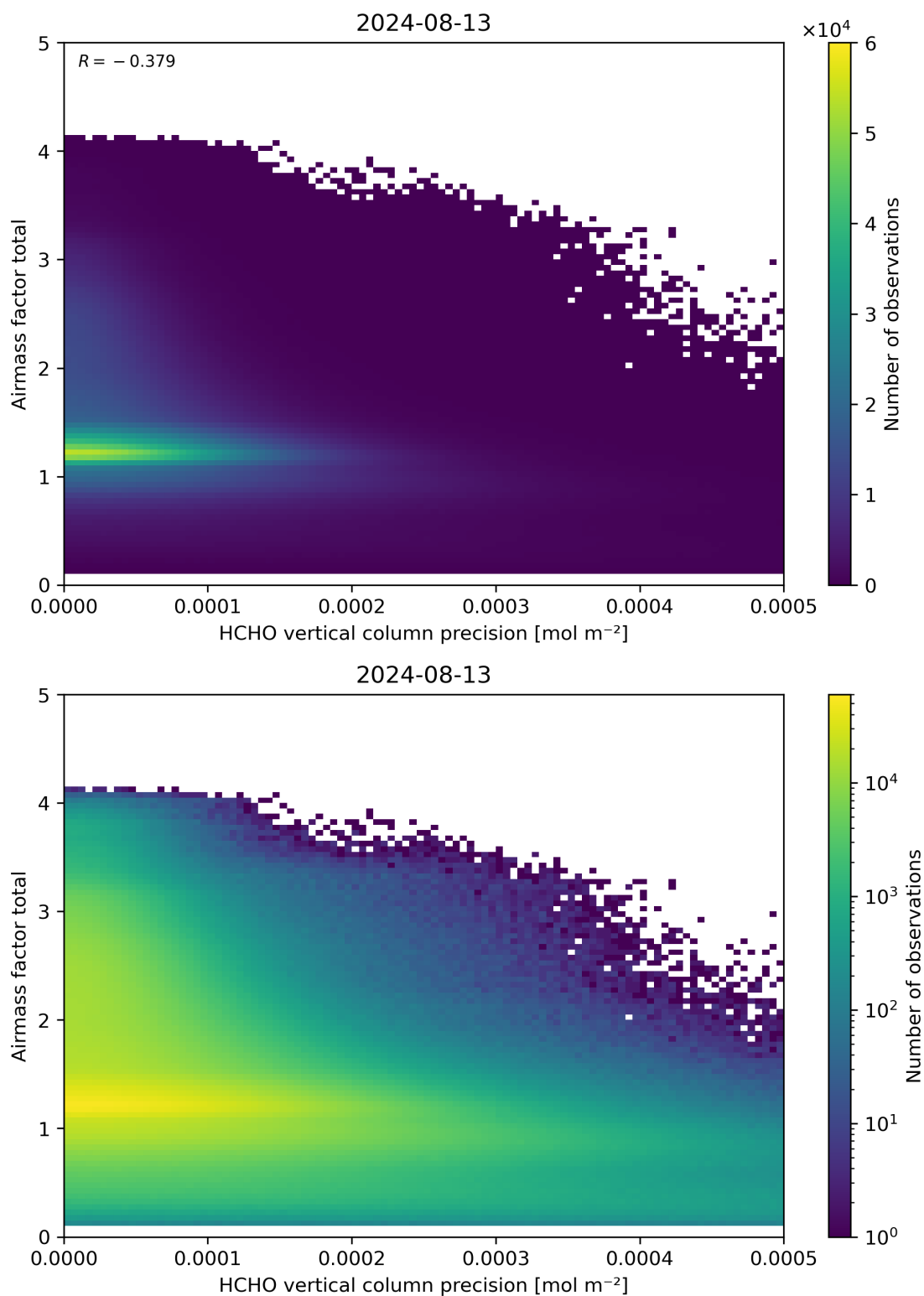
Figure 144: Scatter density plot of “HCHO vertical column precision” against “Airmass factor total” for 2024-08-12 to 2024-08-14.
