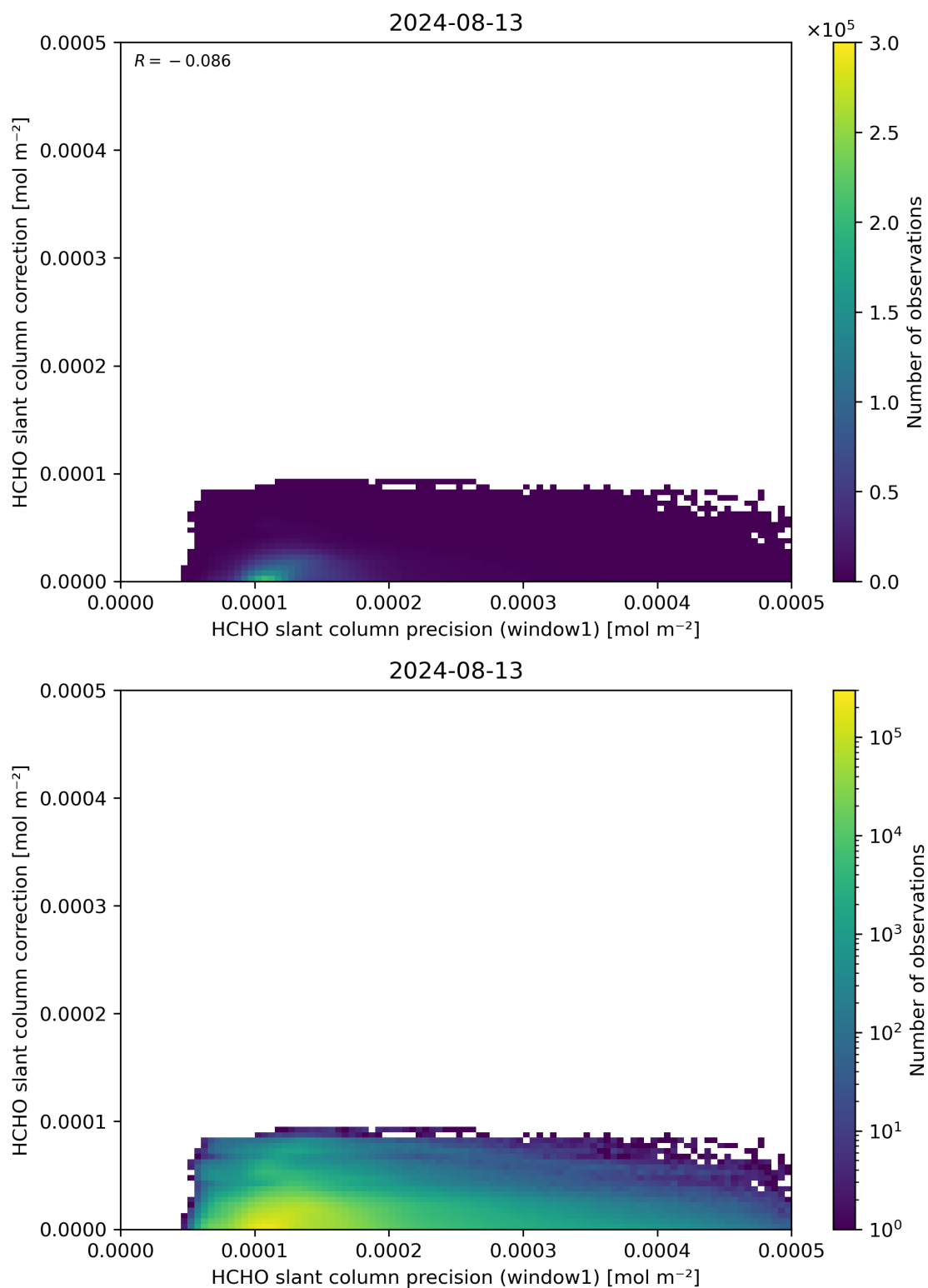
Figure 93: Scatter density plot of “HCHO slant column precision (window1)” against “HCHO slant column correction” for 2024-08-12 to 2024-08-14.
