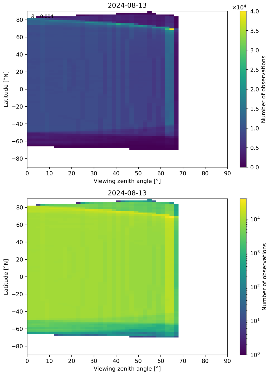
Figure 196: Scatter density plot of “Viewing zenith angle” against “Latitude” for 2024-08-12 to 2024-08-14.
