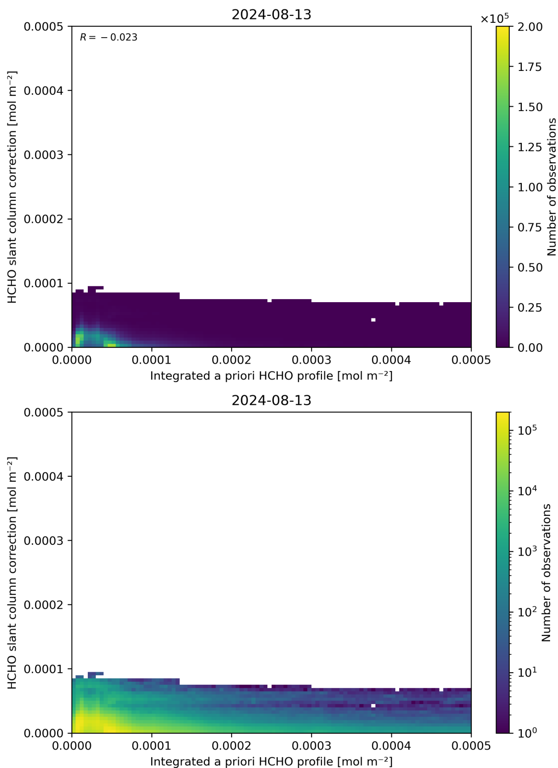
Figure 152: Scatter density plot of “Integrated a priori HCHO profile” against “HCHO slant column correction” for 2024-08-12 to 2024-08-14.
