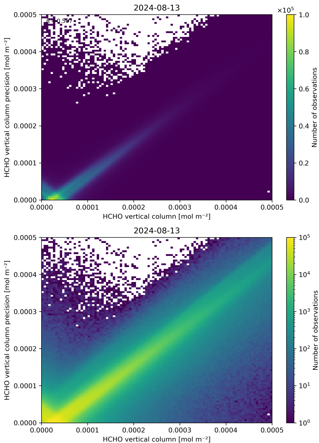
Figure 134: Scatter density plot of “HCHO vertical column” against “HCHO vertical column precision” for 2024-08-12 to 2024-08-14.
