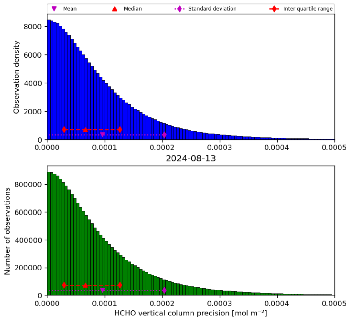
Figure 36: Histogram of “HCHO vertical column precision” for 2024-08-12 to 2024-08-14
