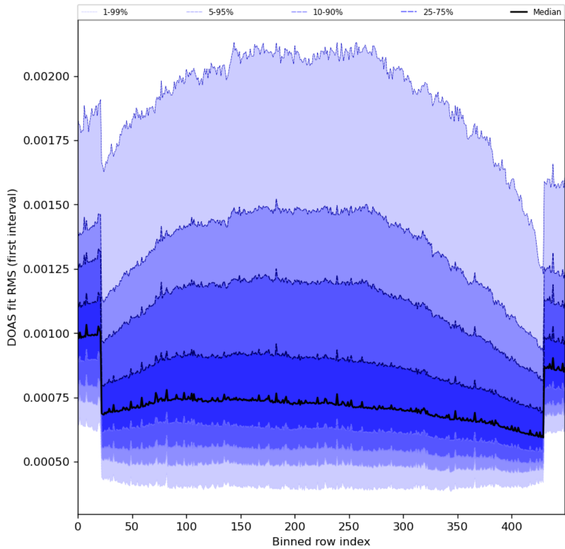
Figure 60: Along track statistics of “DOAS fit RMS (first interval)” for 2024-08-12 to 2024-08-14
