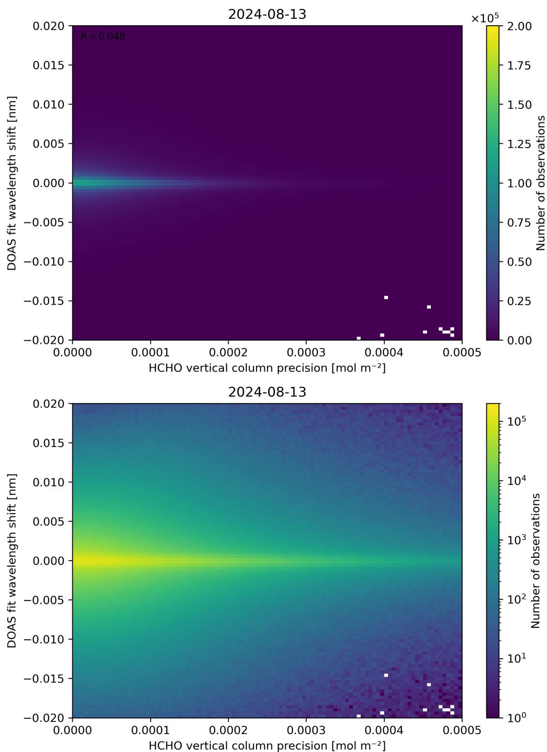
Figure 137: Scatter density plot of “HCHO vertical column precision” against “DOAS fit wavelength shift” for 2024-08-12 to 2024-08-14.
