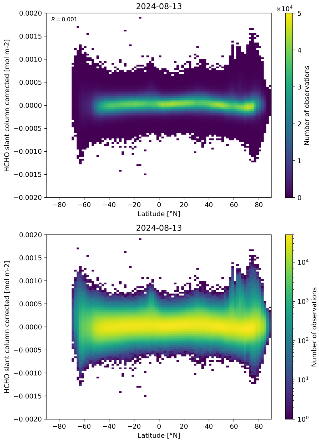
Figure 157: Scatter density plot of “Latitude” against “HCHO slant column corrected” for 2024-08-12 to 2024-08-14.
