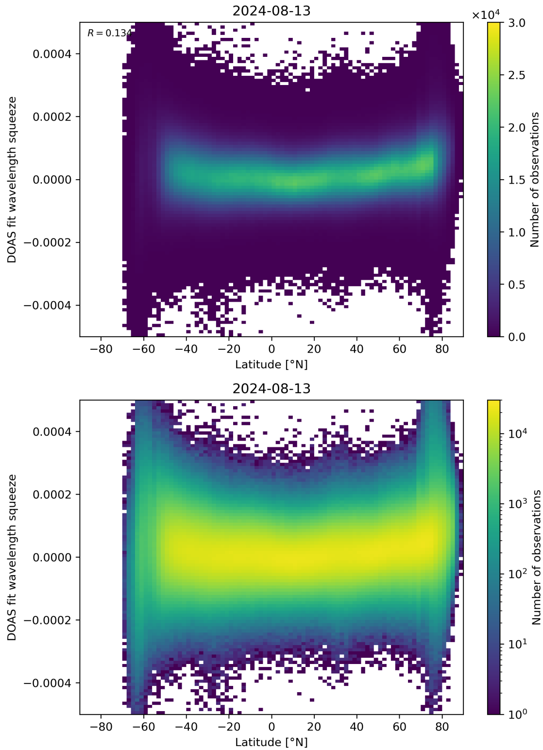
Figure 155: Scatter density plot of “Latitude” against “DOAS fit wavelength squeeze” for 2024-08-12 to 2024-08-14.
