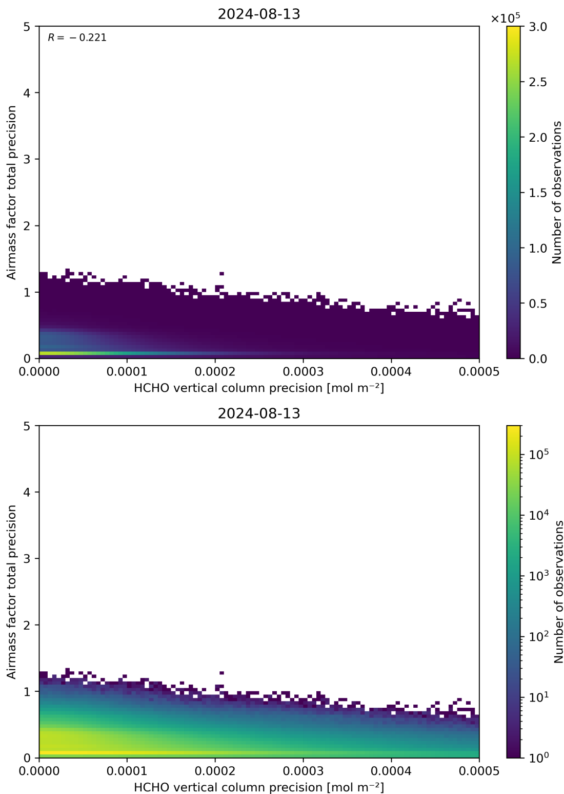
Figure 145: Scatter density plot of “HCHO vertical column precision” against “Airmass factor total precision” for 2024-08-12 to 2024-08-14.
