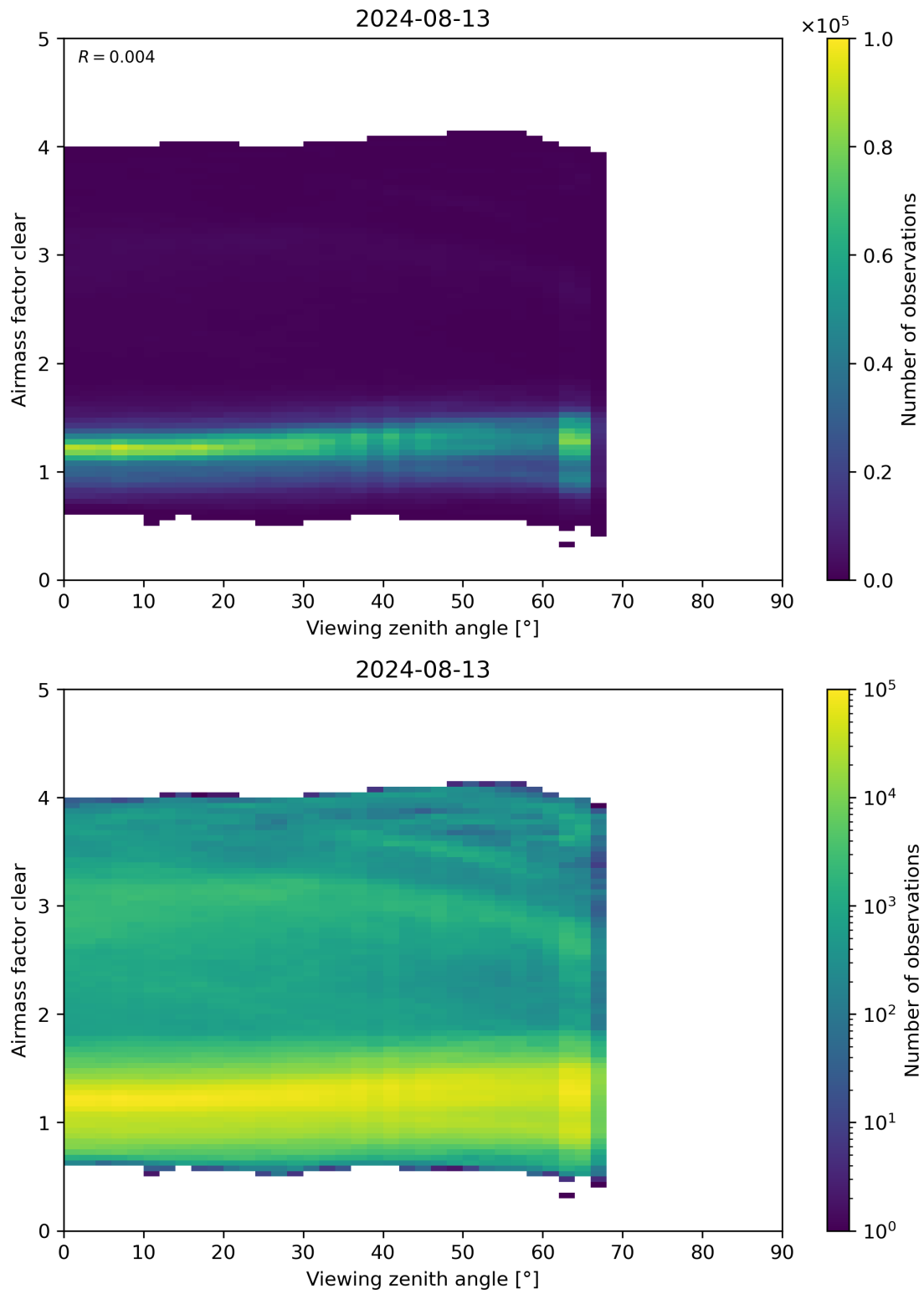
Figure 185: Scatter density plot of “Viewing zenith angle” against “Airmass factor clear” for 2024-08-12 to 2024-08-14.
