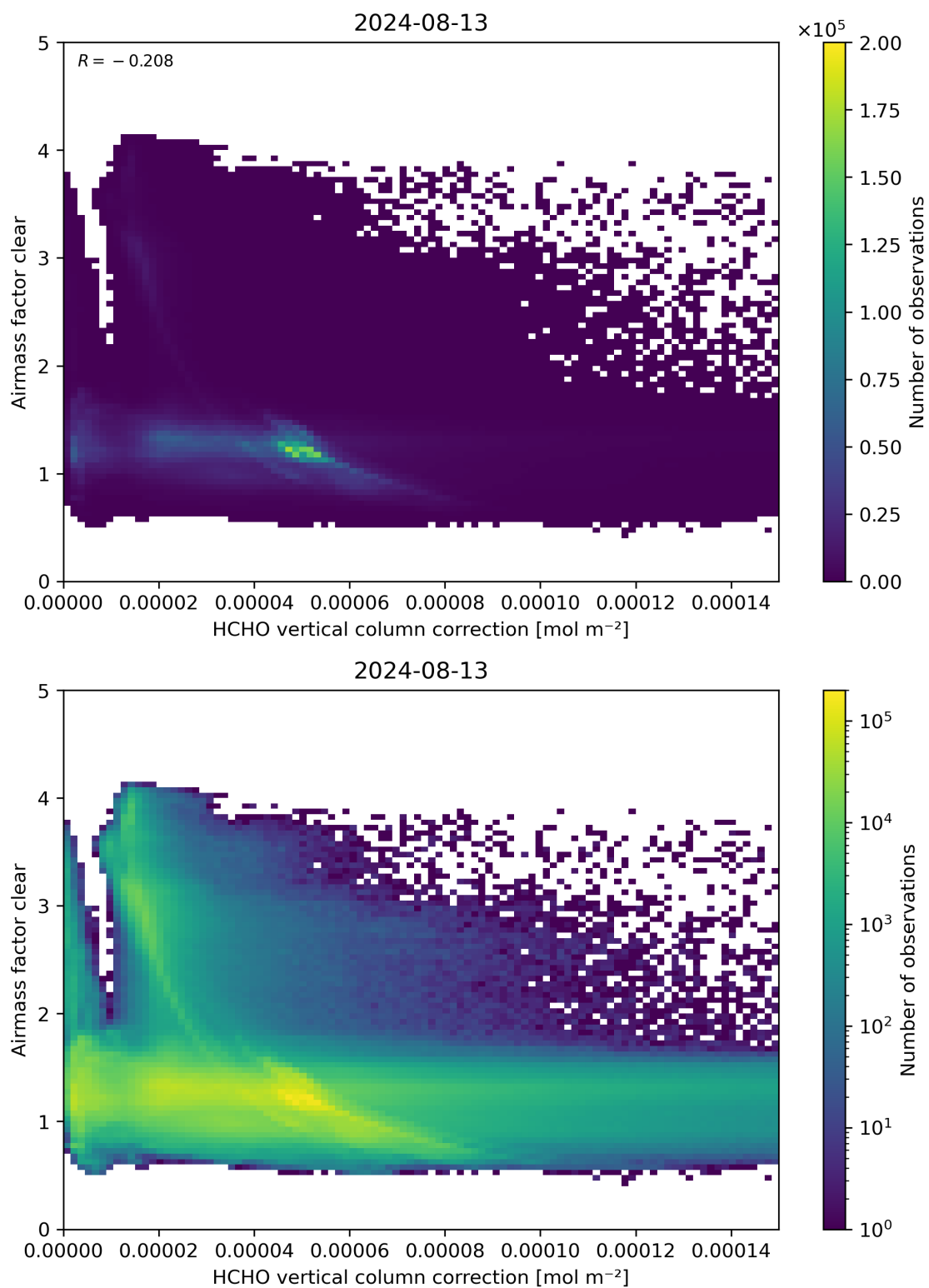
Figure 115: Scatter density plot of “HCHO vertical column correction” against “Airmass factor clear” for 2024-08-12 to 2024-08-14.
