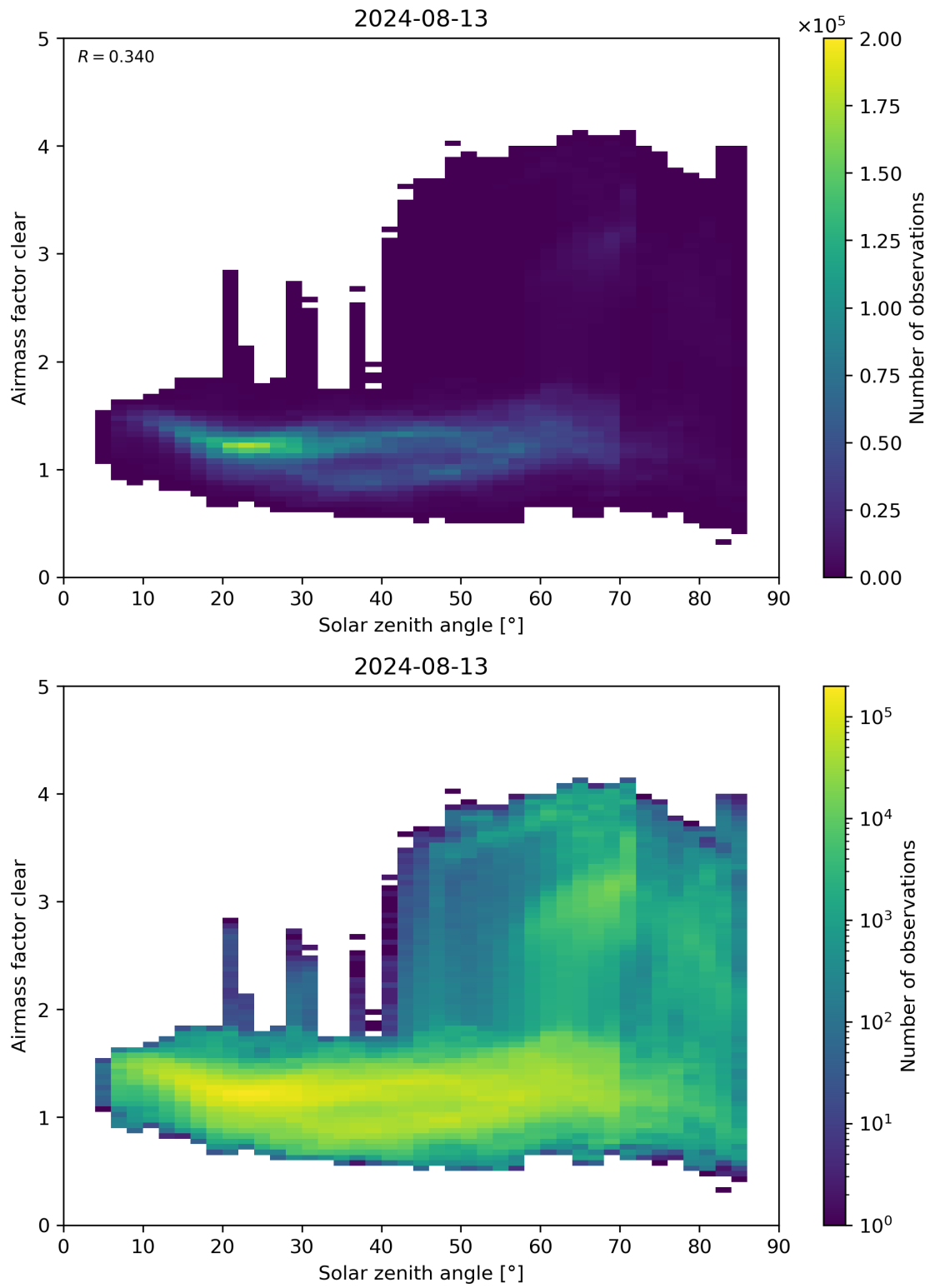
Figure 170: Scatter density plot of “Solar zenith angle” against “Airmass factor clear” for 2024-08-12 to 2024-08-14.
