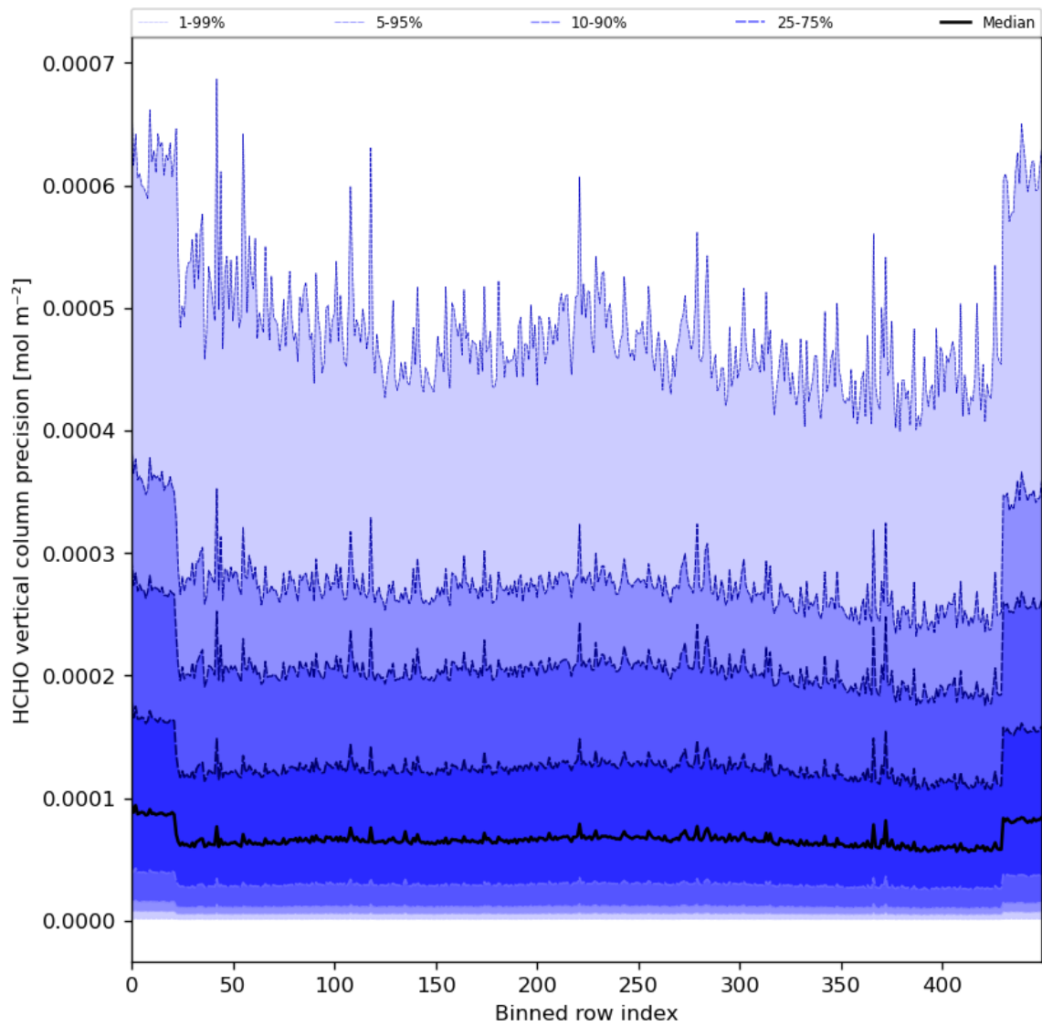
Figure 50: Along track statistics of “HCHO vertical column precision” for 2024-08-12 to 2024-08-14
