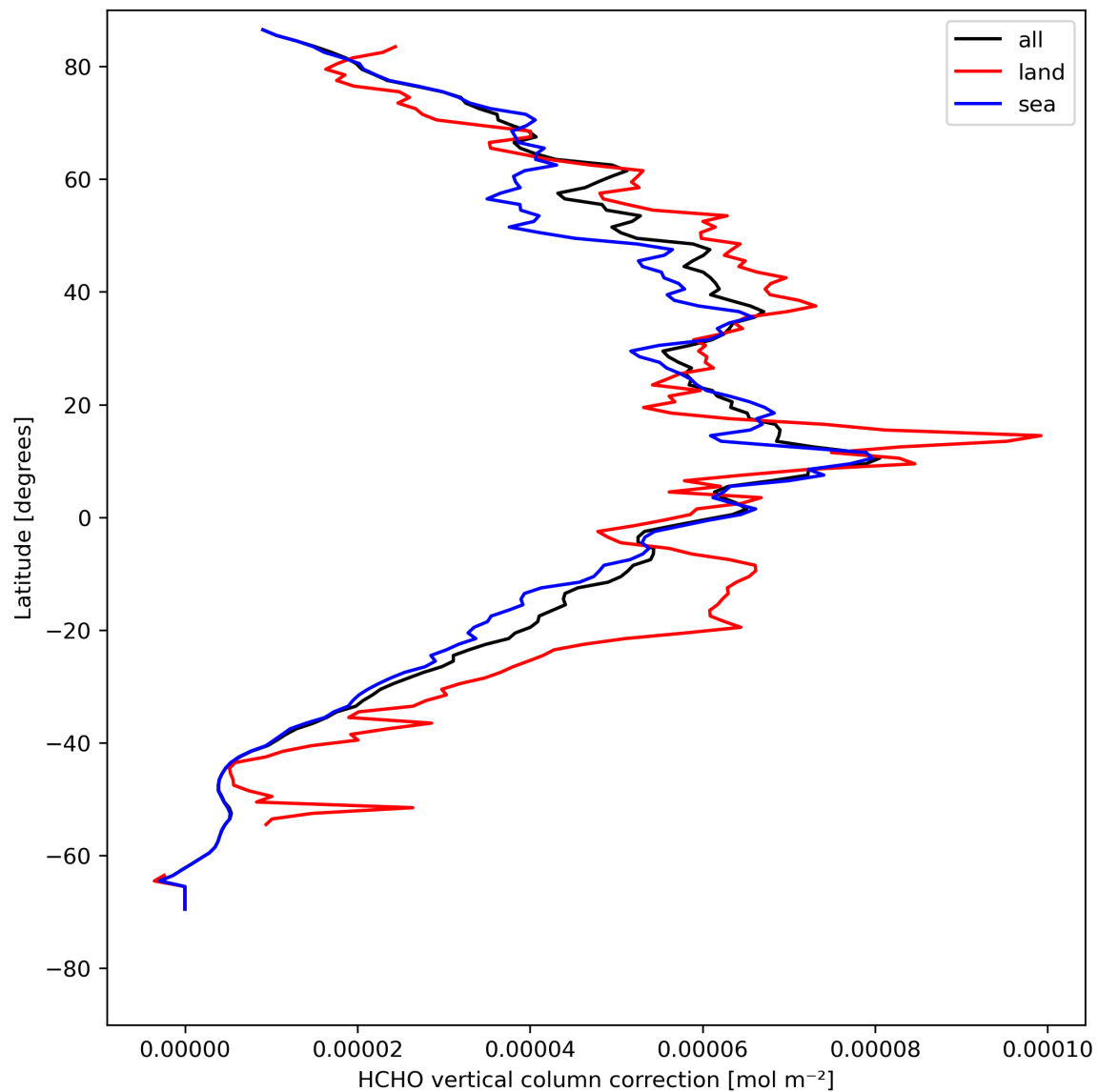
Figure 23: Zonal average of “HCHO vertical column correction” for 2024-08-12 to 2024-08-14.
