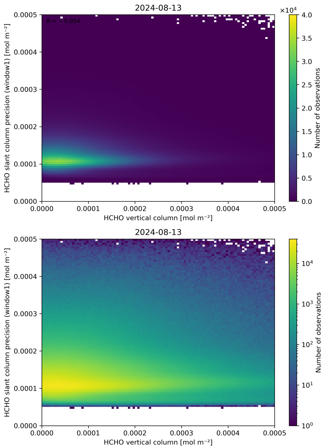
Figure 130: Scatter density plot of “HCHO vertical column” against “HCHO slant column precision (window1)” for 2024-08-12 to 2024-08-14.
