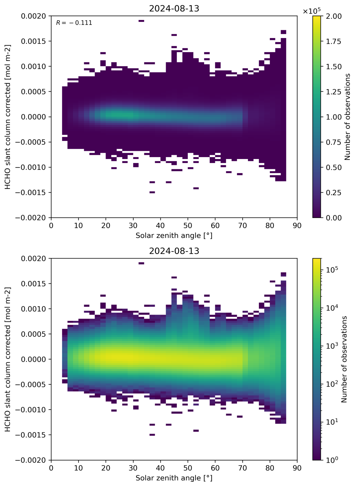
Figure 171: Scatter density plot of “Solar zenith angle” against “HCHO slant column corrected” for 2024-08-12 to 2024-08-14.
