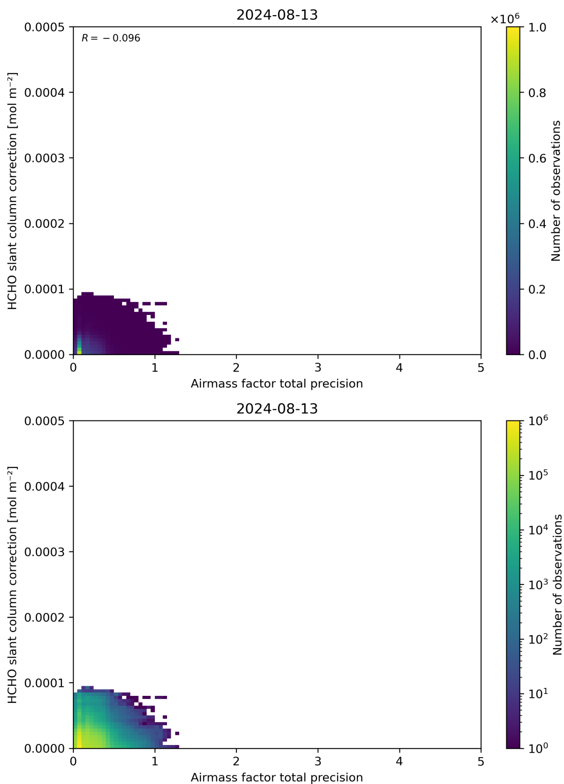
Figure 110: Scatter density plot of “Airmass factor total precision” against “HCHO slant column correction” for 2024-08-12 to 2024-08-14.
