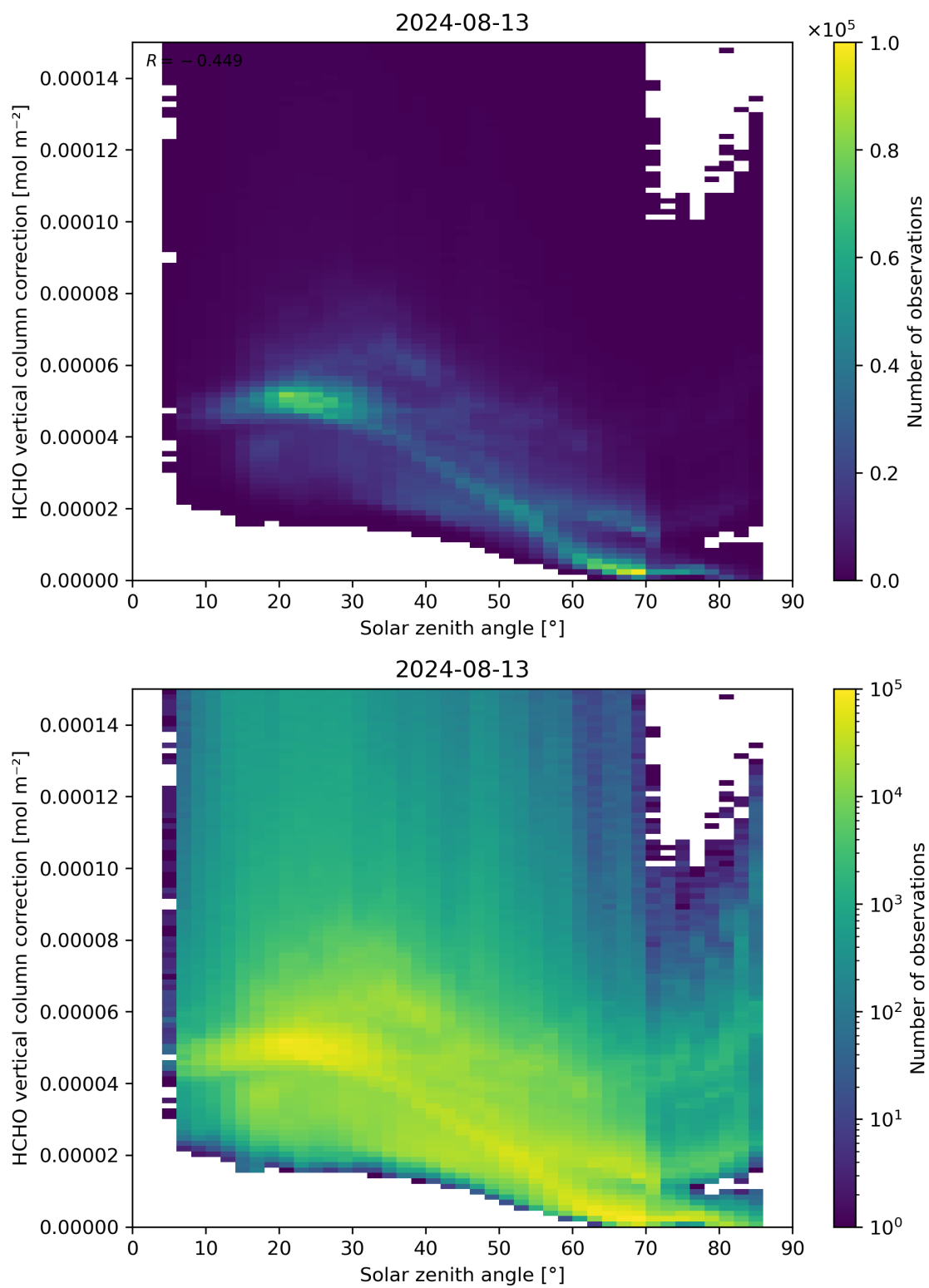
Figure 178: Scatter density plot of “Solar zenith angle” against “HCHO vertical column correction” for 2024-08-12 to 2024-08-14.
