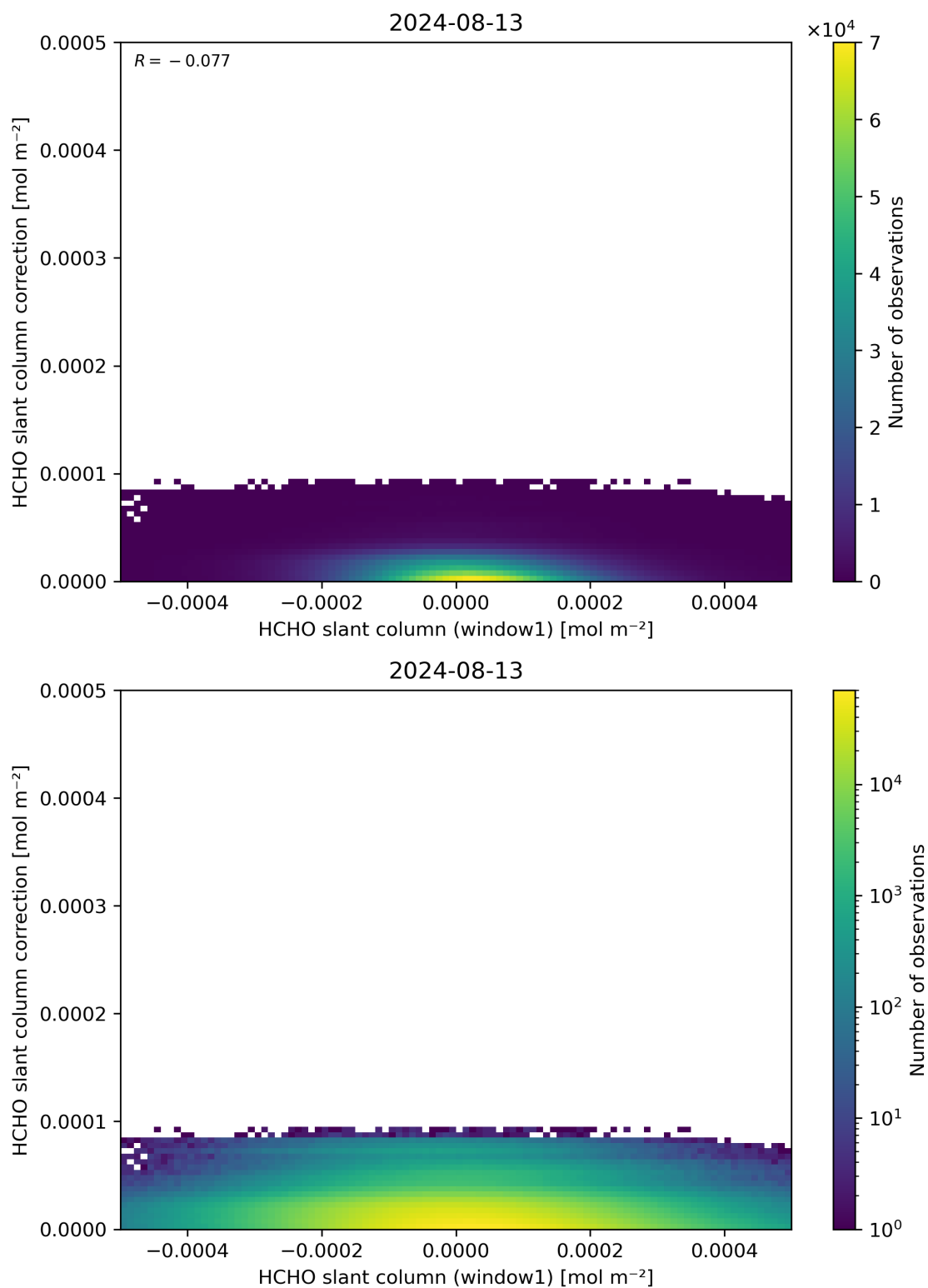
Figure 83: Scatter density plot of “HCHO slant column (window1)” against “HCHO slant column correction” for 2024-08-12 to 2024-08-14.
