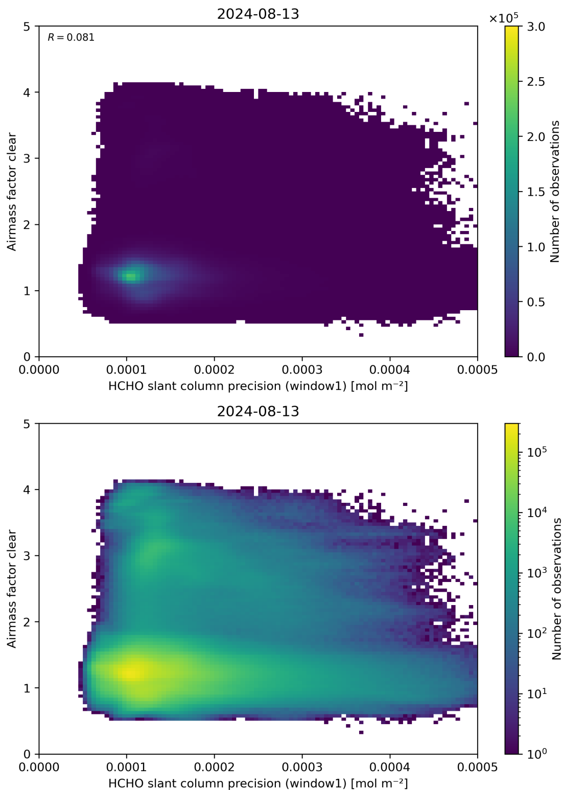
Figure 91: Scatter density plot of “HCHO slant column precision (window1)” against “Airmass factor clear” for 2024-08-12 to 2024-08-14.
