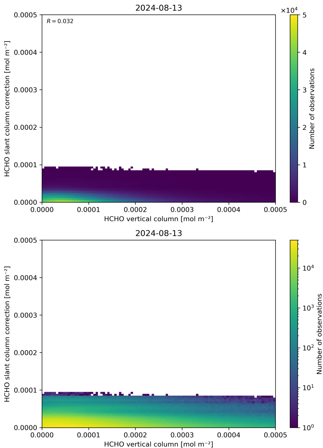
Figure 128: Scatter density plot of “HCHO vertical column” against “HCHO slant column correction” for 2024-08-12 to 2024-08-14.
