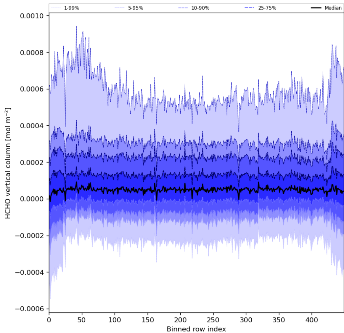
Figure 49: Along track statistics of “HCHO vertical column” for 2024-08-13 to 2024-08-15
