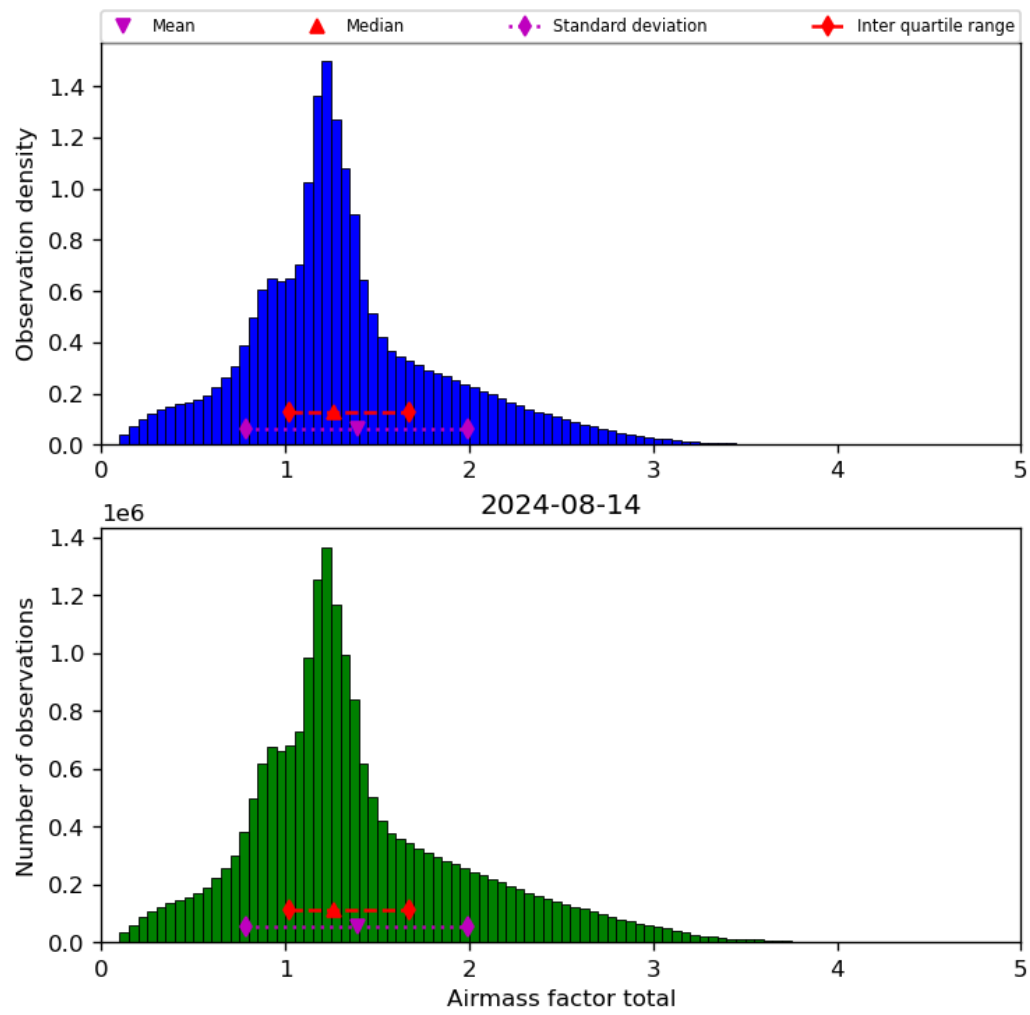
Figure 40: Histogram of “Airmass factor total” for 2024-08-13 to 2024-08-15
