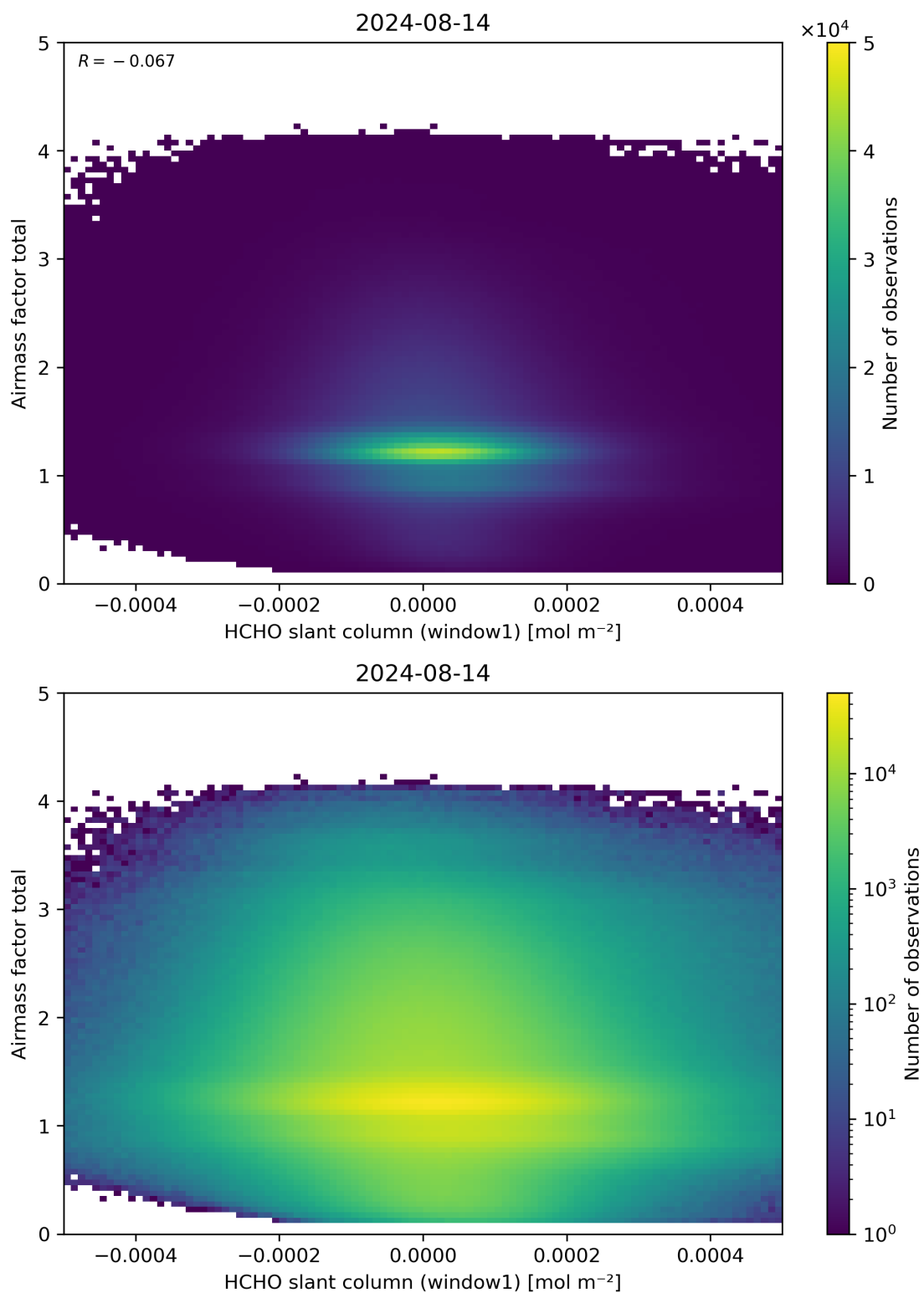
Figure 85: Scatter density plot of “HCHO slant column (window1)” against “Airmass factor total” for 2024-08-13 to 2024-08-15.
