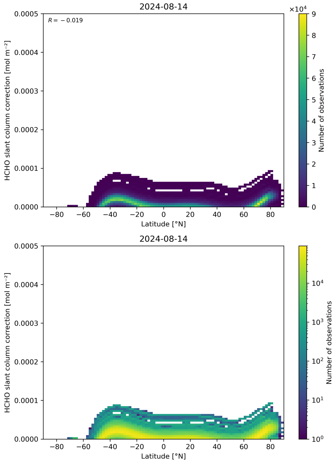
Figure 158: Scatter density plot of “Latitude” against “HCHO slant column correction” for 2024-08-13 to 2024-08-15.
