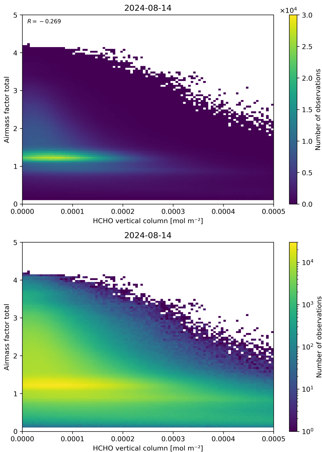
Figure 131: Scatter density plot of “HCHO vertical column” against “Airmass factor total” for 2024-08-13 to 2024-08-15.
