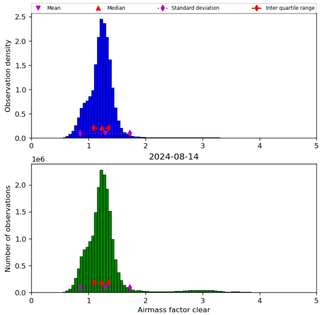
Figure 42: Histogram of “Airmass factor clear” for 2024-08-13 to 2024-08-15
