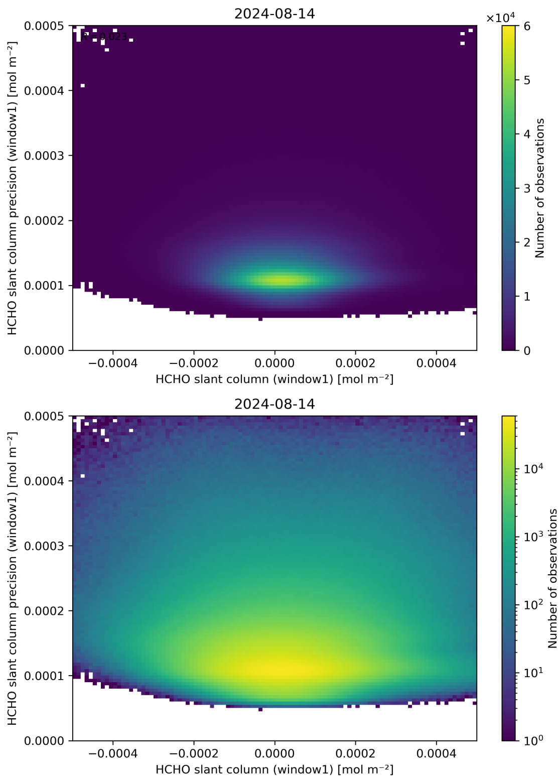
Figure 84: Scatter density plot of “HCHO slant column (window1)” against “HCHO slant column precision (window1)” for 2024-08-13 to 2024-08-15.
