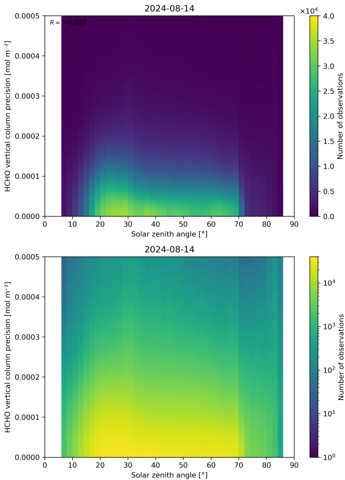
Figure 179: Scatter density plot of “Solar zenith angle” against “HCHO vertical column precision” for 2024-08-13 to 2024-08-15.
