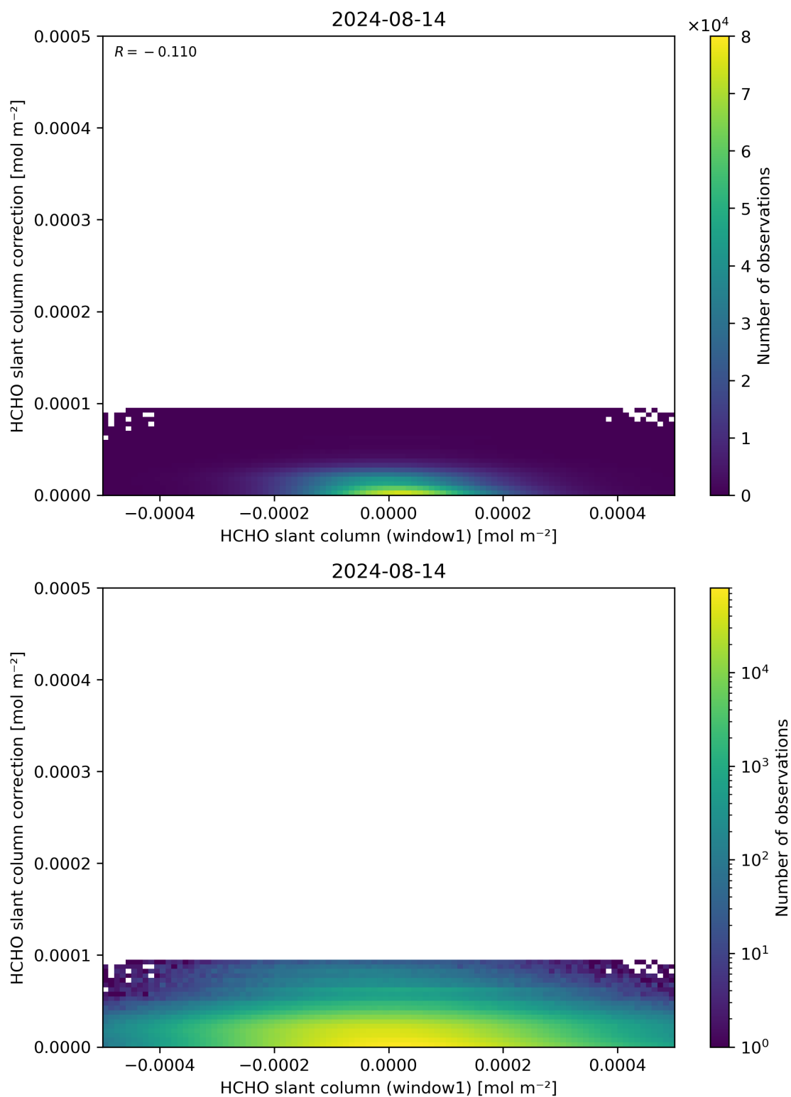
Figure 83: Scatter density plot of “HCHO slant column (window1)” against “HCHO slant column correction” for 2024-08-13 to 2024-08-15.
