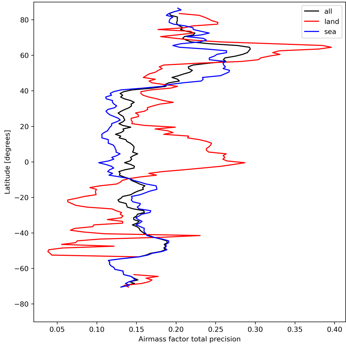
Figure 27: Zonal average of “Airmass factor total precision” for 2024-08-13 to 2024-08-15.
