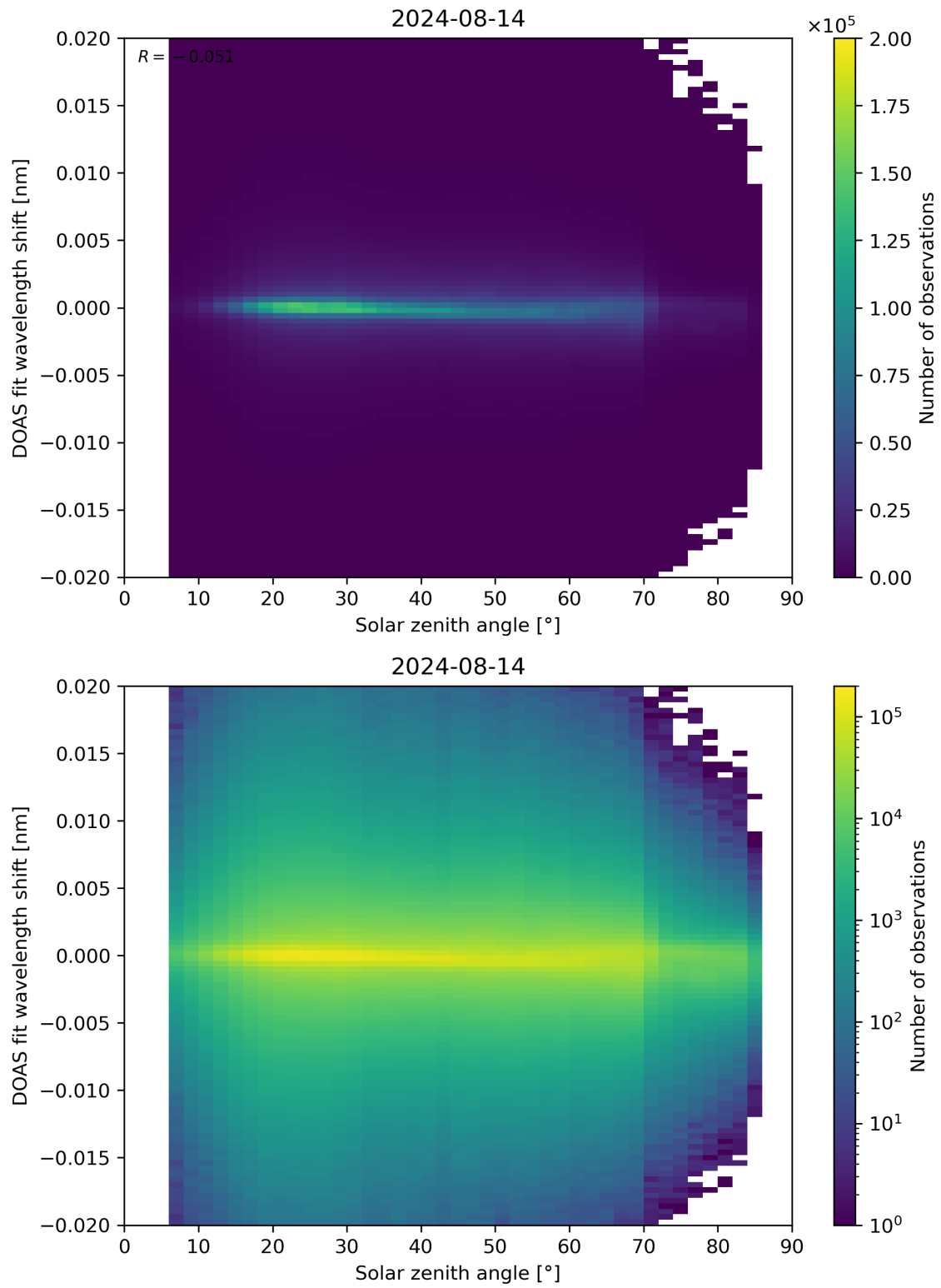
Figure 168: Scatter density plot of “Solar zenith angle” against “DOAS fit wavelength shift” for 2024-08-13 to 2024-08-15.
