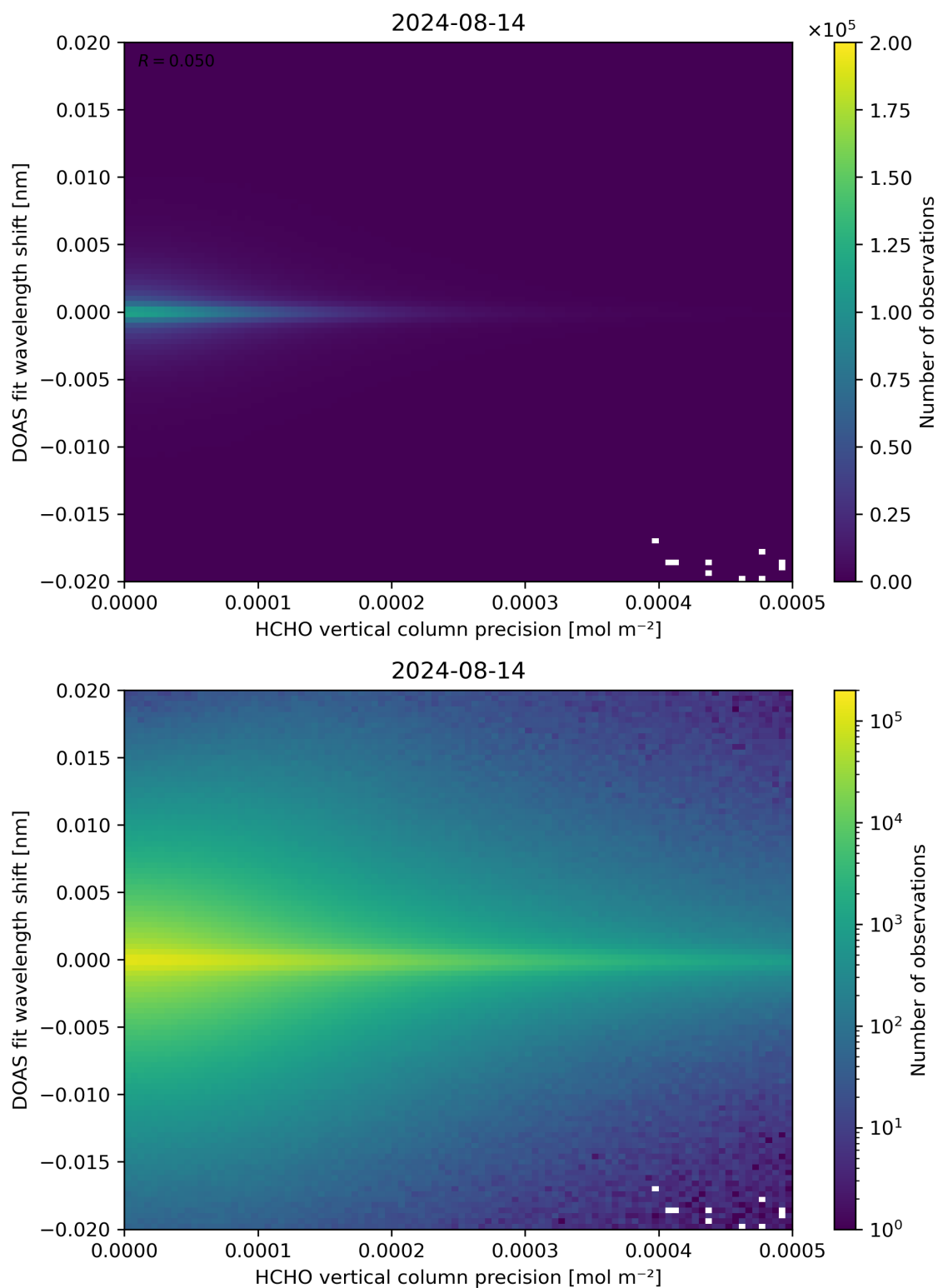
Figure 137: Scatter density plot of “HCHO vertical column precision” against “DOAS fit wavelength shift” for 2024-08-13 to 2024-08-15.
