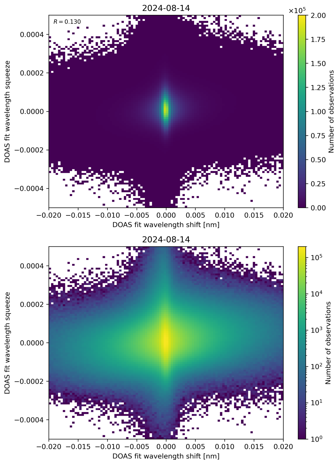
Figure 65: Scatter density plot of “DOAS fit wavelength shift” against “DOAS fit wavelength squeeze” for 2024-08-13 to 2024-08-15.
