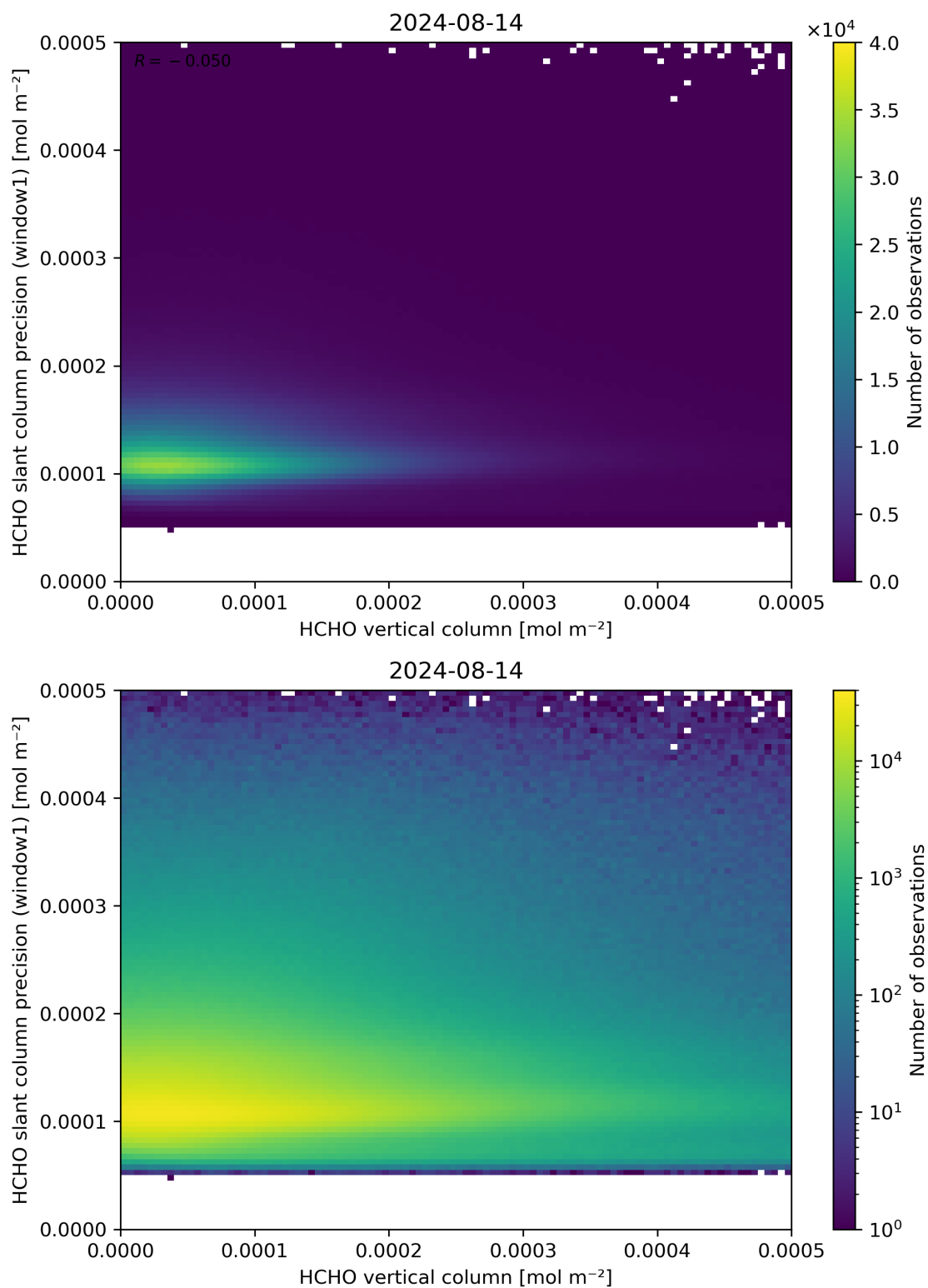
Figure 130: Scatter density plot of “HCHO vertical column” against “HCHO slant column precision (window1)” for 2024-08-13 to 2024-08-15.
