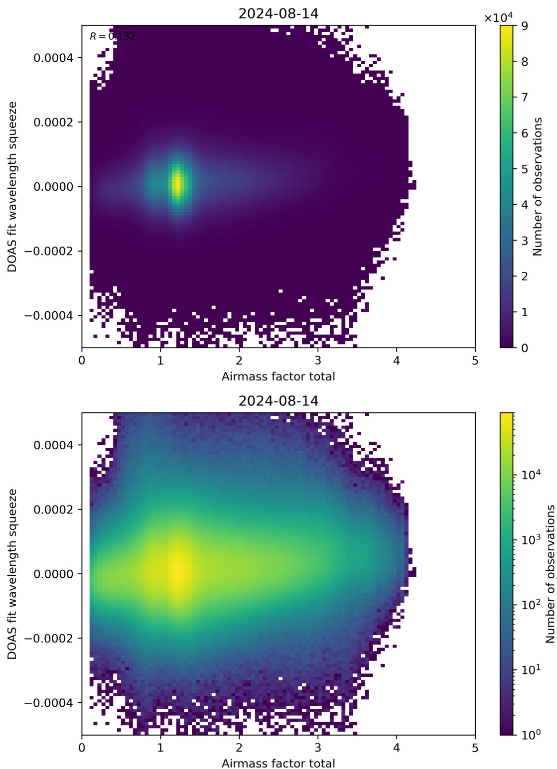
Figure 99: Scatter density plot of “Airmass factor total” against “DOAS fit wavelength squeeze” for 2024-08-13 to 2024-08-15.
