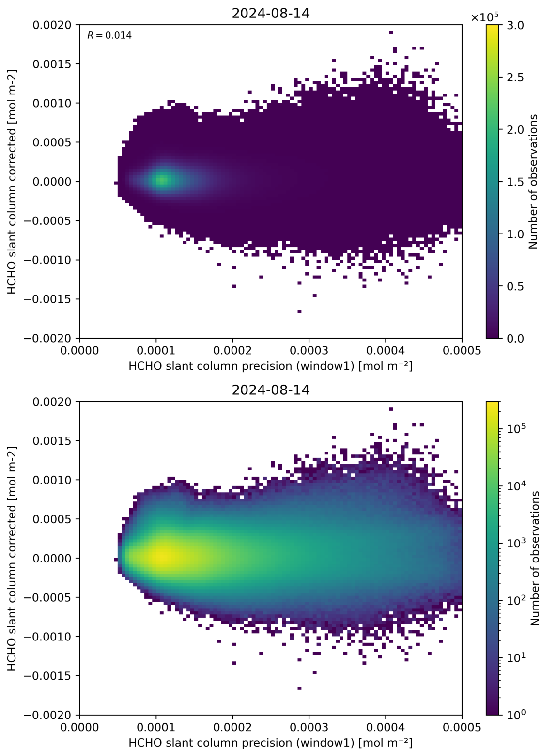
Figure 92: Scatter density plot of “HCHO slant column precision (window1)” against “HCHO slant column corrected” for 2024-08-13 to 2024-08-15.
