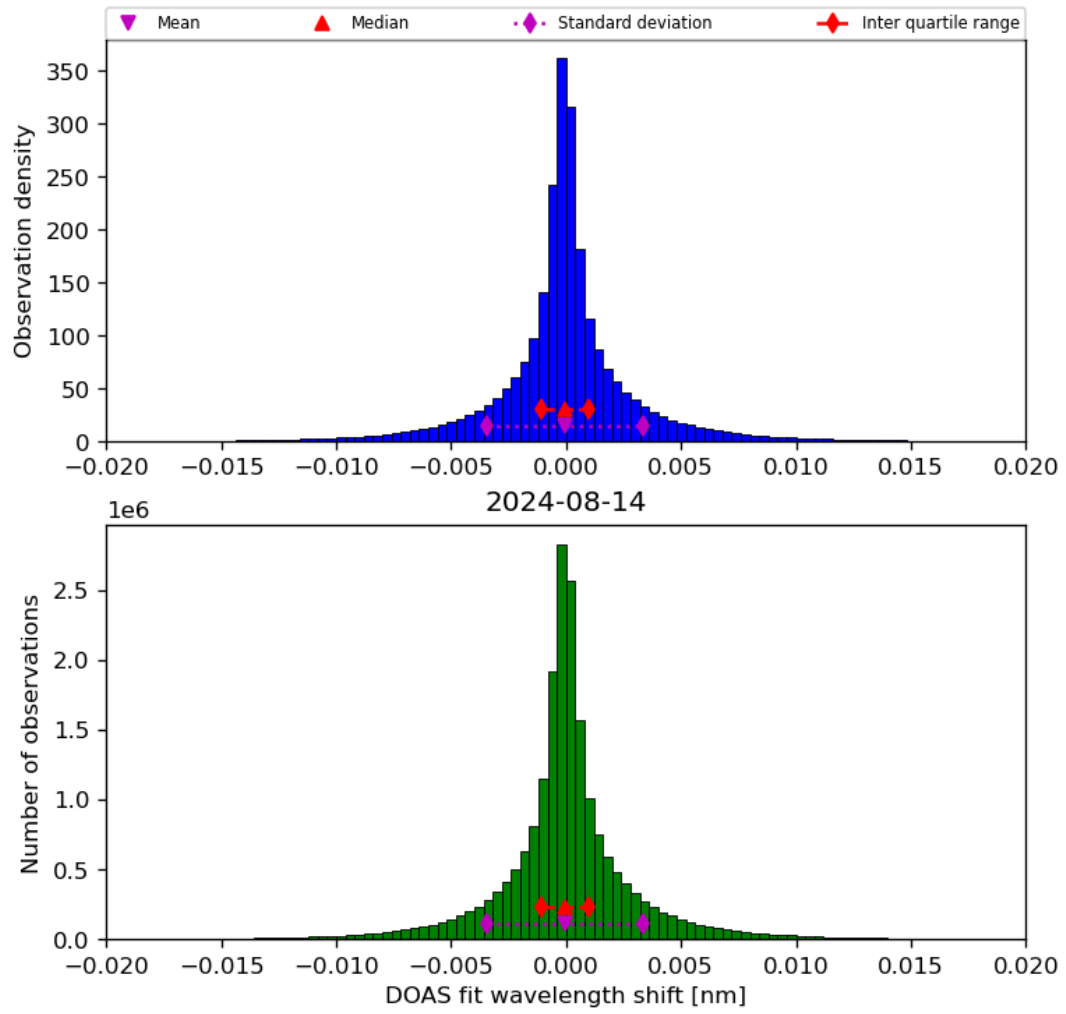
Figure 44: Histogram of “DOAS fit wavelength shift” for 2024-08-13 to 2024-08-15
