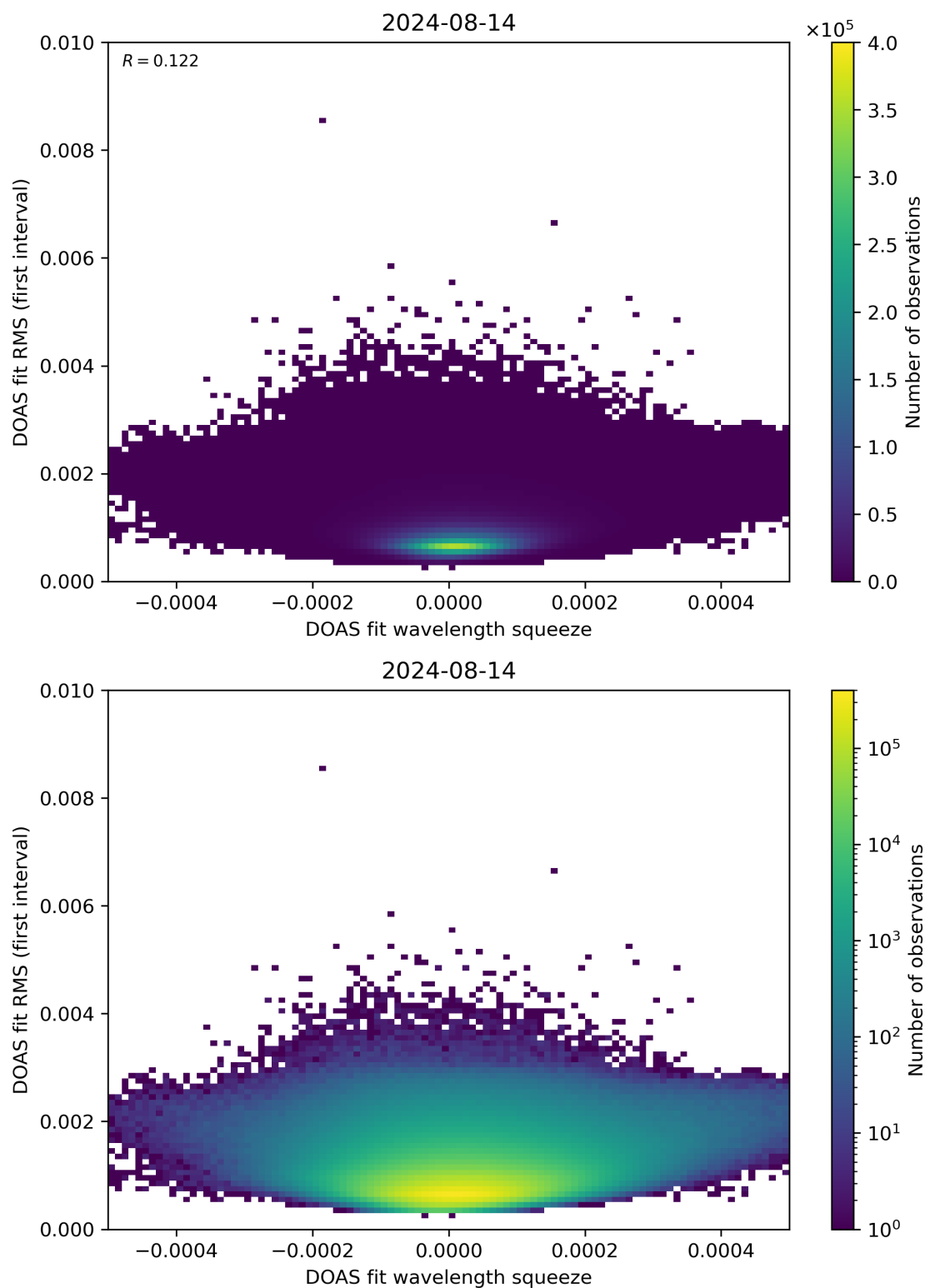
Figure 68: Scatter density plot of “DOAS fit wavelength squeeze” against “DOAS fit RMS (first interval)” for 2024-08-13 to 2024-08-15.
