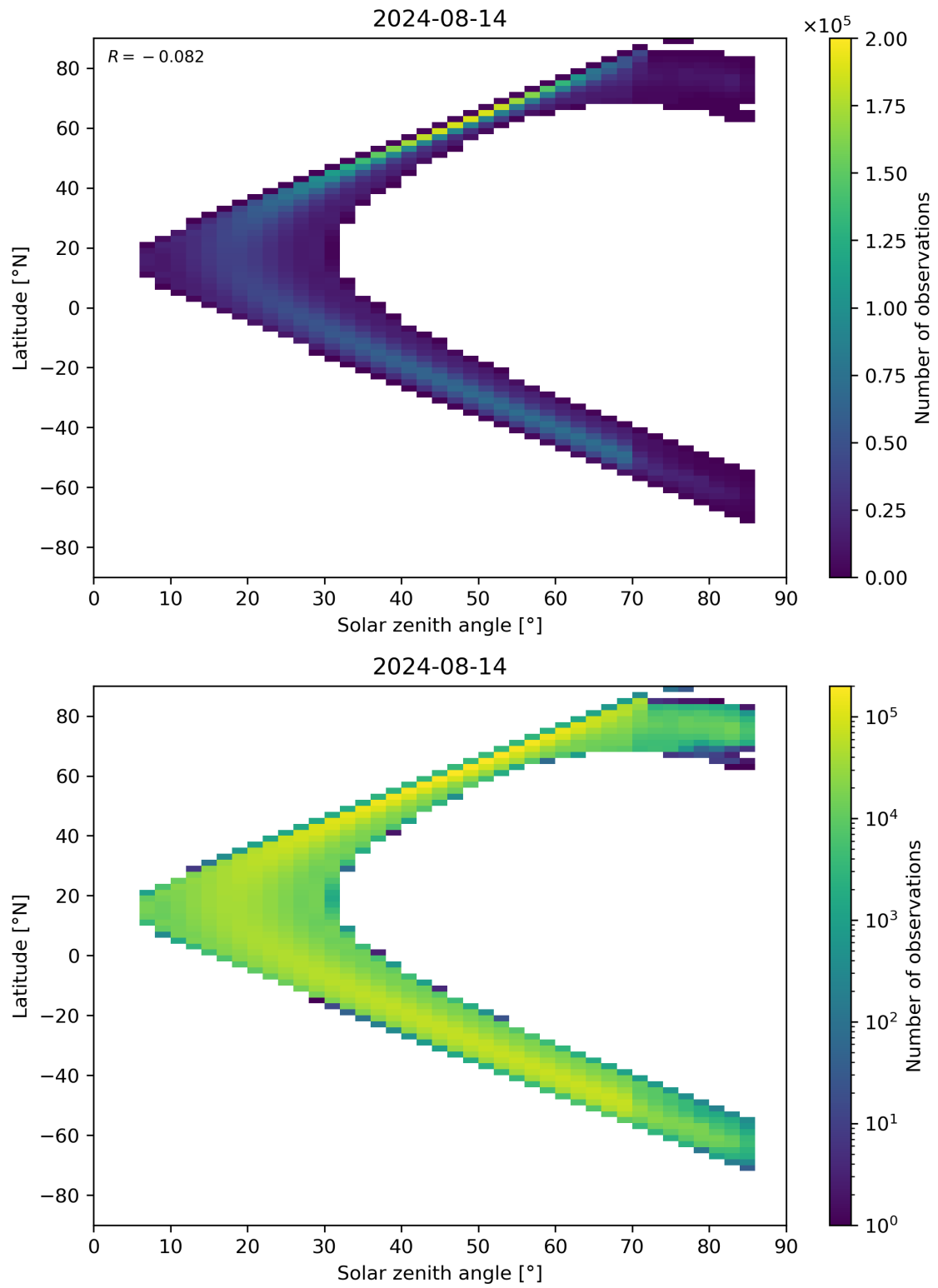
Figure 181: Scatter density plot of “Solar zenith angle” against “Latitude” for 2024-08-13 to 2024-08-15.
