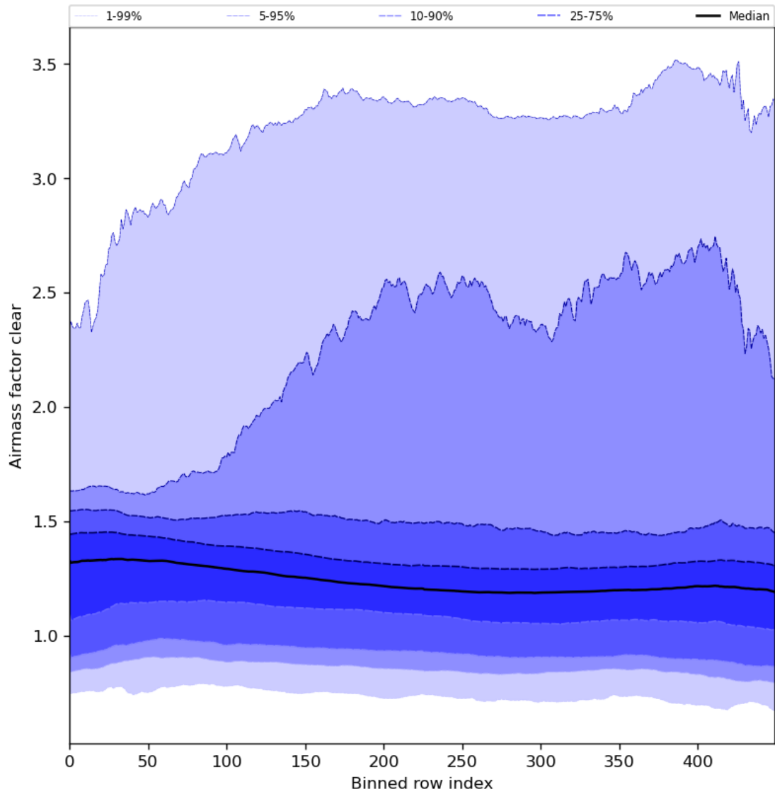
Figure 56: Along track statistics of “Airmass factor clear” for 2024-08-13 to 2024-08-15
