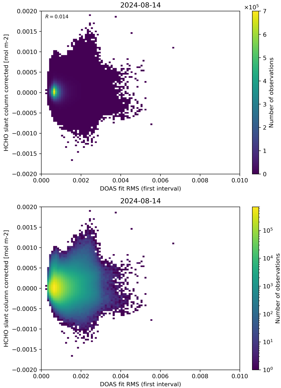
Figure 62: Scatter density plot of “DOAS fit RMS (first interval)” against “HCHO slant column corrected” for 2024-08-13 to 2024-08-15.
