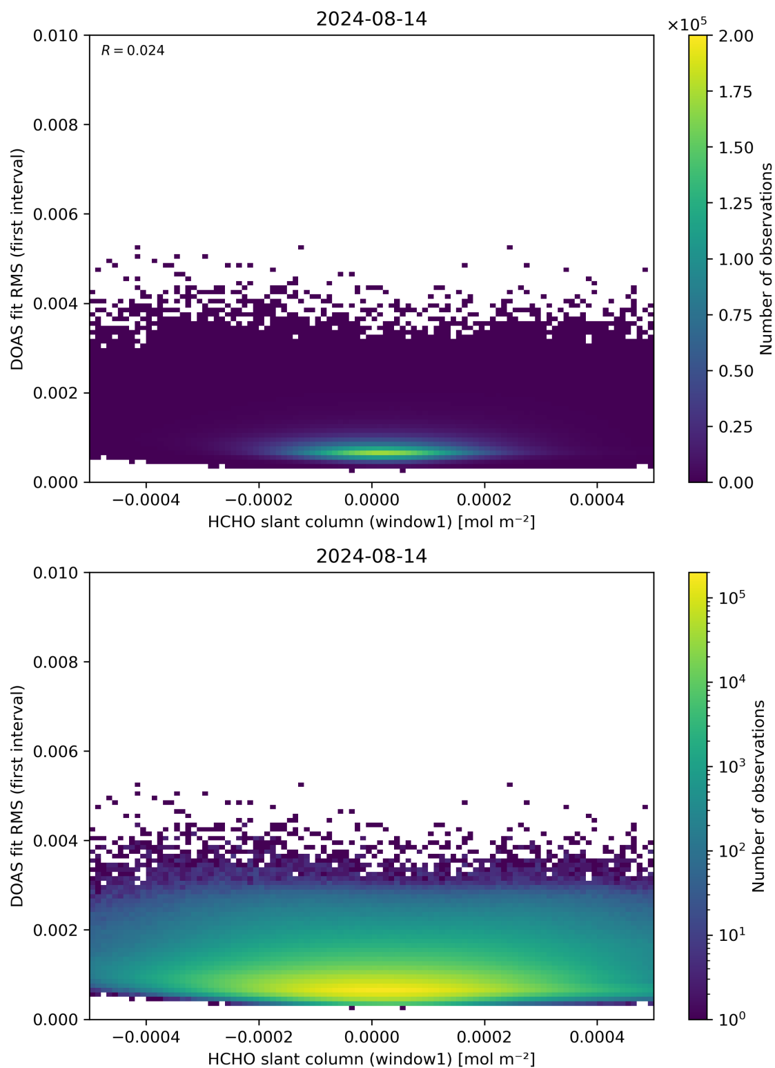
Figure 78: Scatter density plot of “HCHO slant column (window1)” against “DOAS fit RMS (first interval)” for 2024-08-13 to 2024-08-15.
