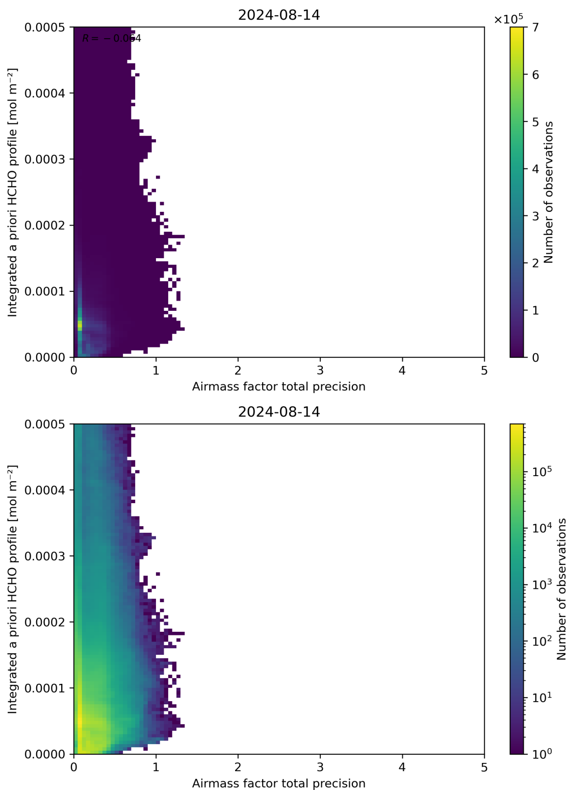
Figure 111: Scatter density plot of “Airmass factor total precision” against “Integrated a priori HCHO profile” for 2024-08-13 to 2024-08-15.
