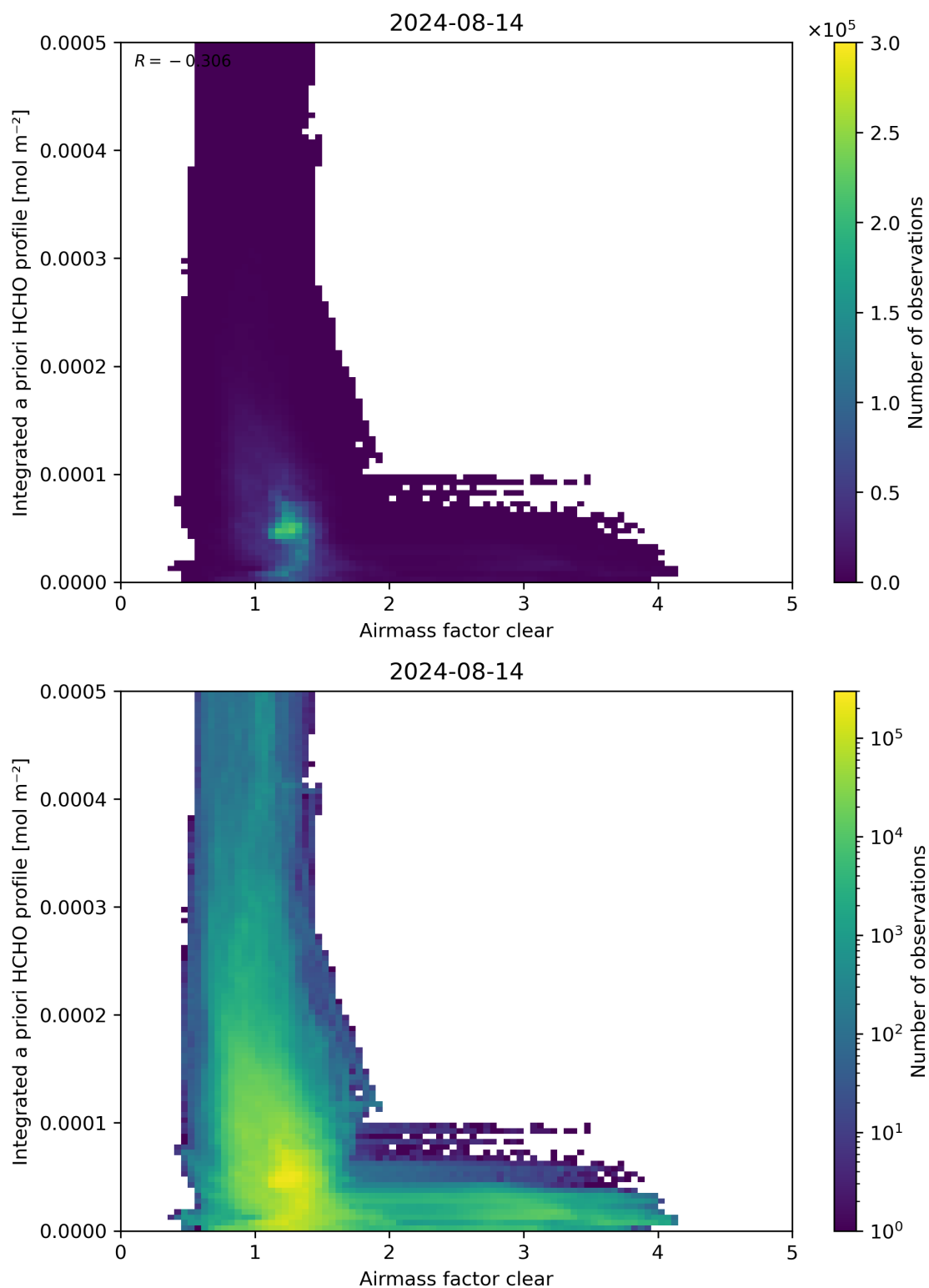
Figure 76: Scatter density plot of “Airmass factor clear” against “Integrated a priori HCHO profile” for 2024-08-13 to 2024-08-15.
