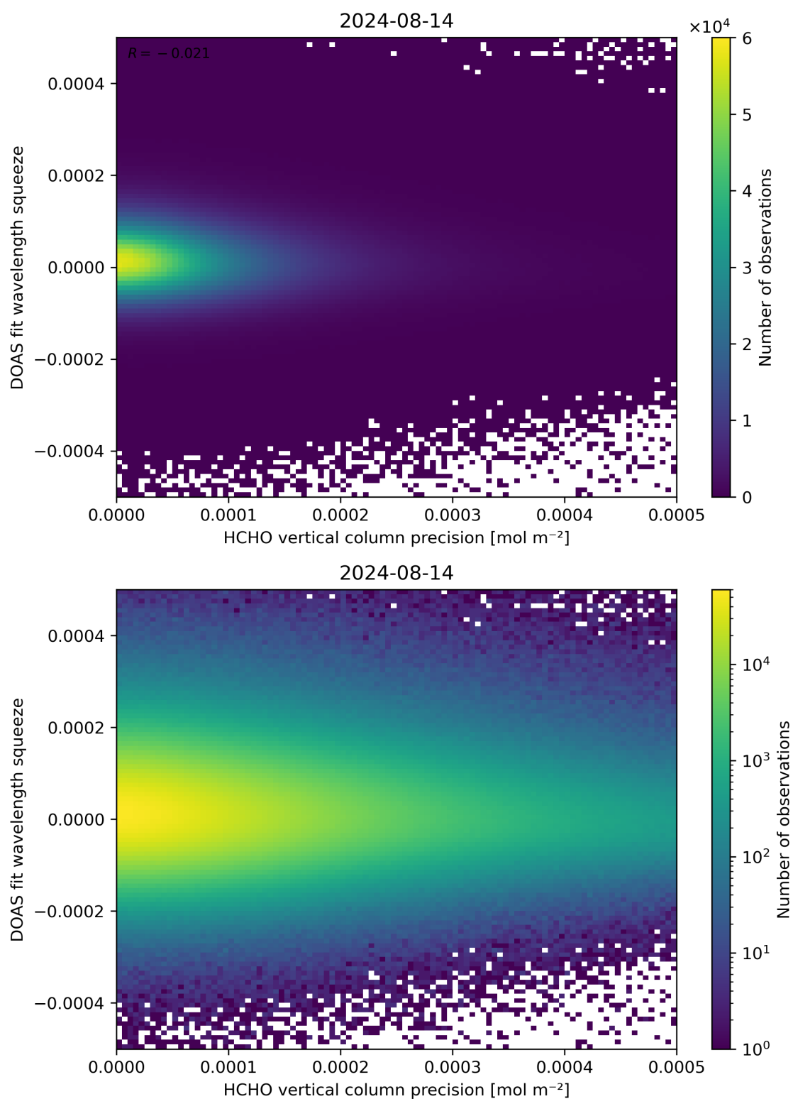
Figure 138: Scatter density plot of “HCHO vertical column precision” against “DOAS fit wavelength squeeze” for 2024-08-13 to 2024-08-15.
