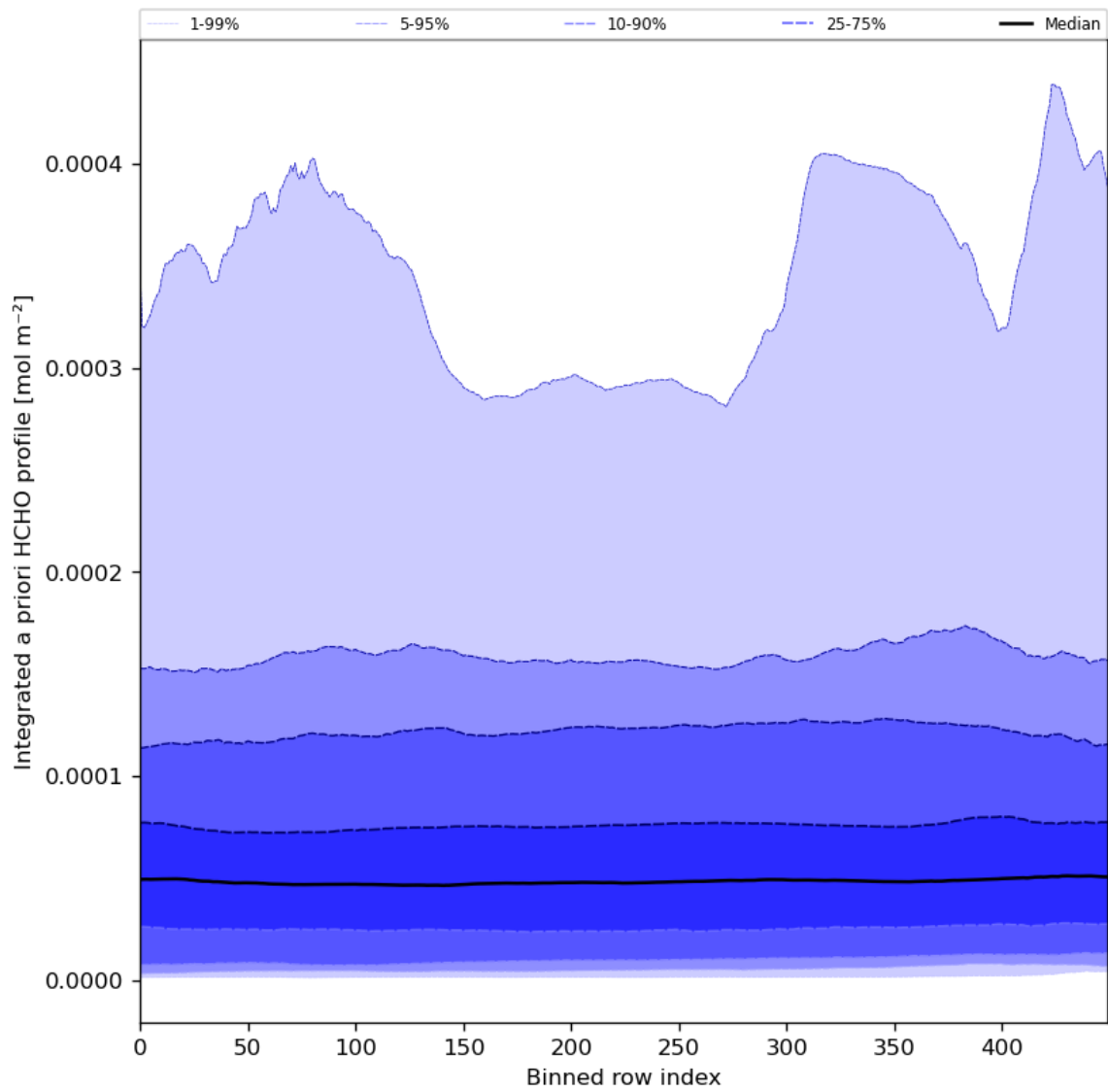
Figure 57: Along track statistics of “Integrated a priori HCHO profile” for 2024-08-13 to 2024-08-15
