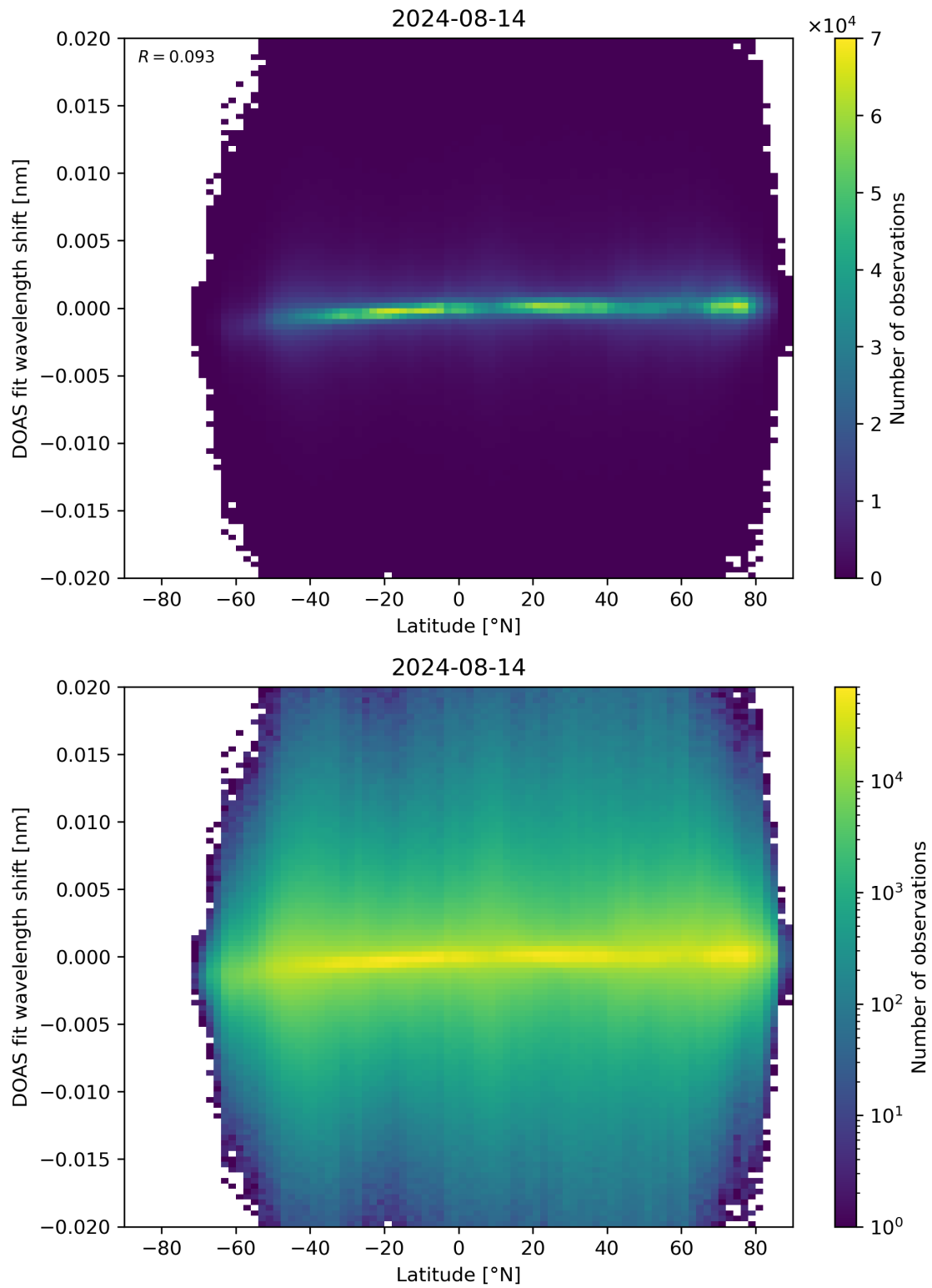
Figure 154: Scatter density plot of “Latitude” against “DOAS fit wavelength shift” for 2024-08-13 to 2024-08-15.
