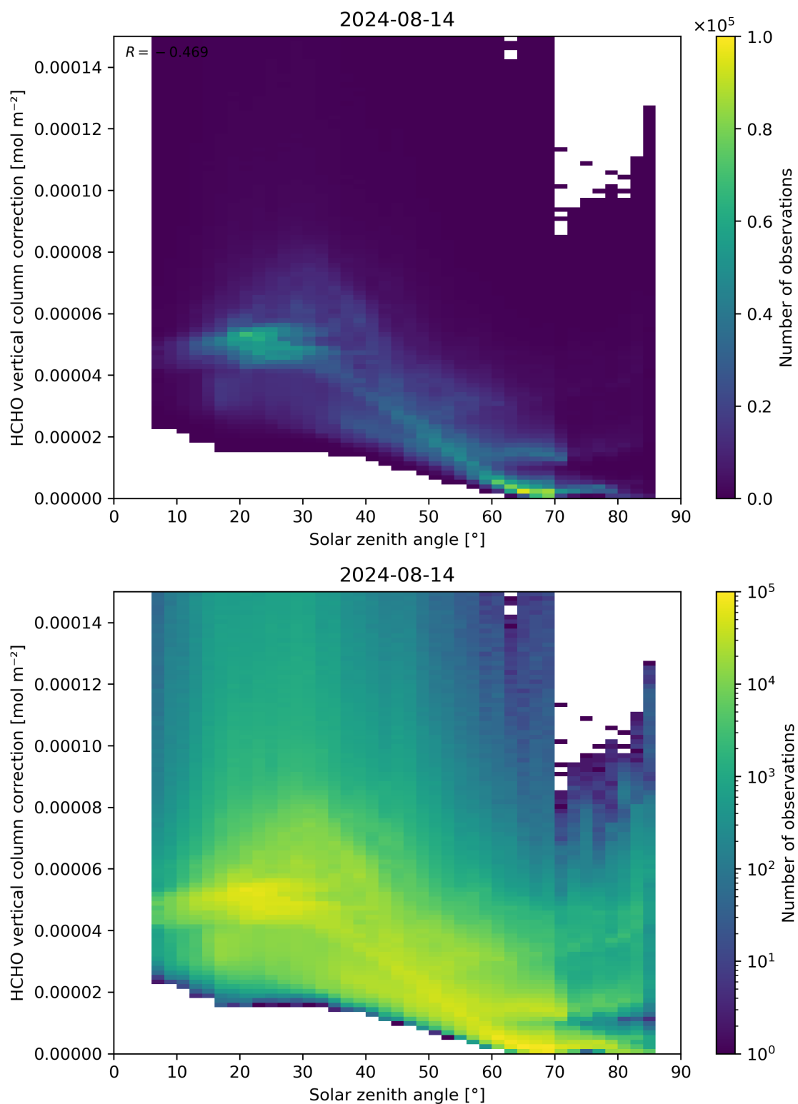
Figure 178: Scatter density plot of “Solar zenith angle” against “HCHO vertical column correction” for 2024-08-13 to 2024-08-15.
