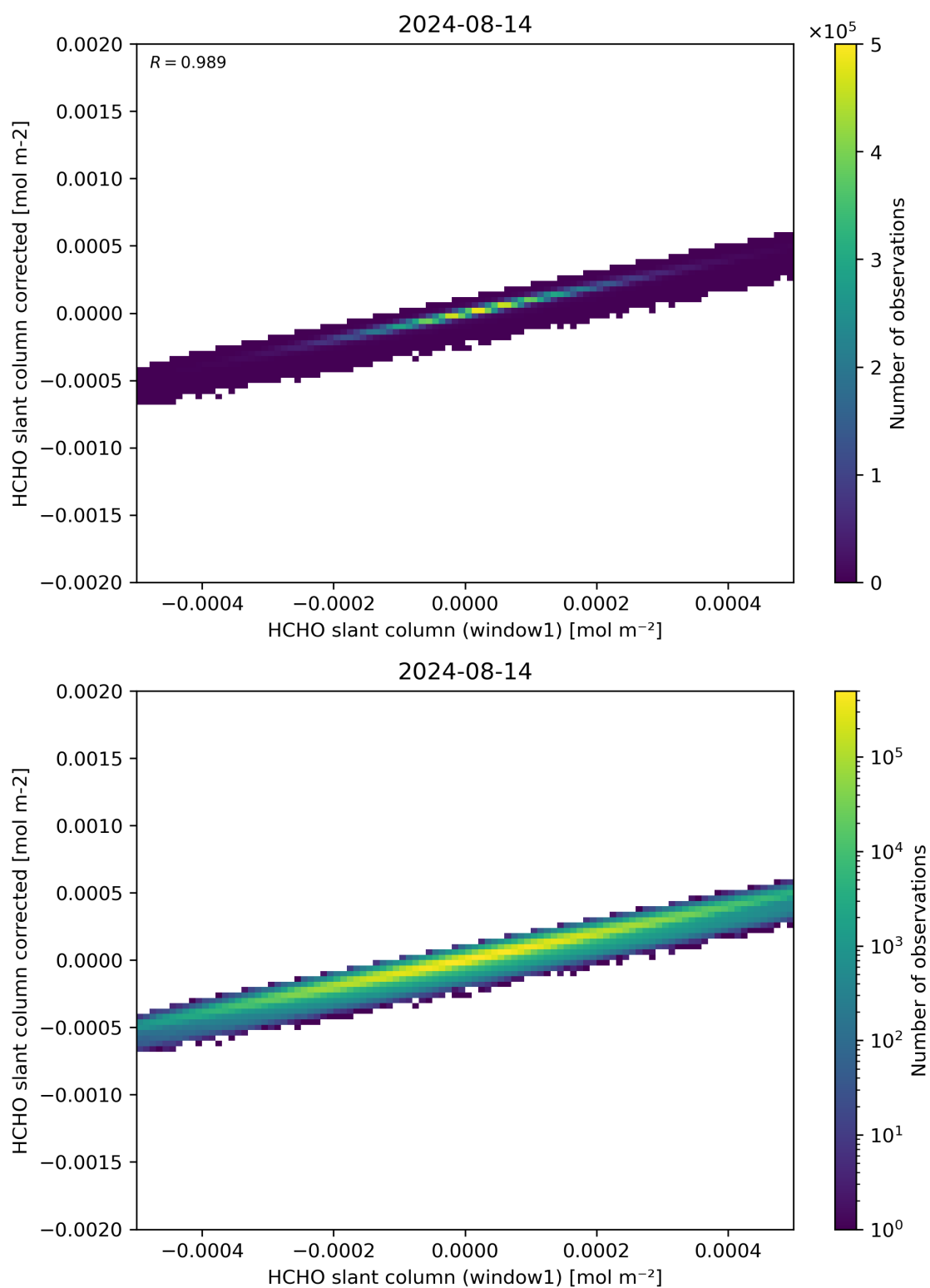
Figure 82: Scatter density plot of “HCHO slant column (window1)” against “HCHO slant column corrected” for 2024-08-13 to 2024-08-15.
