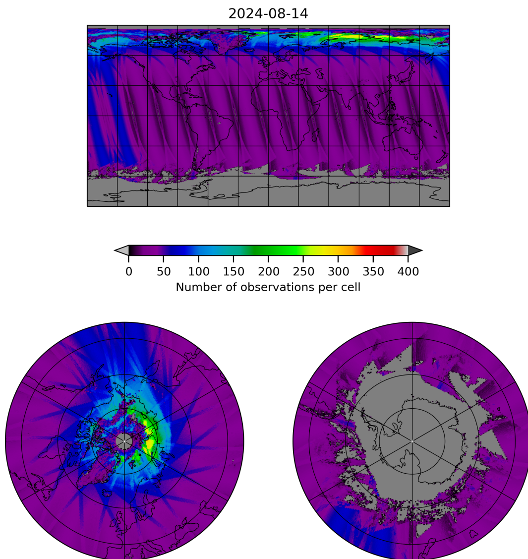
Figure 19: Map of the number of observations for 2024-08-13 to 2024-08-15
