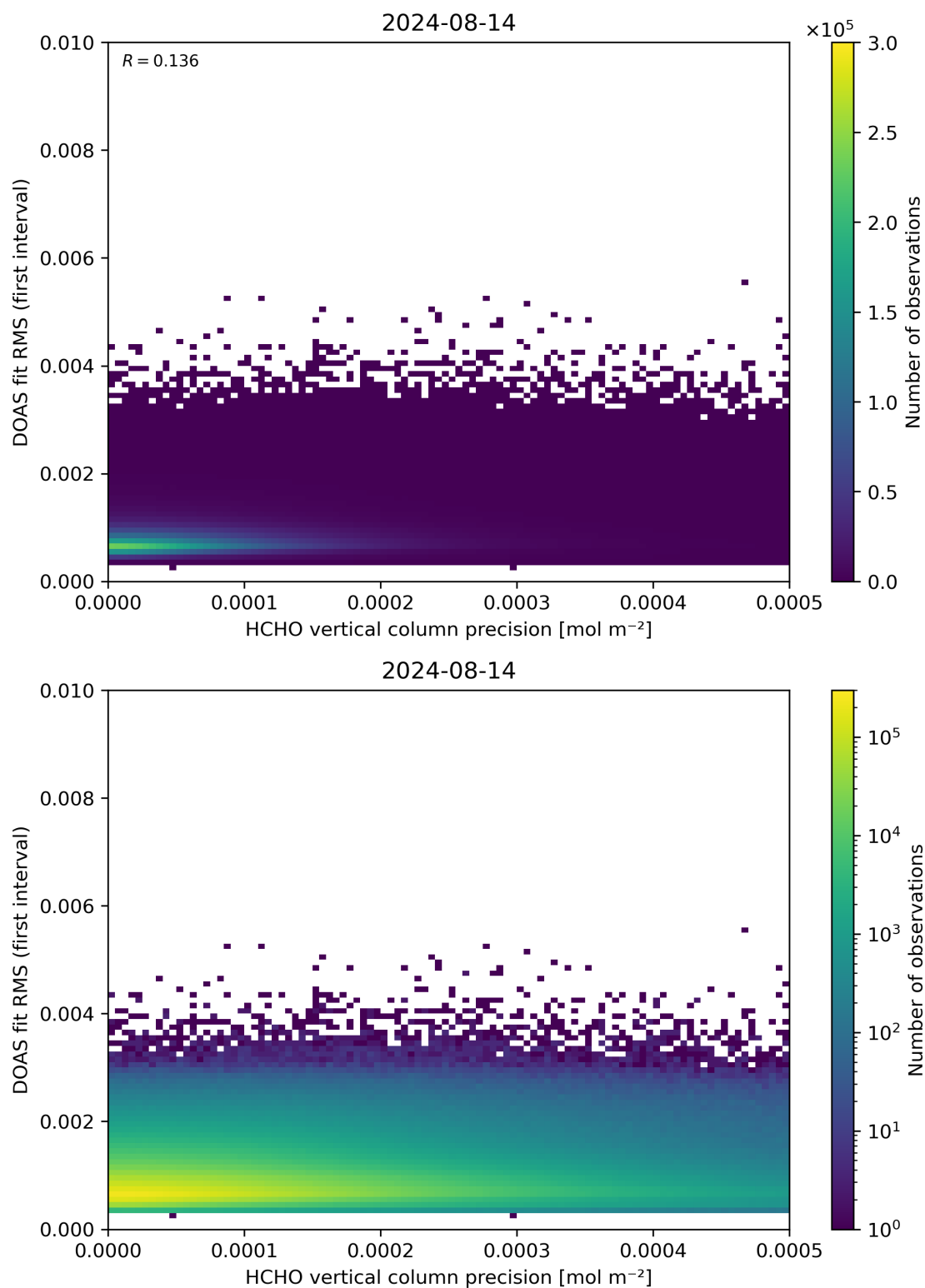
Figure 136: Scatter density plot of “HCHO vertical column precision” against “DOAS fit RMS (first interval)” for 2024-08-13 to 2024-08-15.
