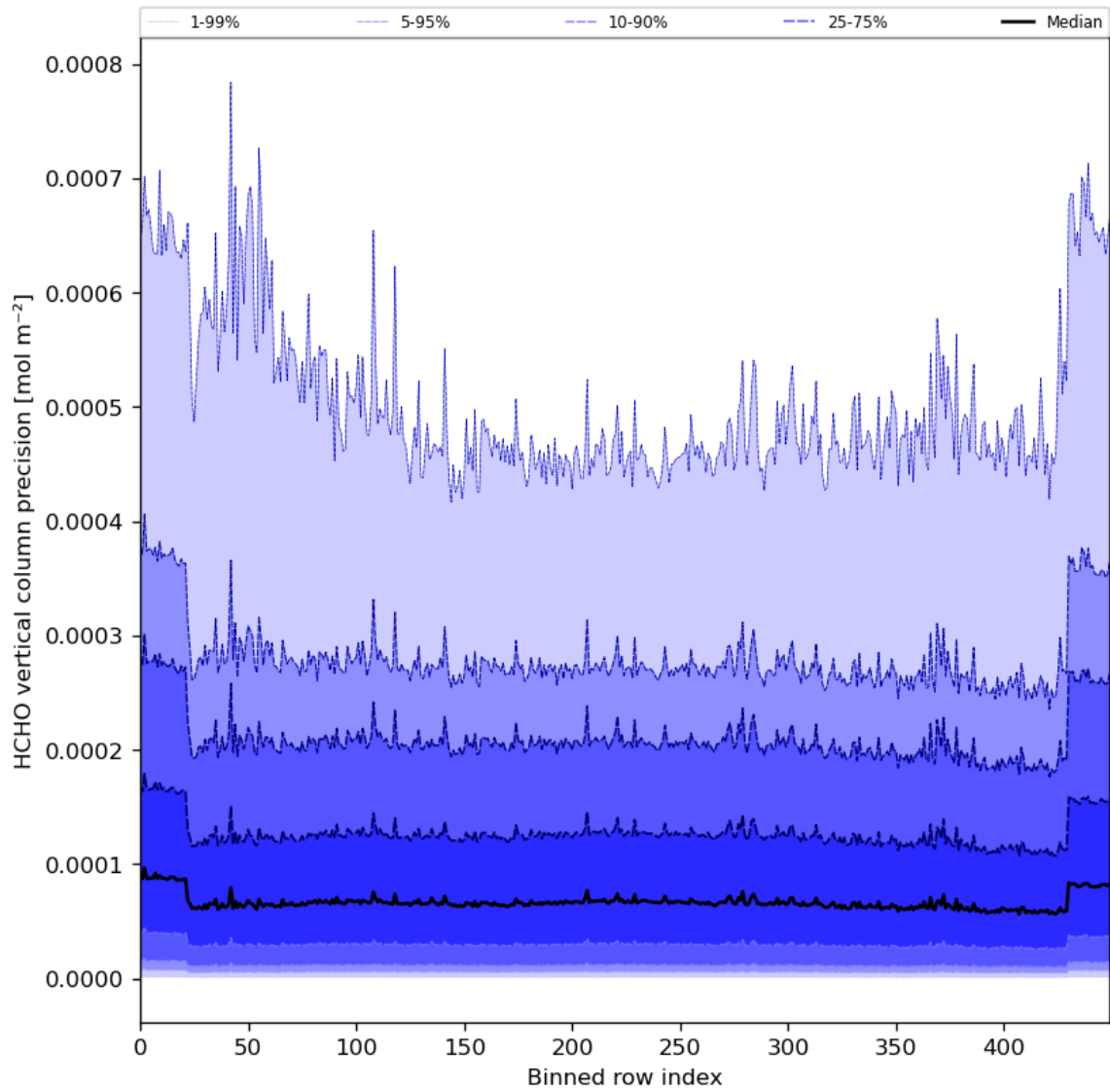
Figure 50: Along track statistics of “HCHO vertical column precision” for 2024-08-13 to 2024-08-15
