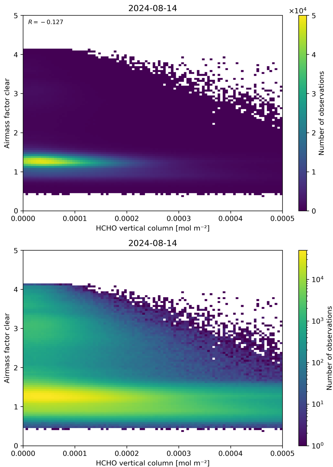
Figure 126: Scatter density plot of “HCHO vertical column” against “Airmass factor clear” for 2024-08-13 to 2024-08-15.
