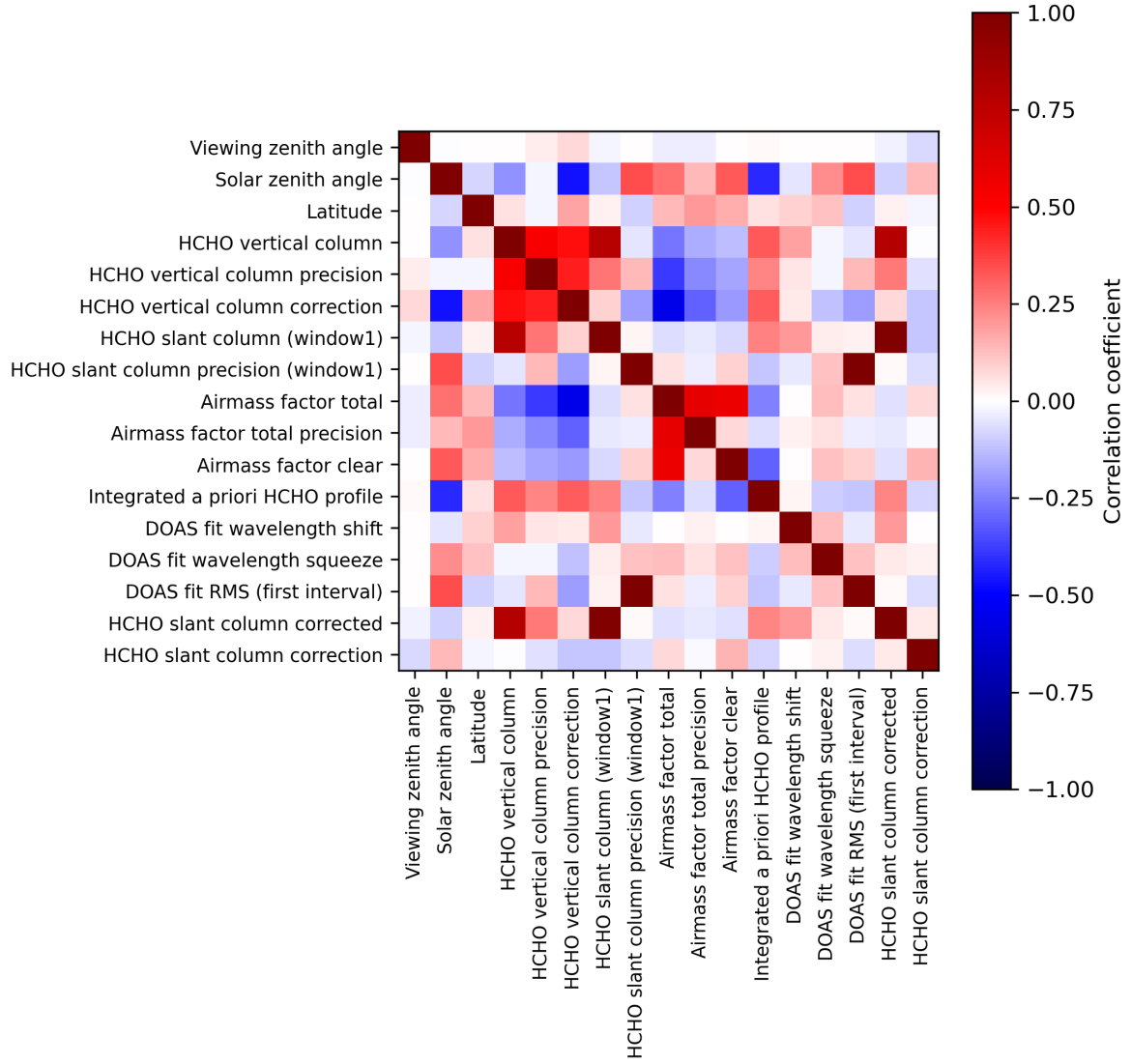
Figure 2: Map of correlation matrix for 2024-08-13 to 2024-08-15.
