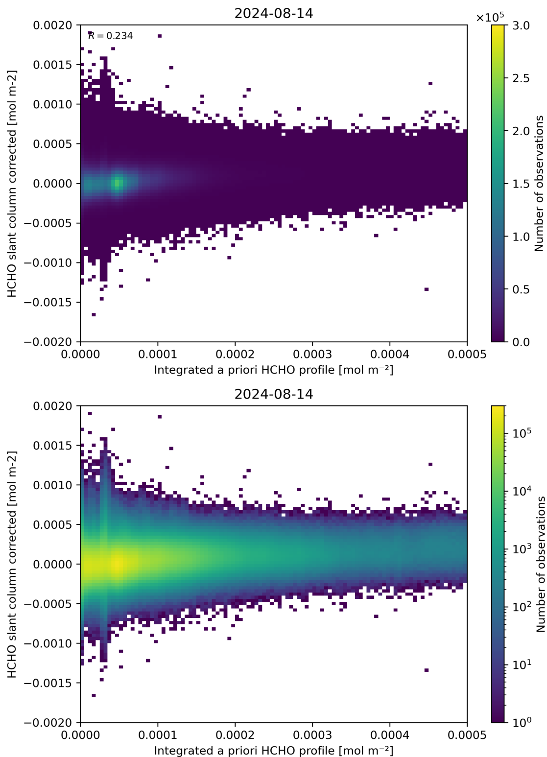
Figure 151: Scatter density plot of “Integrated a priori HCHO profile” against “HCHO slant column corrected” for 2024-08-13 to 2024-08-15.
