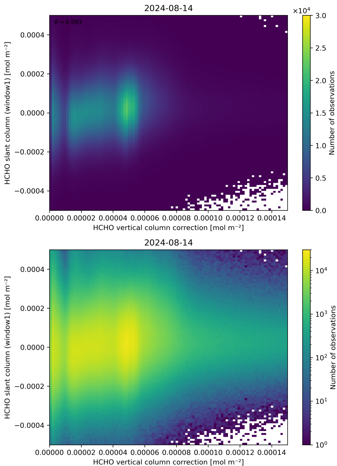
Figure 118: Scatter density plot of “HCHO vertical column correction” against “HCHO slant column (window1)” for 2024-08-13 to 2024-08-15.
