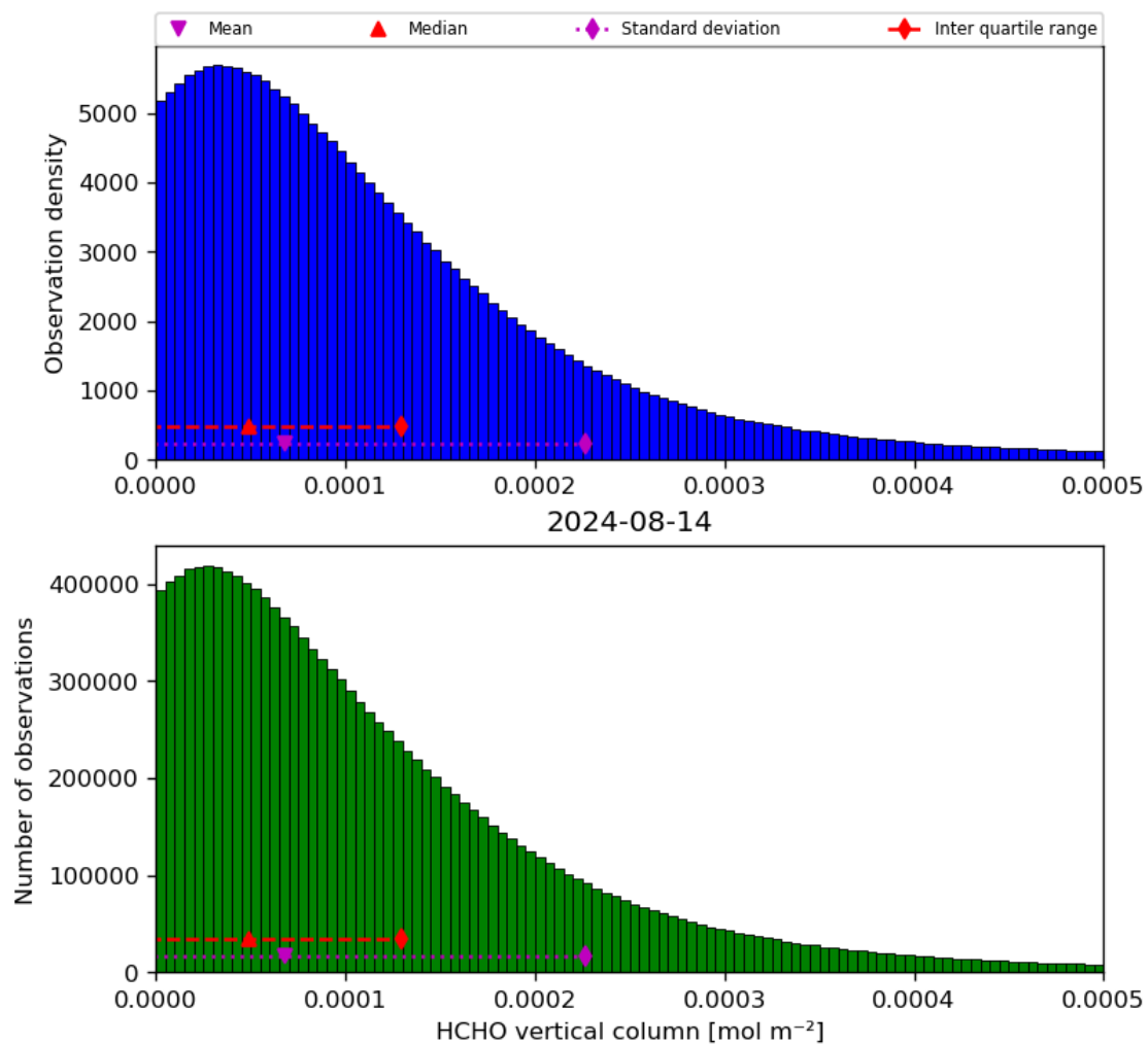
Figure 35: Histogram of “HCHO vertical column” for 2024-08-13 to 2024-08-15
