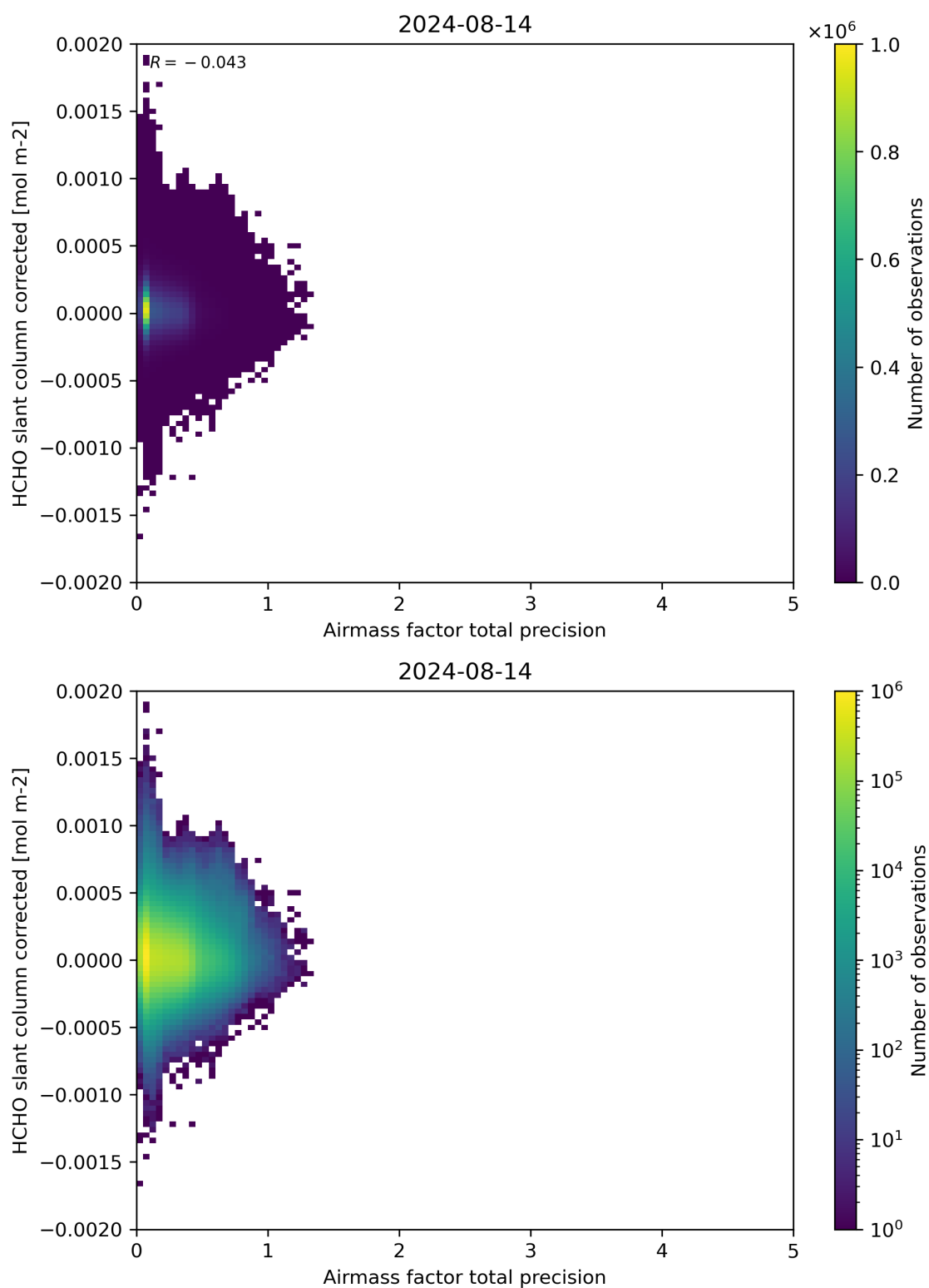
Figure 109: Scatter density plot of “Airmass factor total precision” against “HCHO slant column corrected” for 2024-08-13 to 2024-08-15.
