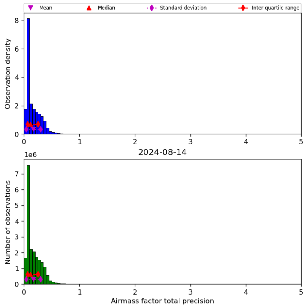
Figure 41: Histogram of “Airmass factor total precision” for 2024-08-13 to 2024-08-15
