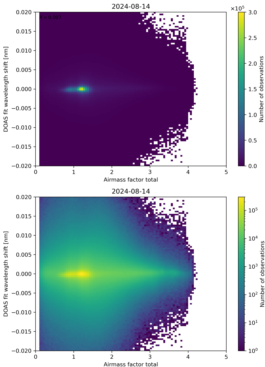
Figure 98: Scatter density plot of “Airmass factor total” against “DOAS fit wavelength shift” for 2024-08-13 to 2024-08-15.
