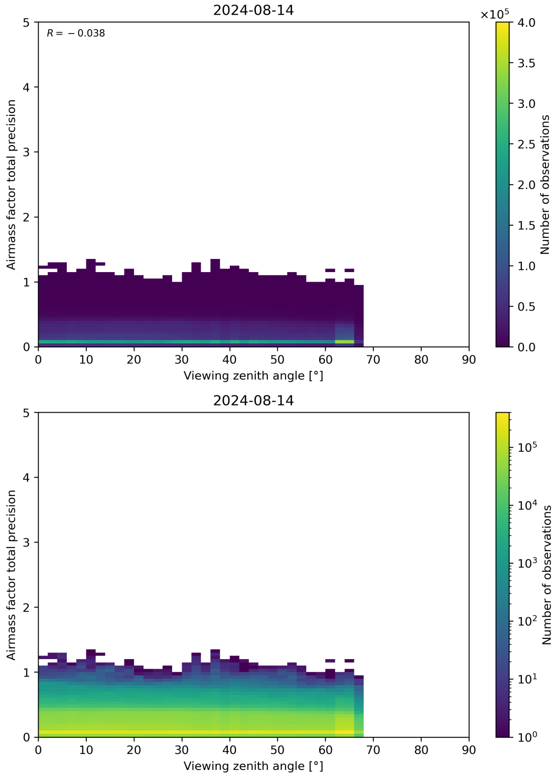
Figure 191: Scatter density plot of “Viewing zenith angle” against “Airmass factor total precision” for 2024-08-13 to 2024-08-15.
