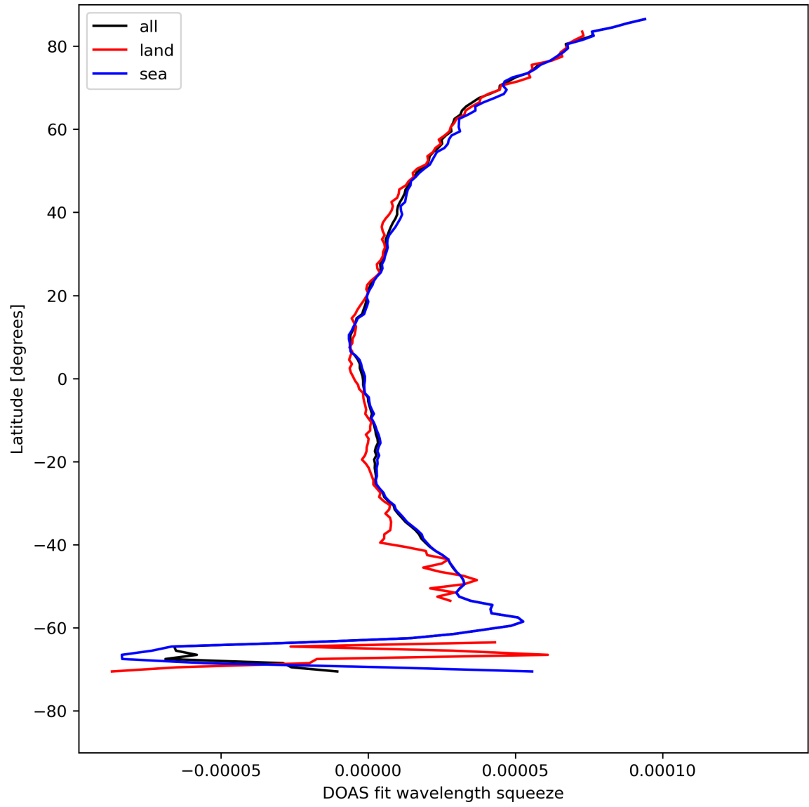
Figure 31: Zonal average of “DOAS fit wavelength squeeze” for 2024-08-13 to 2024-08-15.
