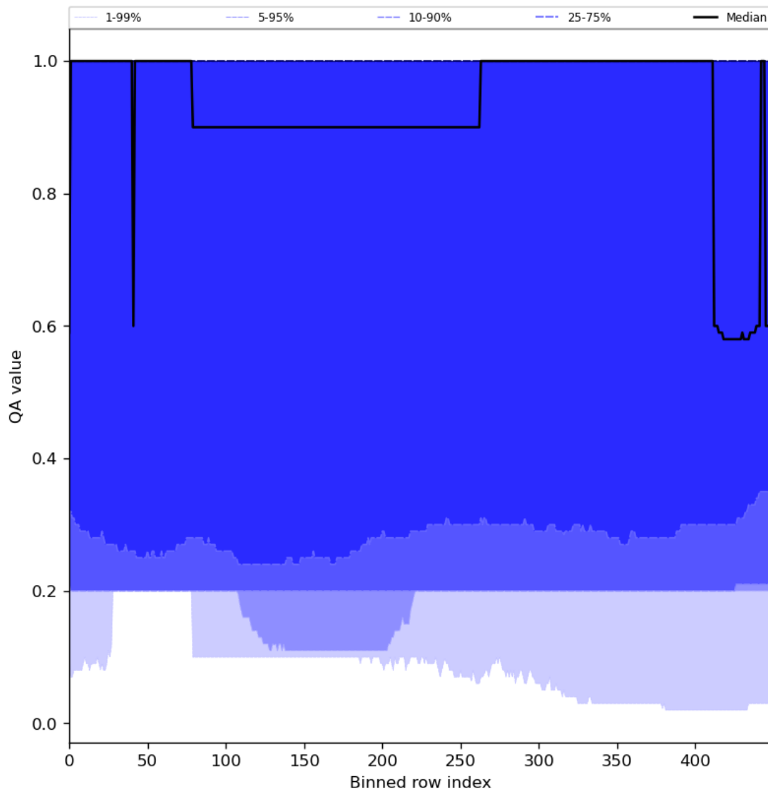
Figure 48: Along track statistics of “QA value” for 2024-08-13 to 2024-08-15
