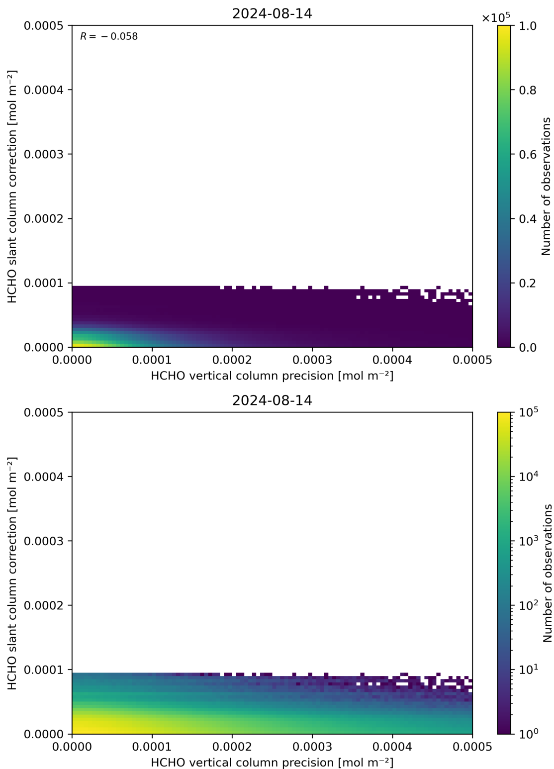
Figure 141: Scatter density plot of “HCHO vertical column precision” against “HCHO slant column correction” for 2024-08-13 to 2024-08-15.
