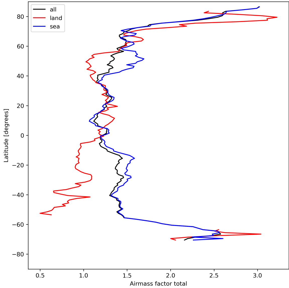
Figure 26: Zonal average of “Airmass factor total” for 2024-08-13 to 2024-08-15.
