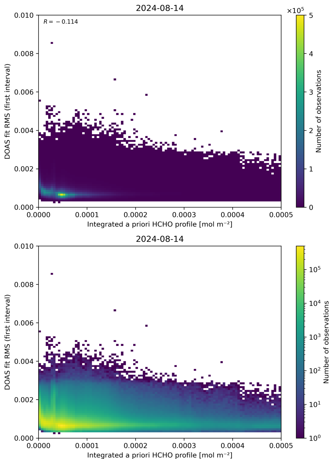
Figure 148: Scatter density plot of “Integrated a priori HCHO profile” against “DOAS fit RMS (first interval)” for 2024-08-13 to 2024-08-15.
