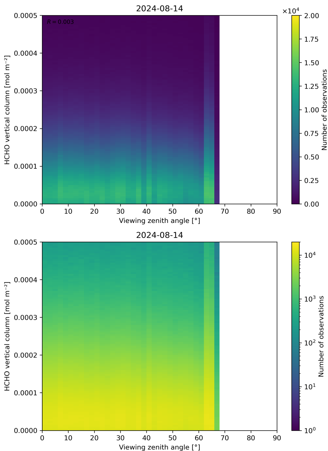
Figure 192: Scatter density plot of “Viewing zenith angle” against “HCHO vertical column” for 2024-08-13 to 2024-08-15.
