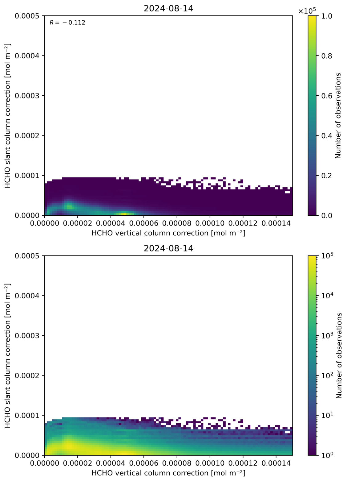
Figure 117: Scatter density plot of “HCHO vertical column correction” against “HCHO slant column correction” for 2024-08-13 to 2024-08-15.
