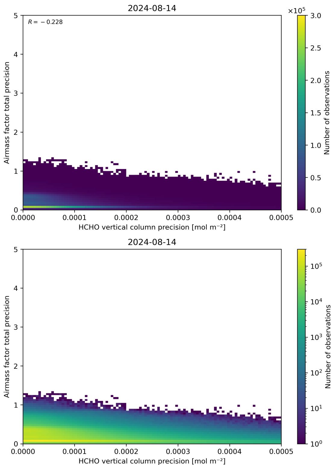
Figure 145: Scatter density plot of “HCHO vertical column precision” against “Airmass factor total precision” for 2024-08-13 to 2024-08-15.
