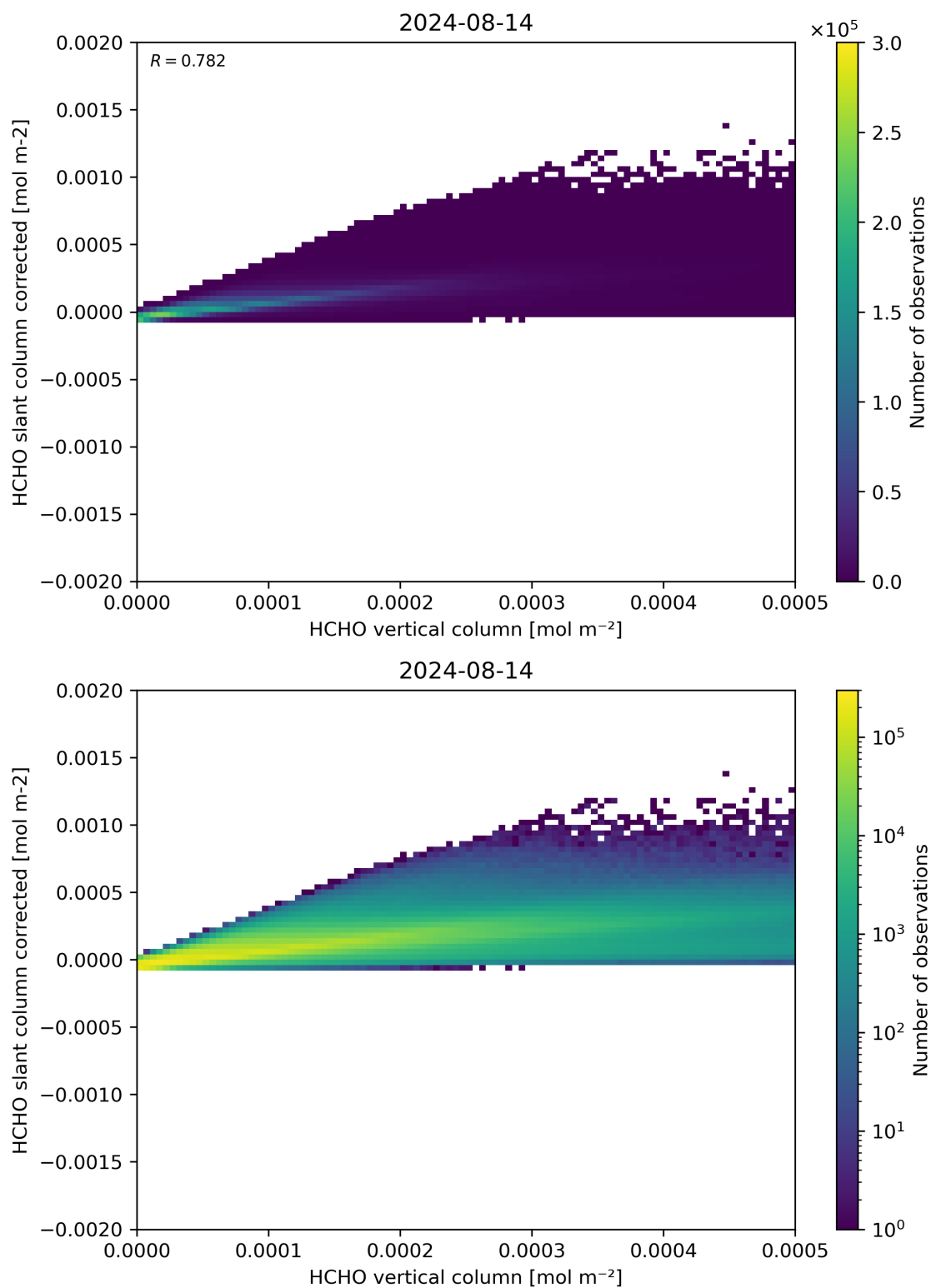
Figure 127: Scatter density plot of “HCHO vertical column” against “HCHO slant column corrected” for 2024-08-13 to 2024-08-15.
