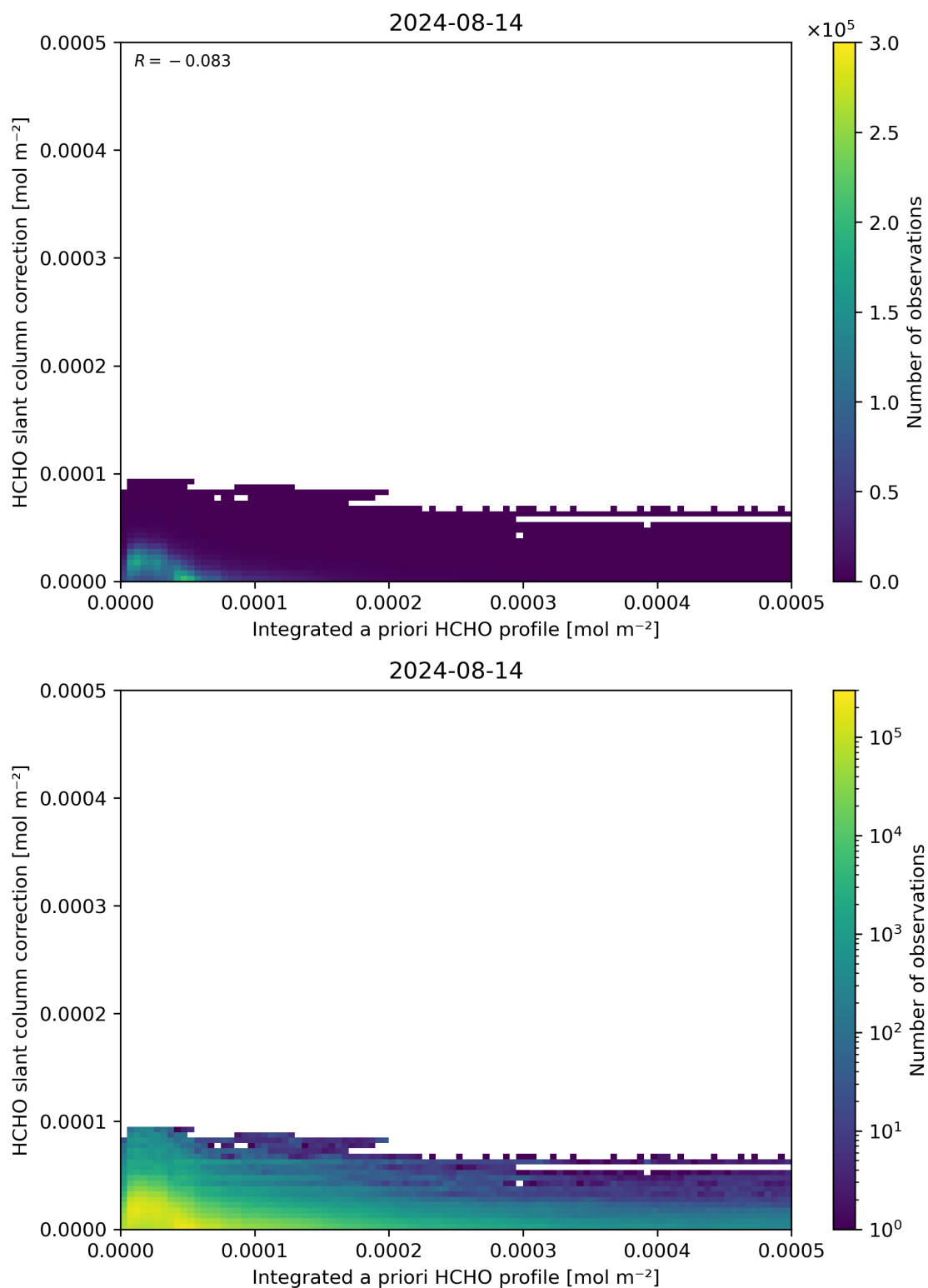
Figure 152: Scatter density plot of “Integrated a priori HCHO profile” against “HCHO slant column correction” for 2024-08-13 to 2024-08-15.
