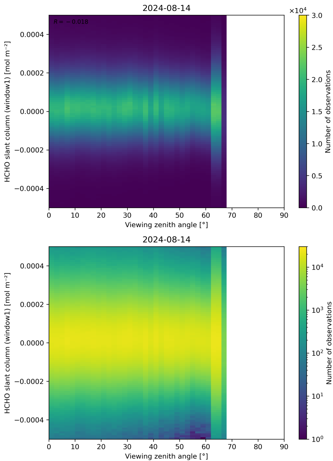
Figure 188: Scatter density plot of “Viewing zenith angle” against “HCHO slant column (window1)” for 2024-08-13 to 2024-08-15.
