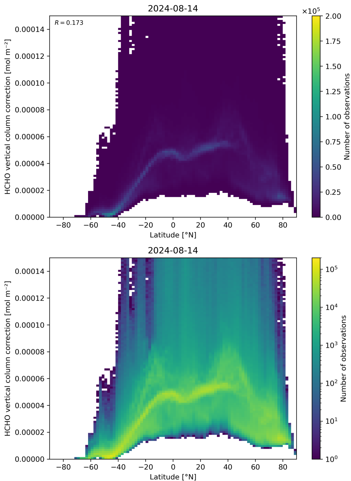
Figure 164: Scatter density plot of “Latitude” against “HCHO vertical column correction” for 2024-08-13 to 2024-08-15.
