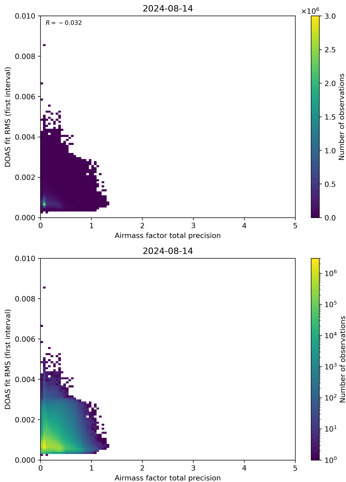
Figure 105: Scatter density plot of “Airmass factor total precision” against “DOAS fit RMS (first interval)” for 2024-08-13 to 2024-08-15.
