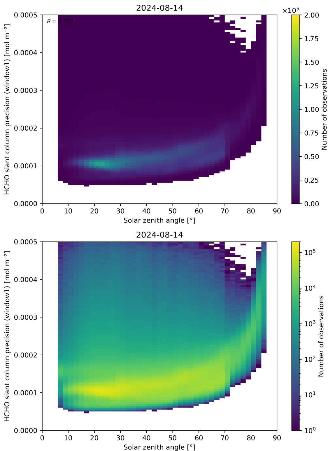
Figure 174: Scatter density plot of “Solar zenith angle” against “HCHO slant column precision (window1)” for 2024-08-13 to 2024-08-15.
