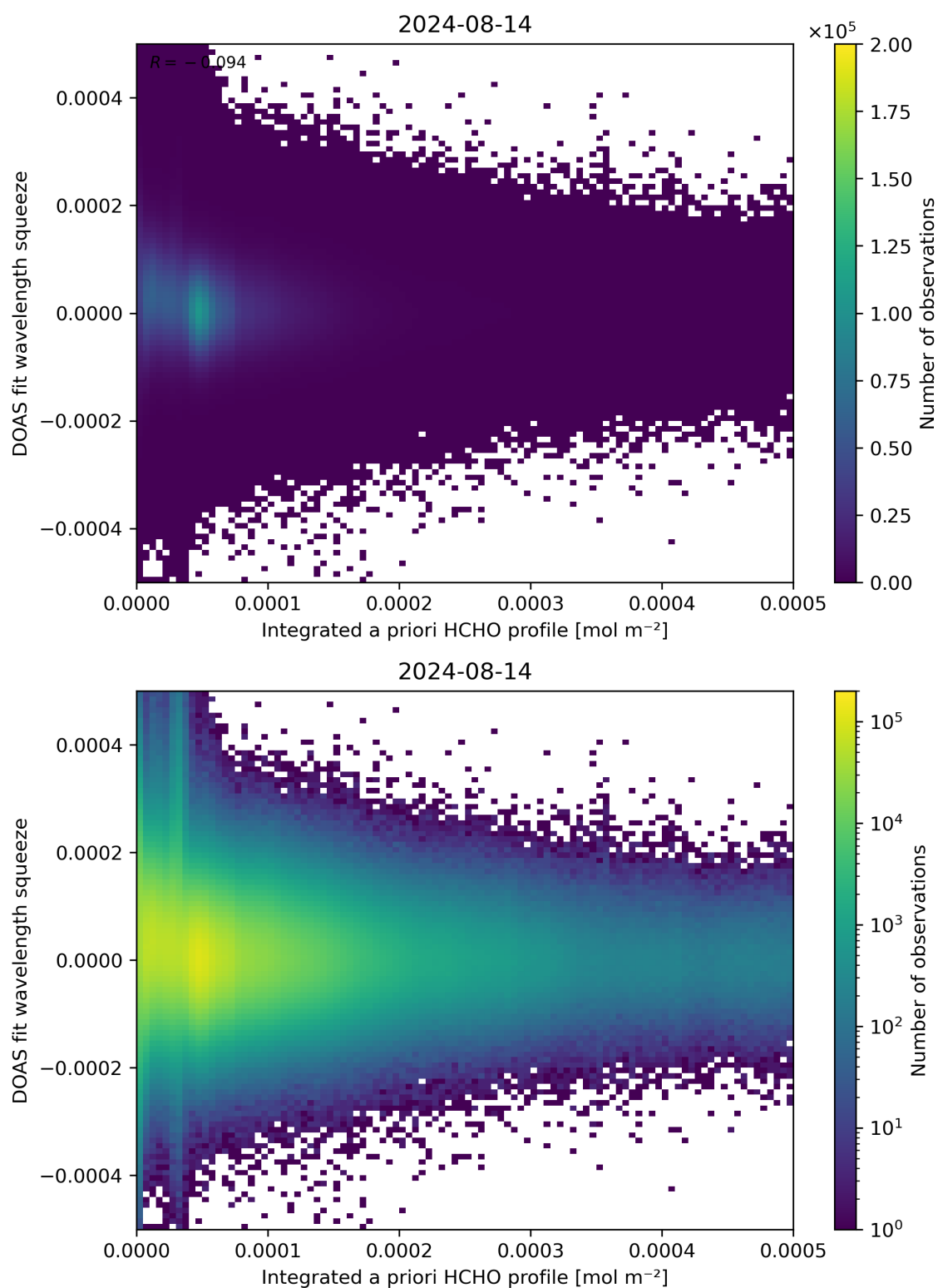
Figure 150: Scatter density plot of “Integrated a priori HCHO profile” against “DOAS fit wavelength squeeze” for 2024-08-13 to 2024-08-15.
