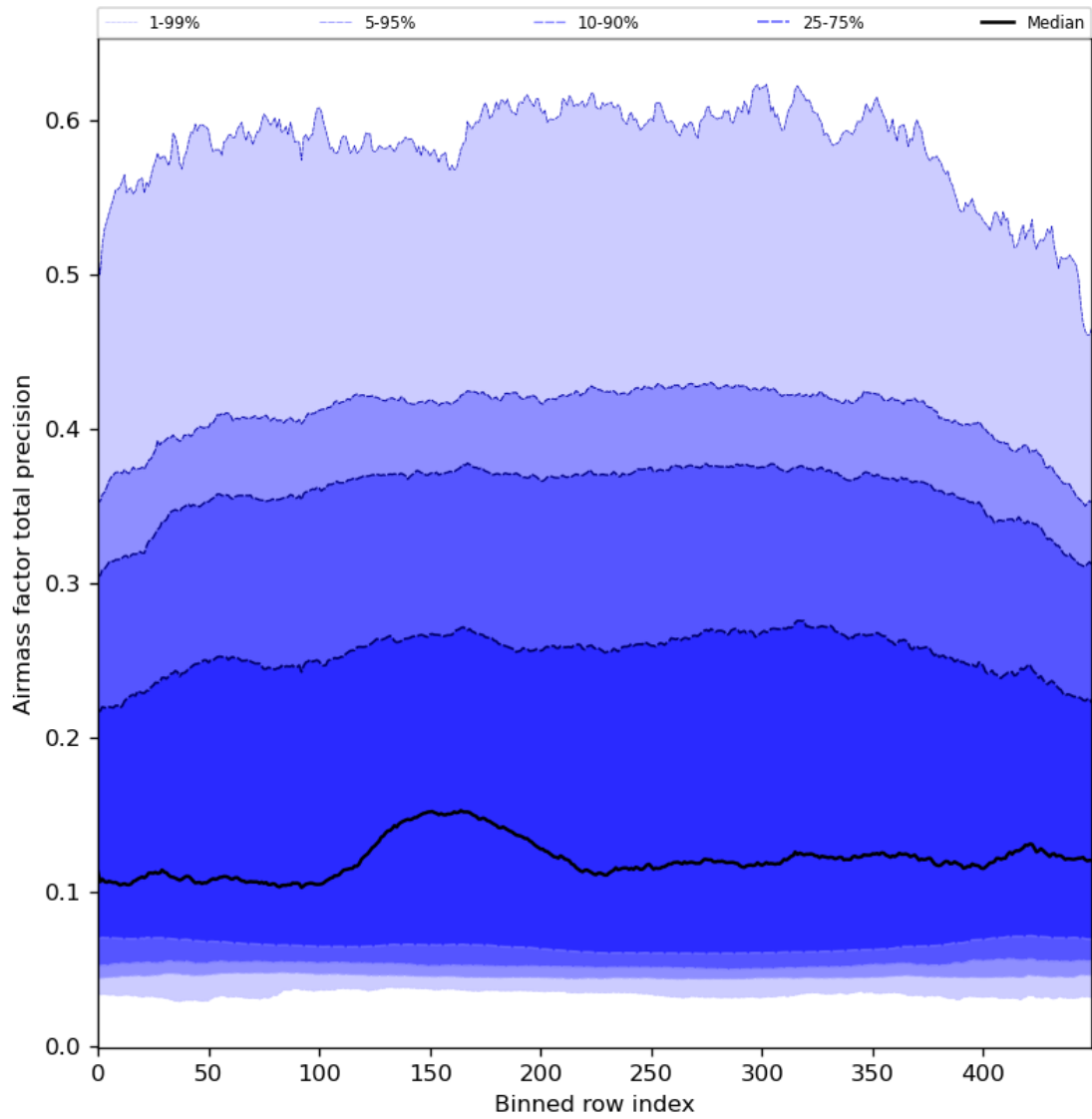
Figure 55: Along track statistics of “Airmass factor total precision” for 2024-08-13 to 2024-08-15
