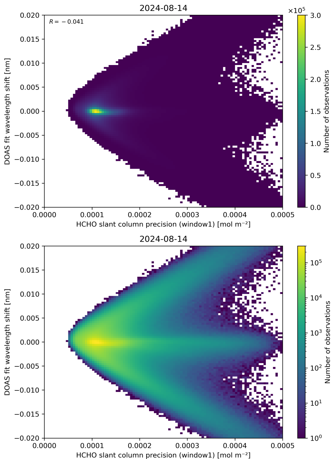
Figure 89: Scatter density plot of “HCHO slant column precision (window1)” against “DOAS fit wavelength shift” for 2024-08-13 to 2024-08-15.
