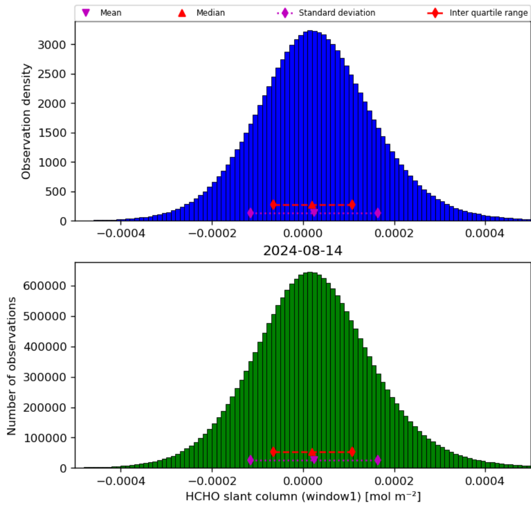
Figure 38: Histogram of “HCHO slant column (window1)” for 2024-08-13 to 2024-08-15
