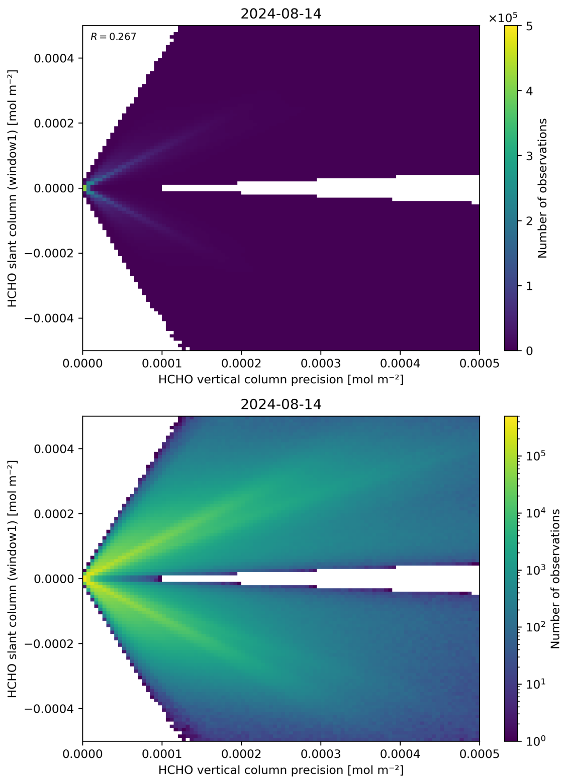
Figure 142: Scatter density plot of “HCHO vertical column precision” against “HCHO slant column (window1)” for 2024-08-13 to 2024-08-15.
