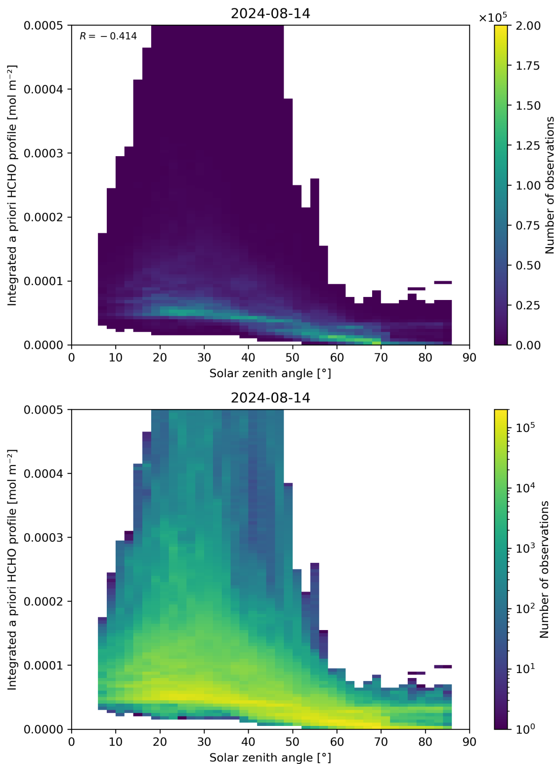
Figure 180: Scatter density plot of “Solar zenith angle” against “Integrated a priori HCHO profile” for 2024-08-13 to 2024-08-15.
