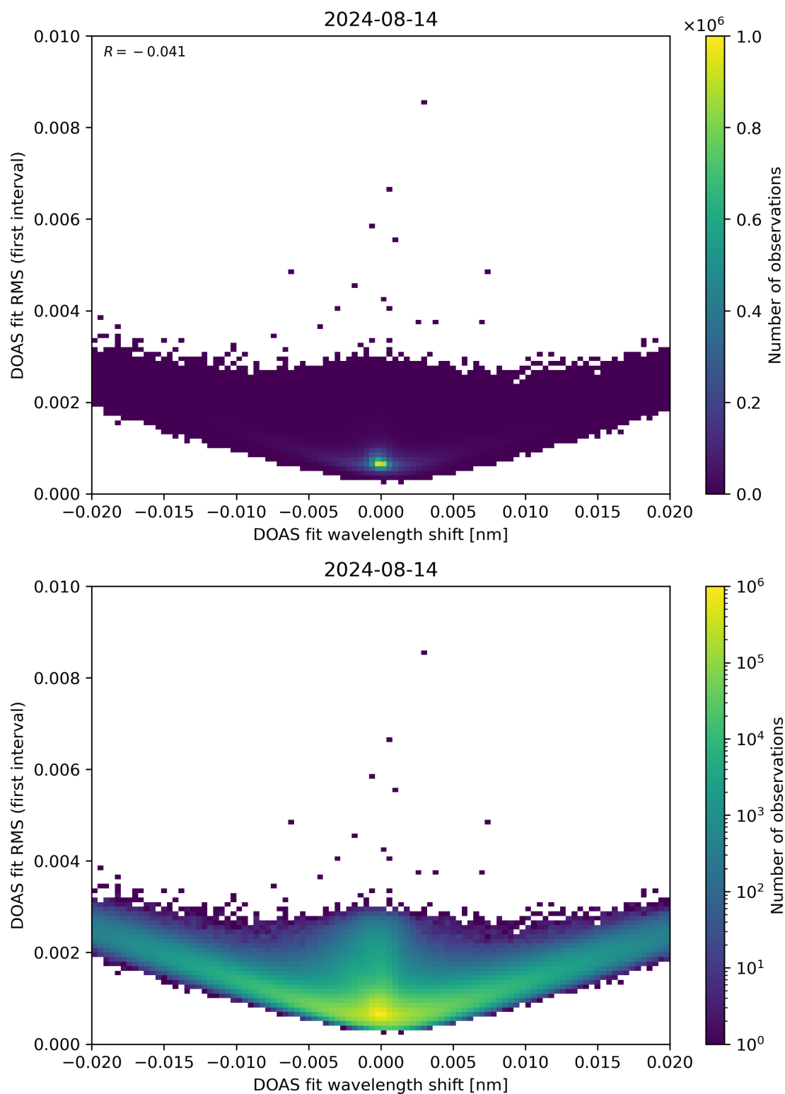
Figure 64: Scatter density plot of “DOAS fit wavelength shift” against “DOAS fit RMS (first interval)” for 2024-08-13 to 2024-08-15.
