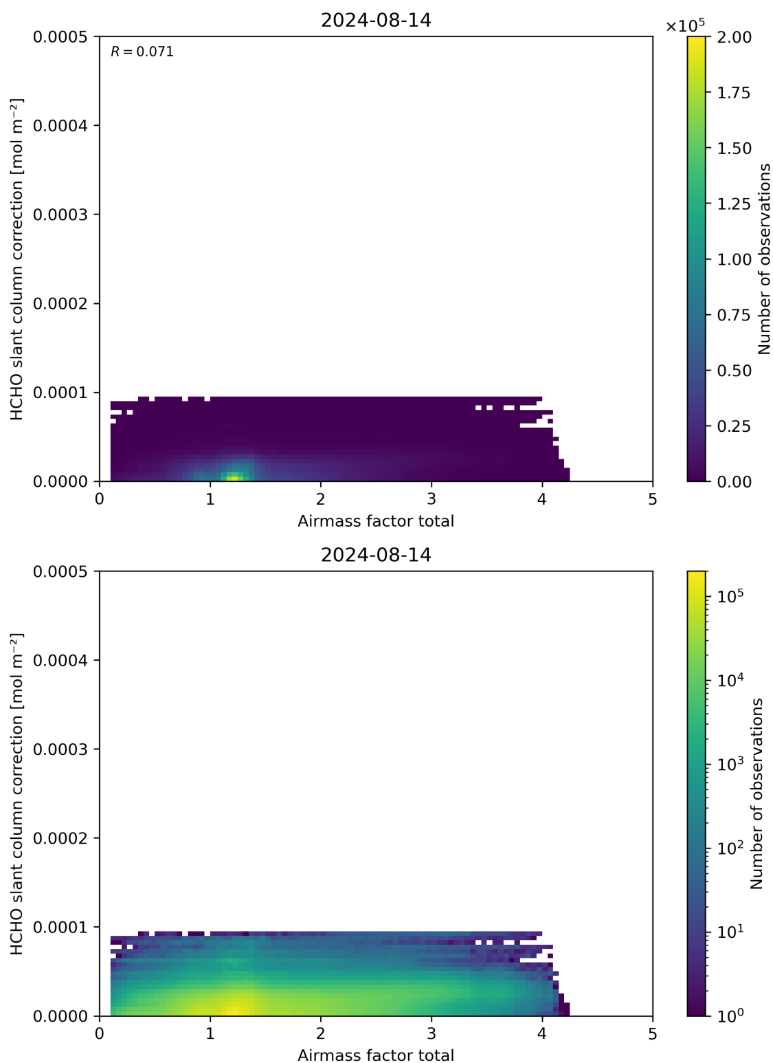
Figure 102: Scatter density plot of “Airmass factor total” against “HCHO slant column correction” for 2024-08-13 to 2024-08-15.
