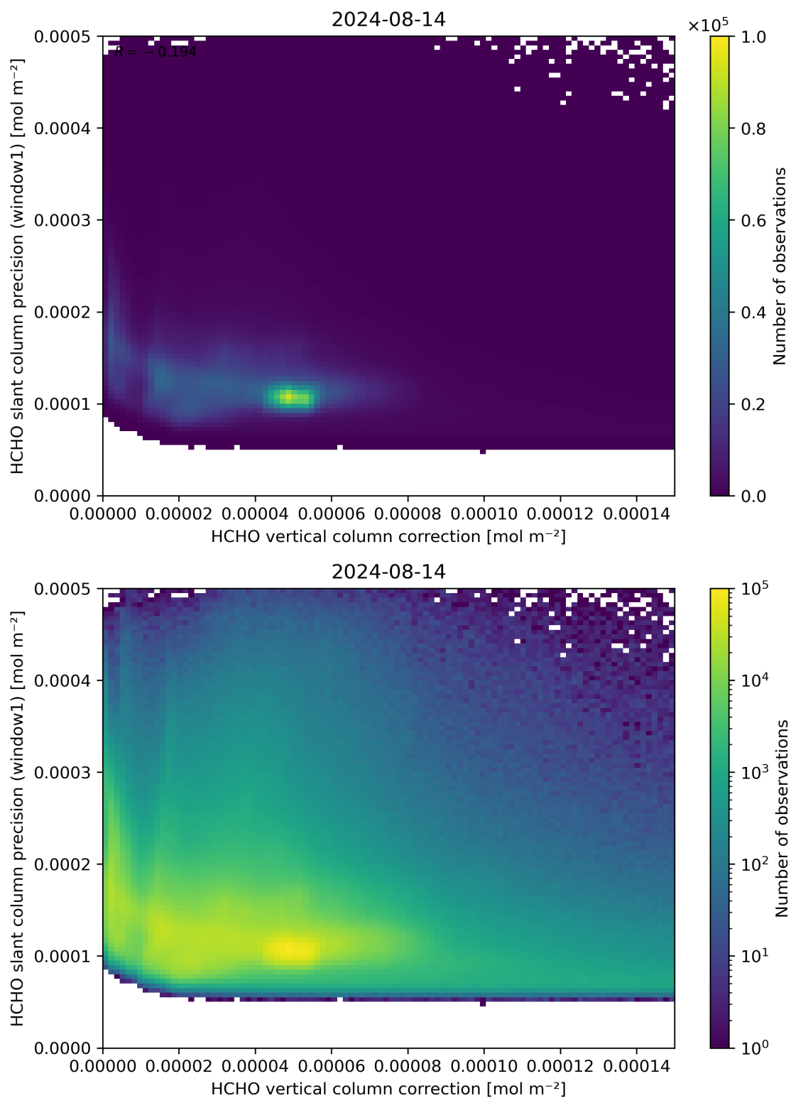
Figure 119: Scatter density plot of “HCHO vertical column correction” against “HCHO slant column precision (window1)” for 2024-08-13 to 2024-08-15.
