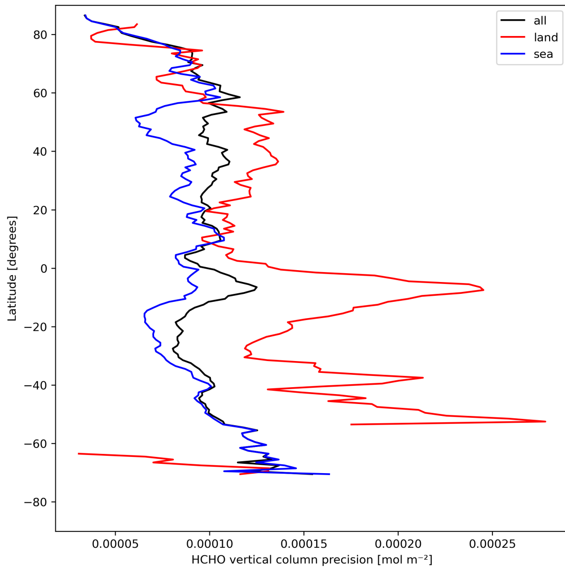
Figure 22: Zonal average of “HCHO vertical column precision” for 2024-08-13 to 2024-08-15.
