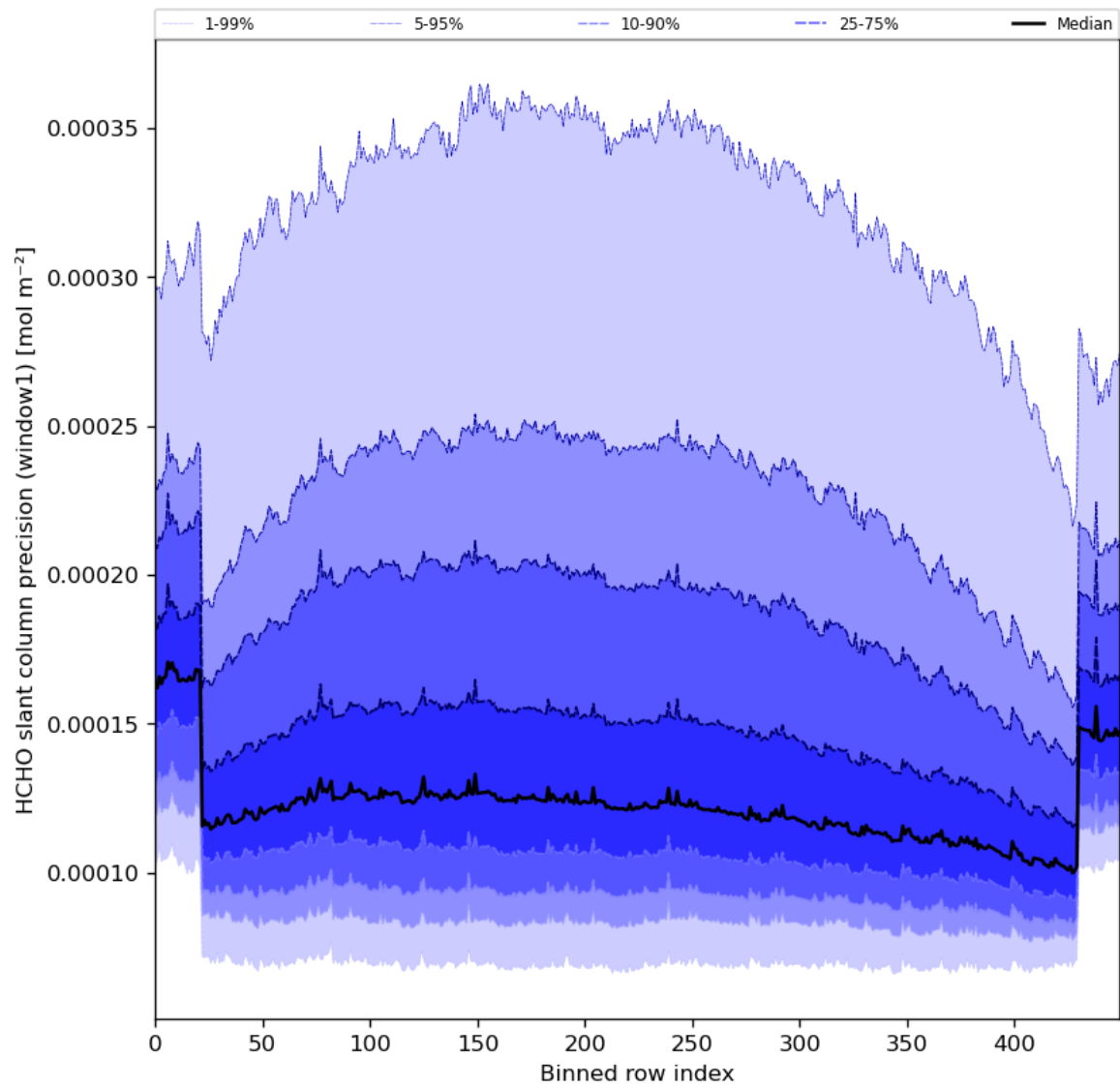
Figure 53: Along track statistics of “HCHO slant column precision (window1)” for 2024-08-13 to 2024-08-15
