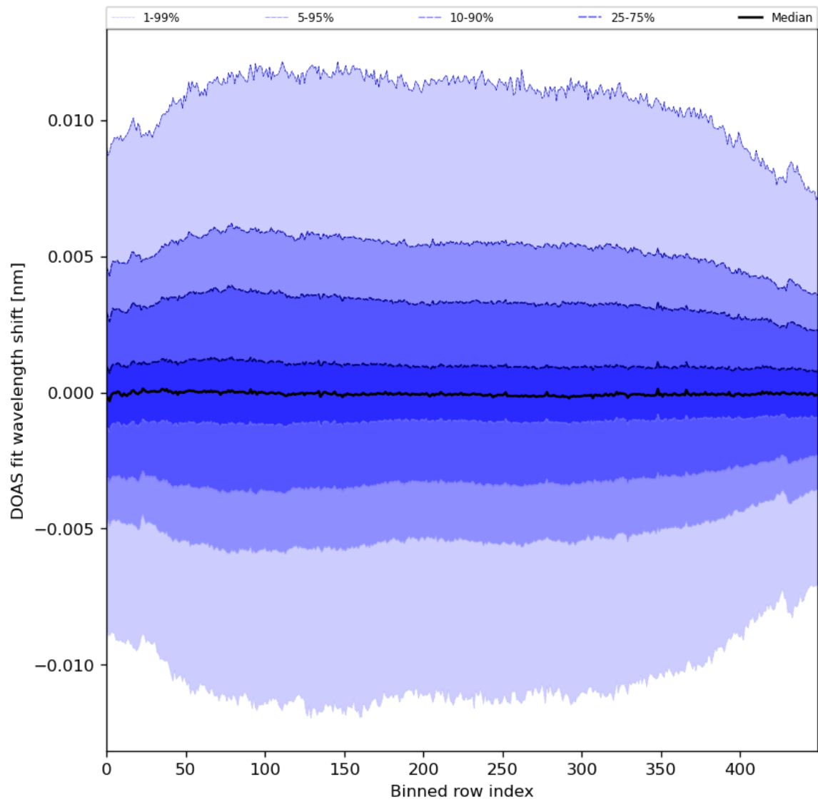
Figure 58: Along track statistics of “DOAS fit wavelength shift” for 2024-08-13 to 2024-08-15
