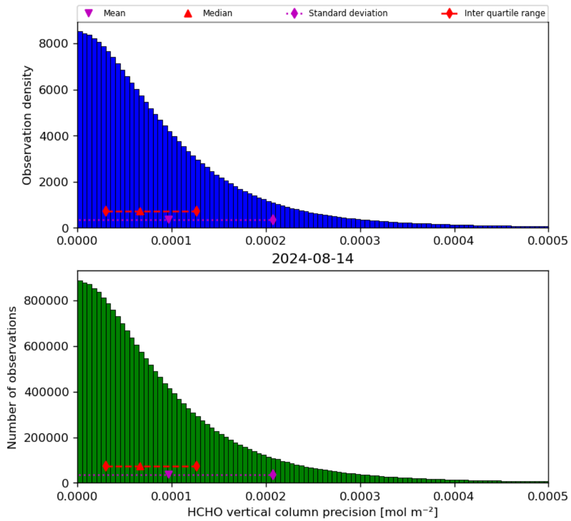
Figure 36: Histogram of “HCHO vertical column precision” for 2024-08-13 to 2024-08-15
