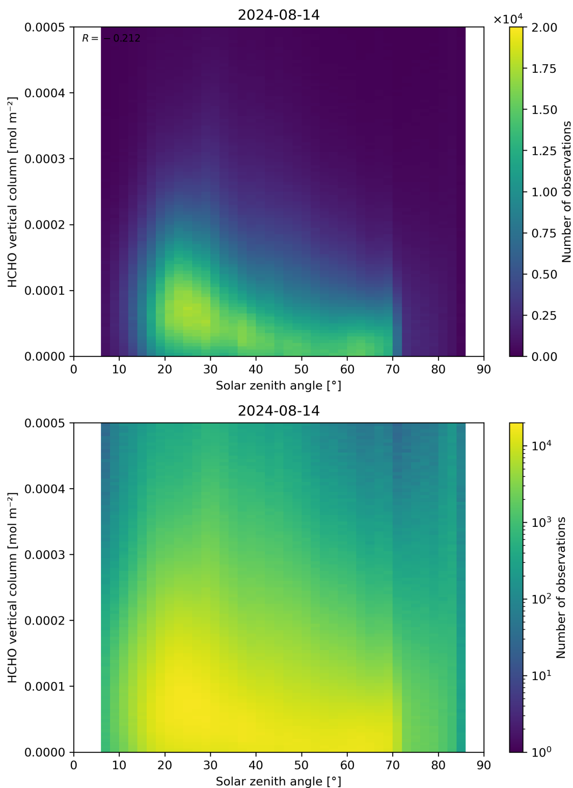
Figure 177: Scatter density plot of “Solar zenith angle” against “HCHO vertical column” for 2024-08-13 to 2024-08-15.
