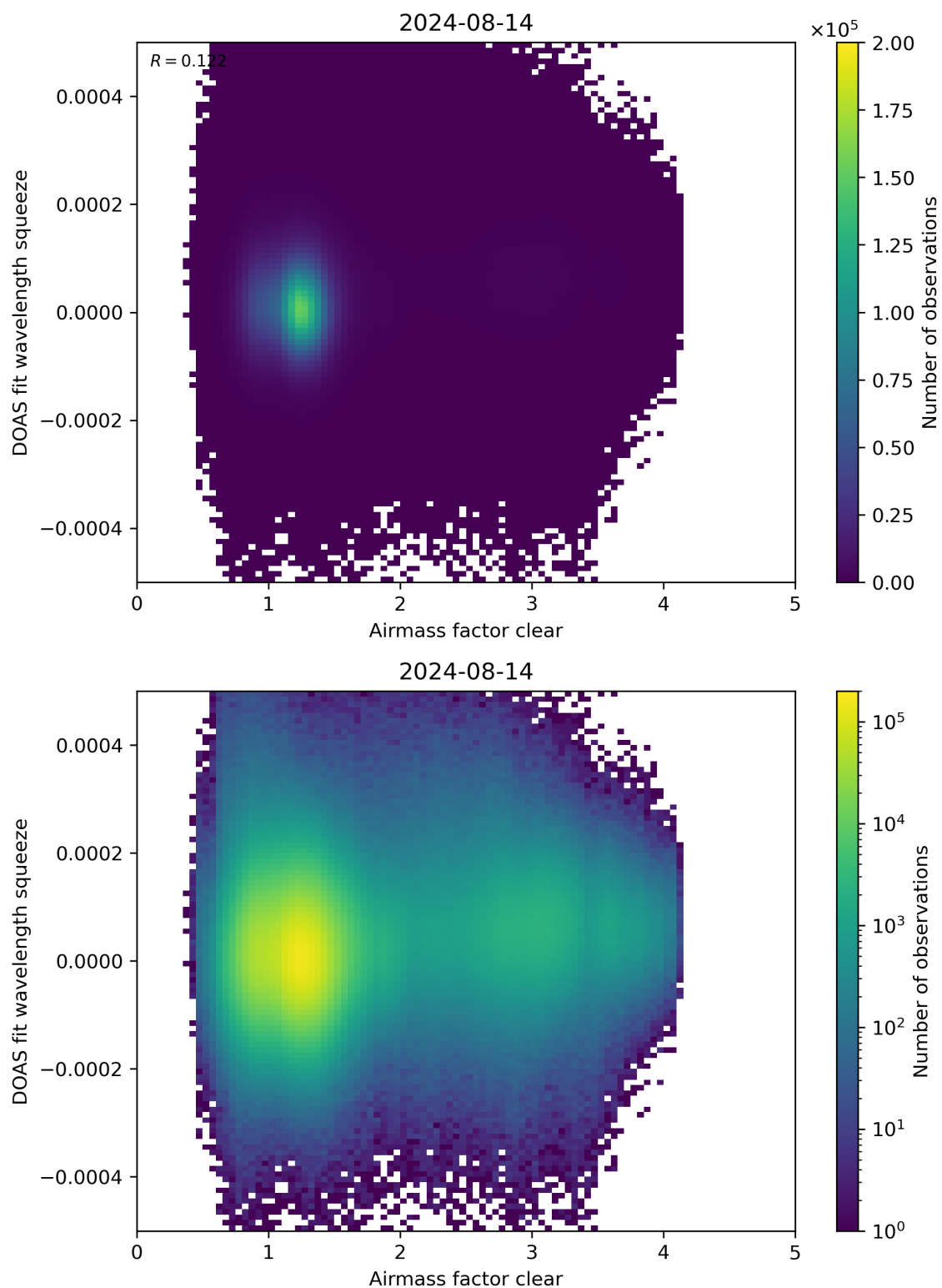
Figure 73: Scatter density plot of “Airmass factor clear” against “DOAS fit wavelength squeeze” for 2024-08-13 to 2024-08-15.
