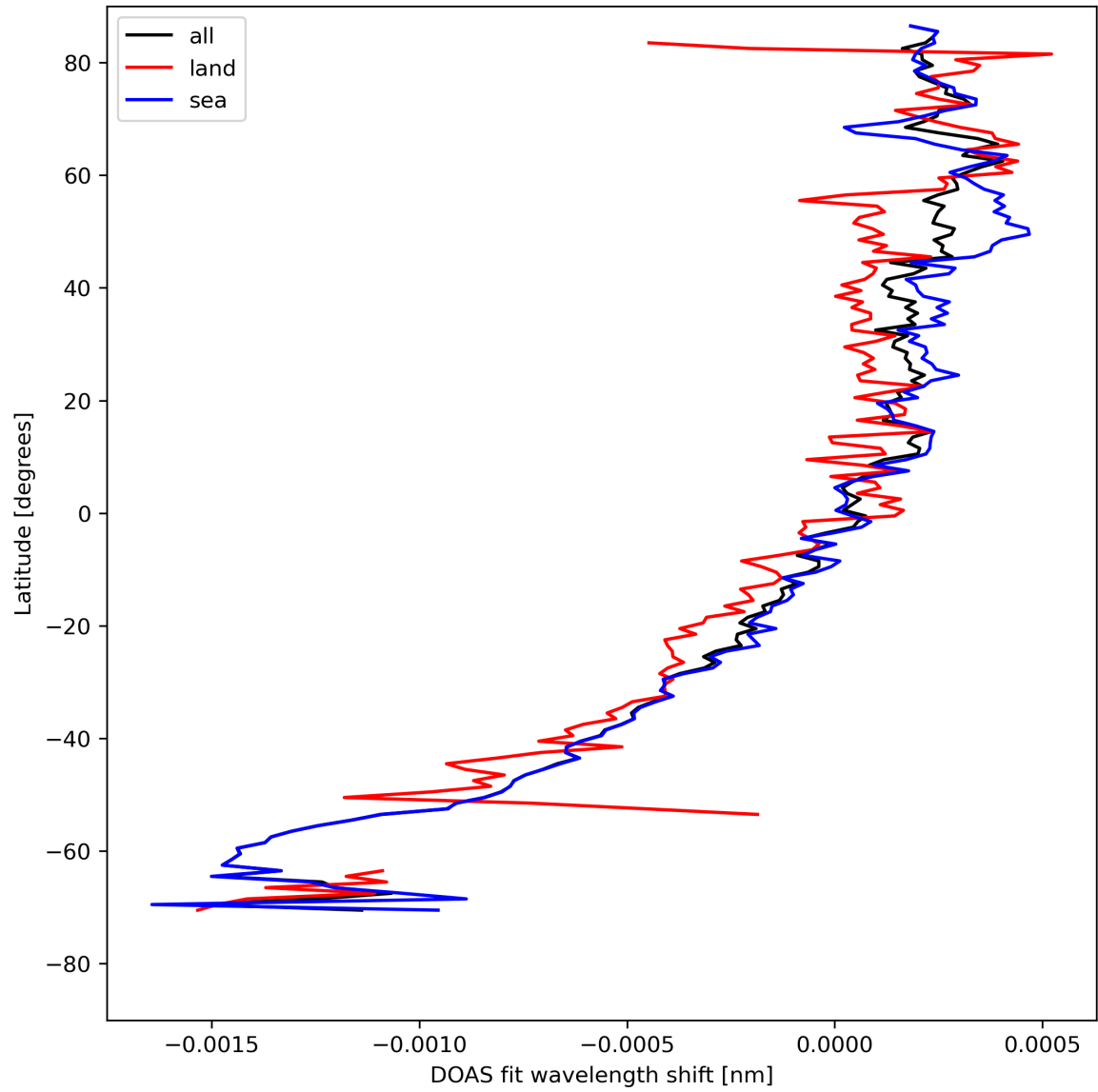
Figure 30: Zonal average of “DOAS fit wavelength shift” for 2024-08-13 to 2024-08-15.
