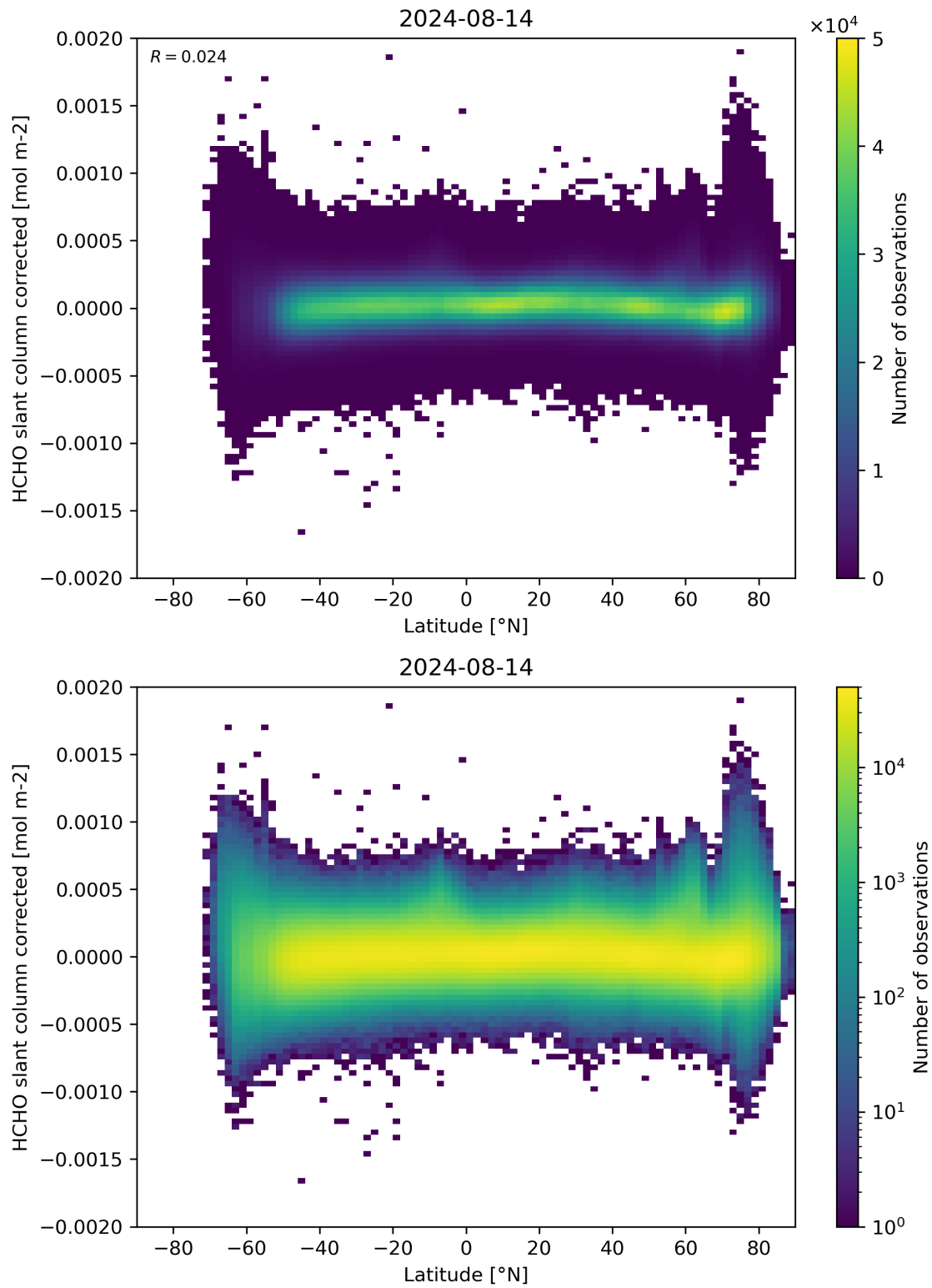
Figure 157: Scatter density plot of “Latitude” against “HCHO slant column corrected” for 2024-08-13 to 2024-08-15.
