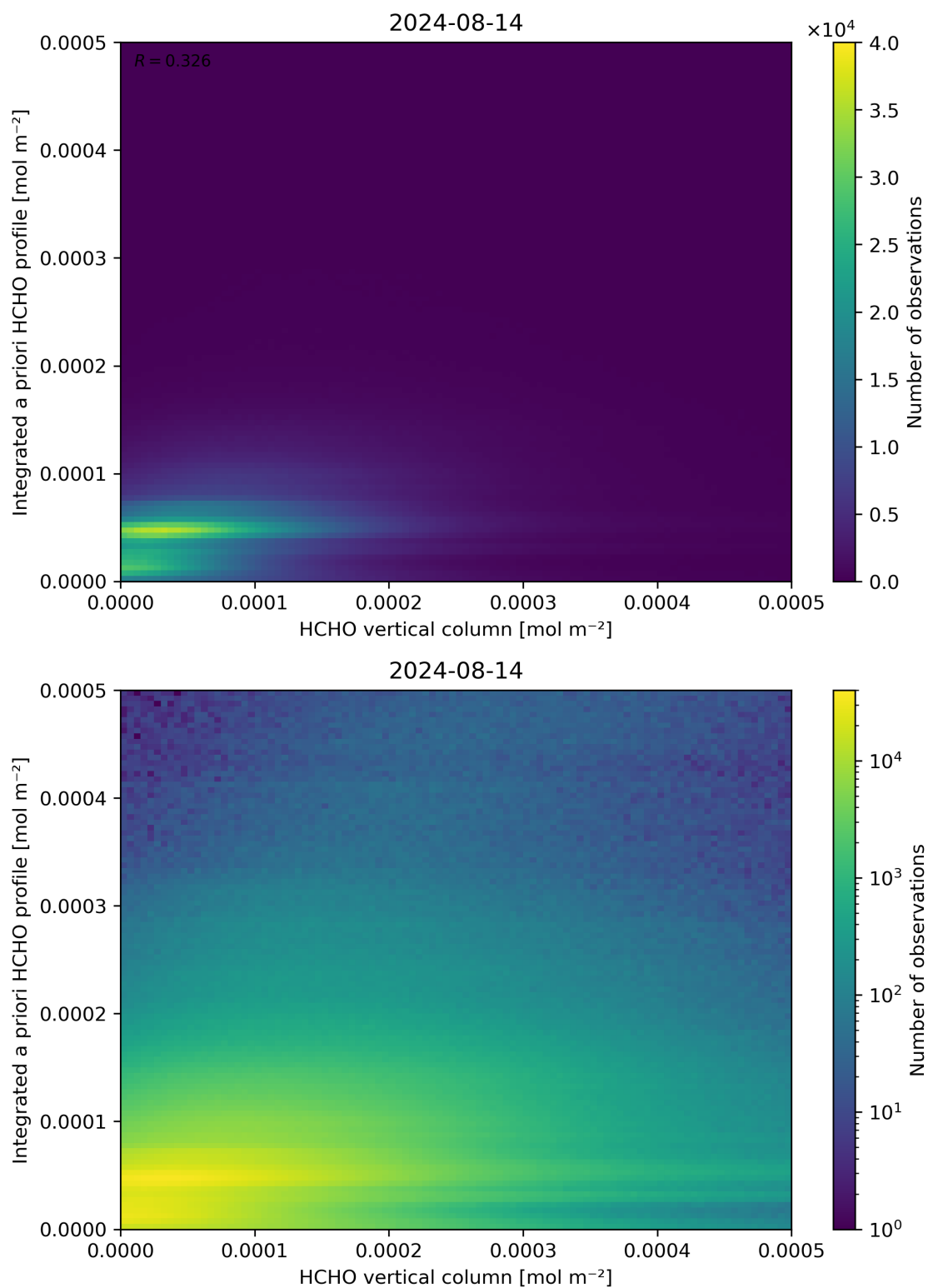
Figure 135: Scatter density plot of “HCHO vertical column” against “Integrated a priori HCHO profile” for 2024-08-13 to 2024-08-15.
