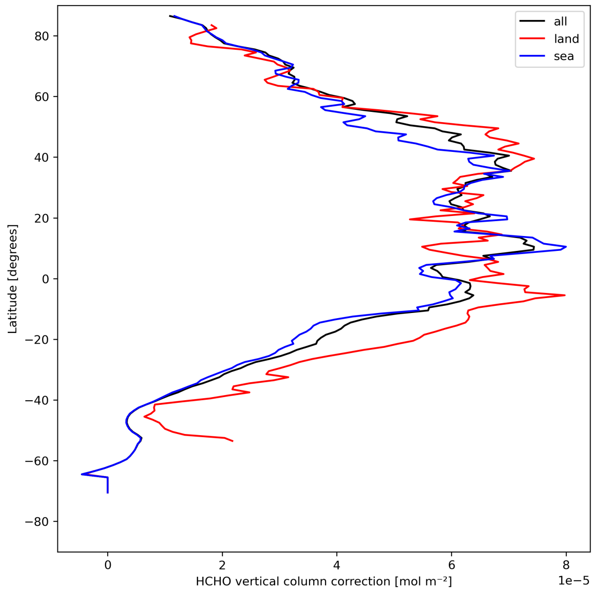
Figure 23: Zonal average of “HCHO vertical column correction” for 2024-08-13 to 2024-08-15.
