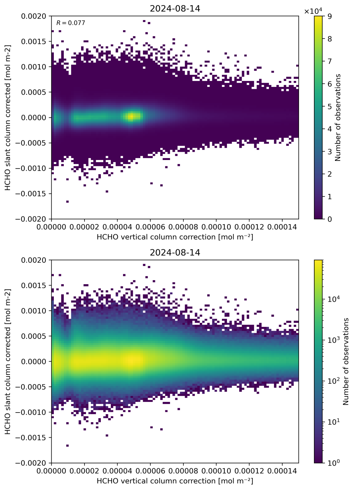
Figure 116: Scatter density plot of “HCHO vertical column correction” against “HCHO slant column corrected” for 2024-08-13 to 2024-08-15.
