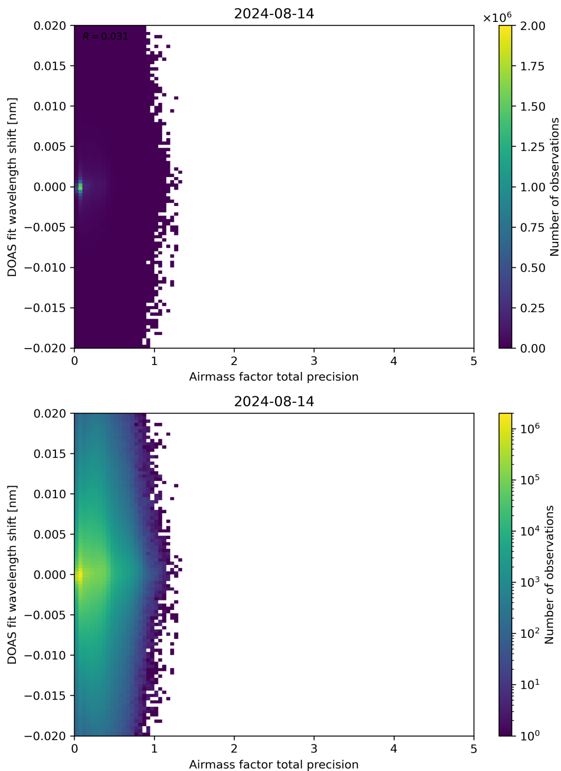
Figure 106: Scatter density plot of “Airmass factor total precision” against “DOAS fit wavelength shift” for 2024-08-13 to 2024-08-15.
