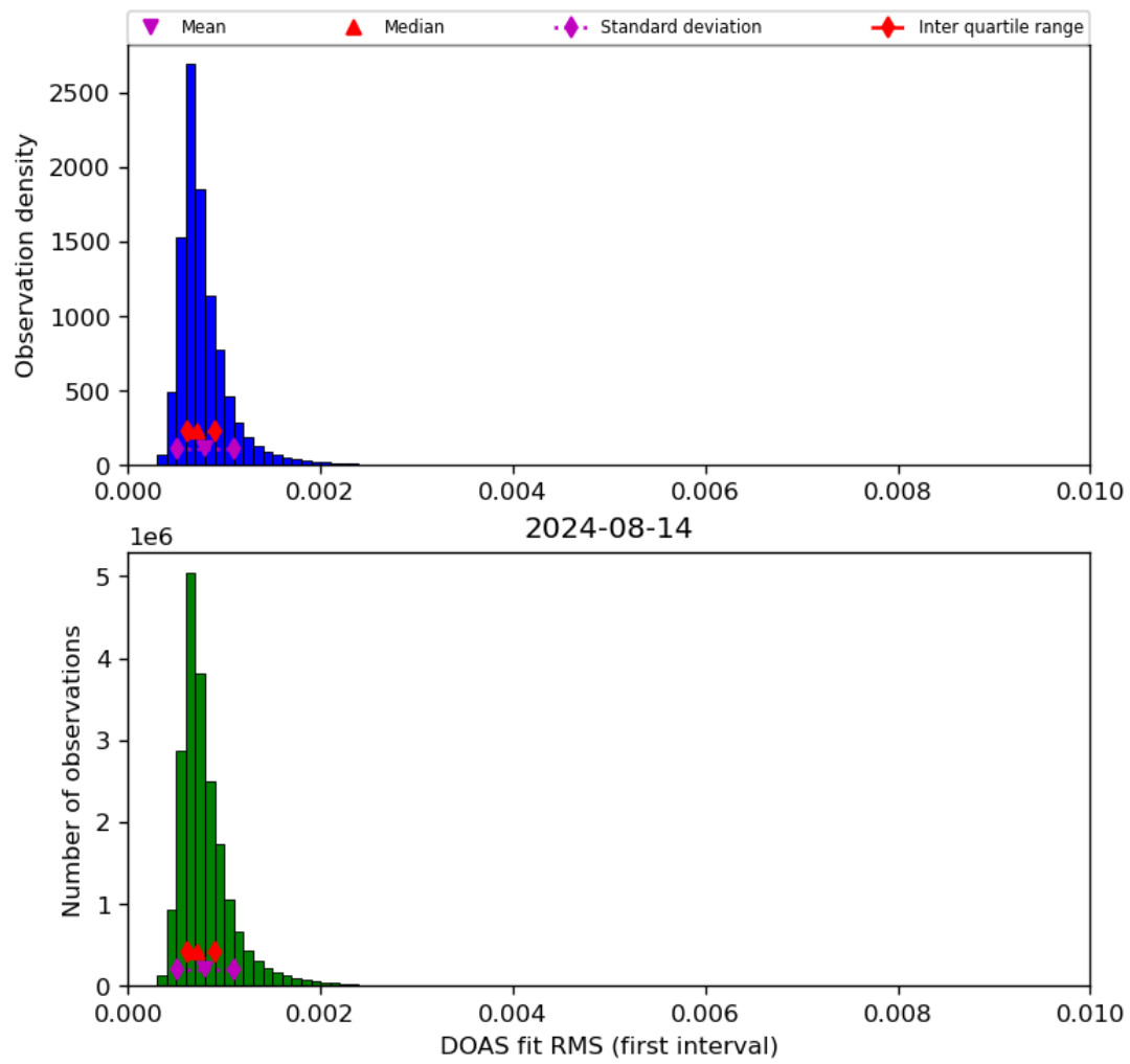
Figure 46: Histogram of “DOAS fit RMS (first interval)” for 2024-08-13 to 2024-08-15
