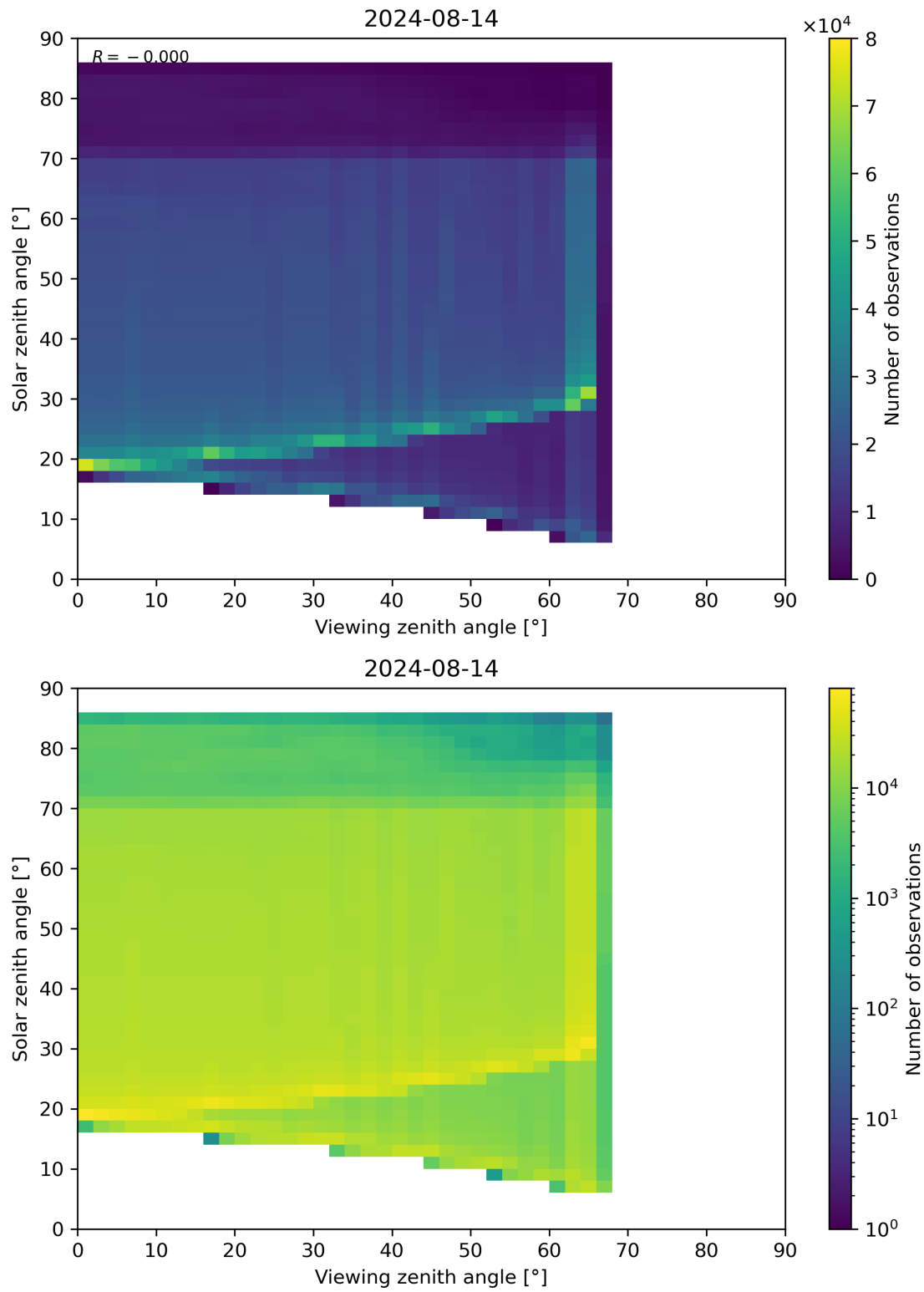
Figure 197: Scatter density plot of “Viewing zenith angle” against “Solar zenith angle” for 2024-08-13 to 2024-08-15.
