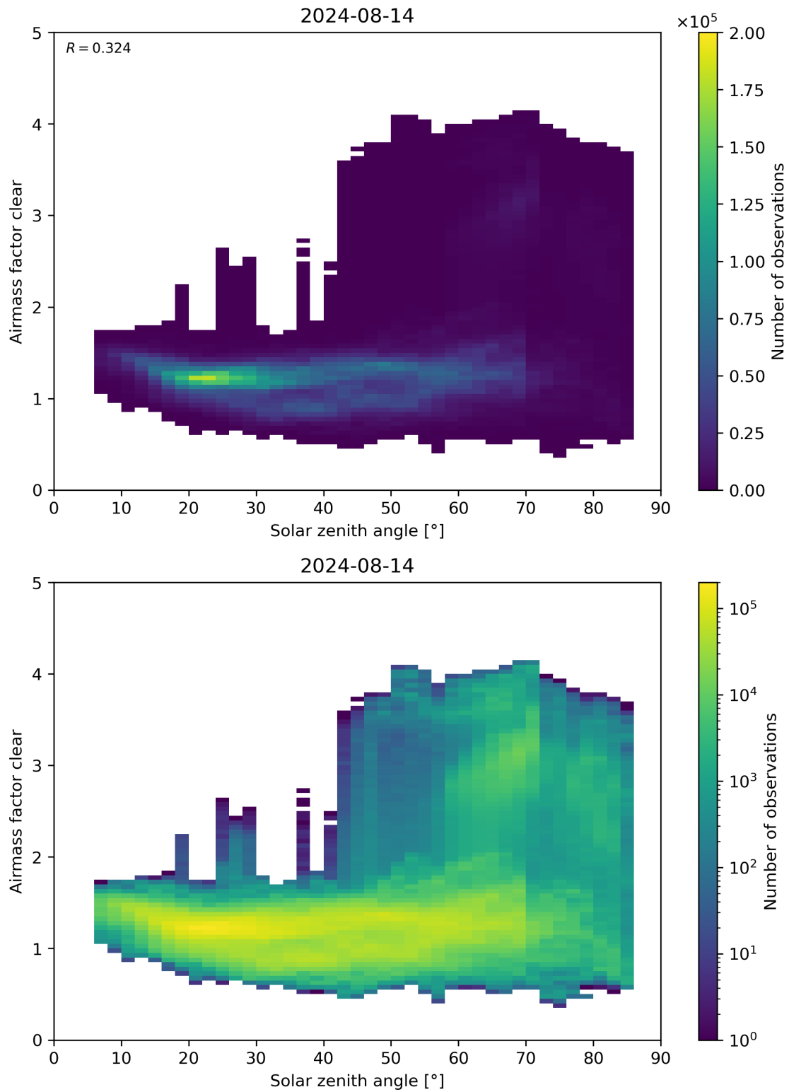
Figure 170: Scatter density plot of “Solar zenith angle” against “Airmass factor clear” for 2024-08-13 to 2024-08-15.
