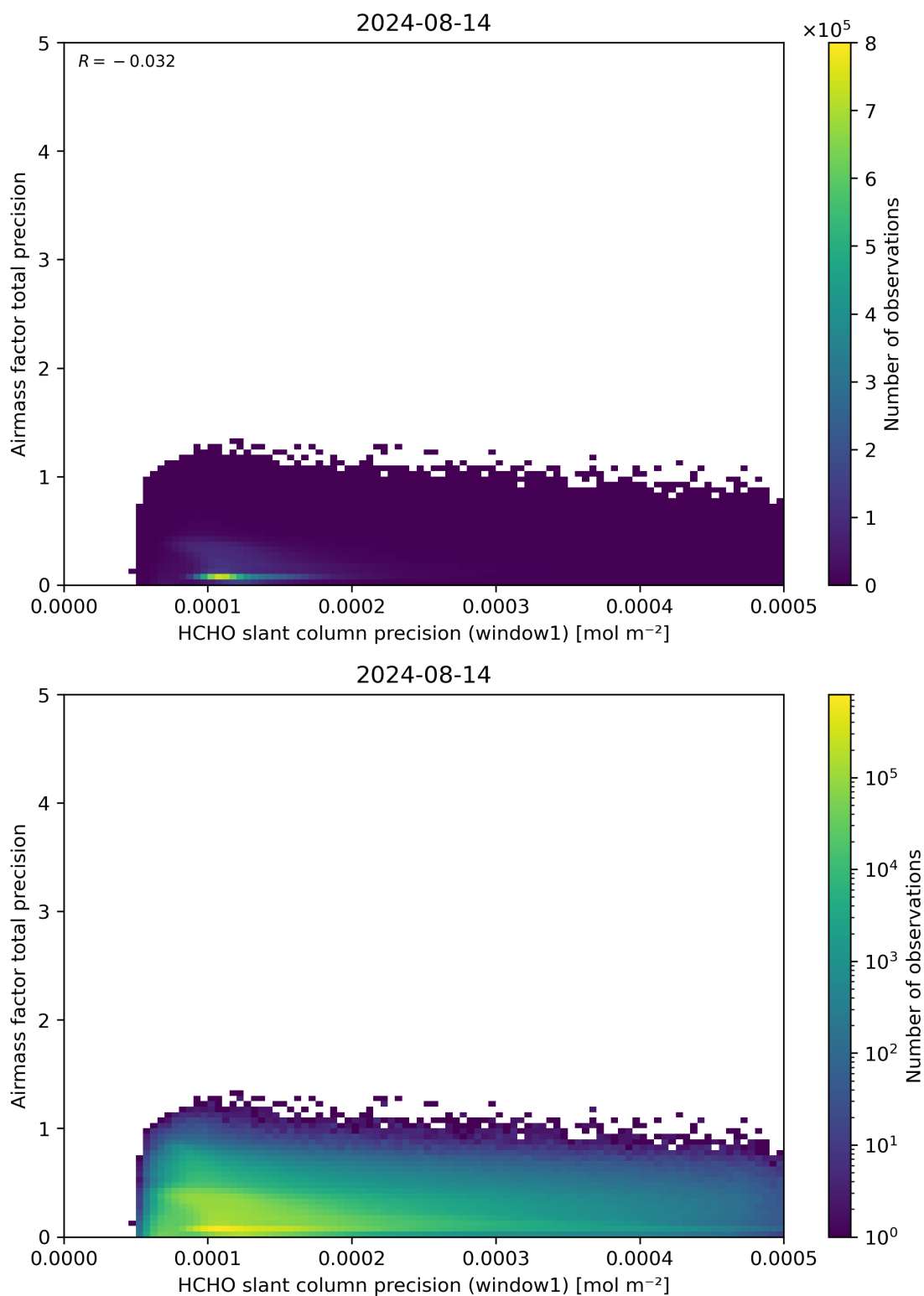
Figure 95: Scatter density plot of “HCHO slant column precision (window1)” against “Airmass factor total precision” for 2024-08-13 to 2024-08-15.
