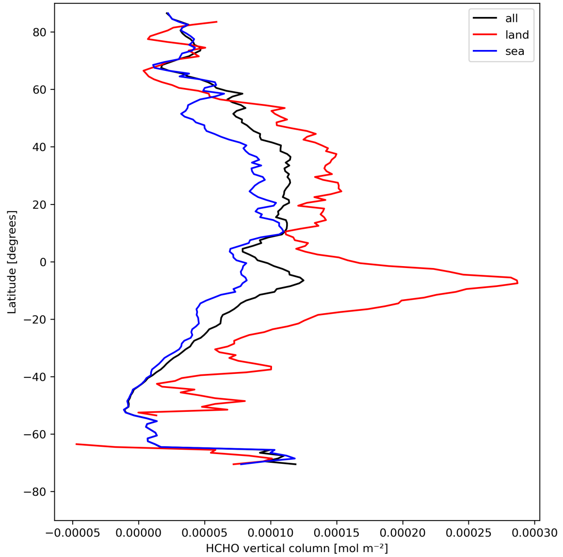
Figure 21: Zonal average of “HCHO vertical column” for 2024-08-13 to 2024-08-15.
