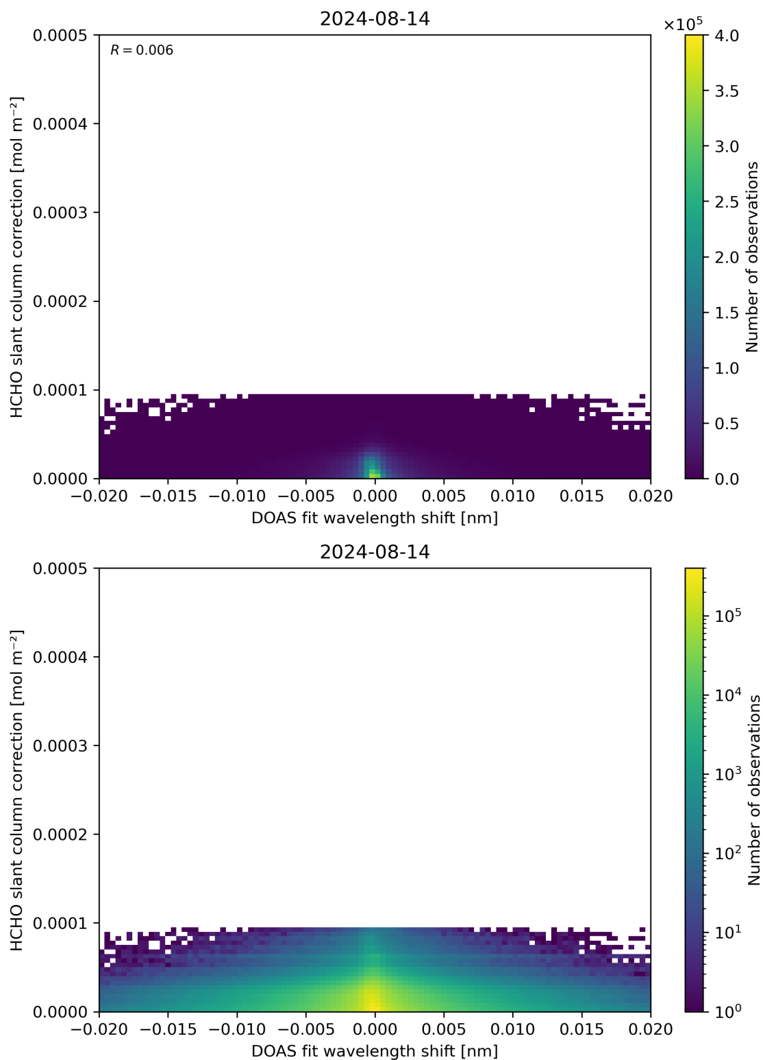
Figure 67: Scatter density plot of “DOAS fit wavelength shift” against “HCHO slant column correction” for 2024-08-13 to 2024-08-15.
