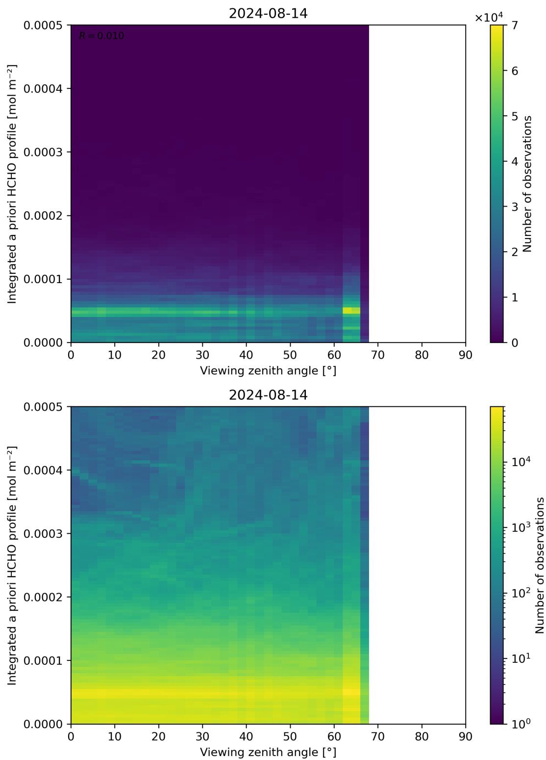
Figure 195: Scatter density plot of “Viewing zenith angle” against “Integrated a priori HCHO profile” for 2024-08-13 to 2024-08-15.
