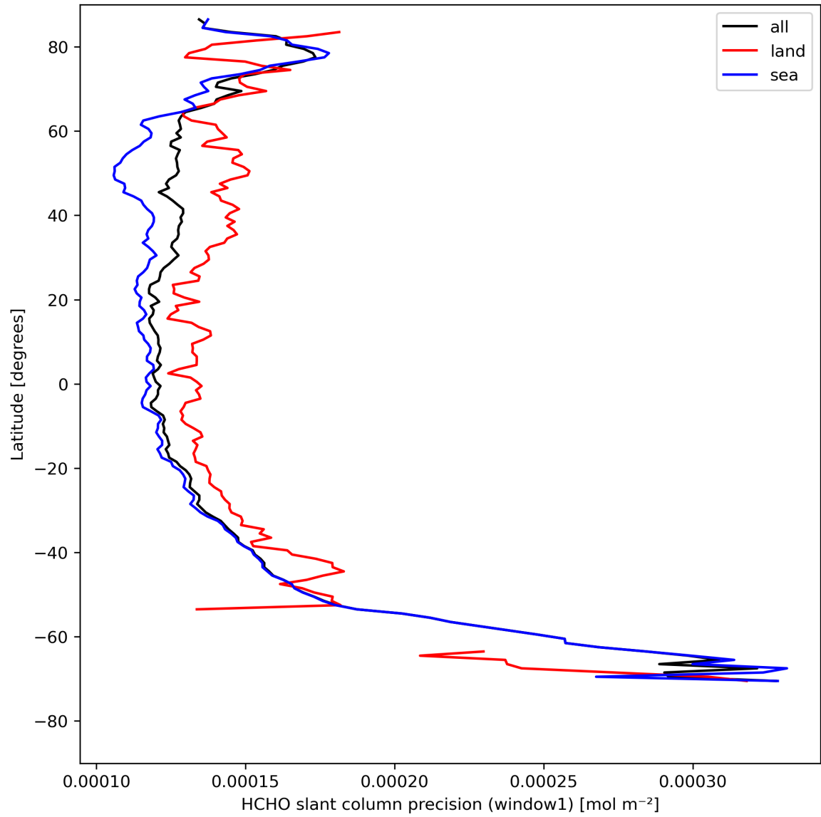
Figure 25: Zonal average of “HCHO slant column precision (window1)” for 2024-08-13 to 2024-08-15.
