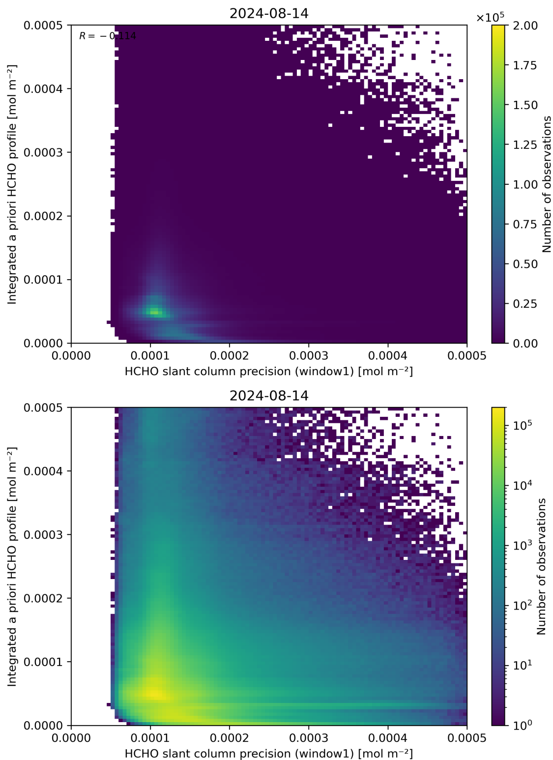
Figure 96: Scatter density plot of “HCHO slant column precision (window1)” against “Integrated a priori HCHO profile” for 2024-08-13 to 2024-08-15.
