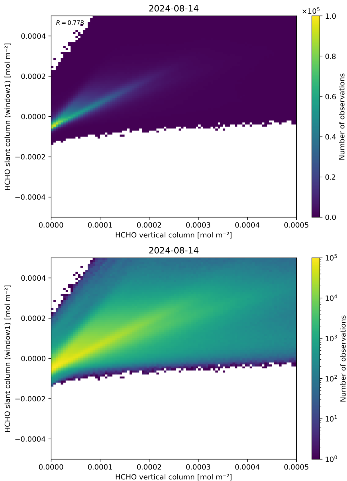
Figure 129: Scatter density plot of “HCHO vertical column” against “HCHO slant column (window1)” for 2024-08-13 to 2024-08-15.
