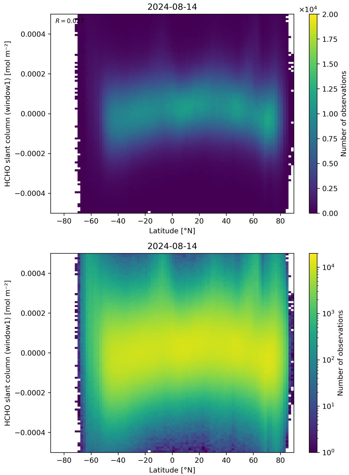
Figure 159: Scatter density plot of “Latitude” against “HCHO slant column (window1)” for 2024-08-13 to 2024-08-15.
