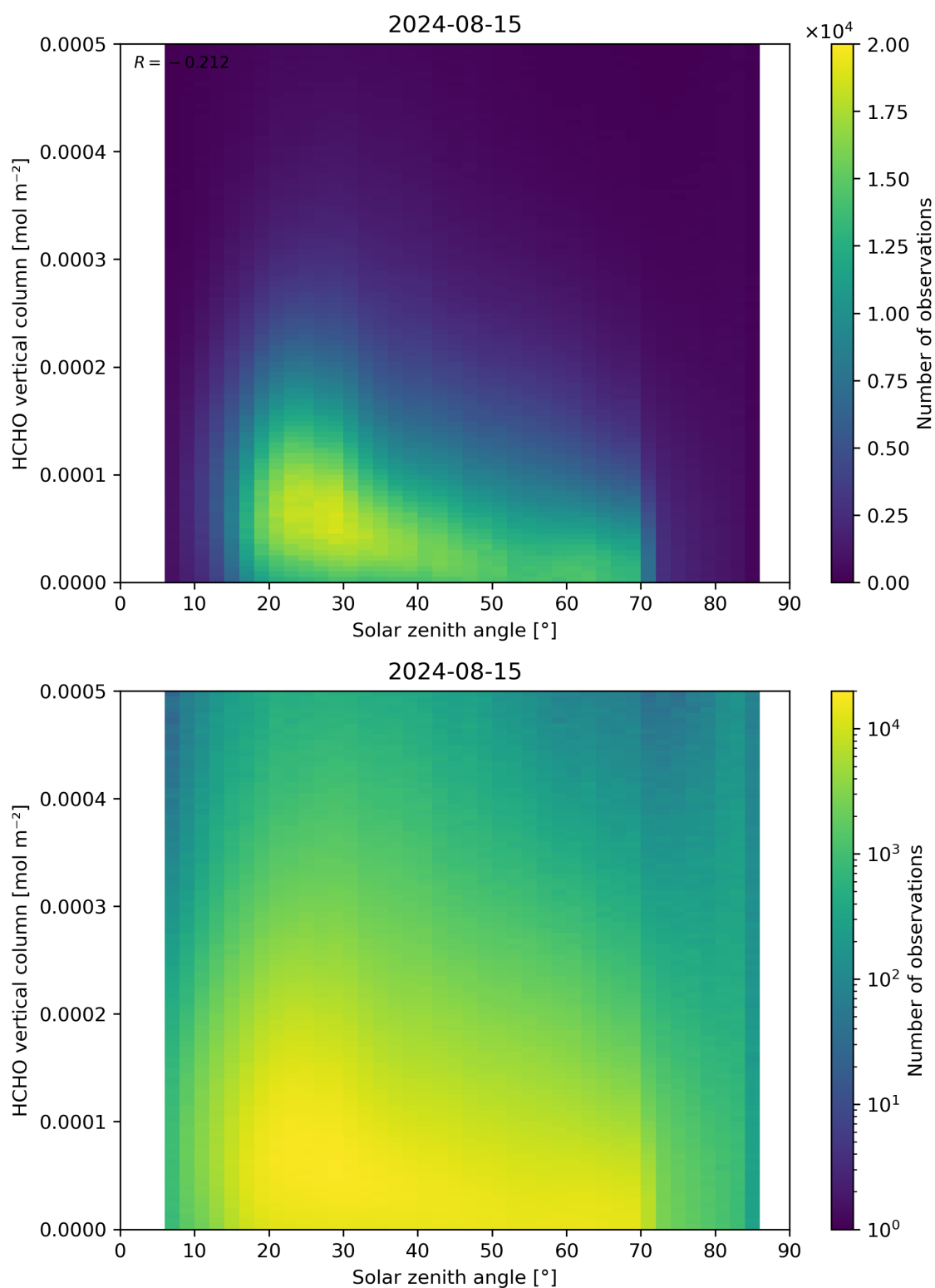
Figure 177: Scatter density plot of “Solar zenith angle” against “HCHO vertical column” for 2024-08-14 to 2024-08-16.
