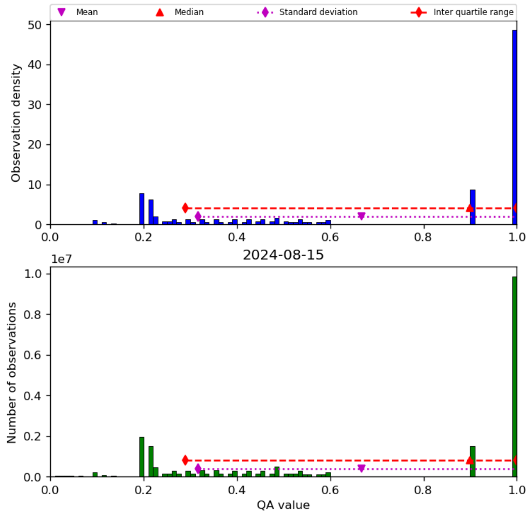
Figure 34: Histogram of “QA value” for 2024-08-14 to 2024-08-16
