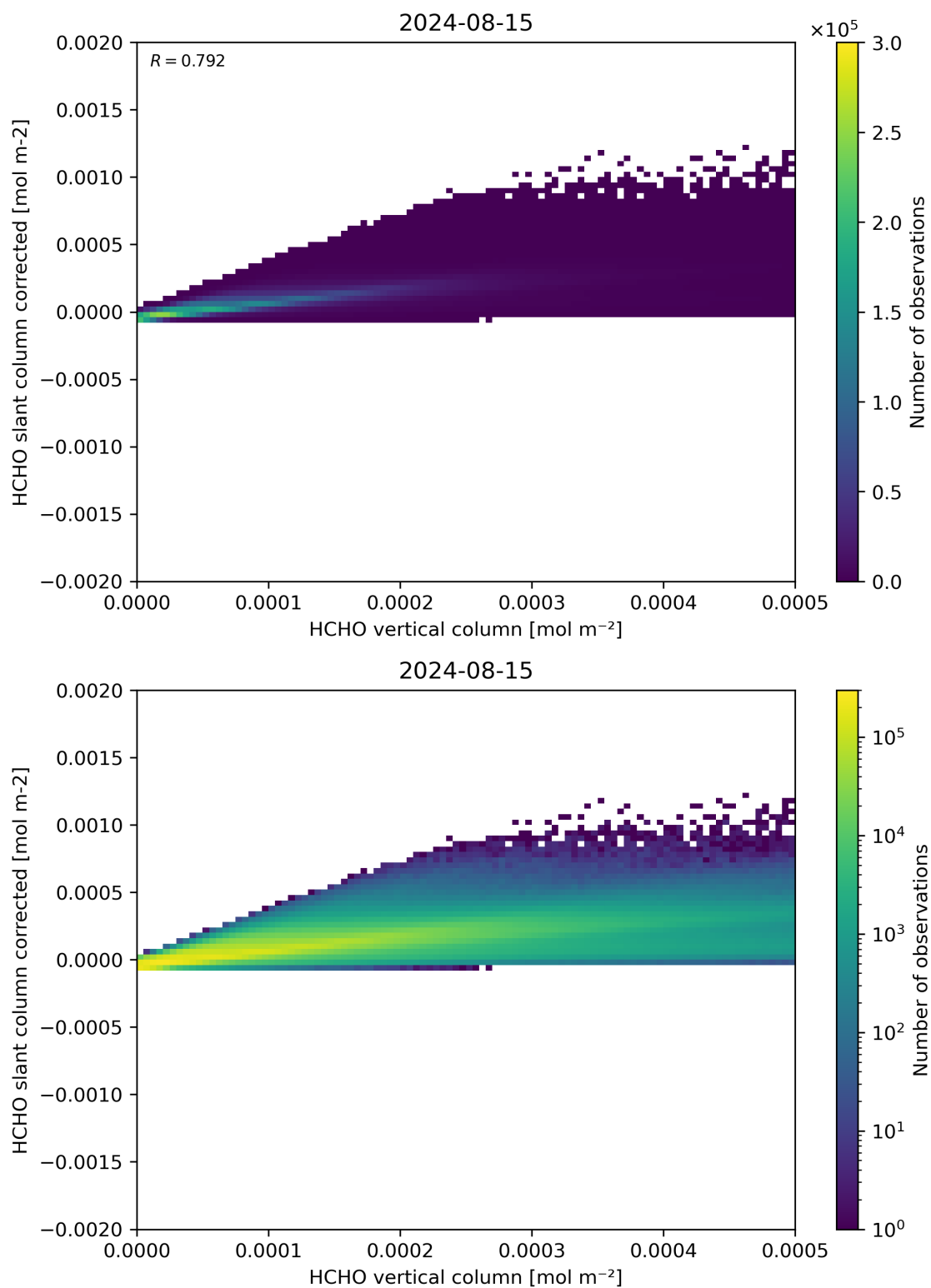
Figure 127: Scatter density plot of “HCHO vertical column” against “HCHO slant column corrected” for 2024-08-14 to 2024-08-16.
