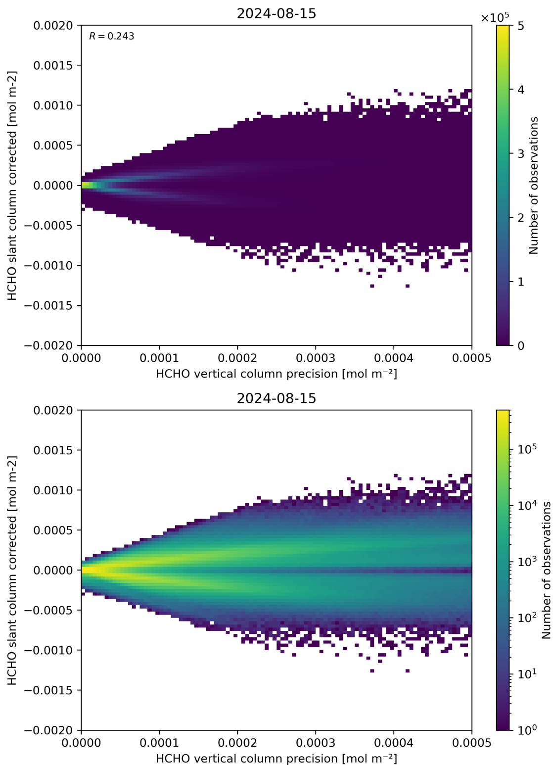
Figure 140: Scatter density plot of “HCHO vertical column precision” against “HCHO slant column corrected” for 2024-08-14 to 2024-08-16.
