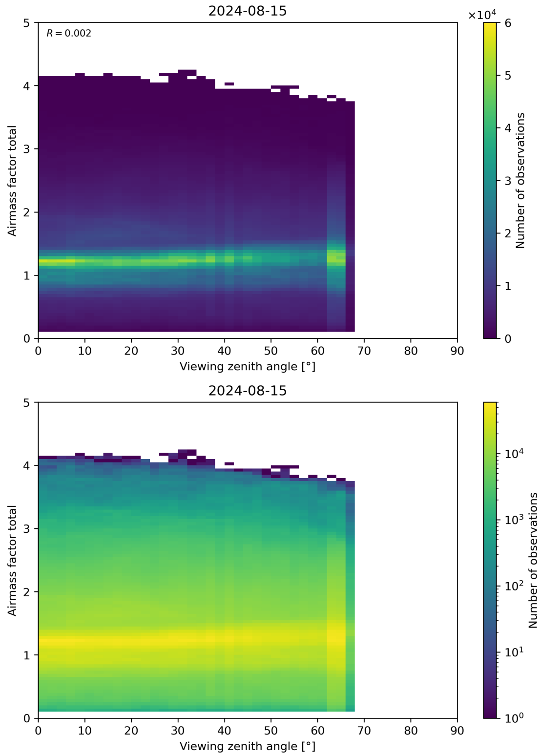
Figure 190: Scatter density plot of “Viewing zenith angle” against “Airmass factor total” for 2024-08-14 to 2024-08-16.
