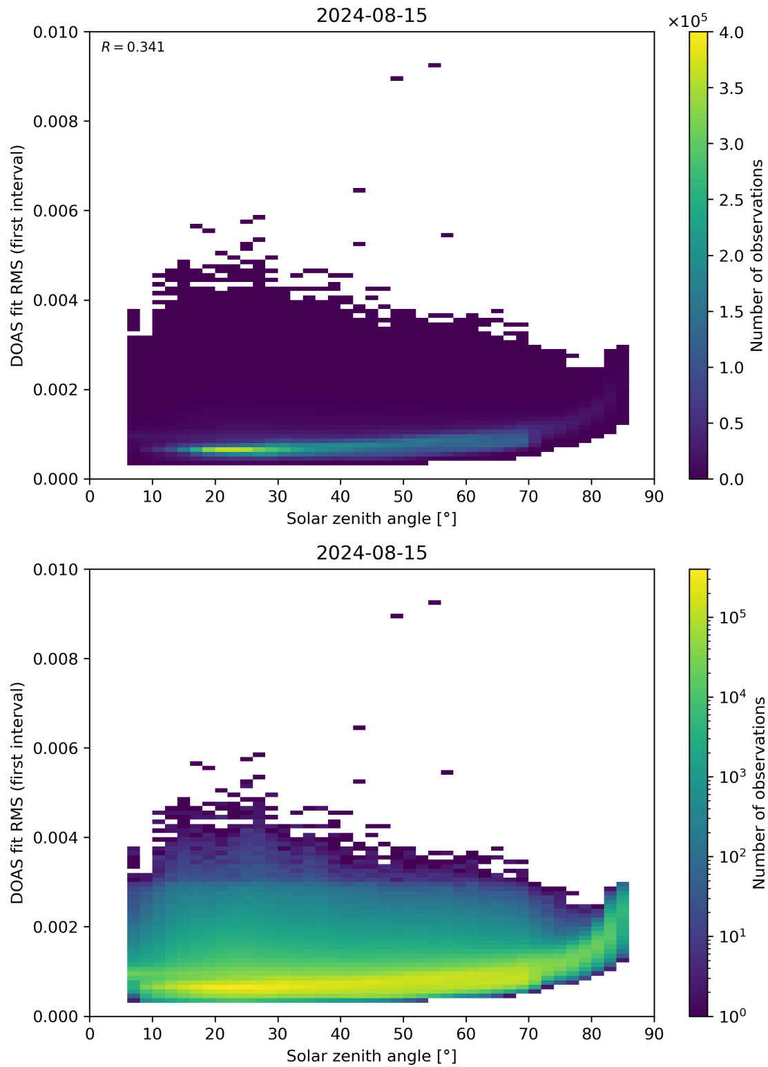
Figure 167: Scatter density plot of “Solar zenith angle” against “DOAS fit RMS (first interval)” for 2024-08-14 to 2024-08-16.
