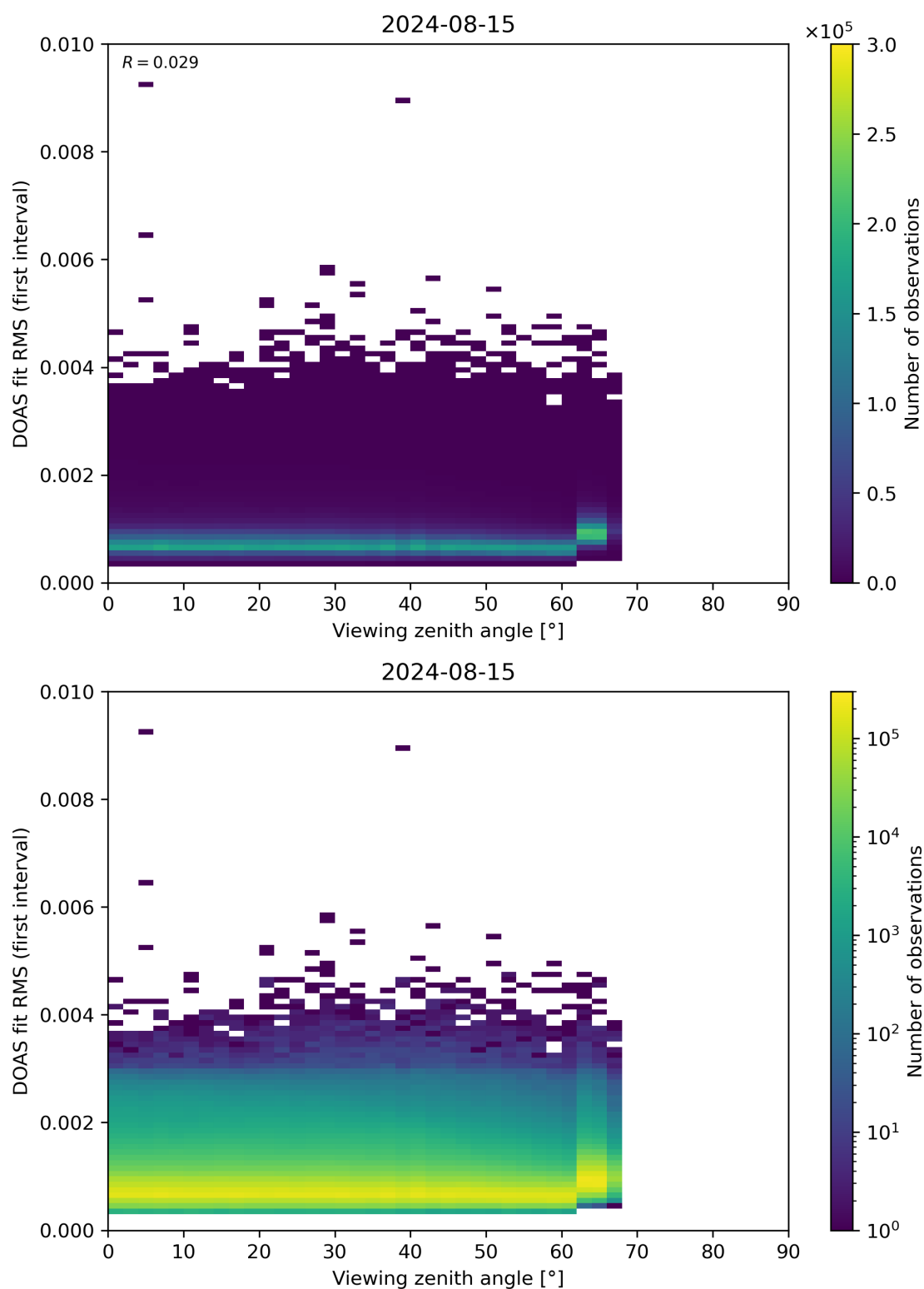
Figure 182: Scatter density plot of “Viewing zenith angle” against “DOAS fit RMS (first interval)” for 2024-08-14 to 2024-08-16.
