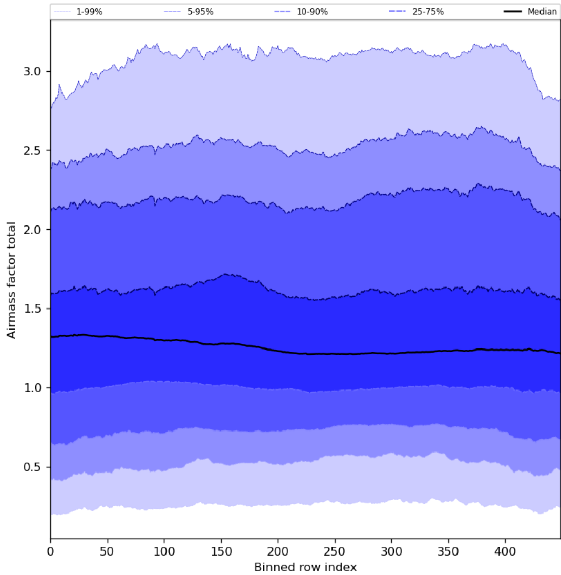
Figure 54: Along track statistics of “Airmass factor total” for 2024-08-14 to 2024-08-16
