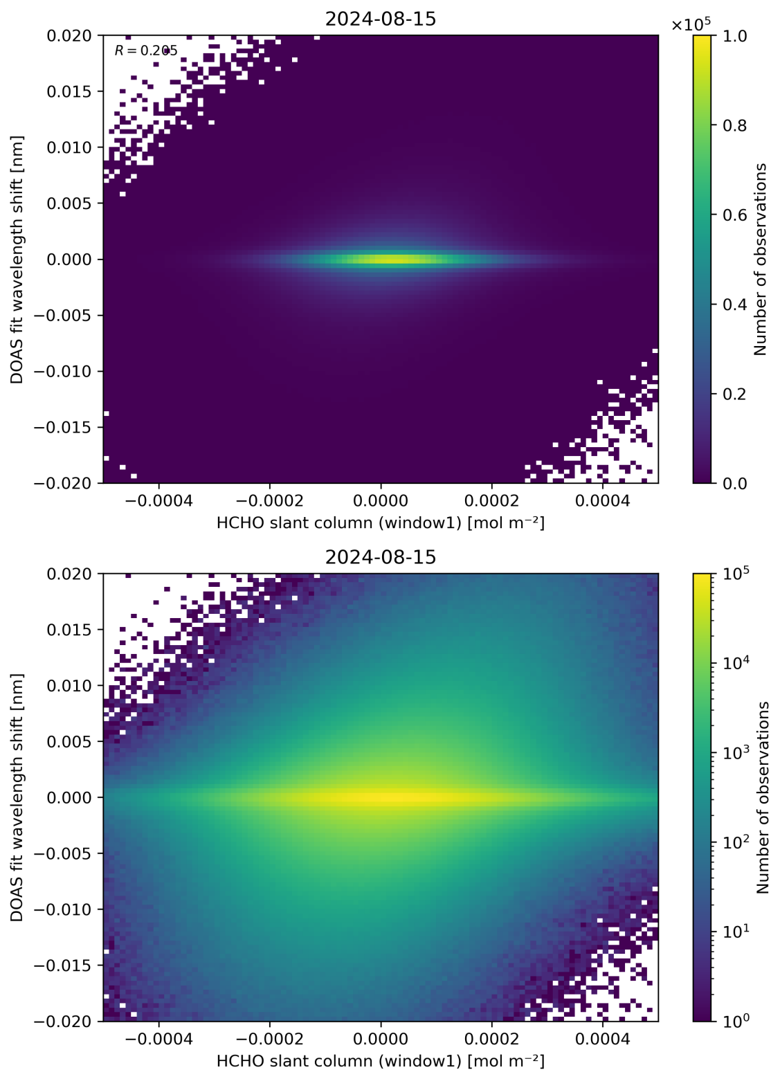
Figure 79: Scatter density plot of “HCHO slant column (window1)” against “DOAS fit wavelength shift” for 2024-08-14 to 2024-08-16.
