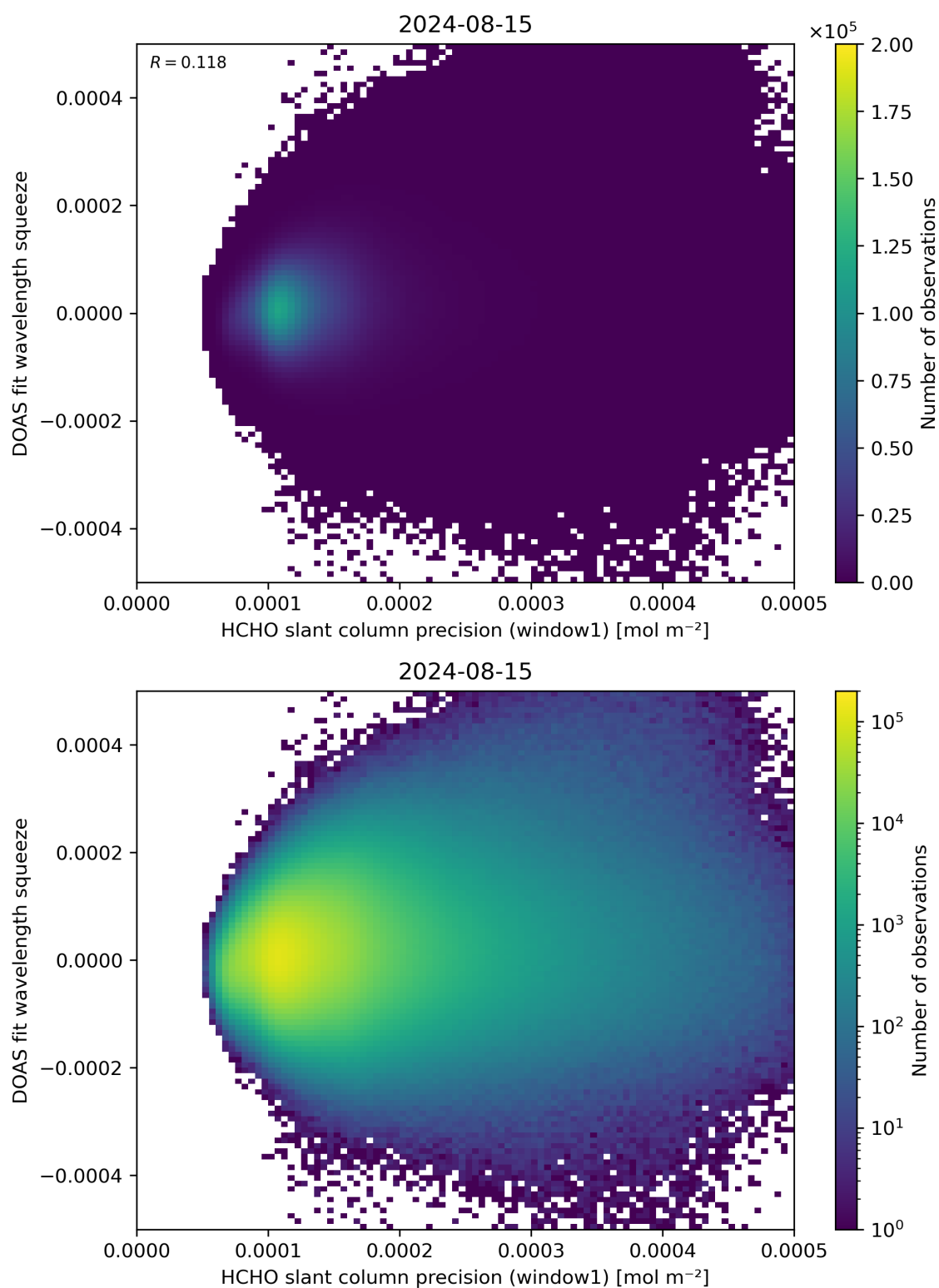
Figure 90: Scatter density plot of “HCHO slant column precision (window1)” against “DOAS fit wavelength squeeze” for 2024-08-14 to 2024-08-16.
