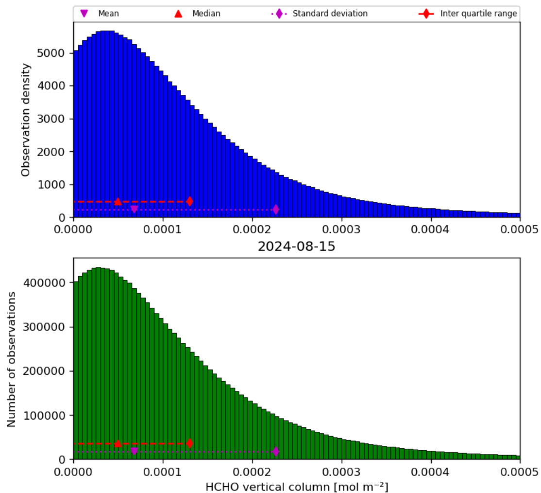
Figure 35: Histogram of “HCHO vertical column” for 2024-08-14 to 2024-08-16
