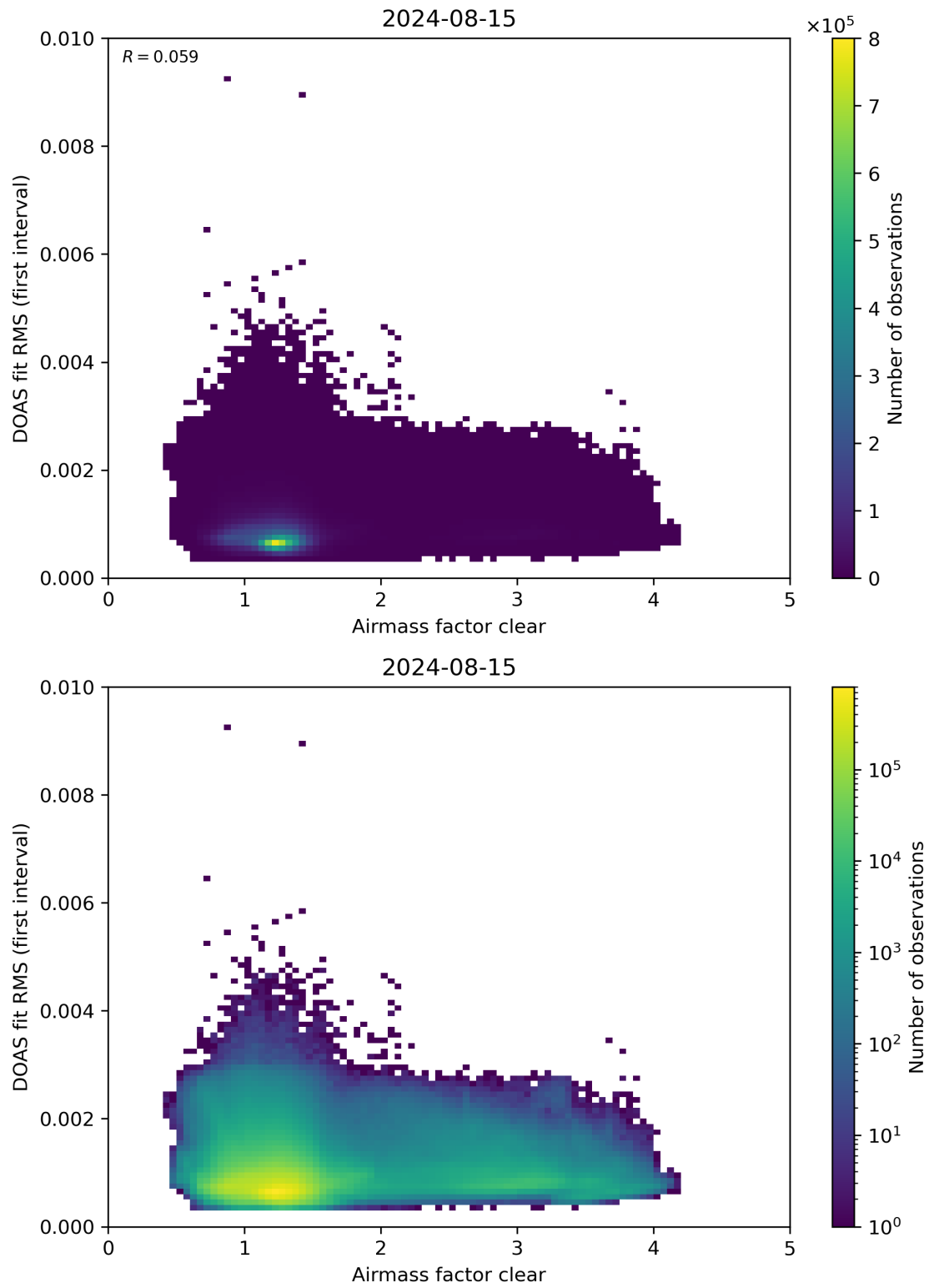
Figure 71: Scatter density plot of “Airmass factor clear” against “DOAS fit RMS (first interval)” for 2024-08-14 to 2024-08-16.
