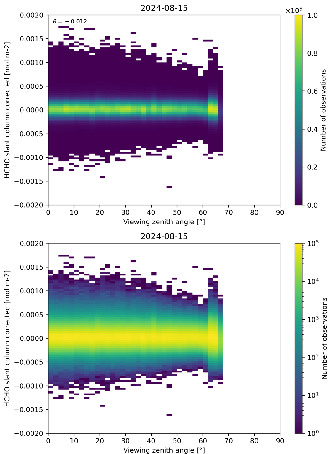
Figure 186: Scatter density plot of “Viewing zenith angle” against “HCHO slant column corrected” for 2024-08-14 to 2024-08-16.
