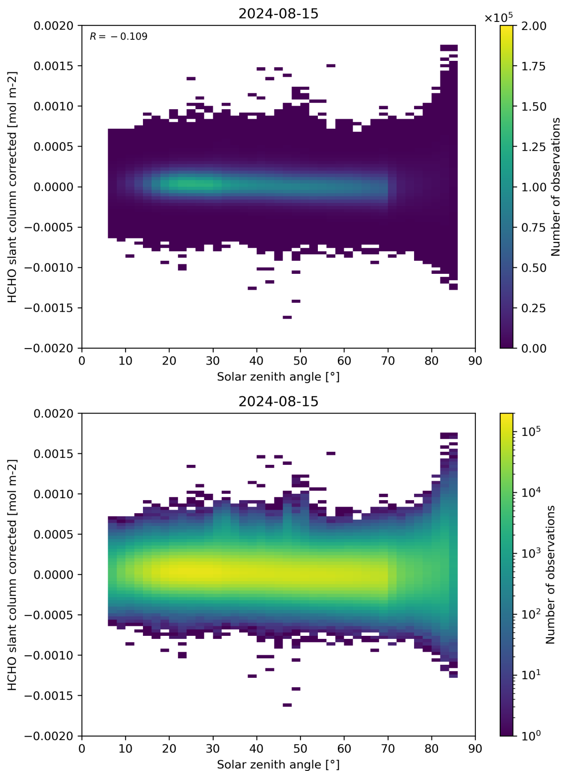
Figure 171: Scatter density plot of “Solar zenith angle” against “HCHO slant column corrected” for 2024-08-14 to 2024-08-16.
