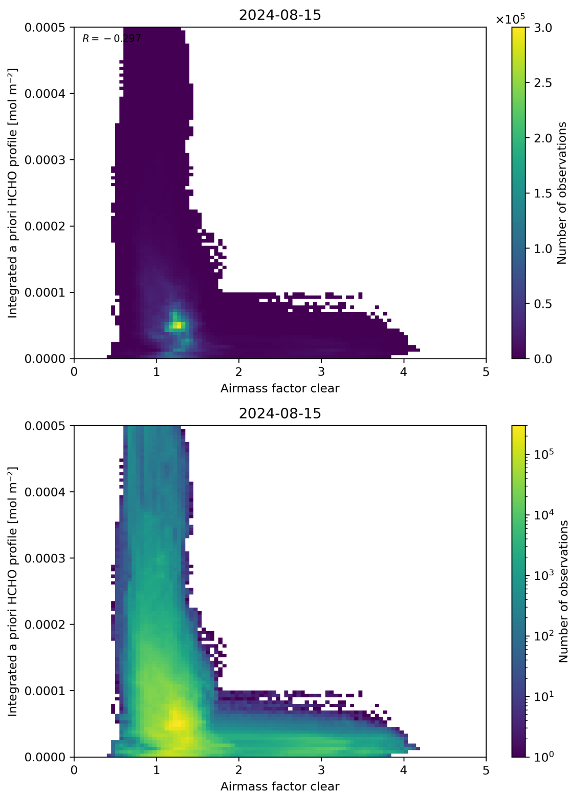
Figure 76: Scatter density plot of “Airmass factor clear” against “Integrated a priori HCHO profile” for 2024-08-14 to 2024-08-16.
