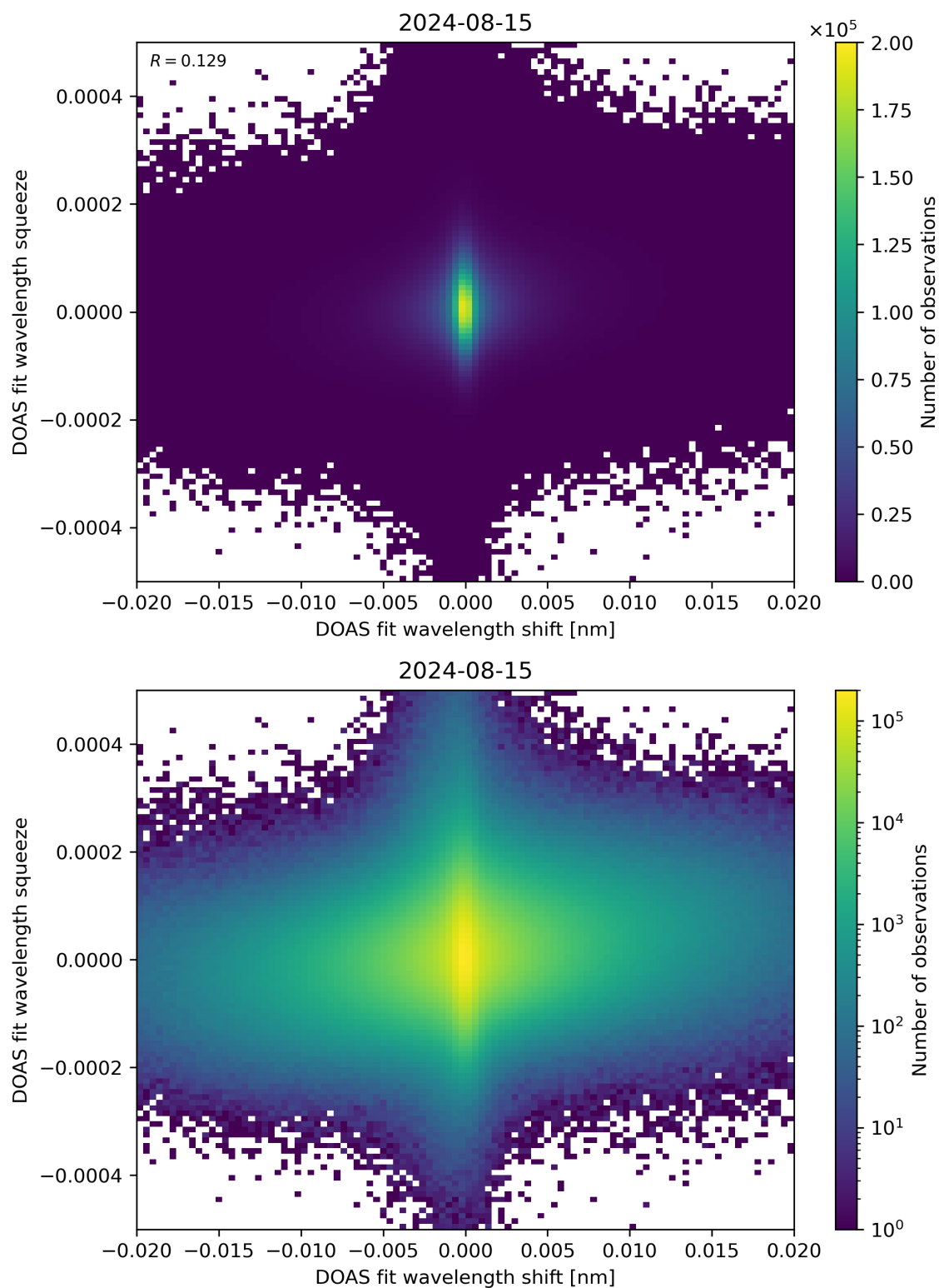
Figure 65: Scatter density plot of “DOAS fit wavelength shift” against “DOAS fit wavelength squeeze” for 2024-08-14 to 2024-08-16.
