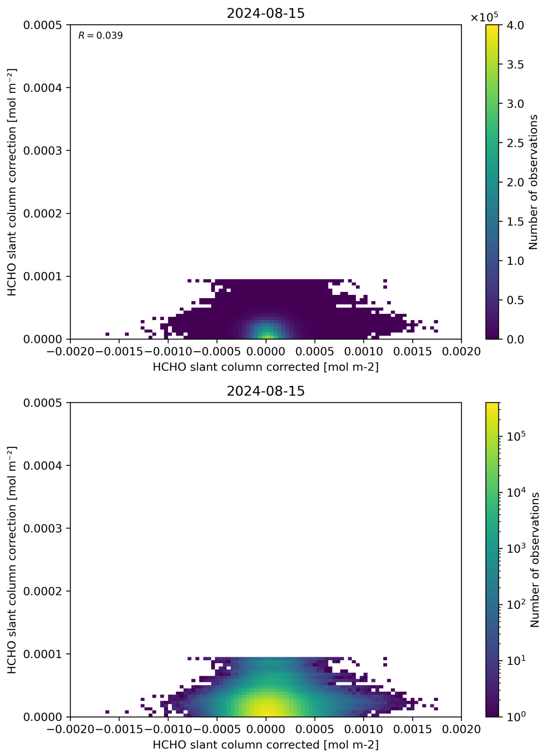
Figure 77: Scatter density plot of “HCHO slant column corrected” against “HCHO slant column correction” for 2024-08-14 to 2024-08-16.
