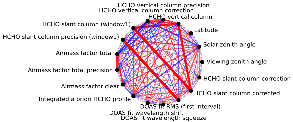
Figure 1: Map of correlation graph for 2024-08-14 to 2024-08-16.
