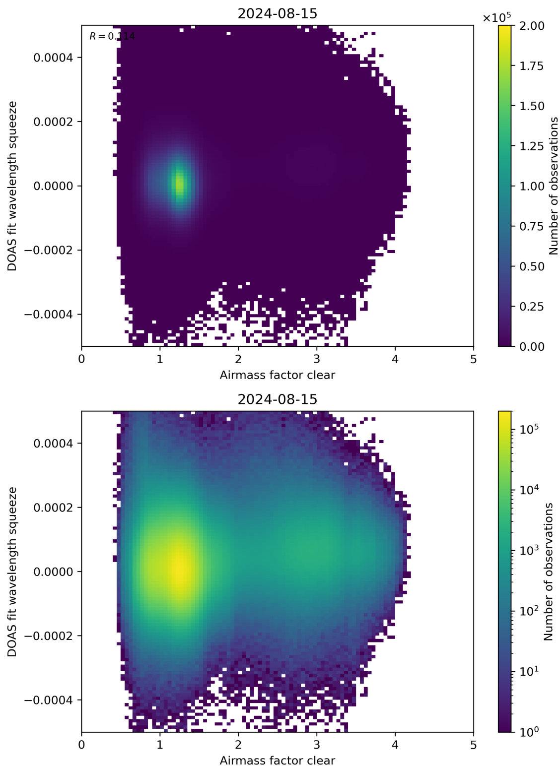
Figure 73: Scatter density plot of “Airmass factor clear” against “DOAS fit wavelength squeeze” for 2024-08-14 to 2024-08-16.
