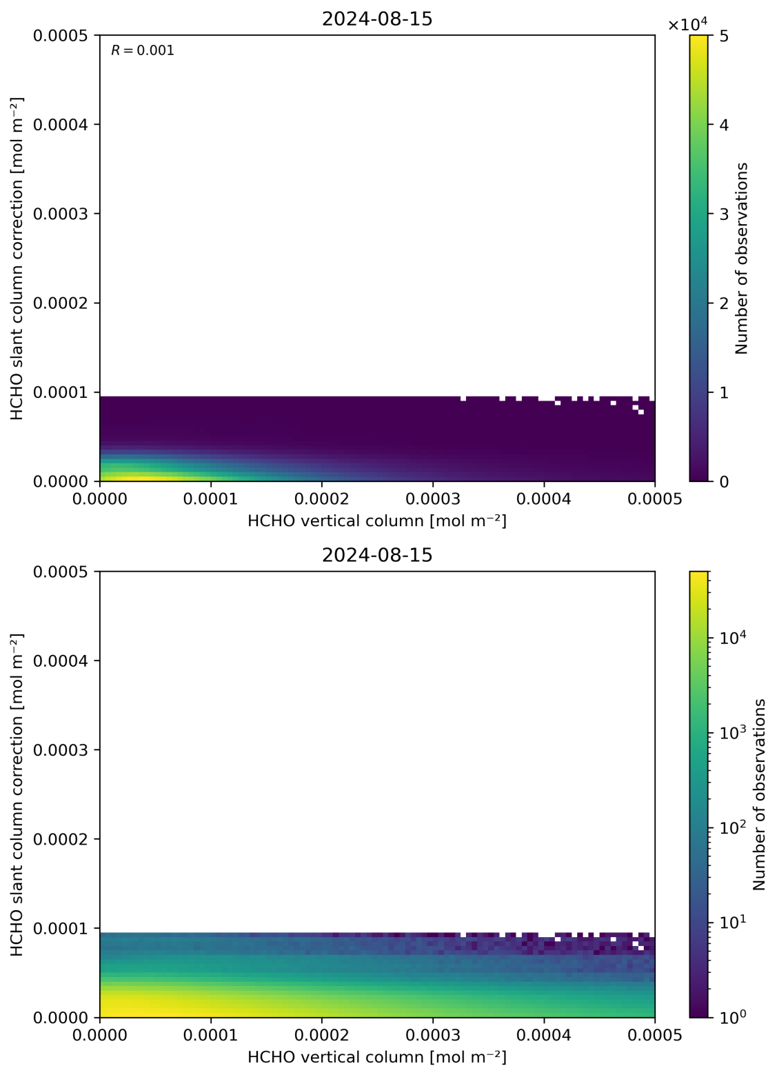
Figure 128: Scatter density plot of “HCHO vertical column” against “HCHO slant column correction” for 2024-08-14 to 2024-08-16.
