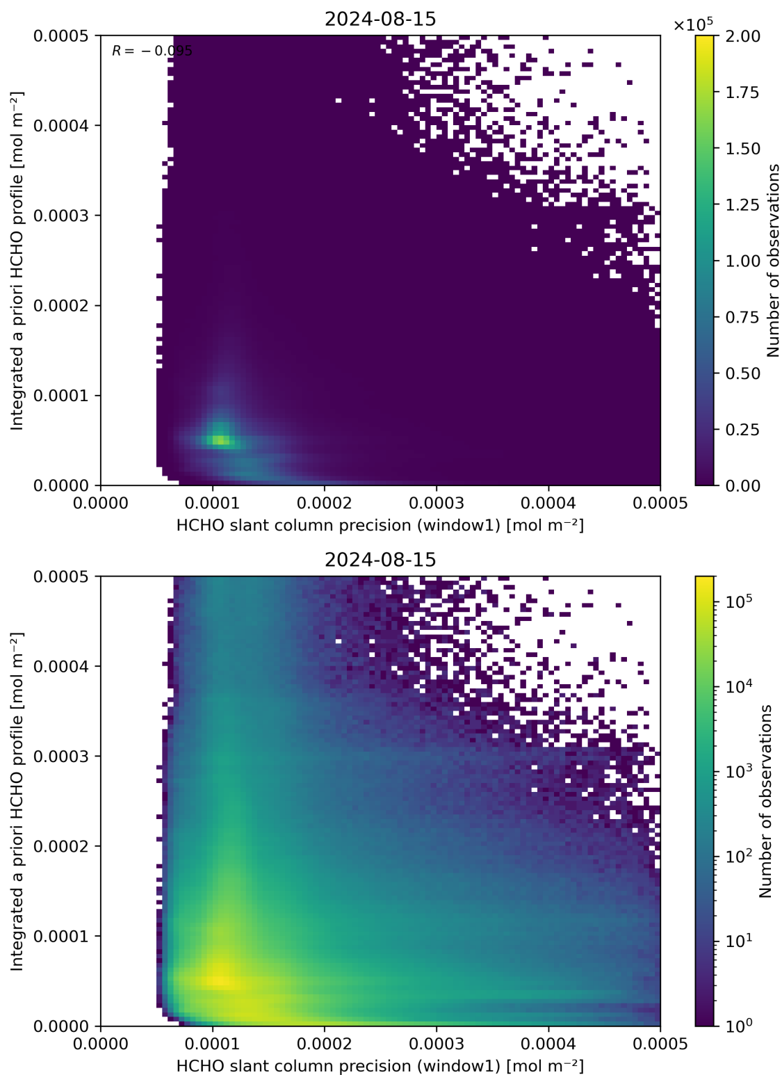
Figure 96: Scatter density plot of “HCHO slant column precision (window1)” against “Integrated a priori HCHO profile” for 2024-08-14 to 2024-08-16.
