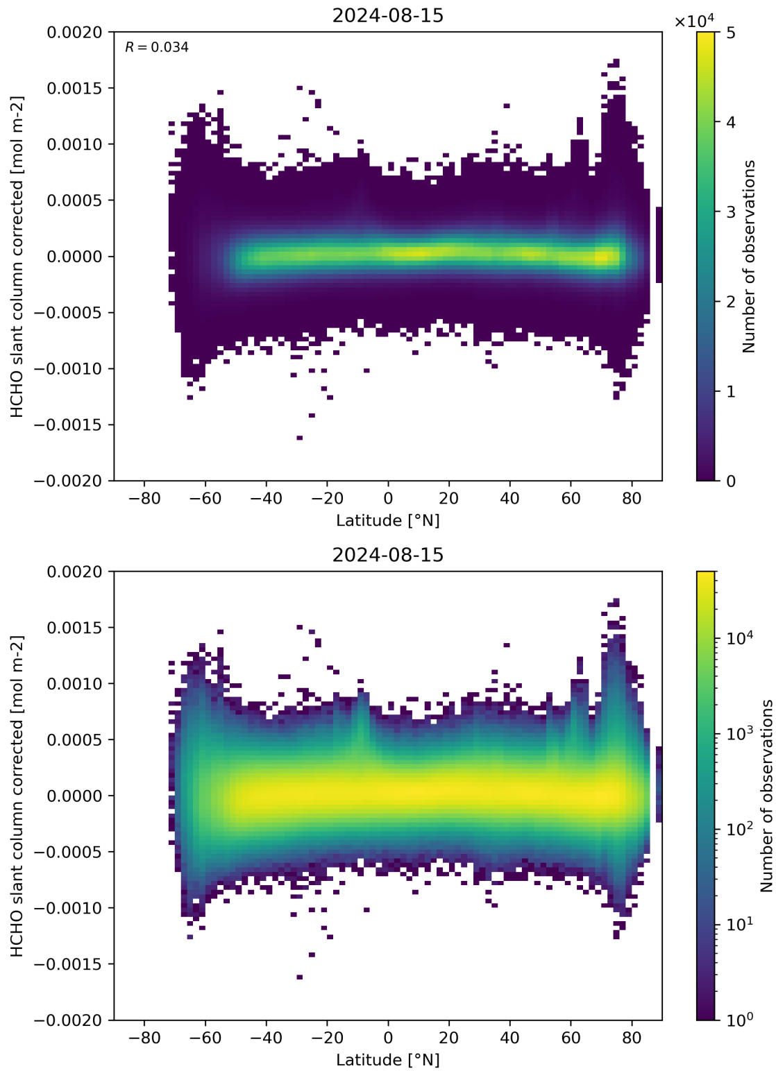
Figure 157: Scatter density plot of “Latitude” against “HCHO slant column corrected” for 2024-08-14 to 2024-08-16.
