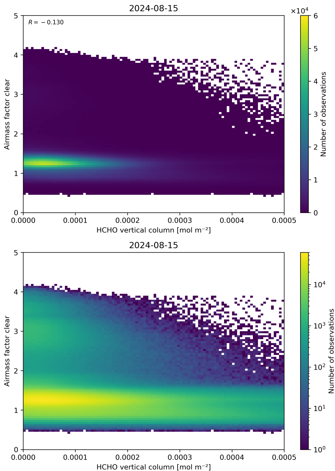
Figure 126: Scatter density plot of “HCHO vertical column” against “Airmass factor clear” for 2024-08-14 to 2024-08-16.
