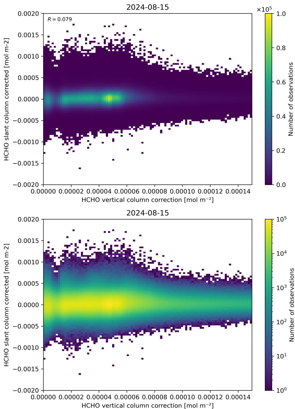
Figure 116: Scatter density plot of “HCHO vertical column correction” against “HCHO slant column corrected” for 2024-08-14 to 2024-08-16.
