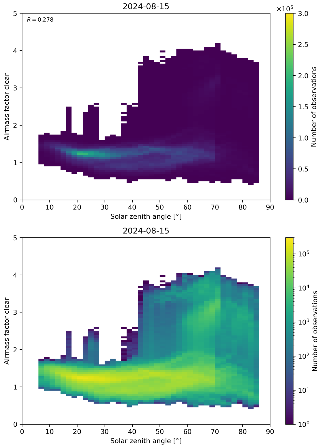
Figure 170: Scatter density plot of “Solar zenith angle” against “Airmass factor clear” for 2024-08-14 to 2024-08-16.
