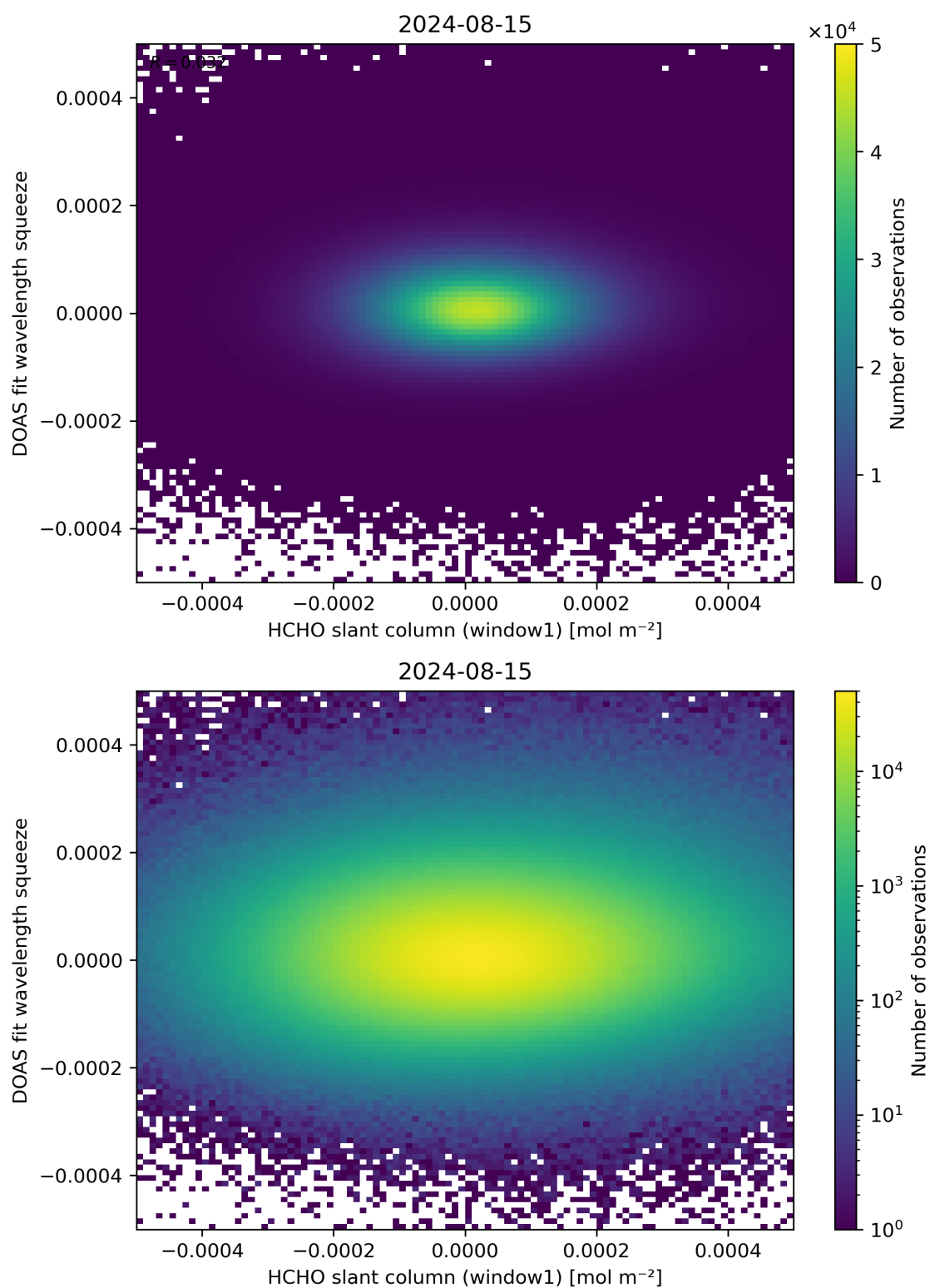
Figure 80: Scatter density plot of “HCHO slant column (window1)” against “DOAS fit wavelength squeeze” for 2024-08-14 to 2024-08-16.
