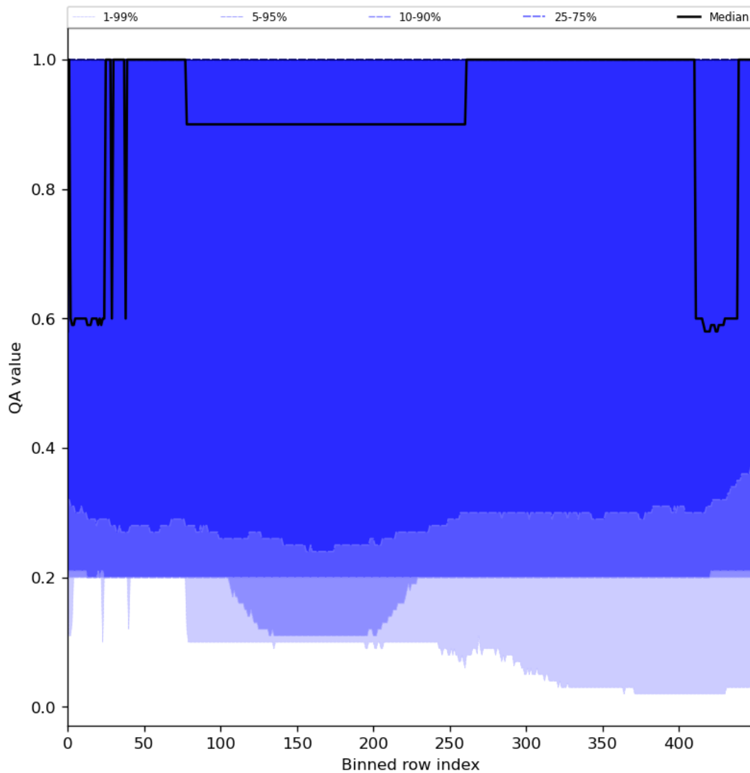
Figure 48: Along track statistics of “QA value” for 2024-08-14 to 2024-08-16
