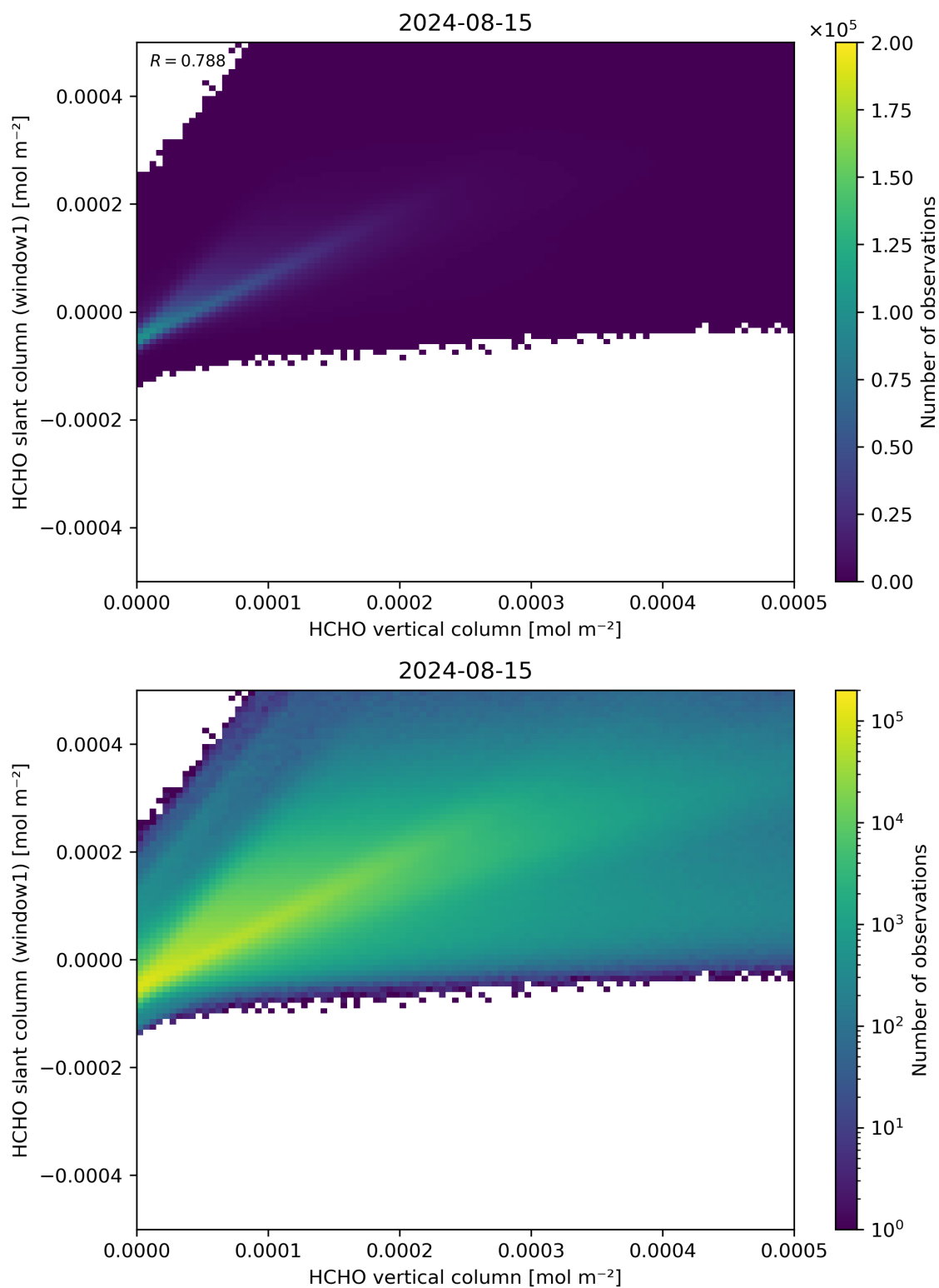
Figure 129: Scatter density plot of “HCHO vertical column” against “HCHO slant column (window1)” for 2024-08-14 to 2024-08-16.
