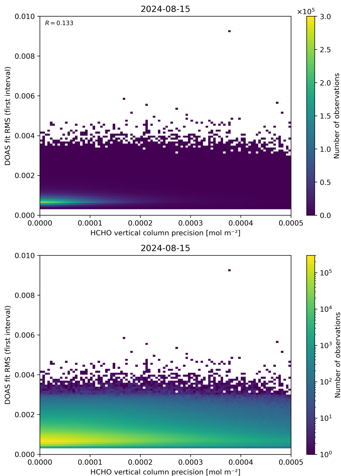
Figure 136: Scatter density plot of “HCHO vertical column precision” against “DOAS fit RMS (first interval)” for 2024-08-14 to 2024-08-16.
