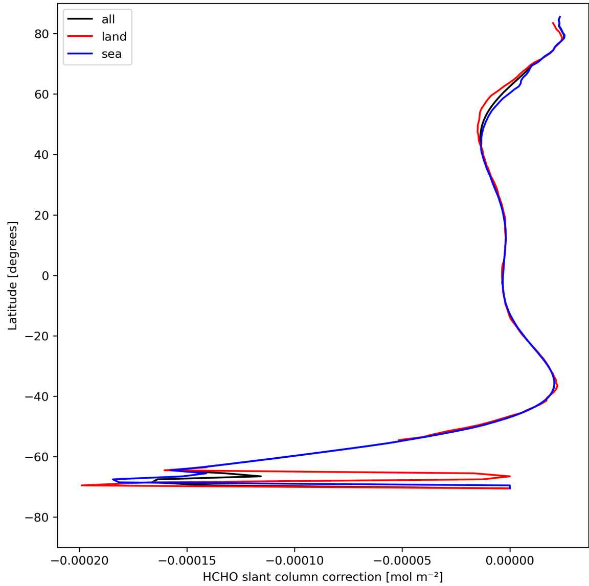
Figure 33: Zonal average of “HCHO slant column correction” for 2024-08-14 to 2024-08-16.
