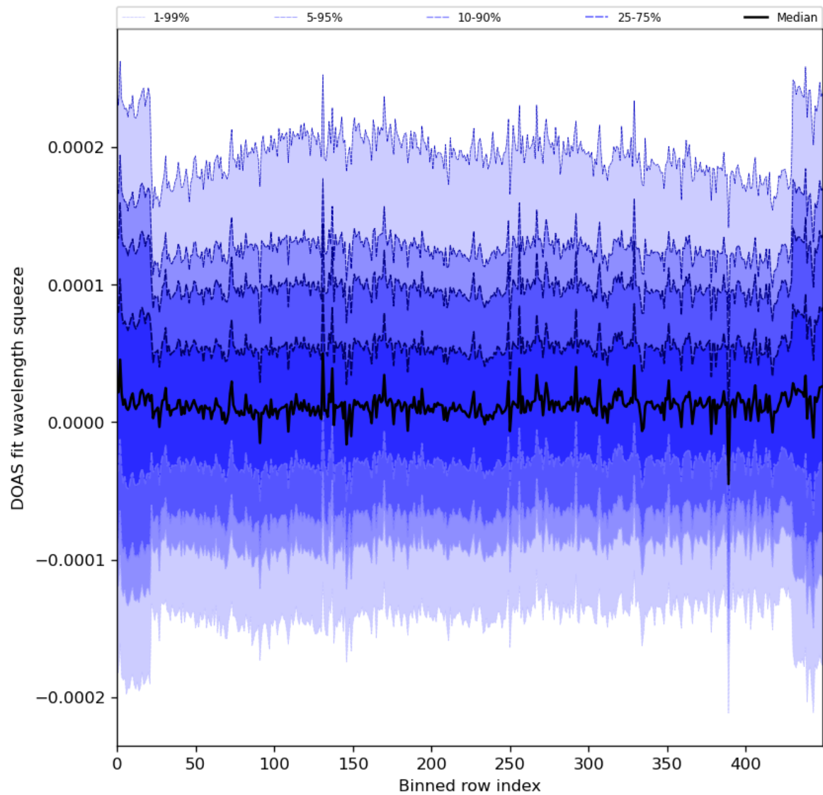
Figure 59: Along track statistics of “DOAS fit wavelength squeeze” for 2024-08-14 to 2024-08-16
