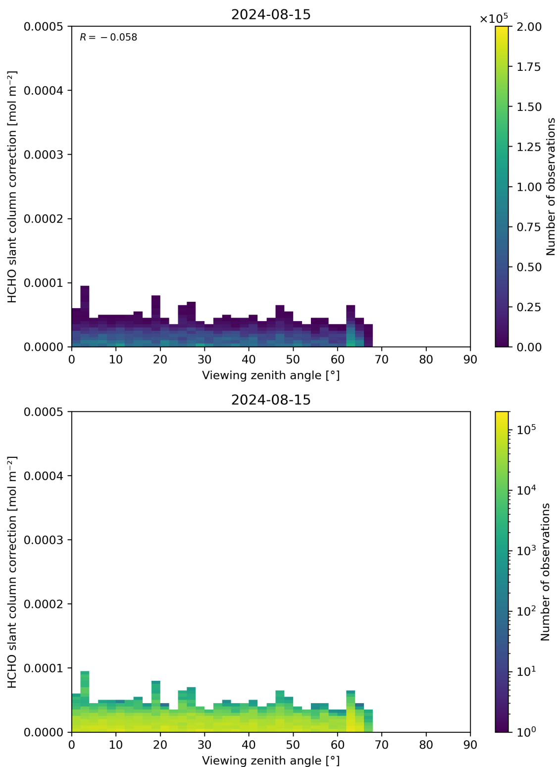
Figure 187: Scatter density plot of “Viewing zenith angle” against “HCHO slant column correction” for 2024-08-14 to 2024-08-16.
