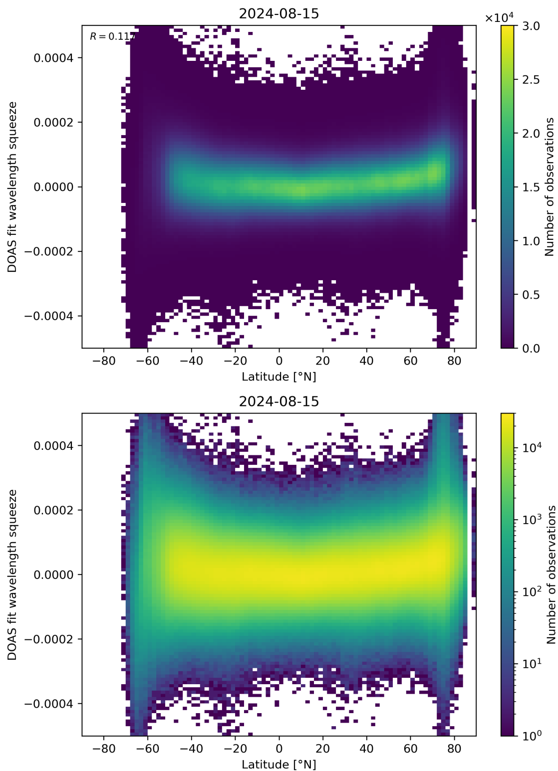
Figure 155: Scatter density plot of “Latitude” against “DOAS fit wavelength squeeze” for 2024-08-14 to 2024-08-16.
