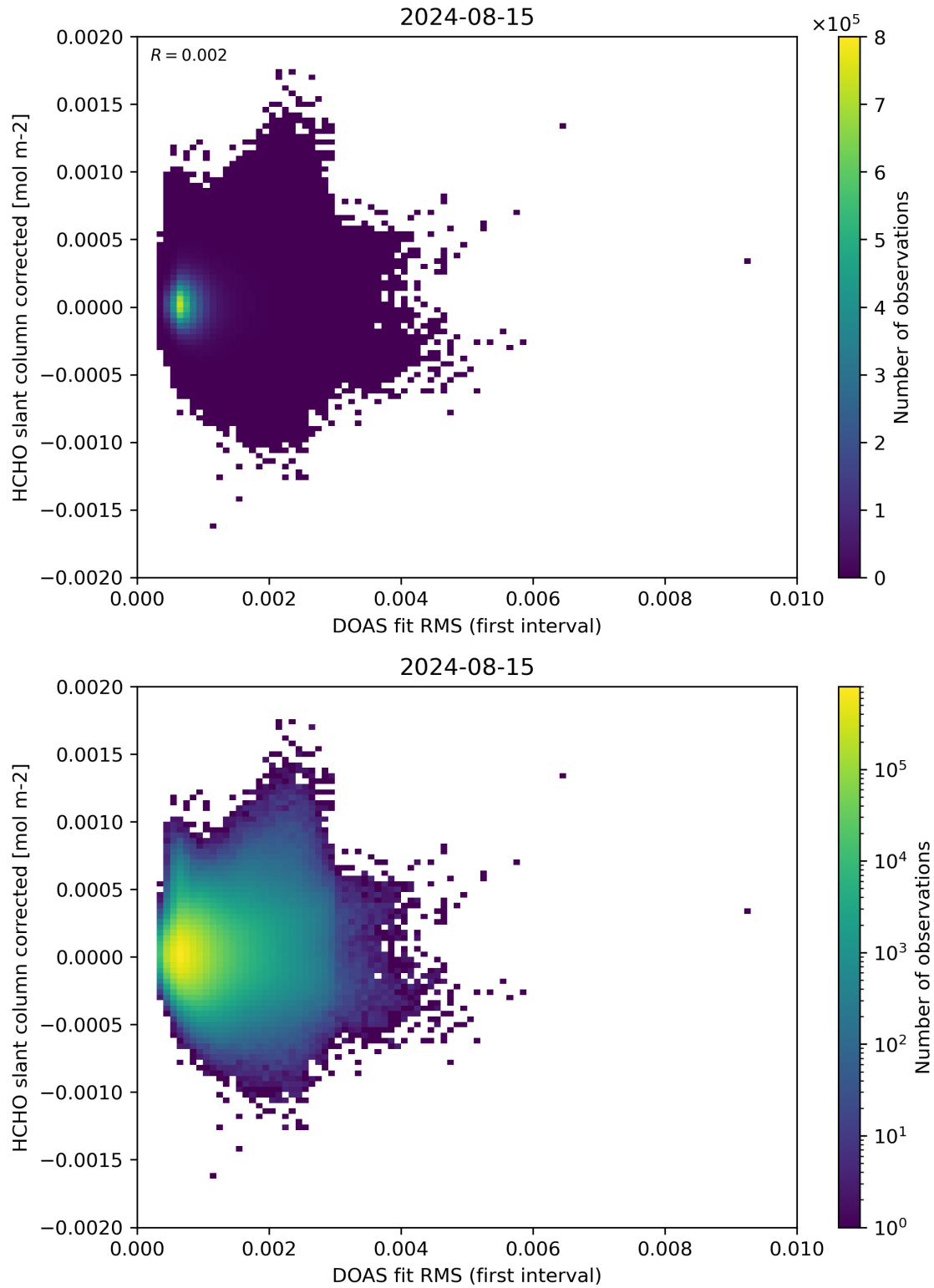
Figure 62: Scatter density plot of “DOAS fit RMS (first interval)” against “HCHO slant column corrected” for 2024-08-14 to 2024-08-16.
