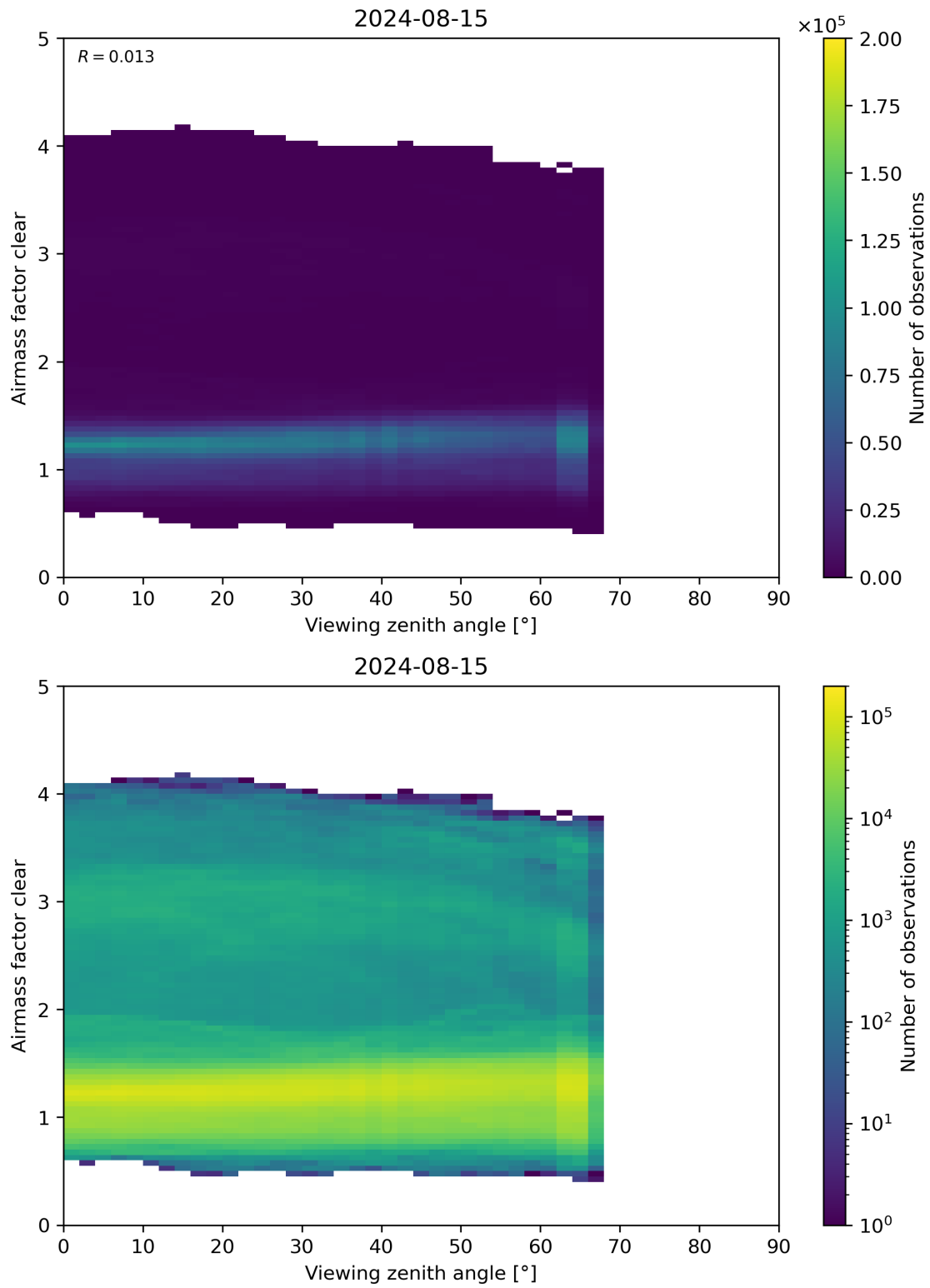
Figure 185: Scatter density plot of “Viewing zenith angle” against “Airmass factor clear” for 2024-08-14 to 2024-08-16.
