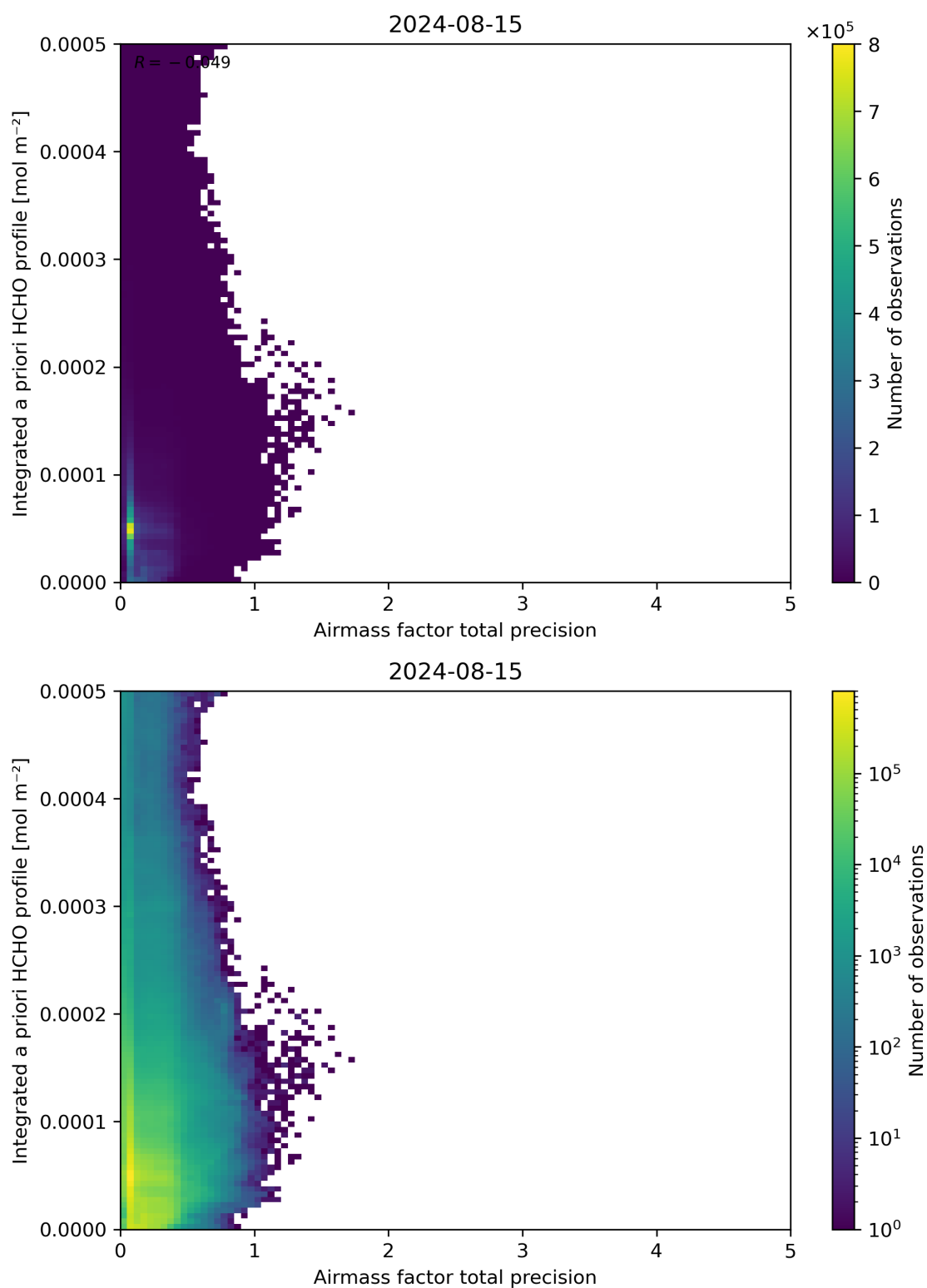
Figure 111: Scatter density plot of “Airmass factor total precision” against “Integrated a priori HCHO profile” for 2024-08-14 to 2024-08-16.
