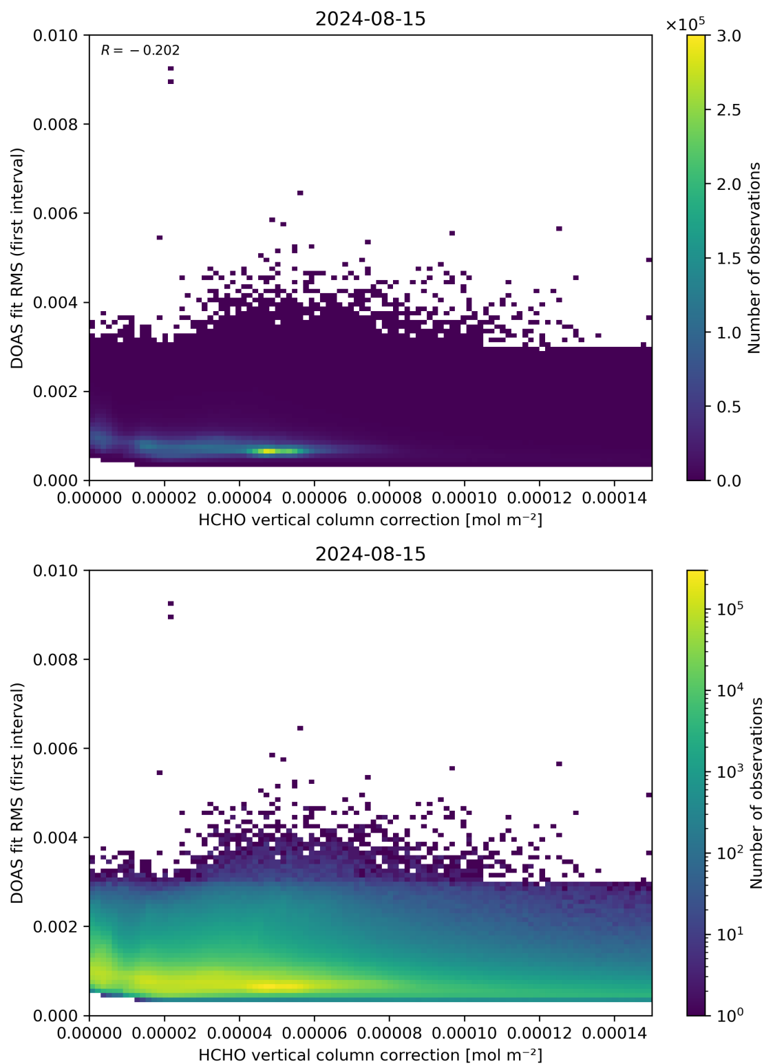
Figure 112: Scatter density plot of “HCHO vertical column correction” against “DOAS fit RMS (first interval)” for 2024-08-14 to 2024-08-16.
