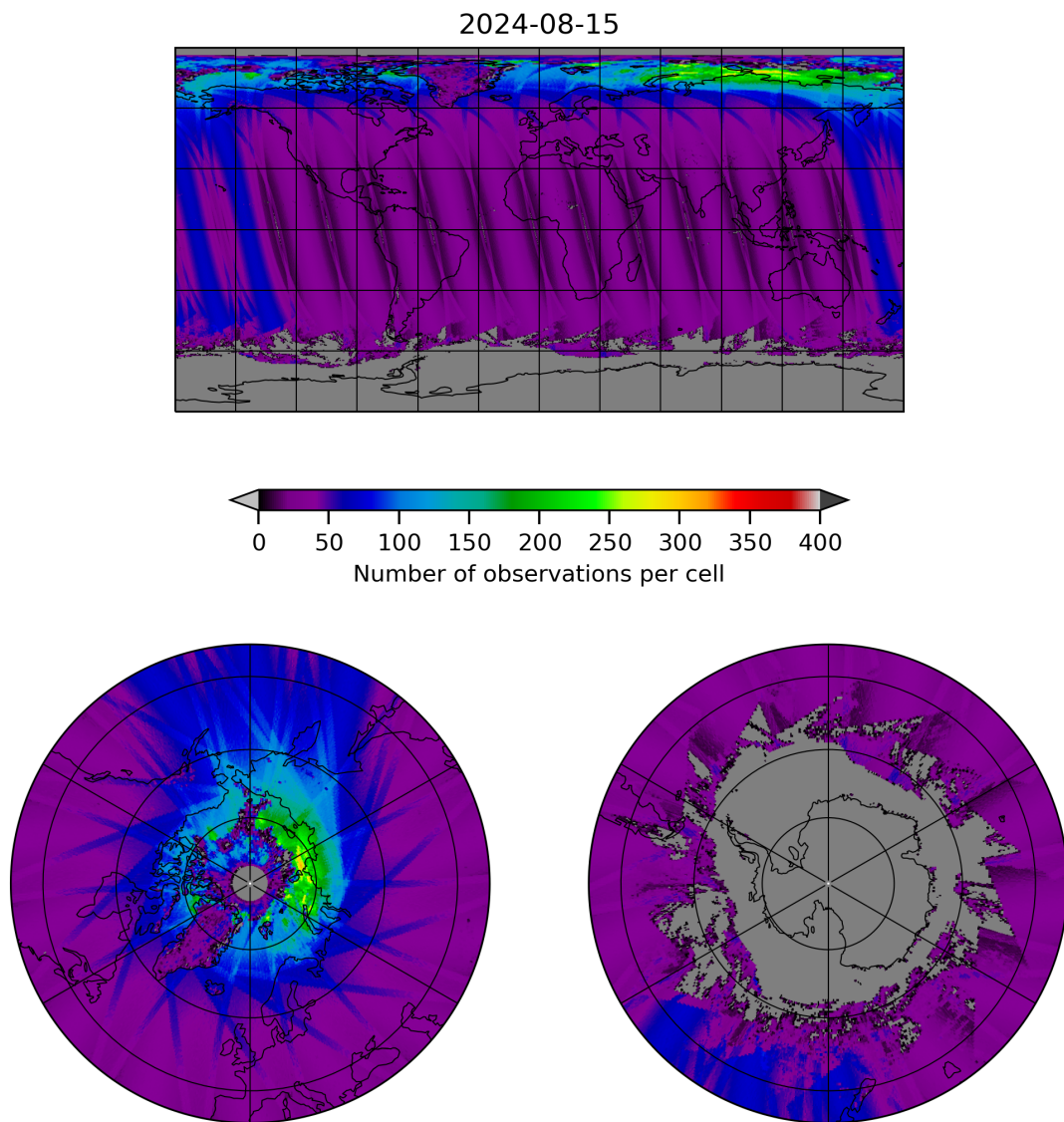
Figure 19: Map of the number of observations for 2024-08-14 to 2024-08-16
