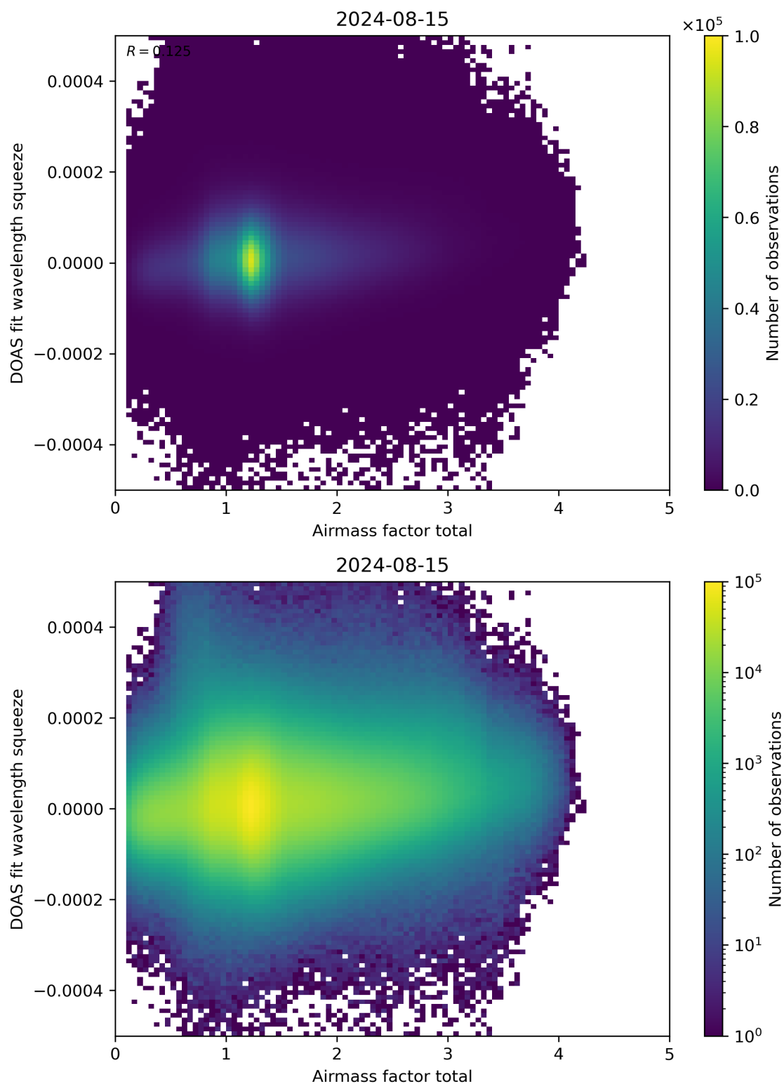
Figure 99: Scatter density plot of “Airmass factor total” against “DOAS fit wavelength squeeze” for 2024-08-14 to 2024-08-16.
