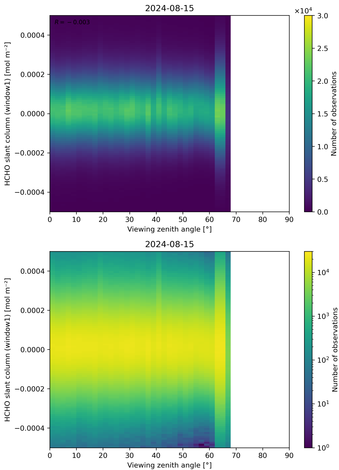
Figure 188: Scatter density plot of “Viewing zenith angle” against “HCHO slant column (window1)” for 2024-08-14 to 2024-08-16.
