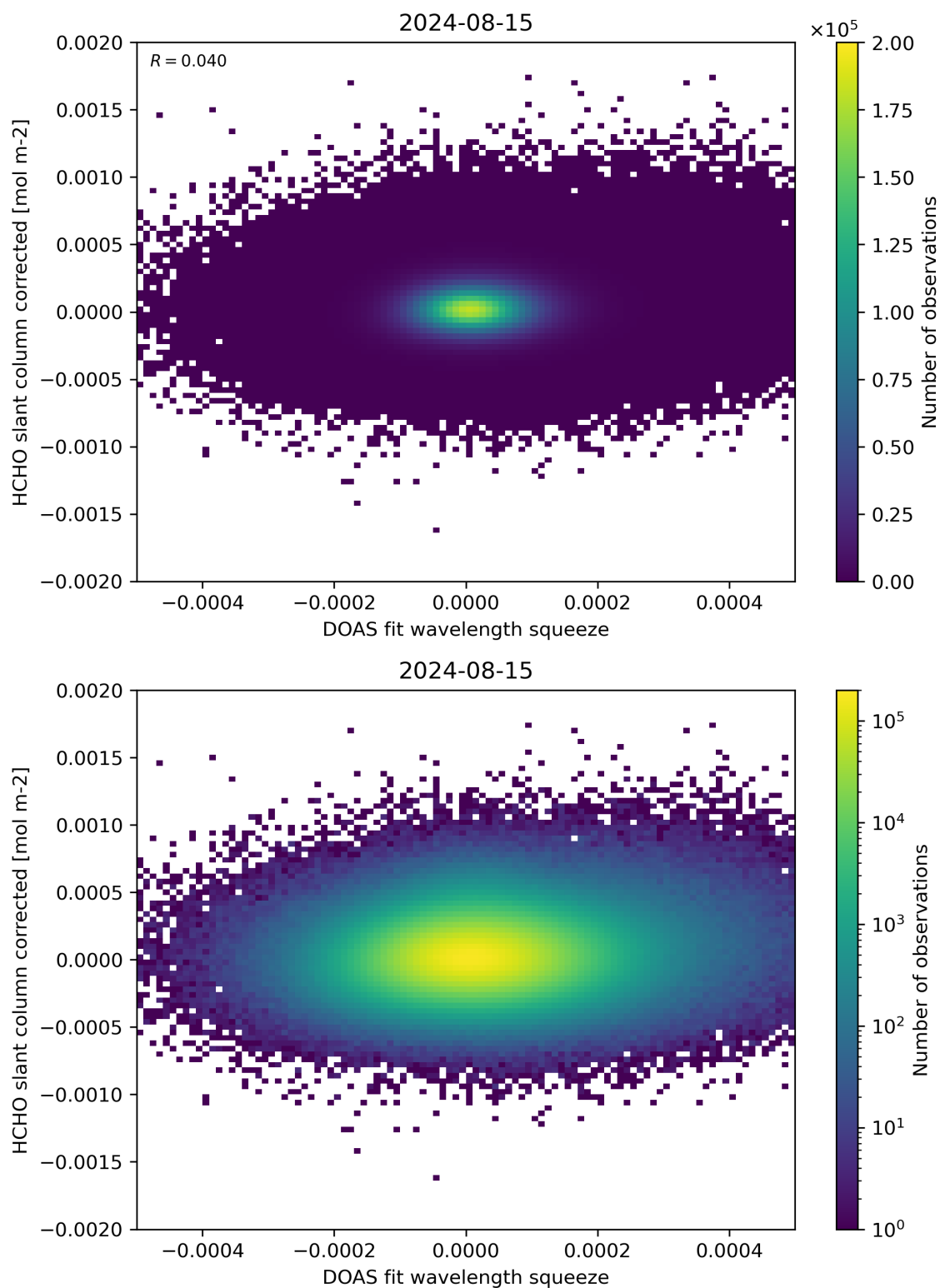
Figure 69: Scatter density plot of “DOAS fit wavelength squeeze” against “HCHO slant column corrected” for 2024-08-14 to 2024-08-16.
