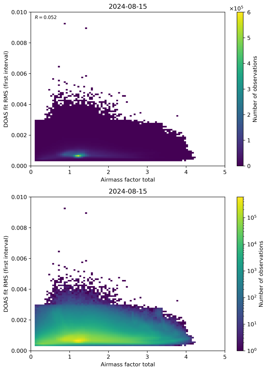
Figure 97: Scatter density plot of “Airmass factor total” against “DOAS fit RMS (first interval)” for 2024-08-14 to 2024-08-16.
