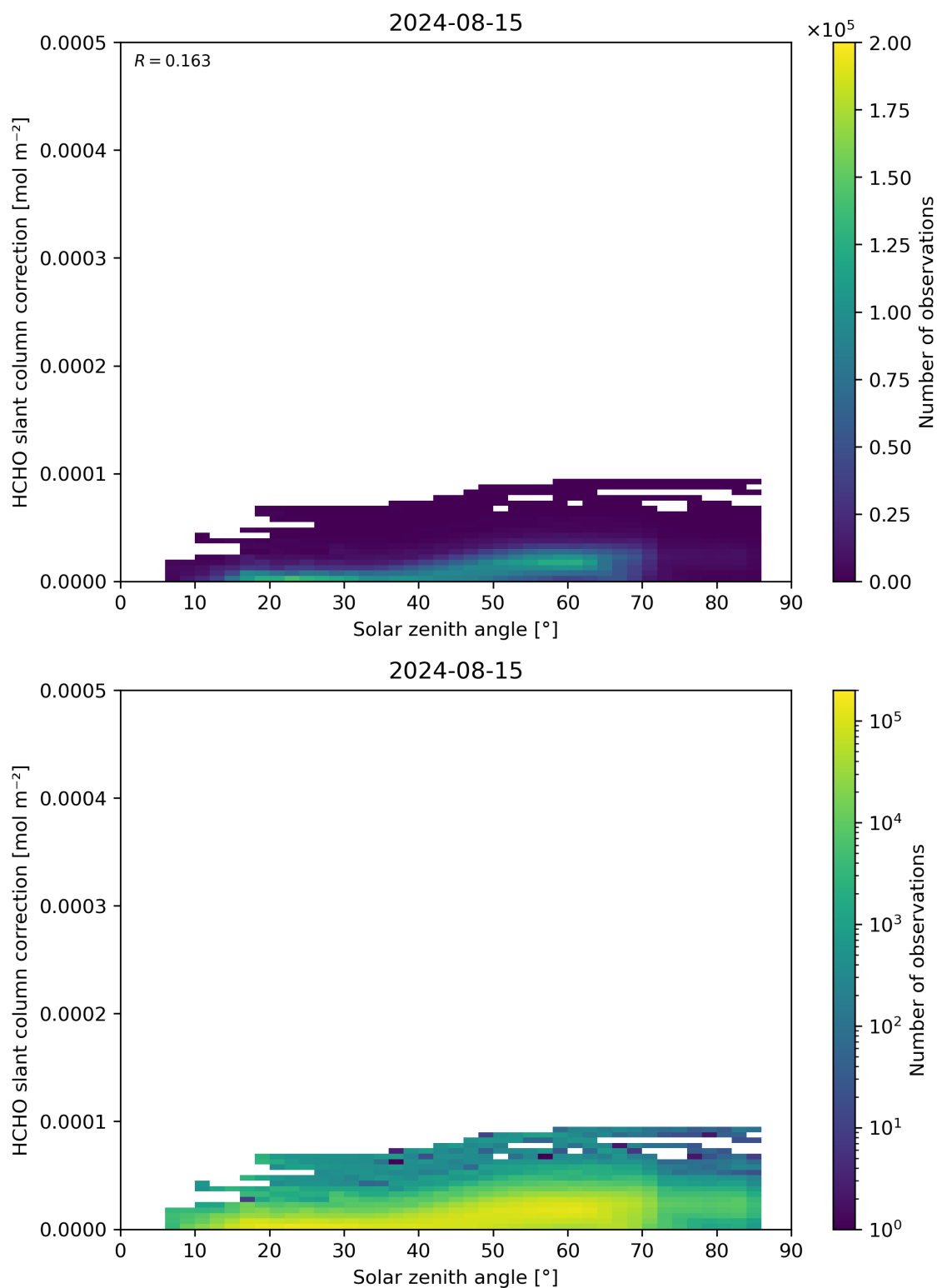
Figure 172: Scatter density plot of “Solar zenith angle” against “HCHO slant column correction” for 2024-08-14 to 2024-08-16.
