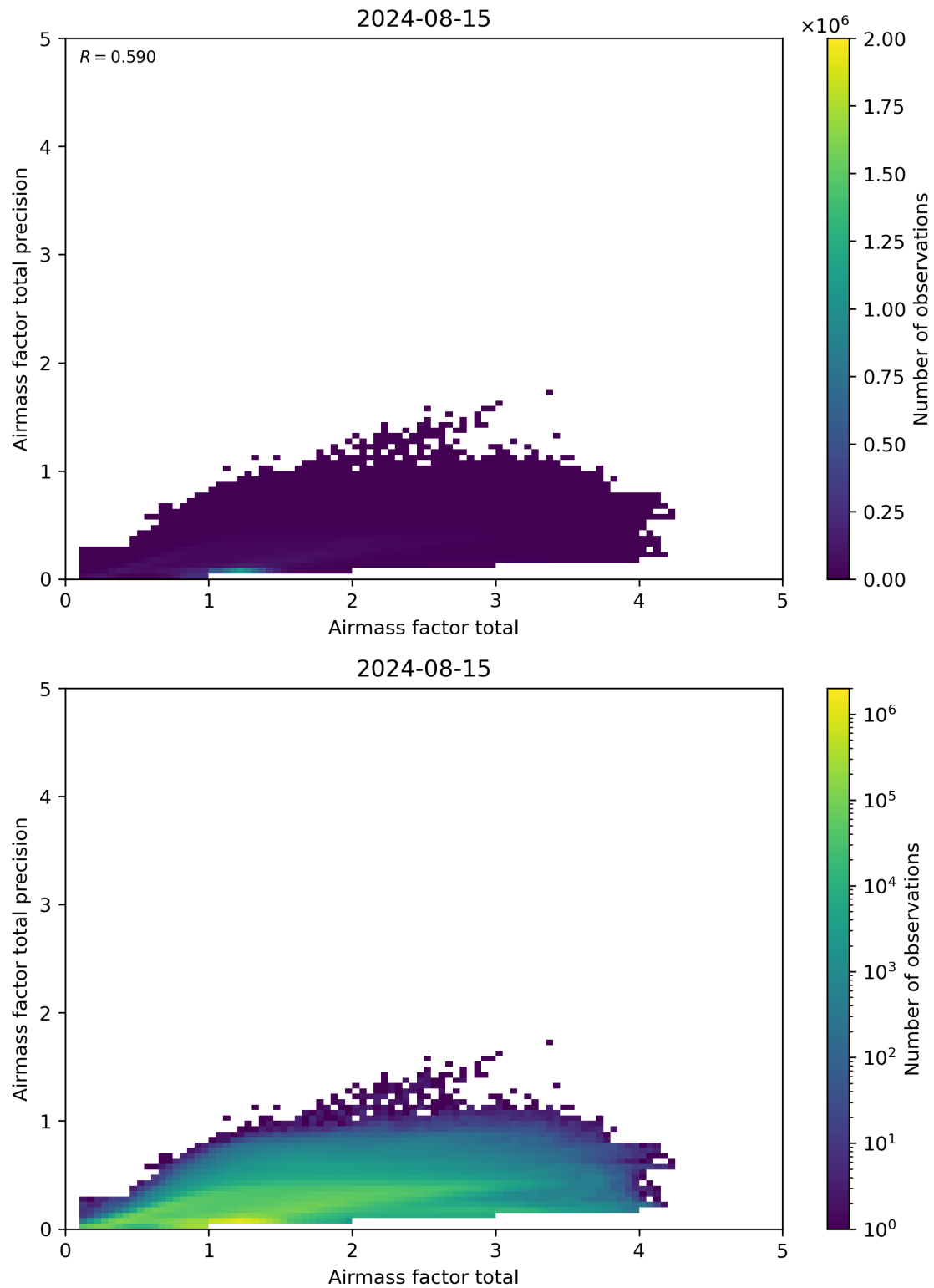
Figure 103: Scatter density plot of “Airmass factor total” against “Airmass factor total precision” for 2024-08-14 to 2024-08-16.
