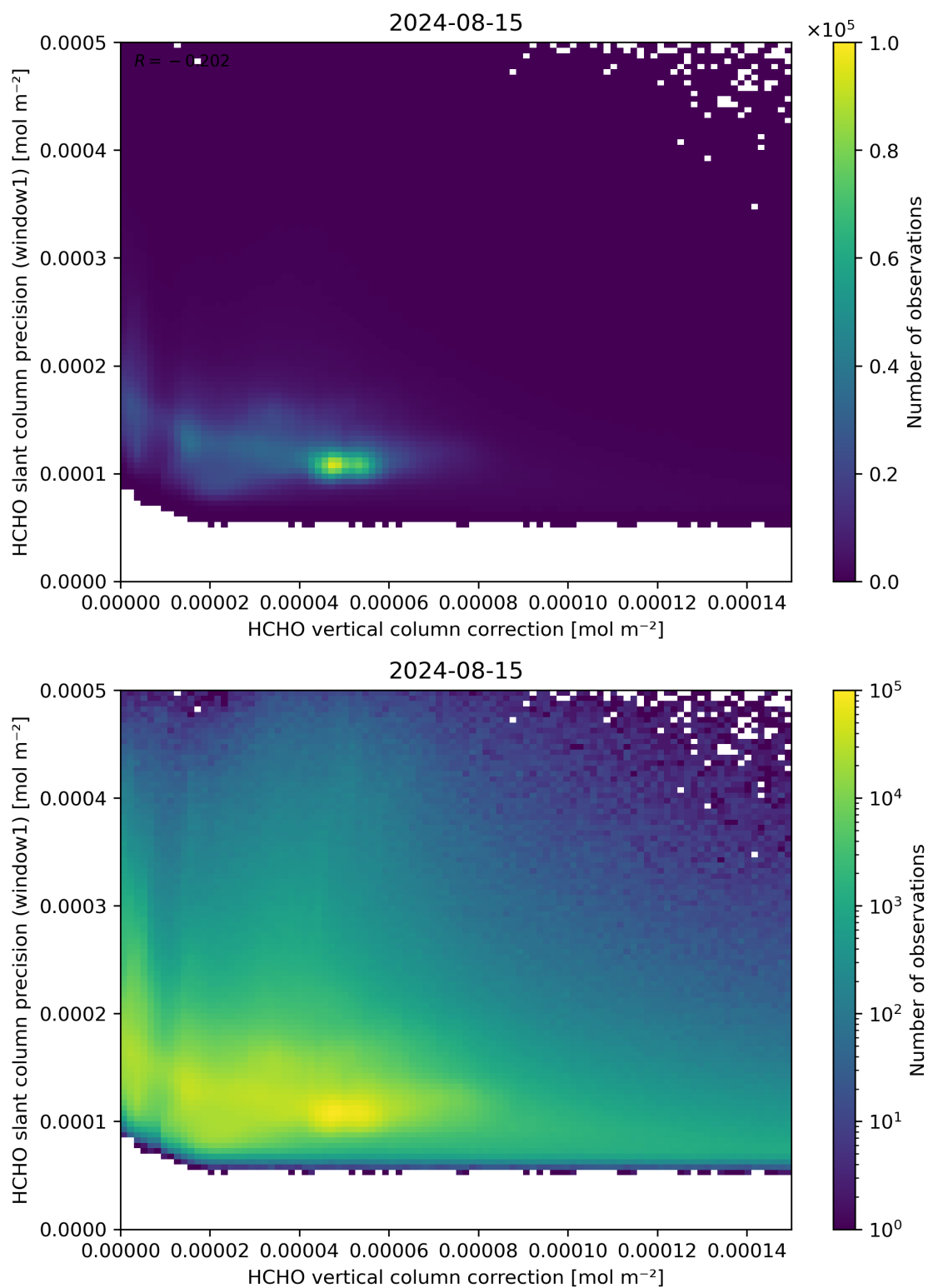
Figure 119: Scatter density plot of “HCHO vertical column correction” against “HCHO slant column precision (window1)” for 2024-08-14 to 2024-08-16.
