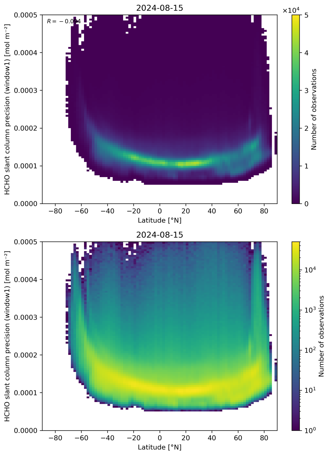
Figure 160: Scatter density plot of “Latitude” against “HCHO slant column precision (window1)” for 2024-08-14 to 2024-08-16.
