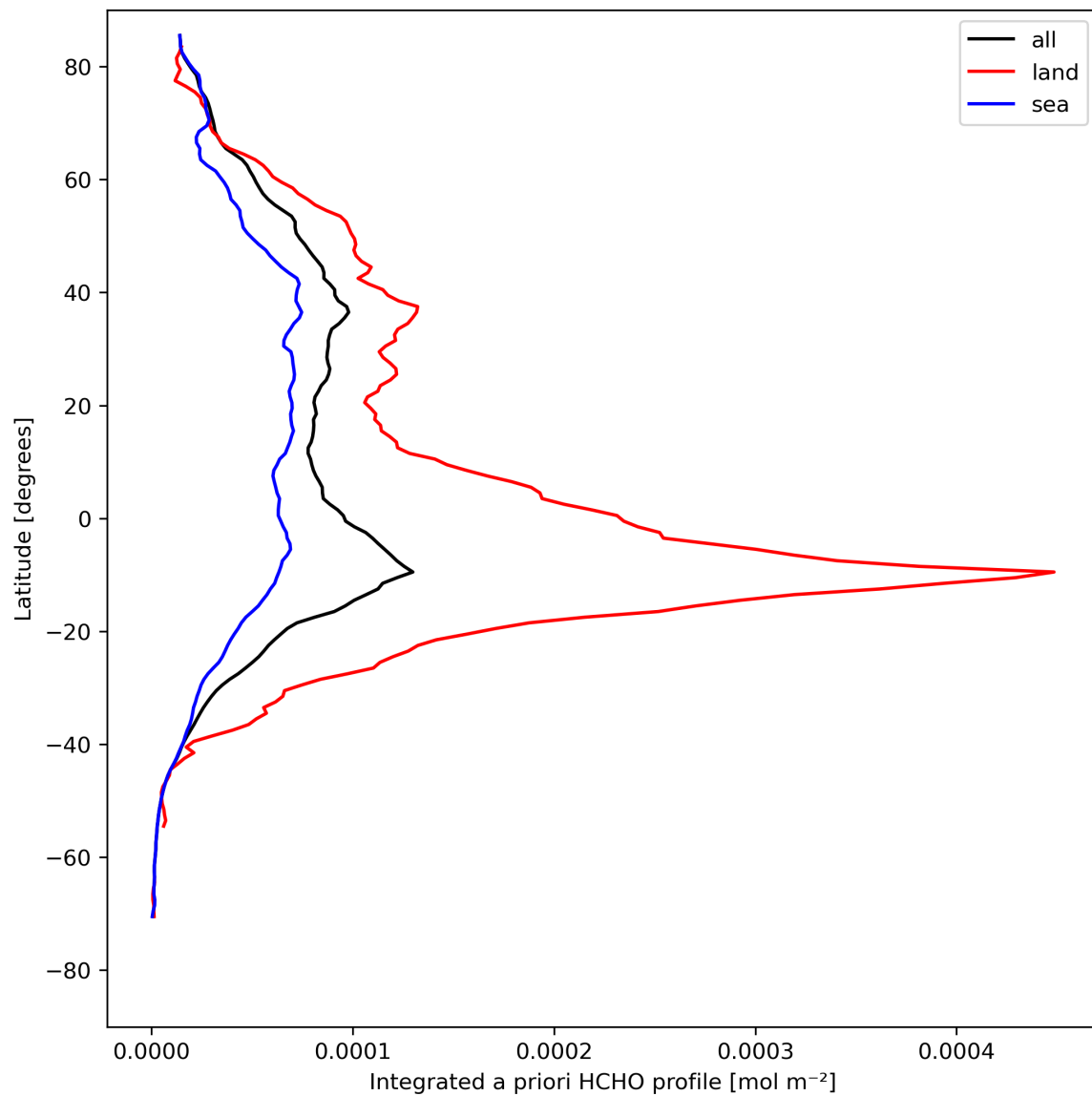
Figure 29: Zonal average of “Integrated a priori HCHO profile” for 2024-08-14 to 2024-08-16.
