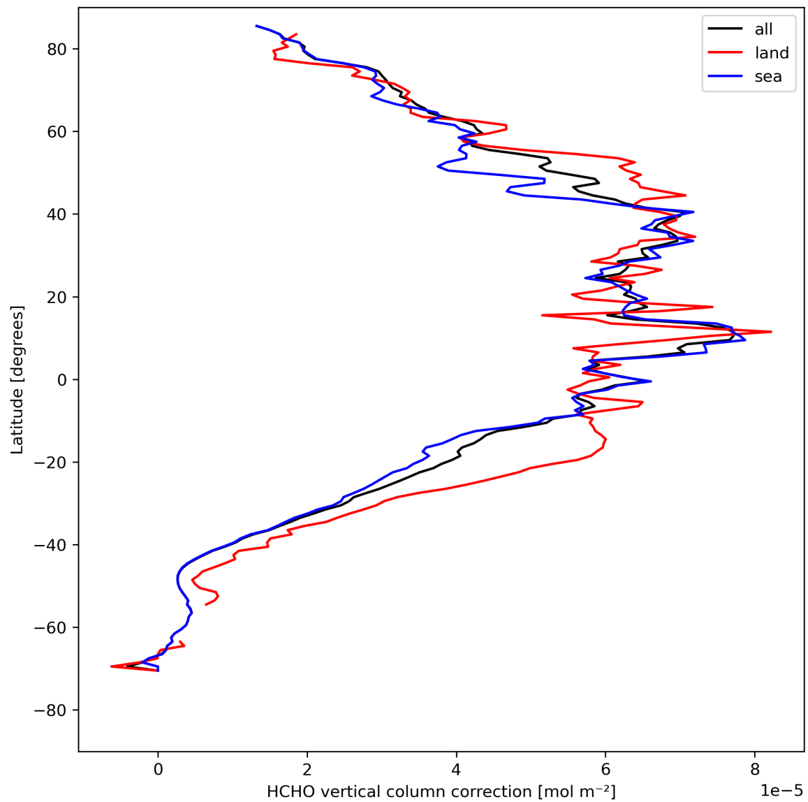
Figure 23: Zonal average of “HCHO vertical column correction” for 2024-08-14 to 2024-08-16.
