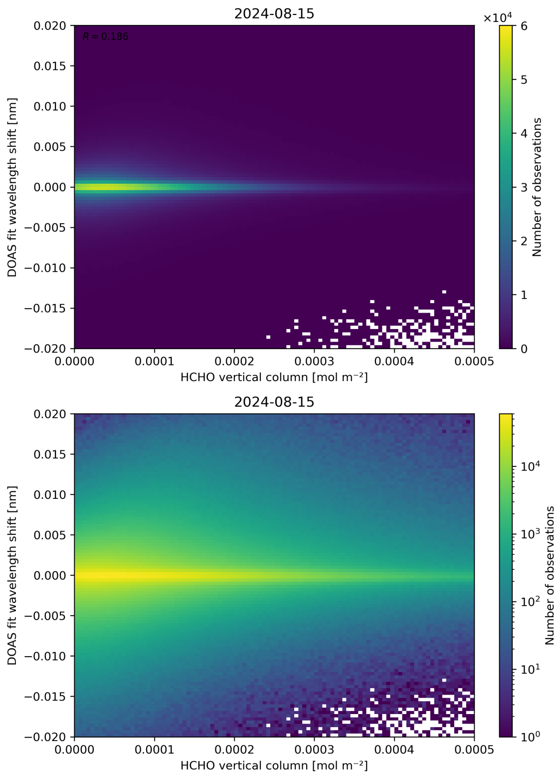
Figure 124: Scatter density plot of “HCHO vertical column” against “DOAS fit wavelength shift” for 2024-08-14 to 2024-08-16.
