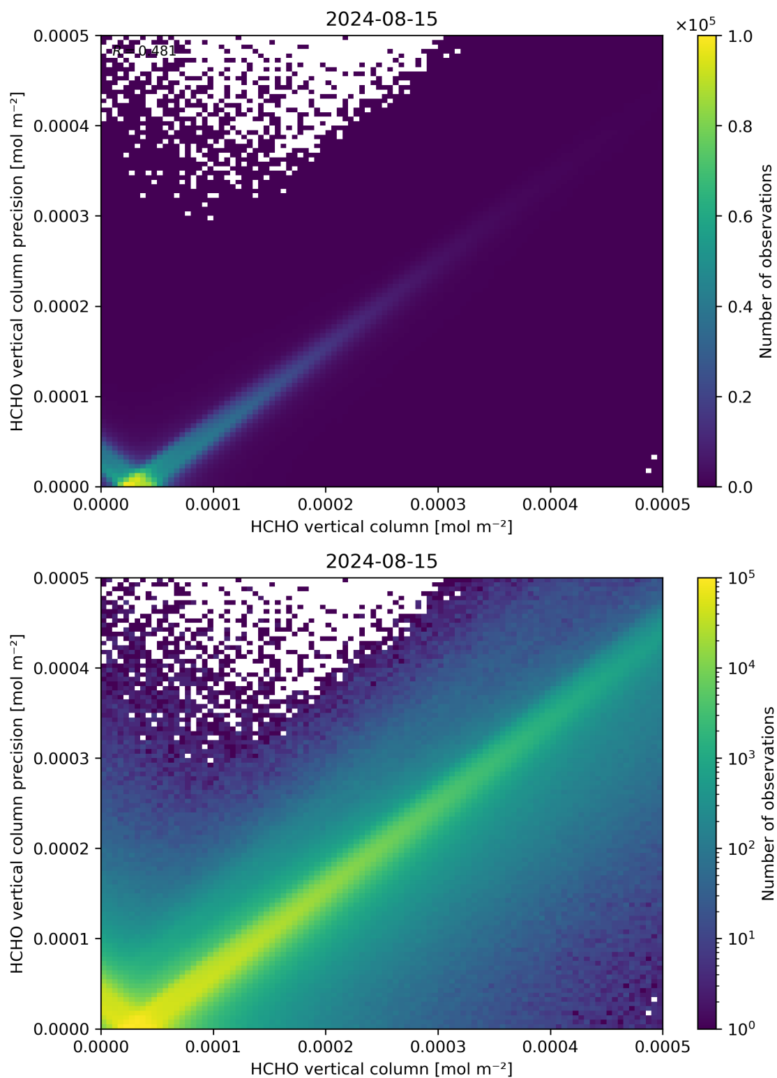
Figure 134: Scatter density plot of “HCHO vertical column” against “HCHO vertical column precision” for 2024-08-14 to 2024-08-16.
