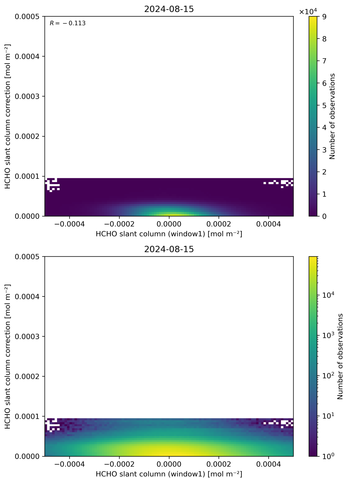
Figure 83: Scatter density plot of “HCHO slant column (window1)” against “HCHO slant column correction” for 2024-08-14 to 2024-08-16.
