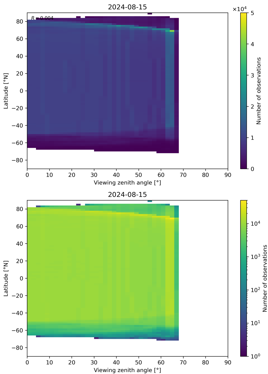
Figure 196: Scatter density plot of “Viewing zenith angle” against “Latitude” for 2024-08-14 to 2024-08-16.
