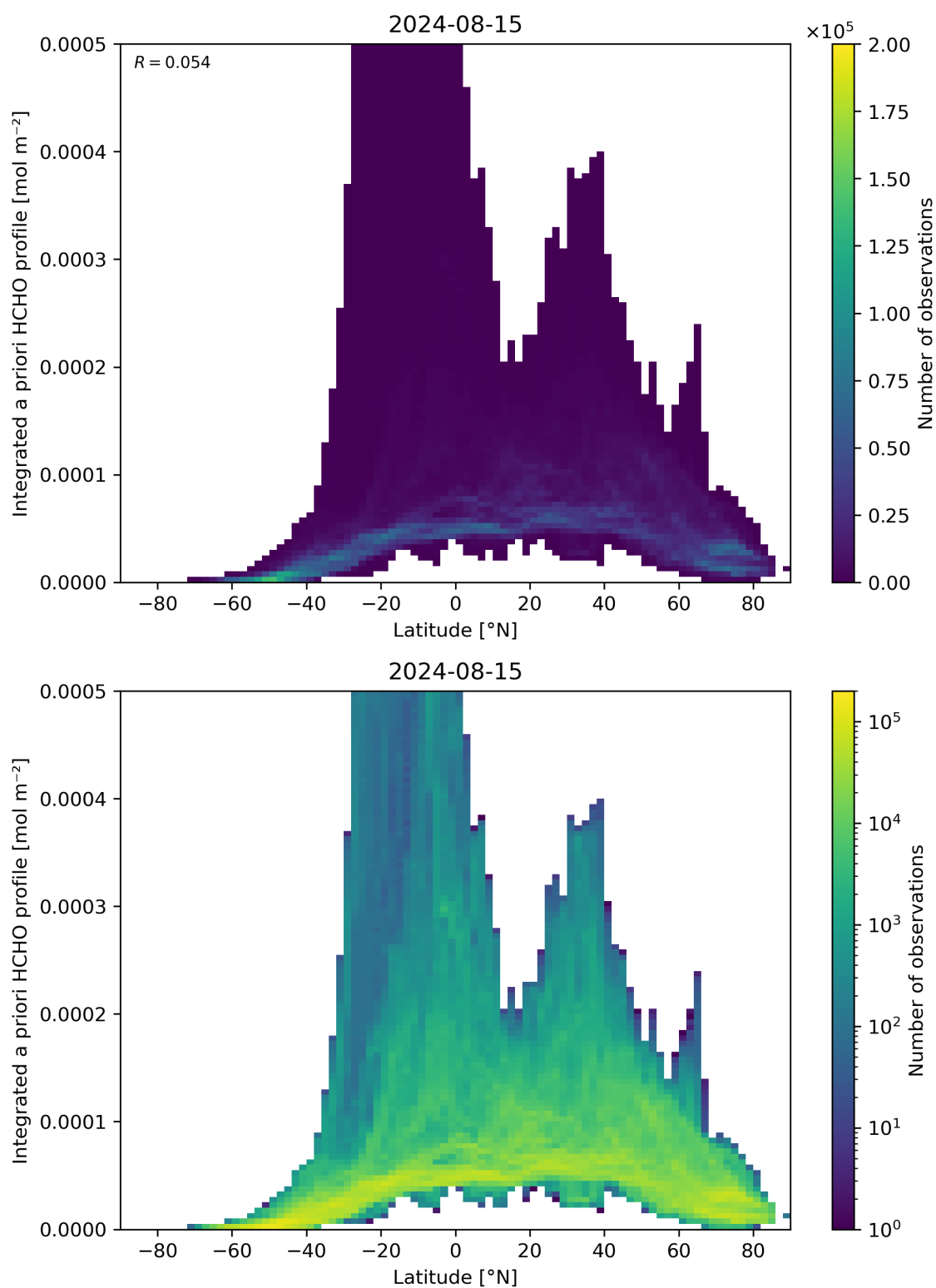
Figure 166: Scatter density plot of “Latitude” against “Integrated a priori HCHO profile” for 2024-08-14 to 2024-08-16.
