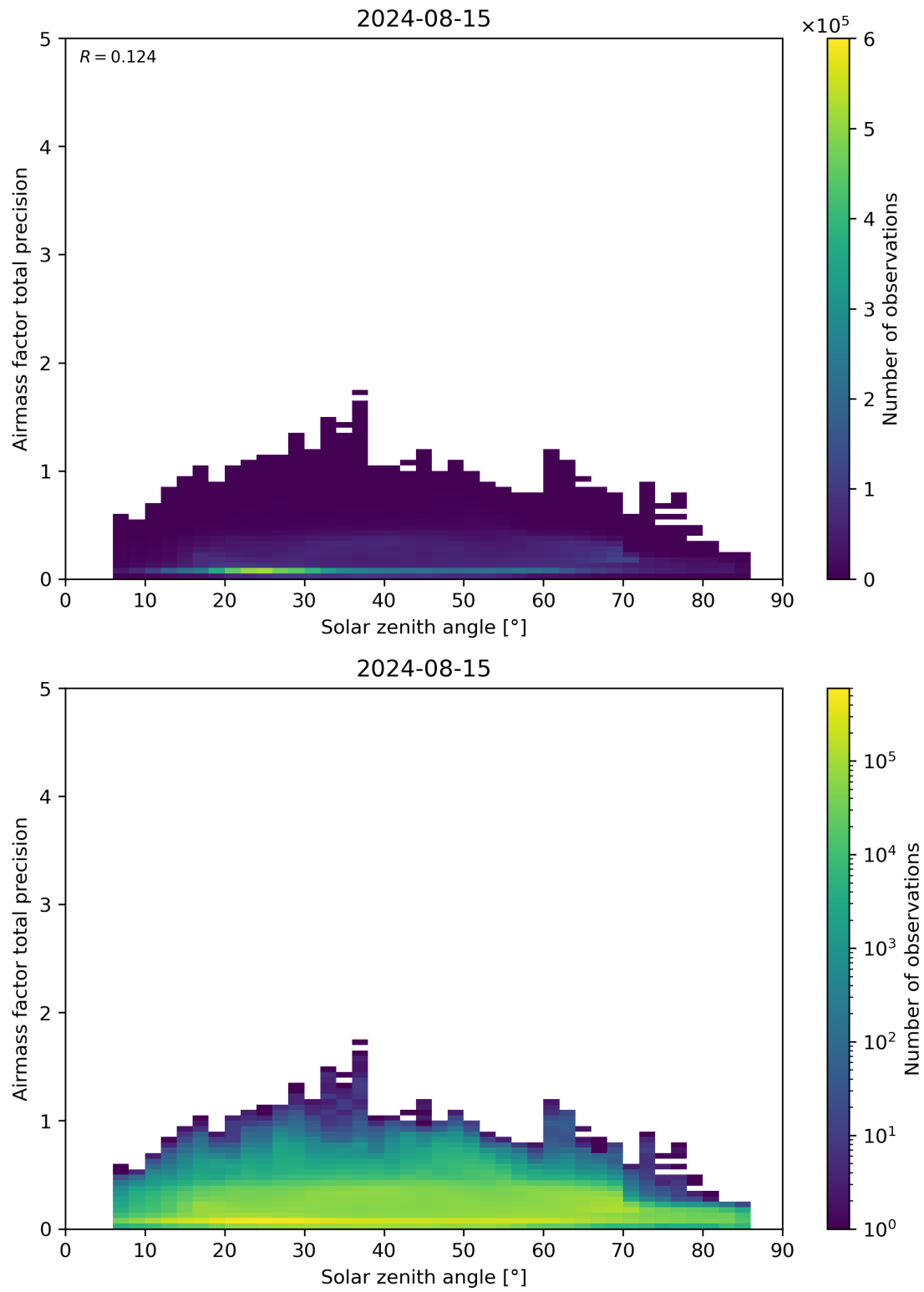
Figure 176: Scatter density plot of “Solar zenith angle” against “Airmass factor total precision” for 2024-08-14 to 2024-08-16.
