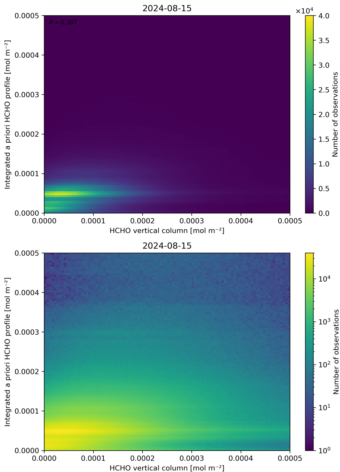
Figure 135: Scatter density plot of “HCHO vertical column” against “Integrated a priori HCHO profile” for 2024-08-14 to 2024-08-16.
