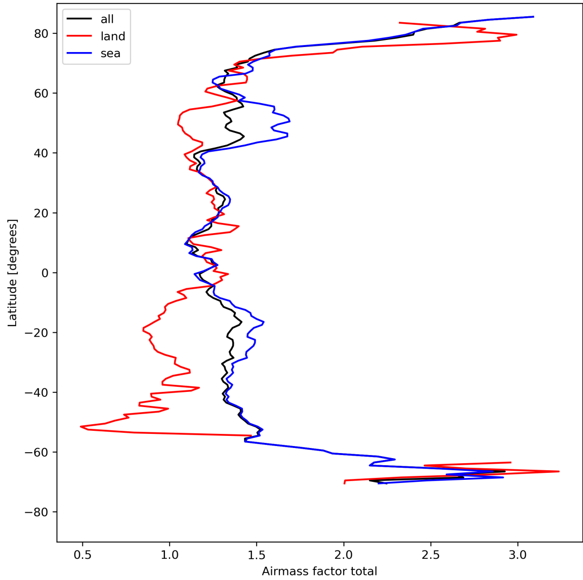
Figure 26: Zonal average of “Airmass factor total” for 2024-08-14 to 2024-08-16.
