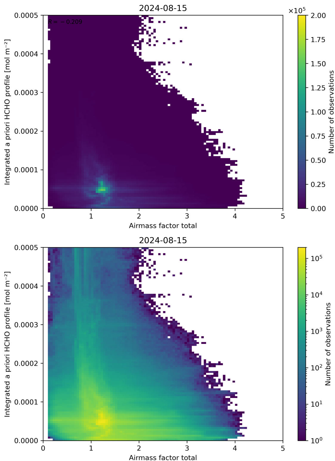
Figure 104: Scatter density plot of “Airmass factor total” against “Integrated a priori HCHO profile” for 2024-08-14 to 2024-08-16.
