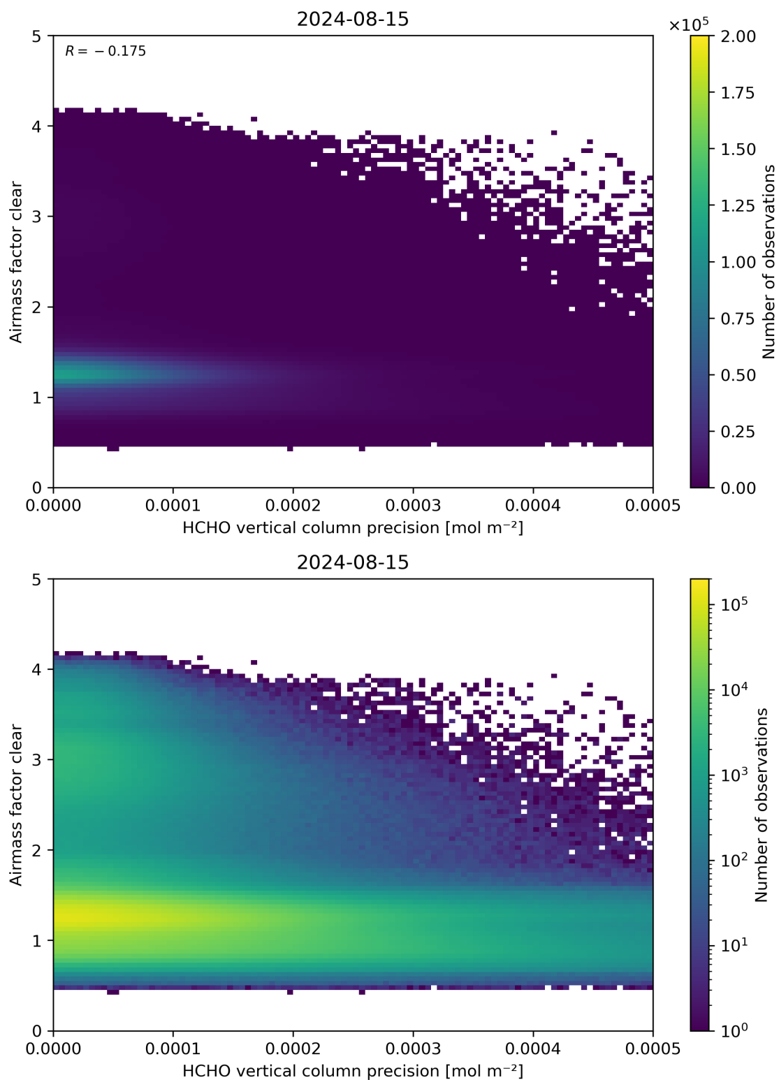
Figure 139: Scatter density plot of “HCHO vertical column precision” against “Airmass factor clear” for 2024-08-14 to 2024-08-16.
