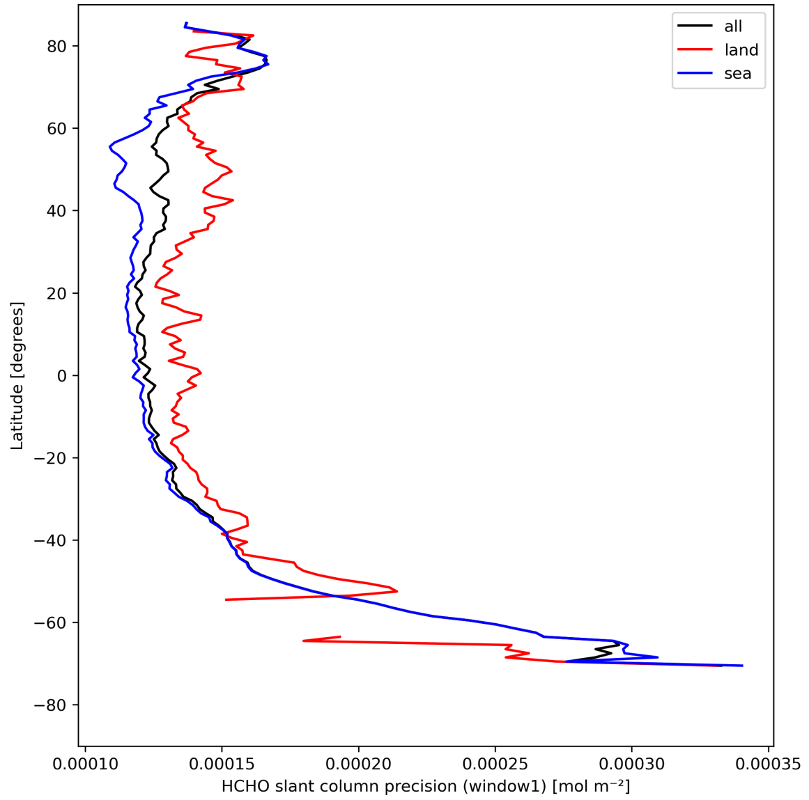
Figure 25: Zonal average of “HCHO slant column precision (window1)” for 2024-08-14 to 2024-08-16.
