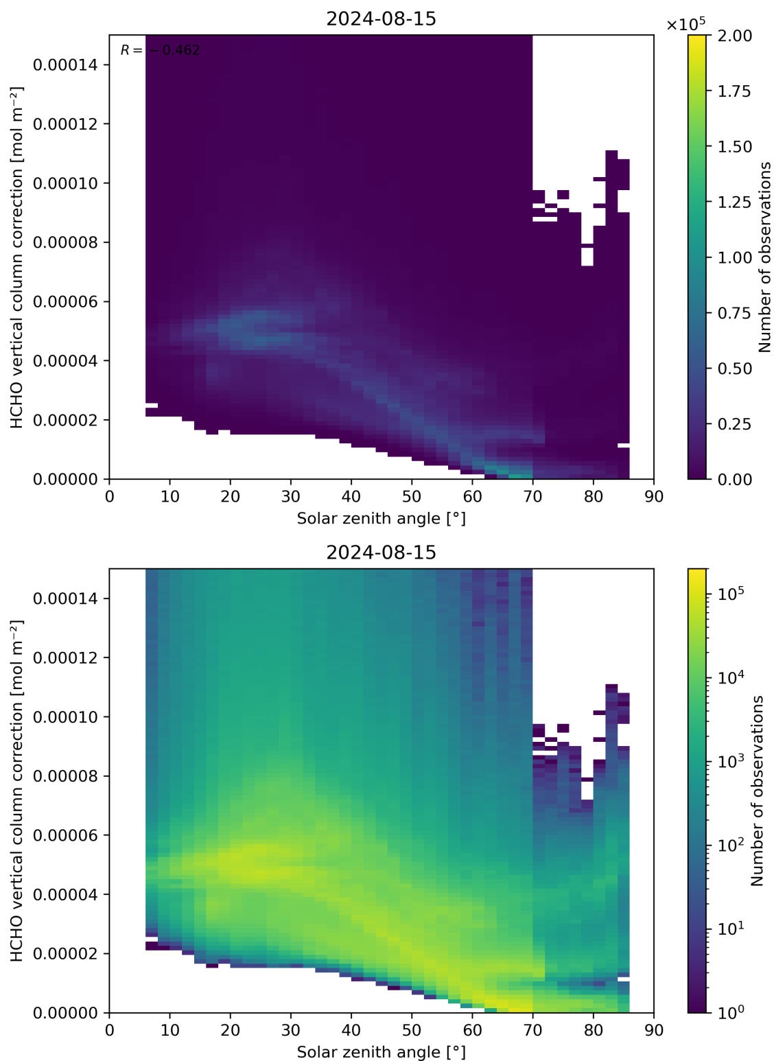
Figure 178: Scatter density plot of “Solar zenith angle” against “HCHO vertical column correction” for 2024-08-14 to 2024-08-16.
