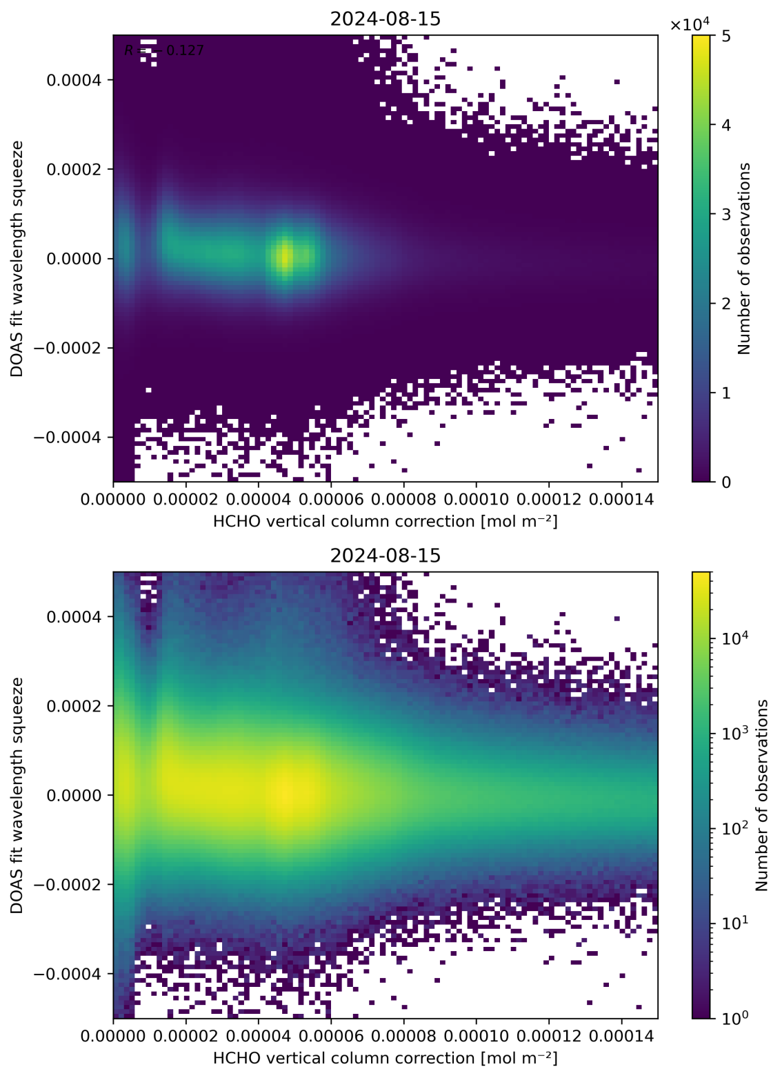
Figure 114: Scatter density plot of “HCHO vertical column correction” against “DOAS fit wavelength squeeze” for 2024-08-14 to 2024-08-16.
