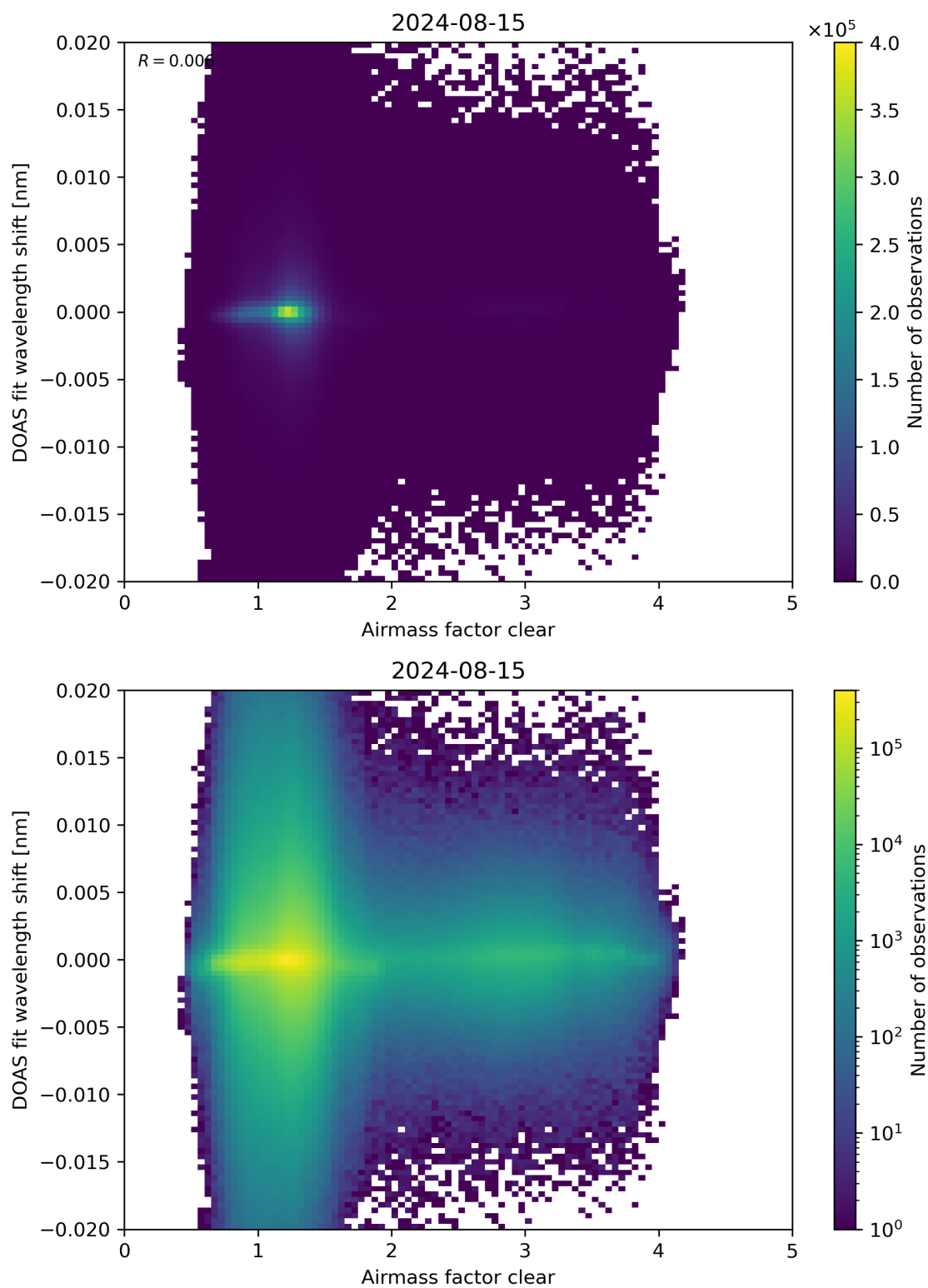
Figure 72: Scatter density plot of “Airmass factor clear” against “DOAS fit wavelength shift” for 2024-08-14 to 2024-08-16.
