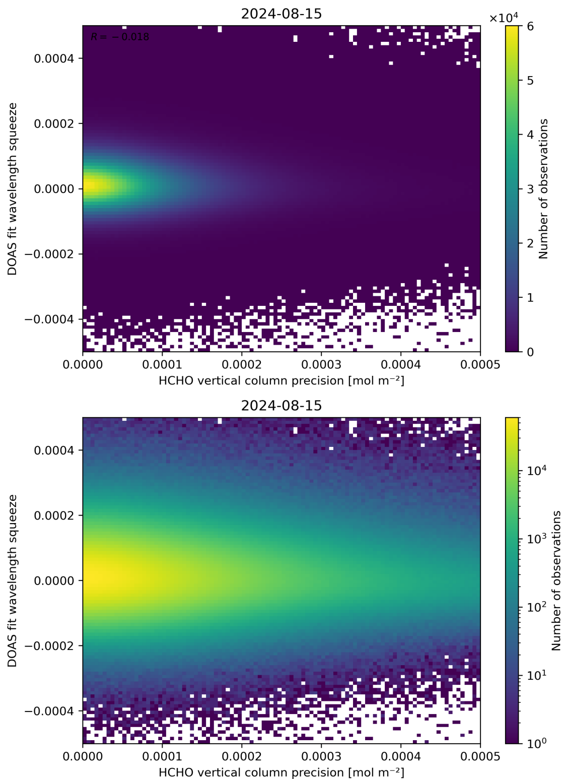
Figure 138: Scatter density plot of “HCHO vertical column precision” against “DOAS fit wavelength squeeze” for 2024-08-14 to 2024-08-16.
