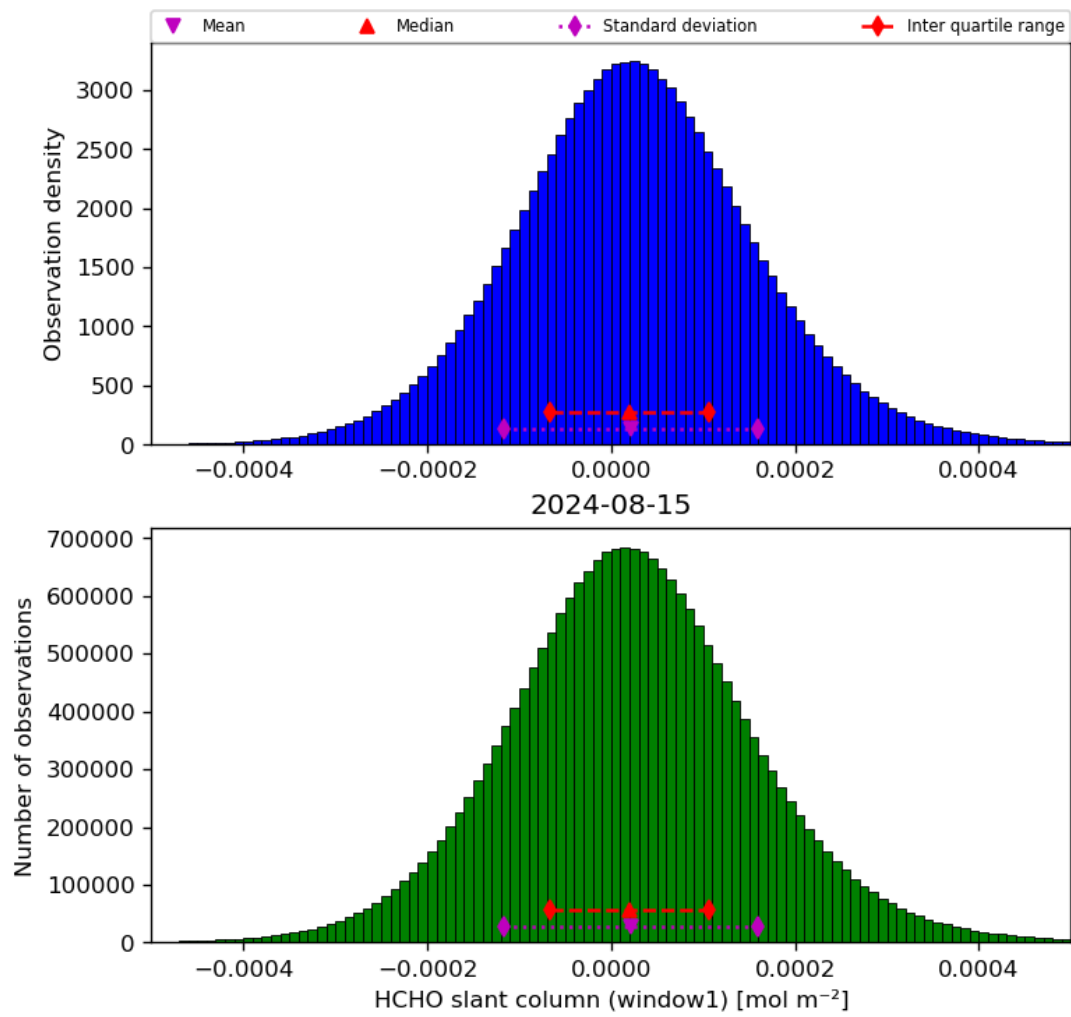
Figure 38: Histogram of “HCHO slant column (window1)” for 2024-08-14 to 2024-08-16
