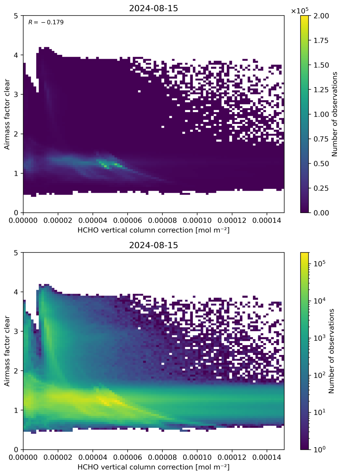
Figure 115: Scatter density plot of “HCHO vertical column correction” against “Airmass factor clear” for 2024-08-14 to 2024-08-16.
