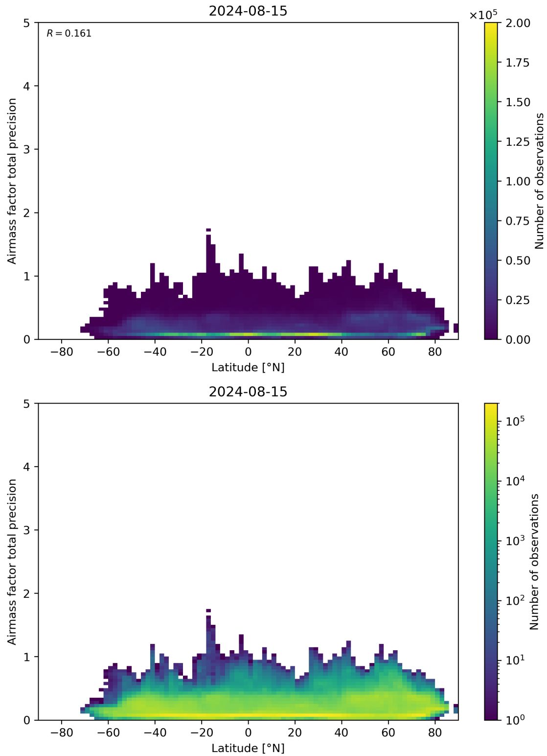
Figure 162: Scatter density plot of “Latitude” against “Airmass factor total precision” for 2024-08-14 to 2024-08-16.
