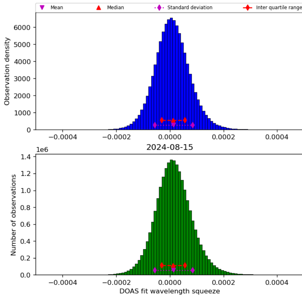
Figure 45: Histogram of “DOAS fit wavelength squeeze” for 2024-08-14 to 2024-08-16
