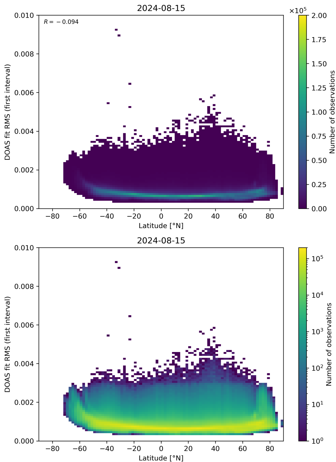
Figure 153: Scatter density plot of “Latitude” against “DOAS fit RMS (first interval)” for 2024-08-14 to 2024-08-16.
