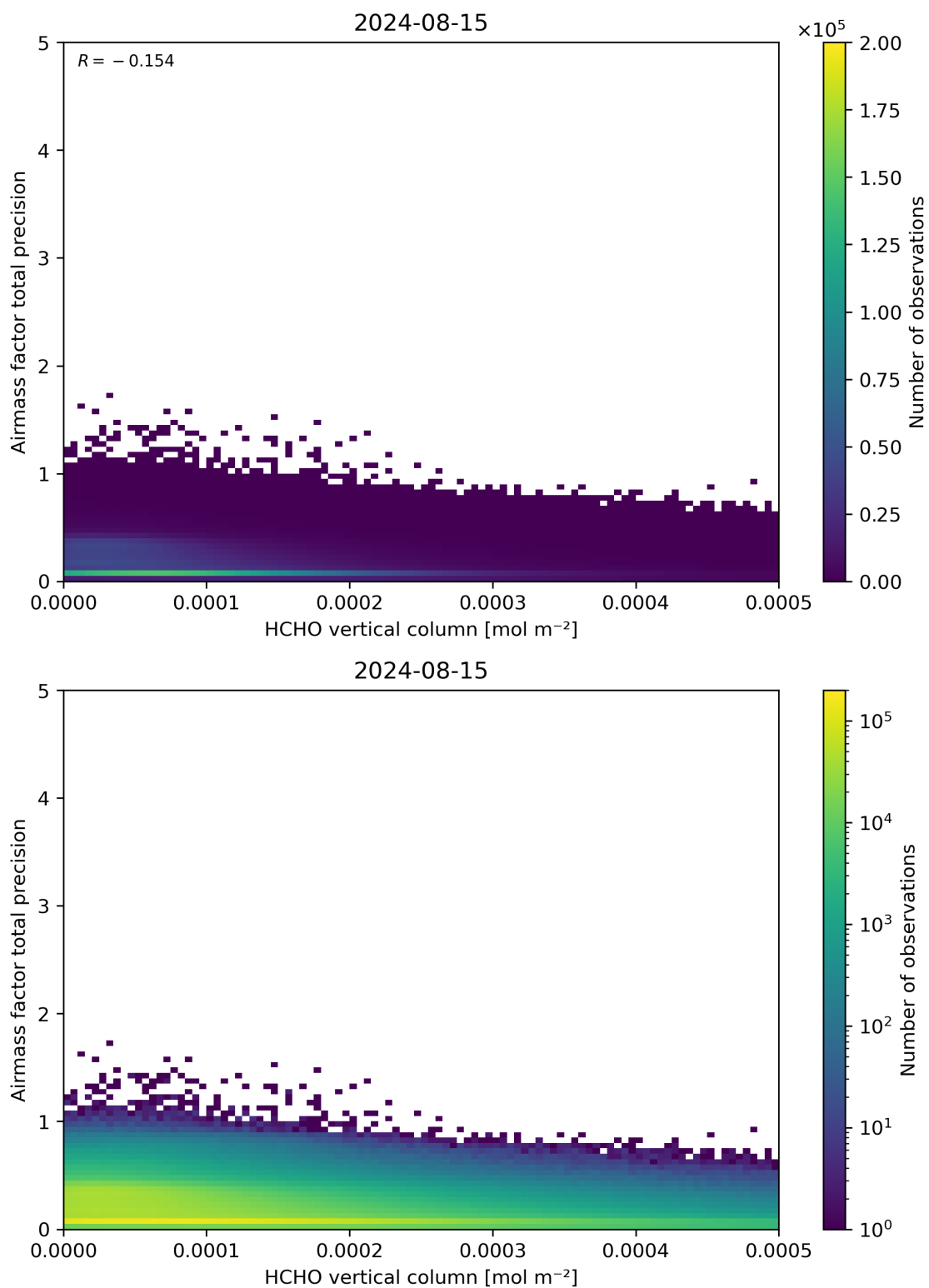
Figure 132: Scatter density plot of “HCHO vertical column” against “Airmass factor total precision” for 2024-08-14 to 2024-08-16.
