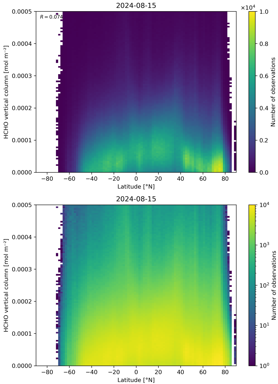
Figure 163: Scatter density plot of “Latitude” against “HCHO vertical column” for 2024-08-14 to 2024-08-16.
