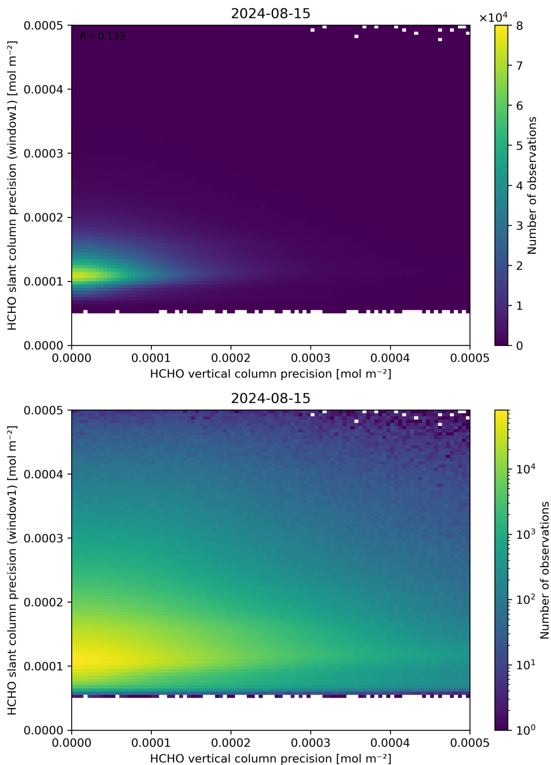
Figure 143: Scatter density plot of “HCHO vertical column precision” against “HCHO slant column precision (window1)” for 2024-08-14 to 2024-08-16.
