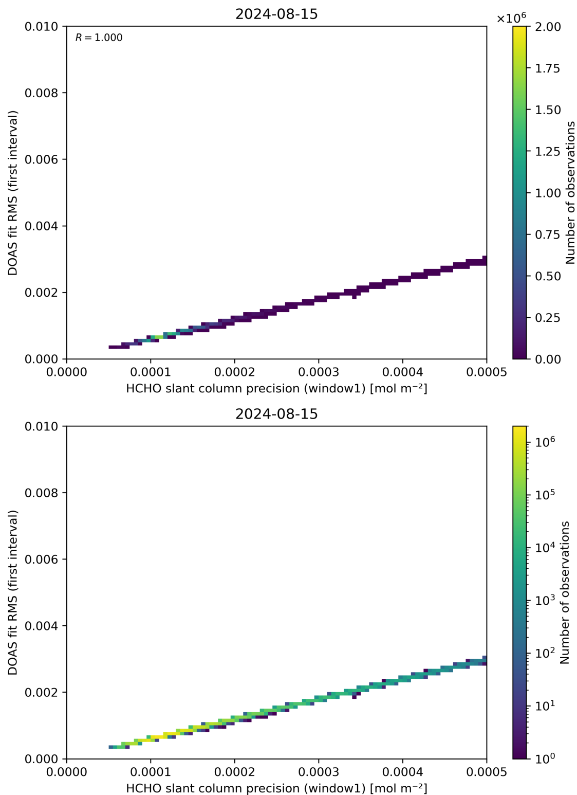
Figure 88: Scatter density plot of “HCHO slant column precision (window1)” against “DOAS fit RMS (first interval)” for 2024-08-14 to 2024-08-16.
