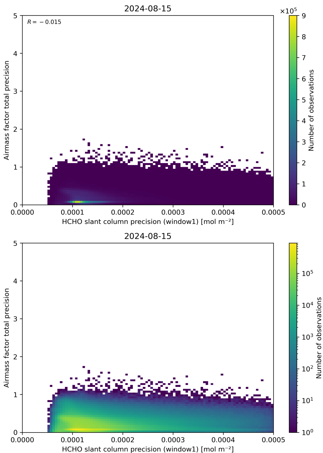
Figure 95: Scatter density plot of “HCHO slant column precision (window1)” against “Airmass factor total precision” for 2024-08-14 to 2024-08-16.
