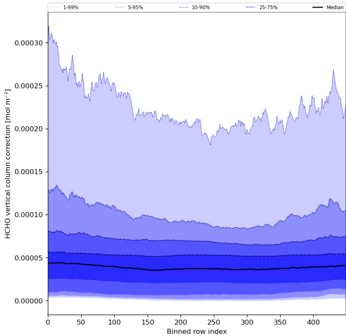
Figure 51: Along track statistics of “HCHO vertical column correction” for 2024-08-14 to 2024-08-16
