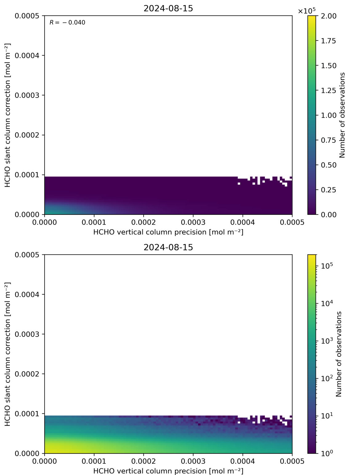
Figure 141: Scatter density plot of “HCHO vertical column precision” against “HCHO slant column correction” for 2024-08-14 to 2024-08-16.
