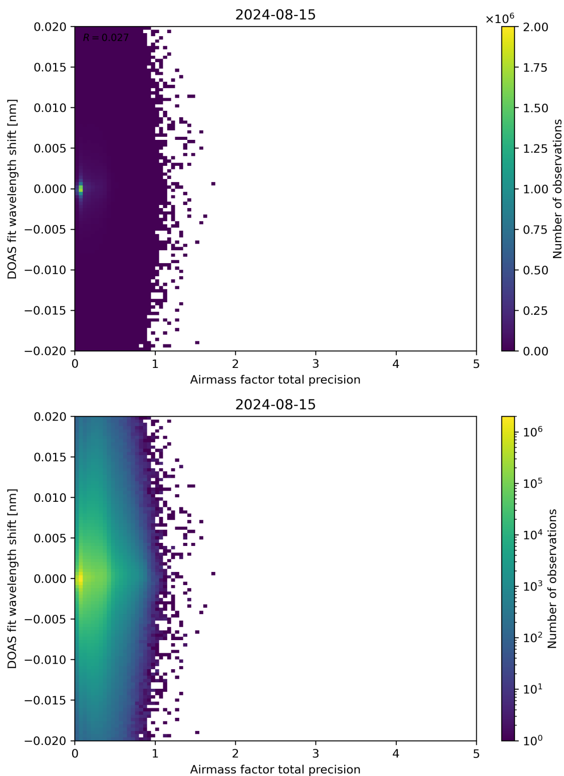
Figure 106: Scatter density plot of “Airmass factor total precision” against “DOAS fit wavelength shift” for 2024-08-14 to 2024-08-16.
