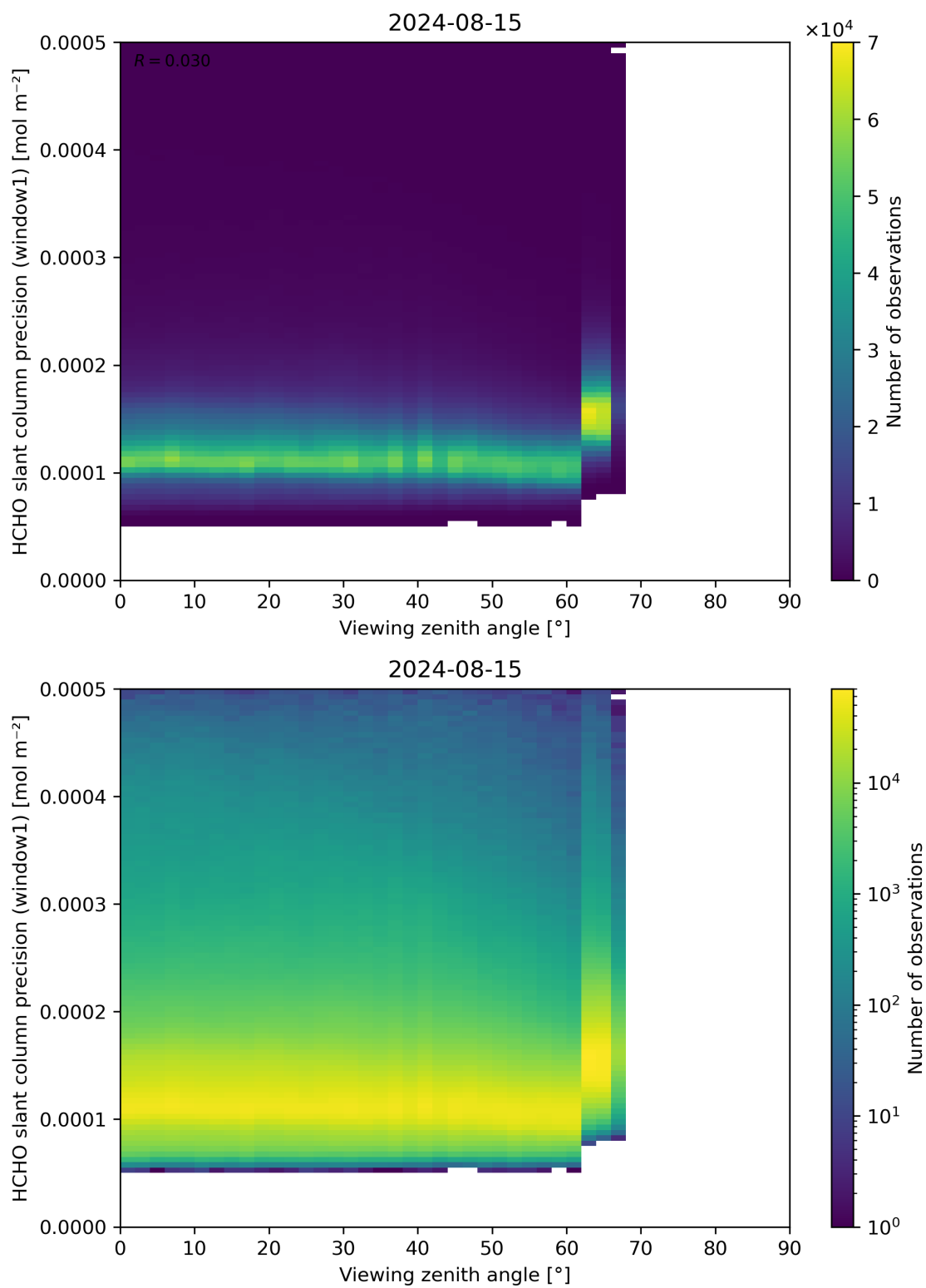
Figure 189: Scatter density plot of “Viewing zenith angle” against “HCHO slant column precision (window1)” for 2024-08-14 to 2024-08-16.
