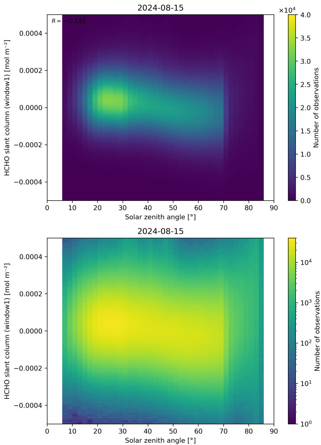
Figure 173: Scatter density plot of “Solar zenith angle” against “HCHO slant column (window1)” for 2024-08-14 to 2024-08-16.
