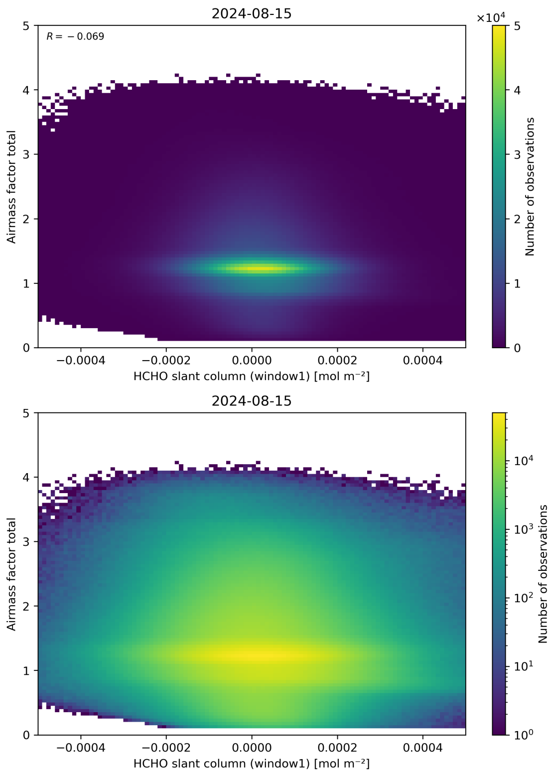
Figure 85: Scatter density plot of “HCHO slant column (window1)” against “Airmass factor total” for 2024-08-14 to 2024-08-16.
