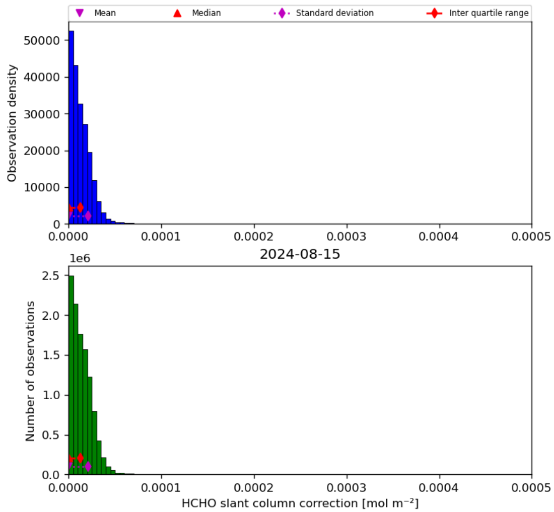
Figure 47: Histogram of “HCHO slant column correction” for 2024-08-14 to 2024-08-16
