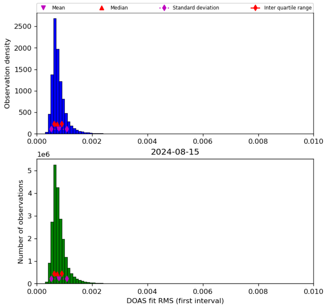
Figure 46: Histogram of “DOAS fit RMS (first interval)” for 2024-08-14 to 2024-08-16
