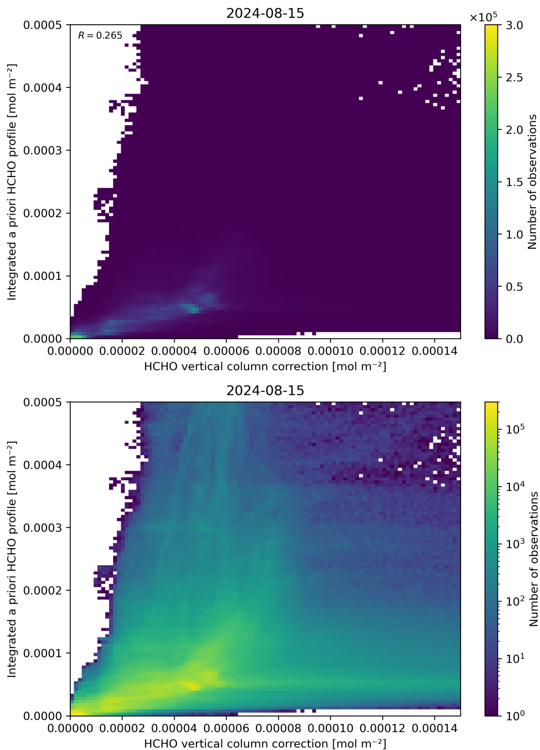
Figure 122: Scatter density plot of “HCHO vertical column correction” against “Integrated a priori HCHO profile” for 2024-08-14 to 2024-08-16.
