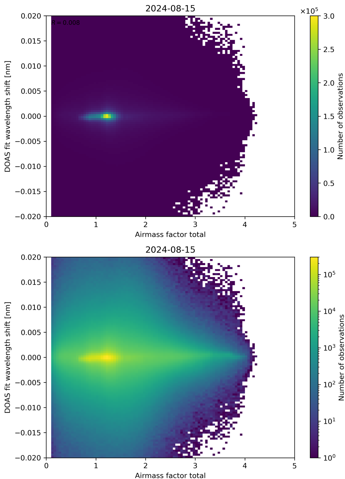
Figure 98: Scatter density plot of “Airmass factor total” against “DOAS fit wavelength shift” for 2024-08-14 to 2024-08-16.
