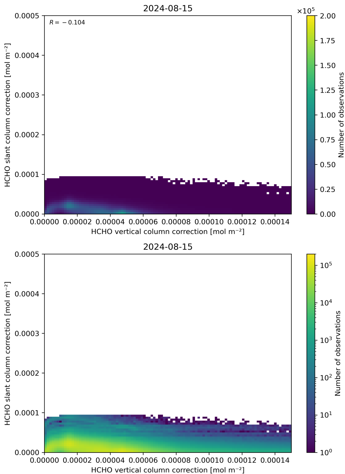
Figure 117: Scatter density plot of “HCHO vertical column correction” against “HCHO slant column correction” for 2024-08-14 to 2024-08-16.
