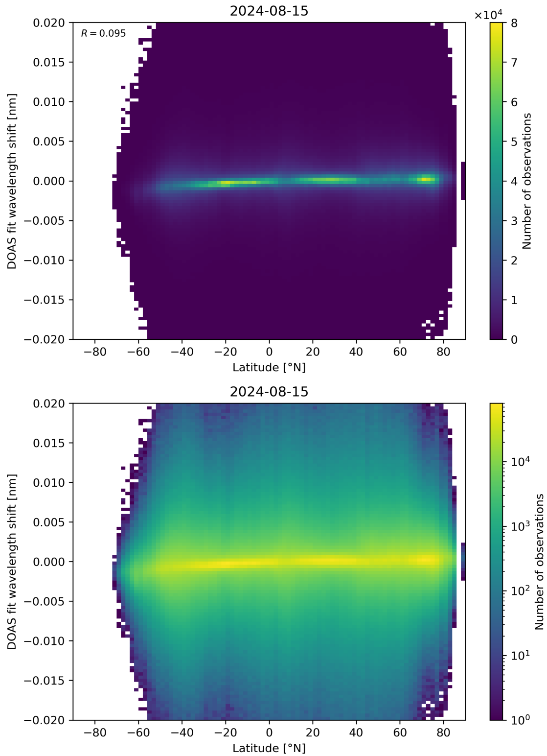
Figure 154: Scatter density plot of “Latitude” against “DOAS fit wavelength shift” for 2024-08-14 to 2024-08-16.
