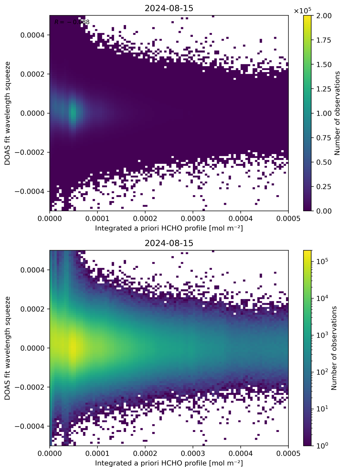
Figure 150: Scatter density plot of “Integrated a priori HCHO profile” against “DOAS fit wavelength squeeze” for 2024-08-14 to 2024-08-16.
