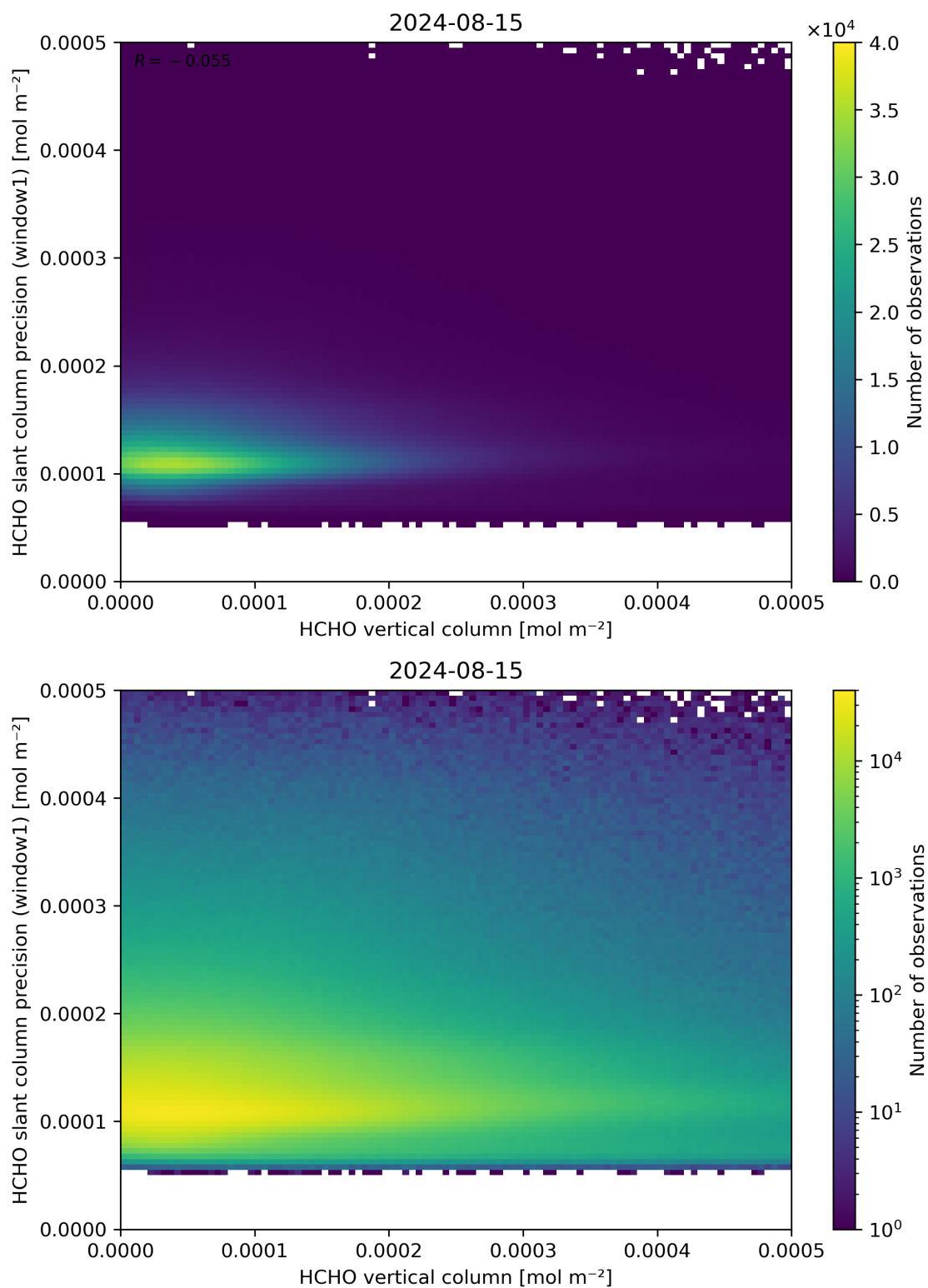
Figure 130: Scatter density plot of “HCHO vertical column” against “HCHO slant column precision (window1)” for 2024-08-14 to 2024-08-16.
