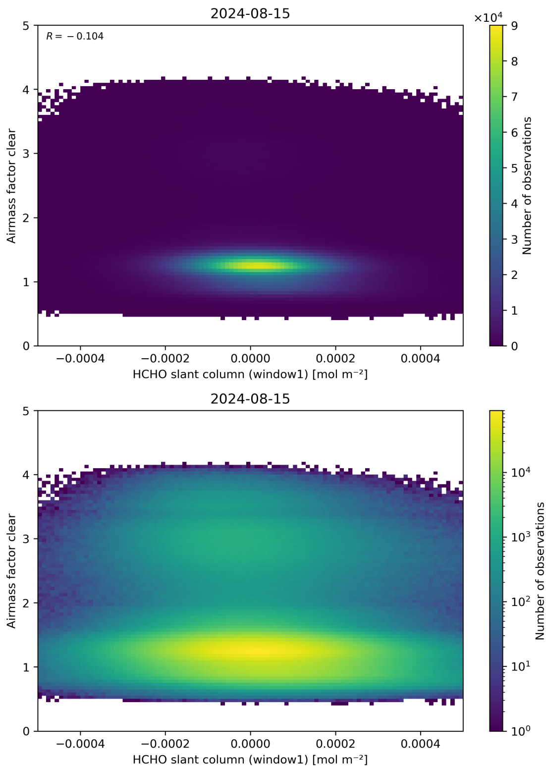
Figure 81: Scatter density plot of “HCHO slant column (window1)” against “Airmass factor clear” for 2024-08-14 to 2024-08-16.
