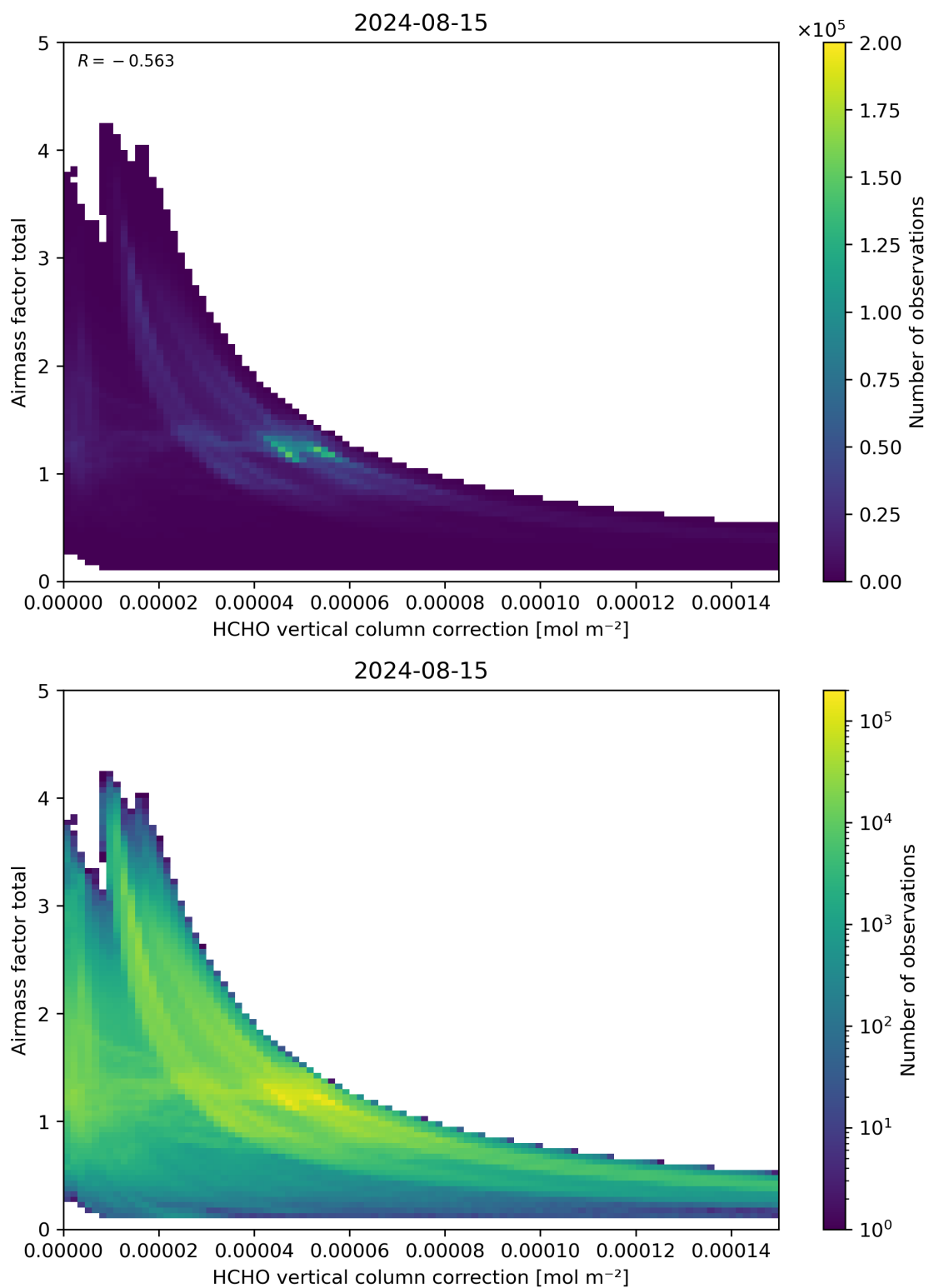
Figure 120: Scatter density plot of “HCHO vertical column correction” against “Airmass factor total” for 2024-08-14 to 2024-08-16.
