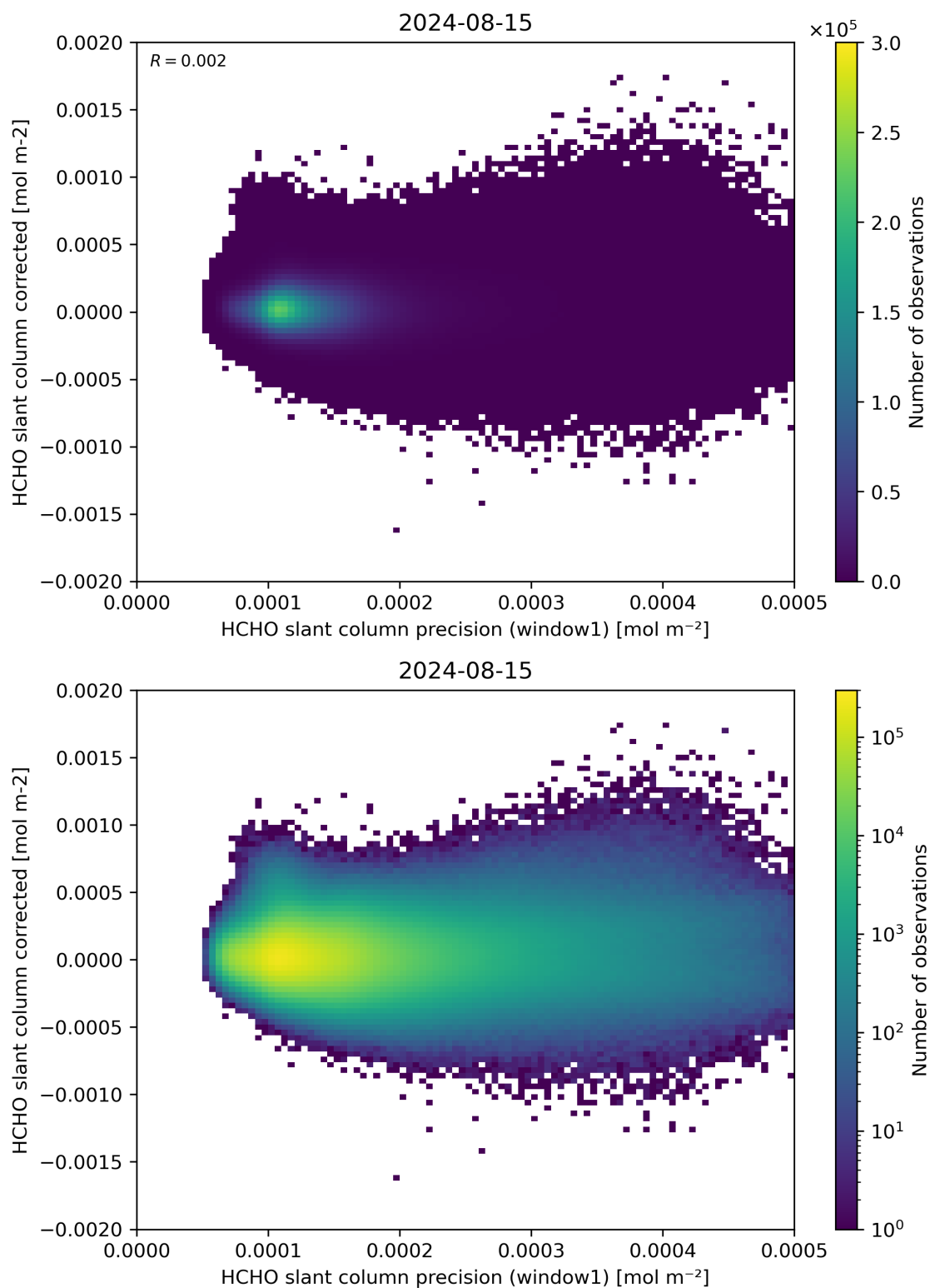
Figure 92: Scatter density plot of “HCHO slant column precision (window1)” against “HCHO slant column corrected” for 2024-08-14 to 2024-08-16.
