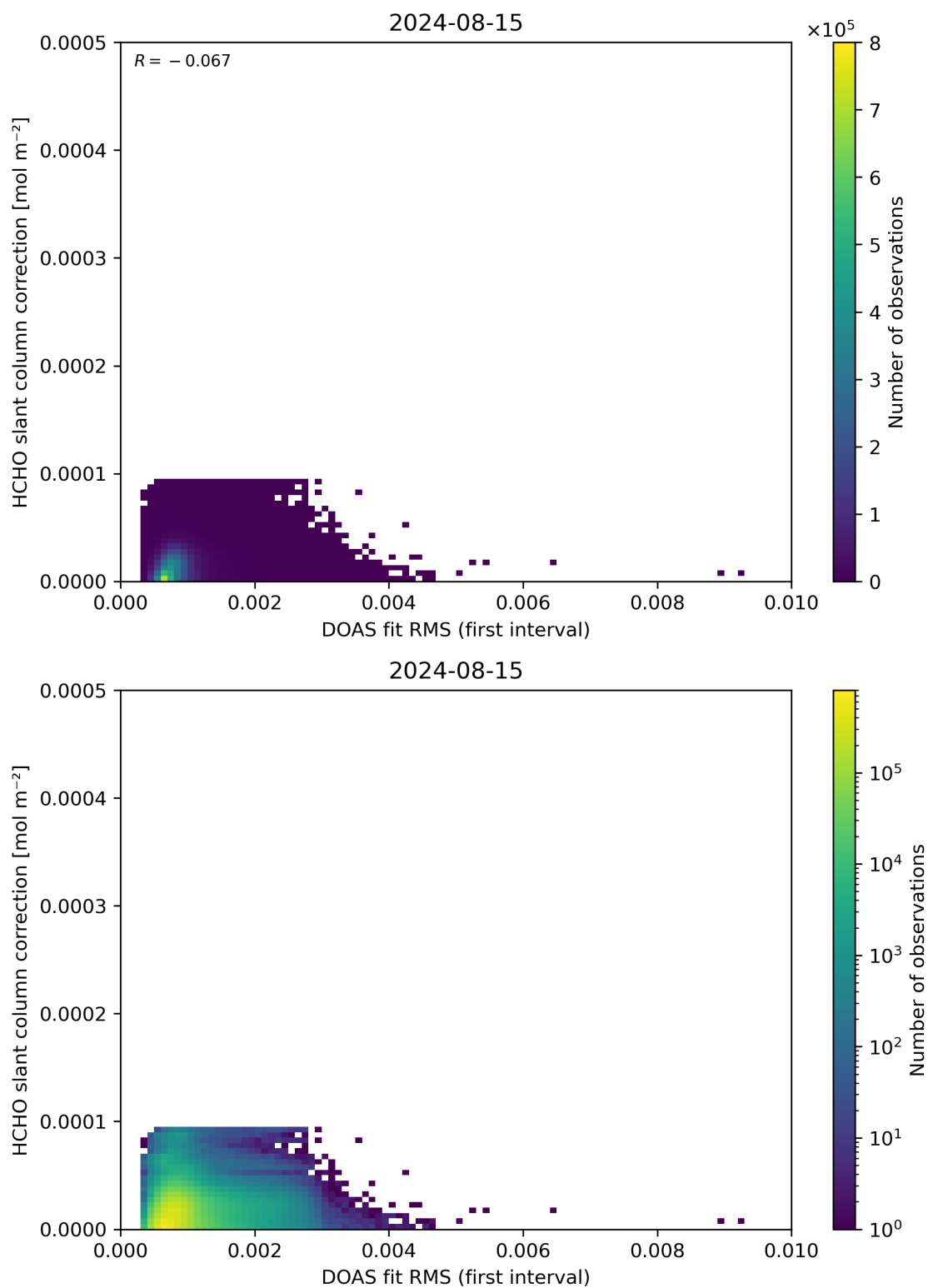
Figure 63: Scatter density plot of “DOAS fit RMS (first interval)” against “HCHO slant column correction” for 2024-08-14 to 2024-08-16.
