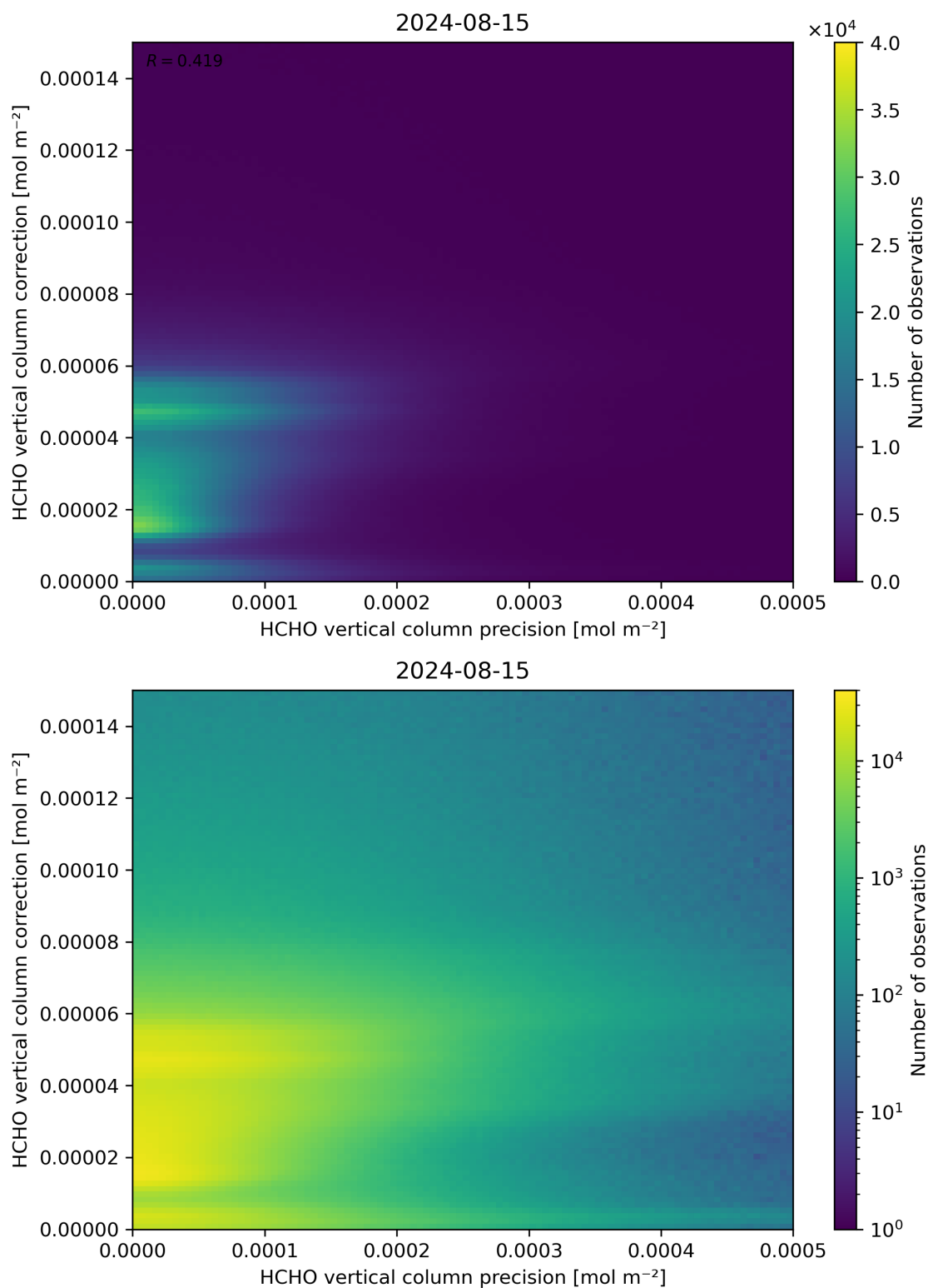
Figure 146: Scatter density plot of “HCHO vertical column precision” against “HCHO vertical column correction” for 2024-08-14 to 2024-08-16.
