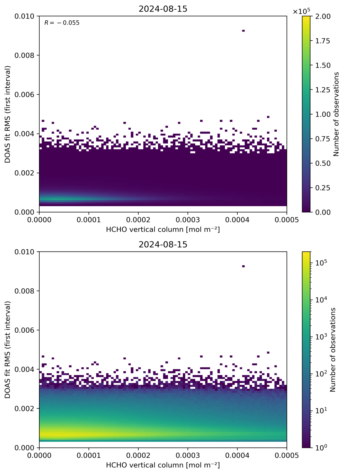
Figure 123: Scatter density plot of “HCHO vertical column” against “DOAS fit RMS (first interval)” for 2024-08-14 to 2024-08-16.
