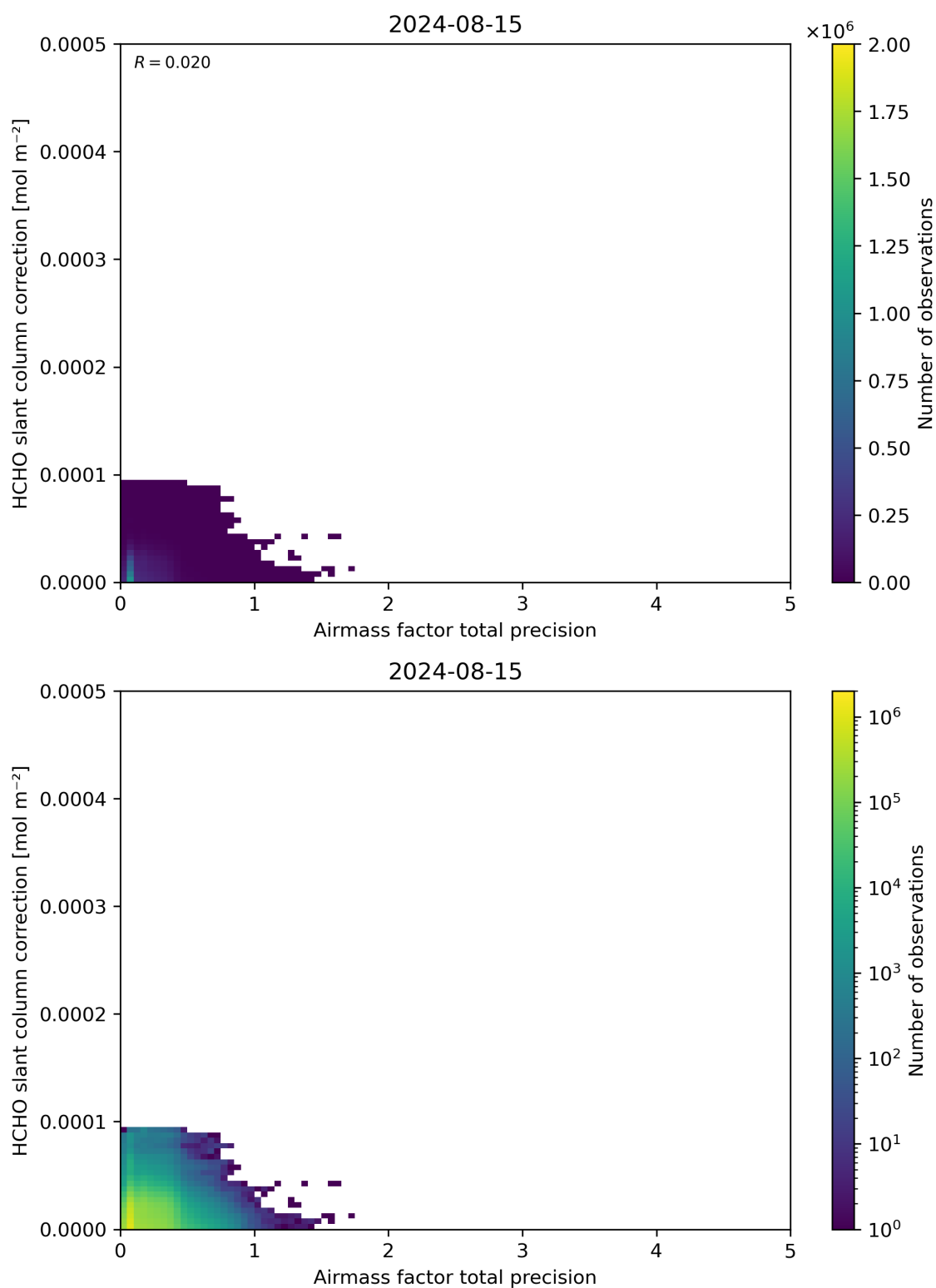
Figure 110: Scatter density plot of “Airmass factor total precision” against “HCHO slant column correction” for 2024-08-14 to 2024-08-16.
