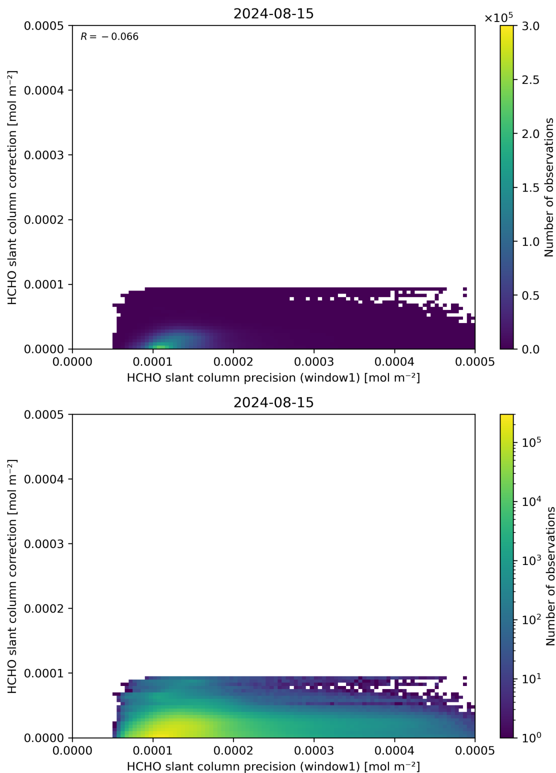
Figure 93: Scatter density plot of “HCHO slant column precision (window1)” against “HCHO slant column correction” for 2024-08-14 to 2024-08-16.
