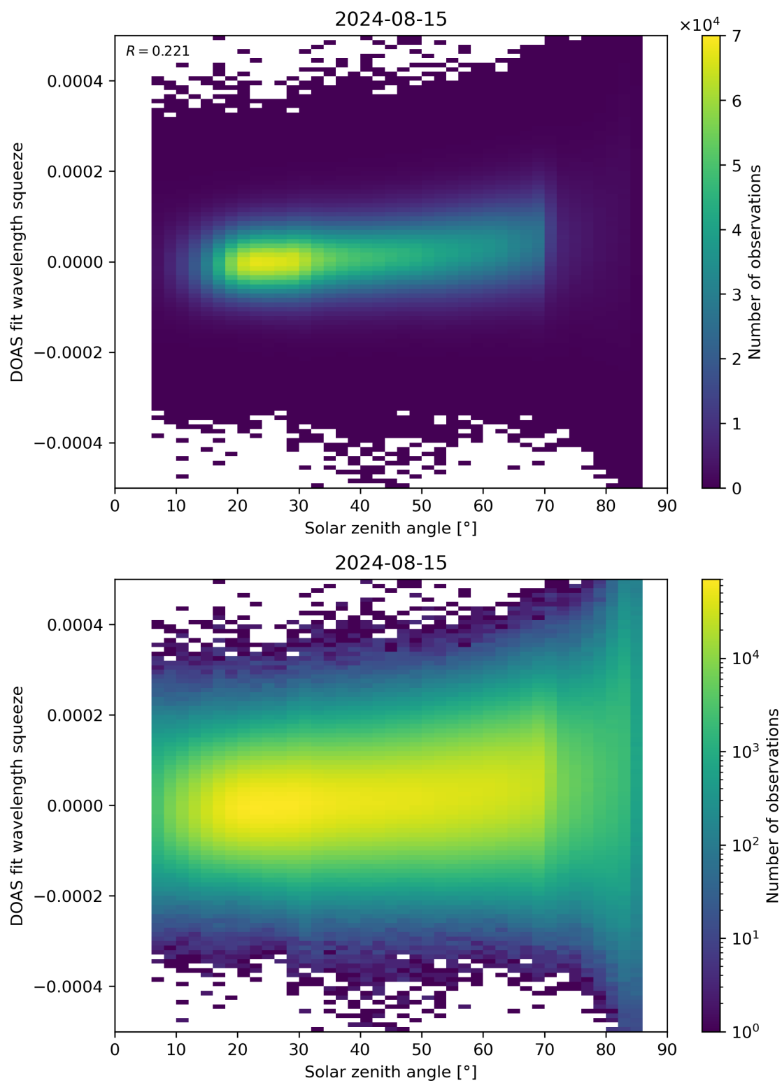
Figure 169: Scatter density plot of “Solar zenith angle” against “DOAS fit wavelength squeeze” for 2024-08-14 to 2024-08-16.
