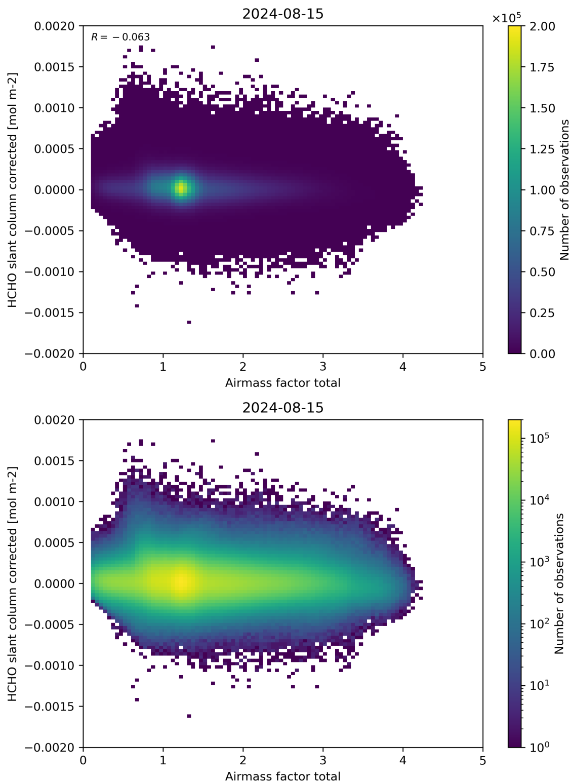
Figure 101: Scatter density plot of “Airmass factor total” against “HCHO slant column corrected” for 2024-08-14 to 2024-08-16.
