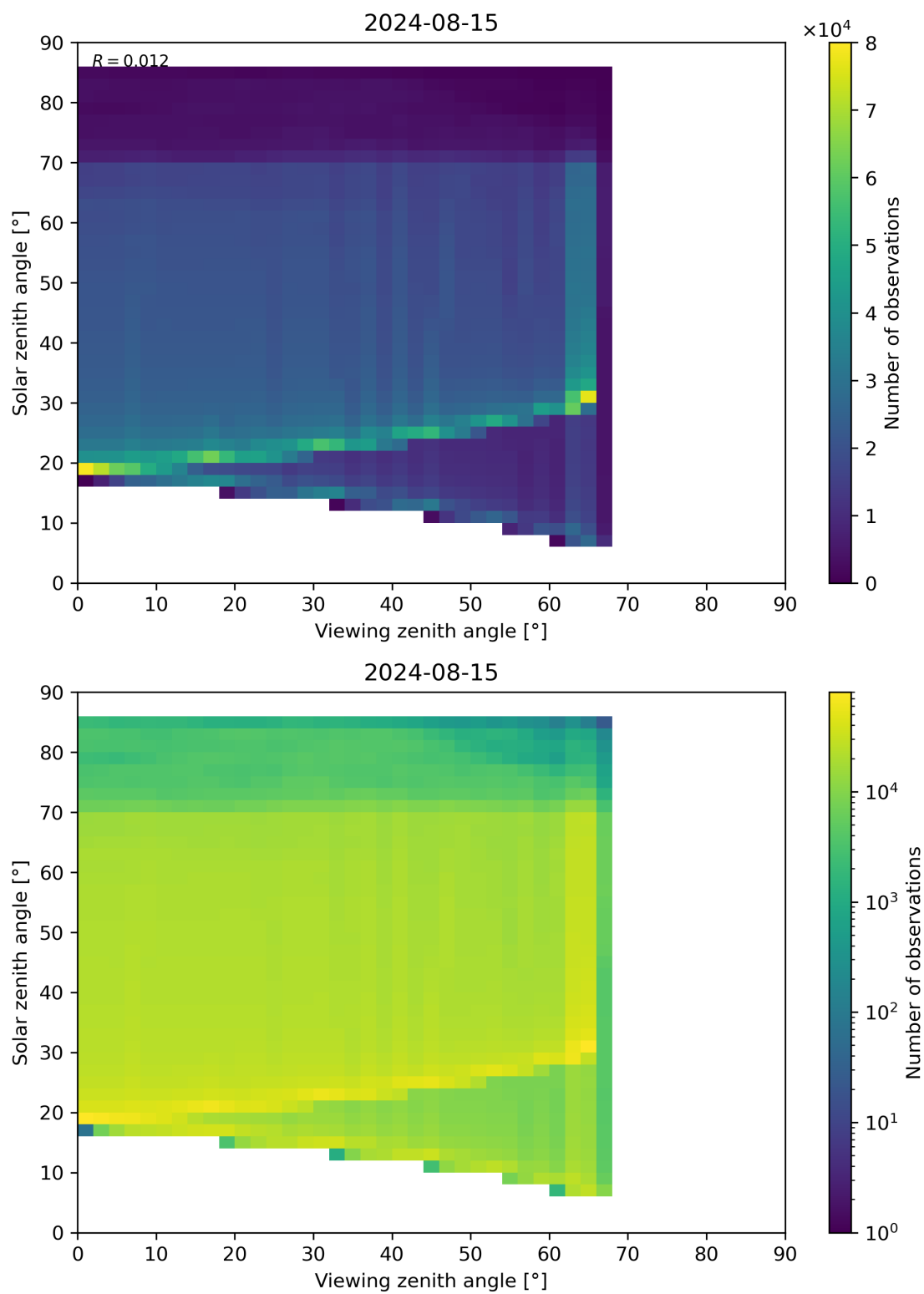
Figure 197: Scatter density plot of “Viewing zenith angle” against “Solar zenith angle” for 2024-08-14 to 2024-08-16.
