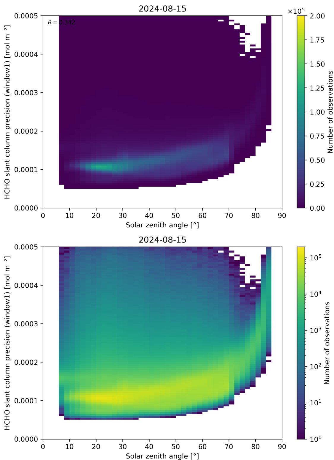
Figure 174: Scatter density plot of “Solar zenith angle” against “HCHO slant column precision (window1)” for 2024-08-14 to 2024-08-16.
