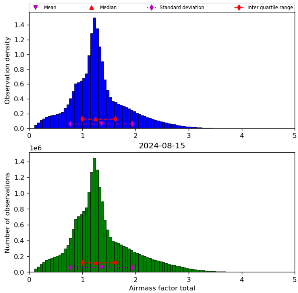
Figure 40: Histogram of “Airmass factor total” for 2024-08-14 to 2024-08-16
