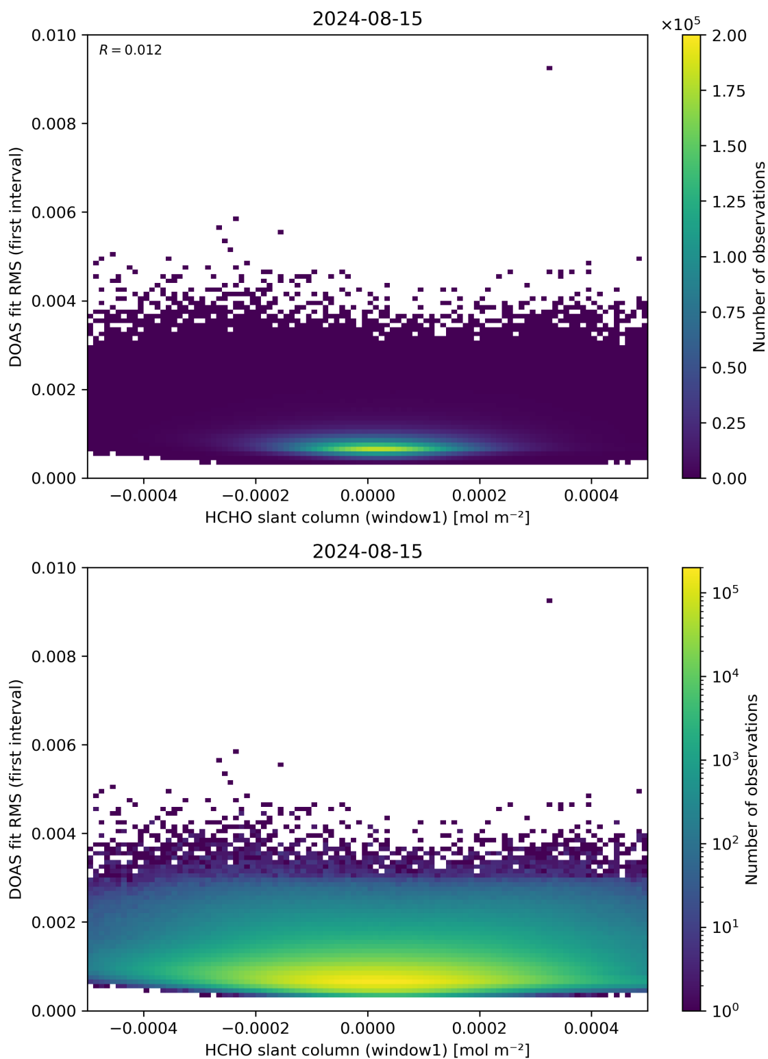
Figure 78: Scatter density plot of “HCHO slant column (window1)” against “DOAS fit RMS (first interval)” for 2024-08-14 to 2024-08-16.
