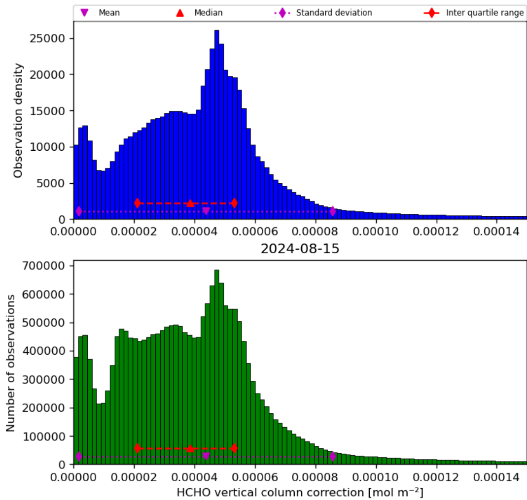
Figure 37: Histogram of “HCHO vertical column correction” for 2024-08-14 to 2024-08-16
