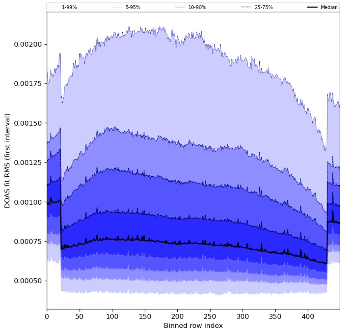
Figure 60: Along track statistics of “DOAS fit RMS (first interval)” for 2024-08-14 to 2024-08-16
