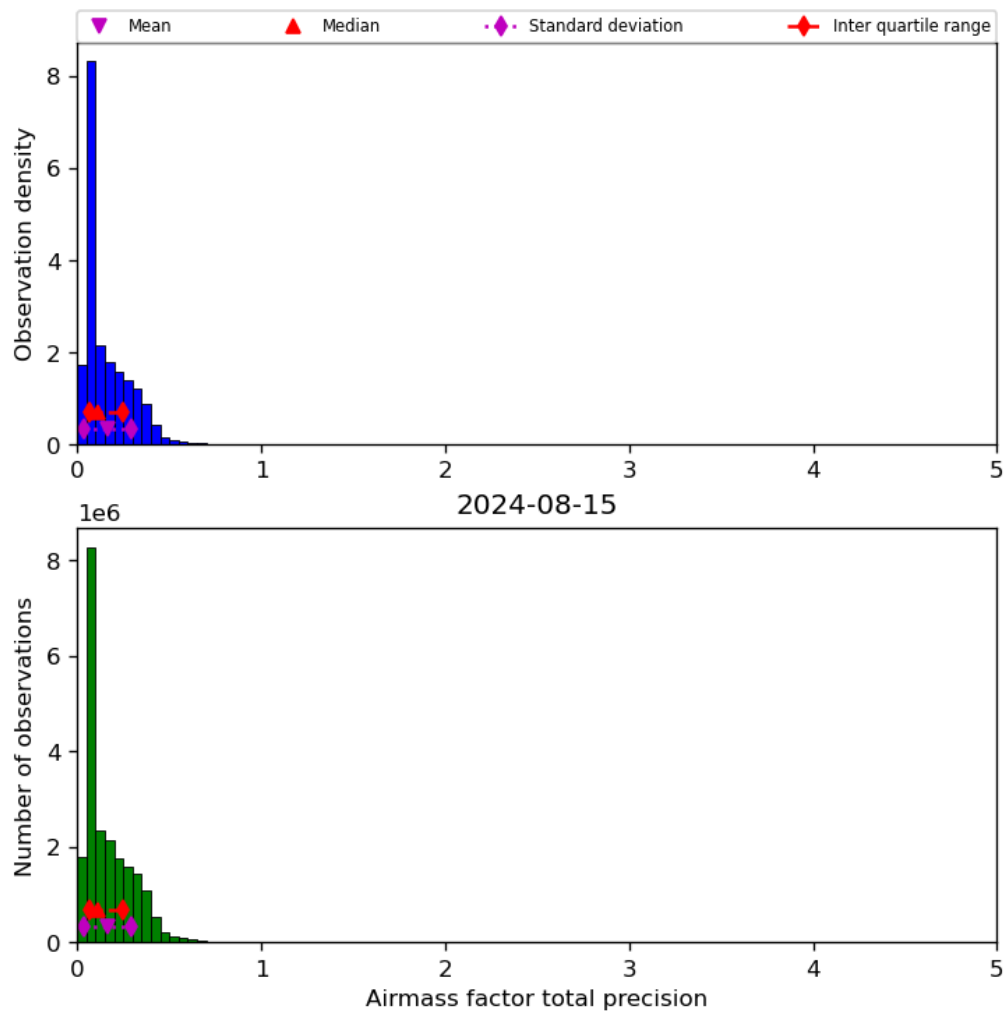
Figure 41: Histogram of “Airmass factor total precision” for 2024-08-14 to 2024-08-16
