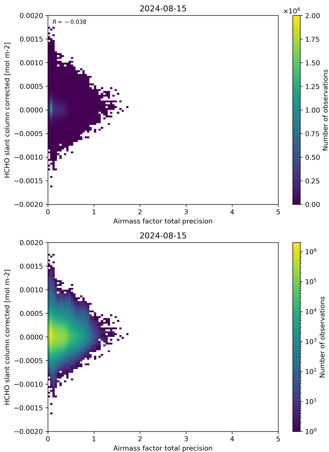
Figure 109: Scatter density plot of “Airmass factor total precision” against “HCHO slant column corrected” for 2024-08-14 to 2024-08-16.
