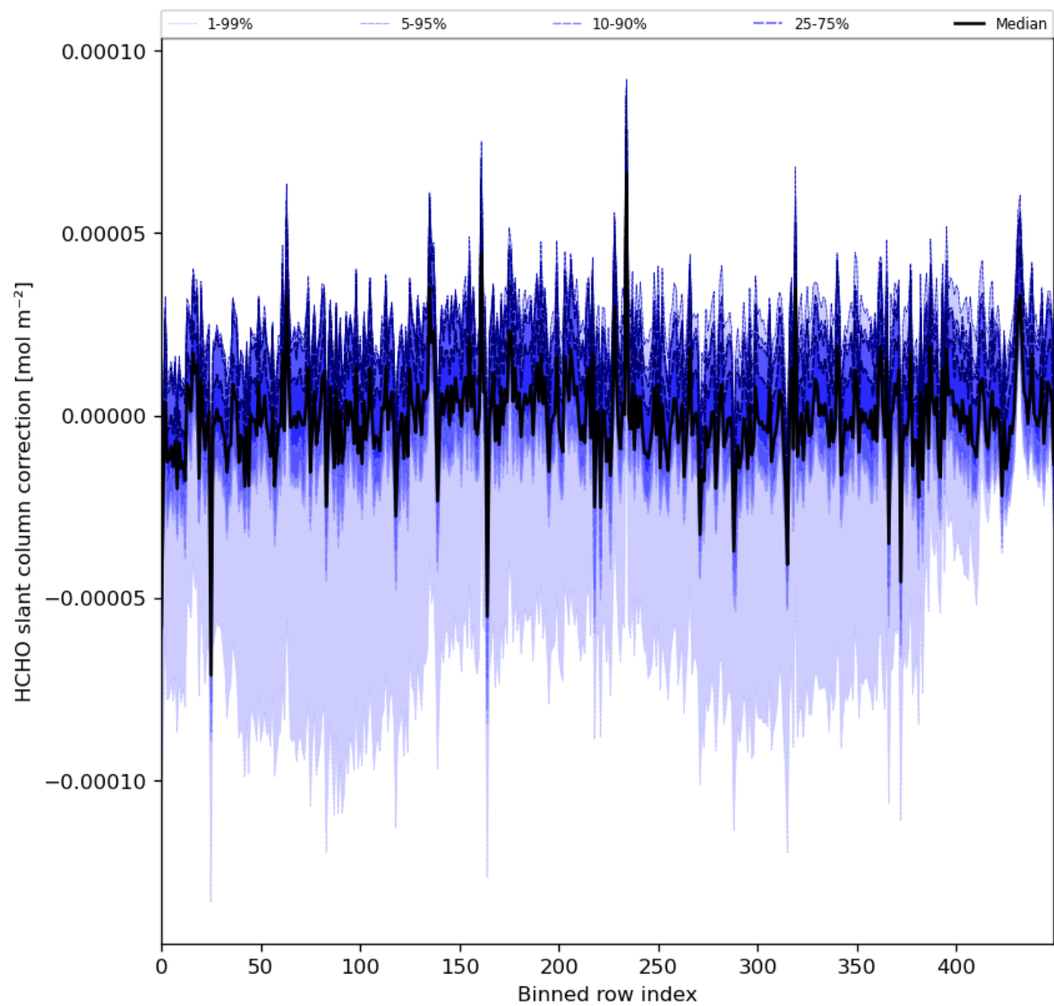
Figure 61: Along track statistics of “HCHO slant column correction” for 2024-08-14 to 2024-08-16
