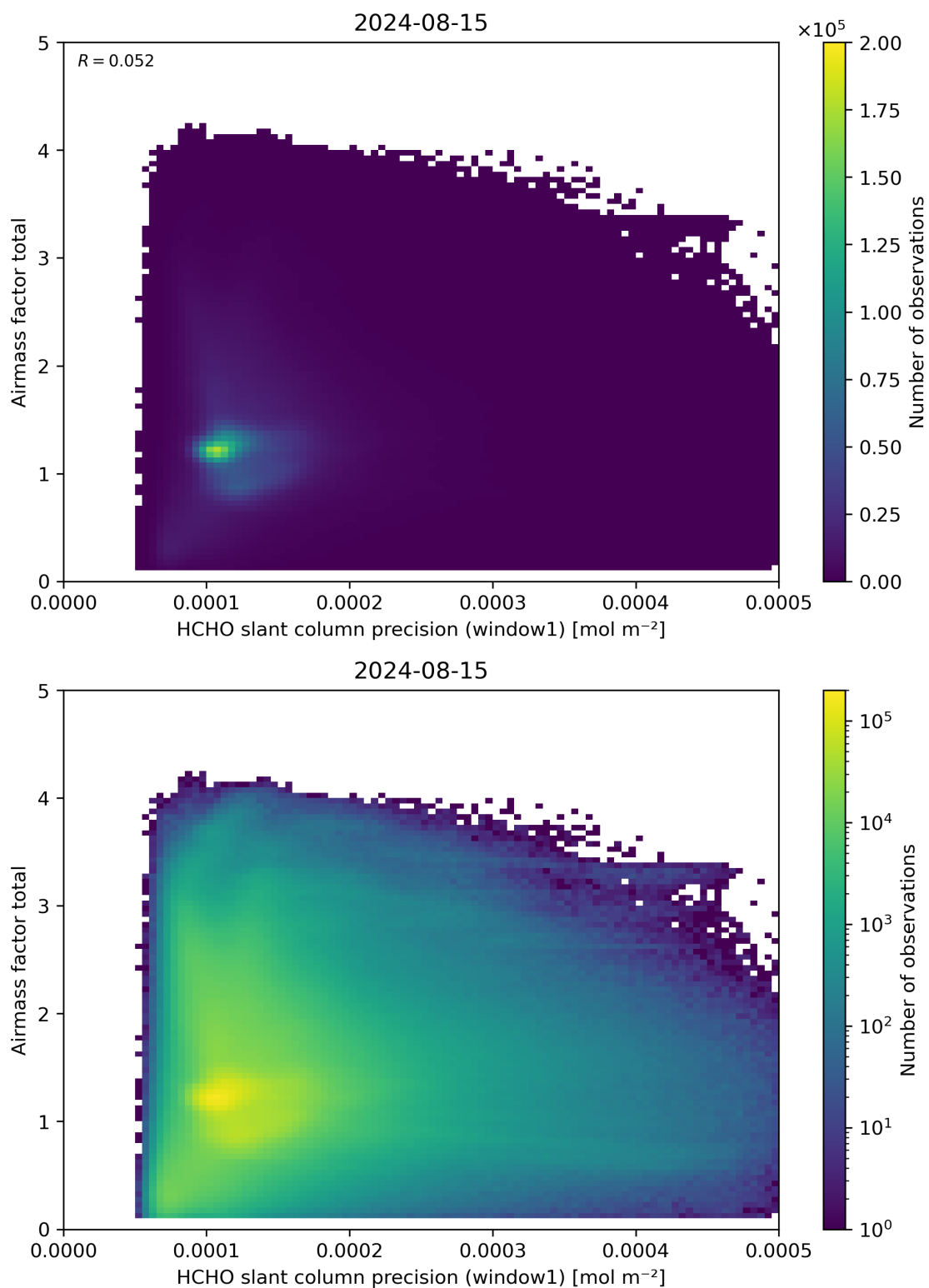
Figure 94: Scatter density plot of “HCHO slant column precision (window1)” against “Airmass factor total” for 2024-08-14 to 2024-08-16.
