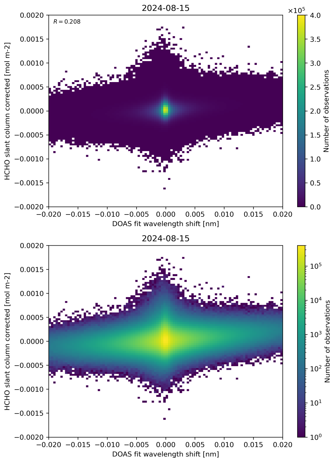
Figure 66: Scatter density plot of “DOAS fit wavelength shift” against “HCHO slant column corrected” for 2024-08-14 to 2024-08-16.
