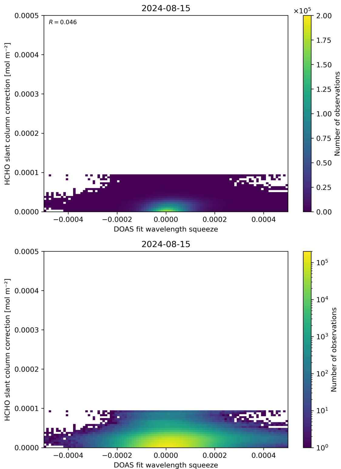
Figure 70: Scatter density plot of “DOAS fit wavelength squeeze” against “HCHO slant column correction” for 2024-08-14 to 2024-08-16.
