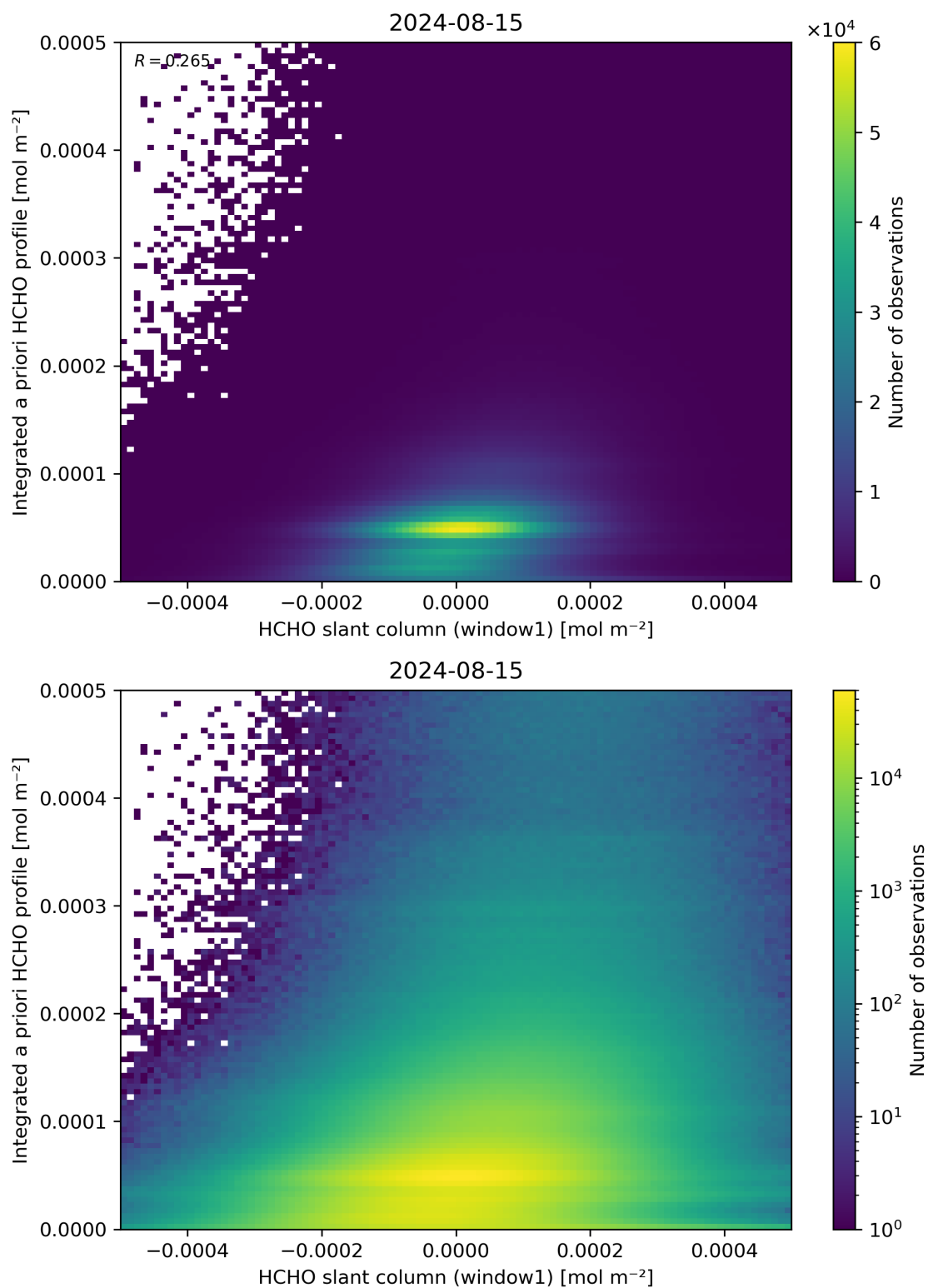
Figure 87: Scatter density plot of “HCHO slant column (window1)” against “Integrated a priori HCHO profile” for 2024-08-14 to 2024-08-16.
