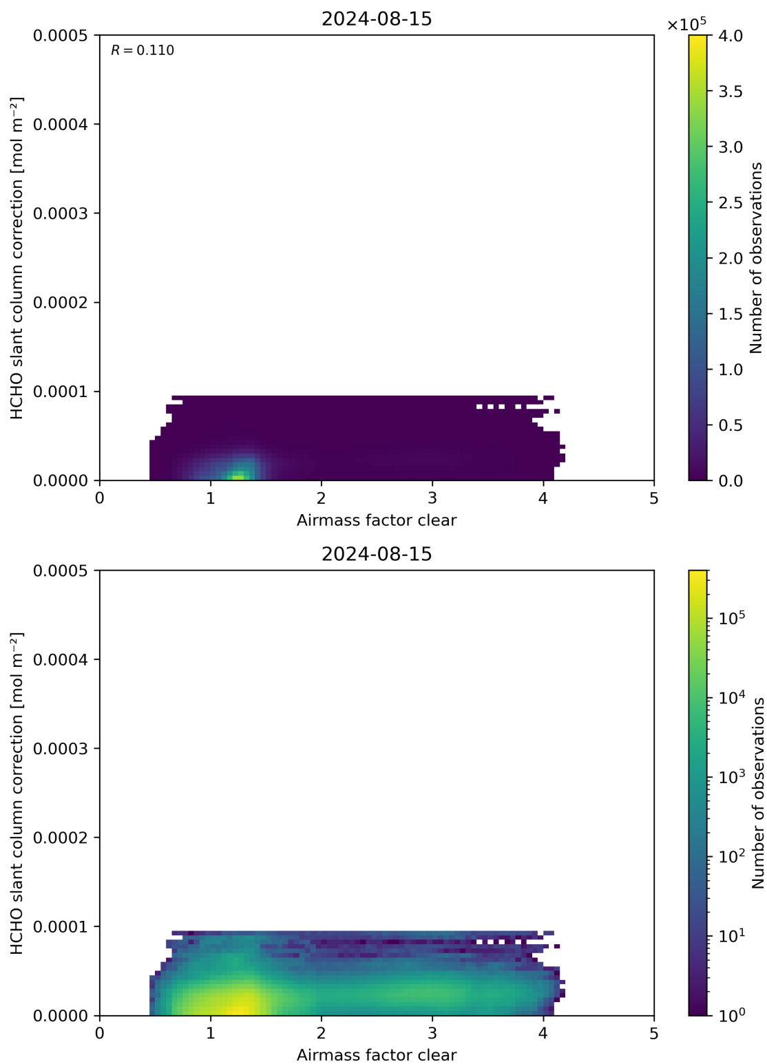
Figure 75: Scatter density plot of “Airmass factor clear” against “HCHO slant column correction” for 2024-08-14 to 2024-08-16.
