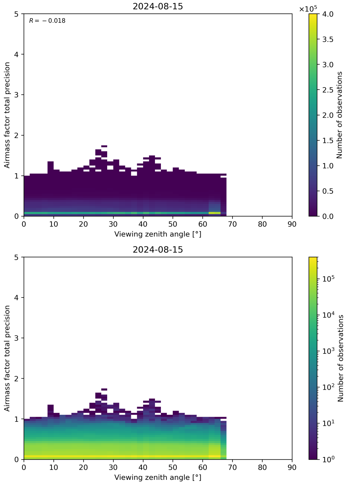
Figure 191: Scatter density plot of “Viewing zenith angle” against “Airmass factor total precision” for 2024-08-14 to 2024-08-16.
