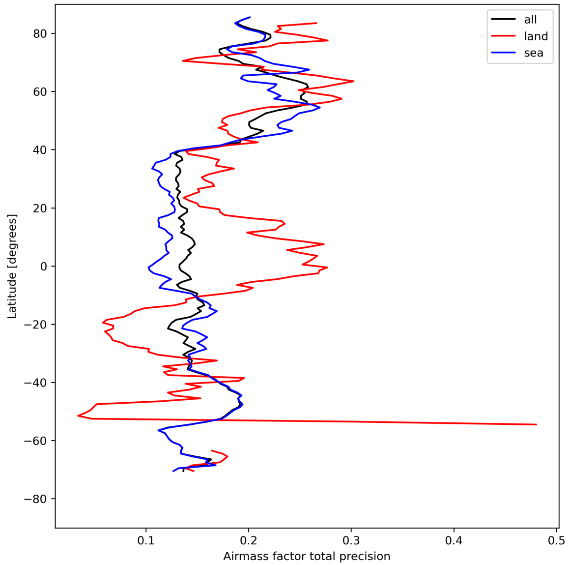
Figure 27: Zonal average of “Airmass factor total precision” for 2024-08-14 to 2024-08-16.
