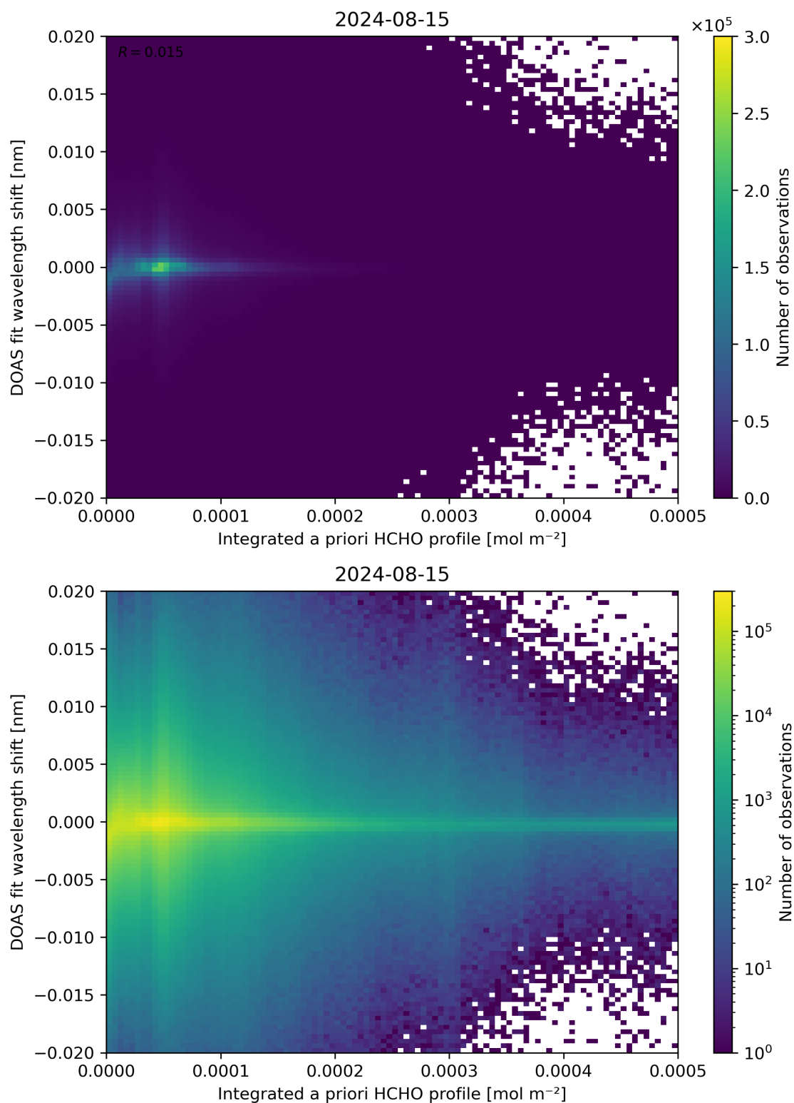
Figure 149: Scatter density plot of “Integrated a priori HCHO profile” against “DOAS fit wavelength shift” for 2024-08-14 to 2024-08-16.
