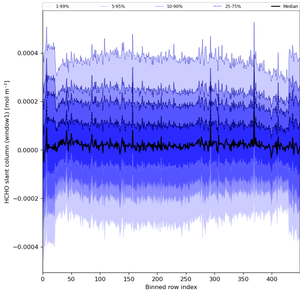
Figure 52: Along track statistics of “HCHO slant column (window1)” for 2024-08-14 to 2024-08-16
