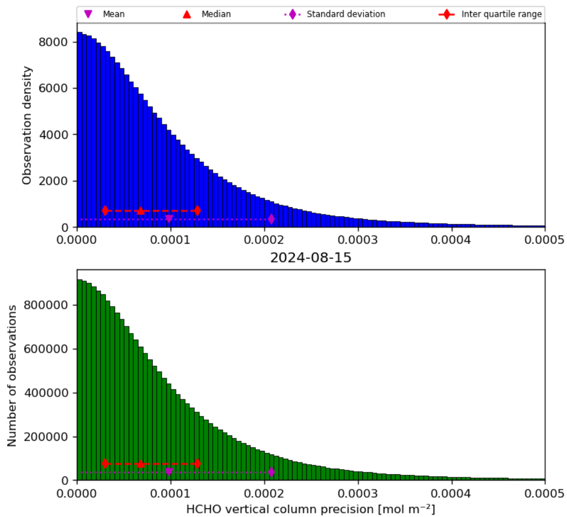
Figure 36: Histogram of “HCHO vertical column precision” for 2024-08-14 to 2024-08-16
