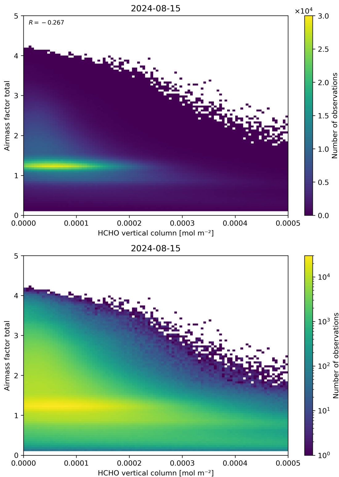
Figure 131: Scatter density plot of “HCHO vertical column” against “Airmass factor total” for 2024-08-14 to 2024-08-16.
