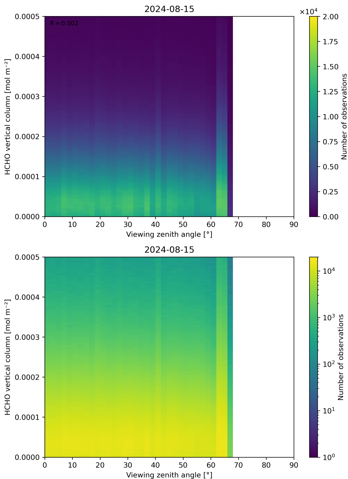
Figure 192: Scatter density plot of “Viewing zenith angle” against “HCHO vertical column” for 2024-08-14 to 2024-08-16.
