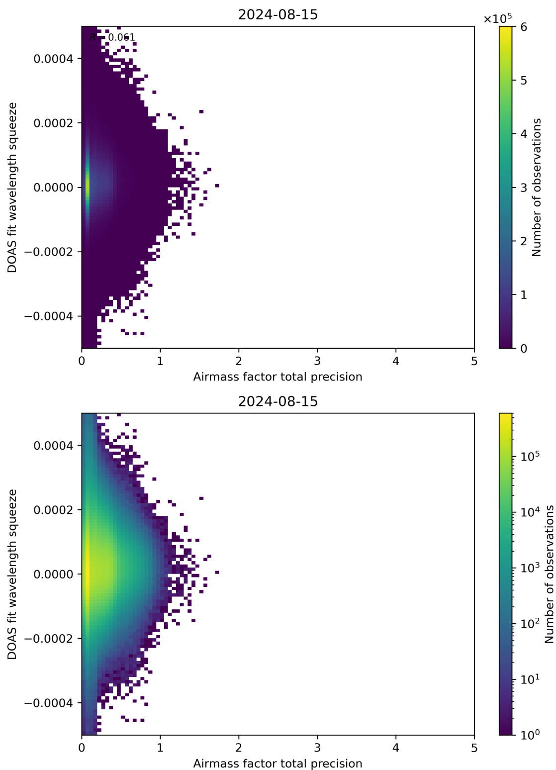
Figure 107: Scatter density plot of “Airmass factor total precision” against “DOAS fit wavelength squeeze” for 2024-08-14 to 2024-08-16.
