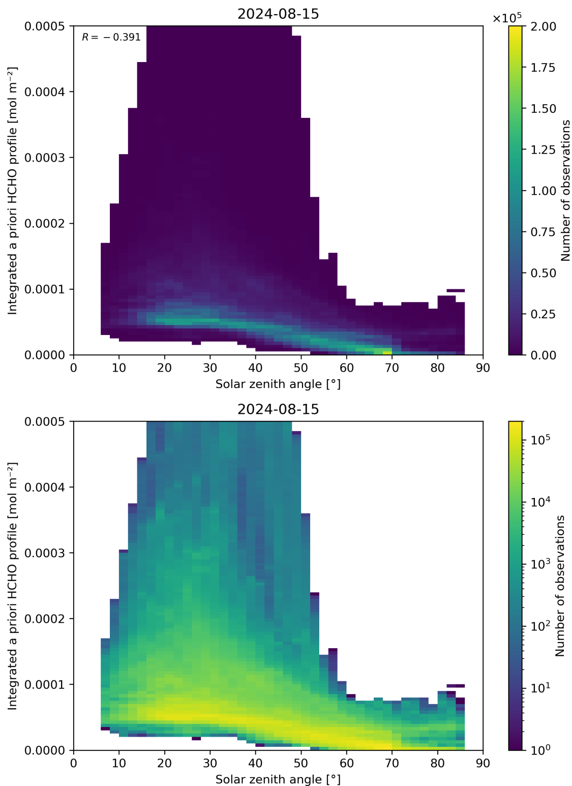
Figure 180: Scatter density plot of “Solar zenith angle” against “Integrated a priori HCHO profile” for 2024-08-14 to 2024-08-16.
