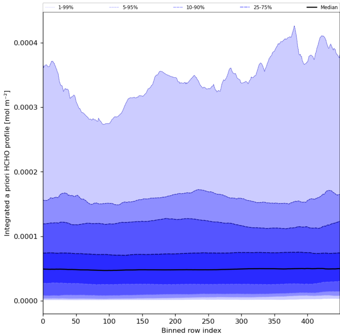
Figure 57: Along track statistics of “Integrated a priori HCHO profile” for 2024-08-14 to 2024-08-16
