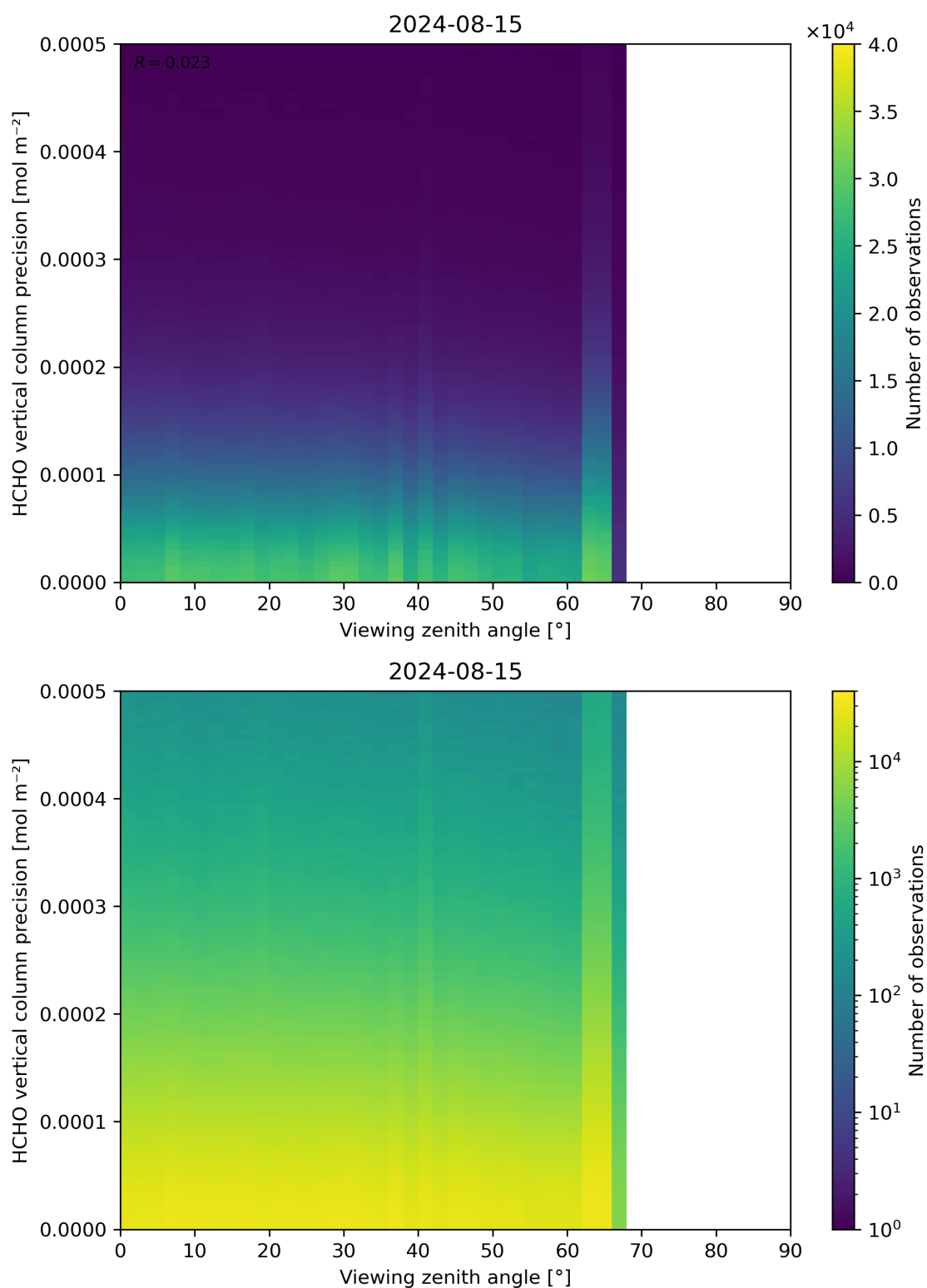
Figure 194: Scatter density plot of “Viewing zenith angle” against “HCHO vertical column precision” for 2024-08-14 to 2024-08-16.
