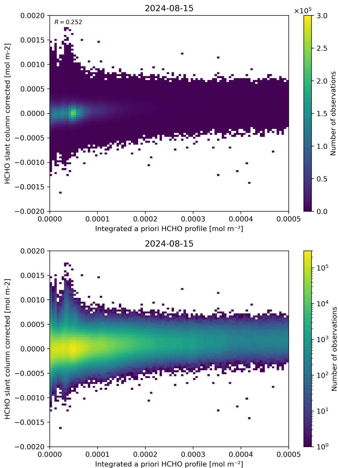
Figure 151: Scatter density plot of “Integrated a priori HCHO profile” against “HCHO slant column corrected” for 2024-08-14 to 2024-08-16.
