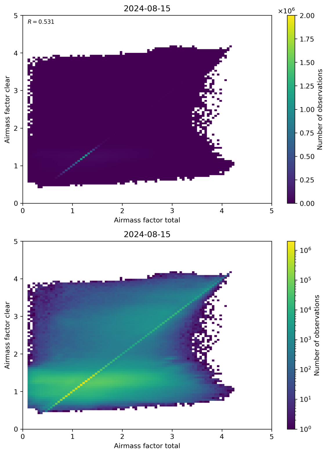
Figure 100: Scatter density plot of “Airmass factor total” against “Airmass factor clear” for 2024-08-14 to 2024-08-16.
