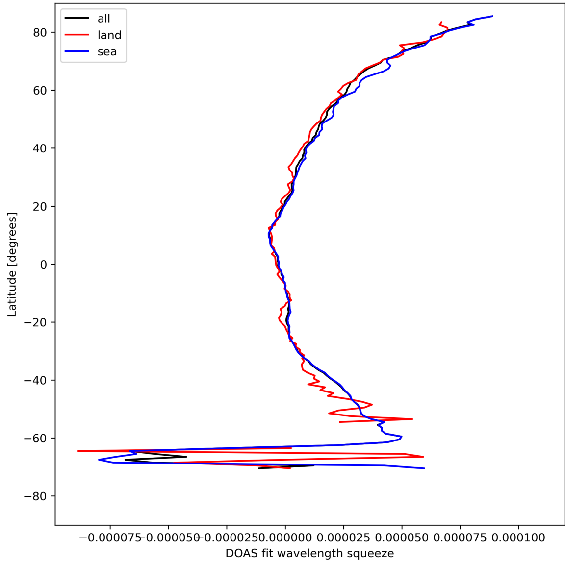
Figure 31: Zonal average of “DOAS fit wavelength squeeze” for 2024-08-14 to 2024-08-16.
