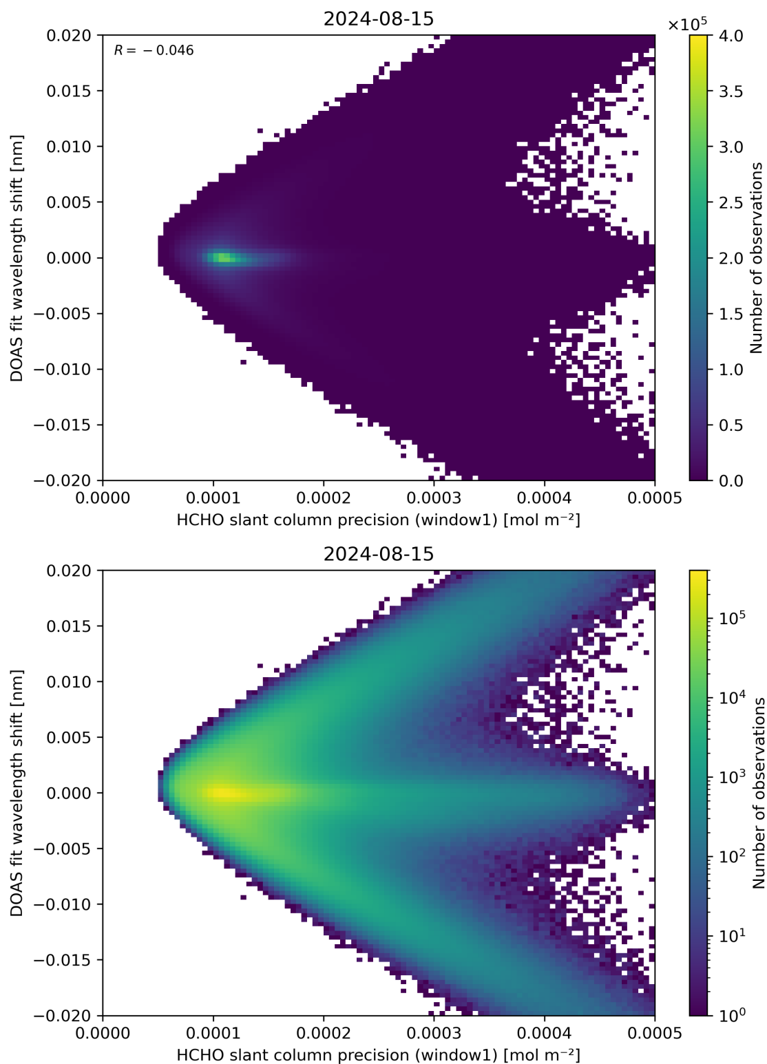
Figure 89: Scatter density plot of “HCHO slant column precision (window1)” against “DOAS fit wavelength shift” for 2024-08-14 to 2024-08-16.
