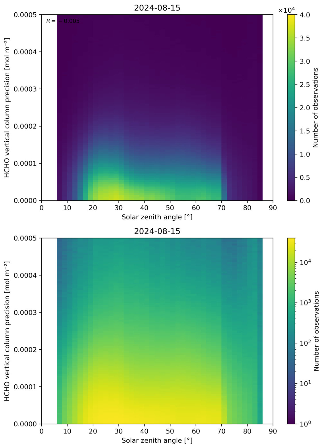
Figure 179: Scatter density plot of “Solar zenith angle” against “HCHO vertical column precision” for 2024-08-14 to 2024-08-16.
