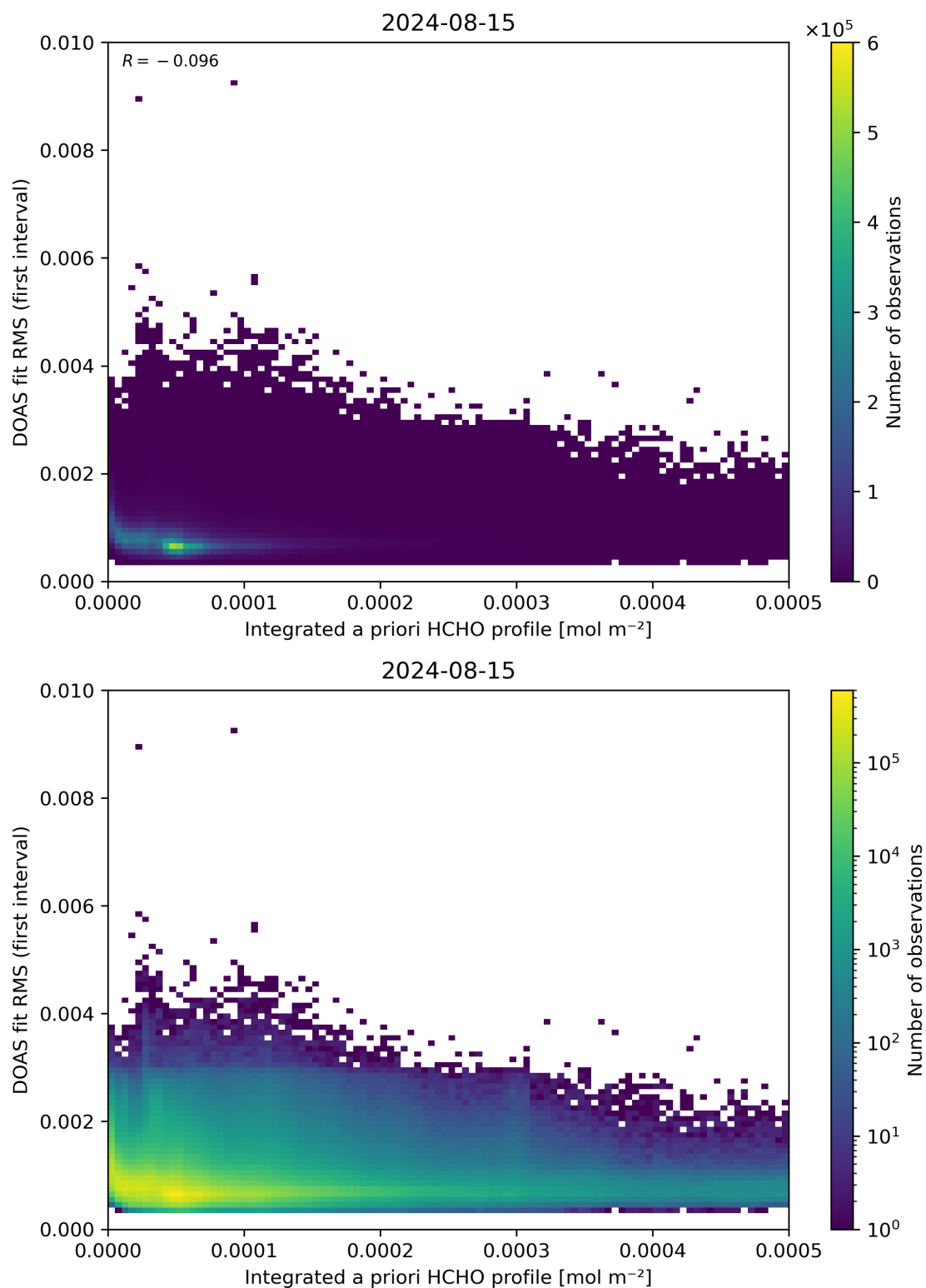
Figure 148: Scatter density plot of “Integrated a priori HCHO profile” against “DOAS fit RMS (first interval)” for 2024-08-14 to 2024-08-16.
