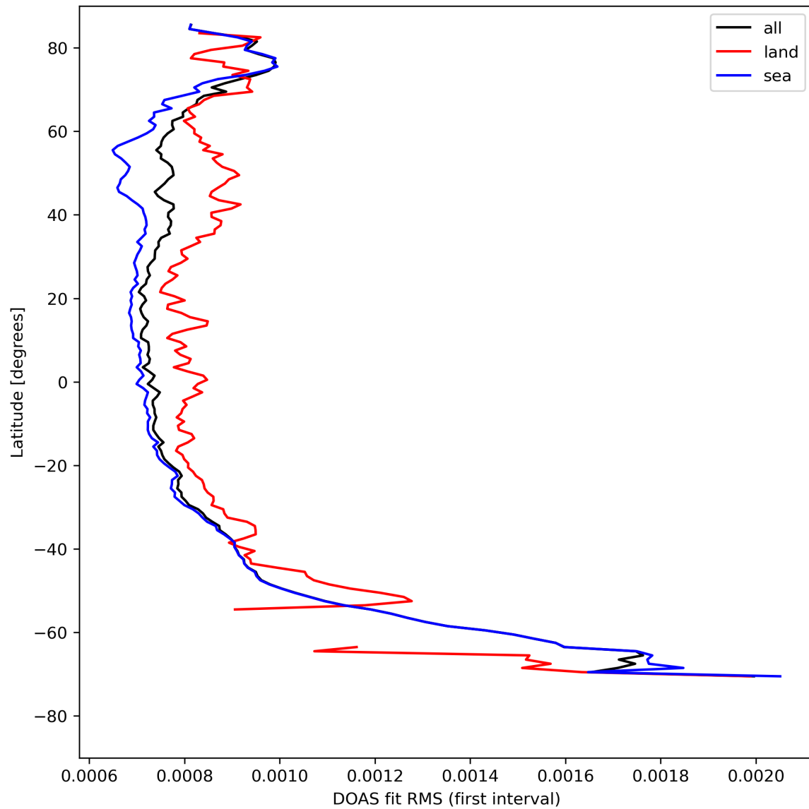
Figure 32: Zonal average of “DOAS fit RMS (first interval)” for 2024-08-14 to 2024-08-16.
