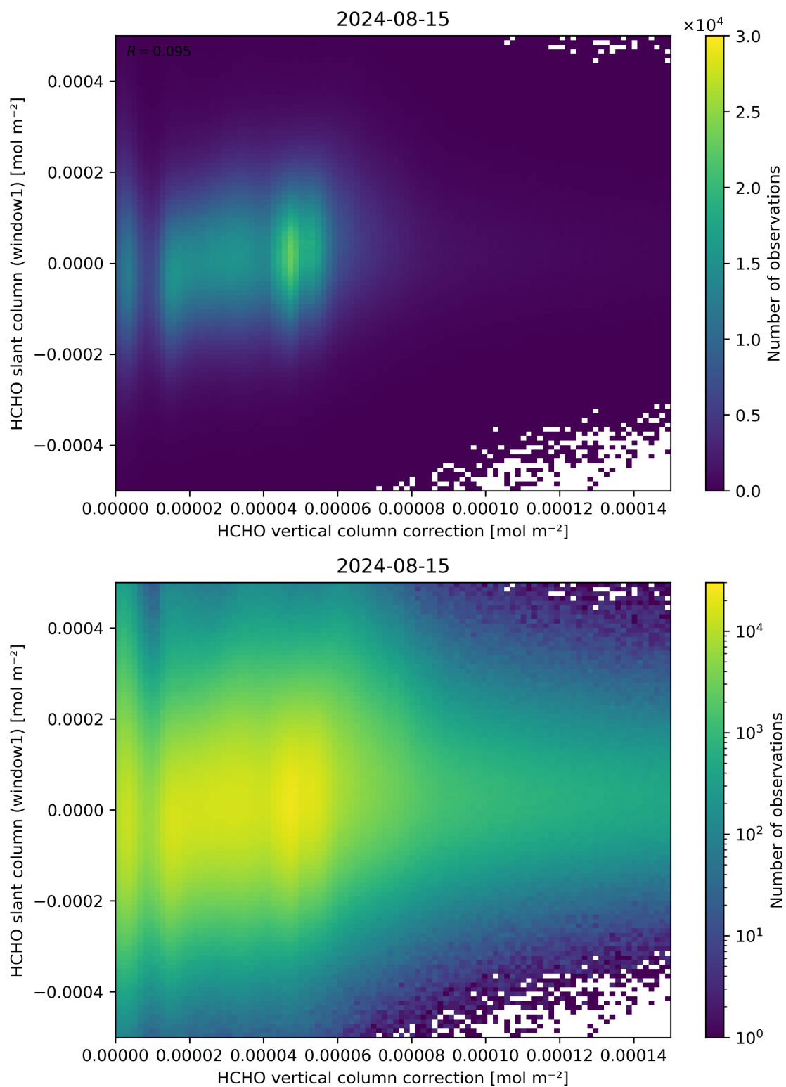
Figure 118: Scatter density plot of “HCHO vertical column correction” against “HCHO slant column (window1)” for 2024-08-14 to 2024-08-16.
