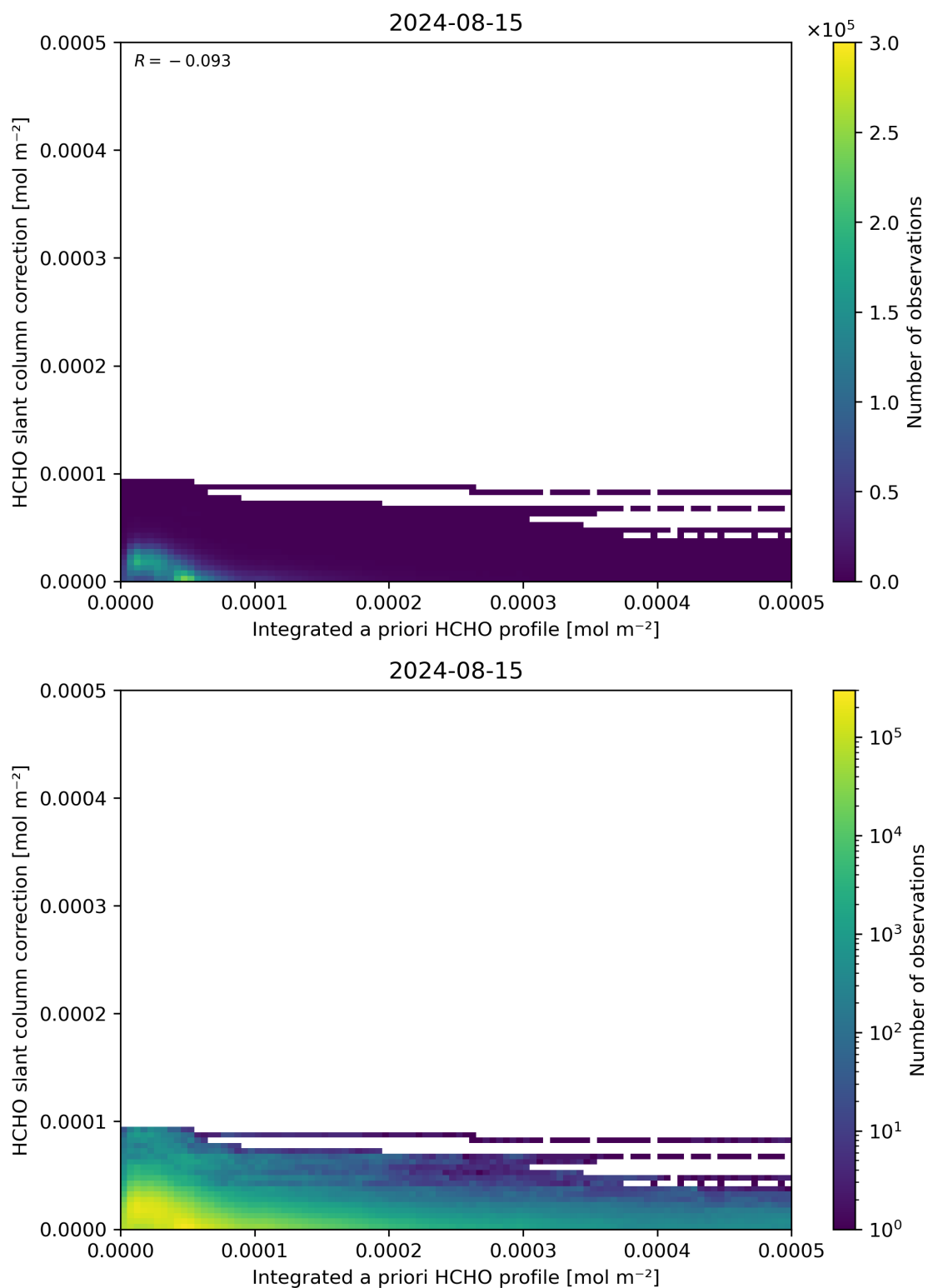
Figure 152: Scatter density plot of “Integrated a priori HCHO profile” against “HCHO slant column correction” for 2024-08-14 to 2024-08-16.
