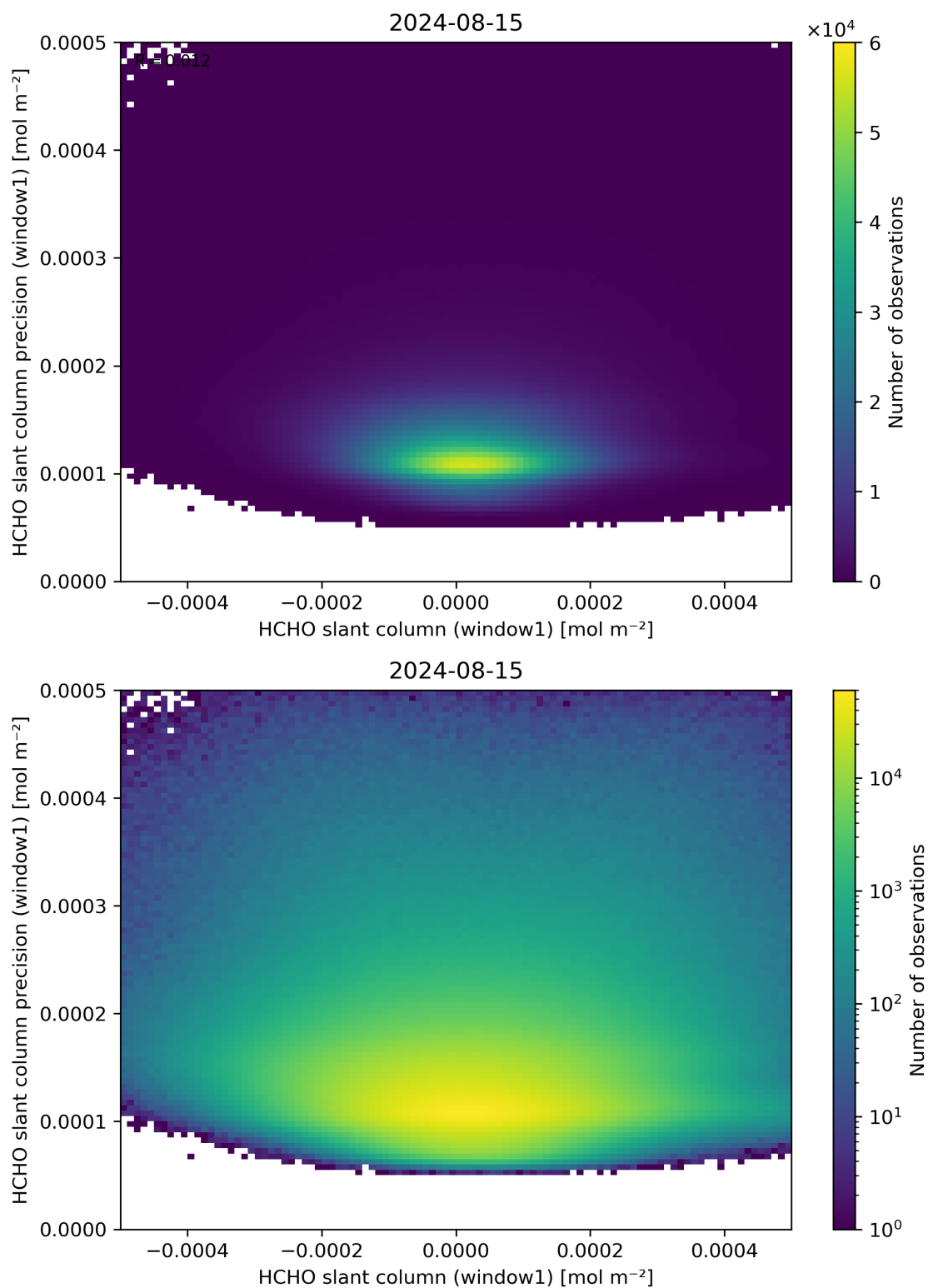
Figure 84: Scatter density plot of “HCHO slant column (window1)” against “HCHO slant column precision (window1)” for 2024-08-14 to 2024-08-16.
