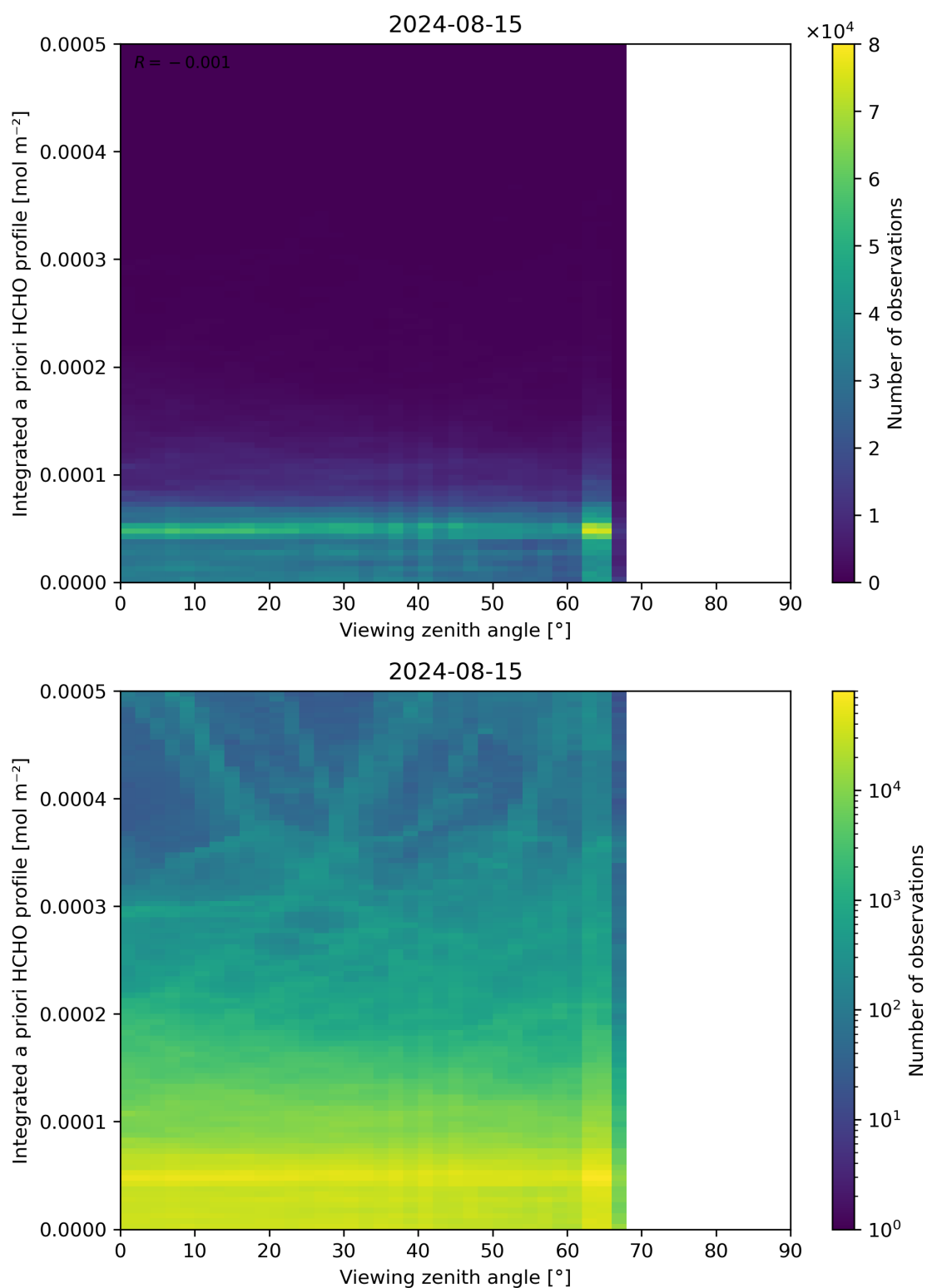
Figure 195: Scatter density plot of “Viewing zenith angle” against “Integrated a priori HCHO profile” for 2024-08-14 to 2024-08-16.
