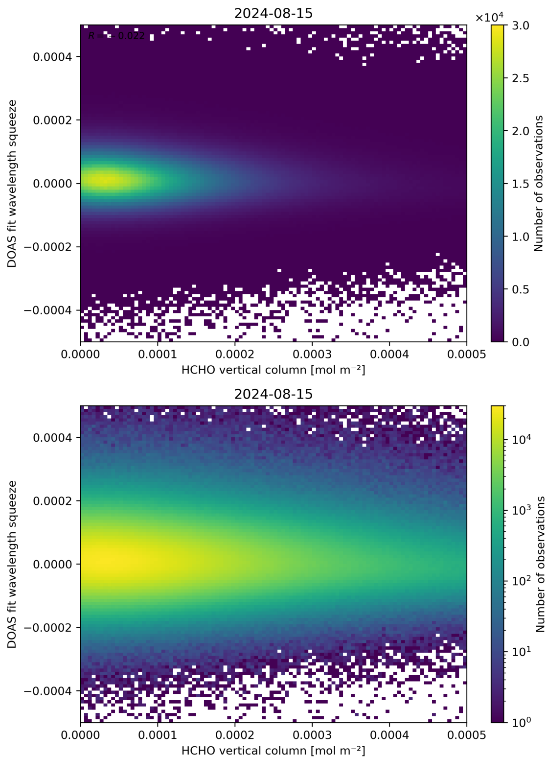
Figure 125: Scatter density plot of “HCHO vertical column” against “DOAS fit wavelength squeeze” for 2024-08-14 to 2024-08-16.
