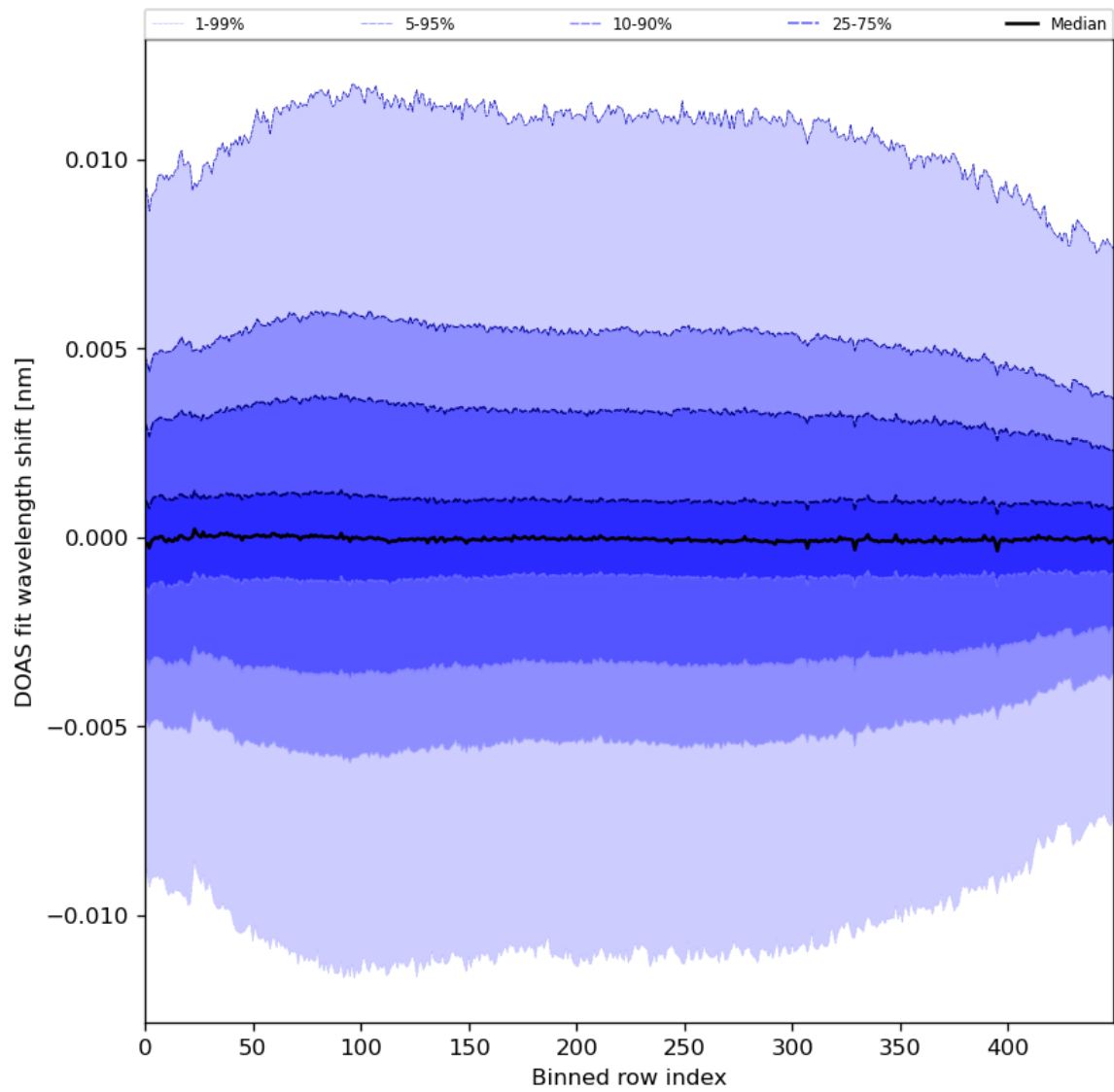
Figure 58: Along track statistics of “DOAS fit wavelength shift” for 2024-08-14 to 2024-08-16
