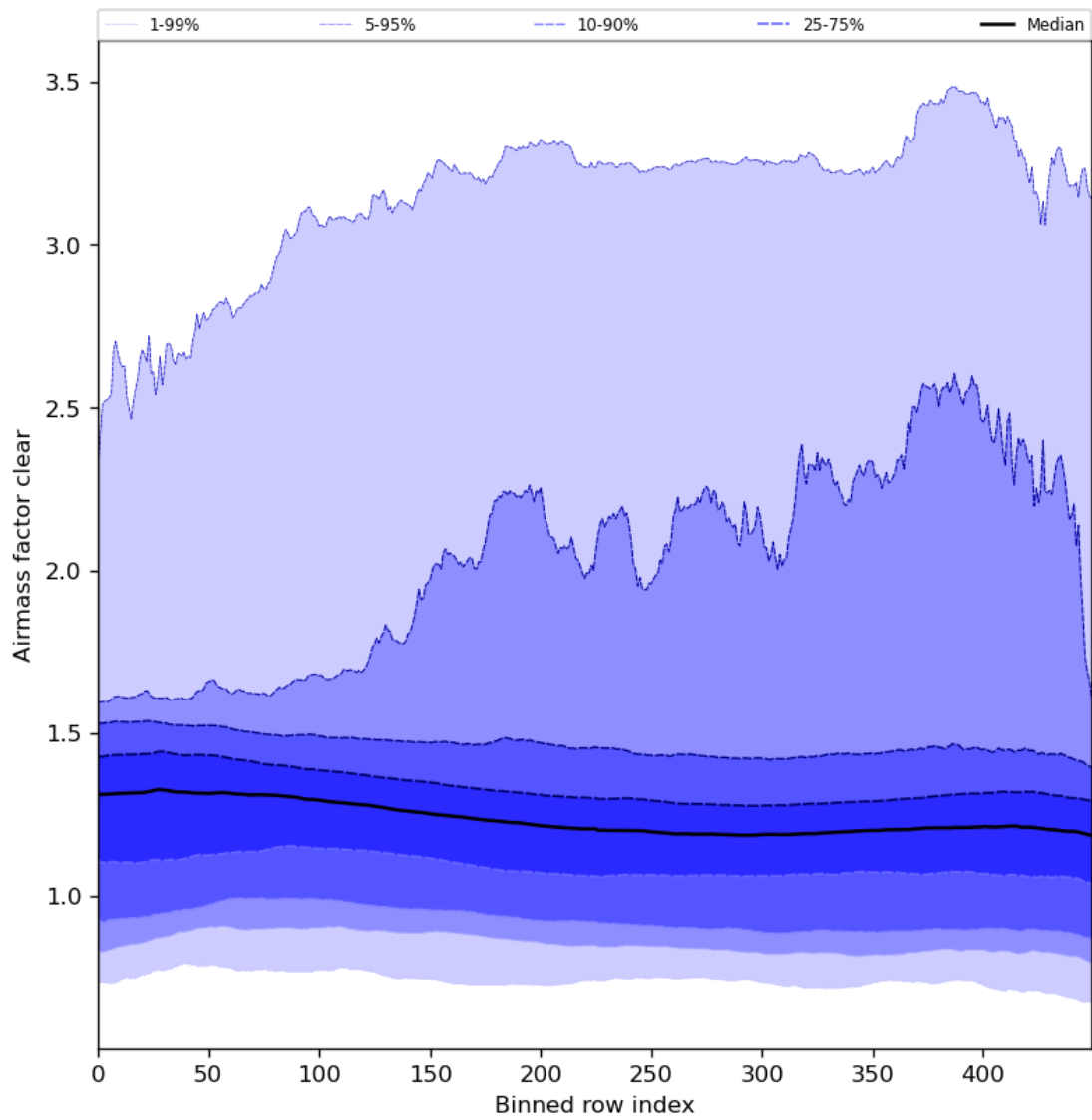
Figure 56: Along track statistics of “Airmass factor clear” for 2024-08-14 to 2024-08-16
