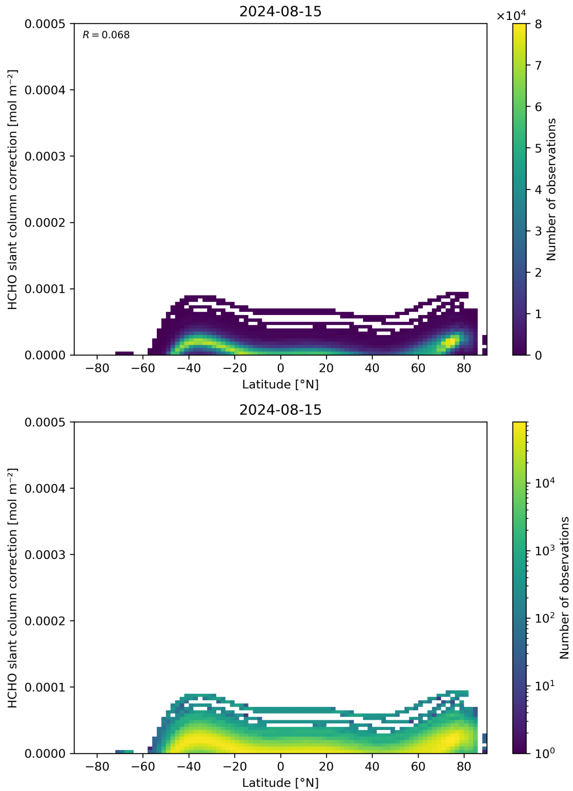
Figure 158: Scatter density plot of “Latitude” against “HCHO slant column correction” for 2024-08-14 to 2024-08-16.
