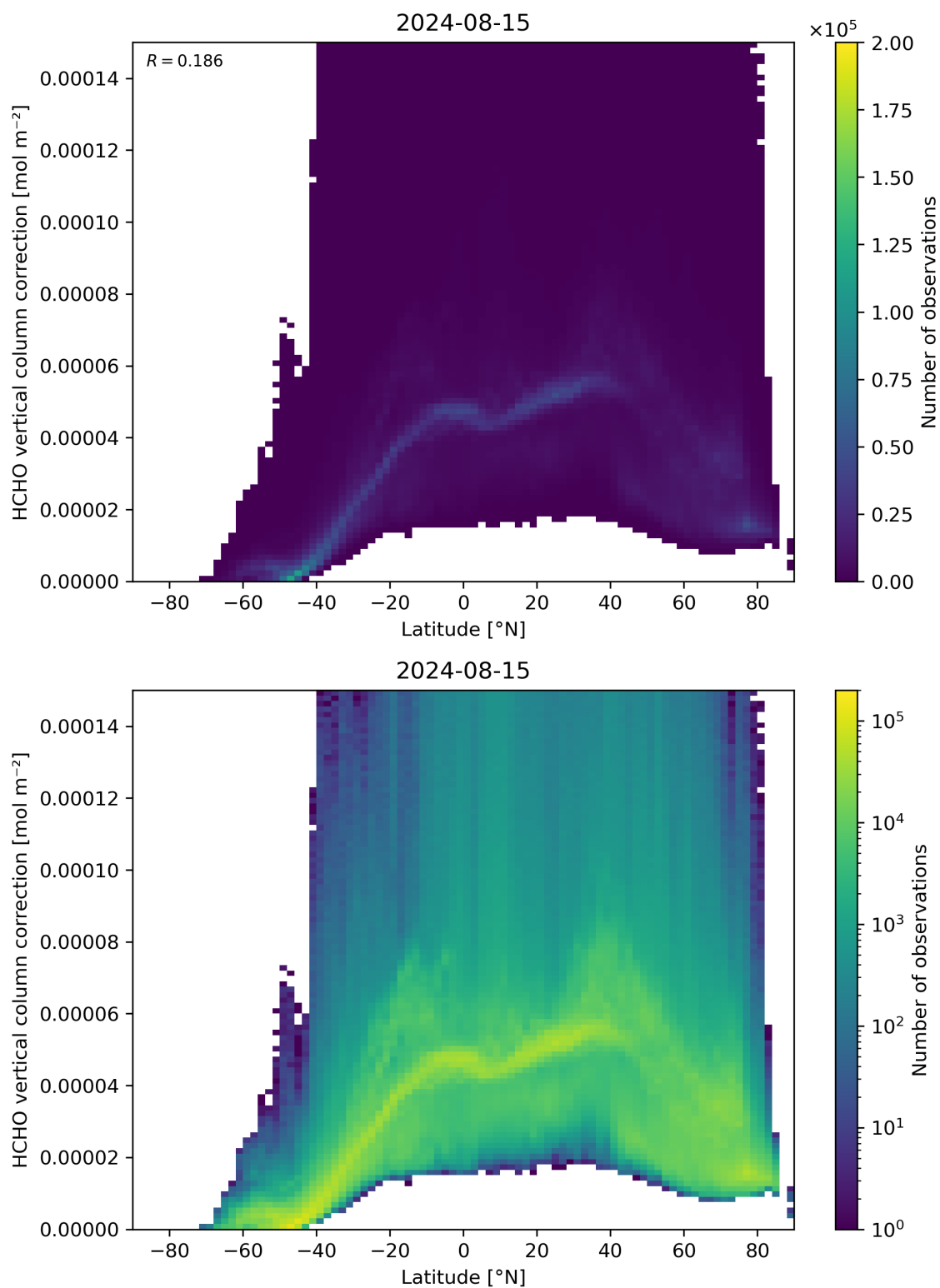
Figure 164: Scatter density plot of “Latitude” against “HCHO vertical column correction” for 2024-08-14 to 2024-08-16.
