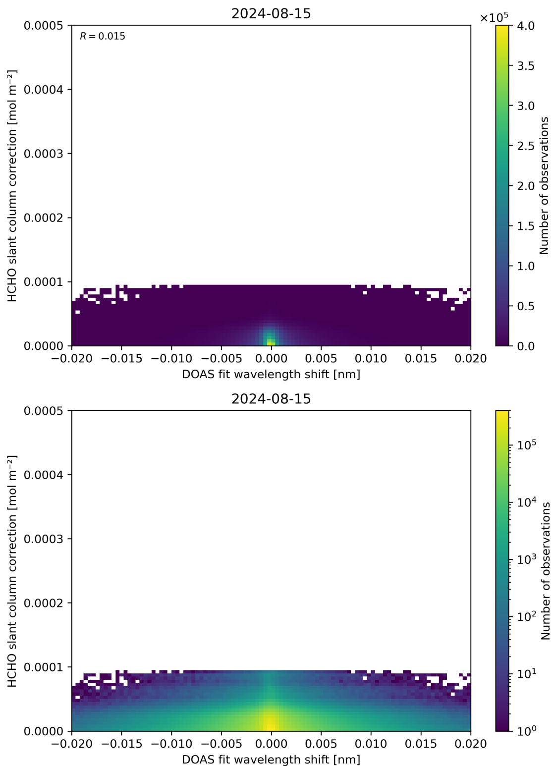
Figure 67: Scatter density plot of “DOAS fit wavelength shift” against “HCHO slant column correction” for 2024-08-14 to 2024-08-16.
