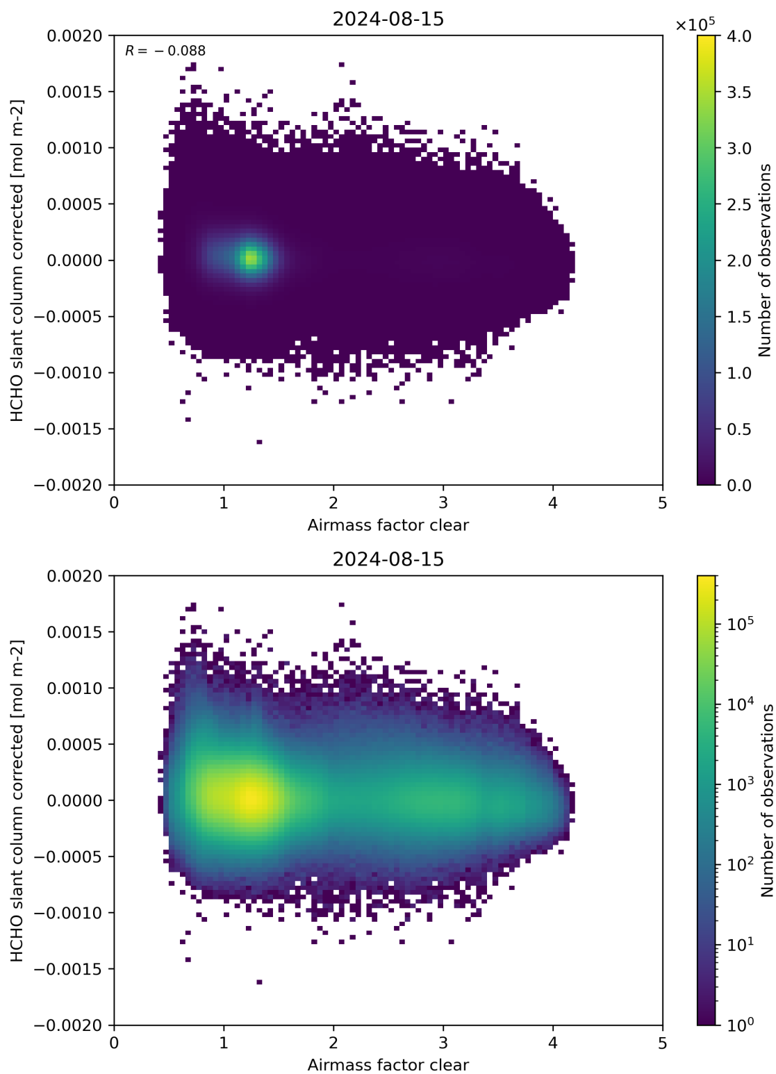
Figure 74: Scatter density plot of “Airmass factor clear” against “HCHO slant column corrected” for 2024-08-14 to 2024-08-16.
