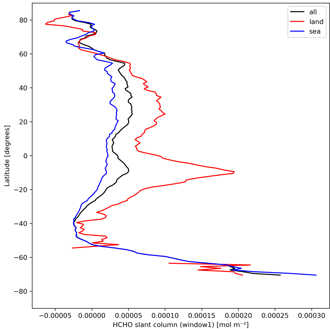
Figure 24: Zonal average of “HCHO slant column (window1)” for 2024-08-14 to 2024-08-16.
