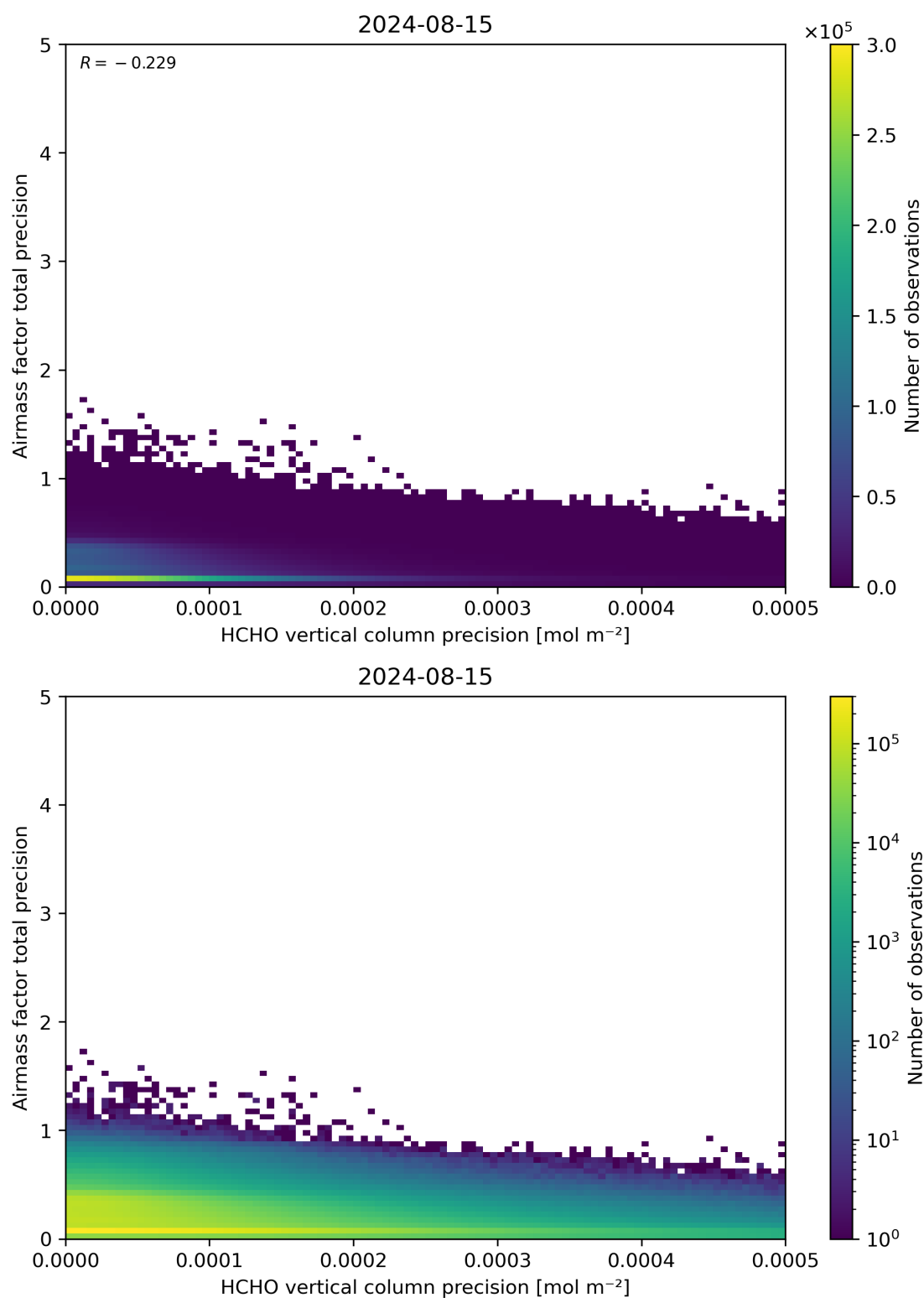
Figure 145: Scatter density plot of “HCHO vertical column precision” against “Airmass factor total precision” for 2024-08-14 to 2024-08-16.
