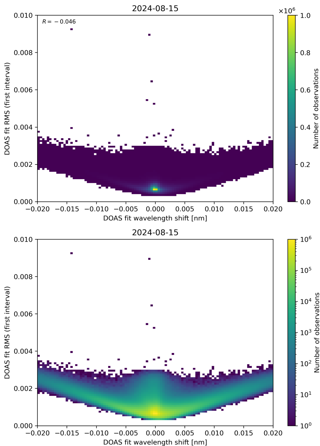
Figure 64: Scatter density plot of “DOAS fit wavelength shift” against “DOAS fit RMS (first interval)” for 2024-08-14 to 2024-08-16.
