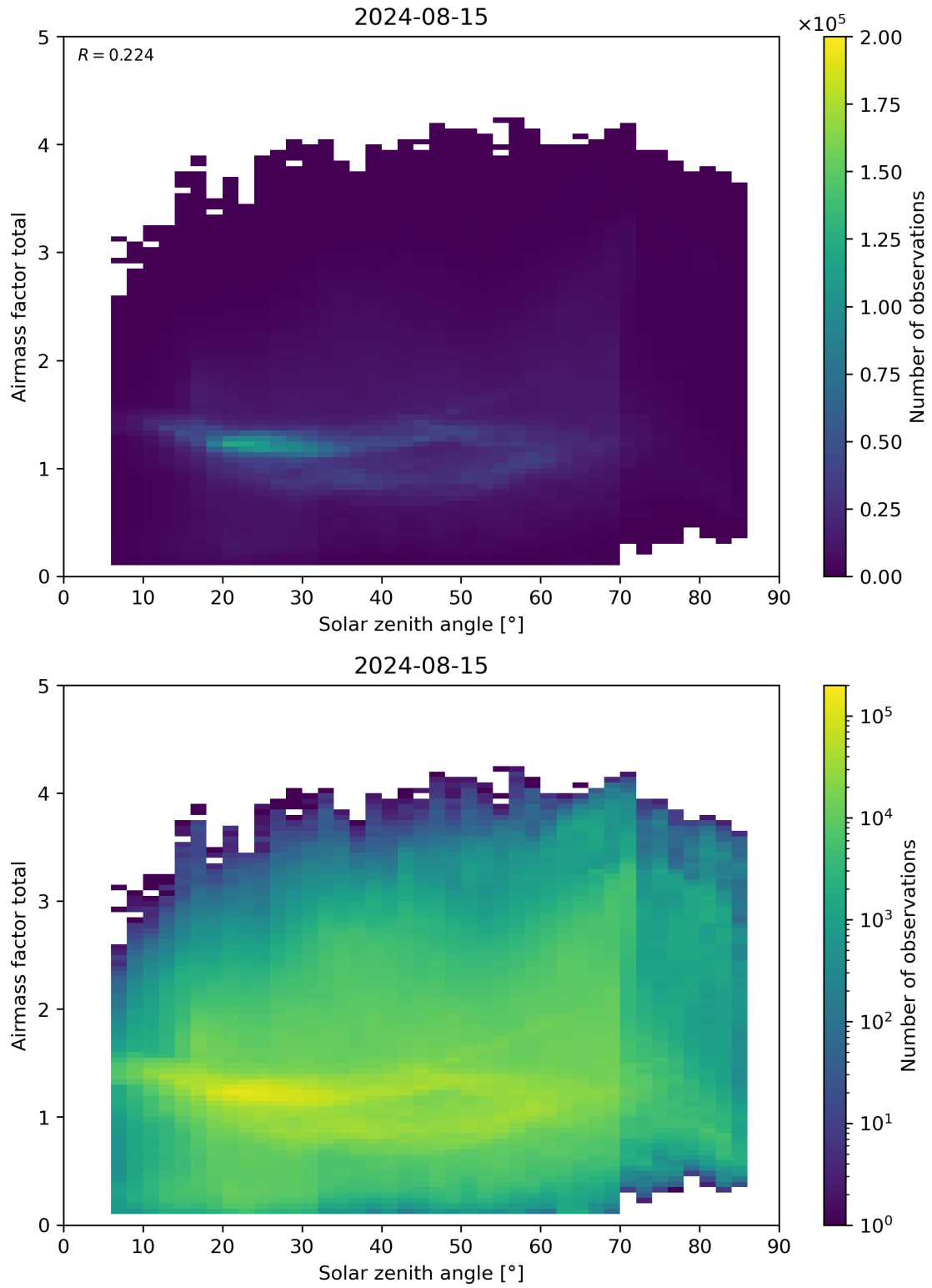
Figure 175: Scatter density plot of “Solar zenith angle” against “Airmass factor total” for 2024-08-14 to 2024-08-16.
