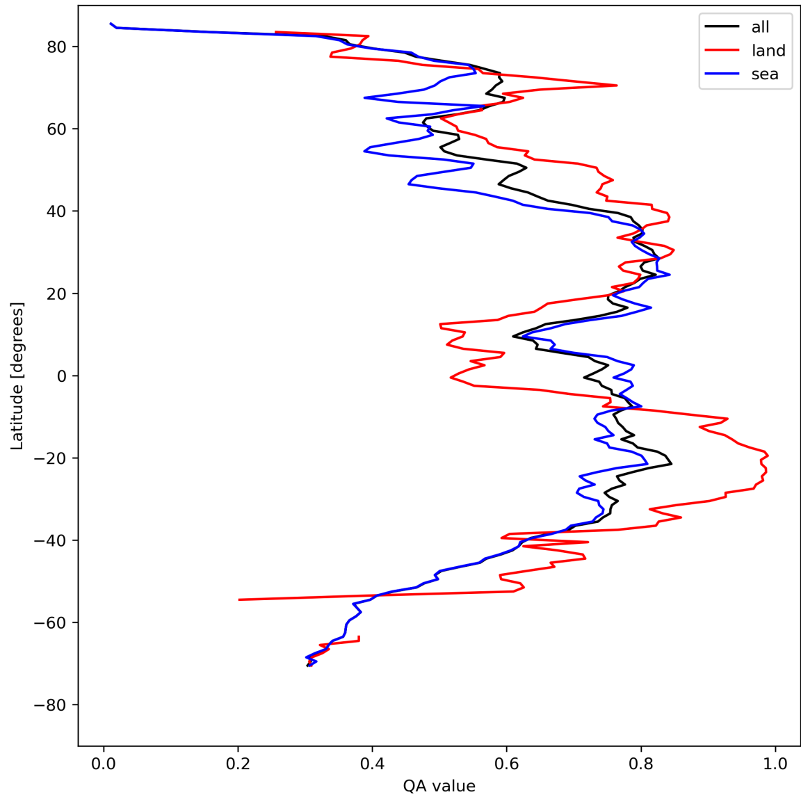
Figure 20: Zonal average of “QA value” for 2024-08-14 to 2024-08-16.
