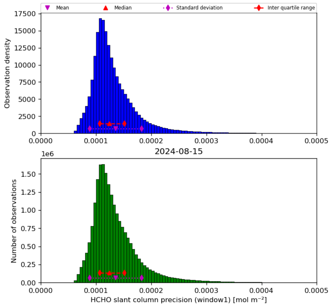
Figure 39: Histogram of “HCHO slant column precision (window1)” for 2024-08-14 to 2024-08-16
