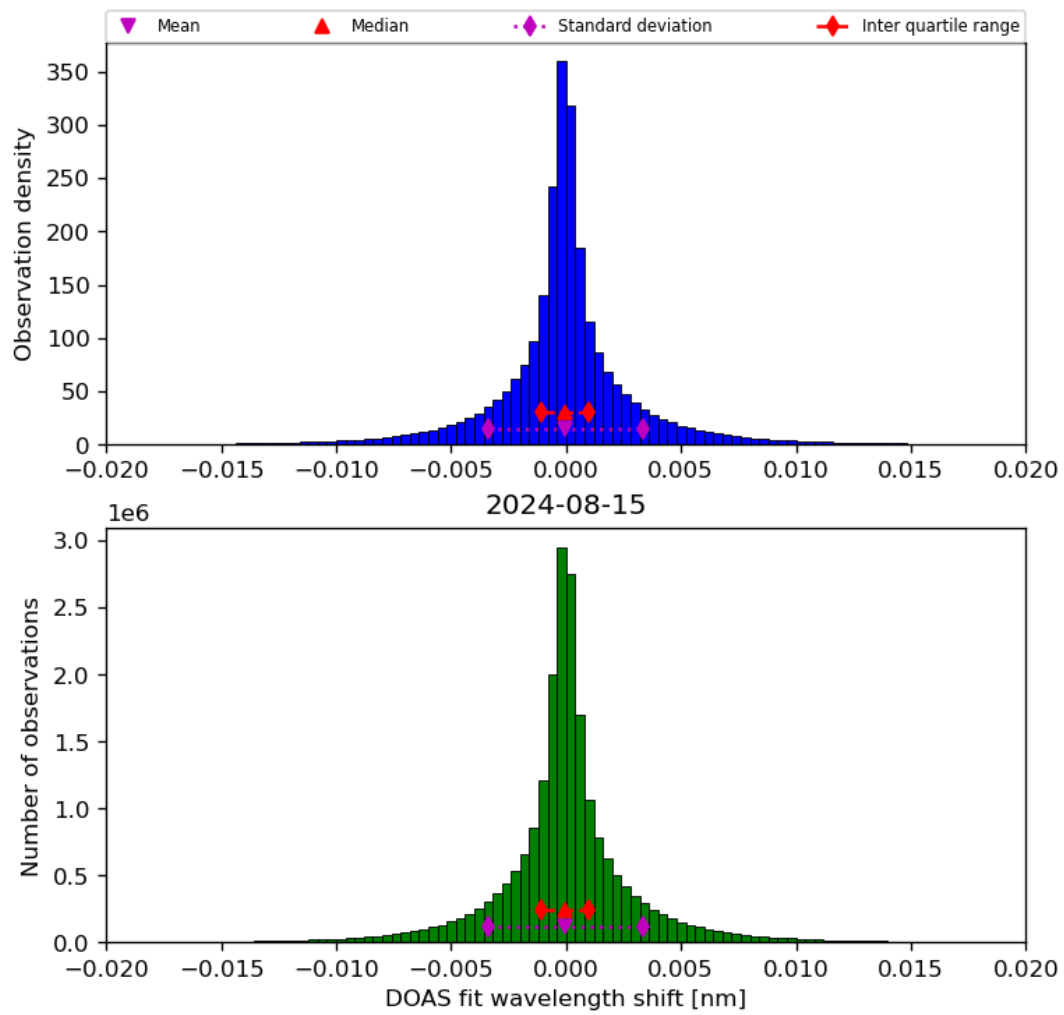
Figure 44: Histogram of “DOAS fit wavelength shift” for 2024-08-14 to 2024-08-16
