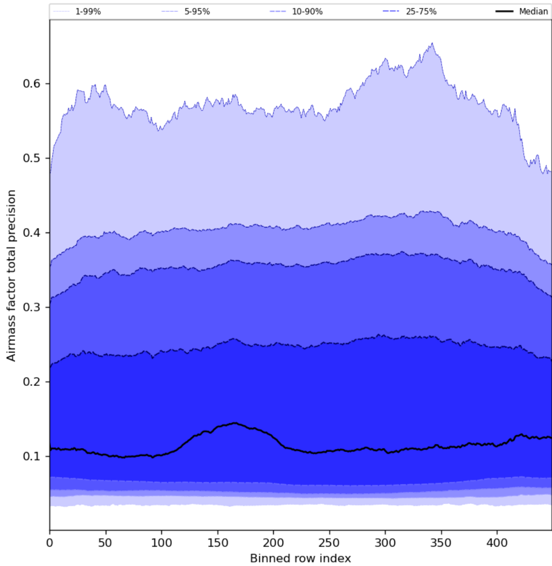
Figure 55: Along track statistics of “Airmass factor total precision” for 2024-08-14 to 2024-08-16
