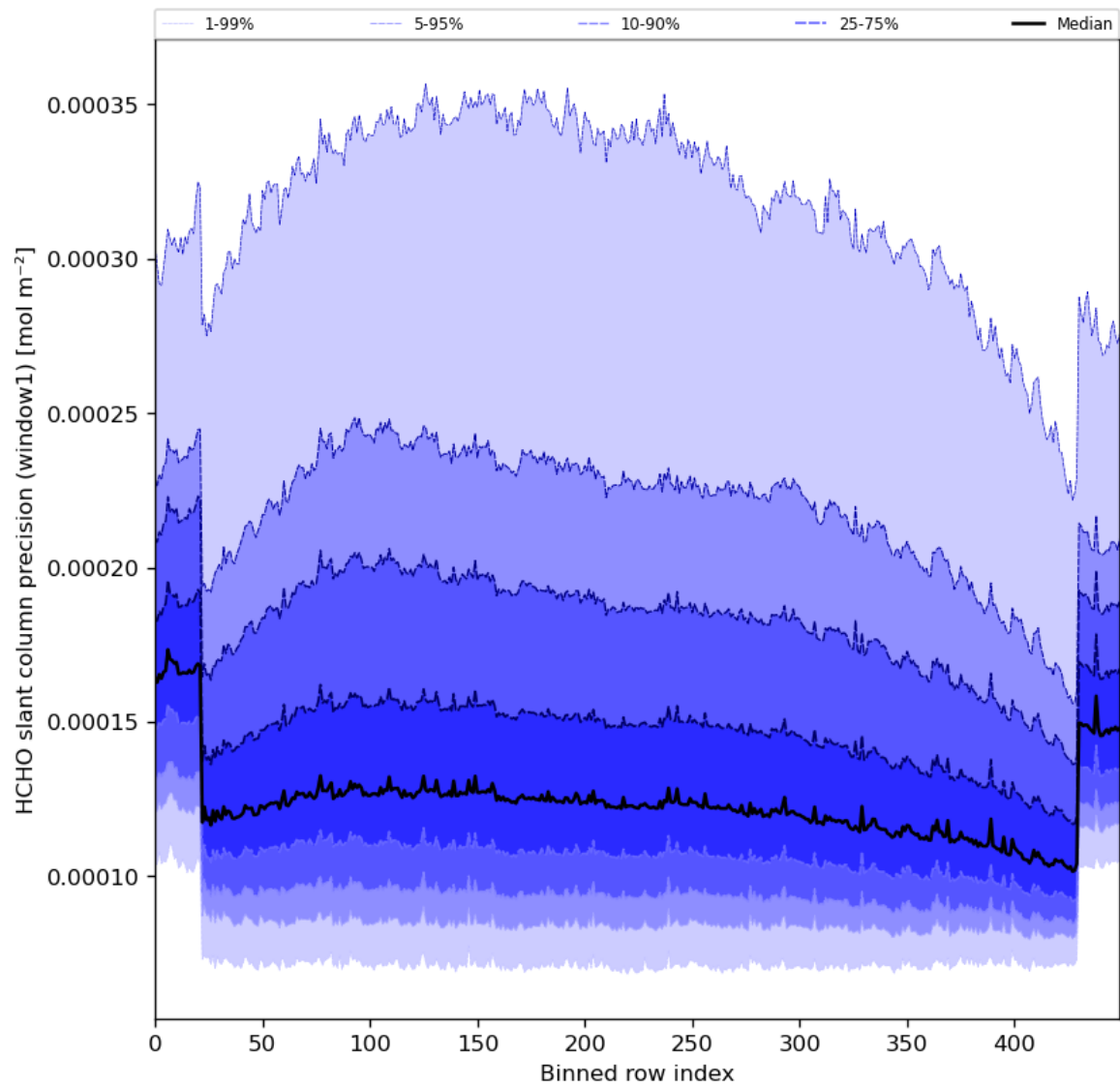
Figure 53: Along track statistics of “HCHO slant column precision (window1)” for 2024-08-14 to 2024-08-16
