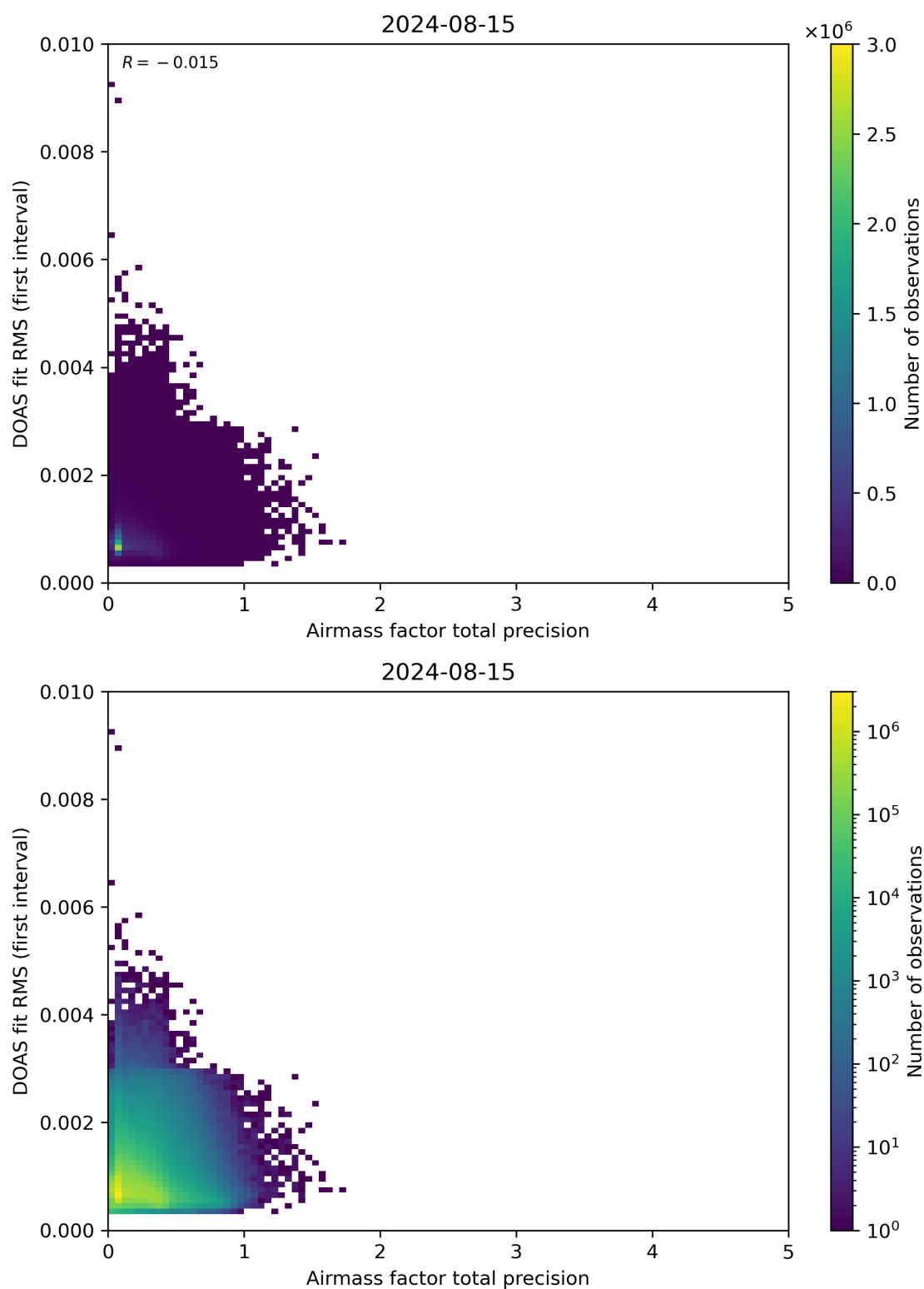
Figure 105: Scatter density plot of “Airmass factor total precision” against “DOAS fit RMS (first interval)” for 2024-08-14 to 2024-08-16.
