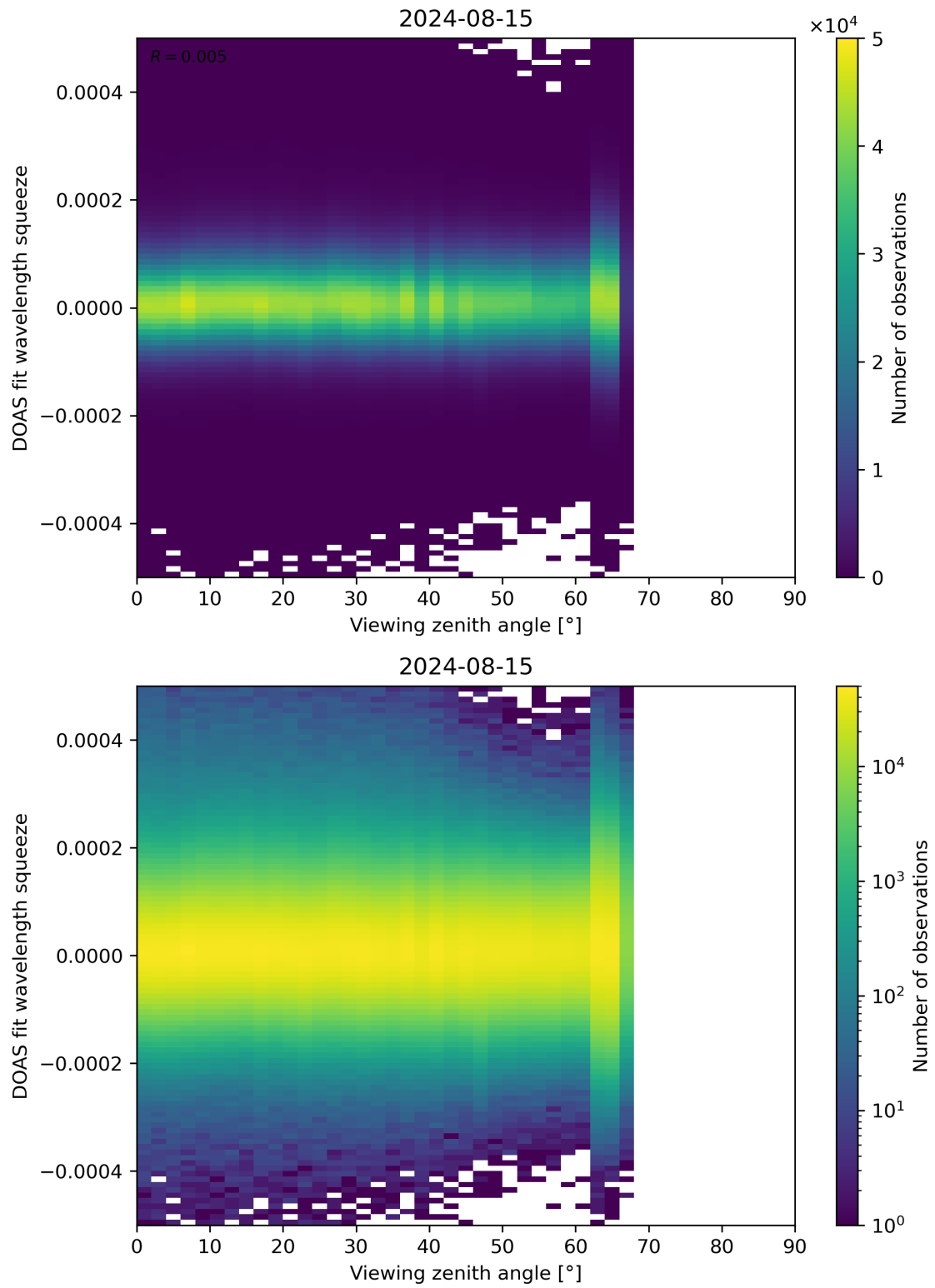
Figure 184: Scatter density plot of “Viewing zenith angle” against “DOAS fit wavelength squeeze” for 2024-08-14 to 2024-08-16.
