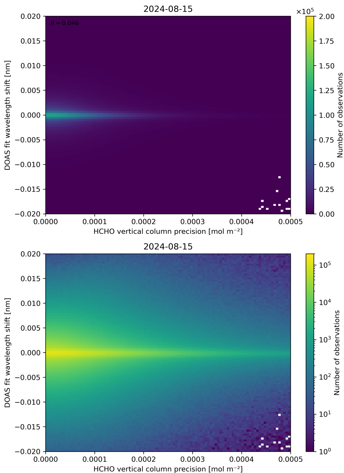
Figure 137: Scatter density plot of “HCHO vertical column precision” against “DOAS fit wavelength shift” for 2024-08-14 to 2024-08-16.
