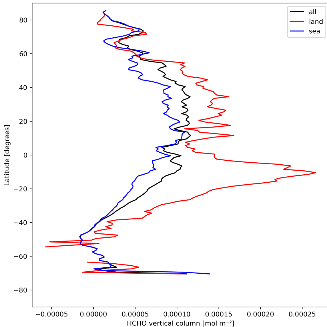
Figure 21: Zonal average of “HCHO vertical column” for 2024-08-14 to 2024-08-16.
