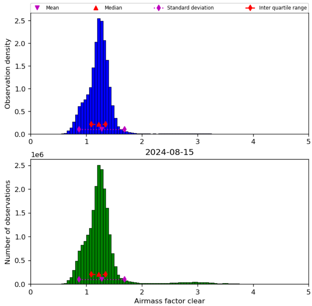
Figure 42: Histogram of “Airmass factor clear” for 2024-08-14 to 2024-08-16
