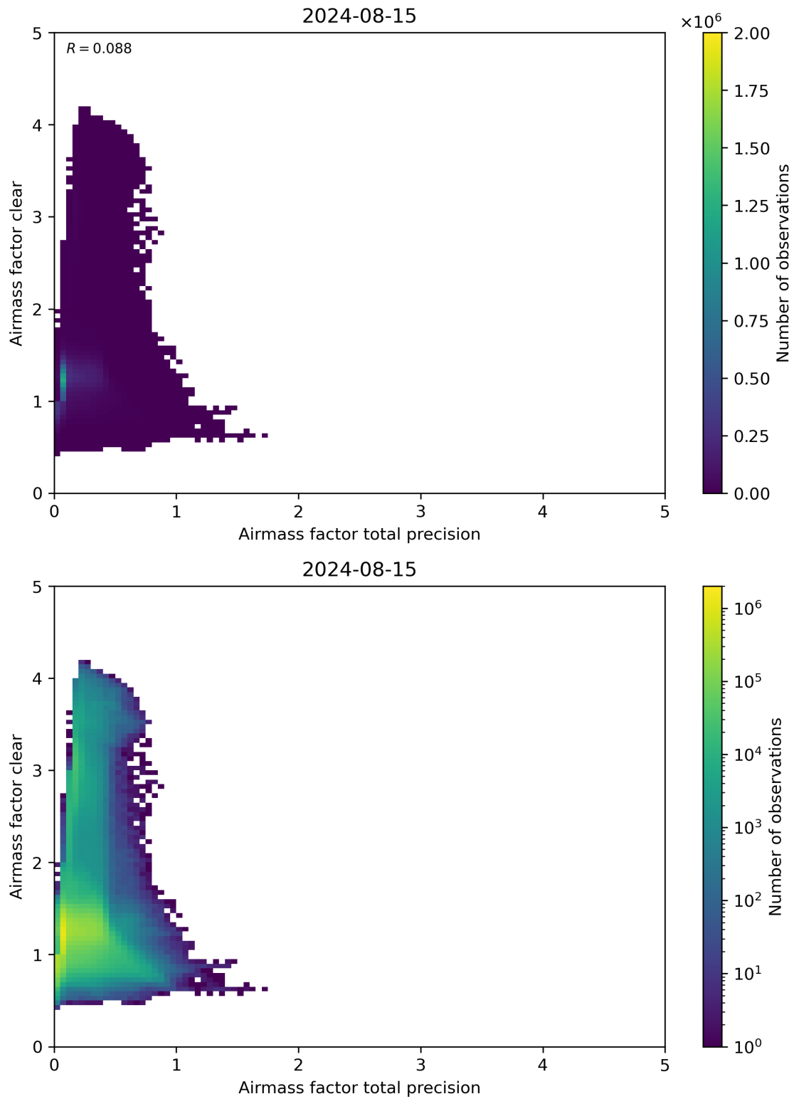
Figure 108: Scatter density plot of “Airmass factor total precision” against “Airmass factor clear” for 2024-08-14 to 2024-08-16.
