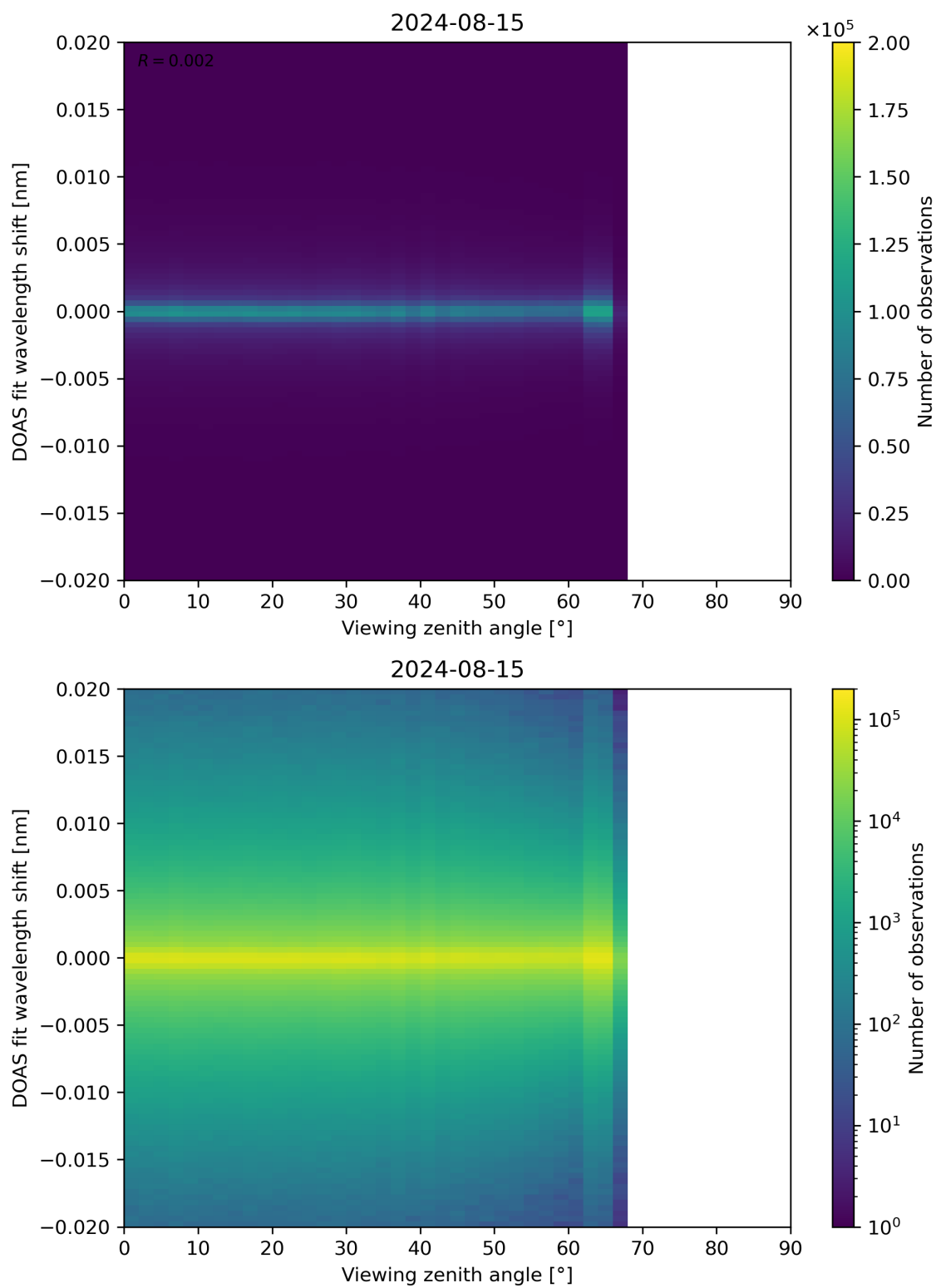
Figure 183: Scatter density plot of “Viewing zenith angle” against “DOAS fit wavelength shift” for 2024-08-14 to 2024-08-16.
