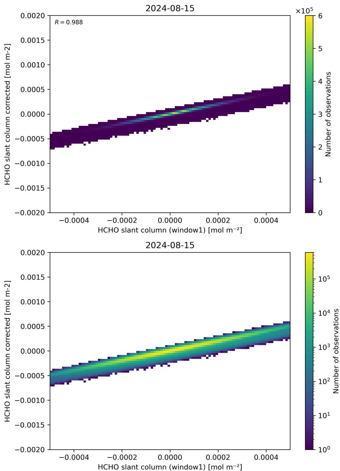
Figure 82: Scatter density plot of “HCHO slant column (window1)” against “HCHO slant column corrected” for 2024-08-14 to 2024-08-16.
