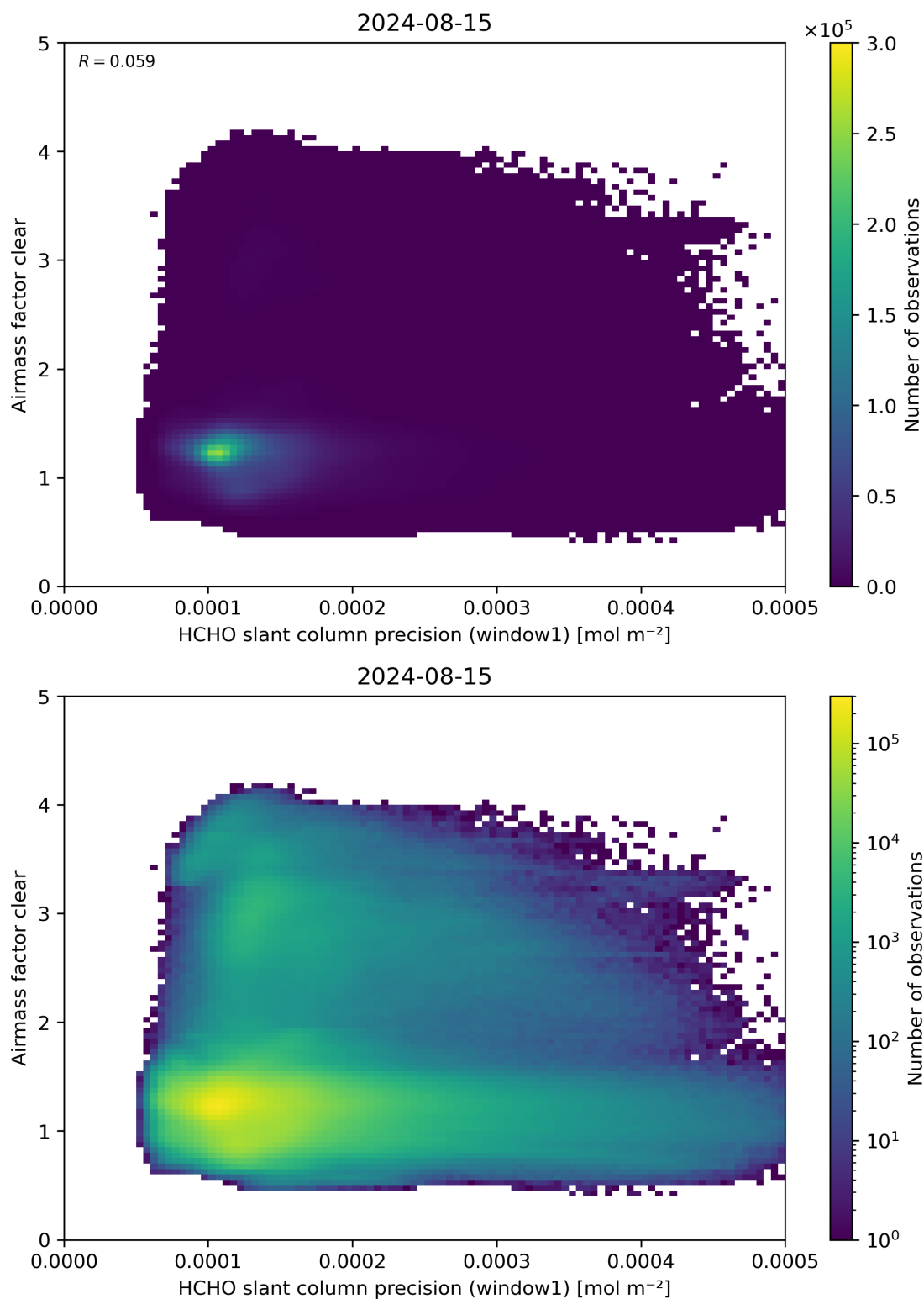
Figure 91: Scatter density plot of “HCHO slant column precision (window1)” against “Airmass factor clear” for 2024-08-14 to 2024-08-16.
