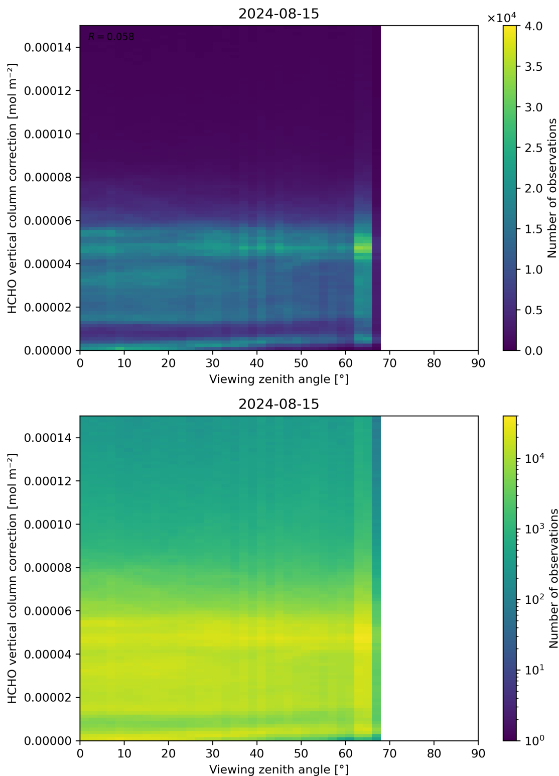
Figure 193: Scatter density plot of “Viewing zenith angle” against “HCHO vertical column correction” for 2024-08-14 to 2024-08-16.
