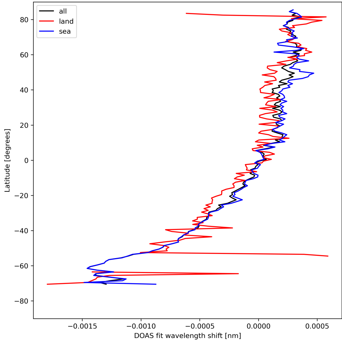
Figure 30: Zonal average of “DOAS fit wavelength shift” for 2024-08-14 to 2024-08-16.
