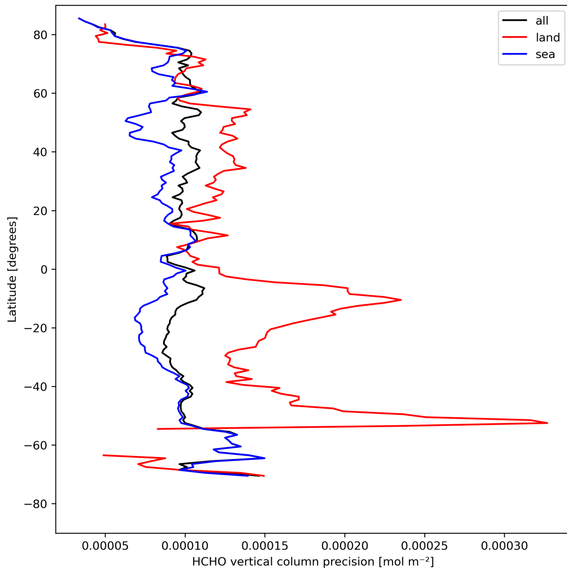
Figure 22: Zonal average of “HCHO vertical column precision” for 2024-08-14 to 2024-08-16.
