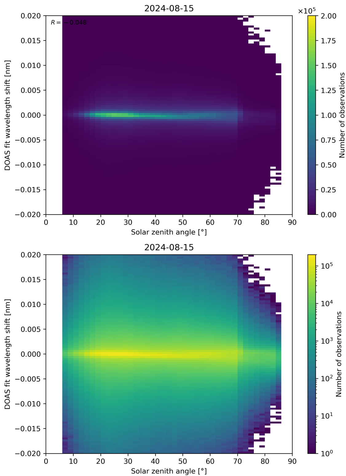
Figure 168: Scatter density plot of “Solar zenith angle” against “DOAS fit wavelength shift” for 2024-08-14 to 2024-08-16.
