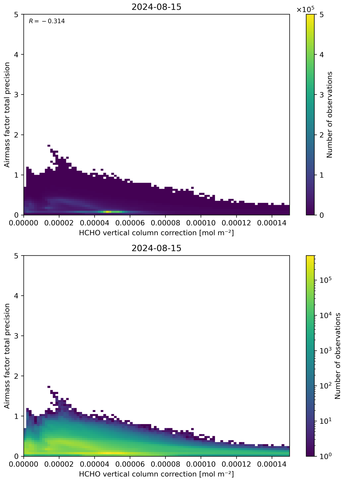
Figure 121: Scatter density plot of “HCHO vertical column correction” against “Airmass factor total precision” for 2024-08-14 to 2024-08-16.
