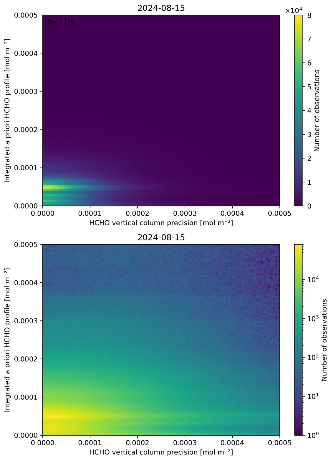
Figure 147: Scatter density plot of “HCHO vertical column precision” against “Integrated a priori HCHO profile” for 2024-08-14 to 2024-08-16.
