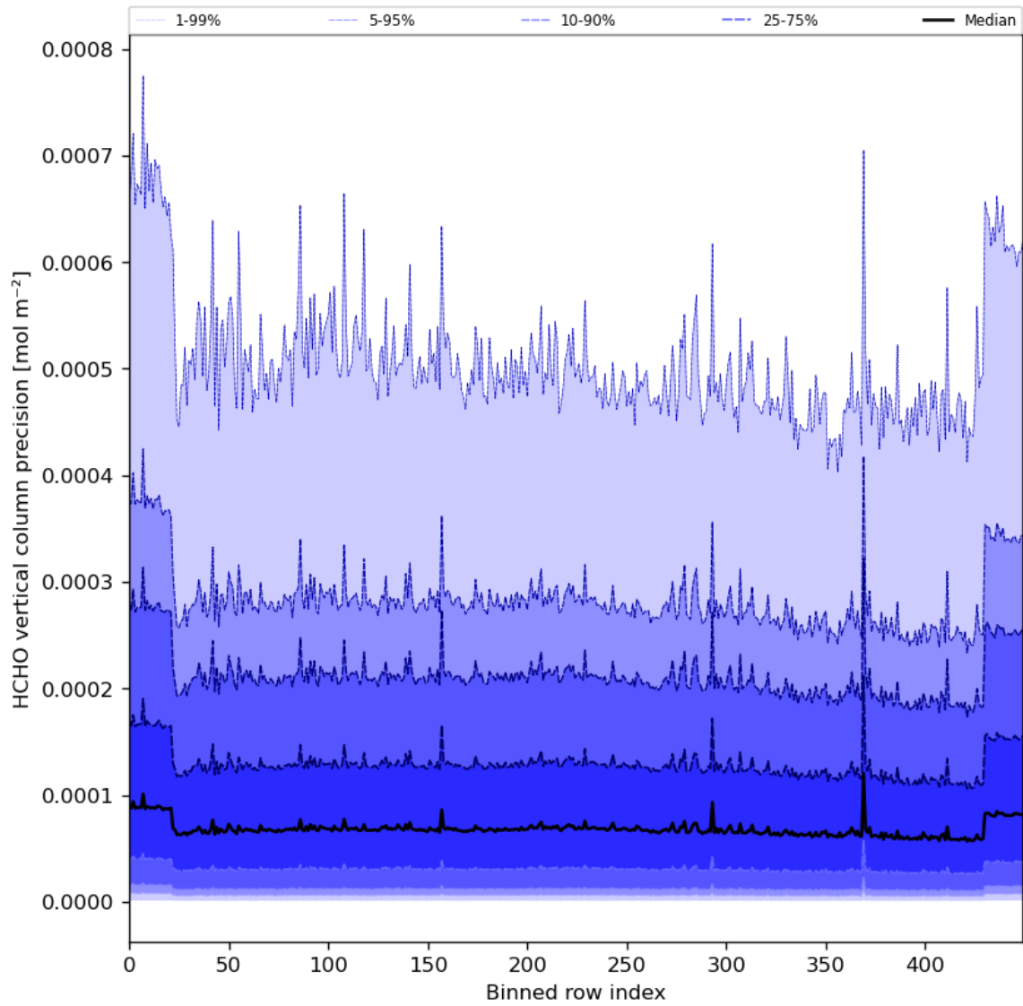
Figure 50: Along track statistics of “HCHO vertical column precision” for 2024-08-14 to 2024-08-16
