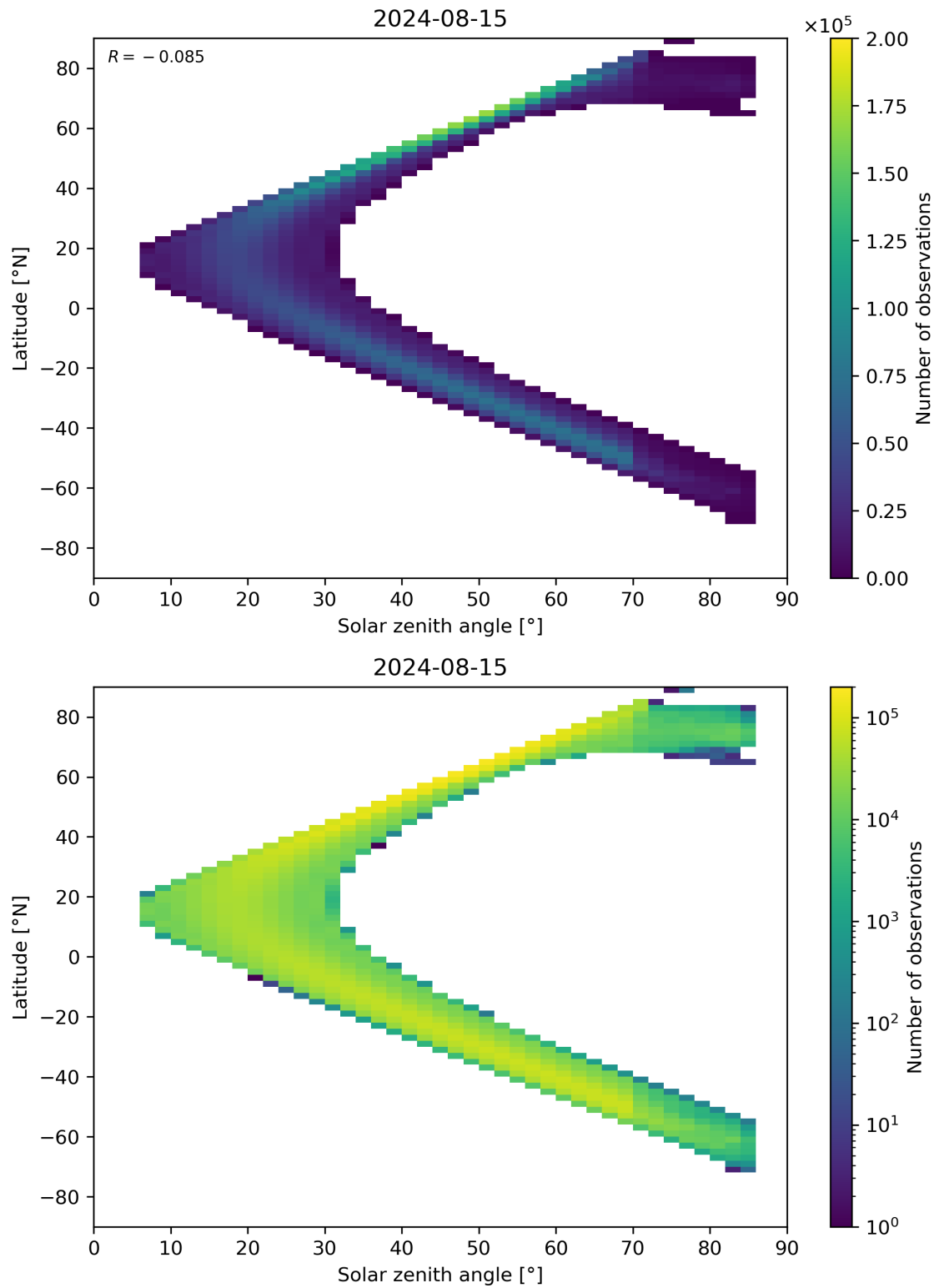
Figure 181: Scatter density plot of “Solar zenith angle” against “Latitude” for 2024-08-14 to 2024-08-16.
