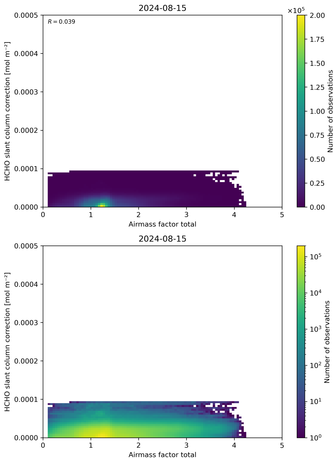
Figure 102: Scatter density plot of “Airmass factor total” against “HCHO slant column correction” for 2024-08-14 to 2024-08-16.
