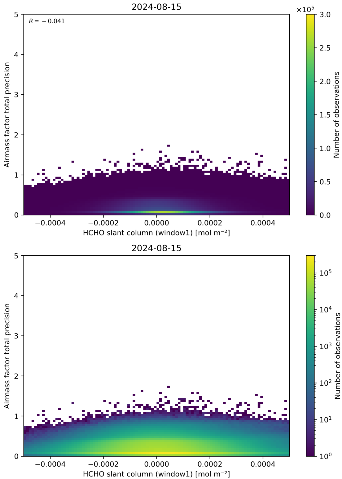
Figure 86: Scatter density plot of “HCHO slant column (window1)” against “Airmass factor total precision” for 2024-08-14 to 2024-08-16.
