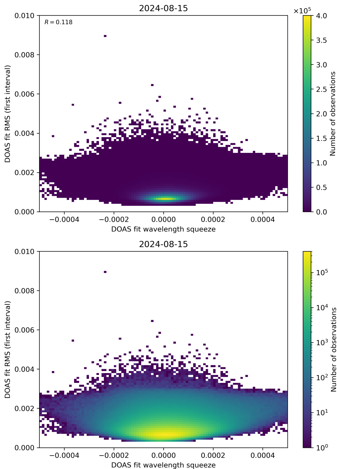
Figure 68: Scatter density plot of “DOAS fit wavelength squeeze” against “DOAS fit RMS (first interval)” for 2024-08-14 to 2024-08-16.
