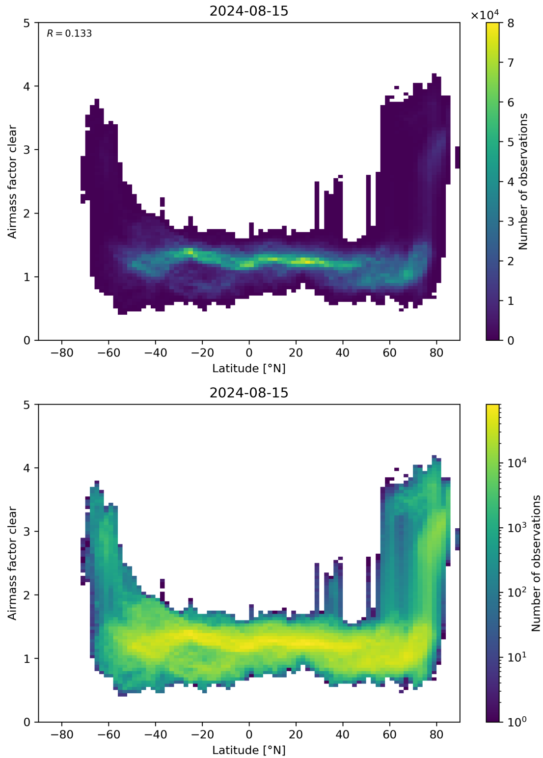
Figure 156: Scatter density plot of “Latitude” against “Airmass factor clear” for 2024-08-14 to 2024-08-16.
