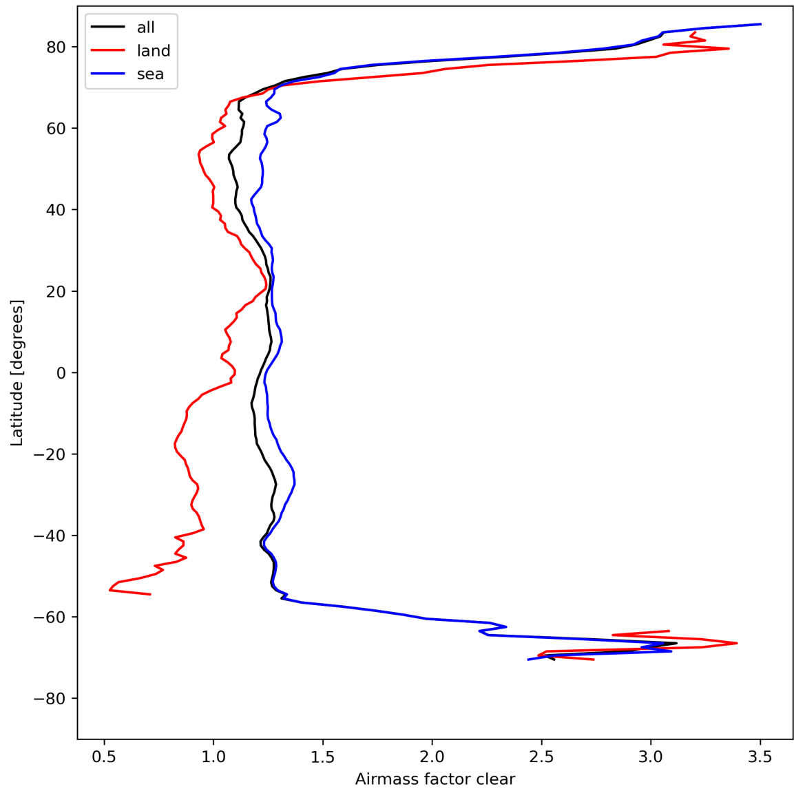
Figure 28: Zonal average of “Airmass factor clear” for 2024-08-14 to 2024-08-16.
