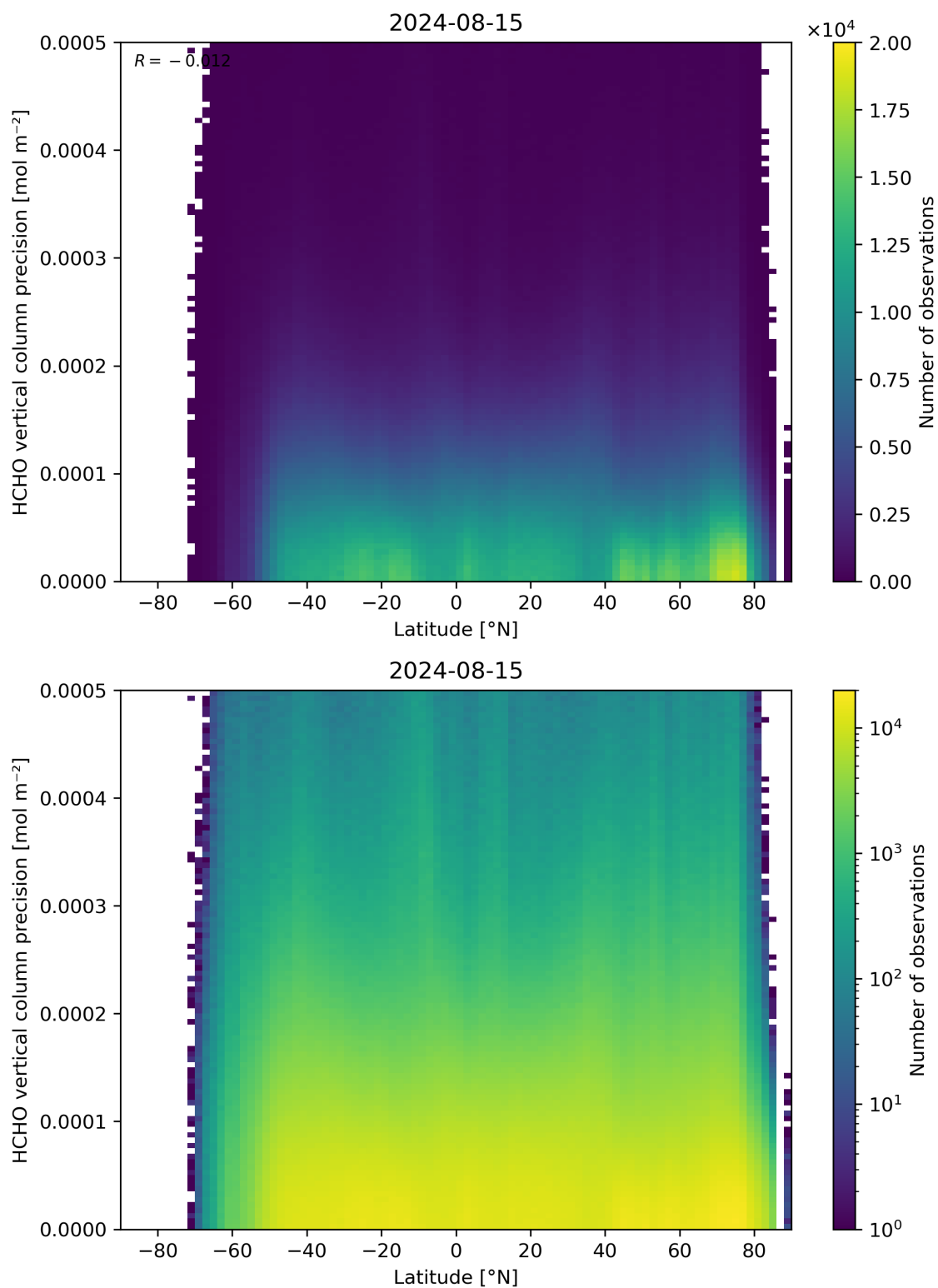
Figure 165: Scatter density plot of “Latitude” against “HCHO vertical column precision” for 2024-08-14 to 2024-08-16.
