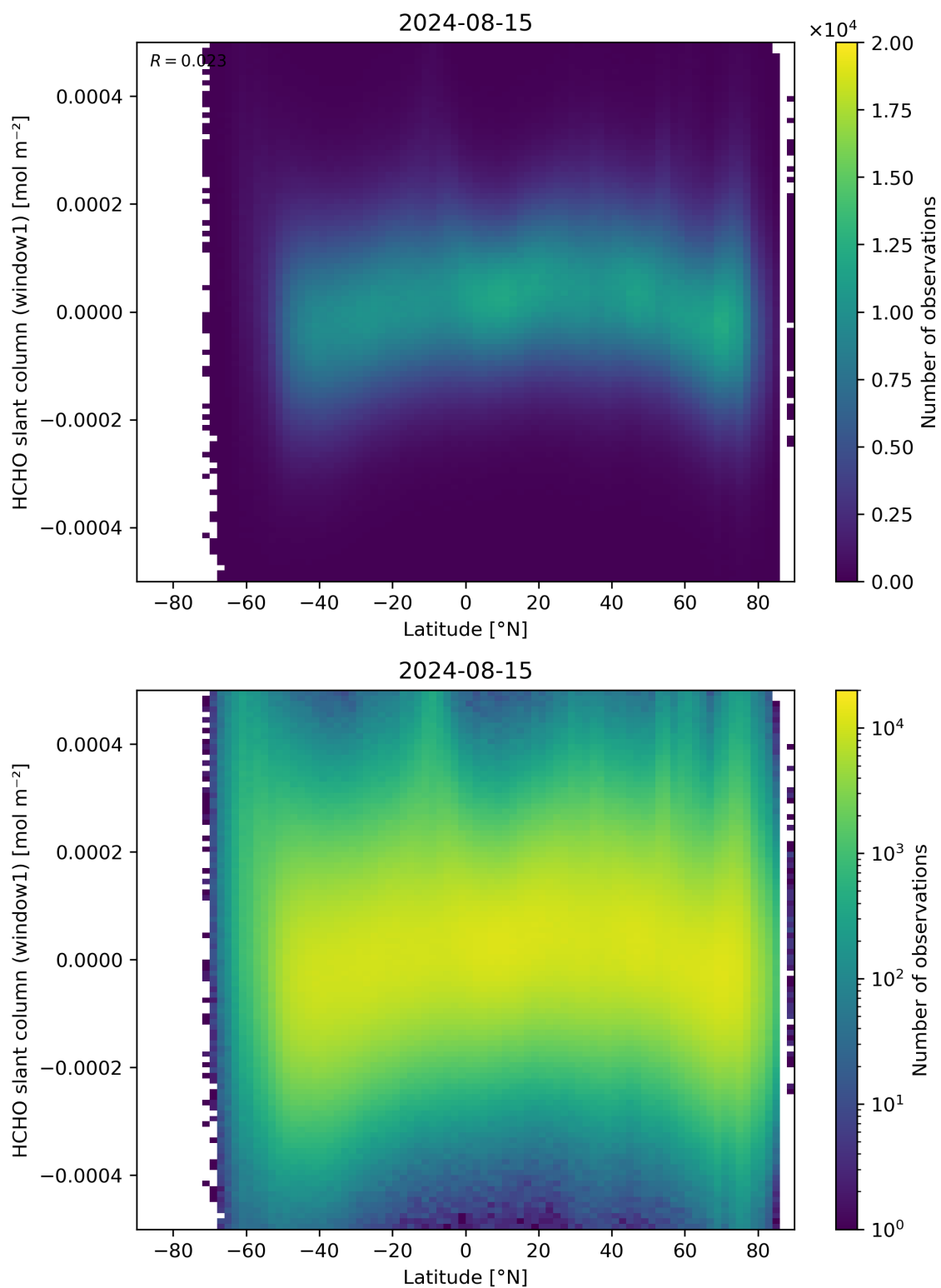
Figure 159: Scatter density plot of “Latitude” against “HCHO slant column (window1)” for 2024-08-14 to 2024-08-16.
