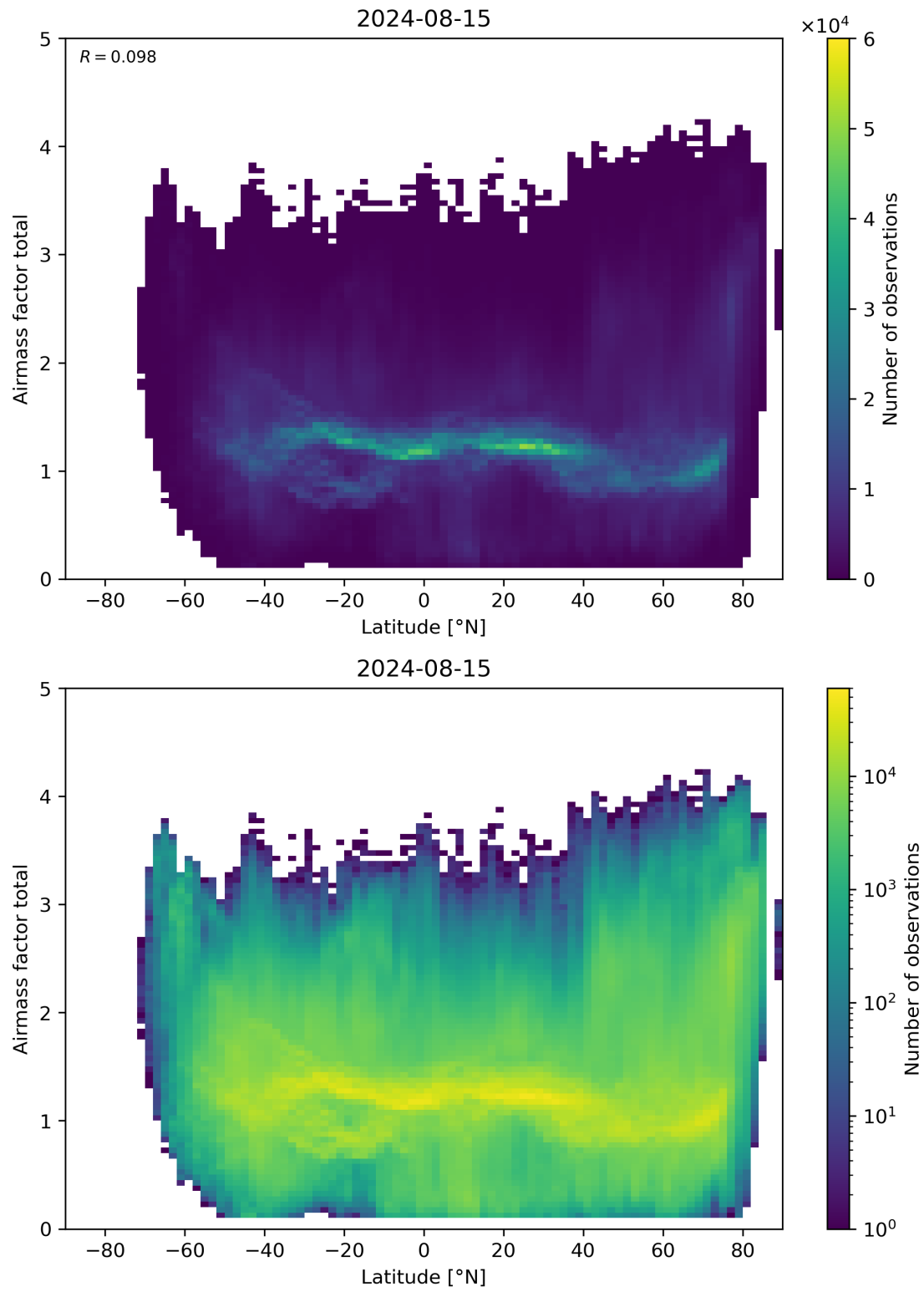
Figure 161: Scatter density plot of “Latitude” against “Airmass factor total” for 2024-08-14 to 2024-08-16.
