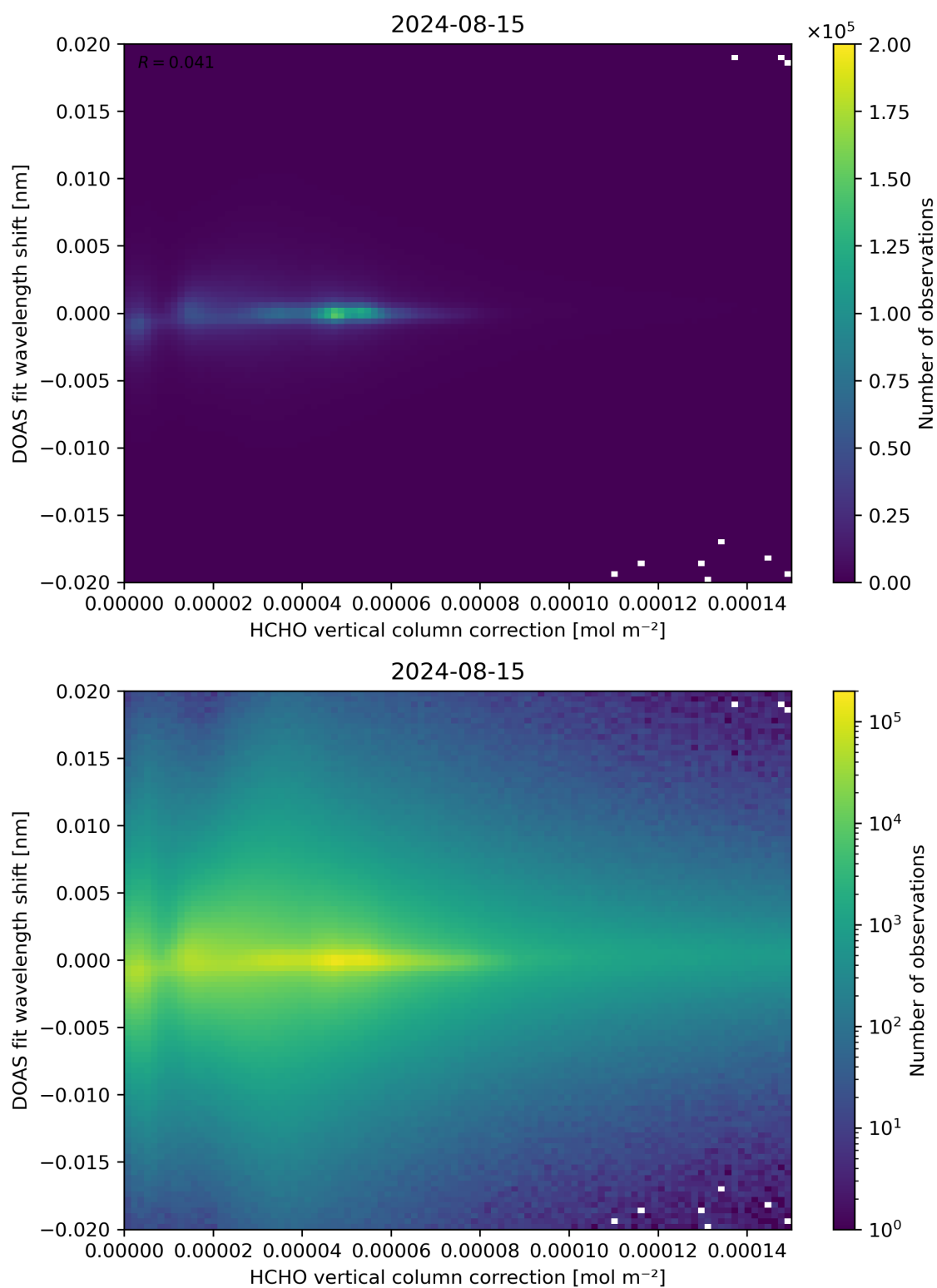
Figure 113: Scatter density plot of “HCHO vertical column correction” against “DOAS fit wavelength shift” for 2024-08-14 to 2024-08-16.
