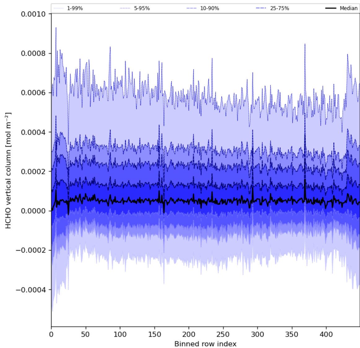
Figure 49: Along track statistics of “HCHO vertical column” for 2024-08-14 to 2024-08-16
