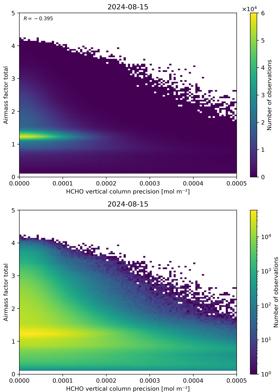
Figure 144: Scatter density plot of “HCHO vertical column precision” against “Airmass factor total” for 2024-08-14 to 2024-08-16.
