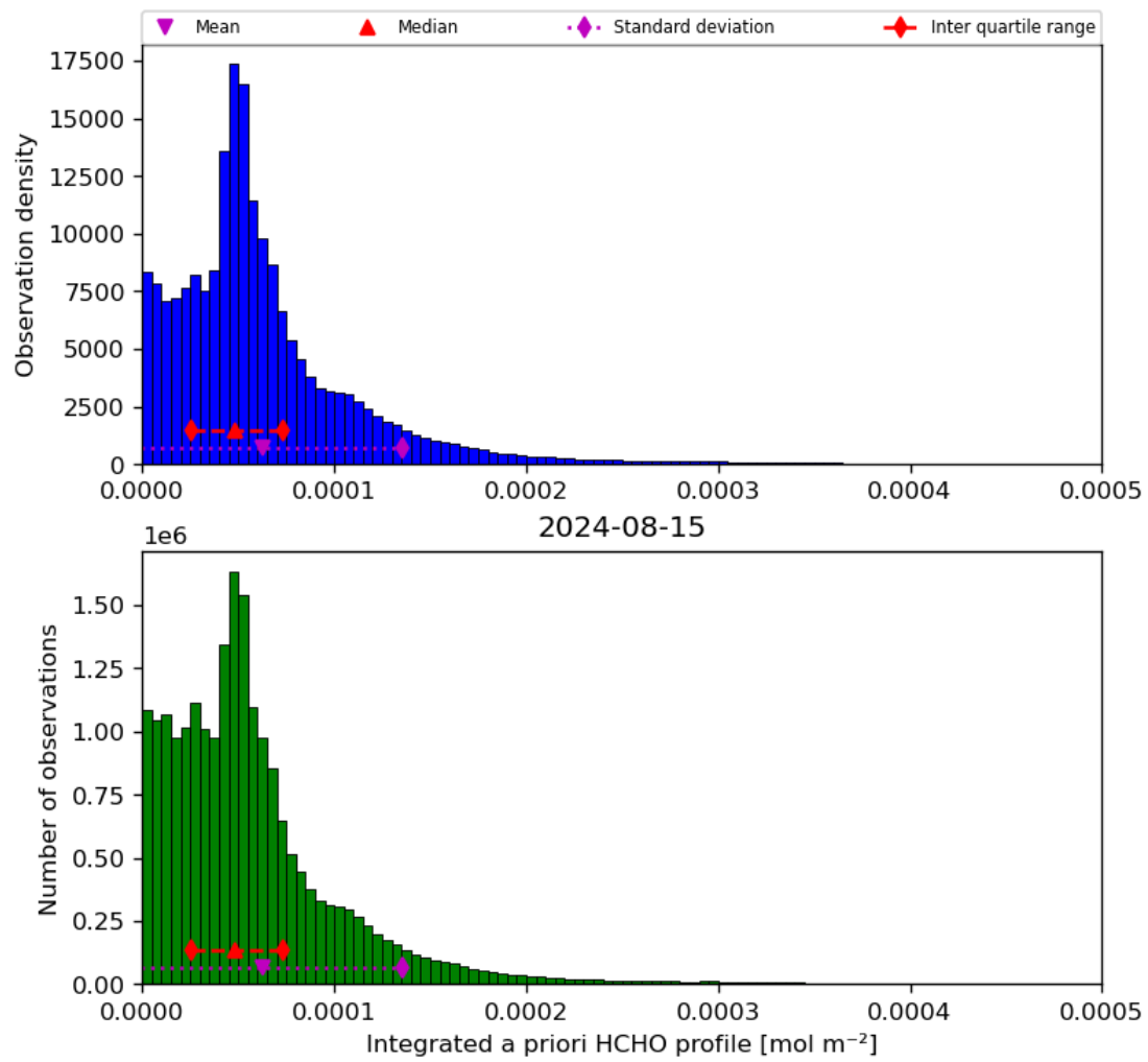
Figure 43: Histogram of “Integrated a priori HCHO profile” for 2024-08-14 to 2024-08-16
