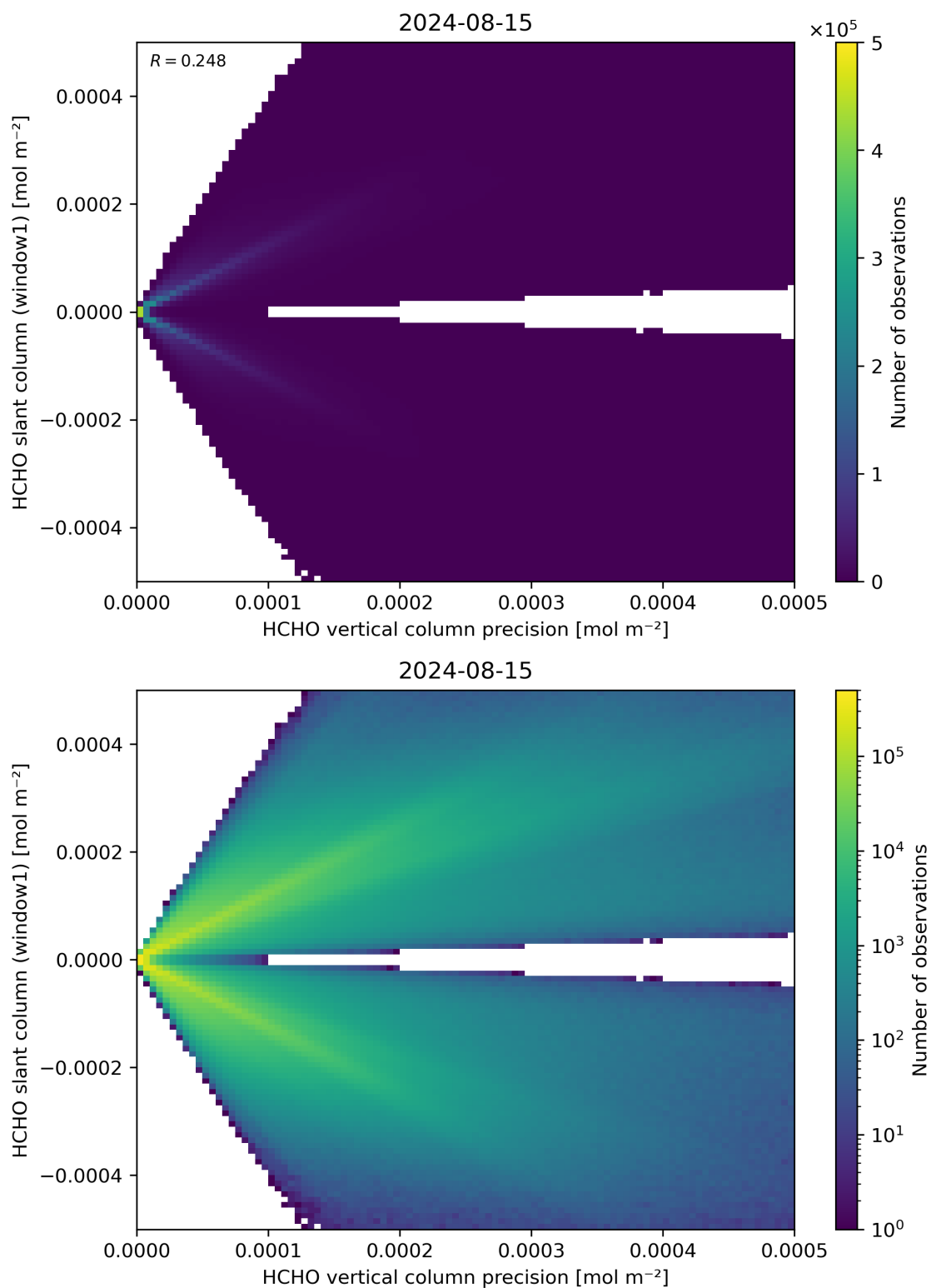
Figure 142: Scatter density plot of “HCHO vertical column precision” against “HCHO slant column (window1)” for 2024-08-14 to 2024-08-16.
