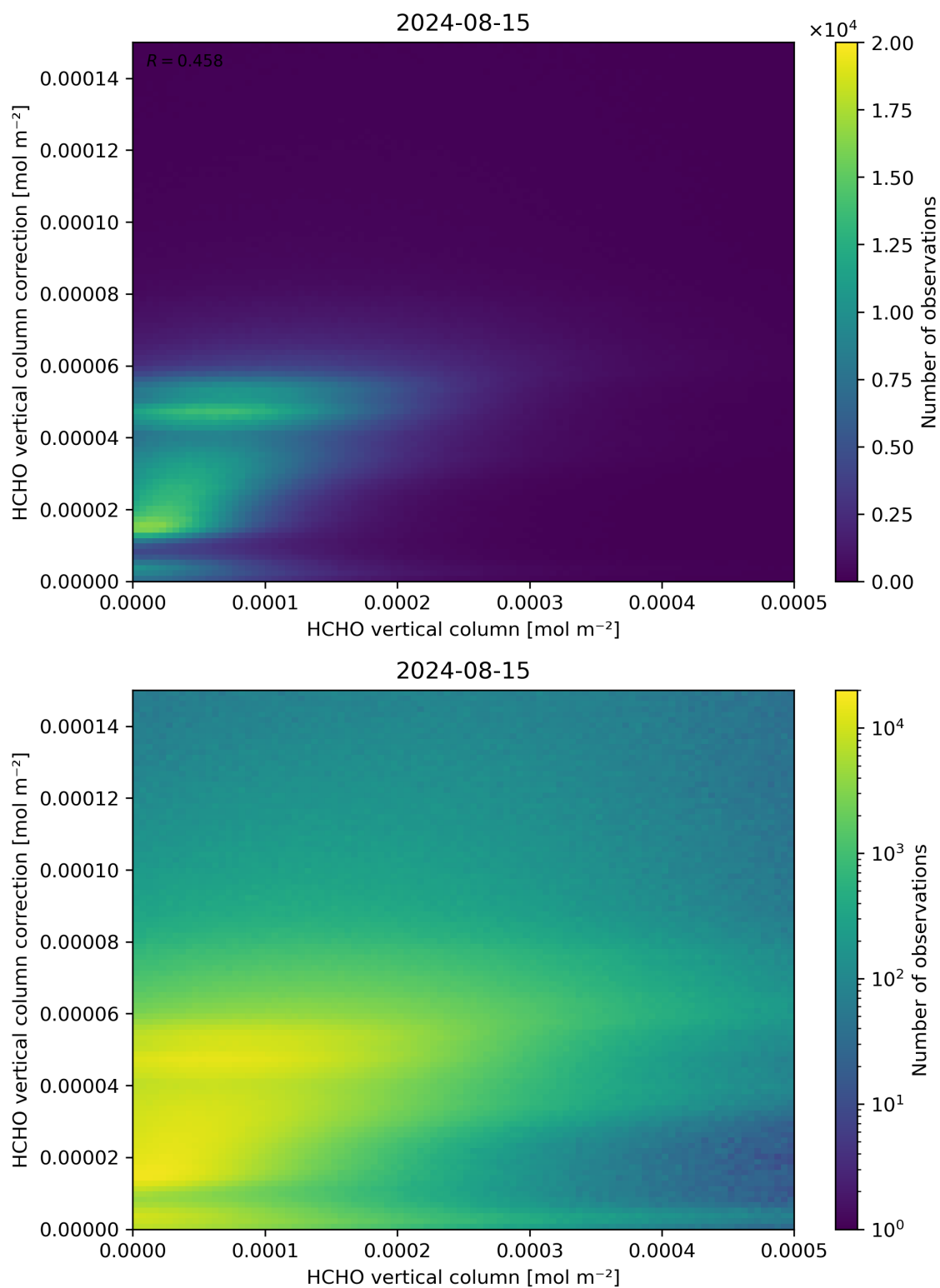
Figure 133: Scatter density plot of “HCHO vertical column” against “HCHO vertical column correction” for 2024-08-14 to 2024-08-16.
