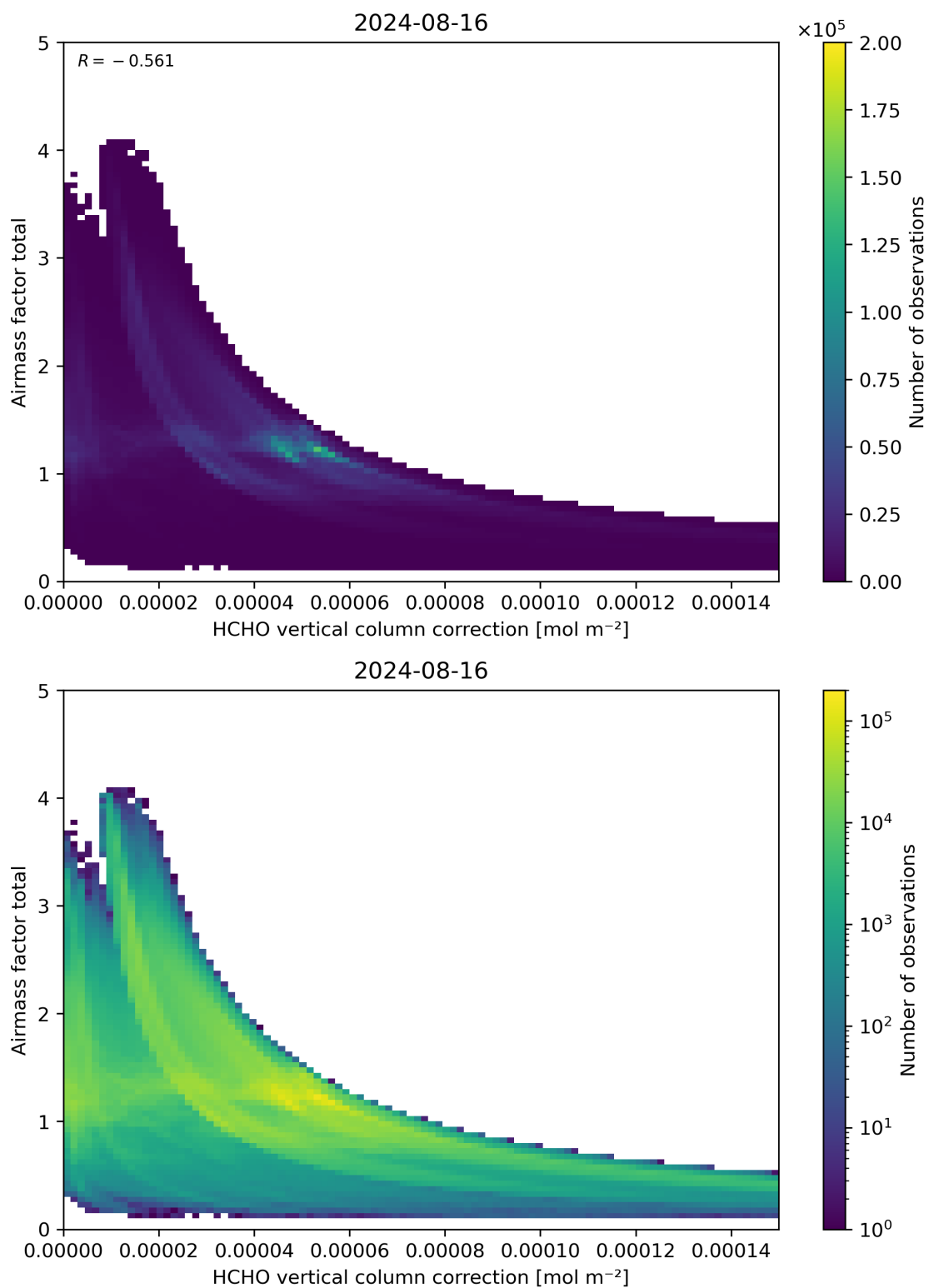
Figure 120: Scatter density plot of “HCHO vertical column correction” against “Airmass factor total” for 2024-08-16 to 2024-08-17.
