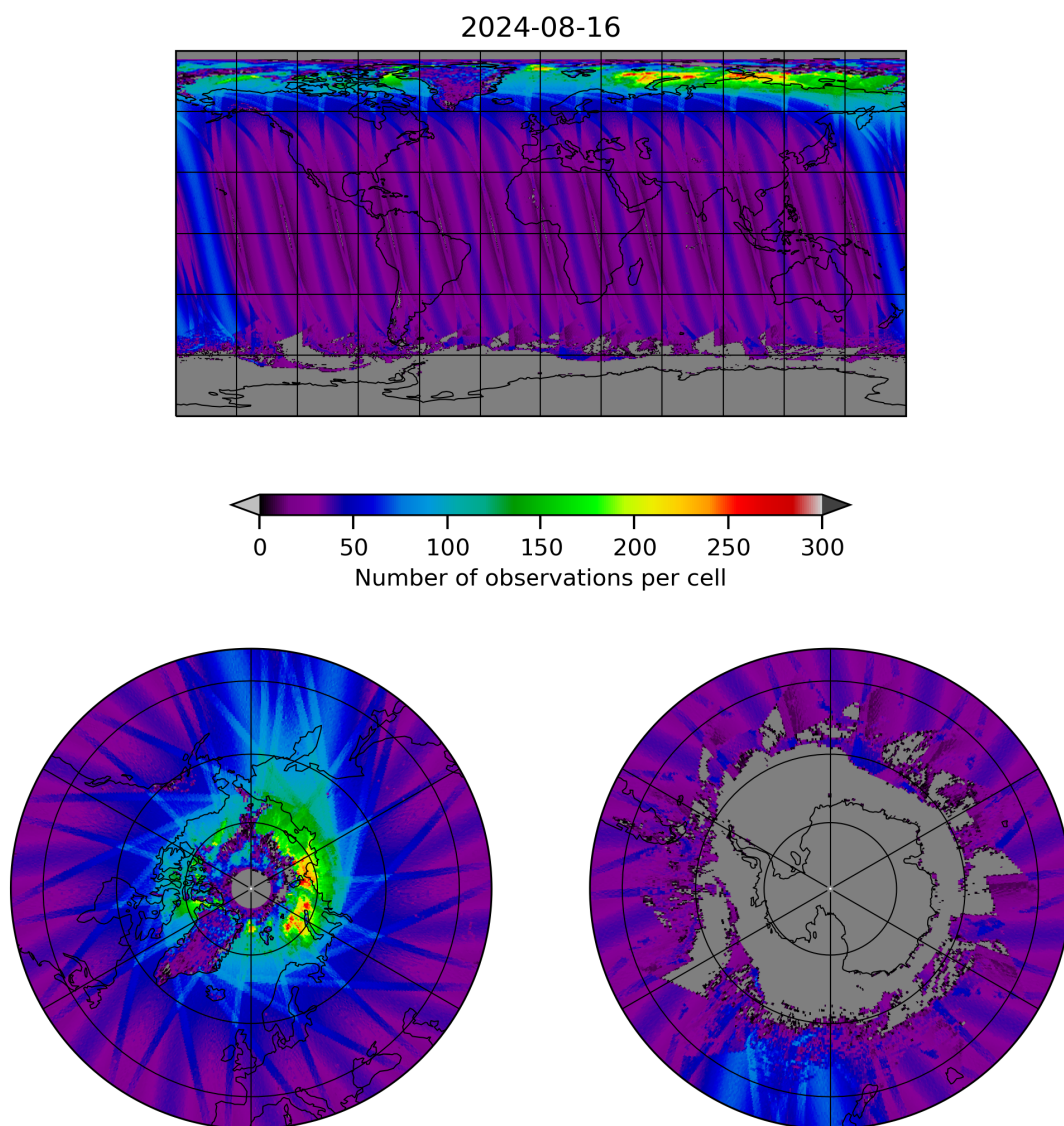
Figure 19: Map of the number of observations for 2024-08-16 to 2024-08-17
