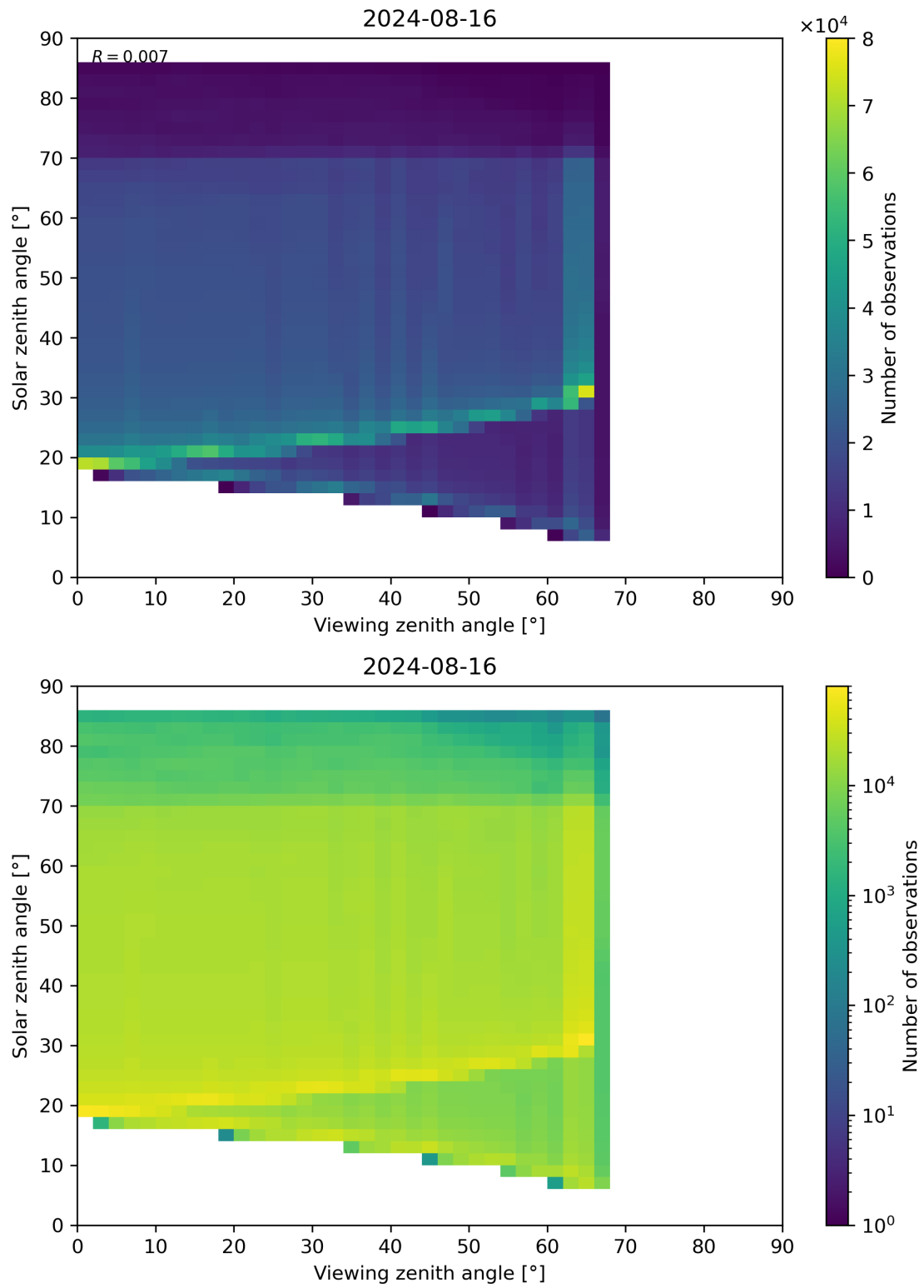
Figure 197: Scatter density plot of “Viewing zenith angle” against “Solar zenith angle” for 2024-08-16 to 2024-08-17.
