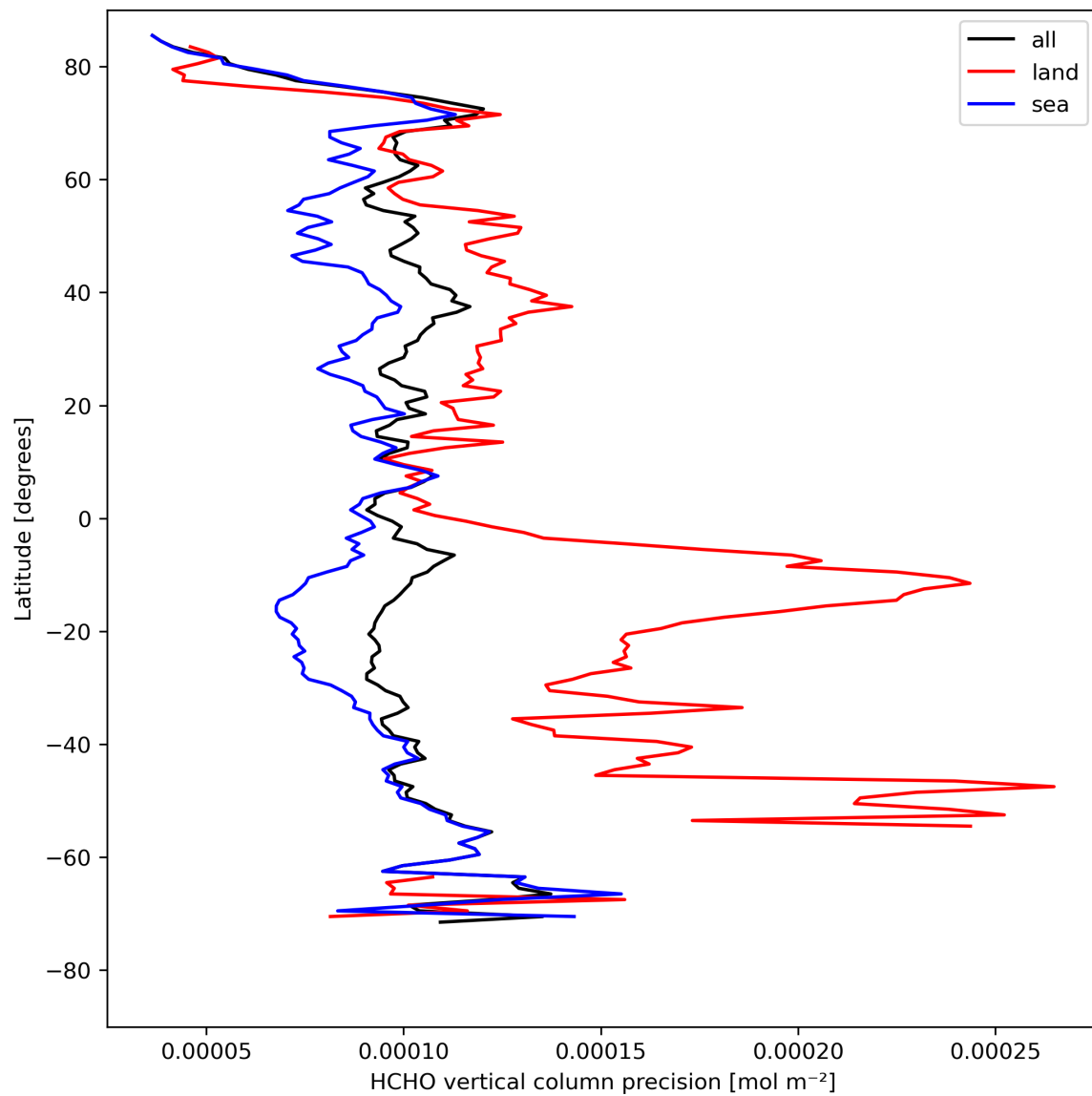
Figure 22: Zonal average of “HCHO vertical column precision” for 2024-08-16 to 2024-08-17.
