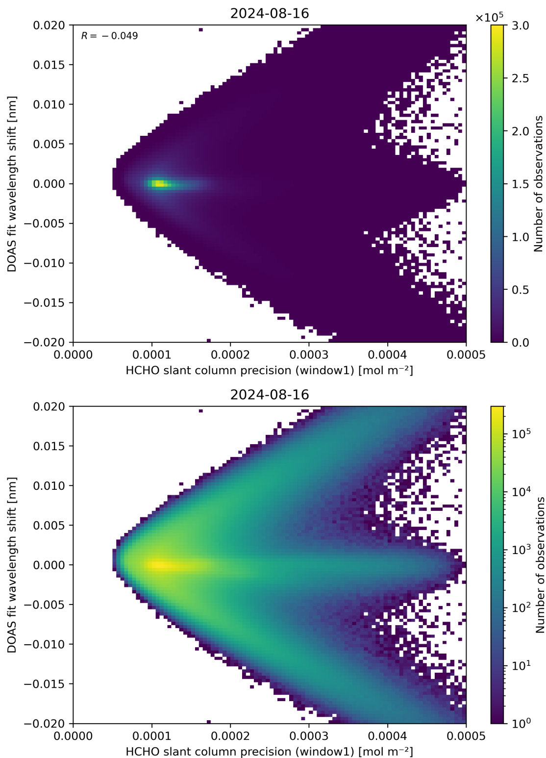
Figure 89: Scatter density plot of “HCHO slant column precision (window1)” against “DOAS fit wavelength shift” for 2024-08-16 to 2024-08-17.
