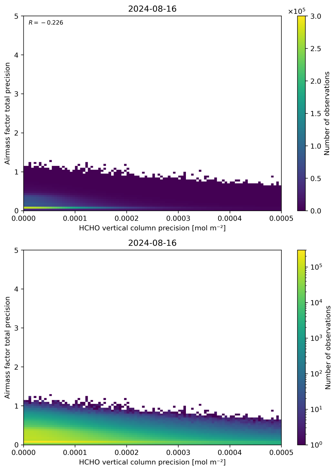
Figure 145: Scatter density plot of “HCHO vertical column precision” against “Airmass factor total precision” for 2024-08-16 to 2024-08-17.
