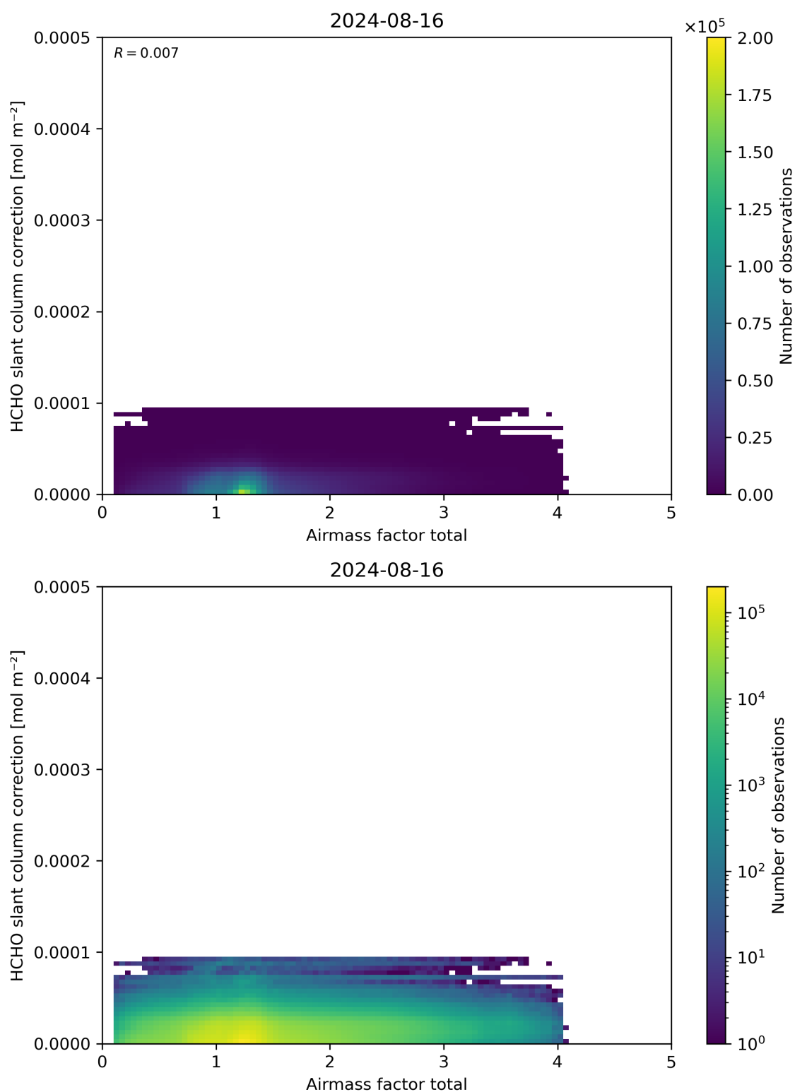
Figure 102: Scatter density plot of “Airmass factor total” against “HCHO slant column correction” for 2024-08-16 to 2024-08-17.
