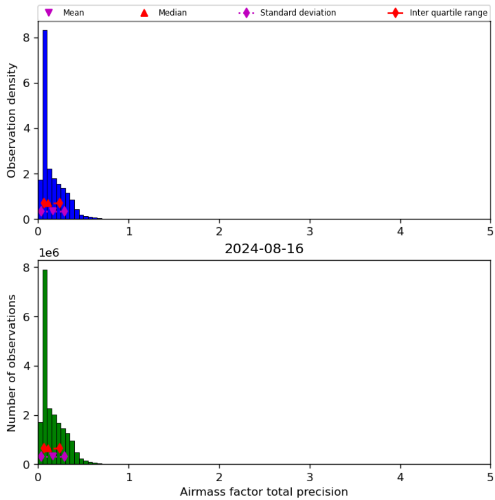
Figure 41: Histogram of “Airmass factor total precision” for 2024-08-16 to 2024-08-17
