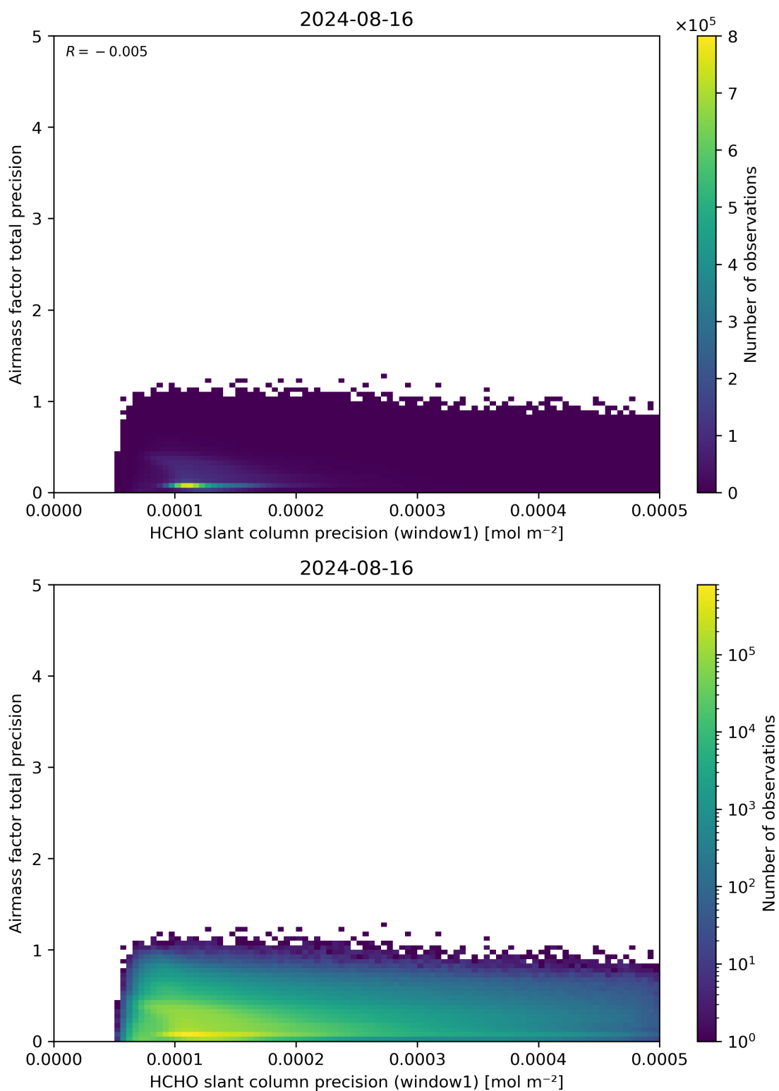
Figure 95: Scatter density plot of “HCHO slant column precision (window1)” against “Airmass factor total precision” for 2024-08-16 to 2024-08-17.
