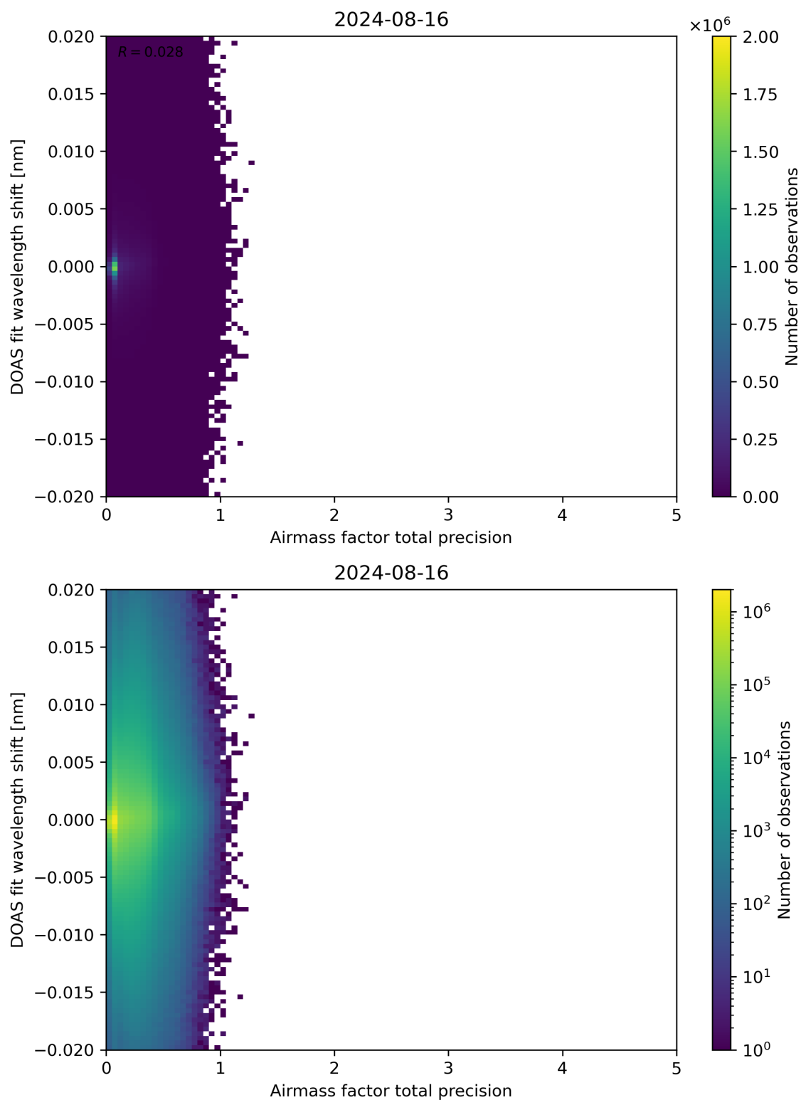
Figure 106: Scatter density plot of “Airmass factor total precision” against “DOAS fit wavelength shift” for 2024-08-16 to 2024-08-17.
