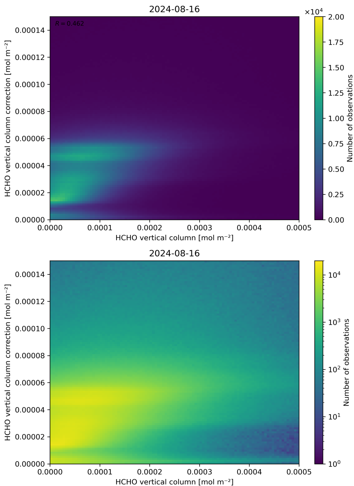
Figure 133: Scatter density plot of “HCHO vertical column” against “HCHO vertical column correction” for 2024-08-16 to 2024-08-17.
