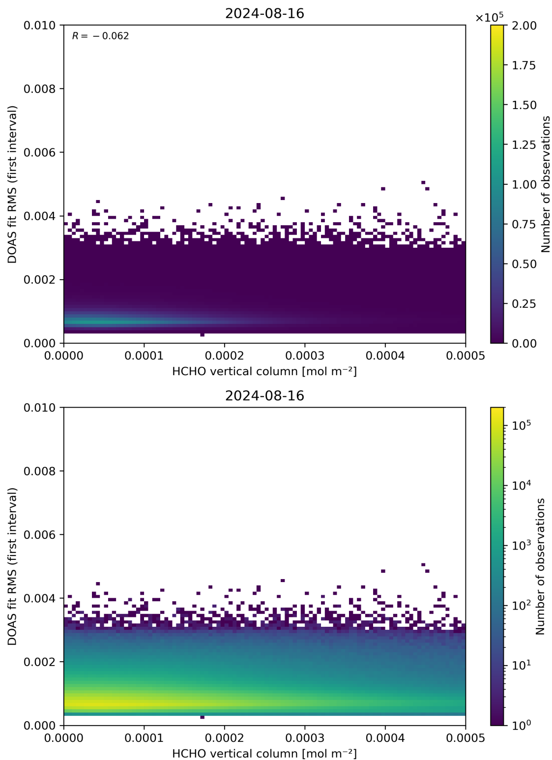
Figure 123: Scatter density plot of “HCHO vertical column” against “DOAS fit RMS (first interval)” for 2024-08-16 to 2024-08-17.
