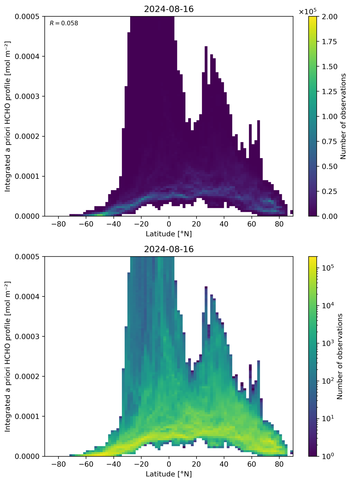
Figure 166: Scatter density plot of “Latitude” against “Integrated a priori HCHO profile” for 2024-08-16 to 2024-08-17.
