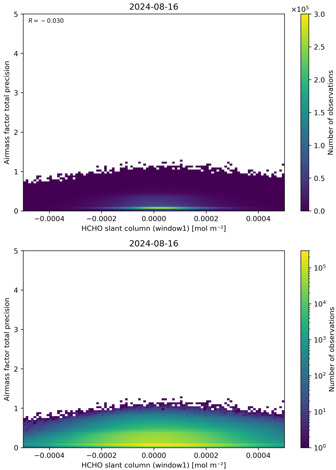
Figure 86: Scatter density plot of “HCHO slant column (window1)” against “Airmass factor total precision” for 2024-08-16 to 2024-08-17.
