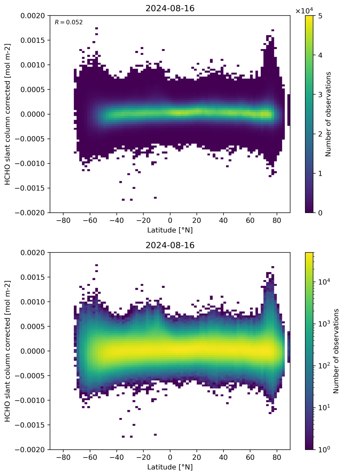
Figure 157: Scatter density plot of “Latitude” against “HCHO slant column corrected” for 2024-08-16 to 2024-08-17.
