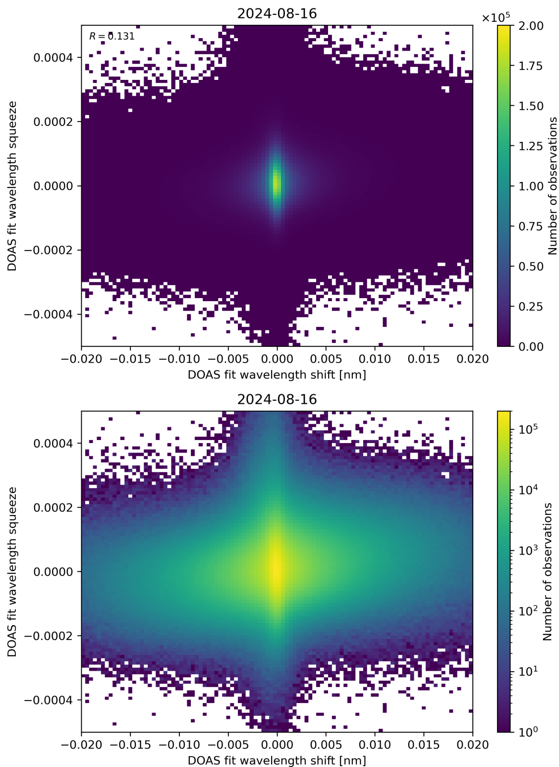
Figure 65: Scatter density plot of “DOAS fit wavelength shift” against “DOAS fit wavelength squeeze” for 2024-08-16 to 2024-08-17.
