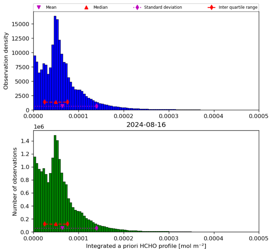
Figure 43: Histogram of “Integrated a priori HCHO profile” for 2024-08-16 to 2024-08-17
