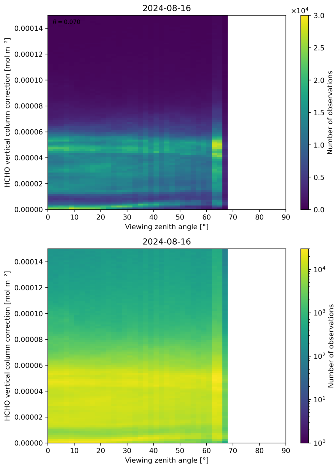
Figure 193: Scatter density plot of “Viewing zenith angle” against “HCHO vertical column correction” for 2024-08-16 to 2024-08-17.
