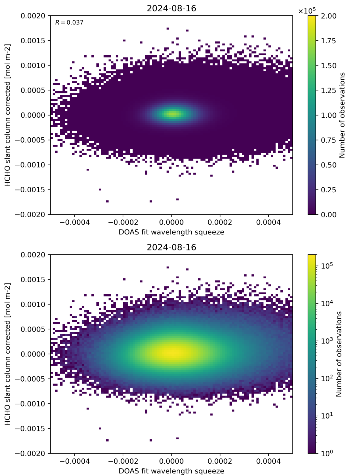
Figure 69: Scatter density plot of “DOAS fit wavelength squeeze” against “HCHO slant column corrected” for 2024-08-16 to 2024-08-17.
