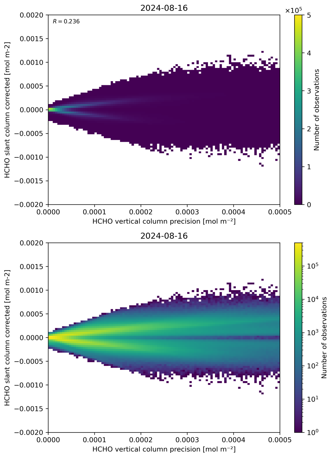
Figure 140: Scatter density plot of “HCHO vertical column precision” against “HCHO slant column corrected” for 2024-08-16 to 2024-08-17.
