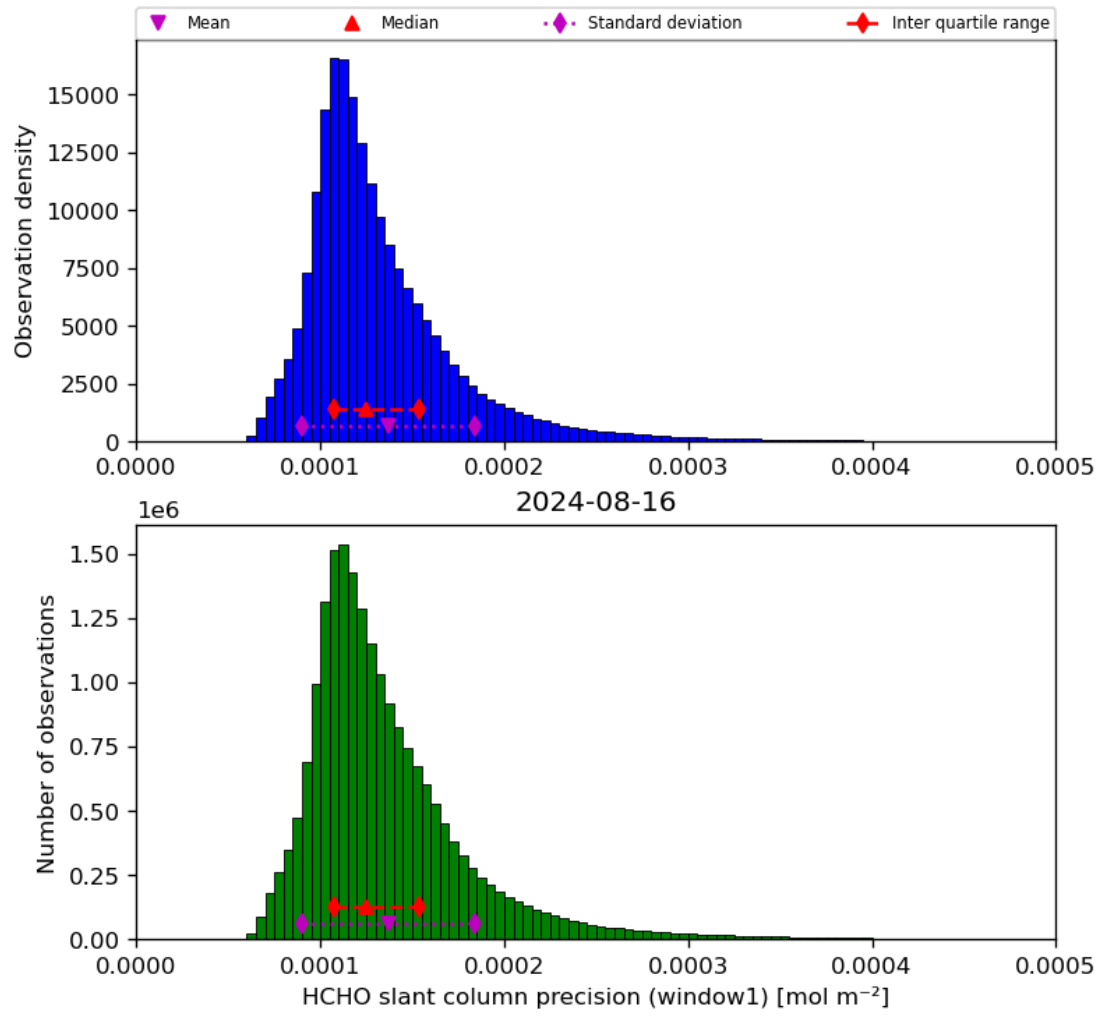
Figure 39: Histogram of “HCHO slant column precision (window1)” for 2024-08-16 to 2024-08-17
