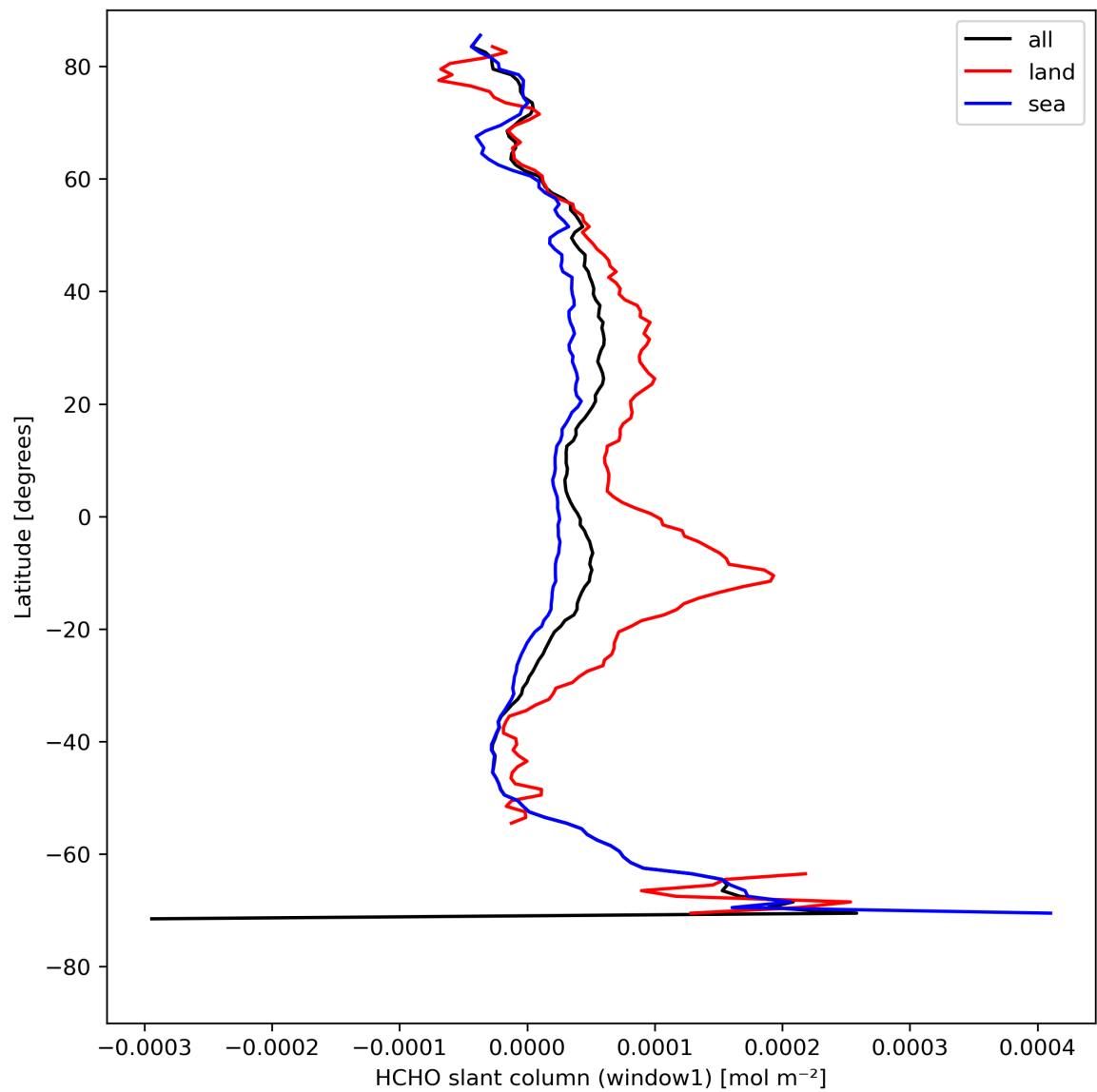
Figure 24: Zonal average of “HCHO slant column (window1)” for 2024-08-16 to 2024-08-17.
