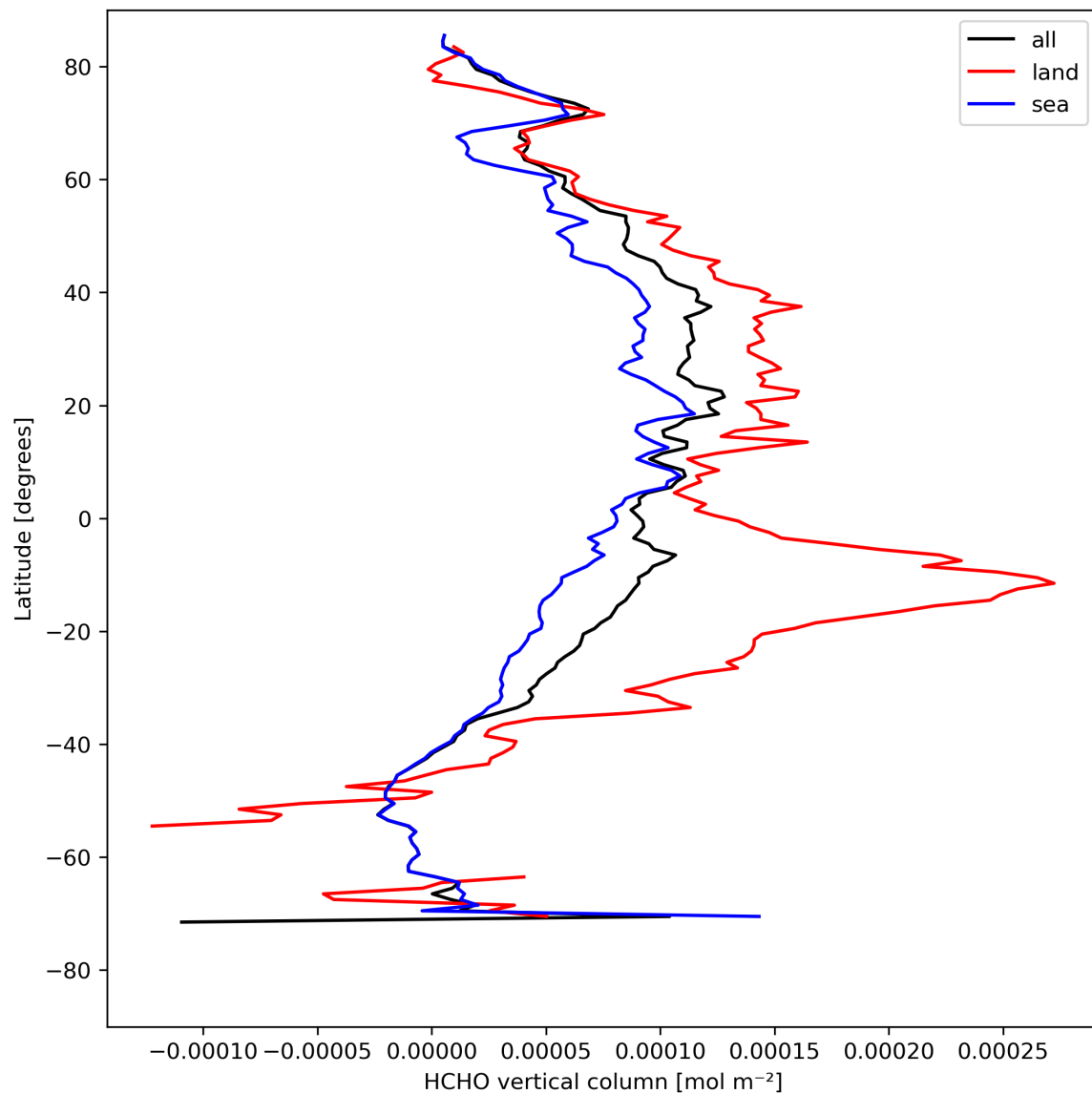
Figure 21: Zonal average of “HCHO vertical column” for 2024-08-16 to 2024-08-17.
