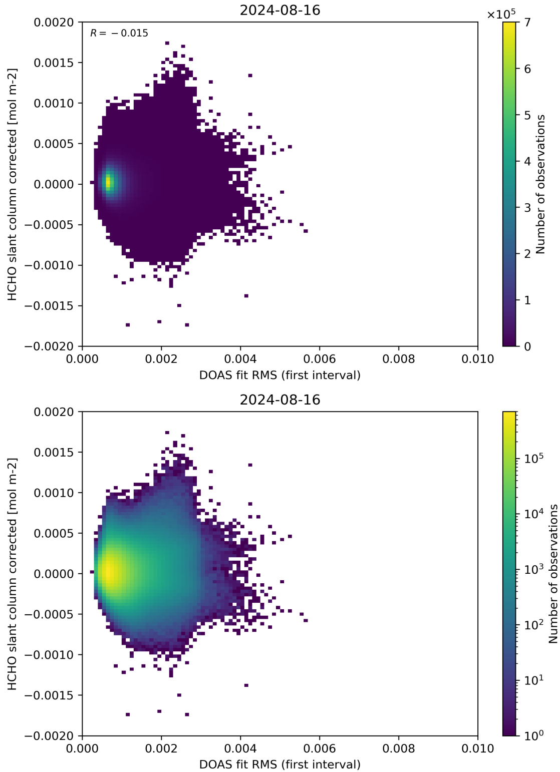
Figure 62: Scatter density plot of “DOAS fit RMS (first interval)” against “HCHO slant column corrected” for 2024-08-16 to 2024-08-17.
