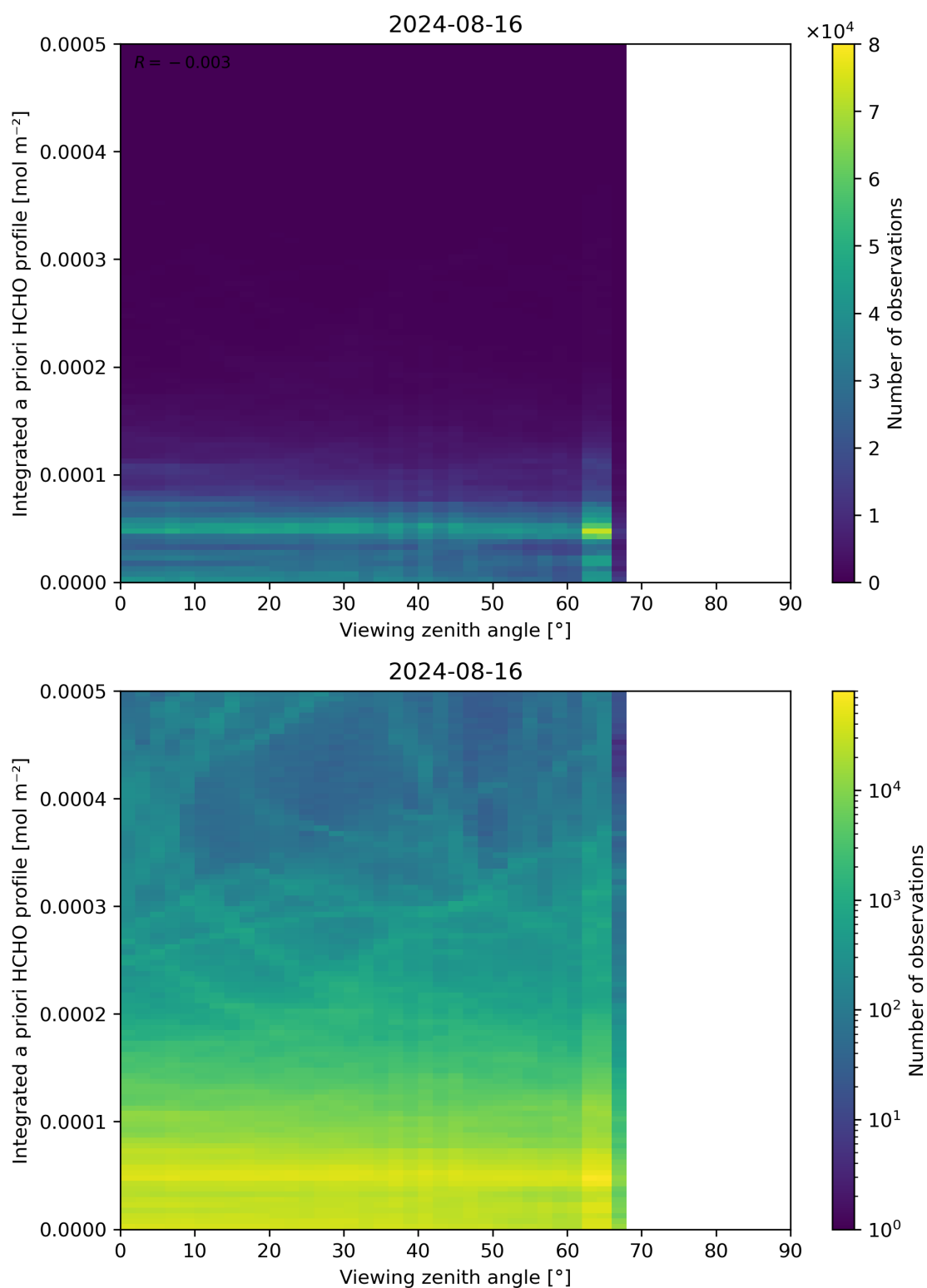
Figure 195: Scatter density plot of “Viewing zenith angle” against “Integrated a priori HCHO profile” for 2024-08-16 to 2024-08-17.
