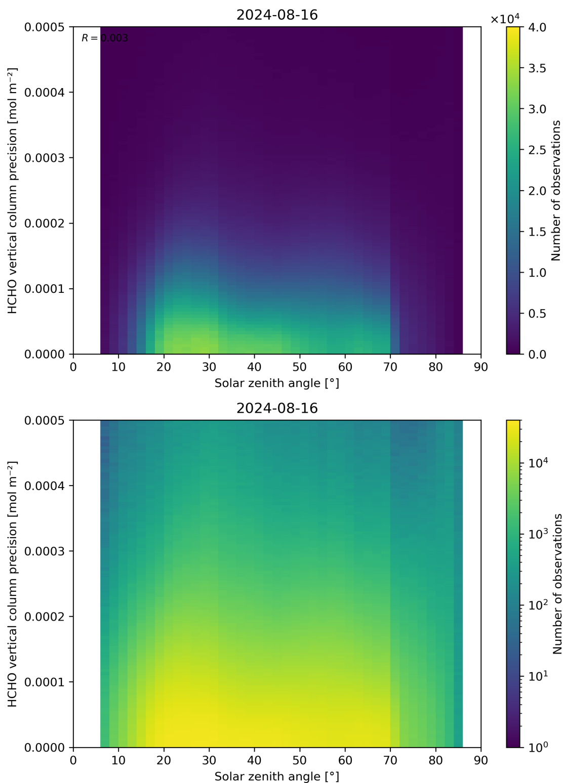
Figure 179: Scatter density plot of “Solar zenith angle” against “HCHO vertical column precision” for 2024-08-16 to 2024-08-17.
