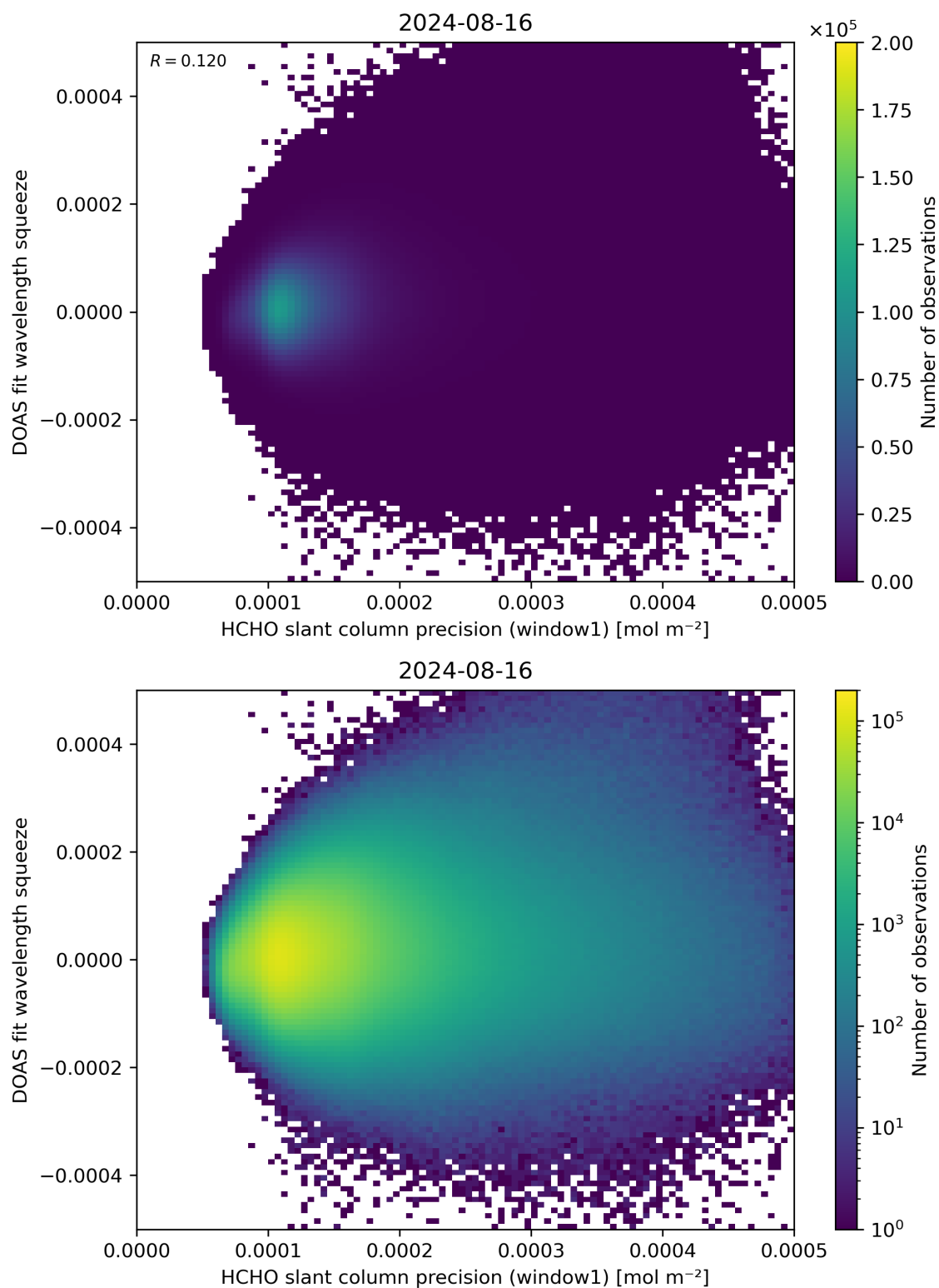
Figure 90: Scatter density plot of “HCHO slant column precision (window1)” against “DOAS fit wavelength squeeze” for 2024-08-16 to 2024-08-17.
