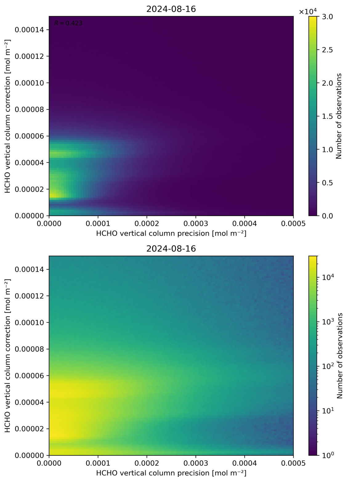
Figure 146: Scatter density plot of “HCHO vertical column precision” against “HCHO vertical column correction” for 2024-08-16 to 2024-08-17.
