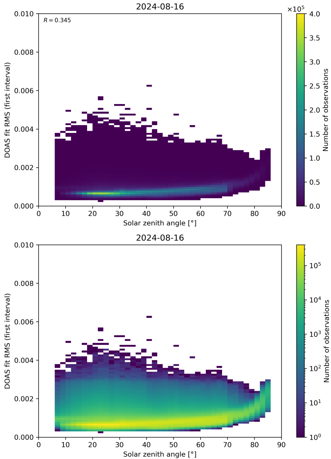
Figure 167: Scatter density plot of “Solar zenith angle” against “DOAS fit RMS (first interval)” for 2024-08-16 to 2024-08-17.
