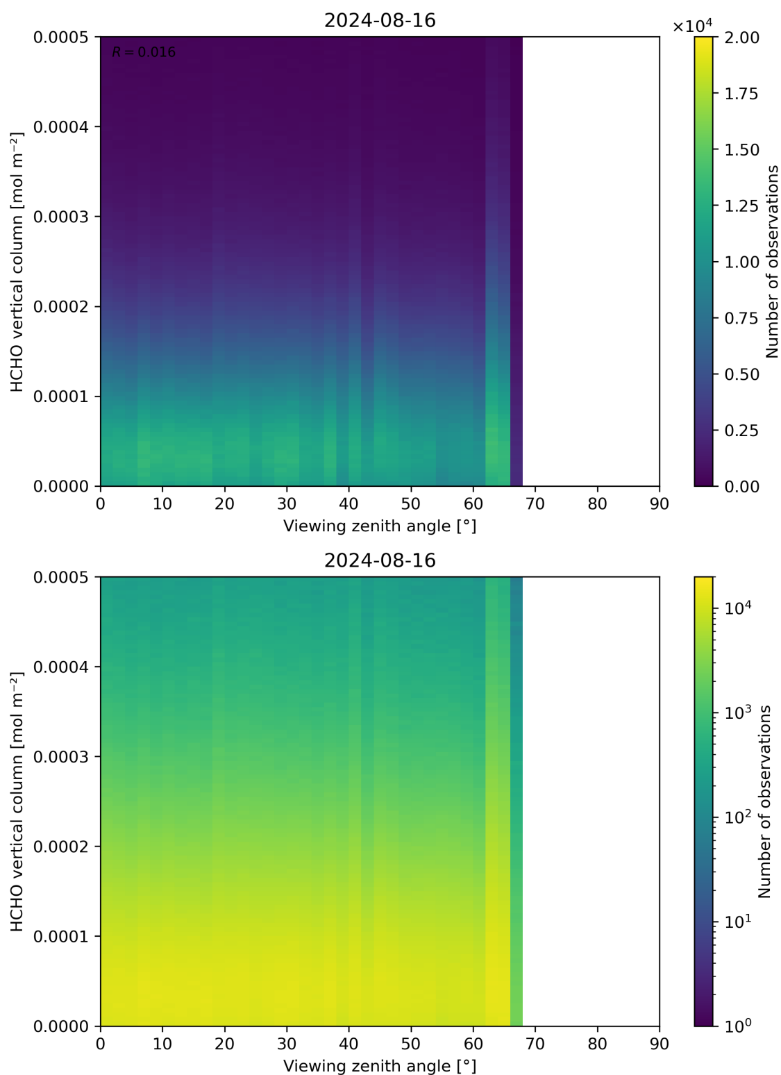
Figure 192: Scatter density plot of “Viewing zenith angle” against “HCHO vertical column” for 2024-08-16 to 2024-08-17.
