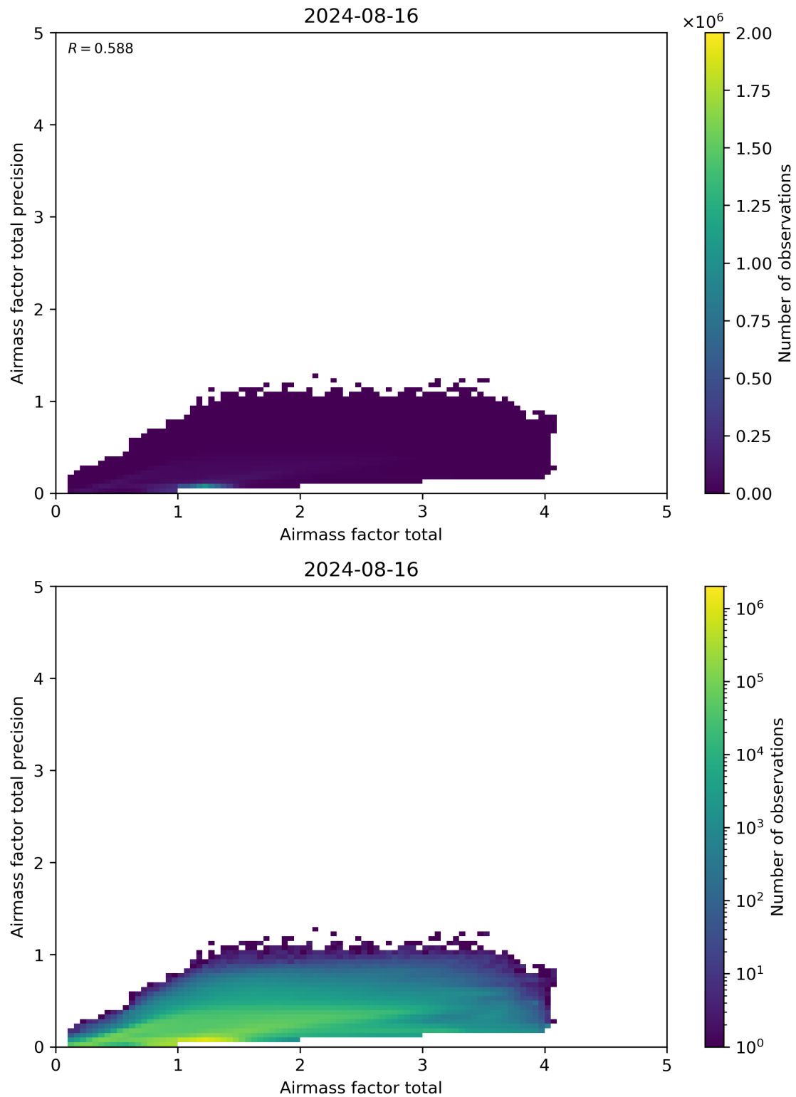
Figure 103: Scatter density plot of “Airmass factor total” against “Airmass factor total precision” for 2024-08-16 to 2024-08-17.
