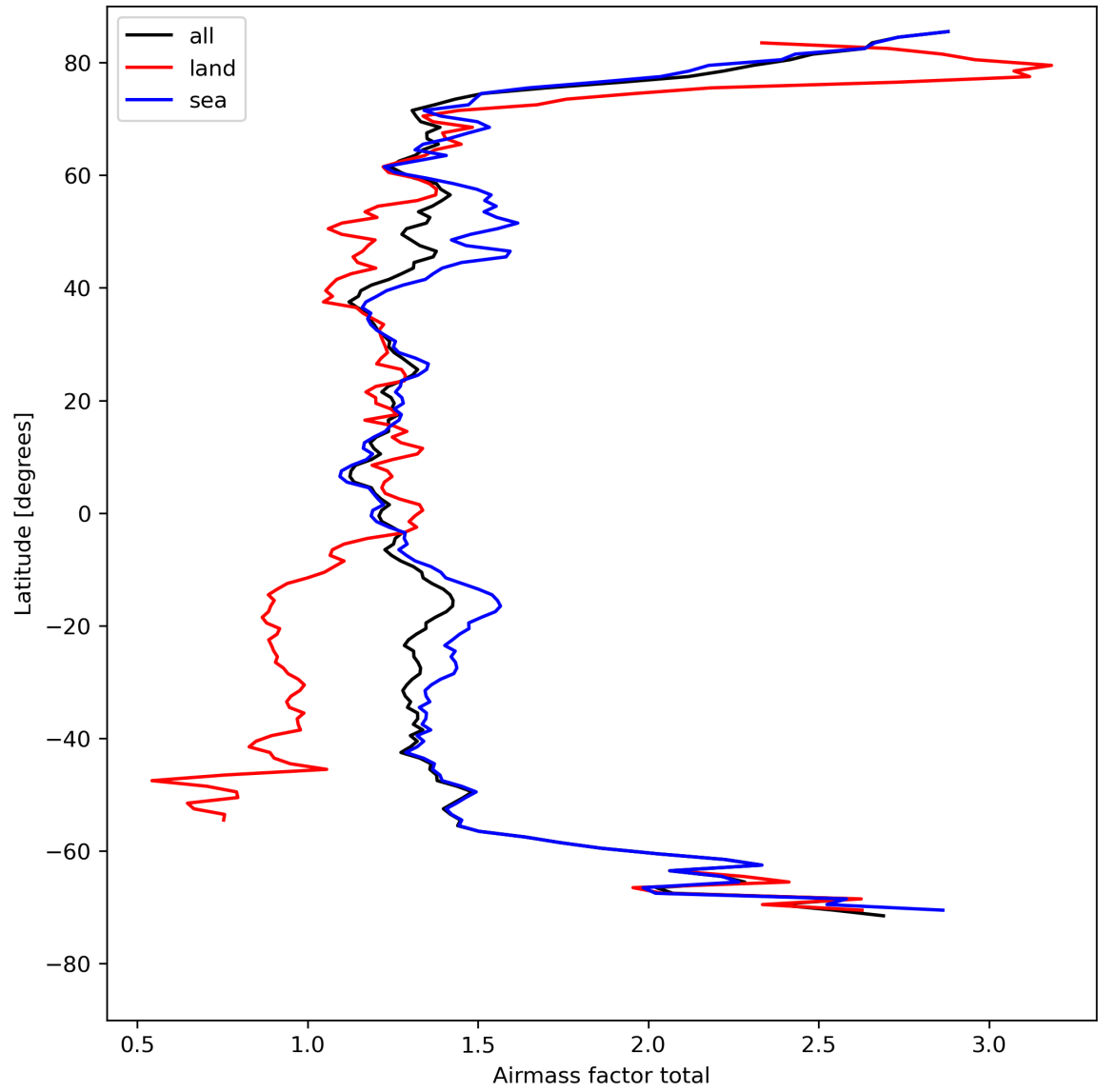
Figure 26: Zonal average of “Airmass factor total” for 2024-08-16 to 2024-08-17.
