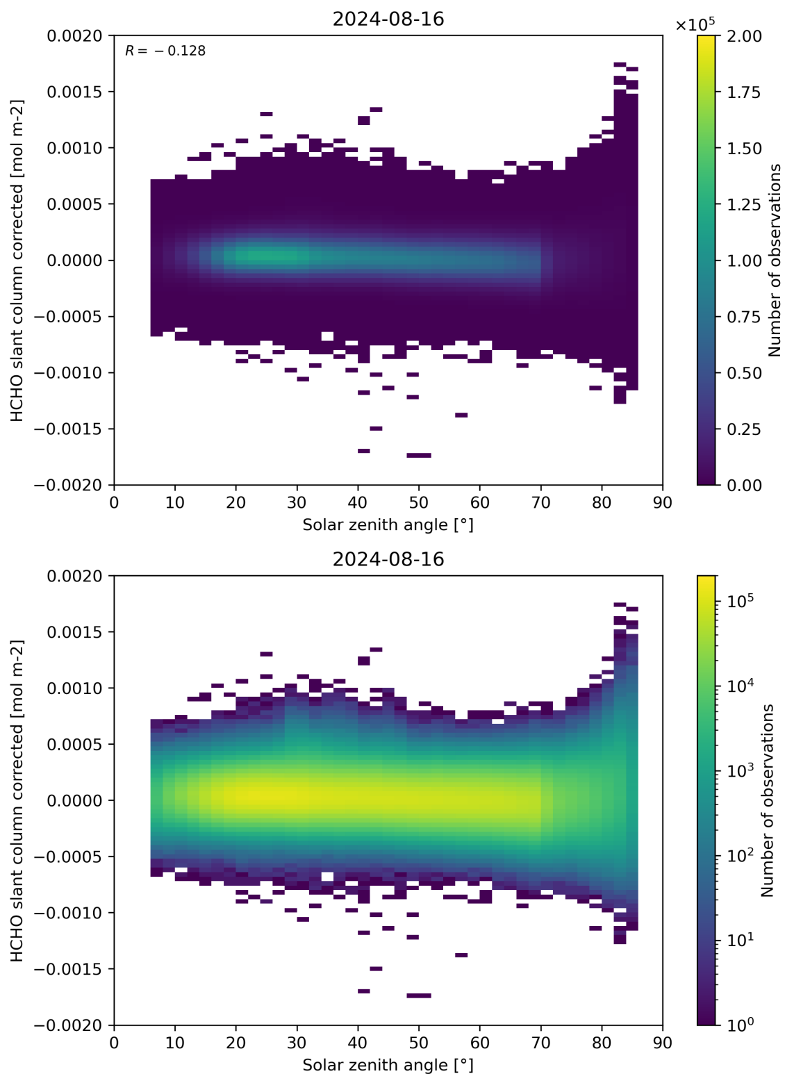
Figure 171: Scatter density plot of “Solar zenith angle” against “HCHO slant column corrected” for 2024-08-16 to 2024-08-17.
