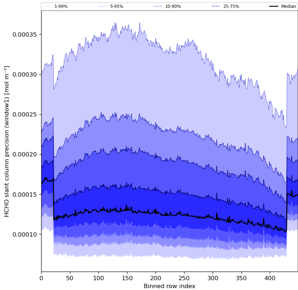
Figure 53: Along track statistics of “HCHO slant column precision (window1)” for 2024-08-16 to 2024-08-17
