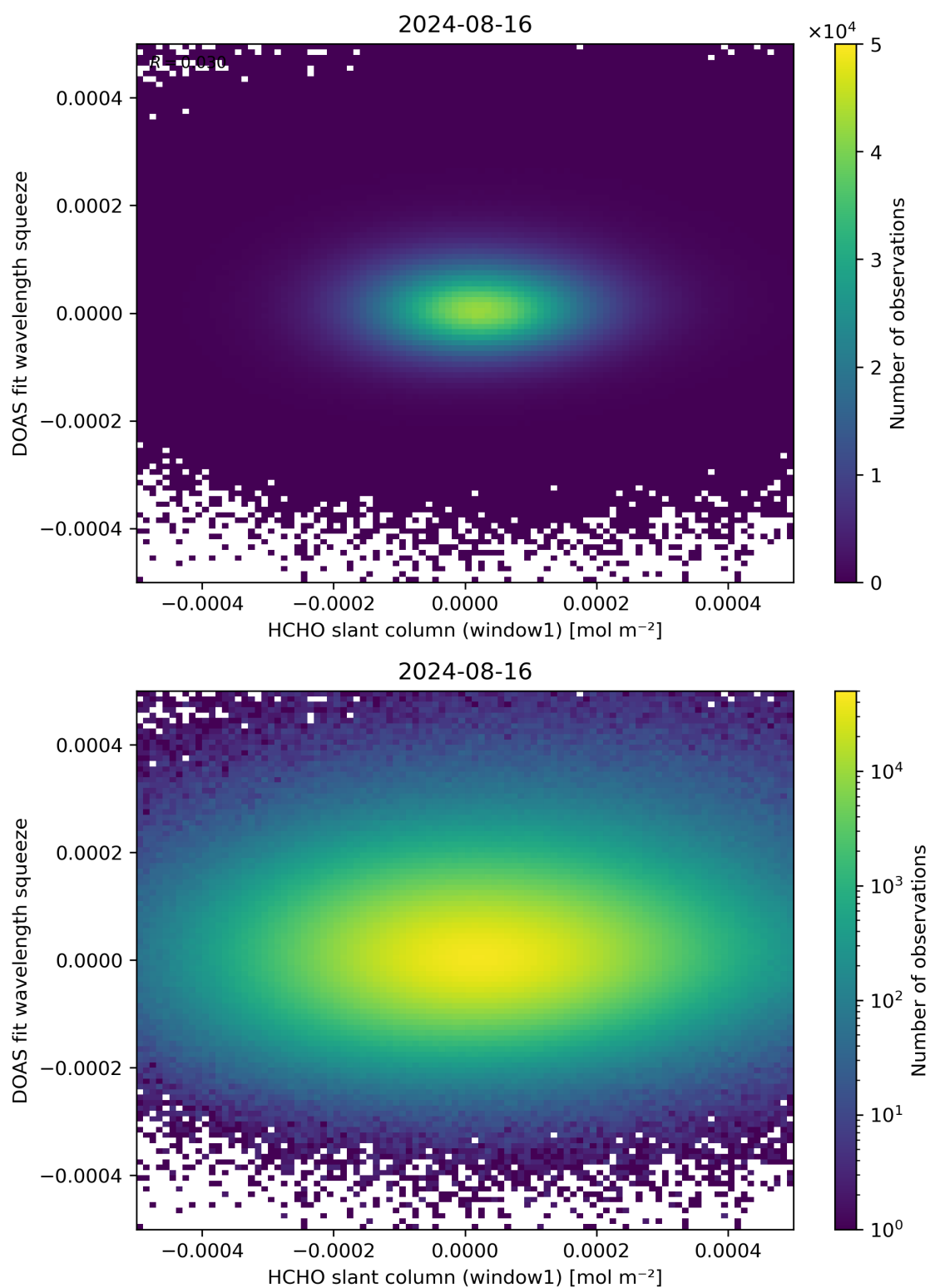
Figure 80: Scatter density plot of “HCHO slant column (window1)” against “DOAS fit wavelength squeeze” for 2024-08-16 to 2024-08-17.
