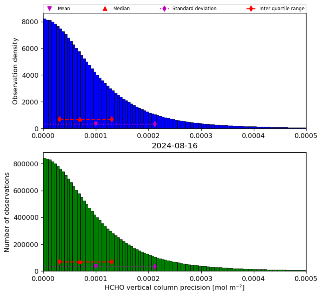
Figure 36: Histogram of “HCHO vertical column precision” for 2024-08-16 to 2024-08-17
