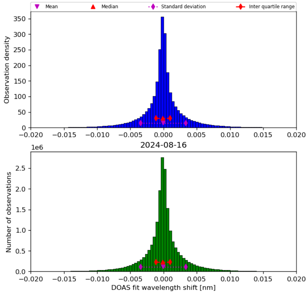
Figure 44: Histogram of “DOAS fit wavelength shift” for 2024-08-16 to 2024-08-17
