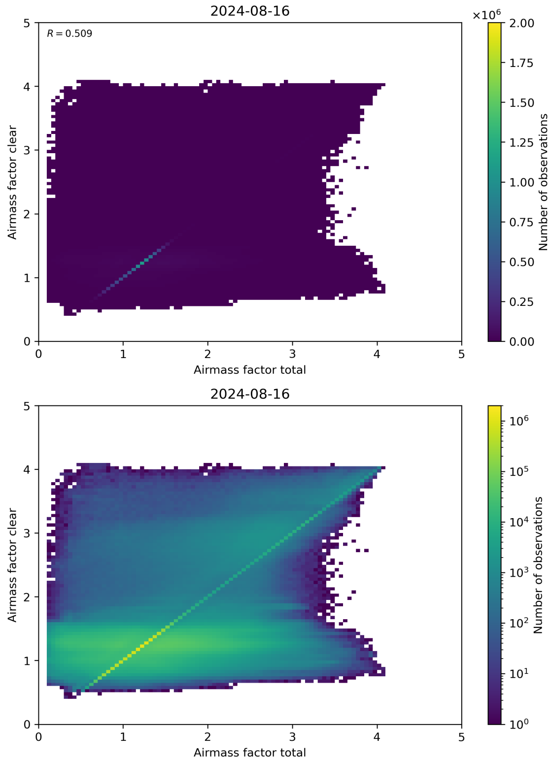
Figure 100: Scatter density plot of “Airmass factor total” against “Airmass factor clear” for 2024-08-16 to 2024-08-17.
