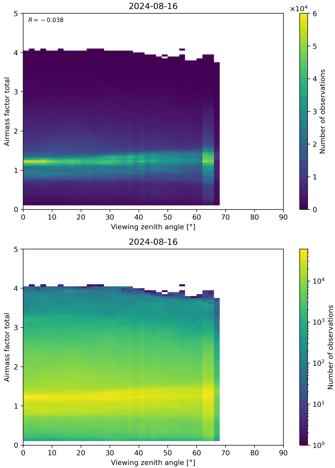
Figure 190: Scatter density plot of “Viewing zenith angle” against “Airmass factor total” for 2024-08-16 to 2024-08-17.
