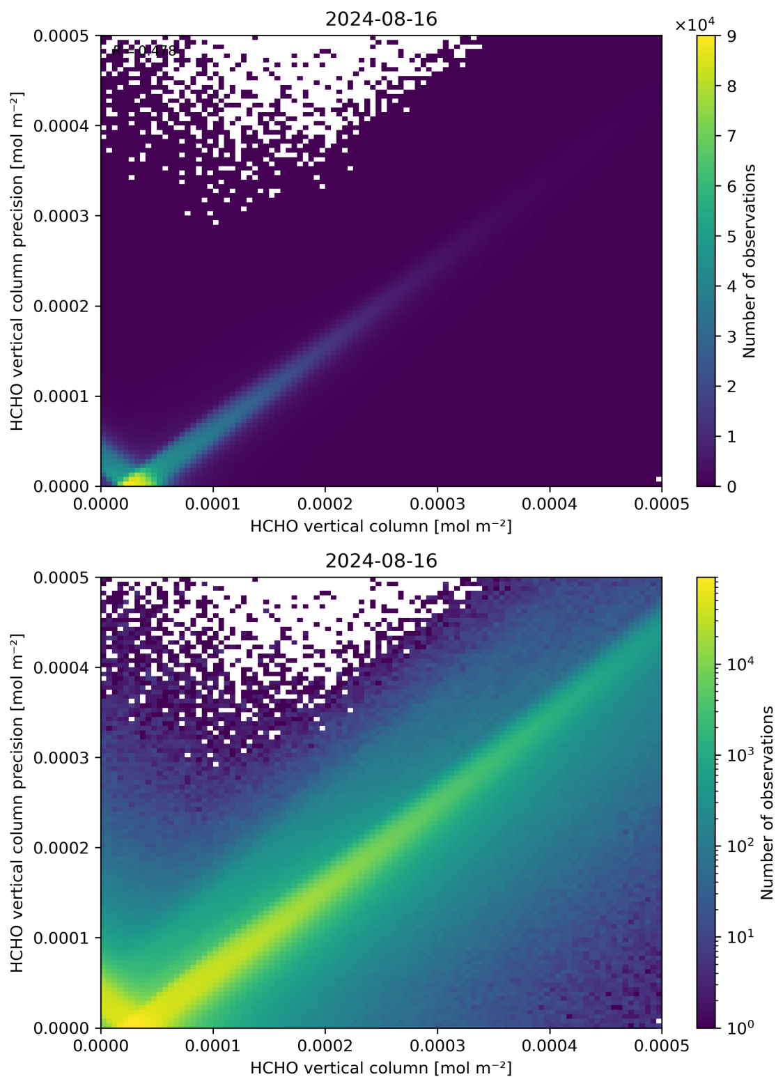
Figure 134: Scatter density plot of “HCHO vertical column” against “HCHO vertical column precision” for 2024-08-16 to 2024-08-17.
