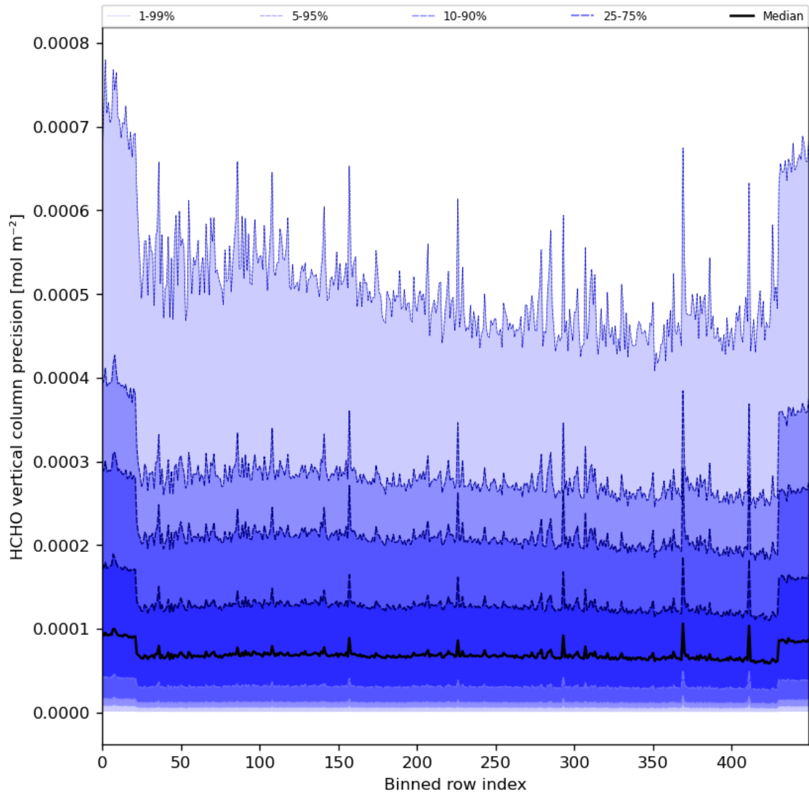
Figure 50: Along track statistics of “HCHO vertical column precision” for 2024-08-16 to 2024-08-17
