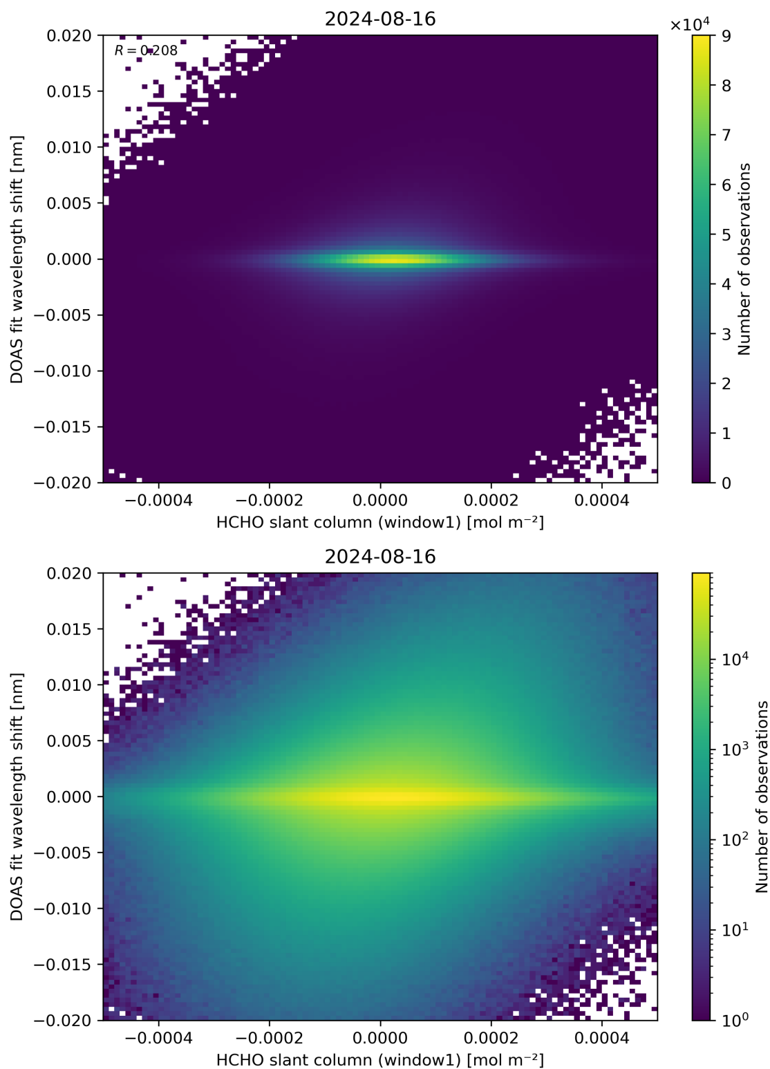
Figure 79: Scatter density plot of “HCHO slant column (window1)” against “DOAS fit wavelength shift” for 2024-08-16 to 2024-08-17.
