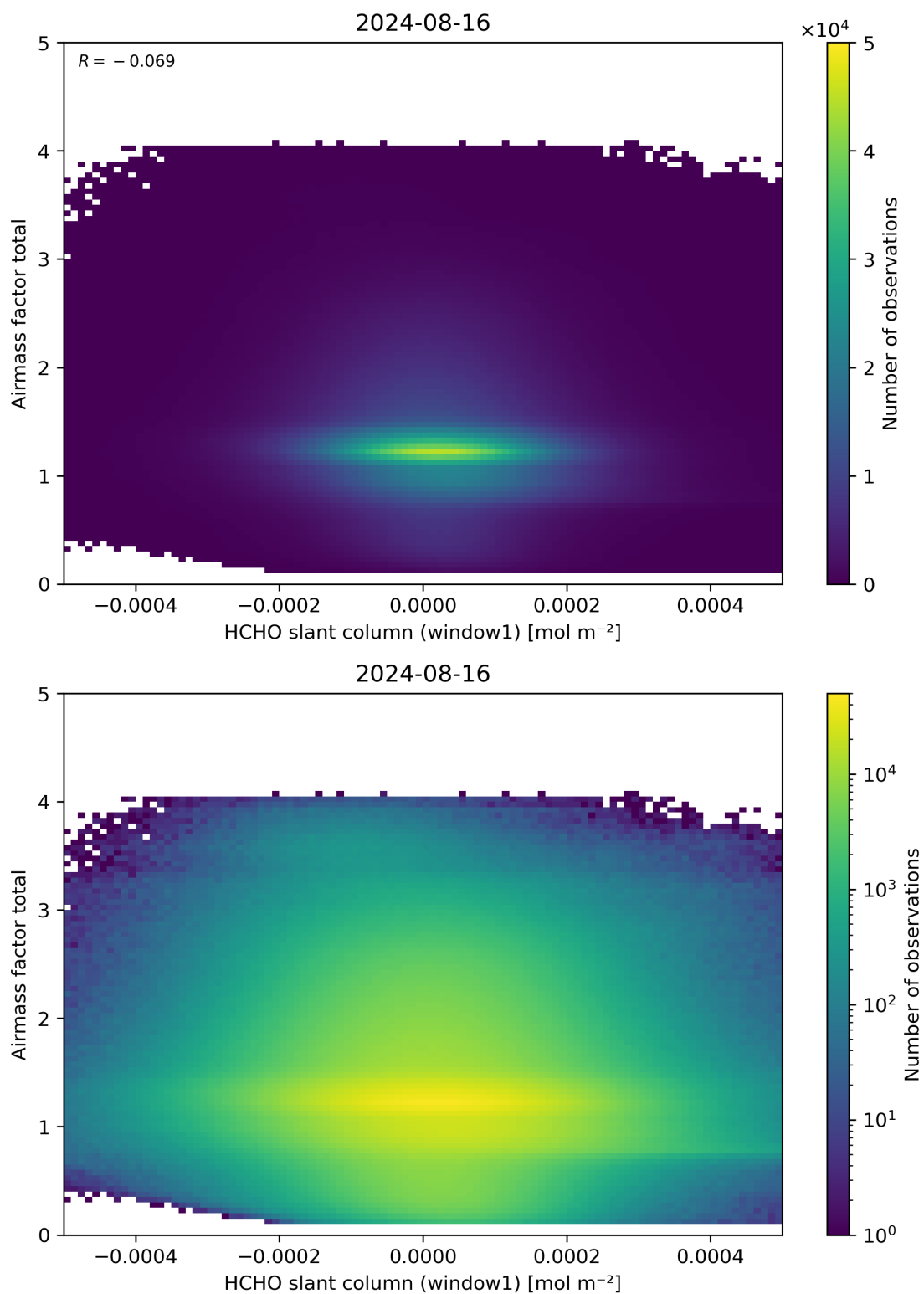
Figure 85: Scatter density plot of “HCHO slant column (window1)” against “Airmass factor total” for 2024-08-16 to 2024-08-17.
