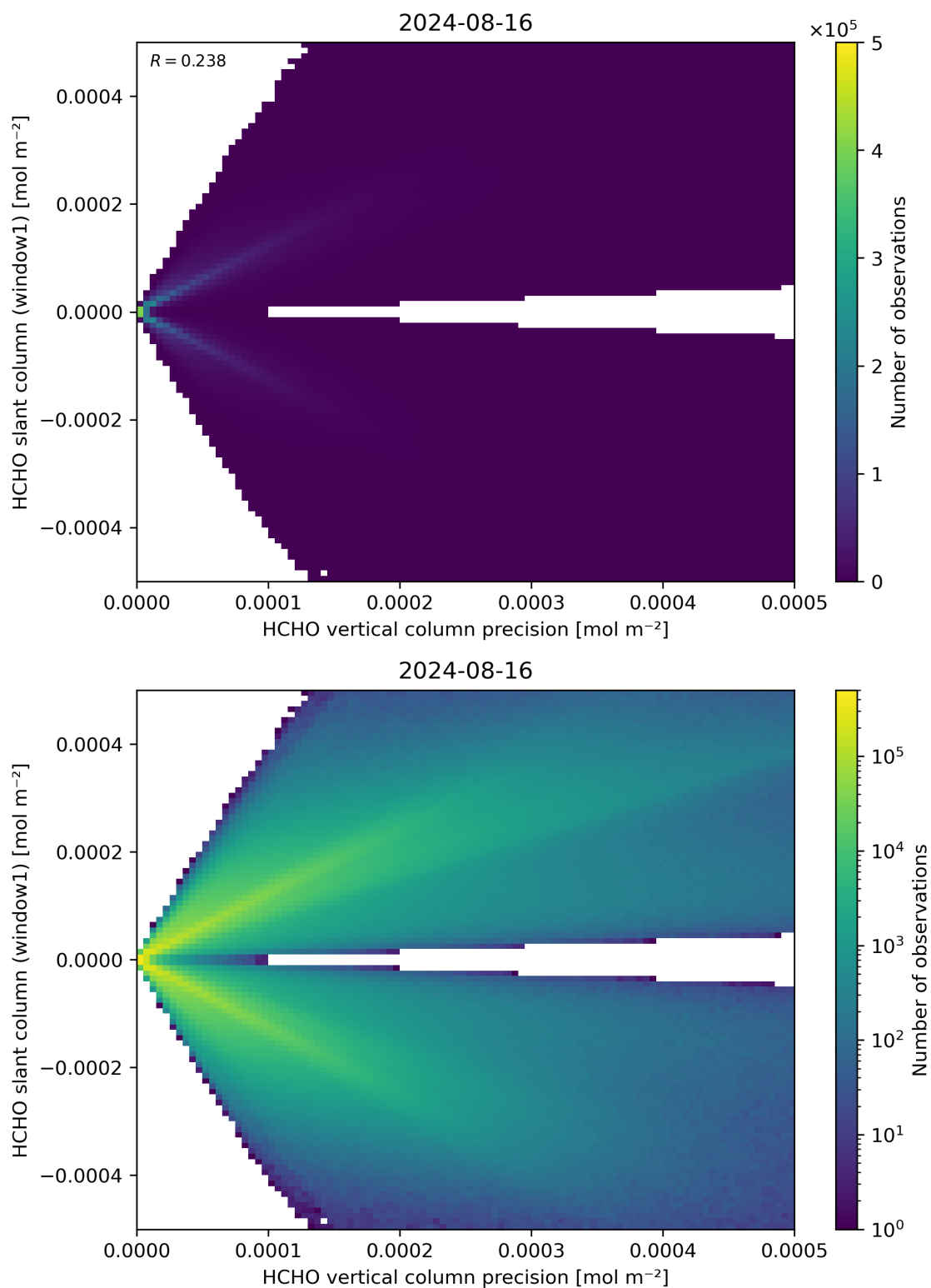
Figure 142: Scatter density plot of “HCHO vertical column precision” against “HCHO slant column (window1)” for 2024-08-16 to 2024-08-17.
