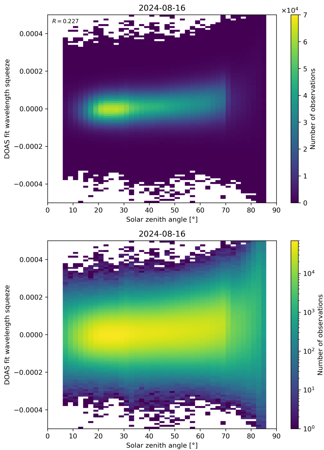
Figure 169: Scatter density plot of “Solar zenith angle” against “DOAS fit wavelength squeeze” for 2024-08-16 to 2024-08-17.
