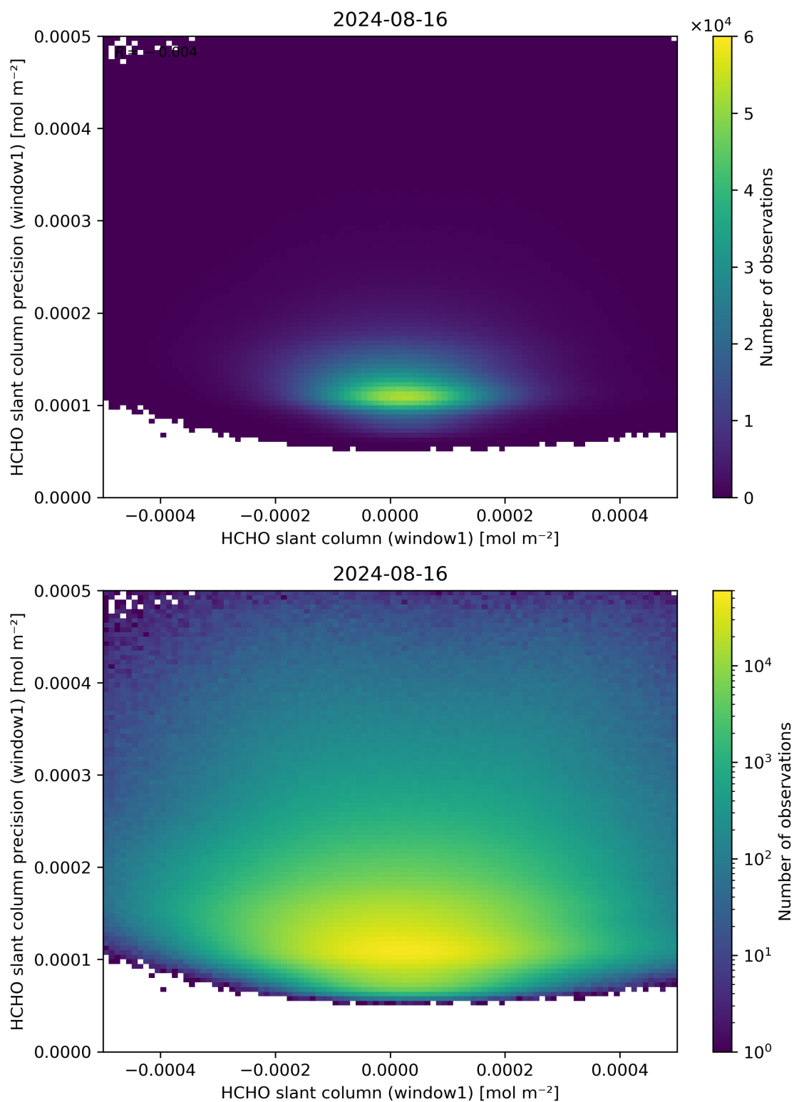
Figure 84: Scatter density plot of “HCHO slant column (window1)” against “HCHO slant column precision (window1)” for 2024-08-16 to 2024-08-17.
