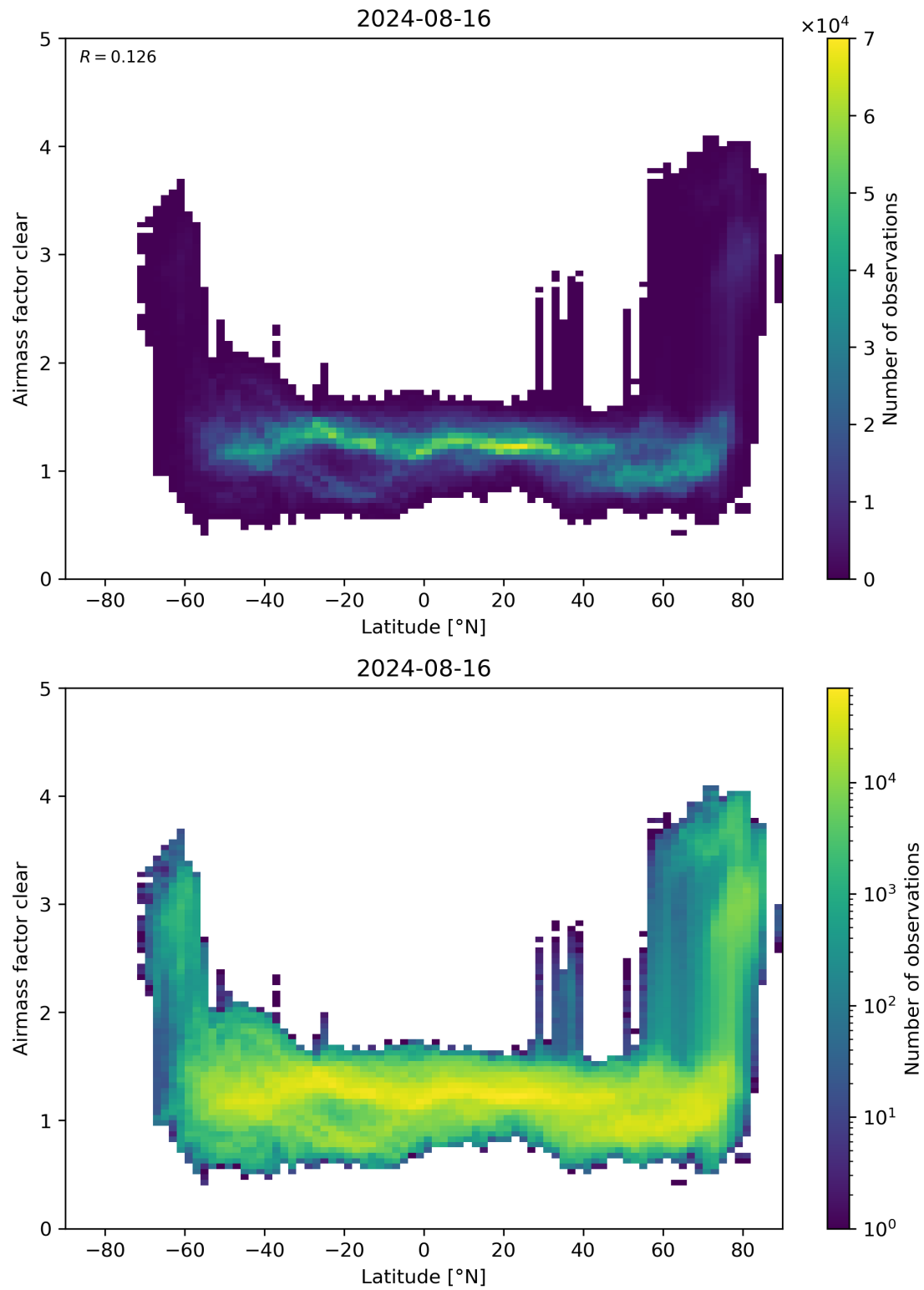
Figure 156: Scatter density plot of “Latitude” against “Airmass factor clear” for 2024-08-16 to 2024-08-17.
