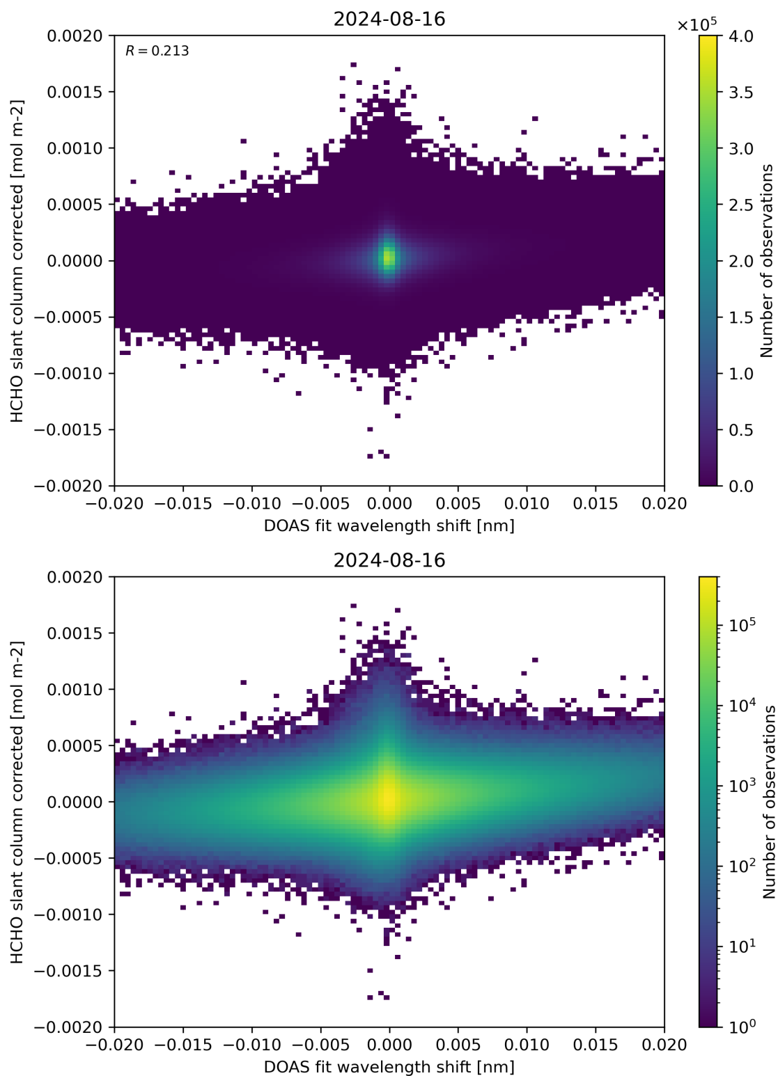
Figure 66: Scatter density plot of “DOAS fit wavelength shift” against “HCHO slant column corrected” for 2024-08-16 to 2024-08-17.
