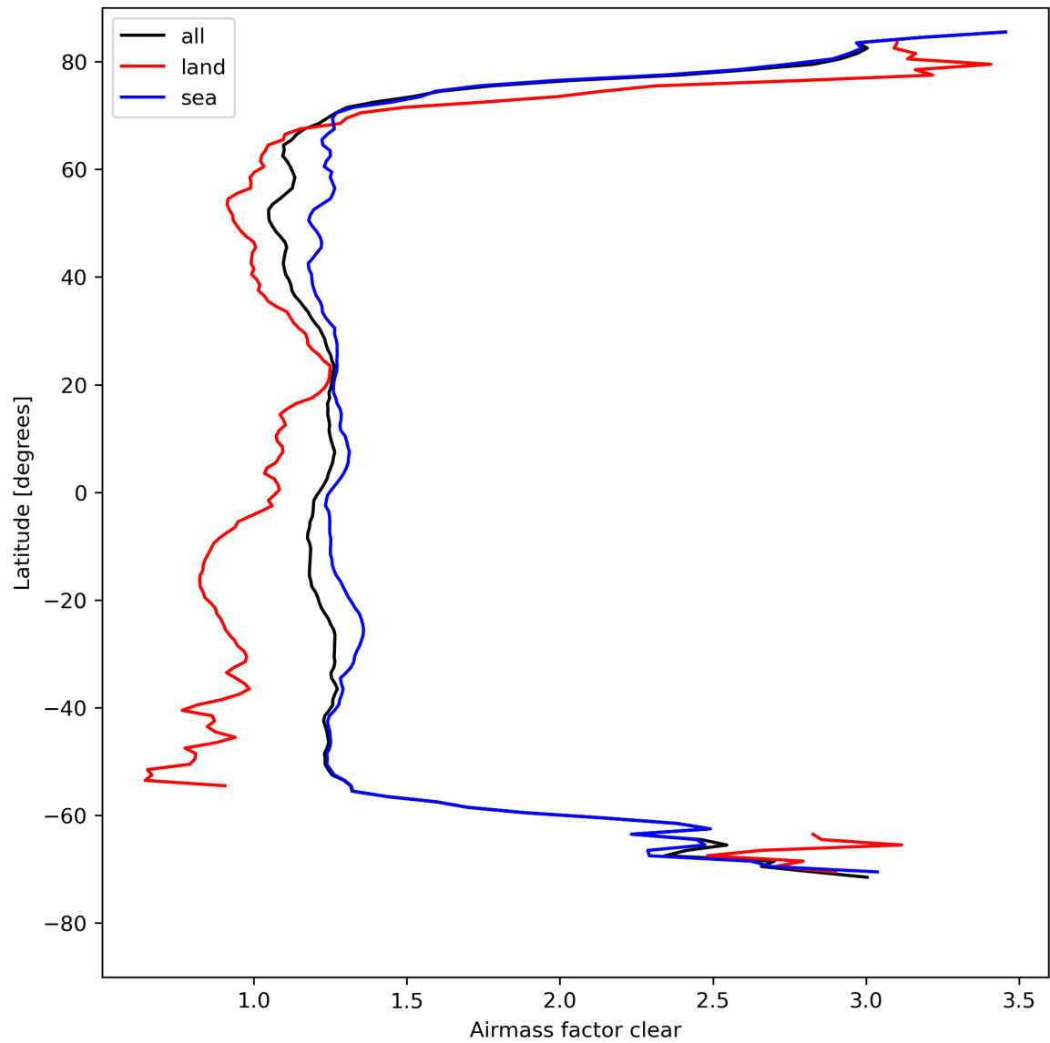
Figure 28: Zonal average of “Airmass factor clear” for 2024-08-16 to 2024-08-17.
