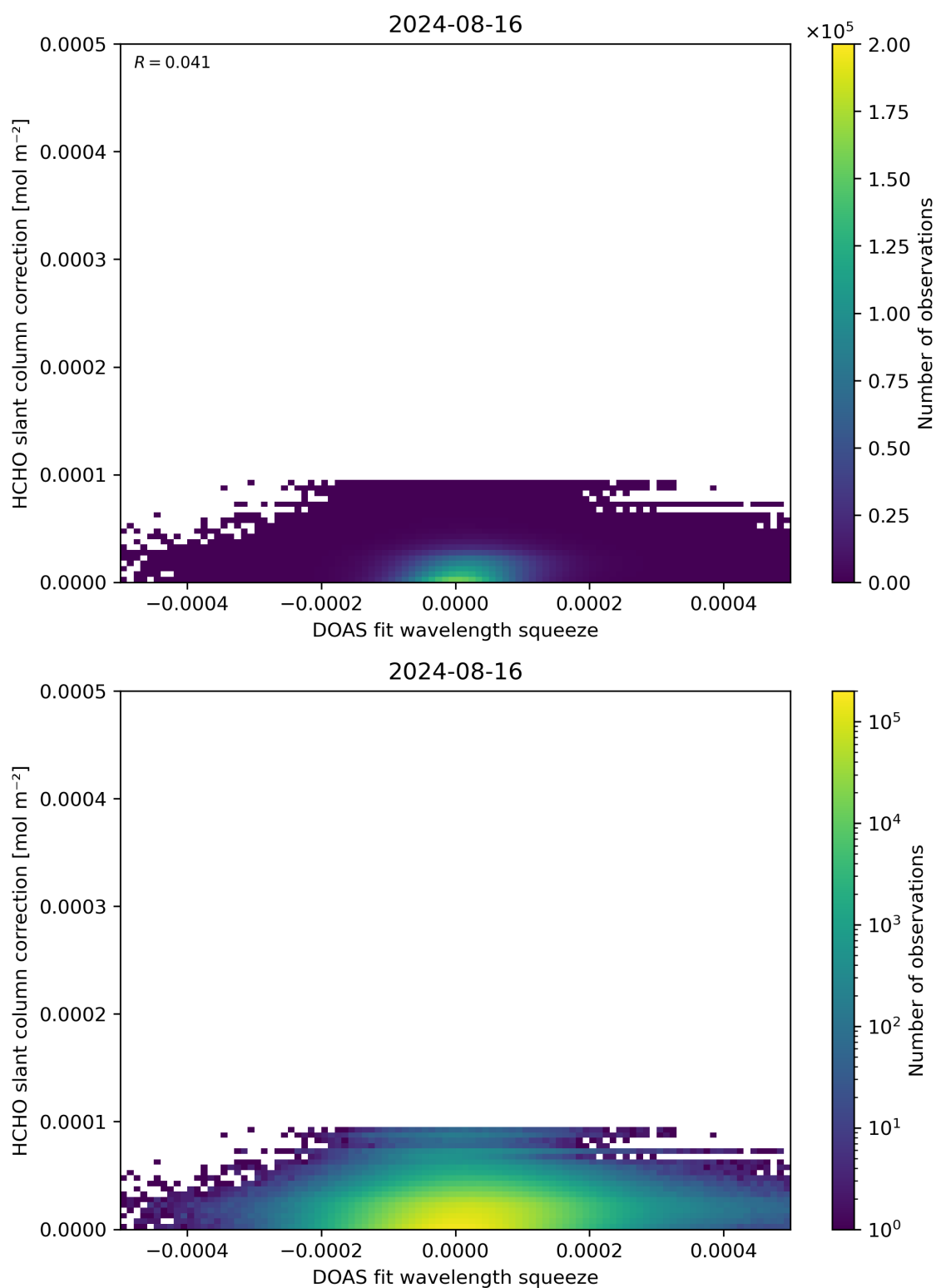
Figure 70: Scatter density plot of “DOAS fit wavelength squeeze” against “HCHO slant column correction” for 2024-08-16 to 2024-08-17.
