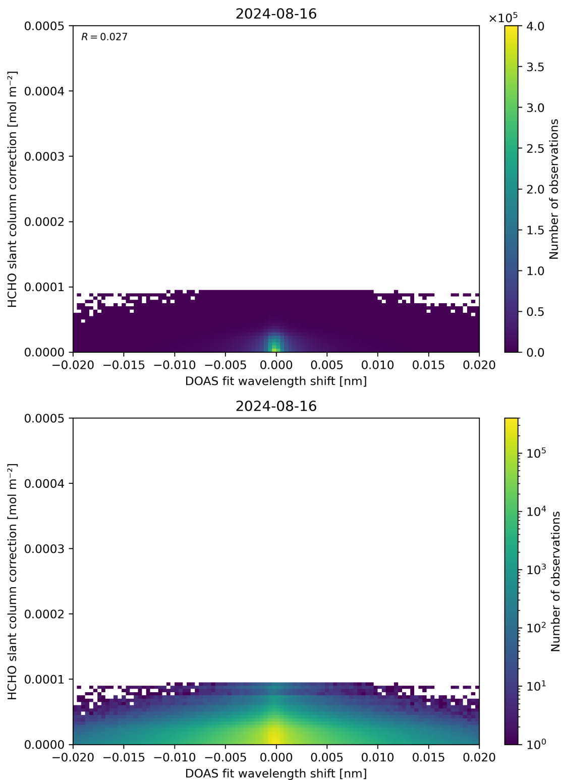
Figure 67: Scatter density plot of “DOAS fit wavelength shift” against “HCHO slant column correction” for 2024-08-16 to 2024-08-17.
