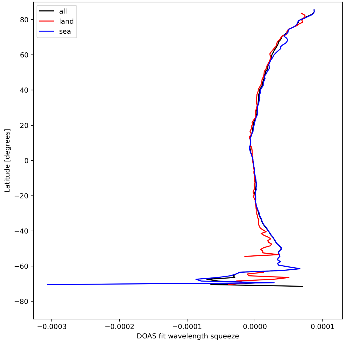
Figure 31: Zonal average of "DOAS fit wavelength squeeze" for 2024-08-16 to 2024-08-17.
