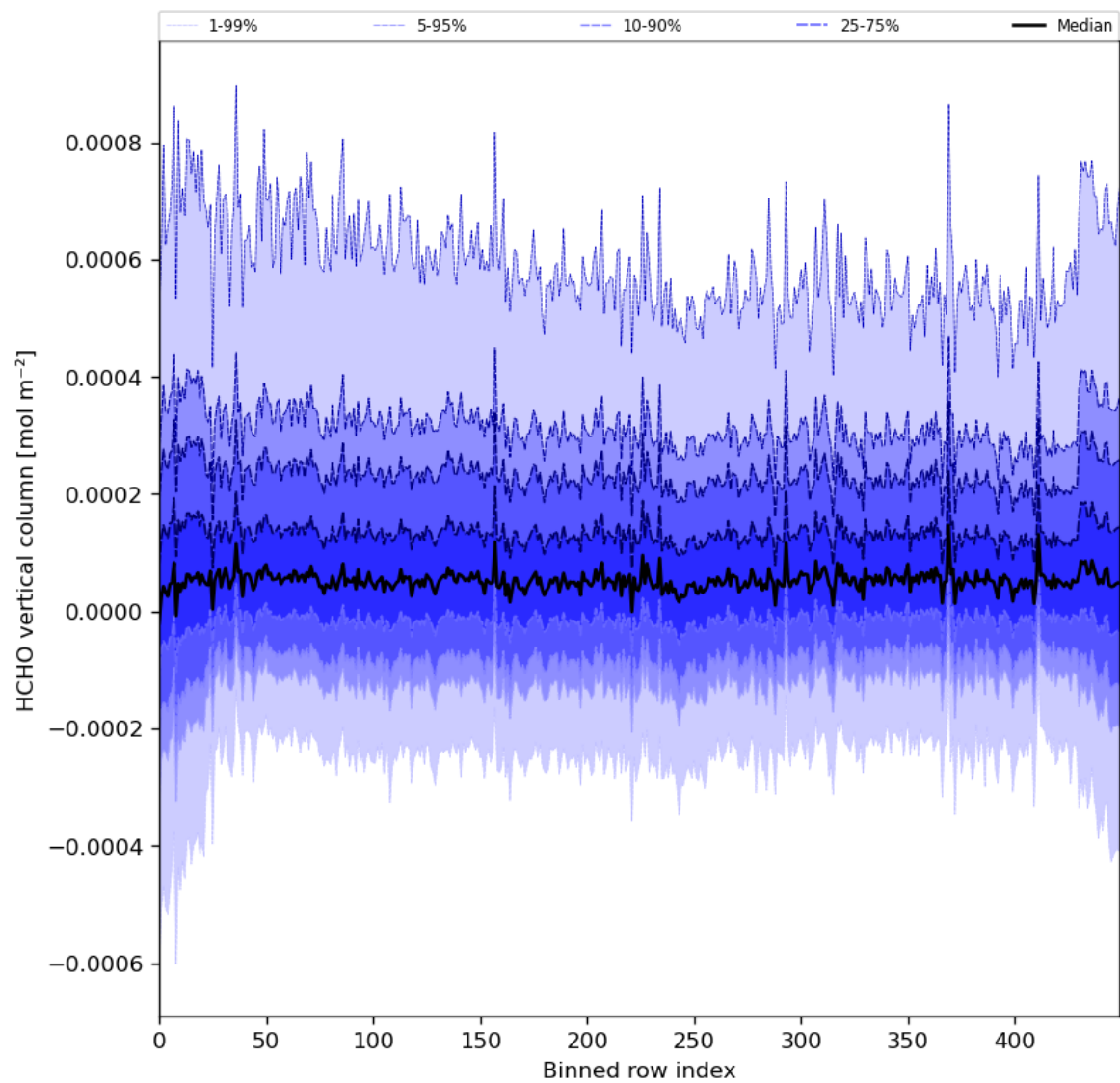
Figure 49: Along track statistics of “HCHO vertical column” for 2024-08-16 to 2024-08-17
