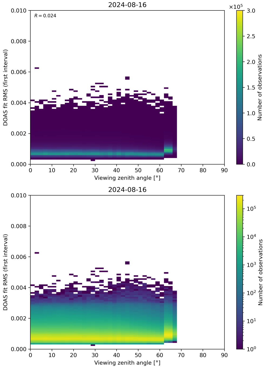
Figure 182: Scatter density plot of “Viewing zenith angle” against “DOAS fit RMS (first interval)” for 2024-08-16 to 2024-08-17.
