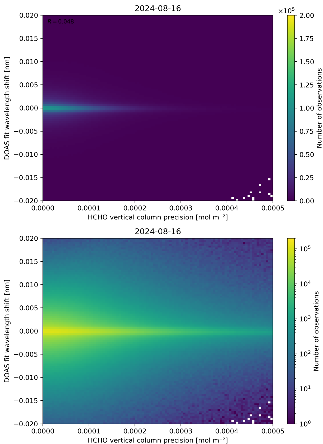
Figure 137: Scatter density plot of “HCHO vertical column precision” against “DOAS fit wavelength shift” for 2024-08-16 to 2024-08-17.
