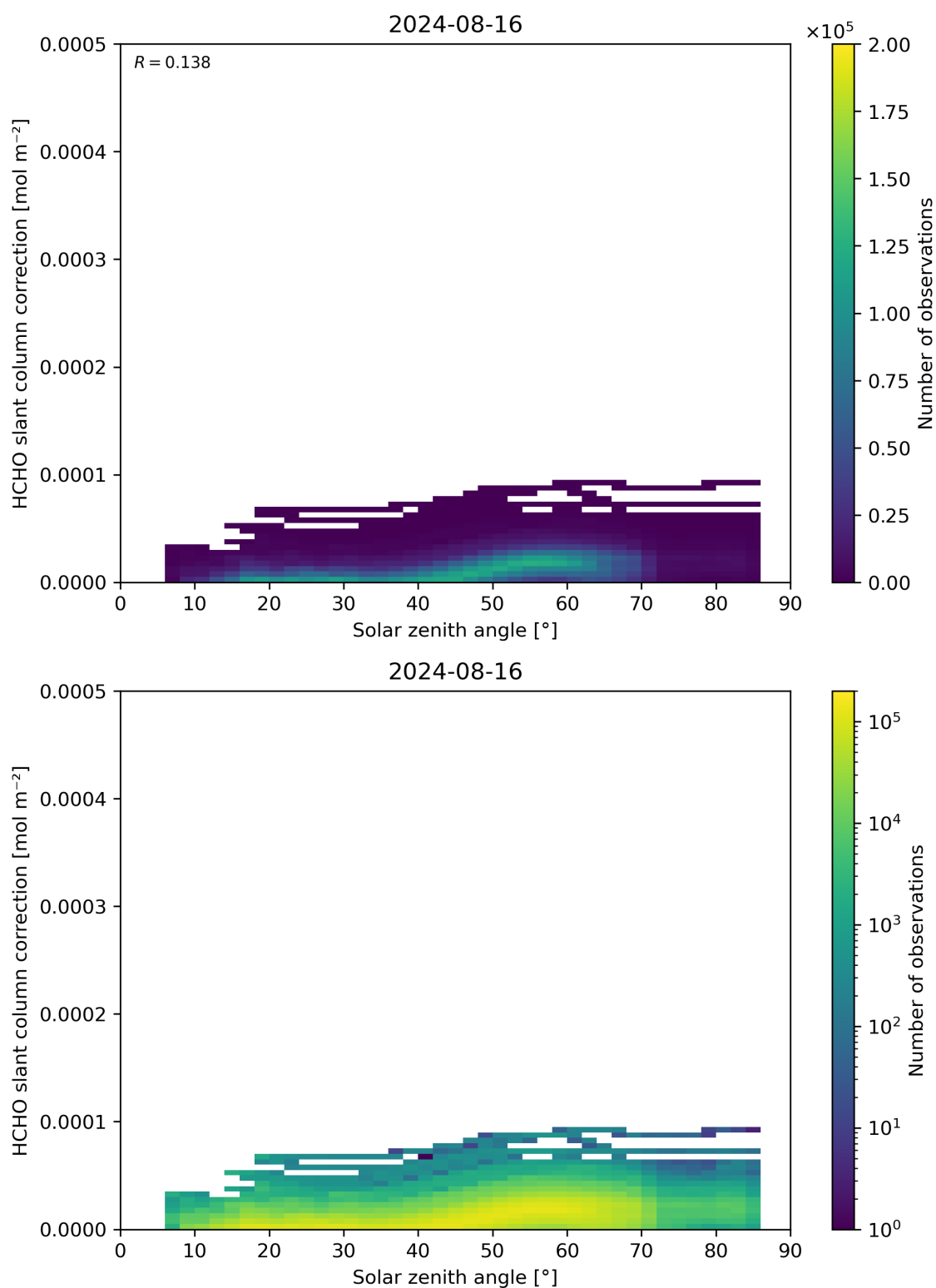
Figure 172: Scatter density plot of “Solar zenith angle” against “HCHO slant column correction” for 2024-08-16 to 2024-08-17.
