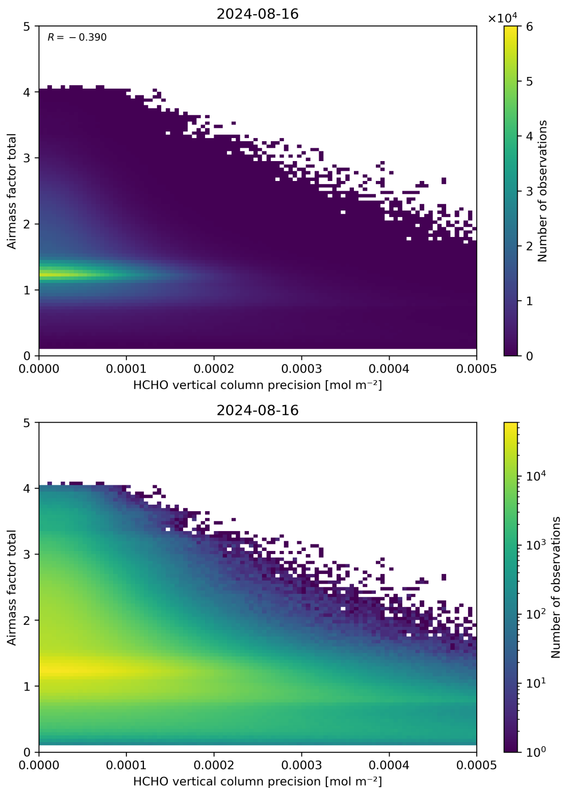
Figure 144: Scatter density plot of “HCHO vertical column precision” against “Airmass factor total” for 2024-08-16 to 2024-08-17.
