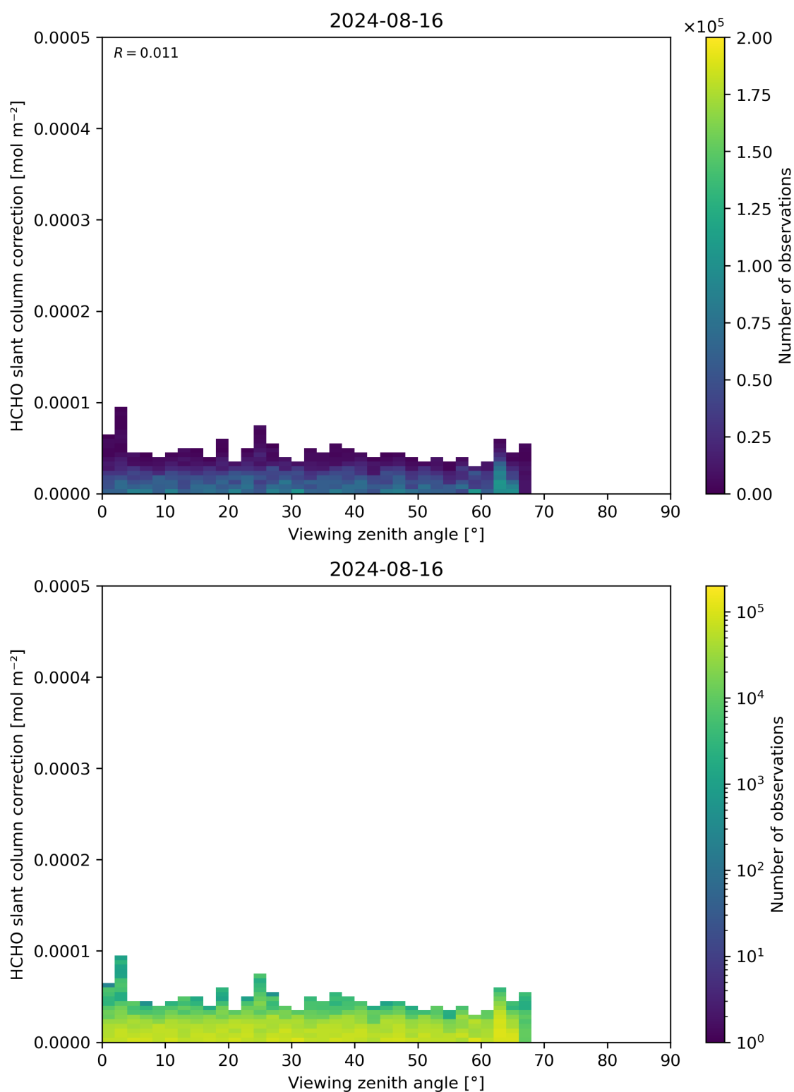
Figure 187: Scatter density plot of “Viewing zenith angle” against “HCHO slant column correction” for 2024-08-16 to 2024-08-17.
