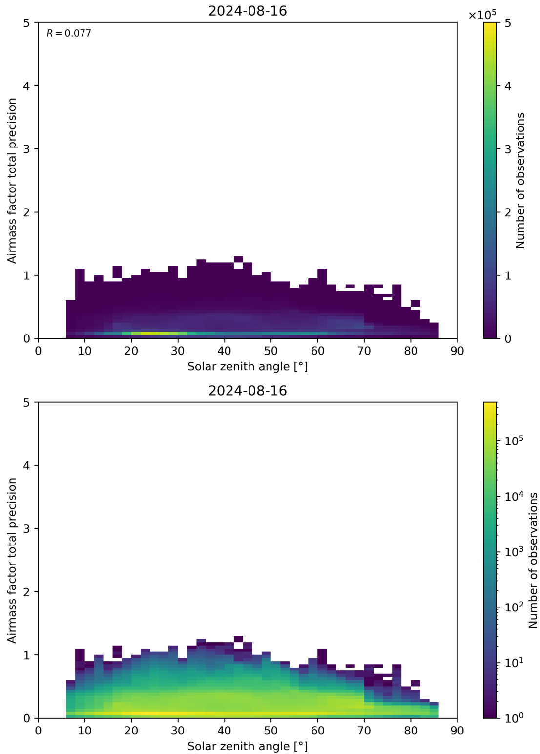
Figure 176: Scatter density plot of “Solar zenith angle” against “Airmass factor total precision” for 2024-08-16 to 2024-08-17.
