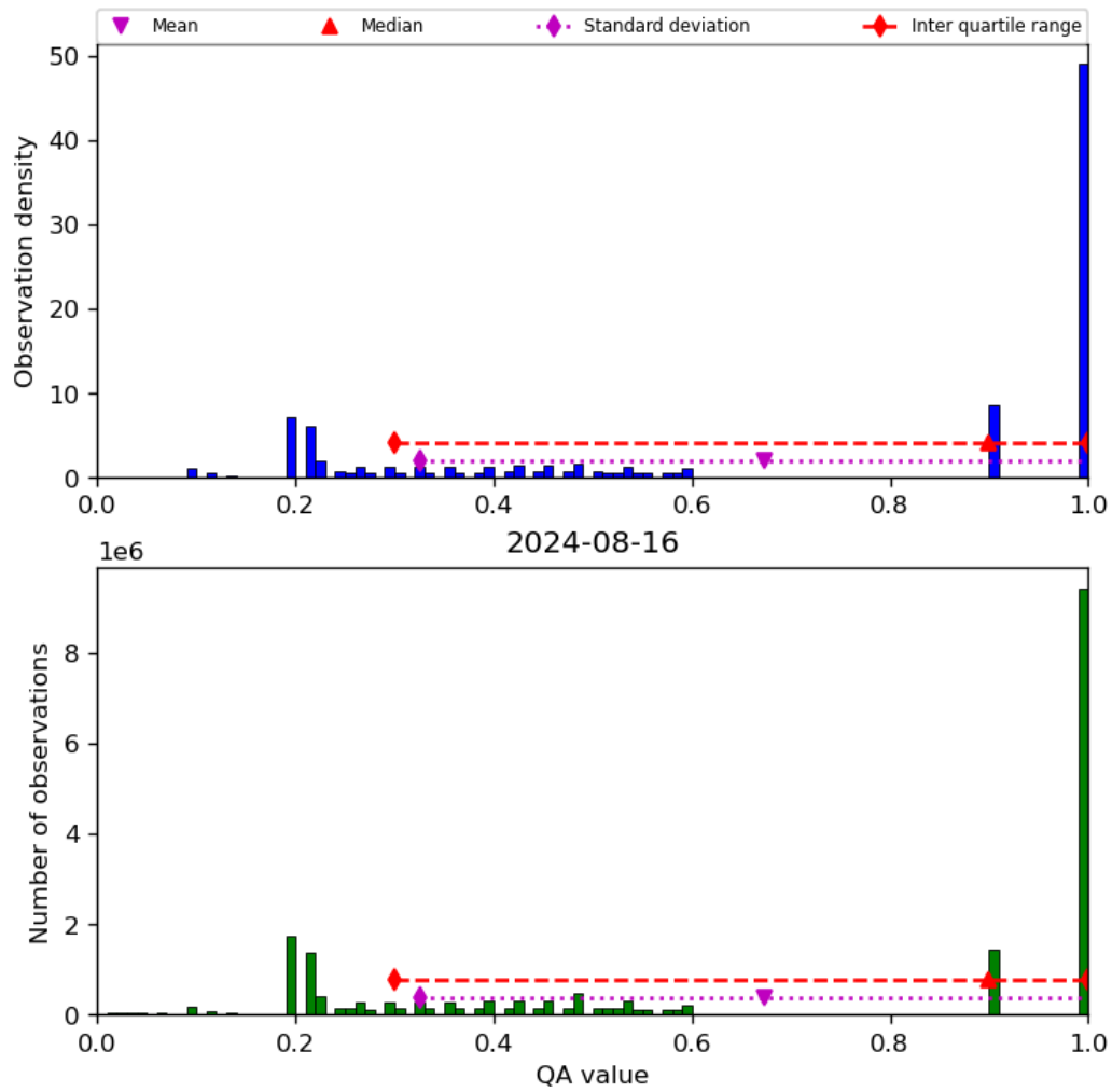
Figure 34: Histogram of “QA value” for 2024-08-16 to 2024-08-17
