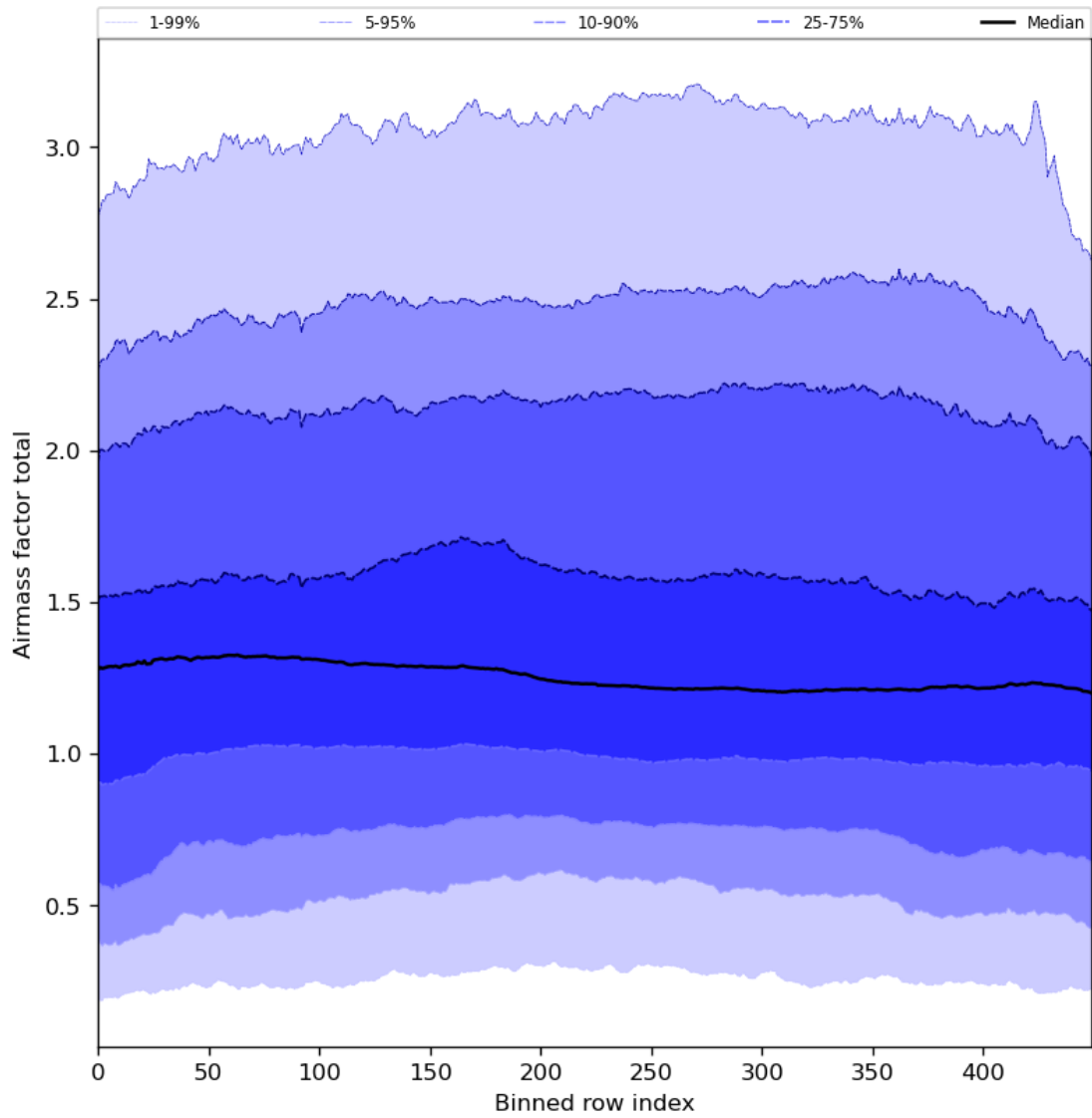
Figure 54: Along track statistics of “Airmass factor total” for 2024-08-16 to 2024-08-17
