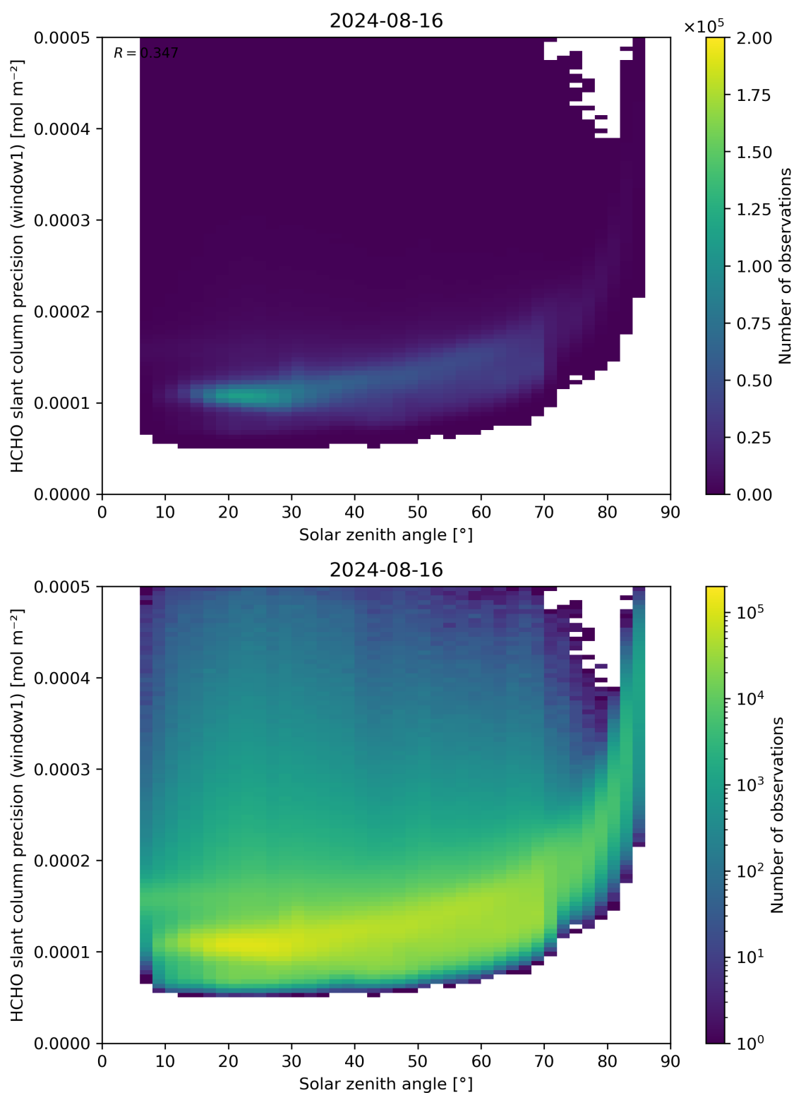
Figure 174: Scatter density plot of “Solar zenith angle” against “HCHO slant column precision (window1)” for 2024-08-16 to 2024-08-17.
