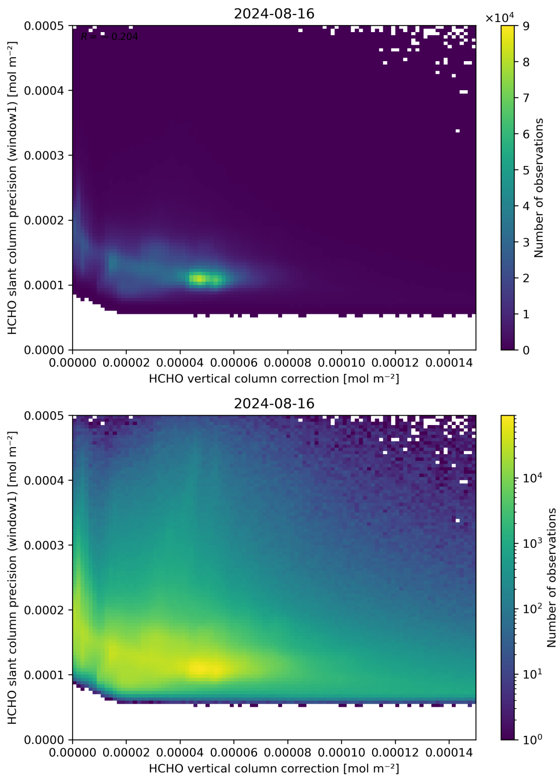
Figure 119: Scatter density plot of “HCHO vertical column correction” against “HCHO slant column precision (window1)” for 2024-08-16 to 2024-08-17.
