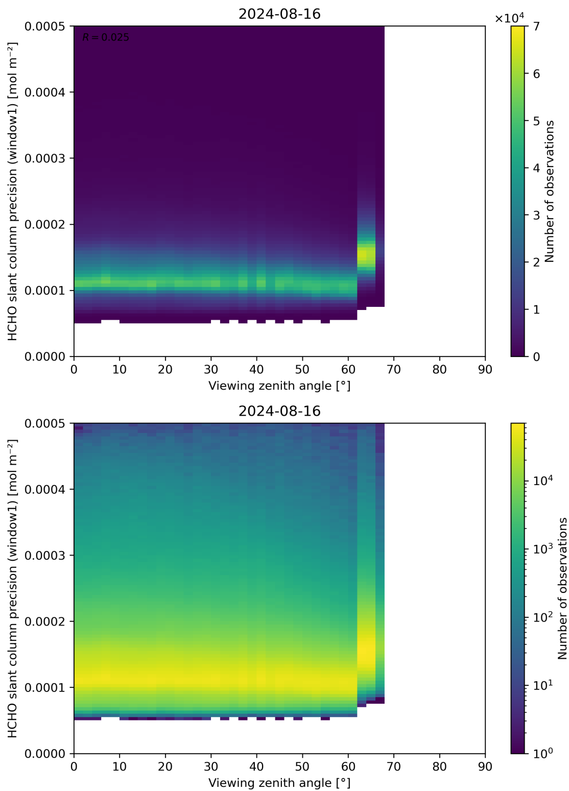
Figure 189: Scatter density plot of “Viewing zenith angle” against “HCHO slant column precision (window1)” for 2024-08-16 to 2024-08-17.
