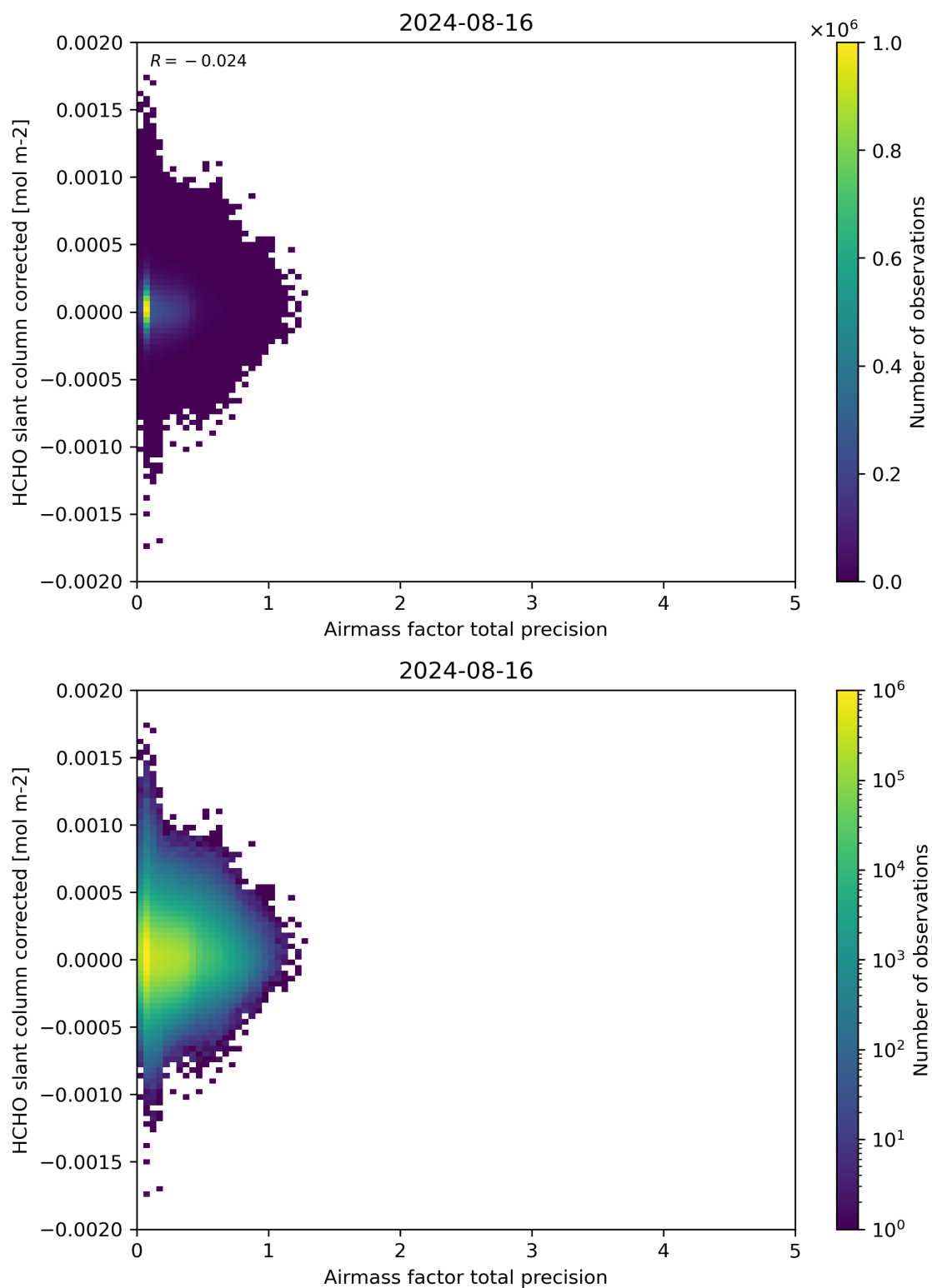
Figure 109: Scatter density plot of “Airmass factor total precision” against “HCHO slant column corrected” for 2024-08-16 to 2024-08-17.
