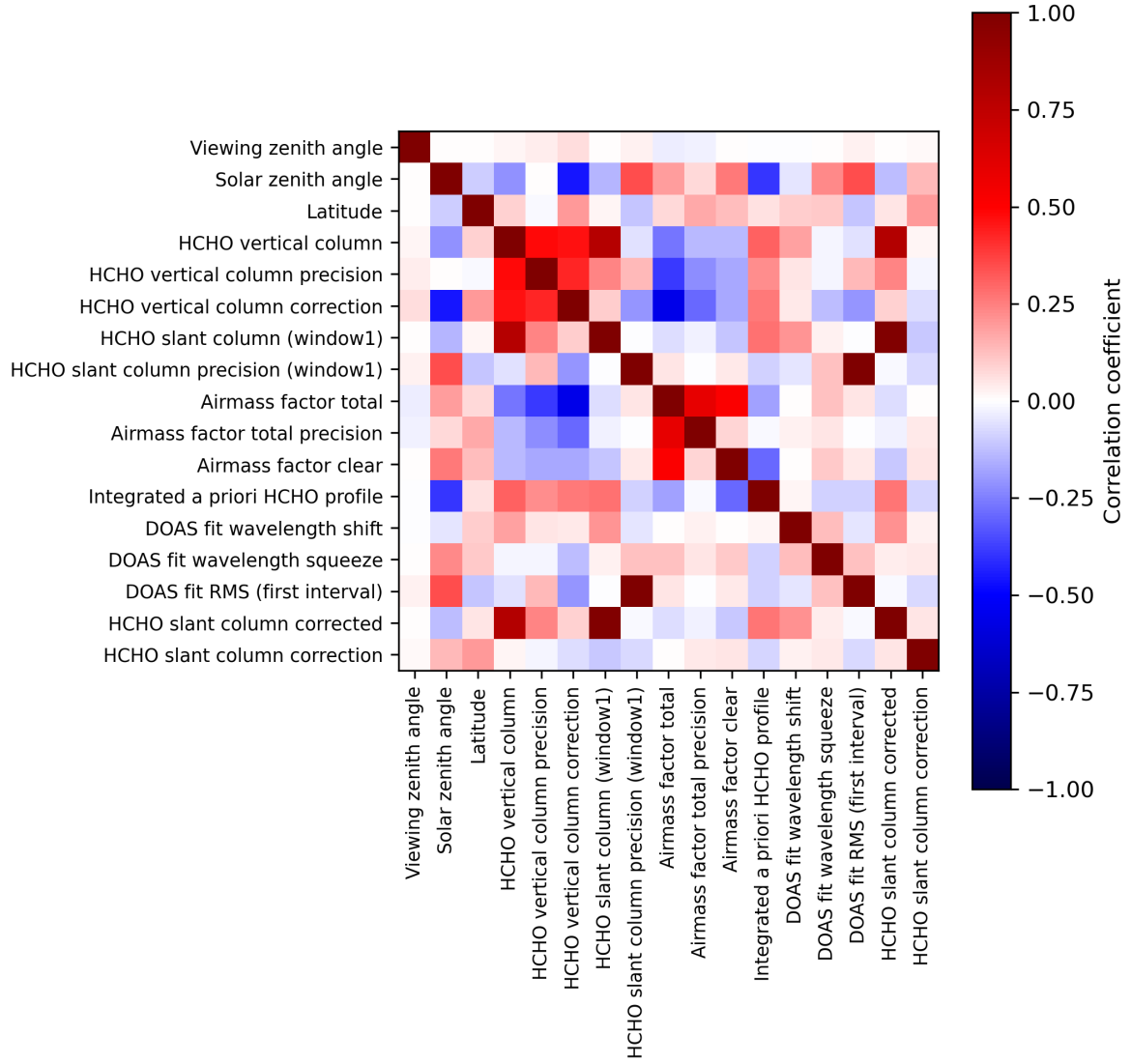
Figure 2: Map of correlation matrix for 2024-08-16 to 2024-08-17.
