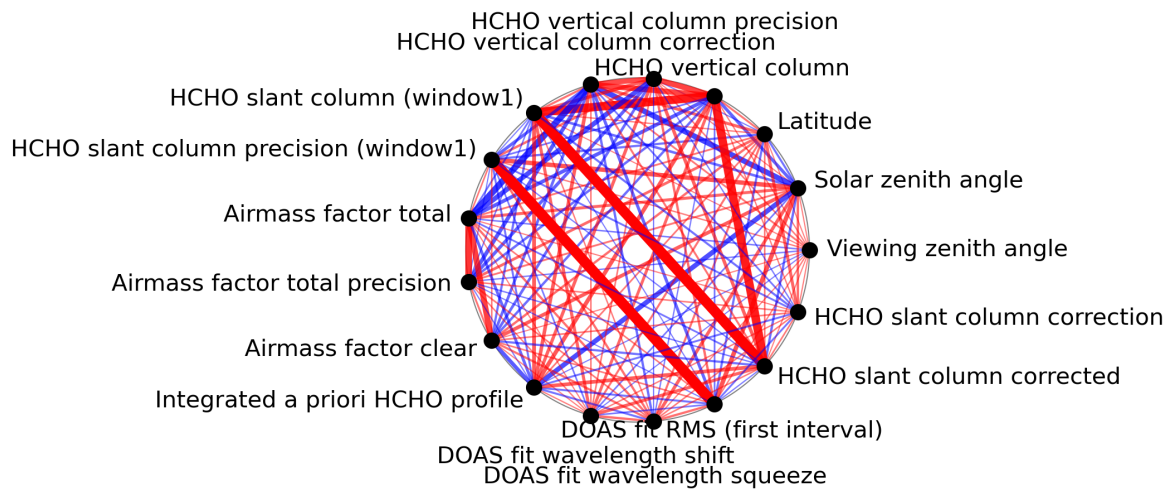
Figure 1: Map of correlation graph for 2024-08-16 to 2024-08-17.
