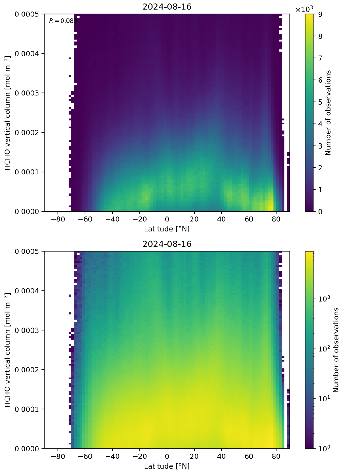
Figure 163: Scatter density plot of “Latitude” against “HCHO vertical column” for 2024-08-16 to 2024-08-17.
