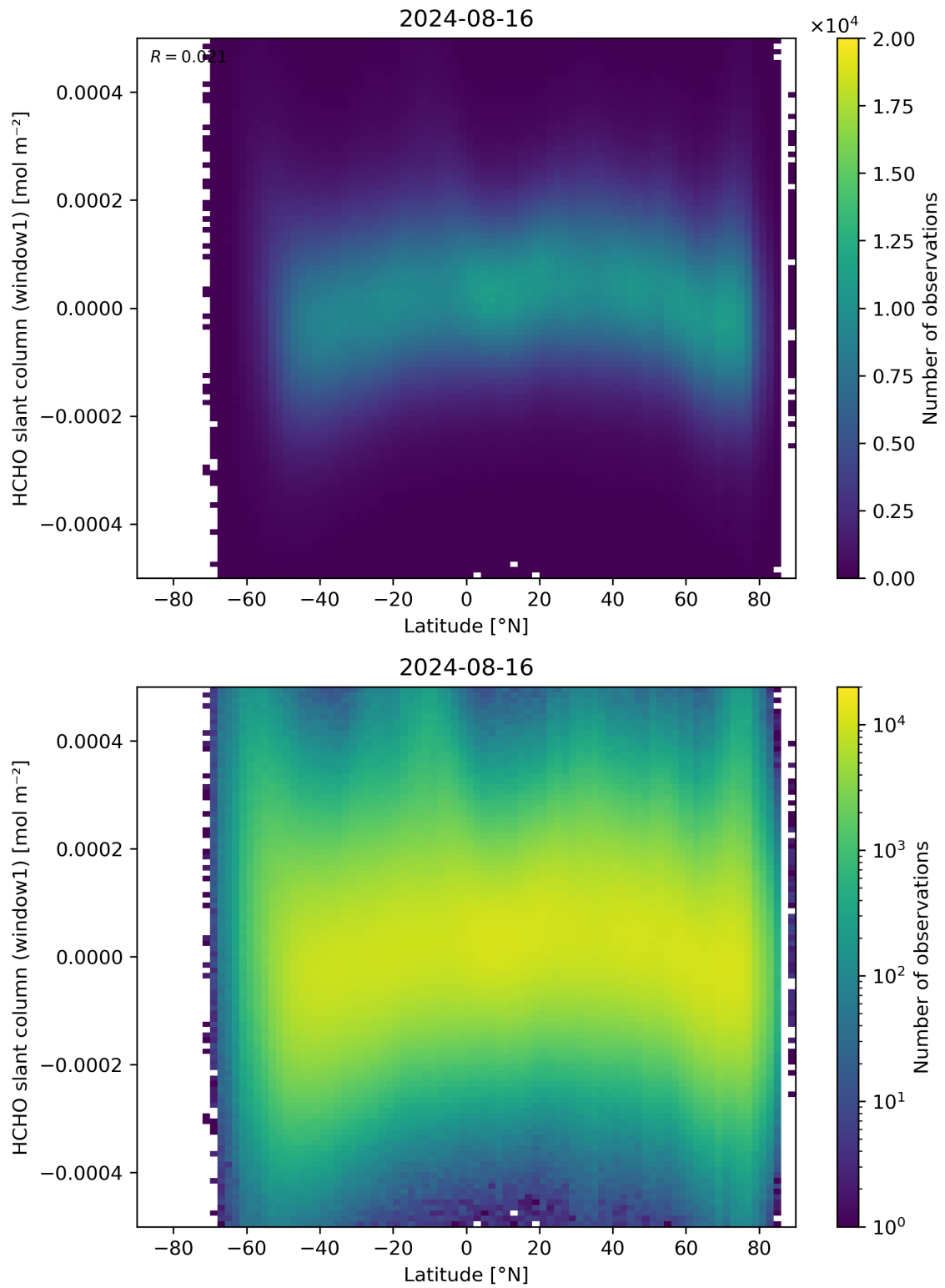
Figure 159: Scatter density plot of “Latitude” against “HCHO slant column (window1)” for 2024-08-16 to 2024-08-17.
