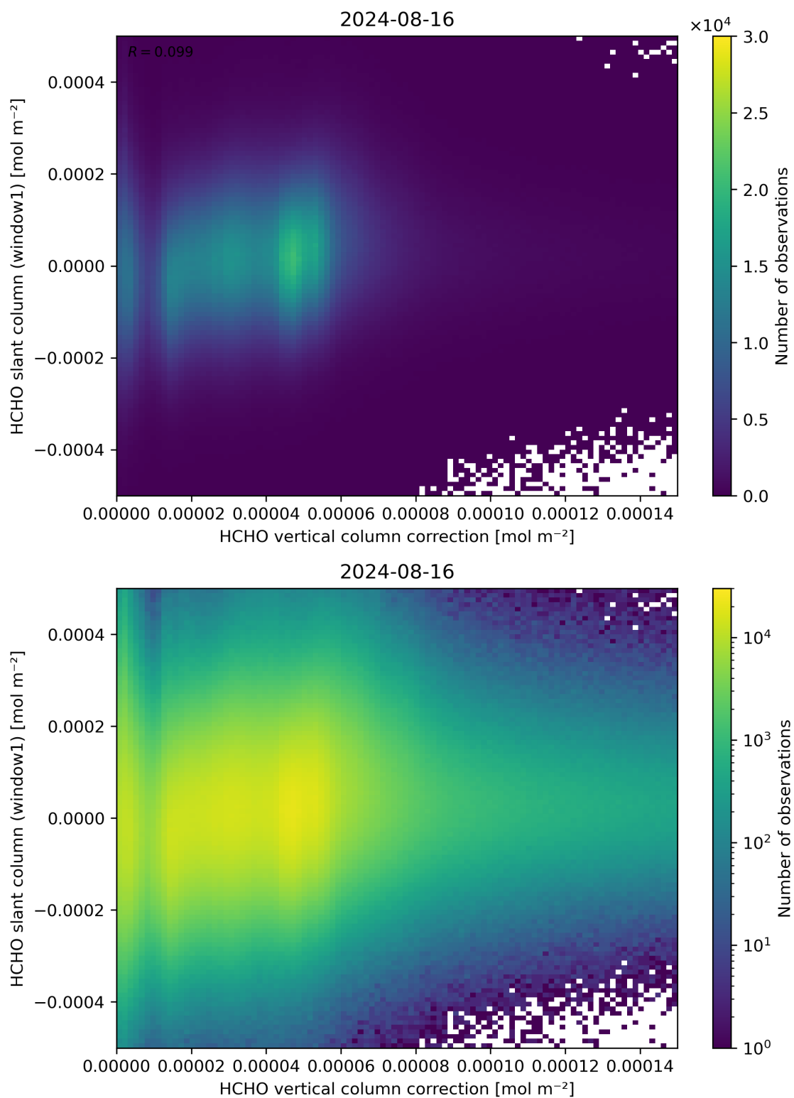
Figure 118: Scatter density plot of “HCHO vertical column correction” against “HCHO slant column (window1)” for 2024-08-16 to 2024-08-17.
