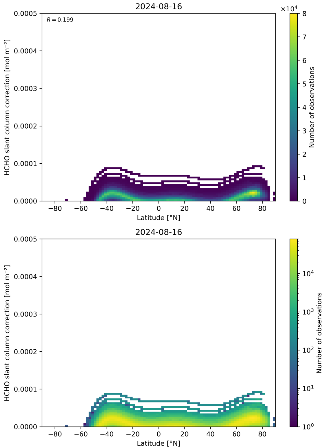
Figure 158: Scatter density plot of “Latitude” against “HCHO slant column correction” for 2024-08-16 to 2024-08-17.
