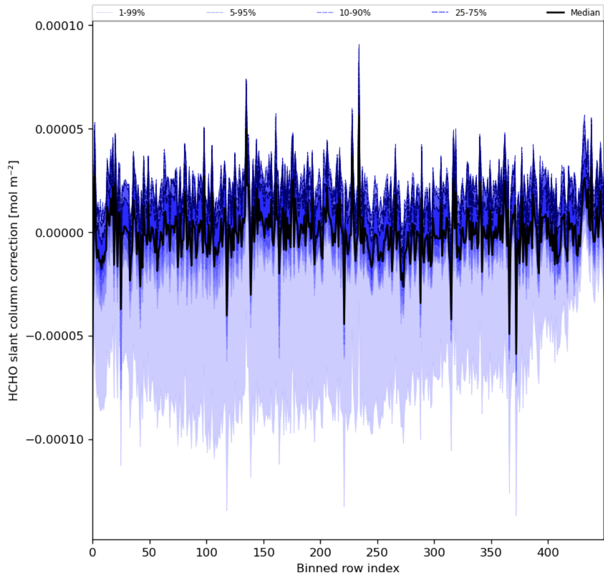
Figure 61: Along track statistics of “HCHO slant column correction” for 2024-08-16 to 2024-08-17
