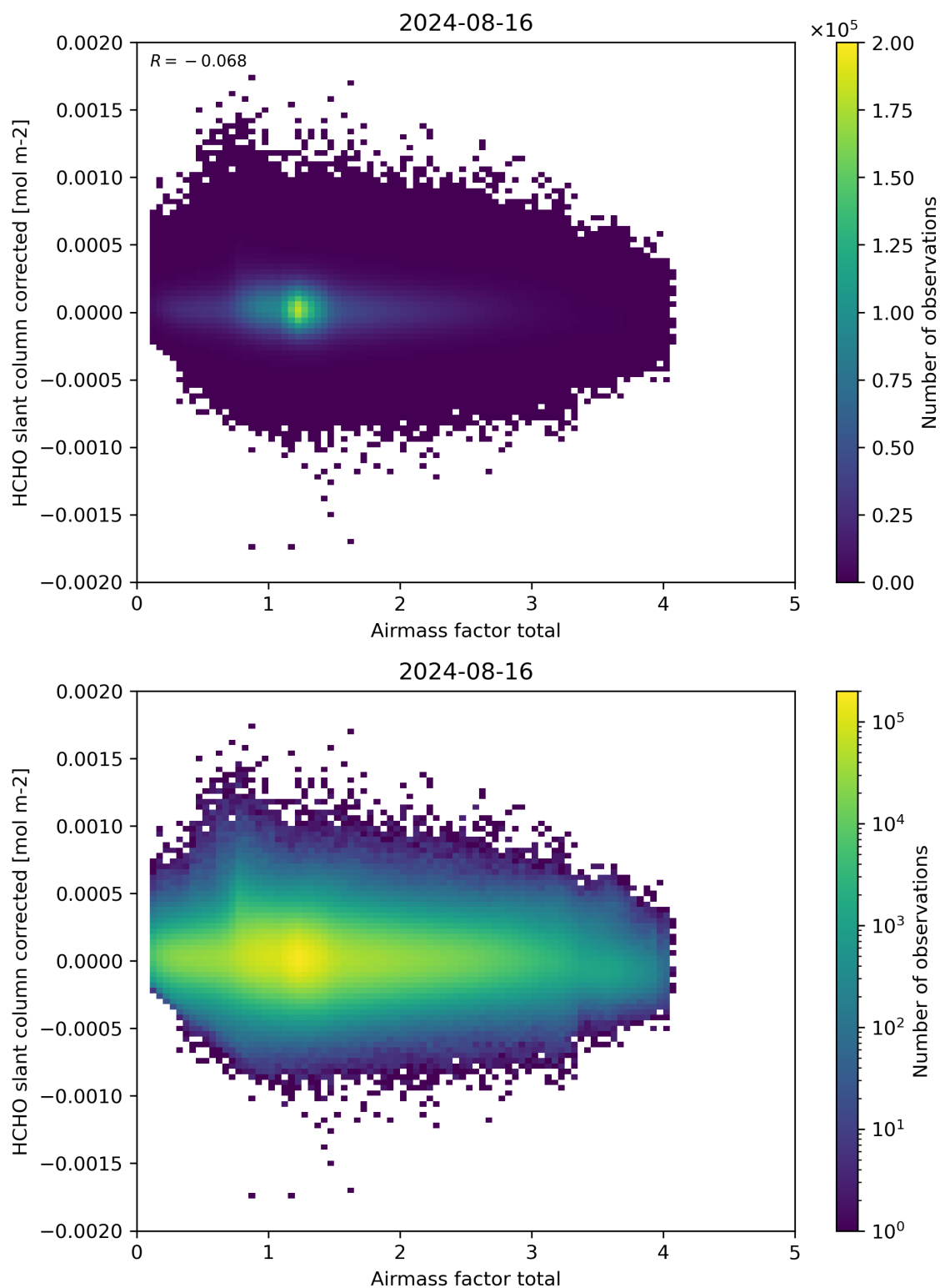
Figure 101: Scatter density plot of “Airmass factor total” against “HCHO slant column corrected” for 2024-08-16 to 2024-08-17.
