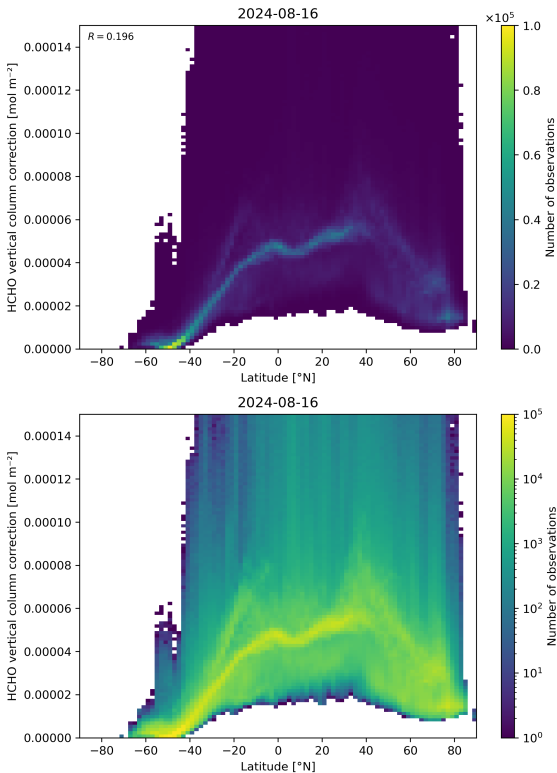
Figure 164: Scatter density plot of “Latitude” against “HCHO vertical column correction” for 2024-08-16 to 2024-08-17.
