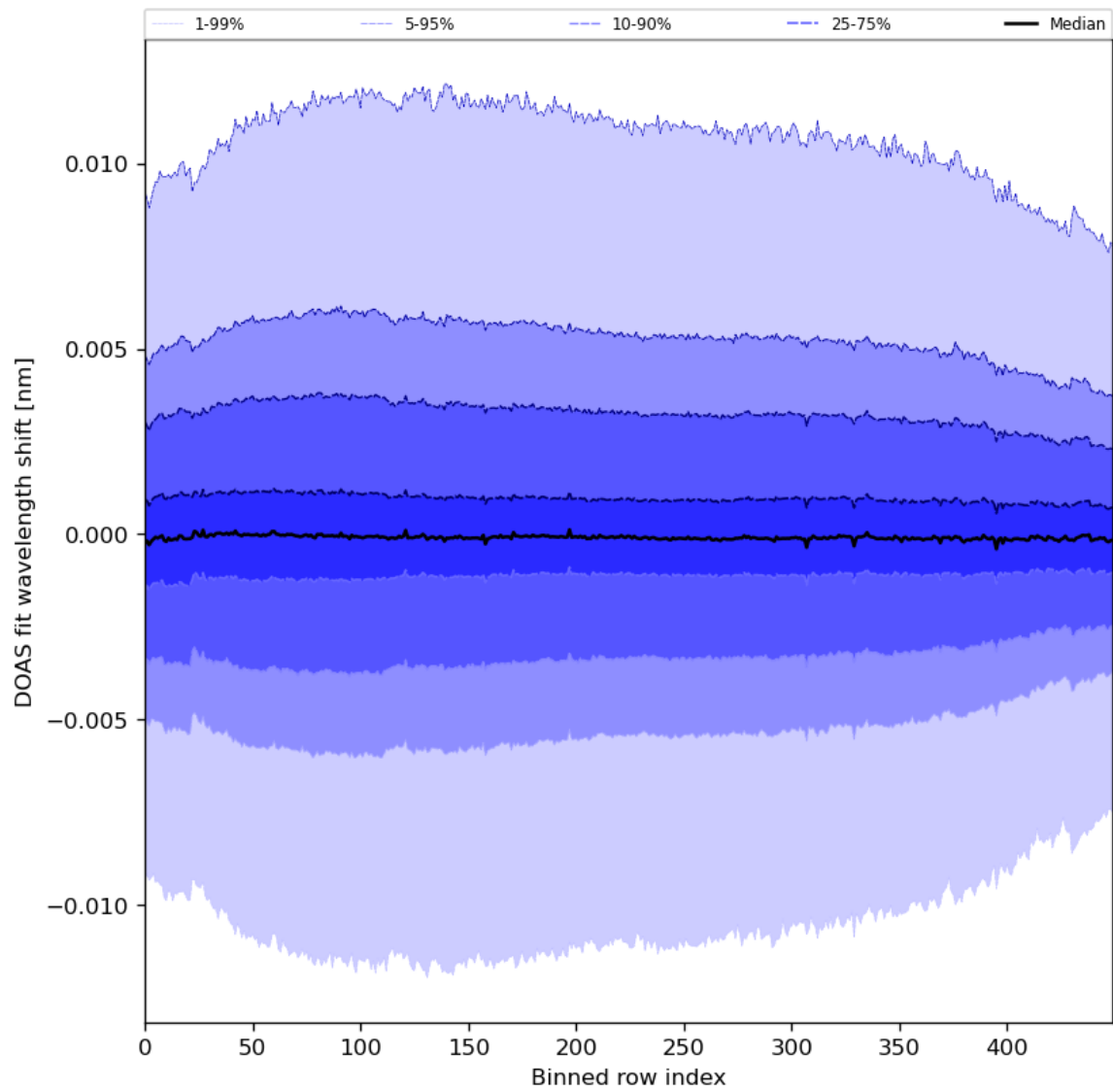
Figure 58: Along track statistics of “DOAS fit wavelength shift” for 2024-08-16 to 2024-08-17
