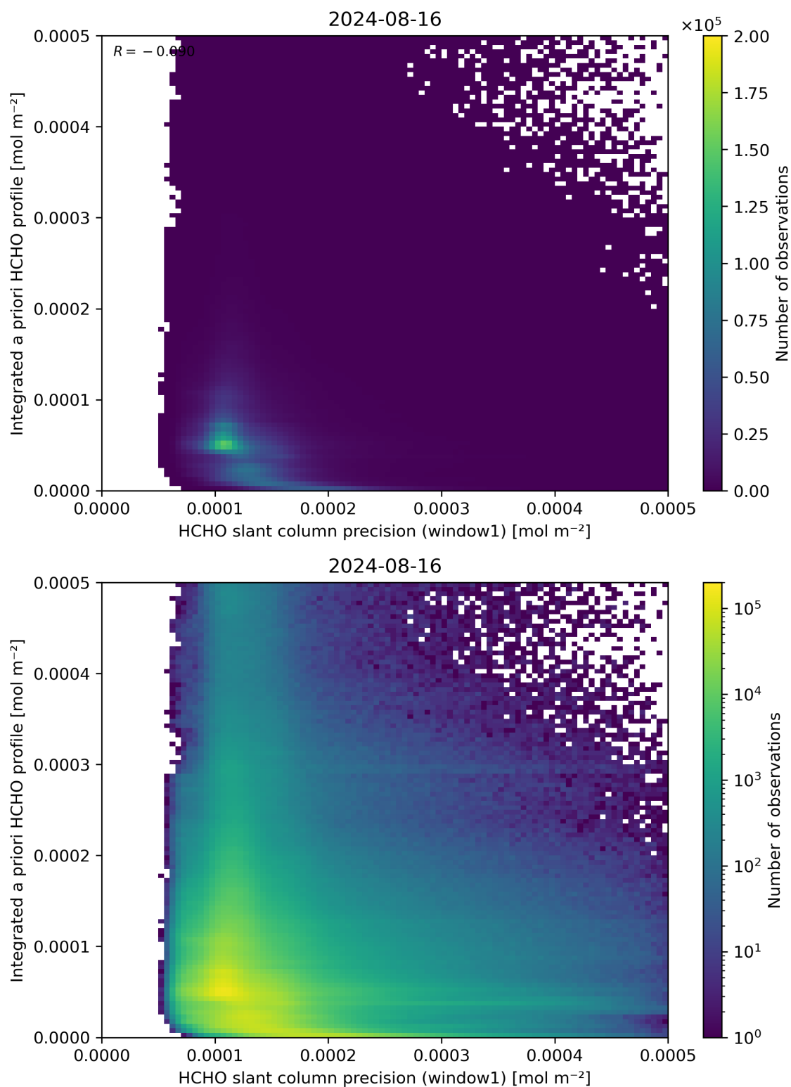
Figure 96: Scatter density plot of “HCHO slant column precision (window1)” against “Integrated a priori HCHO profile” for 2024-08-16 to 2024-08-17.
