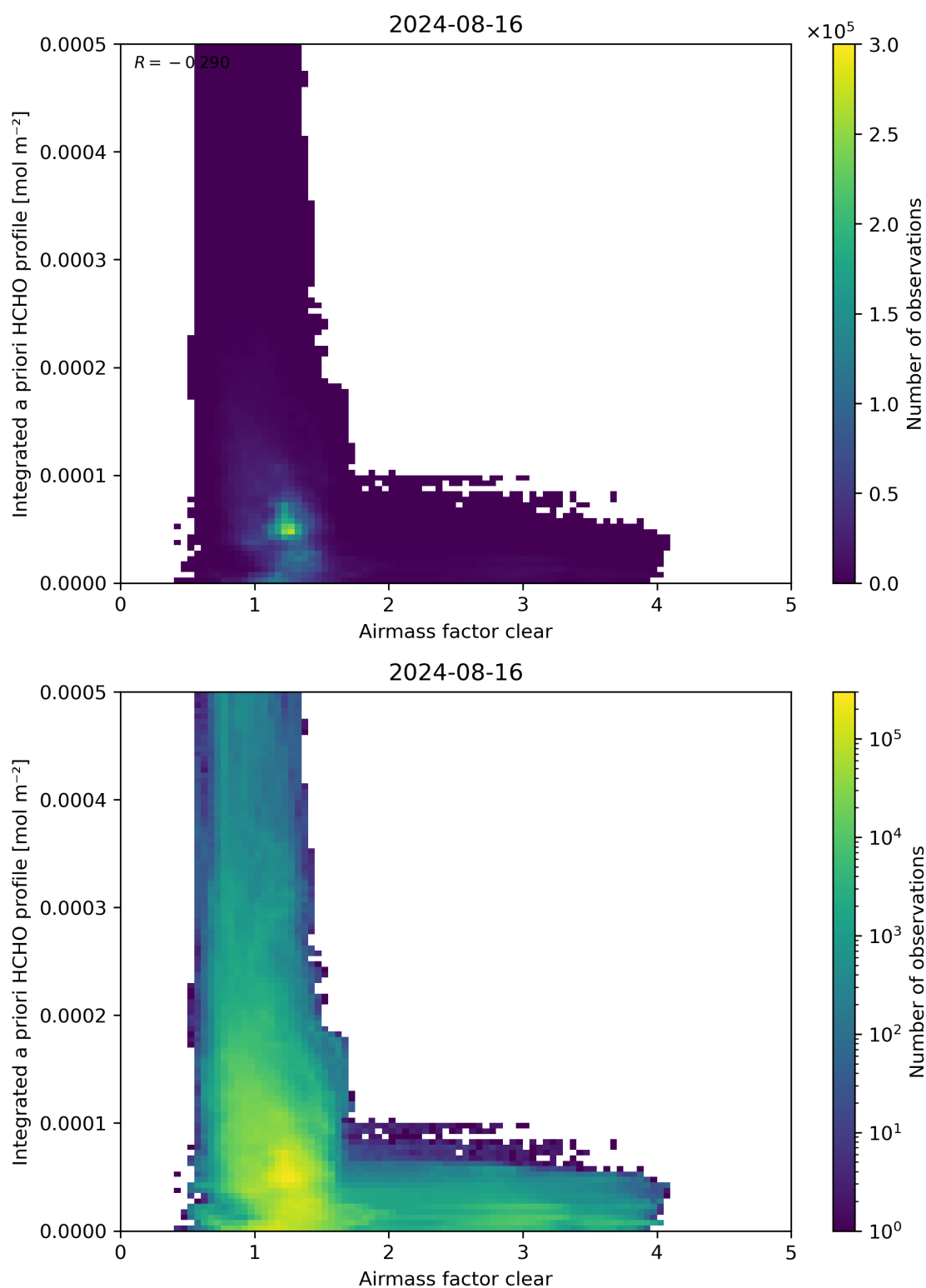
Figure 76: Scatter density plot of “Airmass factor clear” against “Integrated a priori HCHO profile” for 2024-08-16 to 2024-08-17.
