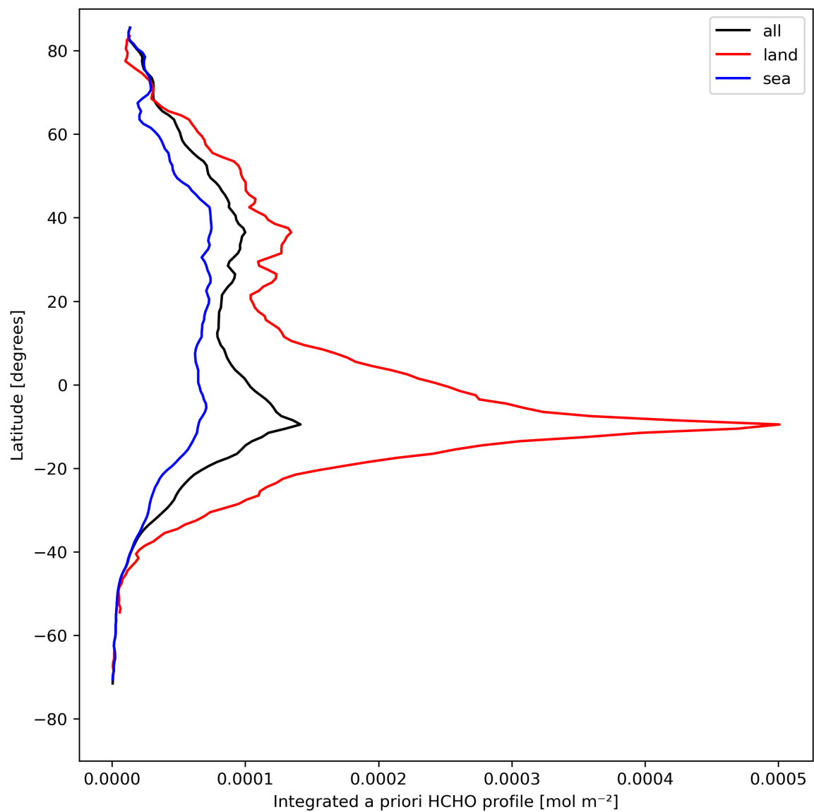
Figure 29: Zonal average of “Integrated a priori HCHO profile” for 2024-08-16 to 2024-08-17.
