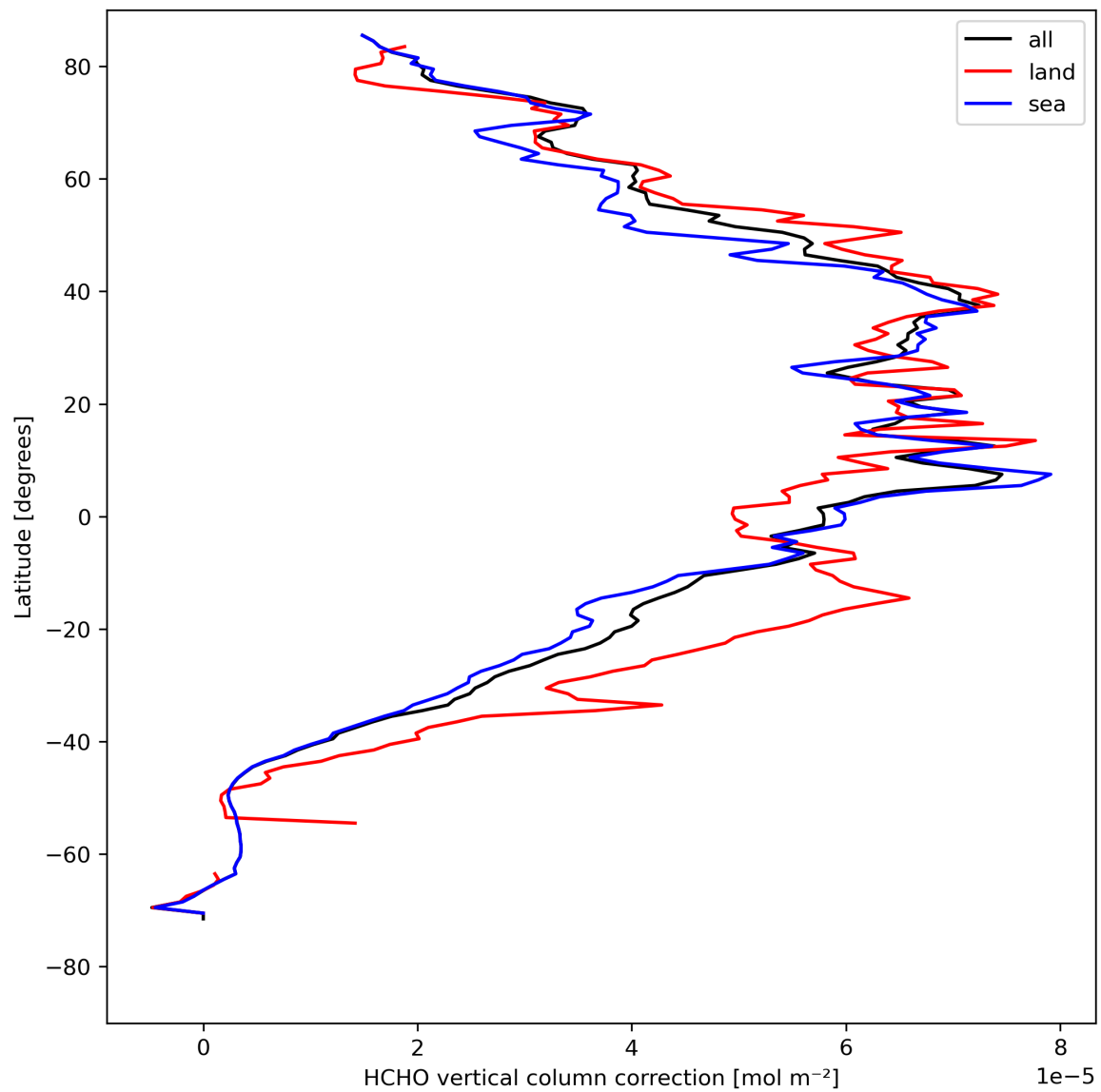
Figure 23: Zonal average of “HCHO vertical column correction” for 2024-08-16 to 2024-08-17.
