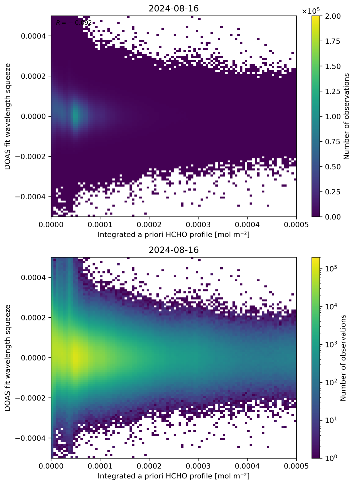
Figure 150: Scatter density plot of “Integrated a priori HCHO profile” against “DOAS fit wavelength squeeze” for 2024-08-16 to 2024-08-17.
