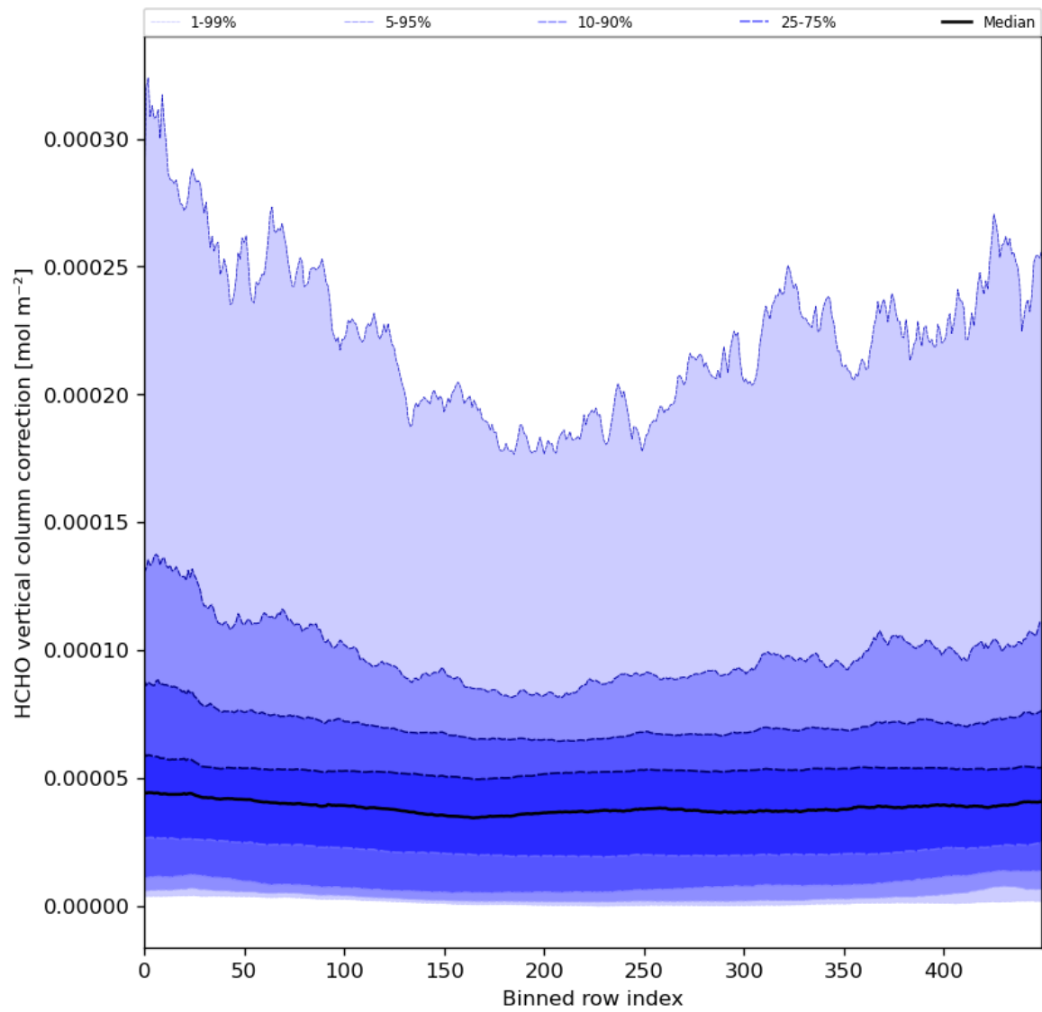
Figure 51: Along track statistics of “HCHO vertical column correction” for 2024-08-16 to 2024-08-17
