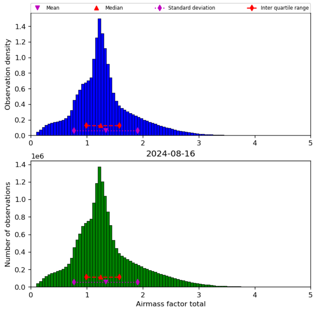
Figure 40: Histogram of “Airmass factor total” for 2024-08-16 to 2024-08-17
