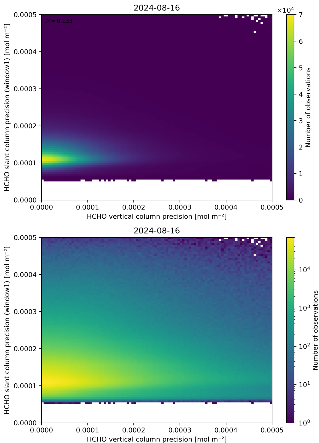
Figure 143: Scatter density plot of “HCHO vertical column precision” against “HCHO slant column precision (window1)” for 2024-08-16 to 2024-08-17.
