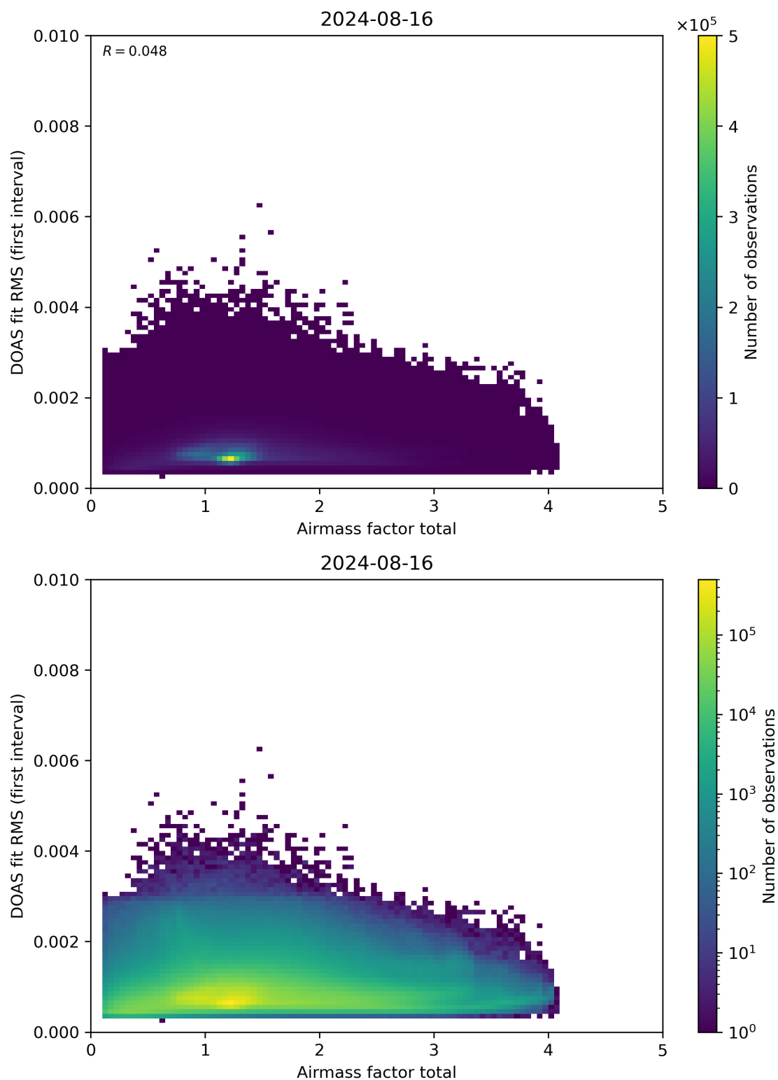
Figure 97: Scatter density plot of “Airmass factor total” against “DOAS fit RMS (first interval)” for 2024-08-16 to 2024-08-17.
