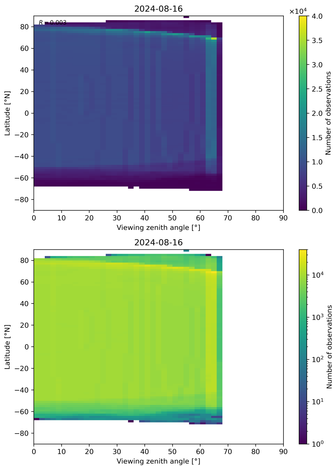
Figure 196: Scatter density plot of “Viewing zenith angle” against “Latitude” for 2024-08-16 to 2024-08-17.
