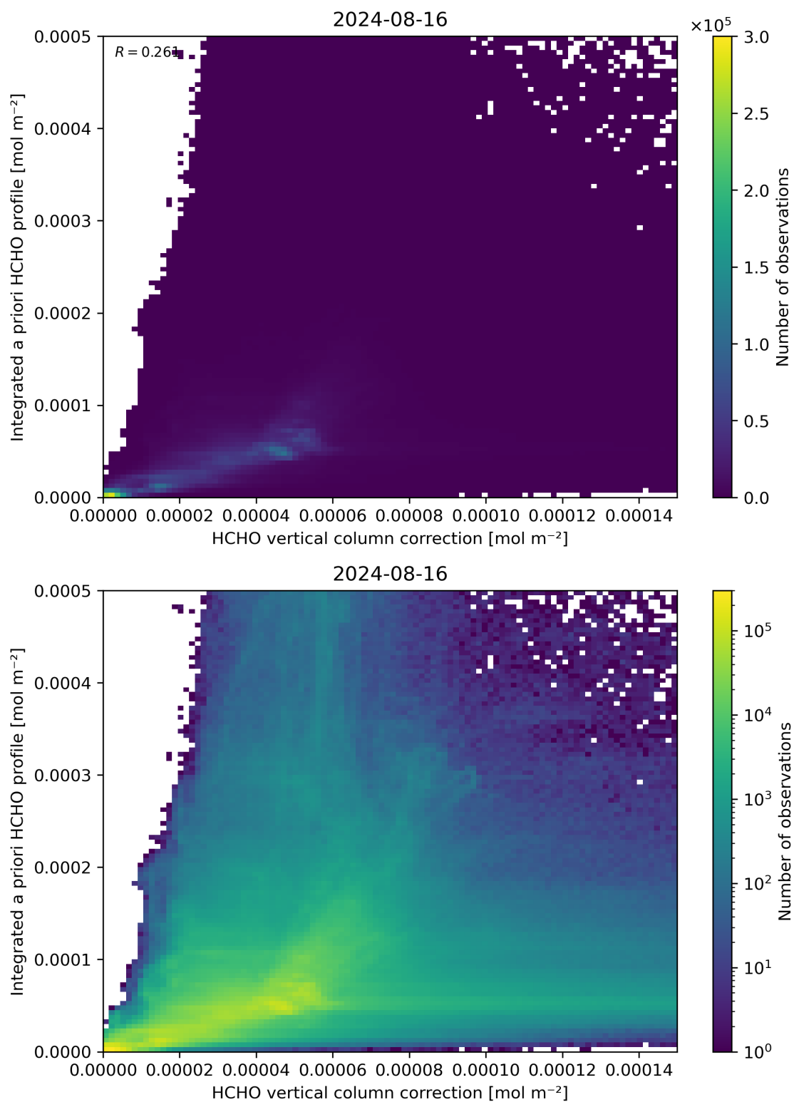
Figure 122: Scatter density plot of “HCHO vertical column correction” against “Integrated a priori HCHO profile” for 2024-08-16 to 2024-08-17.
