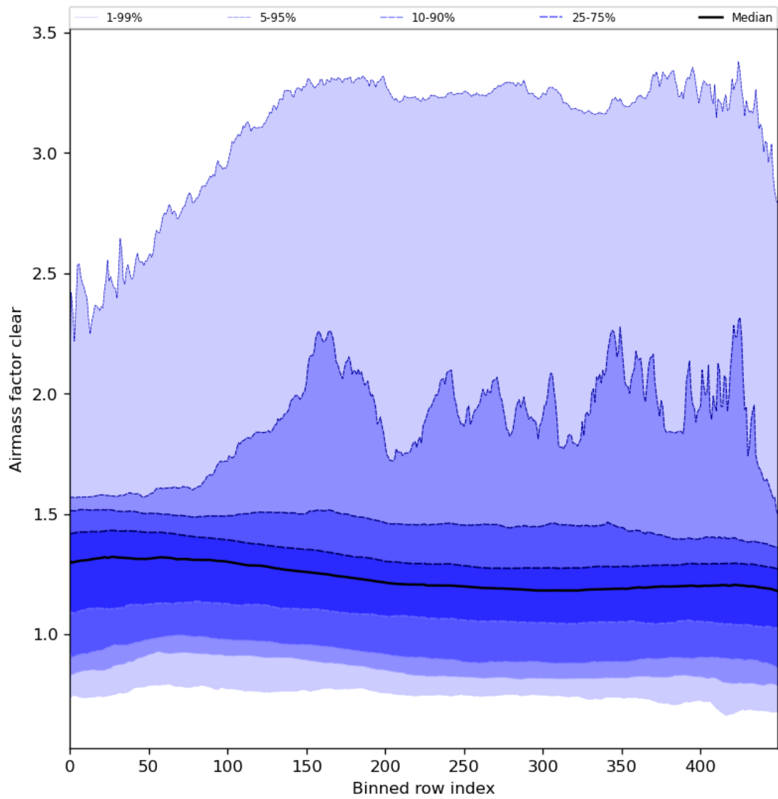
Figure 56: Along track statistics of “Airmass factor clear” for 2024-08-16 to 2024-08-17
