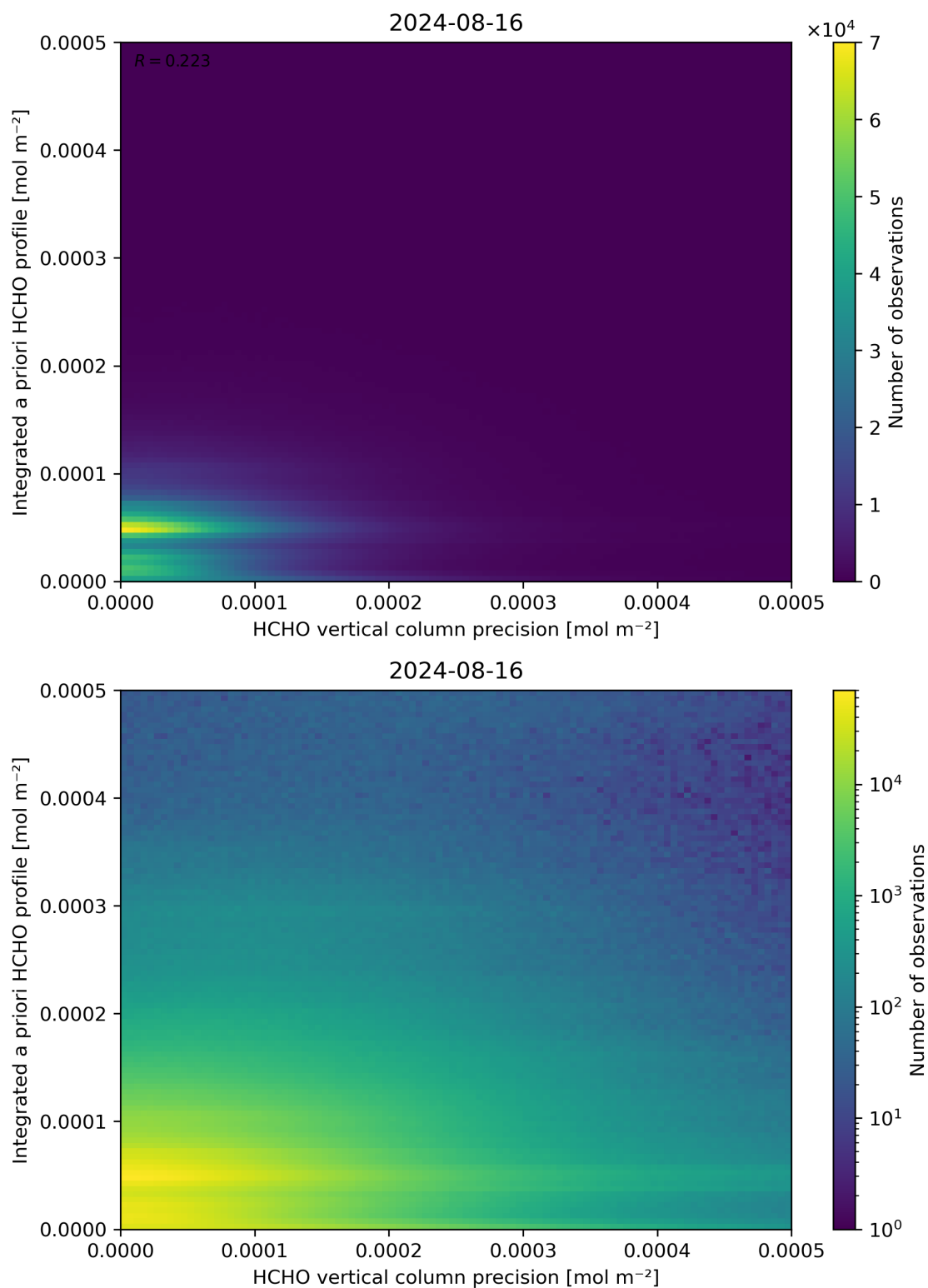
Figure 147: Scatter density plot of “HCHO vertical column precision” against “Integrated a priori HCHO profile” for 2024-08-16 to 2024-08-17.
