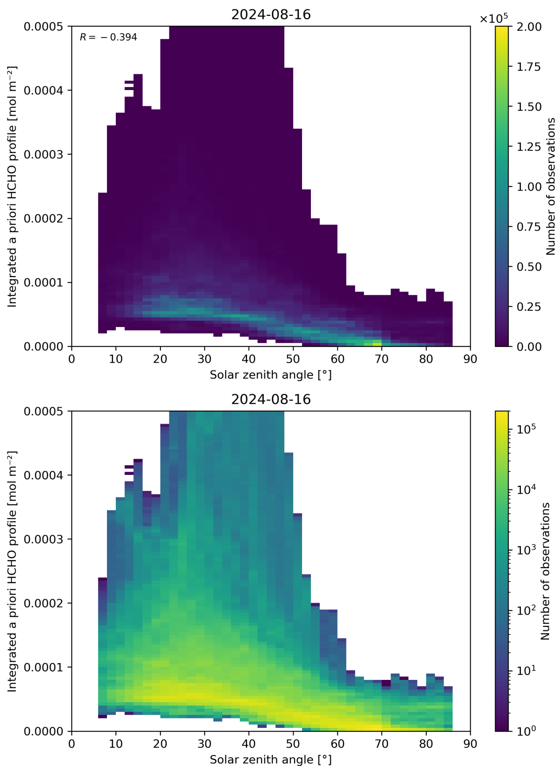
Figure 180: Scatter density plot of “Solar zenith angle” against “Integrated a priori HCHO profile” for 2024-08-16 to 2024-08-17.
