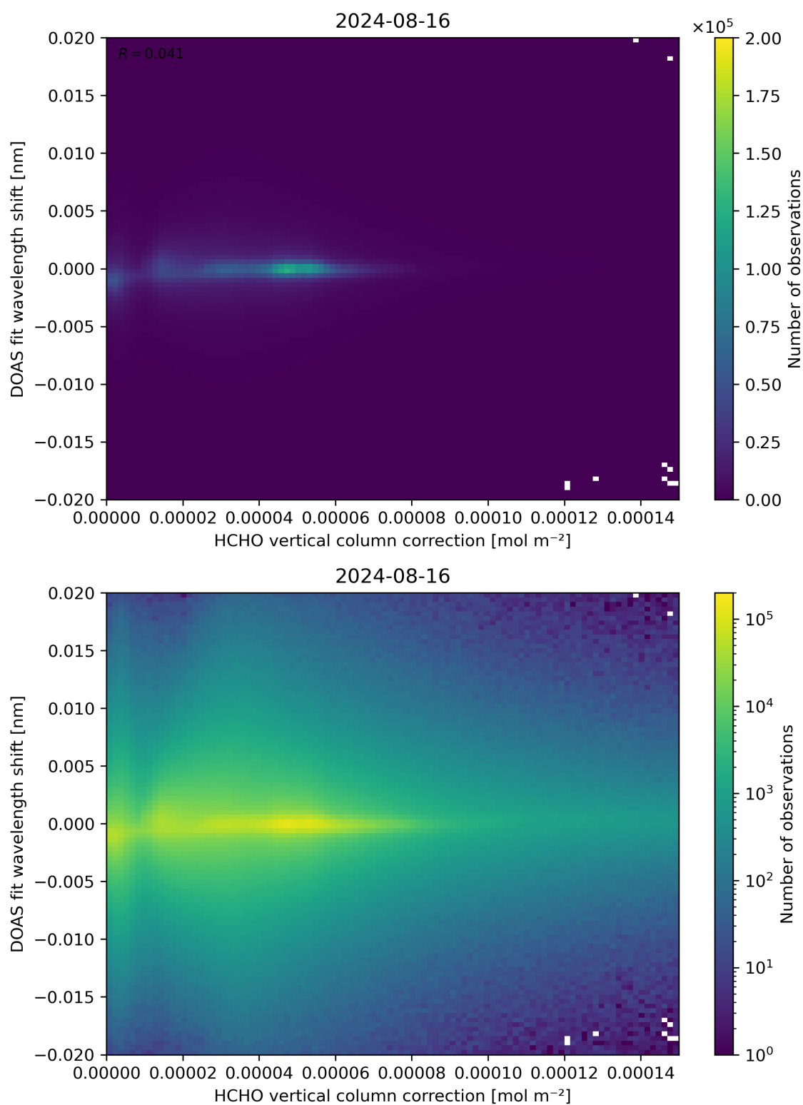
Figure 113: Scatter density plot of “HCHO vertical column correction” against “DOAS fit wavelength shift” for 2024-08-16 to 2024-08-17.
