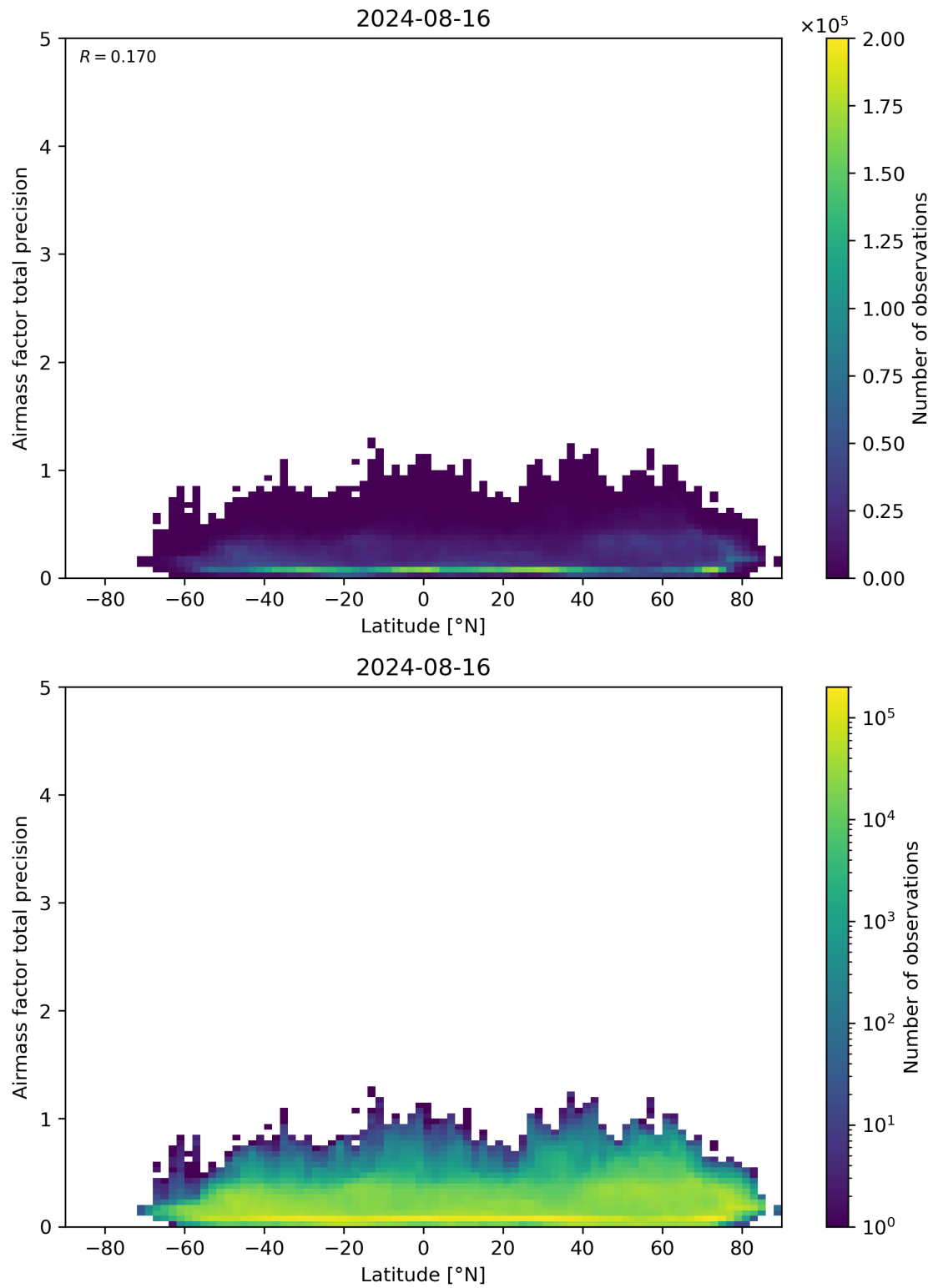
Figure 162: Scatter density plot of “Latitude” against “Airmass factor total precision” for 2024-08-16 to 2024-08-17.
