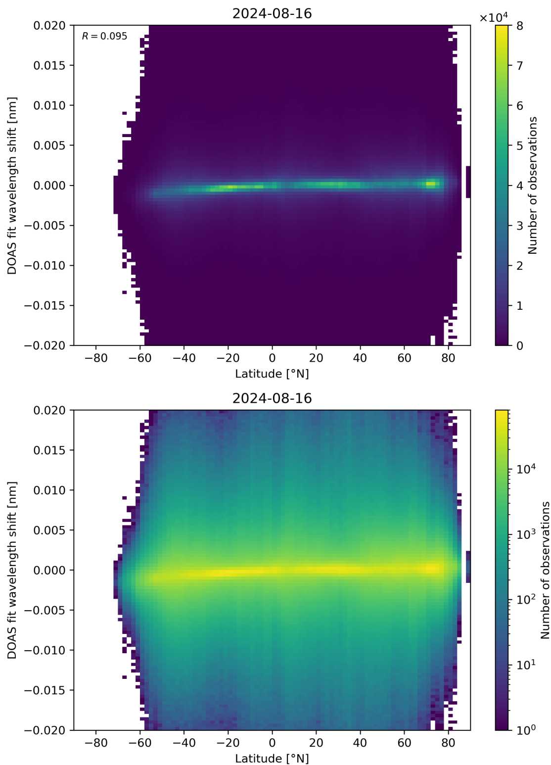
Figure 154: Scatter density plot of “Latitude” against “DOAS fit wavelength shift” for 2024-08-16 to 2024-08-17.
