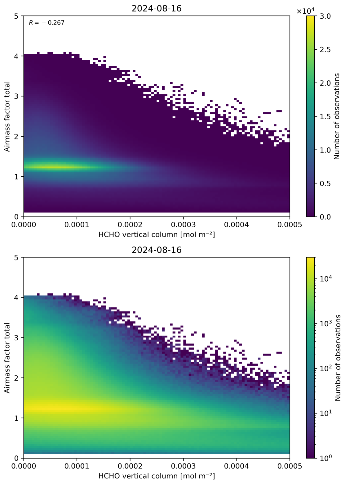
Figure 131: Scatter density plot of “HCHO vertical column” against “Airmass factor total” for 2024-08-16 to 2024-08-17.
