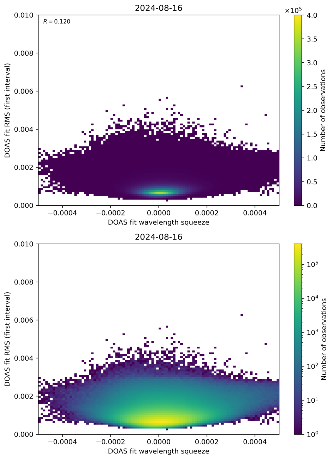
Figure 68: Scatter density plot of “DOAS fit wavelength squeeze” against “DOAS fit RMS (first interval)” for 2024-08-16 to 2024-08-17.
