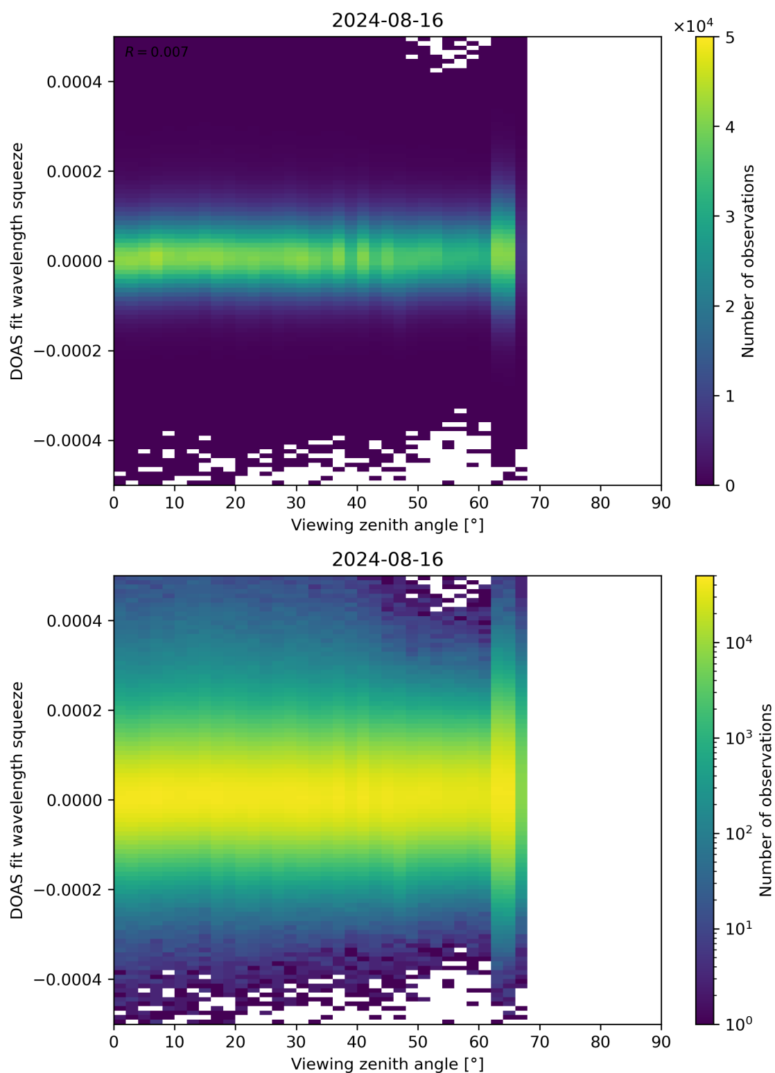
Figure 184: Scatter density plot of “Viewing zenith angle” against “DOAS fit wavelength squeeze” for 2024-08-16 to 2024-08-17.
