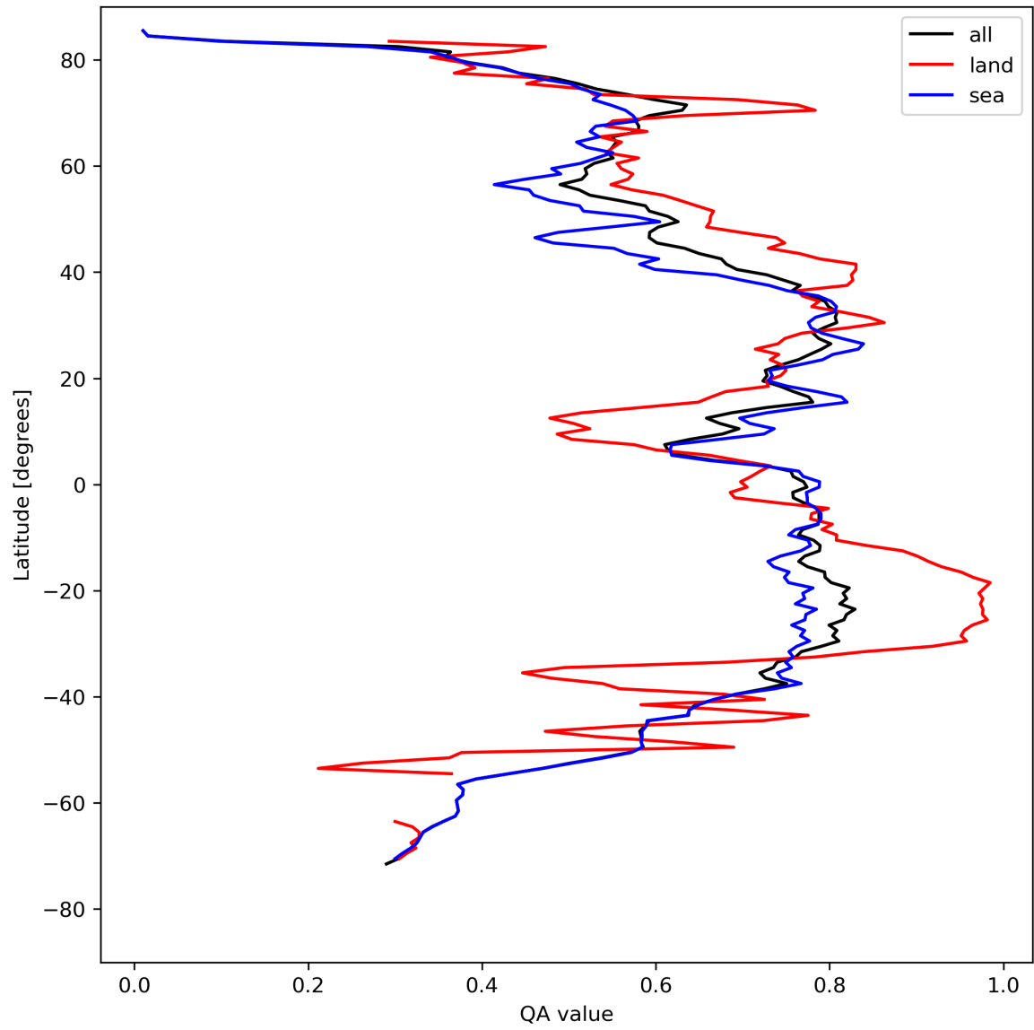
Figure 20: Zonal average of “QA value” for 2024-08-16 to 2024-08-17.
