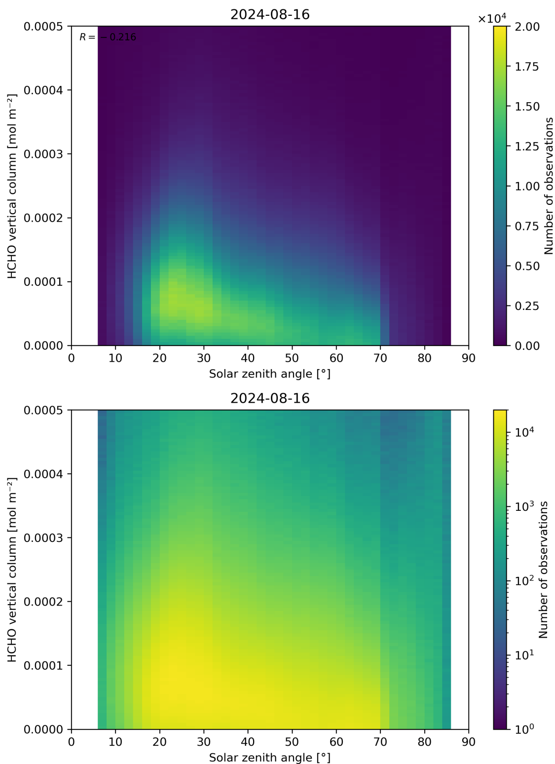
Figure 177: Scatter density plot of “Solar zenith angle” against “HCHO vertical column” for 2024-08-16 to 2024-08-17.
