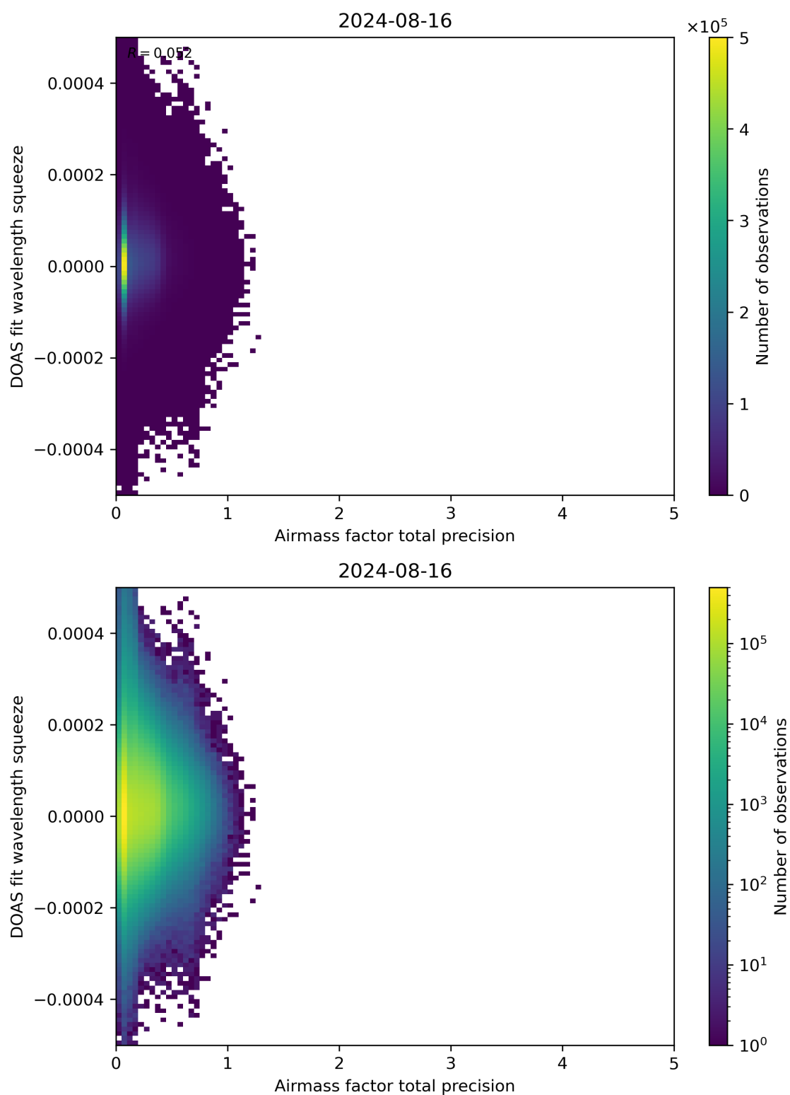
Figure 107: Scatter density plot of “Airmass factor total precision” against “DOAS fit wavelength squeeze” for 2024-08-16 to 2024-08-17.
