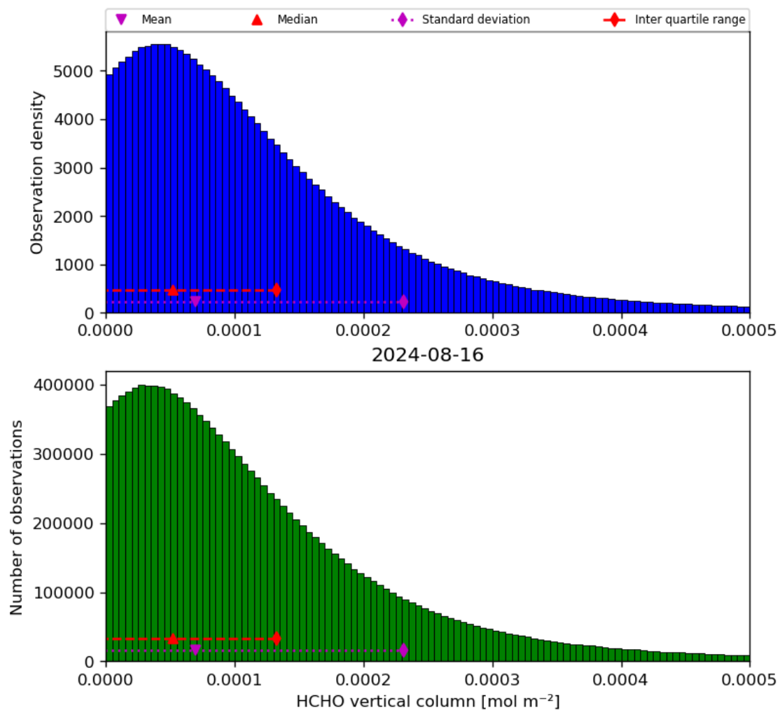
Figure 35: Histogram of “HCHO vertical column” for 2024-08-16 to 2024-08-17
