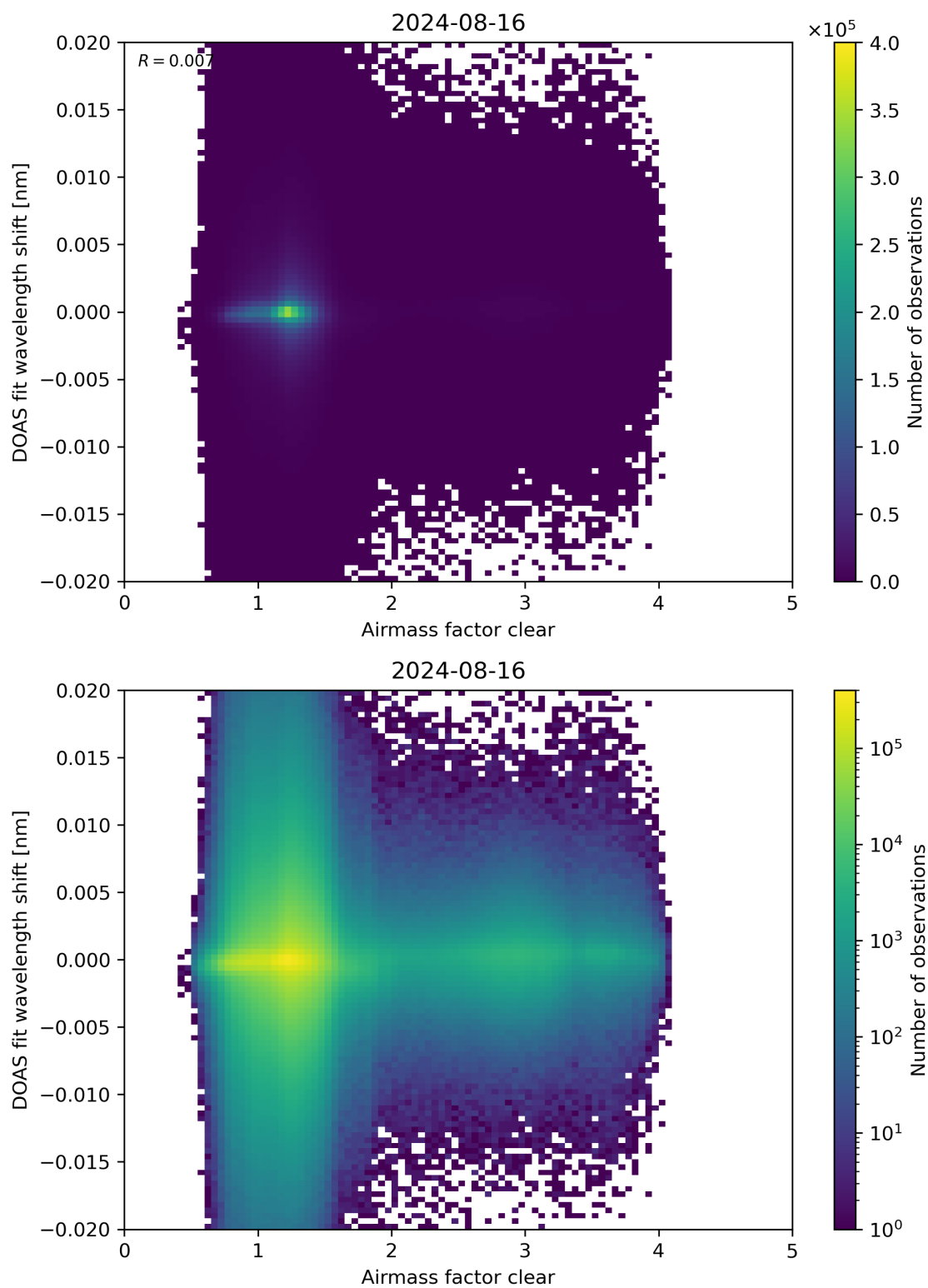
Figure 72: Scatter density plot of “Airmass factor clear” against “DOAS fit wavelength shift” for 2024-08-16 to 2024-08-17.
