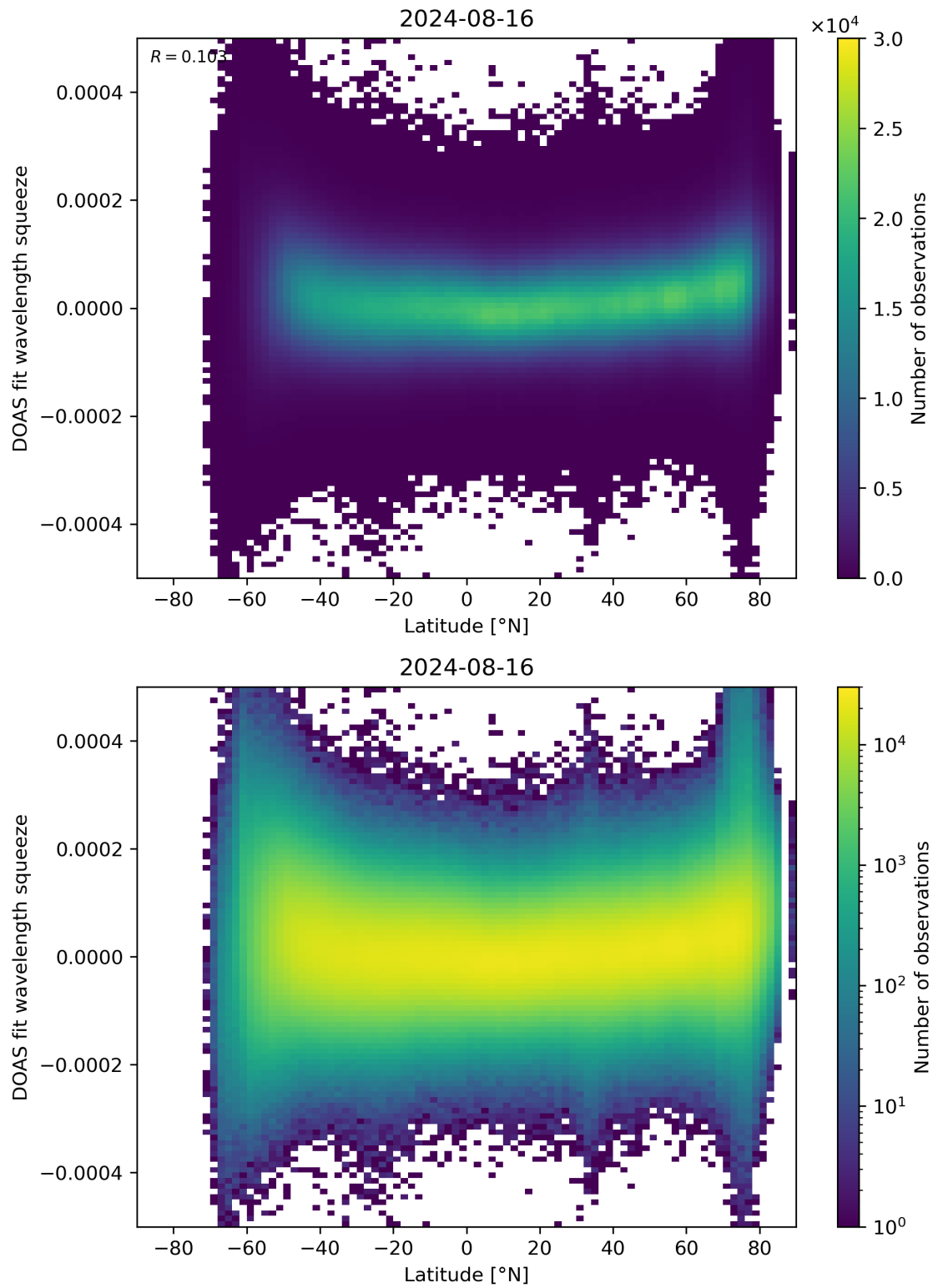
Figure 155: Scatter density plot of “Latitude” against “DOAS fit wavelength squeeze” for 2024-08-16 to 2024-08-17.
