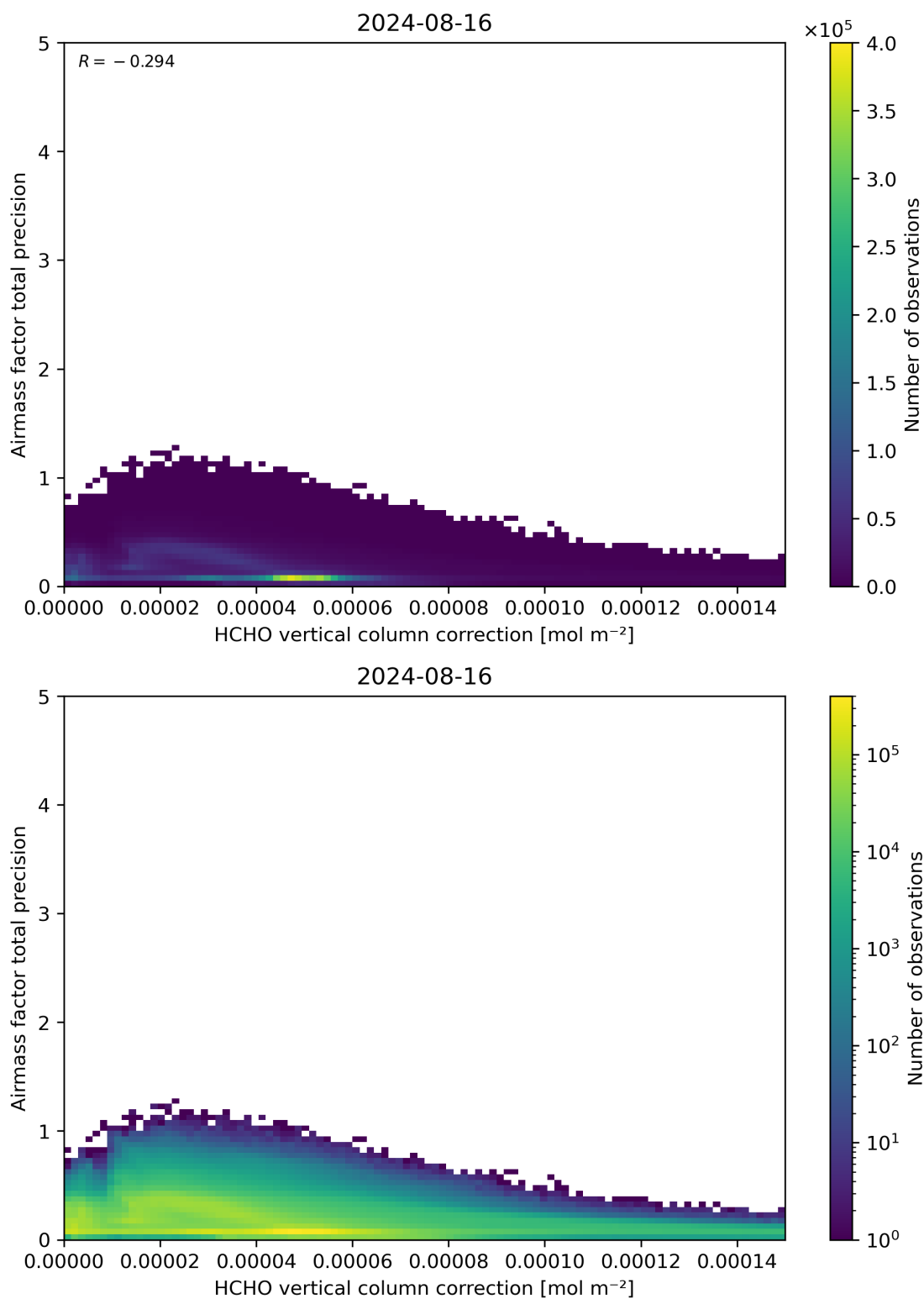
Figure 121: Scatter density plot of “HCHO vertical column correction” against “Airmass factor total precision” for 2024-08-16 to 2024-08-17.
