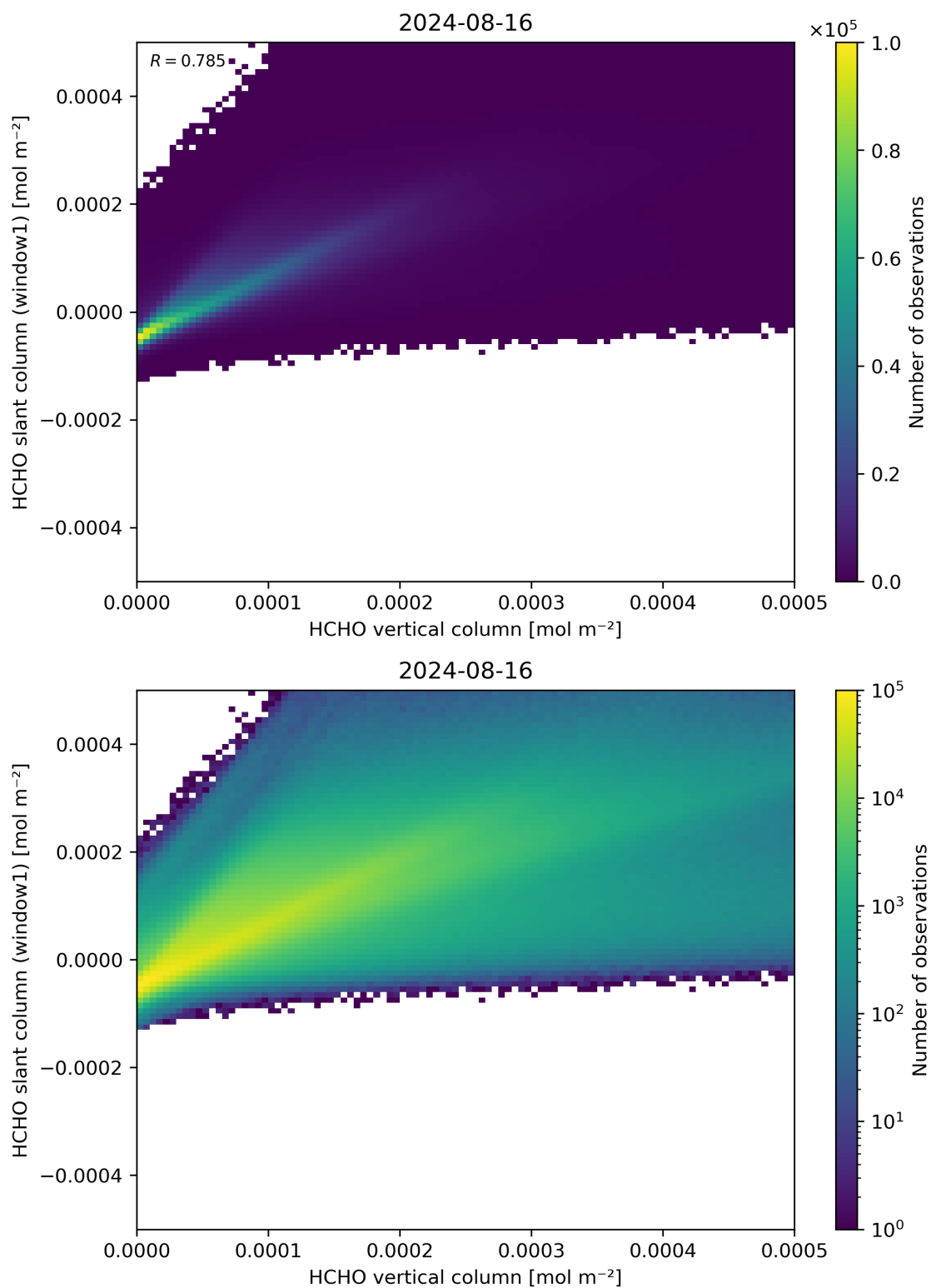
Figure 129: Scatter density plot of “HCHO vertical column” against “HCHO slant column (window1)” for 2024-08-16 to 2024-08-17.
