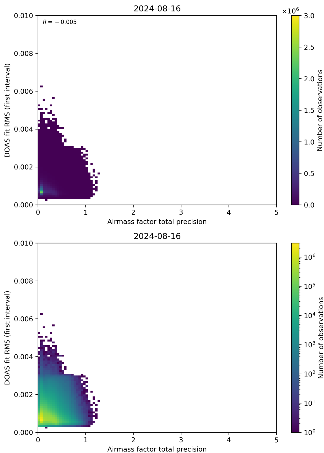
Figure 105: Scatter density plot of “Airmass factor total precision” against “DOAS fit RMS (first interval)” for 2024-08-16 to 2024-08-17.
