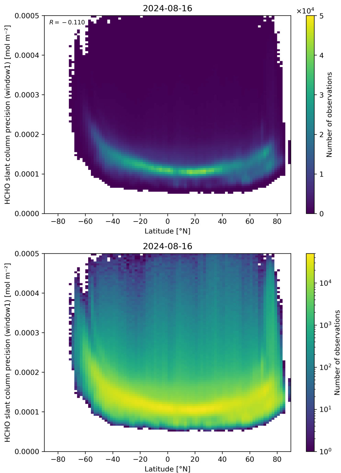
Figure 160: Scatter density plot of “Latitude” against “HCHO slant column precision (window1)” for 2024-08-16 to 2024-08-17.
