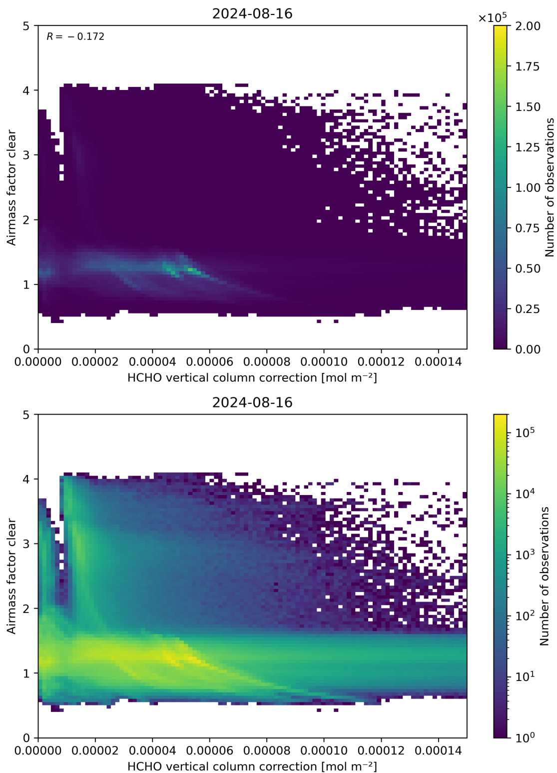
Figure 115: Scatter density plot of “HCHO vertical column correction” against “Airmass factor clear” for 2024-08-16 to 2024-08-17.
