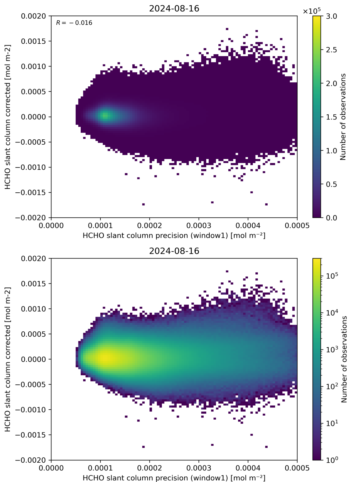
Figure 92: Scatter density plot of “HCHO slant column precision (window1)” against “HCHO slant column corrected” for 2024-08-16 to 2024-08-17.
