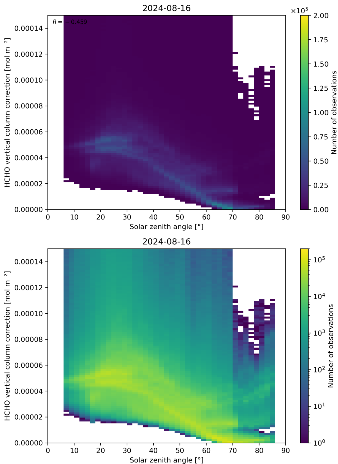
Figure 178: Scatter density plot of “Solar zenith angle” against “HCHO vertical column correction” for 2024-08-16 to 2024-08-17.
