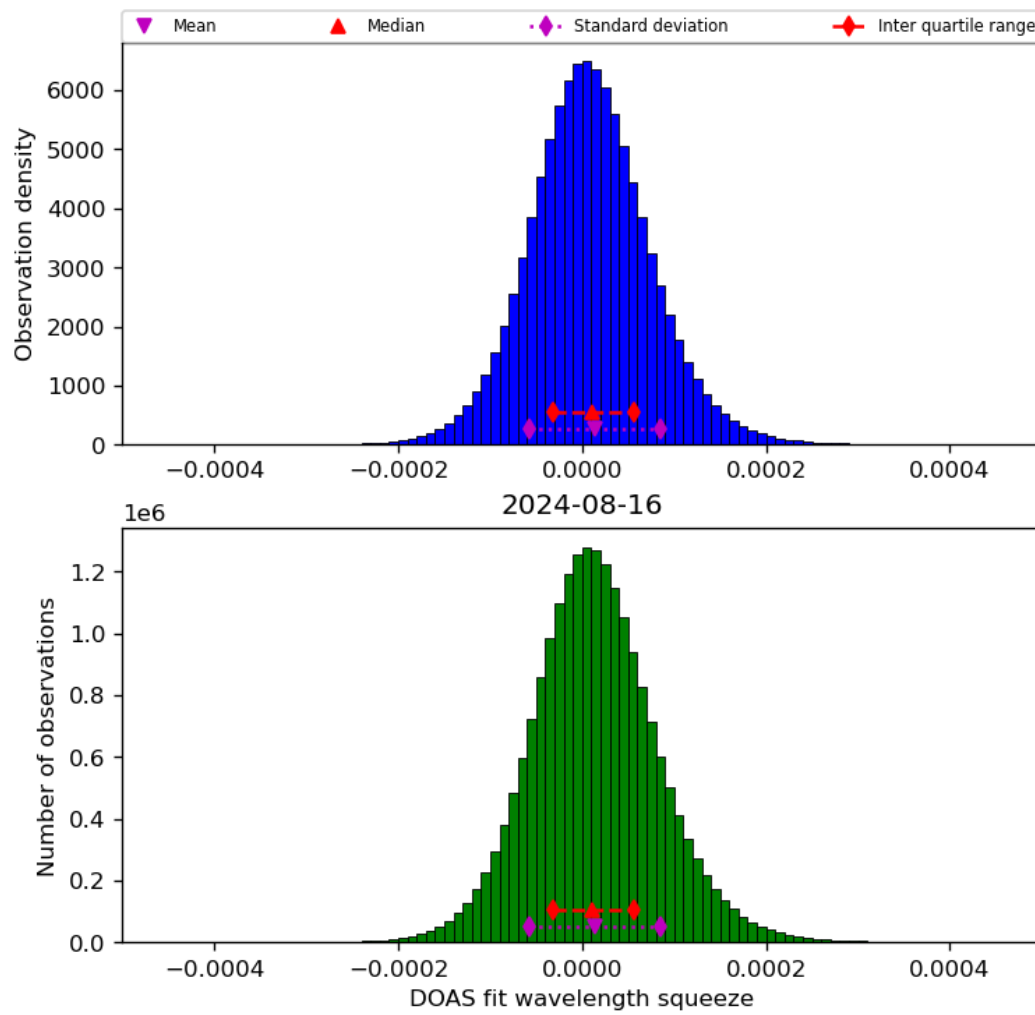
Figure 45: Histogram of “DOAS fit wavelength squeeze” for 2024-08-16 to 2024-08-17
