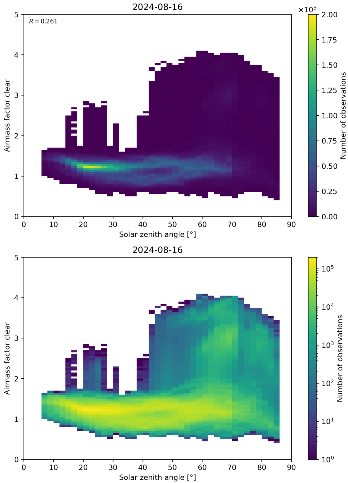
Figure 170: Scatter density plot of “Solar zenith angle” against “Airmass factor clear” for 2024-08-16 to 2024-08-17.
