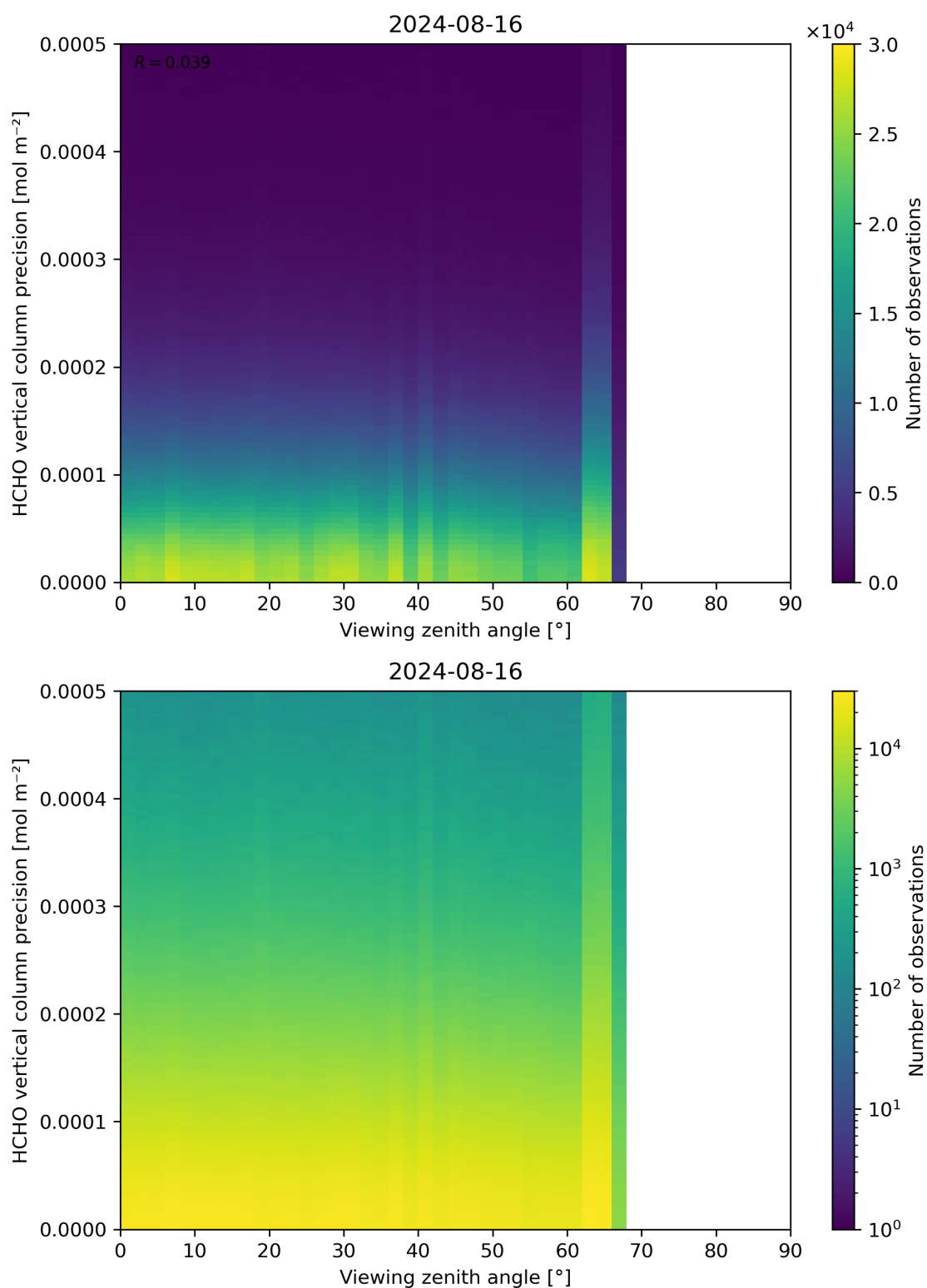
Figure 194: Scatter density plot of “Viewing zenith angle” against “HCHO vertical column precision” for 2024-08-16 to 2024-08-17.
