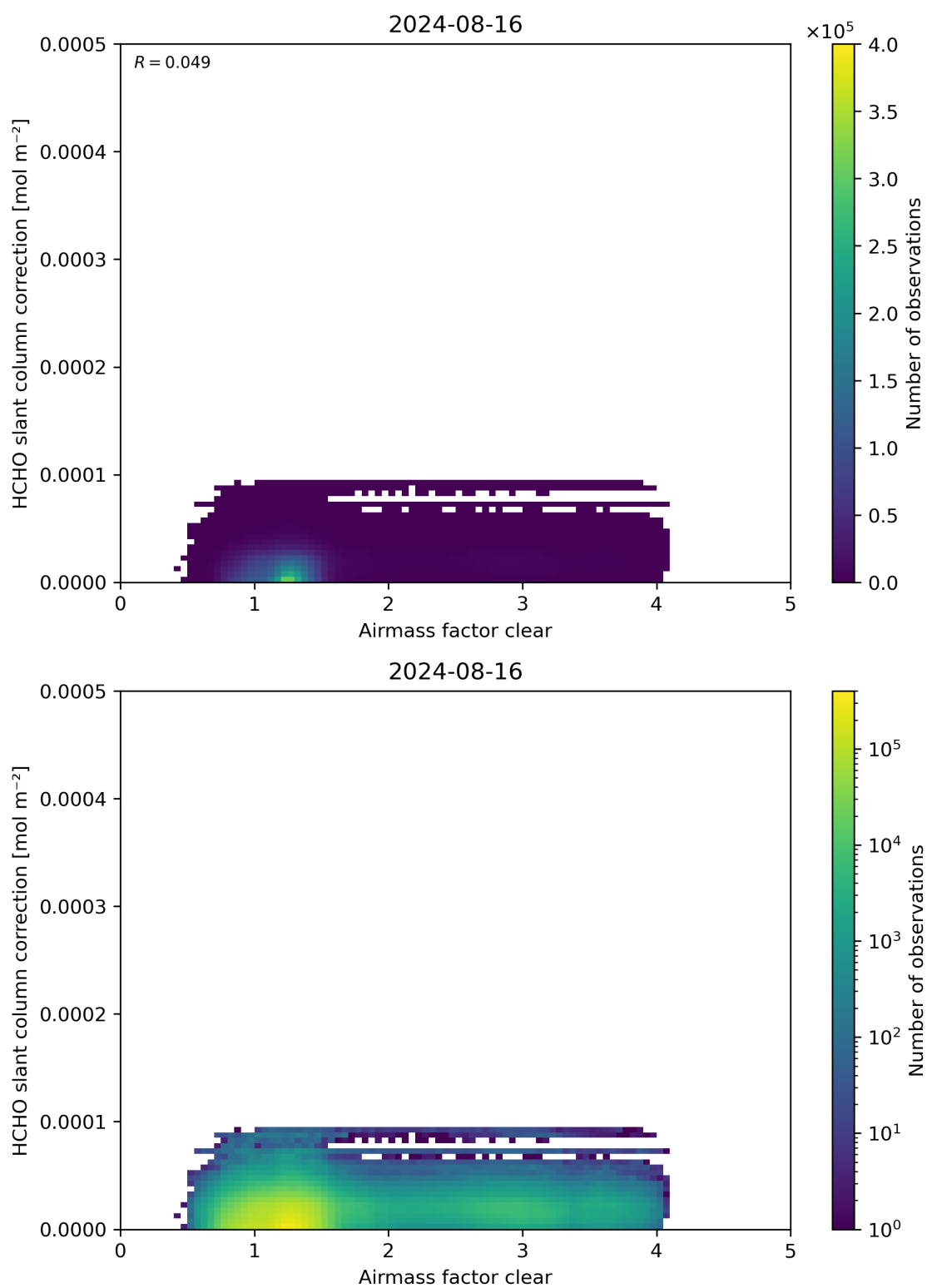
Figure 75: Scatter density plot of “Airmass factor clear” against “HCHO slant column correction” for 2024-08-16 to 2024-08-17.
