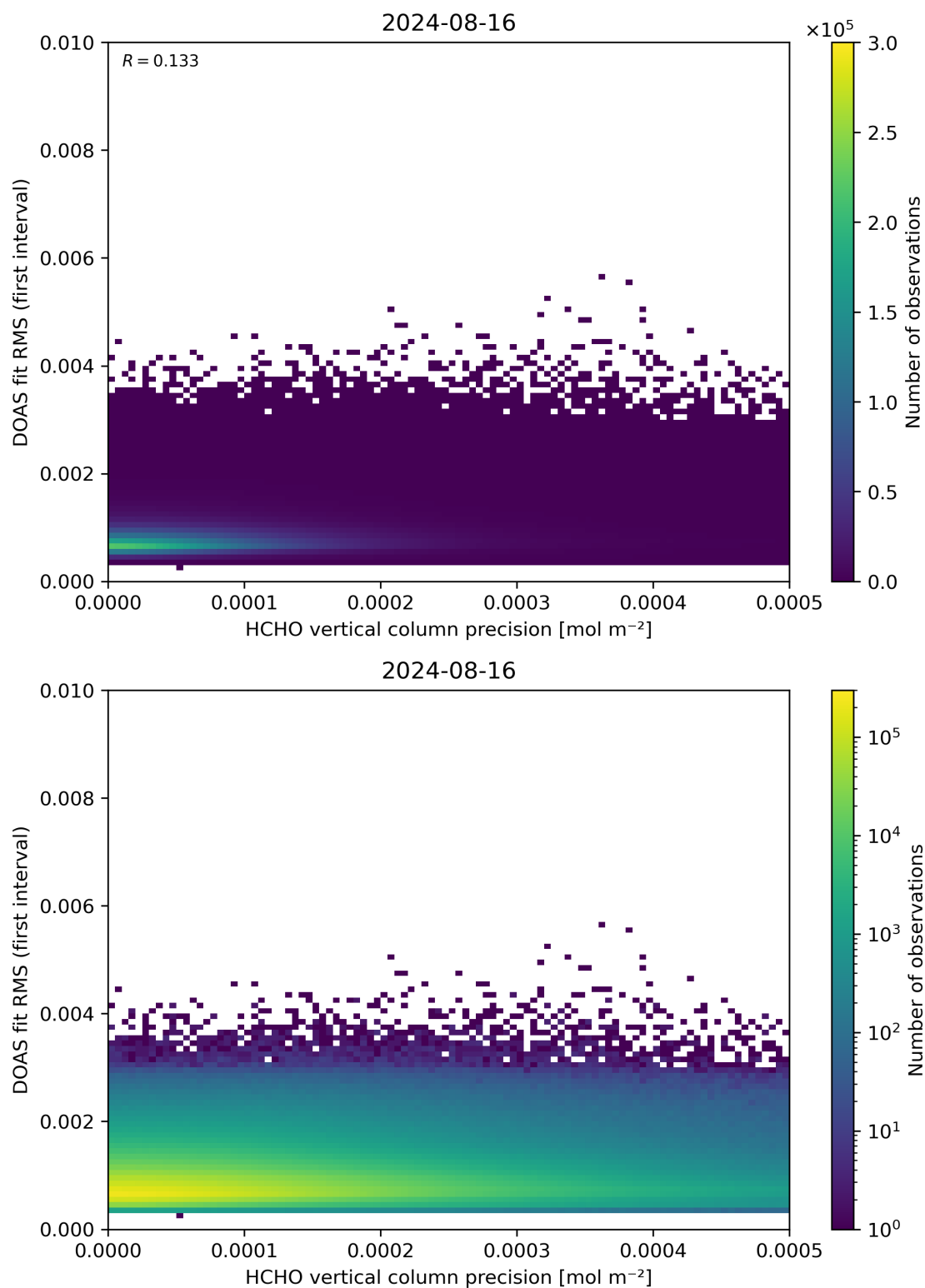
Figure 136: Scatter density plot of “HCHO vertical column precision” against “DOAS fit RMS (first interval)” for 2024-08-16 to 2024-08-17.
