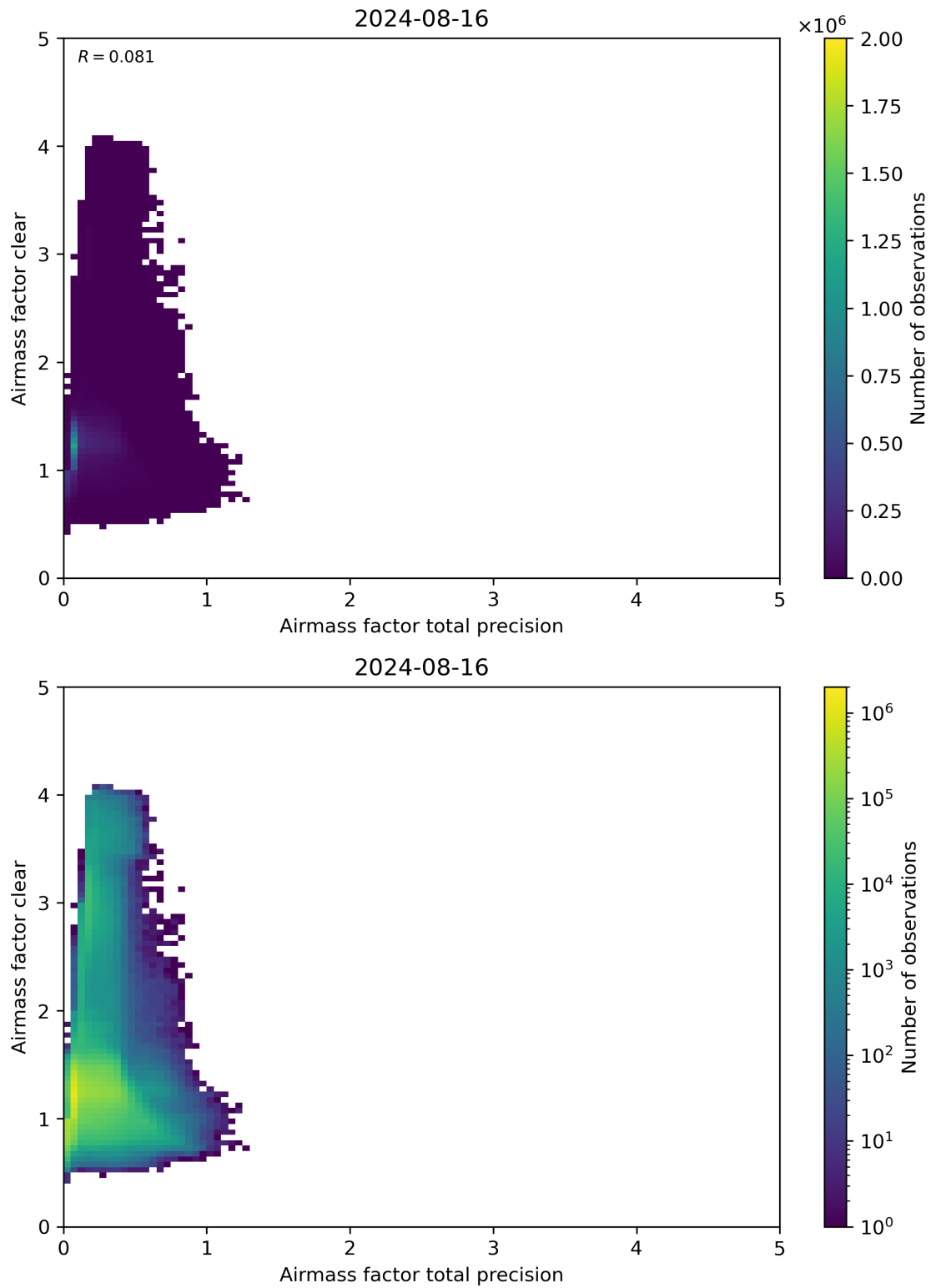
Figure 108: Scatter density plot of “Airmass factor total precision” against “Airmass factor clear” for 2024-08-16 to 2024-08-17.
