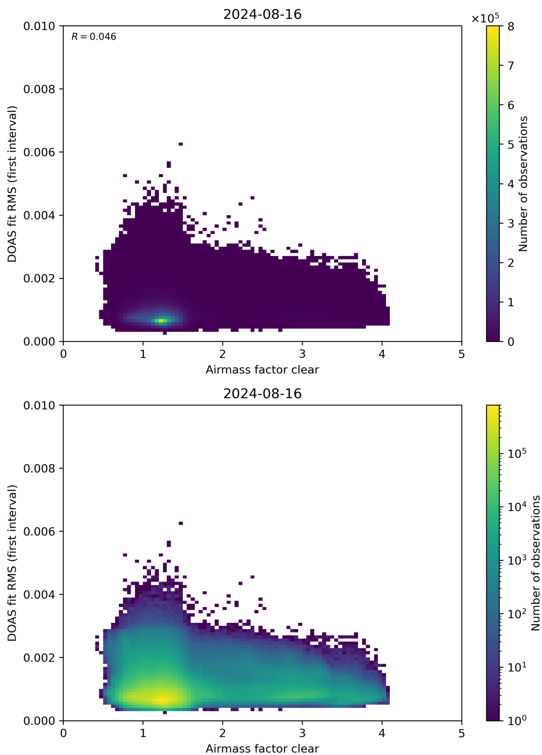
Figure 71: Scatter density plot of “Airmass factor clear” against “DOAS fit RMS (first interval)” for 2024-08-16 to 2024-08-17.
