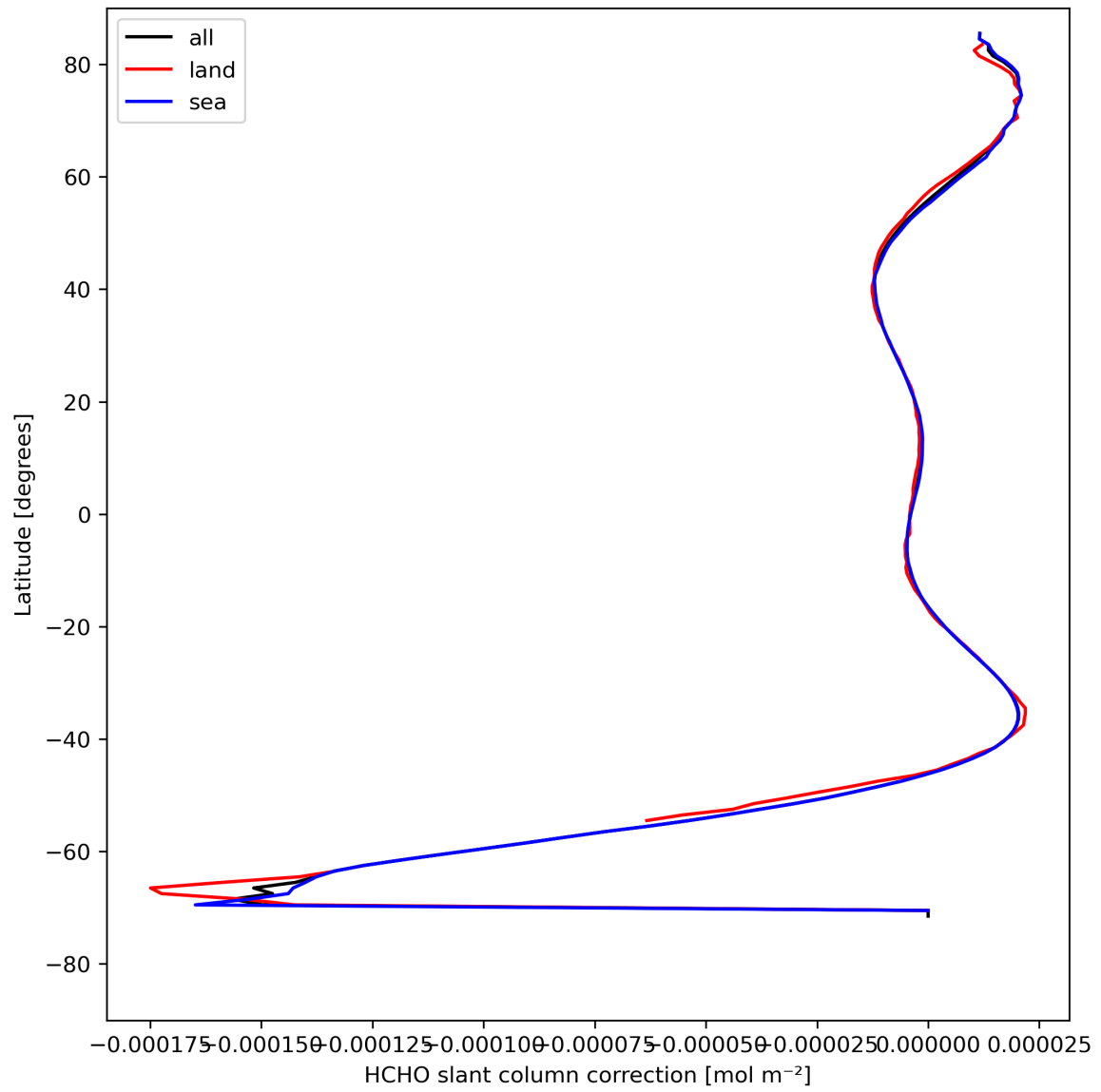
Figure 33: Zonal average of “HCHO slant column correction” for 2024-08-16 to 2024-08-17.
