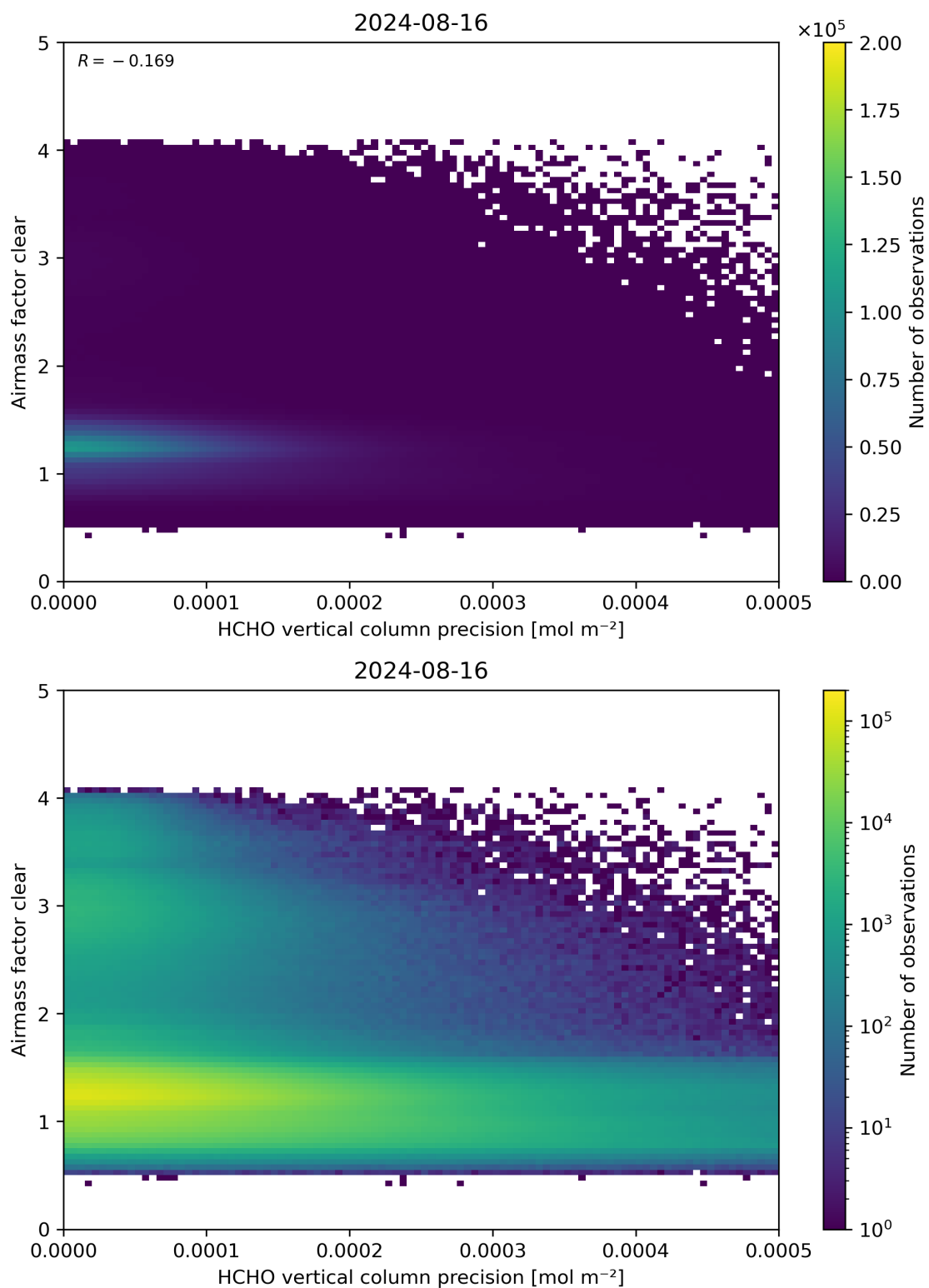
Figure 139: Scatter density plot of “HCHO vertical column precision” against “Airmass factor clear” for 2024-08-16 to 2024-08-17.
