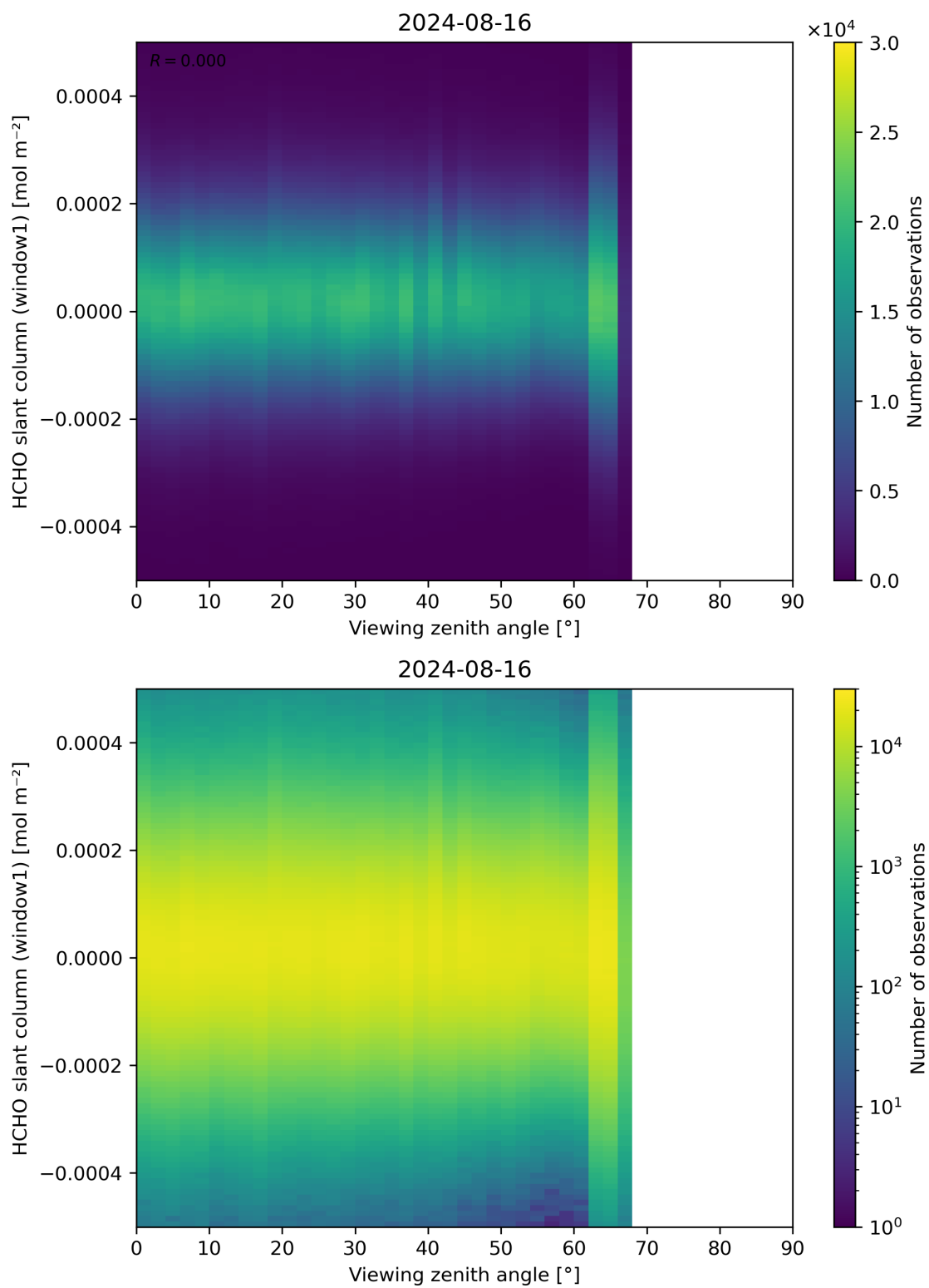
Figure 188: Scatter density plot of “Viewing zenith angle” against “HCHO slant column (window1)” for 2024-08-16 to 2024-08-17.
