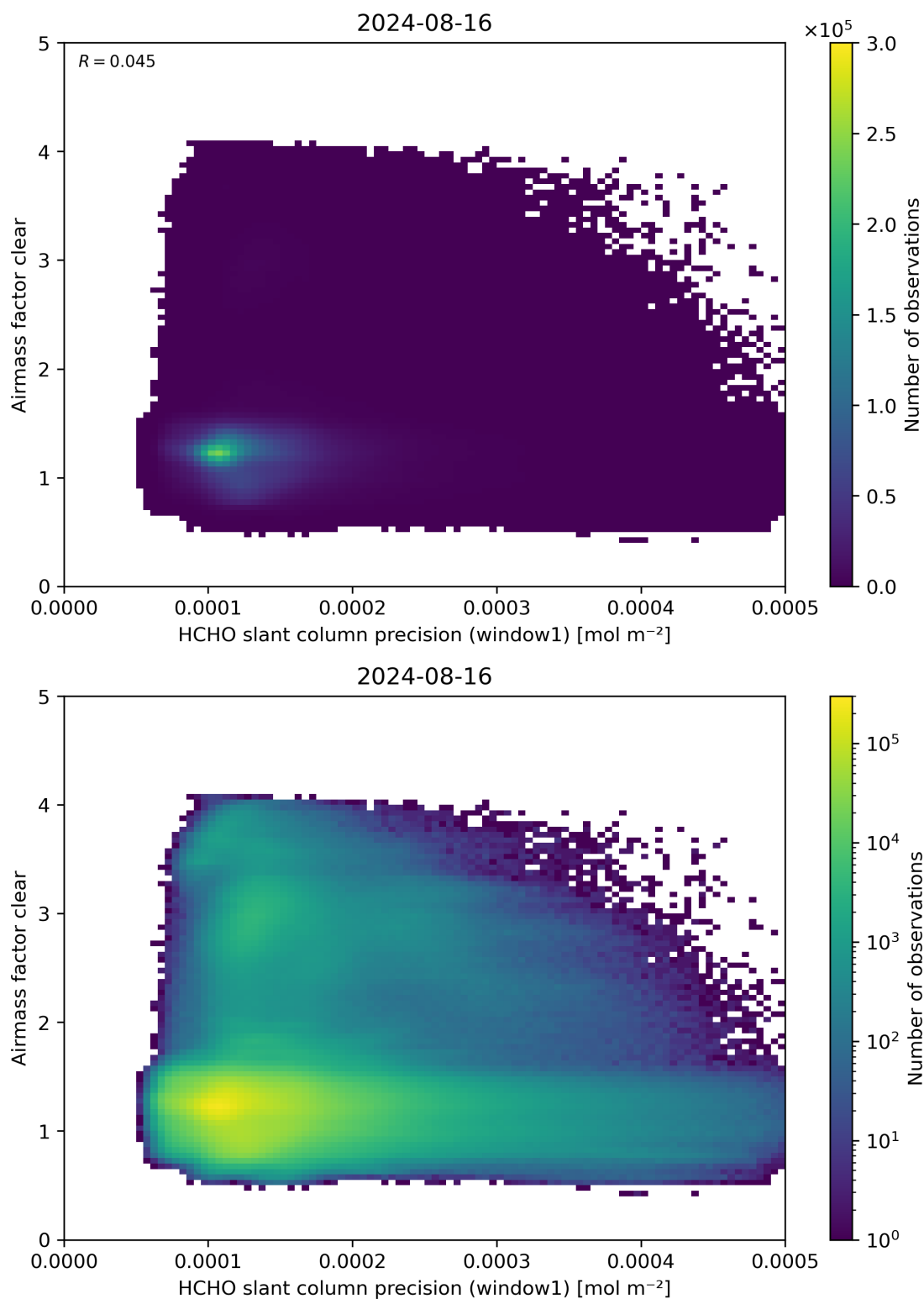
Figure 91: Scatter density plot of “HCHO slant column precision (window1)” against “Airmass factor clear” for 2024-08-16 to 2024-08-17.
