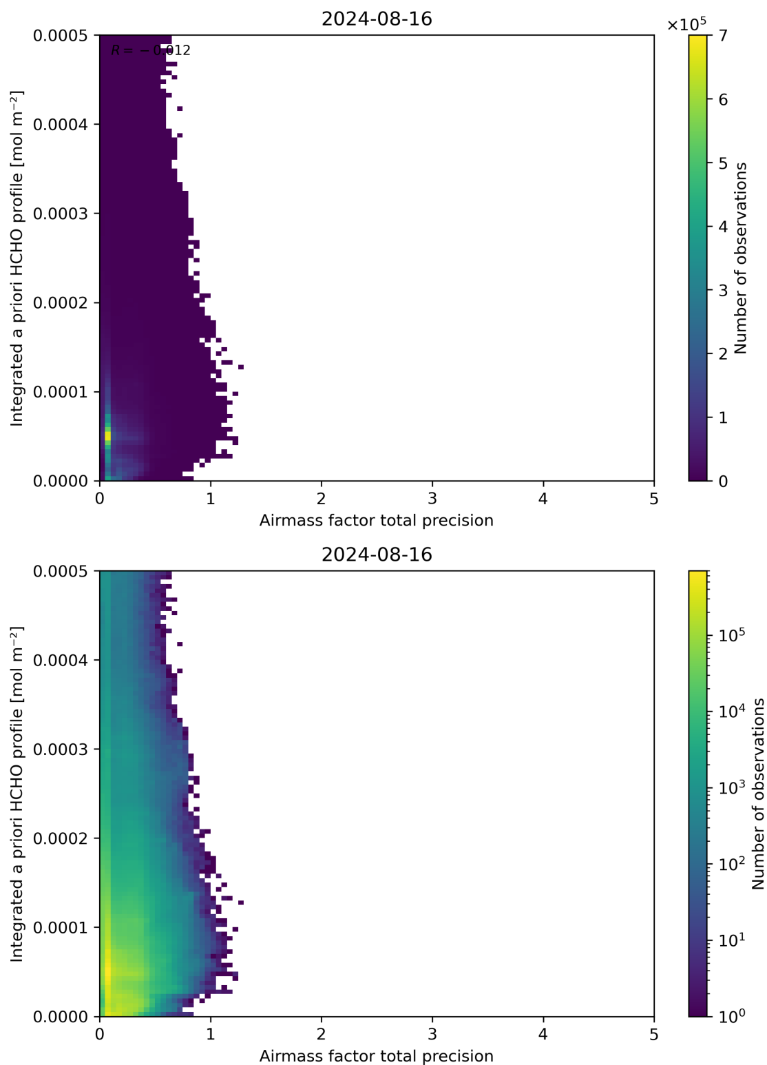
Figure 111: Scatter density plot of “Airmass factor total precision” against “Integrated a priori HCHO profile” for 2024-08-16 to 2024-08-17.
