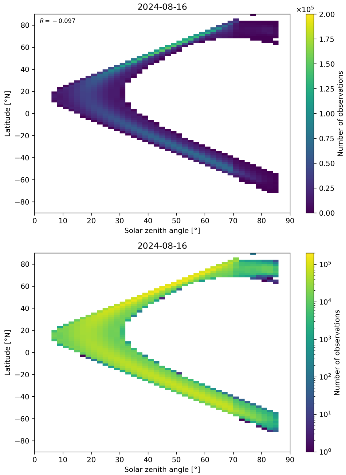
Figure 181: Scatter density plot of “Solar zenith angle” against “Latitude” for 2024-08-16 to 2024-08-17.
