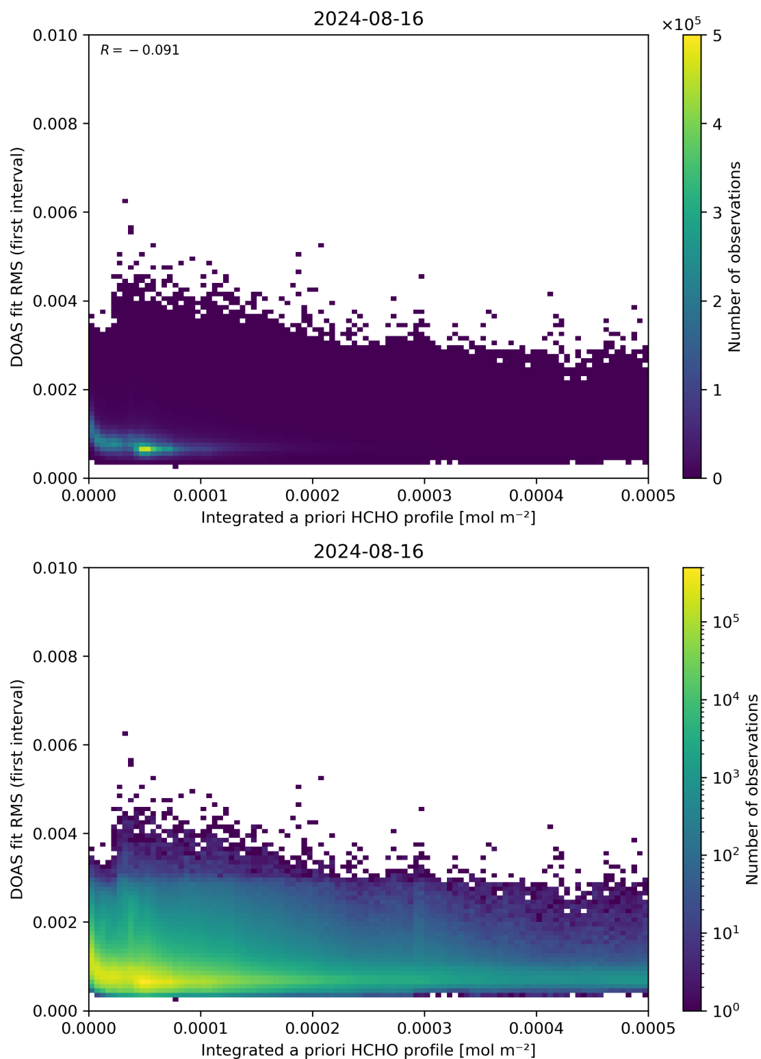
Figure 148: Scatter density plot of “Integrated a priori HCHO profile” against “DOAS fit RMS (first interval)” for 2024-08-16 to 2024-08-17.
