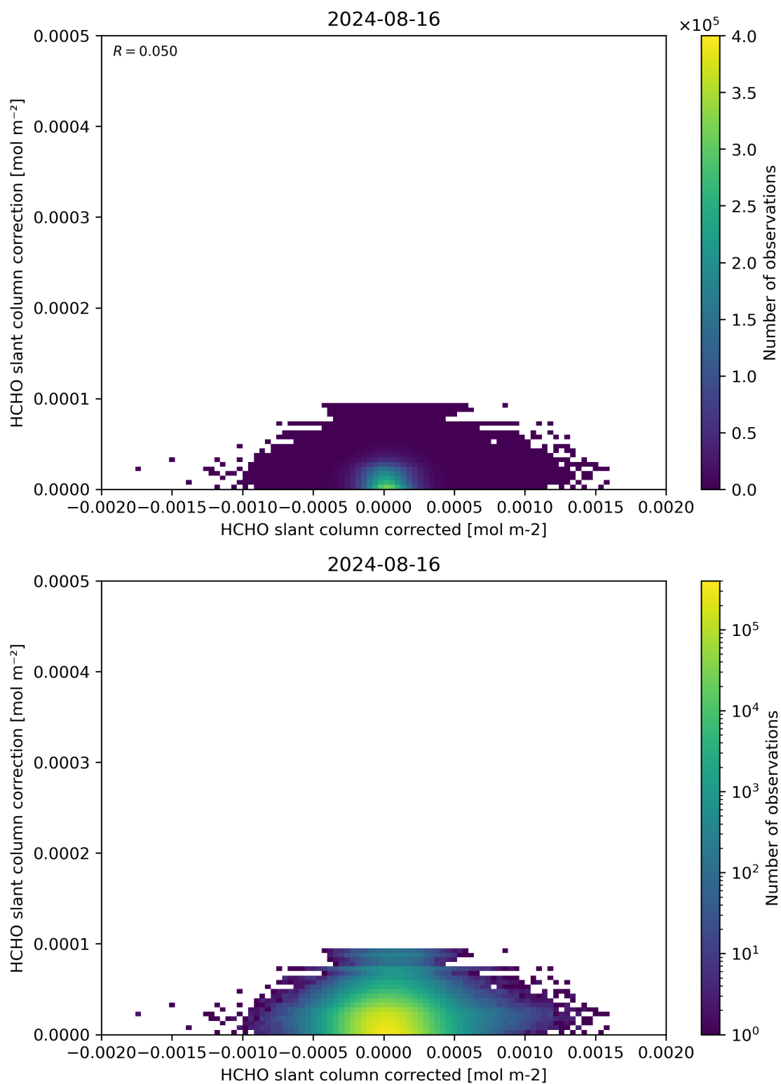
Figure 77: Scatter density plot of “HCHO slant column corrected” against “HCHO slant column correction” for 2024-08-16 to 2024-08-17.
