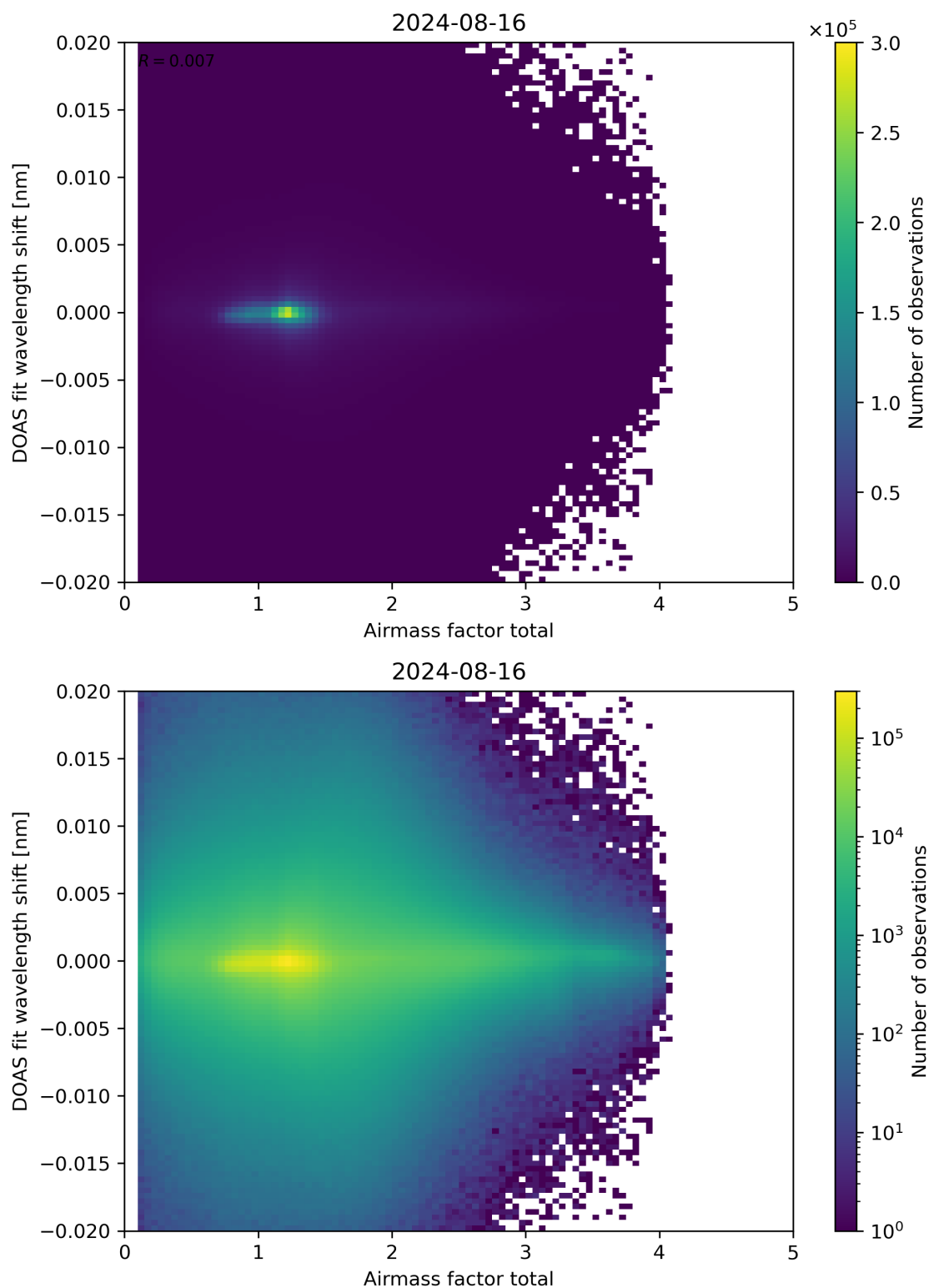
Figure 98: Scatter density plot of “Airmass factor total” against “DOAS fit wavelength shift” for 2024-08-16 to 2024-08-17.
