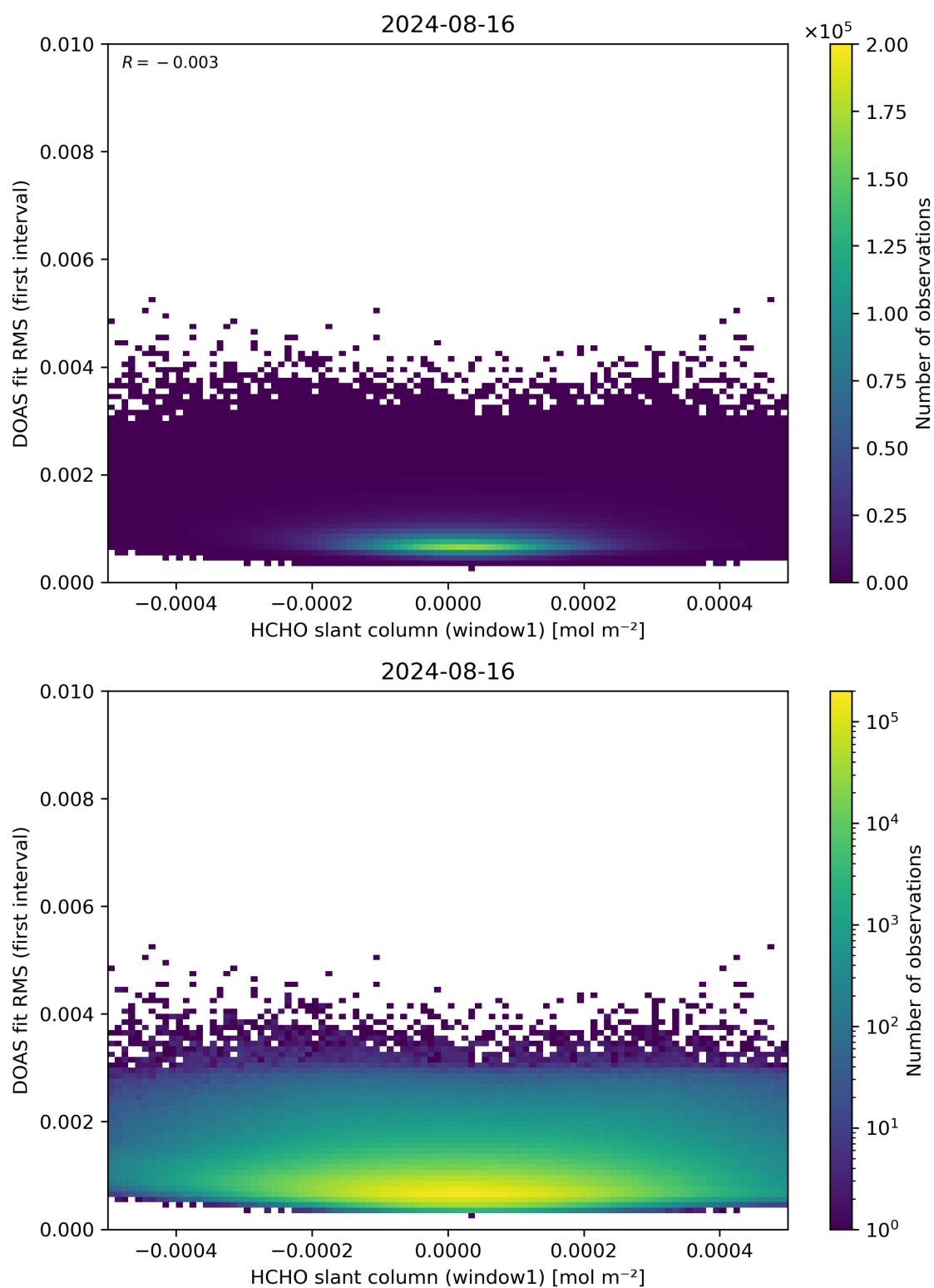
Figure 78: Scatter density plot of “HCHO slant column (window1)” against “DOAS fit RMS (first interval)” for 2024-08-16 to 2024-08-17.
