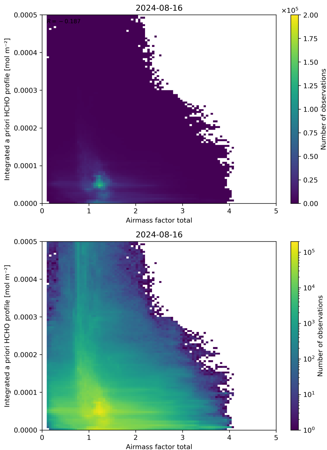
Figure 104: Scatter density plot of “Airmass factor total” against “Integrated a priori HCHO profile” for 2024-08-16 to 2024-08-17.
