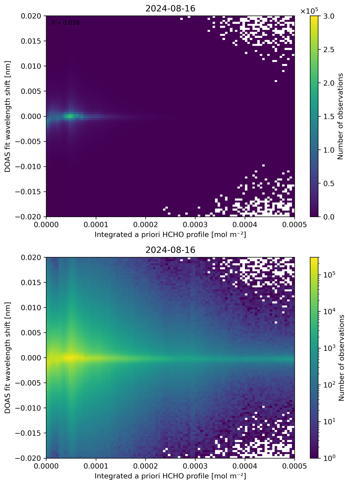
Figure 149: Scatter density plot of “Integrated a priori HCHO profile” against “DOAS fit wavelength shift” for 2024-08-16 to 2024-08-17.
