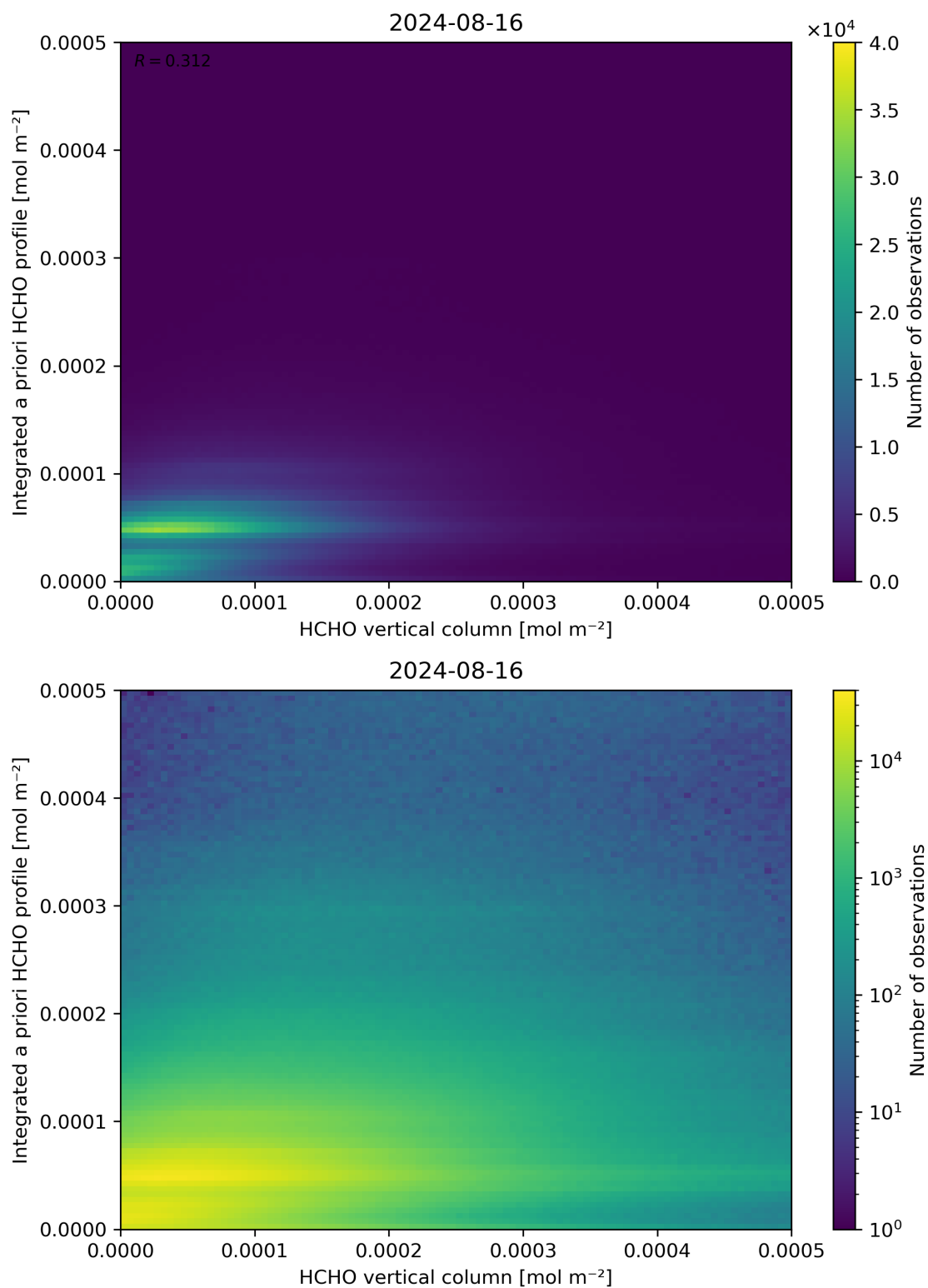
Figure 135: Scatter density plot of “HCHO vertical column” against “Integrated a priori HCHO profile” for 2024-08-16 to 2024-08-17.
