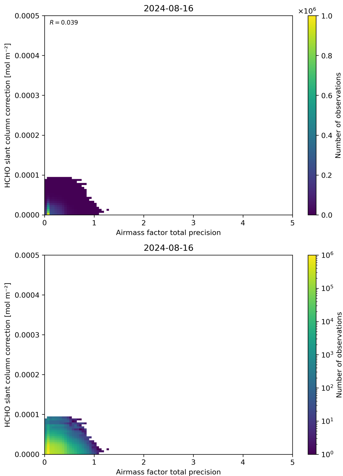
Figure 110: Scatter density plot of “Airmass factor total precision” against “HCHO slant column correction” for 2024-08-16 to 2024-08-17.
