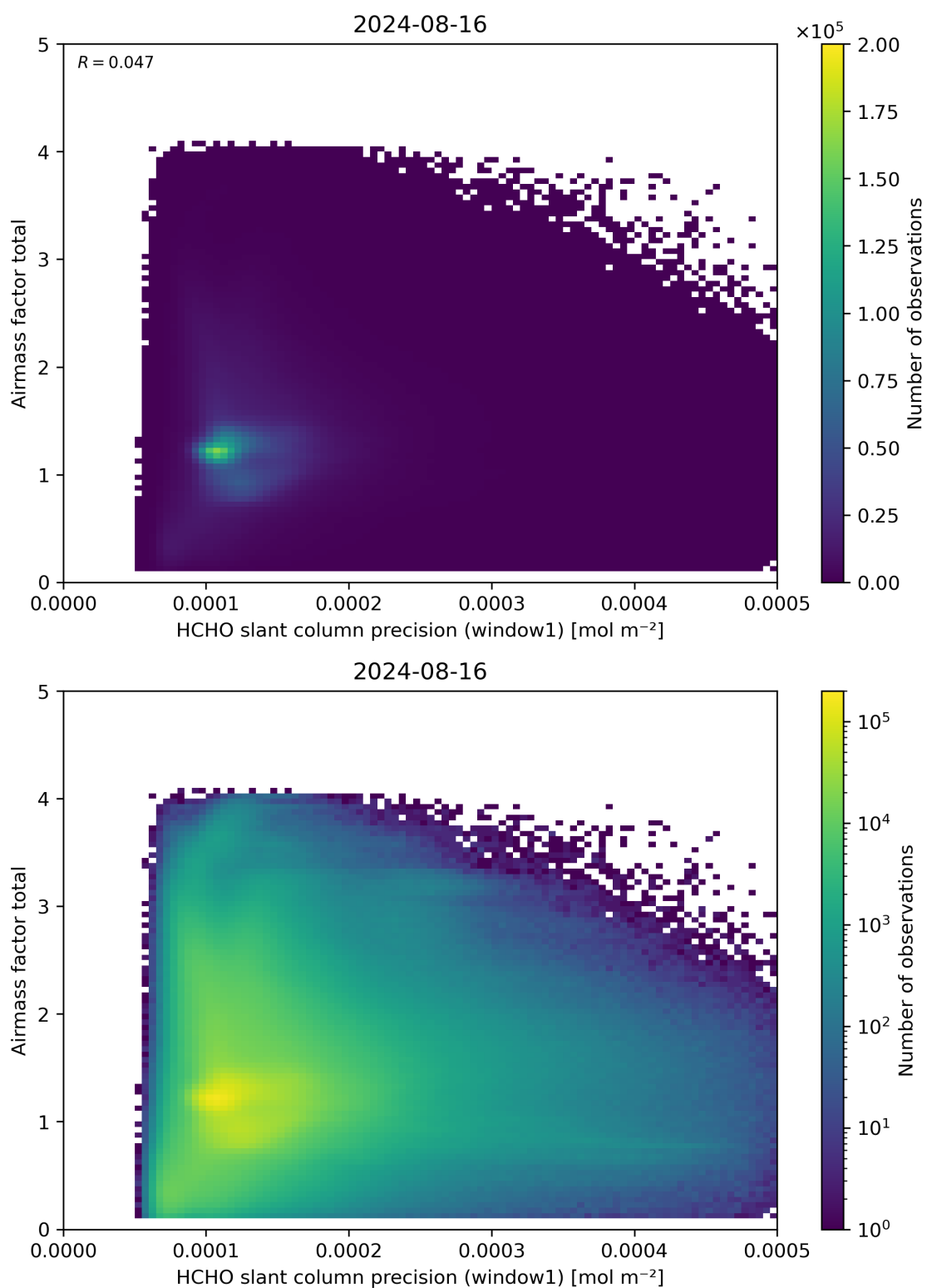
Figure 94: Scatter density plot of “HCHO slant column precision (window1)” against “Airmass factor total” for 2024-08-16 to 2024-08-17.
