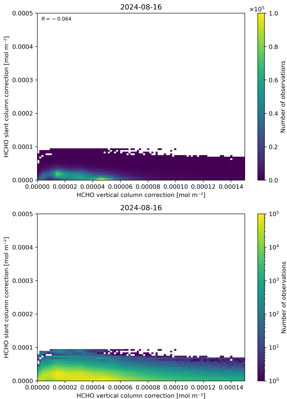
Figure 117: Scatter density plot of “HCHO vertical column correction” against “HCHO slant column correction” for 2024-08-16 to 2024-08-17.
