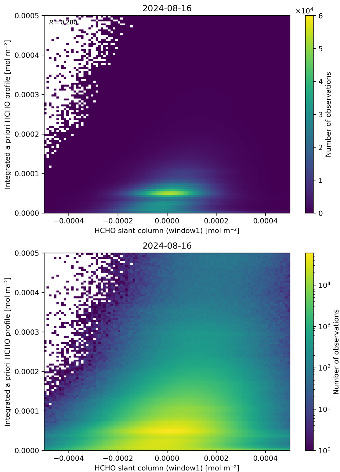
Figure 87: Scatter density plot of “HCHO slant column (window1)” against “Integrated a priori HCHO profile” for 2024-08-16 to 2024-08-17.
