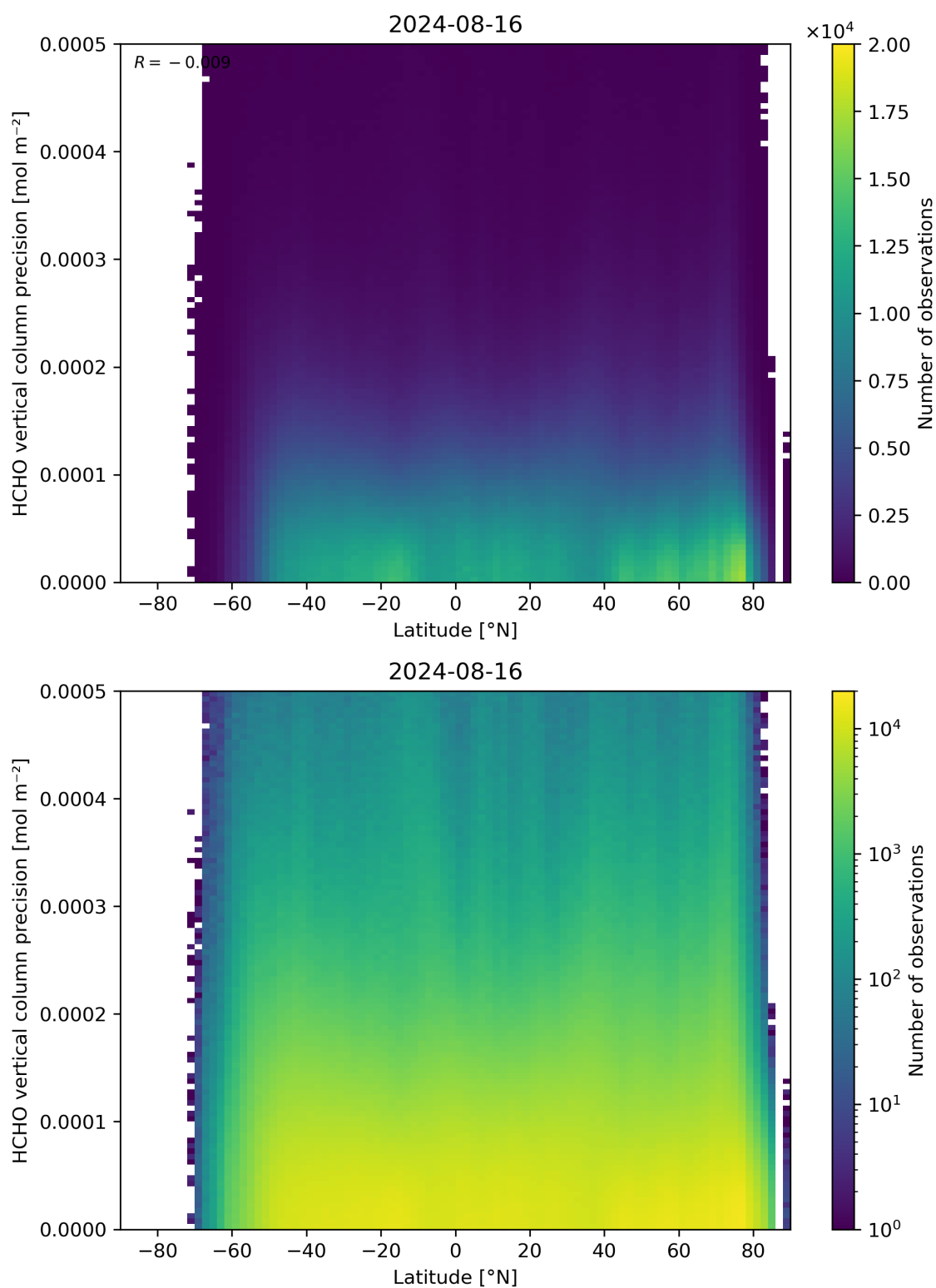
Figure 165: Scatter density plot of “Latitude” against “HCHO vertical column precision” for 2024-08-16 to 2024-08-17.
