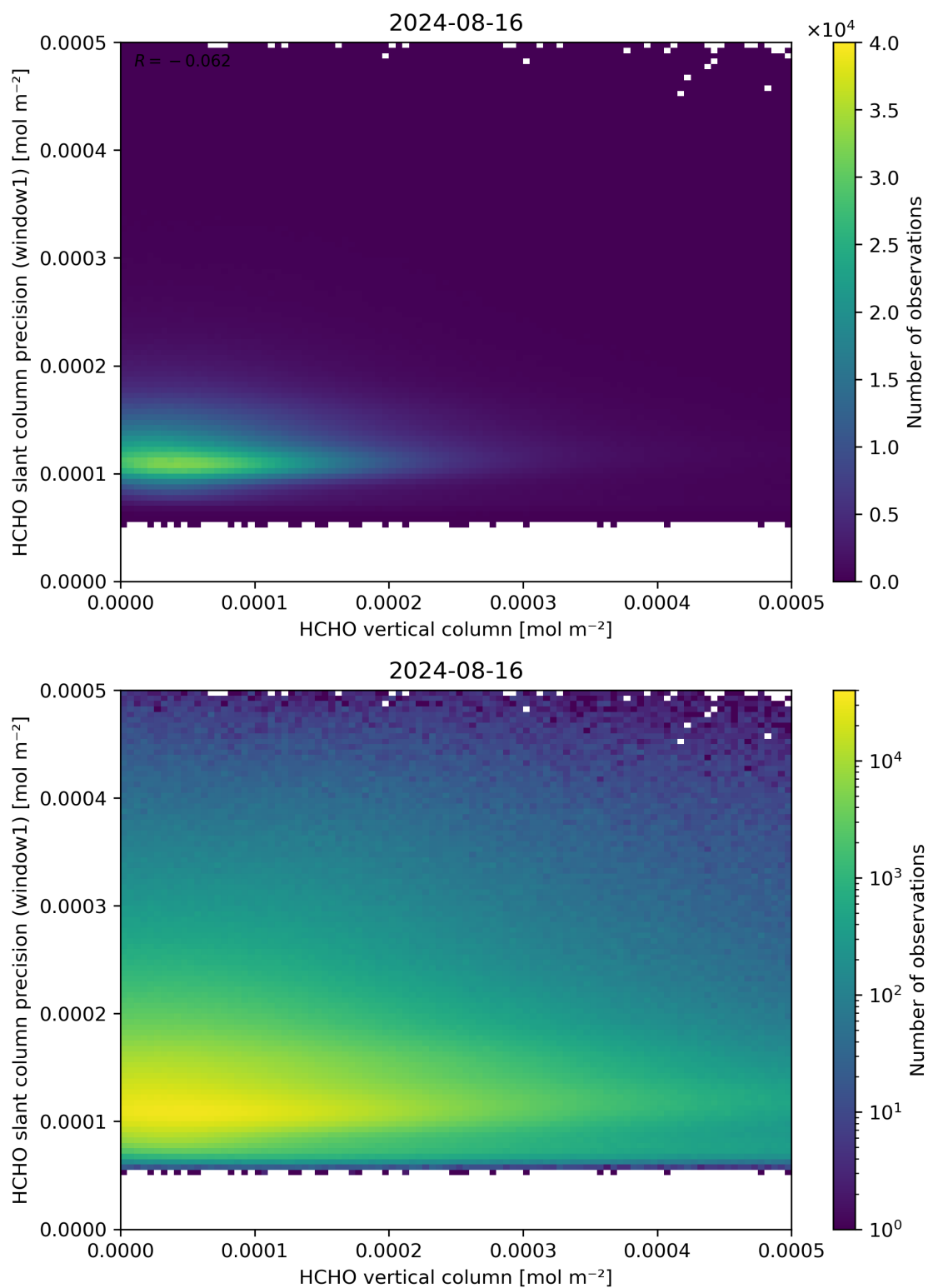
Figure 130: Scatter density plot of “HCHO vertical column” against “HCHO slant column precision (window1)” for 2024-08-16 to 2024-08-17.
