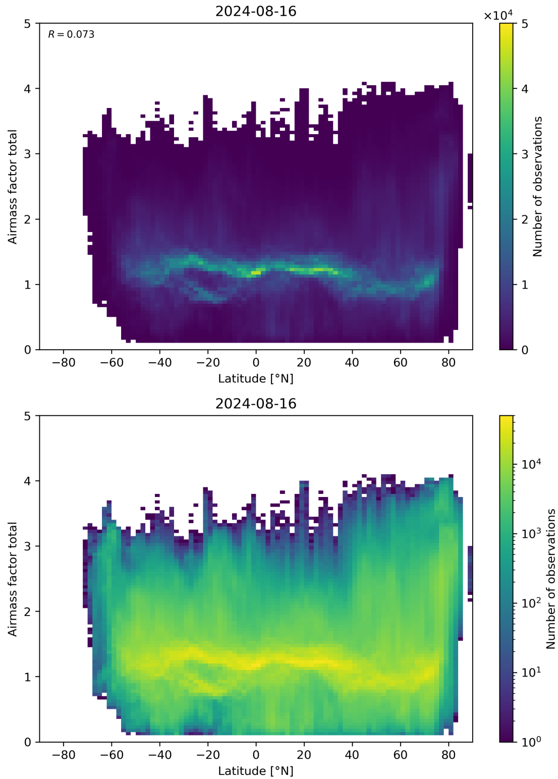
Figure 161: Scatter density plot of “Latitude” against “Airmass factor total” for 2024-08-16 to 2024-08-17.
