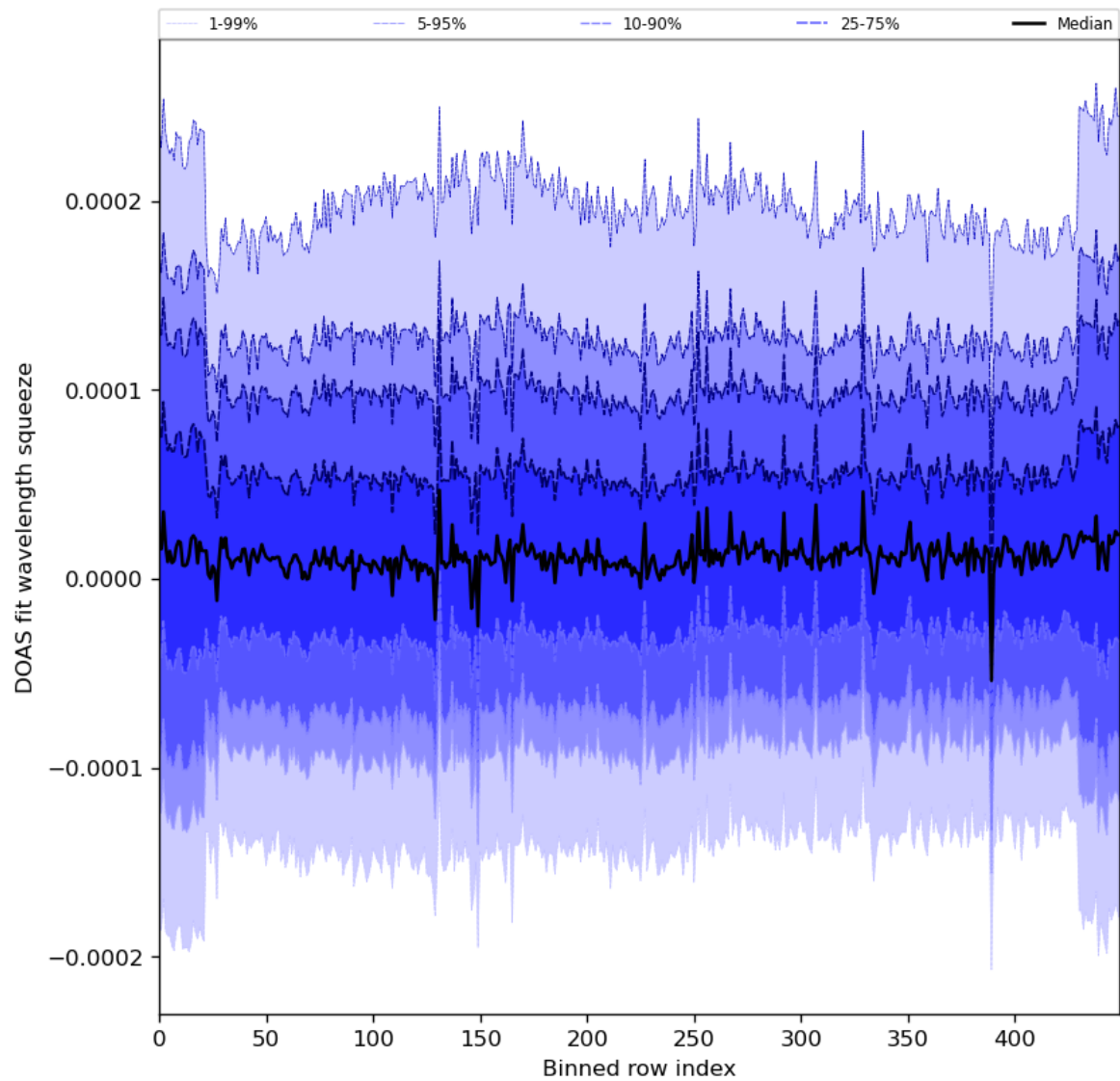
Figure 59: Along track statistics of “DOAS fit wavelength squeeze” for 2024-08-16 to 2024-08-17
