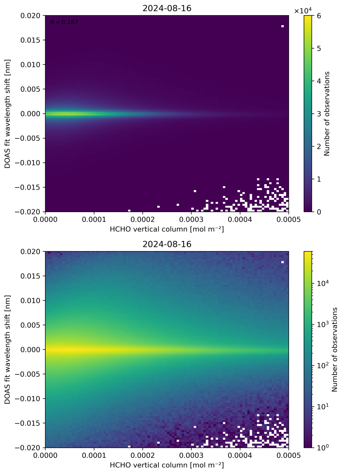
Figure 124: Scatter density plot of “HCHO vertical column” against “DOAS fit wavelength shift” for 2024-08-16 to 2024-08-17.
