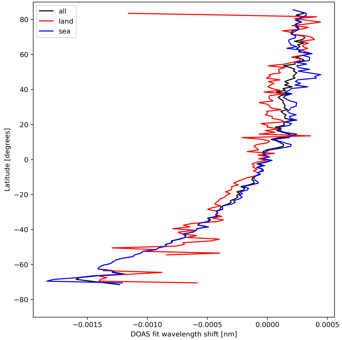
Figure 30: Zonal average of “DOAS fit wavelength shift” for 2024-08-16 to 2024-08-17.
