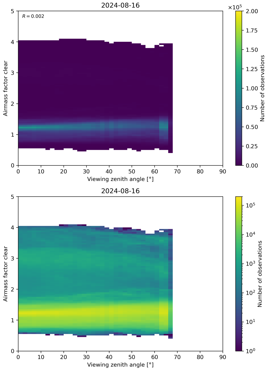
Figure 185: Scatter density plot of “Viewing zenith angle” against “Airmass factor clear” for 2024-08-16 to 2024-08-17.
