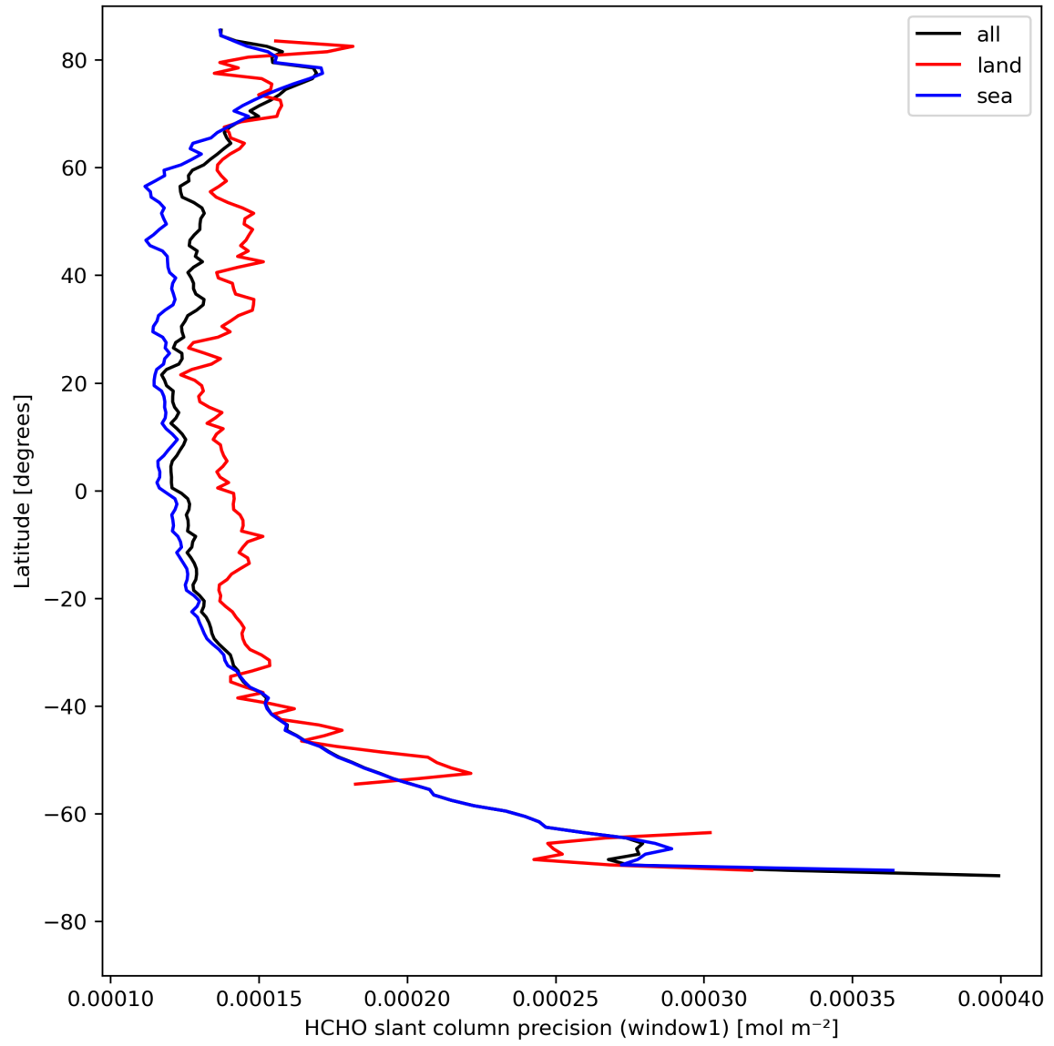
Figure 25: Zonal average of “HCHO slant column precision (window1)” for 2024-08-16 to 2024-08-17.
