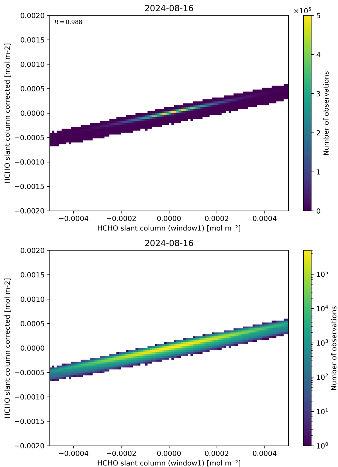
Figure 82: Scatter density plot of “HCHO slant column (window1)” against “HCHO slant column corrected” for 2024-08-16 to 2024-08-17.
