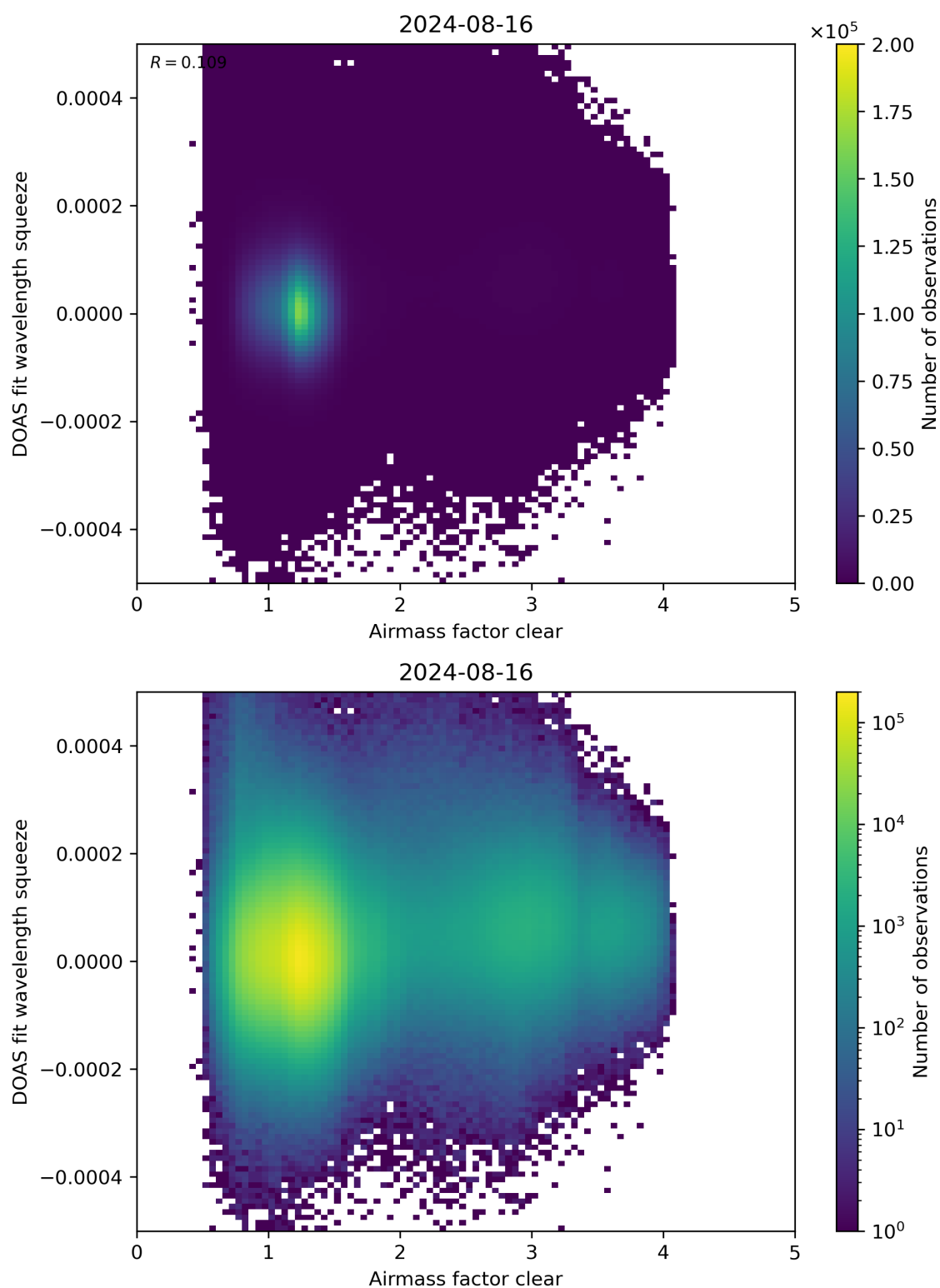
Figure 73: Scatter density plot of “Airmass factor clear” against “DOAS fit wavelength squeeze” for 2024-08-16 to 2024-08-17.
