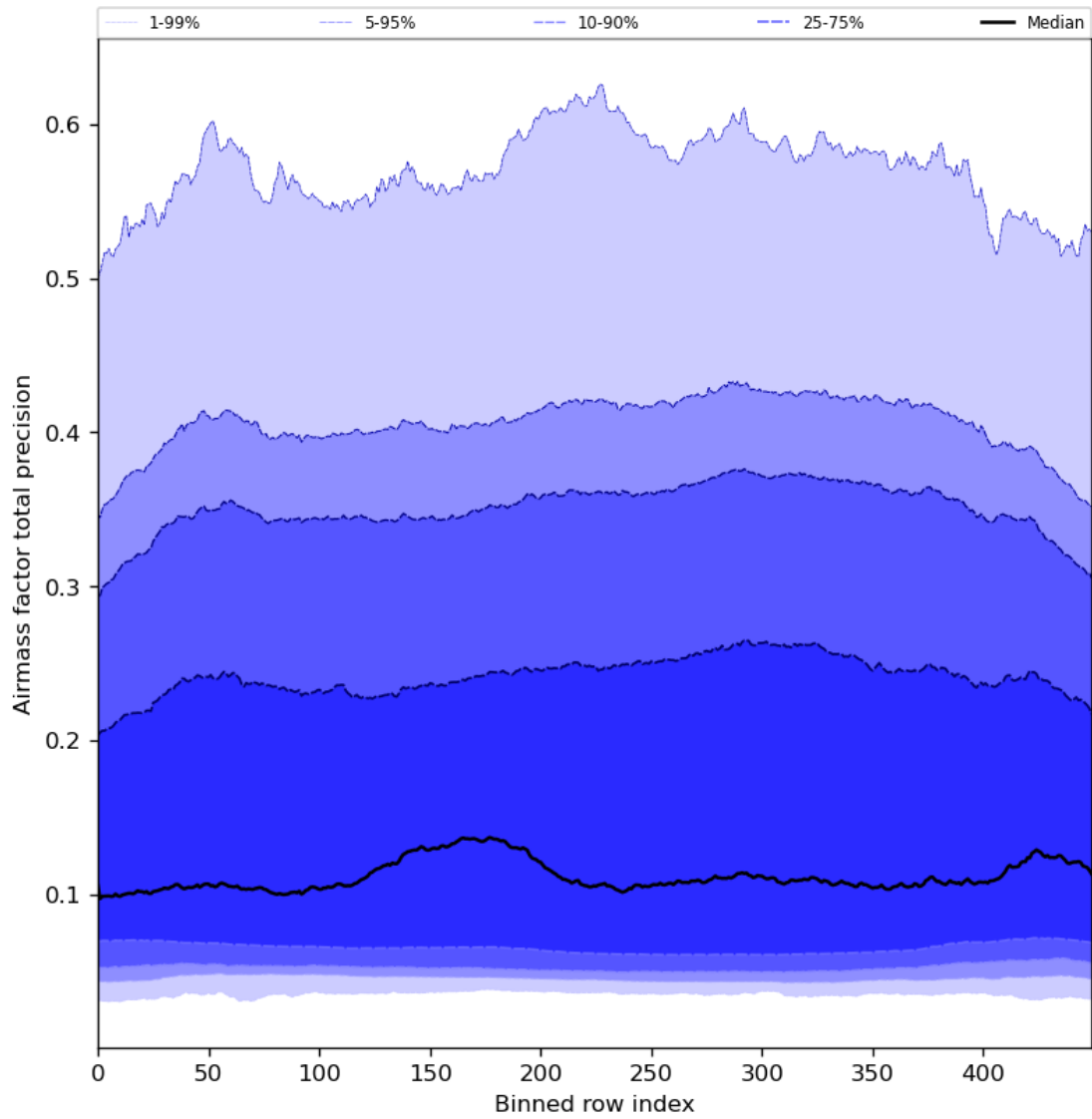
Figure 55: Along track statistics of “Airmass factor total precision” for 2024-08-16 to 2024-08-17
