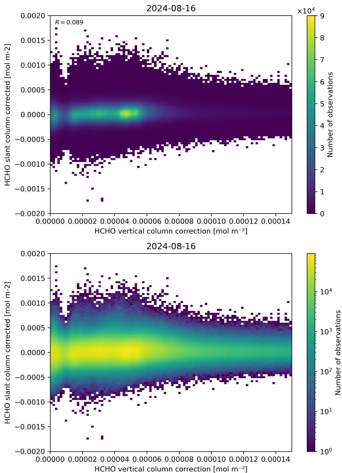
Figure 116: Scatter density plot of “HCHO vertical column correction” against “HCHO slant column corrected” for 2024-08-16 to 2024-08-17.
