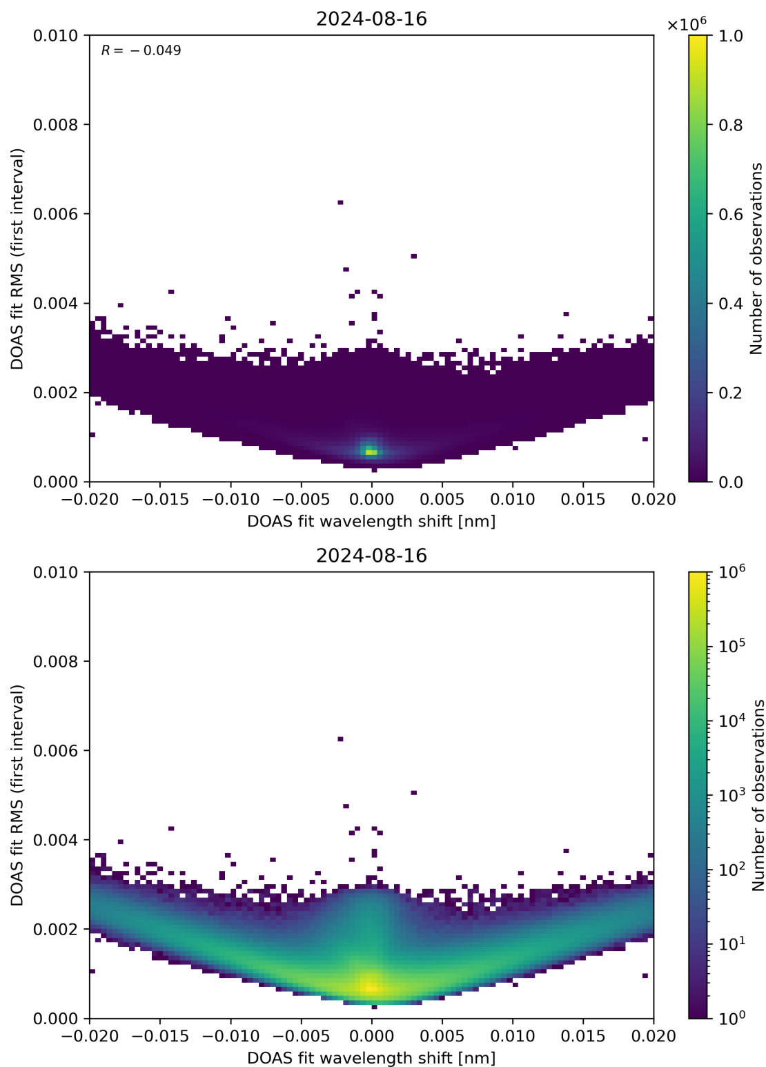
Figure 64: Scatter density plot of “DOAS fit wavelength shift” against “DOAS fit RMS (first interval)” for 2024-08-16 to 2024-08-17.
