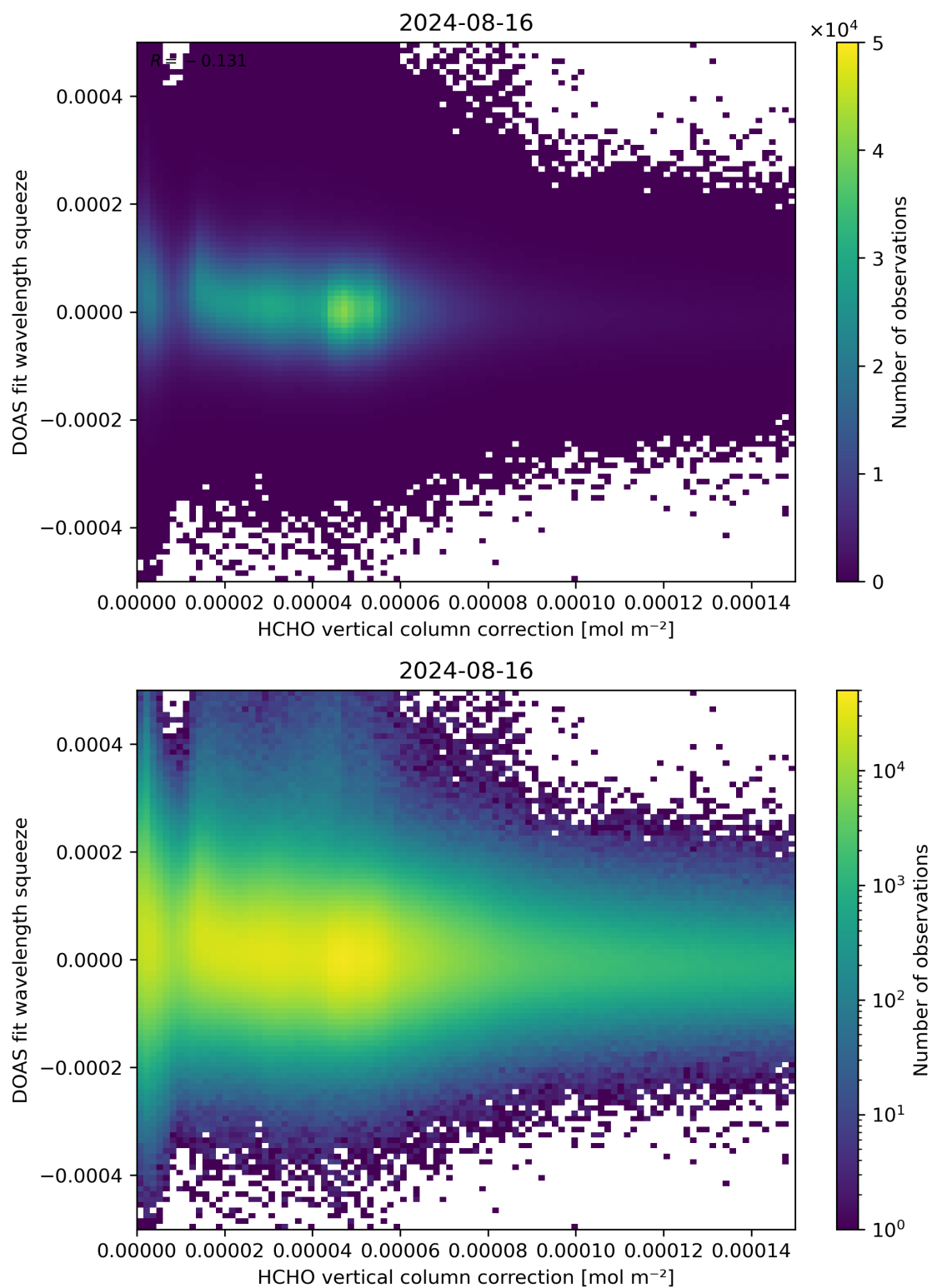
Figure 114: Scatter density plot of “HCHO vertical column correction” against “DOAS fit wavelength squeeze” for 2024-08-16 to 2024-08-17.
