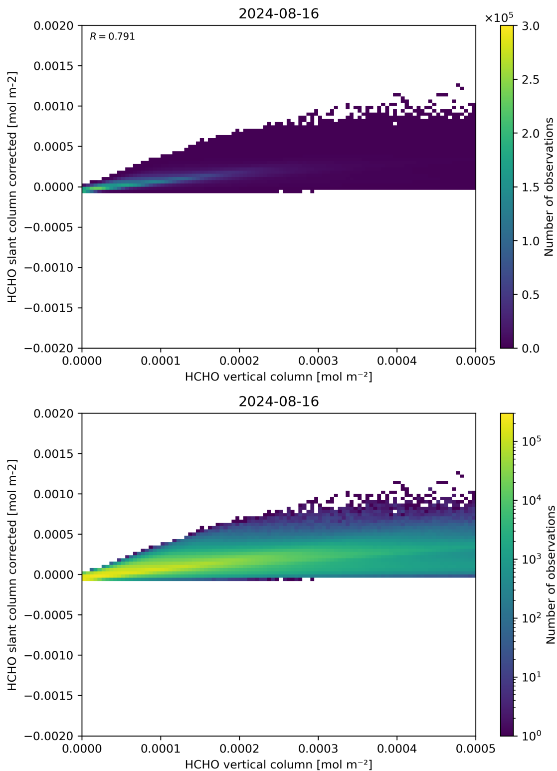
Figure 127: Scatter density plot of “HCHO vertical column” against “HCHO slant column corrected” for 2024-08-16 to 2024-08-17.
