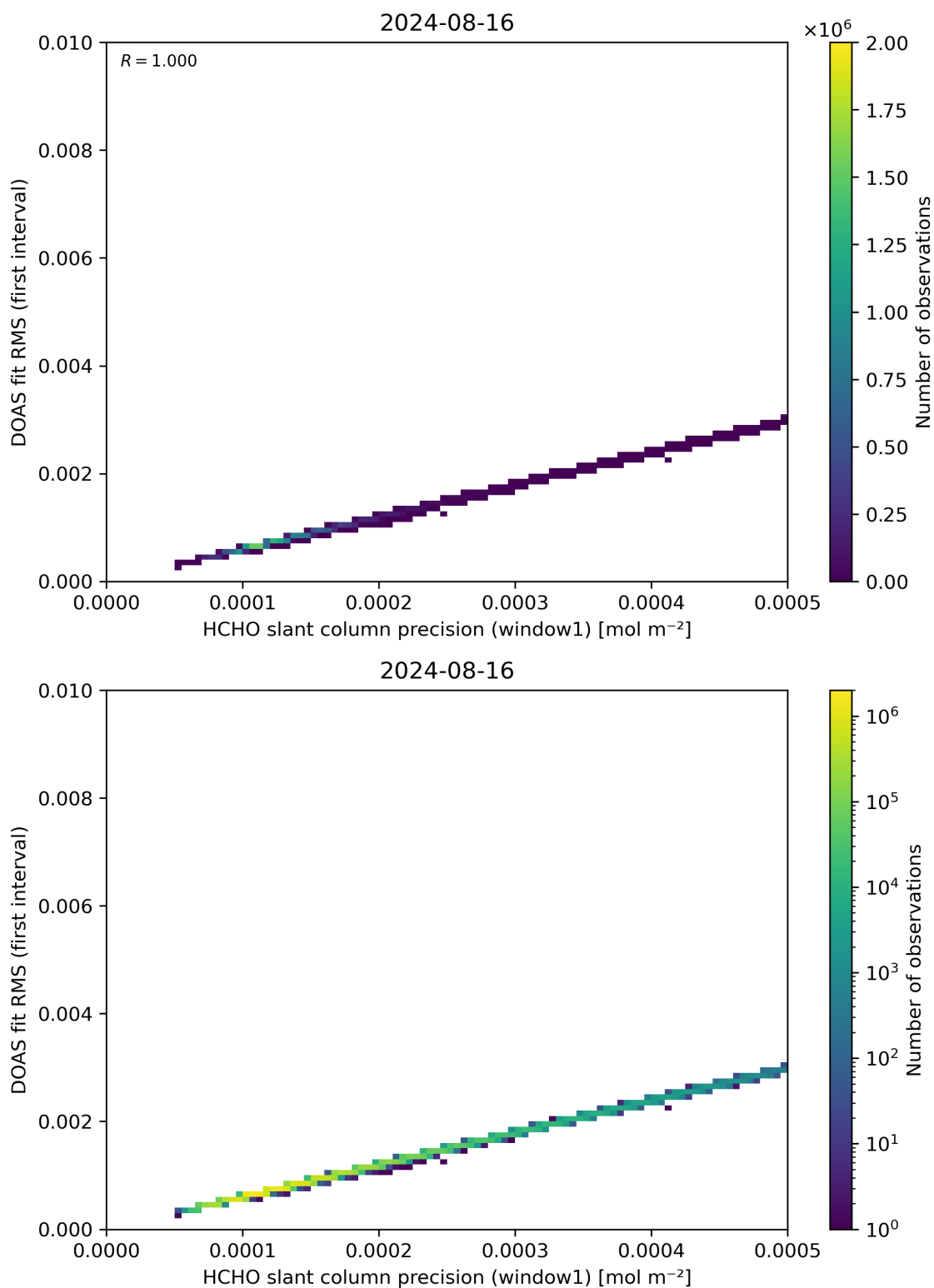
Figure 88: Scatter density plot of “HCHO slant column precision (window1)” against “DOAS fit RMS (first interval)” for 2024-08-16 to 2024-08-17.
