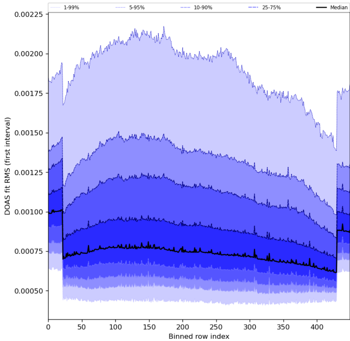
Figure 60: Along track statistics of “DOAS fit RMS (first interval)” for 2024-08-16 to 2024-08-17
