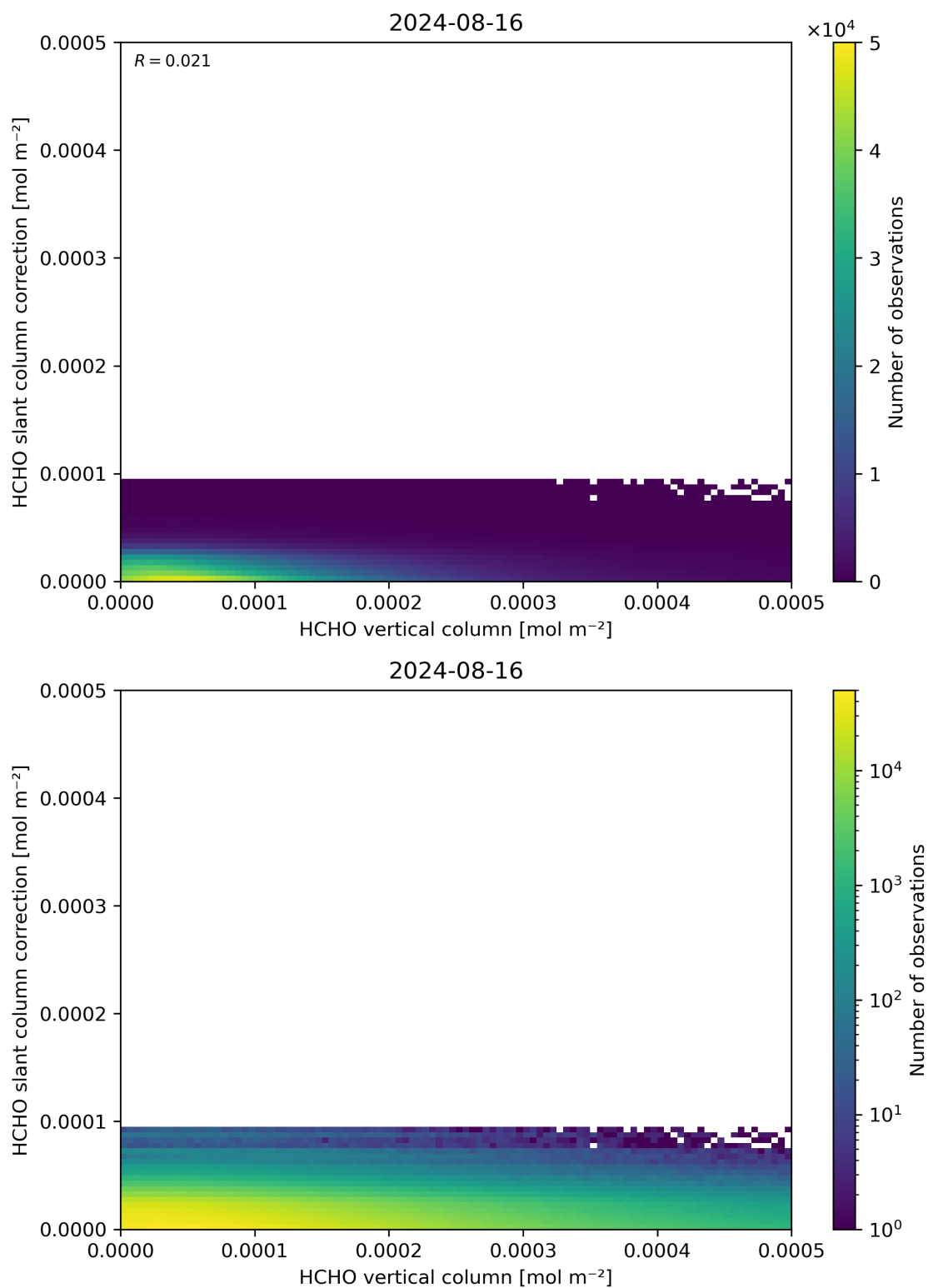
Figure 128: Scatter density plot of “HCHO vertical column” against “HCHO slant column correction” for 2024-08-16 to 2024-08-17.
