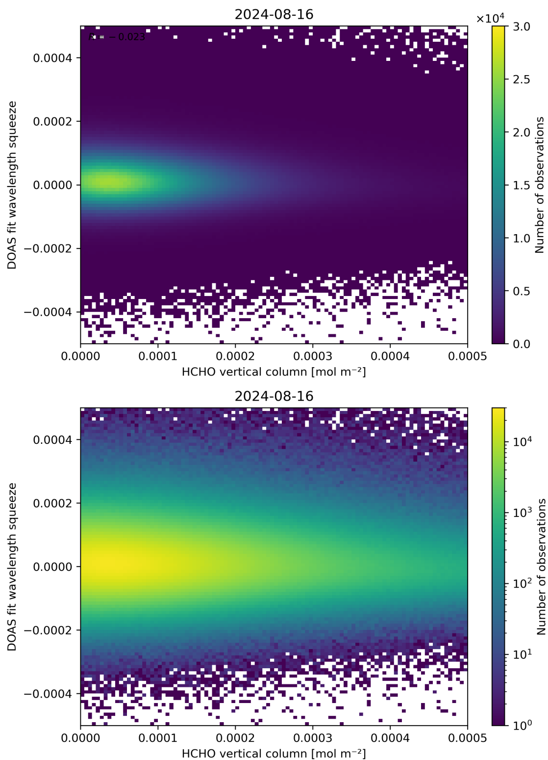
Figure 125: Scatter density plot of “HCHO vertical column” against “DOAS fit wavelength squeeze” for 2024-08-16 to 2024-08-17.
