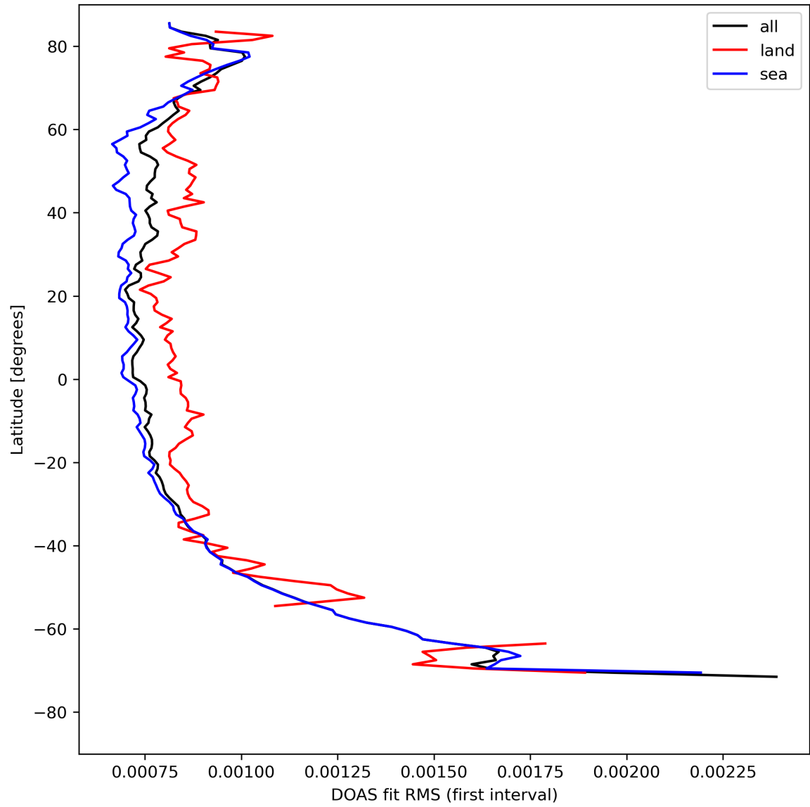
Figure 32: Zonal average of “DOAS fit RMS (first interval)” for 2024-08-16 to 2024-08-17.
