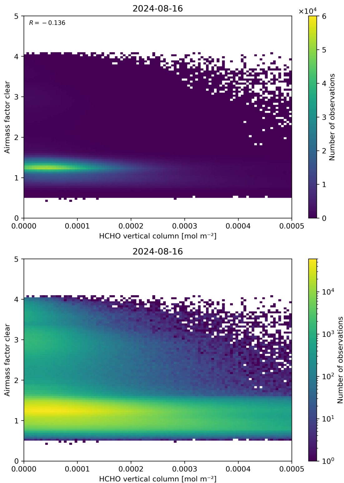
Figure 126: Scatter density plot of “HCHO vertical column” against “Airmass factor clear” for 2024-08-16 to 2024-08-17.
