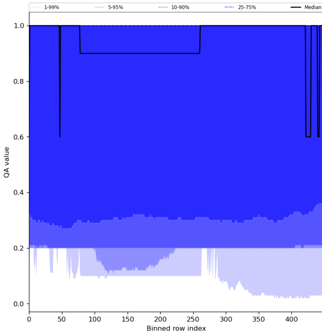
Figure 48: Along track statistics of “QA value” for 2024-08-16 to 2024-08-17
