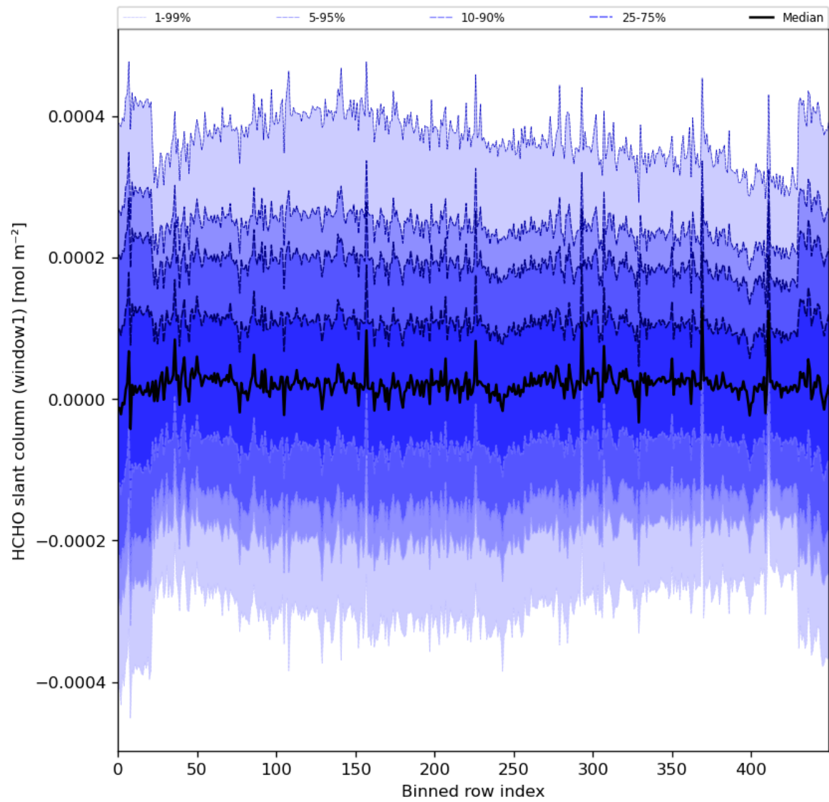
Figure 52: Along track statistics of “HCHO slant column (window1)” for 2024-08-16 to 2024-08-17
