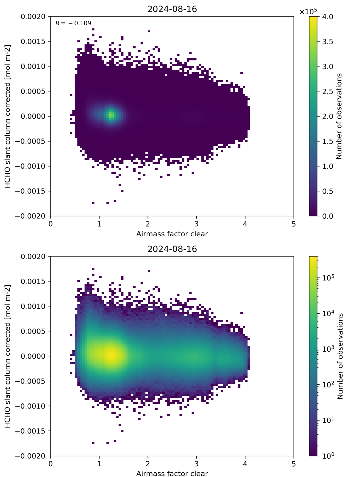
Figure 74: Scatter density plot of “Airmass factor clear” against “HCHO slant column corrected” for 2024-08-16 to 2024-08-17.
