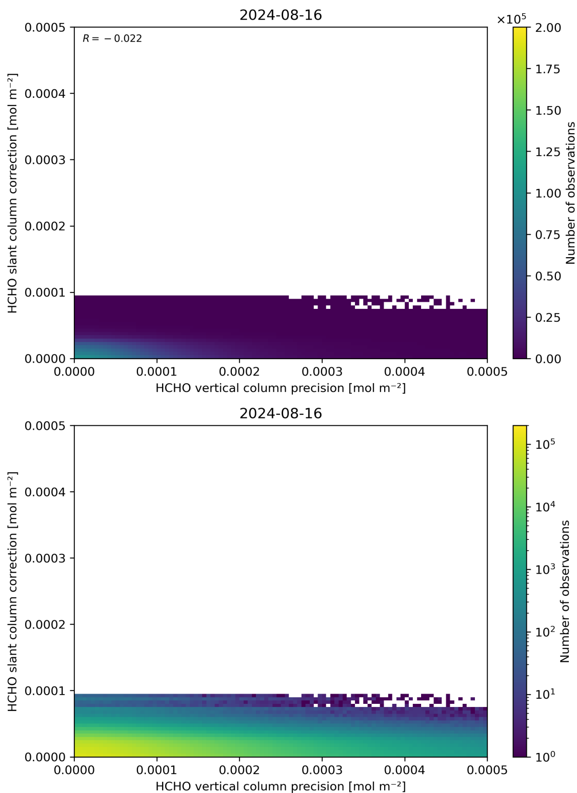
Figure 141: Scatter density plot of “HCHO vertical column precision” against “HCHO slant column correction” for 2024-08-16 to 2024-08-17.
