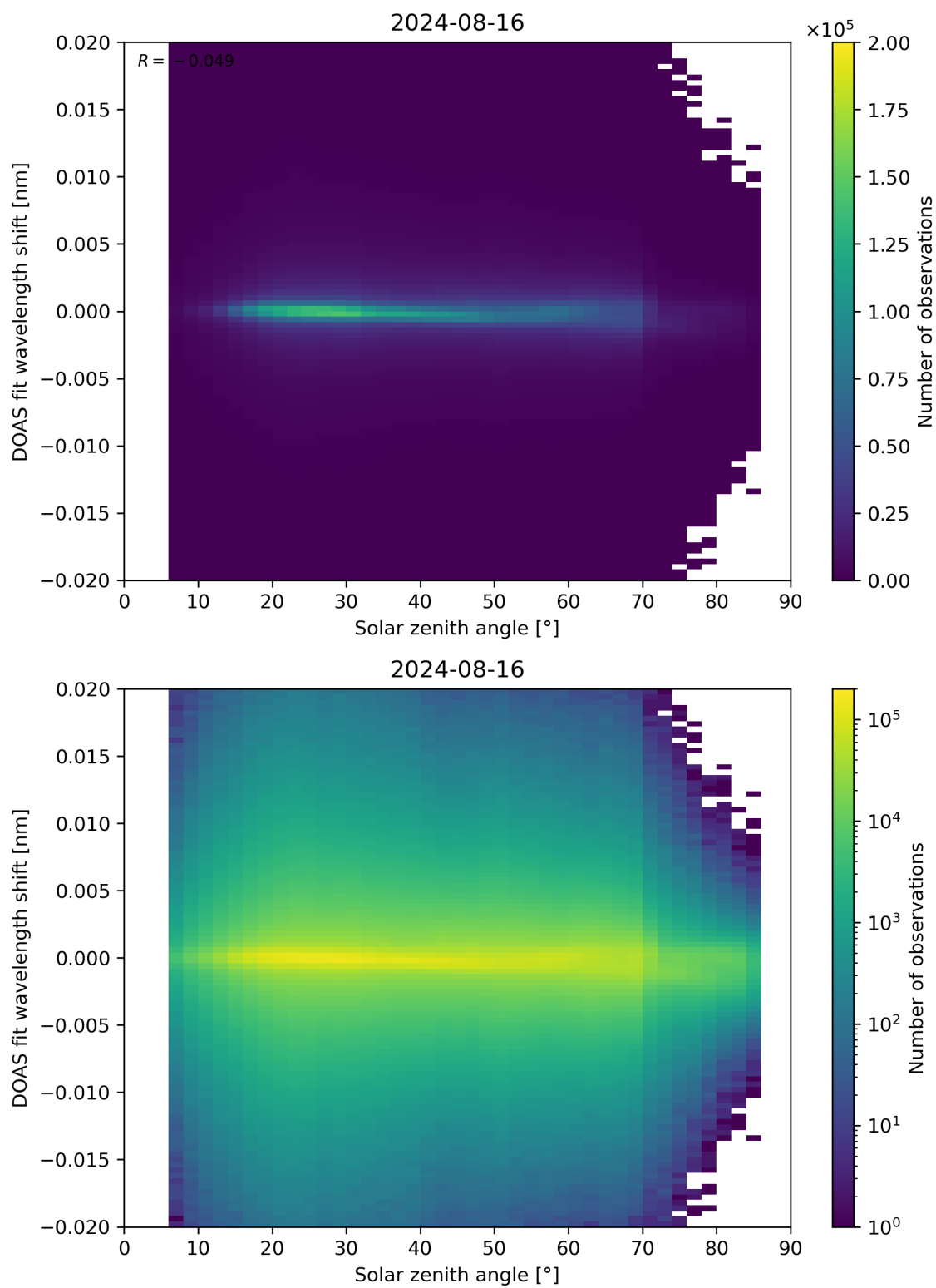
Figure 168: Scatter density plot of “Solar zenith angle” against “DOAS fit wavelength shift” for 2024-08-16 to 2024-08-17.
