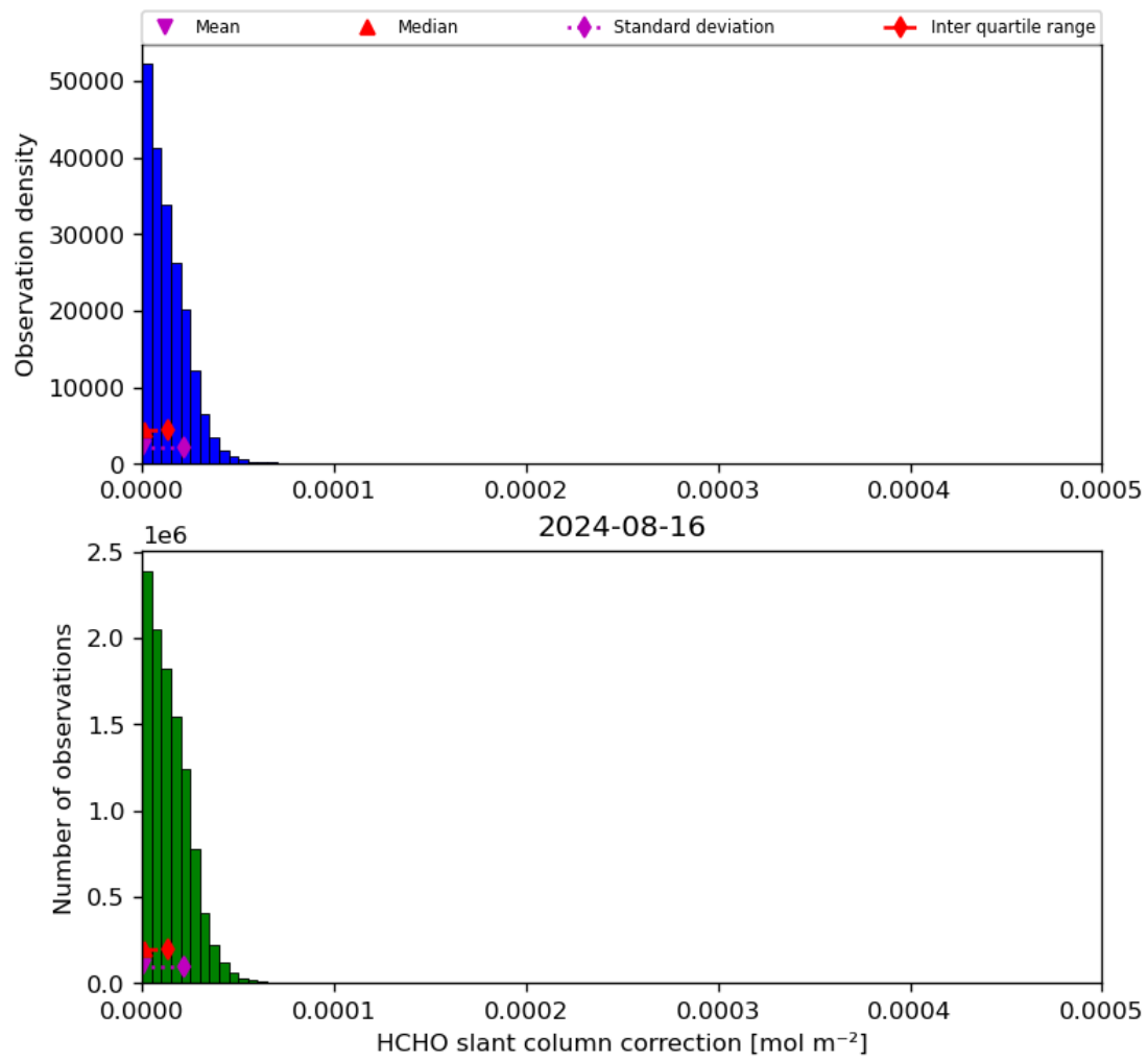
Figure 47: Histogram of “HCHO slant column correction” for 2024-08-16 to 2024-08-17
