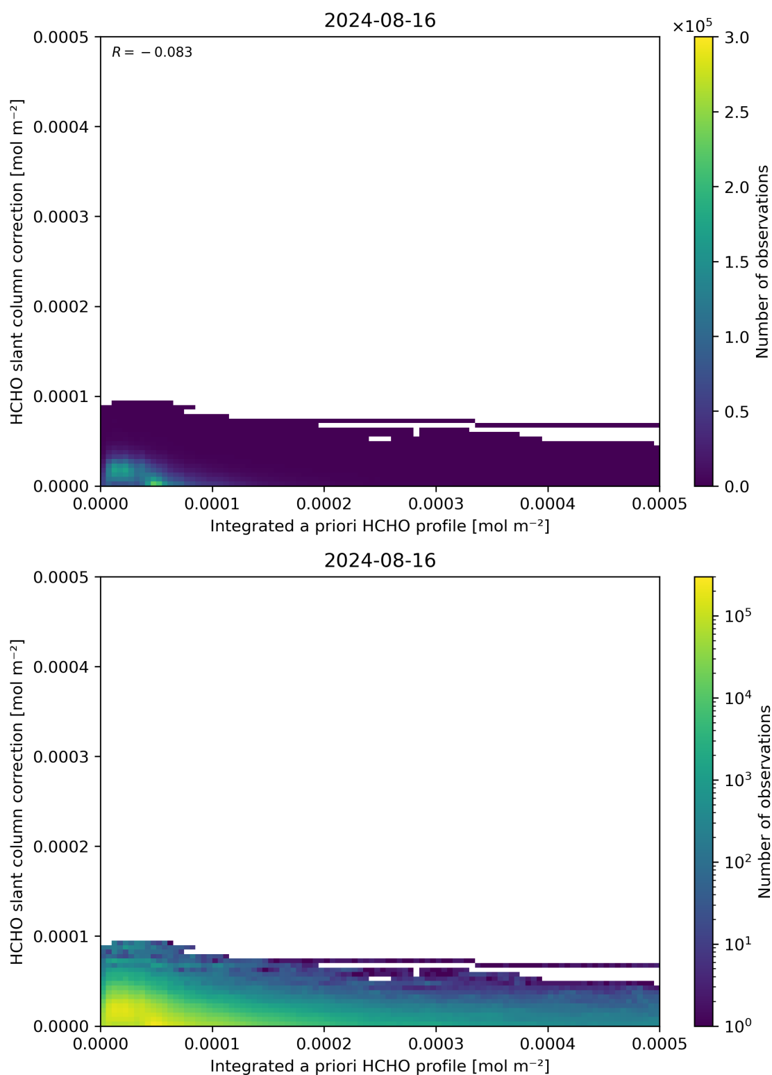
Figure 152: Scatter density plot of “Integrated a priori HCHO profile” against “HCHO slant column correction” for 2024-08-16 to 2024-08-17.
