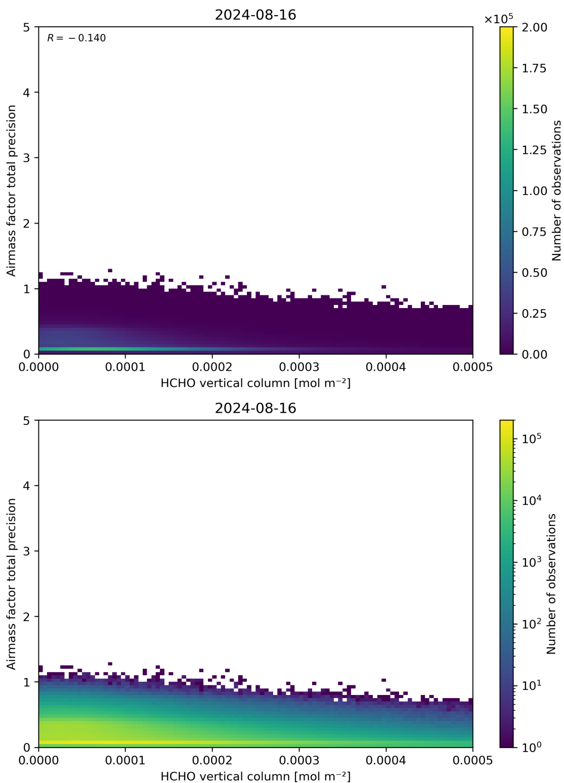
Figure 132: Scatter density plot of “HCHO vertical column” against “Airmass factor total precision” for 2024-08-16 to 2024-08-17.
