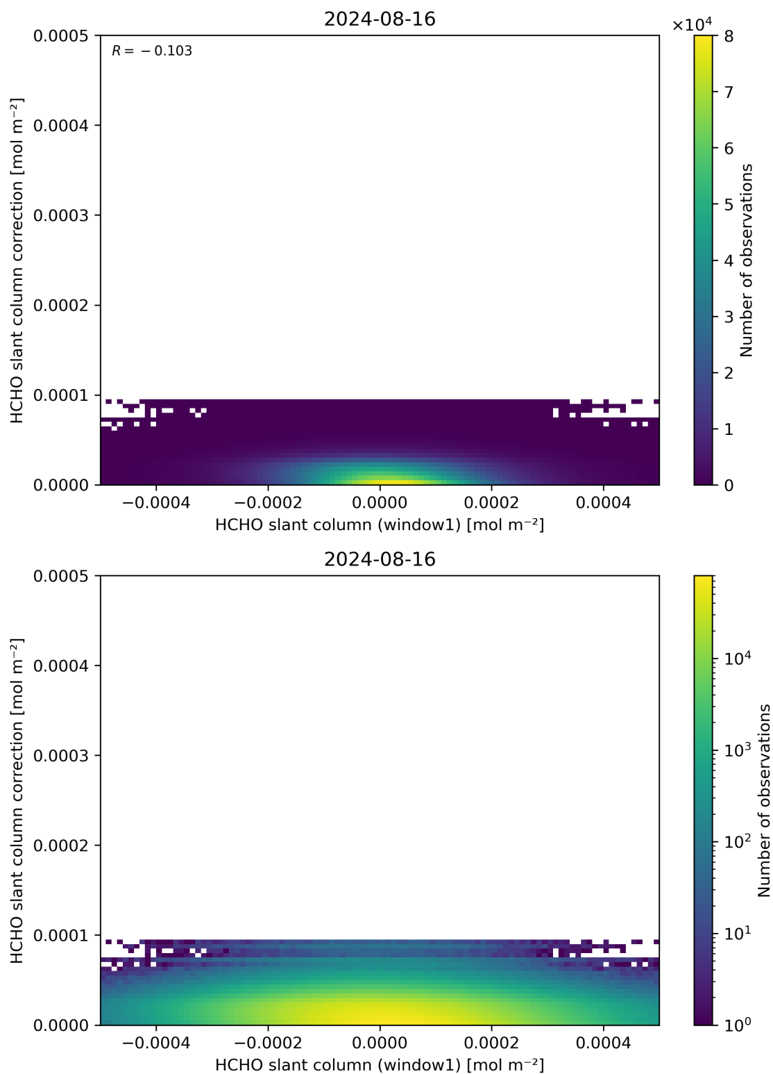
Figure 83: Scatter density plot of “HCHO slant column (window1)” against “HCHO slant column correction” for 2024-08-16 to 2024-08-17.
