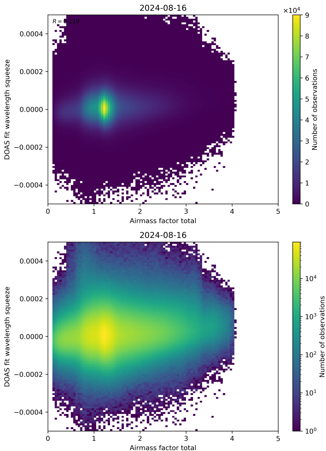
Figure 99: Scatter density plot of “Airmass factor total” against “DOAS fit wavelength squeeze” for 2024-08-16 to 2024-08-17.
