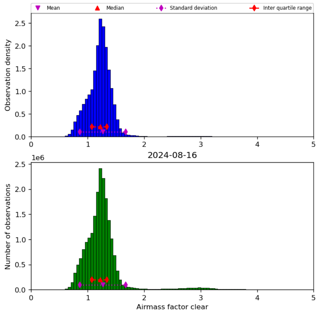
Figure 42: Histogram of “Airmass factor clear” for 2024-08-16 to 2024-08-17
