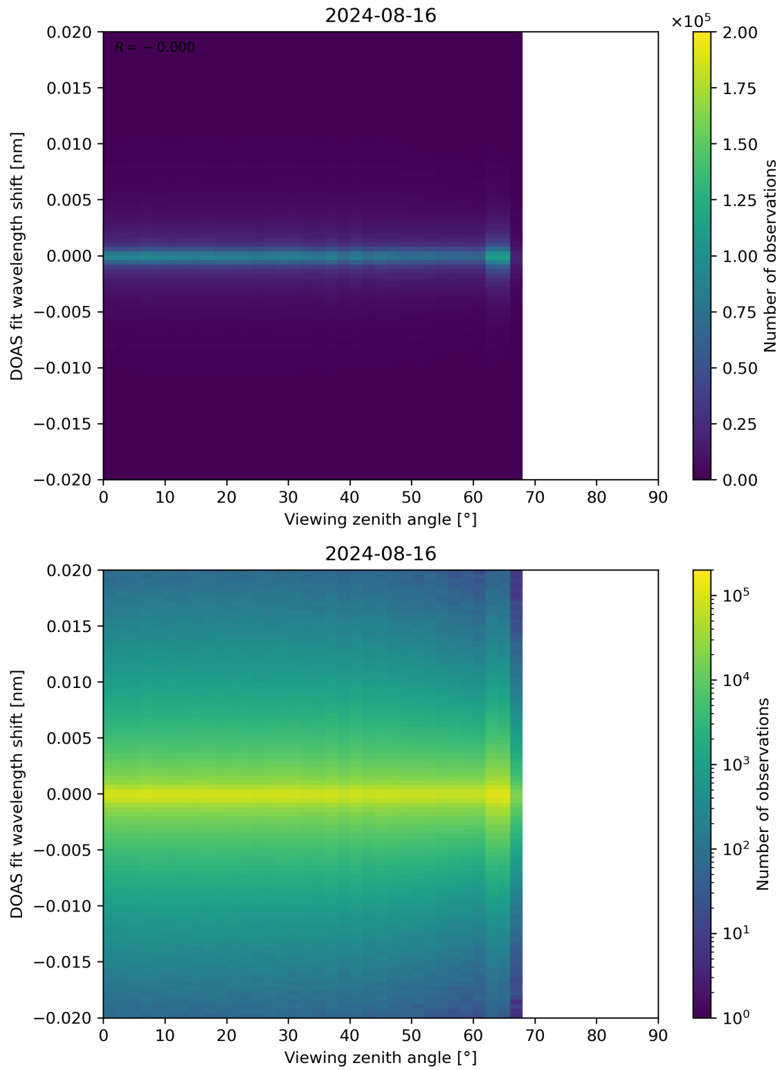
Figure 183: Scatter density plot of “Viewing zenith angle” against “DOAS fit wavelength shift” for 2024-08-16 to 2024-08-17.
