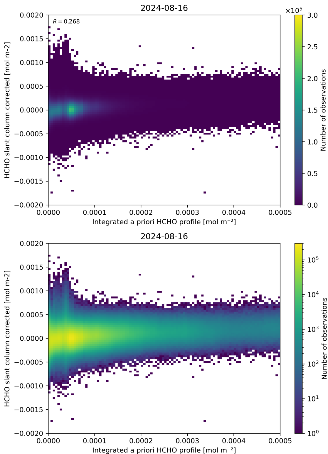
Figure 151: Scatter density plot of “Integrated a priori HCHO profile” against “HCHO slant column corrected” for 2024-08-16 to 2024-08-17.
