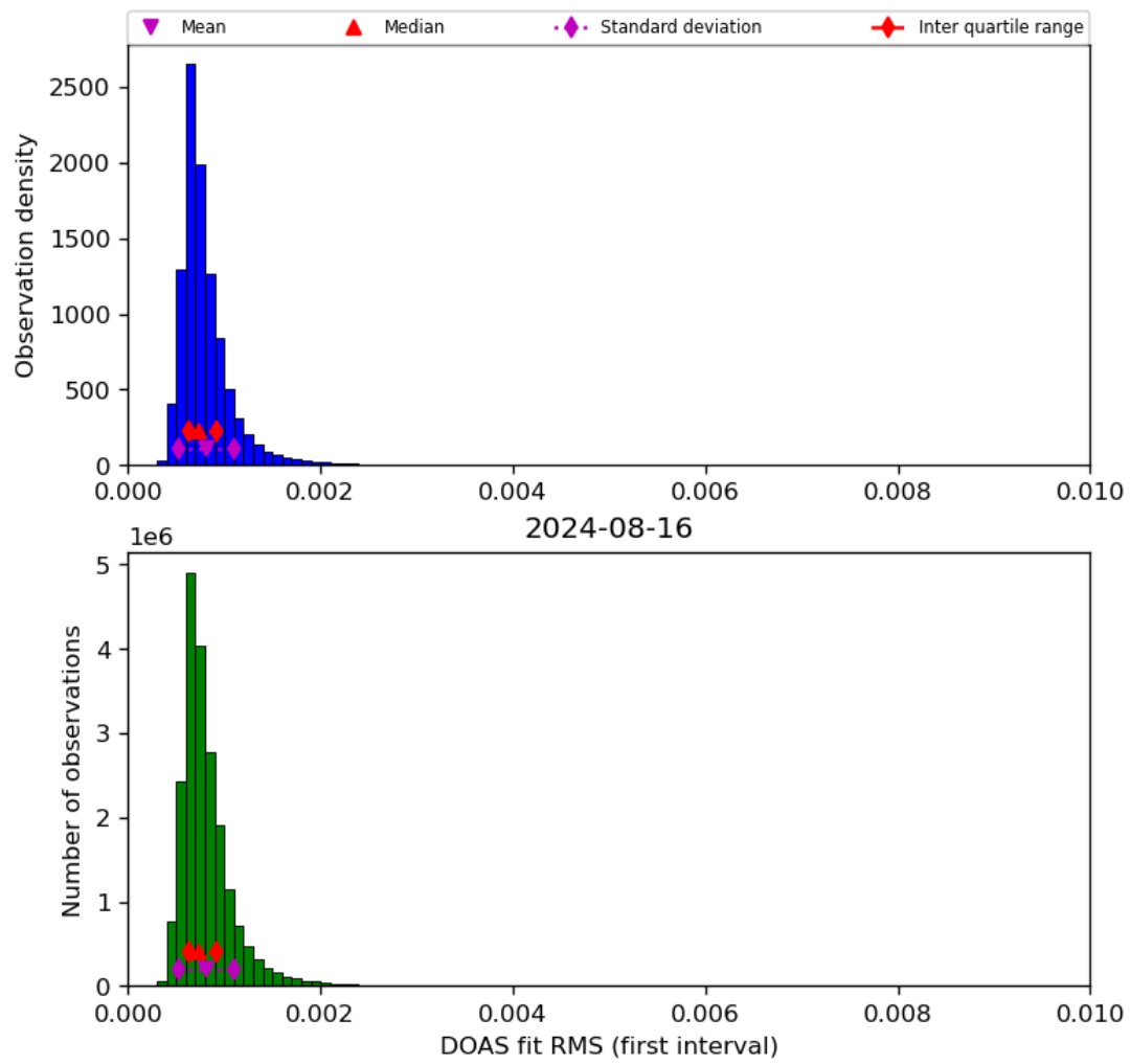
Figure 46: Histogram of “DOAS fit RMS (first interval)” for 2024-08-16 to 2024-08-17
