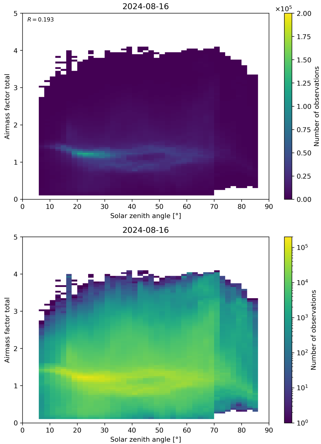
Figure 175: Scatter density plot of “Solar zenith angle” against “Airmass factor total” for 2024-08-16 to 2024-08-17.
