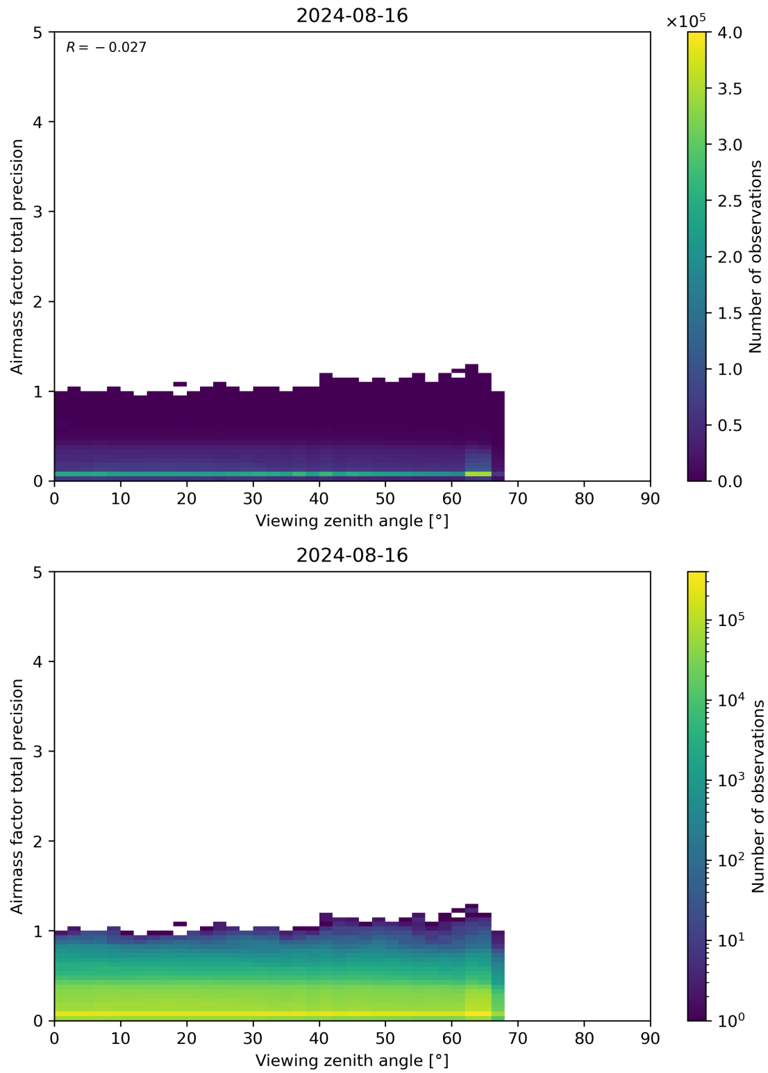
Figure 191: Scatter density plot of “Viewing zenith angle” against “Airmass factor total precision” for 2024-08-16 to 2024-08-17.
