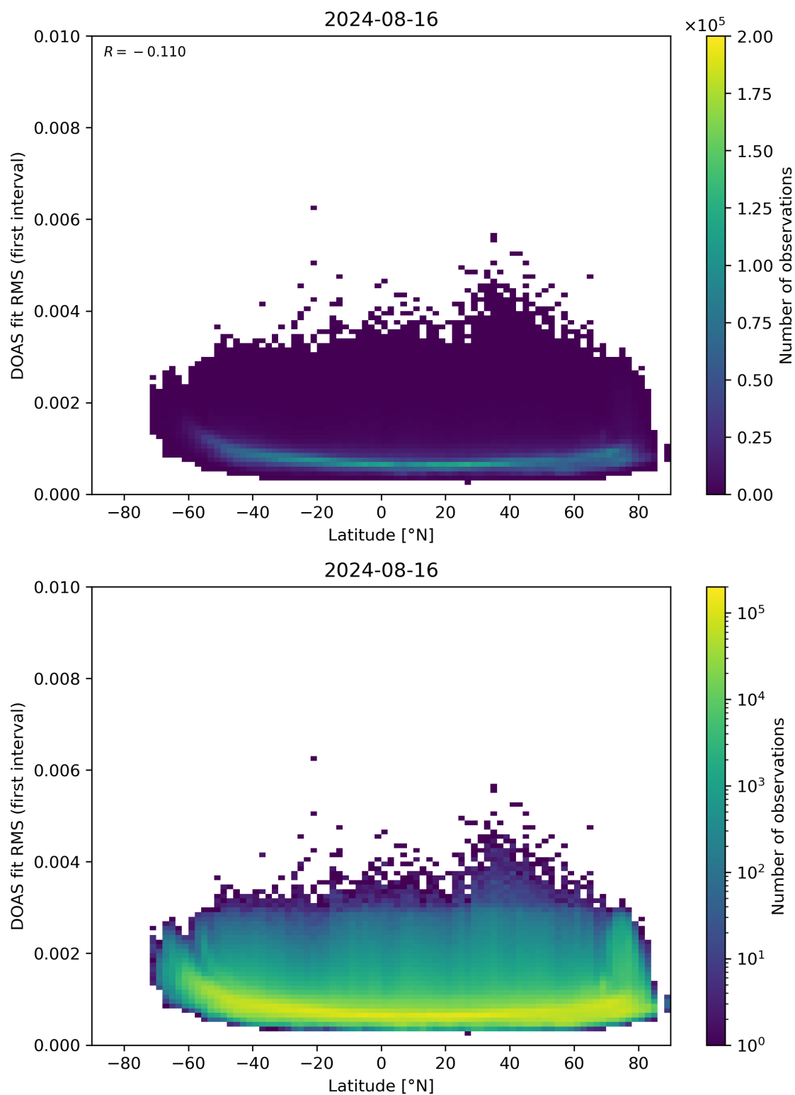
Figure 153: Scatter density plot of “Latitude” against “DOAS fit RMS (first interval)” for 2024-08-16 to 2024-08-17.
