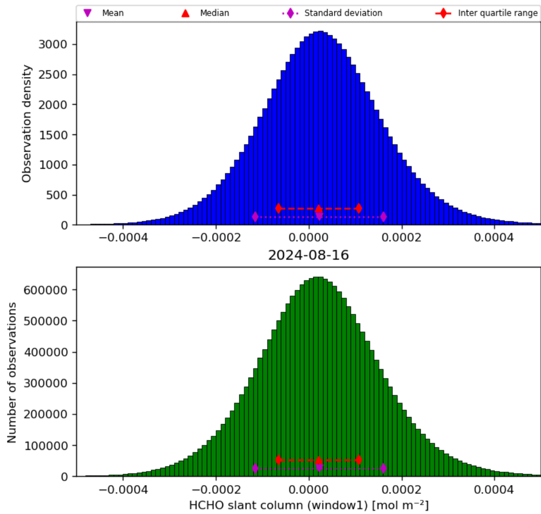
Figure 38: Histogram of “HCHO slant column (window1)” for 2024-08-16 to 2024-08-17
