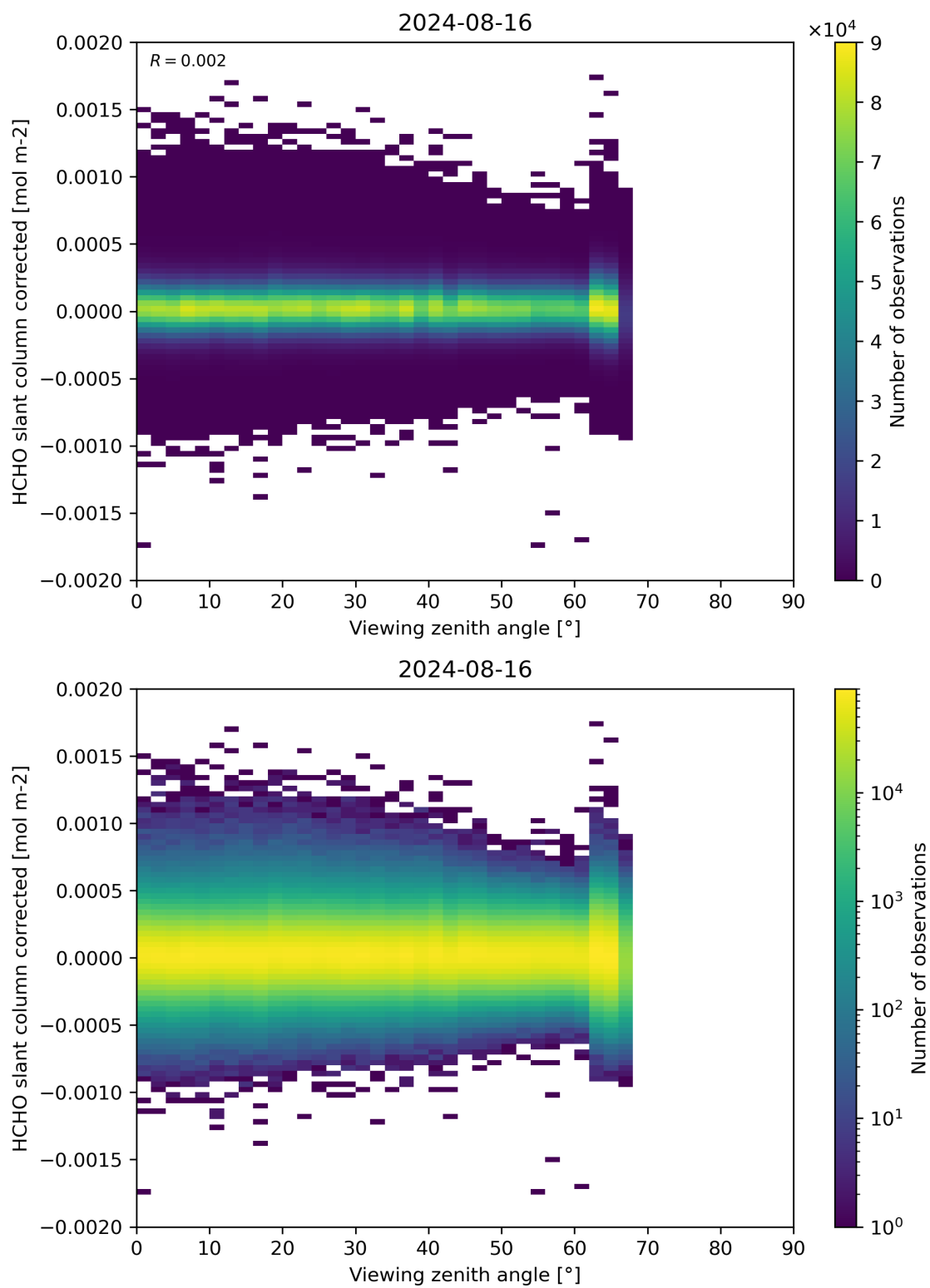
Figure 186: Scatter density plot of “Viewing zenith angle” against “HCHO slant column corrected” for 2024-08-16 to 2024-08-17.
