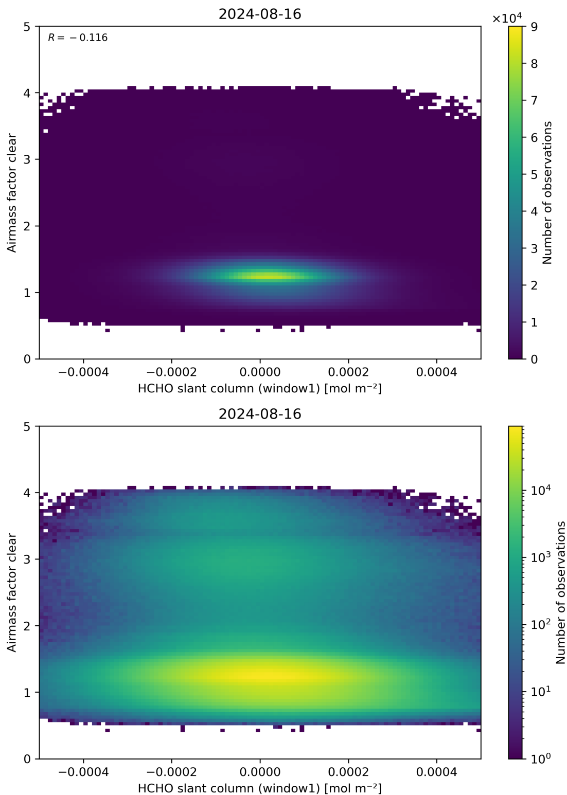
Figure 81: Scatter density plot of “HCHO slant column (window1)” against “Airmass factor clear” for 2024-08-16 to 2024-08-17.
