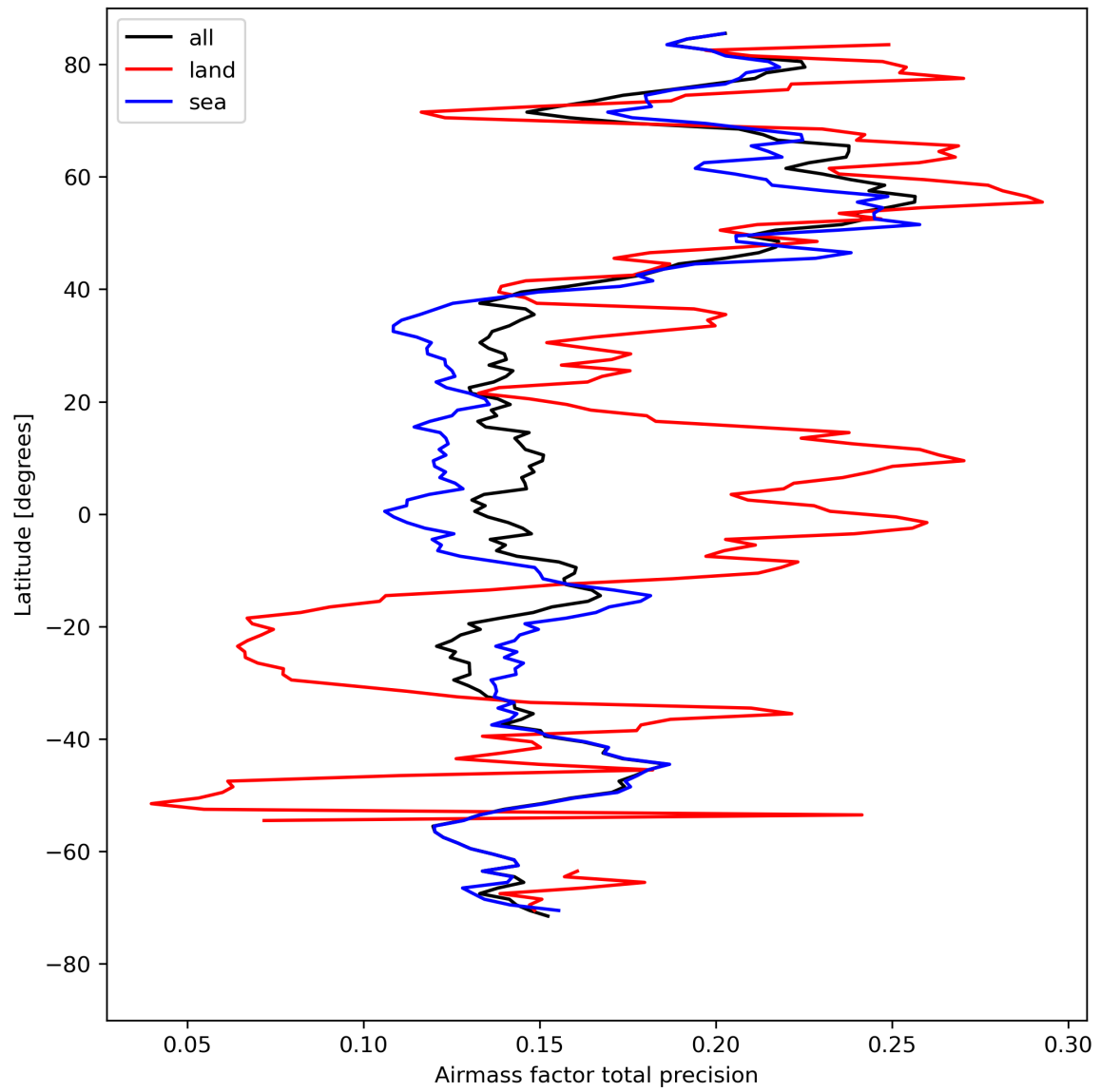
Figure 27: Zonal average of “Airmass factor total precision” for 2024-08-16 to 2024-08-17.
