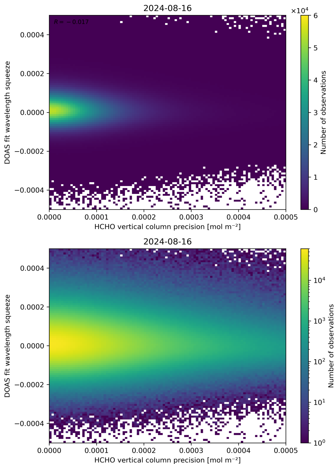
Figure 138: Scatter density plot of “HCHO vertical column precision” against “DOAS fit wavelength squeeze” for 2024-08-16 to 2024-08-17.
