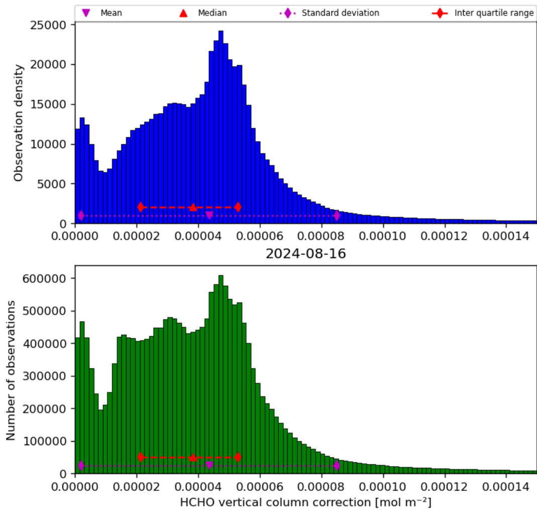
Figure 37: Histogram of “HCHO vertical column correction” for 2024-08-16 to 2024-08-17
