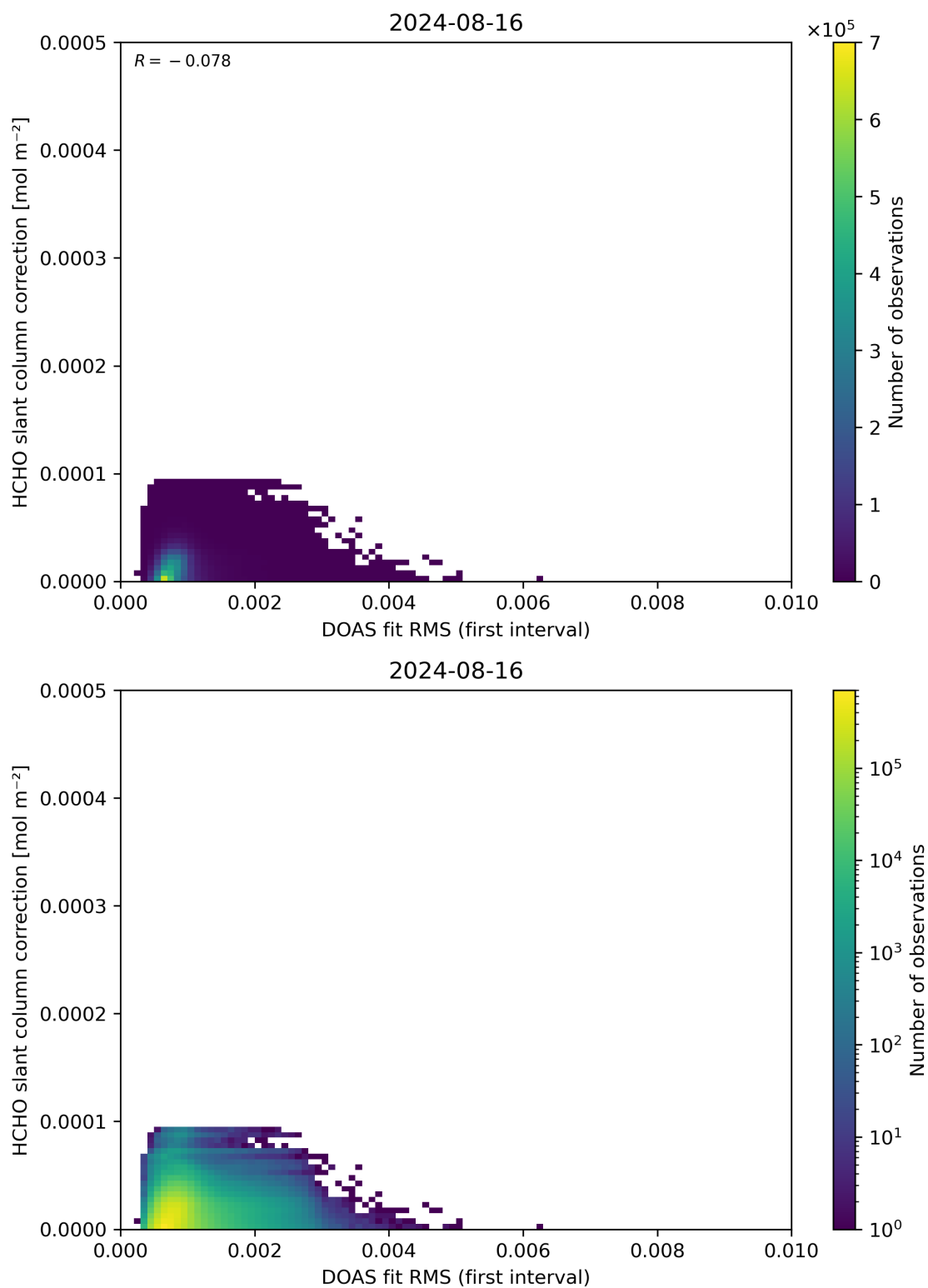
Figure 63: Scatter density plot of “DOAS fit RMS (first interval)” against “HCHO slant column correction” for 2024-08-16 to 2024-08-17.
