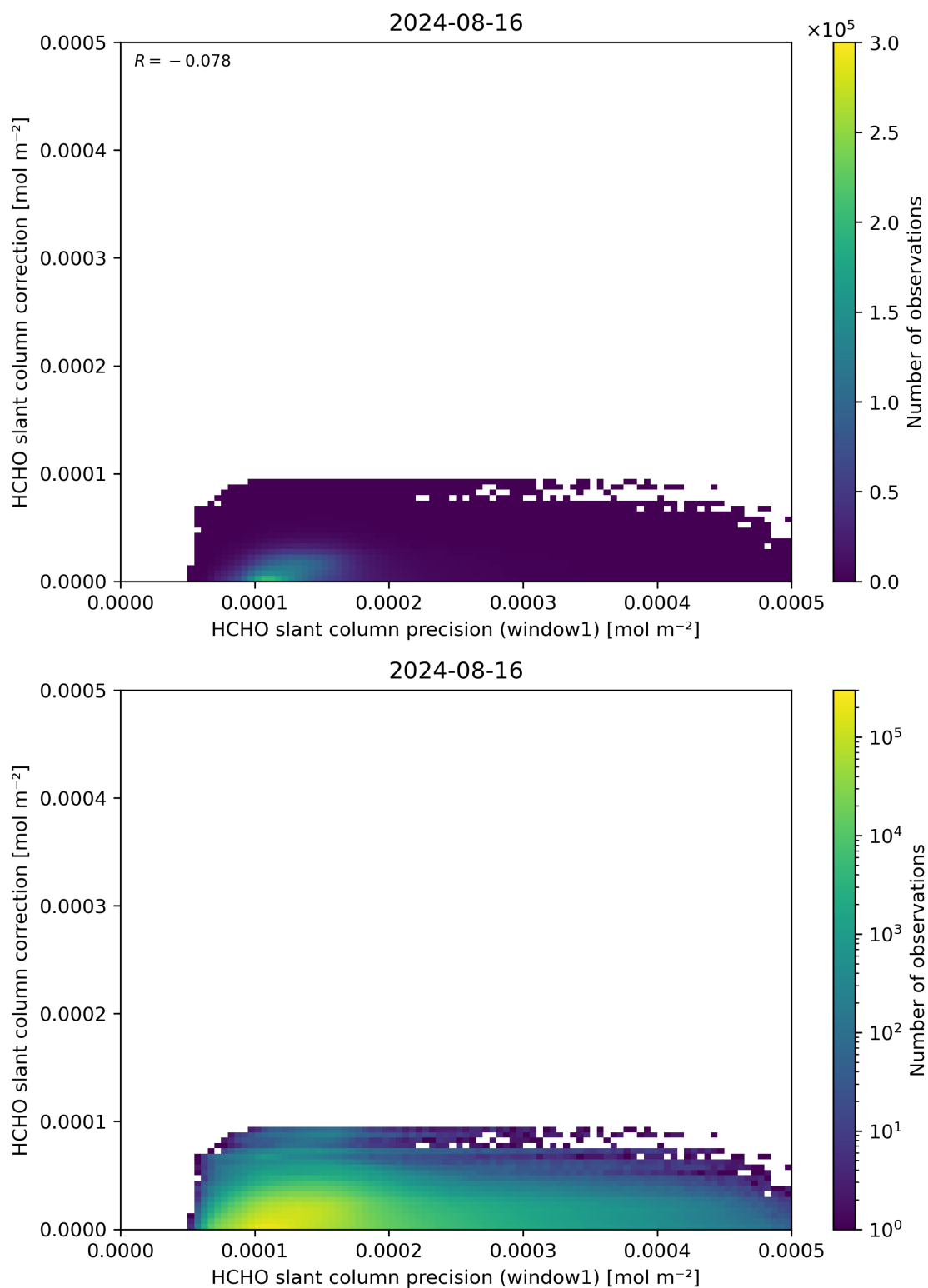
Figure 93: Scatter density plot of “HCHO slant column precision (window1)” against “HCHO slant column correction” for 2024-08-16 to 2024-08-17.
