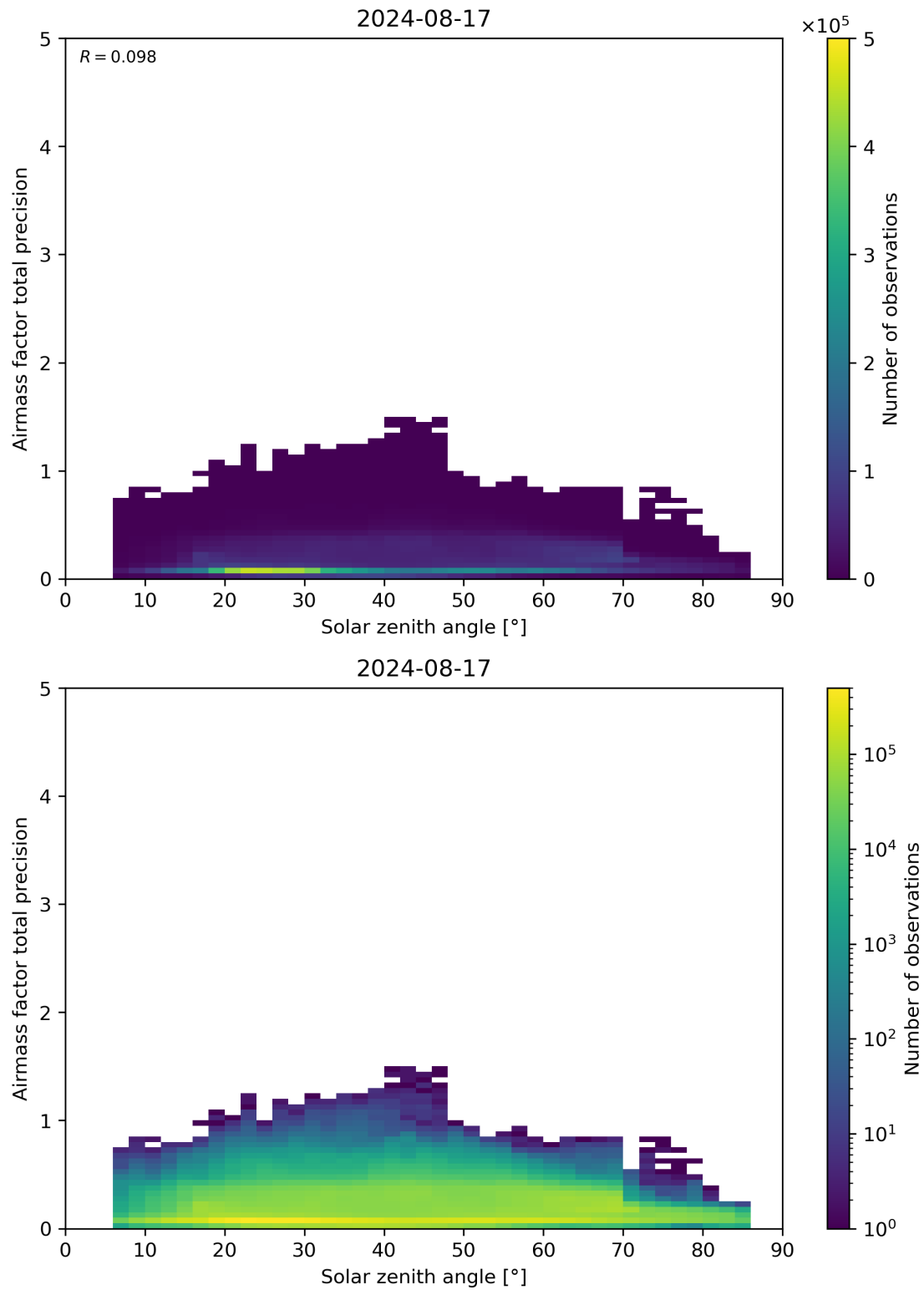
Figure 176: Scatter density plot of “Solar zenith angle” against “Airmass factor total precision” for 2024-08-16 to 2024-08-18.
