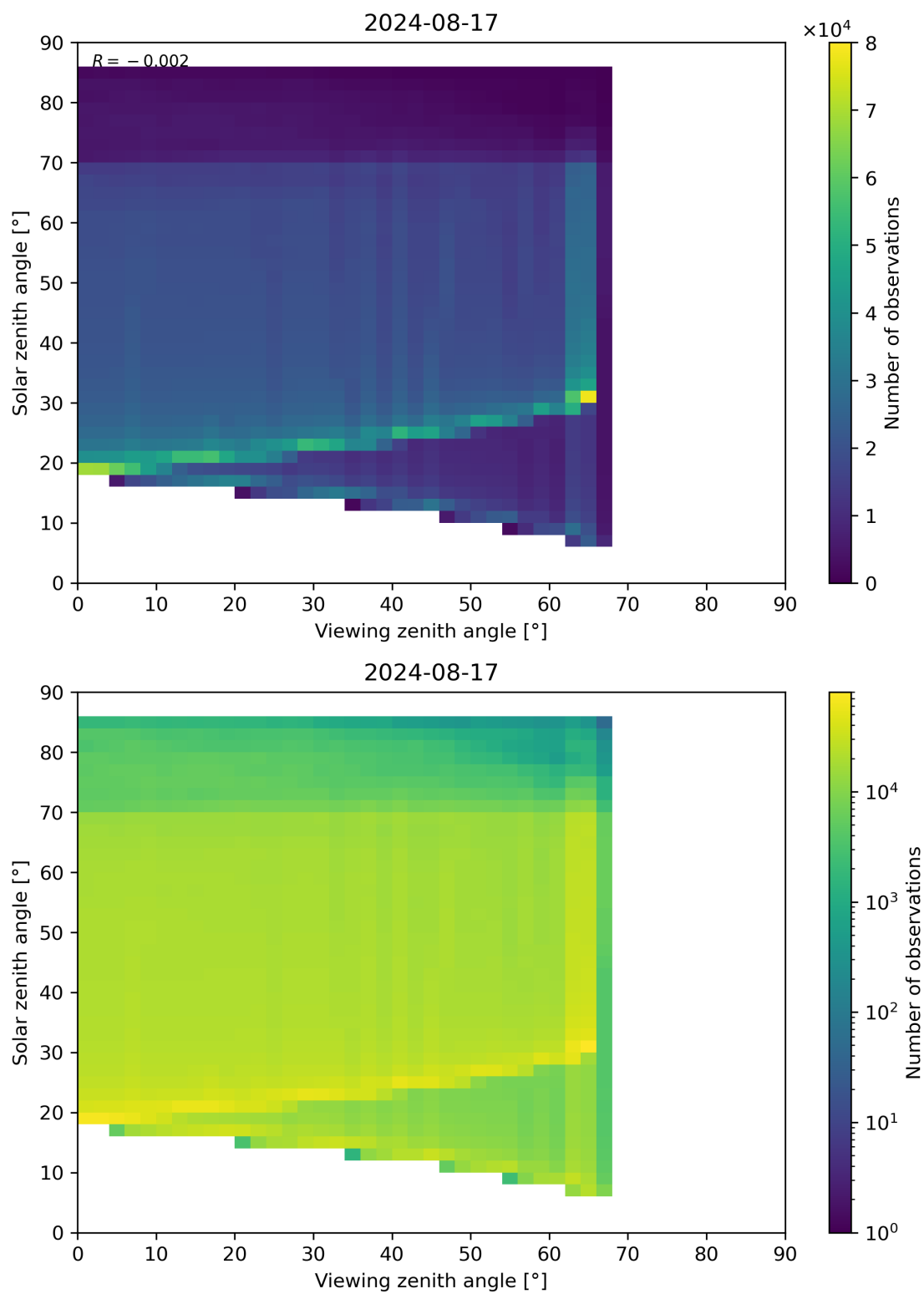
Figure 197: Scatter density plot of “Viewing zenith angle” against “Solar zenith angle” for 2024-08-16 to 2024-08-18.
