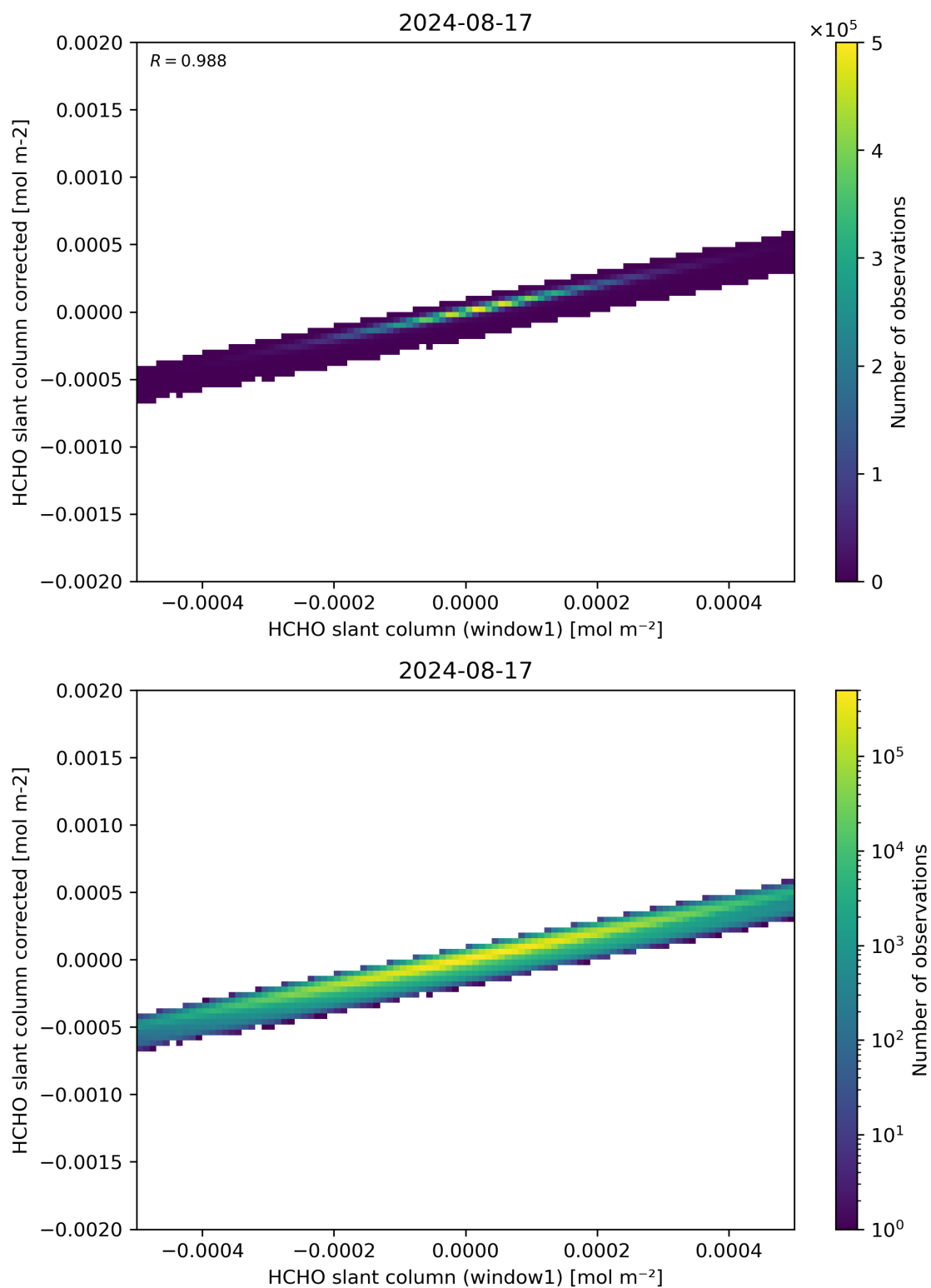
Figure 82: Scatter density plot of “HCHO slant column (window1)” against “HCHO slant column corrected” for 2024-08-16 to 2024-08-18.
