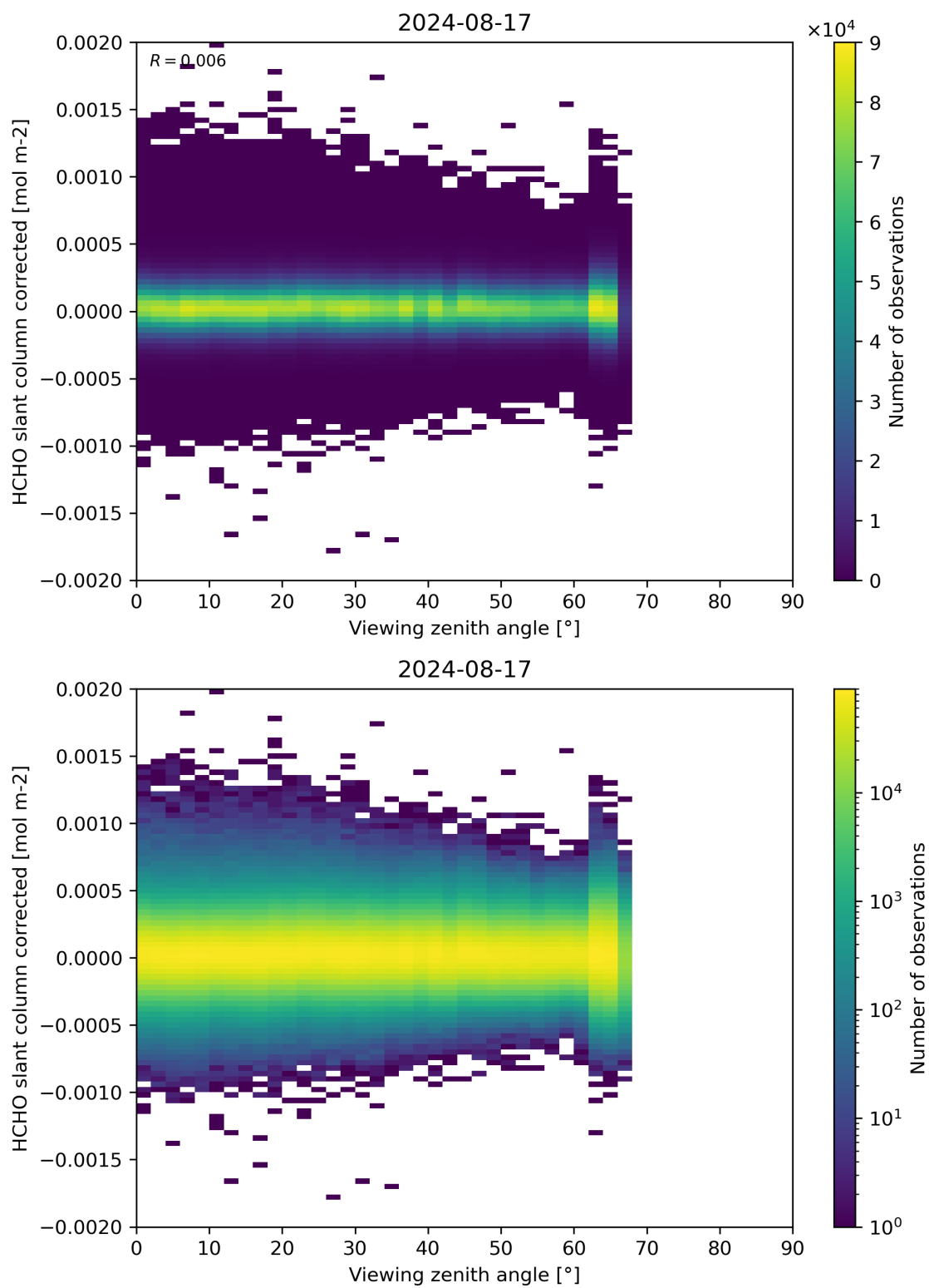
Figure 186: Scatter density plot of “Viewing zenith angle” against “HCHO slant column corrected” for 2024-08-16 to 2024-08-18.
