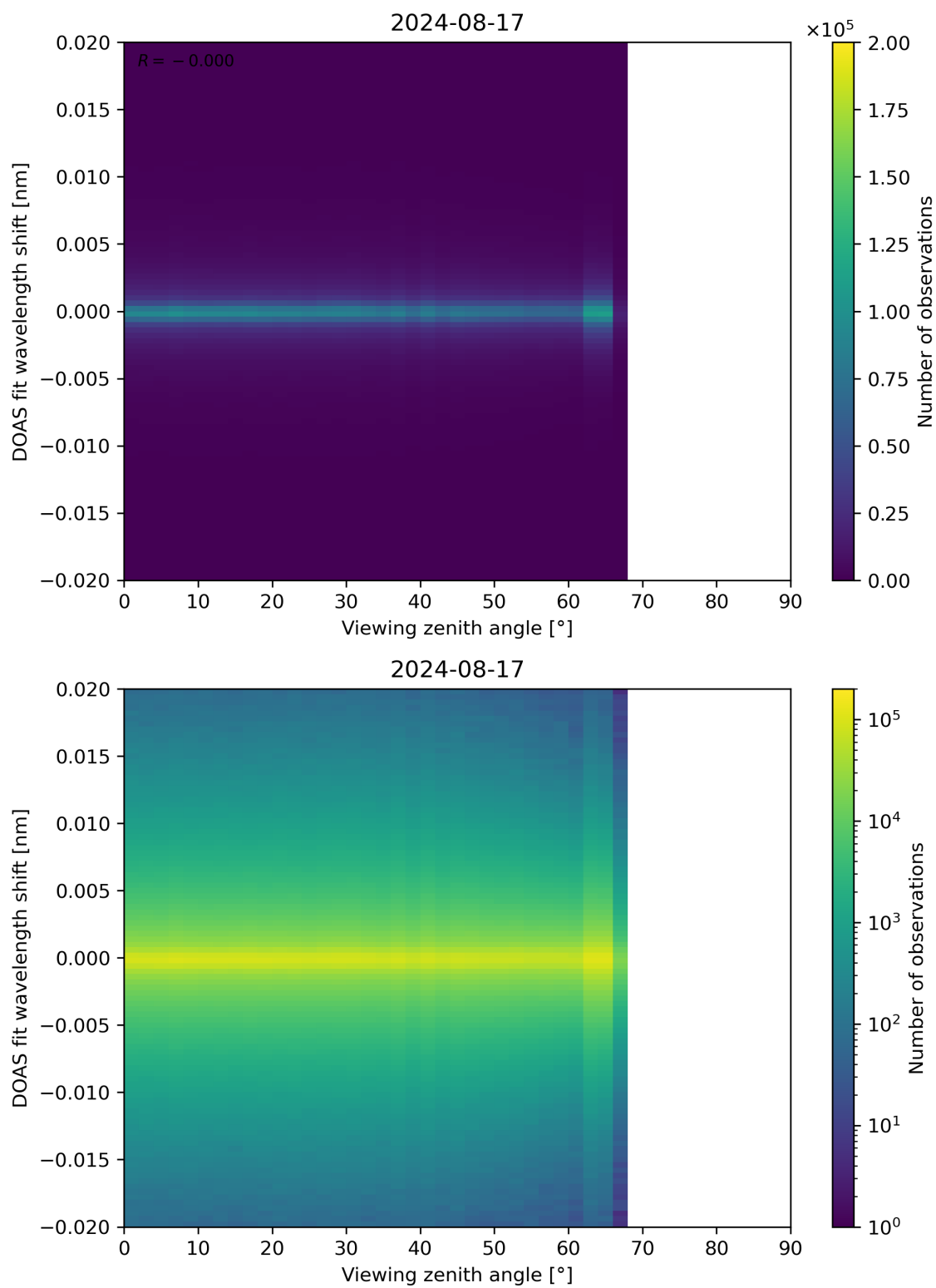
Figure 183: Scatter density plot of “Viewing zenith angle” against “DOAS fit wavelength shift” for 2024-08-16 to 2024-08-18.
