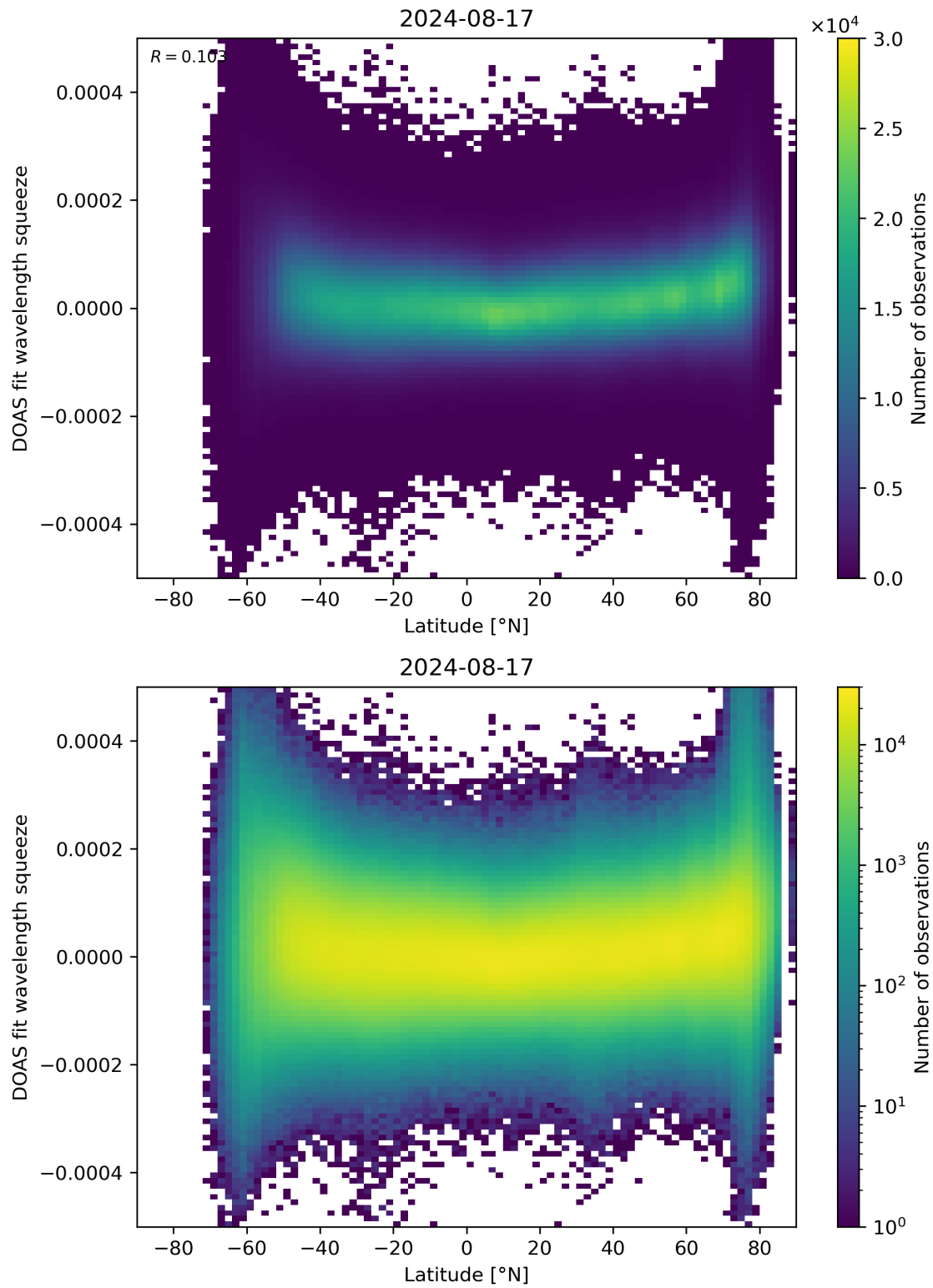
Figure 155: Scatter density plot of “Latitude” against “DOAS fit wavelength squeeze” for 2024-08-16 to 2024-08-18.
