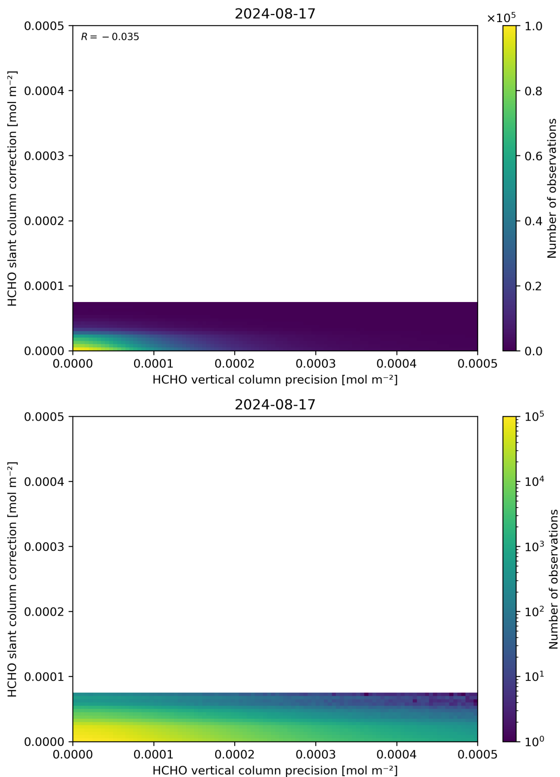
Figure 141: Scatter density plot of “HCHO vertical column precision” against “HCHO slant column correction” for 2024-08-16 to 2024-08-18.
