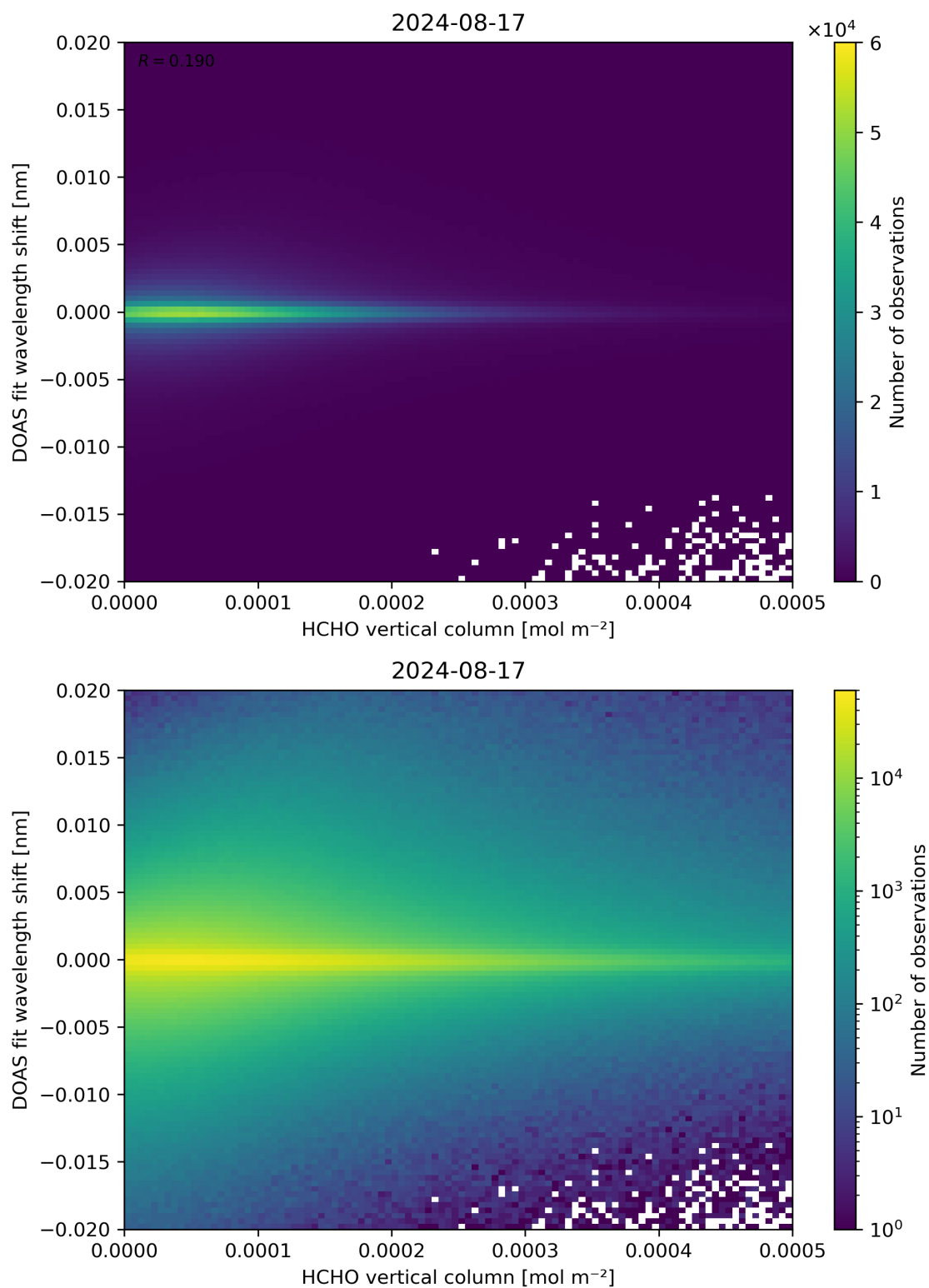
Figure 124: Scatter density plot of “HCHO vertical column” against “DOAS fit wavelength shift” for 2024-08-16 to 2024-08-18.
