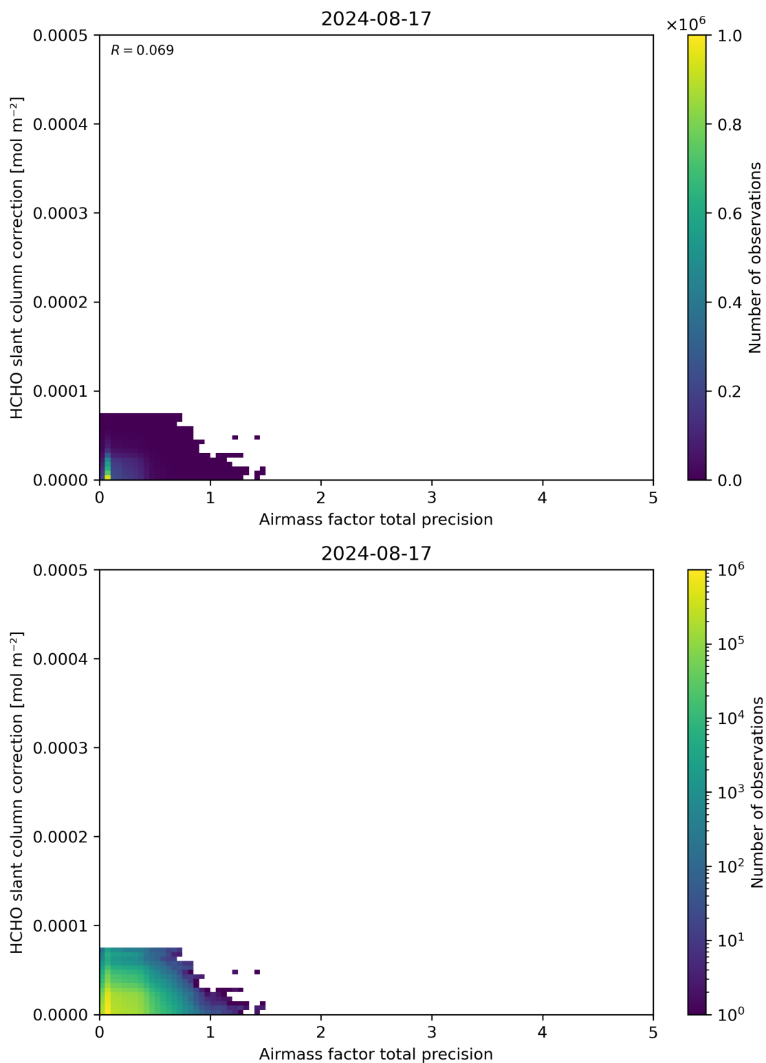
Figure 110: Scatter density plot of “Airmass factor total precision” against “HCHO slant column correction” for 2024-08-16 to 2024-08-18.
