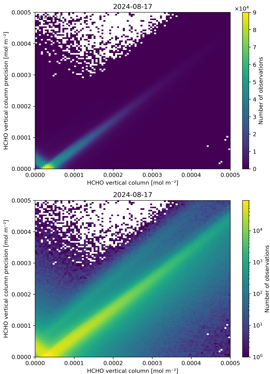
Figure 134: Scatter density plot of “HCHO vertical column” against “HCHO vertical column precision” for 2024-08-16 to 2024-08-18.
