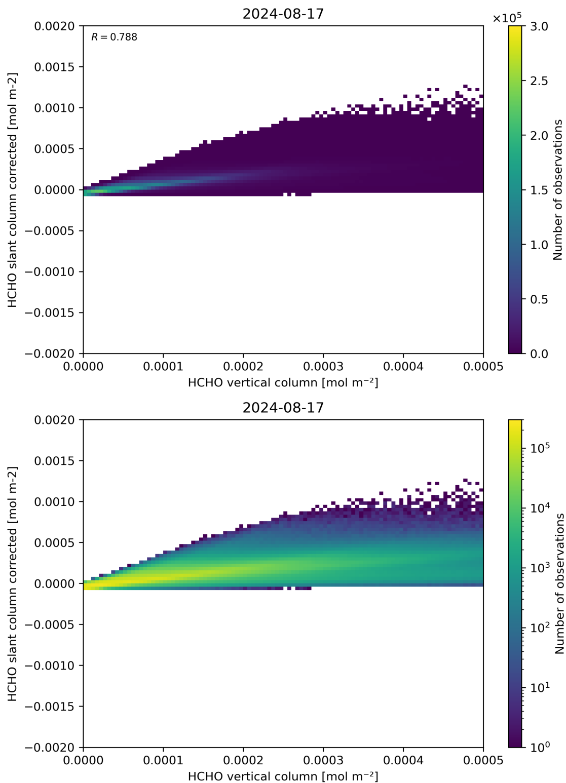
Figure 127: Scatter density plot of “HCHO vertical column” against “HCHO slant column corrected” for 2024-08-16 to 2024-08-18.
