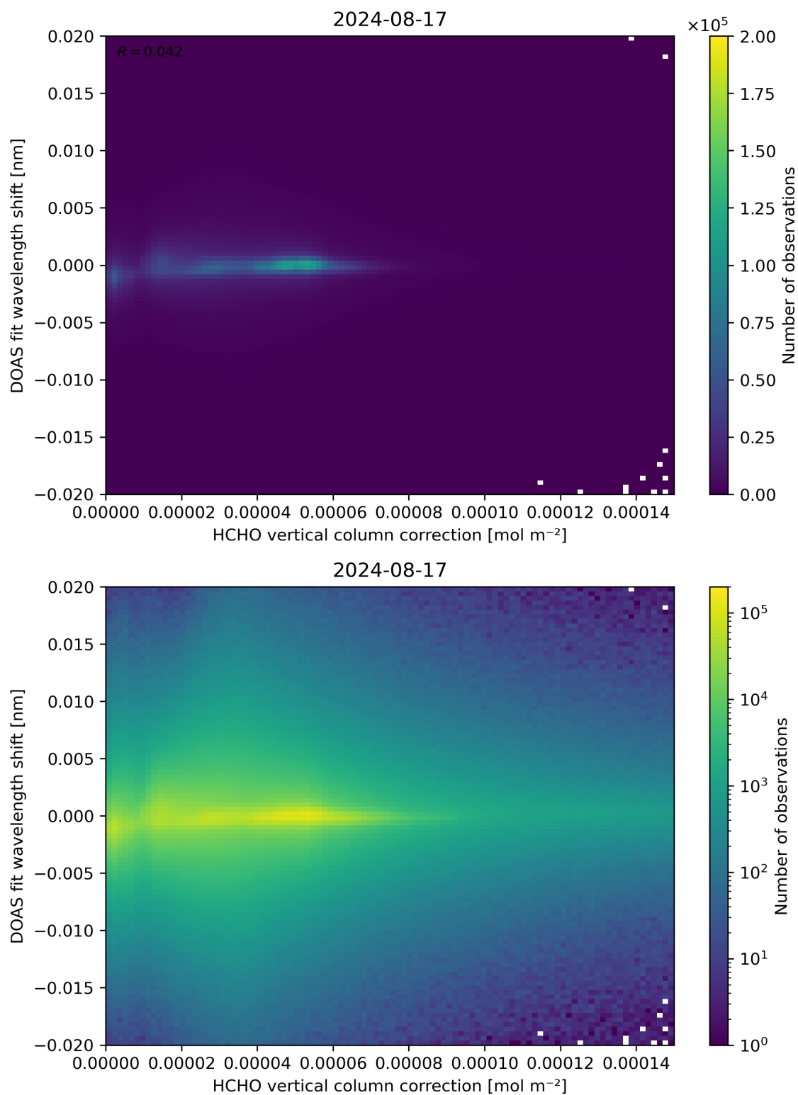
Figure 113: Scatter density plot of “HCHO vertical column correction” against “DOAS fit wavelength shift” for 2024-08-16 to 2024-08-18.
