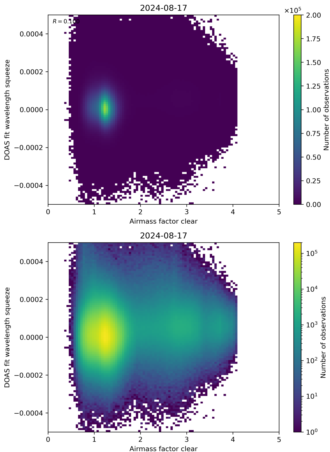
Figure 73: Scatter density plot of “Airmass factor clear” against “DOAS fit wavelength squeeze” for 2024-08-16 to 2024-08-18.
