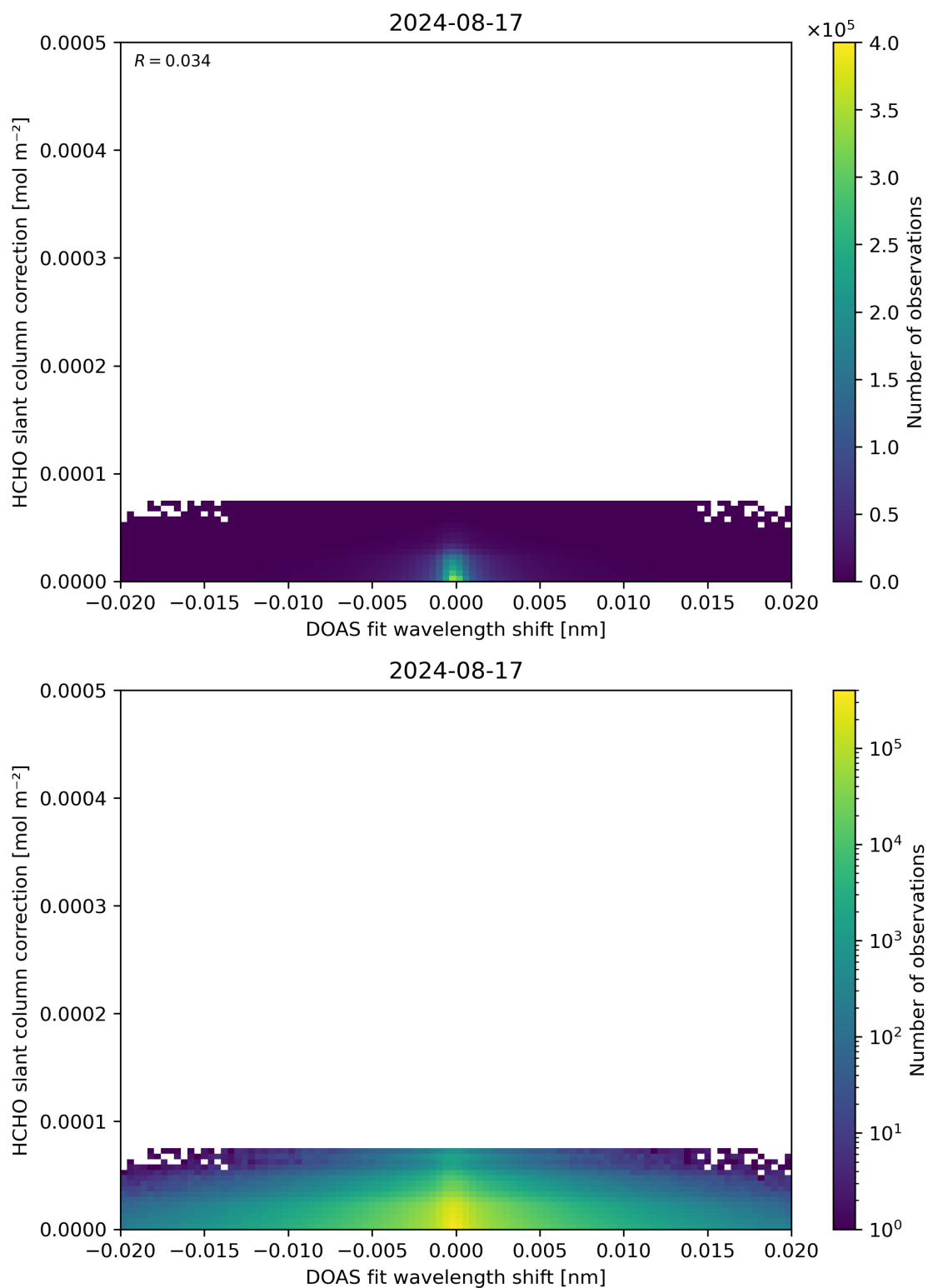
Figure 67: Scatter density plot of “DOAS fit wavelength shift” against “HCHO slant column correction” for 2024-08-16 to 2024-08-18.
