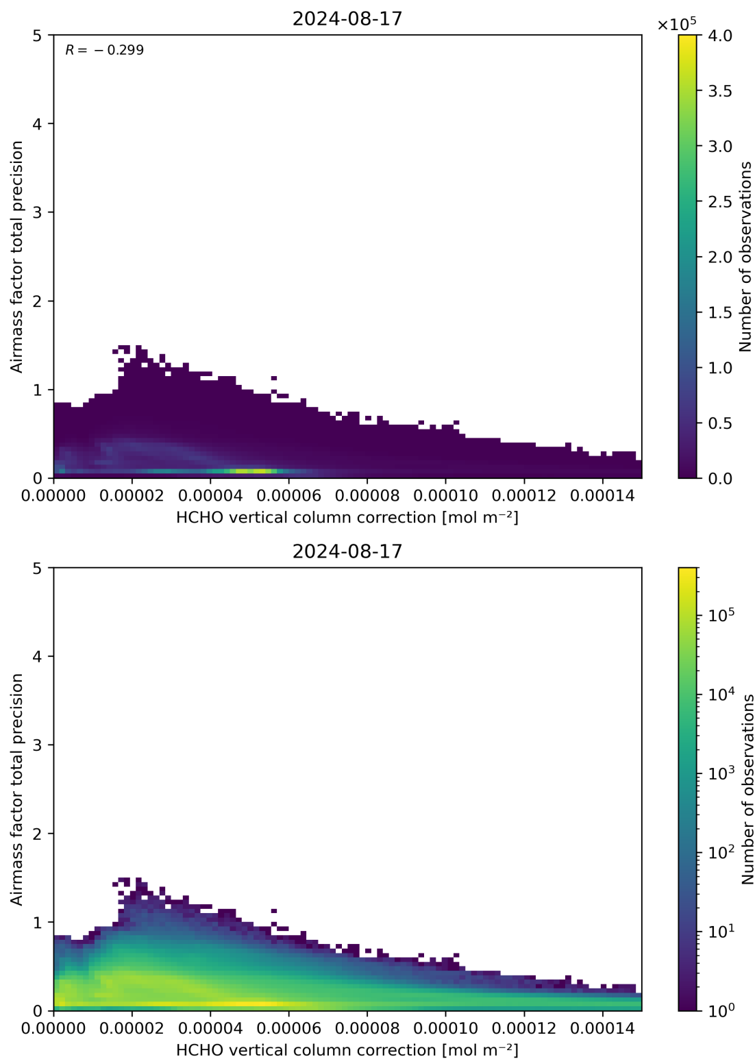
Figure 121: Scatter density plot of “HCHO vertical column correction” against “Airmass factor total precision” for 2024-08-16 to 2024-08-18.
