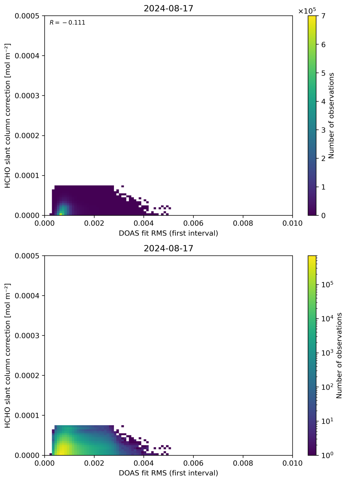
Figure 63: Scatter density plot of “DOAS fit RMS (first interval)” against “HCHO slant column correction” for 2024-08-16 to 2024-08-18.
