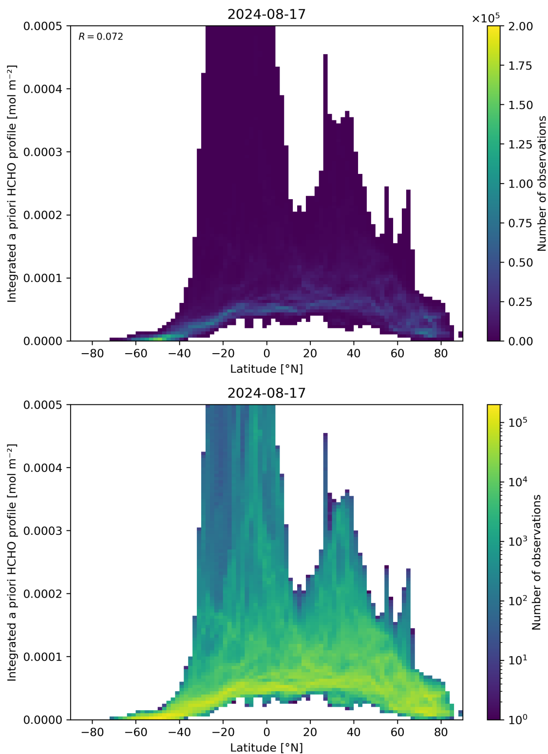
Figure 166: Scatter density plot of “Latitude” against “Integrated a priori HCHO profile” for 2024-08-16 to 2024-08-18.
