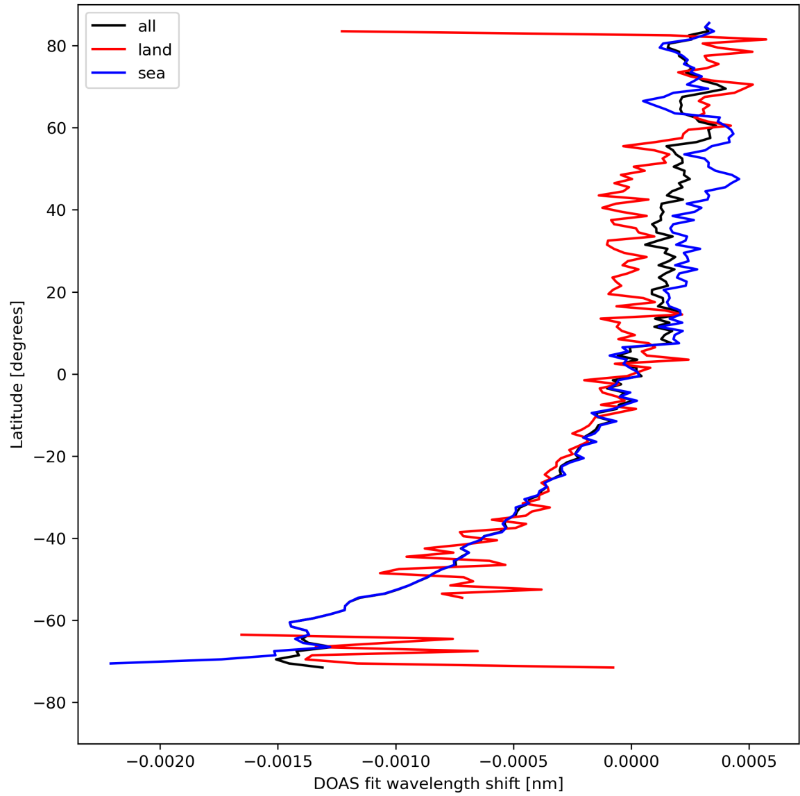
Figure 30: Zonal average of “DOAS fit wavelength shift” for 2024-08-16 to 2024-08-18.
