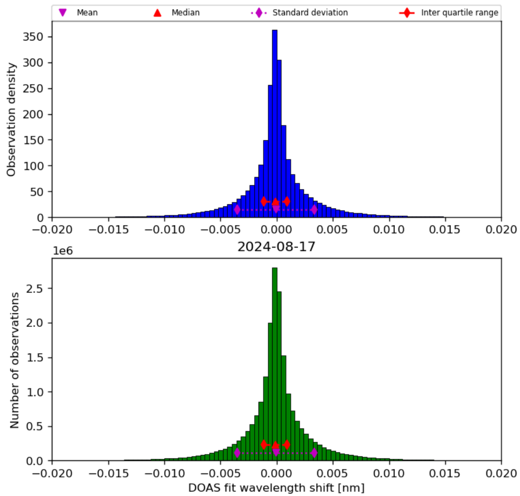
Figure 44: Histogram of “DOAS fit wavelength shift” for 2024-08-16 to 2024-08-18
