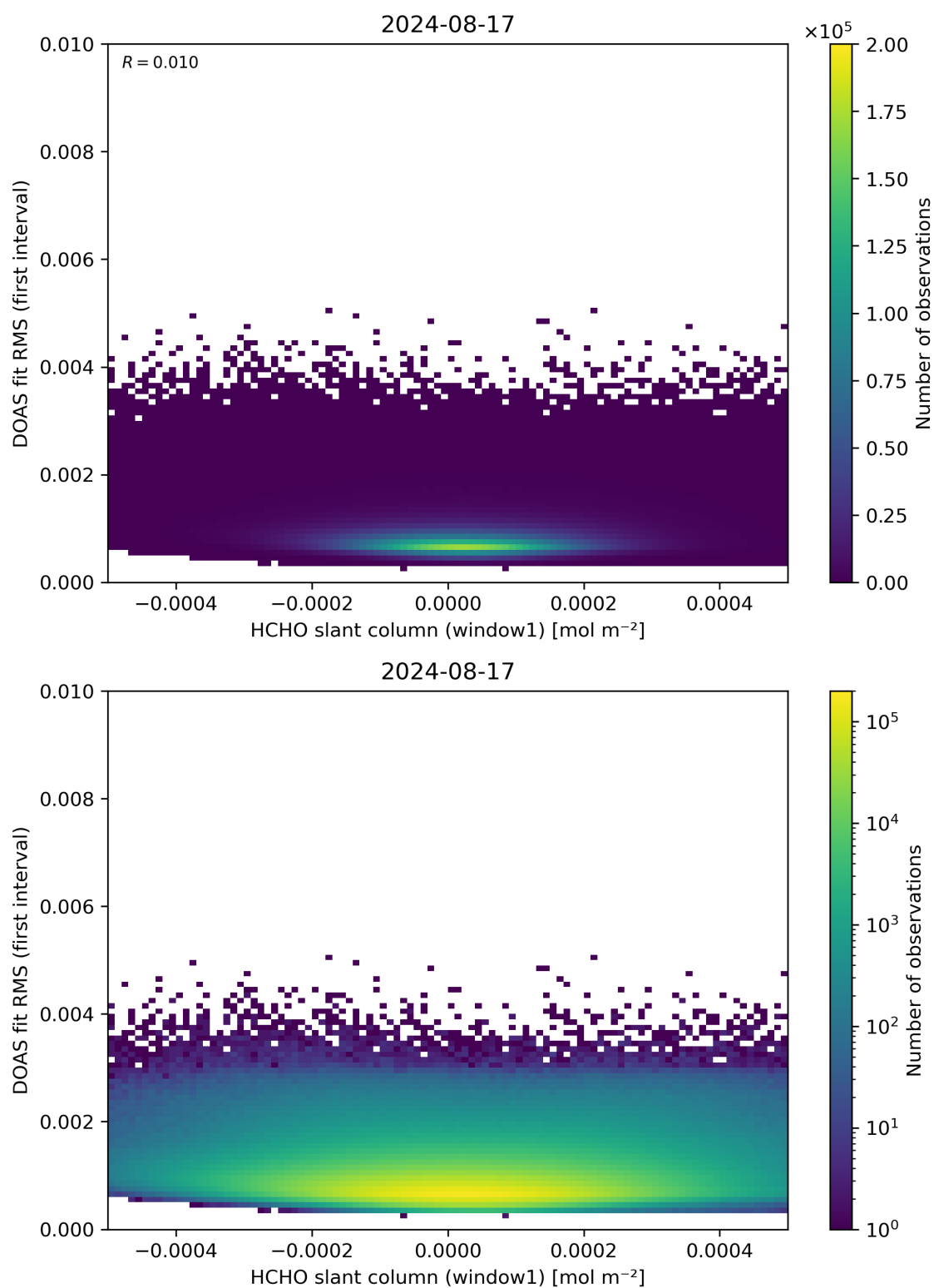
Figure 78: Scatter density plot of “HCHO slant column (window1)” against “DOAS fit RMS (first interval)” for 2024-08-16 to 2024-08-18.
