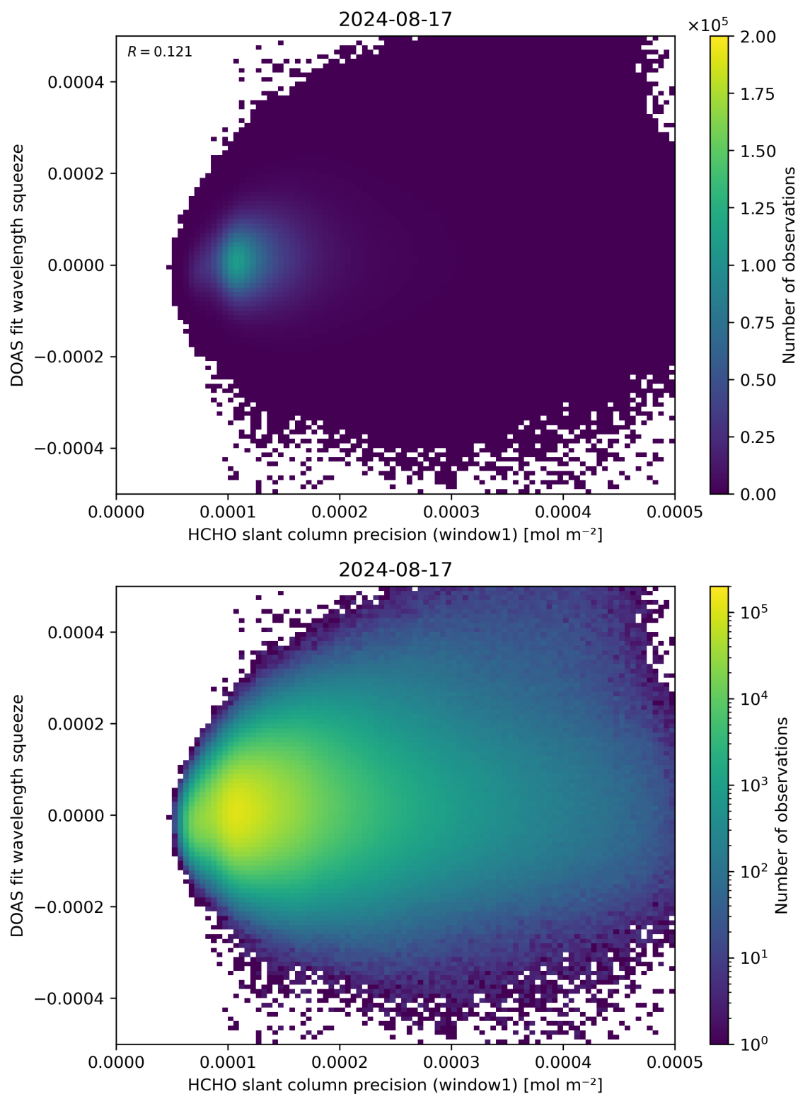
Figure 90: Scatter density plot of “HCHO slant column precision (window1)” against “DOAS fit wavelength squeeze” for 2024-08-16 to 2024-08-18.
