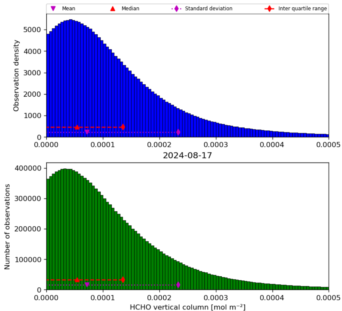
Figure 35: Histogram of “HCHO vertical column” for 2024-08-16 to 2024-08-18
