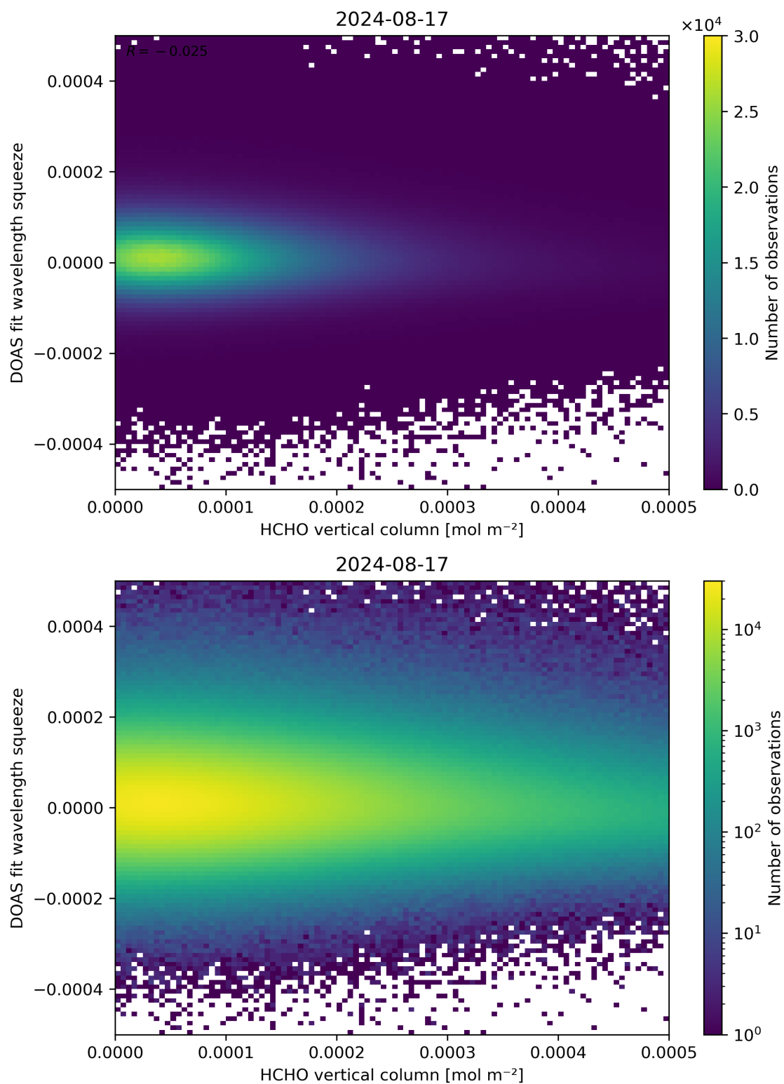
Figure 125: Scatter density plot of “HCHO vertical column” against “DOAS fit wavelength squeeze” for 2024-08-16 to 2024-08-18.
