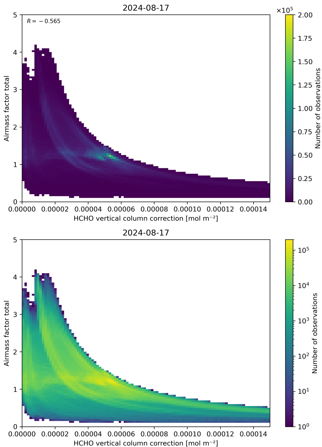
Figure 120: Scatter density plot of “HCHO vertical column correction” against “Airmass factor total” for 2024-08-16 to 2024-08-18.
