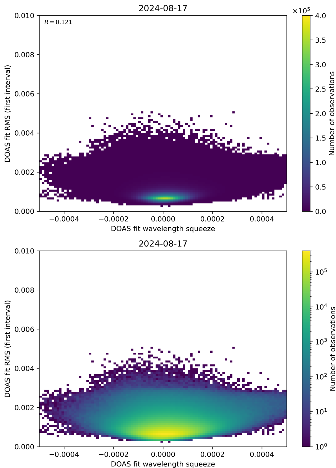
Figure 68: Scatter density plot of “DOAS fit wavelength squeeze” against “DOAS fit RMS (first interval)” for 2024-08-16 to 2024-08-18.
