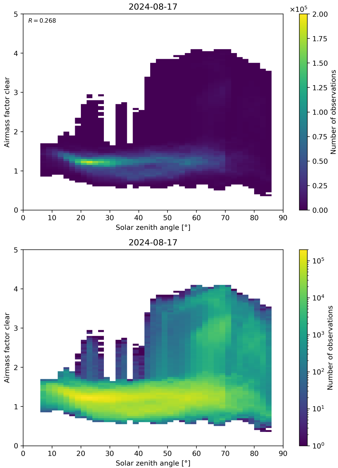
Figure 170: Scatter density plot of “Solar zenith angle” against “Airmass factor clear” for 2024-08-16 to 2024-08-18.
