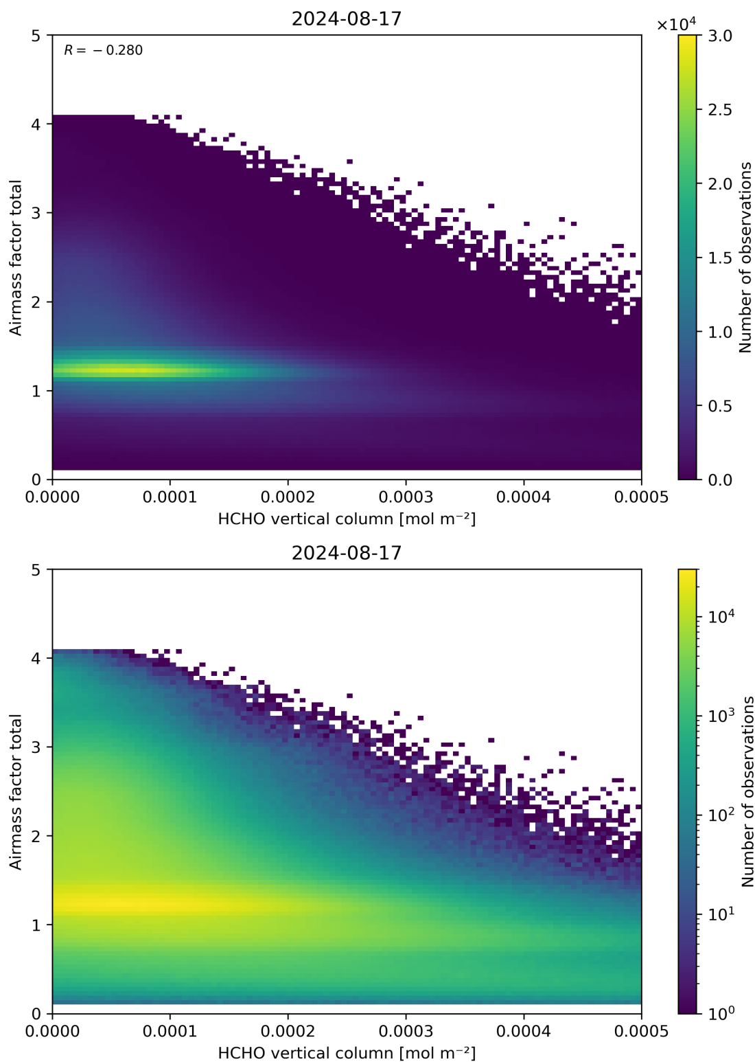
Figure 131: Scatter density plot of “HCHO vertical column” against “Airmass factor total” for 2024-08-16 to 2024-08-18.
