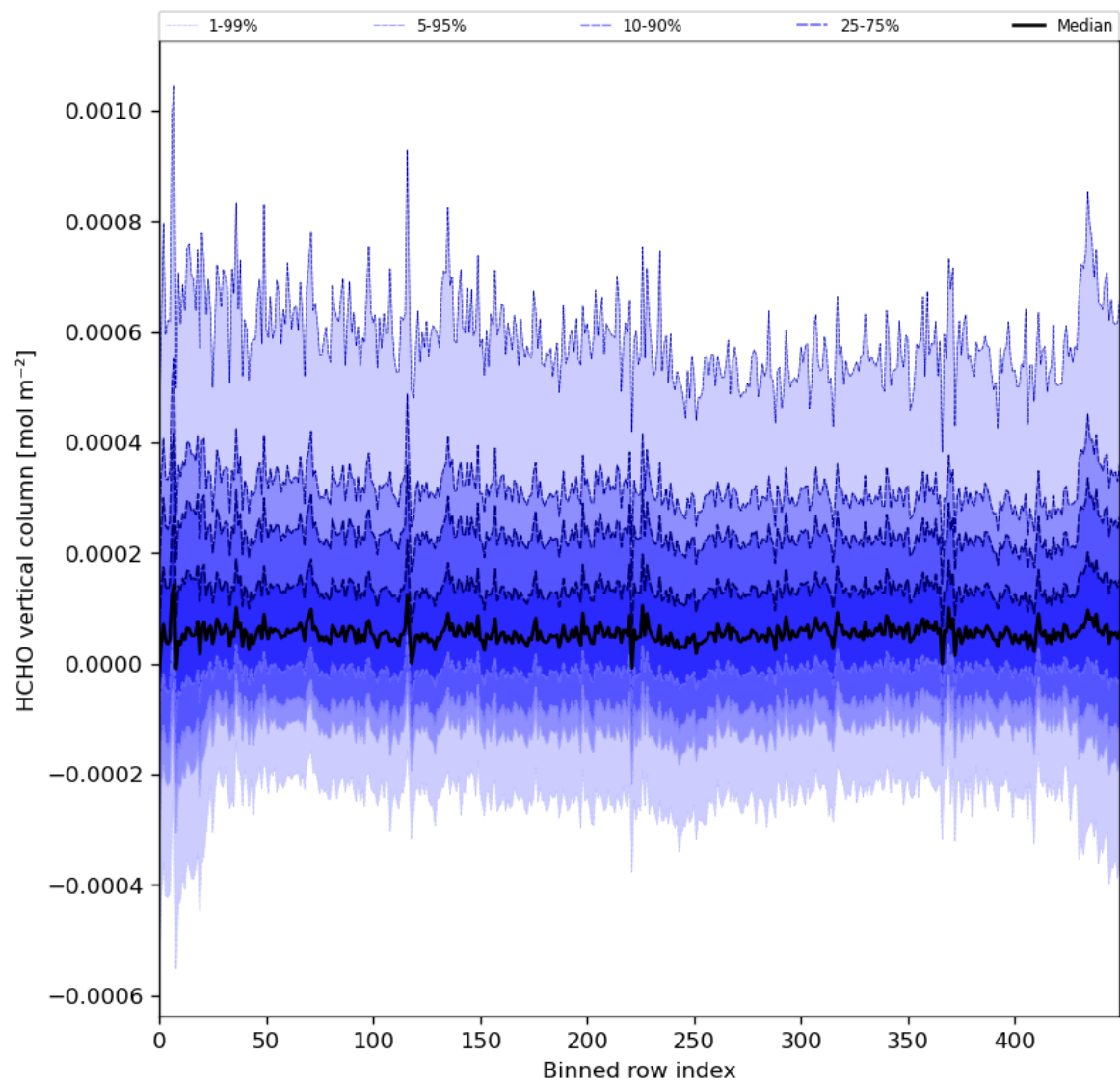
Figure 49: Along track statistics of “HCHO vertical column” for 2024-08-16 to 2024-08-18
