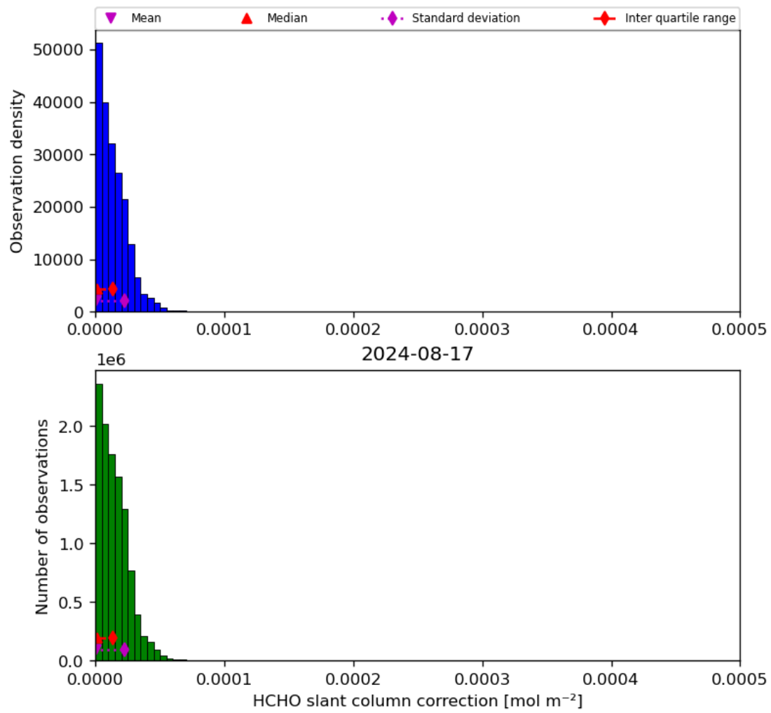
Figure 47: Histogram of “HCHO slant column correction” for 2024-08-16 to 2024-08-18
