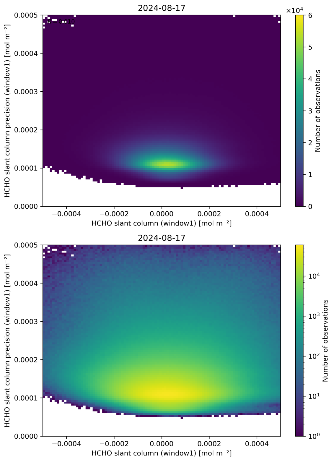
Figure 84: Scatter density plot of “HCHO slant column (window1)” against “HCHO slant column precision (window1)” for 2024-08-16 to 2024-08-18.
