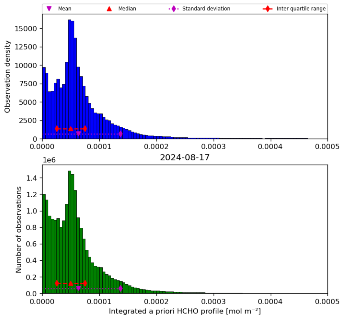
Figure 43: Histogram of “Integrated a priori HCHO profile” for 2024-08-16 to 2024-08-18
