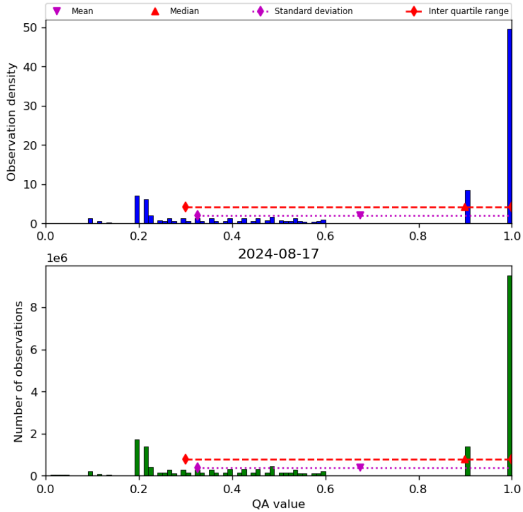
Figure 34: Histogram of “QA value” for 2024-08-16 to 2024-08-18
