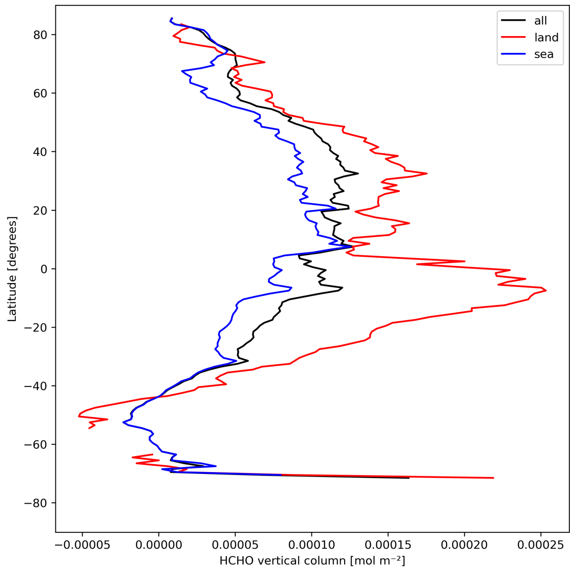
Figure 21: Zonal average of “HCHO vertical column” for 2024-08-16 to 2024-08-18.
