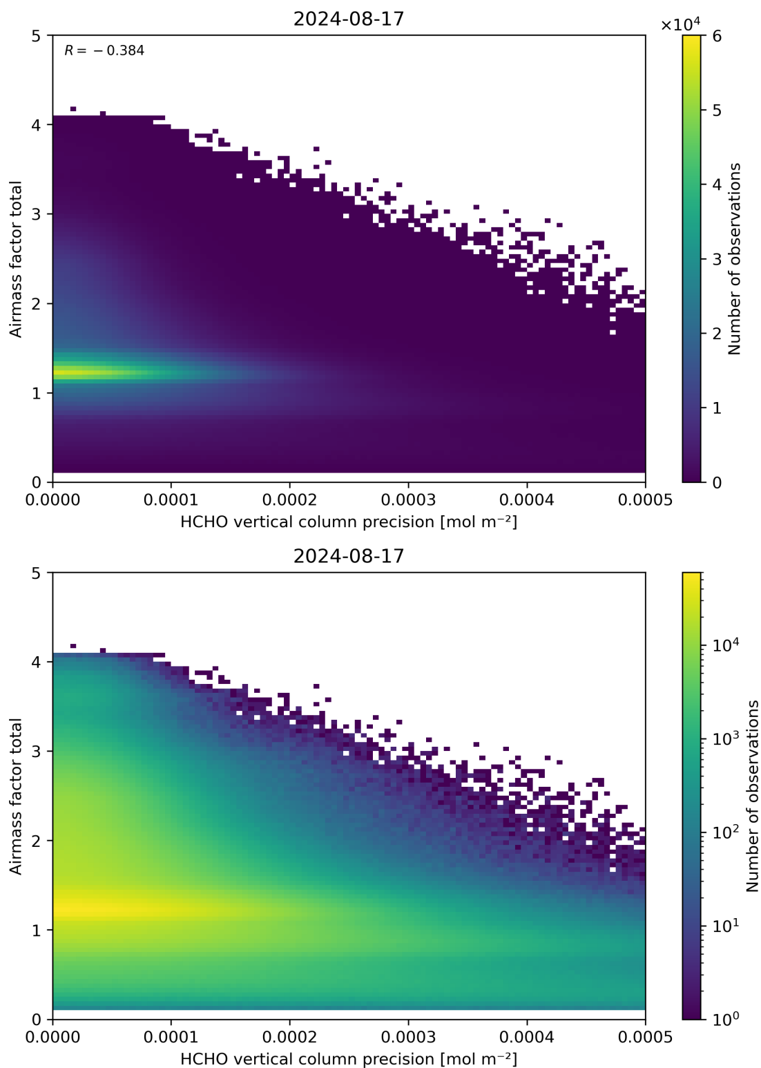
Figure 144: Scatter density plot of “HCHO vertical column precision” against “Airmass factor total” for 2024-08-16 to 2024-08-18.
