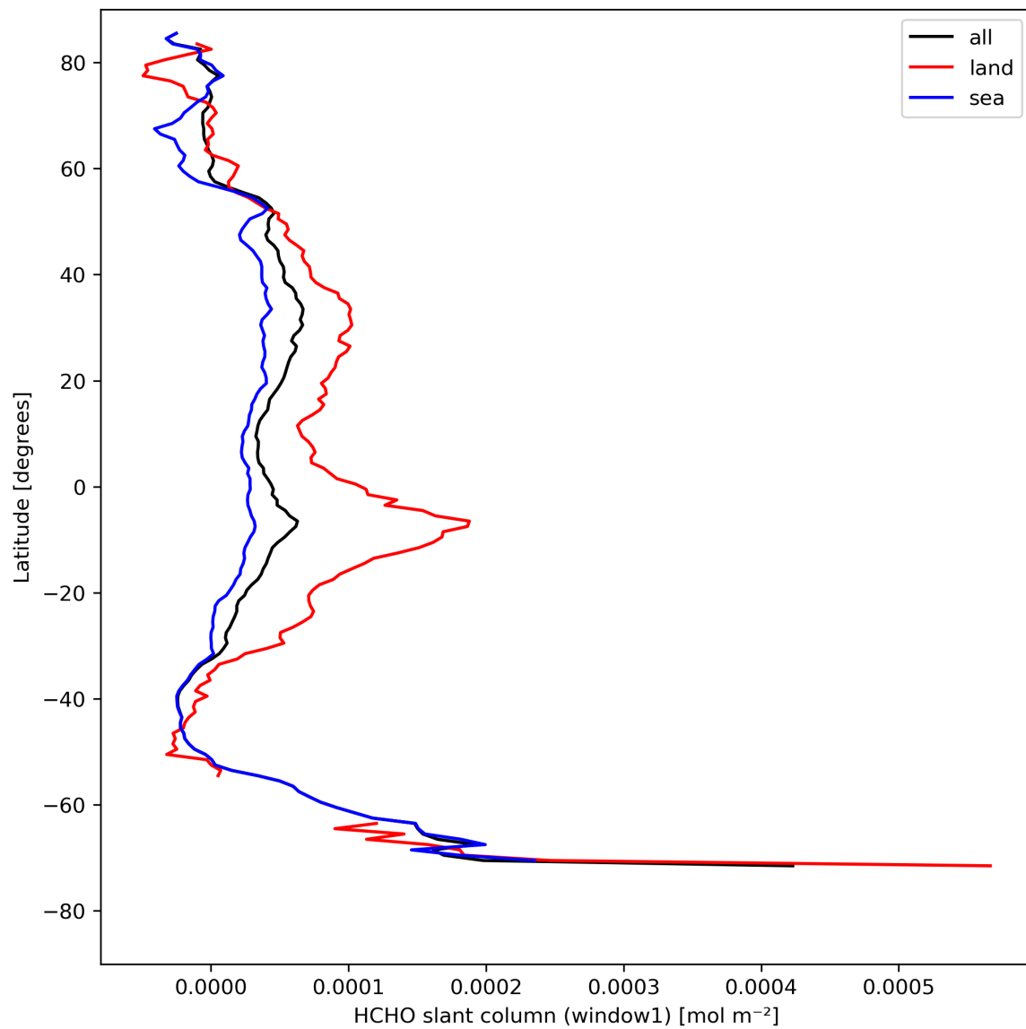
Figure 24: Zonal average of “HCHO slant column (window1)” for 2024-08-16 to 2024-08-18.
