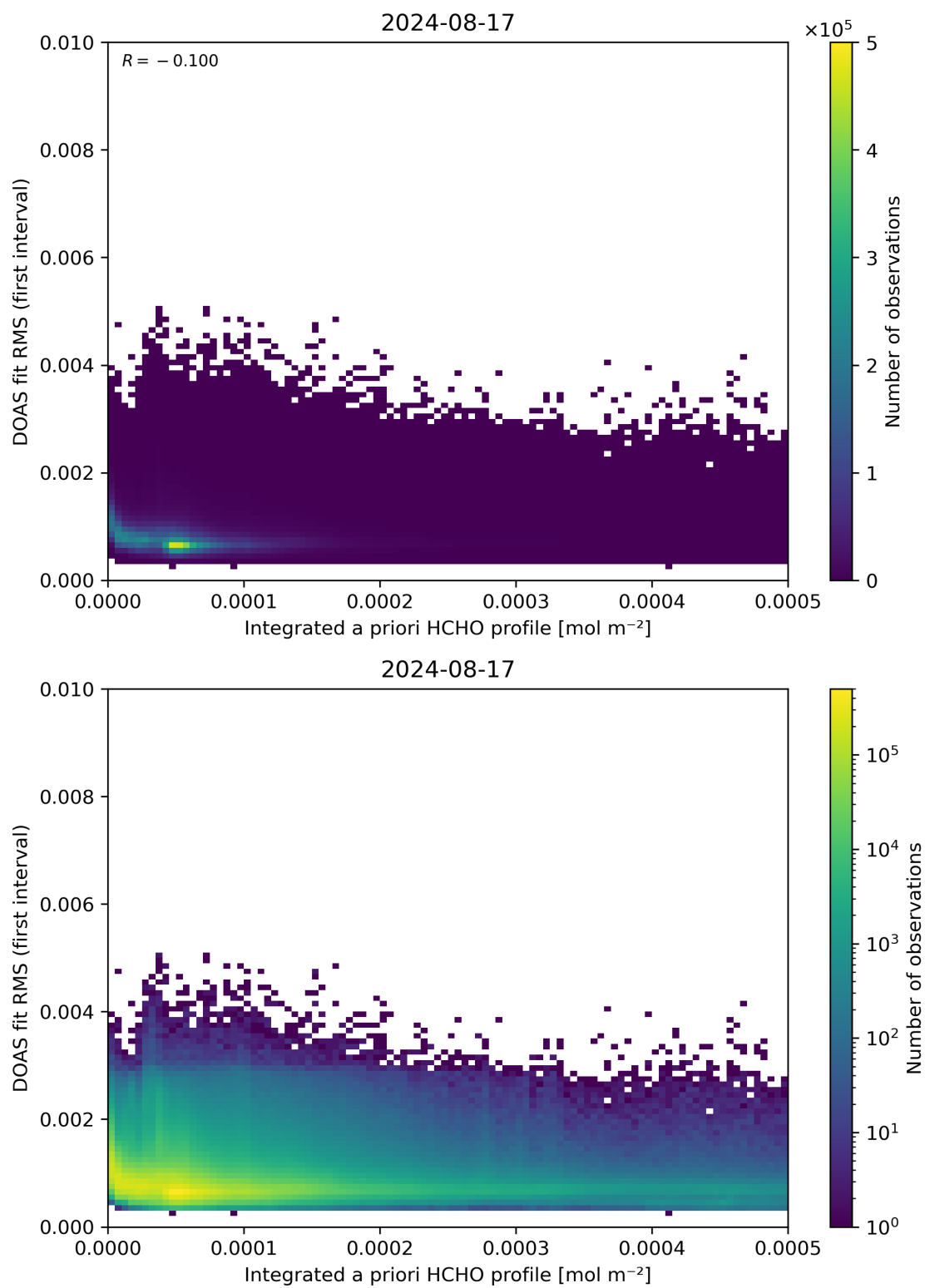
Figure 148: Scatter density plot of “Integrated a priori HCHO profile” against “DOAS fit RMS (first interval)” for 2024-08-16 to 2024-08-18.
