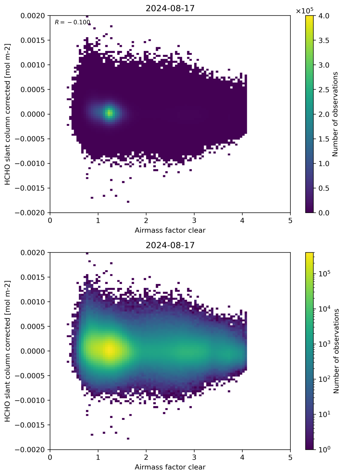
Figure 74: Scatter density plot of “Airmass factor clear” against “HCHO slant column corrected” for 2024-08-16 to 2024-08-18.
