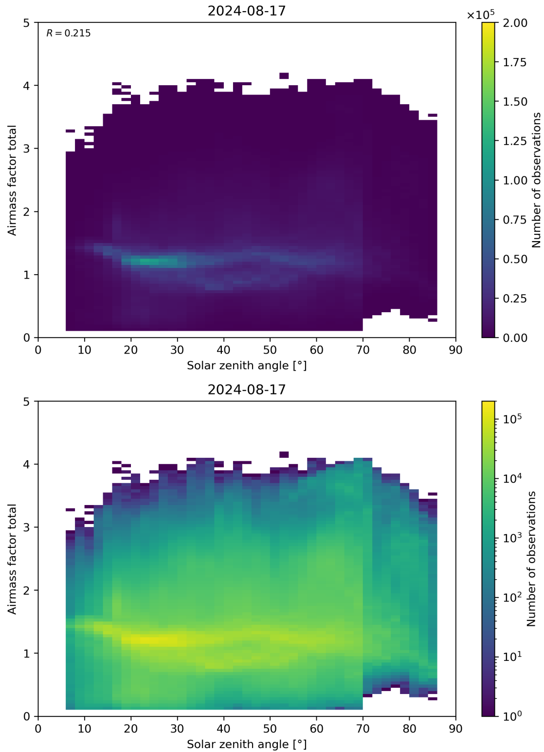
Figure 175: Scatter density plot of “Solar zenith angle” against “Airmass factor total” for 2024-08-16 to 2024-08-18.
