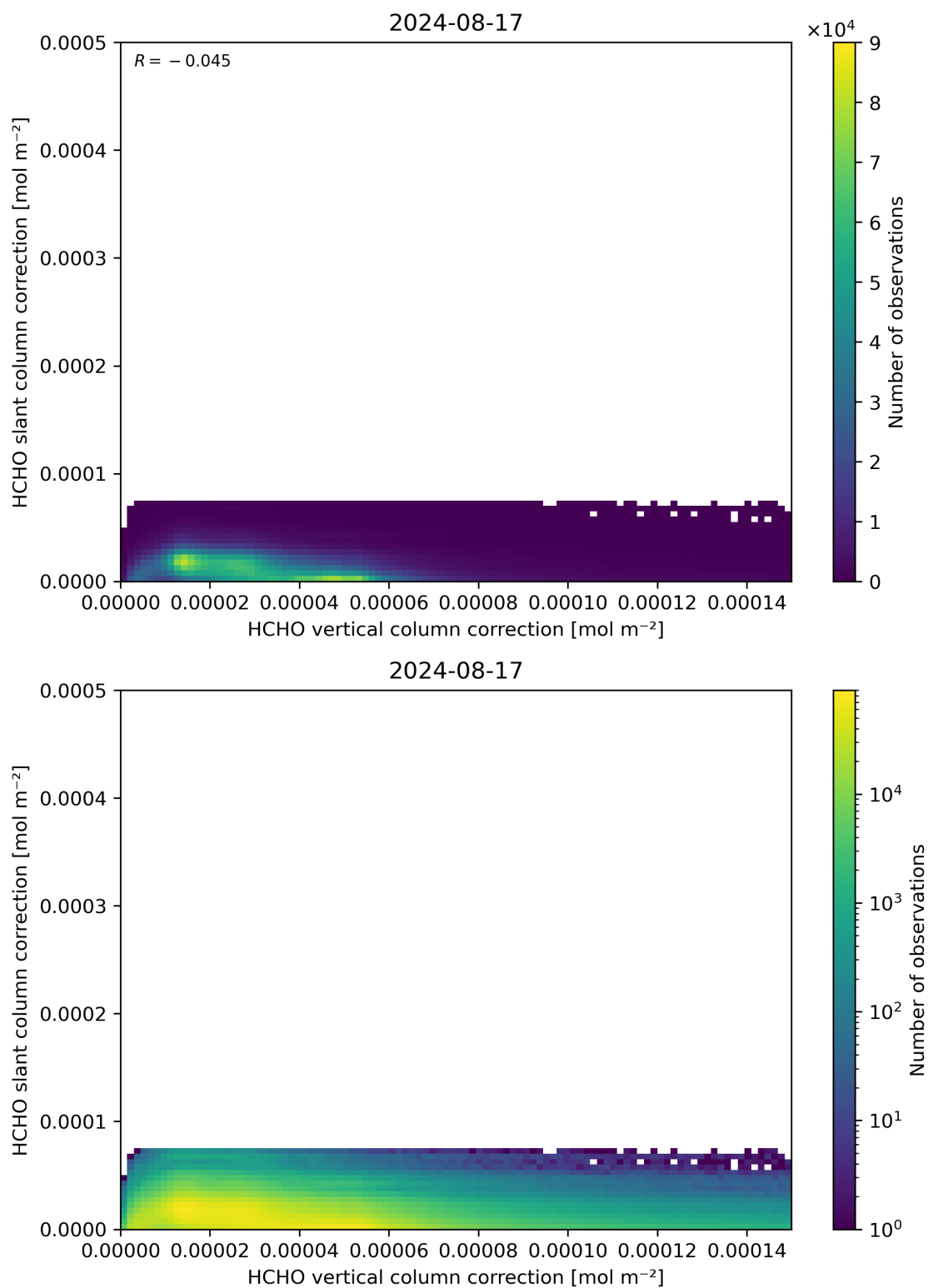
Figure 117: Scatter density plot of “HCHO vertical column correction” against “HCHO slant column correction” for 2024-08-16 to 2024-08-18.
