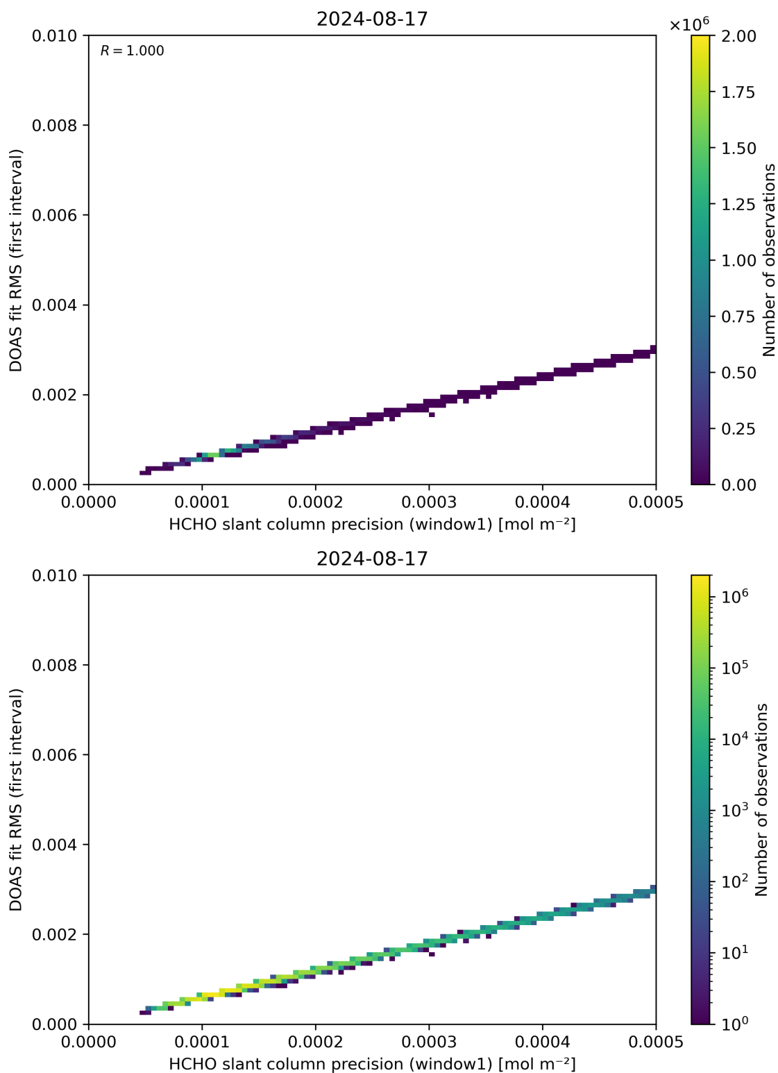
Figure 88: Scatter density plot of “HCHO slant column precision (window1)” against “DOAS fit RMS (first interval)” for 2024-08-16 to 2024-08-18.
