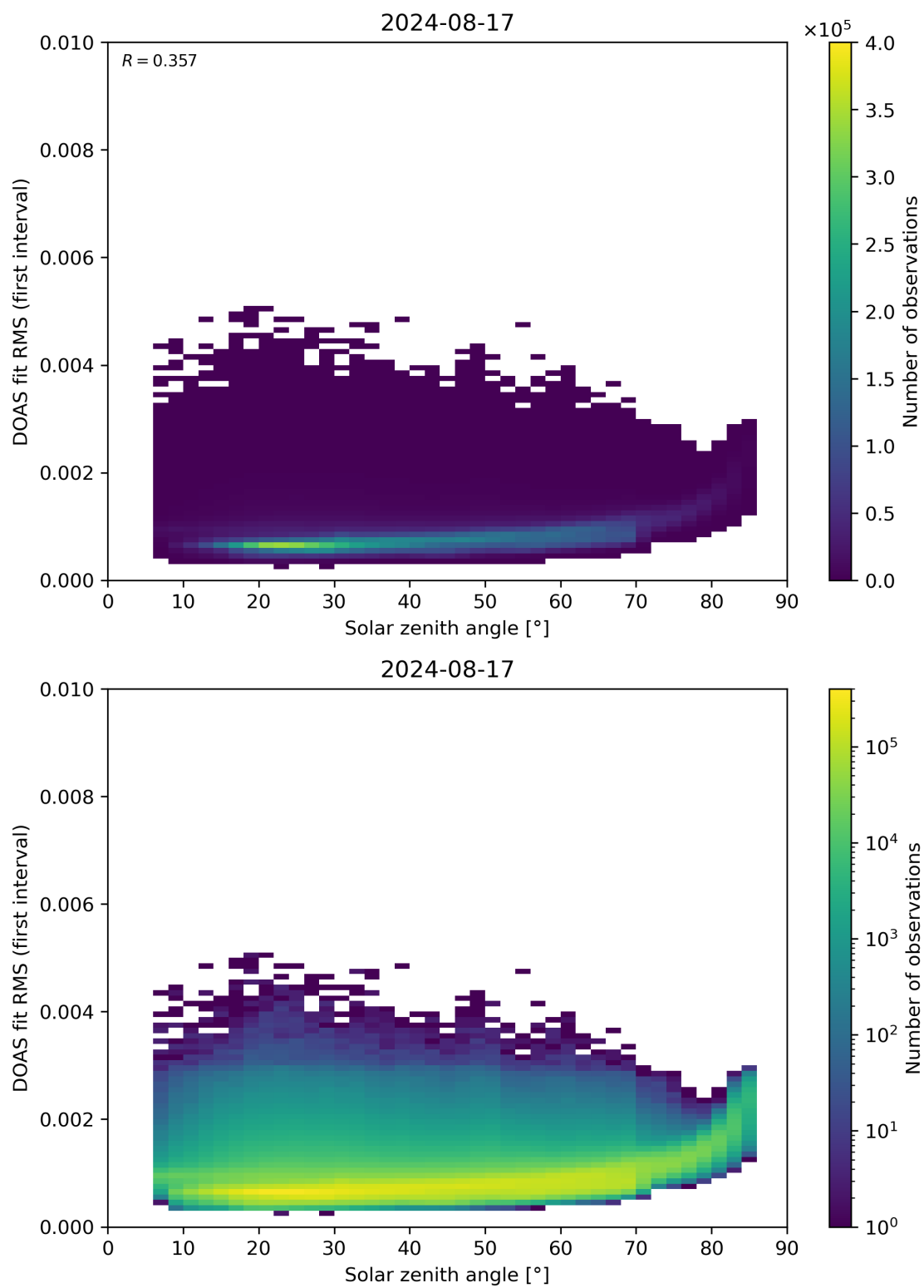
Figure 167: Scatter density plot of “Solar zenith angle” against “DOAS fit RMS (first interval)” for 2024-08-16 to 2024-08-18.
