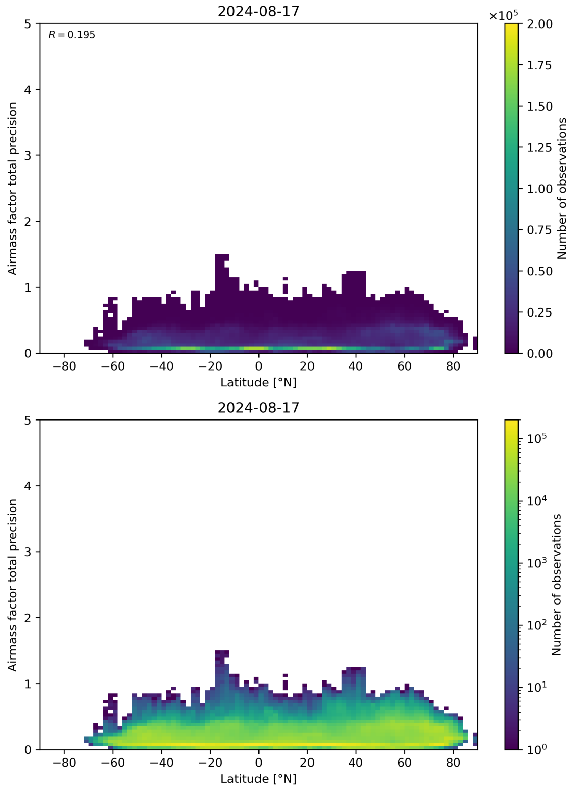
Figure 162: Scatter density plot of “Latitude” against “Airmass factor total precision” for 2024-08-16 to 2024-08-18.
