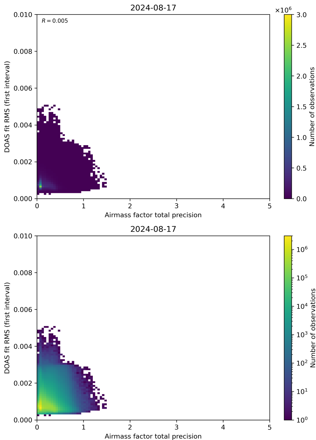
Figure 105: Scatter density plot of “Airmass factor total precision” against “DOAS fit RMS (first interval)” for 2024-08-16 to 2024-08-18.
