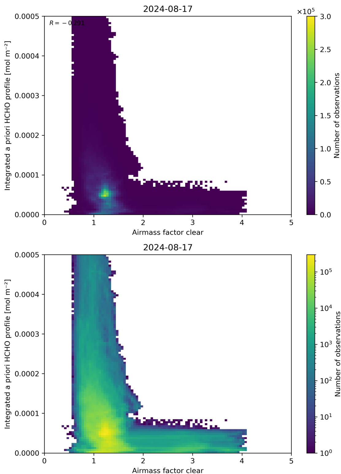
Figure 76: Scatter density plot of “Airmass factor clear” against “Integrated a priori HCHO profile” for 2024-08-16 to 2024-08-18.
