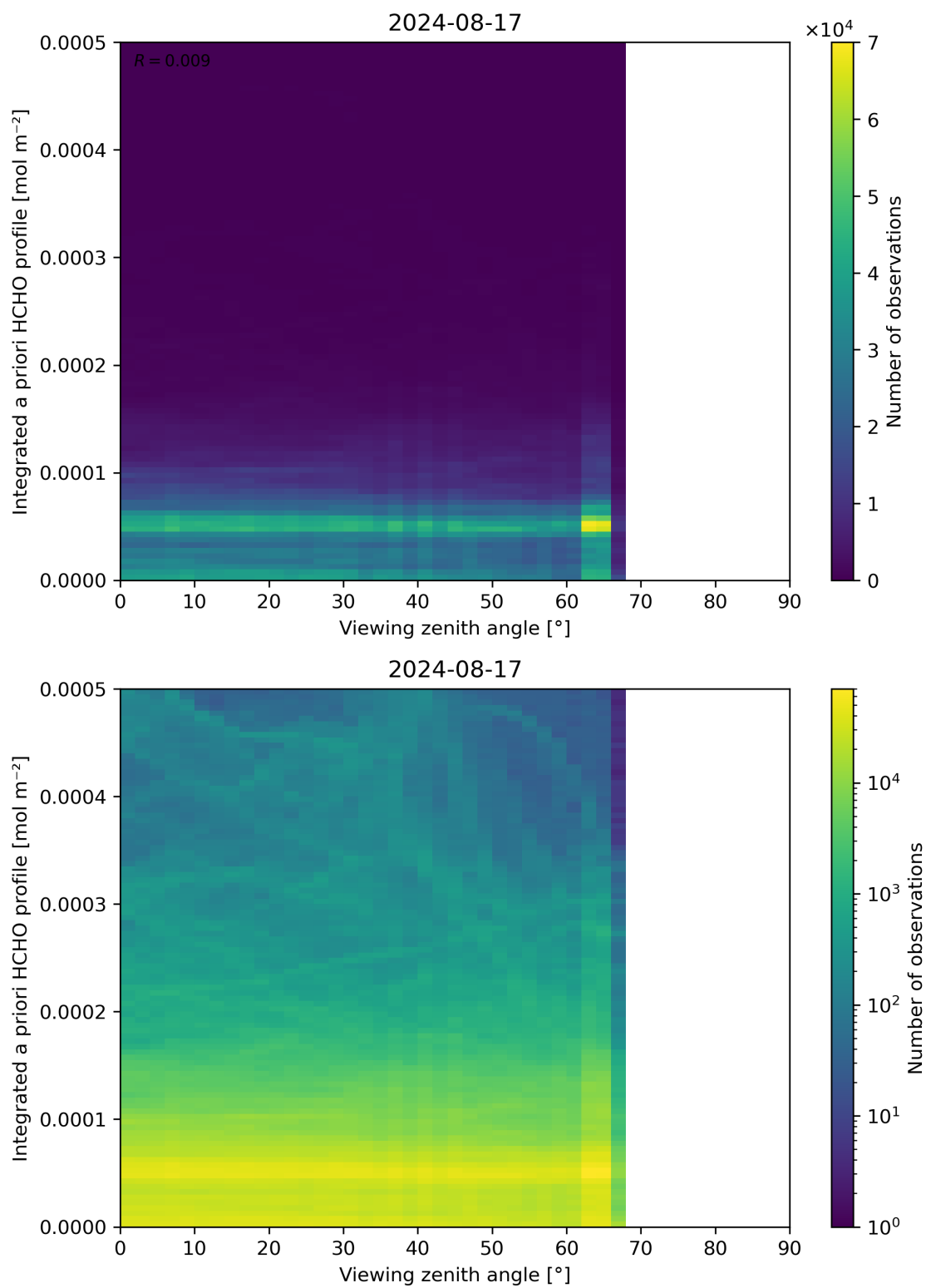
Figure 195: Scatter density plot of “Viewing zenith angle” against “Integrated a priori HCHO profile” for 2024-08-16 to 2024-08-18.
