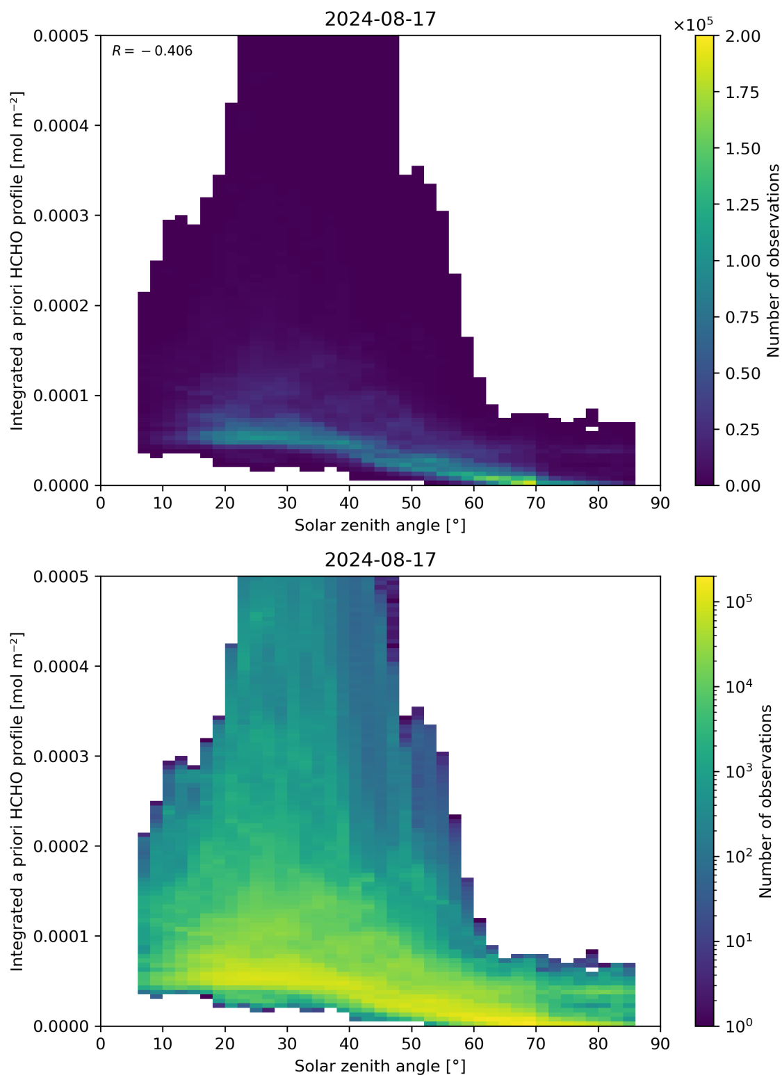
Figure 180: Scatter density plot of “Solar zenith angle” against “Integrated a priori HCHO profile” for 2024-08-16 to 2024-08-18.
