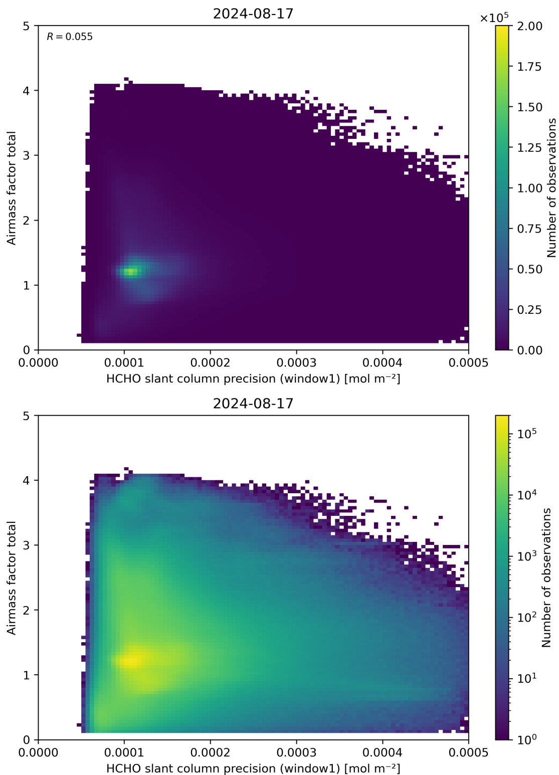
Figure 94: Scatter density plot of “HCHO slant column precision (window1)” against “Airmass factor total” for 2024-08-16 to 2024-08-18.
