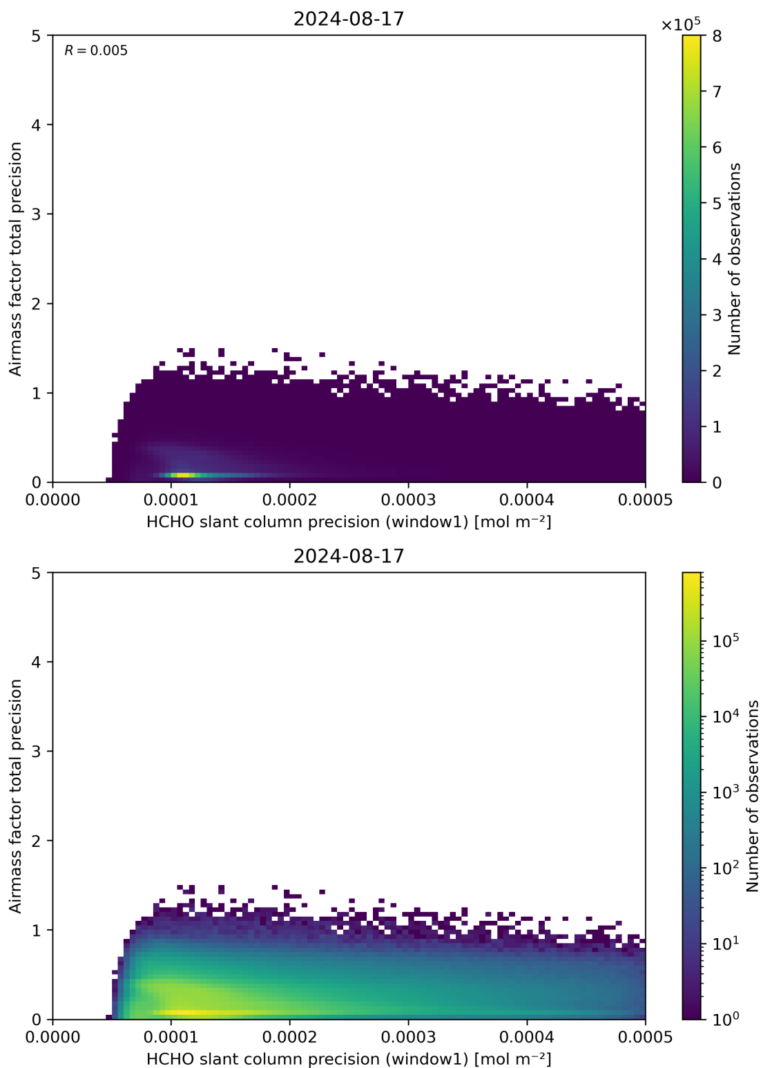
Figure 95: Scatter density plot of “HCHO slant column precision (window1)” against “Airmass factor total precision” for 2024-08-16 to 2024-08-18.
