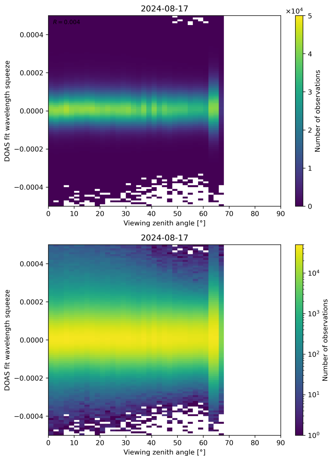
Figure 184: Scatter density plot of “Viewing zenith angle” against “DOAS fit wavelength squeeze” for 2024-08-16 to 2024-08-18.
