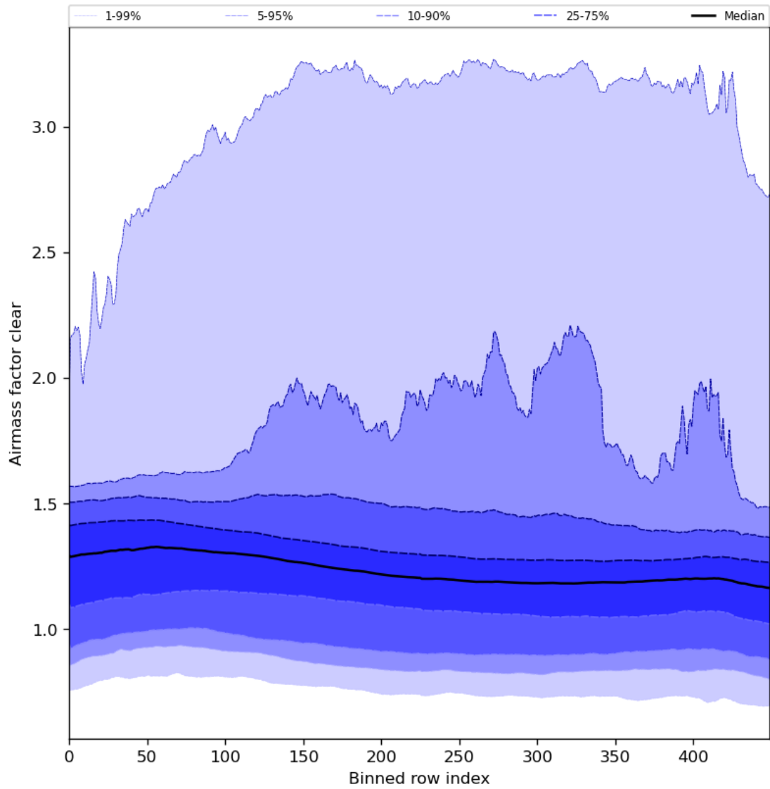
Figure 56: Along track statistics of “Airmass factor clear” for 2024-08-16 to 2024-08-18
