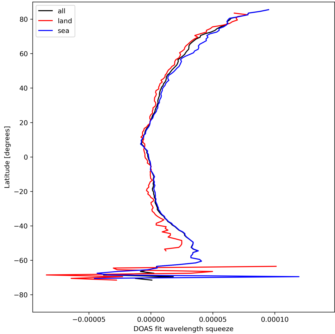
Figure 31: Zonal average of “DOAS fit wavelength squeeze” for 2024-08-16 to 2024-08-18.
