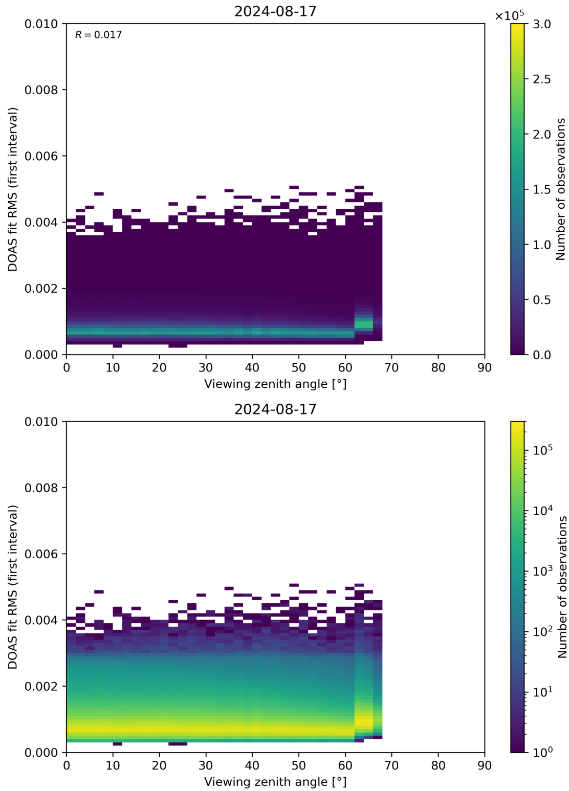
Figure 182: Scatter density plot of “Viewing zenith angle” against “DOAS fit RMS (first interval)” for 2024-08-16 to 2024-08-18.
