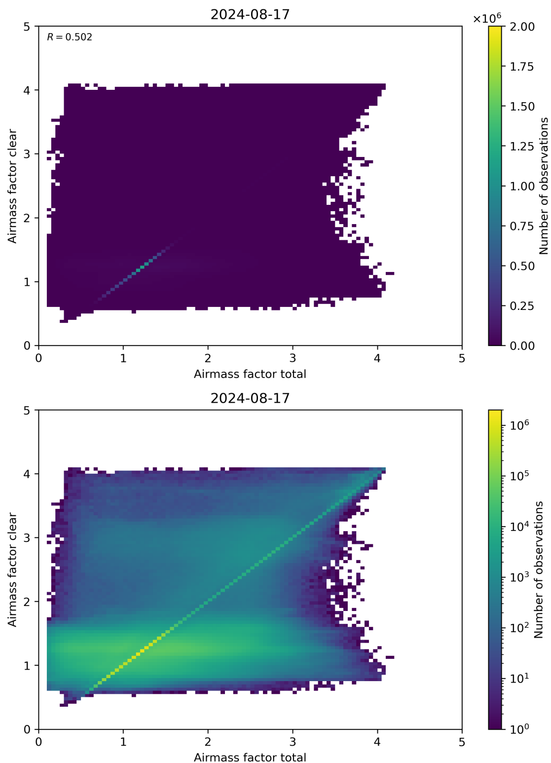
Figure 100: Scatter density plot of “Airmass factor total” against “Airmass factor clear” for 2024-08-16 to 2024-08-18.
