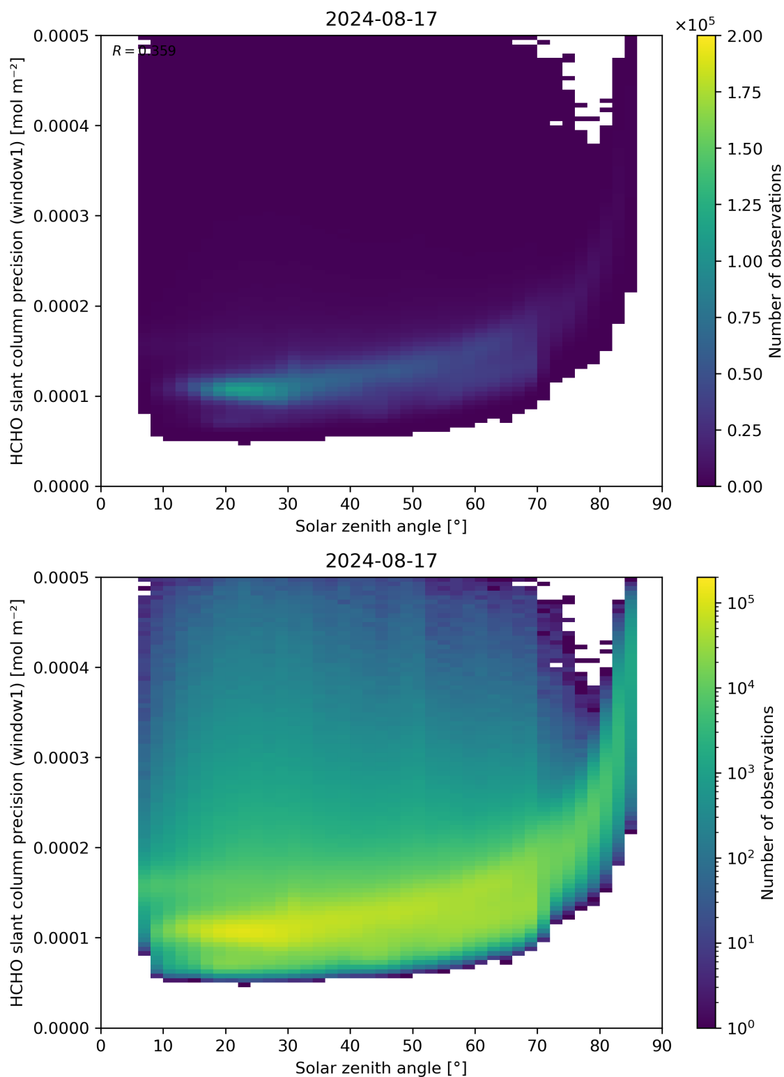
Figure 174: Scatter density plot of “Solar zenith angle” against “HCHO slant column precision (window1)” for 2024-08-16 to 2024-08-18.
