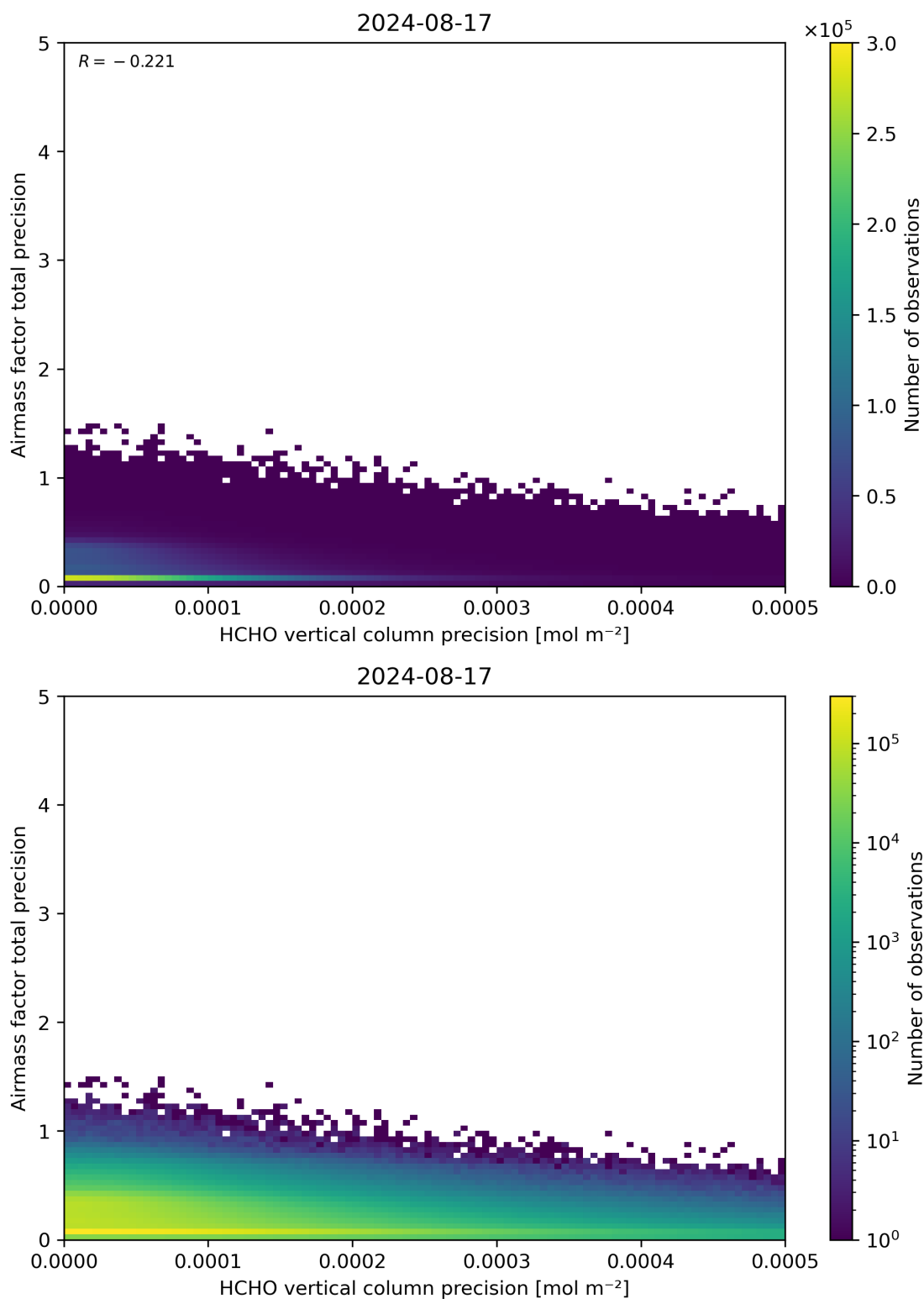
Figure 145: Scatter density plot of “HCHO vertical column precision” against “Airmass factor total precision” for 2024-08-16 to 2024-08-18.
