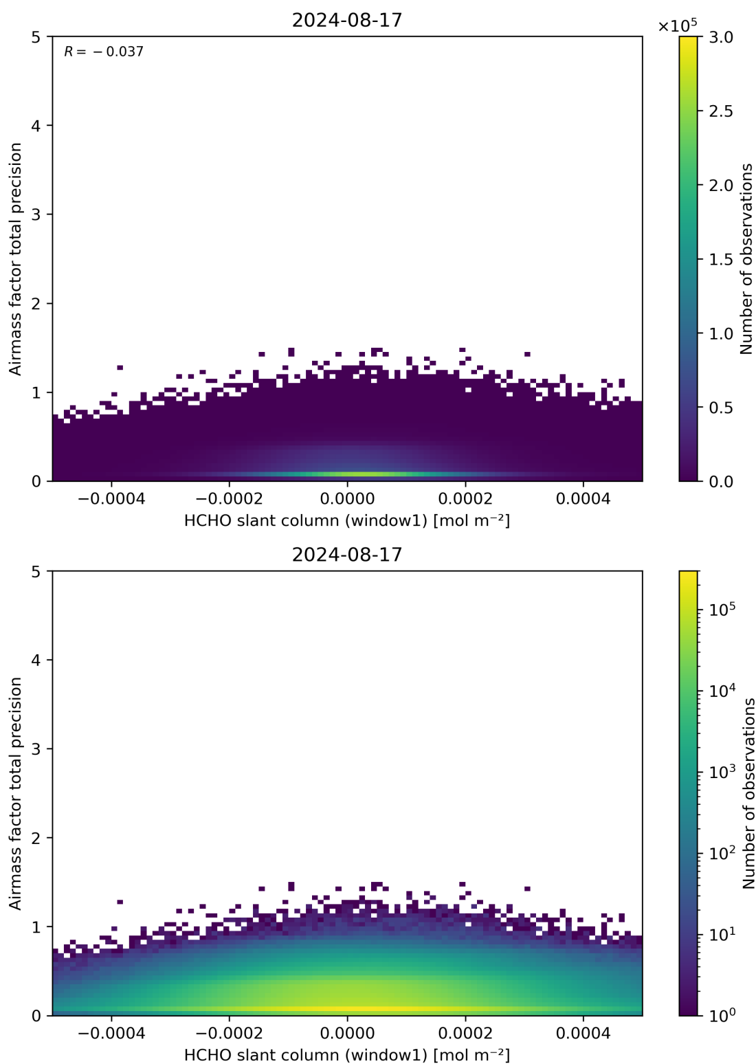
Figure 86: Scatter density plot of “HCHO slant column (window1)” against “Airmass factor total precision” for 2024-08-16 to 2024-08-18.
