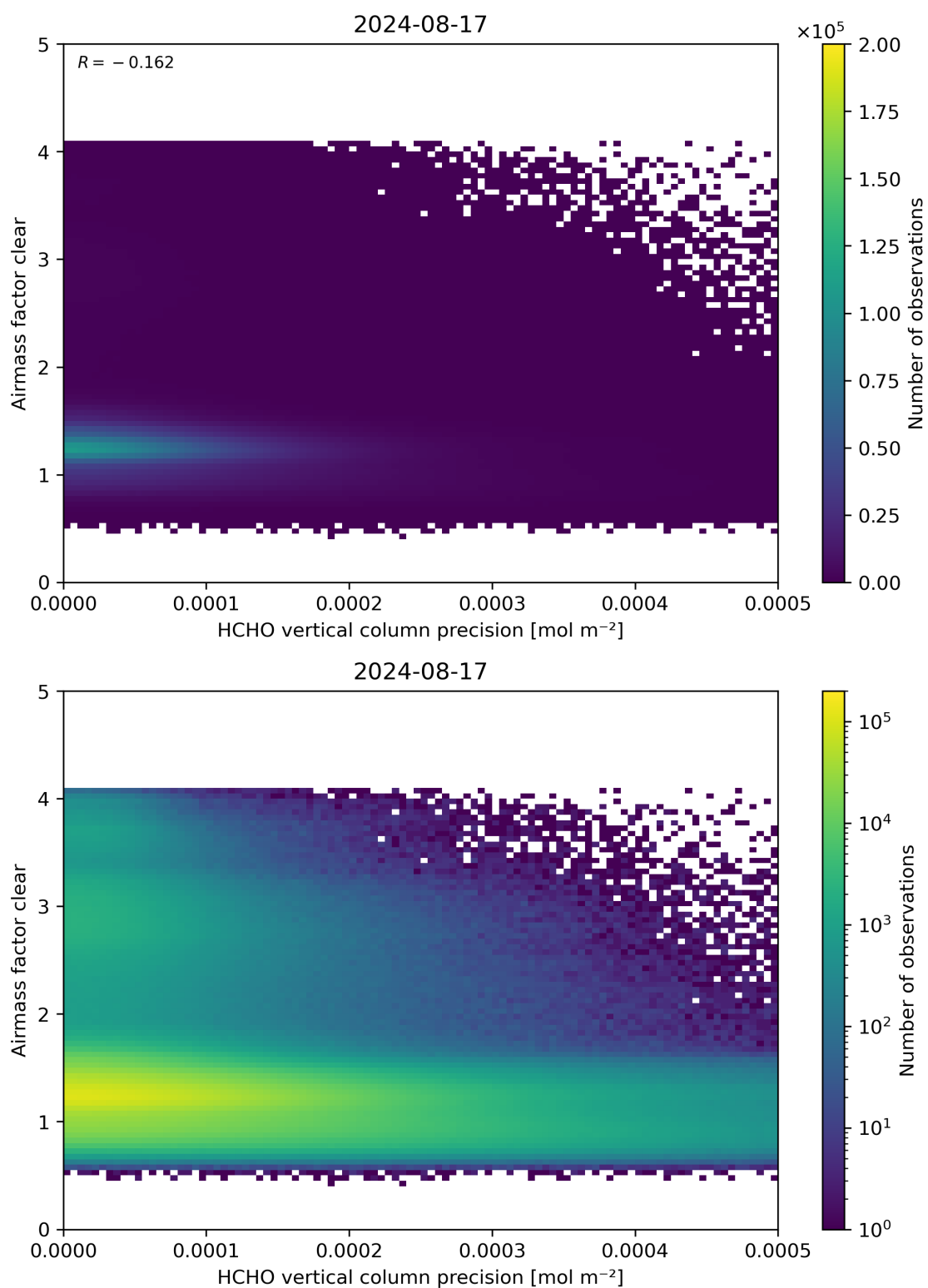
Figure 139: Scatter density plot of “HCHO vertical column precision” against “Airmass factor clear” for 2024-08-16 to 2024-08-18.
