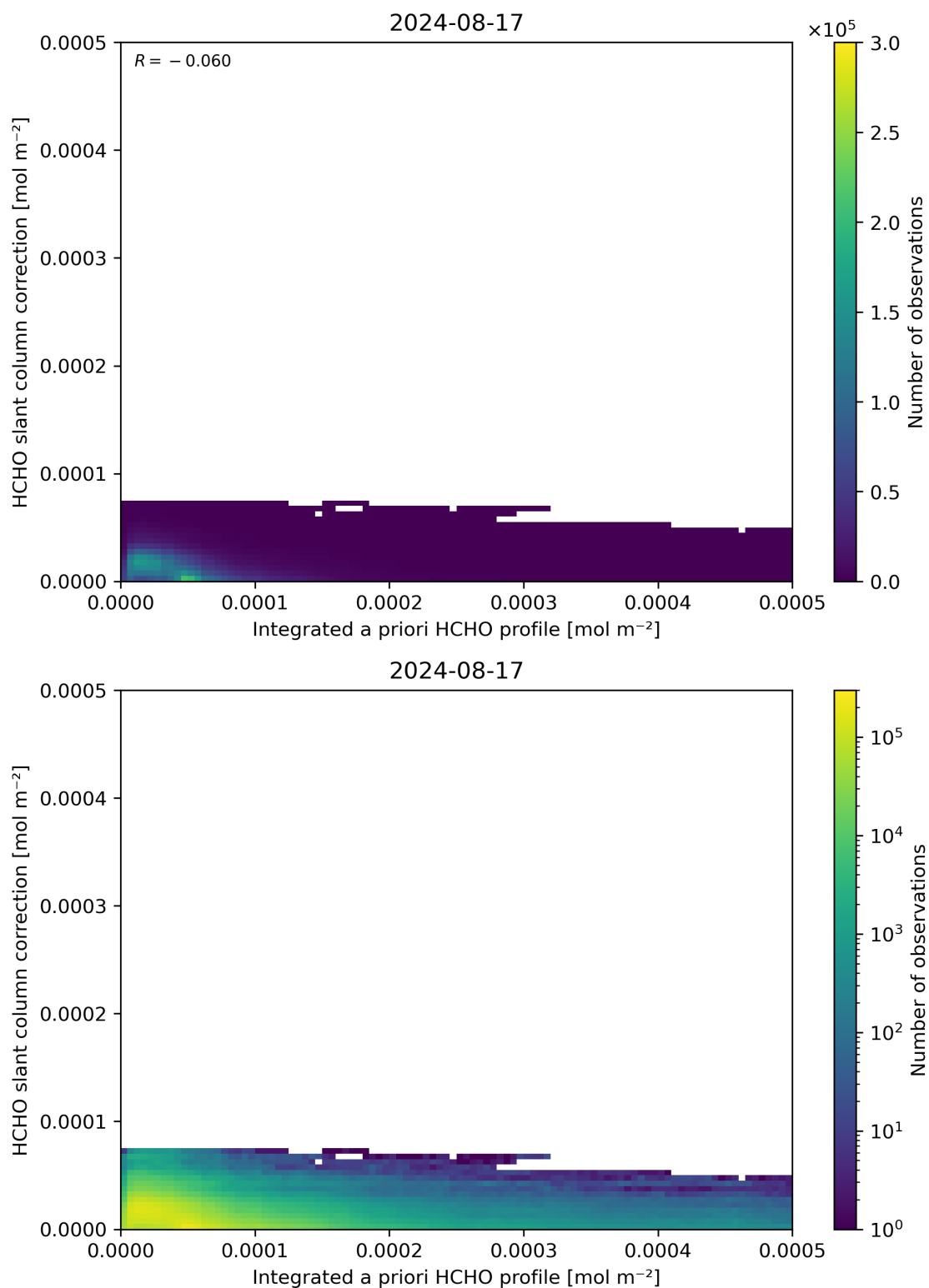
Figure 152: Scatter density plot of “Integrated a priori HCHO profile” against “HCHO slant column correction” for 2024-08-16 to 2024-08-18.
