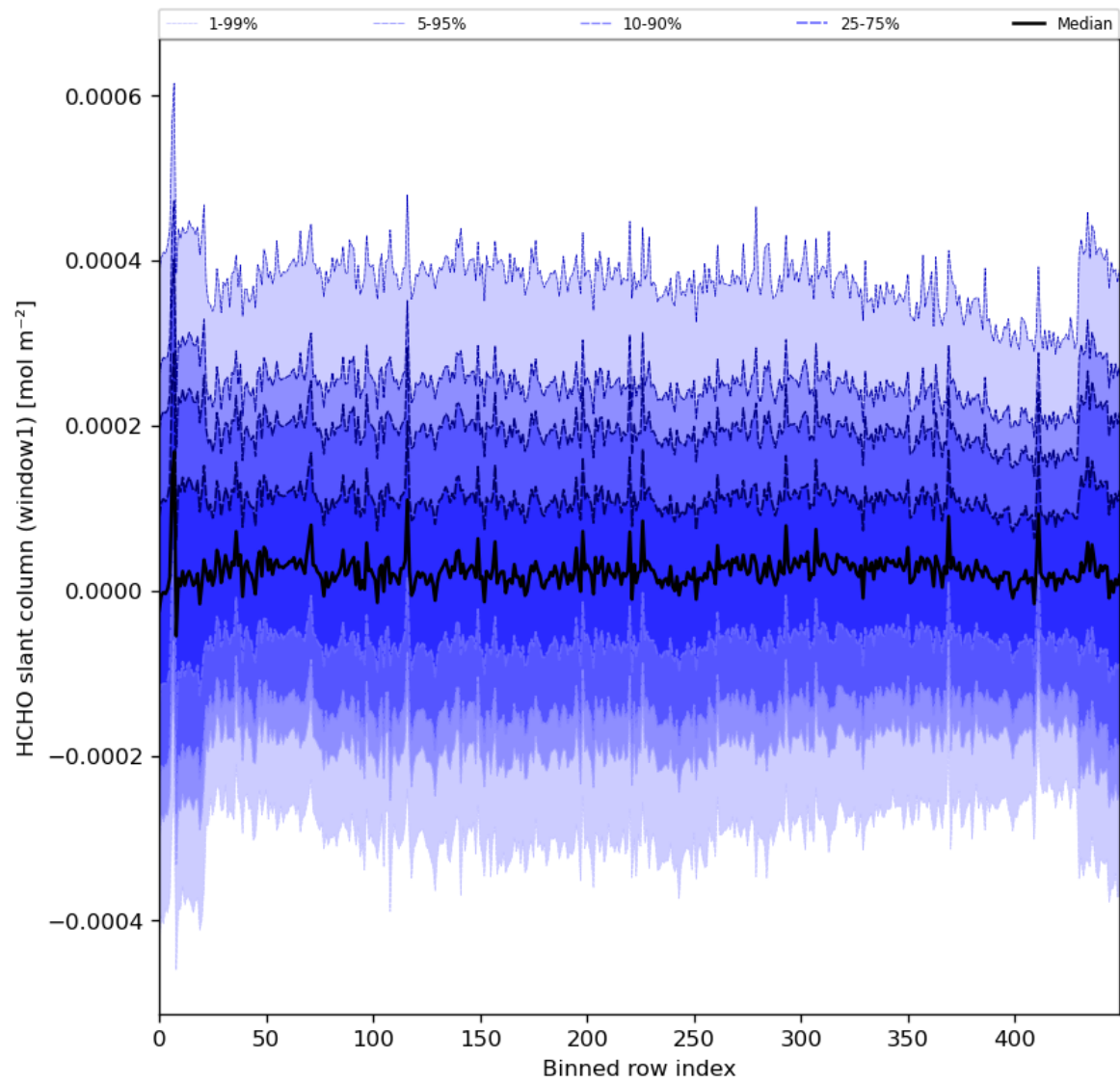
Figure 52: Along track statistics of “HCHO slant column (window1)” for 2024-08-16 to 2024-08-18
