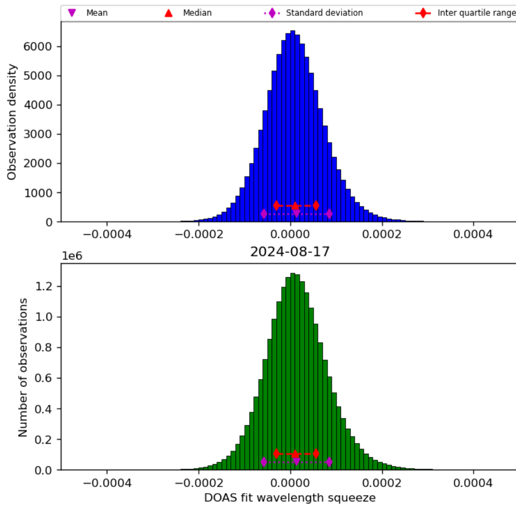
Figure 45: Histogram of “DOAS fit wavelength squeeze” for 2024-08-16 to 2024-08-18
