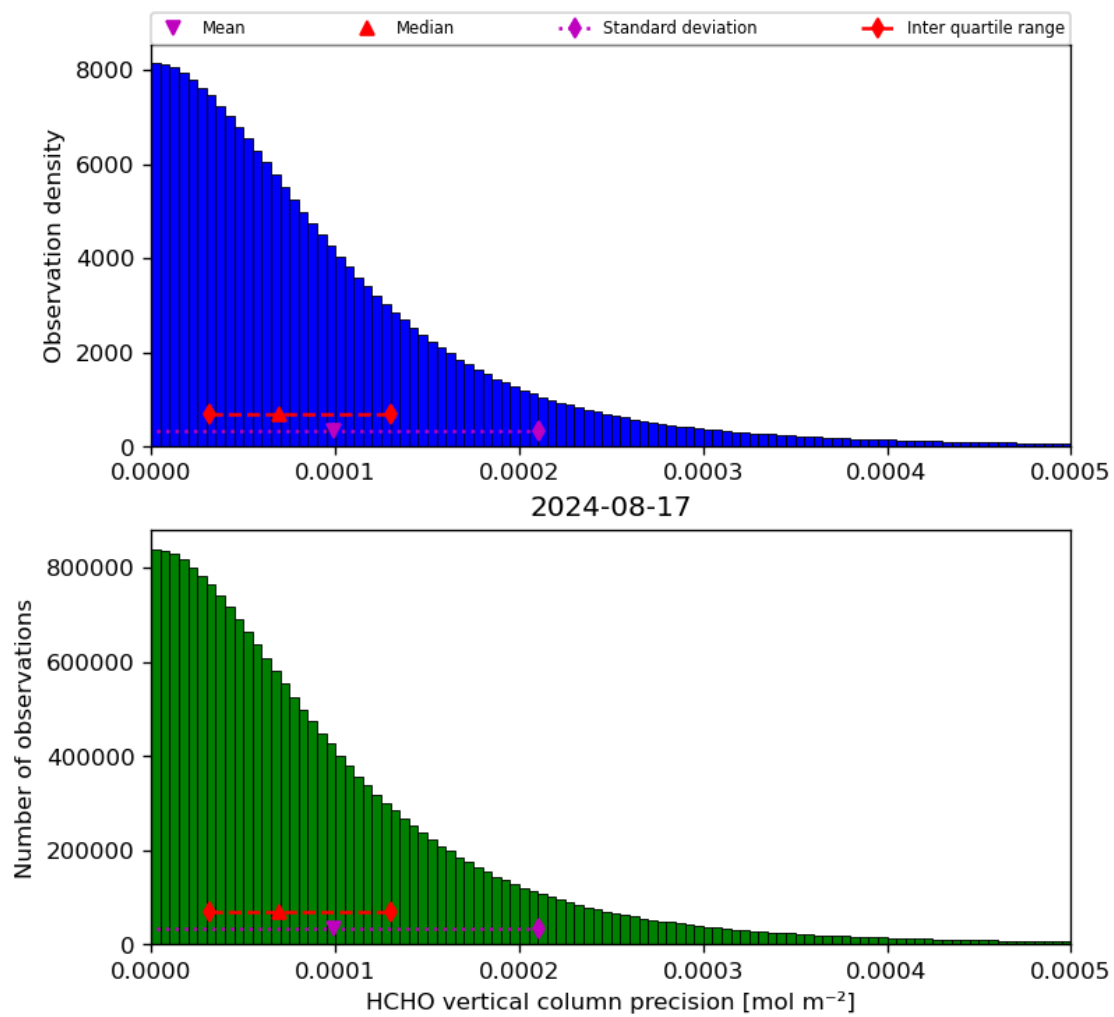
Figure 36: Histogram of “HCHO vertical column precision” for 2024-08-16 to 2024-08-18
