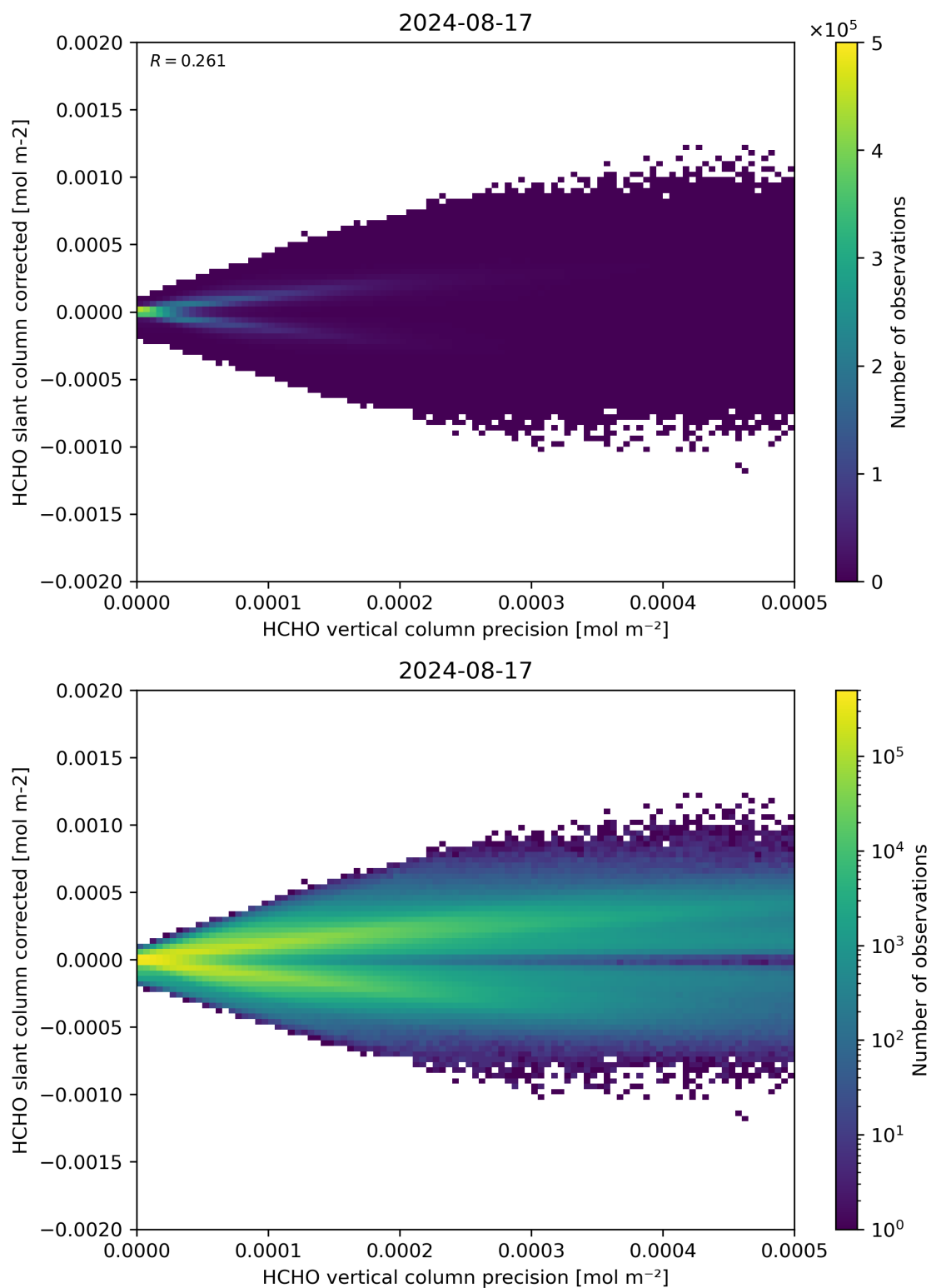
Figure 140: Scatter density plot of “HCHO vertical column precision” against “HCHO slant column corrected” for 2024-08-16 to 2024-08-18.
