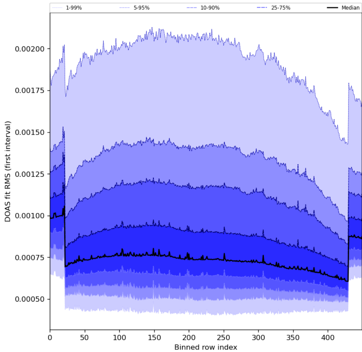
Figure 60: Along track statistics of “DOAS fit RMS (first interval)” for 2024-08-16 to 2024-08-18
