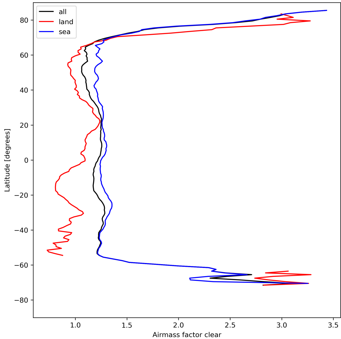
Figure 28: Zonal average of “Airmass factor clear” for 2024-08-16 to 2024-08-18.
