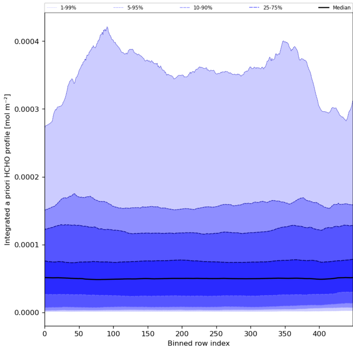
Figure 57: Along track statistics of “Integrated a priori HCHO profile” for 2024-08-16 to 2024-08-18
