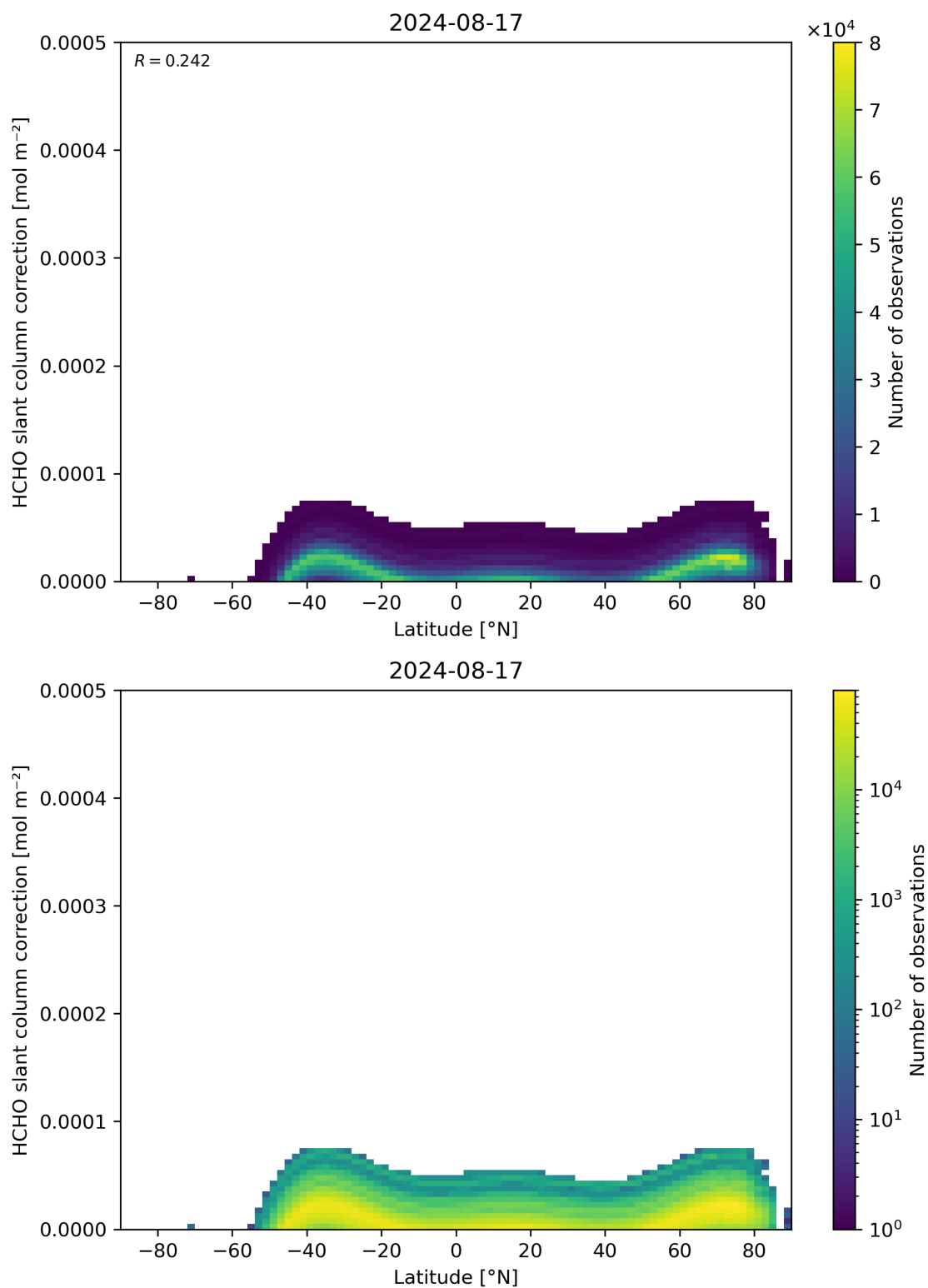
Figure 158: Scatter density plot of “Latitude” against “HCHO slant column correction” for 2024-08-16 to 2024-08-18.
