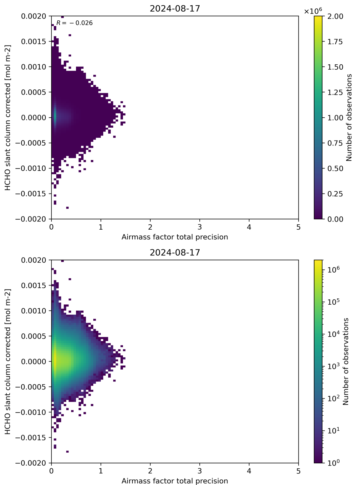
Figure 109: Scatter density plot of “Airmass factor total precision” against “HCHO slant column corrected” for 2024-08-16 to 2024-08-18.
