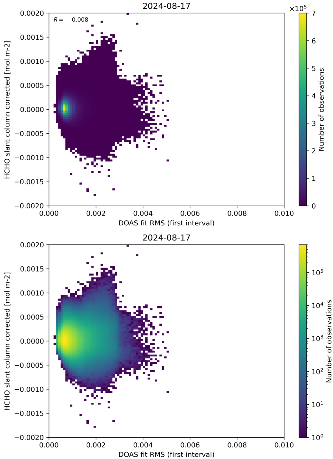
Figure 62: Scatter density plot of “DOAS fit RMS (first interval)” against “HCHO slant column corrected” for 2024-08-16 to 2024-08-18.
