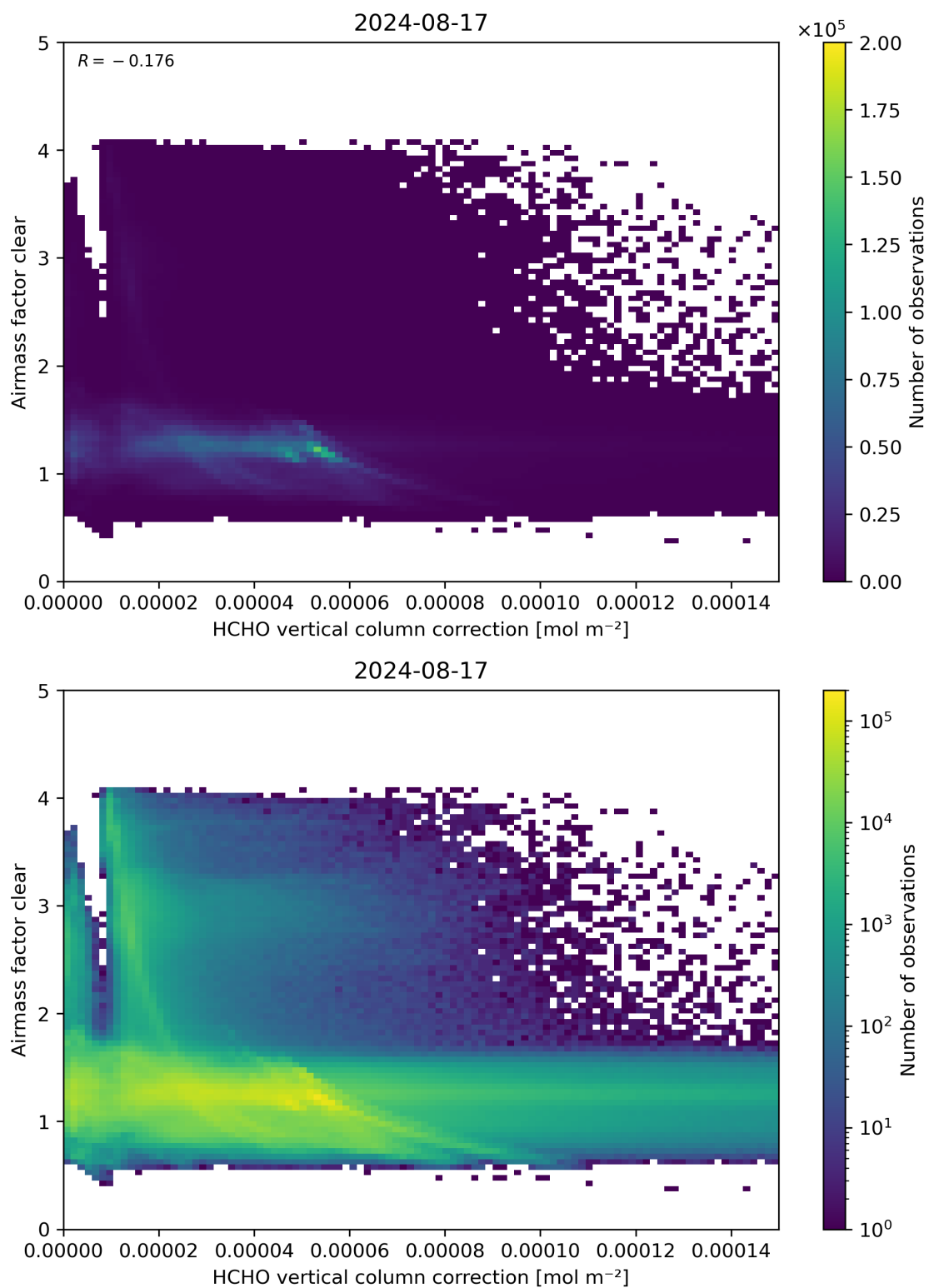
Figure 115: Scatter density plot of “HCHO vertical column correction” against “Airmass factor clear” for 2024-08-16 to 2024-08-18.
