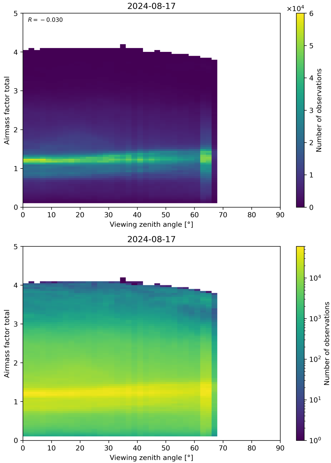
Figure 190: Scatter density plot of “Viewing zenith angle” against “Airmass factor total” for 2024-08-16 to 2024-08-18.
