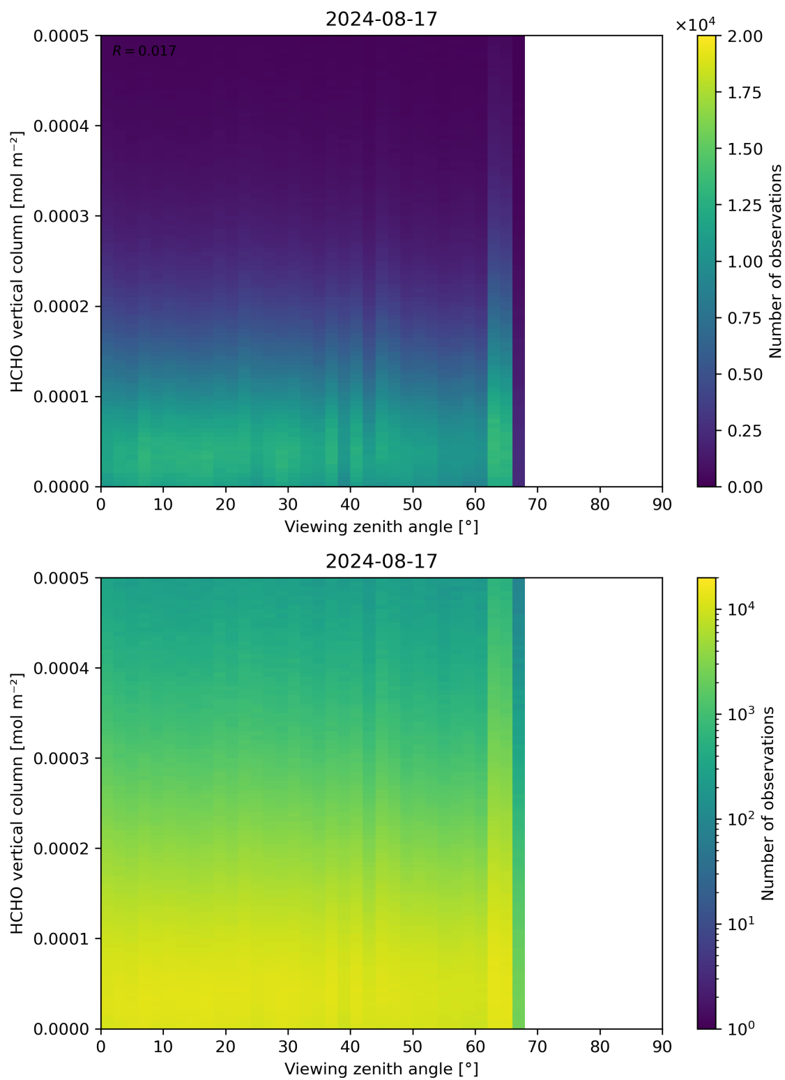
Figure 192: Scatter density plot of “Viewing zenith angle” against “HCHO vertical column” for 2024-08-16 to 2024-08-18.
