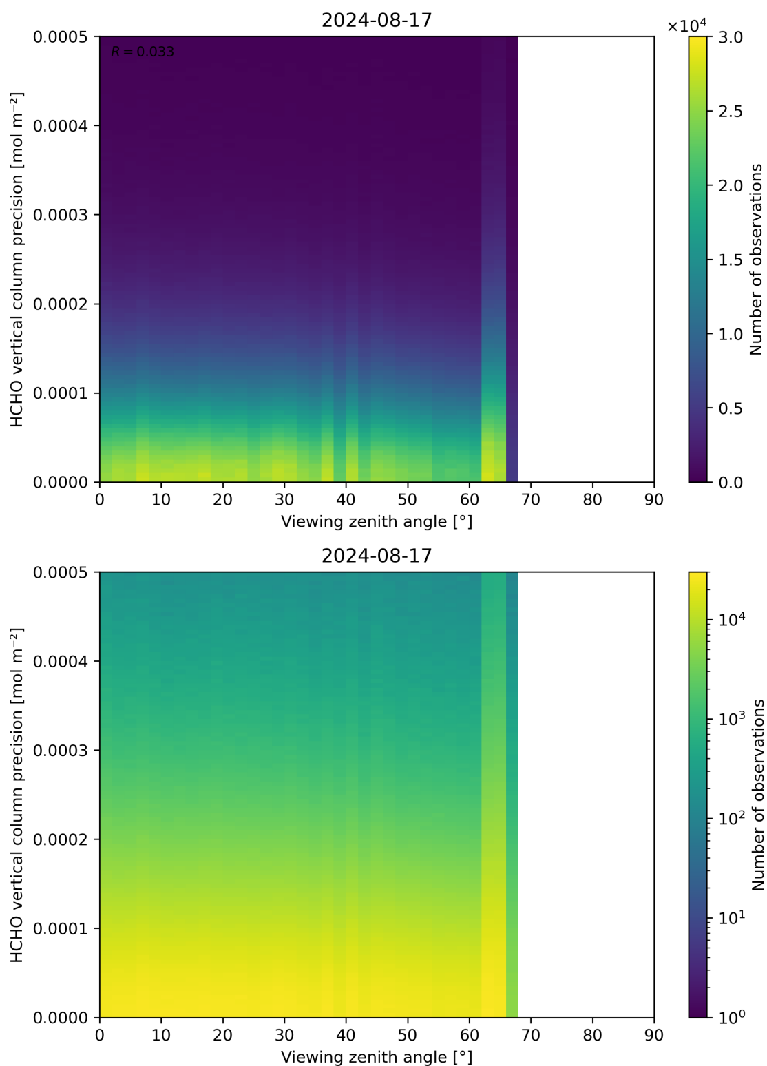
Figure 194: Scatter density plot of “Viewing zenith angle” against “HCHO vertical column precision” for 2024-08-16 to 2024-08-18.
