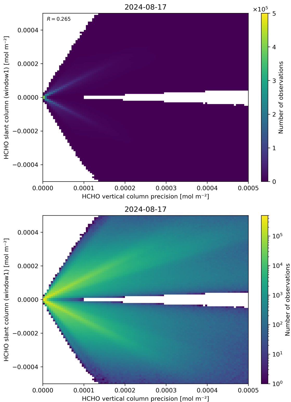
Figure 142: Scatter density plot of “HCHO vertical column precision” against “HCHO slant column (window1)” for 2024-08-16 to 2024-08-18.
