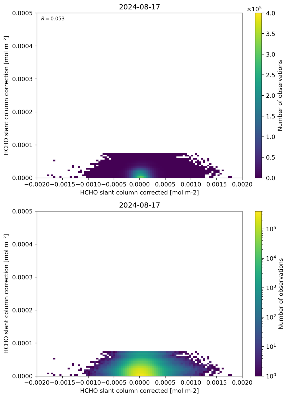
Figure 77: Scatter density plot of “HCHO slant column corrected” against “HCHO slant column correction” for 2024-08-16 to 2024-08-18.
