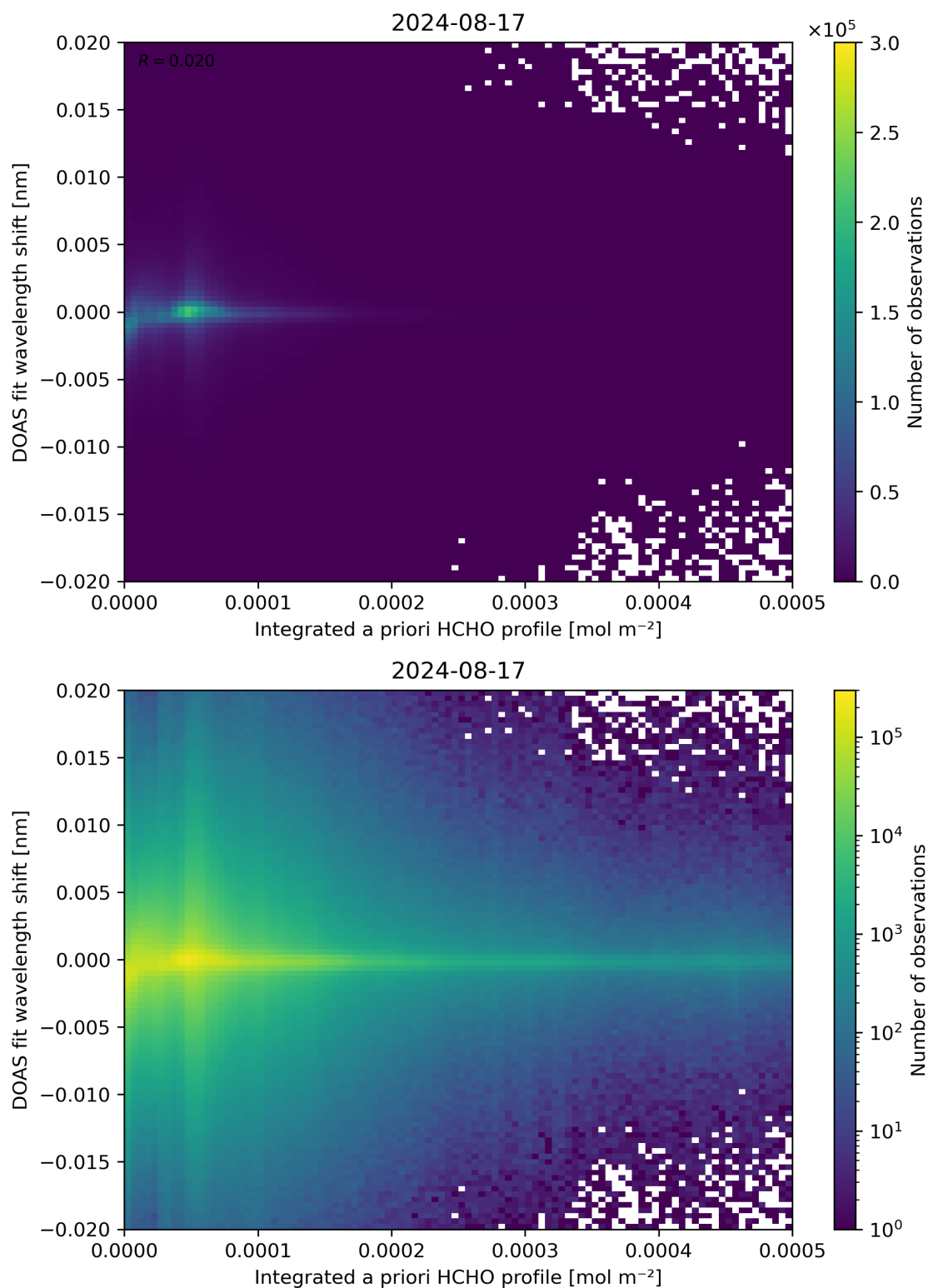
Figure 149: Scatter density plot of “Integrated a priori HCHO profile” against “DOAS fit wavelength shift” for 2024-08-16 to 2024-08-18.
