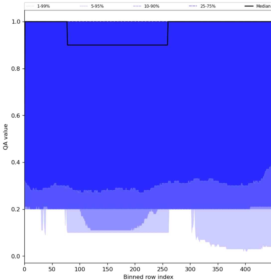
Figure 48: Along track statistics of “QA value” for 2024-08-16 to 2024-08-18
