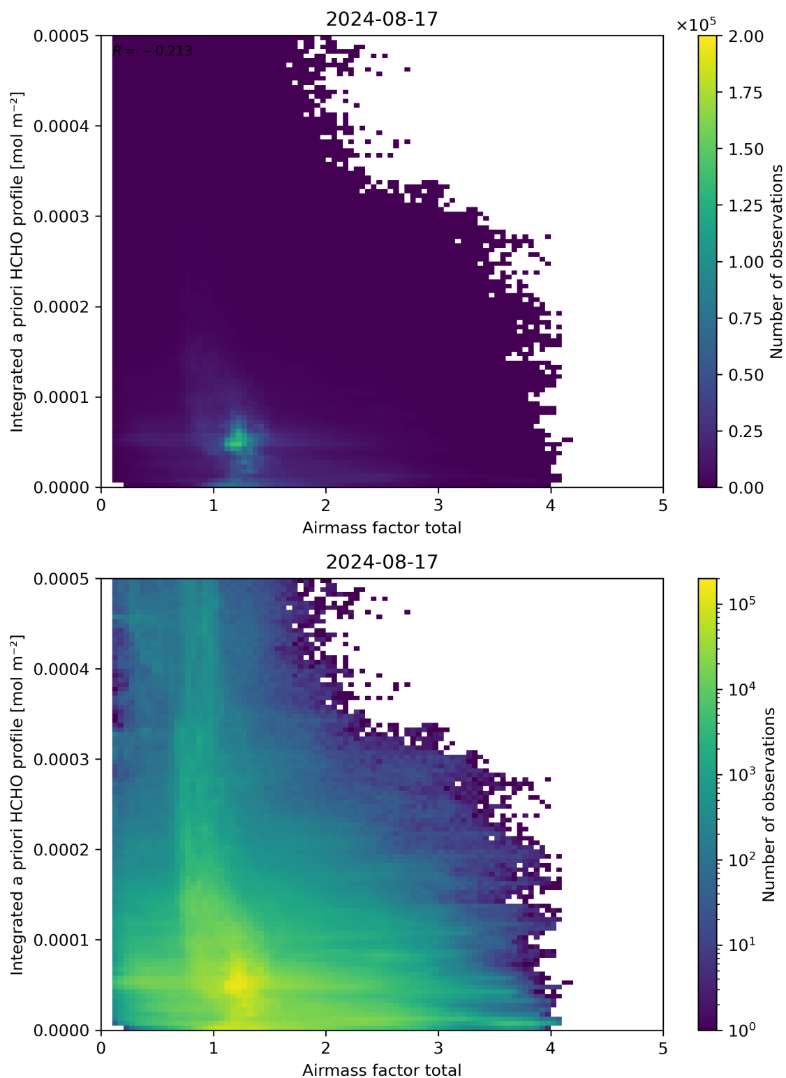
Figure 104: Scatter density plot of “Airmass factor total” against “Integrated a priori HCHO profile” for 2024-08-16 to 2024-08-18.
