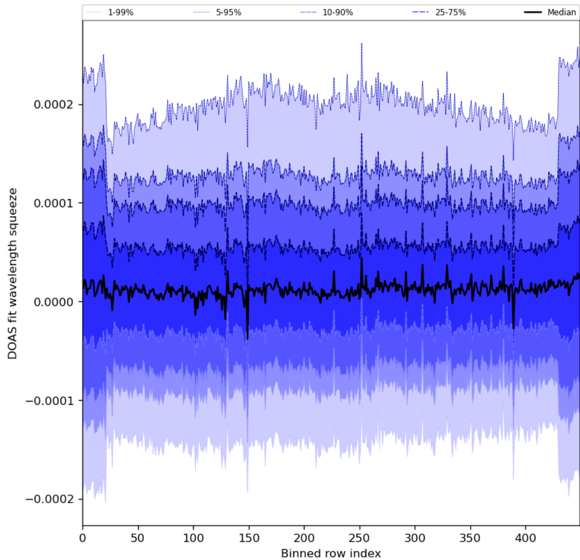
Figure 59: Along track statistics of “DOAS fit wavelength squeeze” for 2024-08-16 to 2024-08-18
