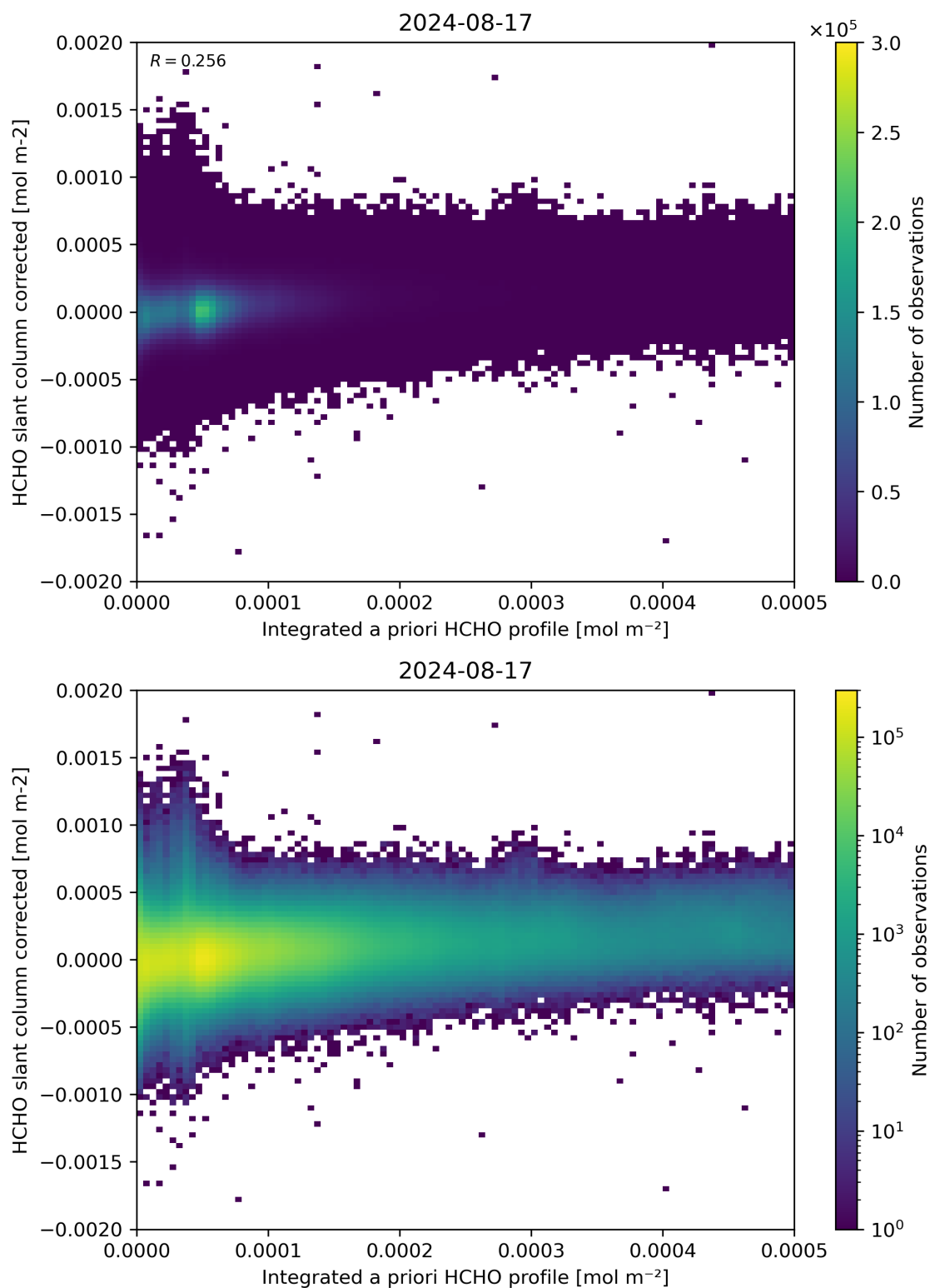
Figure 151: Scatter density plot of “Integrated a priori HCHO profile” against “HCHO slant column corrected” for 2024-08-16 to 2024-08-18.
