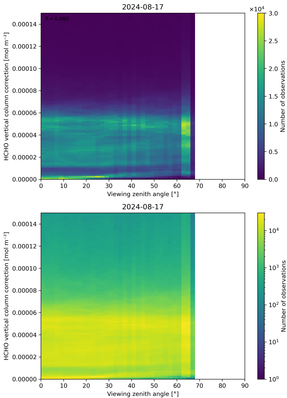
Figure 193: Scatter density plot of “Viewing zenith angle” against “HCHO vertical column correction” for 2024-08-16 to 2024-08-18.
