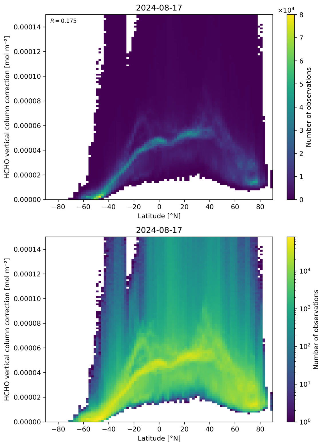
Figure 164: Scatter density plot of “Latitude” against “HCHO vertical column correction” for 2024-08-16 to 2024-08-18.
