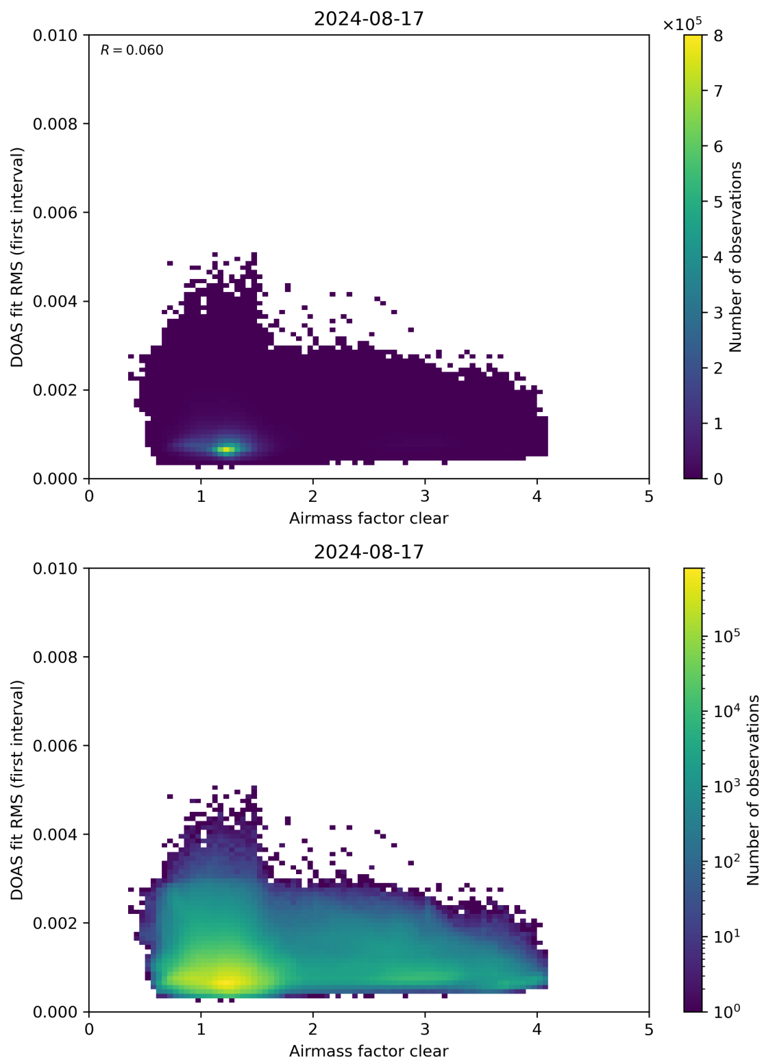
Figure 71: Scatter density plot of “Airmass factor clear” against “DOAS fit RMS (first interval)” for 2024-08-16 to 2024-08-18.
