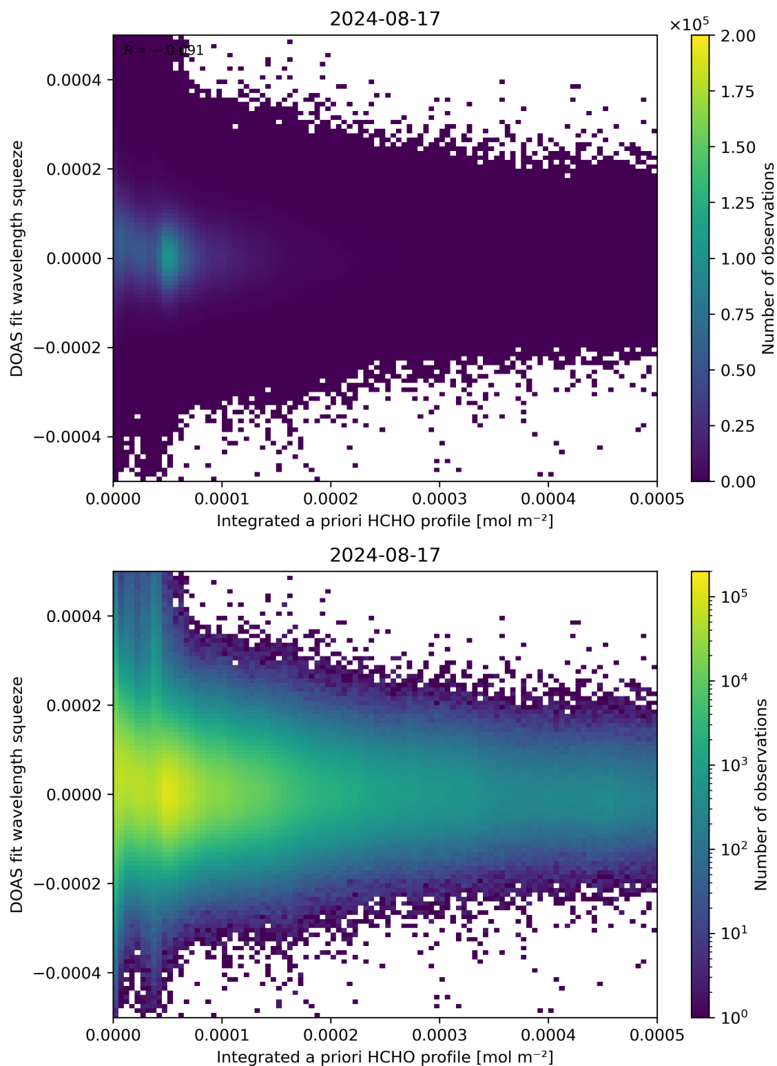
Figure 150: Scatter density plot of “Integrated a priori HCHO profile” against “DOAS fit wavelength squeeze” for 2024-08-16 to 2024-08-18.
