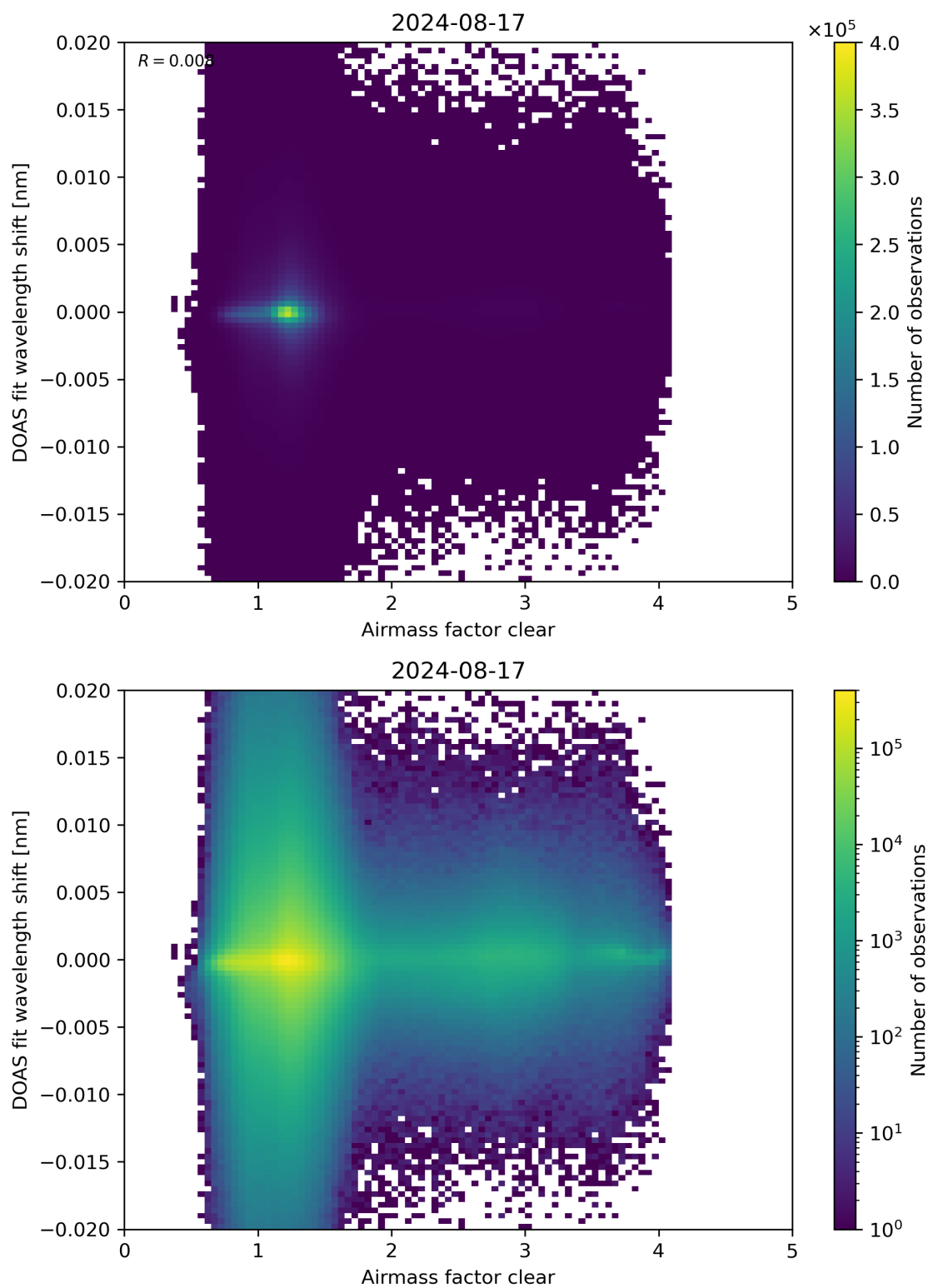
Figure 72: Scatter density plot of “Airmass factor clear” against “DOAS fit wavelength shift” for 2024-08-16 to 2024-08-18.
