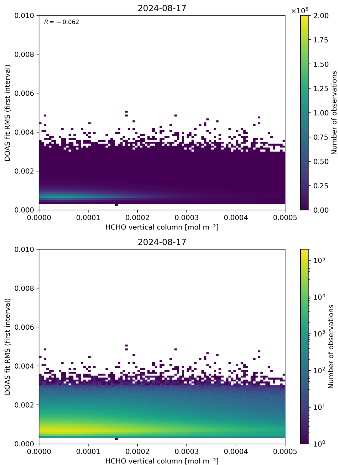
Figure 123: Scatter density plot of “HCHO vertical column” against “DOAS fit RMS (first interval)” for 2024-08-16 to 2024-08-18.
