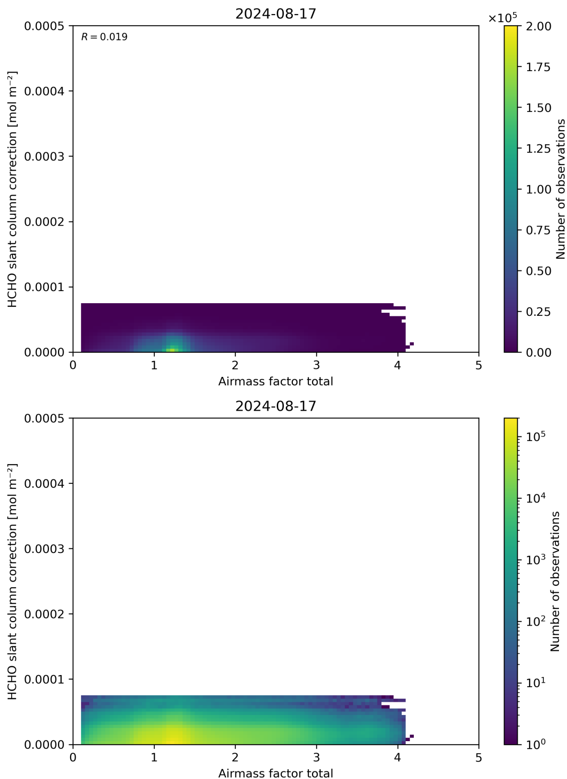
Figure 102: Scatter density plot of “Airmass factor total” against “HCHO slant column correction” for 2024-08-16 to 2024-08-18.
