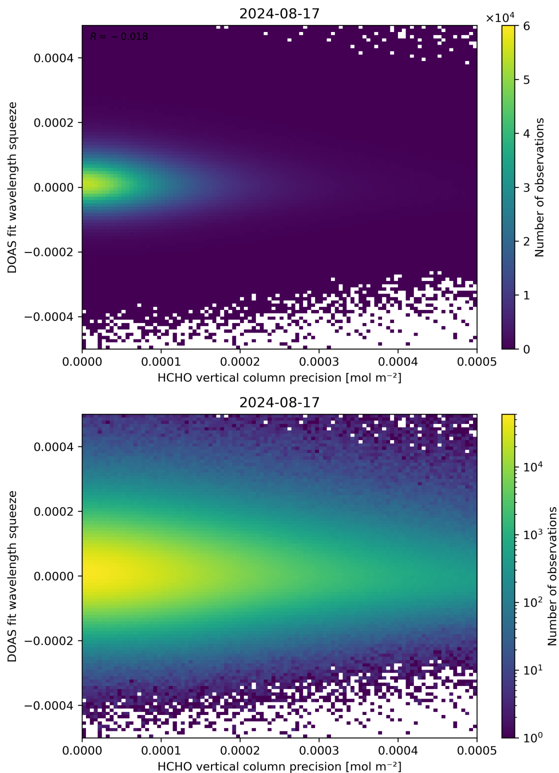
Figure 138: Scatter density plot of “HCHO vertical column precision” against “DOAS fit wavelength squeeze” for 2024-08-16 to 2024-08-18.
