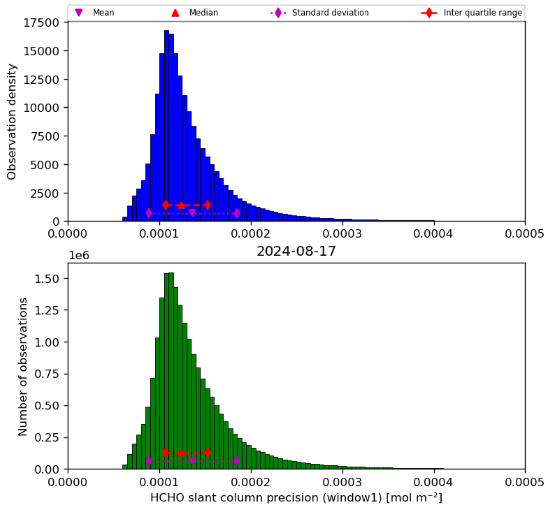
Figure 39: Histogram of “HCHO slant column precision (window1)” for 2024-08-16 to 2024-08-18
