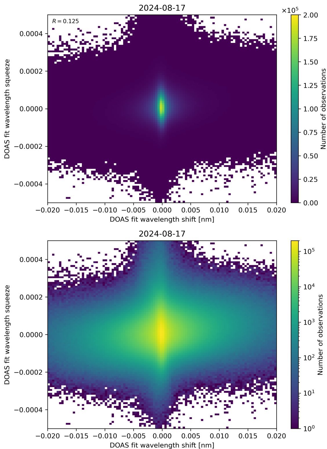
Figure 65: Scatter density plot of “DOAS fit wavelength shift” against “DOAS fit wavelength squeeze” for 2024-08-16 to 2024-08-18.
