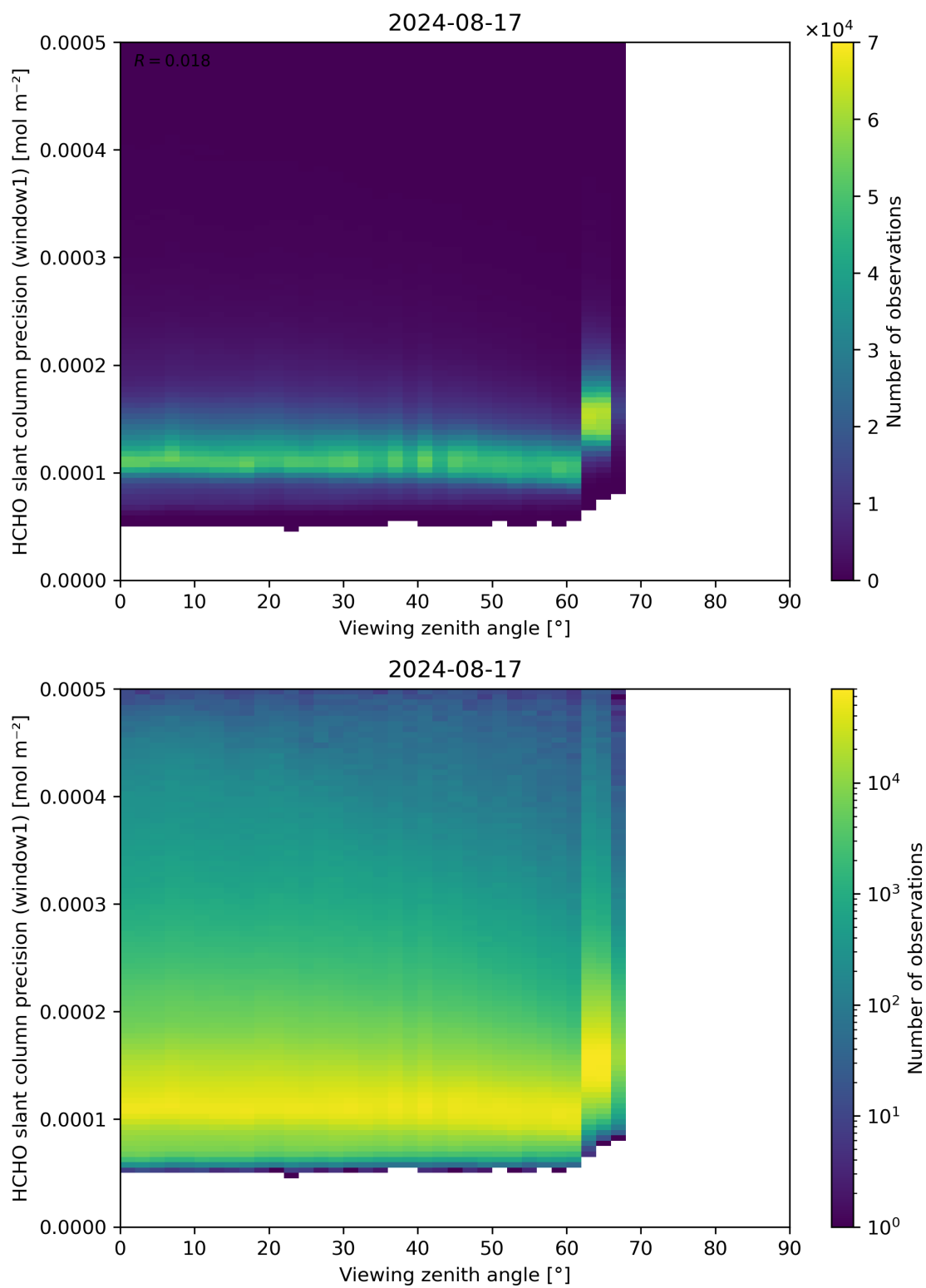
Figure 189: Scatter density plot of “Viewing zenith angle” against “HCHO slant column precision (window1)” for 2024-08-16 to 2024-08-18.
