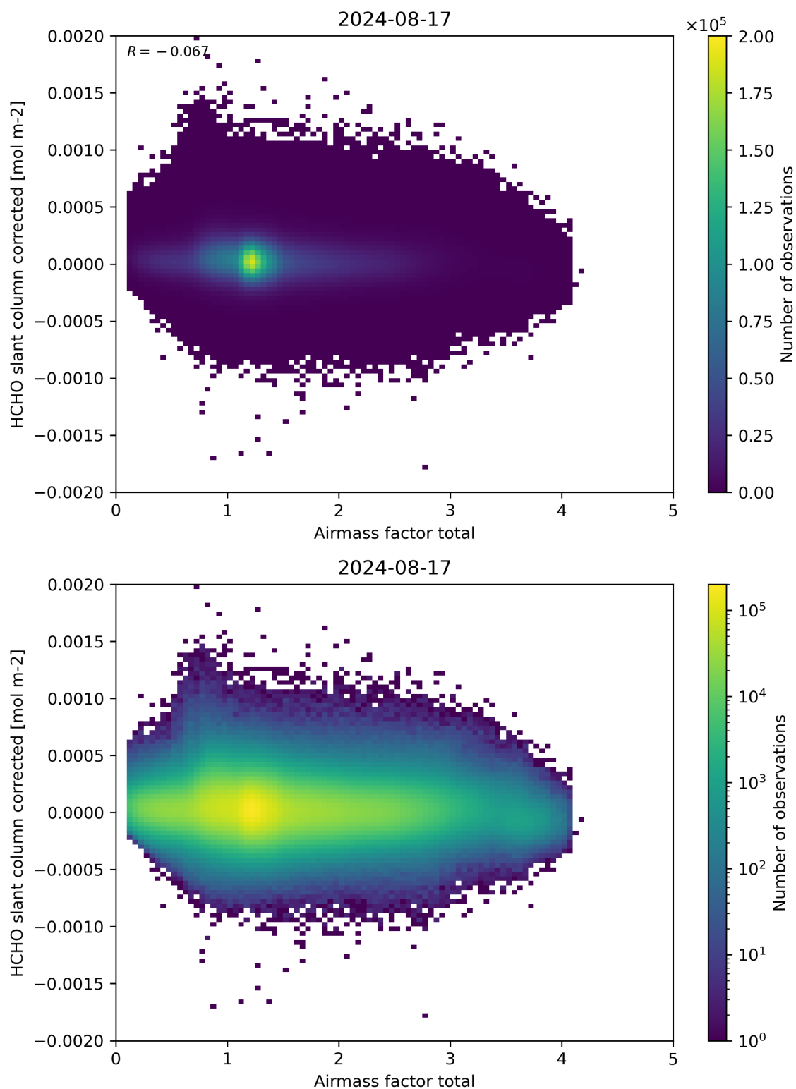
Figure 101: Scatter density plot of “Airmass factor total” against “HCHO slant column corrected” for 2024-08-16 to 2024-08-18.
