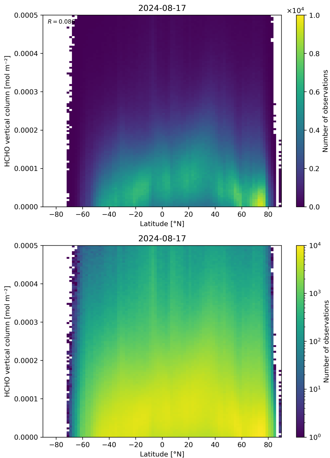
Figure 163: Scatter density plot of “Latitude” against “HCHO vertical column” for 2024-08-16 to 2024-08-18.
