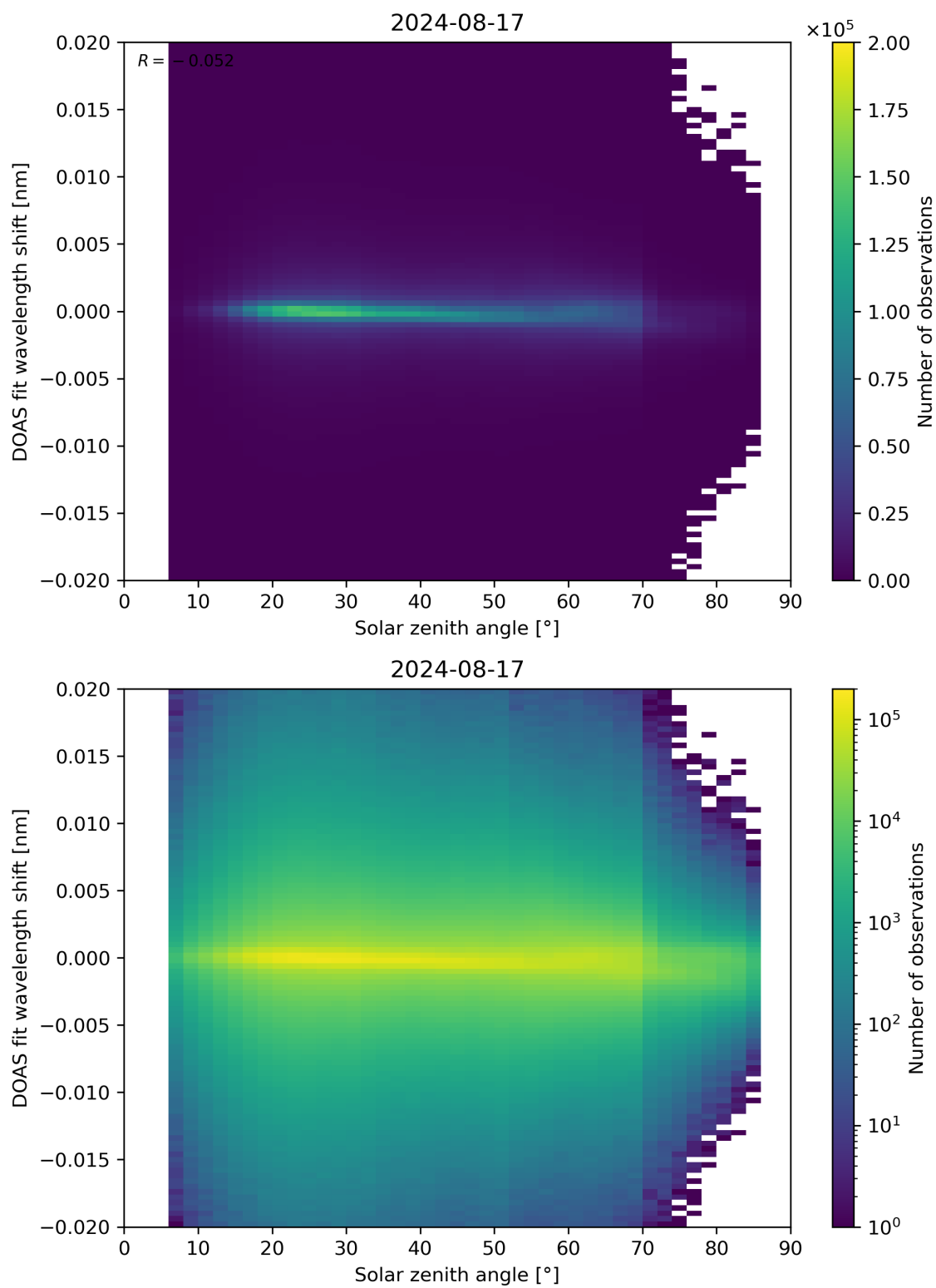
Figure 168: Scatter density plot of “Solar zenith angle” against “DOAS fit wavelength shift” for 2024-08-16 to 2024-08-18.
