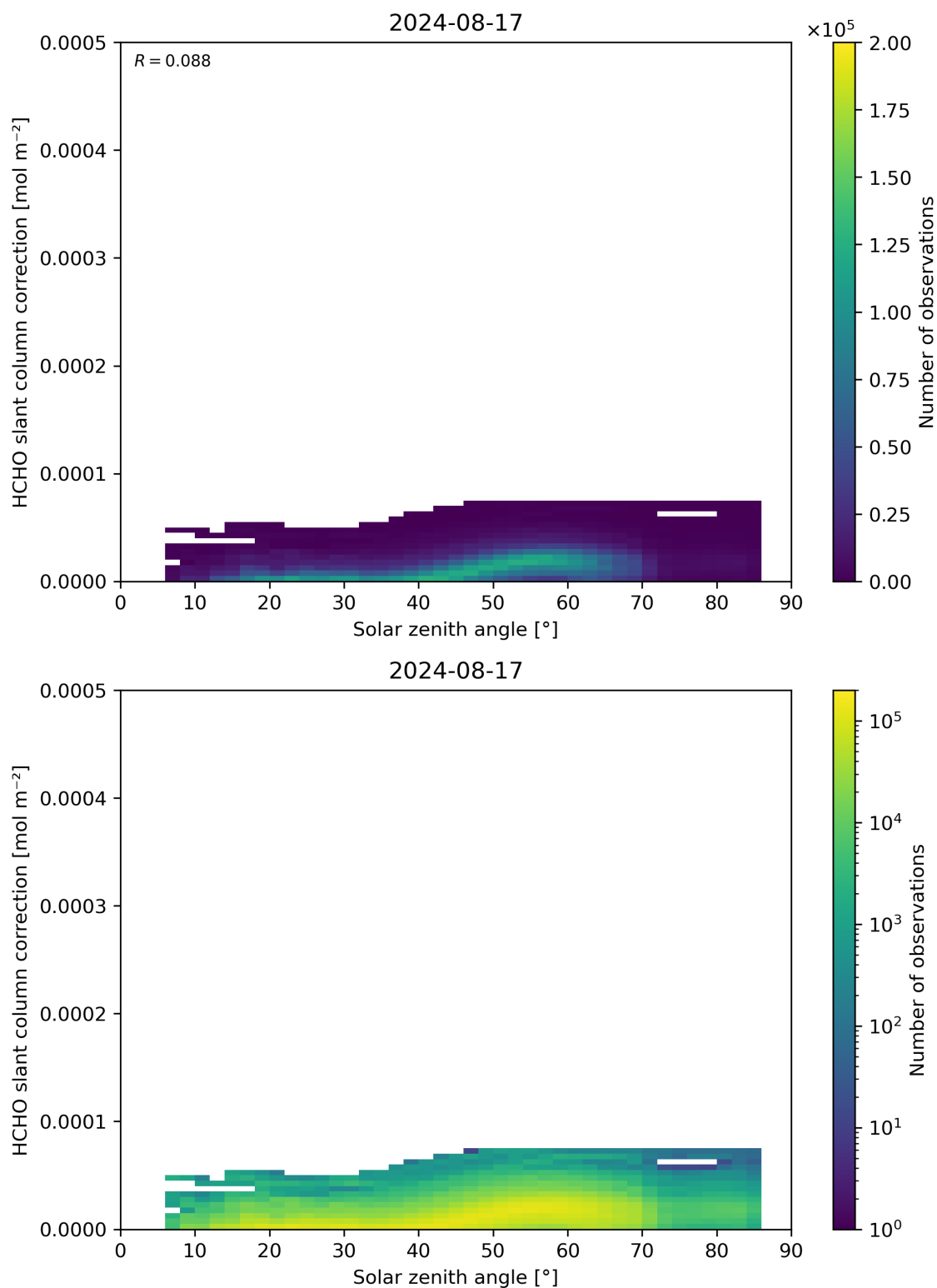
Figure 172: Scatter density plot of “Solar zenith angle” against “HCHO slant column correction” for 2024-08-16 to 2024-08-18.
