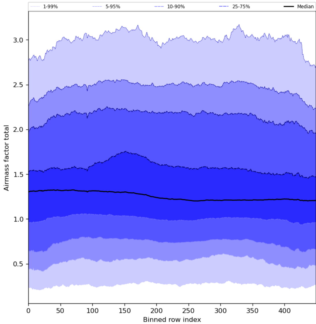
Figure 54: Along track statistics of “Airmass factor total” for 2024-08-16 to 2024-08-18
