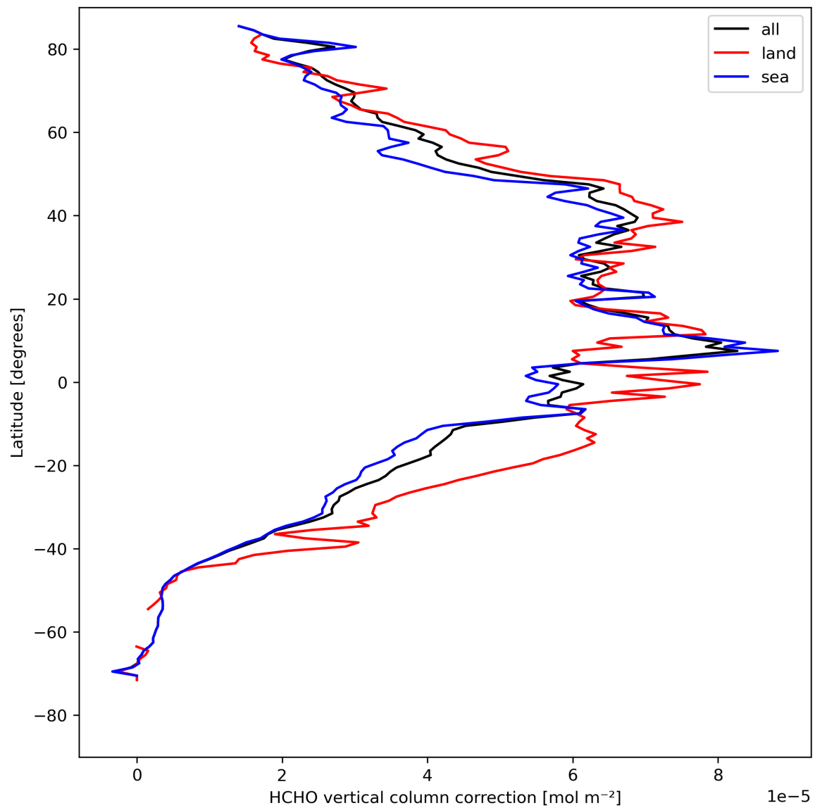
Figure 23: Zonal average of “HCHO vertical column correction” for 2024-08-16 to 2024-08-18.
