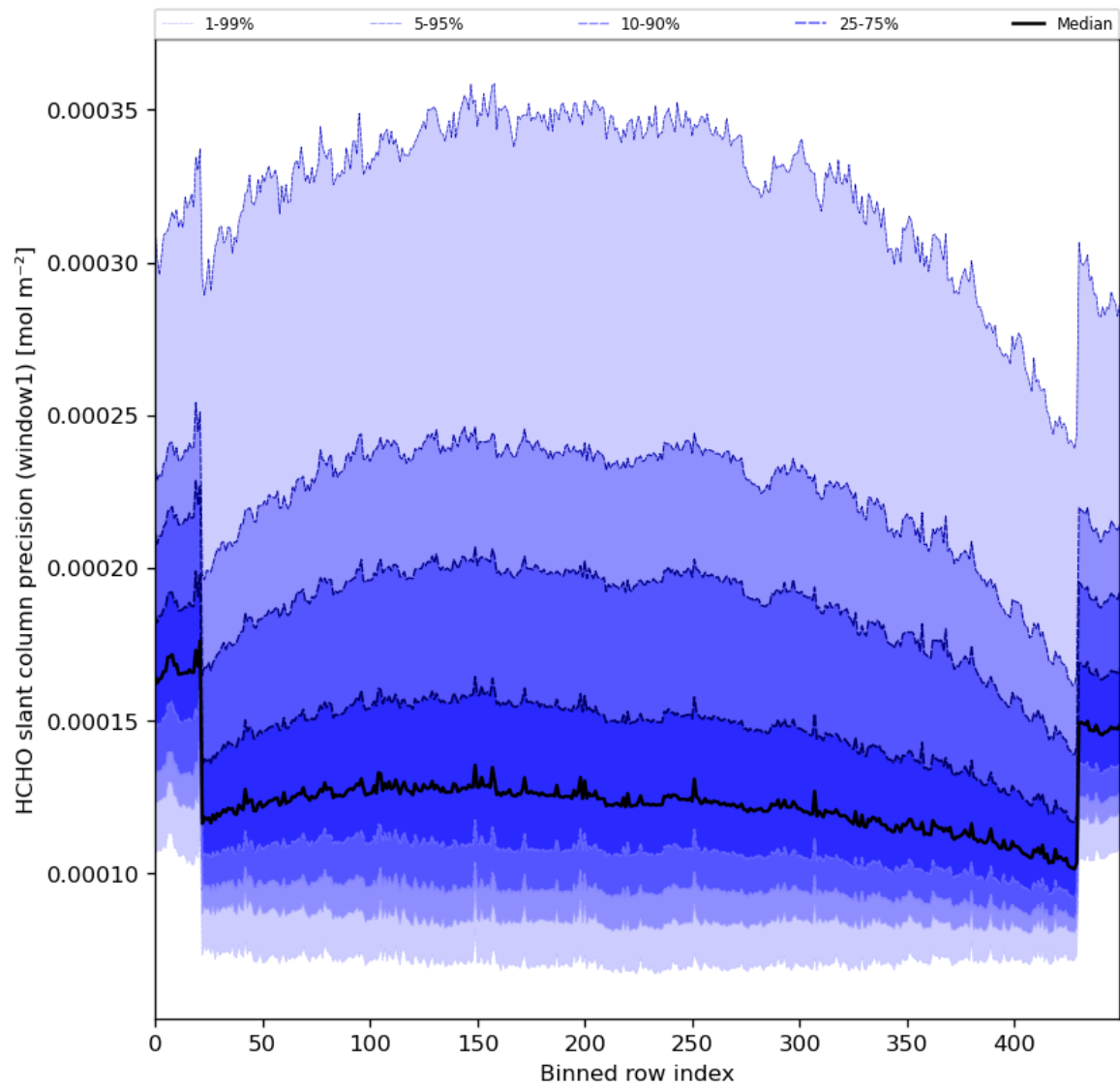
Figure 53: Along track statistics of “HCHO slant column precision (window1)” for 2024-08-16 to 2024-08-18
