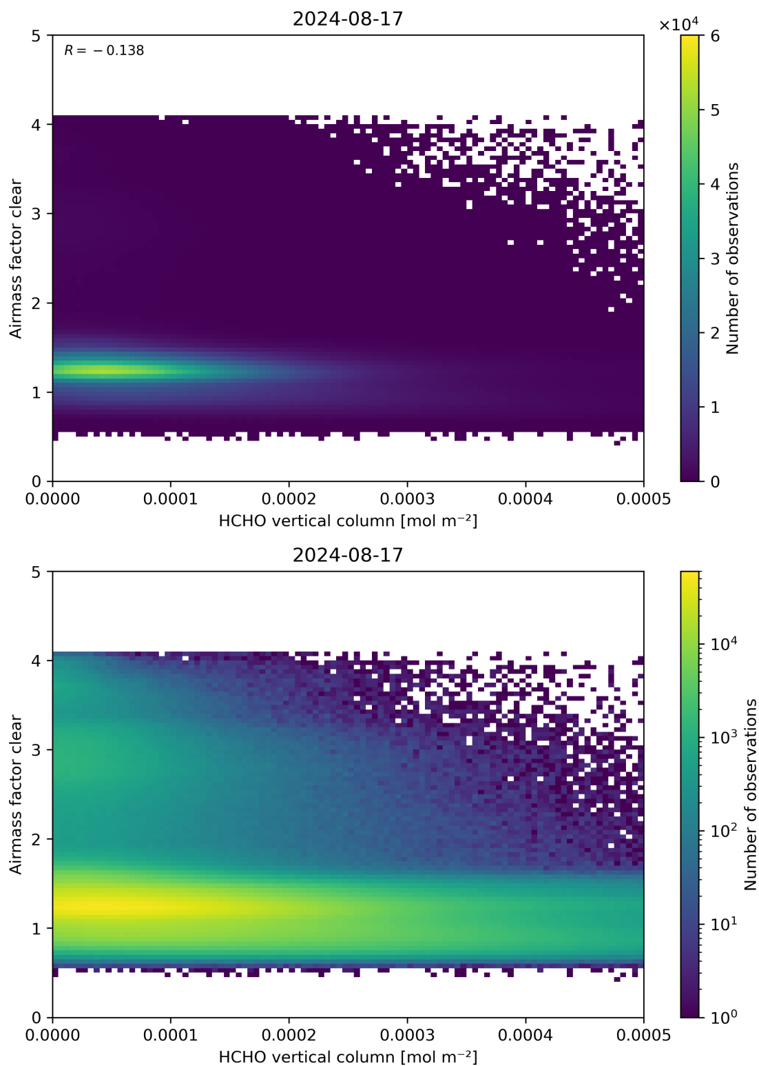
Figure 126: Scatter density plot of “HCHO vertical column” against “Airmass factor clear” for 2024-08-16 to 2024-08-18.
