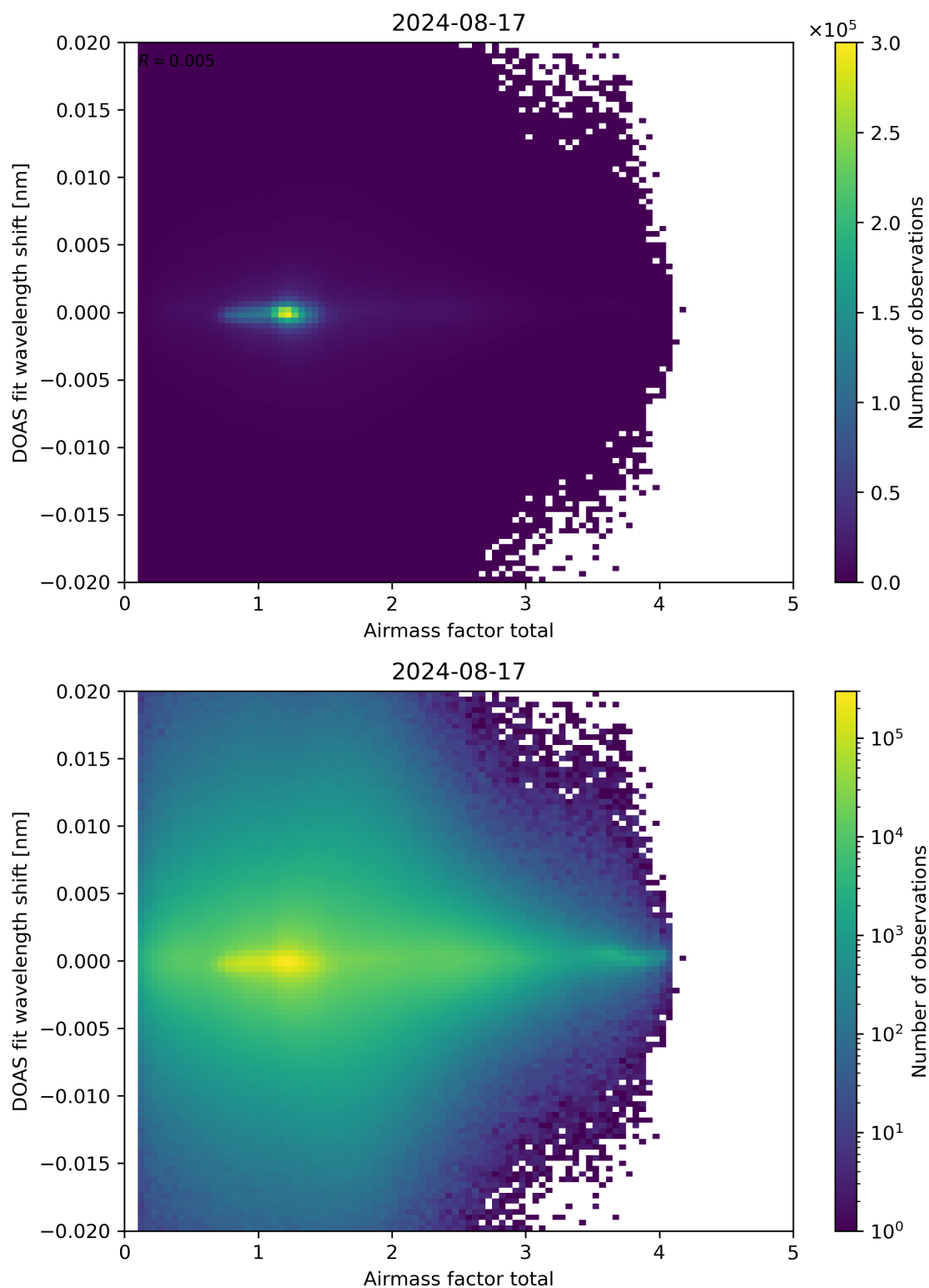
Figure 98: Scatter density plot of “Airmass factor total” against “DOAS fit wavelength shift” for 2024-08-16 to 2024-08-18.
