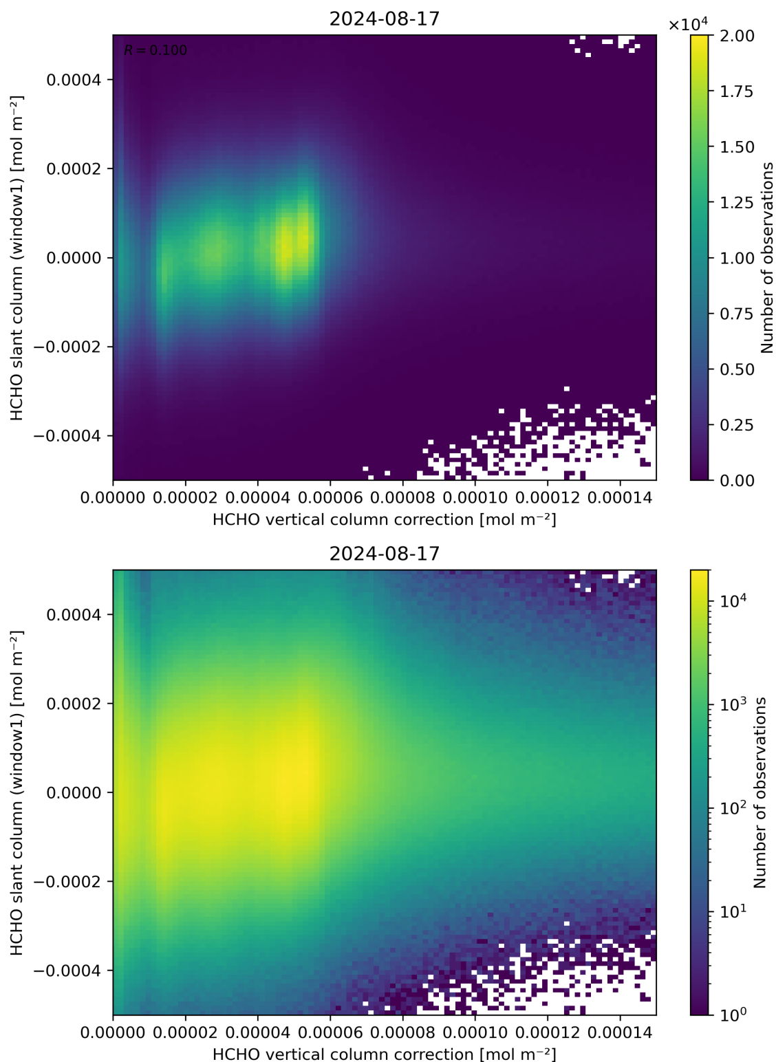
Figure 118: Scatter density plot of “HCHO vertical column correction” against “HCHO slant column (window1)” for 2024-08-16 to 2024-08-18.
