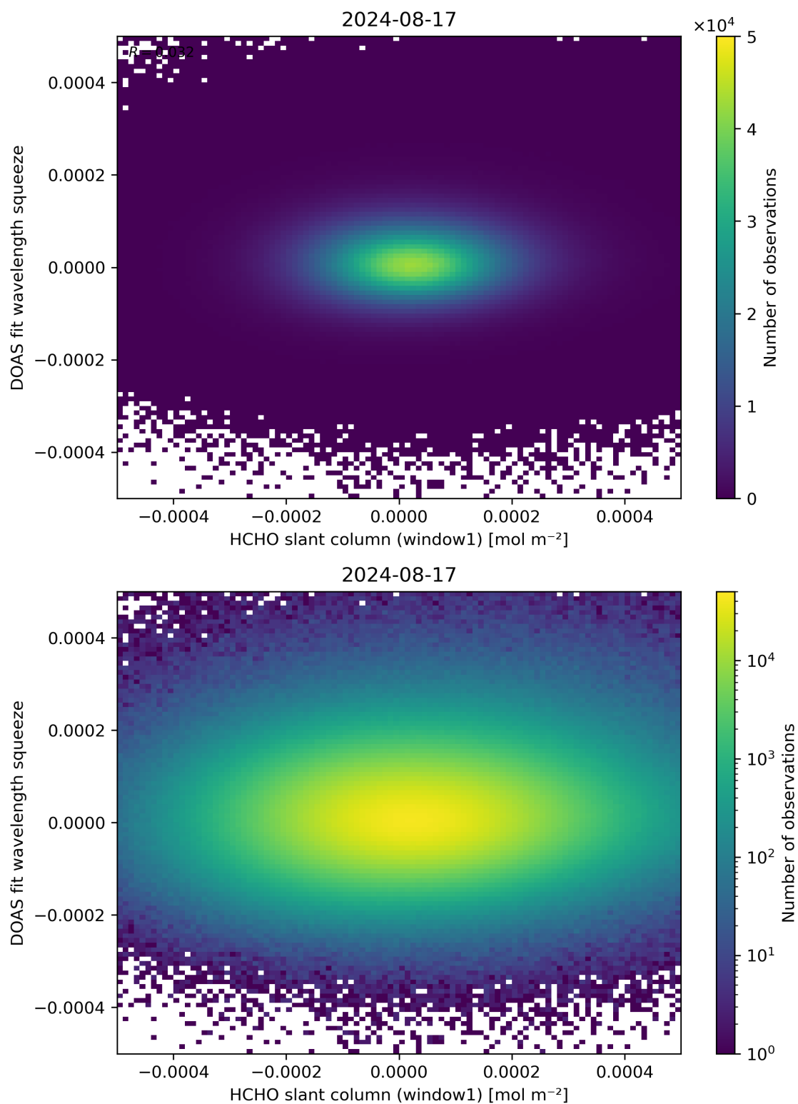
Figure 80: Scatter density plot of “HCHO slant column (window1)” against “DOAS fit wavelength squeeze” for 2024-08-16 to 2024-08-18.
