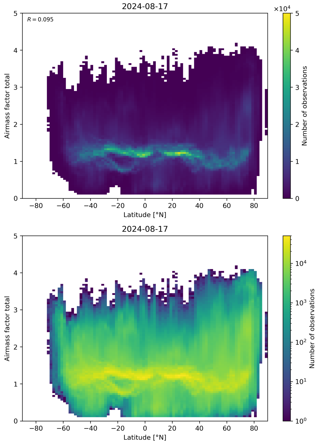
Figure 161: Scatter density plot of “Latitude” against “Airmass factor total” for 2024-08-16 to 2024-08-18.
