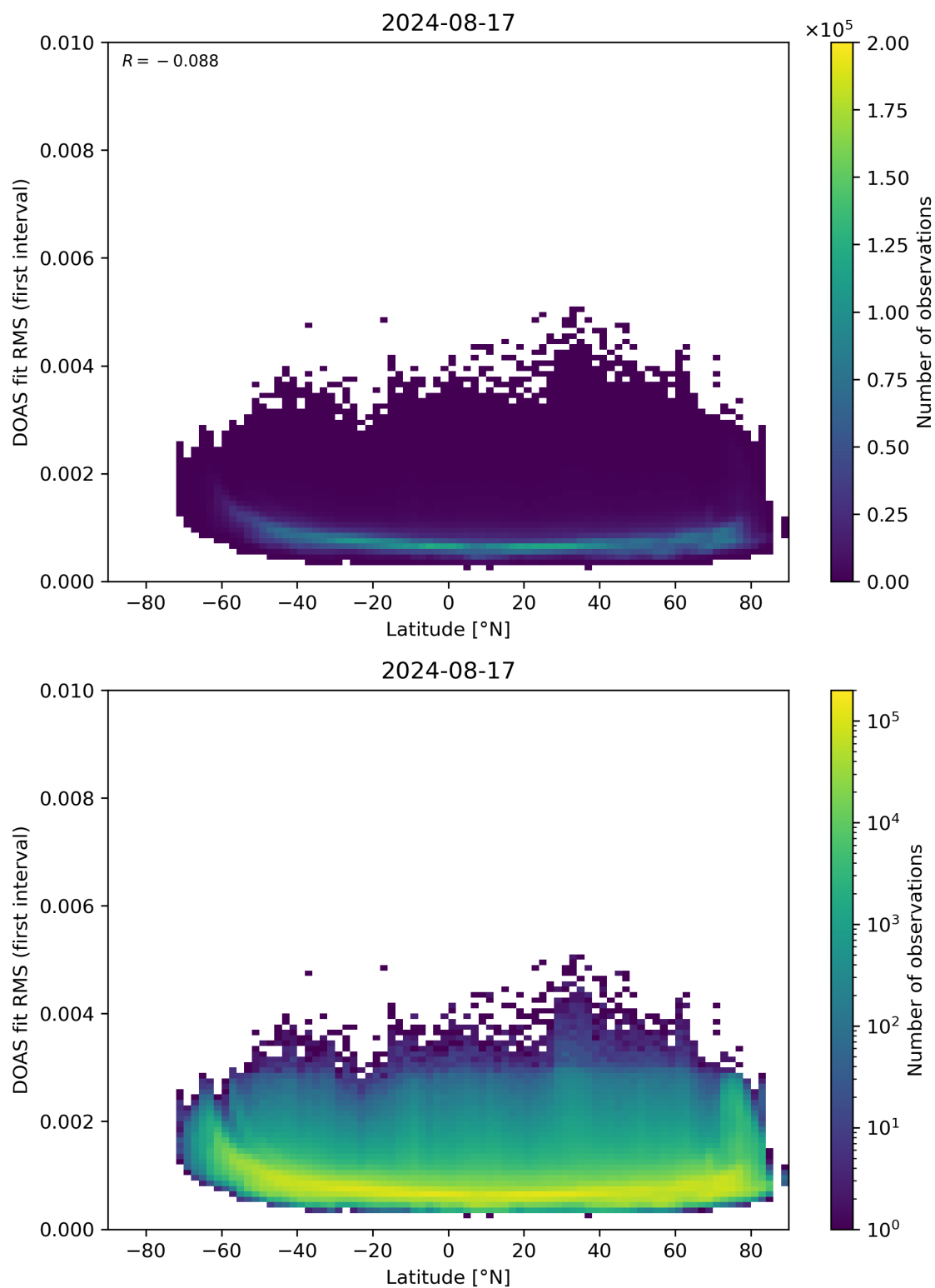
Figure 153: Scatter density plot of “Latitude” against “DOAS fit RMS (first interval)” for 2024-08-16 to 2024-08-18.
