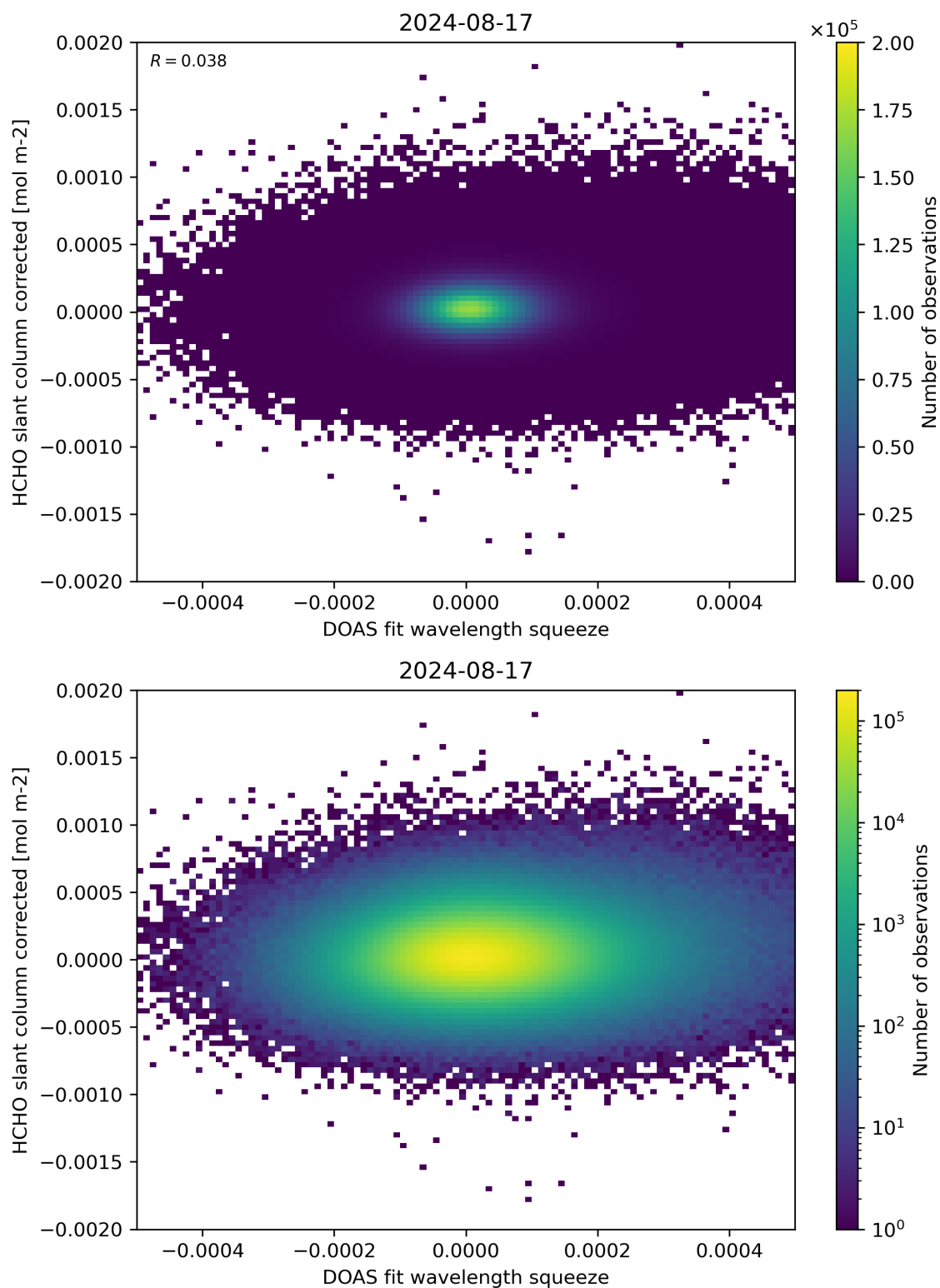
Figure 69: Scatter density plot of “DOAS fit wavelength squeeze” against “HCHO slant column corrected” for 2024-08-16 to 2024-08-18.
