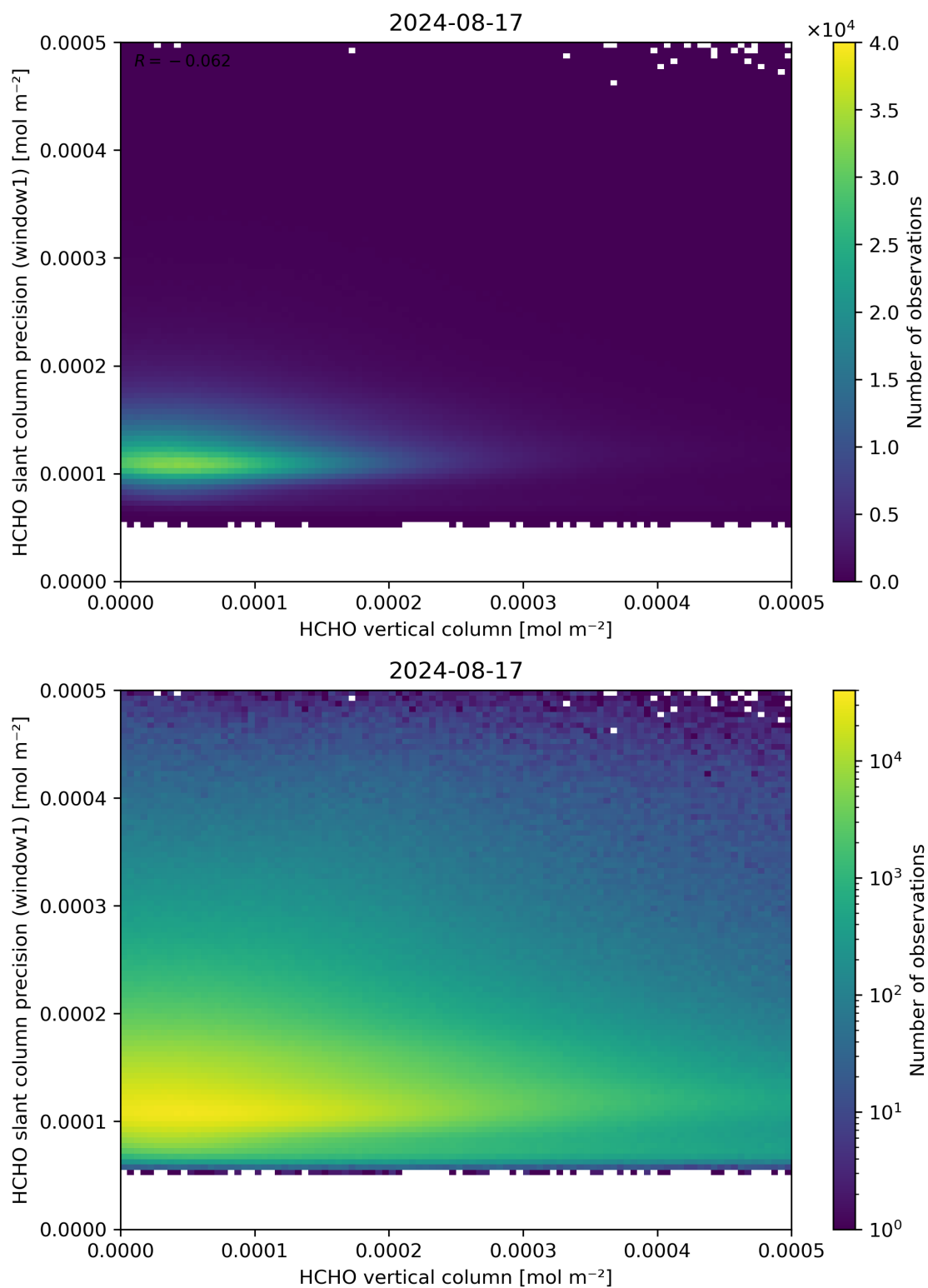
Figure 130: Scatter density plot of “HCHO vertical column” against “HCHO slant column precision (window1)” for 2024-08-16 to 2024-08-18.
