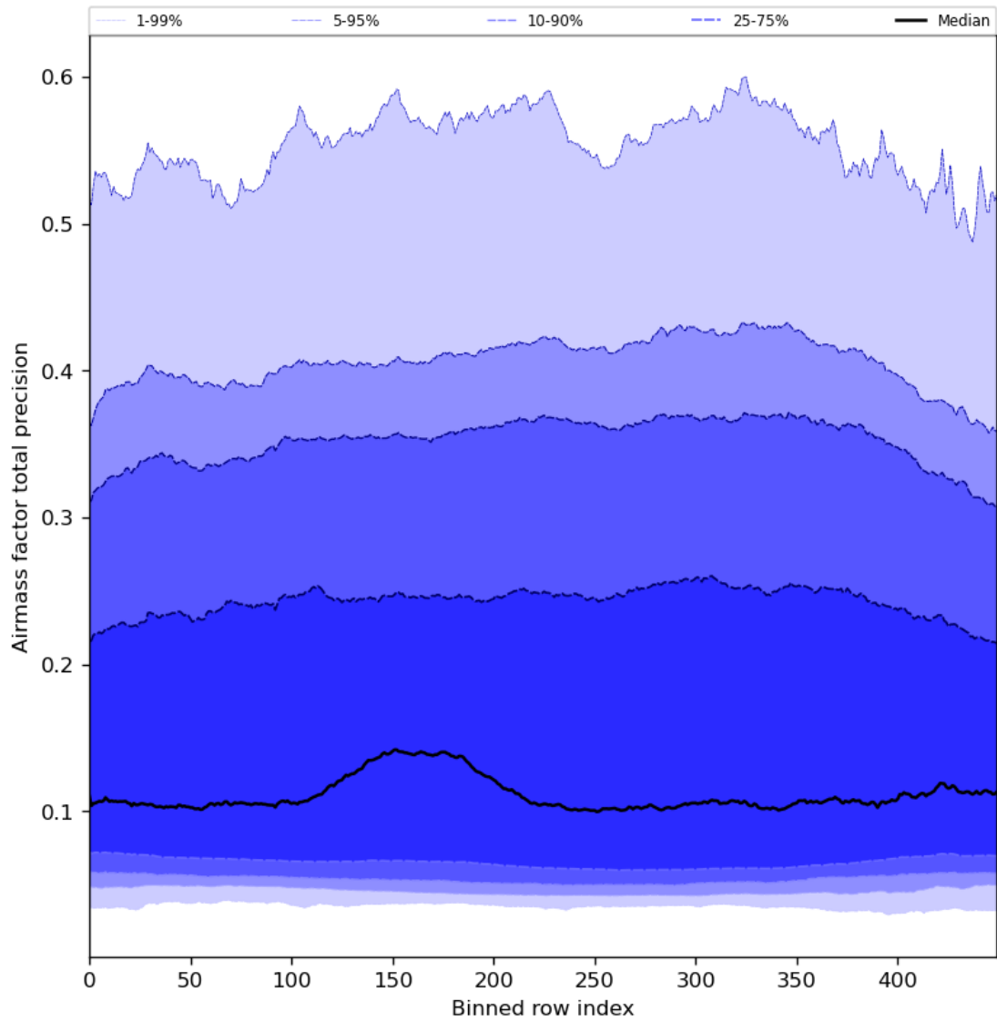
Figure 55: Along track statistics of “Airmass factor total precision” for 2024-08-16 to 2024-08-18
