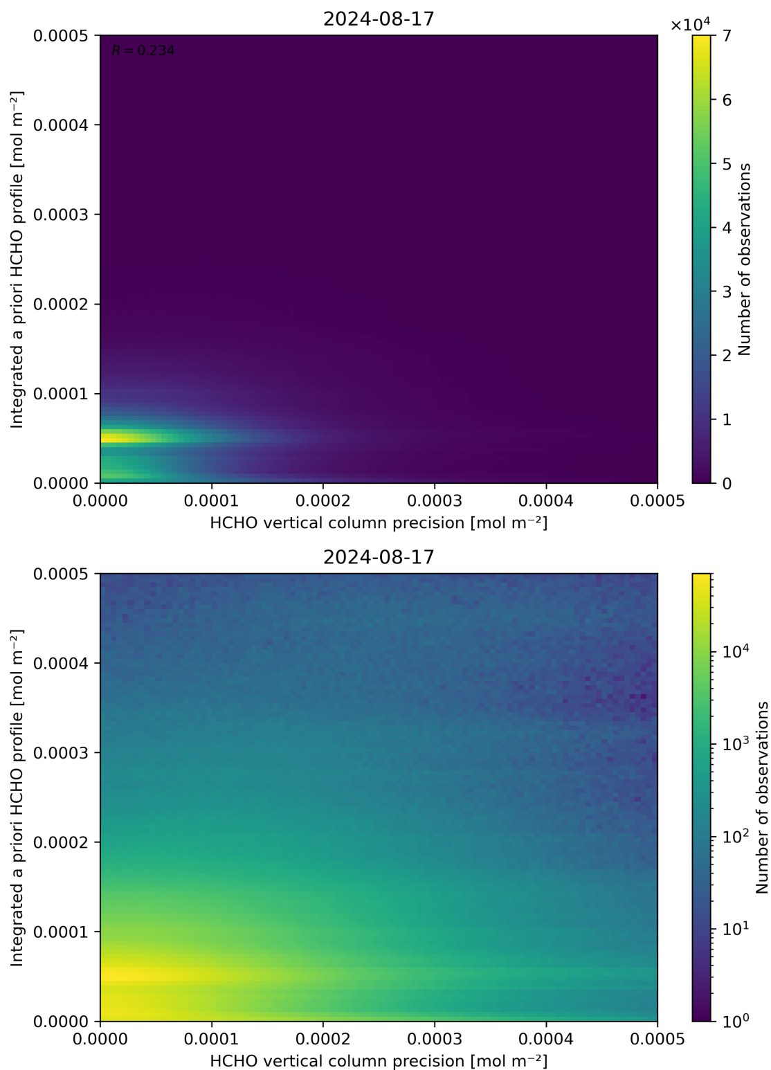
Figure 147: Scatter density plot of “HCHO vertical column precision” against “Integrated a priori HCHO profile” for 2024-08-16 to 2024-08-18.
