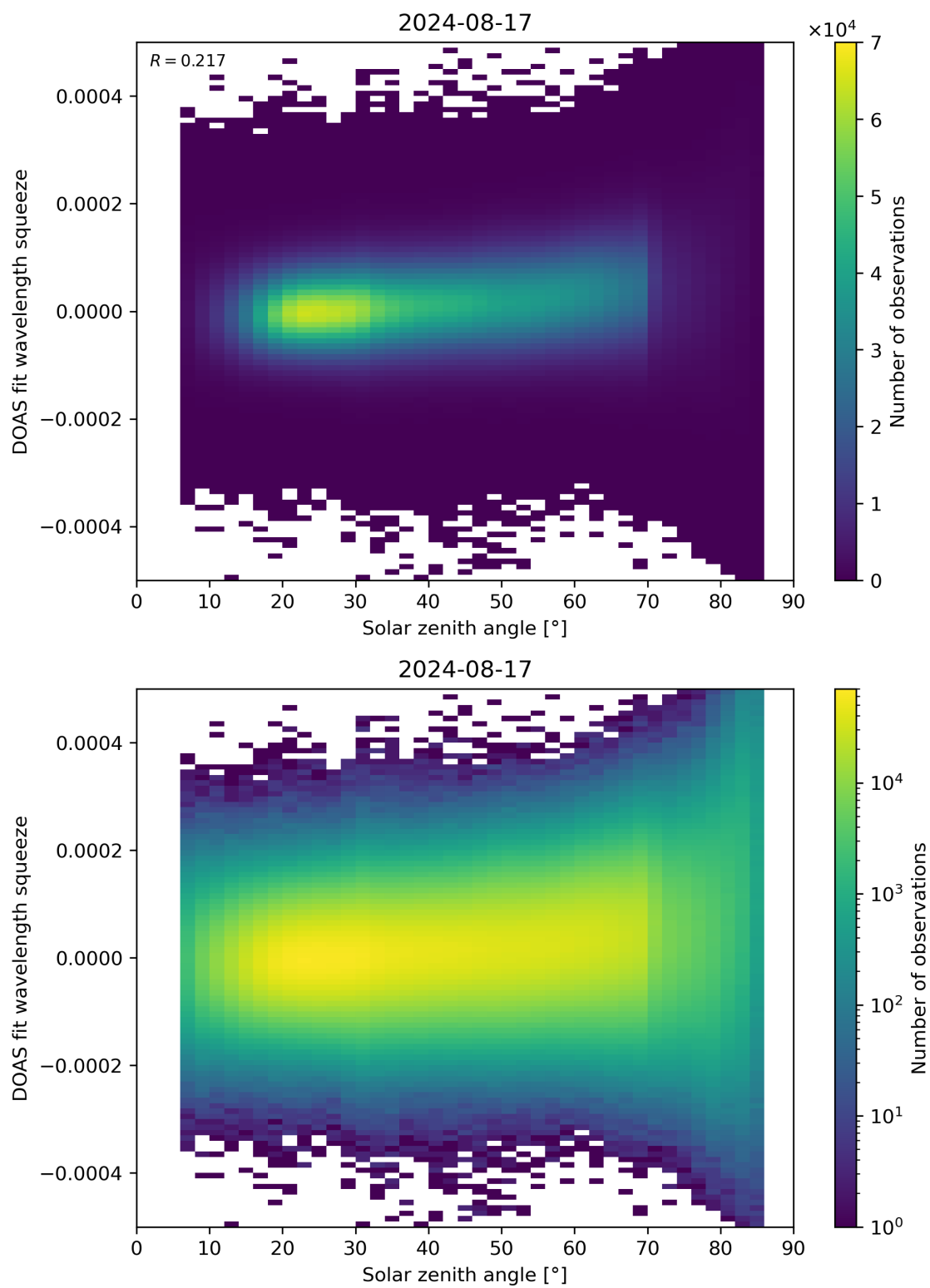
Figure 169: Scatter density plot of “Solar zenith angle” against “DOAS fit wavelength squeeze” for 2024-08-16 to 2024-08-18.
