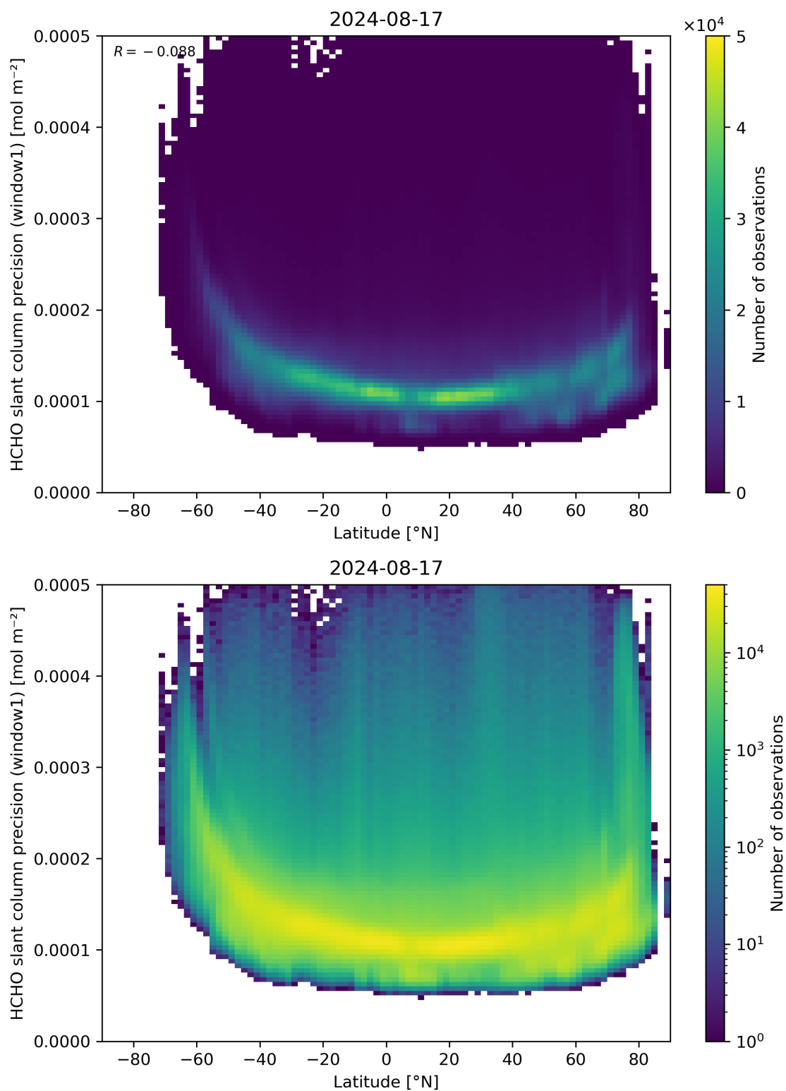
Figure 160: Scatter density plot of “Latitude” against “HCHO slant column precision (window1)” for 2024-08-16 to 2024-08-18.
