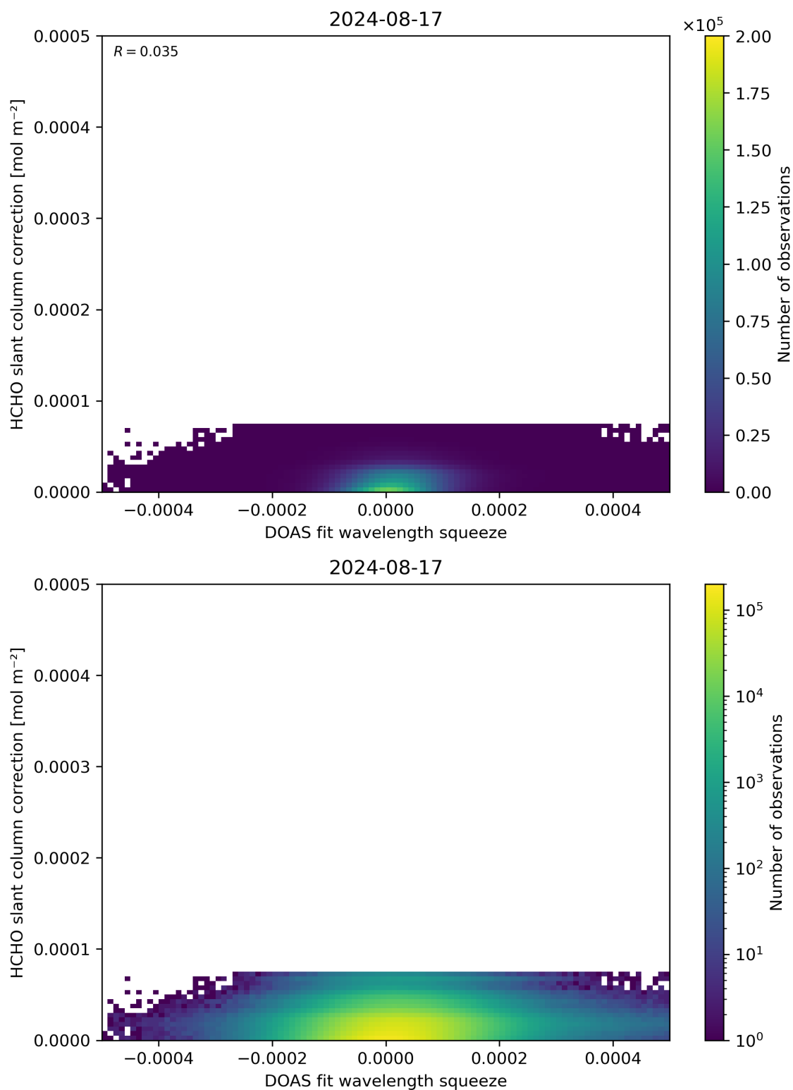
Figure 70: Scatter density plot of “DOAS fit wavelength squeeze” against “HCHO slant column correction” for 2024-08-16 to 2024-08-18.
