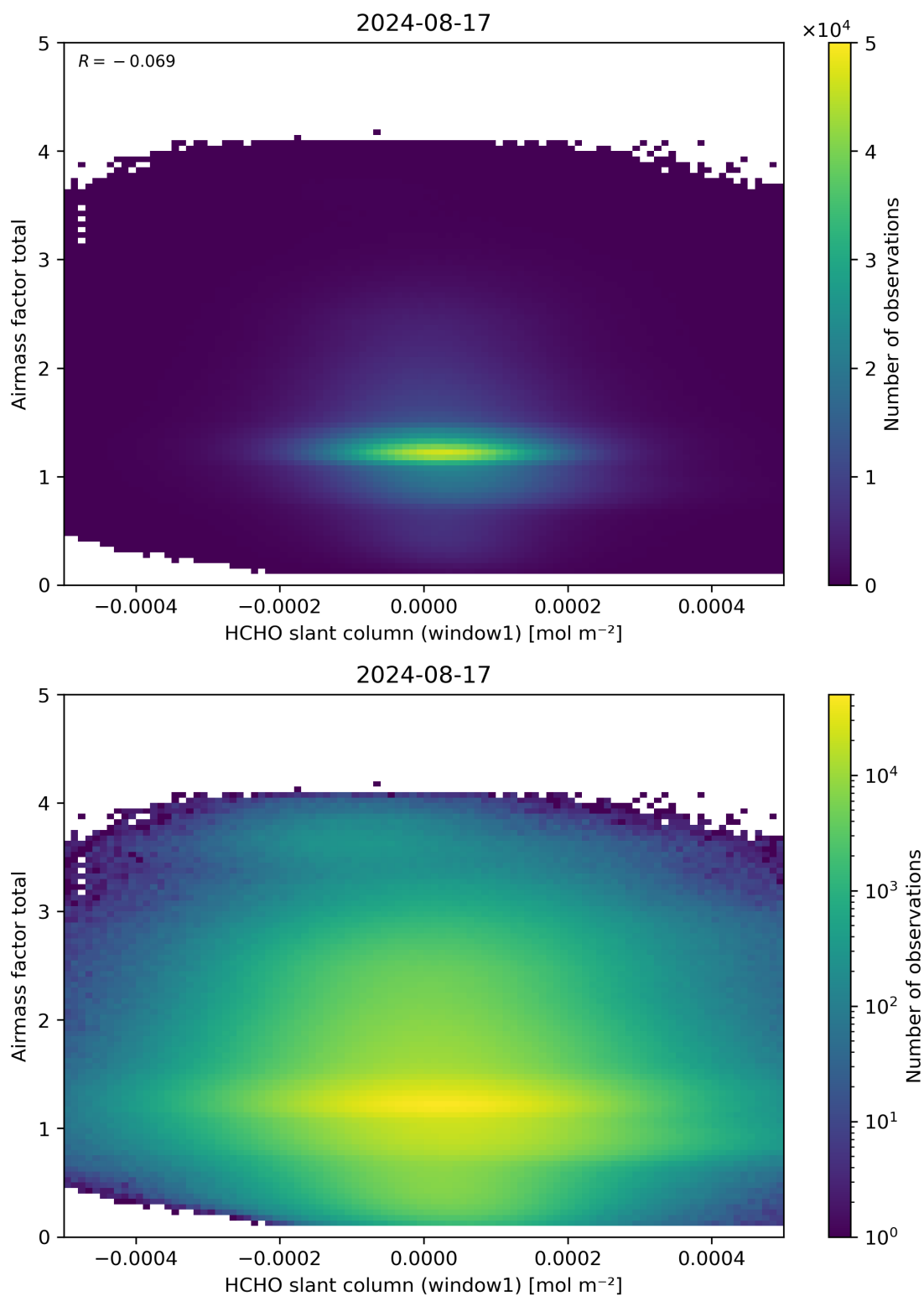
Figure 85: Scatter density plot of “HCHO slant column (window1)” against “Airmass factor total” for 2024-08-16 to 2024-08-18.
