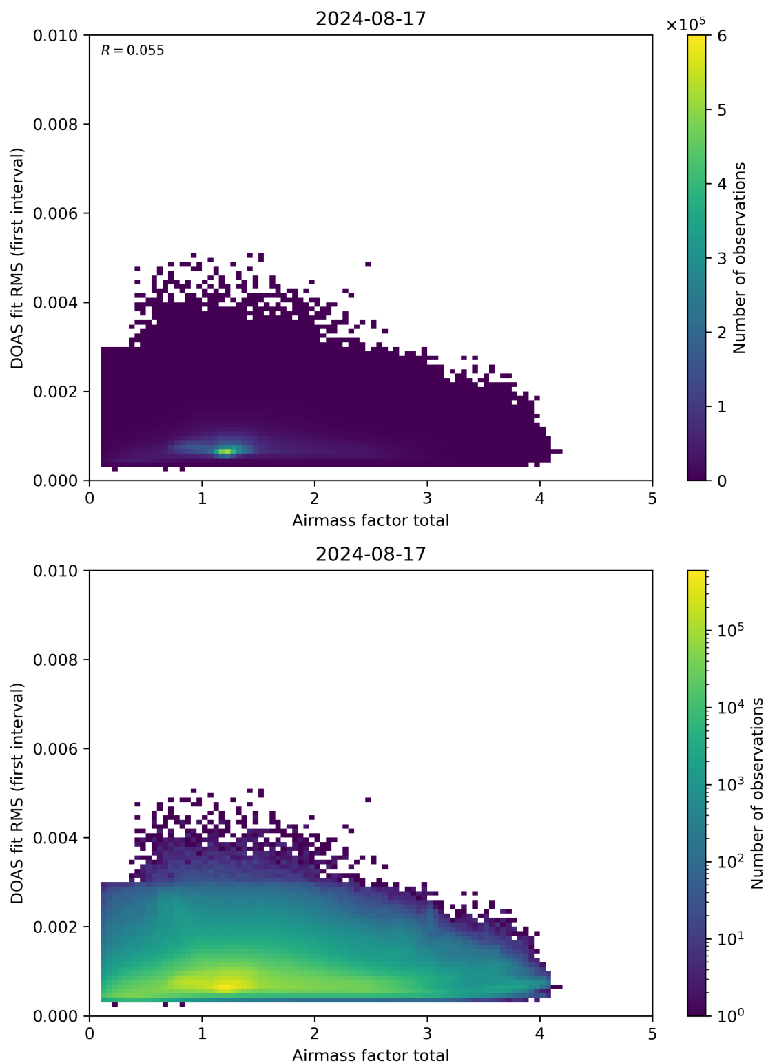
Figure 97: Scatter density plot of “Airmass factor total” against “DOAS fit RMS (first interval)” for 2024-08-16 to 2024-08-18.
