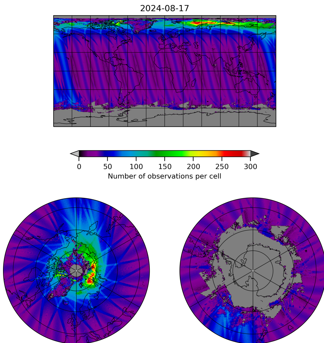
Figure 19: Map of the number of observations for 2024-08-16 to 2024-08-18
