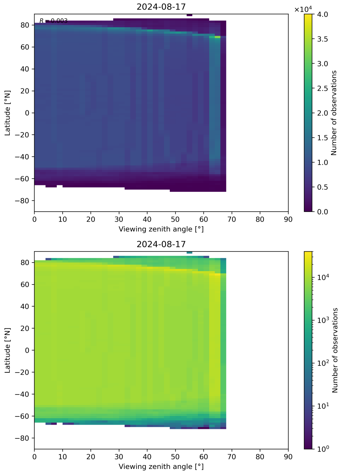
Figure 196: Scatter density plot of “Viewing zenith angle” against “Latitude” for 2024-08-16 to 2024-08-18.
