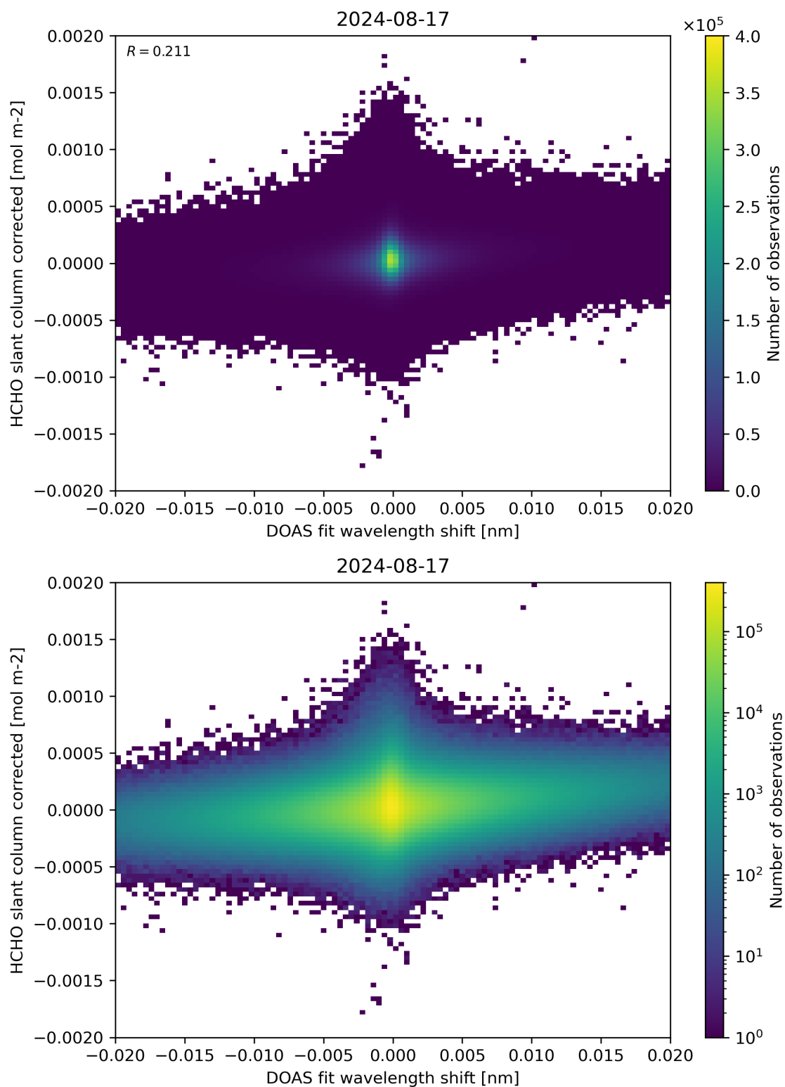
Figure 66: Scatter density plot of “DOAS fit wavelength shift” against “HCHO slant column corrected” for 2024-08-16 to 2024-08-18.
