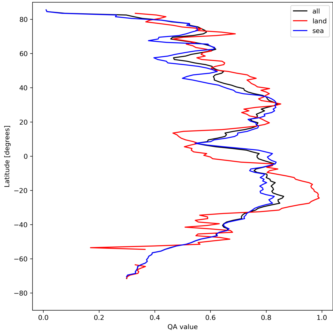
Figure 20: Zonal average of “QA value” for 2024-08-16 to 2024-08-18.
