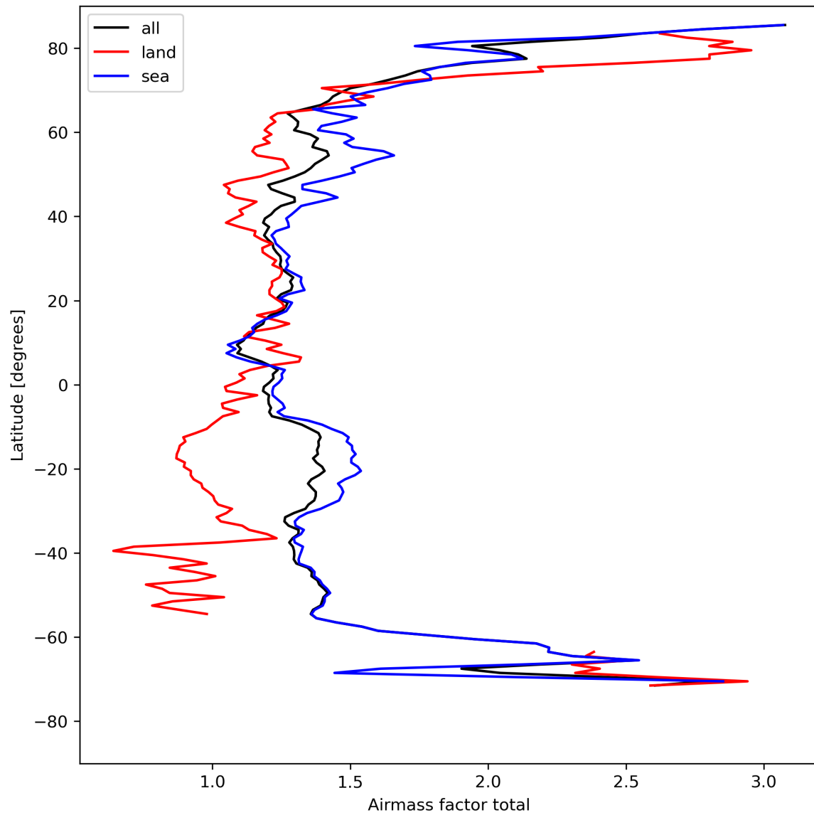
Figure 26: Zonal average of “Airmass factor total” for 2024-08-16 to 2024-08-18.
