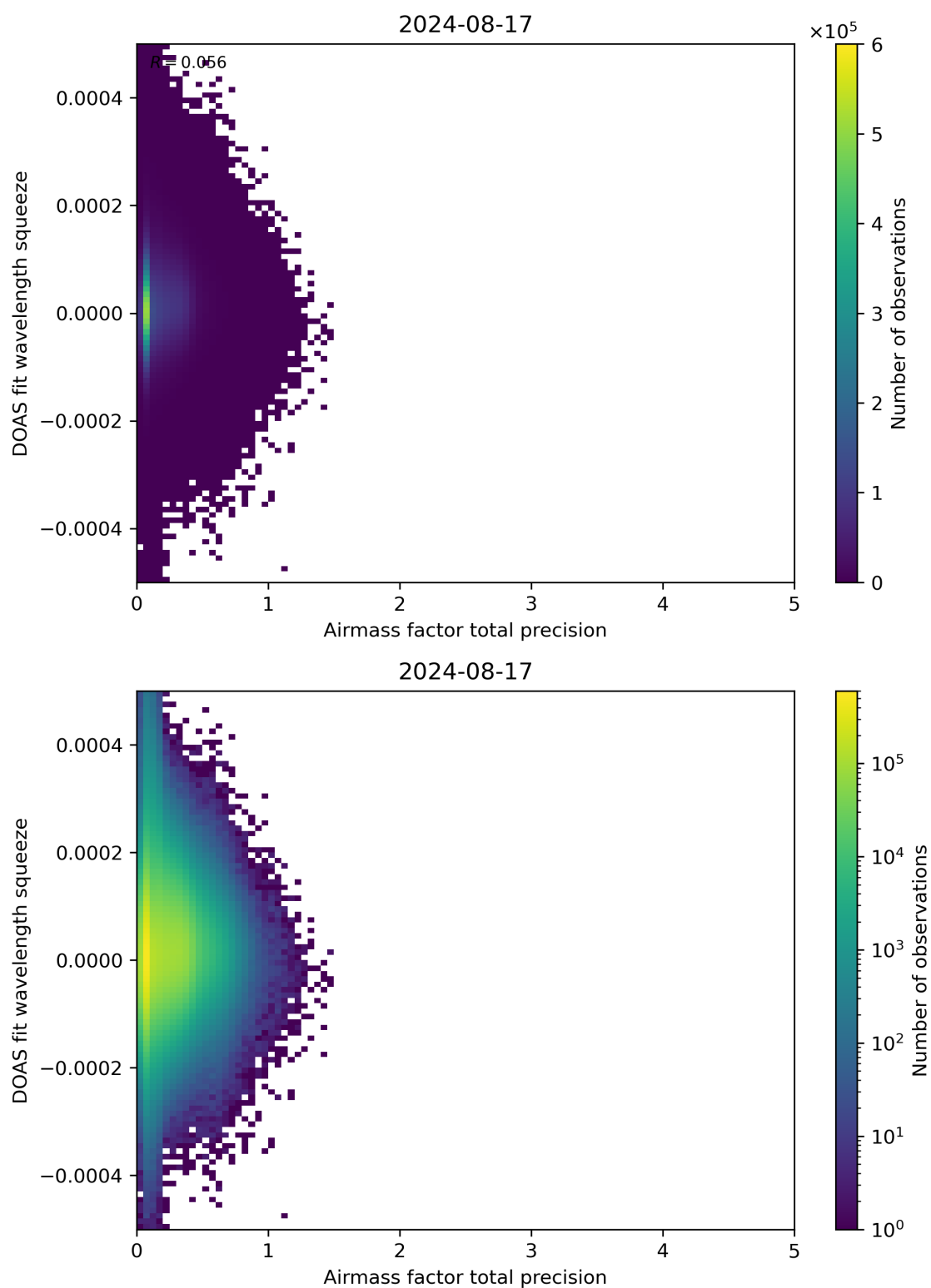
Figure 107: Scatter density plot of “Airmass factor total precision” against “DOAS fit wavelength squeeze” for 2024-08-16 to 2024-08-18.
