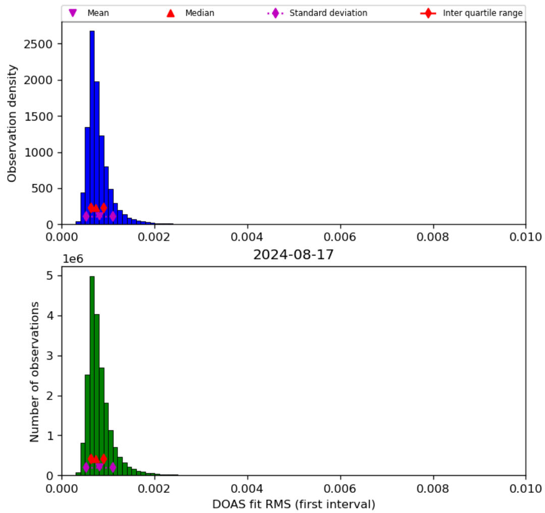
Figure 46: Histogram of “DOAS fit RMS (first interval)” for 2024-08-16 to 2024-08-18
