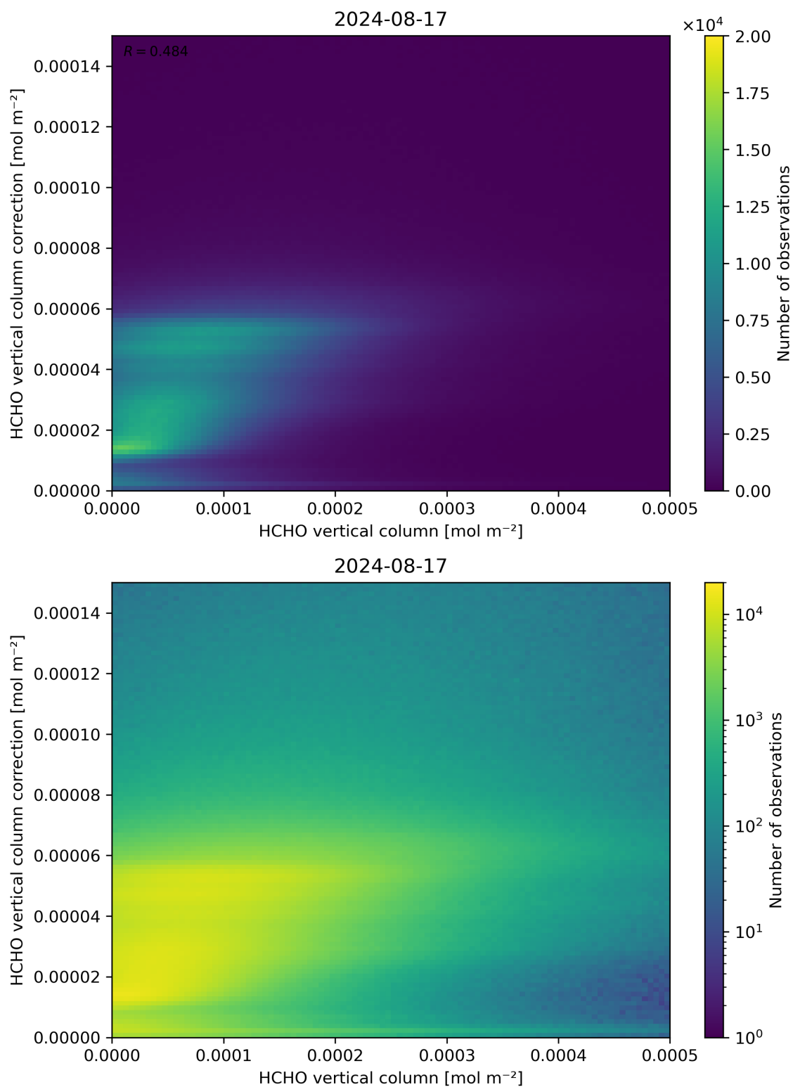
Figure 133: Scatter density plot of “HCHO vertical column” against “HCHO vertical column correction” for 2024-08-16 to 2024-08-18.
