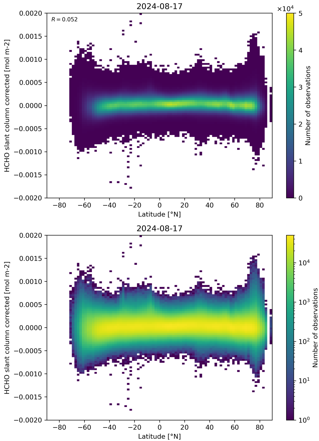
Figure 157: Scatter density plot of “Latitude” against “HCHO slant column corrected” for 2024-08-16 to 2024-08-18.
