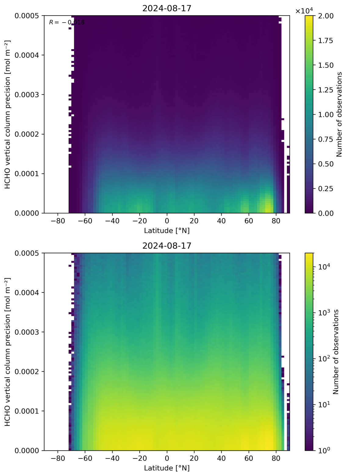
Figure 165: Scatter density plot of “Latitude” against “HCHO vertical column precision” for 2024-08-16 to 2024-08-18.
