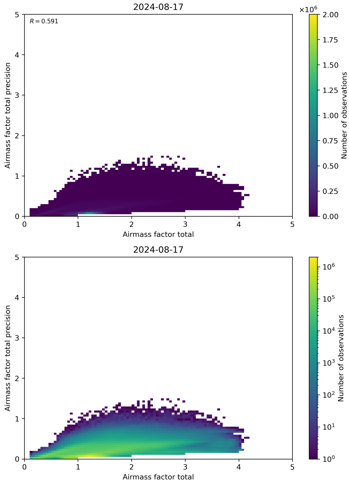
Figure 103: Scatter density plot of “Airmass factor total” against “Airmass factor total precision” for 2024-08-16 to 2024-08-18.
