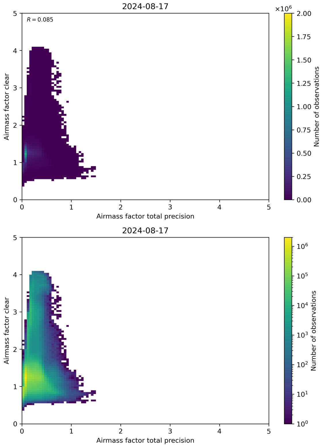
Figure 108: Scatter density plot of “Airmass factor total precision” against “Airmass factor clear” for 2024-08-16 to 2024-08-18.
