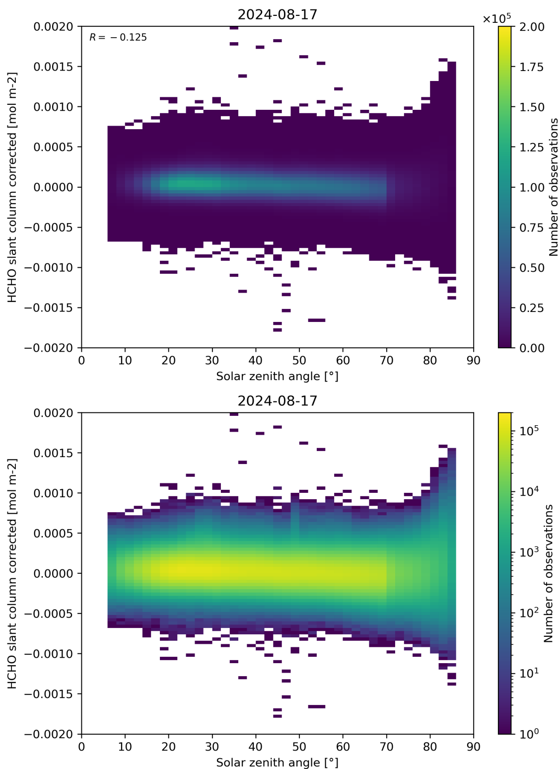
Figure 171: Scatter density plot of “Solar zenith angle” against “HCHO slant column corrected” for 2024-08-16 to 2024-08-18.
