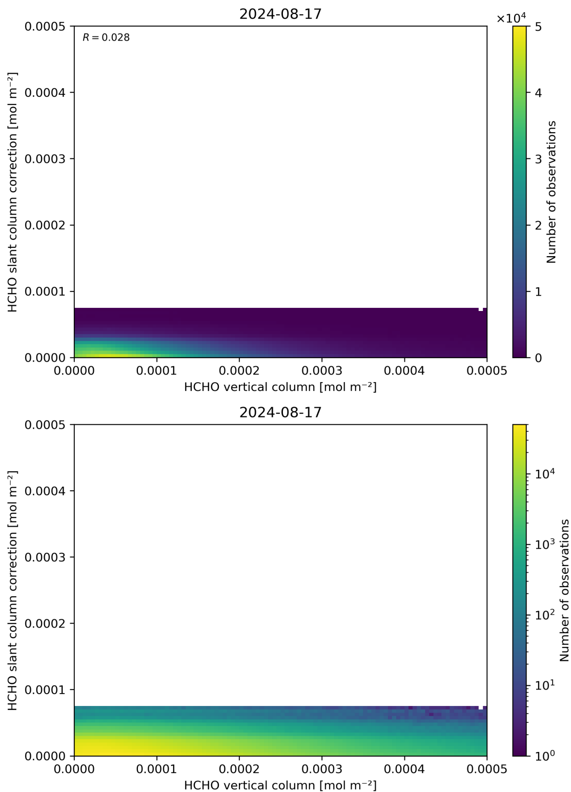
Figure 128: Scatter density plot of “HCHO vertical column” against “HCHO slant column correction” for 2024-08-16 to 2024-08-18.
