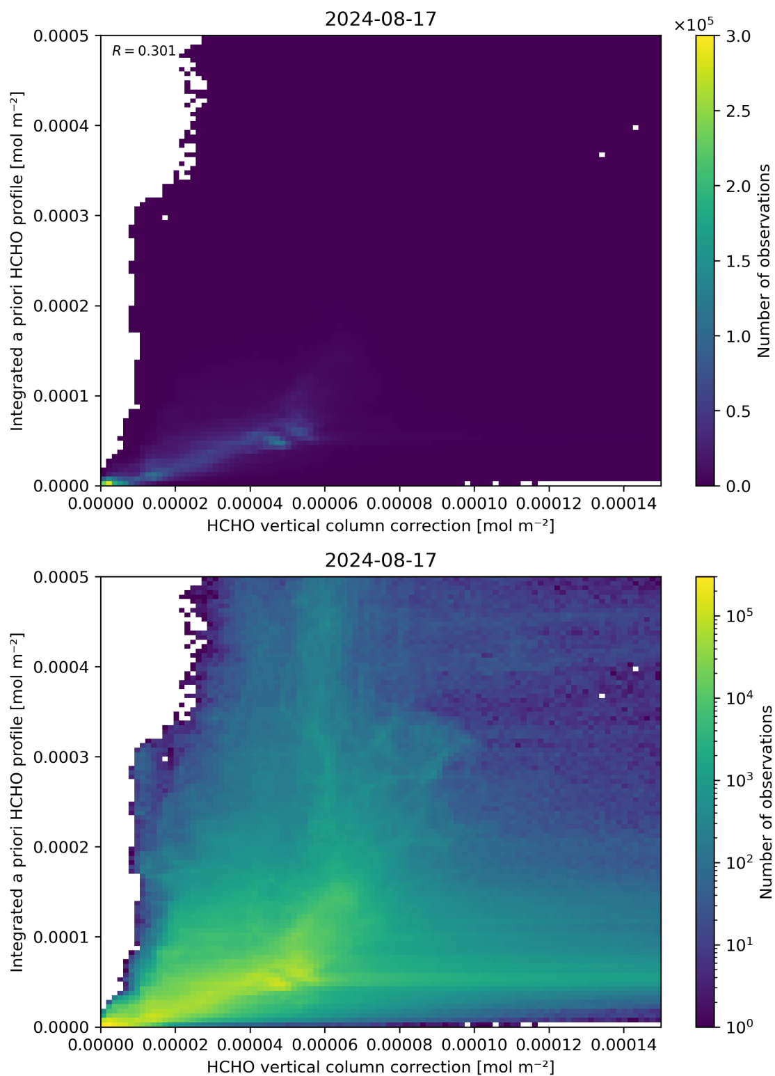
Figure 122: Scatter density plot of “HCHO vertical column correction” against “Integrated a priori HCHO profile” for 2024-08-16 to 2024-08-18.
