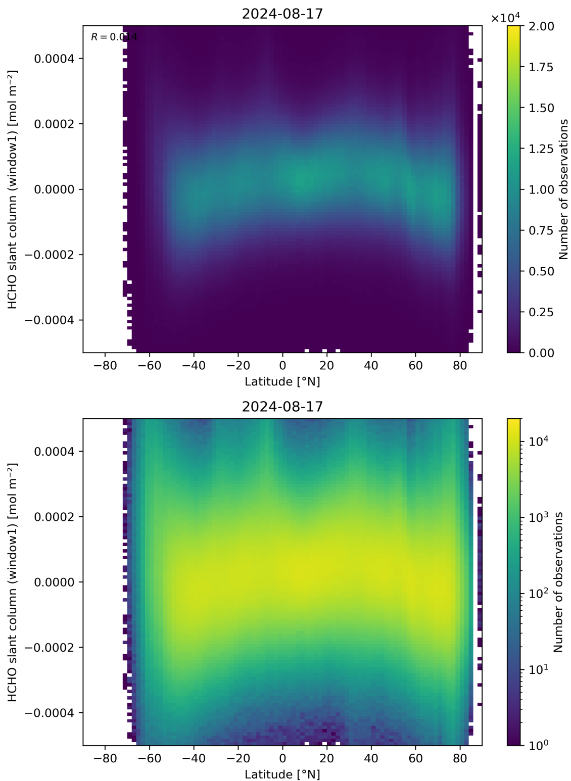
Figure 159: Scatter density plot of “Latitude” against “HCHO slant column (window1)” for 2024-08-16 to 2024-08-18.
