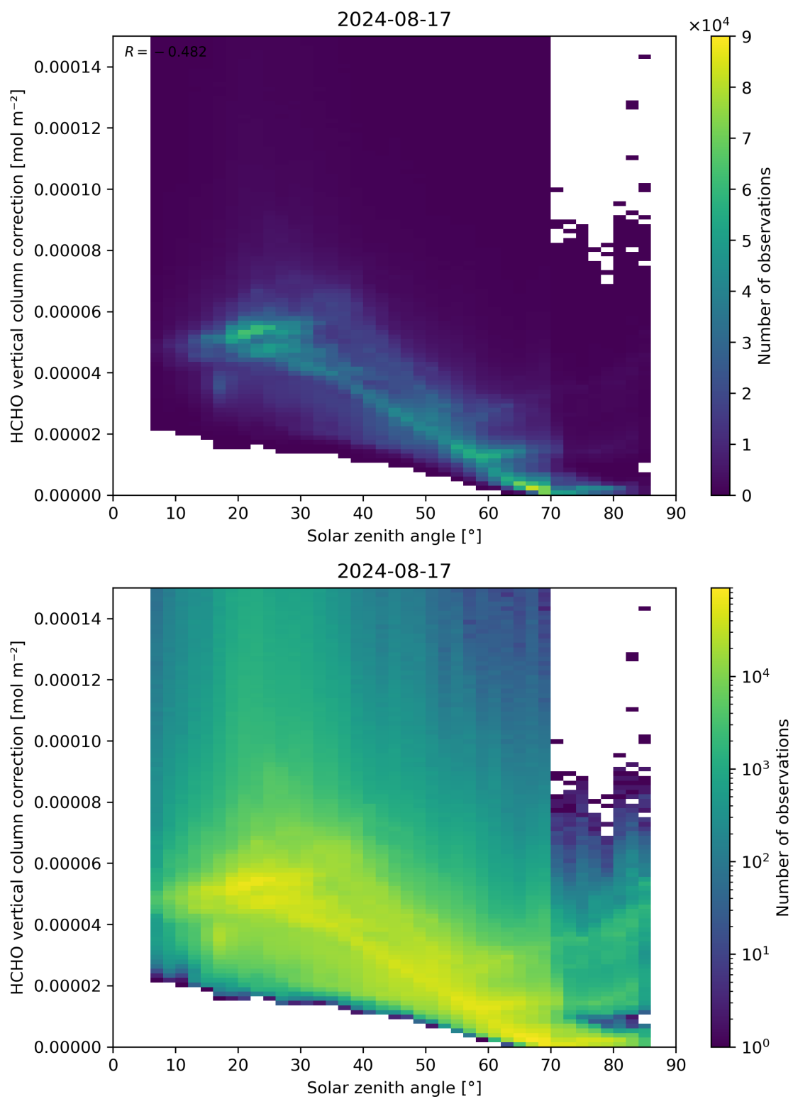
Figure 178: Scatter density plot of “Solar zenith angle” against “HCHO vertical column correction” for 2024-08-16 to 2024-08-18.
