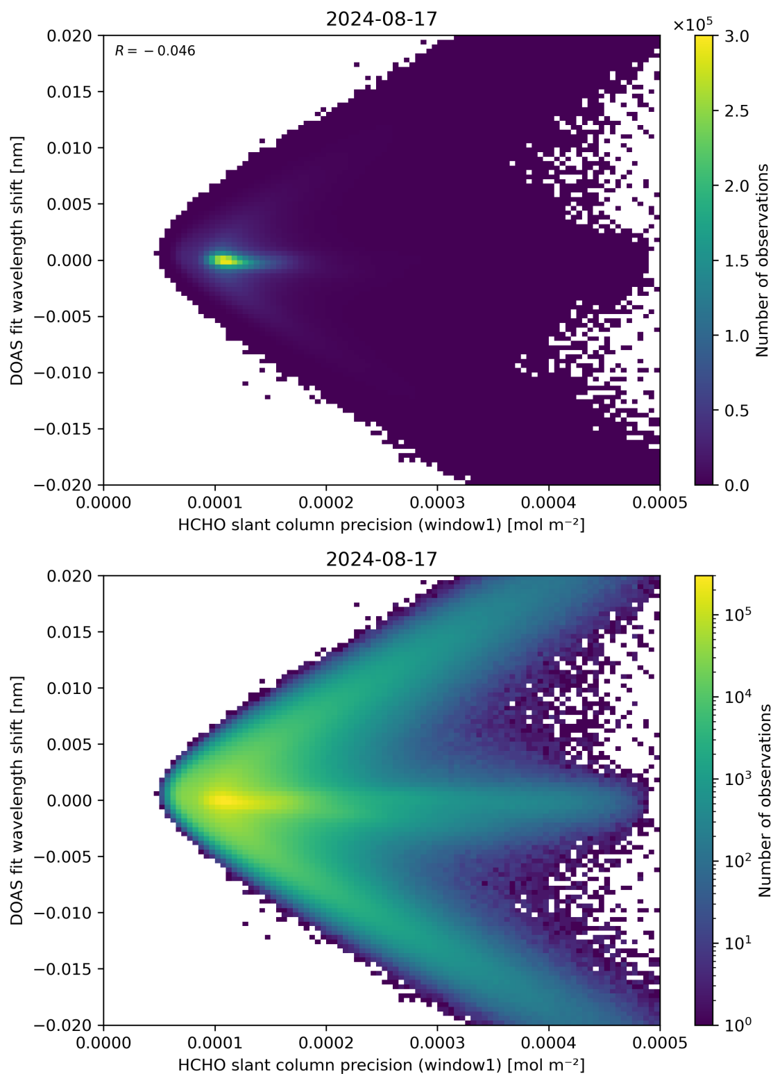
Figure 89: Scatter density plot of “HCHO slant column precision (window1)” against “DOAS fit wavelength shift” for 2024-08-16 to 2024-08-18.
