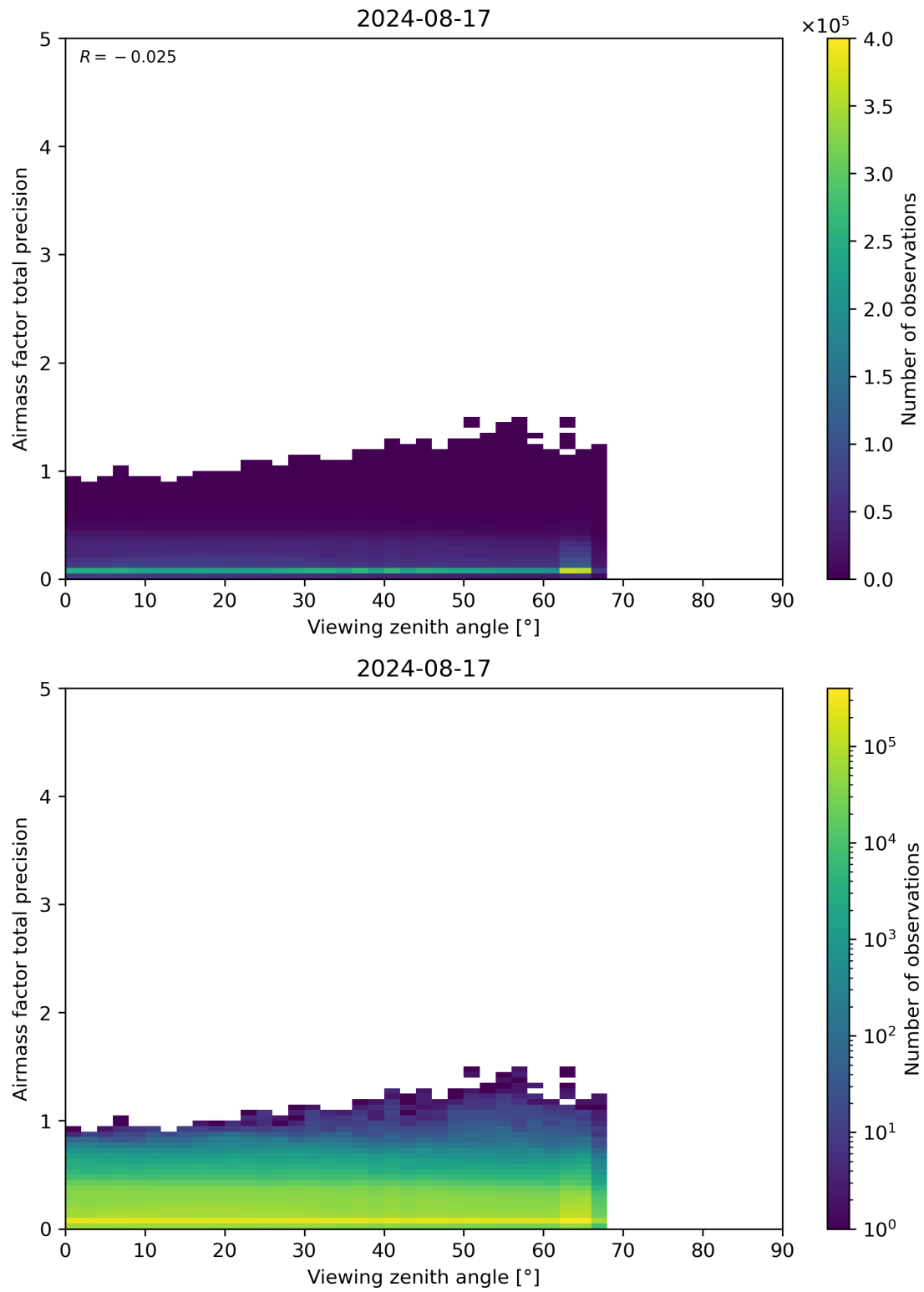
Figure 191: Scatter density plot of “Viewing zenith angle” against “Airmass factor total precision” for 2024-08-16 to 2024-08-18.
