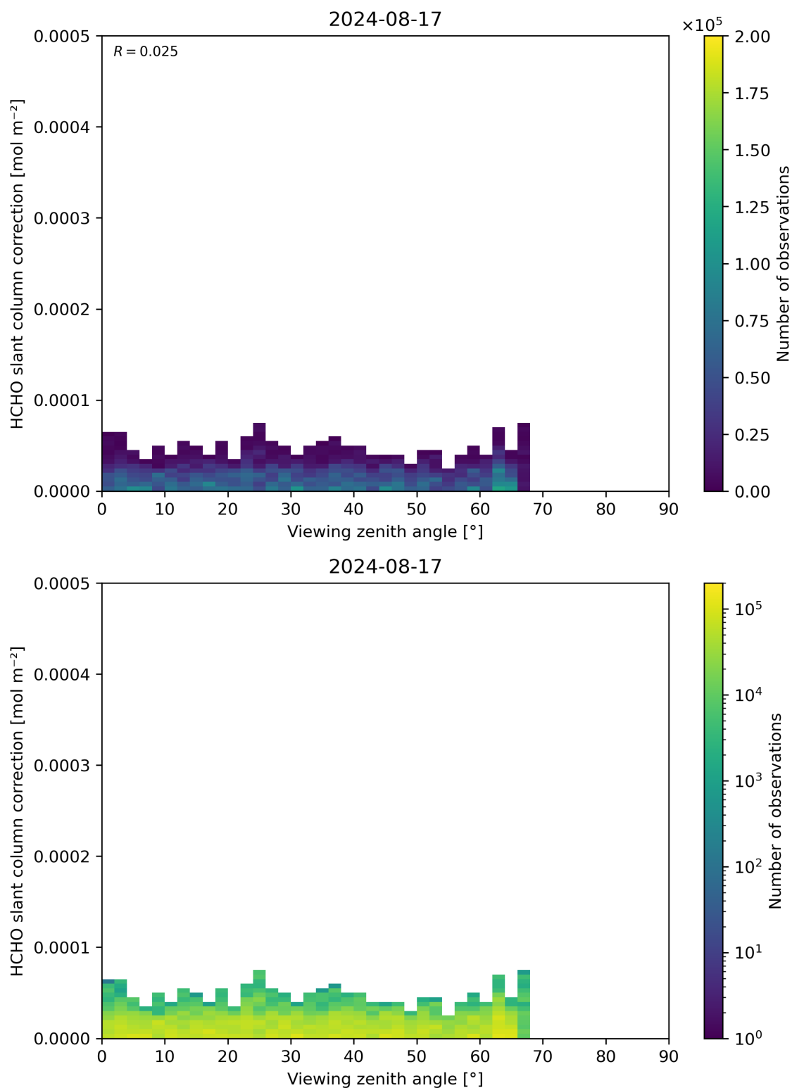
Figure 187: Scatter density plot of “Viewing zenith angle” against “HCHO slant column correction” for 2024-08-16 to 2024-08-18.
