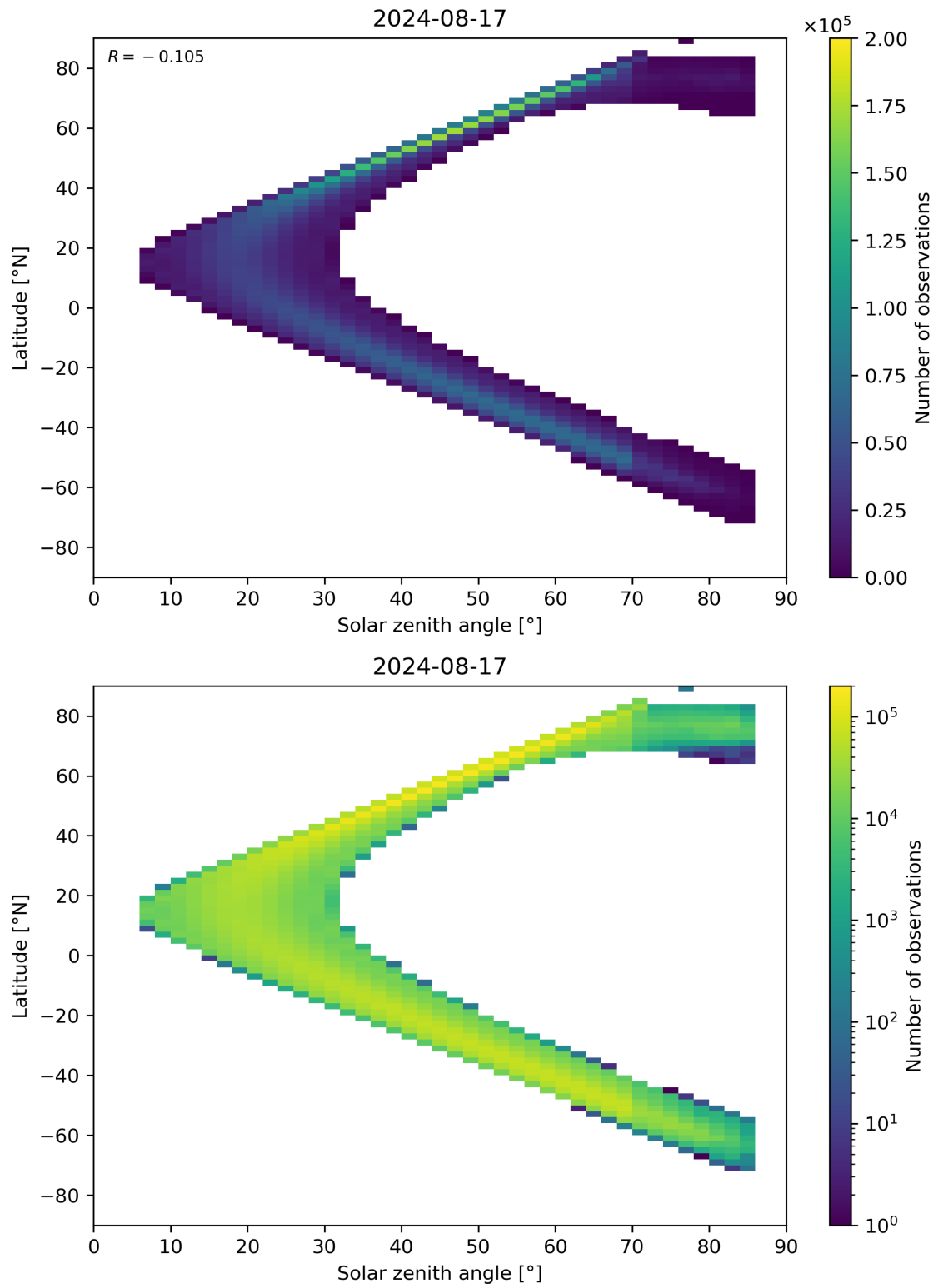
Figure 181: Scatter density plot of “Solar zenith angle” against “Latitude” for 2024-08-16 to 2024-08-18.
