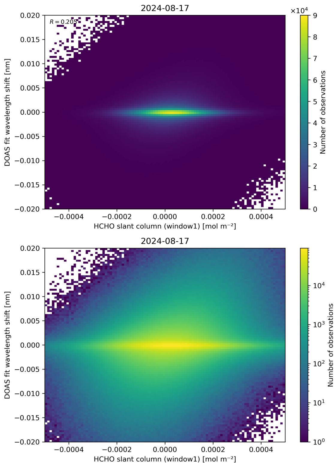
Figure 79: Scatter density plot of “HCHO slant column (window1)” against “DOAS fit wavelength shift” for 2024-08-16 to 2024-08-18.
