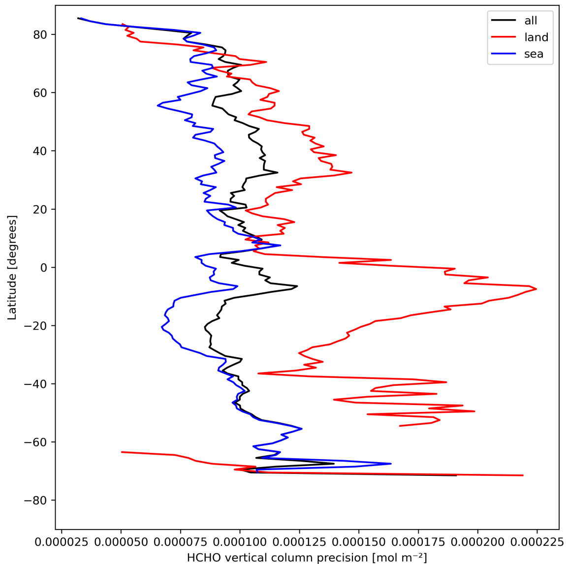
Figure 22: Zonal average of “HCHO vertical column precision” for 2024-08-16 to 2024-08-18.
