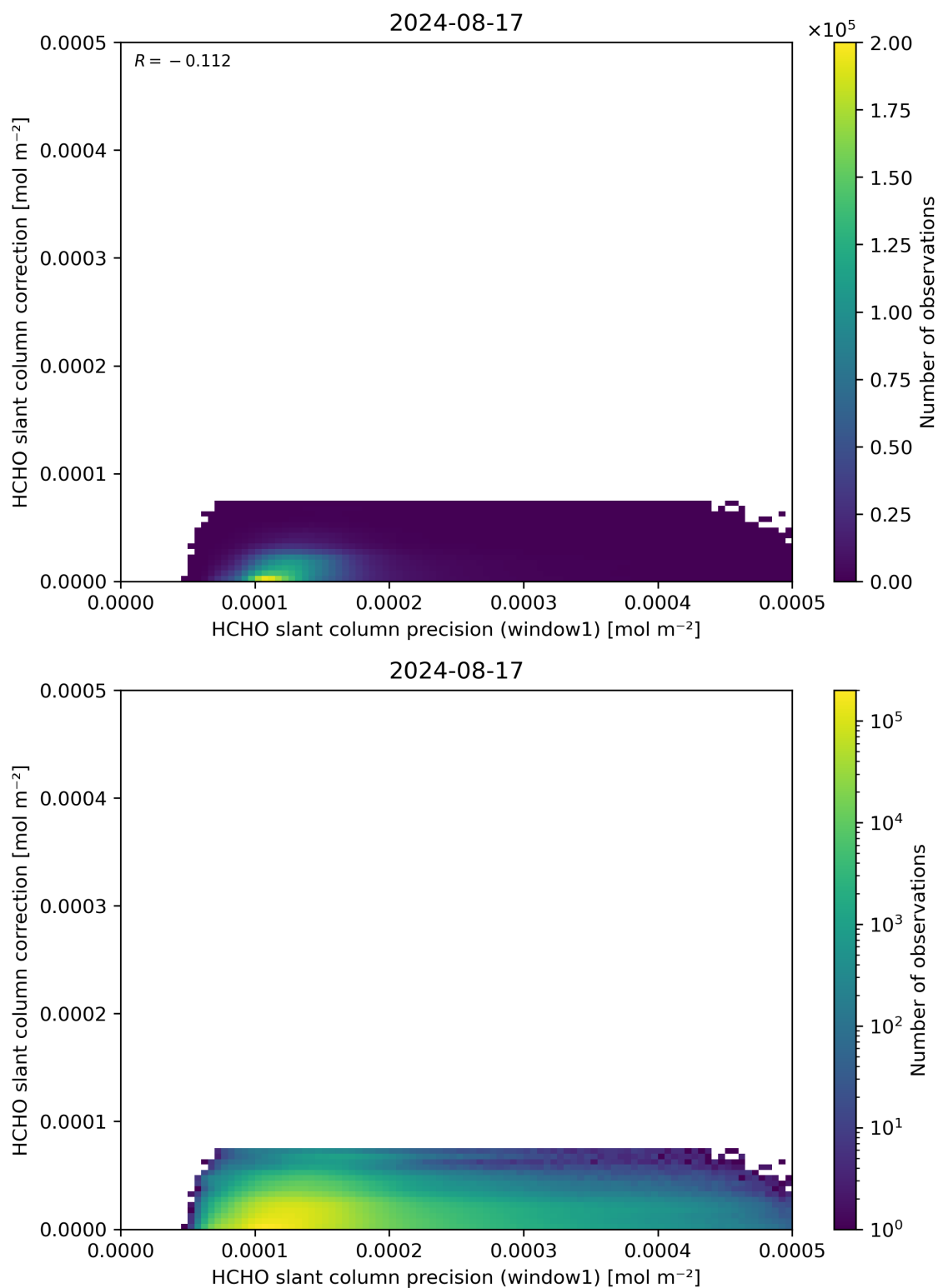
Figure 93: Scatter density plot of “HCHO slant column precision (window1)” against “HCHO slant column correction” for 2024-08-16 to 2024-08-18.
