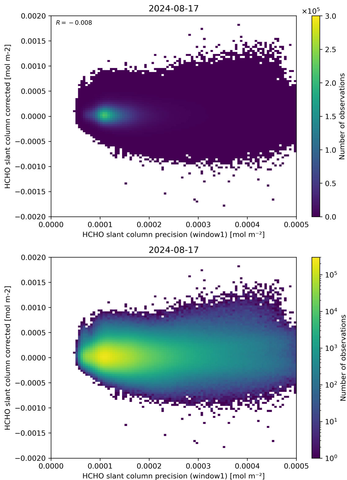
Figure 92: Scatter density plot of “HCHO slant column precision (window1)” against “HCHO slant column corrected” for 2024-08-16 to 2024-08-18.
