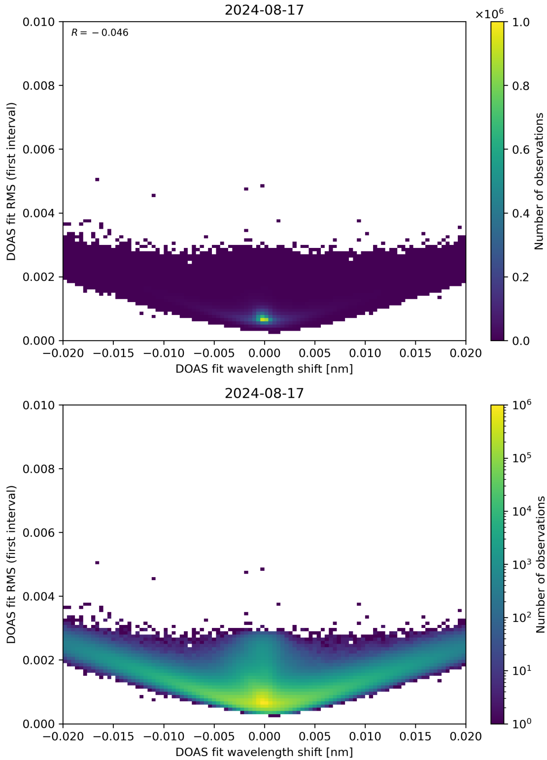
Figure 64: Scatter density plot of “DOAS fit wavelength shift” against “DOAS fit RMS (first interval)” for 2024-08-16 to 2024-08-18.
