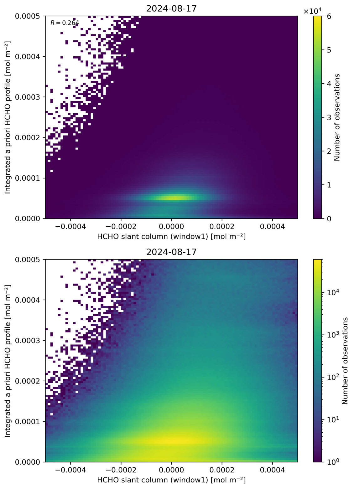
Figure 87: Scatter density plot of “HCHO slant column (window1)” against “Integrated a priori HCHO profile” for 2024-08-16 to 2024-08-18.
