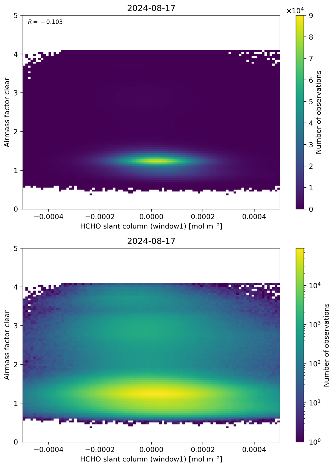
Figure 81: Scatter density plot of “HCHO slant column (window1)” against “Airmass factor clear” for 2024-08-16 to 2024-08-18.
