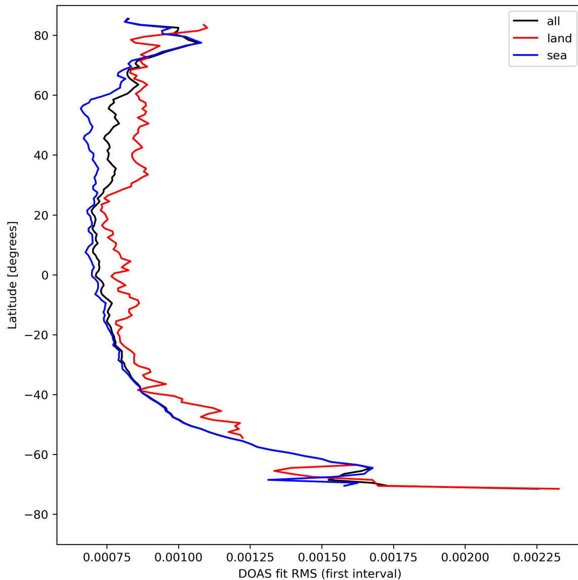
Figure 32: Zonal average of “DOAS fit RMS (first interval)” for 2024-08-16 to 2024-08-18.
