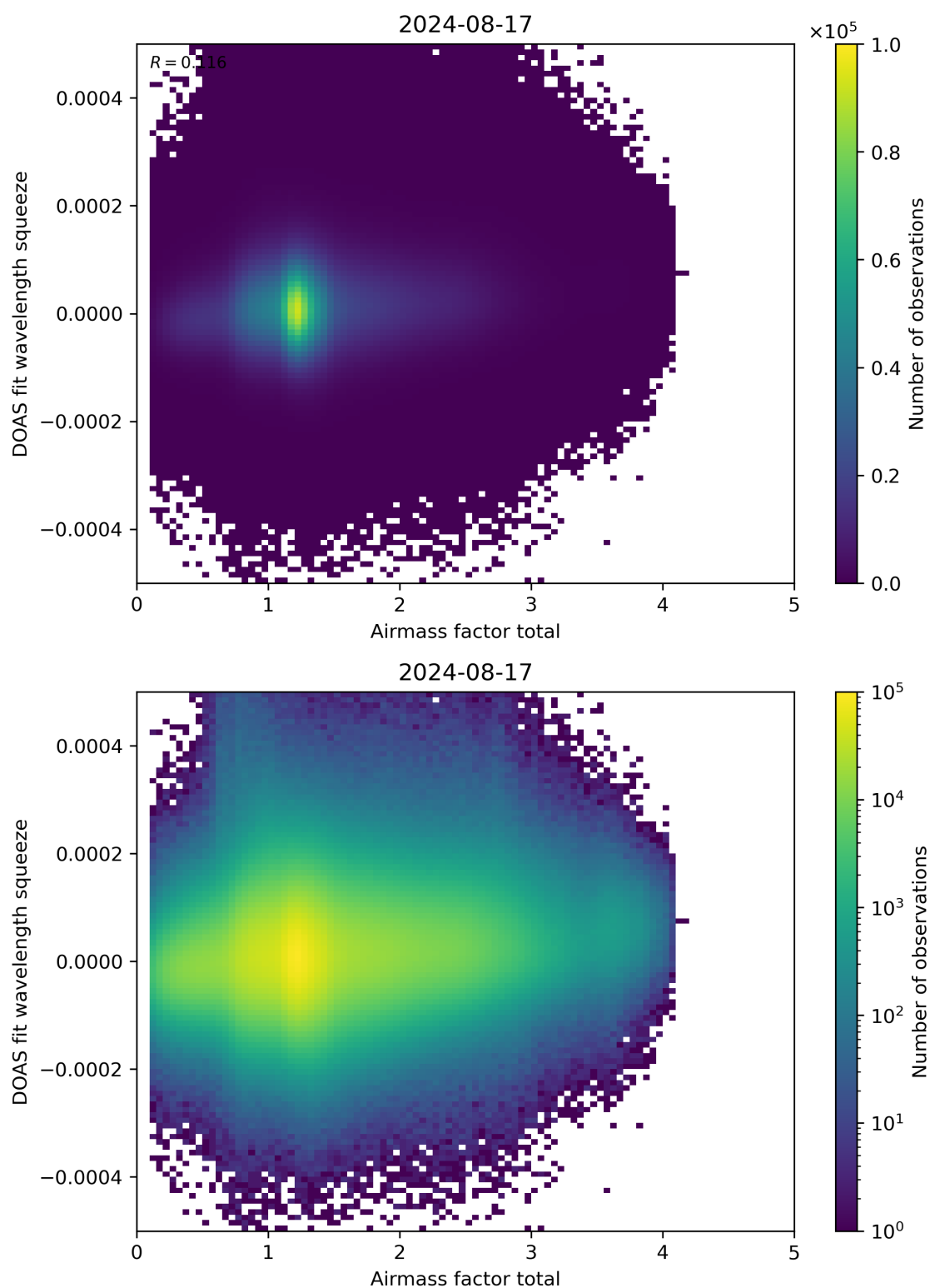
Figure 99: Scatter density plot of “Airmass factor total” against “DOAS fit wavelength squeeze” for 2024-08-16 to 2024-08-18.
