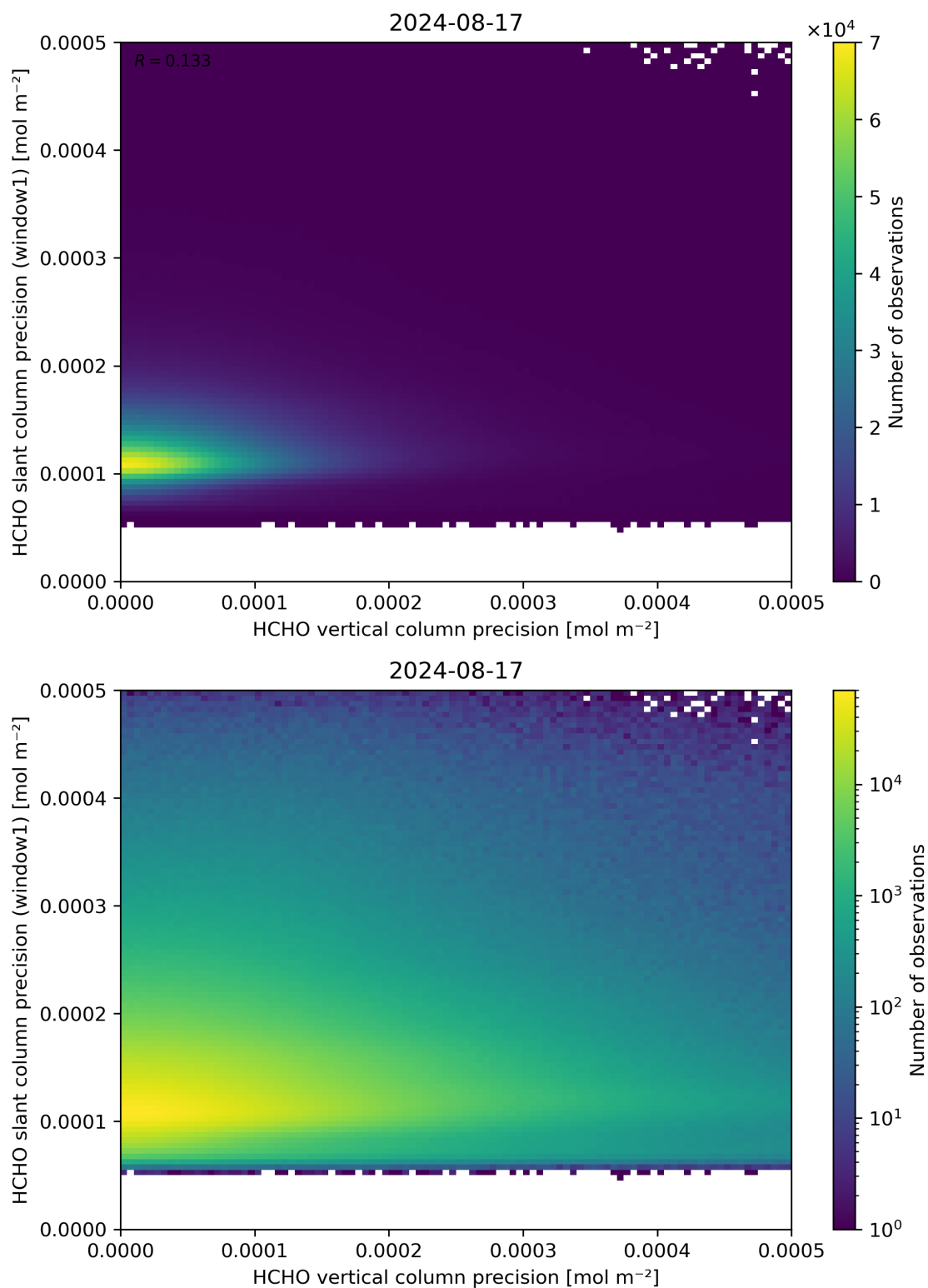
Figure 143: Scatter density plot of “HCHO vertical column precision” against “HCHO slant column precision (window1)” for 2024-08-16 to 2024-08-18.
