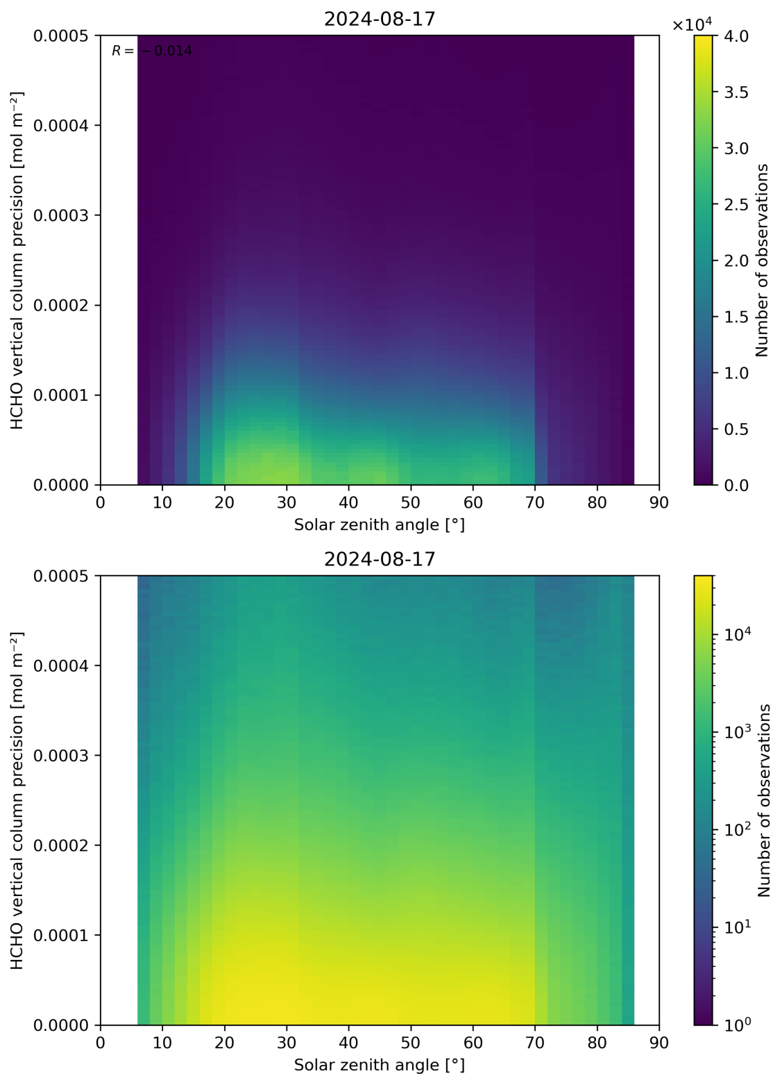
Figure 179: Scatter density plot of “Solar zenith angle” against “HCHO vertical column precision” for 2024-08-16 to 2024-08-18.
