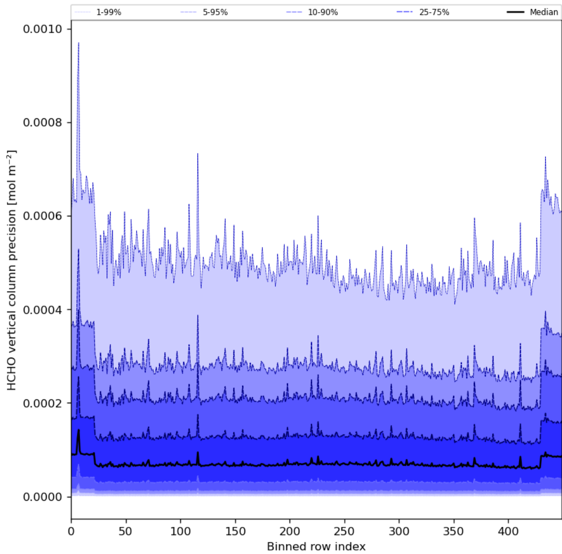
Figure 50: Along track statistics of “HCHO vertical column precision” for 2024-08-16 to 2024-08-18
