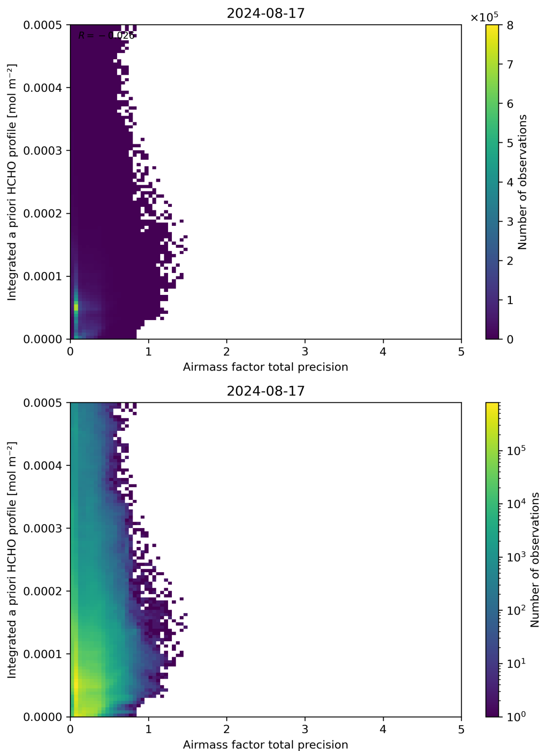
Figure 111: Scatter density plot of “Airmass factor total precision” against “Integrated a priori HCHO profile” for 2024-08-16 to 2024-08-18.
