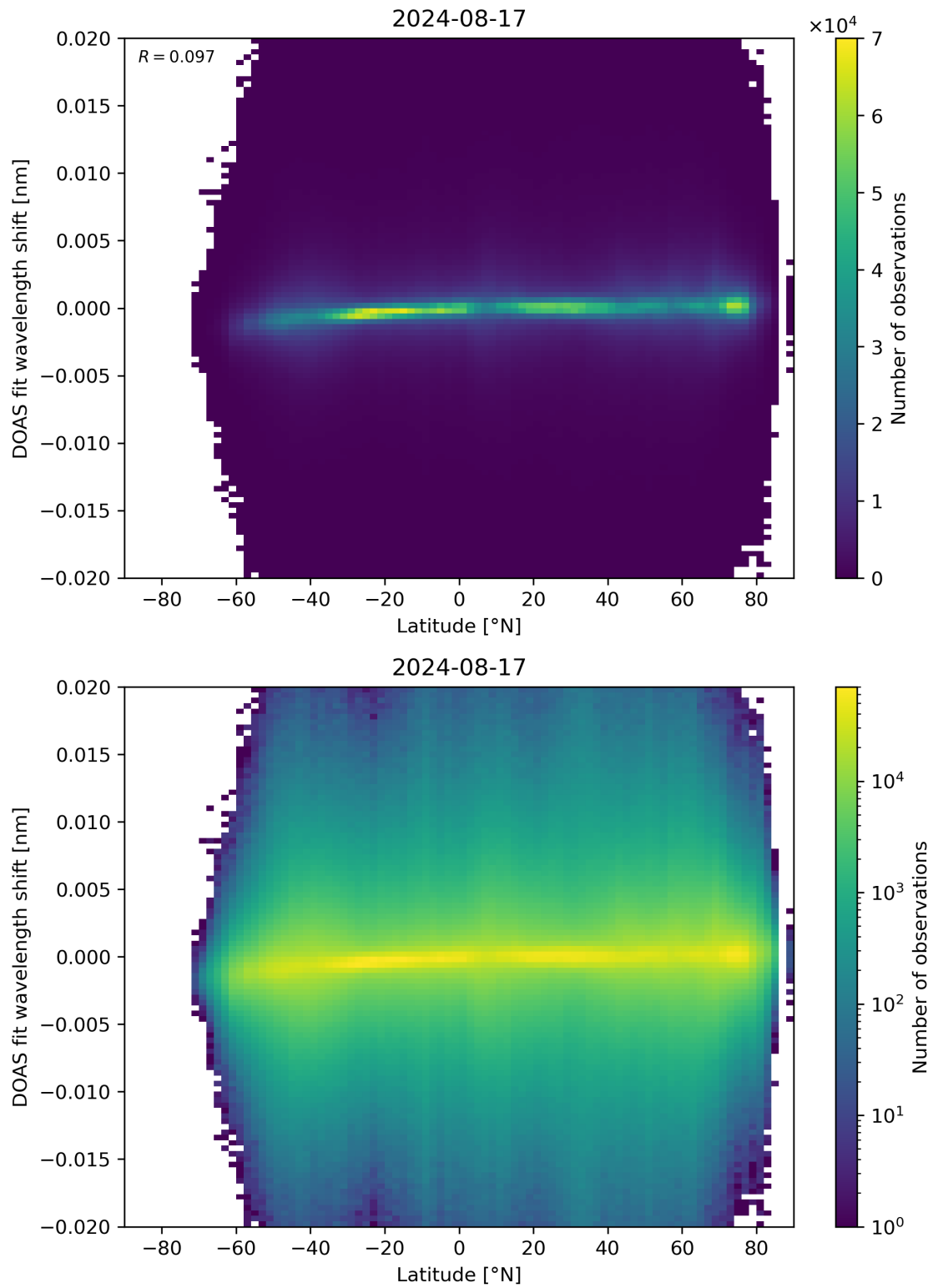
Figure 154: Scatter density plot of “Latitude” against “DOAS fit wavelength shift” for 2024-08-16 to 2024-08-18.
