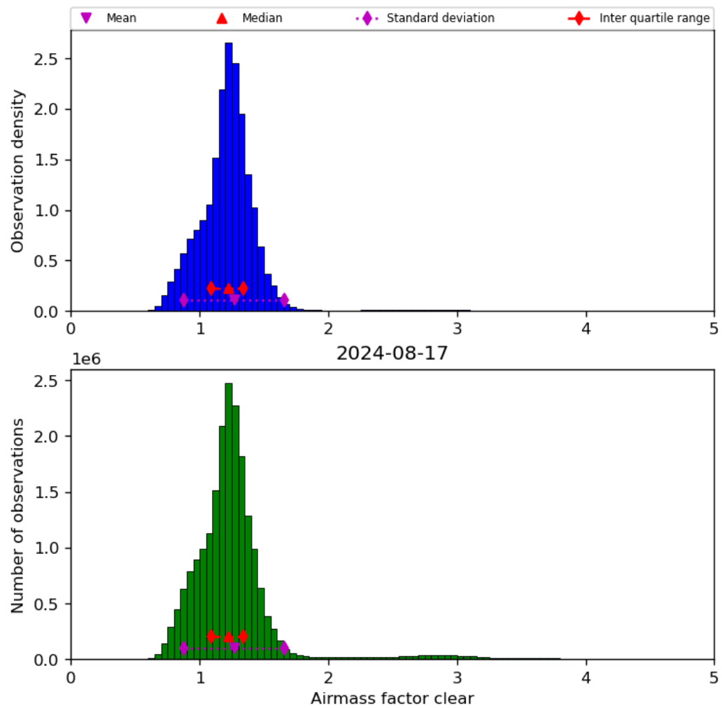
Figure 42: Histogram of “Airmass factor clear” for 2024-08-16 to 2024-08-18
