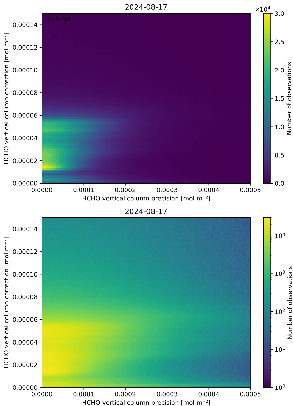
Figure 146: Scatter density plot of “HCHO vertical column precision” against “HCHO vertical column correction” for 2024-08-16 to 2024-08-18.
