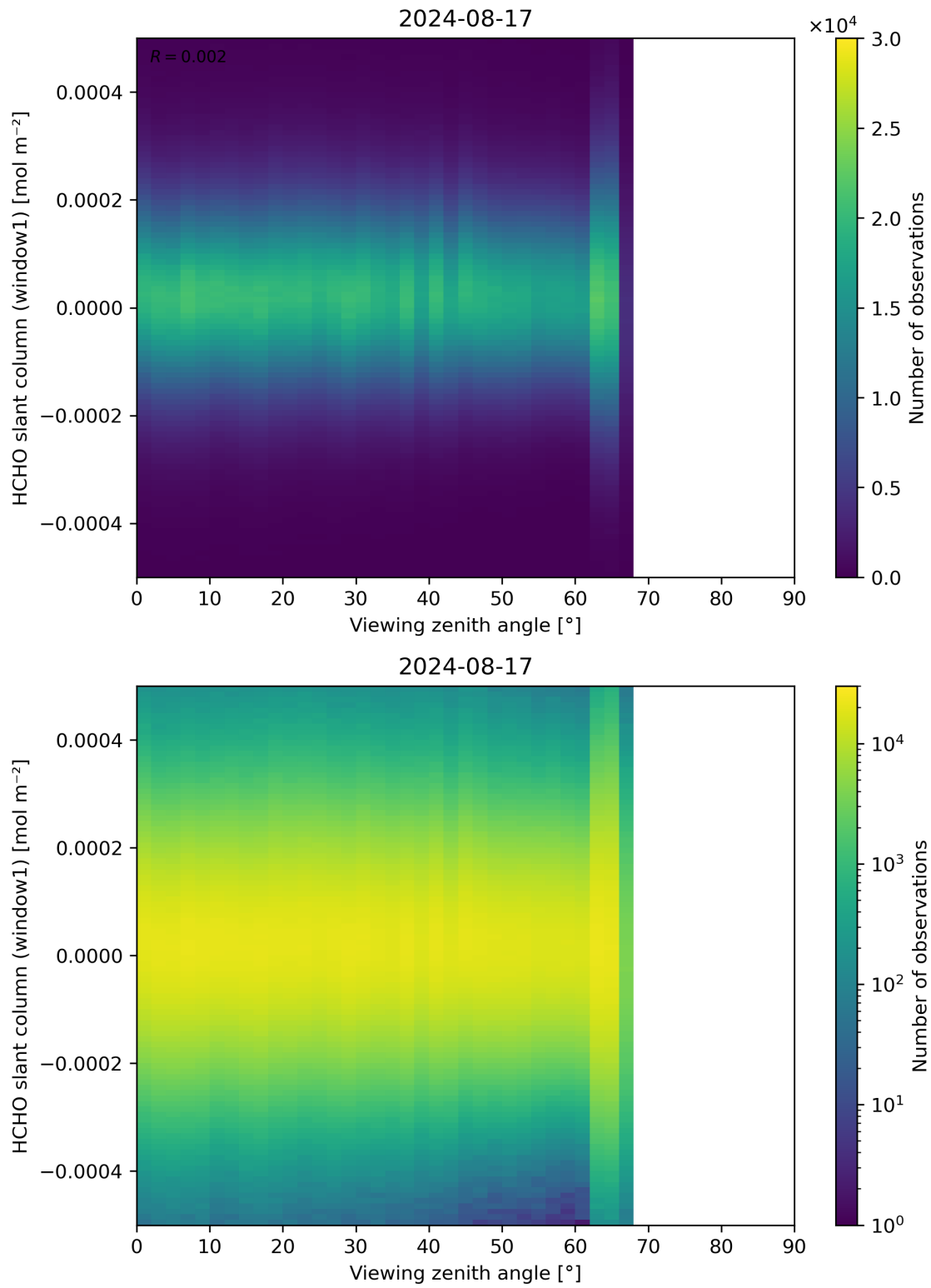
Figure 188: Scatter density plot of “Viewing zenith angle” against “HCHO slant column (window1)” for 2024-08-16 to 2024-08-18.
