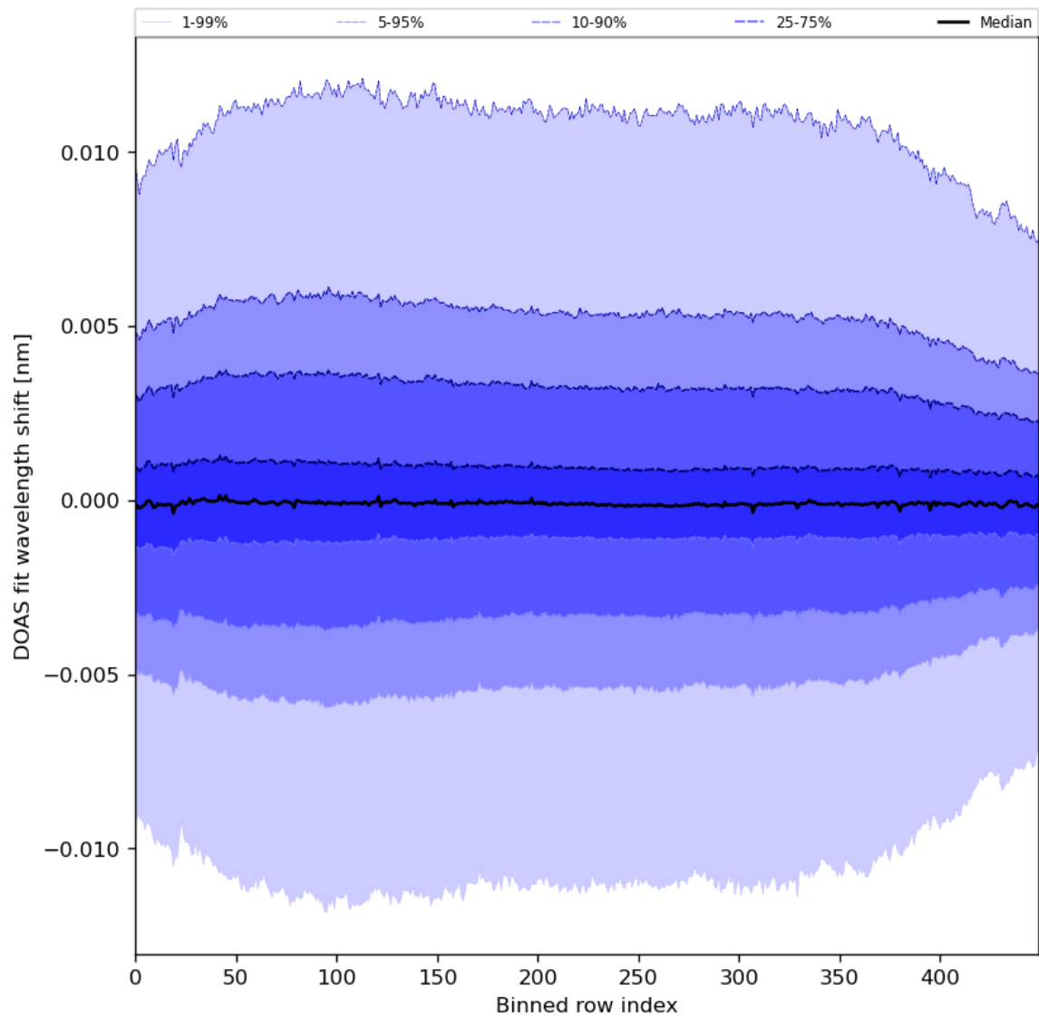
Figure 58: Along track statistics of “DOAS fit wavelength shift” for 2024-08-16 to 2024-08-18
