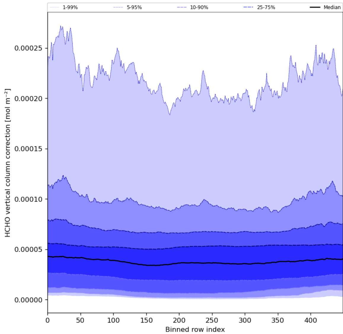
Figure 51: Along track statistics of “HCHO vertical column correction” for 2024-08-16 to 2024-08-18
