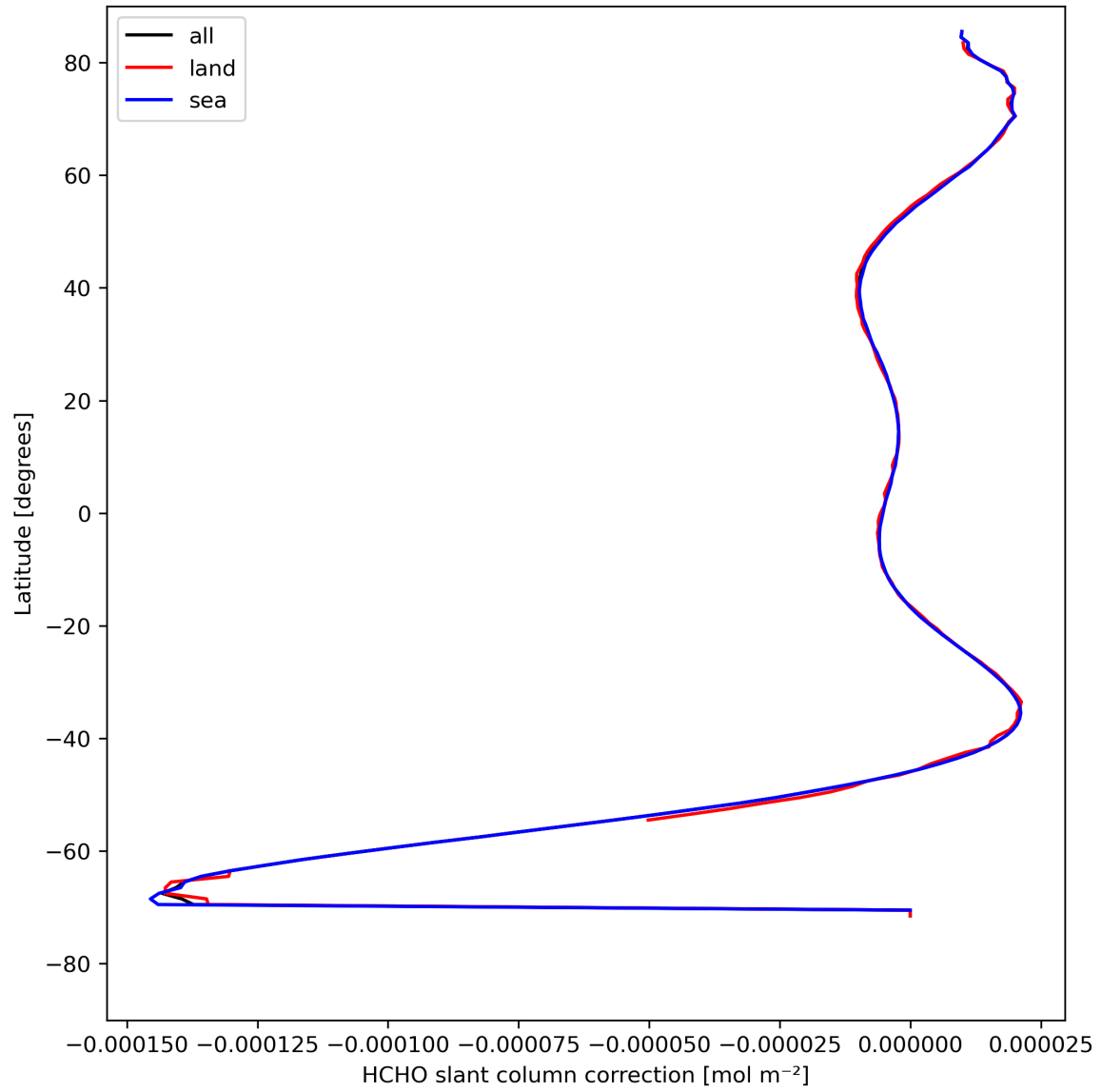
Figure 33: Zonal average of “HCHO slant column correction” for 2024-08-16 to 2024-08-18.
