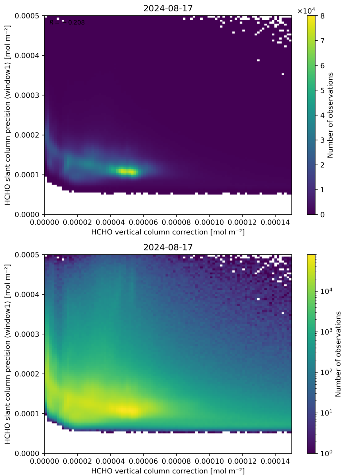
Figure 119: Scatter density plot of “HCHO vertical column correction” against “HCHO slant column precision (window1)” for 2024-08-16 to 2024-08-18.
