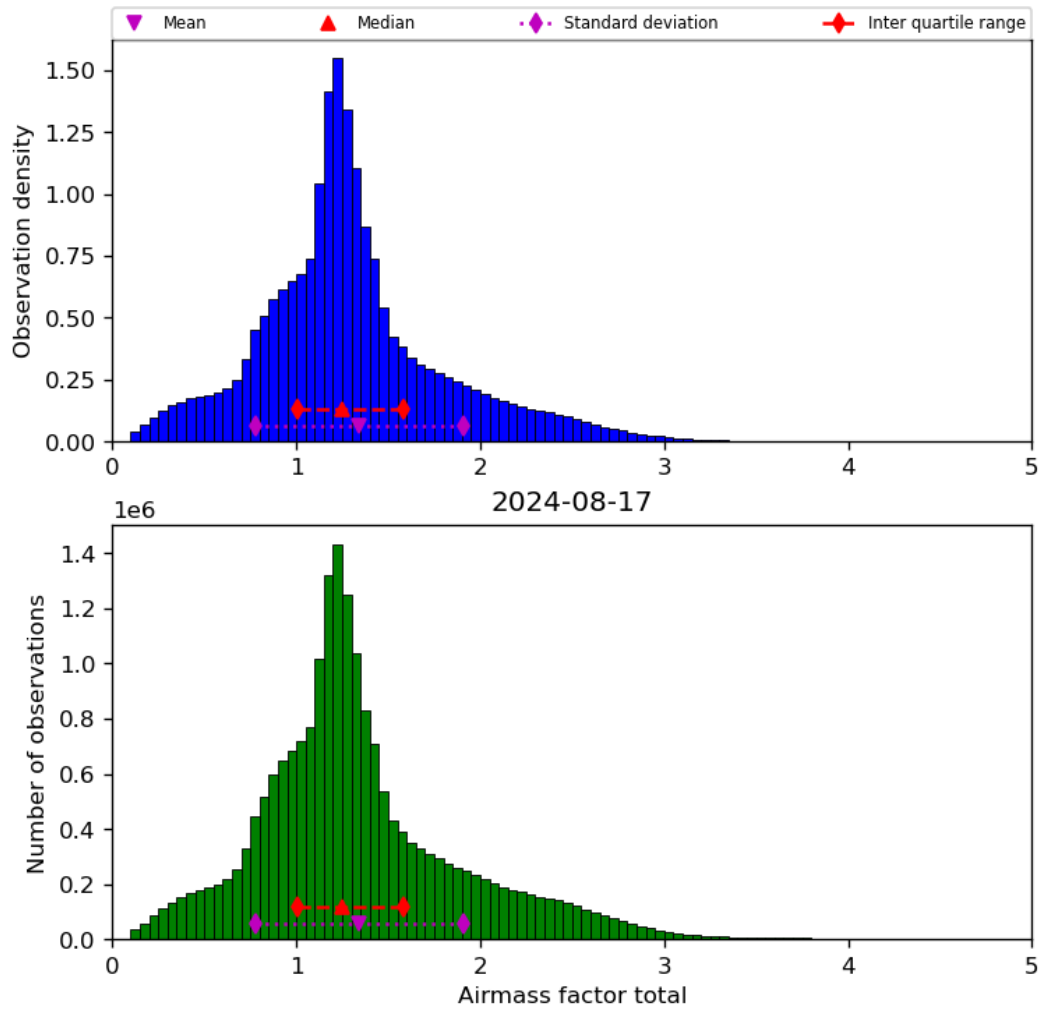
Figure 40: Histogram of “Airmass factor total” for 2024-08-16 to 2024-08-18
