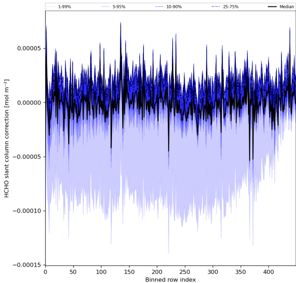
Figure 61: Along track statistics of “HCHO slant column correction” for 2024-08-16 to 2024-08-18
