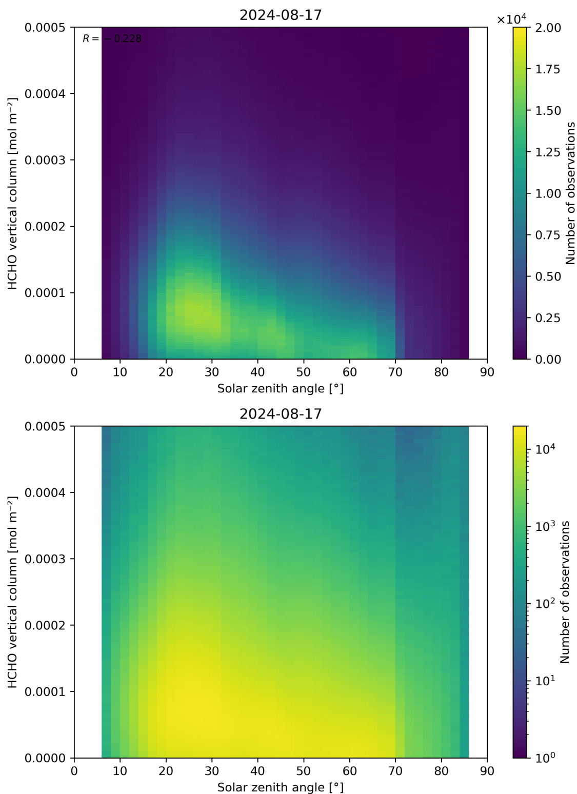
Figure 177: Scatter density plot of “Solar zenith angle” against “HCHO vertical column” for 2024-08-16 to 2024-08-18.
