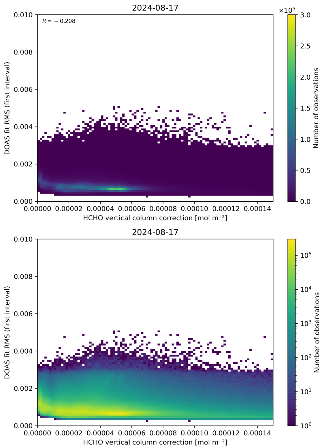
Figure 112: Scatter density plot of “HCHO vertical column correction” against “DOAS fit RMS (first interval)” for 2024-08-16 to 2024-08-18.
