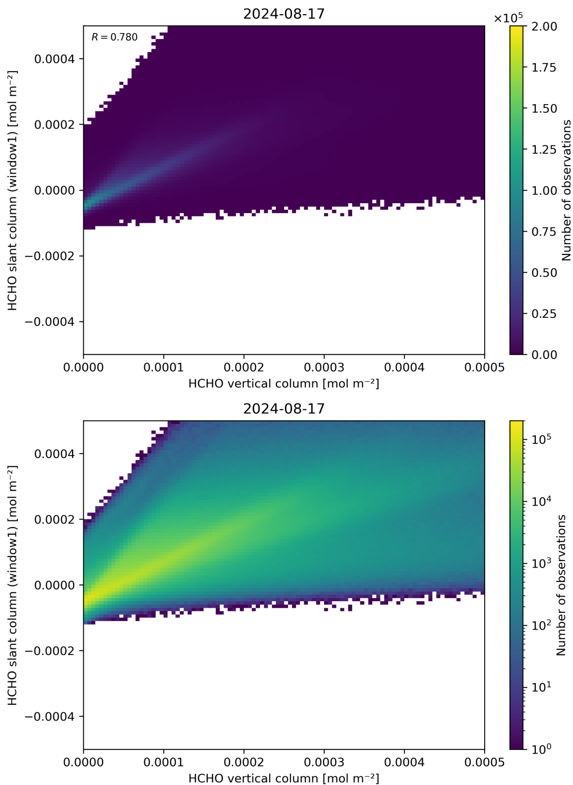
Figure 129: Scatter density plot of “HCHO vertical column” against “HCHO slant column (window1)” for 2024-08-16 to 2024-08-18.
