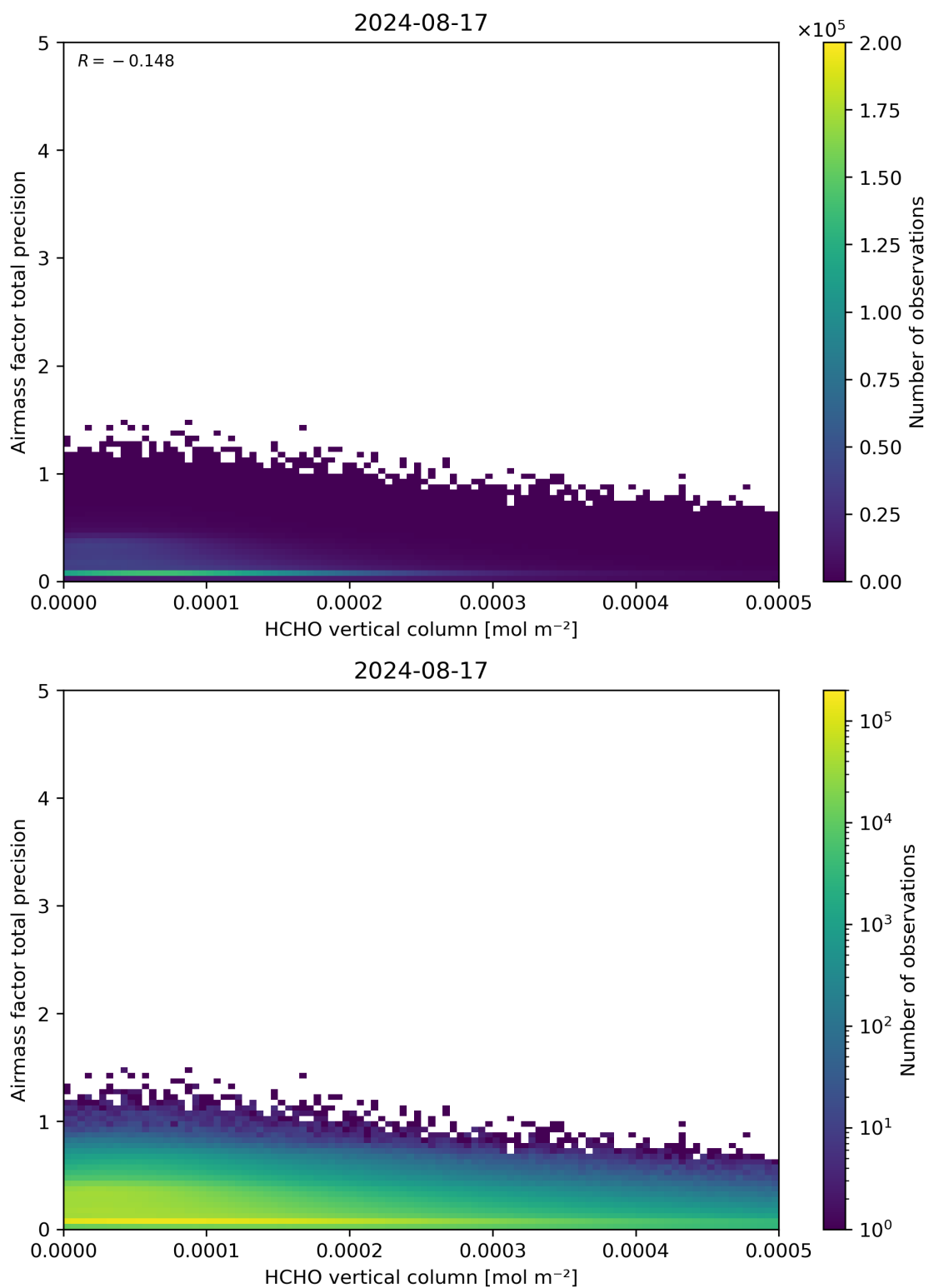
Figure 132: Scatter density plot of “HCHO vertical column” against “Airmass factor total precision” for 2024-08-16 to 2024-08-18.
