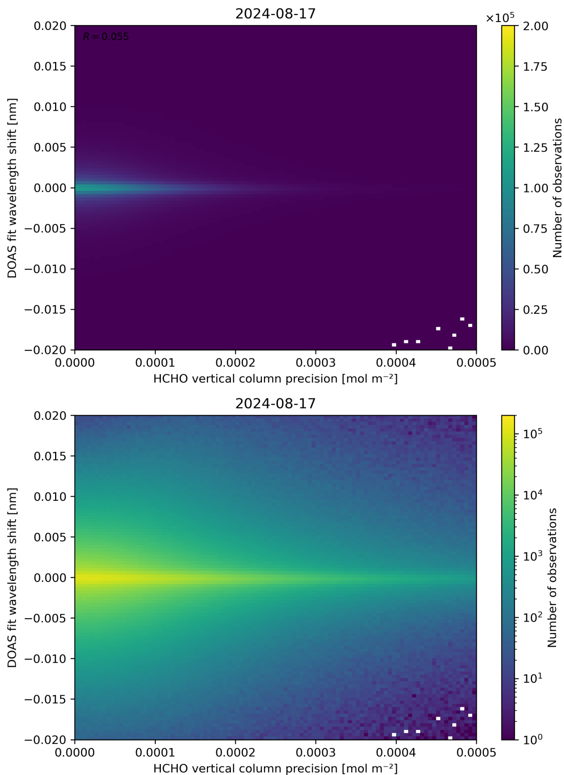
Figure 137: Scatter density plot of “HCHO vertical column precision” against “DOAS fit wavelength shift” for 2024-08-16 to 2024-08-18.
