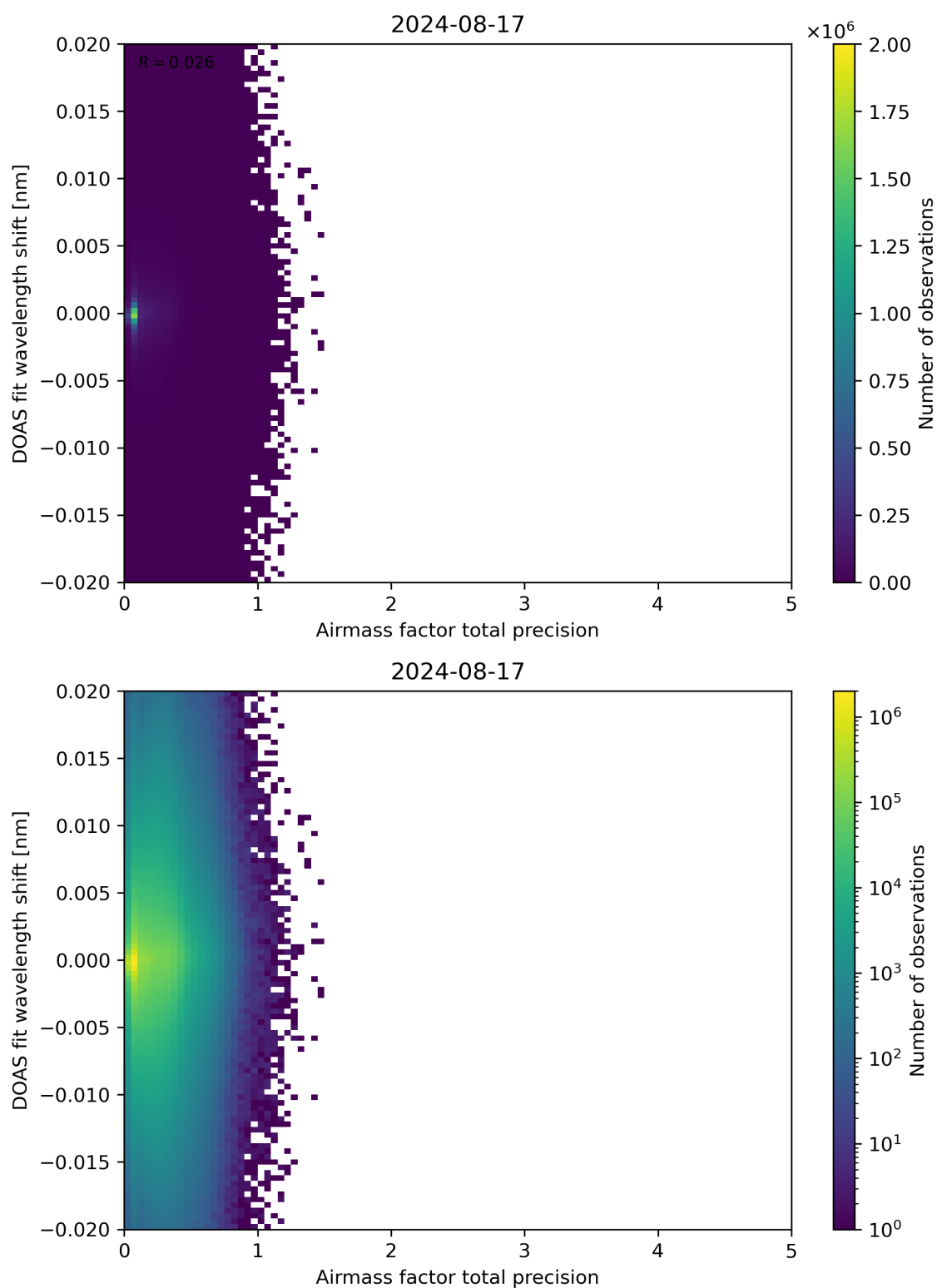
Figure 106: Scatter density plot of “Airmass factor total precision” against “DOAS fit wavelength shift” for 2024-08-16 to 2024-08-18.
