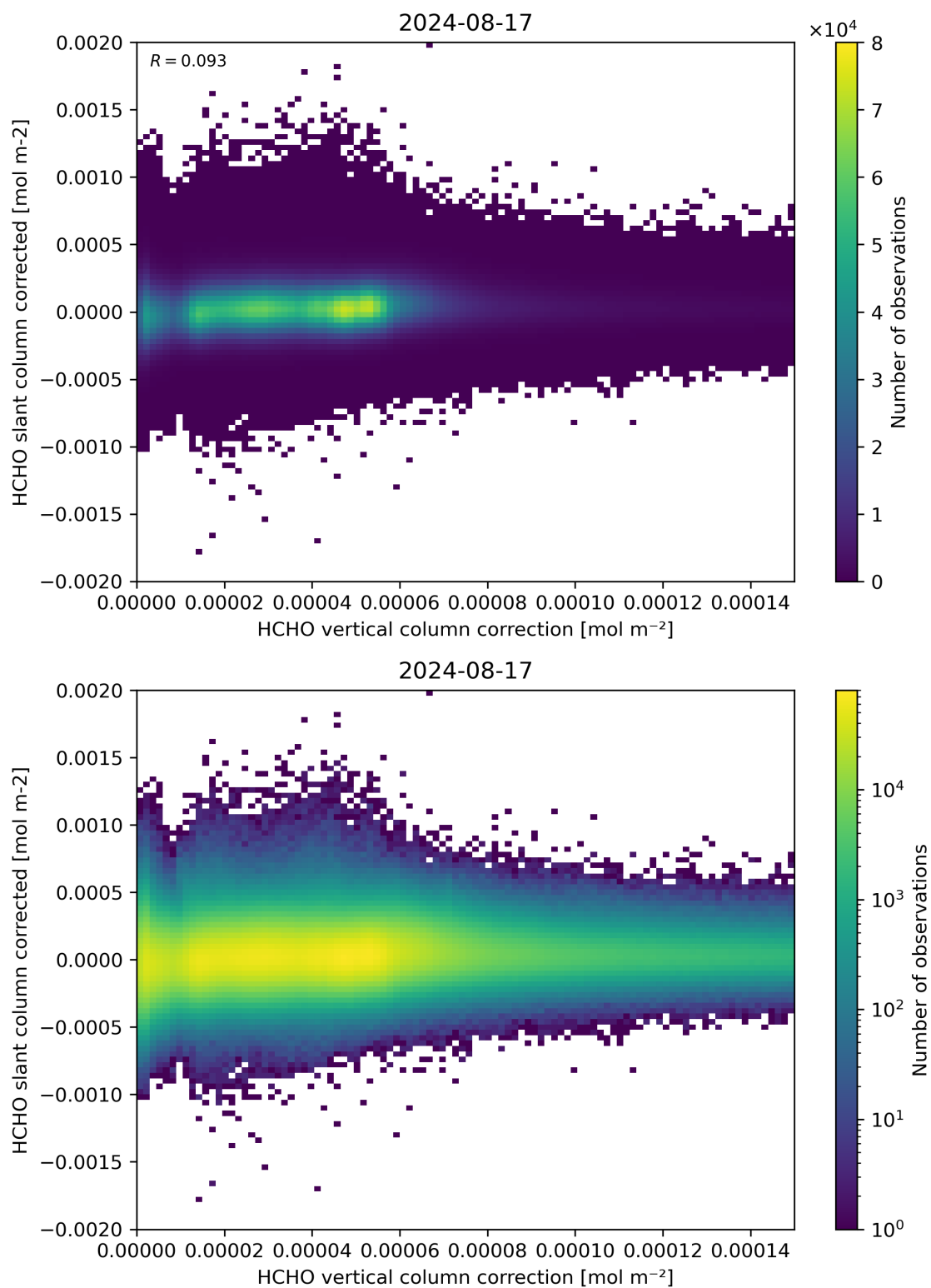
Figure 116: Scatter density plot of “HCHO vertical column correction” against “HCHO slant column corrected” for 2024-08-16 to 2024-08-18.
