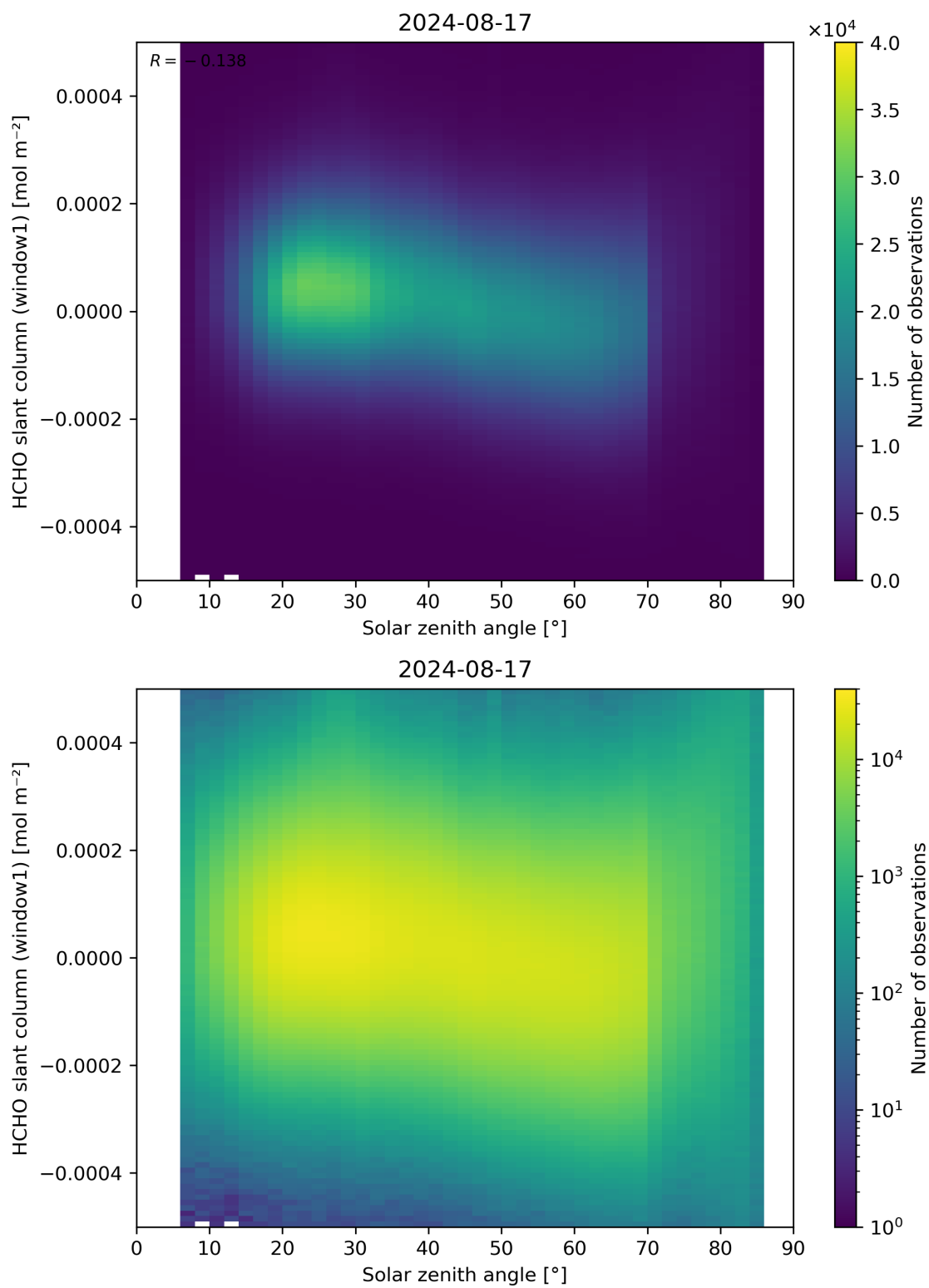
Figure 173: Scatter density plot of “Solar zenith angle” against “HCHO slant column (window1)” for 2024-08-16 to 2024-08-18.
