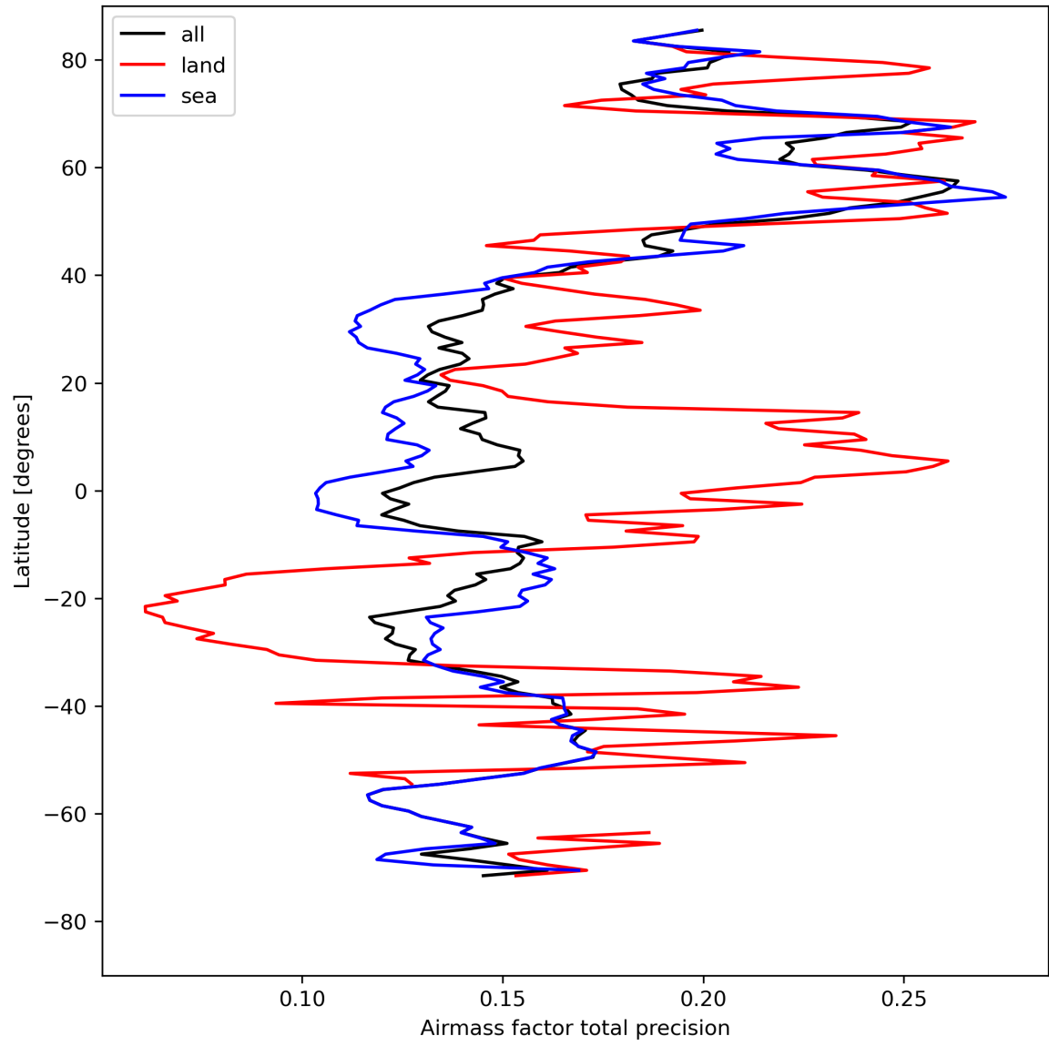
Figure 27: Zonal average of “Airmass factor total precision” for 2024-08-16 to 2024-08-18.
