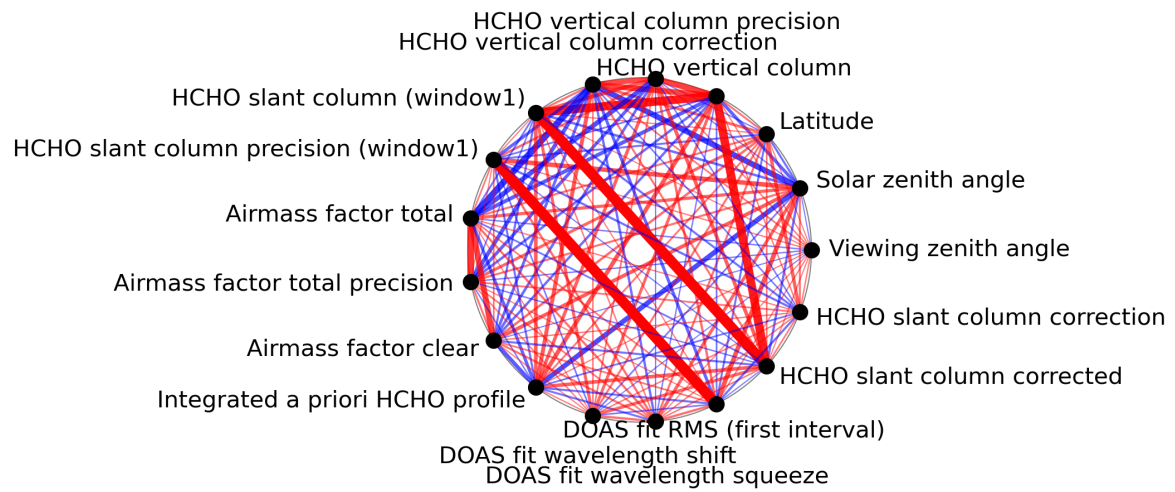
Figure 1: Map of correlation graph for 2024-08-16 to 2024-08-18.
