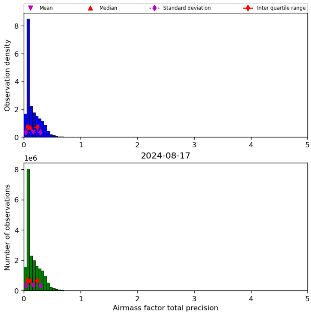
Figure 41: Histogram of “Airmass factor total precision” for 2024-08-16 to 2024-08-18
