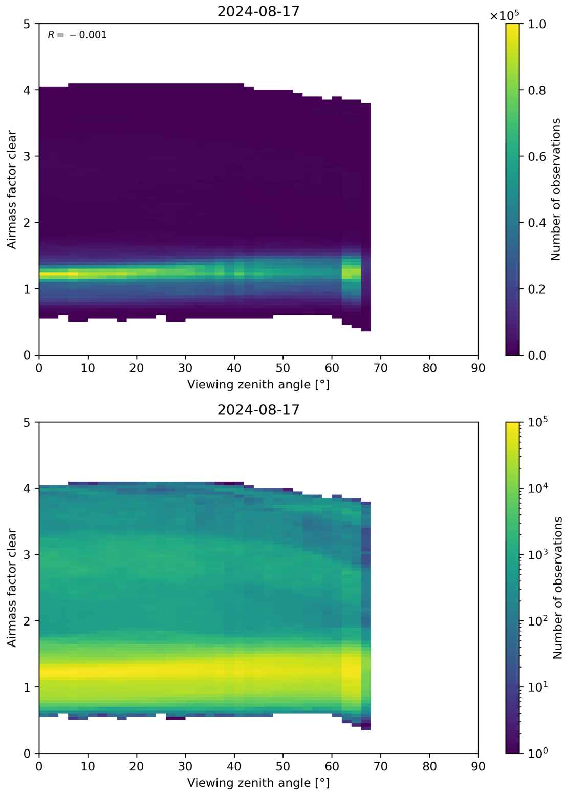
Figure 185: Scatter density plot of “Viewing zenith angle” against “Airmass factor clear” for 2024-08-16 to 2024-08-18.
