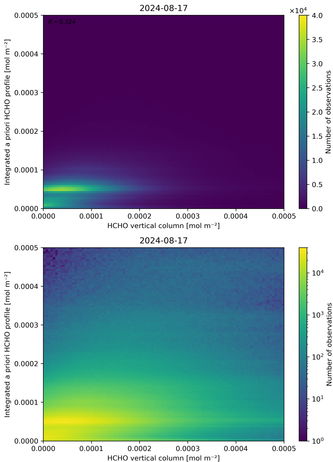
Figure 135: Scatter density plot of “HCHO vertical column” against “Integrated a priori HCHO profile” for 2024-08-16 to 2024-08-18.
