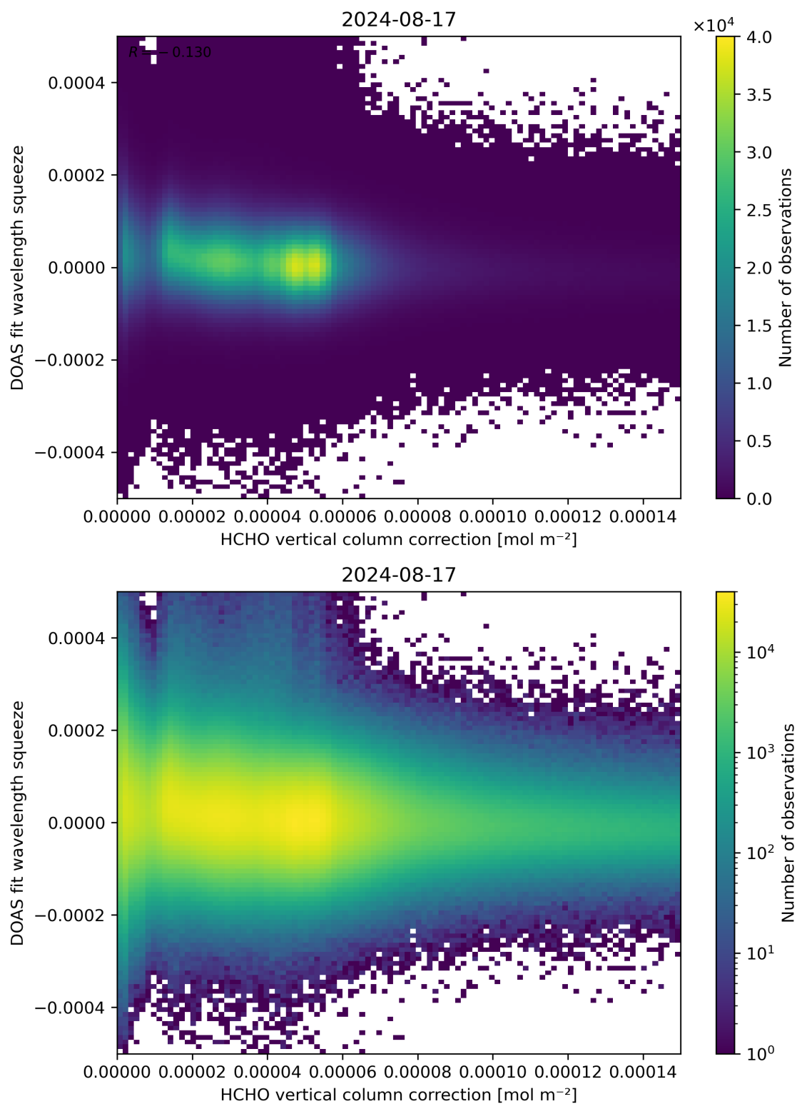
Figure 114: Scatter density plot of “HCHO vertical column correction” against “DOAS fit wavelength squeeze” for 2024-08-16 to 2024-08-18.
