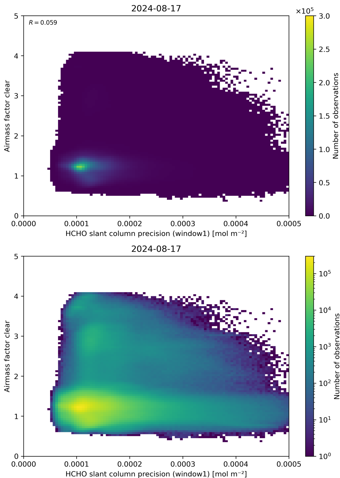
Figure 91: Scatter density plot of “HCHO slant column precision (window1)” against “Airmass factor clear” for 2024-08-16 to 2024-08-18.
