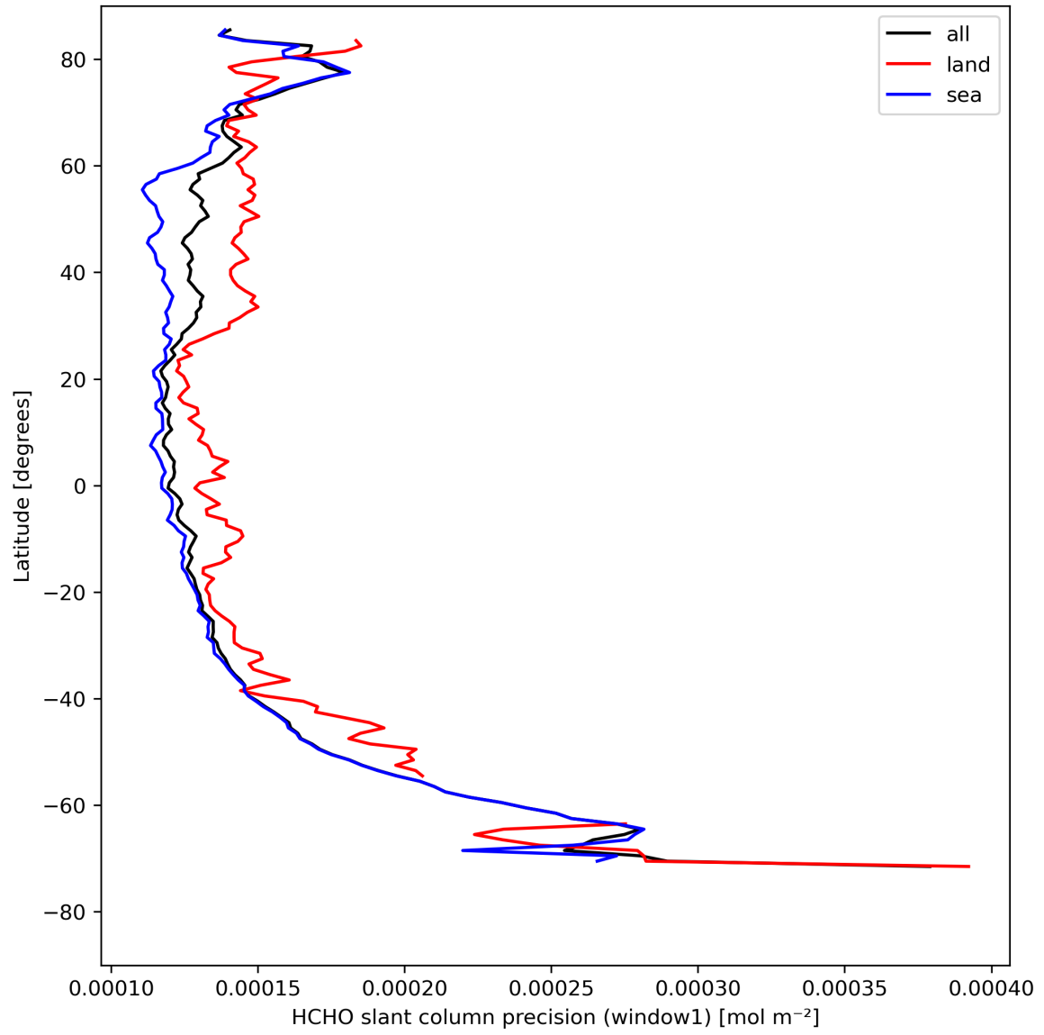
Figure 25: Zonal average of “HCHO slant column precision (window1)” for 2024-08-16 to 2024-08-18.
