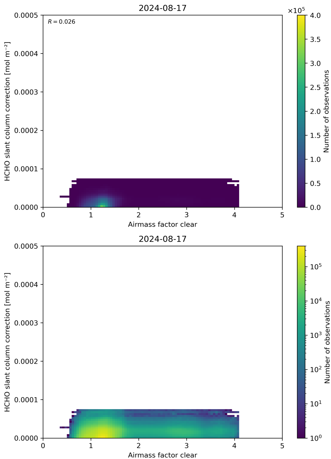
Figure 75: Scatter density plot of “Airmass factor clear” against “HCHO slant column correction” for 2024-08-16 to 2024-08-18.
