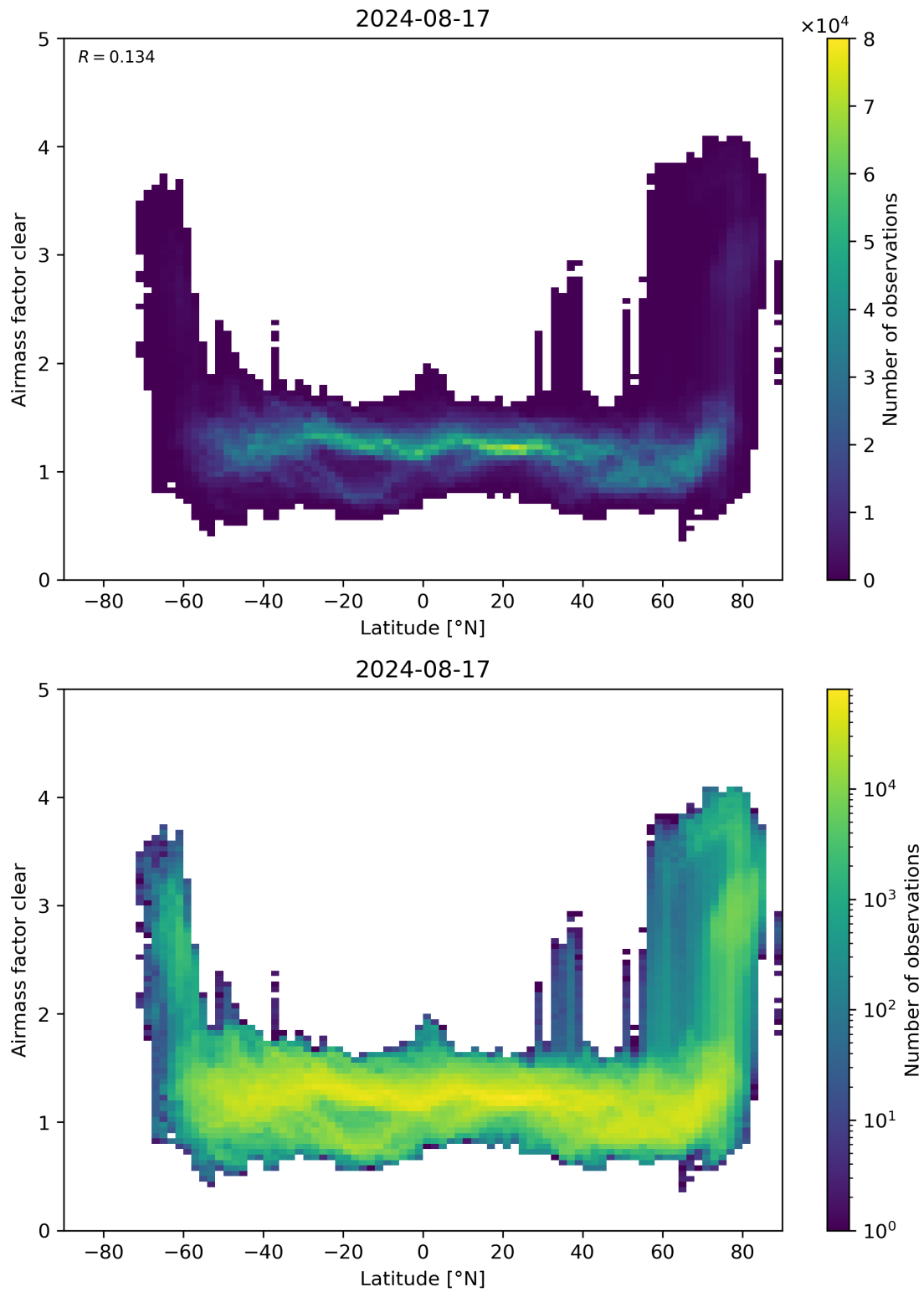
Figure 156: Scatter density plot of “Latitude” against “Airmass factor clear” for 2024-08-16 to 2024-08-18.
