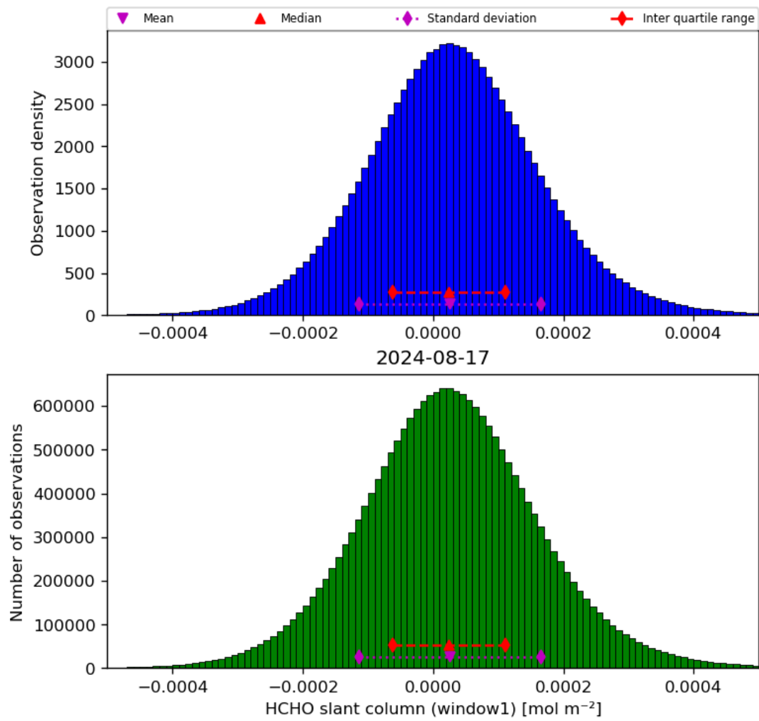
Figure 38: Histogram of “HCHO slant column (window1)” for 2024-08-16 to 2024-08-18
