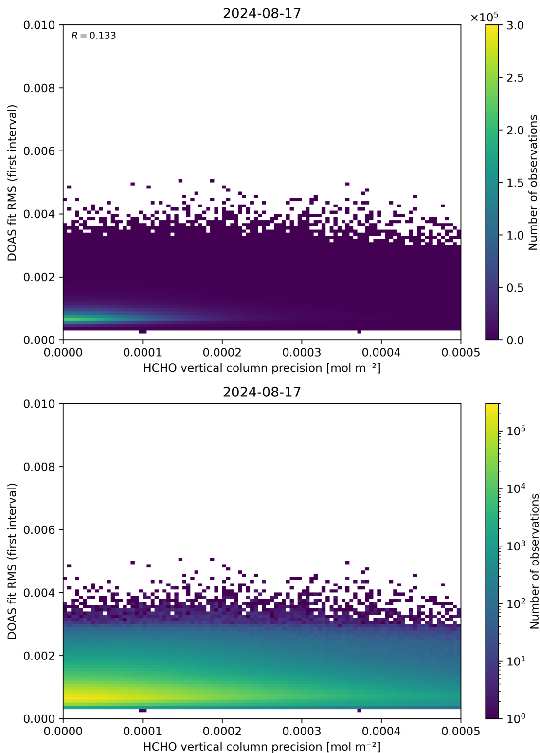
Figure 136: Scatter density plot of “HCHO vertical column precision” against “DOAS fit RMS (first interval)” for 2024-08-16 to 2024-08-18.
