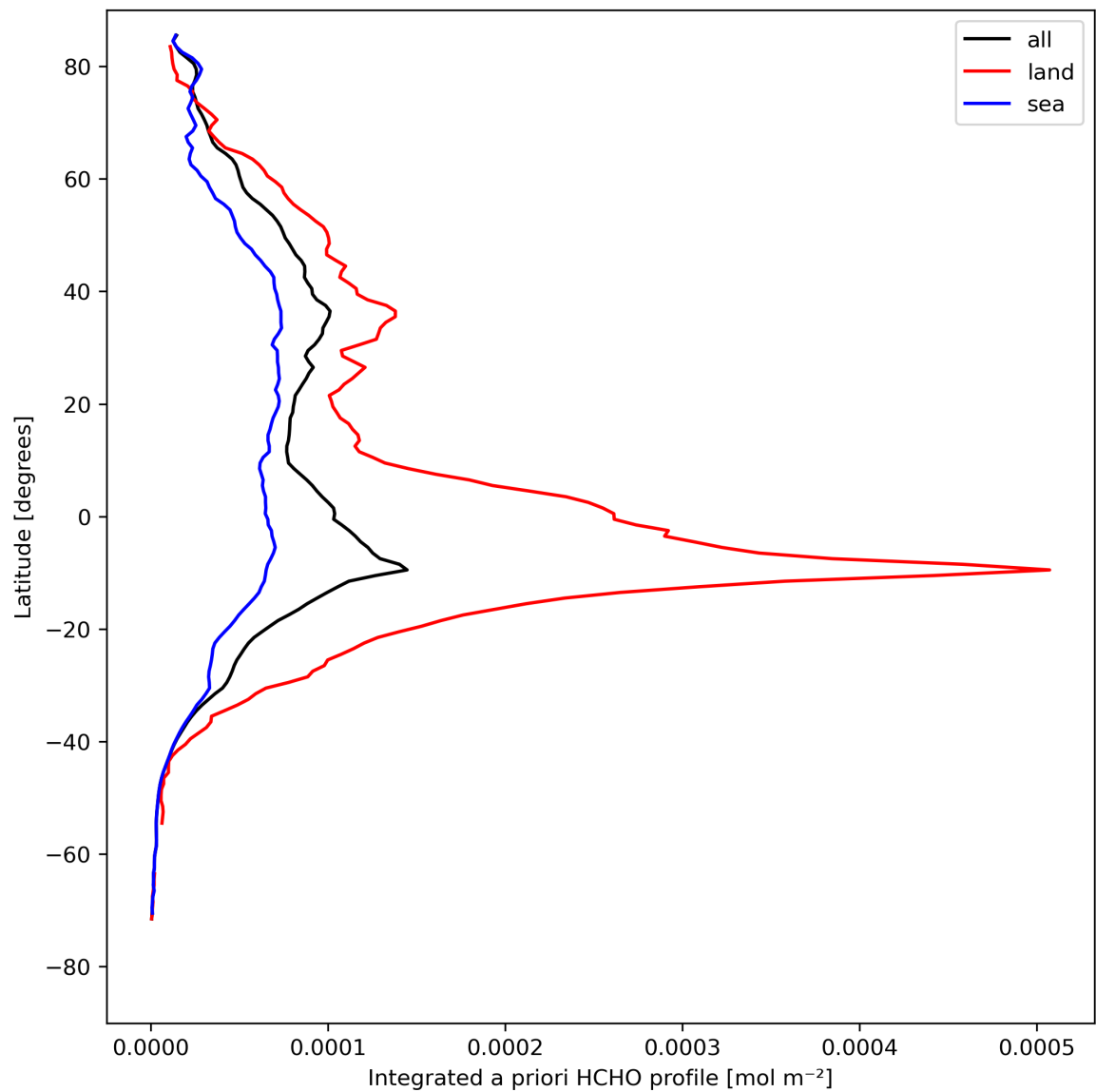
Figure 29: Zonal average of “Integrated a priori HCHO profile” for 2024-08-16 to 2024-08-18.
