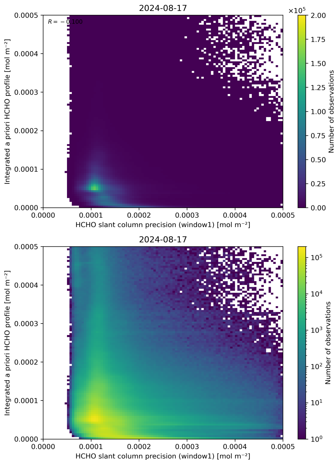
Figure 96: Scatter density plot of “HCHO slant column precision (window1)” against “Integrated a priori HCHO profile” for 2024-08-16 to 2024-08-18.
