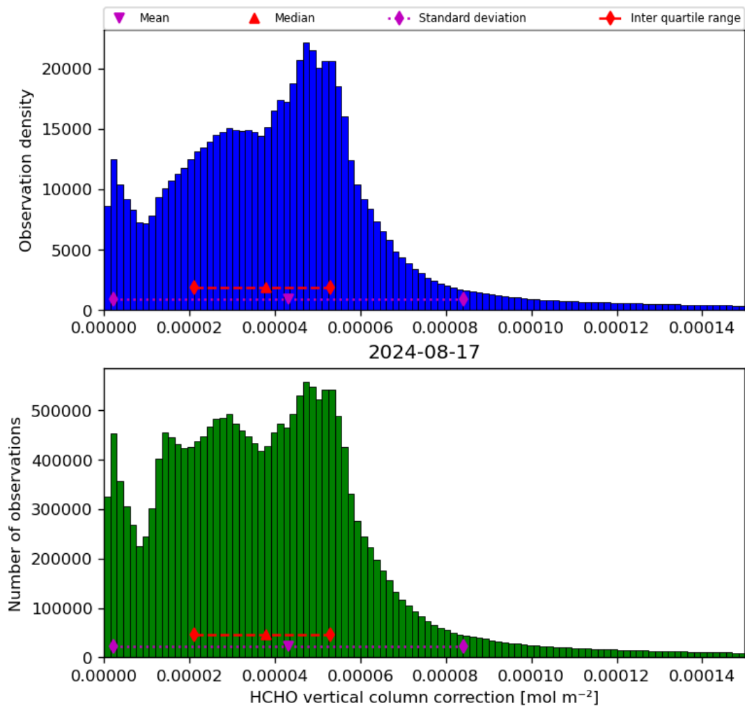
Figure 37: Histogram of “HCHO vertical column correction” for 2024-08-16 to 2024-08-18
