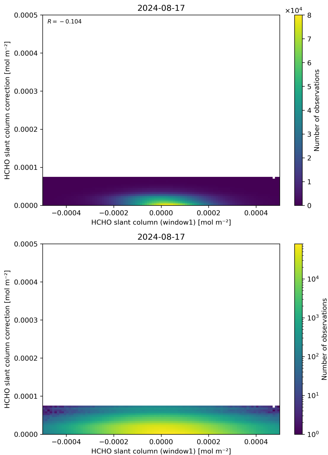
Figure 83: Scatter density plot of “HCHO slant column (window1)” against “HCHO slant column correction” for 2024-08-16 to 2024-08-18.
