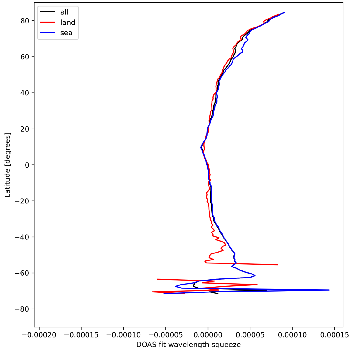
Figure 31: Zonal average of "DOAS fit wavelength squeeze" for 2024-08-17 to 2024-08-19.
