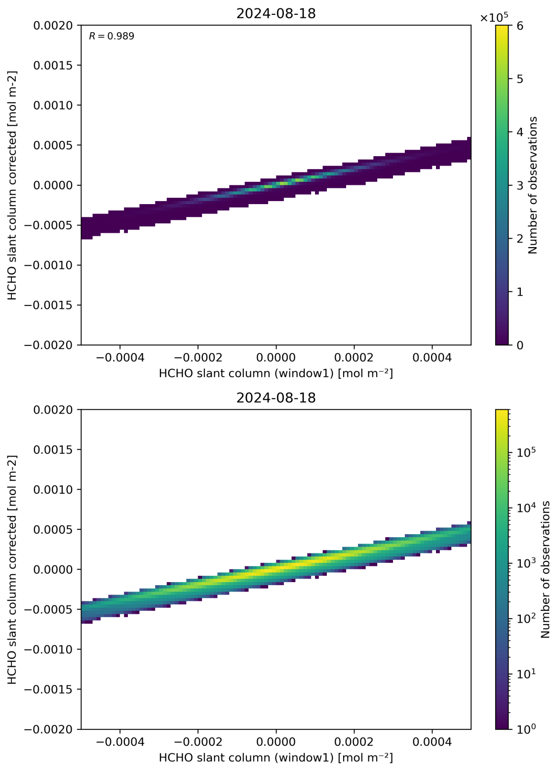
Figure 82: Scatter density plot of “HCHO slant column (window1)” against “HCHO slant column corrected” for 2024-08-17 to 2024-08-19.
