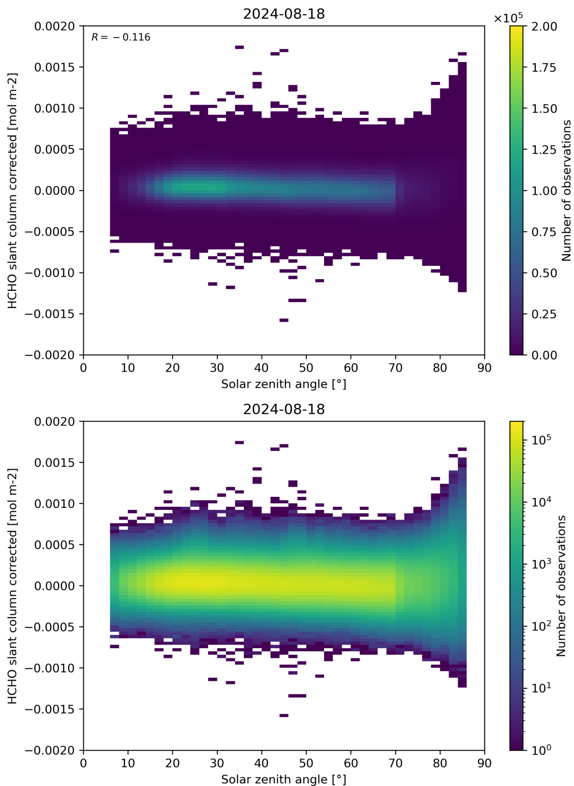
Figure 171: Scatter density plot of “Solar zenith angle” against “HCHO slant column corrected” for 2024-08-17 to 2024-08-19.
