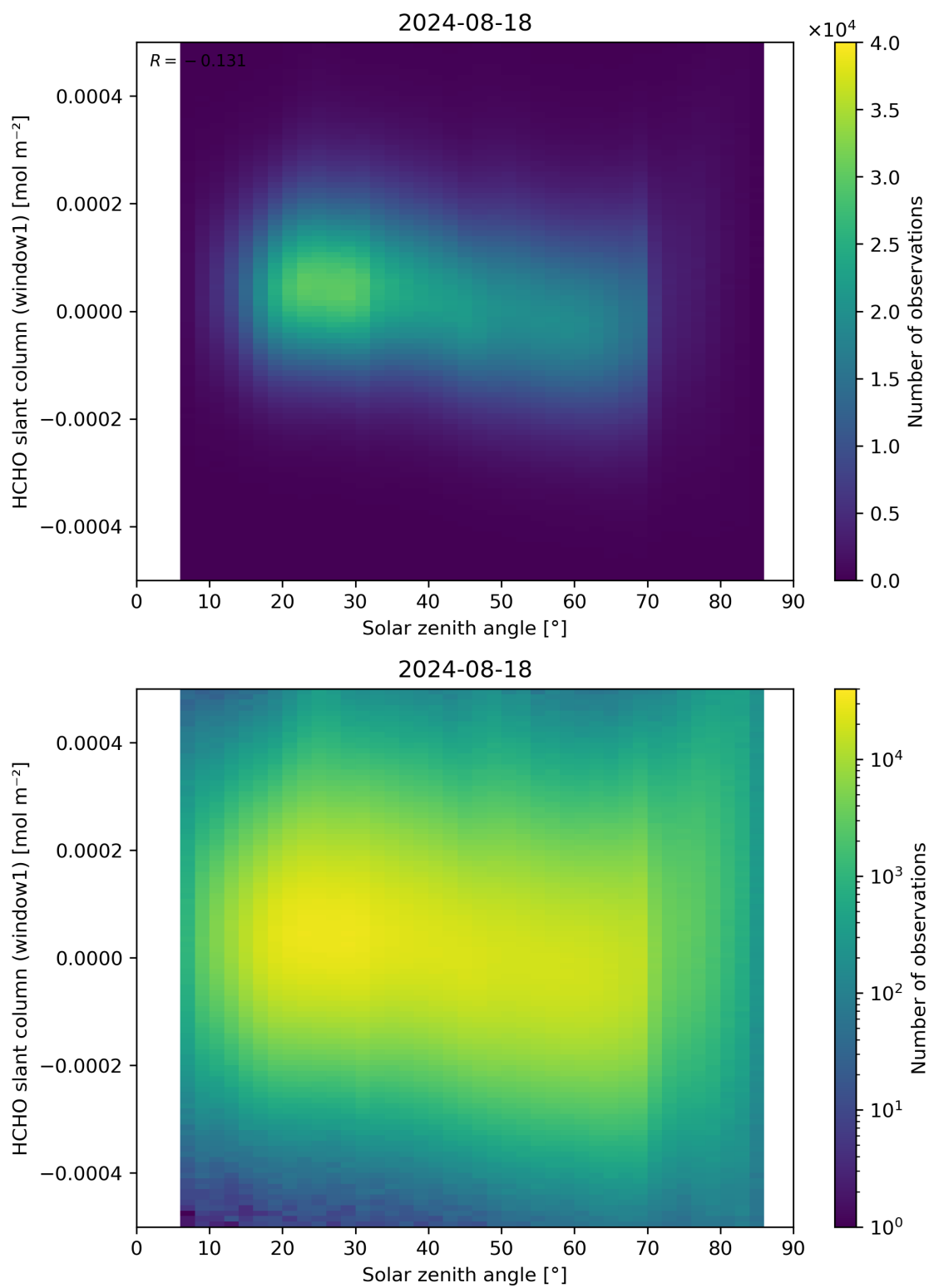
Figure 173: Scatter density plot of “Solar zenith angle” against “HCHO slant column (window1)” for 2024-08-17 to 2024-08-19.
