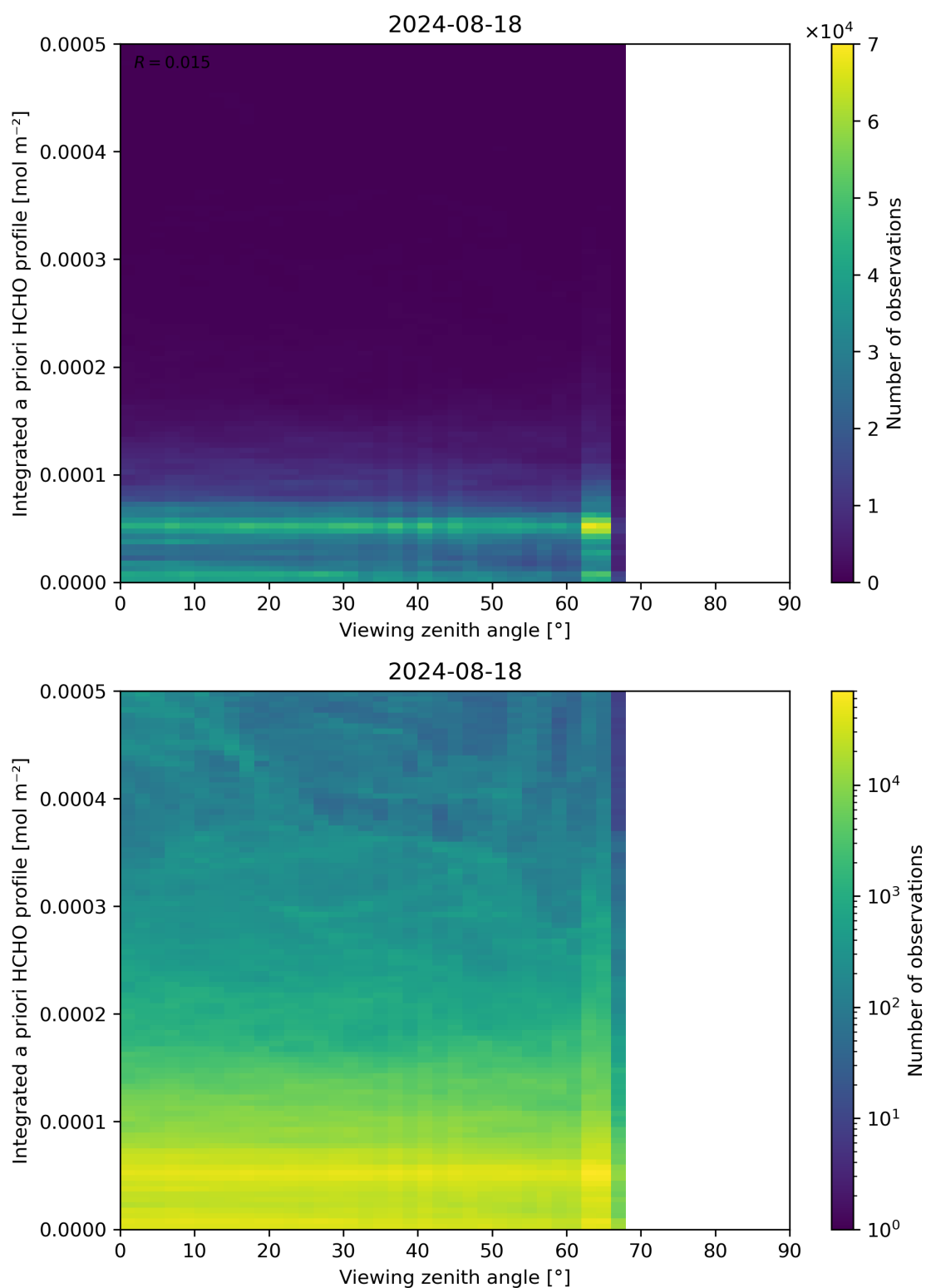
Figure 195: Scatter density plot of “Viewing zenith angle” against “Integrated a priori HCHO profile” for 2024-08-17 to 2024-08-19.
