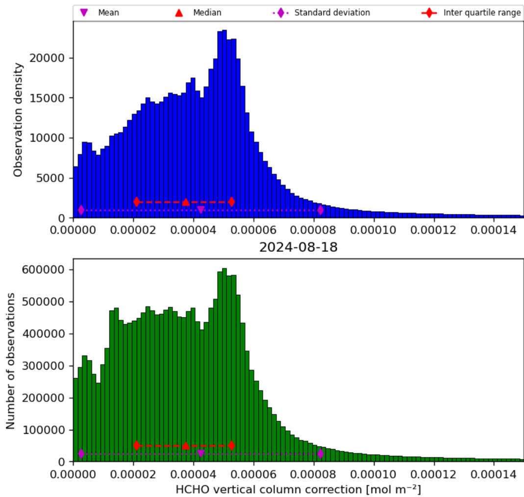
Figure 37: Histogram of “HCHO vertical column correction” for 2024-08-17 to 2024-08-19
