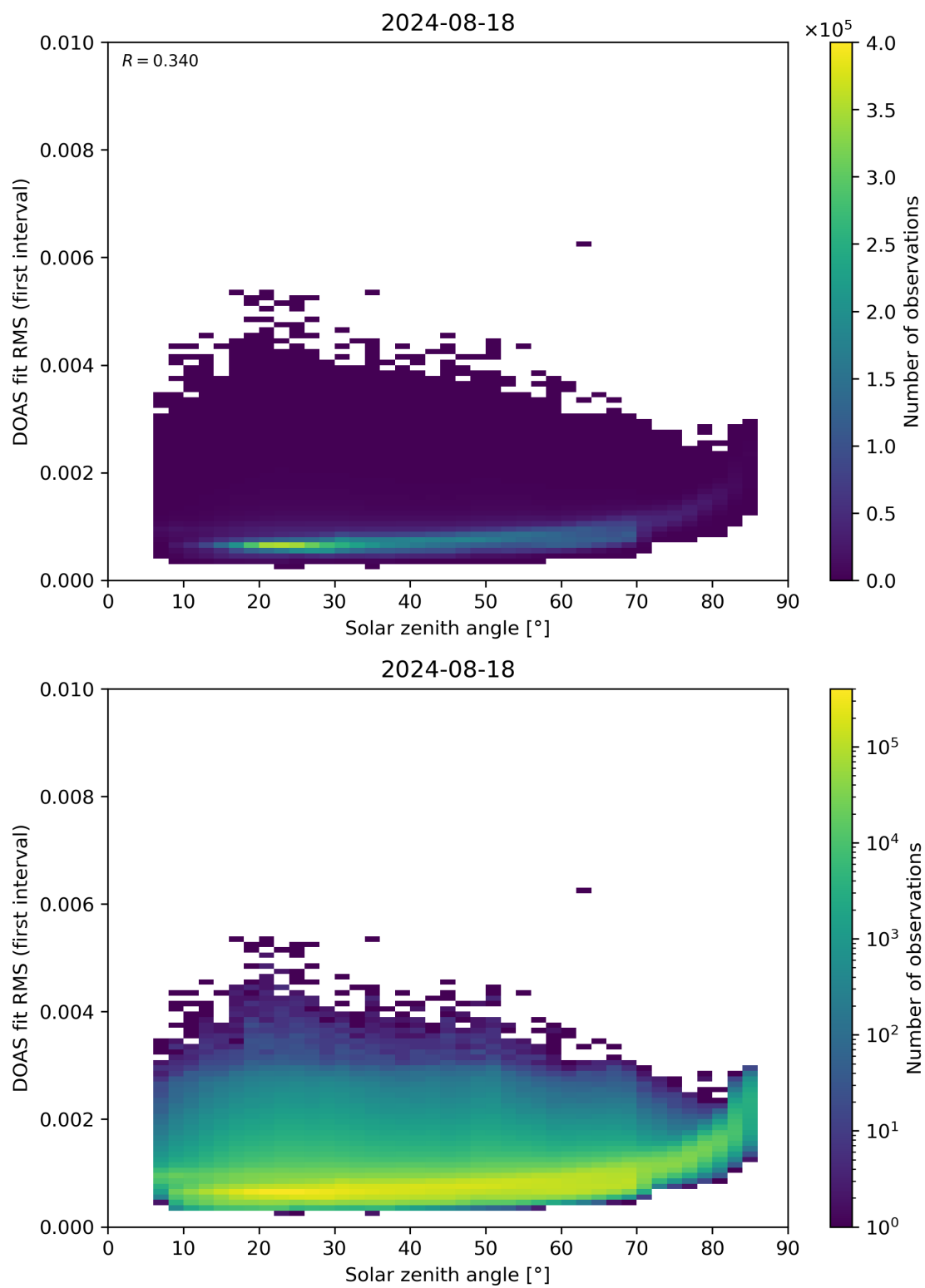
Figure 167: Scatter density plot of “Solar zenith angle” against “DOAS fit RMS (first interval)” for 2024-08-17 to 2024-08-19.
