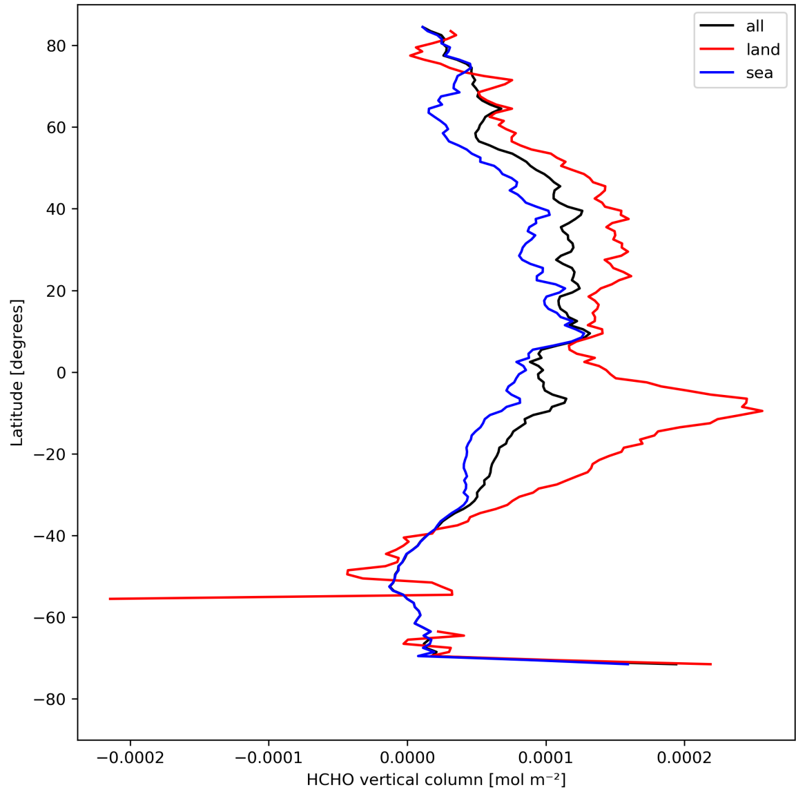
Figure 21: Zonal average of “HCHO vertical column” for 2024-08-17 to 2024-08-19.
