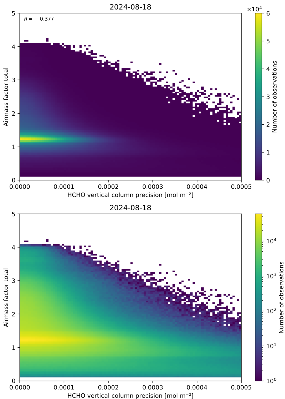
Figure 144: Scatter density plot of “HCHO vertical column precision” against “Airmass factor total” for 2024-08-17 to 2024-08-19.
