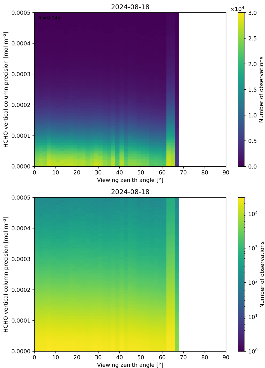
Figure 194: Scatter density plot of “Viewing zenith angle” against “HCHO vertical column precision” for 2024-08-17 to 2024-08-19.
