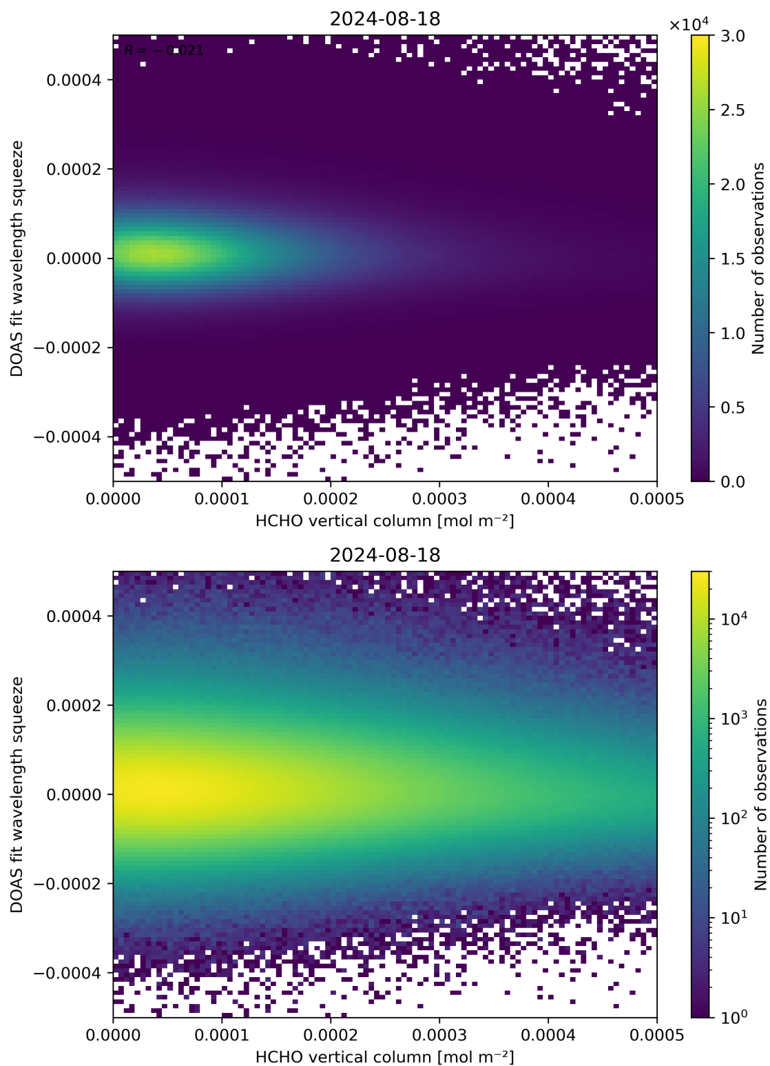
Figure 125: Scatter density plot of “HCHO vertical column” against “DOAS fit wavelength squeeze” for 2024-08-17 to 2024-08-19.
