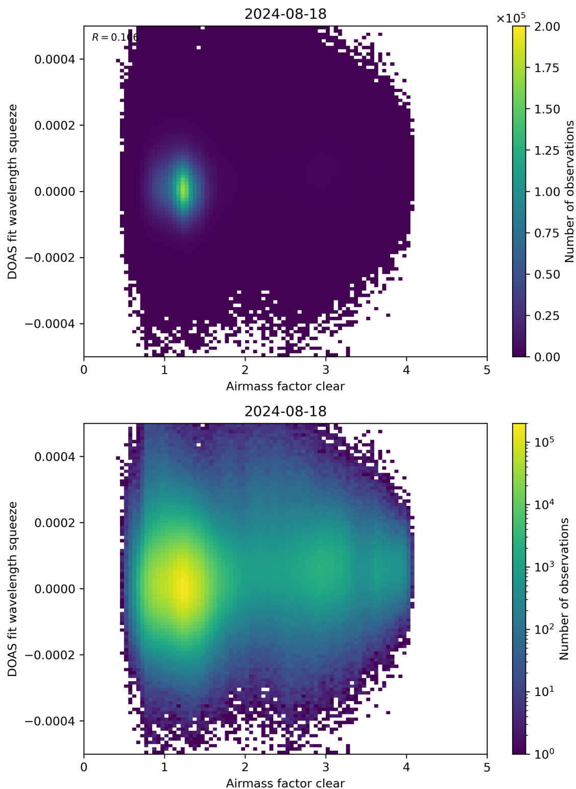
Figure 73: Scatter density plot of “Airmass factor clear” against “DOAS fit wavelength squeeze” for 2024-08-17 to 2024-08-19.
