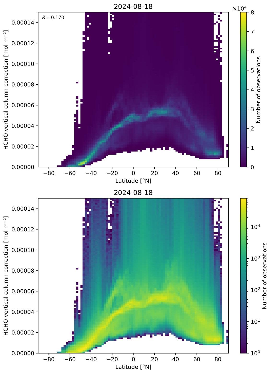
Figure 164: Scatter density plot of “Latitude” against “HCHO vertical column correction” for 2024-08-17 to 2024-08-19.
