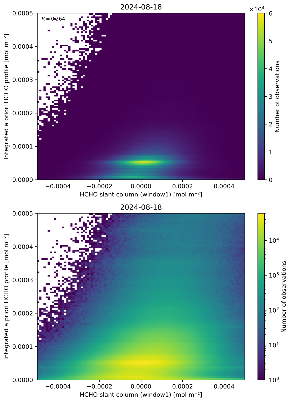
Figure 87: Scatter density plot of “HCHO slant column (window1)” against “Integrated a priori HCHO profile” for 2024-08-17 to 2024-08-19.
