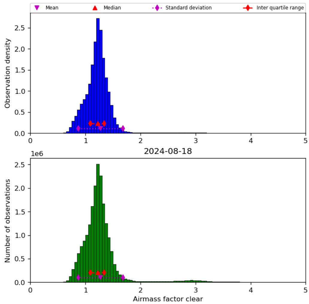
Figure 42: Histogram of “Airmass factor clear” for 2024-08-17 to 2024-08-19
