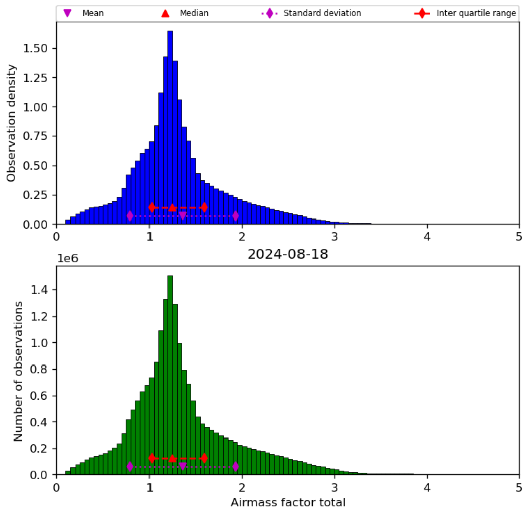
Figure 40: Histogram of “Airmass factor total” for 2024-08-17 to 2024-08-19
