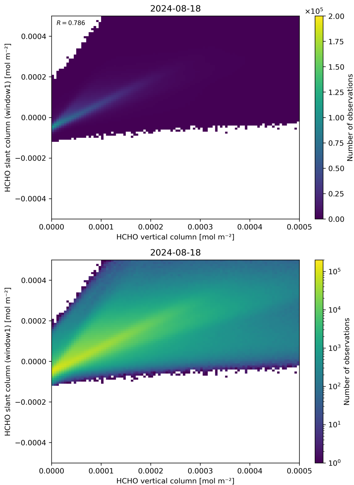
Figure 129: Scatter density plot of “HCHO vertical column” against “HCHO slant column (window1)” for 2024-08-17 to 2024-08-19.
