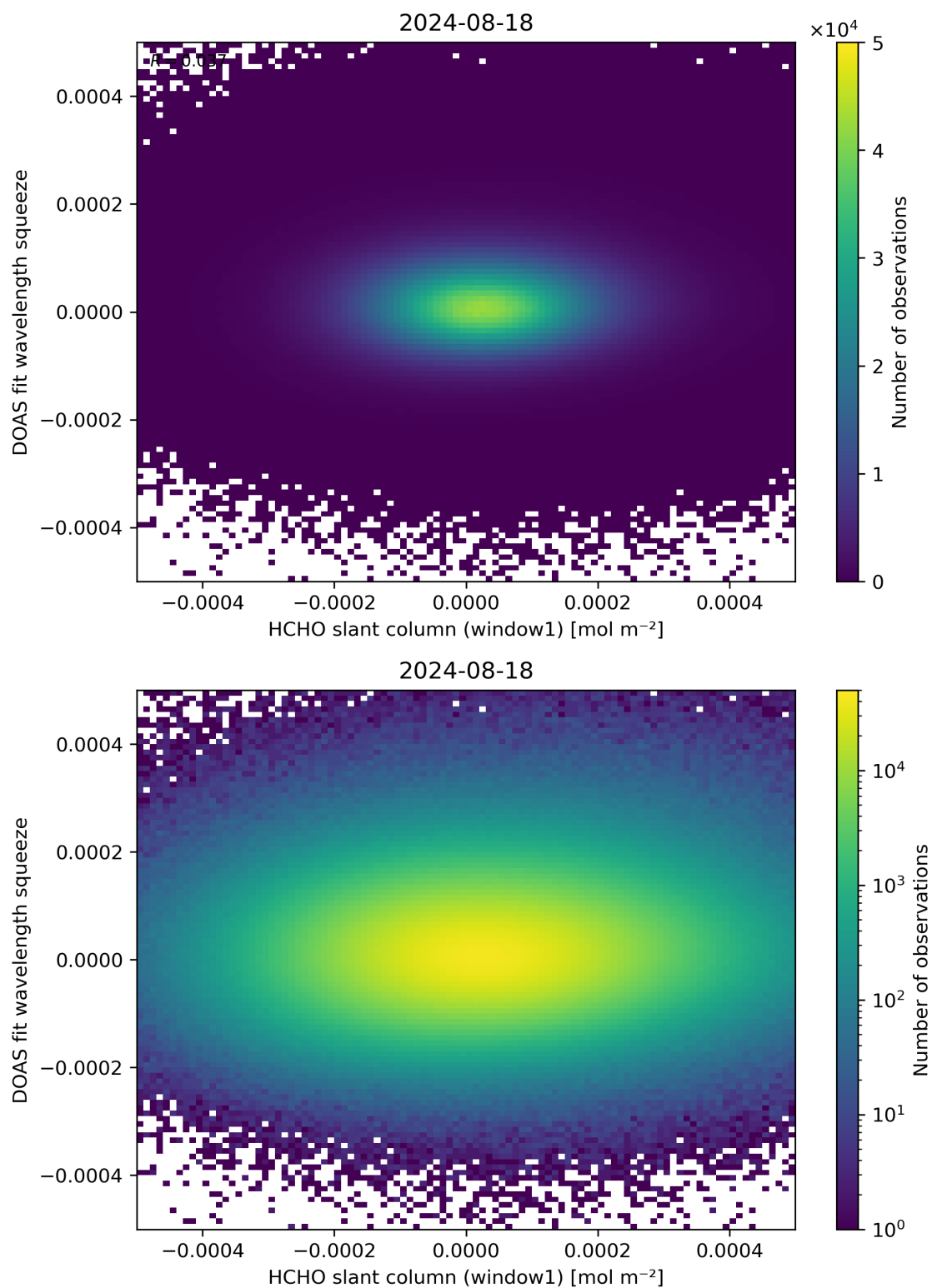
Figure 80: Scatter density plot of “HCHO slant column (window1)” against “DOAS fit wavelength squeeze” for 2024-08-17 to 2024-08-19.
