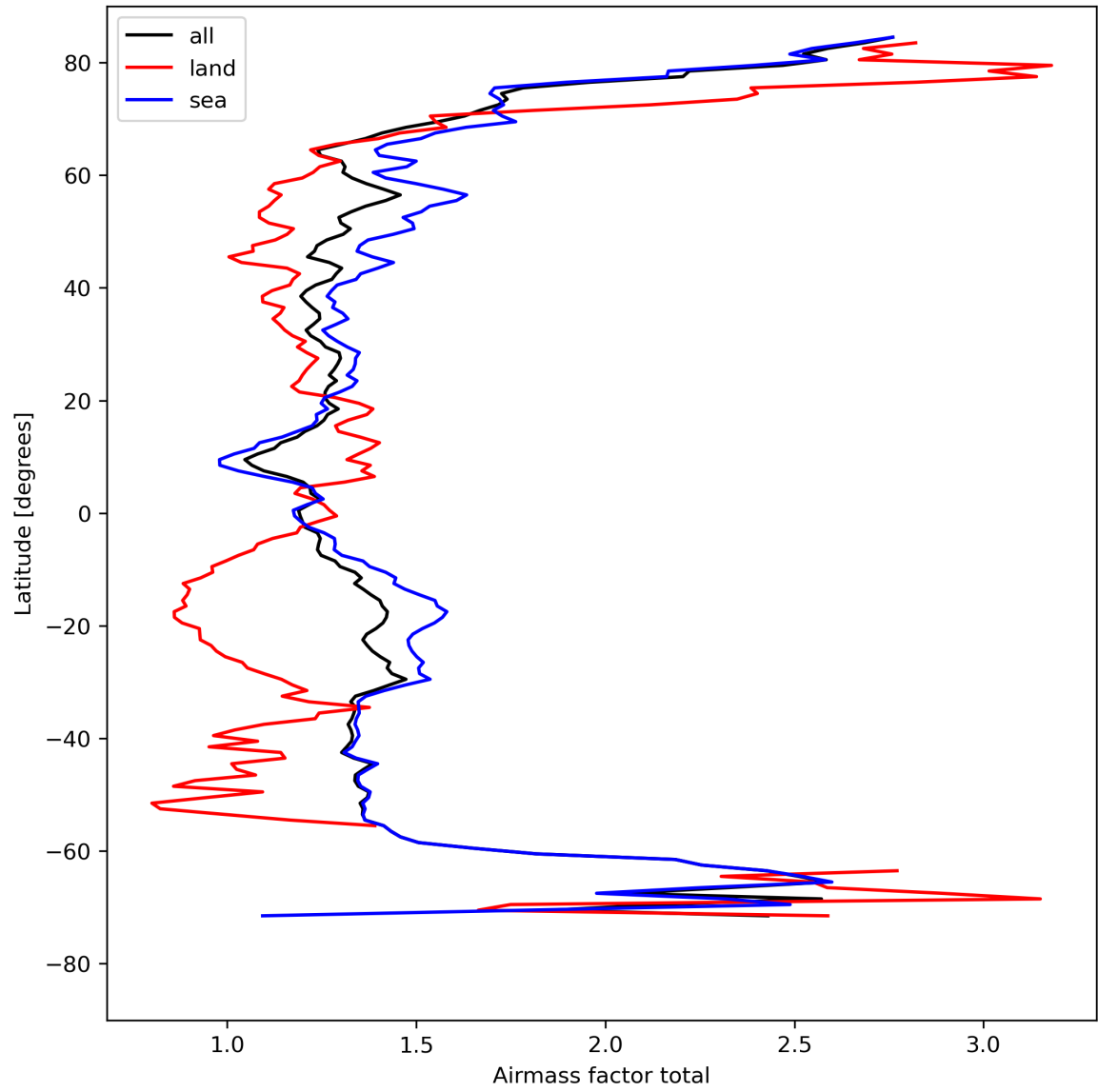
Figure 26: Zonal average of “Airmass factor total” for 2024-08-17 to 2024-08-19.
