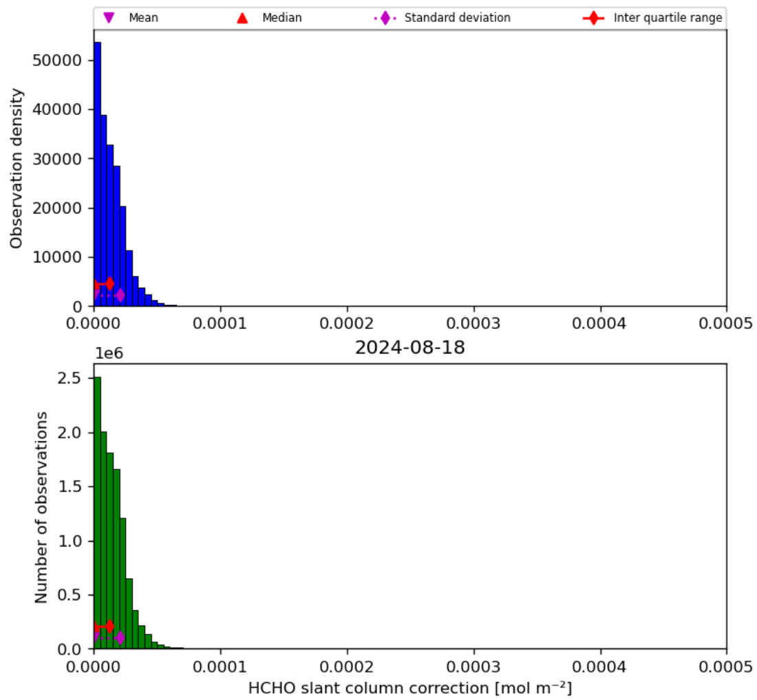
Figure 47: Histogram of “HCHO slant column correction” for 2024-08-17 to 2024-08-19
