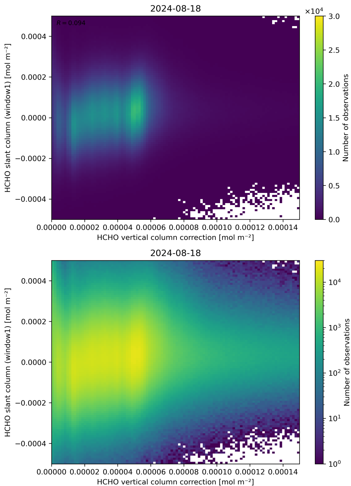
Figure 118: Scatter density plot of “HCHO vertical column correction” against “HCHO slant column (window1)” for 2024-08-17 to 2024-08-19.
