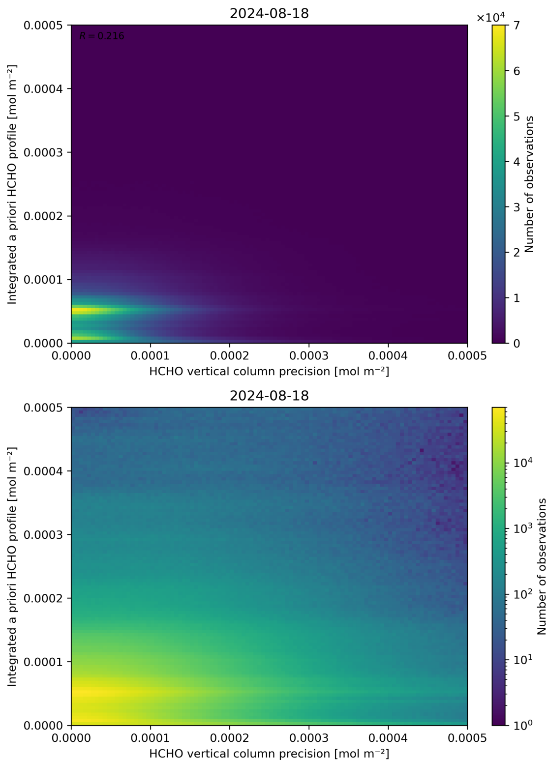
Figure 147: Scatter density plot of “HCHO vertical column precision” against “Integrated a priori HCHO profile” for 2024-08-17 to 2024-08-19.
