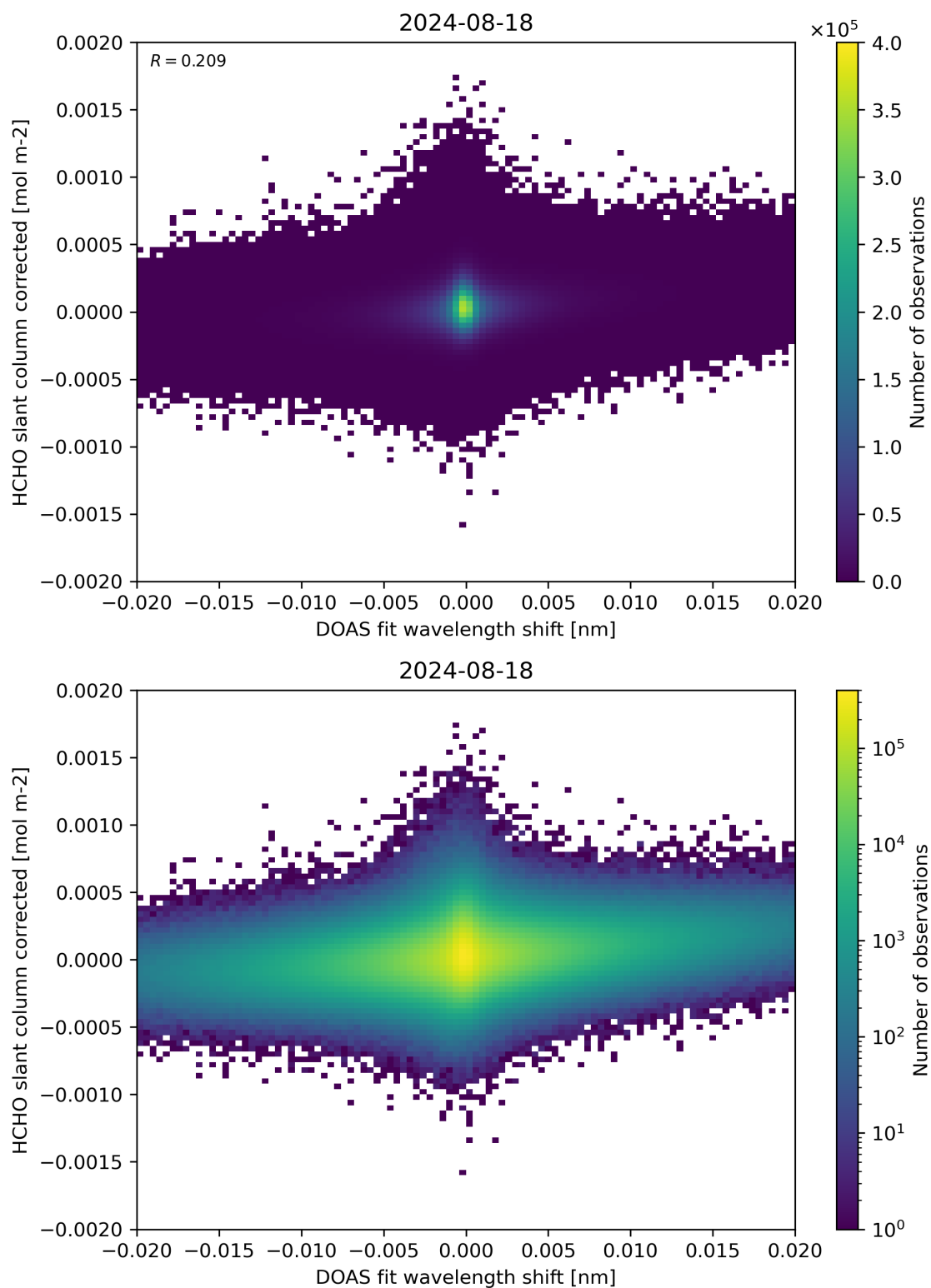
Figure 66: Scatter density plot of “DOAS fit wavelength shift” against “HCHO slant column corrected” for 2024-08-17 to 2024-08-19.
