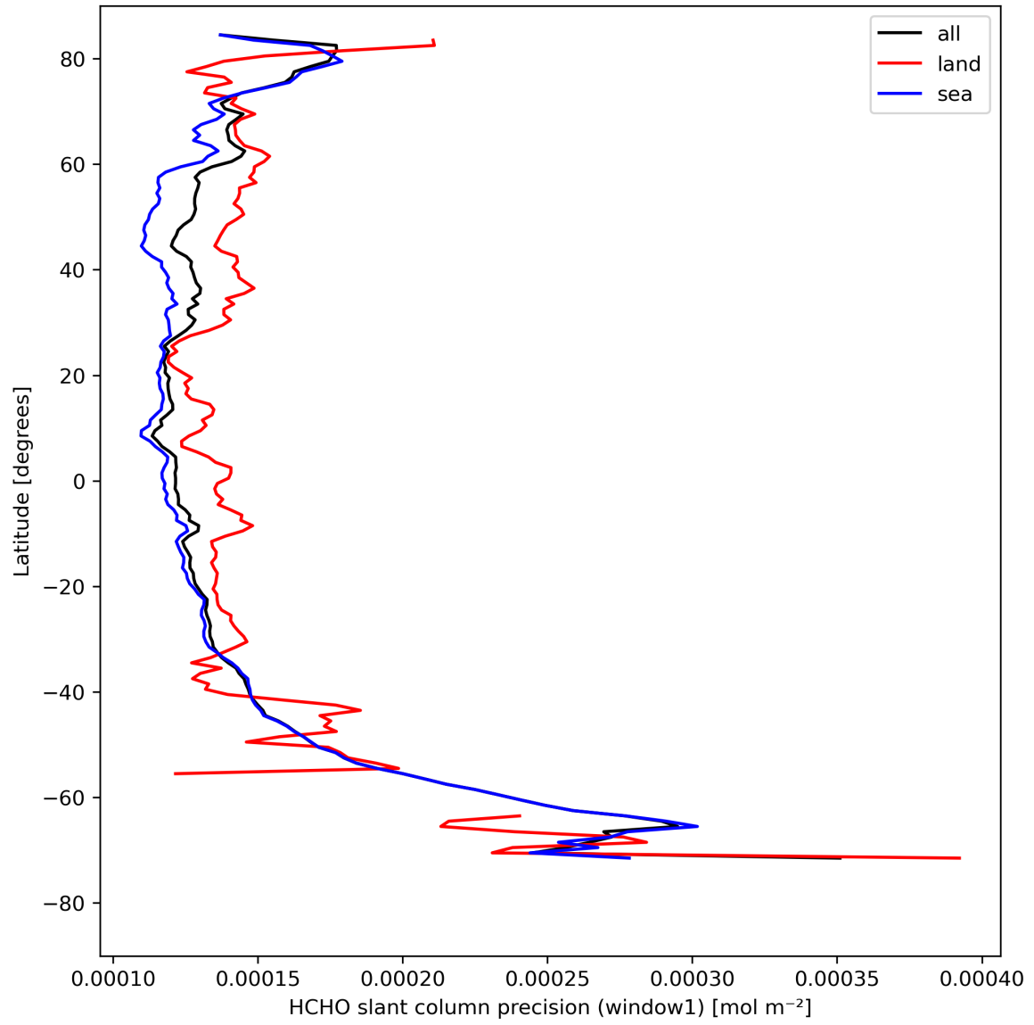
Figure 25: Zonal average of “HCHO slant column precision (window1)” for 2024-08-17 to 2024-08-19.
