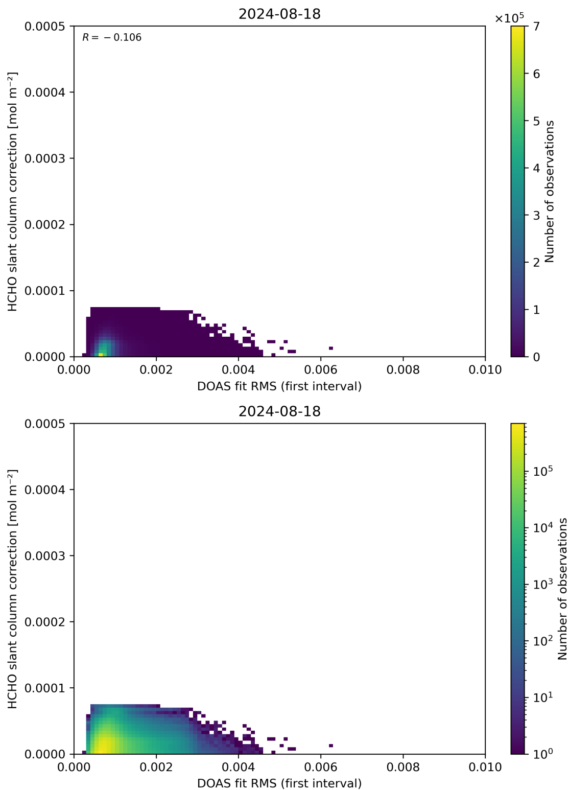
Figure 63: Scatter density plot of “DOAS fit RMS (first interval)” against “HCHO slant column correction” for 2024-08-17 to 2024-08-19.
