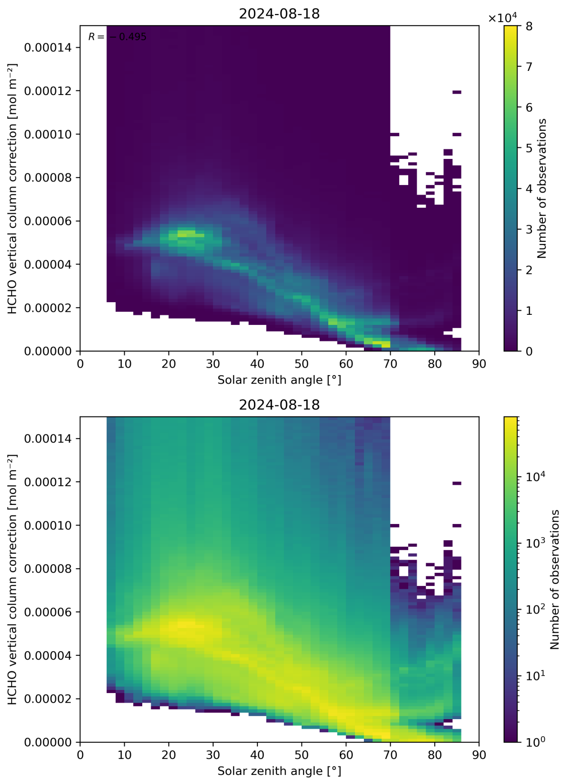
Figure 178: Scatter density plot of “Solar zenith angle” against “HCHO vertical column correction” for 2024-08-17 to 2024-08-19.
