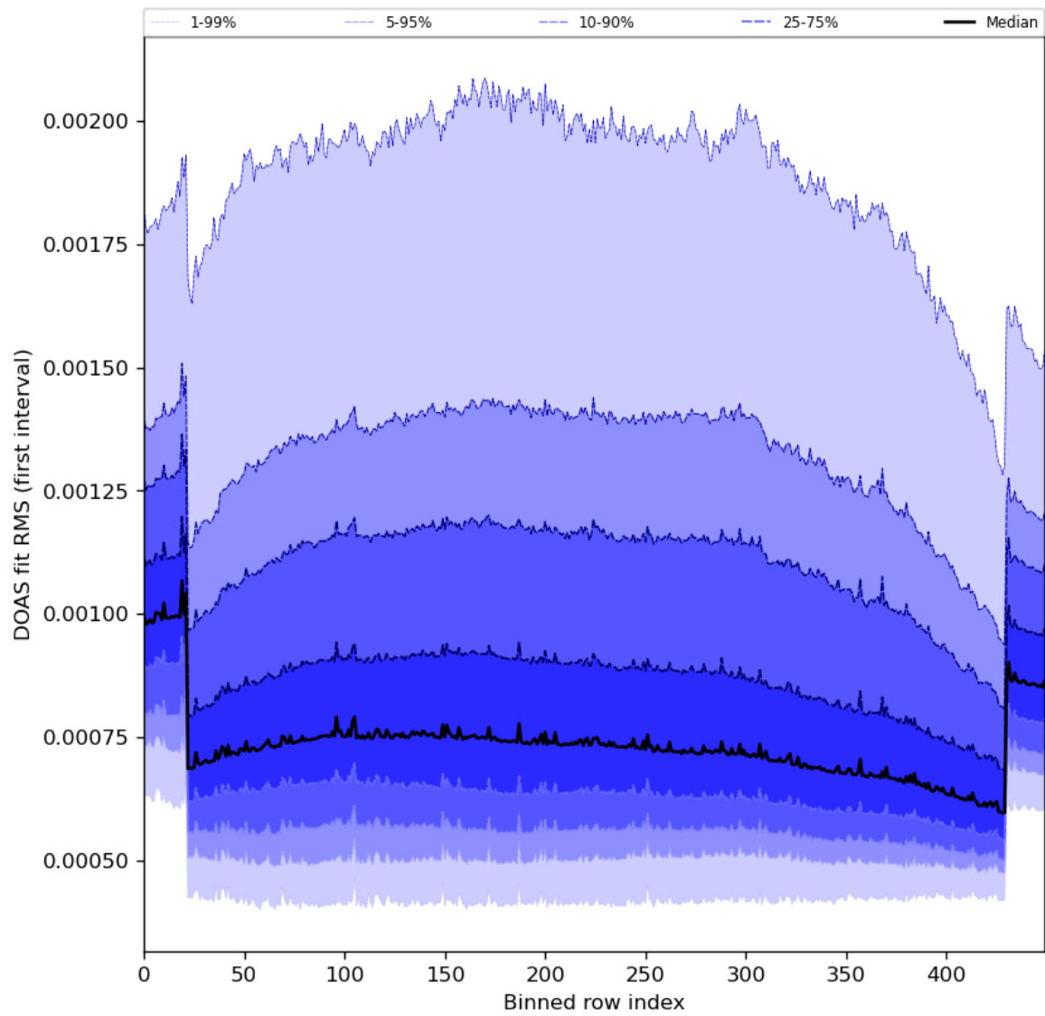
Figure 60: Along track statistics of “DOAS fit RMS (first interval)” for 2024-08-17 to 2024-08-19
