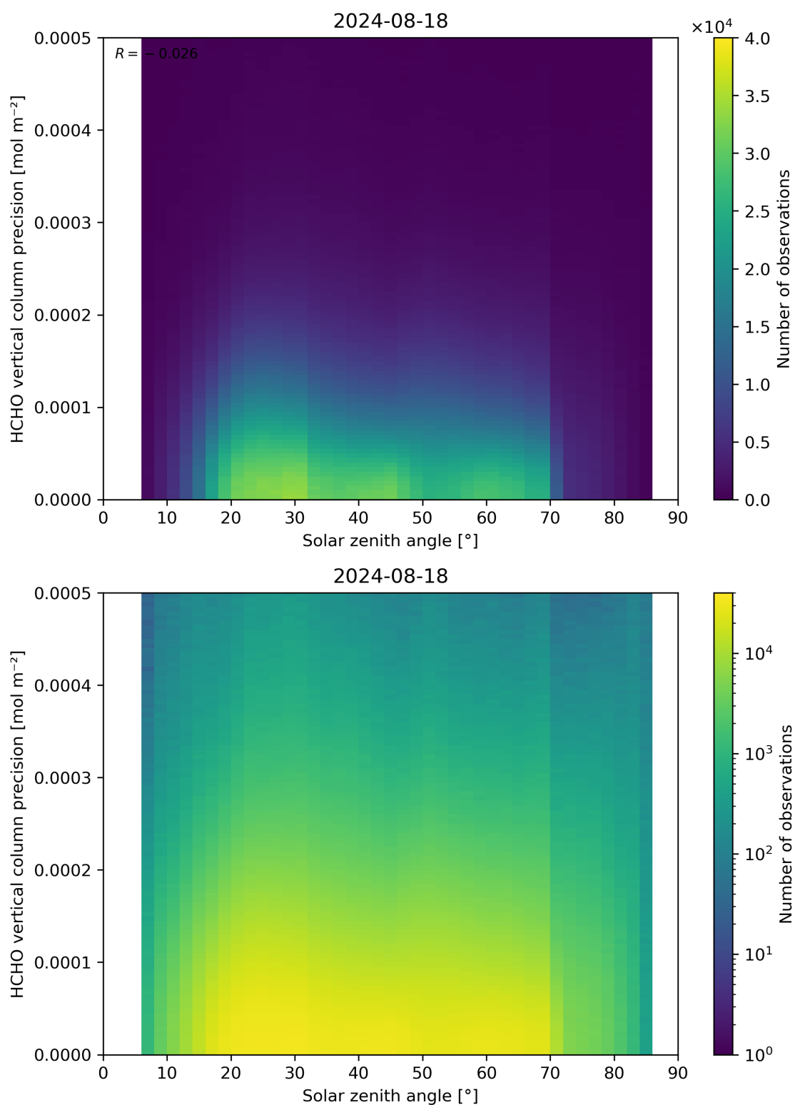
Figure 179: Scatter density plot of “Solar zenith angle” against “HCHO vertical column precision” for 2024-08-17 to 2024-08-19.
