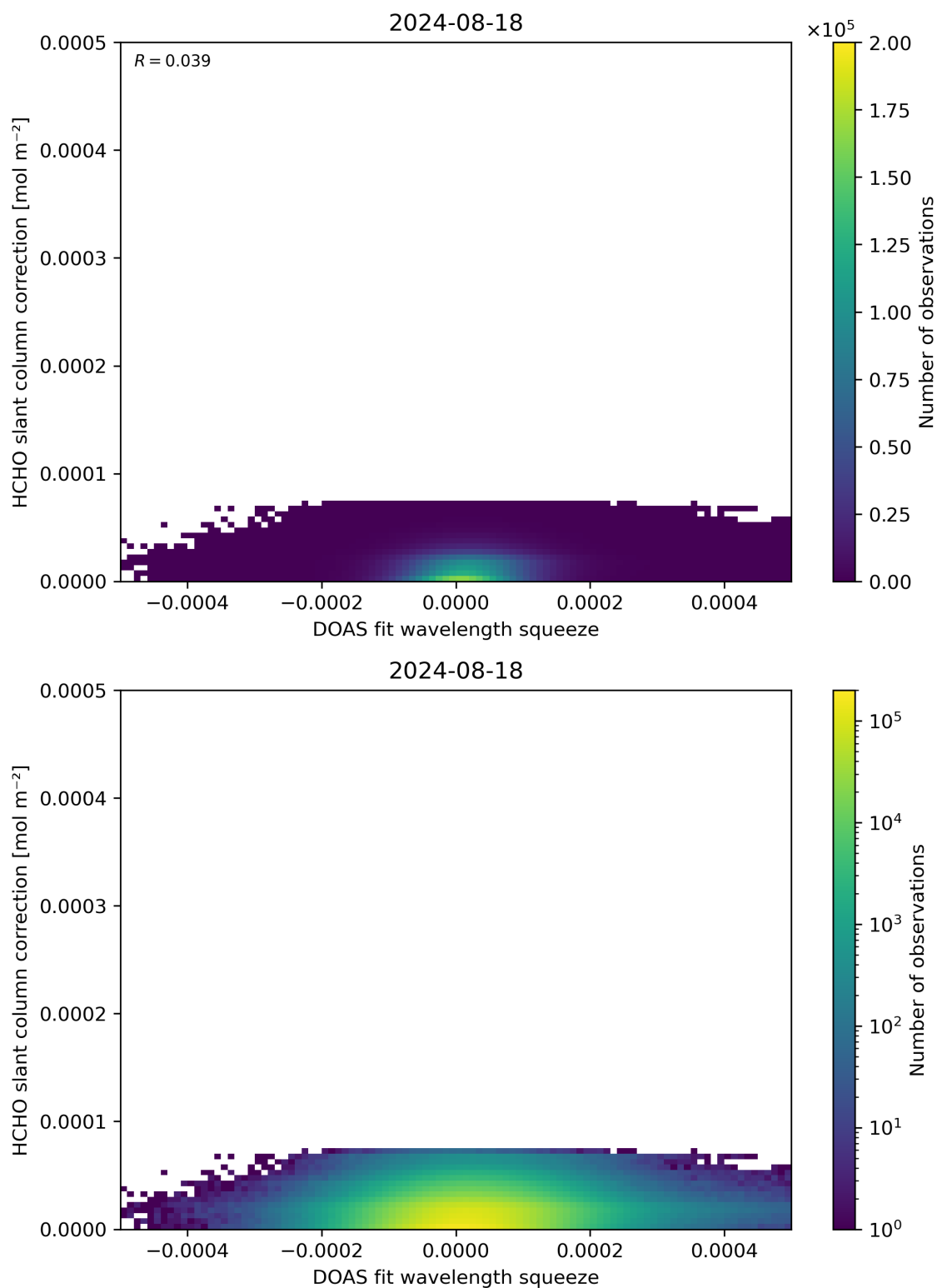
Figure 70: Scatter density plot of “DOAS fit wavelength squeeze” against “HCHO slant column correction” for 2024-08-17 to 2024-08-19.
