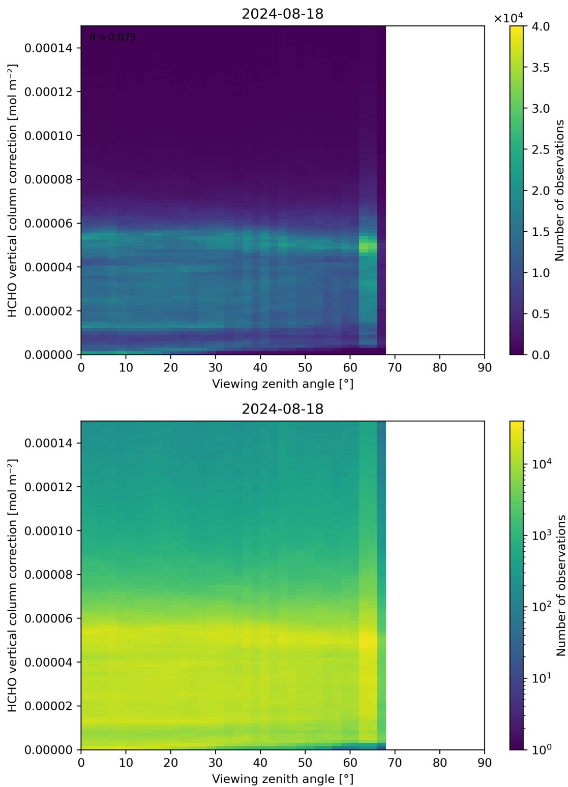
Figure 193: Scatter density plot of “Viewing zenith angle” against “HCHO vertical column correction” for 2024-08-17 to 2024-08-19.
