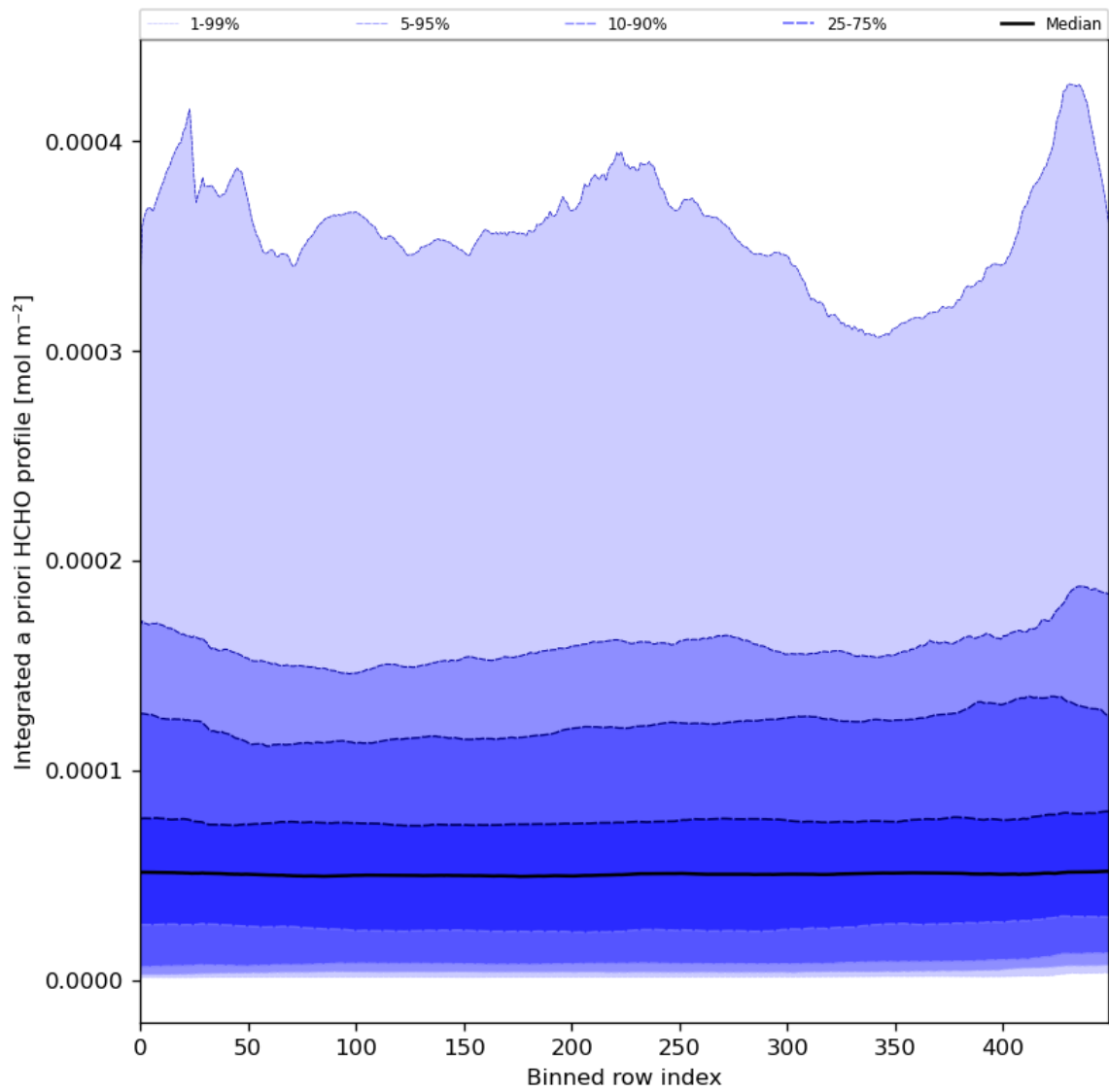
Figure 57: Along track statistics of "Integrated a priori HCHO profile" for 2024-08-17 to 2024-08-19
