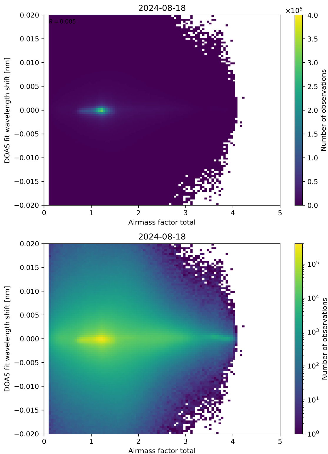
Figure 98: Scatter density plot of “Airmass factor total” against “DOAS fit wavelength shift” for 2024-08-17 to 2024-08-19.
