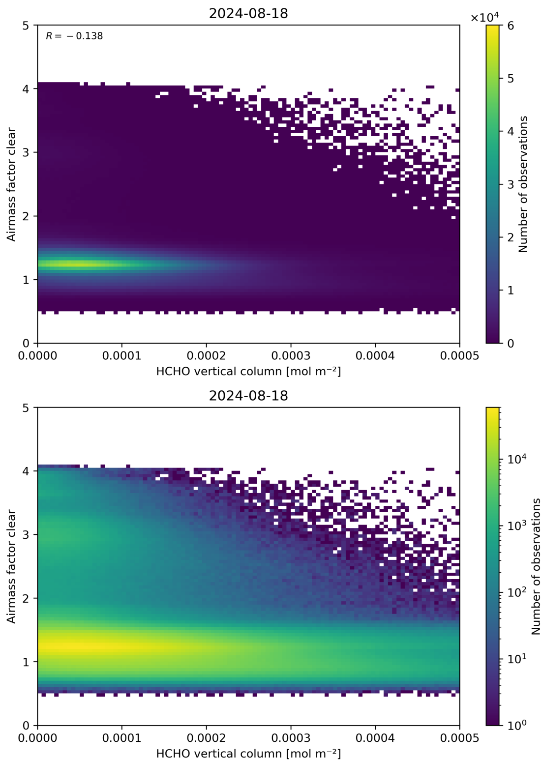
Figure 126: Scatter density plot of “HCHO vertical column” against “Airmass factor clear” for 2024-08-17 to 2024-08-19.
