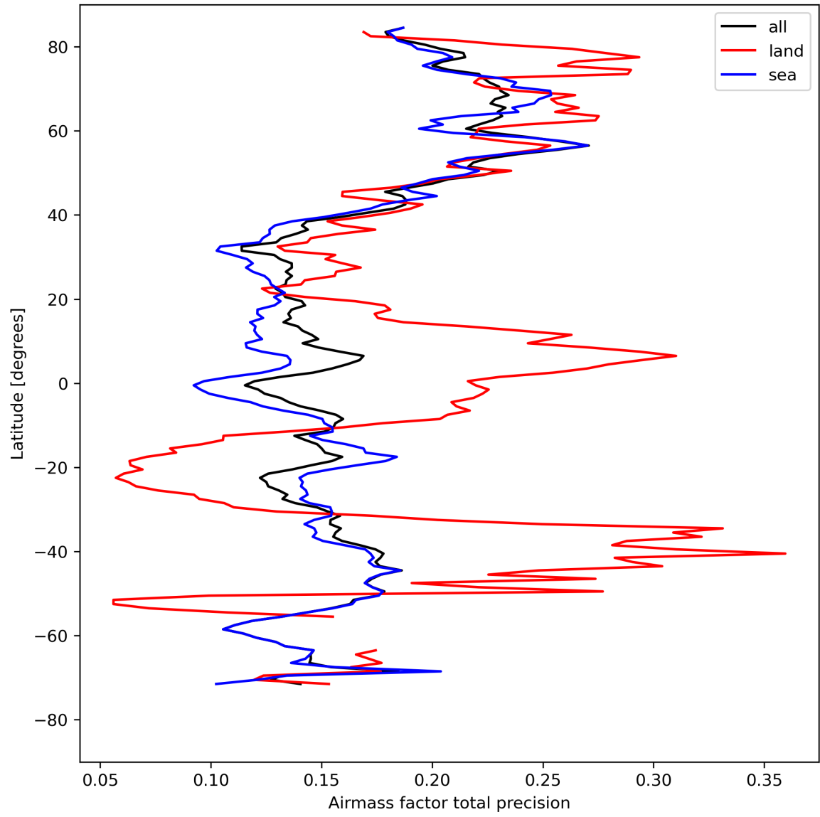
Figure 27: Zonal average of “Airmass factor total precision” for 2024-08-17 to 2024-08-19.
