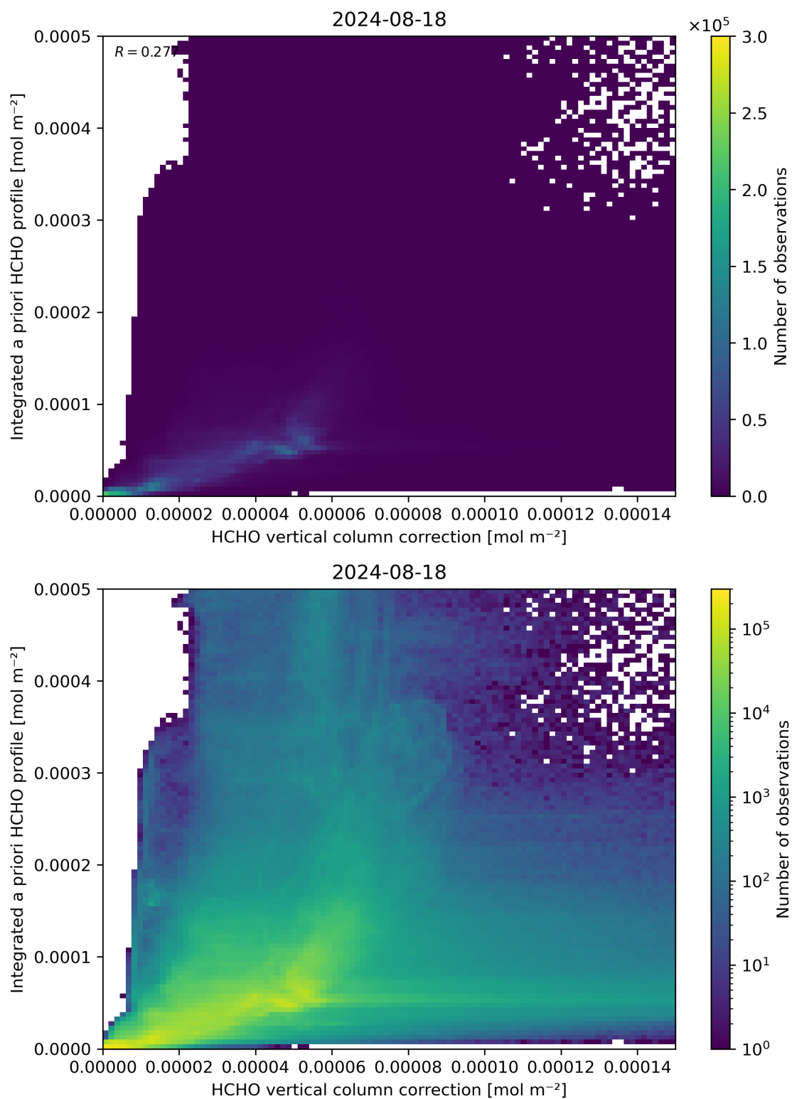
Figure 122: Scatter density plot of “HCHO vertical column correction” against “Integrated a priori HCHO profile” for 2024-08-17 to 2024-08-19.
