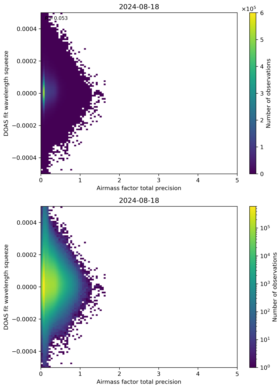
Figure 107: Scatter density plot of “Airmass factor total precision” against “DOAS fit wavelength squeeze” for 2024-08-17 to 2024-08-19.
