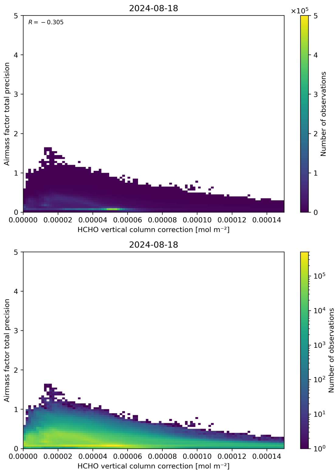
Figure 121: Scatter density plot of “HCHO vertical column correction” against “Airmass factor total precision” for 2024-08-17 to 2024-08-19.
