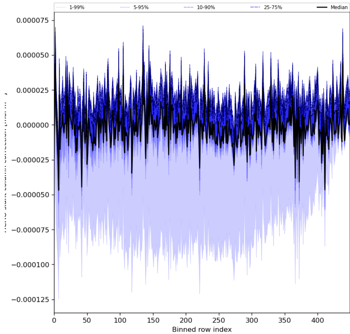
Figure 61: Along track statistics of “HCHO slant column correction” for 2024-08-17 to 2024-08-19
