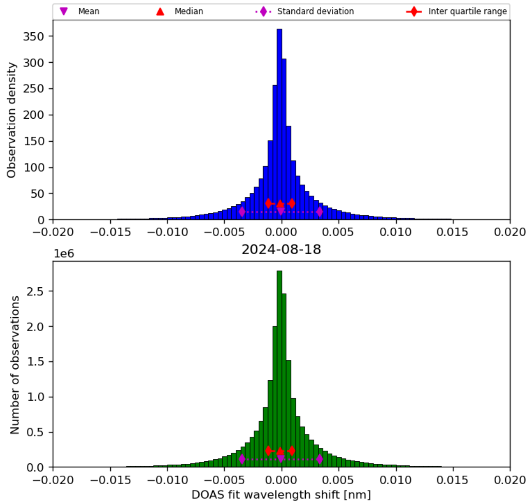
Figure 44: Histogram of “DOAS fit wavelength shift” for 2024-08-17 to 2024-08-19
