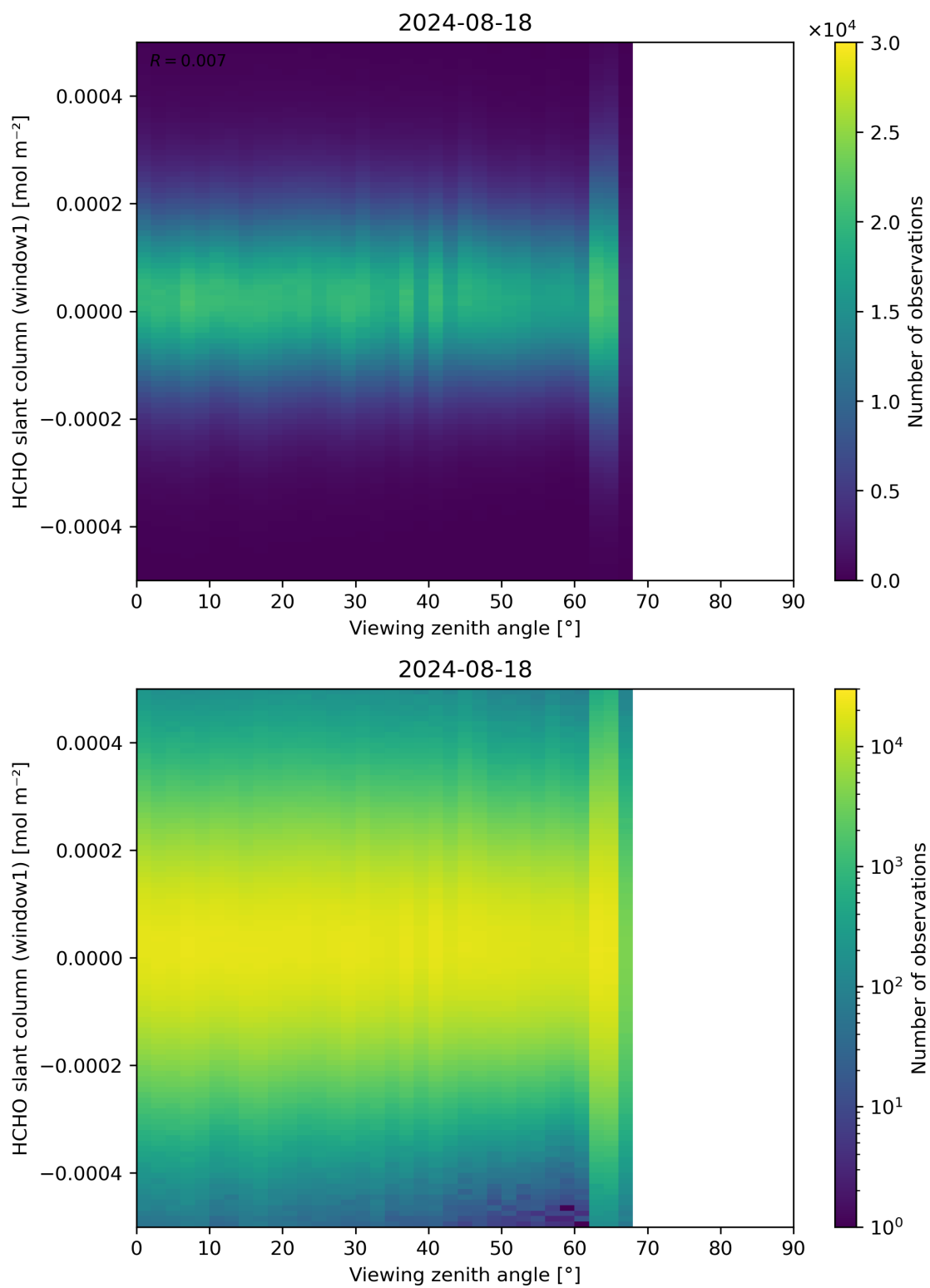
Figure 188: Scatter density plot of “Viewing zenith angle” against “HCHO slant column (window1)” for 2024-08-17 to 2024-08-19.
