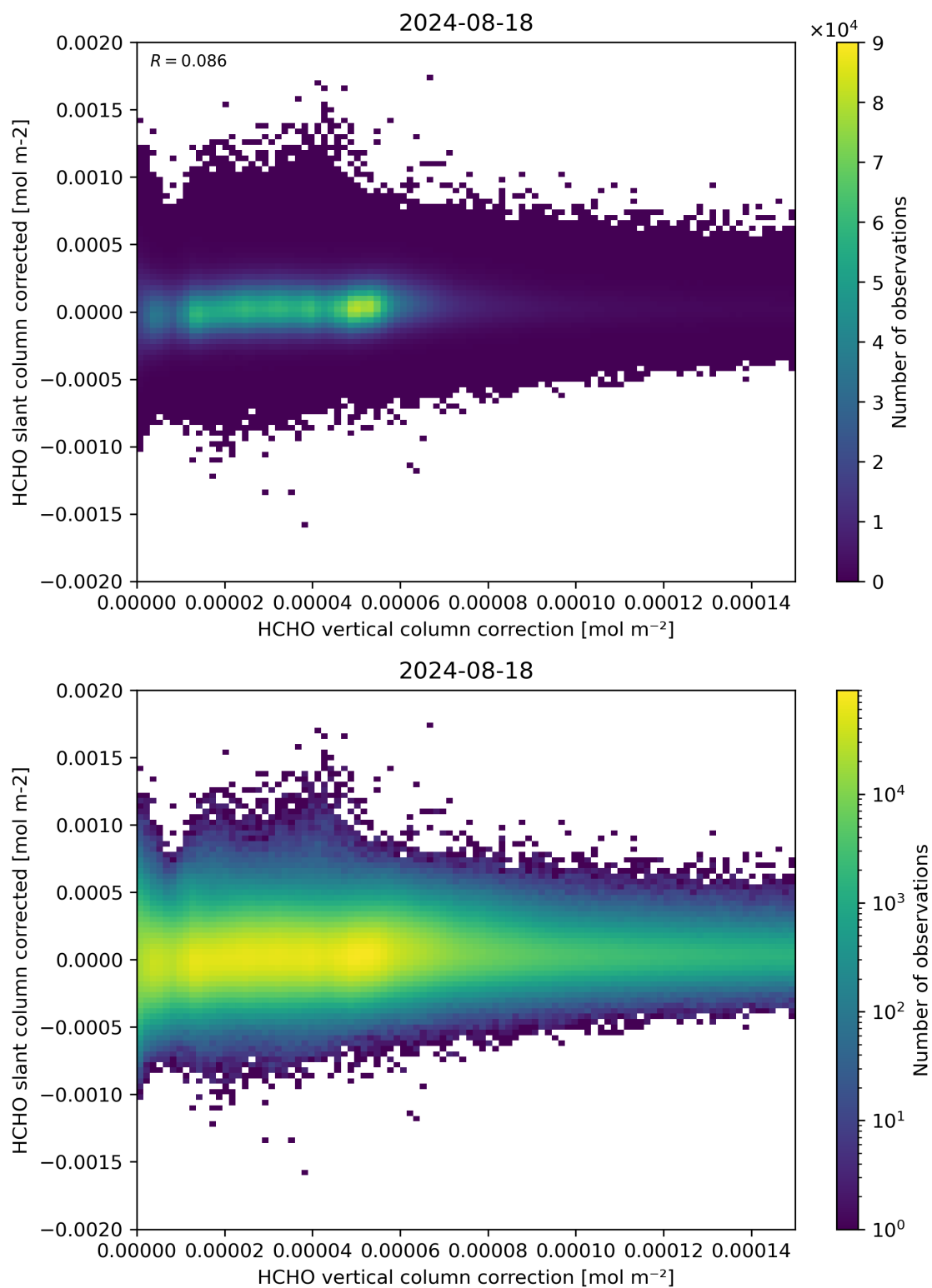
Figure 116: Scatter density plot of “HCHO vertical column correction” against “HCHO slant column corrected” for 2024-08-17 to 2024-08-19.
