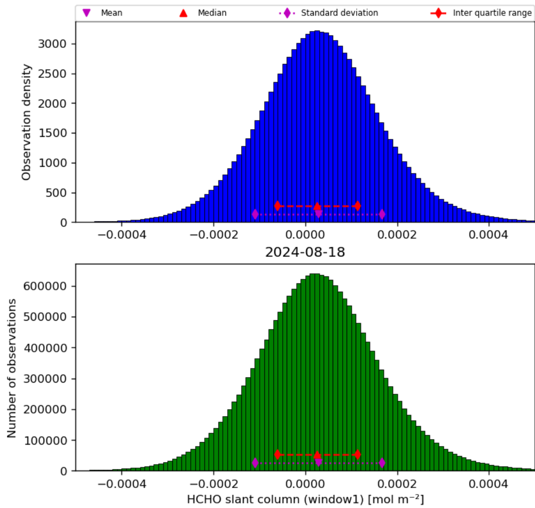
Figure 38: Histogram of “HCHO slant column (window1)” for 2024-08-17 to 2024-08-19
