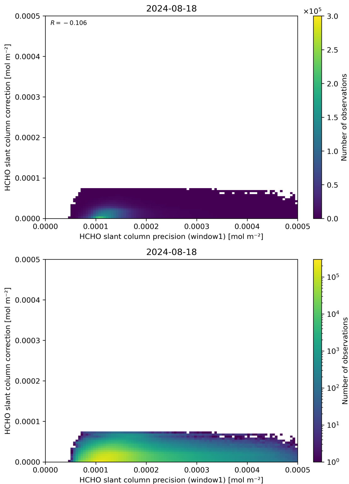
Figure 93: Scatter density plot of “HCHO slant column precision (window1)” against “HCHO slant column correction” for 2024-08-17 to 2024-08-19.
