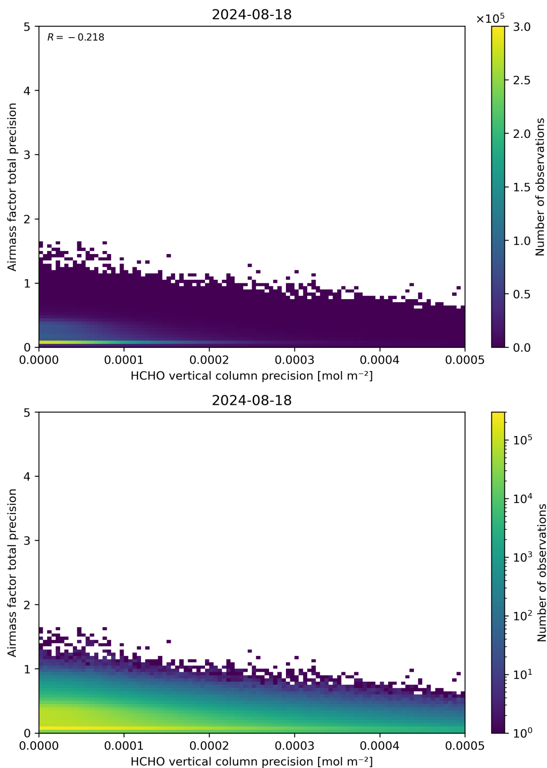
Figure 145: Scatter density plot of “HCHO vertical column precision” against “Airmass factor total precision” for 2024-08-17 to 2024-08-19.
