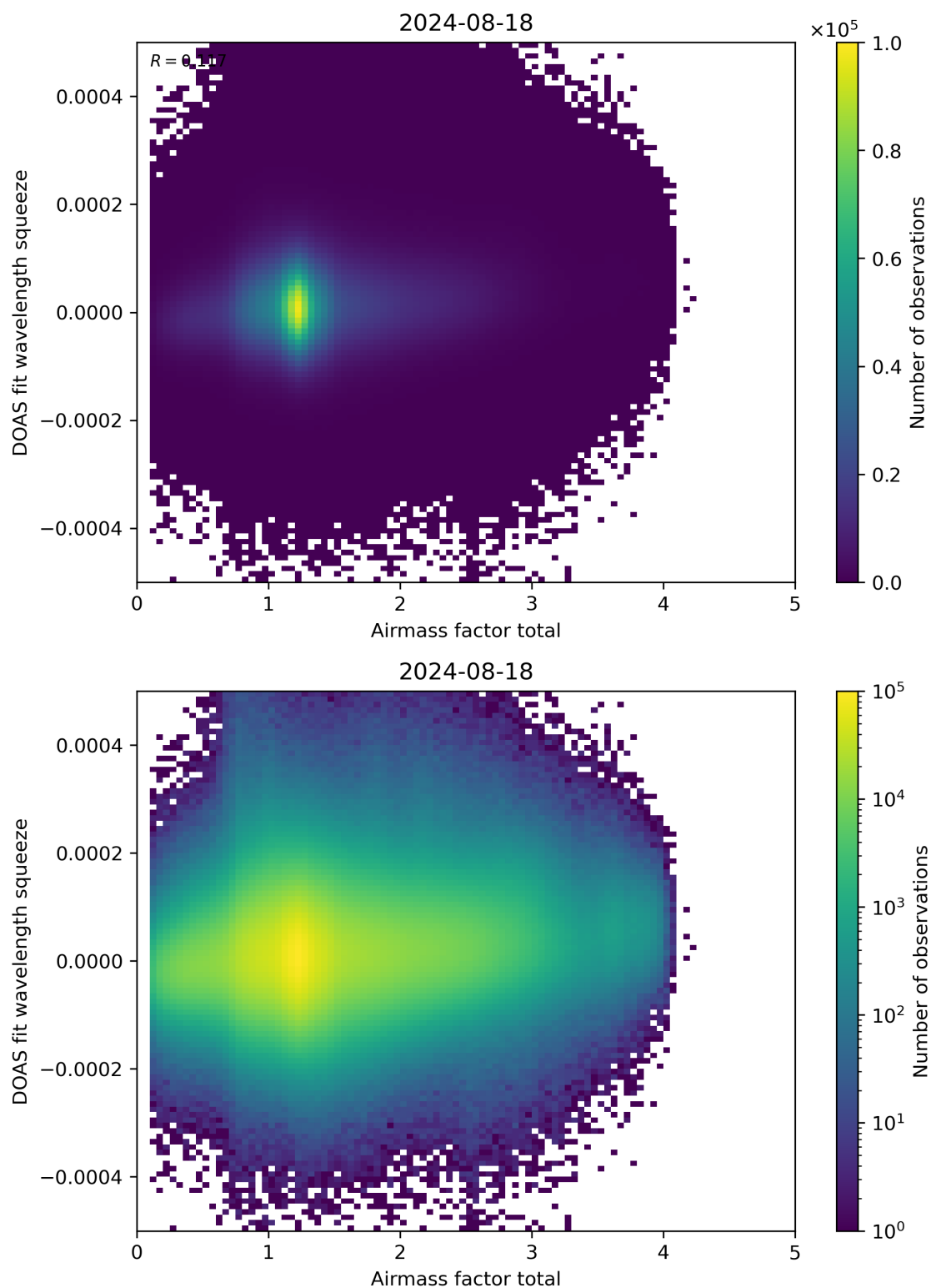
Figure 99: Scatter density plot of “Airmass factor total” against “DOAS fit wavelength squeeze” for 2024-08-17 to 2024-08-19.
