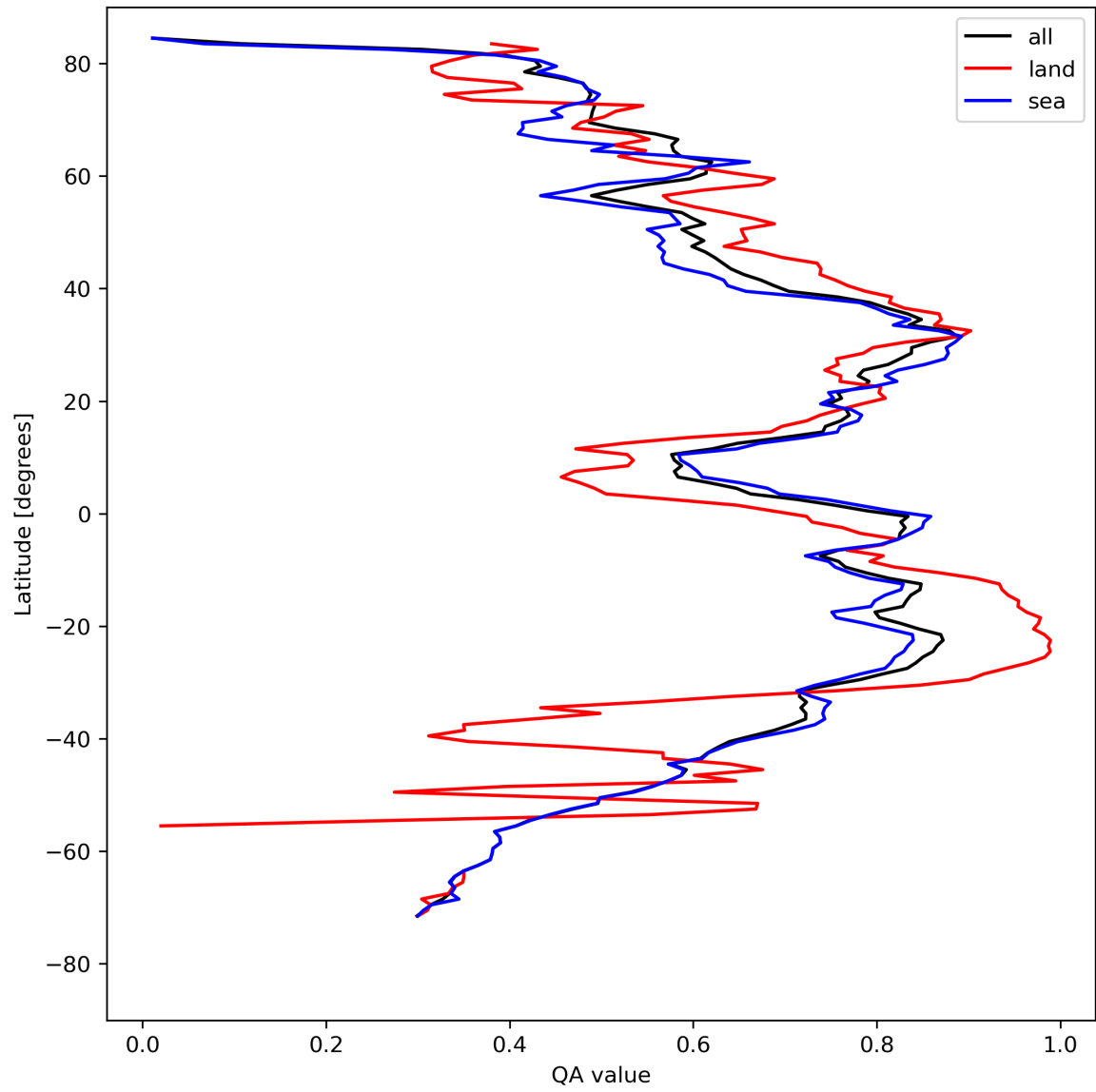
Figure 20: Zonal average of “QA value” for 2024-08-17 to 2024-08-19.
