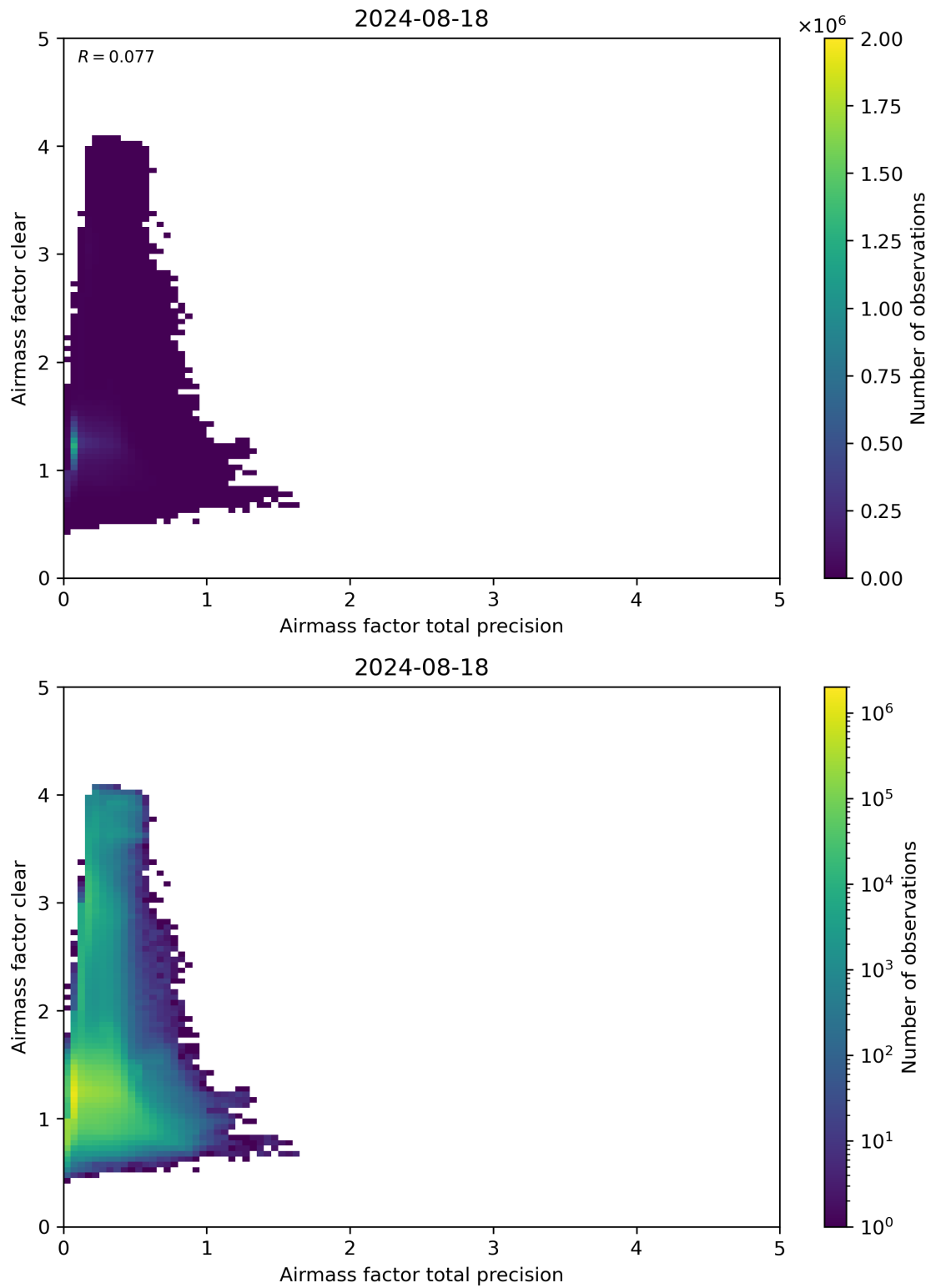
Figure 108: Scatter density plot of “Airmass factor total precision” against “Airmass factor clear” for 2024-08-17 to 2024-08-19.
