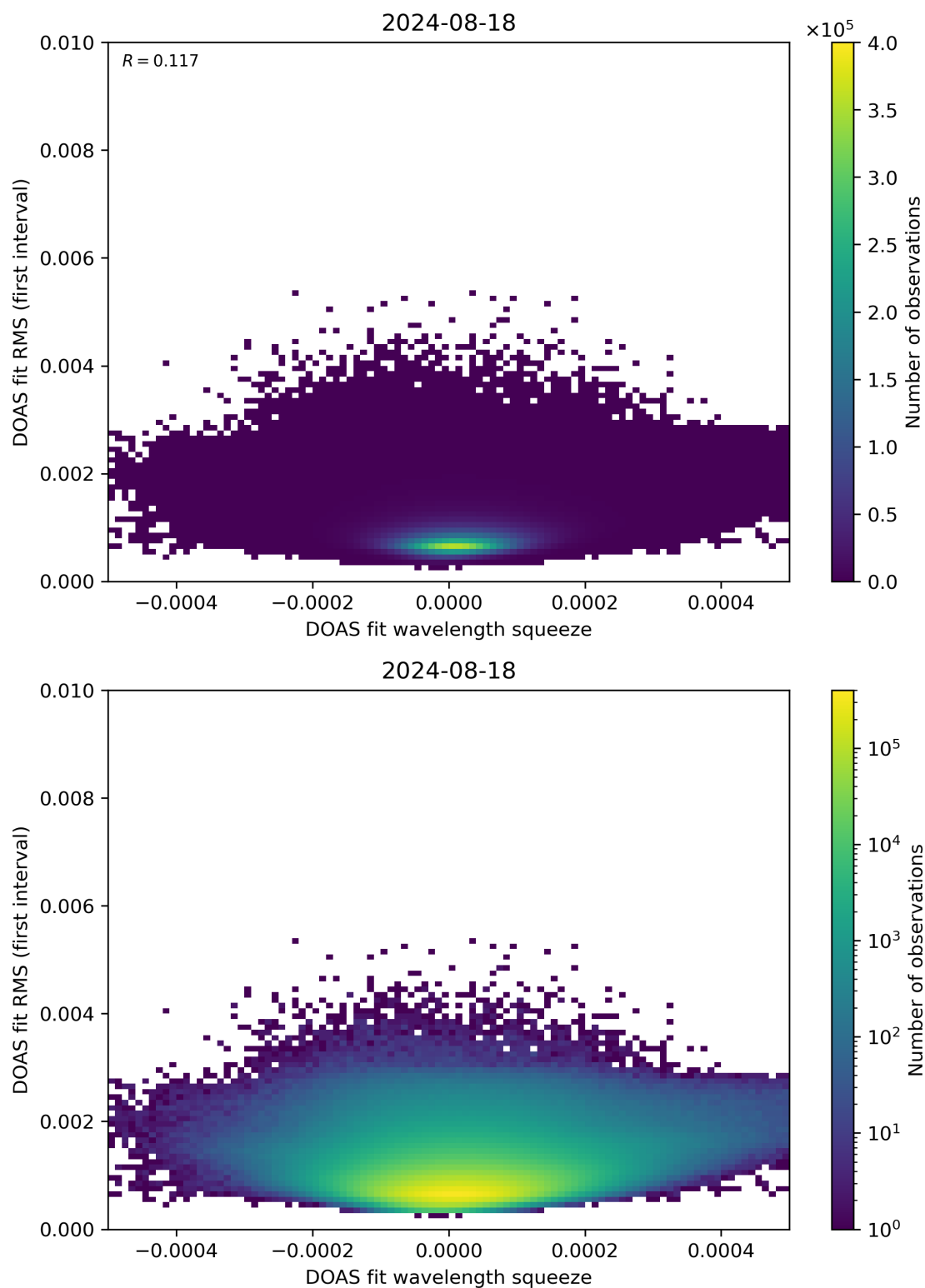
Figure 68: Scatter density plot of “DOAS fit wavelength squeeze” against “DOAS fit RMS (first interval)” for 2024-08-17 to 2024-08-19.
