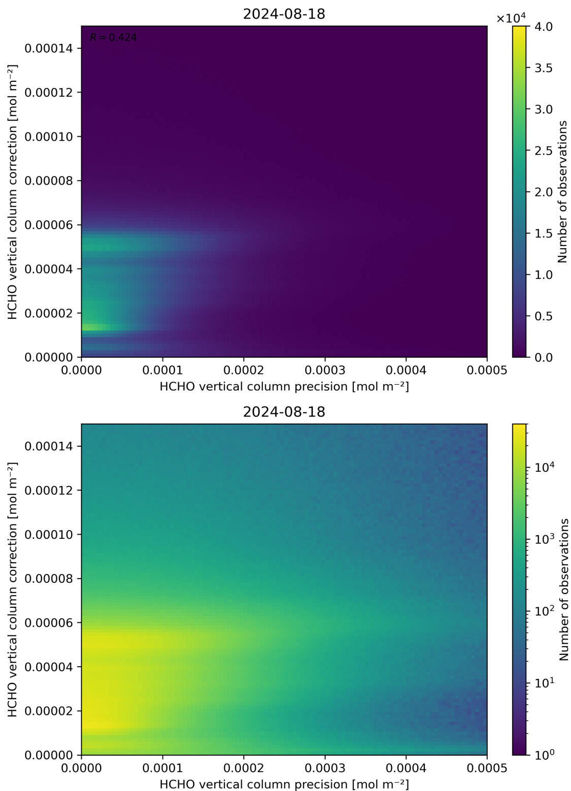
Figure 146: Scatter density plot of “HCHO vertical column precision” against “HCHO vertical column correction” for 2024-08-17 to 2024-08-19.
