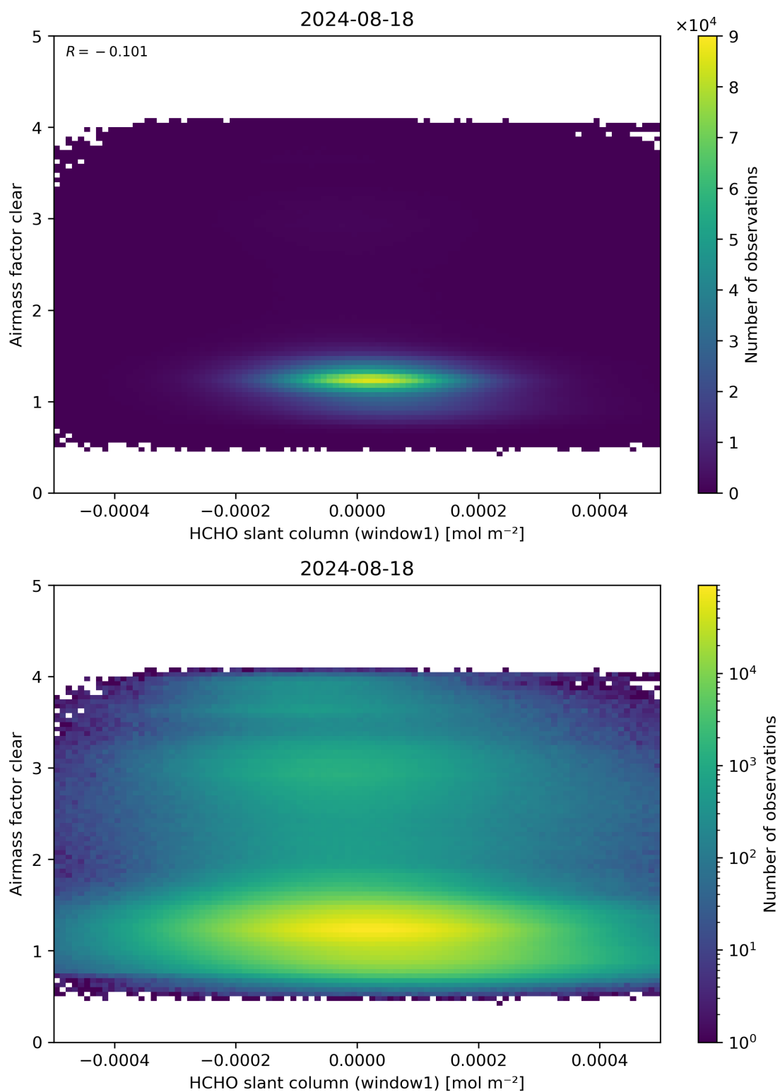
Figure 81: Scatter density plot of “HCHO slant column (window1)” against “Airmass factor clear” for 2024-08-17 to 2024-08-19.
