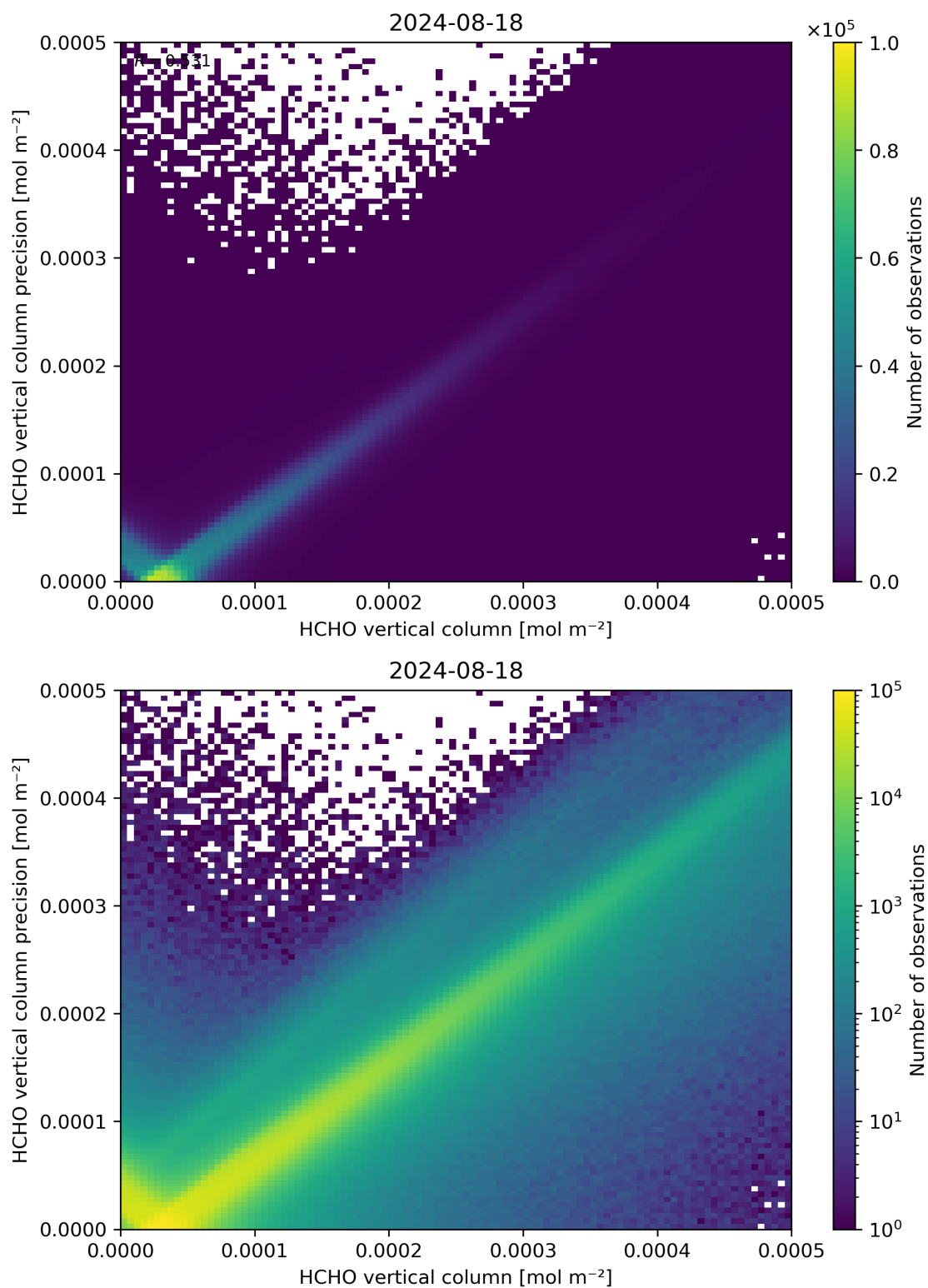
Figure 134: Scatter density plot of “HCHO vertical column” against “HCHO vertical column precision” for 2024-08-17 to 2024-08-19.
