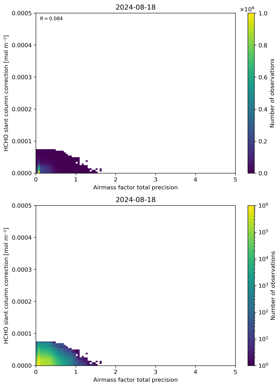
Figure 110: Scatter density plot of “Airmass factor total precision” against “HCHO slant column correction” for 2024-08-17 to 2024-08-19.
