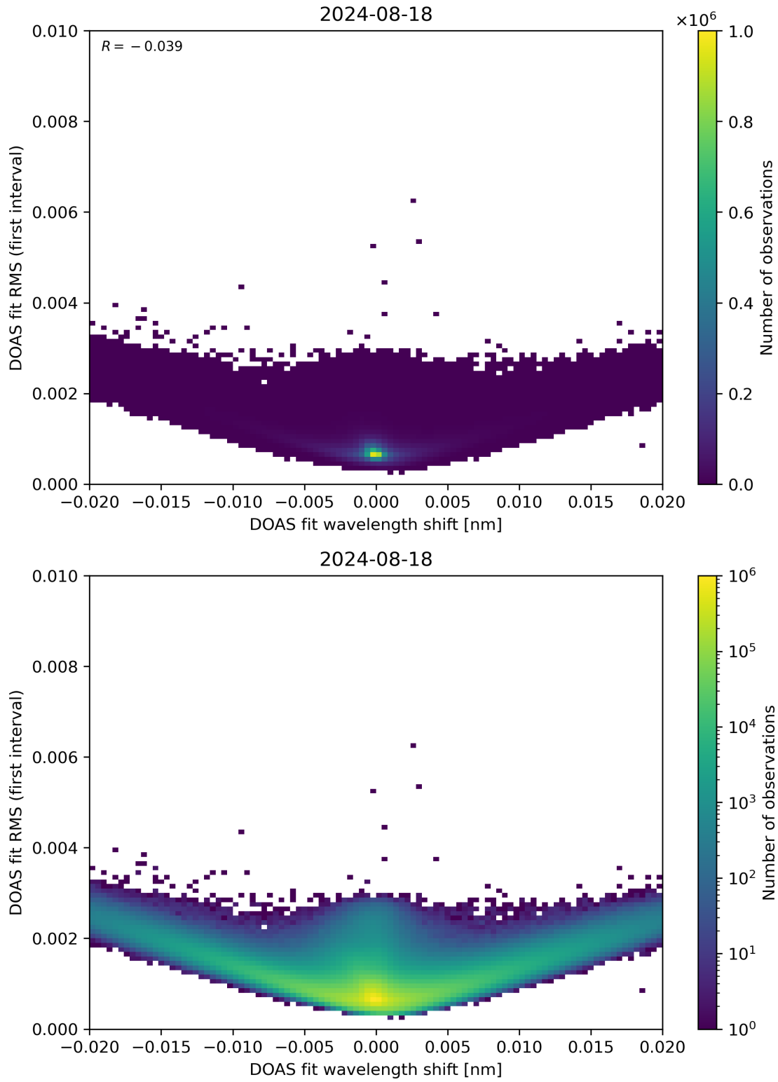
Figure 64: Scatter density plot of “DOAS fit wavelength shift” against “DOAS fit RMS (first interval)” for 2024-08-17 to 2024-08-19.
