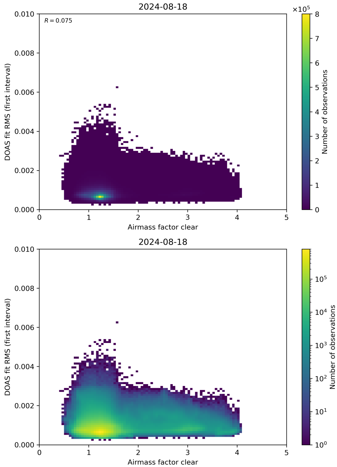
Figure 71: Scatter density plot of “Airmass factor clear” against “DOAS fit RMS (first interval)” for 2024-08-17 to 2024-08-19.
