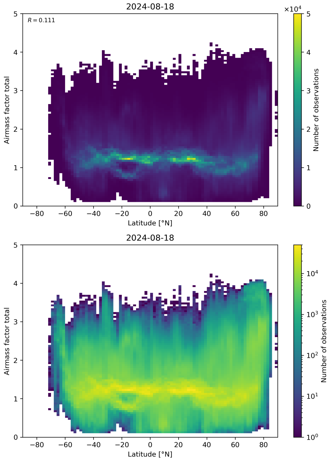
Figure 161: Scatter density plot of “Latitude” against “Airmass factor total” for 2024-08-17 to 2024-08-19.
