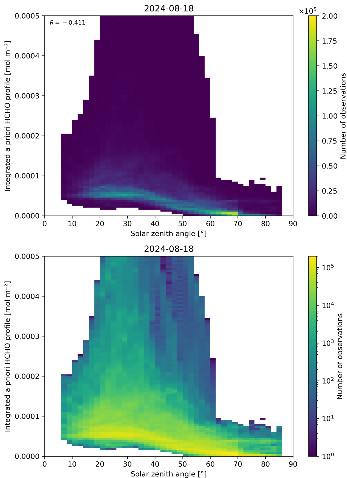
Figure 180: Scatter density plot of “Solar zenith angle” against “Integrated a priori HCHO profile” for 2024-08-17 to 2024-08-19.
