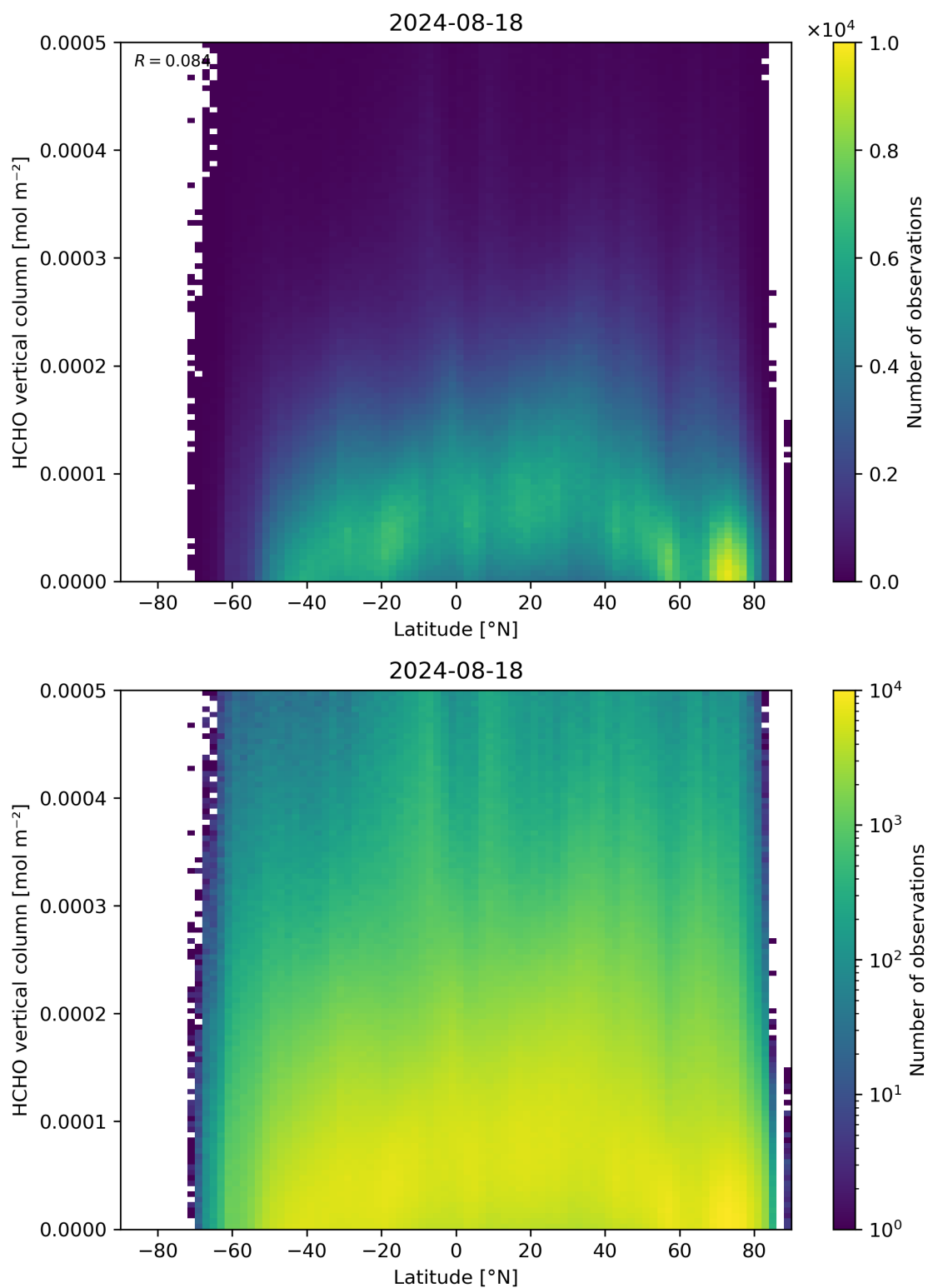
Figure 163: Scatter density plot of “Latitude” against “HCHO vertical column” for 2024-08-17 to 2024-08-19.
