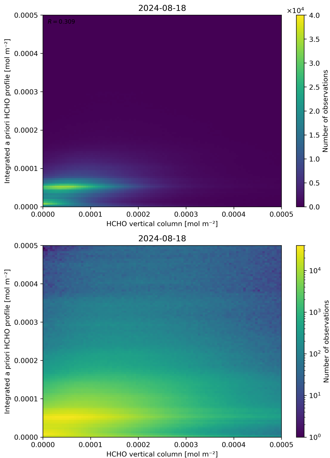
Figure 135: Scatter density plot of “HCHO vertical column” against “Integrated a priori HCHO profile” for 2024-08-17 to 2024-08-19.
