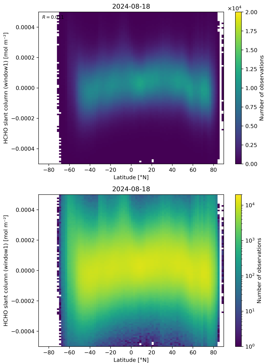
Figure 159: Scatter density plot of “Latitude” against “HCHO slant column (window1)” for 2024-08-17 to 2024-08-19.
