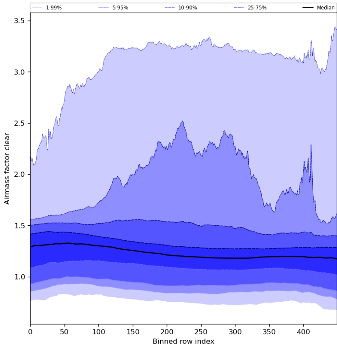
Figure 56: Along track statistics of “Airmass factor clear” for 2024-08-17 to 2024-08-19
