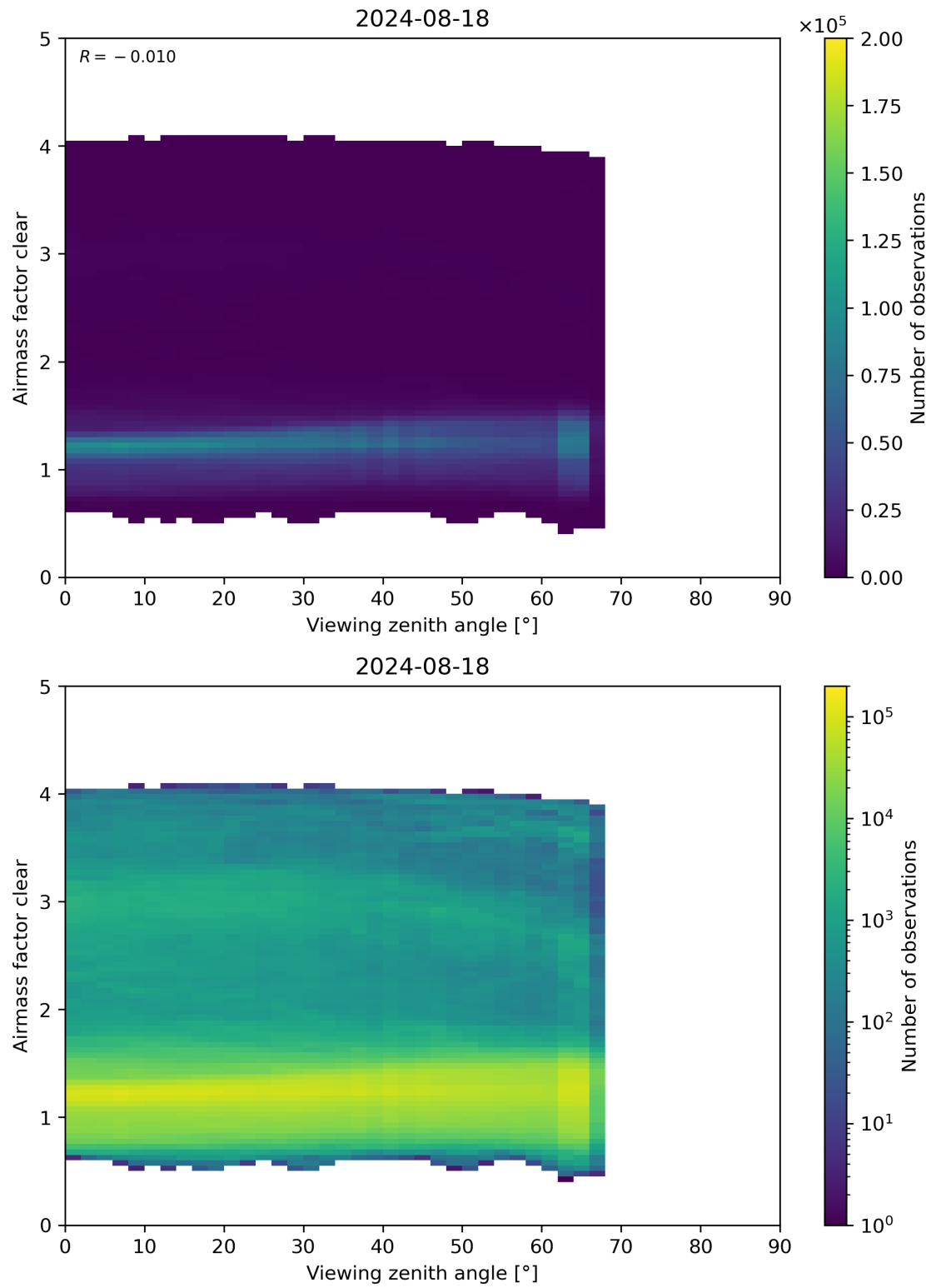
Figure 185: Scatter density plot of “Viewing zenith angle” against “Airmass factor clear” for 2024-08-17 to 2024-08-19.
