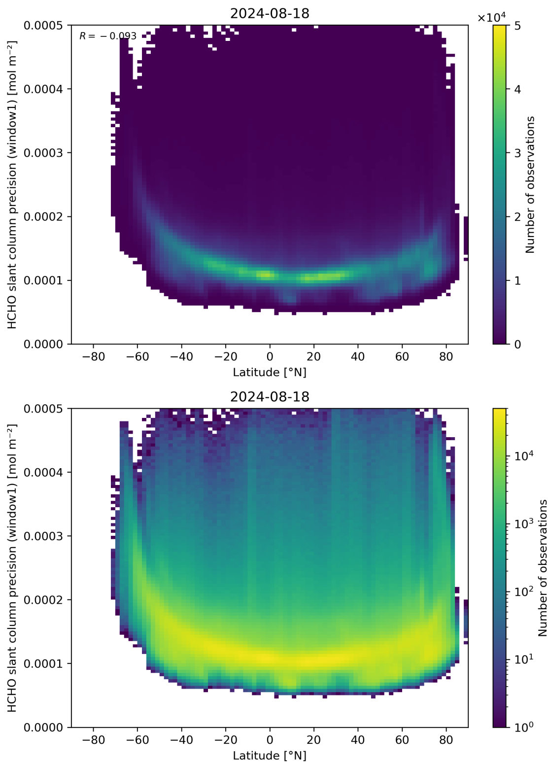
Figure 160: Scatter density plot of “Latitude” against “HCHO slant column precision (window1)” for 2024-08-17 to 2024-08-19.
