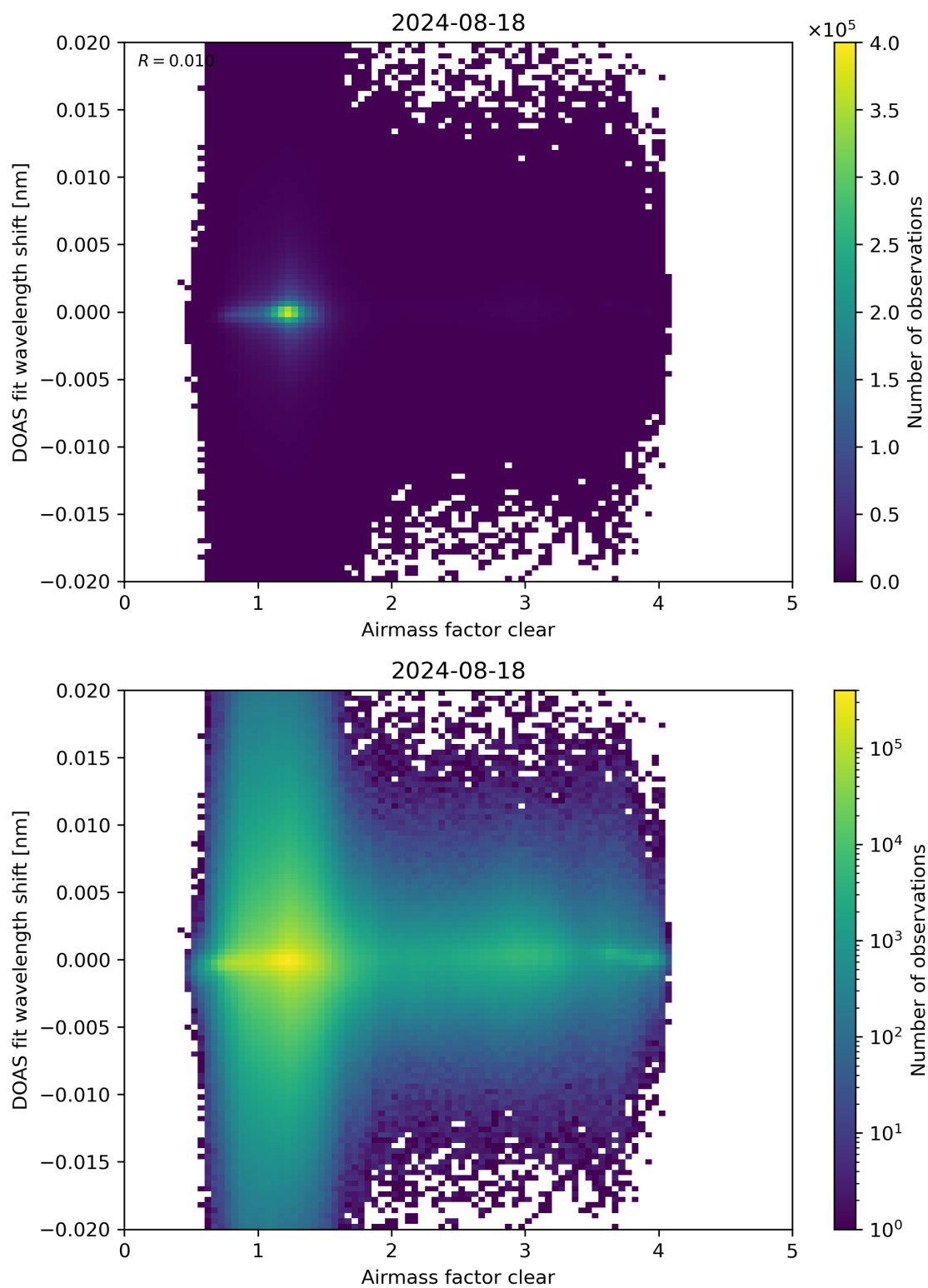
Figure 72: Scatter density plot of “Airmass factor clear” against “DOAS fit wavelength shift” for 2024-08-17 to 2024-08-19.
