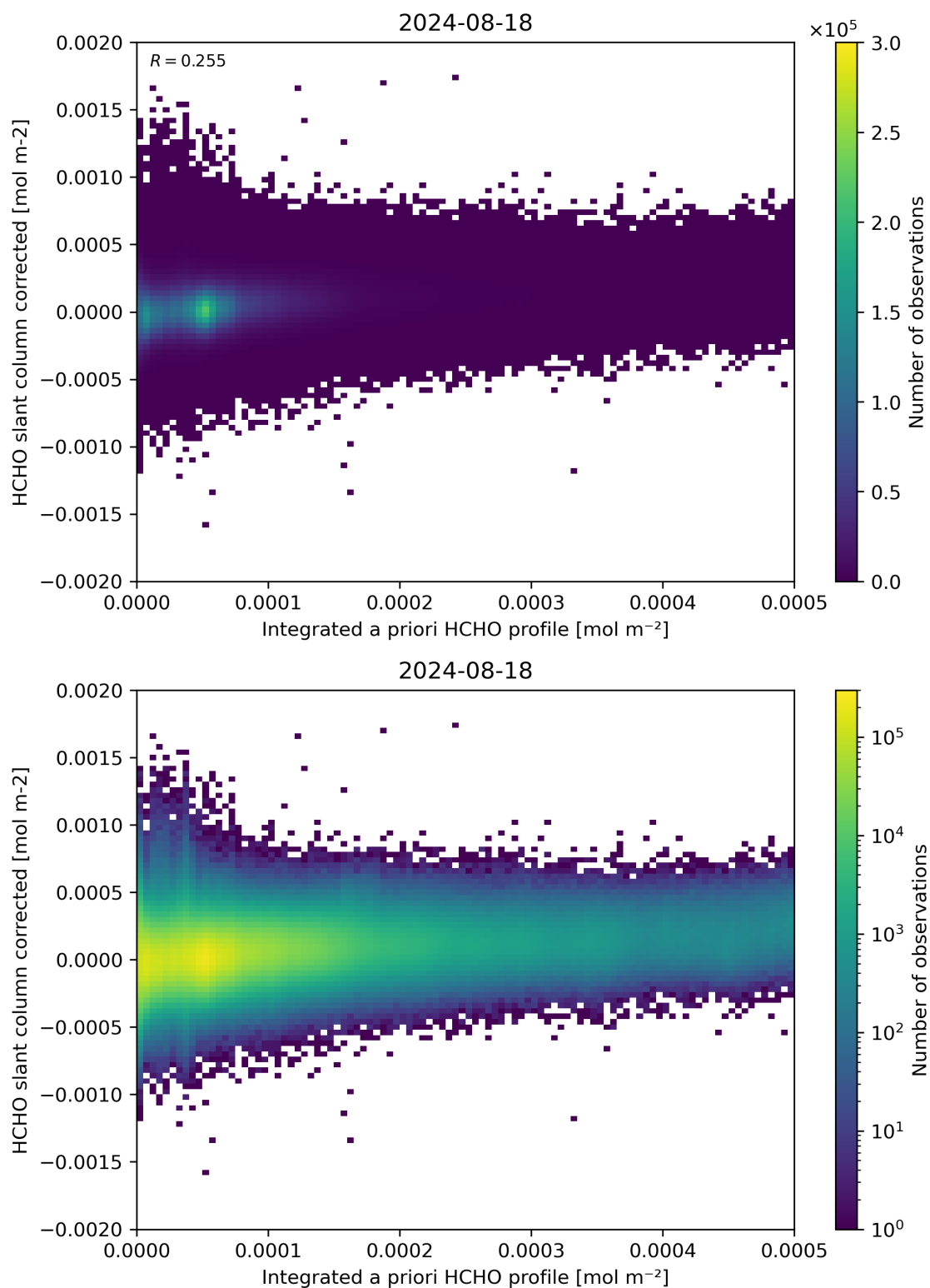
Figure 151: Scatter density plot of “Integrated a priori HCHO profile” against “HCHO slant column corrected” for 2024-08-17 to 2024-08-19.
