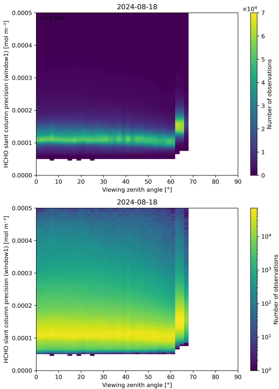
Figure 189: Scatter density plot of “Viewing zenith angle” against “HCHO slant column precision (window1)” for 2024-08-17 to 2024-08-19.
