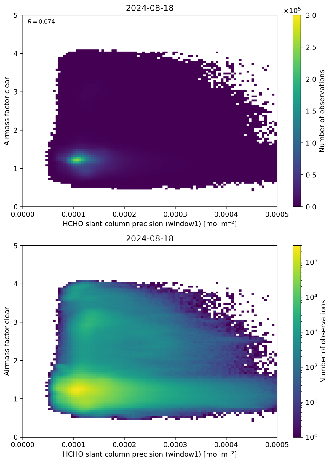
Figure 91: Scatter density plot of “HCHO slant column precision (window1)” against “Airmass factor clear” for 2024-08-17 to 2024-08-19.
