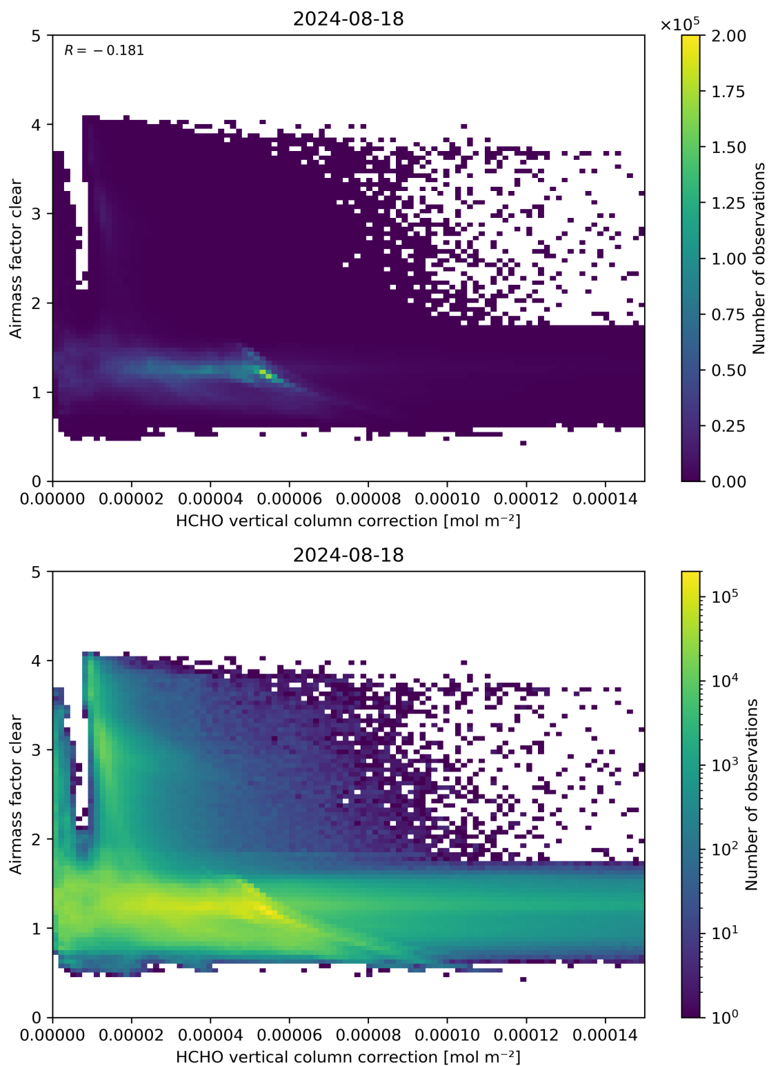
Figure 115: Scatter density plot of “HCHO vertical column correction” against “Airmass factor clear” for 2024-08-17 to 2024-08-19.
