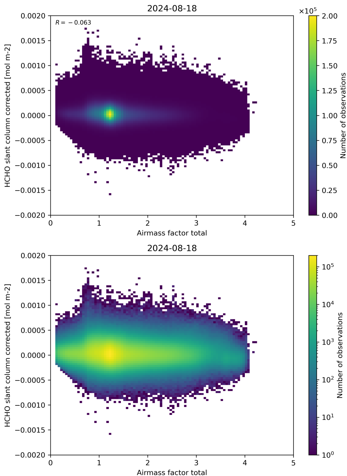
Figure 101: Scatter density plot of “Airmass factor total” against “HCHO slant column corrected” for 2024-08-17 to 2024-08-19.
