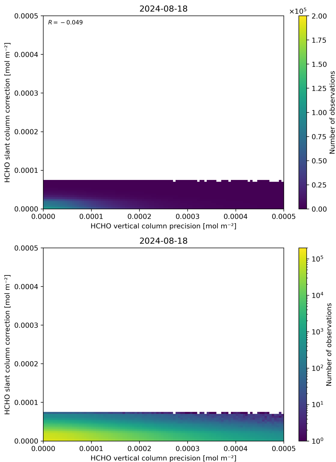
Figure 141: Scatter density plot of “HCHO vertical column precision” against “HCHO slant column correction” for 2024-08-17 to 2024-08-19.
