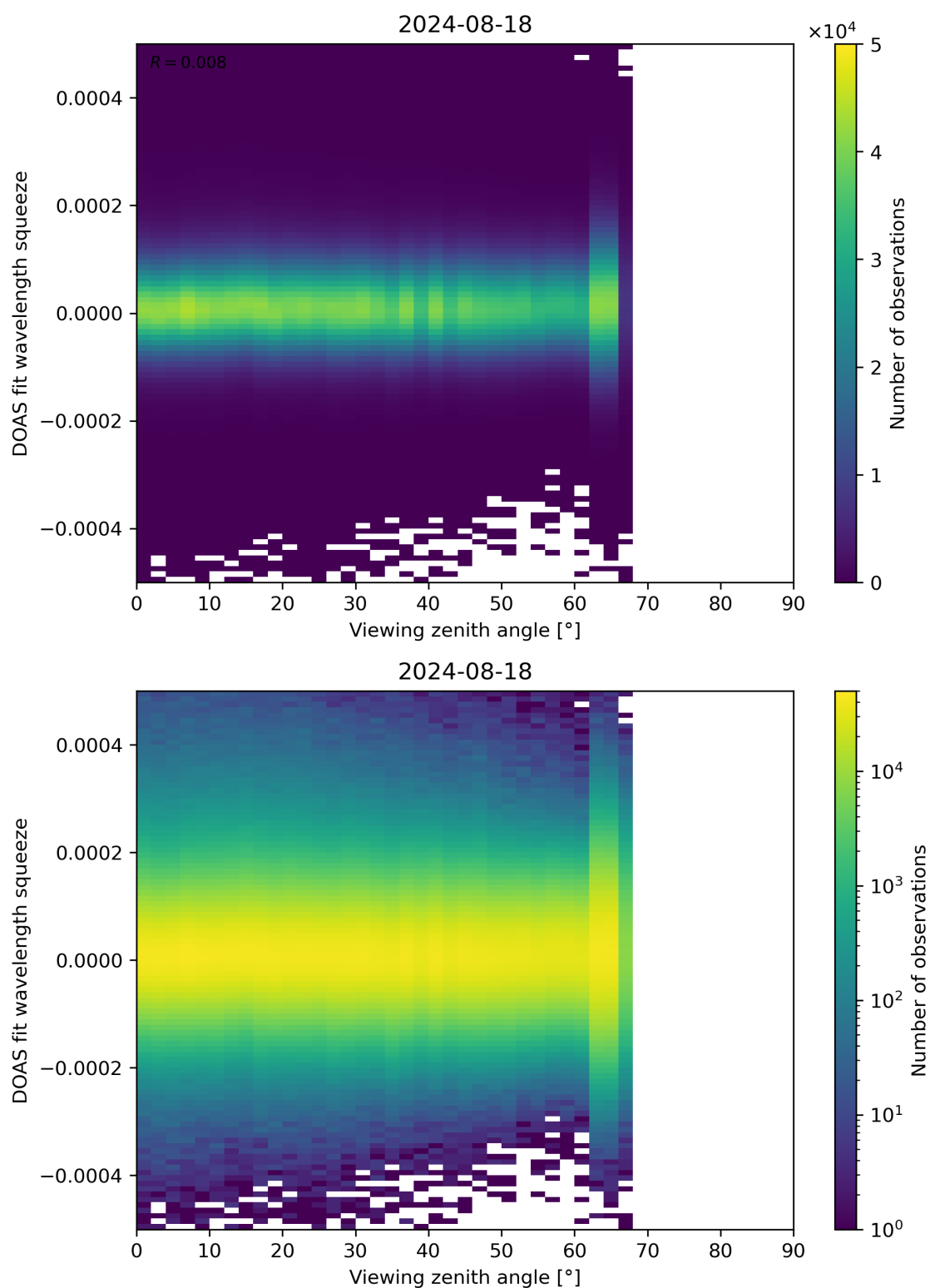
Figure 184: Scatter density plot of “Viewing zenith angle” against “DOAS fit wavelength squeeze” for 2024-08-17 to 2024-08-19.
