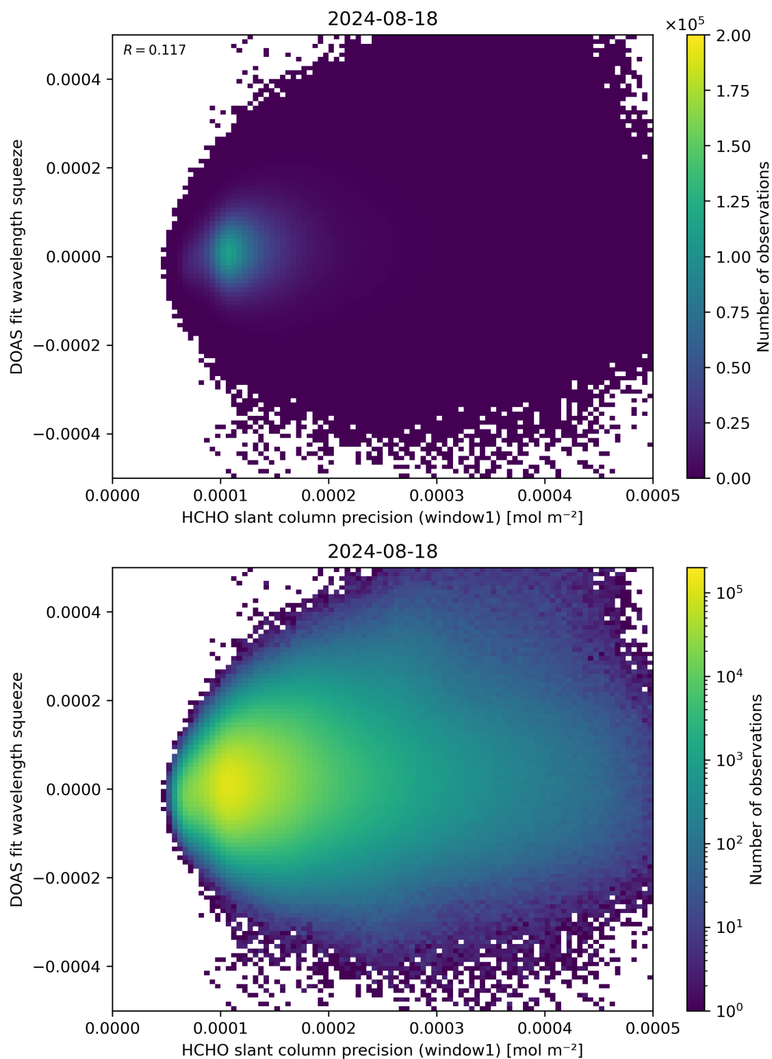
Figure 90: Scatter density plot of “HCHO slant column precision (window1)” against “DOAS fit wavelength squeeze” for 2024-08-17 to 2024-08-19.
