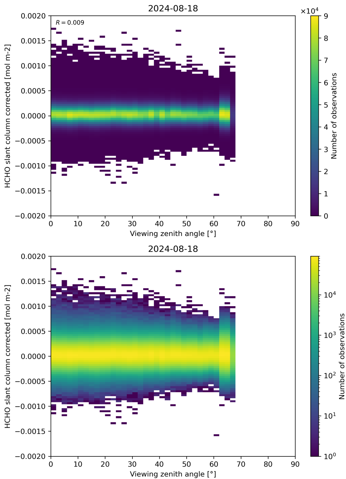
Figure 186: Scatter density plot of “Viewing zenith angle” against “HCHO slant column corrected” for 2024-08-17 to 2024-08-19.
