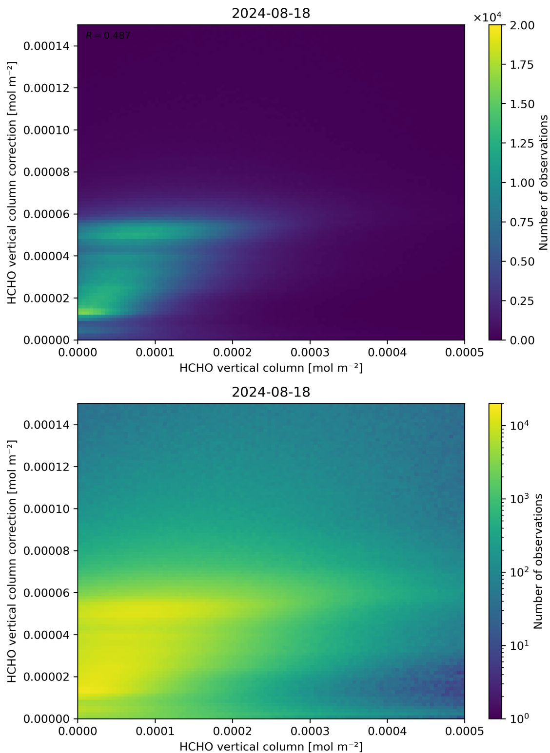
Figure 133: Scatter density plot of “HCHO vertical column” against “HCHO vertical column correction” for 2024-08-17 to 2024-08-19.
