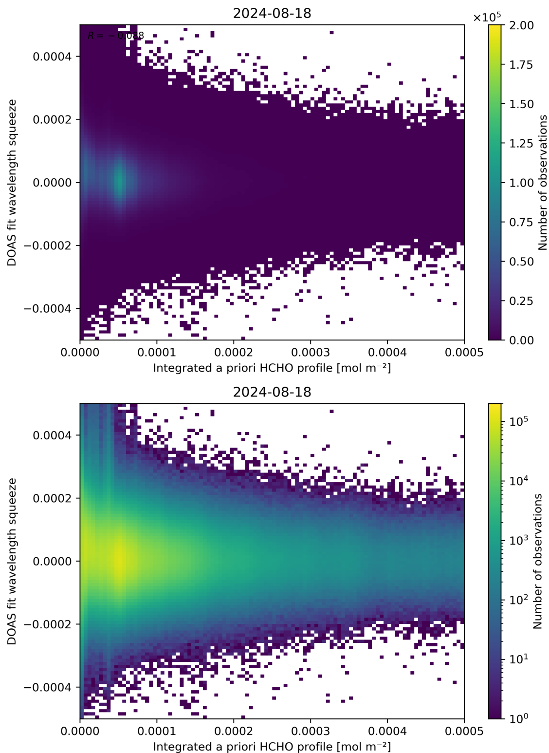
Figure 150: Scatter density plot of “Integrated a priori HCHO profile” against “DOAS fit wavelength squeeze” for 2024-08-17 to 2024-08-19.
