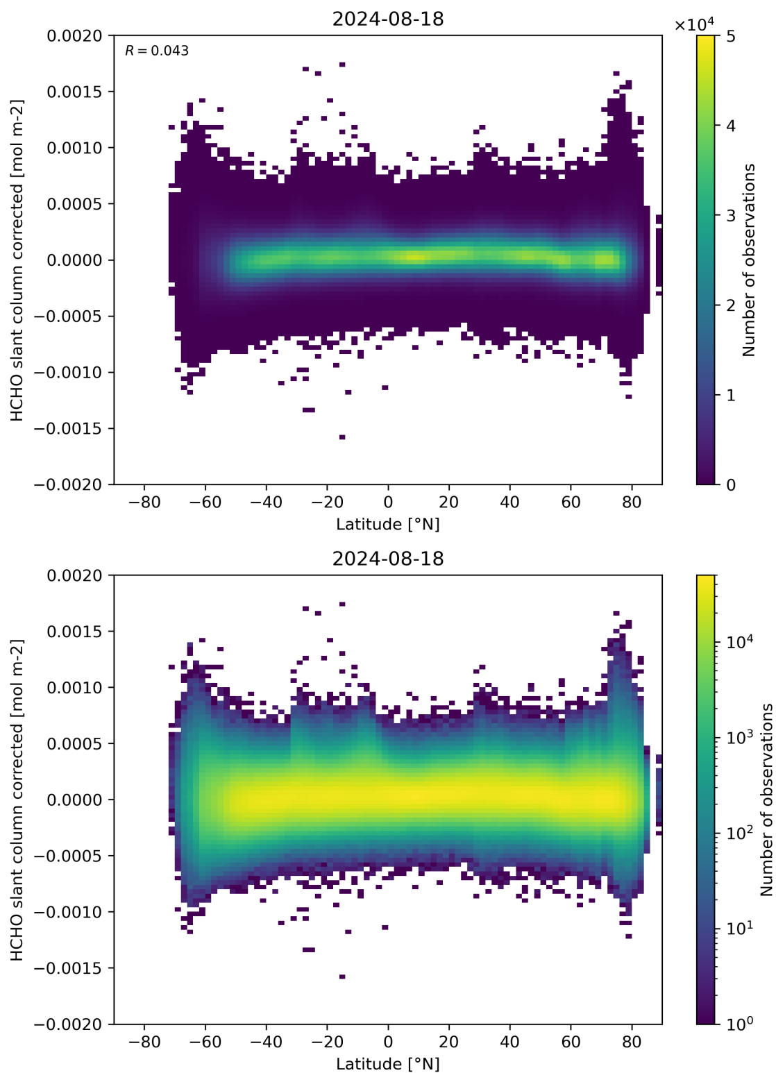
Figure 157: Scatter density plot of “Latitude” against “HCHO slant column corrected” for 2024-08-17 to 2024-08-19.
