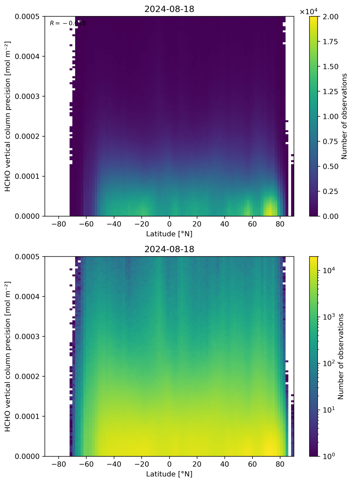
Figure 165: Scatter density plot of “Latitude” against “HCHO vertical column precision” for 2024-08-17 to 2024-08-19.
