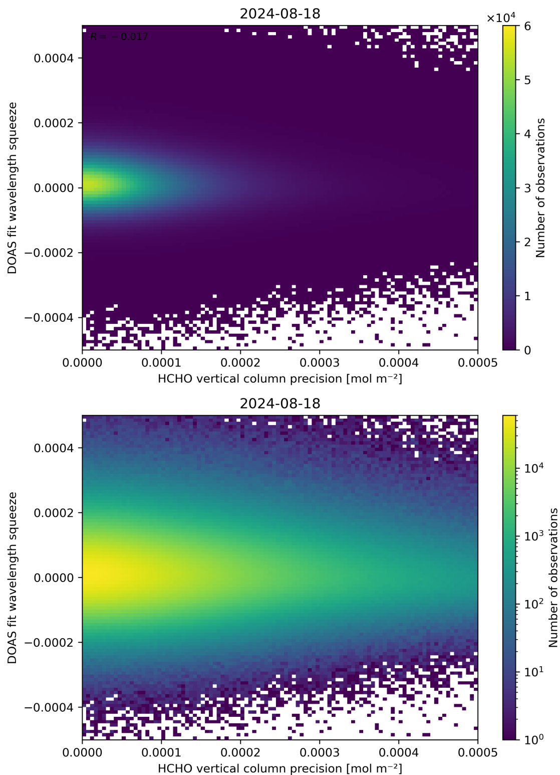
Figure 138: Scatter density plot of “HCHO vertical column precision” against “DOAS fit wavelength squeeze” for 2024-08-17 to 2024-08-19.
