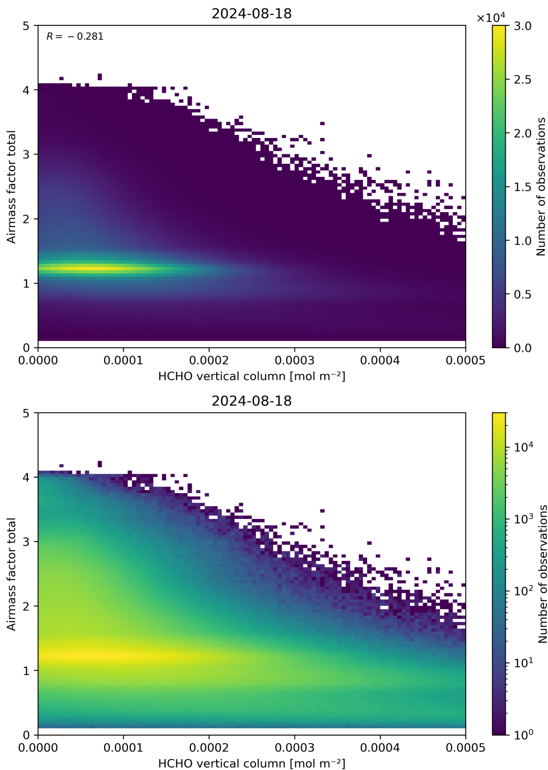
Figure 131: Scatter density plot of “HCHO vertical column” against “Airmass factor total” for 2024-08-17 to 2024-08-19.
