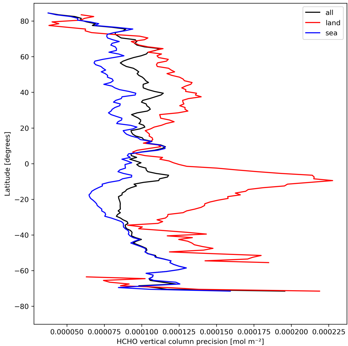
Figure 22: Zonal average of “HCHO vertical column precision” for 2024-08-17 to 2024-08-19.
