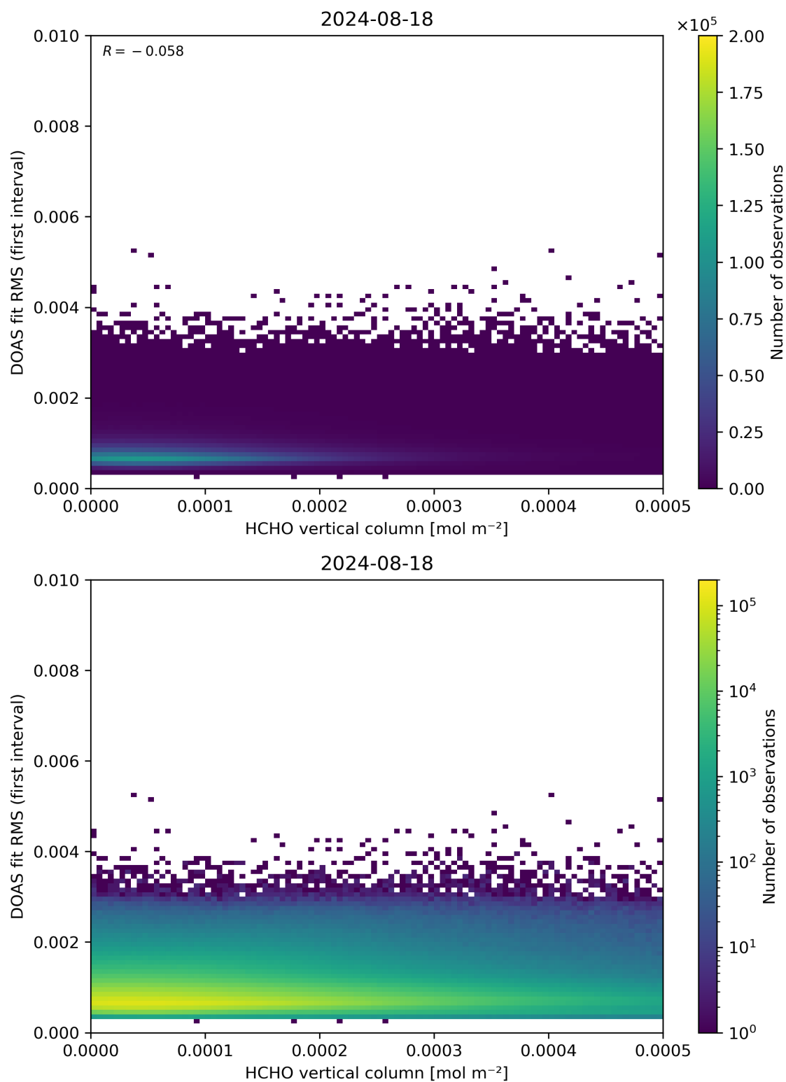
Figure 123: Scatter density plot of “HCHO vertical column” against “DOAS fit RMS (first interval)” for 2024-08-17 to 2024-08-19.
