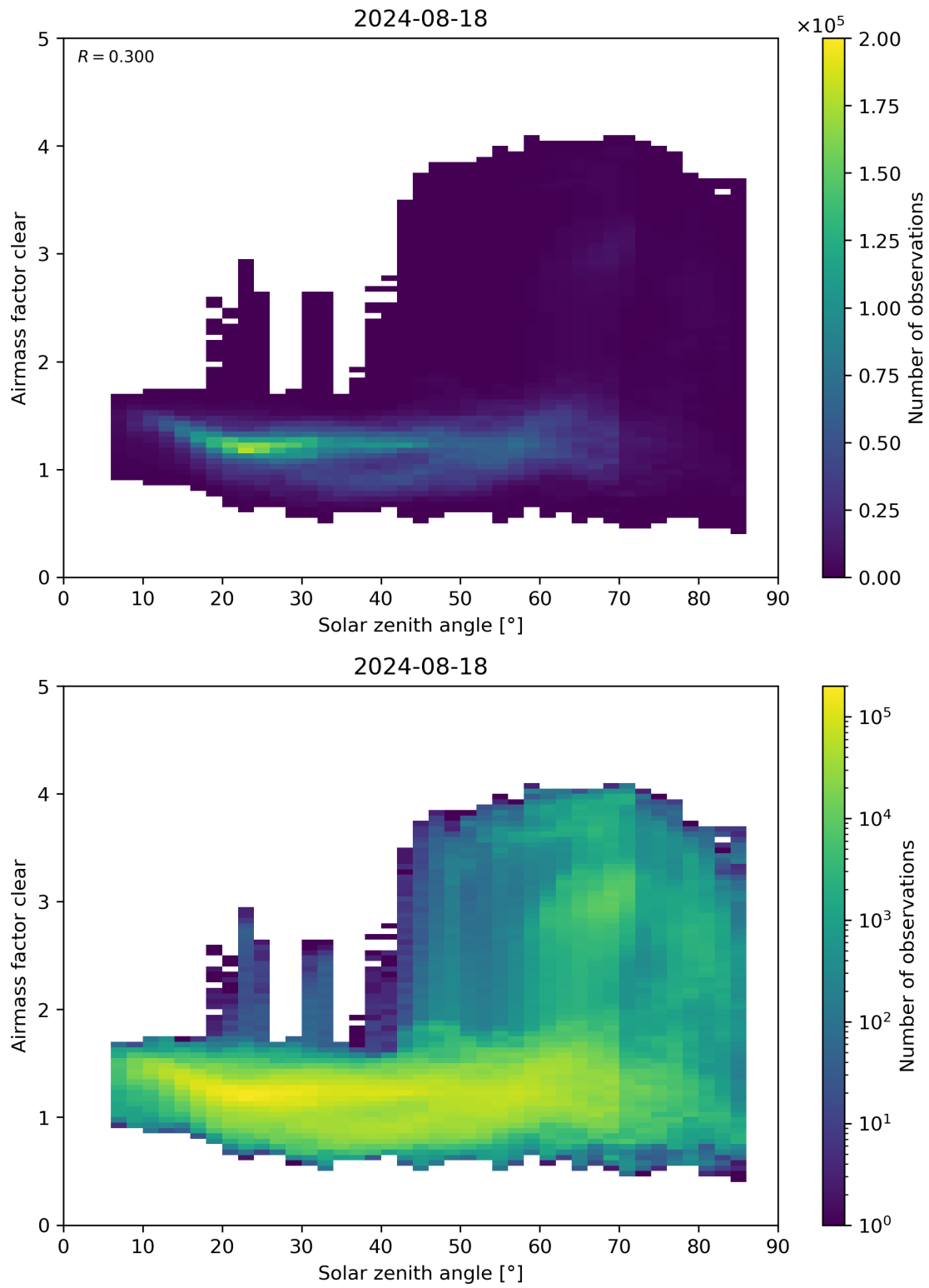
Figure 170: Scatter density plot of “Solar zenith angle” against “Airmass factor clear” for 2024-08-17 to 2024-08-19.
