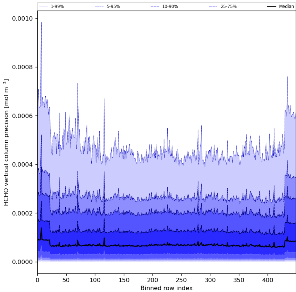
Figure 50: Along track statistics of “HCHO vertical column precision” for 2024-08-17 to 2024-08-19
