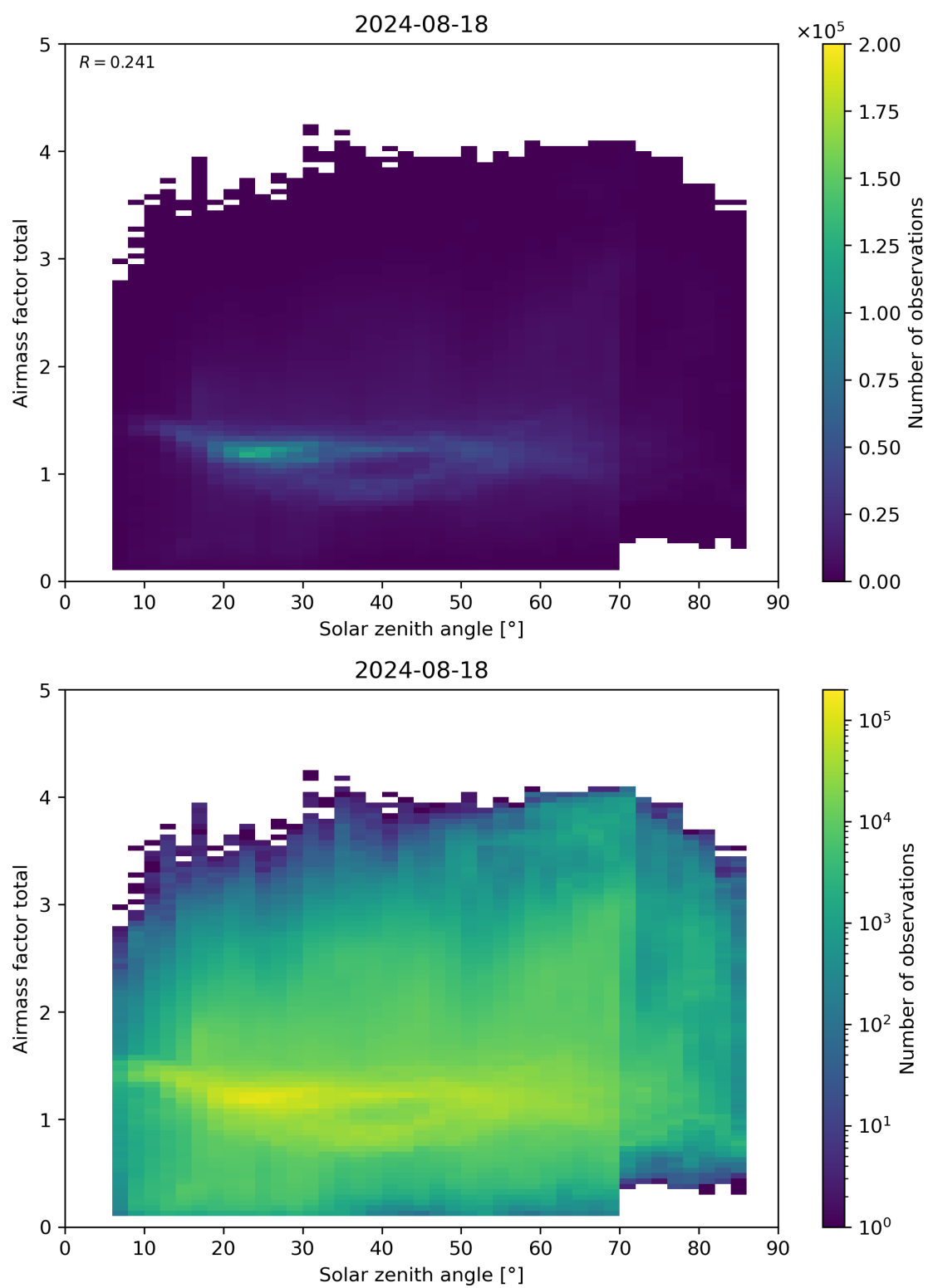
Figure 175: Scatter density plot of “Solar zenith angle” against “Airmass factor total” for 2024-08-17 to 2024-08-19.
