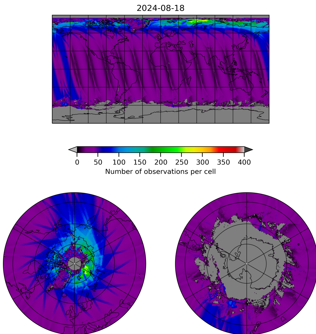
Figure 19: Map of the number of observations for 2024-08-17 to 2024-08-19
