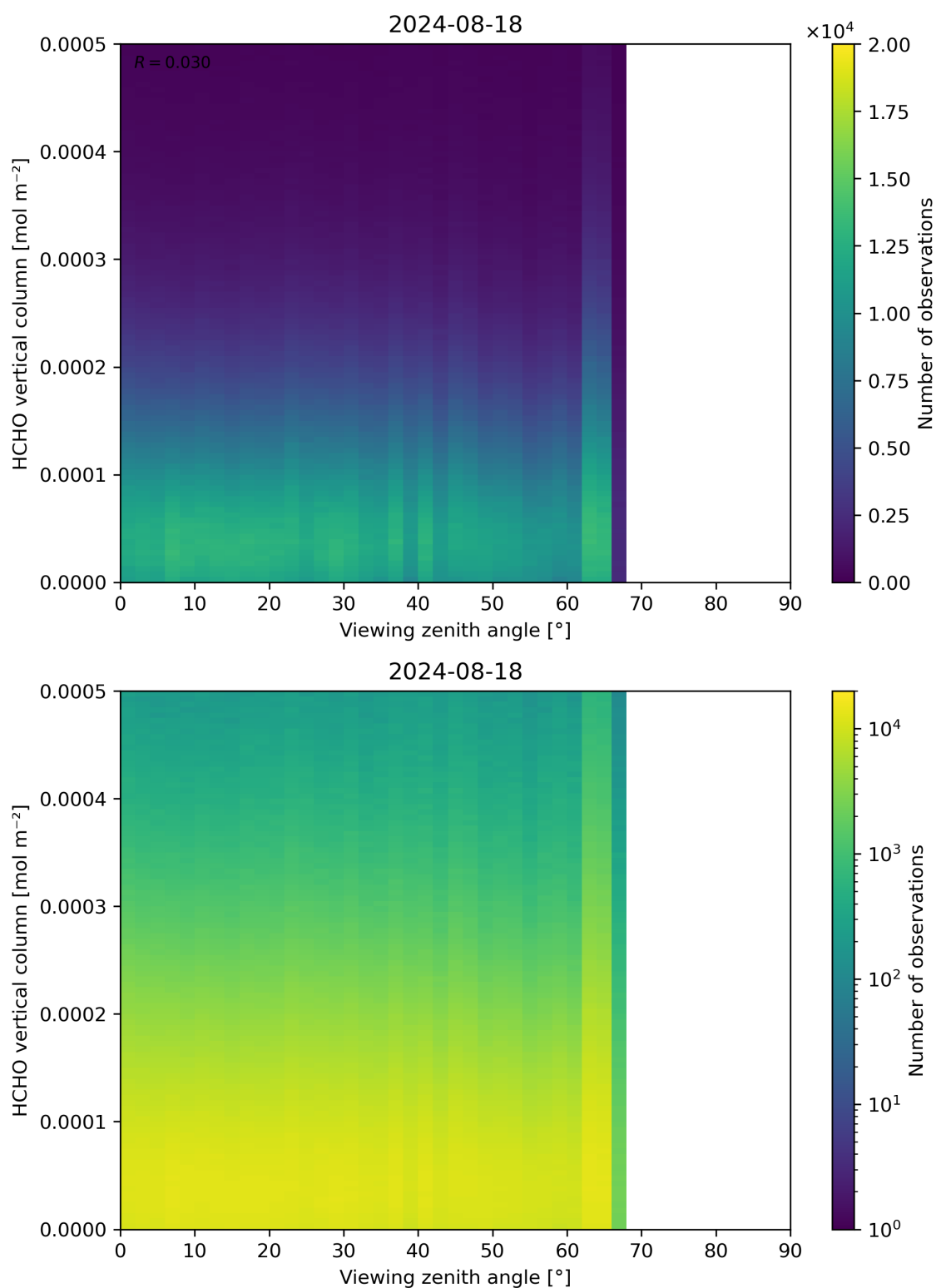
Figure 192: Scatter density plot of “Viewing zenith angle” against “HCHO vertical column” for 2024-08-17 to 2024-08-19.
