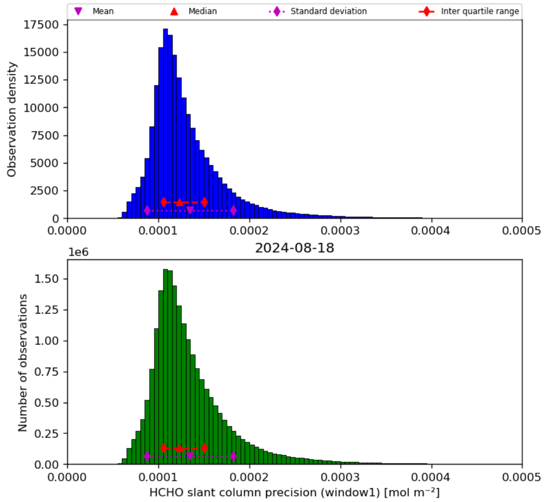
Figure 39: Histogram of “HCHO slant column precision (window1)” for 2024-08-17 to 2024-08-19
