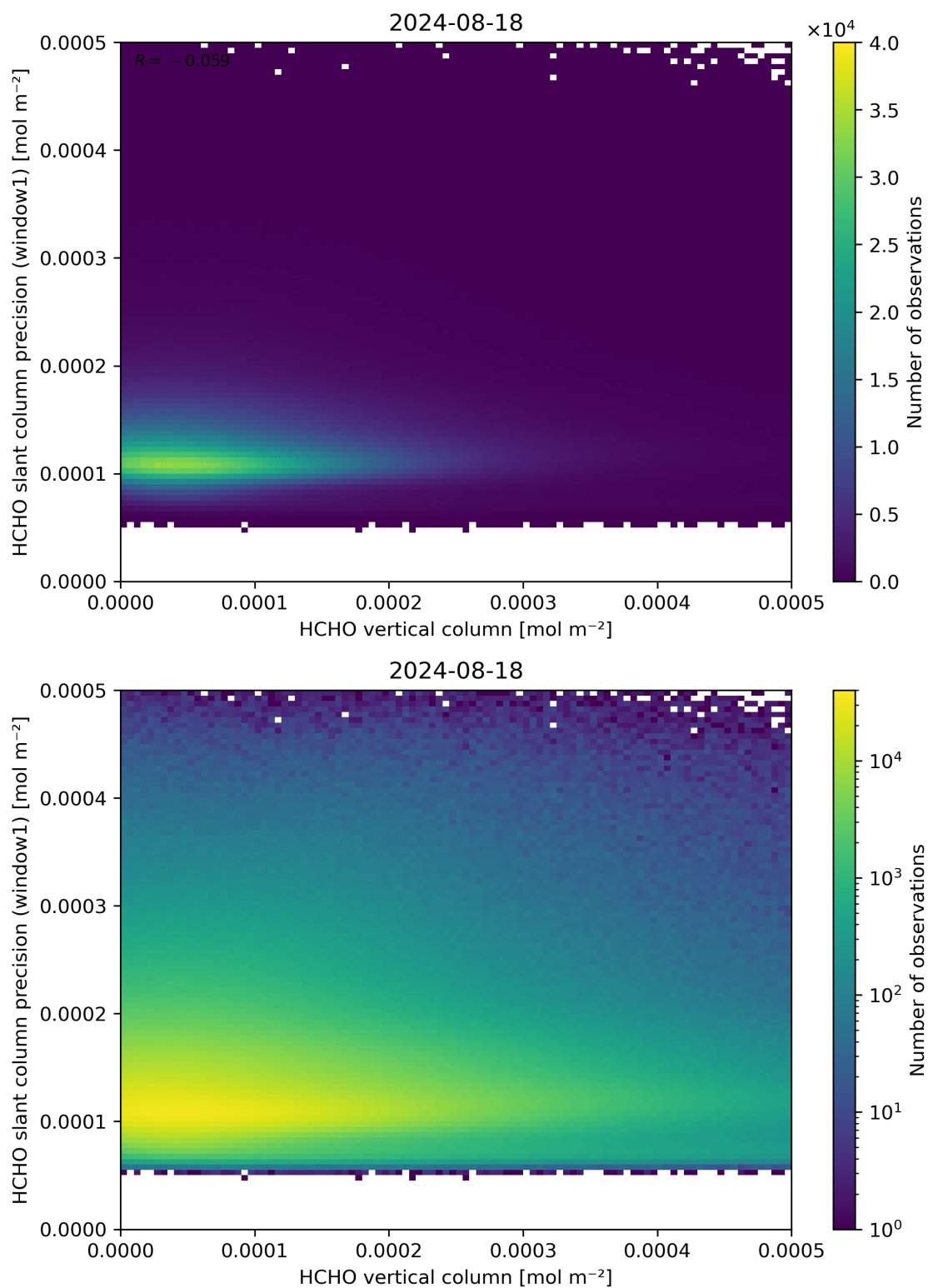
Figure 130: Scatter density plot of “HCHO vertical column” against “HCHO slant column precision (window1)” for 2024-08-17 to 2024-08-19.
