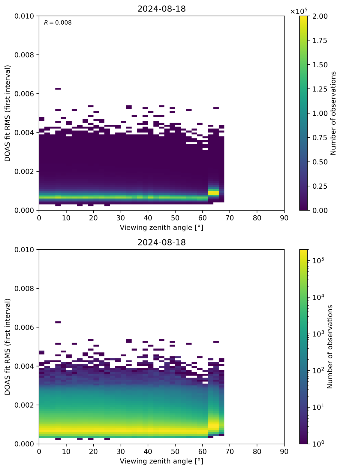
Figure 182: Scatter density plot of “Viewing zenith angle” against “DOAS fit RMS (first interval)” for 2024-08-17 to 2024-08-19.
