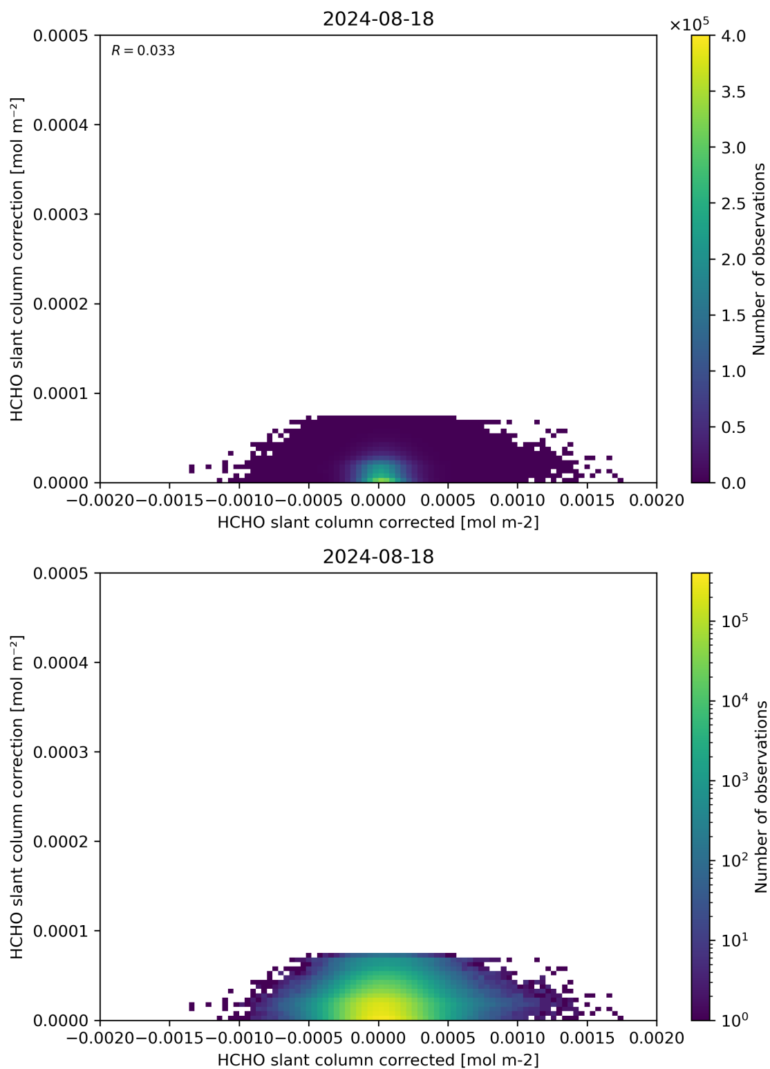
Figure 77: Scatter density plot of “HCHO slant column corrected” against “HCHO slant column correction” for 2024-08-17 to 2024-08-19.
