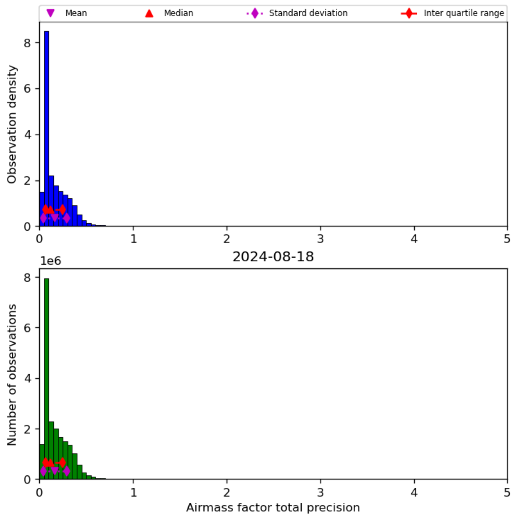
Figure 41: Histogram of "Airmass factor total precision" for 2024-08-17 to 2024-08-19
