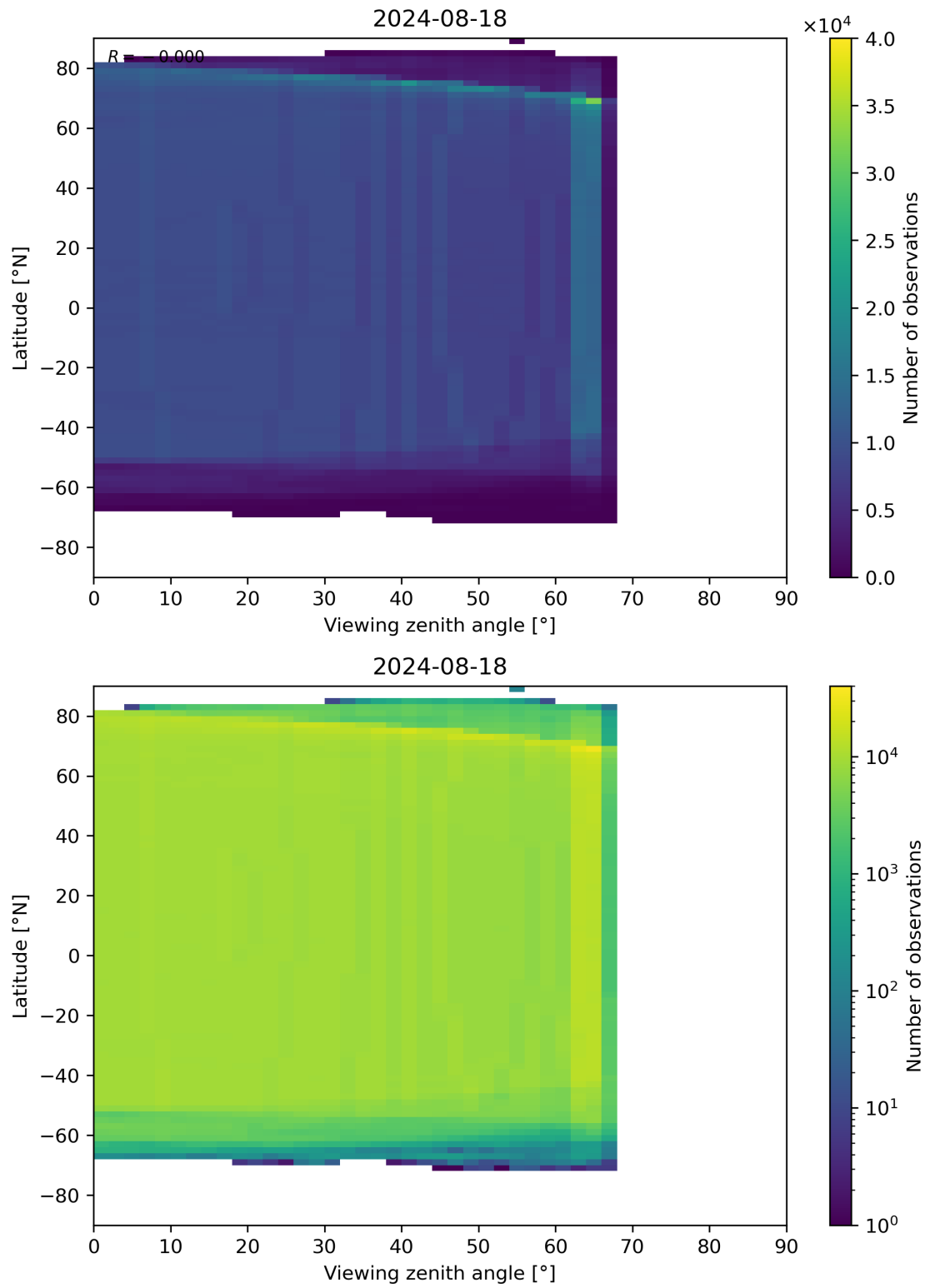
Figure 196: Scatter density plot of “Viewing zenith angle” against “Latitude” for 2024-08-17 to 2024-08-19.
