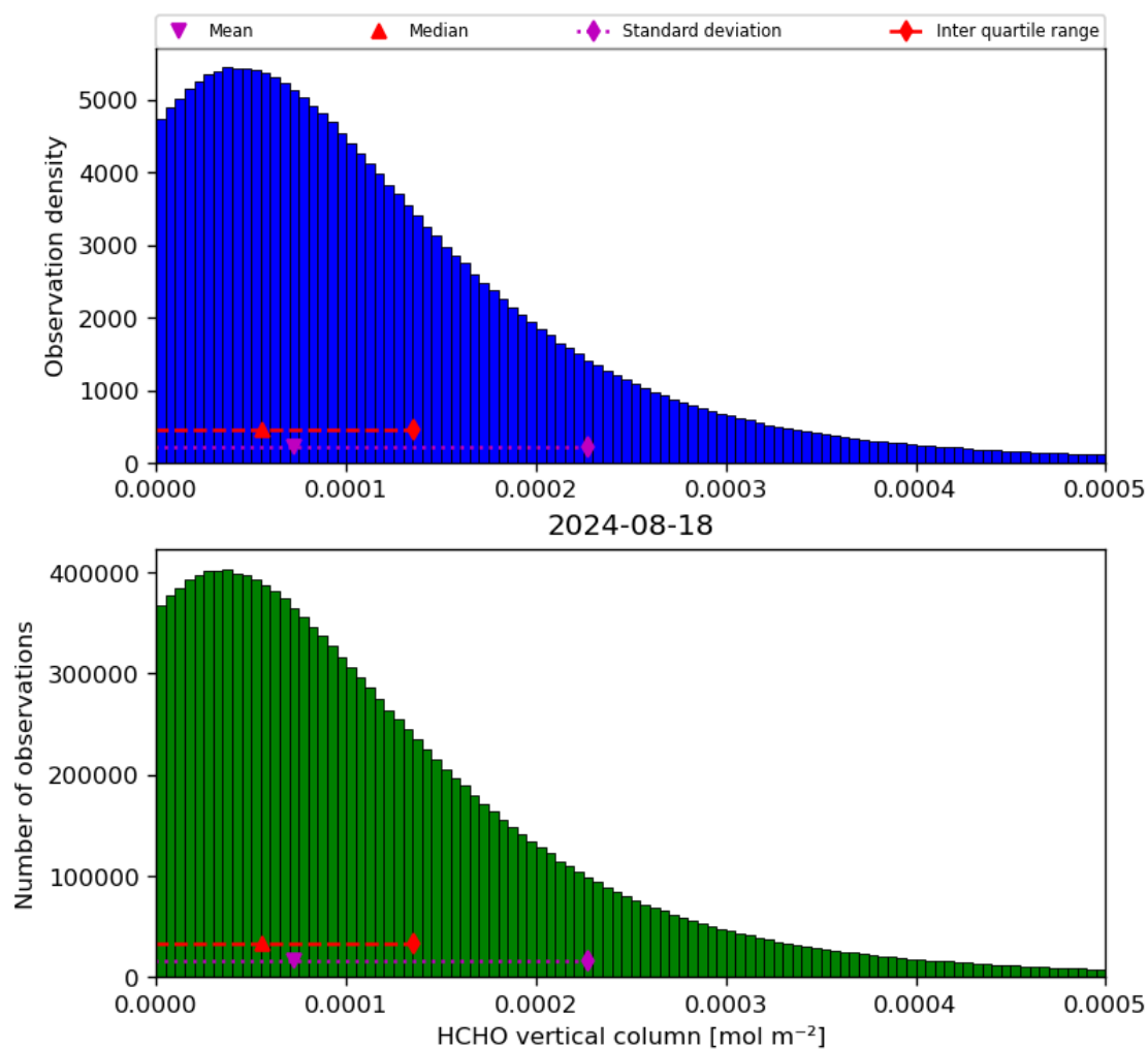
Figure 35: Histogram of “HCHO vertical column” for 2024-08-17 to 2024-08-19
