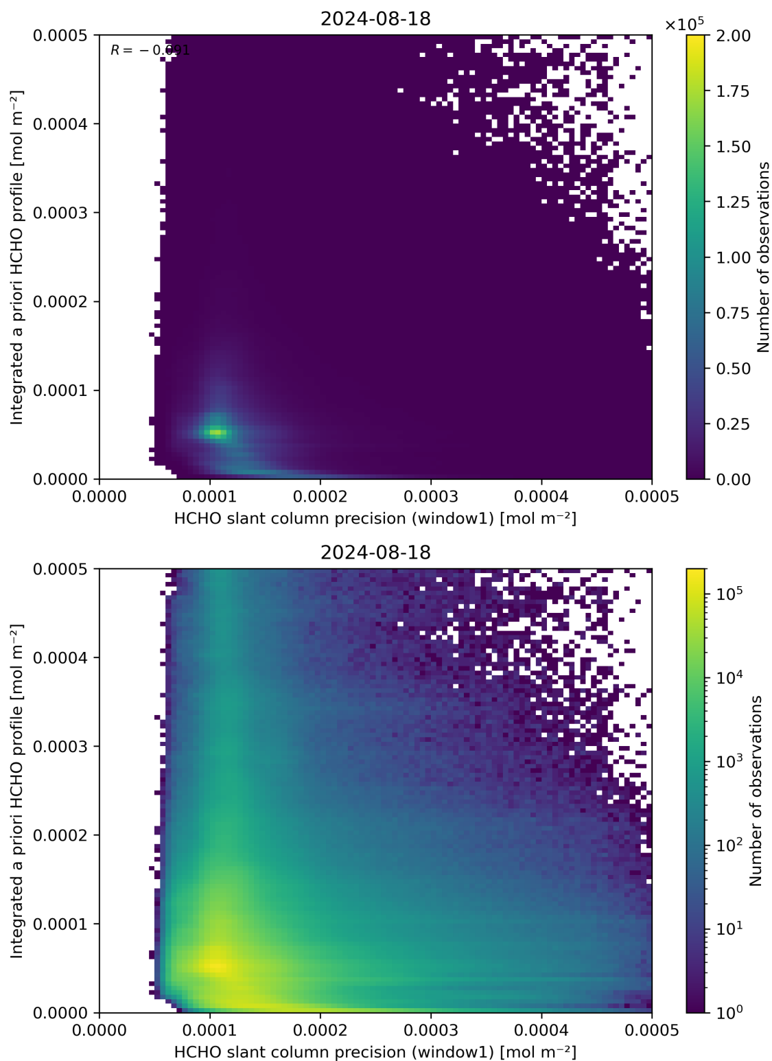
Figure 96: Scatter density plot of “HCHO slant column precision (window1)” against “Integrated a priori HCHO profile” for 2024-08-17 to 2024-08-19.
