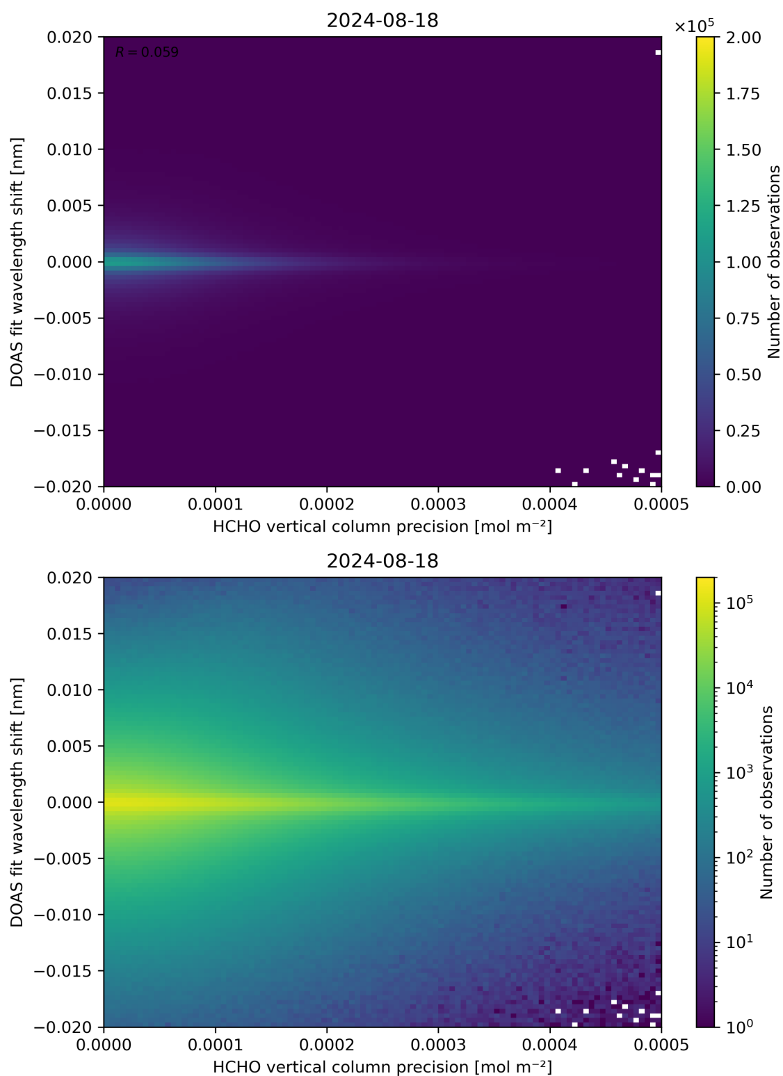
Figure 137: Scatter density plot of “HCHO vertical column precision” against “DOAS fit wavelength shift” for 2024-08-17 to 2024-08-19.
