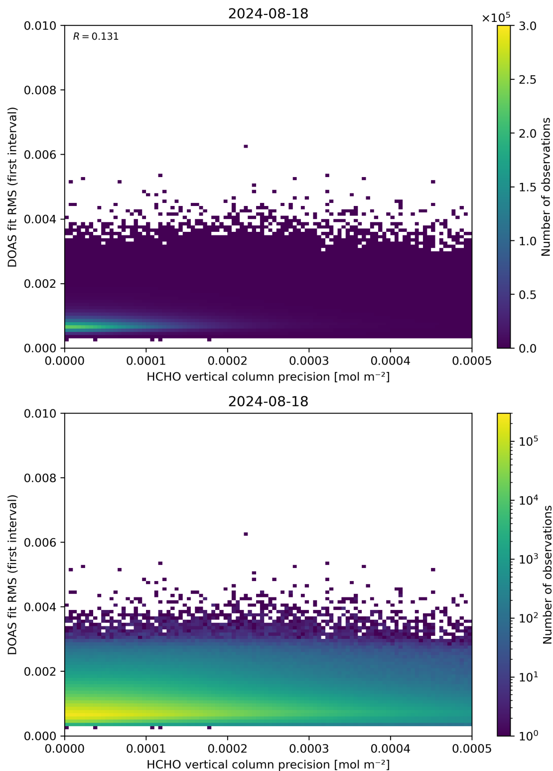
Figure 136: Scatter density plot of “HCHO vertical column precision” against “DOAS fit RMS (first interval)” for 2024-08-17 to 2024-08-19.
