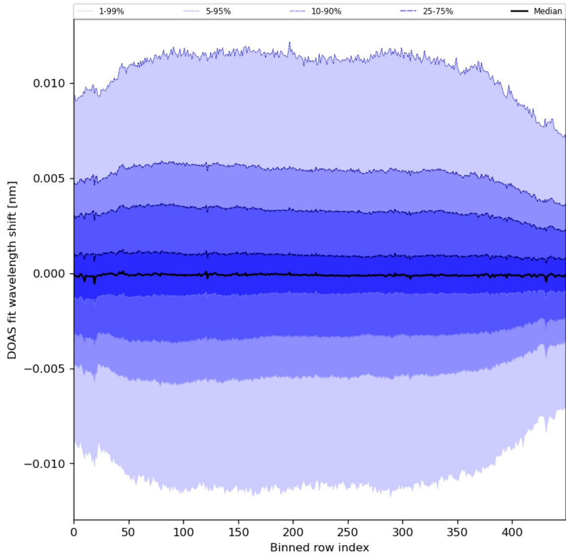
Figure 58: Along track statistics of “DOAS fit wavelength shift” for 2024-08-17 to 2024-08-19
