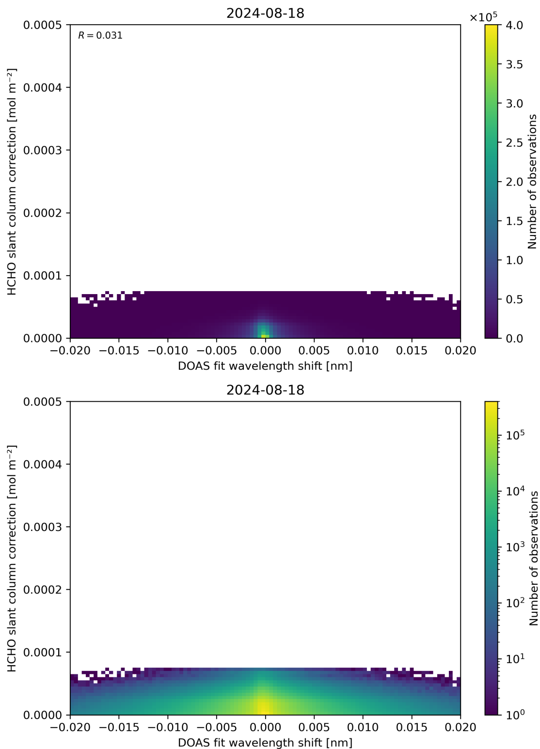
Figure 67: Scatter density plot of “DOAS fit wavelength shift” against “HCHO slant column correction” for 2024-08-17 to 2024-08-19.
