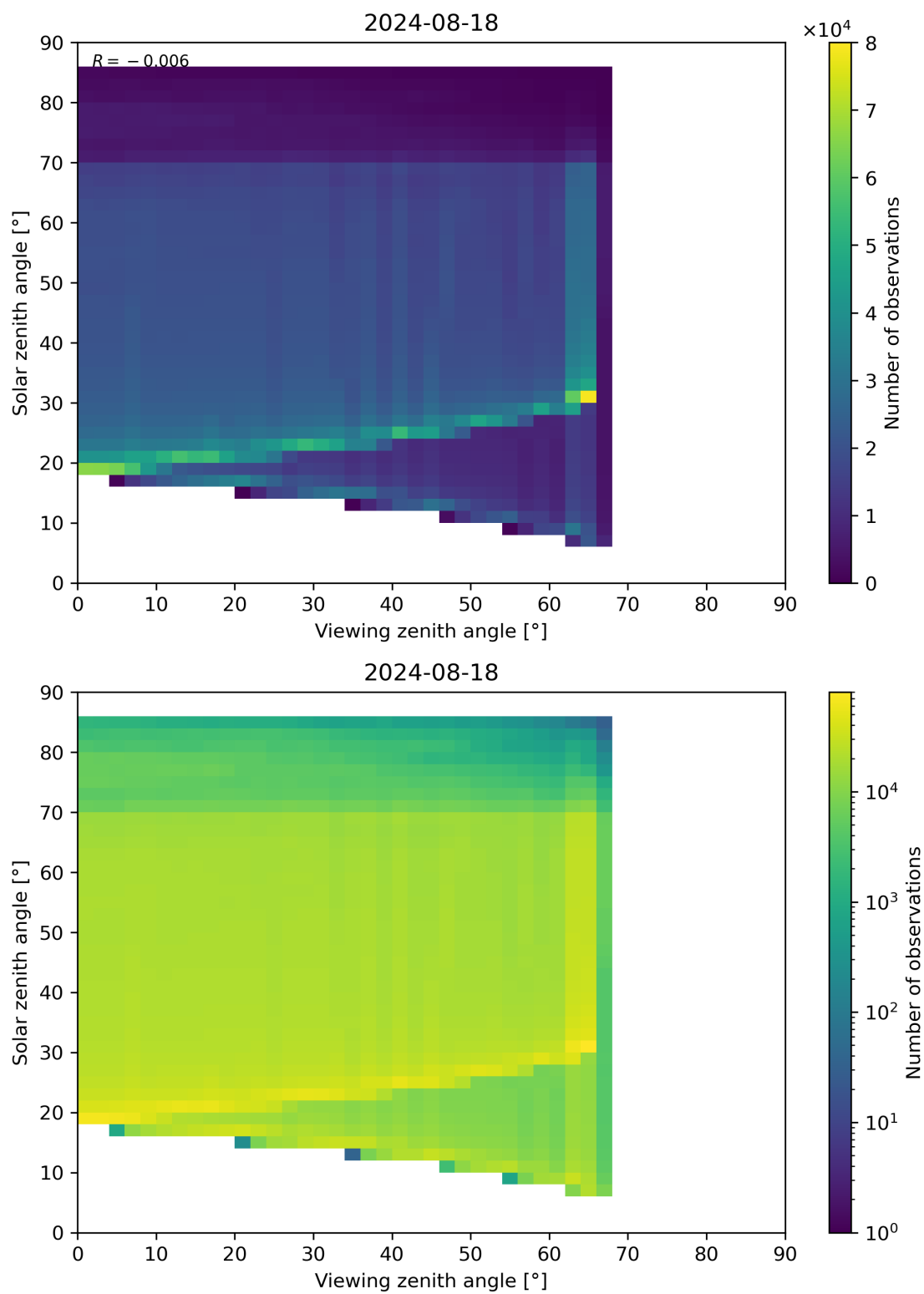
Figure 197: Scatter density plot of “Viewing zenith angle” against “Solar zenith angle” for 2024-08-17 to 2024-08-19.
