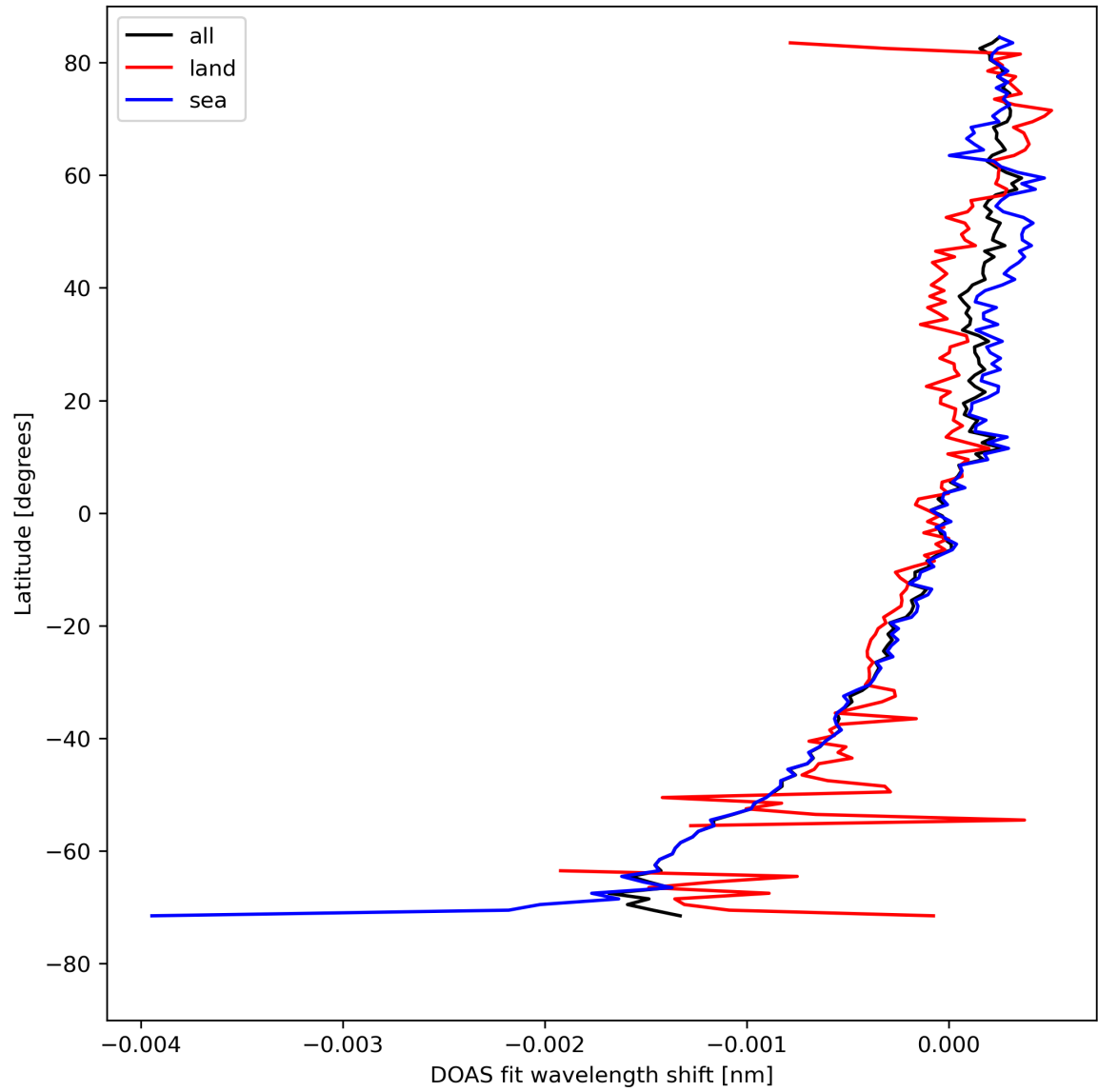
Figure 30: Zonal average of “DOAS fit wavelength shift” for 2024-08-17 to 2024-08-19.
