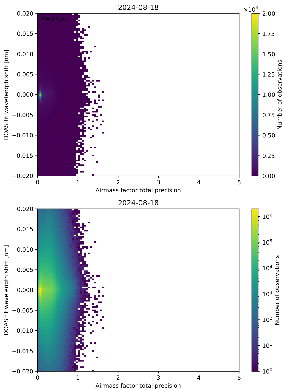
Figure 106: Scatter density plot of “Airmass factor total precision” against “DOAS fit wavelength shift” for 2024-08-17 to 2024-08-19.
