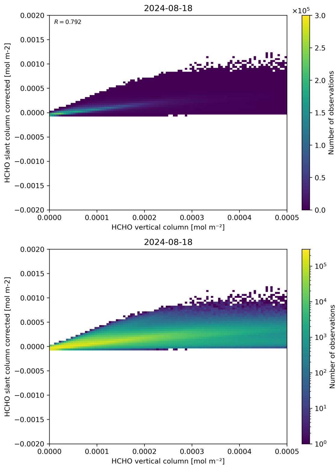
Figure 127: Scatter density plot of “HCHO vertical column” against “HCHO slant column corrected” for 2024-08-17 to 2024-08-19.
