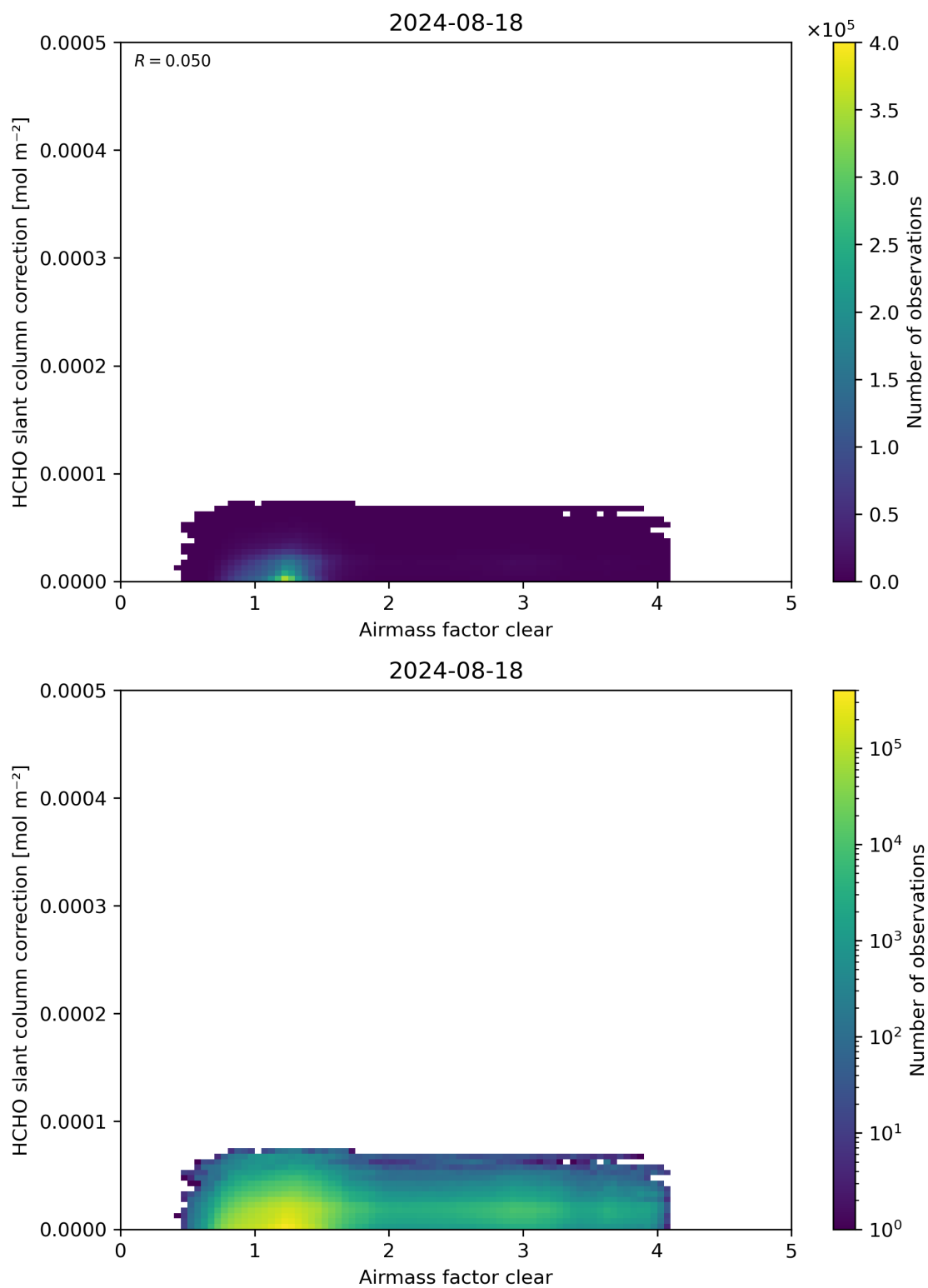
Figure 75: Scatter density plot of “Airmass factor clear” against “HCHO slant column correction” for 2024-08-17 to 2024-08-19.
