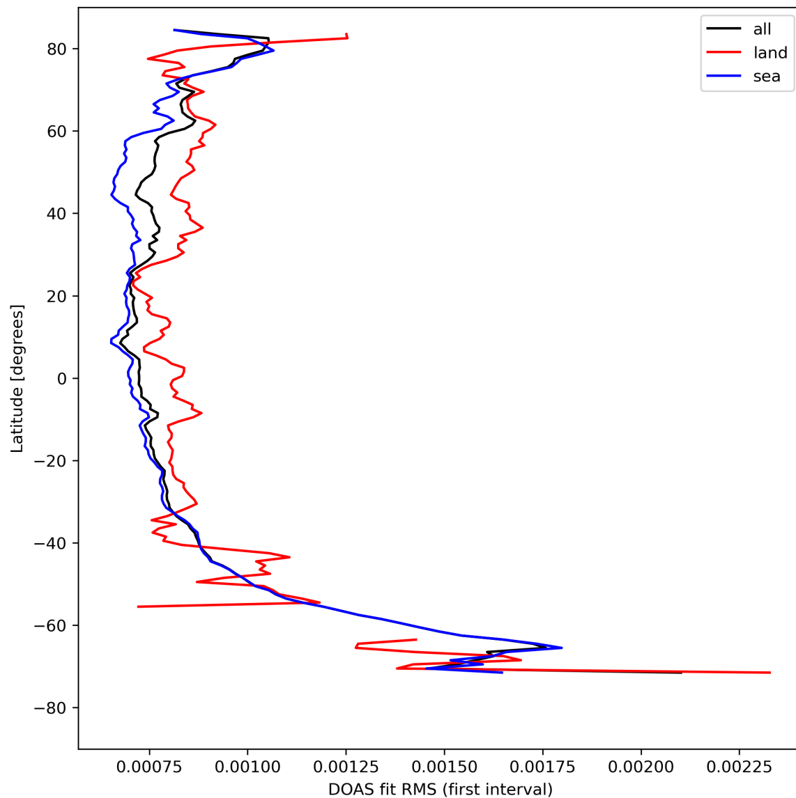
Figure 32: Zonal average of "DOAS fit RMS (first interval)" for 2024-08-17 to 2024-08-19.
