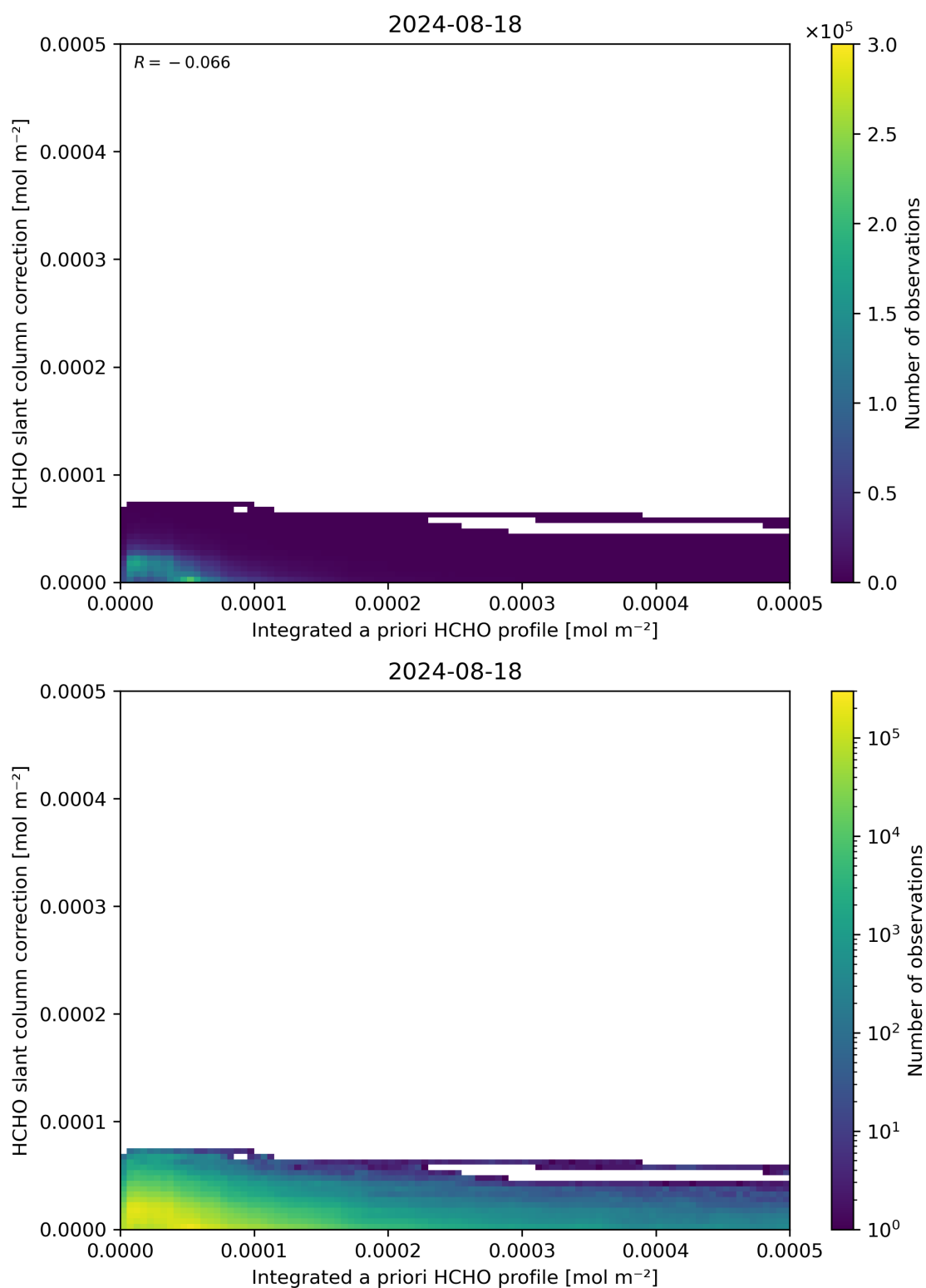
Figure 152: Scatter density plot of “Integrated a priori HCHO profile” against “HCHO slant column correction” for 2024-08-17 to 2024-08-19.
