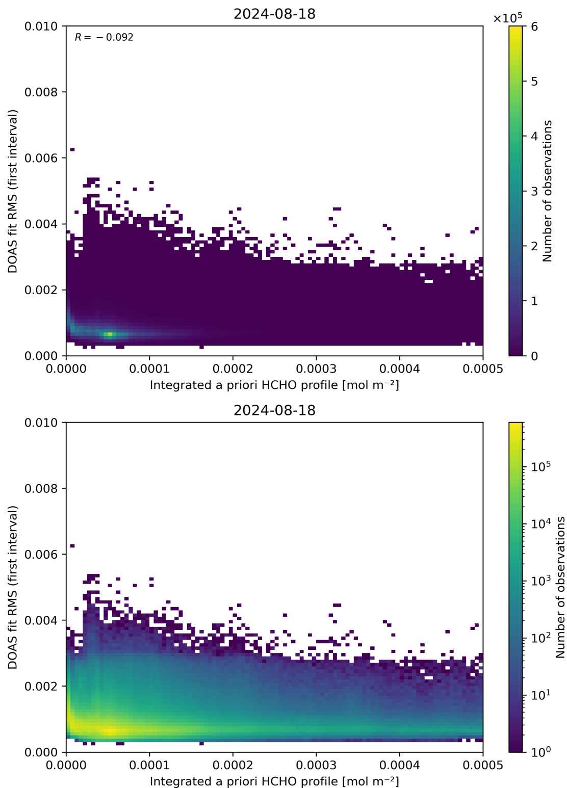
Figure 148: Scatter density plot of “Integrated a priori HCHO profile” against “DOAS fit RMS (first interval)” for 2024-08-17 to 2024-08-19.
