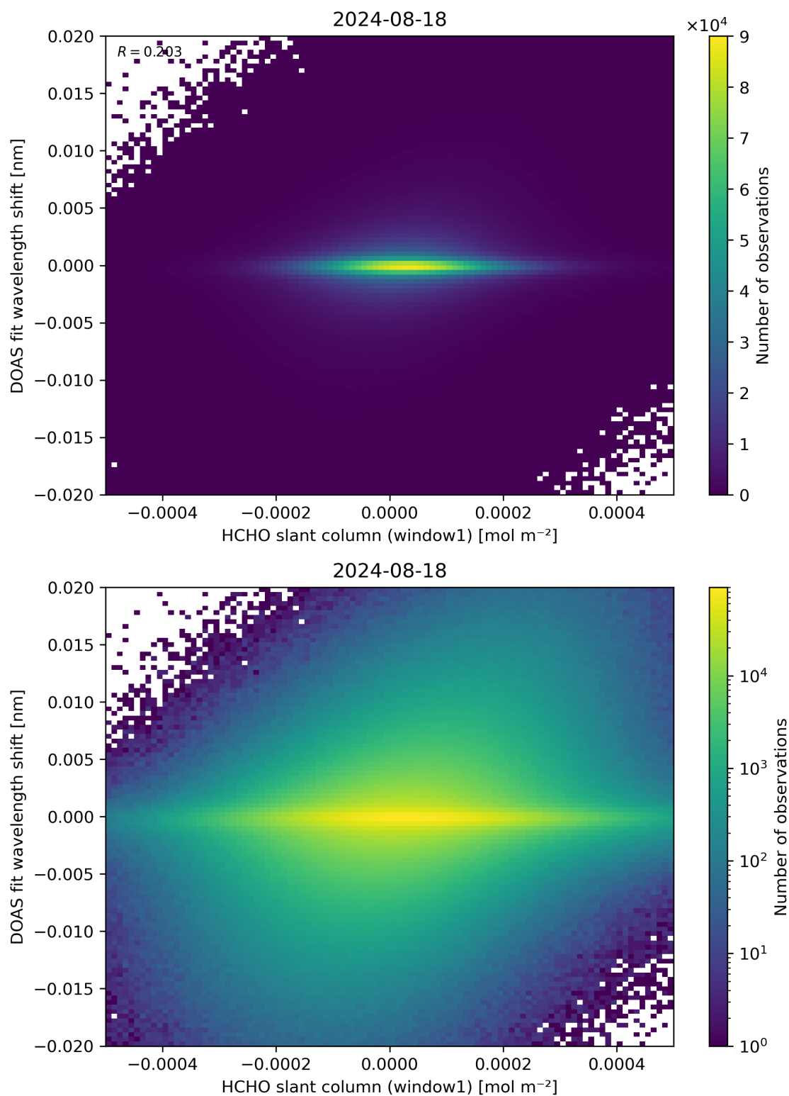
Figure 79: Scatter density plot of “HCHO slant column (window1)” against “DOAS fit wavelength shift” for 2024-08-17 to 2024-08-19.
