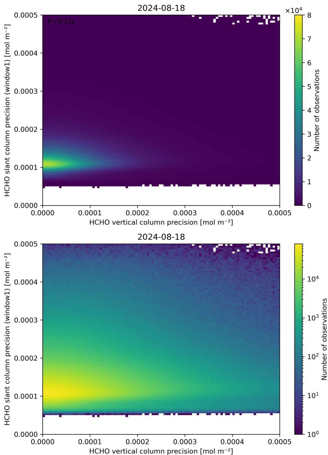
Figure 143: Scatter density plot of “HCHO vertical column precision” against “HCHO slant column precision (window1)” for 2024-08-17 to 2024-08-19.
