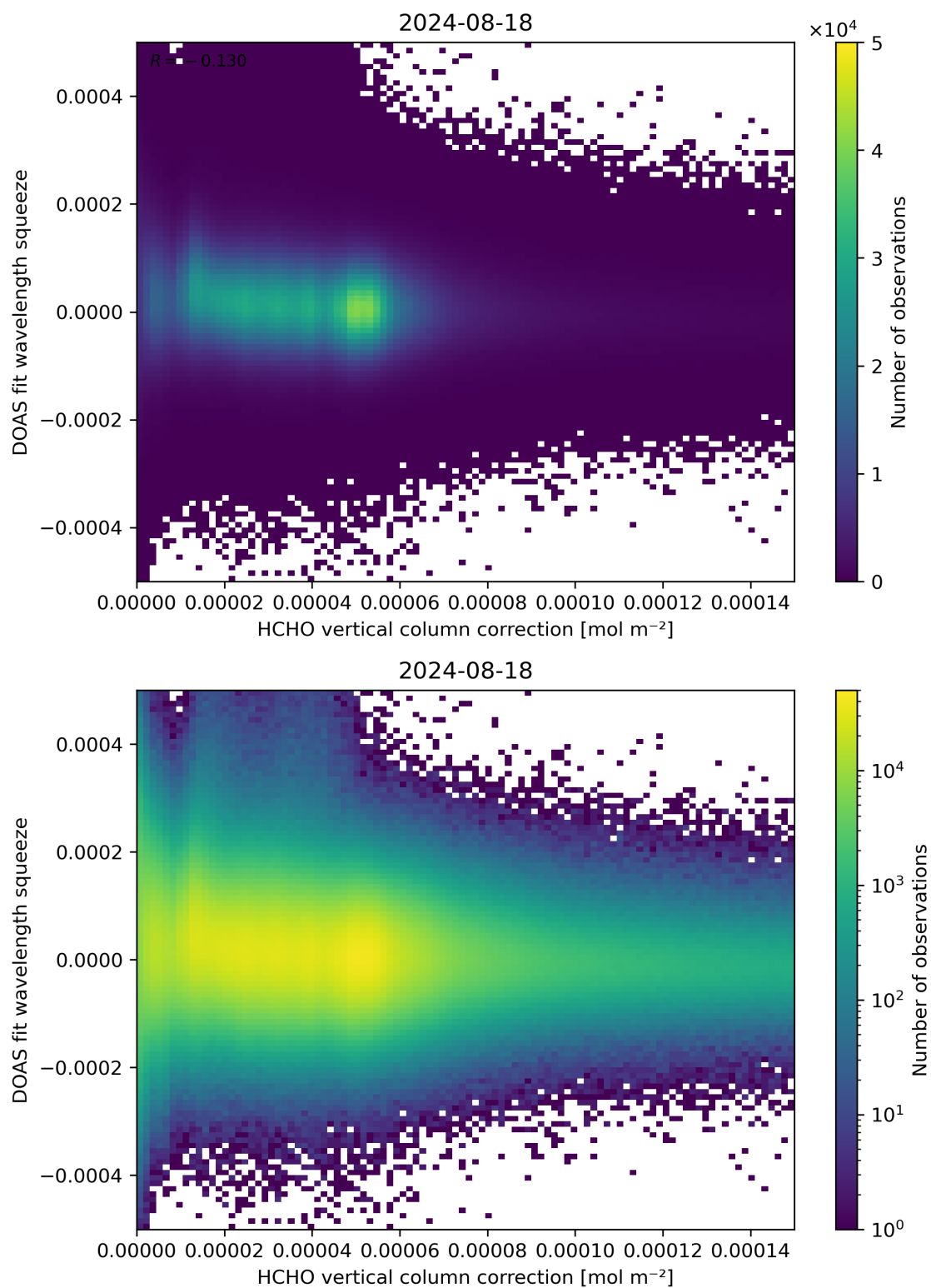
Figure 114: Scatter density plot of “HCHO vertical column correction” against “DOAS fit wavelength squeeze” for 2024-08-17 to 2024-08-19.
