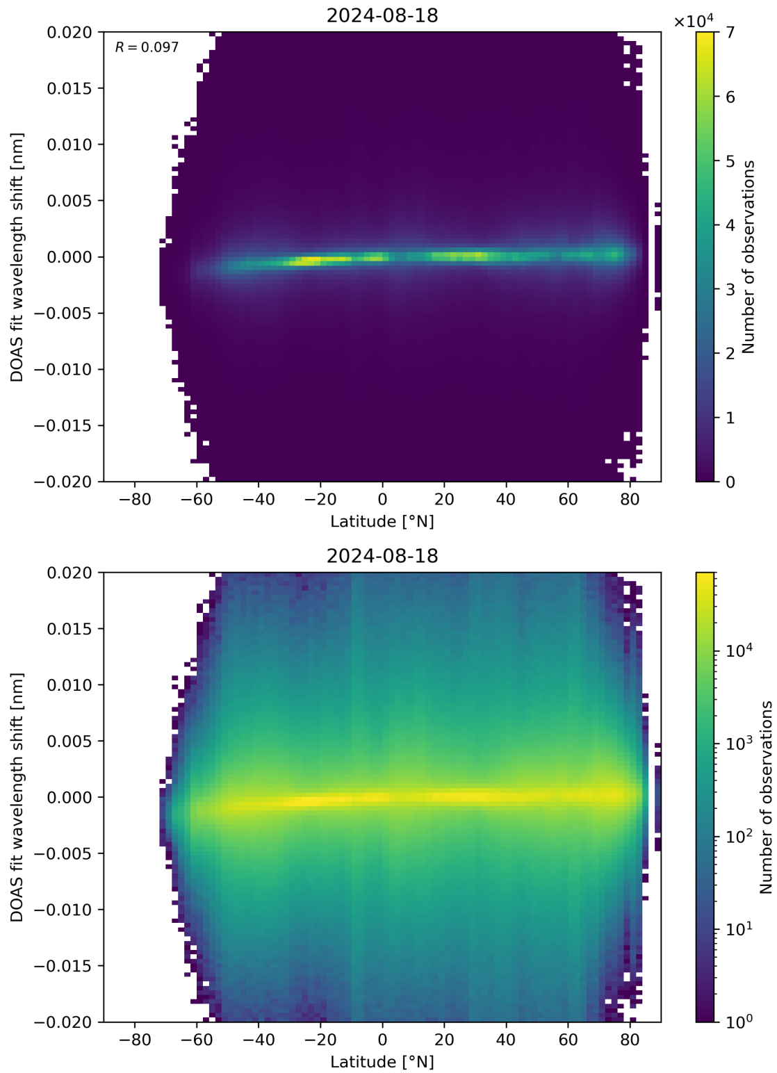
Figure 154: Scatter density plot of “Latitude” against “DOAS fit wavelength shift” for 2024-08-17 to 2024-08-19.
