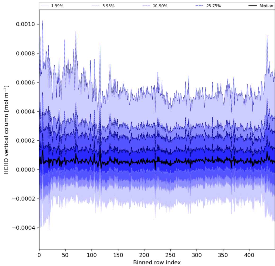
Figure 49: Along track statistics of “HCHO vertical column” for 2024-08-17 to 2024-08-19
