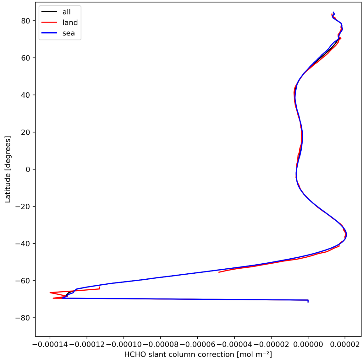
Figure 33: Zonal average of “HCHO slant column correction” for 2024-08-17 to 2024-08-19.
