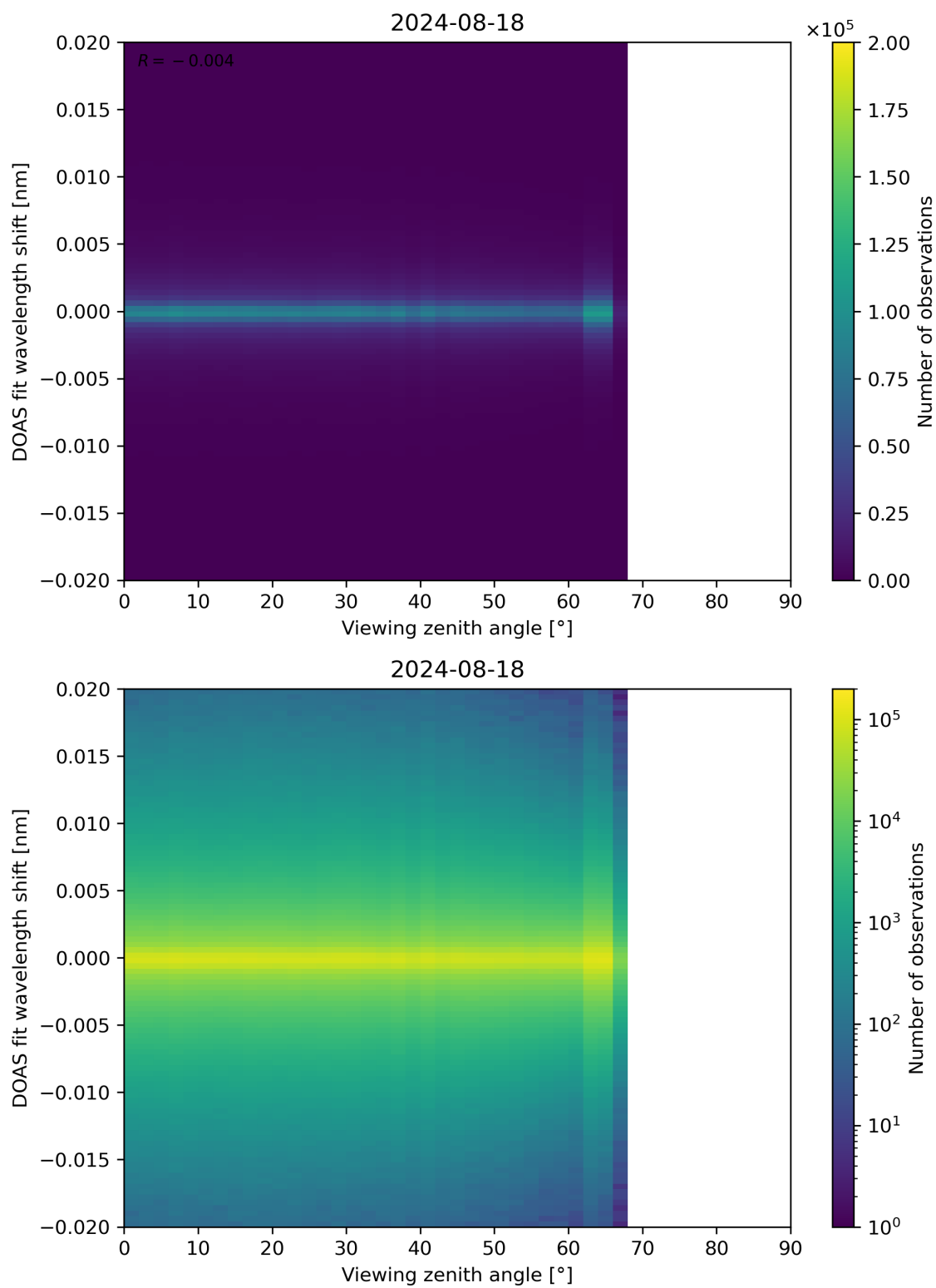
Figure 183: Scatter density plot of “Viewing zenith angle” against “DOAS fit wavelength shift” for 2024-08-17 to 2024-08-19.
