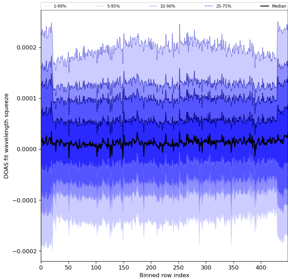
Figure 59: Along track statistics of “DOAS fit wavelength squeeze” for 2024-08-17 to 2024-08-19
