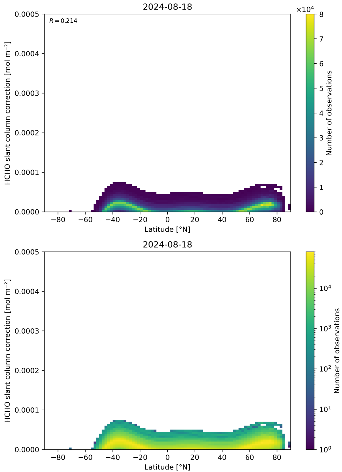
Figure 158: Scatter density plot of “Latitude” against “HCHO slant column correction” for 2024-08-17 to 2024-08-19.
