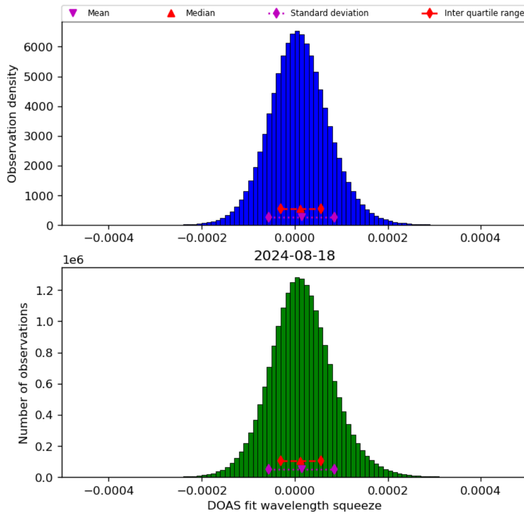
Figure 45: Histogram of “DOAS fit wavelength squeeze” for 2024-08-17 to 2024-08-19
