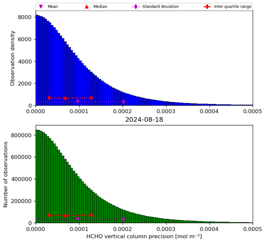
Figure 36: Histogram of “HCHO vertical column precision” for 2024-08-17 to 2024-08-19
