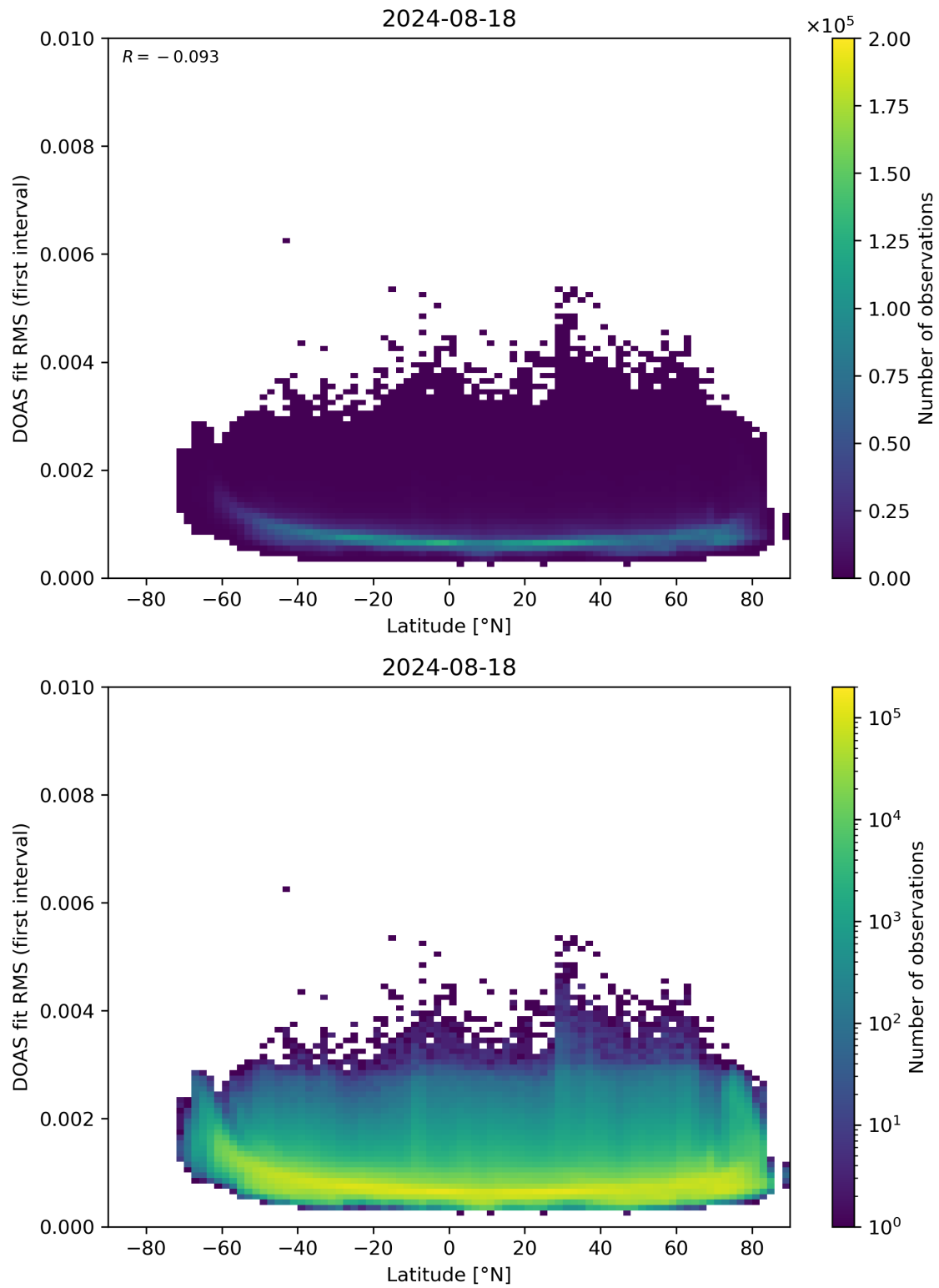
Figure 153: Scatter density plot of “Latitude” against “DOAS fit RMS (first interval)” for 2024-08-17 to 2024-08-19.
