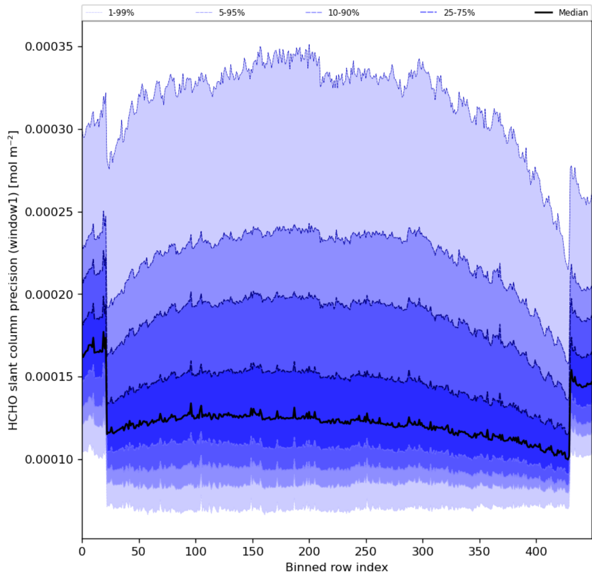
Figure 53: Along track statistics of “HCHO slant column precision (window1)” for 2024-08-17 to 2024-08-19
