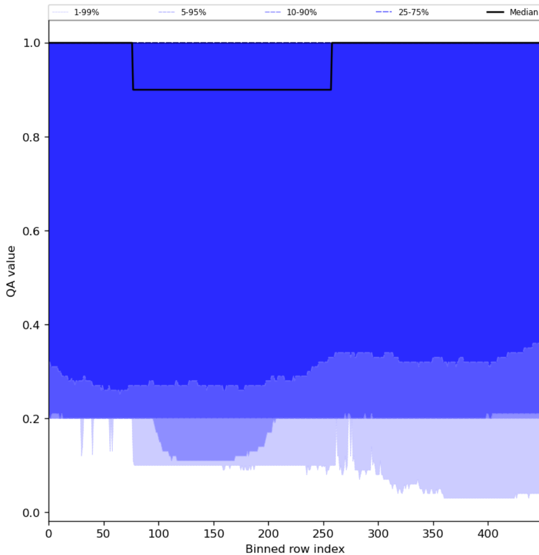
Figure 48: Along track statistics of “QA value” for 2024-08-17 to 2024-08-19
