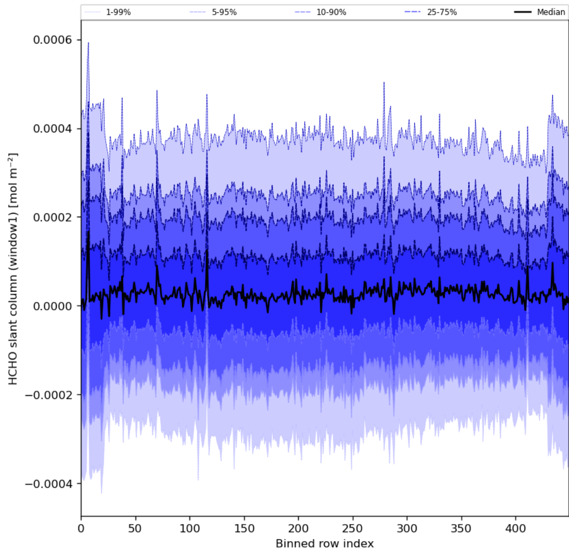
Figure 52: Along track statistics of “HCHO slant column (window1)” for 2024-08-17 to 2024-08-19
