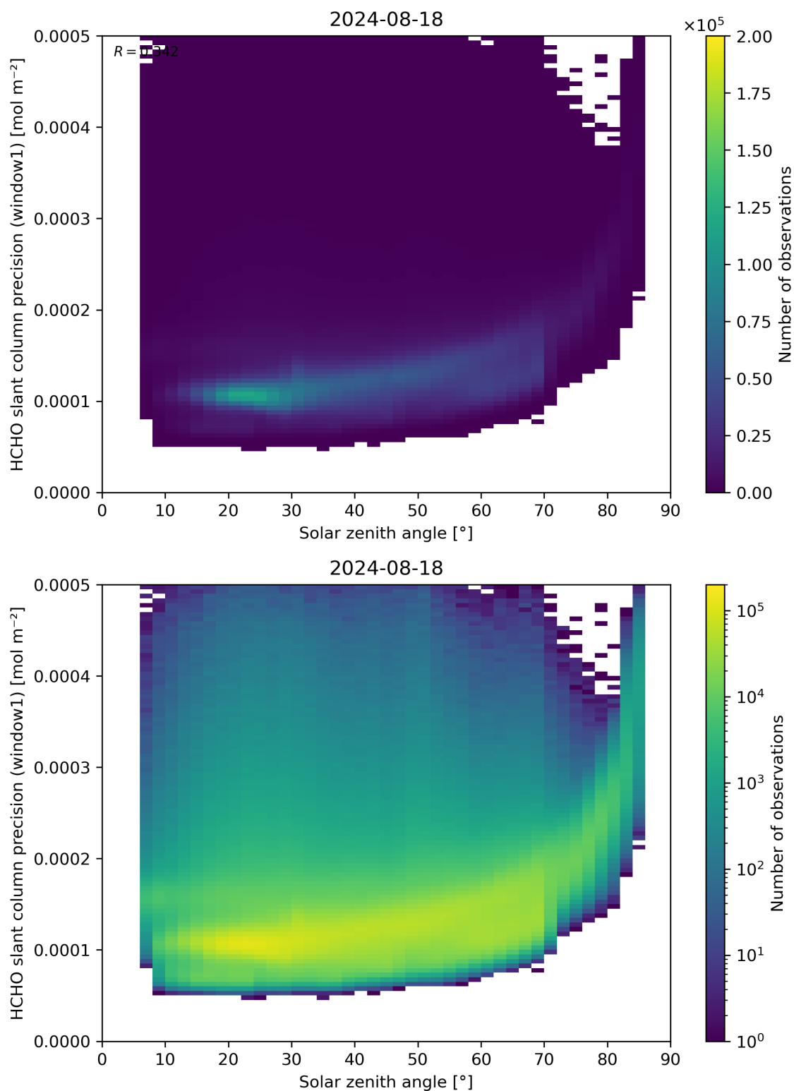
Figure 174: Scatter density plot of “Solar zenith angle” against “HCHO slant column precision (window1)” for 2024-08-17 to 2024-08-19.
