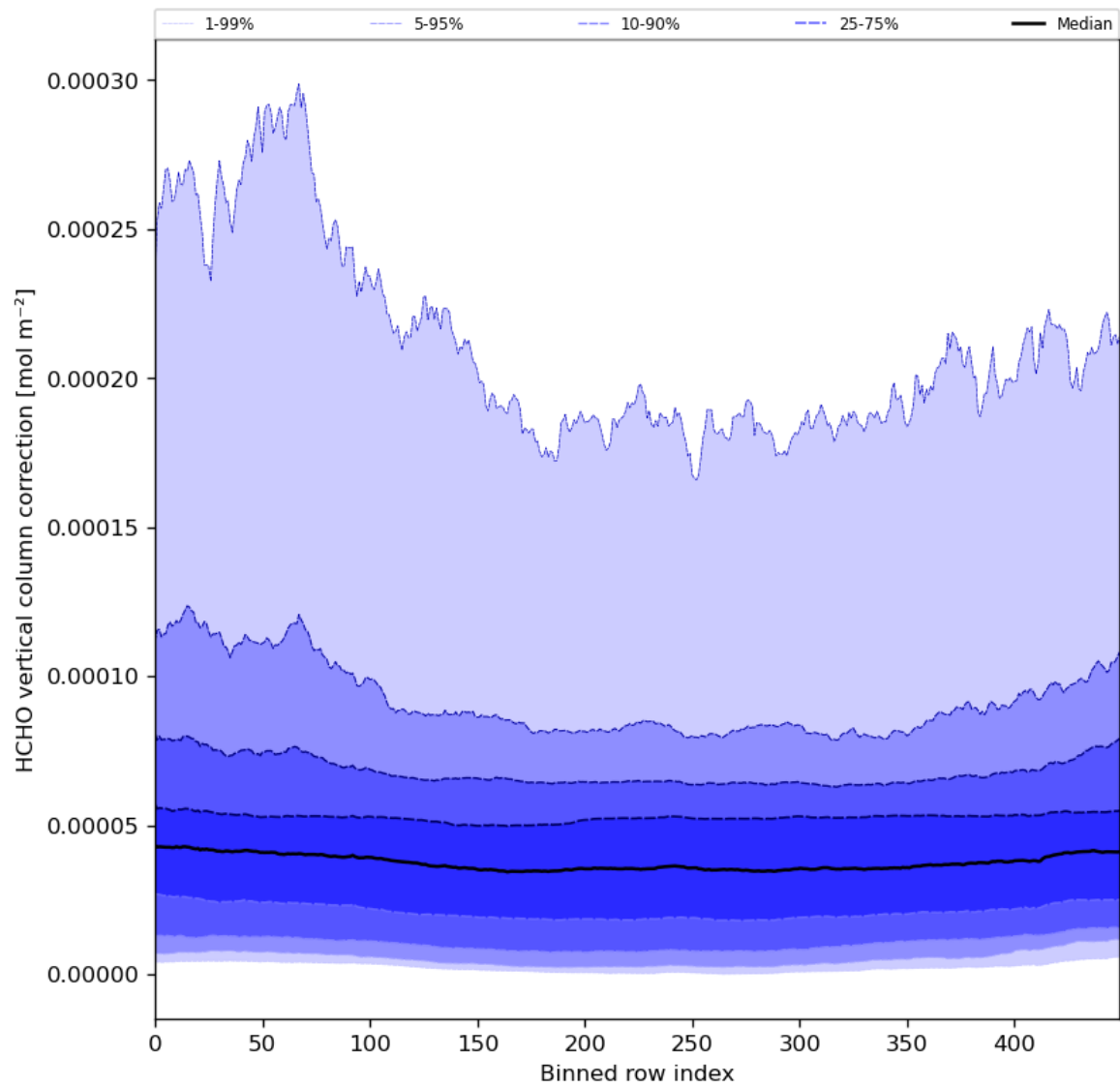
Figure 51: Along track statistics of “HCHO vertical column correction” for 2024-08-17 to 2024-08-19
