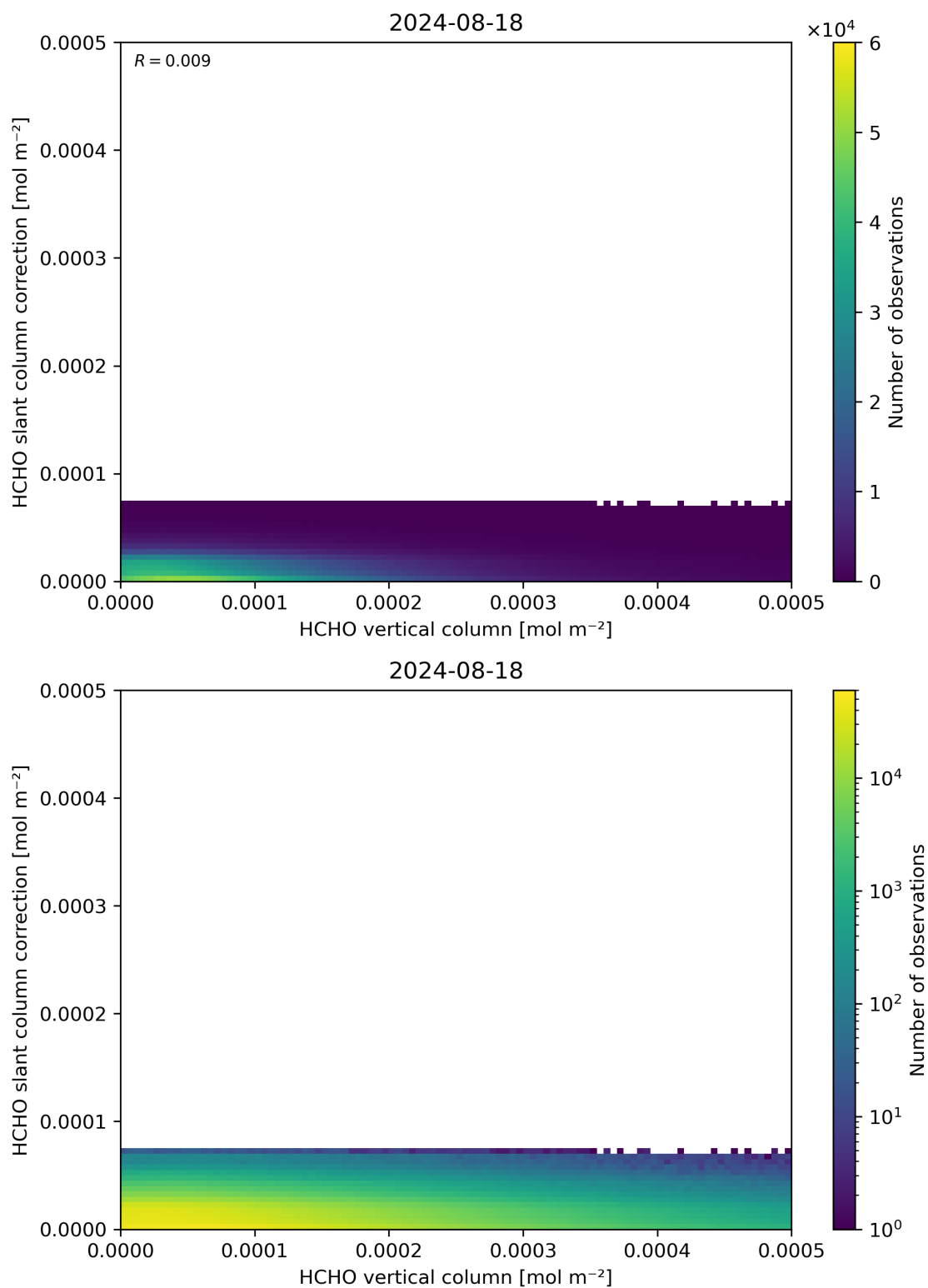
Figure 128: Scatter density plot of “HCHO vertical column” against “HCHO slant column correction” for 2024-08-17 to 2024-08-19.
