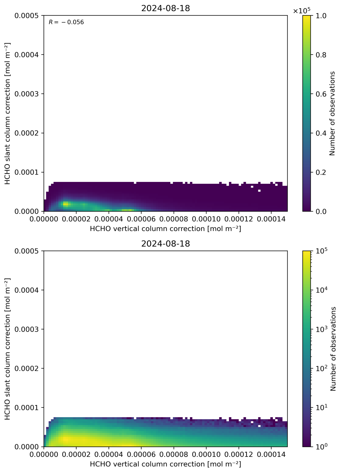
Figure 117: Scatter density plot of “HCHO vertical column correction” against “HCHO slant column correction” for 2024-08-17 to 2024-08-19.
