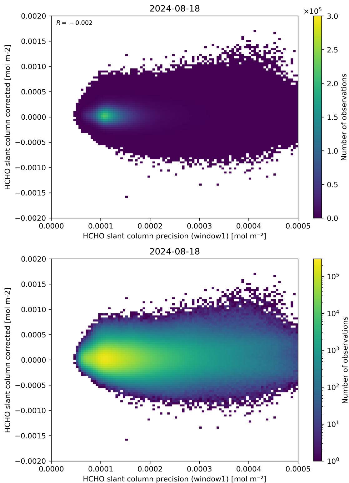
Figure 92: Scatter density plot of “HCHO slant column precision (window1)” against “HCHO slant column corrected” for 2024-08-17 to 2024-08-19.
