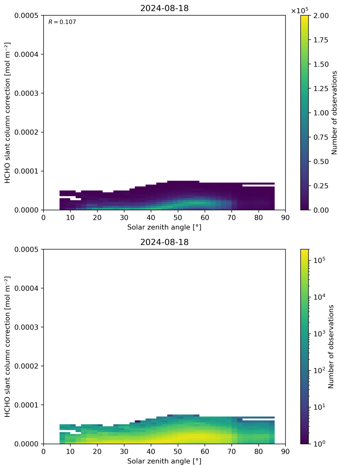
Figure 172: Scatter density plot of “Solar zenith angle” against “HCHO slant column correction” for 2024-08-17 to 2024-08-19.
