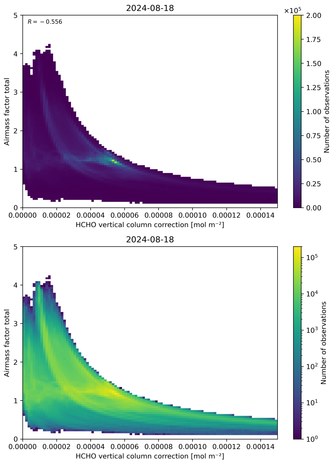
Figure 120: Scatter density plot of “HCHO vertical column correction” against “Airmass factor total” for 2024-08-17 to 2024-08-19.
