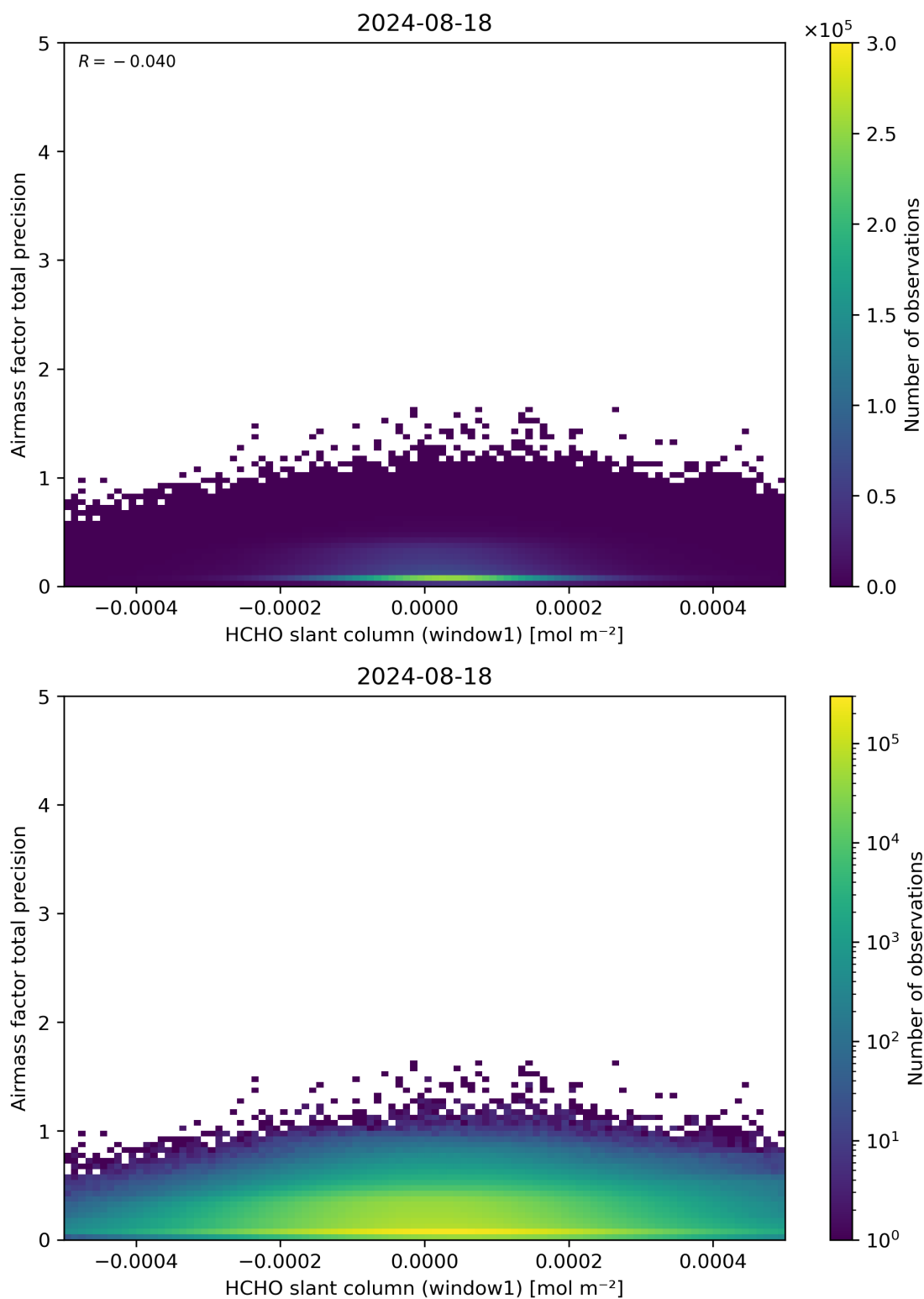
Figure 86: Scatter density plot of “HCHO slant column (window1)” against “Airmass factor total precision” for 2024-08-17 to 2024-08-19.
