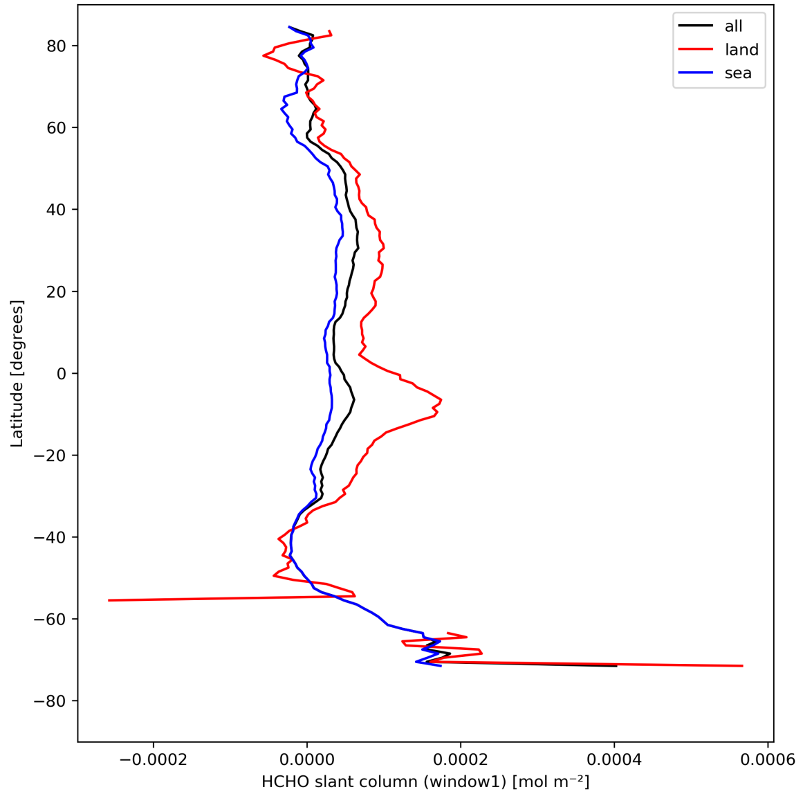
Figure 24: Zonal average of “HCHO slant column (window1)” for 2024-08-17 to 2024-08-19.
