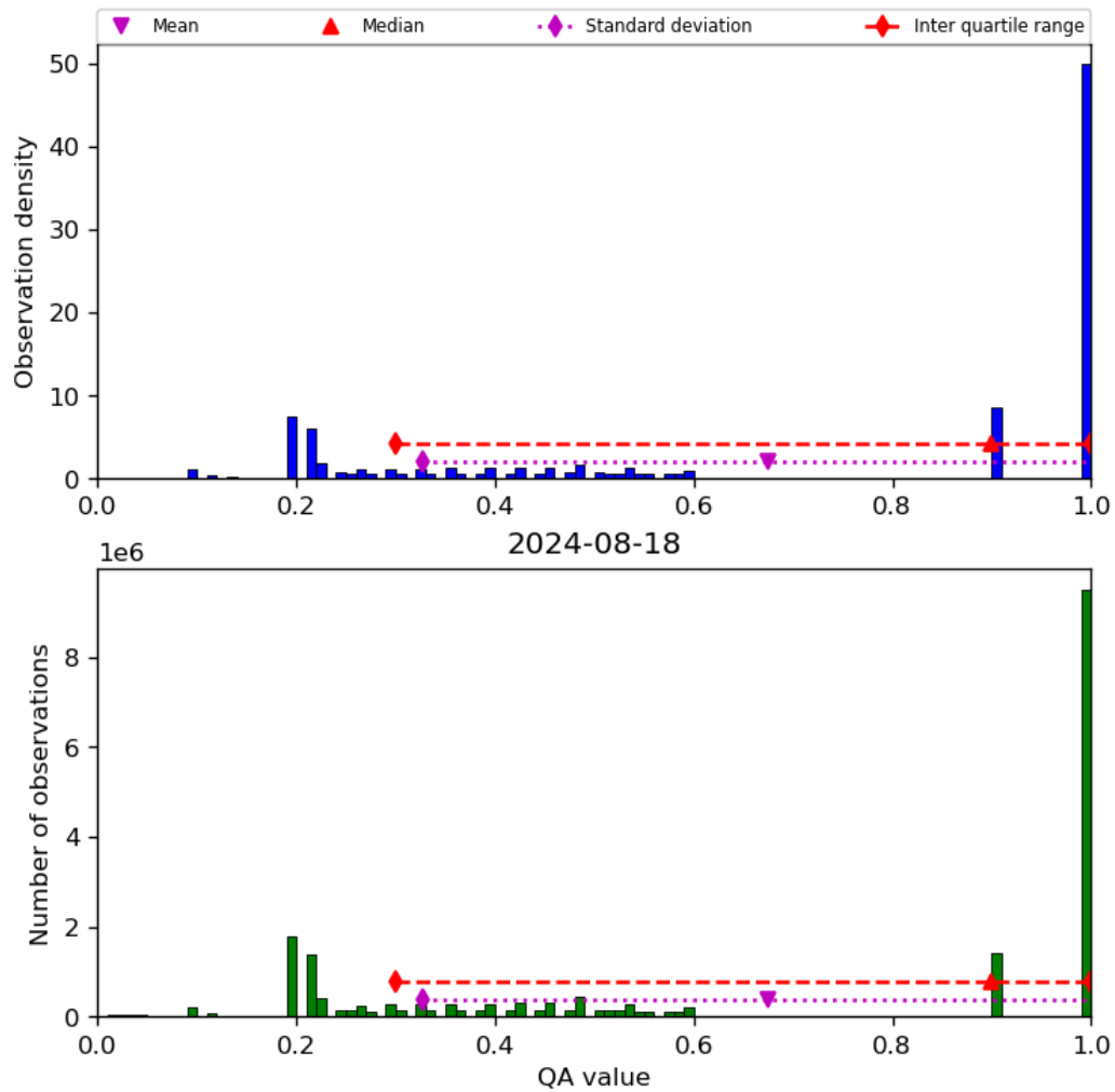
Figure 34: Histogram of “QA value” for 2024-08-17 to 2024-08-19
