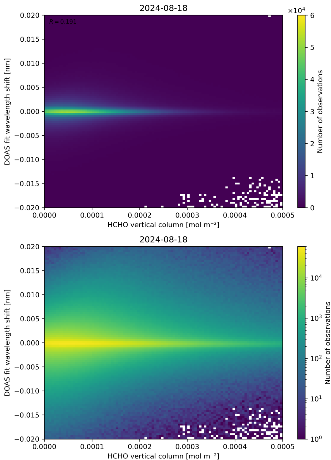
Figure 124: Scatter density plot of “HCHO vertical column” against “DOAS fit wavelength shift” for 2024-08-17 to 2024-08-19.
