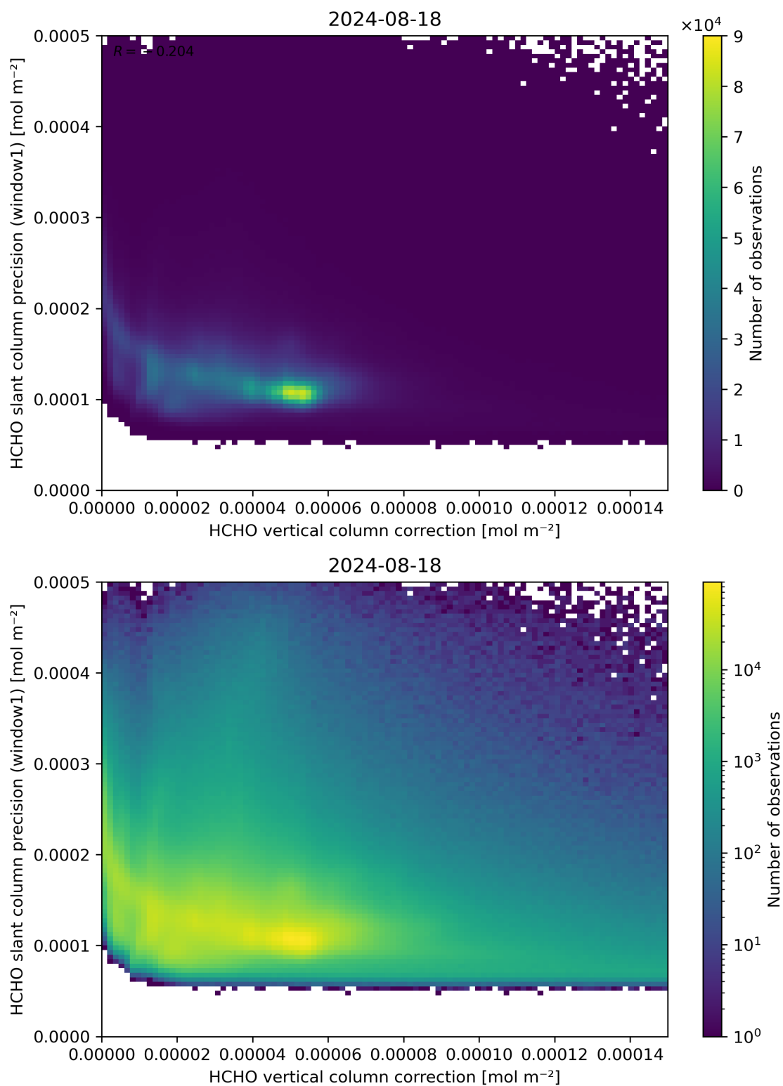
Figure 119: Scatter density plot of “HCHO vertical column correction” against “HCHO slant column precision (window1)” for 2024-08-17 to 2024-08-19.
