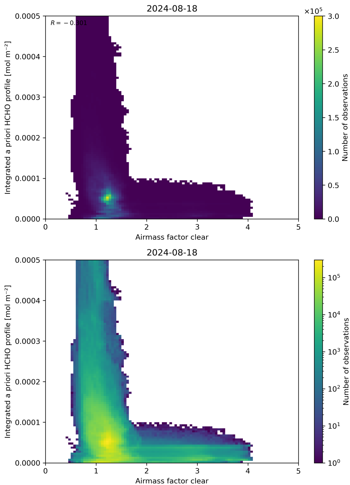
Figure 76: Scatter density plot of “Airmass factor clear” against “Integrated a priori HCHO profile” for 2024-08-17 to 2024-08-19.
