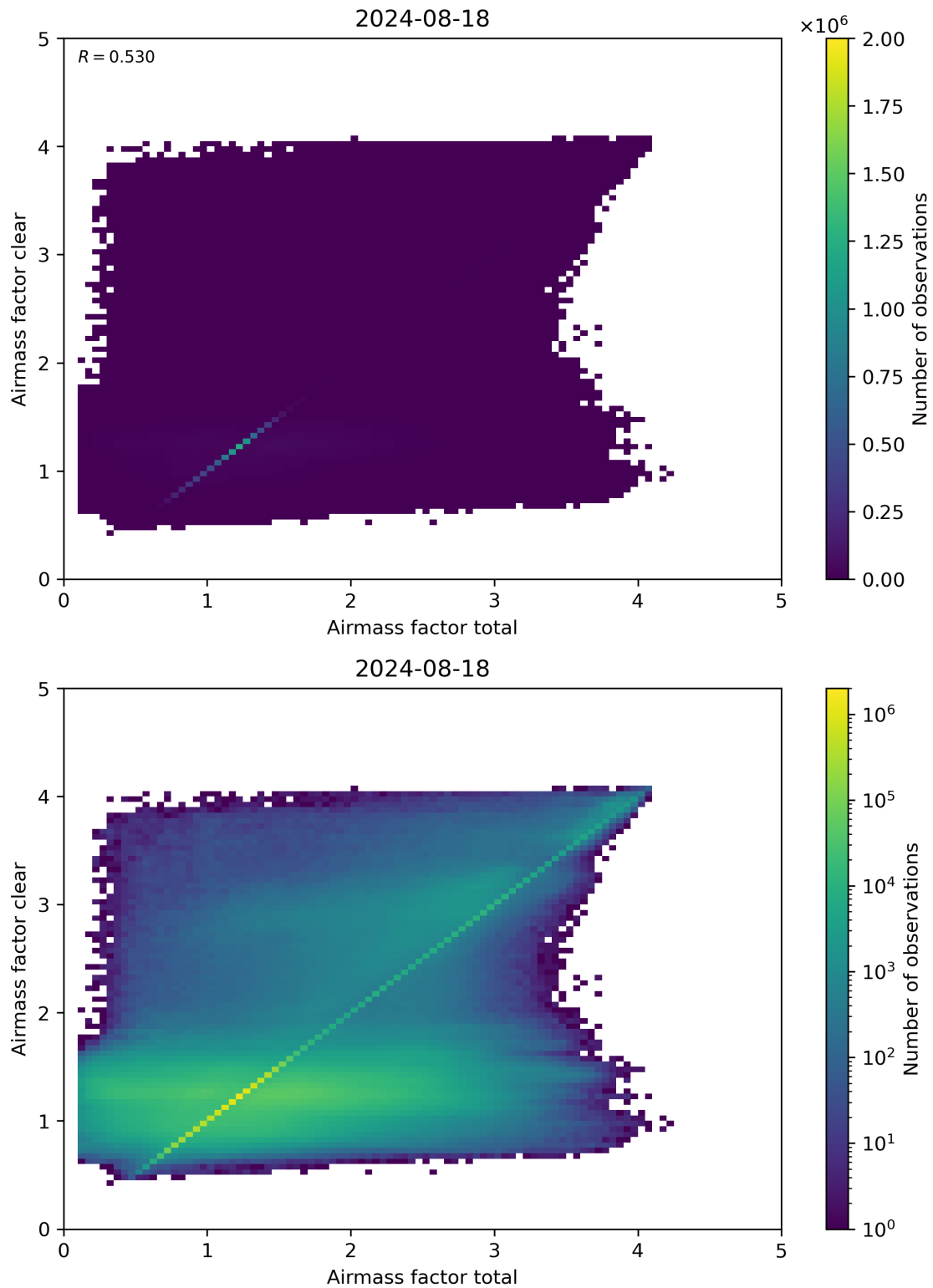
Figure 100: Scatter density plot of “Airmass factor total” against “Airmass factor clear” for 2024-08-17 to 2024-08-19.
