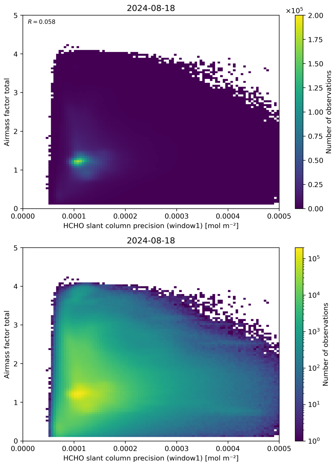
Figure 94: Scatter density plot of “HCHO slant column precision (window1)” against “Airmass factor total” for 2024-08-17 to 2024-08-19.
