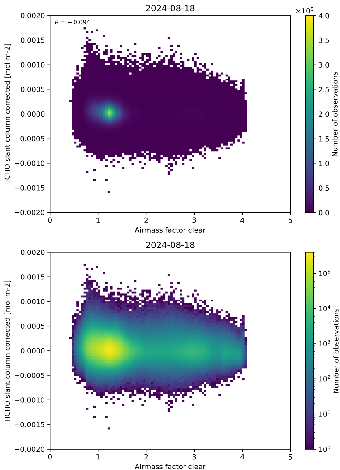
Figure 74: Scatter density plot of “Airmass factor clear” against “HCHO slant column corrected” for 2024-08-17 to 2024-08-19.
