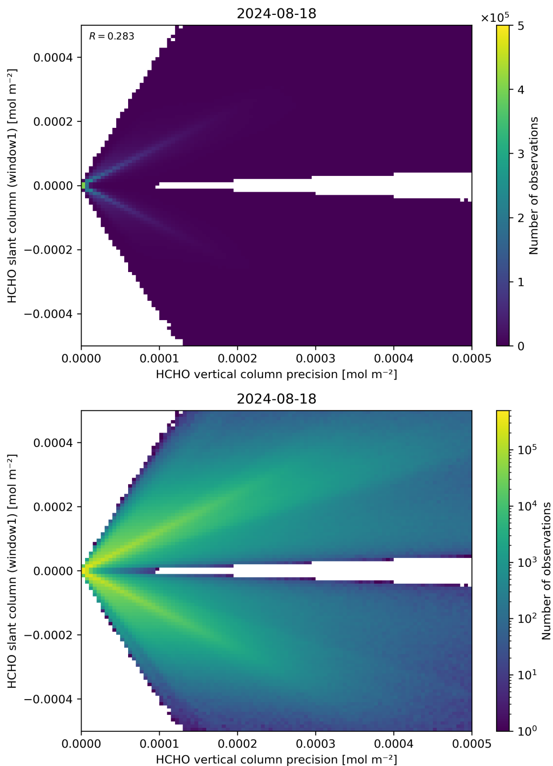
Figure 142: Scatter density plot of “HCHO vertical column precision” against “HCHO slant column (window1)” for 2024-08-17 to 2024-08-19.
