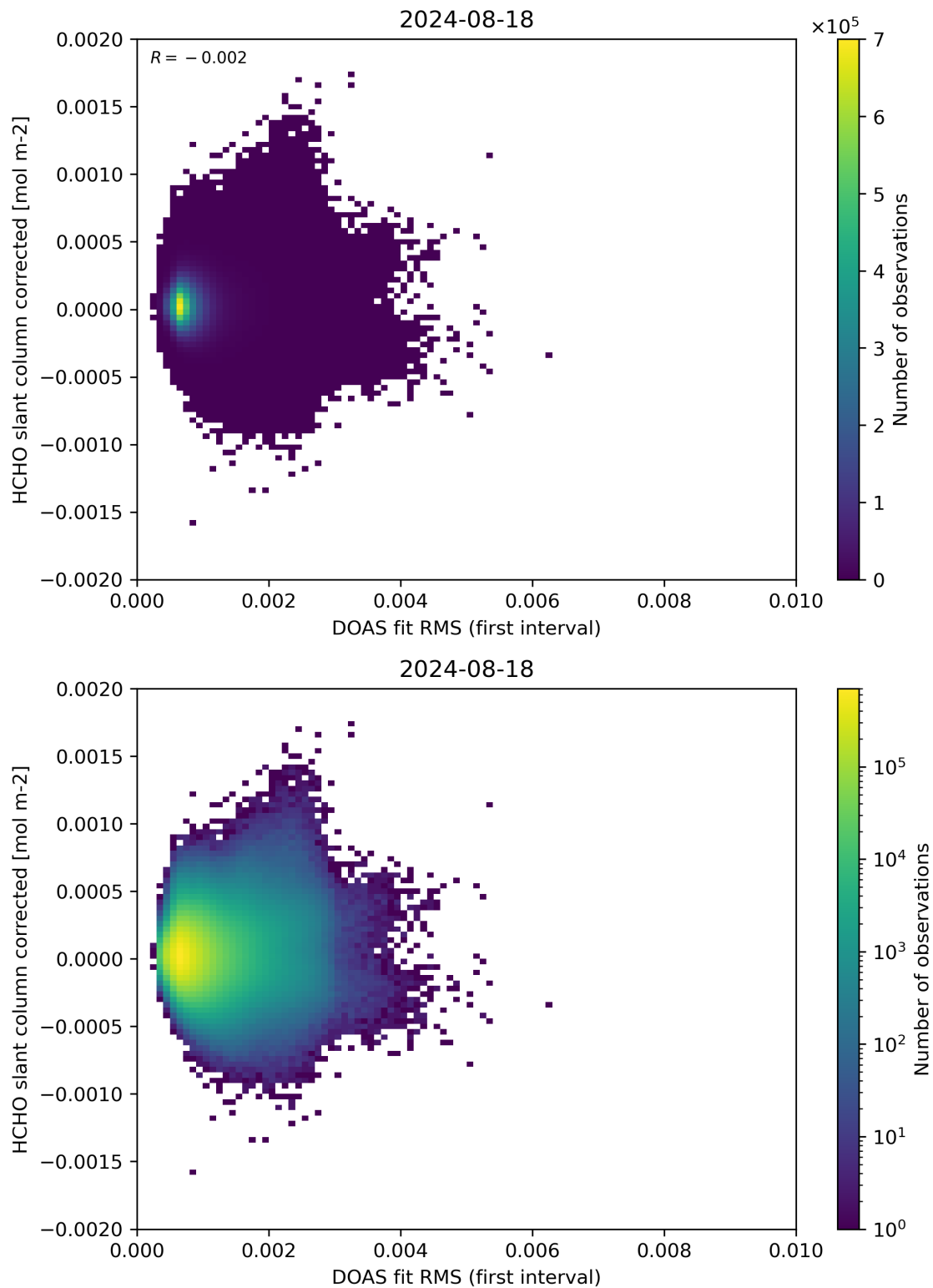
Figure 62: Scatter density plot of “DOAS fit RMS (first interval)” against “HCHO slant column corrected” for 2024-08-17 to 2024-08-19.
