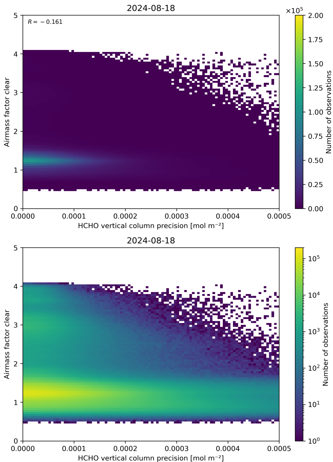
Figure 139: Scatter density plot of “HCHO vertical column precision” against “Airmass factor clear” for 2024-08-17 to 2024-08-19.
