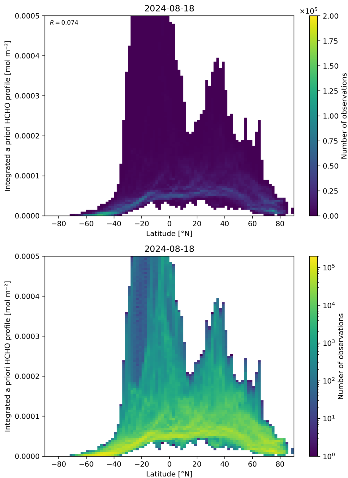
Figure 166: Scatter density plot of “Latitude” against “Integrated a priori HCHO profile” for 2024-08-17 to 2024-08-19.
