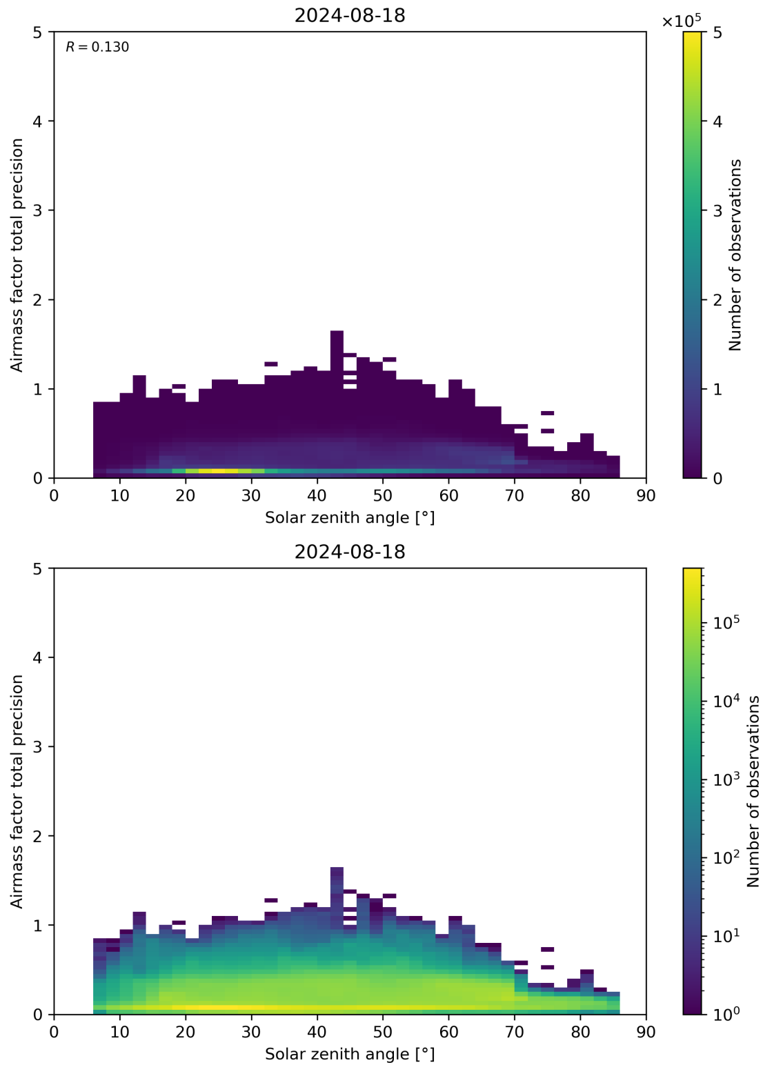
Figure 176: Scatter density plot of “Solar zenith angle” against “Airmass factor total precision” for 2024-08-17 to 2024-08-19.
