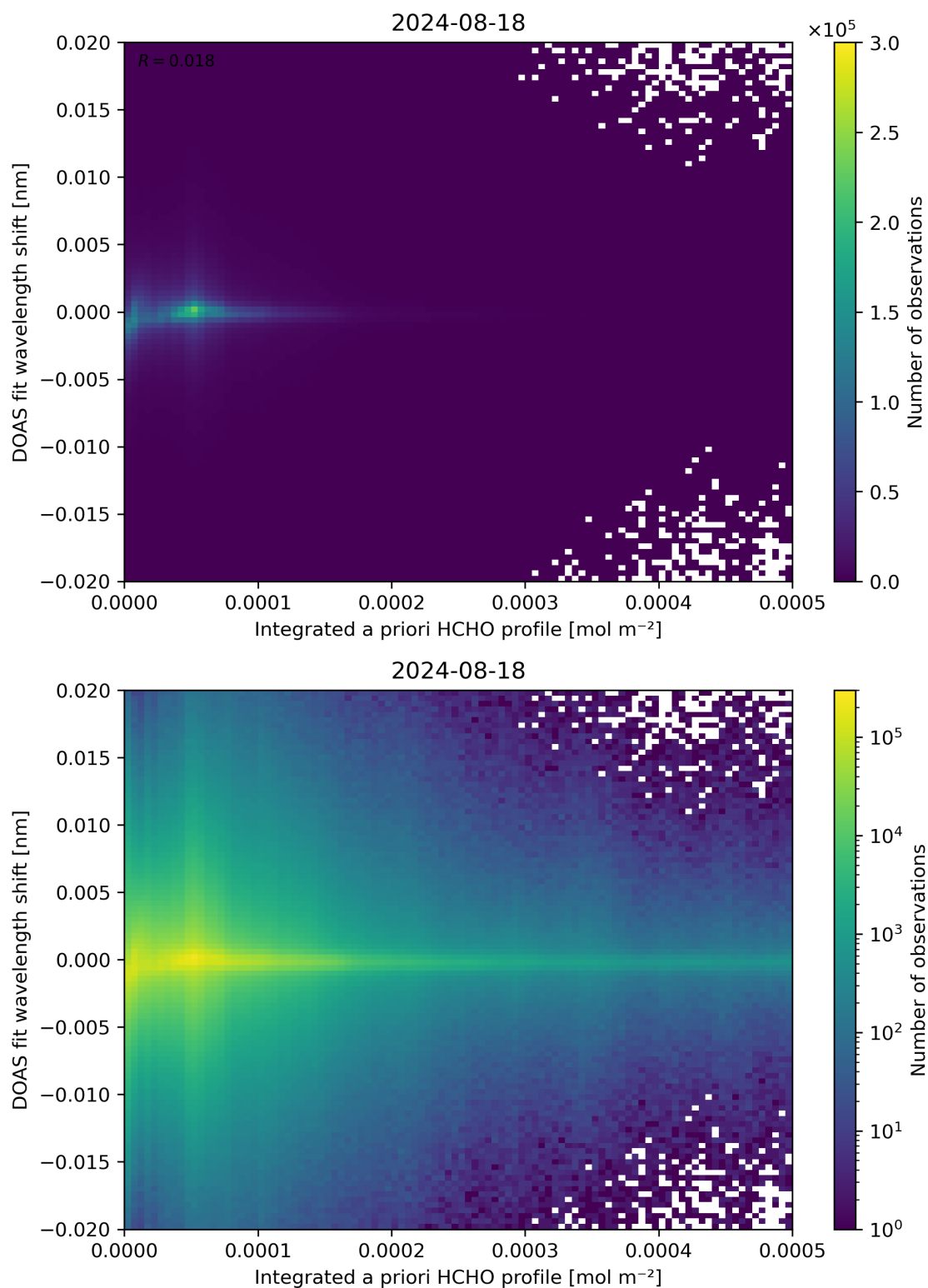
Figure 149: Scatter density plot of “Integrated a priori HCHO profile” against “DOAS fit wavelength shift” for 2024-08-17 to 2024-08-19.
