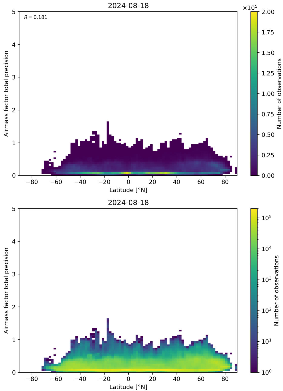
Figure 162: Scatter density plot of “Latitude” against “Airmass factor total precision” for 2024-08-17 to 2024-08-19.
