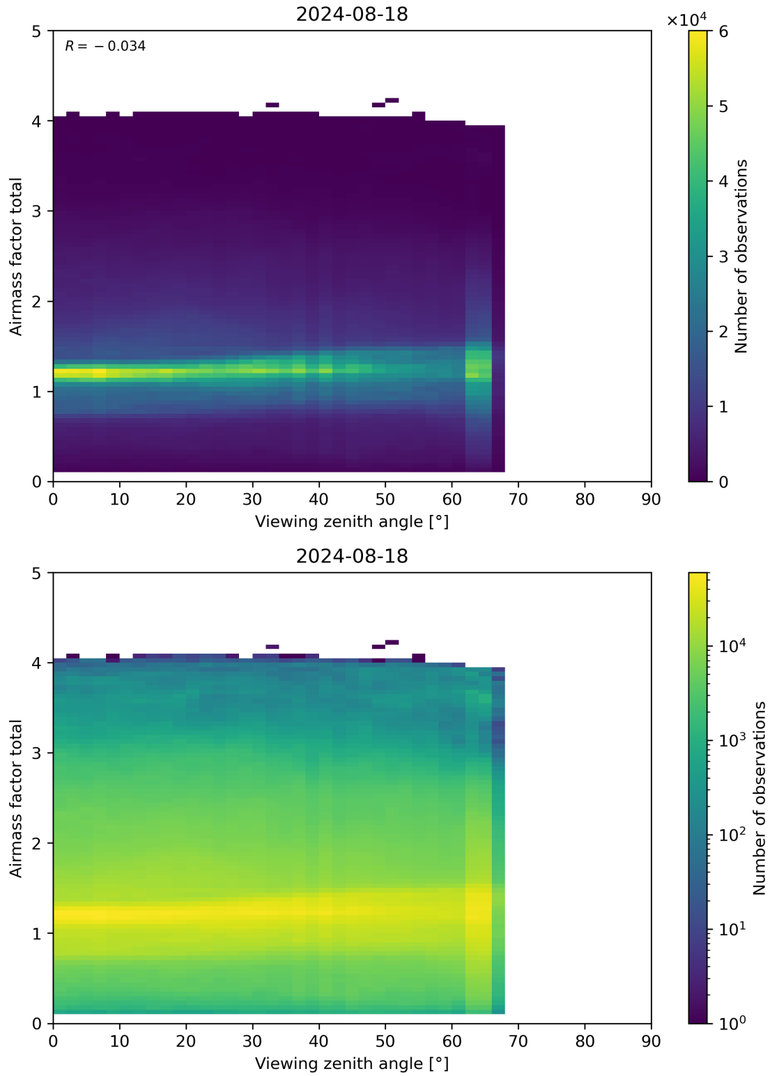
Figure 190: Scatter density plot of “Viewing zenith angle” against “Airmass factor total” for 2024-08-17 to 2024-08-19.
