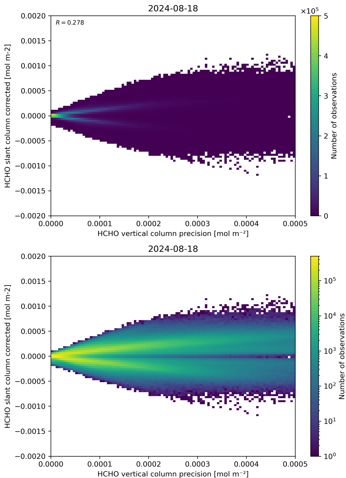
Figure 140: Scatter density plot of “HCHO vertical column precision” against “HCHO slant column corrected” for 2024-08-17 to 2024-08-19.
