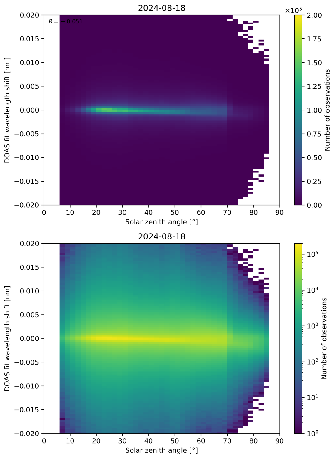
Figure 168: Scatter density plot of “Solar zenith angle” against “DOAS fit wavelength shift” for 2024-08-17 to 2024-08-19.
