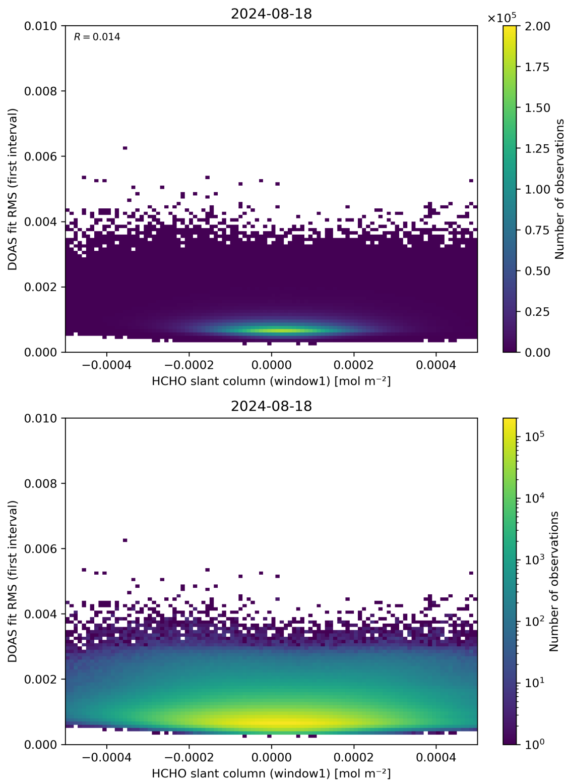
Figure 78: Scatter density plot of “HCHO slant column (window1)” against “DOAS fit RMS (first interval)” for 2024-08-17 to 2024-08-19.
