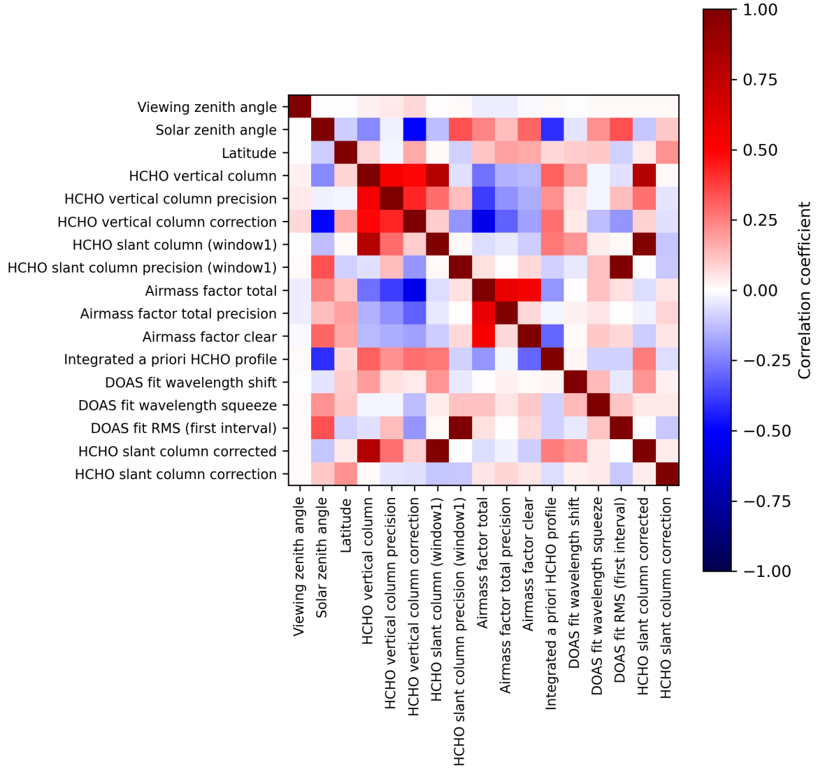
Figure 2: Map of correlation matrix for 2024-08-17 to 2024-08-19.
