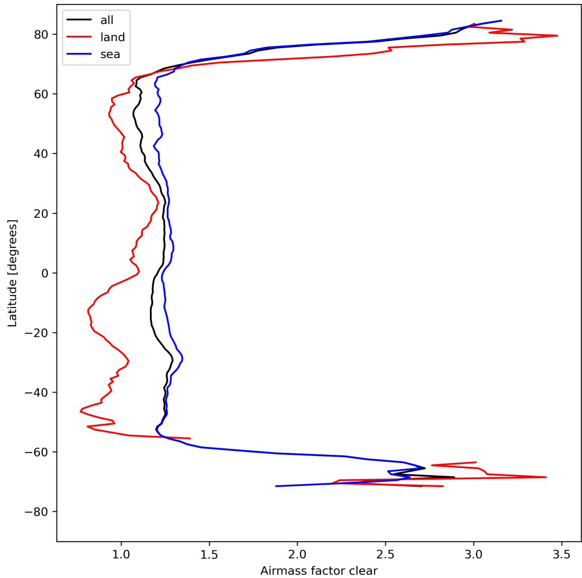
Figure 28: Zonal average of “Airmass factor clear” for 2024-08-17 to 2024-08-19.
