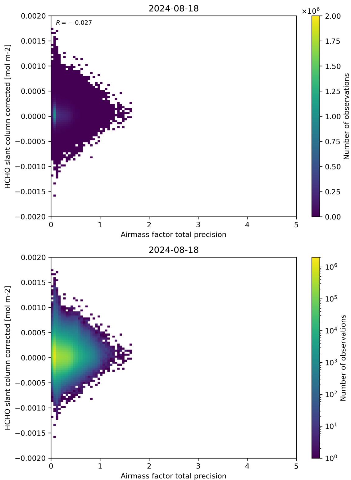
Figure 109: Scatter density plot of “Airmass factor total precision” against “HCHO slant column corrected” for 2024-08-17 to 2024-08-19.
