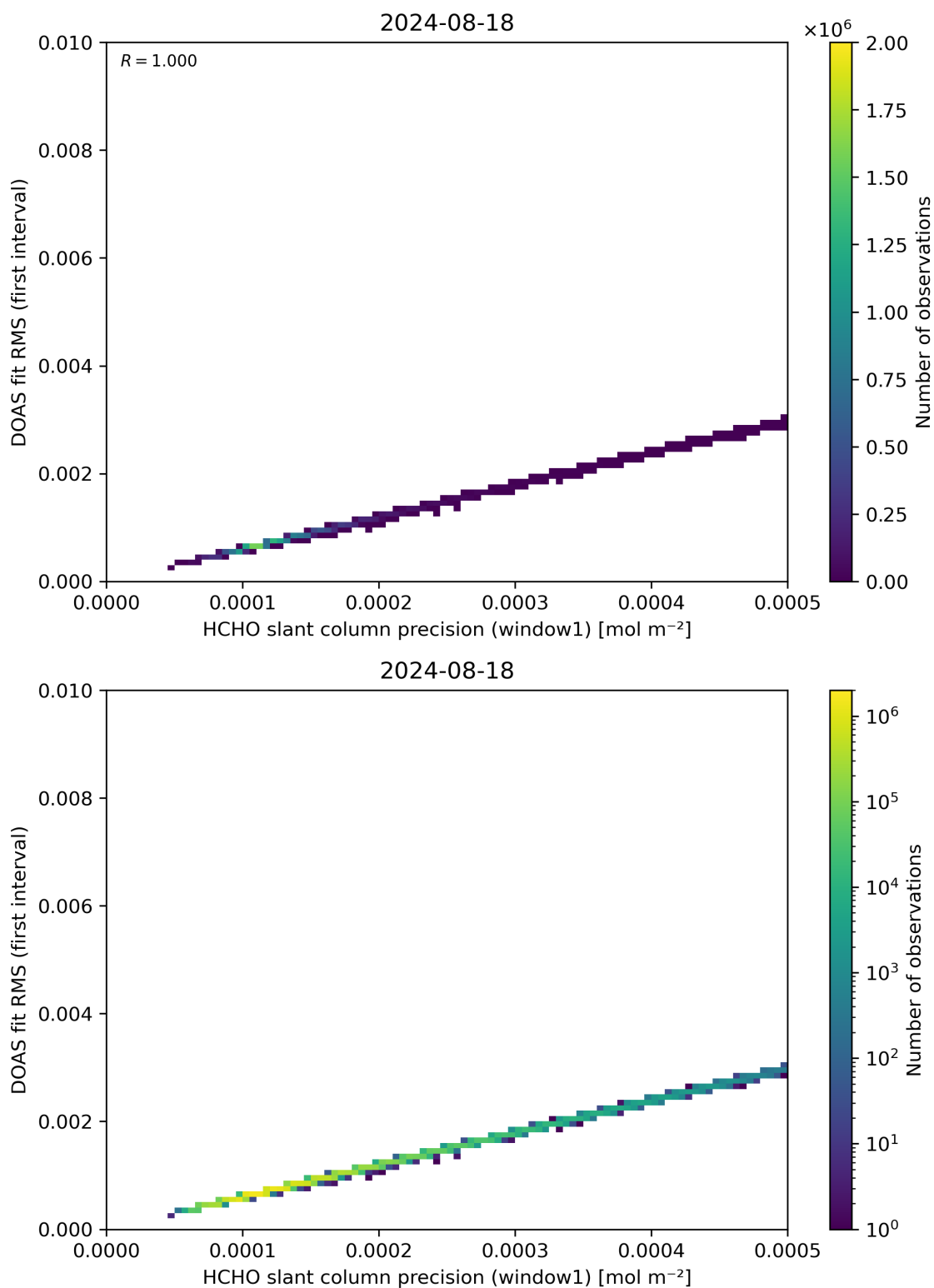
Figure 88: Scatter density plot of “HCHO slant column precision (window1)” against “DOAS fit RMS (first interval)” for 2024-08-17 to 2024-08-19.
