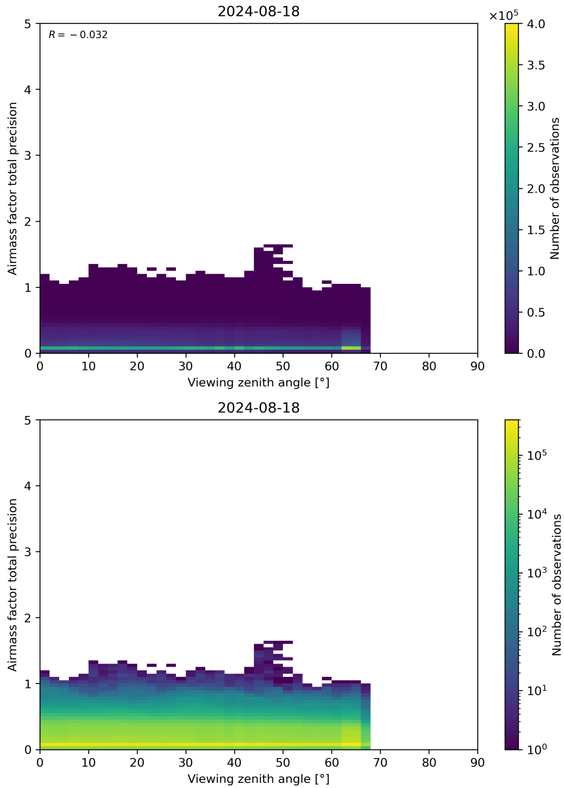
Figure 191: Scatter density plot of “Viewing zenith angle” against “Airmass factor total precision” for 2024-08-17 to 2024-08-19.
