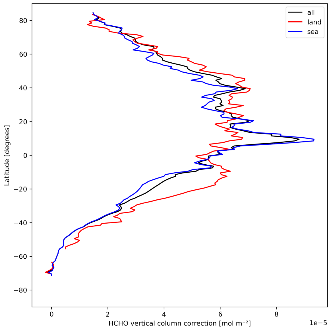
Figure 23: Zonal average of “HCHO vertical column correction” for 2024-08-17 to 2024-08-19.
