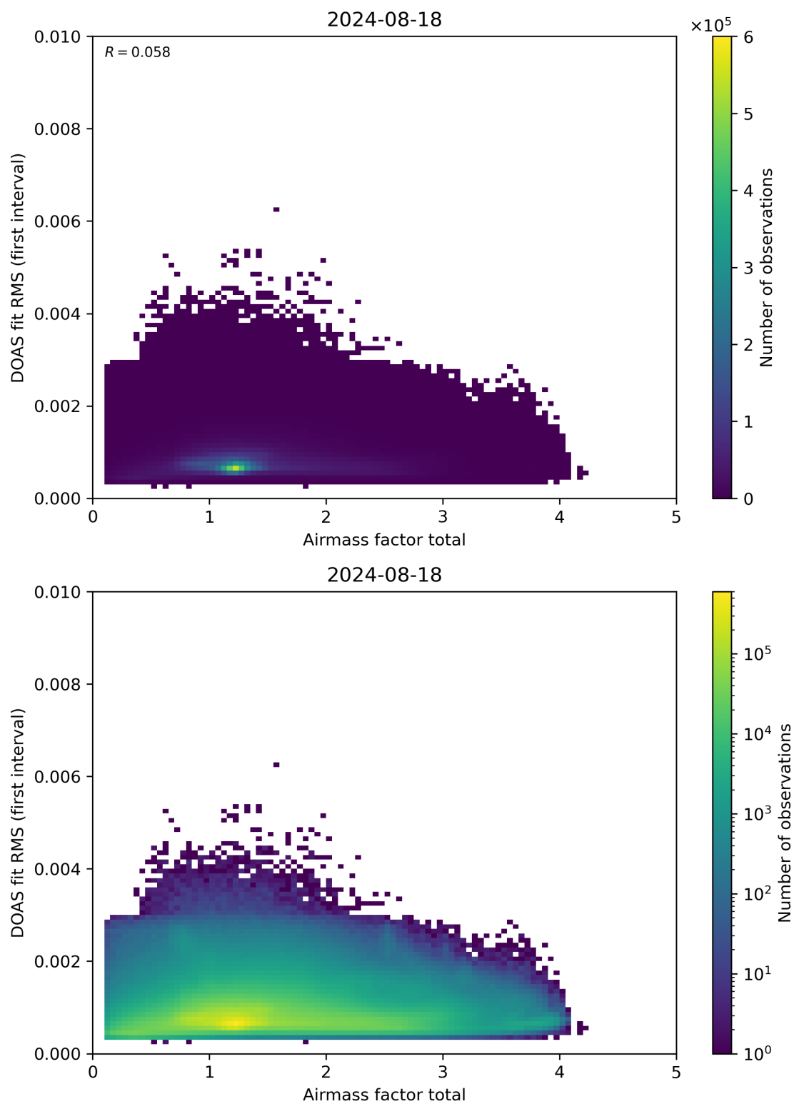
Figure 97: Scatter density plot of “Airmass factor total” against “DOAS fit RMS (first interval)” for 2024-08-17 to 2024-08-19.
