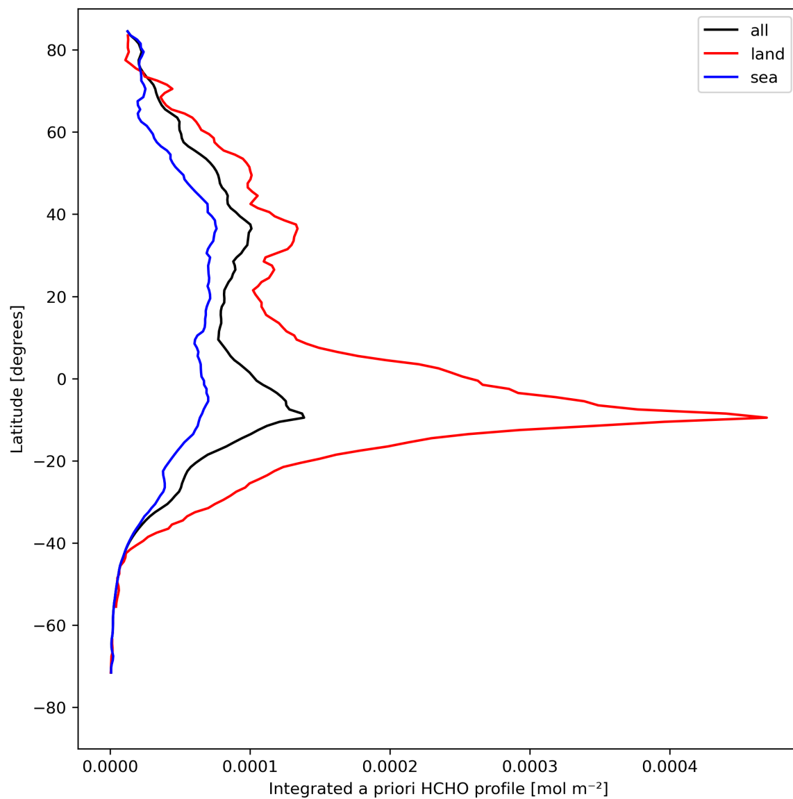
Figure 29: Zonal average of “Integrated a priori HCHO profile” for 2024-08-17 to 2024-08-19.
