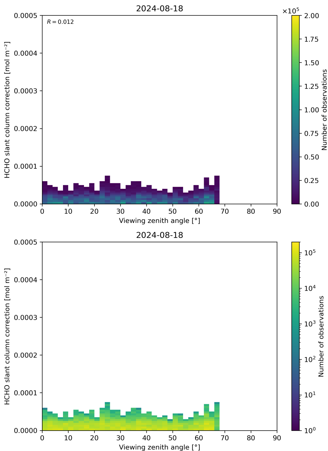
Figure 187: Scatter density plot of “Viewing zenith angle” against “HCHO slant column correction” for 2024-08-17 to 2024-08-19.
