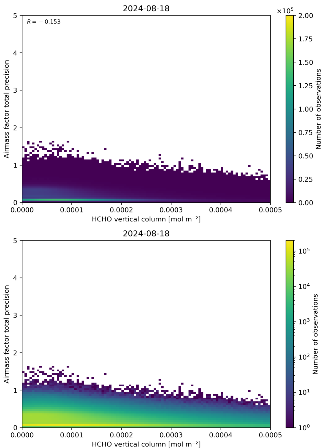
Figure 132: Scatter density plot of “HCHO vertical column” against “Airmass factor total precision” for 2024-08-17 to 2024-08-19.
