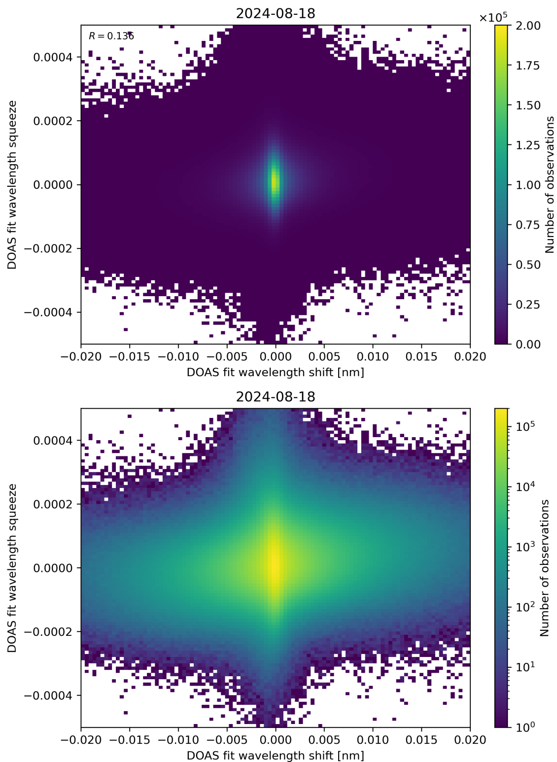
Figure 65: Scatter density plot of “DOAS fit wavelength shift” against “DOAS fit wavelength squeeze” for 2024-08-17 to 2024-08-19.
