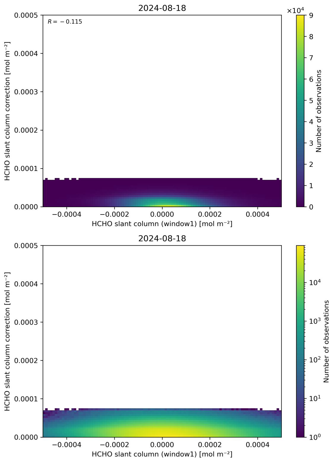
Figure 83: Scatter density plot of “HCHO slant column (window1)” against “HCHO slant column correction” for 2024-08-17 to 2024-08-19.
