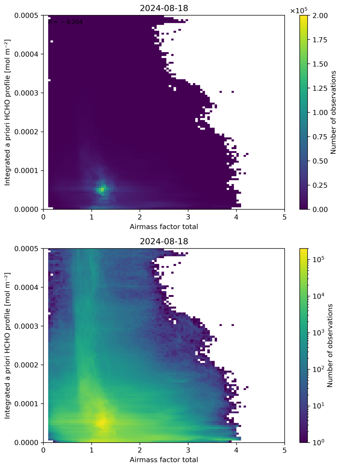
Figure 104: Scatter density plot of “Airmass factor total” against “Integrated a priori HCHO profile” for 2024-08-17 to 2024-08-19.
