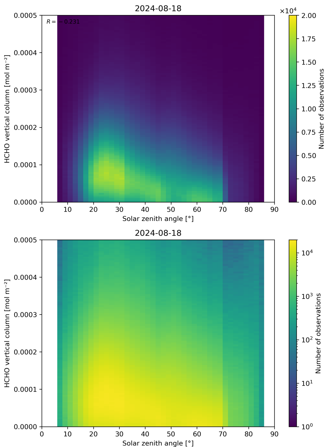
Figure 177: Scatter density plot of “Solar zenith angle” against “HCHO vertical column” for 2024-08-17 to 2024-08-19.
