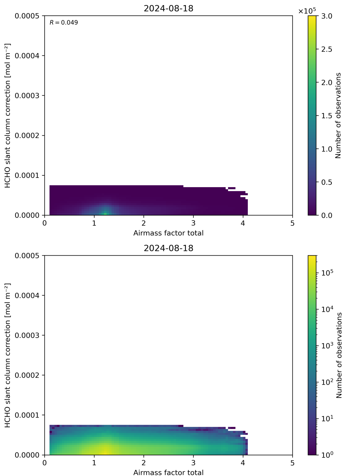
Figure 102: Scatter density plot of “Airmass factor total” against “HCHO slant column correction” for 2024-08-17 to 2024-08-19.
