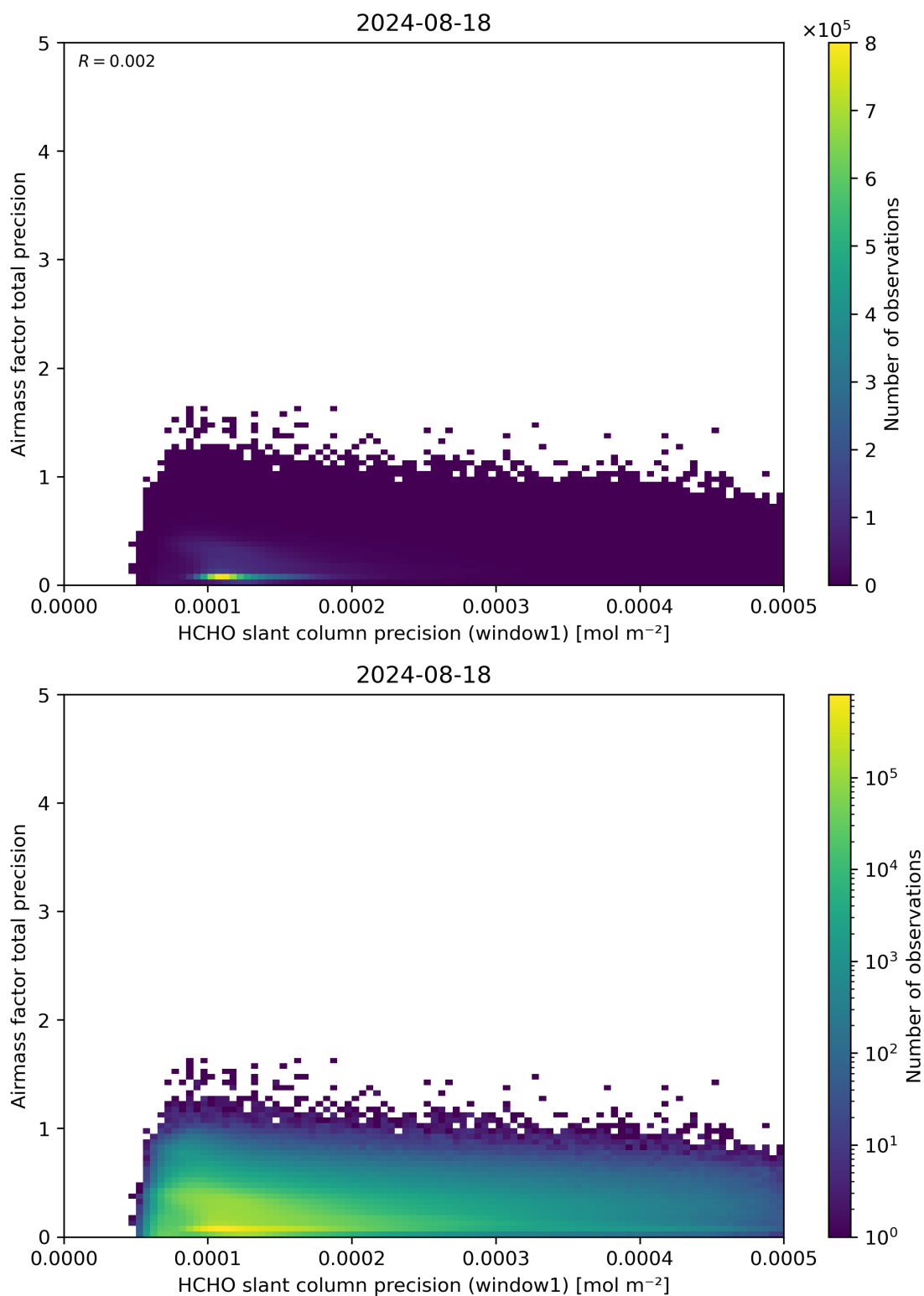
Figure 95: Scatter density plot of “HCHO slant column precision (window1)” against “Airmass factor total precision” for 2024-08-17 to 2024-08-19.
