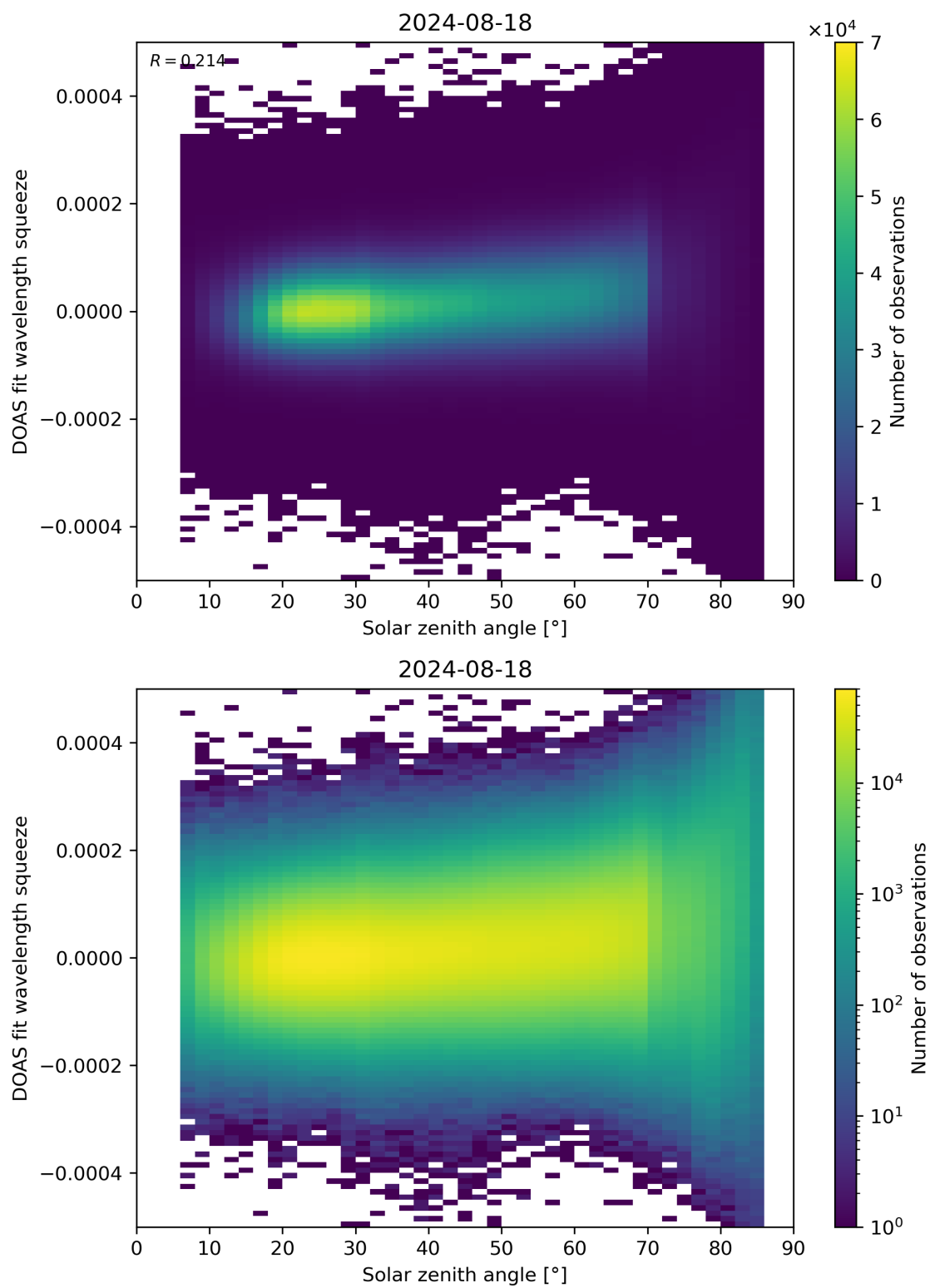
Figure 169: Scatter density plot of “Solar zenith angle” against “DOAS fit wavelength squeeze” for 2024-08-17 to 2024-08-19.
