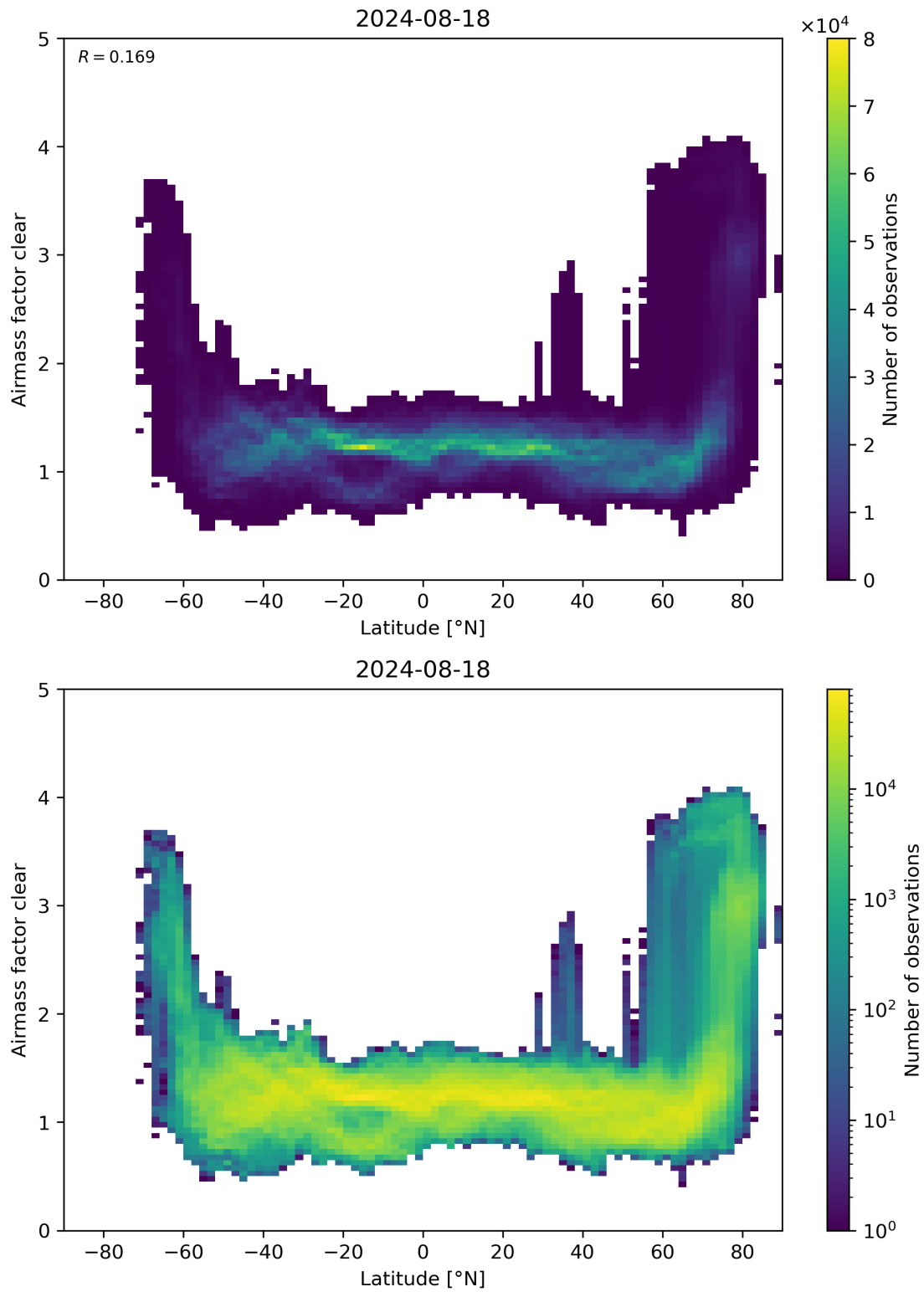
Figure 156: Scatter density plot of “Latitude” against “Airmass factor clear” for 2024-08-17 to 2024-08-19.
