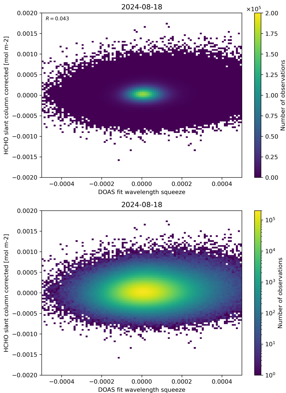
Figure 69: Scatter density plot of “DOAS fit wavelength squeeze” against “HCHO slant column corrected” for 2024-08-17 to 2024-08-19.
