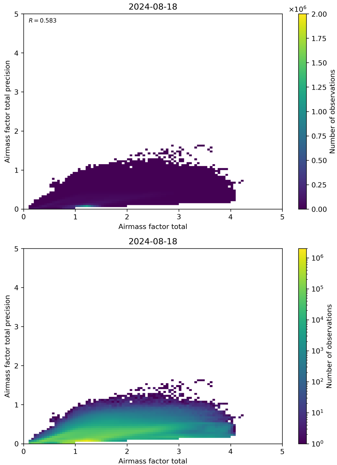
Figure 103: Scatter density plot of “Airmass factor total” against “Airmass factor total precision” for 2024-08-17 to 2024-08-19.
