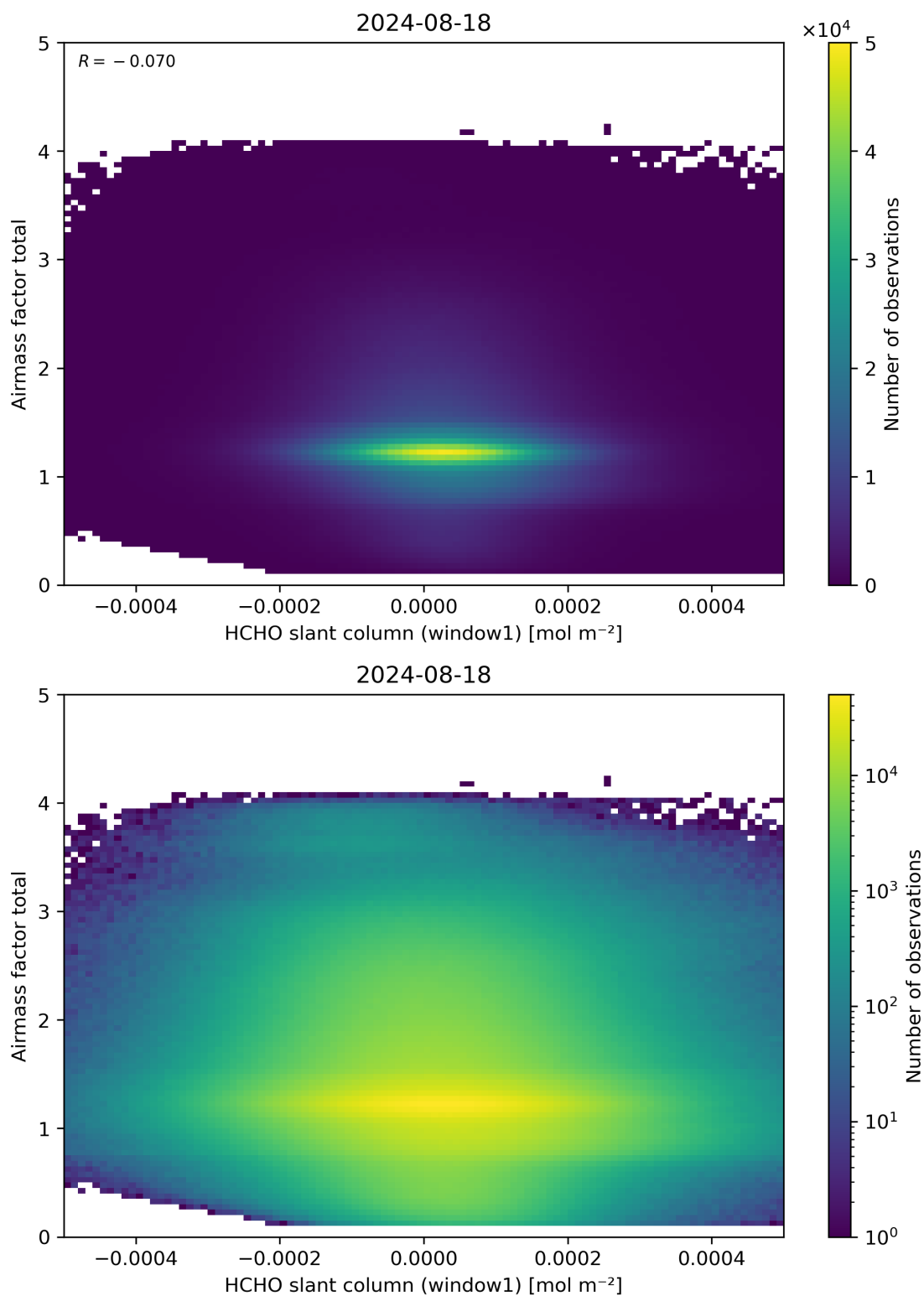
Figure 85: Scatter density plot of “HCHO slant column (window1)” against “Airmass factor total” for 2024-08-17 to 2024-08-19.
