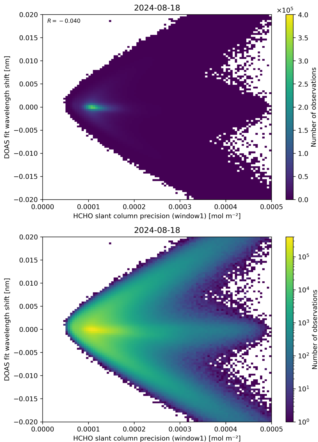
Figure 89: Scatter density plot of “HCHO slant column precision (window1)” against “DOAS fit wavelength shift” for 2024-08-17 to 2024-08-19.
