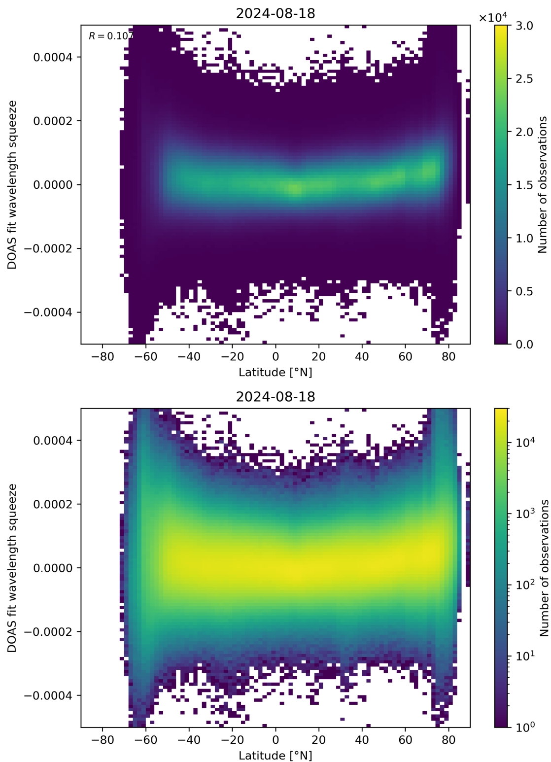
Figure 155: Scatter density plot of “Latitude” against “DOAS fit wavelength squeeze” for 2024-08-17 to 2024-08-19.
