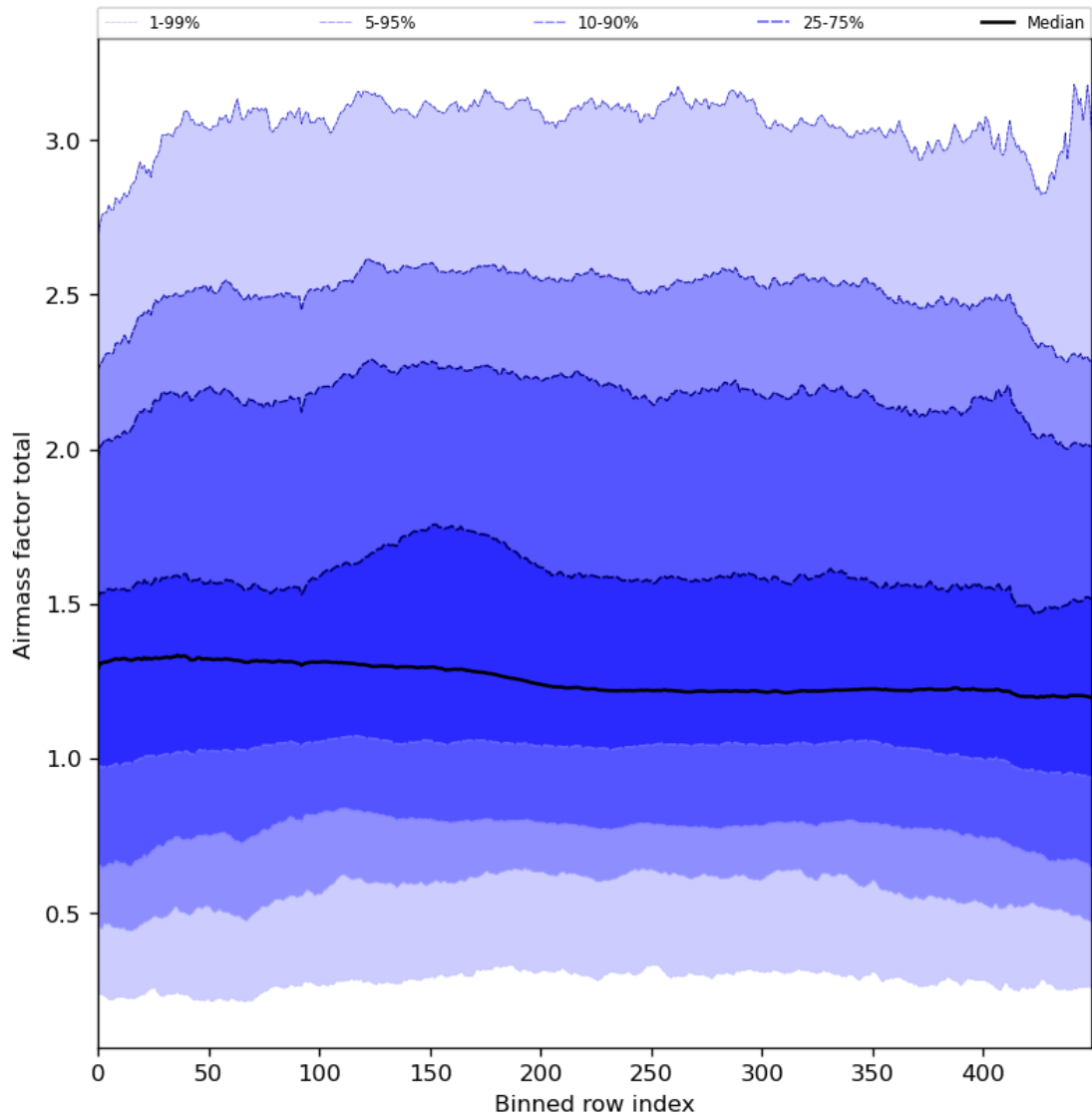
Figure 54: Along track statistics of “Airmass factor total” for 2024-08-17 to 2024-08-19
