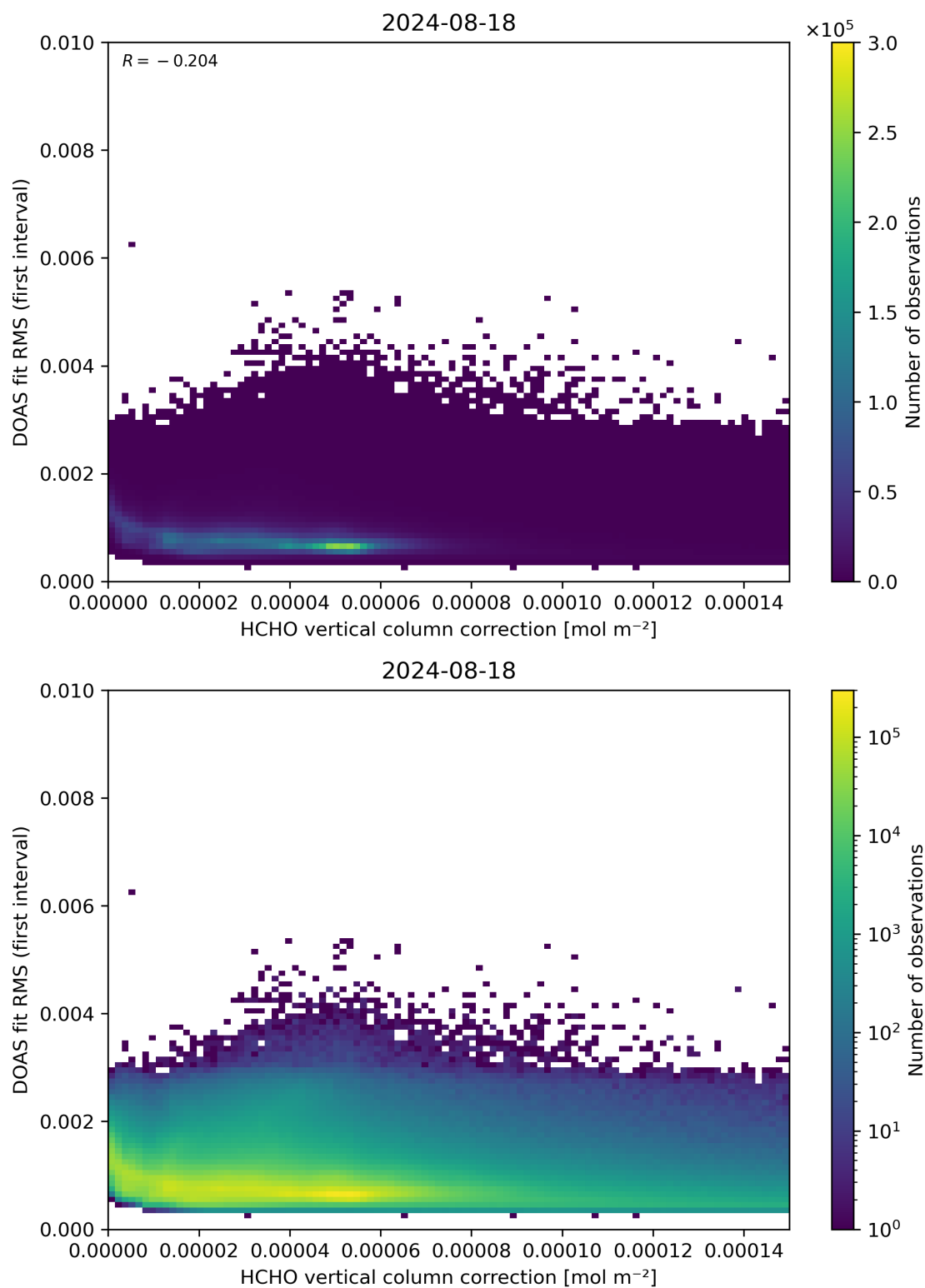
Figure 112: Scatter density plot of “HCHO vertical column correction” against “DOAS fit RMS (first interval)” for 2024-08-17 to 2024-08-19.
