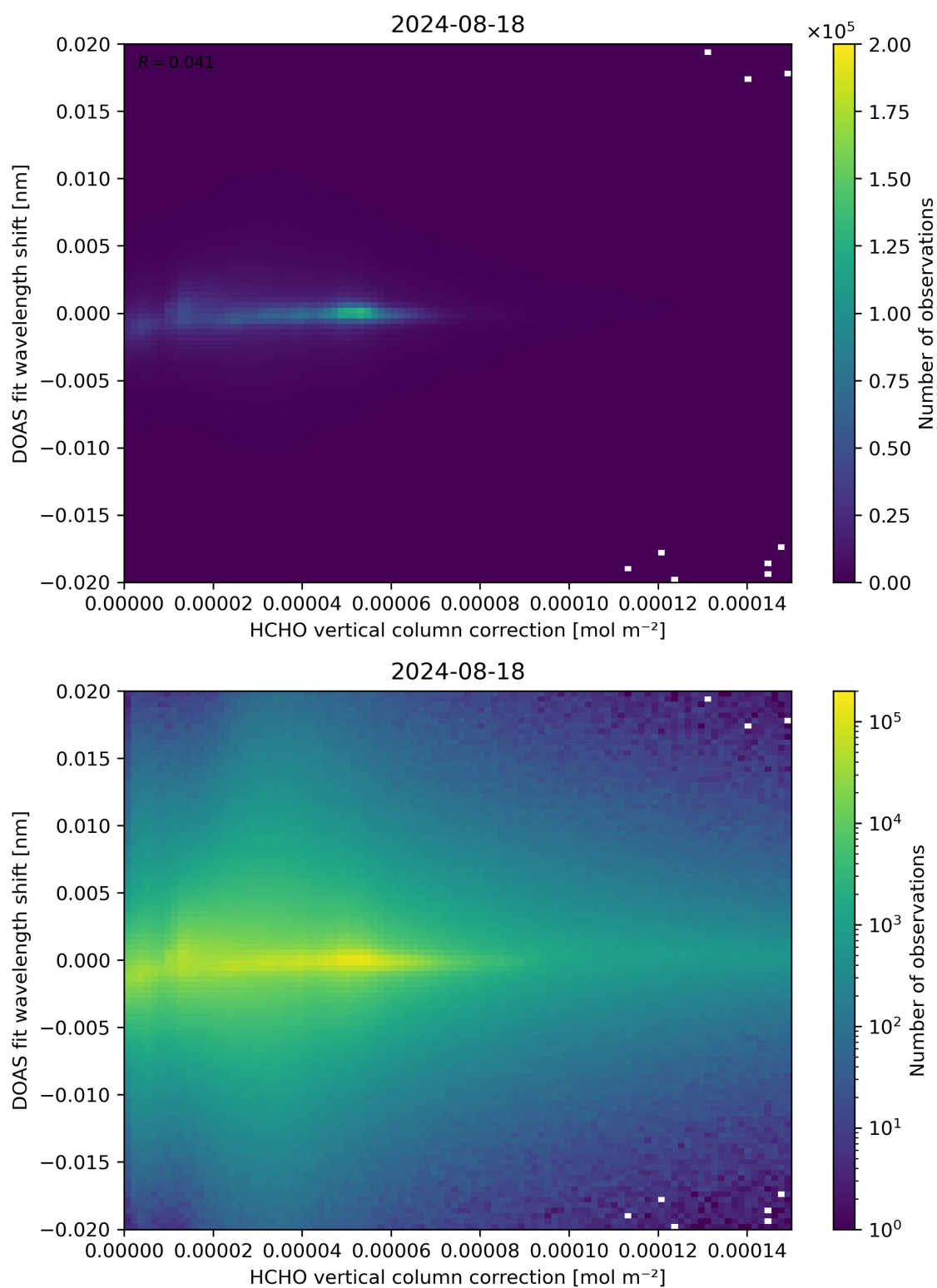
Figure 113: Scatter density plot of “HCHO vertical column correction” against “DOAS fit wavelength shift” for 2024-08-17 to 2024-08-19.
