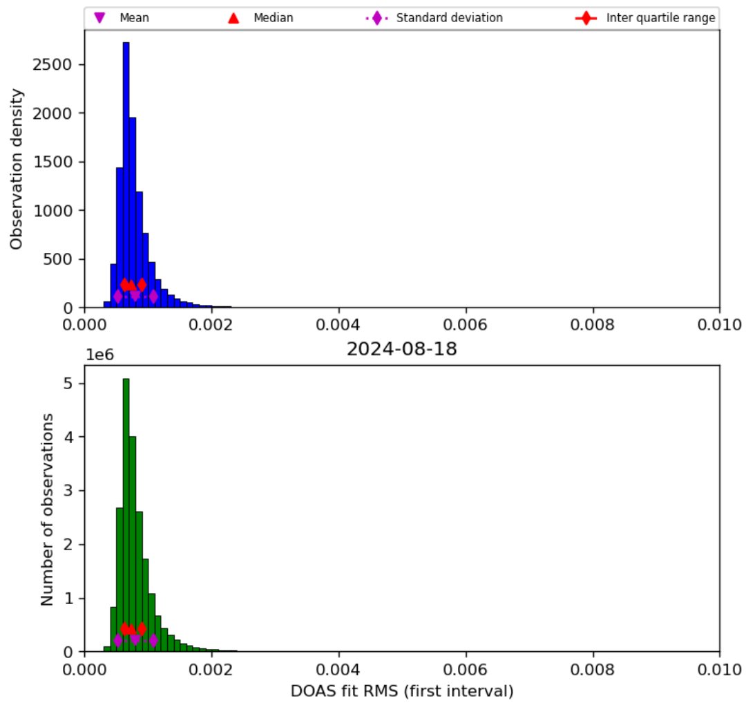
Figure 46: Histogram of “DOAS fit RMS (first interval)” for 2024-08-17 to 2024-08-19
