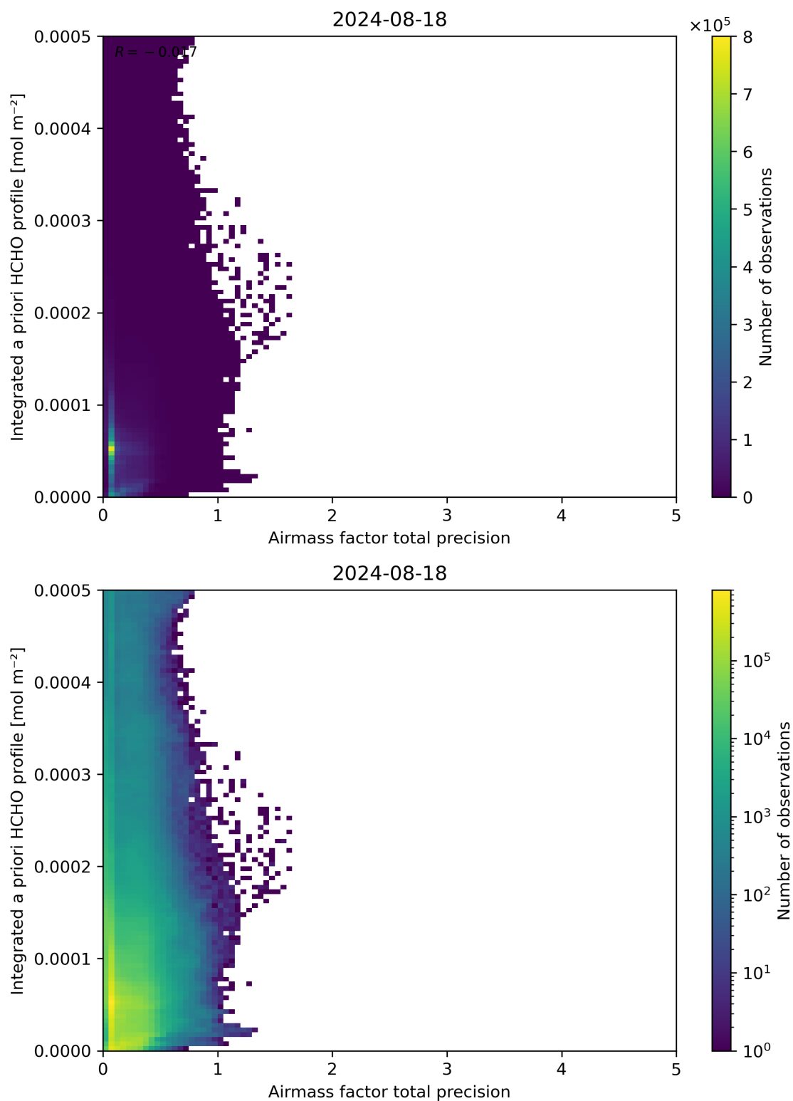
Figure 111: Scatter density plot of “Airmass factor total precision” against “Integrated a priori HCHO profile” for 2024-08-17 to 2024-08-19.
