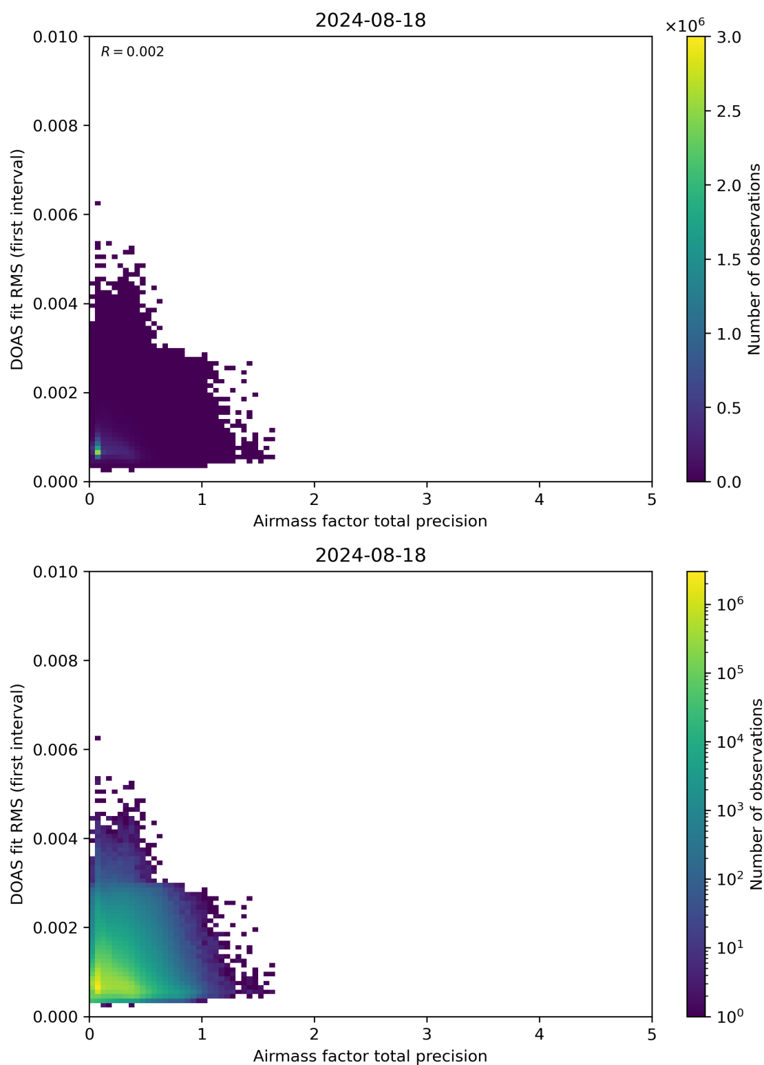
Figure 105: Scatter density plot of “Airmass factor total precision” against “DOAS fit RMS (first interval)” for 2024-08-17 to 2024-08-19.
