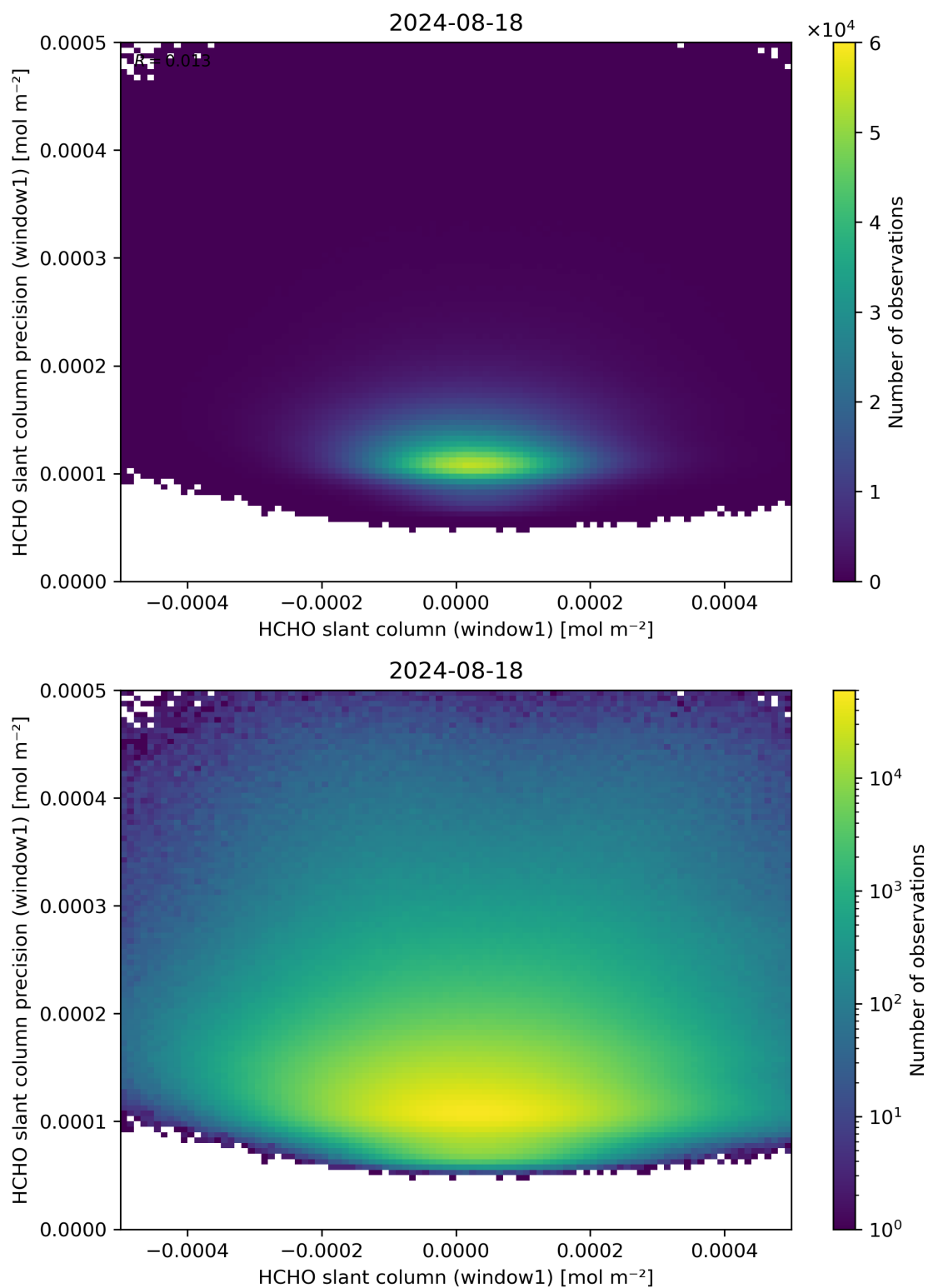
Figure 84: Scatter density plot of “HCHO slant column (window1)” against “HCHO slant column precision (window1)” for 2024-08-17 to 2024-08-19.
