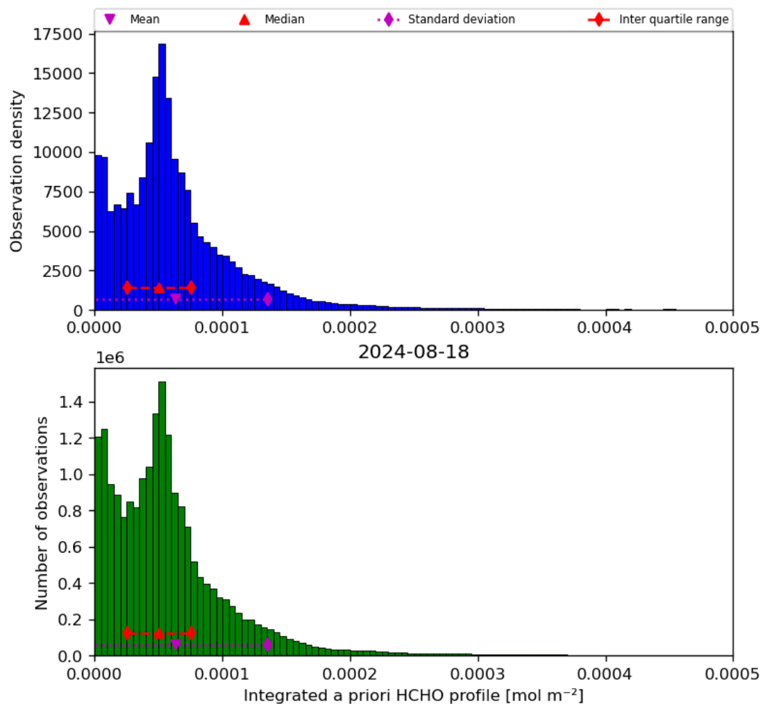
Figure 43: Histogram of “Integrated a priori HCHO profile” for 2024-08-17 to 2024-08-19
