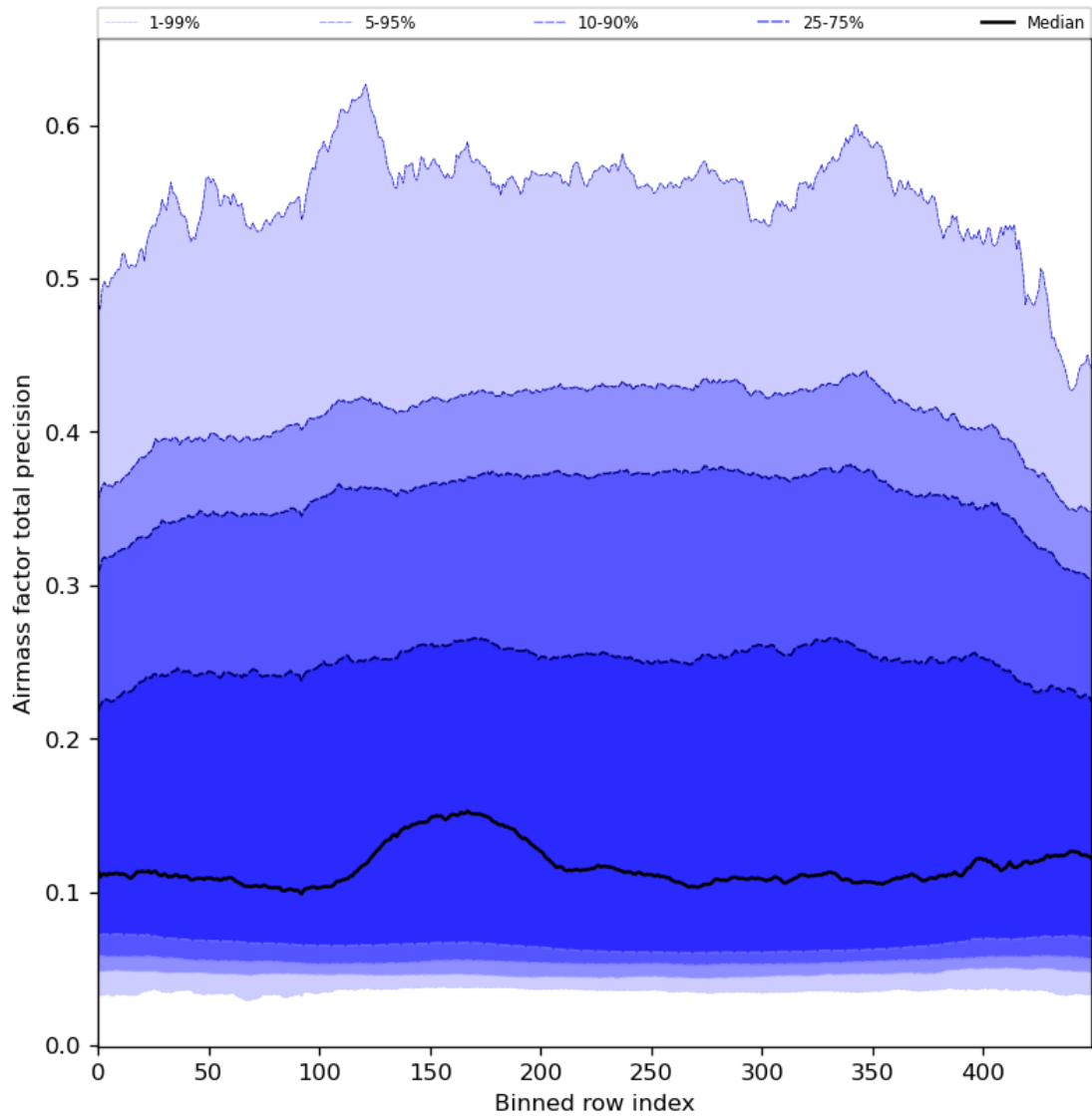
Figure 55: Along track statistics of “Airmass factor total precision” for 2024-08-17 to 2024-08-19
