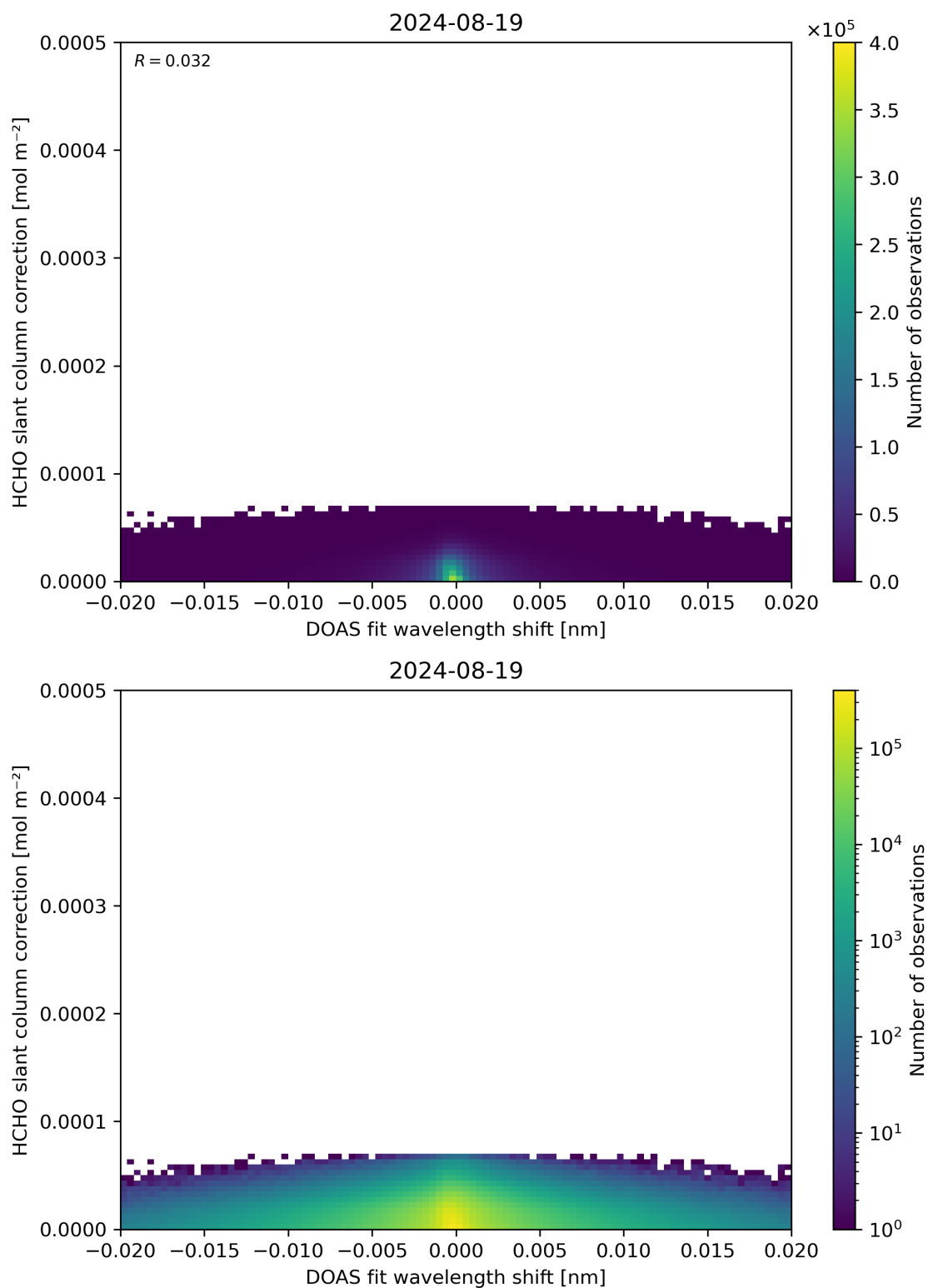
Figure 67: Scatter density plot of “DOAS fit wavelength shift” against “HCHO slant column correction” for 2024-08-18 to 2024-08-20.
