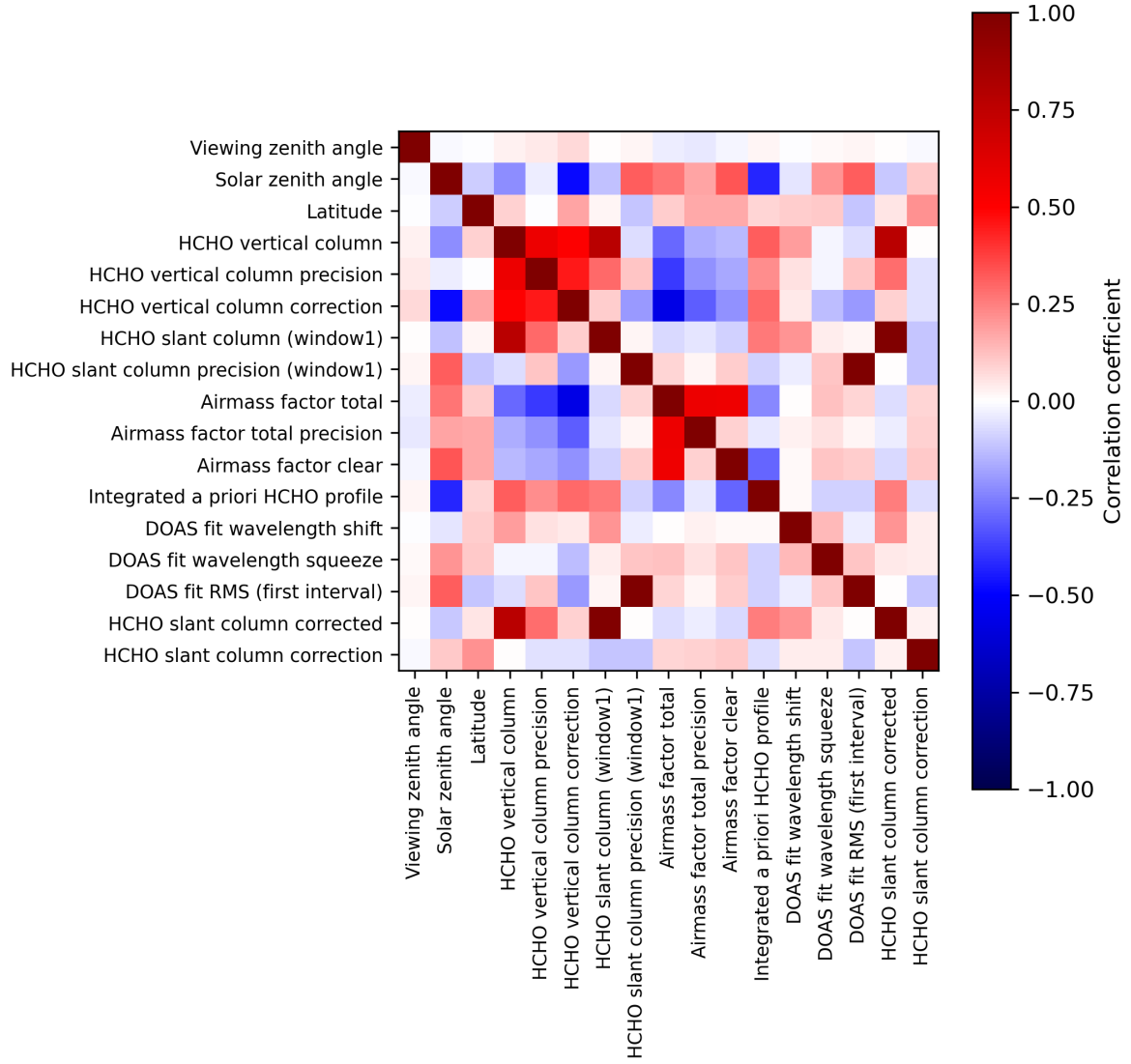
Figure 2: Map of correlation matrix for 2024-08-18 to 2024-08-20.
