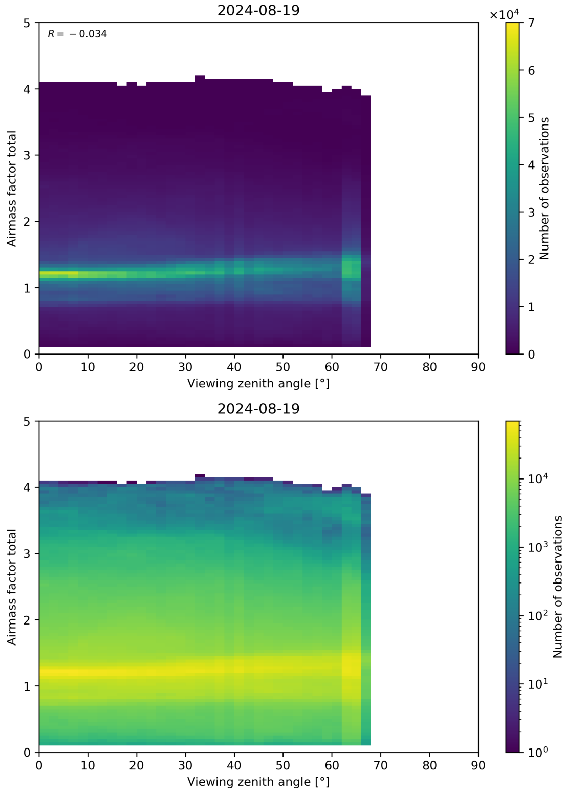
Figure 190: Scatter density plot of “Viewing zenith angle” against “Airmass factor total” for 2024-08-18 to 2024-08-20.
