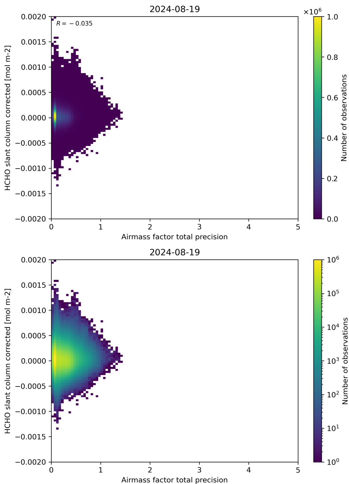
Figure 109: Scatter density plot of “Airmass factor total precision” against “HCHO slant column corrected” for 2024-08-18 to 2024-08-20.
