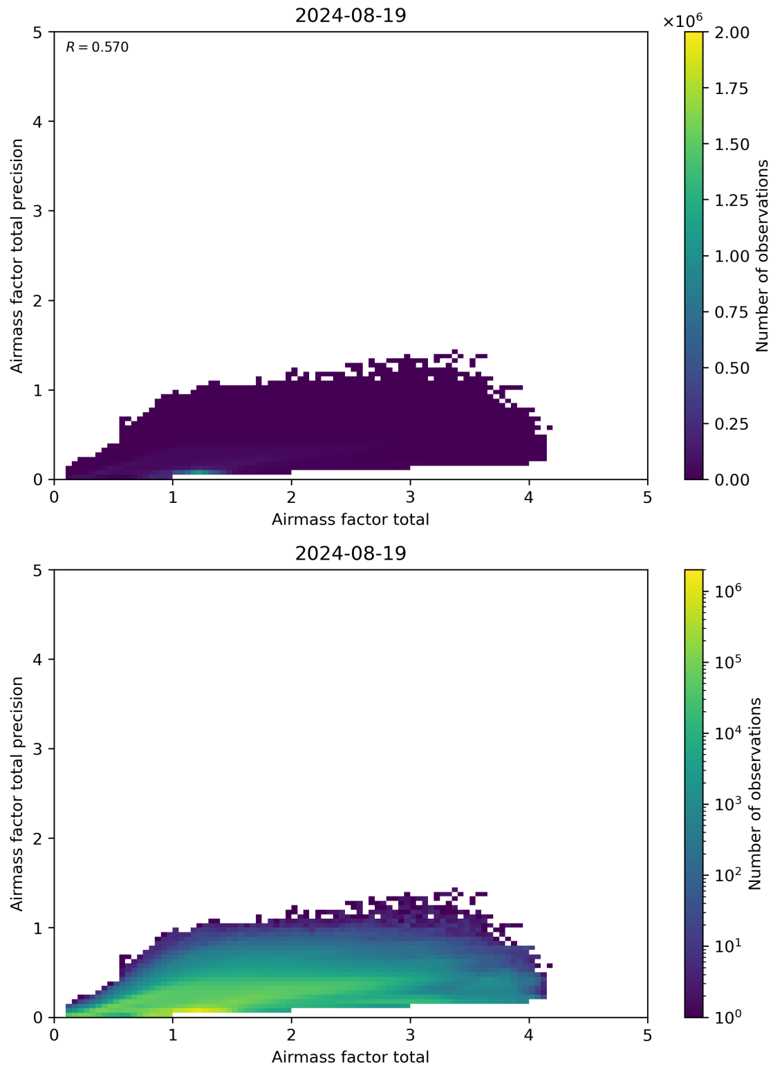
Figure 103: Scatter density plot of “Airmass factor total” against “Airmass factor total precision” for 2024-08-18 to 2024-08-20.
