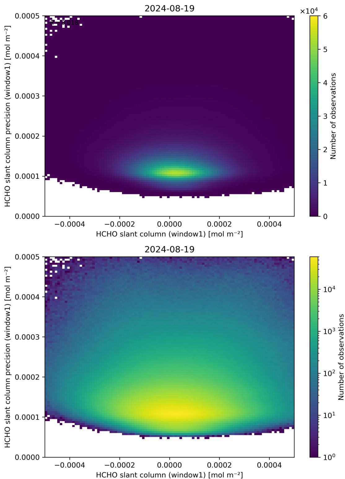
Figure 84: Scatter density plot of “HCHO slant column (window1)” against “HCHO slant column precision (window1)” for 2024-08-18 to 2024-08-20.
