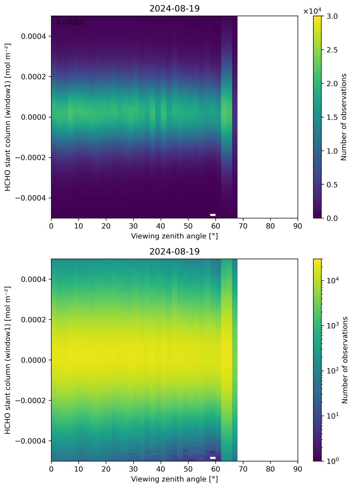
Figure 188: Scatter density plot of “Viewing zenith angle” against “HCHO slant column (window1)” for 2024-08-18 to 2024-08-20.
