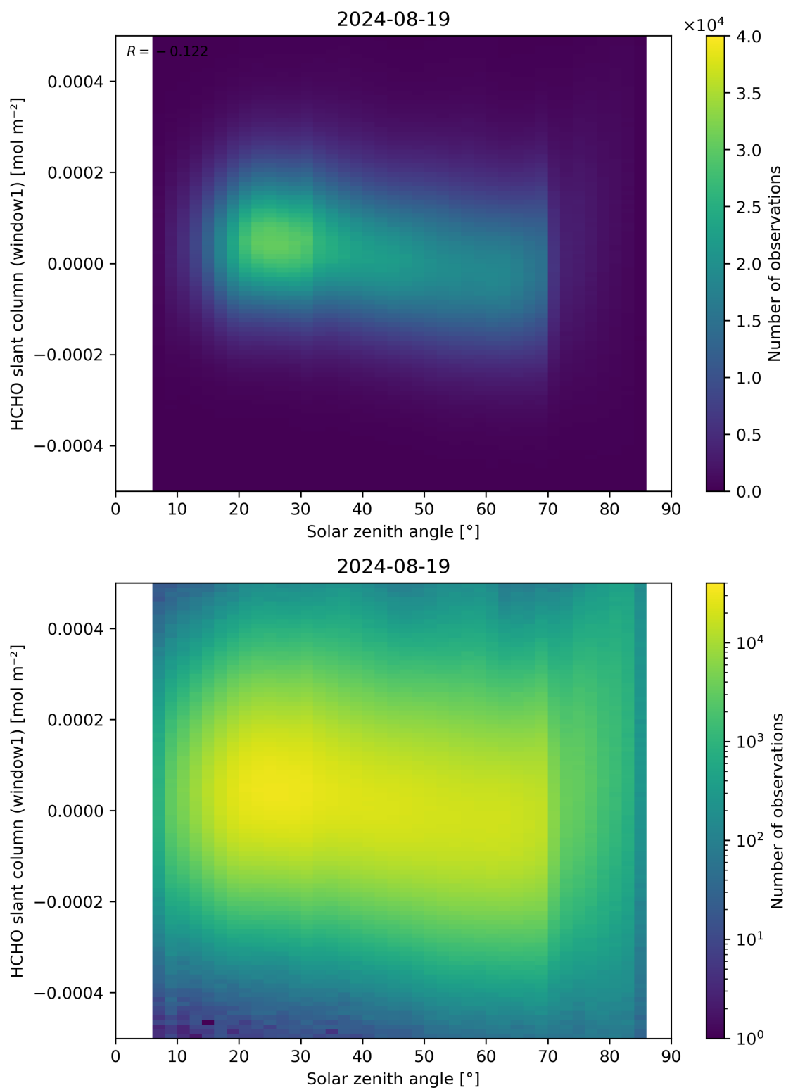
Figure 173: Scatter density plot of “Solar zenith angle” against “HCHO slant column (window1)” for 2024-08-18 to 2024-08-20.
