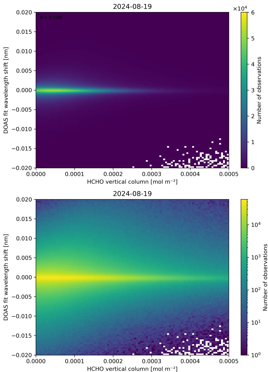
Figure 124: Scatter density plot of “HCHO vertical column” against “DOAS fit wavelength shift” for 2024-08-18 to 2024-08-20.
