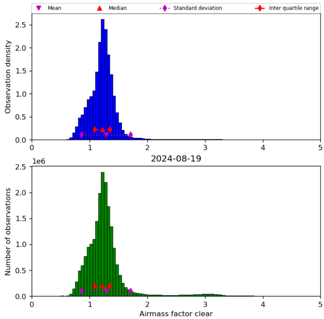
Figure 42: Histogram of “Airmass factor clear” for 2024-08-18 to 2024-08-20
