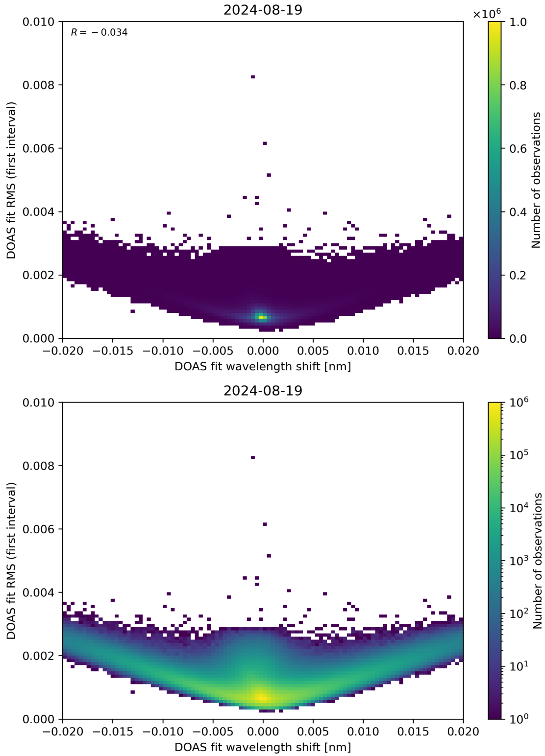
Figure 64: Scatter density plot of “DOAS fit wavelength shift” against “DOAS fit RMS (first interval)” for 2024-08-18 to 2024-08-20.
