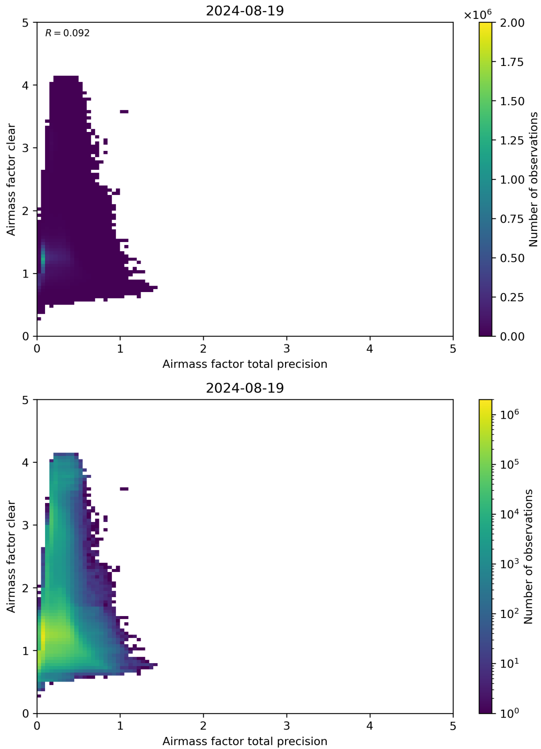
Figure 108: Scatter density plot of “Airmass factor total precision” against “Airmass factor clear” for 2024-08-18 to 2024-08-20.
