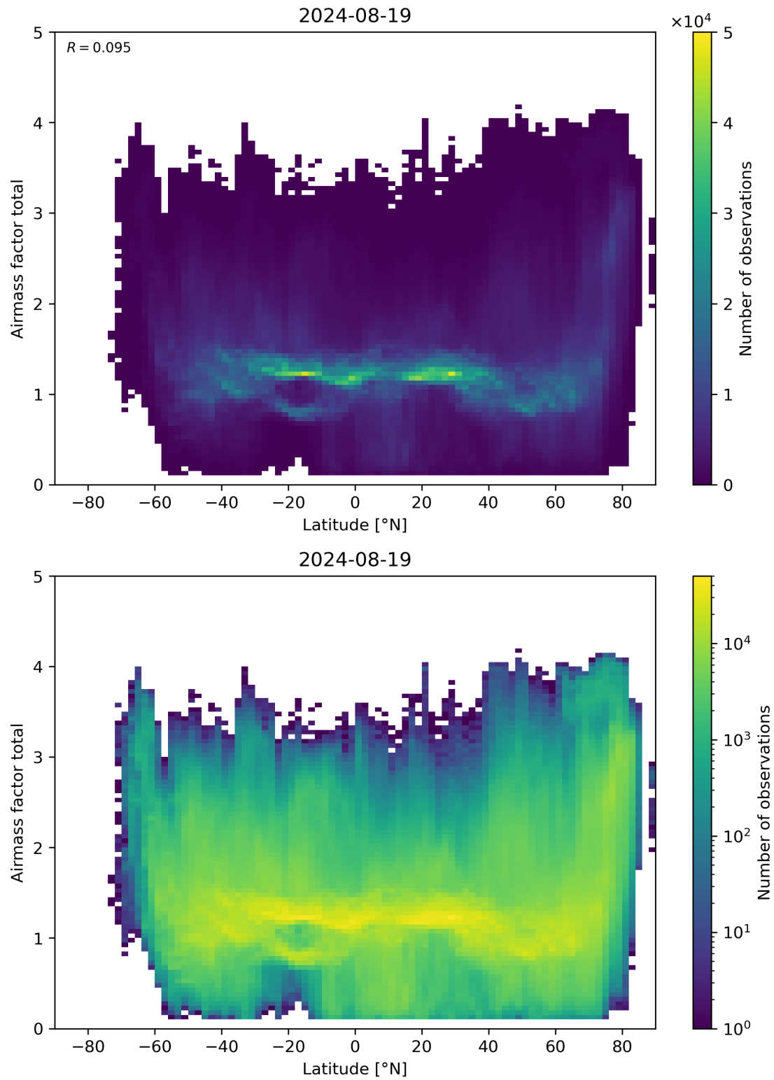
Figure 161: Scatter density plot of “Latitude” against “Airmass factor total” for 2024-08-18 to 2024-08-20.
