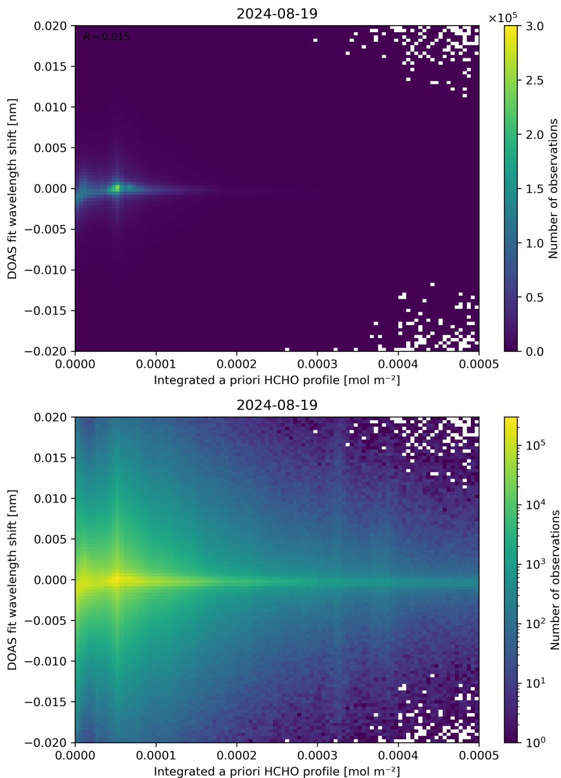
Figure 149: Scatter density plot of “Integrated a priori HCHO profile” against “DOAS fit wavelength shift” for 2024-08-18 to 2024-08-20.
