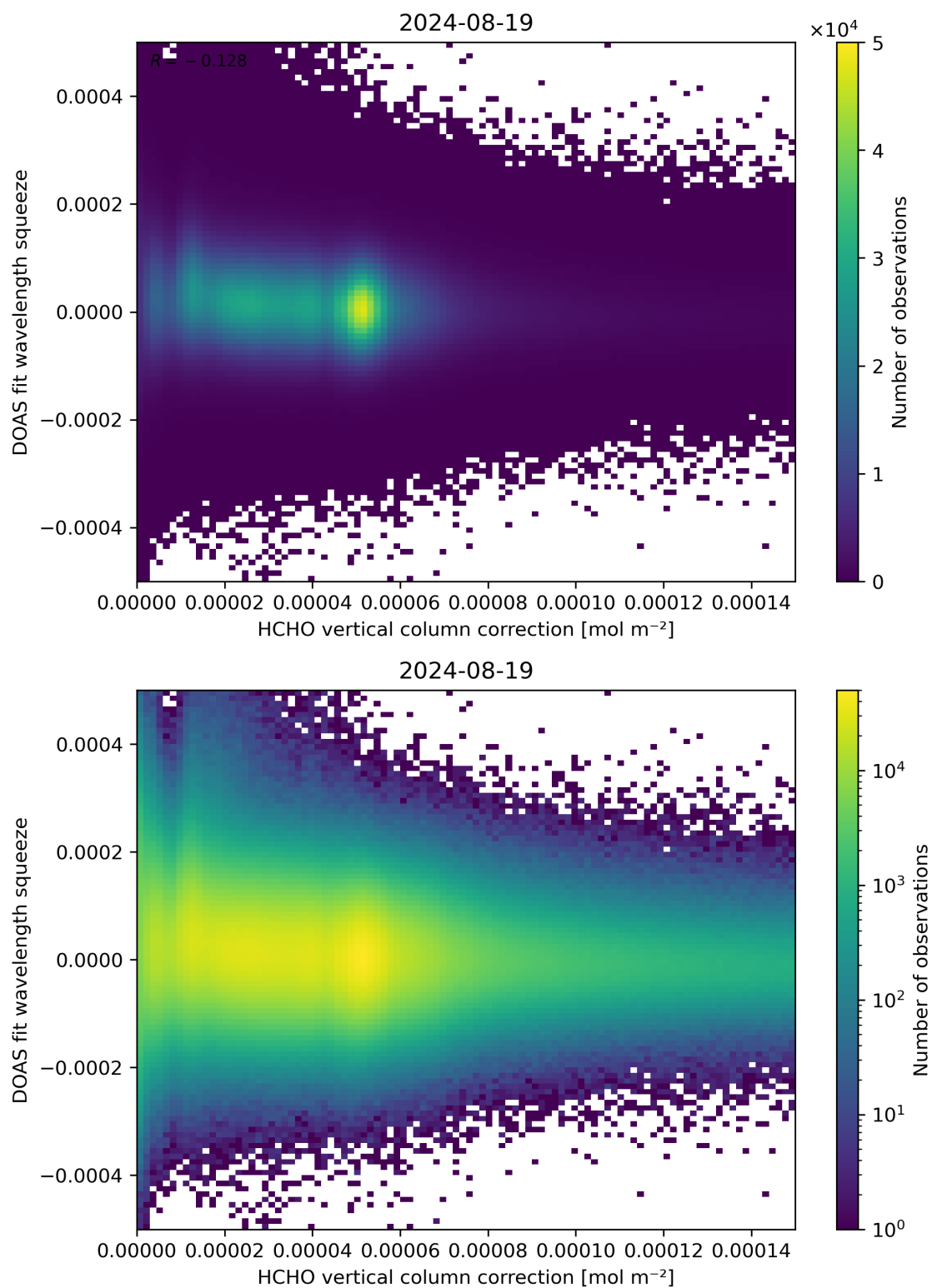
Figure 114: Scatter density plot of “HCHO vertical column correction” against “DOAS fit wavelength squeeze” for 2024-08-18 to 2024-08-20.
