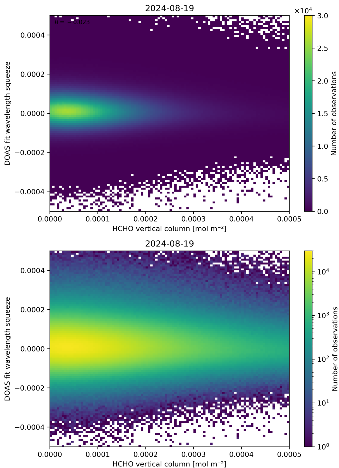
Figure 125: Scatter density plot of “HCHO vertical column” against “DOAS fit wavelength squeeze” for 2024-08-18 to 2024-08-20.
