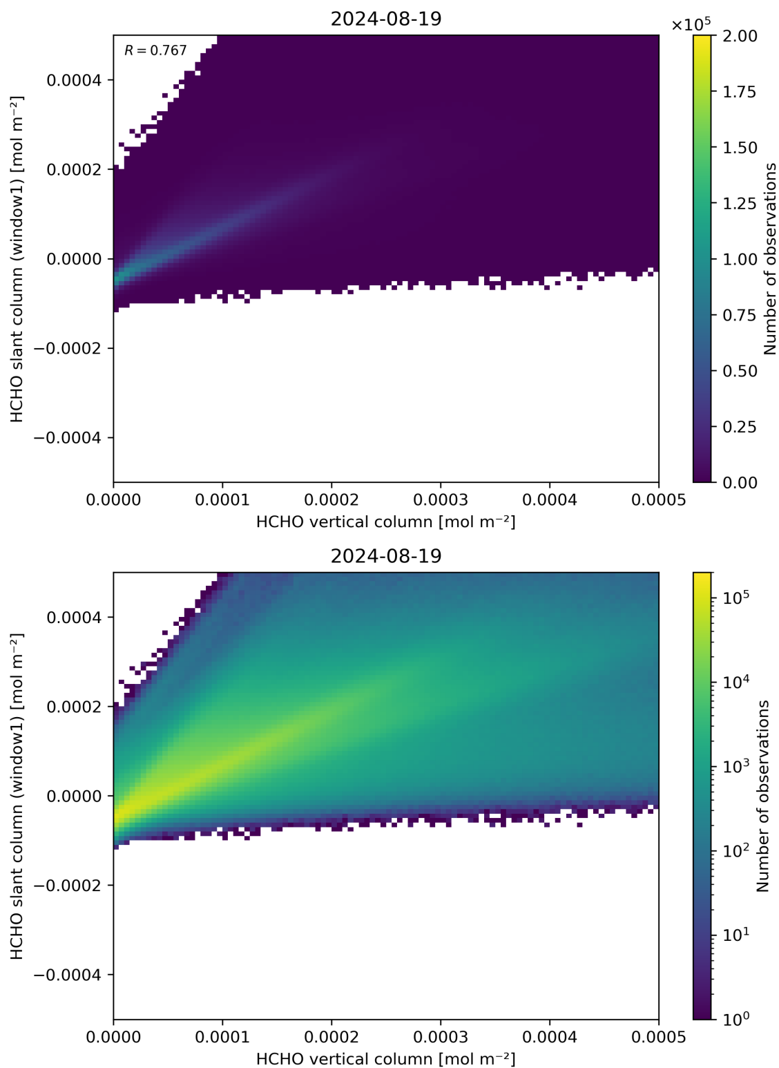
Figure 129: Scatter density plot of “HCHO vertical column” against “HCHO slant column (window1)” for 2024-08-18 to 2024-08-20.
