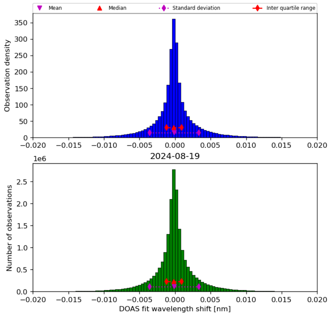
Figure 44: Histogram of “DOAS fit wavelength shift” for 2024-08-18 to 2024-08-20
