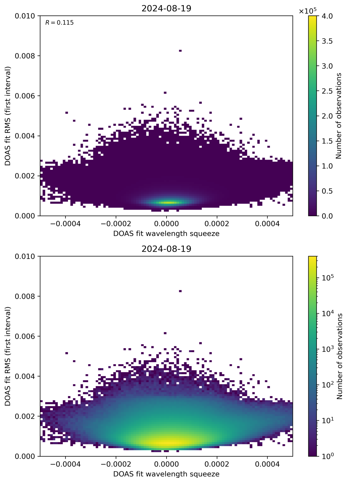
Figure 68: Scatter density plot of “DOAS fit wavelength squeeze” against “DOAS fit RMS (first interval)” for 2024-08-18 to 2024-08-20.
