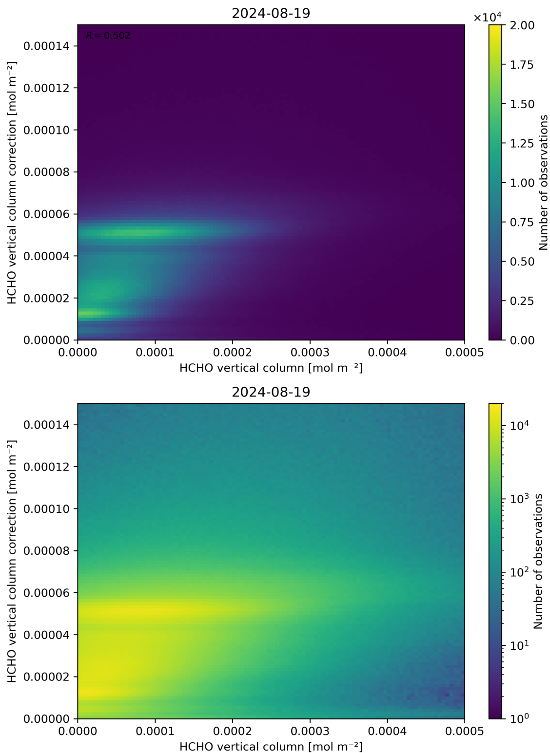
Figure 133: Scatter density plot of “HCHO vertical column” against “HCHO vertical column correction” for 2024-08-18 to 2024-08-20.
