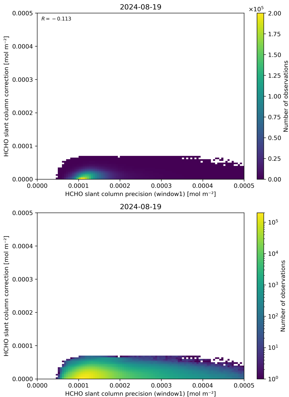
Figure 93: Scatter density plot of “HCHO slant column precision (window1)” against “HCHO slant column correction” for 2024-08-18 to 2024-08-20.
