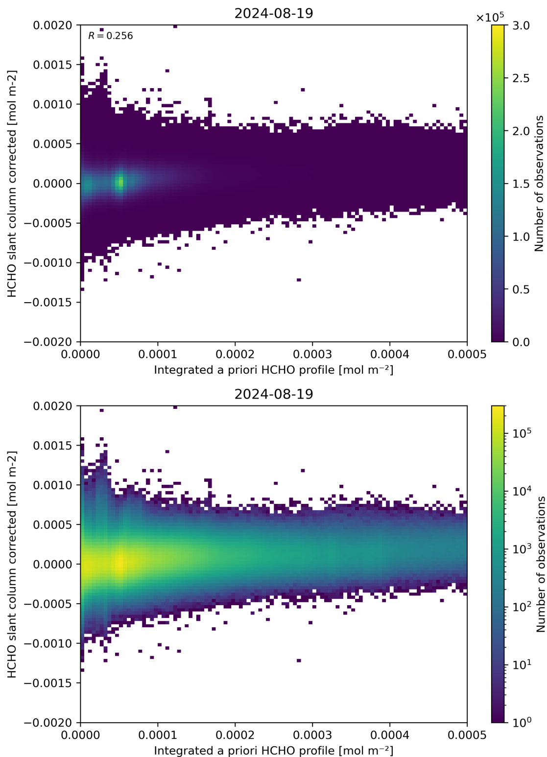
Figure 151: Scatter density plot of “Integrated a priori HCHO profile” against “HCHO slant column corrected” for 2024-08-18 to 2024-08-20.
