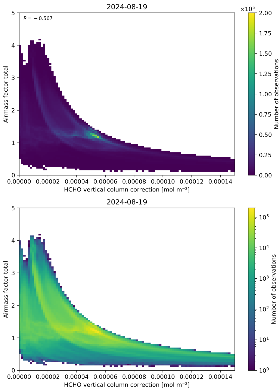
Figure 120: Scatter density plot of “HCHO vertical column correction” against “Airmass factor total” for 2024-08-18 to 2024-08-20.
