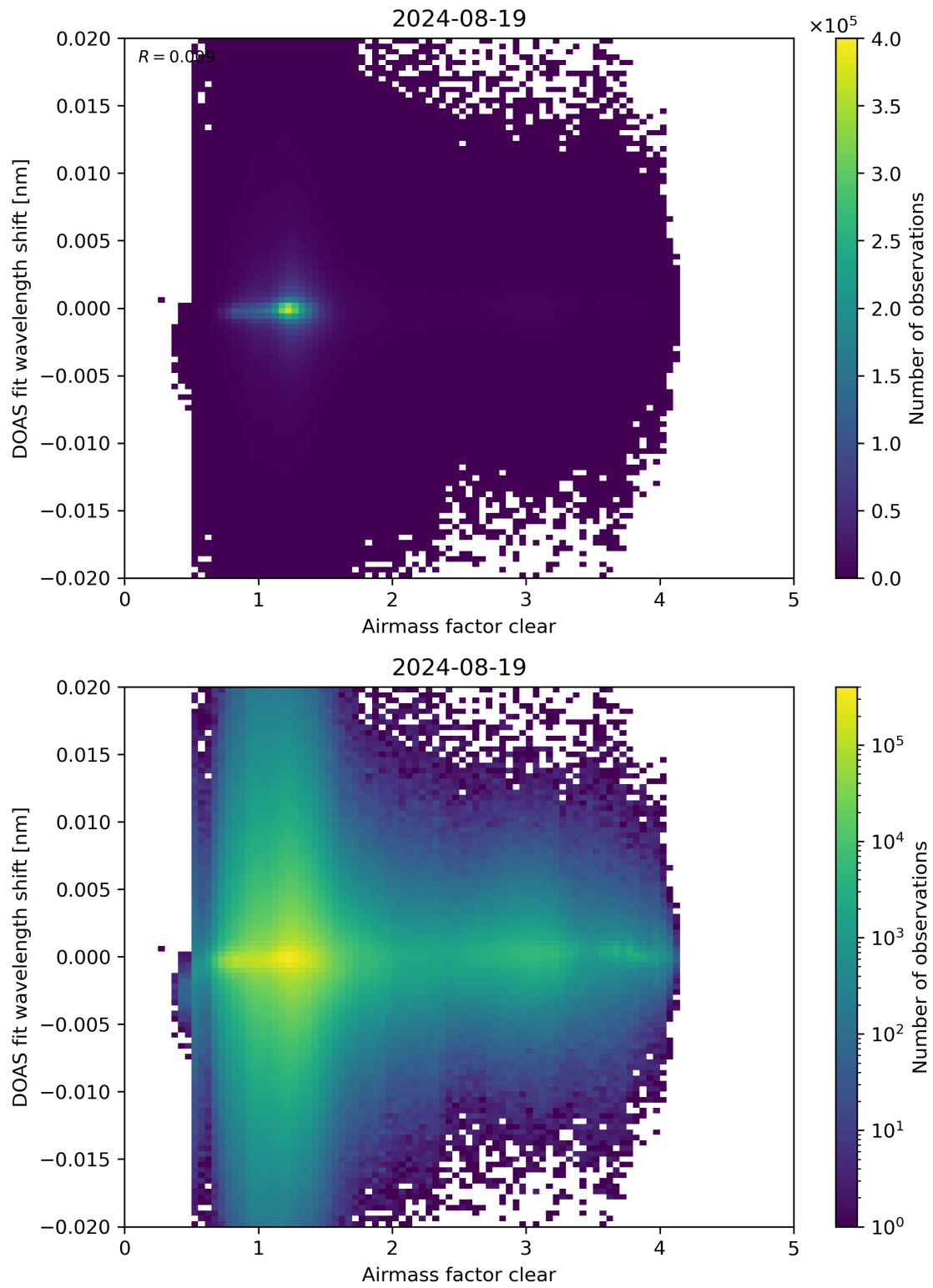
Figure 72: Scatter density plot of “Airmass factor clear” against “DOAS fit wavelength shift” for 2024-08-18 to 2024-08-20.
