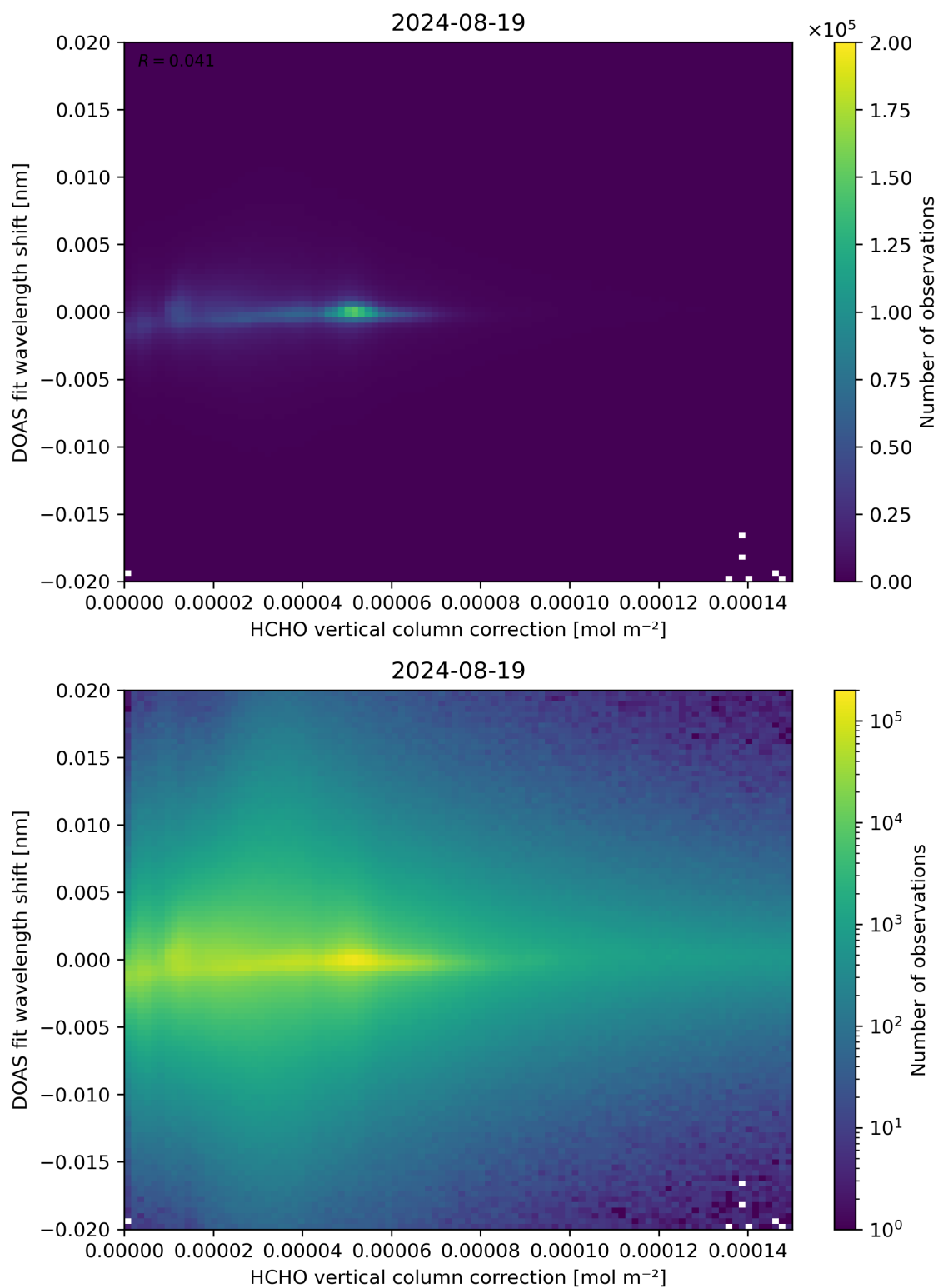
Figure 113: Scatter density plot of “HCHO vertical column correction” against “DOAS fit wavelength shift” for 2024-08-18 to 2024-08-20.
