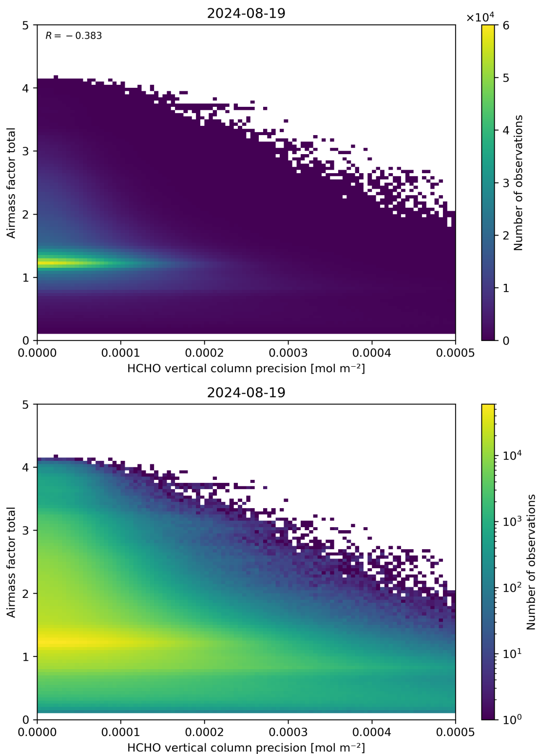
Figure 144: Scatter density plot of “HCHO vertical column precision” against “Airmass factor total” for 2024-08-18 to 2024-08-20.
