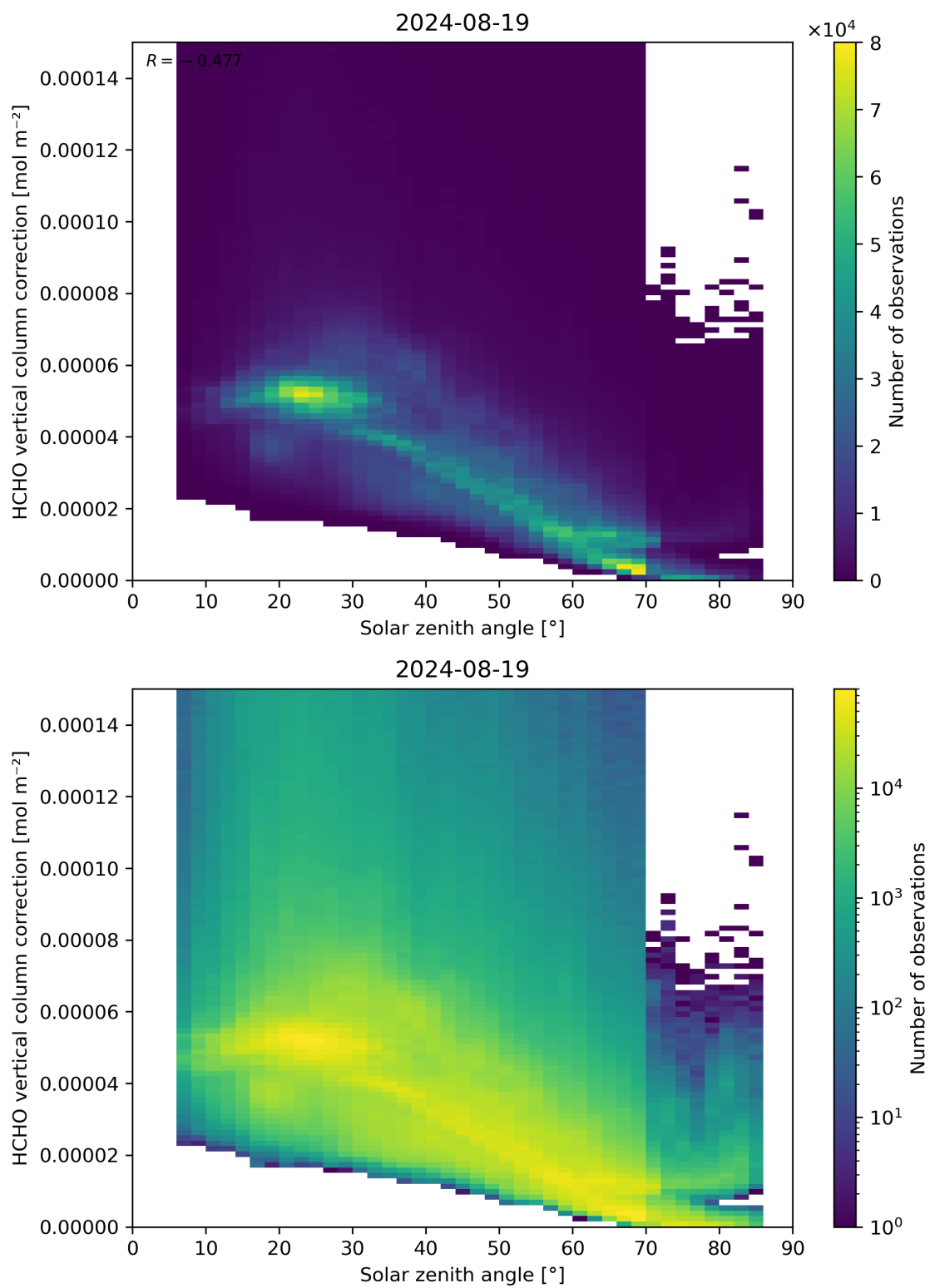
Figure 178: Scatter density plot of “Solar zenith angle” against “HCHO vertical column correction” for 2024-08-18 to 2024-08-20.
