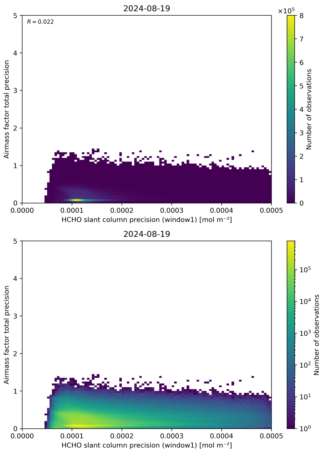
Figure 95: Scatter density plot of “HCHO slant column precision (window1)” against “Airmass factor total precision” for 2024-08-18 to 2024-08-20.
