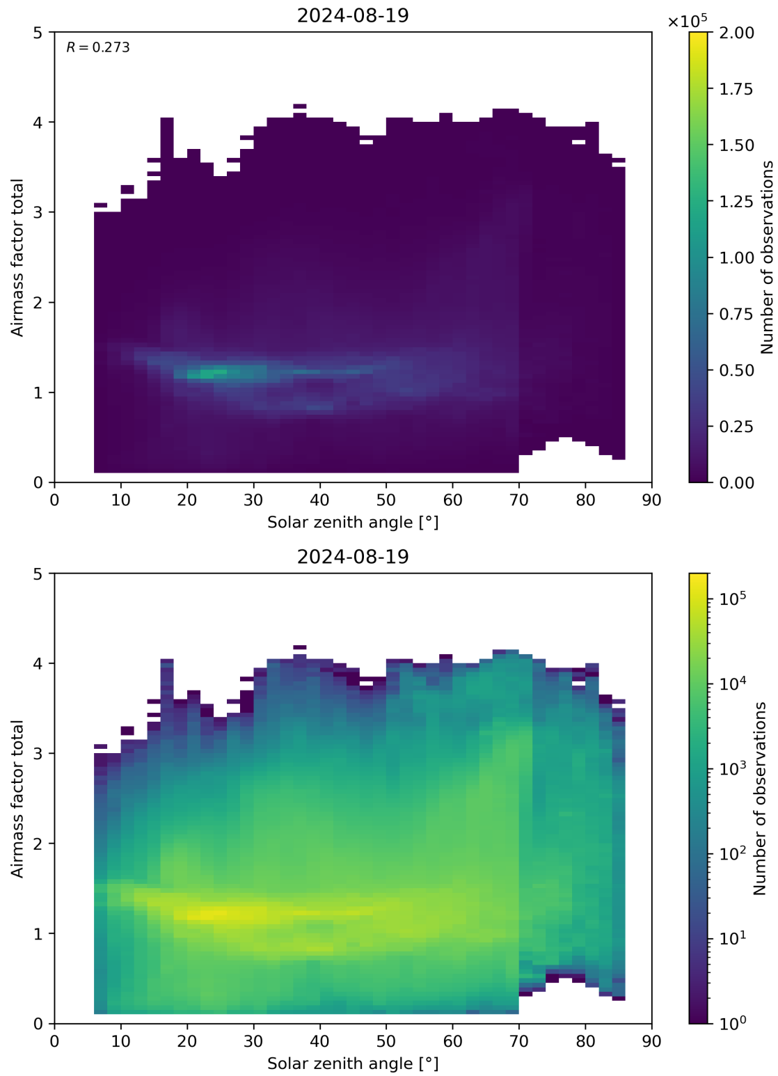
Figure 175: Scatter density plot of “Solar zenith angle” against “Airmass factor total” for 2024-08-18 to 2024-08-20.
