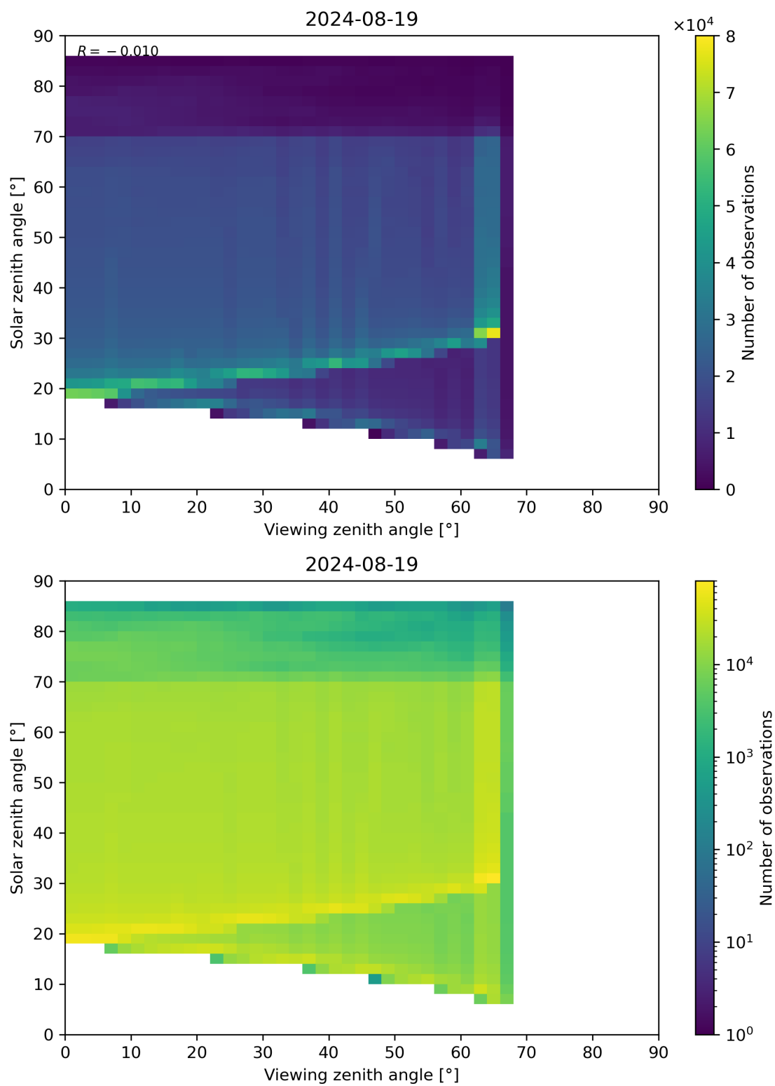
Figure 197: Scatter density plot of “Viewing zenith angle” against “Solar zenith angle” for 2024-08-18 to 2024-08-20.
