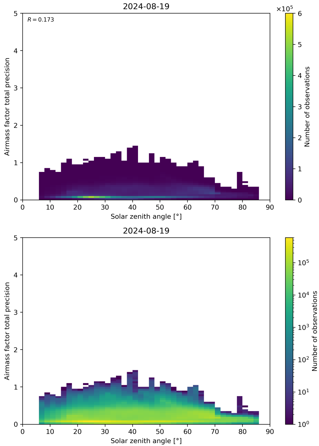
Figure 176: Scatter density plot of “Solar zenith angle” against “Airmass factor total precision” for 2024-08-18 to 2024-08-20.
