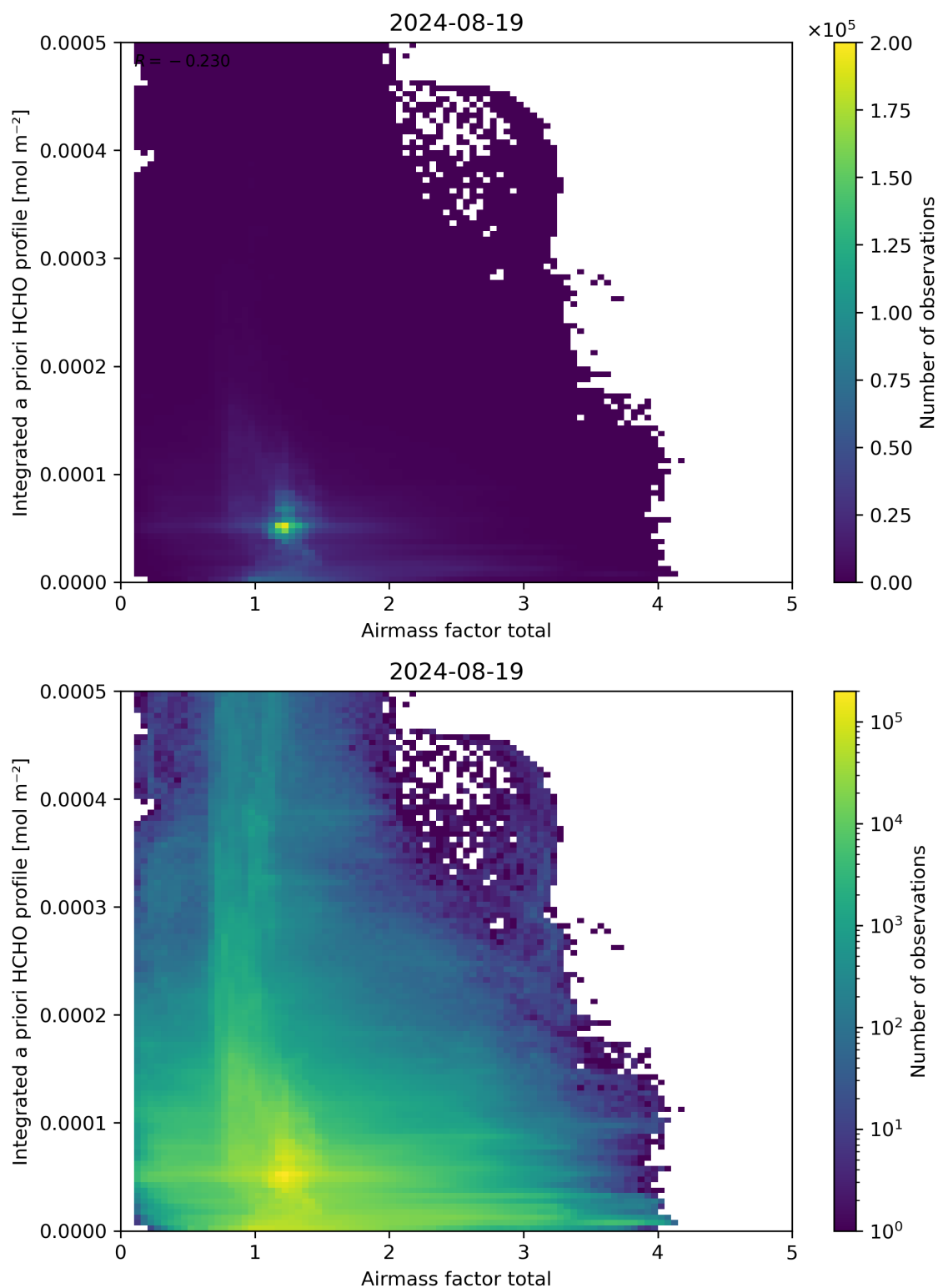
Figure 104: Scatter density plot of “Airmass factor total” against “Integrated a priori HCHO profile” for 2024-08-18 to 2024-08-20.
