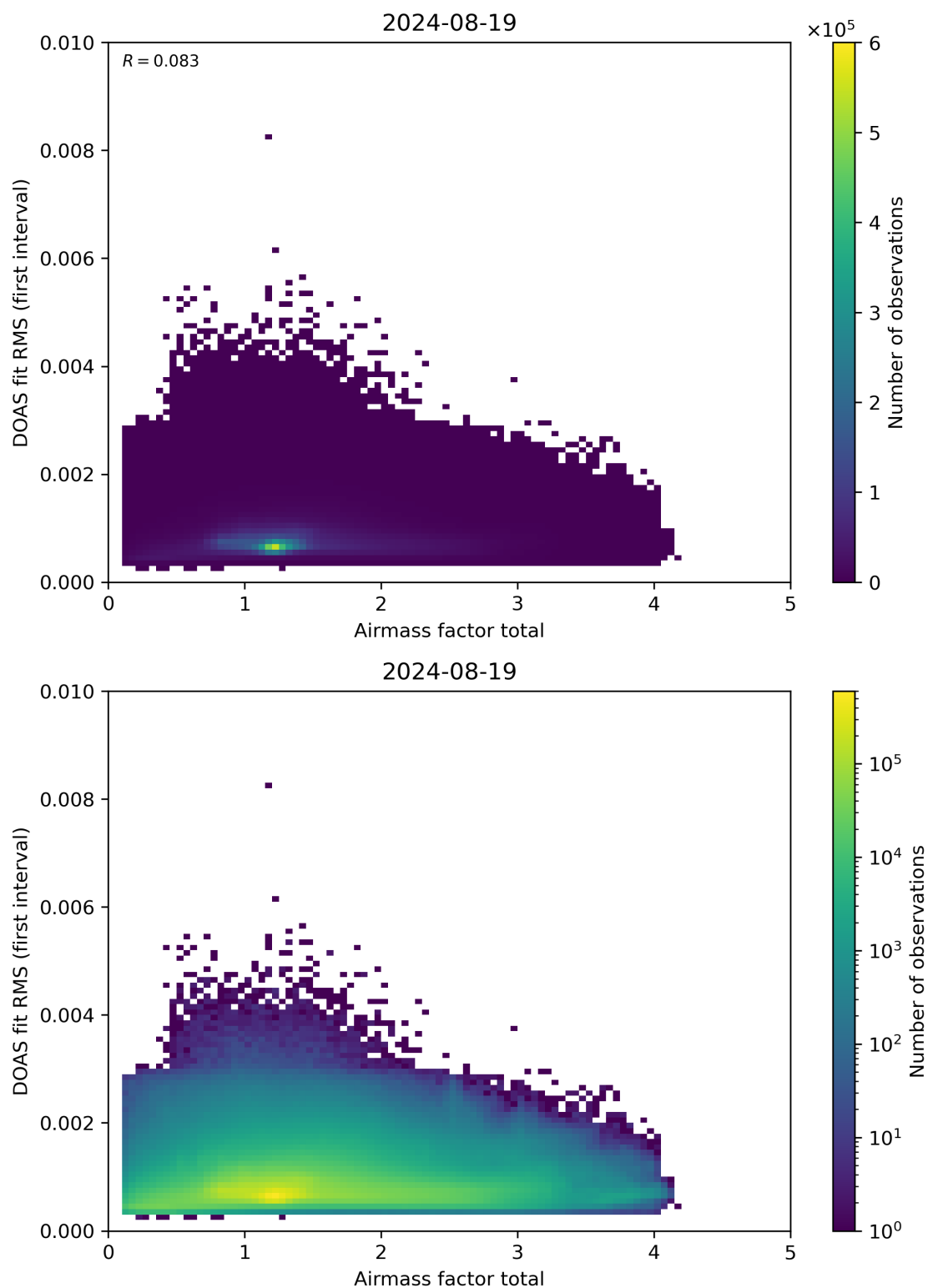
Figure 97: Scatter density plot of “Airmass factor total” against “DOAS fit RMS (first interval)” for 2024-08-18 to 2024-08-20.
