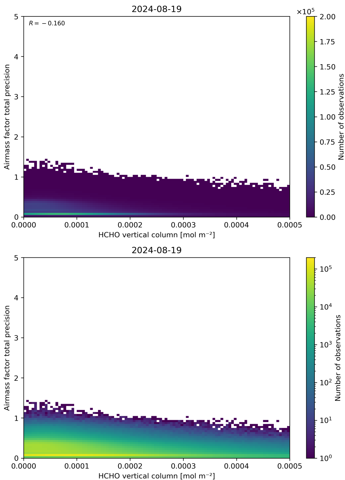
Figure 132: Scatter density plot of “HCHO vertical column” against “Airmass factor total precision” for 2024-08-18 to 2024-08-20.
