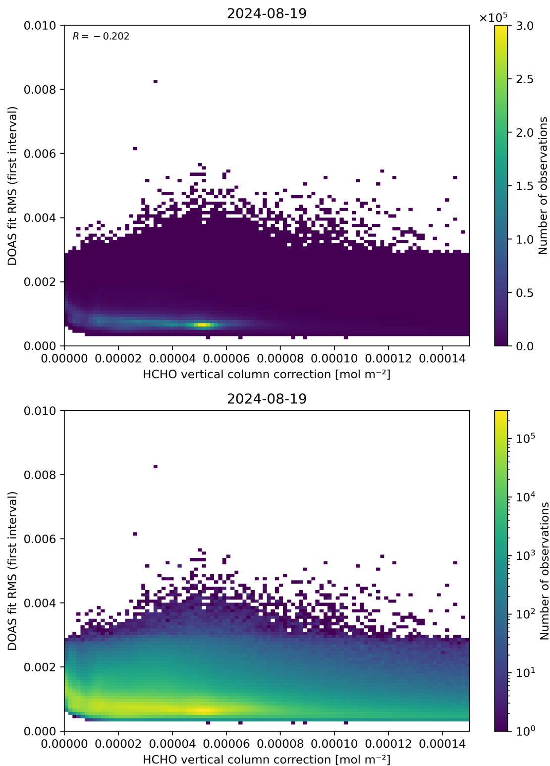
Figure 112: Scatter density plot of “HCHO vertical column correction” against “DOAS fit RMS (first interval)” for 2024-08-18 to 2024-08-20.
