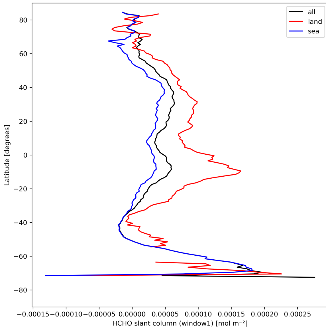
Figure 24: Zonal average of “HCHO slant column (window1)” for 2024-08-18 to 2024-08-20.
