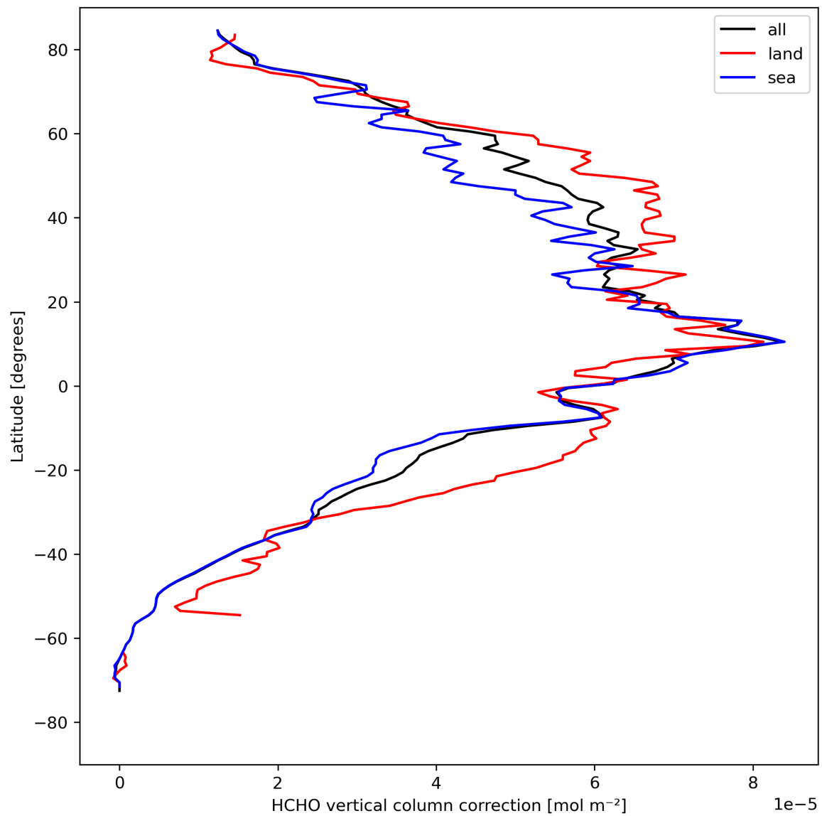
Figure 23: Zonal average of “HCHO vertical column correction” for 2024-08-18 to 2024-08-20.
