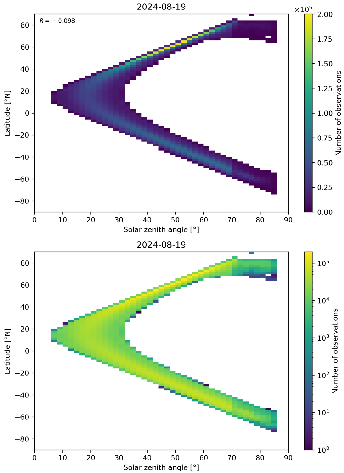
Figure 181: Scatter density plot of “Solar zenith angle” against “Latitude” for 2024-08-18 to 2024-08-20.
