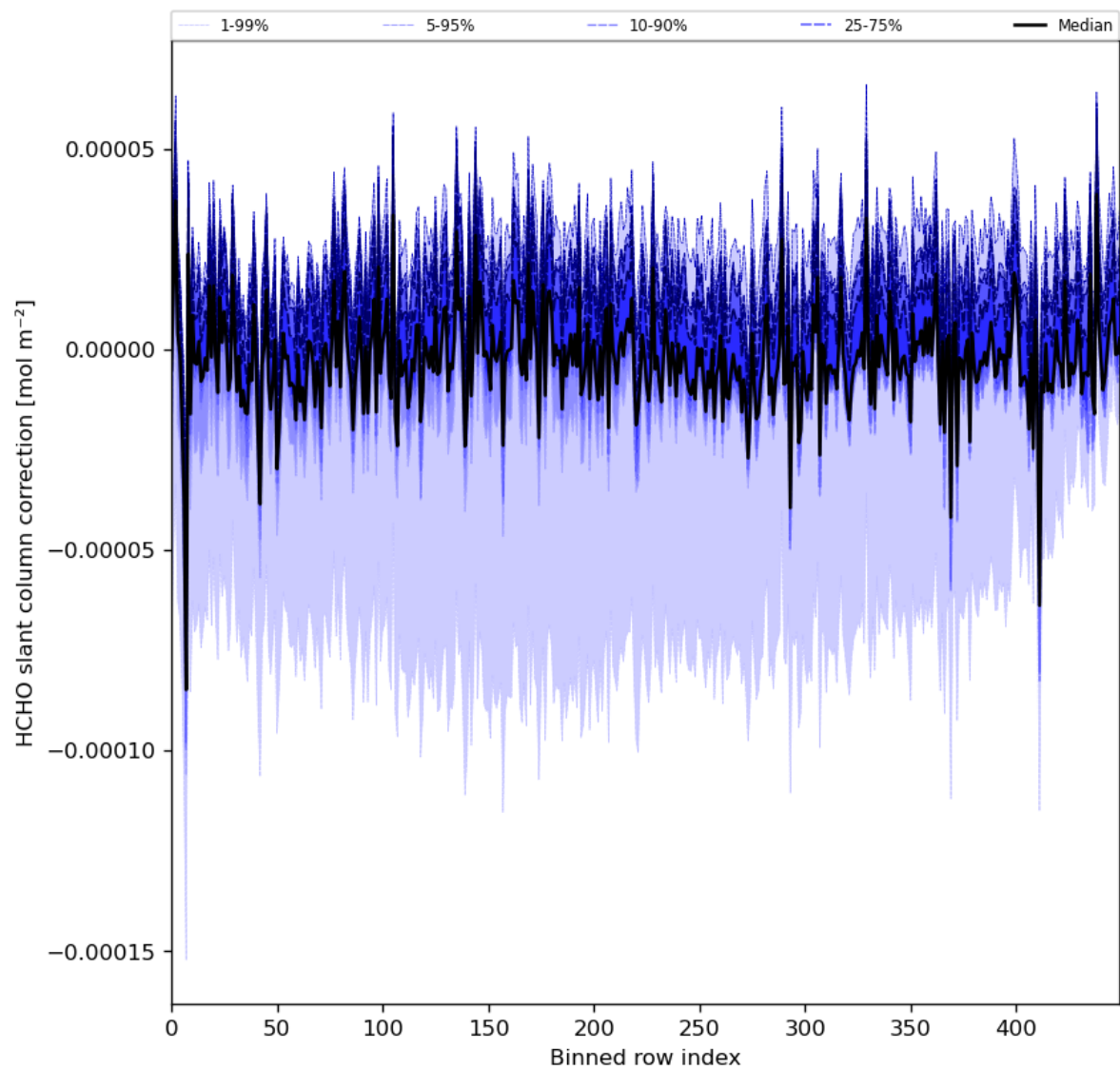
Figure 61: Along track statistics of “HCHO slant column correction” for 2024-08-18 to 2024-08-20
