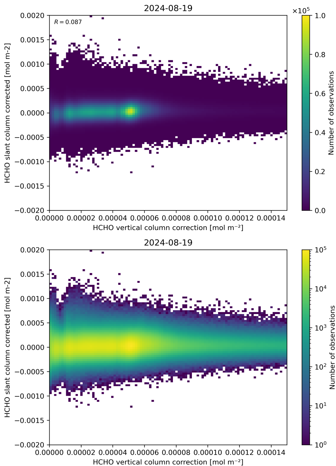
Figure 116: Scatter density plot of “HCHO vertical column correction” against “HCHO slant column corrected” for 2024-08-18 to 2024-08-20.
