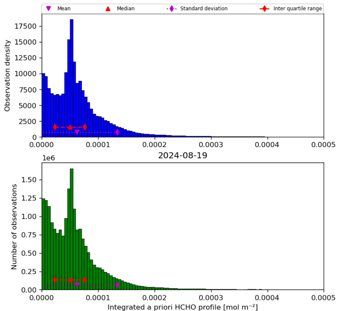
Figure 43: Histogram of “Integrated a priori HCHO profile” for 2024-08-18 to 2024-08-20
