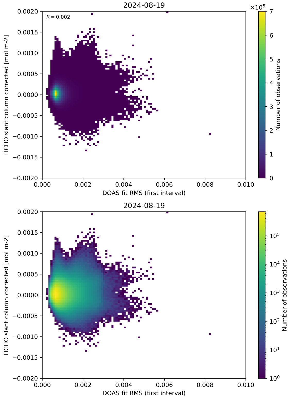
Figure 62: Scatter density plot of “DOAS fit RMS (first interval)” against “HCHO slant column corrected” for 2024-08-18 to 2024-08-20.
