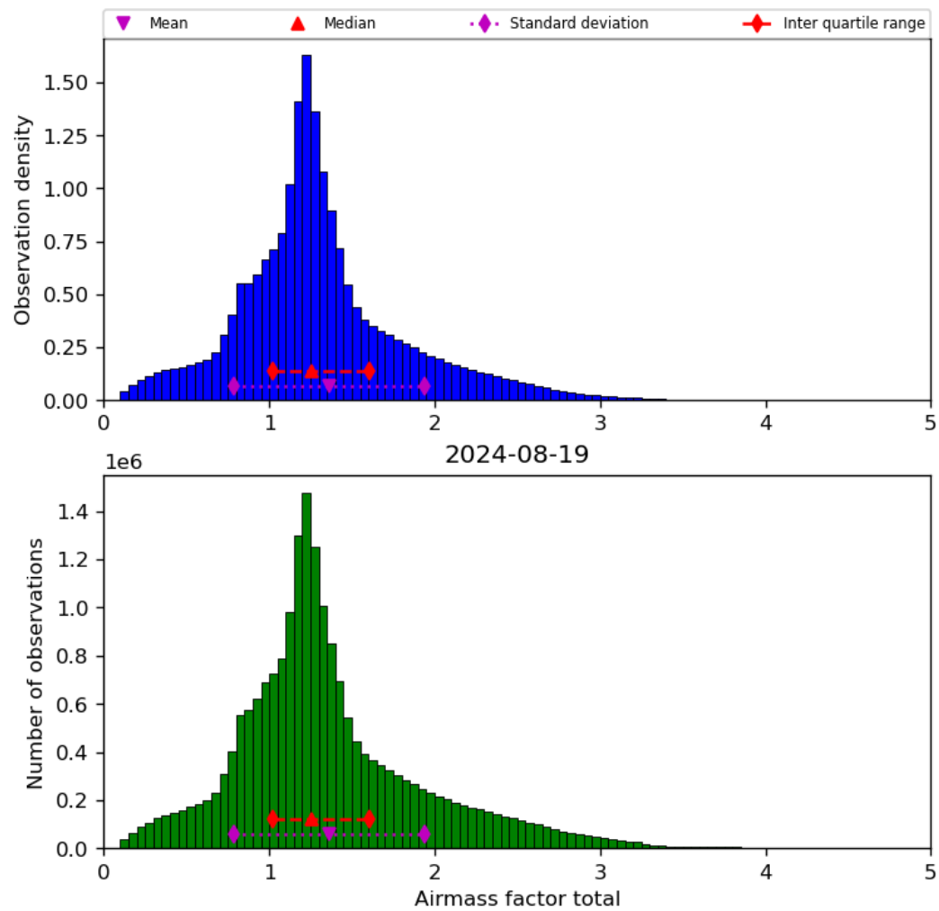
Figure 40: Histogram of “Airmass factor total” for 2024-08-18 to 2024-08-20
