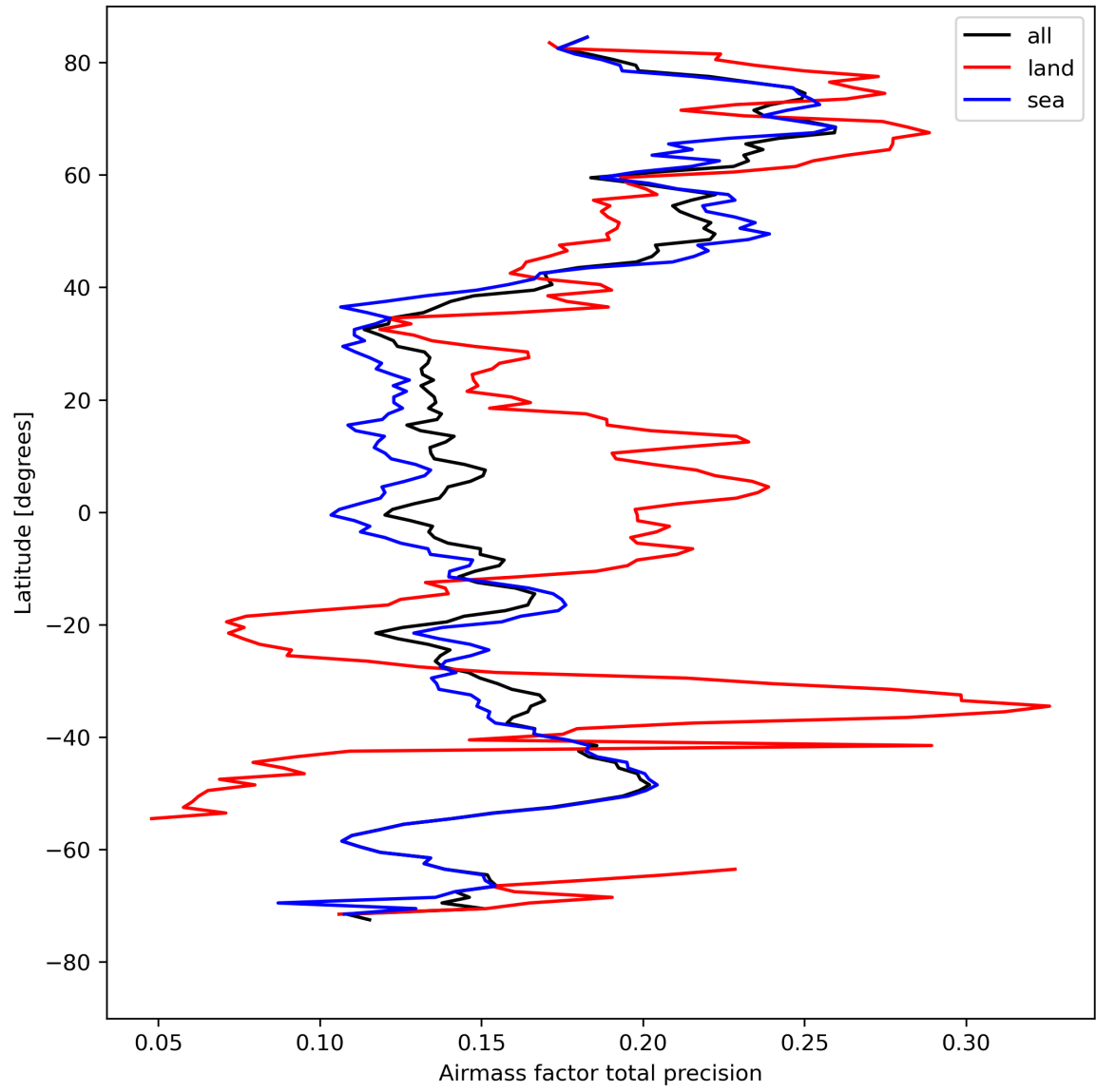
Figure 27: Zonal average of “Airmass factor total precision” for 2024-08-18 to 2024-08-20.
