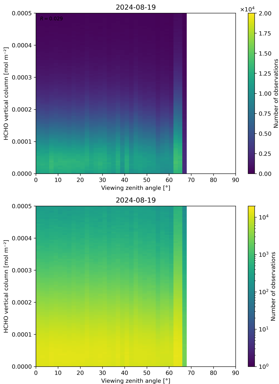
Figure 192: Scatter density plot of “Viewing zenith angle” against “HCHO vertical column” for 2024-08-18 to 2024-08-20.
