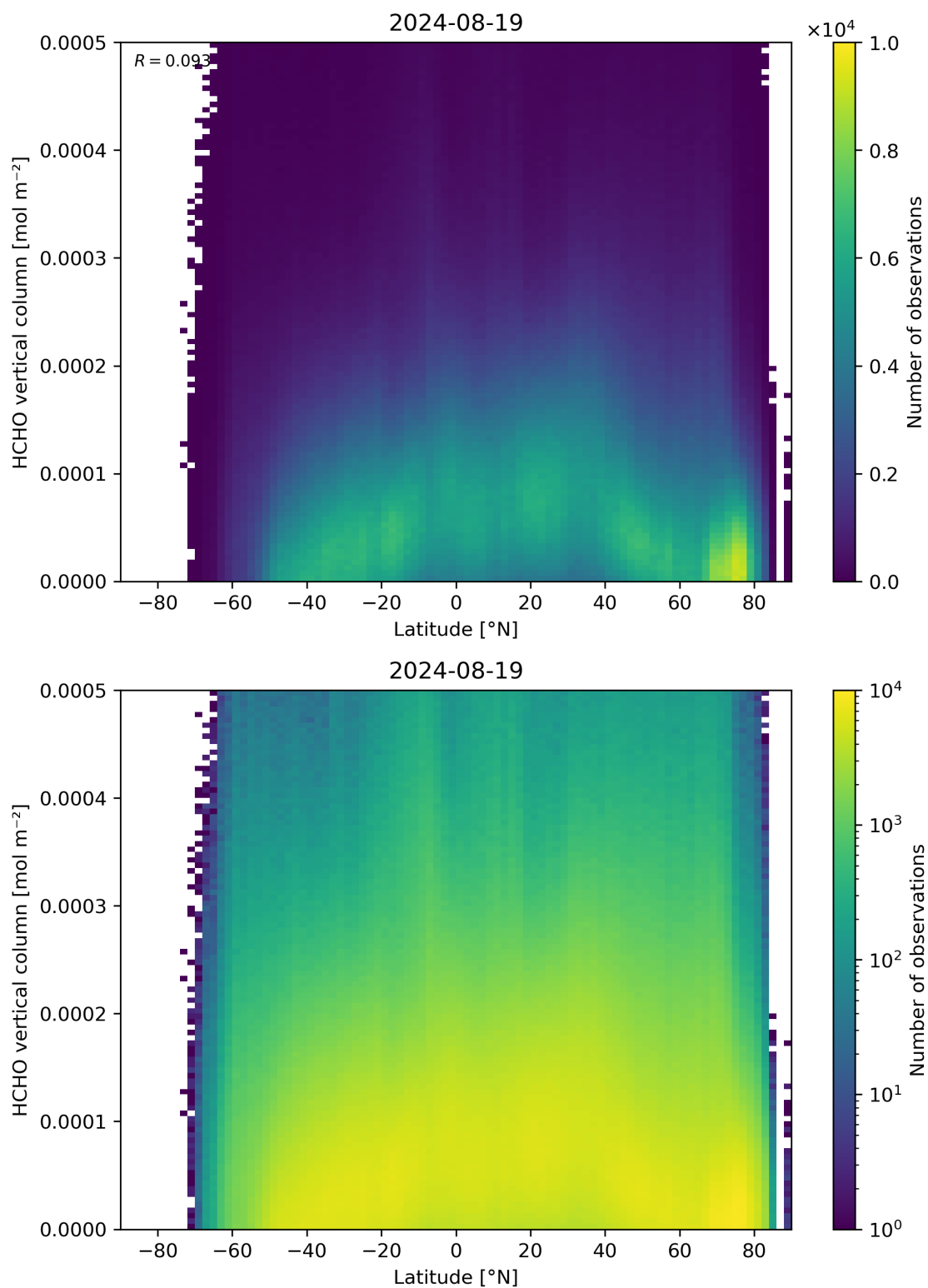
Figure 163: Scatter density plot of “Latitude” against “HCHO vertical column” for 2024-08-18 to 2024-08-20.
