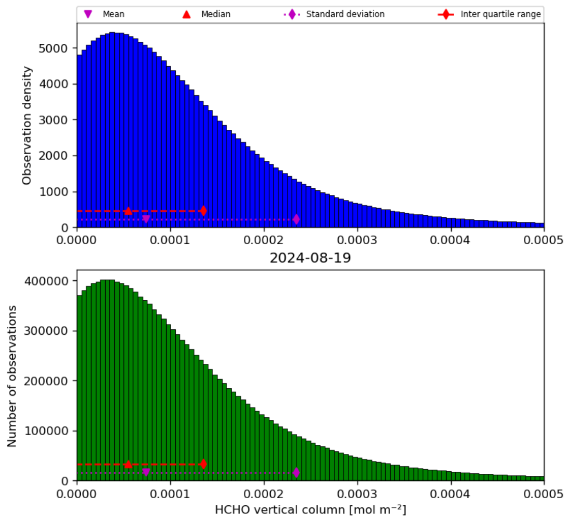
Figure 35: Histogram of “HCHO vertical column” for 2024-08-18 to 2024-08-20
