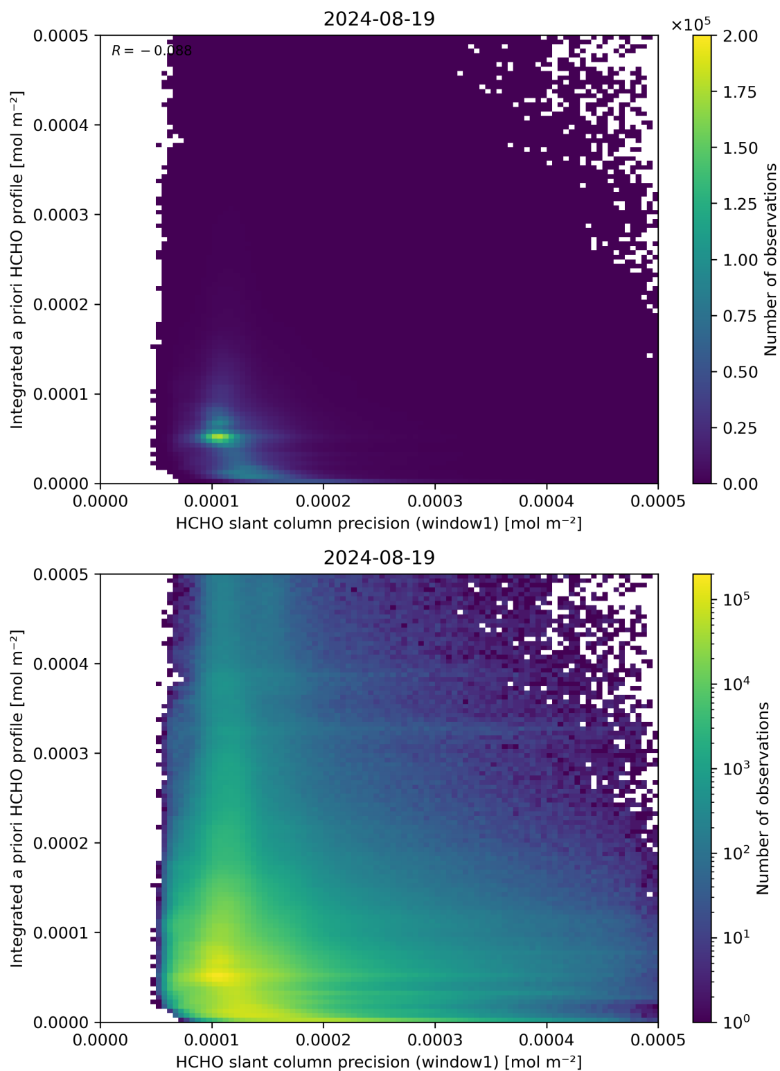
Figure 96: Scatter density plot of “HCHO slant column precision (window1)” against “Integrated a priori HCHO profile” for 2024-08-18 to 2024-08-20.
