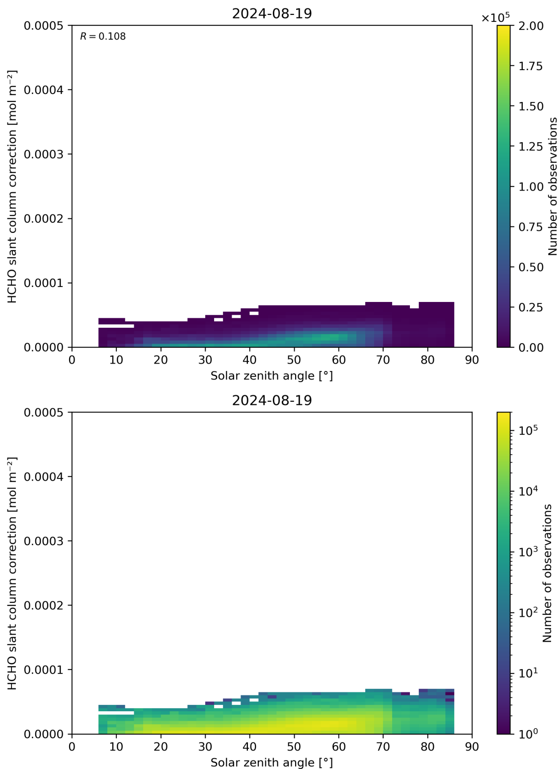
Figure 172: Scatter density plot of “Solar zenith angle” against “HCHO slant column correction” for 2024-08-18 to 2024-08-20.
