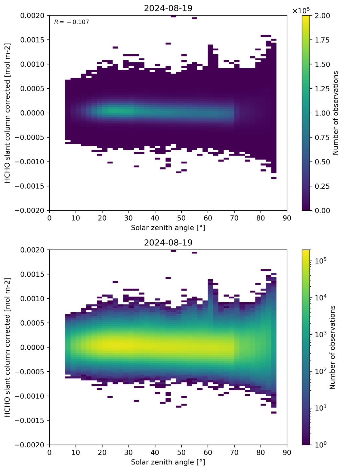
Figure 171: Scatter density plot of “Solar zenith angle” against “HCHO slant column corrected” for 2024-08-18 to 2024-08-20.
