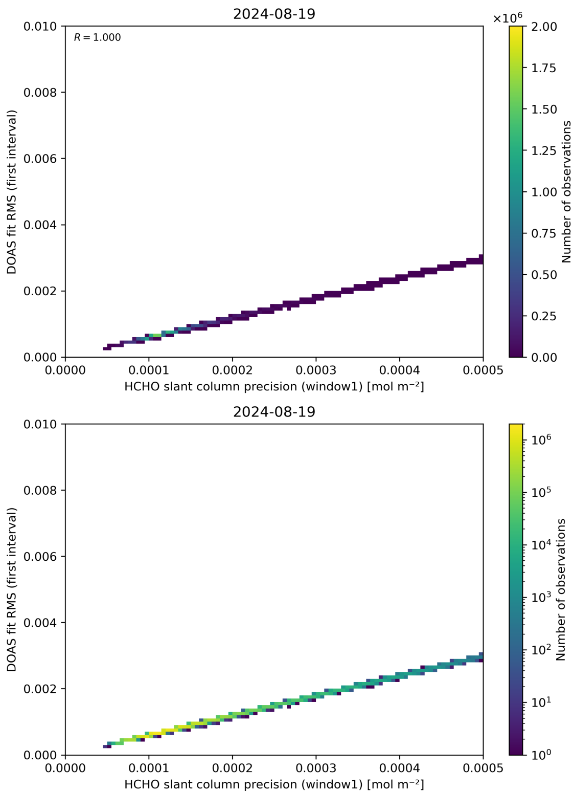
Figure 88: Scatter density plot of “HCHO slant column precision (window1)” against “DOAS fit RMS (first interval)” for 2024-08-18 to 2024-08-20.
