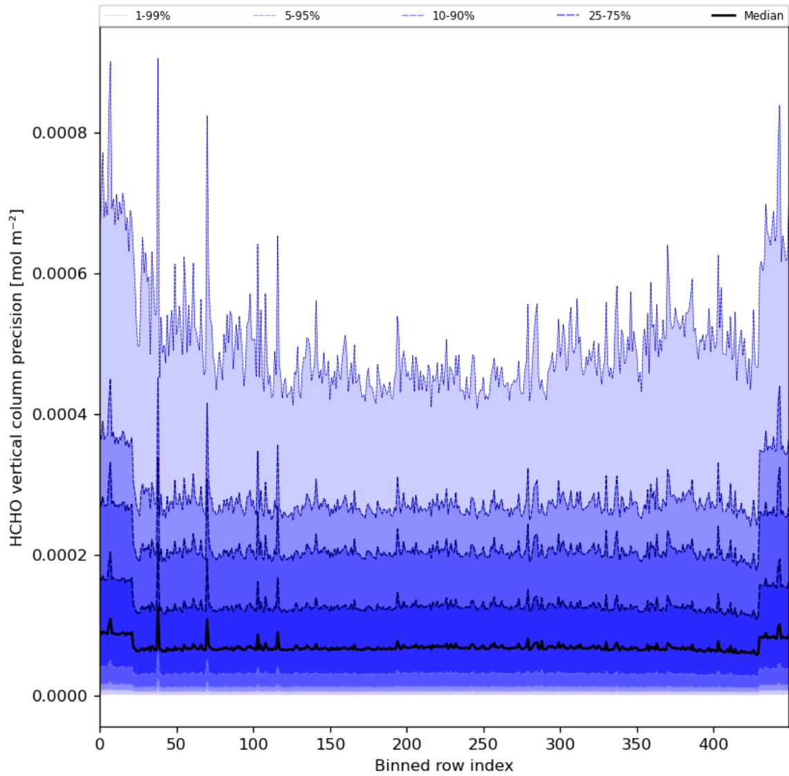
Figure 50: Along track statistics of “HCHO vertical column precision” for 2024-08-18 to 2024-08-20
