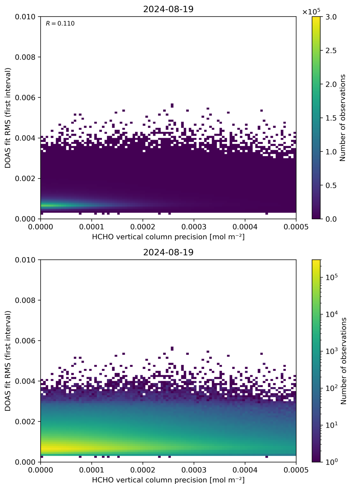
Figure 136: Scatter density plot of “HCHO vertical column precision” against “DOAS fit RMS (first interval)” for 2024-08-18 to 2024-08-20.
