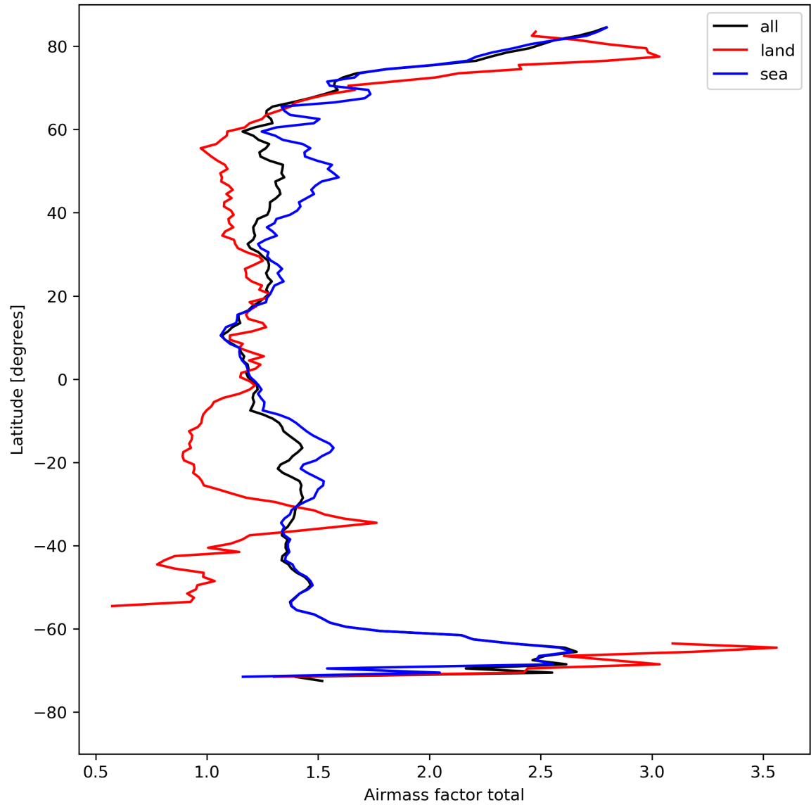
Figure 26: Zonal average of “Airmass factor total” for 2024-08-18 to 2024-08-20.
