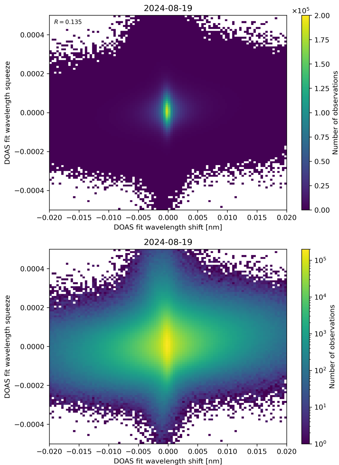
Figure 65: Scatter density plot of “DOAS fit wavelength shift” against “DOAS fit wavelength squeeze” for 2024-08-18 to 2024-08-20.
