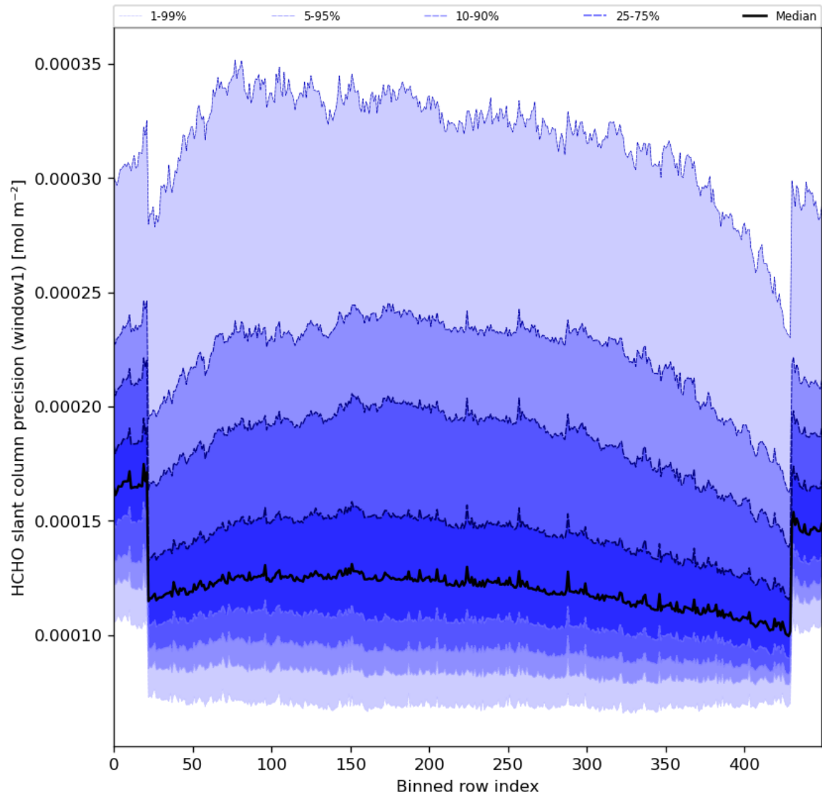
Figure 53: Along track statistics of “HCHO slant column precision (window1)” for 2024-08-18 to 2024-08-20
