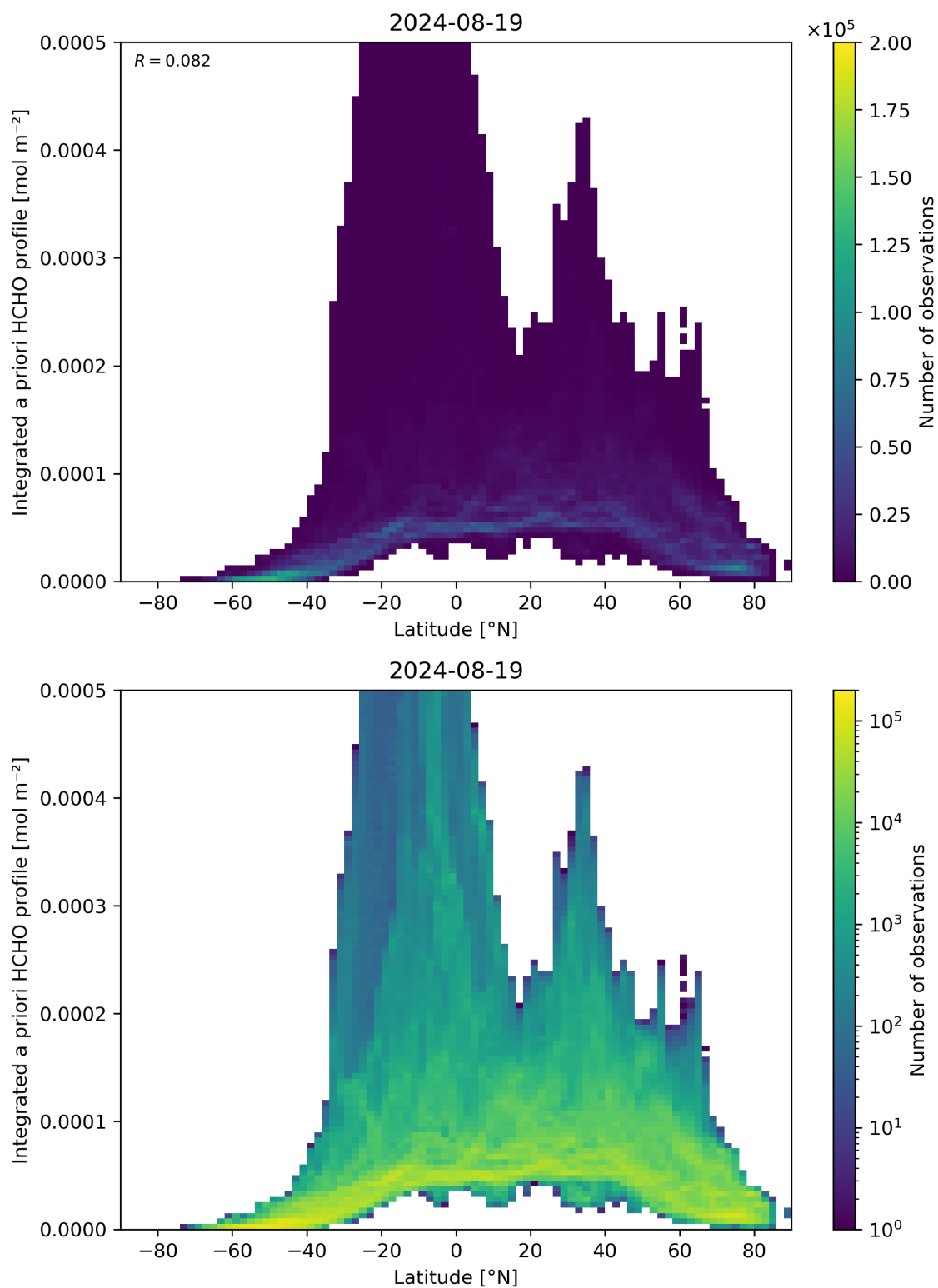
Figure 166: Scatter density plot of “Latitude” against “Integrated a priori HCHO profile” for 2024-08-18 to 2024-08-20.
