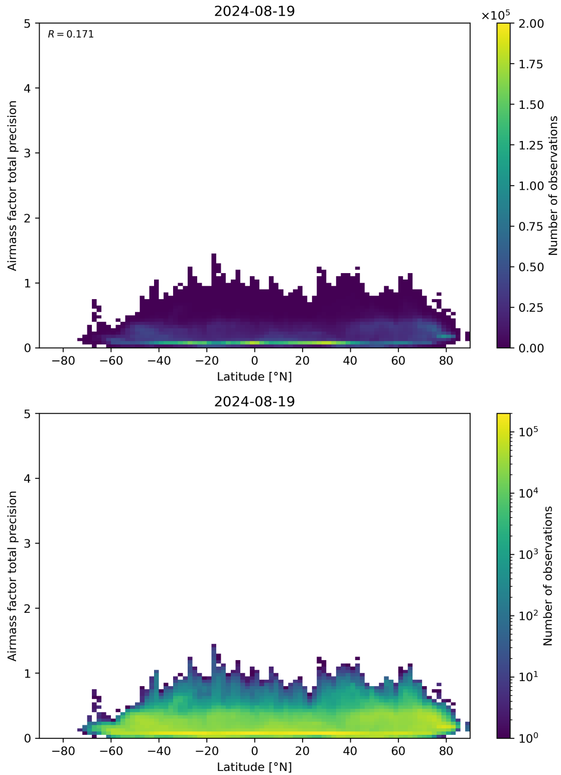
Figure 162: Scatter density plot of “Latitude” against “Airmass factor total precision” for 2024-08-18 to 2024-08-20.
