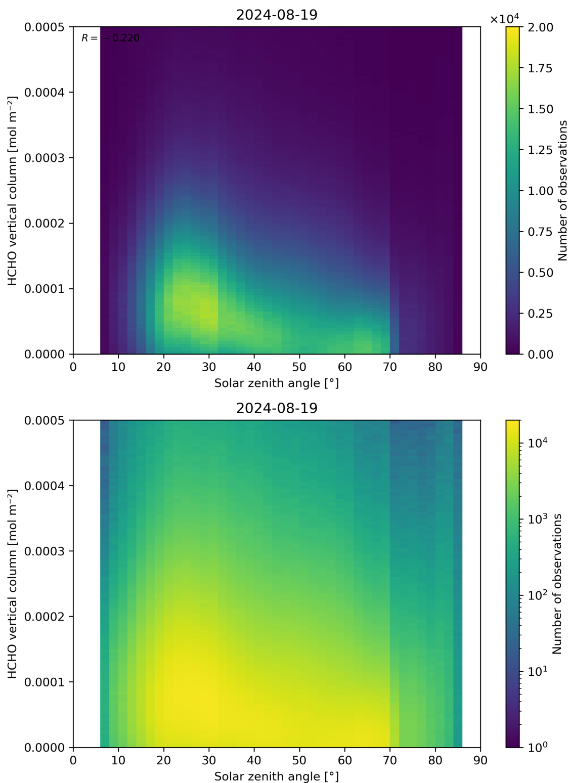
Figure 177: Scatter density plot of “Solar zenith angle” against “HCHO vertical column” for 2024-08-18 to 2024-08-20.
