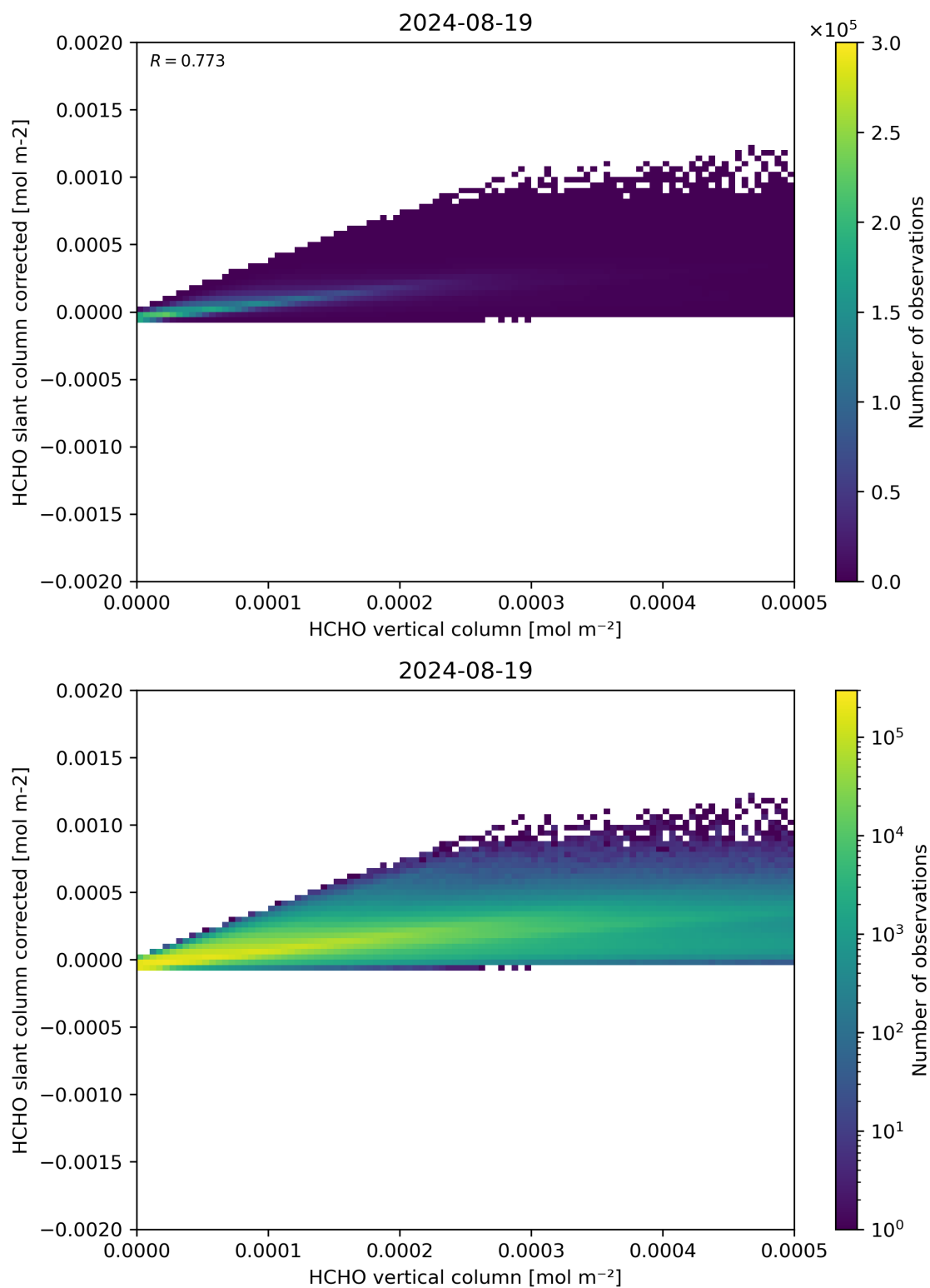
Figure 127: Scatter density plot of “HCHO vertical column” against “HCHO slant column corrected” for 2024-08-18 to 2024-08-20.
