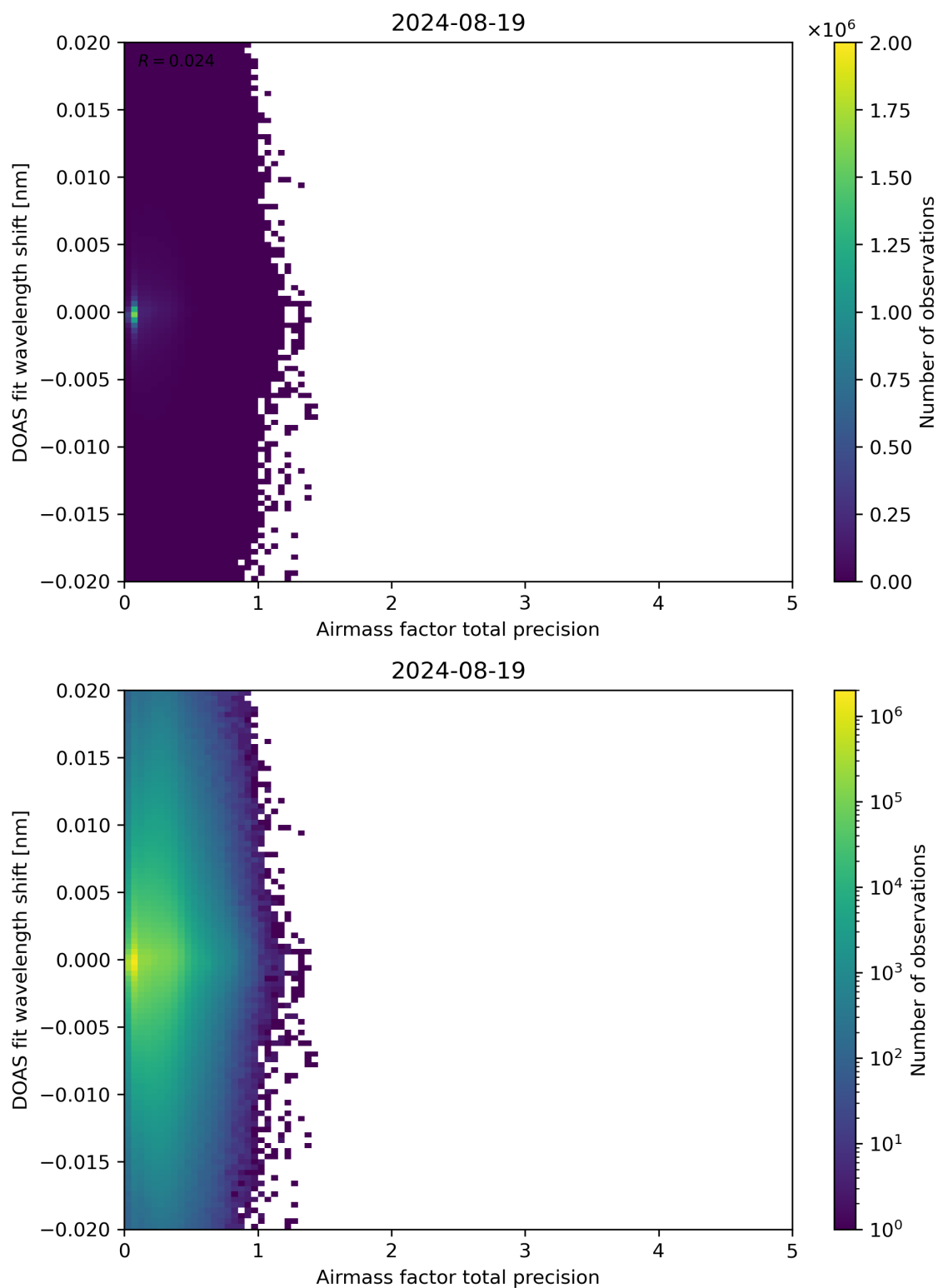
Figure 106: Scatter density plot of “Airmass factor total precision” against “DOAS fit wavelength shift” for 2024-08-18 to 2024-08-20.
