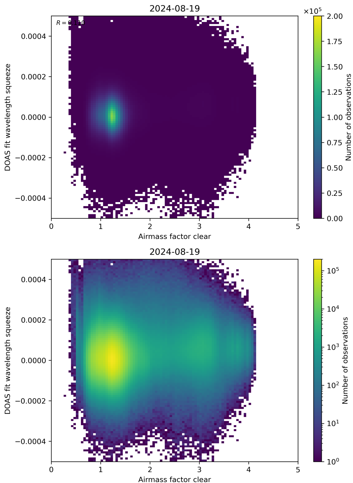
Figure 73: Scatter density plot of “Airmass factor clear” against “DOAS fit wavelength squeeze” for 2024-08-18 to 2024-08-20.
