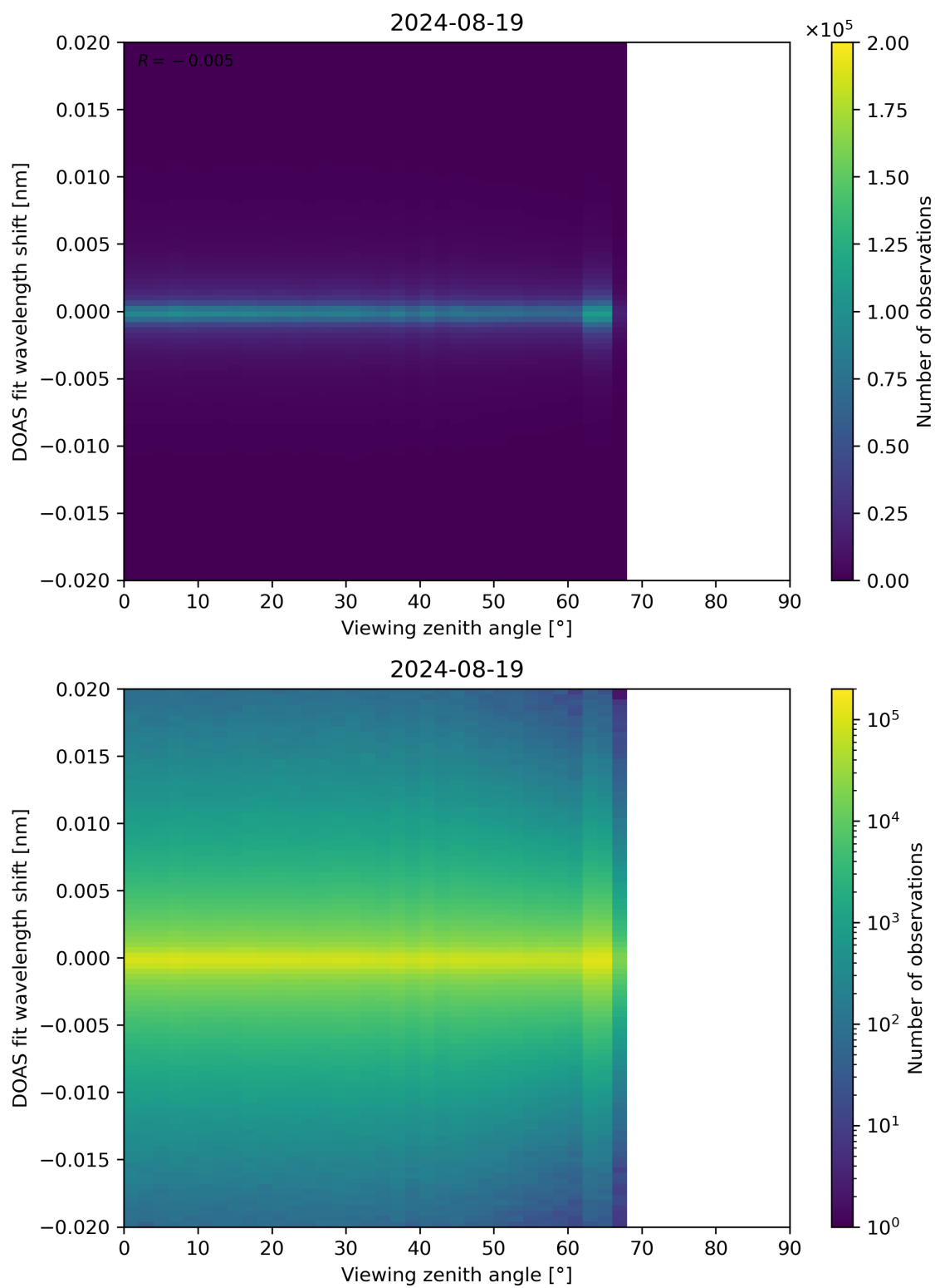
Figure 183: Scatter density plot of “Viewing zenith angle” against “DOAS fit wavelength shift” for 2024-08-18 to 2024-08-20.
