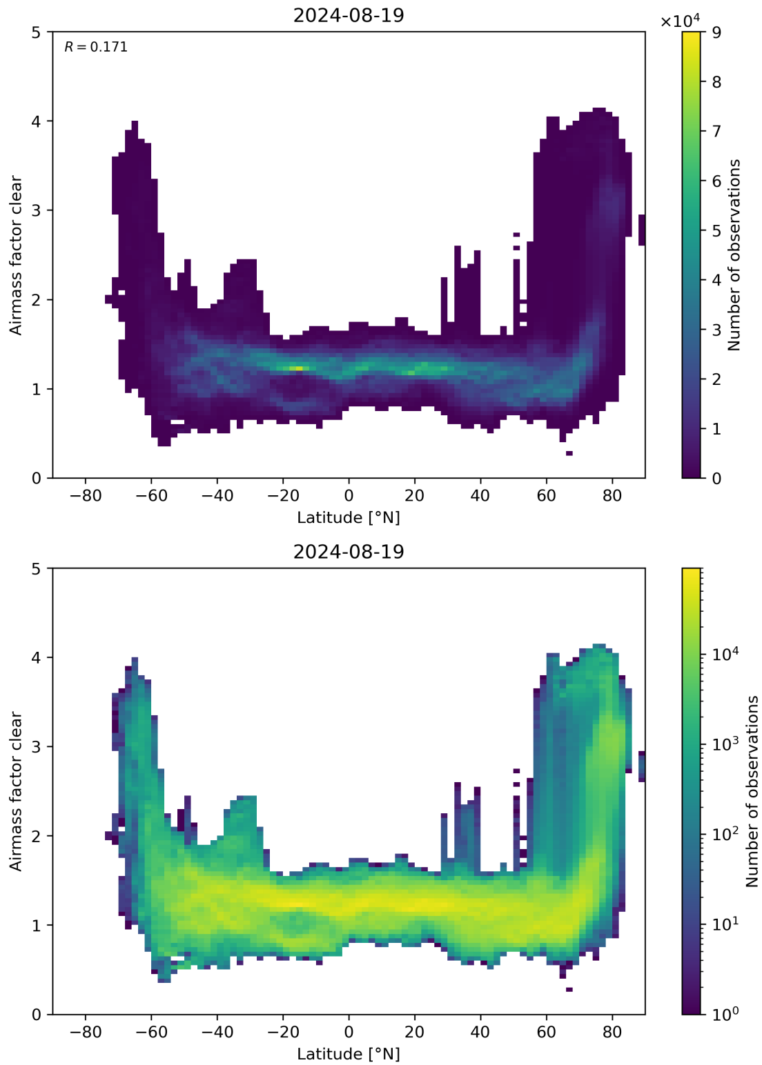
Figure 156: Scatter density plot of “Latitude” against “Airmass factor clear” for 2024-08-18 to 2024-08-20.
