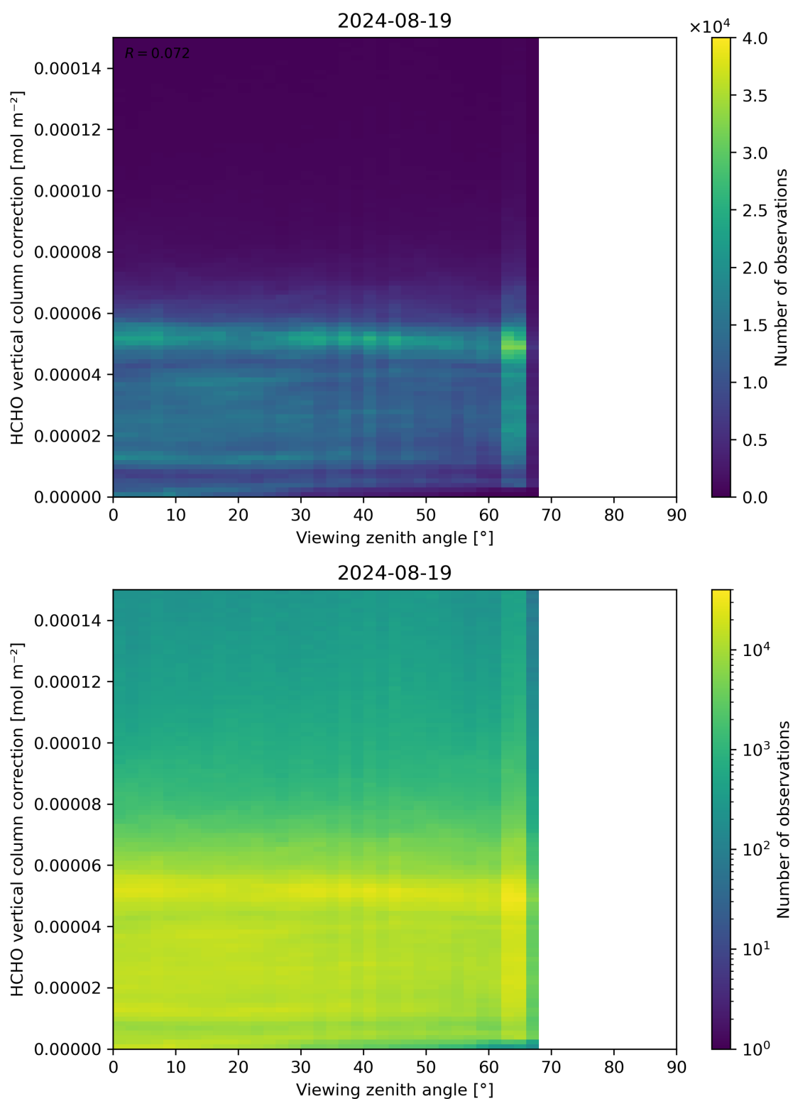
Figure 193: Scatter density plot of “Viewing zenith angle” against “HCHO vertical column correction” for 2024-08-18 to 2024-08-20.
