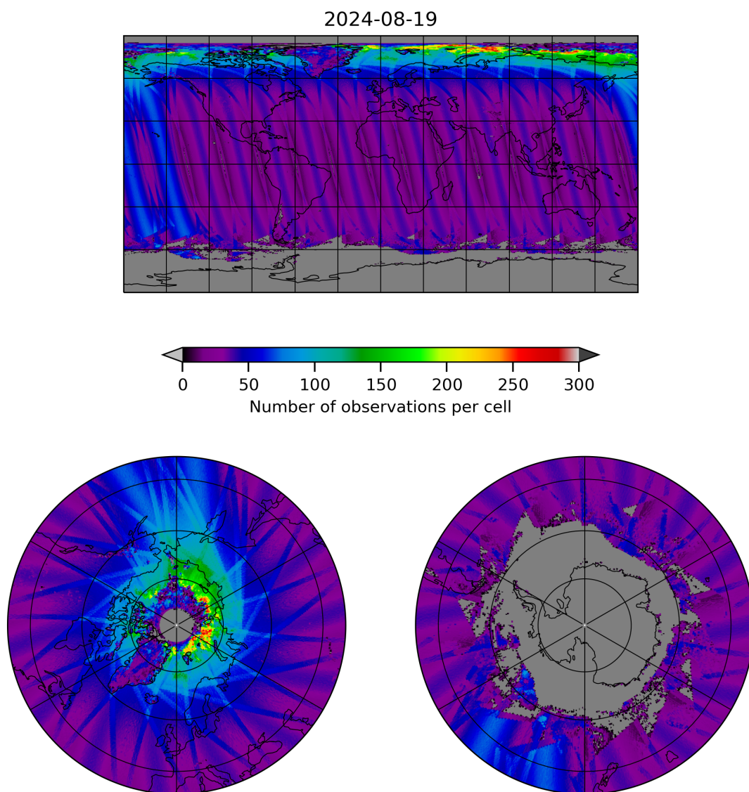
Figure 19: Map of the number of observations for 2024-08-18 to 2024-08-20
