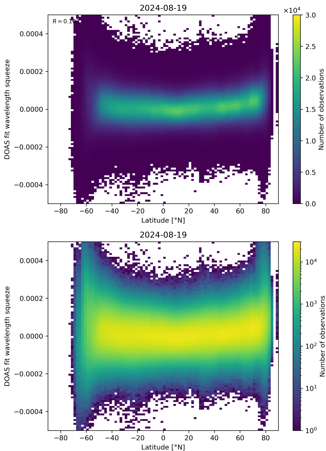
Figure 155: Scatter density plot of “Latitude” against “DOAS fit wavelength squeeze” for 2024-08-18 to 2024-08-20.
