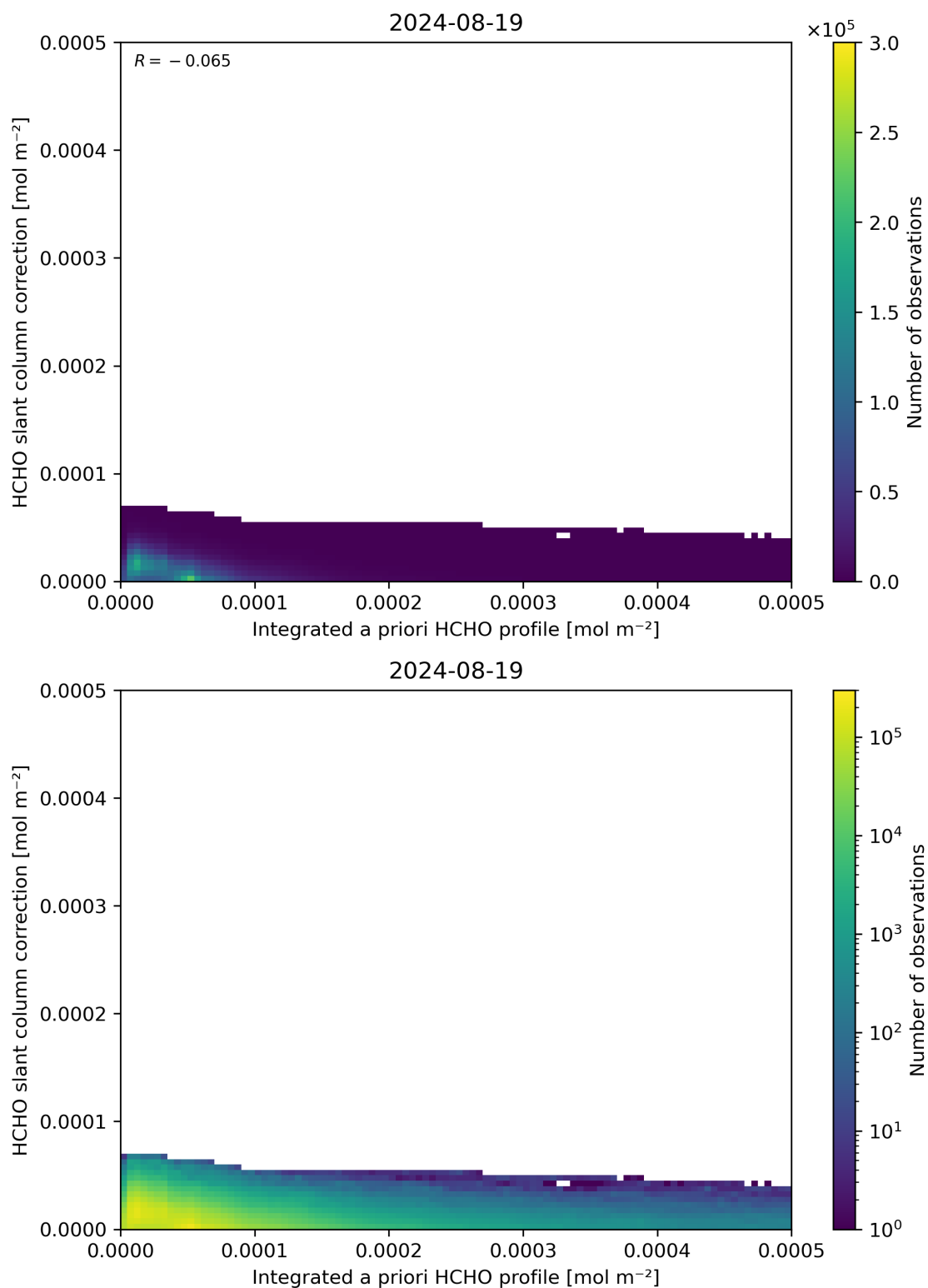
Figure 152: Scatter density plot of “Integrated a priori HCHO profile” against “HCHO slant column correction” for 2024-08-18 to 2024-08-20.
