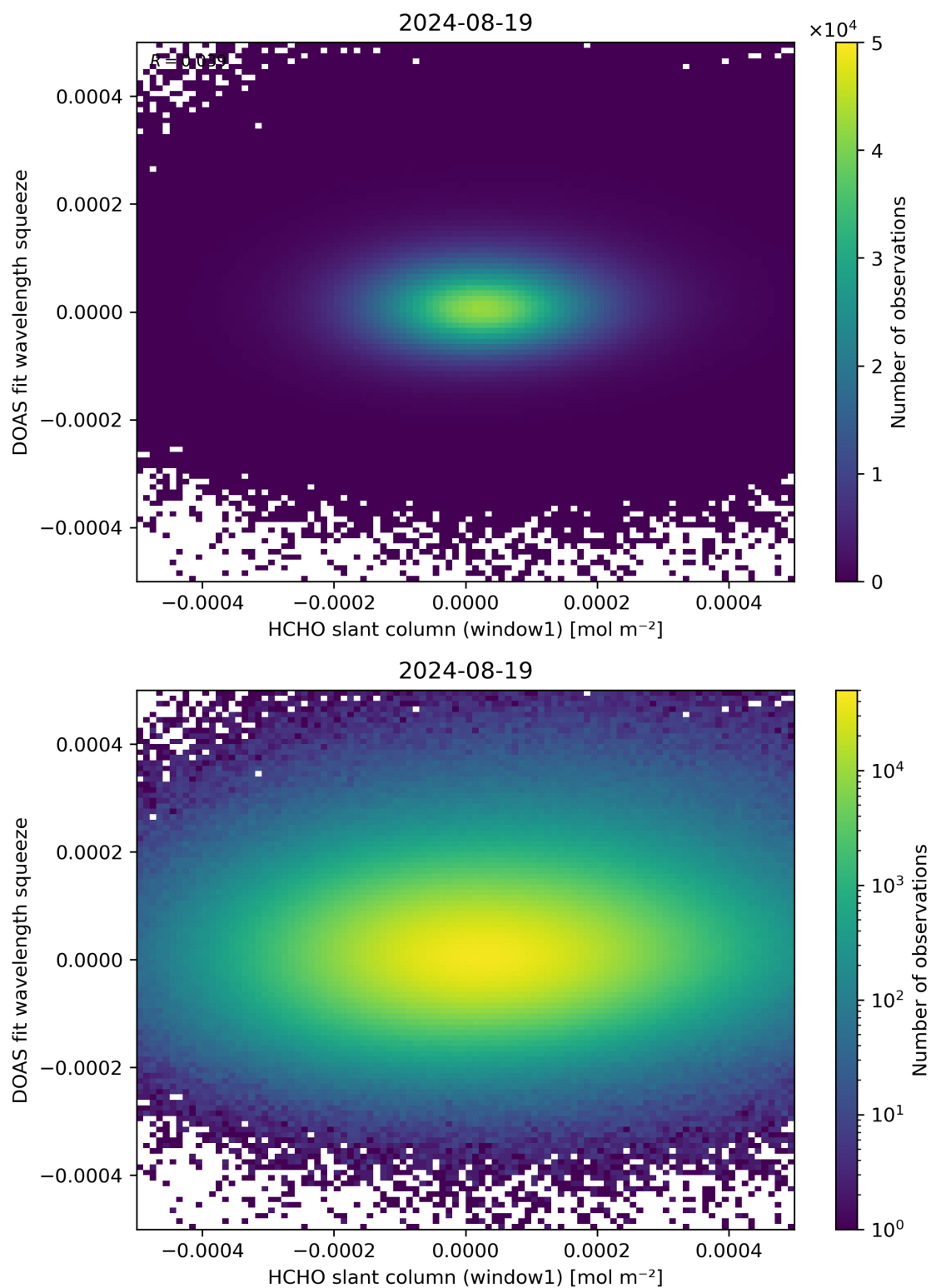
Figure 80: Scatter density plot of “HCHO slant column (window1)” against “DOAS fit wavelength squeeze” for 2024-08-18 to 2024-08-20.
