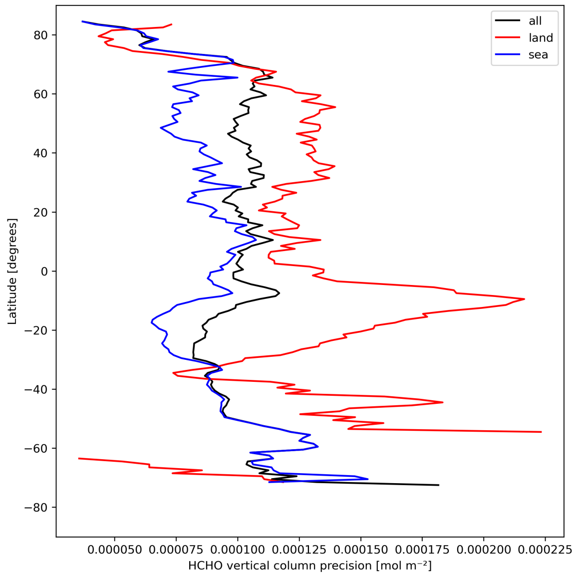
Figure 22: Zonal average of “HCHO vertical column precision” for 2024-08-18 to 2024-08-20.
