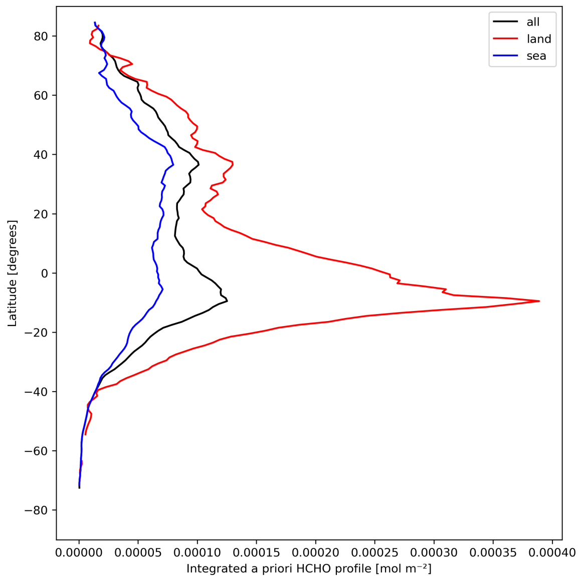
Figure 29: Zonal average of “Integrated a priori HCHO profile” for 2024-08-18 to 2024-08-20.
