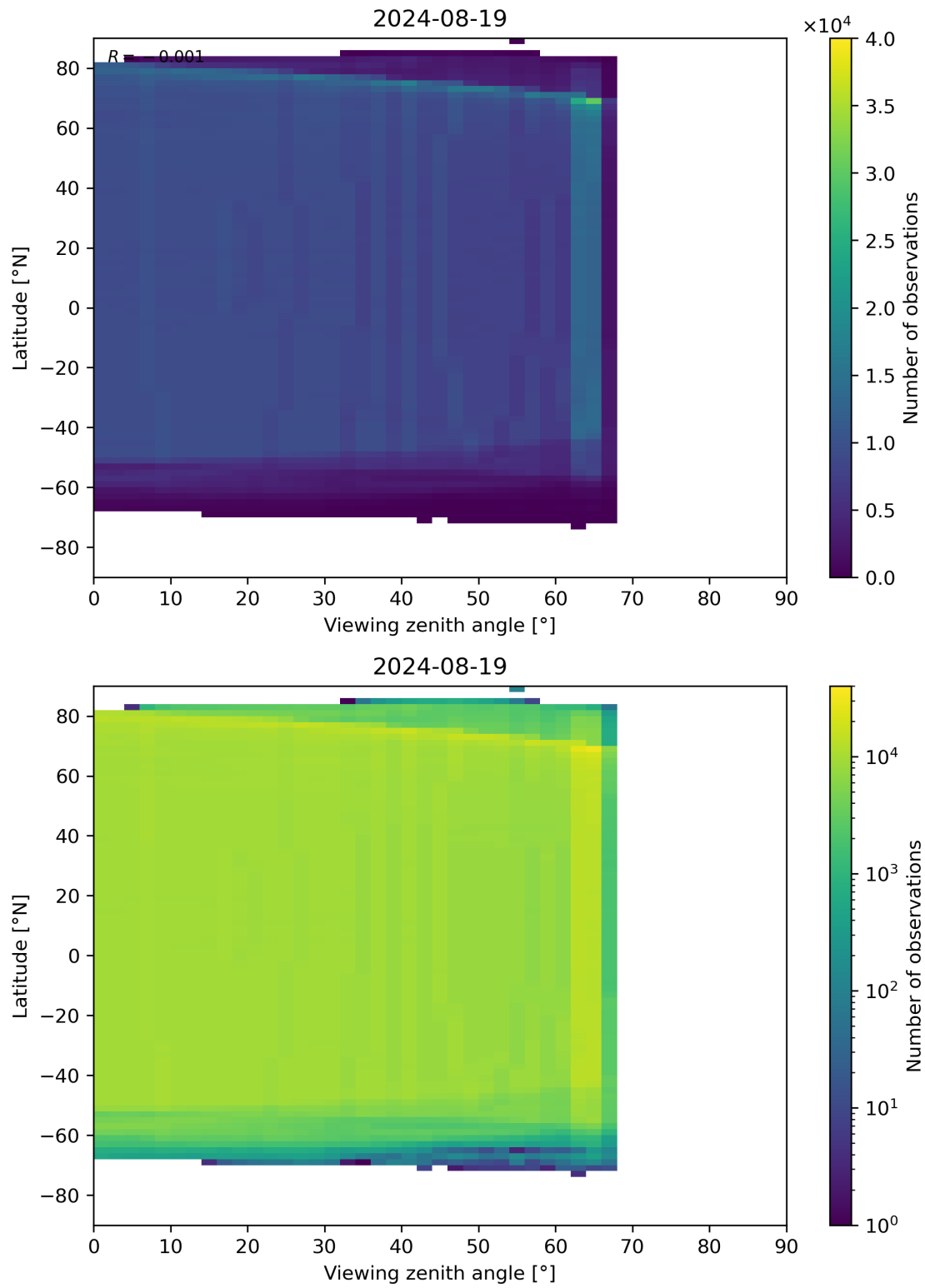
Figure 196: Scatter density plot of “Viewing zenith angle” against “Latitude” for 2024-08-18 to 2024-08-20.
