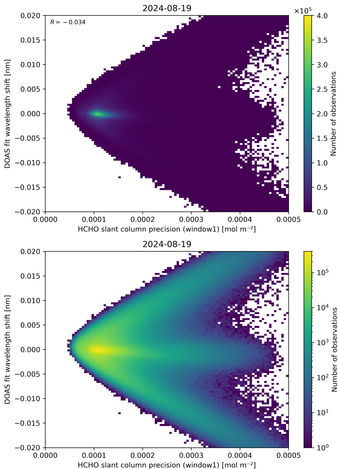
Figure 89: Scatter density plot of “HCHO slant column precision (window1)” against “DOAS fit wavelength shift” for 2024-08-18 to 2024-08-20.
