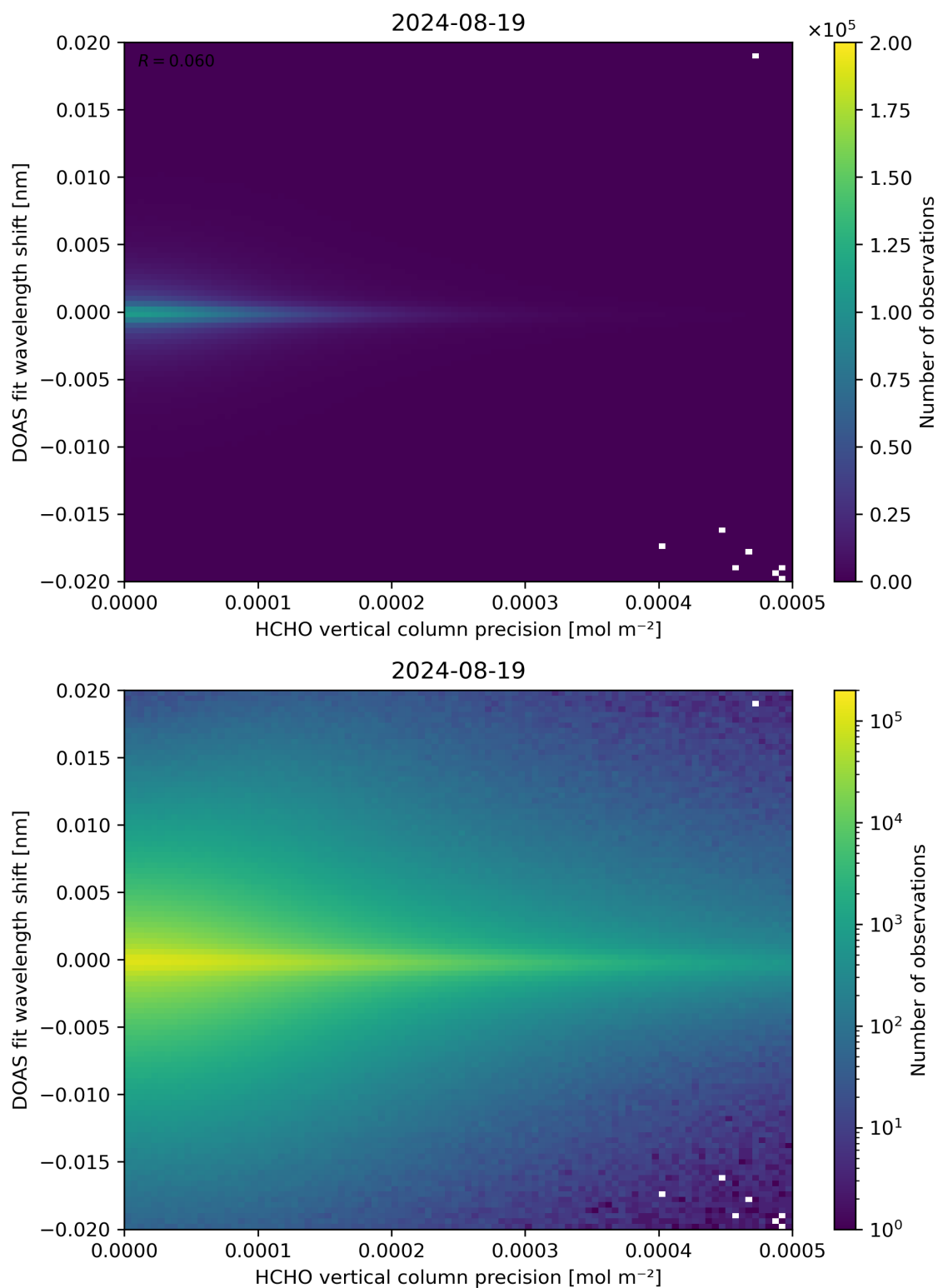
Figure 137: Scatter density plot of “HCHO vertical column precision” against “DOAS fit wavelength shift” for 2024-08-18 to 2024-08-20.
