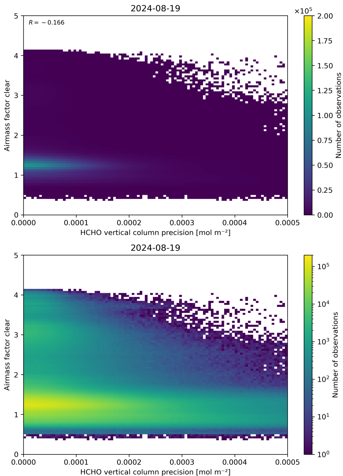
Figure 139: Scatter density plot of “HCHO vertical column precision” against “Airmass factor clear” for 2024-08-18 to 2024-08-20.
