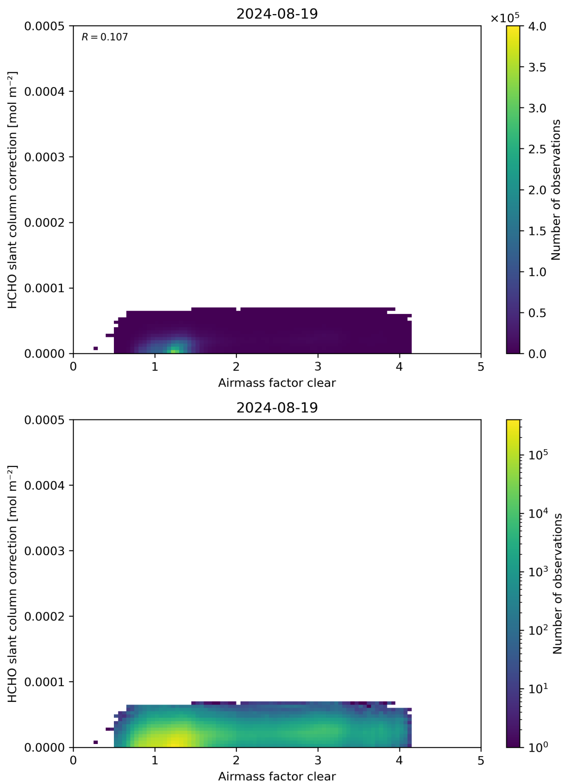
Figure 75: Scatter density plot of “Airmass factor clear” against “HCHO slant column correction” for 2024-08-18 to 2024-08-20.
