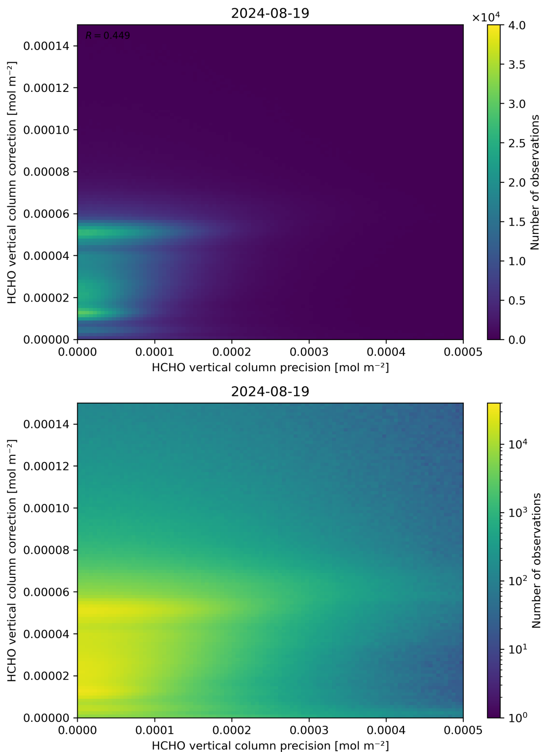
Figure 146: Scatter density plot of “HCHO vertical column precision” against “HCHO vertical column correction” for 2024-08-18 to 2024-08-20.
