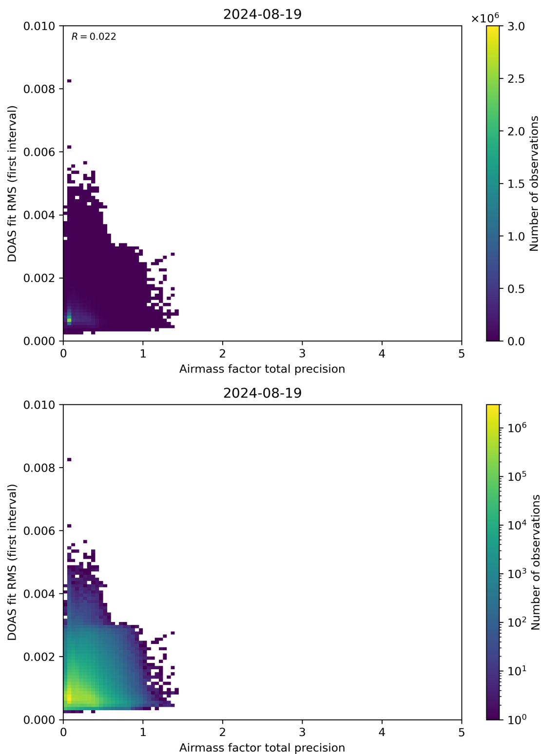
Figure 105: Scatter density plot of “Airmass factor total precision” against “DOAS fit RMS (first interval)” for 2024-08-18 to 2024-08-20.
