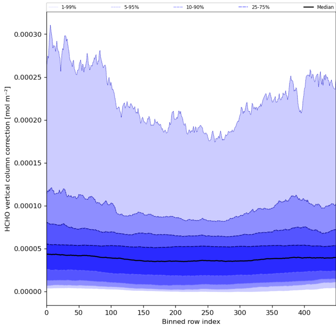
Figure 51: Along track statistics of “HCHO vertical column correction” for 2024-08-18 to 2024-08-20
