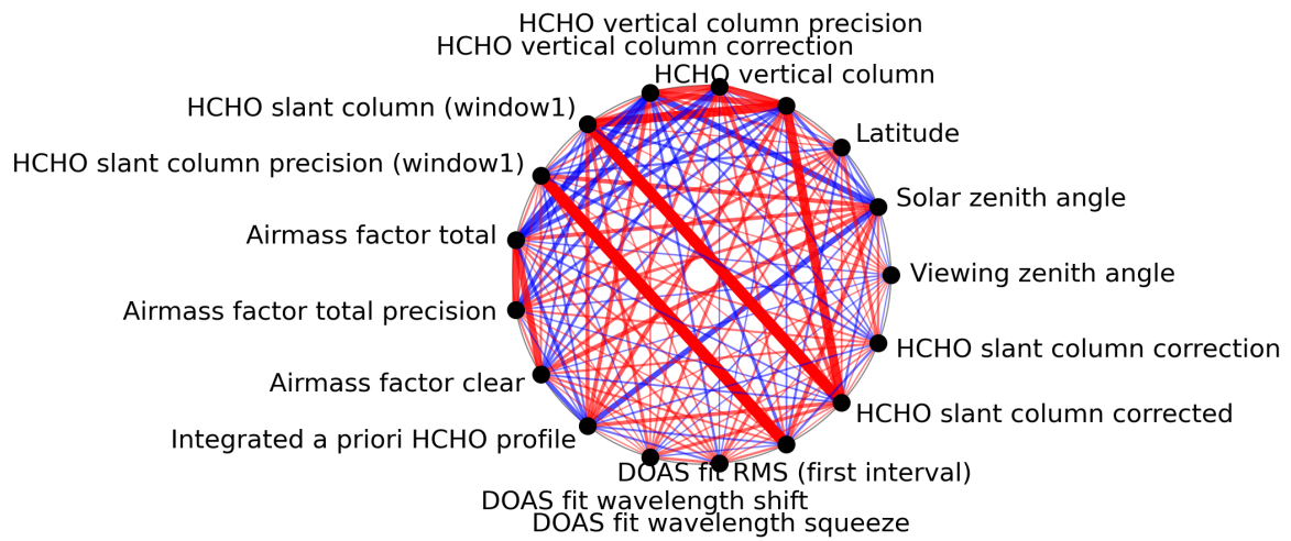
Figure 1: Map of correlation graph for 2024-08-18 to 2024-08-20.
