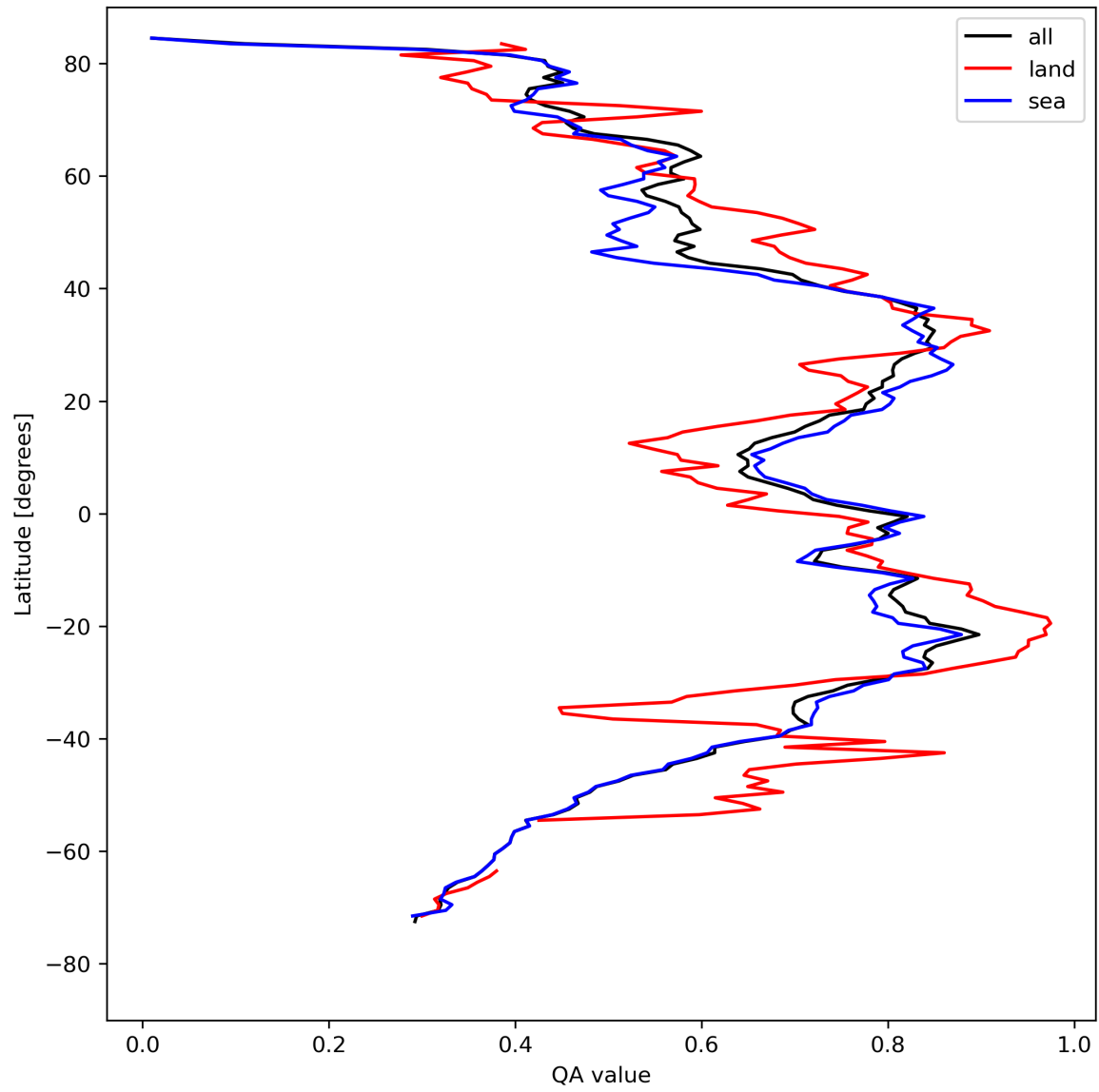
Figure 20: Zonal average of “QA value” for 2024-08-18 to 2024-08-20.
