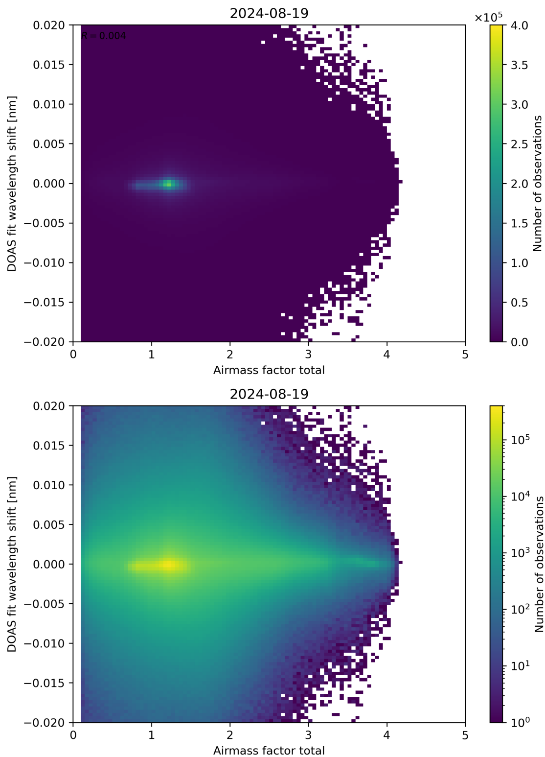
Figure 98: Scatter density plot of “Airmass factor total” against “DOAS fit wavelength shift” for 2024-08-18 to 2024-08-20.
