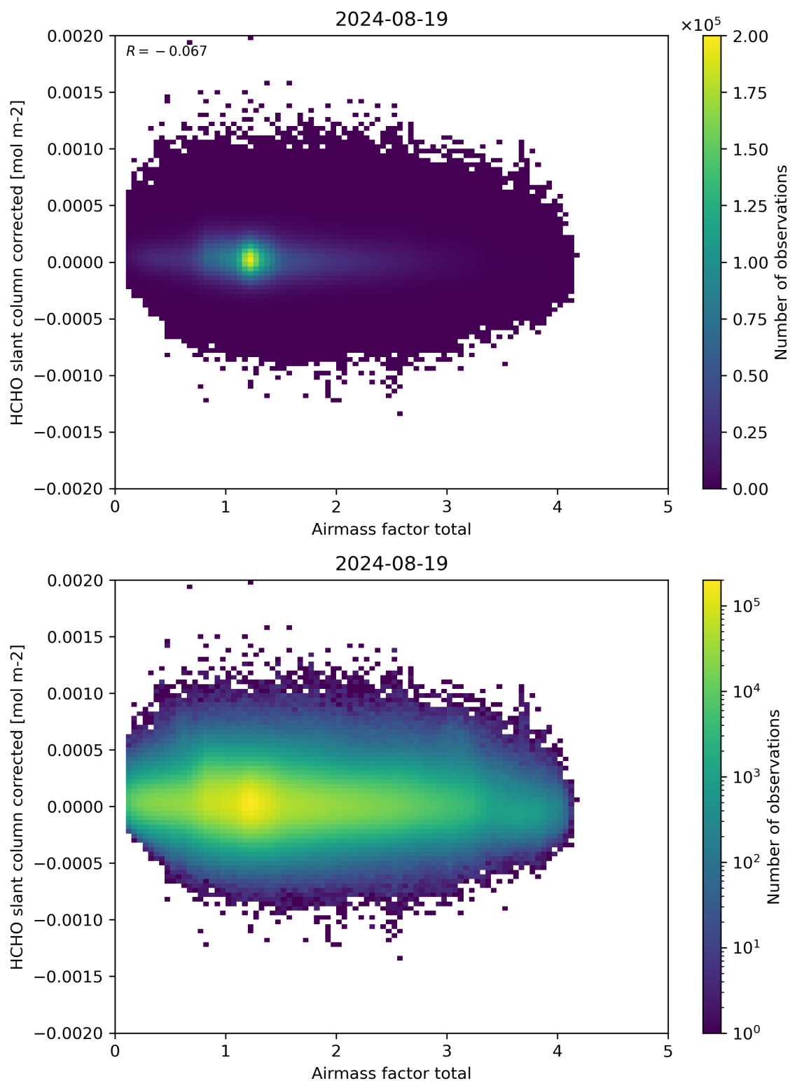
Figure 101: Scatter density plot of “Airmass factor total” against “HCHO slant column corrected” for 2024-08-18 to 2024-08-20.
