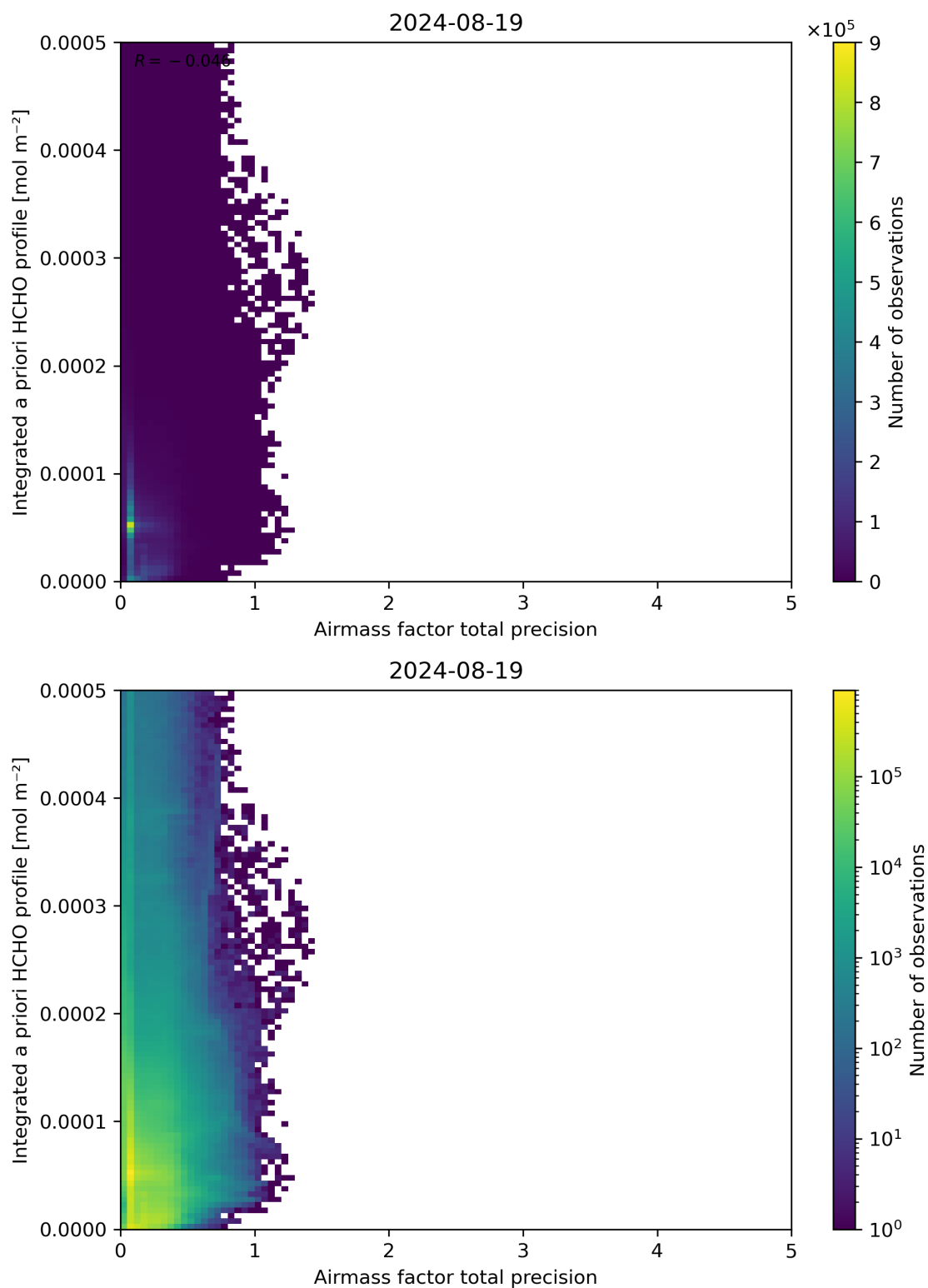
Figure 111: Scatter density plot of “Airmass factor total precision” against “Integrated a priori HCHO profile” for 2024-08-18 to 2024-08-20.
