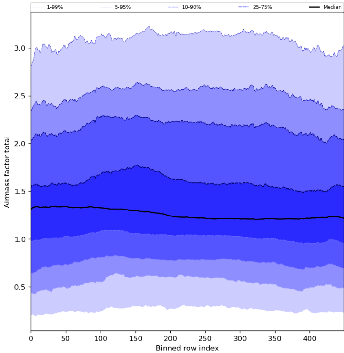
Figure 54: Along track statistics of “Airmass factor total” for 2024-08-18 to 2024-08-20
