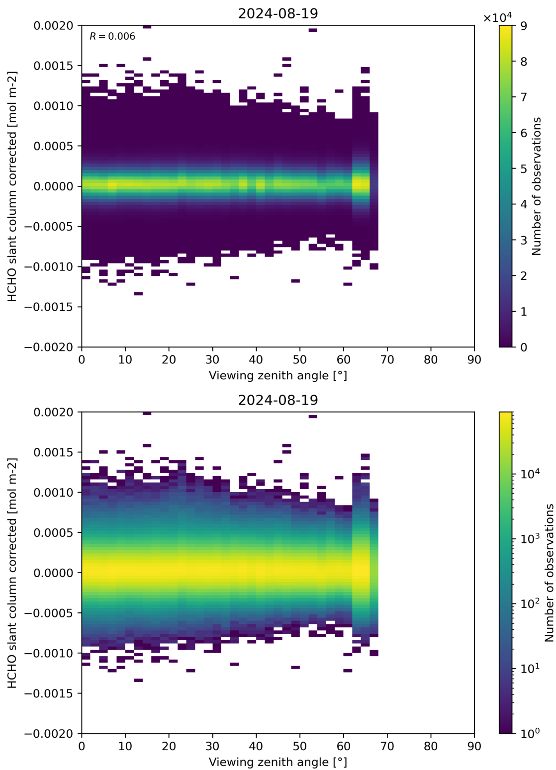
Figure 186: Scatter density plot of “Viewing zenith angle” against “HCHO slant column corrected” for 2024-08-18 to 2024-08-20.
