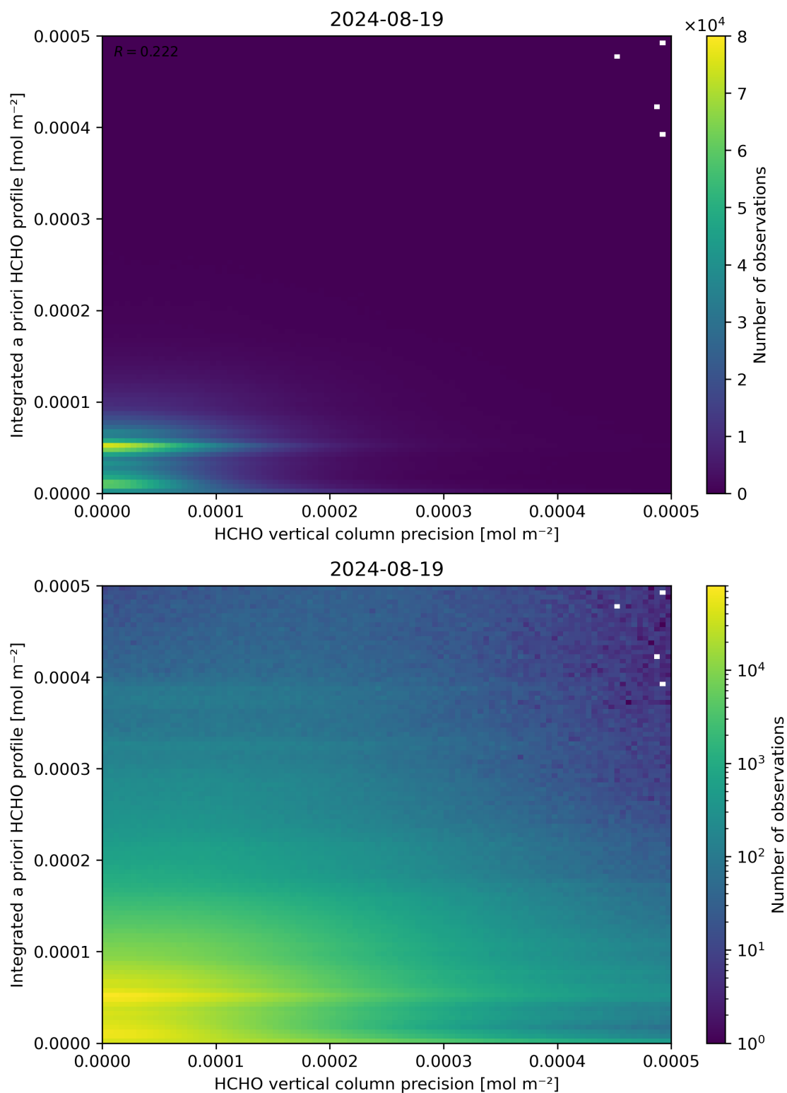
Figure 147: Scatter density plot of “HCHO vertical column precision” against “Integrated a priori HCHO profile” for 2024-08-18 to 2024-08-20.
