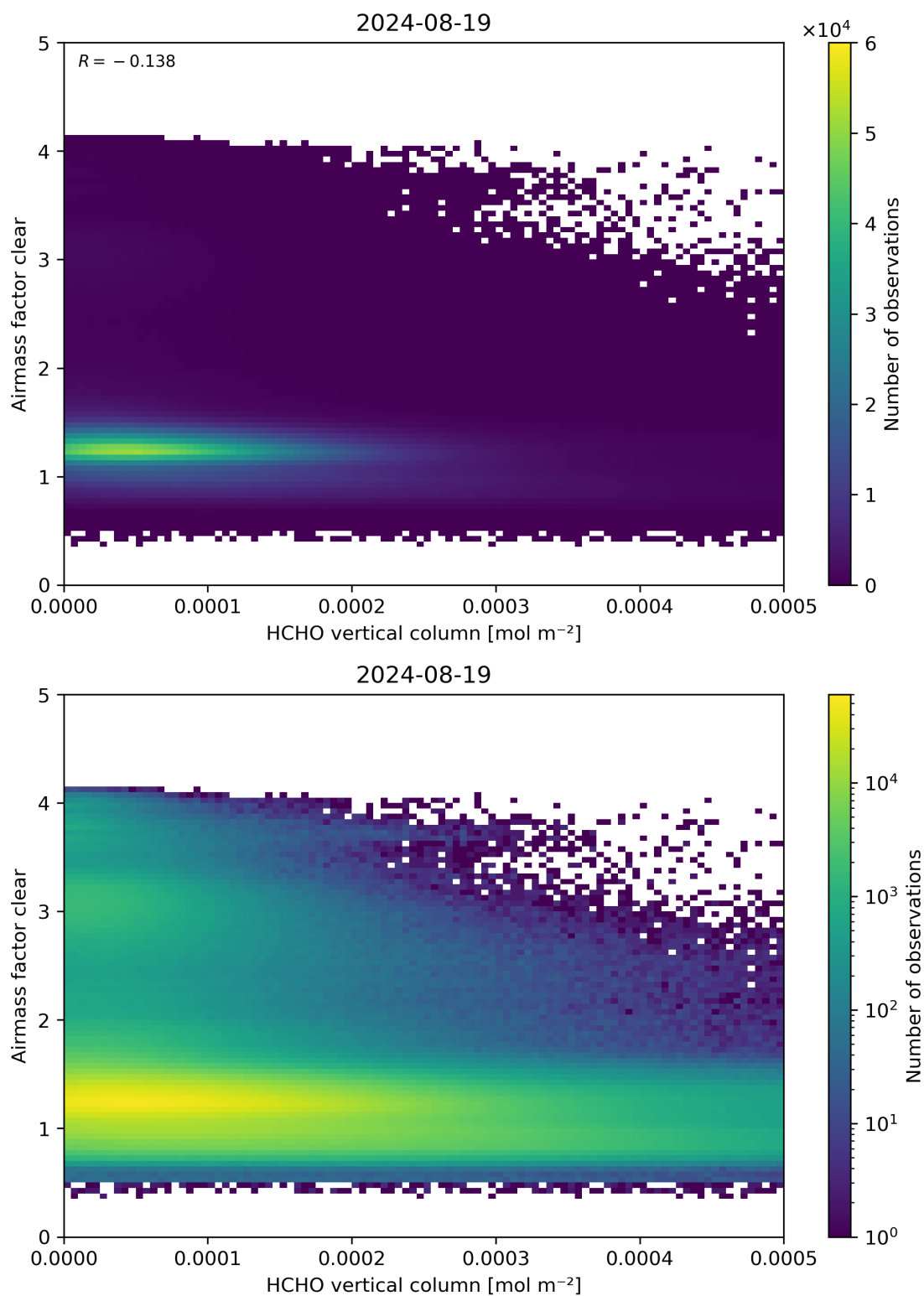
Figure 126: Scatter density plot of “HCHO vertical column” against “Airmass factor clear” for 2024-08-18 to 2024-08-20.
