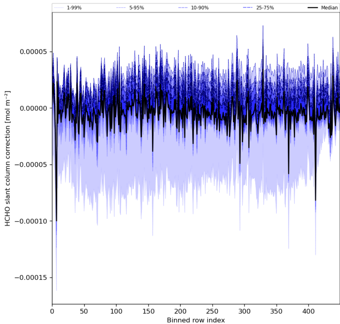
Figure 61: Along track statistics of “HCHO slant column correction” for 2024-08-19 to 2024-08-21
