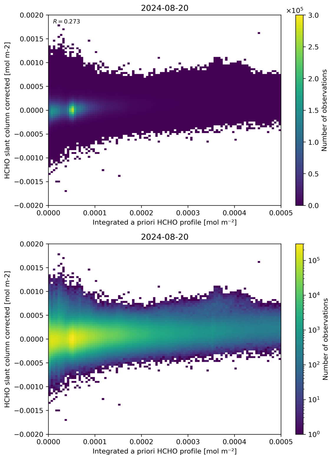
Figure 151: Scatter density plot of “Integrated a priori HCHO profile” against “HCHO slant column corrected” for 2024-08-19 to 2024-08-21.
