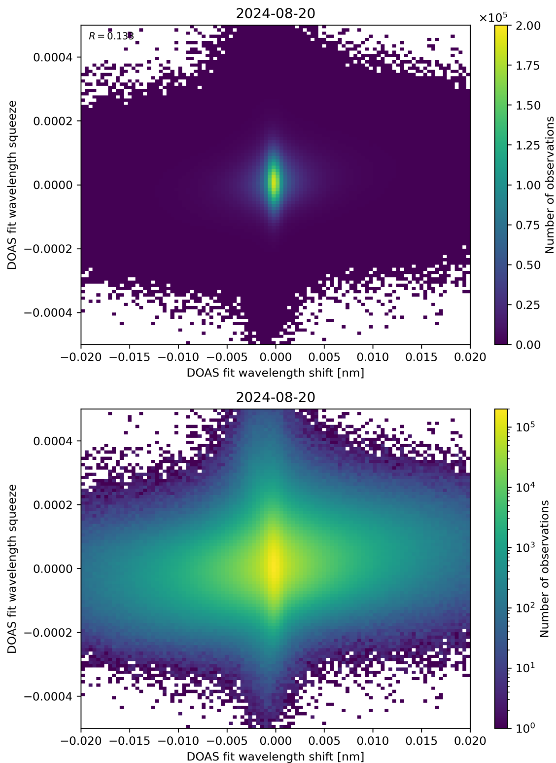
Figure 65: Scatter density plot of “DOAS fit wavelength shift” against “DOAS fit wavelength squeeze” for 2024-08-19 to 2024-08-21.
