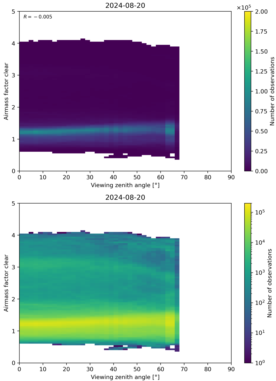
Figure 185: Scatter density plot of “Viewing zenith angle” against “Airmass factor clear” for 2024-08-19 to 2024-08-21.
