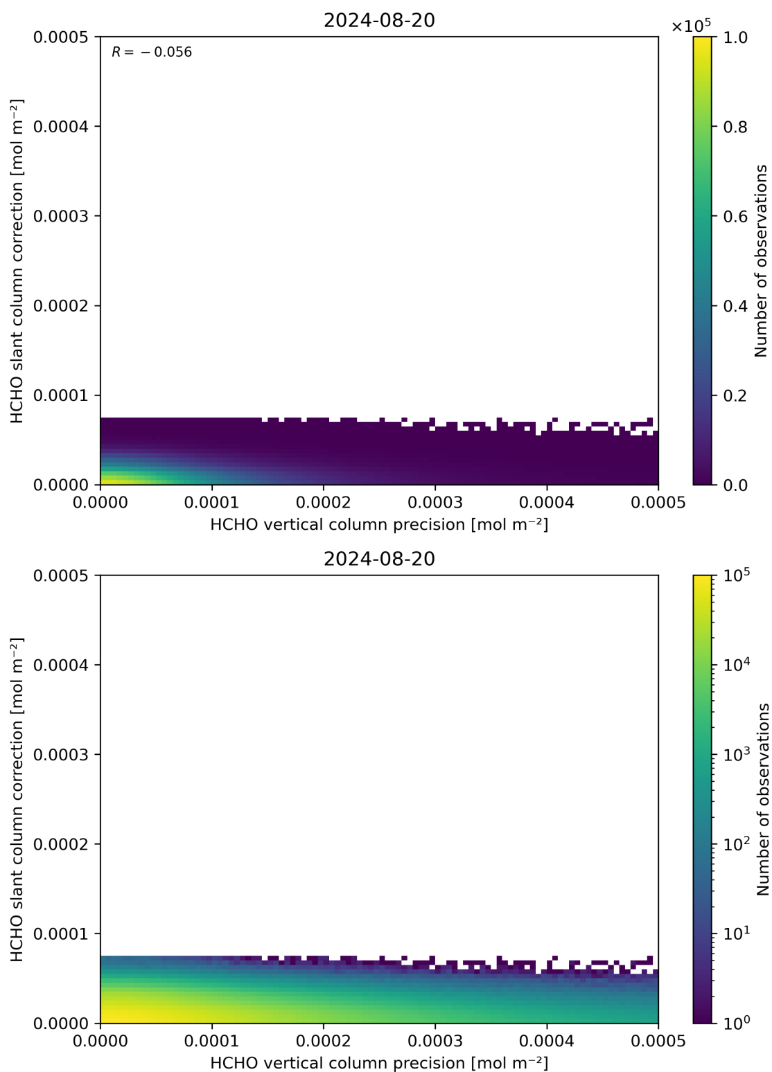
Figure 141: Scatter density plot of “HCHO vertical column precision” against “HCHO slant column correction” for 2024-08-19 to 2024-08-21.
