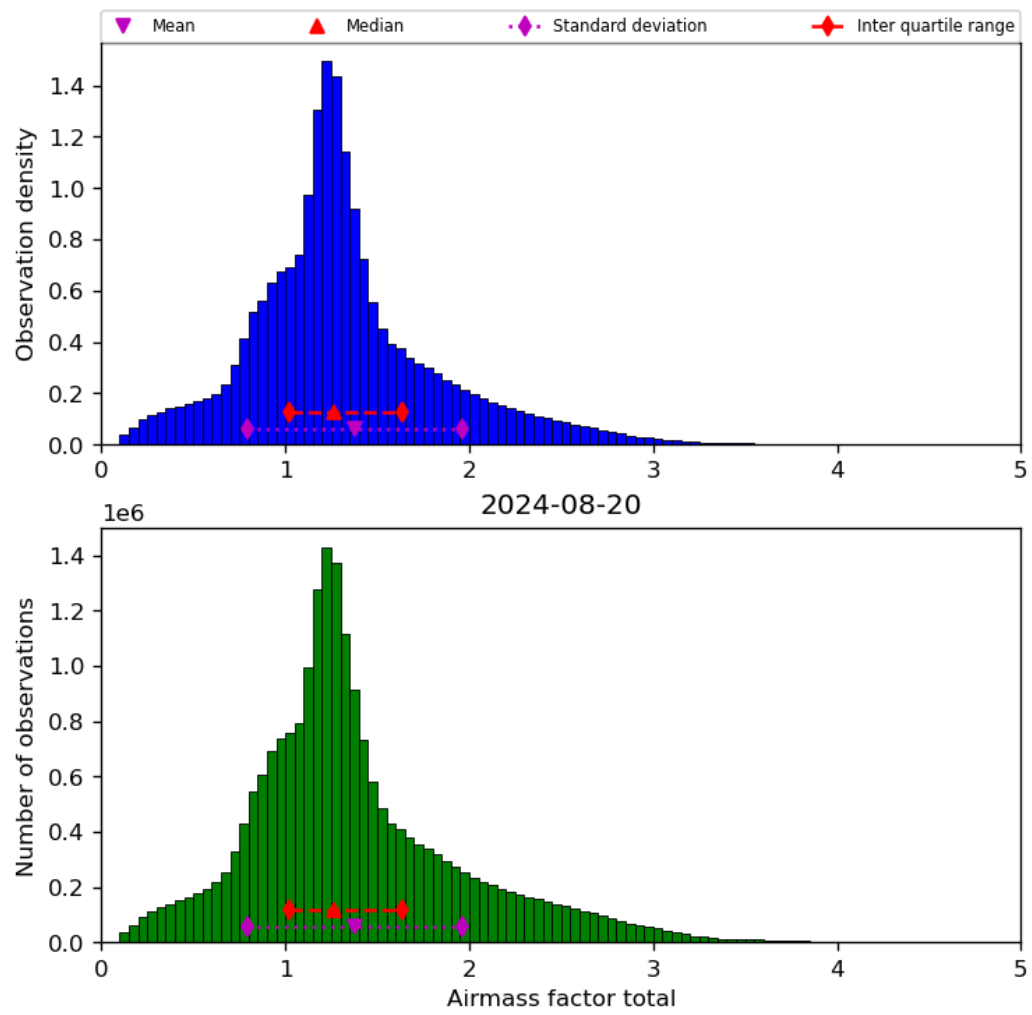
Figure 40: Histogram of “Airmass factor total” for 2024-08-19 to 2024-08-21
