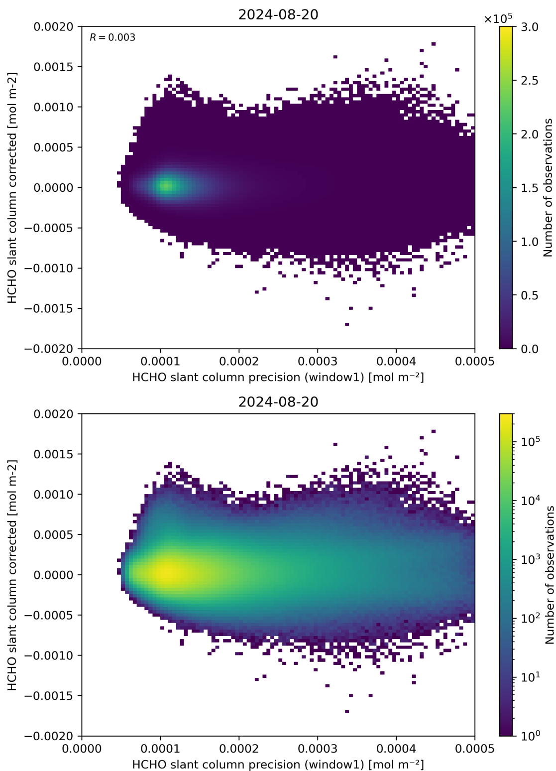
Figure 92: Scatter density plot of “HCHO slant column precision (window1)” against “HCHO slant column corrected” for 2024-08-19 to 2024-08-21.
