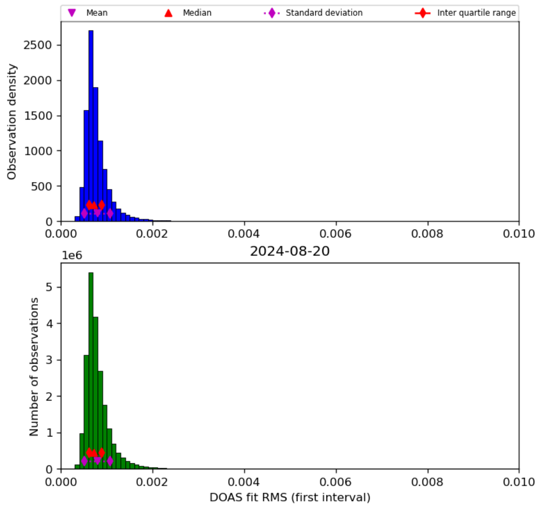
Figure 46: Histogram of “DOAS fit RMS (first interval)” for 2024-08-19 to 2024-08-21
