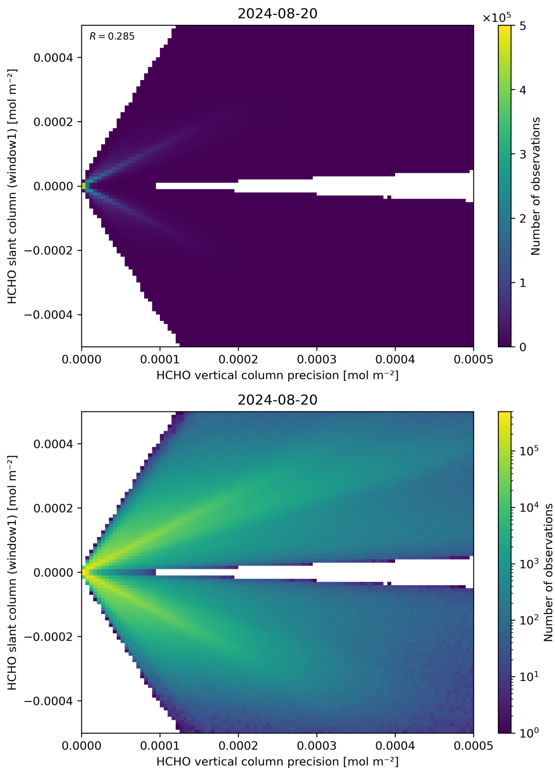
Figure 142: Scatter density plot of “HCHO vertical column precision” against “HCHO slant column (window1)” for 2024-08-19 to 2024-08-21.
