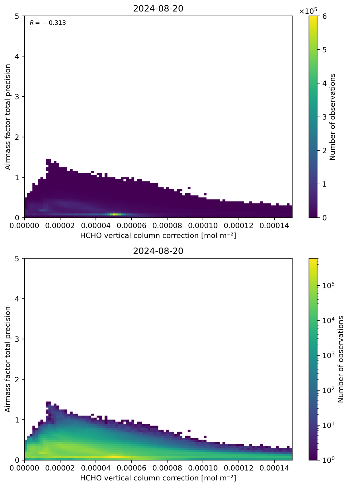
Figure 121: Scatter density plot of “HCHO vertical column correction” against “Airmass factor total precision” for 2024-08-19 to 2024-08-21.
