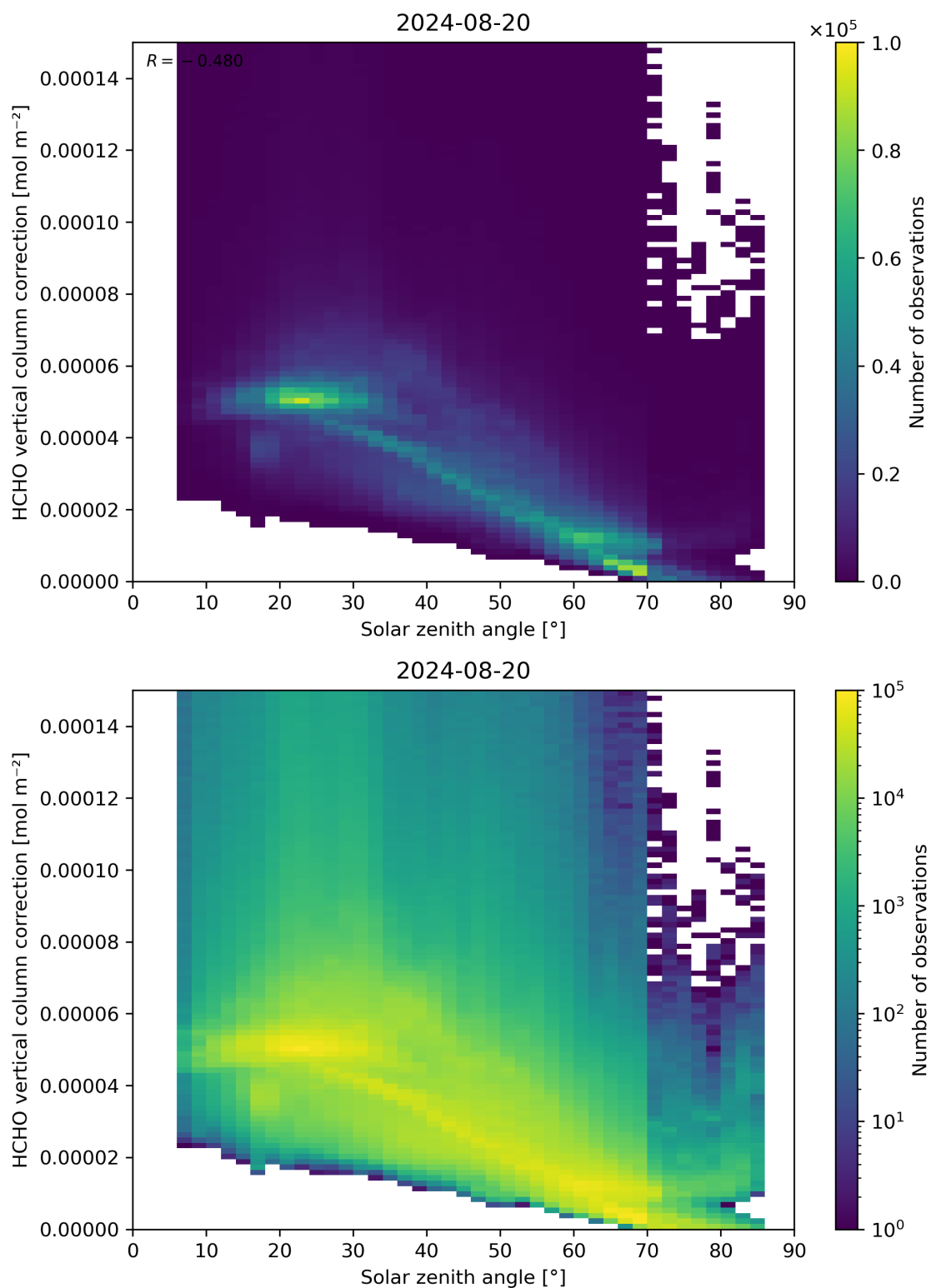
Figure 178: Scatter density plot of “Solar zenith angle” against “HCHO vertical column correction” for 2024-08-19 to 2024-08-21.
