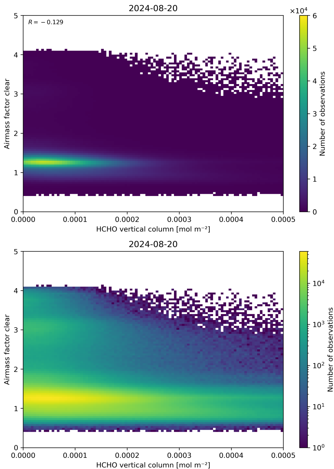
Figure 126: Scatter density plot of “HCHO vertical column” against “Airmass factor clear” for 2024-08-19 to 2024-08-21.
