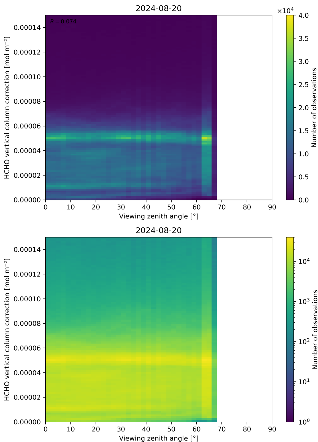
Figure 193: Scatter density plot of “Viewing zenith angle” against “HCHO vertical column correction” for 2024-08-19 to 2024-08-21.
