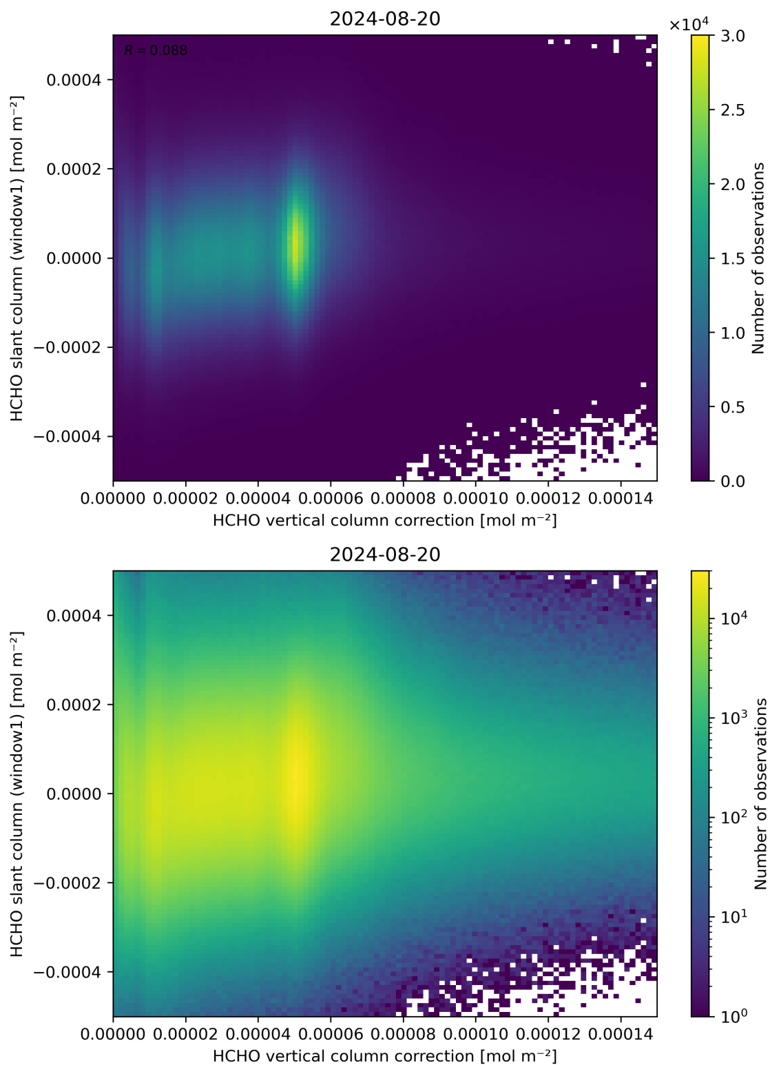
Figure 118: Scatter density plot of “HCHO vertical column correction” against “HCHO slant column (window1)” for 2024-08-19 to 2024-08-21.
