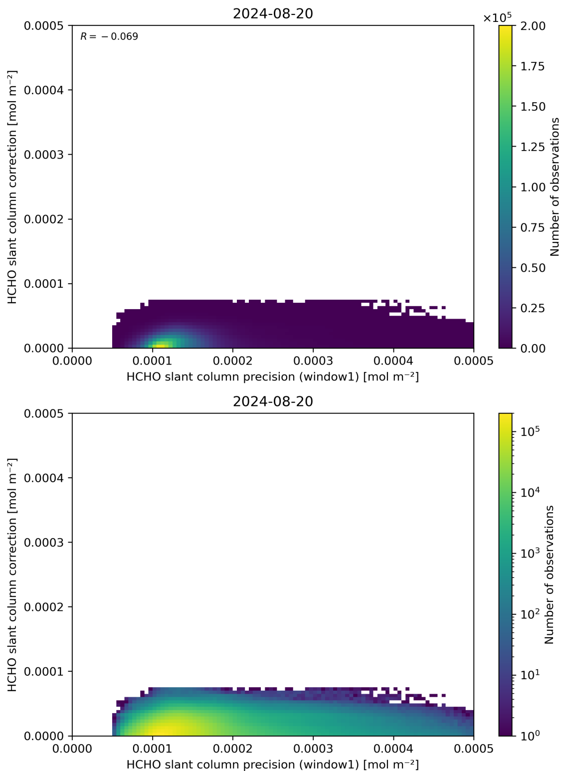
Figure 93: Scatter density plot of “HCHO slant column precision (window1)” against “HCHO slant column correction” for 2024-08-19 to 2024-08-21.
