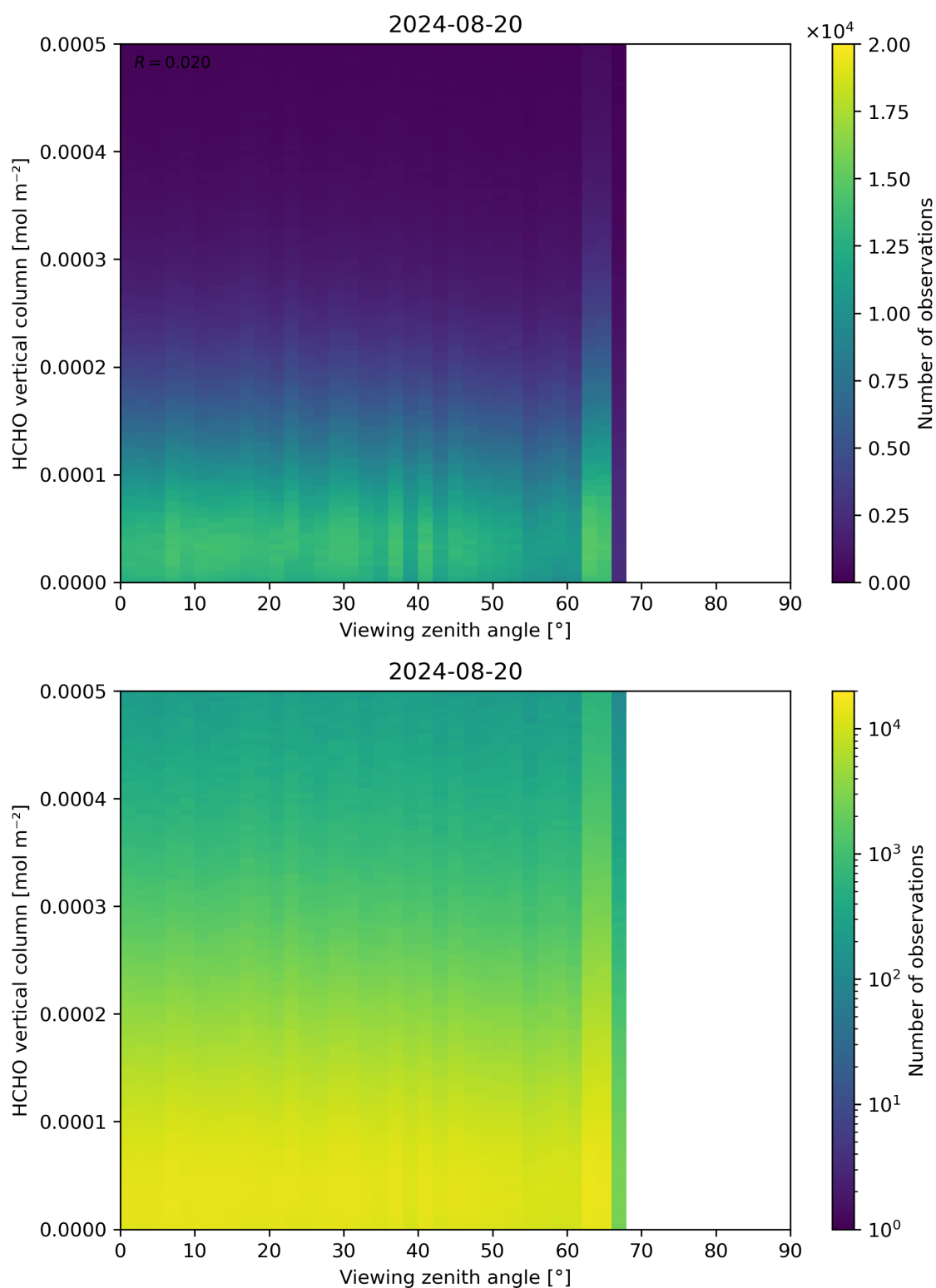
Figure 192: Scatter density plot of “Viewing zenith angle” against “HCHO vertical column” for 2024-08-19 to 2024-08-21.
