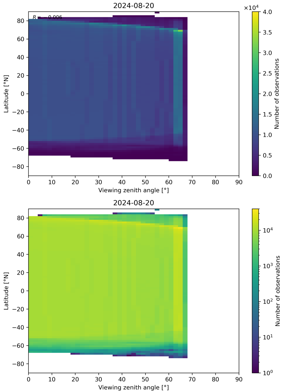
Figure 196: Scatter density plot of “Viewing zenith angle” against “Latitude” for 2024-08-19 to 2024-08-21.
