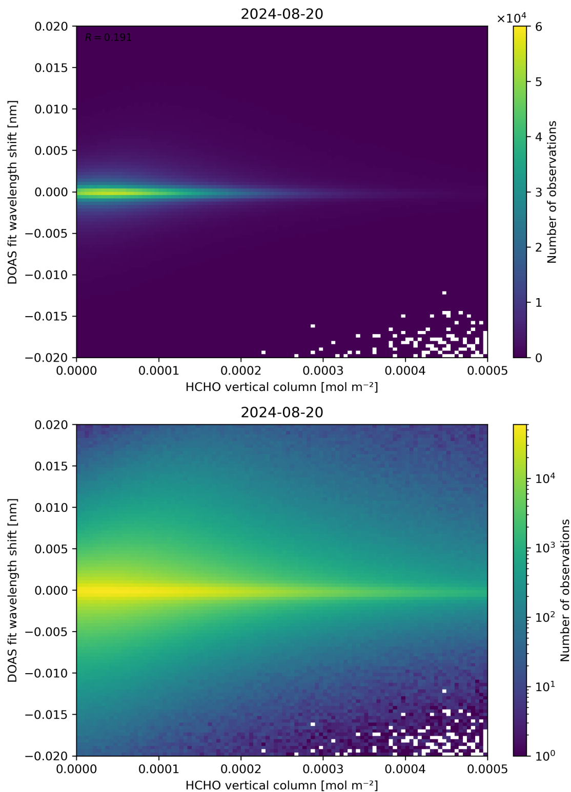
Figure 124: Scatter density plot of “HCHO vertical column” against “DOAS fit wavelength shift” for 2024-08-19 to 2024-08-21.
