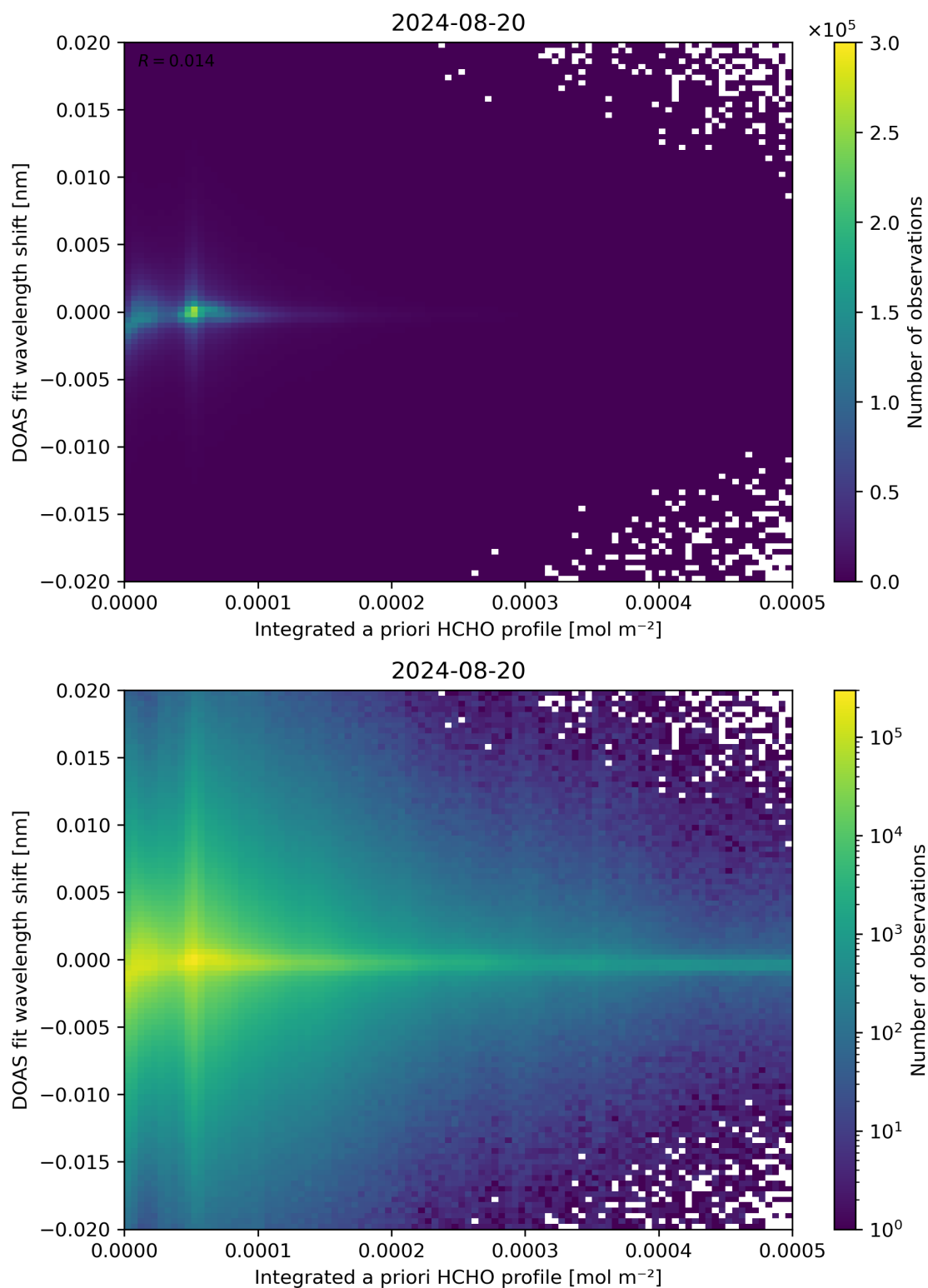
Figure 149: Scatter density plot of “Integrated a priori HCHO profile” against “DOAS fit wavelength shift” for 2024-08-19 to 2024-08-21.
