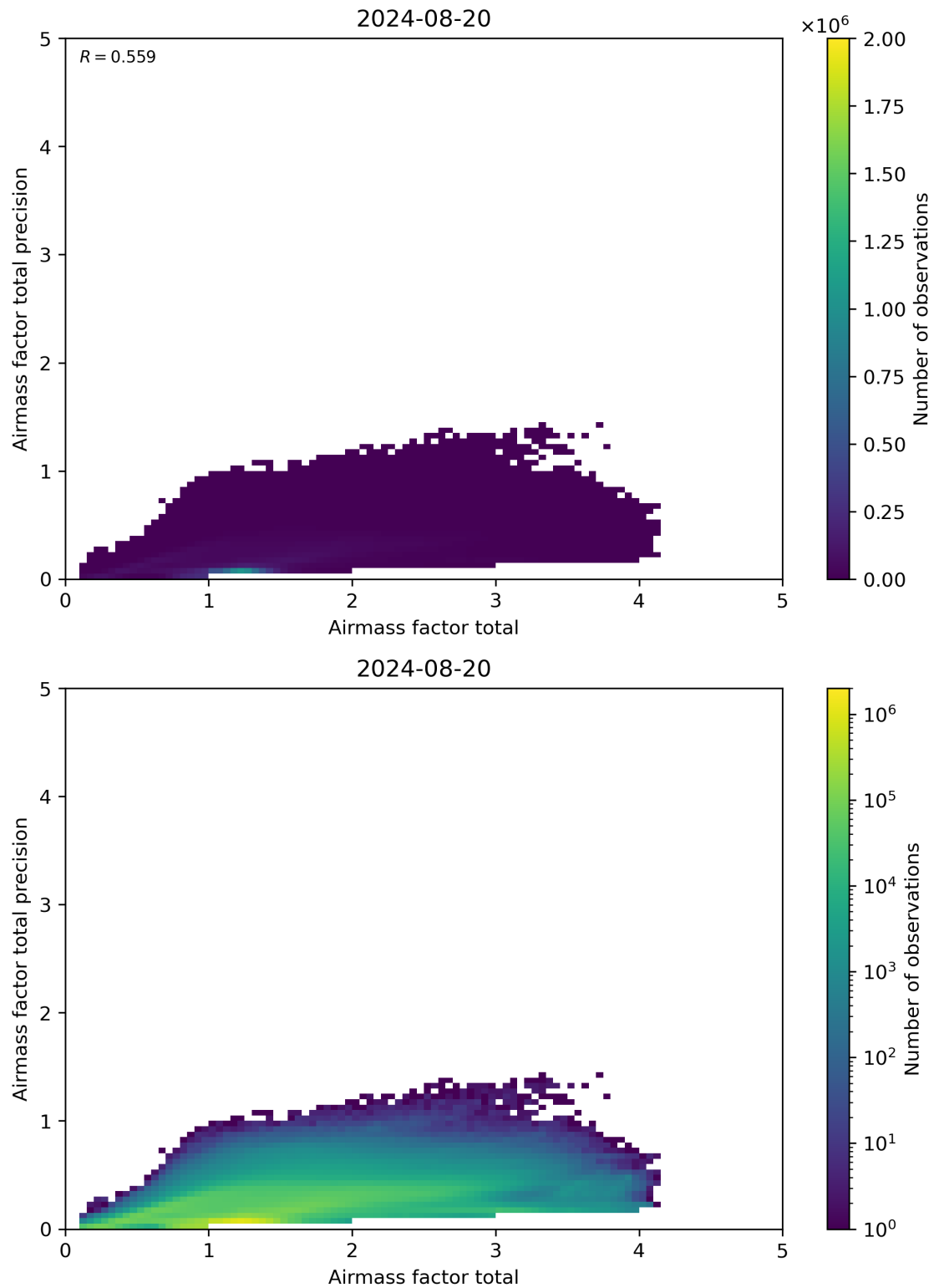
Figure 103: Scatter density plot of “Airmass factor total” against “Airmass factor total precision” for 2024-08-19 to 2024-08-21.
