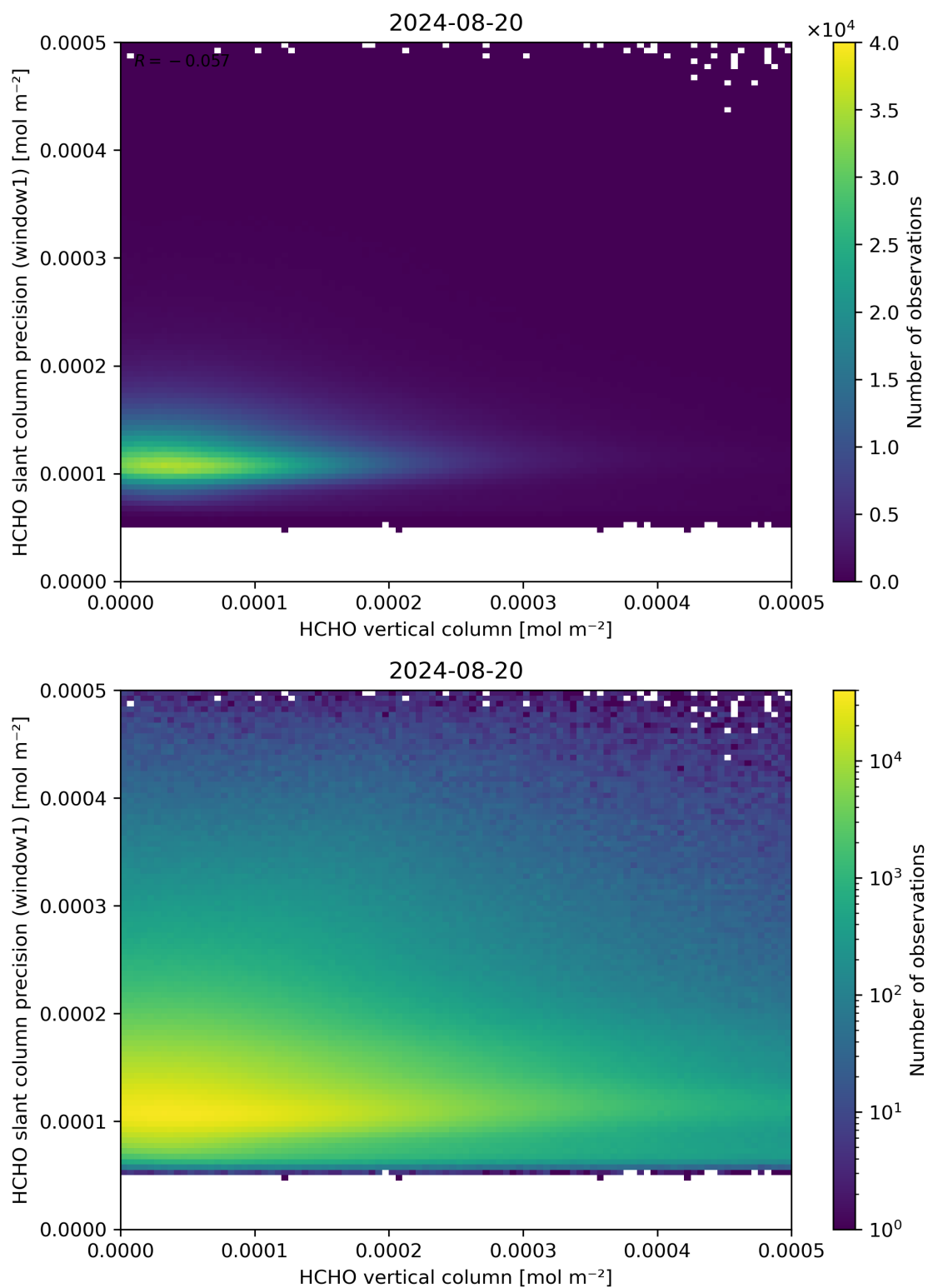
Figure 130: Scatter density plot of “HCHO vertical column” against “HCHO slant column precision (window1)” for 2024-08-19 to 2024-08-21.
