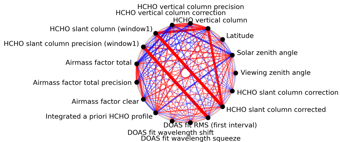
Figure 1: Map of correlation graph for 2024-08-19 to 2024-08-21.
