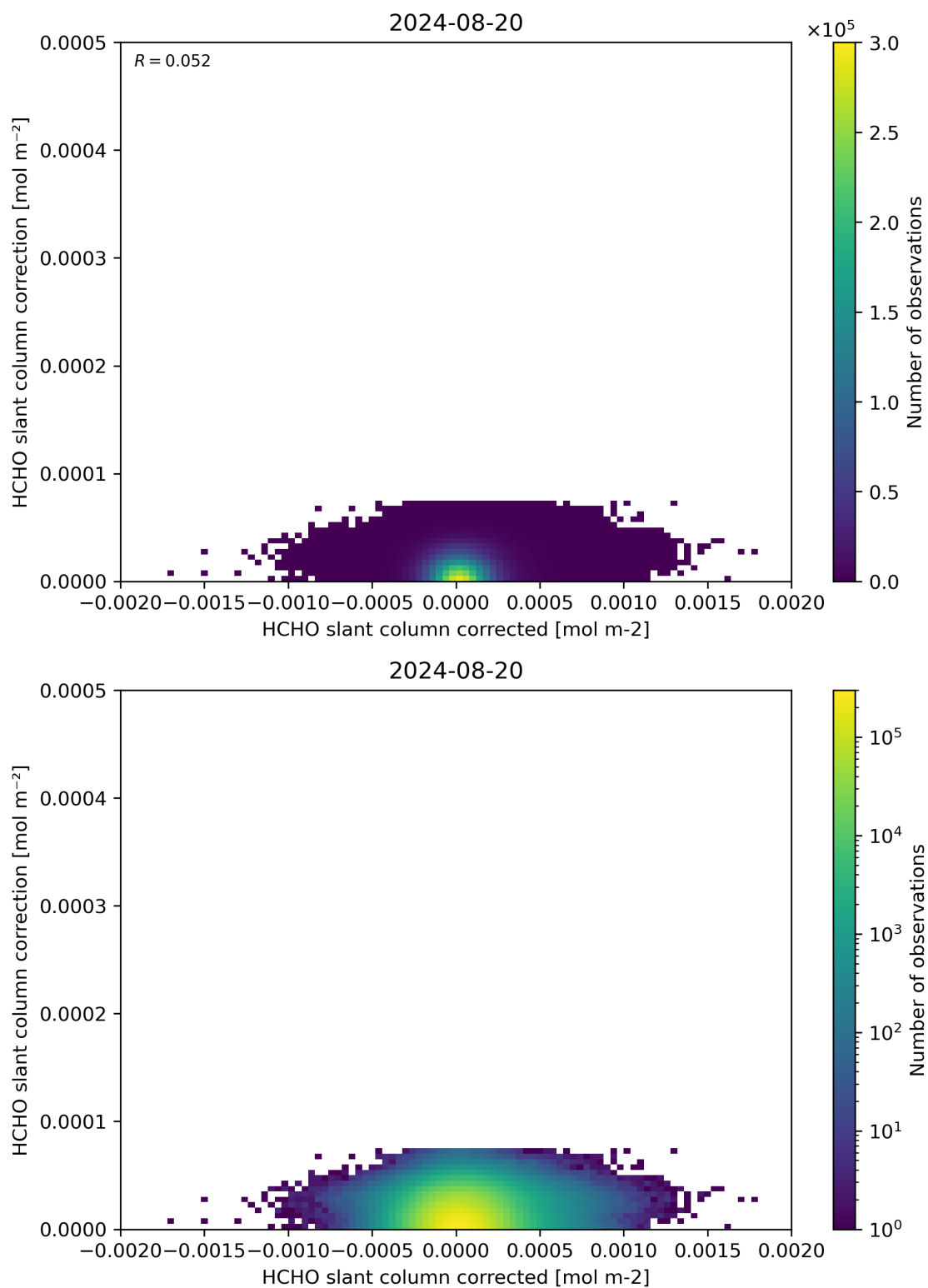
Figure 77: Scatter density plot of “HCHO slant column corrected” against “HCHO slant column correction” for 2024-08-19 to 2024-08-21.
