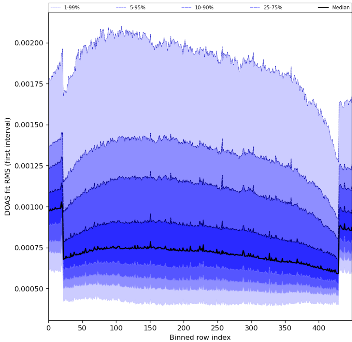
Figure 60: Along track statistics of “DOAS fit RMS (first interval)” for 2024-08-19 to 2024-08-21
