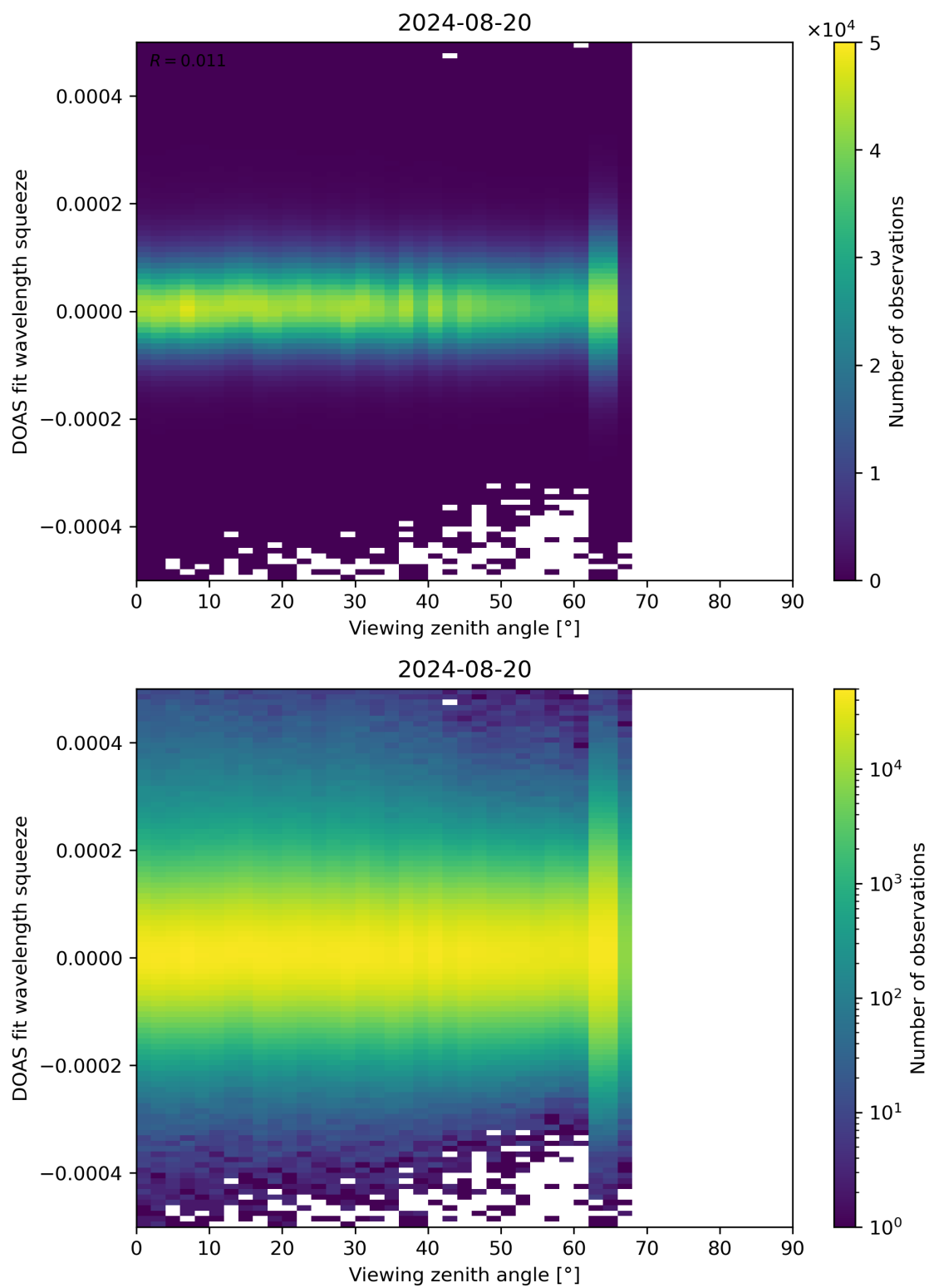
Figure 184: Scatter density plot of “Viewing zenith angle” against “DOAS fit wavelength squeeze” for 2024-08-19 to 2024-08-21.
