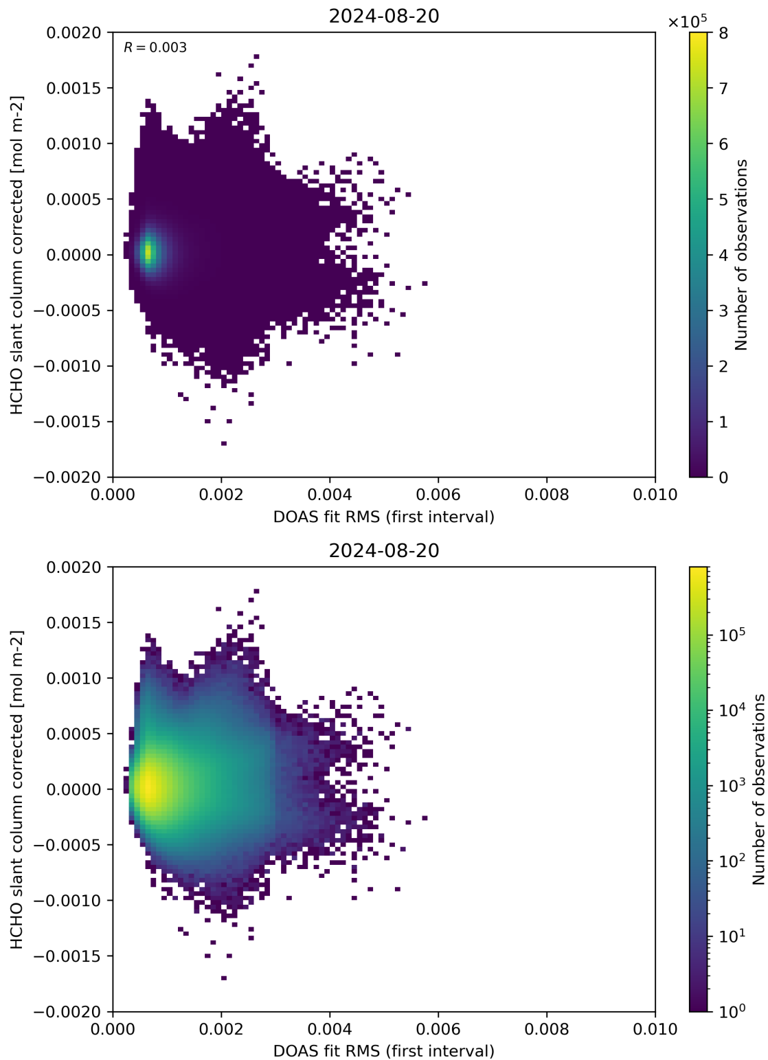
Figure 62: Scatter density plot of “DOAS fit RMS (first interval)” against “HCHO slant column corrected” for 2024-08-19 to 2024-08-21.
