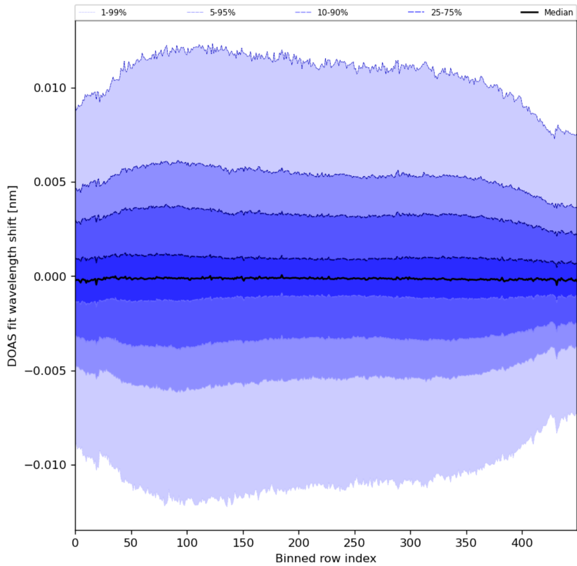
Figure 58: Along track statistics of “DOAS fit wavelength shift” for 2024-08-19 to 2024-08-21
