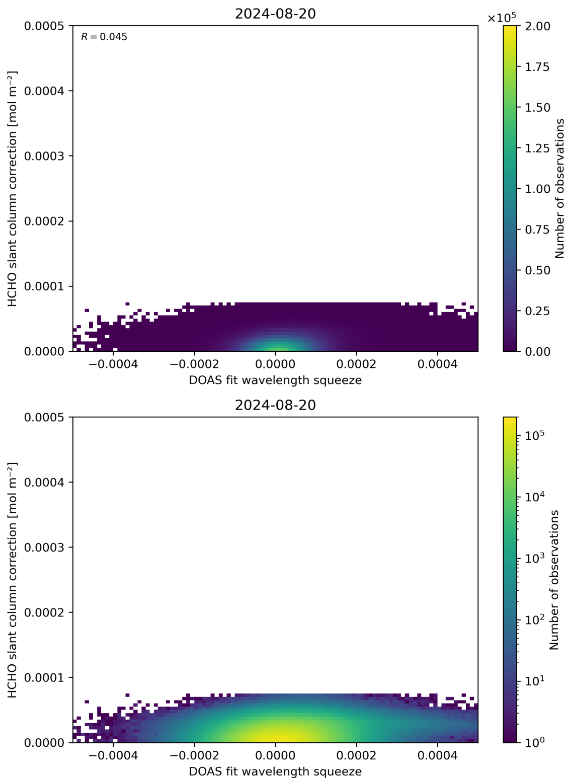
Figure 70: Scatter density plot of “DOAS fit wavelength squeeze” against “HCHO slant column correction” for 2024-08-19 to 2024-08-21.
