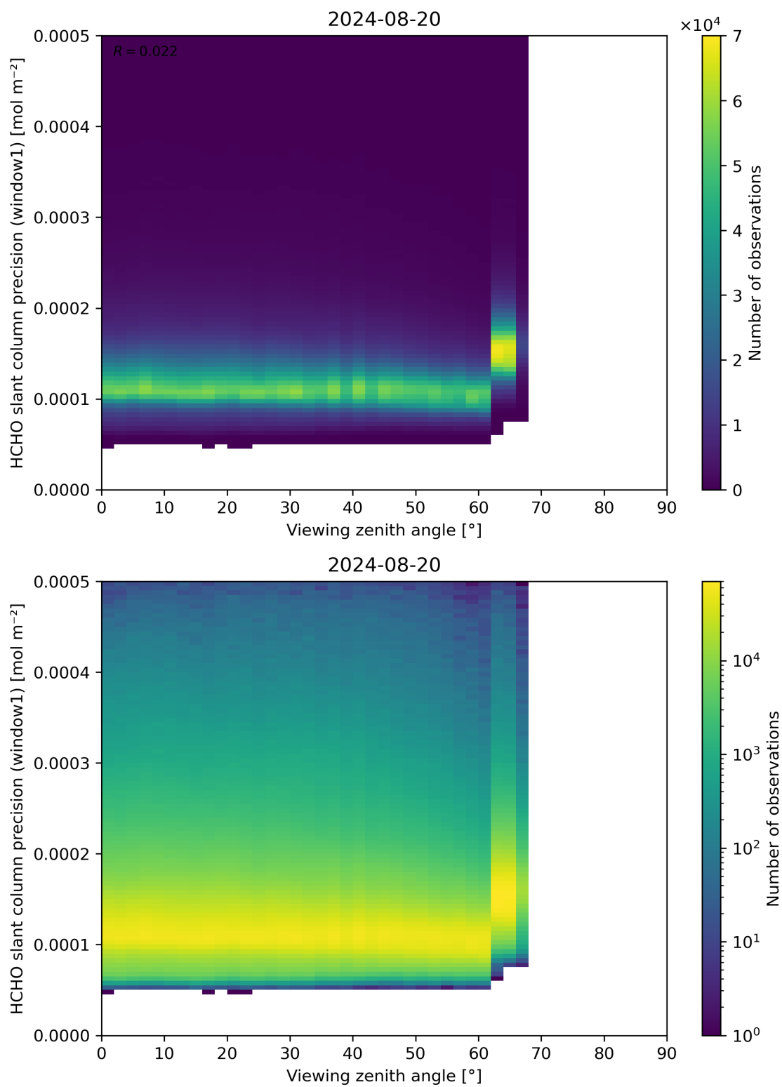
Figure 189: Scatter density plot of “Viewing zenith angle” against “HCHO slant column precision (window1)” for 2024-08-19 to 2024-08-21.
