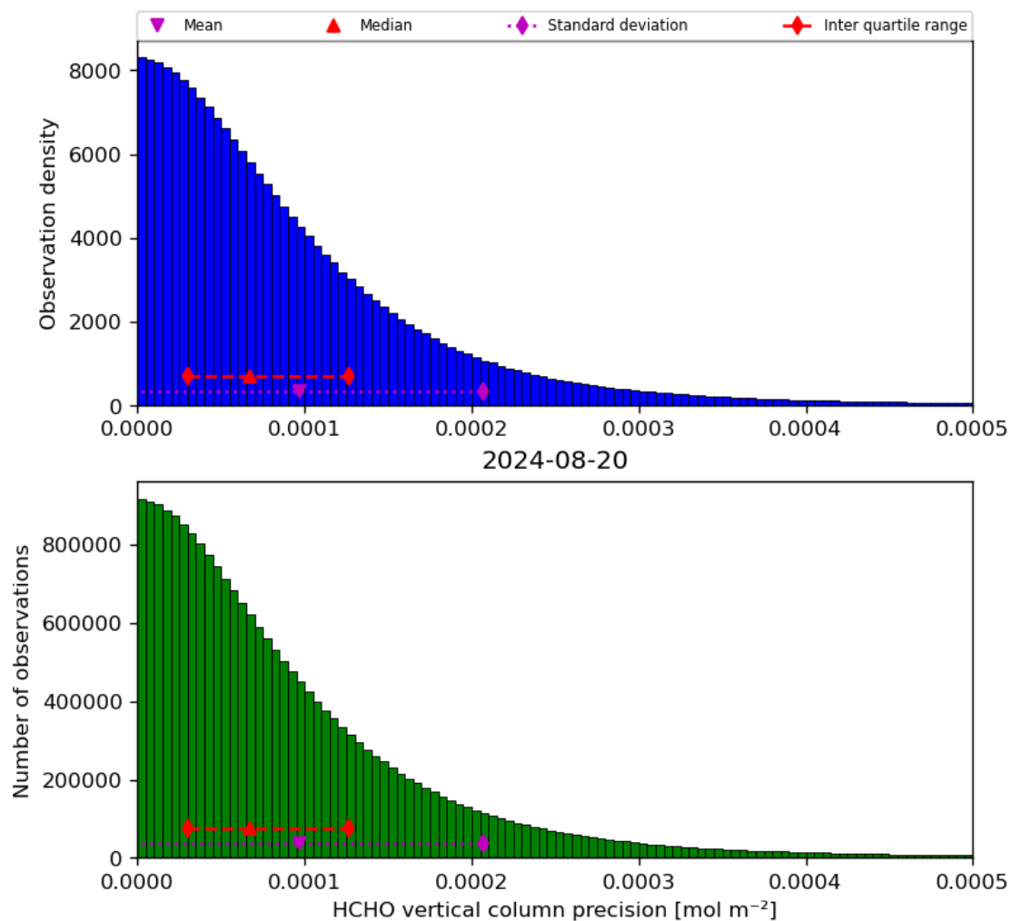
Figure 36: Histogram of “HCHO vertical column precision” for 2024-08-19 to 2024-08-21
