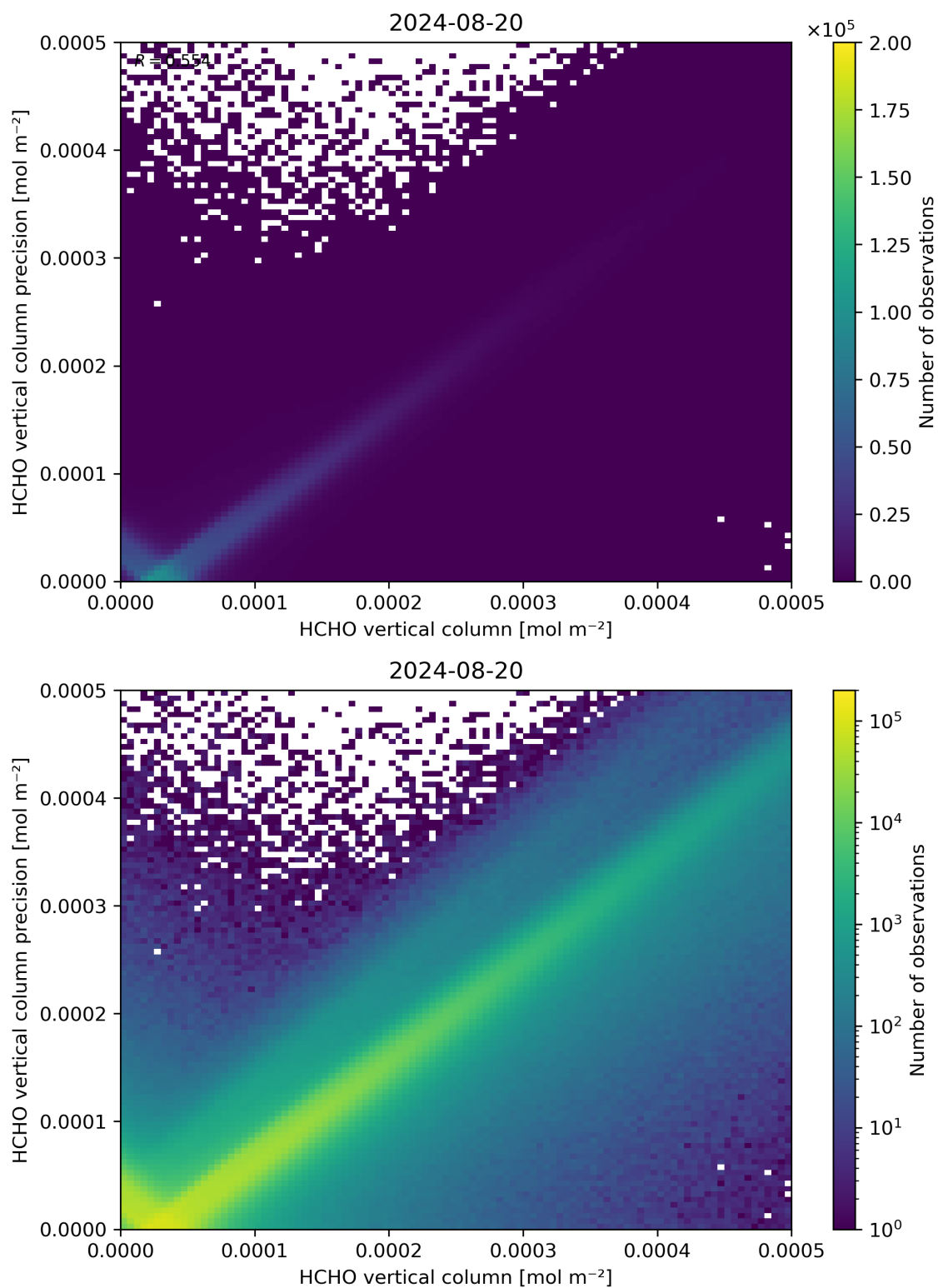
Figure 134: Scatter density plot of “HCHO vertical column” against “HCHO vertical column precision” for 2024-08-19 to 2024-08-21.
