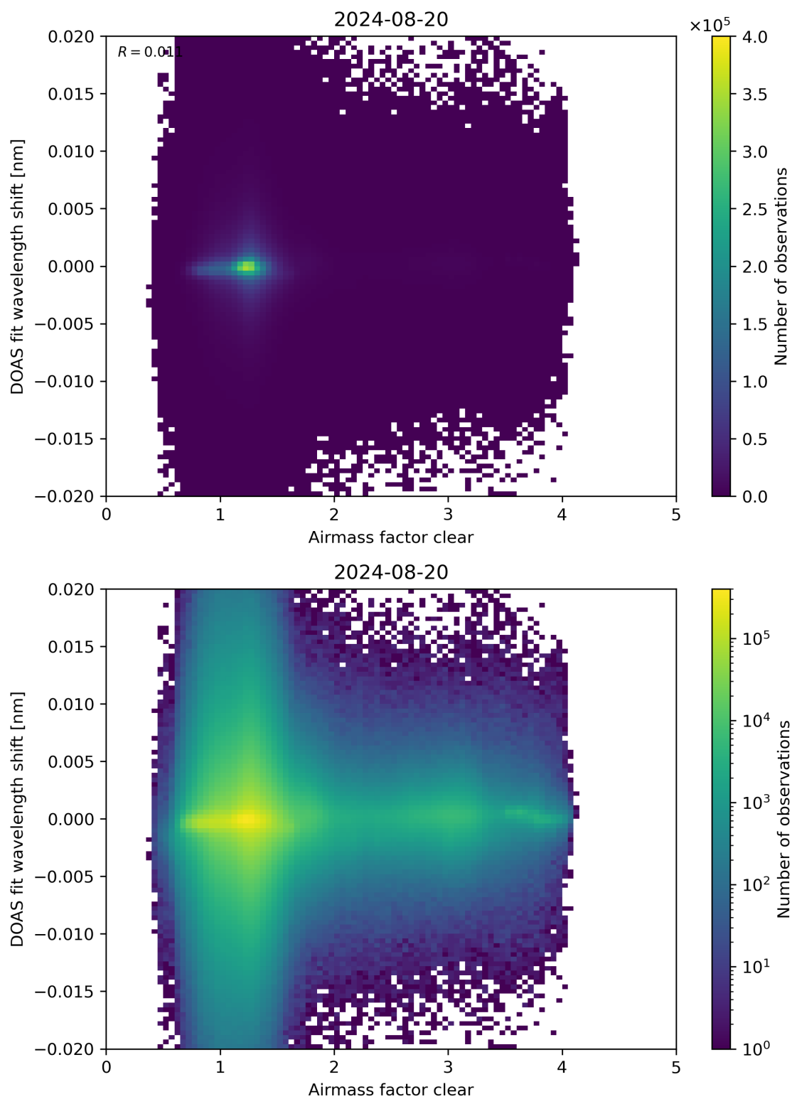
Figure 72: Scatter density plot of “Airmass factor clear” against “DOAS fit wavelength shift” for 2024-08-19 to 2024-08-21.
