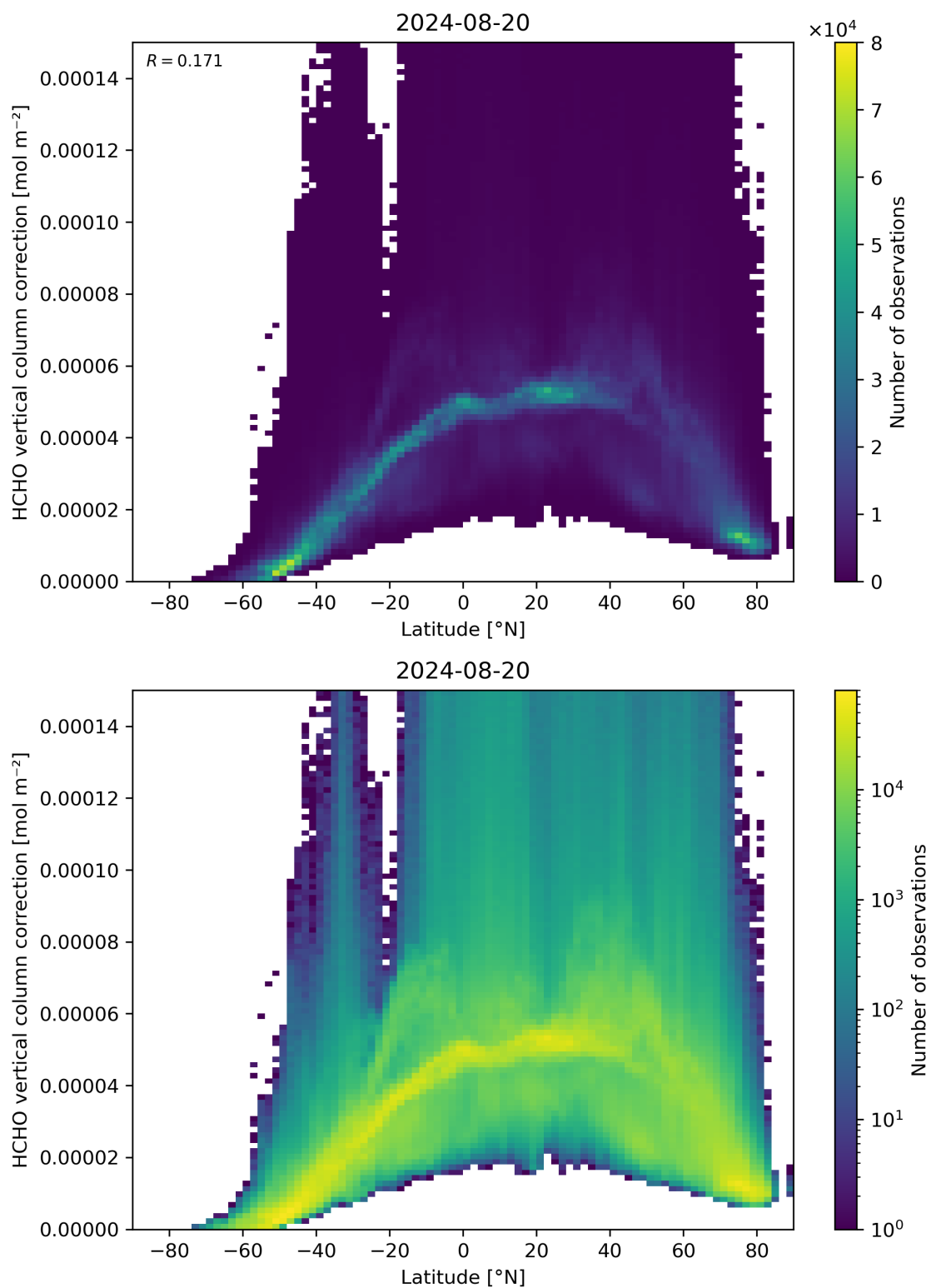
Figure 164: Scatter density plot of “Latitude” against “HCHO vertical column correction” for 2024-08-19 to 2024-08-21.
