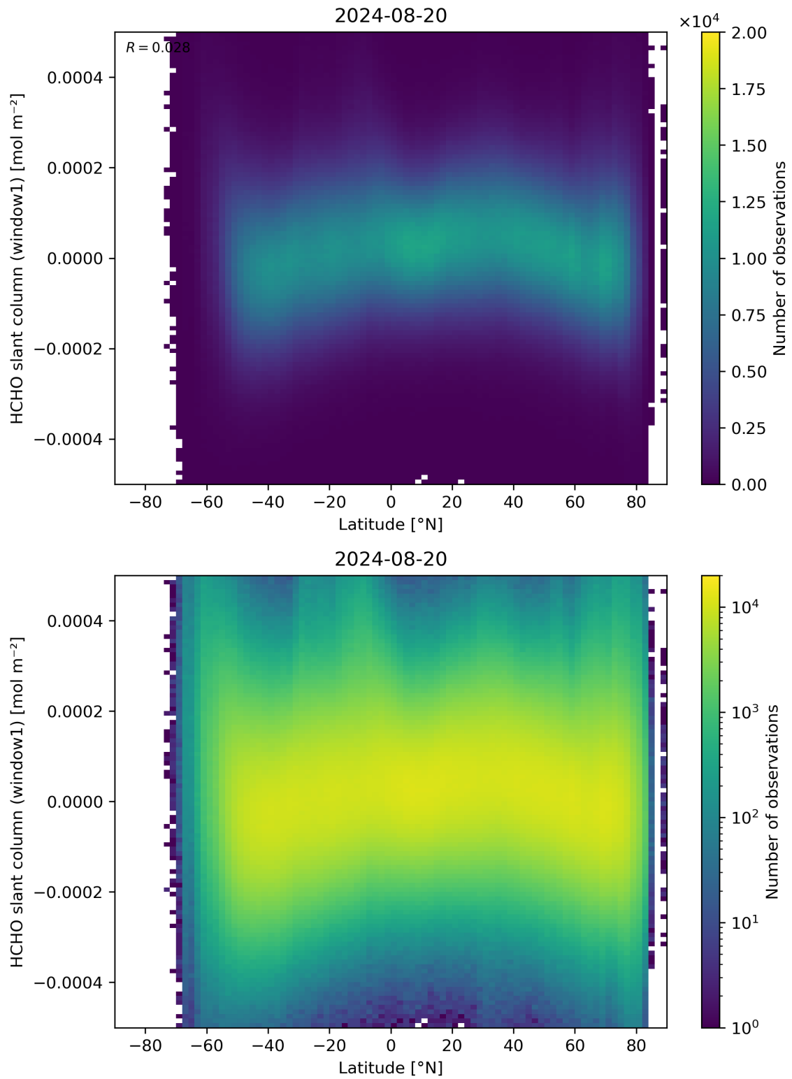
Figure 159: Scatter density plot of “Latitude” against “HCHO slant column (window1)” for 2024-08-19 to 2024-08-21.
