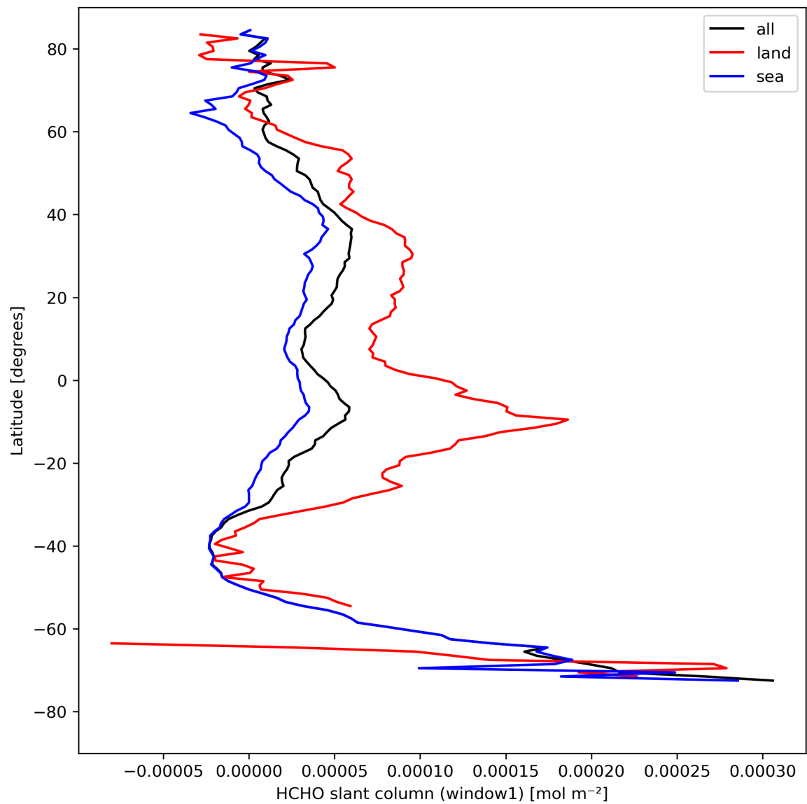
Figure 24: Zonal average of “HCHO slant column (window1)” for 2024-08-19 to 2024-08-21.
