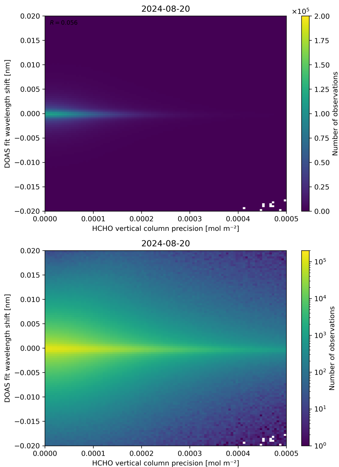
Figure 137: Scatter density plot of “HCHO vertical column precision” against “DOAS fit wavelength shift” for 2024-08-19 to 2024-08-21.
