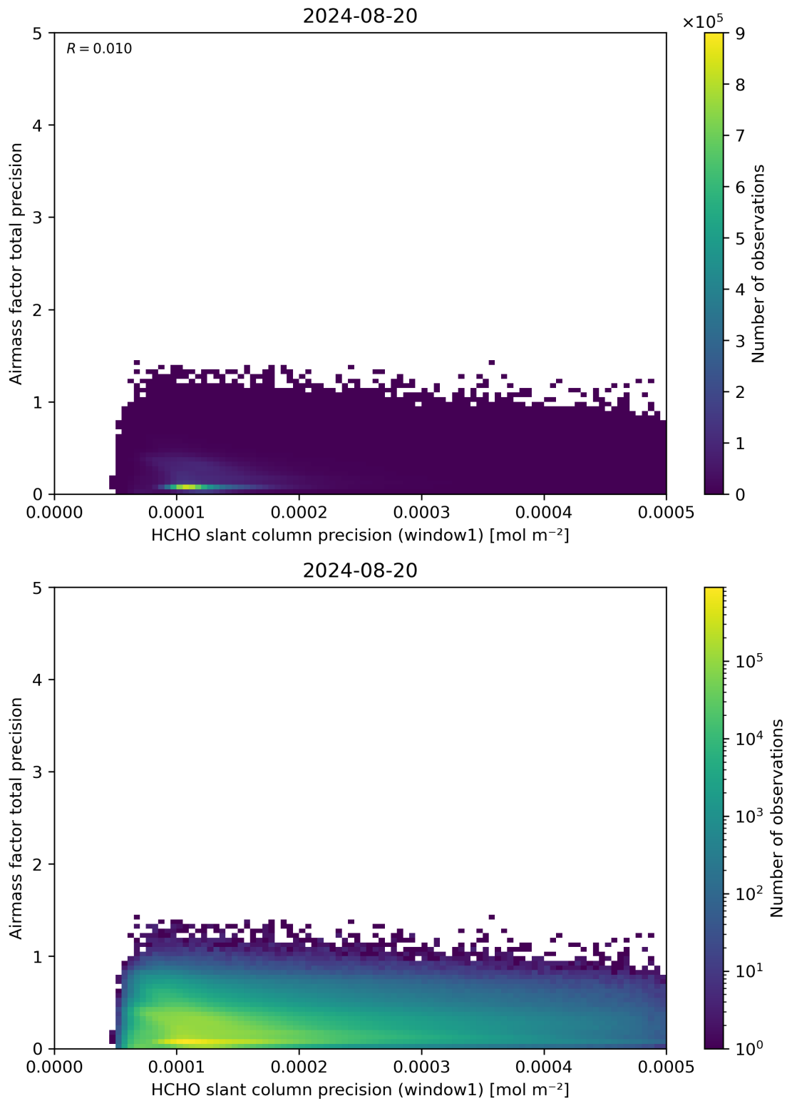
Figure 95: Scatter density plot of “HCHO slant column precision (window1)” against “Airmass factor total precision” for 2024-08-19 to 2024-08-21.
