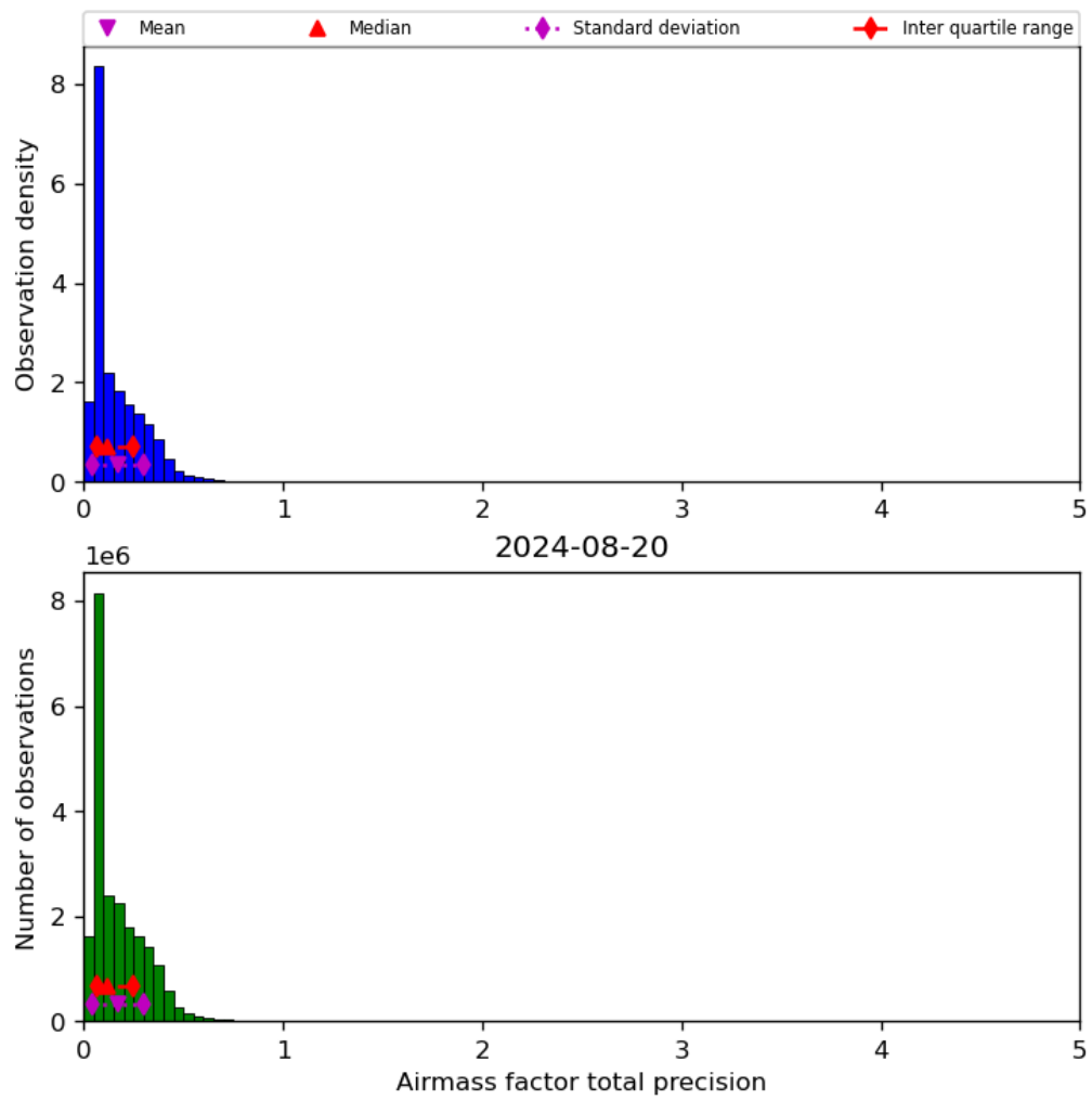
Figure 41: Histogram of "Airmass factor total precision" for 2024-08-19 to 2024-08-21
