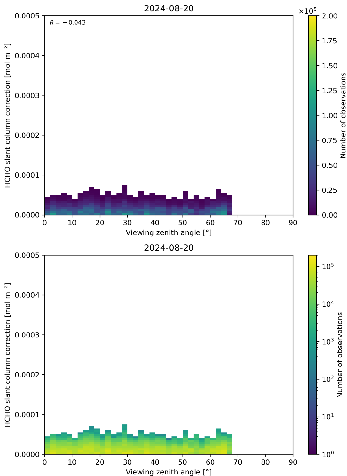
Figure 187: Scatter density plot of “Viewing zenith angle” against “HCHO slant column correction” for 2024-08-19 to 2024-08-21.
