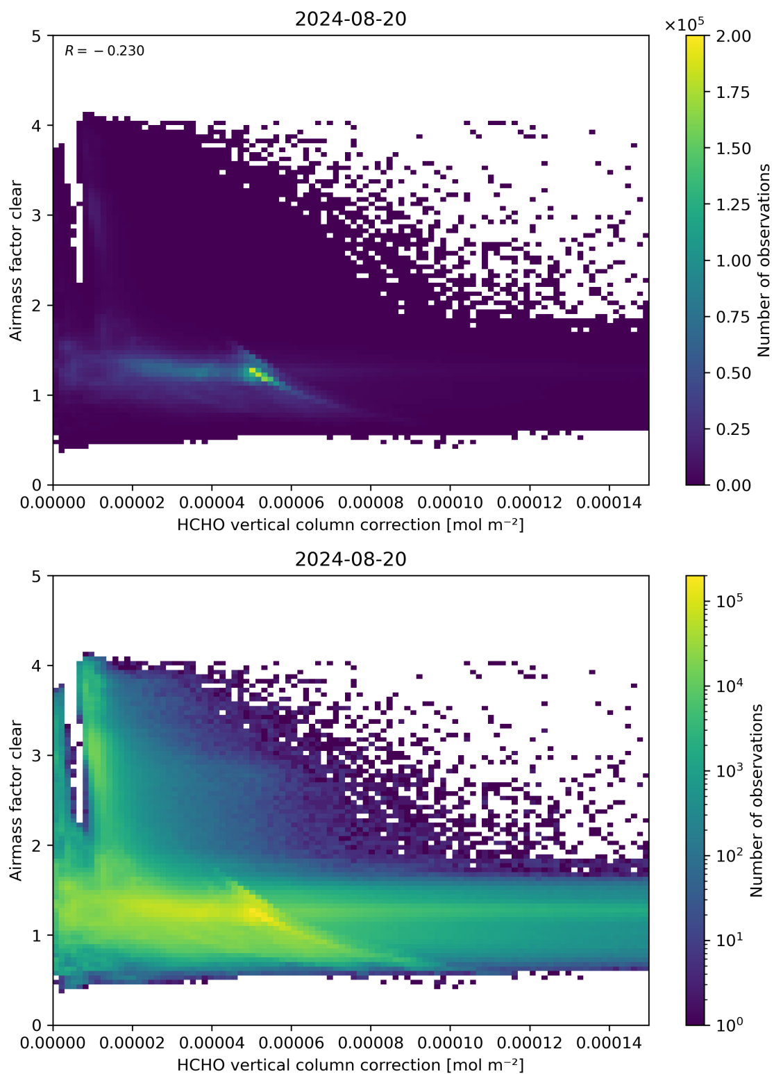
Figure 115: Scatter density plot of “HCHO vertical column correction” against “Airmass factor clear” for 2024-08-19 to 2024-08-21.
