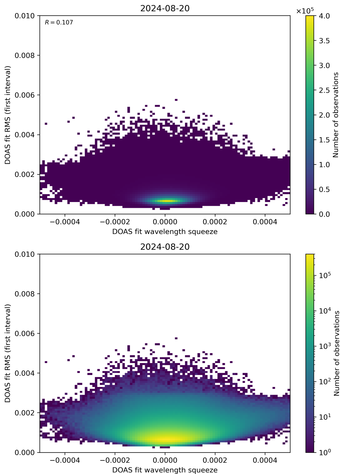
Figure 68: Scatter density plot of “DOAS fit wavelength squeeze” against “DOAS fit RMS (first interval)” for 2024-08-19 to 2024-08-21.
