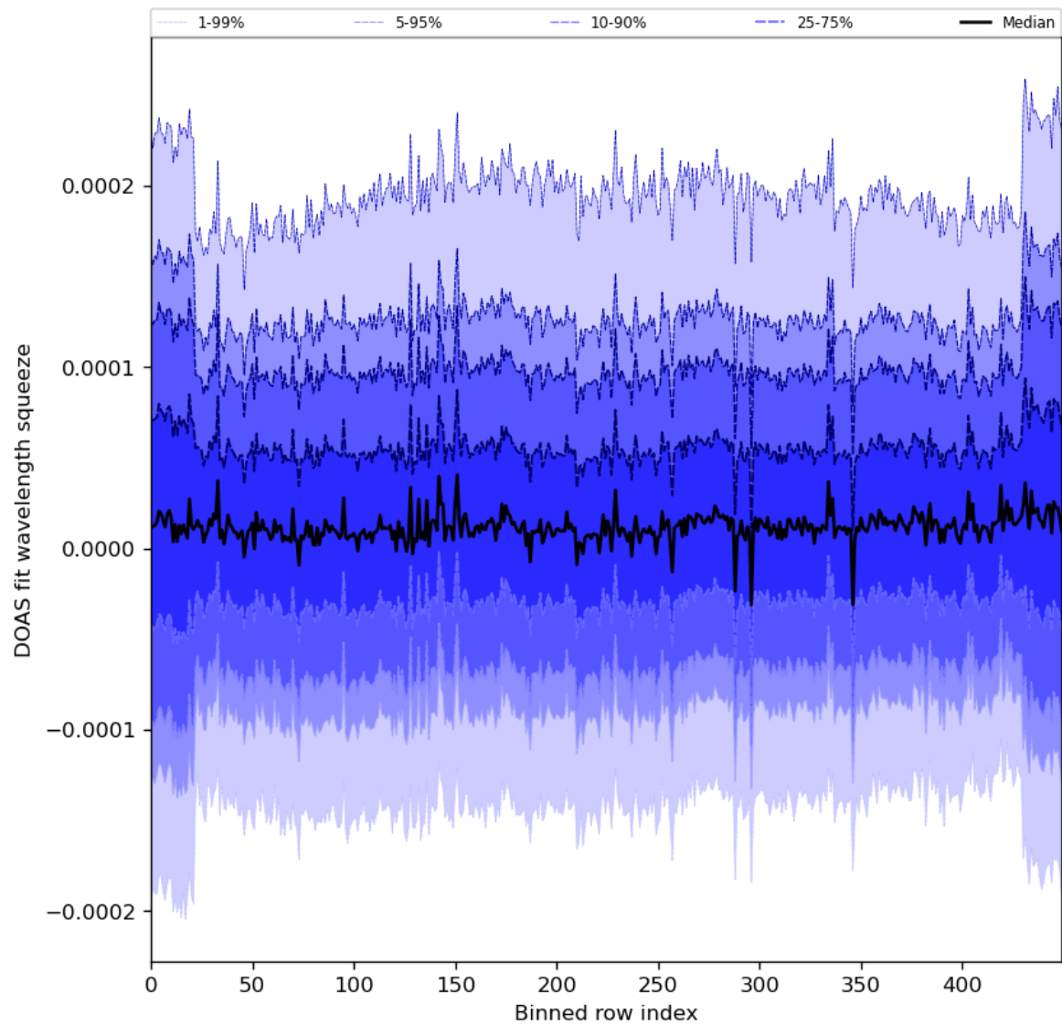
Figure 59: Along track statistics of “DOAS fit wavelength squeeze” for 2024-08-19 to 2024-08-21
