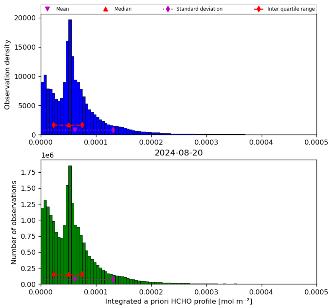
Figure 43: Histogram of “Integrated a priori HCHO profile” for 2024-08-19 to 2024-08-21
