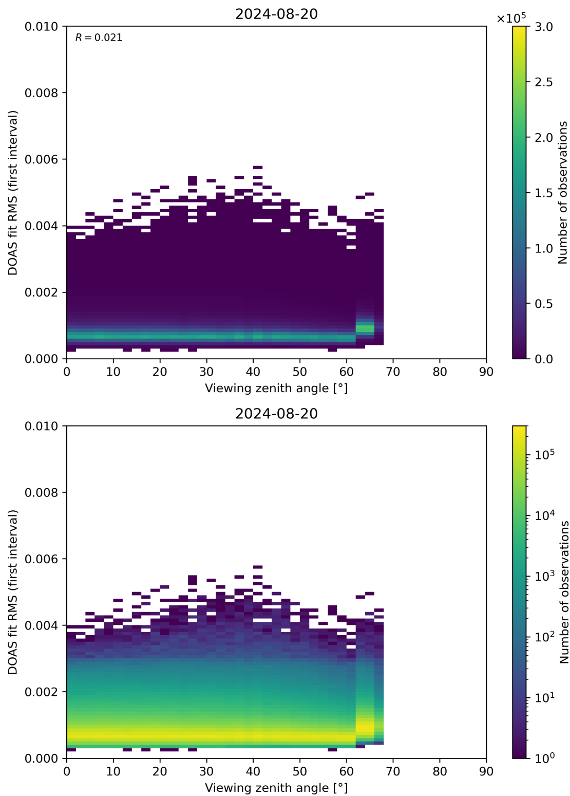
Figure 182: Scatter density plot of “Viewing zenith angle” against “DOAS fit RMS (first interval)” for 2024-08-19 to 2024-08-21.
