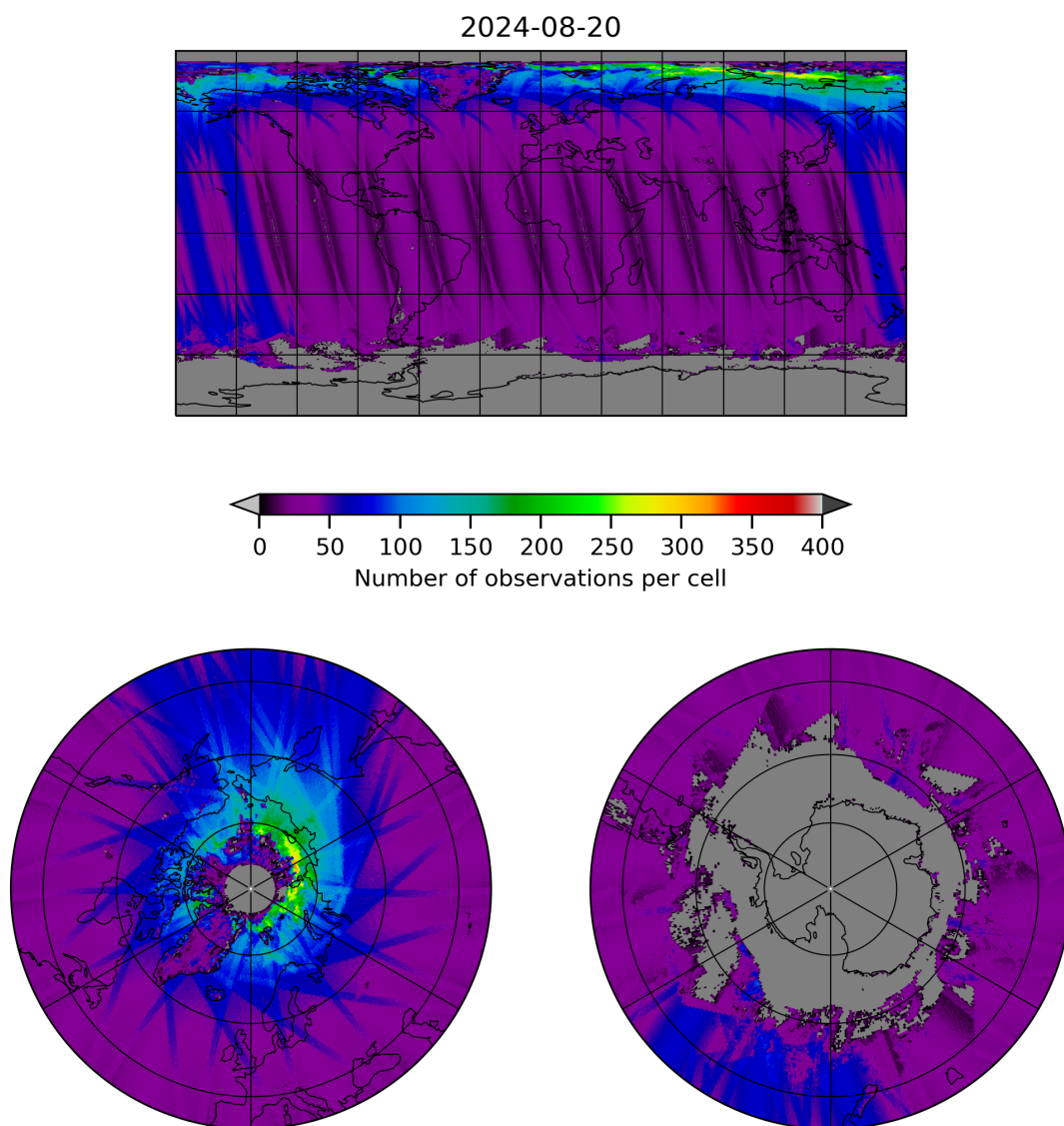
Figure 19: Map of the number of observations for 2024-08-19 to 2024-08-21
