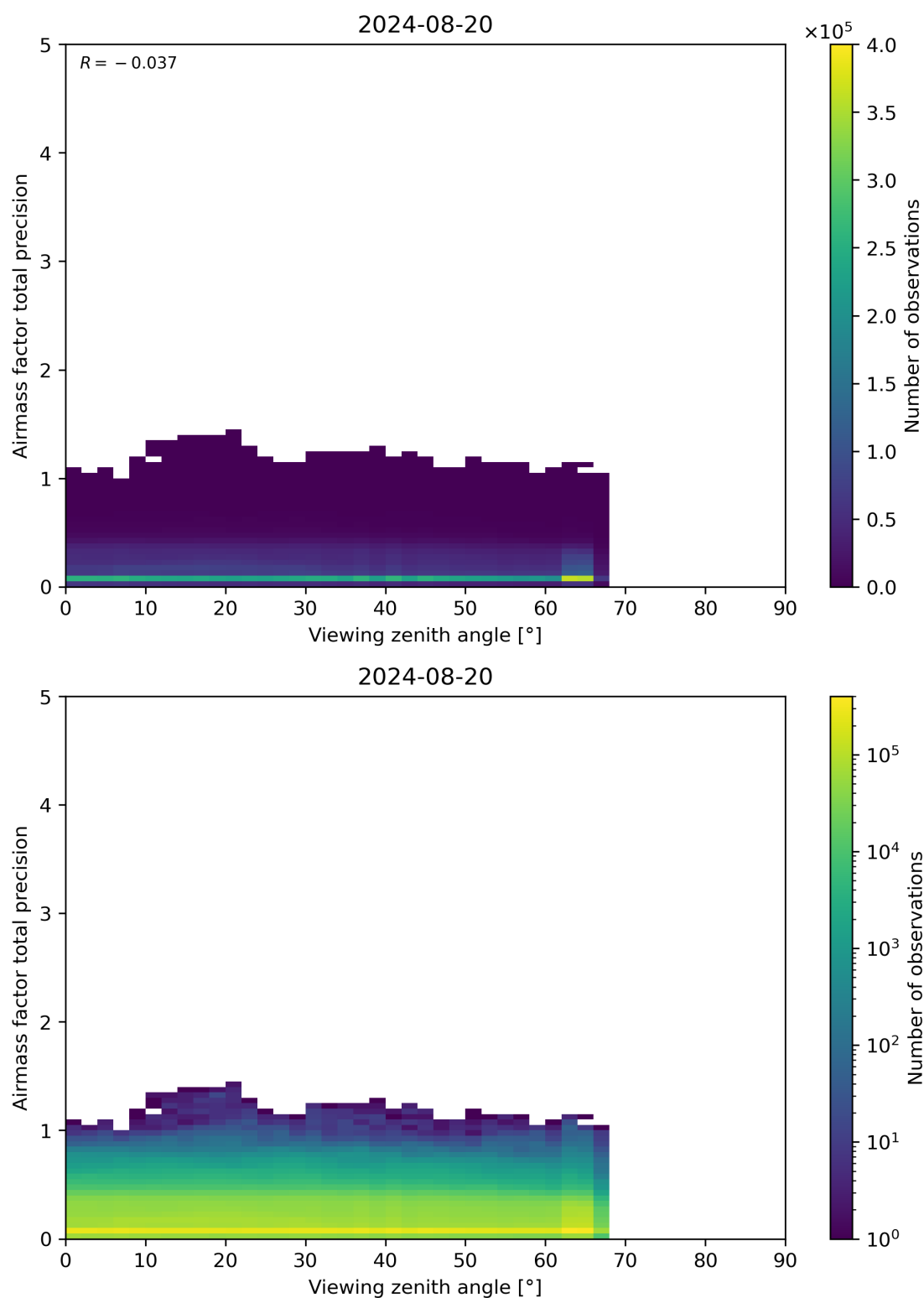
Figure 191: Scatter density plot of “Viewing zenith angle” against “Airmass factor total precision” for 2024-08-19 to 2024-08-21.
