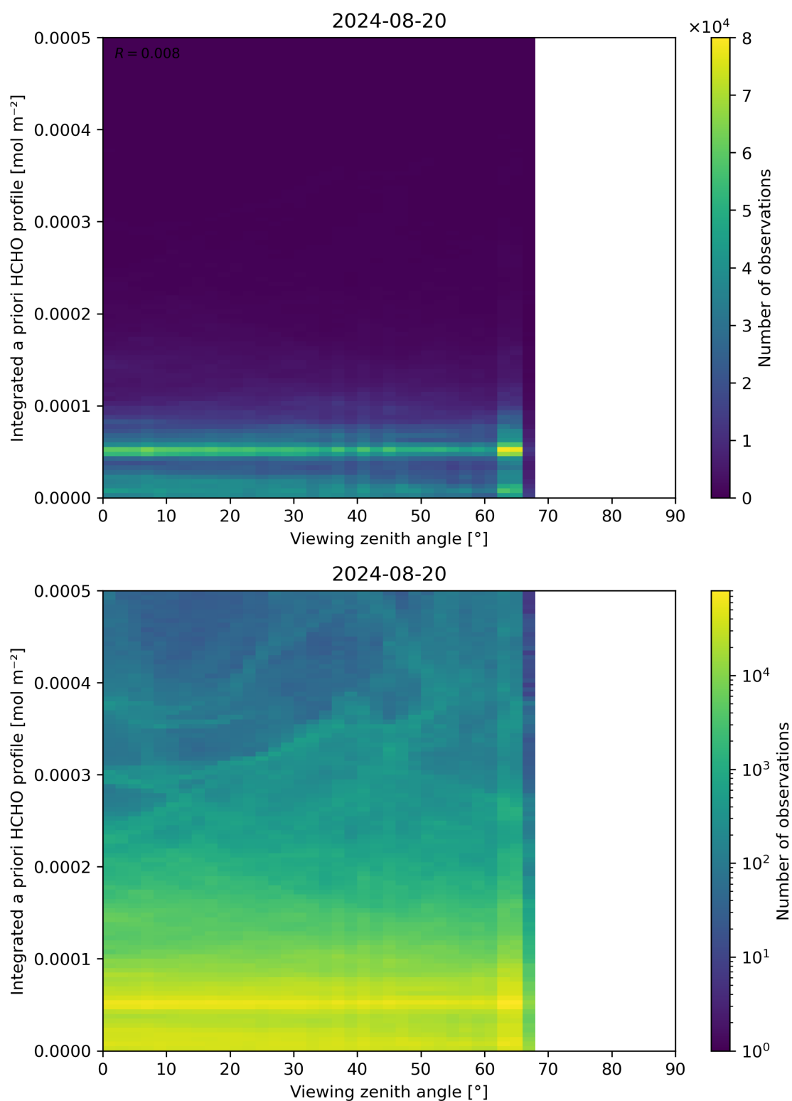
Figure 195: Scatter density plot of “Viewing zenith angle” against “Integrated a priori HCHO profile” for 2024-08-19 to 2024-08-21.
