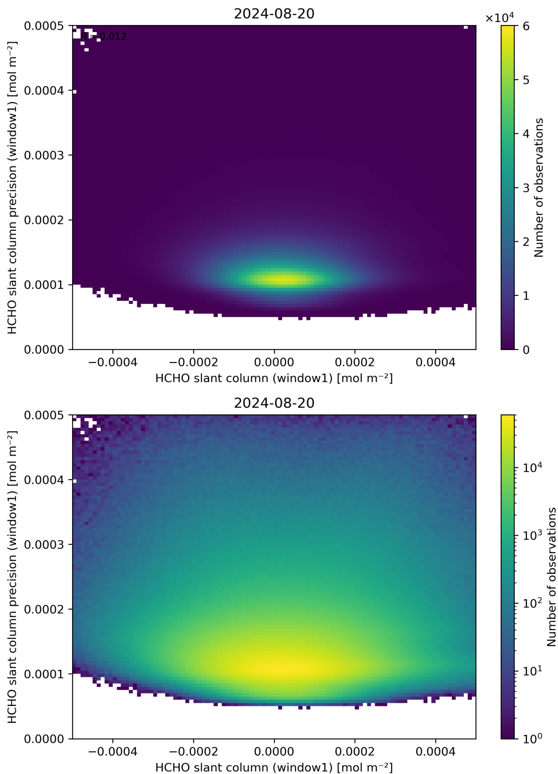
Figure 84: Scatter density plot of “HCHO slant column (window1)” against “HCHO slant column precision (window1)” for 2024-08-19 to 2024-08-21.
