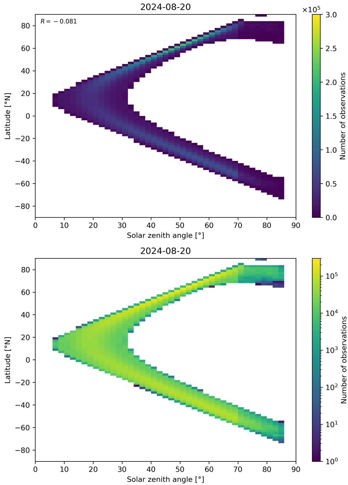
Figure 181: Scatter density plot of “Solar zenith angle” against “Latitude” for 2024-08-19 to 2024-08-21.
