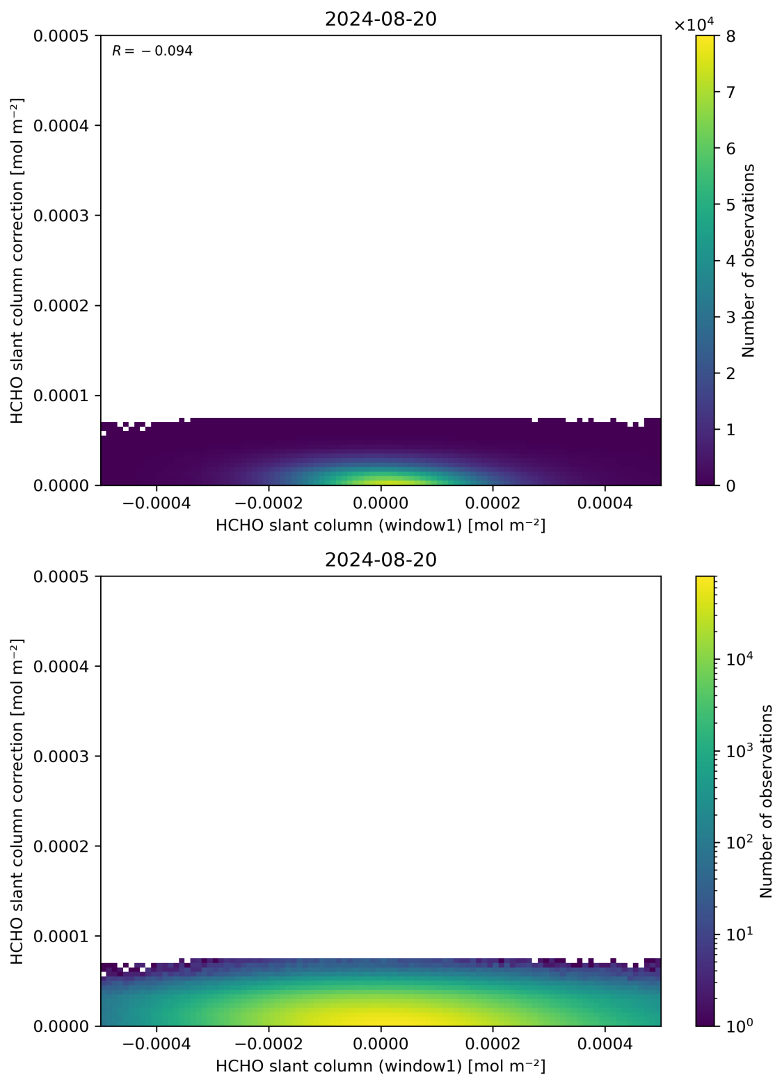
Figure 83: Scatter density plot of “HCHO slant column (window1)” against “HCHO slant column correction” for 2024-08-19 to 2024-08-21.
