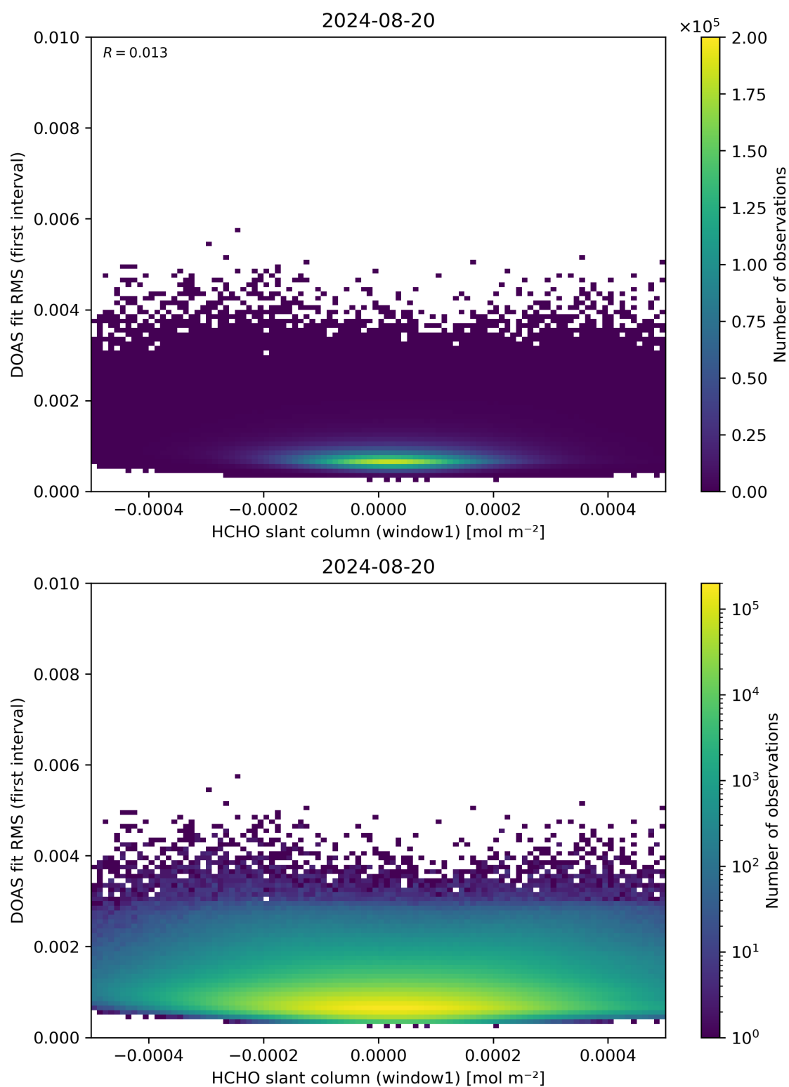
Figure 78: Scatter density plot of “HCHO slant column (window1)” against “DOAS fit RMS (first interval)” for 2024-08-19 to 2024-08-21.
