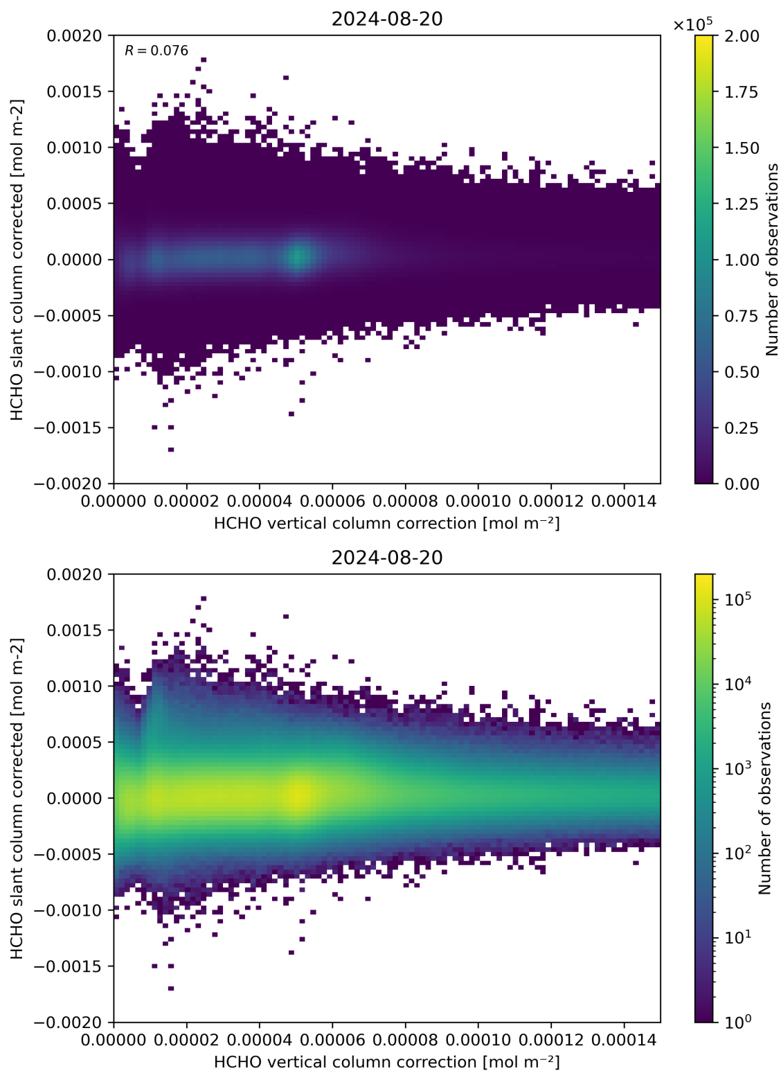
Figure 116: Scatter density plot of “HCHO vertical column correction” against “HCHO slant column corrected” for 2024-08-19 to 2024-08-21.
