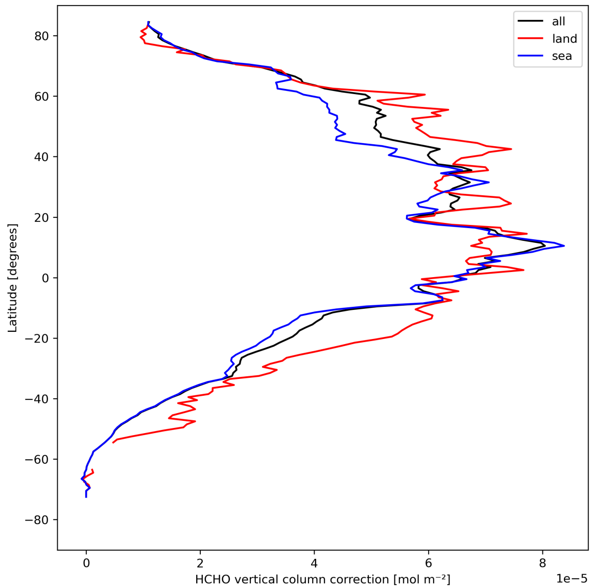
Figure 23: Zonal average of “HCHO vertical column correction” for 2024-08-19 to 2024-08-21.
