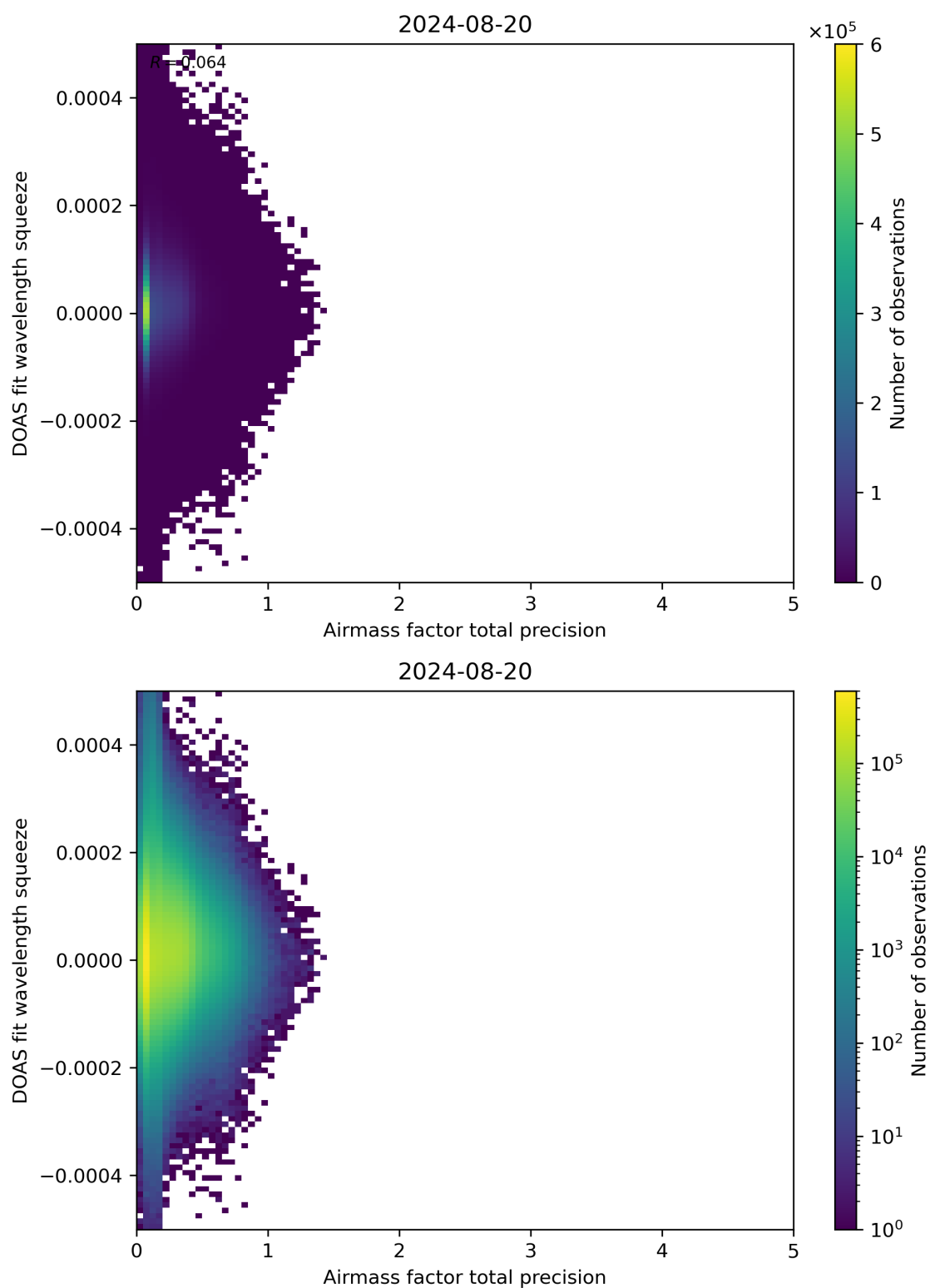
Figure 107: Scatter density plot of “Airmass factor total precision” against “DOAS fit wavelength squeeze” for 2024-08-19 to 2024-08-21.
