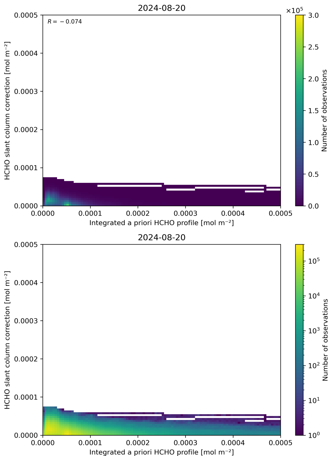
Figure 152: Scatter density plot of “Integrated a priori HCHO profile” against “HCHO slant column correction” for 2024-08-19 to 2024-08-21.
