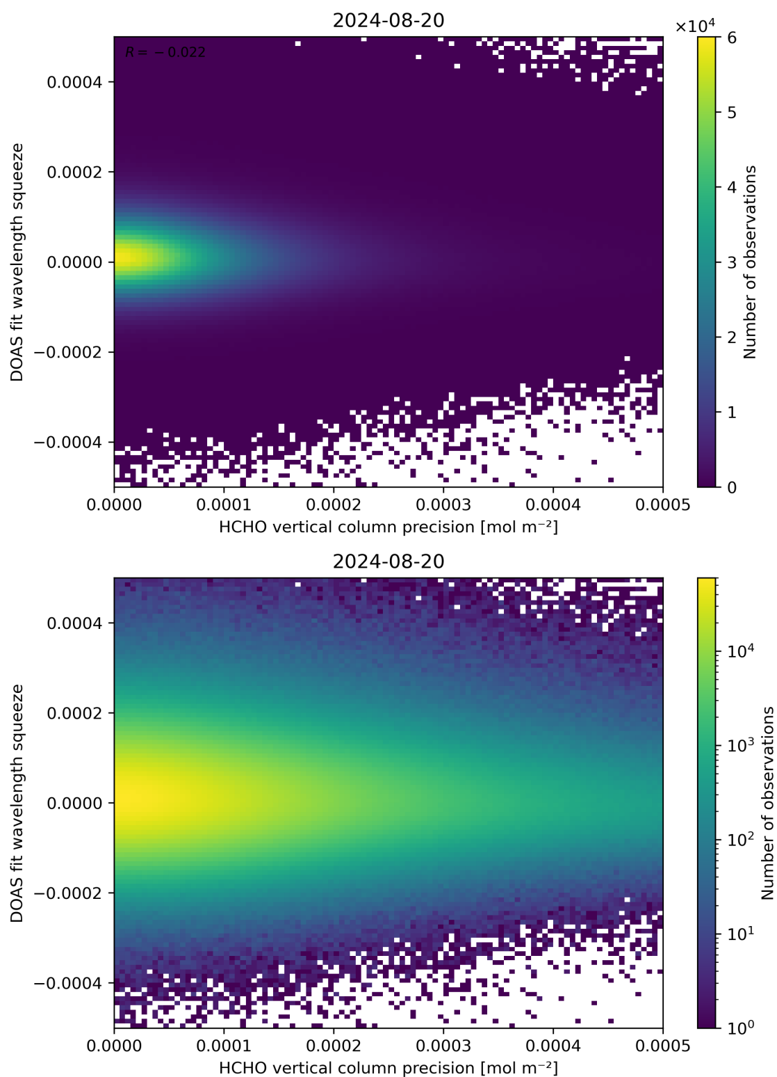
Figure 138: Scatter density plot of “HCHO vertical column precision” against “DOAS fit wavelength squeeze” for 2024-08-19 to 2024-08-21.
