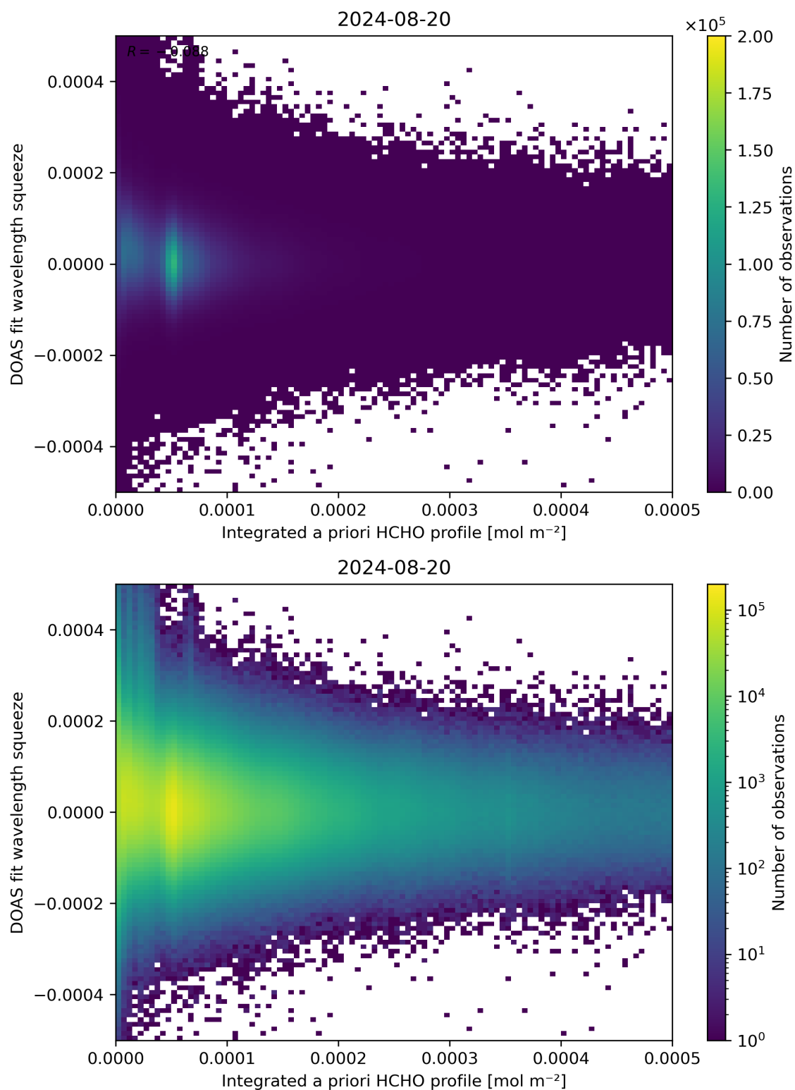
Figure 150: Scatter density plot of “Integrated a priori HCHO profile” against “DOAS fit wavelength squeeze” for 2024-08-19 to 2024-08-21.
