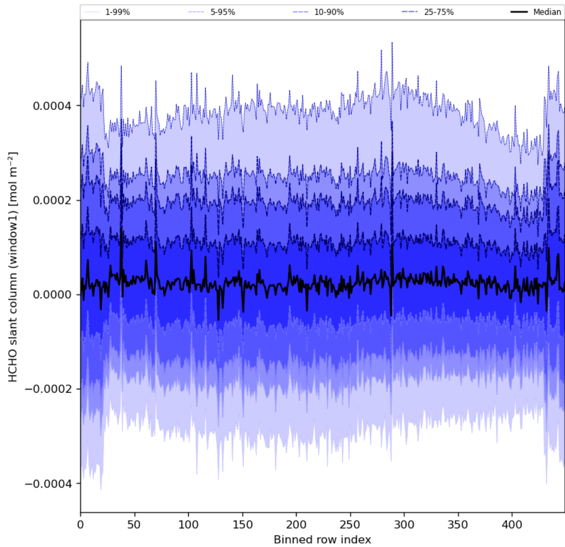
Figure 52: Along track statistics of “HCHO slant column (window1)” for 2024-08-19 to 2024-08-21
