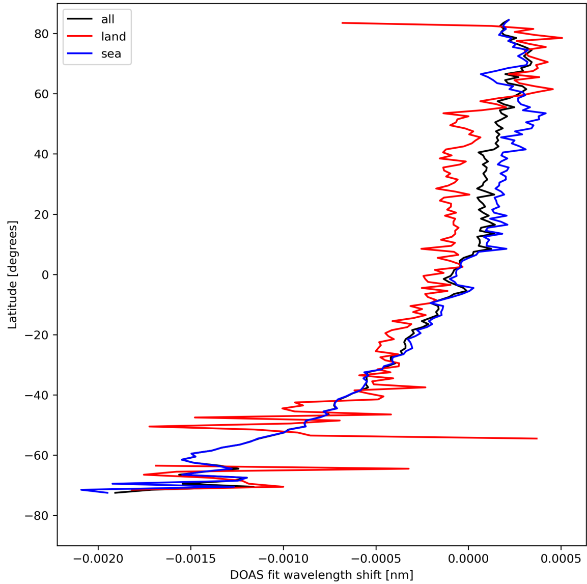
Figure 30: Zonal average of “DOAS fit wavelength shift” for 2024-08-19 to 2024-08-21.
