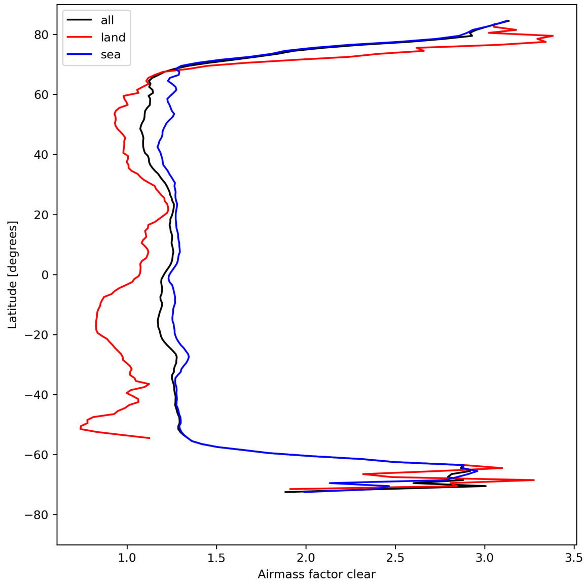
Figure 28: Zonal average of “Airmass factor clear” for 2024-08-19 to 2024-08-21.
