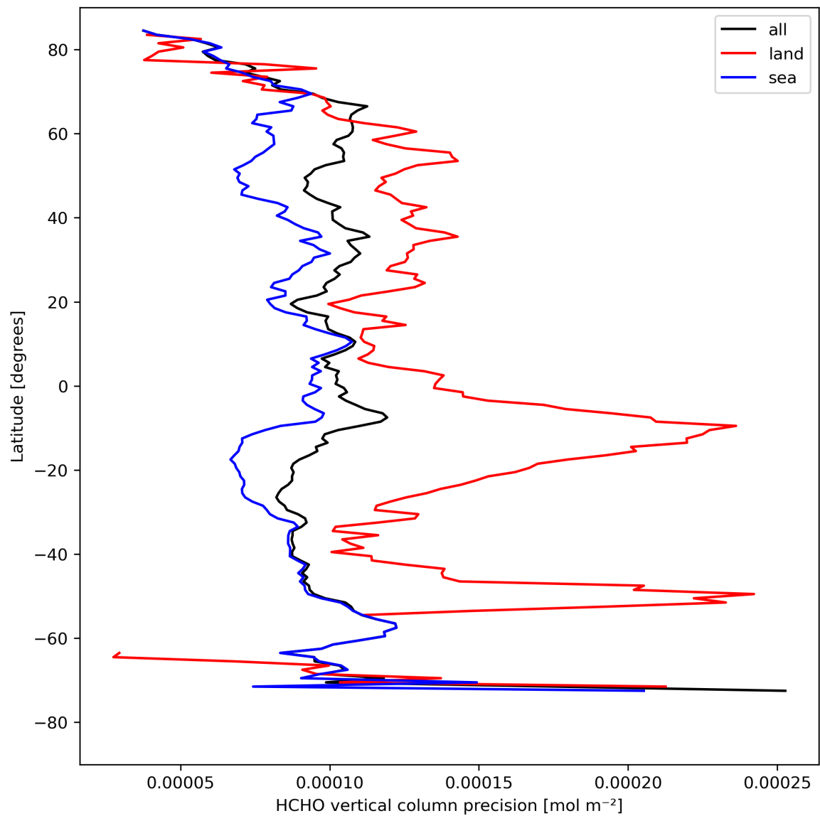
Figure 22: Zonal average of “HCHO vertical column precision” for 2024-08-19 to 2024-08-21.
