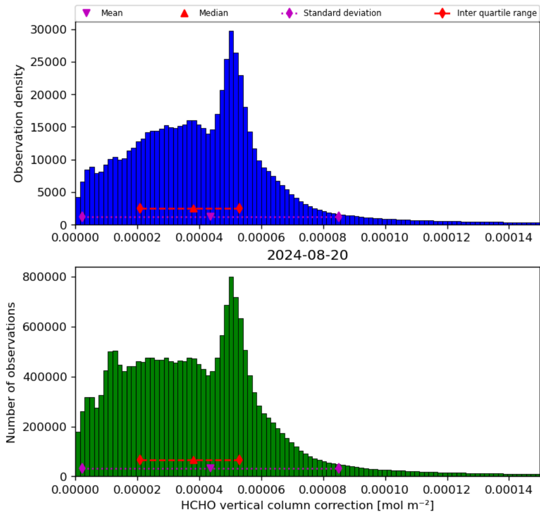
Figure 37: Histogram of “HCHO vertical column correction” for 2024-08-19 to 2024-08-21
