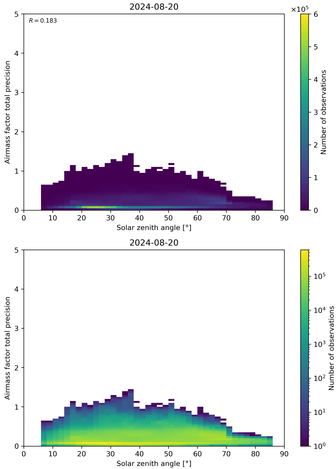
Figure 176: Scatter density plot of “Solar zenith angle” against “Airmass factor total precision” for 2024-08-19 to 2024-08-21.
