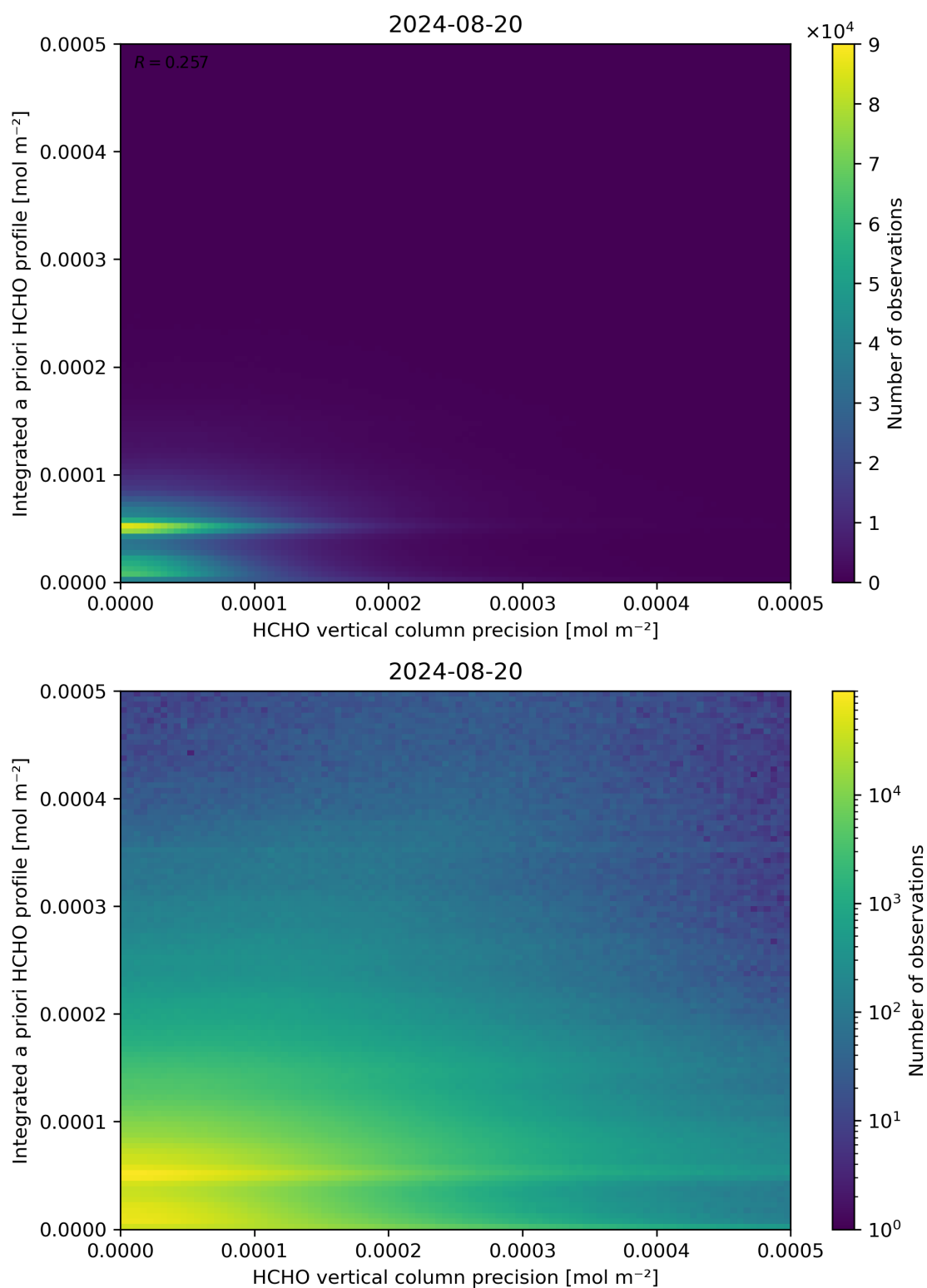
Figure 147: Scatter density plot of “HCHO vertical column precision” against “Integrated a priori HCHO profile” for 2024-08-19 to 2024-08-21.
