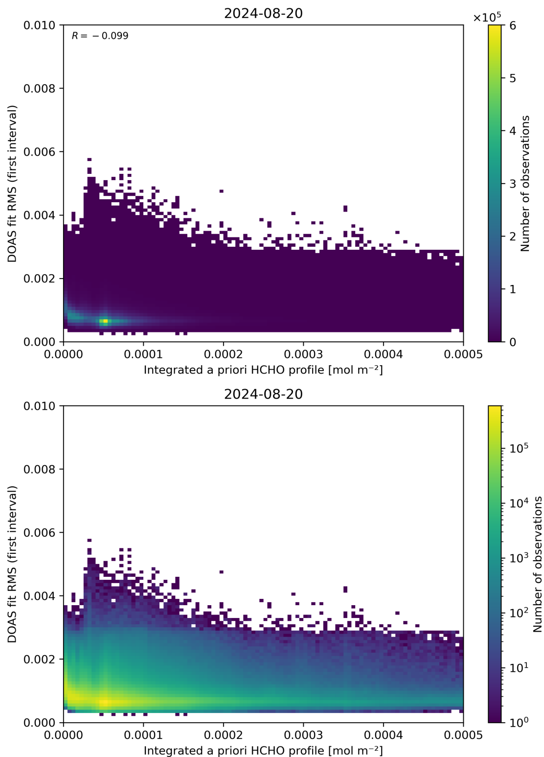
Figure 148: Scatter density plot of “Integrated a priori HCHO profile” against “DOAS fit RMS (first interval)” for 2024-08-19 to 2024-08-21.
