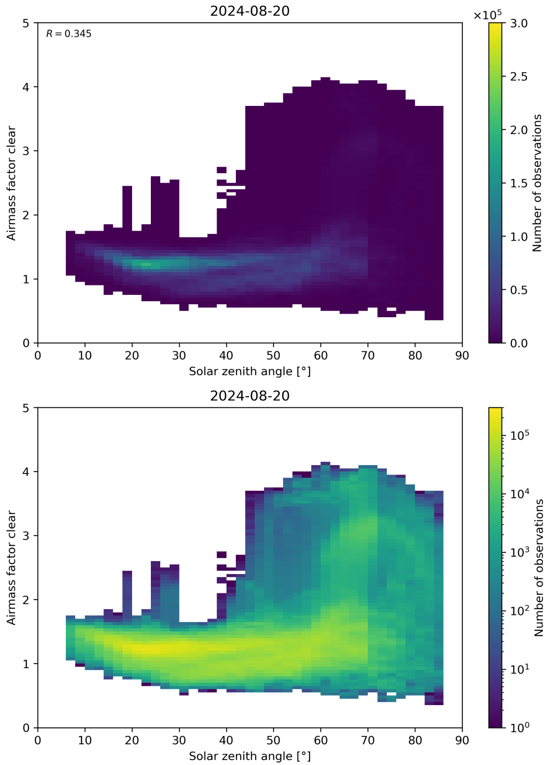
Figure 170: Scatter density plot of “Solar zenith angle” against “Airmass factor clear” for 2024-08-19 to 2024-08-21.
