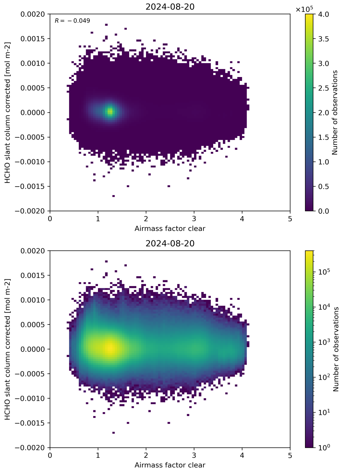
Figure 74: Scatter density plot of “Airmass factor clear” against “HCHO slant column corrected” for 2024-08-19 to 2024-08-21.
