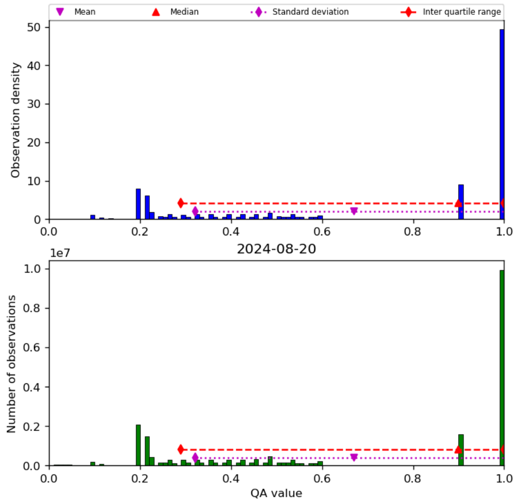
Figure 34: Histogram of “QA value” for 2024-08-19 to 2024-08-21
