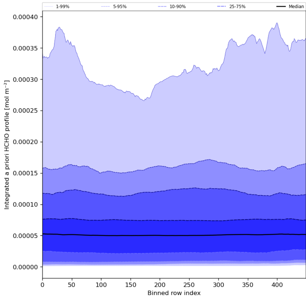
Figure 57: Along track statistics of "Integrated a priori HCHO profile" for 2024-08-19 to 2024-08-21
