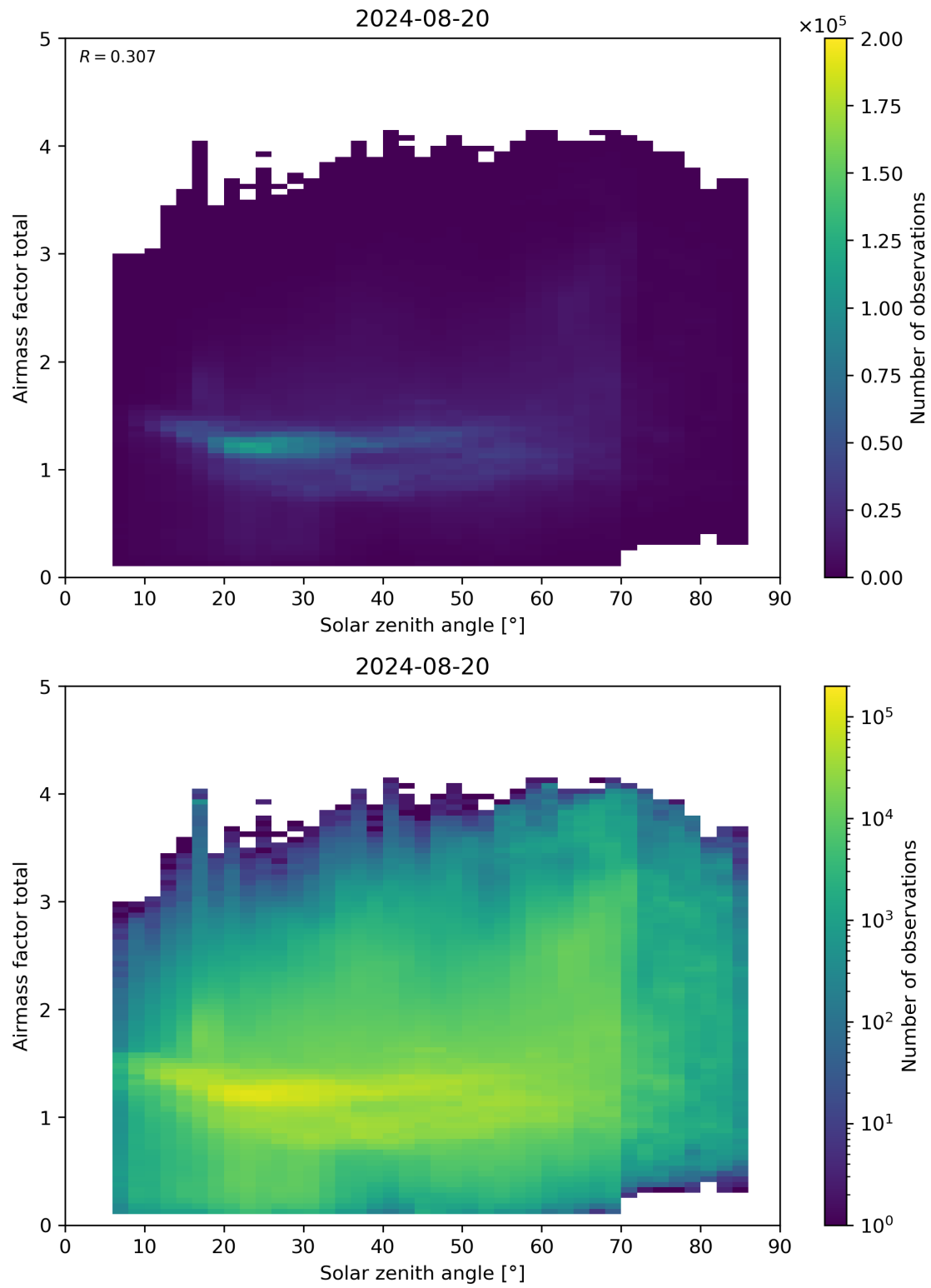
Figure 175: Scatter density plot of “Solar zenith angle” against “Airmass factor total” for 2024-08-19 to 2024-08-21.
