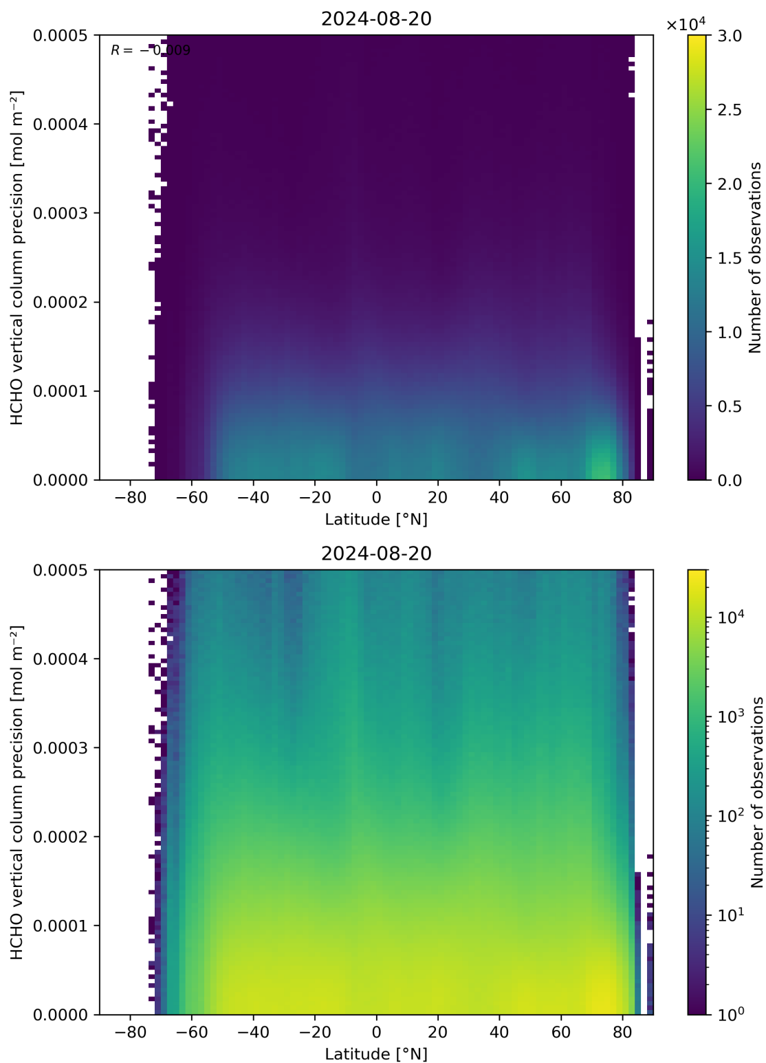
Figure 165: Scatter density plot of “Latitude” against “HCHO vertical column precision” for 2024-08-19 to 2024-08-21.
