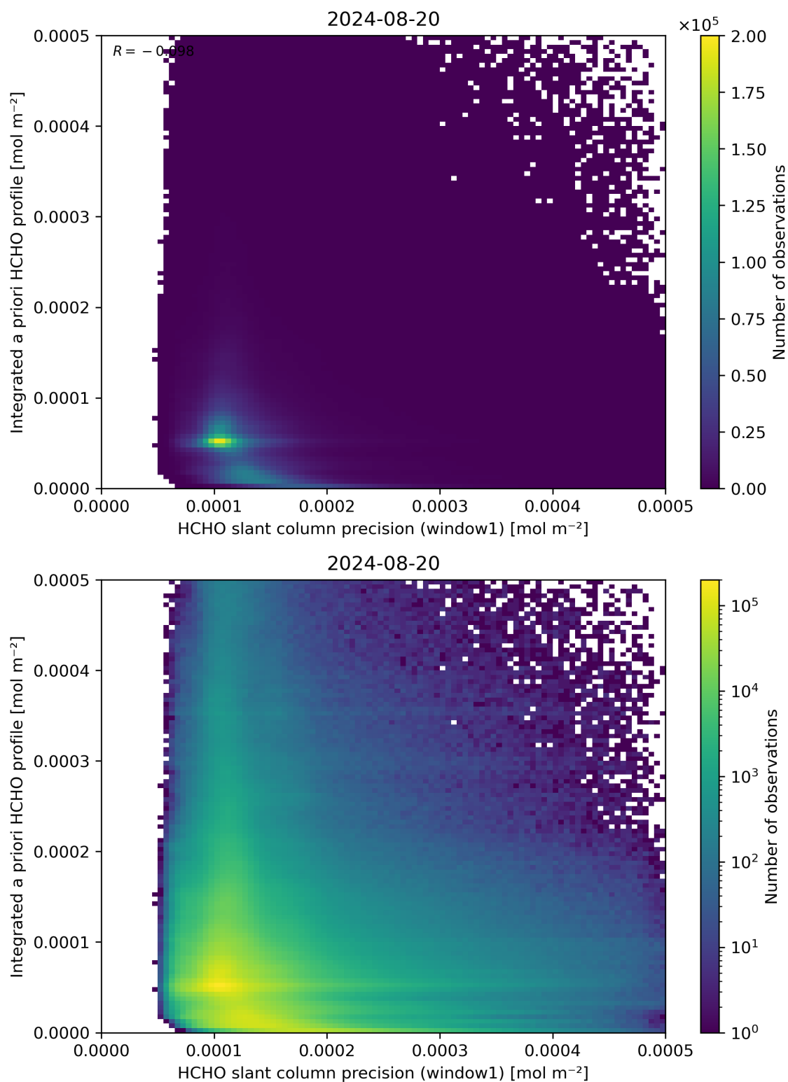
Figure 96: Scatter density plot of “HCHO slant column precision (window1)” against “Integrated a priori HCHO profile” for 2024-08-19 to 2024-08-21.
