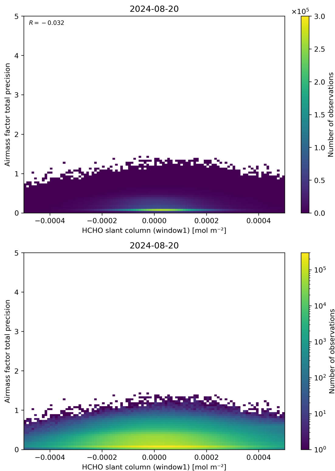
Figure 86: Scatter density plot of “HCHO slant column (window1)” against “Airmass factor total precision” for 2024-08-19 to 2024-08-21.
