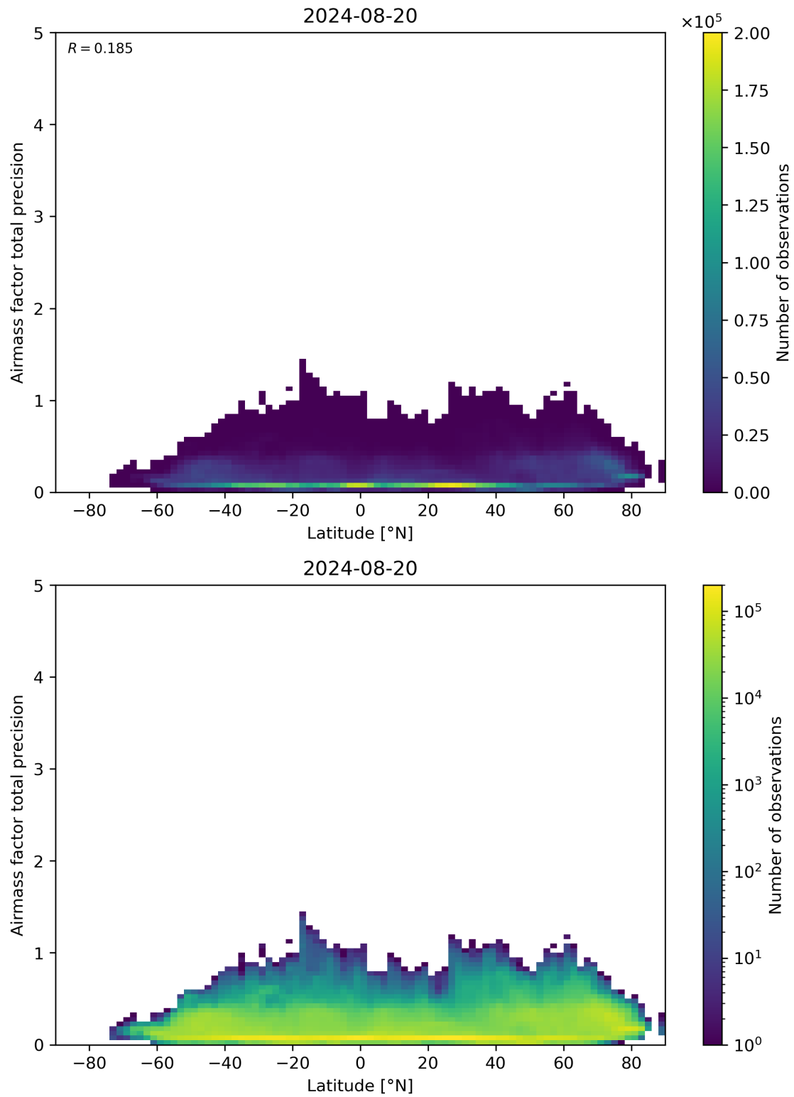
Figure 162: Scatter density plot of “Latitude” against “Airmass factor total precision” for 2024-08-19 to 2024-08-21.
