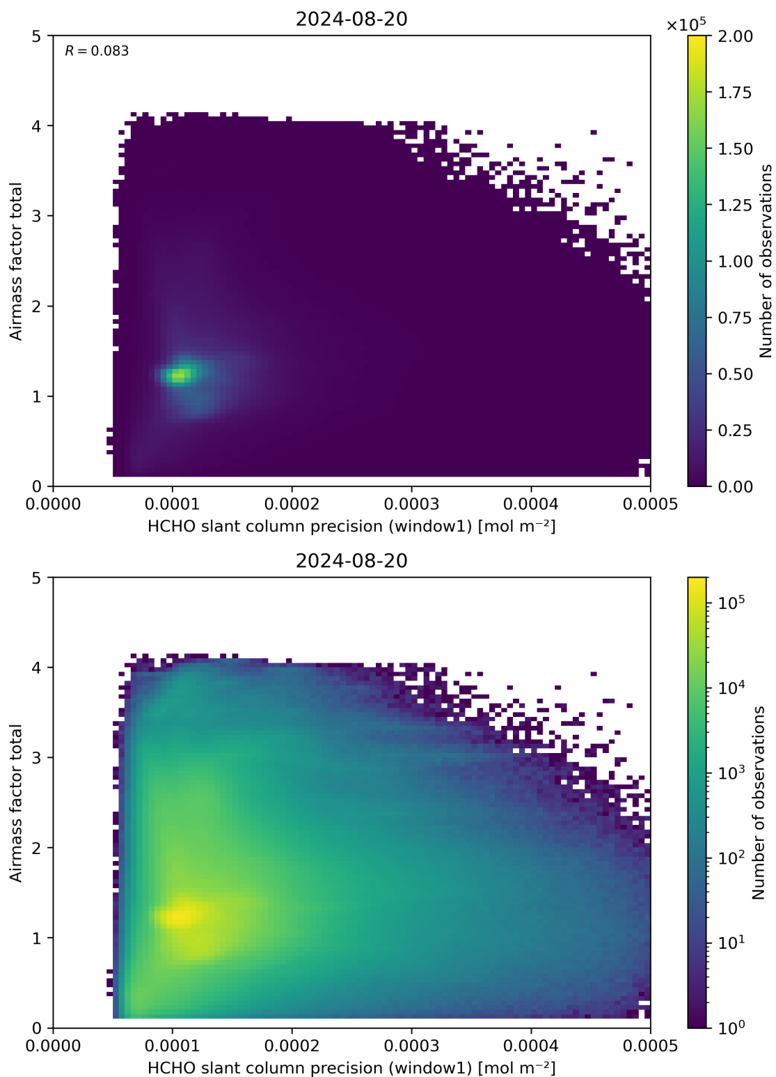
Figure 94: Scatter density plot of “HCHO slant column precision (window1)” against “Airmass factor total” for 2024-08-19 to 2024-08-21.
