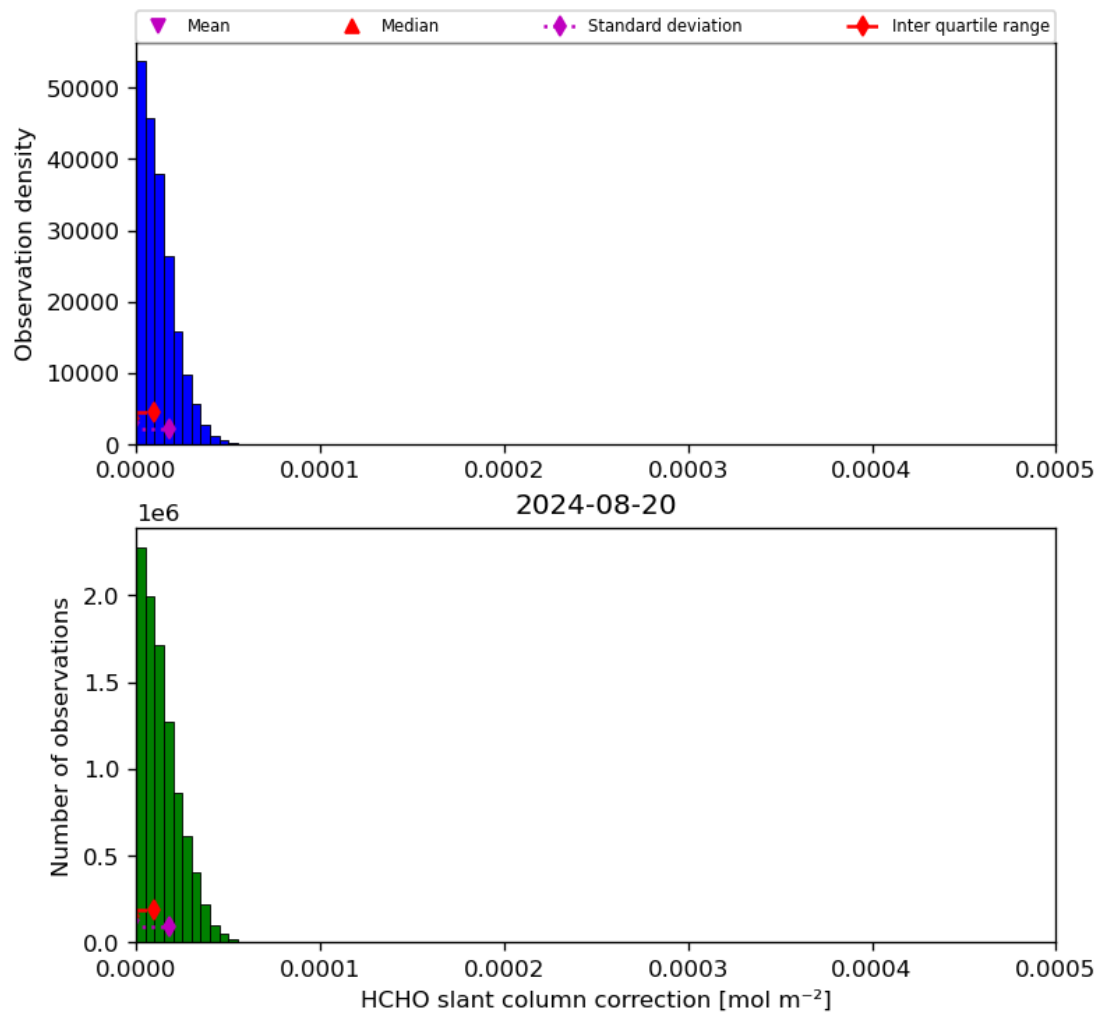
Figure 47: Histogram of “HCHO slant column correction” for 2024-08-19 to 2024-08-21
