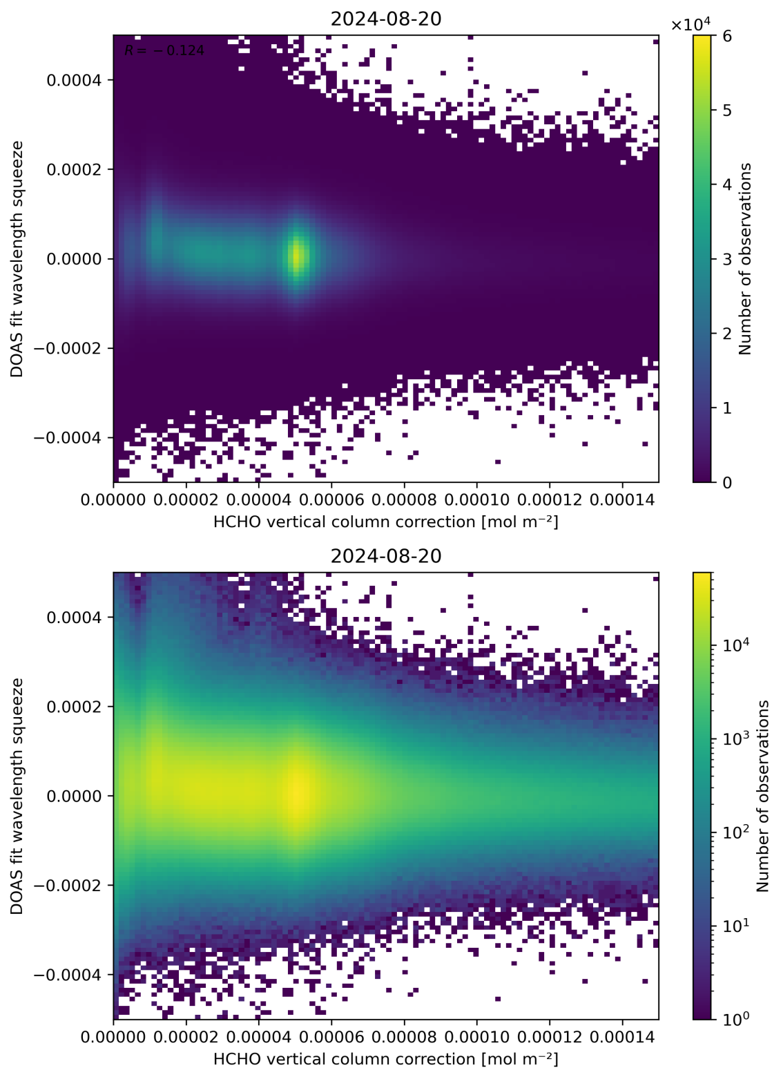
Figure 114: Scatter density plot of “HCHO vertical column correction” against “DOAS fit wavelength squeeze” for 2024-08-19 to 2024-08-21.
