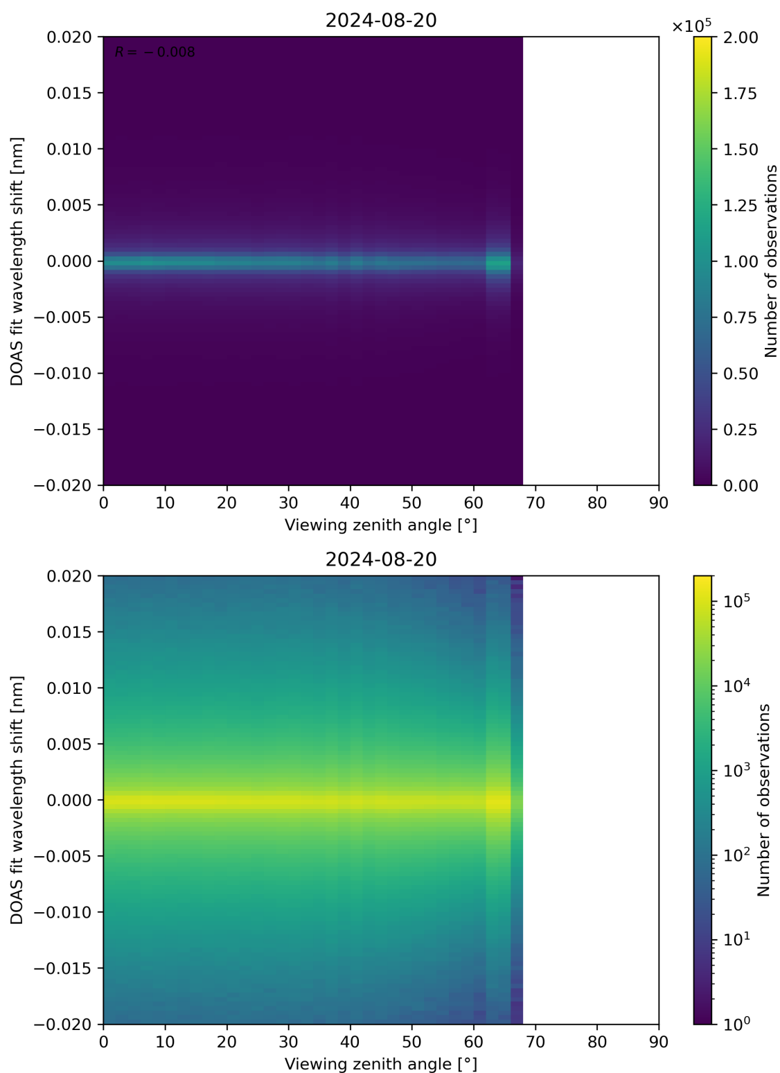
Figure 183: Scatter density plot of “Viewing zenith angle” against “DOAS fit wavelength shift” for 2024-08-19 to 2024-08-21.
