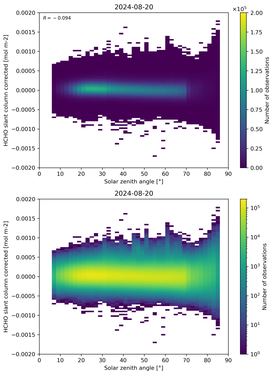
Figure 171: Scatter density plot of “Solar zenith angle” against “HCHO slant column corrected” for 2024-08-19 to 2024-08-21.
