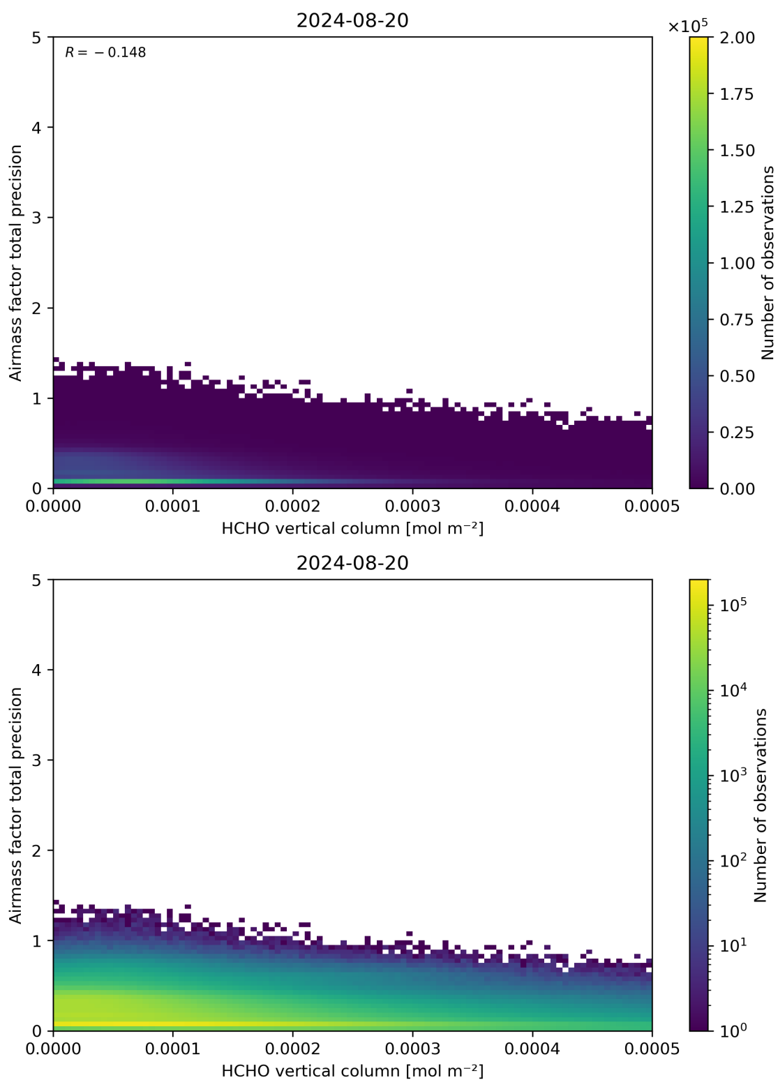
Figure 132: Scatter density plot of “HCHO vertical column” against “Airmass factor total precision” for 2024-08-19 to 2024-08-21.
