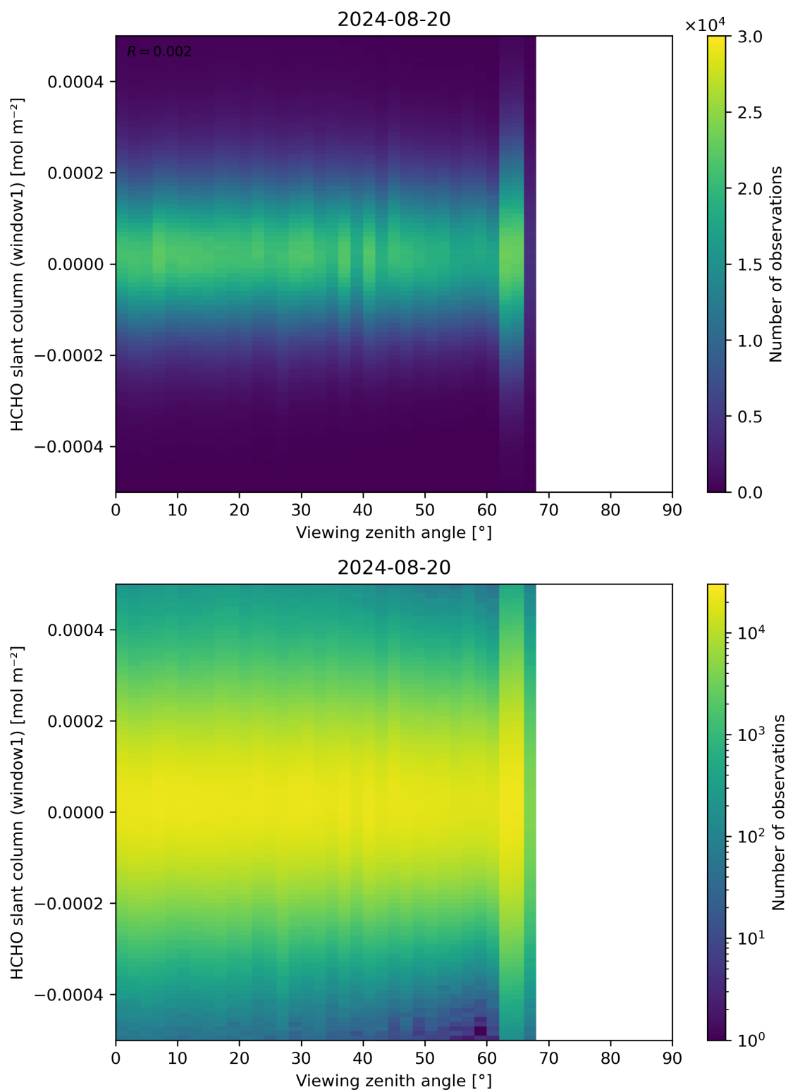
Figure 188: Scatter density plot of “Viewing zenith angle” against “HCHO slant column (window1)” for 2024-08-19 to 2024-08-21.
