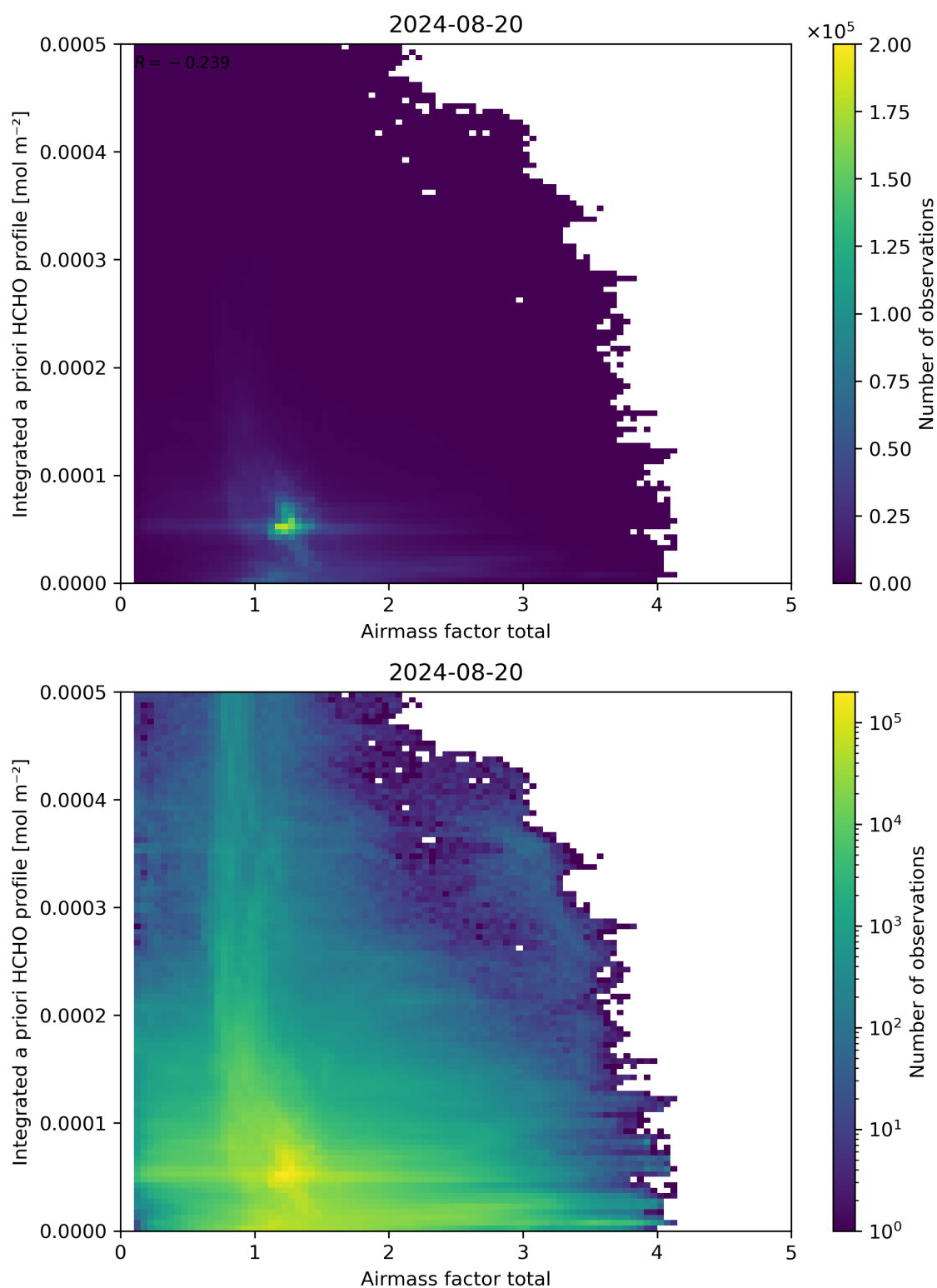
Figure 104: Scatter density plot of “Airmass factor total” against “Integrated a priori HCHO profile” for 2024-08-19 to 2024-08-21.
