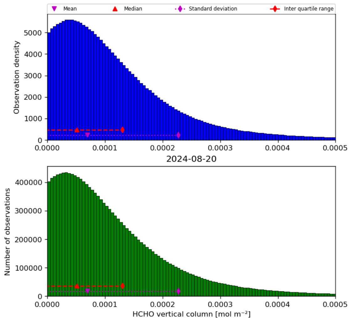
Figure 35: Histogram of “HCHO vertical column” for 2024-08-19 to 2024-08-21
