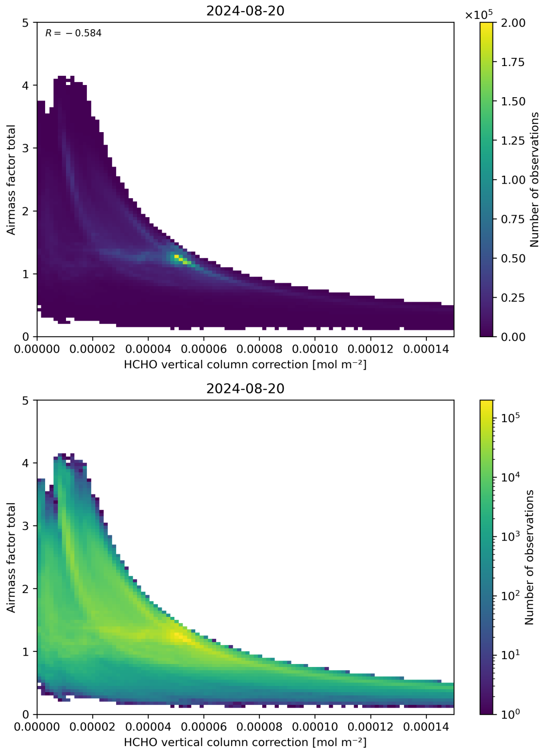
Figure 120: Scatter density plot of “HCHO vertical column correction” against “Airmass factor total” for 2024-08-19 to 2024-08-21.
