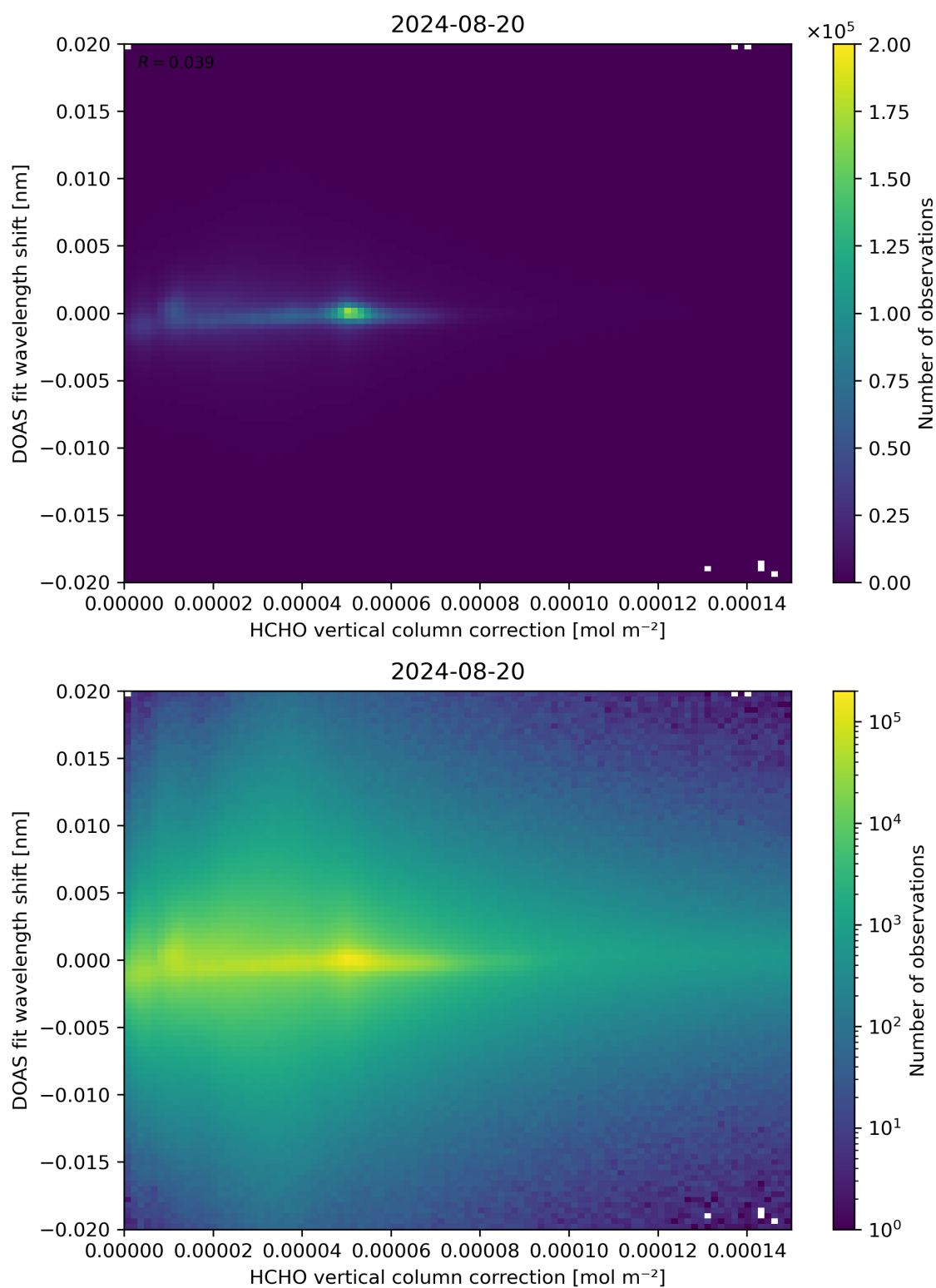
Figure 113: Scatter density plot of “HCHO vertical column correction” against “DOAS fit wavelength shift” for 2024-08-19 to 2024-08-21.
