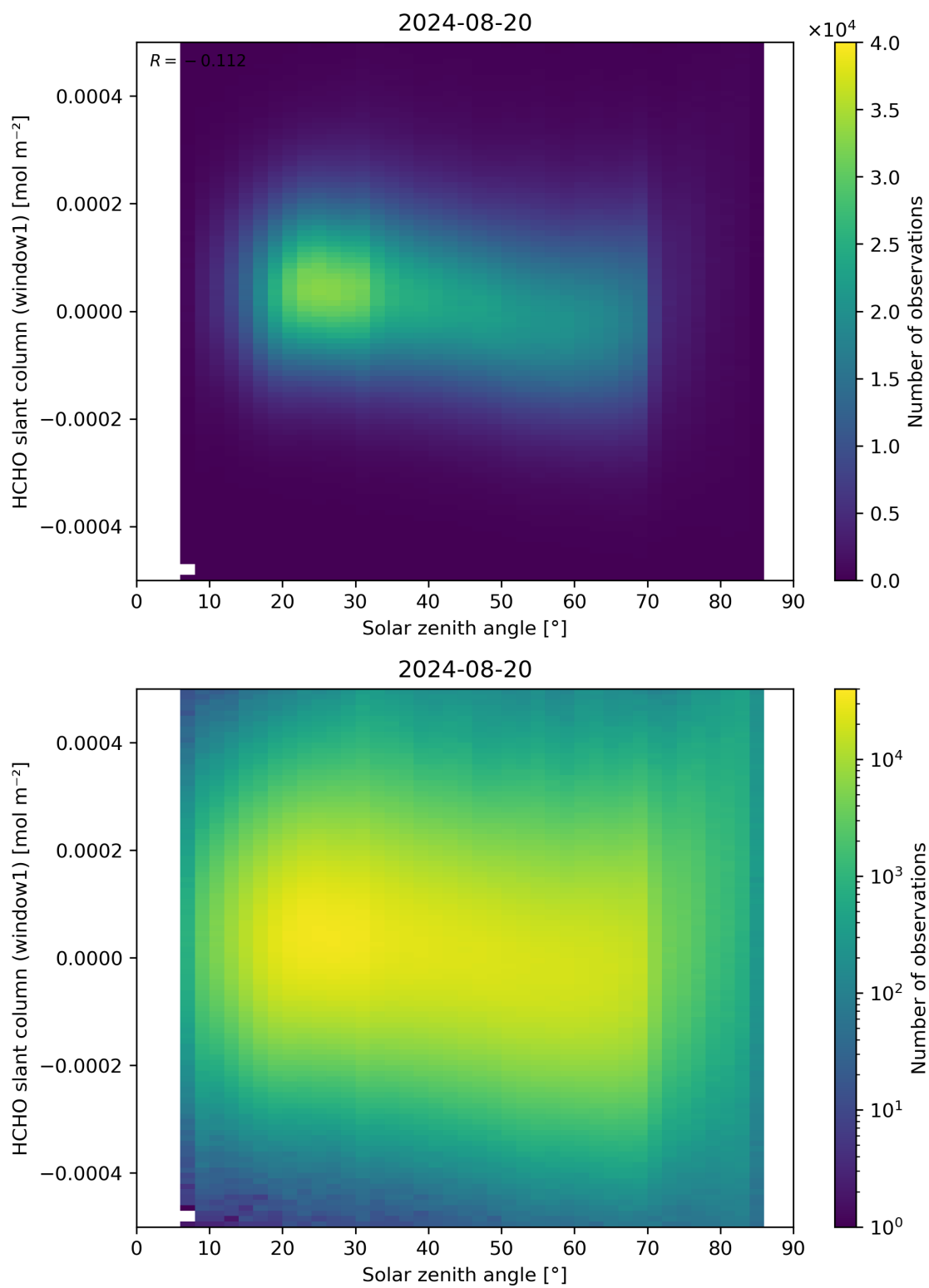
Figure 173: Scatter density plot of “Solar zenith angle” against “HCHO slant column (window1)” for 2024-08-19 to 2024-08-21.
