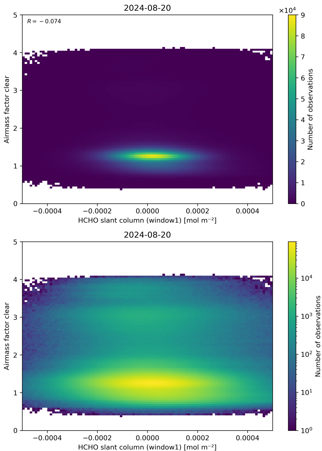
Figure 81: Scatter density plot of “HCHO slant column (window1)” against “Airmass factor clear” for 2024-08-19 to 2024-08-21.
