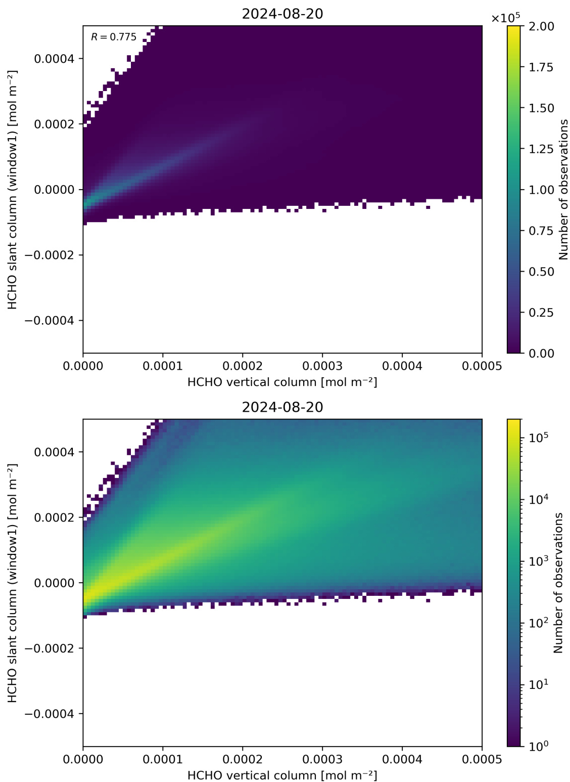
Figure 129: Scatter density plot of “HCHO vertical column” against “HCHO slant column (window1)” for 2024-08-19 to 2024-08-21.
