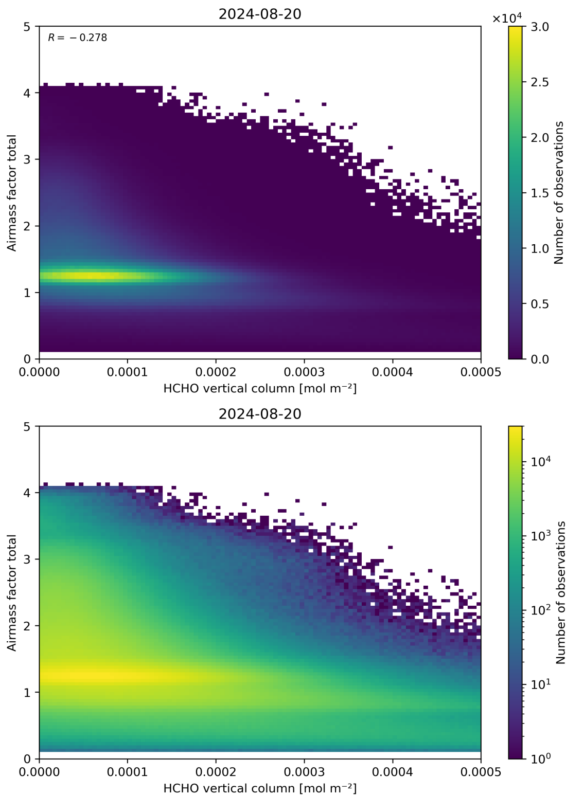
Figure 131: Scatter density plot of “HCHO vertical column” against “Airmass factor total” for 2024-08-19 to 2024-08-21.
