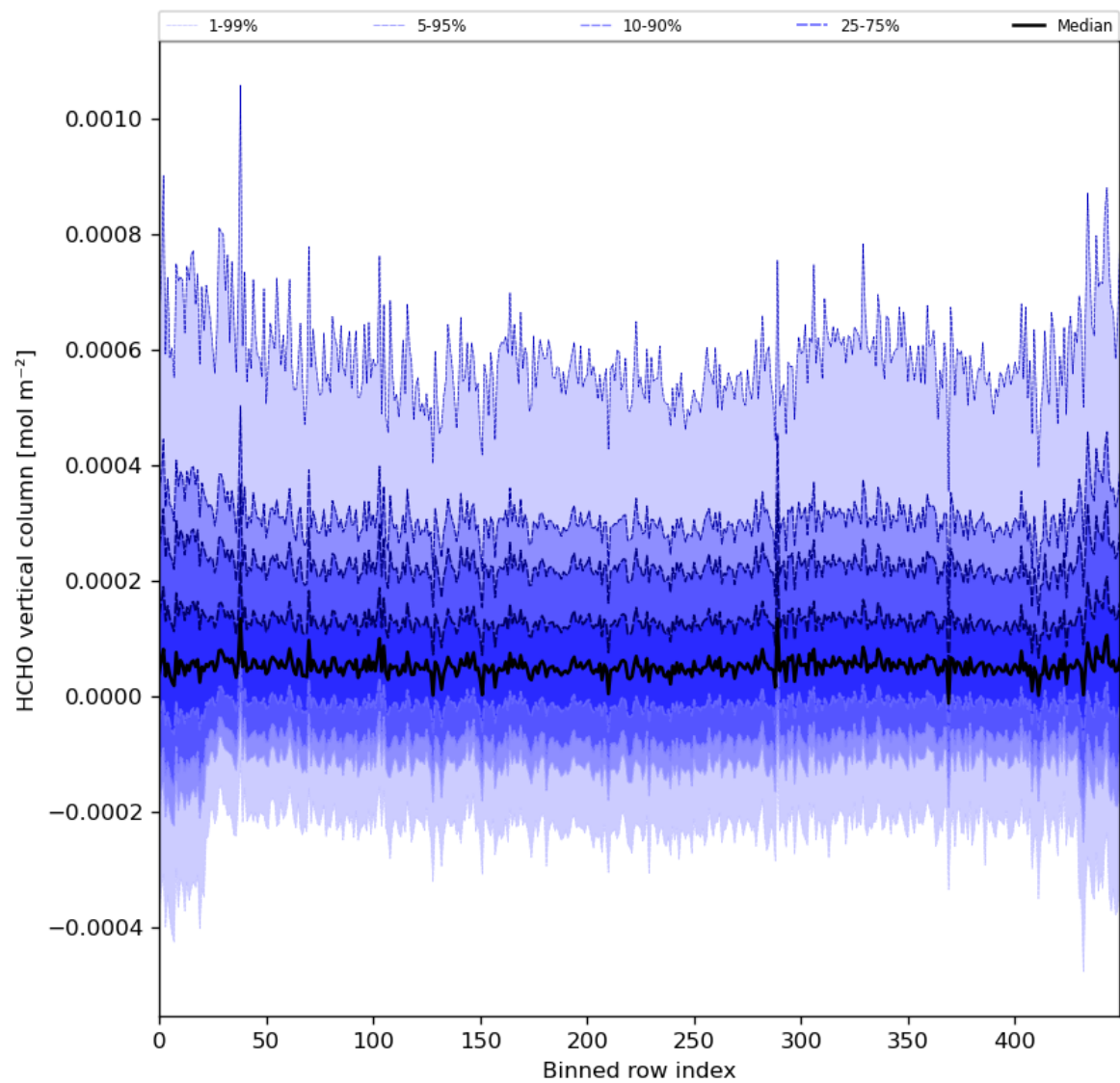
Figure 49: Along track statistics of “HCHO vertical column” for 2024-08-19 to 2024-08-21
