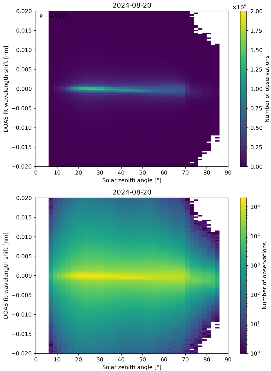
Figure 168: Scatter density plot of “Solar zenith angle” against “DOAS fit wavelength shift” for 2024-08-19 to 2024-08-21.
