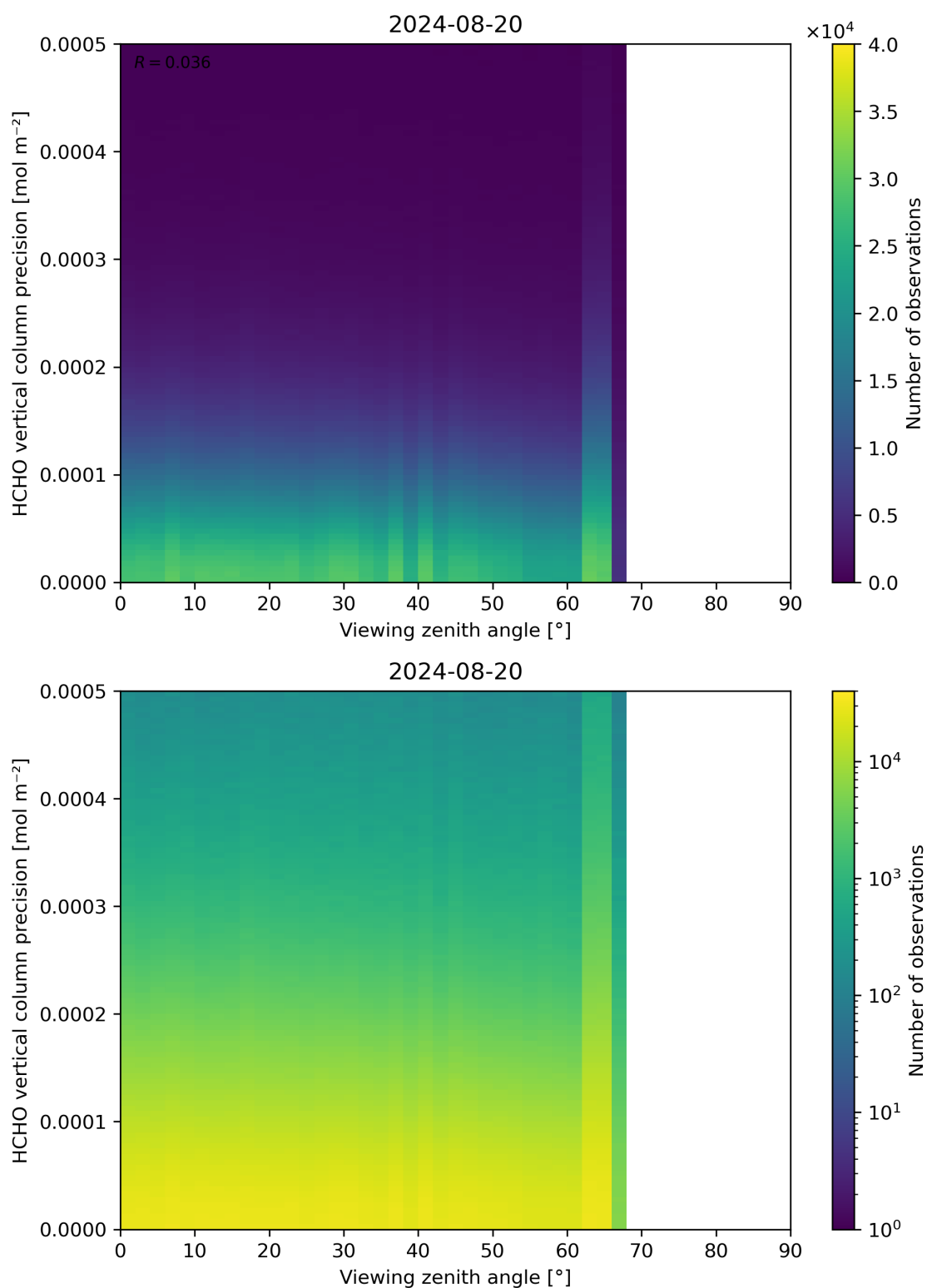
Figure 194: Scatter density plot of “Viewing zenith angle” against “HCHO vertical column precision” for 2024-08-19 to 2024-08-21.
