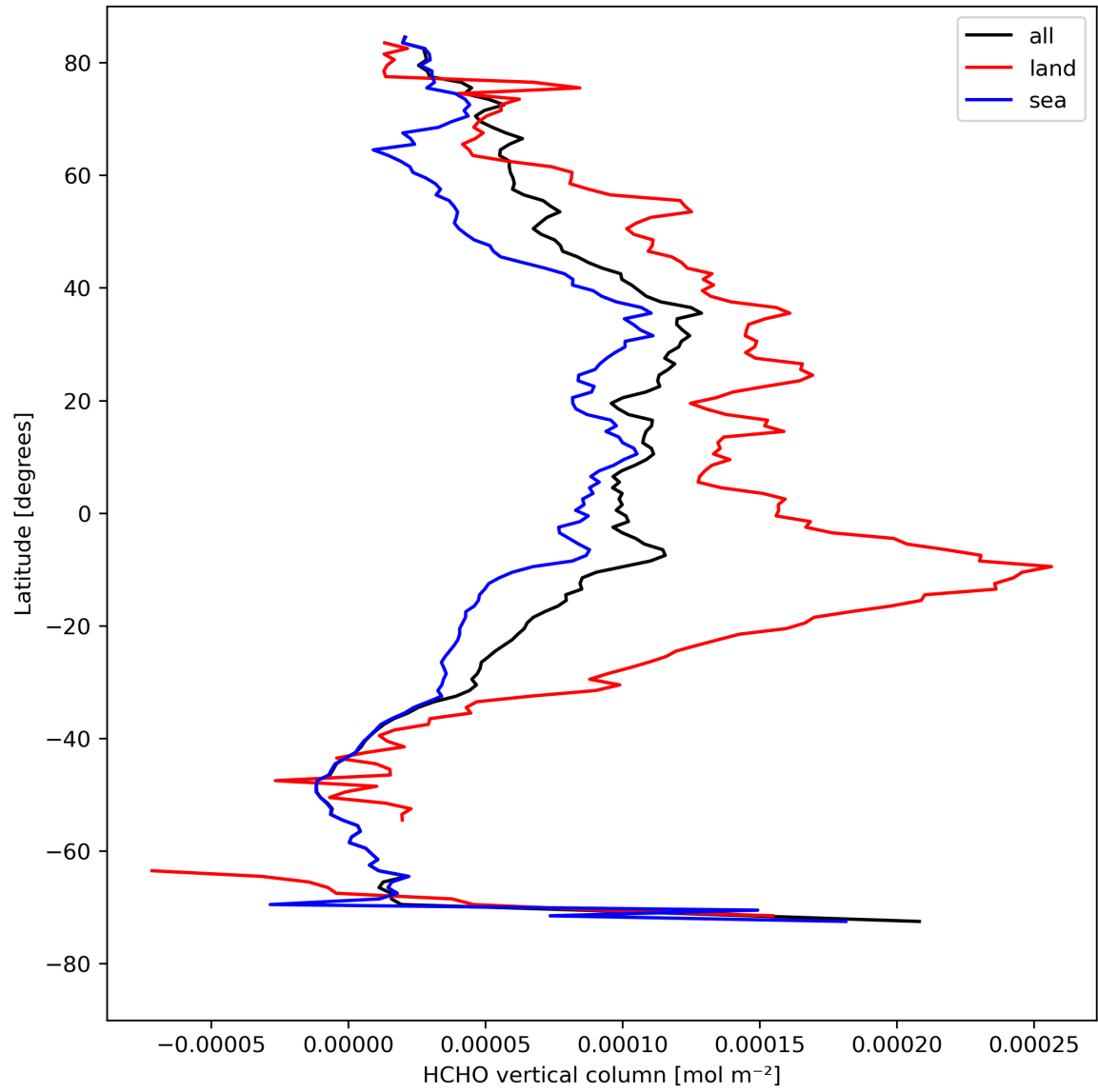
Figure 21: Zonal average of “HCHO vertical column” for 2024-08-19 to 2024-08-21.
