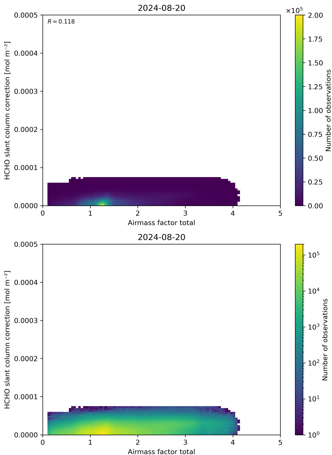
Figure 102: Scatter density plot of “Airmass factor total” against “HCHO slant column correction” for 2024-08-19 to 2024-08-21.
