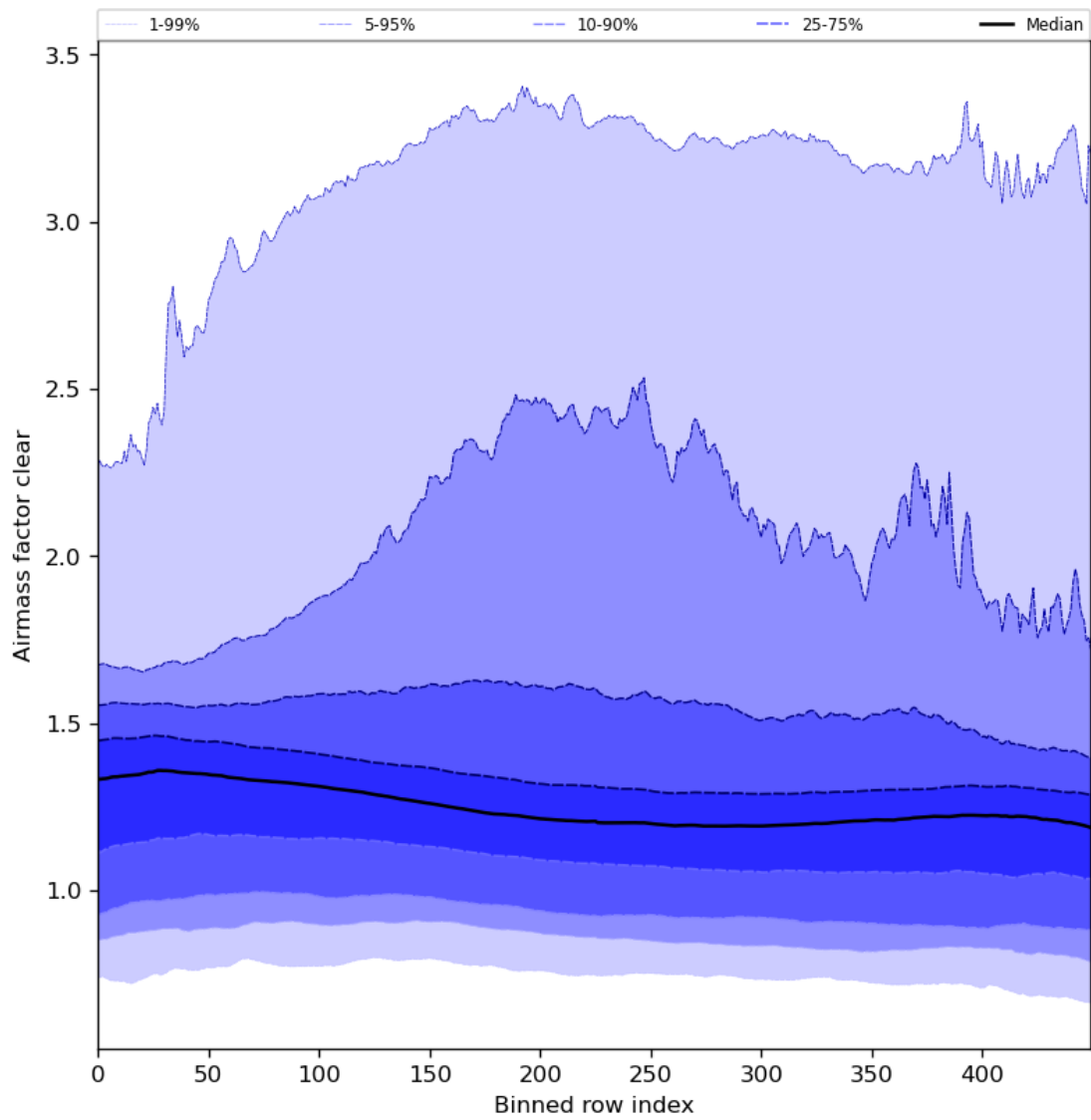
Figure 56: Along track statistics of “Air mass factor clear” for 2024-08-19 to 2024-08-21
