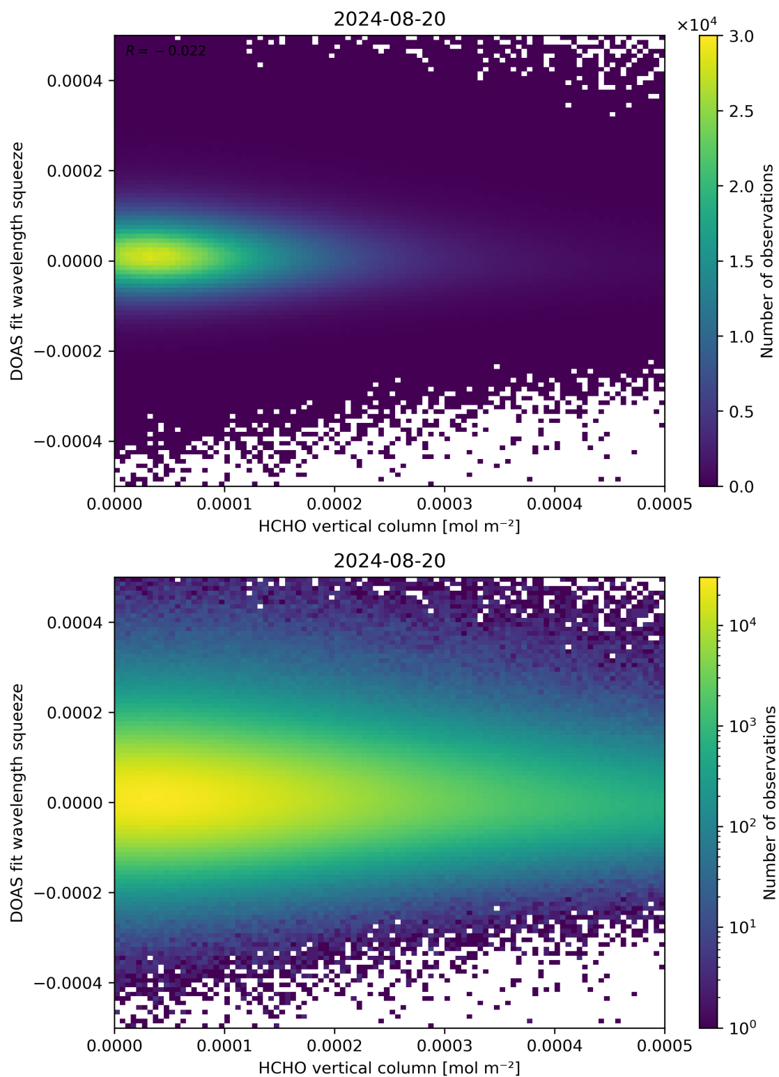
Figure 125: Scatter density plot of “HCHO vertical column” against “DOAS fit wavelength squeeze” for 2024-08-19 to 2024-08-21.
