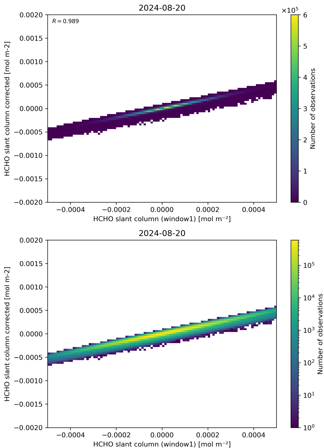
Figure 82: Scatter density plot of “HCHO slant column (window1)” against “HCHO slant column corrected” for 2024-08-19 to 2024-08-21.
