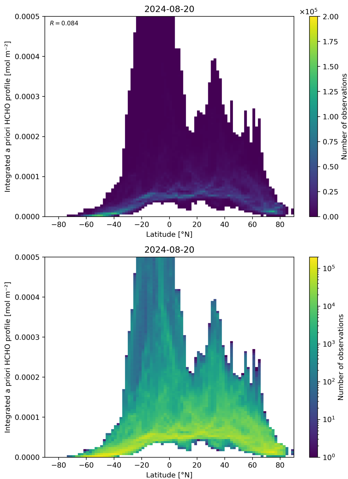
Figure 166: Scatter density plot of “Latitude” against “Integrated a priori HCHO profile” for 2024-08-19 to 2024-08-21.
