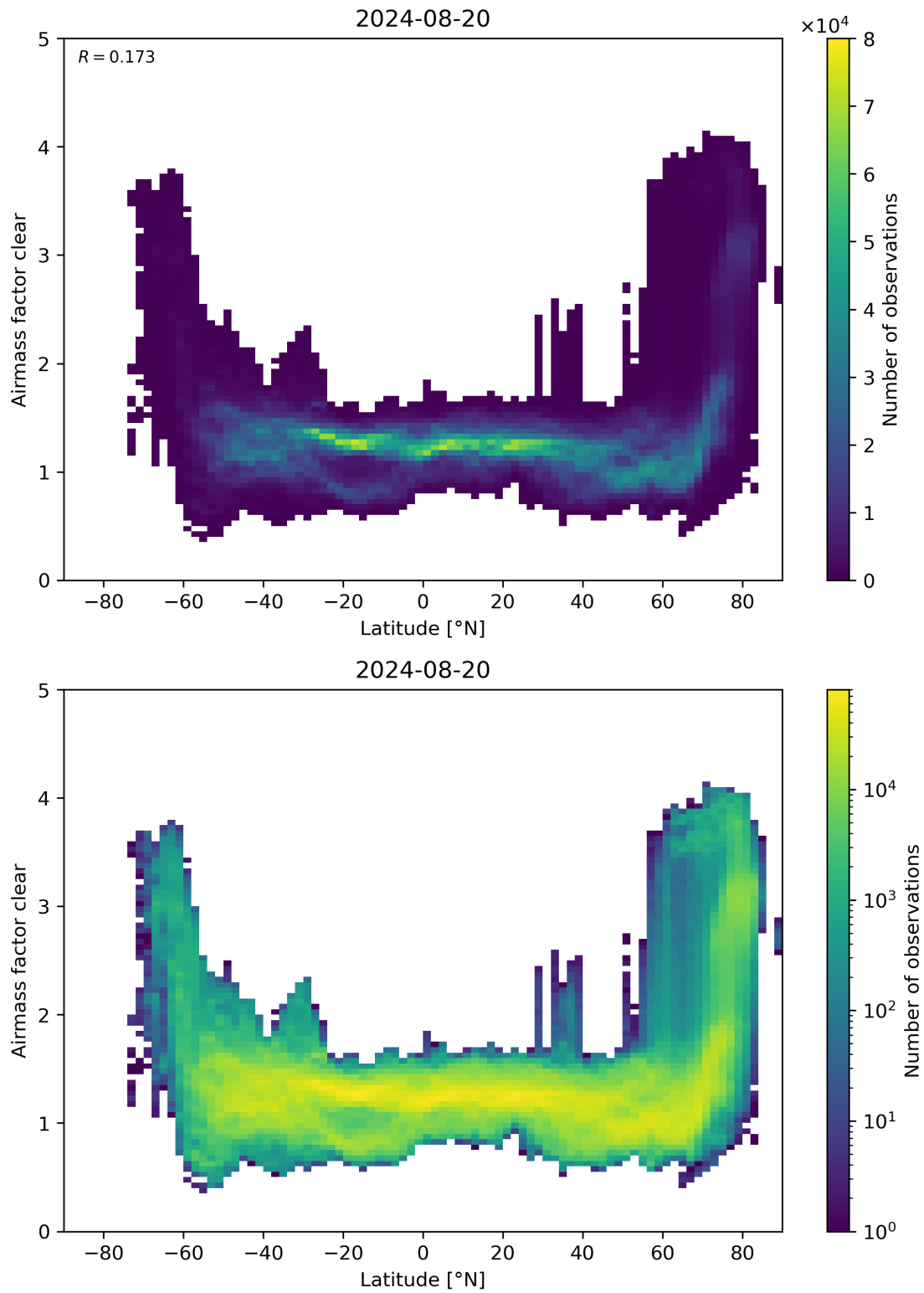
Figure 156: Scatter density plot of “Latitude” against “Airmass factor clear” for 2024-08-19 to 2024-08-21.
