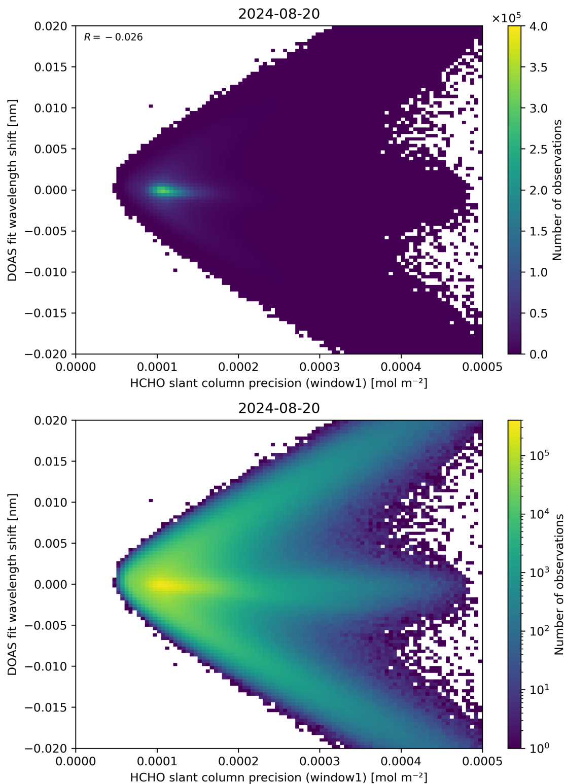
Figure 89: Scatter density plot of “HCHO slant column precision (window1)” against “DOAS fit wavelength shift” for 2024-08-19 to 2024-08-21.
