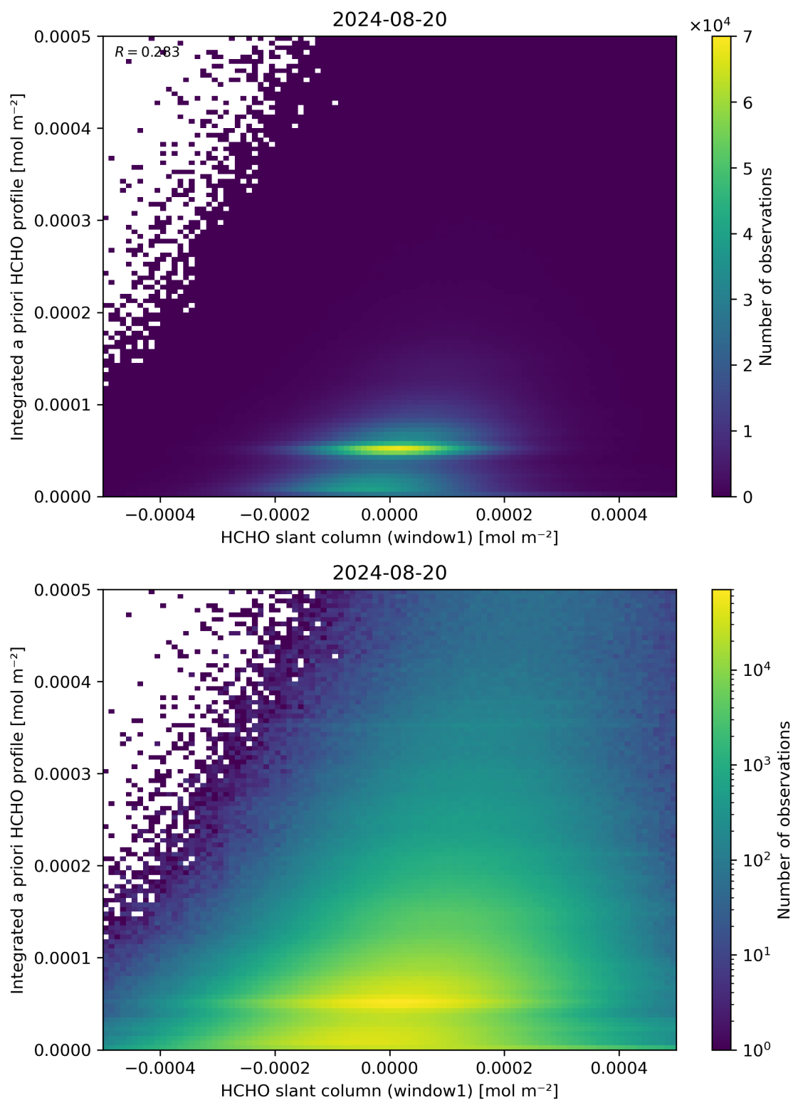
Figure 87: Scatter density plot of “HCHO slant column (window1)” against “Integrated a priori HCHO profile” for 2024-08-19 to 2024-08-21.
