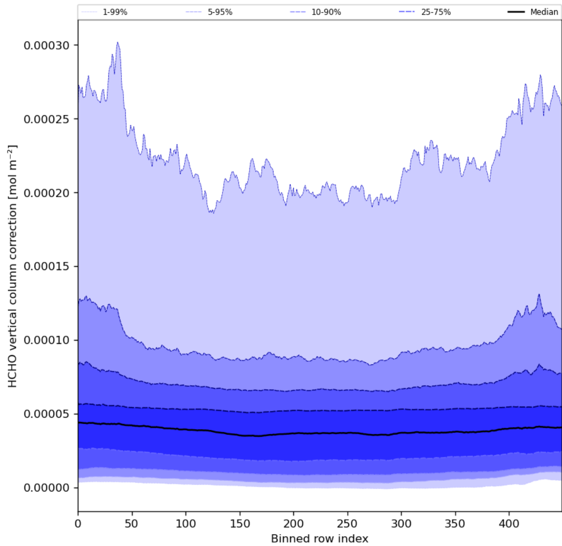
Figure 51: Along track statistics of “HCHO vertical column correction” for 2024-08-19 to 2024-08-21
