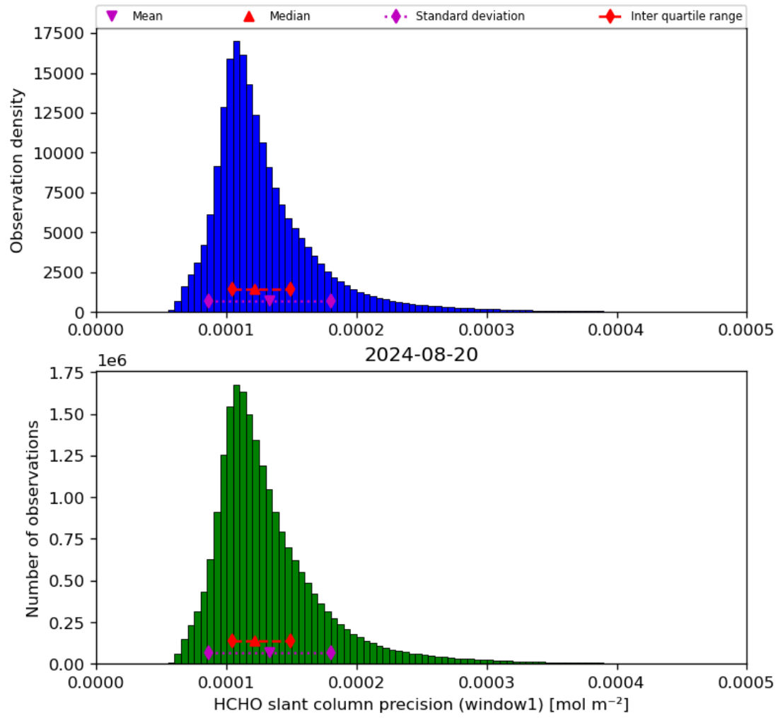
Figure 39: Histogram of “HCHO slant column precision (window1)” for 2024-08-19 to 2024-08-21
