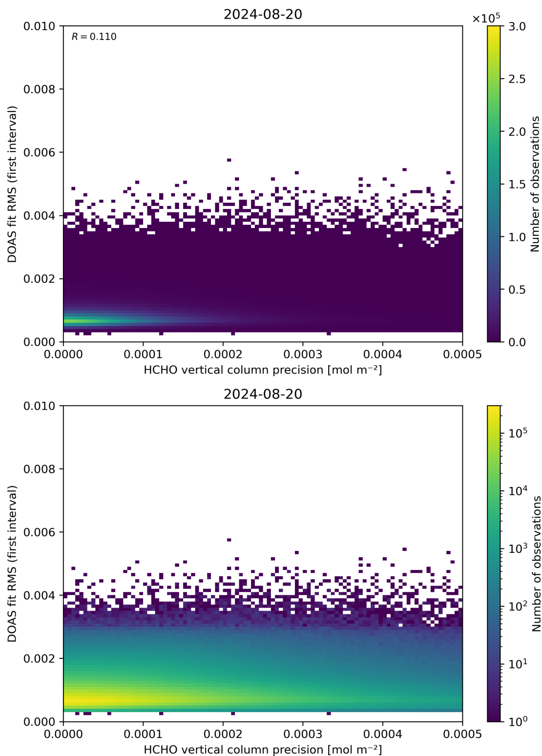
Figure 136: Scatter density plot of “HCHO vertical column precision” against “DOAS fit RMS (first interval)” for 2024-08-19 to 2024-08-21.
