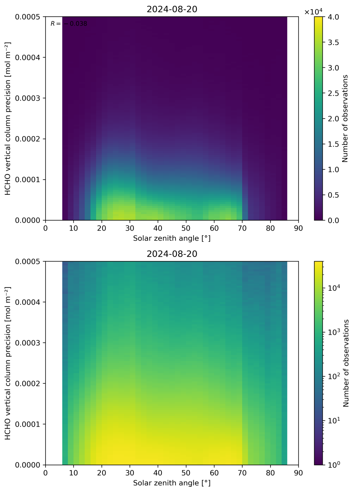
Figure 179: Scatter density plot of “Solar zenith angle” against “HCHO vertical column precision” for 2024-08-19 to 2024-08-21.
