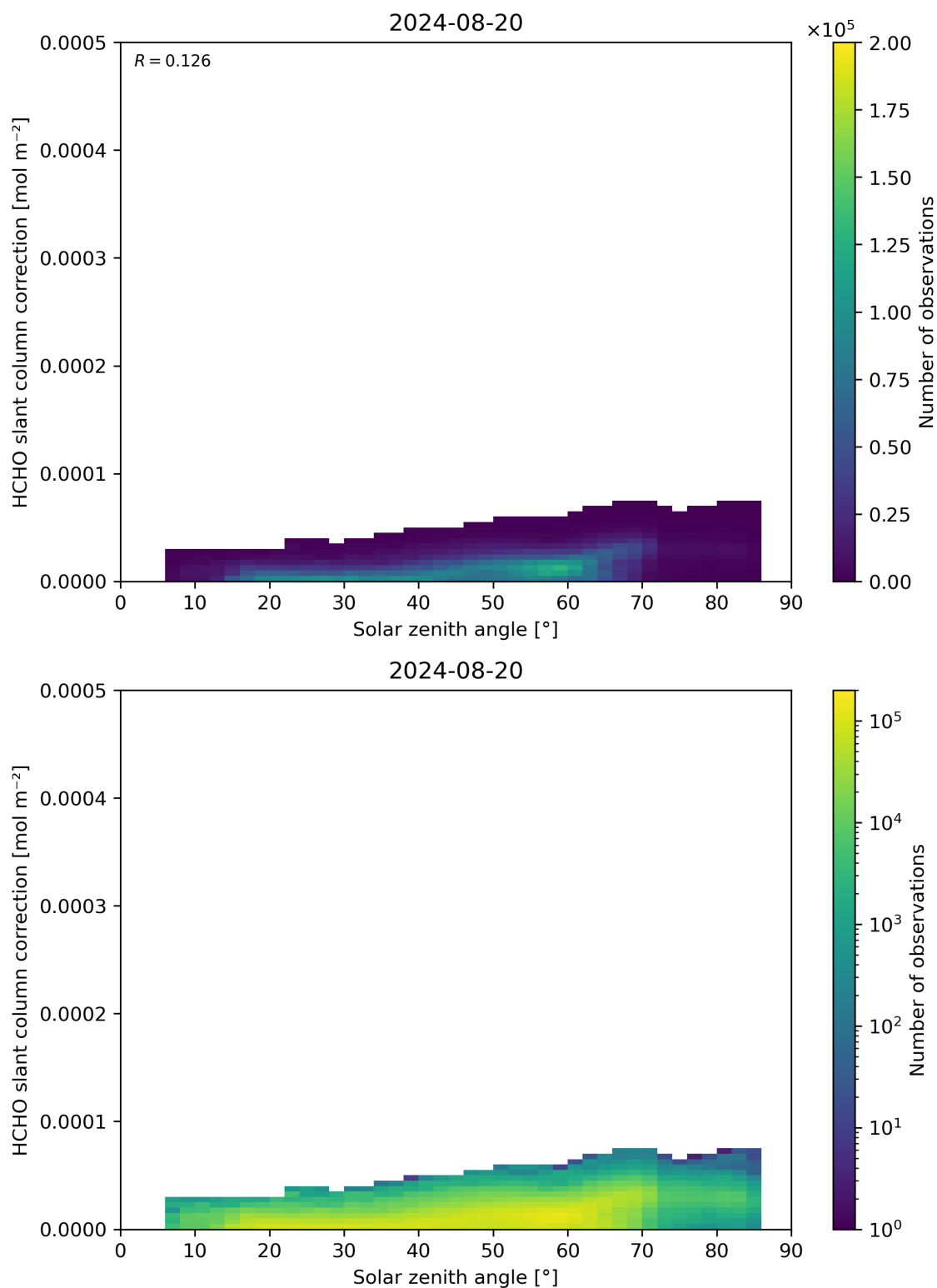
Figure 172: Scatter density plot of “Solar zenith angle” against “HCHO slant column correction” for 2024-08-19 to 2024-08-21.
