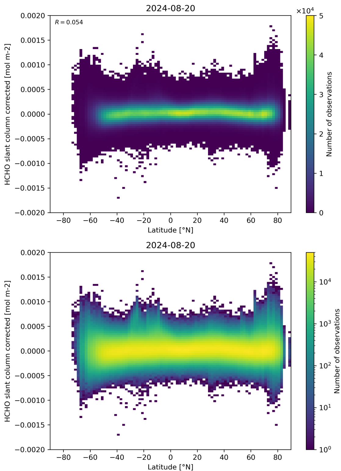
Figure 157: Scatter density plot of “Latitude” against “HCHO slant column corrected” for 2024-08-19 to 2024-08-21.
