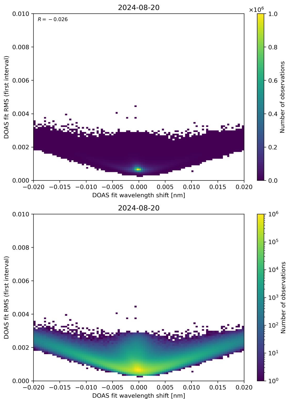
Figure 64: Scatter density plot of “DOAS fit wavelength shift” against “DOAS fit RMS (first interval)” for 2024-08-19 to 2024-08-21.
