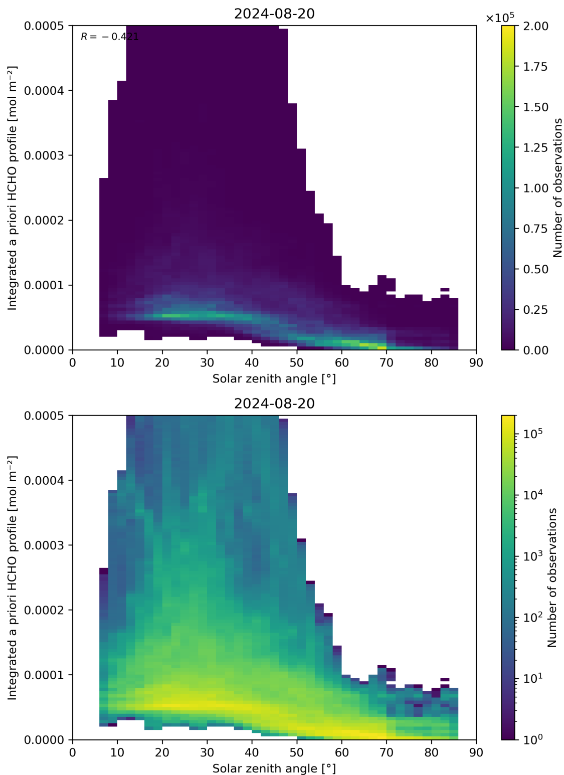
Figure 180: Scatter density plot of “Solar zenith angle” against “Integrated a priori HCHO profile” for 2024-08-19 to 2024-08-21.
