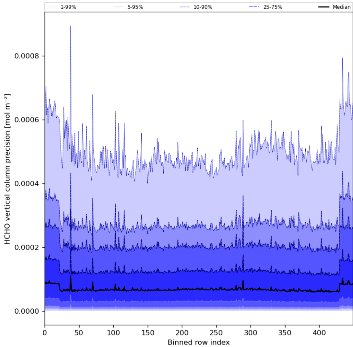
Figure 50: Along track statistics of “HCHO vertical column precision” for 2024-08-19 to 2024-08-21
