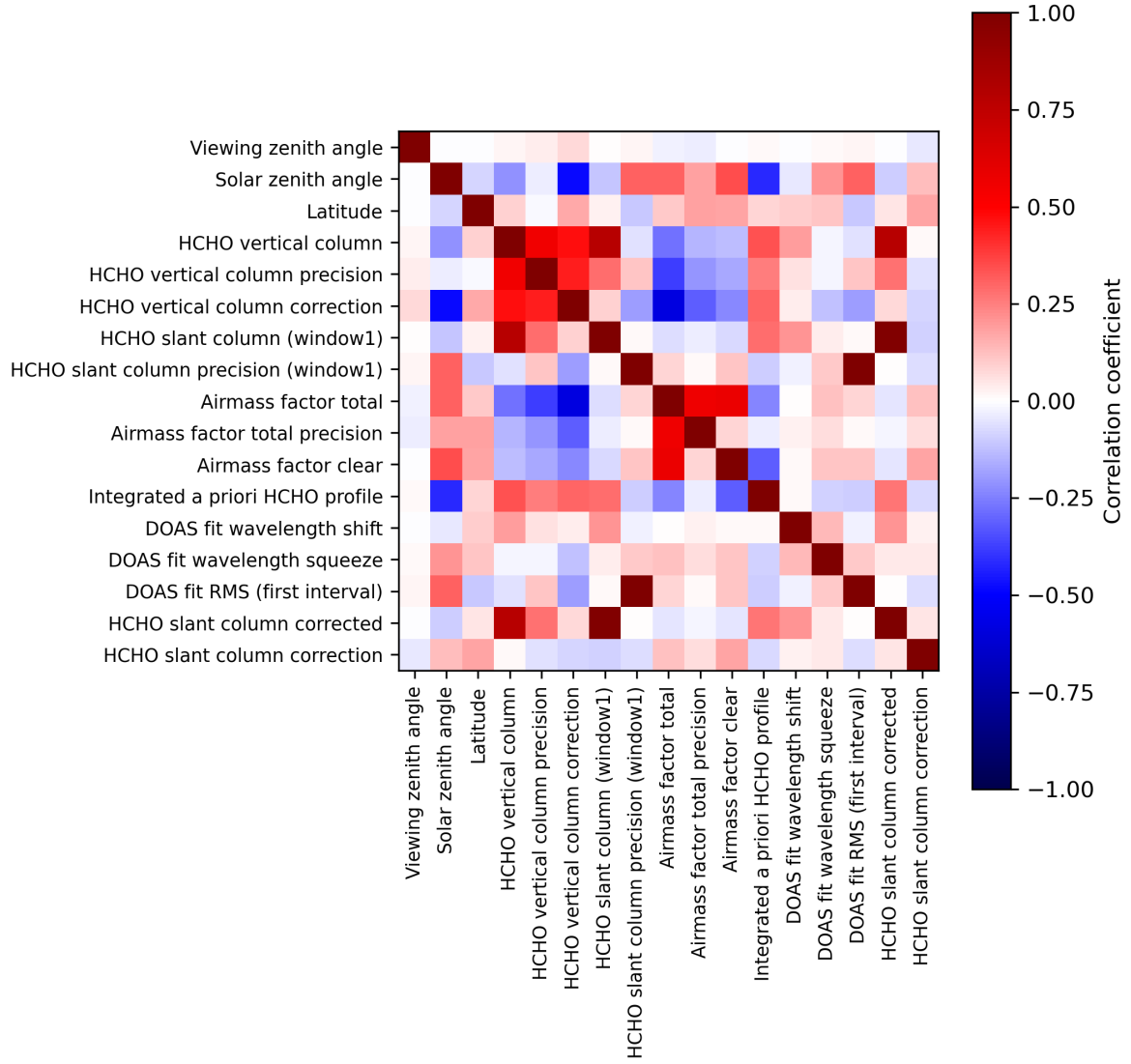
Figure 2: Map of correlation matrix for 2024-08-19 to 2024-08-21.
