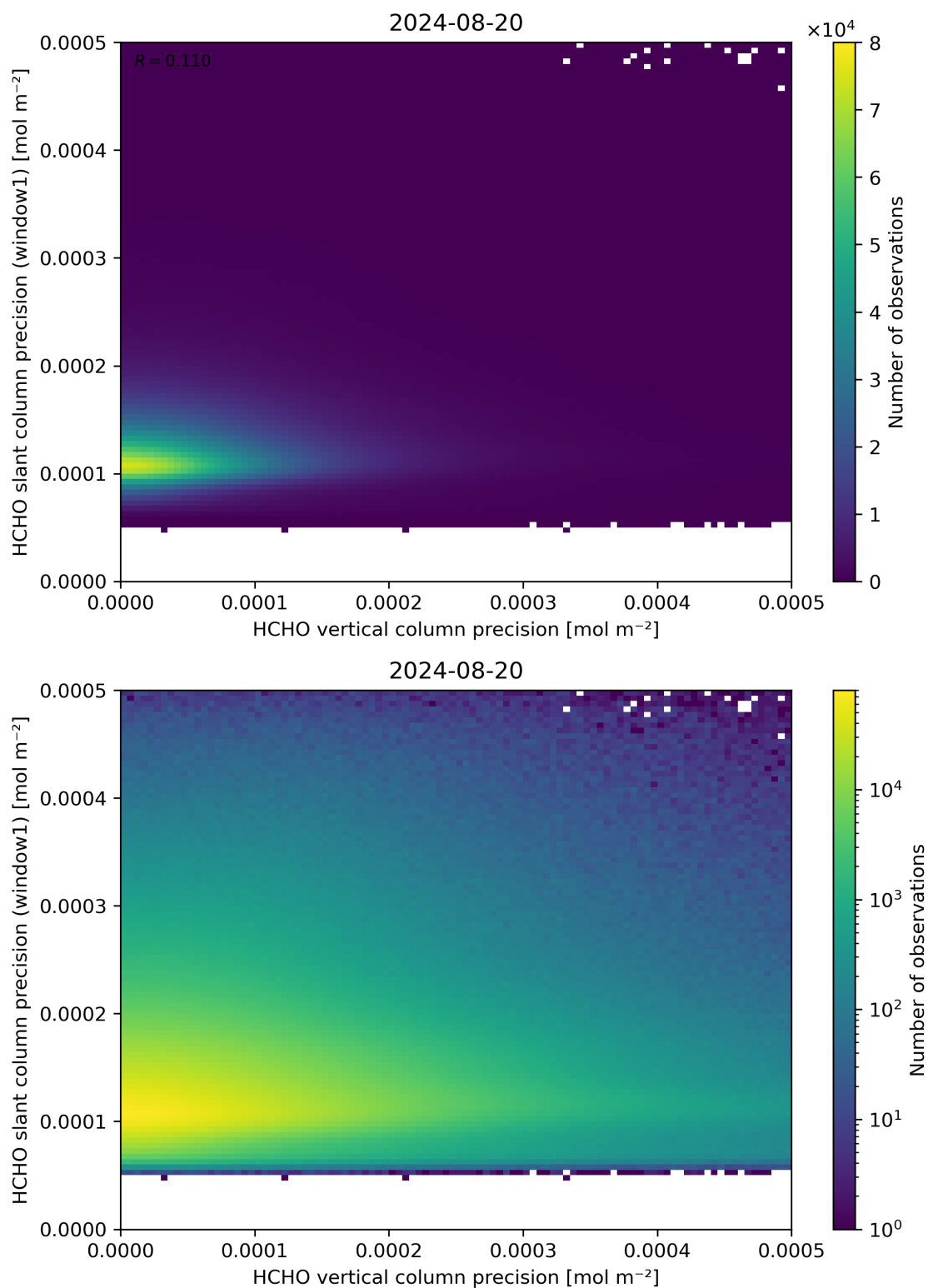
Figure 143: Scatter density plot of “HCHO vertical column precision” against “HCHO slant column precision (window1)” for 2024-08-19 to 2024-08-21.
