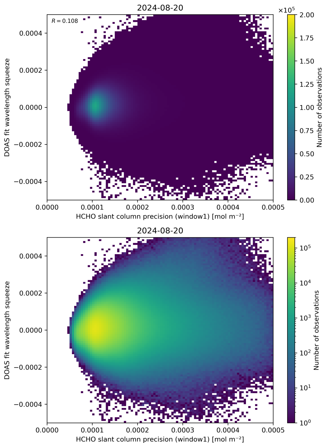
Figure 90: Scatter density plot of “HCHO slant column precision (window1)” against “DOAS fit wavelength squeeze” for 2024-08-19 to 2024-08-21.
