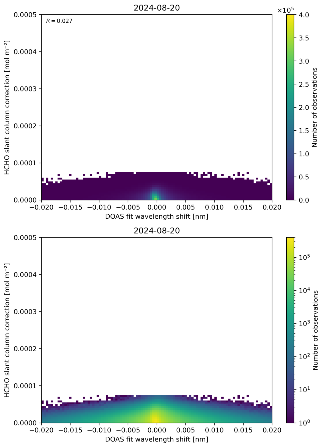
Figure 67: Scatter density plot of “DOAS fit wavelength shift” against “HCHO slant column correction” for 2024-08-19 to 2024-08-21.
