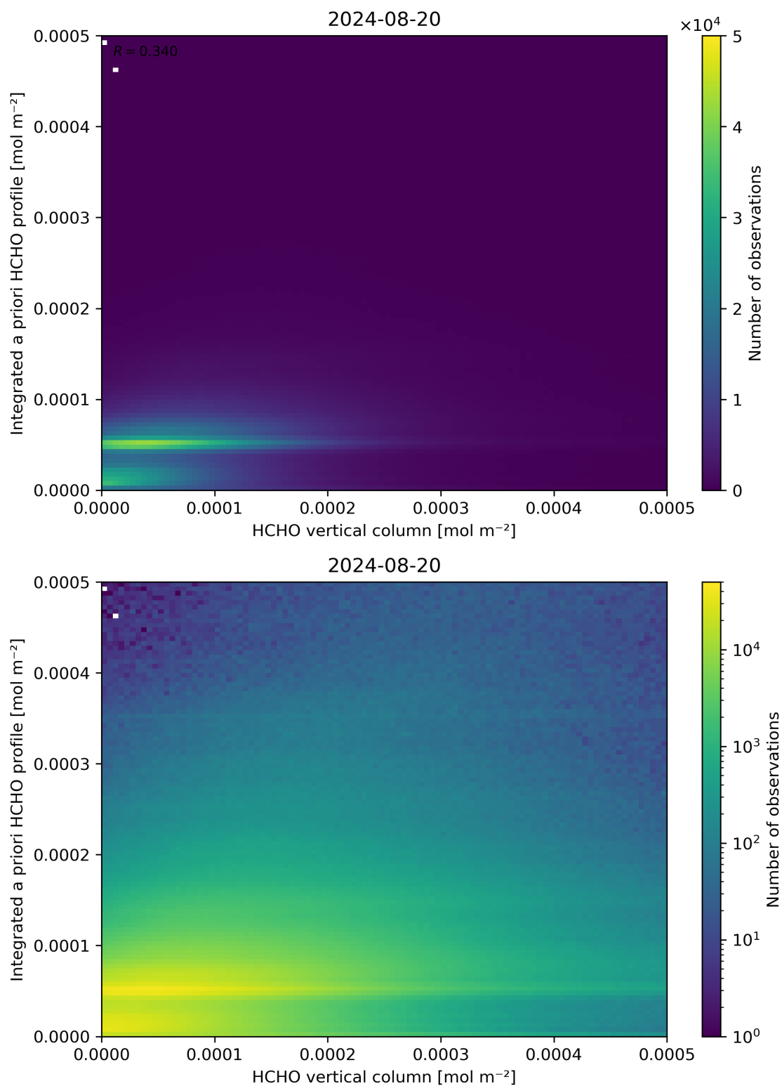
Figure 135: Scatter density plot of “HCHO vertical column” against “Integrated a priori HCHO profile” for 2024-08-19 to 2024-08-21.
