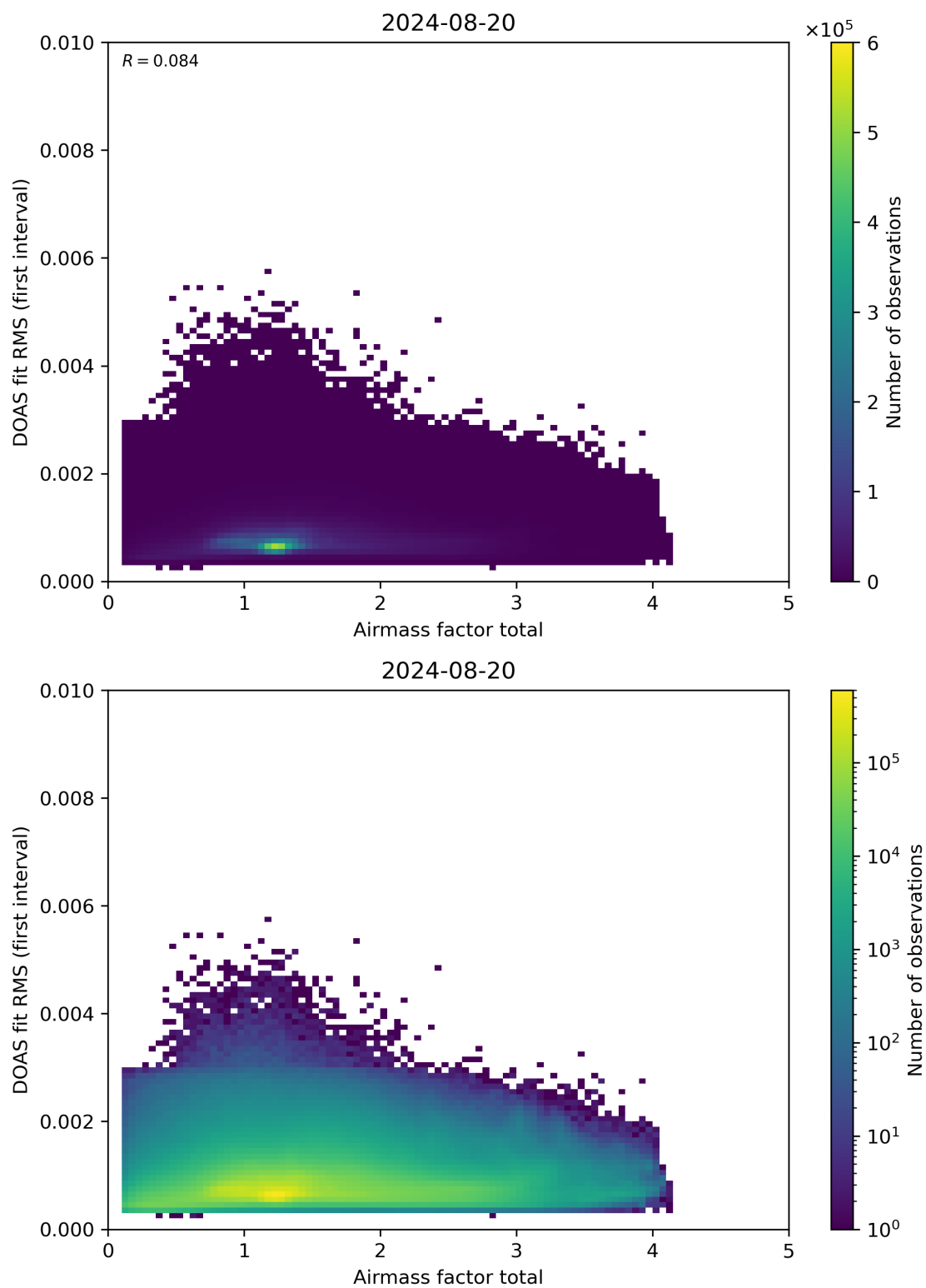
Figure 97: Scatter density plot of “Airmass factor total” against “DOAS fit RMS (first interval)” for 2024-08-19 to 2024-08-21.
