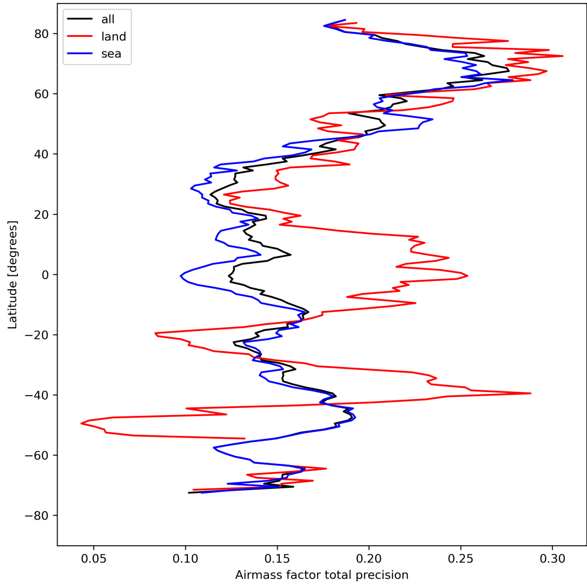
Figure 27: Zonal average of “Airmass factor total precision” for 2024-08-19 to 2024-08-21.
