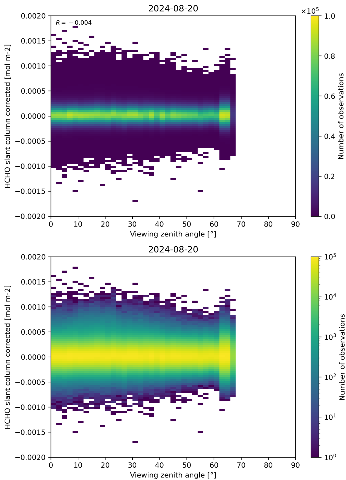
Figure 186: Scatter density plot of “Viewing zenith angle” against “HCHO slant column corrected” for 2024-08-19 to 2024-08-21.
