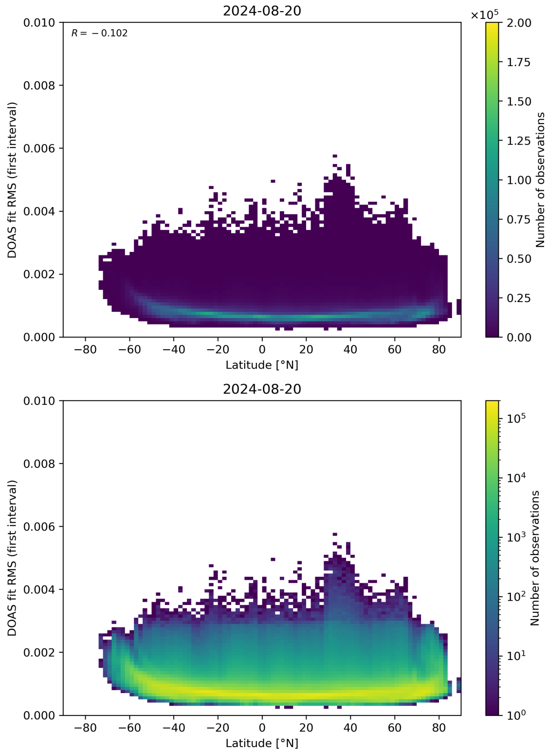
Figure 153: Scatter density plot of “Latitude” against “DOAS fit RMS (first interval)” for 2024-08-19 to 2024-08-21.
