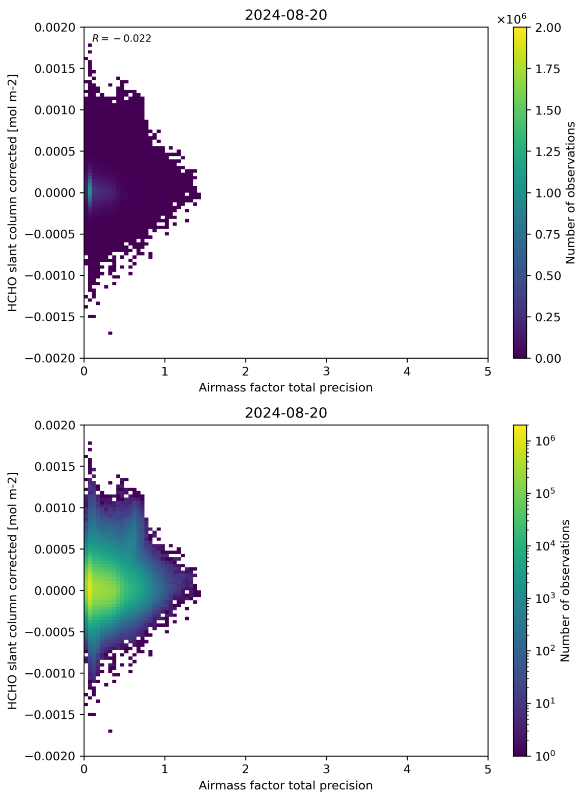
Figure 109: Scatter density plot of “Airmass factor total precision” against “HCHO slant column corrected” for 2024-08-19 to 2024-08-21.
