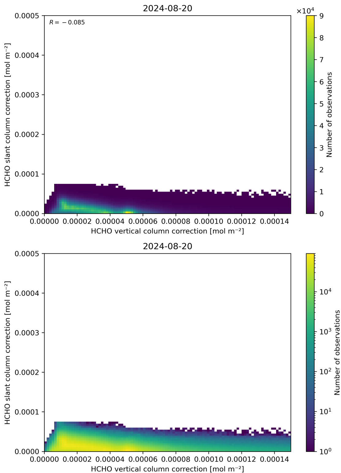
Figure 117: Scatter density plot of “HCHO vertical column correction” against “HCHO slant column correction” for 2024-08-19 to 2024-08-21.
