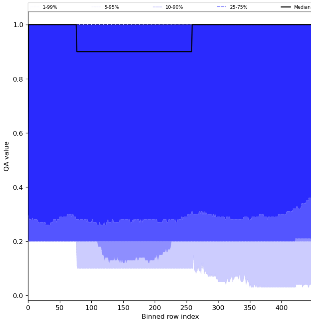
Figure 48: Along track statistics of “QA value” for 2024-08-19 to 2024-08-21
