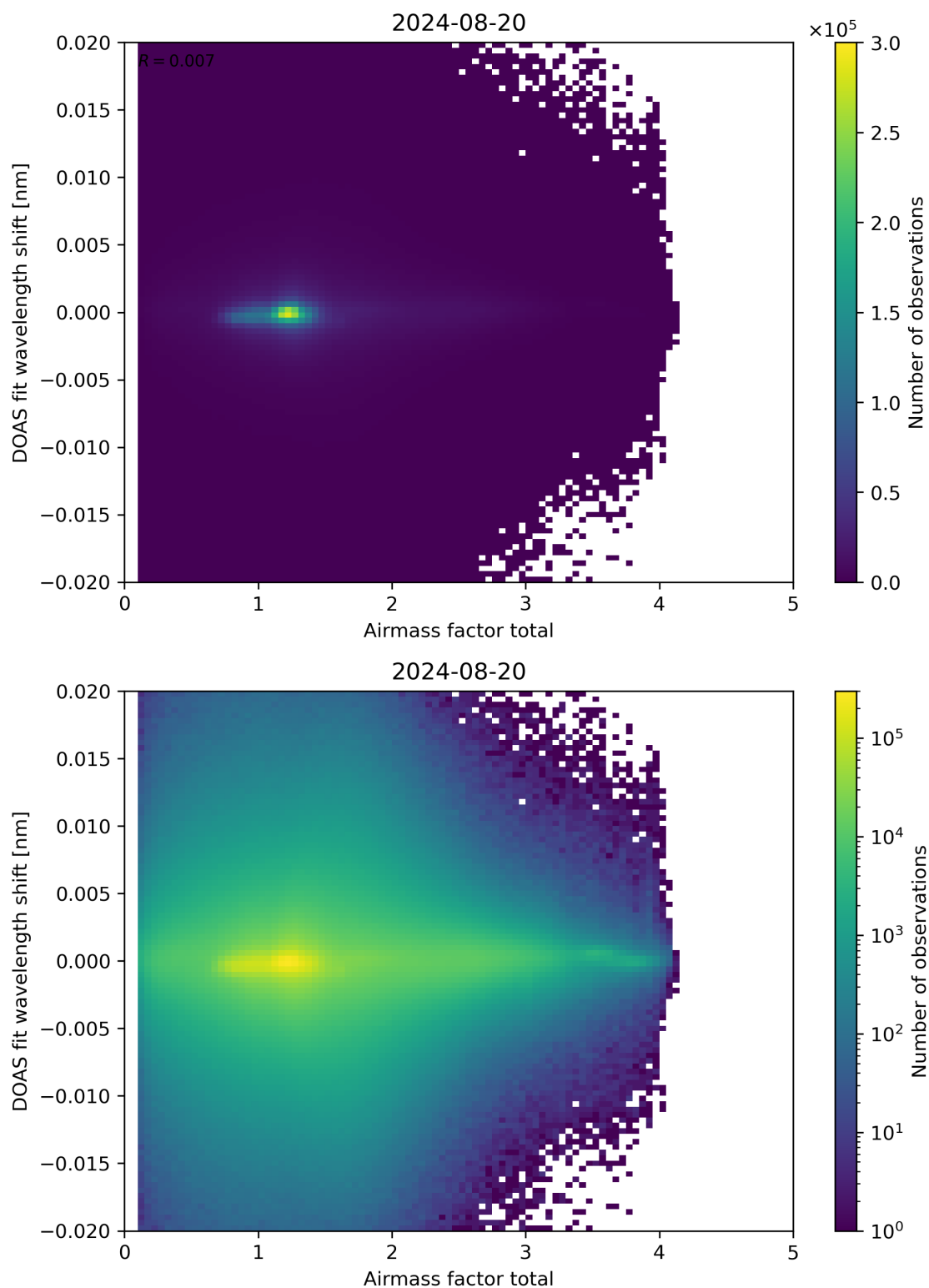
Figure 98: Scatter density plot of “Airmass factor total” against “DOAS fit wavelength shift” for 2024-08-19 to 2024-08-21.
