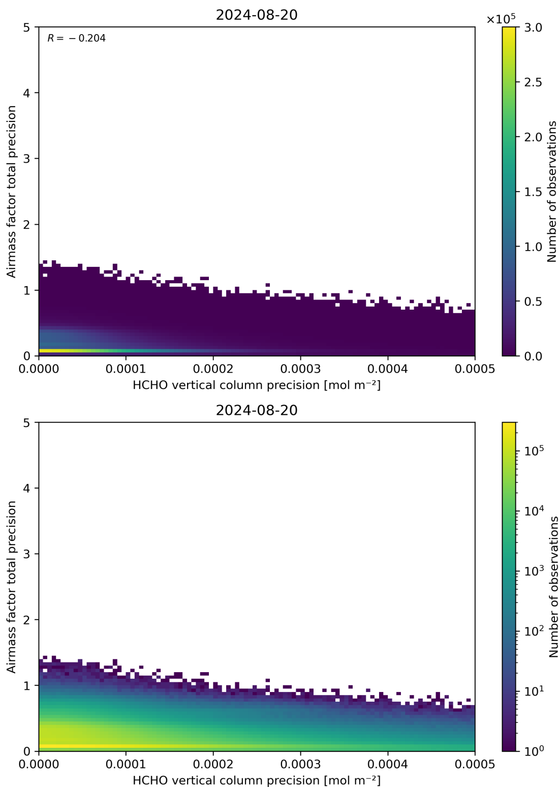
Figure 145: Scatter density plot of “HCHO vertical column precision” against “Airmass factor total precision” for 2024-08-19 to 2024-08-21.
