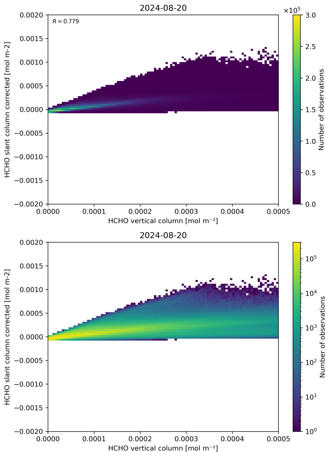
Figure 127: Scatter density plot of “HCHO vertical column” against “HCHO slant column corrected” for 2024-08-19 to 2024-08-21.
