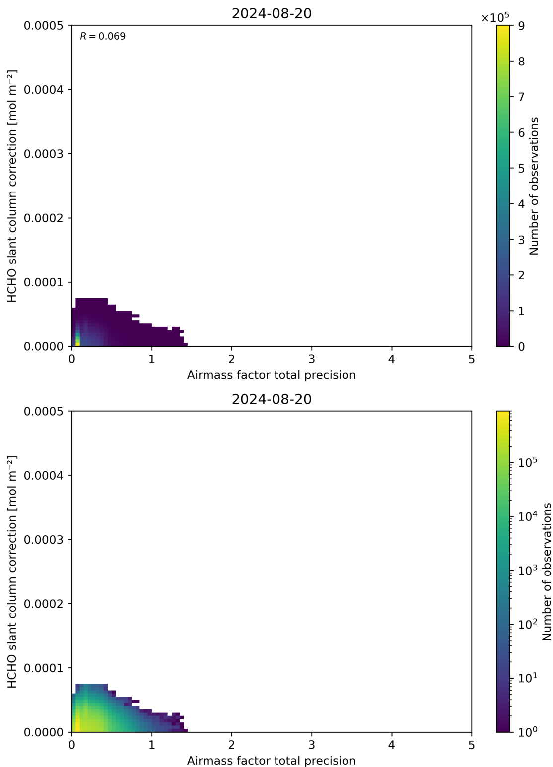
Figure 110: Scatter density plot of “Airmass factor total precision” against “HCHO slant column correction” for 2024-08-19 to 2024-08-21.
