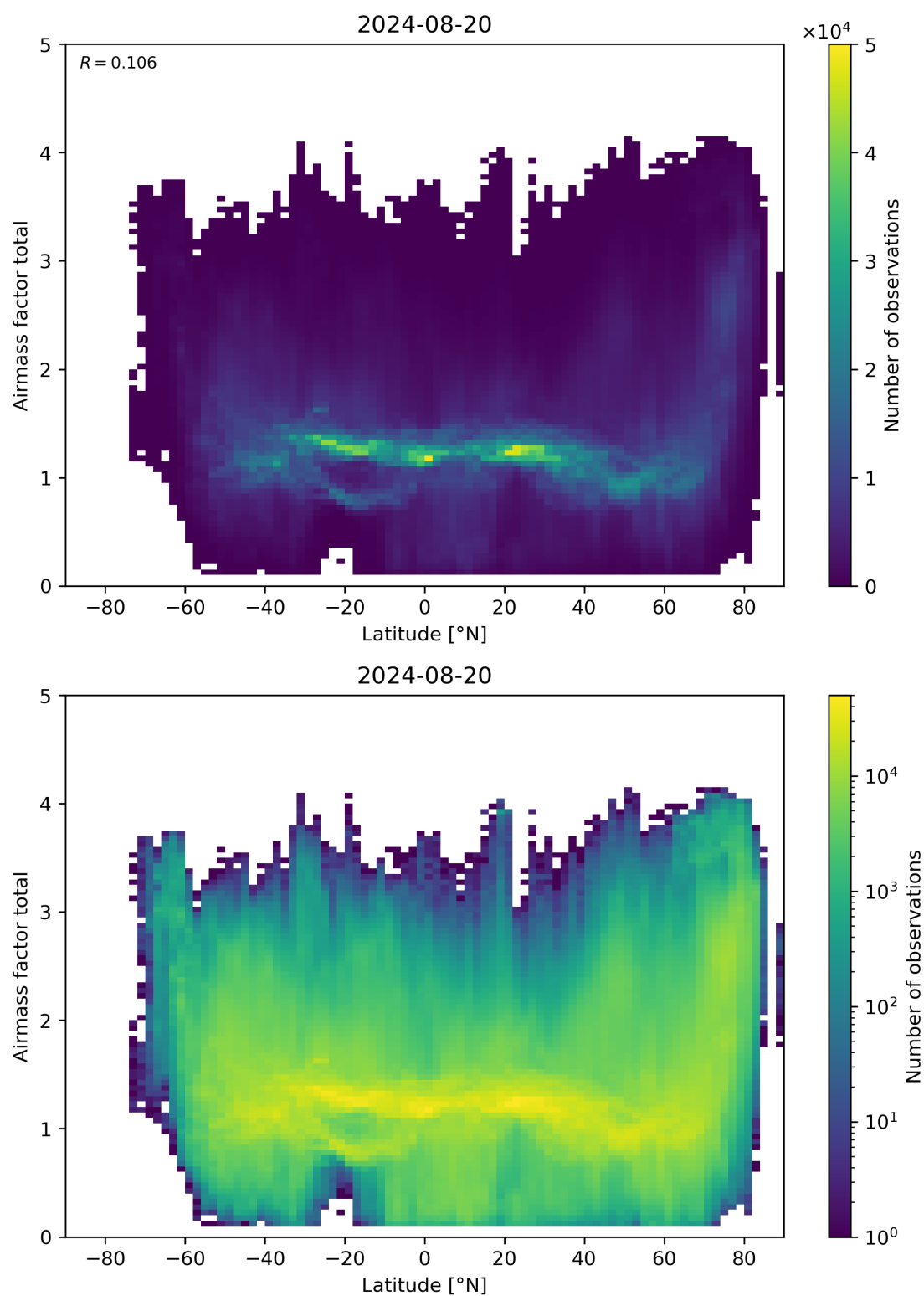
Figure 161: Scatter density plot of “Latitude” against “Airmass factor total” for 2024-08-19 to 2024-08-21.
