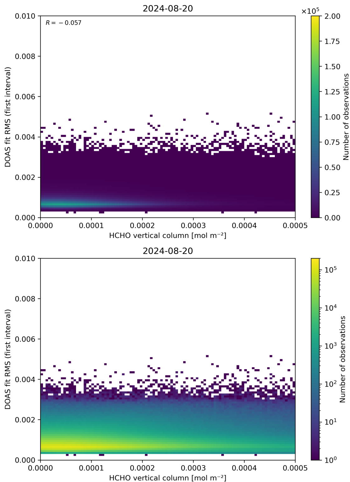
Figure 123: Scatter density plot of “HCHO vertical column” against “DOAS fit RMS (first interval)” for 2024-08-19 to 2024-08-21.
