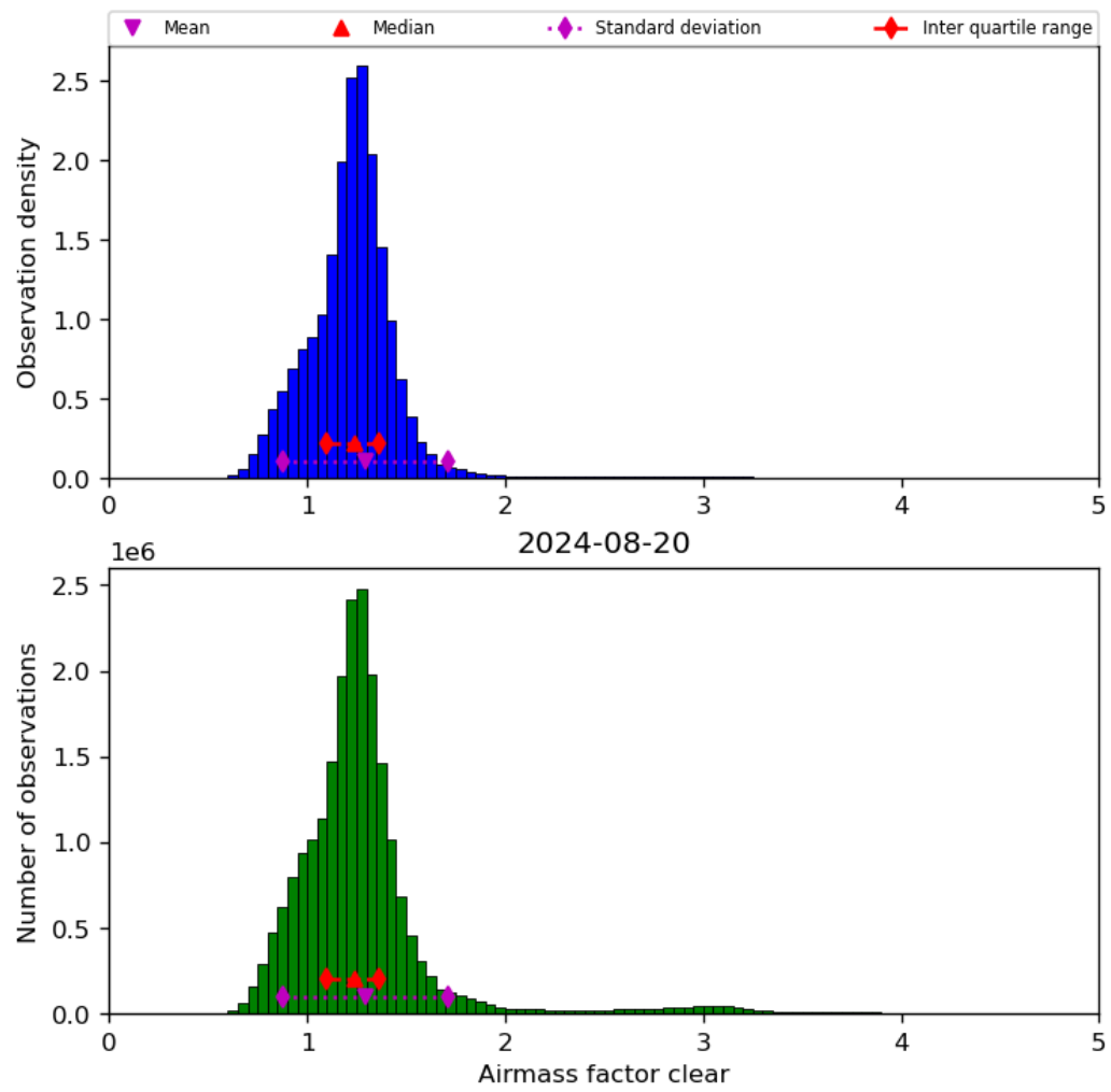
Figure 42: Histogram of “Airmass factor clear” for 2024-08-19 to 2024-08-21
