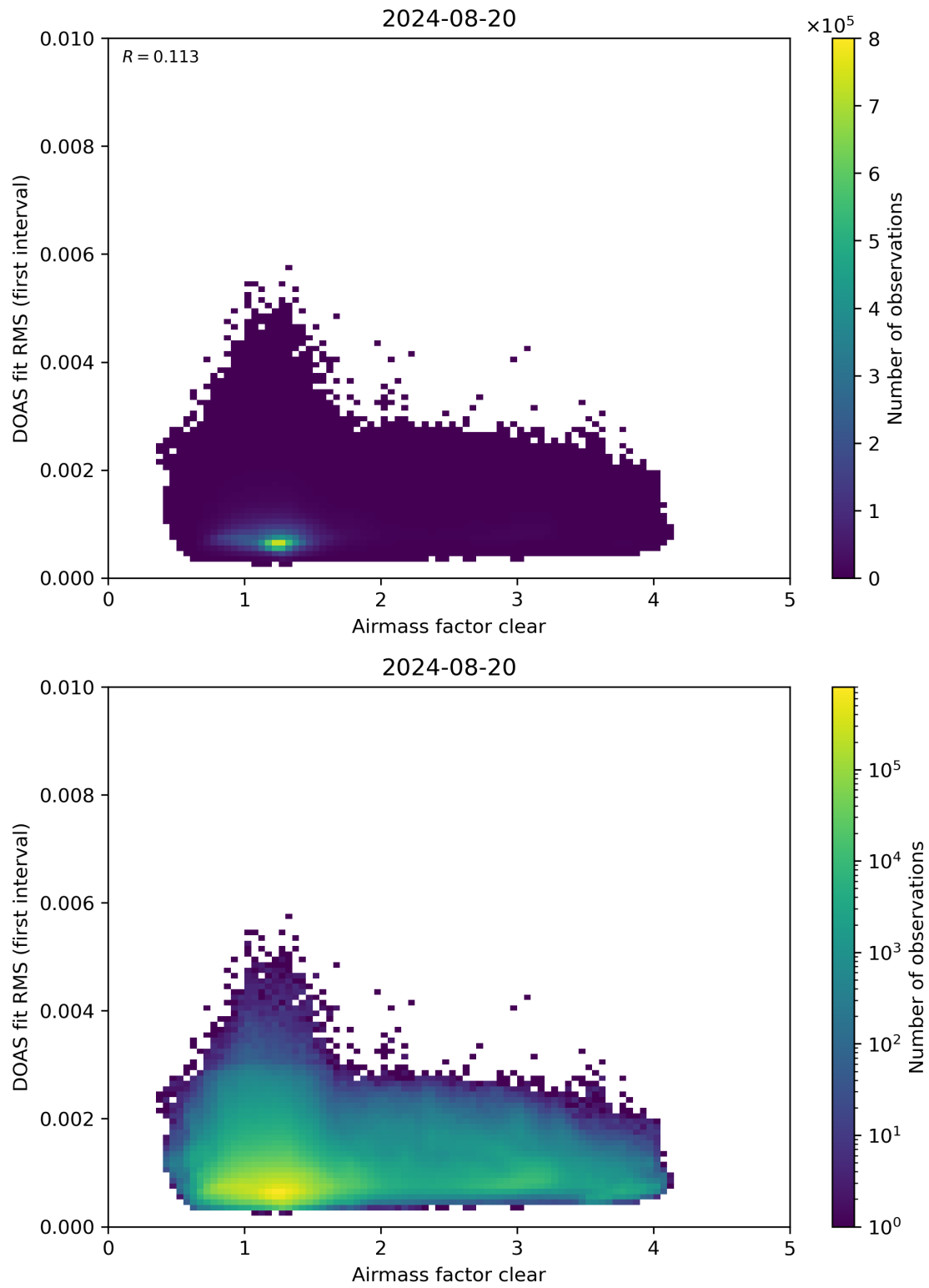
Figure 71: Scatter density plot of “Airmass factor clear” against “DOAS fit RMS (first interval)” for 2024-08-19 to 2024-08-21.
