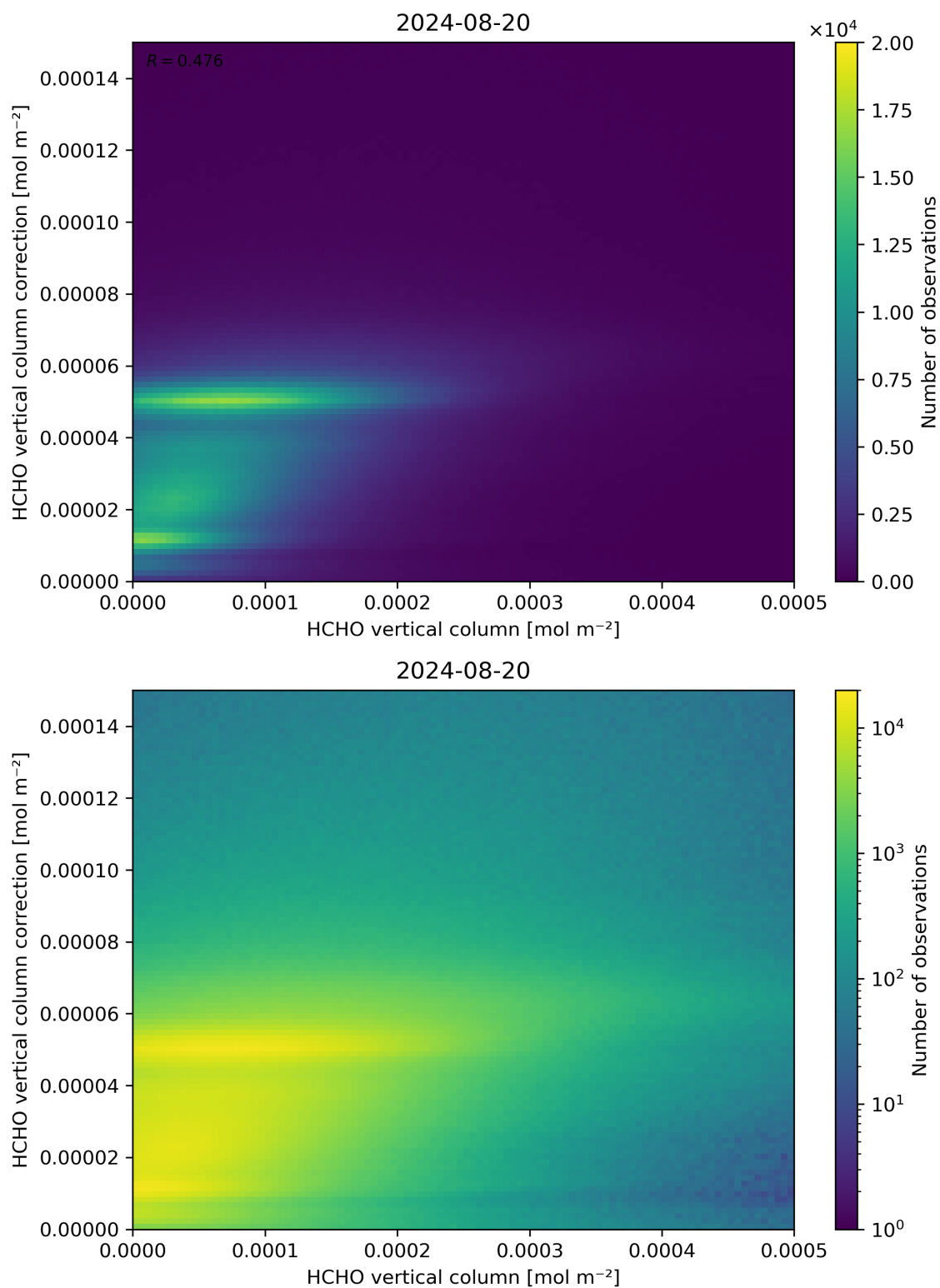
Figure 133: Scatter density plot of “HCHO vertical column” against “HCHO vertical column correction” for 2024-08-19 to 2024-08-21.
