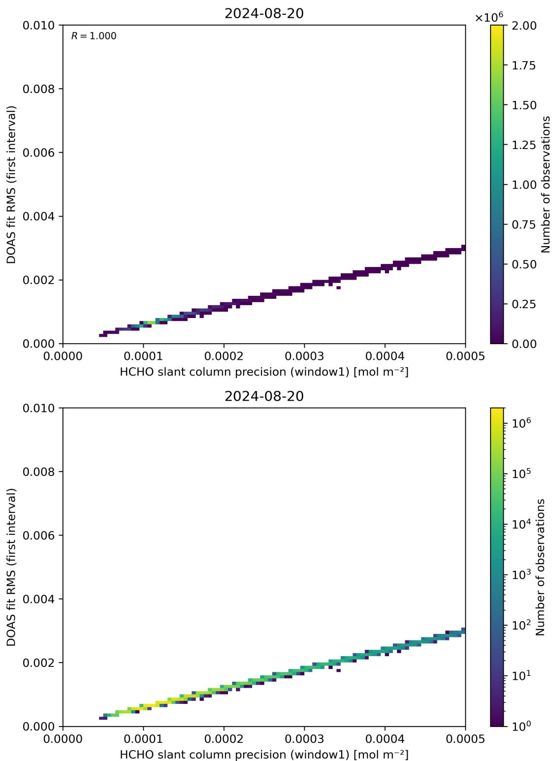
Figure 88: Scatter density plot of “HCHO slant column precision (window1)” against “DOAS fit RMS (first interval)” for 2024-08-19 to 2024-08-21.
