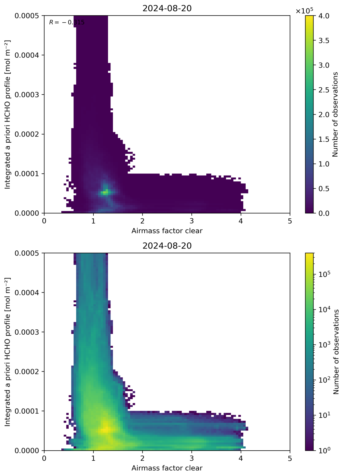
Figure 76: Scatter density plot of “Airmass factor clear” against “Integrated a priori HCHO profile” for 2024-08-19 to 2024-08-21.
