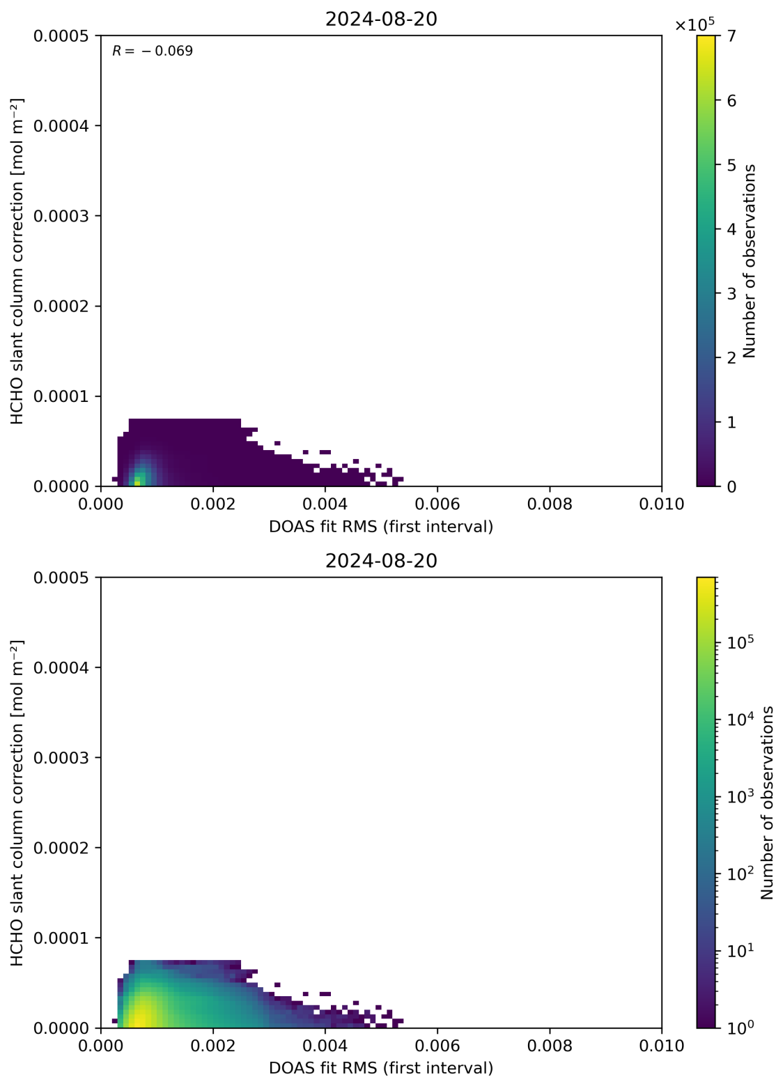
Figure 63: Scatter density plot of “DOAS fit RMS (first interval)” against “HCHO slant column correction” for 2024-08-19 to 2024-08-21.
