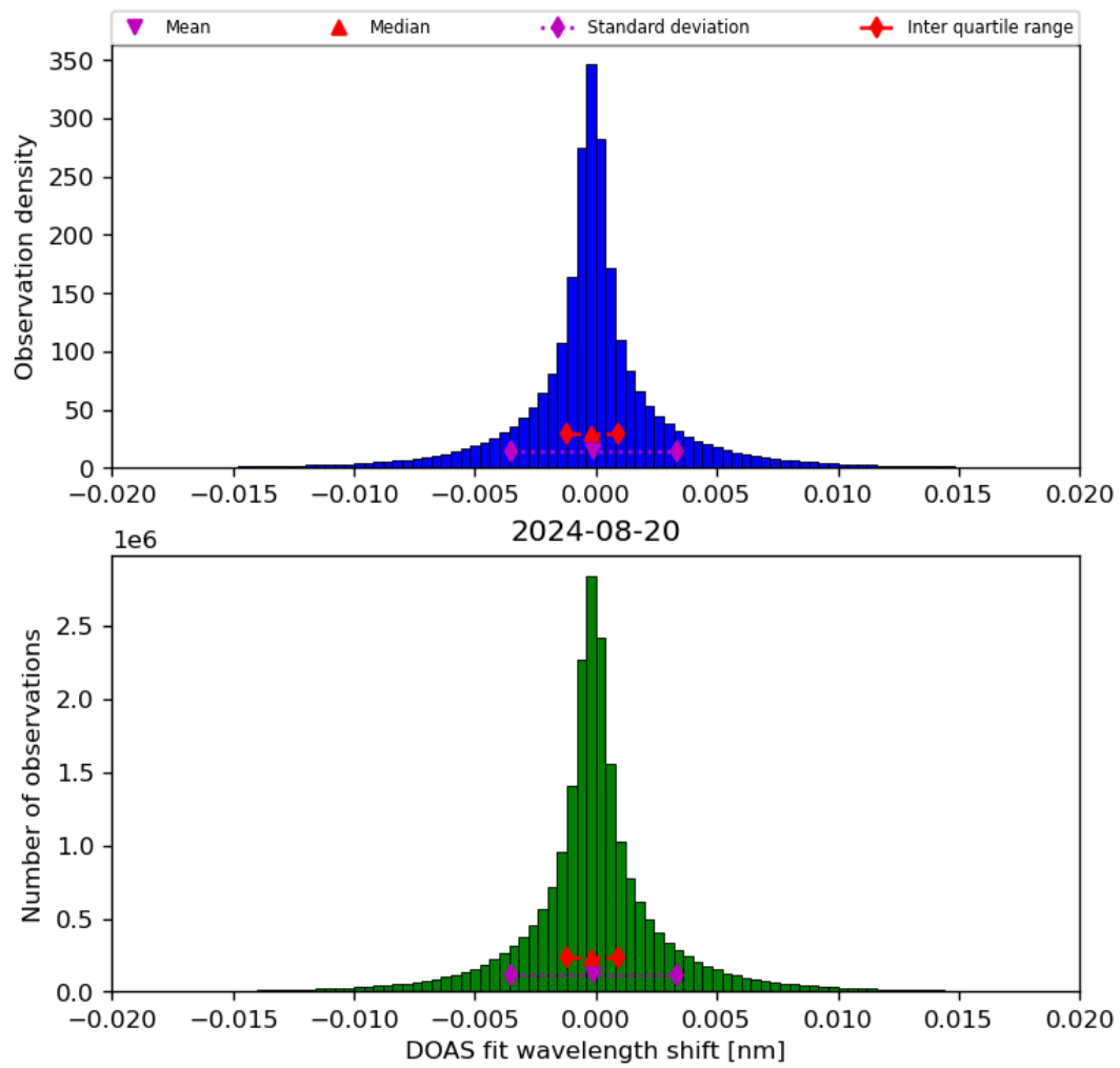
Figure 44: Histogram of “DOAS fit wavelength shift” for 2024-08-19 to 2024-08-21
