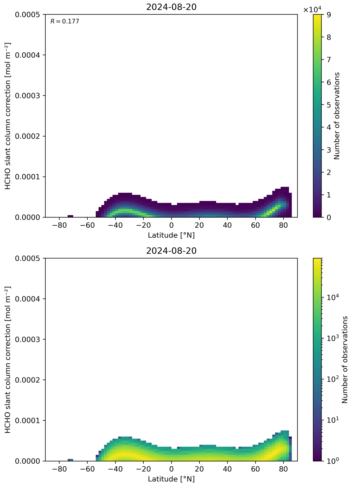
Figure 158: Scatter density plot of “Latitude” against “HCHO slant column correction” for 2024-08-19 to 2024-08-21.
