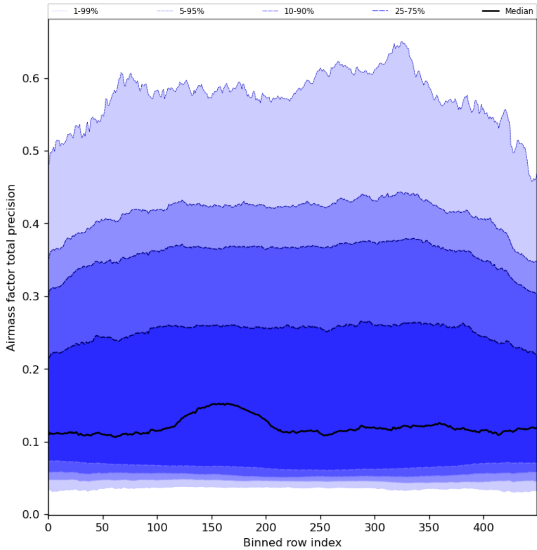
Figure 55: Along track statistics of “Airmass factor total precision” for 2024-08-19 to 2024-08-21
