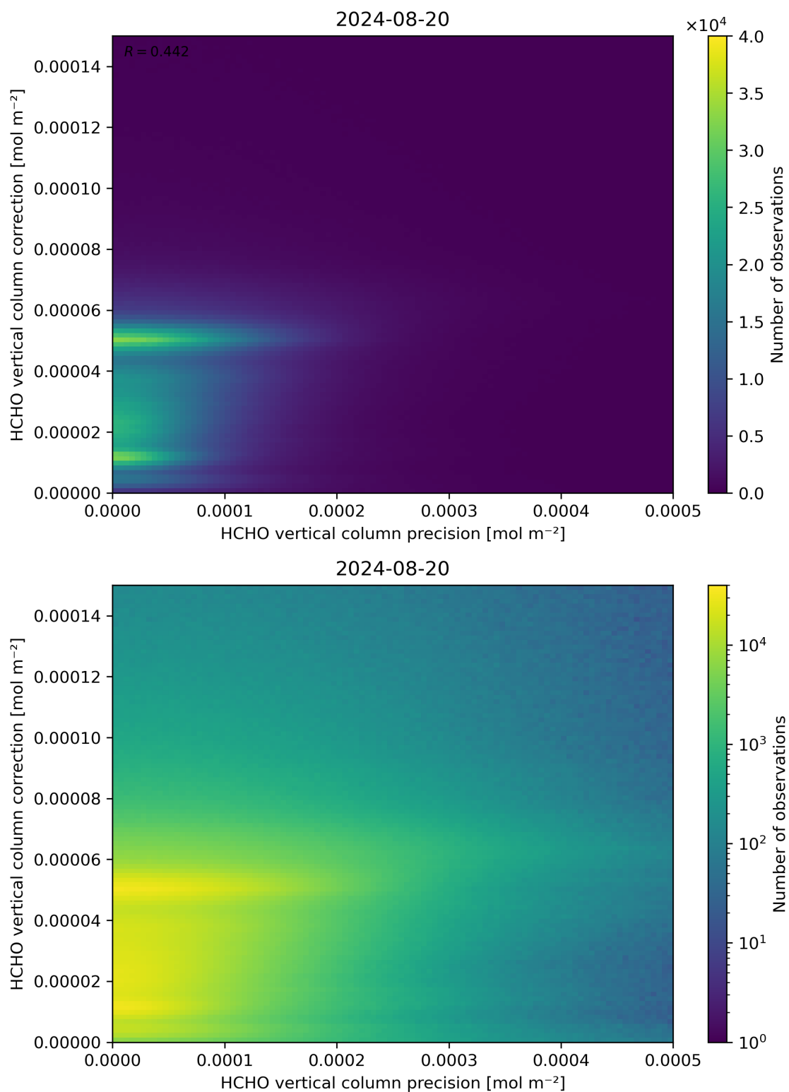
Figure 146: Scatter density plot of “HCHO vertical column precision” against “HCHO vertical column correction” for 2024-08-19 to 2024-08-21.
