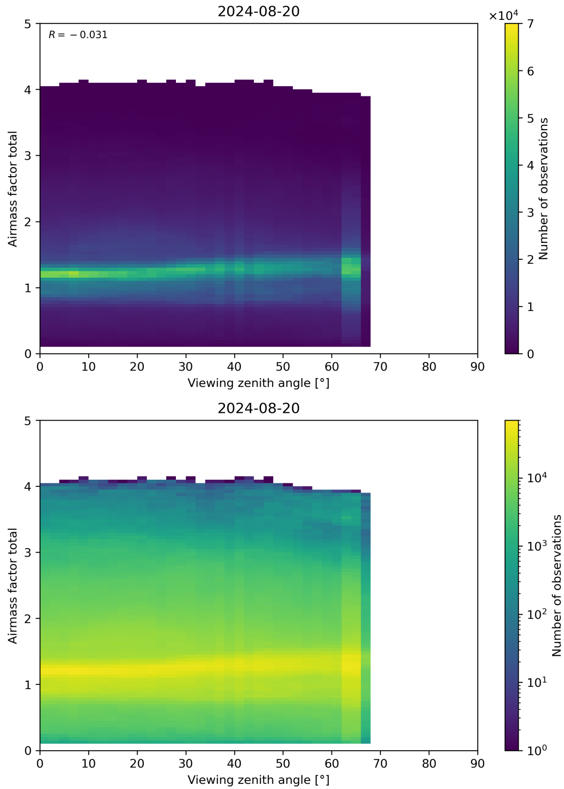
Figure 190: Scatter density plot of “Viewing zenith angle” against “Airmass factor total” for 2024-08-19 to 2024-08-21.
