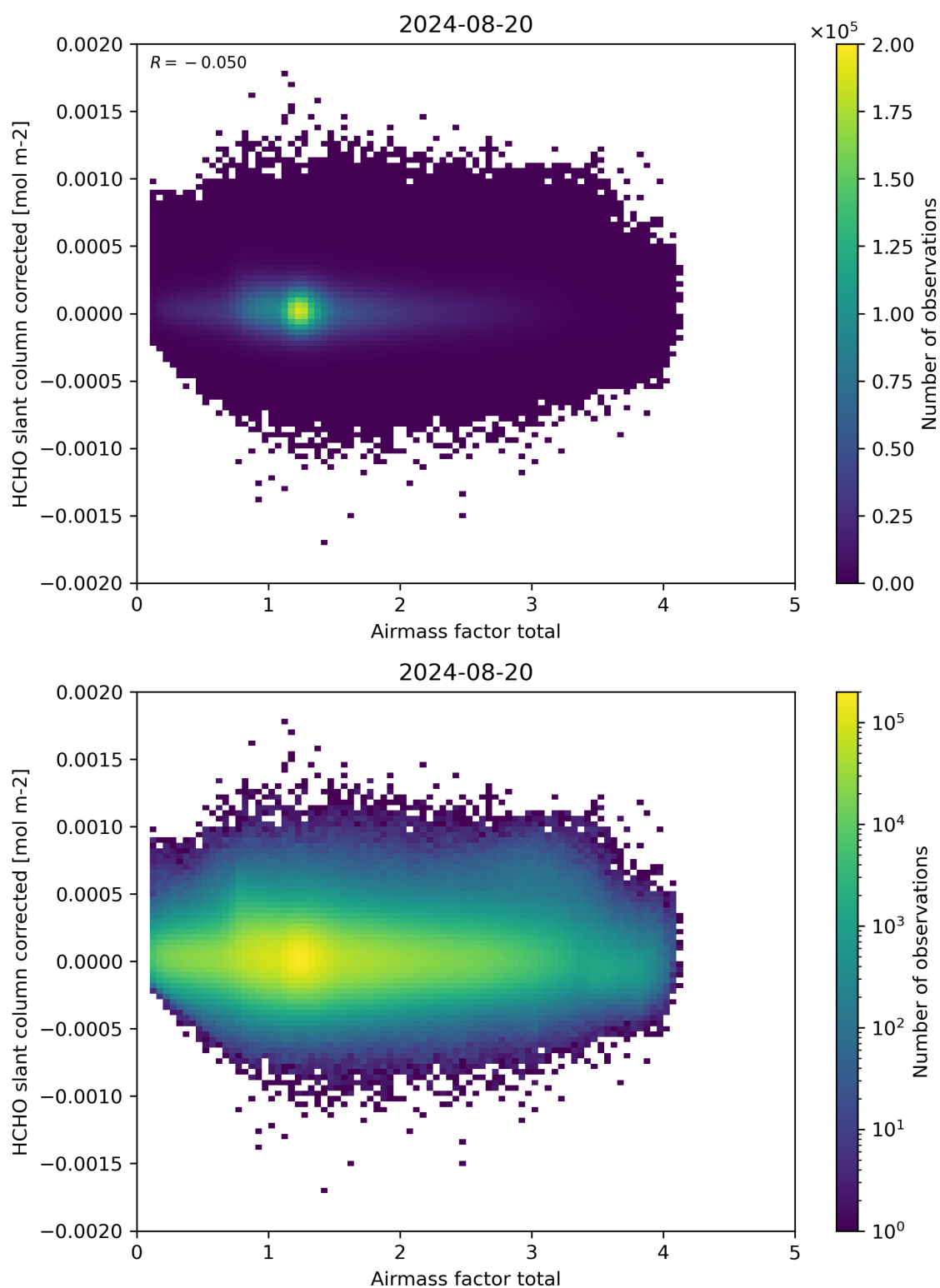
Figure 101: Scatter density plot of “Airmass factor total” against “HCHO slant column corrected” for 2024-08-19 to 2024-08-21.
