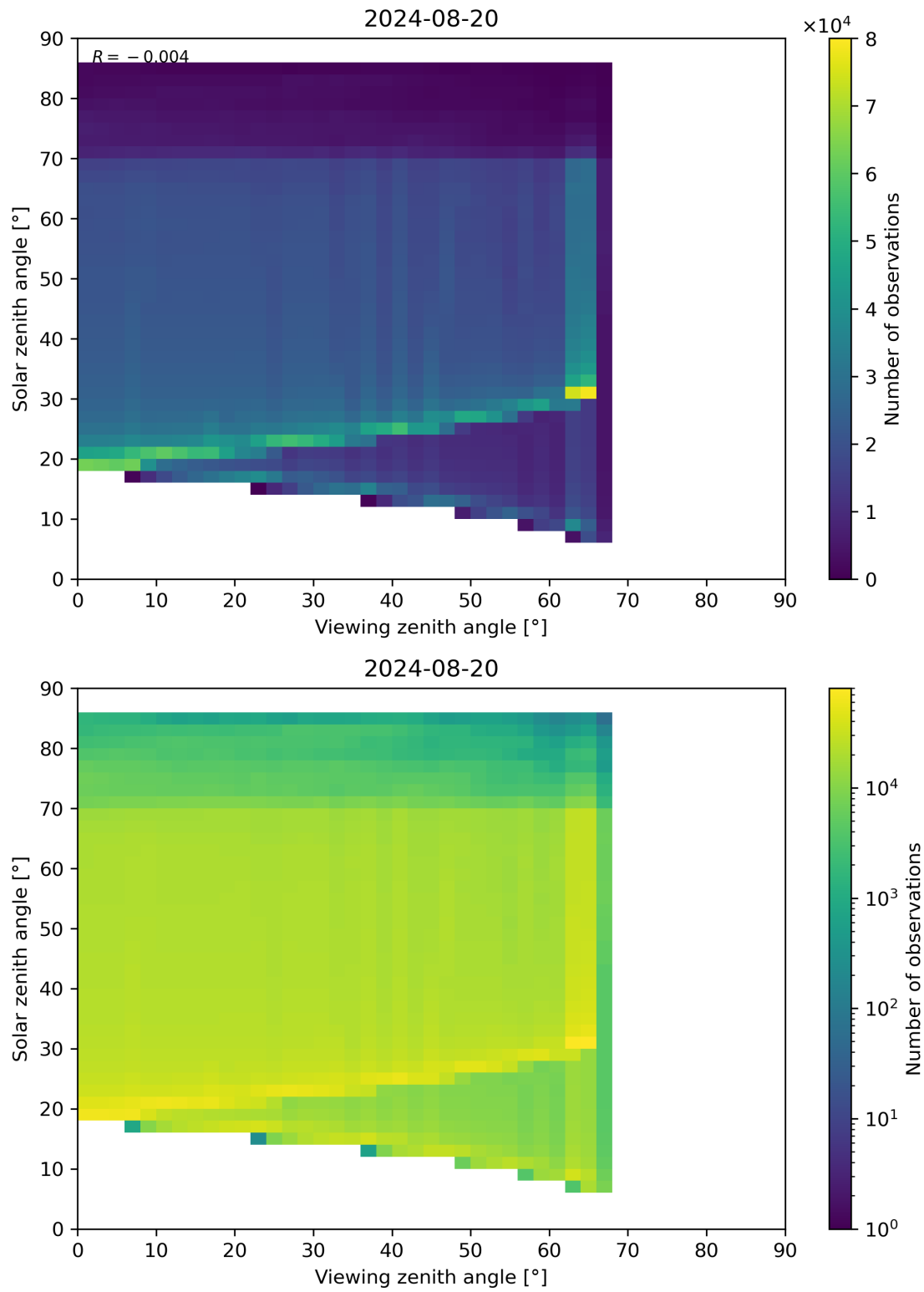
Figure 197: Scatter density plot of “Viewing zenith angle” against “Solar zenith angle” for 2024-08-19 to 2024-08-21.
