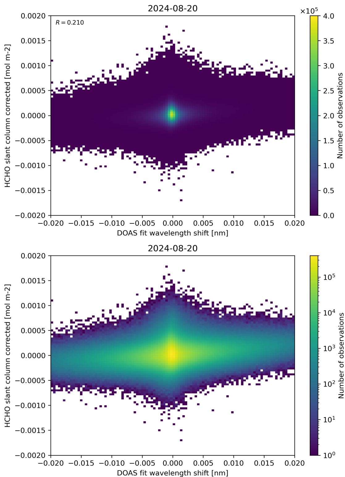
Figure 66: Scatter density plot of “DOAS fit wavelength shift” against “HCHO slant column corrected” for 2024-08-19 to 2024-08-21.
