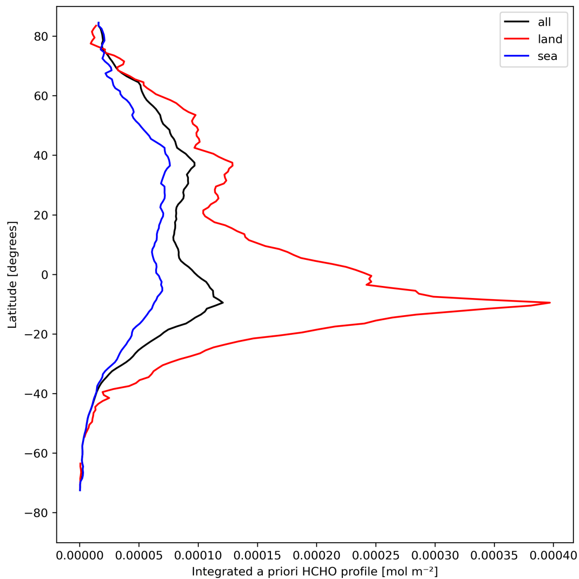
Figure 29: Zonal average of “Integrated a priori HCHO profile” for 2024-08-19 to 2024-08-21.
