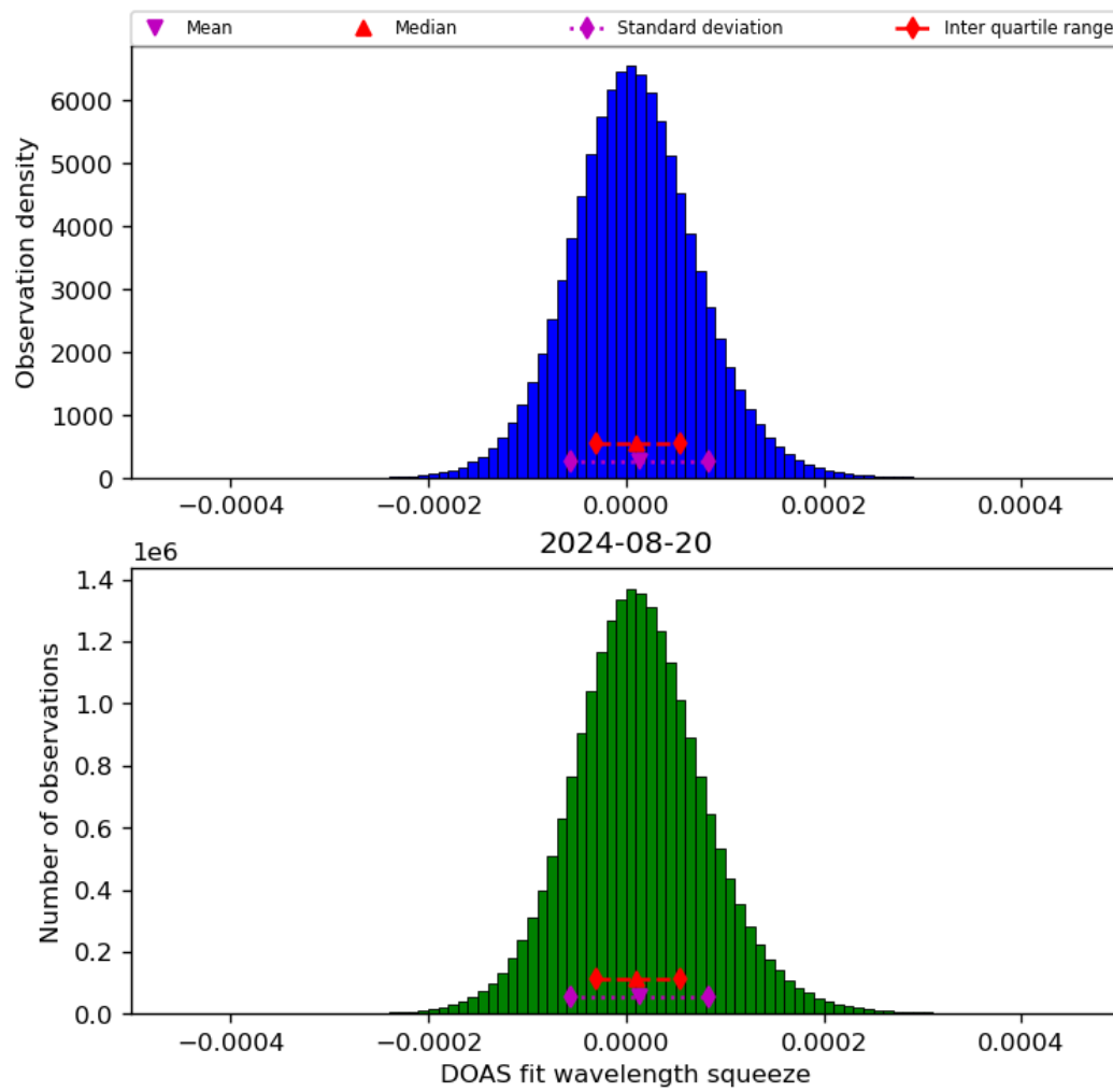
Figure 45: Histogram of “DOAS fit wavelength squeeze” for 2024-08-19 to 2024-08-21
