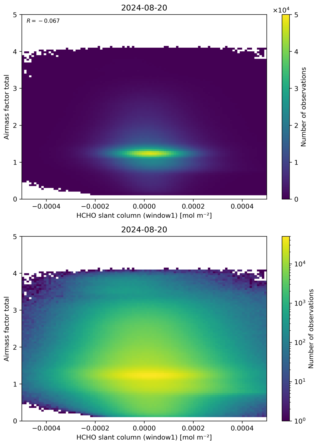
Figure 85: Scatter density plot of “HCHO slant column (window1)” against “Airmass factor total” for 2024-08-19 to 2024-08-21.
