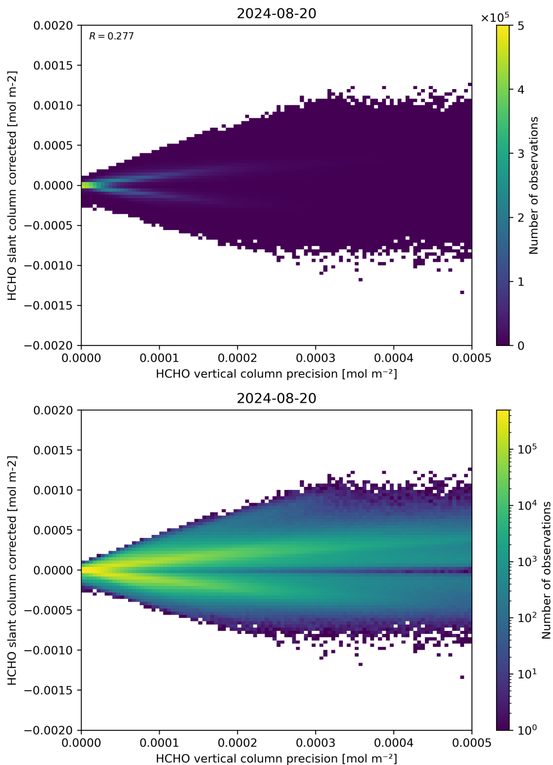
Figure 140: Scatter density plot of “HCHO vertical column precision” against “HCHO slant column corrected” for 2024-08-19 to 2024-08-21.
