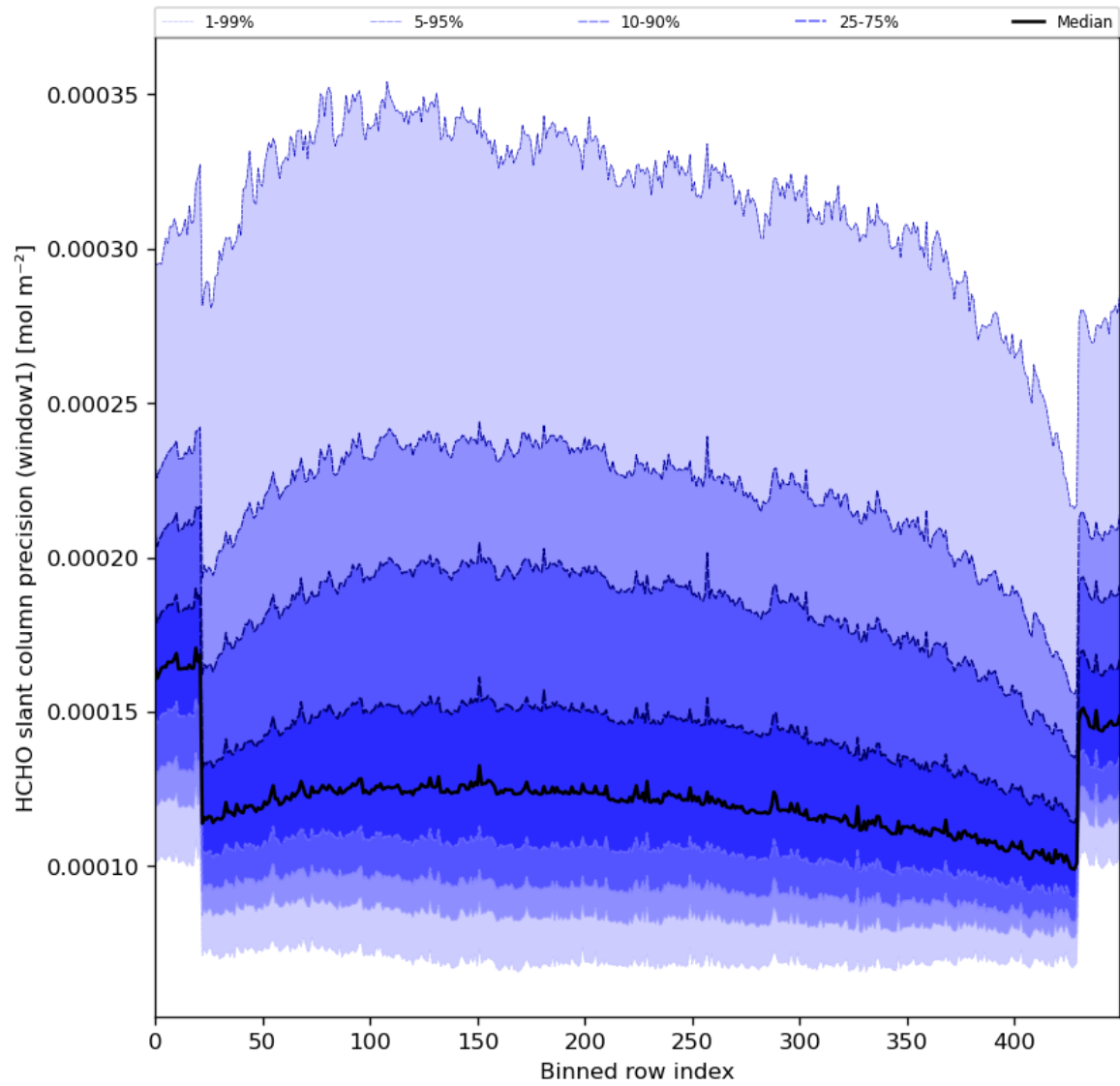
Figure 53: Along track statistics of “HCHO slant column precision (window1)” for 2024-08-19 to 2024-08-21
