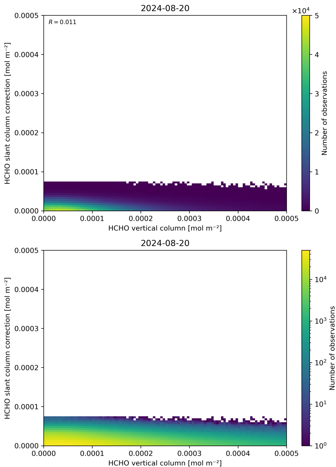
Figure 128: Scatter density plot of “HCHO vertical column” against “HCHO slant column correction” for 2024-08-19 to 2024-08-21.
