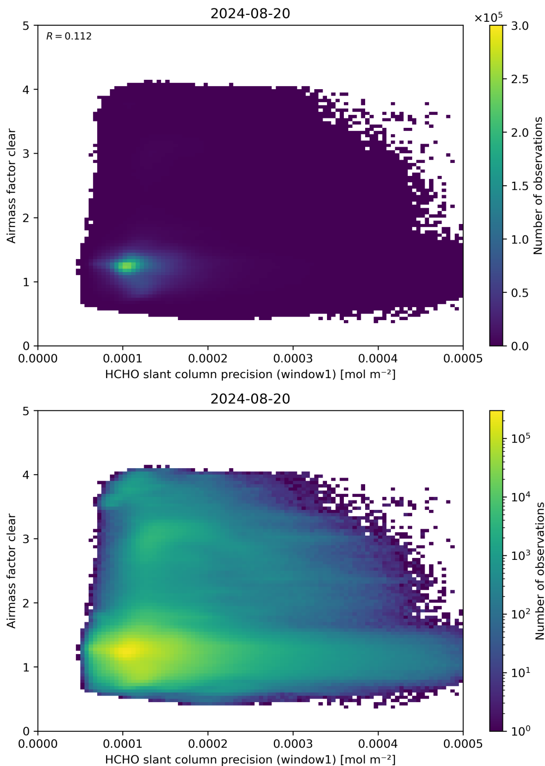
Figure 91: Scatter density plot of “HCHO slant column precision (window1)” against “Airmass factor clear” for 2024-08-19 to 2024-08-21.
