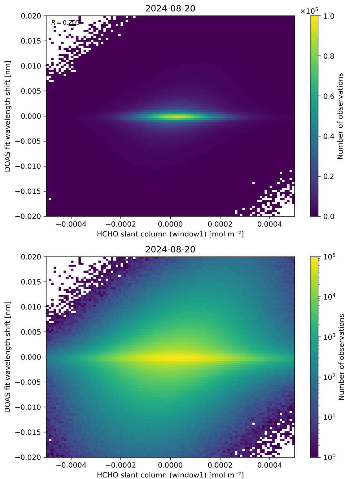
Figure 79: Scatter density plot of “HCHO slant column (window1)” against “DOAS fit wavelength shift” for 2024-08-19 to 2024-08-21.
