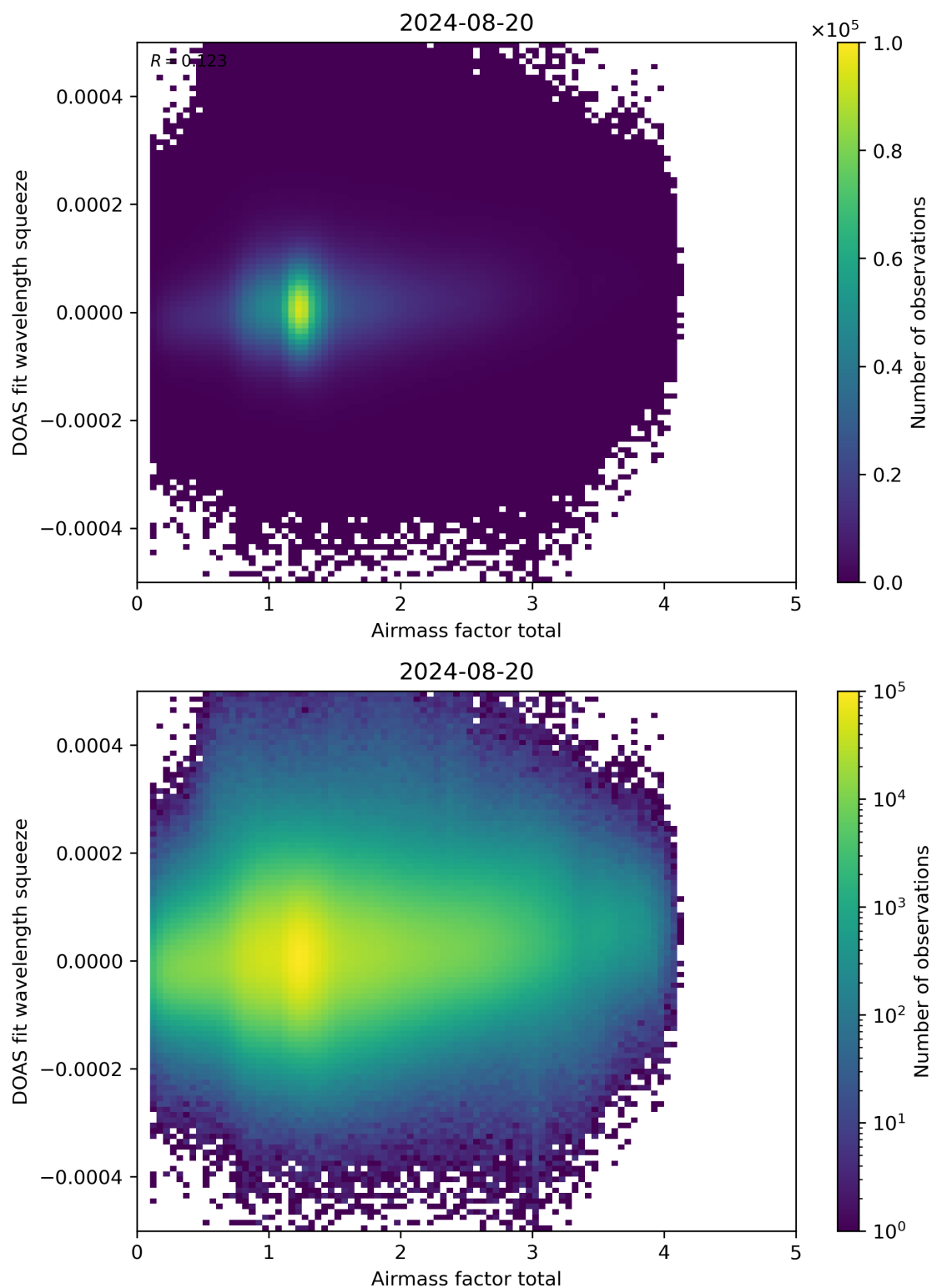
Figure 99: Scatter density plot of “Airmass factor total” against “DOAS fit wavelength squeeze” for 2024-08-19 to 2024-08-21.
