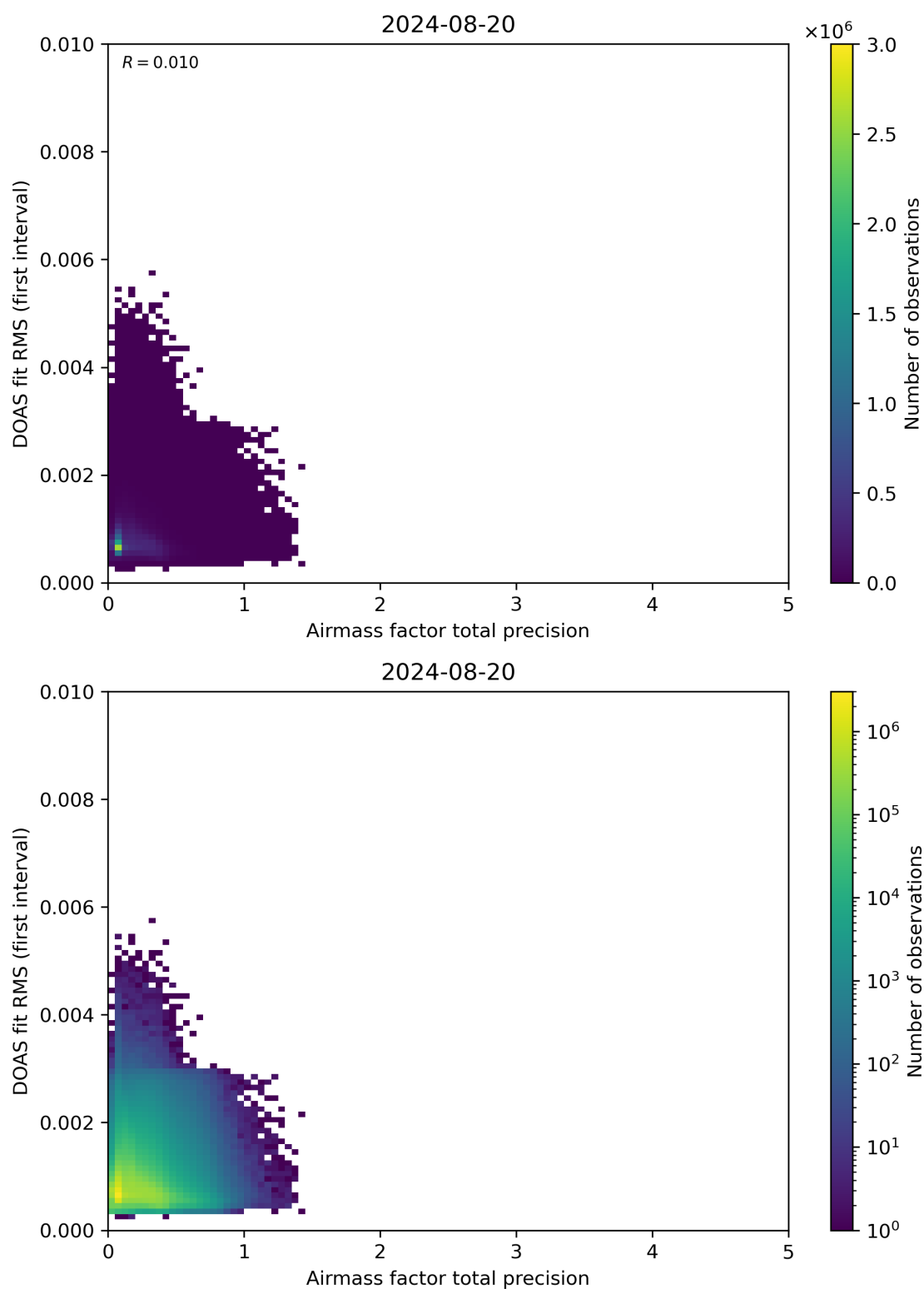
Figure 105: Scatter density plot of “Airmass factor total precision” against “DOAS fit RMS (first interval)” for 2024-08-19 to 2024-08-21.
