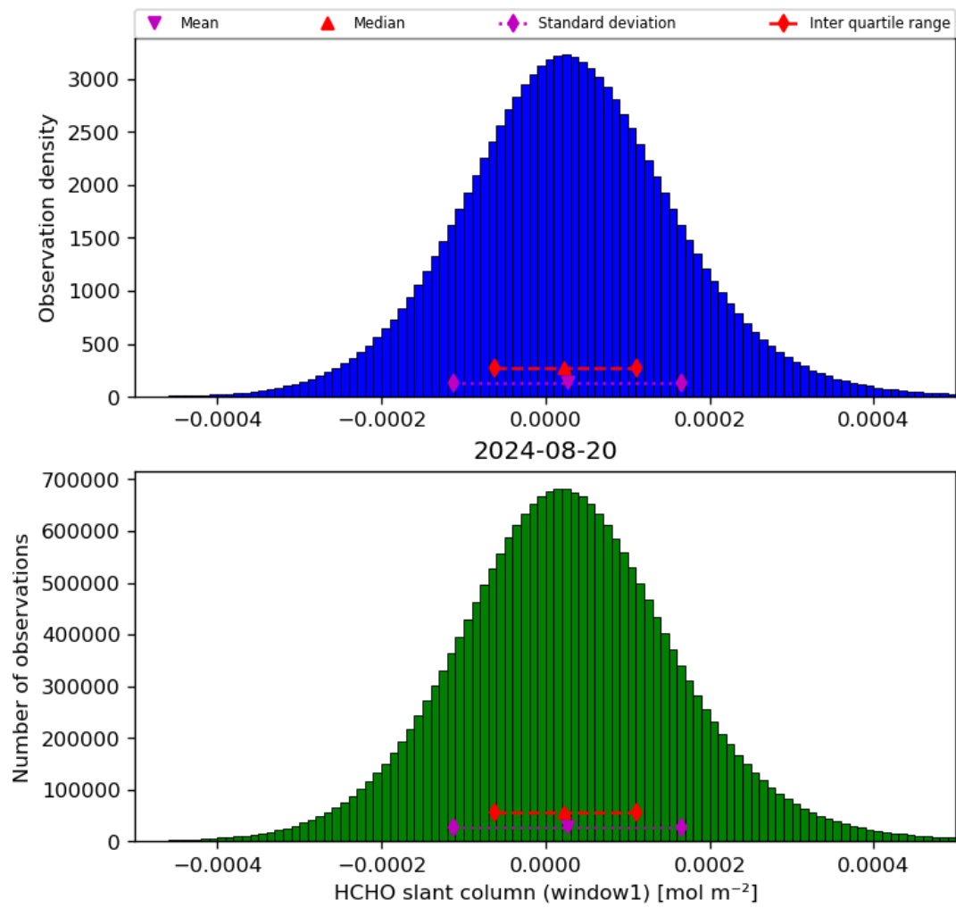
Figure 38: Histogram of “HCHO slant column (window1)” for 2024-08-19 to 2024-08-21
