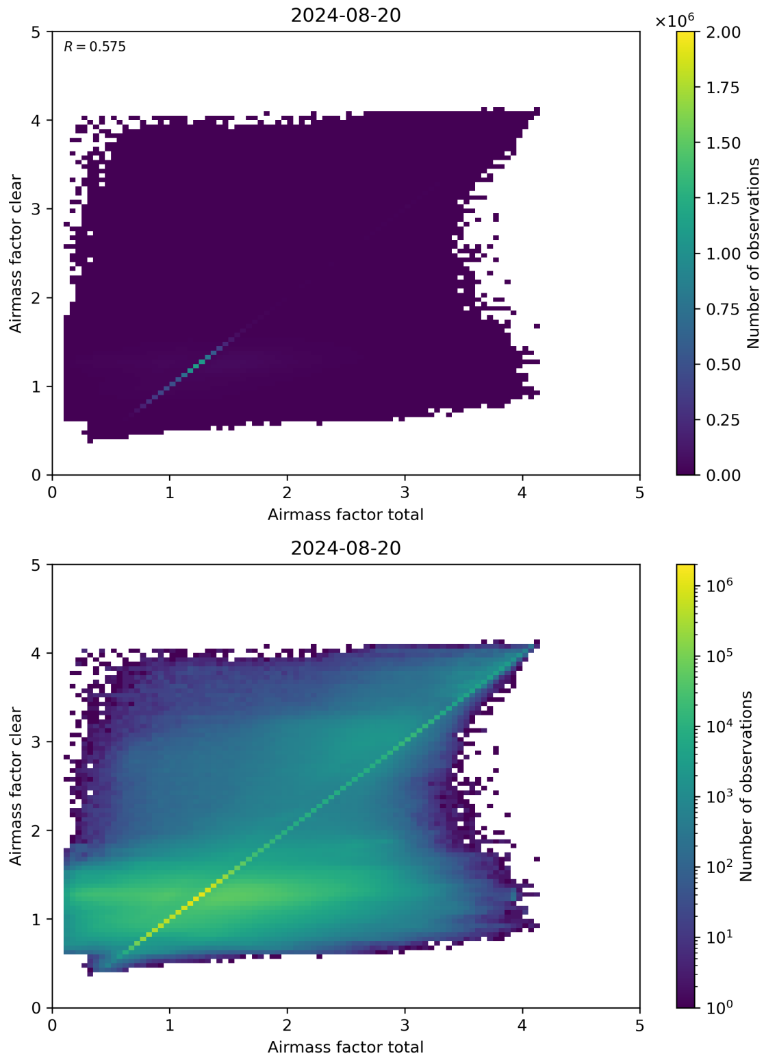
Figure 100: Scatter density plot of “Airmass factor total” against “Airmass factor clear” for 2024-08-19 to 2024-08-21.
