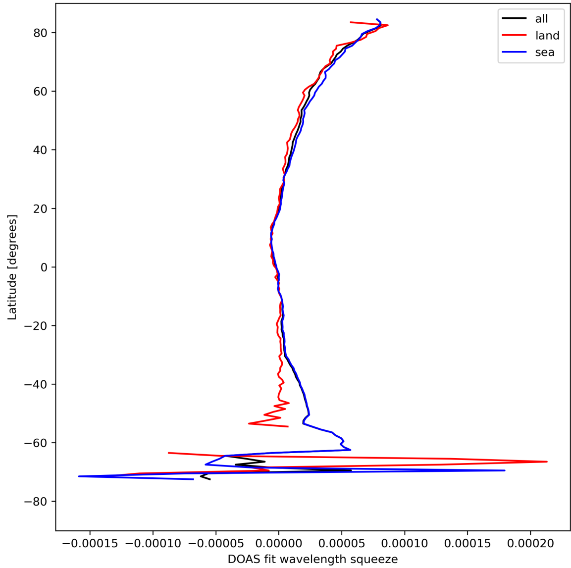
Figure 31: Zonal average of “DOAS fit wavelength squeeze” for 2024-08-19 to 2024-08-21.
