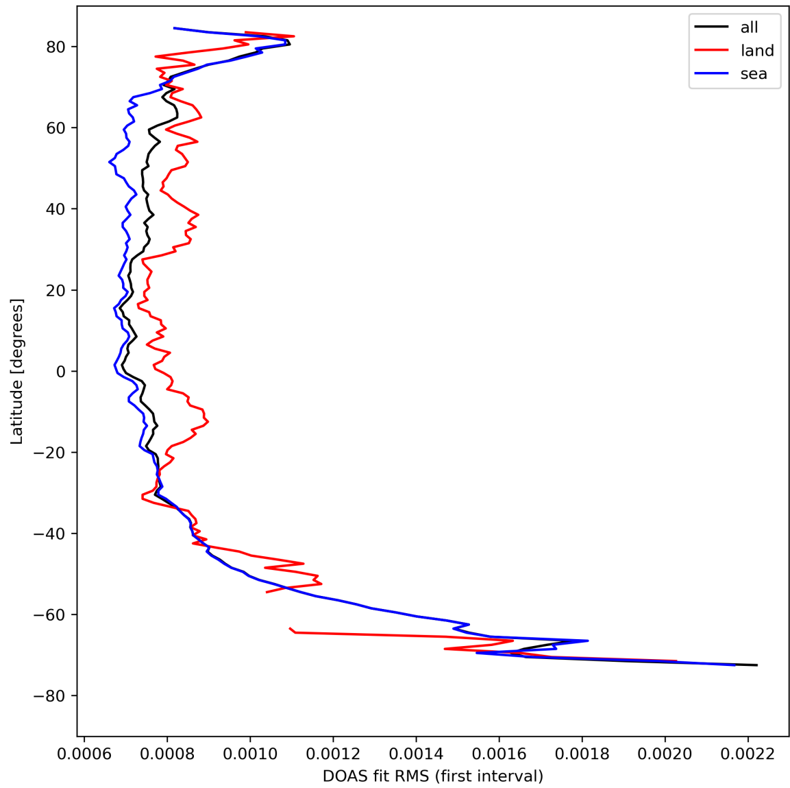
Figure 32: Zonal average of “DOAS fit RMS (first interval)” for 2024-08-19 to 2024-08-21.
