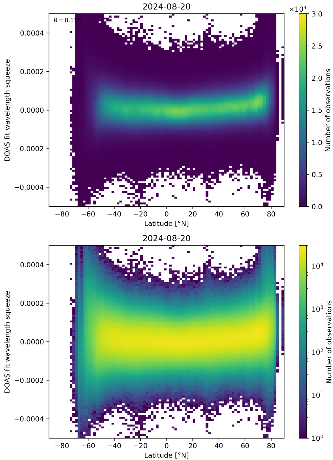
Figure 155: Scatter density plot of “Latitude” against “DOAS fit wavelength squeeze” for 2024-08-19 to 2024-08-21.
