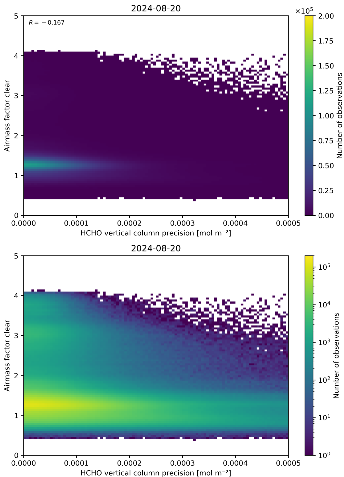
Figure 139: Scatter density plot of “HCHO vertical column precision” against “Airmass factor clear” for 2024-08-19 to 2024-08-21.
