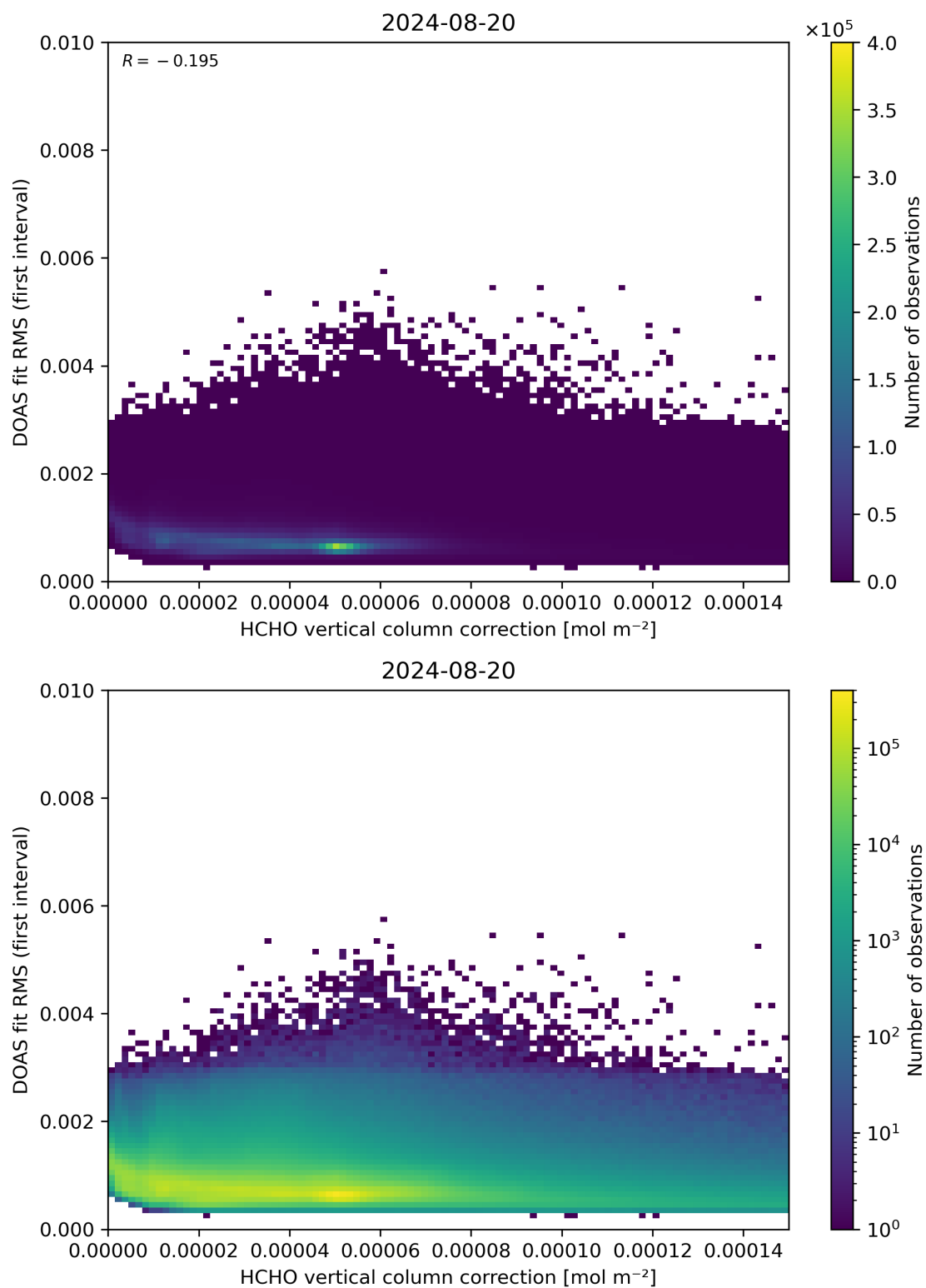
Figure 112: Scatter density plot of “HCHO vertical column correction” against “DOAS fit RMS (first interval)” for 2024-08-19 to 2024-08-21.
