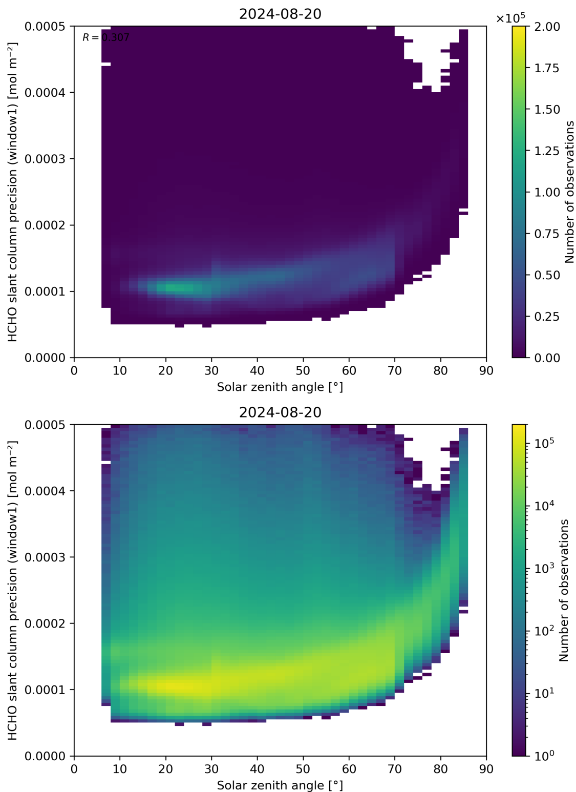
Figure 174: Scatter density plot of “Solar zenith angle” against “HCHO slant column precision (window1)” for 2024-08-19 to 2024-08-21.
