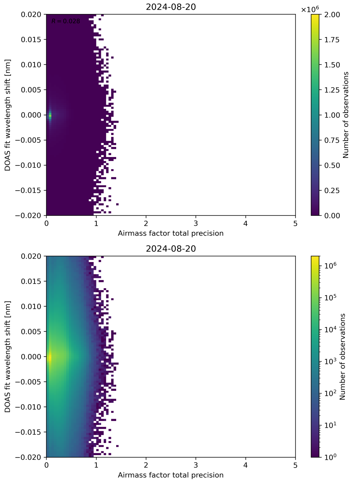
Figure 106: Scatter density plot of “Airmass factor total precision” against “DOAS fit wavelength shift” for 2024-08-19 to 2024-08-21.
