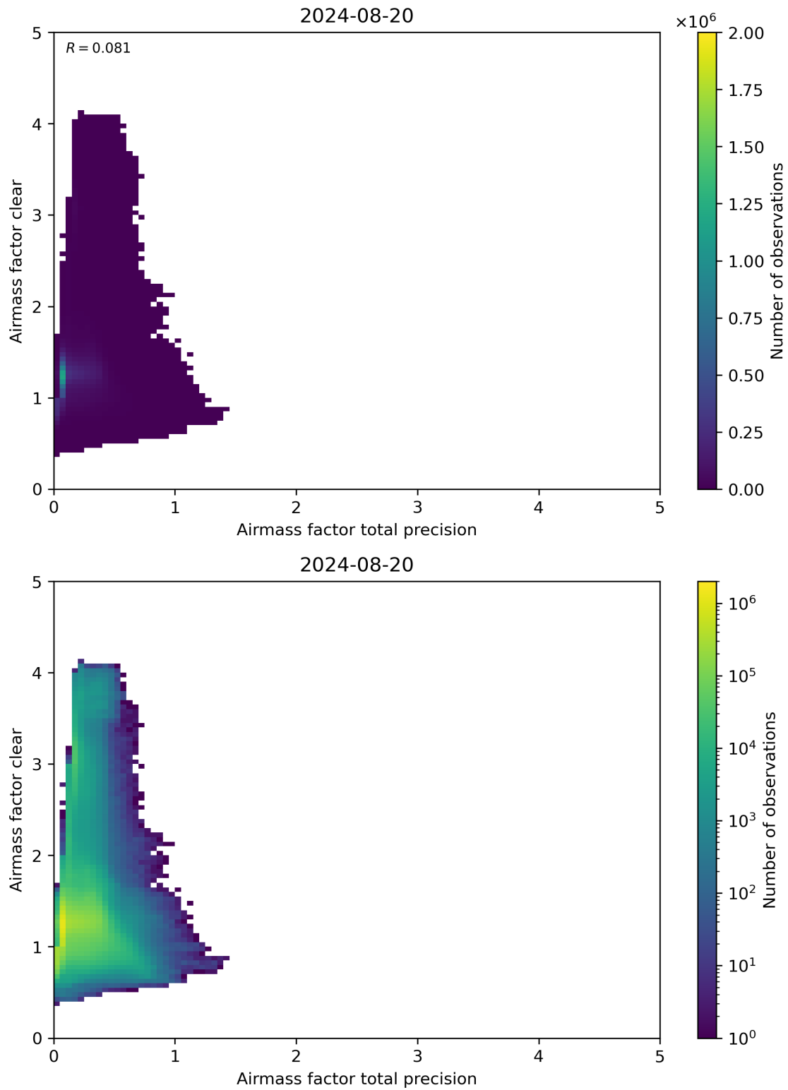
Figure 108: Scatter density plot of “Airmass factor total precision” against “Airmass factor clear” for 2024-08-19 to 2024-08-21.
