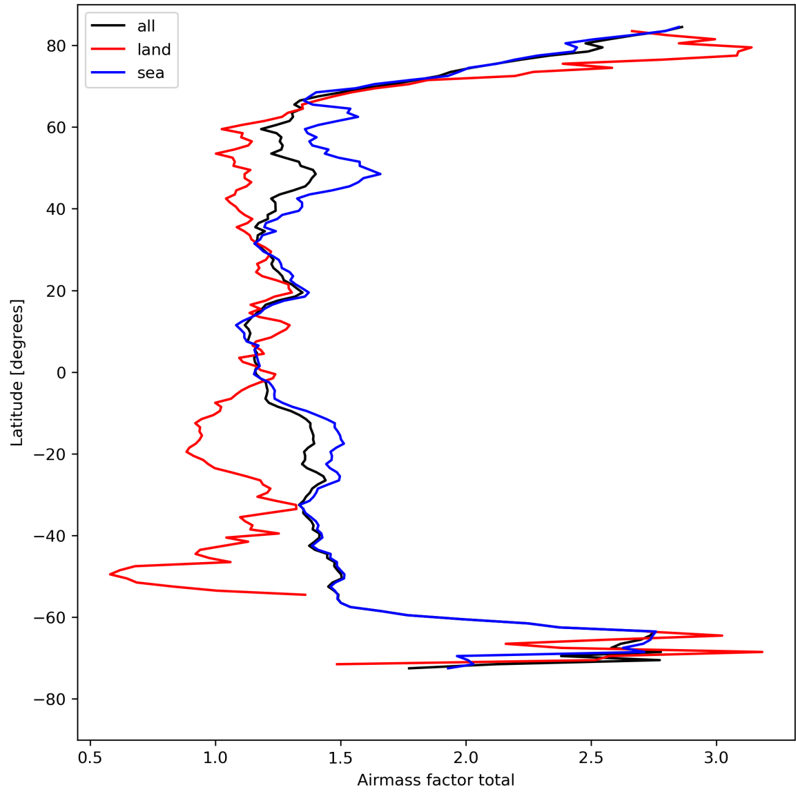
Figure 26: Zonal average of “Airmass factor total” for 2024-08-19 to 2024-08-21.
