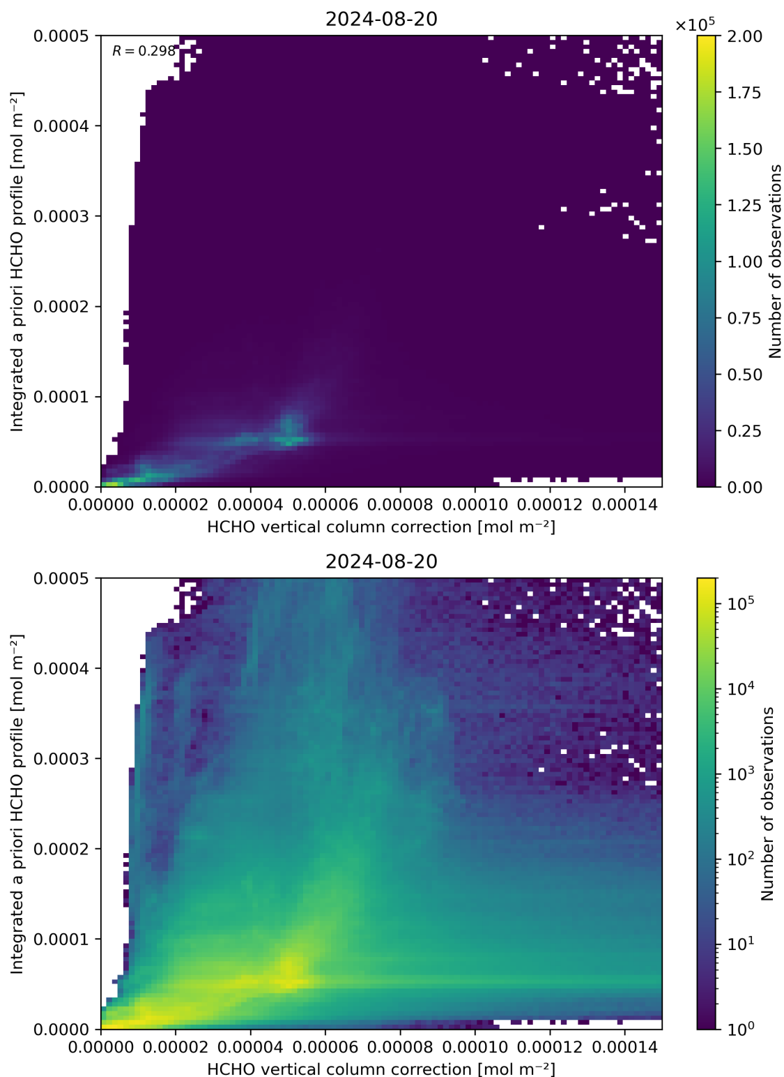
Figure 122: Scatter density plot of “HCHO vertical column correction” against “Integrated a priori HCHO profile” for 2024-08-19 to 2024-08-21.
