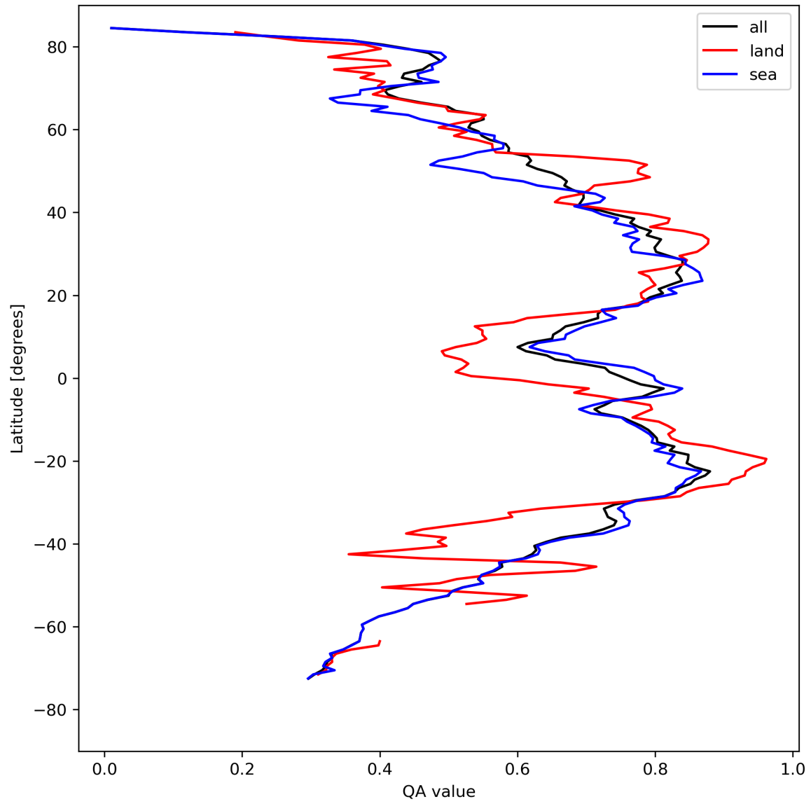
Figure 20: Zonal average of “QA value” for 2024-08-19 to 2024-08-21.
