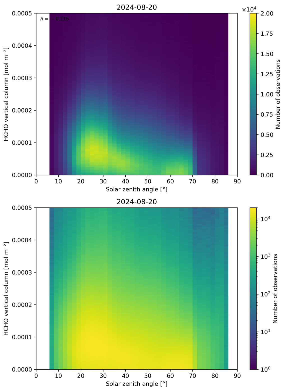
Figure 177: Scatter density plot of “Solar zenith angle” against “HCHO vertical column” for 2024-08-19 to 2024-08-21.
