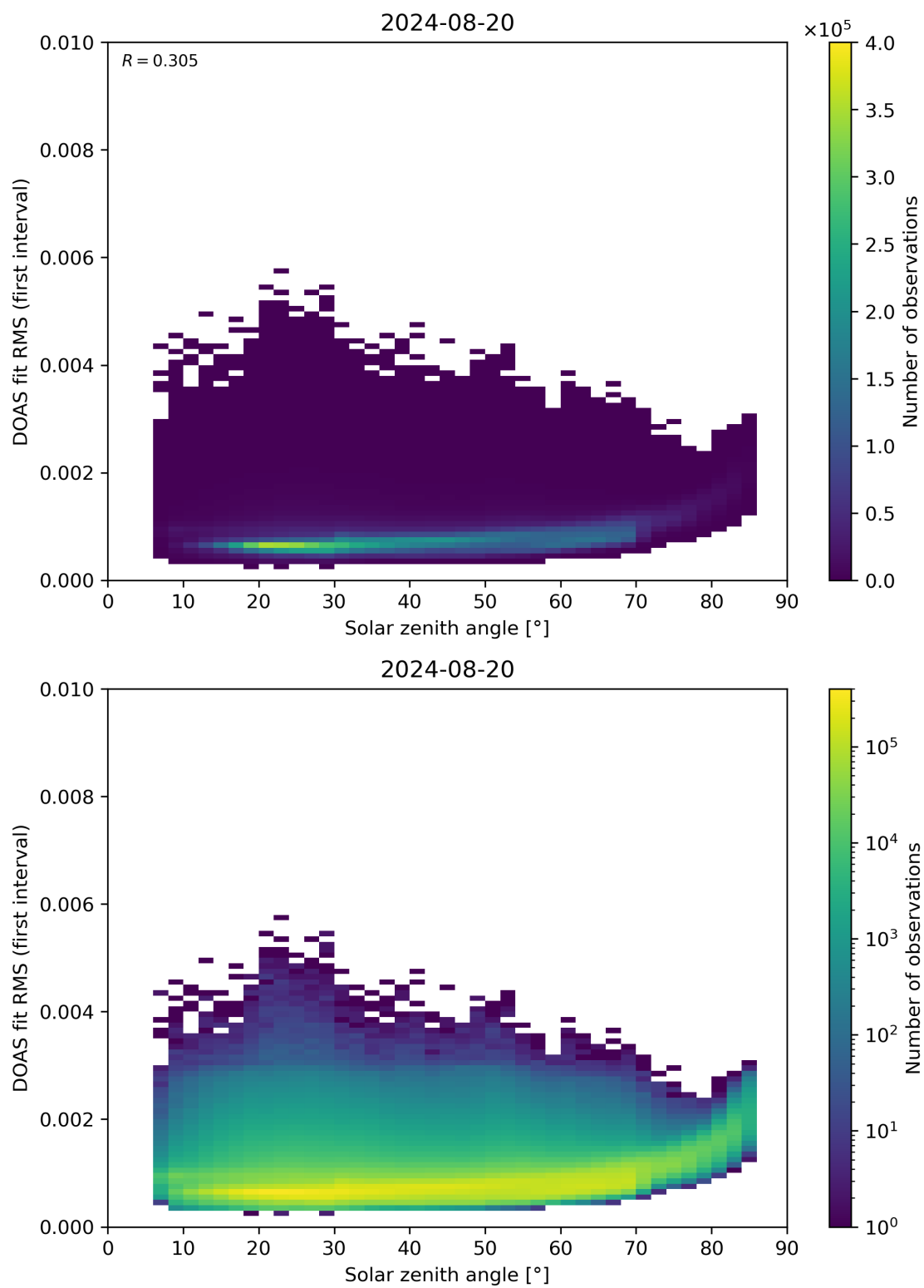
Figure 167: Scatter density plot of “Solar zenith angle” against “DOAS fit RMS (first interval)” for 2024-08-19 to 2024-08-21.
