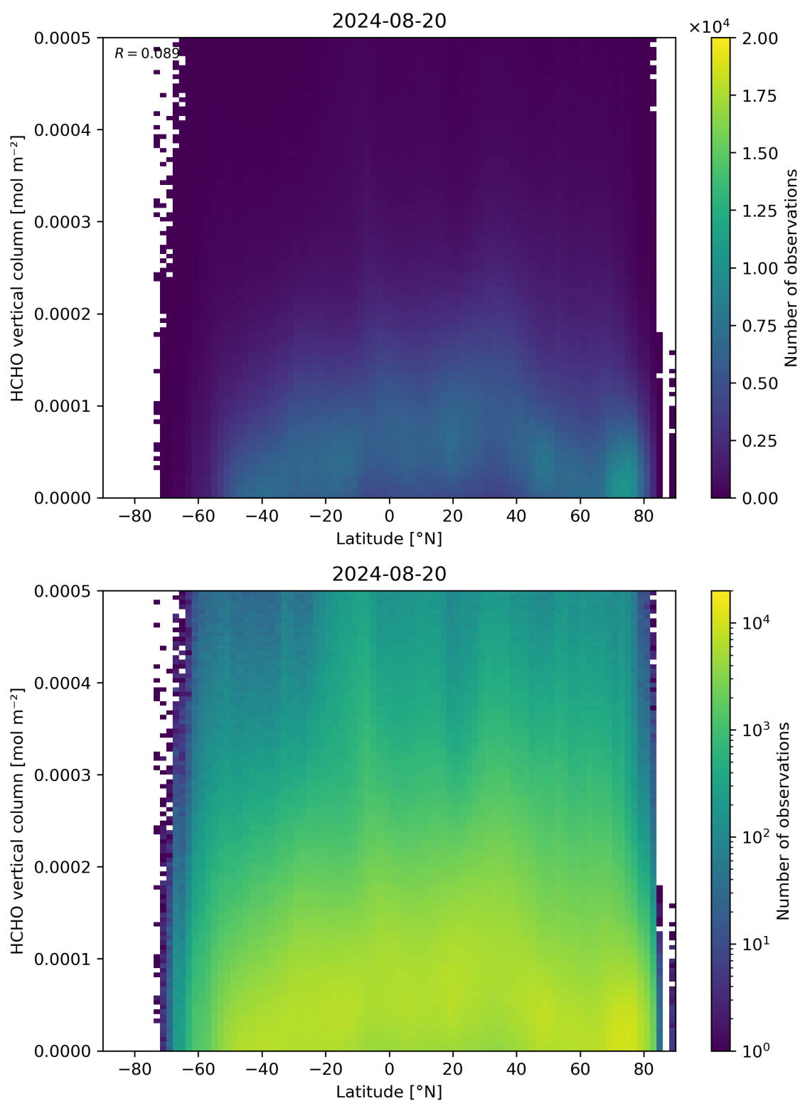
Figure 163: Scatter density plot of “Latitude” against “HCHO vertical column” for 2024-08-19 to 2024-08-21.
