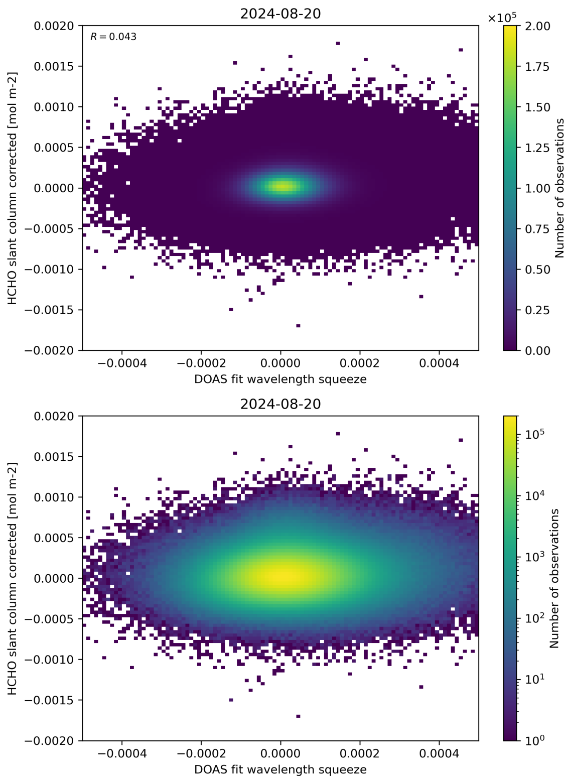
Figure 69: Scatter density plot of “DOAS fit wavelength squeeze” against “HCHO slant column corrected” for 2024-08-19 to 2024-08-21.
