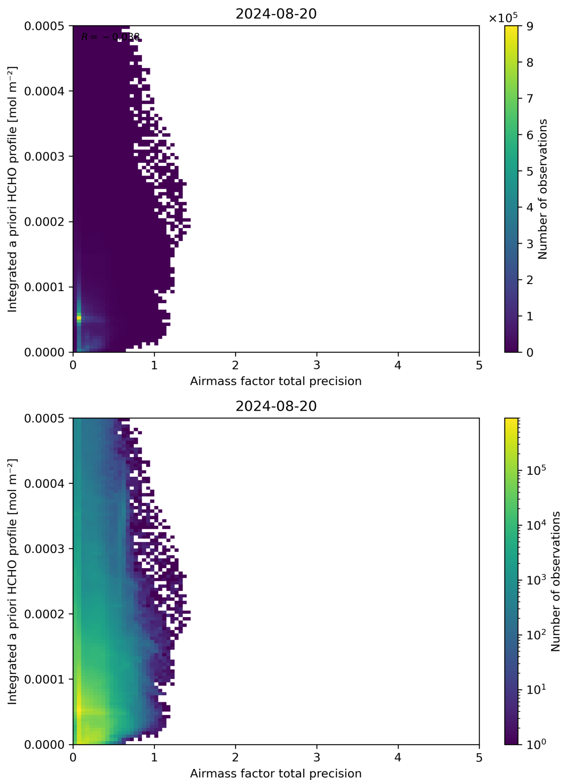
Figure 111: Scatter density plot of “Airmass factor total precision” against “Integrated a priori HCHO profile” for 2024-08-19 to 2024-08-21.
