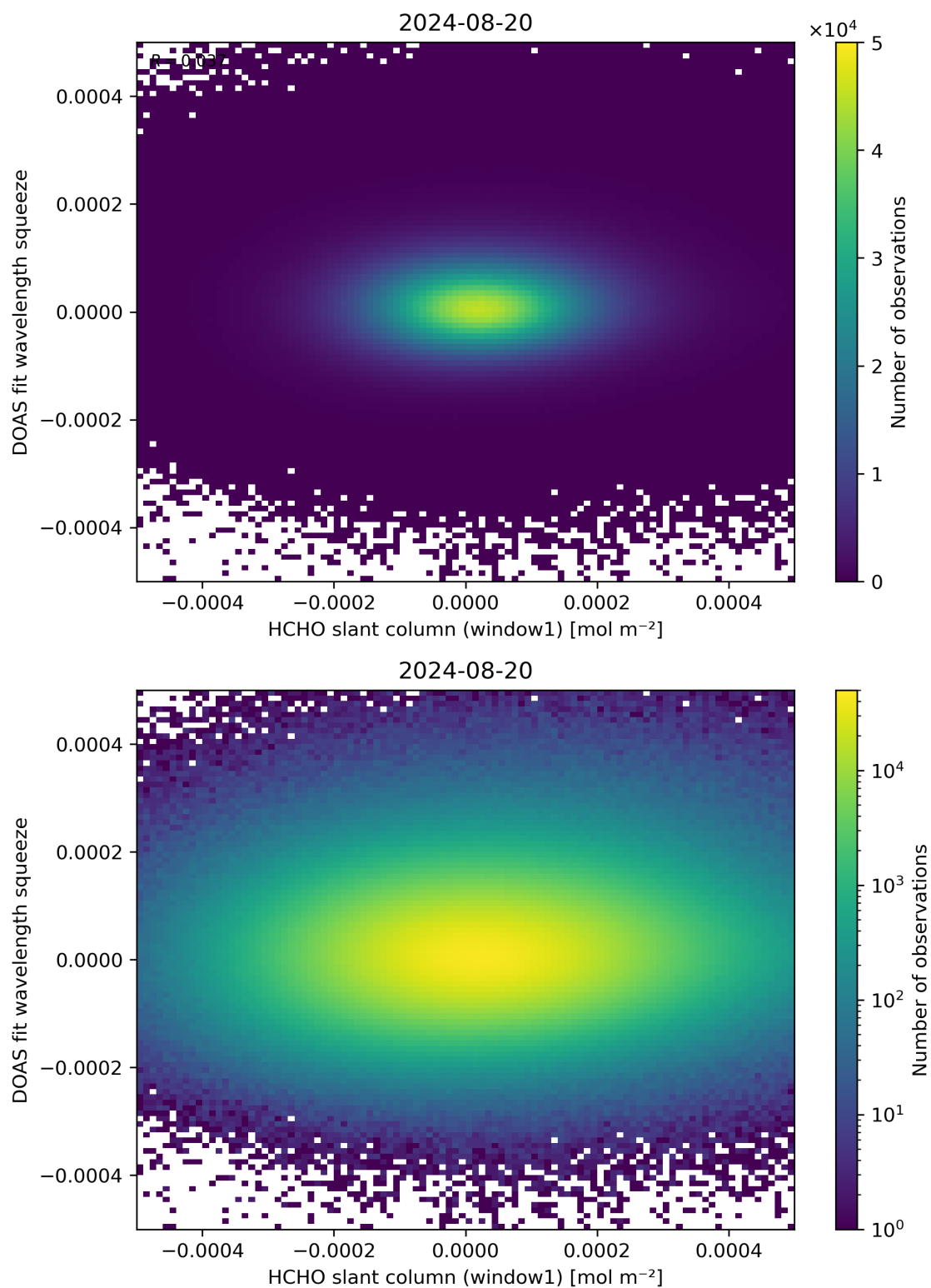
Figure 80: Scatter density plot of “HCHO slant column (window1)” against “DOAS fit wavelength squeeze” for 2024-08-19 to 2024-08-21.
