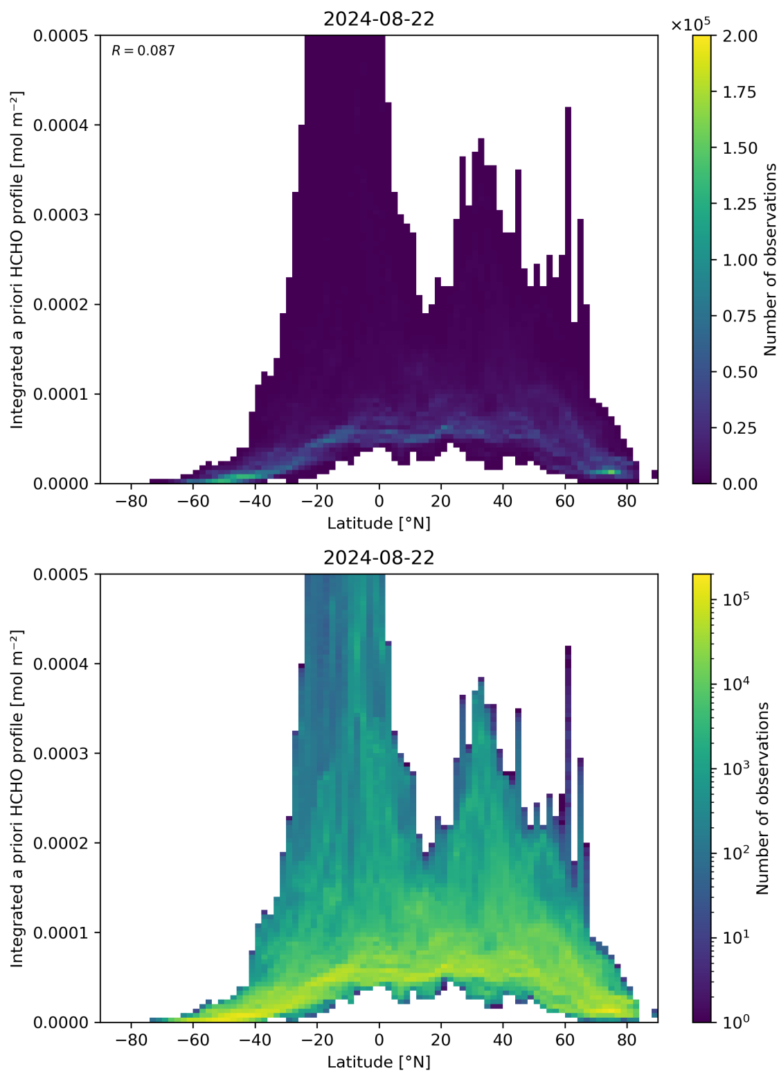
Figure 166: Scatter density plot of “Latitude” against “Integrated a priori HCHO profile” for 2024-08-22 to 2024-08-23.
