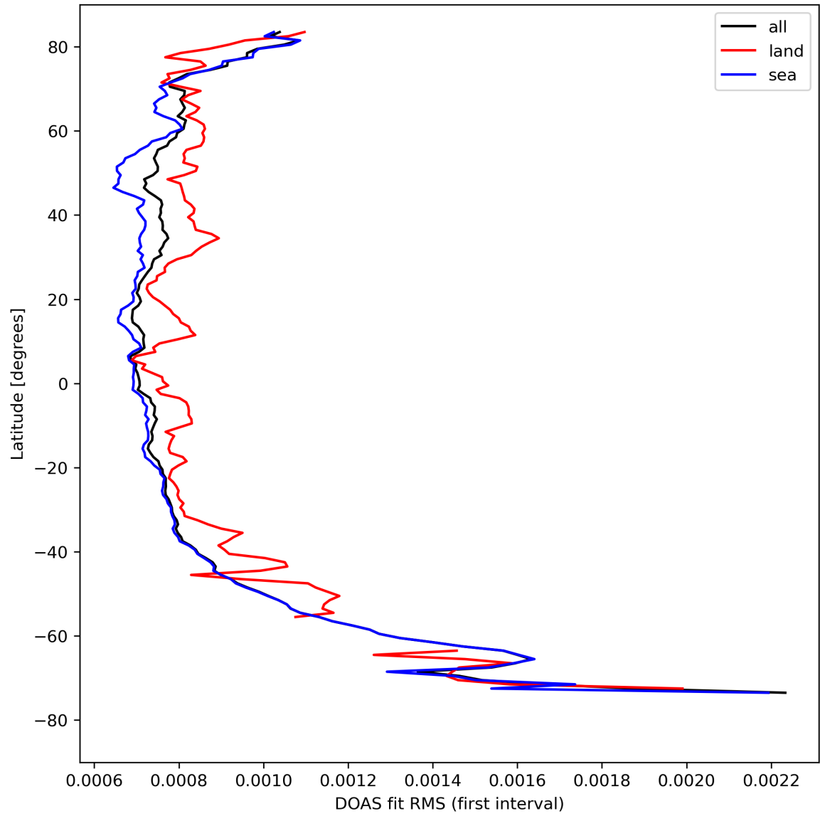
Figure 32: Zonal average of "DOAS fit RMS (first interval)" for 2024-08-22 to 2024-08-23.
