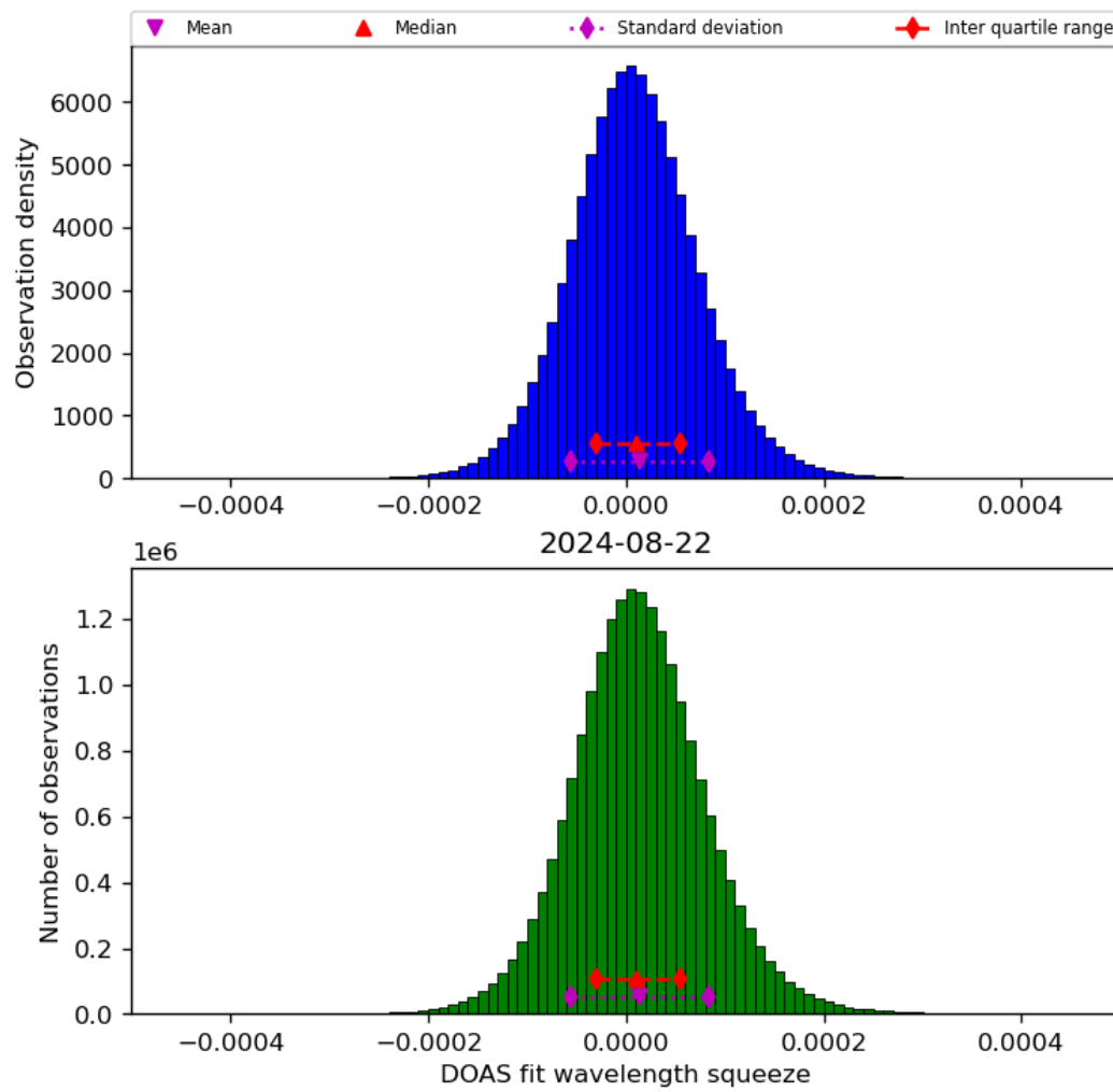
Figure 45: Histogram of “DOAS fit wavelength squeeze” for 2024-08-22 to 2024-08-23
