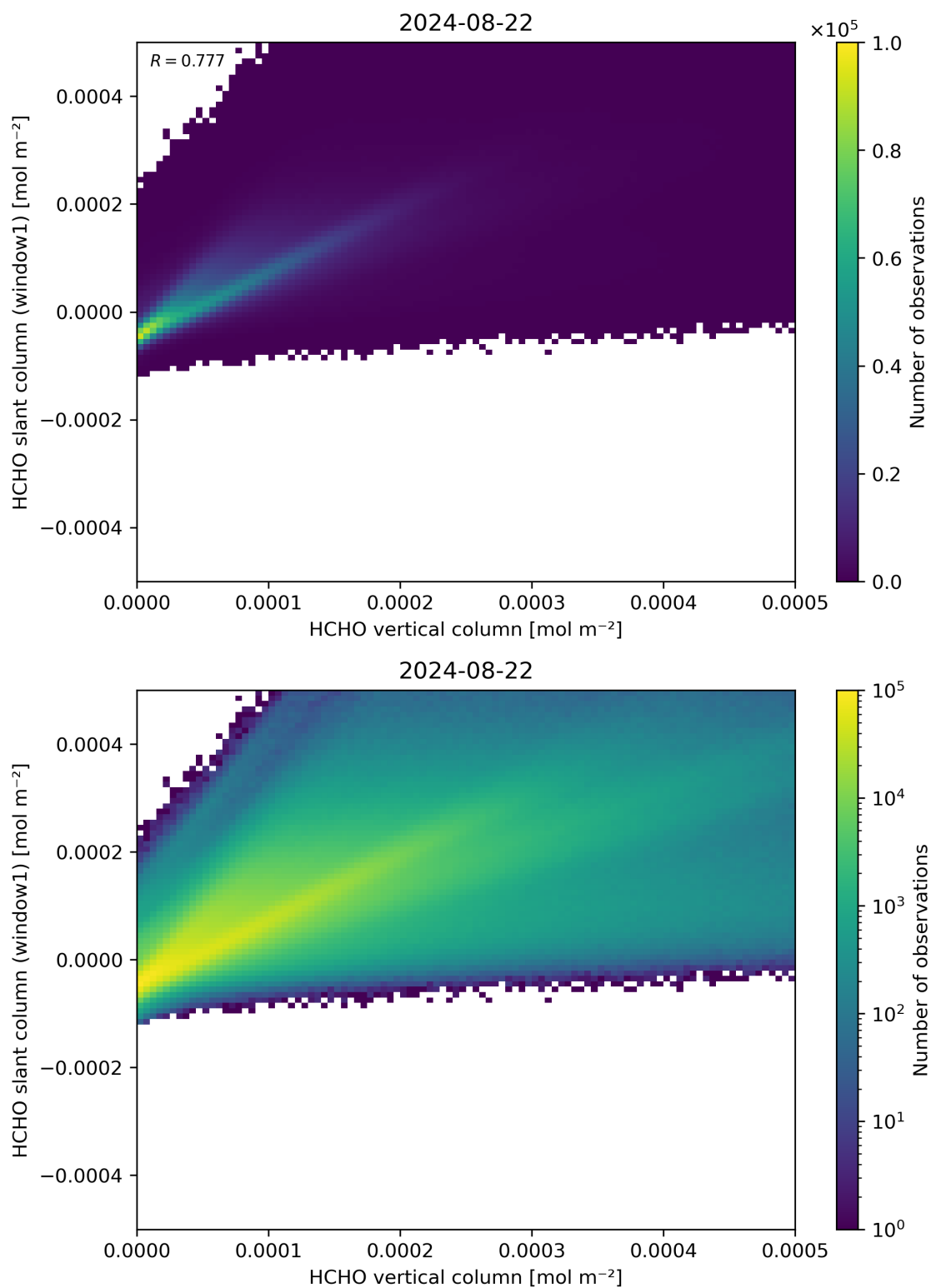
Figure 129: Scatter density plot of “HCHO vertical column” against “HCHO slant column (window1)” for 2024-08-22 to 2024-08-23.
