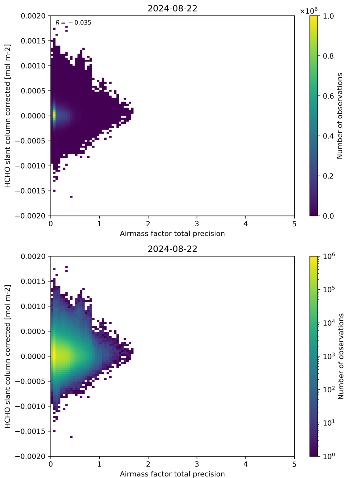
Figure 109: Scatter density plot of “Airmass factor total precision” against “HCHO slant column corrected” for 2024-08-22 to 2024-08-23.
