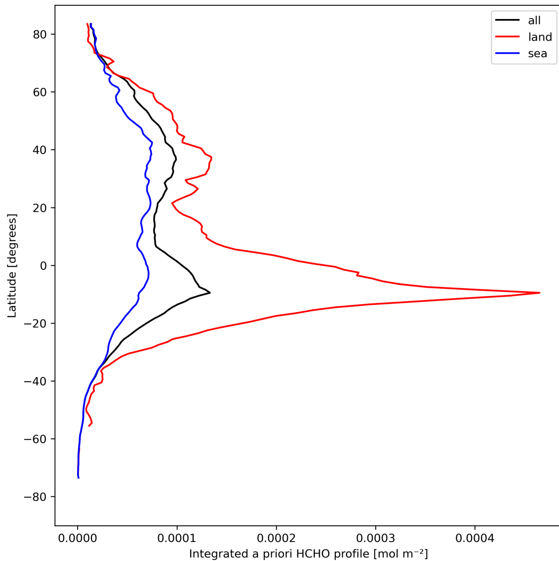
Figure 29: Zonal average of “Integrated a priori HCHO profile” for 2024-08-22 to 2024-08-23.
