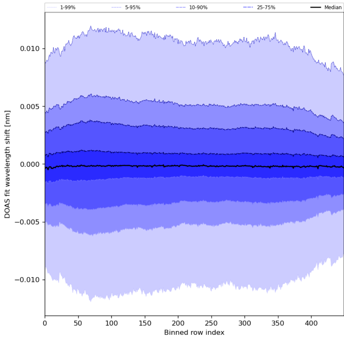
Figure 58: Along track statistics of “DOAS fit wavelength shift” for 2024-08-22 to 2024-08-23
