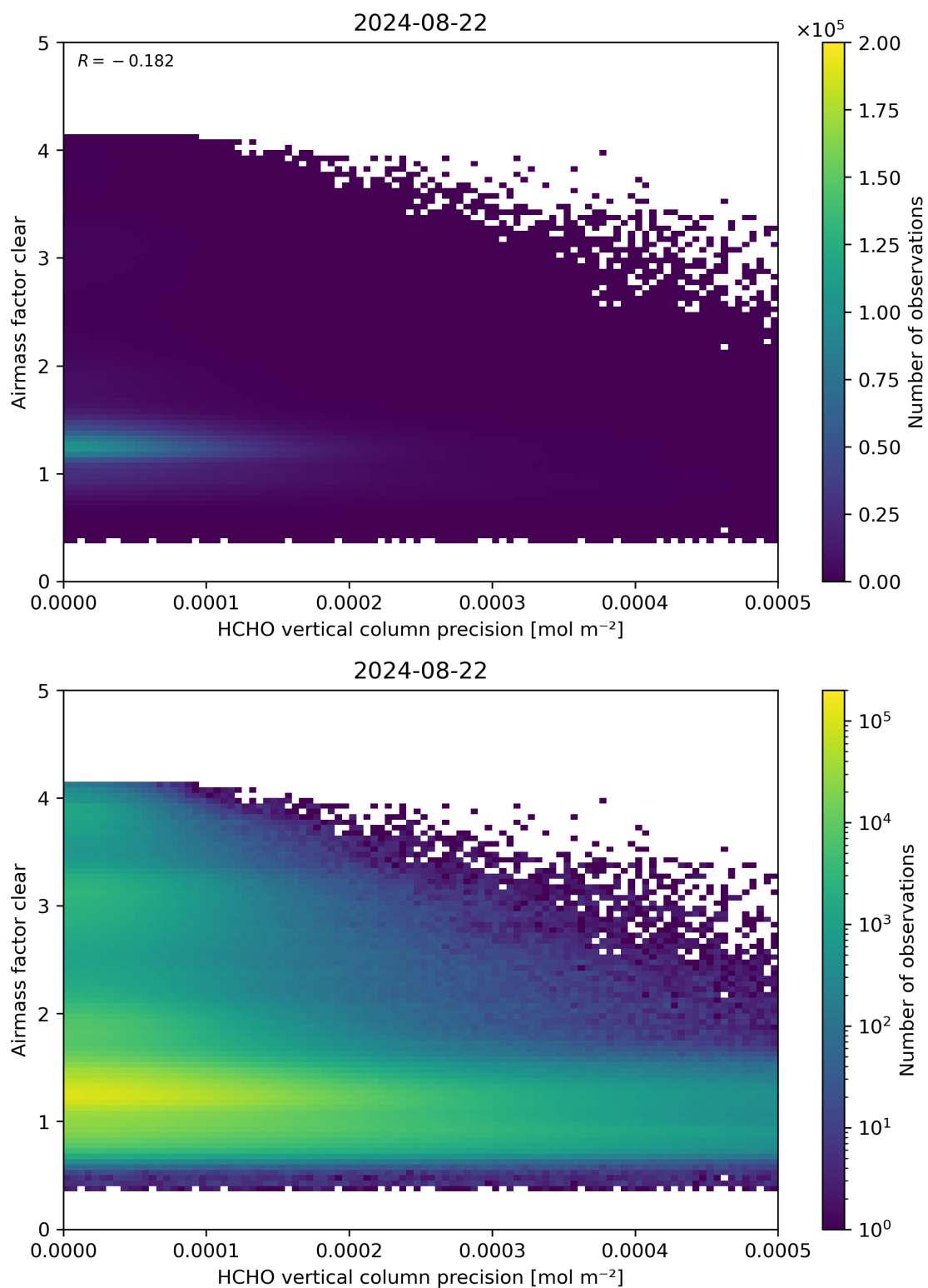
Figure 139: Scatter density plot of “HCHO vertical column precision” against “Airmass factor clear” for 2024-08-22 to 2024-08-23.
