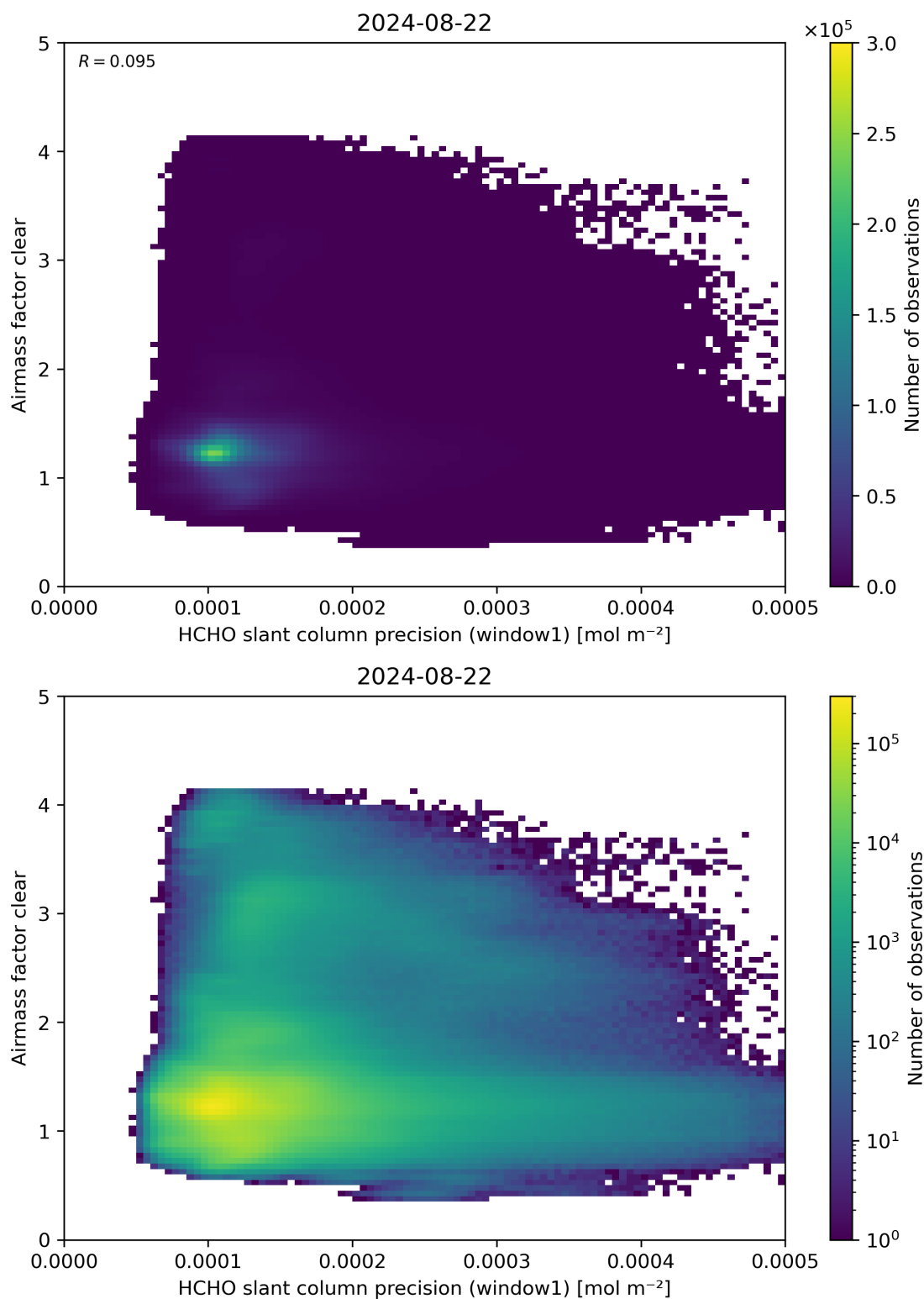
Figure 91: Scatter density plot of “HCHO slant column precision (window1)” against “Airmass factor clear” for 2024-08-22 to 2024-08-23.
