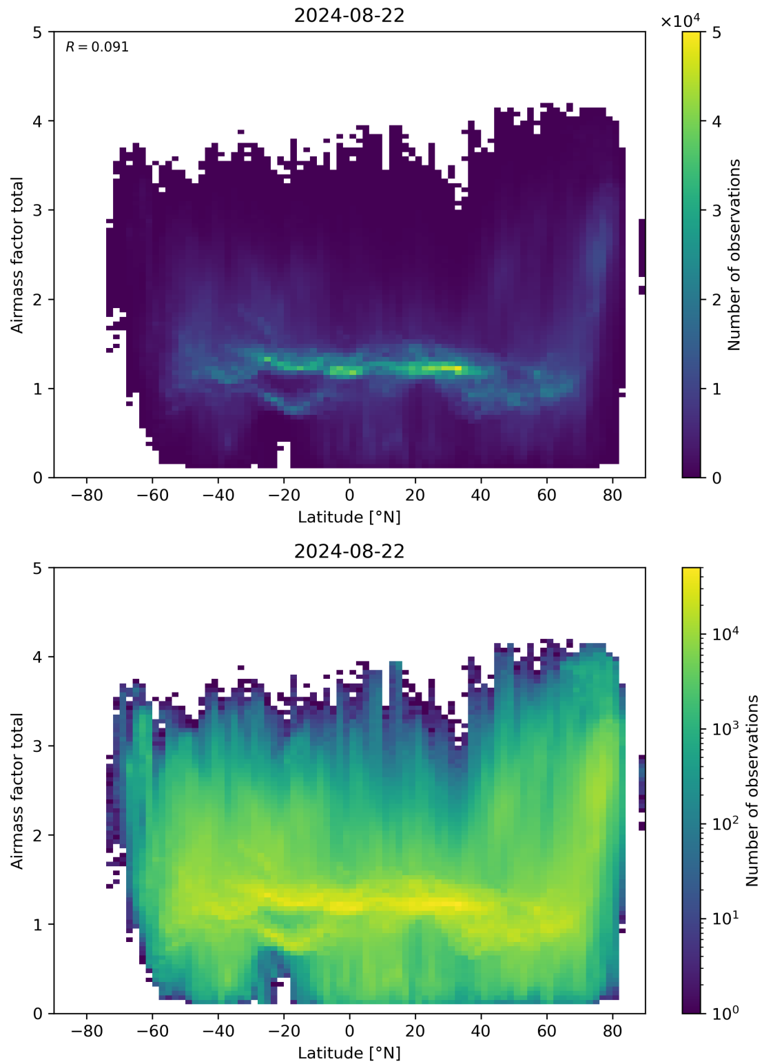
Figure 161: Scatter density plot of “Latitude” against “Airmass factor total” for 2024-08-22 to 2024-08-23.
