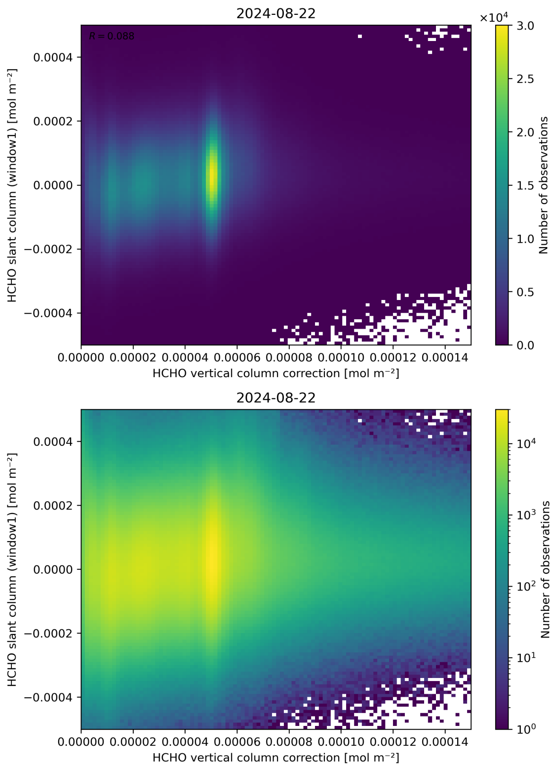
Figure 118: Scatter density plot of “HCHO vertical column correction” against “HCHO slant column (window1)” for 2024-08-22 to 2024-08-23.
