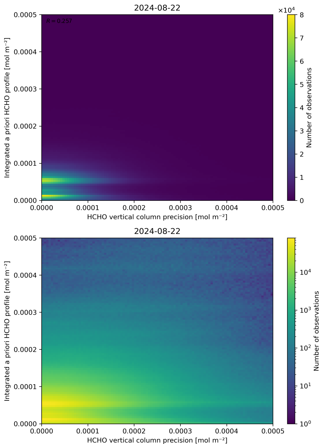
Figure 147: Scatter density plot of “HCHO vertical column precision” against “Integrated a priori HCHO profile” for 2024-08-22 to 2024-08-23.
