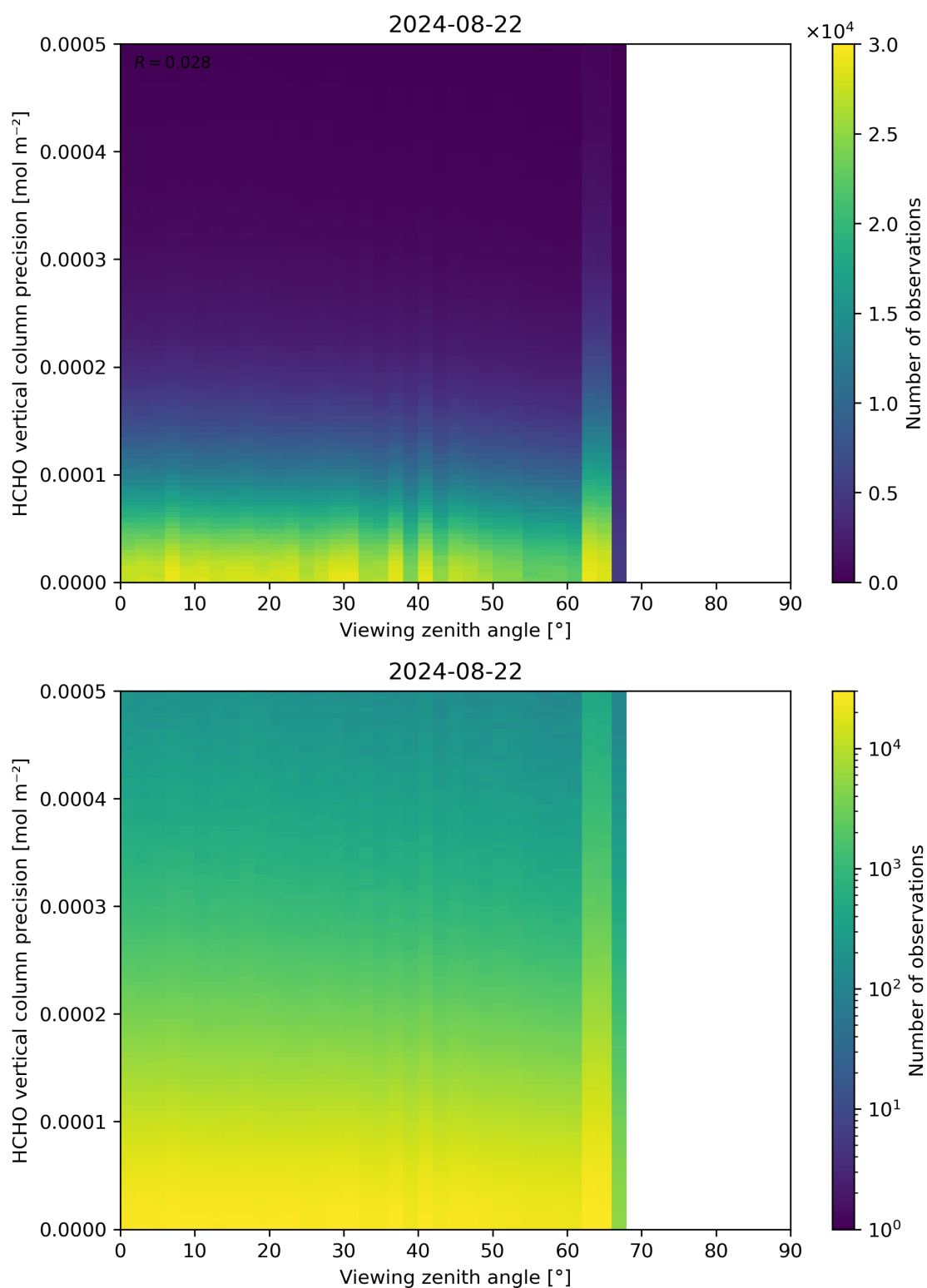
Figure 194: Scatter density plot of “Viewing zenith angle” against “HCHO vertical column precision” for 2024-08-22 to 2024-08-23.
