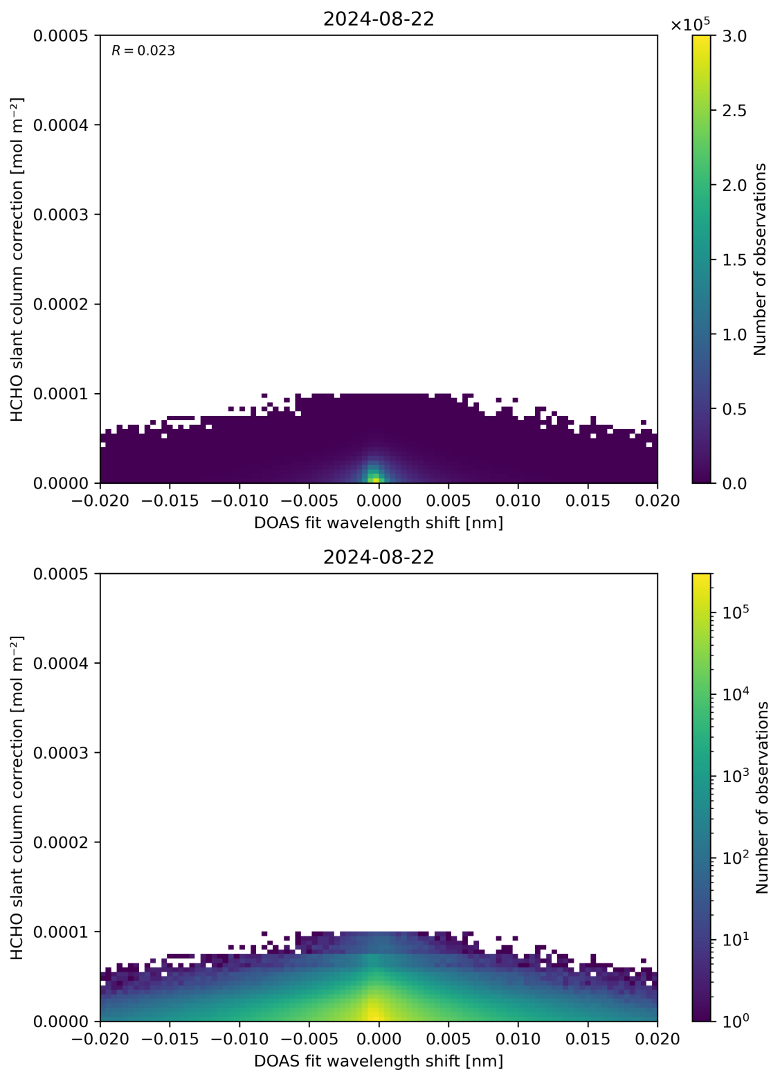
Figure 67: Scatter density plot of “DOAS fit wavelength shift” against “HCHO slant column correction” for 2024-08-22 to 2024-08-23.
