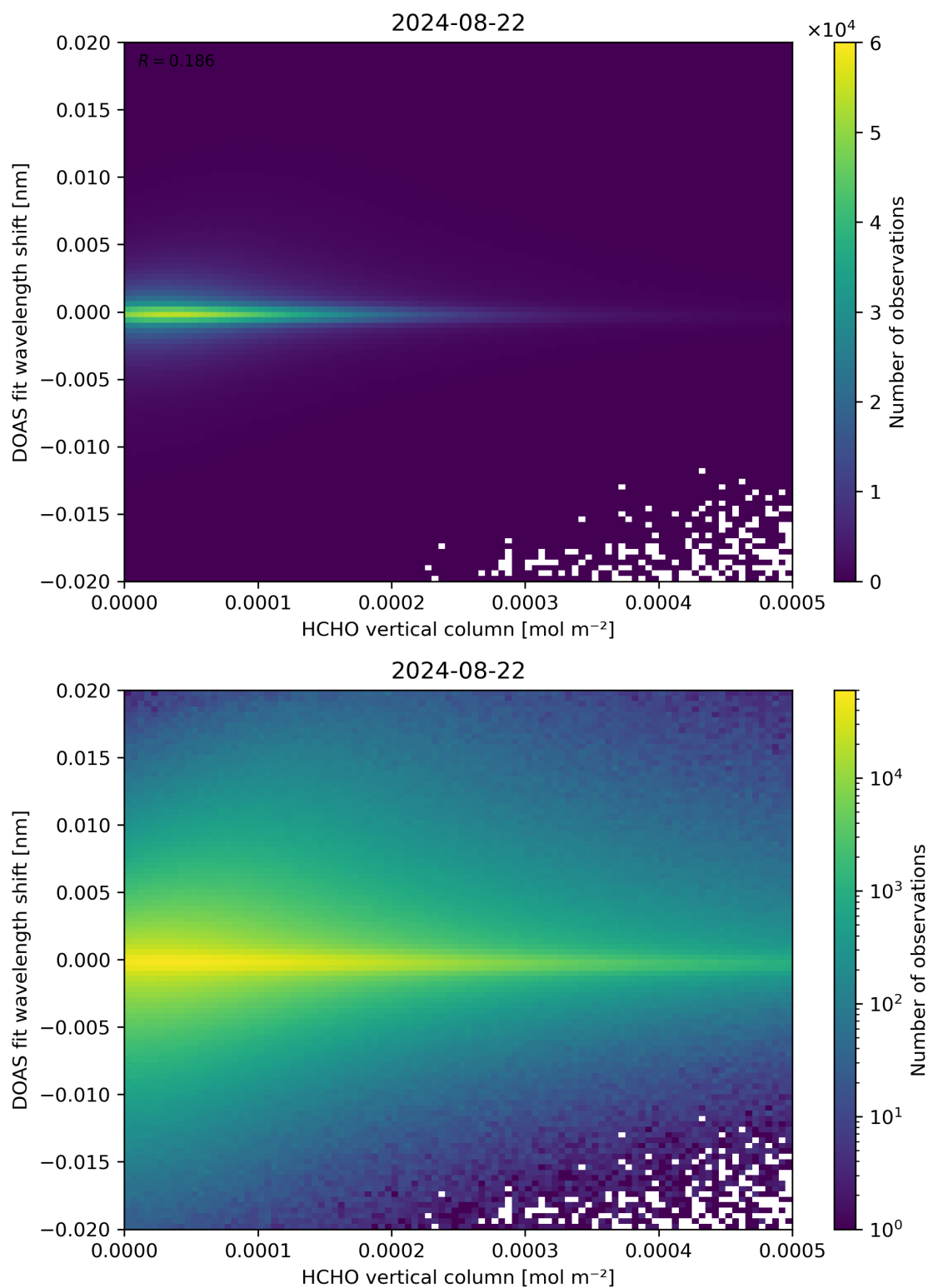
Figure 124: Scatter density plot of “HCHO vertical column” against “DOAS fit wavelength shift” for 2024-08-22 to 2024-08-23.
