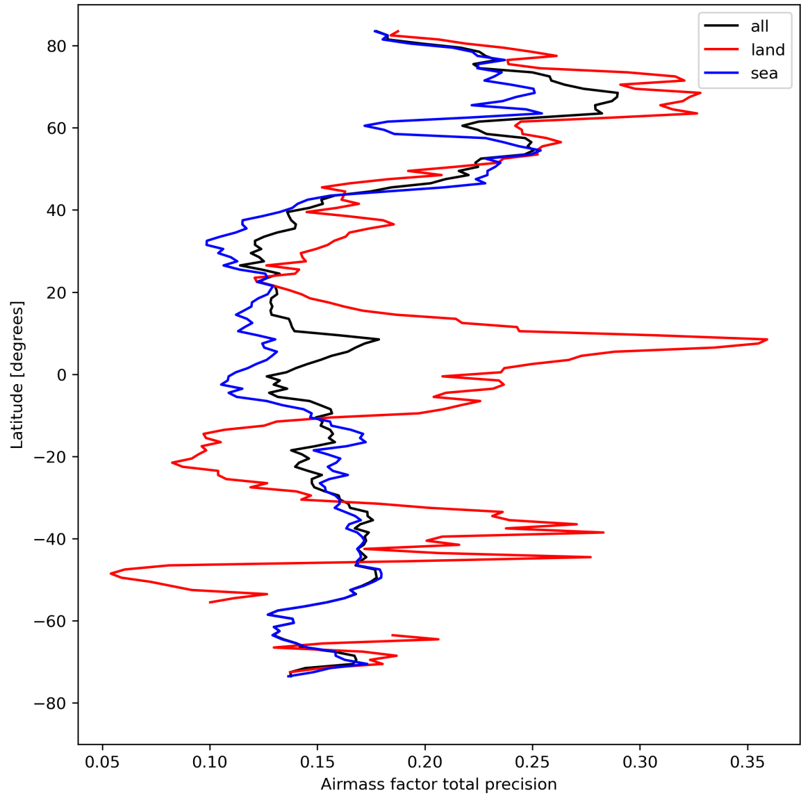
Figure 27: Zonal average of “Airmass factor total precision” for 2024-08-22 to 2024-08-23.
