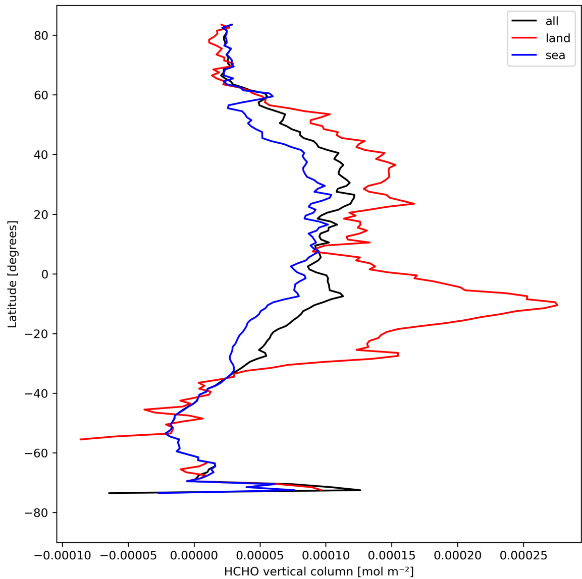
Figure 21: Zonal average of “HCHO vertical column” for 2024-08-22 to 2024-08-23.
