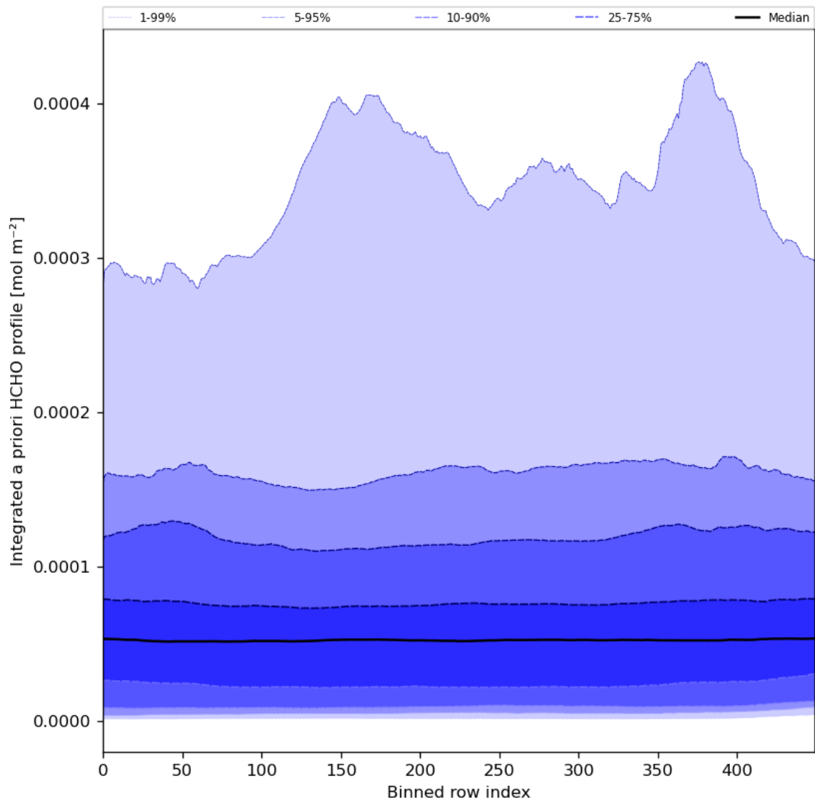
Figure 57: Along track statistics of "Integrated a priori HCHO profile" for 2024-08-22 to 2024-08-23
