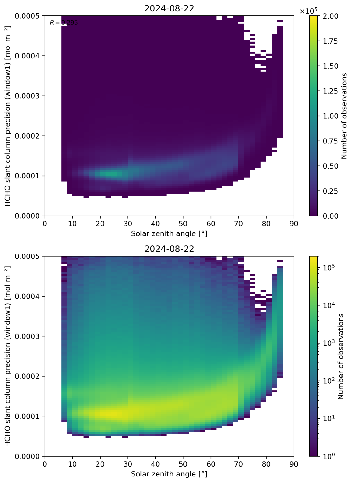
Figure 174: Scatter density plot of “Solar zenith angle” against “HCHO slant column precision (window1)” for 2024-08-22 to 2024-08-23.
