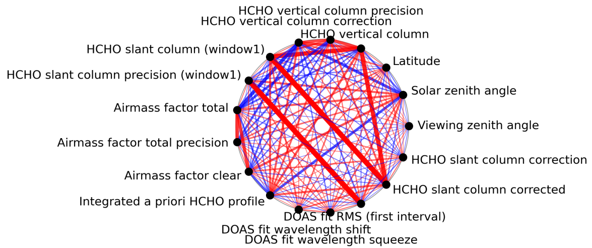
Figure 1: Map of correlation graph for 2024-08-22 to 2024-08-23.
