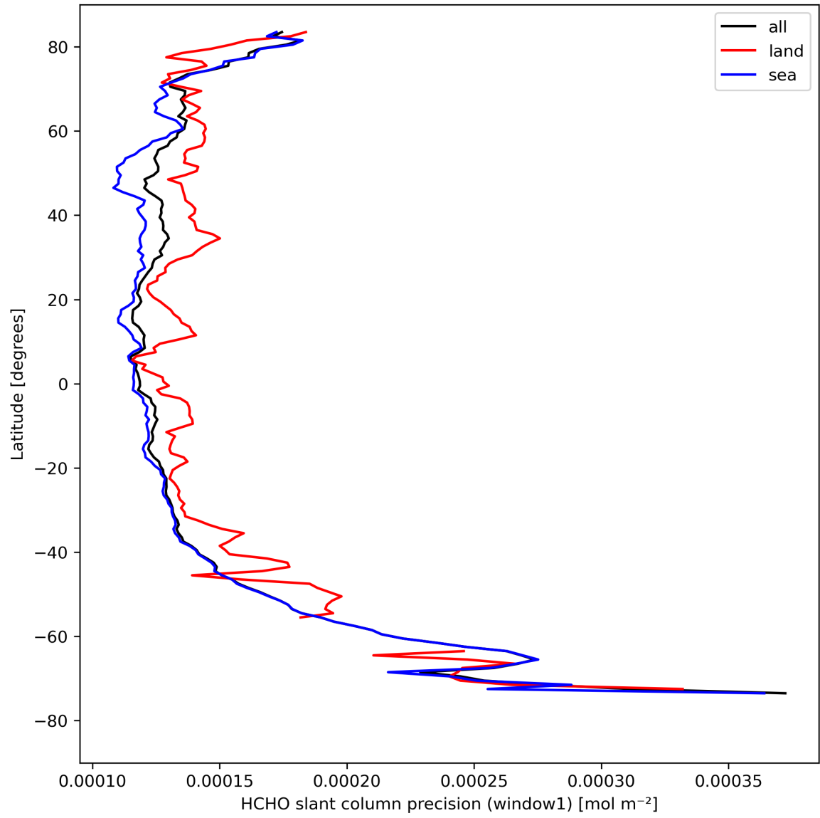
Figure 25: Zonal average of “HCHO slant column precision (window1)” for 2024-08-22 to 2024-08-23.
