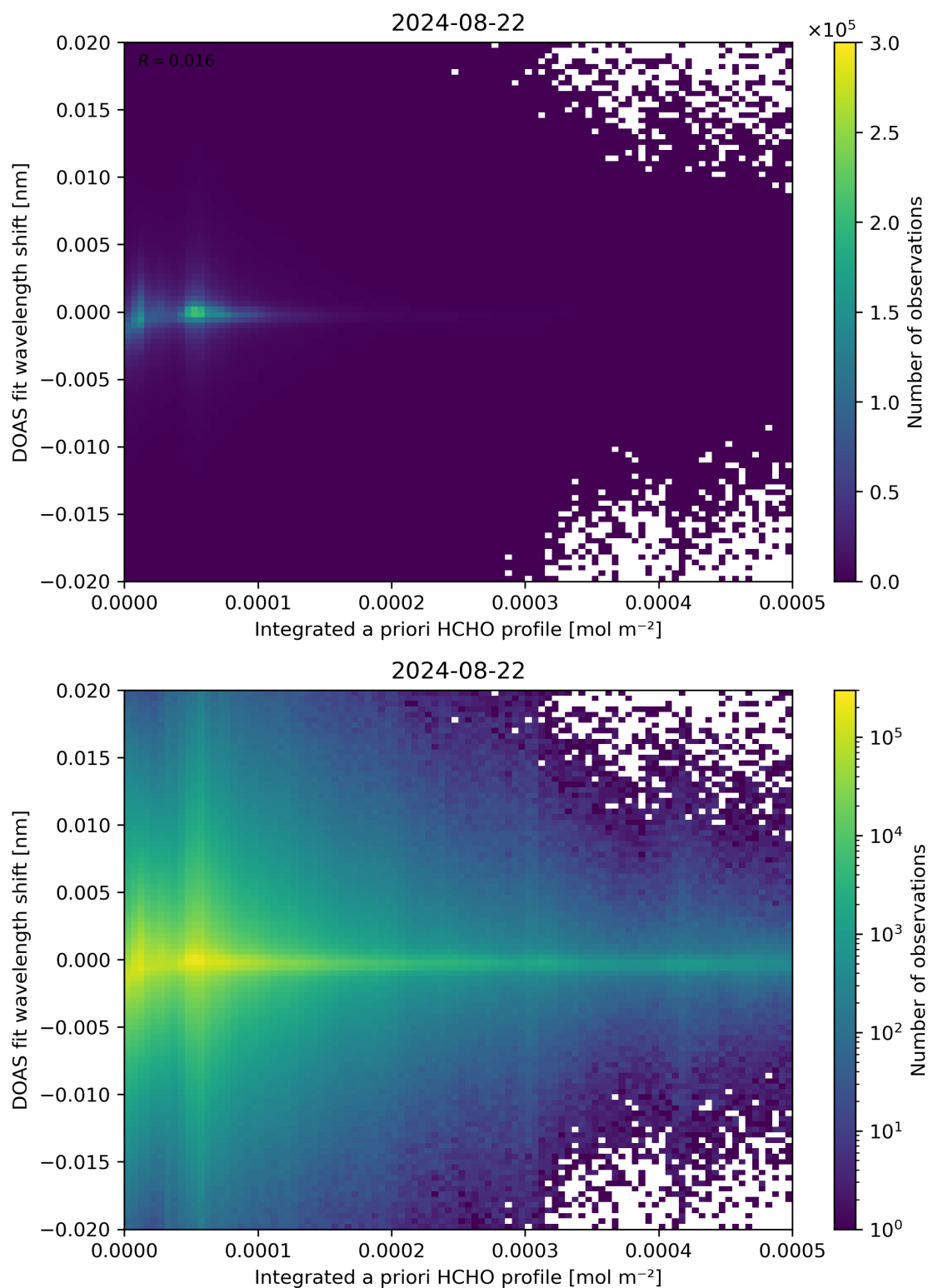
Figure 149: Scatter density plot of “Integrated a priori HCHO profile” against “DOAS fit wavelength shift” for 2024-08-22 to 2024-08-23.
