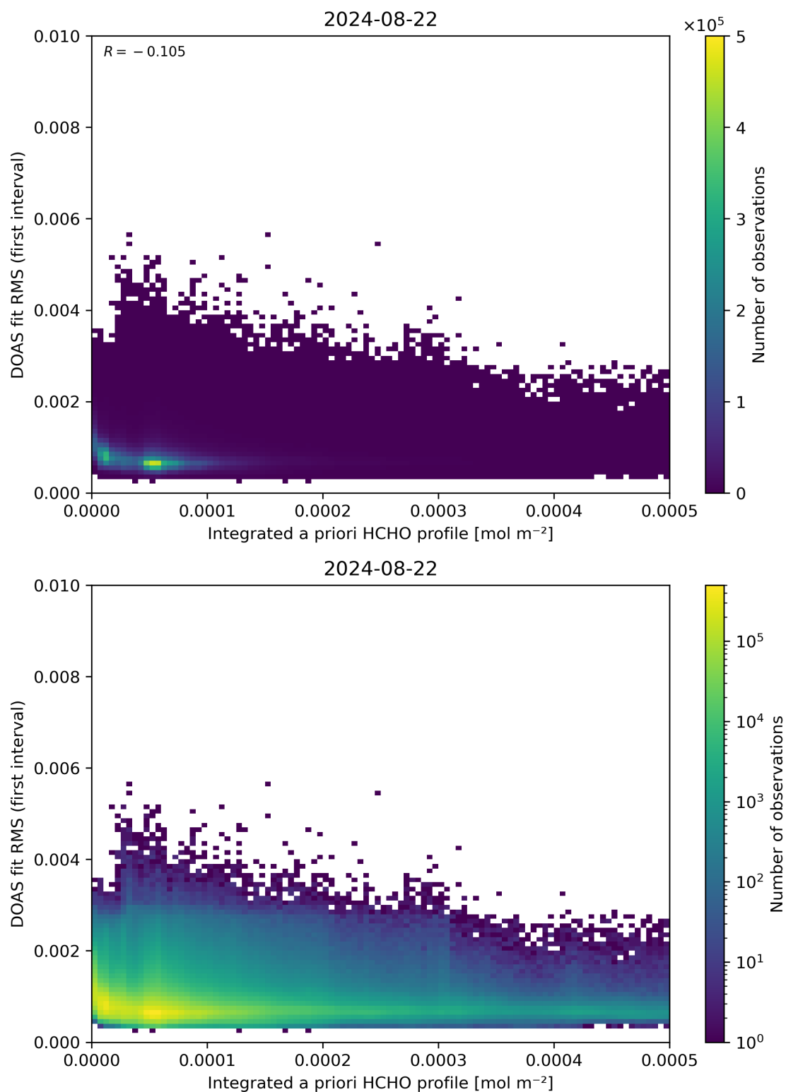
Figure 148: Scatter density plot of “Integrated a priori HCHO profile” against “DOAS fit RMS (first interval)” for 2024-08-22 to 2024-08-23.
