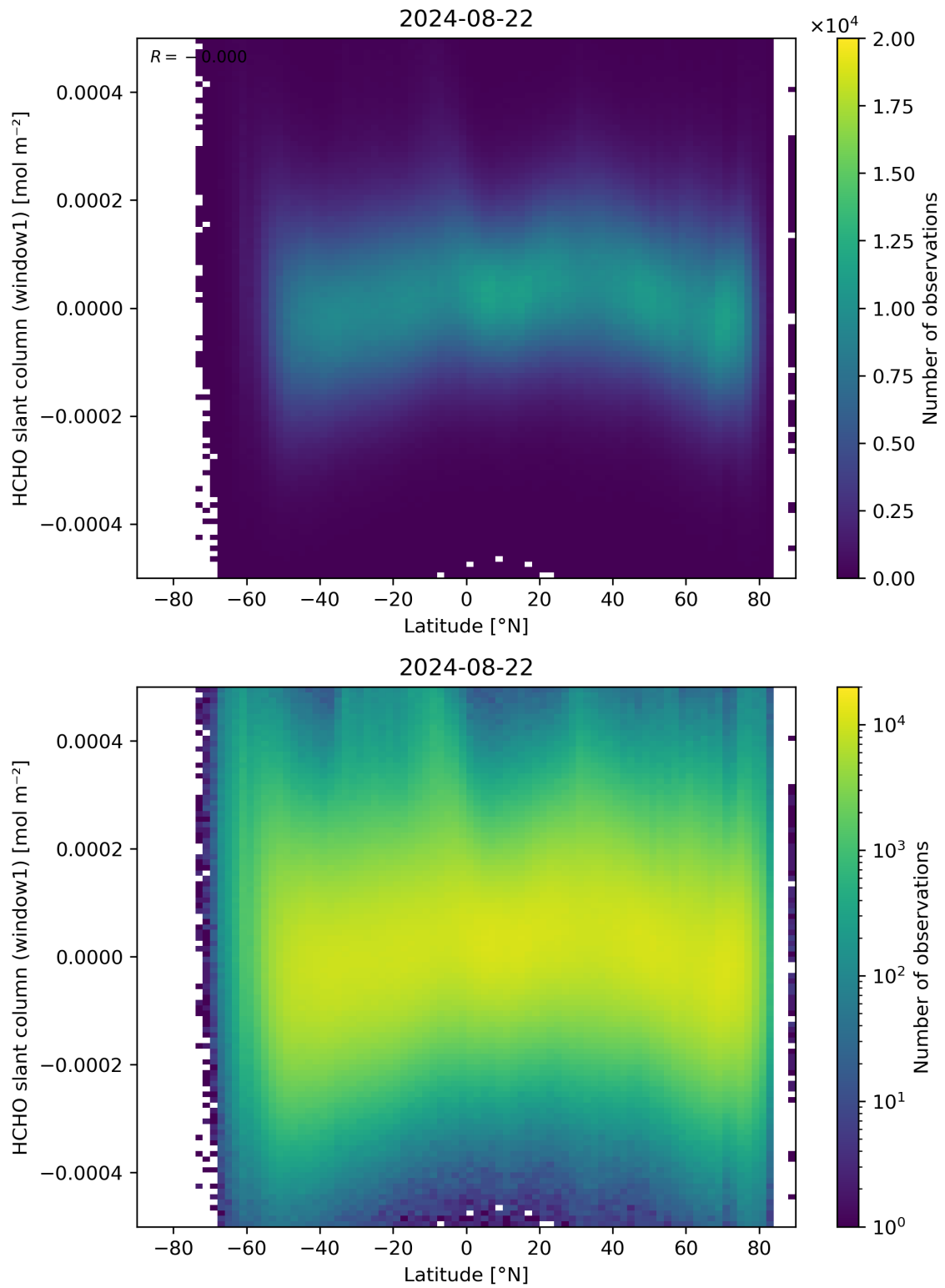
Figure 159: Scatter density plot of “Latitude” against “HCHO slant column (window1)” for 2024-08-22 to 2024-08-23.
