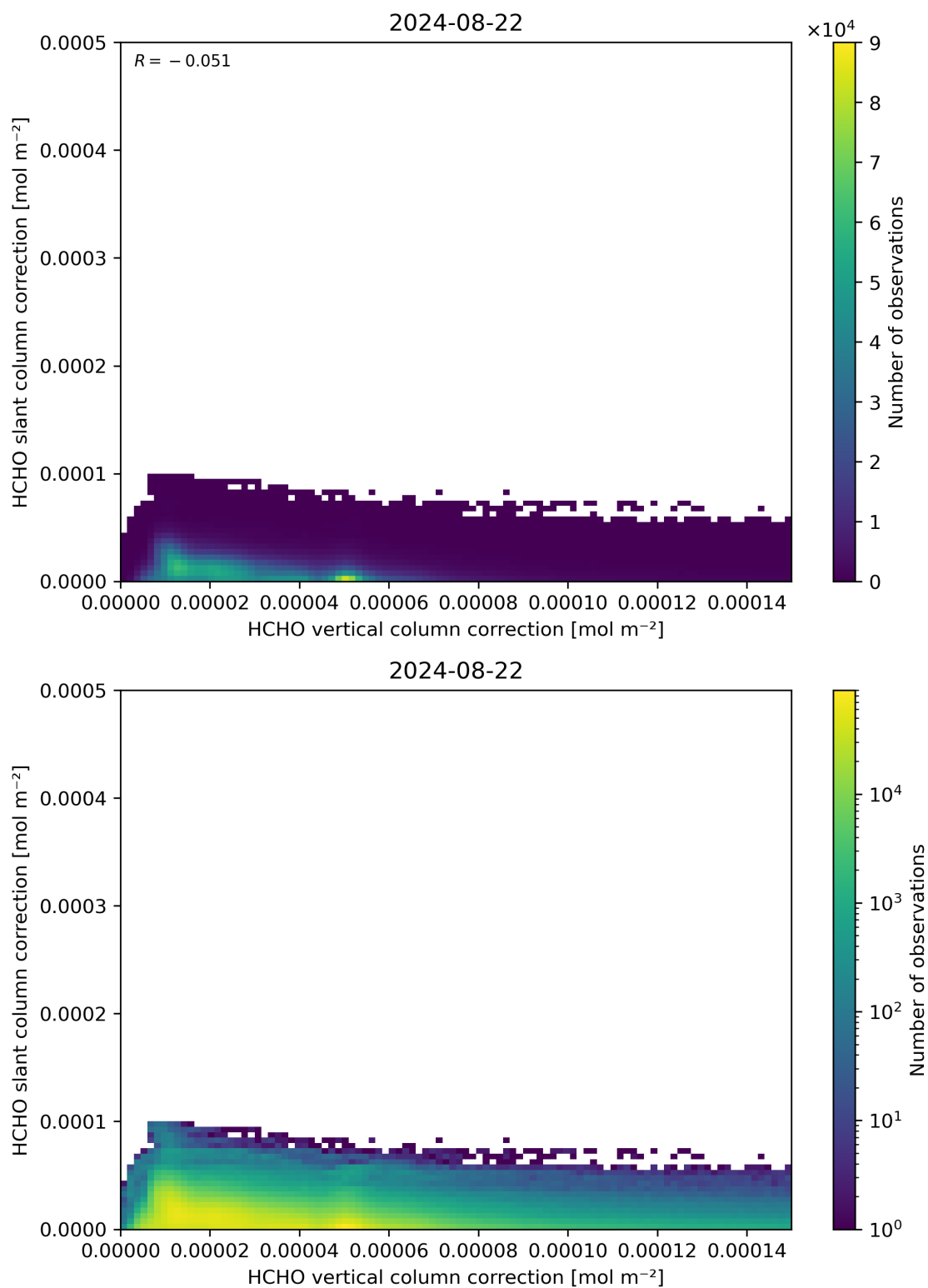
Figure 117: Scatter density plot of “HCHO vertical column correction” against “HCHO slant column correction” for 2024-08-22 to 2024-08-23.
