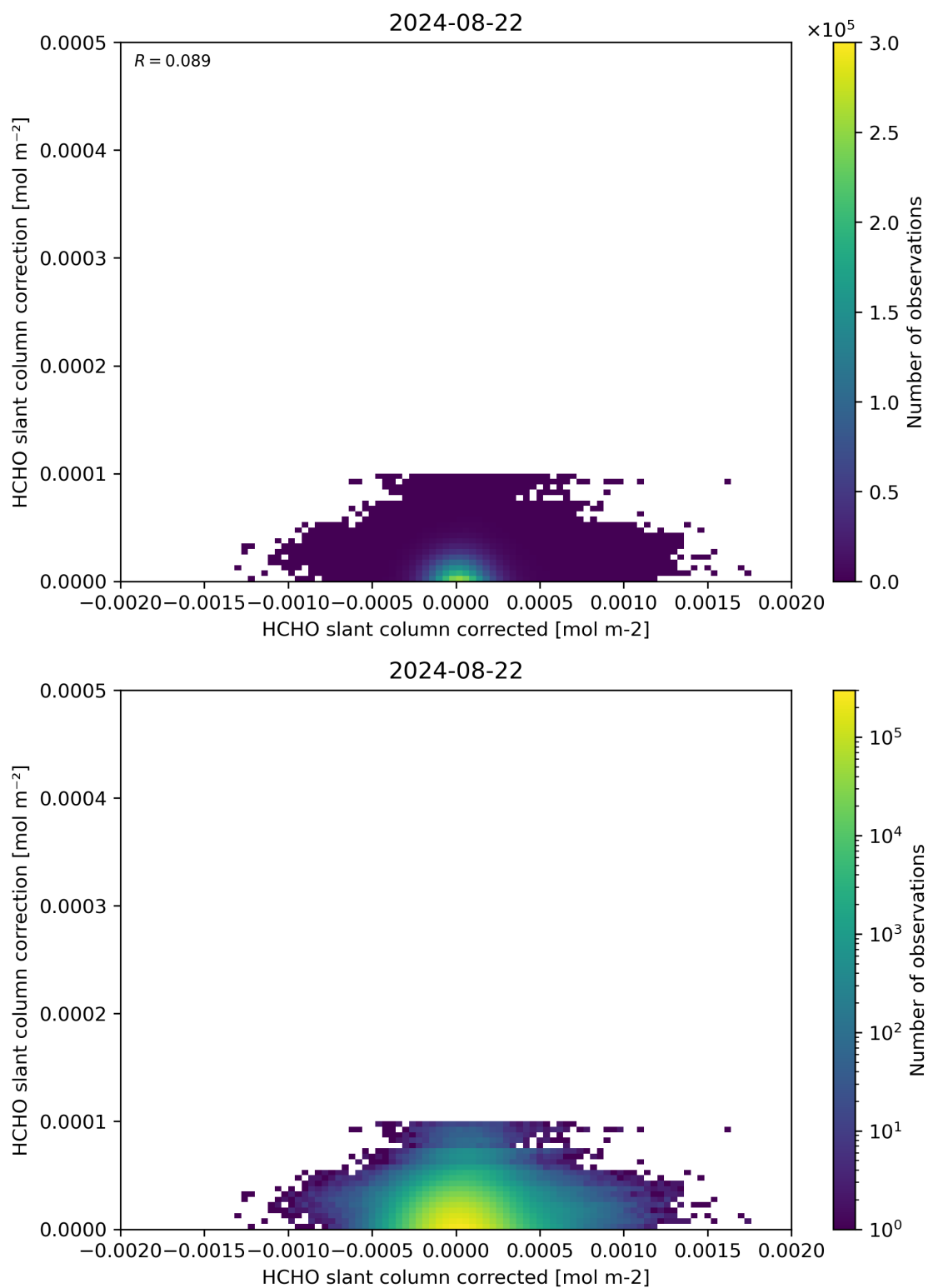
Figure 77: Scatter density plot of “HCHO slant column corrected” against “HCHO slant column correction” for 2024-08-22 to 2024-08-23.
