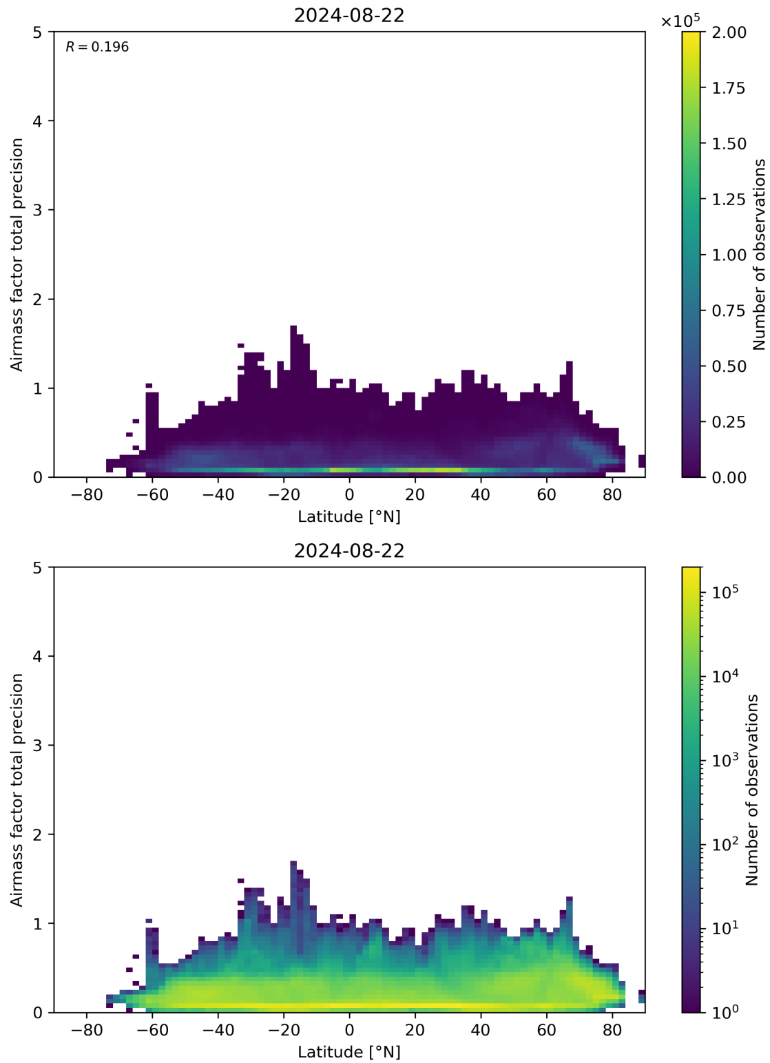
Figure 162: Scatter density plot of “Latitude” against “Airmass factor total precision” for 2024-08-22 to 2024-08-23.
