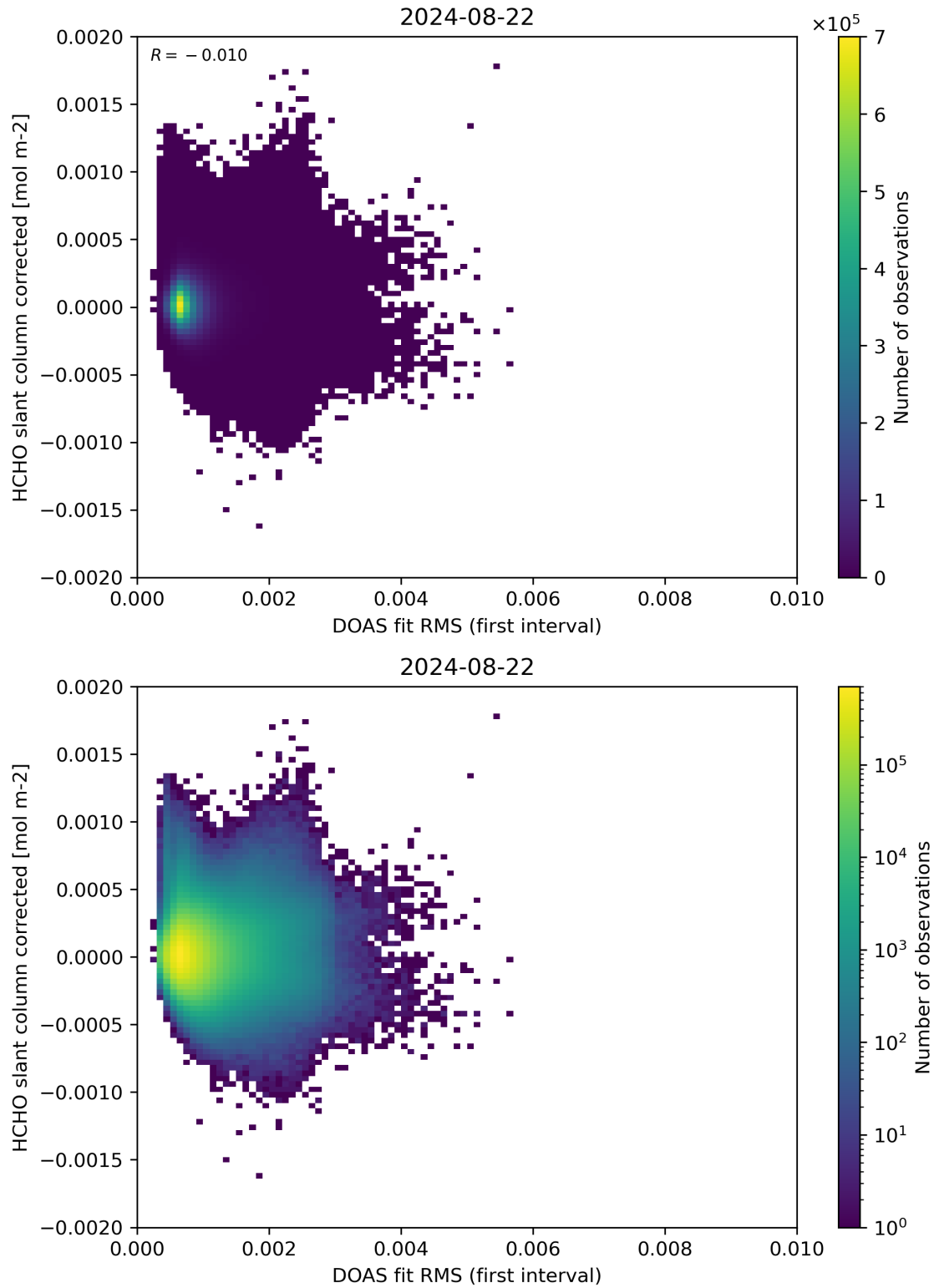
Figure 62: Scatter density plot of “DOAS fit RMS (first interval)” against “HCHO slant column corrected” for 2024-08-22 to 2024-08-23.
