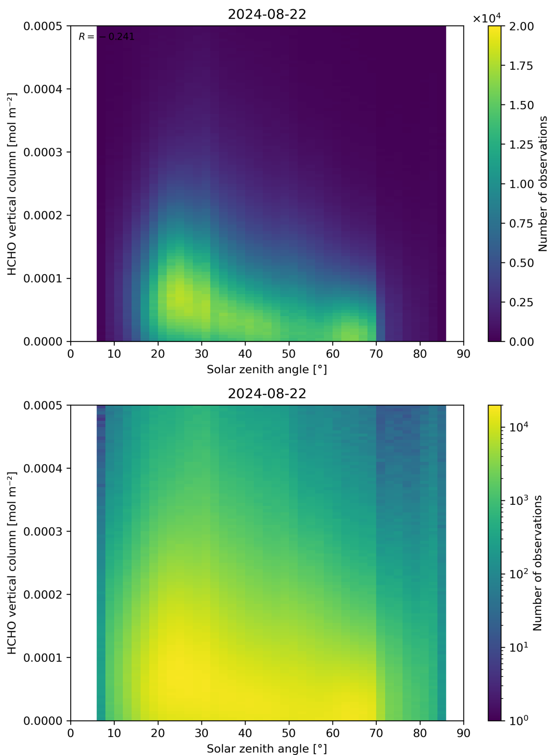
Figure 177: Scatter density plot of “Solar zenith angle” against “HCHO vertical column” for 2024-08-22 to 2024-08-23.
