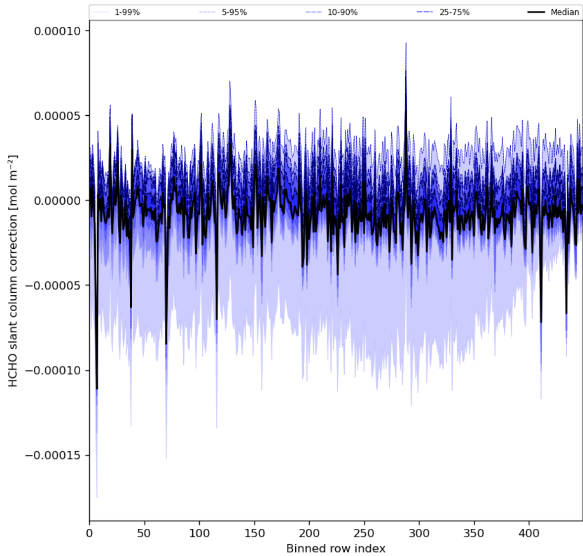
Figure 61: Along track statistics of “HCHO slant column correction” for 2024-08-22 to 2024-08-23
