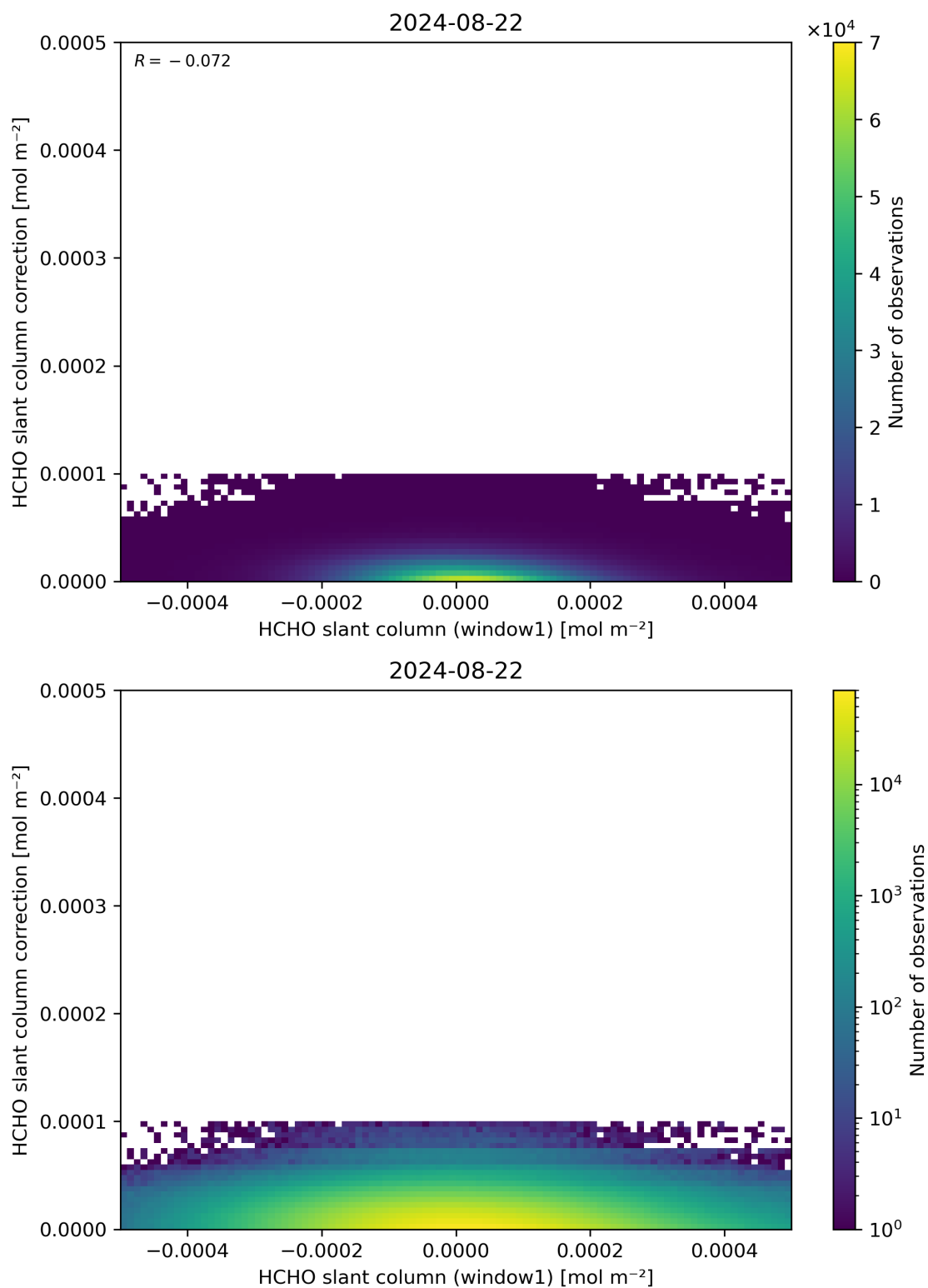
Figure 83: Scatter density plot of “HCHO slant column (window1)” against “HCHO slant column correction” for 2024-08-22 to 2024-08-23.
