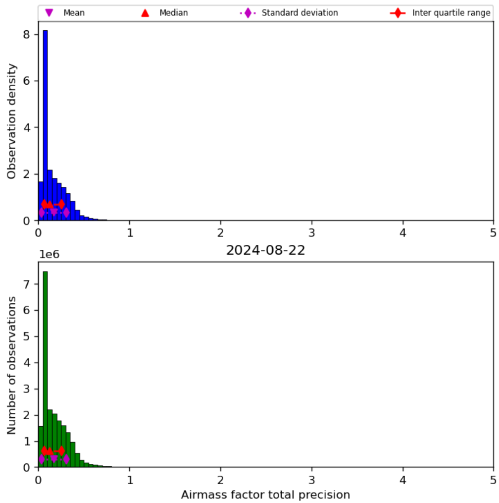
Figure 41: Histogram of “Airmass factor total precision” for 2024-08-22 to 2024-08-23
