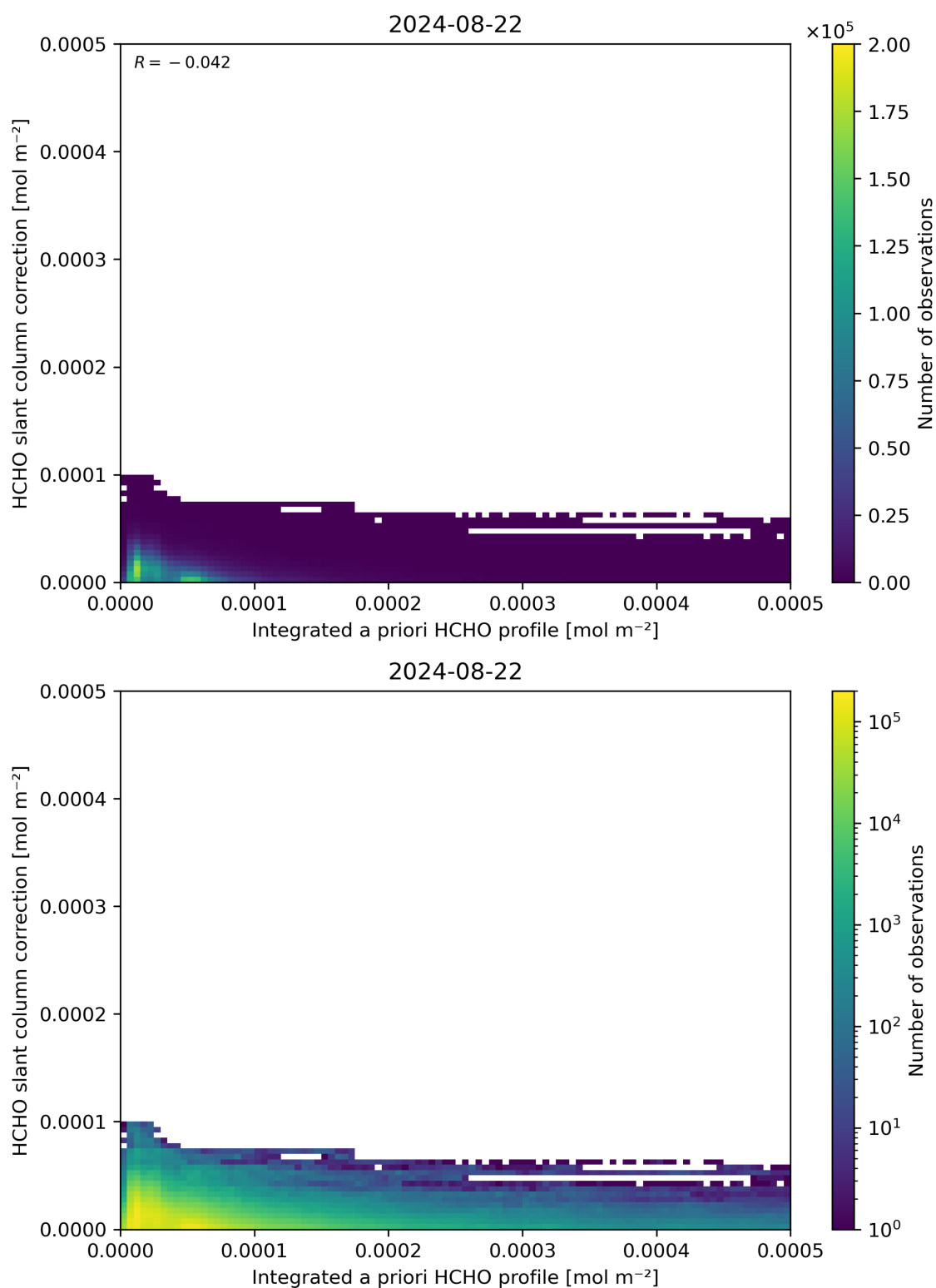
Figure 152: Scatter density plot of “Integrated a priori HCHO profile” against “HCHO slant column correction” for 2024-08-22 to 2024-08-23.
