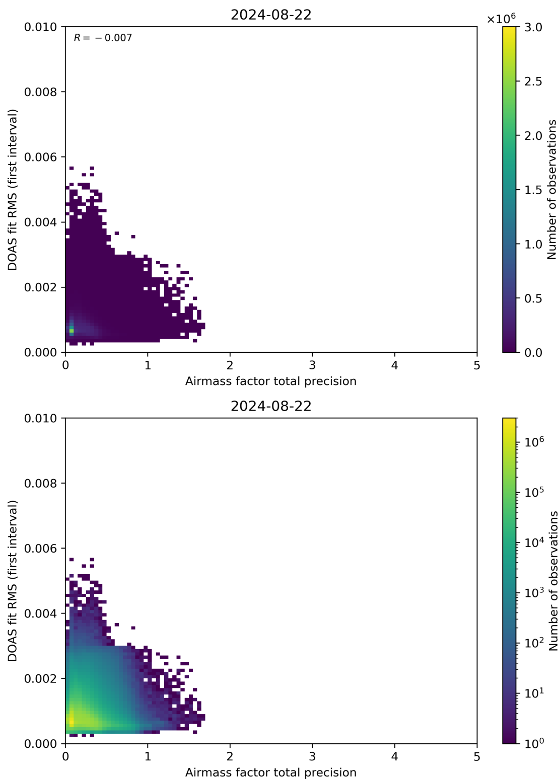
Figure 105: Scatter density plot of “Airmass factor total precision” against “DOAS fit RMS (first interval)” for 2024-08-22 to 2024-08-23.
