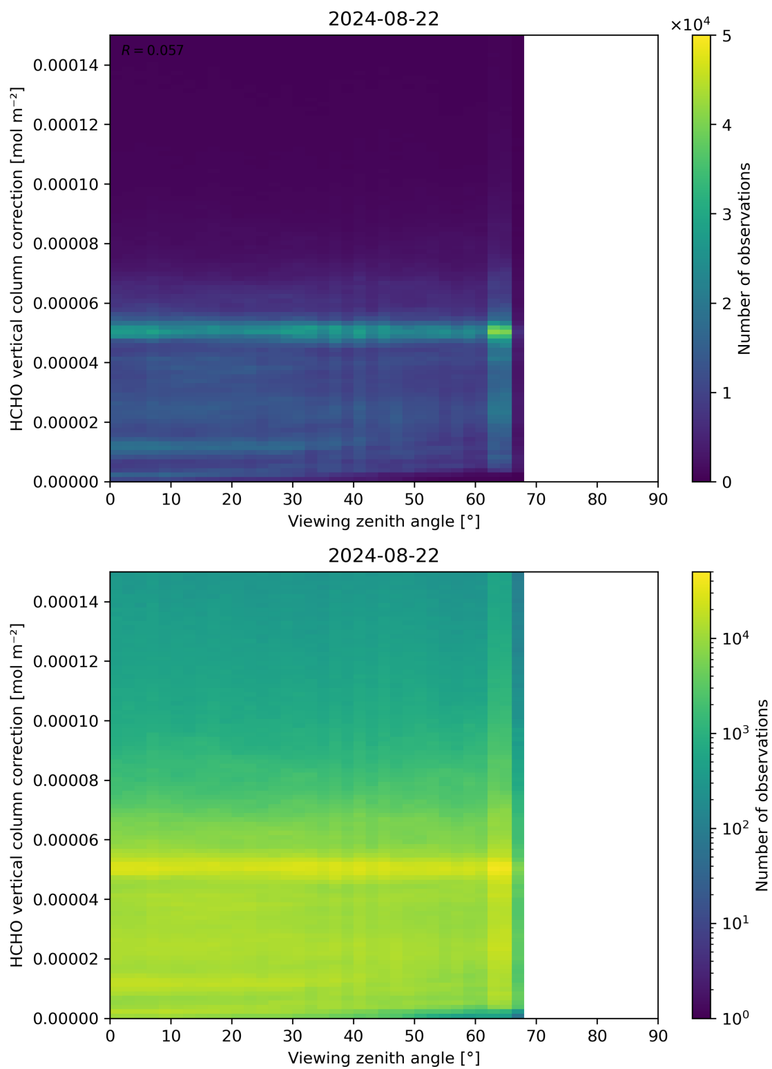
Figure 193: Scatter density plot of “Viewing zenith angle” against “HCHO vertical column correction” for 2024-08-22 to 2024-08-23.
