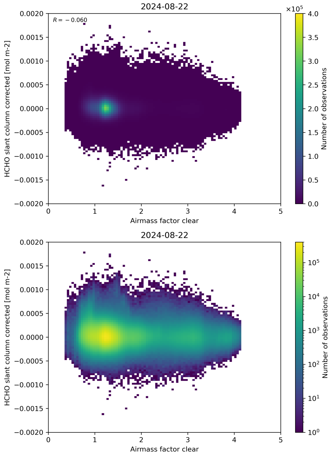
Figure 74: Scatter density plot of “Airmass factor clear” against “HCHO slant column corrected” for 2024-08-22 to 2024-08-23.
