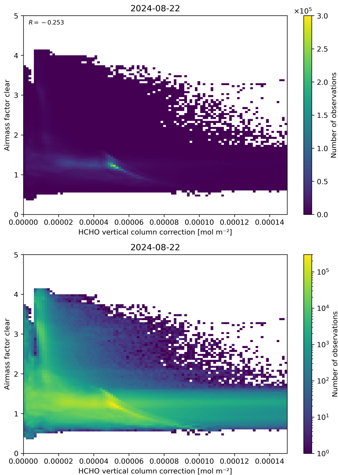
Figure 115: Scatter density plot of “HCHO vertical column correction” against “Airmass factor clear” for 2024-08-22 to 2024-08-23.
