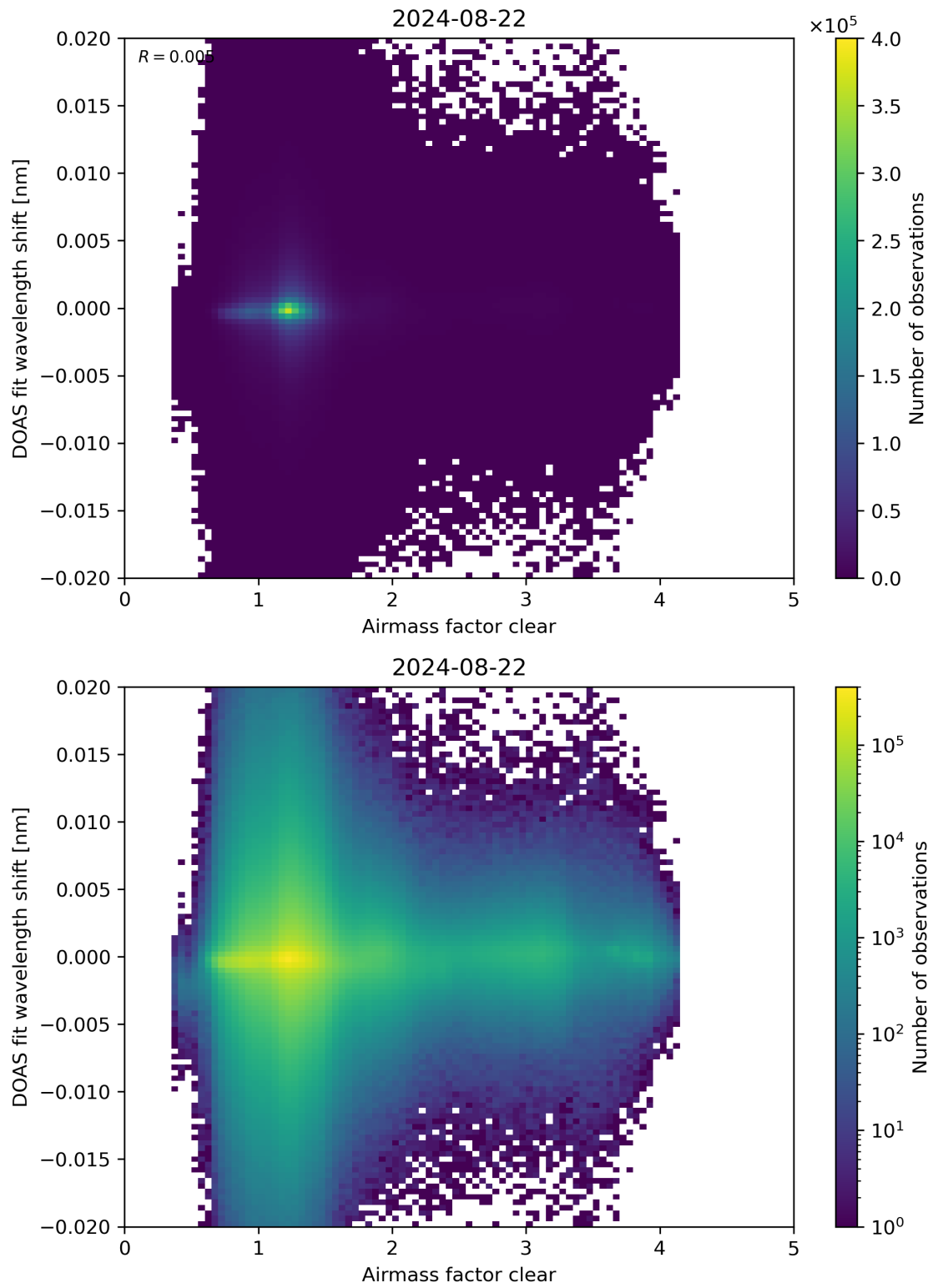
Figure 72: Scatter density plot of “Airmass factor clear” against “DOAS fit wavelength shift” for 2024-08-22 to 2024-08-23.
