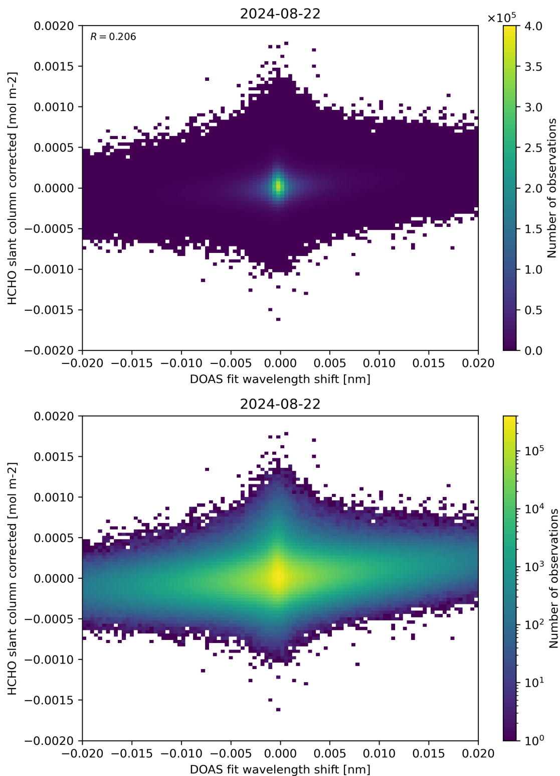
Figure 66: Scatter density plot of “DOAS fit wavelength shift” against “HCHO slant column corrected” for 2024-08-22 to 2024-08-23.
