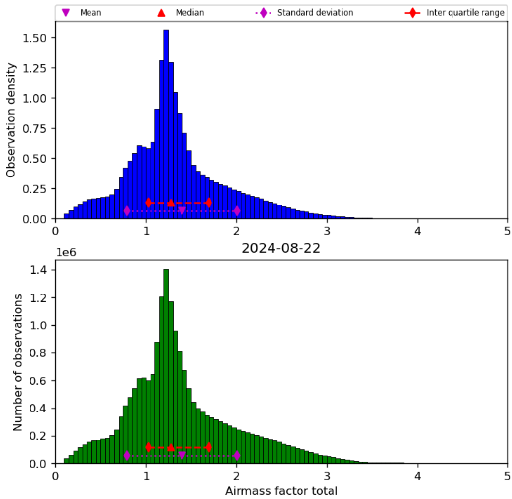
Figure 40: Histogram of “Airmass factor total” for 2024-08-22 to 2024-08-23
