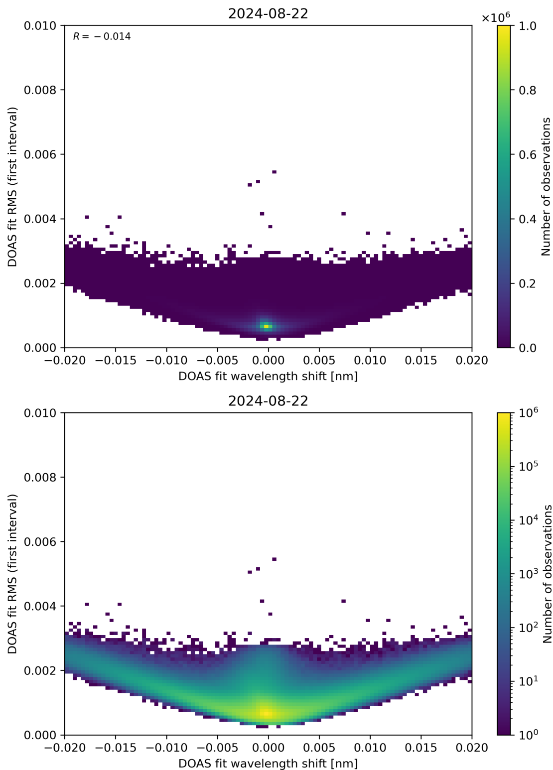
Figure 64: Scatter density plot of “DOAS fit wavelength shift” against “DOAS fit RMS (first interval)” for 2024-08-22 to 2024-08-23.
