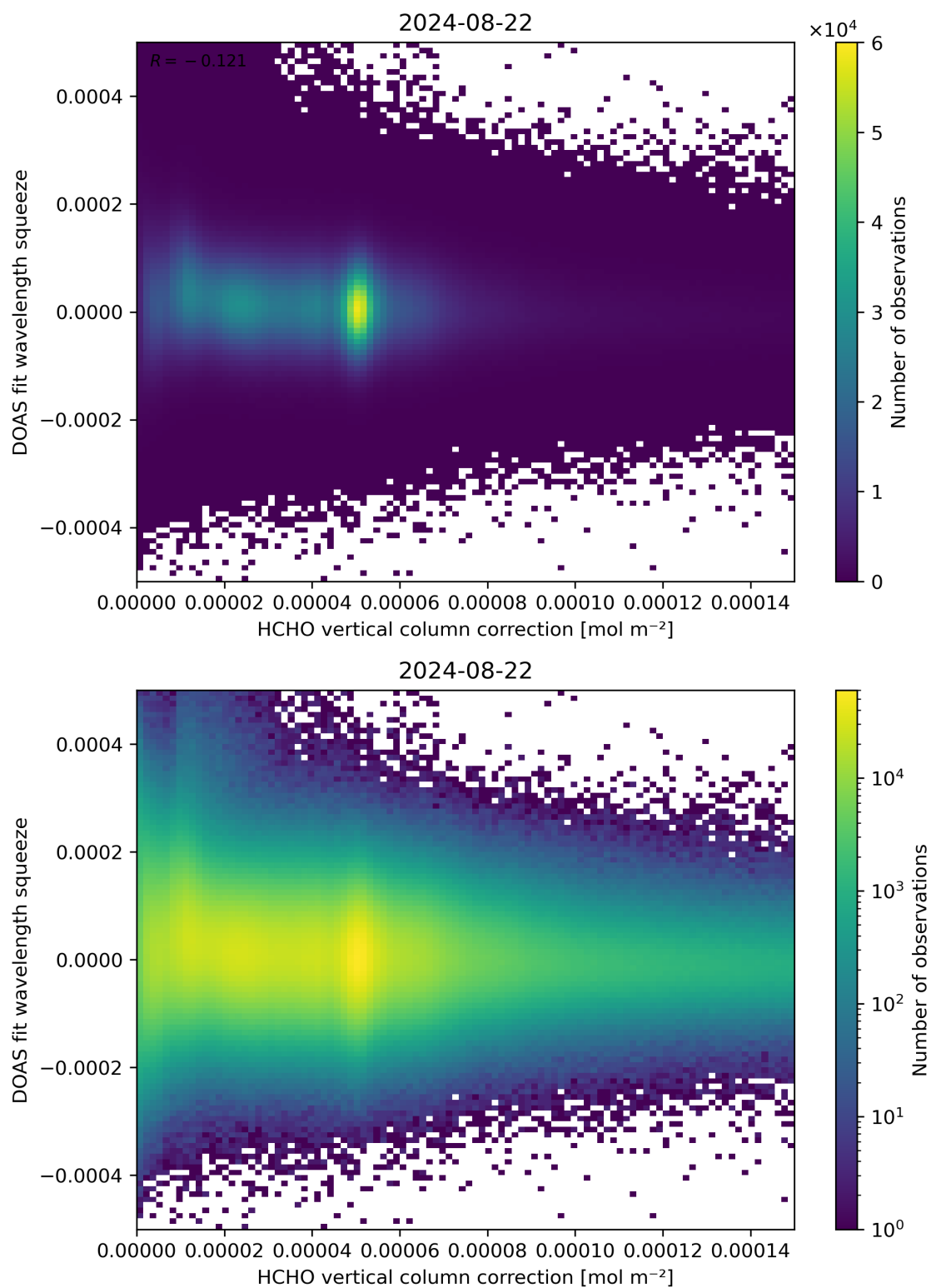
Figure 114: Scatter density plot of “HCHO vertical column correction” against “DOAS fit wavelength squeeze” for 2024-08-22 to 2024-08-23.
