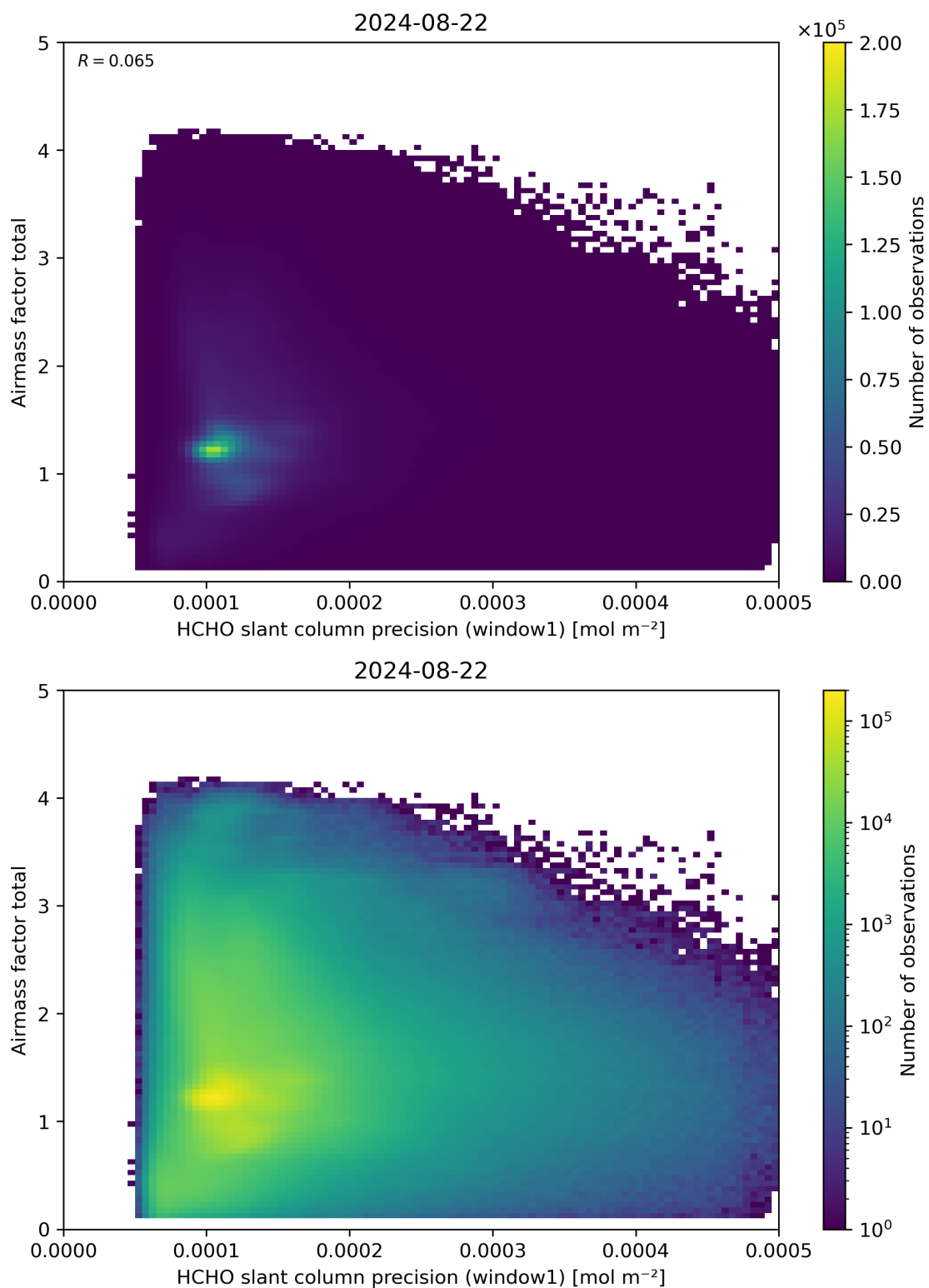
Figure 94: Scatter density plot of “HCHO slant column precision (window1)” against “Airmass factor total” for 2024-08-22 to 2024-08-23.
