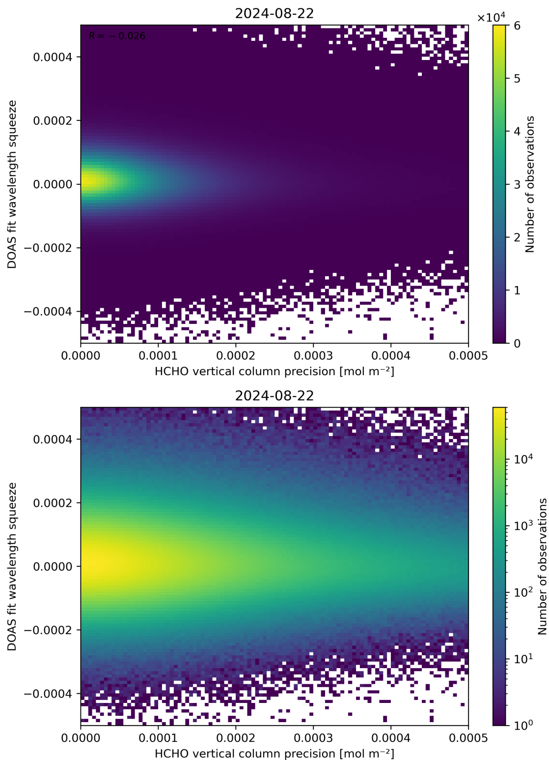
Figure 138: Scatter density plot of “HCHO vertical column precision” against “DOAS fit wavelength squeeze” for 2024-08-22 to 2024-08-23.
