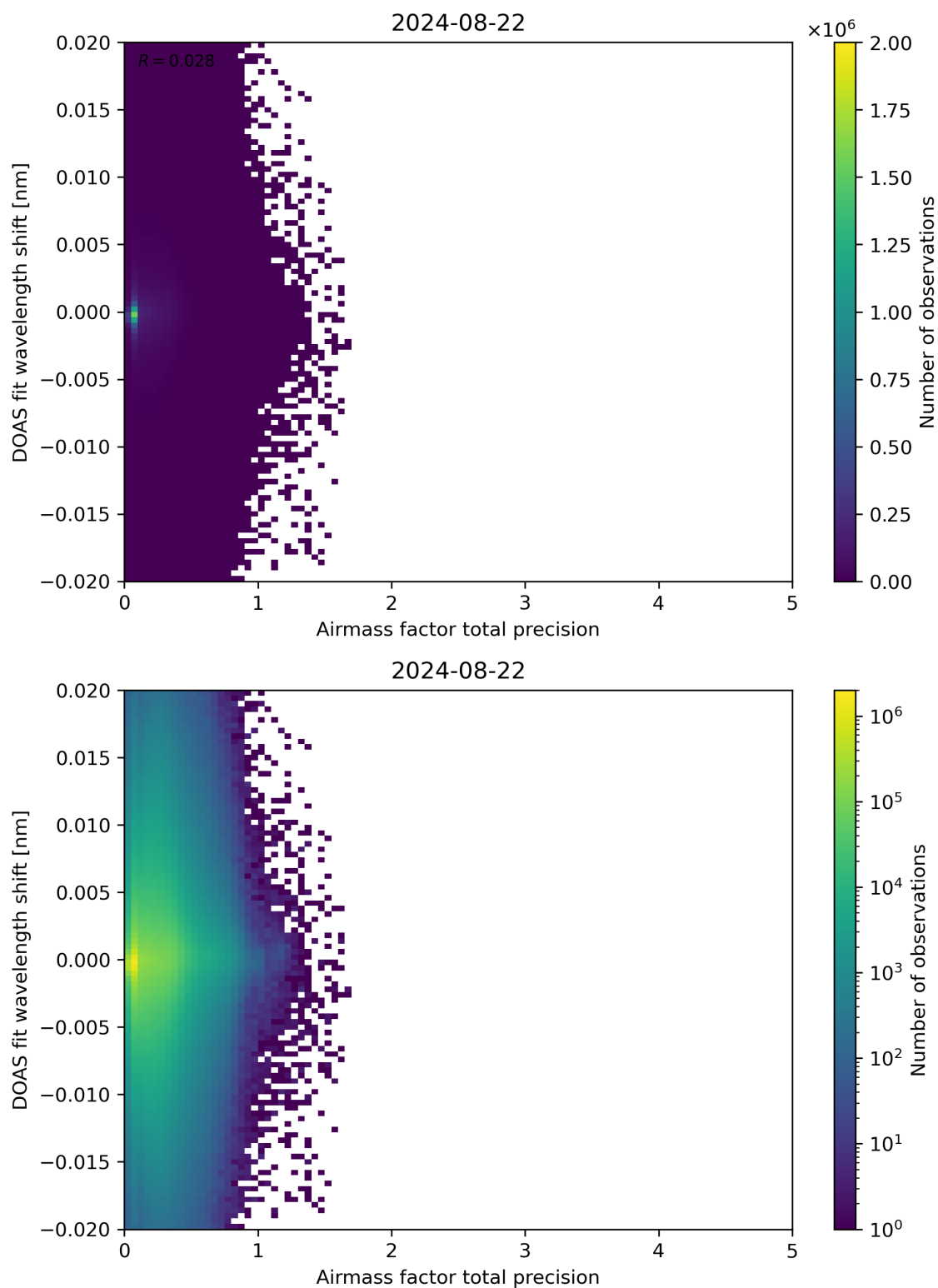
Figure 106: Scatter density plot of “Airmass factor total precision” against “DOAS fit wavelength shift” for 2024-08-22 to 2024-08-23.
