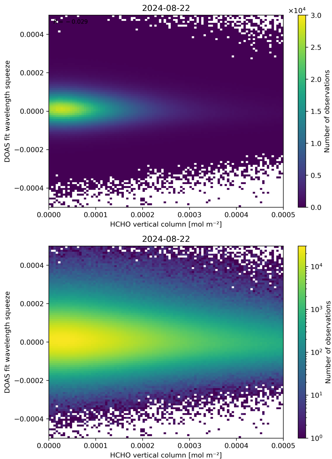
Figure 125: Scatter density plot of “HCHO vertical column” against “DOAS fit wavelength squeeze” for 2024-08-22 to 2024-08-23.
