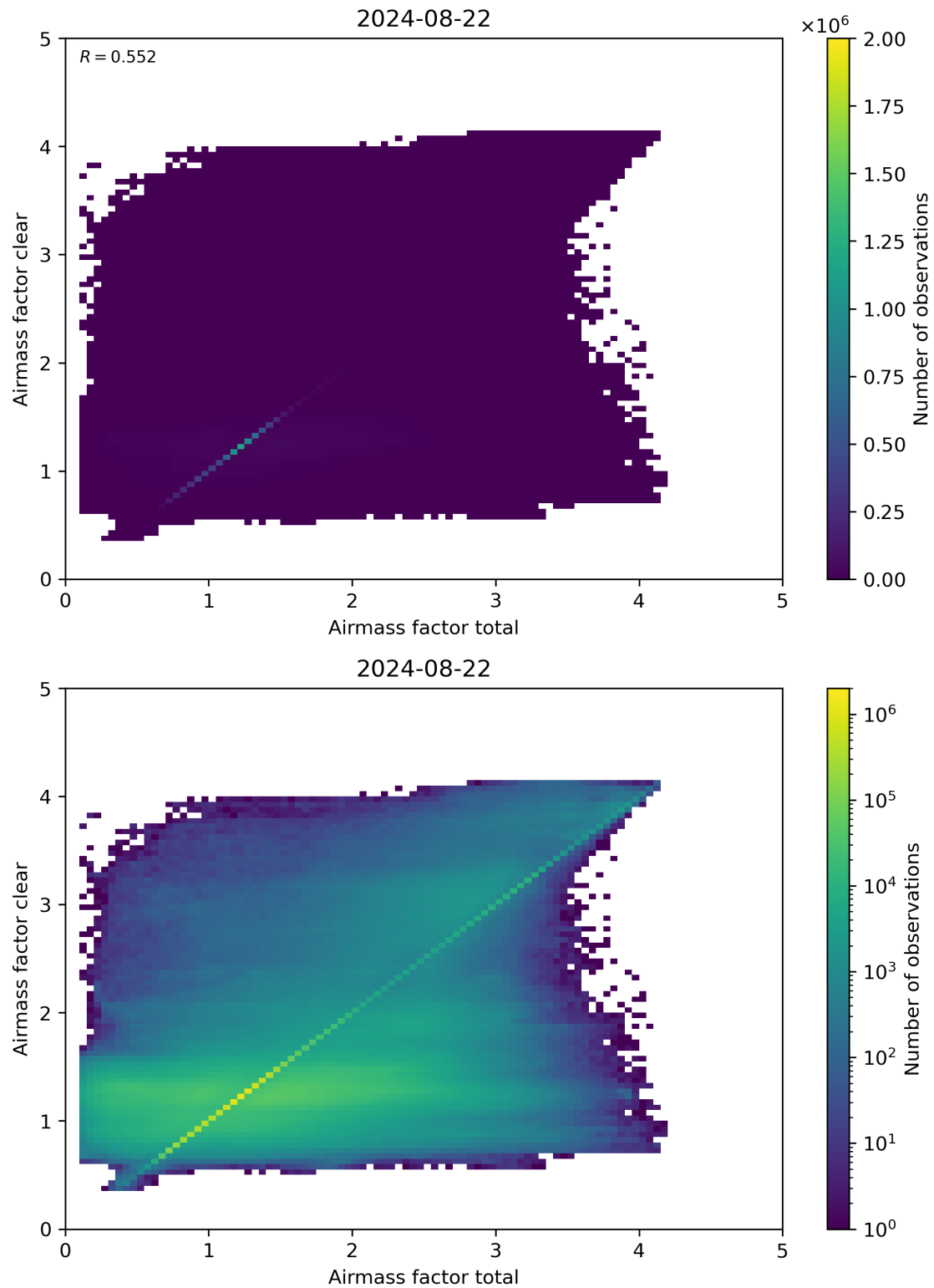
Figure 100: Scatter density plot of “Airmass factor total” against “Airmass factor clear” for 2024-08-22 to 2024-08-23.
