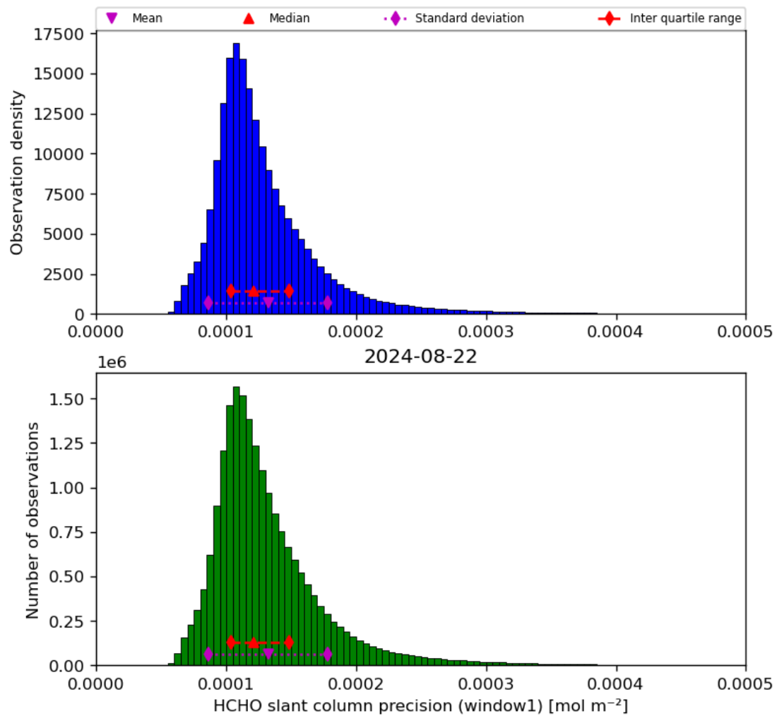
Figure 39: Histogram of “HCHO slant column precision (window1)” for 2024-08-22 to 2024-08-23
