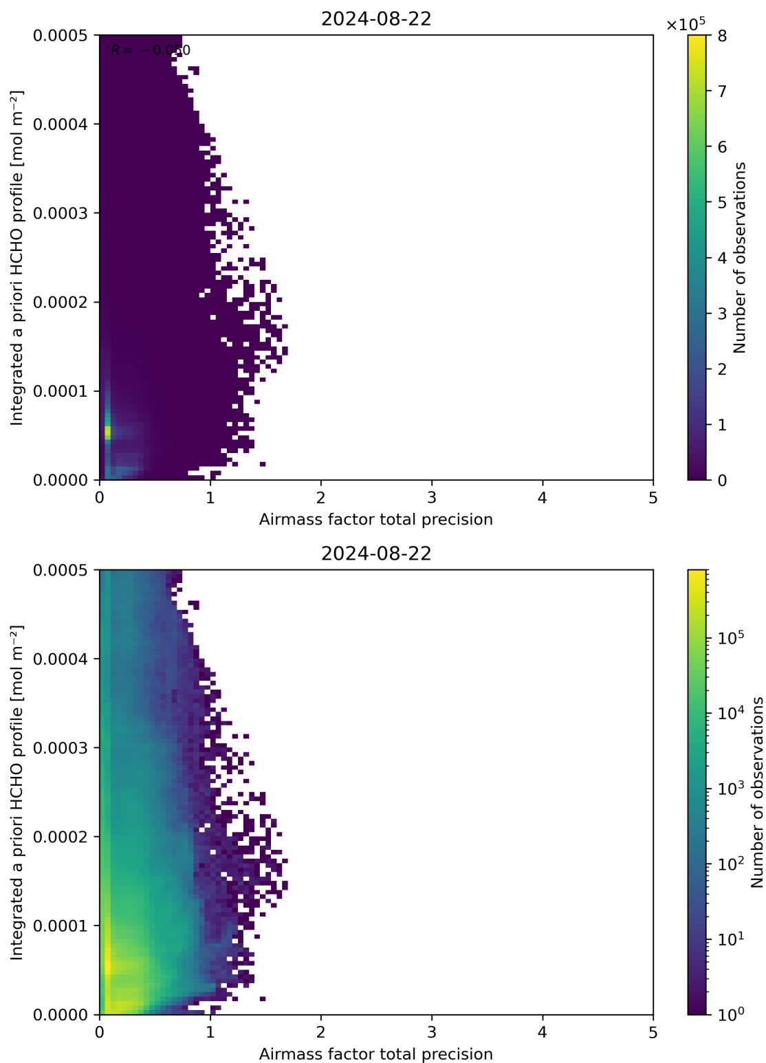
Figure 111: Scatter density plot of “Airmass factor total precision” against “Integrated a priori HCHO profile” for 2024-08-22 to 2024-08-23.
