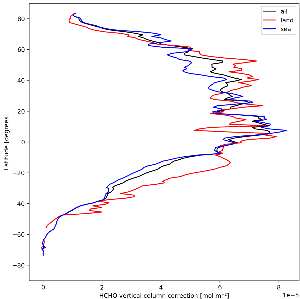
Figure 23: Zonal average of "HCHO vertical column correction" for 2024-08-22 to 2024-08-23.
