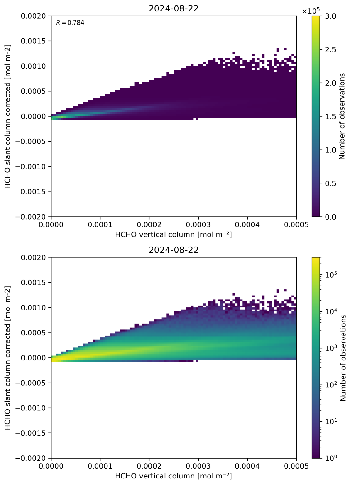
Figure 127: Scatter density plot of “HCHO vertical column” against “HCHO slant column corrected” for 2024-08-22 to 2024-08-23.
