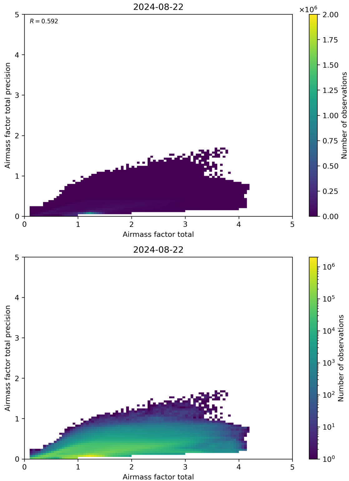
Figure 103: Scatter density plot of “Airmass factor total” against “Airmass factor total precision” for 2024-08-22 to 2024-08-23.
