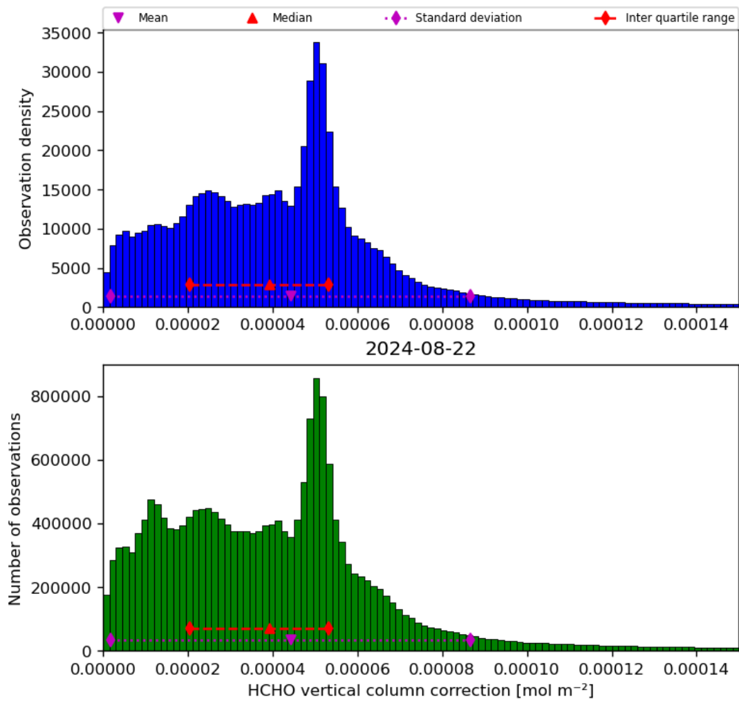
Figure 37: Histogram of “HCHO vertical column correction” for 2024-08-22 to 2024-08-23
