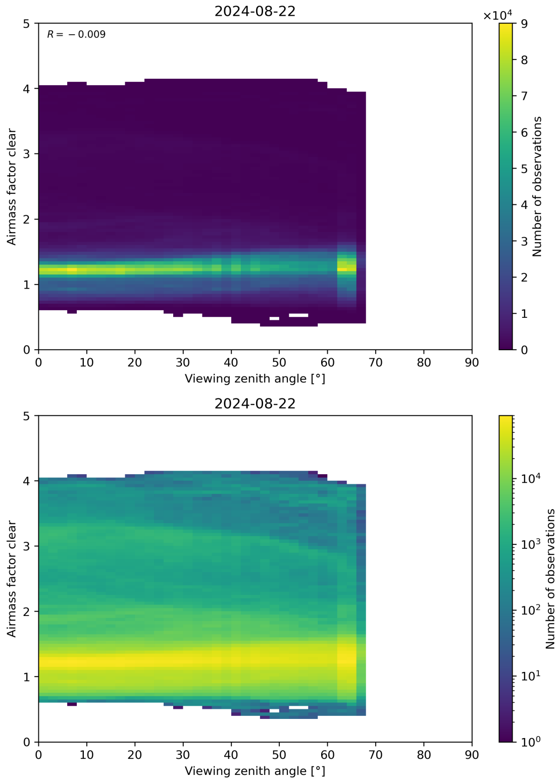
Figure 185: Scatter density plot of “Viewing zenith angle” against “Airmass factor clear” for 2024-08-22 to 2024-08-23.
