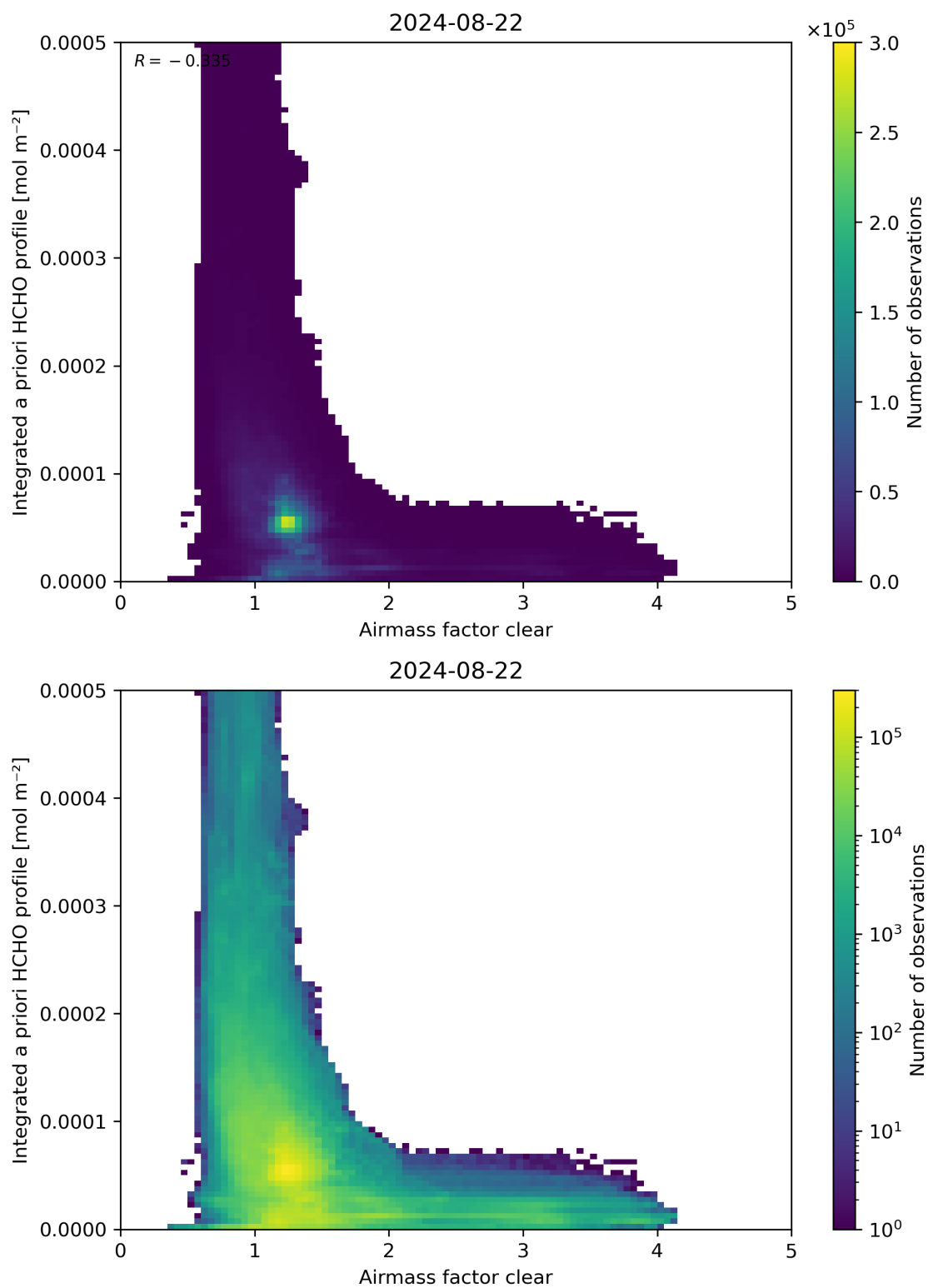
Figure 76: Scatter density plot of “Airmass factor clear” against “Integrated a priori HCHO profile” for 2024-08-22 to 2024-08-23.
