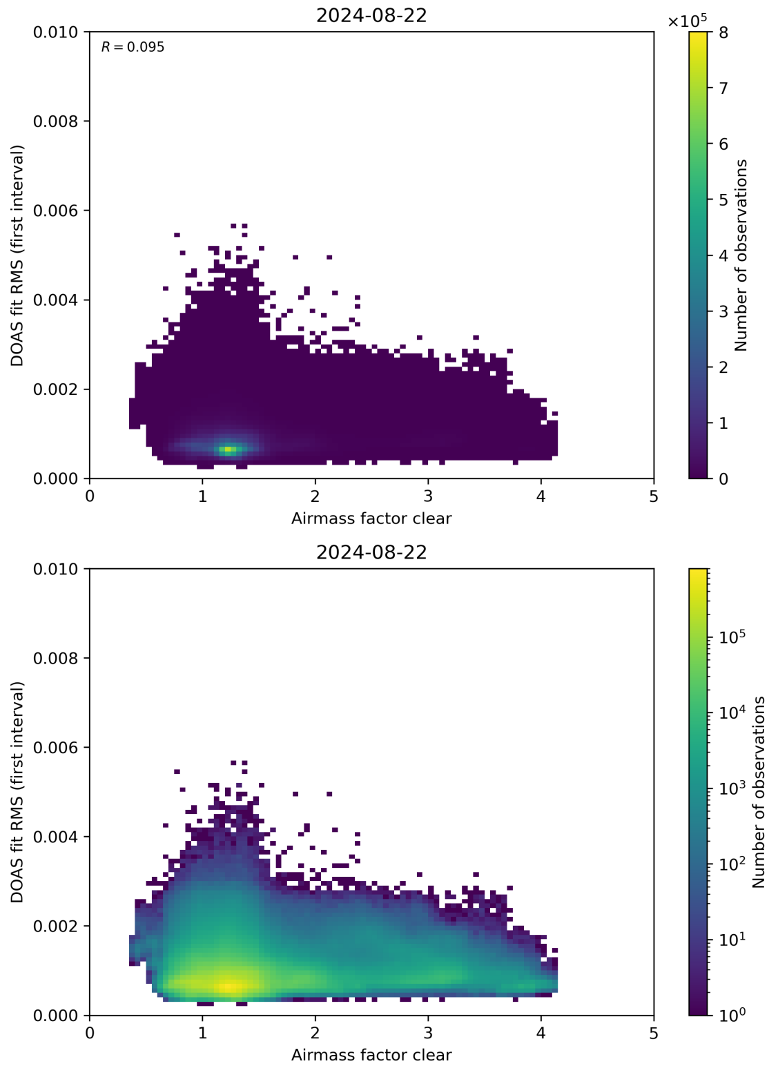
Figure 71: Scatter density plot of “Airmass factor clear” against “DOAS fit RMS (first interval)” for 2024-08-22 to 2024-08-23.
