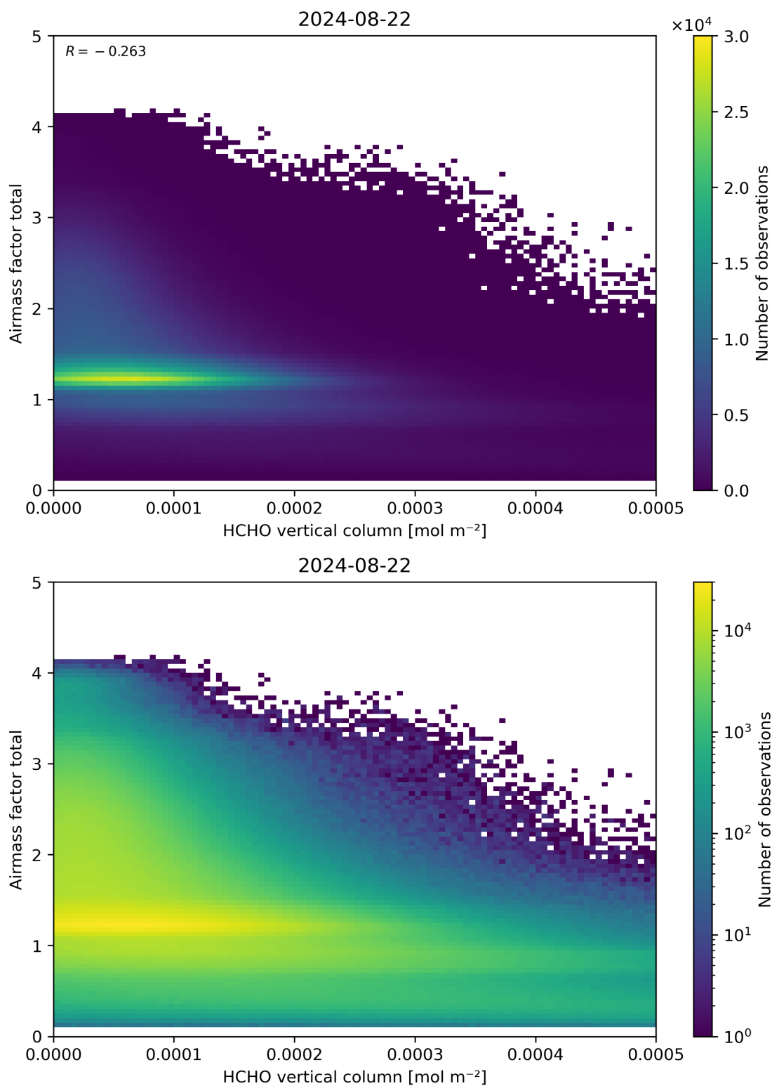
Figure 131: Scatter density plot of “HCHO vertical column” against “Airmass factor total” for 2024-08-22 to 2024-08-23.
