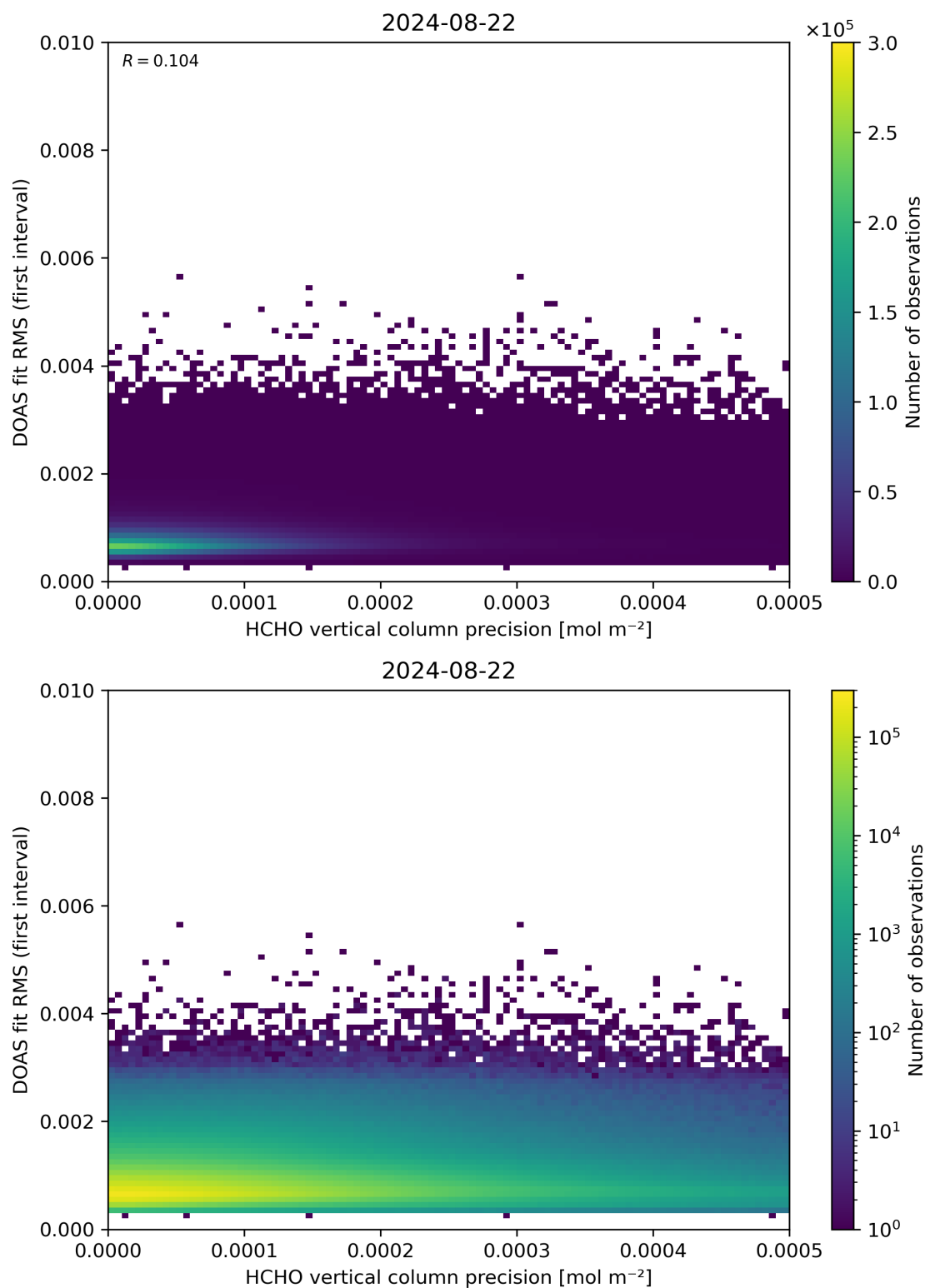
Figure 136: Scatter density plot of “HCHO vertical column precision” against “DOAS fit RMS (first interval)” for 2024-08-22 to 2024-08-23.
