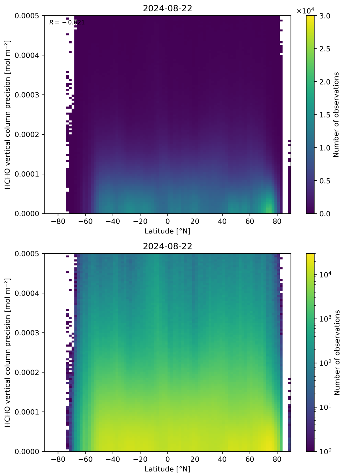
Figure 165: Scatter density plot of “Latitude” against “HCHO vertical column precision” for 2024-08-22 to 2024-08-23.
