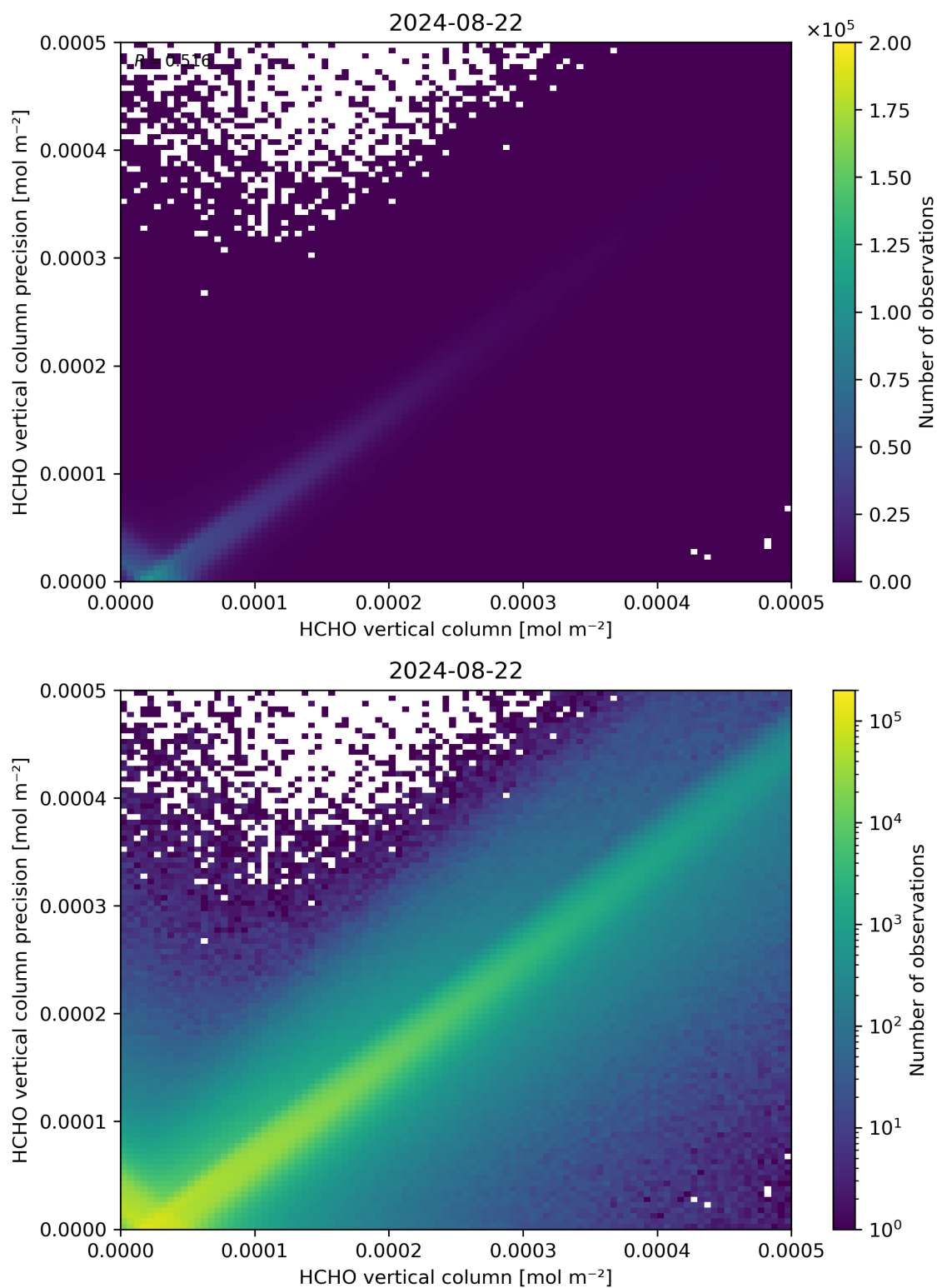
Figure 134: Scatter density plot of “HCHO vertical column” against “HCHO vertical column precision” for 2024-08-22 to 2024-08-23.
