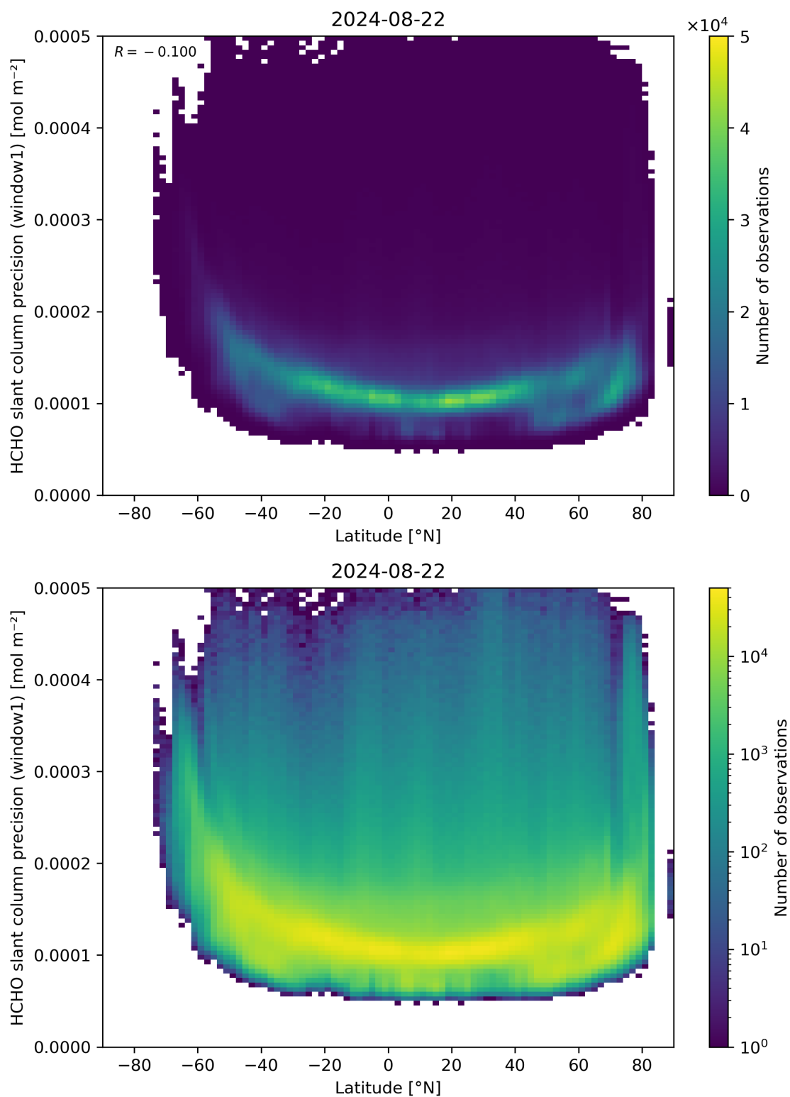
Figure 160: Scatter density plot of “Latitude” against “HCHO slant column precision (window1)” for 2024-08-22 to 2024-08-23.
