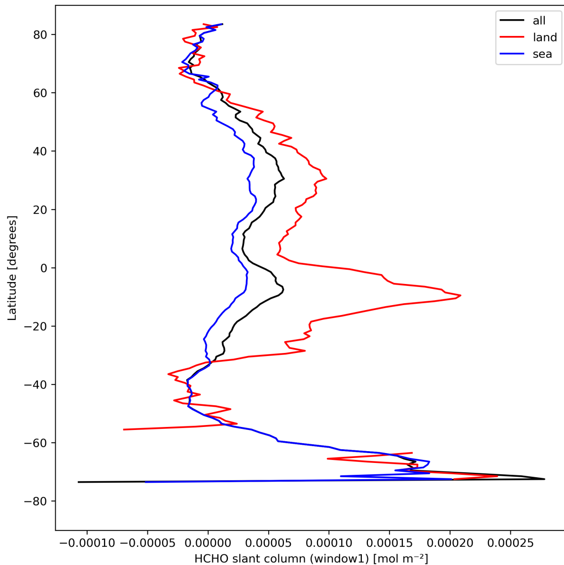
Figure 24: Zonal average of “HCHO slant column (window1)” for 2024-08-22 to 2024-08-23.
