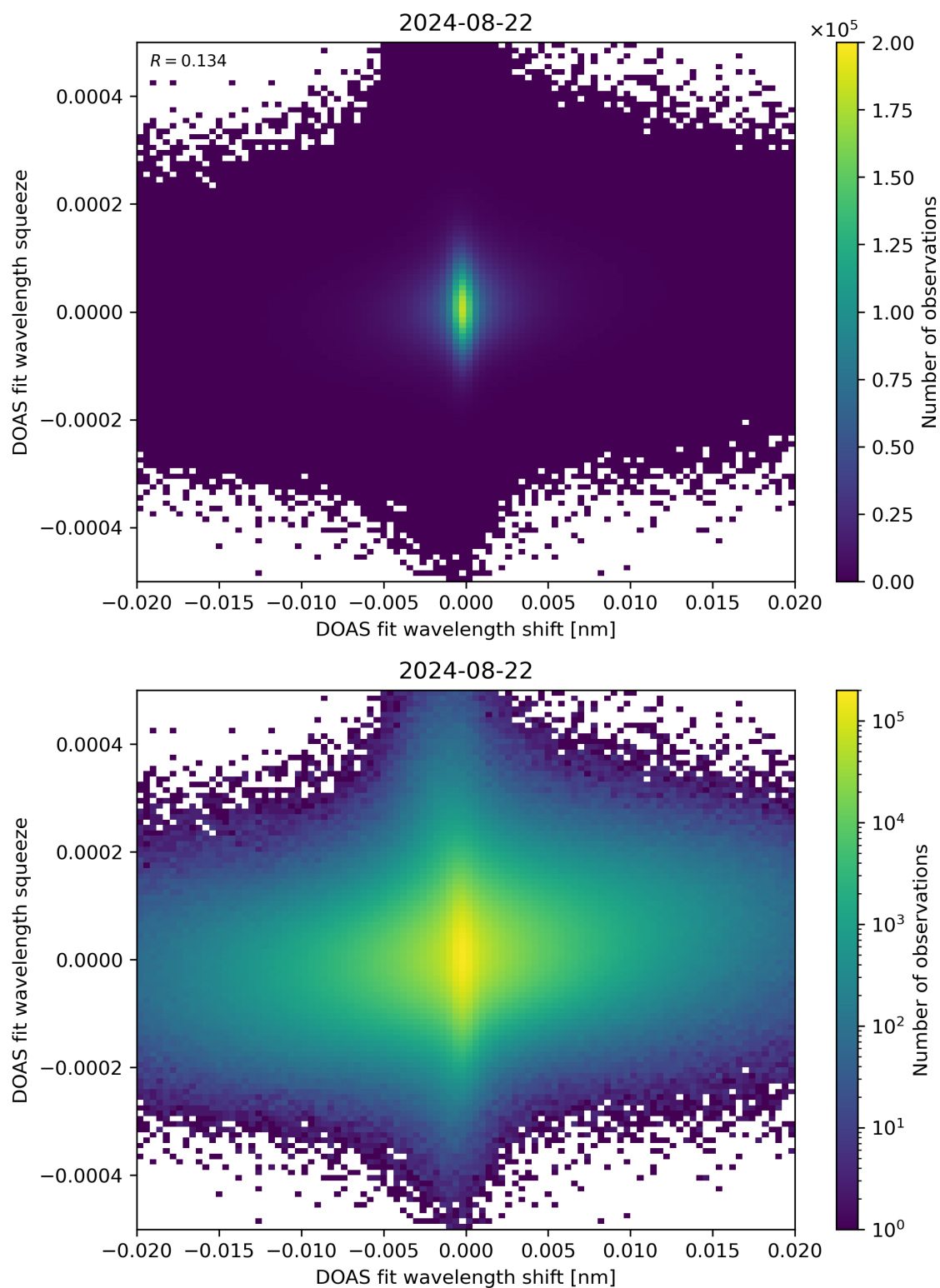
Figure 65: Scatter density plot of “DOAS fit wavelength shift” against “DOAS fit wavelength squeeze” for 2024-08-22 to 2024-08-23.
