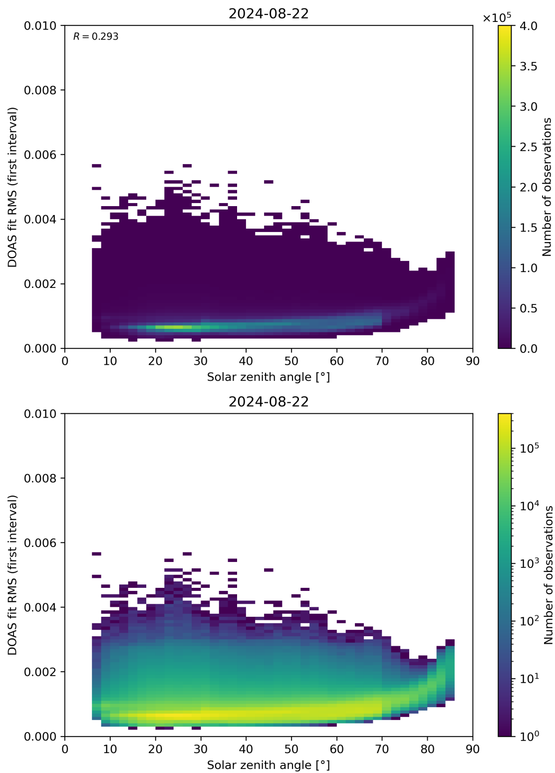
Figure 167: Scatter density plot of “Solar zenith angle” against “DOAS fit RMS (first interval)” for 2024-08-22 to 2024-08-23.
