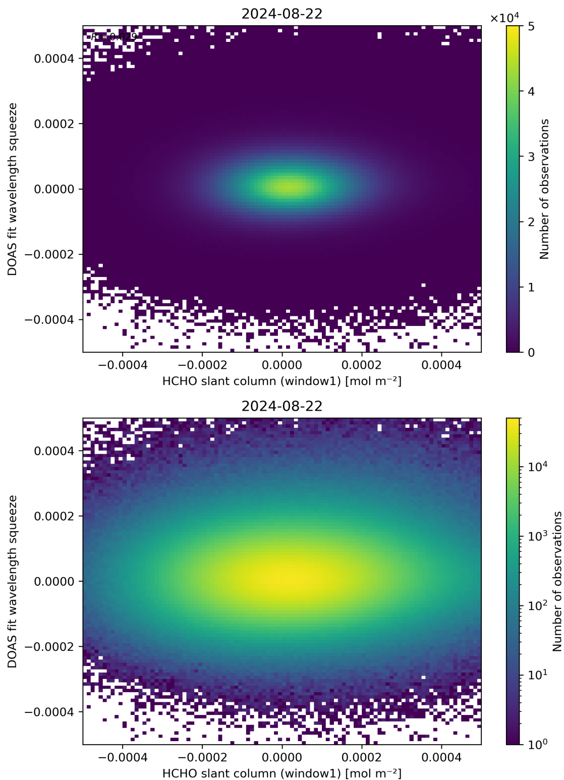
Figure 80: Scatter density plot of “HCHO slant column (window1)” against “DOAS fit wavelength squeeze” for 2024-08-22 to 2024-08-23.
