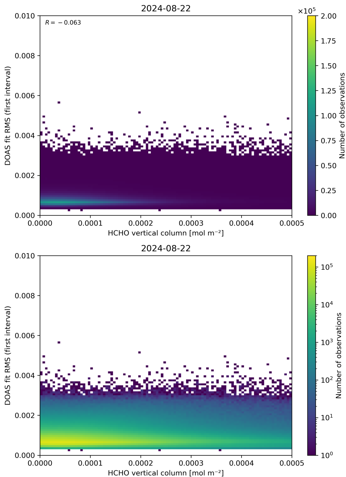
Figure 123: Scatter density plot of “HCHO vertical column” against “DOAS fit RMS (first interval)” for 2024-08-22 to 2024-08-23.
