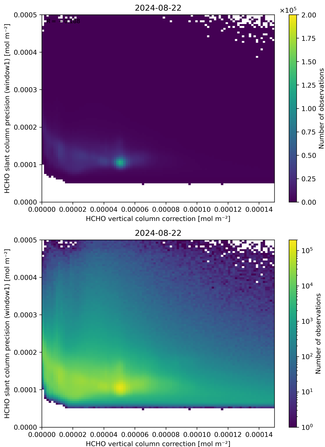
Figure 119: Scatter density plot of “HCHO vertical column correction” against “HCHO slant column precision (window1)” for 2024-08-22 to 2024-08-23.
