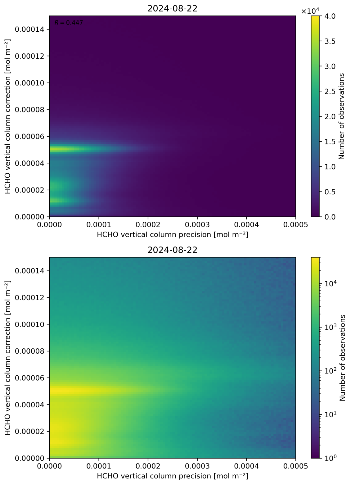
Figure 146: Scatter density plot of “HCHO vertical column precision” against “HCHO vertical column correction” for 2024-08-22 to 2024-08-23.
