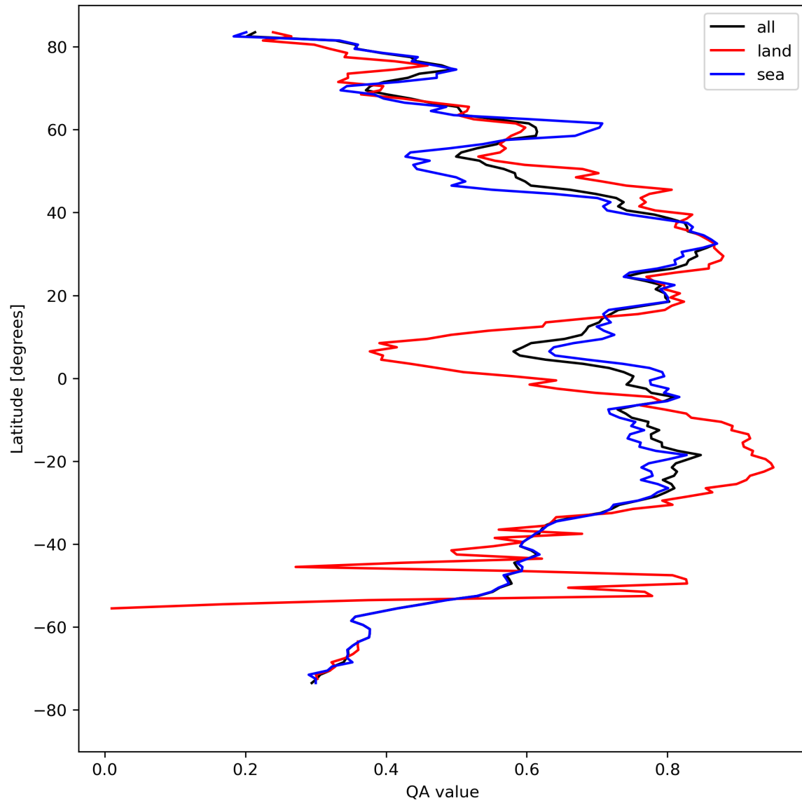
Figure 20: Zonal average of “QA value” for 2024-08-22 to 2024-08-23.
