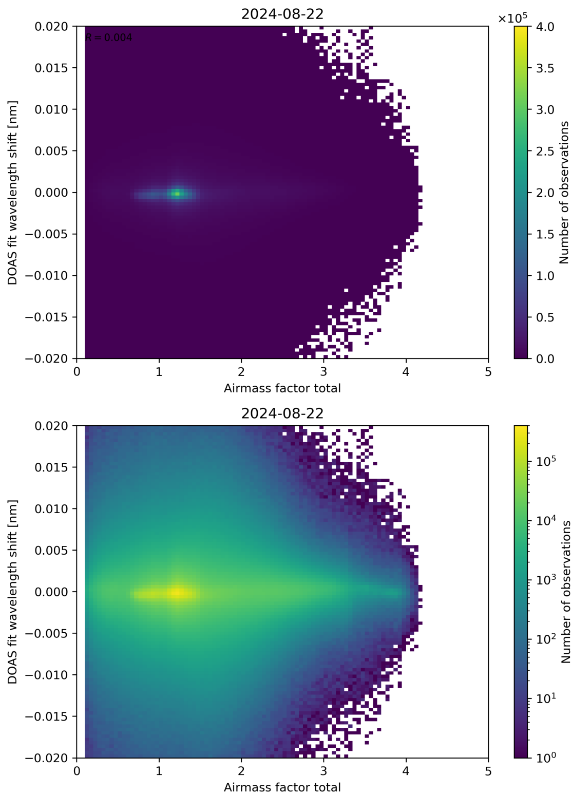
Figure 98: Scatter density plot of “Airmass factor total” against “DOAS fit wavelength shift” for 2024-08-22 to 2024-08-23.
