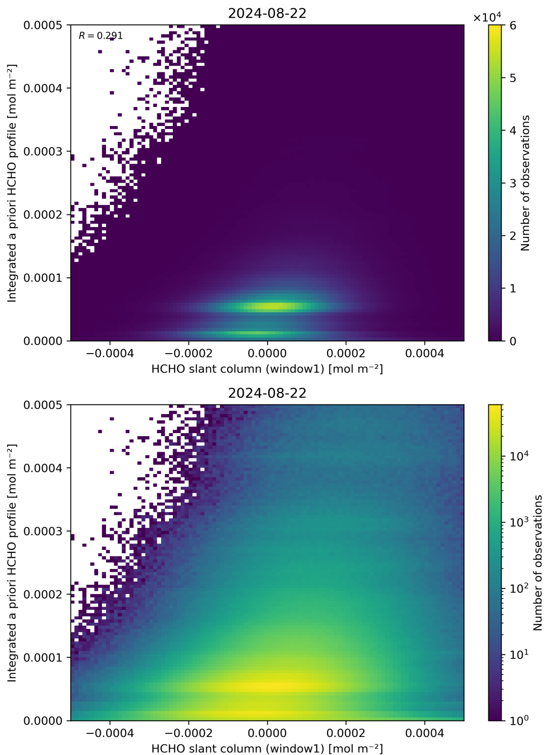
Figure 87: Scatter density plot of “HCHO slant column (window1)” against “Integrated a priori HCHO profile” for 2024-08-22 to 2024-08-23.
