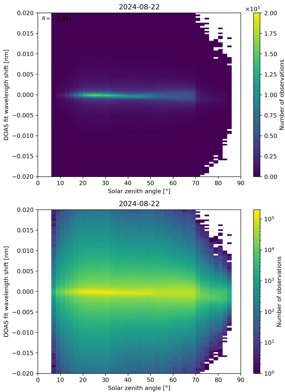
Figure 168: Scatter density plot of “Solar zenith angle” against “DOAS fit wavelength shift” for 2024-08-22 to 2024-08-23.
