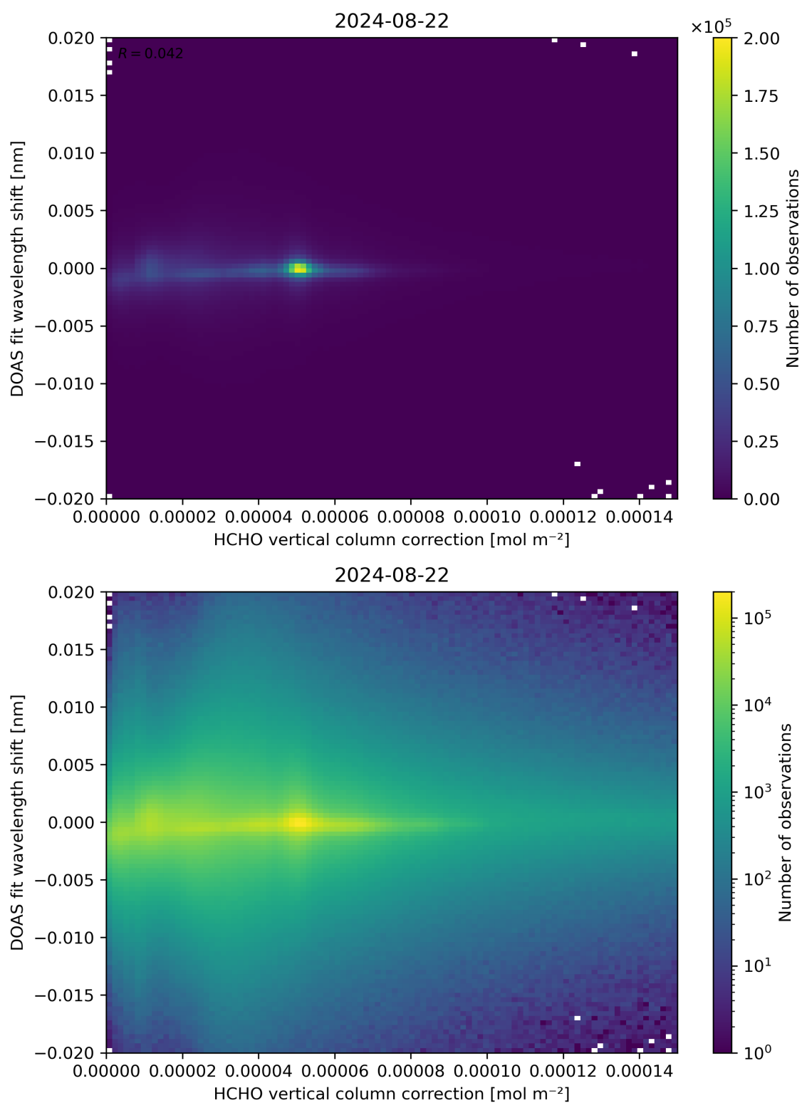
Figure 113: Scatter density plot of “HCHO vertical column correction” against “DOAS fit wavelength shift” for 2024-08-22 to 2024-08-23.
