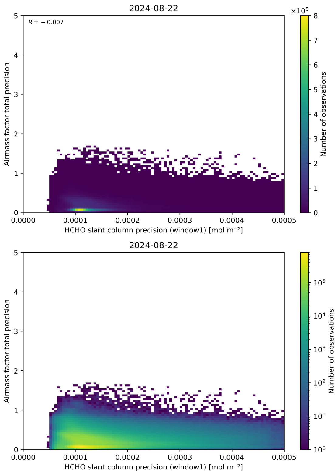
Figure 95: Scatter density plot of “HCHO slant column precision (window1)” against “Airmass factor total precision” for 2024-08-22 to 2024-08-23.
