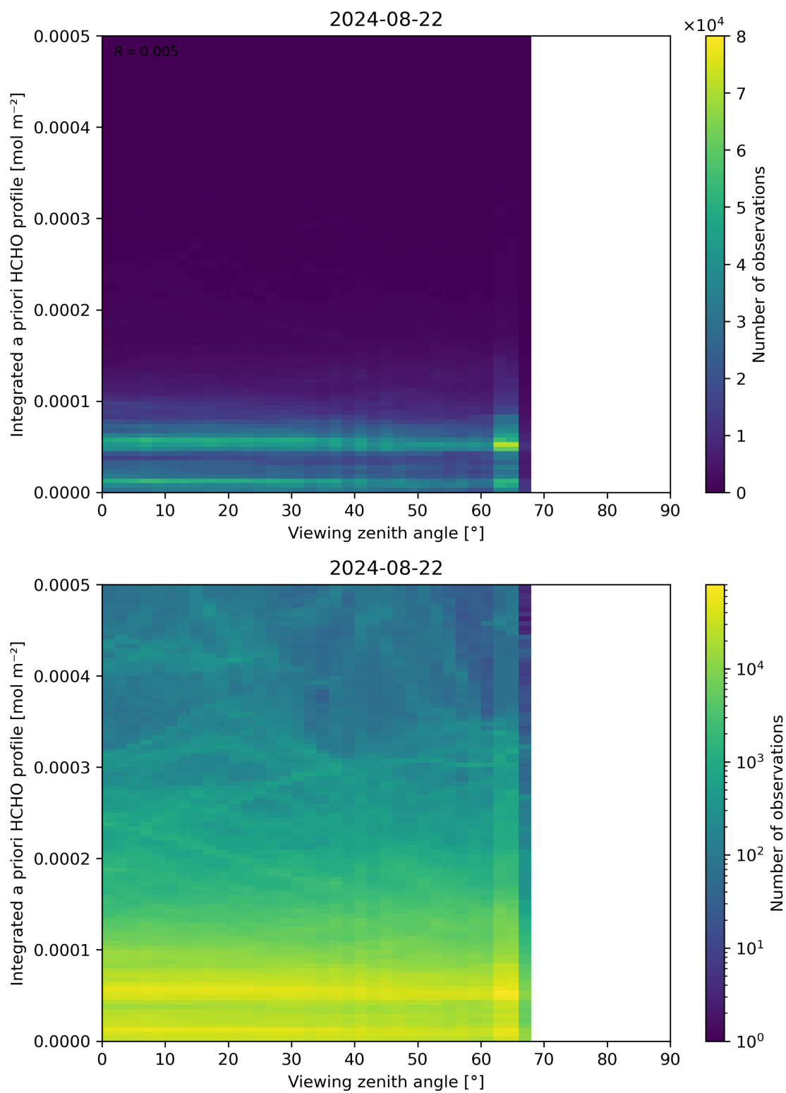
Figure 195: Scatter density plot of “Viewing zenith angle” against “Integrated a priori HCHO profile” for 2024-08-22 to 2024-08-23.
