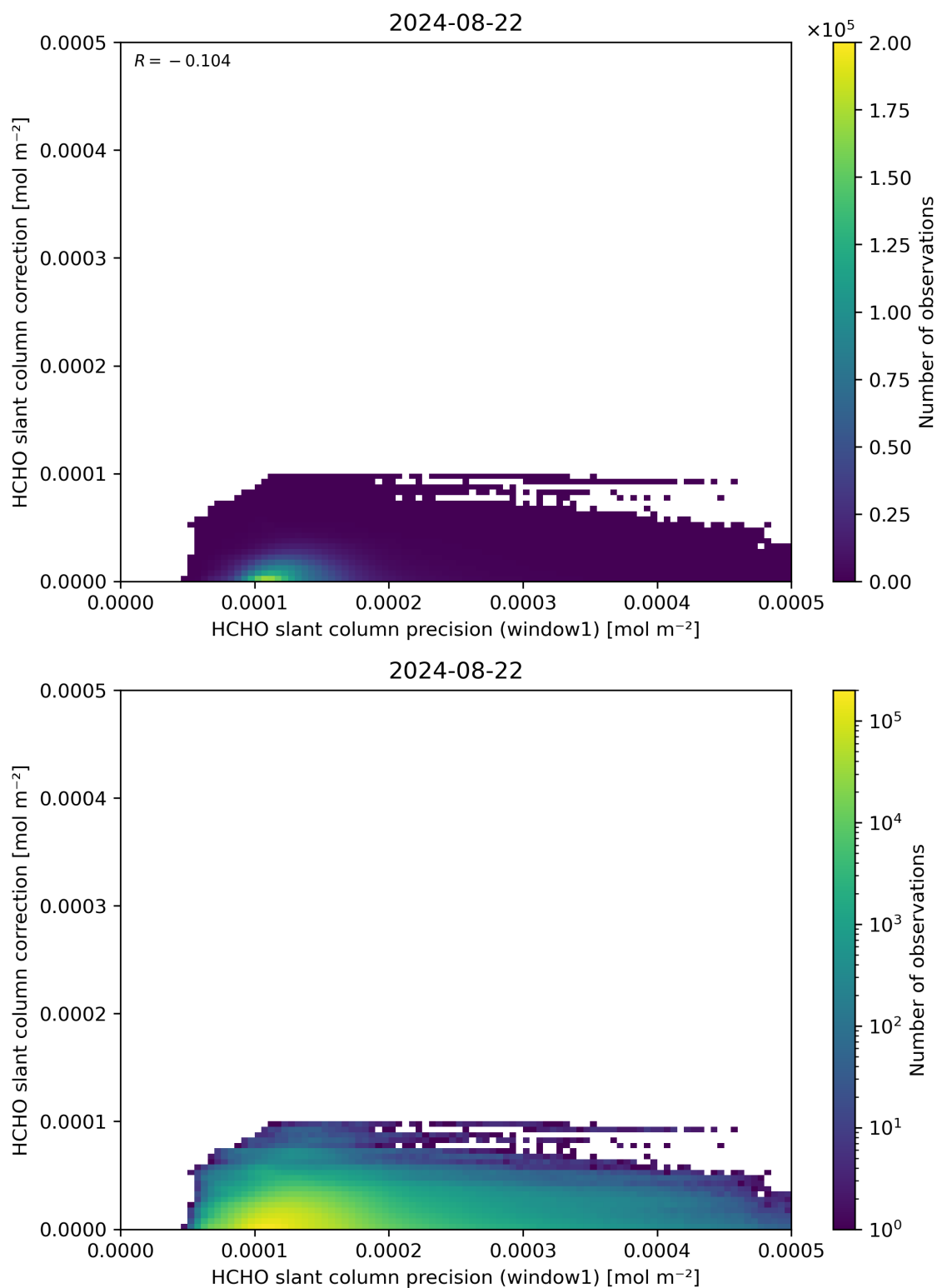
Figure 93: Scatter density plot of “HCHO slant column precision (window1)” against “HCHO slant column correction” for 2024-08-22 to 2024-08-23.
