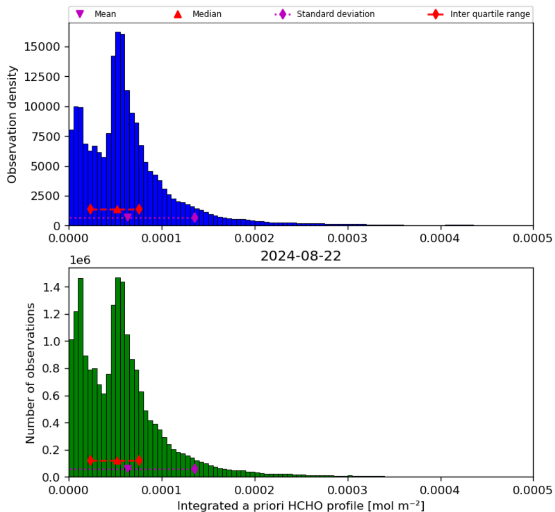
Figure 43: Histogram of “Integrated a priori HCHO profile” for 2024-08-22 to 2024-08-23
