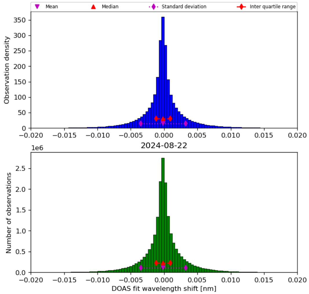
Figure 44: Histogram of “DOAS fit wavelength shift” for 2024-08-22 to 2024-08-23
