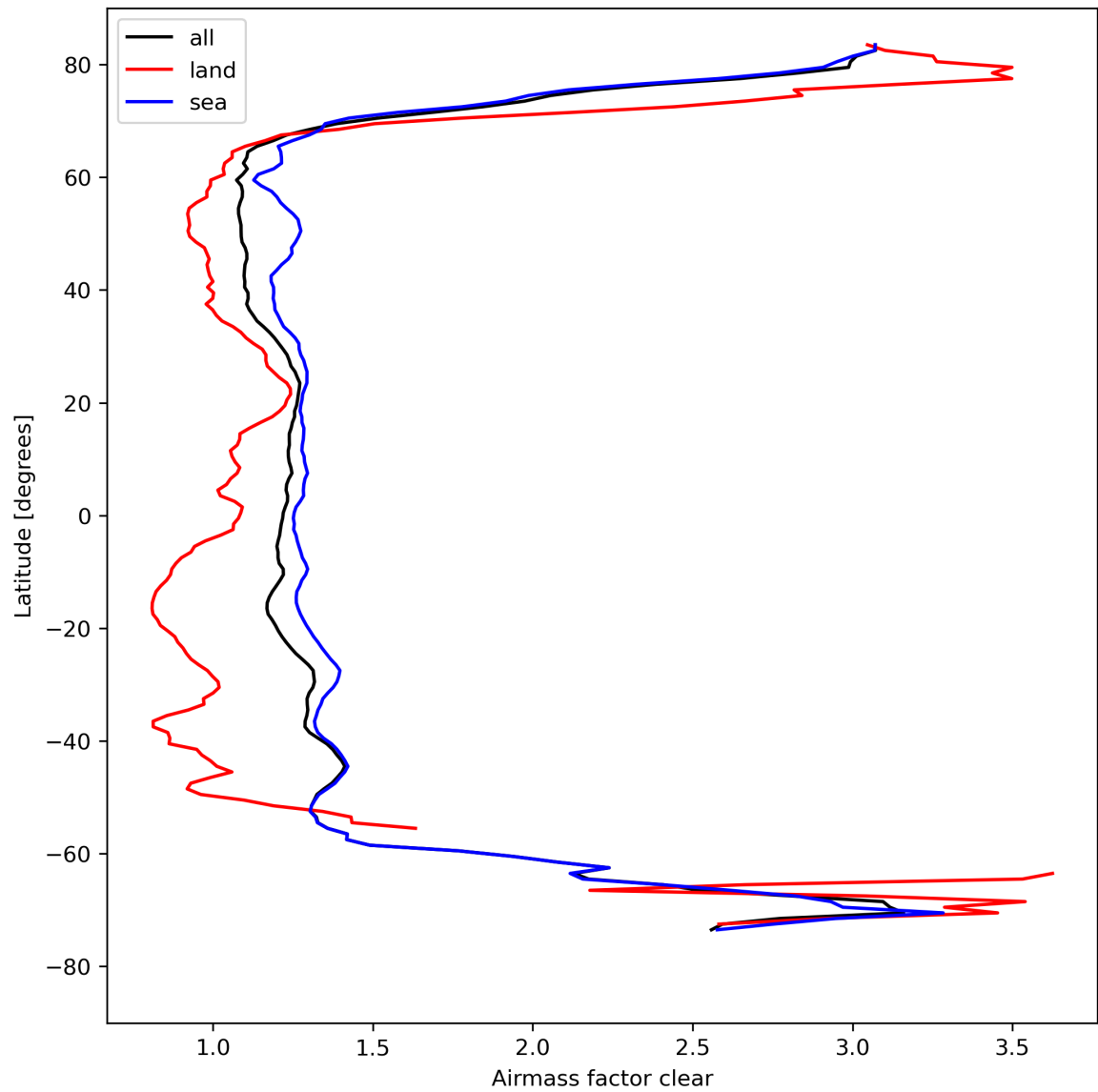
Figure 28: Zonal average of “Airmass factor clear” for 2024-08-22 to 2024-08-23.
