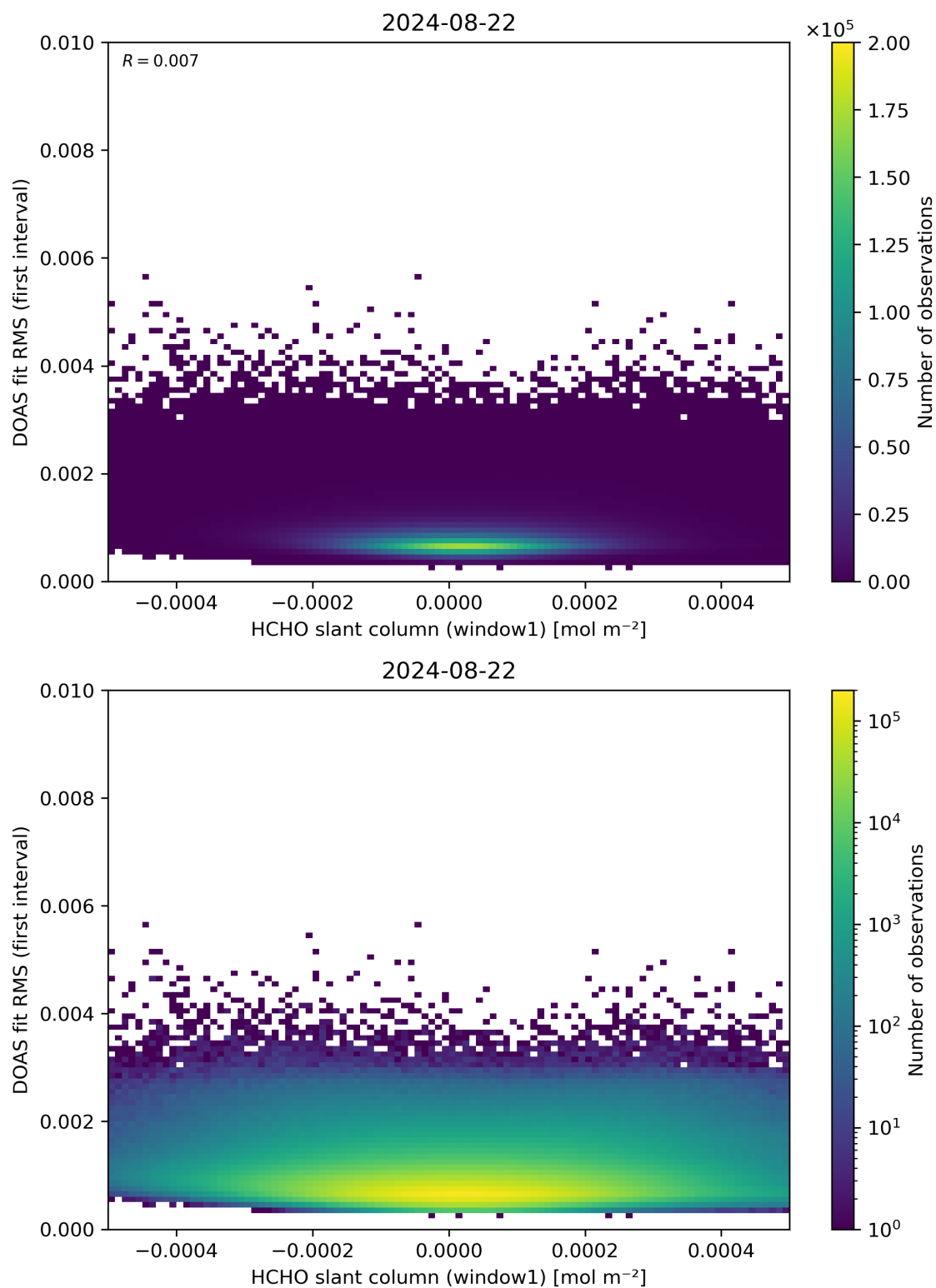
Figure 78: Scatter density plot of “HCHO slant column (window1)” against “DOAS fit RMS (first interval)” for 2024-08-22 to 2024-08-23.
