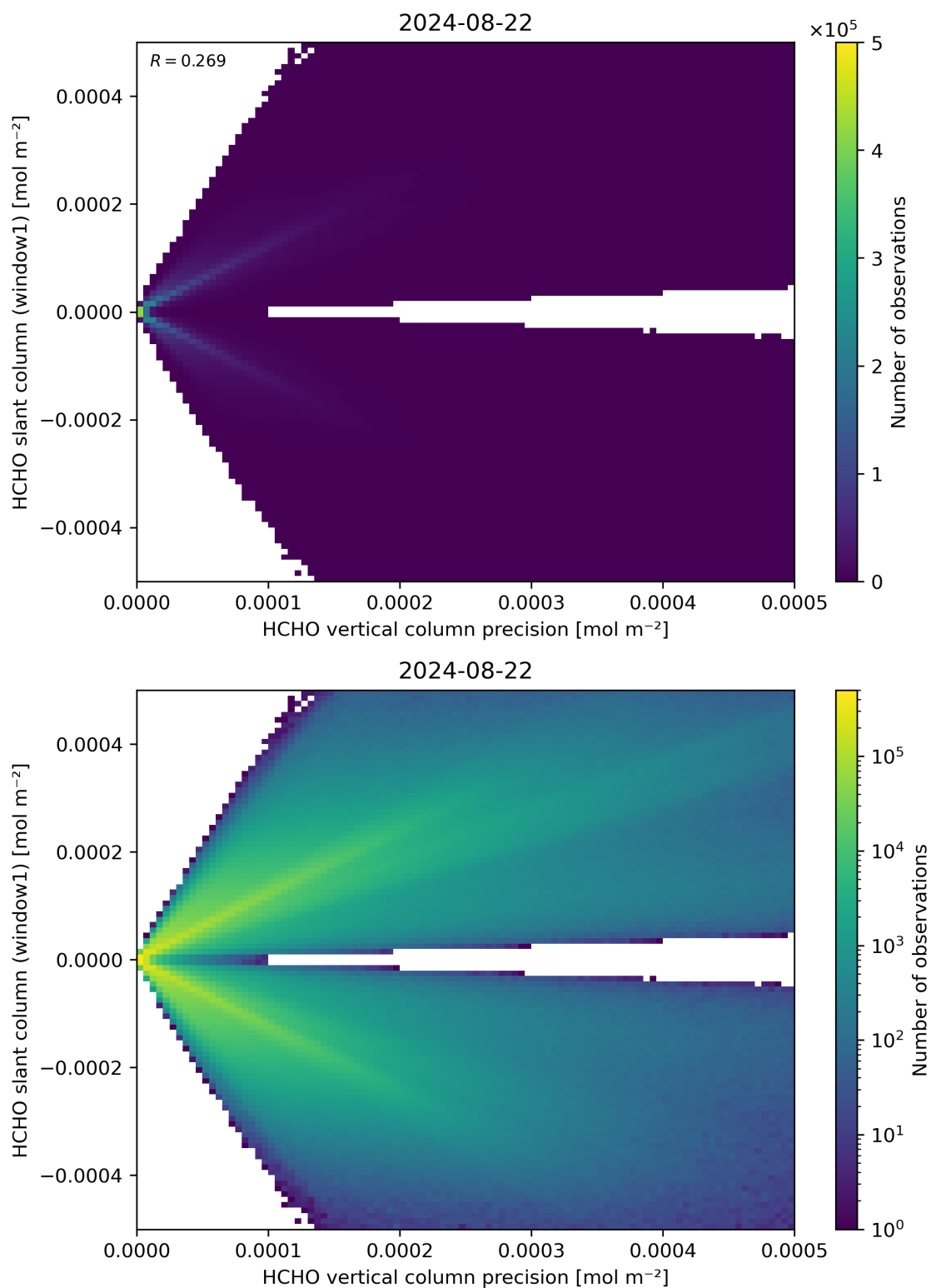
Figure 142: Scatter density plot of “HCHO vertical column precision” against “HCHO slant column (window1)” for 2024-08-22 to 2024-08-23.
