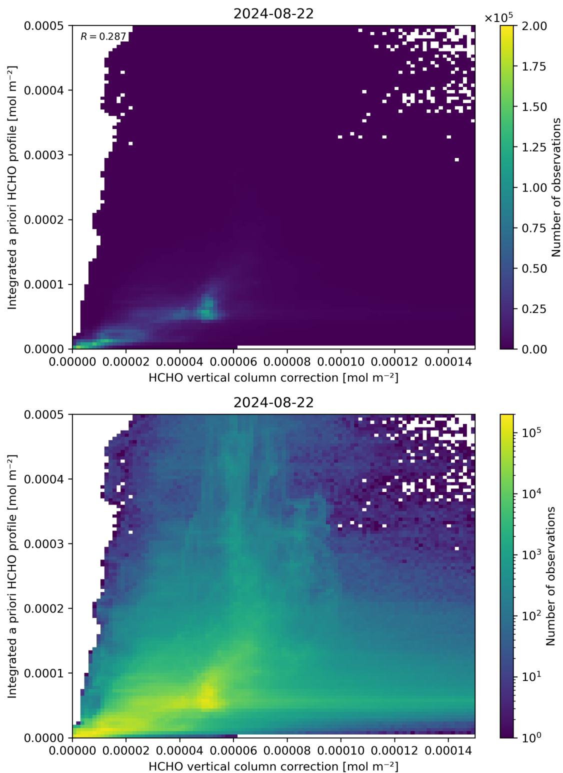
Figure 122: Scatter density plot of “HCHO vertical column correction” against “Integrated a priori HCHO profile” for 2024-08-22 to 2024-08-23.
