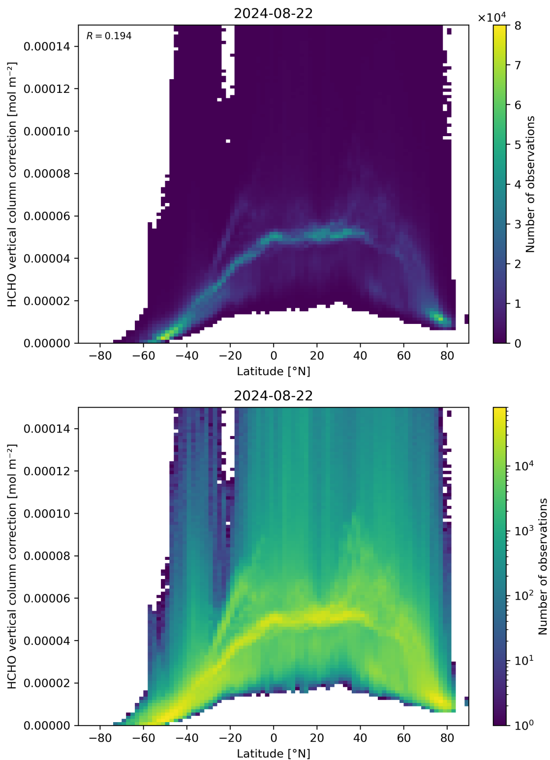
Figure 164: Scatter density plot of “Latitude” against “HCHO vertical column correction” for 2024-08-22 to 2024-08-23.
