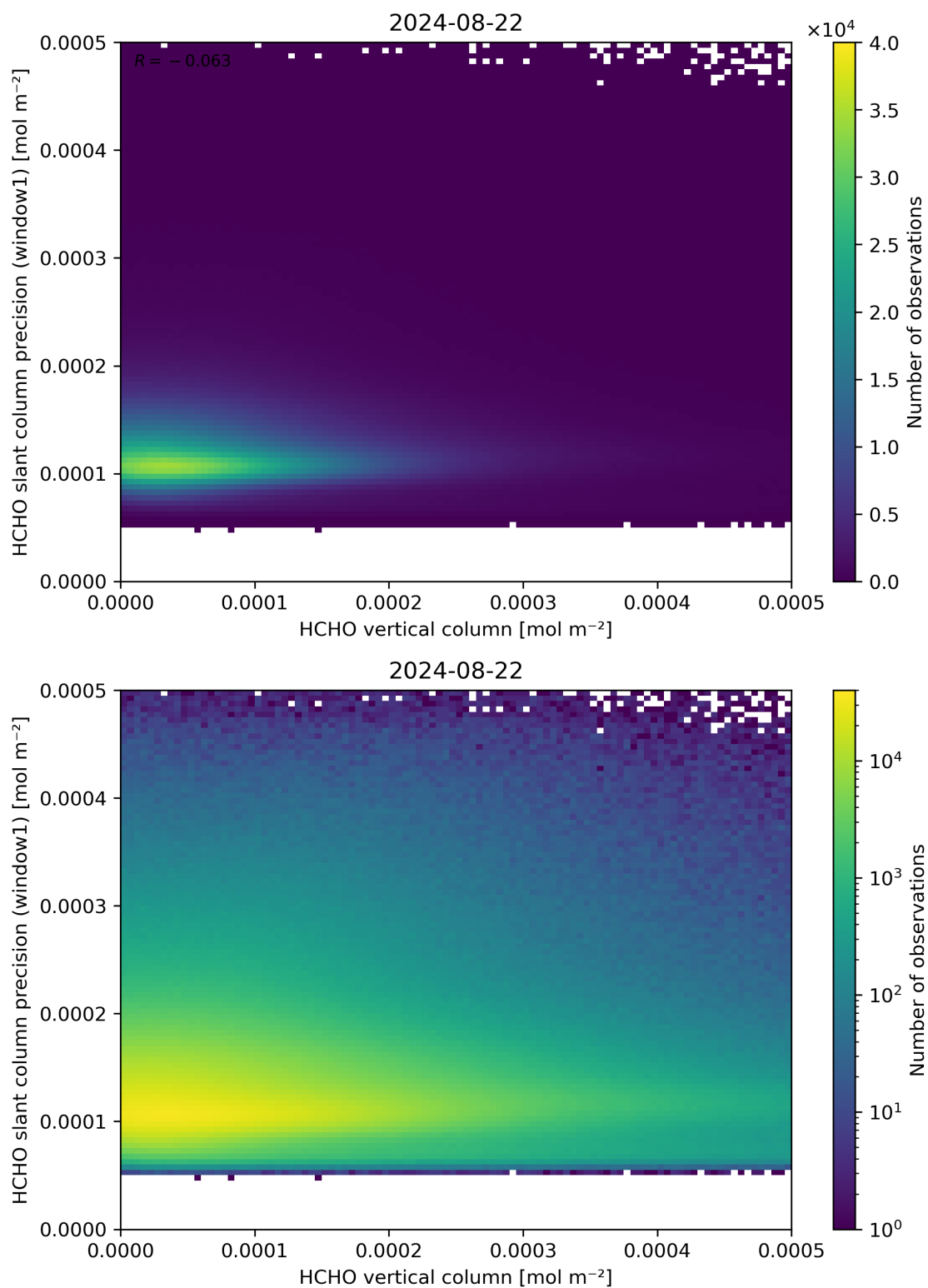
Figure 130: Scatter density plot of “HCHO vertical column” against “HCHO slant column precision (window1)” for 2024-08-22 to 2024-08-23.
