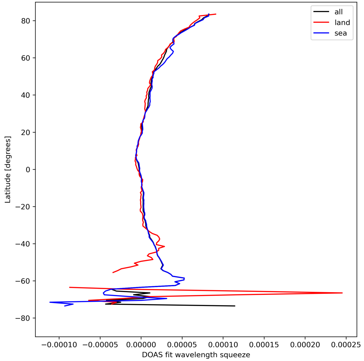
Figure 31: Zonal average of “DOAS fit wavelength squeeze” for 2024-08-22 to 2024-08-23.
