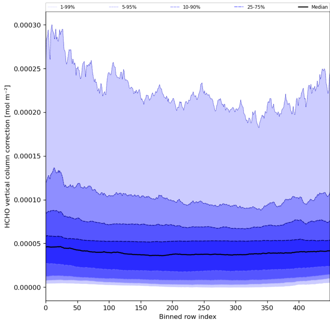
Figure 51: Along track statistics of “HCHO vertical column correction” for 2024-08-22 to 2024-08-23
