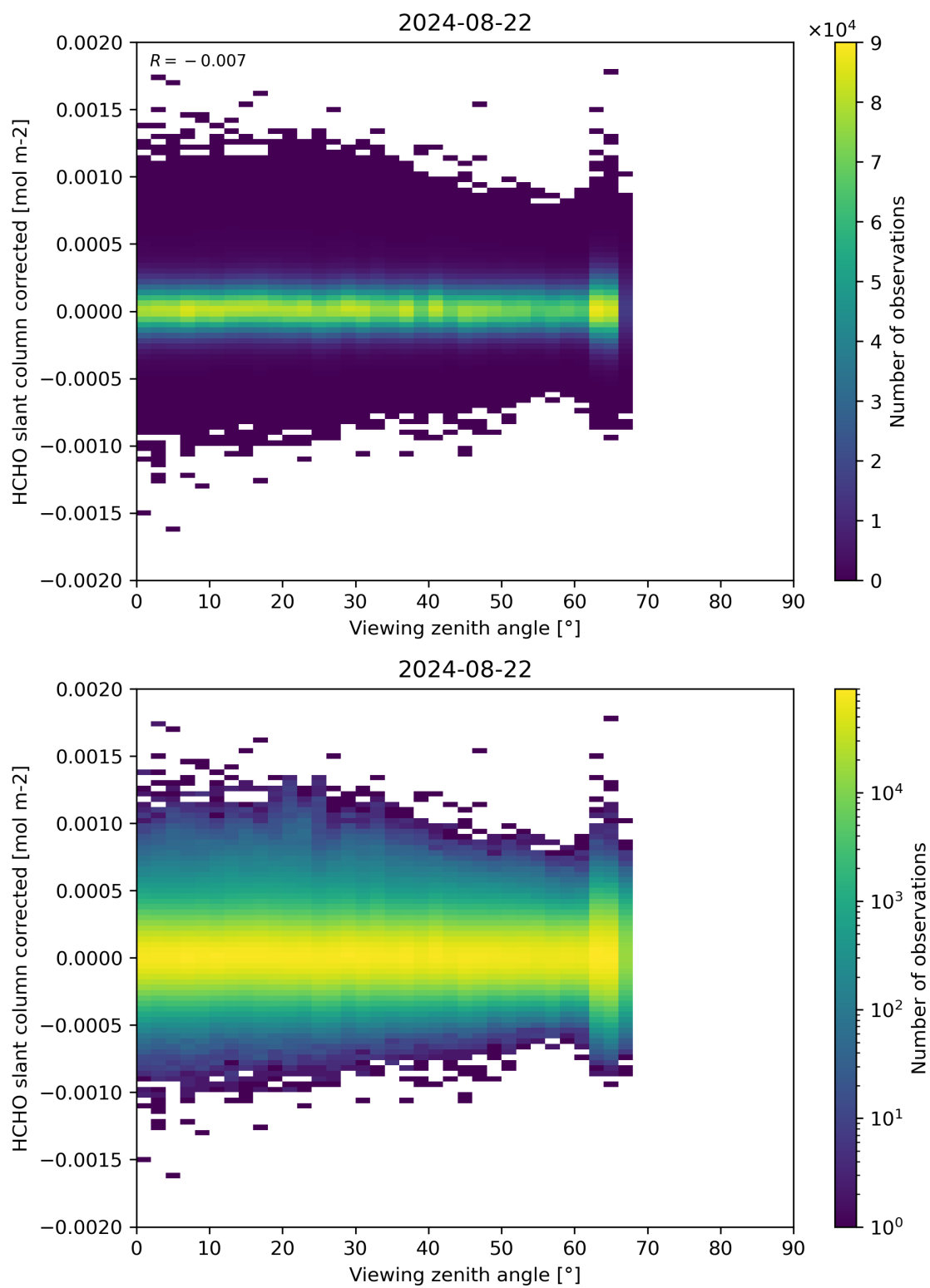
Figure 186: Scatter density plot of “Viewing zenith angle” against “HCHO slant column corrected” for 2024-08-22 to 2024-08-23.
