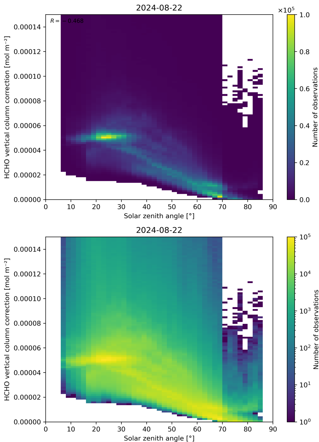
Figure 178: Scatter density plot of “Solar zenith angle” against “HCHO vertical column correction” for 2024-08-22 to 2024-08-23.
