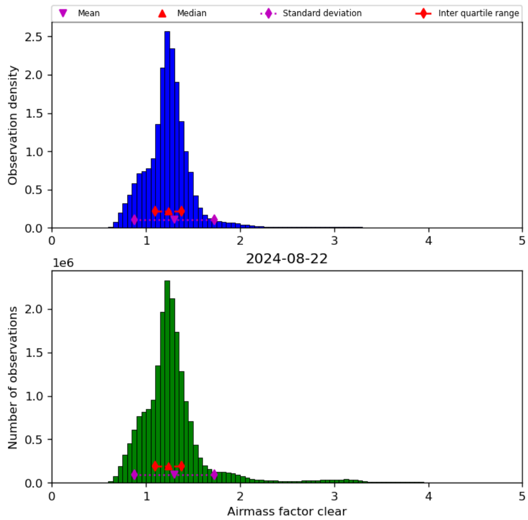
Figure 42: Histogram of “Airmass factor clear” for 2024-08-22 to 2024-08-23
