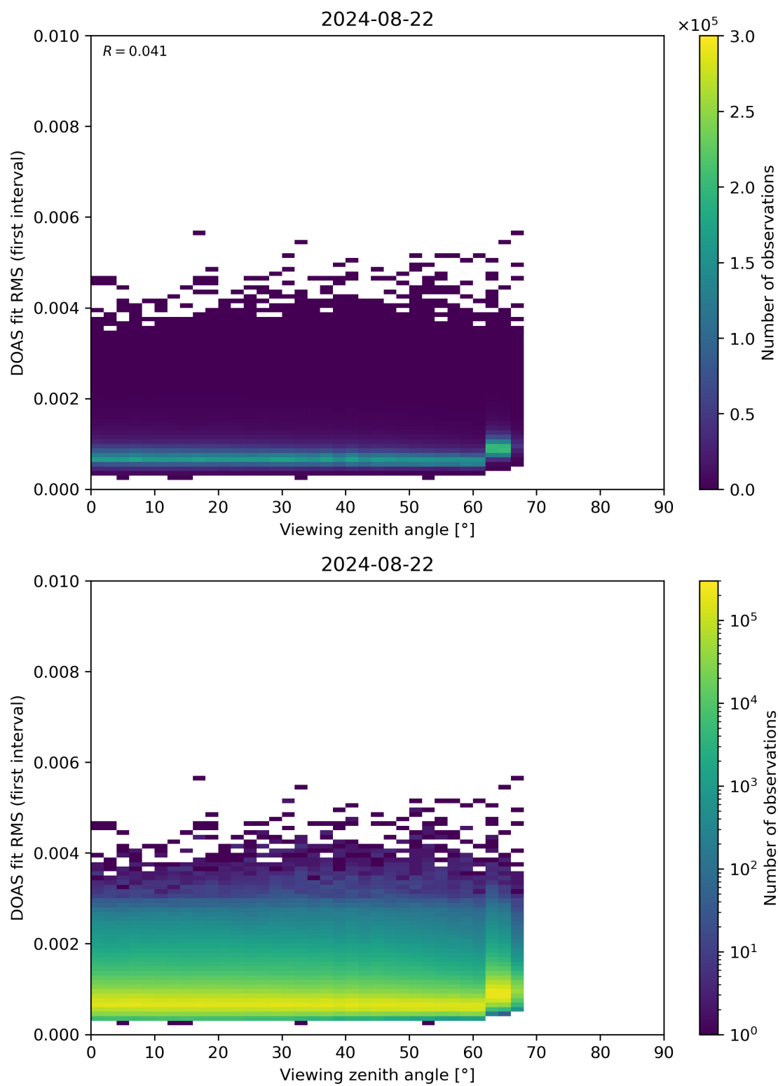
Figure 182: Scatter density plot of “Viewing zenith angle” against “DOAS fit RMS (first interval)” for 2024-08-22 to 2024-08-23.
