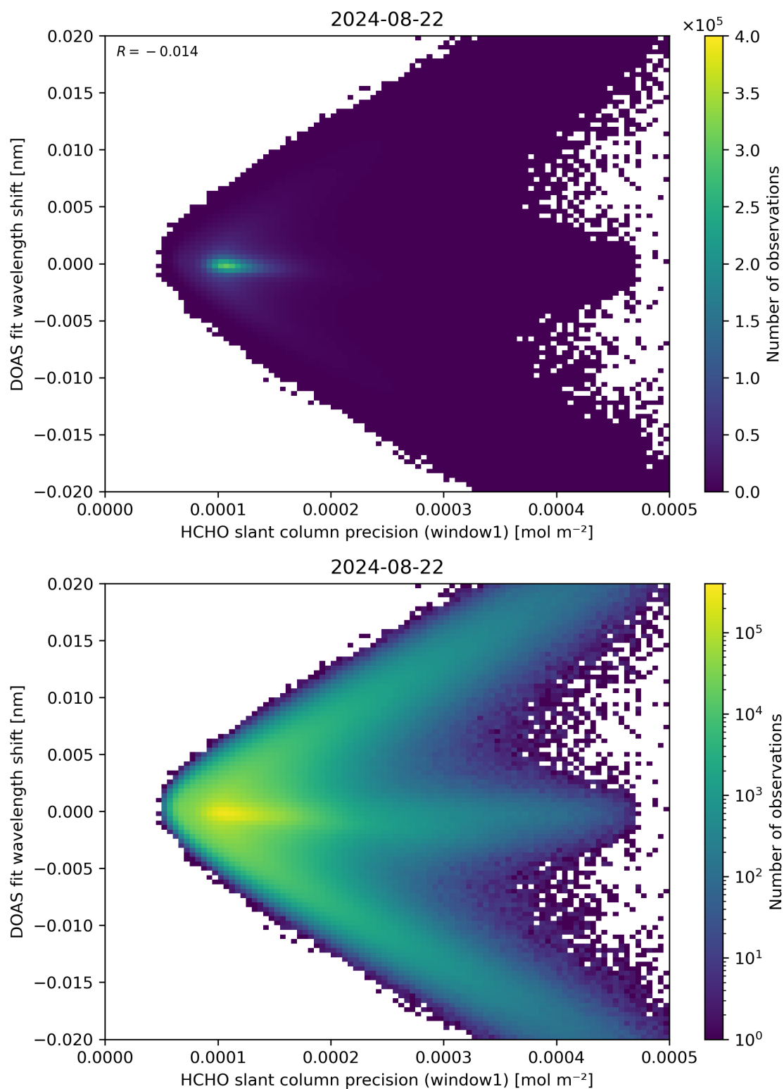
Figure 89: Scatter density plot of “HCHO slant column precision (window1)” against “DOAS fit wavelength shift” for 2024-08-22 to 2024-08-23.
