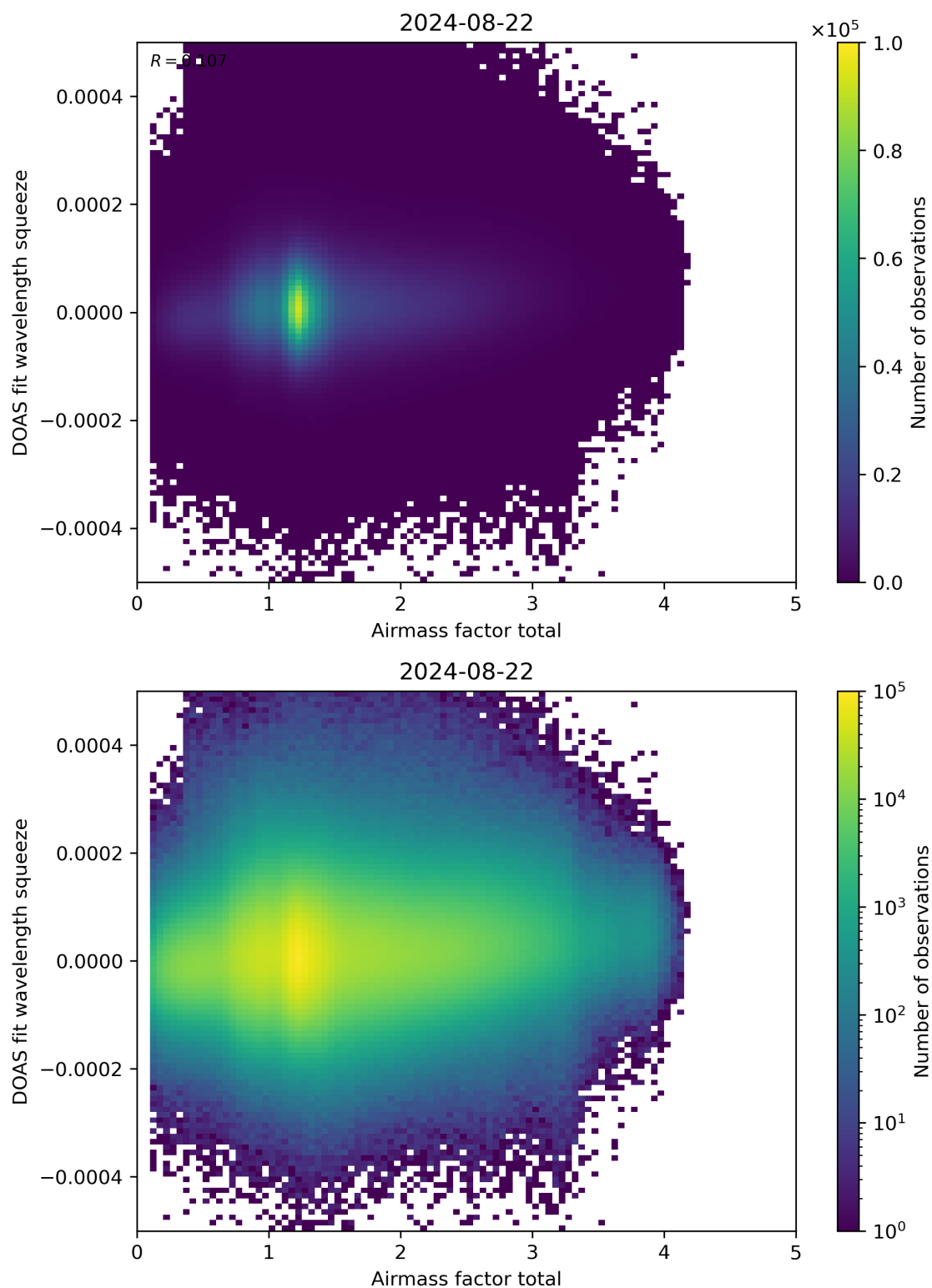
Figure 99: Scatter density plot of “Airmass factor total” against “DOAS fit wavelength squeeze” for 2024-08-22 to 2024-08-23.
