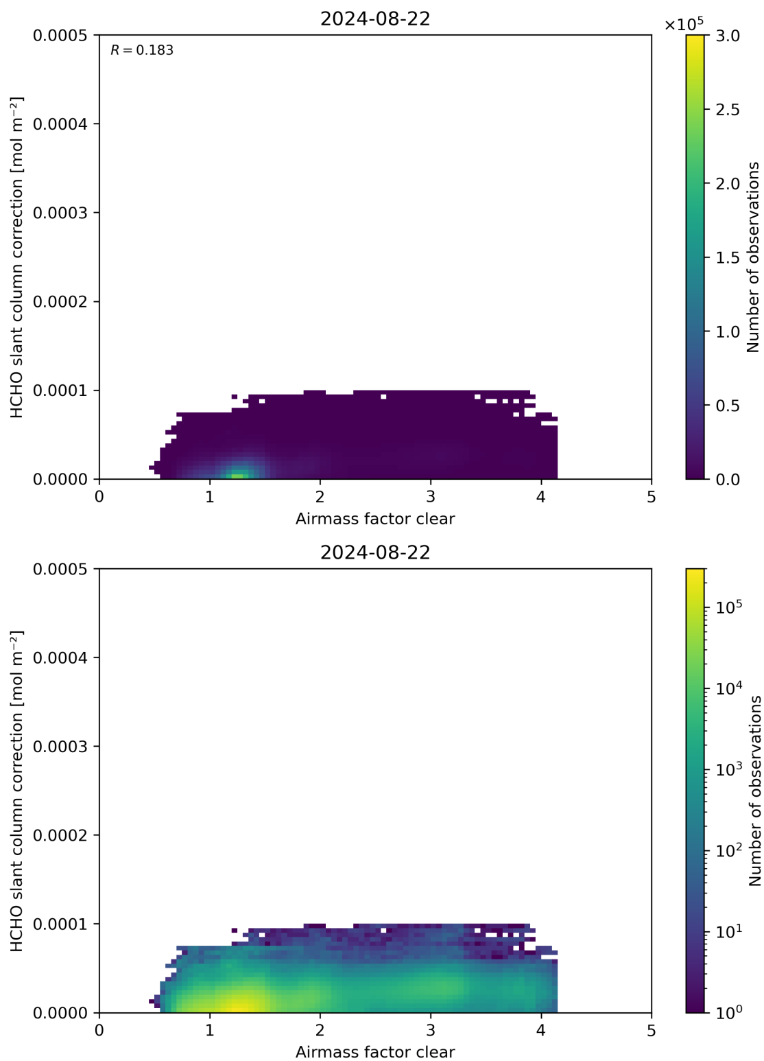
Figure 75: Scatter density plot of “Airmass factor clear” against “HCHO slant column correction” for 2024-08-22 to 2024-08-23.
