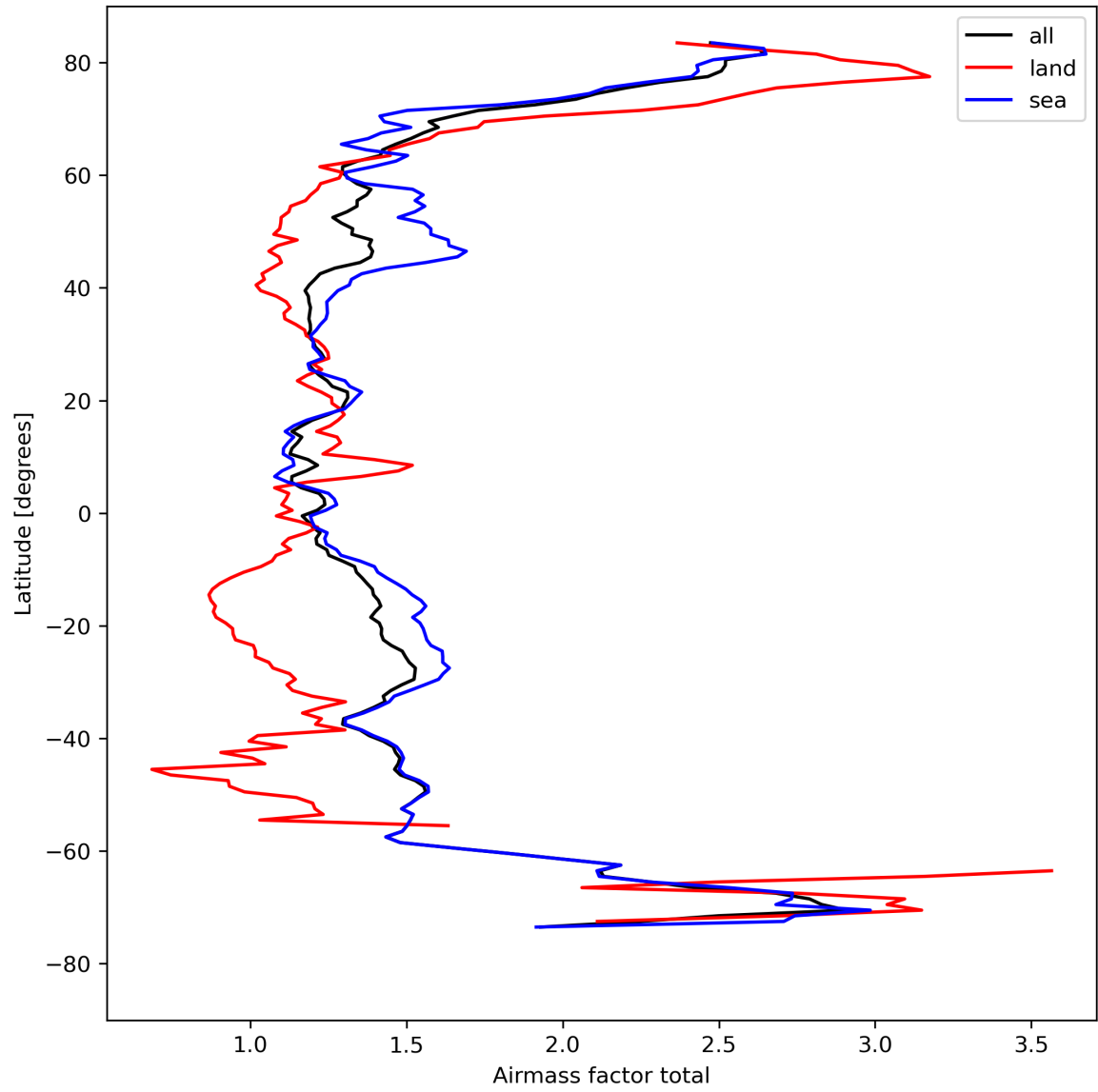
Figure 26: Zonal average of “Airmass factor total” for 2024-08-22 to 2024-08-23.
