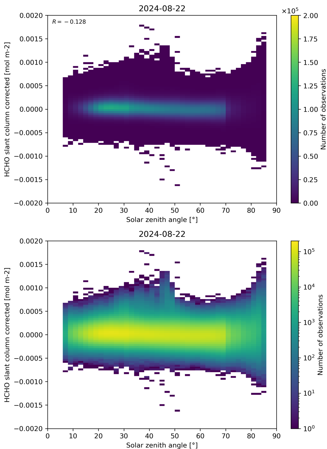
Figure 171: Scatter density plot of “Solar zenith angle” against “HCHO slant column corrected” for 2024-08-22 to 2024-08-23.
