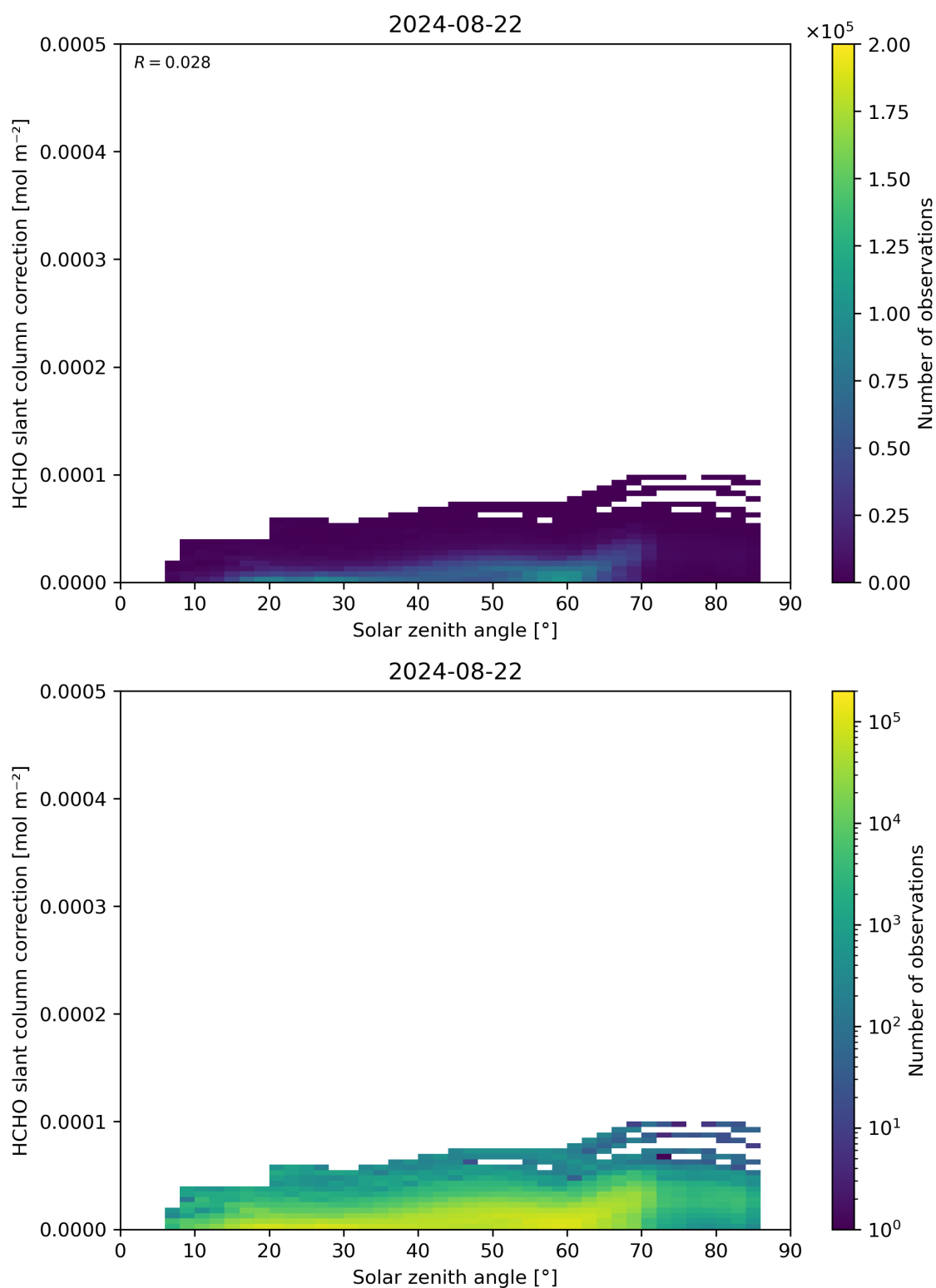
Figure 172: Scatter density plot of “Solar zenith angle” against “HCHO slant column correction” for 2024-08-22 to 2024-08-23.
