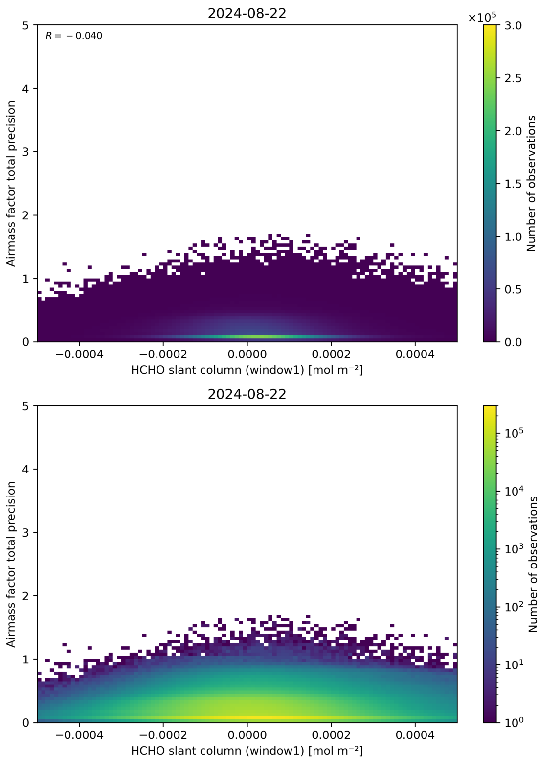
Figure 86: Scatter density plot of “HCHO slant column (window1)” against “Airmass factor total precision” for 2024-08-22 to 2024-08-23.
