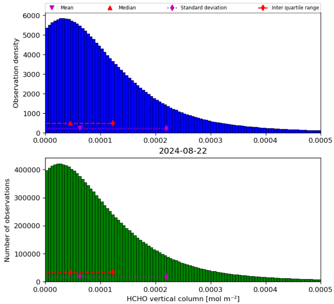
Figure 35: Histogram of “HCHO vertical column” for 2024-08-22 to 2024-08-23
