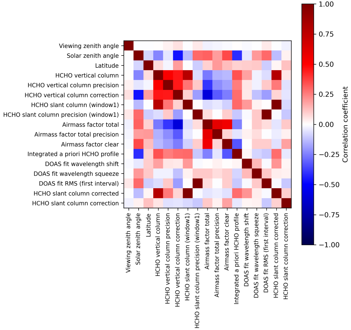
Figure 2: Map of correlation matrix for 2024-08-22 to 2024-08-23.
