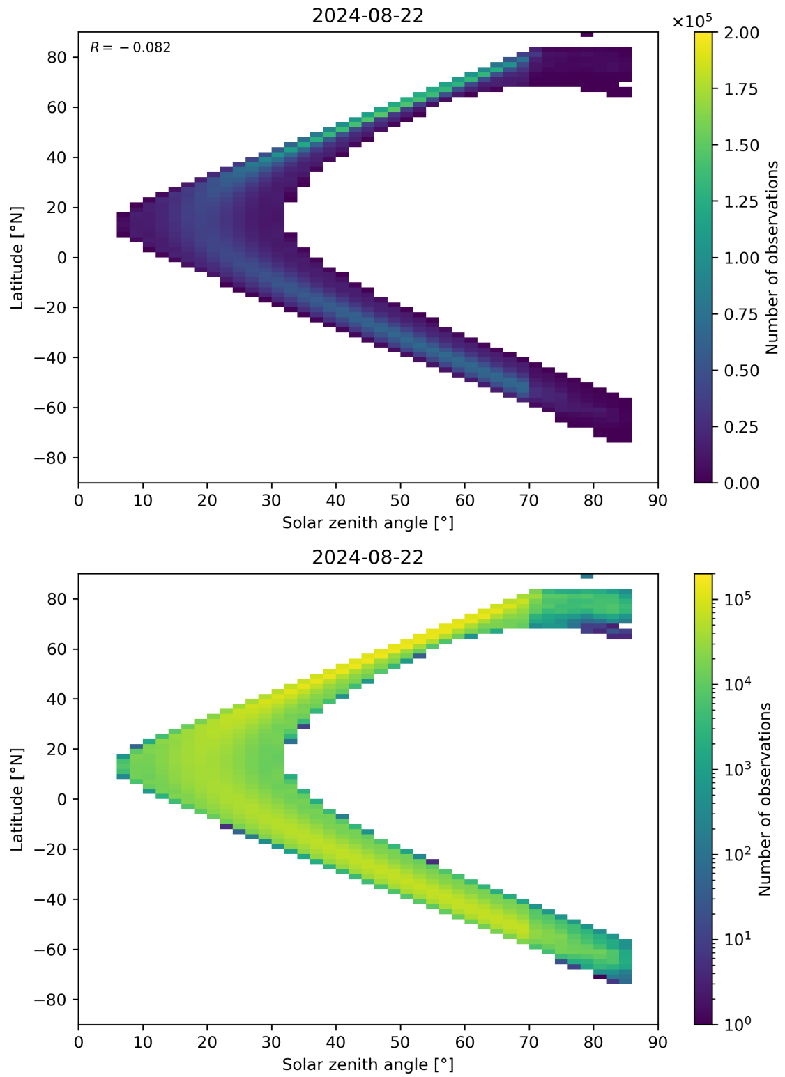
Figure 181: Scatter density plot of “Solar zenith angle” against “Latitude” for 2024-08-22 to 2024-08-23.
