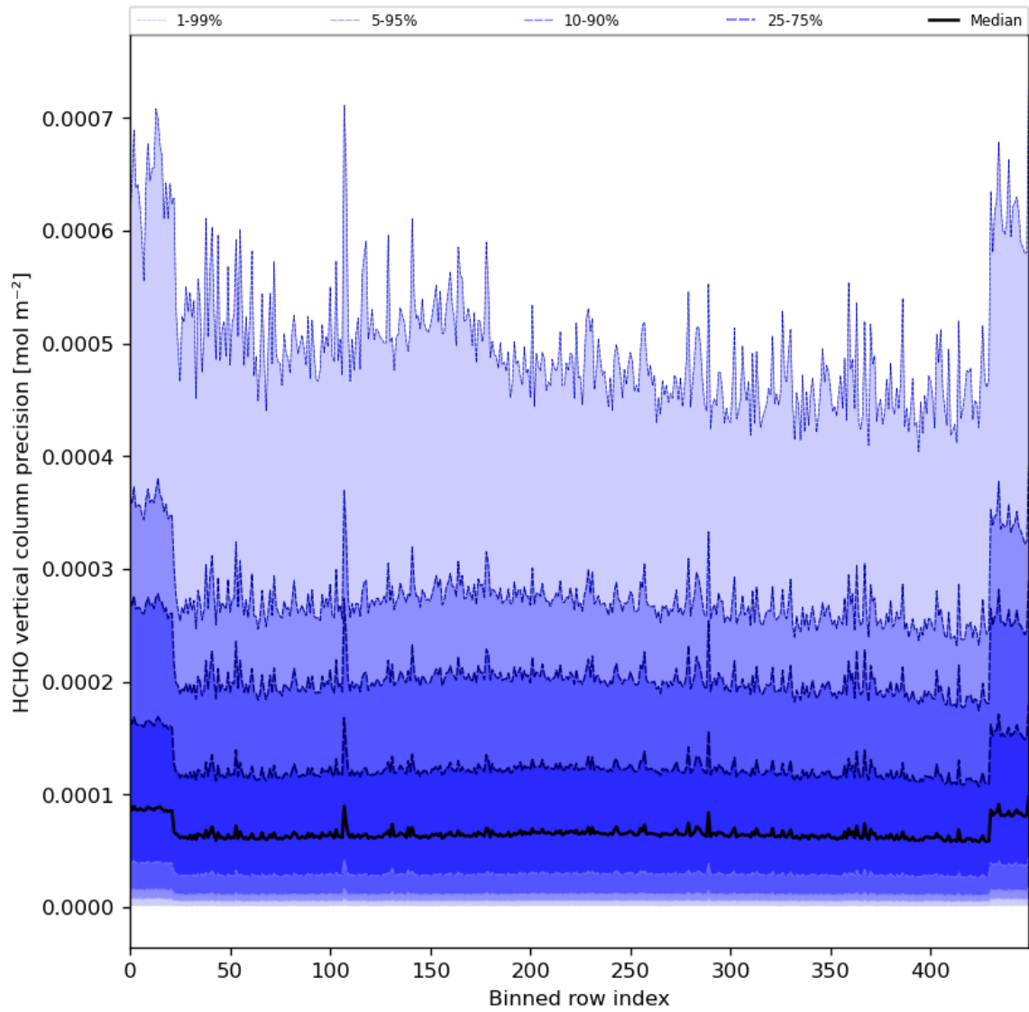
Figure 50: Along track statistics of “HCHO vertical column precision” for 2024-08-22 to 2024-08-23
