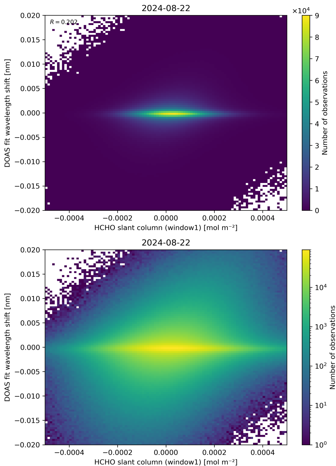
Figure 79: Scatter density plot of “HCHO slant column (window1)” against “DOAS fit wavelength shift” for 2024-08-22 to 2024-08-23.
