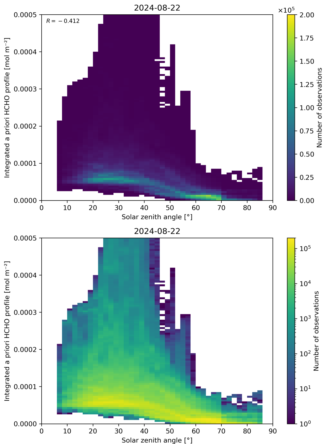
Figure 180: Scatter density plot of “Solar zenith angle” against “Integrated a priori HCHO profile” for 2024-08-22 to 2024-08-23.
