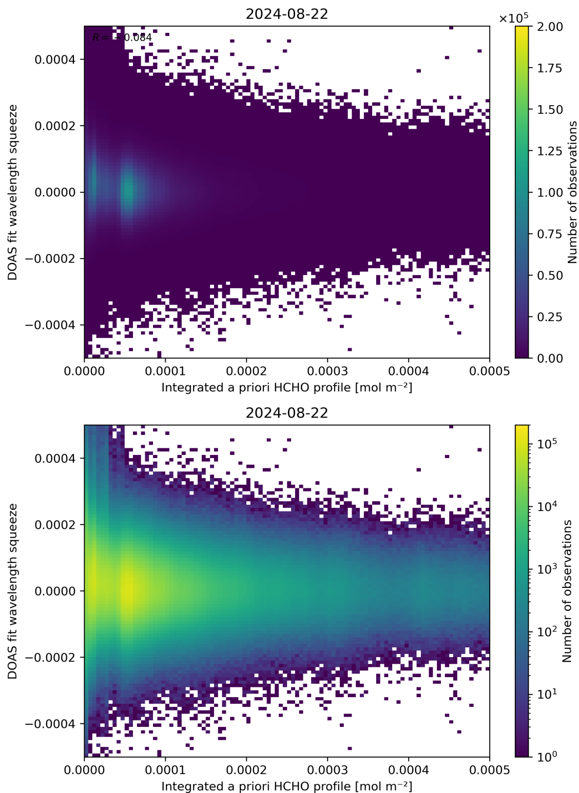
Figure 150: Scatter density plot of “Integrated a priori HCHO profile” against “DOAS fit wavelength squeeze” for 2024-08-22 to 2024-08-23.
