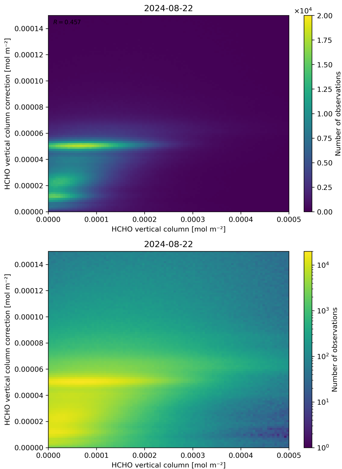
Figure 133: Scatter density plot of “HCHO vertical column” against “HCHO vertical column correction” for 2024-08-22 to 2024-08-23.
