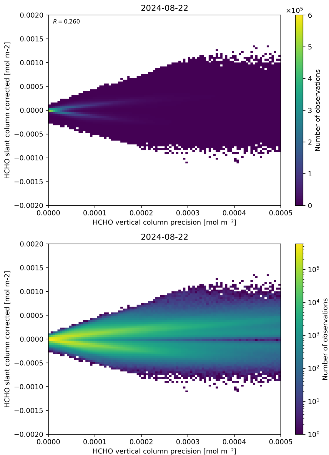
Figure 140: Scatter density plot of “HCHO vertical column precision” against “HCHO slant column corrected” for 2024-08-22 to 2024-08-23.
