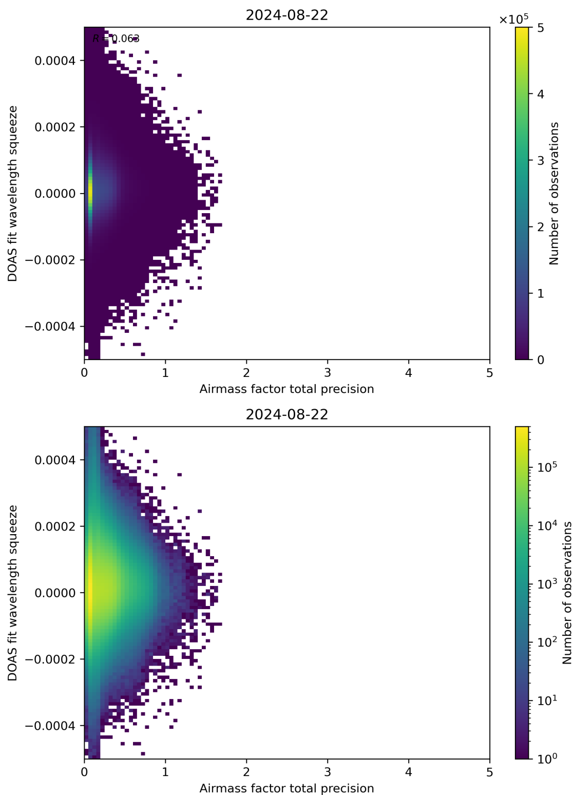
Figure 107: Scatter density plot of “Airmass factor total precision” against “DOAS fit wavelength squeeze” for 2024-08-22 to 2024-08-23.
