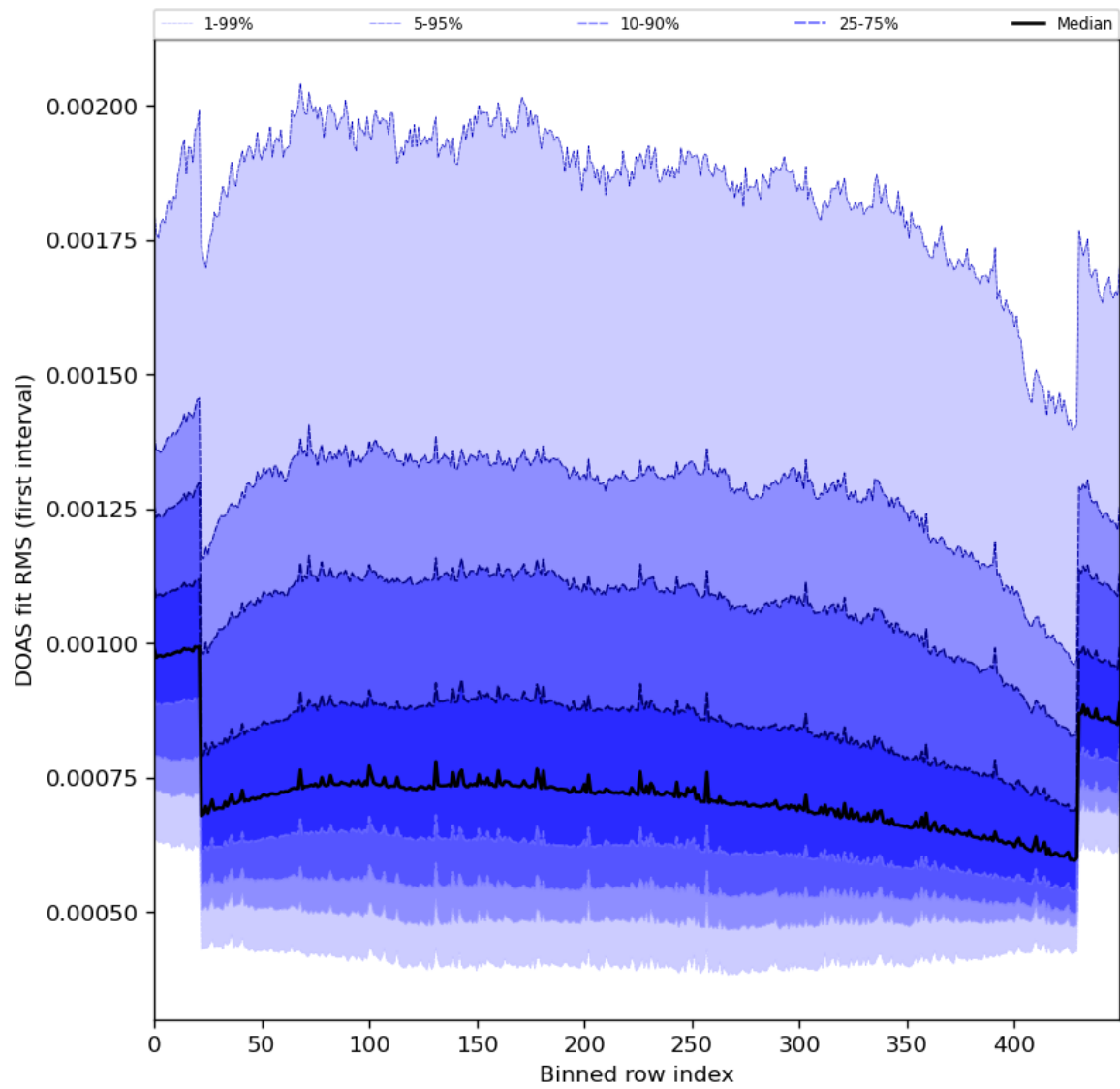
Figure 60: Along track statistics of “DOAS fit RMS (first interval)” for 2024-08-22 to 2024-08-23
