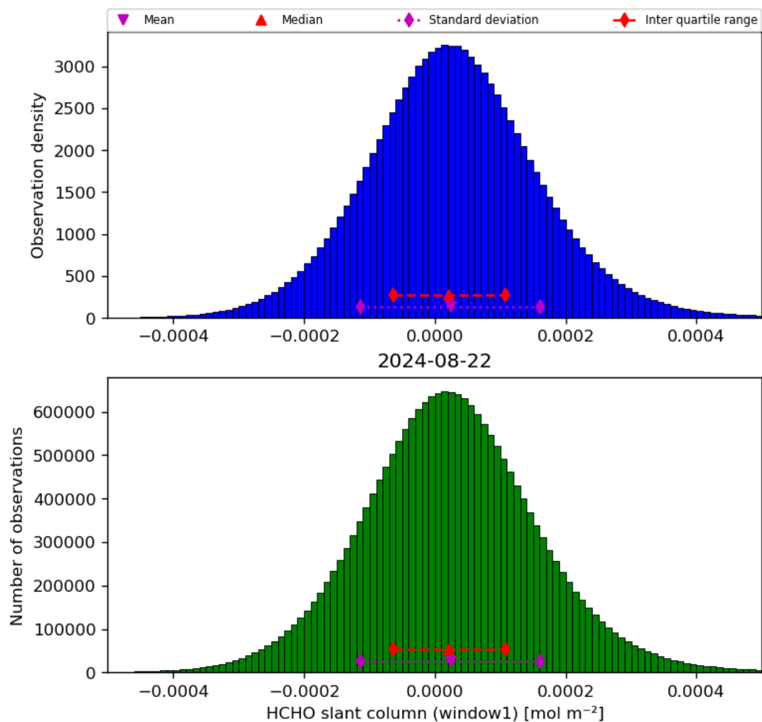
Figure 38: Histogram of “HCHO slant column (window1)” for 2024-08-22 to 2024-08-23
