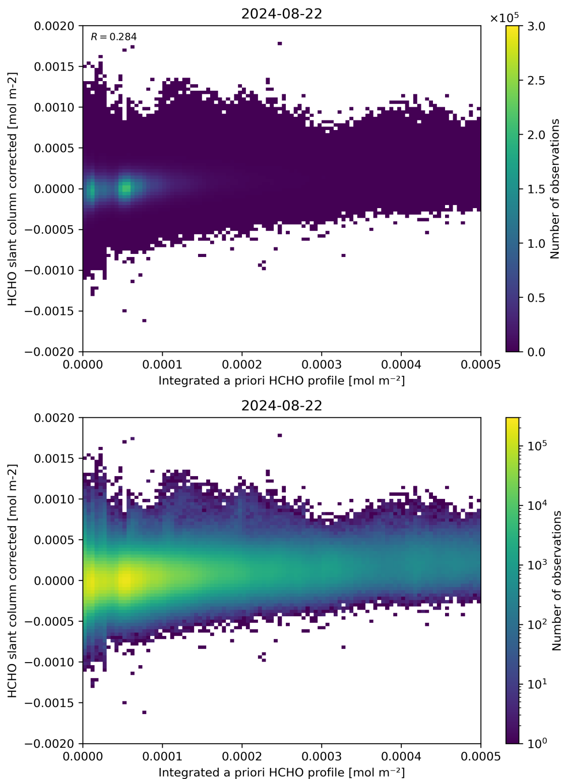
Figure 151: Scatter density plot of “Integrated a priori HCHO profile” against “HCHO slant column corrected” for 2024-08-22 to 2024-08-23.
