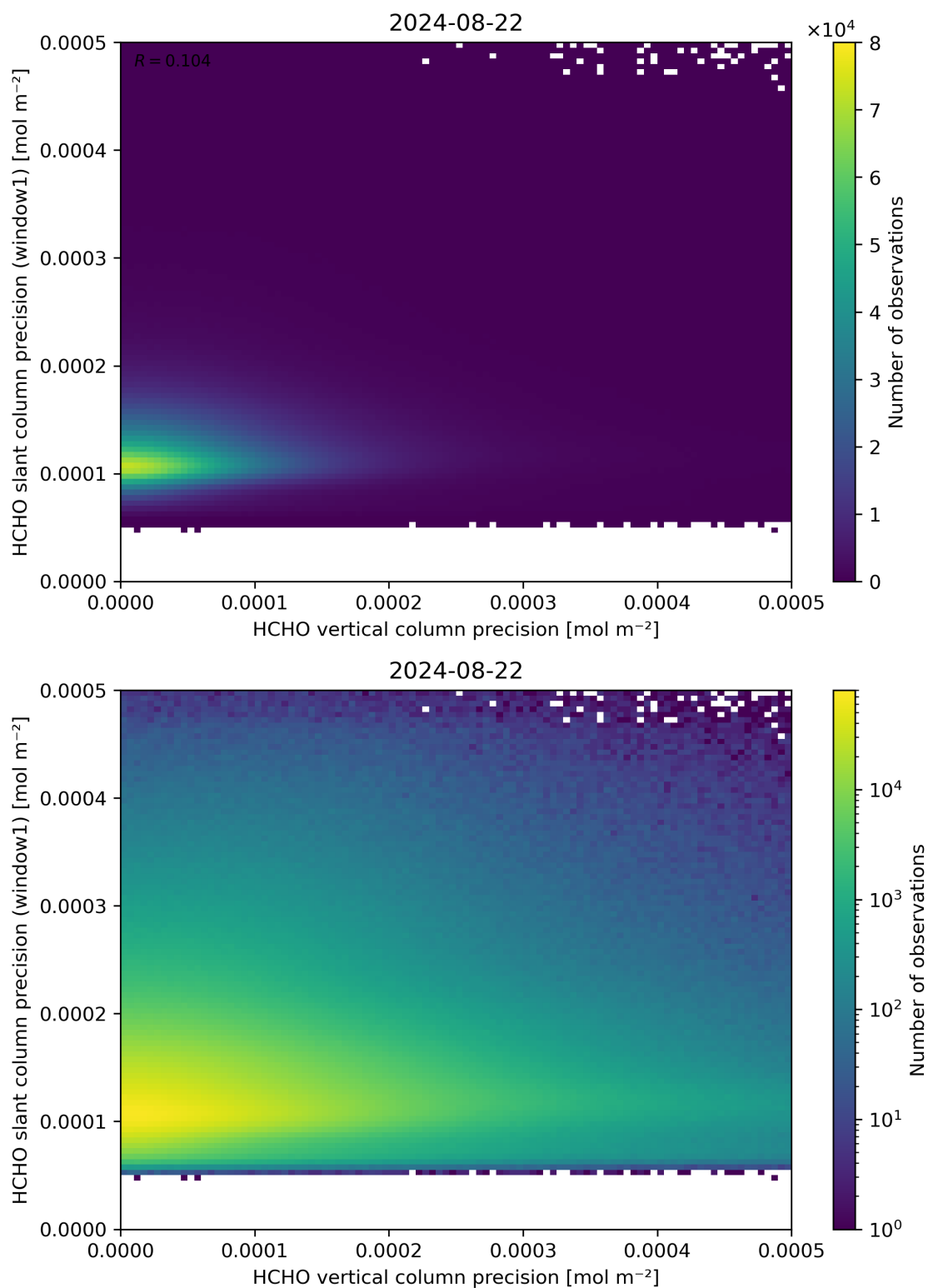
Figure 143: Scatter density plot of “HCHO vertical column precision” against “HCHO slant column precision (window1)” for 2024-08-22 to 2024-08-23.
