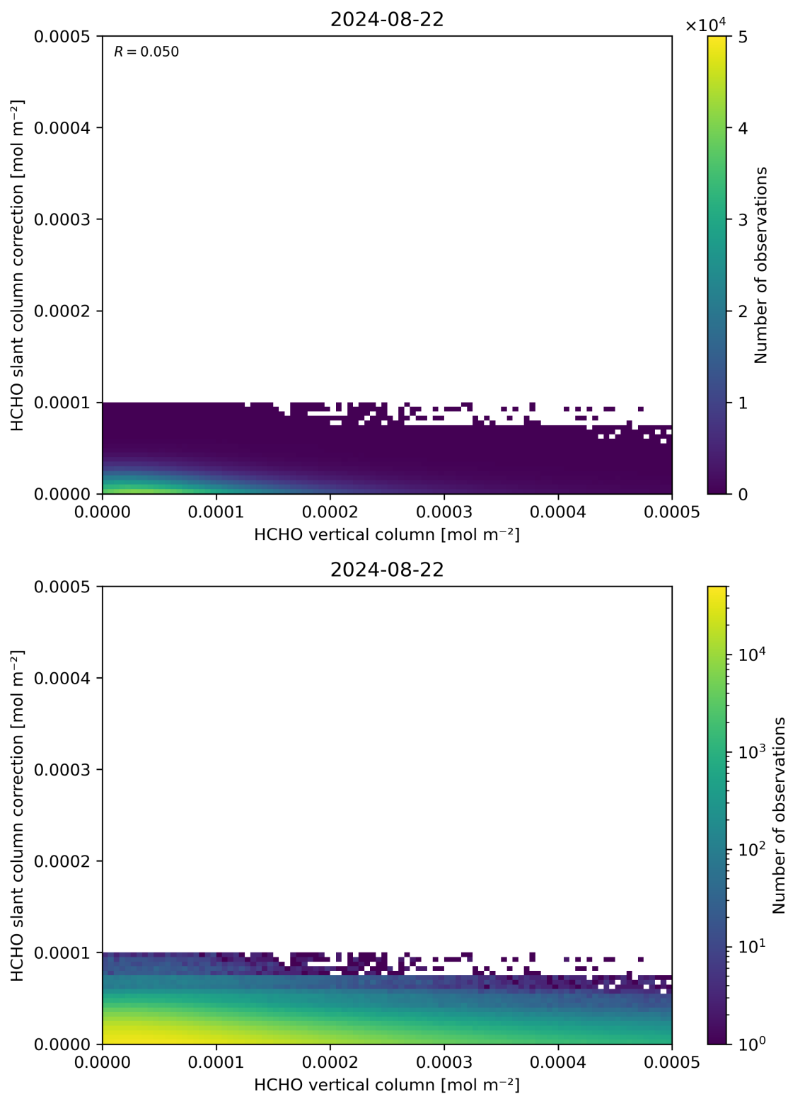
Figure 128: Scatter density plot of “HCHO vertical column” against “HCHO slant column correction” for 2024-08-22 to 2024-08-23.
