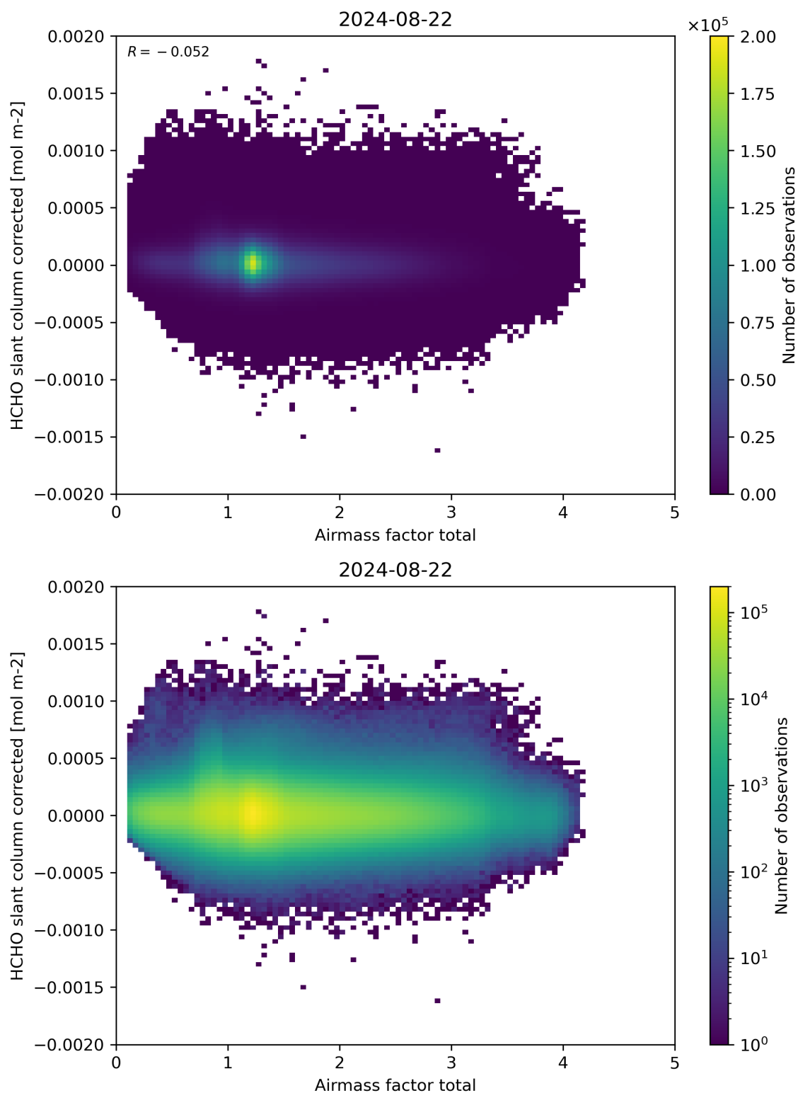
Figure 101: Scatter density plot of “Airmass factor total” against “HCHO slant column corrected” for 2024-08-22 to 2024-08-23.
