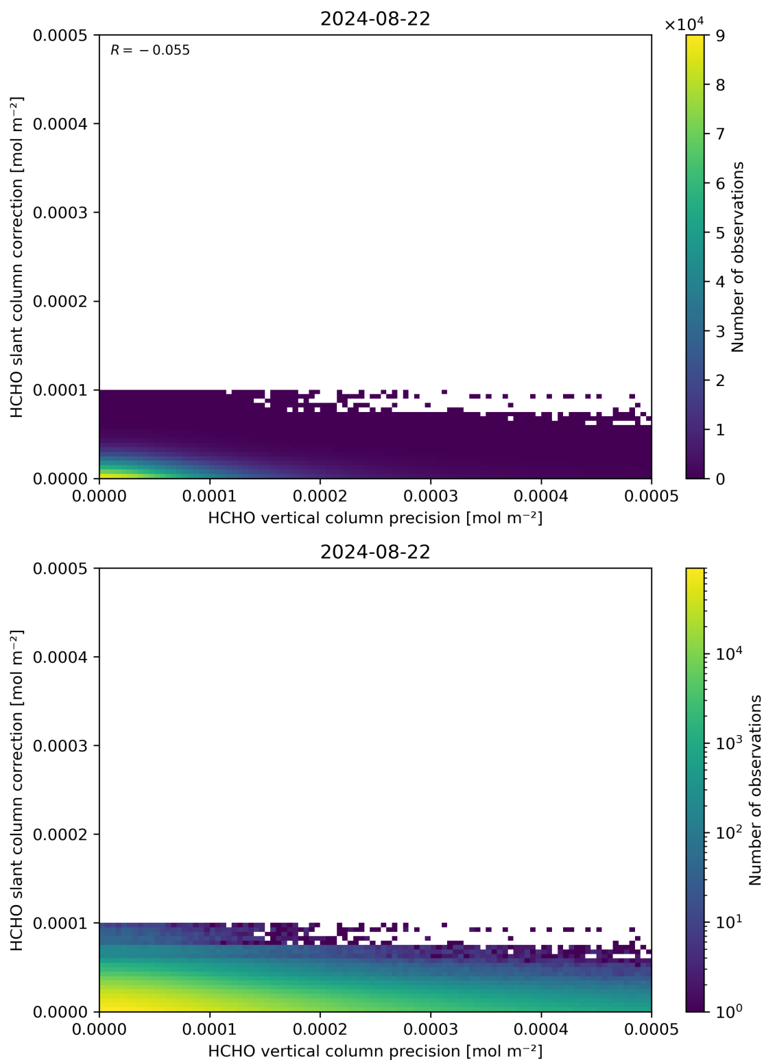
Figure 141: Scatter density plot of “HCHO vertical column precision” against “HCHO slant column correction” for 2024-08-22 to 2024-08-23.
