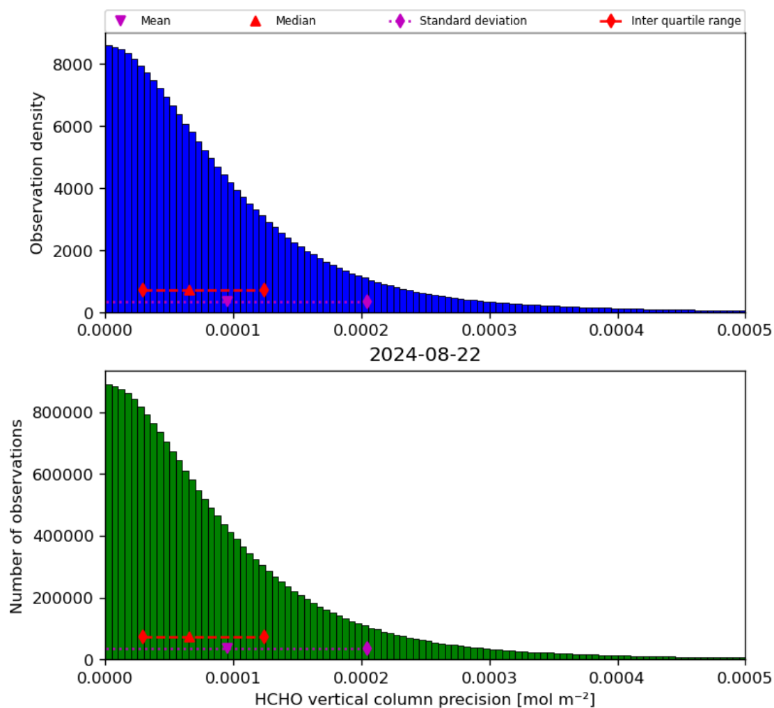
Figure 36: Histogram of “HCHO vertical column precision” for 2024-08-22 to 2024-08-23
