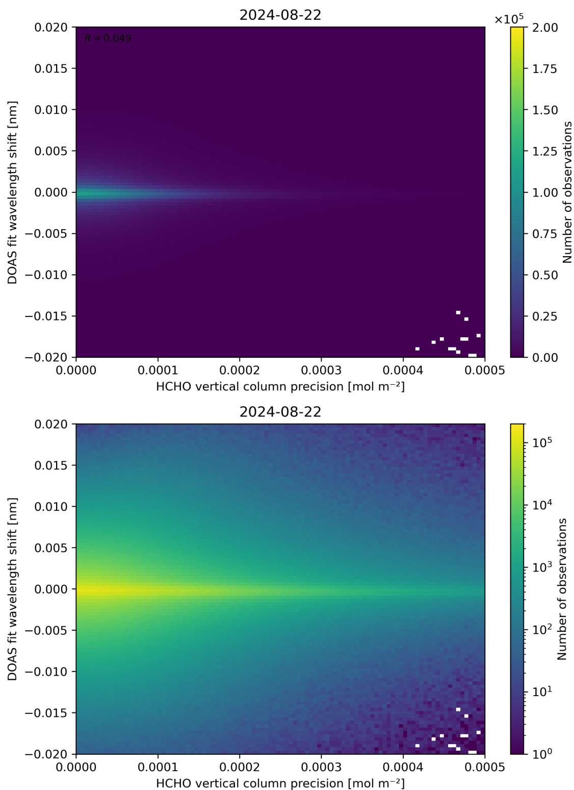
Figure 137: Scatter density plot of “HCHO vertical column precision” against “DOAS fit wavelength shift” for 2024-08-22 to 2024-08-23.
