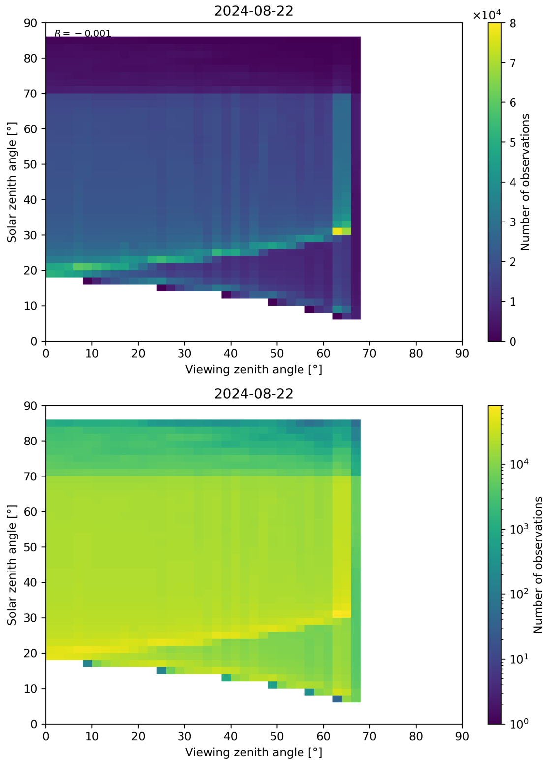
Figure 197: Scatter density plot of “Viewing zenith angle” against “Solar zenith angle” for 2024-08-22 to 2024-08-23.
