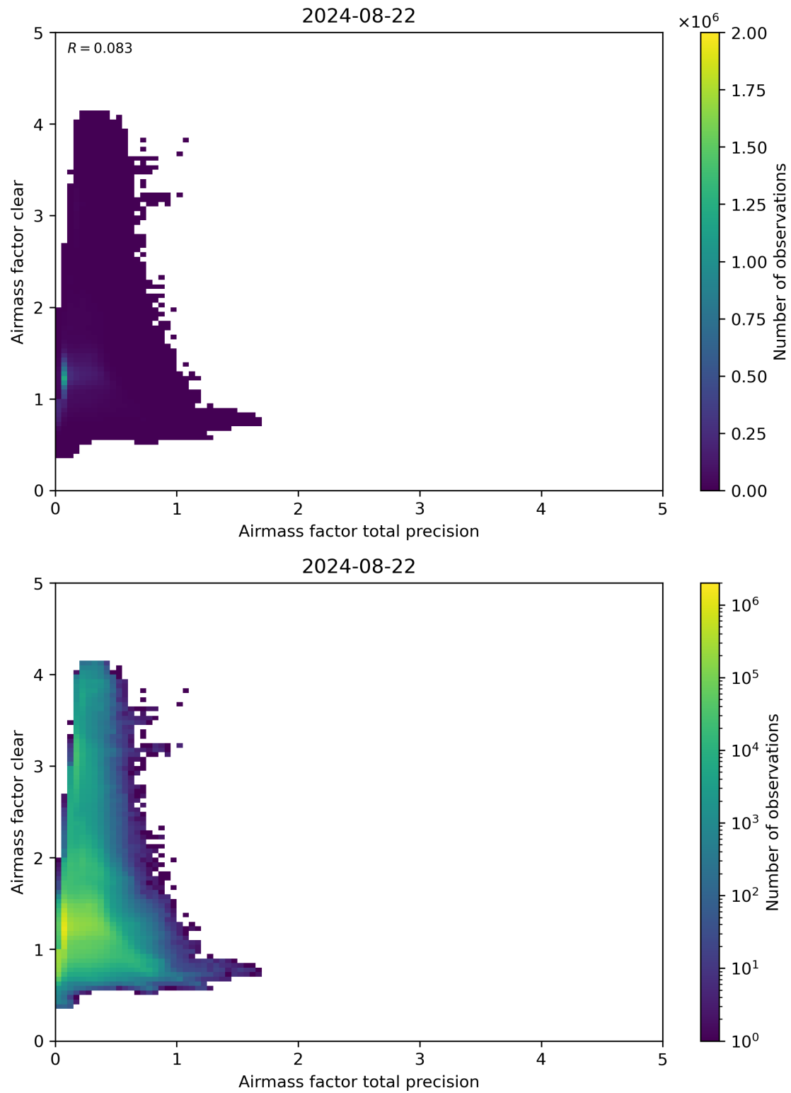
Figure 108: Scatter density plot of “Airmass factor total precision” against “Airmass factor clear” for 2024-08-22 to 2024-08-23.
