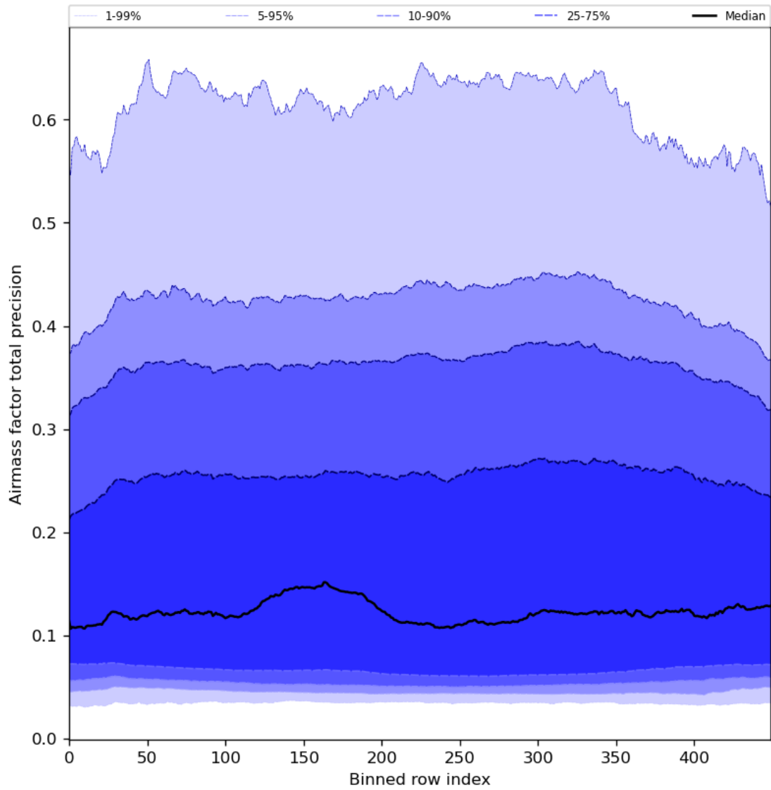
Figure 55: Along track statistics of “Airmass factor total precision” for 2024-08-22 to 2024-08-23
