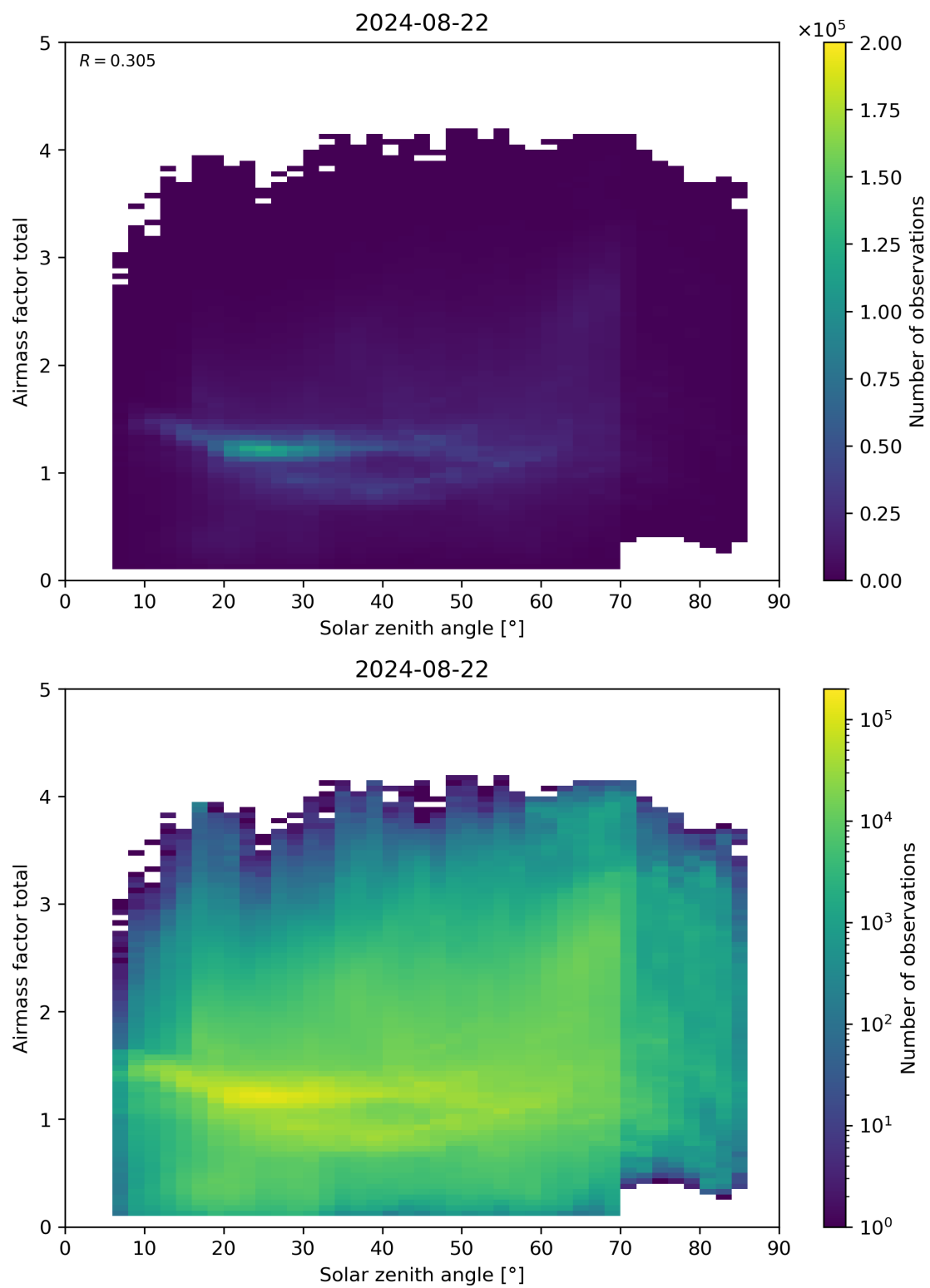
Figure 175: Scatter density plot of “Solar zenith angle” against “Airmass factor total” for 2024-08-22 to 2024-08-23.
