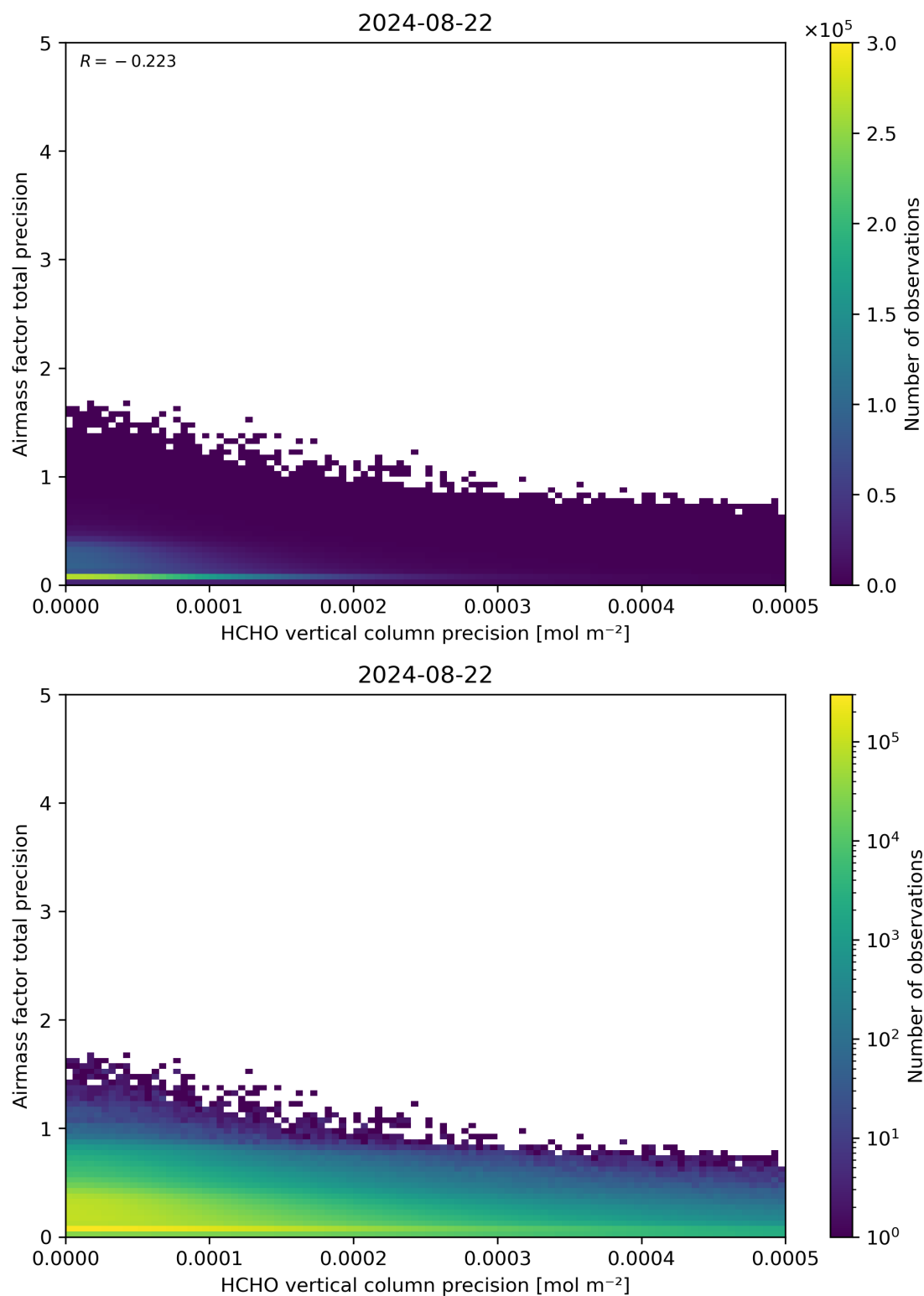
Figure 145: Scatter density plot of “HCHO vertical column precision” against “Airmass factor total precision” for 2024-08-22 to 2024-08-23.
