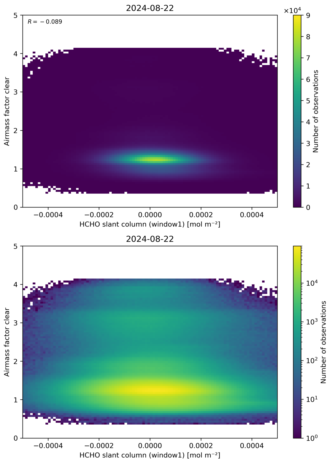
Figure 81: Scatter density plot of “HCHO slant column (window1)” against “Airmass factor clear” for 2024-08-22 to 2024-08-23.
