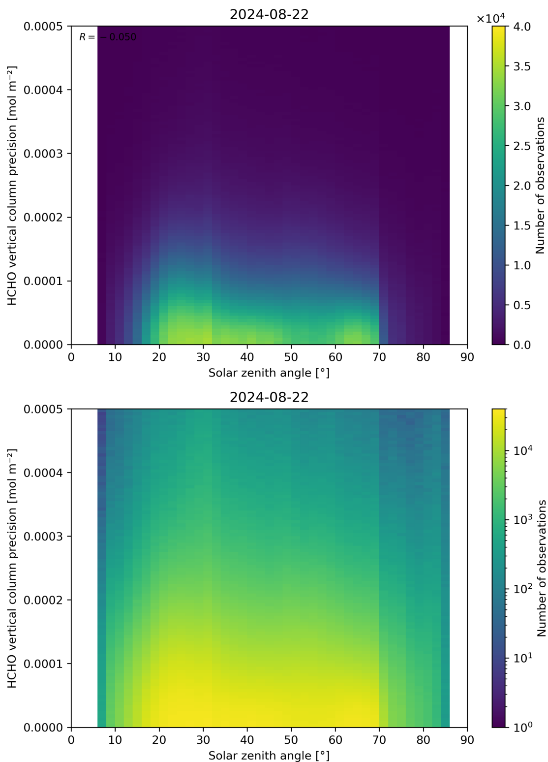
Figure 179: Scatter density plot of “Solar zenith angle” against “HCHO vertical column precision” for 2024-08-22 to 2024-08-23.
