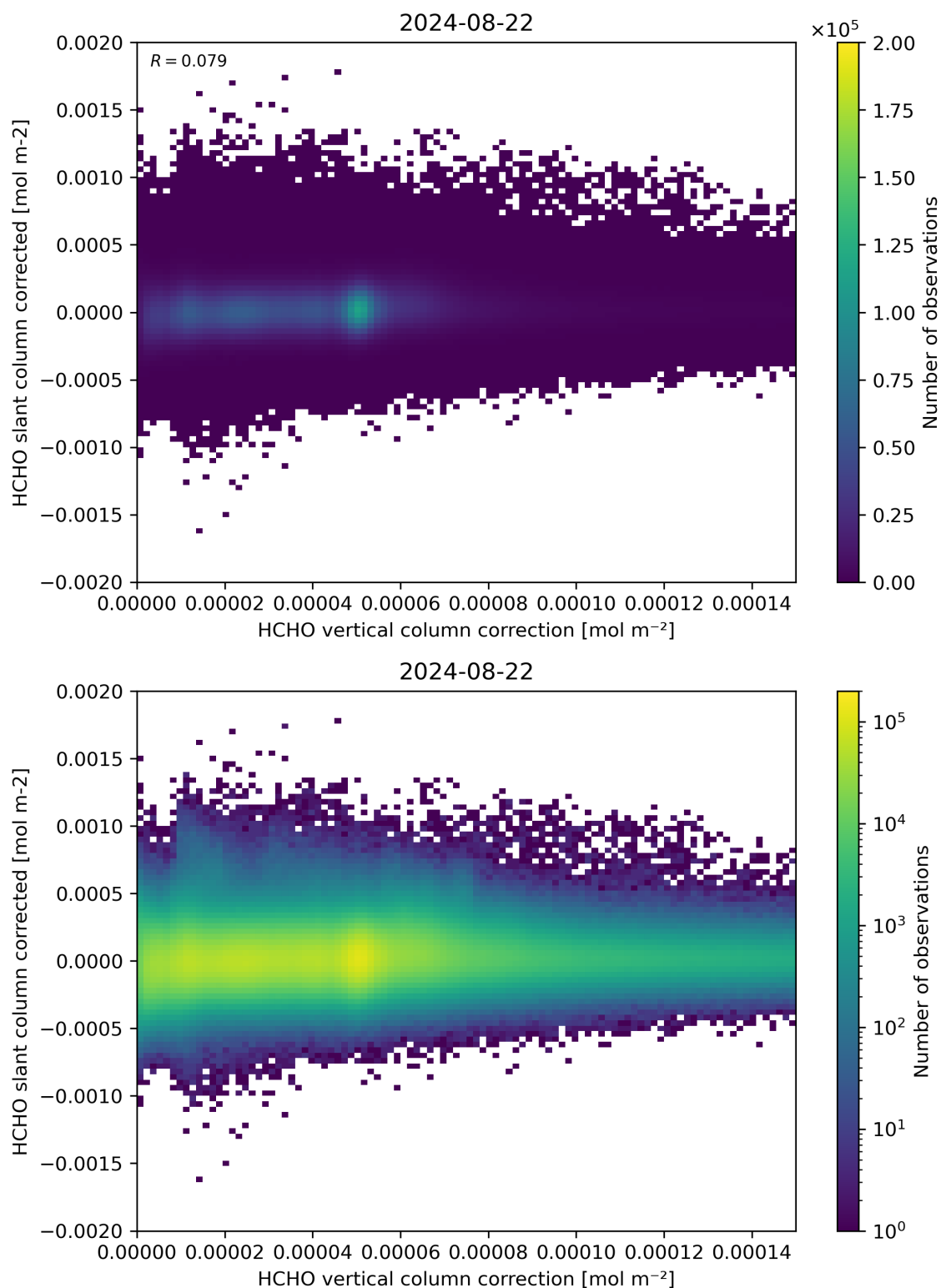
Figure 116: Scatter density plot of “HCHO vertical column correction” against “HCHO slant column corrected” for 2024-08-22 to 2024-08-23.
