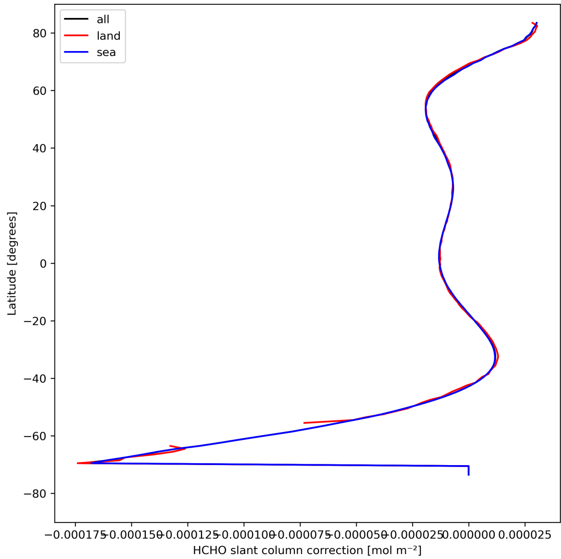
Figure 33: Zonal average of “HCHO slant column correction” for 2024-08-22 to 2024-08-23.
