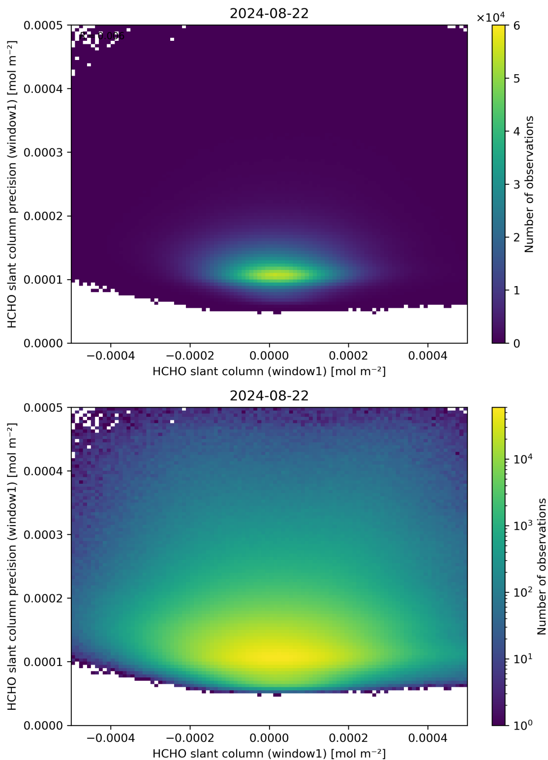
Figure 84: Scatter density plot of “HCHO slant column (window1)” against “HCHO slant column precision (window1)” for 2024-08-22 to 2024-08-23.
