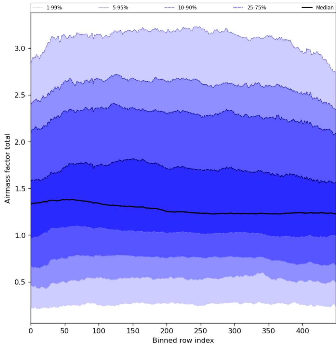
Figure 54: Along track statistics of “Airmass factor total” for 2024-08-22 to 2024-08-23
