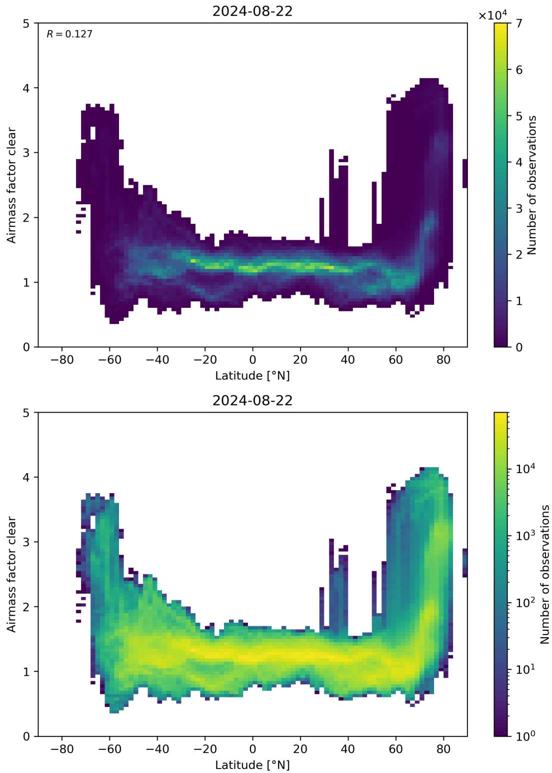
Figure 156: Scatter density plot of “Latitude” against “Airmass factor clear” for 2024-08-22 to 2024-08-23.
