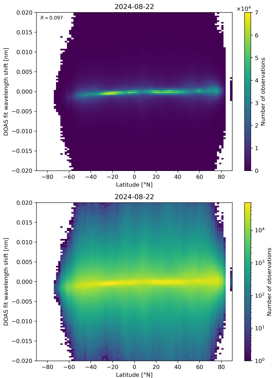
Figure 154: Scatter density plot of “Latitude” against “DOAS fit wavelength shift” for 2024-08-22 to 2024-08-23.
