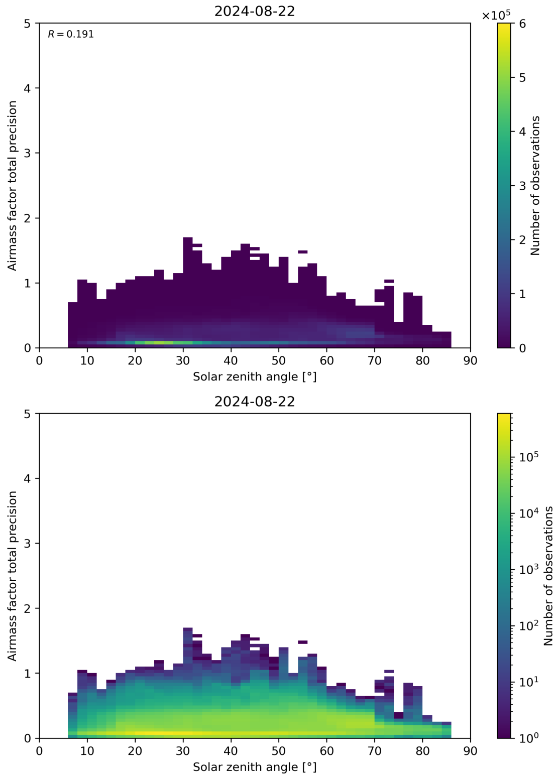
Figure 176: Scatter density plot of “Solar zenith angle” against “Airmass factor total precision” for 2024-08-22 to 2024-08-23.
