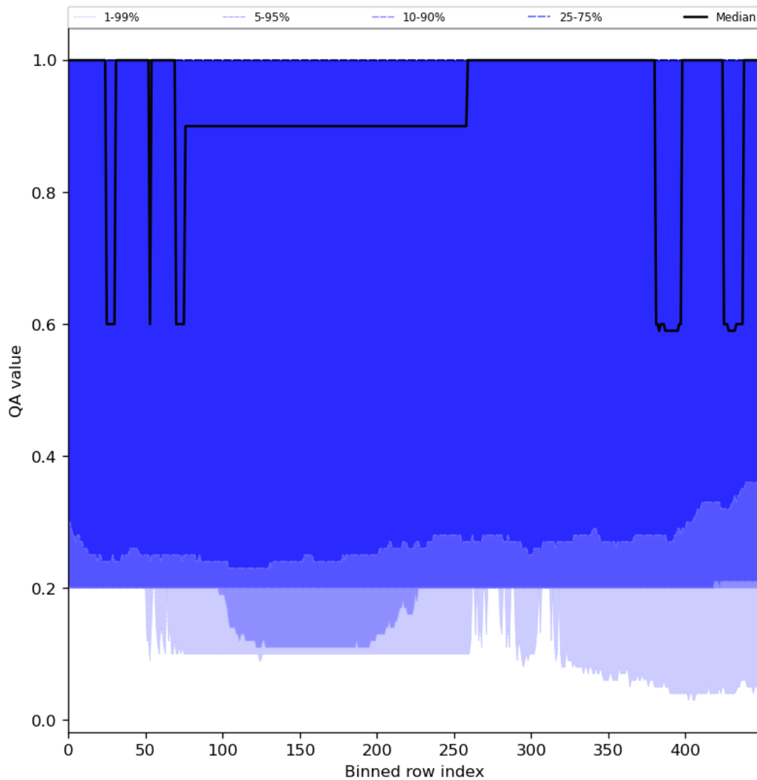
Figure 48: Along track statistics of “QA value” for 2024-08-22 to 2024-08-23
