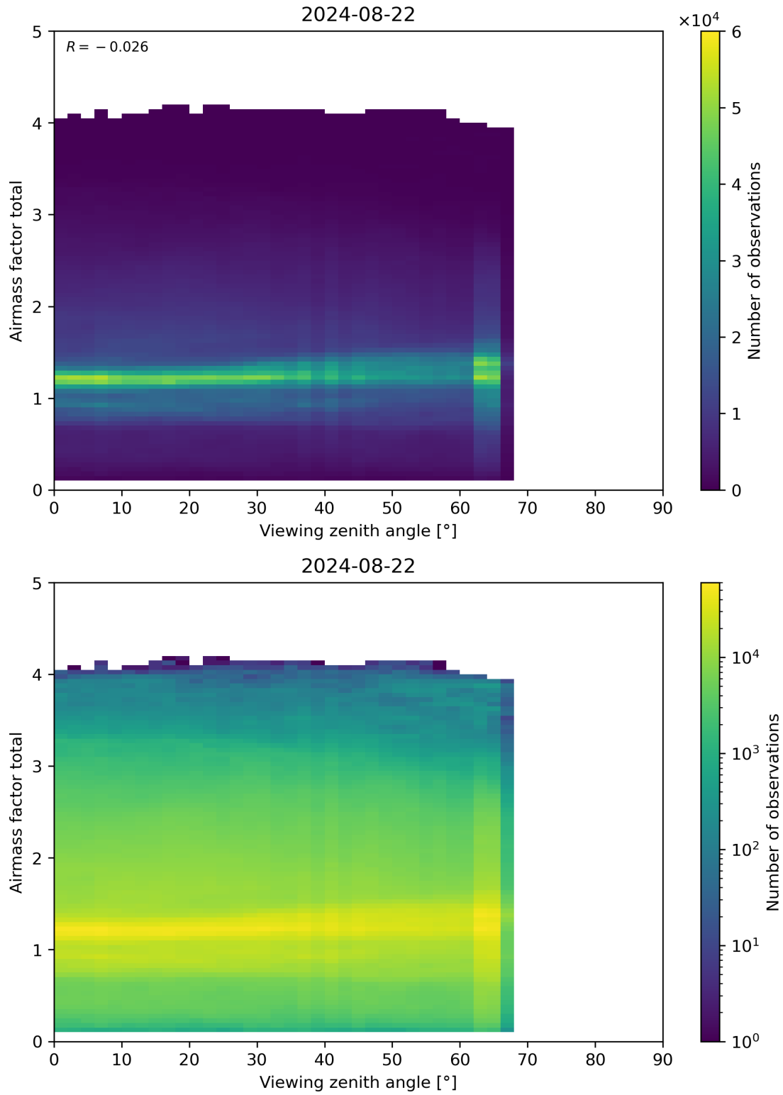
Figure 190: Scatter density plot of “Viewing zenith angle” against “Airmass factor total” for 2024-08-22 to 2024-08-23.
