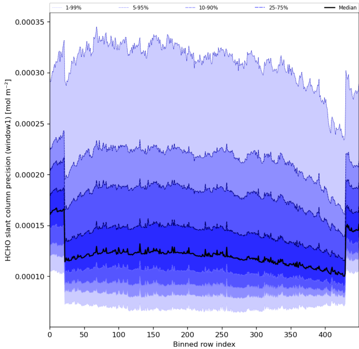
Figure 53: Along track statistics of “HCHO slant column precision (window1)” for 2024-08-22 to 2024-08-23
