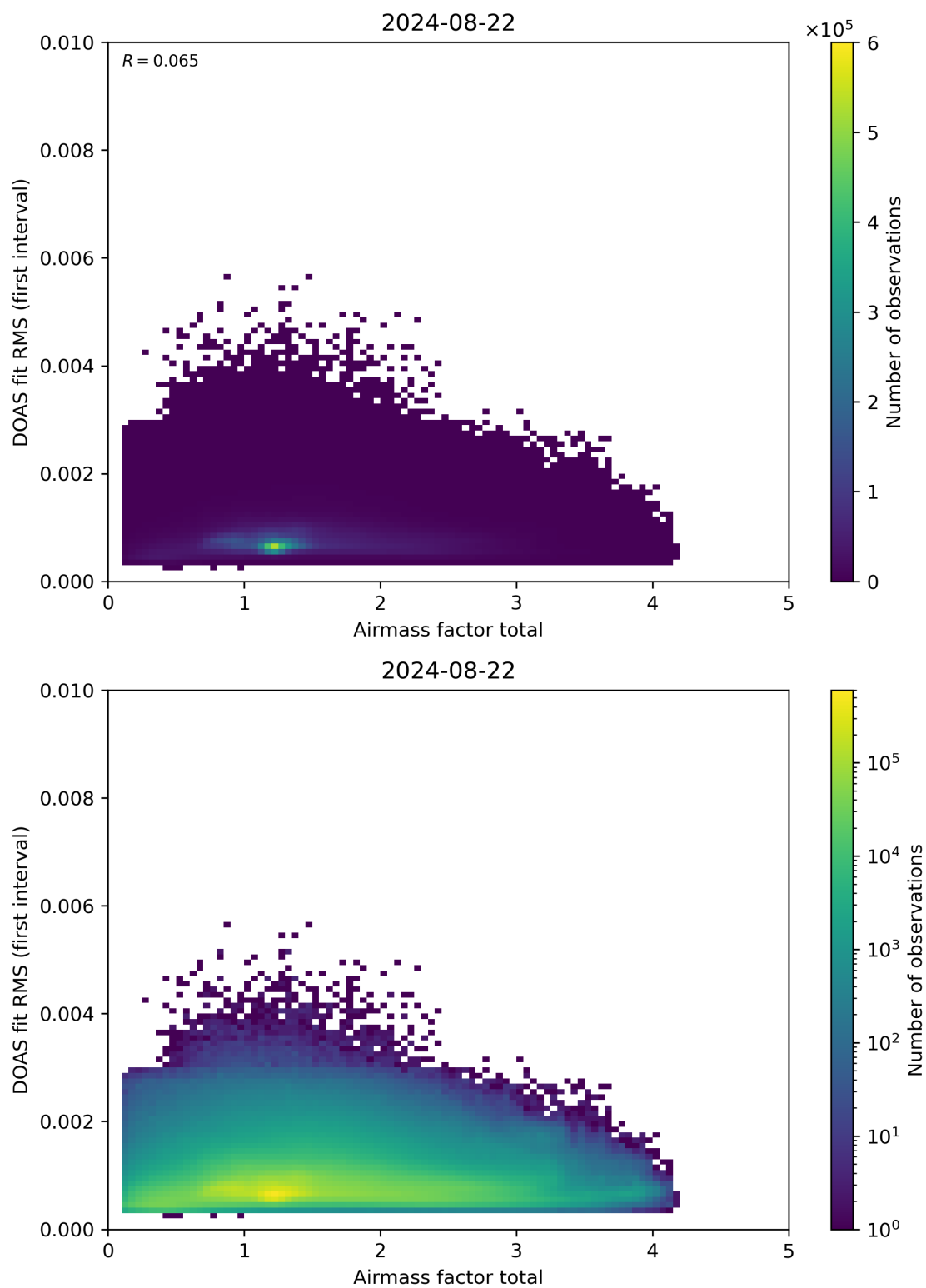
Figure 97: Scatter density plot of “Airmass factor total” against “DOAS fit RMS (first interval)” for 2024-08-22 to 2024-08-23.
