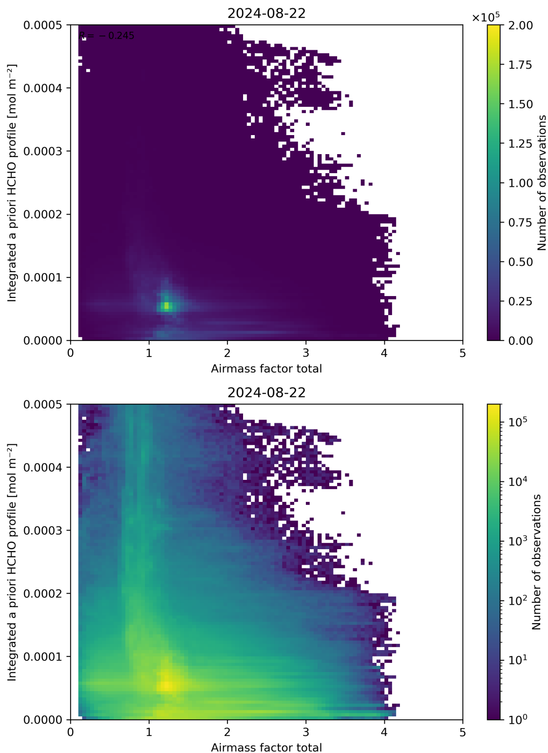
Figure 104: Scatter density plot of “Airmass factor total” against “Integrated a priori HCHO profile” for 2024-08-22 to 2024-08-23.
