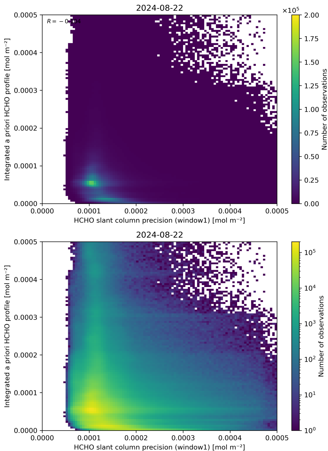
Figure 96: Scatter density plot of “HCHO slant column precision (window1)” against “Integrated a priori HCHO profile” for 2024-08-22 to 2024-08-23.
