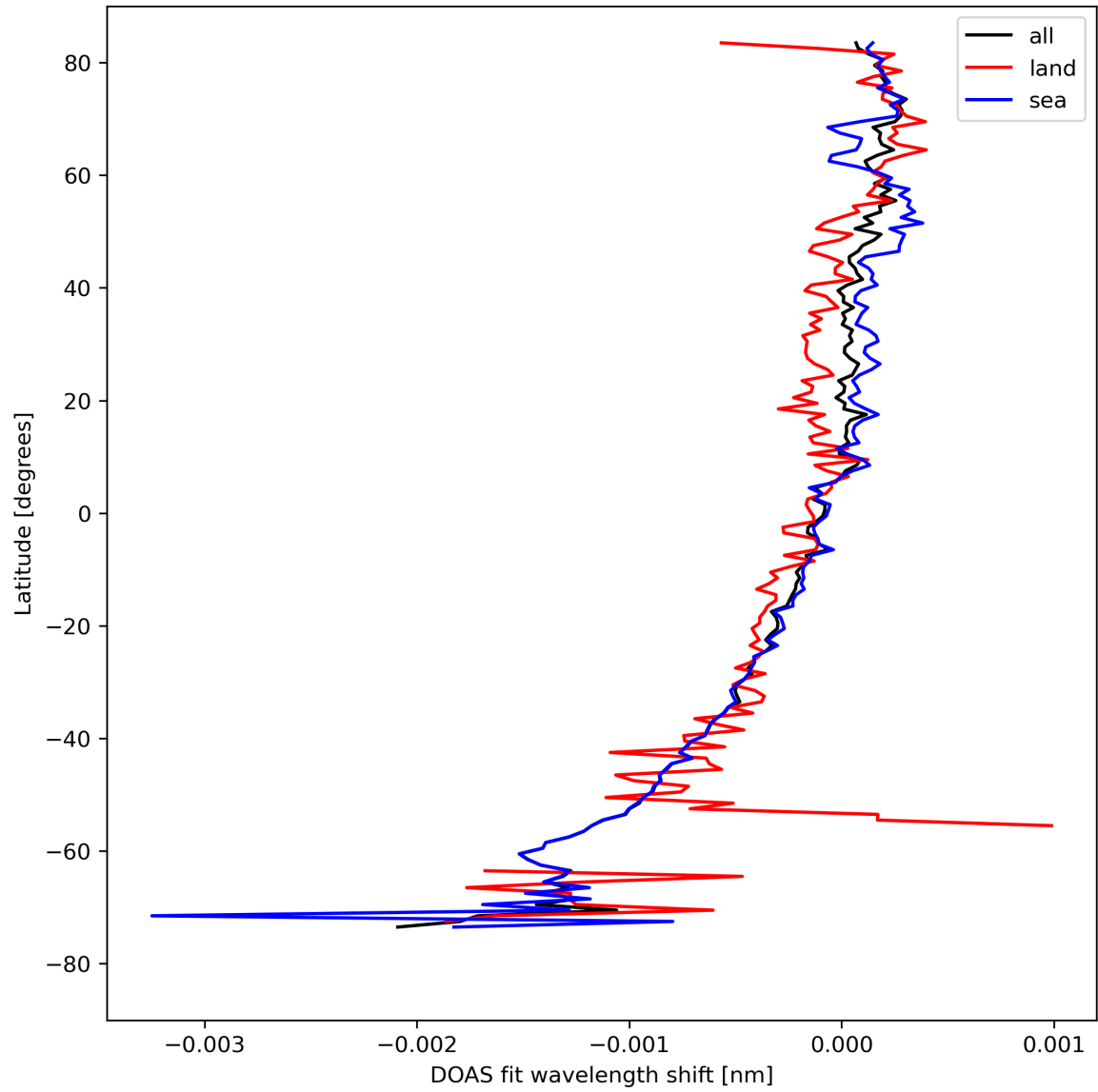
Figure 30: Zonal average of “DOAS fit wavelength shift” for 2024-08-22 to 2024-08-23.
