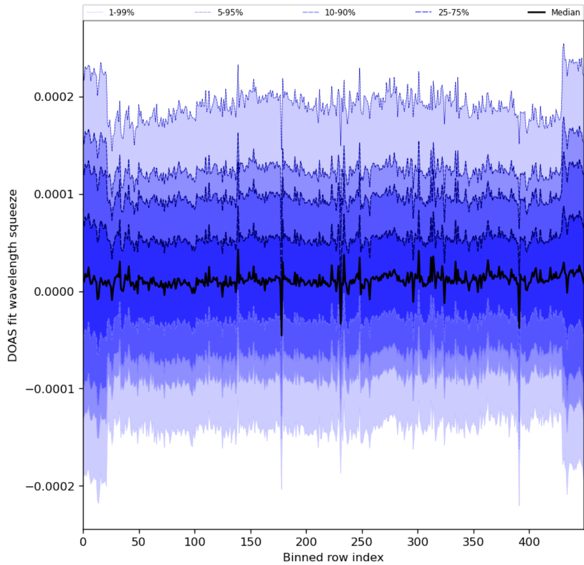
Figure 59: Along track statistics of “DOAS fit wavelength squeeze” for 2024-08-22 to 2024-08-23
