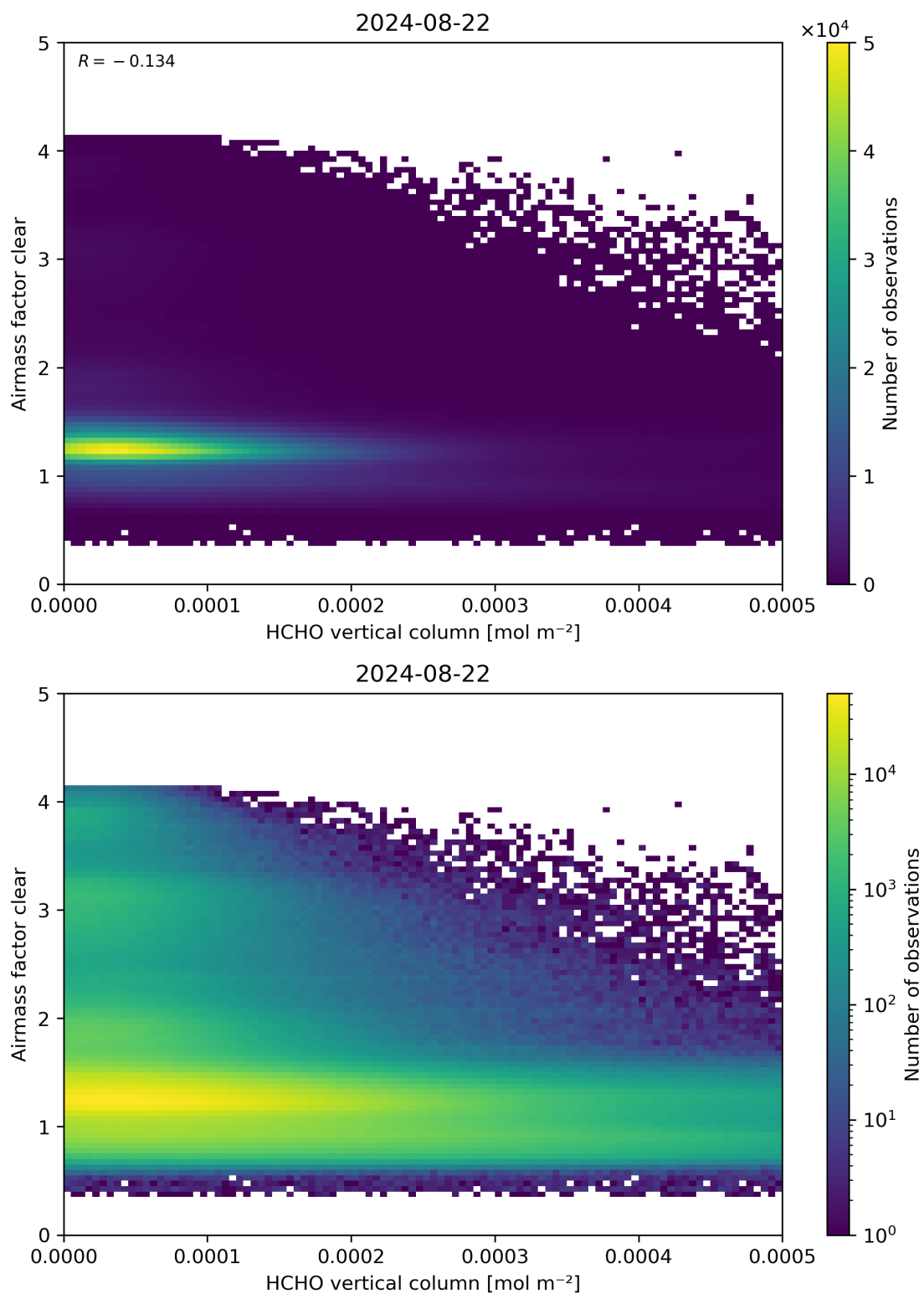
Figure 126: Scatter density plot of “HCHO vertical column” against “Airmass factor clear” for 2024-08-22 to 2024-08-23.
