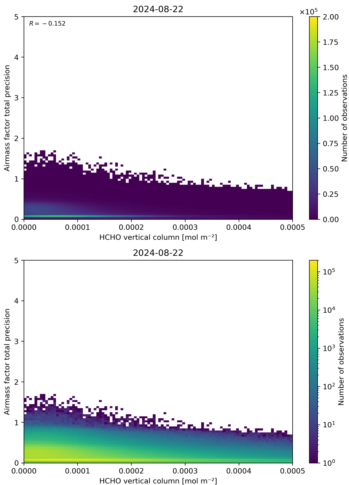
Figure 132: Scatter density plot of “HCHO vertical column” against “Airmass factor total precision” for 2024-08-22 to 2024-08-23.
