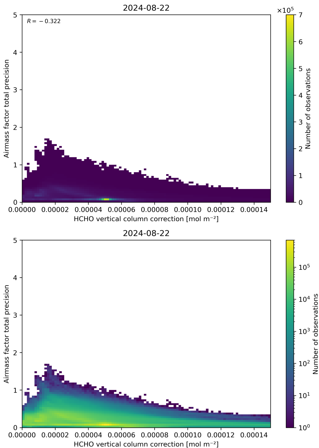
Figure 121: Scatter density plot of “HCHO vertical column correction” against “Airmass factor total precision” for 2024-08-22 to 2024-08-23.
