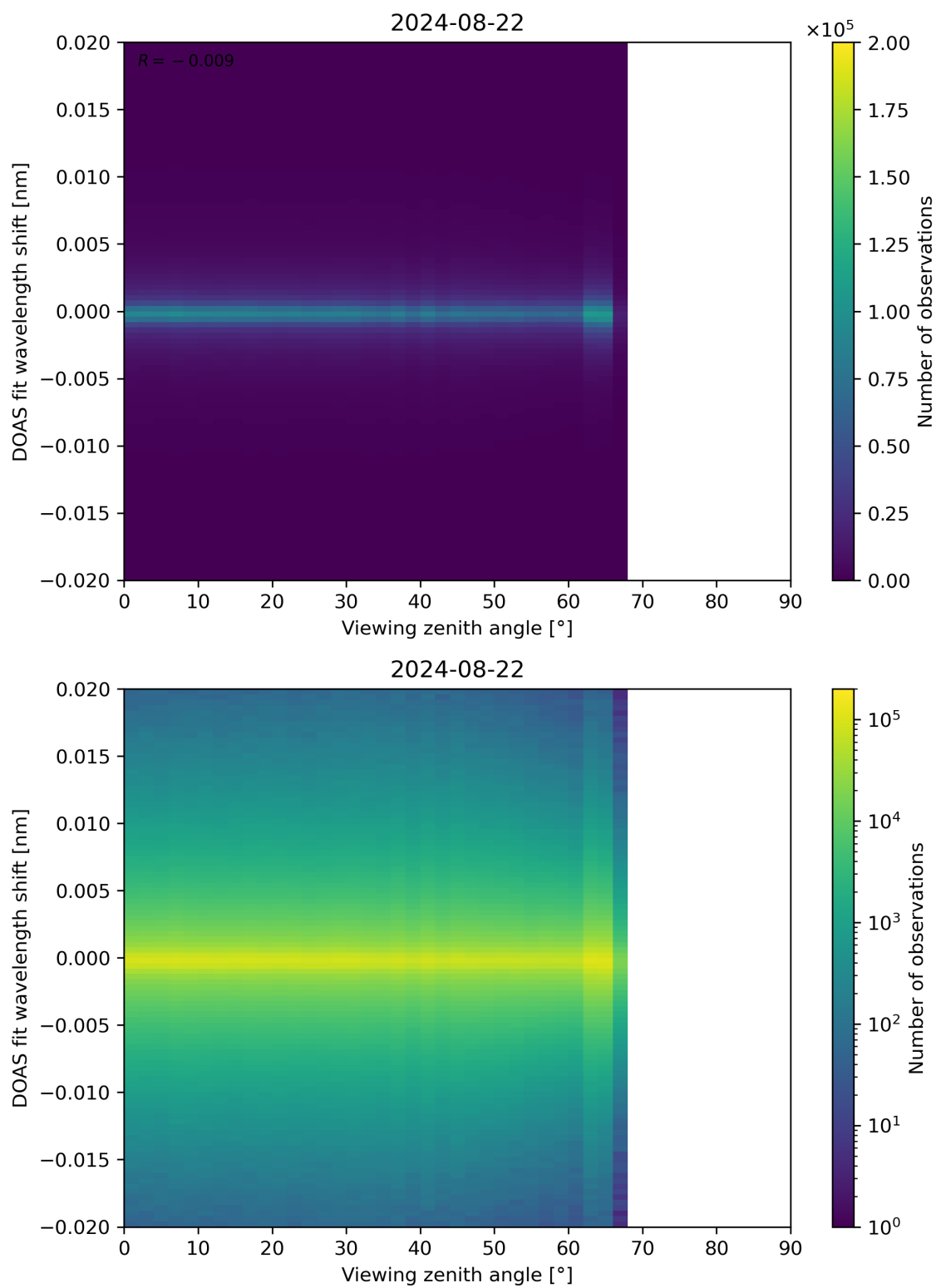
Figure 183: Scatter density plot of “Viewing zenith angle” against “DOAS fit wavelength shift” for 2024-08-22 to 2024-08-23.
