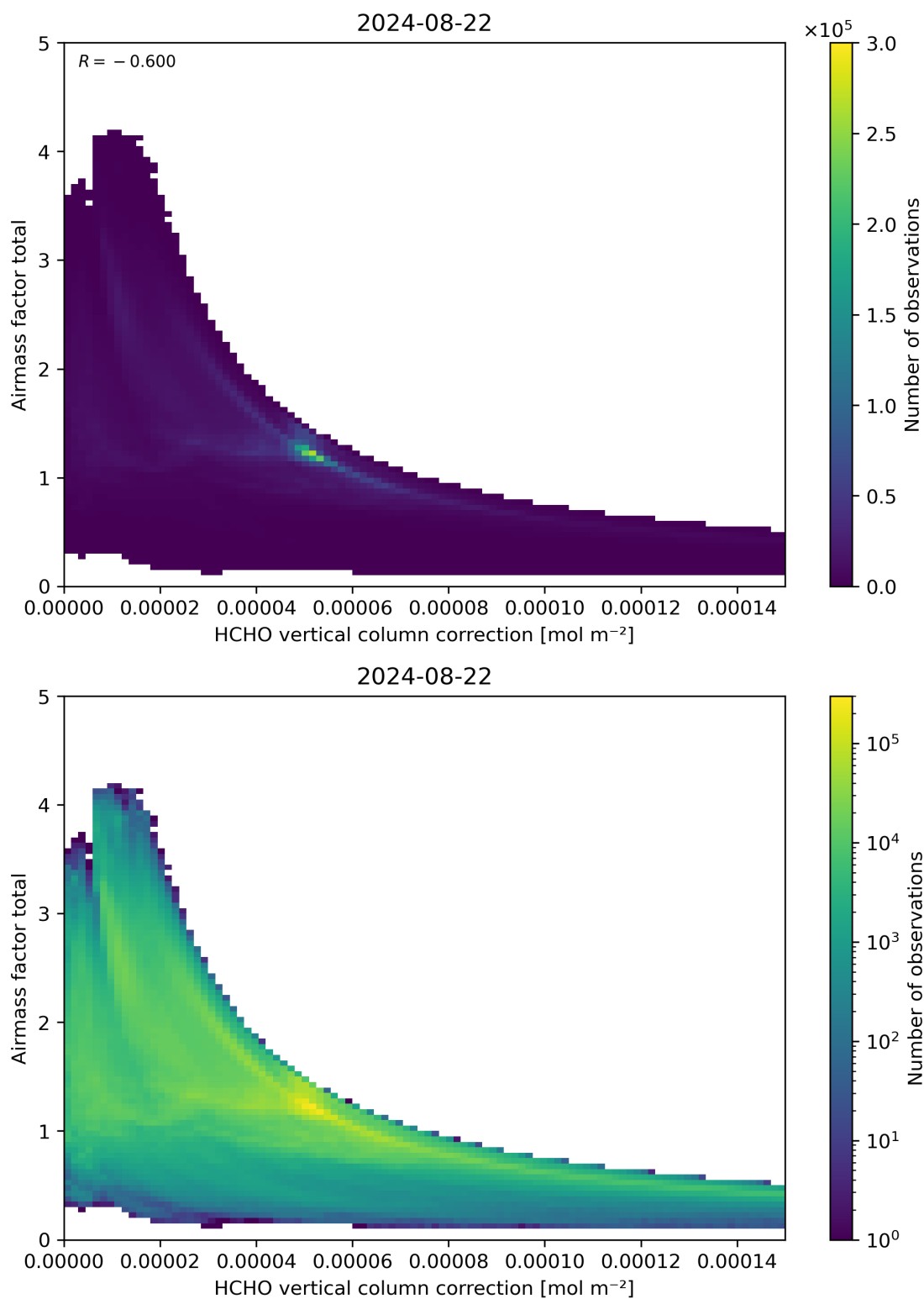
Figure 120: Scatter density plot of “HCHO vertical column correction” against “Airmass factor total” for 2024-08-22 to 2024-08-23.
