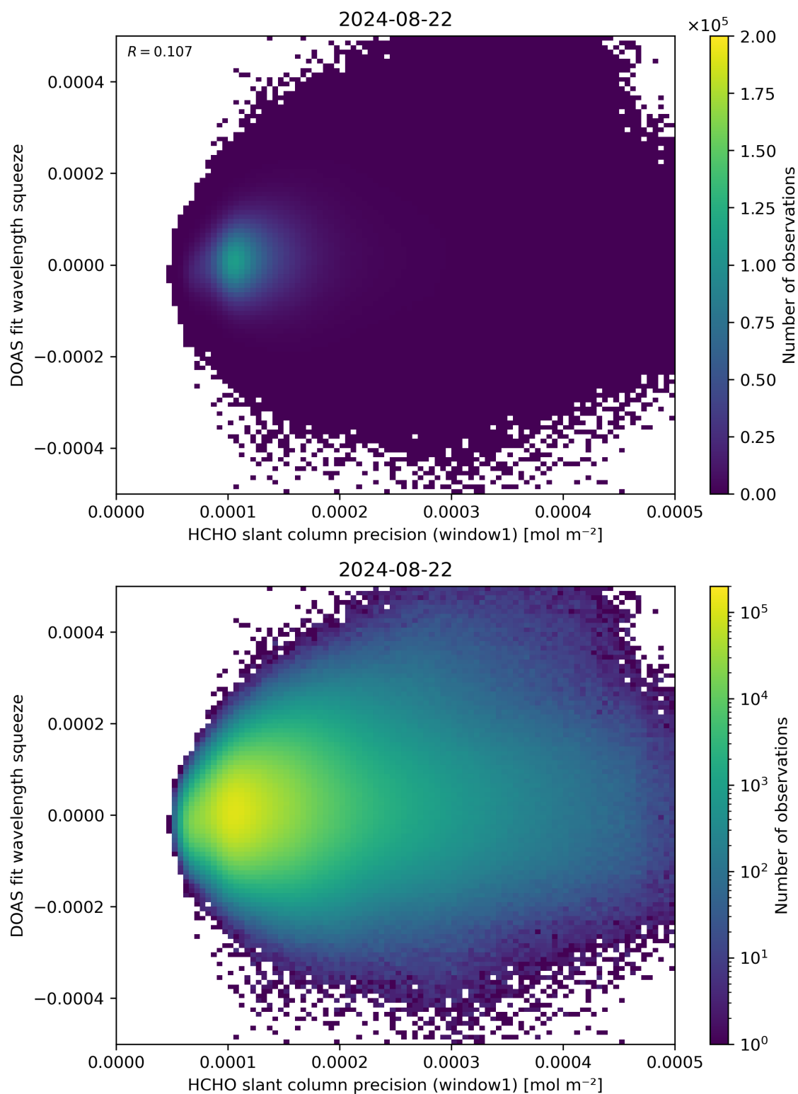
Figure 90: Scatter density plot of “HCHO slant column precision (window1)” against “DOAS fit wavelength squeeze” for 2024-08-22 to 2024-08-23.
