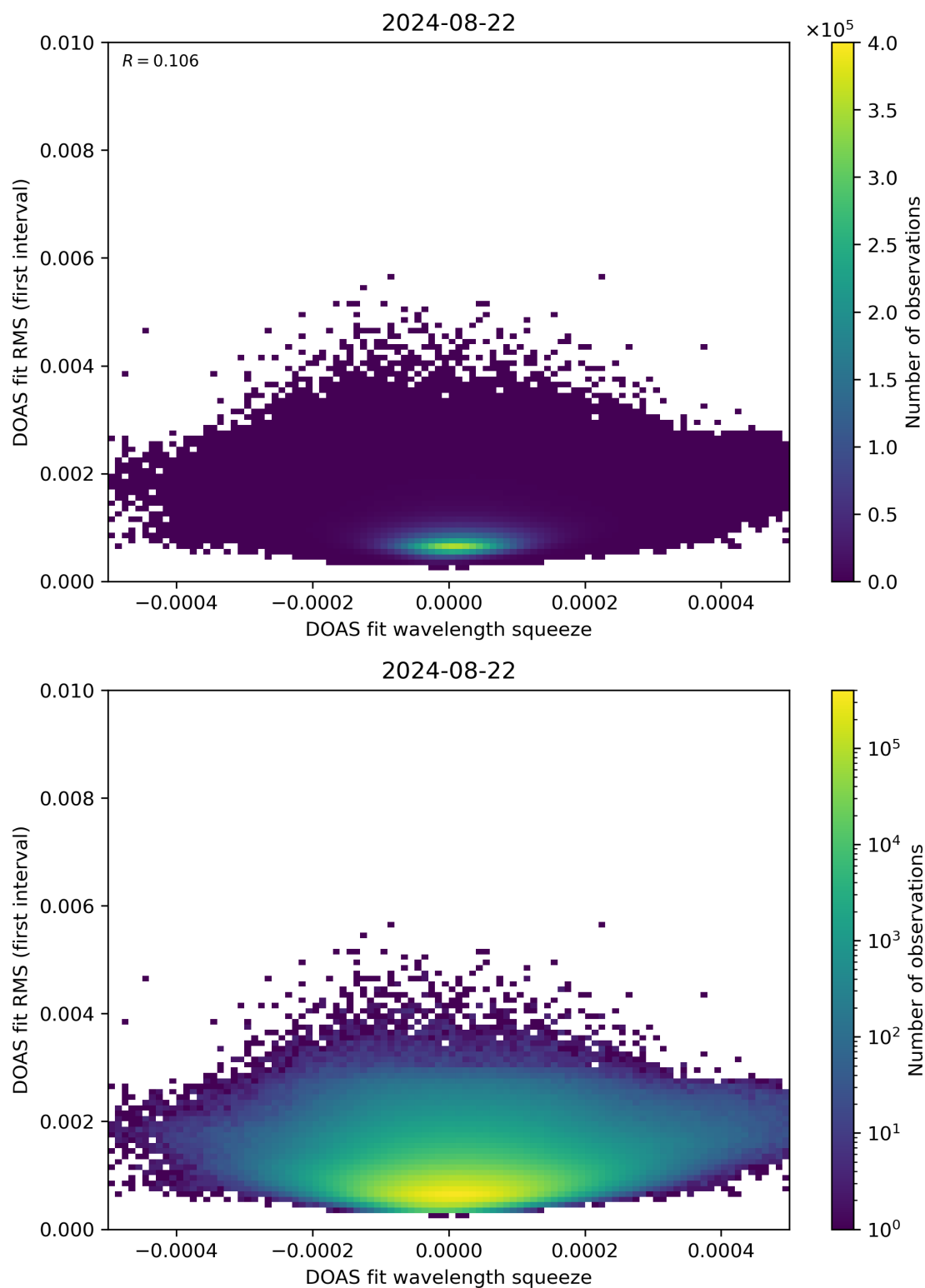
Figure 68: Scatter density plot of “DOAS fit wavelength squeeze” against “DOAS fit RMS (first interval)” for 2024-08-22 to 2024-08-23.
