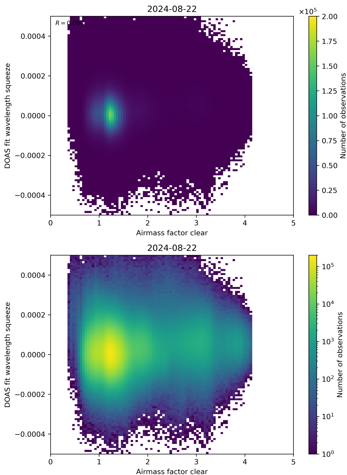
Figure 73: Scatter density plot of “Airmass factor clear” against “DOAS fit wavelength squeeze” for 2024-08-22 to 2024-08-23.
