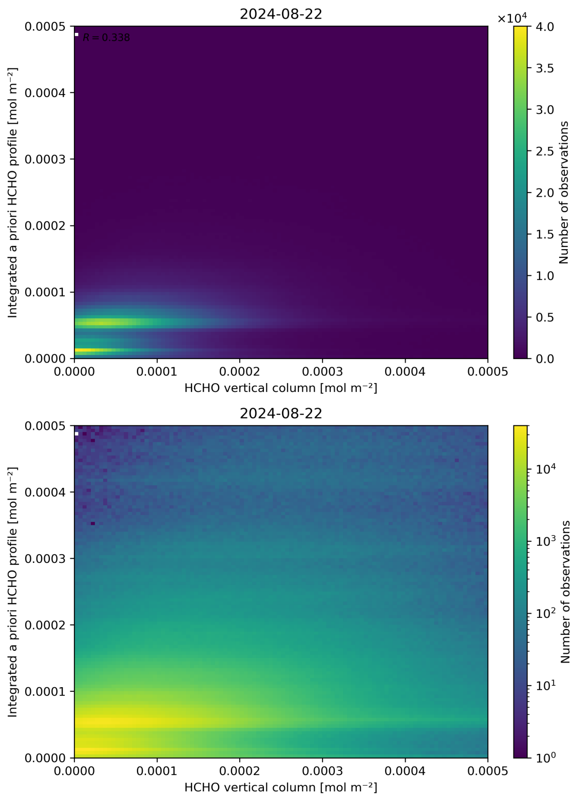
Figure 135: Scatter density plot of “HCHO vertical column” against “Integrated a priori HCHO profile” for 2024-08-22 to 2024-08-23.
