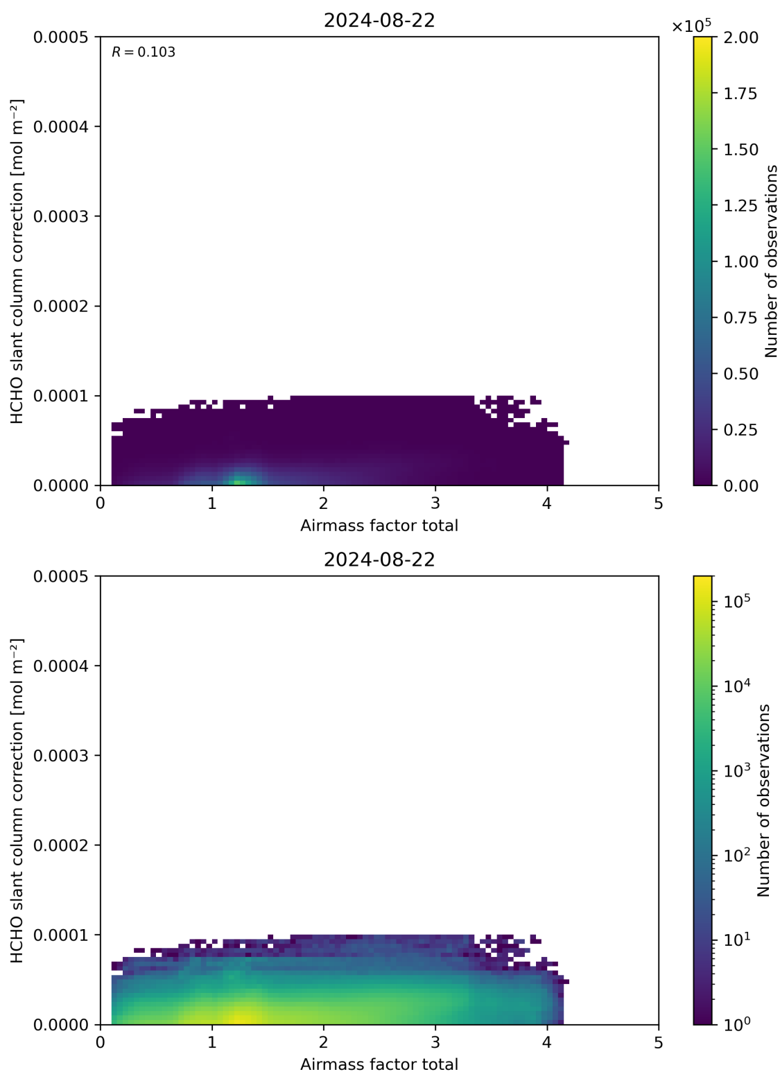
Figure 102: Scatter density plot of “Airmass factor total” against “HCHO slant column correction” for 2024-08-22 to 2024-08-23.
