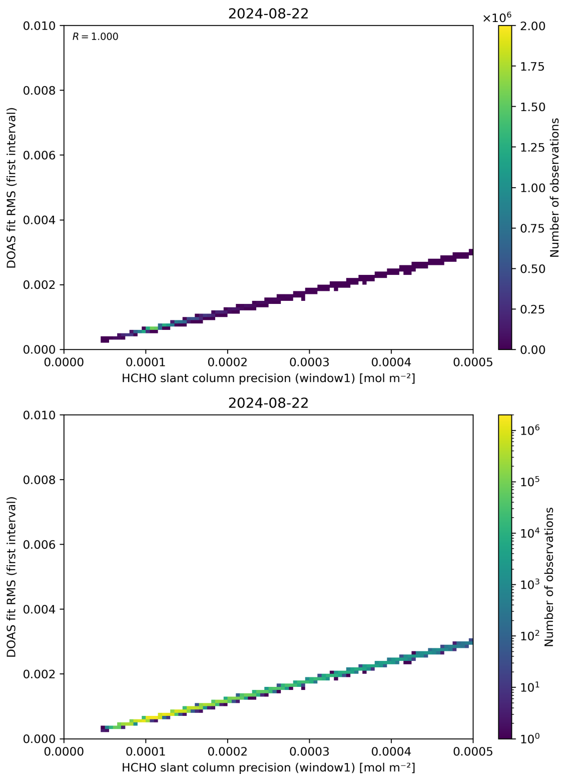
Figure 88: Scatter density plot of “HCHO slant column precision (window1)” against “DOAS fit RMS (first interval)” for 2024-08-22 to 2024-08-23.
