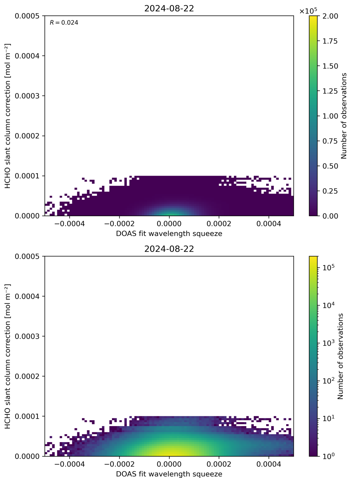
Figure 70: Scatter density plot of “DOAS fit wavelength squeeze” against “HCHO slant column correction” for 2024-08-22 to 2024-08-23.
