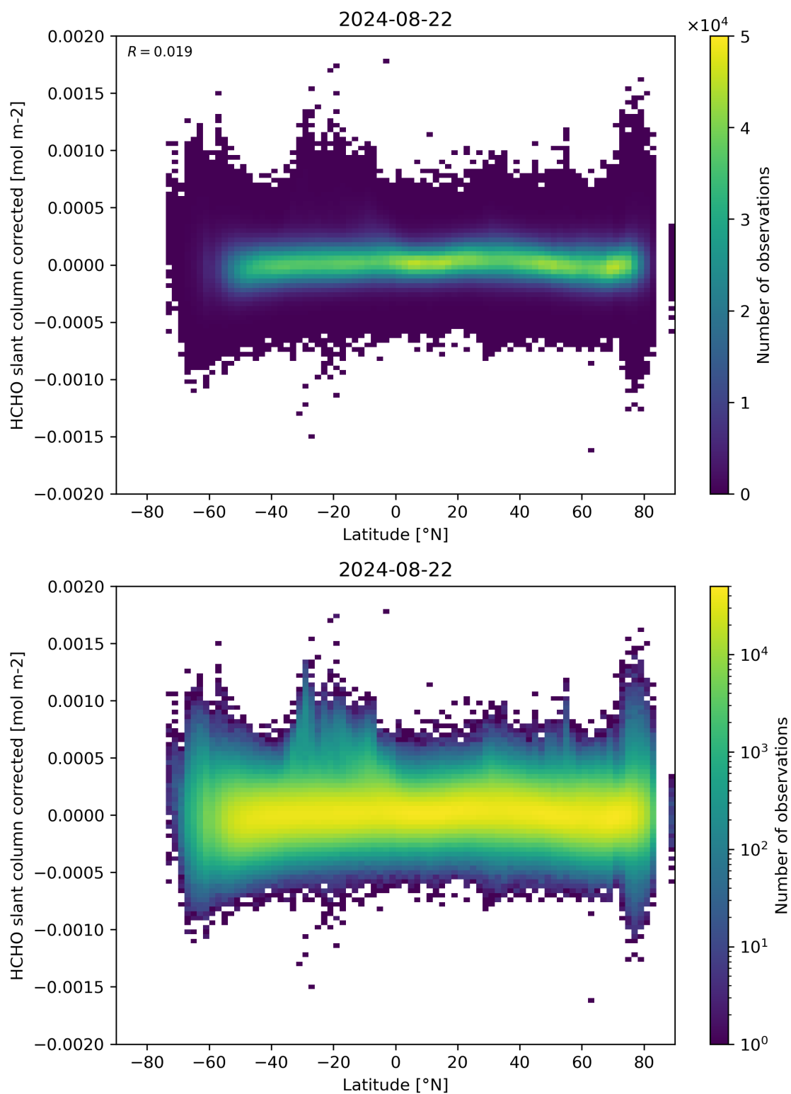
Figure 157: Scatter density plot of “Latitude” against “HCHO slant column corrected” for 2024-08-22 to 2024-08-23.
