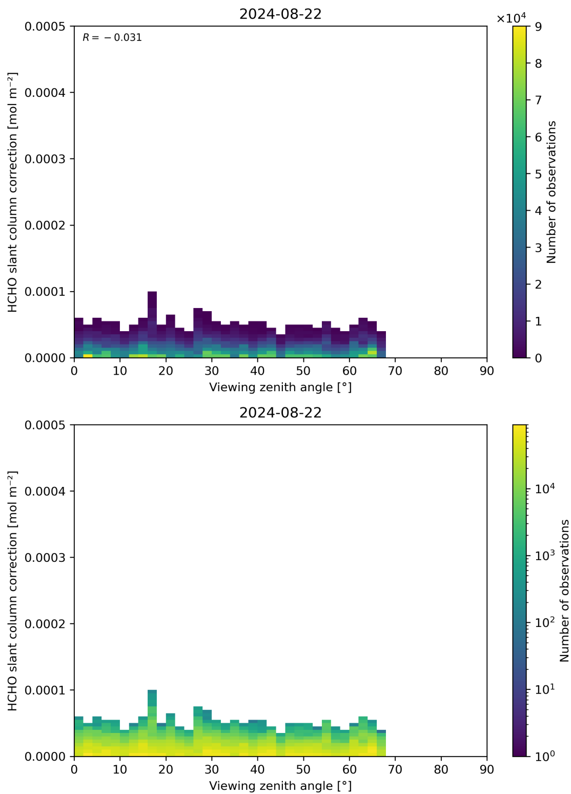
Figure 187: Scatter density plot of “Viewing zenith angle” against “HCHO slant column correction” for 2024-08-22 to 2024-08-23.
