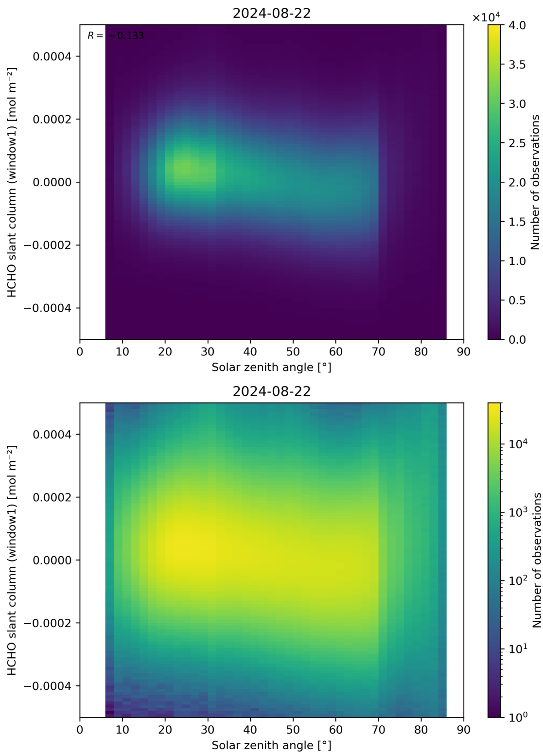
Figure 173: Scatter density plot of “Solar zenith angle” against “HCHO slant column (window1)” for 2024-08-22 to 2024-08-23.
