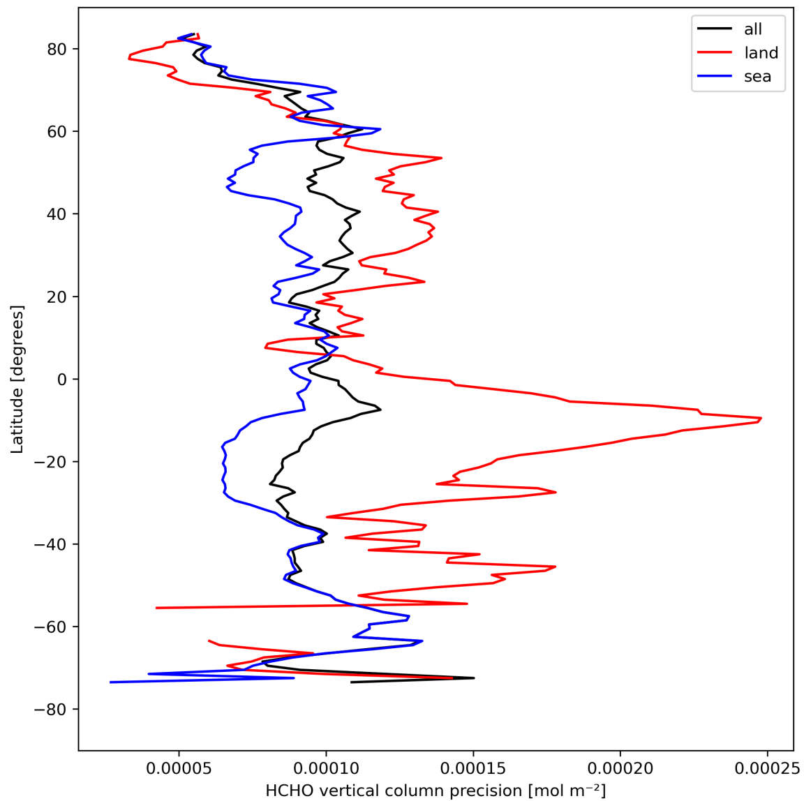
Figure 22: Zonal average of “HCHO vertical column precision” for 2024-08-22 to 2024-08-23.
