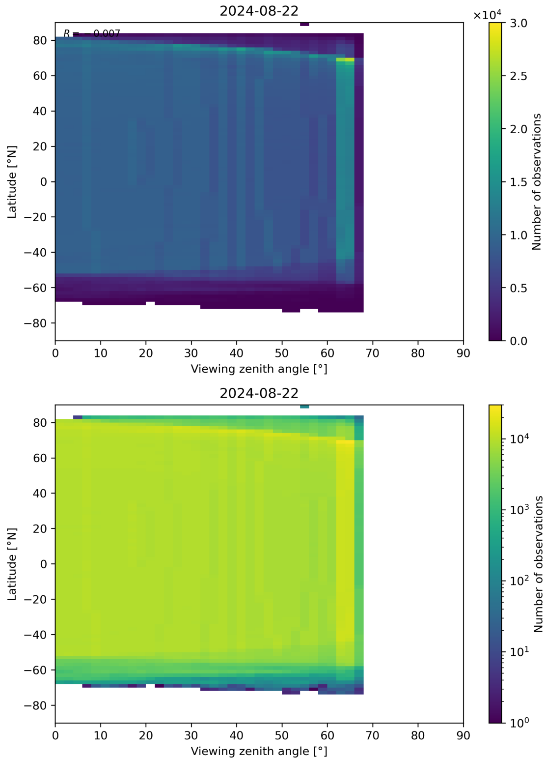
Figure 196: Scatter density plot of “Viewing zenith angle” against “Latitude” for 2024-08-22 to 2024-08-23.
