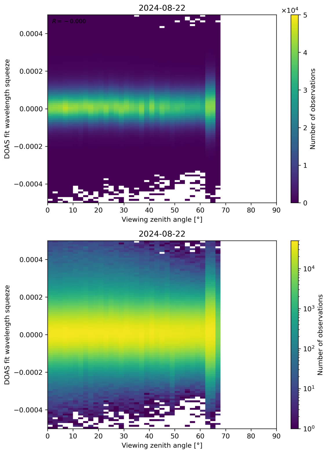
Figure 184: Scatter density plot of “Viewing zenith angle” against “DOAS fit wavelength squeeze” for 2024-08-22 to 2024-08-23.
