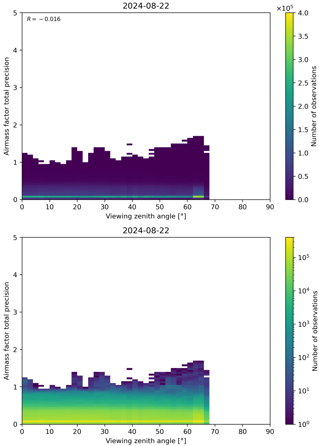
Figure 191: Scatter density plot of “Viewing zenith angle” against “Airmass factor total precision” for 2024-08-22 to 2024-08-23.
