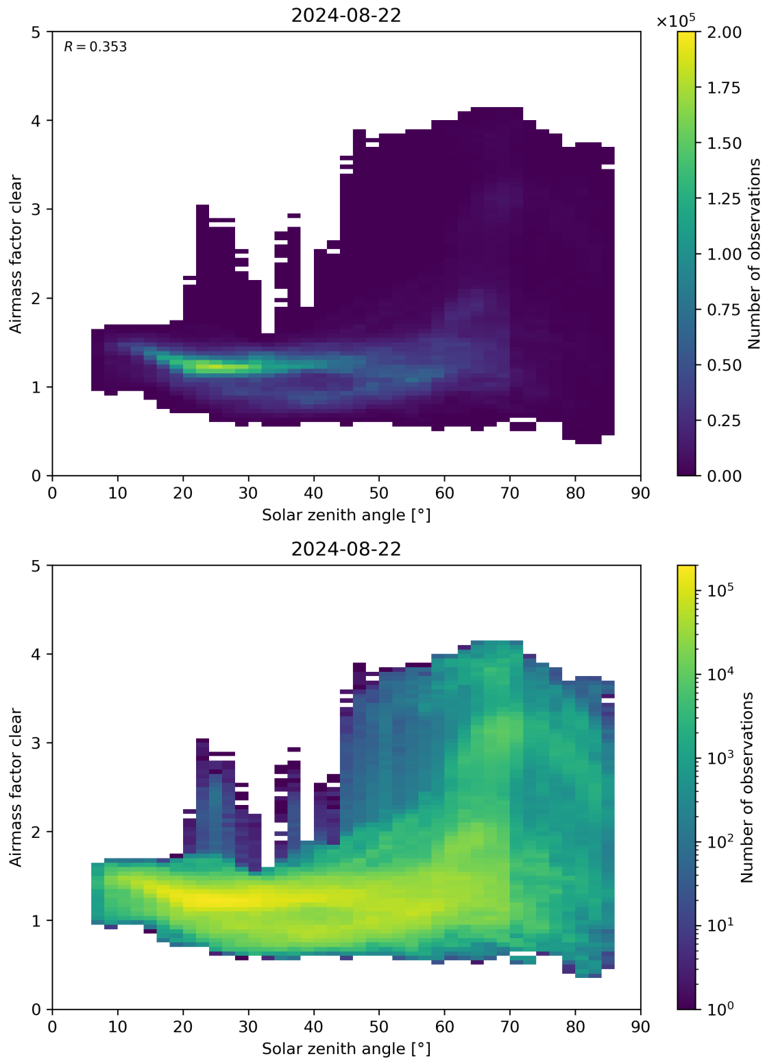
Figure 170: Scatter density plot of “Solar zenith angle” against “Airmass factor clear” for 2024-08-22 to 2024-08-23.
