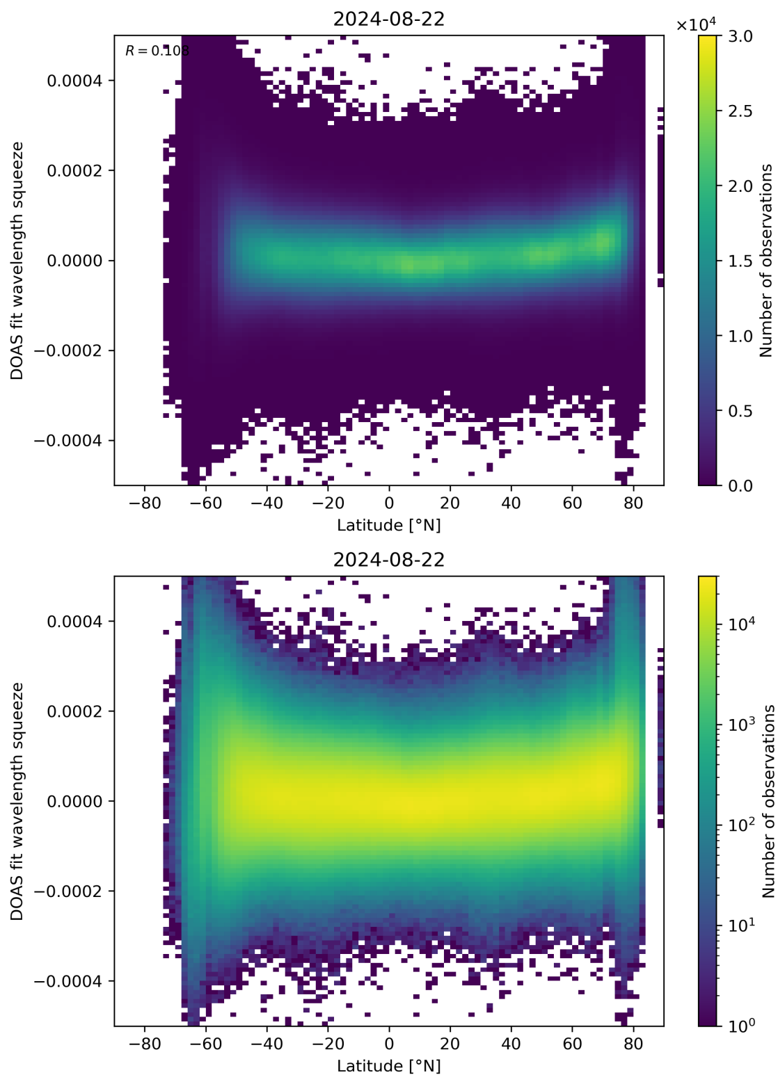
Figure 155: Scatter density plot of “Latitude” against “DOAS fit wavelength squeeze” for 2024-08-22 to 2024-08-23.
