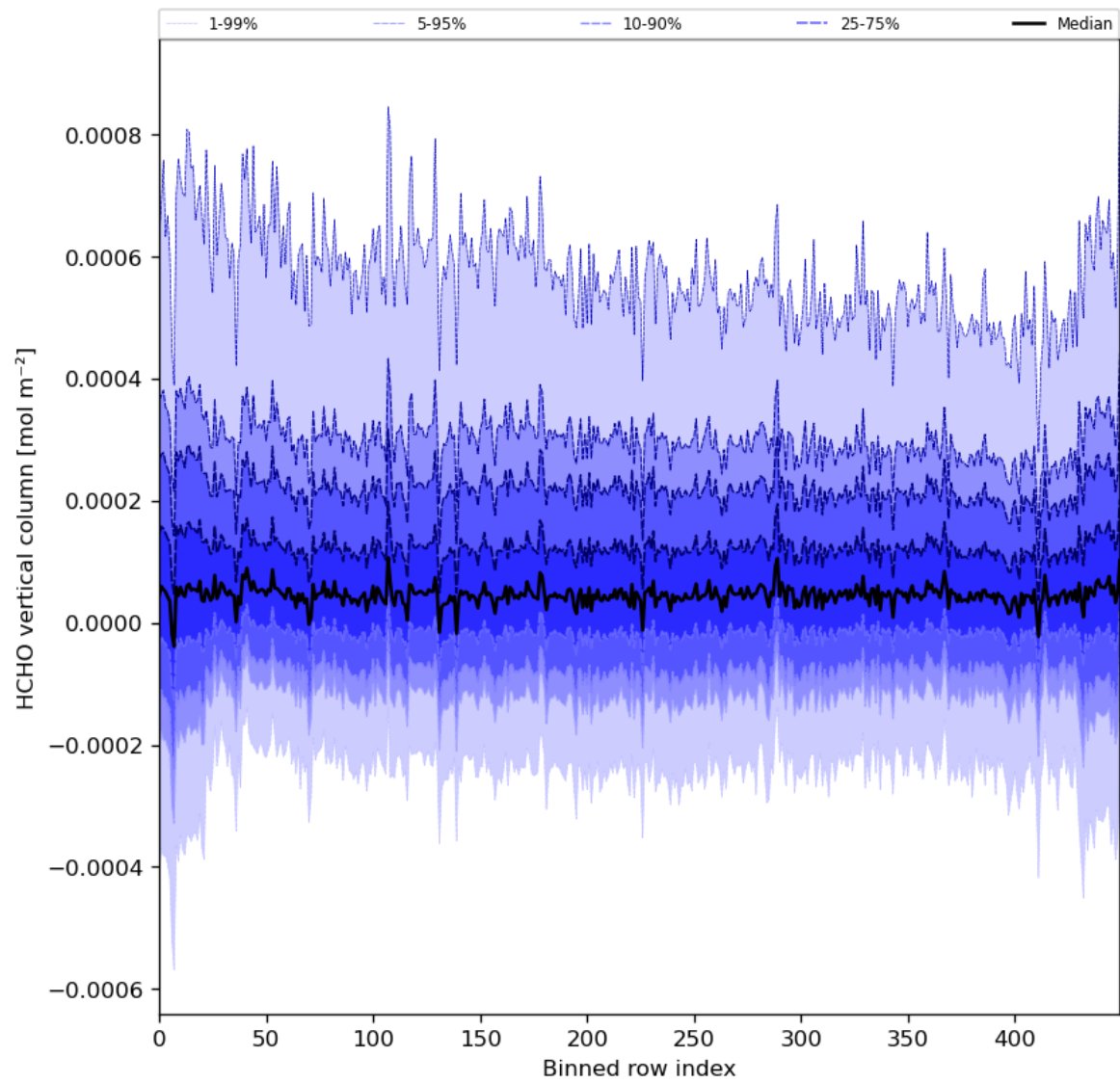
Figure 49: Along track statistics of “HCHO vertical column” for 2024-08-22 to 2024-08-23
