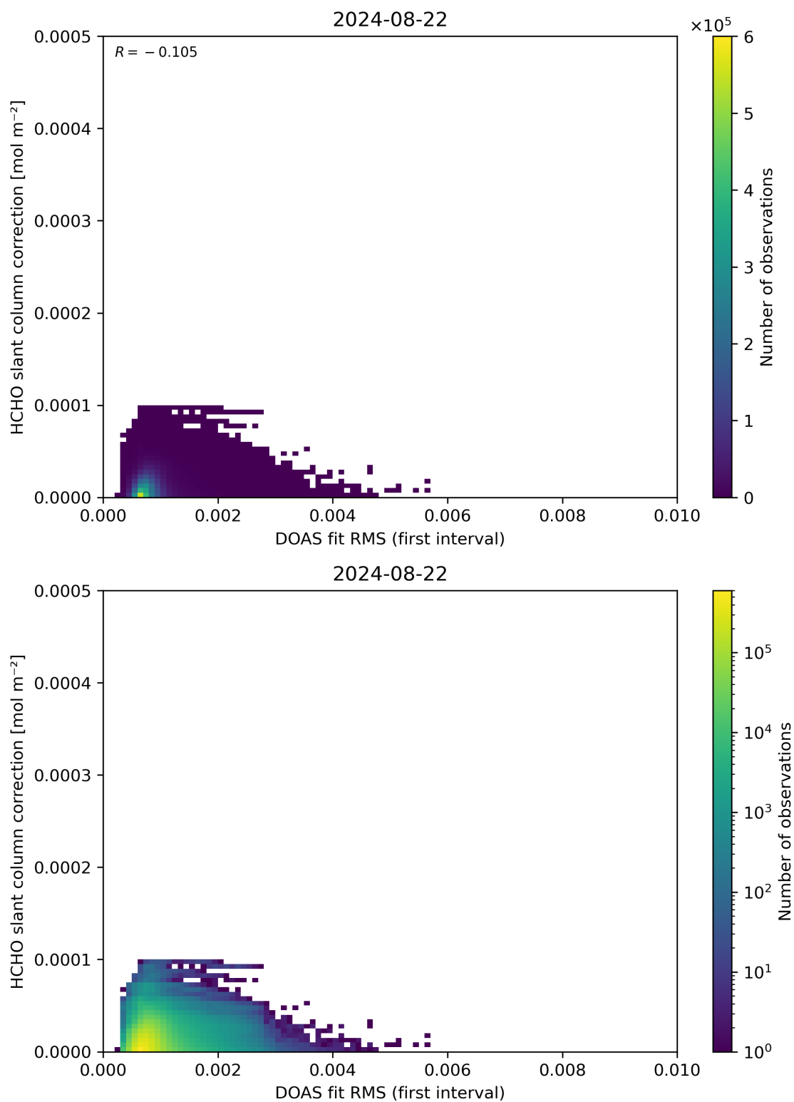
Figure 63: Scatter density plot of “DOAS fit RMS (first interval)” against “HCHO slant column correction” for 2024-08-22 to 2024-08-23.
