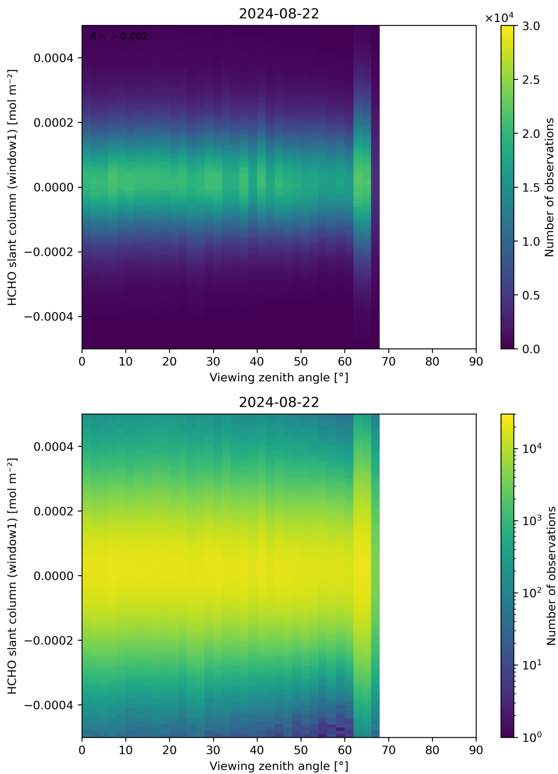
Figure 188: Scatter density plot of “Viewing zenith angle” against “HCHO slant column (window1)” for 2024-08-22 to 2024-08-23.
