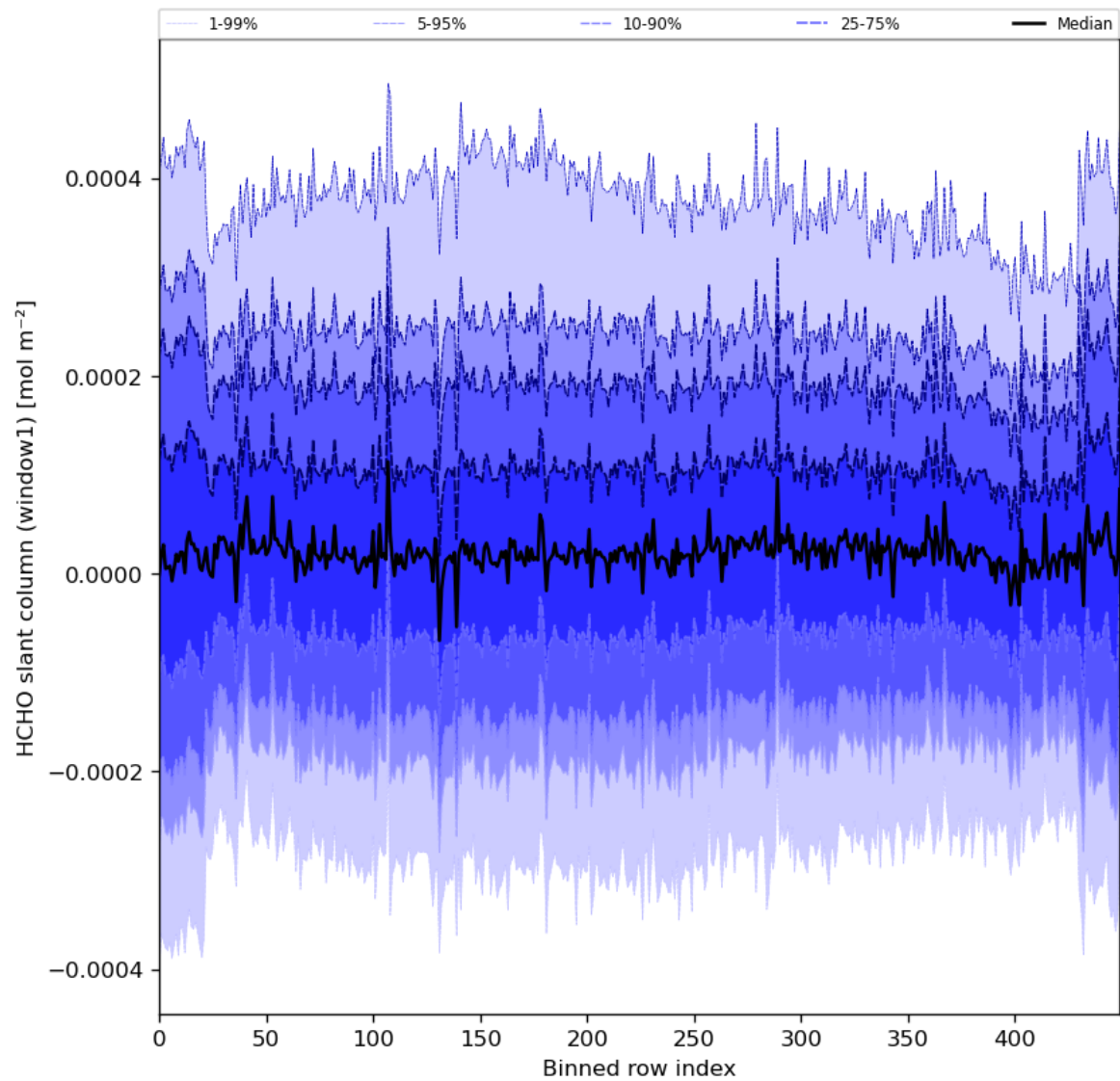
Figure 52: Along track statistics of “HCHO slant column (window1)” for 2024-08-22 to 2024-08-23
