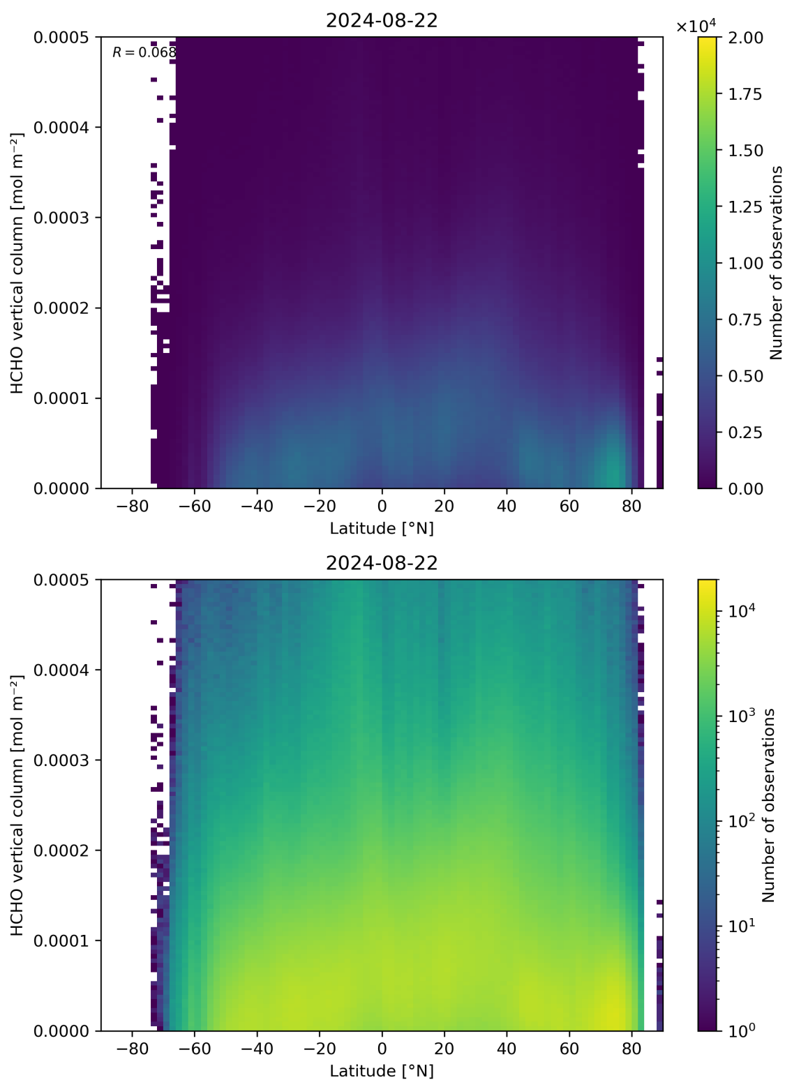
Figure 163: Scatter density plot of “Latitude” against “HCHO vertical column” for 2024-08-22 to 2024-08-23.
