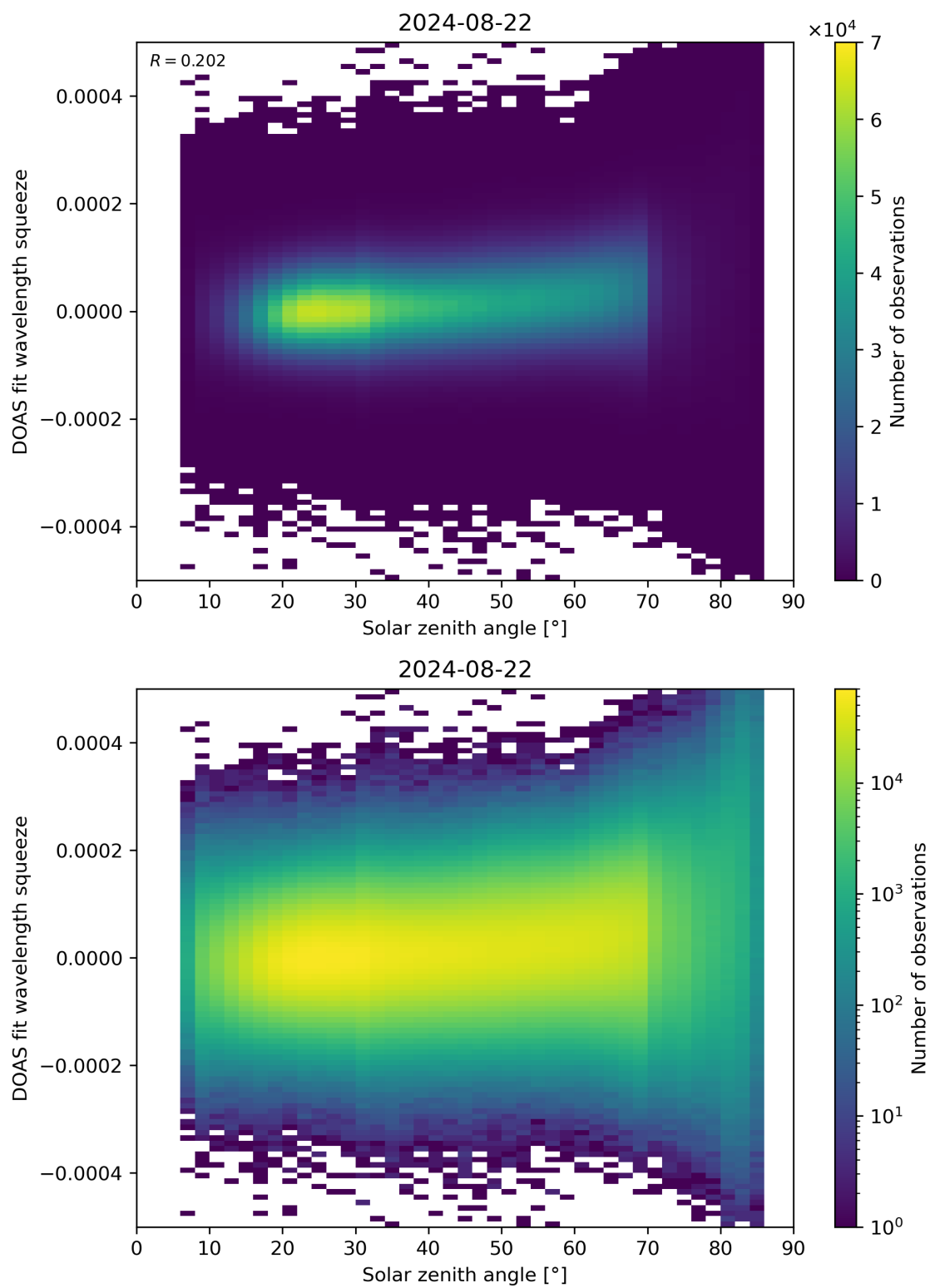
Figure 169: Scatter density plot of “Solar zenith angle” against “DOAS fit wavelength squeeze” for 2024-08-22 to 2024-08-23.
