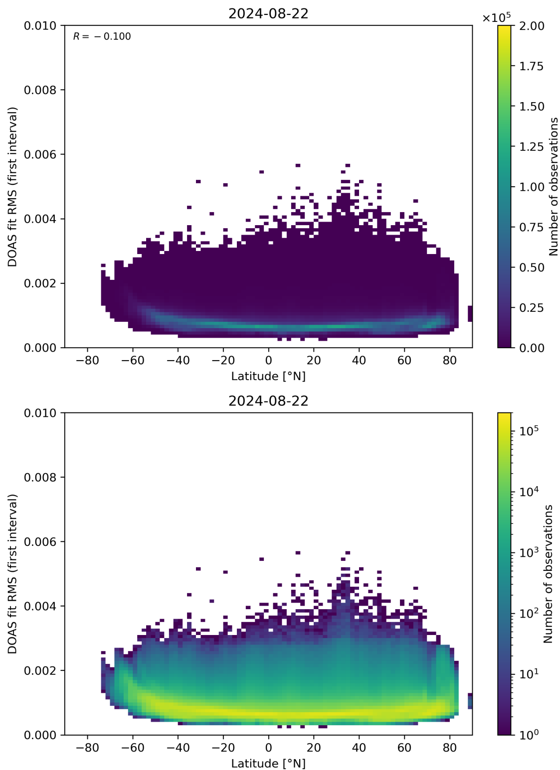
Figure 153: Scatter density plot of “Latitude” against “DOAS fit RMS (first interval)” for 2024-08-22 to 2024-08-23.
