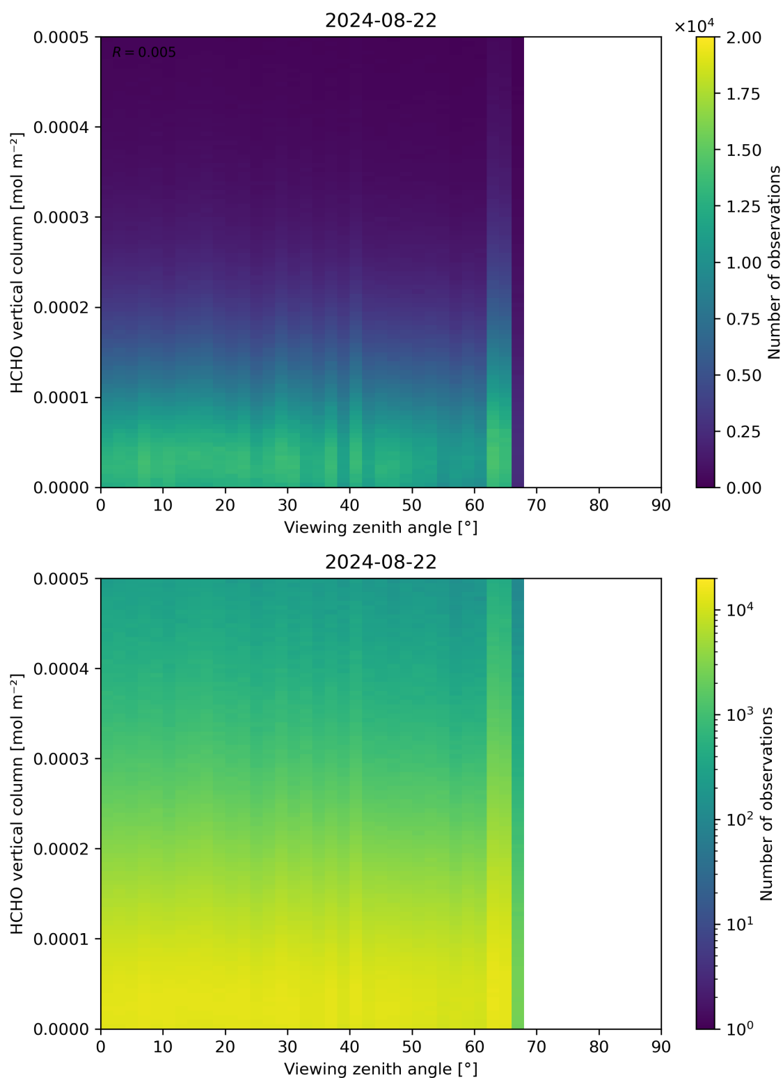
Figure 192: Scatter density plot of “Viewing zenith angle” against “HCHO vertical column” for 2024-08-22 to 2024-08-23.
