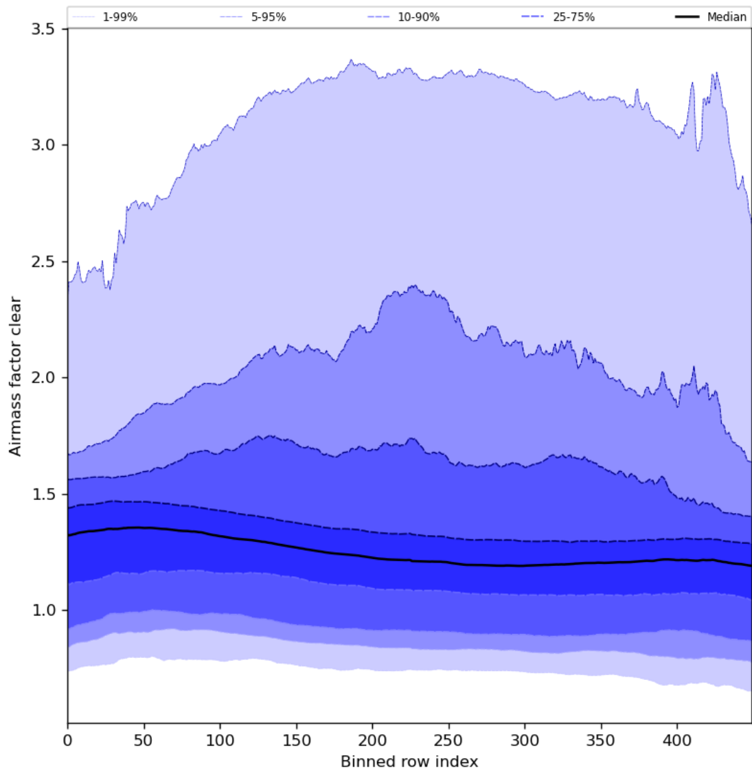
Figure 56: Along track statistics of “Air mass factor clear” for 2024-08-22 to 2024-08-23
