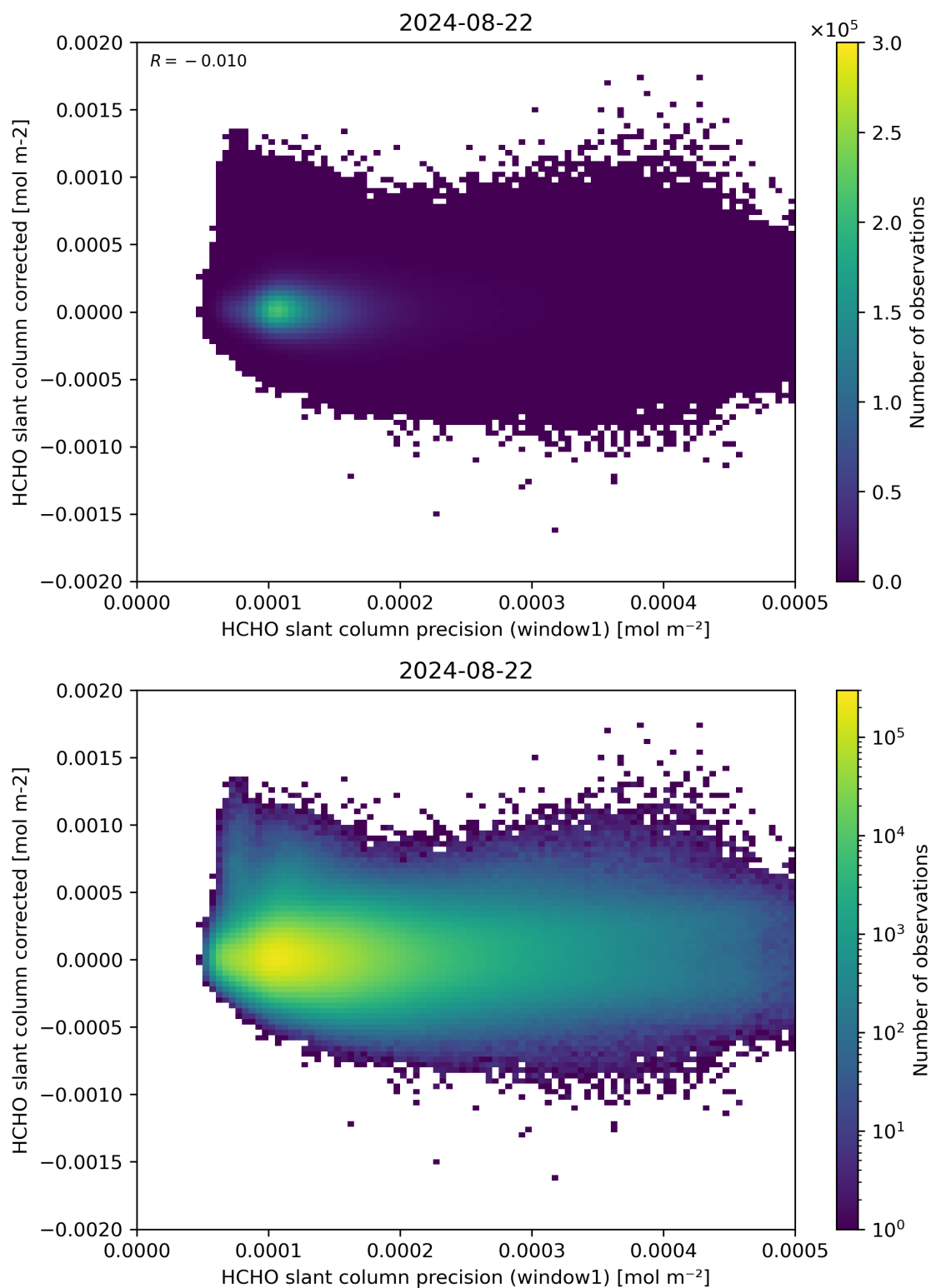
Figure 92: Scatter density plot of “HCHO slant column precision (window1)” against “HCHO slant column corrected” for 2024-08-22 to 2024-08-23.
