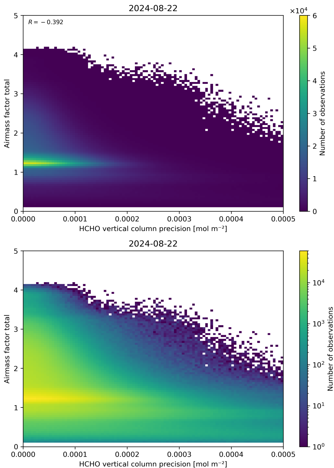
Figure 144: Scatter density plot of “HCHO vertical column precision” against “Airmass factor total” for 2024-08-22 to 2024-08-23.
