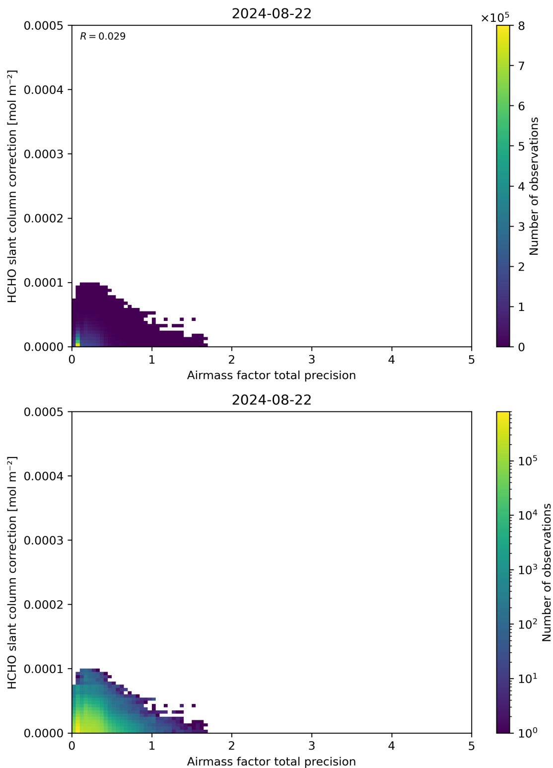
Figure 110: Scatter density plot of “Airmass factor total precision” against “HCHO slant column correction” for 2024-08-22 to 2024-08-23.
