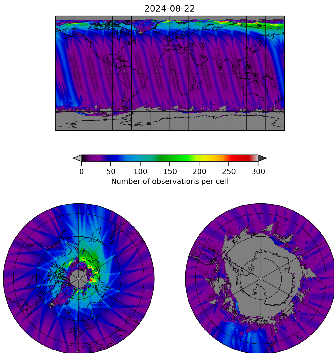
Figure 19: Map of the number of observations for 2024-08-22 to 2024-08-23
