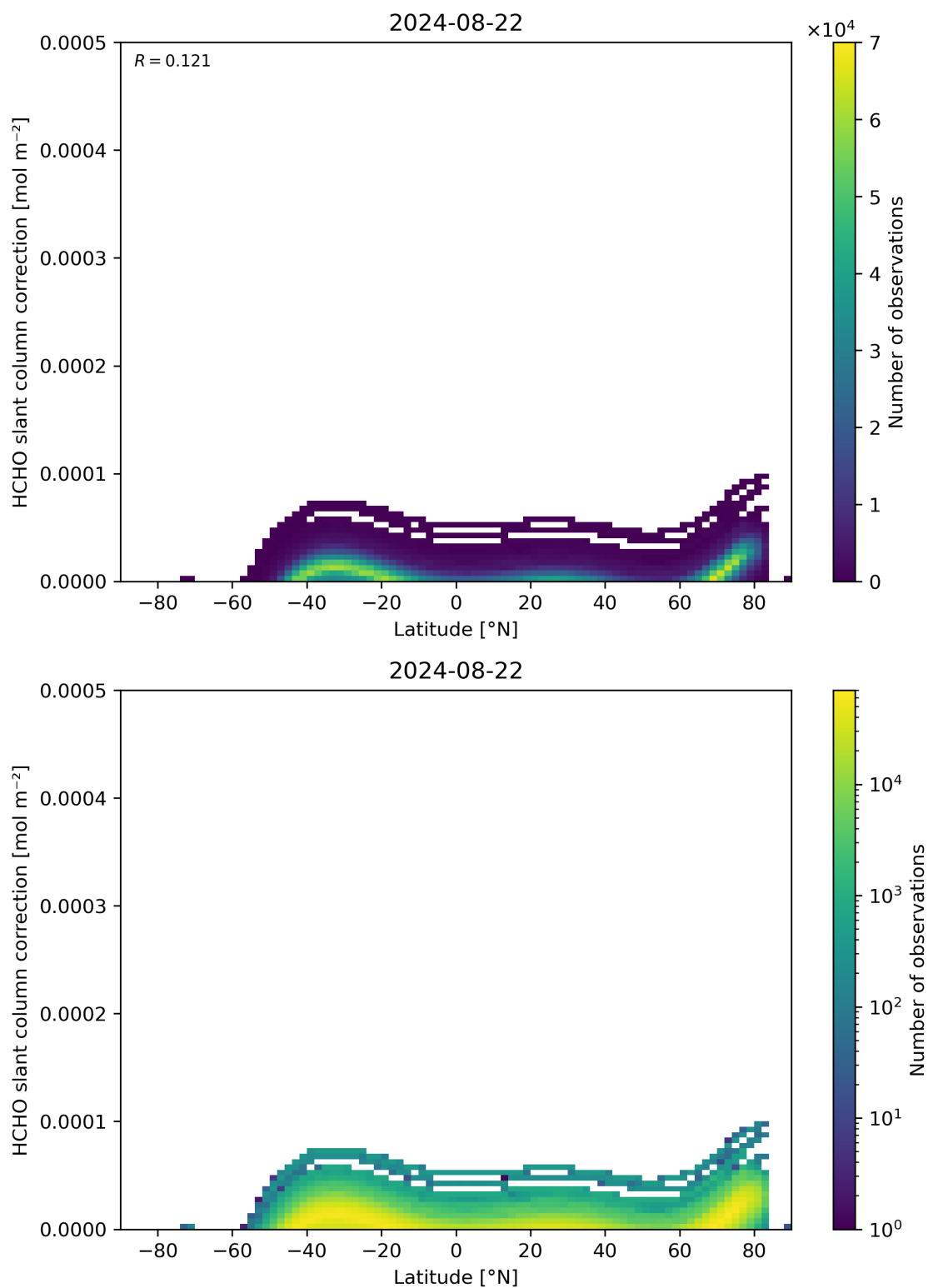
Figure 158: Scatter density plot of “Latitude” against “HCHO slant column correction” for 2024-08-22 to 2024-08-23.
