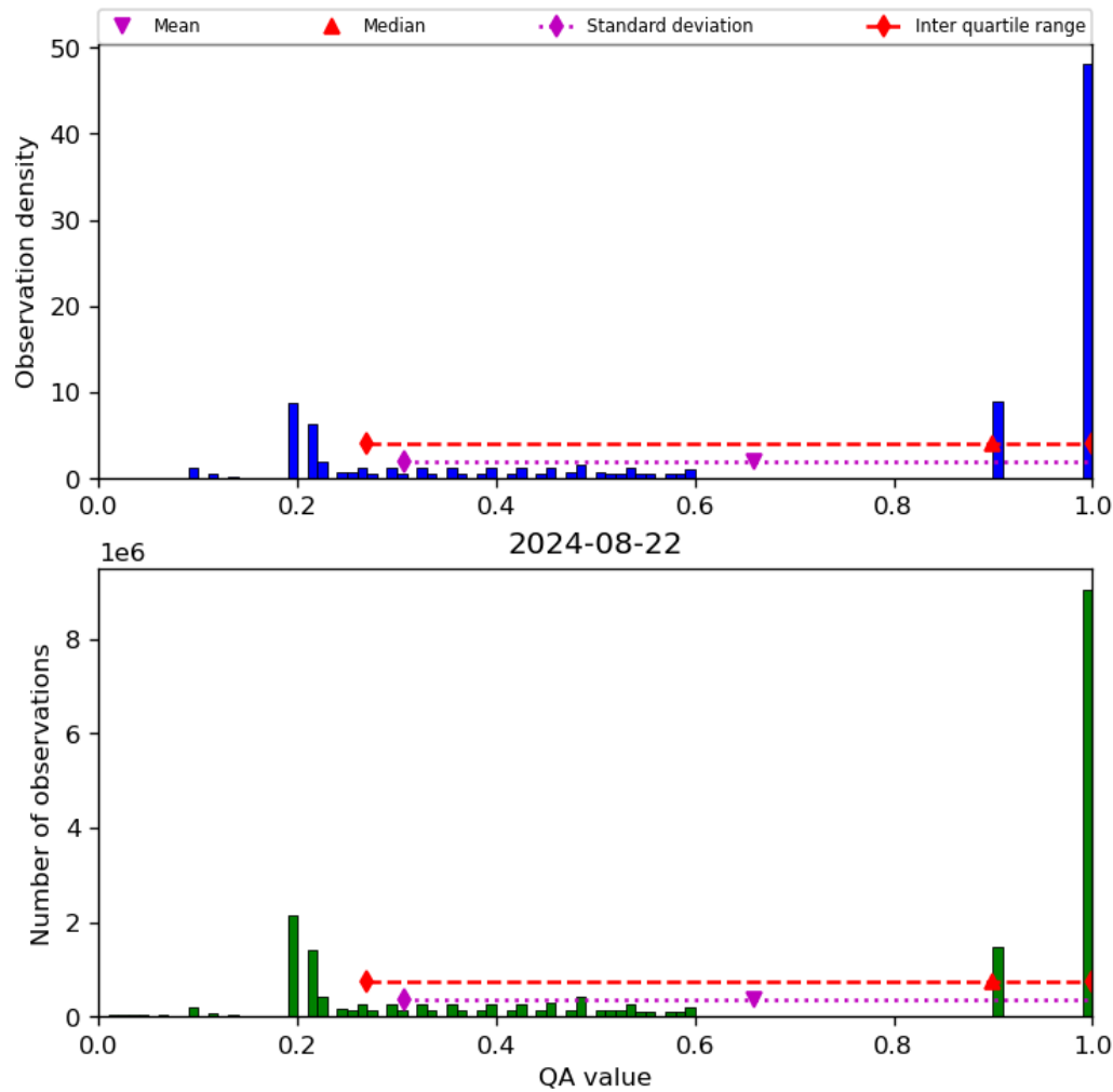
Figure 34: Histogram of “QA value” for 2024-08-22 to 2024-08-23
