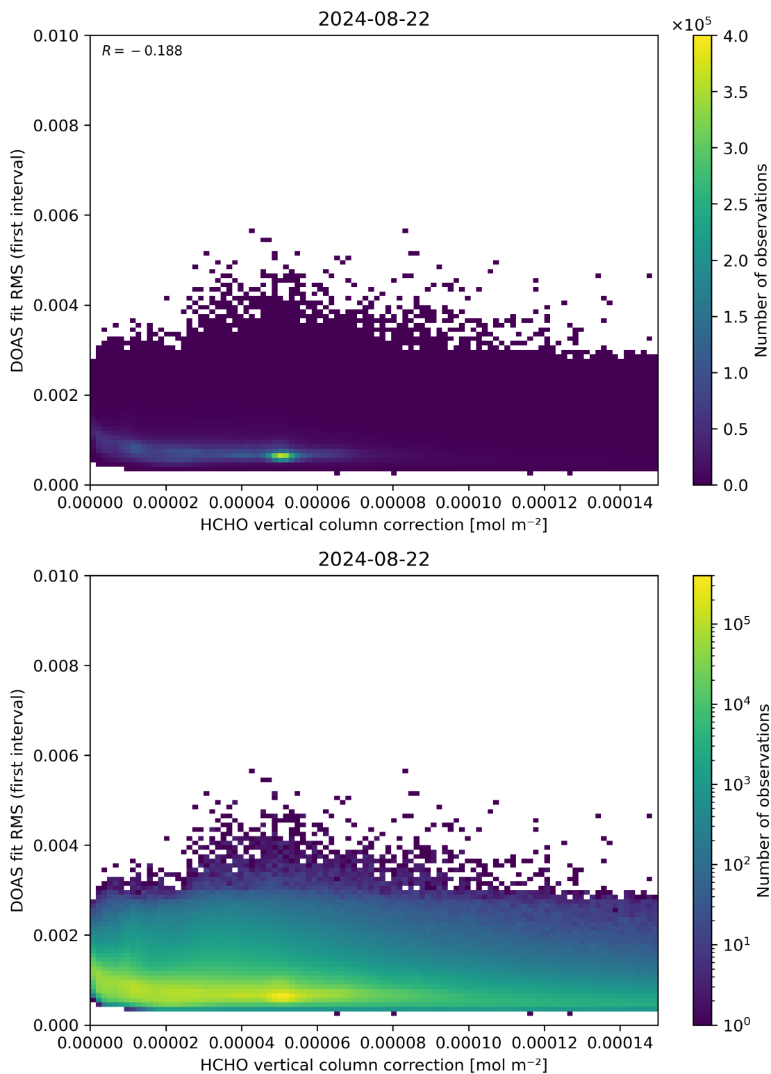
Figure 112: Scatter density plot of “HCHO vertical column correction” against “DOAS fit RMS (first interval)” for 2024-08-22 to 2024-08-23.
