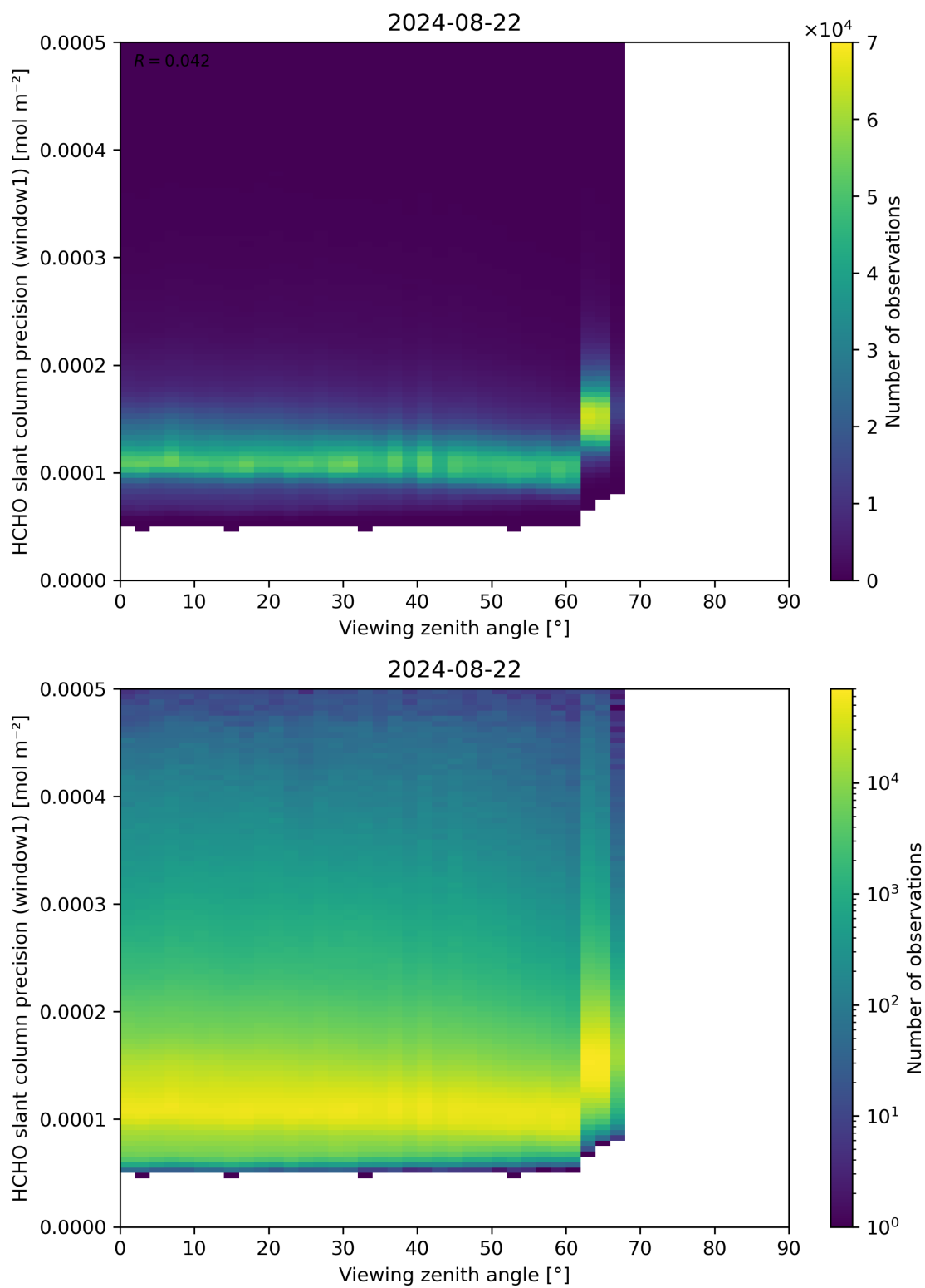
Figure 189: Scatter density plot of “Viewing zenith angle” against “HCHO slant column precision (window1)” for 2024-08-22 to 2024-08-23.
