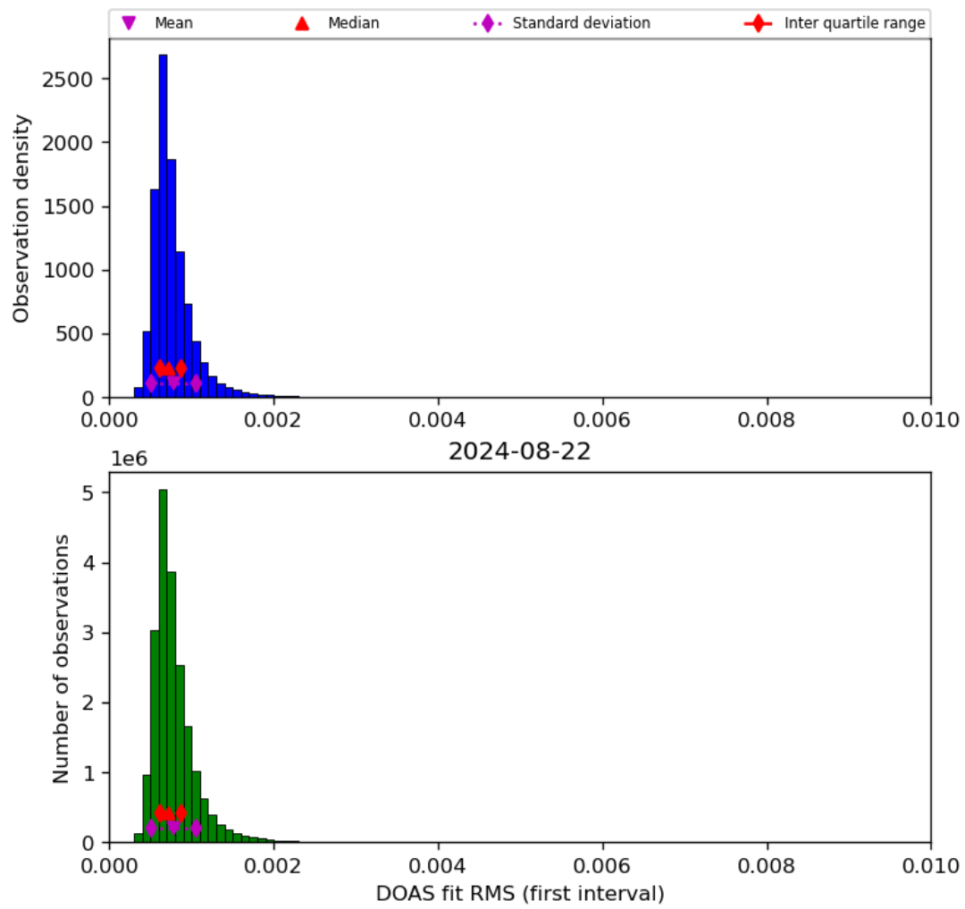
Figure 46: Histogram of “DOAS fit RMS (first interval)” for 2024-08-22 to 2024-08-23
