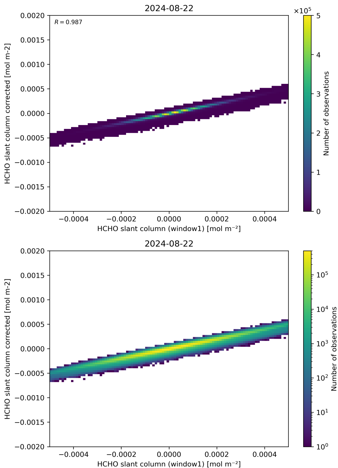
Figure 82: Scatter density plot of “HCHO slant column (window1)” against “HCHO slant column corrected” for 2024-08-22 to 2024-08-23.
