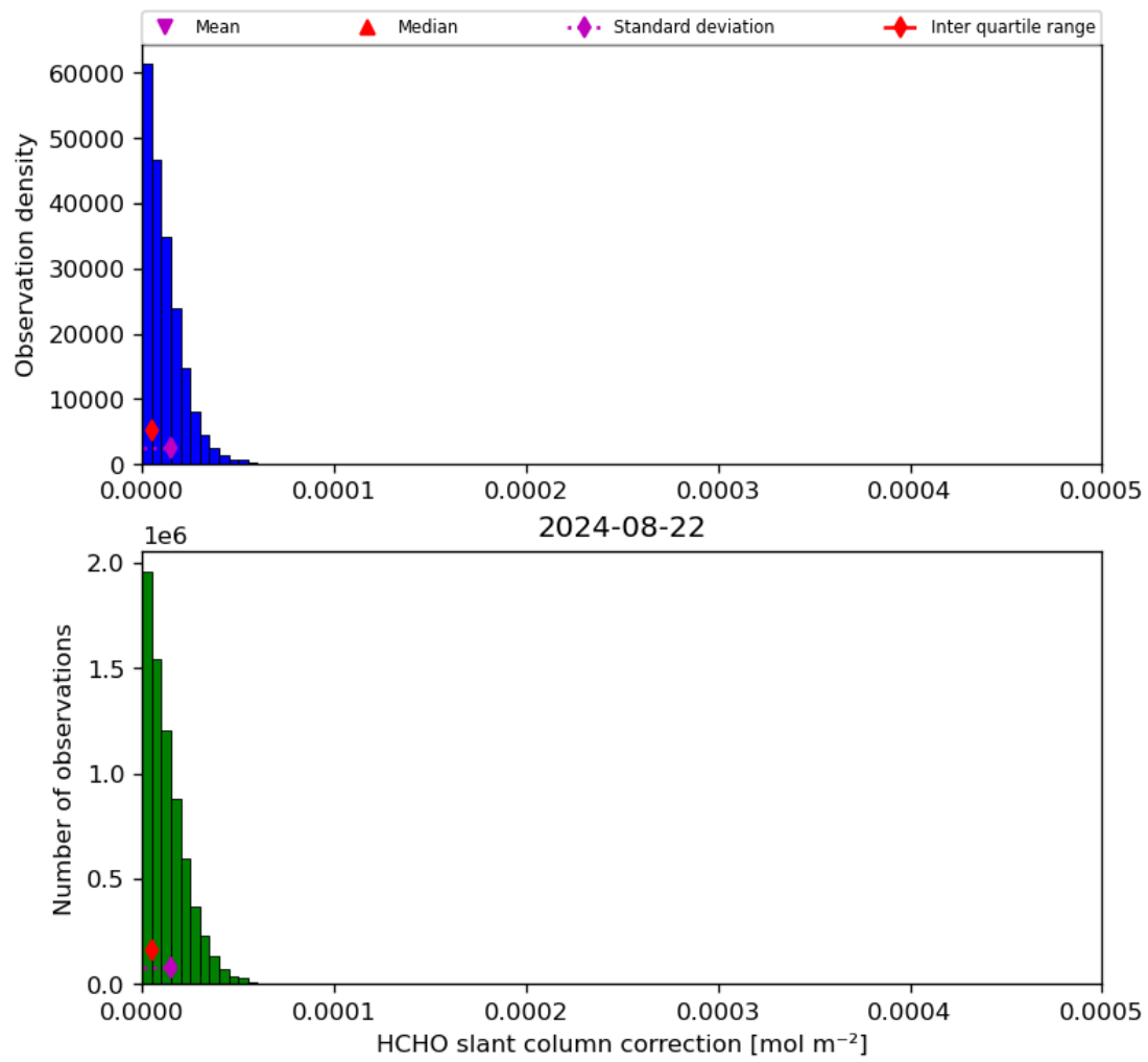
Figure 47: Histogram of “HCHO slant column correction” for 2024-08-22 to 2024-08-23
