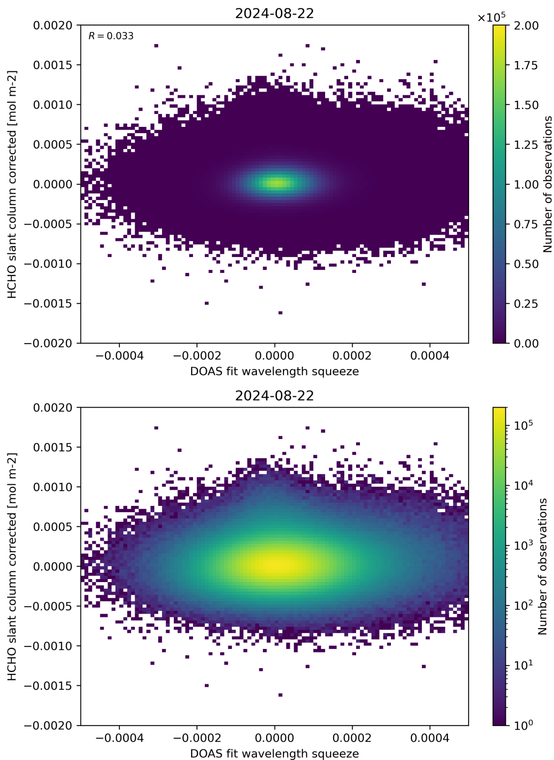
Figure 69: Scatter density plot of “DOAS fit wavelength squeeze” against “HCHO slant column corrected” for 2024-08-22 to 2024-08-23.
