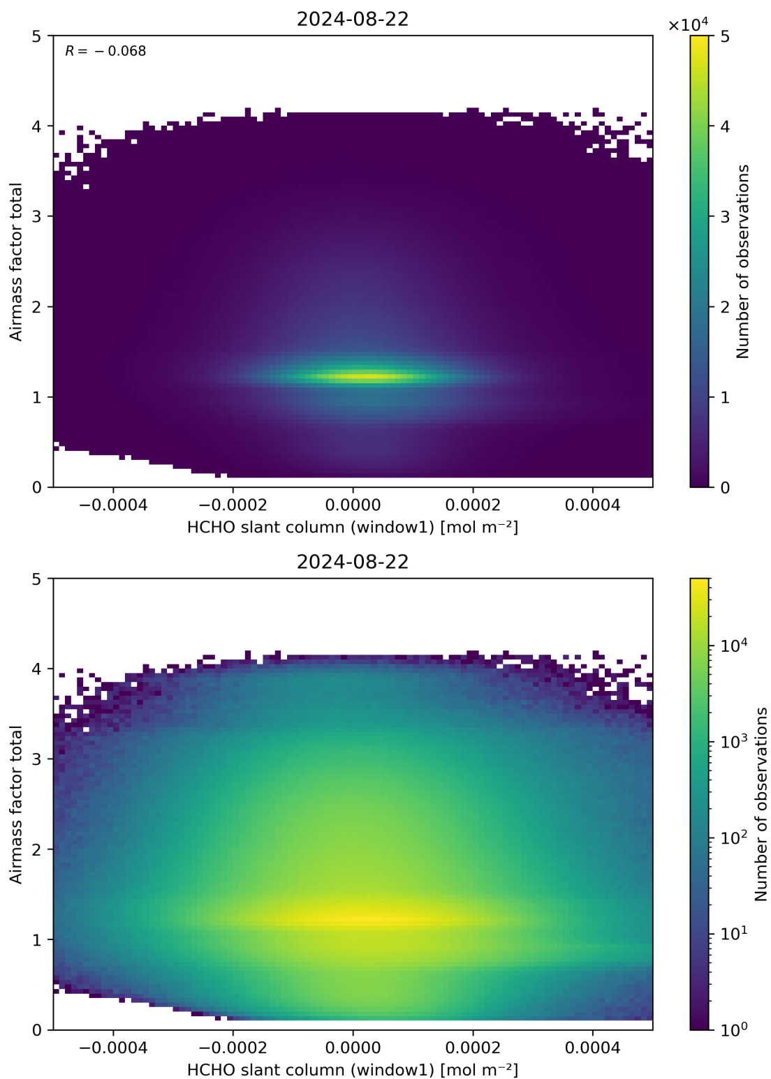
Figure 85: Scatter density plot of “HCHO slant column (window1)” against “Airmass factor total” for 2024-08-22 to 2024-08-23.
