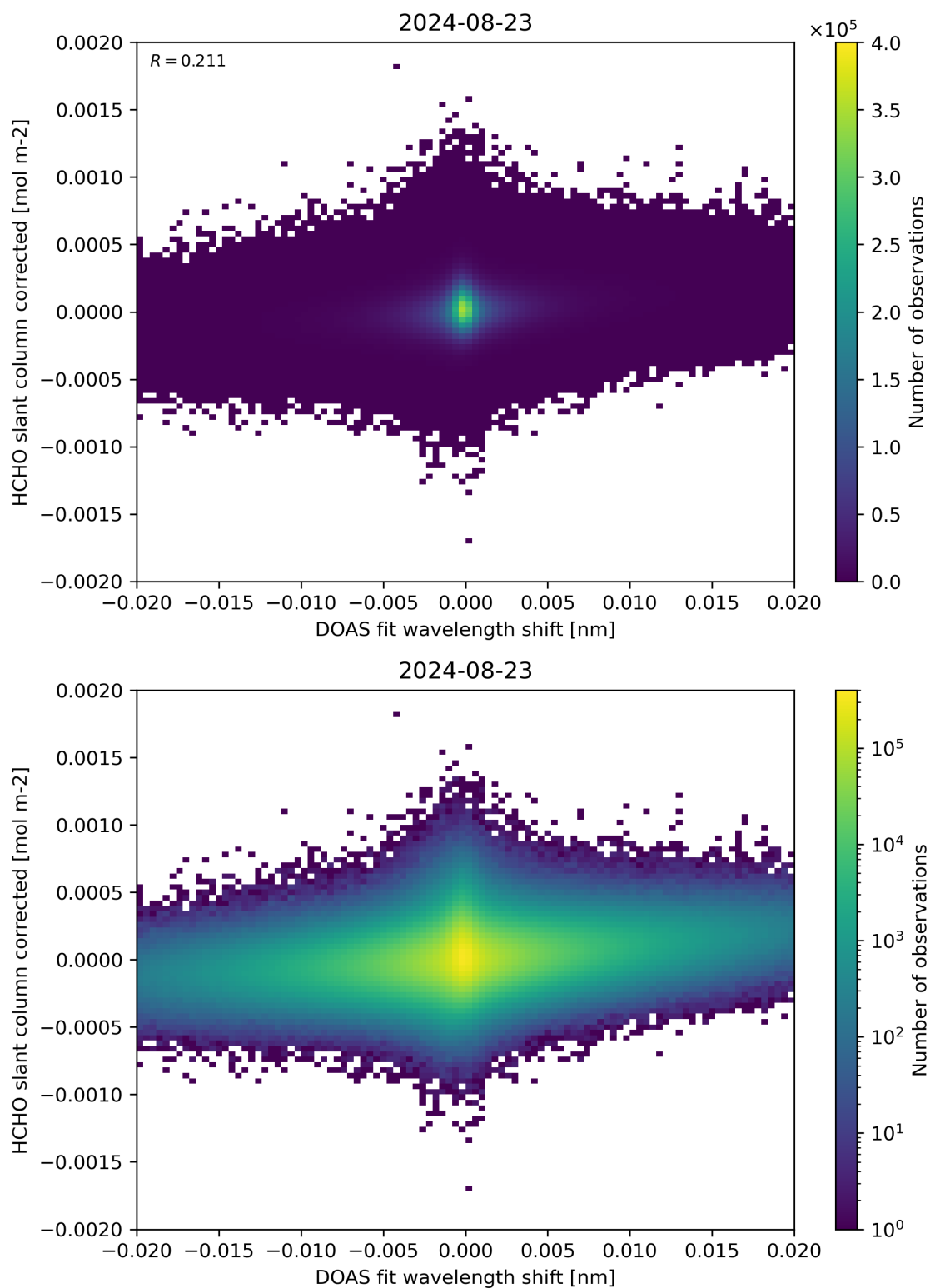
Figure 66: Scatter density plot of “DOAS fit wavelength shift” against “HCHO slant column corrected” for 2024-08-22 to 2024-08-24.
