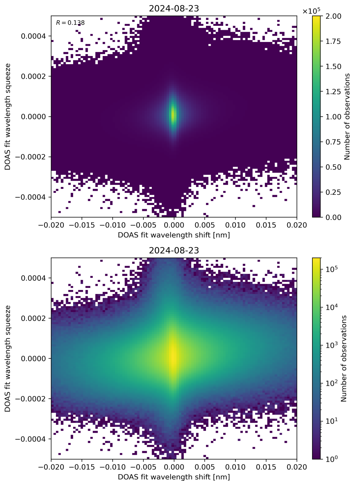
Figure 65: Scatter density plot of “DOAS fit wavelength shift” against “DOAS fit wavelength squeeze” for 2024-08-22 to 2024-08-24.
