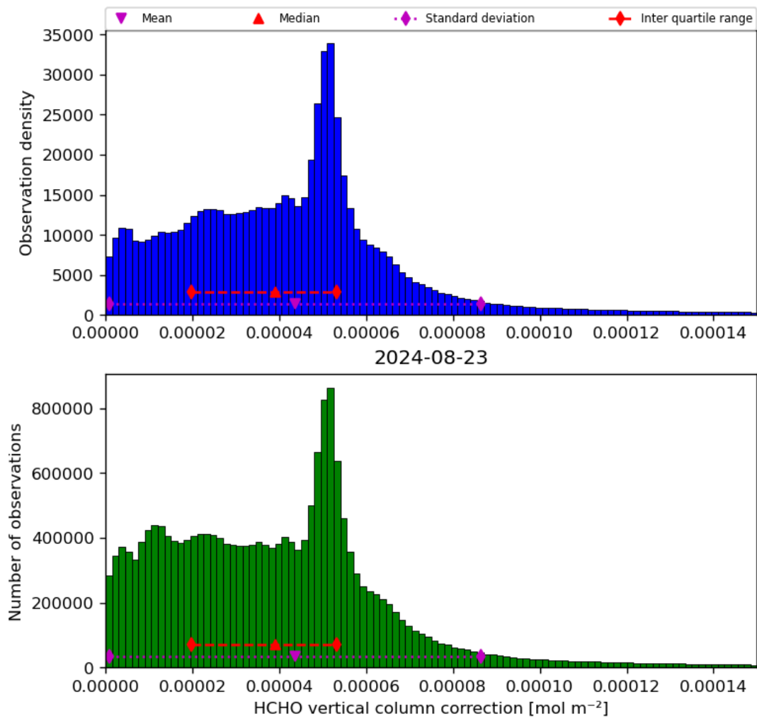
Figure 37: Histogram of “HCHO vertical column correction” for 2024-08-22 to 2024-08-24
