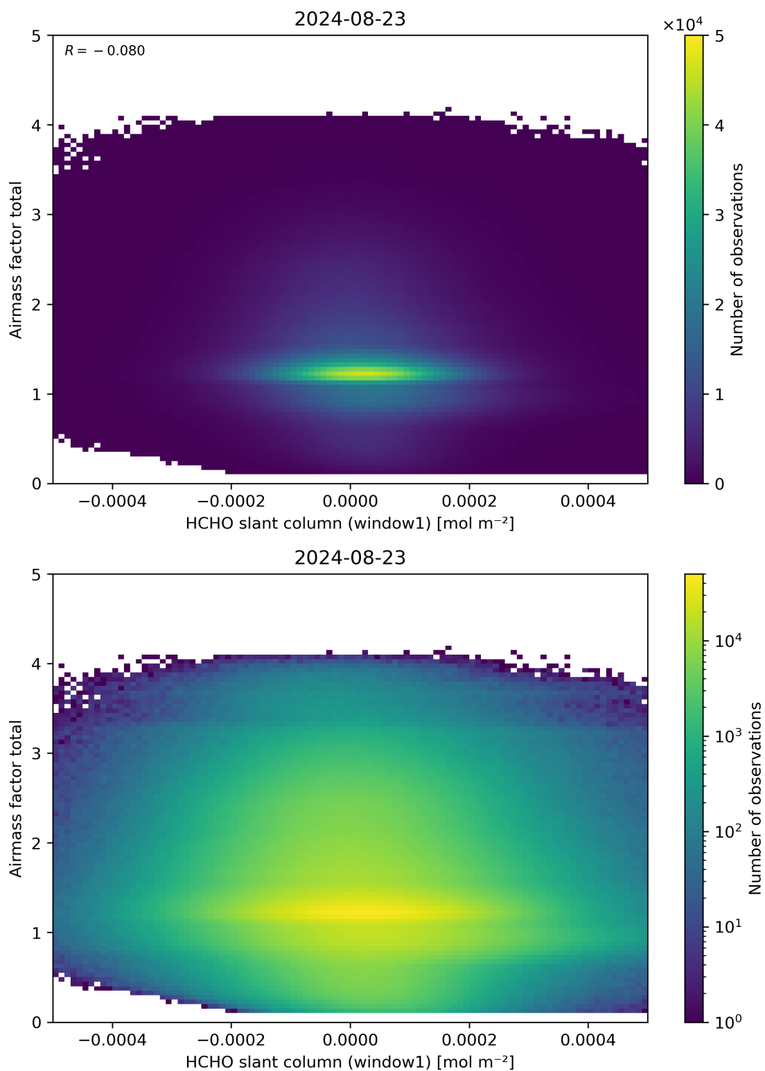
Figure 85: Scatter density plot of “HCHO slant column (window1)” against “Airmass factor total” for 2024-08-22 to 2024-08-24.
