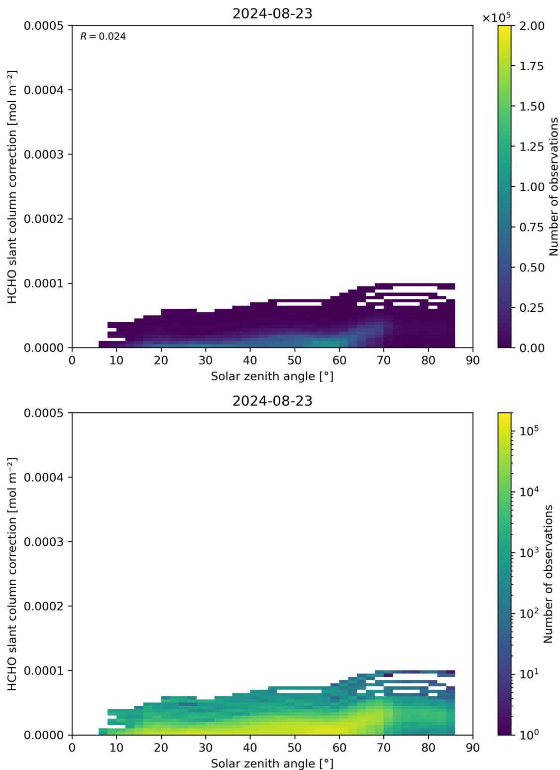
Figure 172: Scatter density plot of “Solar zenith angle” against “HCHO slant column correction” for 2024-08-22 to 2024-08-24.
