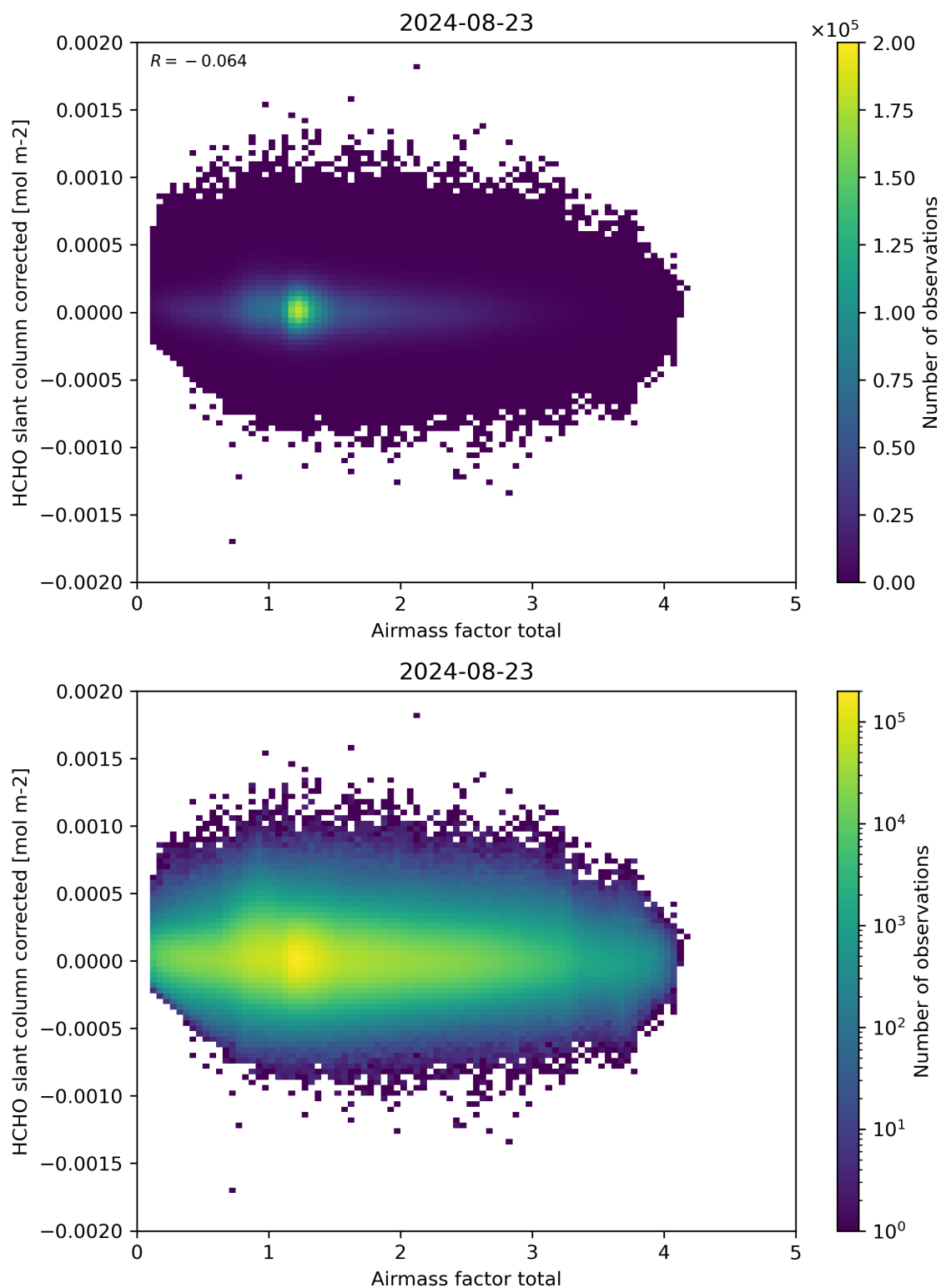
Figure 101: Scatter density plot of “Airmass factor total” against “HCHO slant column corrected” for 2024-08-22 to 2024-08-24.
