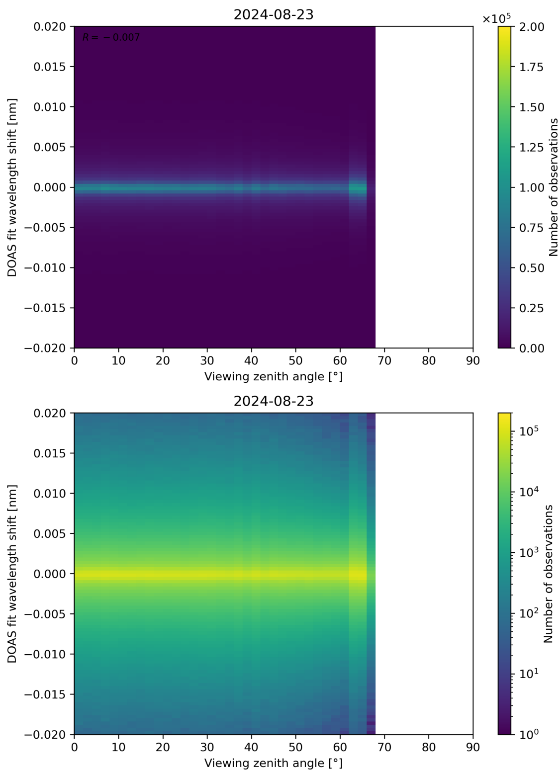
Figure 183: Scatter density plot of “Viewing zenith angle” against “DOAS fit wavelength shift” for 2024-08-22 to 2024-08-24.
