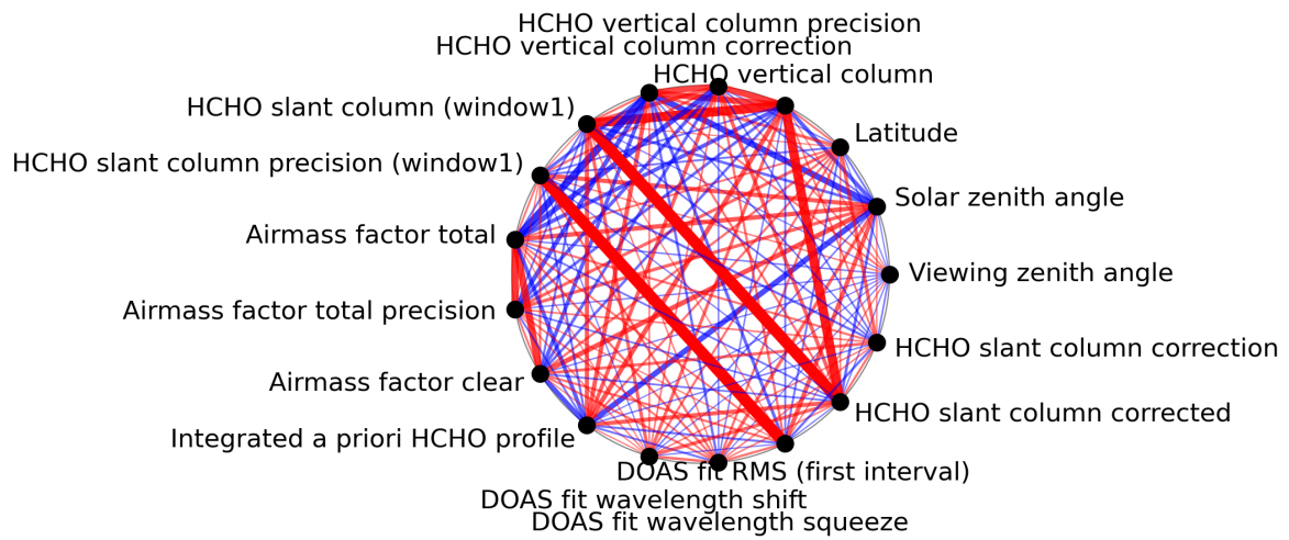
Figure 1: Map of correlation graph for 2024-08-22 to 2024-08-24.
