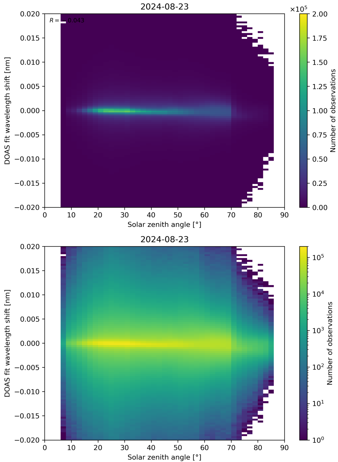
Figure 168: Scatter density plot of “Solar zenith angle” against “DOAS fit wavelength shift” for 2024-08-22 to 2024-08-24.
