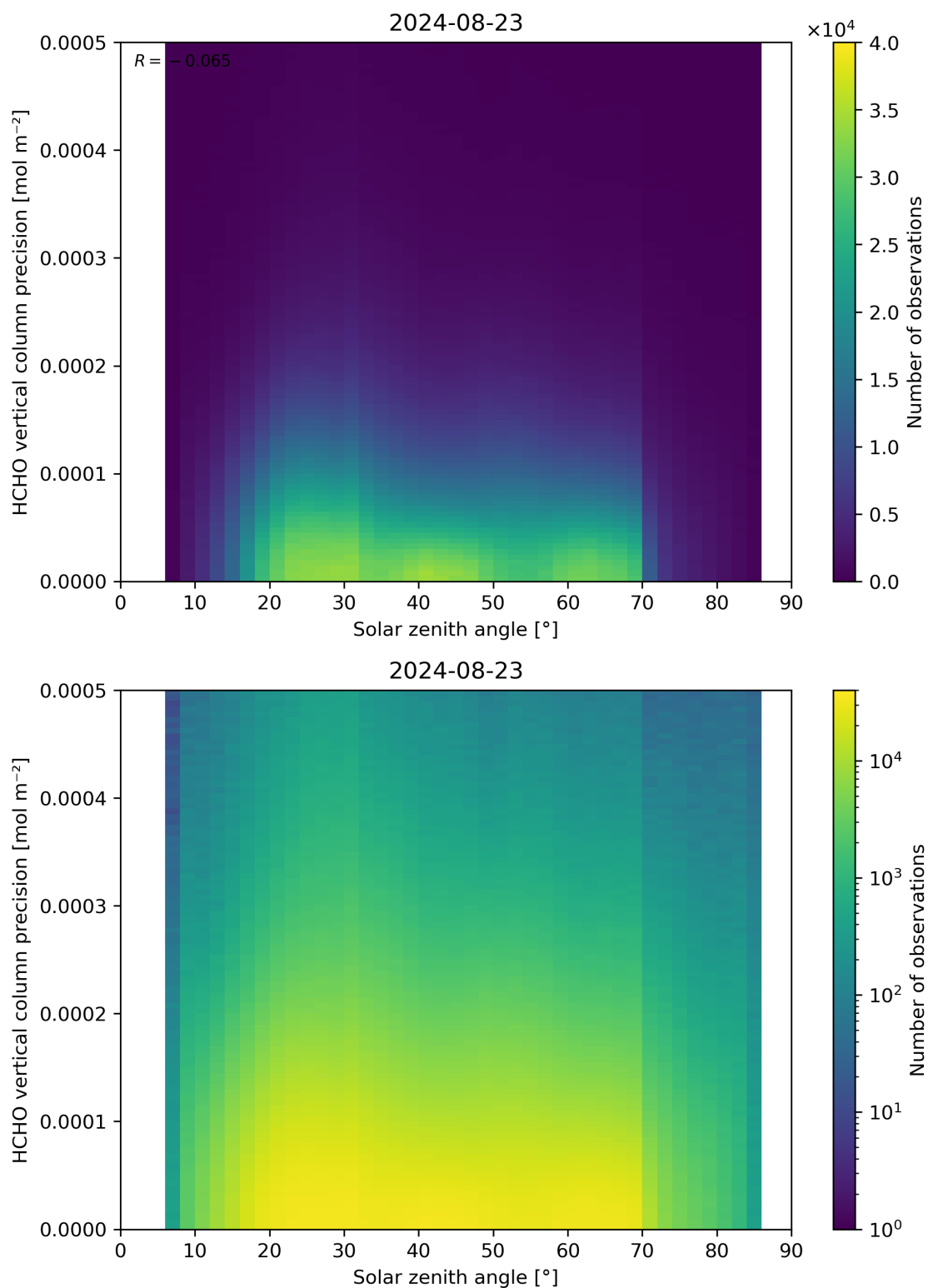
Figure 179: Scatter density plot of “Solar zenith angle” against “HCHO vertical column precision” for 2024-08-22 to 2024-08-24.
