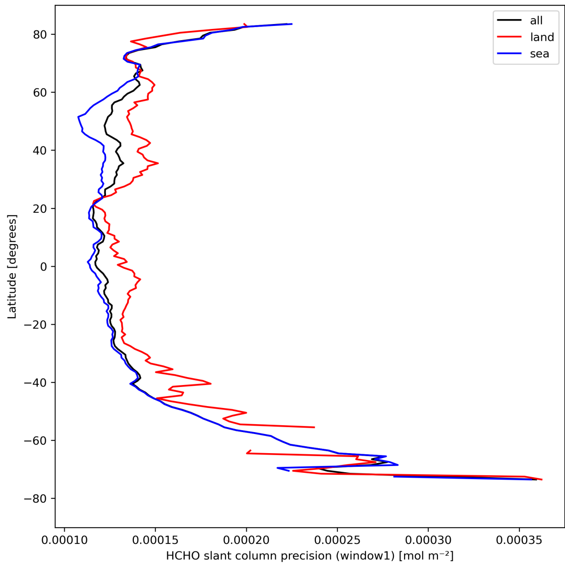
Figure 25: Zonal average of “HCHO slant column precision (window1)” for 2024-08-22 to 2024-08-24.
