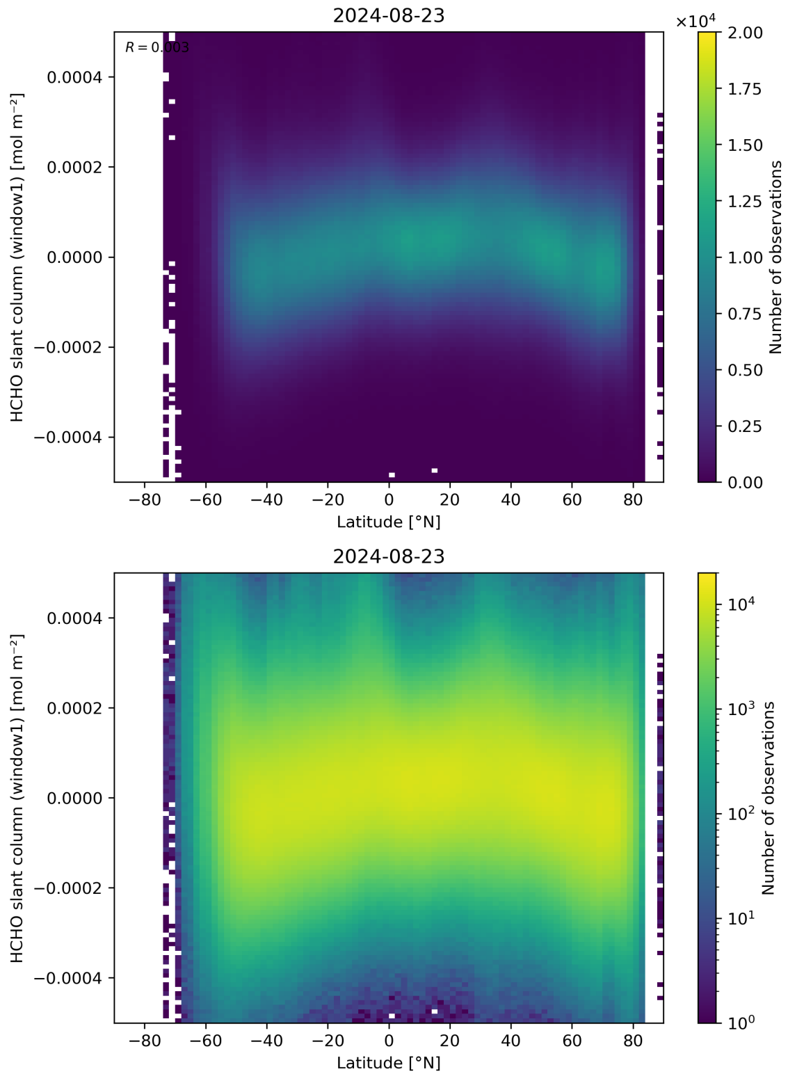
Figure 159: Scatter density plot of “Latitude” against “HCHO slant column (window1)” for 2024-08-22 to 2024-08-24.
