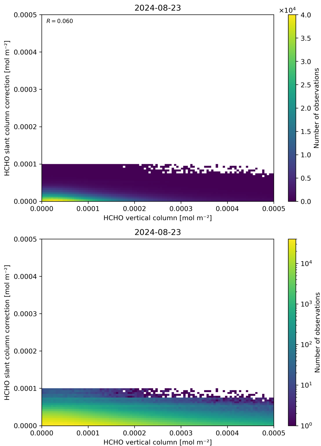
Figure 128: Scatter density plot of “HCHO vertical column” against “HCHO slant column correction” for 2024-08-22 to 2024-08-24.
