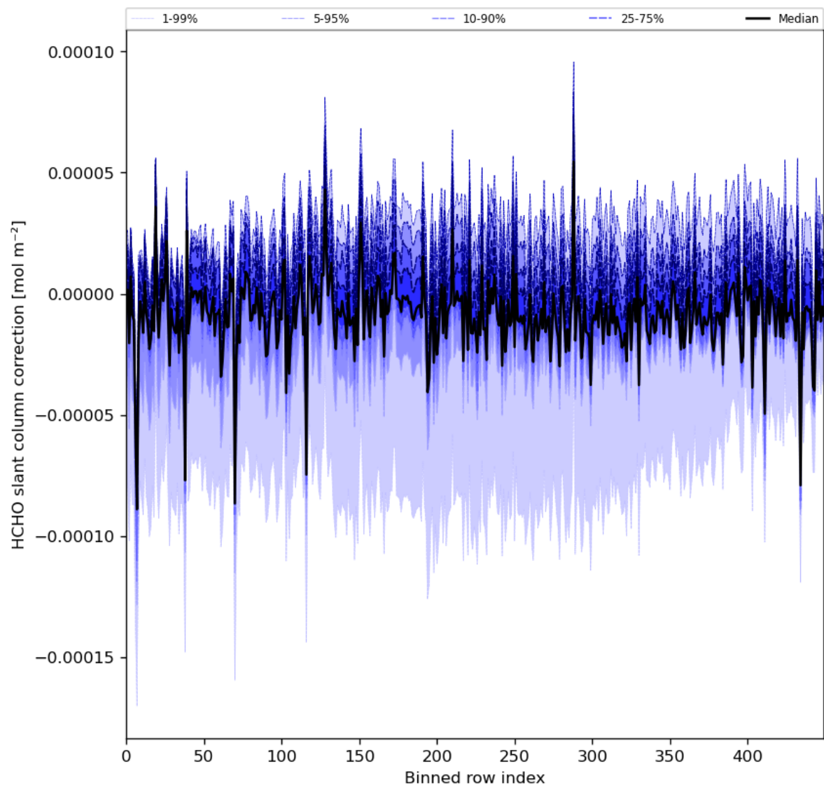
Figure 61: Along track statistics of “HCHO slant column correction” for 2024-08-22 to 2024-08-24
