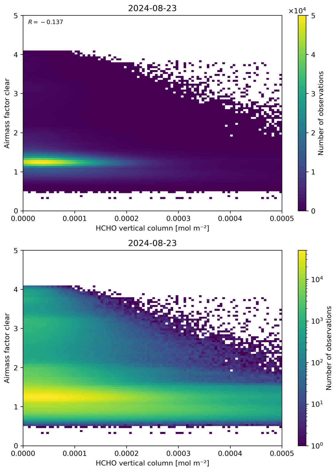
Figure 126: Scatter density plot of “HCHO vertical column” against “Airmass factor clear” for 2024-08-22 to 2024-08-24.
