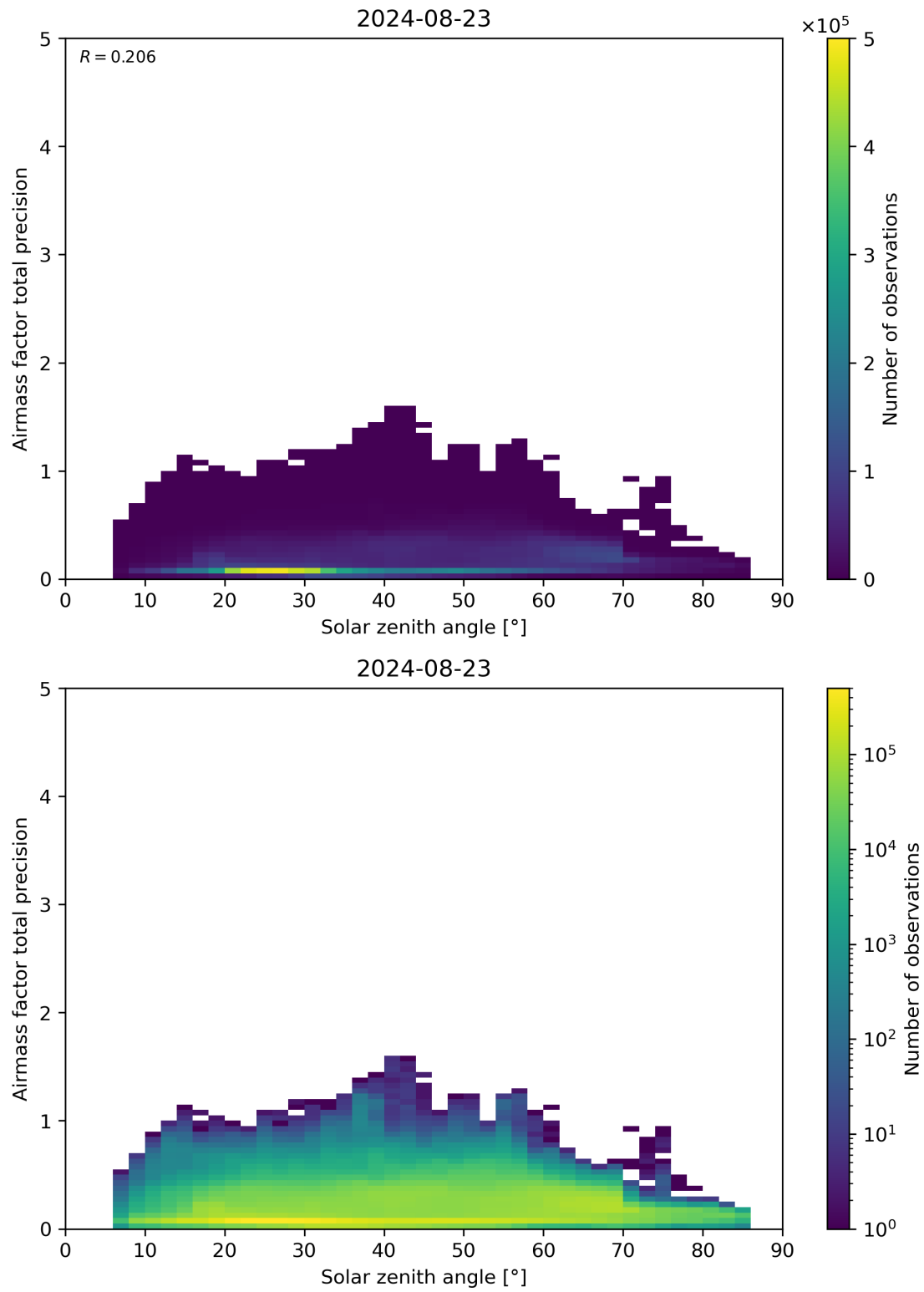
Figure 176: Scatter density plot of “Solar zenith angle” against “Airmass factor total precision” for 2024-08-22 to 2024-08-24.
