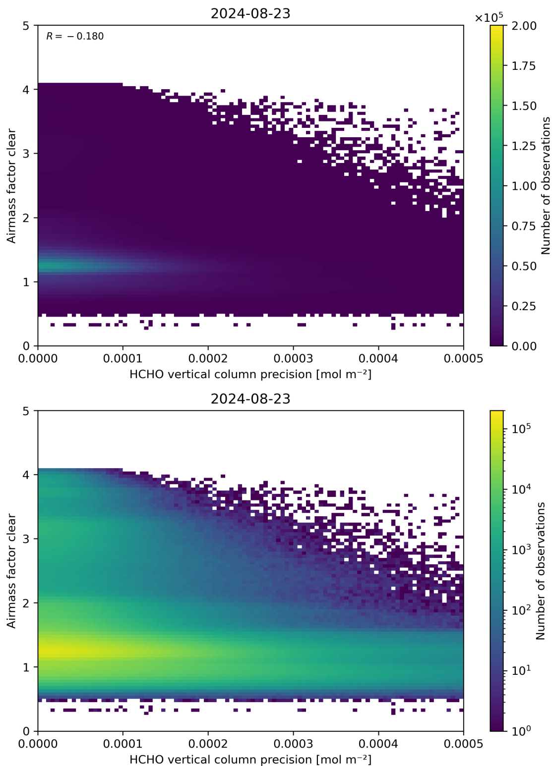
Figure 139: Scatter density plot of “HCHO vertical column precision” against “Airmass factor clear” for 2024-08-22 to 2024-08-24.
