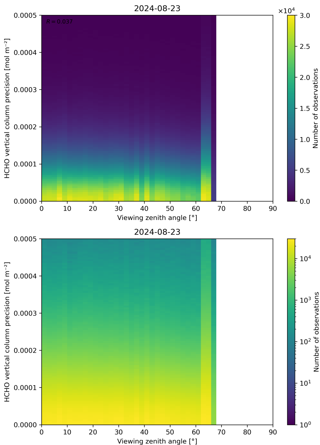
Figure 194: Scatter density plot of “Viewing zenith angle” against “HCHO vertical column precision” for 2024-08-22 to 2024-08-24.
