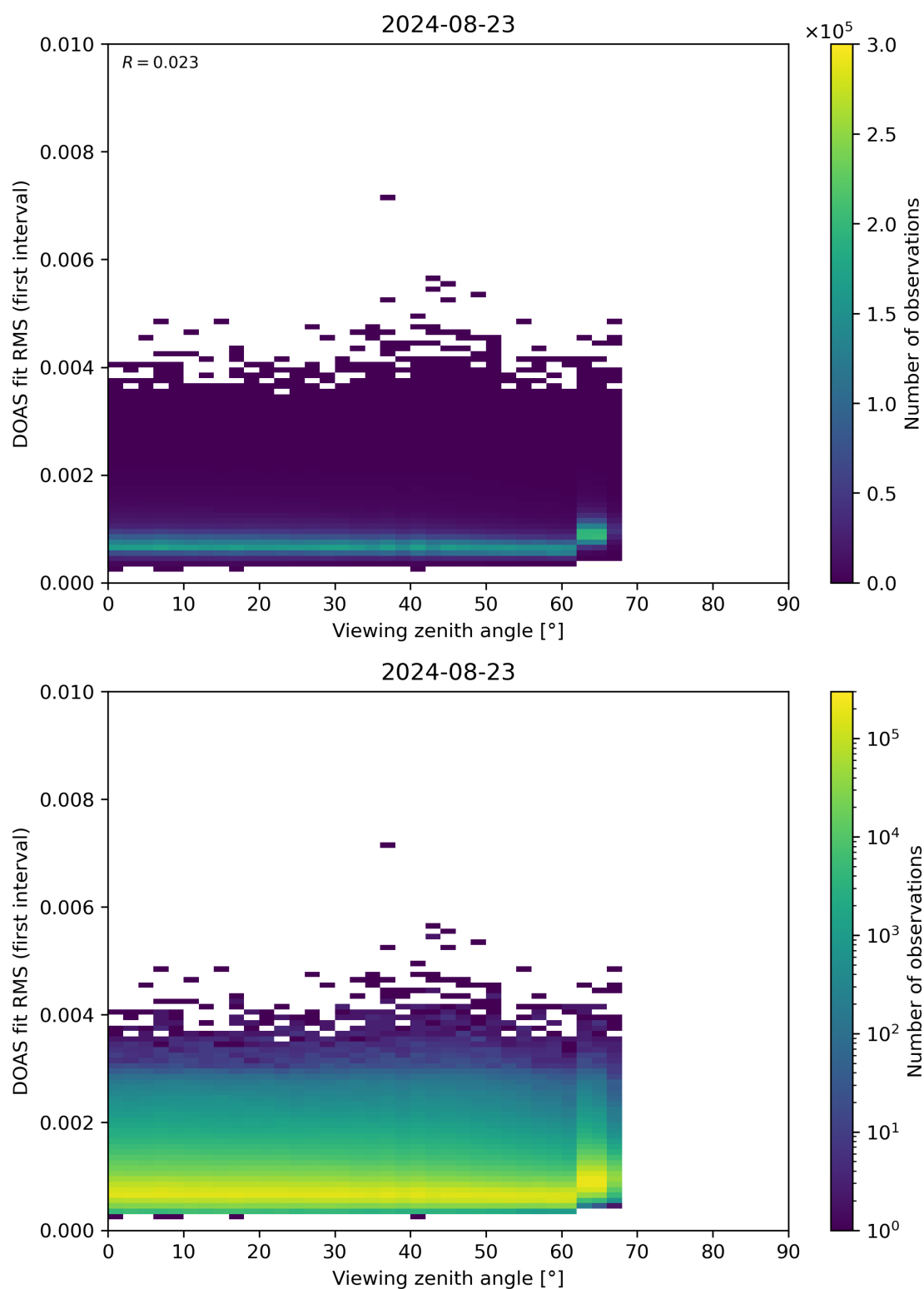
Figure 182: Scatter density plot of “Viewing zenith angle” against “DOAS fit RMS (first interval)” for 2024-08-22 to 2024-08-24.
