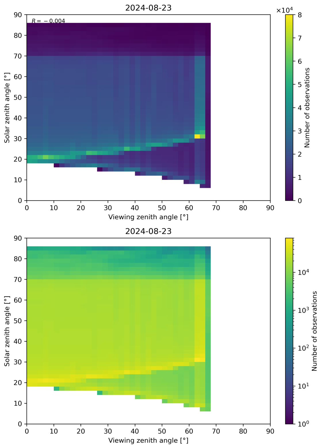
Figure 197: Scatter density plot of “Viewing zenith angle” against “Solar zenith angle” for 2024-08-22 to 2024-08-24.
