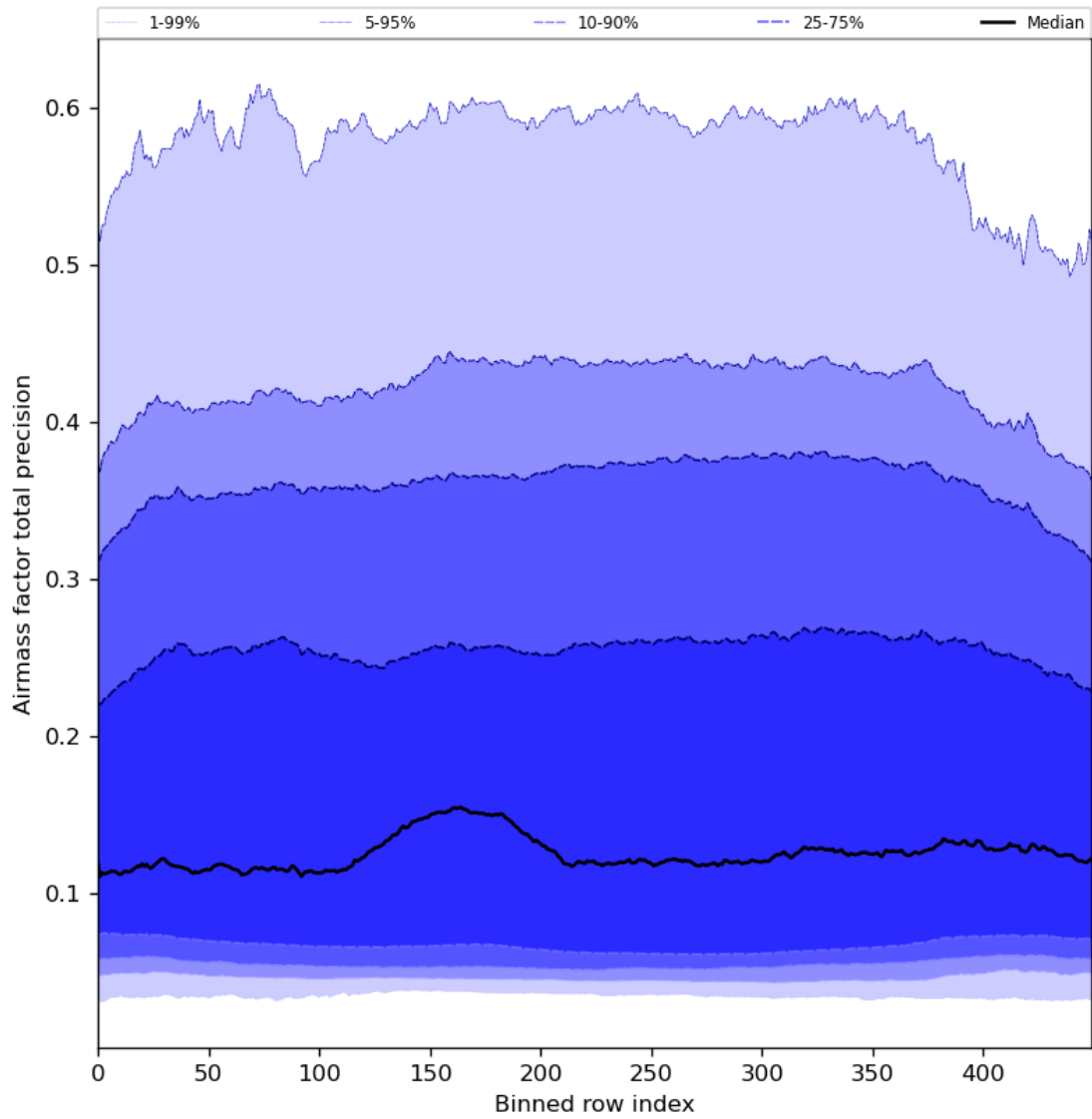
Figure 55: Along track statistics of “Airmass factor total precision” for 2024-08-22 to 2024-08-24
