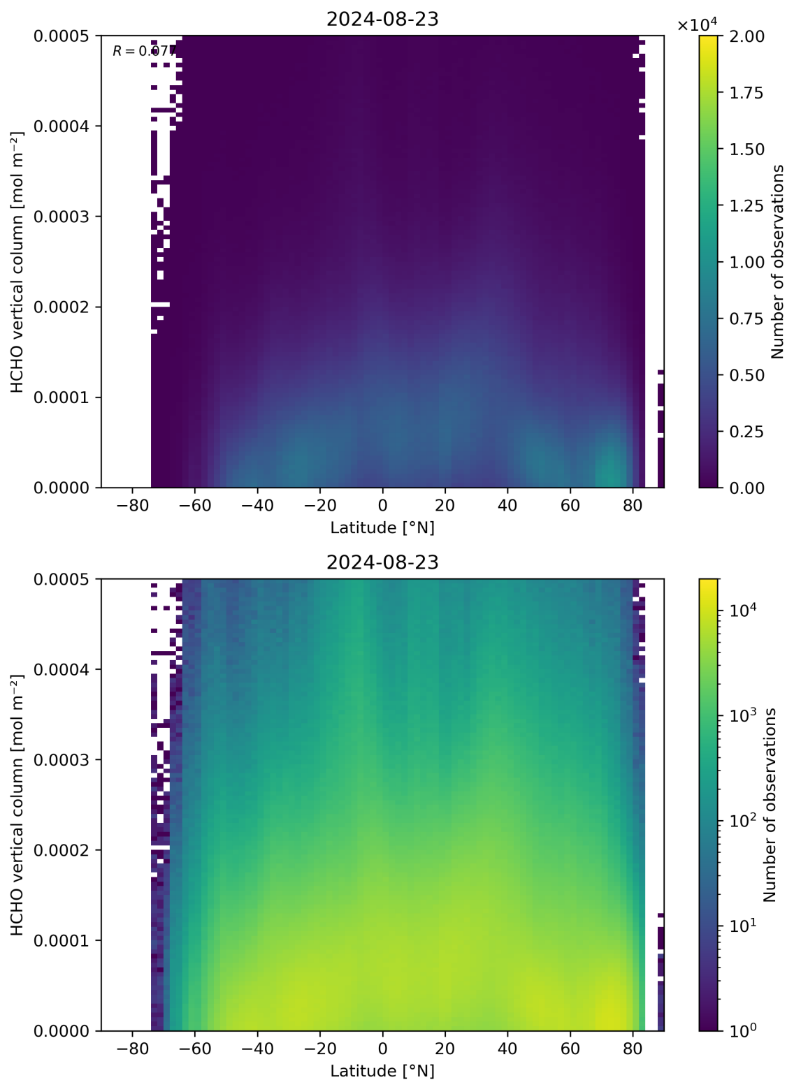
Figure 163: Scatter density plot of “Latitude” against “HCHO vertical column” for 2024-08-22 to 2024-08-24.
