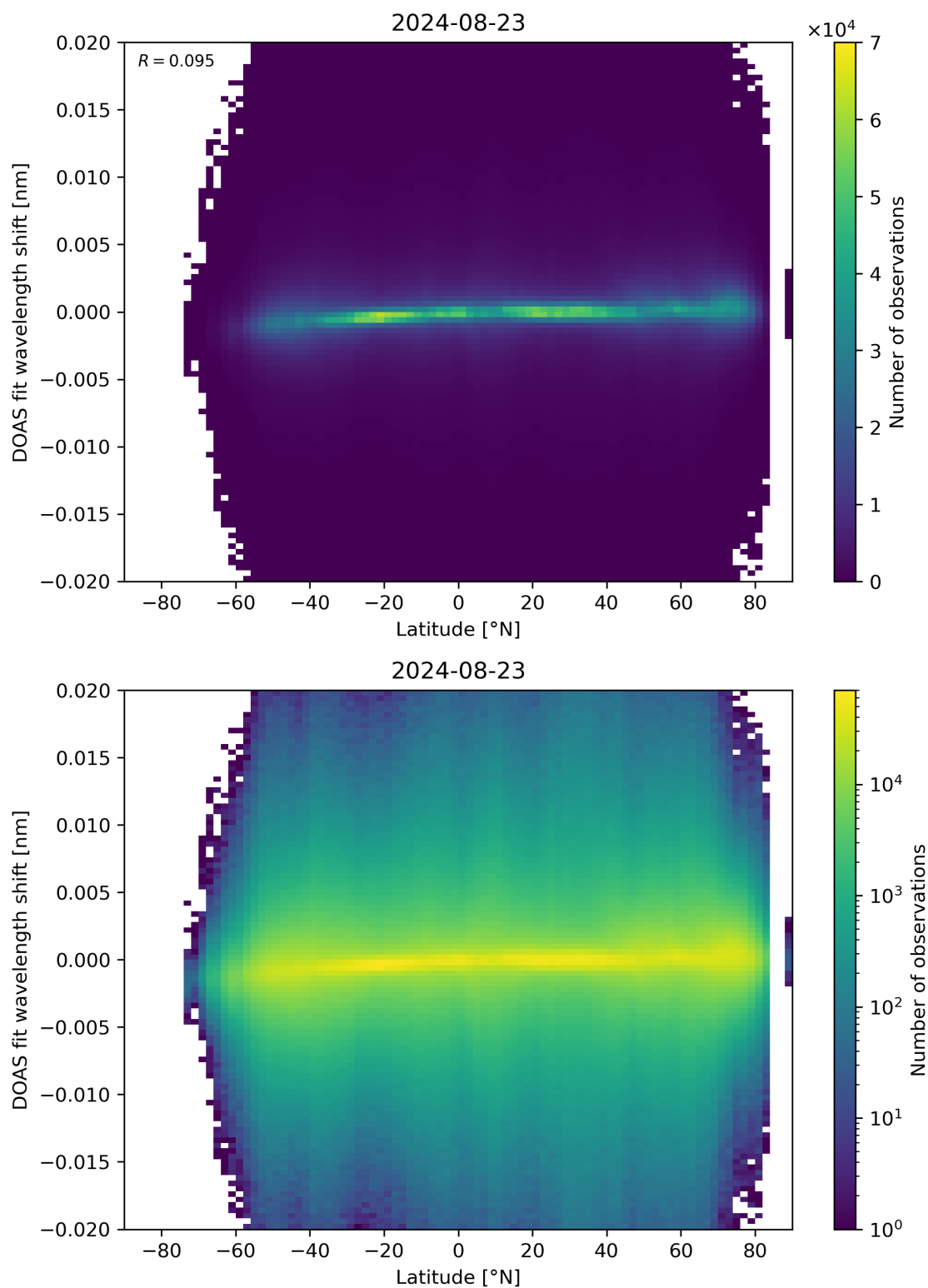
Figure 154: Scatter density plot of “Latitude” against “DOAS fit wavelength shift” for 2024-08-22 to 2024-08-24.
