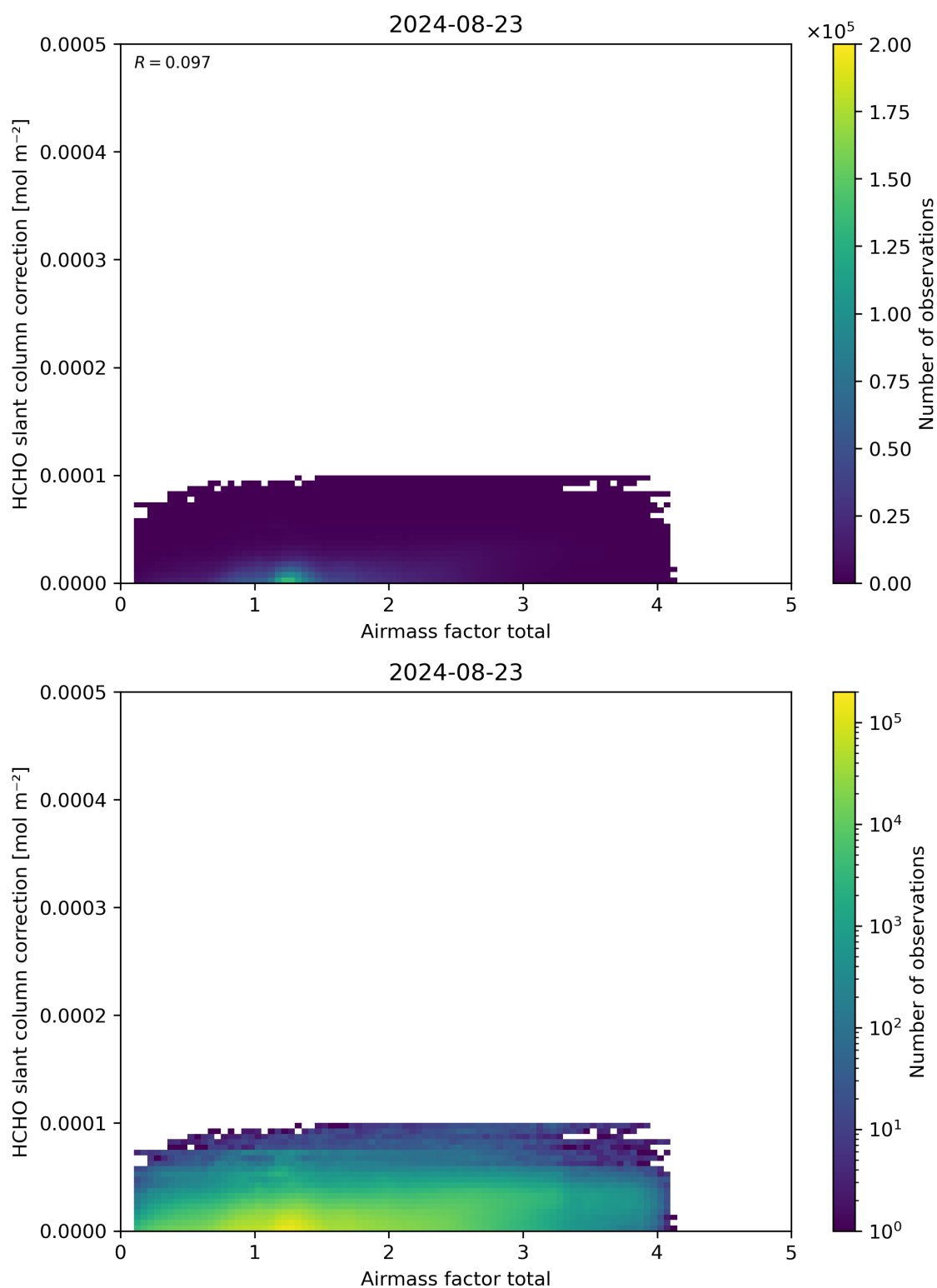
Figure 102: Scatter density plot of “Airmass factor total” against “HCHO slant column correction” for 2024-08-22 to 2024-08-24.
