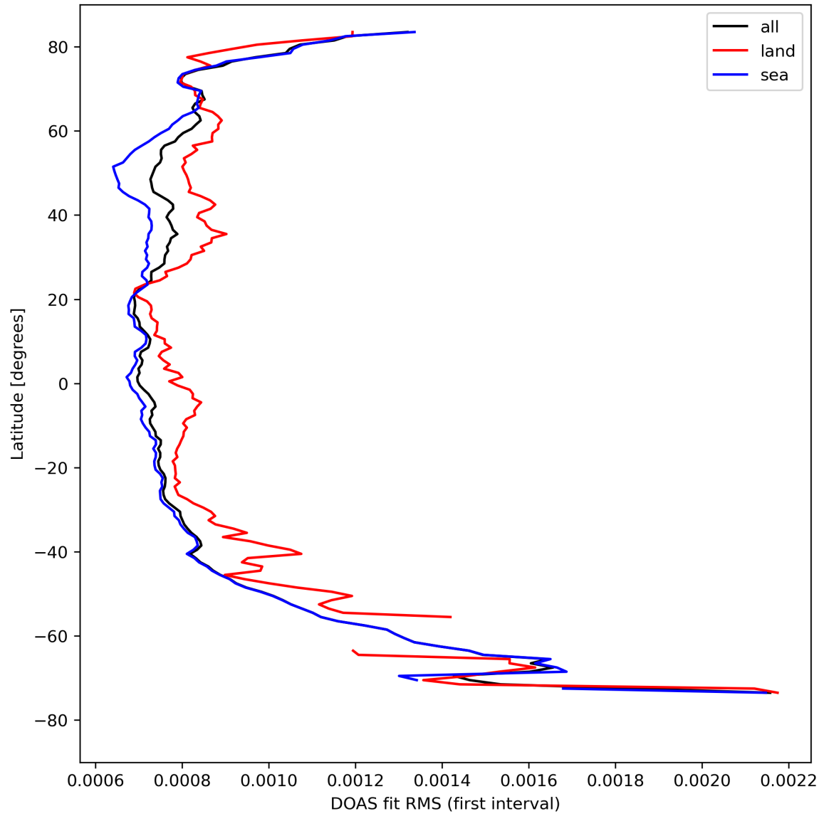
Figure 32: Zonal average of “DOAS fit RMS (first interval)” for 2024-08-22 to 2024-08-24.
