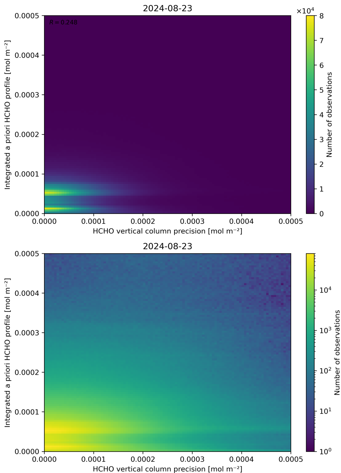
Figure 147: Scatter density plot of “HCHO vertical column precision” against “Integrated a priori HCHO profile” for 2024-08-22 to 2024-08-24.
