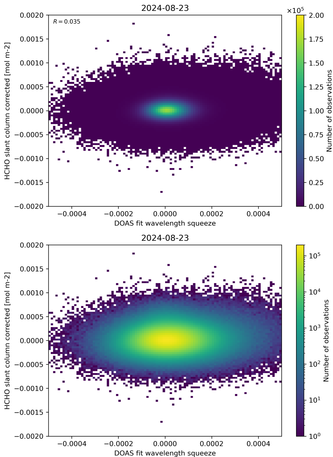
Figure 69: Scatter density plot of “DOAS fit wavelength squeeze” against “HCHO slant column corrected” for 2024-08-22 to 2024-08-24.
