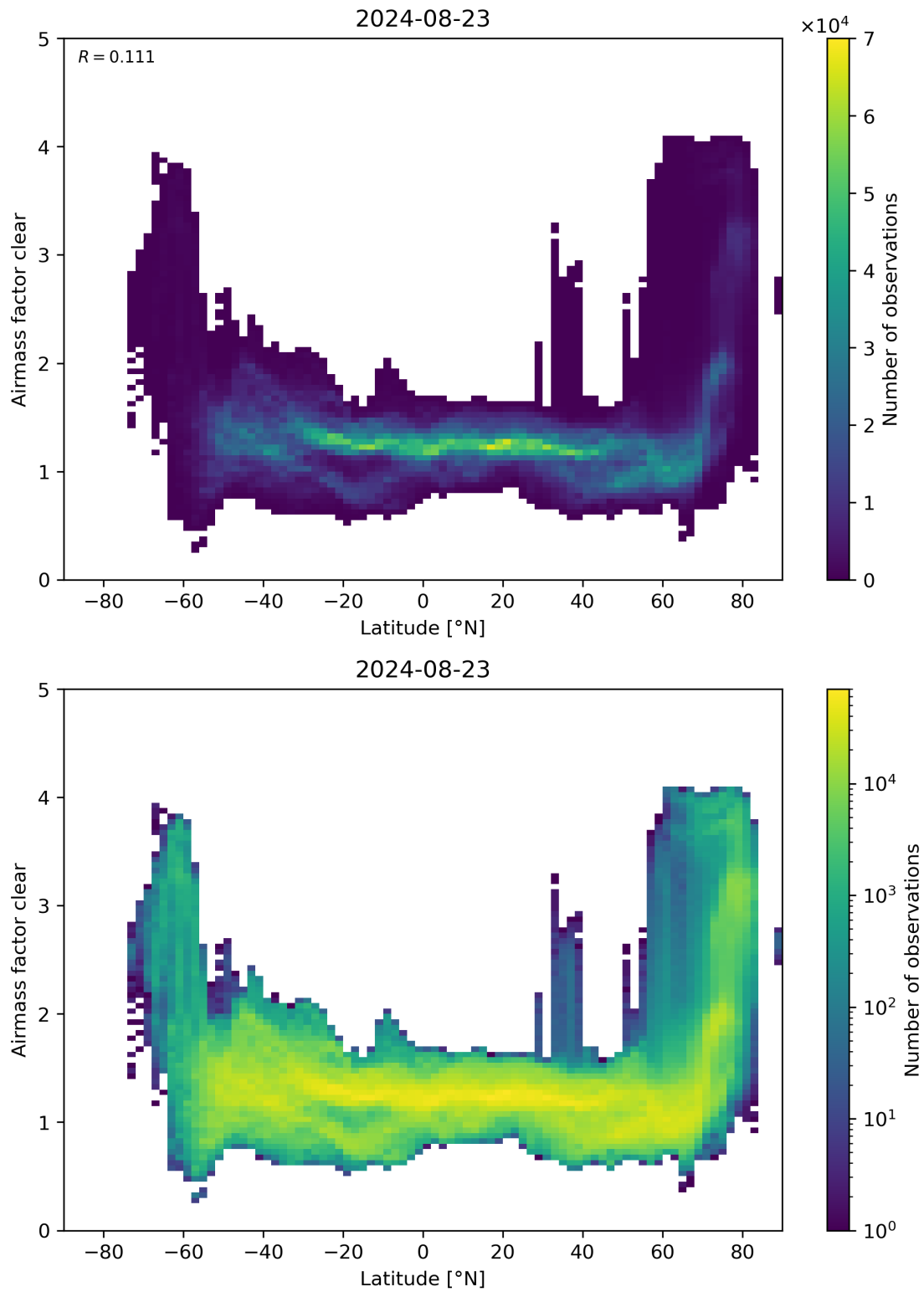
Figure 156: Scatter density plot of “Latitude” against “Airmass factor clear” for 2024-08-22 to 2024-08-24.
