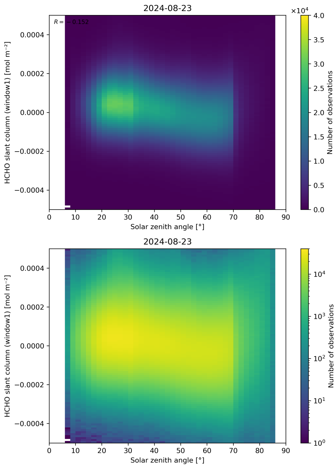
Figure 173: Scatter density plot of “Solar zenith angle” against “HCHO slant column (window1)” for 2024-08-22 to 2024-08-24.
