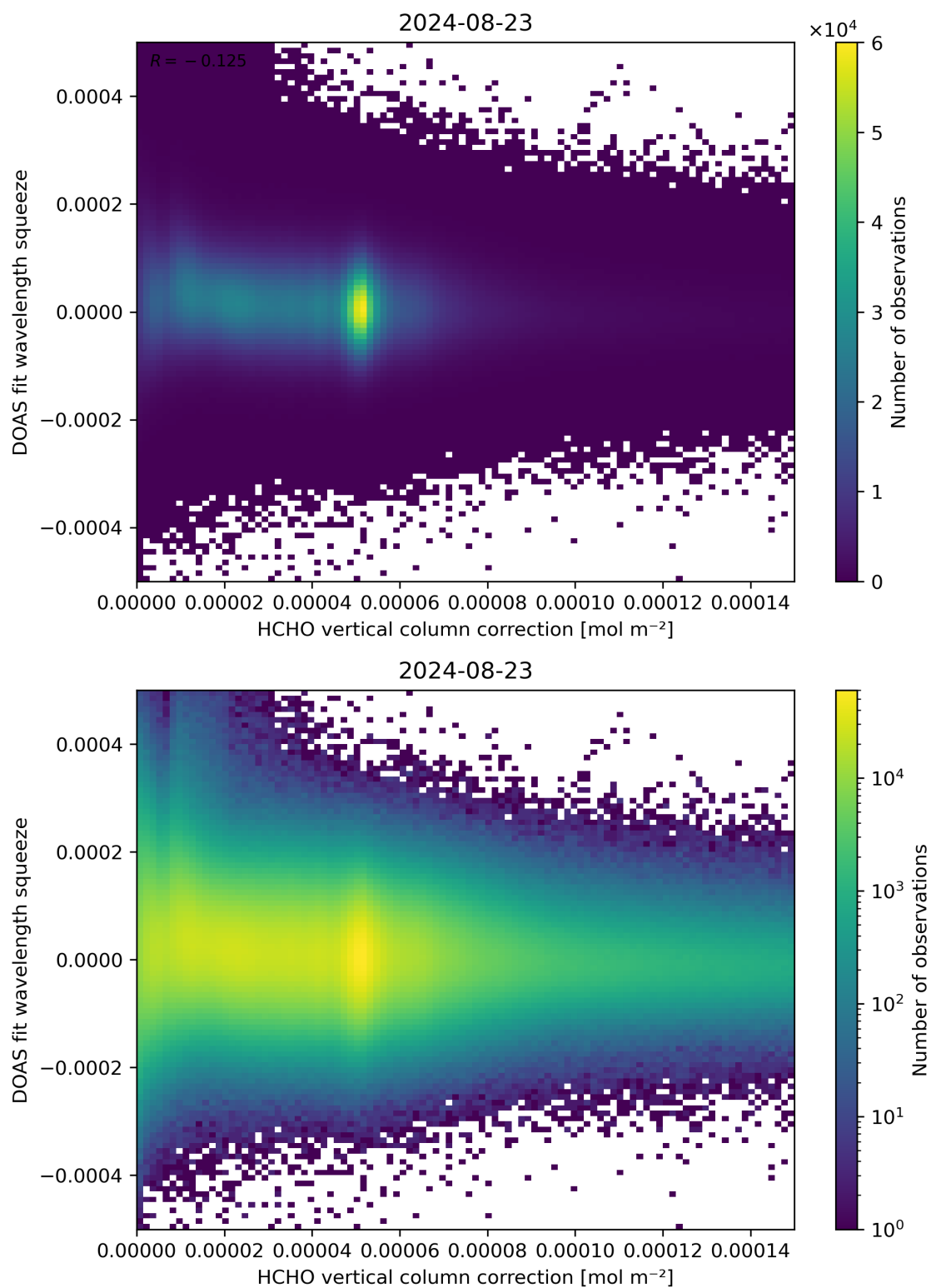
Figure 114: Scatter density plot of “HCHO vertical column correction” against “DOAS fit wavelength squeeze” for 2024-08-22 to 2024-08-24.
