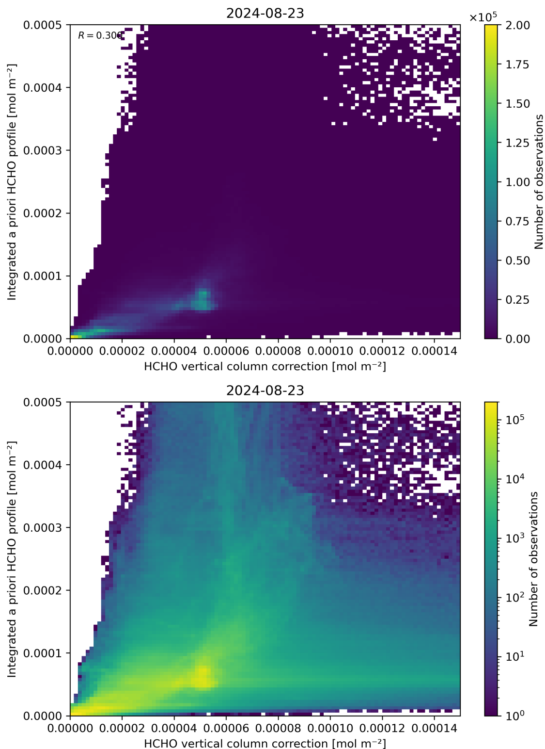
Figure 122: Scatter density plot of “HCHO vertical column correction” against “Integrated a priori HCHO profile” for 2024-08-22 to 2024-08-24.
