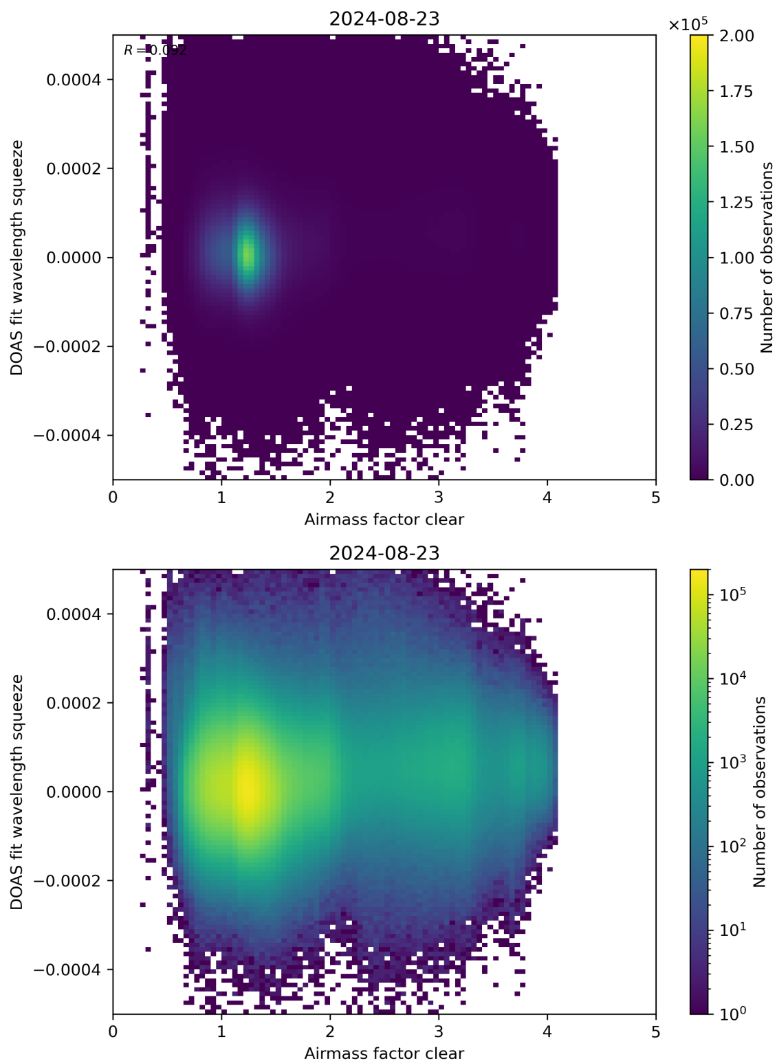
Figure 73: Scatter density plot of “Airmass factor clear” against “DOAS fit wavelength squeeze” for 2024-08-22 to 2024-08-24.
