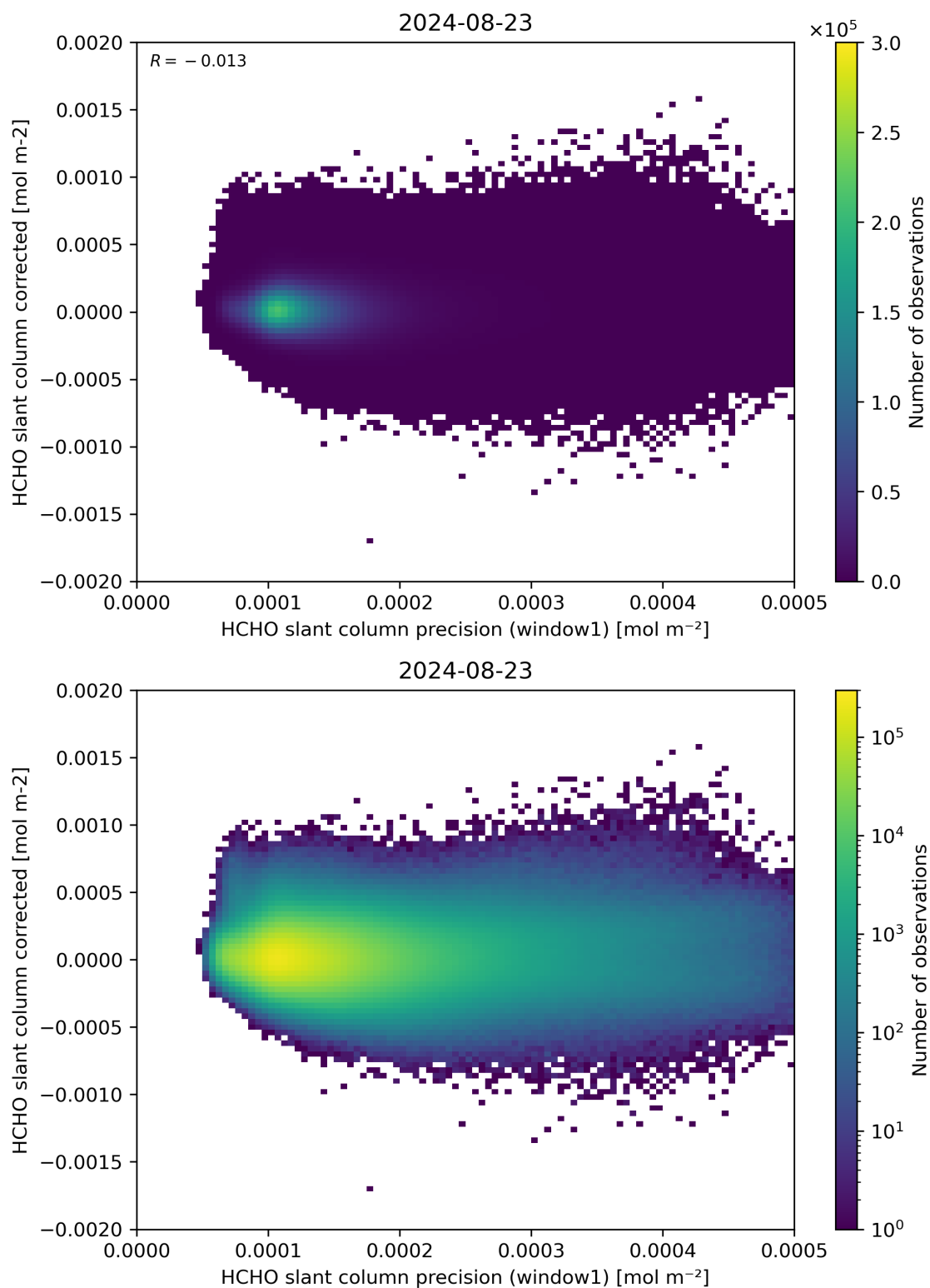
Figure 92: Scatter density plot of “HCHO slant column precision (window1)” against “HCHO slant column corrected” for 2024-08-22 to 2024-08-24.
