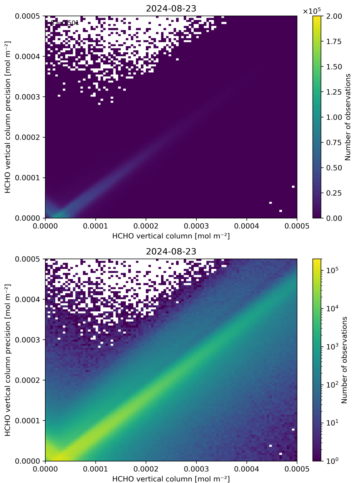
Figure 134: Scatter density plot of “HCHO vertical column” against “HCHO vertical column precision” for 2024-08-22 to 2024-08-24.
