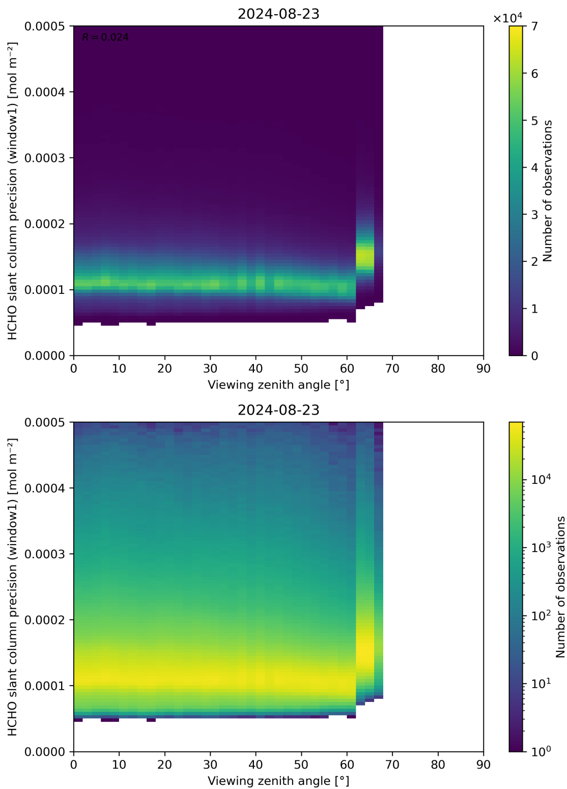
Figure 189: Scatter density plot of “Viewing zenith angle” against “HCHO slant column precision (window1)” for 2024-08-22 to 2024-08-24.
