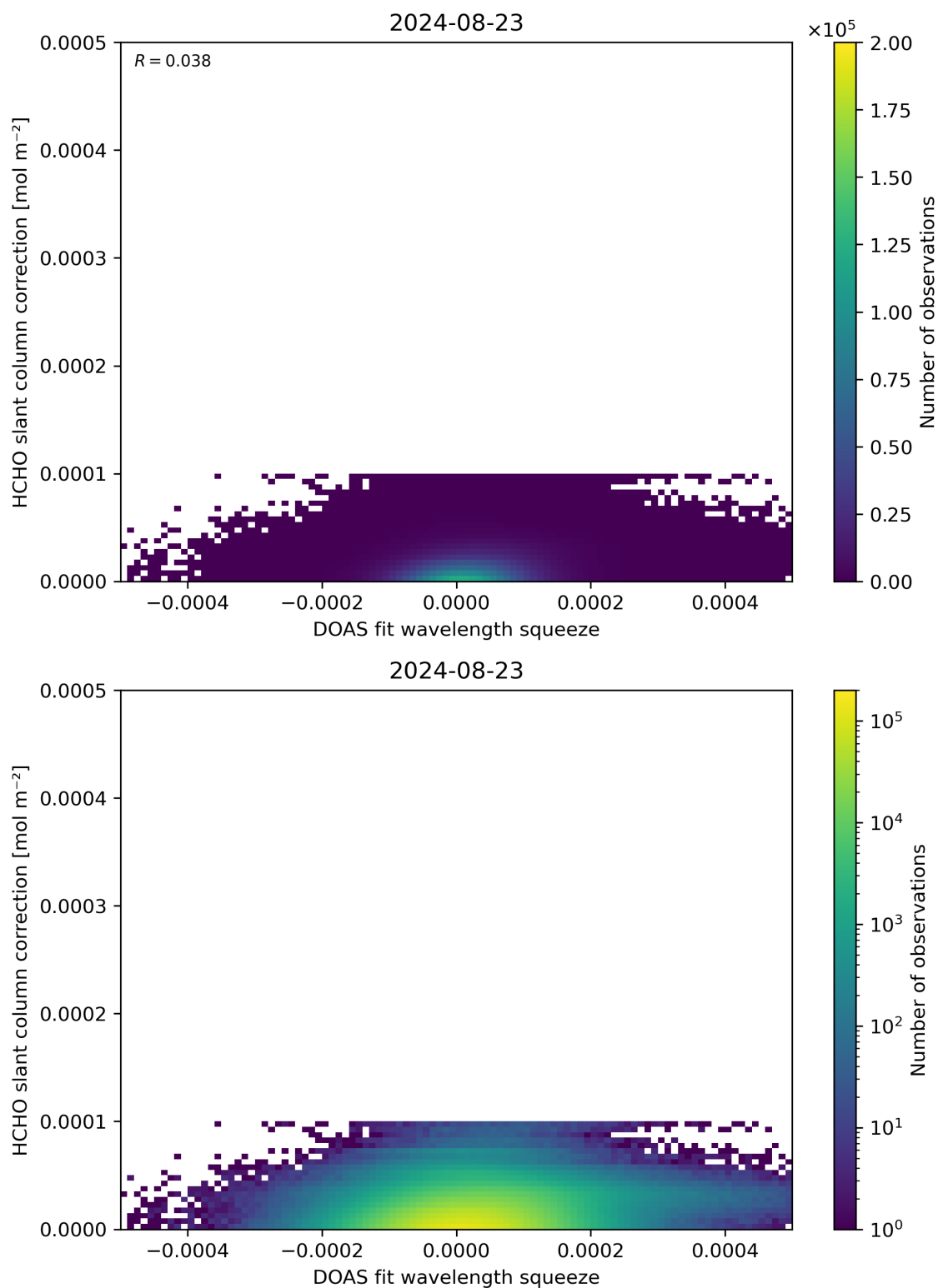
Figure 70: Scatter density plot of “DOAS fit wavelength squeeze” against “HCHO slant column correction” for 2024-08-22 to 2024-08-24.
