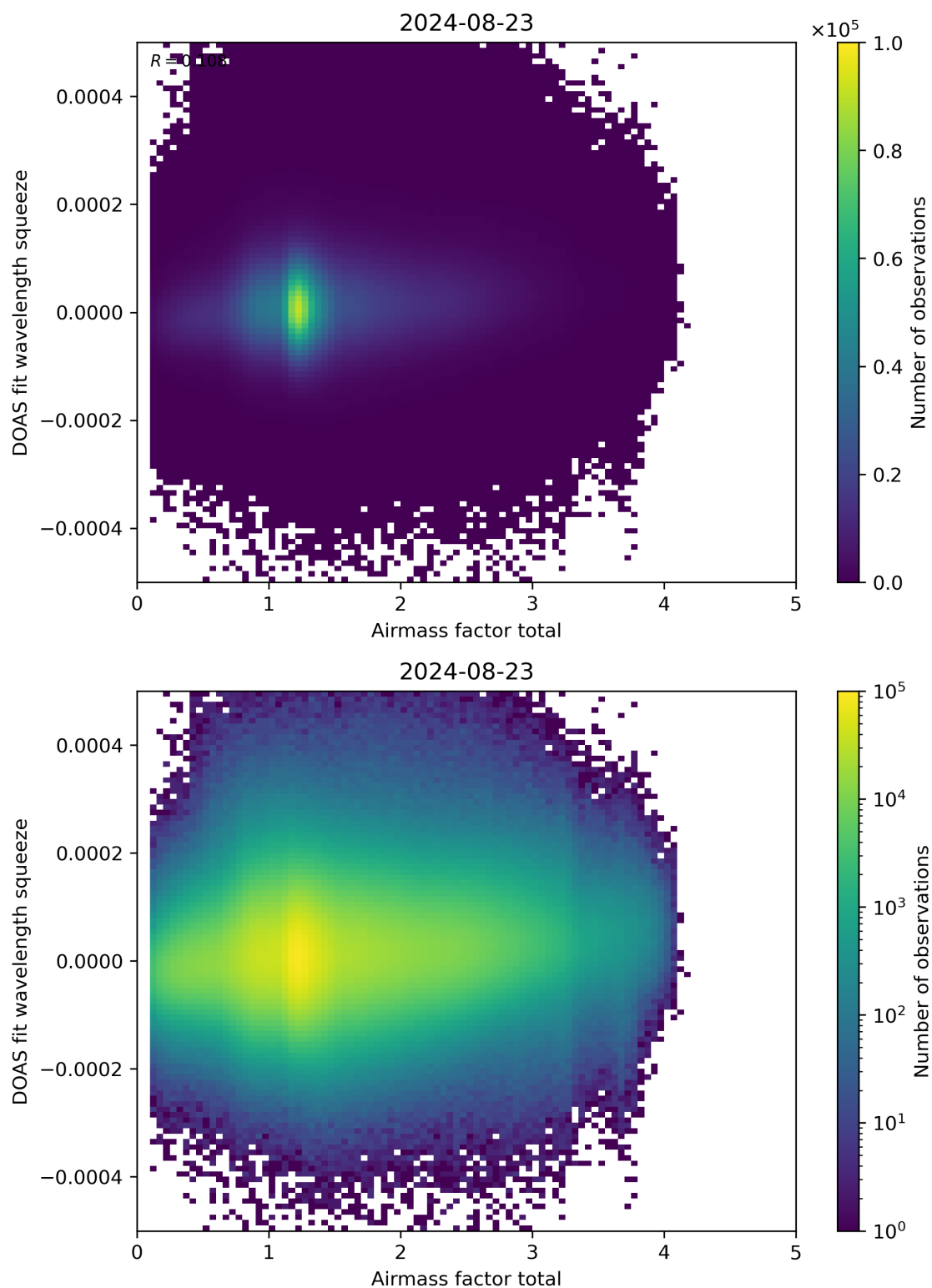
Figure 99: Scatter density plot of “Airmass factor total” against “DOAS fit wavelength squeeze” for 2024-08-22 to 2024-08-24.
