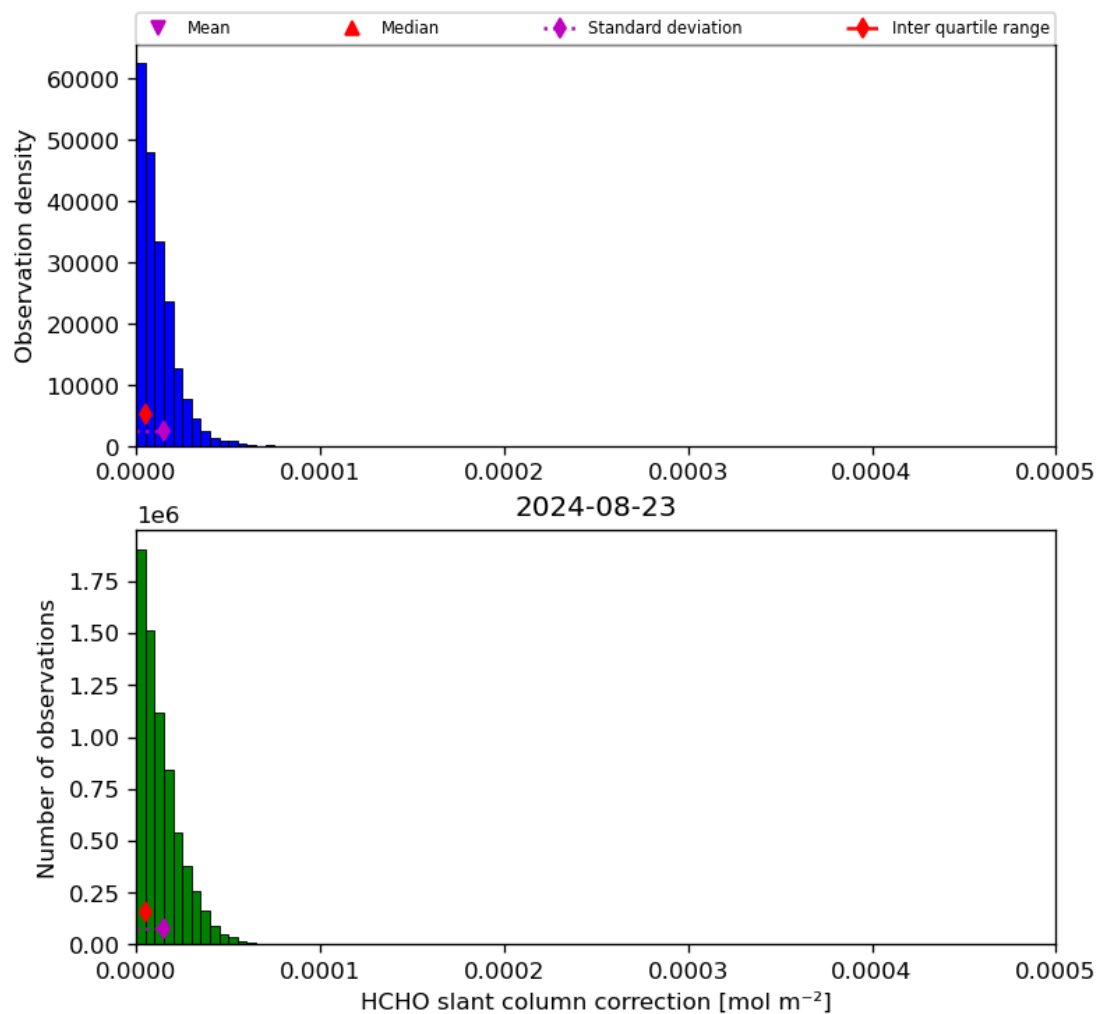
Figure 47: Histogram of “HCHO slant column correction” for 2024-08-22 to 2024-08-24
