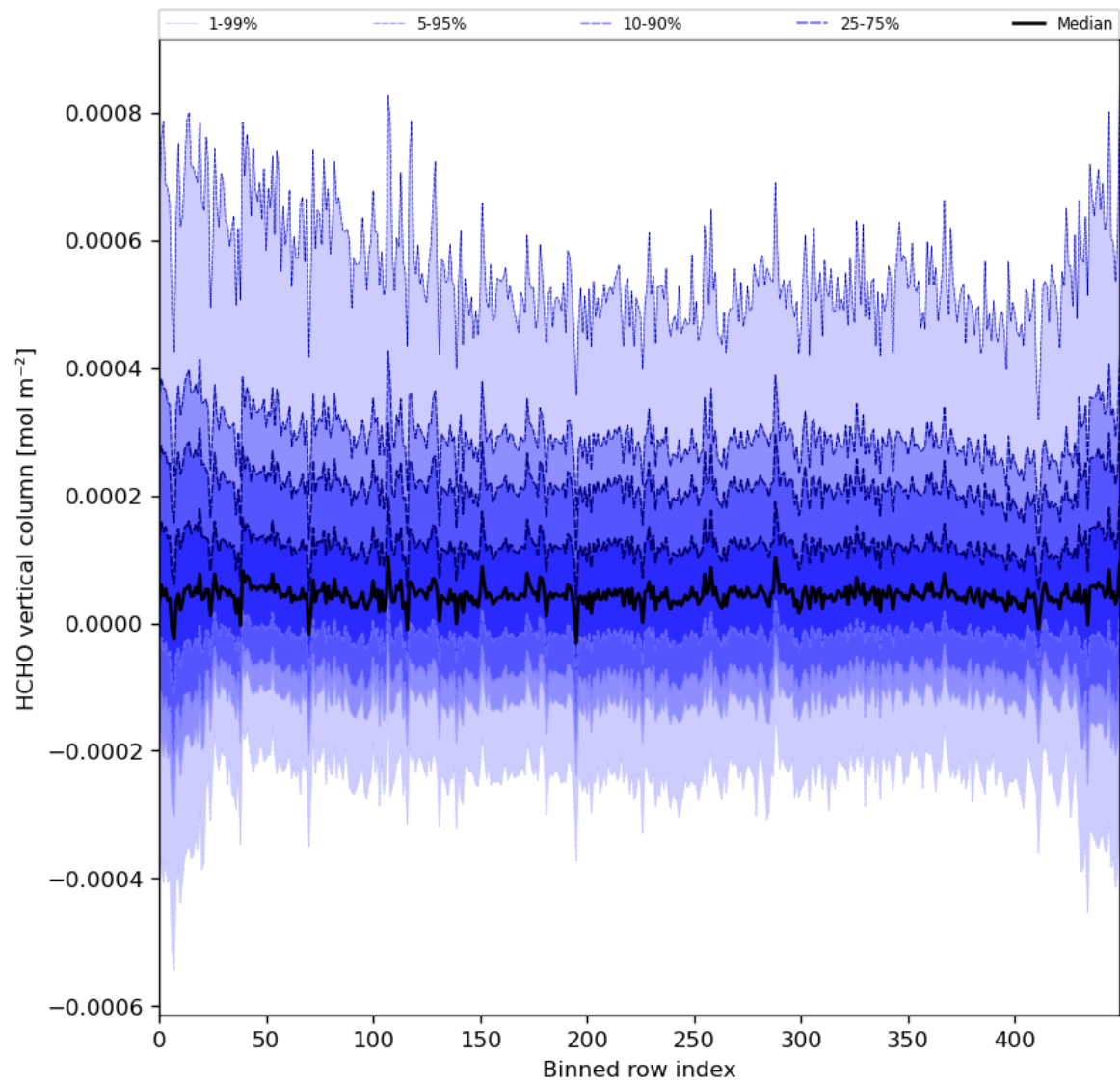
Figure 49: Along track statistics of “HCHO vertical column” for 2024-08-22 to 2024-08-24
