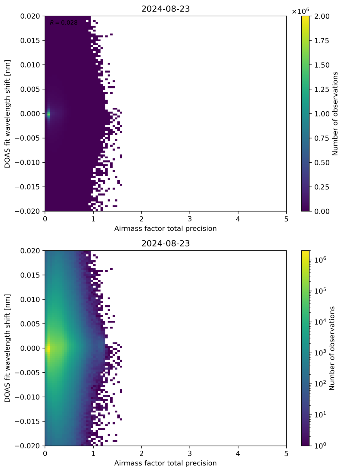
Figure 106: Scatter density plot of “Airmass factor total precision” against “DOAS fit wavelength shift” for 2024-08-22 to 2024-08-24.
