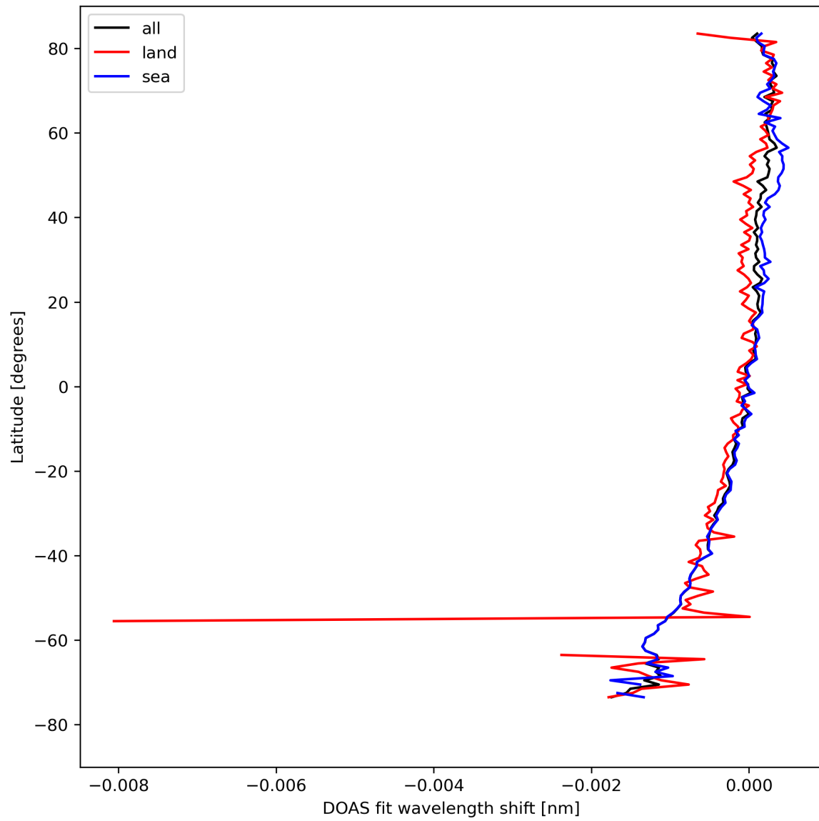
Figure 30: Zonal average of "DOAS fit wavelength shift" for 2024-08-22 to 2024-08-24.
