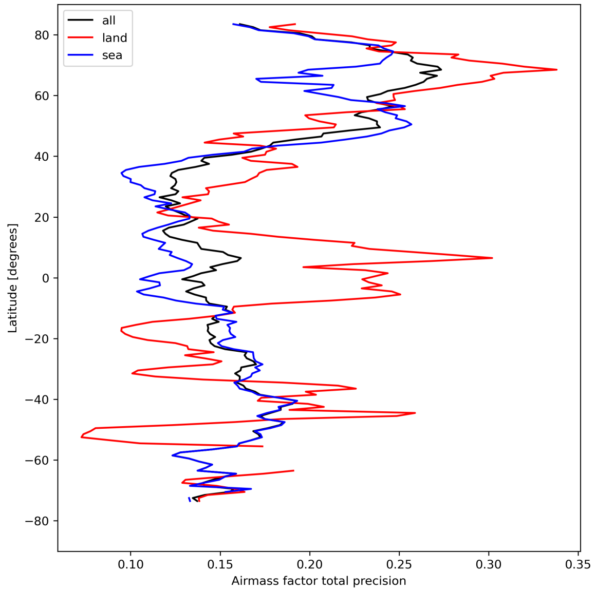
Figure 27: Zonal average of “Airmass factor total precision” for 2024-08-22 to 2024-08-24.
