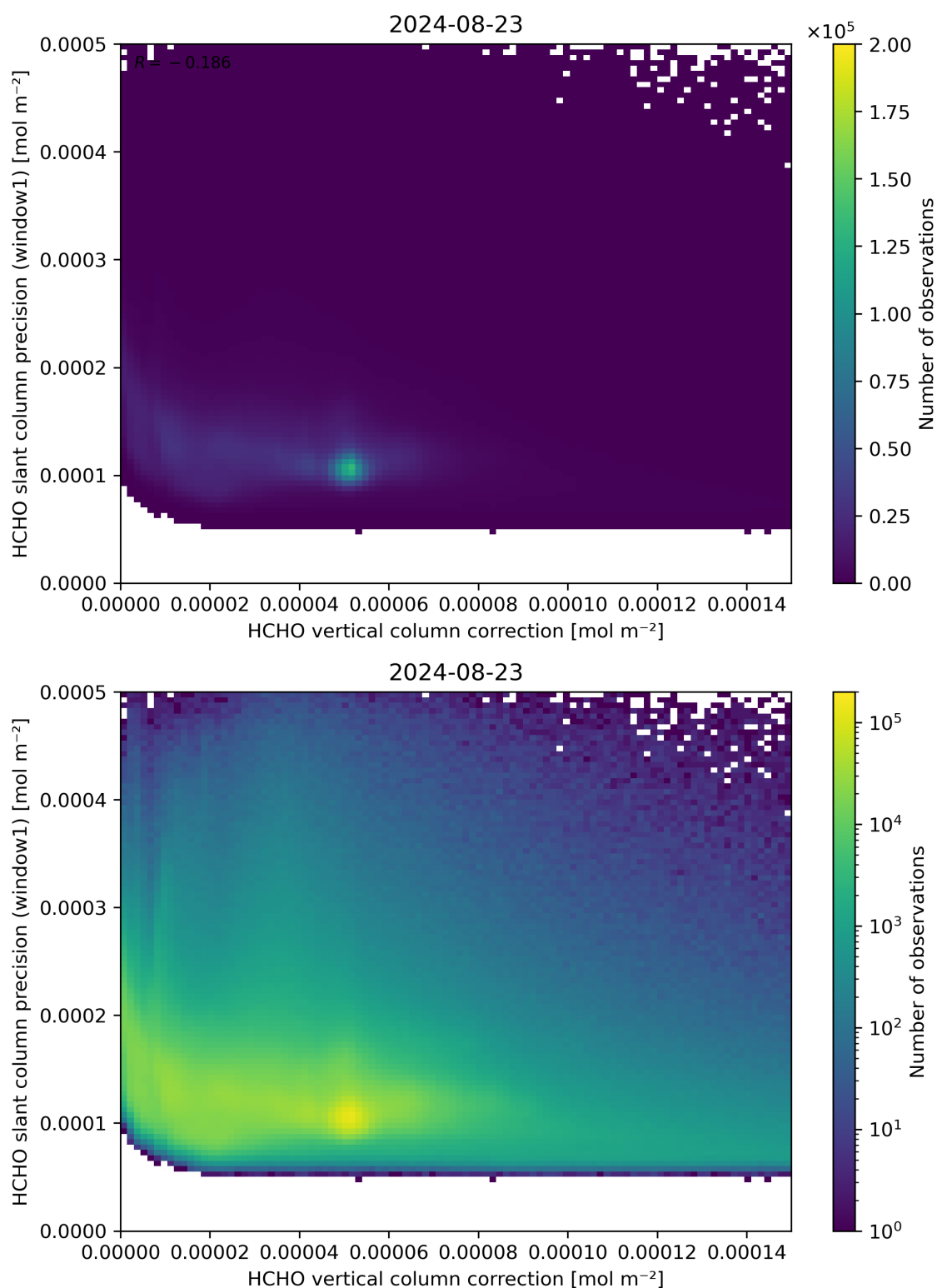
Figure 119: Scatter density plot of “HCHO vertical column correction” against “HCHO slant column precision (window1)” for 2024-08-22 to 2024-08-24.
