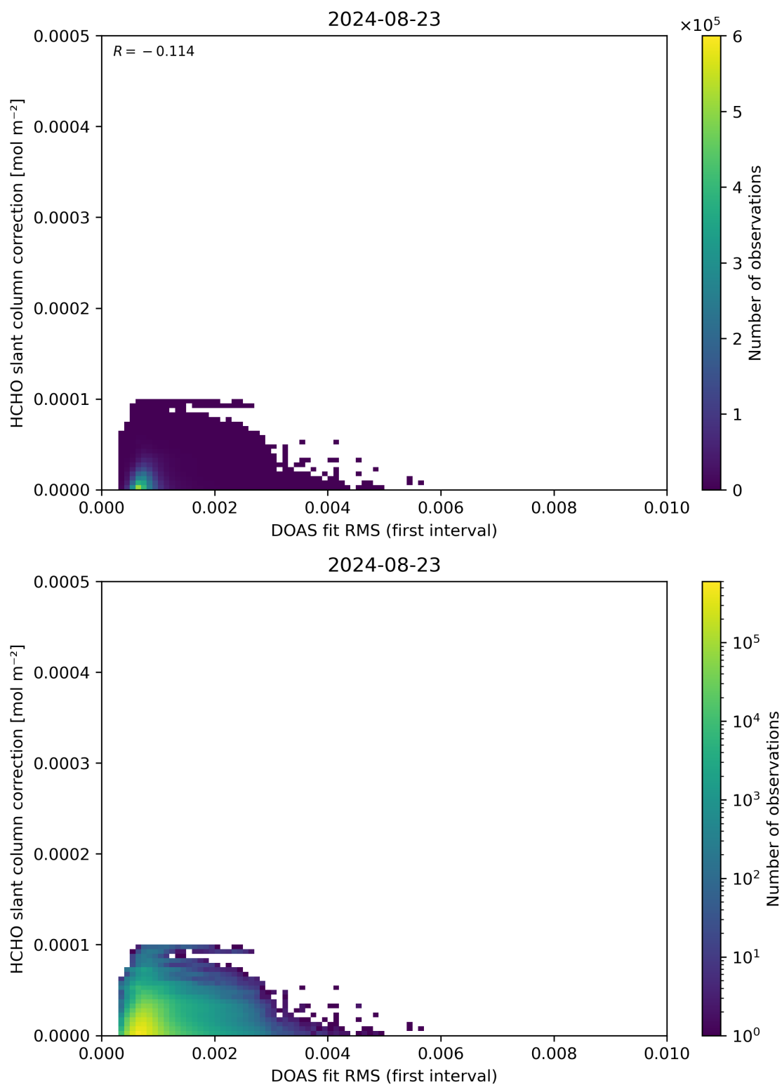
Figure 63: Scatter density plot of “DOAS fit RMS (first interval)” against “HCHO slant column correction” for 2024-08-22 to 2024-08-24.
