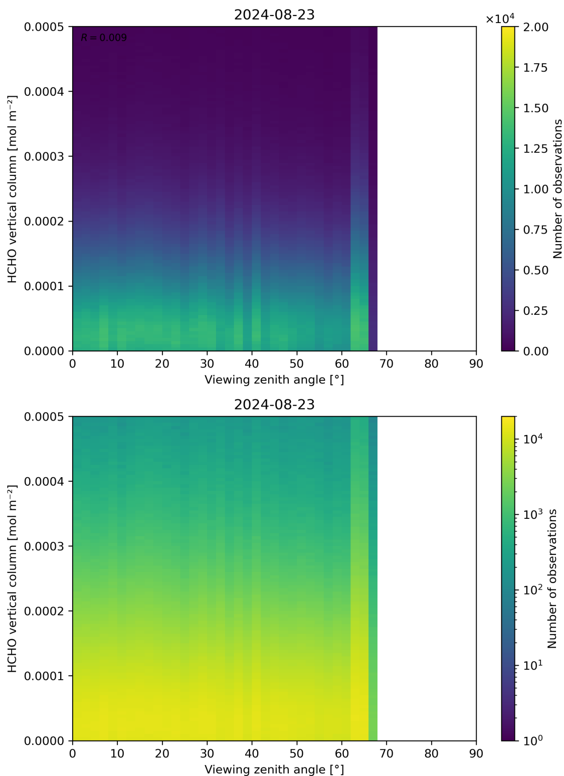
Figure 192: Scatter density plot of “Viewing zenith angle” against “HCHO vertical column” for 2024-08-22 to 2024-08-24.
