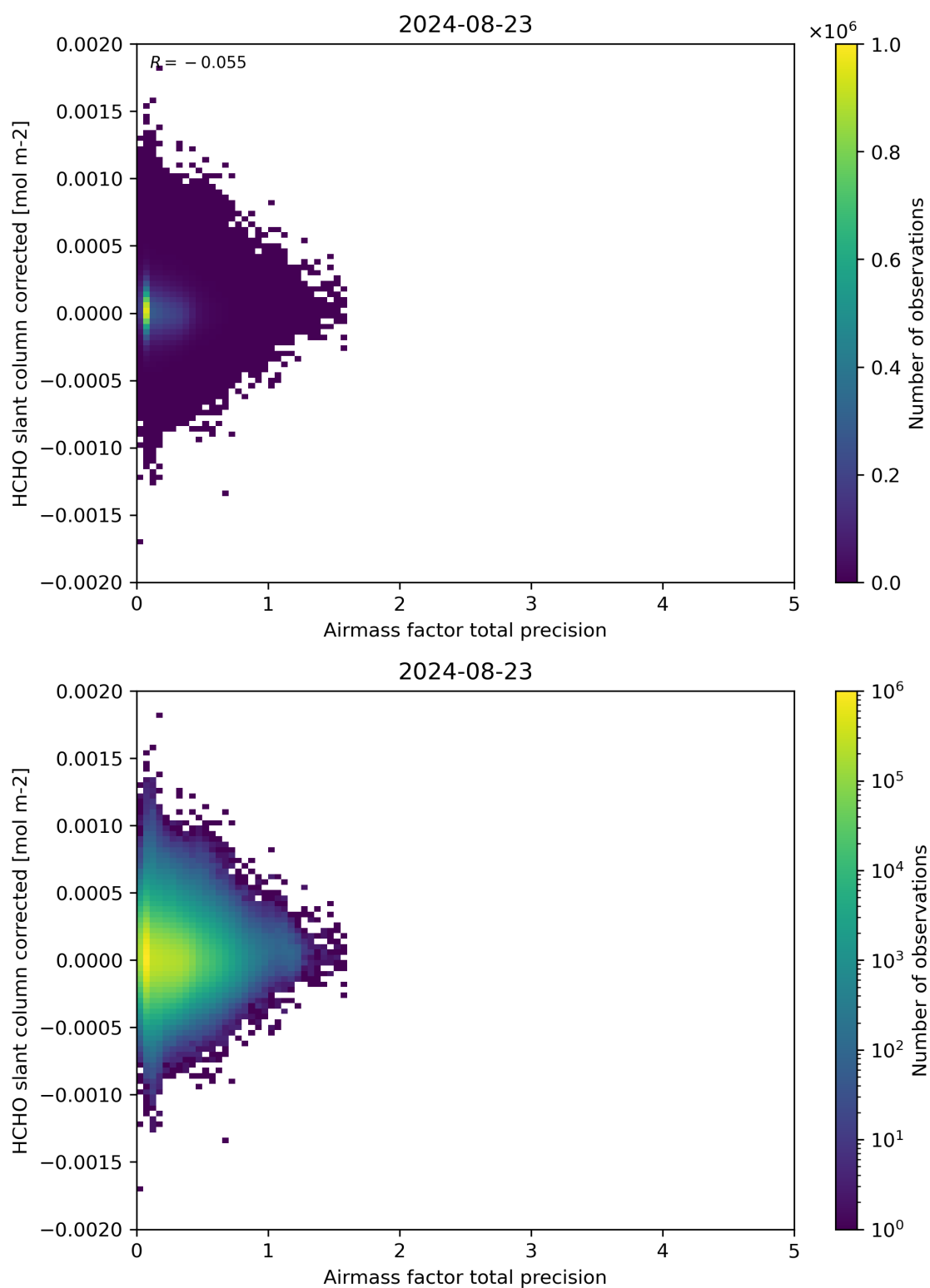
Figure 109: Scatter density plot of “Airmass factor total precision” against “HCHO slant column corrected” for 2024-08-22 to 2024-08-24.
