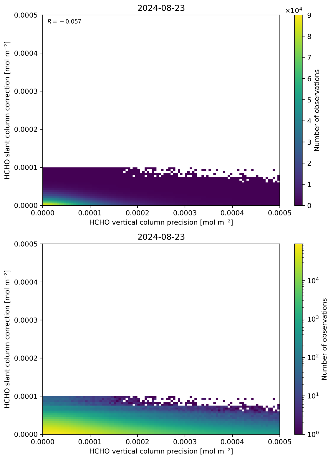
Figure 141: Scatter density plot of “HCHO vertical column precision” against “HCHO slant column correction” for 2024-08-22 to 2024-08-24.
