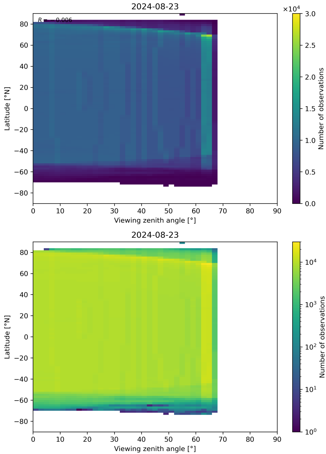
Figure 196: Scatter density plot of “Viewing zenith angle” against “Latitude” for 2024-08-22 to 2024-08-24.
