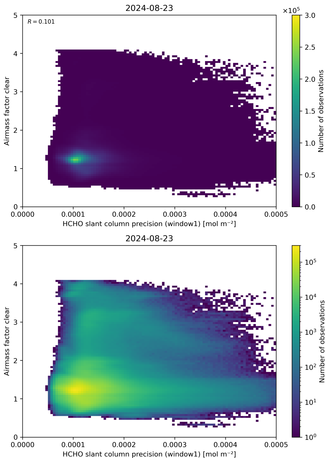
Figure 91: Scatter density plot of “HCHO slant column precision (window1)” against “Airmass factor clear” for 2024-08-22 to 2024-08-24.
