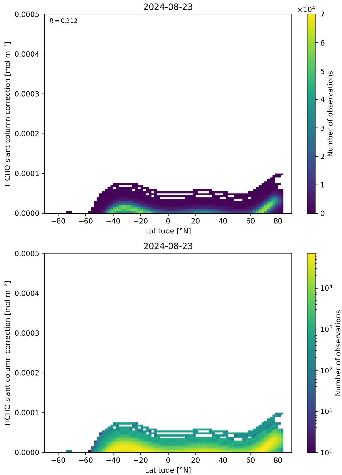
Figure 158: Scatter density plot of “Latitude” against “HCHO slant column correction” for 2024-08-22 to 2024-08-24.
