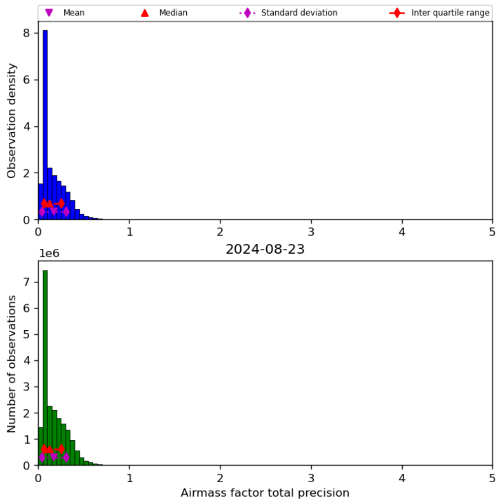
Figure 41: Histogram of “Airmass factor total precision” for 2024-08-22 to 2024-08-24
