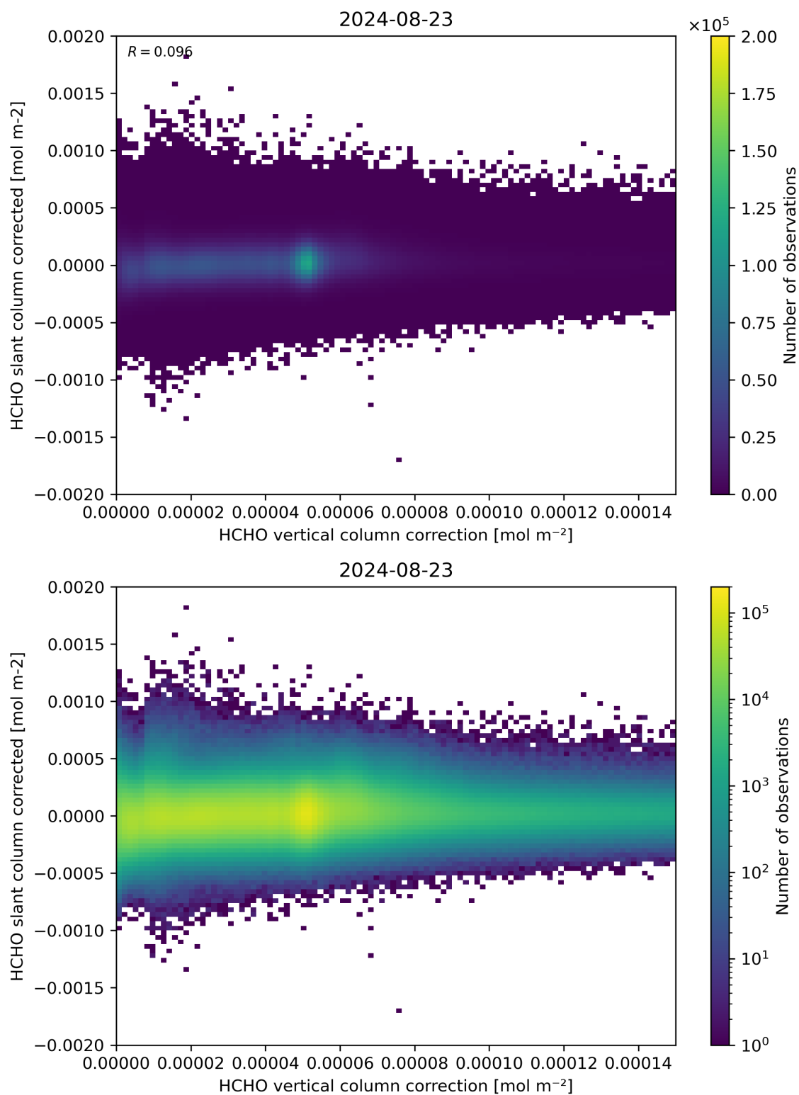
Figure 116: Scatter density plot of “HCHO vertical column correction” against “HCHO slant column corrected” for 2024-08-22 to 2024-08-24.
