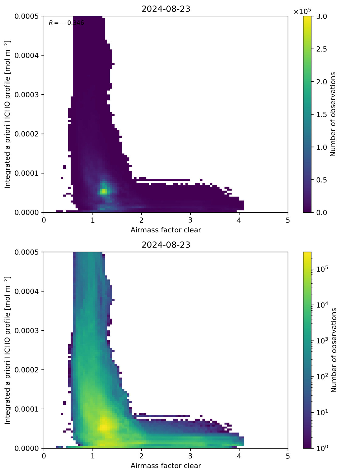
Figure 76: Scatter density plot of “Airmass factor clear” against “Integrated a priori HCHO profile” for 2024-08-22 to 2024-08-24.
