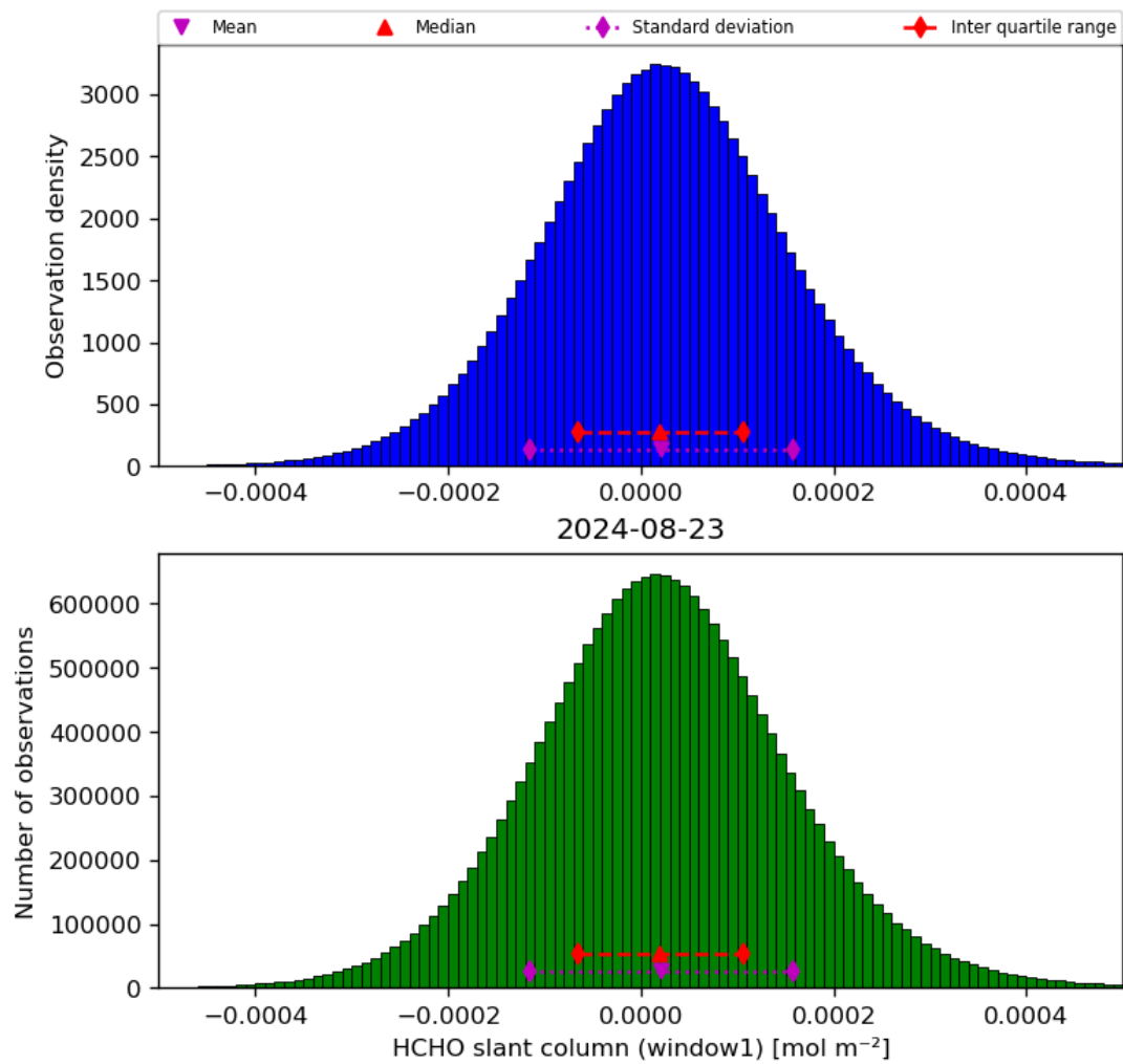
Figure 38: Histogram of “HCHO slant column (window1)” for 2024-08-22 to 2024-08-24
