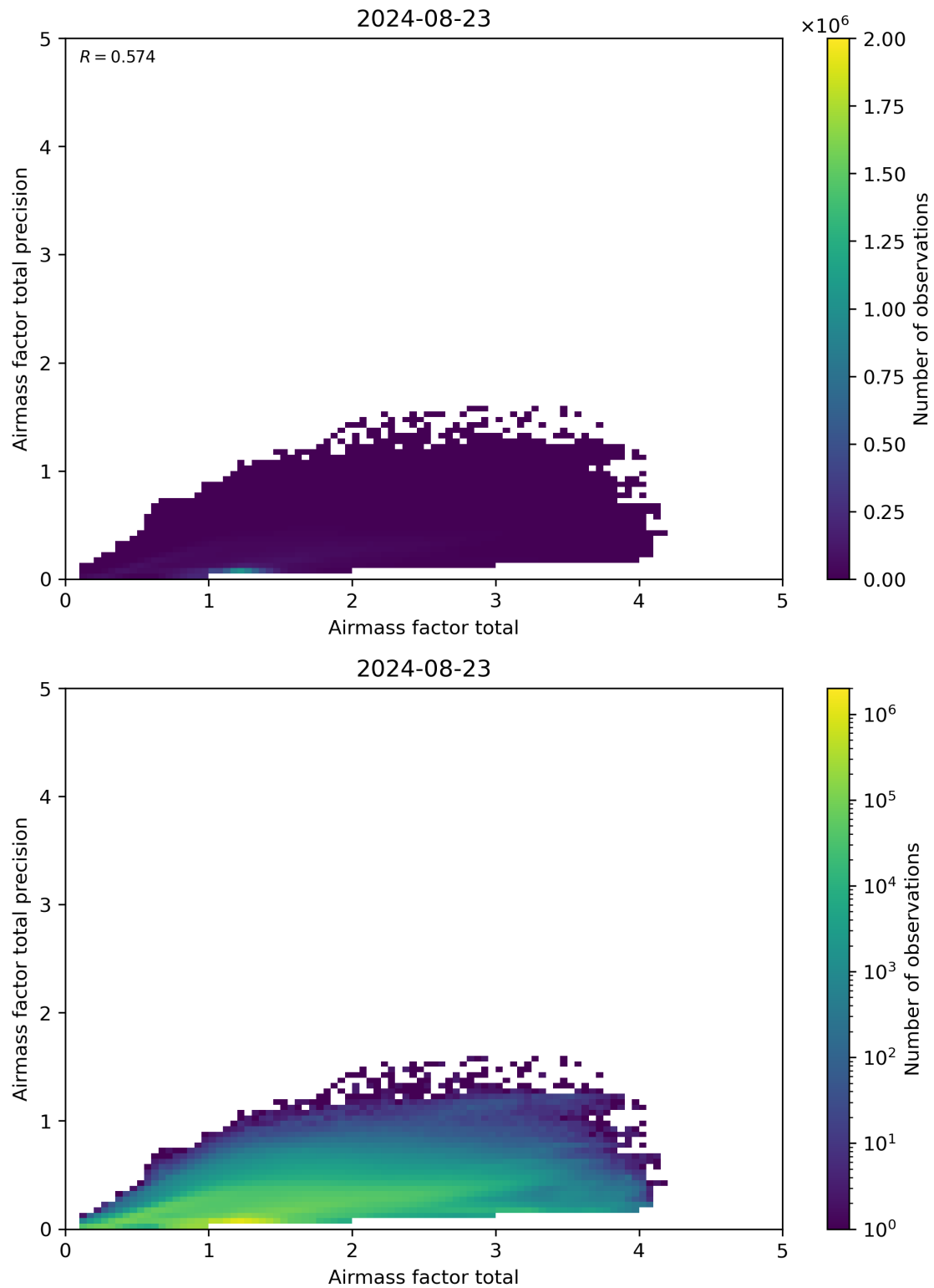
Figure 103: Scatter density plot of “Airmass factor total” against “Airmass factor total precision” for 2024-08-22 to 2024-08-24.
