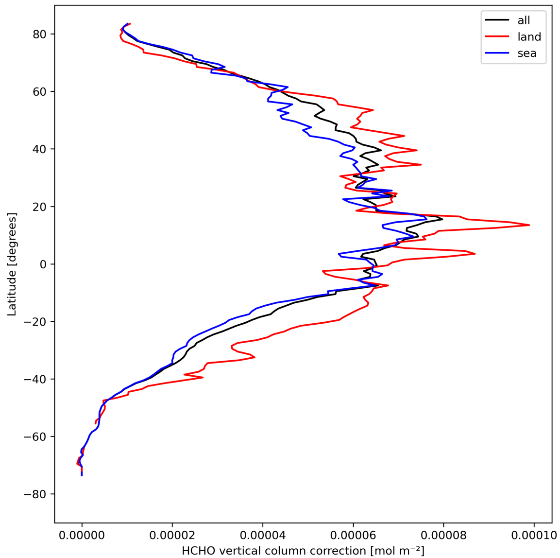
Figure 23: Zonal average of “HCHO vertical column correction” for 2024-08-22 to 2024-08-24.
