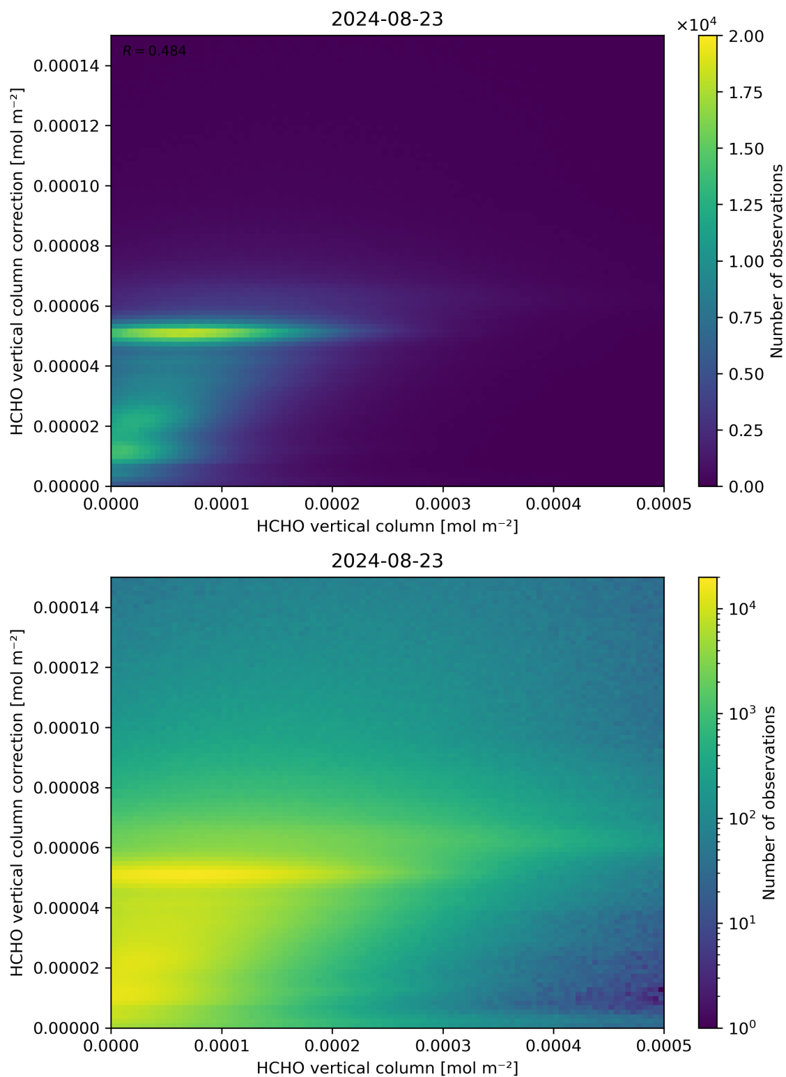
Figure 133: Scatter density plot of “HCHO vertical column” against “HCHO vertical column correction” for 2024-08-22 to 2024-08-24.
