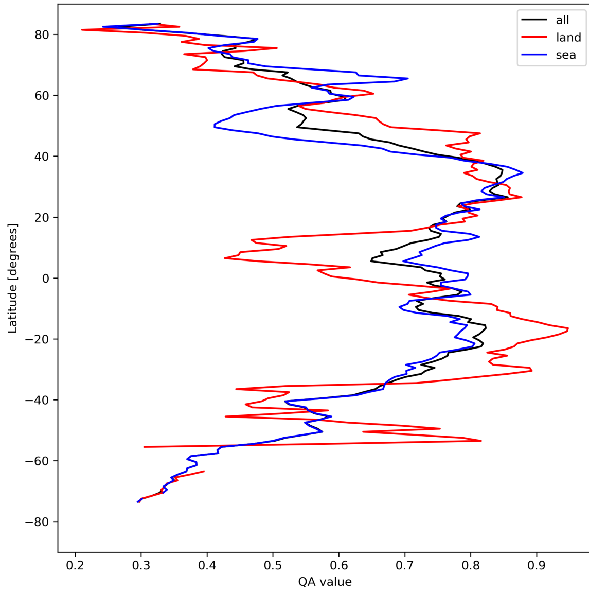
Figure 20: Zonal average of “QA value” for 2024-08-22 to 2024-08-24.
