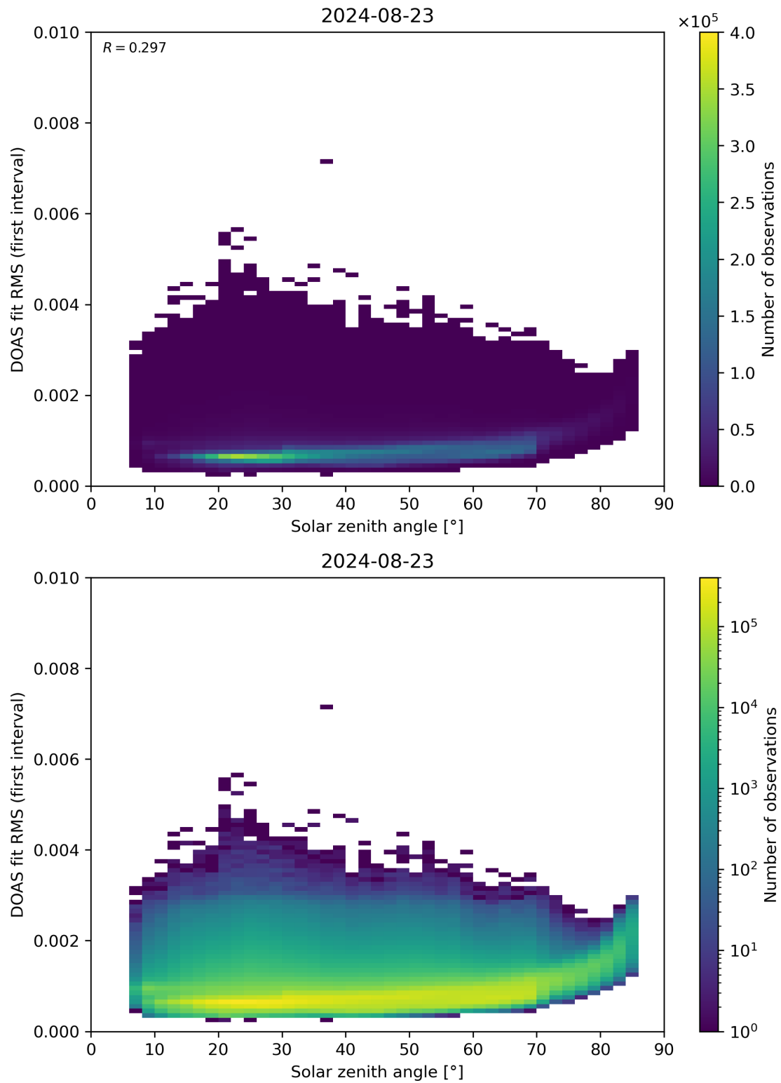
Figure 167: Scatter density plot of “Solar zenith angle” against “DOAS fit RMS (first interval)” for 2024-08-22 to 2024-08-24.
