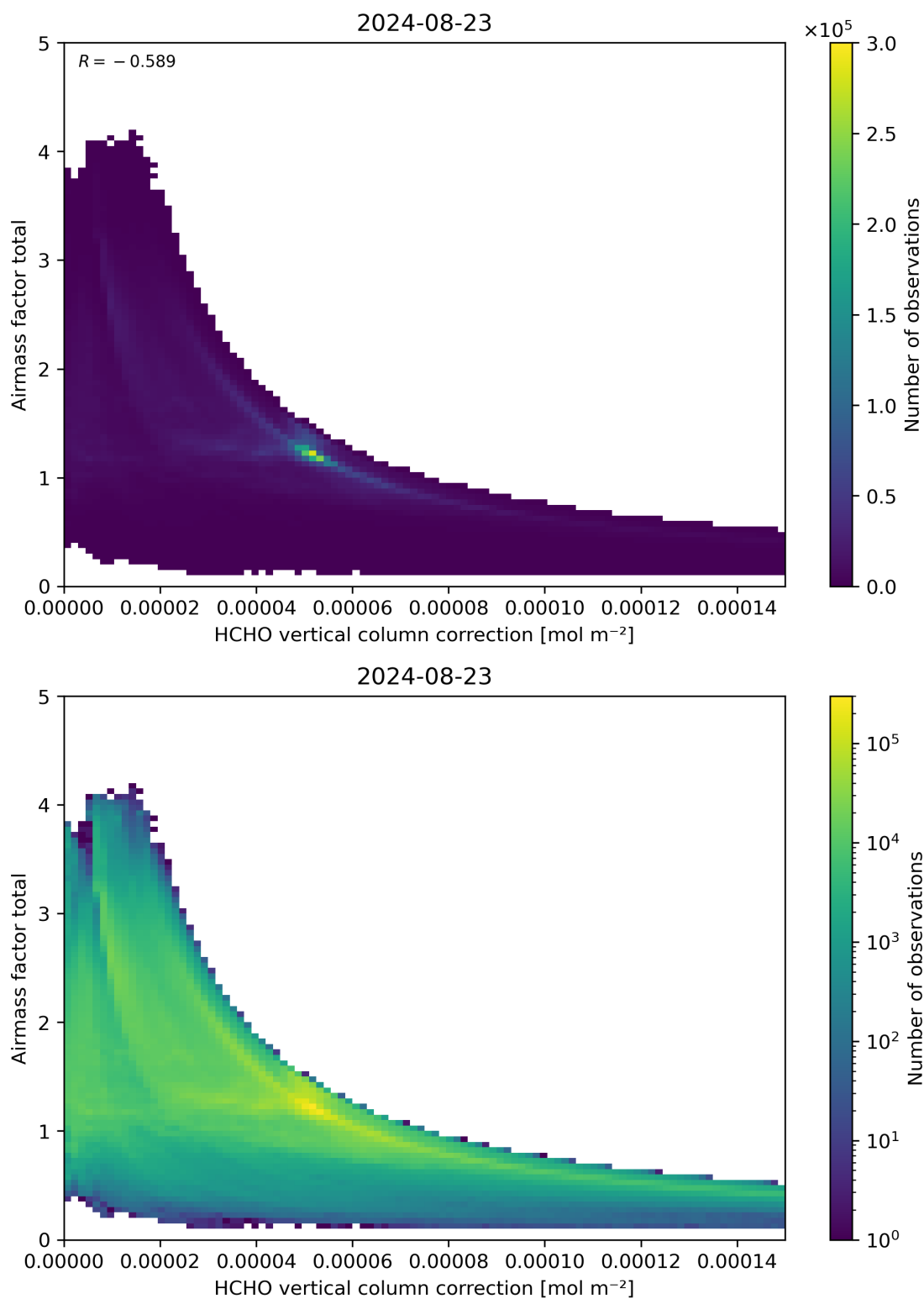
Figure 120: Scatter density plot of “HCHO vertical column correction” against “Airmass factor total” for 2024-08-22 to 2024-08-24.
