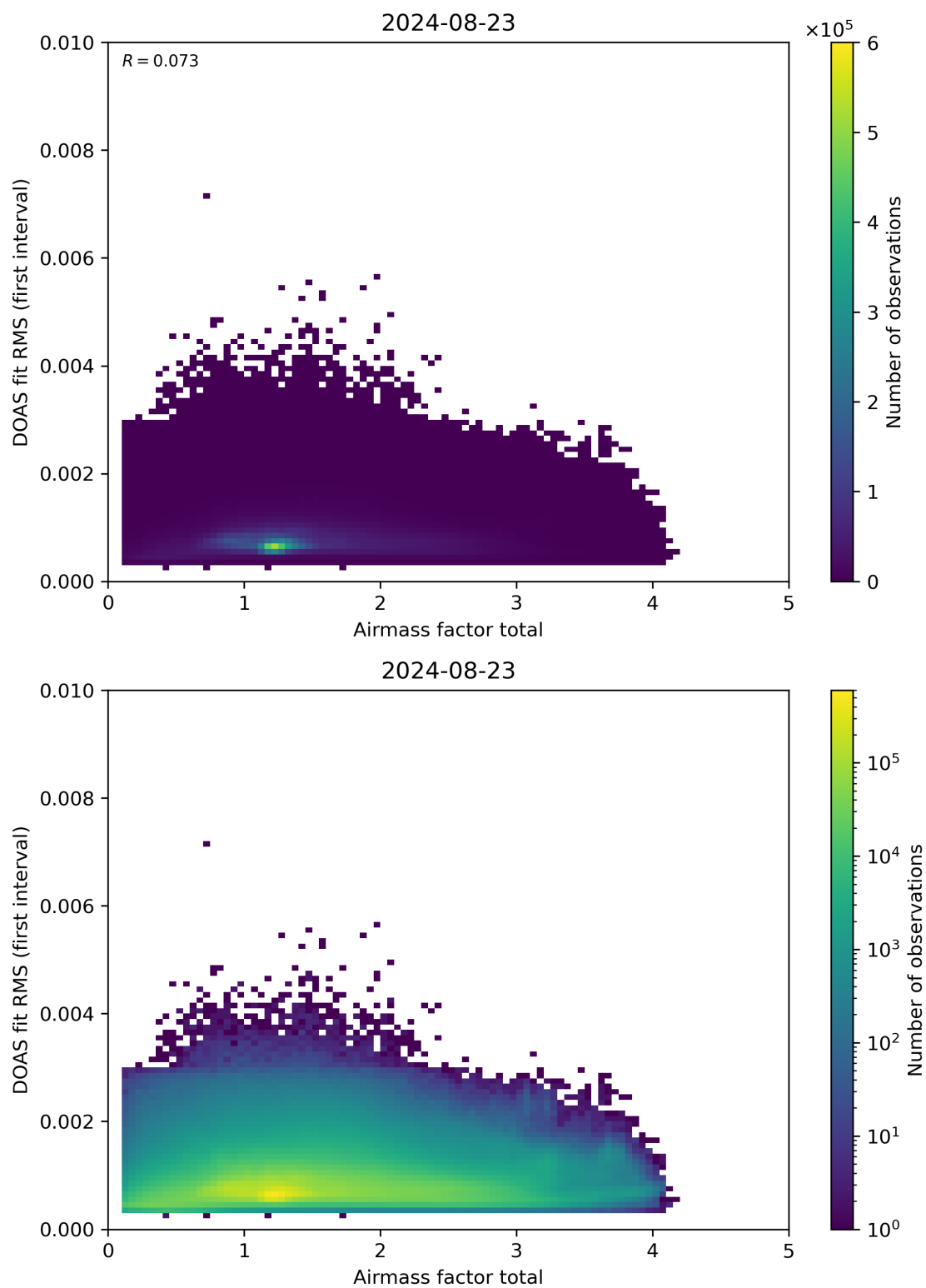
Figure 97: Scatter density plot of “Airmass factor total” against “DOAS fit RMS (first interval)” for 2024-08-22 to 2024-08-24.
