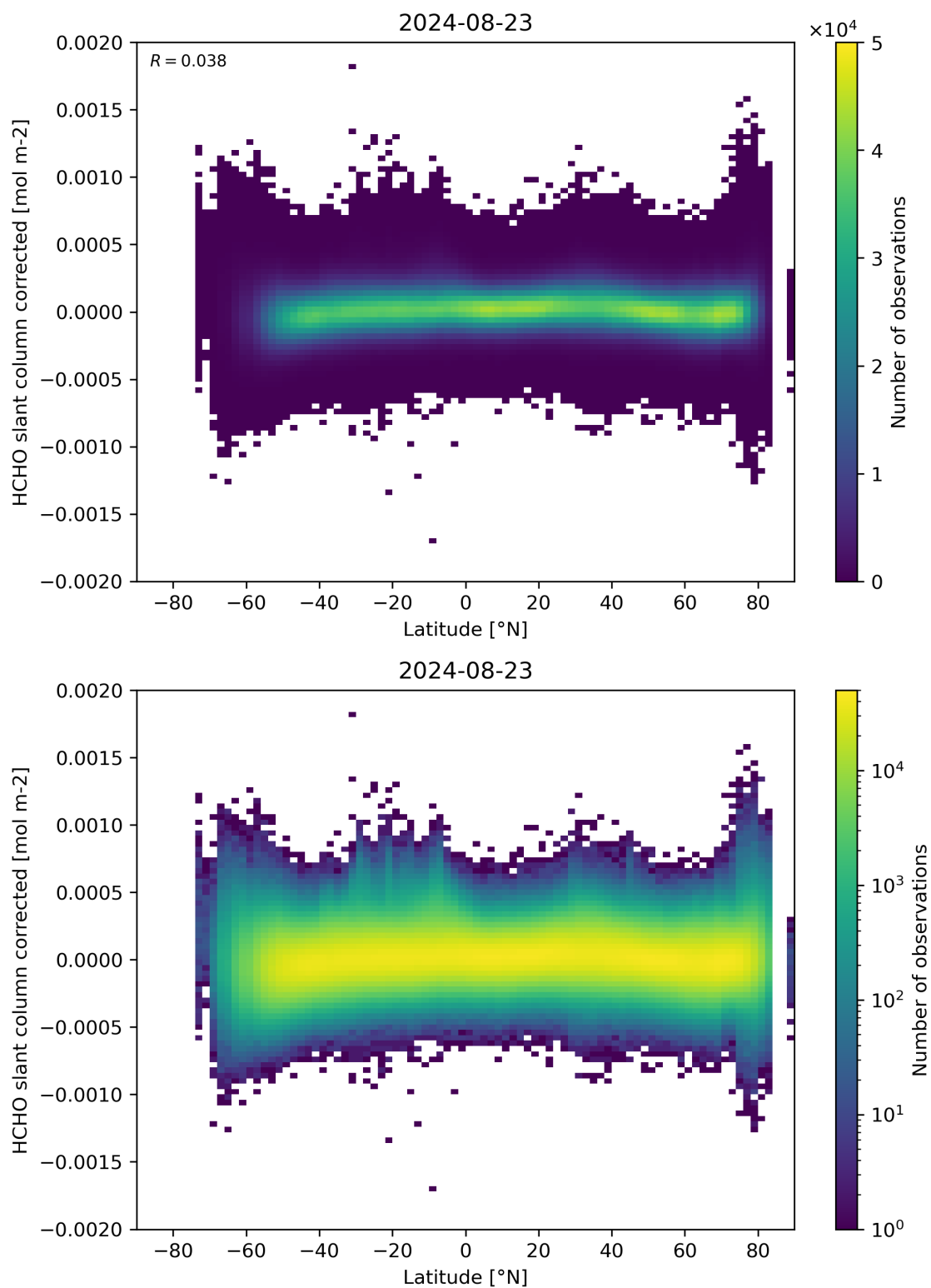
Figure 157: Scatter density plot of “Latitude” against “HCHO slant column corrected” for 2024-08-22 to 2024-08-24.
