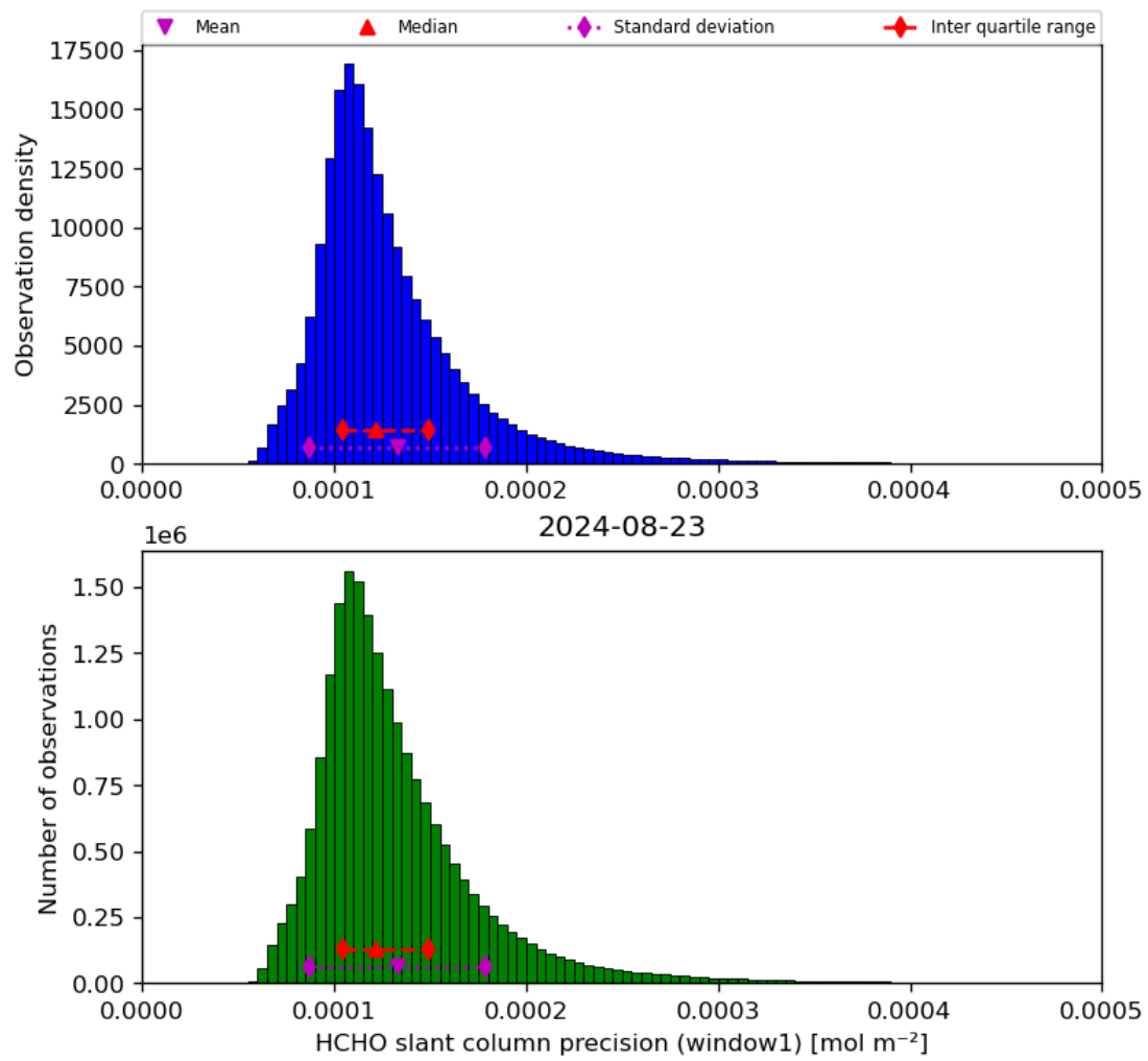
Figure 39: Histogram of “HCHO slant column precision (window1)” for 2024-08-22 to 2024-08-24
