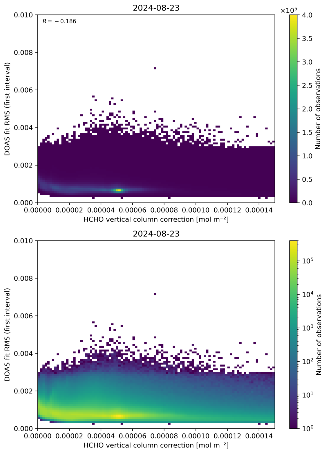
Figure 112: Scatter density plot of “HCHO vertical column correction” against “DOAS fit RMS (first interval)” for 2024-08-22 to 2024-08-24.
