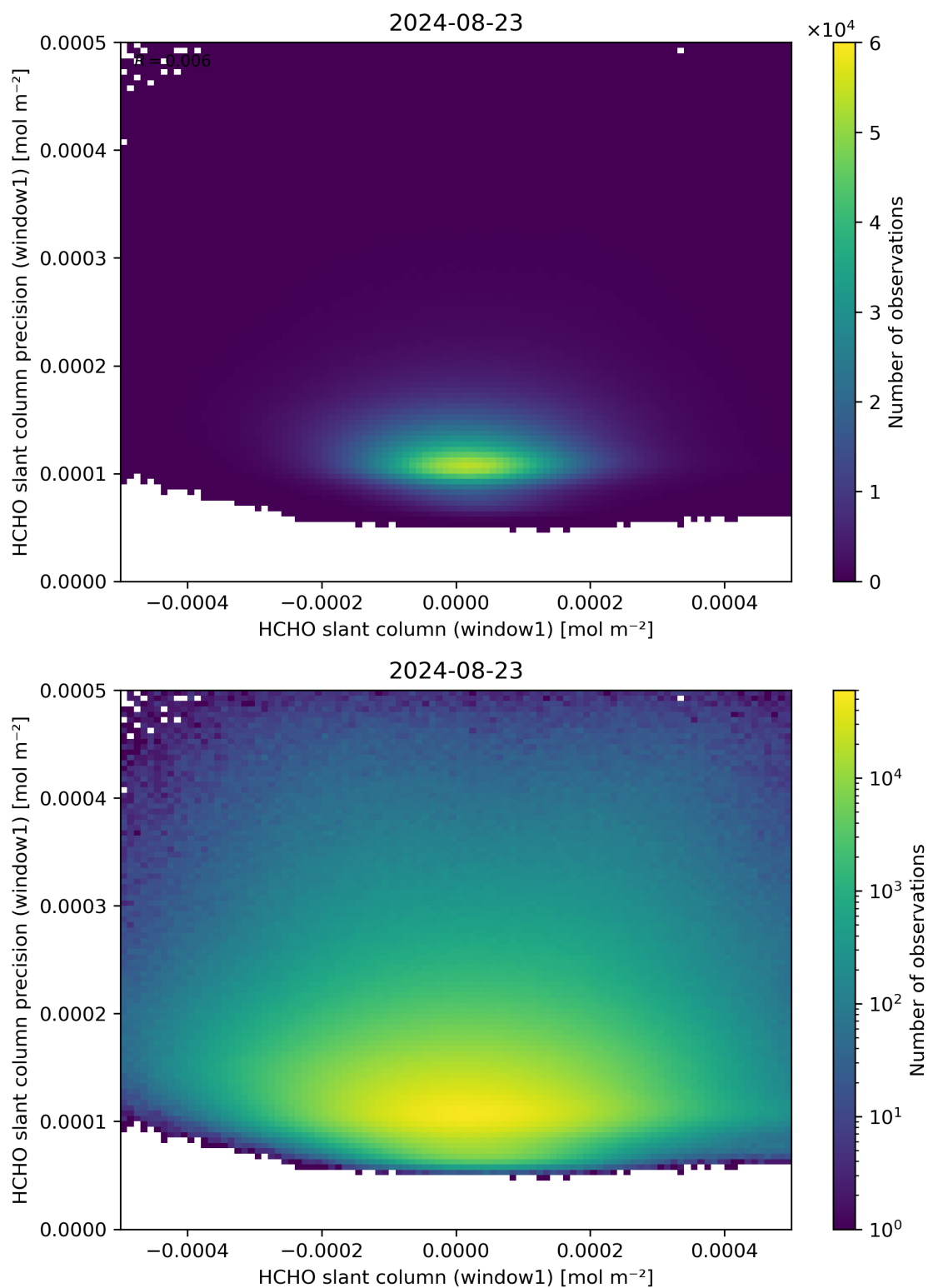
Figure 84: Scatter density plot of “HCHO slant column (window1)” against “HCHO slant column precision (window1)” for 2024-08-22 to 2024-08-24.
