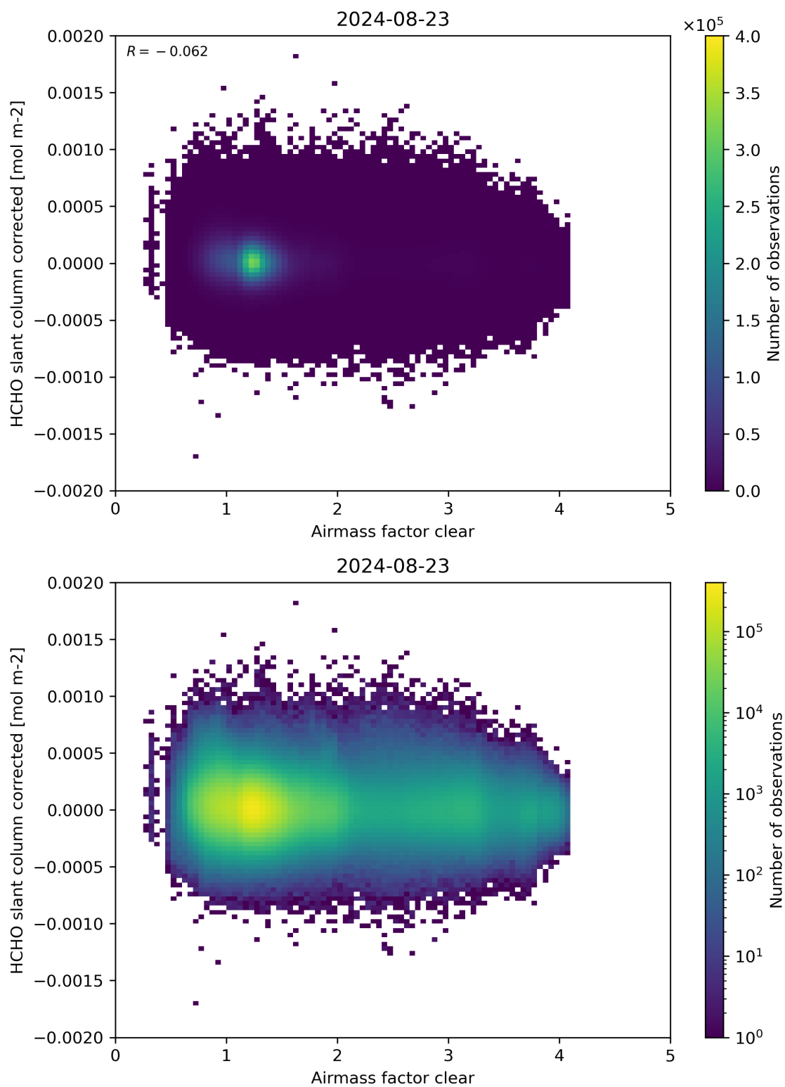
Figure 74: Scatter density plot of “Airmass factor clear” against “HCHO slant column corrected” for 2024-08-22 to 2024-08-24.
