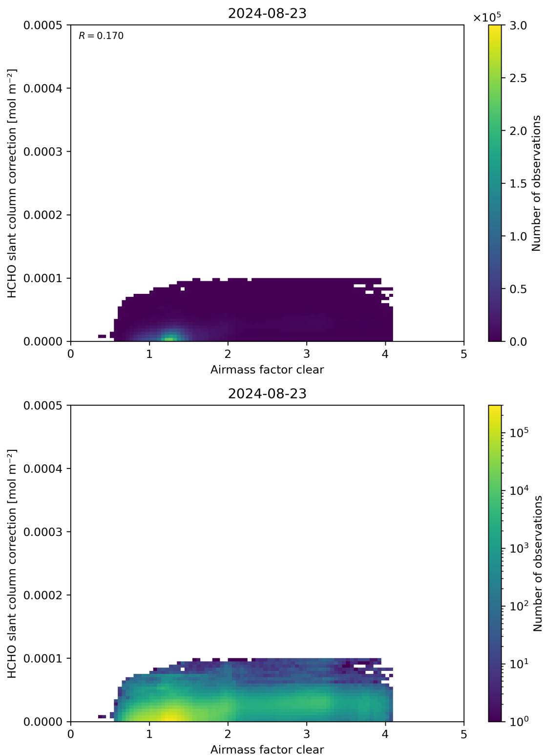
Figure 75: Scatter density plot of “Airmass factor clear” against “HCHO slant column correction” for 2024-08-22 to 2024-08-24.
