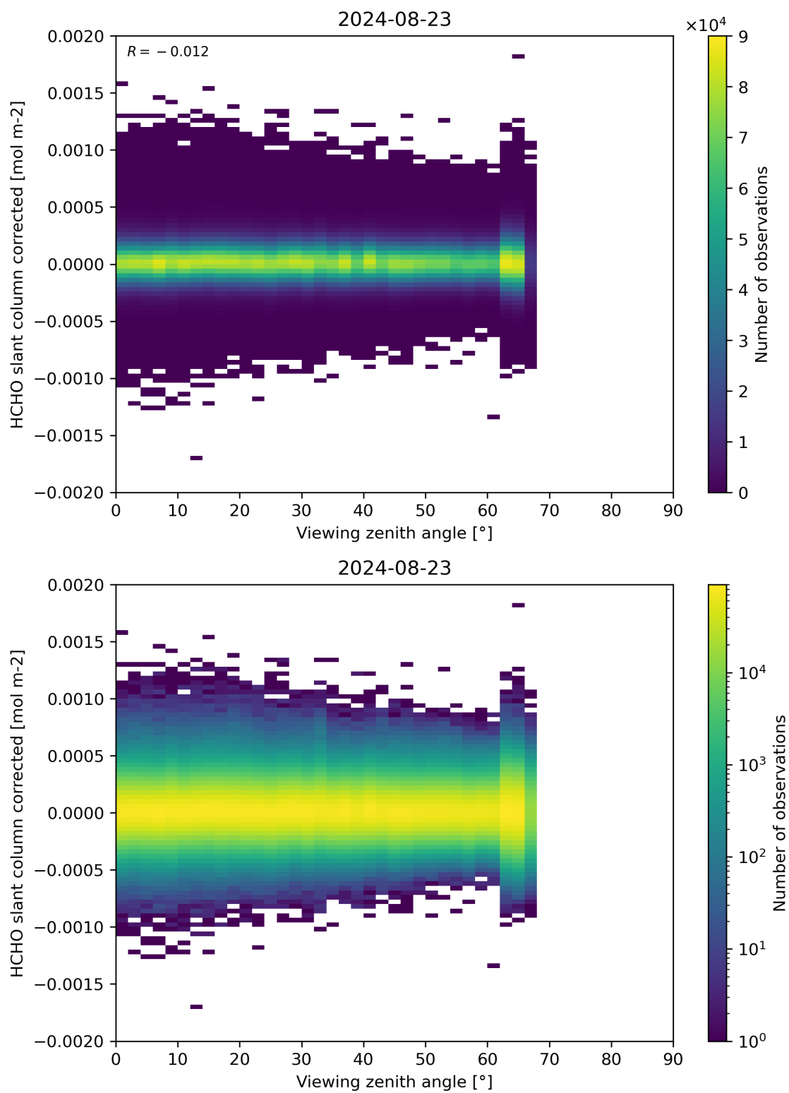
Figure 186: Scatter density plot of “Viewing zenith angle” against “HCHO slant column corrected” for 2024-08-22 to 2024-08-24.
