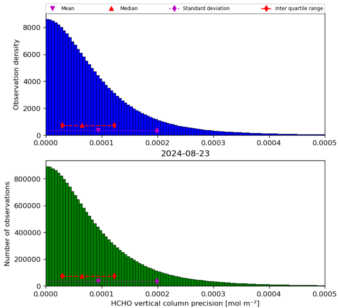
Figure 36: Histogram of “HCHO vertical column precision” for 2024-08-22 to 2024-08-24
