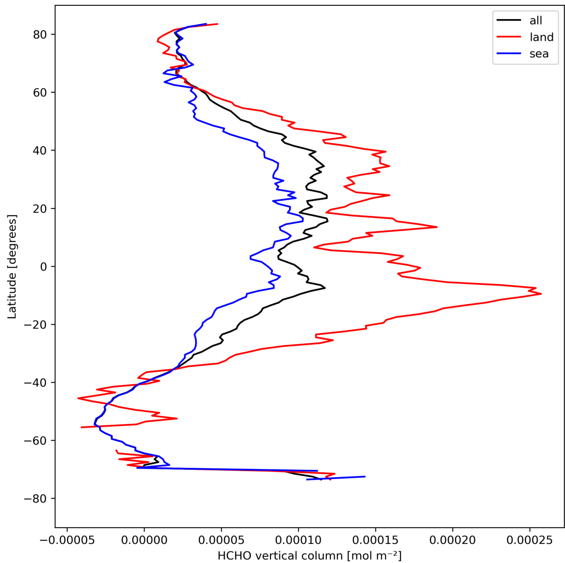
Figure 21: Zonal average of “HCHO vertical column” for 2024-08-22 to 2024-08-24.
