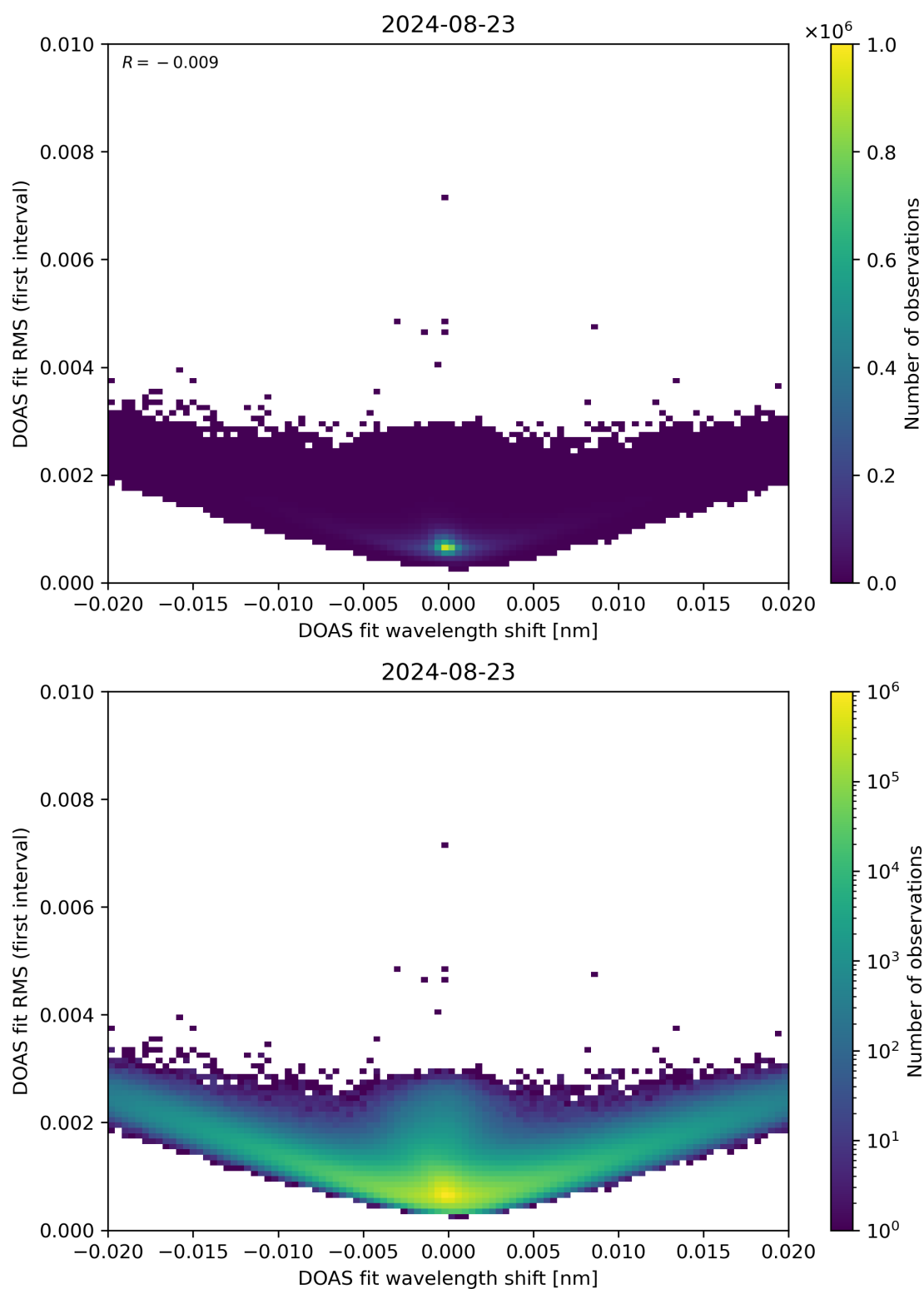
Figure 64: Scatter density plot of “DOAS fit wavelength shift” against “DOAS fit RMS (first interval)” for 2024-08-22 to 2024-08-24.
