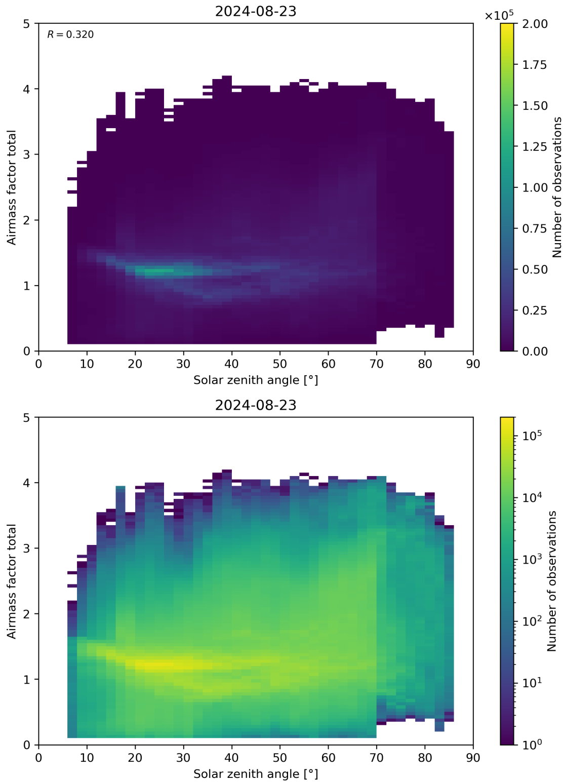
Figure 175: Scatter density plot of “Solar zenith angle” against “Airmass factor total” for 2024-08-22 to 2024-08-24.
