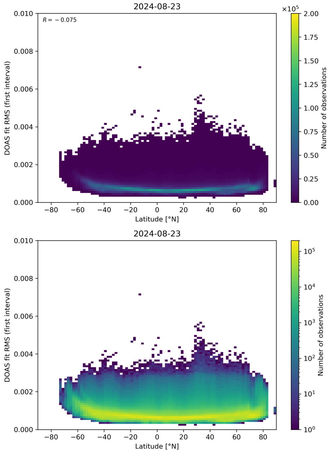
Figure 153: Scatter density plot of “Latitude” against “DOAS fit RMS (first interval)” for 2024-08-22 to 2024-08-24.
