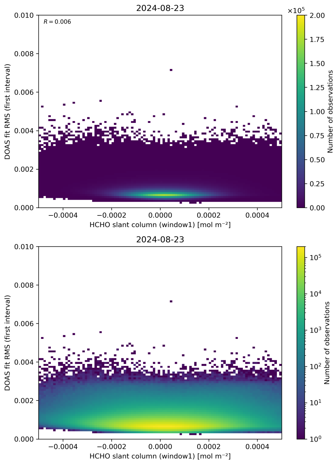
Figure 78: Scatter density plot of “HCHO slant column (window1)” against “DOAS fit RMS (first interval)” for 2024-08-22 to 2024-08-24.
