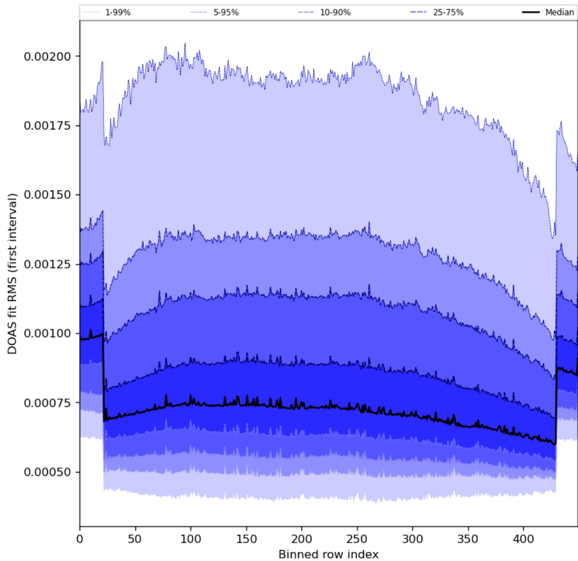
Figure 60: Along track statistics of “DOAS fit RMS (first interval)” for 2024-08-22 to 2024-08-24
