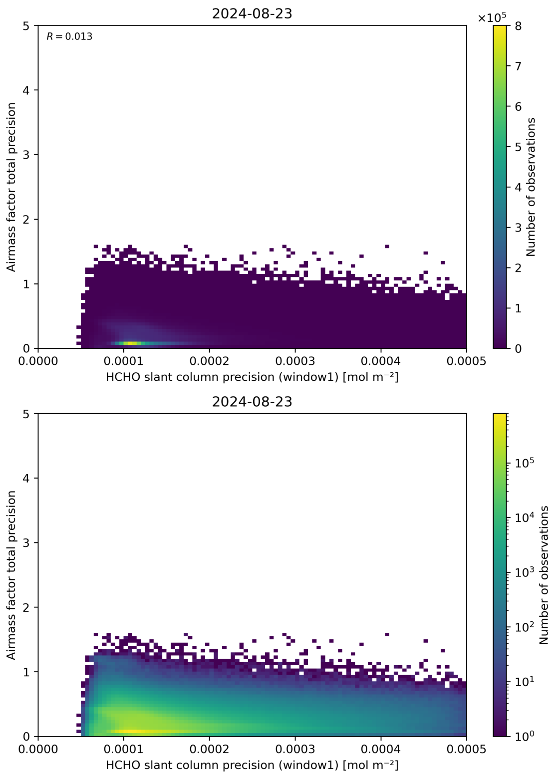
Figure 95: Scatter density plot of “HCHO slant column precision (window1)” against “Airmass factor total precision” for 2024-08-22 to 2024-08-24.
