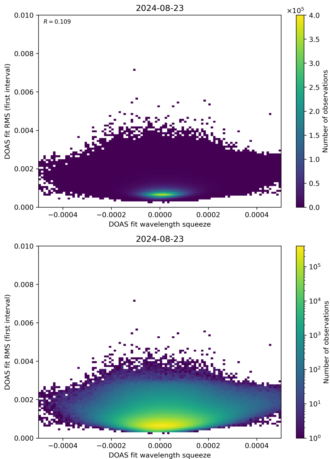
Figure 68: Scatter density plot of “DOAS fit wavelength squeeze” against “DOAS fit RMS (first interval)” for 2024-08-22 to 2024-08-24.
