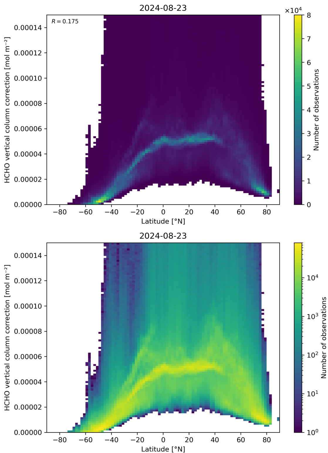
Figure 164: Scatter density plot of “Latitude” against “HCHO vertical column correction” for 2024-08-22 to 2024-08-24.
