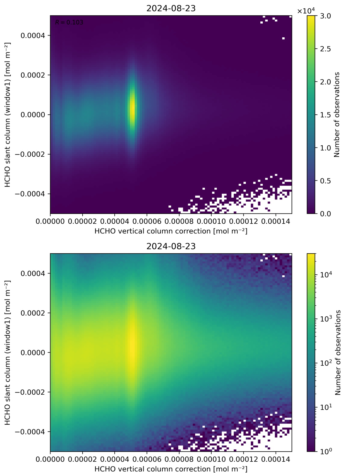
Figure 118: Scatter density plot of “HCHO vertical column correction” against “HCHO slant column (window1)” for 2024-08-22 to 2024-08-24.
