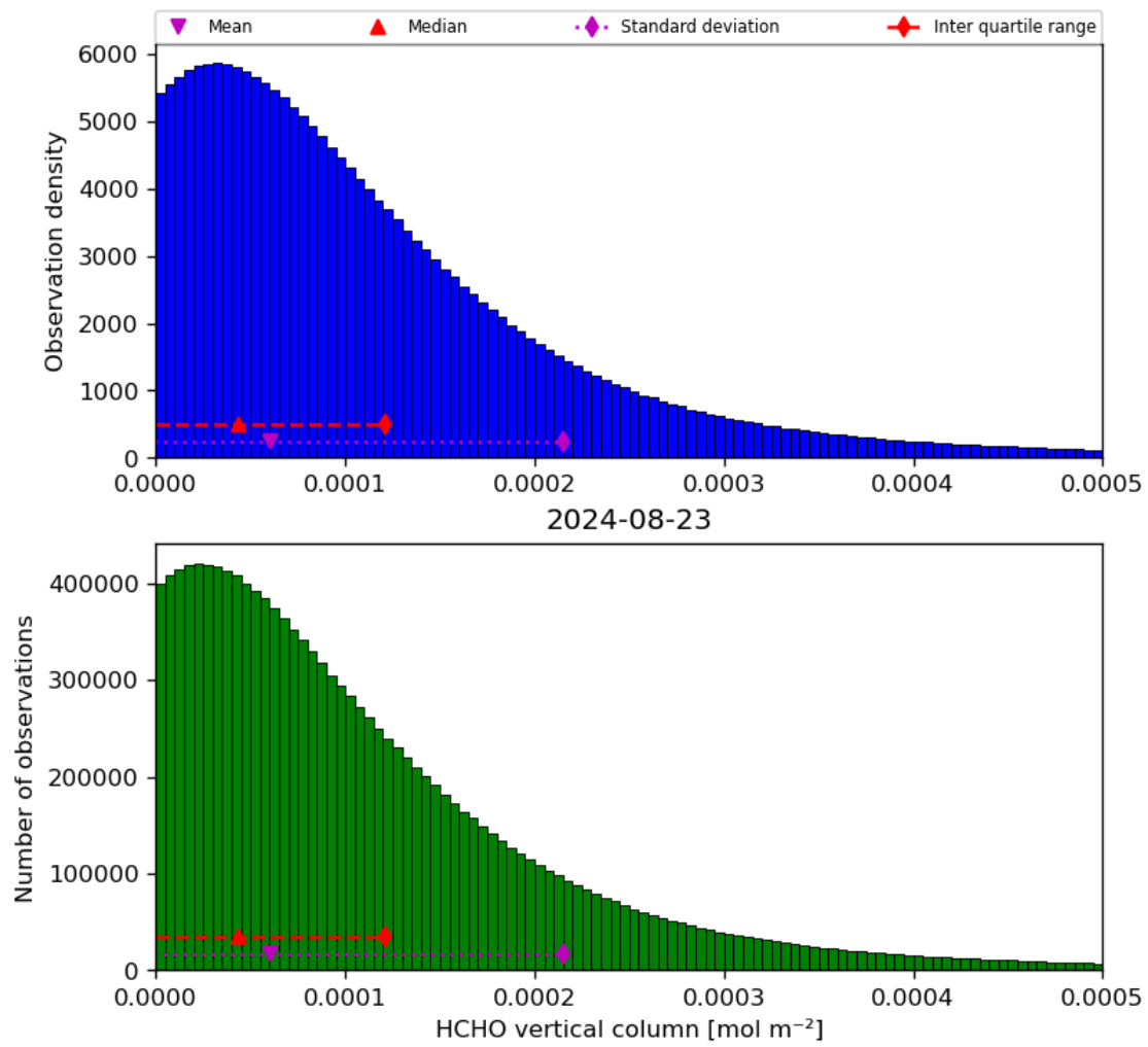
Figure 35: Histogram of “HCHO vertical column” for 2024-08-22 to 2024-08-24
