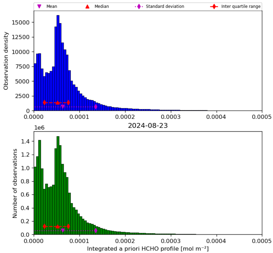
Figure 43: Histogram of “Integrated a priori HCHO profile” for 2024-08-22 to 2024-08-24
