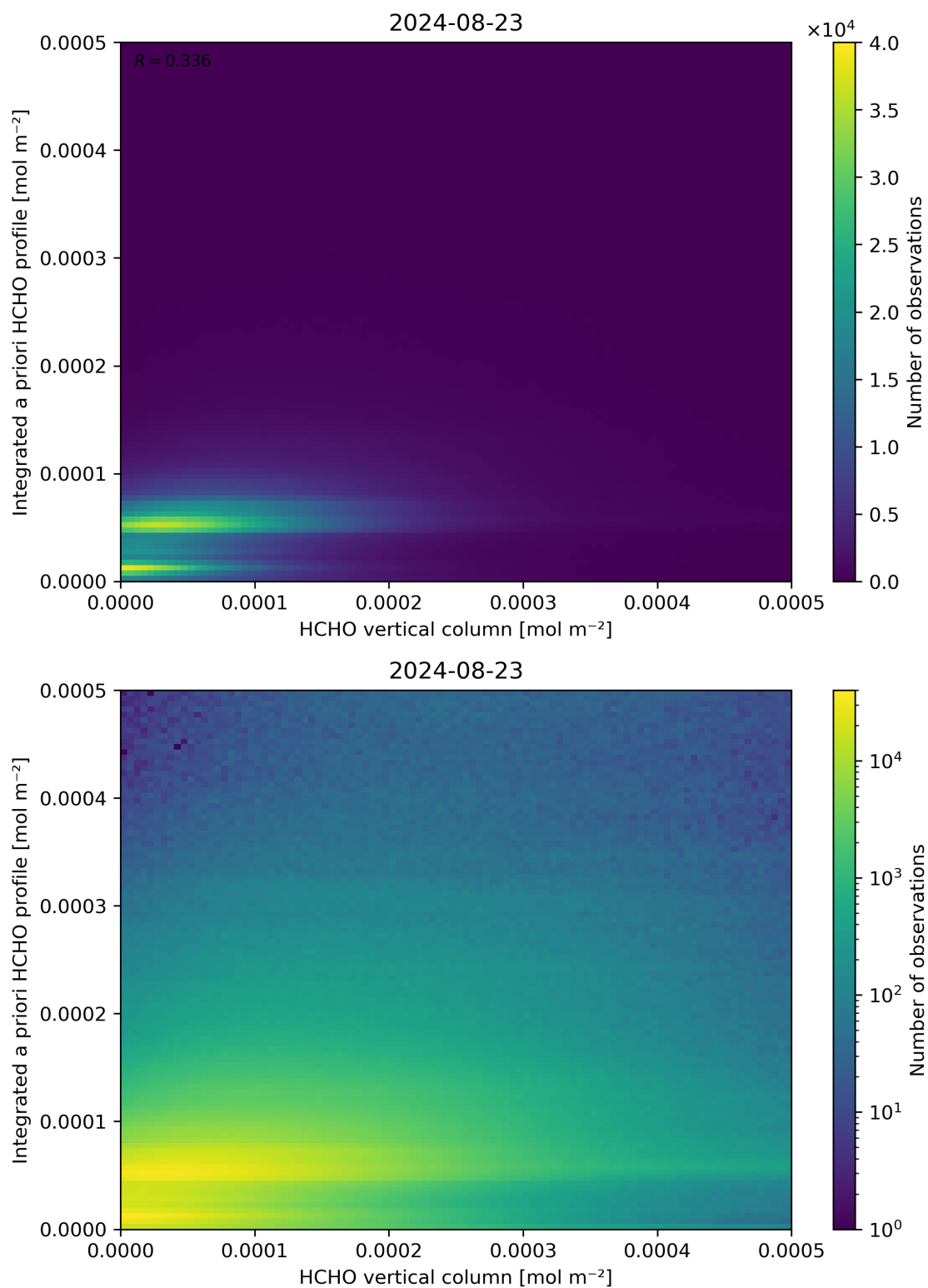
Figure 135: Scatter density plot of “HCHO vertical column” against “Integrated a priori HCHO profile” for 2024-08-22 to 2024-08-24.
