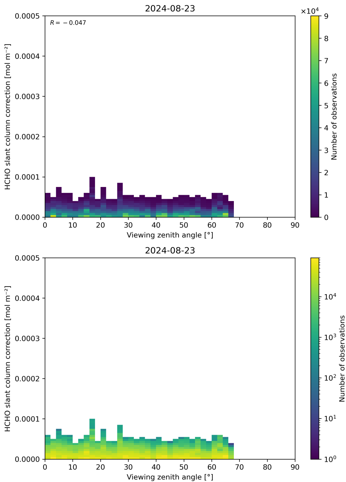
Figure 187: Scatter density plot of “Viewing zenith angle” against “HCHO slant column correction” for 2024-08-22 to 2024-08-24.
