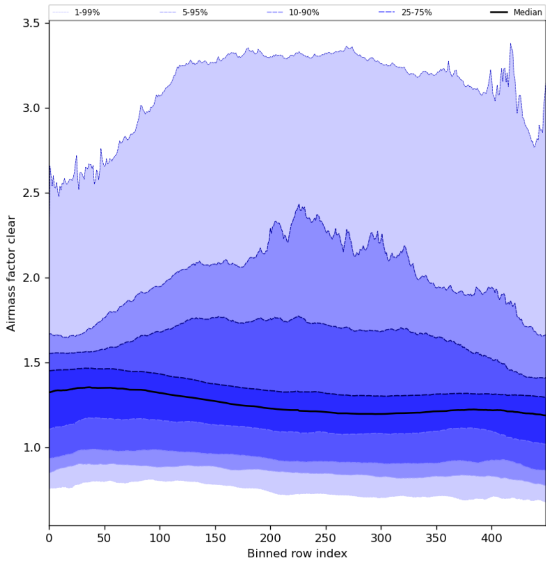
Figure 56: Along track statistics of “Airmass factor clear” for 2024-08-22 to 2024-08-24
