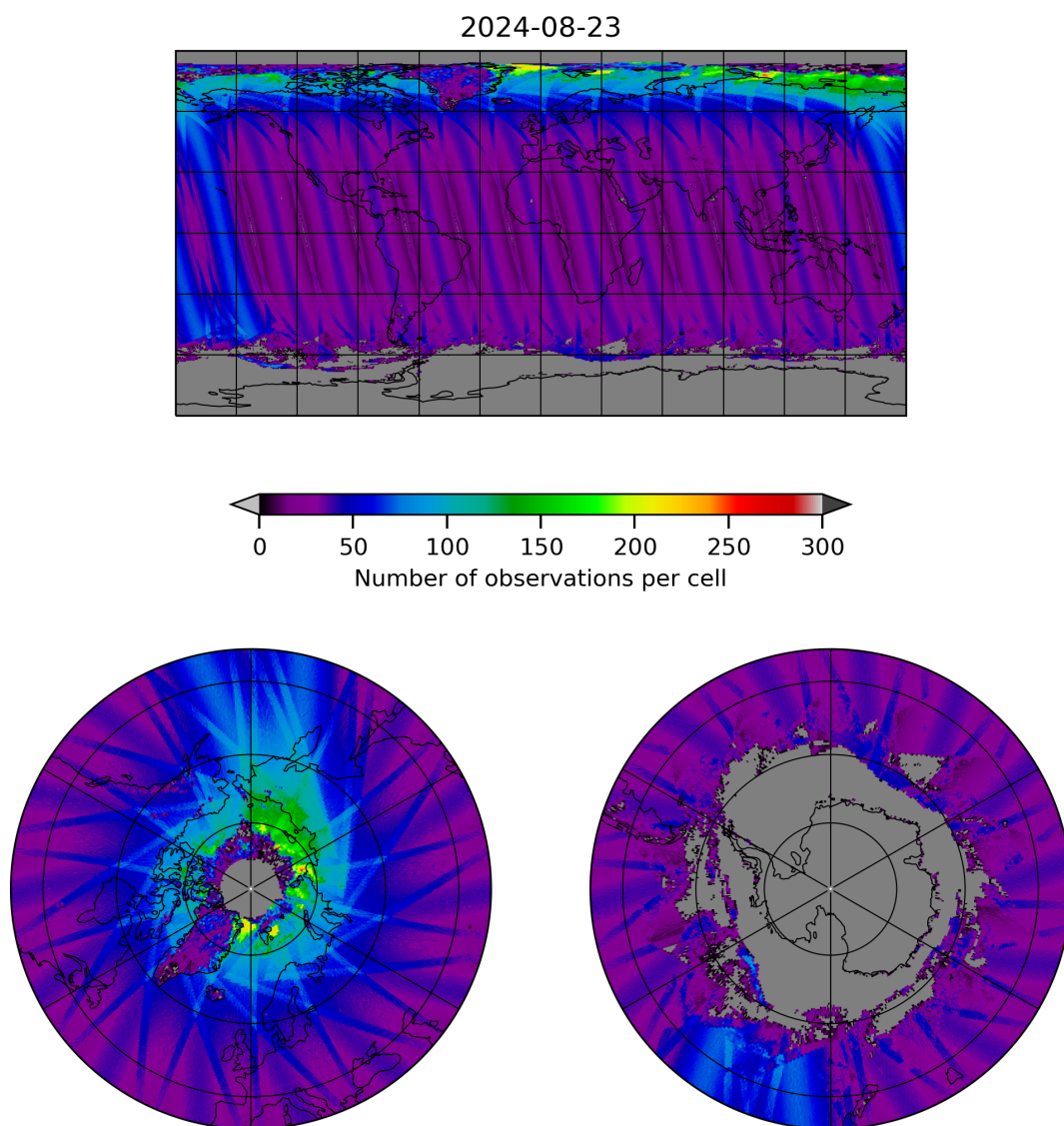
Figure 19: Map of the number of observations for 2024-08-22 to 2024-08-24
