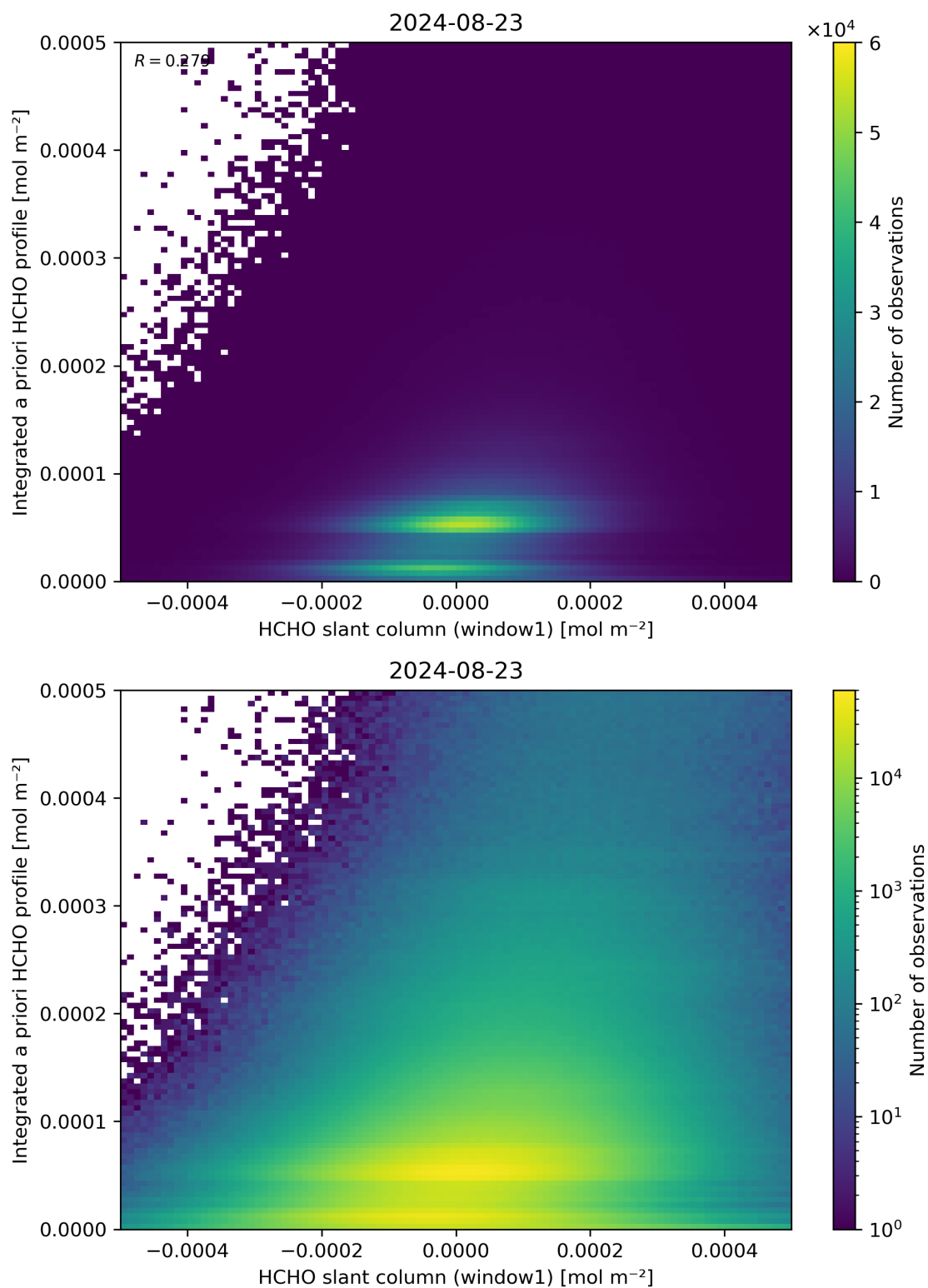
Figure 87: Scatter density plot of “HCHO slant column (window1)” against “Integrated a priori HCHO profile” for 2024-08-22 to 2024-08-24.
