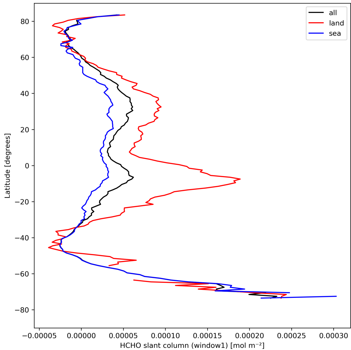
Figure 24: Zonal average of “HCHO slant column (window1)” for 2024-08-22 to 2024-08-24.
