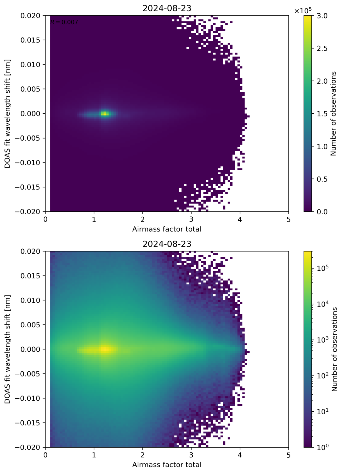
Figure 98: Scatter density plot of “Airmass factor total” against “DOAS fit wavelength shift” for 2024-08-22 to 2024-08-24.
