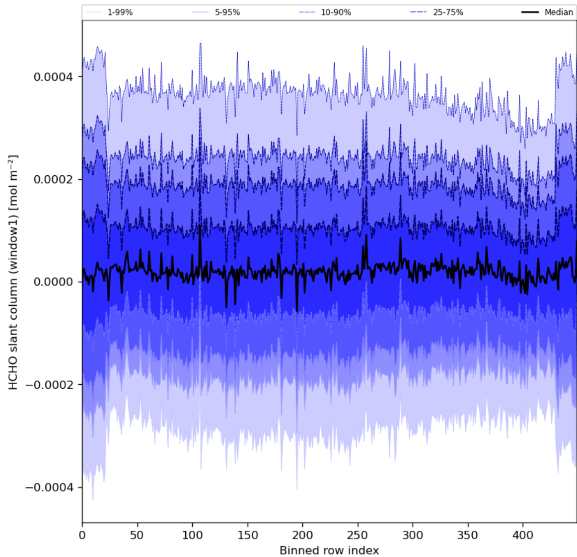
Figure 52: Along track statistics of “HCHO slant column (window1)” for 2024-08-22 to 2024-08-24
