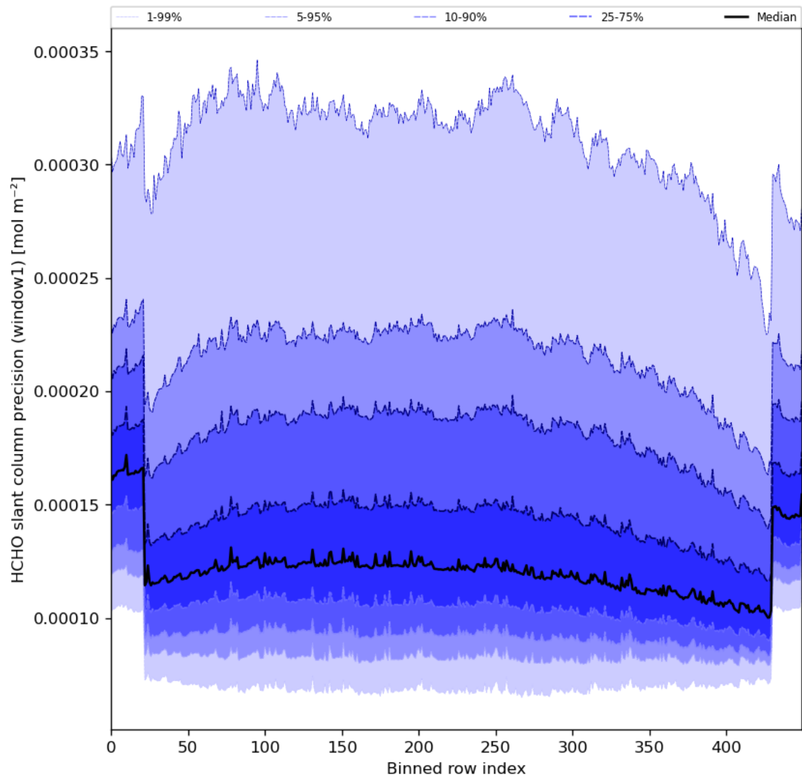
Figure 53: Along track statistics of “HCHO slant column precision (window1)” for 2024-08-22 to 2024-08-24
