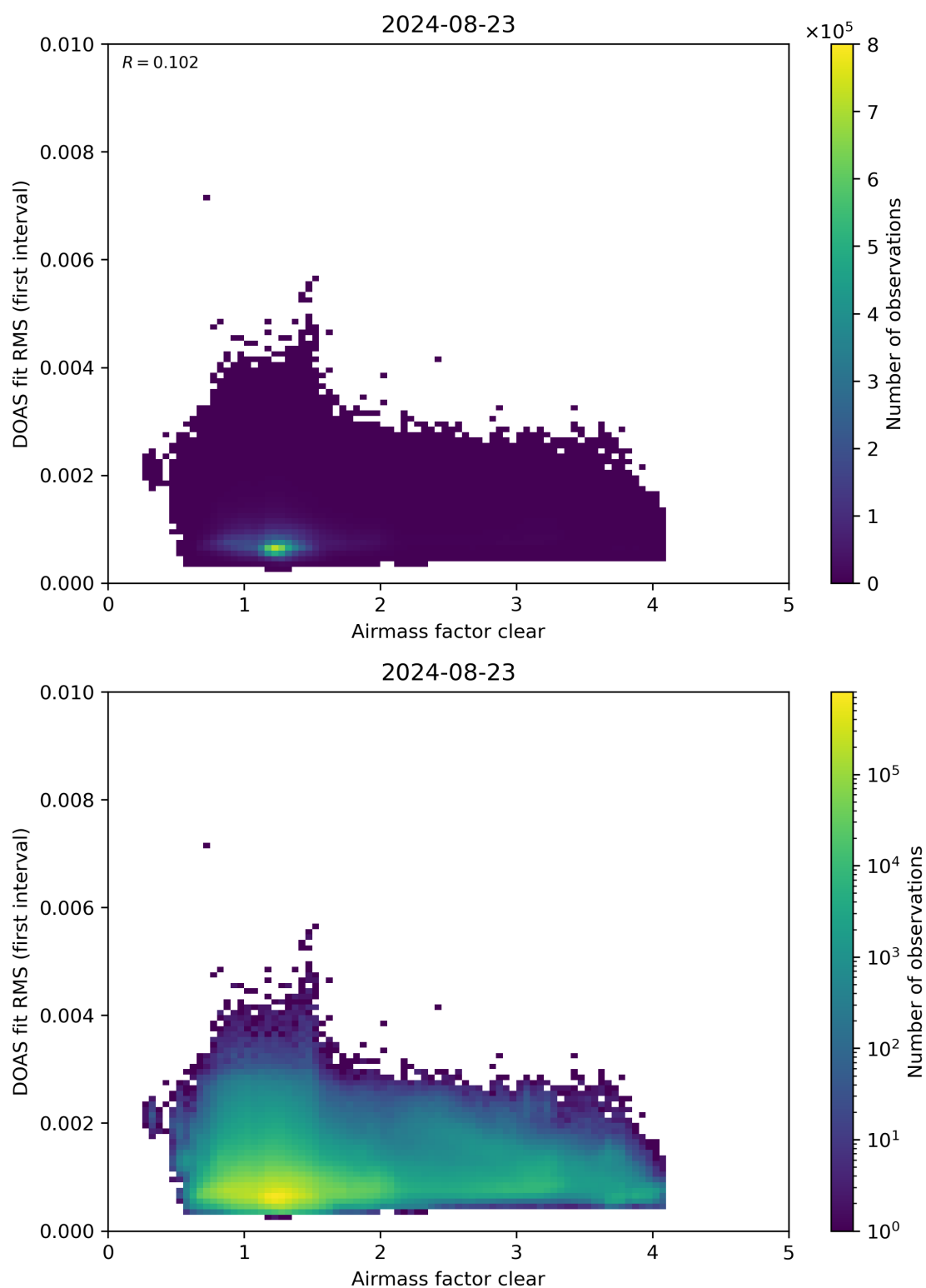
Figure 71: Scatter density plot of “Airmass factor clear” against “DOAS fit RMS (first interval)” for 2024-08-22 to 2024-08-24.
