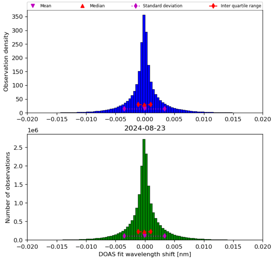
Figure 44: Histogram of “DOAS fit wavelength shift” for 2024-08-22 to 2024-08-24
