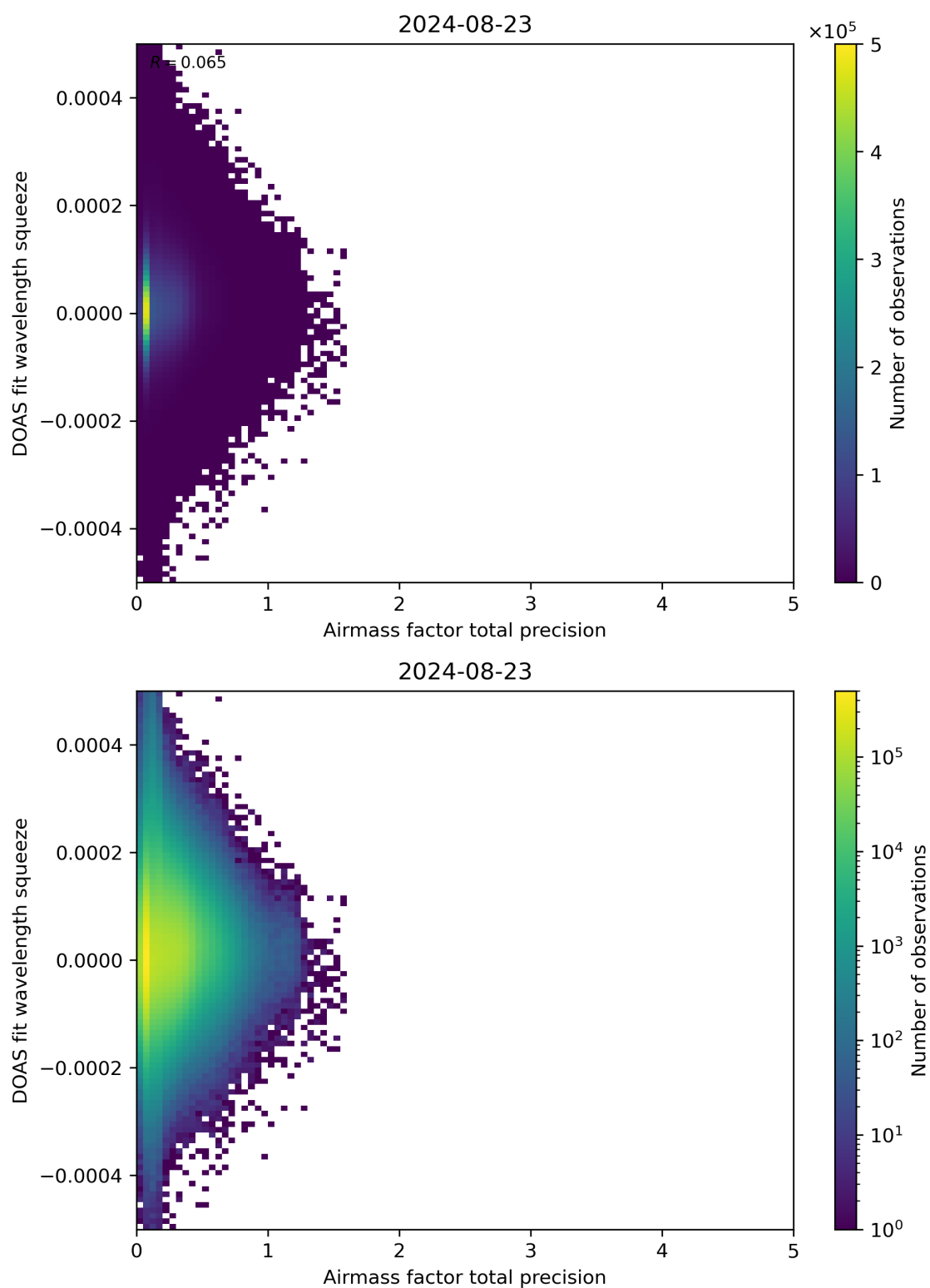
Figure 107: Scatter density plot of “Airmass factor total precision” against “DOAS fit wavelength squeeze” for 2024-08-22 to 2024-08-24.
