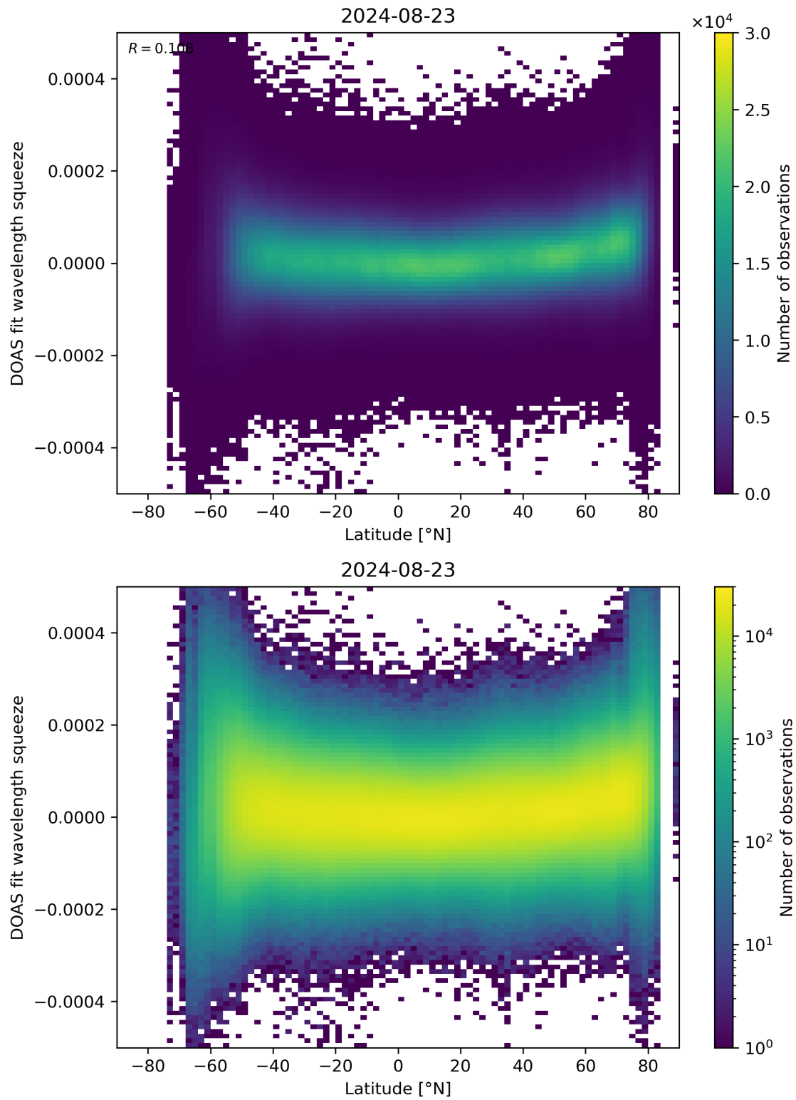
Figure 155: Scatter density plot of “Latitude” against “DOAS fit wavelength squeeze” for 2024-08-22 to 2024-08-24.
