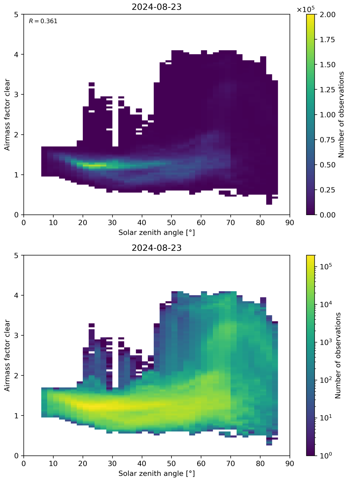
Figure 170: Scatter density plot of “Solar zenith angle” against “Airmass factor clear” for 2024-08-22 to 2024-08-24.
