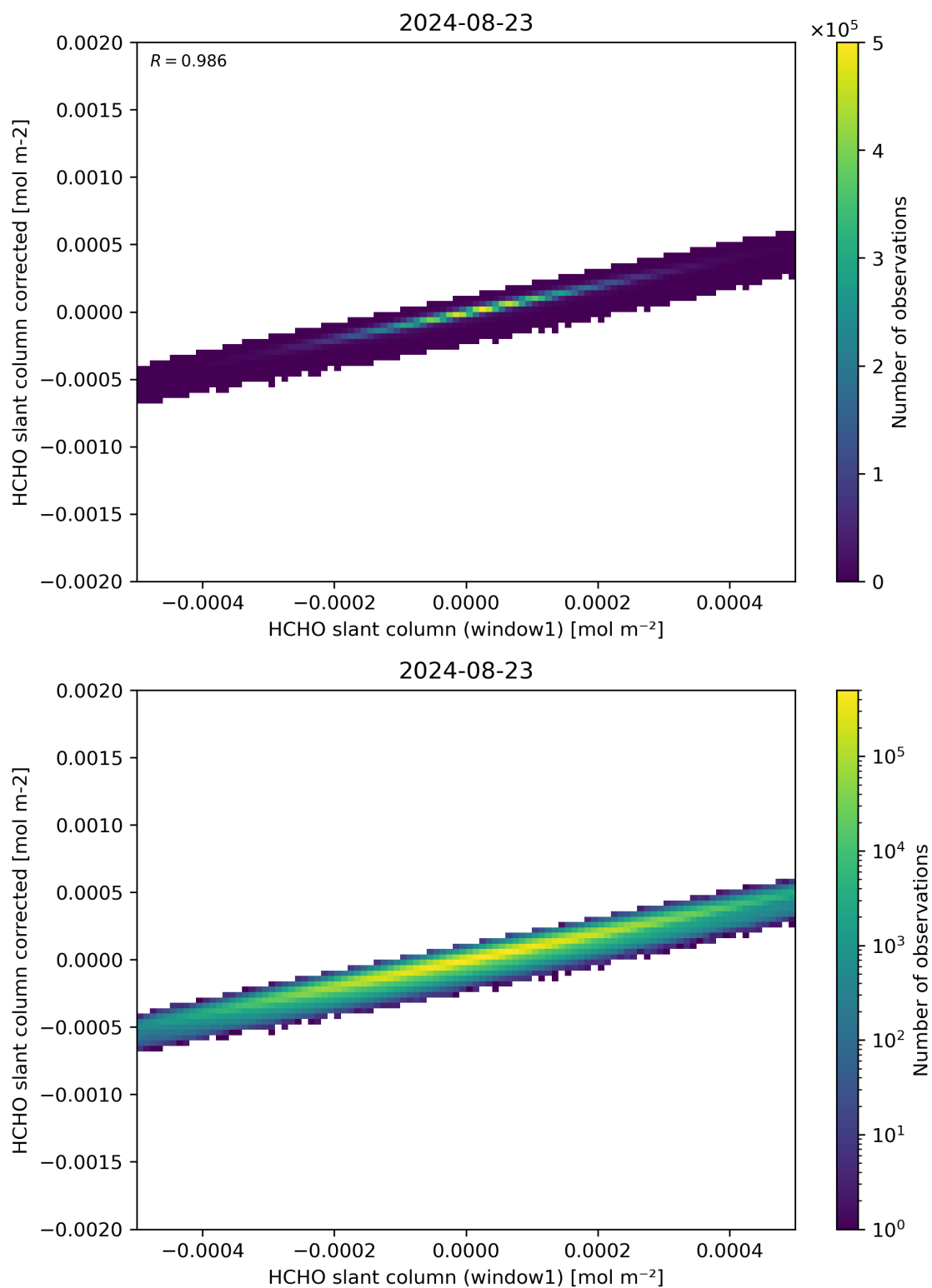
Figure 82: Scatter density plot of “HCHO slant column (window1)” against “HCHO slant column corrected” for 2024-08-22 to 2024-08-24.
