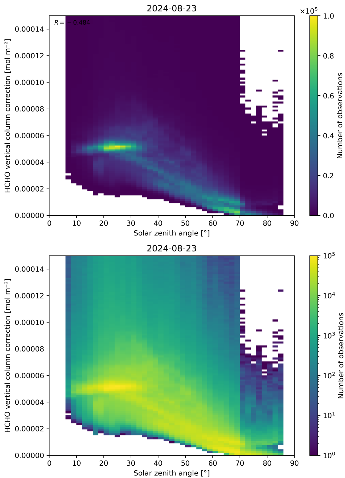
Figure 178: Scatter density plot of “Solar zenith angle” against “HCHO vertical column correction” for 2024-08-22 to 2024-08-24.
