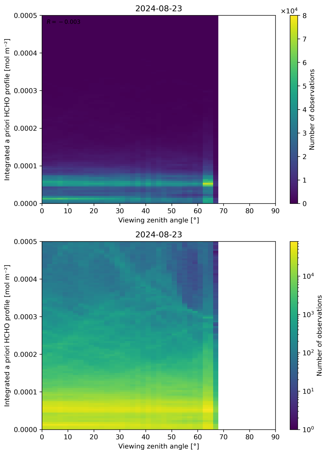
Figure 195: Scatter density plot of “Viewing zenith angle” against “Integrated a priori HCHO profile” for 2024-08-22 to 2024-08-24.
