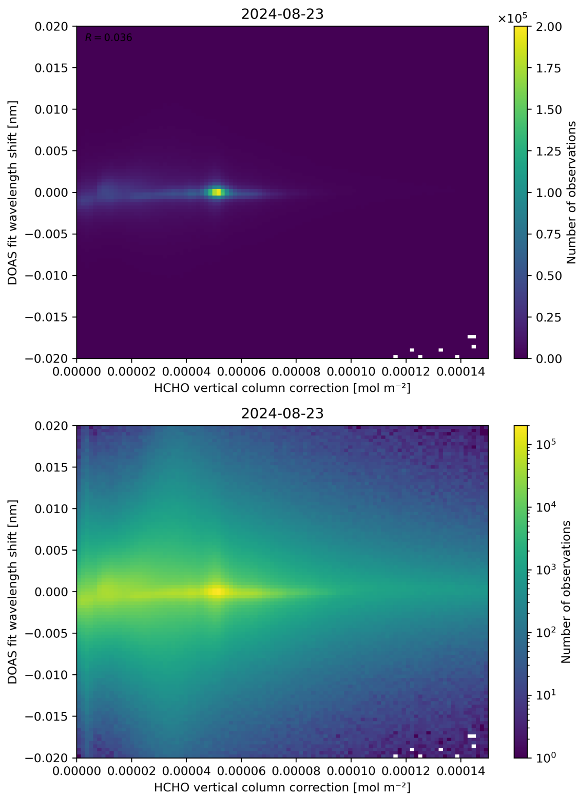
Figure 113: Scatter density plot of “HCHO vertical column correction” against “DOAS fit wavelength shift” for 2024-08-22 to 2024-08-24.
