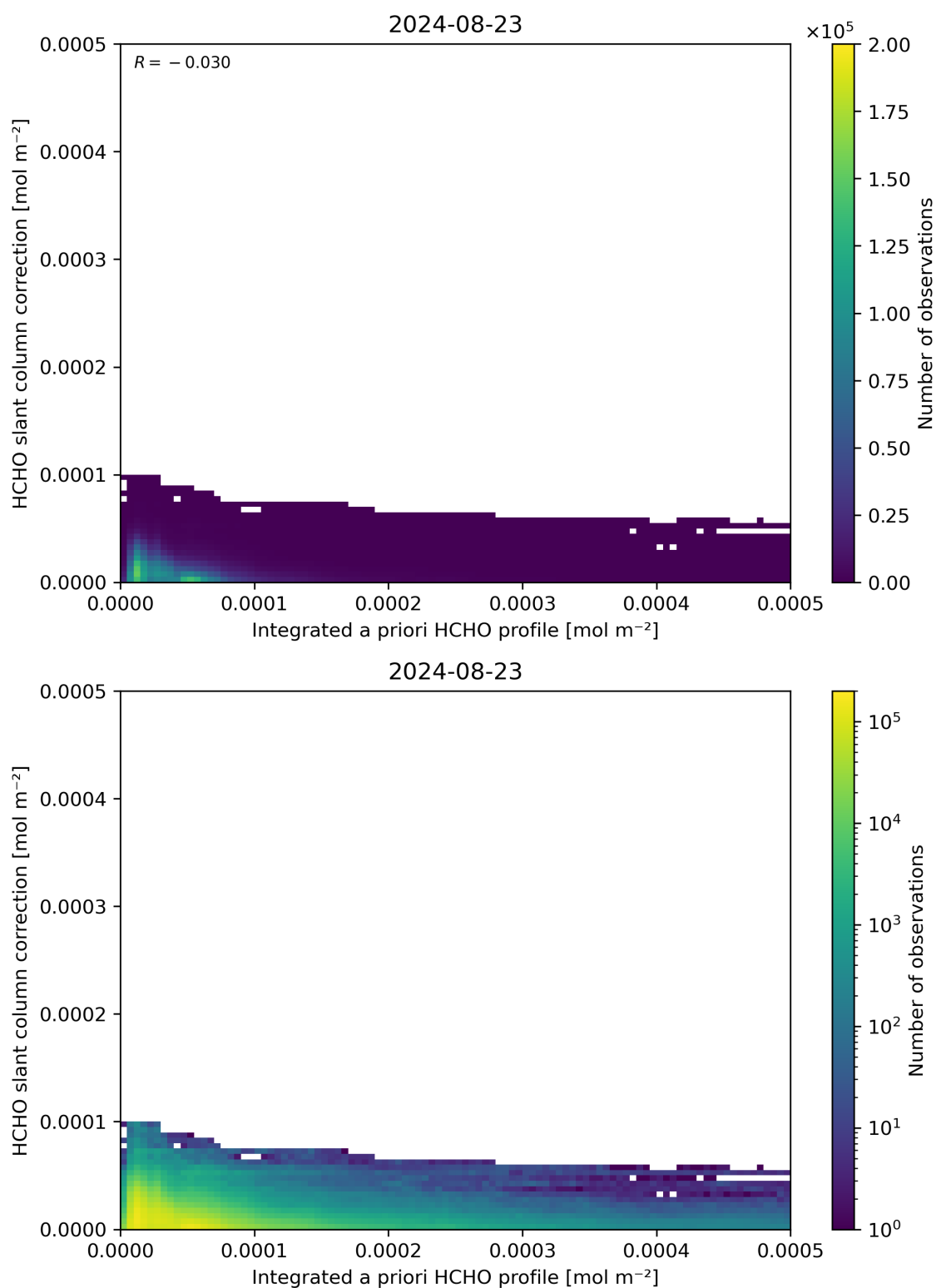
Figure 152: Scatter density plot of “Integrated a priori HCHO profile” against “HCHO slant column correction” for 2024-08-22 to 2024-08-24.
