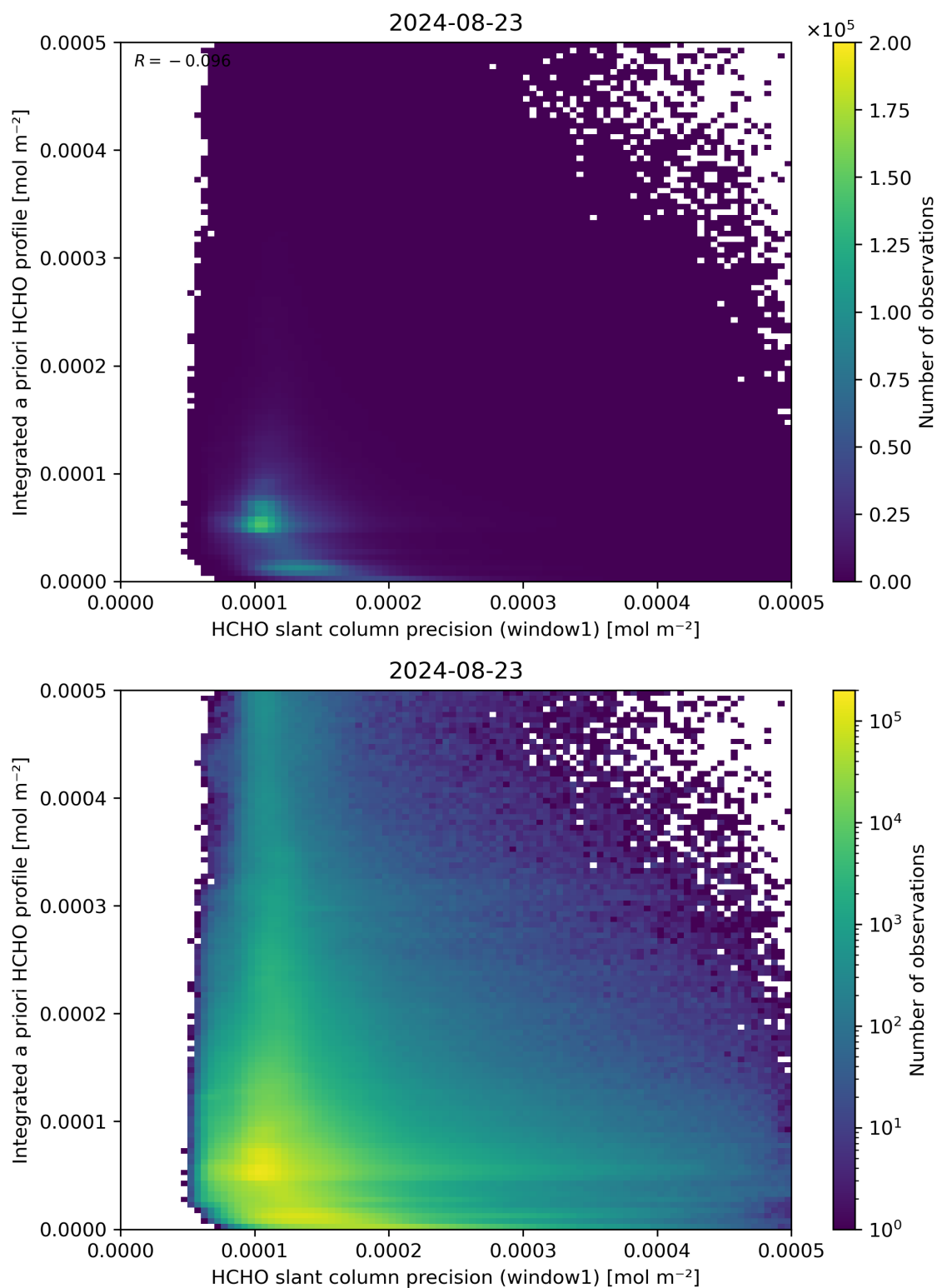
Figure 96: Scatter density plot of “HCHO slant column precision (window1)” against “Integrated a priori HCHO profile” for 2024-08-22 to 2024-08-24.
