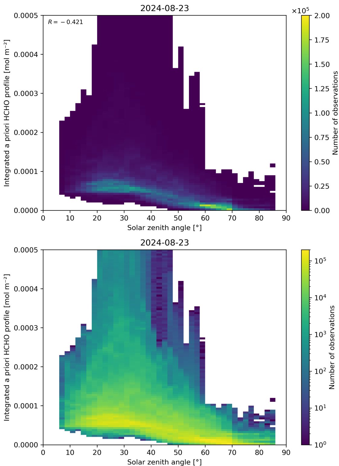
Figure 180: Scatter density plot of “Solar zenith angle” against “Integrated a priori HCHO profile” for 2024-08-22 to 2024-08-24.
