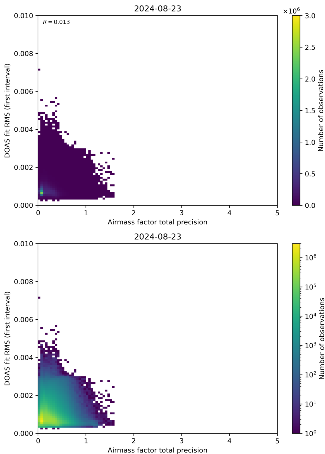
Figure 105: Scatter density plot of “Airmass factor total precision” against “DOAS fit RMS (first interval)” for 2024-08-22 to 2024-08-24.
