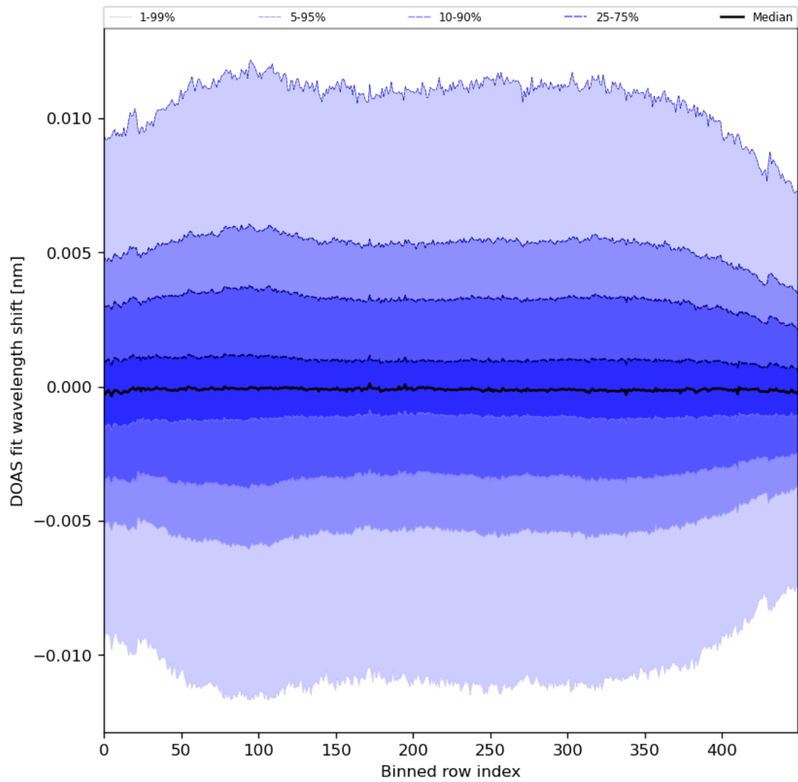
Figure 58: Along track statistics of “DOAS fit wavelength shift” for 2024-08-22 to 2024-08-24
