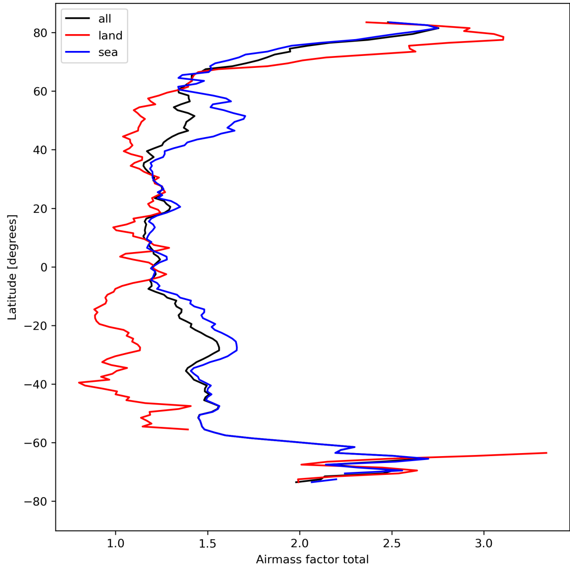
Figure 26: Zonal average of “Airmass factor total” for 2024-08-22 to 2024-08-24.
