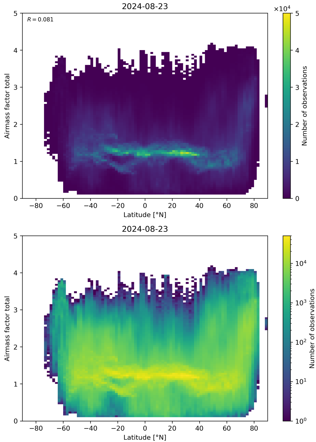
Figure 161: Scatter density plot of “Latitude” against “Airmass factor total” for 2024-08-22 to 2024-08-24.
