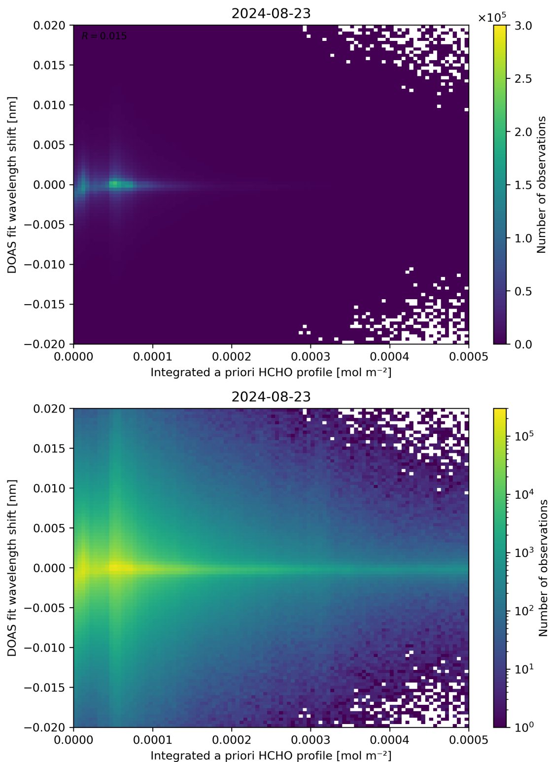
Figure 149: Scatter density plot of “Integrated a priori HCHO profile” against “DOAS fit wavelength shift” for 2024-08-22 to 2024-08-24.
