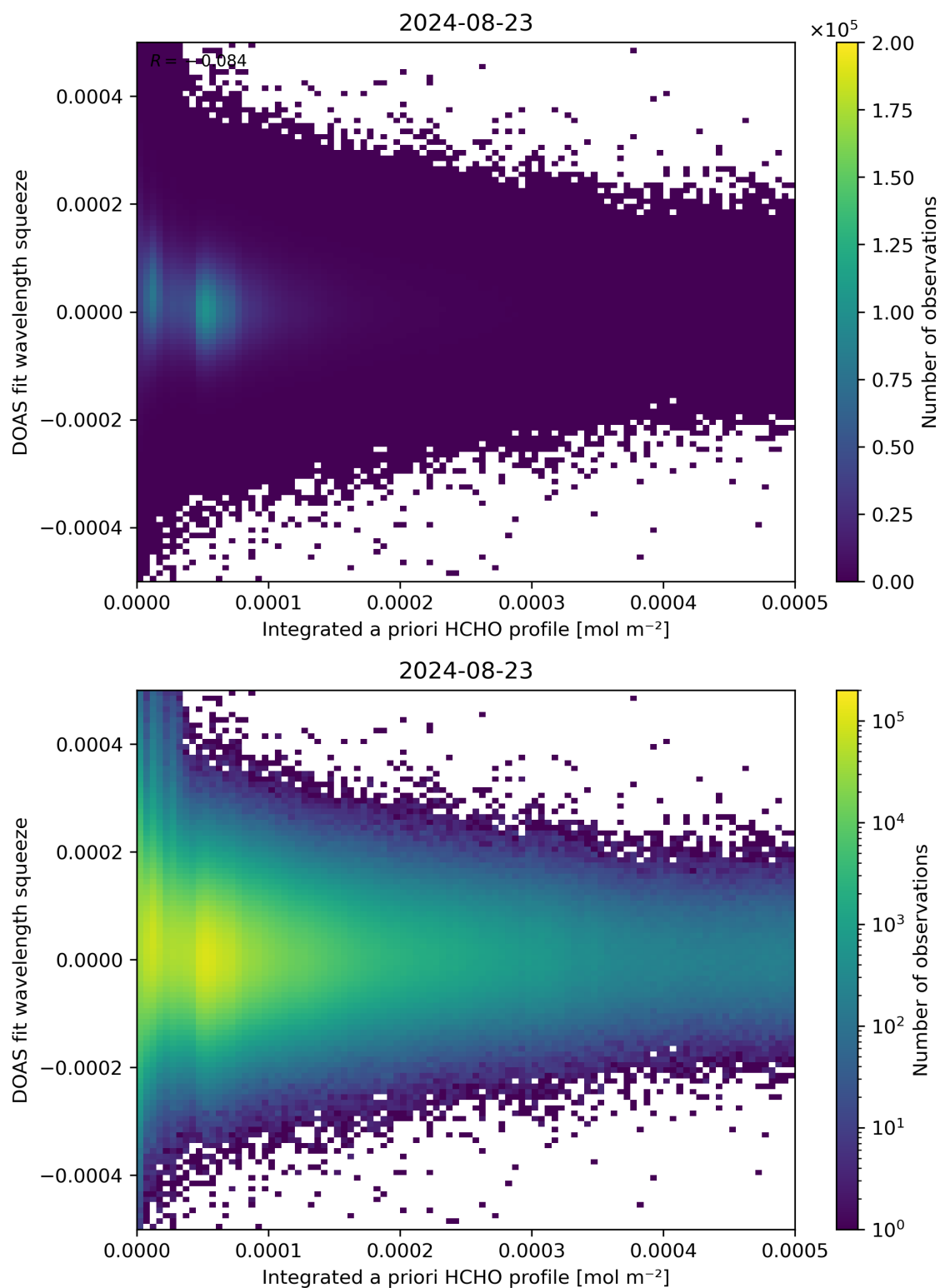
Figure 150: Scatter density plot of “Integrated a priori HCHO profile” against “DOAS fit wavelength squeeze” for 2024-08-22 to 2024-08-24.
