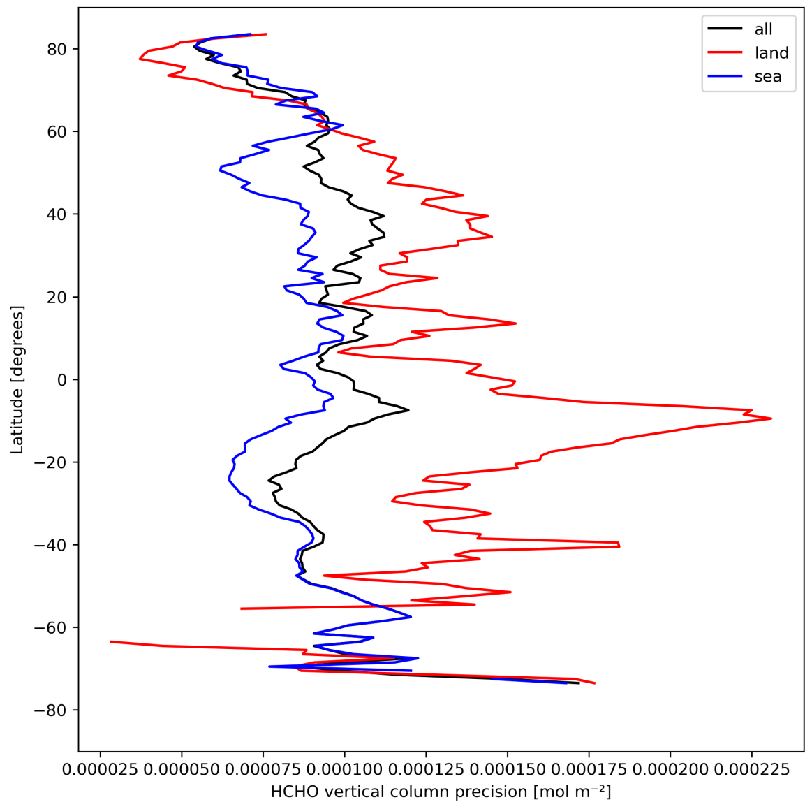
Figure 22: Zonal average of “HCHO vertical column precision” for 2024-08-22 to 2024-08-24.
