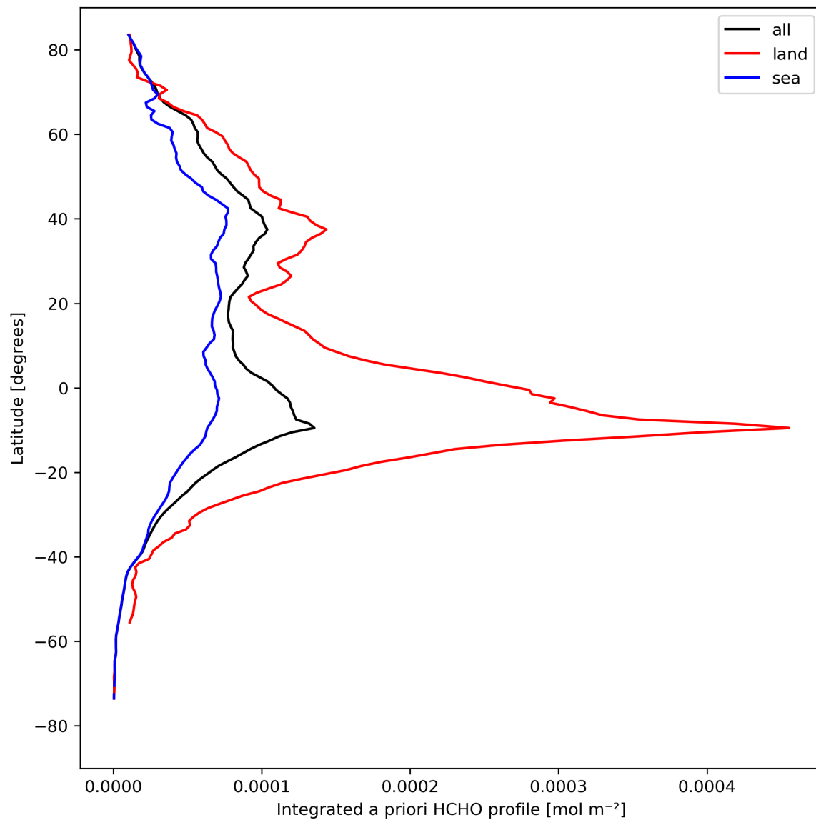
Figure 29: Zonal average of “Integrated a priori HCHO profile” for 2024-08-22 to 2024-08-24.
