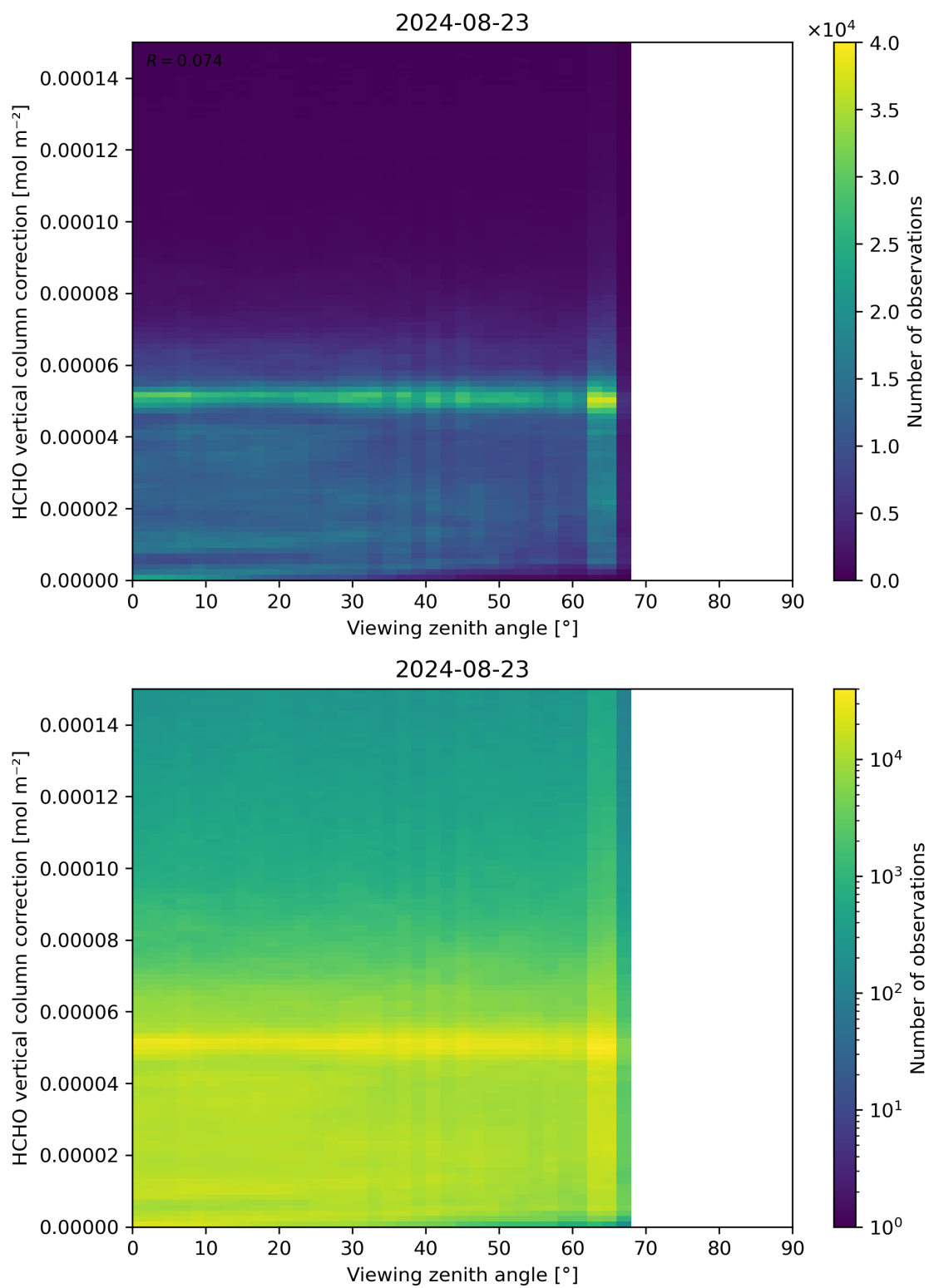
Figure 193: Scatter density plot of “Viewing zenith angle” against “HCHO vertical column correction” for 2024-08-22 to 2024-08-24.
