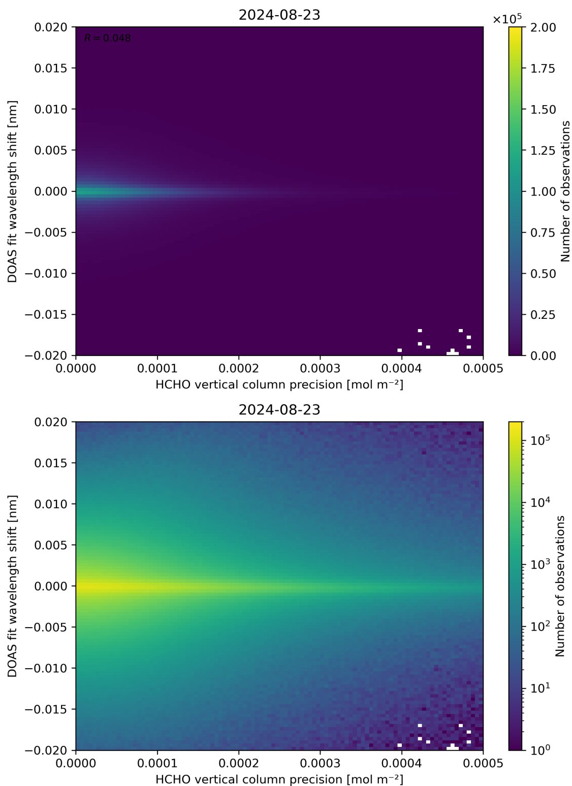
Figure 137: Scatter density plot of “HCHO vertical column precision” against “DOAS fit wavelength shift” for 2024-08-22 to 2024-08-24.
