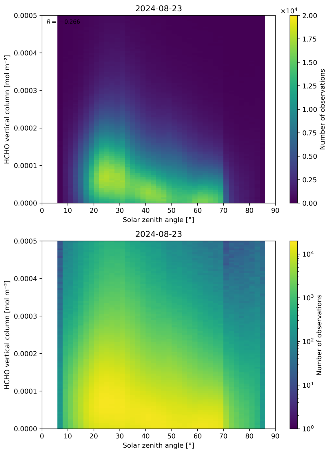
Figure 177: Scatter density plot of “Solar zenith angle” against “HCHO vertical column” for 2024-08-22 to 2024-08-24.
