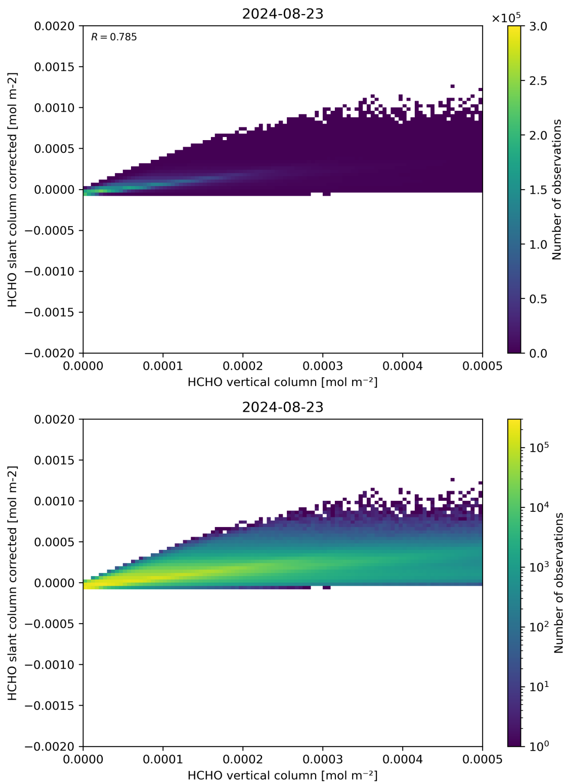
Figure 127: Scatter density plot of “HCHO vertical column” against “HCHO slant column corrected” for 2024-08-22 to 2024-08-24.
