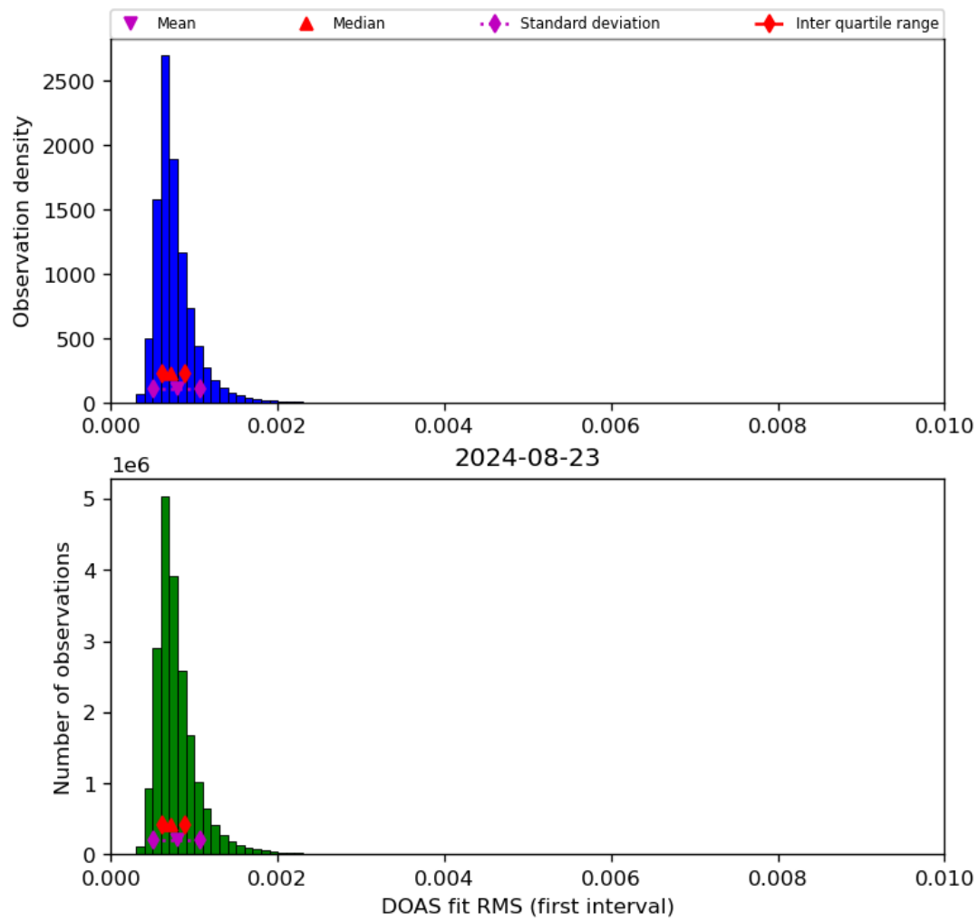
Figure 46: Histogram of “DOAS fit RMS (first interval)” for 2024-08-22 to 2024-08-24
