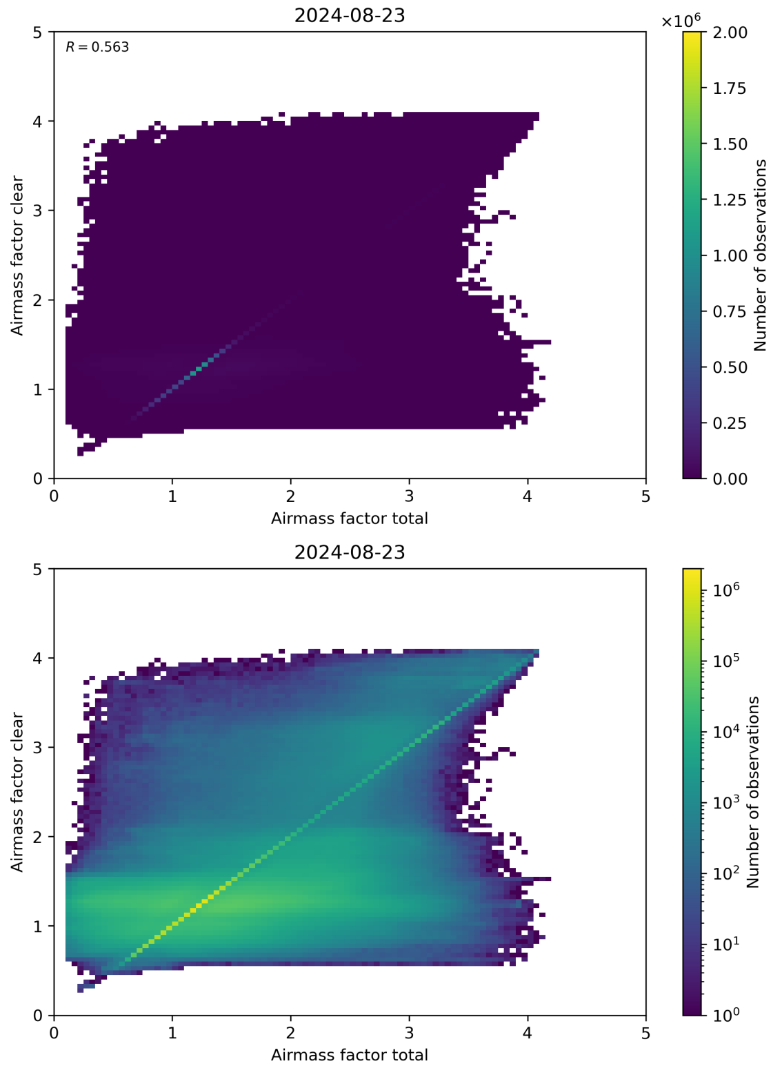
Figure 100: Scatter density plot of “Airmass factor total” against “Airmass factor clear” for 2024-08-22 to 2024-08-24.
