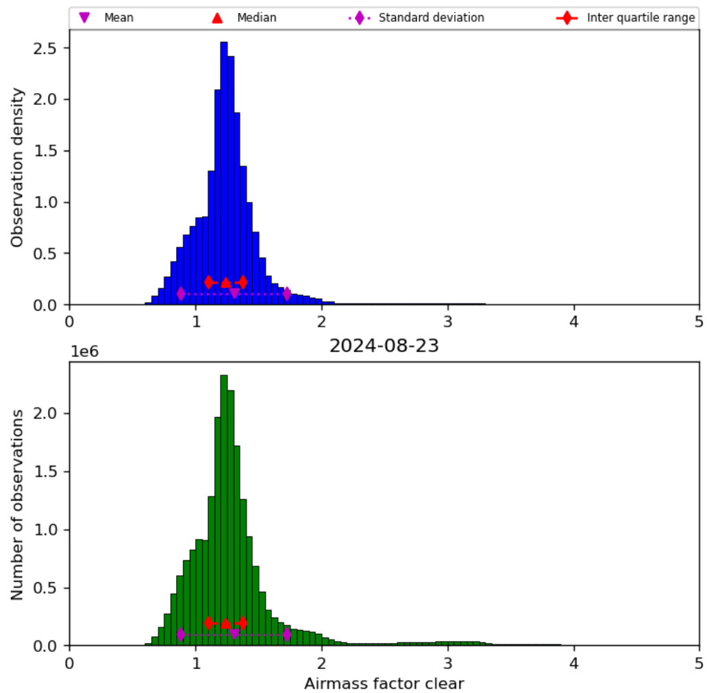
Figure 42: Histogram of “Airmass factor clear” for 2024-08-22 to 2024-08-24
