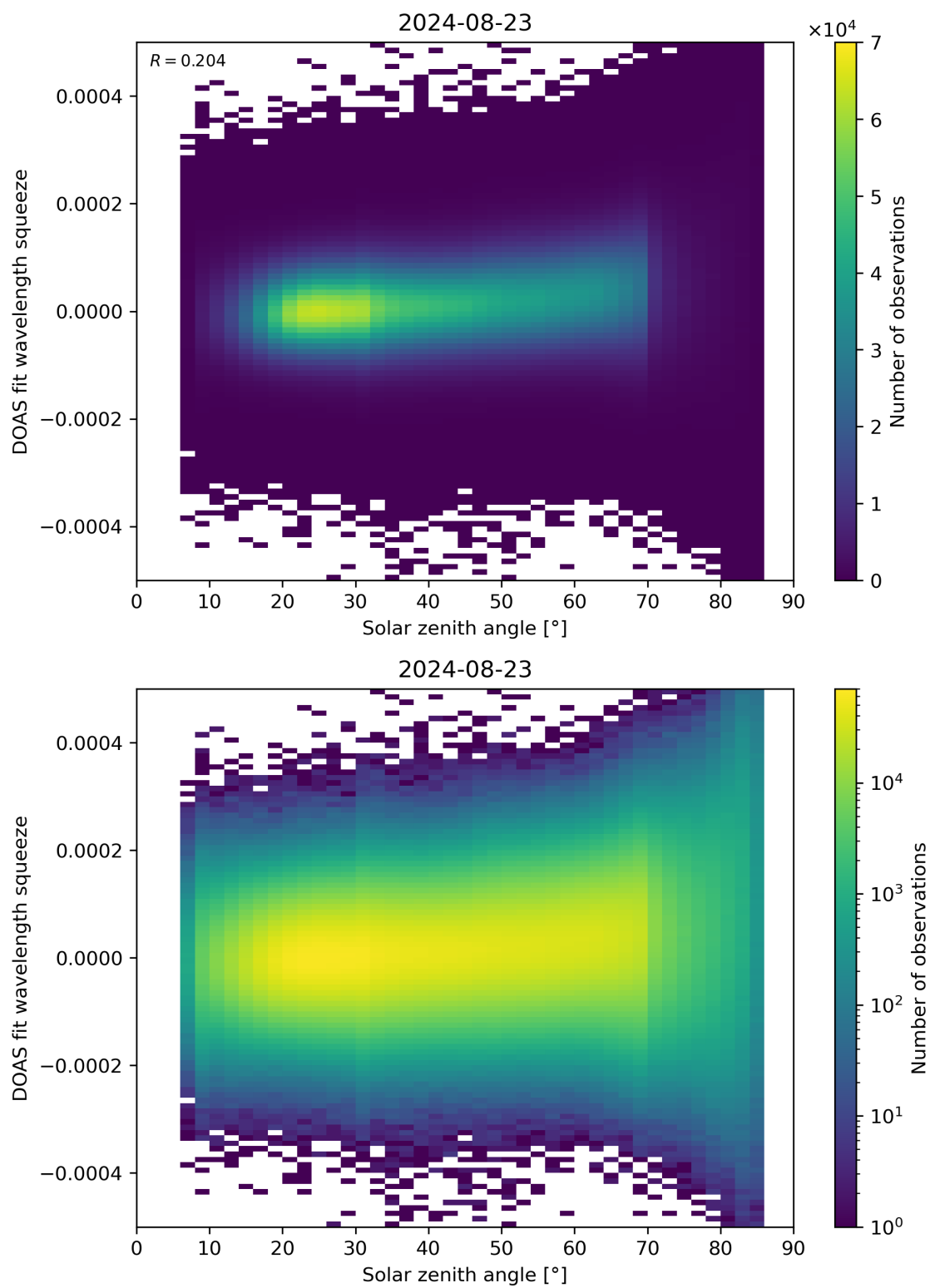
Figure 169: Scatter density plot of “Solar zenith angle” against “DOAS fit wavelength squeeze” for 2024-08-22 to 2024-08-24.
