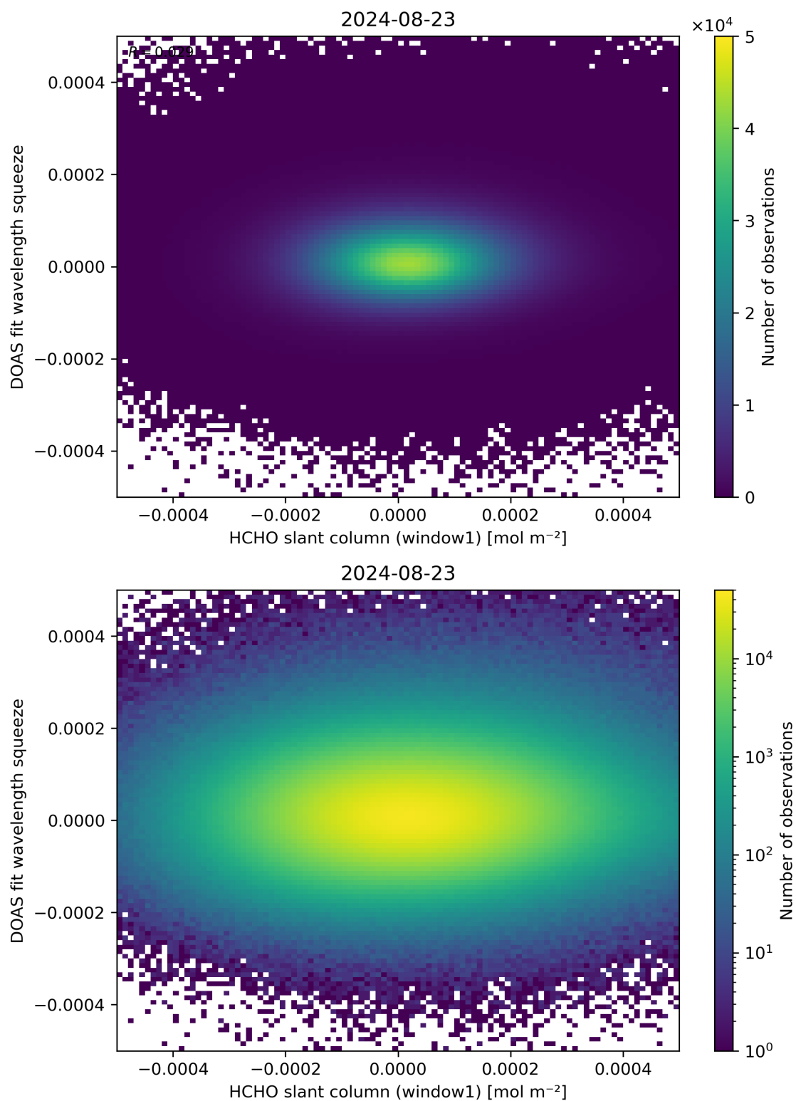
Figure 80: Scatter density plot of “HCHO slant column (window1)” against “DOAS fit wavelength squeeze” for 2024-08-22 to 2024-08-24.
