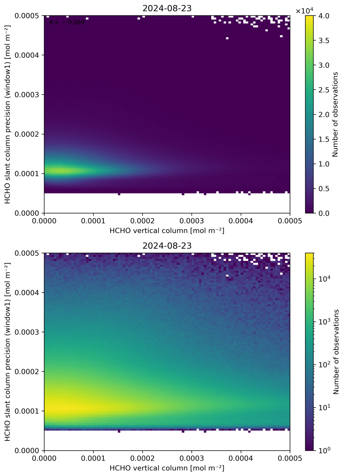
Figure 130: Scatter density plot of “HCHO vertical column” against “HCHO slant column precision (window1)” for 2024-08-22 to 2024-08-24.
