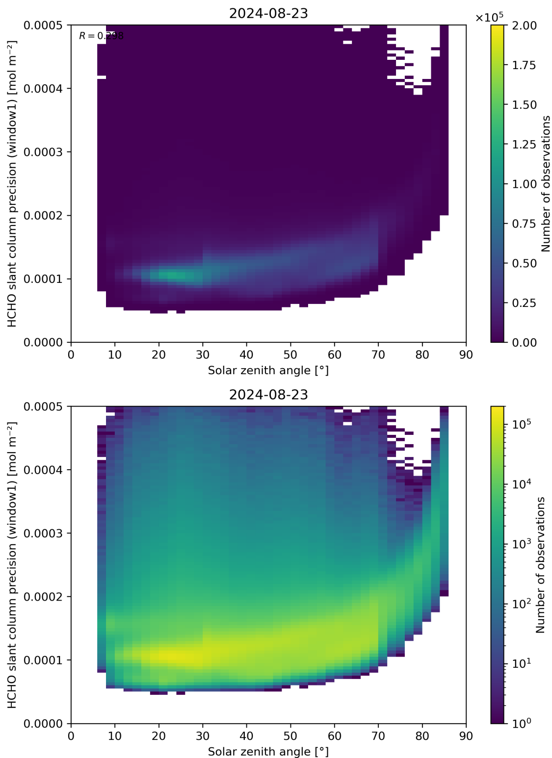
Figure 174: Scatter density plot of “Solar zenith angle” against “HCHO slant column precision (window1)” for 2024-08-22 to 2024-08-24.
