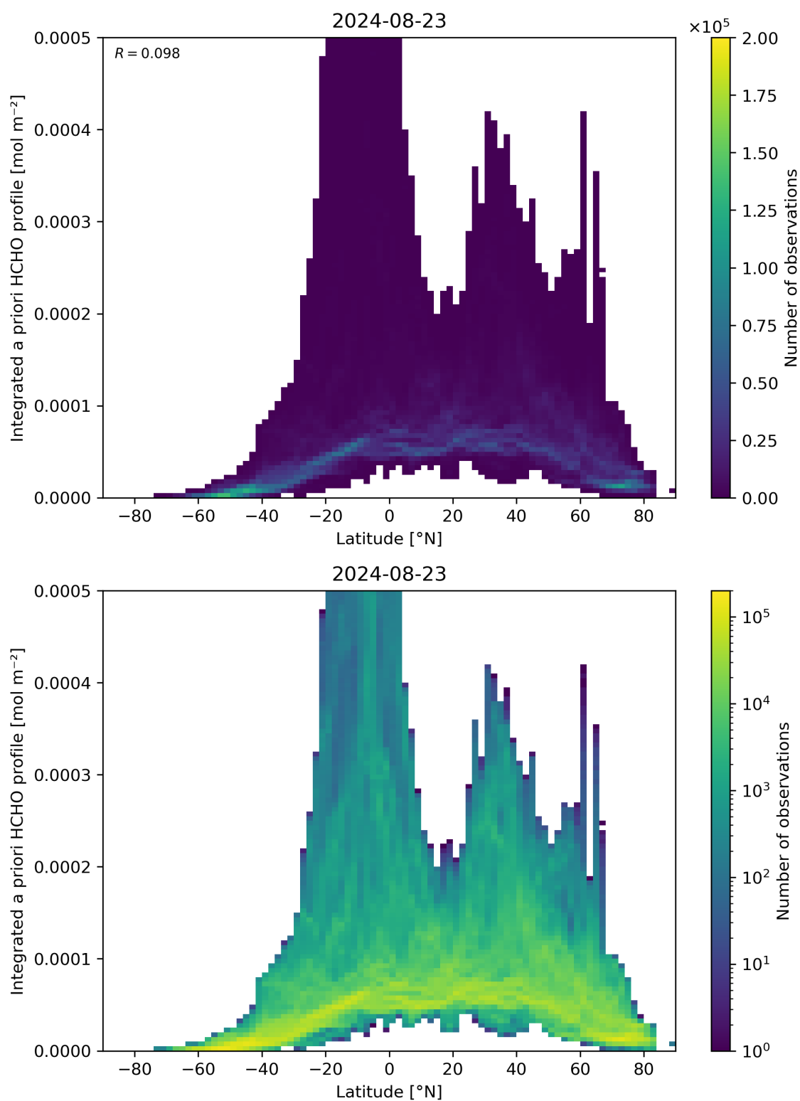
Figure 166: Scatter density plot of “Latitude” against “Integrated a priori HCHO profile” for 2024-08-22 to 2024-08-24.
