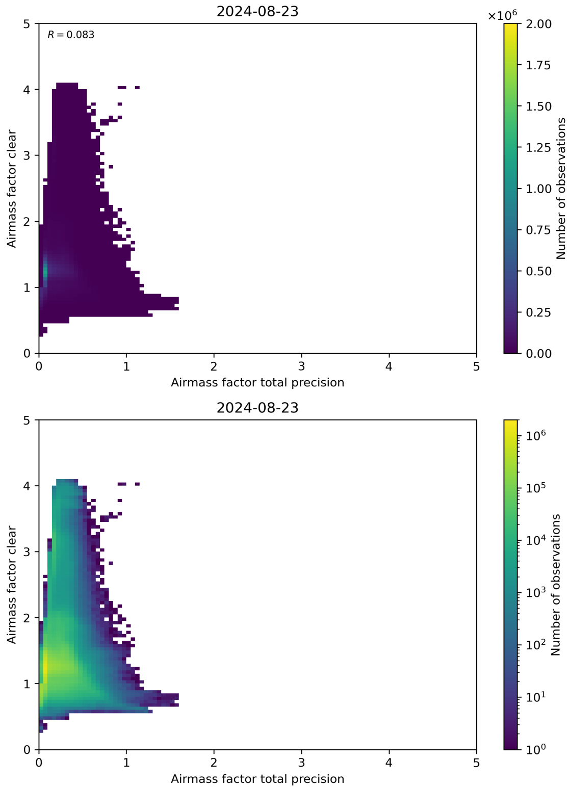
Figure 108: Scatter density plot of “Airmass factor total precision” against “Airmass factor clear” for 2024-08-22 to 2024-08-24.
