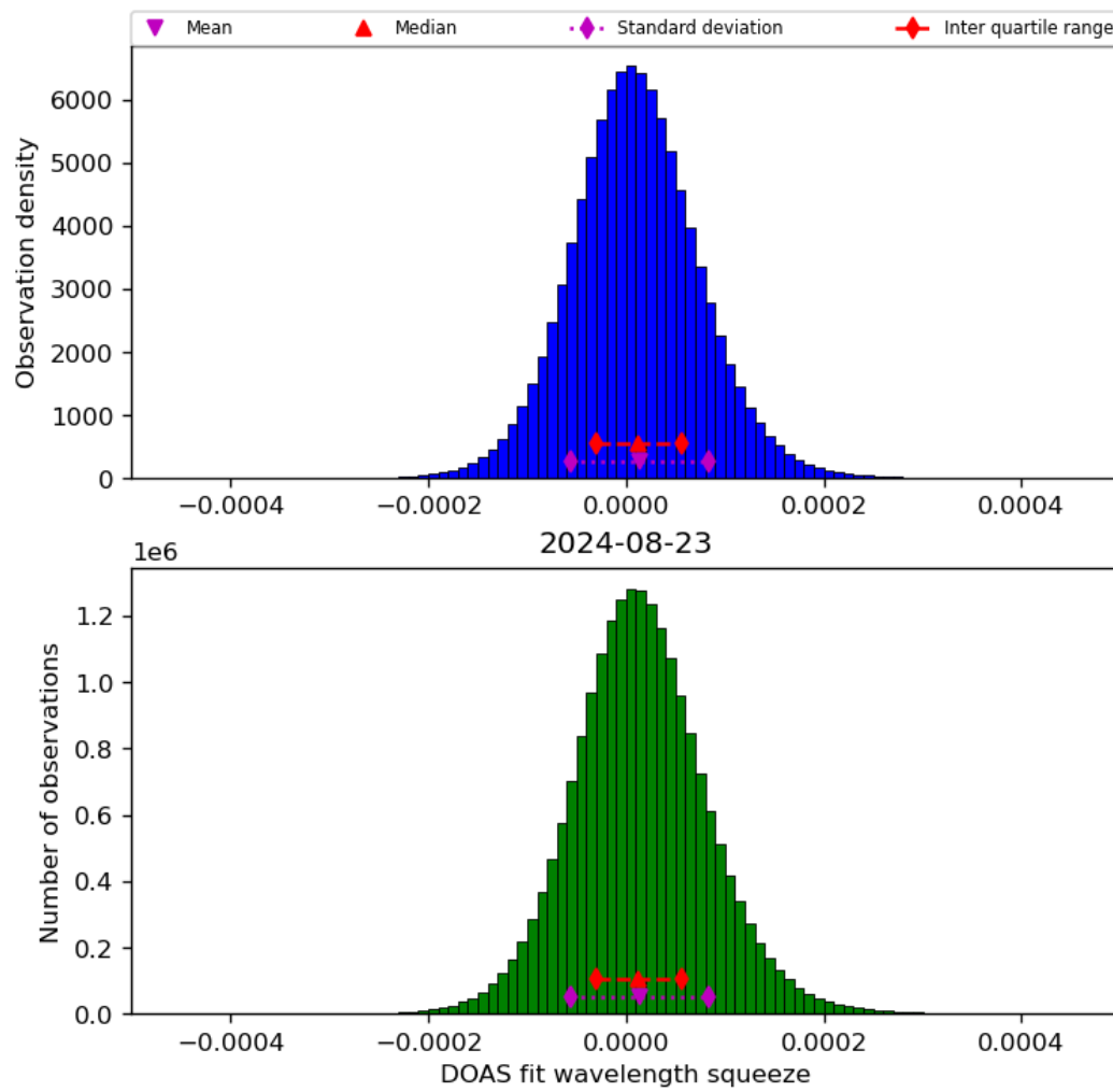
Figure 45: Histogram of “DOAS fit wavelength squeeze” for 2024-08-22 to 2024-08-24
