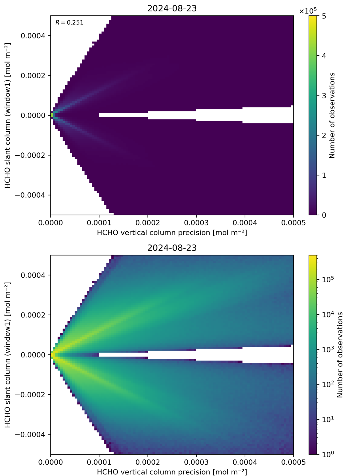
Figure 142: Scatter density plot of “HCHO vertical column precision” against “HCHO slant column (window1)” for 2024-08-22 to 2024-08-24.
