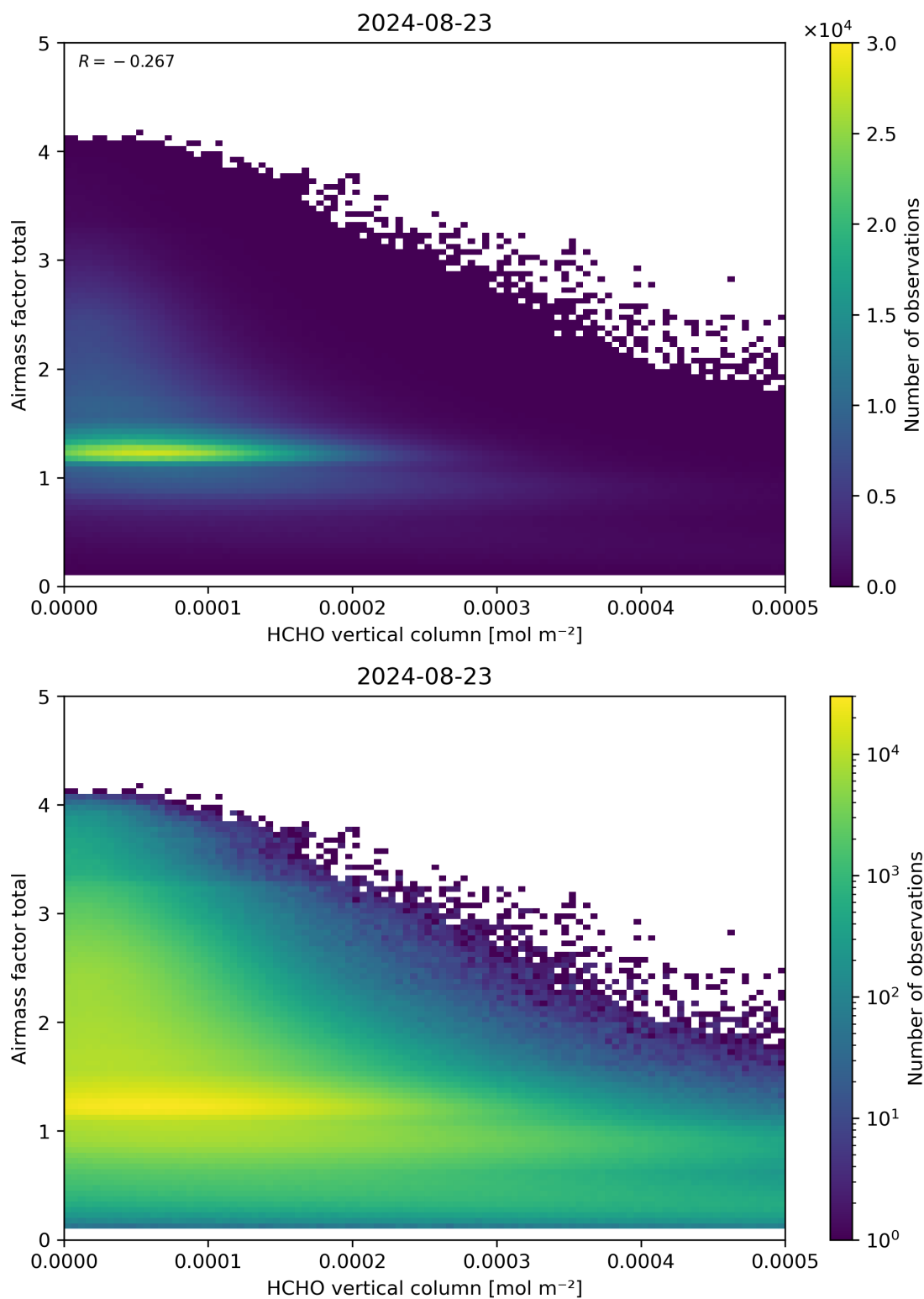
Figure 131: Scatter density plot of “HCHO vertical column” against “Airmass factor total” for 2024-08-22 to 2024-08-24.
