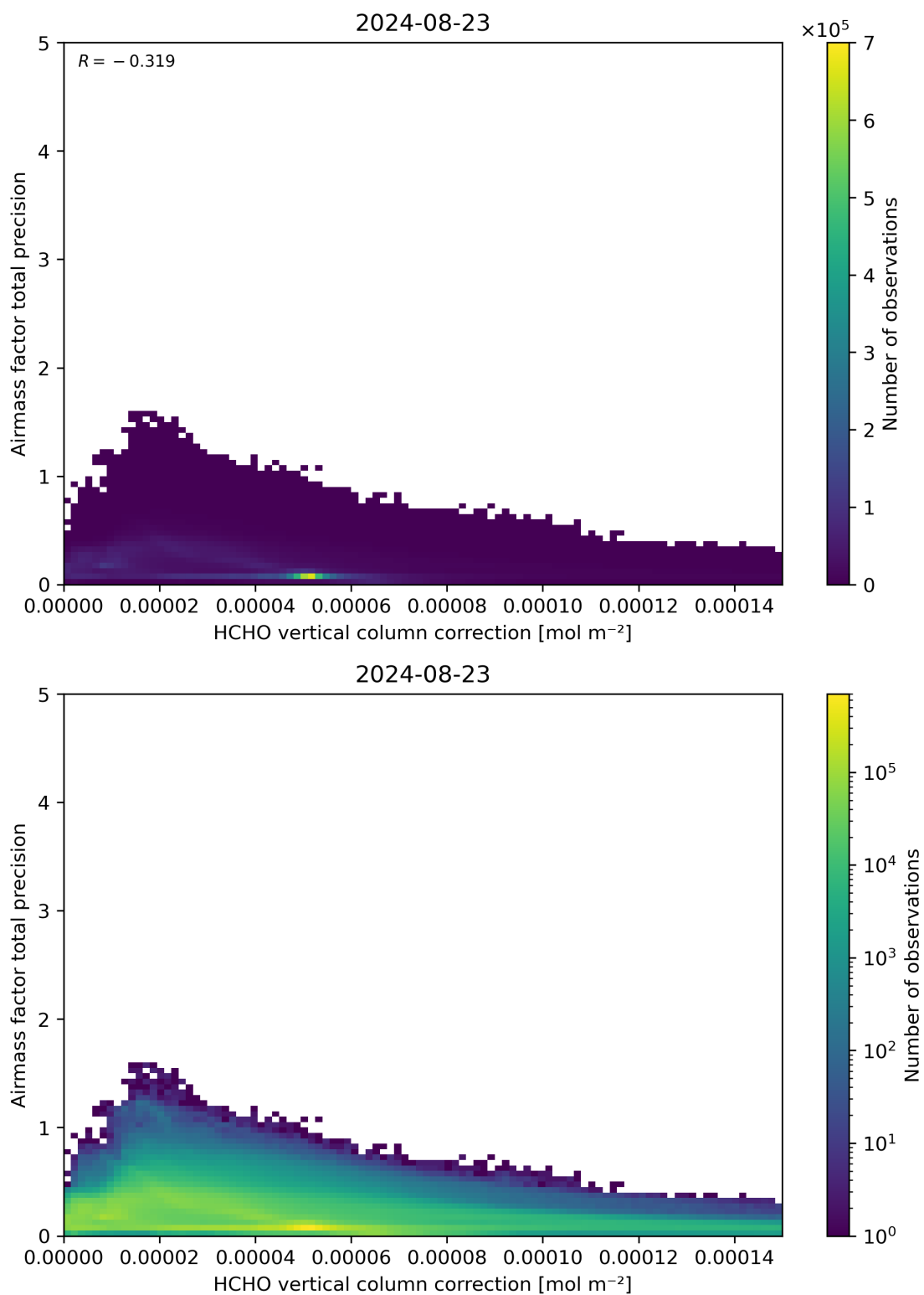
Figure 121: Scatter density plot of “HCHO vertical column correction” against “Airmass factor total precision” for 2024-08-22 to 2024-08-24.
