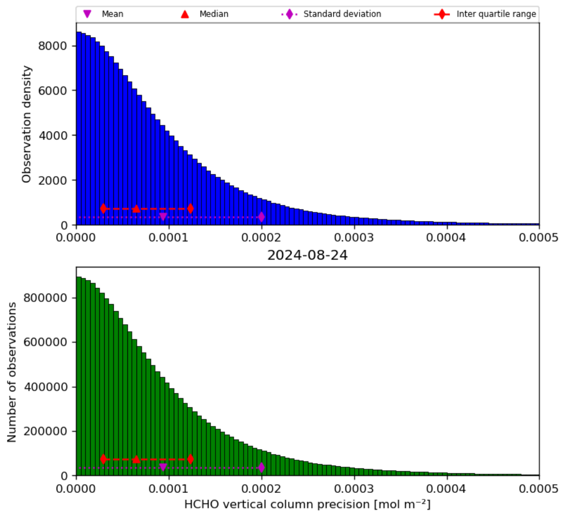
Figure 36: Histogram of “HCHO vertical column precision” for 2024-08-23 to 2024-08-25
