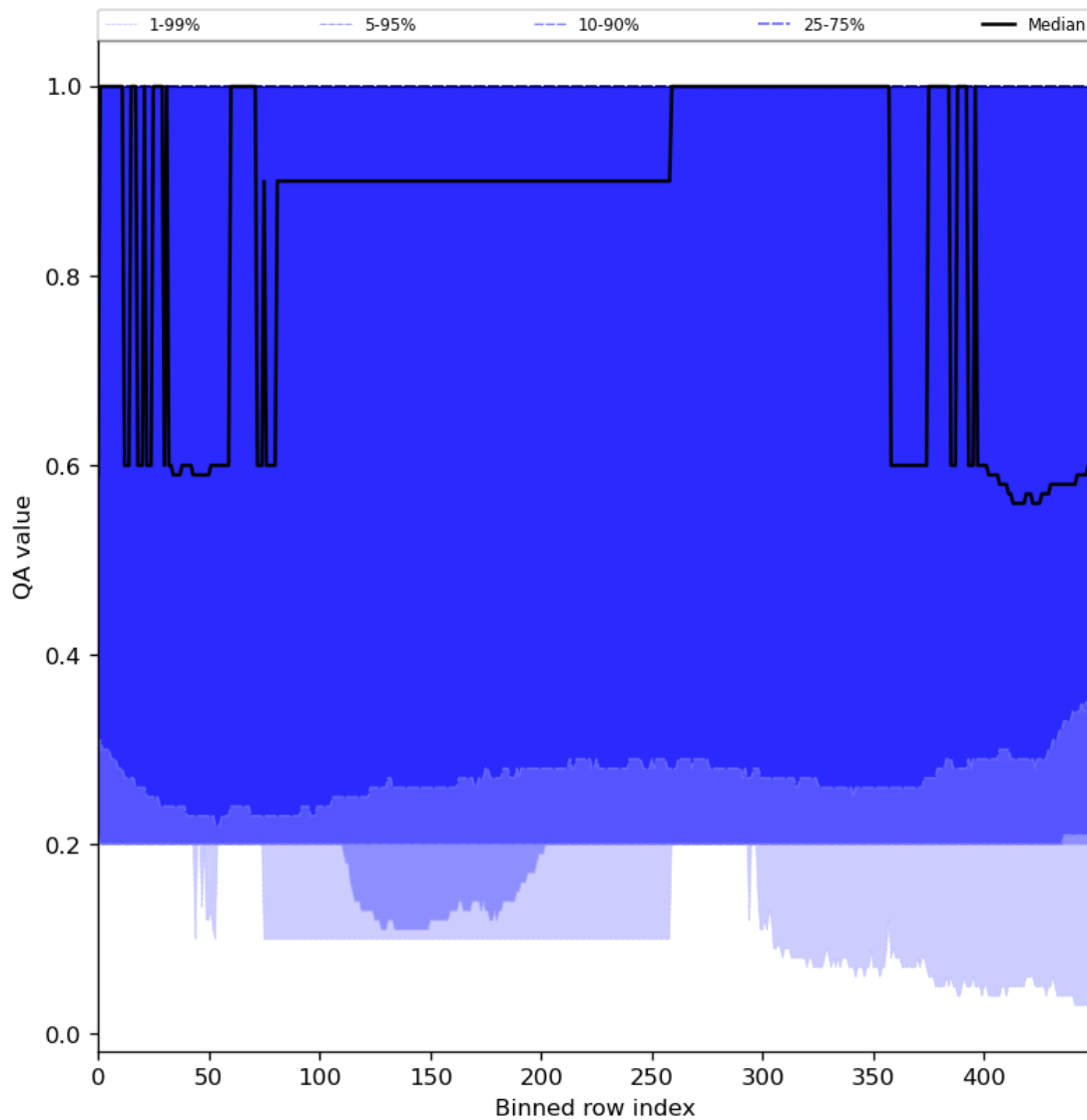
Figure 48: Along track statistics of “QA value” for 2024-08-23 to 2024-08-25
