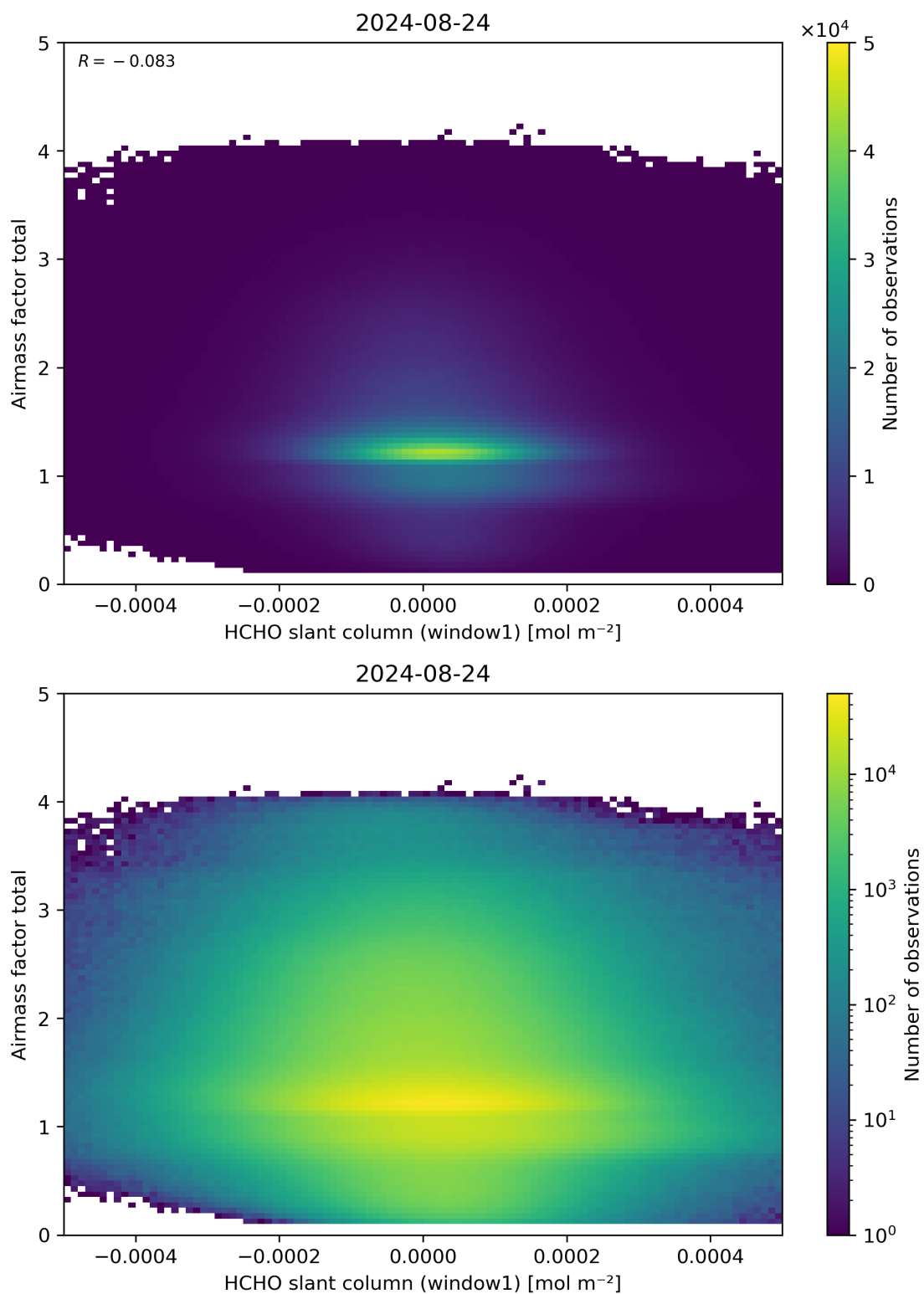
Figure 85: Scatter density plot of “HCHO slant column (window1)” against “Airmass factor total” for 2024-08-23 to 2024-08-25.
