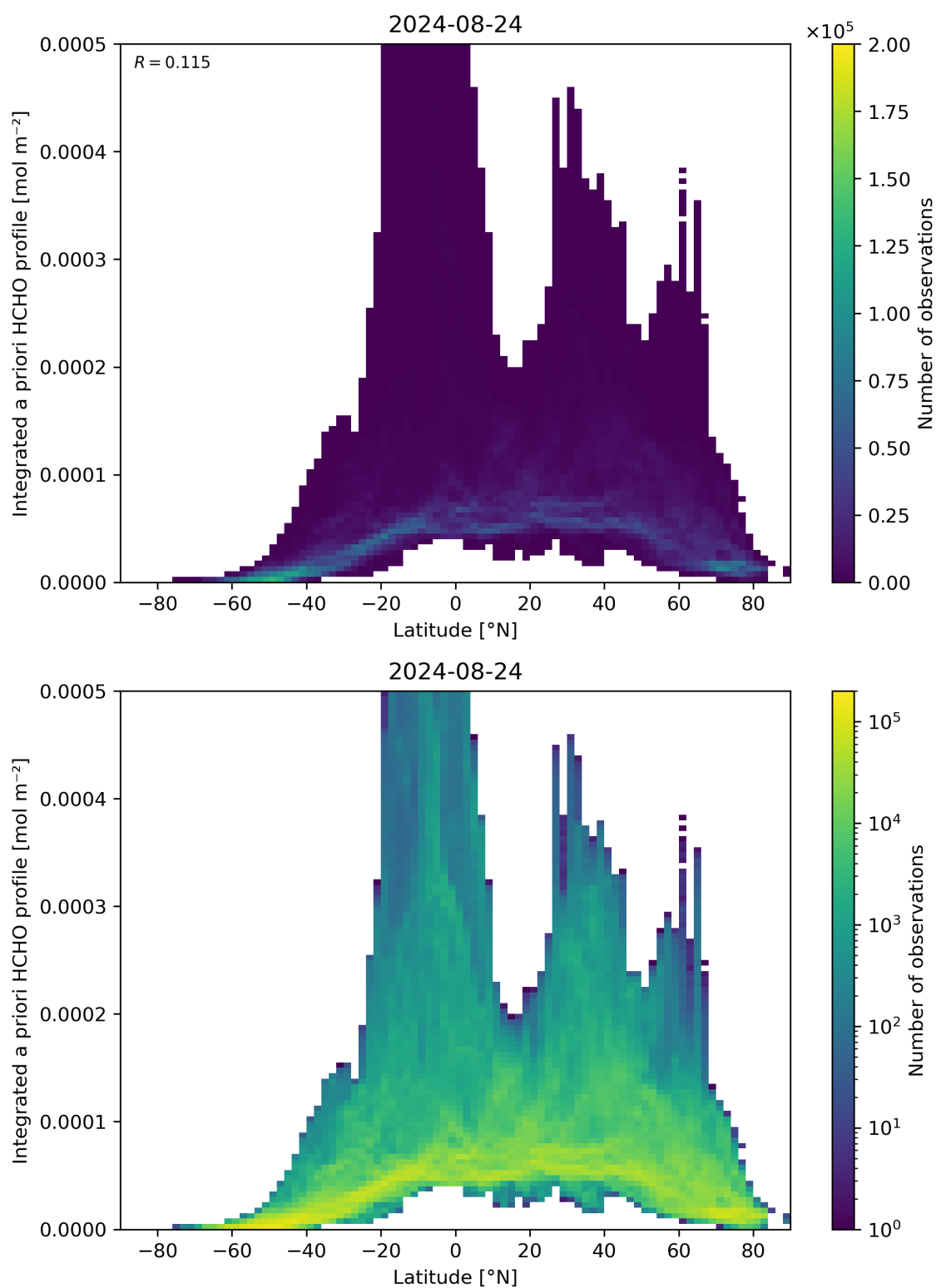
Figure 166: Scatter density plot of “Latitude” against “Integrated a priori HCHO profile” for 2024-08-23 to 2024-08-25.
