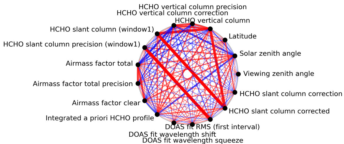
Figure 1: Map of correlation graph for 2024-08-23 to 2024-08-25.
