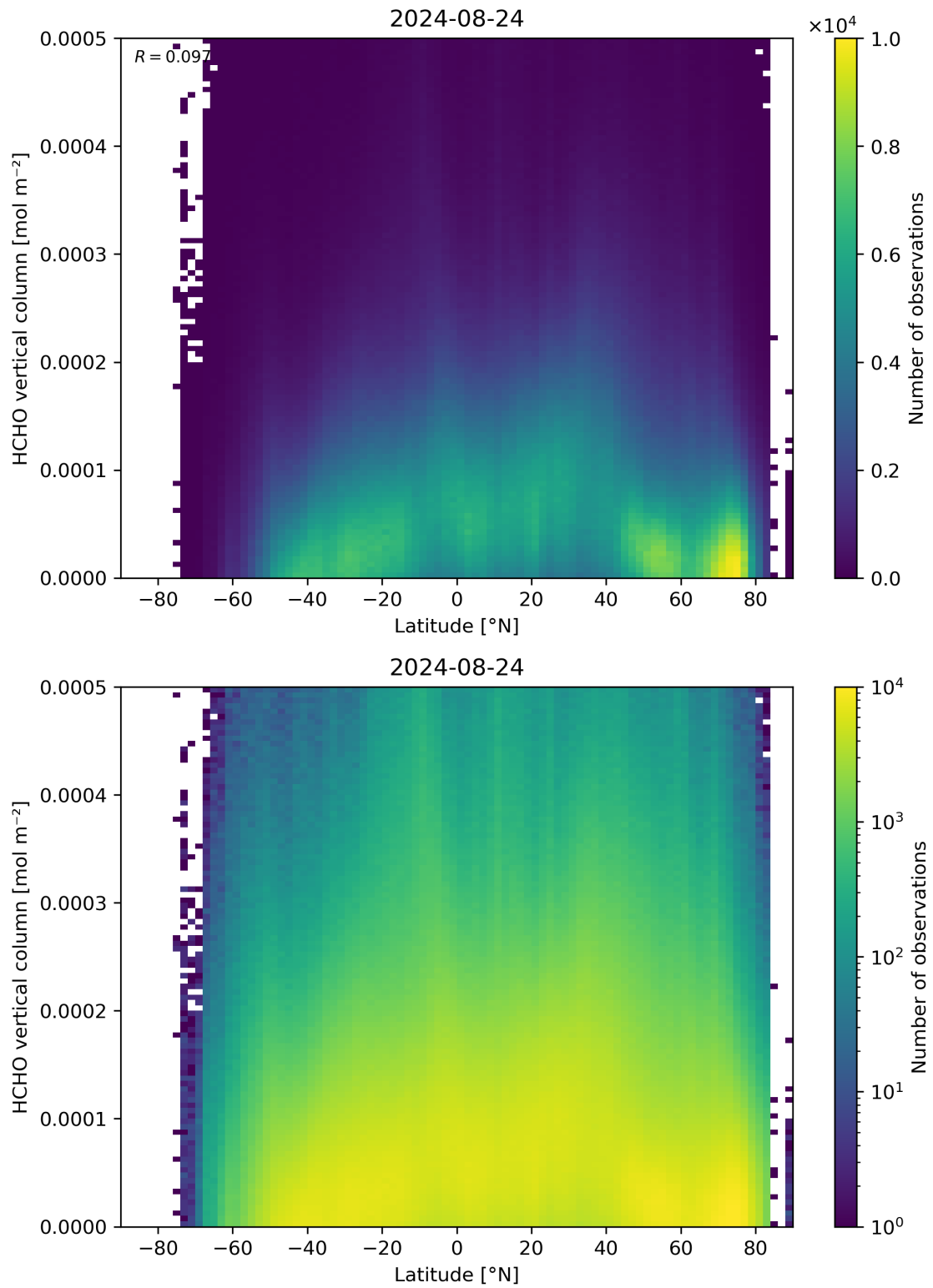
Figure 163: Scatter density plot of “Latitude” against “HCHO vertical column” for 2024-08-23 to 2024-08-25.
