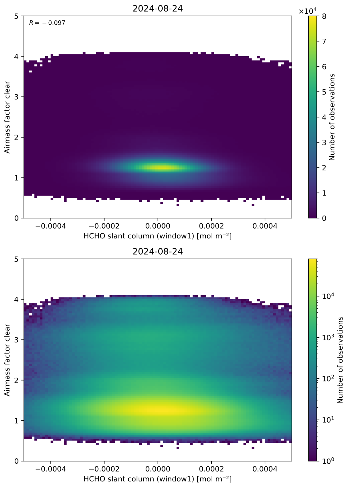
Figure 81: Scatter density plot of “HCHO slant column (window1)” against “Airmass factor clear” for 2024-08-23 to 2024-08-25.
