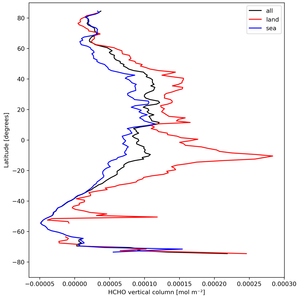
Figure 21: Zonal average of “HCHO vertical column” for 2024-08-23 to 2024-08-25.
