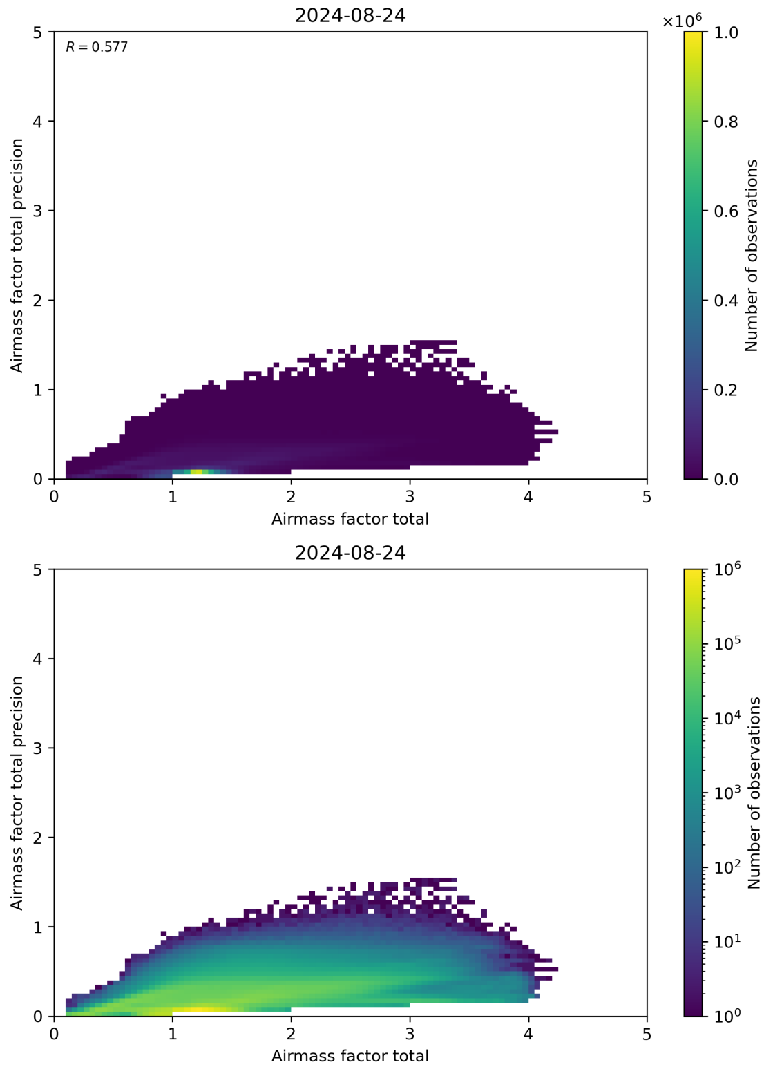
Figure 103: Scatter density plot of “Airmass factor total” against “Airmass factor total precision” for 2024-08-23 to 2024-08-25.
