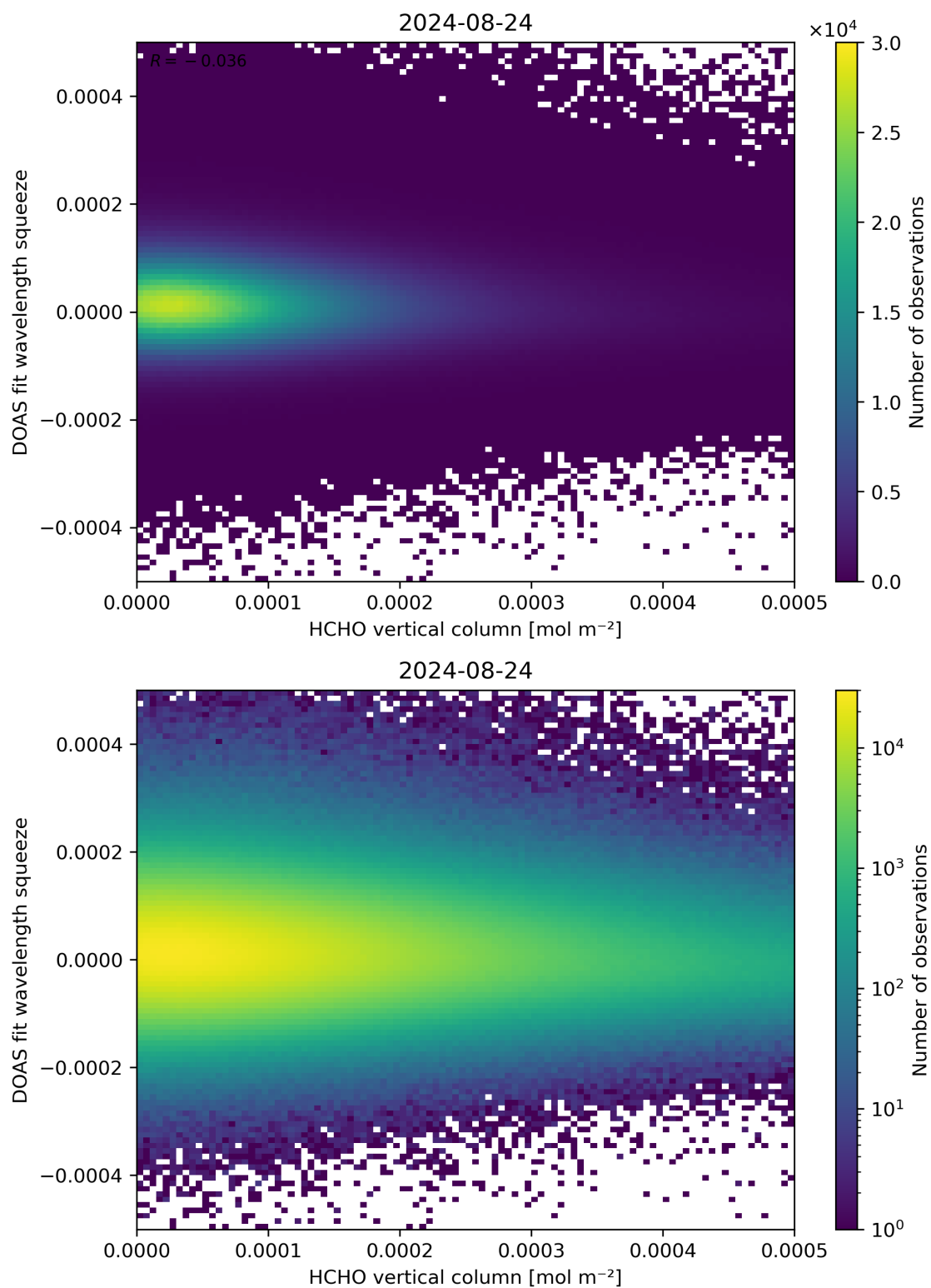
Figure 125: Scatter density plot of “HCHO vertical column” against “DOAS fit wavelength squeeze” for 2024-08-23 to 2024-08-25.
