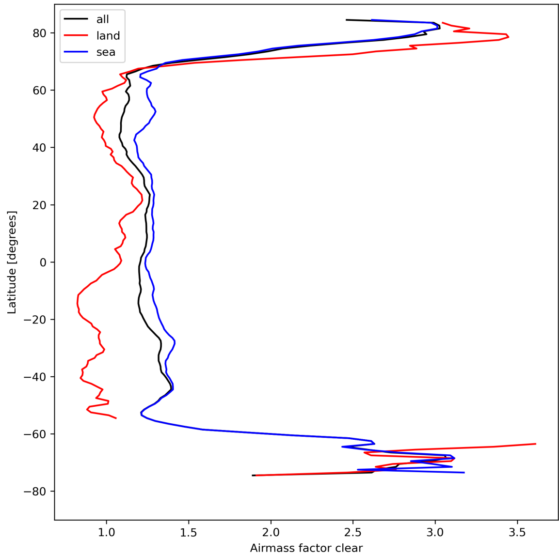
Figure 28: Zonal average of “Airmass factor clear” for 2024-08-23 to 2024-08-25.
