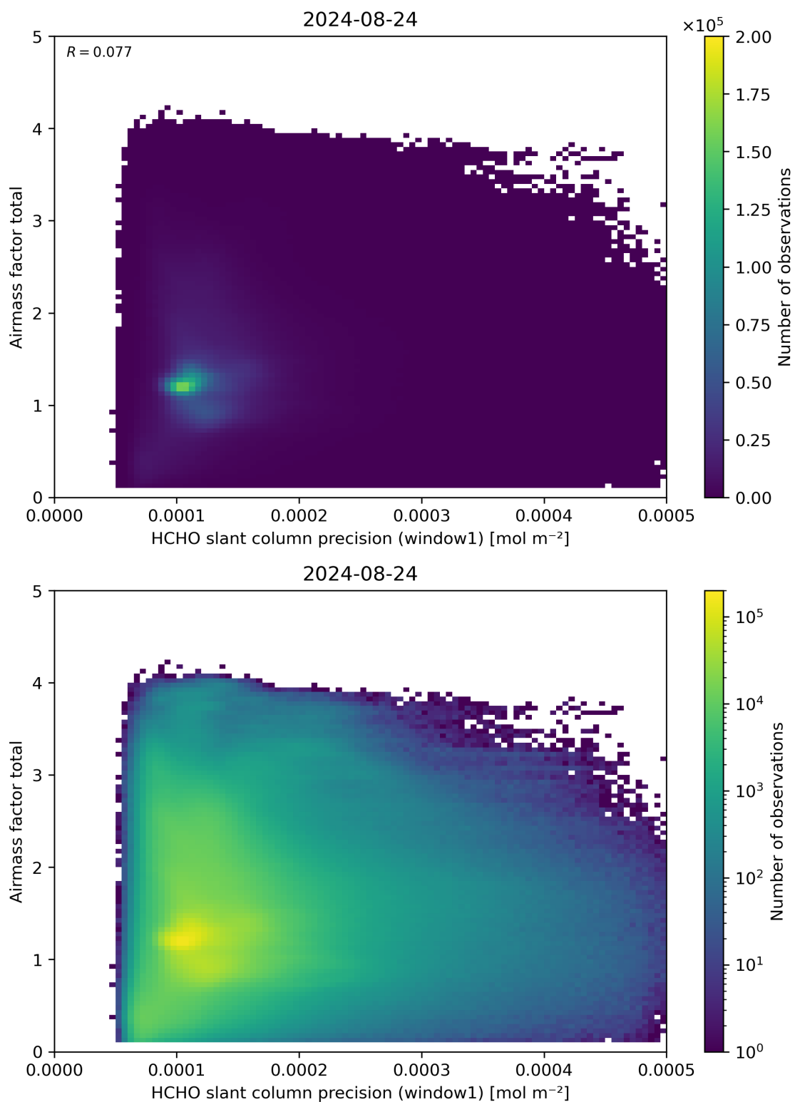
Figure 94: Scatter density plot of “HCHO slant column precision (window1)” against “Airmass factor total” for 2024-08-23 to 2024-08-25.
