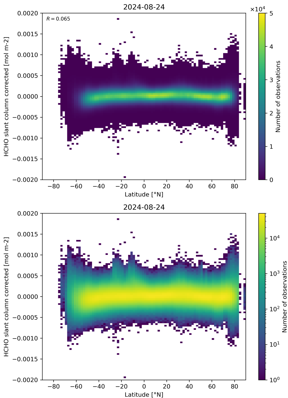
Figure 157: Scatter density plot of “Latitude” against “HCHO slant column corrected” for 2024-08-23 to 2024-08-25.
