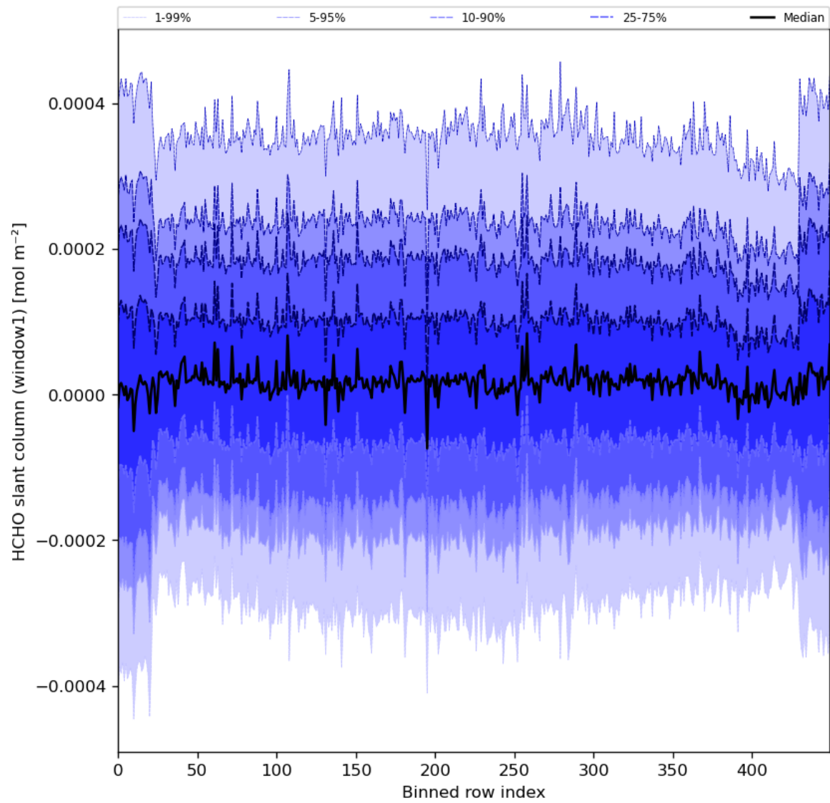
Figure 52: Along track statistics of “HCHO slant column (window1)” for 2024-08-23 to 2024-08-25
