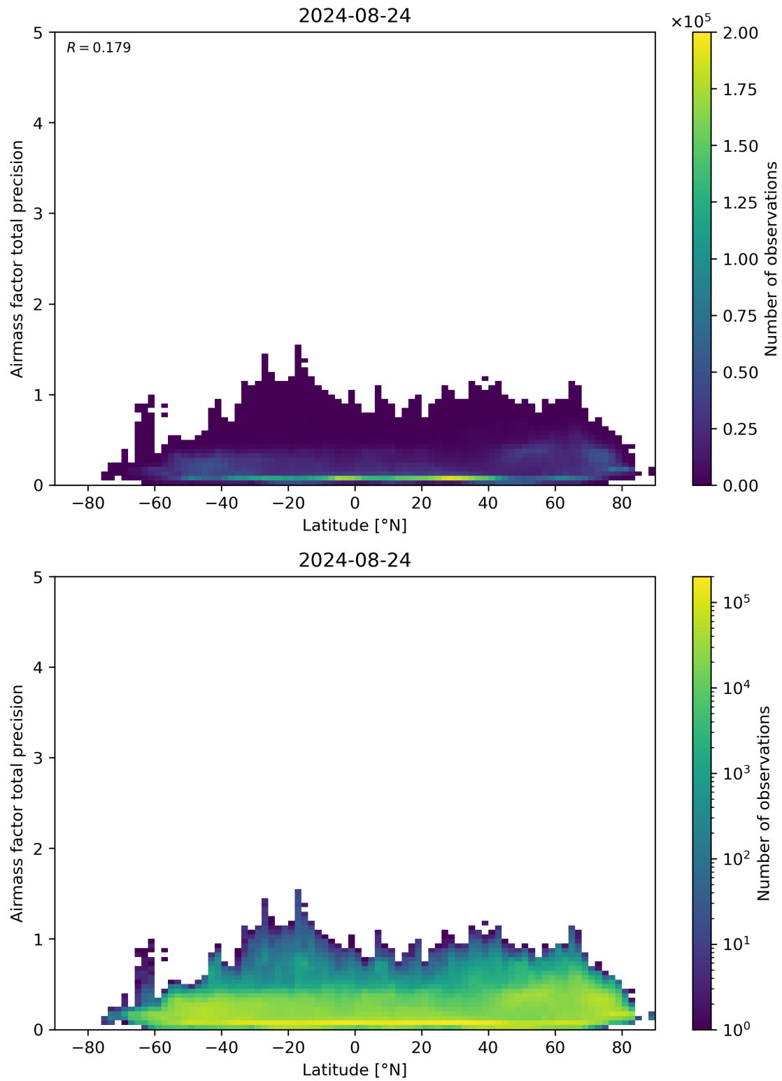
Figure 162: Scatter density plot of “Latitude” against “Airmass factor total precision” for 2024-08-23 to 2024-08-25.
