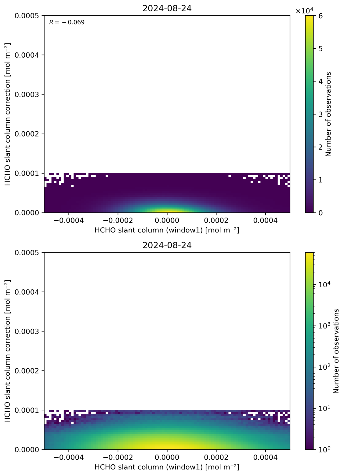
Figure 83: Scatter density plot of “HCHO slant column (window1)” against “HCHO slant column correction” for 2024-08-23 to 2024-08-25.
