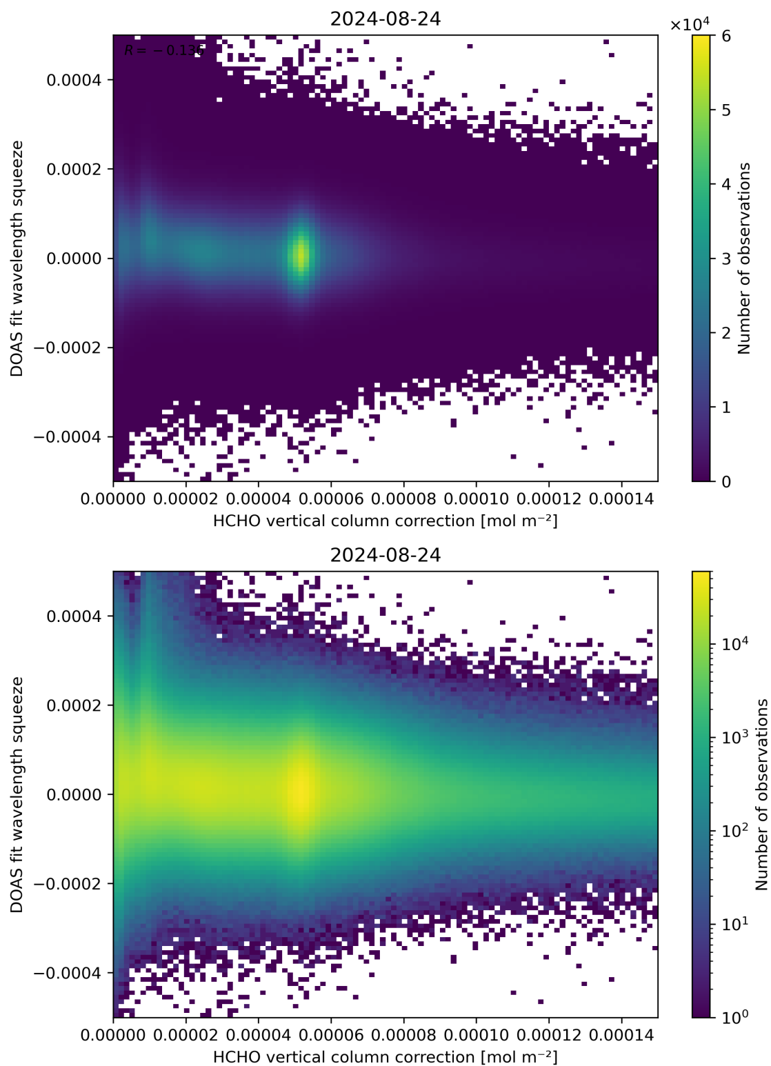
Figure 114: Scatter density plot of “HCHO vertical column correction” against “DOAS fit wavelength squeeze” for 2024-08-23 to 2024-08-25.
