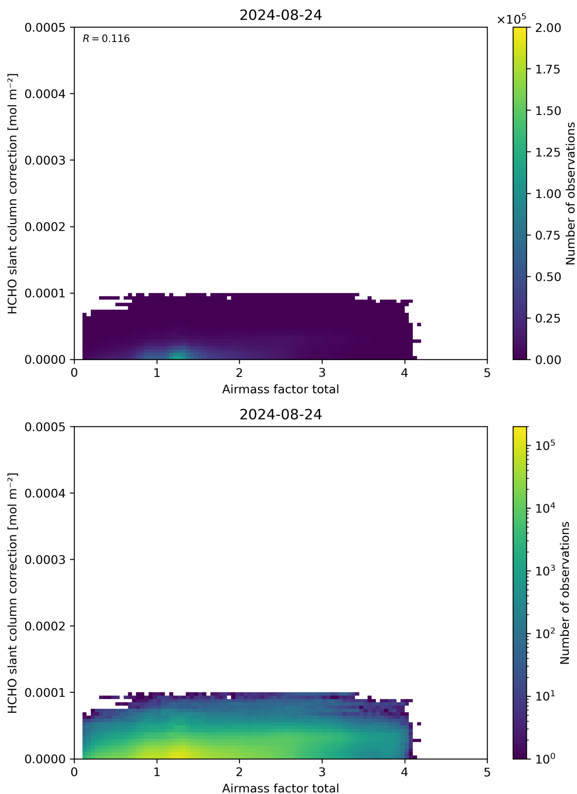
Figure 102: Scatter density plot of “Airmass factor total” against “HCHO slant column correction” for 2024-08-23 to 2024-08-25.
