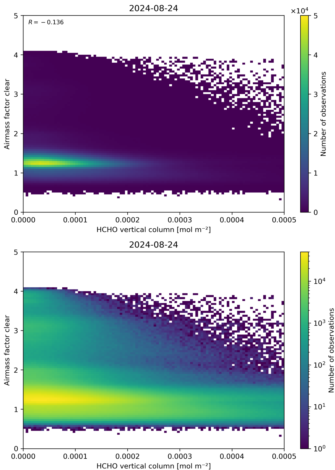
Figure 126: Scatter density plot of “HCHO vertical column” against “Airmass factor clear” for 2024-08-23 to 2024-08-25.
