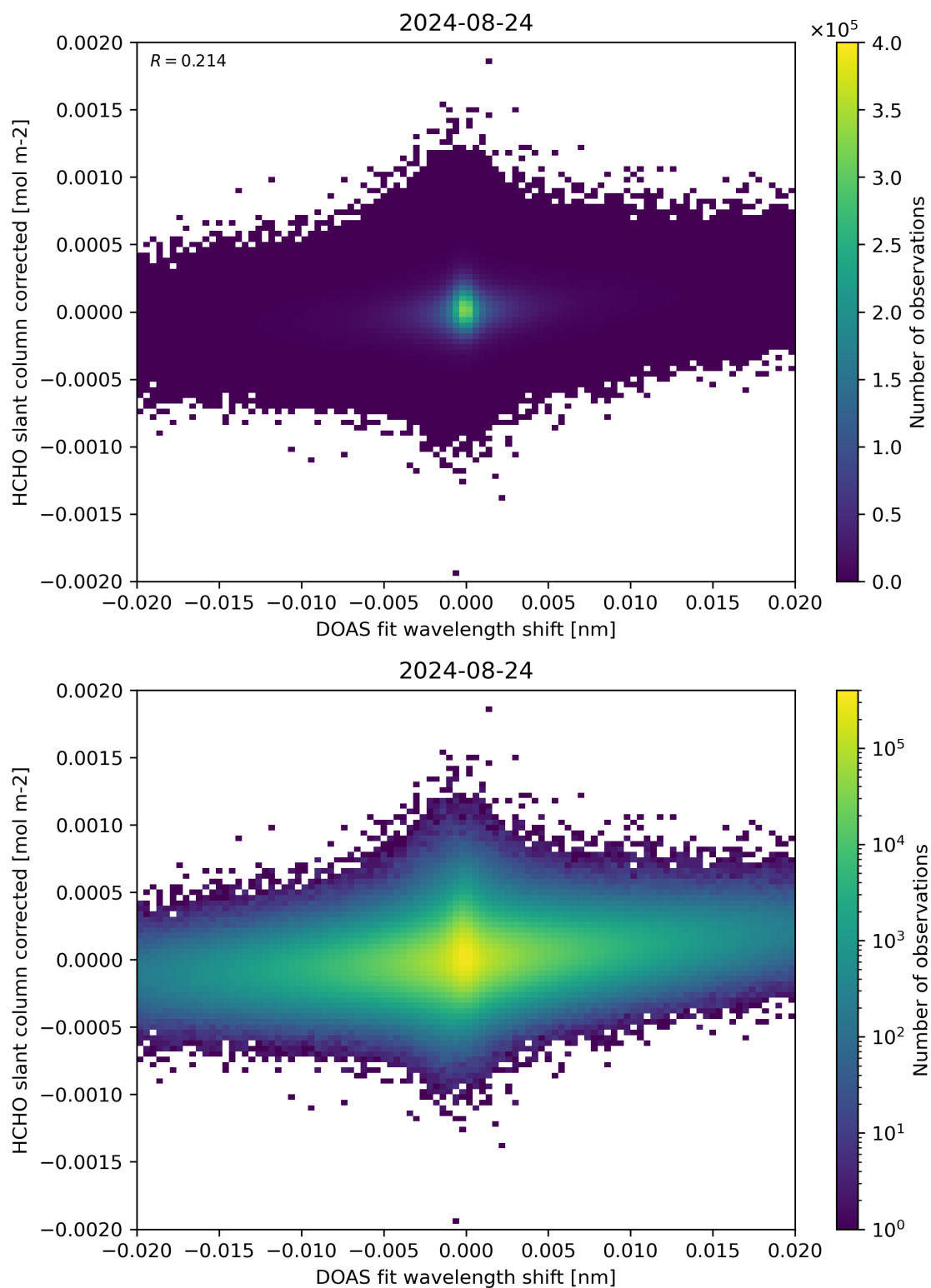
Figure 66: Scatter density plot of “DOAS fit wavelength shift” against “HCHO slant column corrected” for 2024-08-23 to 2024-08-25.
