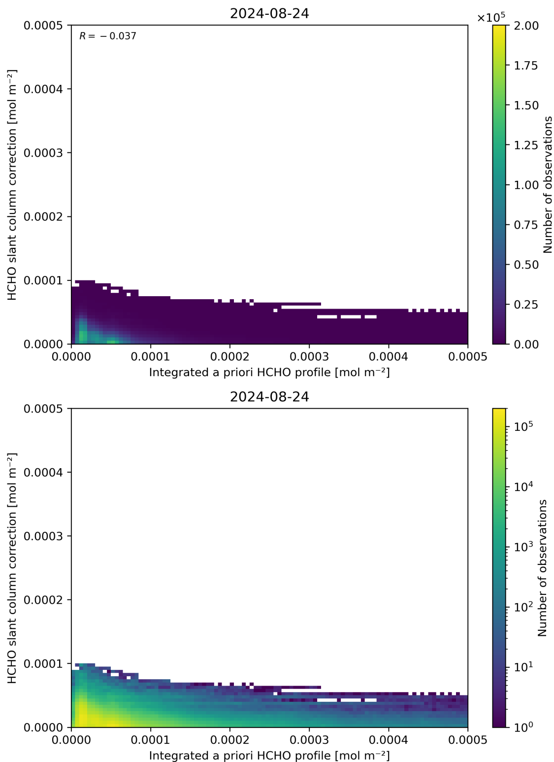
Figure 152: Scatter density plot of “Integrated a priori HCHO profile” against “HCHO slant column correction” for 2024-08-23 to 2024-08-25.
