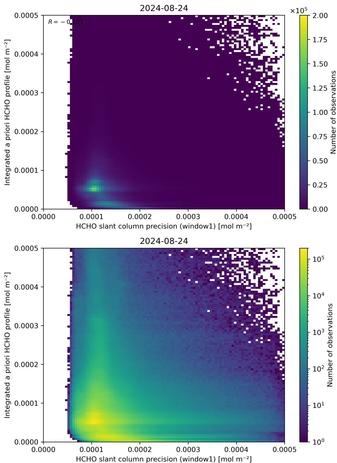
Figure 96: Scatter density plot of “HCHO slant column precision (window1)” against “Integrated a priori HCHO profile” for 2024-08-23 to 2024-08-25.
