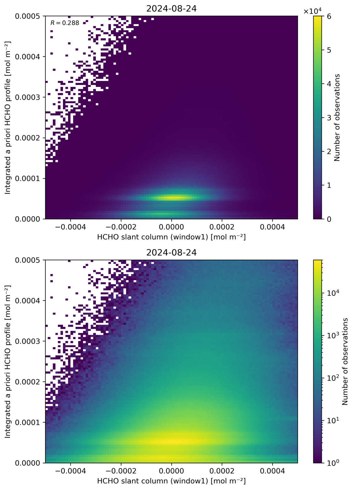
Figure 87: Scatter density plot of “HCHO slant column (window1)” against “Integrated a priori HCHO profile” for 2024-08-23 to 2024-08-25.
