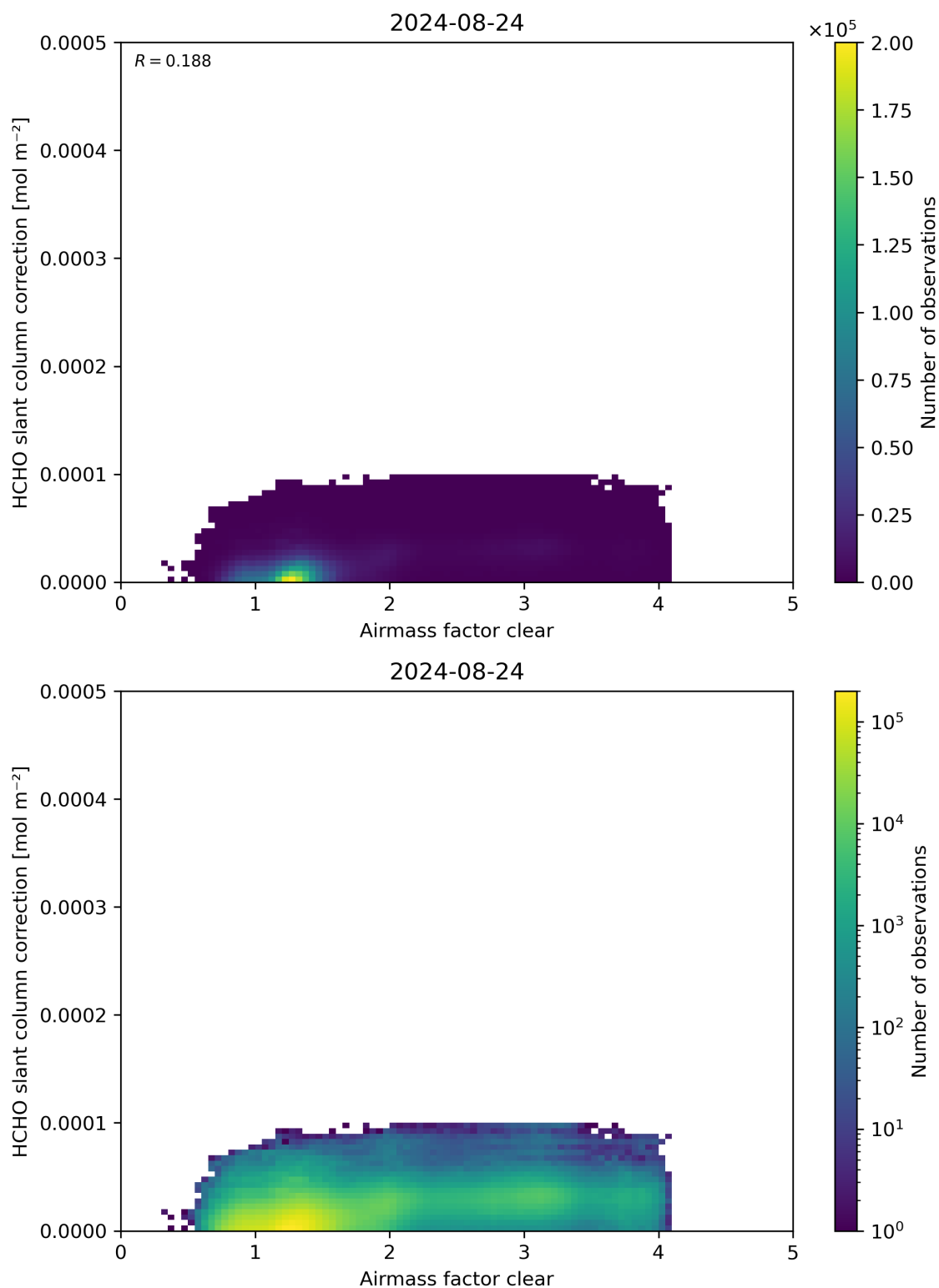
Figure 75: Scatter density plot of “Airmass factor clear” against “HCHO slant column correction” for 2024-08-23 to 2024-08-25.
