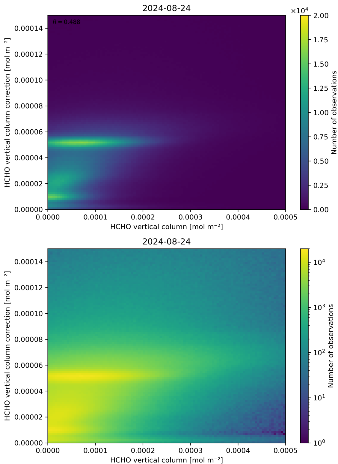
Figure 133: Scatter density plot of “HCHO vertical column” against “HCHO vertical column correction” for 2024-08-23 to 2024-08-25.
