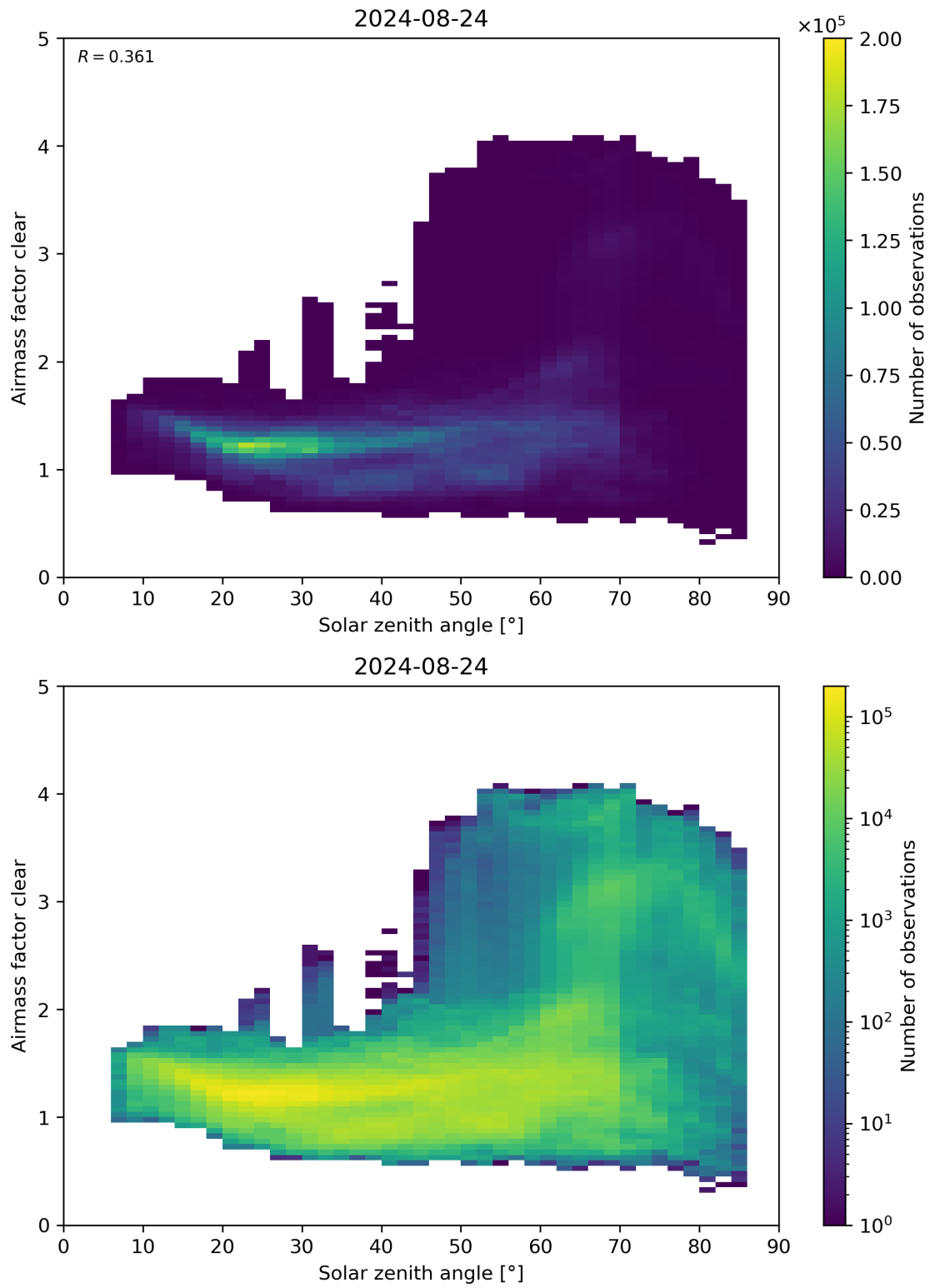
Figure 170: Scatter density plot of “Solar zenith angle” against “Airmass factor clear” for 2024-08-23 to 2024-08-25.
