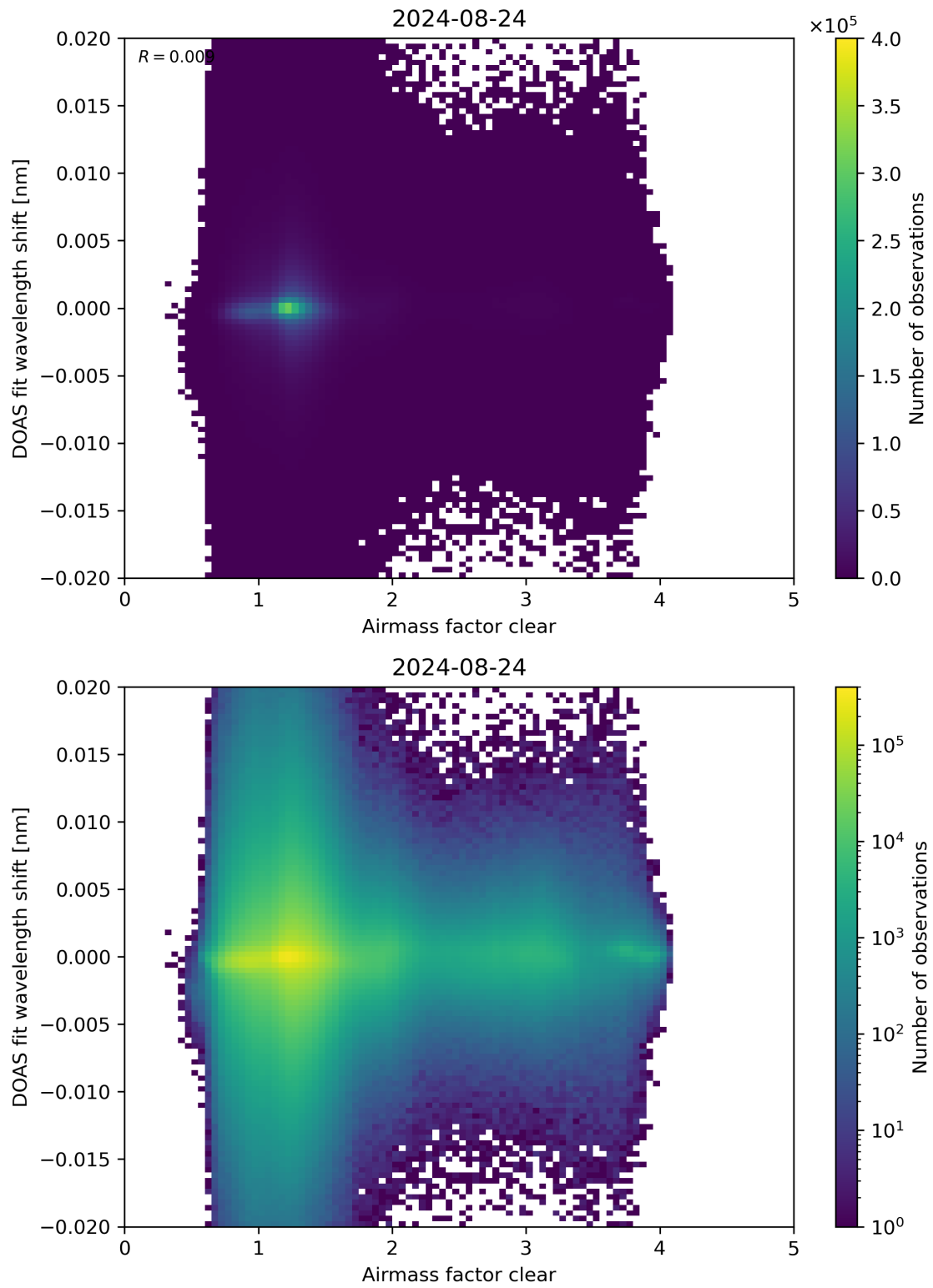
Figure 72: Scatter density plot of “Airmass factor clear” against “DOAS fit wavelength shift” for 2024-08-23 to 2024-08-25.
