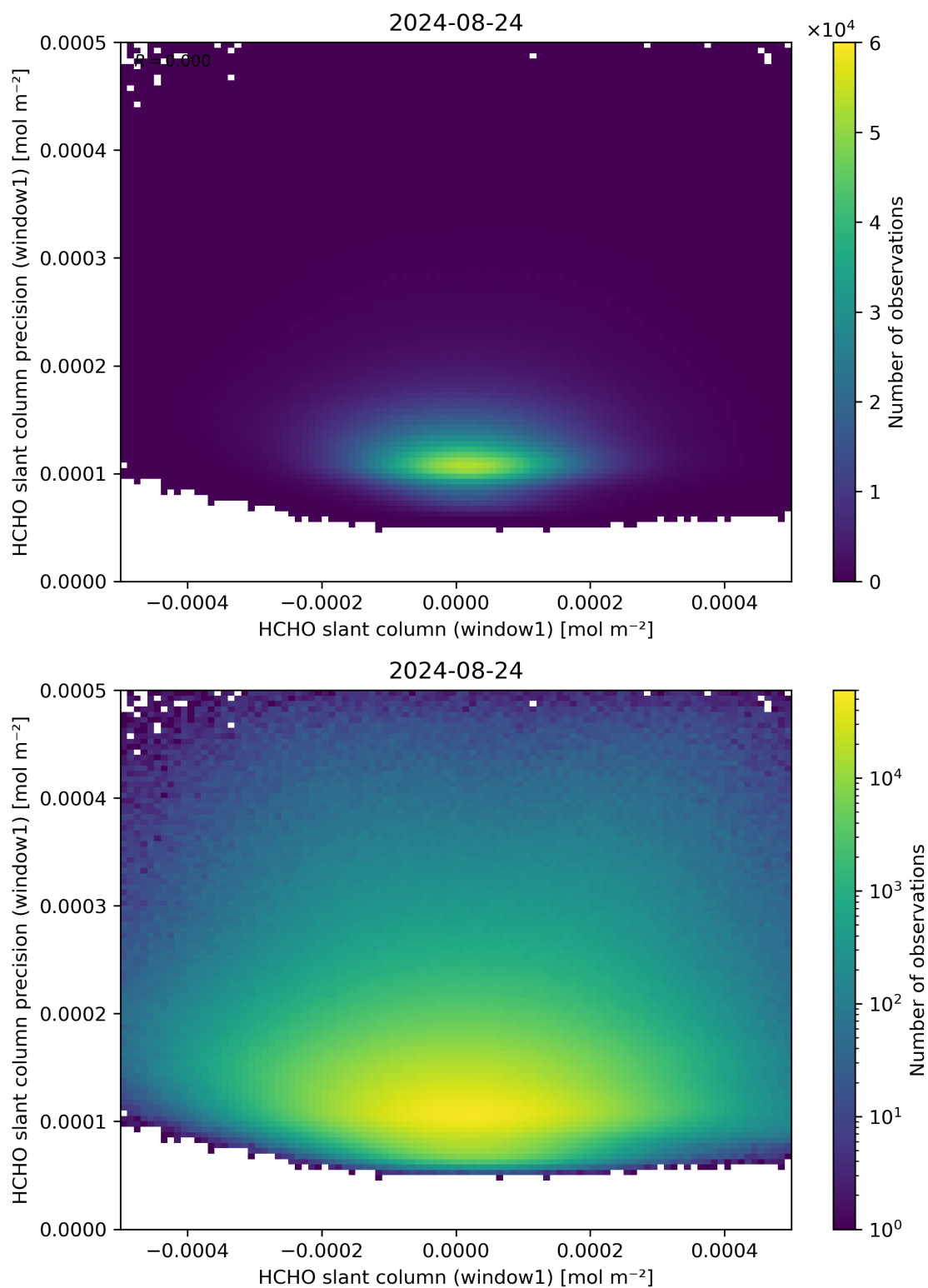
Figure 84: Scatter density plot of “HCHO slant column (window1)” against “HCHO slant column precision (window1)” for 2024-08-23 to 2024-08-25.
