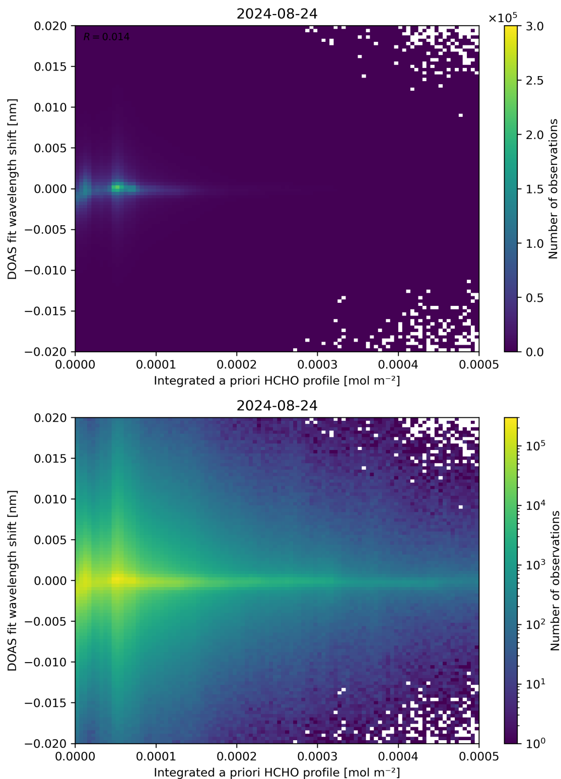
Figure 149: Scatter density plot of “Integrated a priori HCHO profile” against “DOAS fit wavelength shift” for 2024-08-23 to 2024-08-25.
