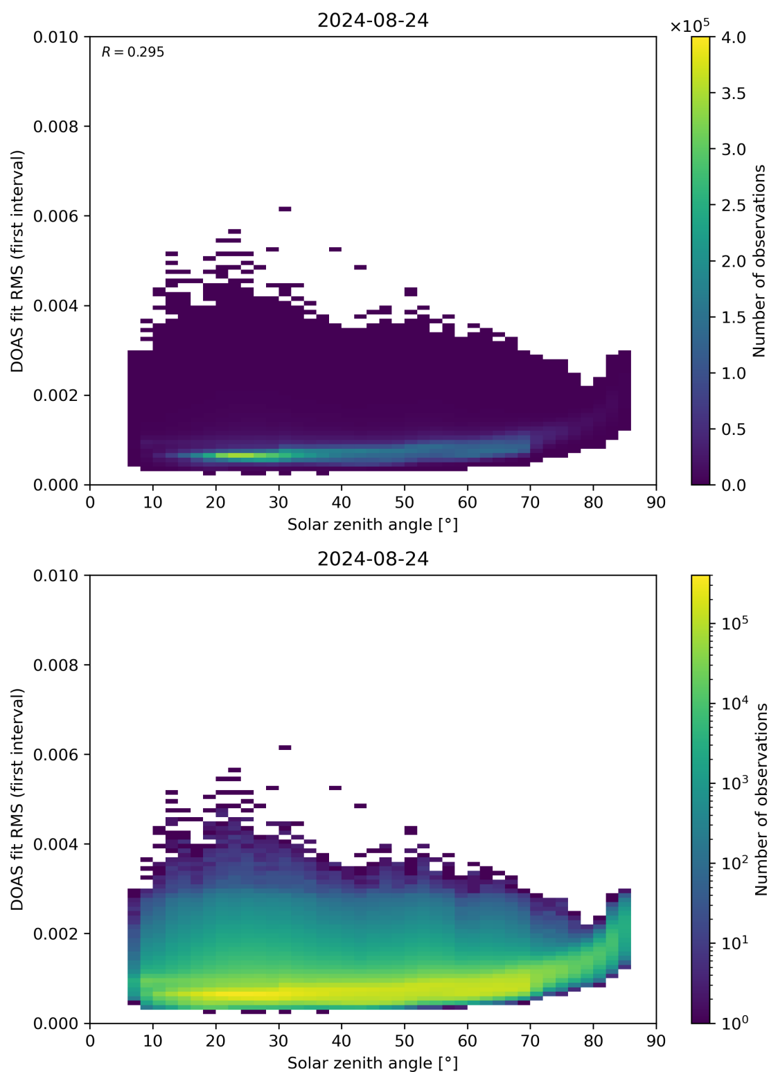
Figure 167: Scatter density plot of “Solar zenith angle” against “DOAS fit RMS (first interval)” for 2024-08-23 to 2024-08-25.
