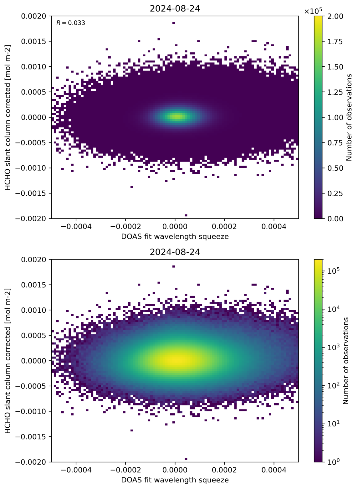
Figure 69: Scatter density plot of “DOAS fit wavelength squeeze” against “HCHO slant column corrected” for 2024-08-23 to 2024-08-25.
