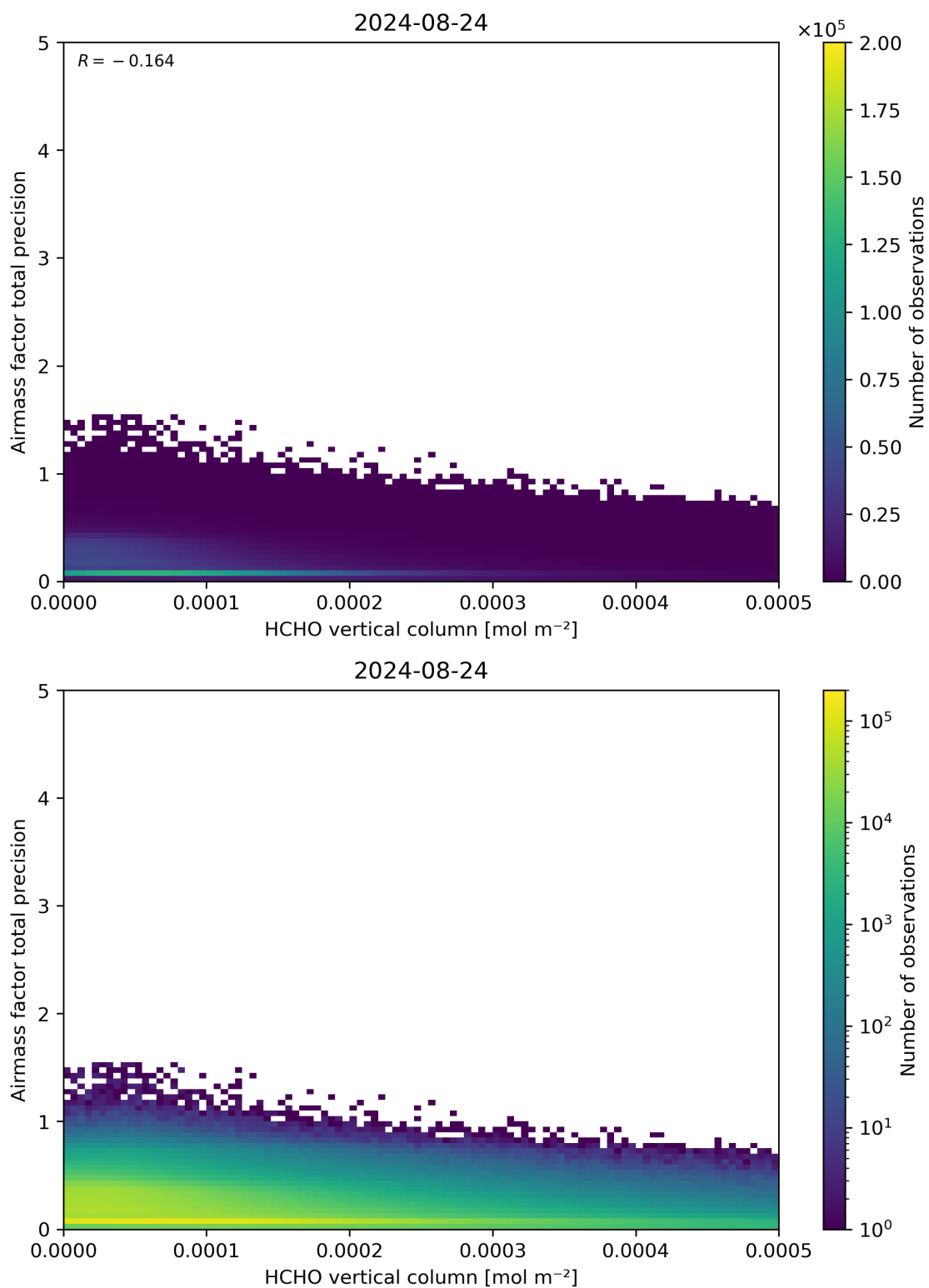
Figure 132: Scatter density plot of “HCHO vertical column” against “Airmass factor total precision” for 2024-08-23 to 2024-08-25.
