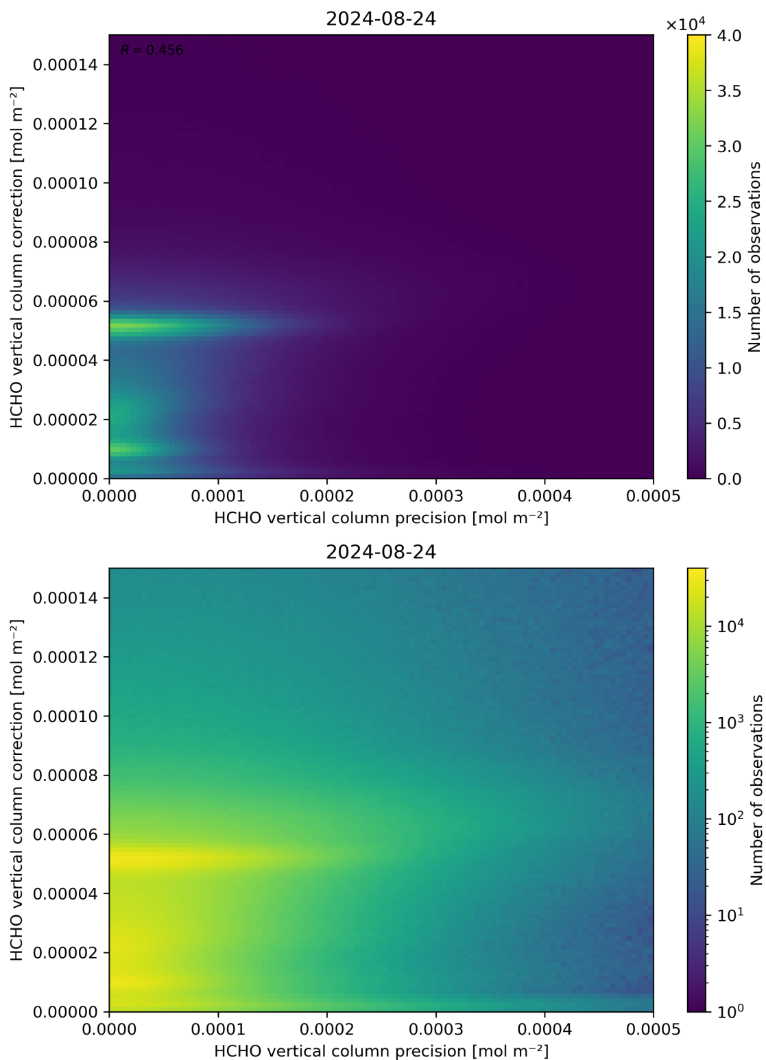
Figure 146: Scatter density plot of “HCHO vertical column precision” against “HCHO vertical column correction” for 2024-08-23 to 2024-08-25.
