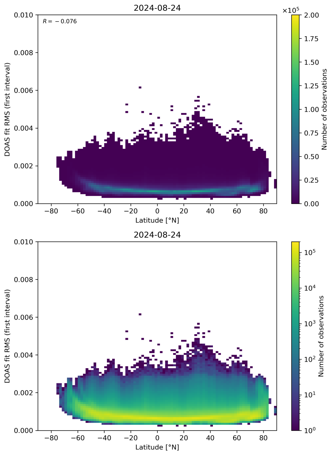
Figure 153: Scatter density plot of “Latitude” against “DOAS fit RMS (first interval)” for 2024-08-23 to 2024-08-25.
