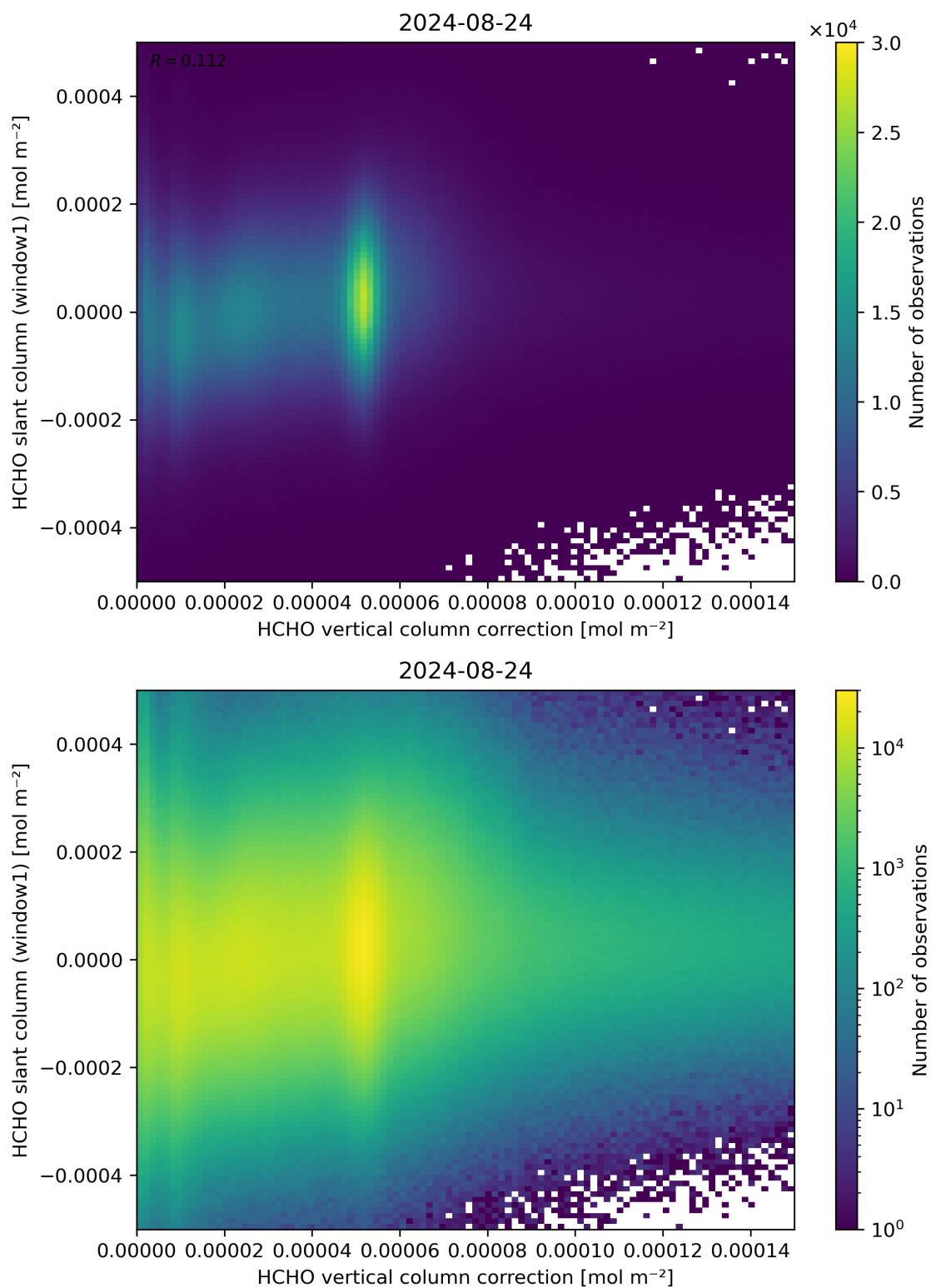
Figure 118: Scatter density plot of “HCHO vertical column correction” against “HCHO slant column (window1)” for 2024-08-23 to 2024-08-25.
