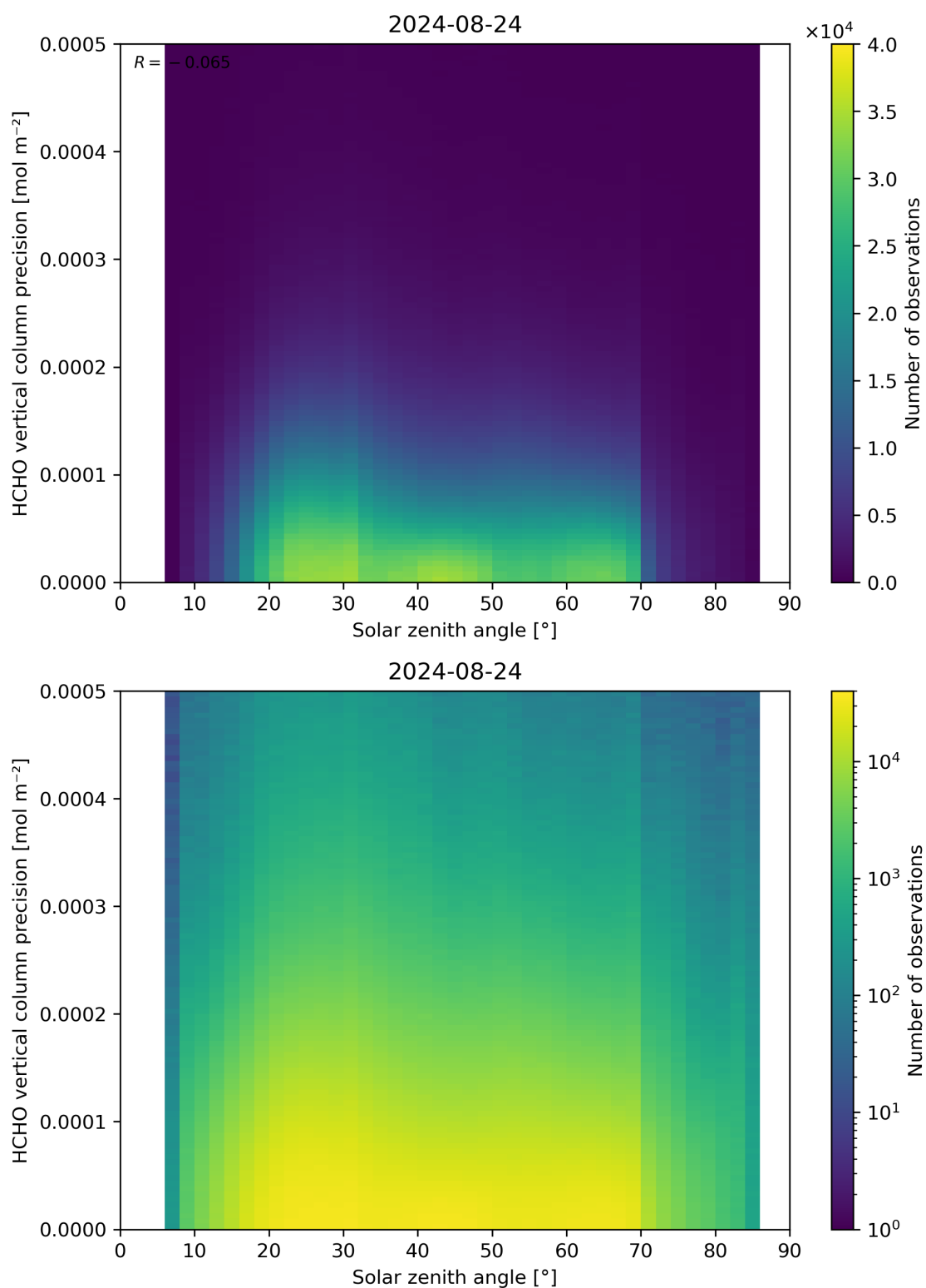
Figure 179: Scatter density plot of “Solar zenith angle” against “HCHO vertical column precision” for 2024-08-23 to 2024-08-25.
