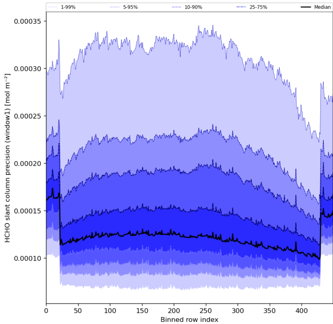
Figure 53: Along track statistics of “HCHO slant column precision (window1)” for 2024-08-23 to 2024-08-25
