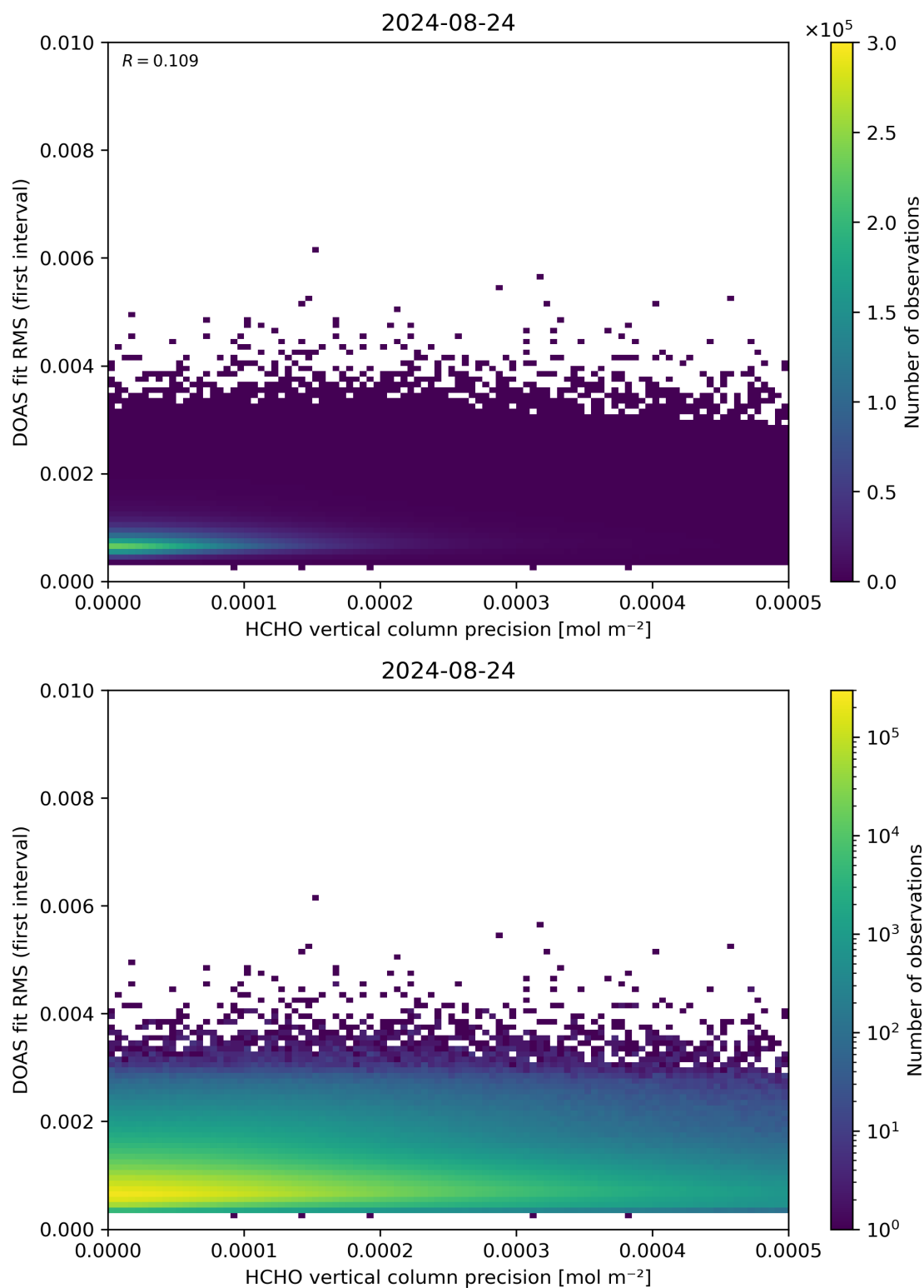
Figure 136: Scatter density plot of “HCHO vertical column precision” against “DOAS fit RMS (first interval)” for 2024-08-23 to 2024-08-25.
