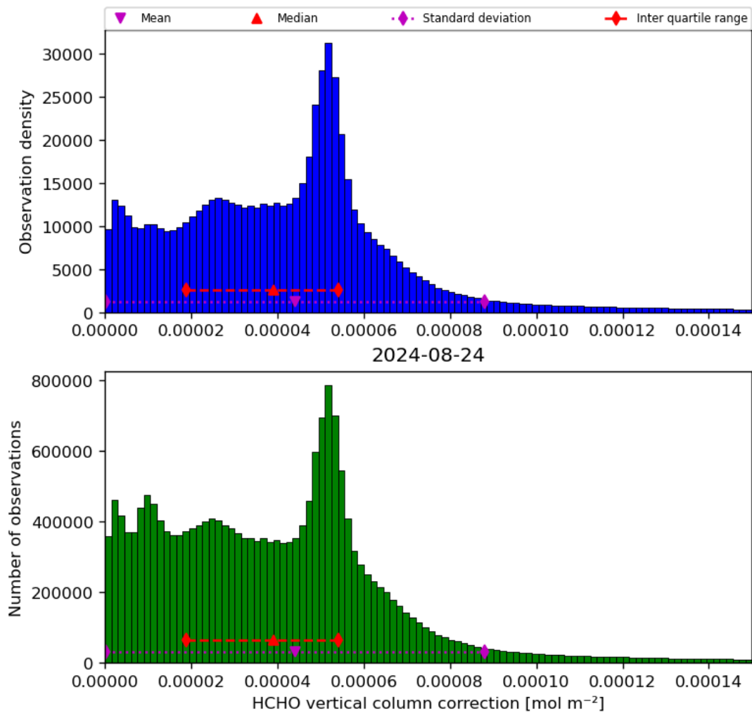
Figure 37: Histogram of “HCHO vertical column correction” for 2024-08-23 to 2024-08-25
