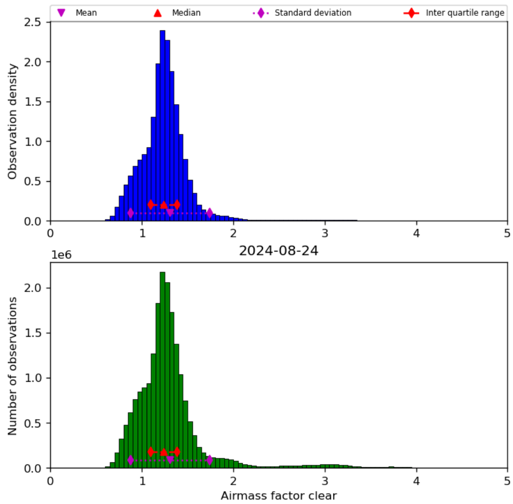
Figure 42: Histogram of “Airmass factor clear” for 2024-08-23 to 2024-08-25
