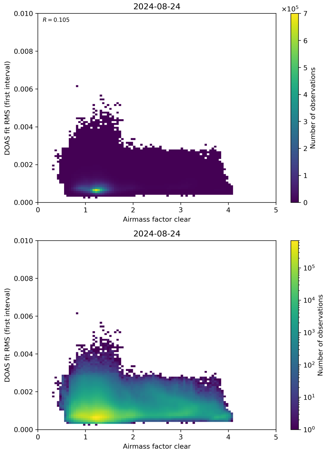
Figure 71: Scatter density plot of “Airmass factor clear” against “DOAS fit RMS (first interval)” for 2024-08-23 to 2024-08-25.
