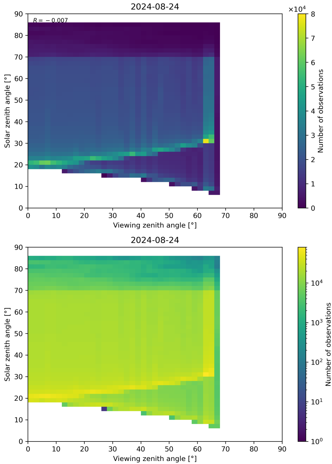
Figure 197: Scatter density plot of “Viewing zenith angle” against “Solar zenith angle” for 2024-08-23 to 2024-08-25.
