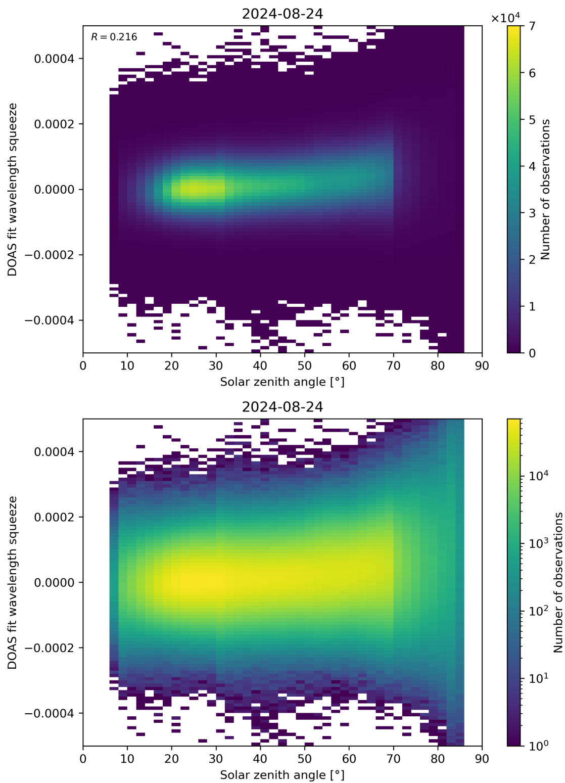
Figure 169: Scatter density plot of “Solar zenith angle” against “DOAS fit wavelength squeeze” for 2024-08-23 to 2024-08-25.
