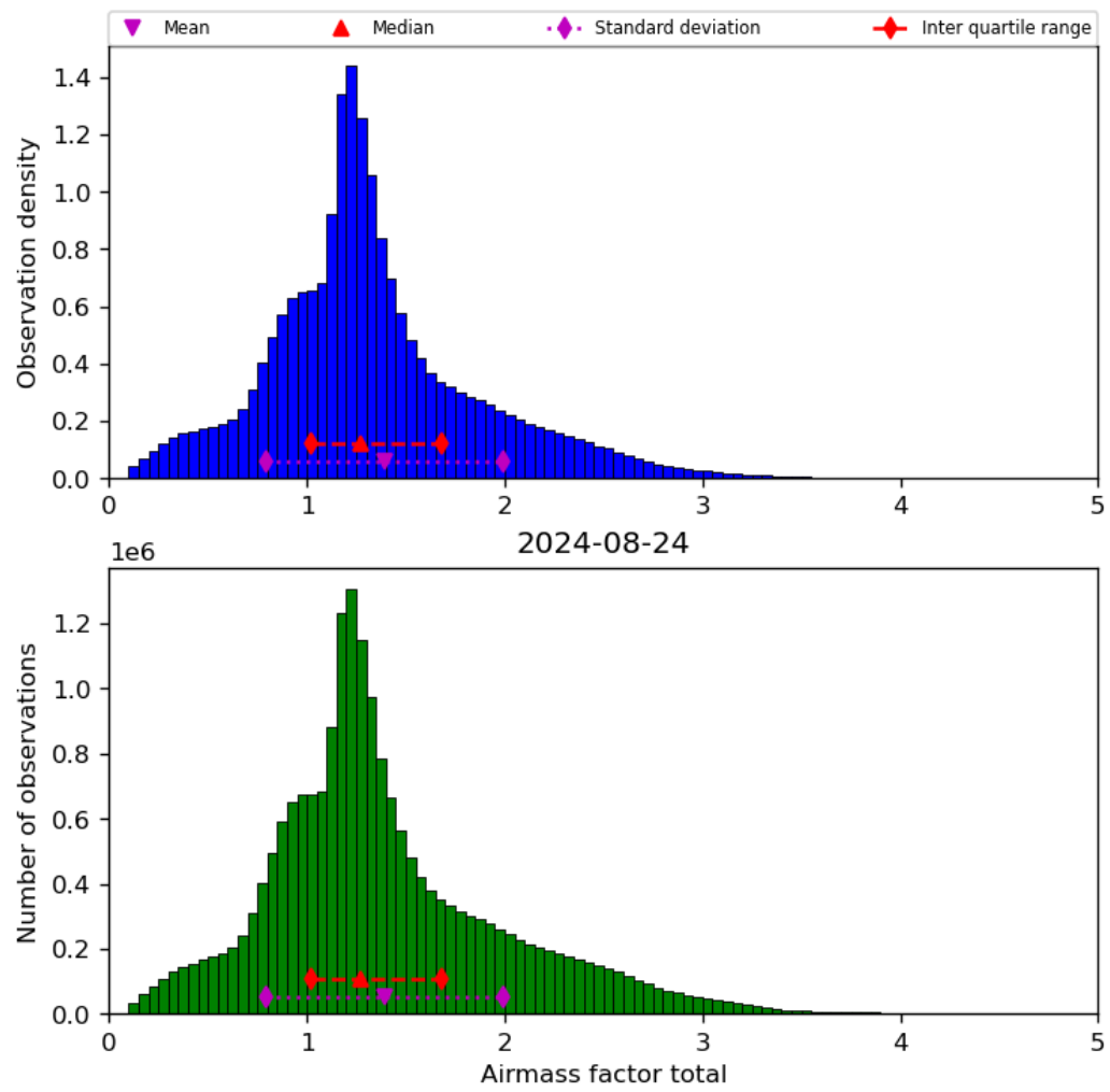
Figure 40: Histogram of “Airmass factor total” for 2024-08-23 to 2024-08-25
