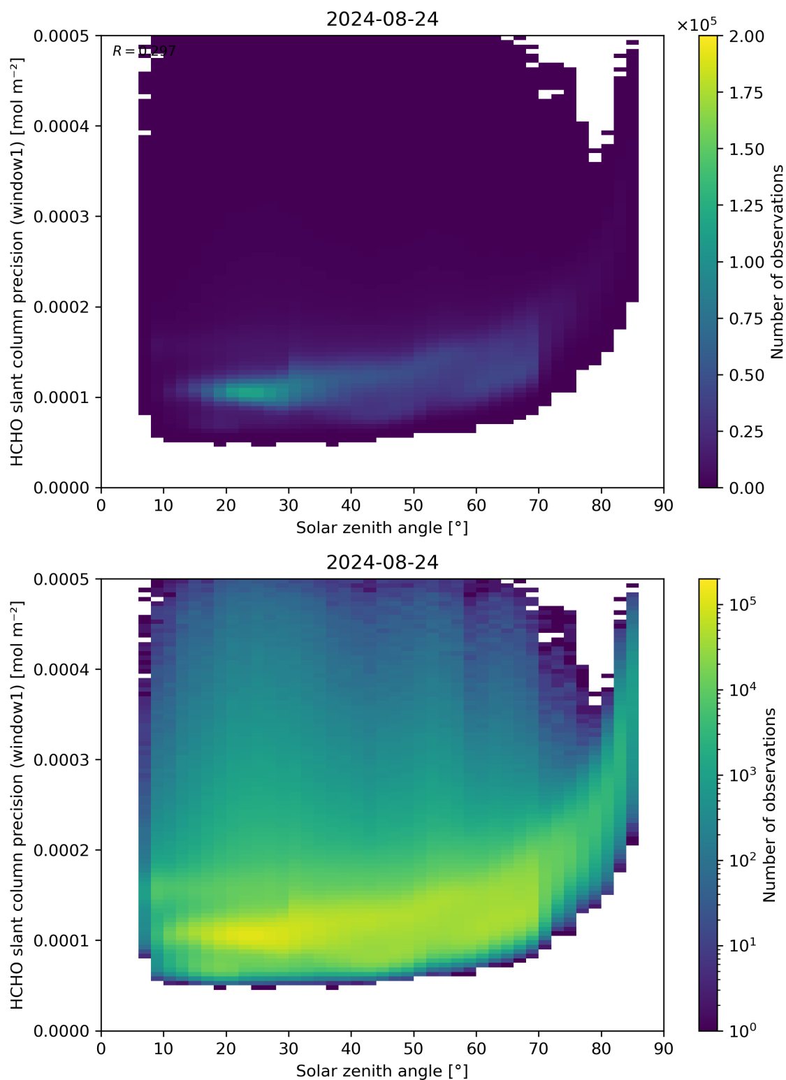
Figure 174: Scatter density plot of “Solar zenith angle” against “HCHO slant column precision (window1)” for 2024-08-23 to 2024-08-25.
