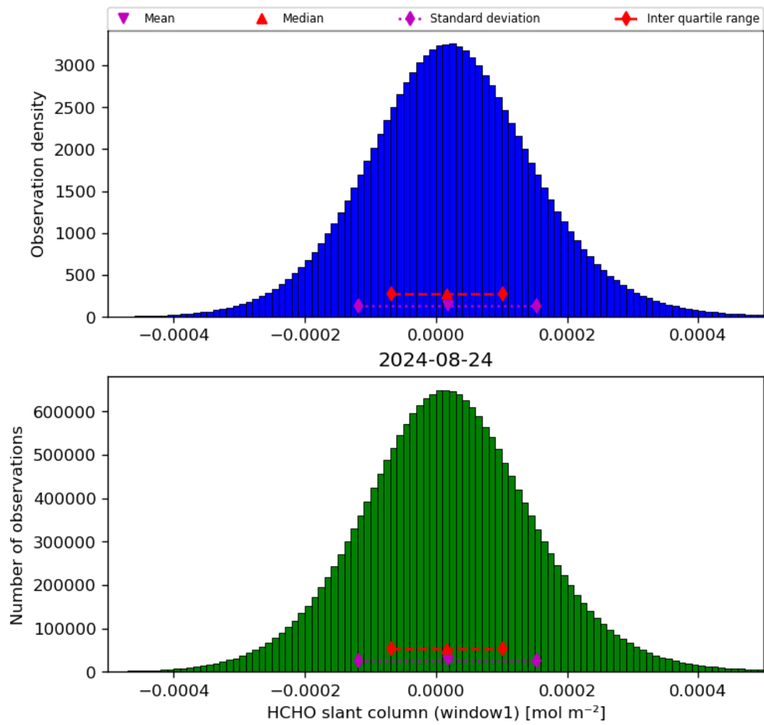
Figure 38: Histogram of “HCHO slant column (window1)” for 2024-08-23 to 2024-08-25
