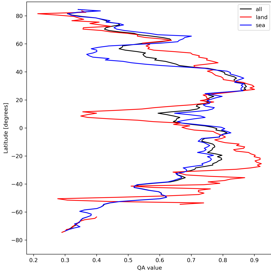
Figure 20: Zonal average of “QA value” for 2024-08-23 to 2024-08-25.
