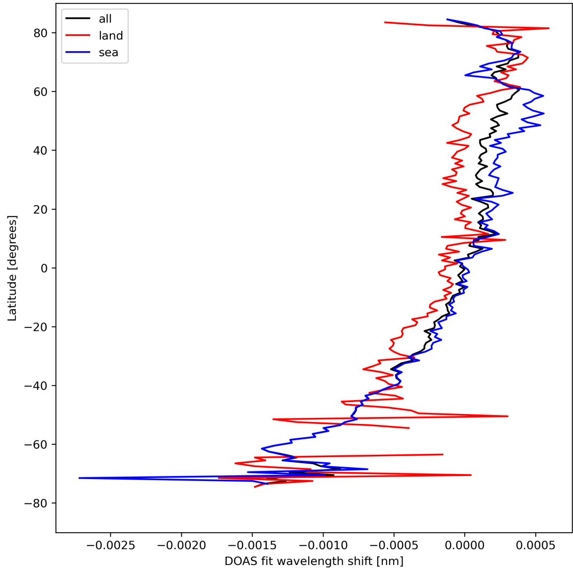
Figure 30: Zonal average of “DOAS fit wavelength shift” for 2024-08-23 to 2024-08-25.
