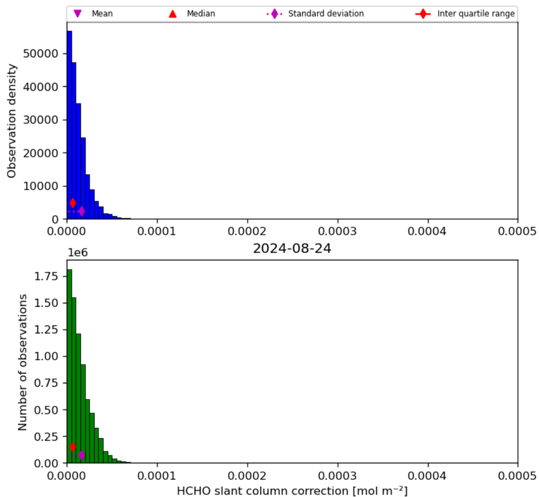
Figure 47: Histogram of “HCHO slant column correction” for 2024-08-23 to 2024-08-25
