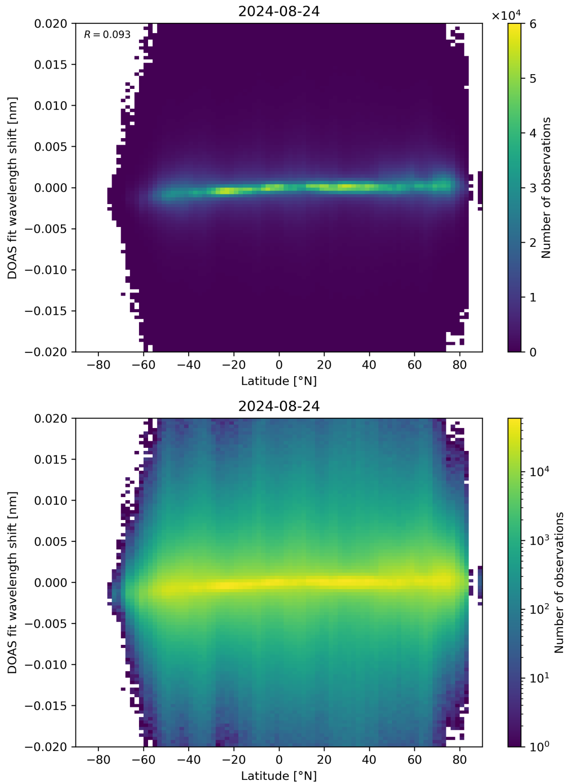
Figure 154: Scatter density plot of “Latitude” against “DOAS fit wavelength shift” for 2024-08-23 to 2024-08-25.
