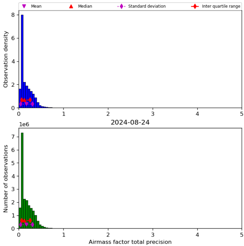
Figure 41: Histogram of “Airmass factor total precision” for 2024-08-23 to 2024-08-25
