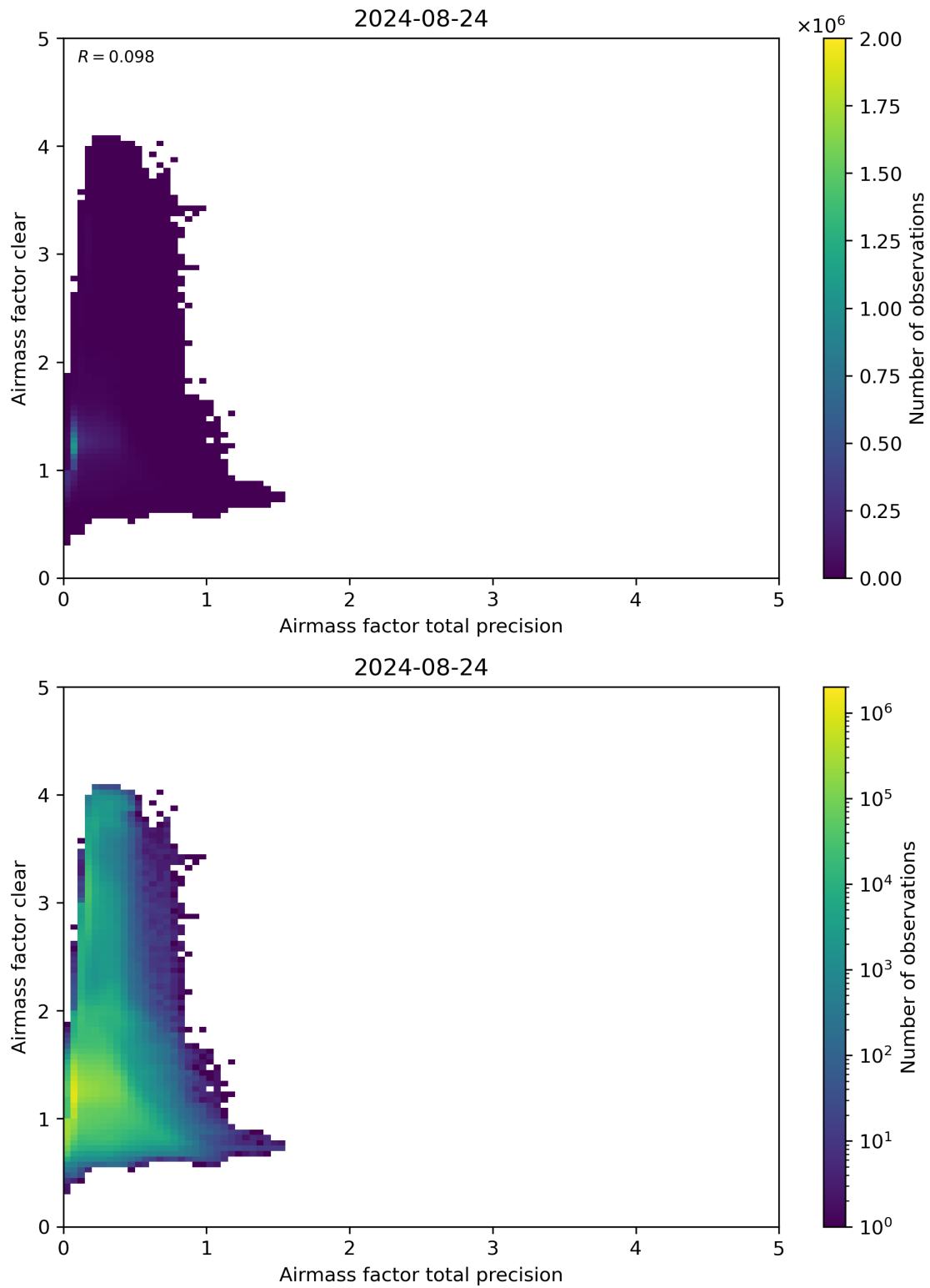
Figure 108: Scatter density plot of “Airmass factor total precision” against “Airmass factor clear” for 2024-08-23 to 2024-08-25.
