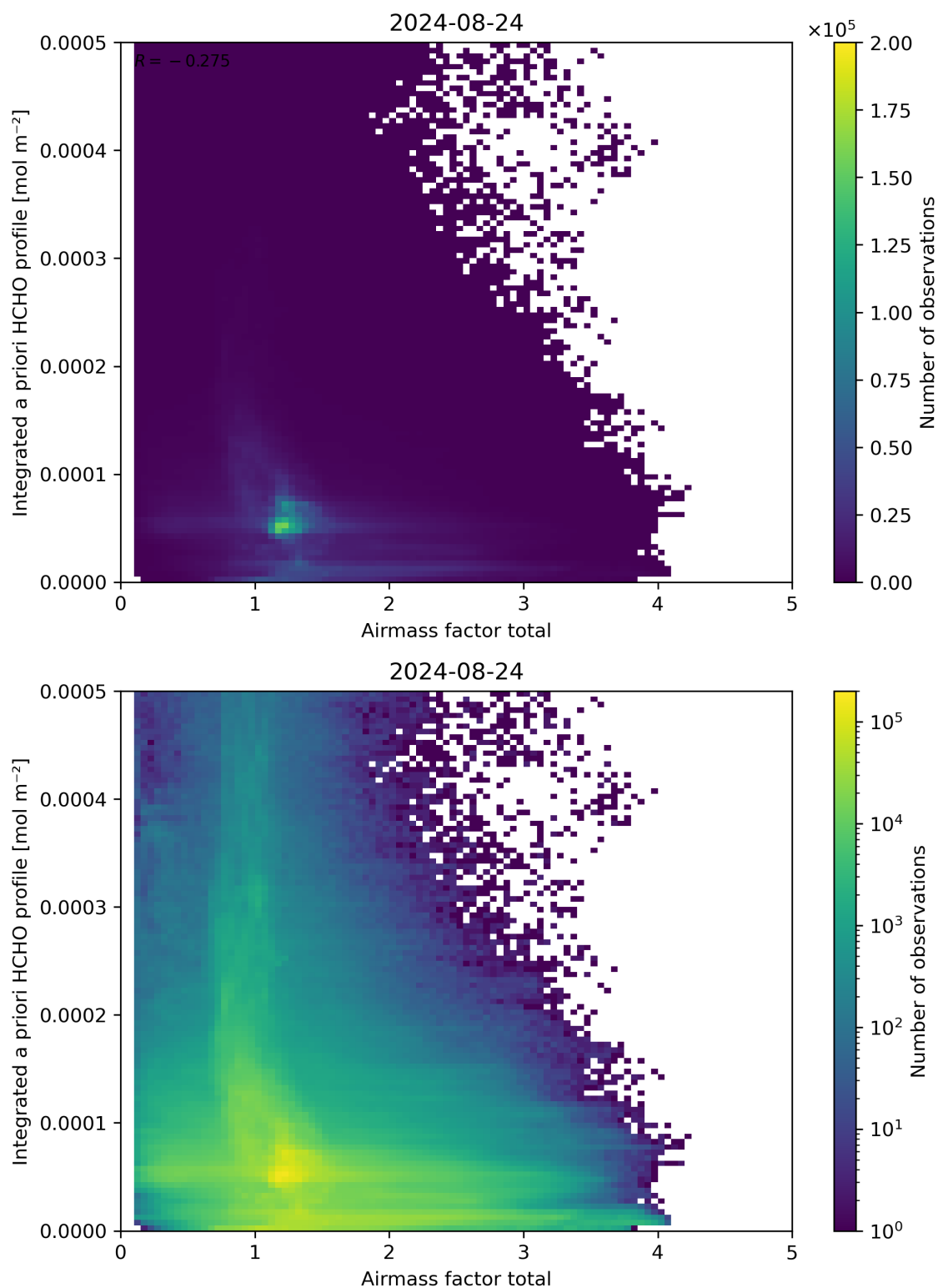
Figure 104: Scatter density plot of “Airmass factor total” against “Integrated a priori HCHO profile” for 2024-08-23 to 2024-08-25.
