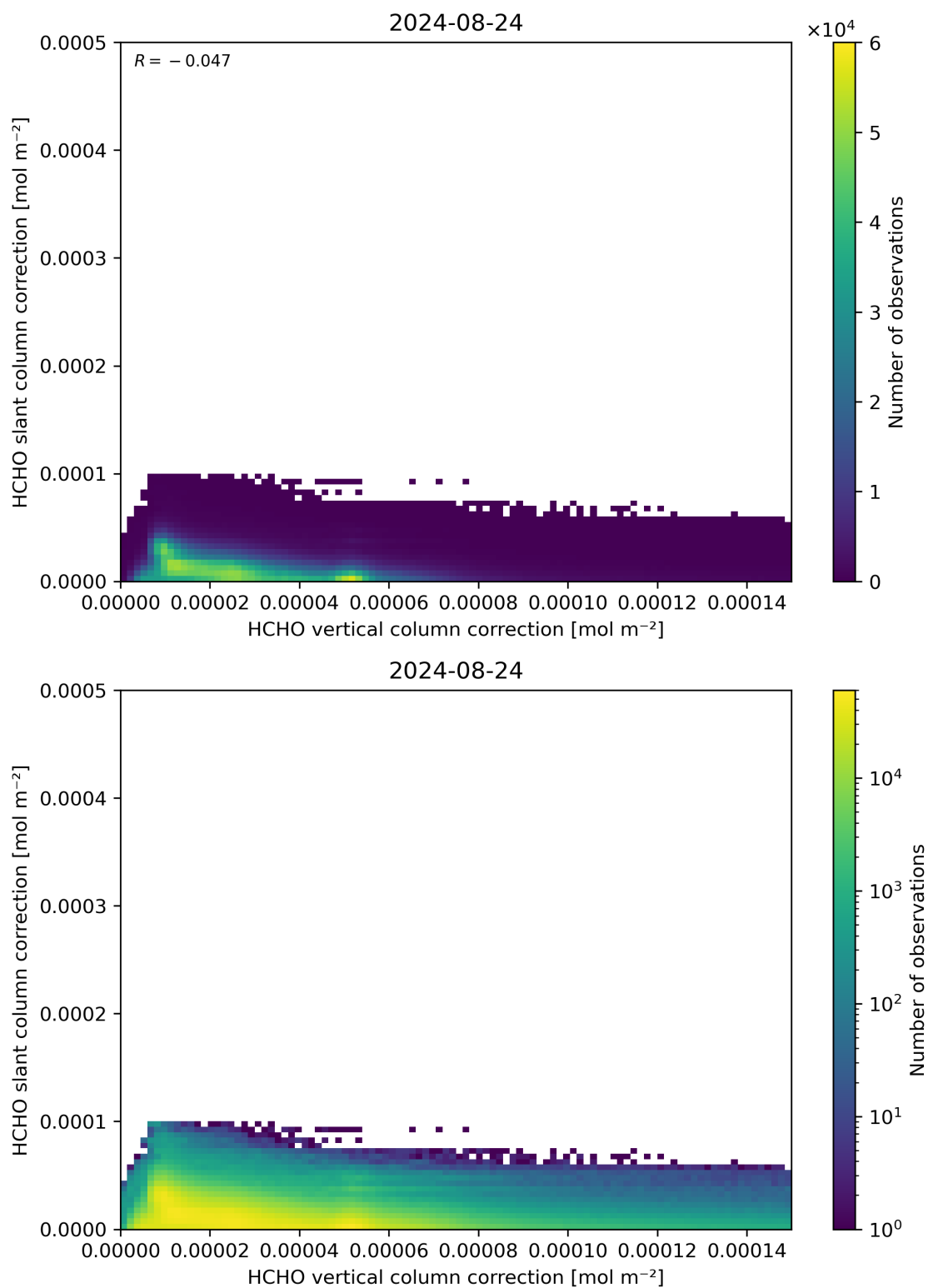
Figure 117: Scatter density plot of “HCHO vertical column correction” against “HCHO slant column correction” for 2024-08-23 to 2024-08-25.
