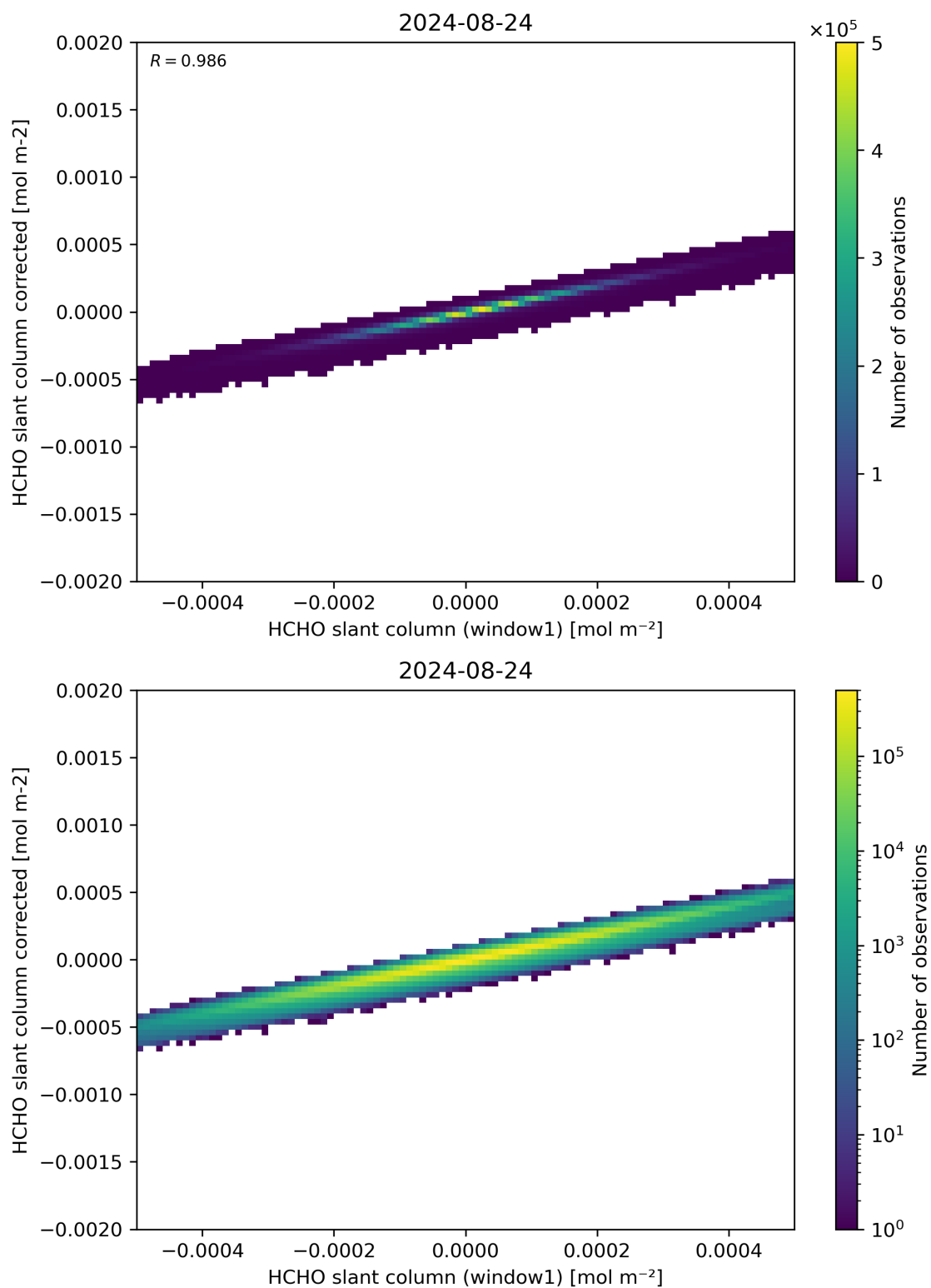
Figure 82: Scatter density plot of “HCHO slant column (window1)” against “HCHO slant column corrected” for 2024-08-23 to 2024-08-25.
