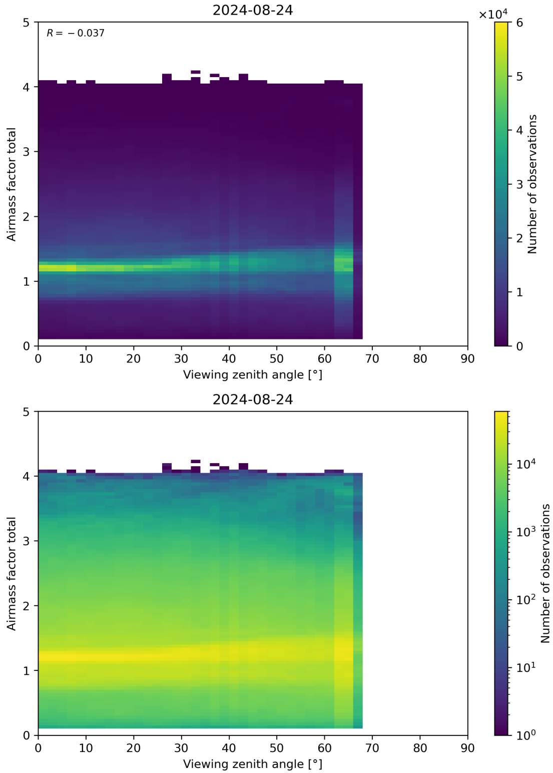
Figure 190: Scatter density plot of “Viewing zenith angle” against “Airmass factor total” for 2024-08-23 to 2024-08-25.
