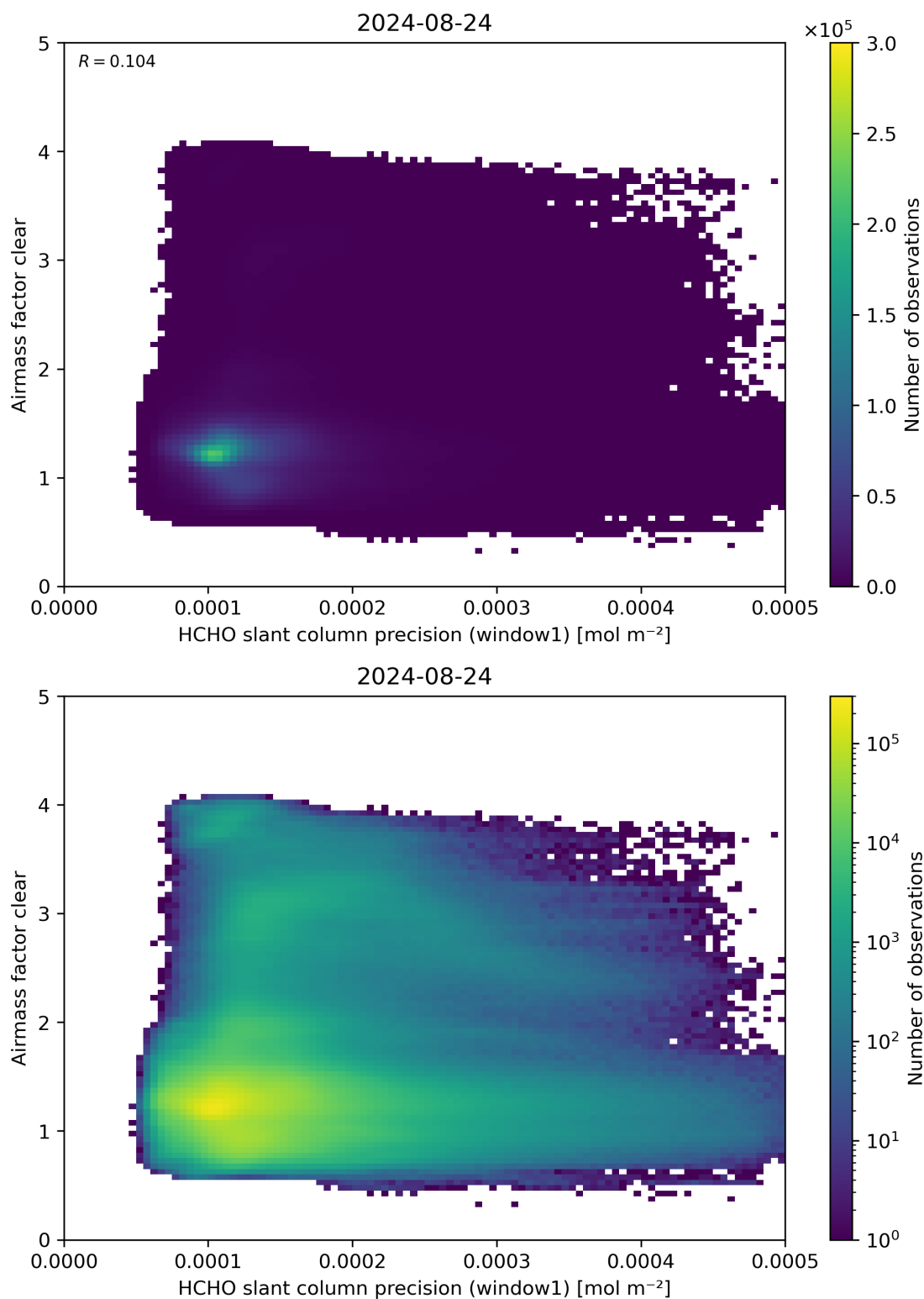
Figure 91: Scatter density plot of “HCHO slant column precision (window1)” against “Airmass factor clear” for 2024-08-23 to 2024-08-25.
