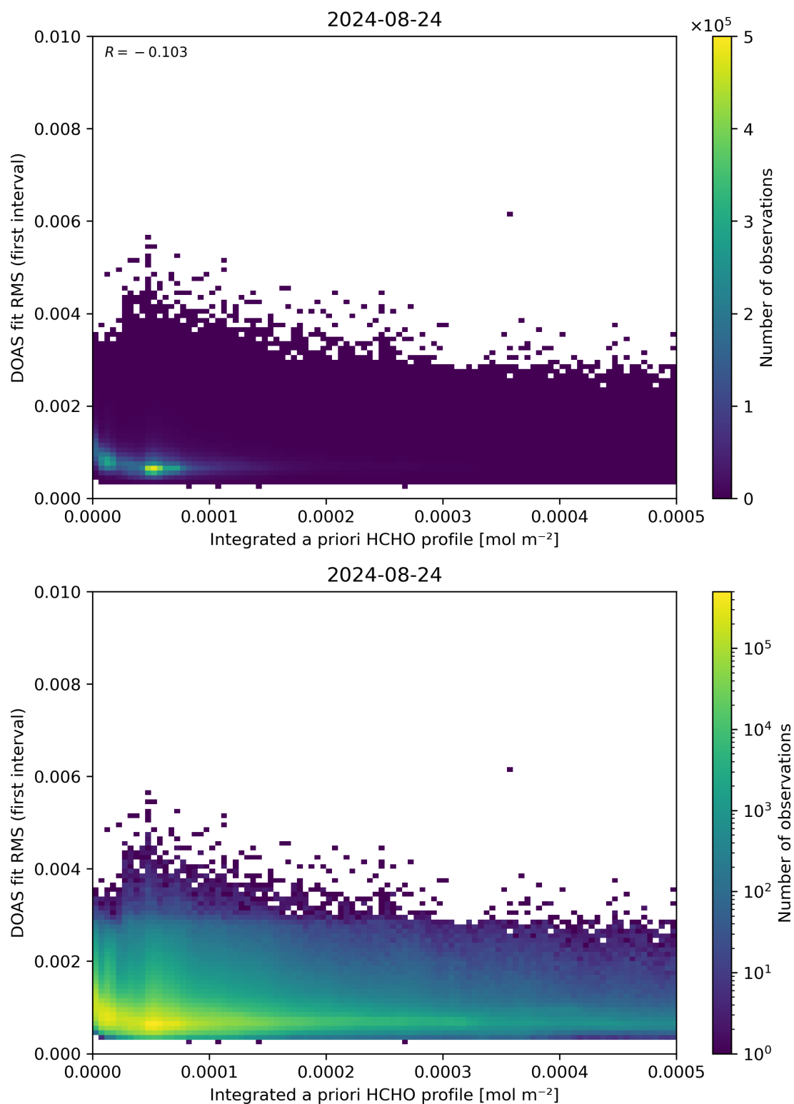
Figure 148: Scatter density plot of “Integrated a priori HCHO profile” against “DOAS fit RMS (first interval)” for 2024-08-23 to 2024-08-25.
