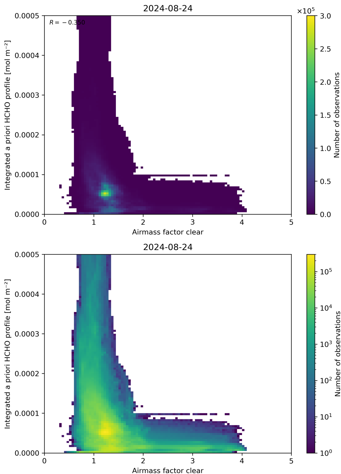
Figure 76: Scatter density plot of “Airmass factor clear” against “Integrated a priori HCHO profile” for 2024-08-23 to 2024-08-25.
