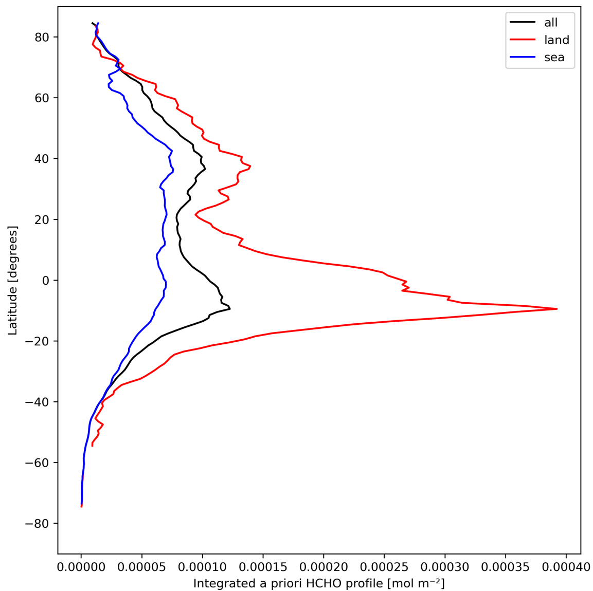
Figure 29: Zonal average of “Integrated a priori HCHO profile” for 2024-08-23 to 2024-08-25.
