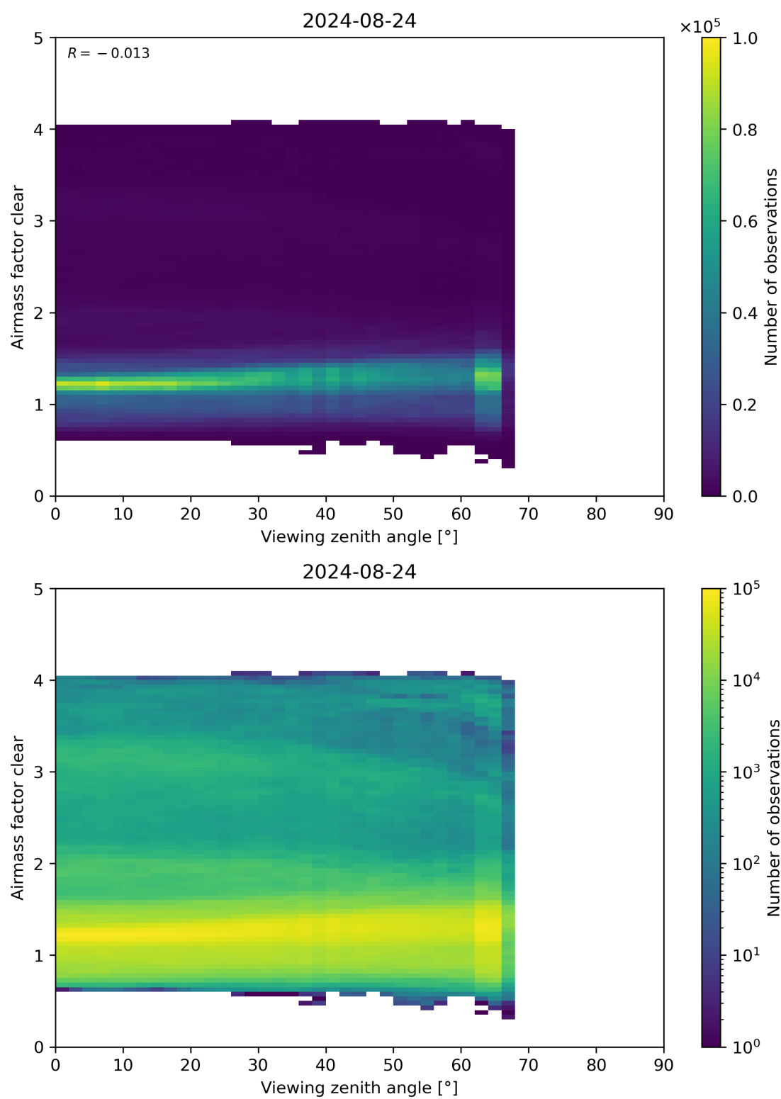
Figure 185: Scatter density plot of “Viewing zenith angle” against “Airmass factor clear” for 2024-08-23 to 2024-08-25.
