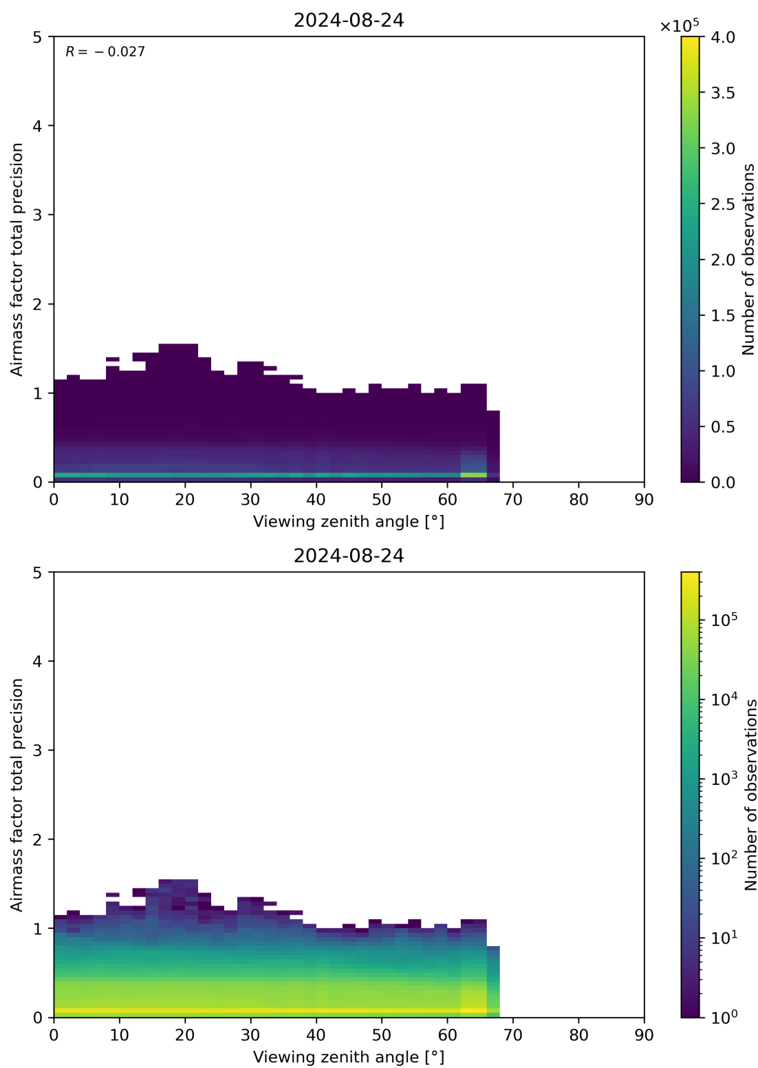
Figure 191: Scatter density plot of “Viewing zenith angle” against “Airmass factor total precision” for 2024-08-23 to 2024-08-25.
