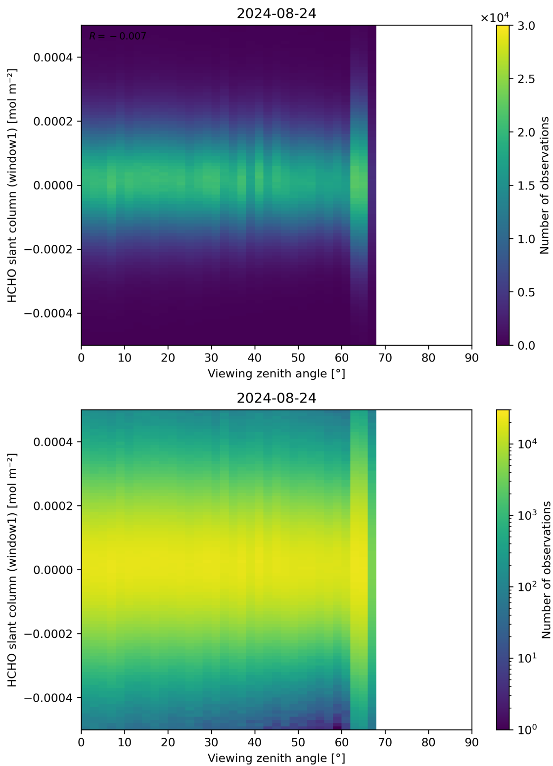
Figure 188: Scatter density plot of “Viewing zenith angle” against “HCHO slant column (window1)” for 2024-08-23 to 2024-08-25.
