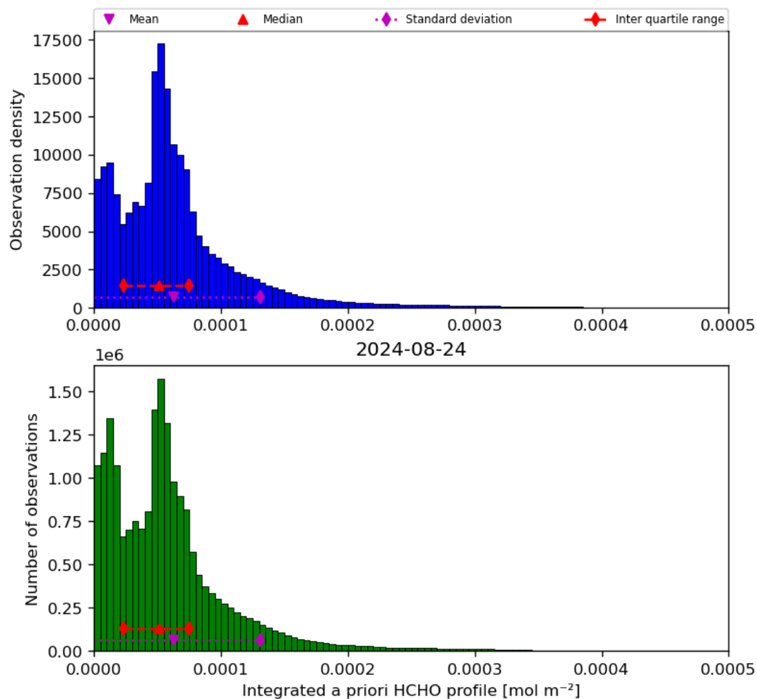
Figure 43: Histogram of “Integrated a priori HCHO profile” for 2024-08-23 to 2024-08-25
