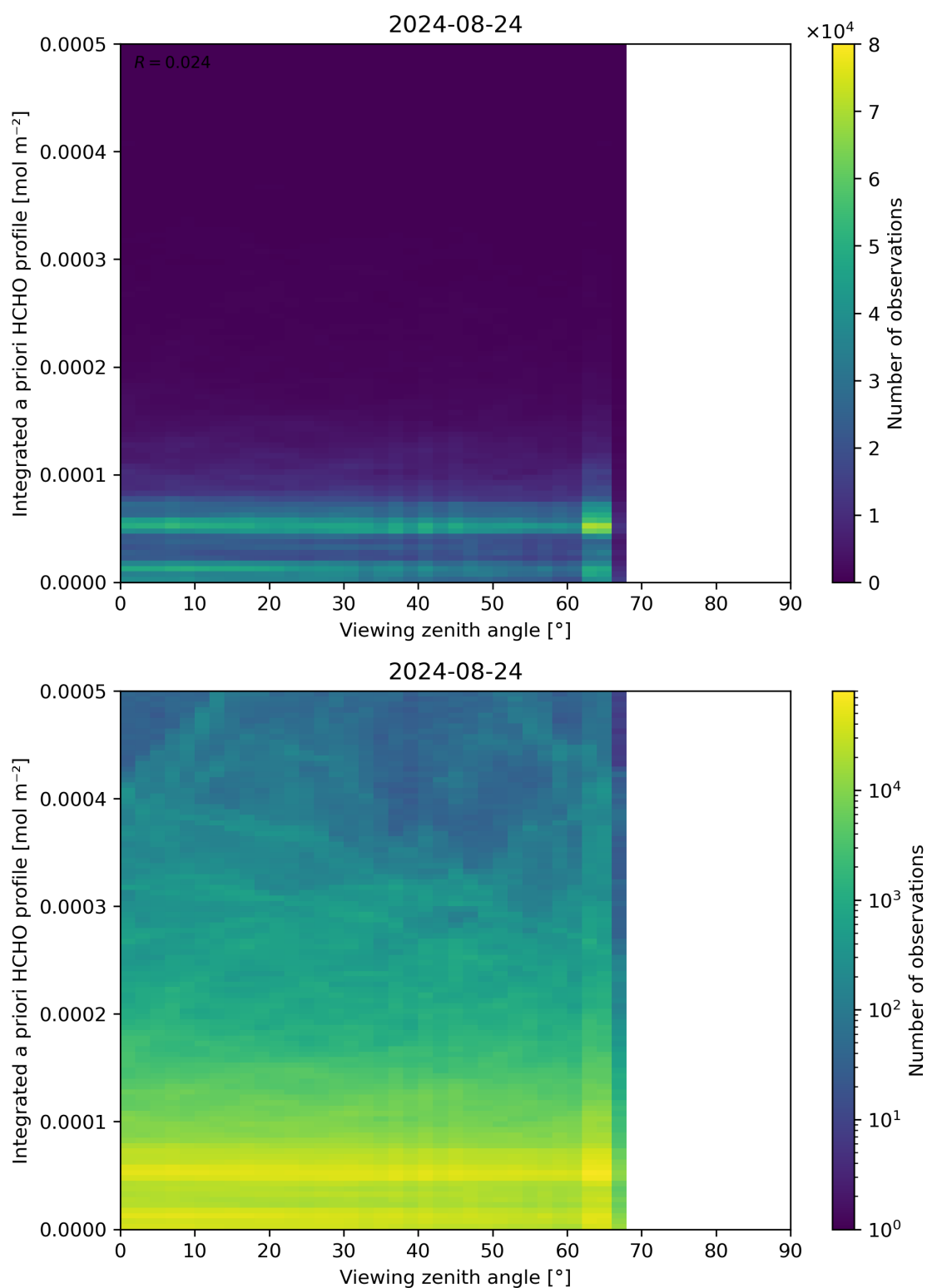
Figure 195: Scatter density plot of “Viewing zenith angle” against “Integrated a priori HCHO profile” for 2024-08-23 to 2024-08-25.
