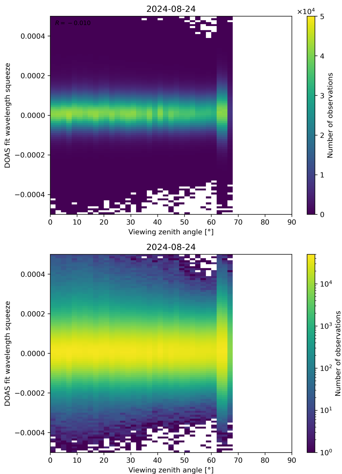
Figure 184: Scatter density plot of “Viewing zenith angle” against “DOAS fit wavelength squeeze” for 2024-08-23 to 2024-08-25.
