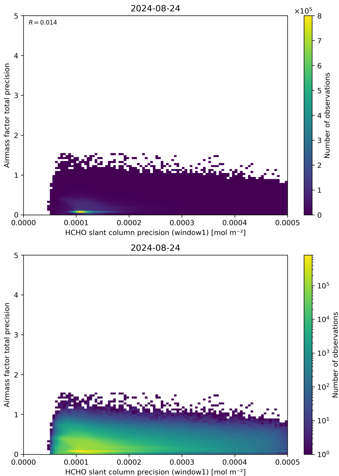
Figure 95: Scatter density plot of “HCHO slant column precision (window1)” against “Airmass factor total precision” for 2024-08-23 to 2024-08-25.
