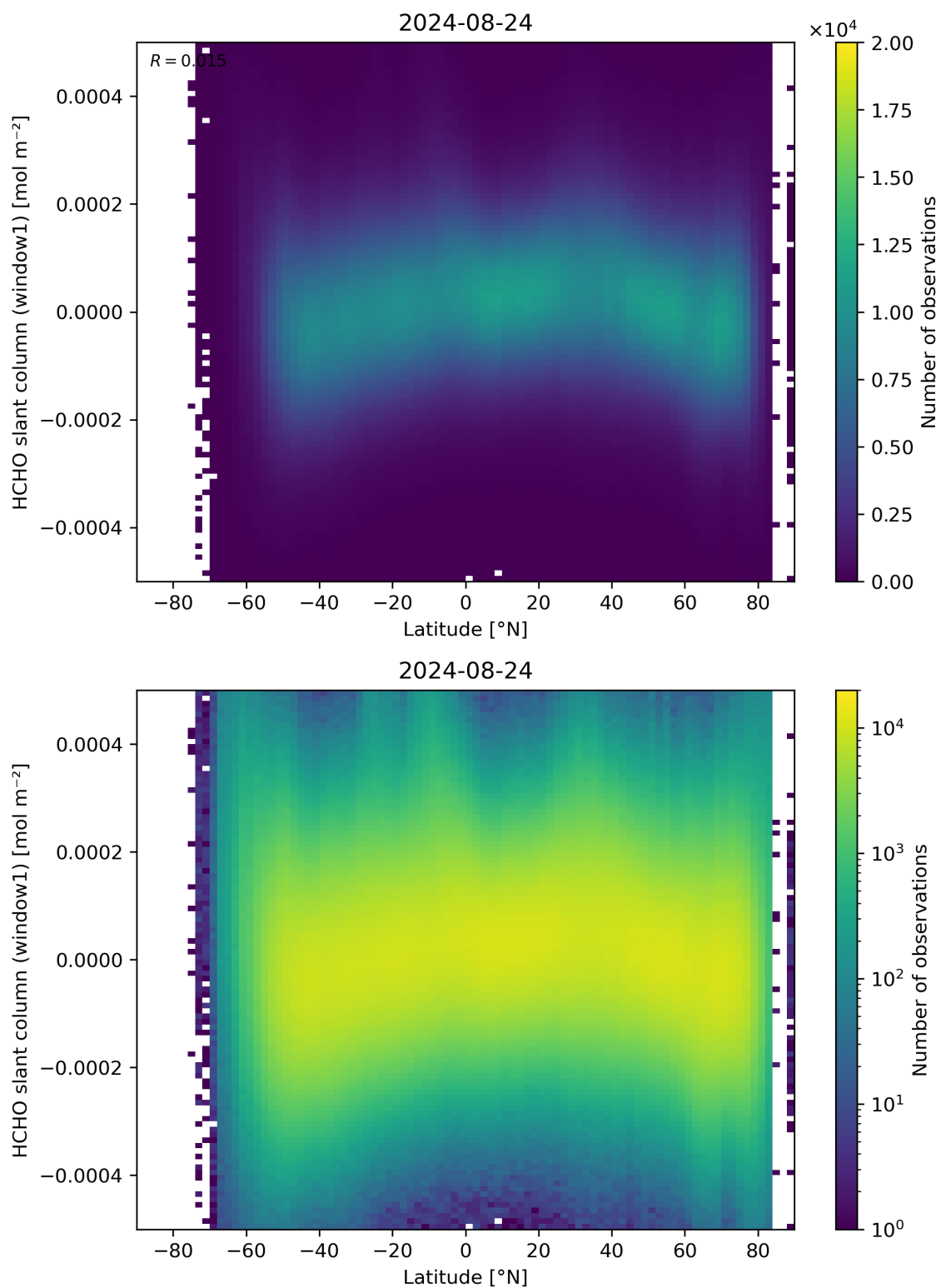
Figure 159: Scatter density plot of “Latitude” against “HCHO slant column (window1)” for 2024-08-23 to 2024-08-25.
