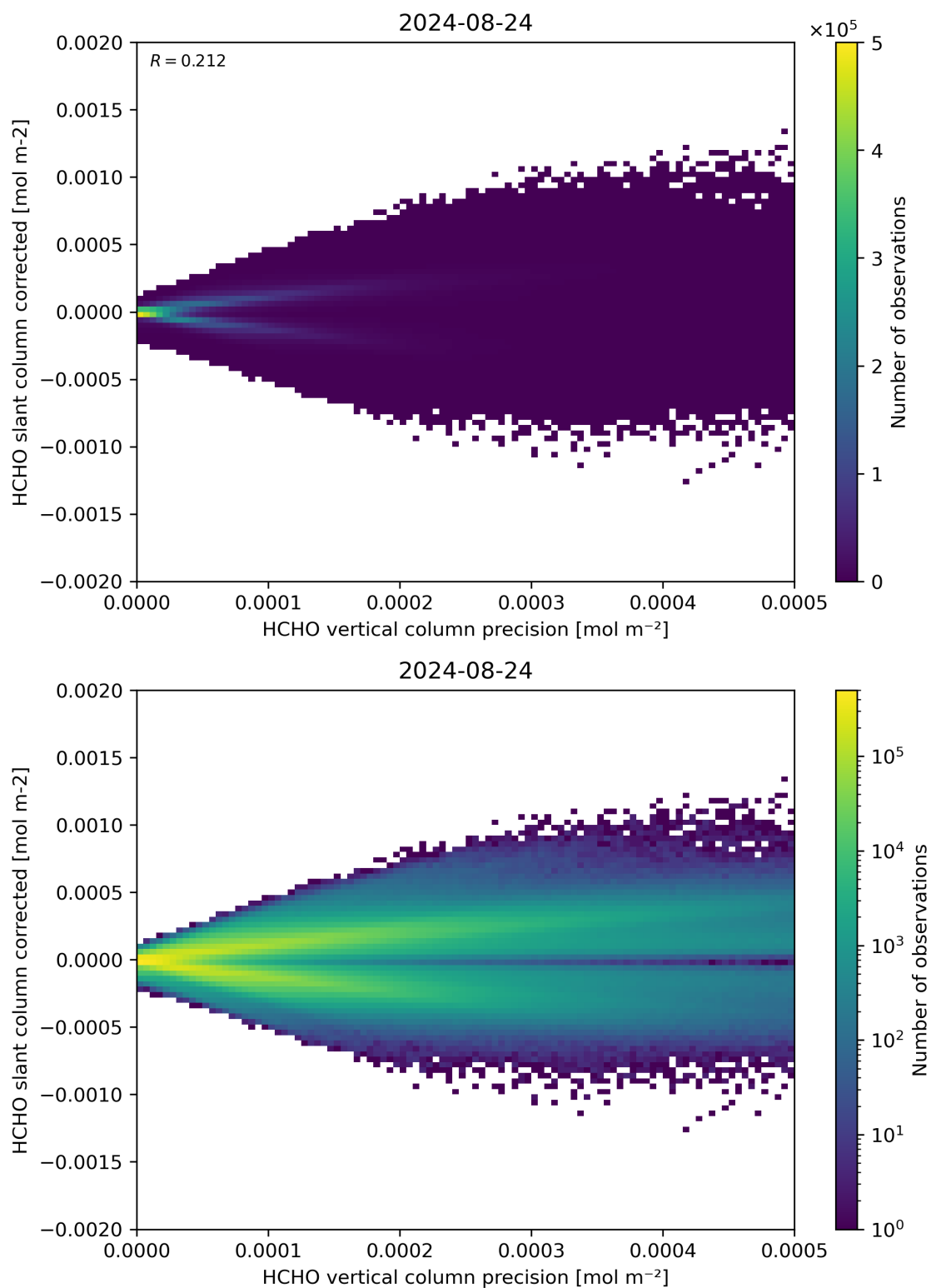
Figure 140: Scatter density plot of “HCHO vertical column precision” against “HCHO slant column corrected” for 2024-08-23 to 2024-08-25.
