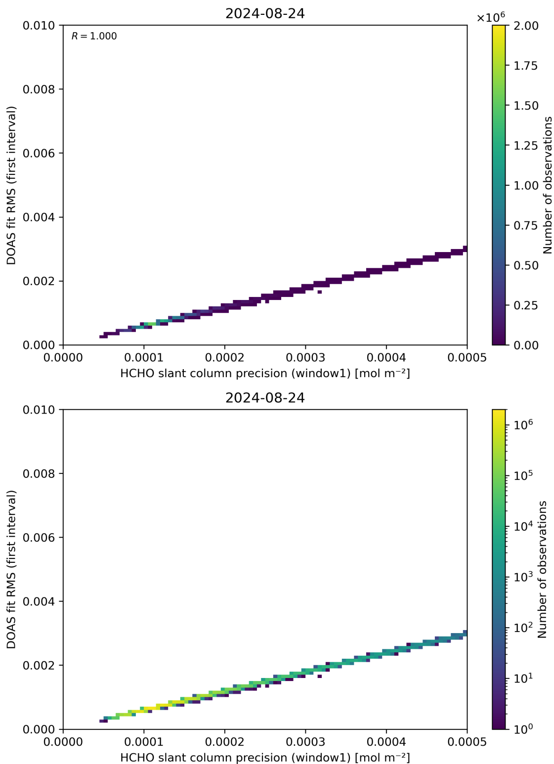
Figure 88: Scatter density plot of “HCHO slant column precision (window1)” against “DOAS fit RMS (first interval)” for 2024-08-23 to 2024-08-25.
