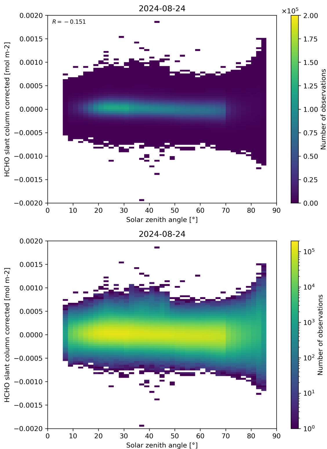
Figure 171: Scatter density plot of “Solar zenith angle” against “HCHO slant column corrected” for 2024-08-23 to 2024-08-25.
