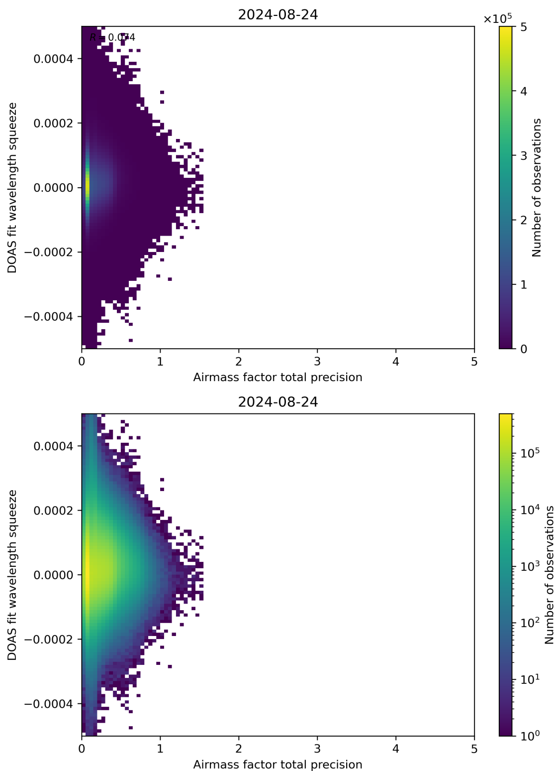
Figure 107: Scatter density plot of “Airmass factor total precision” against “DOAS fit wavelength squeeze” for 2024-08-23 to 2024-08-25.
