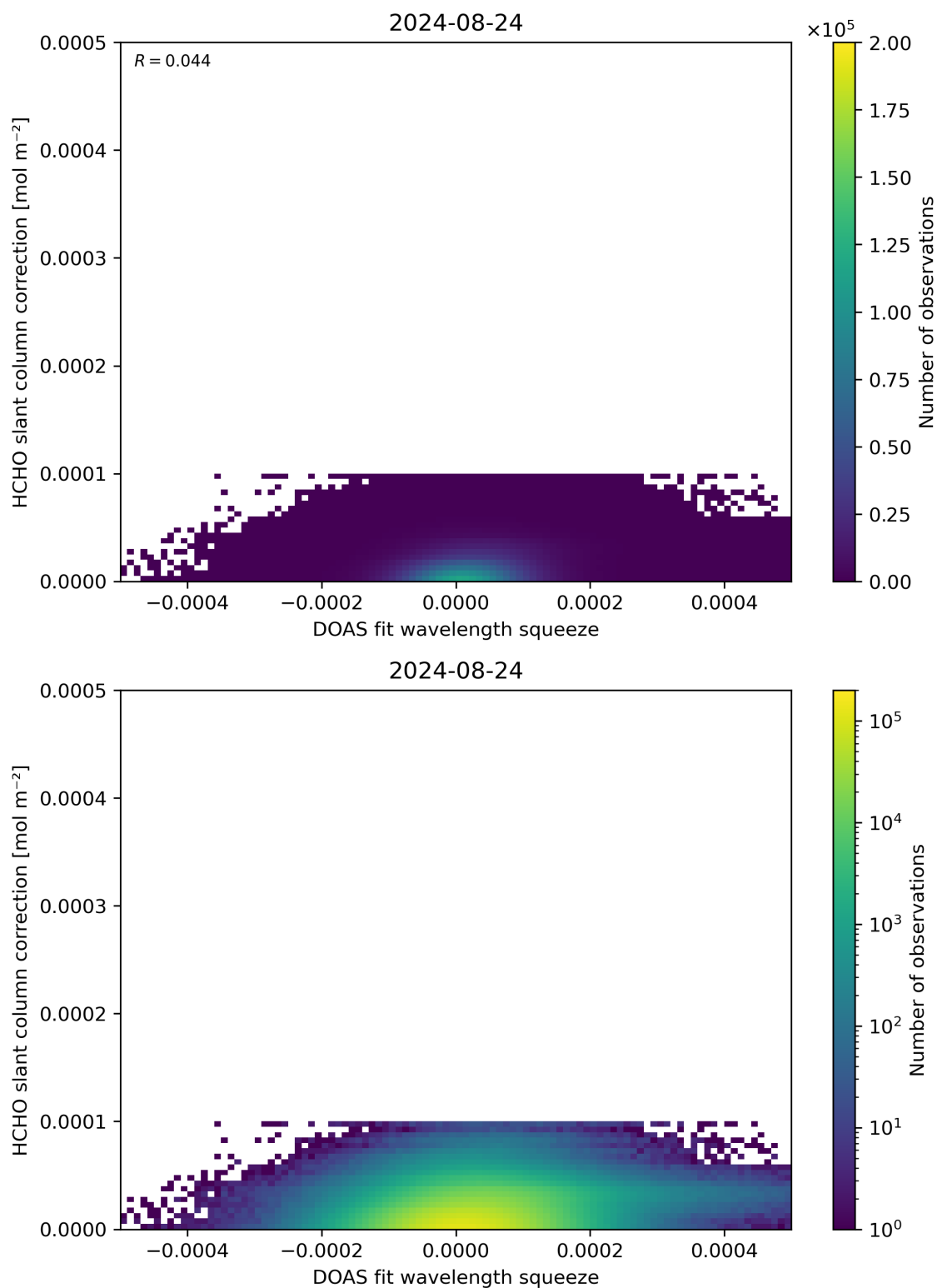
Figure 70: Scatter density plot of “DOAS fit wavelength squeeze” against “HCHO slant column correction” for 2024-08-23 to 2024-08-25.
