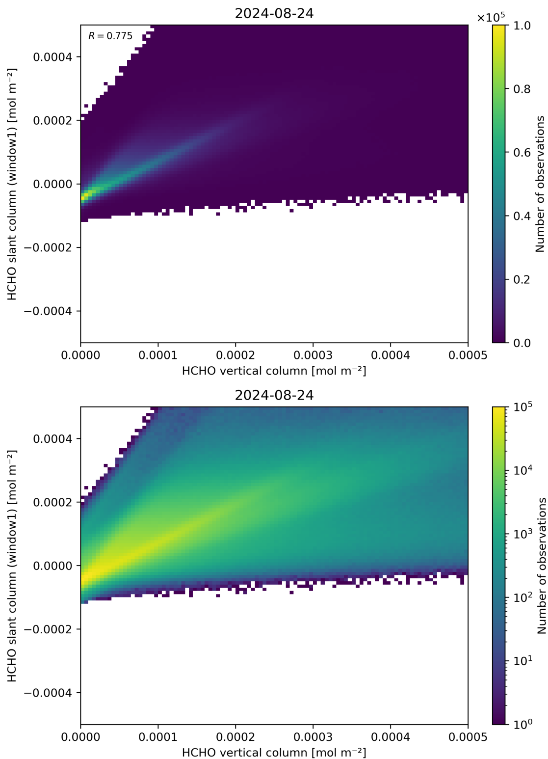
Figure 129: Scatter density plot of “HCHO vertical column” against “HCHO slant column (window1)” for 2024-08-23 to 2024-08-25.
