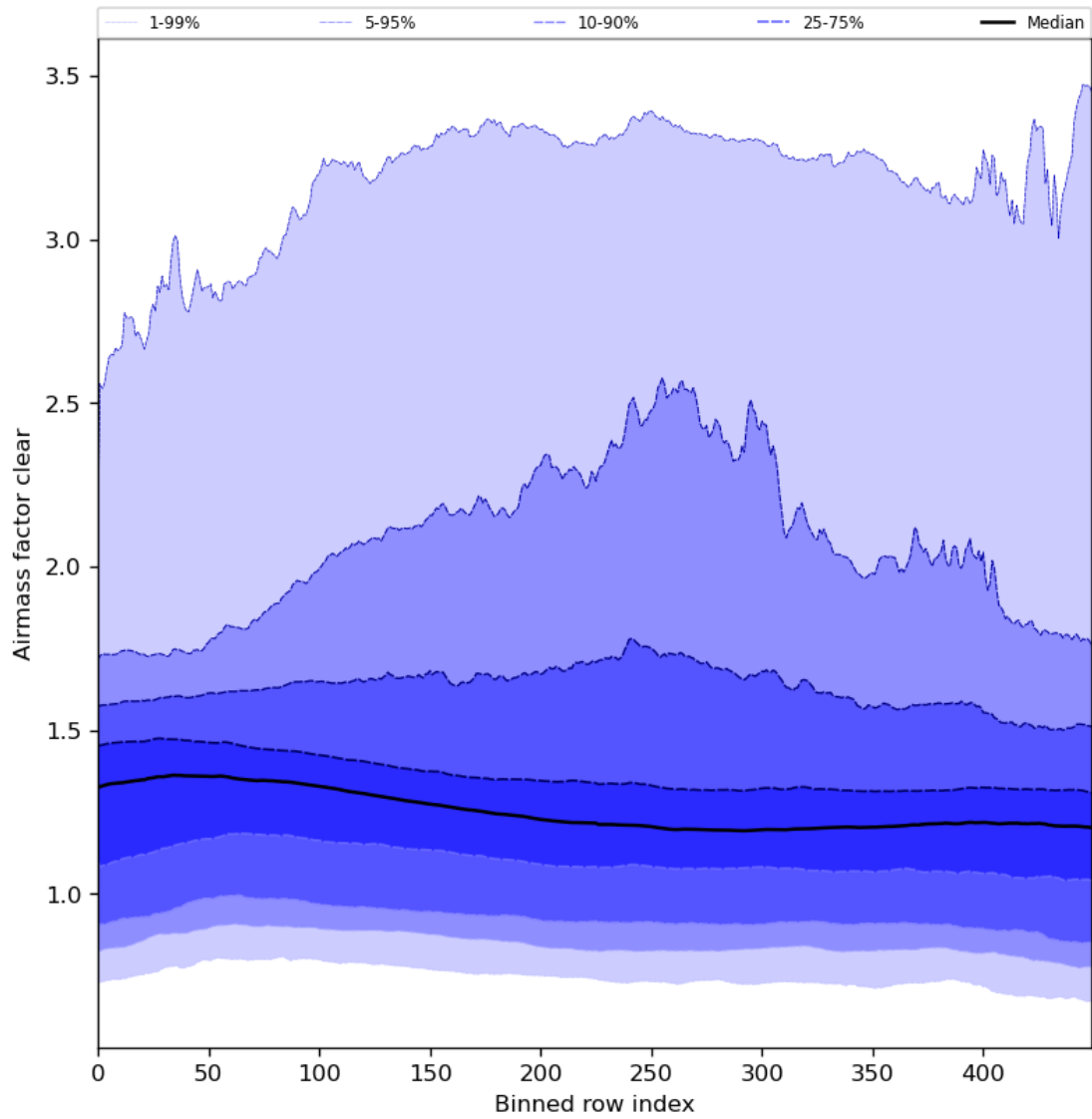
Figure 56: Along track statistics of “Airmass factor clear” for 2024-08-23 to 2024-08-25
