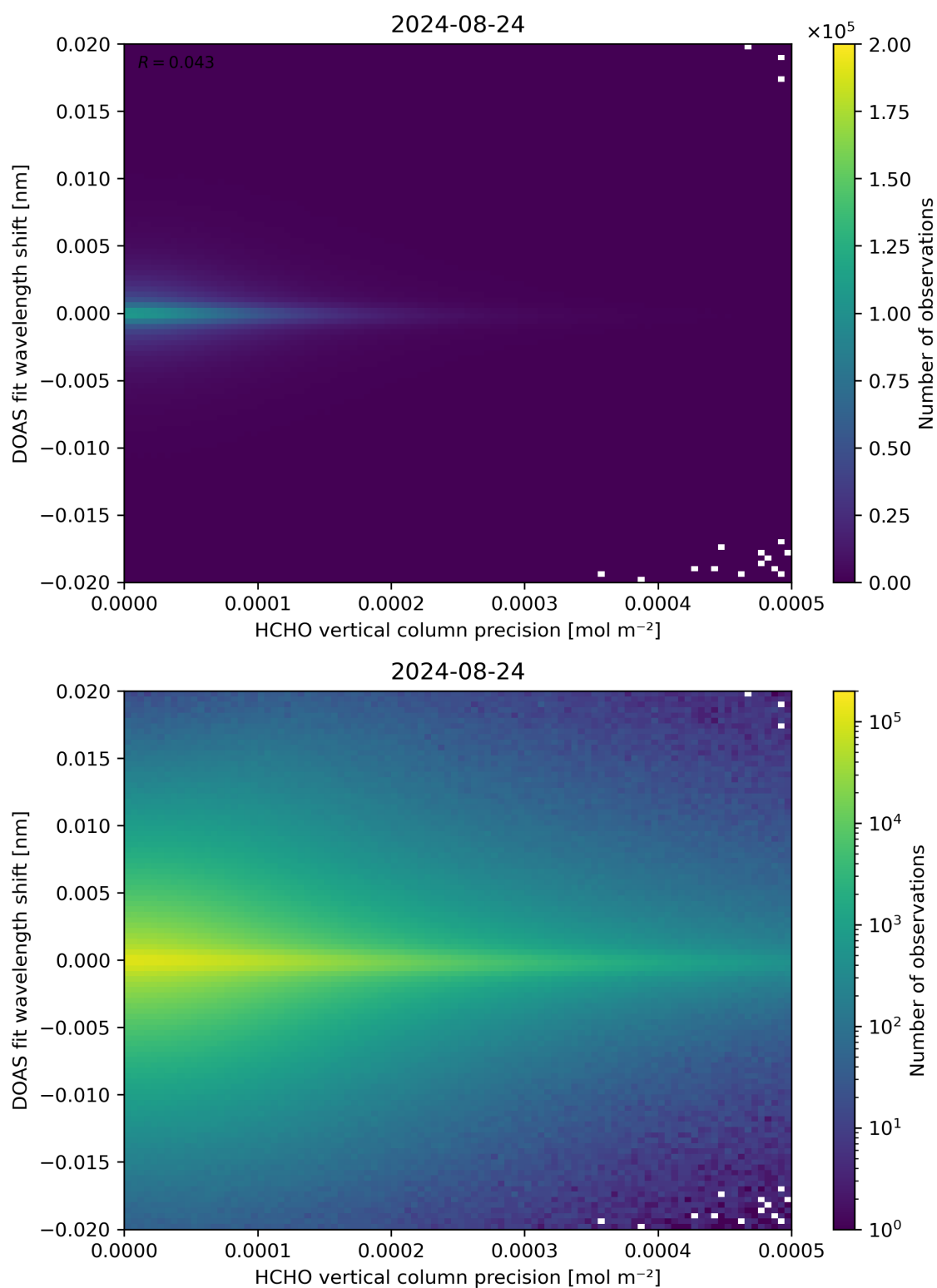
Figure 137: Scatter density plot of “HCHO vertical column precision” against “DOAS fit wavelength shift” for 2024-08-23 to 2024-08-25.
