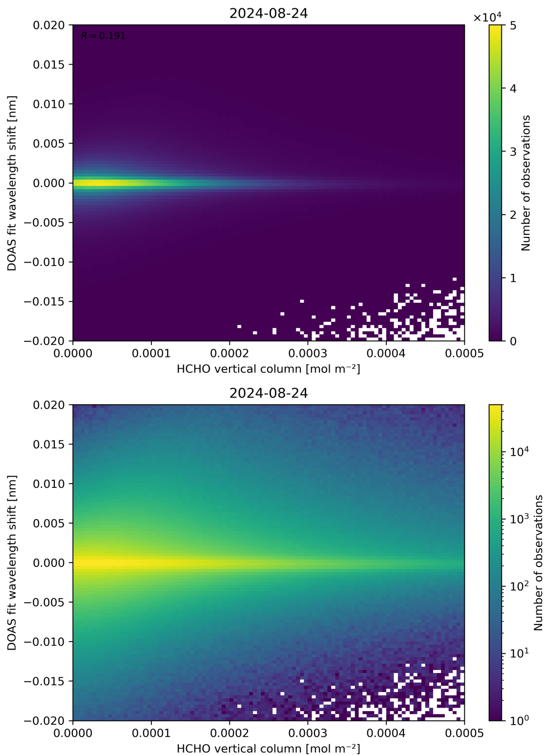
Figure 124: Scatter density plot of “HCHO vertical column” against “DOAS fit wavelength shift” for 2024-08-23 to 2024-08-25.
