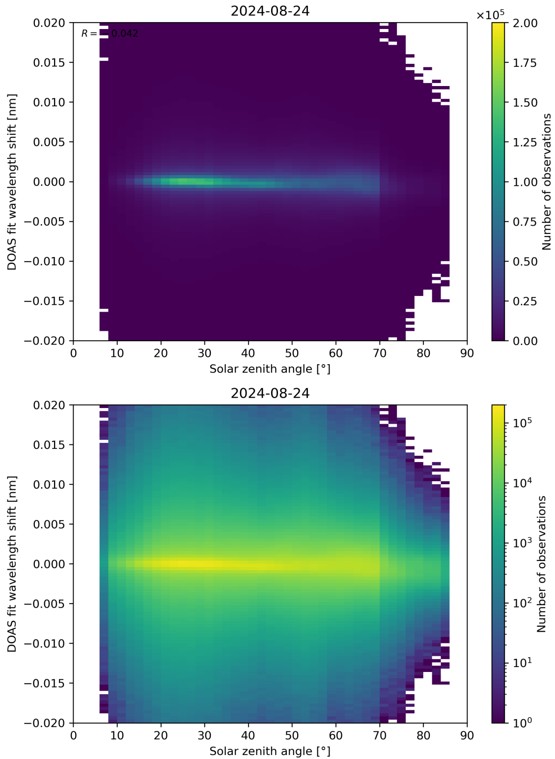
Figure 168: Scatter density plot of “Solar zenith angle” against “DOAS fit wavelength shift” for 2024-08-23 to 2024-08-25.
