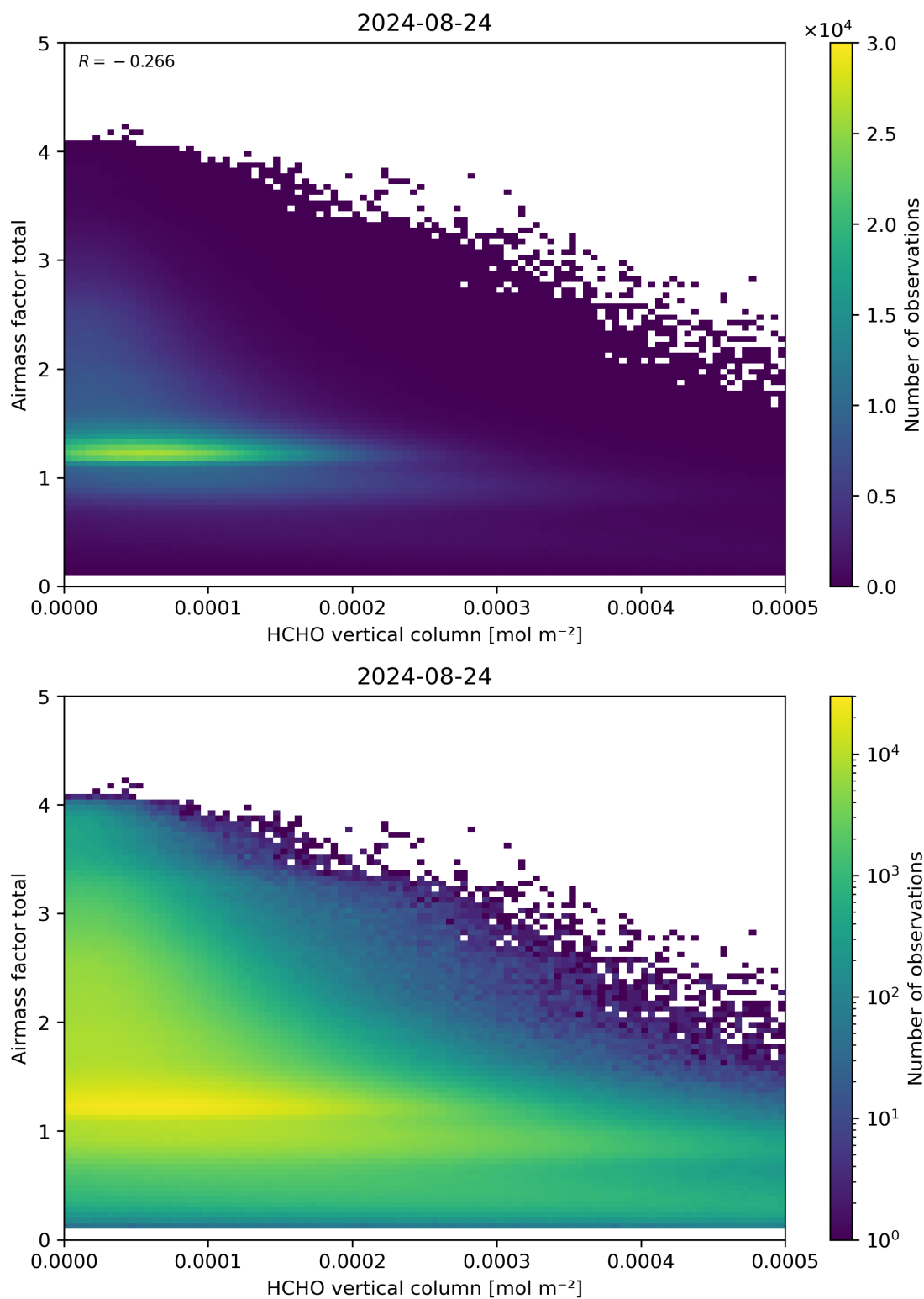
Figure 131: Scatter density plot of “HCHO vertical column” against “Airmass factor total” for 2024-08-23 to 2024-08-25.
