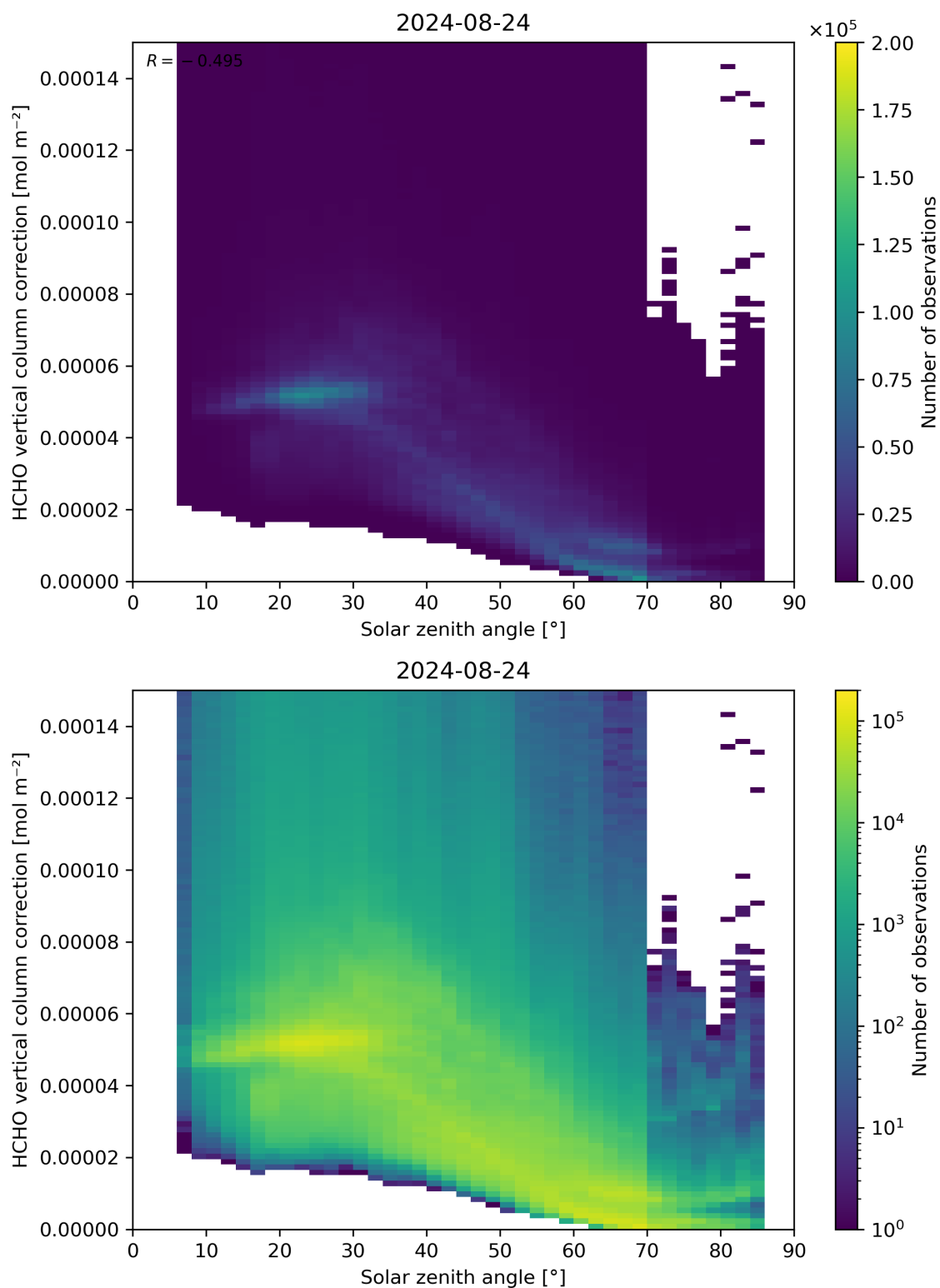
Figure 178: Scatter density plot of “Solar zenith angle” against “HCHO vertical column correction” for 2024-08-23 to 2024-08-25.
