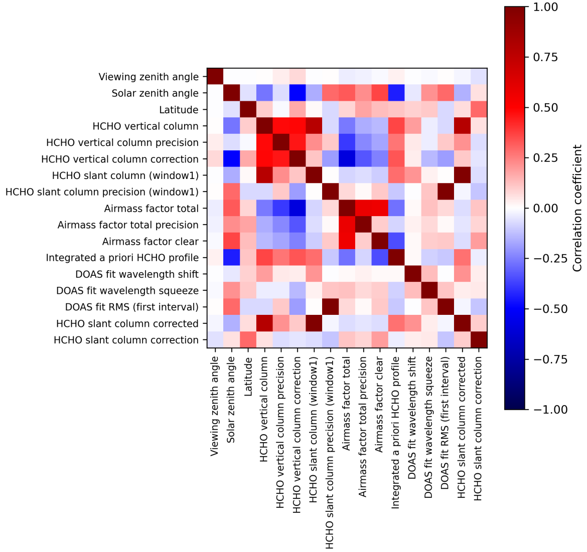
Figure 2: Map of correlation matrix for 2024-08-23 to 2024-08-25.
