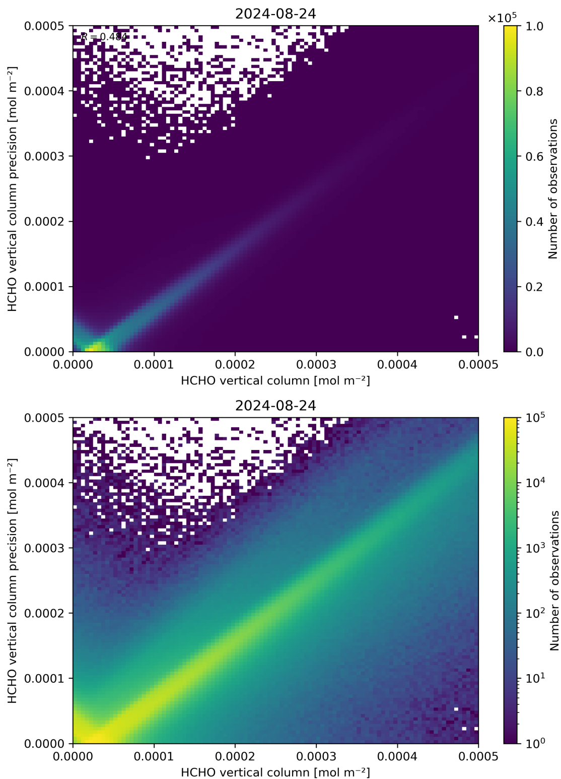
Figure 134: Scatter density plot of “HCHO vertical column” against “HCHO vertical column precision” for 2024-08-23 to 2024-08-25.
