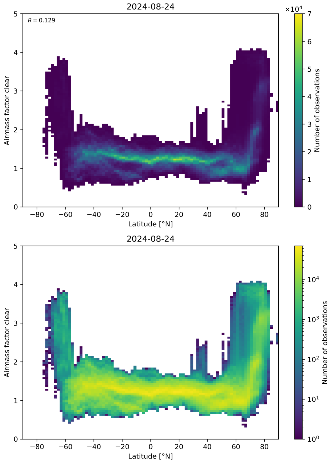
Figure 156: Scatter density plot of “Latitude” against “Airmass factor clear” for 2024-08-23 to 2024-08-25.
