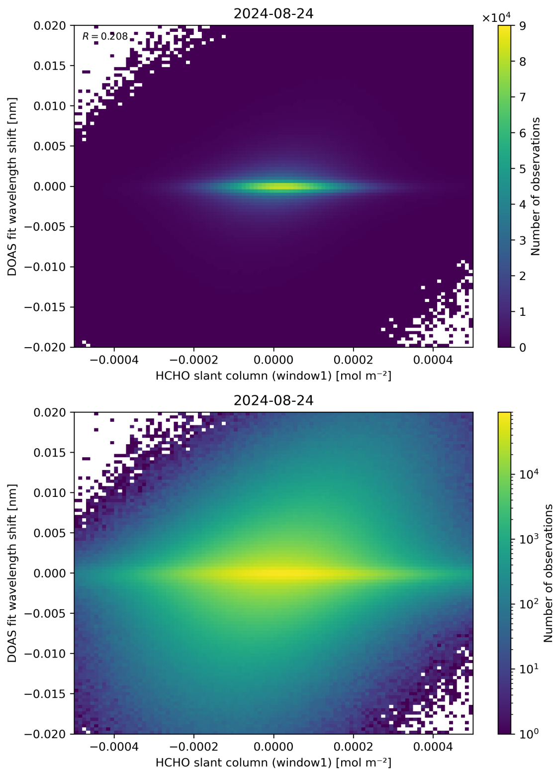
Figure 79: Scatter density plot of “HCHO slant column (window1)” against “DOAS fit wavelength shift” for 2024-08-23 to 2024-08-25.
