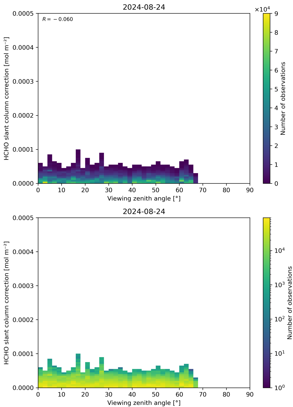
Figure 187: Scatter density plot of “Viewing zenith angle” against “HCHO slant column correction” for 2024-08-23 to 2024-08-25.
