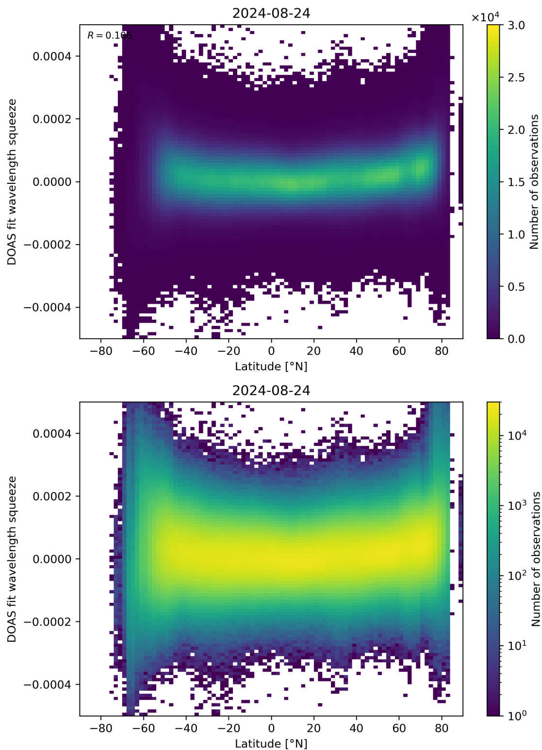
Figure 155: Scatter density plot of “Latitude” against “DOAS fit wavelength squeeze” for 2024-08-23 to 2024-08-25.
