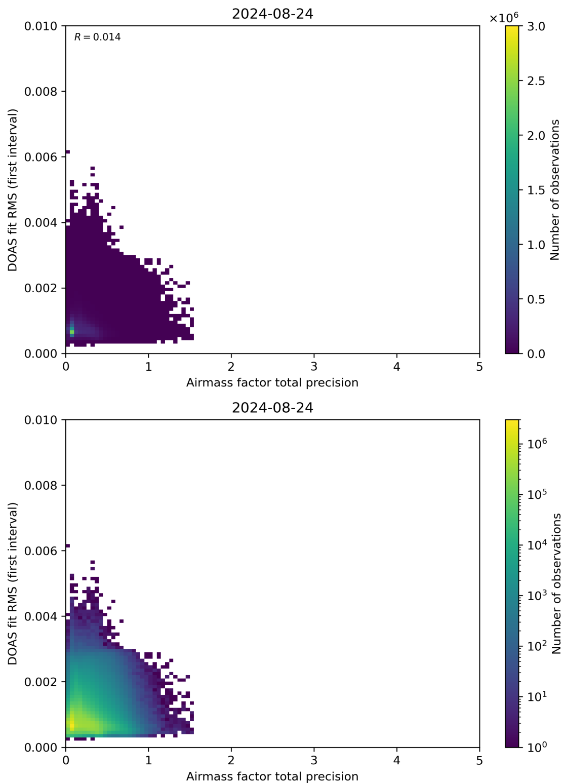
Figure 105: Scatter density plot of “Airmass factor total precision” against “DOAS fit RMS (first interval)” for 2024-08-23 to 2024-08-25.
