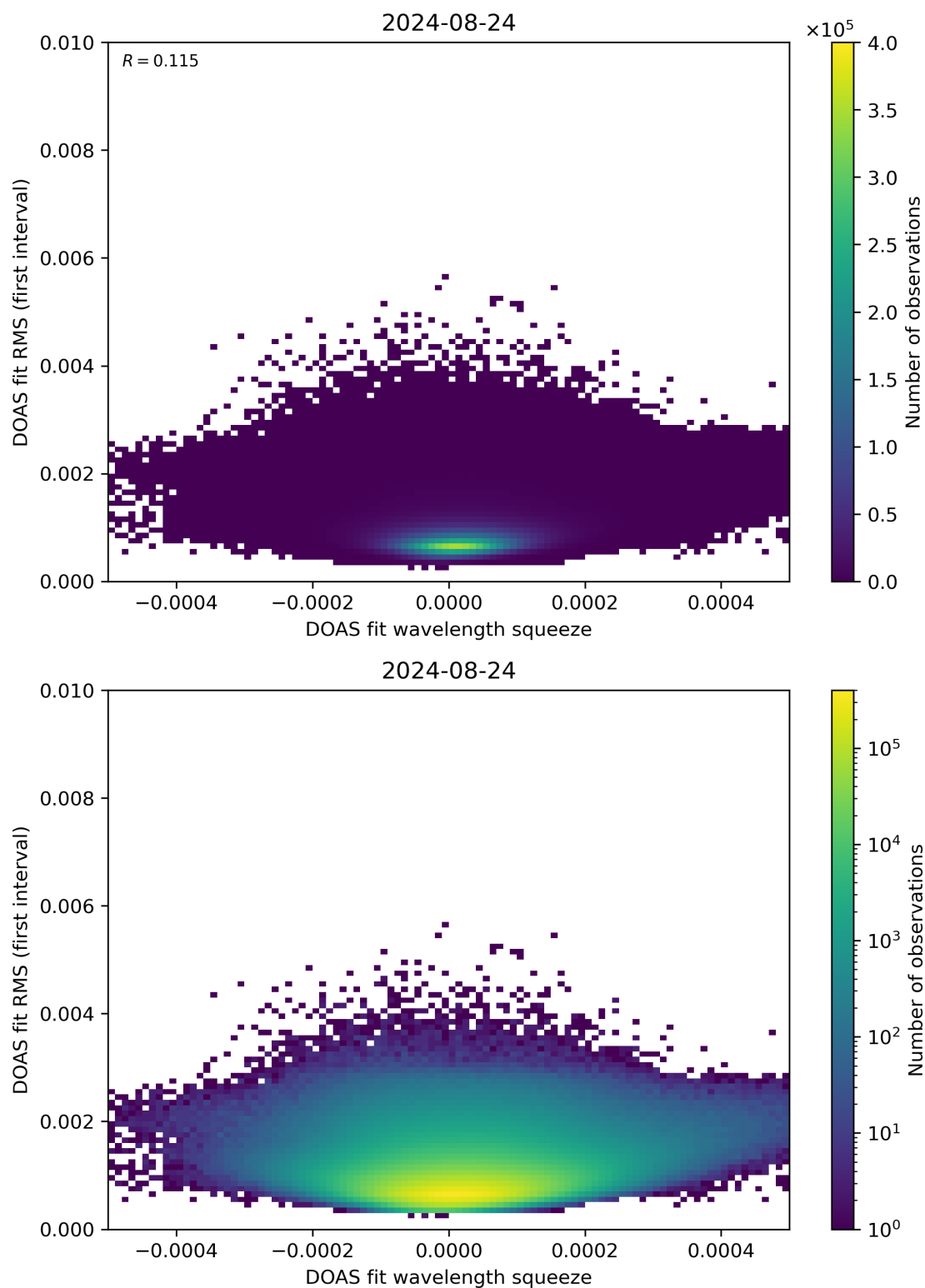
Figure 68: Scatter density plot of “DOAS fit wavelength squeeze” against “DOAS fit RMS (first interval)” for 2024-08-23 to 2024-08-25.
