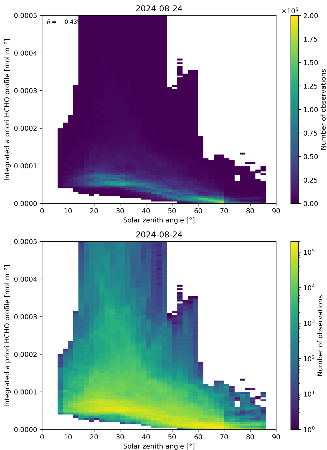
Figure 180: Scatter density plot of “Solar zenith angle” against “Integrated a priori HCHO profile” for 2024-08-23 to 2024-08-25.
