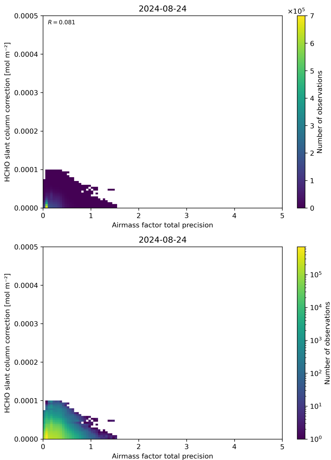
Figure 110: Scatter density plot of “Airmass factor total precision” against “HCHO slant column correction” for 2024-08-23 to 2024-08-25.
