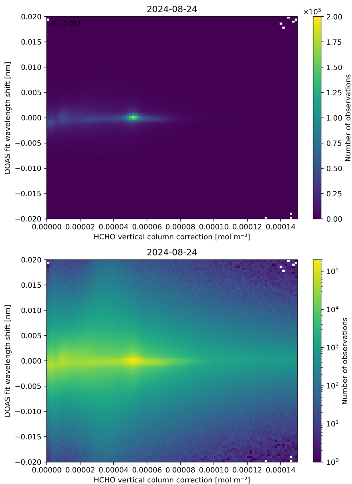
Figure 113: Scatter density plot of “HCHO vertical column correction” against “DOAS fit wavelength shift” for 2024-08-23 to 2024-08-25.
