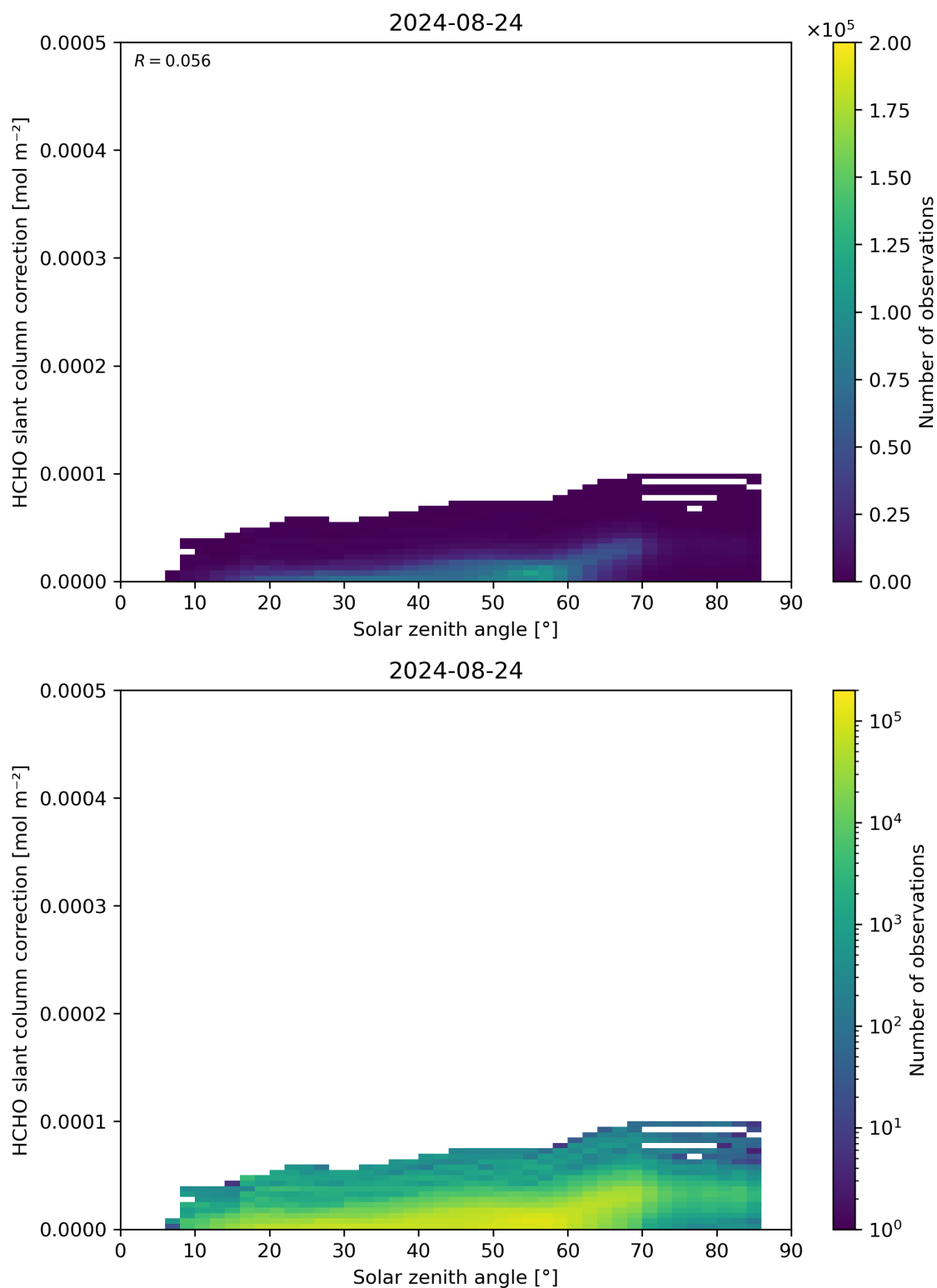
Figure 172: Scatter density plot of “Solar zenith angle” against “HCHO slant column correction” for 2024-08-23 to 2024-08-25.
