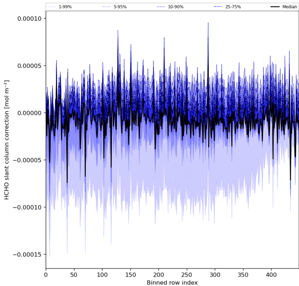
Figure 61: Along track statistics of “HCHO slant column correction” for 2024-08-23 to 2024-08-25
