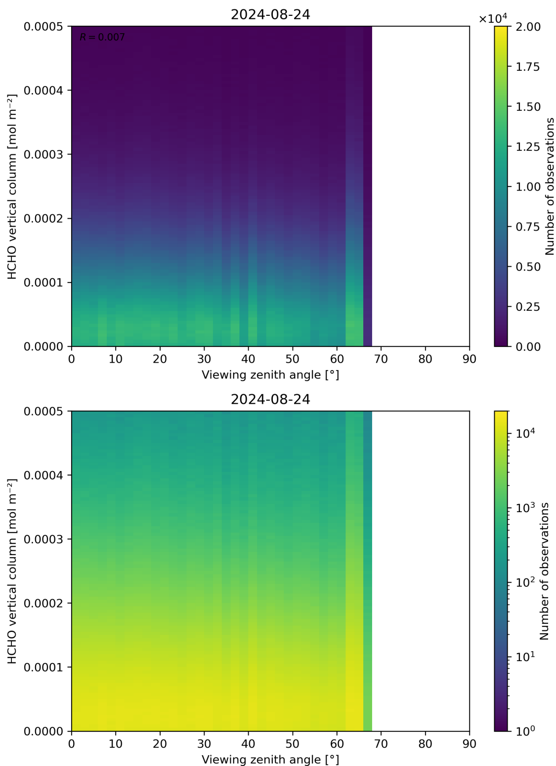
Figure 192: Scatter density plot of “Viewing zenith angle” against “HCHO vertical column” for 2024-08-23 to 2024-08-25.
