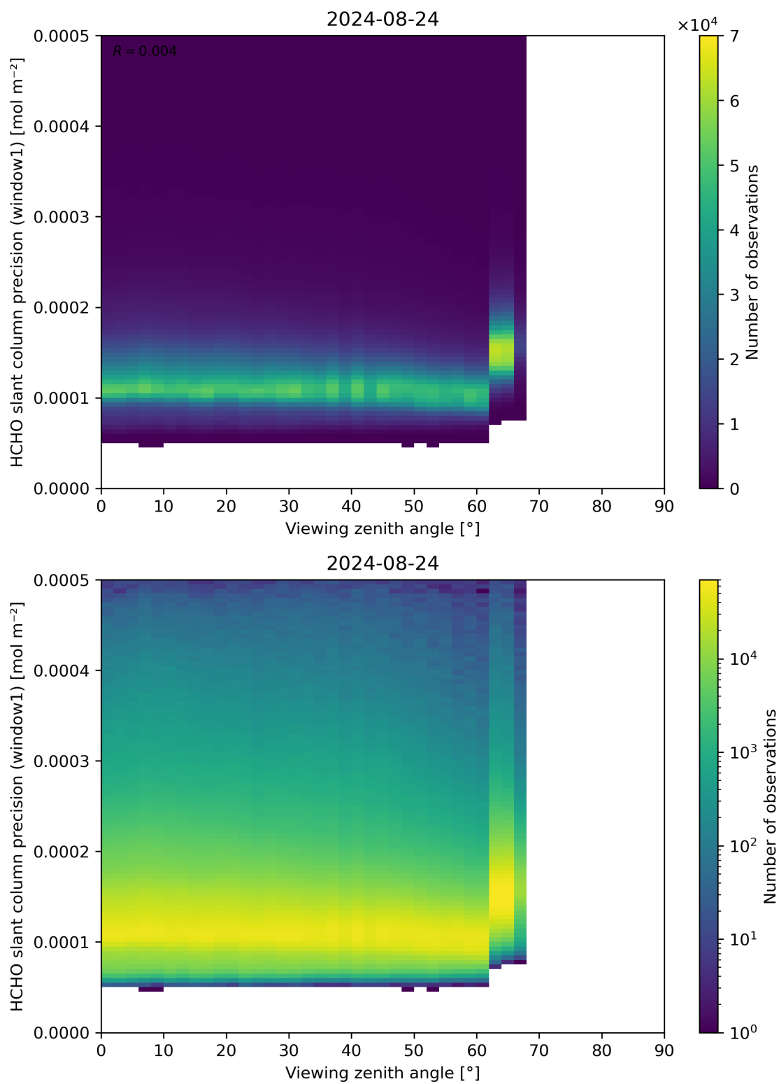
Figure 189: Scatter density plot of “Viewing zenith angle” against “HCHO slant column precision (window1)” for 2024-08-23 to 2024-08-25.
