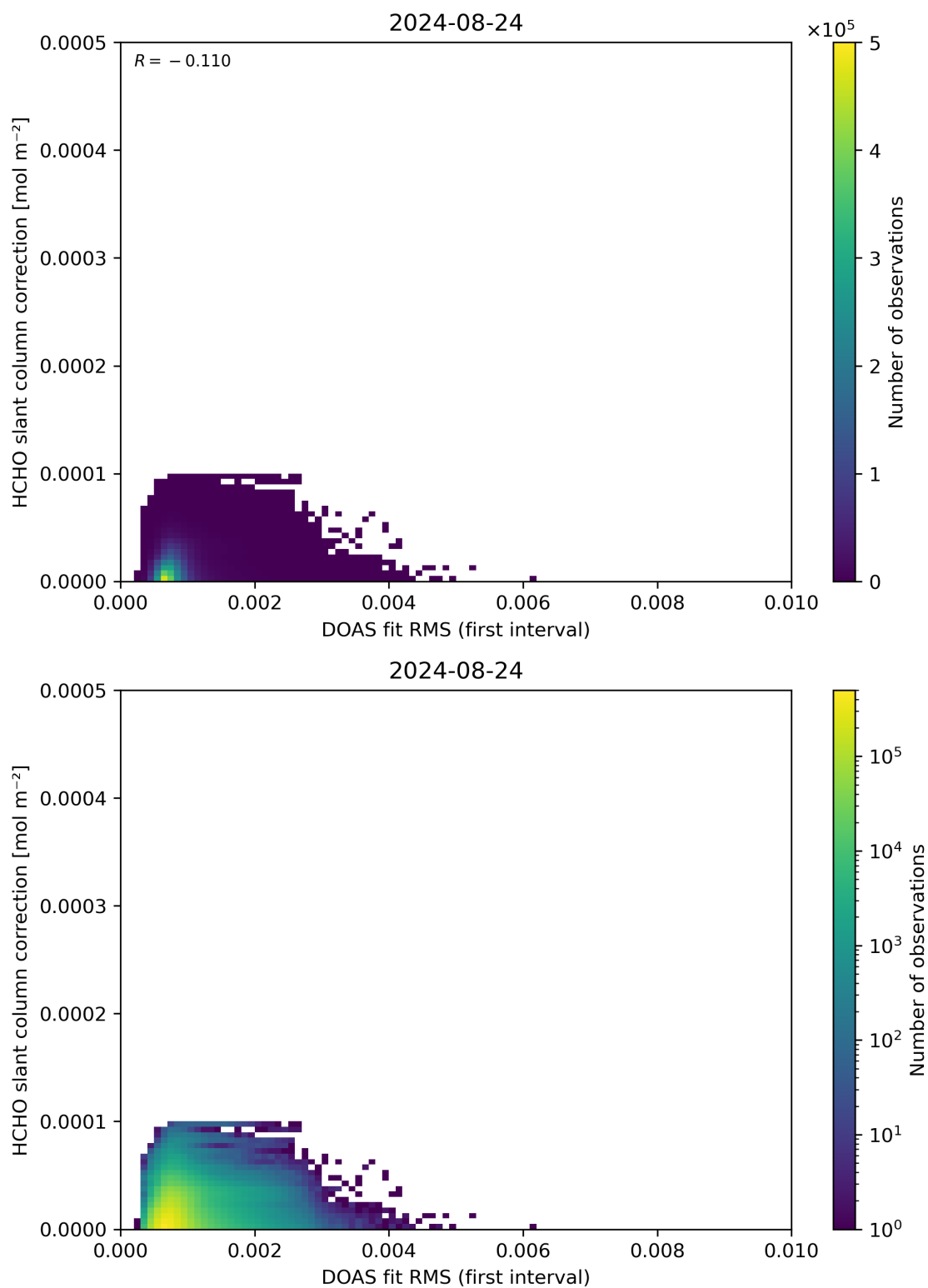
Figure 63: Scatter density plot of “DOAS fit RMS (first interval)” against “HCHO slant column correction” for 2024-08-23 to 2024-08-25.
