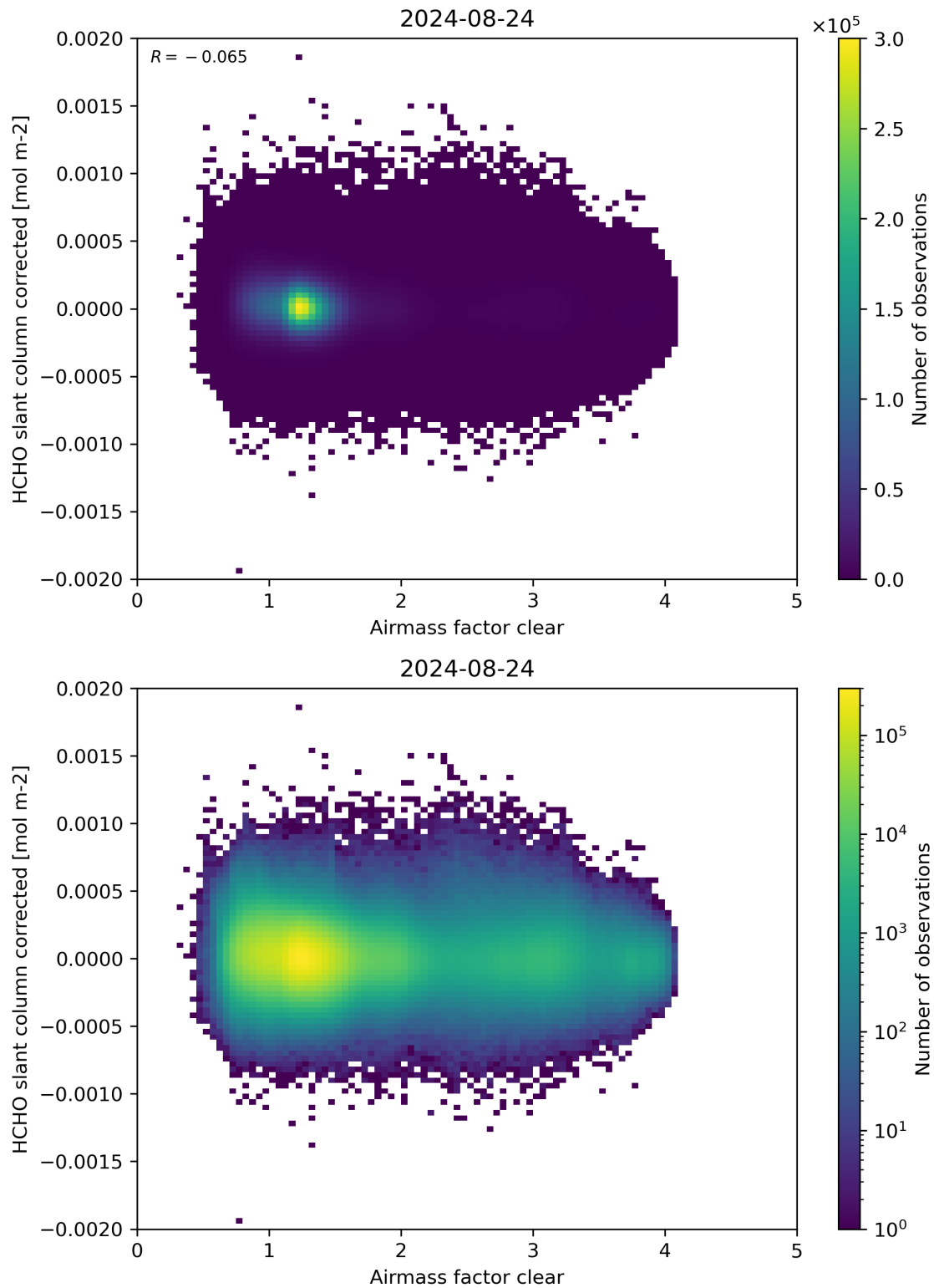
Figure 74: Scatter density plot of “Airmass factor clear” against “HCHO slant column corrected” for 2024-08-23 to 2024-08-25.
