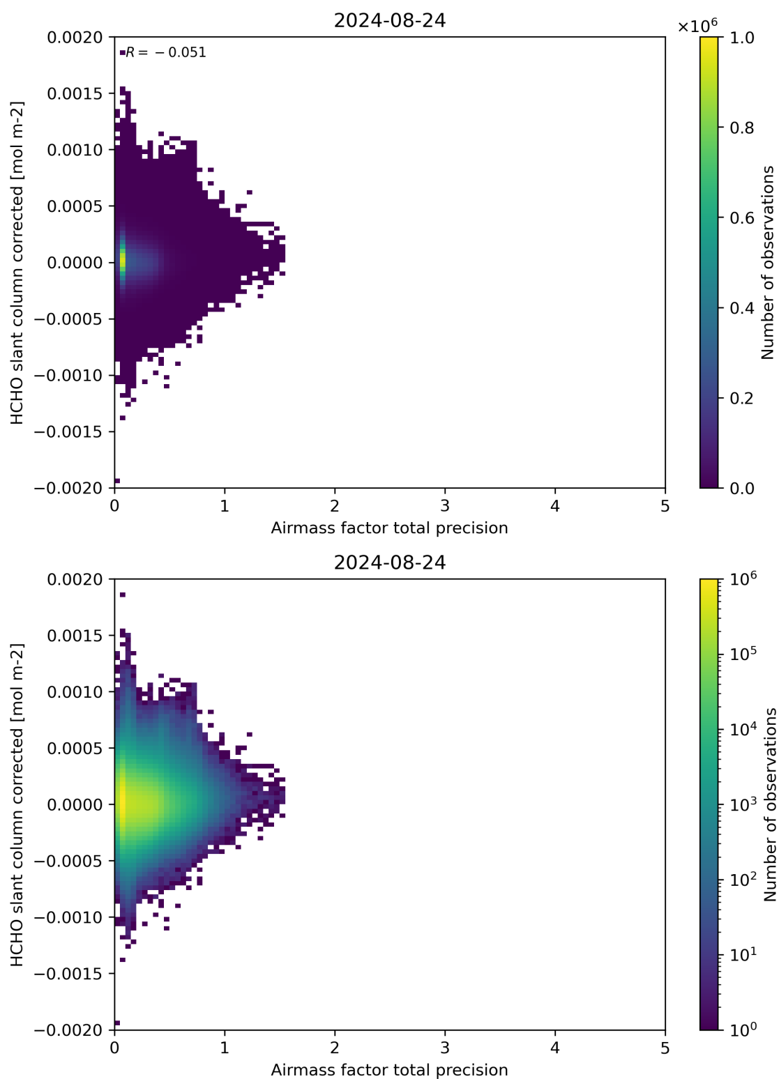
Figure 109: Scatter density plot of “Airmass factor total precision” against “HCHO slant column corrected” for 2024-08-23 to 2024-08-25.
