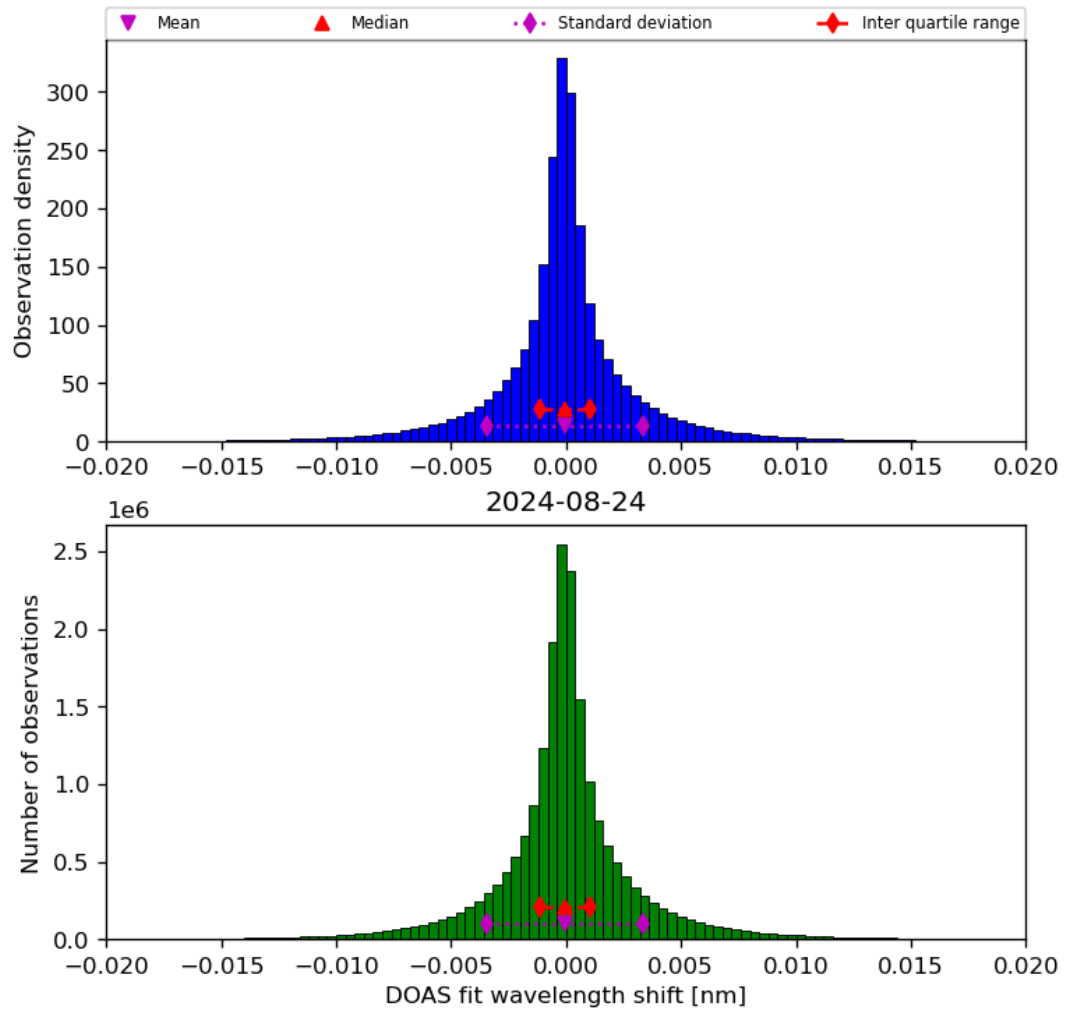
Figure 44: Histogram of “DOAS fit wavelength shift” for 2024-08-23 to 2024-08-25
