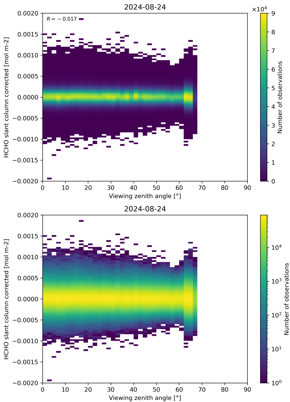
Figure 186: Scatter density plot of “Viewing zenith angle” against “HCHO slant column corrected” for 2024-08-23 to 2024-08-25.
