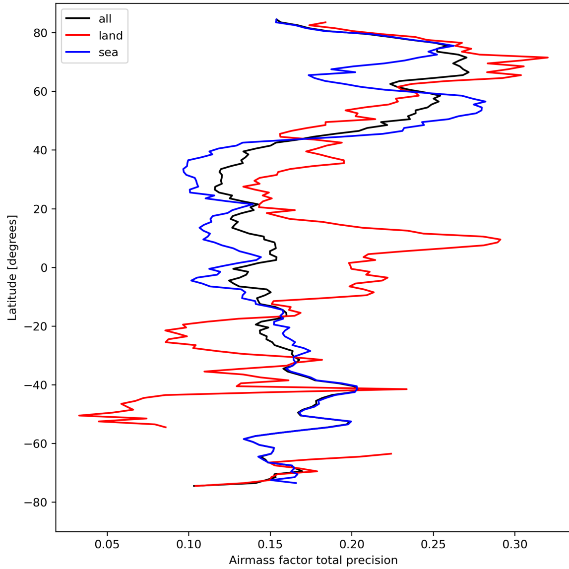
Figure 27: Zonal average of “Airmass factor total precision” for 2024-08-23 to 2024-08-25.
