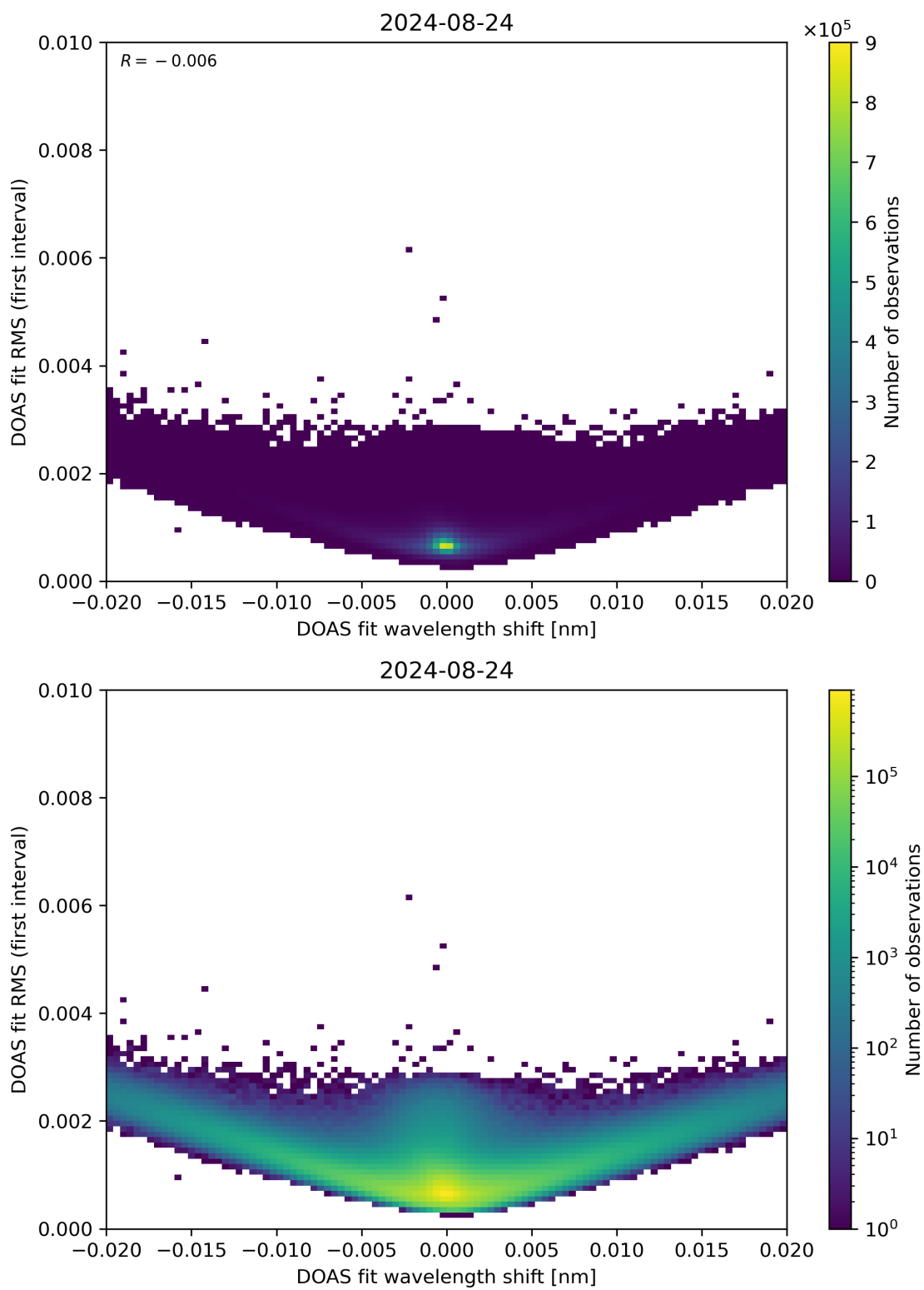
Figure 64: Scatter density plot of “DOAS fit wavelength shift” against “DOAS fit RMS (first interval)” for 2024-08-23 to 2024-08-25.
