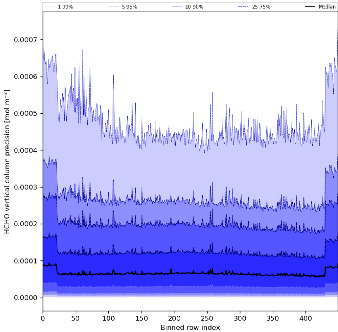
Figure 50: Along track statistics of “HCHO vertical column precision” for 2024-08-23 to 2024-08-25
