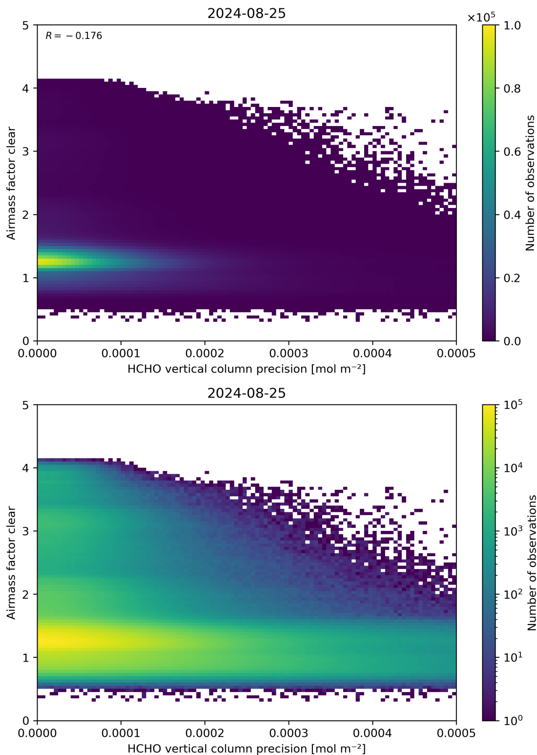
Figure 139: Scatter density plot of “HCHO vertical column precision” against “Airmass factor clear” for 2024-08-24 to 2024-08-26.
