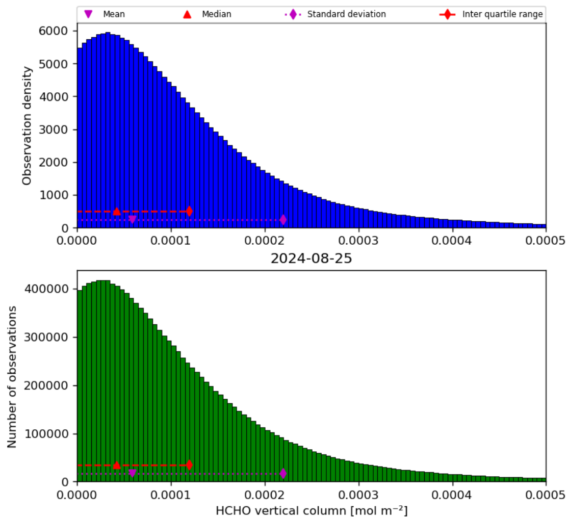
Figure 35: Histogram of “HCHO vertical column” for 2024-08-24 to 2024-08-26
