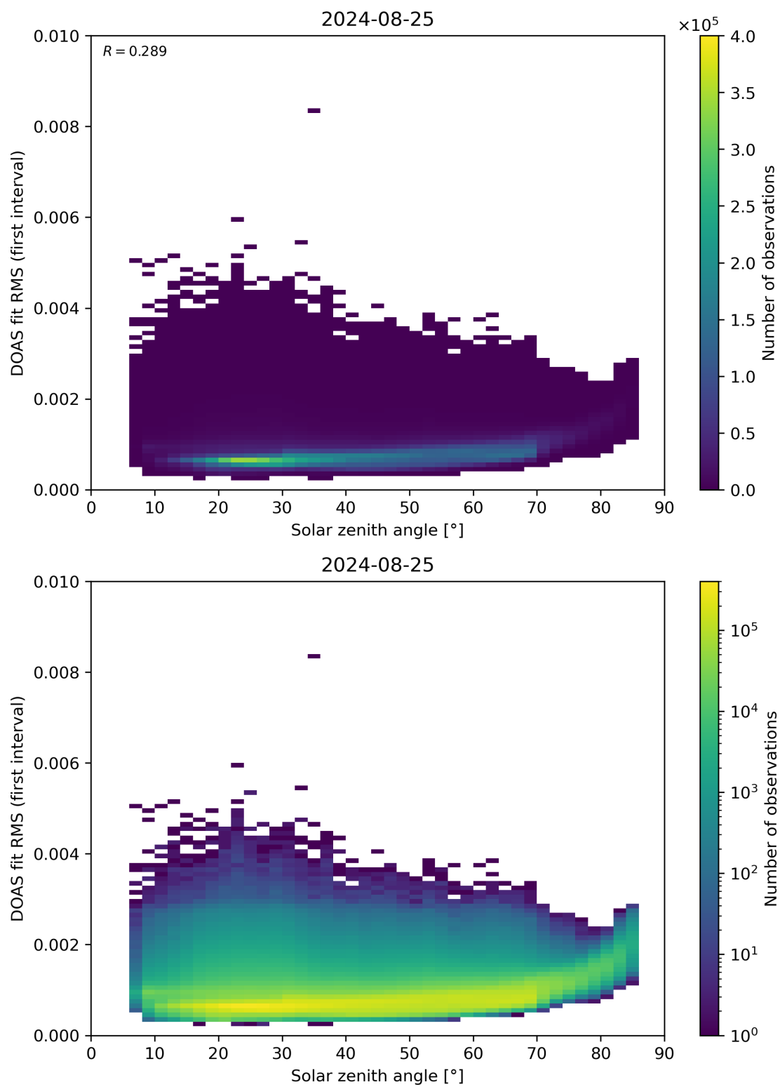
Figure 167: Scatter density plot of “Solar zenith angle” against “DOAS fit RMS (first interval)” for 2024-08-24 to 2024-08-26.
