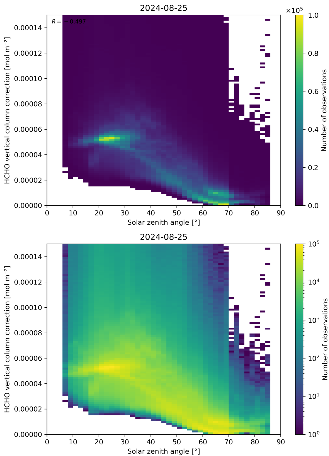
Figure 178: Scatter density plot of “Solar zenith angle” against “HCHO vertical column correction” for 2024-08-24 to 2024-08-26.
