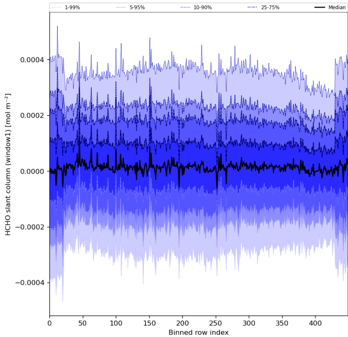
Figure 52: Along track statistics of "HCHO slant column (window1)" for 2024-08-24 to 2024-08-26
