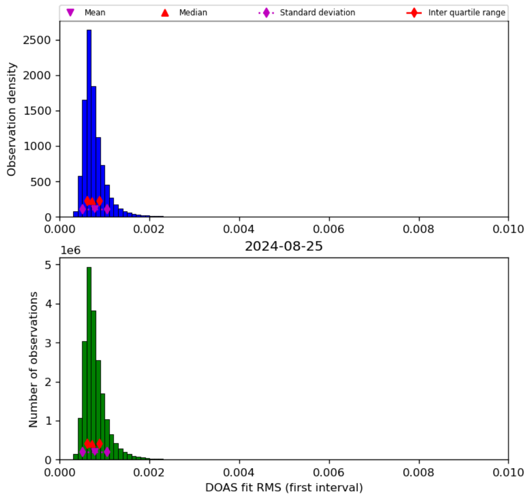
Figure 46: Histogram of “DOAS fit RMS (first interval)” for 2024-08-24 to 2024-08-26
