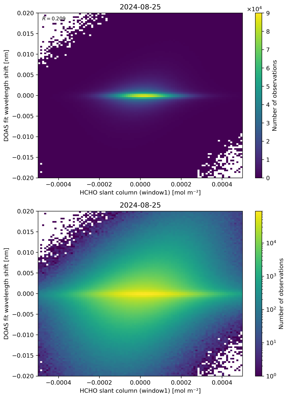
Figure 79: Scatter density plot of “HCHO slant column (window1)” against “DOAS fit wavelength shift” for 2024-08-24 to 2024-08-26.
