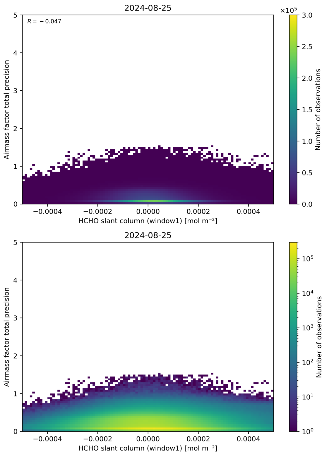
Figure 86: Scatter density plot of “HCHO slant column (window1)” against “Airmass factor total precision” for 2024-08-24 to 2024-08-26.
