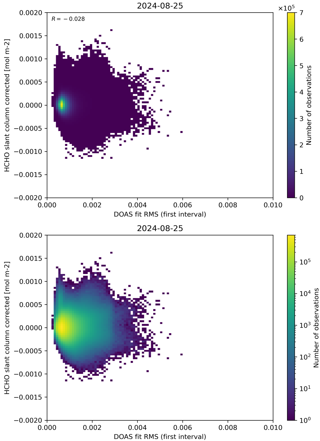
Figure 62: Scatter density plot of “DOAS fit RMS (first interval)” against “HCHO slant column corrected” for 2024-08-24 to 2024-08-26.
