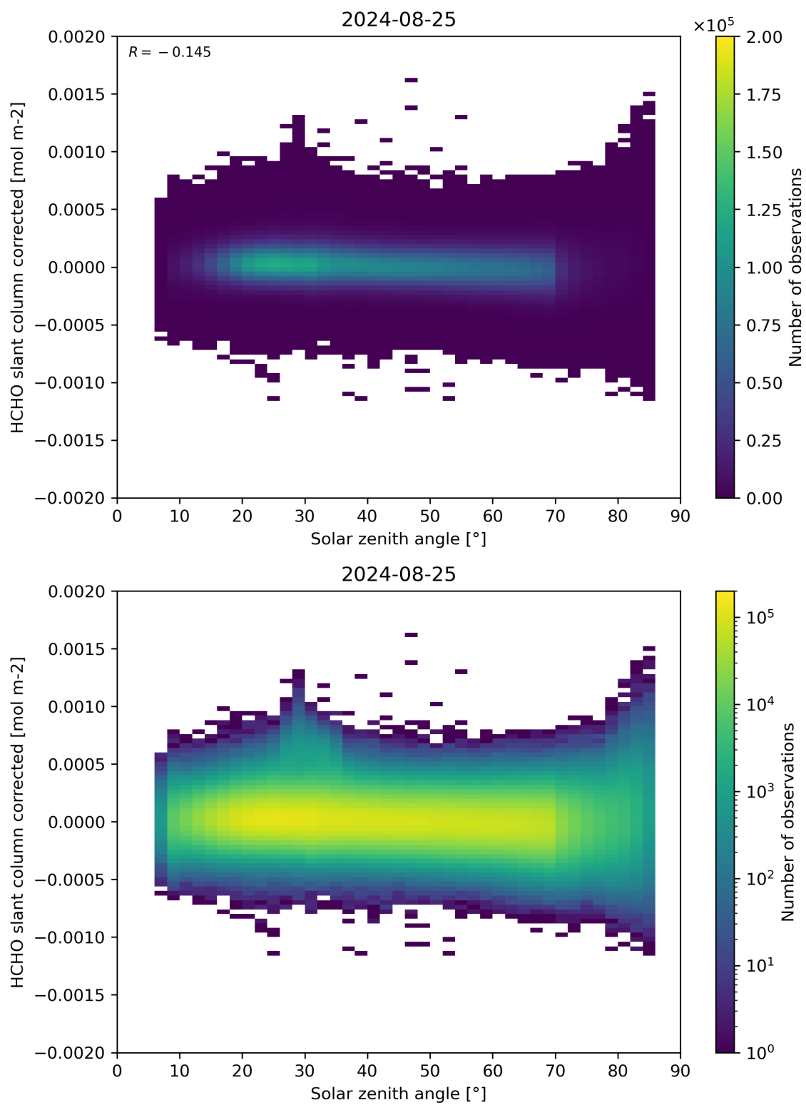
Figure 171: Scatter density plot of “Solar zenith angle” against “HCHO slant column corrected” for 2024-08-24 to 2024-08-26.
