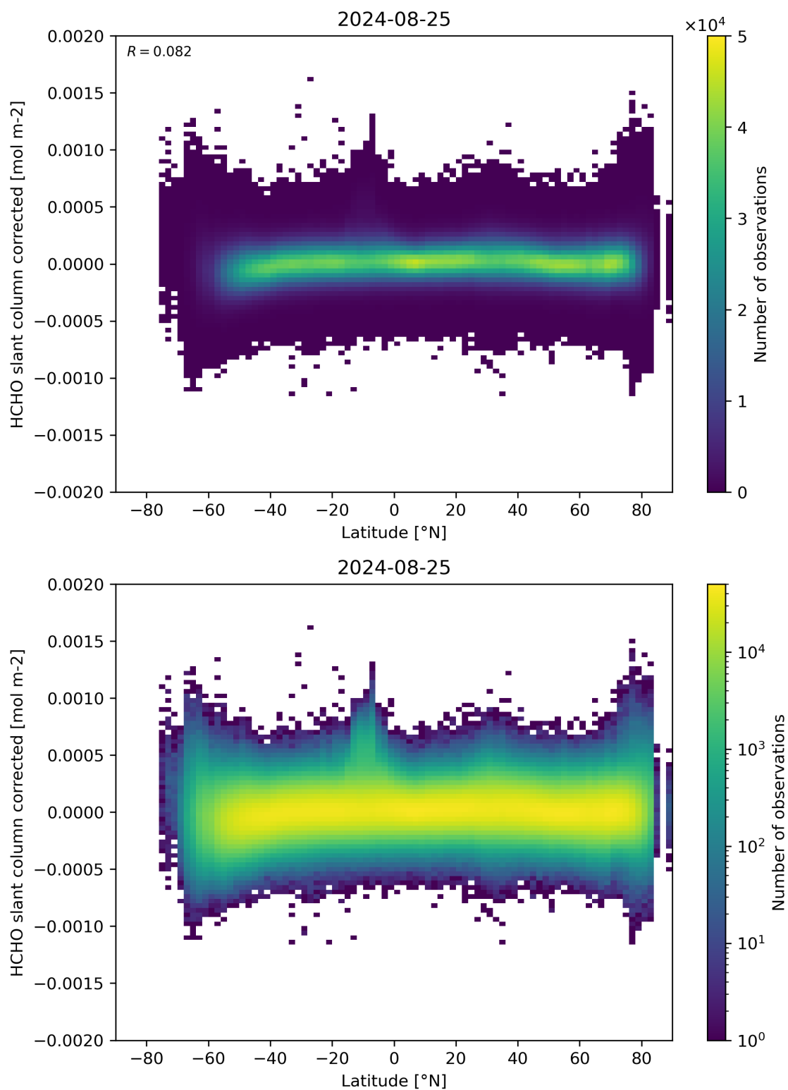
Figure 157: Scatter density plot of “Latitude” against “HCHO slant column corrected” for 2024-08-24 to 2024-08-26.
