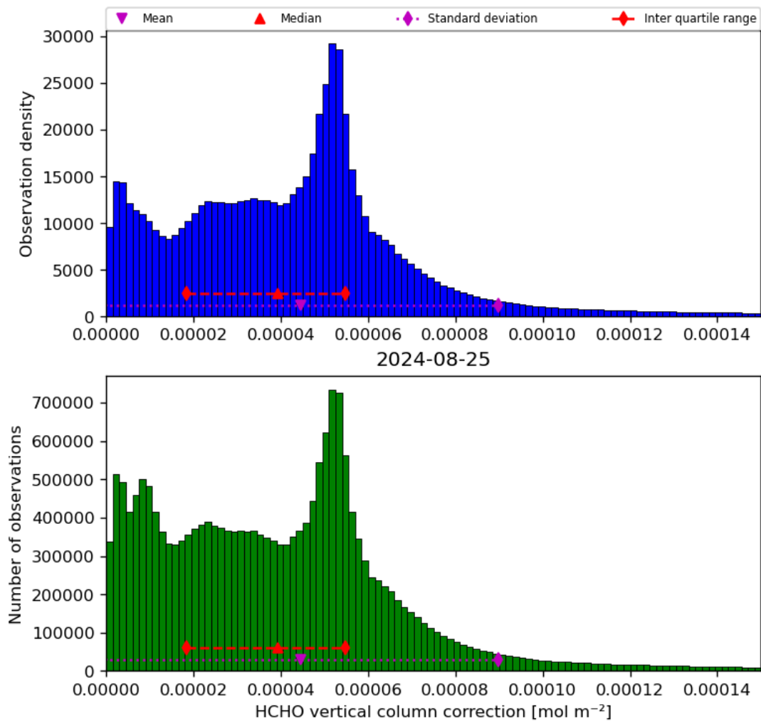
Figure 37: Histogram of “HCHO vertical column correction” for 2024-08-24 to 2024-08-26
