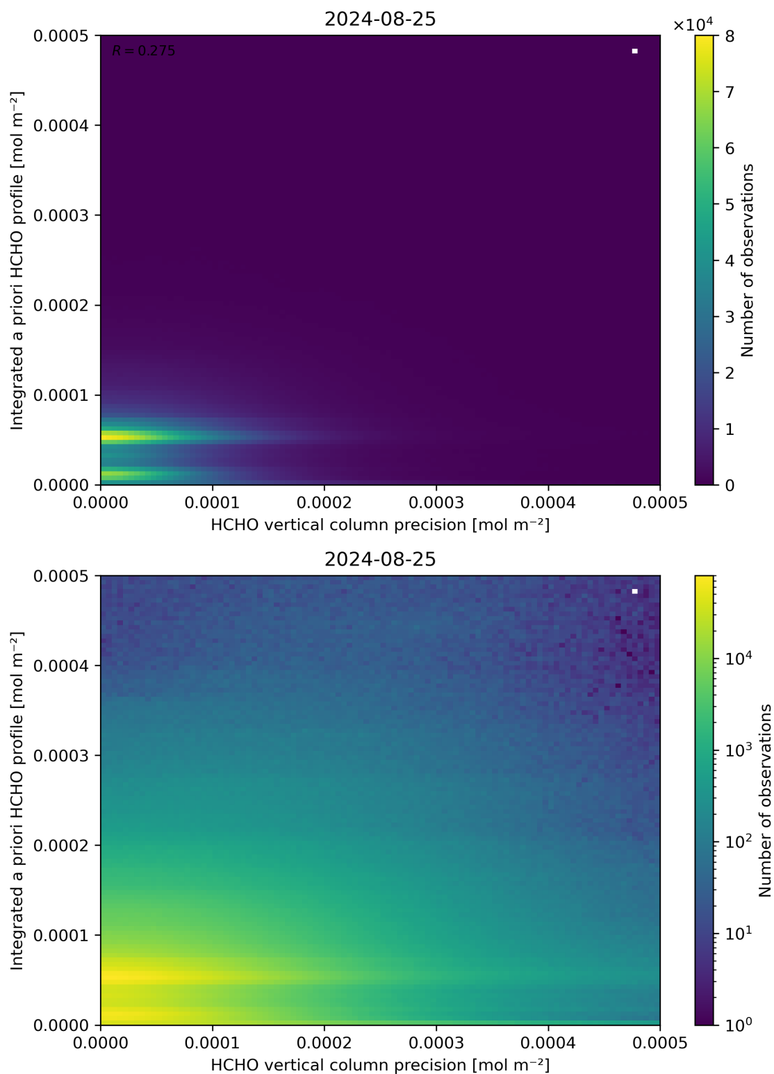
Figure 147: Scatter density plot of “HCHO vertical column precision” against “Integrated a priori HCHO profile” for 2024-08-24 to 2024-08-26.
