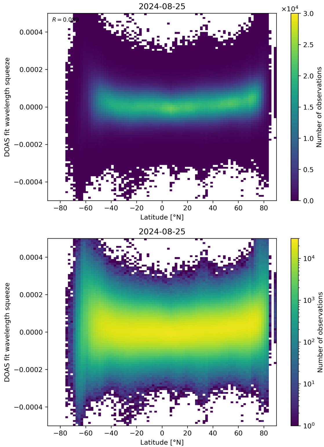
Figure 155: Scatter density plot of “Latitude” against “DOAS fit wavelength squeeze” for 2024-08-24 to 2024-08-26.
