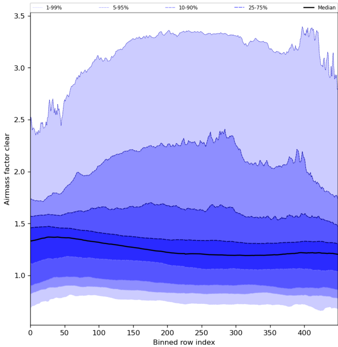
Figure 56: Along track statistics of “Air mass factor clear” for 2024-08-24 to 2024-08-26
