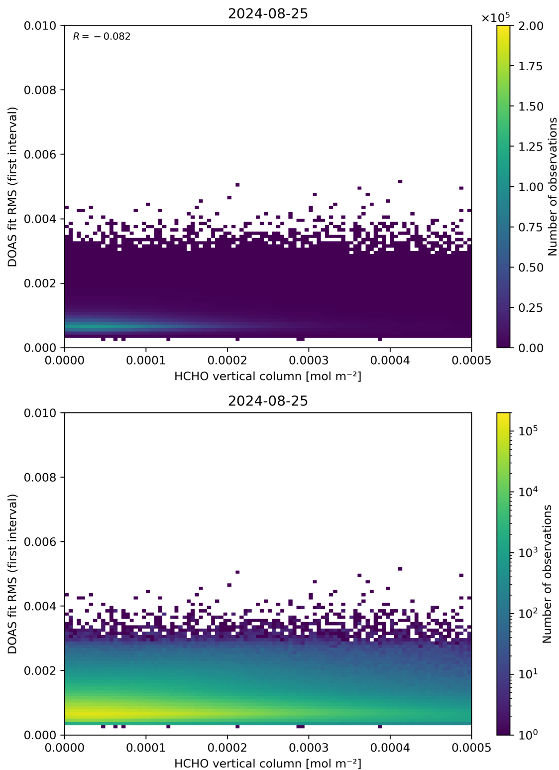
Figure 123: Scatter density plot of “HCHO vertical column” against “DOAS fit RMS (first interval)” for 2024-08-24 to 2024-08-26.
