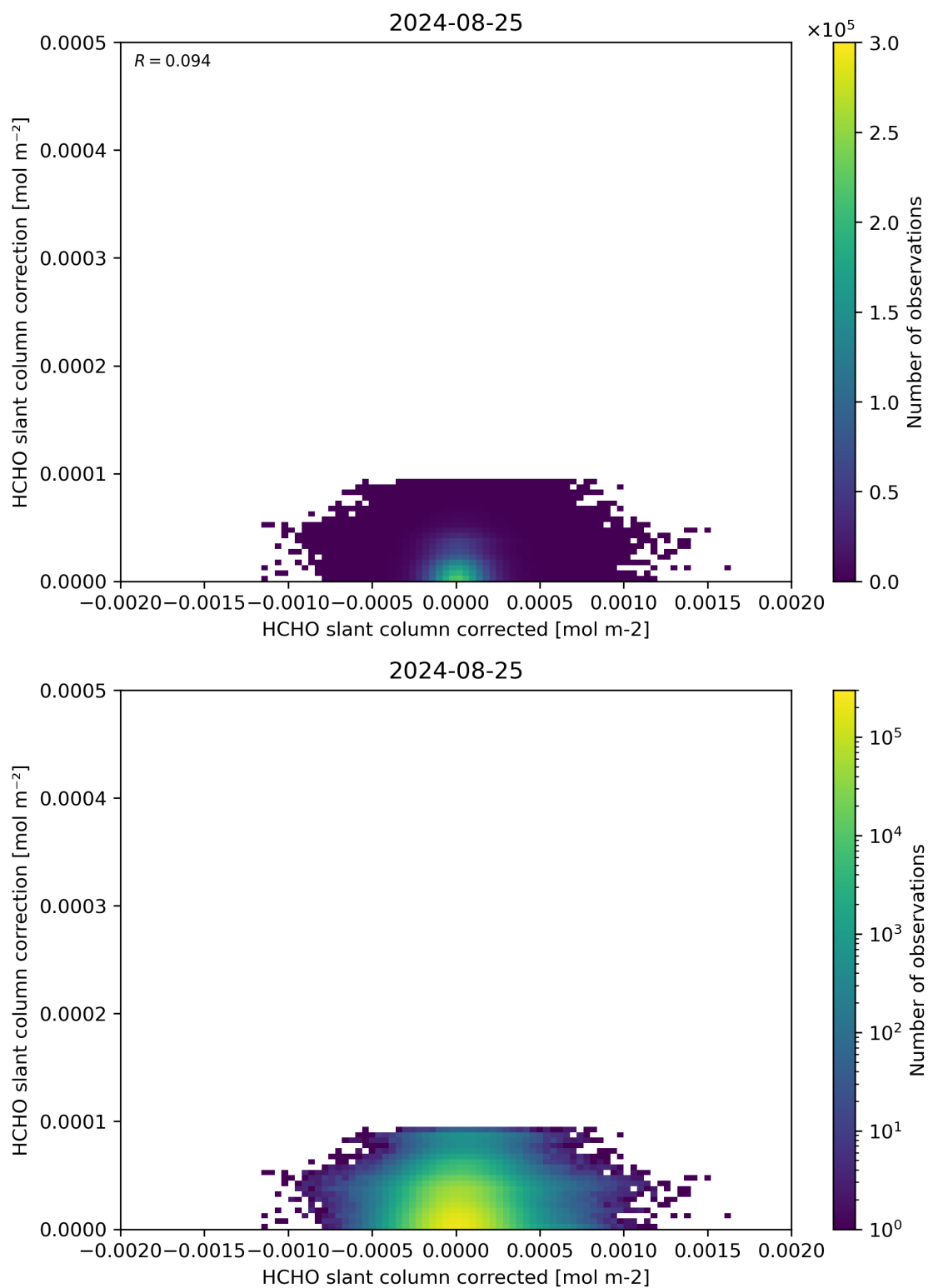
Figure 77: Scatter density plot of “HCHO slant column corrected” against “HCHO slant column correction” for 2024-08-24 to 2024-08-26.
