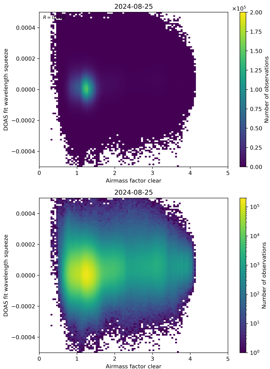
Figure 73: Scatter density plot of “Airmass factor clear” against “DOAS fit wavelength squeeze” for 2024-08-24 to 2024-08-26.
