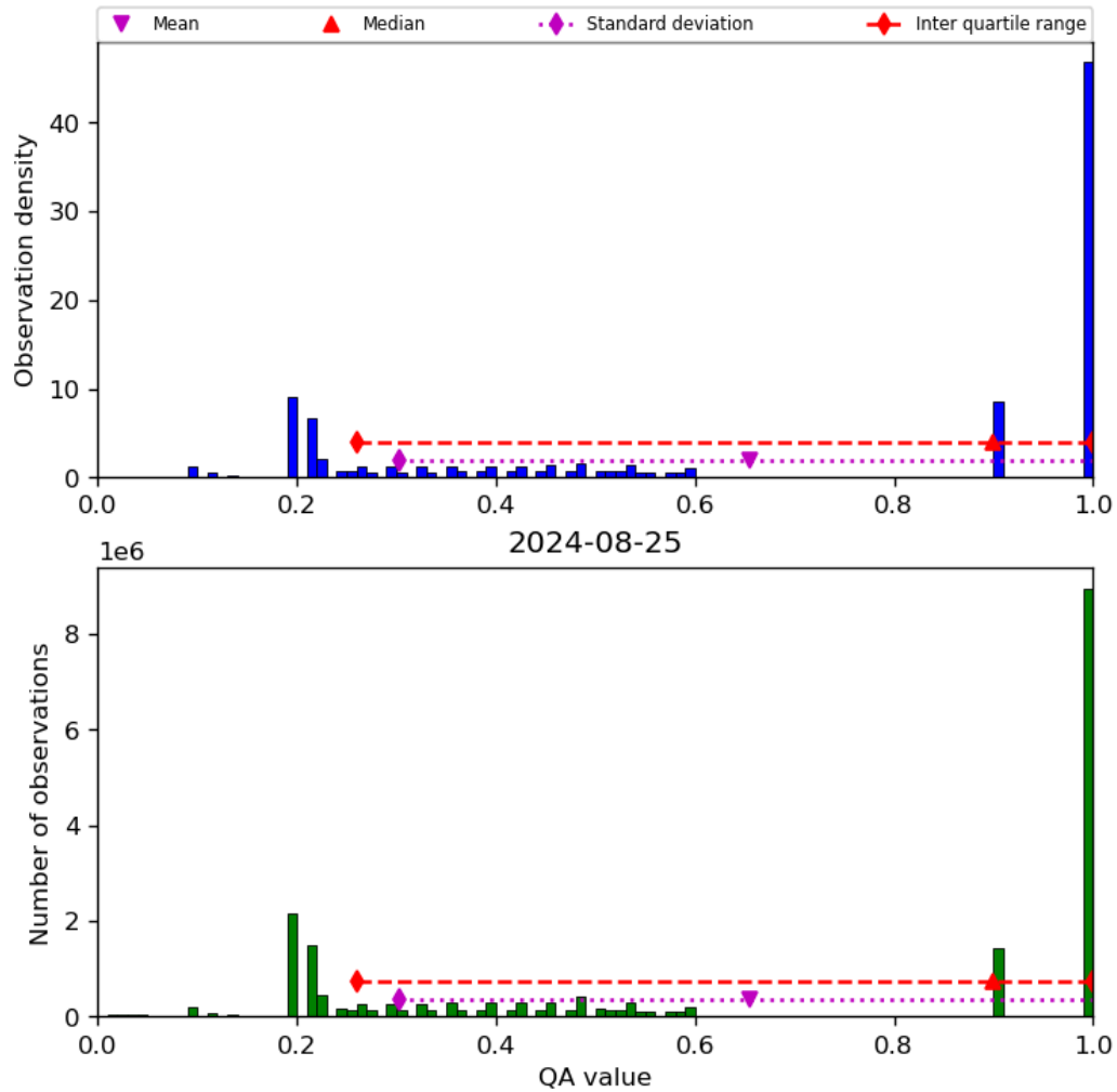
Figure 34: Histogram of “QA value” for 2024-08-24 to 2024-08-26
