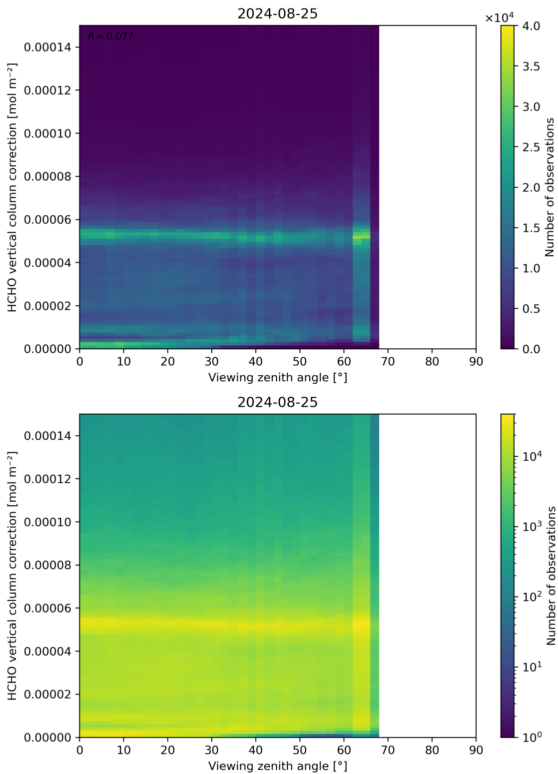
Figure 193: Scatter density plot of “Viewing zenith angle” against “HCHO vertical column correction” for 2024-08-24 to 2024-08-26.
