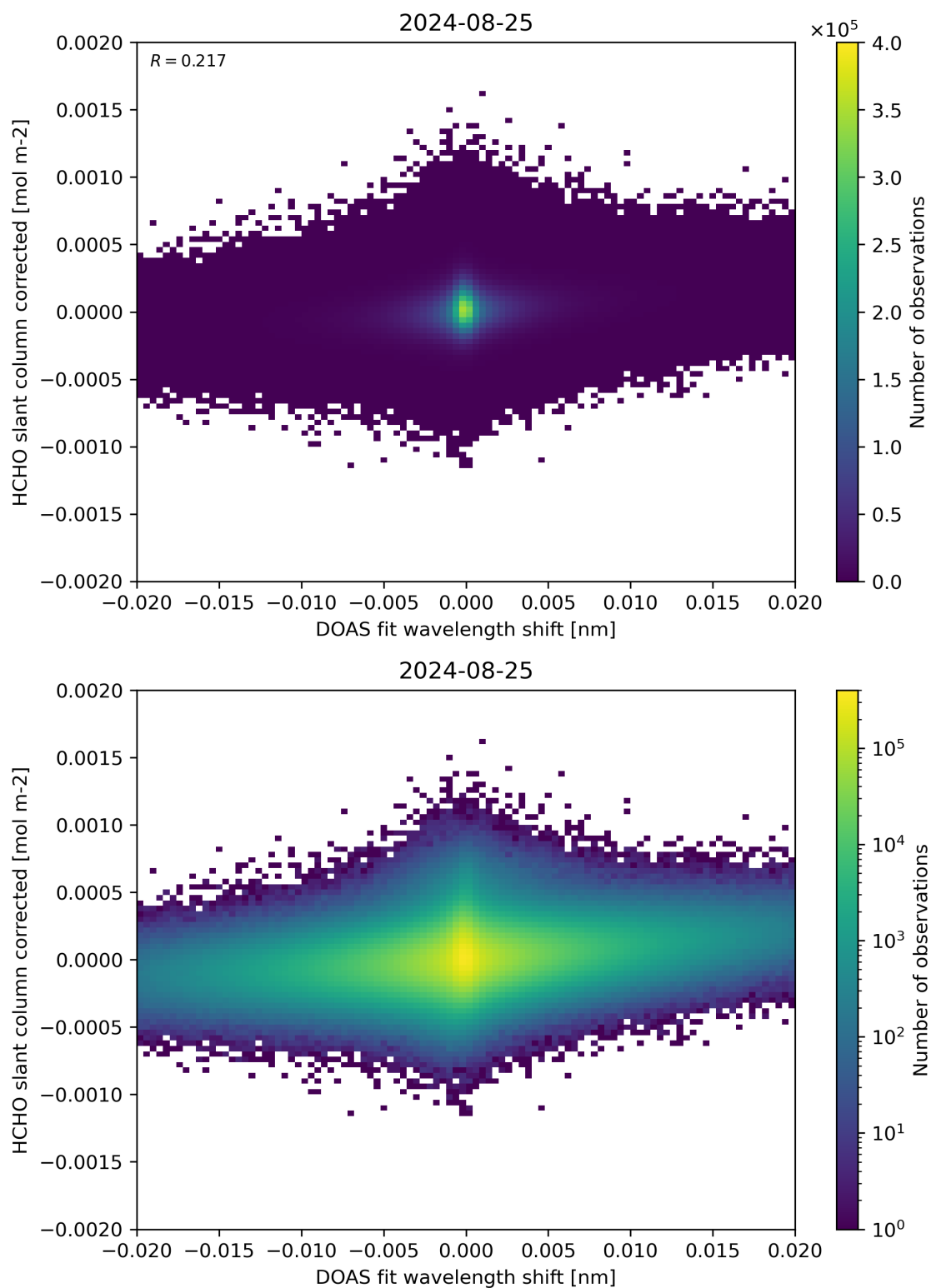
Figure 66: Scatter density plot of “DOAS fit wavelength shift” against “HCHO slant column corrected” for 2024-08-24 to 2024-08-26.
