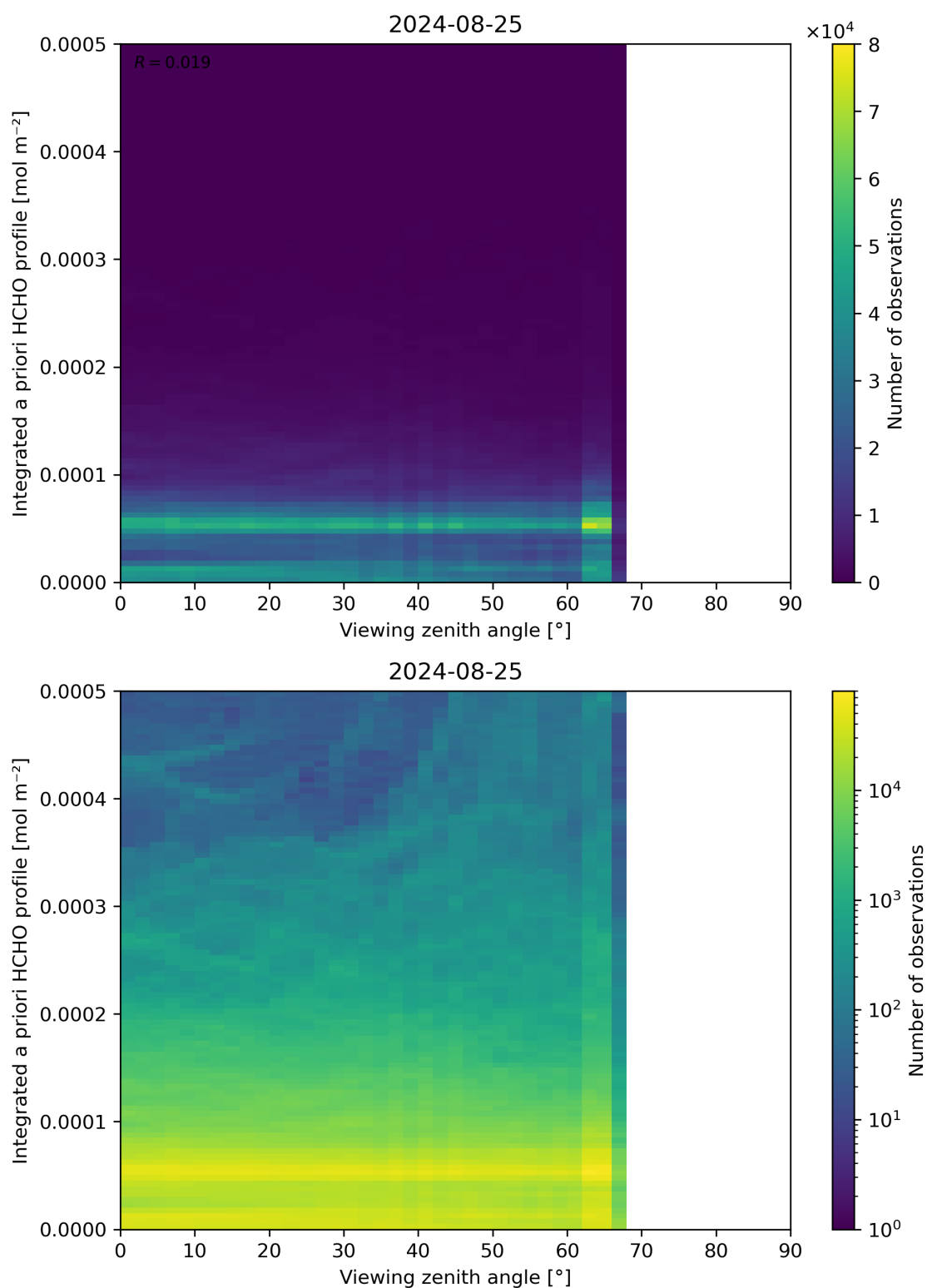
Figure 195: Scatter density plot of “Viewing zenith angle” against “Integrated a priori HCHO profile” for 2024-08-24 to 2024-08-26.
