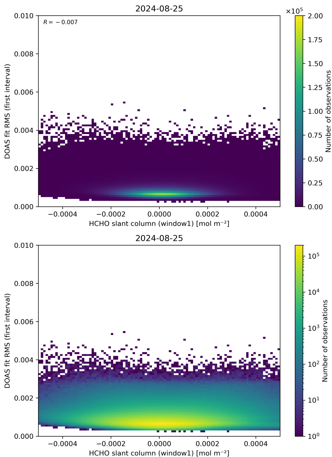
Figure 78: Scatter density plot of “HCHO slant column (window1)” against “DOAS fit RMS (first interval)” for 2024-08-24 to 2024-08-26.
