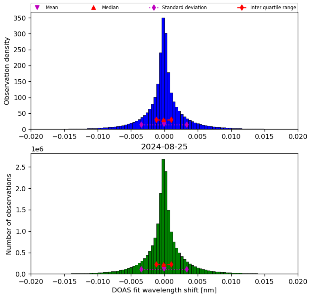
Figure 44: Histogram of “DOAS fit wavelength shift” for 2024-08-24 to 2024-08-26
