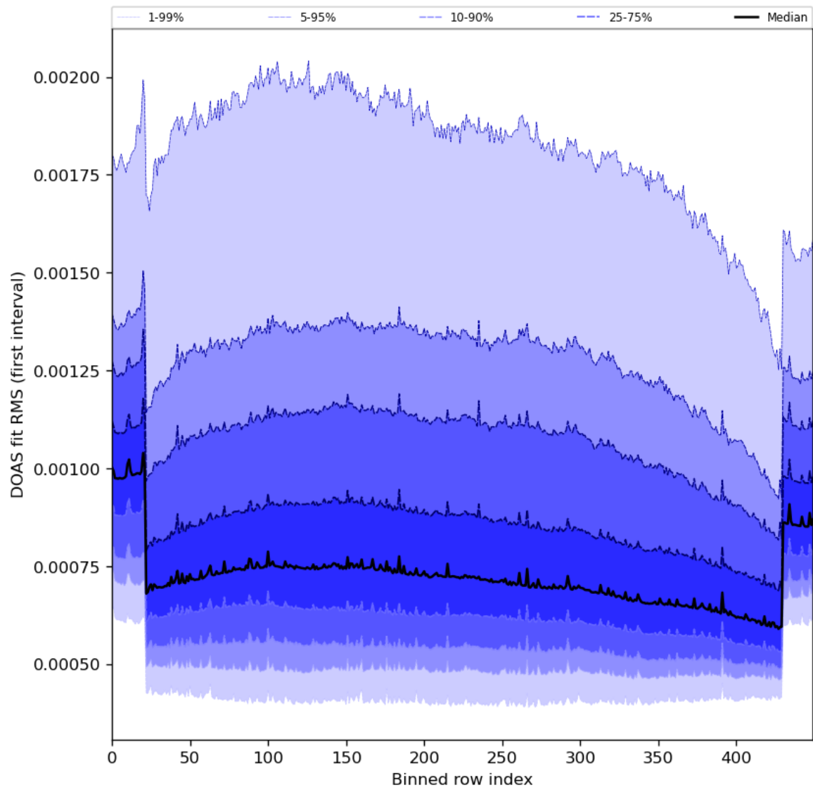
Figure 60: Along track statistics of “DOAS fit RMS (first interval)” for 2024-08-24 to 2024-08-26
