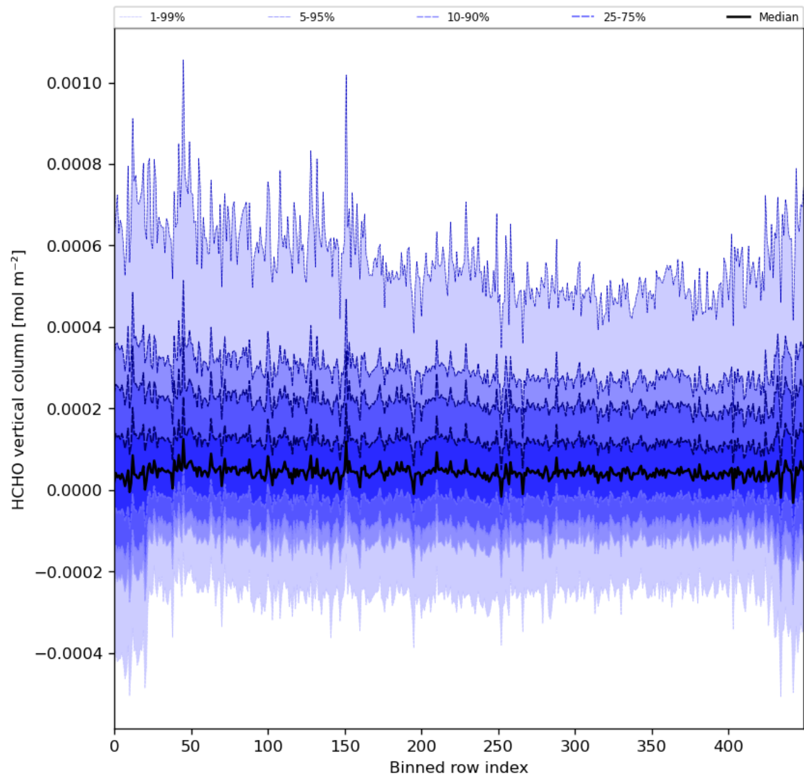
Figure 49: Along track statistics of “HCHO vertical column” for 2024-08-24 to 2024-08-26
