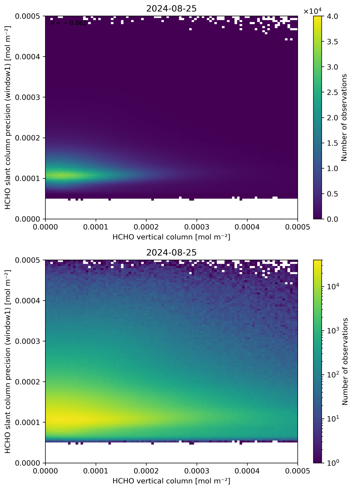
Figure 130: Scatter density plot of “HCHO vertical column” against “HCHO slant column precision (window1)” for 2024-08-24 to 2024-08-26.
