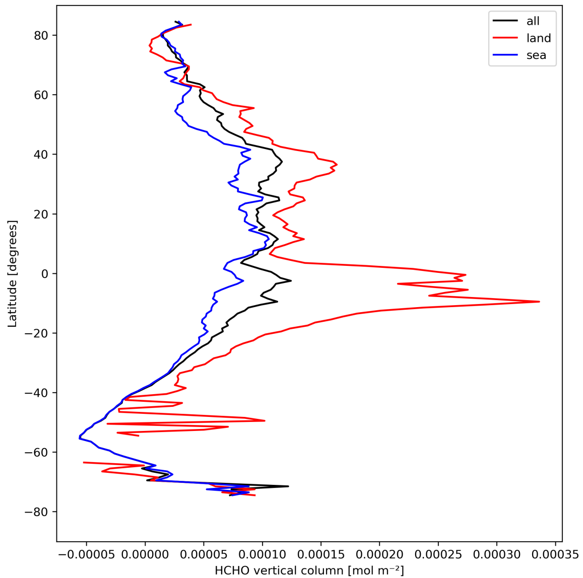
Figure 21: Zonal average of “HCHO vertical column” for 2024-08-24 to 2024-08-26.
