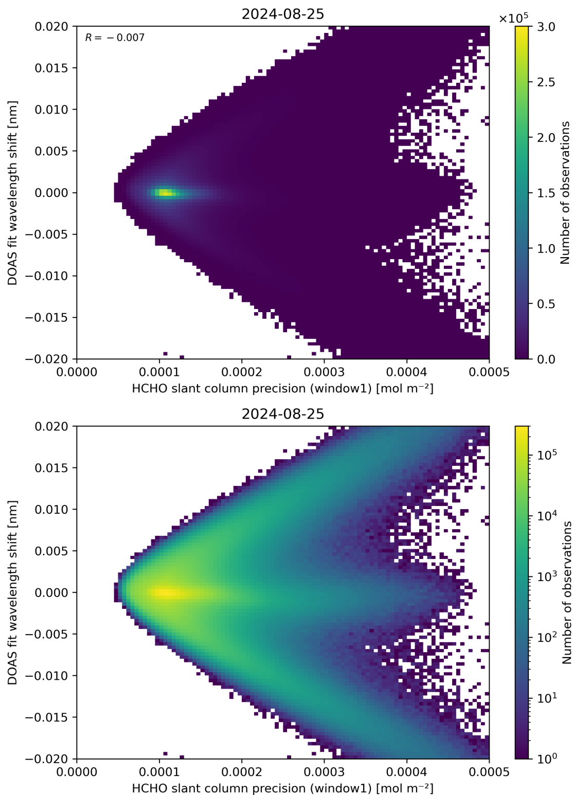
Figure 89: Scatter density plot of “HCHO slant column precision (window1)” against “DOAS fit wavelength shift” for 2024-08-24 to 2024-08-26.
