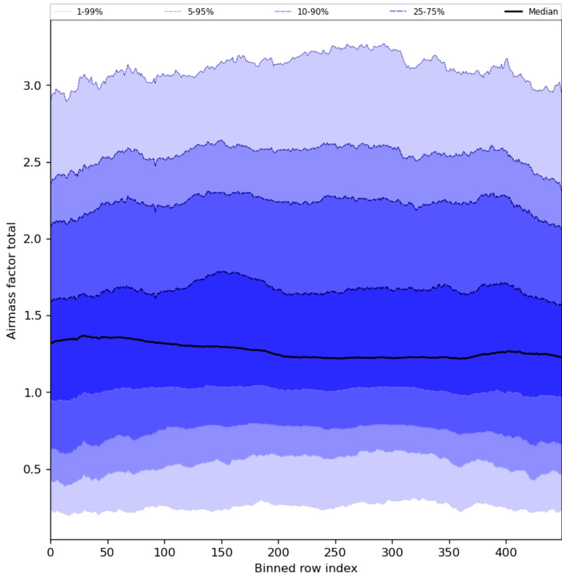
Figure 54: Along track statistics of “Airmass factor total” for 2024-08-24 to 2024-08-26
