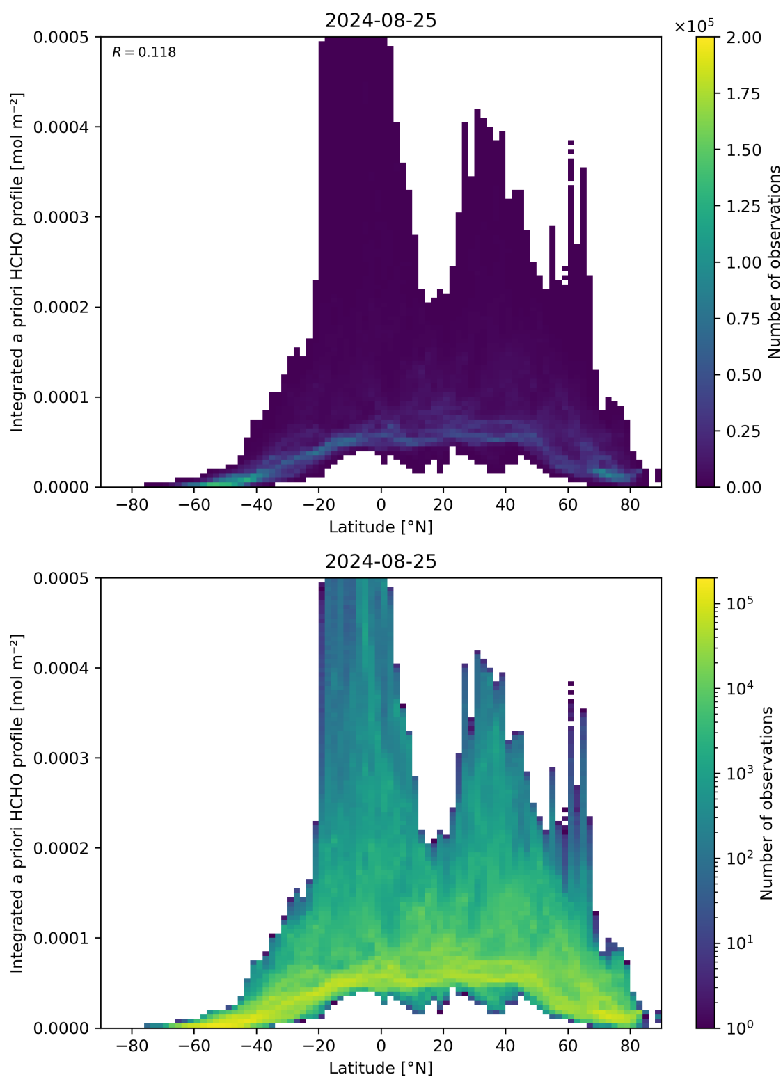
Figure 166: Scatter density plot of “Latitude” against “Integrated a priori HCHO profile” for 2024-08-24 to 2024-08-26.
