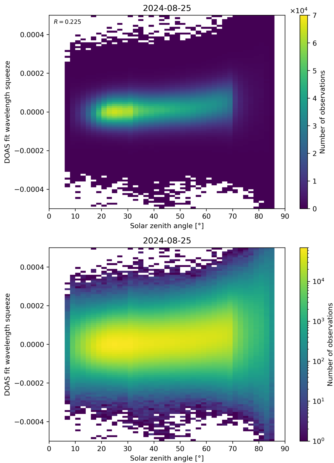
Figure 169: Scatter density plot of “Solar zenith angle” against “DOAS fit wavelength squeeze” for 2024-08-24 to 2024-08-26.
