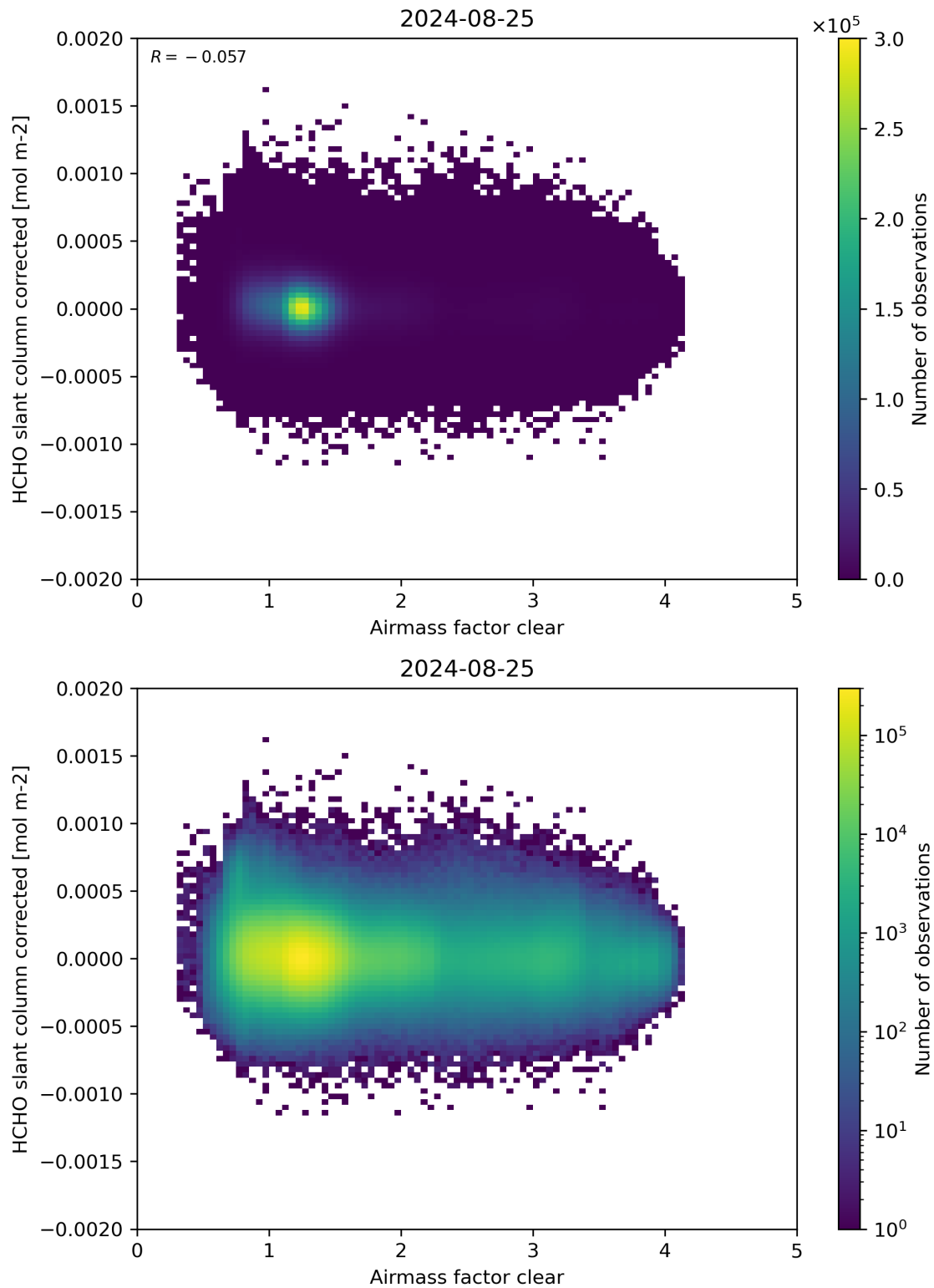
Figure 74: Scatter density plot of “Airmass factor clear” against “HCHO slant column corrected” for 2024-08-24 to 2024-08-26.
