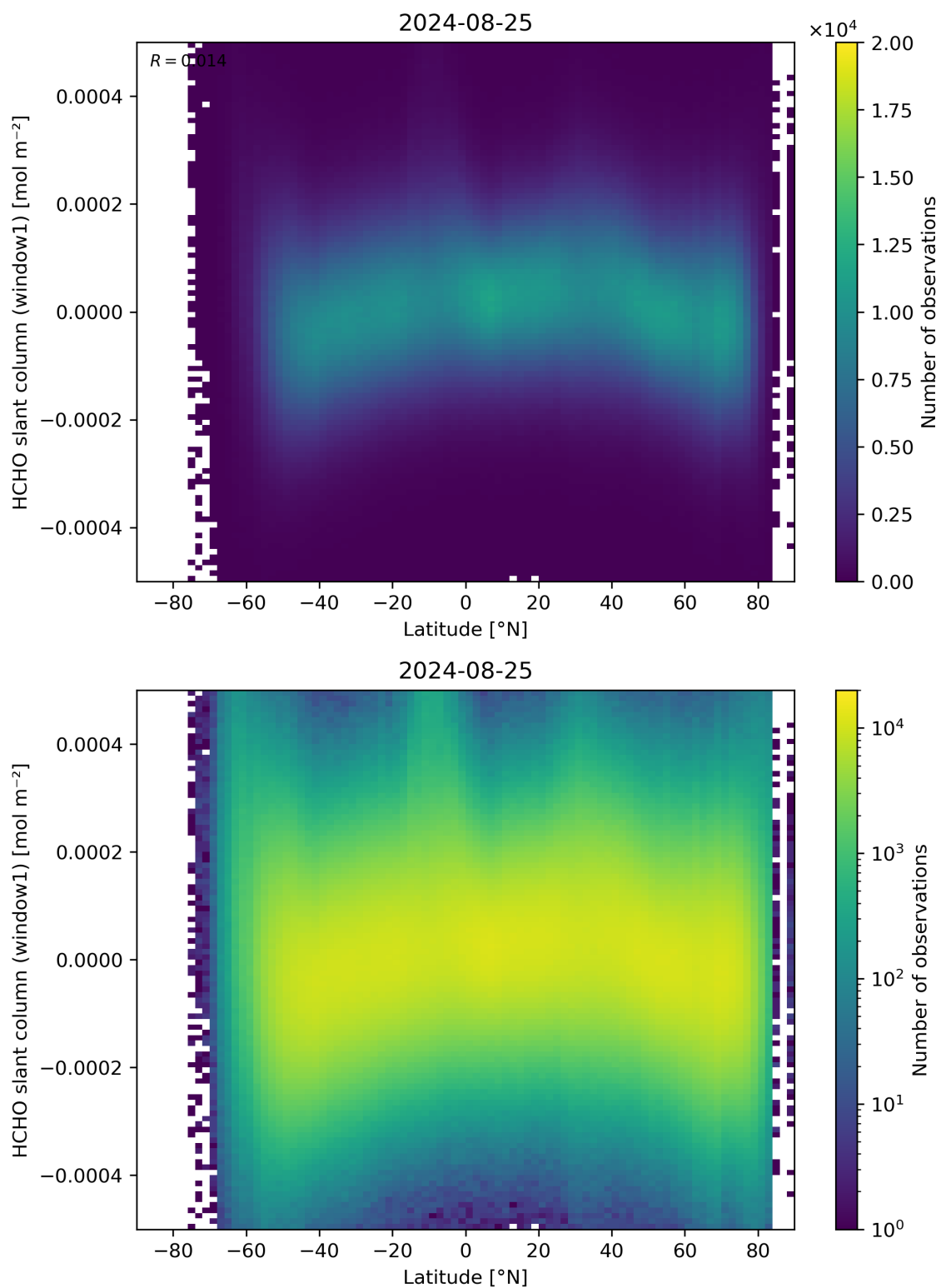
Figure 159: Scatter density plot of “Latitude” against “HCHO slant column (window1)” for 2024-08-24 to 2024-08-26.
