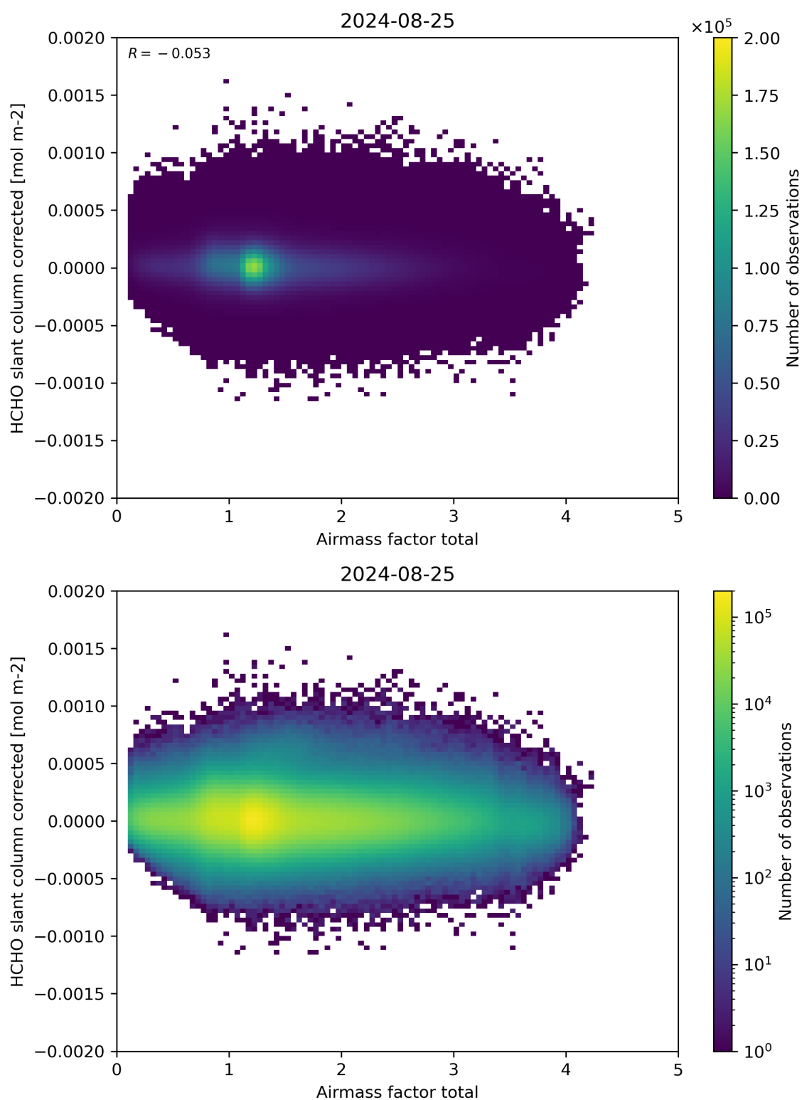
Figure 101: Scatter density plot of “Airmass factor total” against “HCHO slant column corrected” for 2024-08-24 to 2024-08-26.
