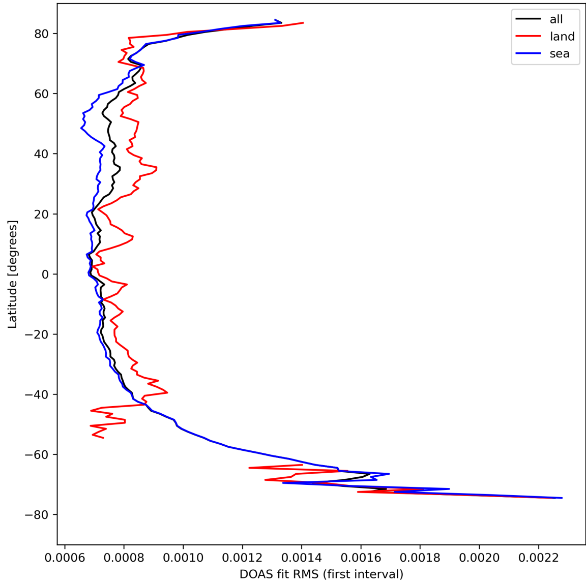
Figure 32: Zonal average of “DOAS fit RMS (first interval)” for 2024-08-24 to 2024-08-26.
