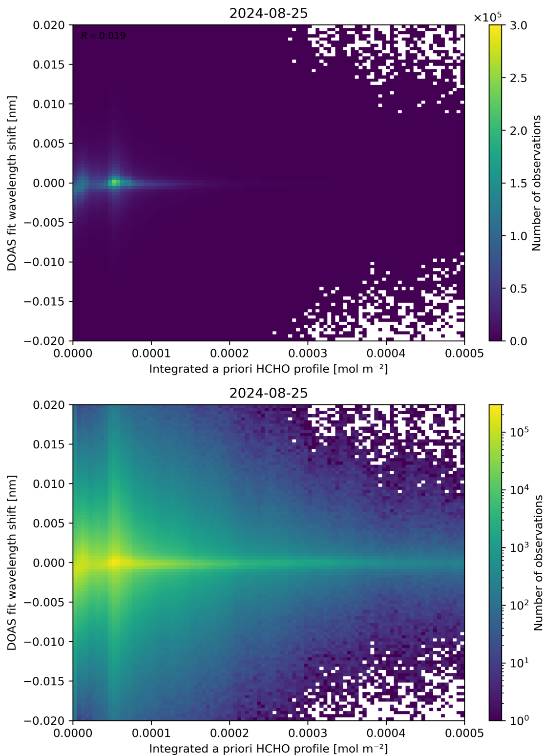
Figure 149: Scatter density plot of “Integrated a priori HCHO profile” against “DOAS fit wavelength shift” for 2024-08-24 to 2024-08-26.
