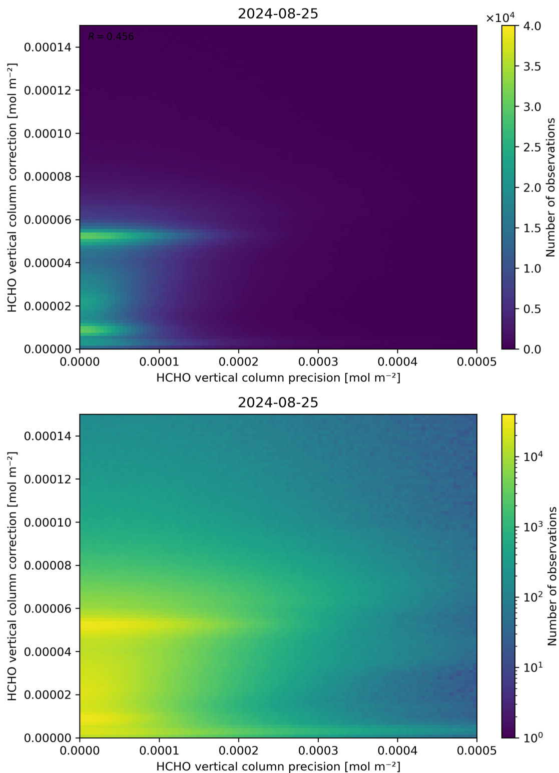
Figure 146: Scatter density plot of “HCHO vertical column precision” against “HCHO vertical column correction” for 2024-08-24 to 2024-08-26.
