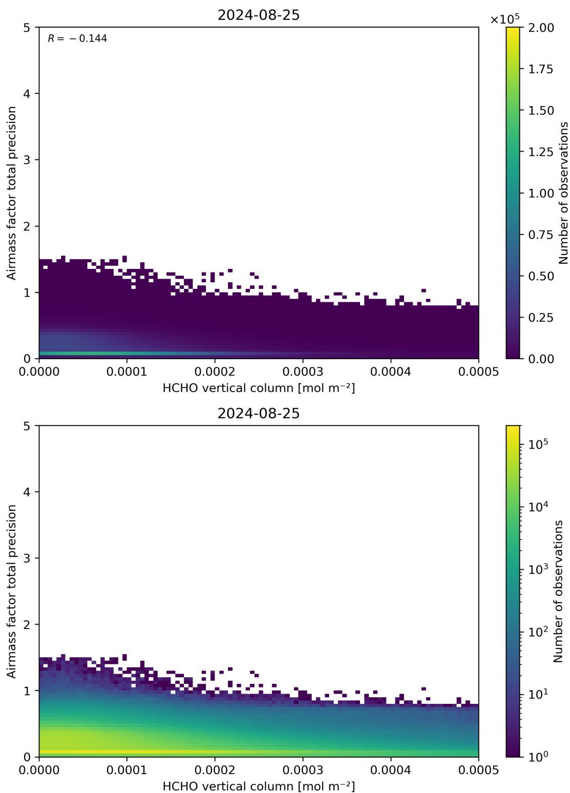
Figure 132: Scatter density plot of “HCHO vertical column” against “Airmass factor total precision” for 2024-08-24 to 2024-08-26.
