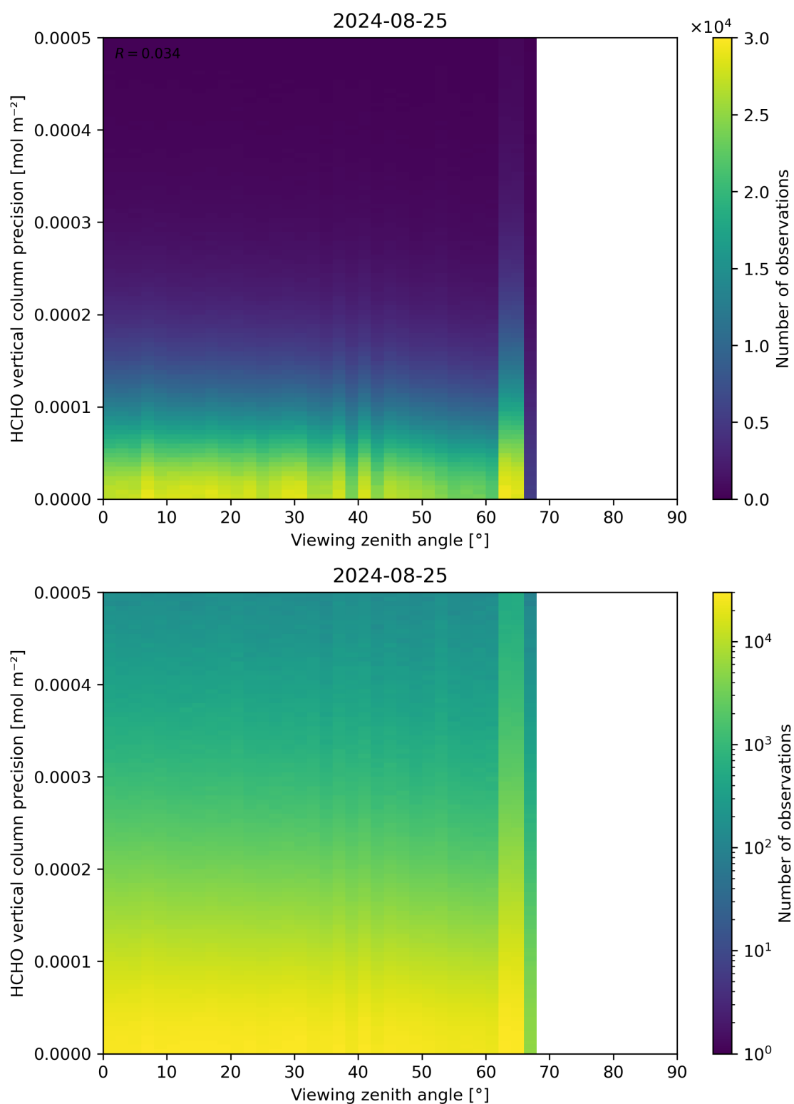
Figure 194: Scatter density plot of “Viewing zenith angle” against “HCHO vertical column precision” for 2024-08-24 to 2024-08-26.
