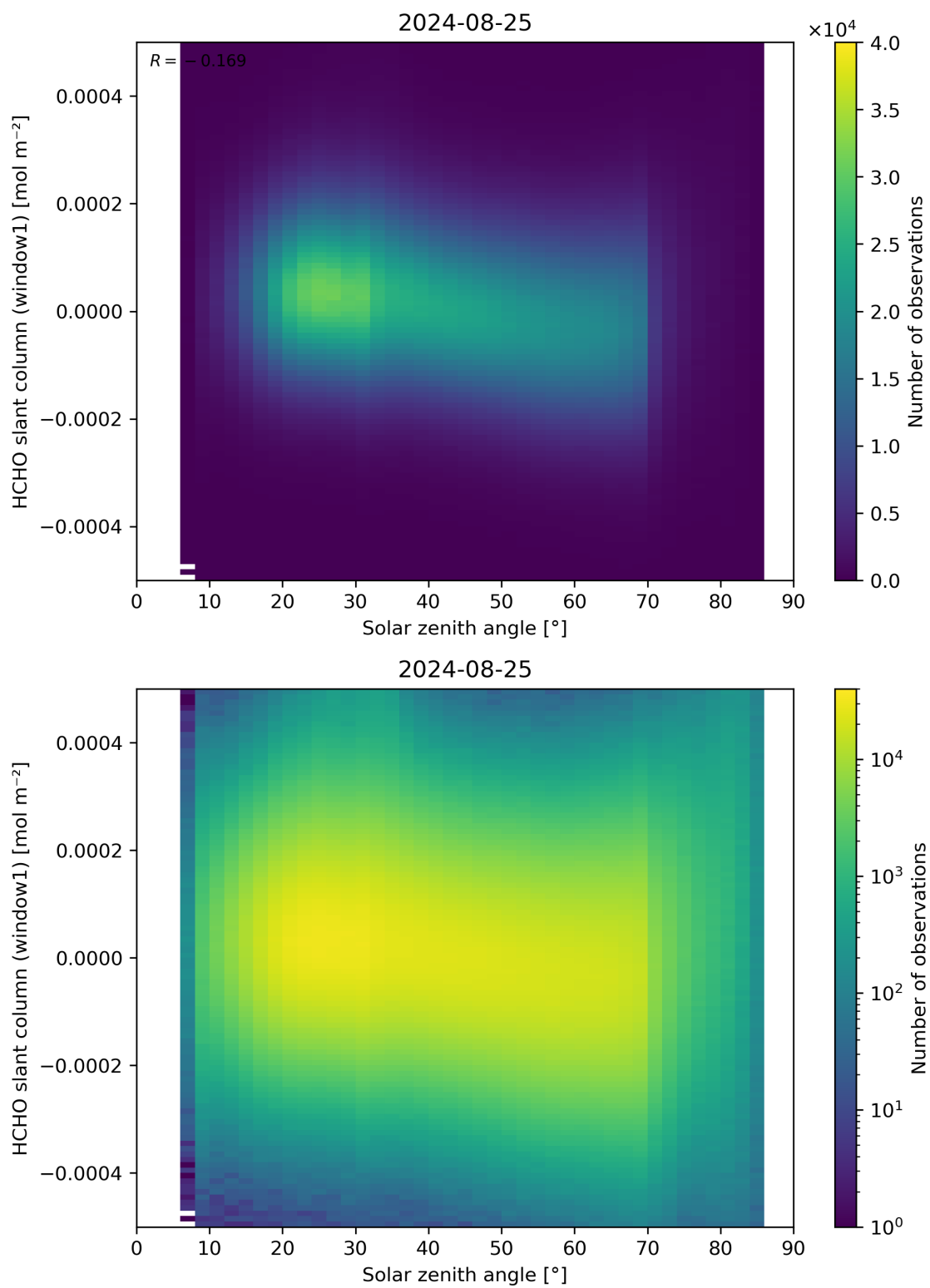
Figure 173: Scatter density plot of “Solar zenith angle” against “HCHO slant column (window1)” for 2024-08-24 to 2024-08-26.
