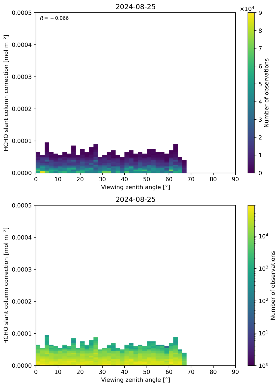
Figure 187: Scatter density plot of “Viewing zenith angle” against “HCHO slant column correction” for 2024-08-24 to 2024-08-26.
