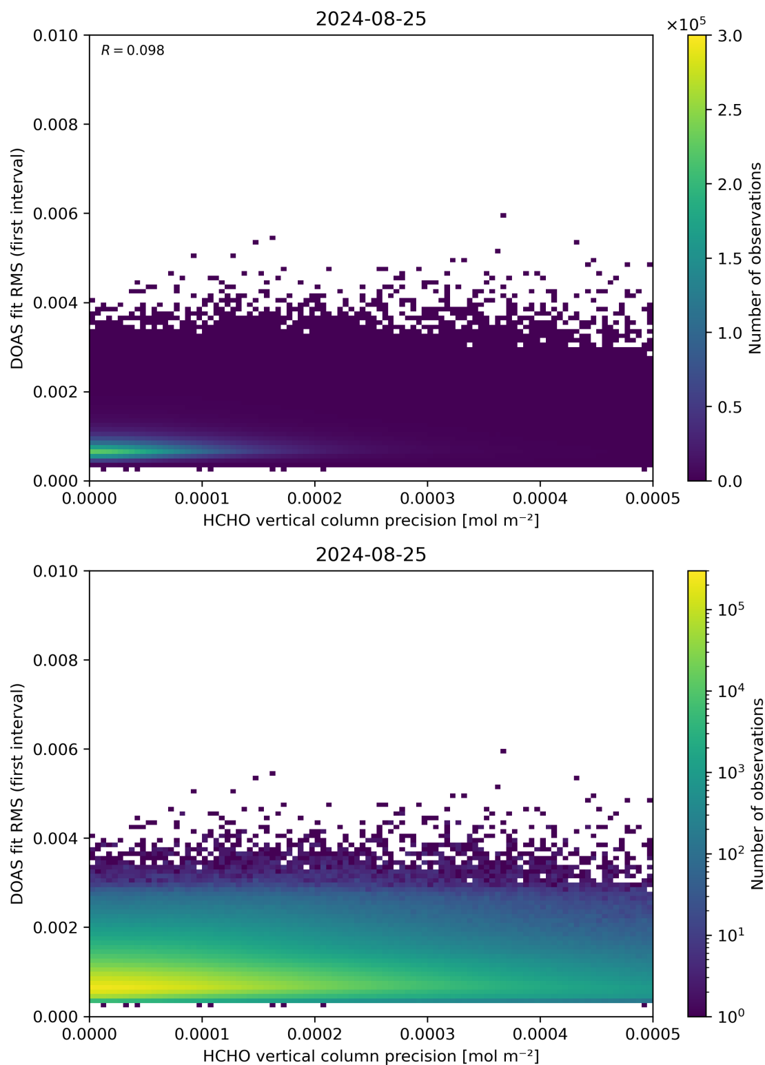
Figure 136: Scatter density plot of “HCHO vertical column precision” against “DOAS fit RMS (first interval)” for 2024-08-24 to 2024-08-26.
