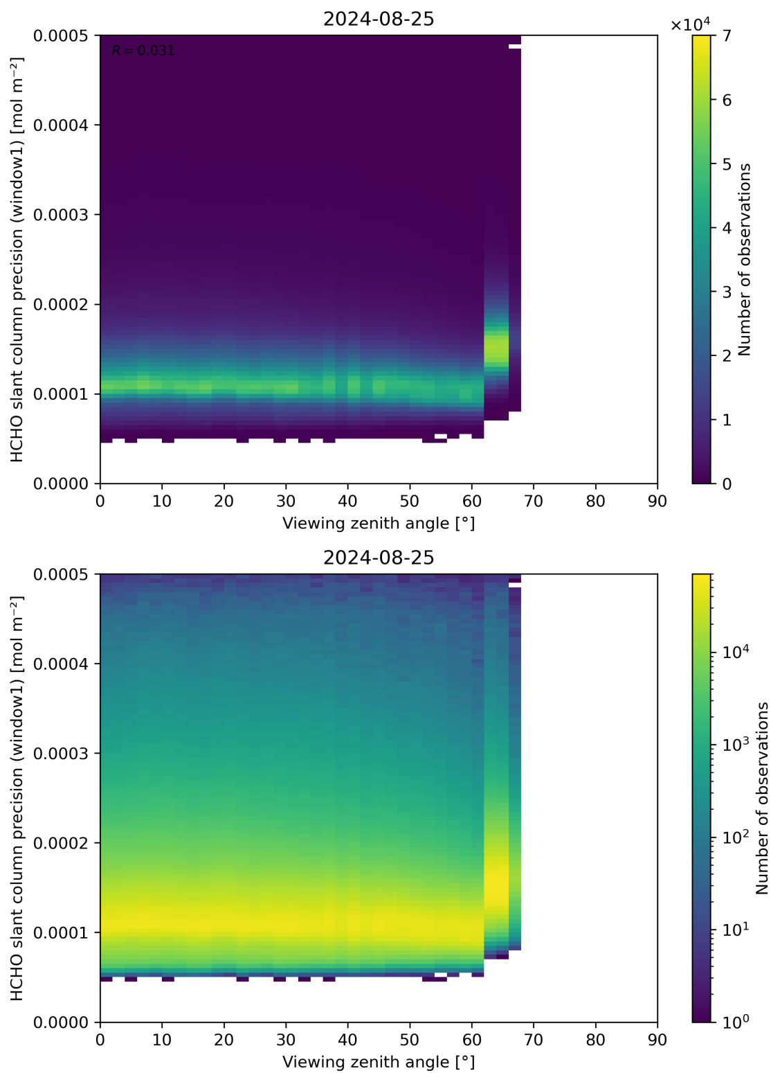
Figure 189: Scatter density plot of “Viewing zenith angle” against “HCHO slant column precision (window1)” for 2024-08-24 to 2024-08-26.
