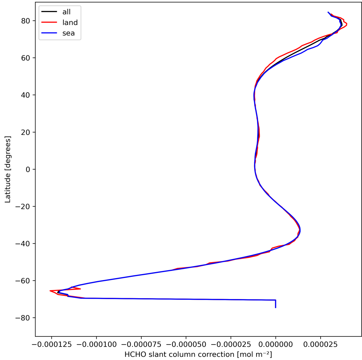
Figure 33: Zonal average of “HCHO slant column correction” for 2024-08-24 to 2024-08-26.
