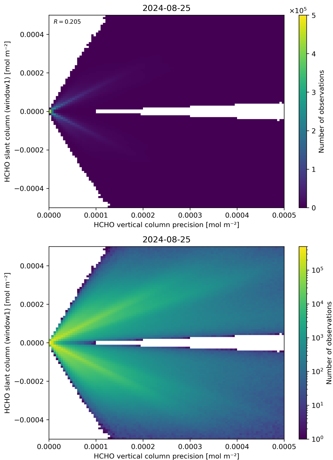
Figure 142: Scatter density plot of “HCHO vertical column precision” against “HCHO slant column (window1)” for 2024-08-24 to 2024-08-26.
