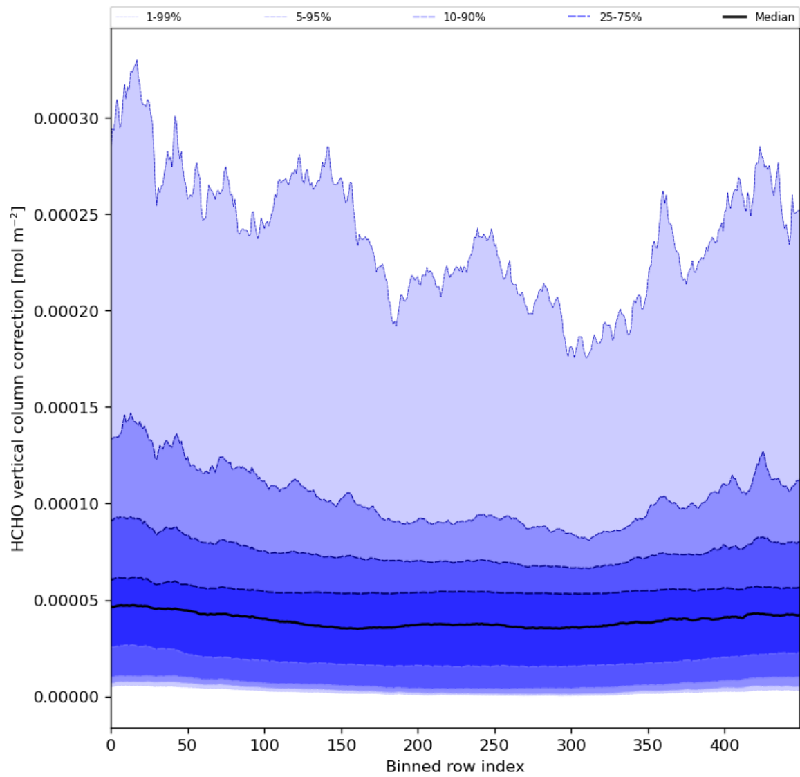
Figure 51: Along track statistics of “HCHO vertical column correction” for 2024-08-24 to 2024-08-26
