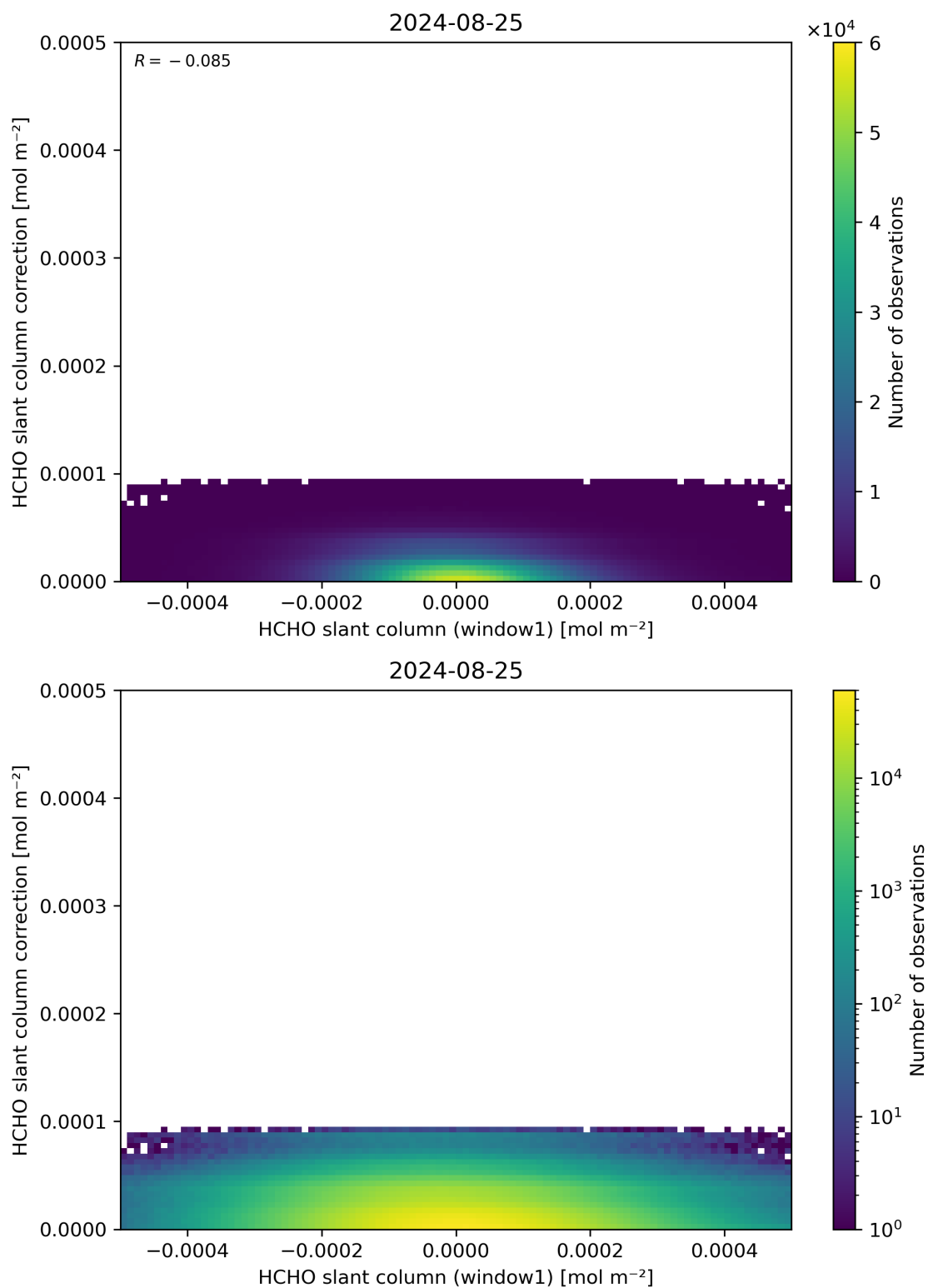
Figure 83: Scatter density plot of “HCHO slant column (window1)” against “HCHO slant column correction” for 2024-08-24 to 2024-08-26.
