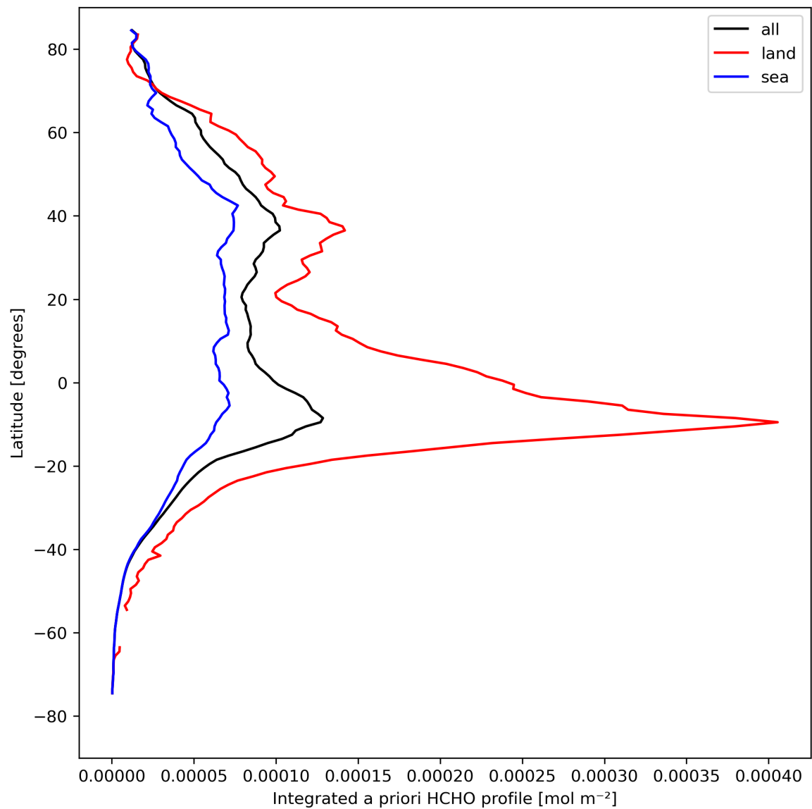
Figure 29: Zonal average of “Integrated a priori HCHO profile” for 2024-08-24 to 2024-08-26.
