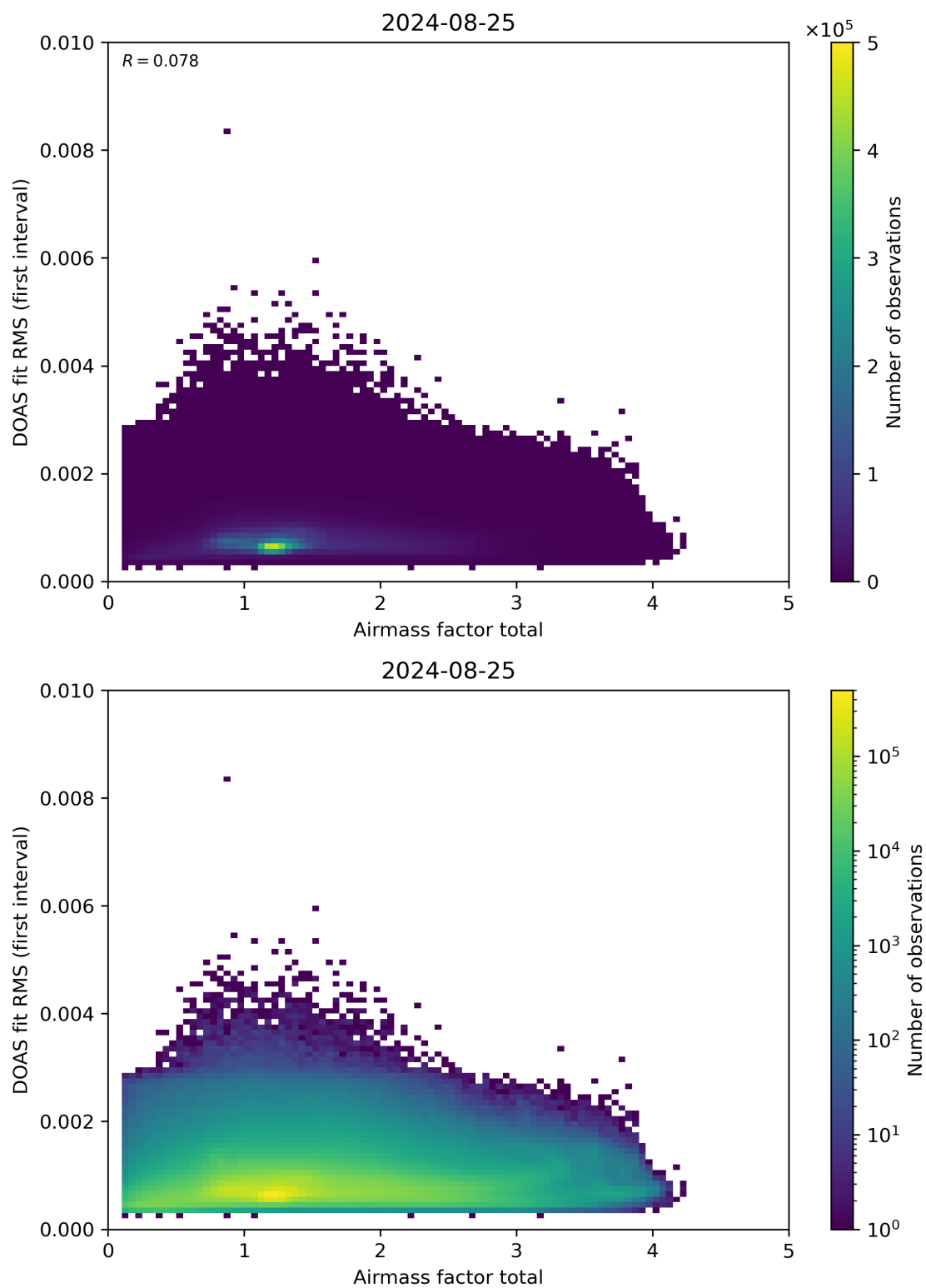
Figure 97: Scatter density plot of “Airmass factor total” against “DOAS fit RMS (first interval)” for 2024-08-24 to 2024-08-26.
