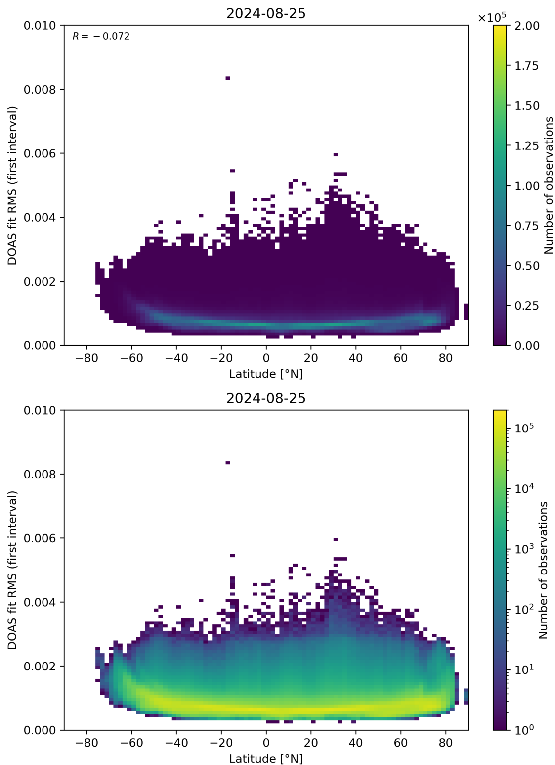
Figure 153: Scatter density plot of “Latitude” against “DOAS fit RMS (first interval)” for 2024-08-24 to 2024-08-26.
