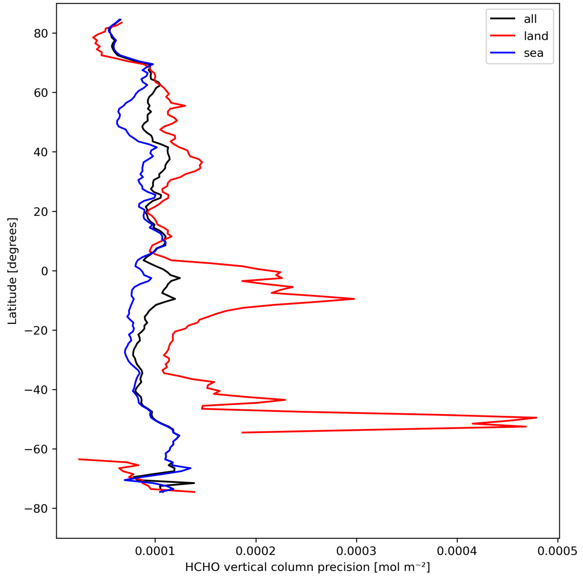
Figure 22: Zonal average of "HCHO vertical column precision" for 2024-08-24 to 2024-08-26.
