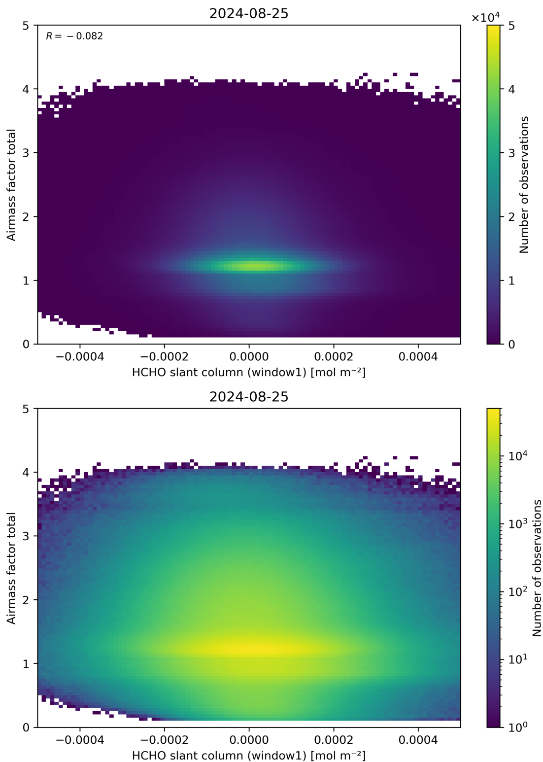
Figure 85: Scatter density plot of “HCHO slant column (window1)” against “Airmass factor total” for 2024-08-24 to 2024-08-26.
