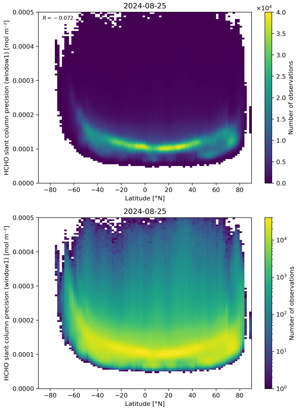
Figure 160: Scatter density plot of “Latitude” against “HCHO slant column precision (window1)” for 2024-08-24 to 2024-08-26.
