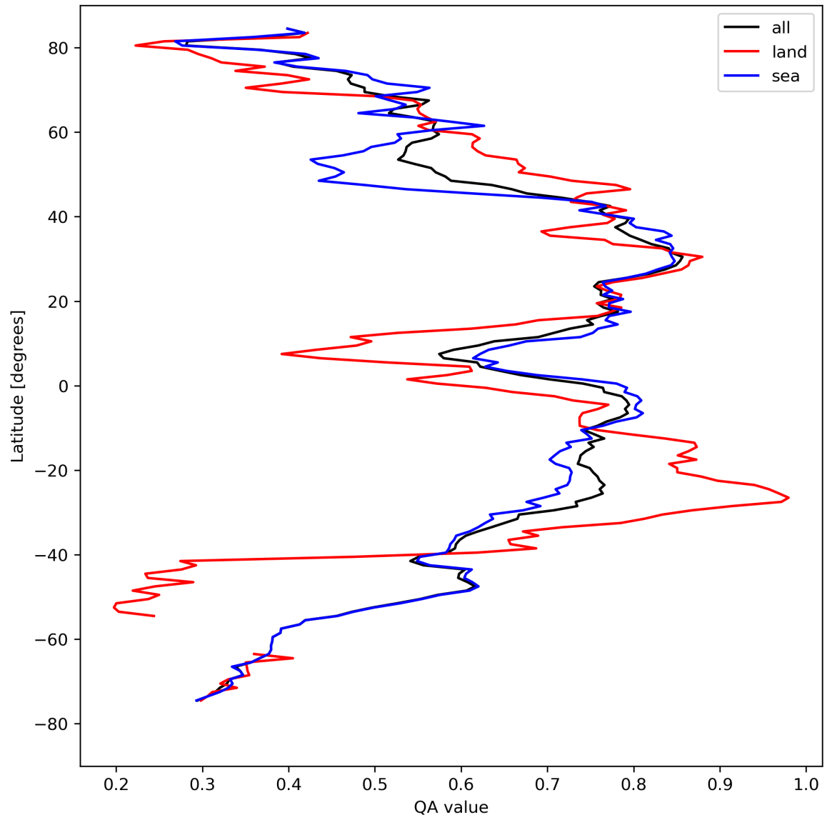
Figure 20: Zonal average of “QA value” for 2024-08-24 to 2024-08-26.
