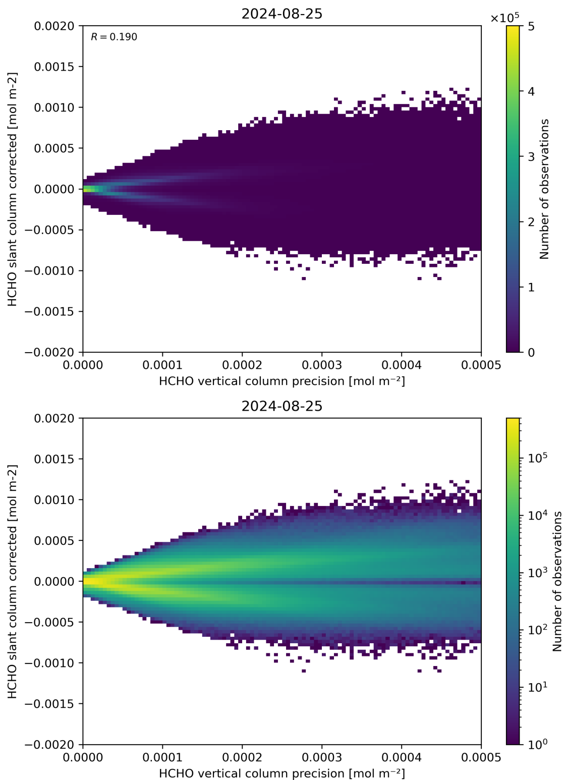
Figure 140: Scatter density plot of “HCHO vertical column precision” against “HCHO slant column corrected” for 2024-08-24 to 2024-08-26.
