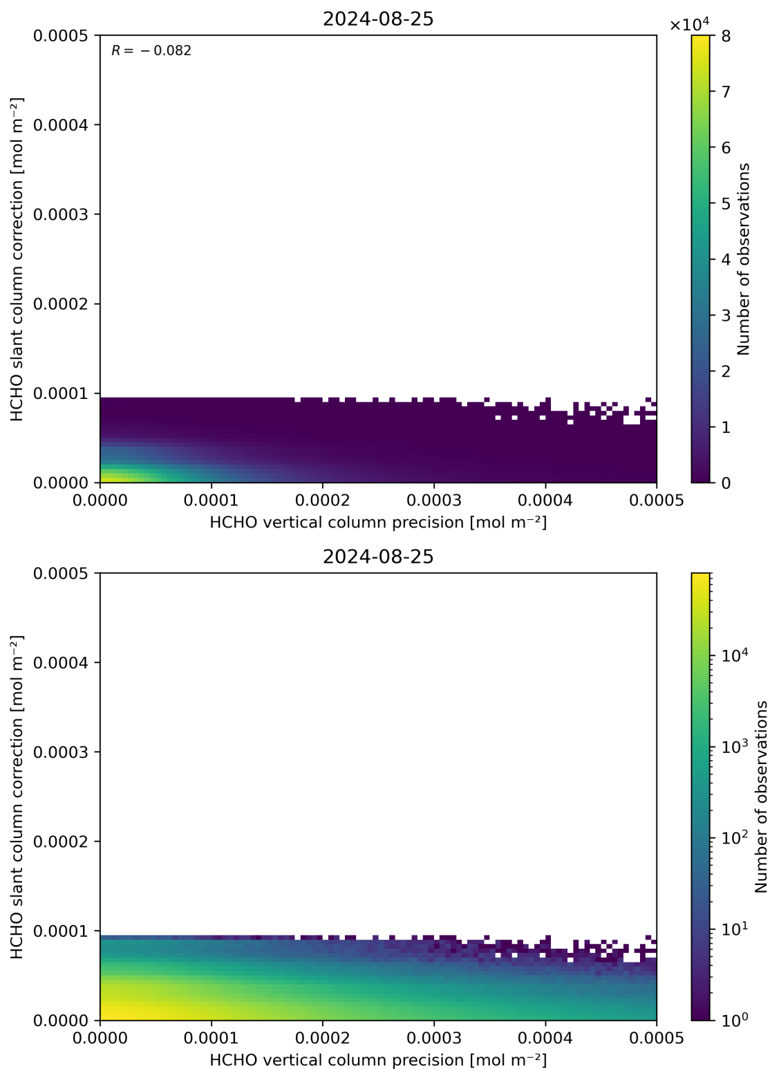
Figure 141: Scatter density plot of “HCHO vertical column precision” against “HCHO slant column correction” for 2024-08-24 to 2024-08-26.
