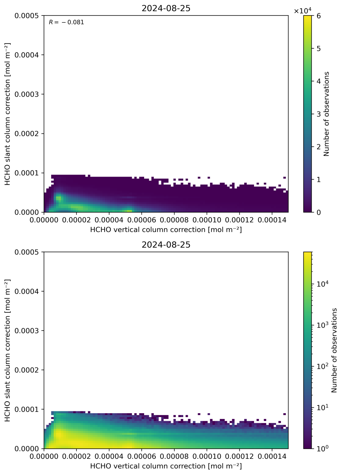
Figure 117: Scatter density plot of “HCHO vertical column correction” against “HCHO slant column correction” for 2024-08-24 to 2024-08-26.
