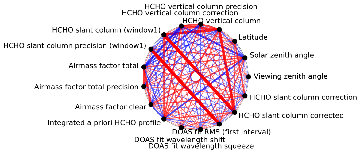
Figure 1: Map of correlation graph for 2024-08-24 to 2024-08-26.
