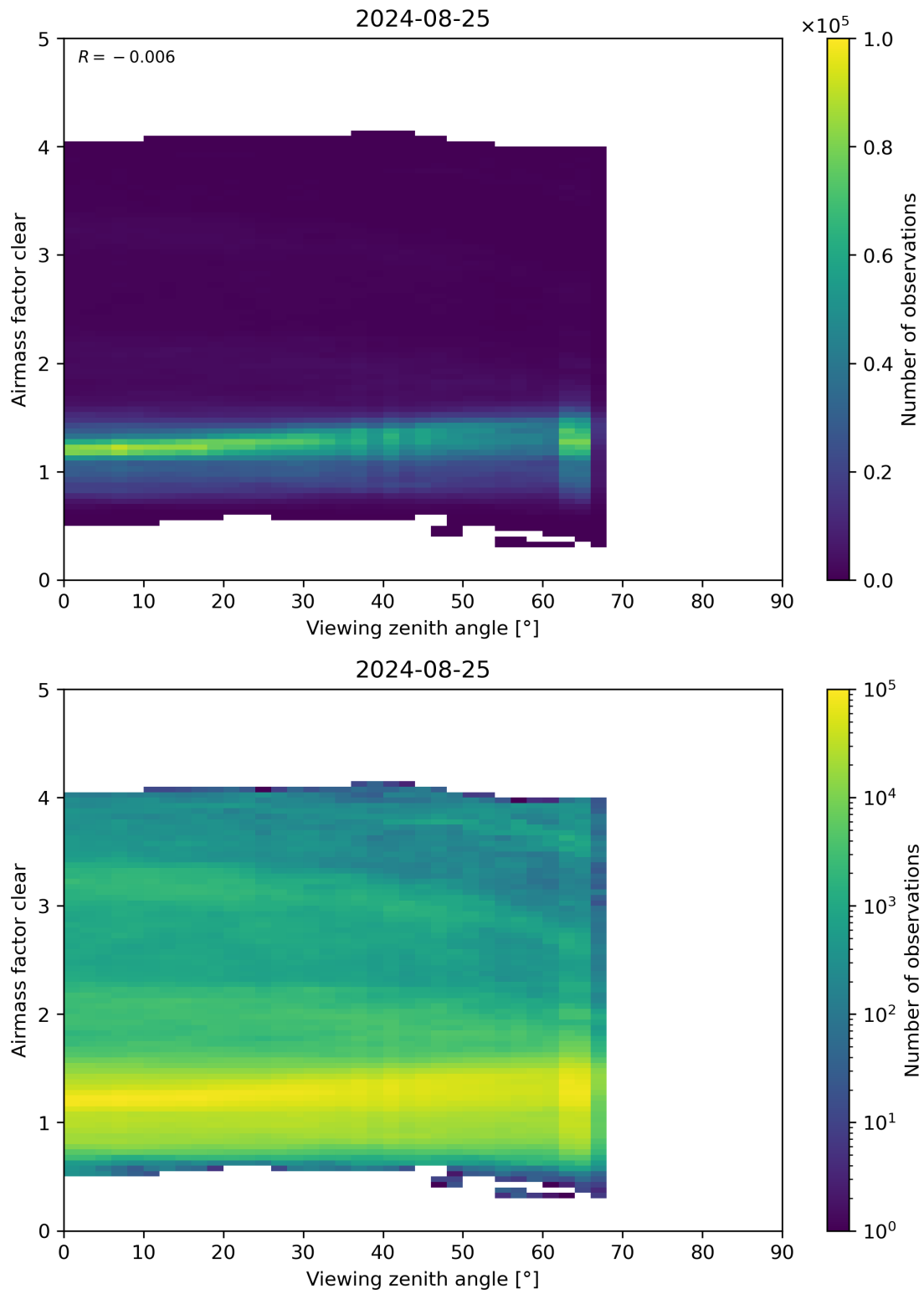
Figure 185: Scatter density plot of “Viewing zenith angle” against “Airmass factor clear” for 2024-08-24 to 2024-08-26.
