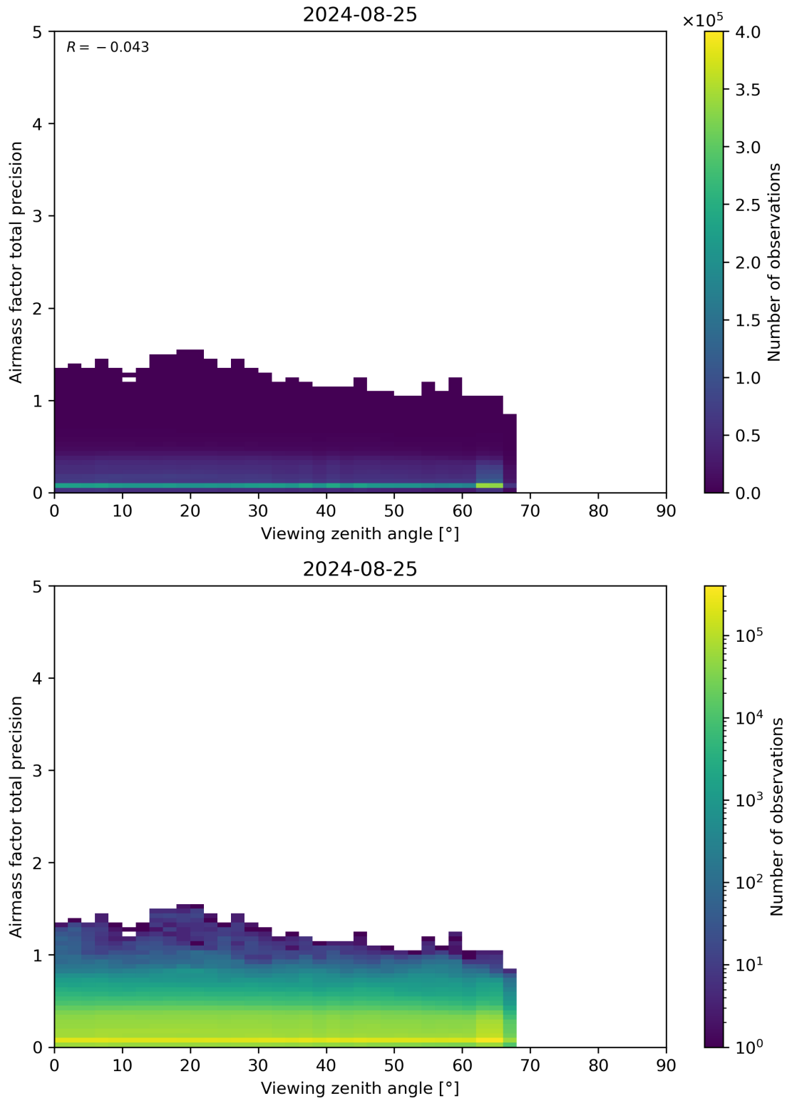
Figure 191: Scatter density plot of “Viewing zenith angle” against “Airmass factor total precision” for 2024-08-24 to 2024-08-26.
