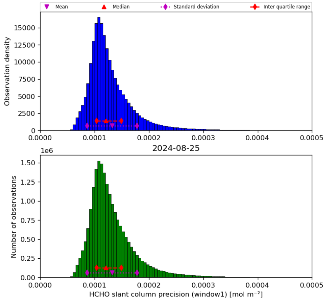
Figure 39: Histogram of “HCHO slant column precision (window1)” for 2024-08-24 to 2024-08-26
