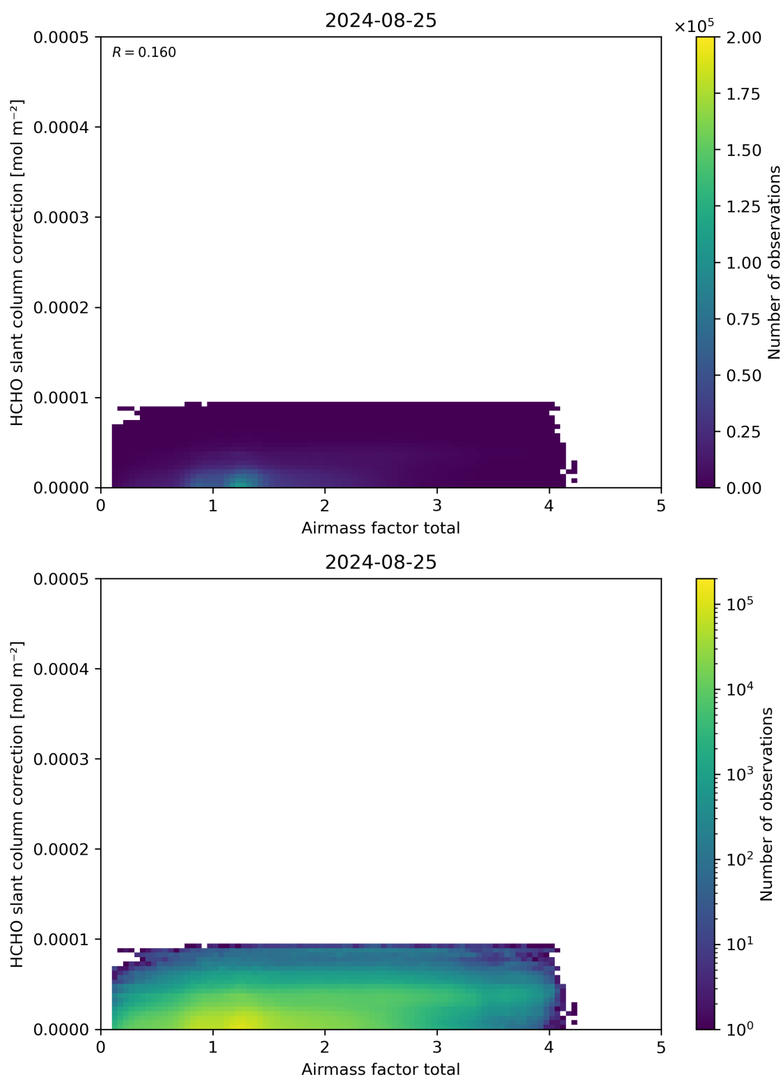
Figure 102: Scatter density plot of “Airmass factor total” against “HCHO slant column correction” for 2024-08-24 to 2024-08-26.
