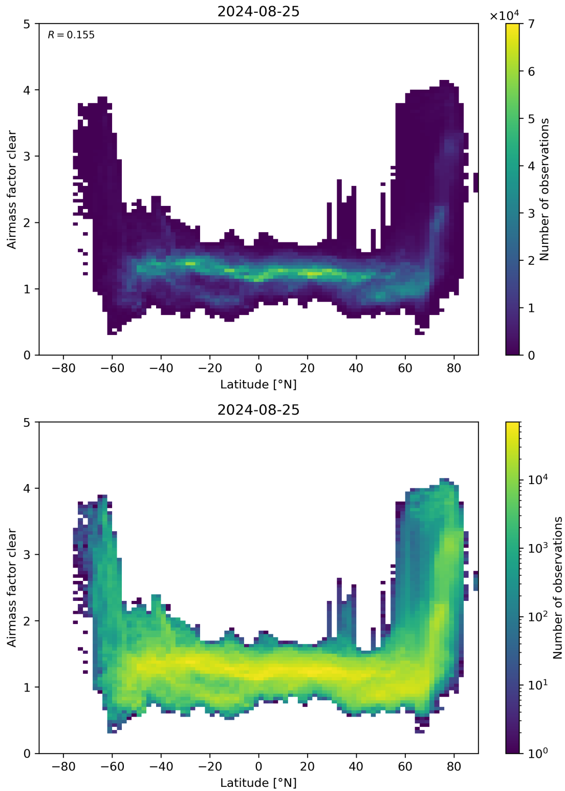
Figure 156: Scatter density plot of “Latitude” against “Airmass factor clear” for 2024-08-24 to 2024-08-26.
