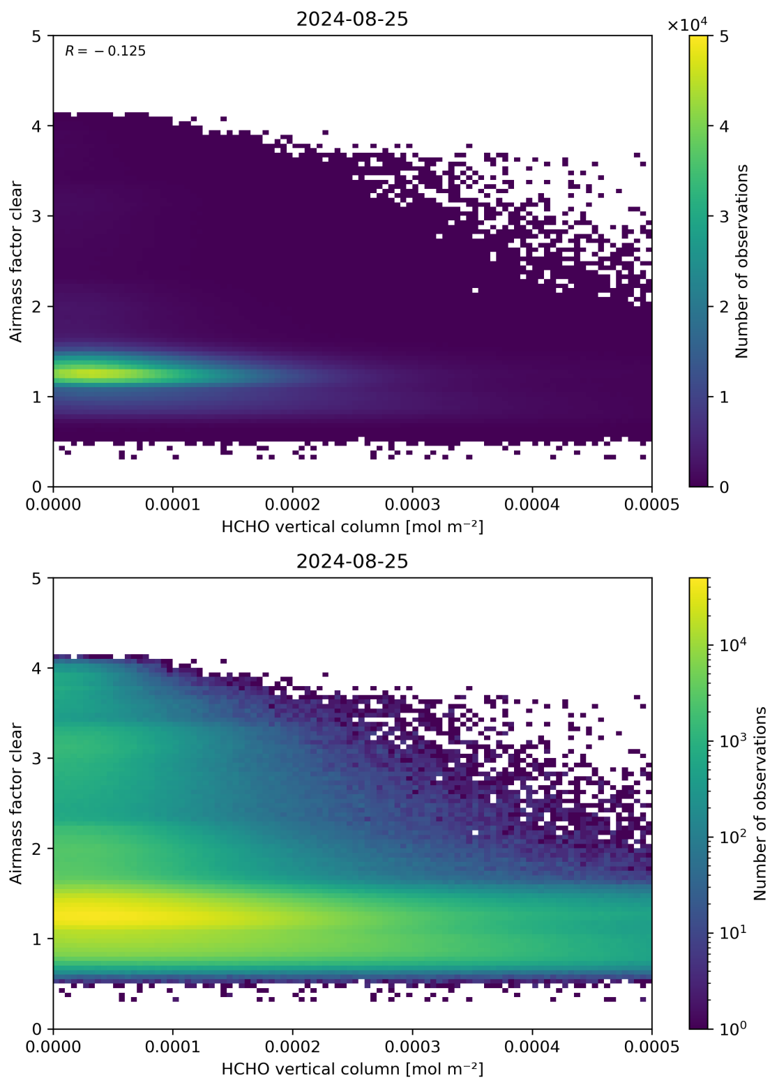
Figure 126: Scatter density plot of “HCHO vertical column” against “Airmass factor clear” for 2024-08-24 to 2024-08-26.
