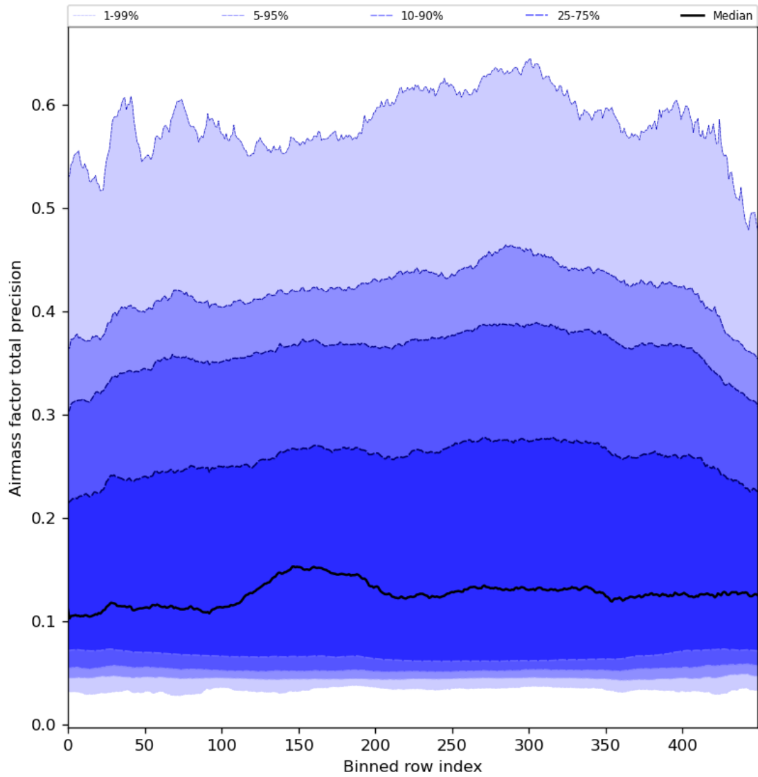
Figure 55: Along track statistics of “Airmass factor total precision” for 2024-08-24 to 2024-08-26
