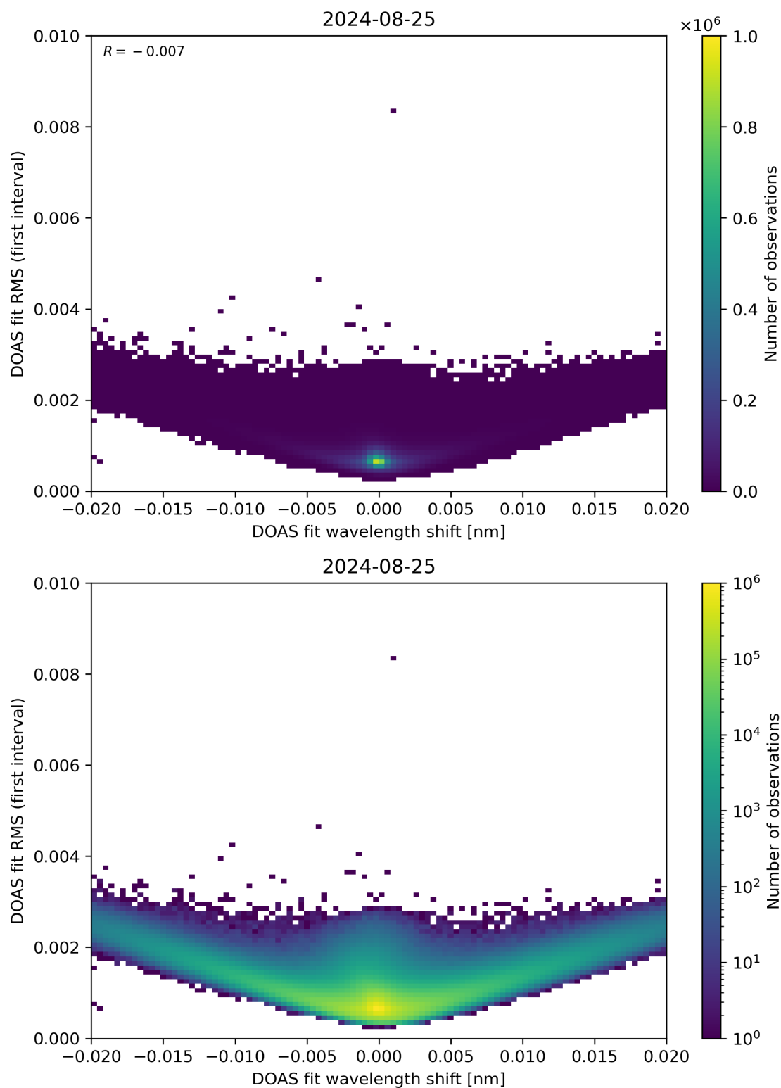
Figure 64: Scatter density plot of “DOAS fit wavelength shift” against “DOAS fit RMS (first interval)” for 2024-08-24 to 2024-08-26.
