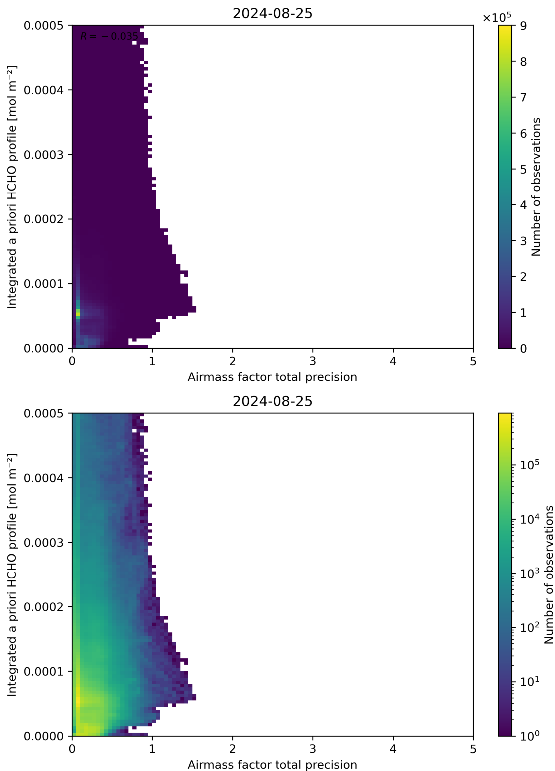
Figure 111: Scatter density plot of “Airmass factor total precision” against “Integrated a priori HCHO profile” for 2024-08-24 to 2024-08-26.
