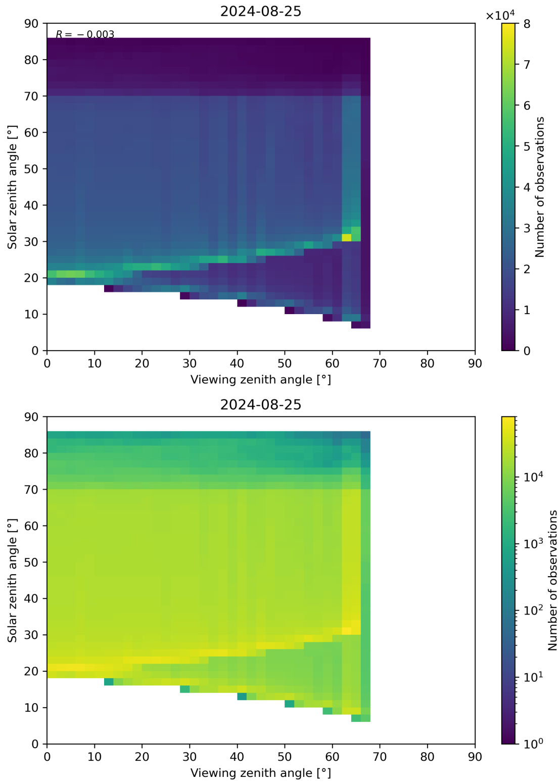
Figure 197: Scatter density plot of “Viewing zenith angle” against “Solar zenith angle” for 2024-08-24 to 2024-08-26.
