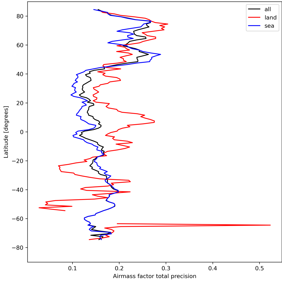
Figure 27: Zonal average of “Airmass factor total precision” for 2024-08-24 to 2024-08-26.
