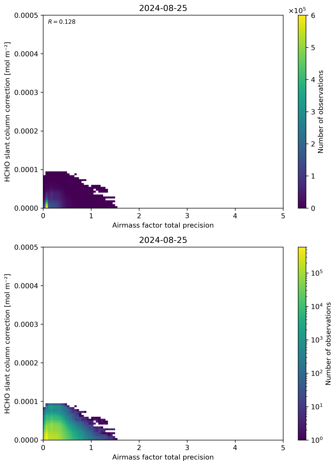
Figure 110: Scatter density plot of “Airmass factor total precision” against “HCHO slant column correction” for 2024-08-24 to 2024-08-26.
