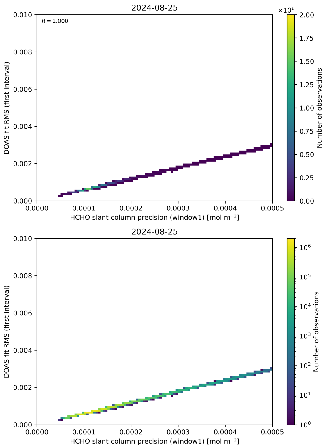
Figure 88: Scatter density plot of “HCHO slant column precision (window1)” against “DOAS fit RMS (first interval)” for 2024-08-24 to 2024-08-26.
