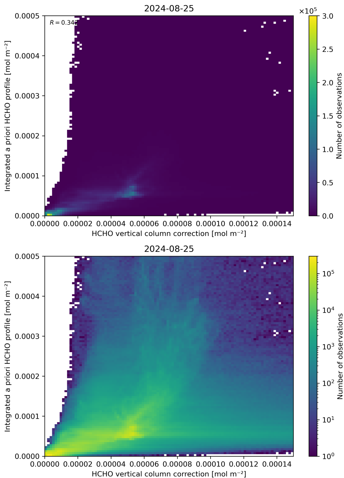
Figure 122: Scatter density plot of “HCHO vertical column correction” against “Integrated a priori HCHO profile” for 2024-08-24 to 2024-08-26.
