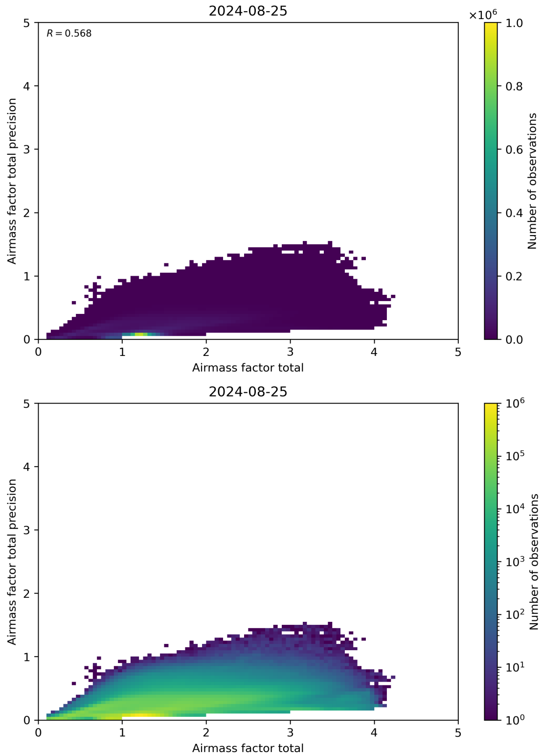
Figure 103: Scatter density plot of “Airmass factor total” against “Airmass factor total precision” for 2024-08-24 to 2024-08-26.
