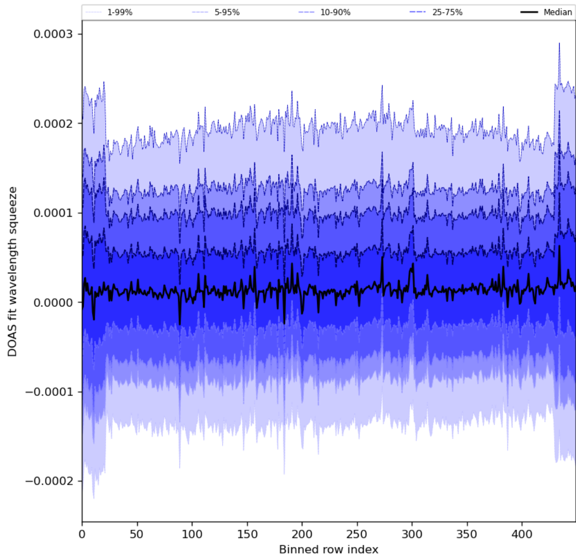
Figure 59: Along track statistics of “DOAS fit wavelength squeeze” for 2024-08-24 to 2024-08-26
