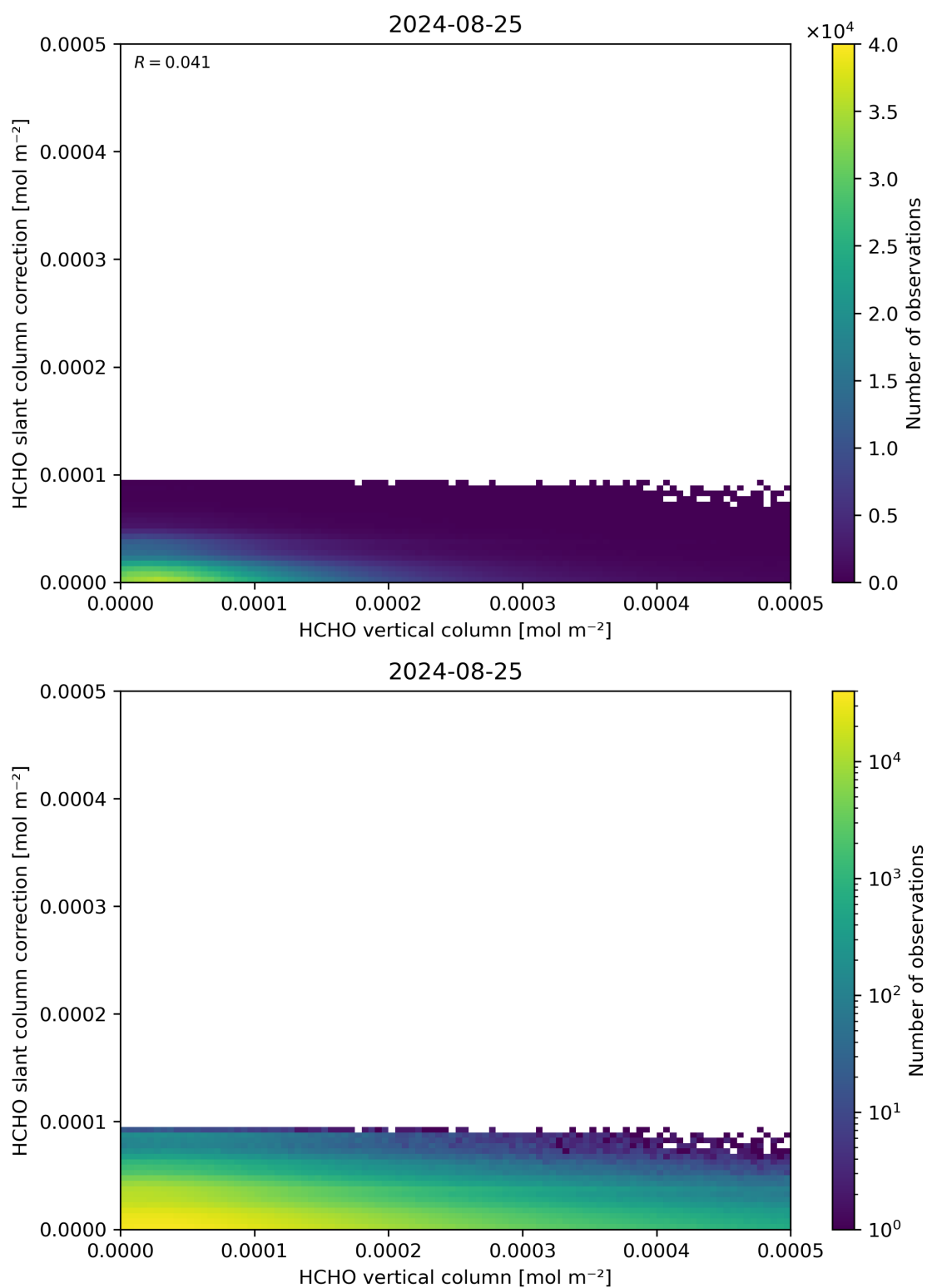
Figure 128: Scatter density plot of “HCHO vertical column” against “HCHO slant column correction” for 2024-08-24 to 2024-08-26.
