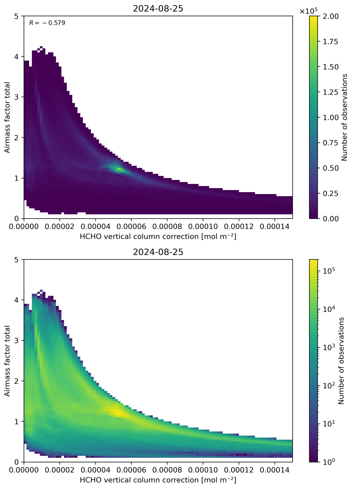
Figure 120: Scatter density plot of “HCHO vertical column correction” against “Airmass factor total” for 2024-08-24 to 2024-08-26.
