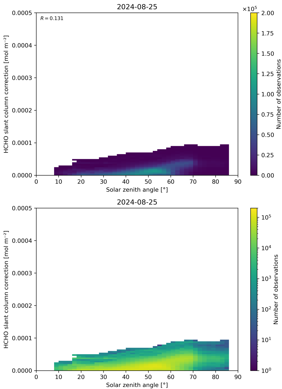
Figure 172: Scatter density plot of “Solar zenith angle” against “HCHO slant column correction” for 2024-08-24 to 2024-08-26.
