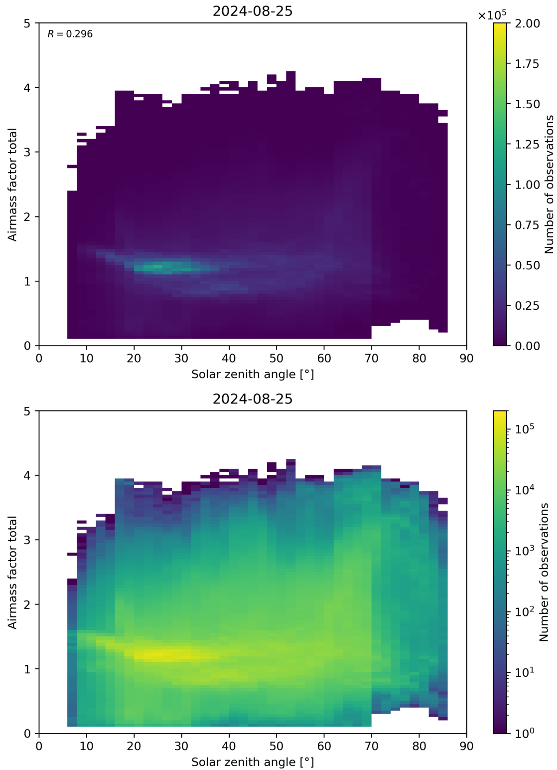
Figure 175: Scatter density plot of “Solar zenith angle” against “Airmass factor total” for 2024-08-24 to 2024-08-26.
