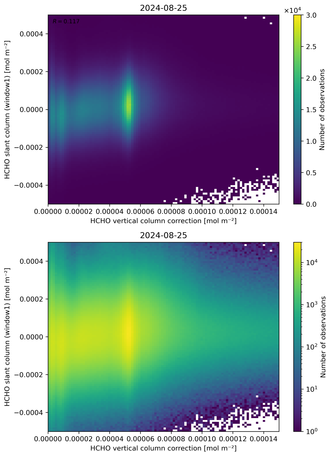
Figure 118: Scatter density plot of “HCHO vertical column correction” against “HCHO slant column (window1)” for 2024-08-24 to 2024-08-26.
