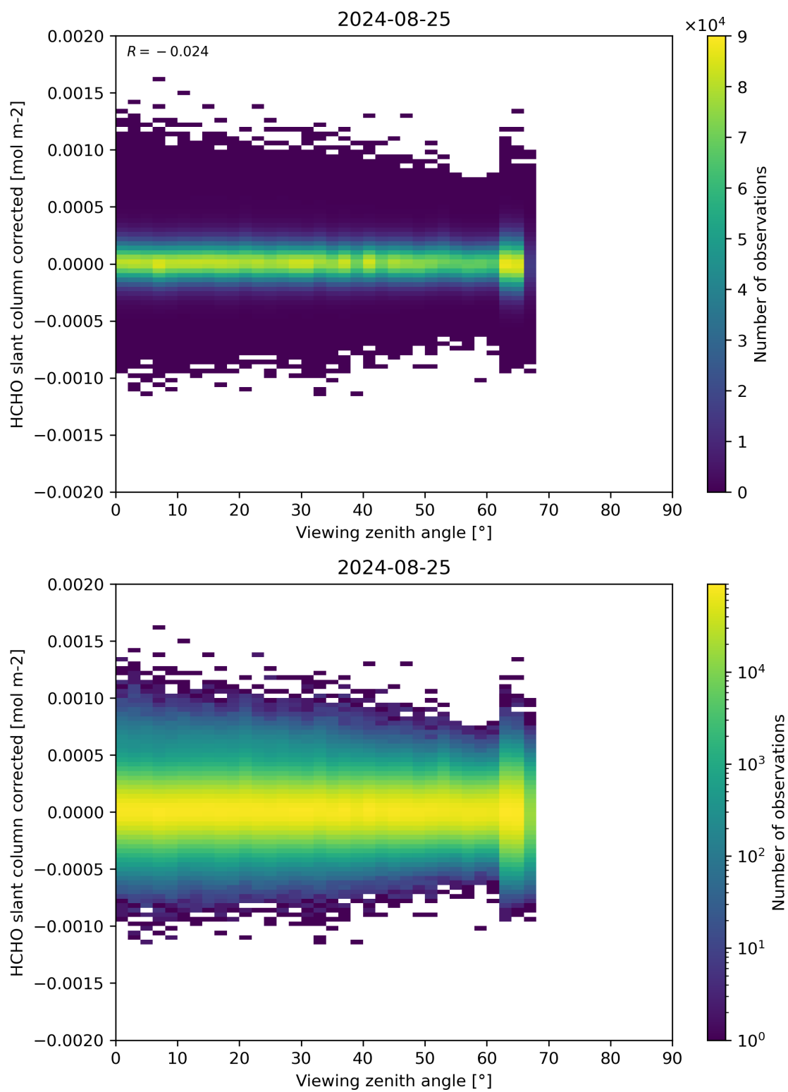
Figure 186: Scatter density plot of “Viewing zenith angle” against “HCHO slant column corrected” for 2024-08-24 to 2024-08-26.
