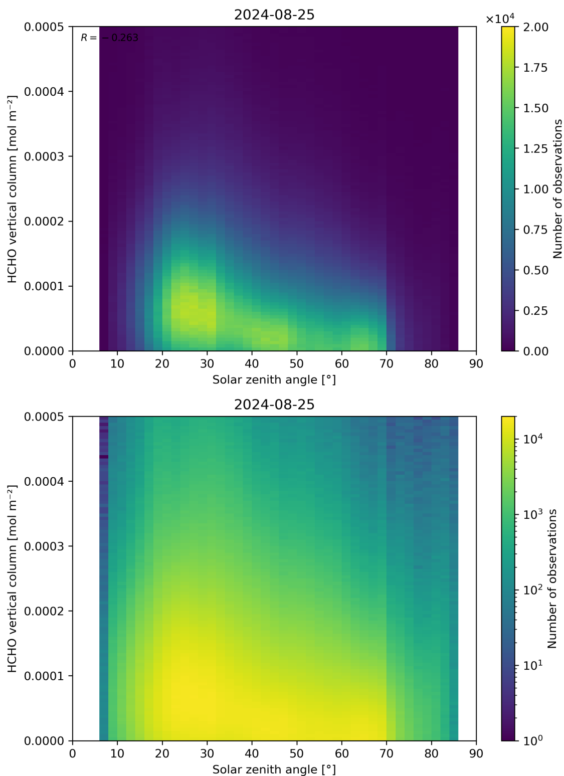
Figure 177: Scatter density plot of “Solar zenith angle” against “HCHO vertical column” for 2024-08-24 to 2024-08-26.
