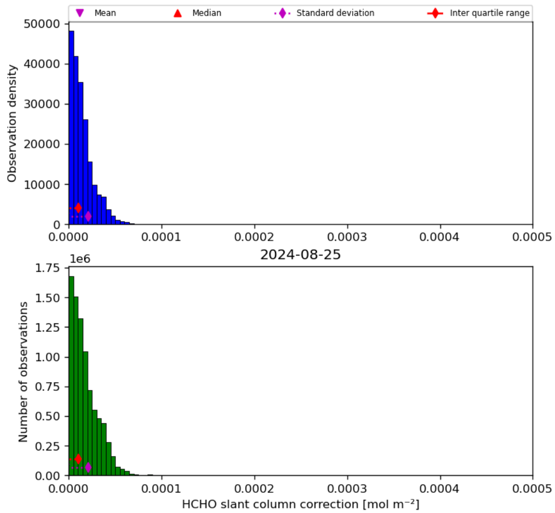
Figure 47: Histogram of “HCHO slant column correction” for 2024-08-24 to 2024-08-26
