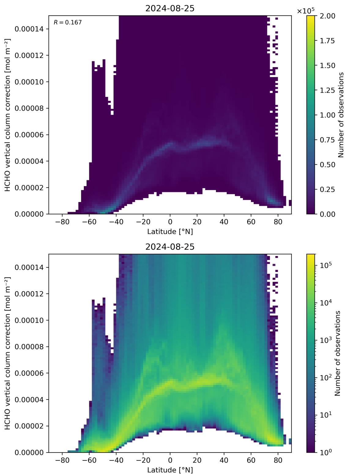
Figure 164: Scatter density plot of “Latitude” against “HCHO vertical column correction” for 2024-08-24 to 2024-08-26.
