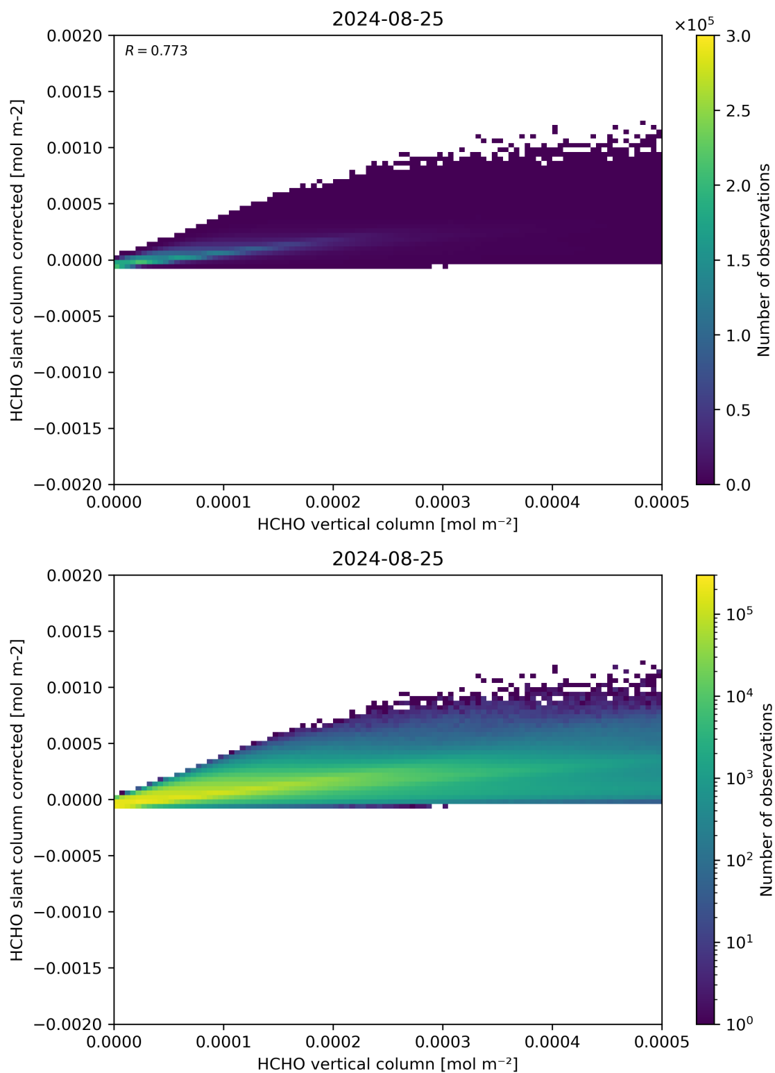
Figure 127: Scatter density plot of “HCHO vertical column” against “HCHO slant column corrected” for 2024-08-24 to 2024-08-26.
