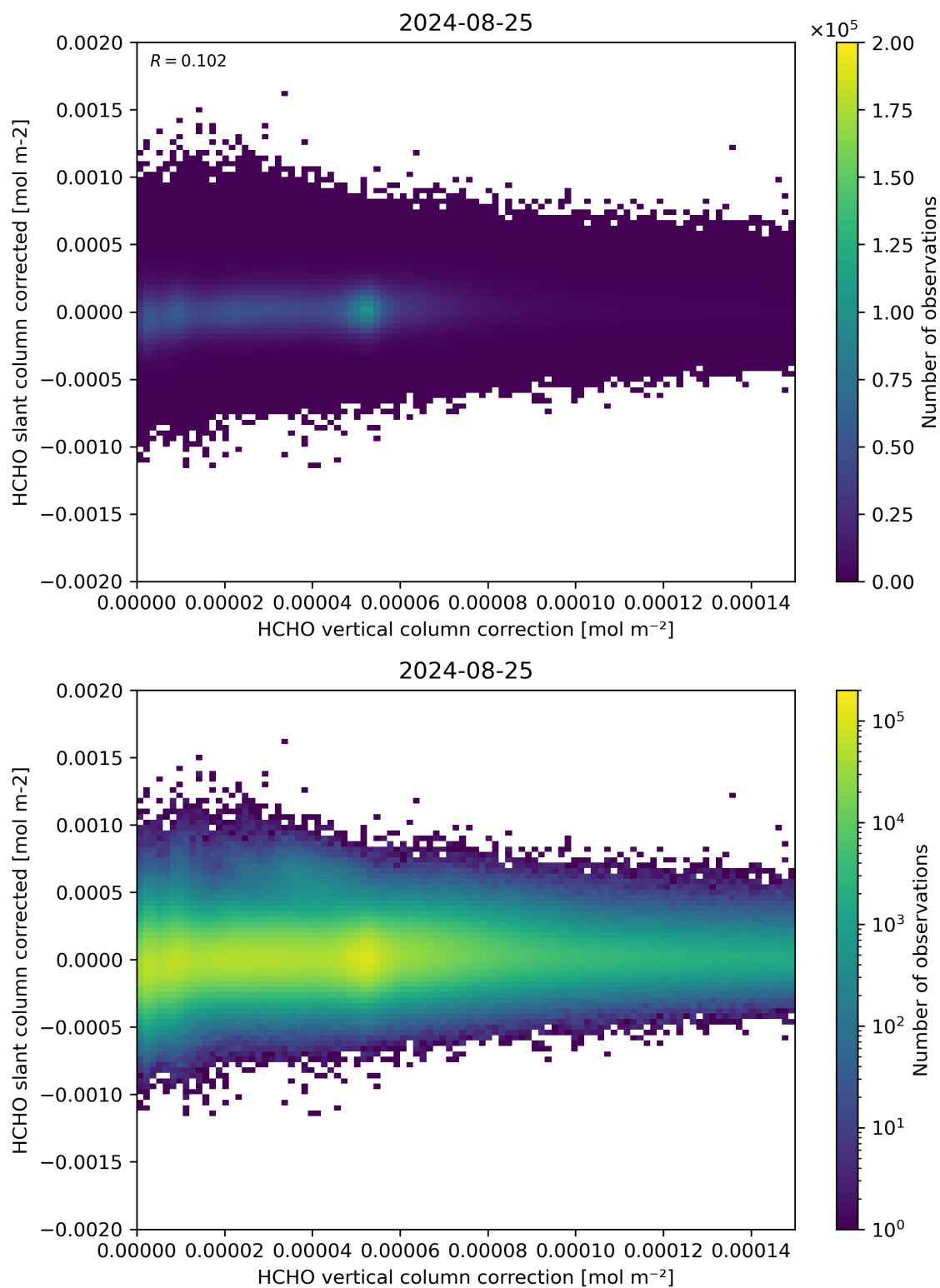
Figure 116: Scatter density plot of “HCHO vertical column correction” against “HCHO slant column corrected” for 2024-08-24 to 2024-08-26.
