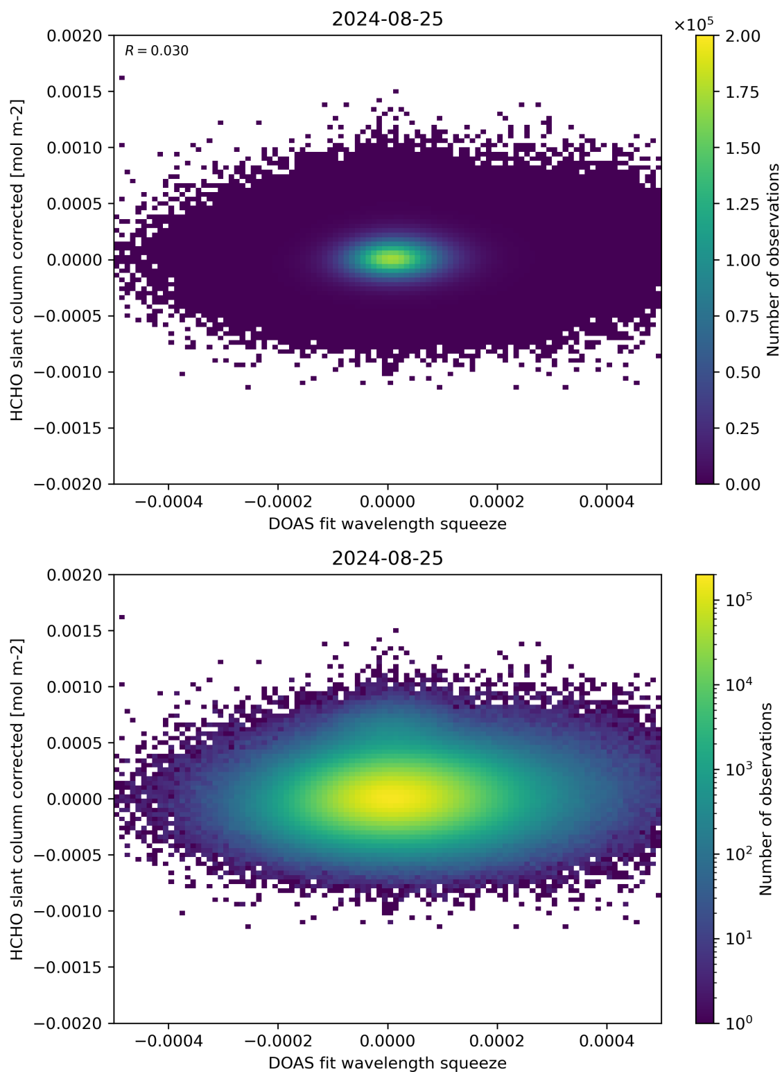
Figure 69: Scatter density plot of “DOAS fit wavelength squeeze” against “HCHO slant column corrected” for 2024-08-24 to 2024-08-26.
