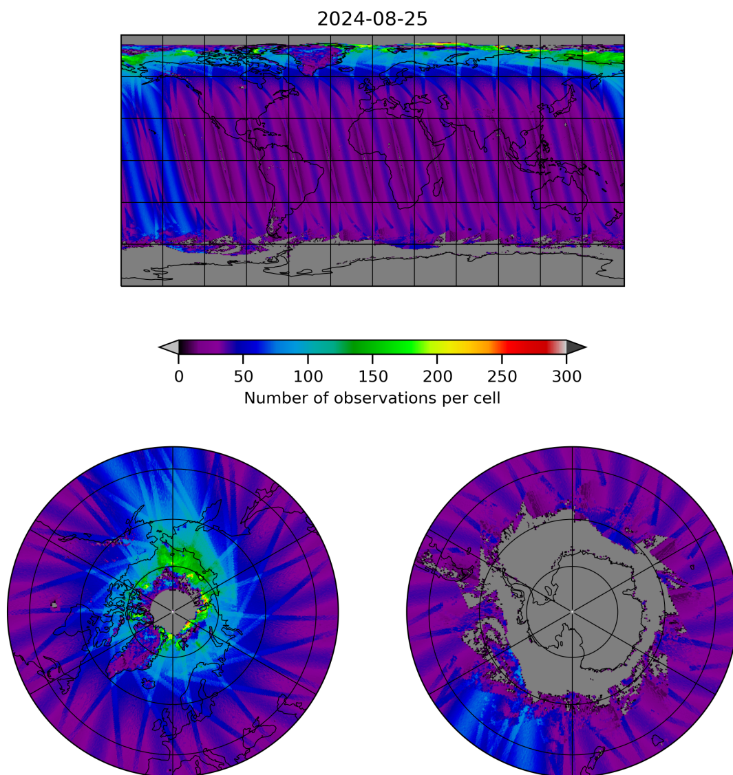
Figure 19: Map of the number of observations for 2024-08-24 to 2024-08-26
