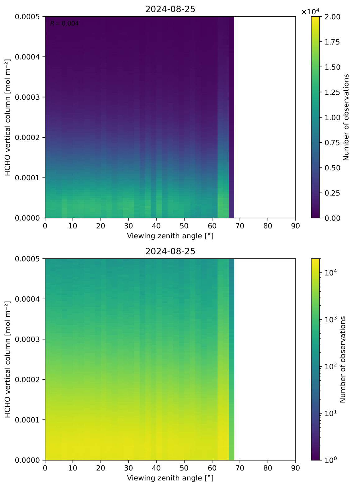
Figure 192: Scatter density plot of “Viewing zenith angle” against “HCHO vertical column” for 2024-08-24 to 2024-08-26.
