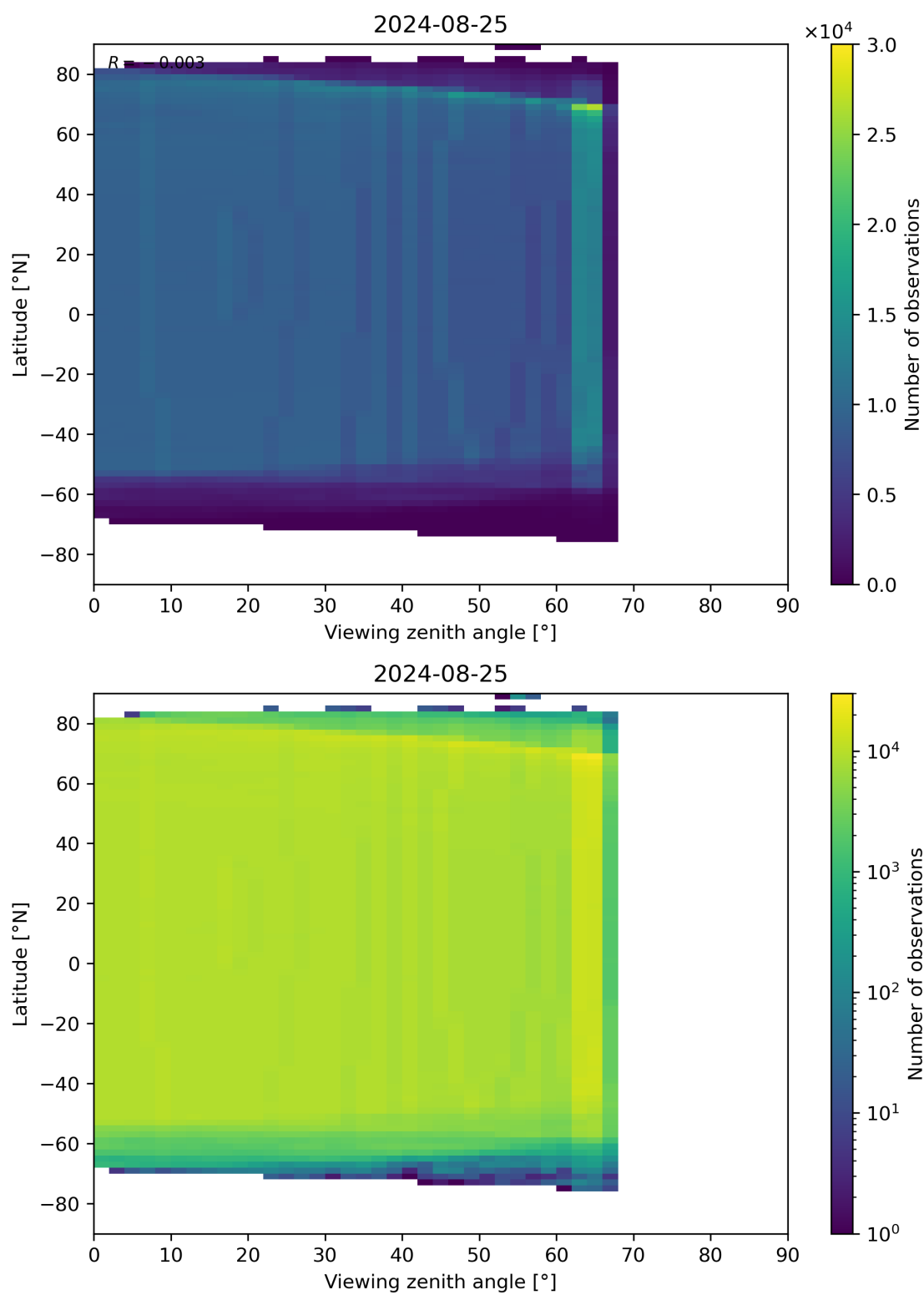
Figure 196: Scatter density plot of “Viewing zenith angle” against “Latitude” for 2024-08-24 to 2024-08-26.
