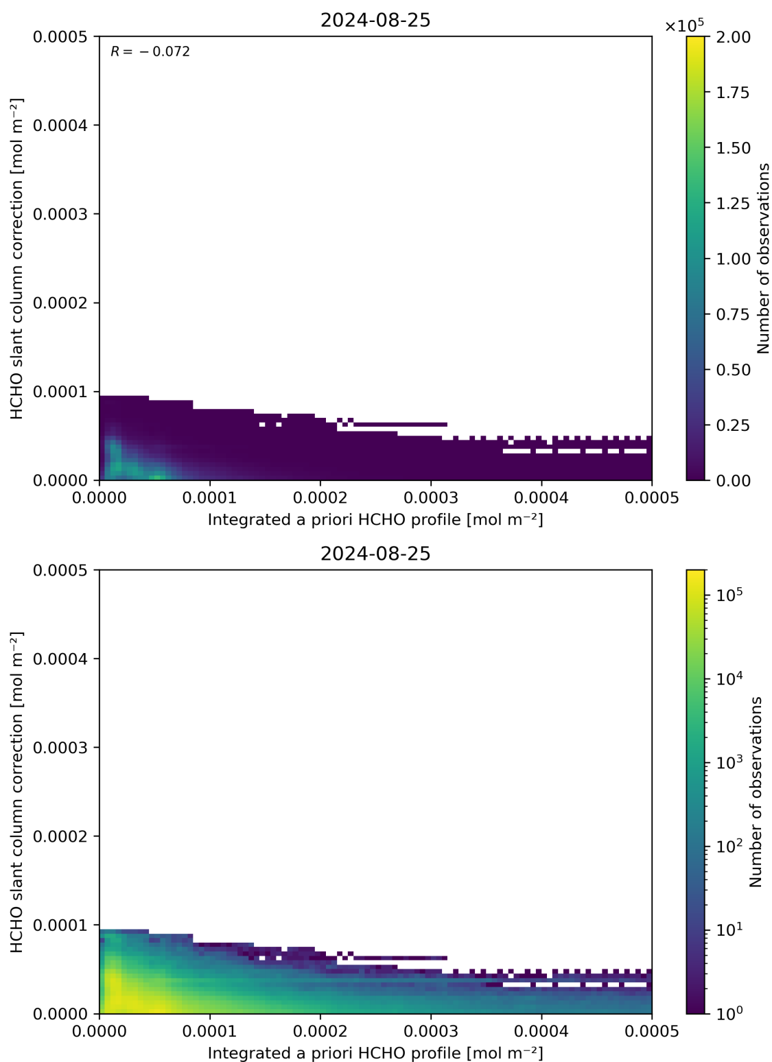
Figure 152: Scatter density plot of “Integrated a priori HCHO profile” against “HCHO slant column correction” for 2024-08-24 to 2024-08-26.
