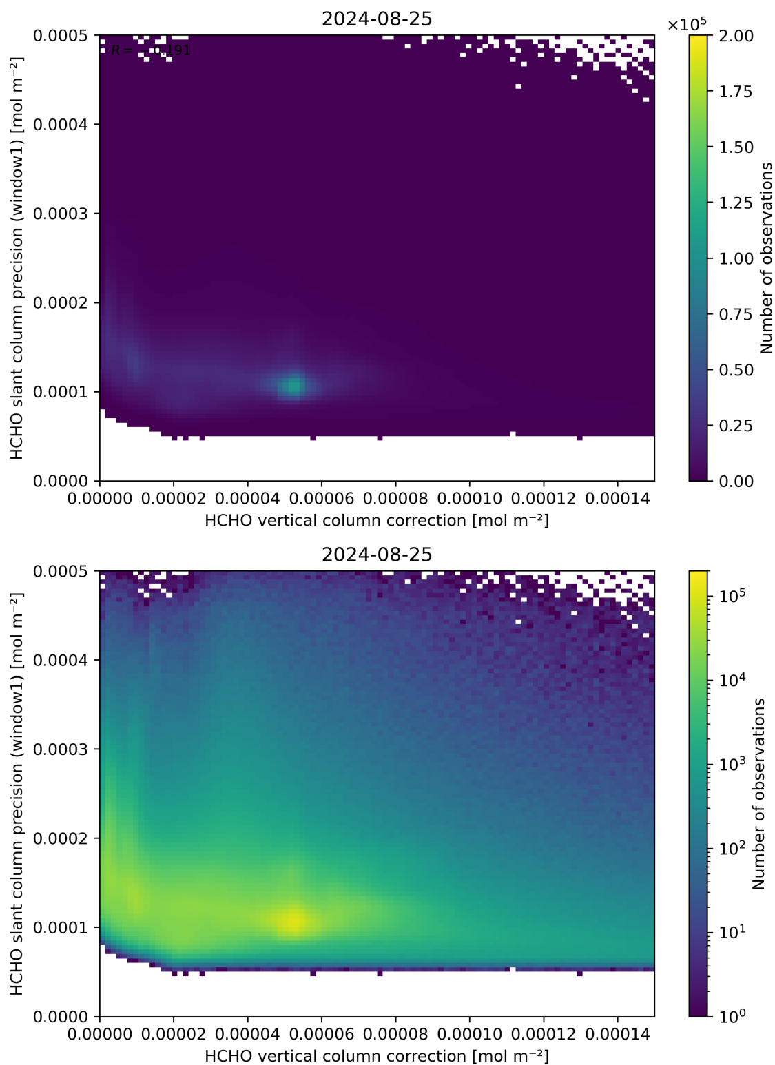
Figure 119: Scatter density plot of “HCHO vertical column correction” against “HCHO slant column precision (window1)” for 2024-08-24 to 2024-08-26.
