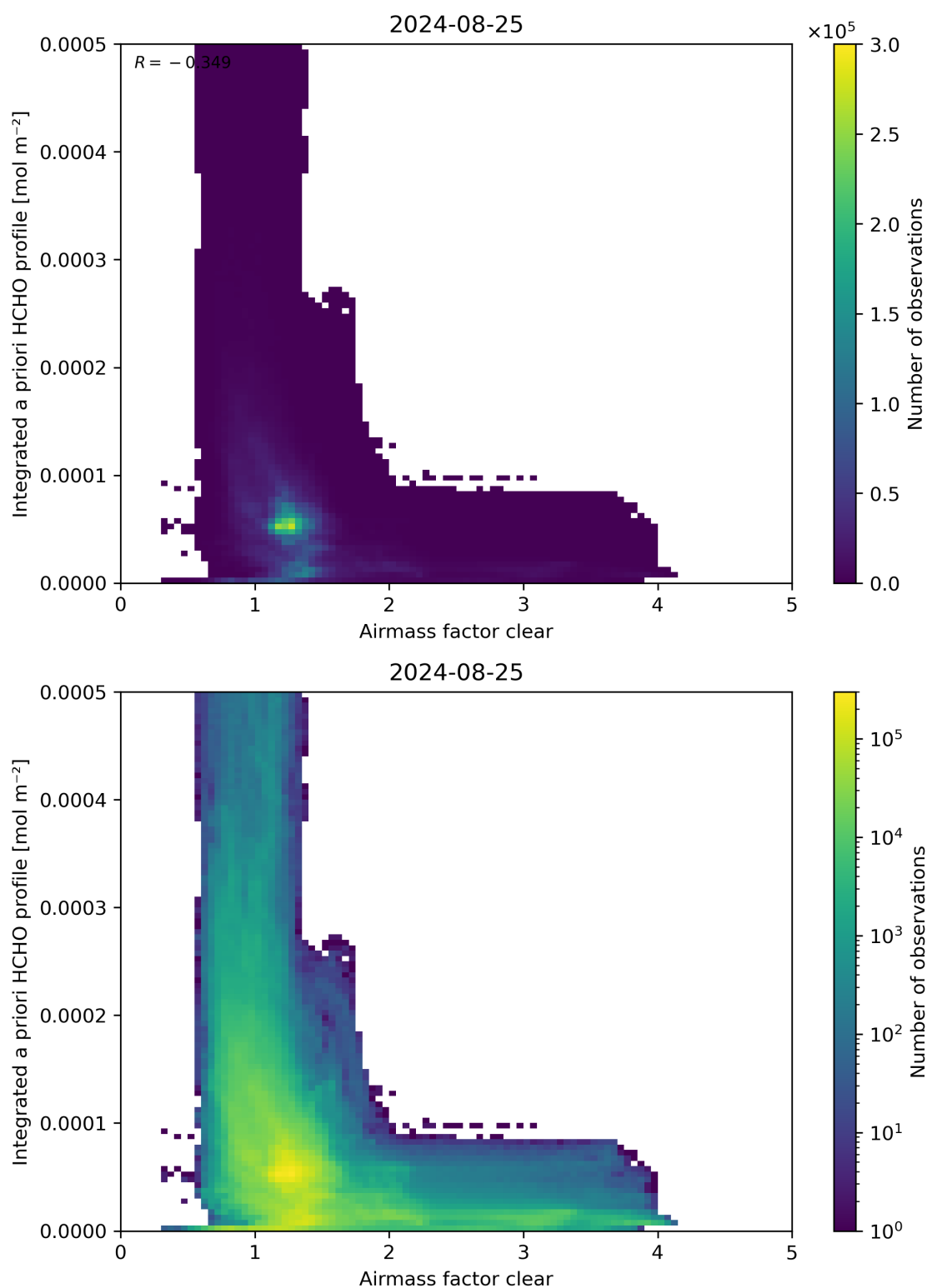
Figure 76: Scatter density plot of “Airmass factor clear” against “Integrated a priori HCHO profile” for 2024-08-24 to 2024-08-26.
