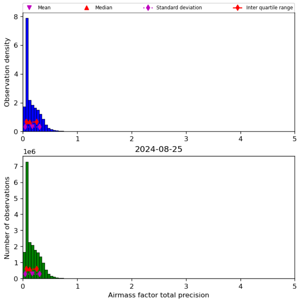
Figure 41: Histogram of “Airmass factor total precision” for 2024-08-24 to 2024-08-26
