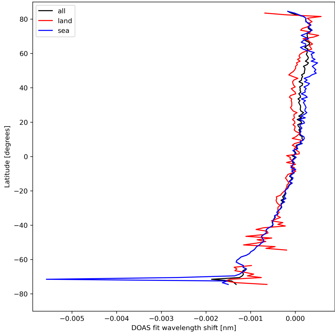
Figure 30: Zonal average of “DOAS fit wavelength shift” for 2024-08-24 to 2024-08-26.
