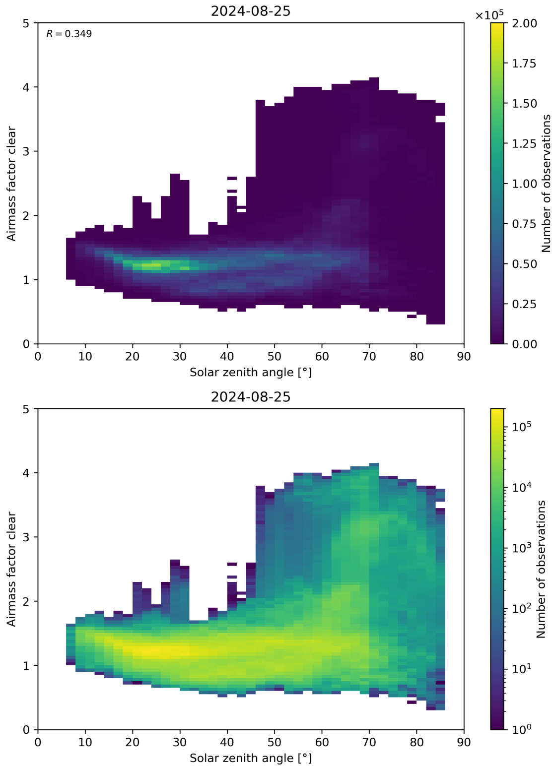
Figure 170: Scatter density plot of “Solar zenith angle” against “Airmass factor clear” for 2024-08-24 to 2024-08-26.
