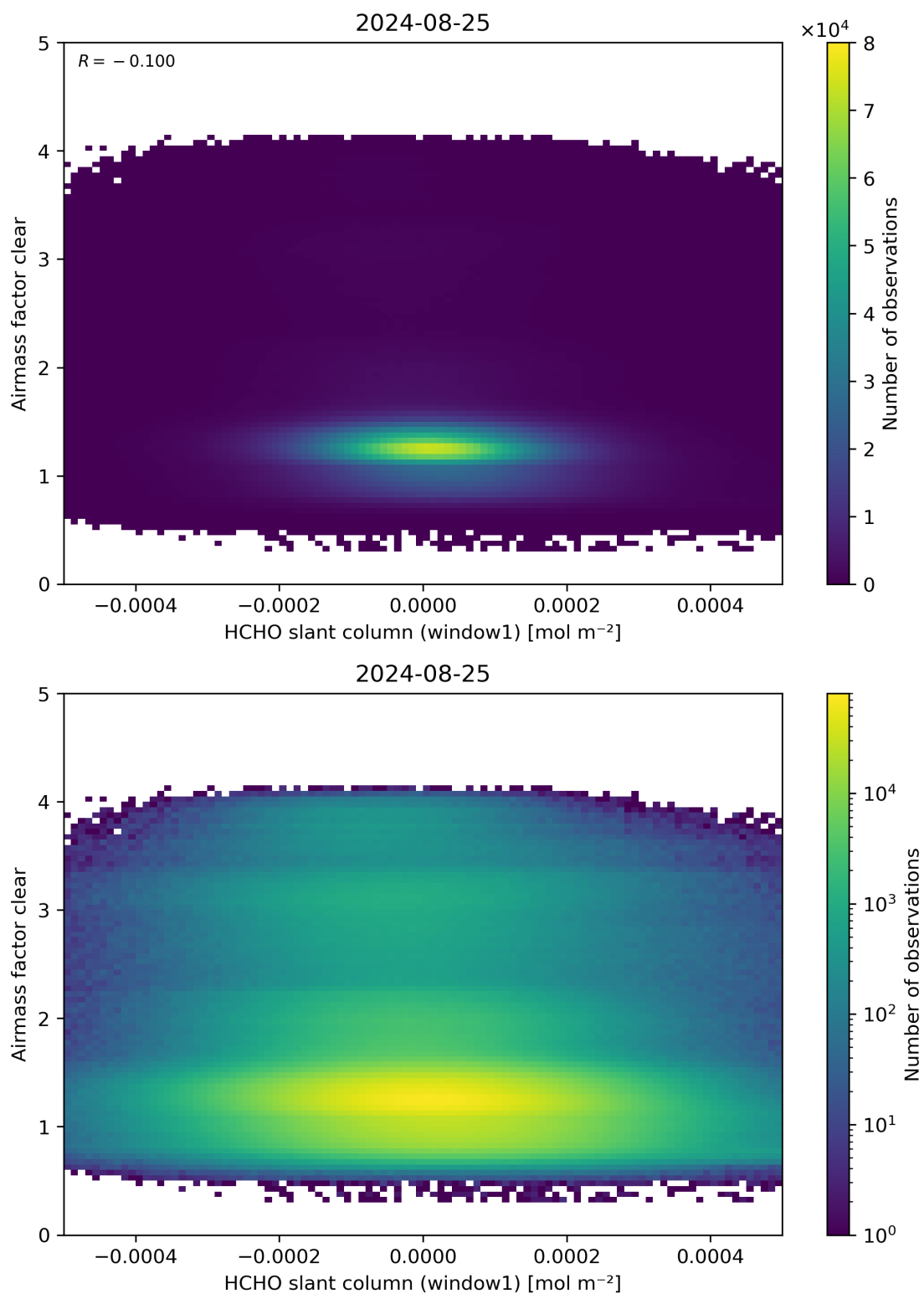
Figure 81: Scatter density plot of “HCHO slant column (window1)” against “Airmass factor clear” for 2024-08-24 to 2024-08-26.
