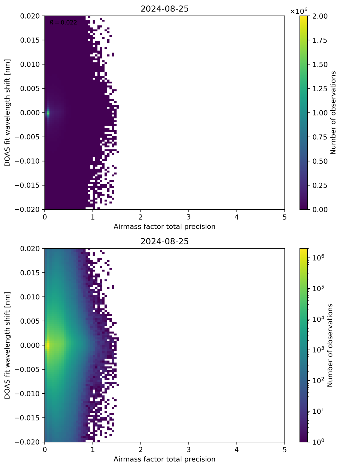
Figure 106: Scatter density plot of “Airmass factor total precision” against “DOAS fit wavelength shift” for 2024-08-24 to 2024-08-26.
