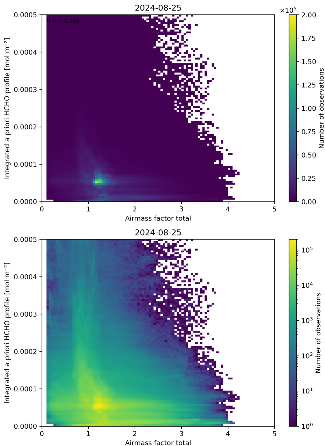
Figure 104: Scatter density plot of “Airmass factor total” against “Integrated a priori HCHO profile” for 2024-08-24 to 2024-08-26.
