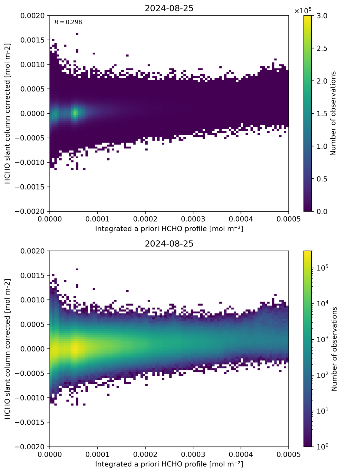
Figure 151: Scatter density plot of “Integrated a priori HCHO profile” against “HCHO slant column corrected” for 2024-08-24 to 2024-08-26.
