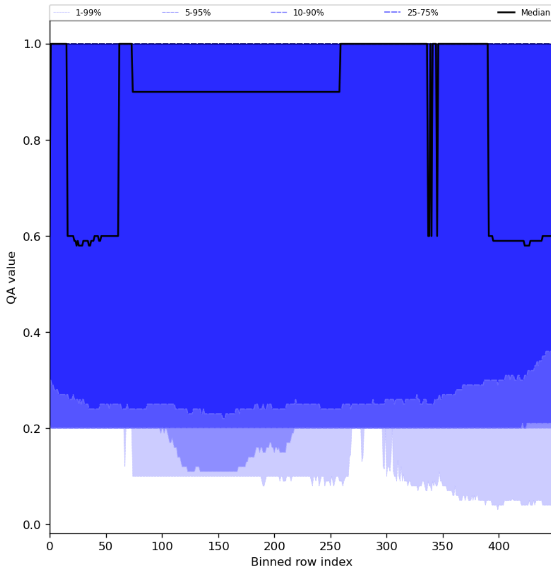
Figure 48: Along track statistics of “QA value” for 2024-08-24 to 2024-08-26
