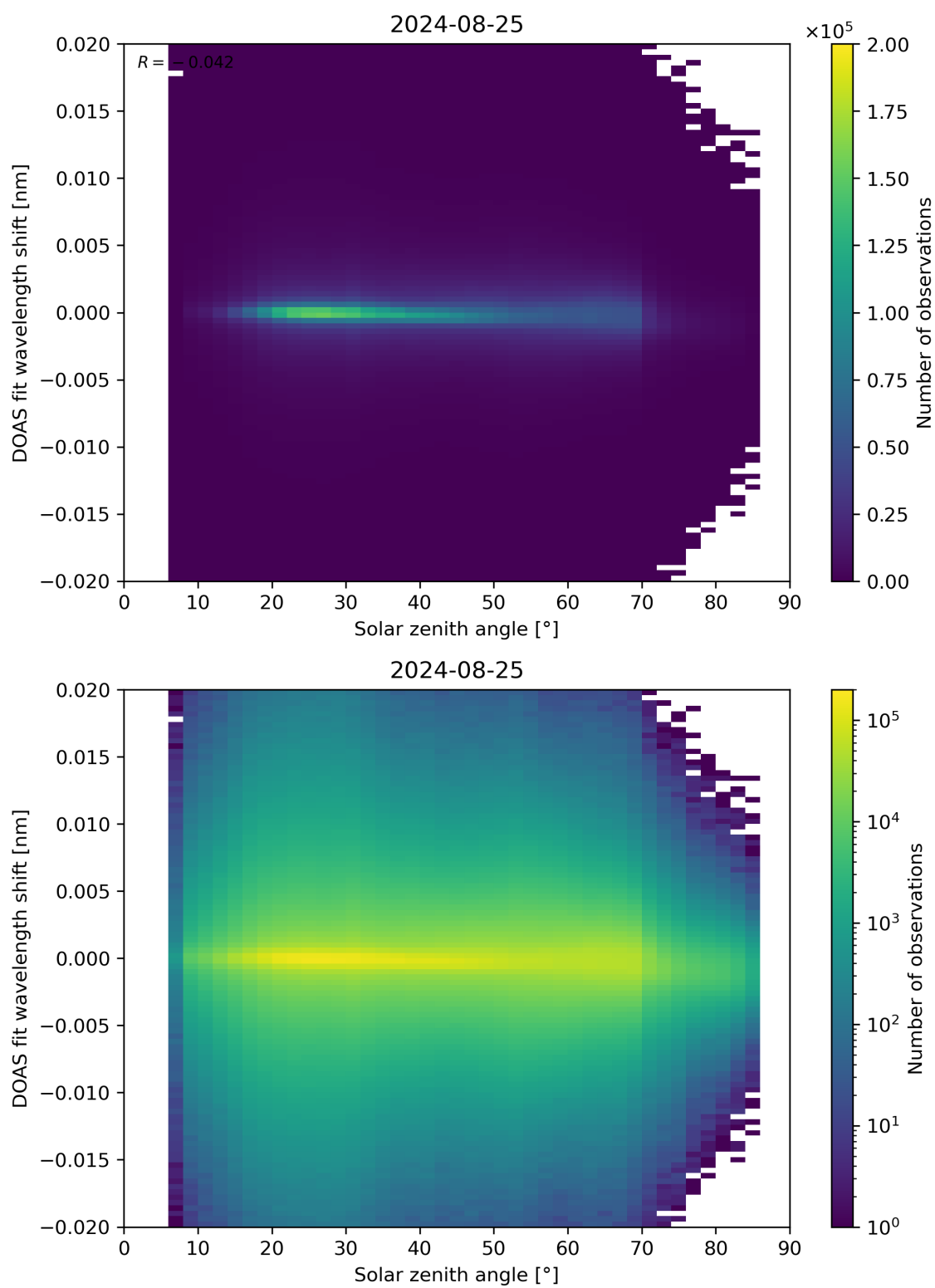
Figure 168: Scatter density plot of “Solar zenith angle” against “DOAS fit wavelength shift” for 2024-08-24 to 2024-08-26.
