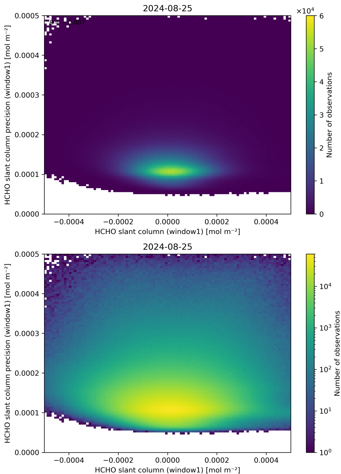
Figure 84: Scatter density plot of “HCHO slant column (window1)” against “HCHO slant column precision (window1)” for 2024-08-24 to 2024-08-26.
