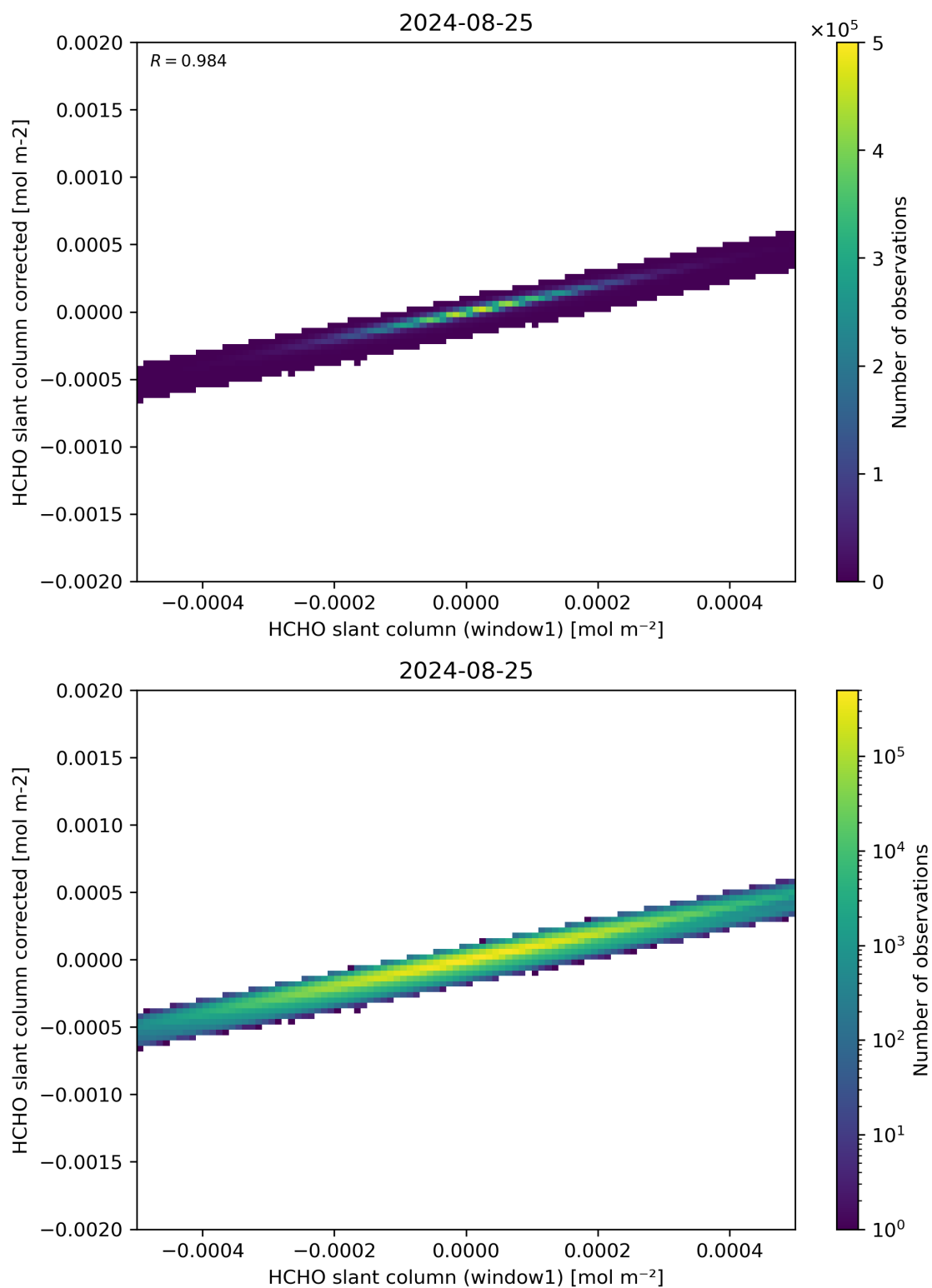
Figure 82: Scatter density plot of “HCHO slant column (window1)” against “HCHO slant column corrected” for 2024-08-24 to 2024-08-26.
