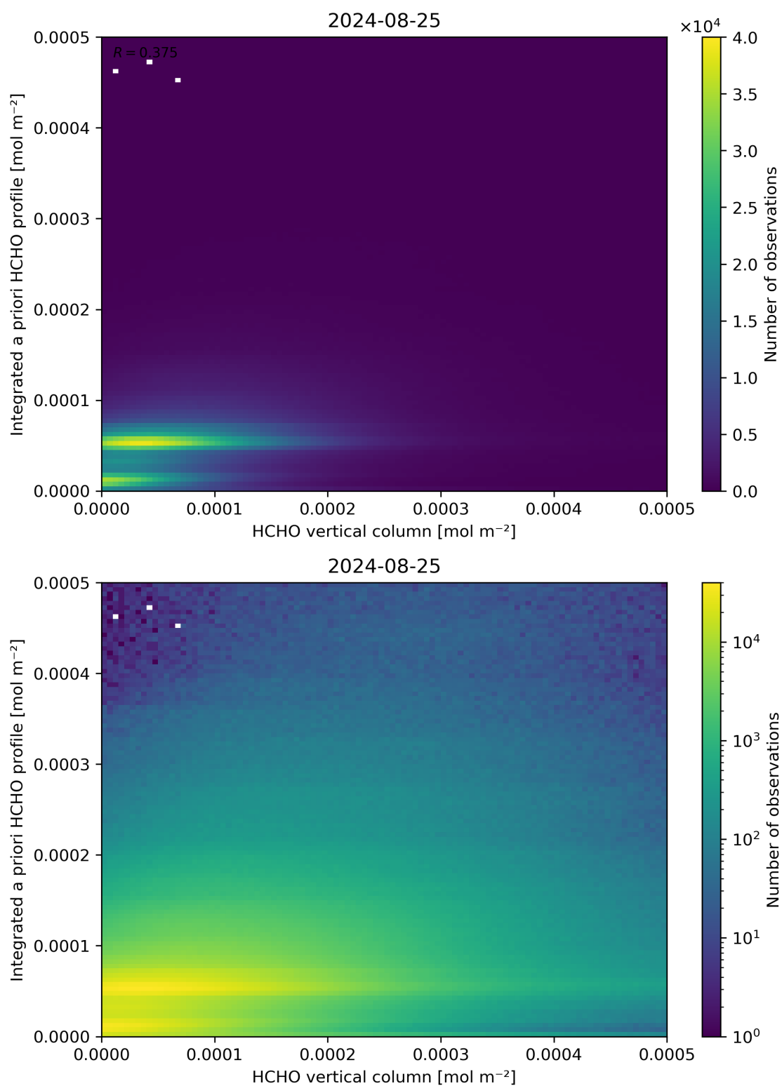
Figure 135: Scatter density plot of “HCHO vertical column” against “Integrated a priori HCHO profile” for 2024-08-24 to 2024-08-26.
