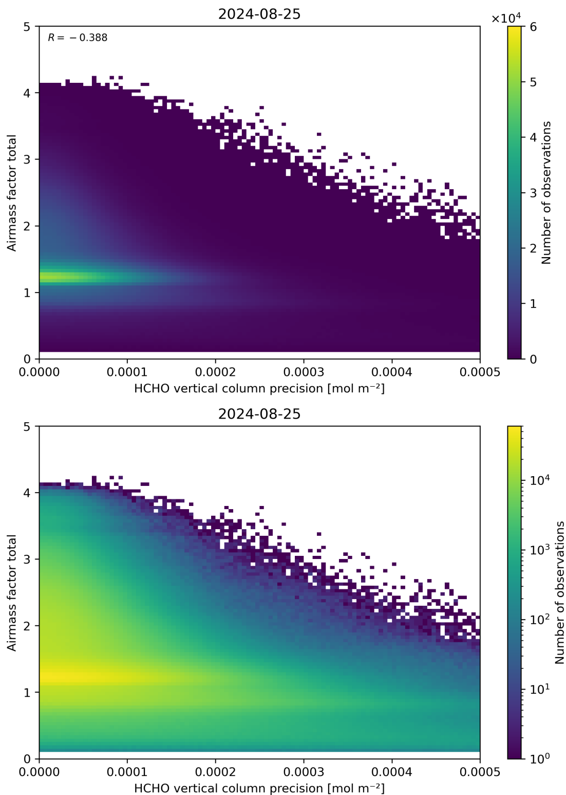
Figure 144: Scatter density plot of “HCHO vertical column precision” against “Airmass factor total” for 2024-08-24 to 2024-08-26.
