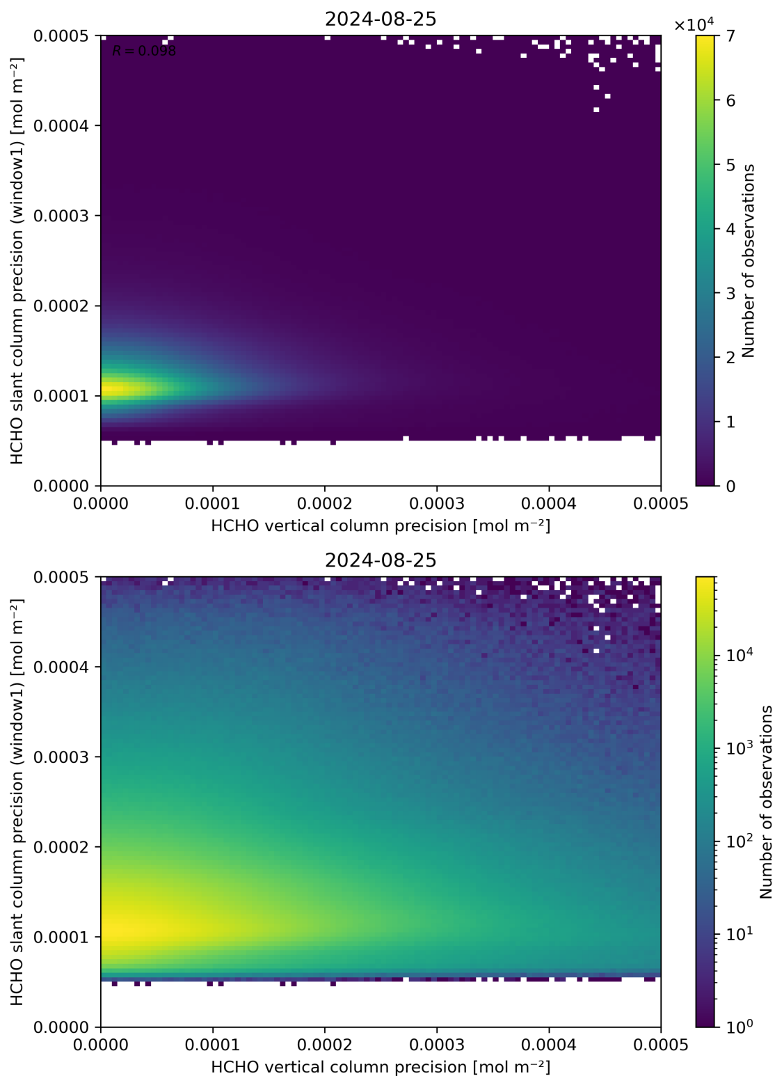
Figure 143: Scatter density plot of “HCHO vertical column precision” against “HCHO slant column precision (window1)” for 2024-08-24 to 2024-08-26.
