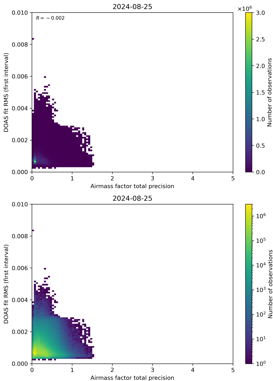
Figure 105: Scatter density plot of “Airmass factor total precision” against “DOAS fit RMS (first interval)” for 2024-08-24 to 2024-08-26.
