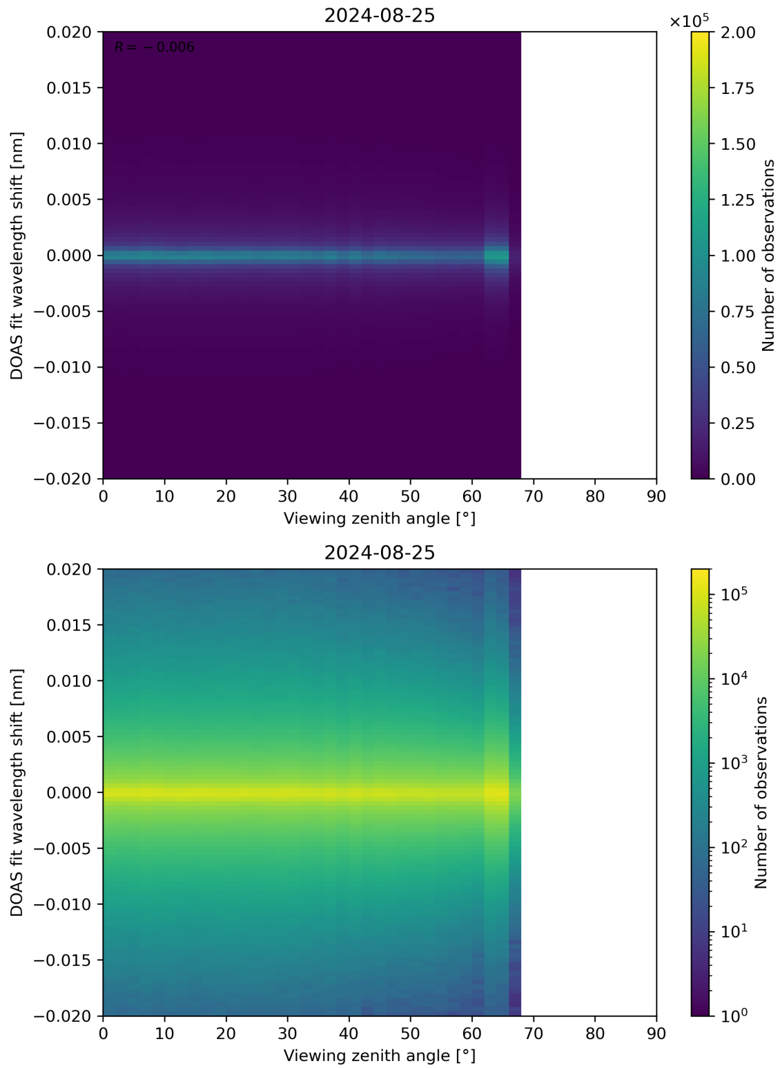
Figure 183: Scatter density plot of “Viewing zenith angle” against “DOAS fit wavelength shift” for 2024-08-24 to 2024-08-26.
