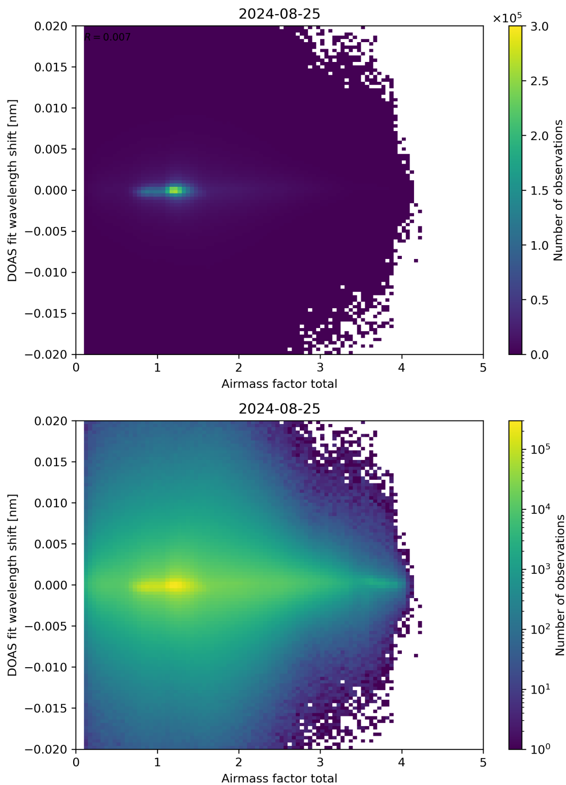
Figure 98: Scatter density plot of “Airmass factor total” against “DOAS fit wavelength shift” for 2024-08-24 to 2024-08-26.
