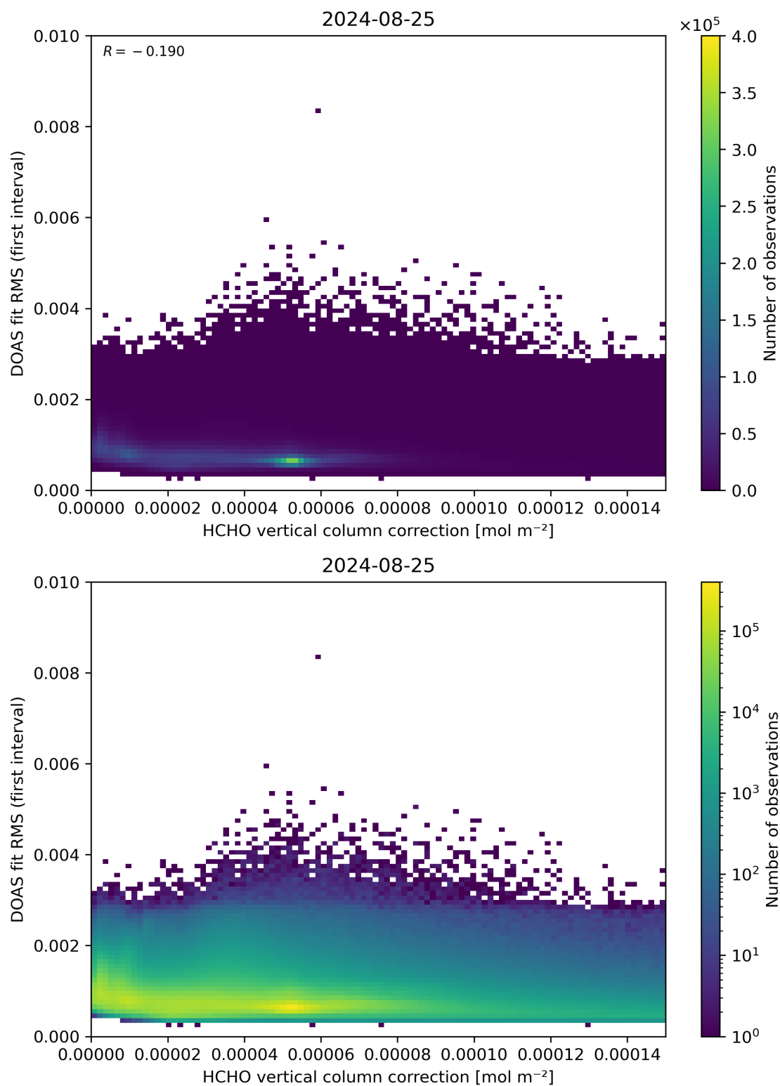
Figure 112: Scatter density plot of “HCHO vertical column correction” against “DOAS fit RMS (first interval)” for 2024-08-24 to 2024-08-26.
