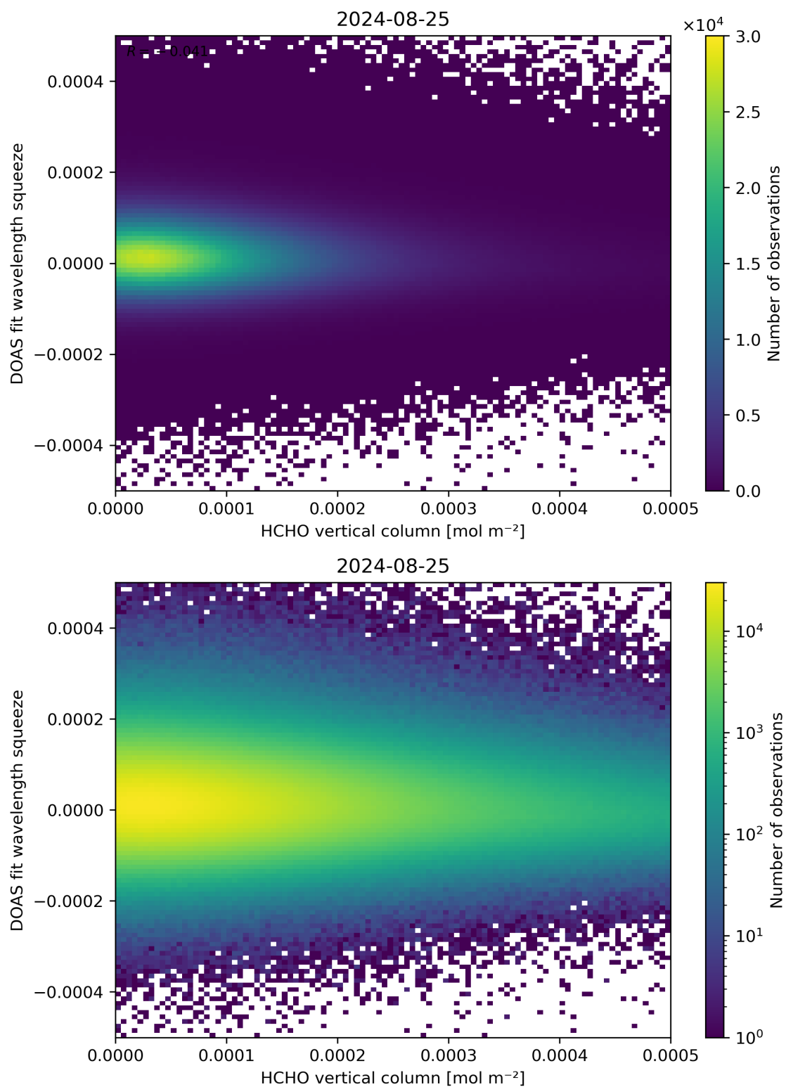
Figure 125: Scatter density plot of “HCHO vertical column” against “DOAS fit wavelength squeeze” for 2024-08-24 to 2024-08-26.
