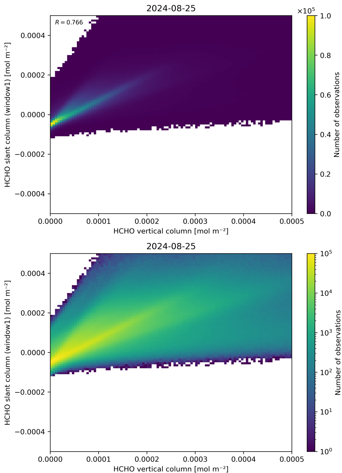
Figure 129: Scatter density plot of “HCHO vertical column” against “HCHO slant column (window1)” for 2024-08-24 to 2024-08-26.
