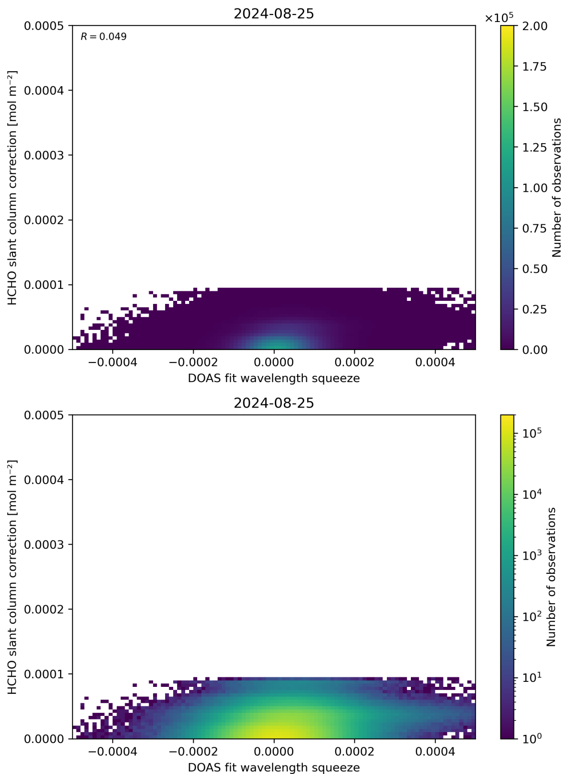
Figure 70: Scatter density plot of “DOAS fit wavelength squeeze” against “HCHO slant column correction” for 2024-08-24 to 2024-08-26.
