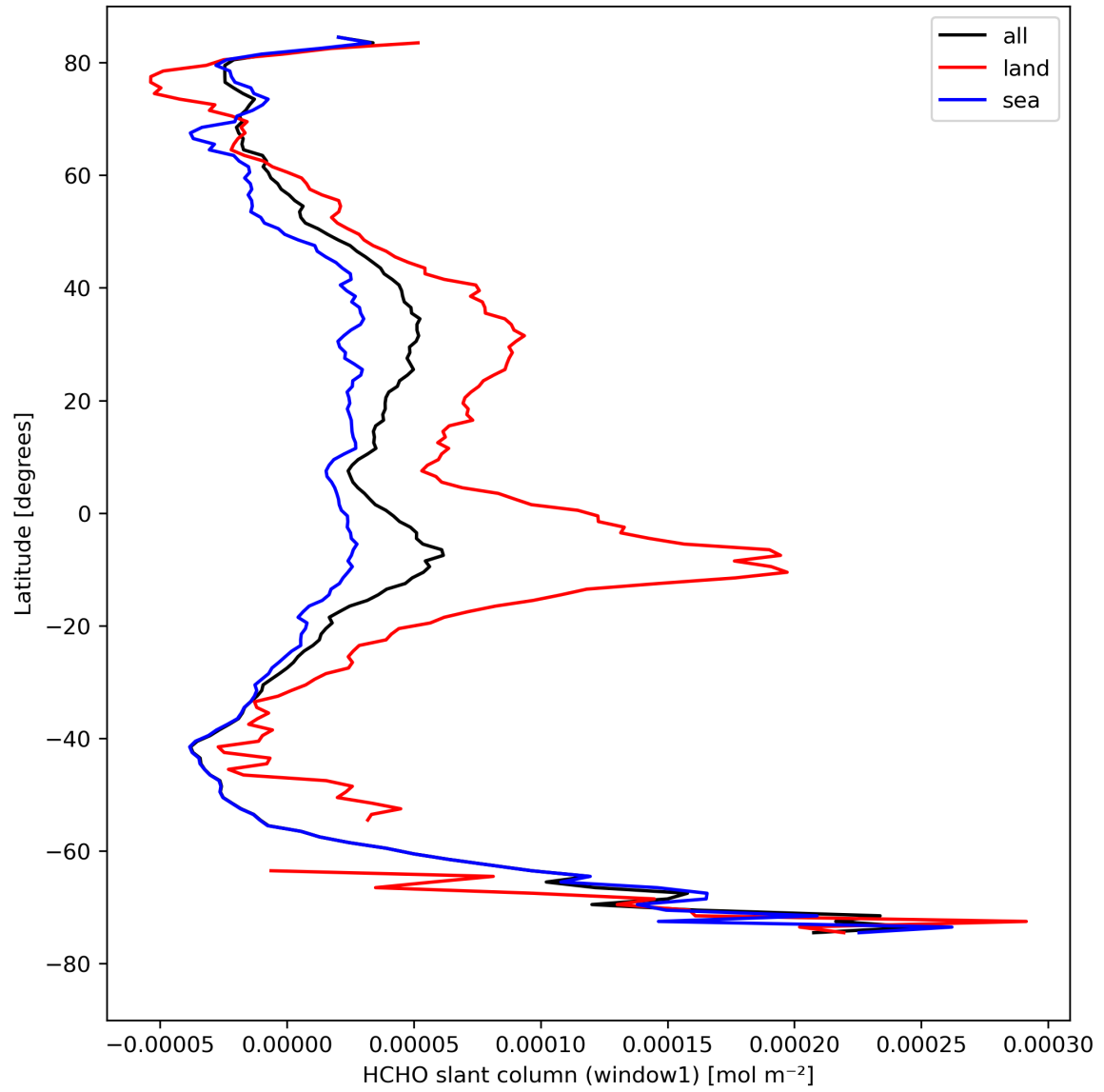
Figure 24: Zonal average of “HCHO slant column (window1)” for 2024-08-24 to 2024-08-26.
