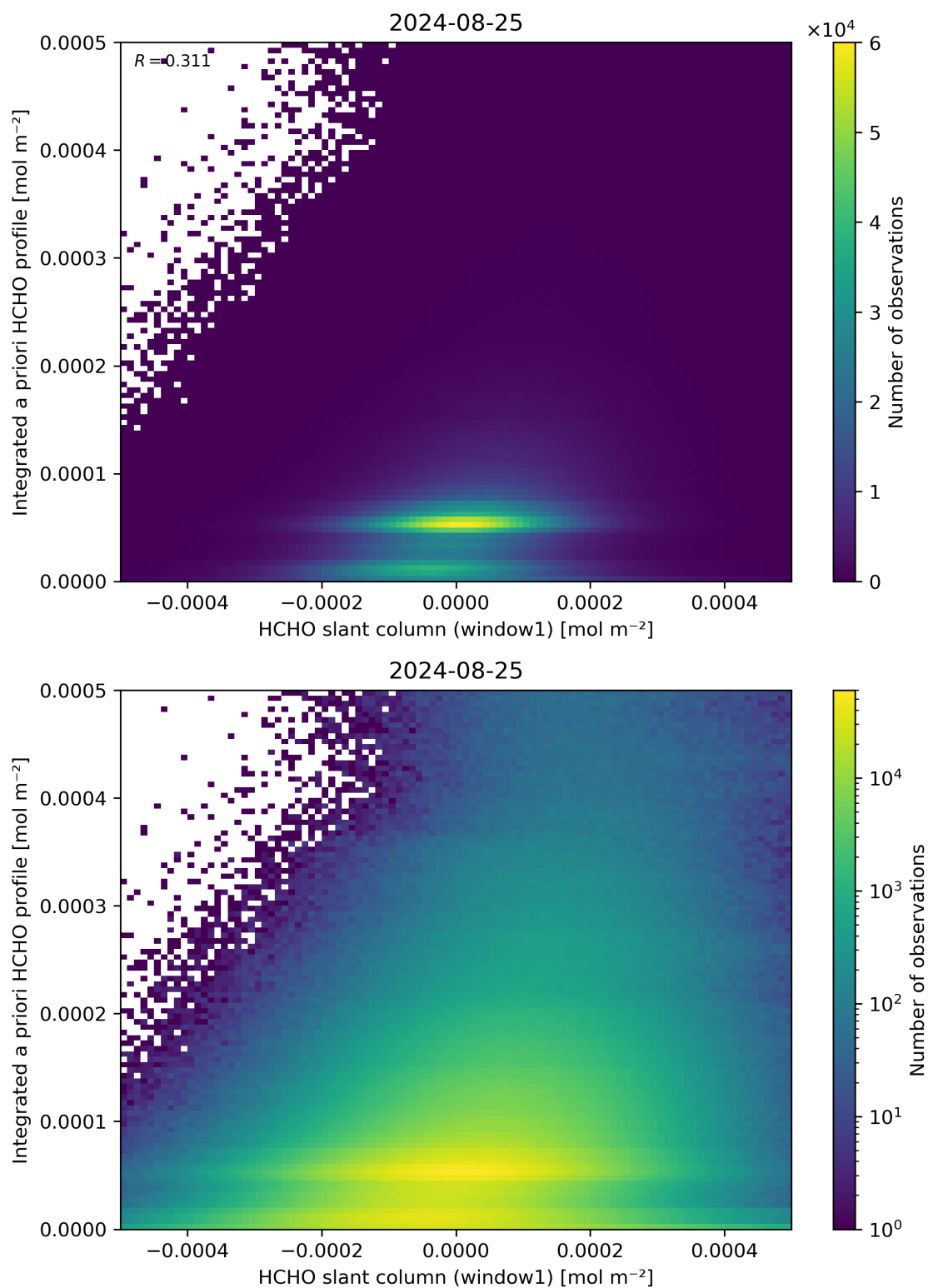
Figure 87: Scatter density plot of “HCHO slant column (window1)” against “Integrated a priori HCHO profile” for 2024-08-24 to 2024-08-26.
