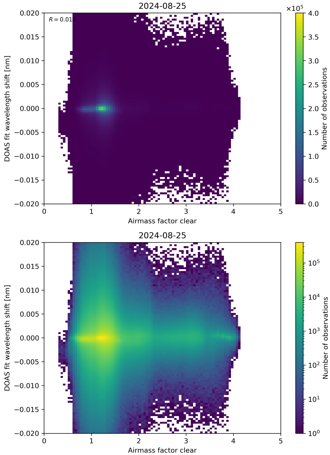
Figure 72: Scatter density plot of “Airmass factor clear” against “DOAS fit wavelength shift” for 2024-08-24 to 2024-08-26.
