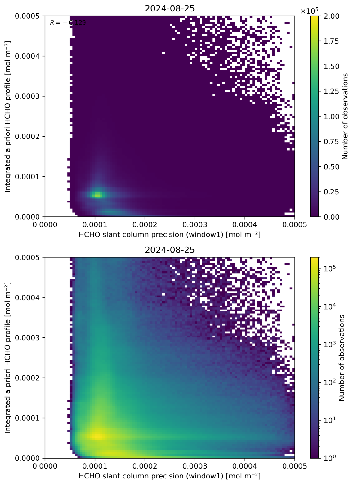
Figure 96: Scatter density plot of “HCHO slant column precision (window1)” against “Integrated a priori HCHO profile” for 2024-08-24 to 2024-08-26.
