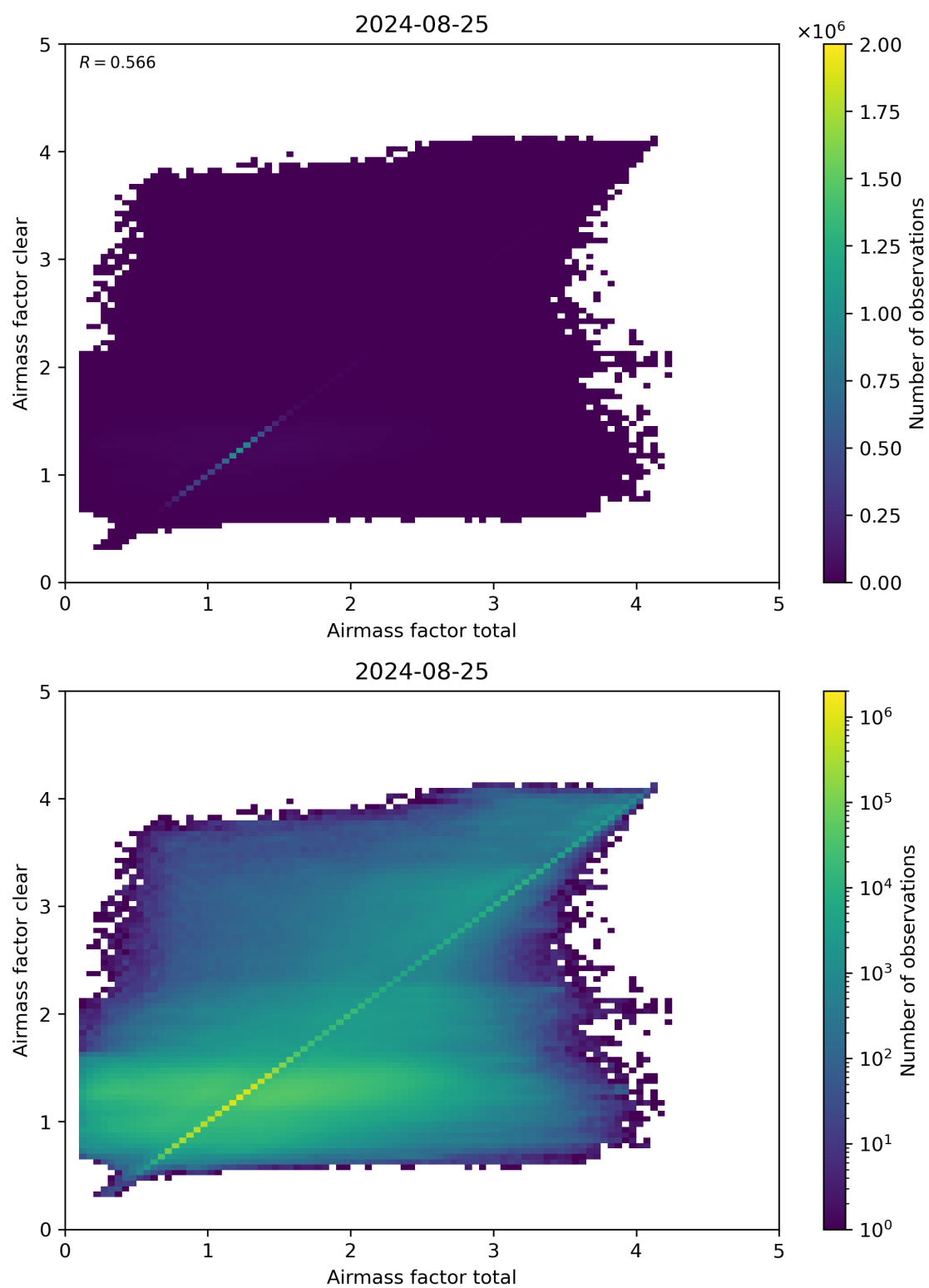
Figure 100: Scatter density plot of “Airmass factor total” against “Airmass factor clear” for 2024-08-24 to 2024-08-26.
