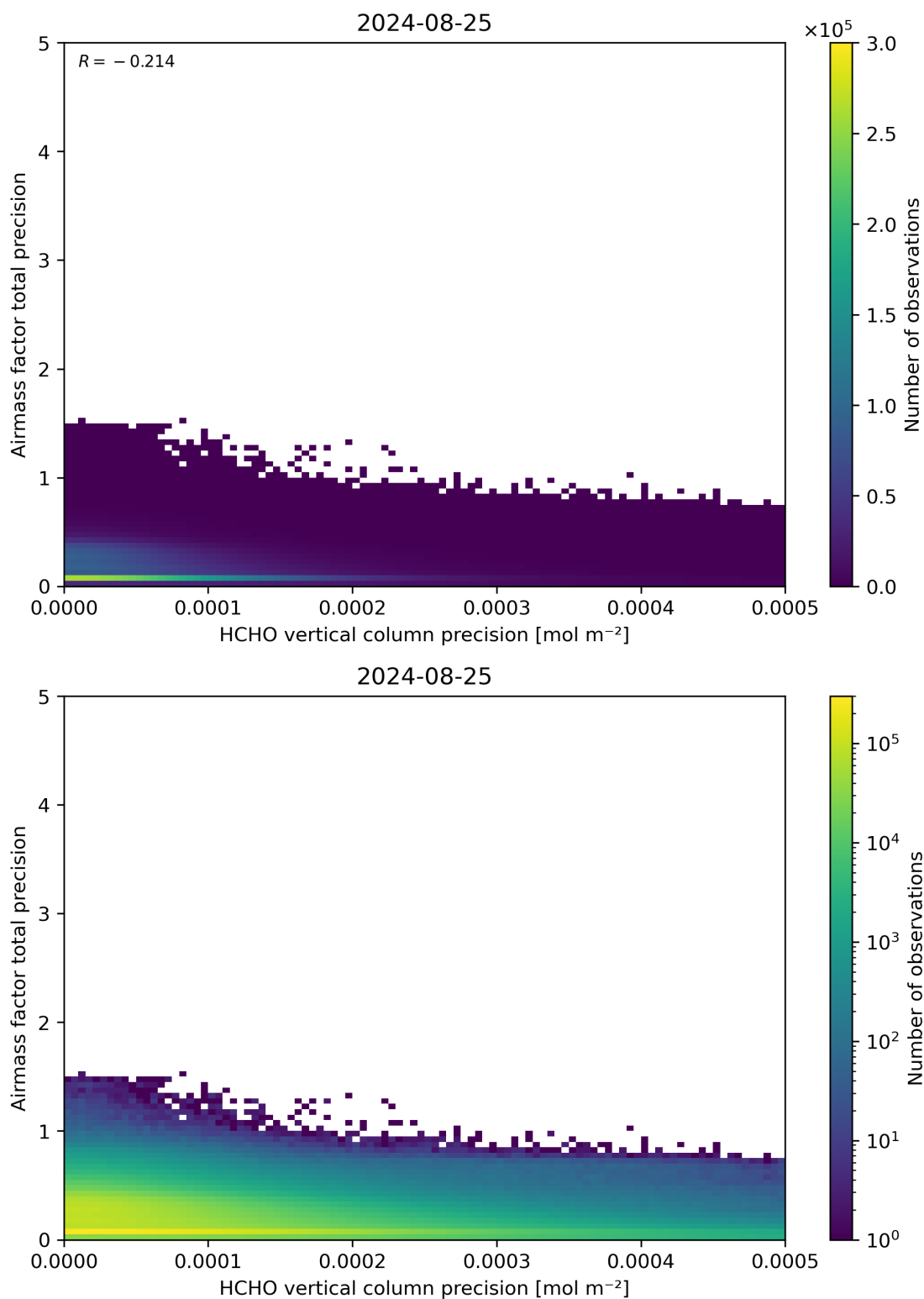
Figure 145: Scatter density plot of “HCHO vertical column precision” against “Airmass factor total precision” for 2024-08-24 to 2024-08-26.
