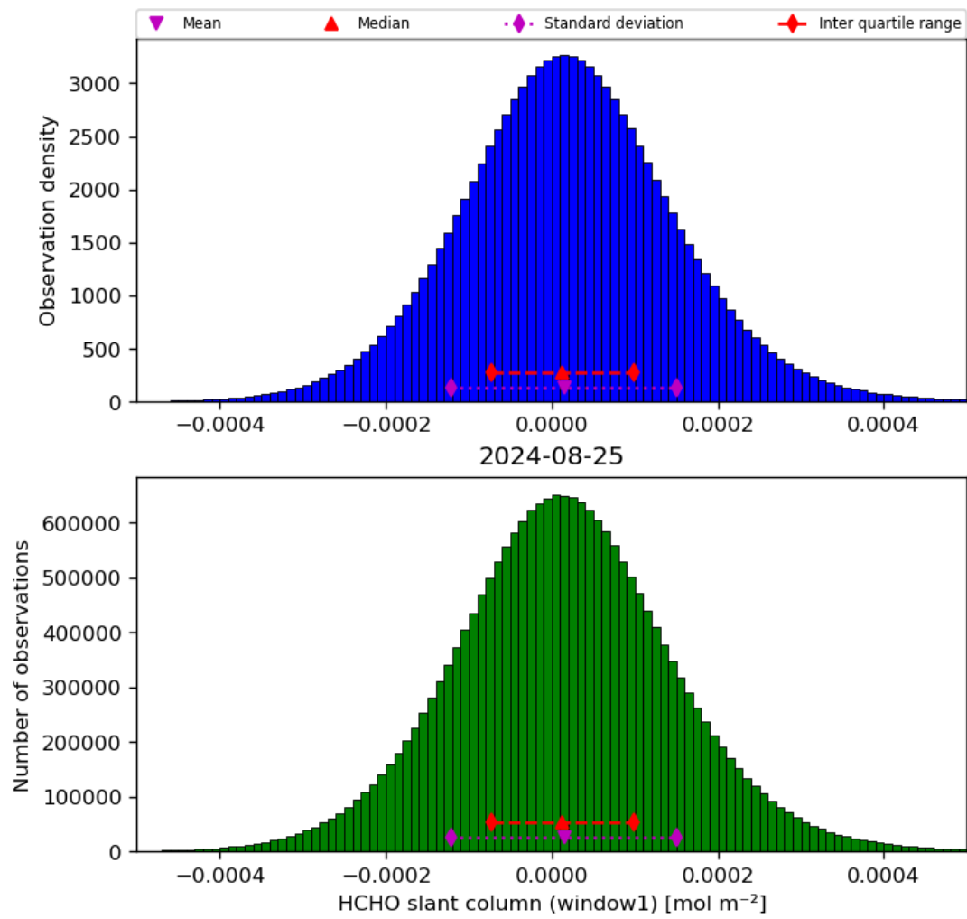
Figure 38: Histogram of “HCHO slant column (window1)” for 2024-08-24 to 2024-08-26
