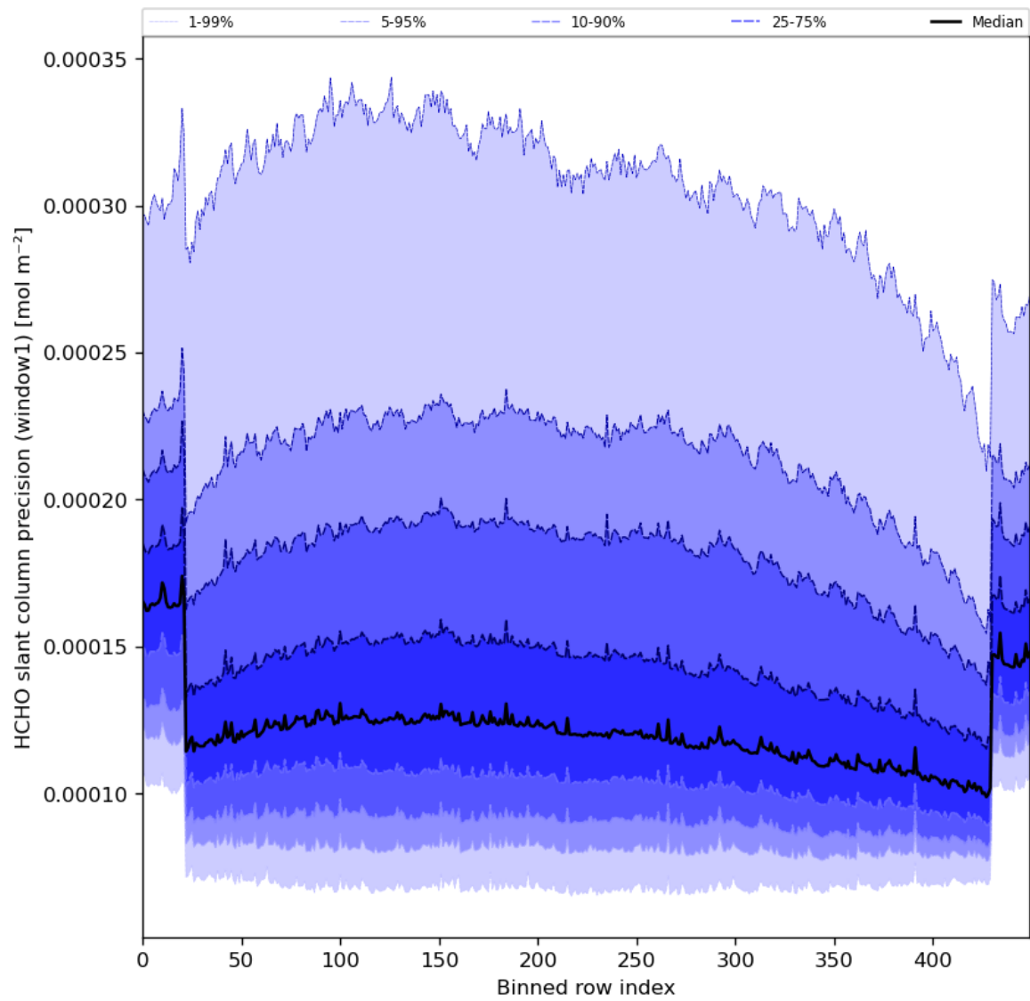
Figure 53: Along track statistics of “HCHO slant column precision (window1)” for 2024-08-24 to 2024-08-26
