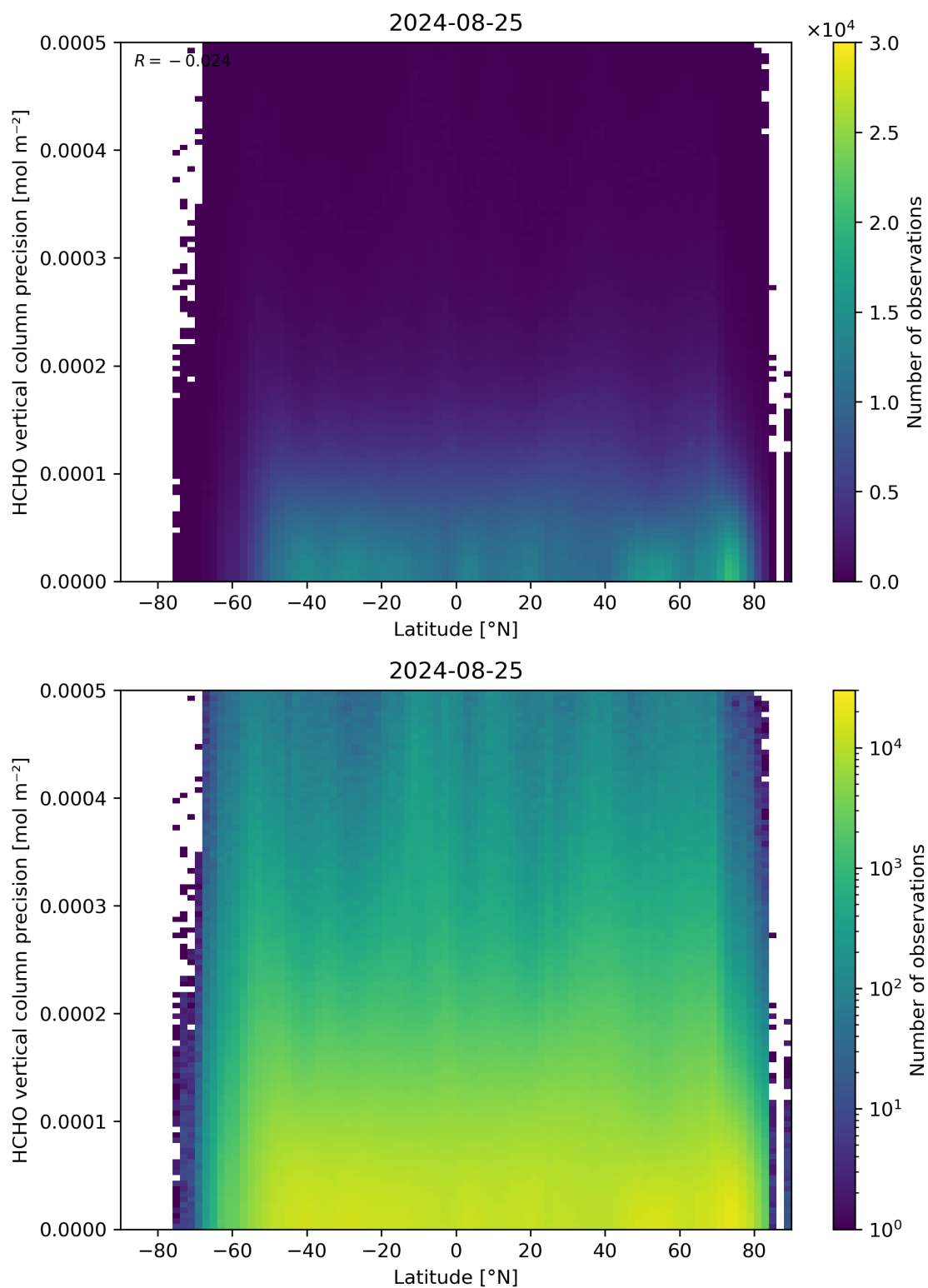
Figure 165: Scatter density plot of “Latitude” against “HCHO vertical column precision” for 2024-08-24 to 2024-08-26.
