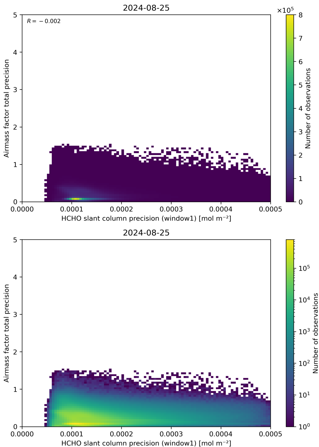
Figure 95: Scatter density plot of “HCHO slant column precision (window1)” against “Airmass factor total precision” for 2024-08-24 to 2024-08-26.
