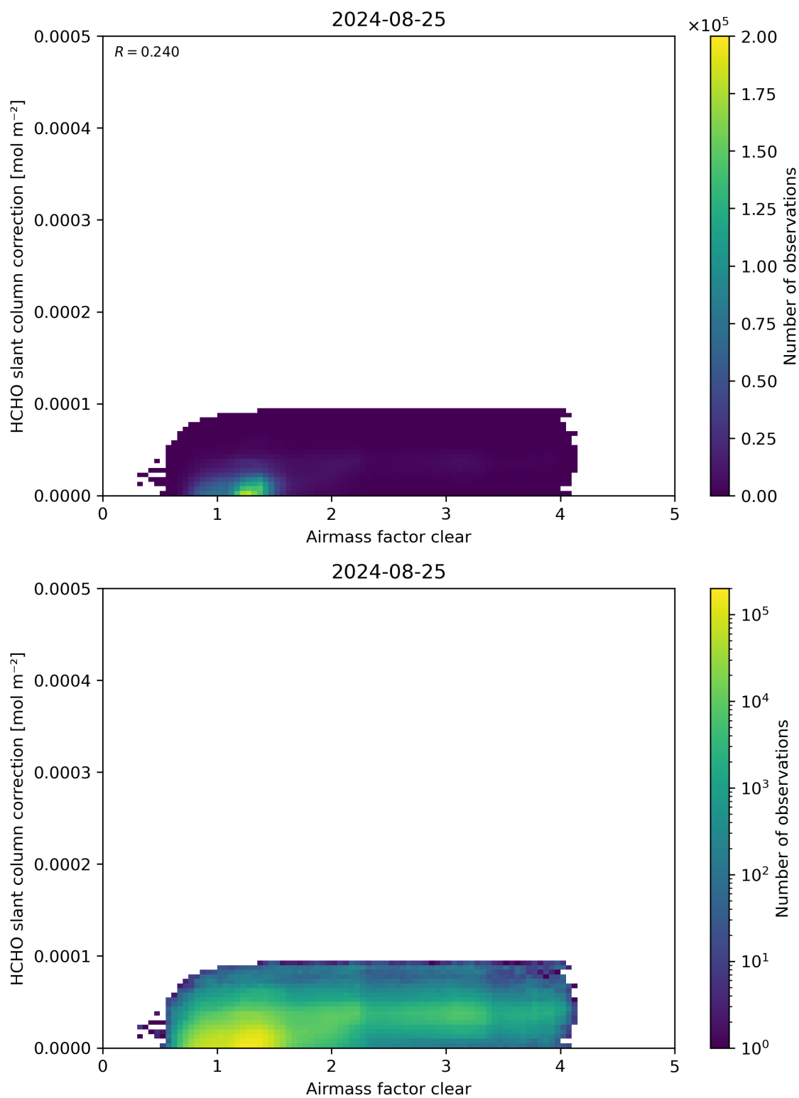
Figure 75: Scatter density plot of “Airmass factor clear” against “HCHO slant column correction” for 2024-08-24 to 2024-08-26.
