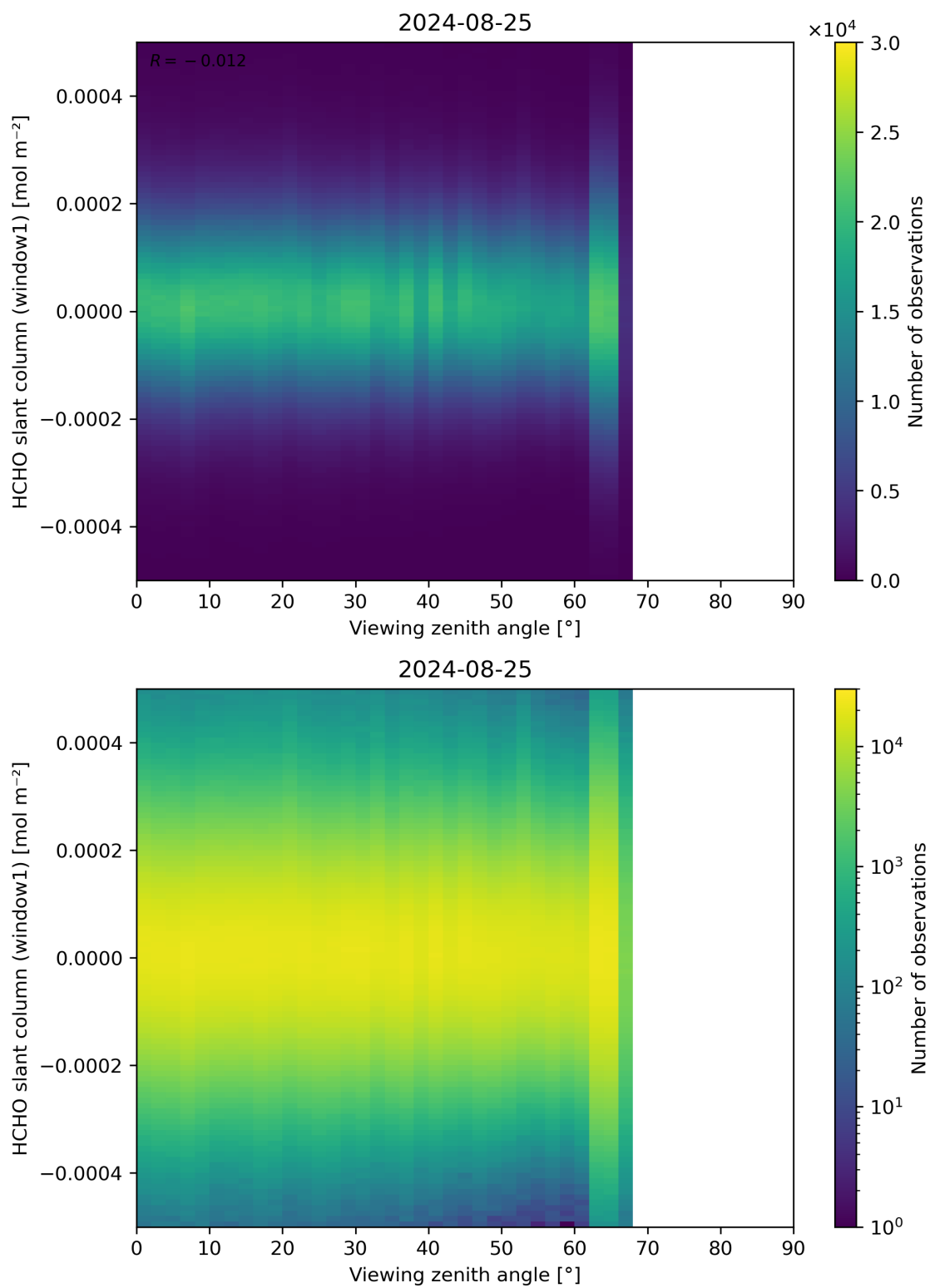
Figure 188: Scatter density plot of “Viewing zenith angle” against “HCHO slant column (window1)” for 2024-08-24 to 2024-08-26.
