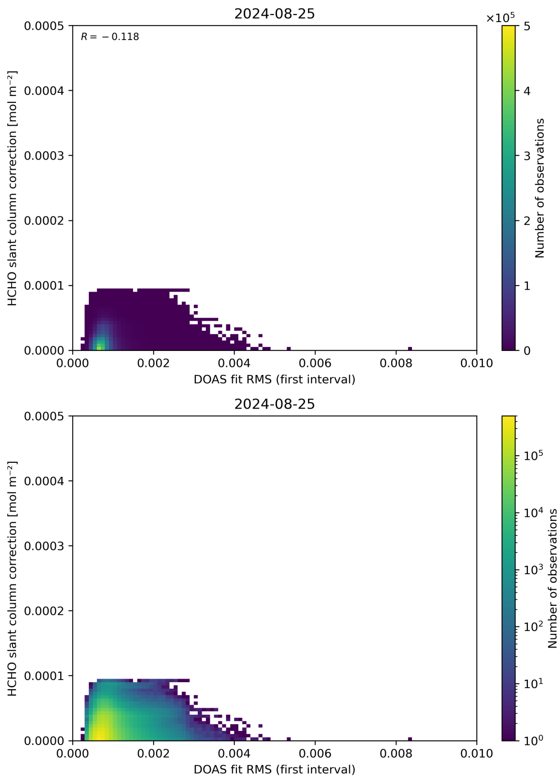
Figure 63: Scatter density plot of “DOAS fit RMS (first interval)” against “HCHO slant column correction” for 2024-08-24 to 2024-08-26.
