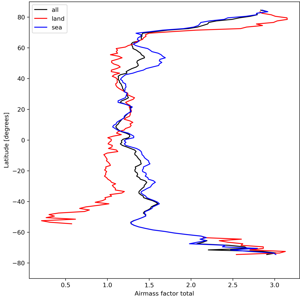
Figure 26: Zonal average of “Airmass factor total” for 2024-08-24 to 2024-08-26.
