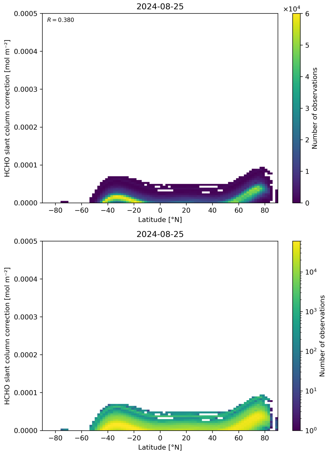
Figure 158: Scatter density plot of “Latitude” against “HCHO slant column correction” for 2024-08-24 to 2024-08-26.
