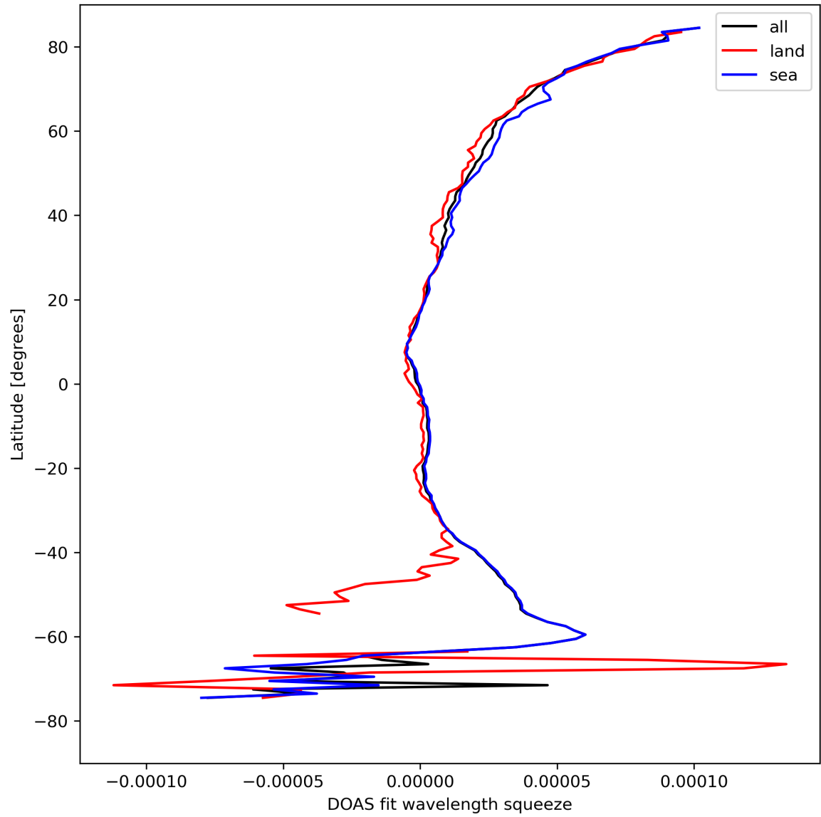
Figure 31: Zonal average of “DOAS fit wavelength squeeze” for 2024-08-24 to 2024-08-26.
