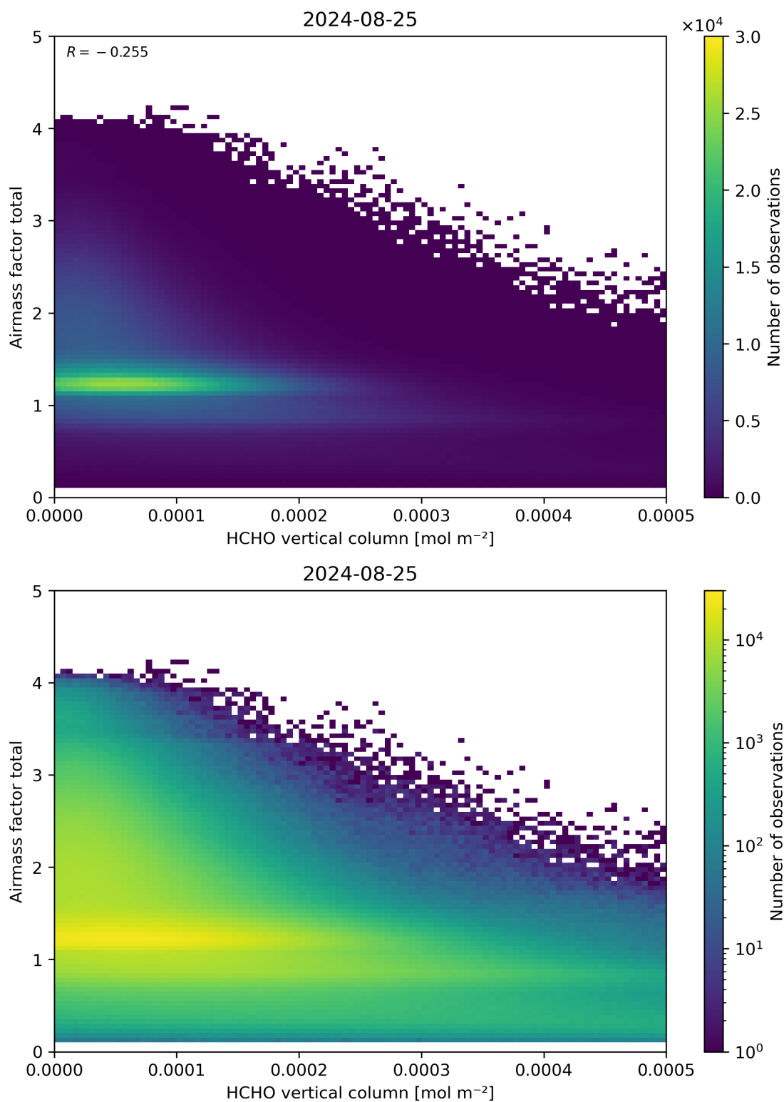
Figure 131: Scatter density plot of “HCHO vertical column” against “Airmass factor total” for 2024-08-24 to 2024-08-26.
