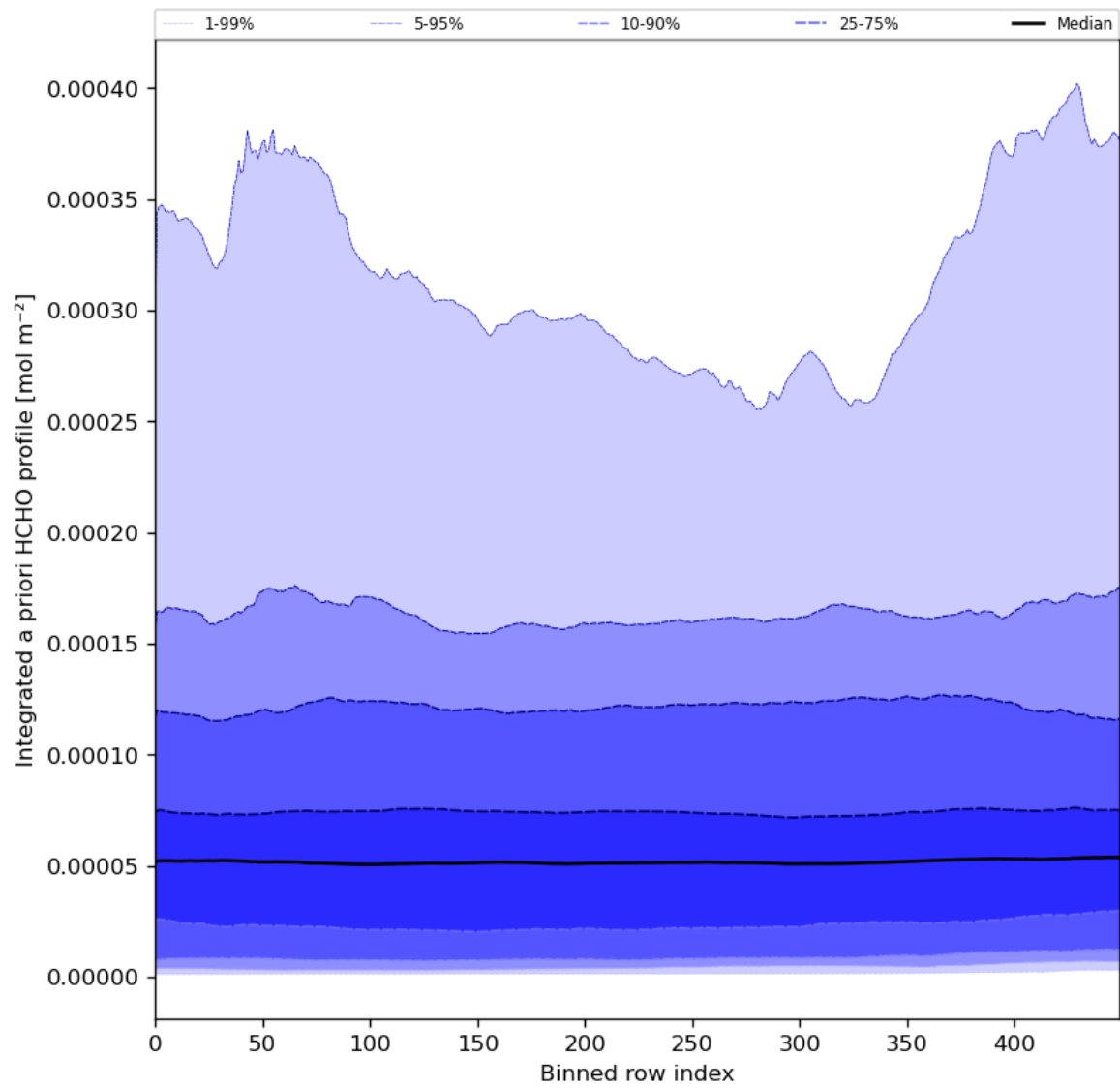
Figure 57: Along track statistics of “Integrated a priori HCHO profile” for 2024-08-24 to 2024-08-26
