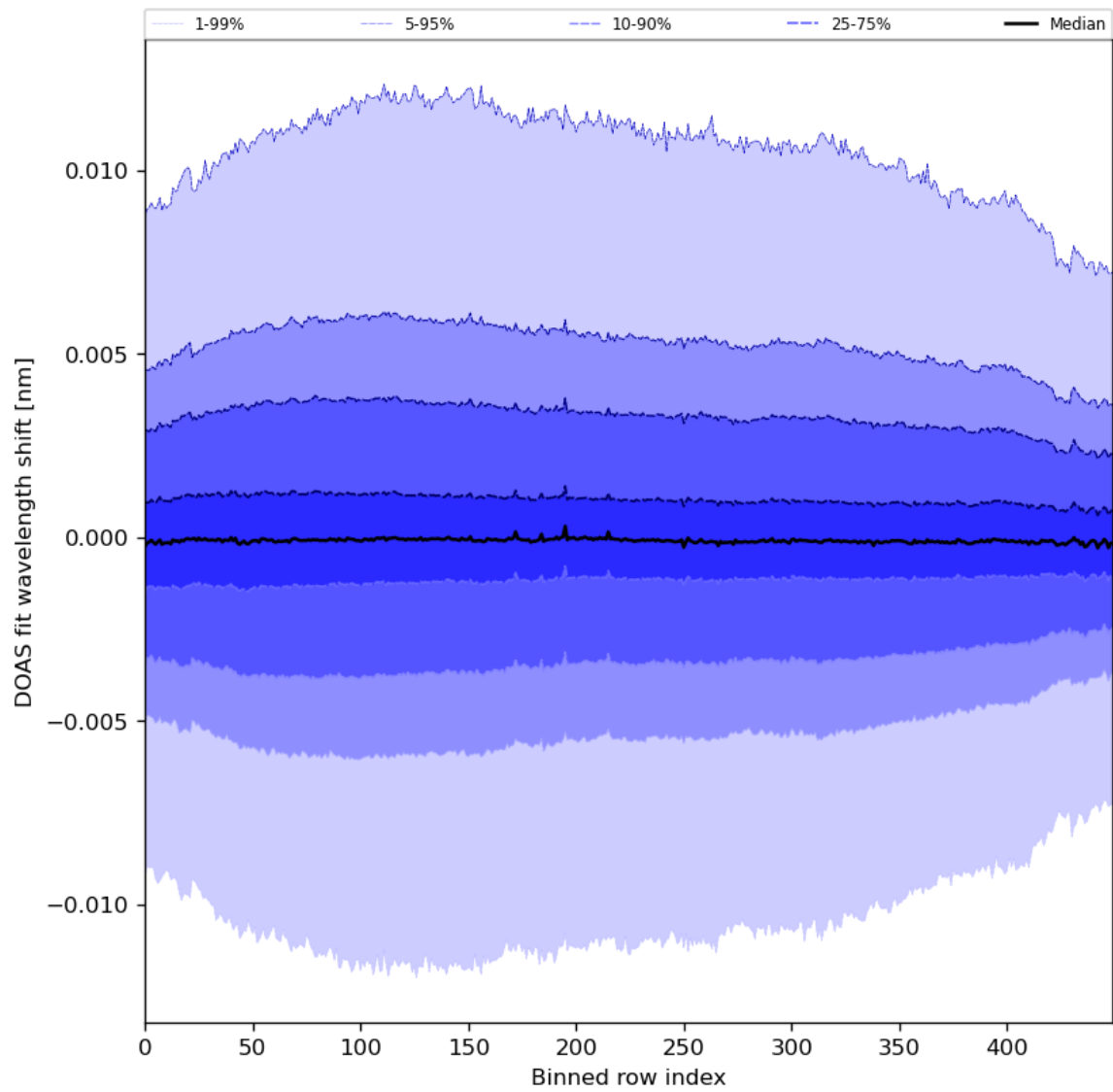
Figure 58: Along track statistics of “DOAS fit wavelength shift” for 2024-08-24 to 2024-08-26
