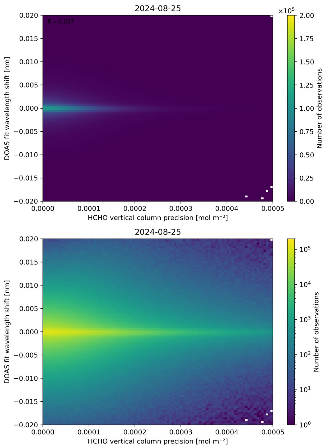
Figure 137: Scatter density plot of “HCHO vertical column precision” against “DOAS fit wavelength shift” for 2024-08-24 to 2024-08-26.
