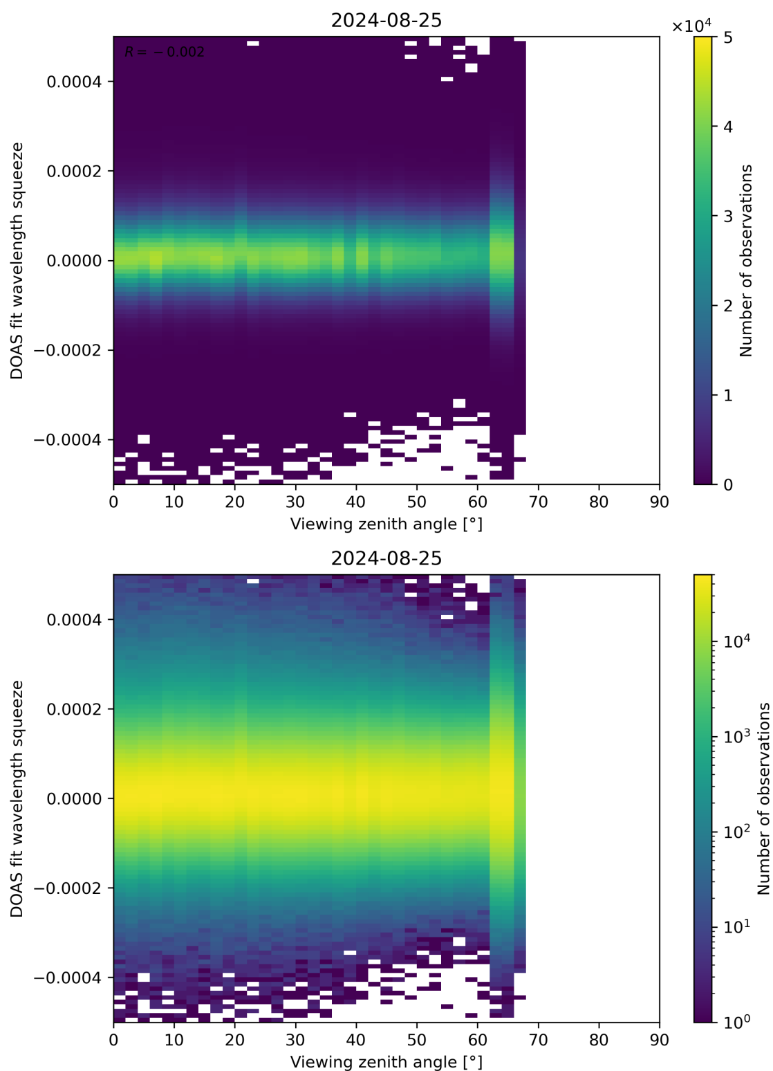
Figure 184: Scatter density plot of “Viewing zenith angle” against “DOAS fit wavelength squeeze” for 2024-08-24 to 2024-08-26.
