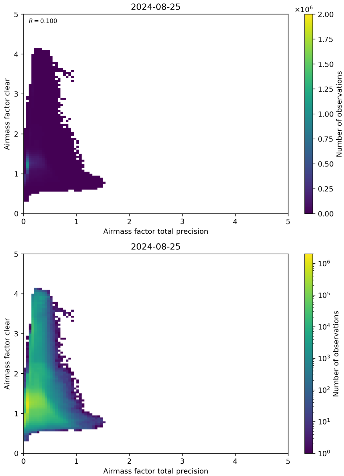
Figure 108: Scatter density plot of “Airmass factor total precision” against “Airmass factor clear” for 2024-08-24 to 2024-08-26.
