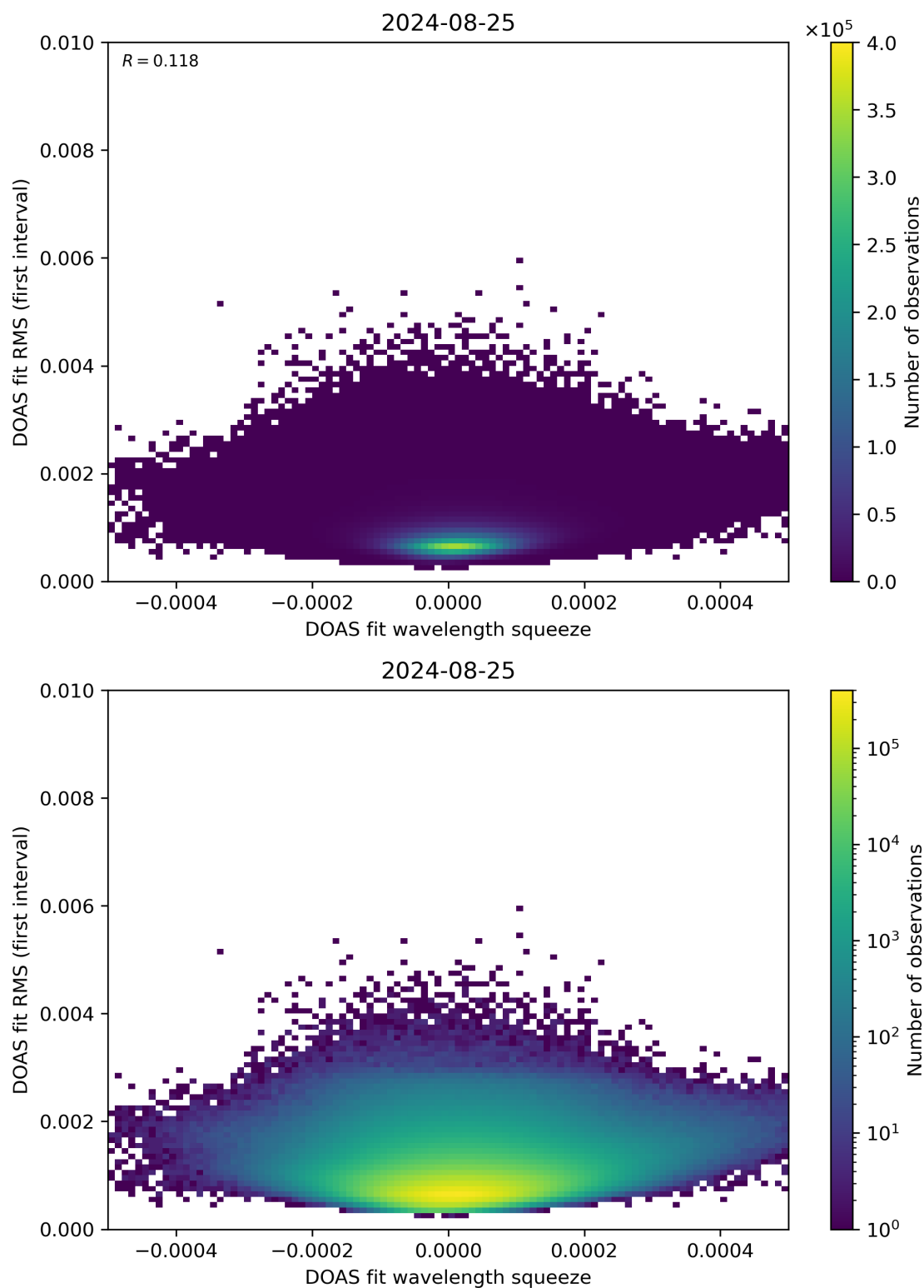
Figure 68: Scatter density plot of “DOAS fit wavelength squeeze” against “DOAS fit RMS (first interval)” for 2024-08-24 to 2024-08-26.
