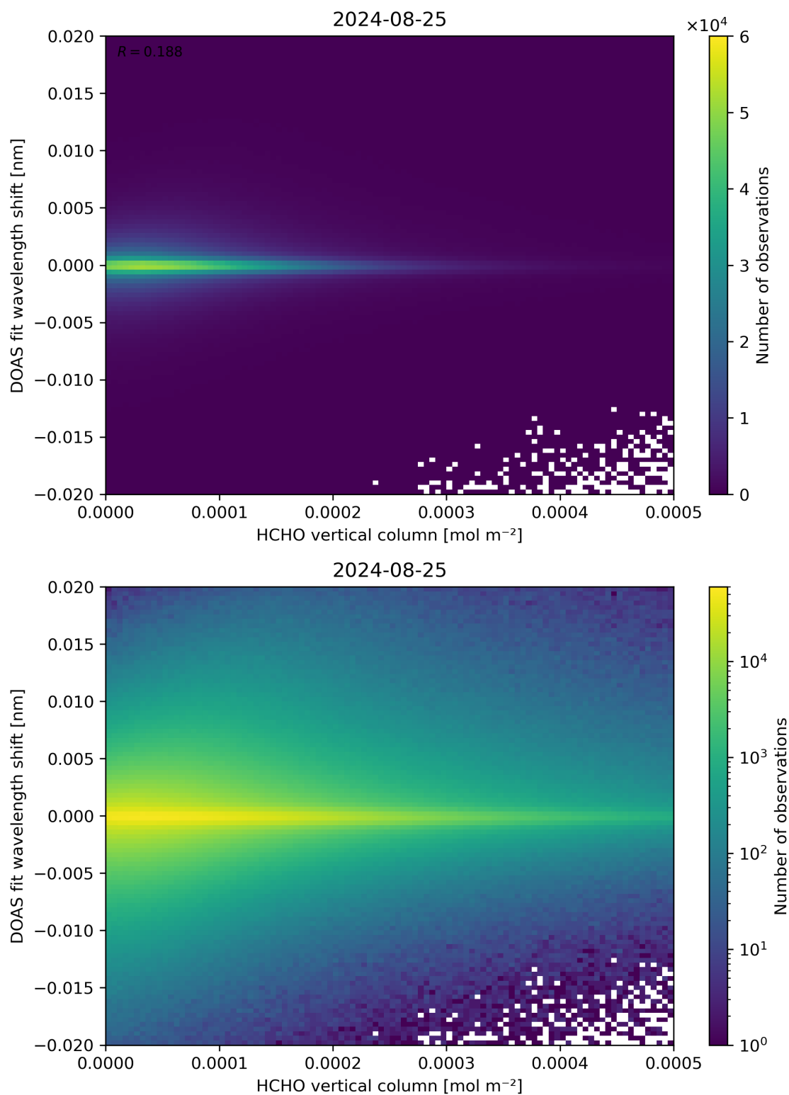
Figure 124: Scatter density plot of “HCHO vertical column” against “DOAS fit wavelength shift” for 2024-08-24 to 2024-08-26.
