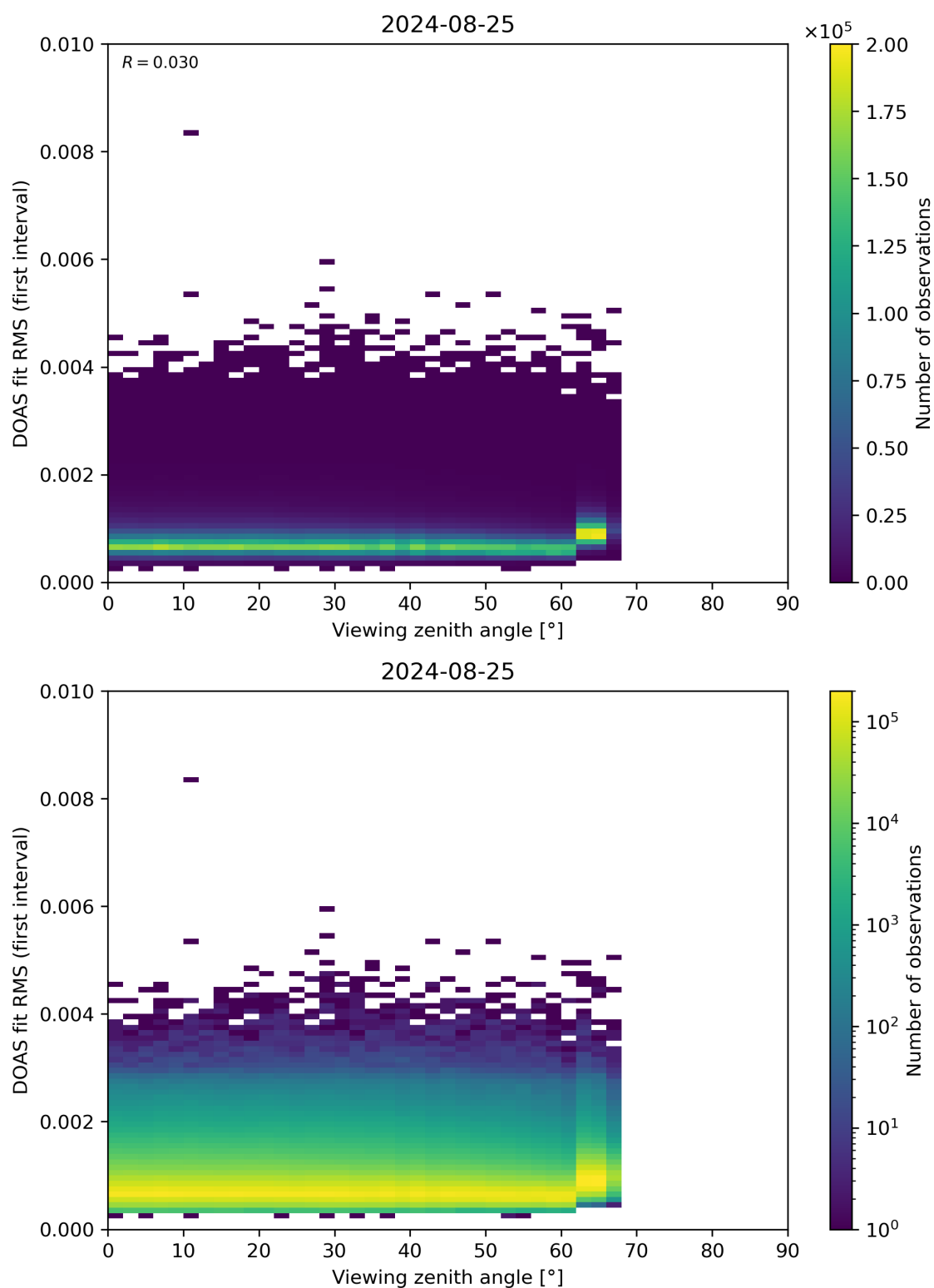
Figure 182: Scatter density plot of “Viewing zenith angle” against “DOAS fit RMS (first interval)” for 2024-08-24 to 2024-08-26.
