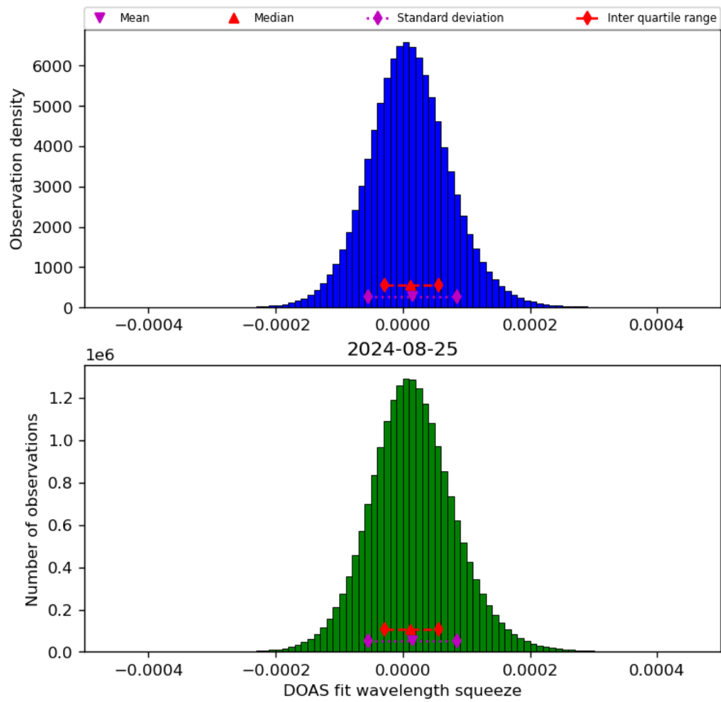
Figure 45: Histogram of “DOAS fit wavelength squeeze” for 2024-08-24 to 2024-08-26
