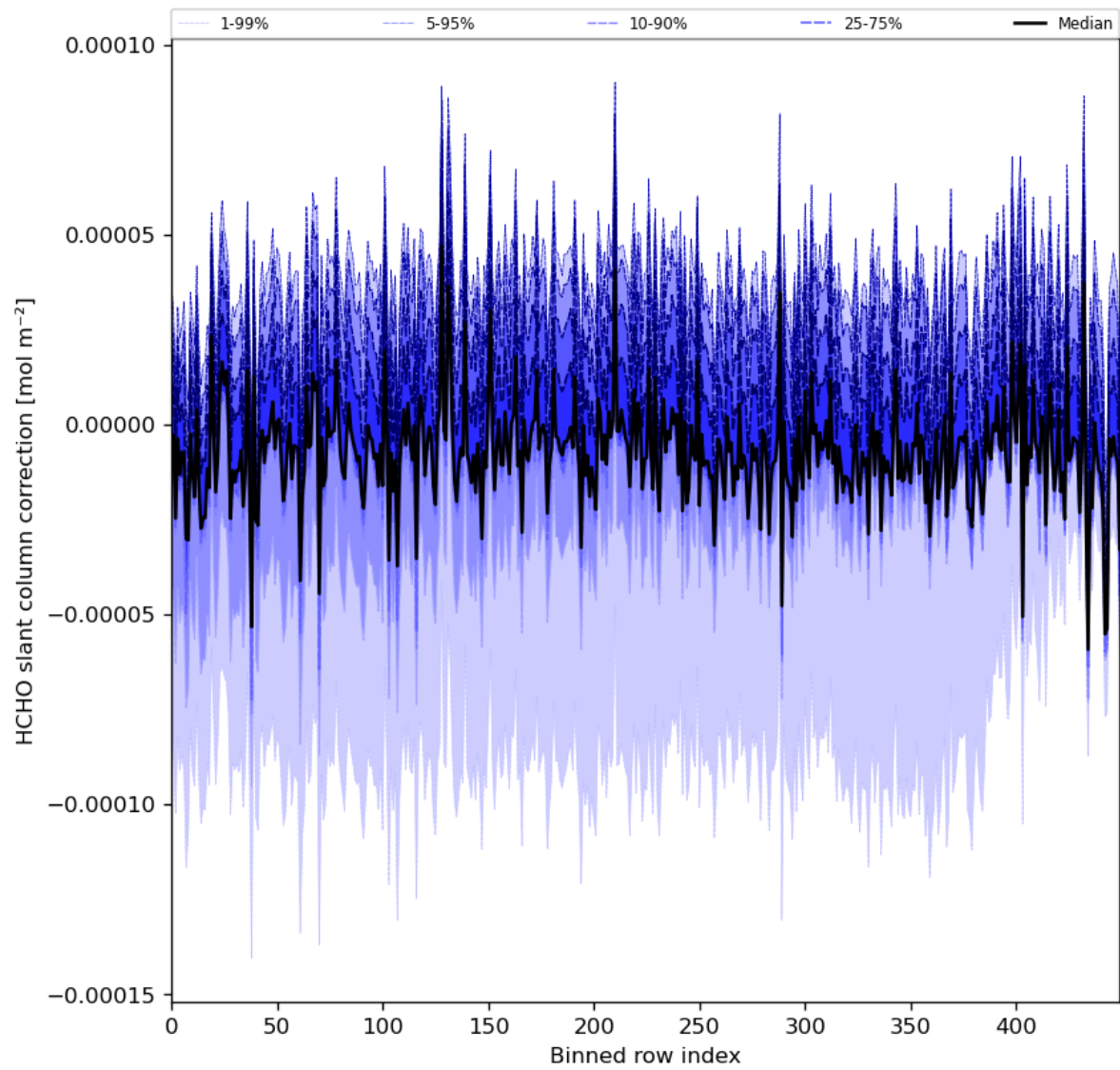
Figure 61: Along track statistics of “HCHO slant column correction” for 2024-08-24 to 2024-08-26
