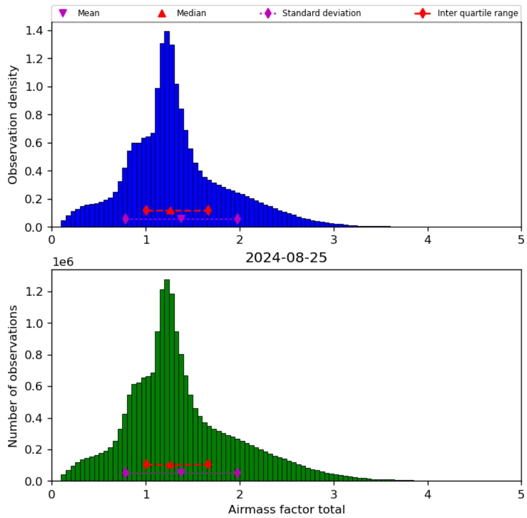
Figure 40: Histogram of “Airmass factor total” for 2024-08-24 to 2024-08-26
