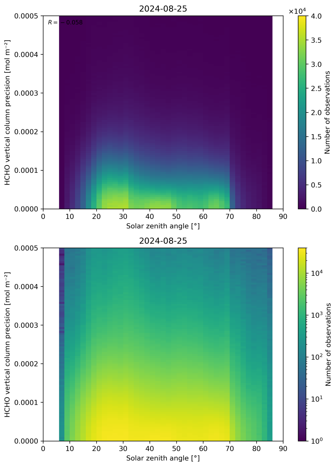
Figure 179: Scatter density plot of “Solar zenith angle” against “HCHO vertical column precision” for 2024-08-24 to 2024-08-26.
