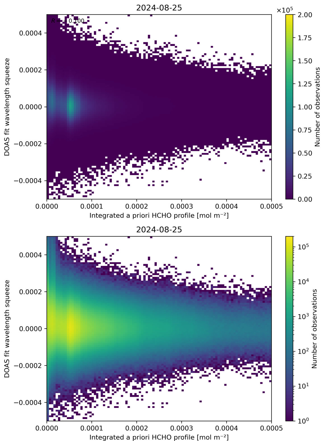
Figure 150: Scatter density plot of “Integrated a priori HCHO profile” against “DOAS fit wavelength squeeze” for 2024-08-24 to 2024-08-26.
