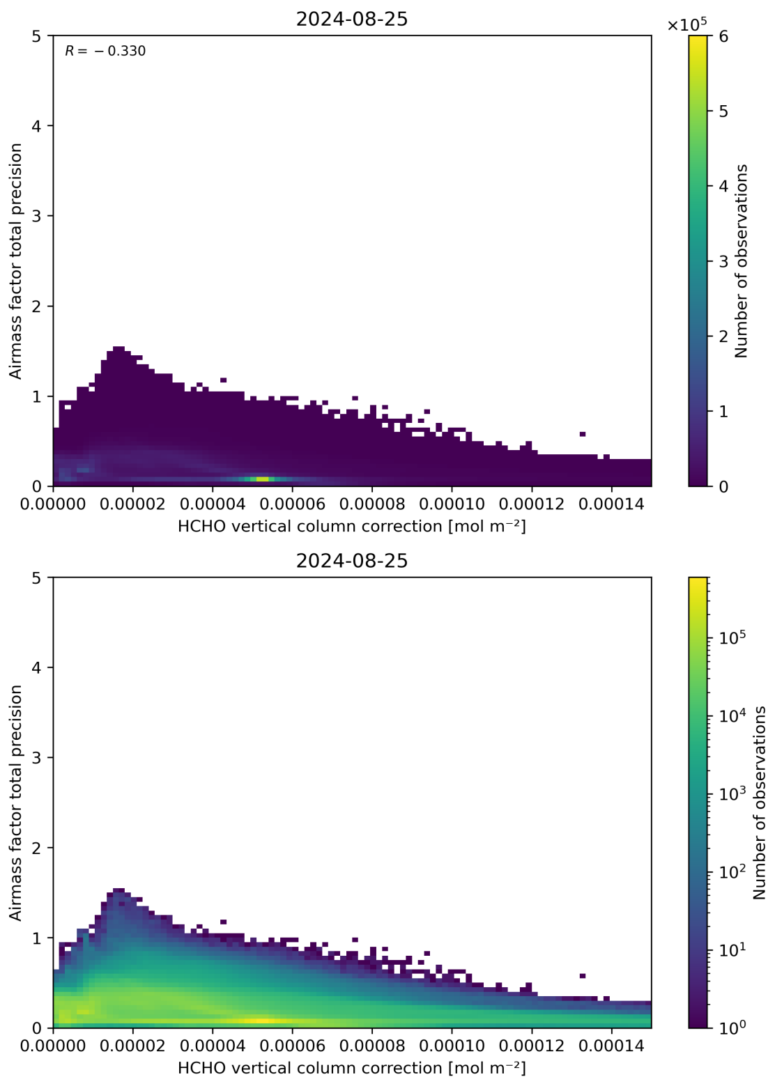
Figure 121: Scatter density plot of “HCHO vertical column correction” against “Airmass factor total precision” for 2024-08-24 to 2024-08-26.
