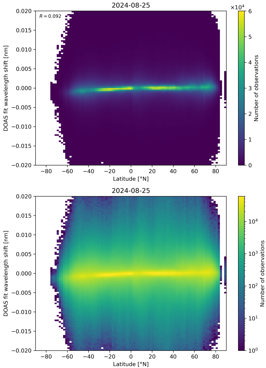
Figure 154: Scatter density plot of “Latitude” against “DOAS fit wavelength shift” for 2024-08-24 to 2024-08-26.
