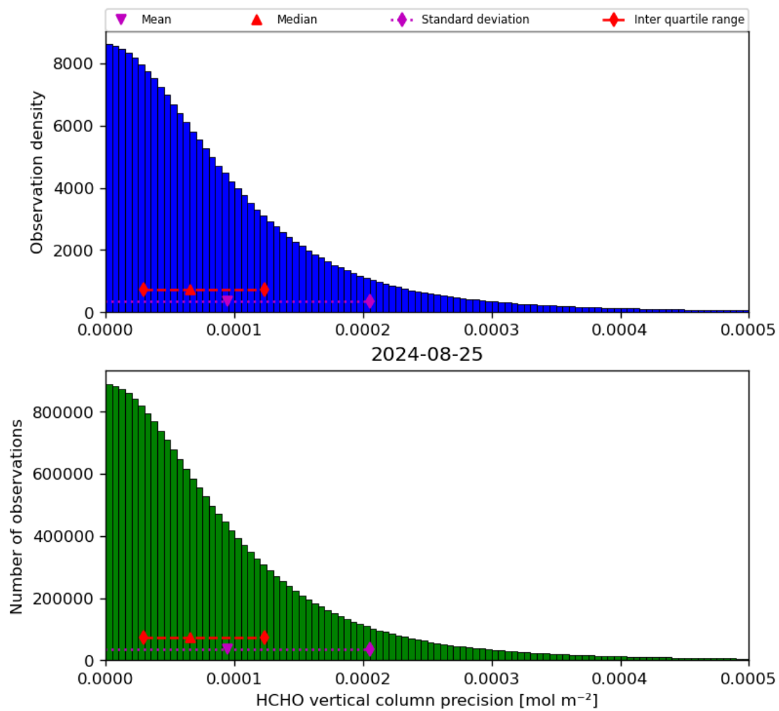
Figure 36: Histogram of “HCHO vertical column precision” for 2024-08-24 to 2024-08-26
