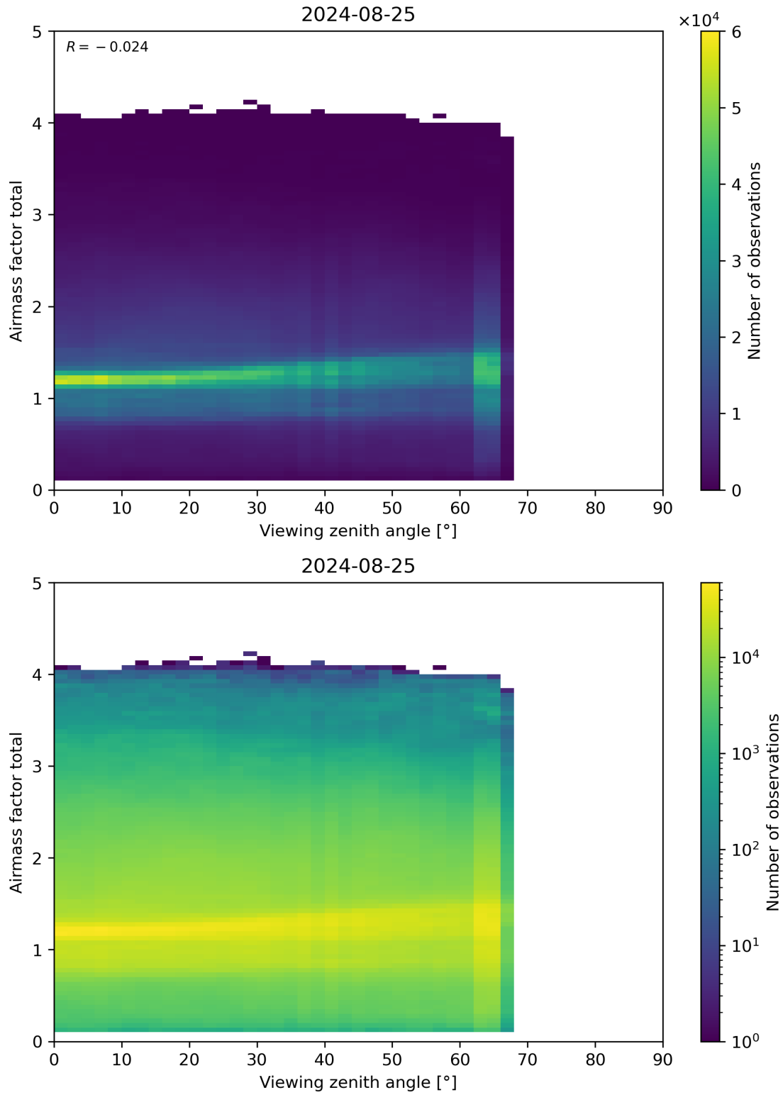
Figure 190: Scatter density plot of “Viewing zenith angle” against “Airmass factor total” for 2024-08-24 to 2024-08-26.
