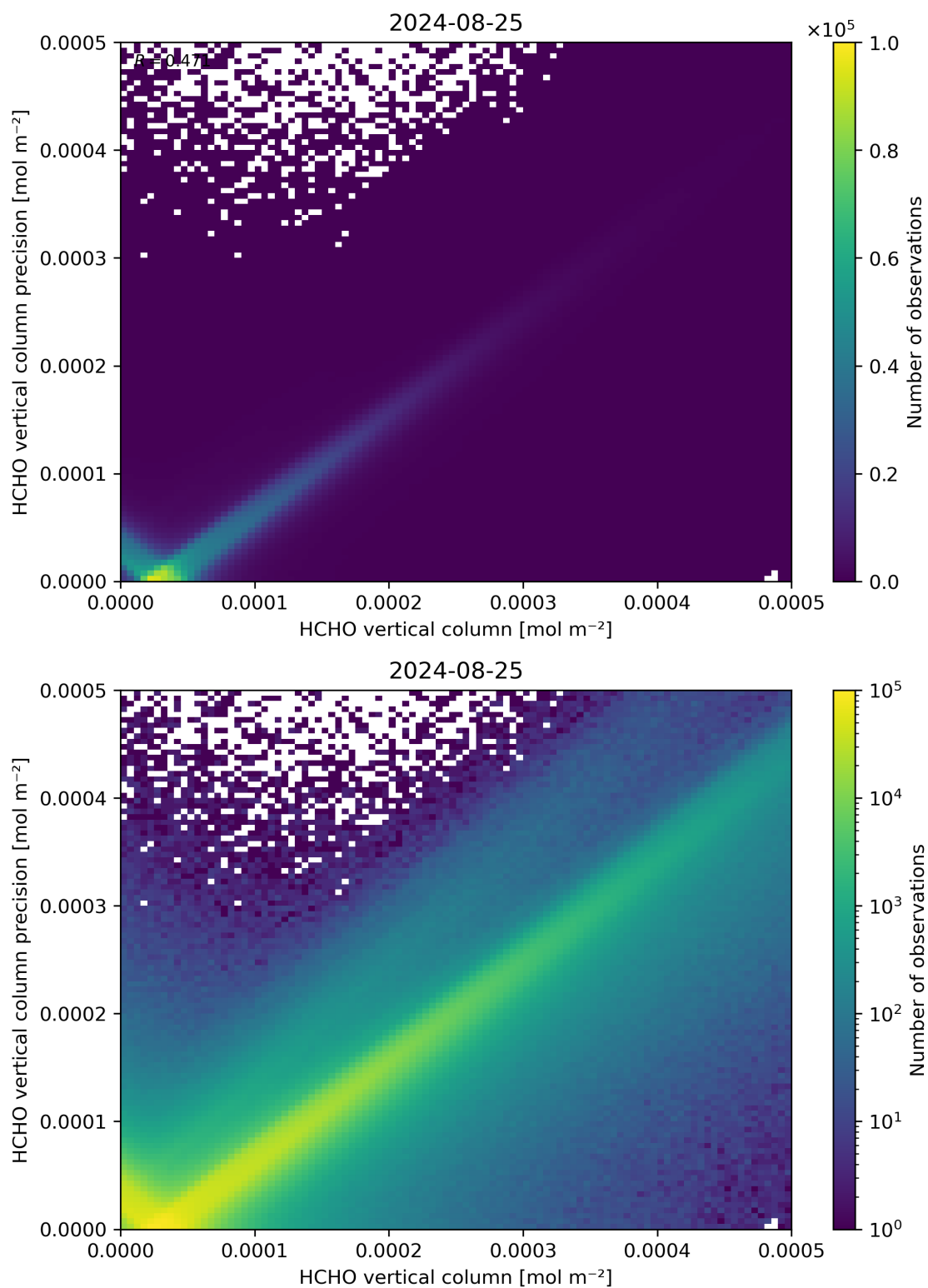
Figure 134: Scatter density plot of “HCHO vertical column” against “HCHO vertical column precision” for 2024-08-24 to 2024-08-26.
