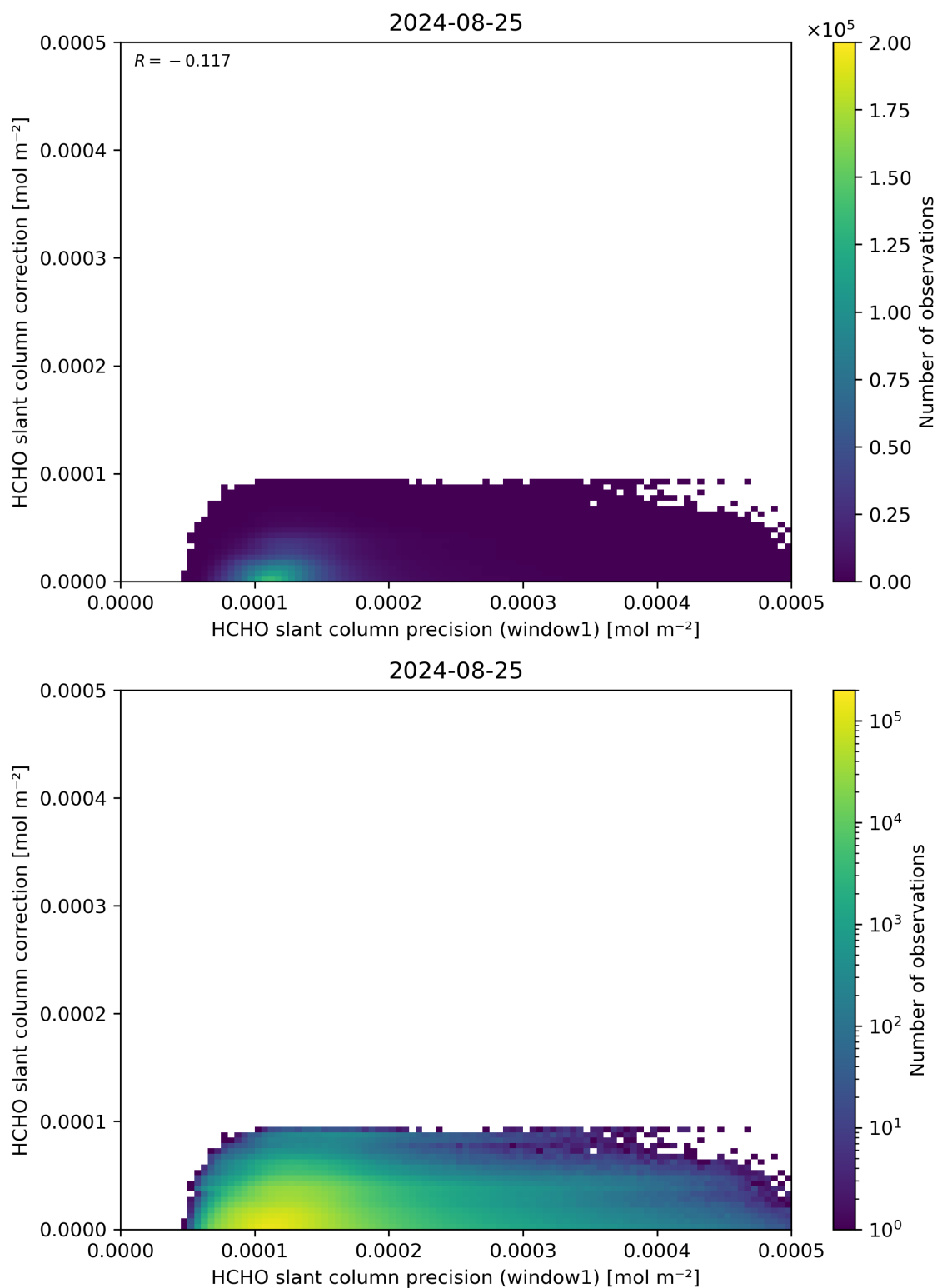
Figure 93: Scatter density plot of “HCHO slant column precision (window1)” against “HCHO slant column correction” for 2024-08-24 to 2024-08-26.
