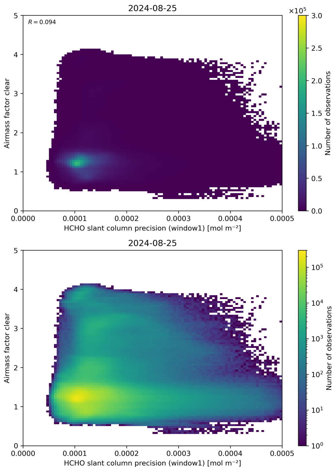
Figure 91: Scatter density plot of “HCHO slant column precision (window1)” against “Airmass factor clear” for 2024-08-24 to 2024-08-26.
