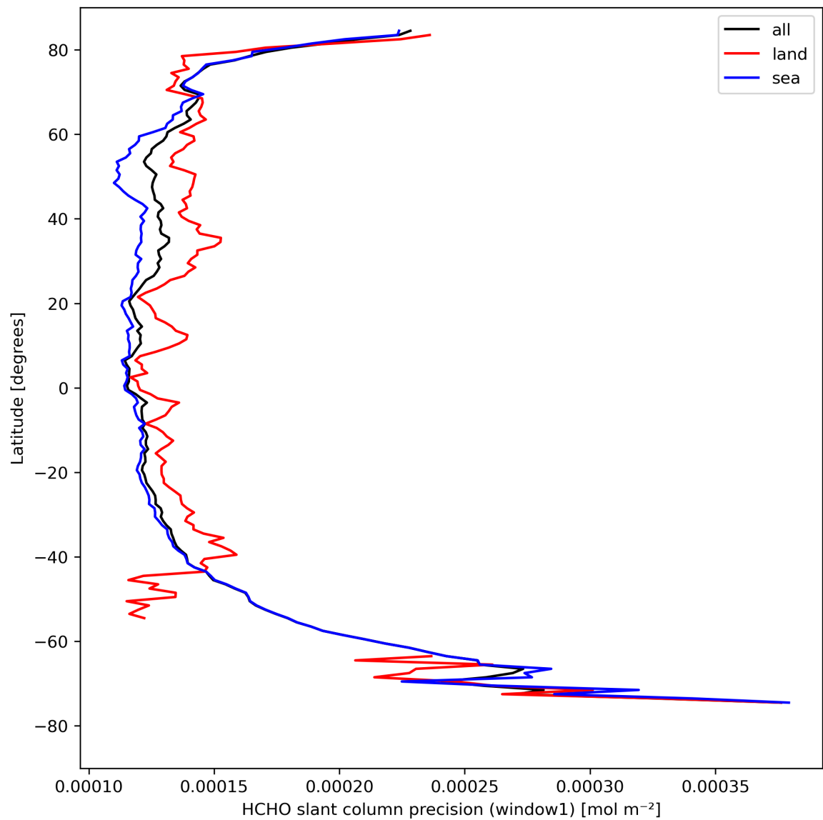
Figure 25: Zonal average of “HCHO slant column precision (window1)” for 2024-08-24 to 2024-08-26.
