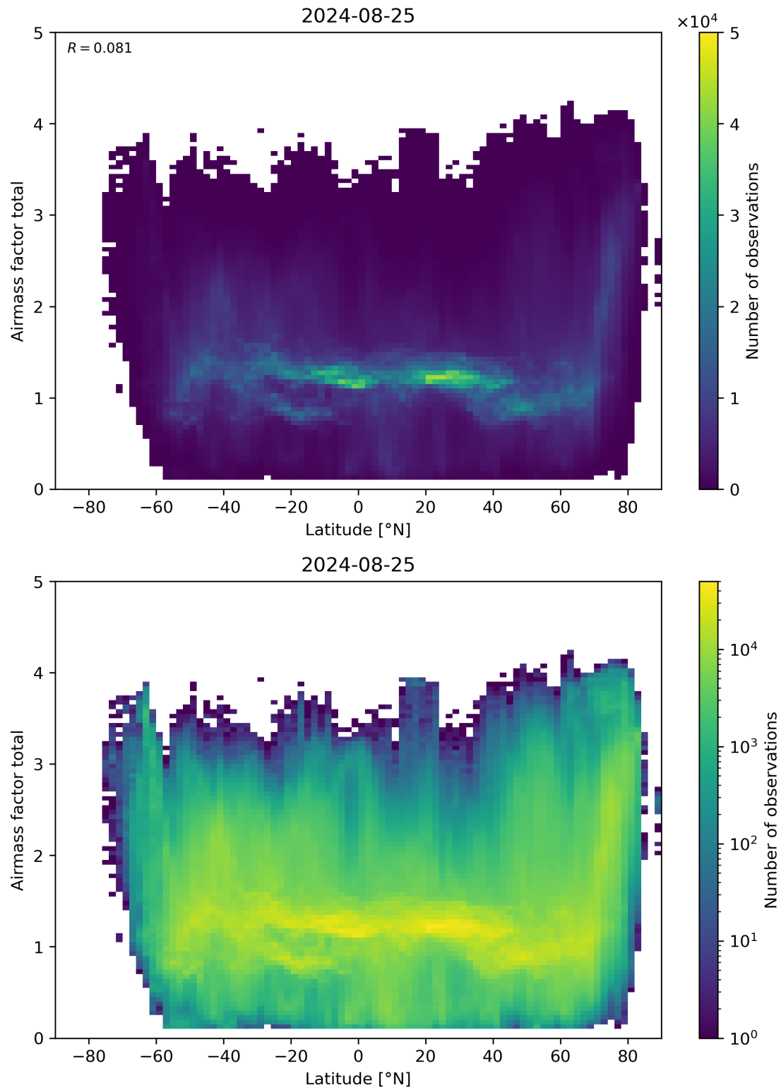
Figure 161: Scatter density plot of “Latitude” against “Airmass factor total” for 2024-08-24 to 2024-08-26.
