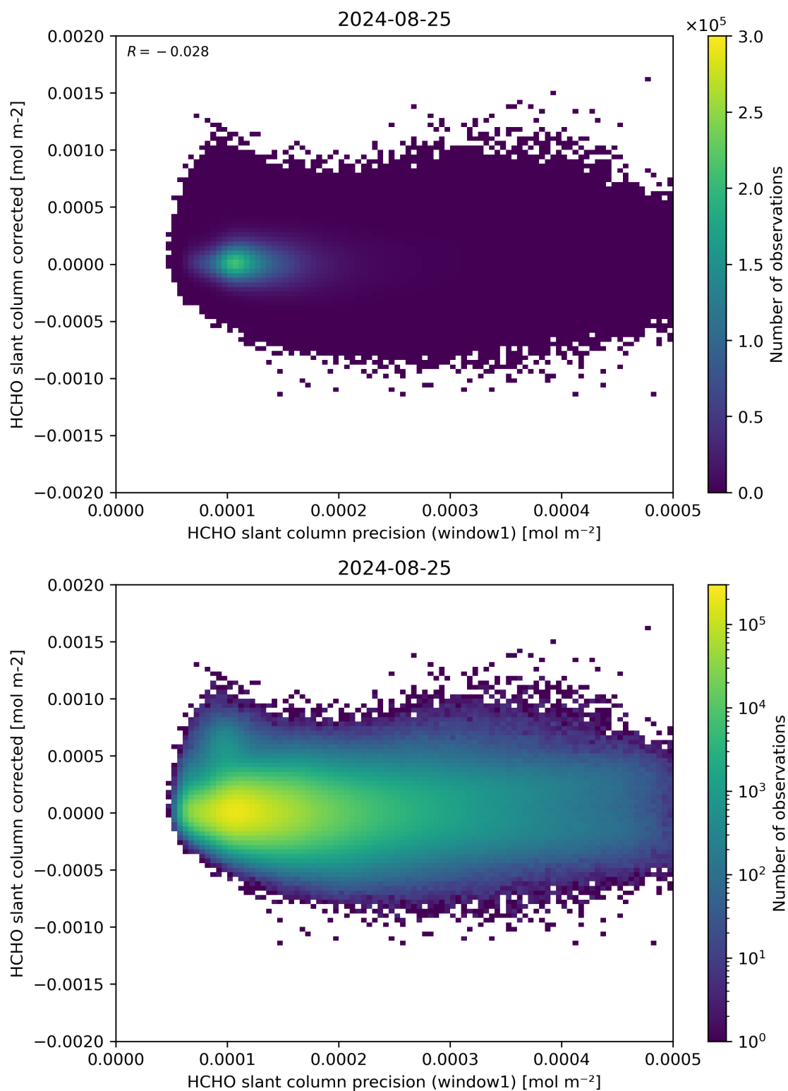
Figure 92: Scatter density plot of “HCHO slant column precision (window1)” against “HCHO slant column corrected” for 2024-08-24 to 2024-08-26.
