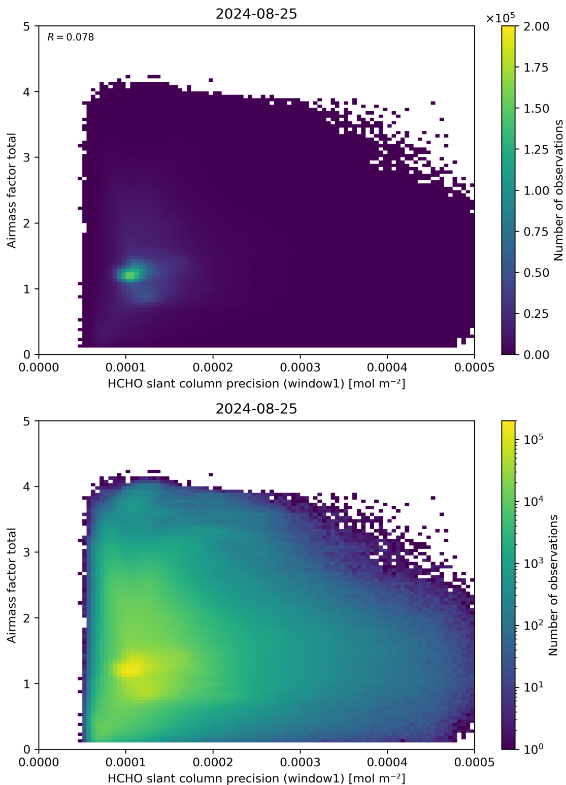
Figure 94: Scatter density plot of “HCHO slant column precision (window1)” against “Airmass factor total” for 2024-08-24 to 2024-08-26.
