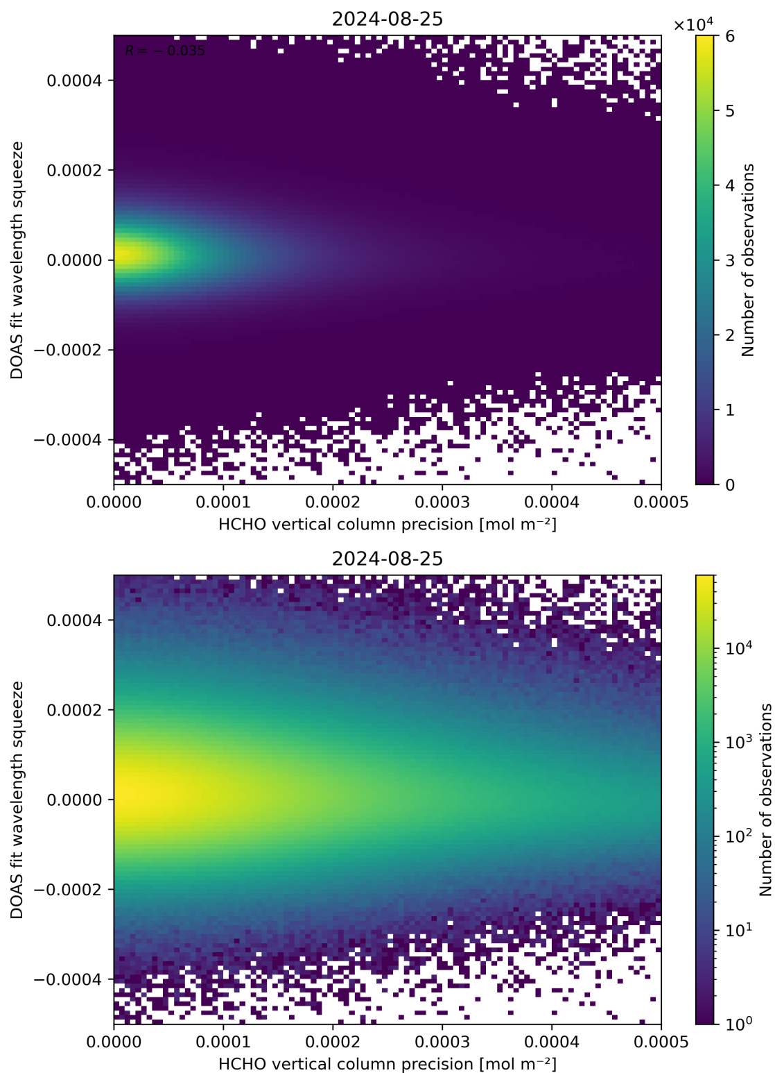
Figure 138: Scatter density plot of “HCHO vertical column precision” against “DOAS fit wavelength squeeze” for 2024-08-24 to 2024-08-26.
