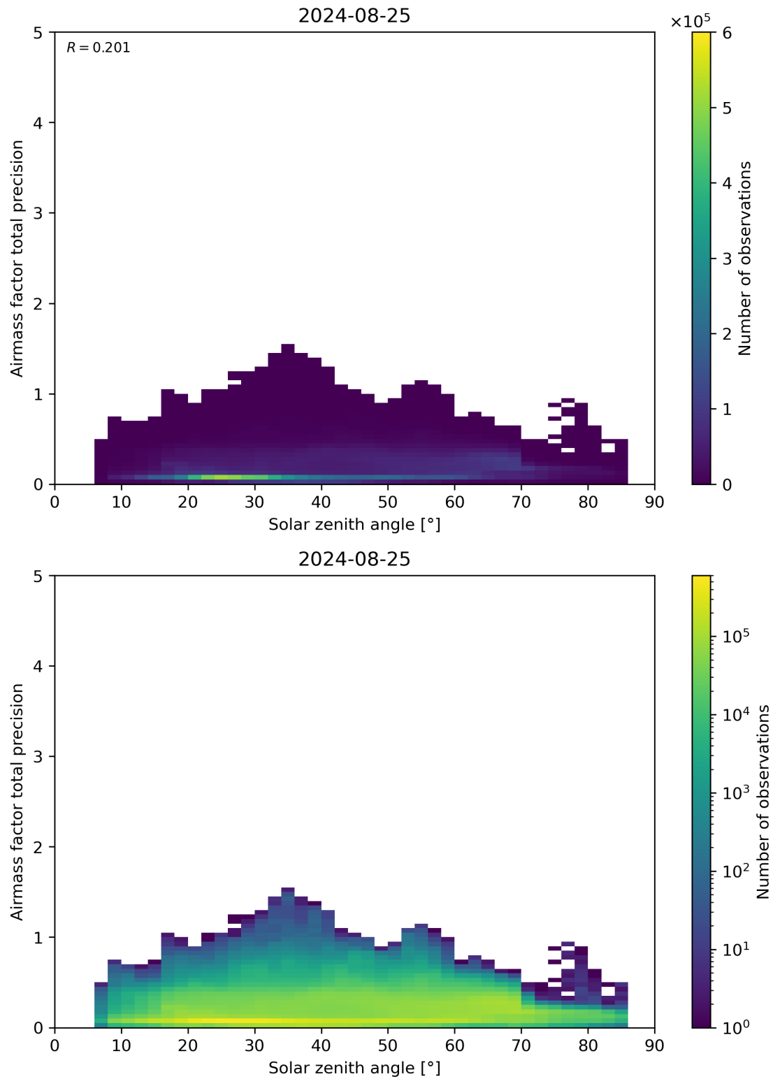
Figure 176: Scatter density plot of “Solar zenith angle” against “Airmass factor total precision” for 2024-08-24 to 2024-08-26.
