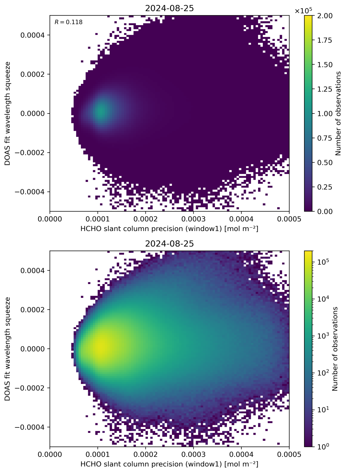
Figure 90: Scatter density plot of “HCHO slant column precision (window1)” against “DOAS fit wavelength squeeze” for 2024-08-24 to 2024-08-26.
