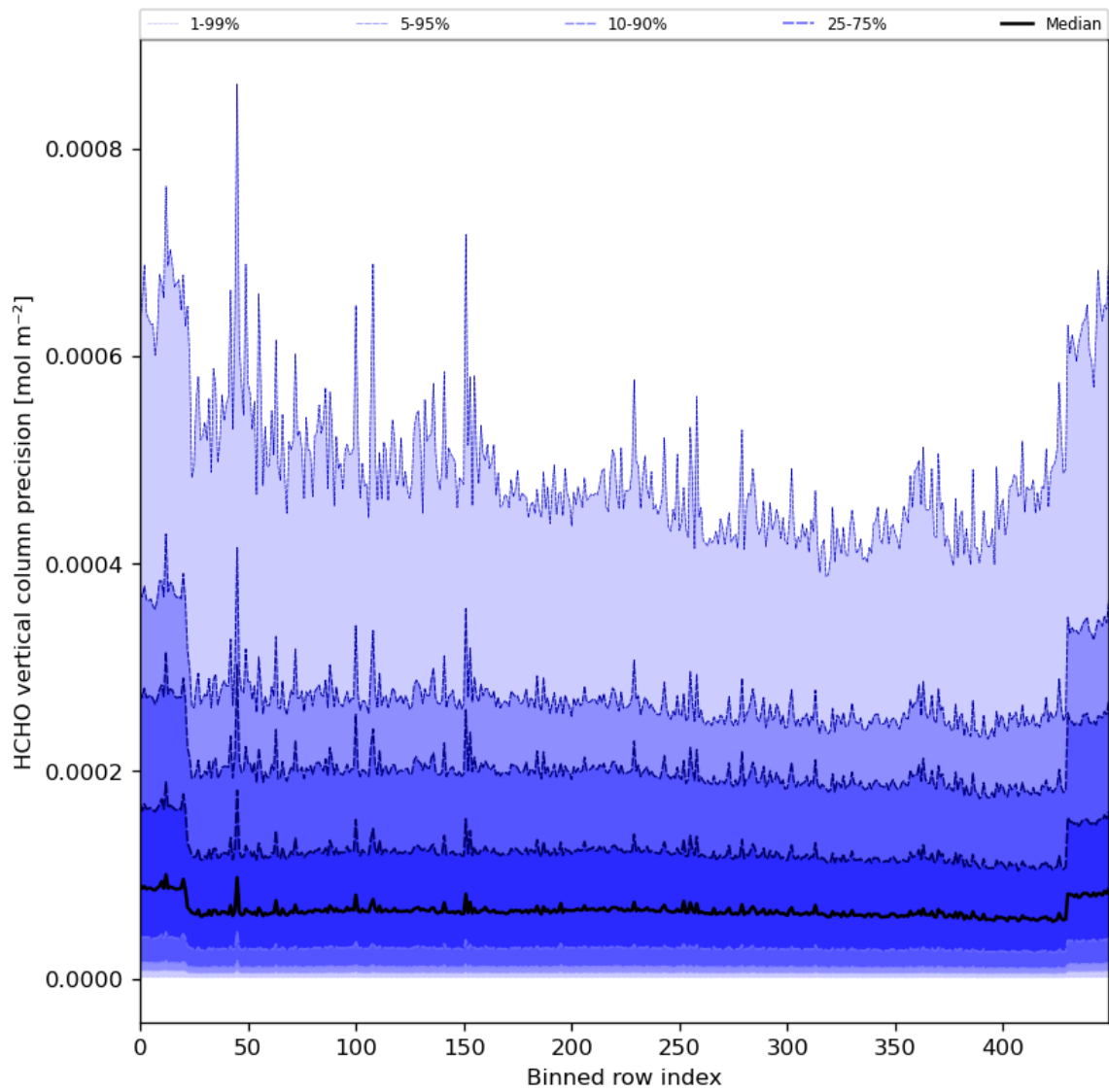
Figure 50: Along track statistics of “HCHO vertical column precision” for 2024-08-24 to 2024-08-26
