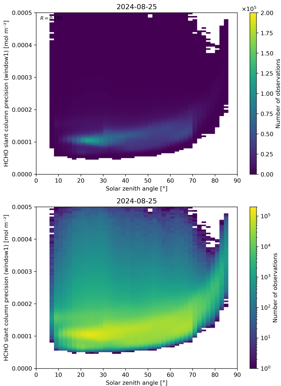
Figure 174: Scatter density plot of “Solar zenith angle” against “HCHO slant column precision (window1)” for 2024-08-24 to 2024-08-26.
