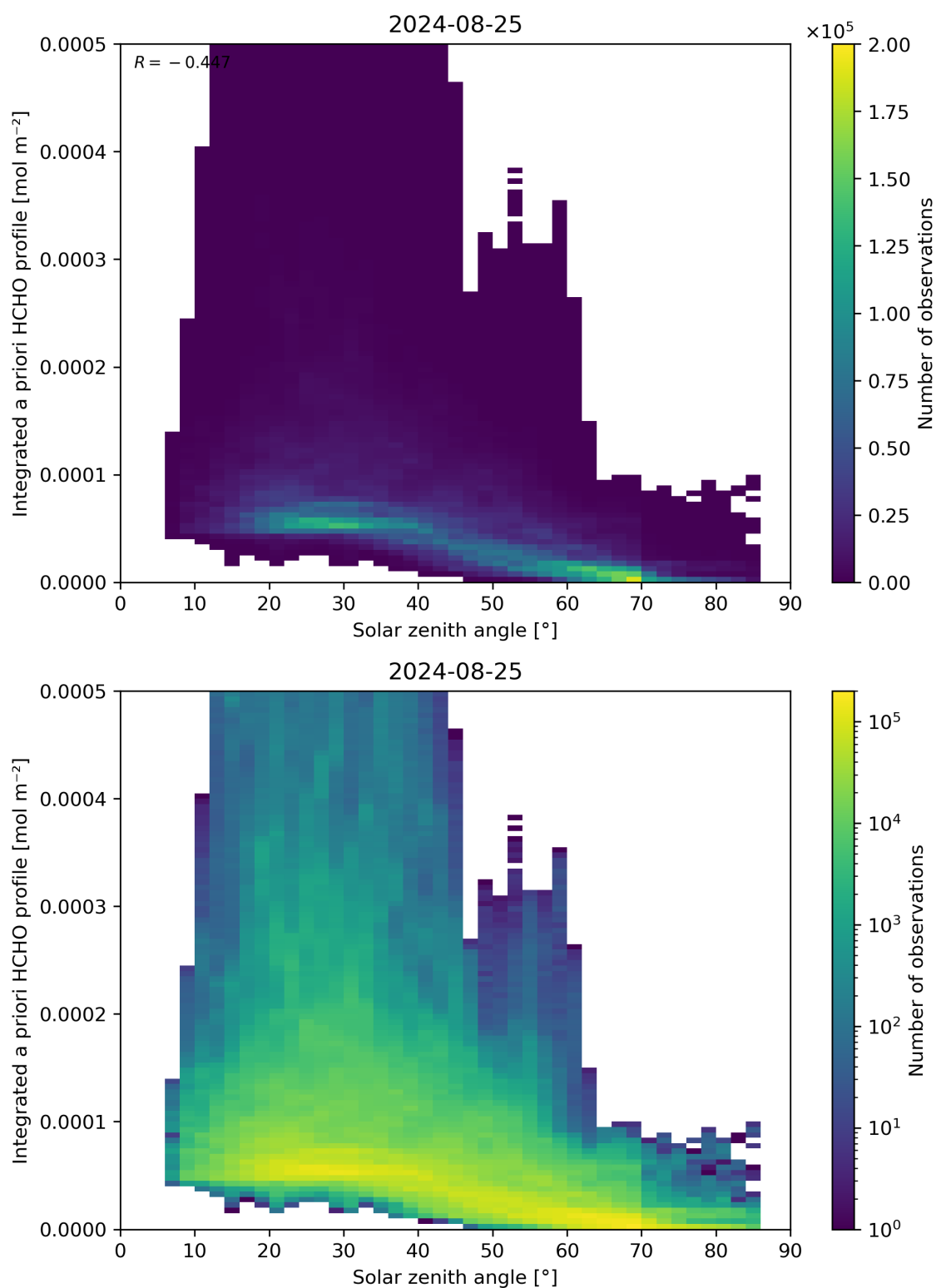
Figure 180: Scatter density plot of “Solar zenith angle” against “Integrated a priori HCHO profile” for 2024-08-24 to 2024-08-26.
