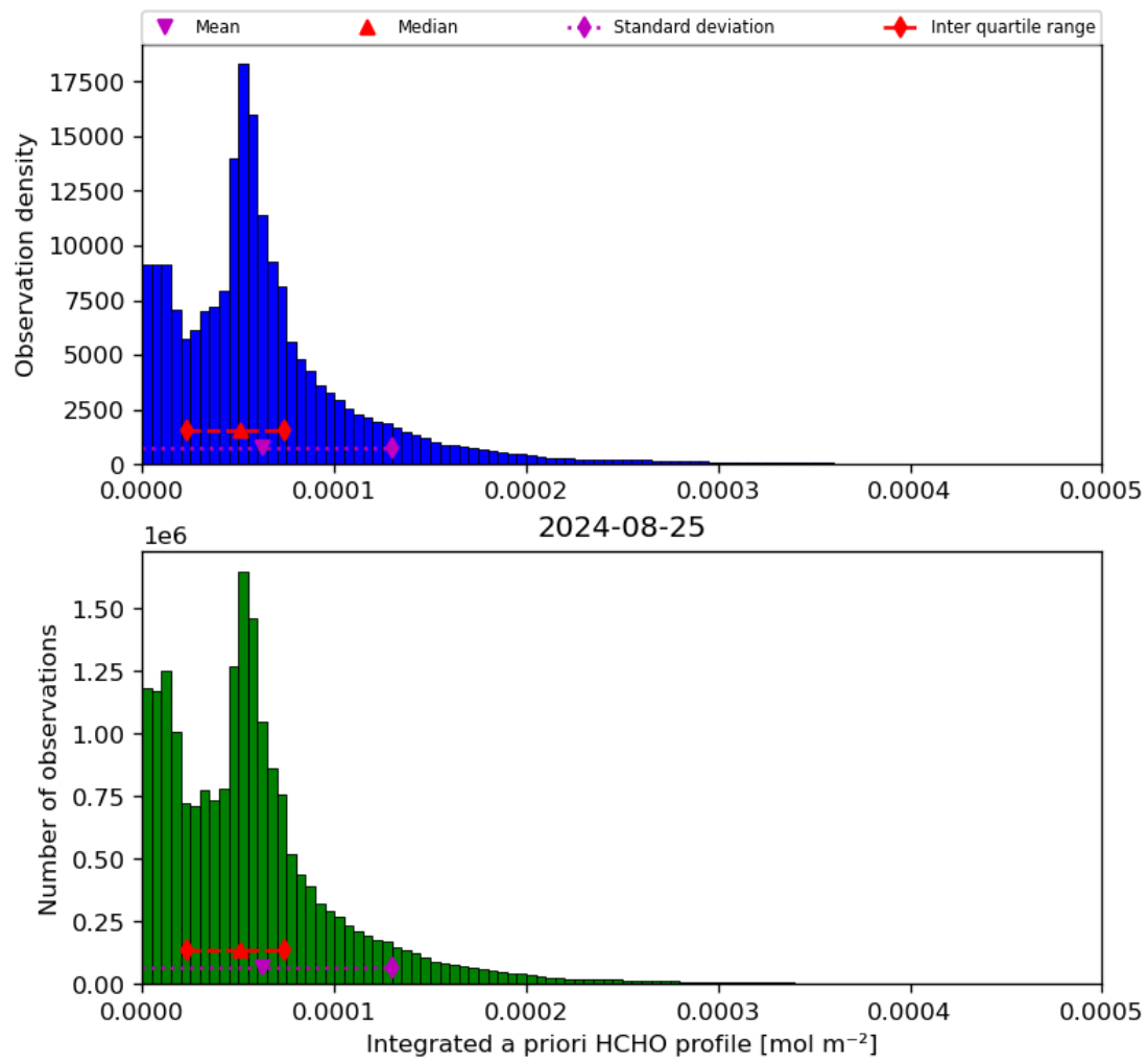
Figure 43: Histogram of “Integrated a priori HCHO profile” for 2024-08-24 to 2024-08-26
