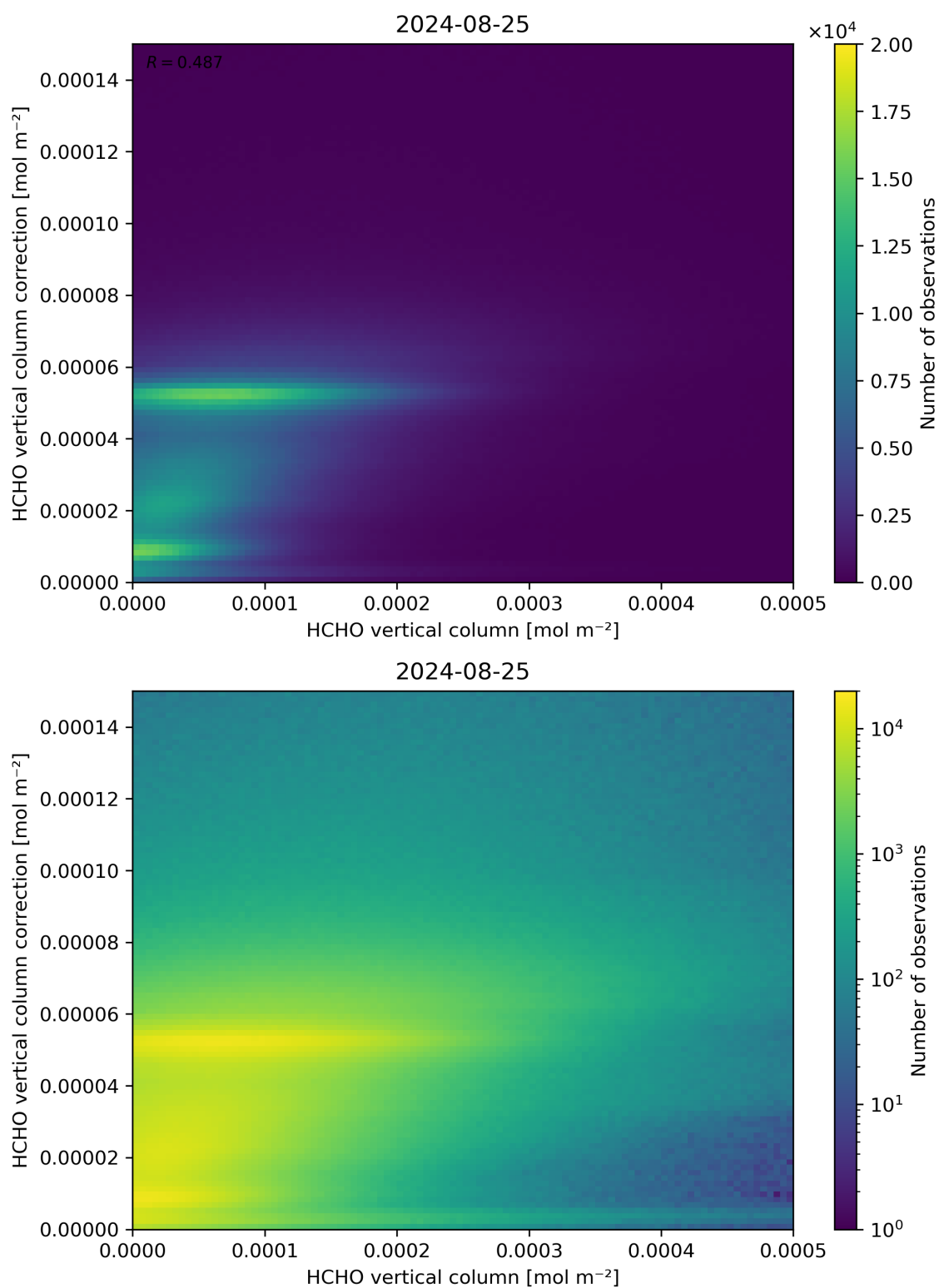
Figure 133: Scatter density plot of “HCHO vertical column” against “HCHO vertical column correction” for 2024-08-24 to 2024-08-26.
