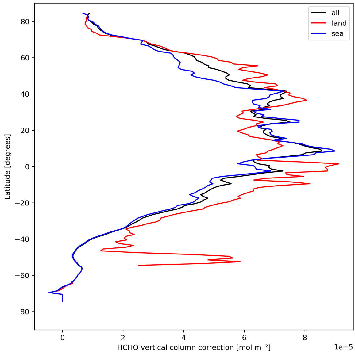
Figure 23: Zonal average of “HCHO vertical column correction” for 2024-08-24 to 2024-08-26.
