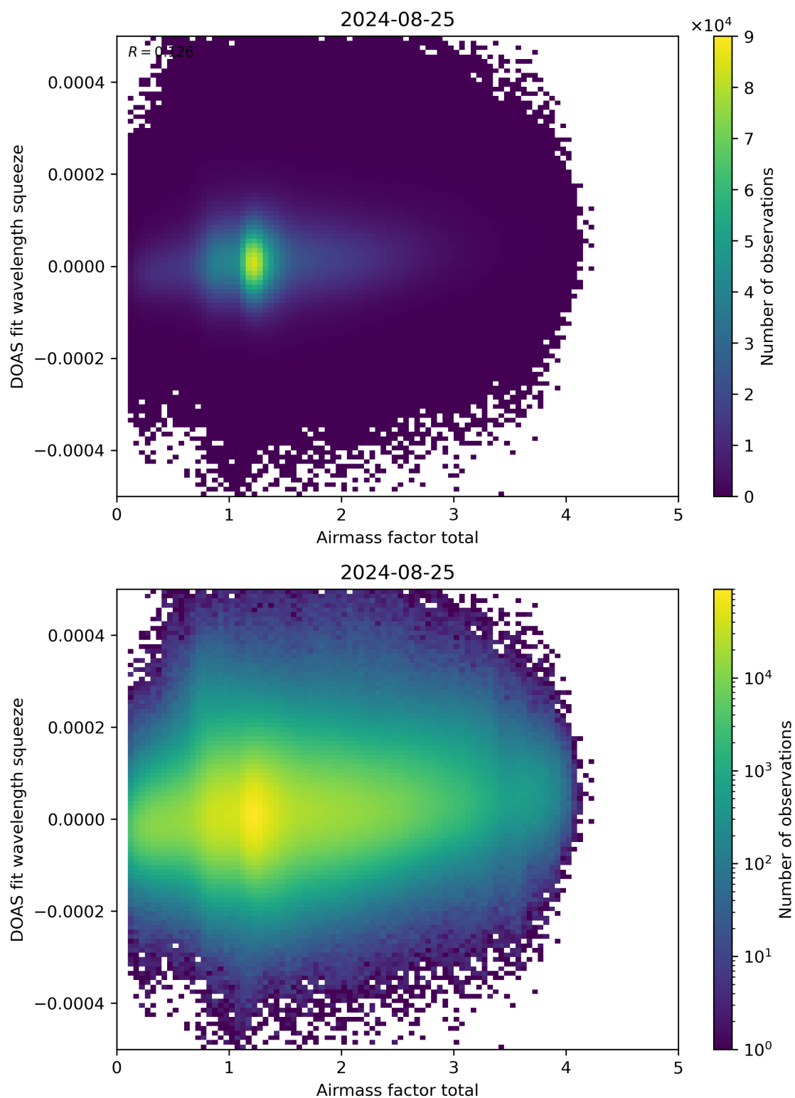
Figure 99: Scatter density plot of “Airmass factor total” against “DOAS fit wavelength squeeze” for 2024-08-24 to 2024-08-26.
