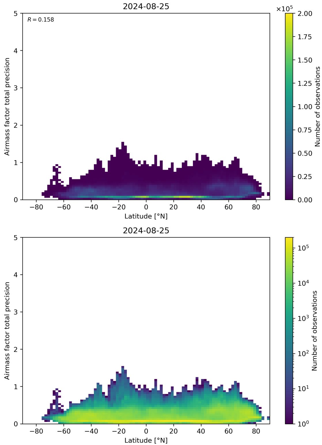
Figure 162: Scatter density plot of “Latitude” against “Airmass factor total precision” for 2024-08-24 to 2024-08-26.
