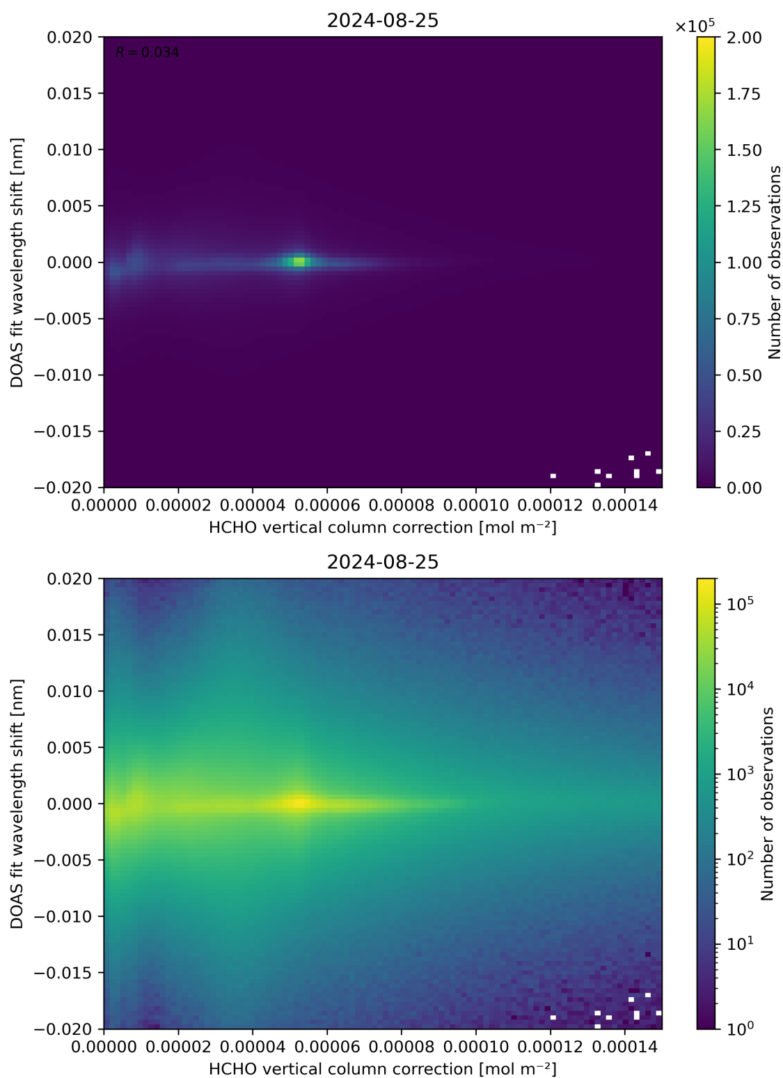
Figure 113: Scatter density plot of “HCHO vertical column correction” against “DOAS fit wavelength shift” for 2024-08-24 to 2024-08-26.
