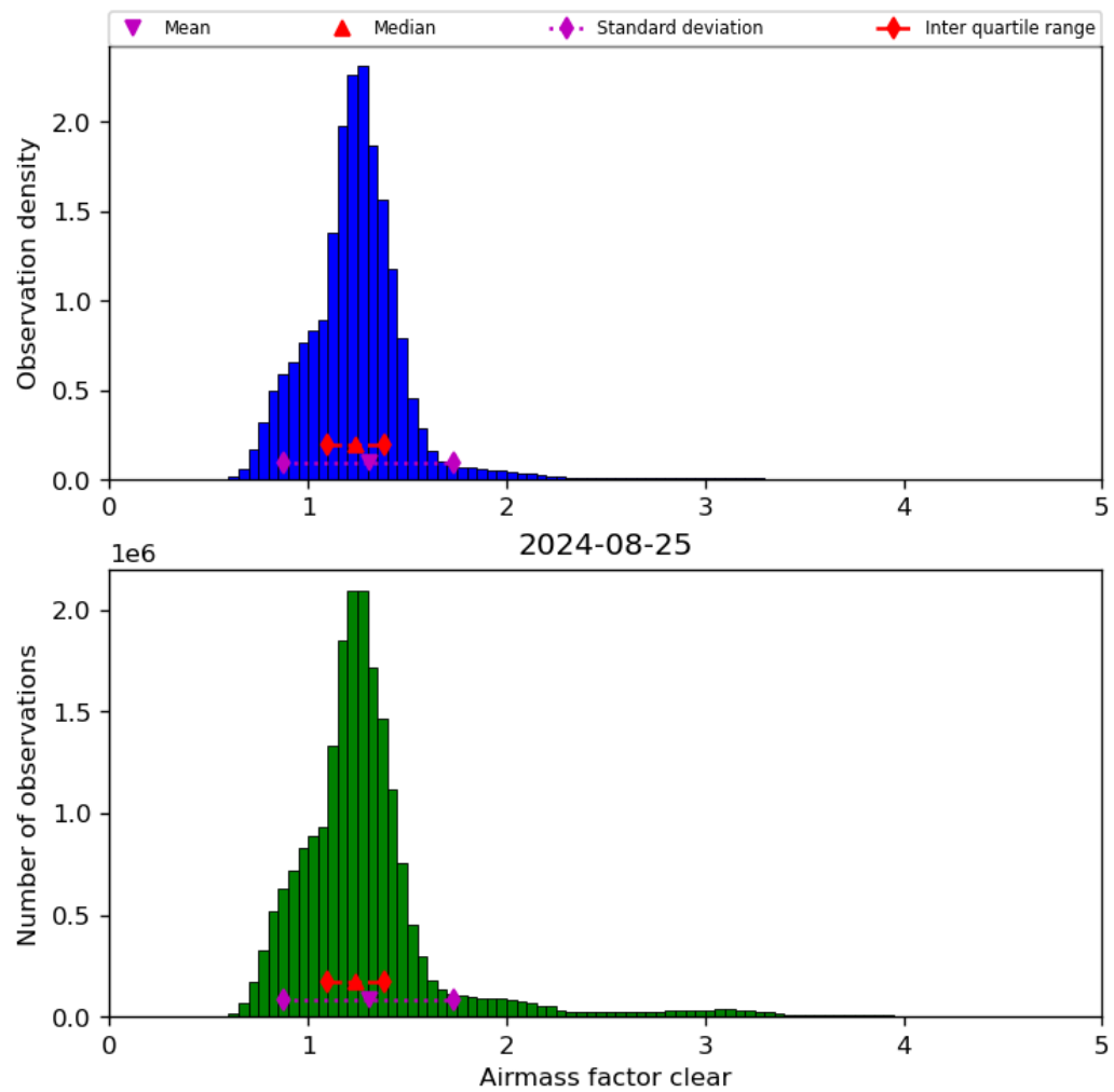
Figure 42: Histogram of “Airmass factor clear” for 2024-08-24 to 2024-08-26
