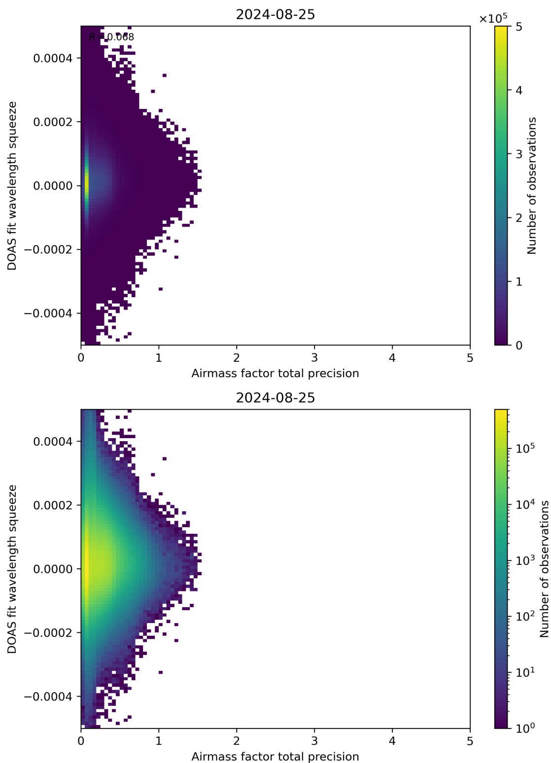
Figure 107: Scatter density plot of “Airmass factor total precision” against “DOAS fit wavelength squeeze” for 2024-08-24 to 2024-08-26.
