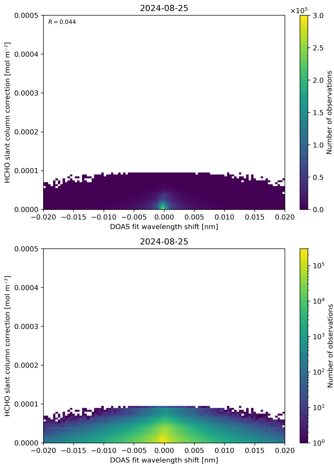
Figure 67: Scatter density plot of “DOAS fit wavelength shift” against “HCHO slant column correction” for 2024-08-24 to 2024-08-26.
