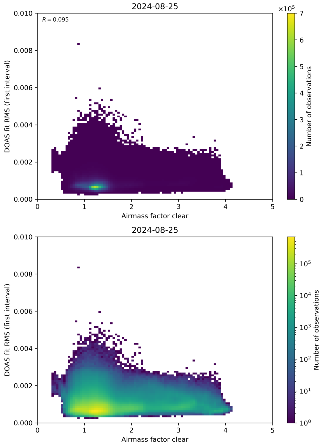
Figure 71: Scatter density plot of “Airmass factor clear” against “DOAS fit RMS (first interval)” for 2024-08-24 to 2024-08-26.
