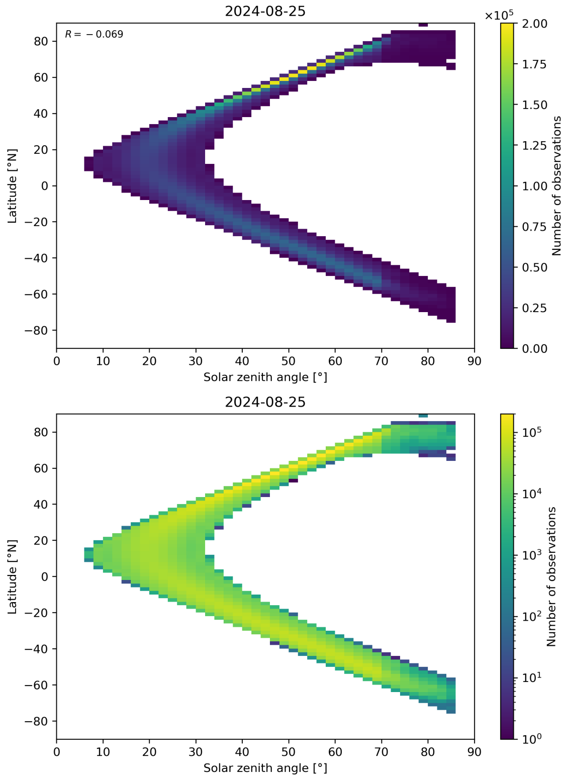
Figure 181: Scatter density plot of “Solar zenith angle” against “Latitude” for 2024-08-24 to 2024-08-26.
