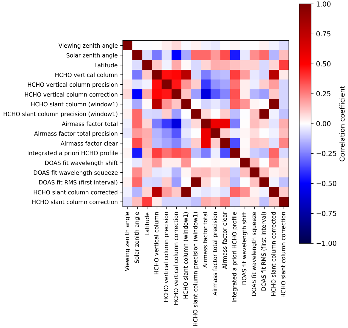
Figure 2: Map of correlation matrix for 2024-08-24 to 2024-08-26.
