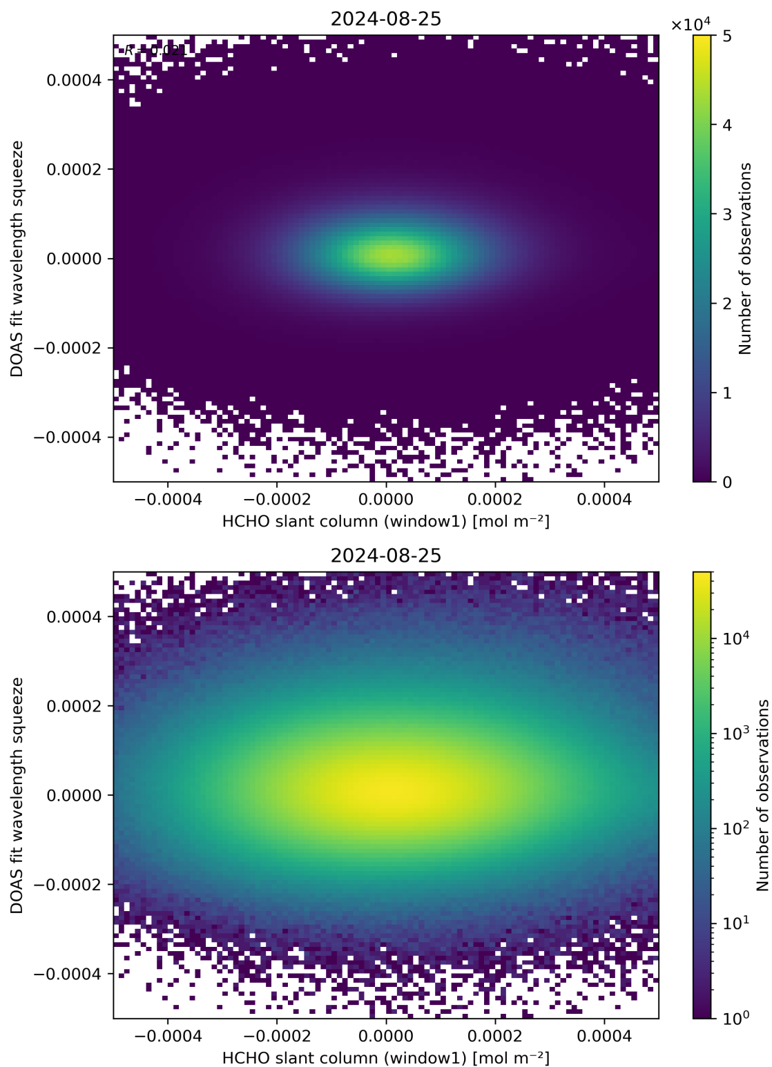
Figure 80: Scatter density plot of “HCHO slant column (window1)” against “DOAS fit wavelength squeeze” for 2024-08-24 to 2024-08-26.
