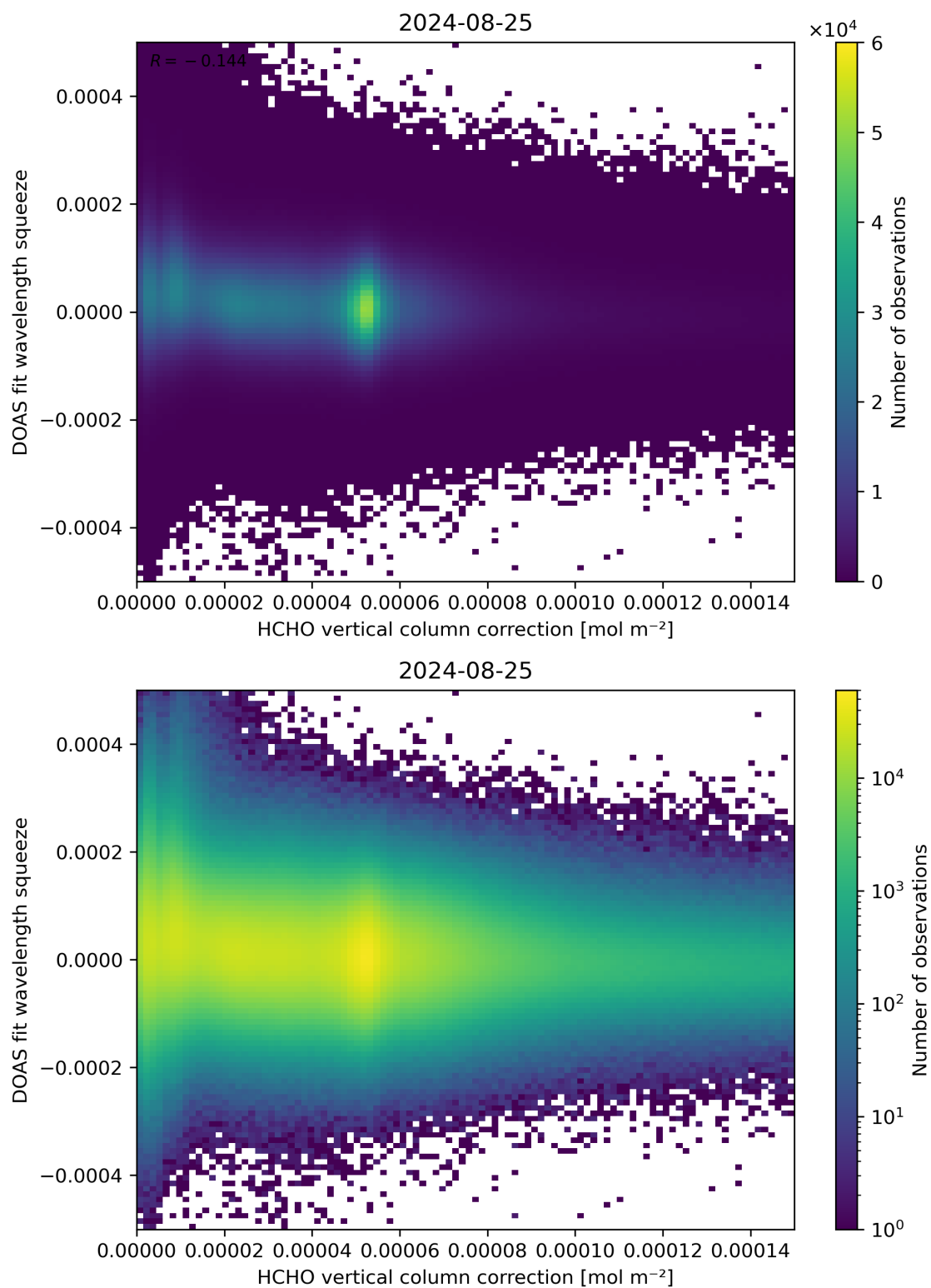
Figure 114: Scatter density plot of “HCHO vertical column correction” against “DOAS fit wavelength squeeze” for 2024-08-24 to 2024-08-26.
