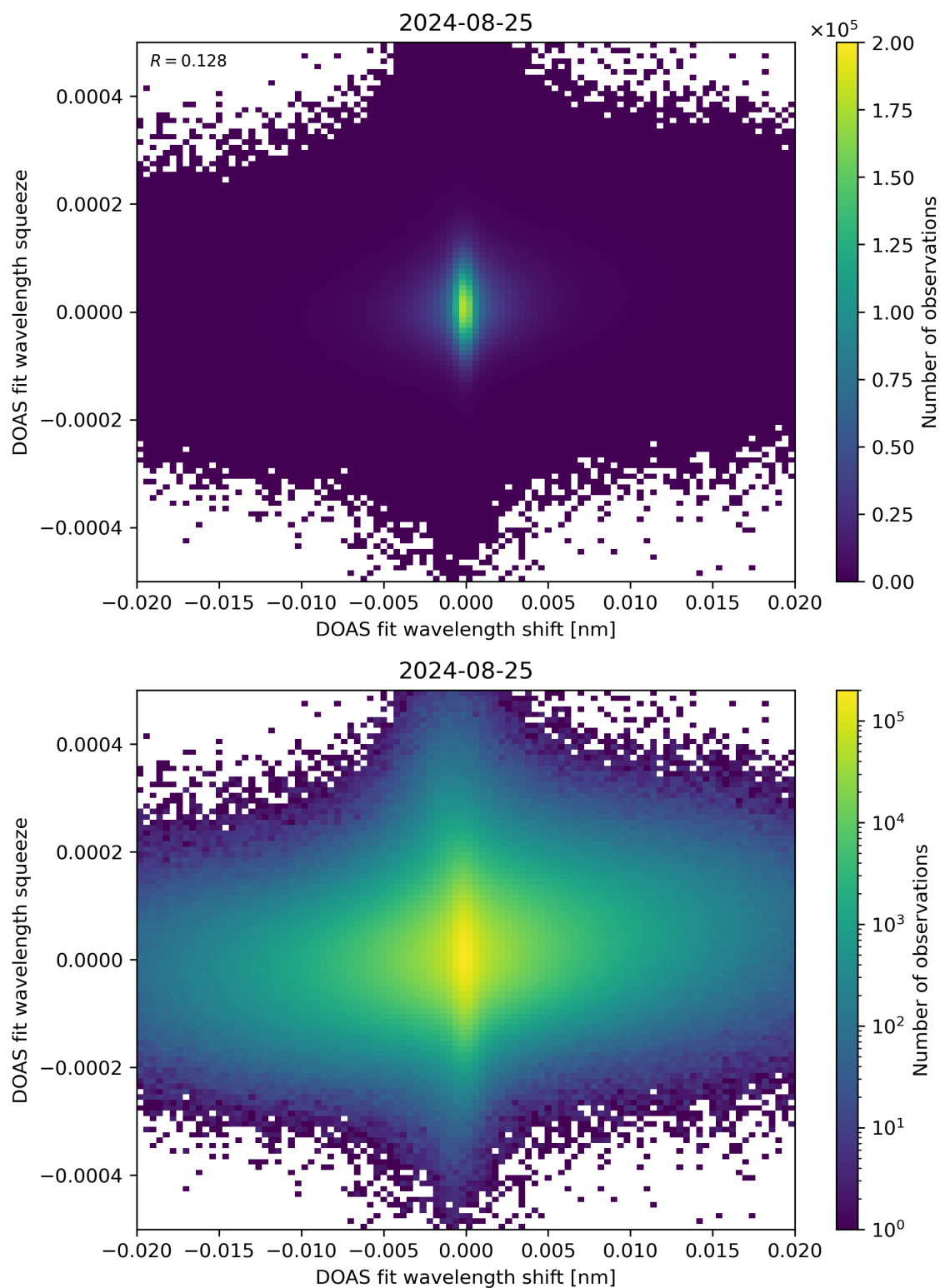
Figure 65: Scatter density plot of “DOAS fit wavelength shift” against “DOAS fit wavelength squeeze” for 2024-08-24 to 2024-08-26.
