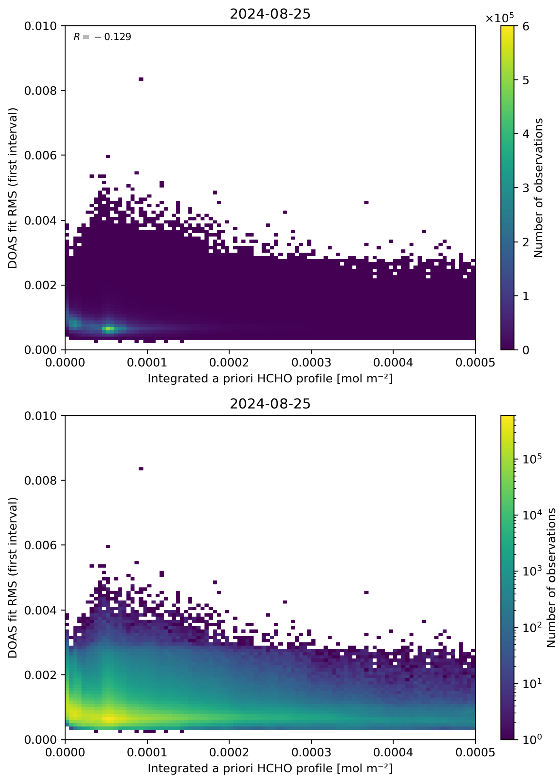
Figure 148: Scatter density plot of “Integrated a priori HCHO profile” against “DOAS fit RMS (first interval)” for 2024-08-24 to 2024-08-26.
