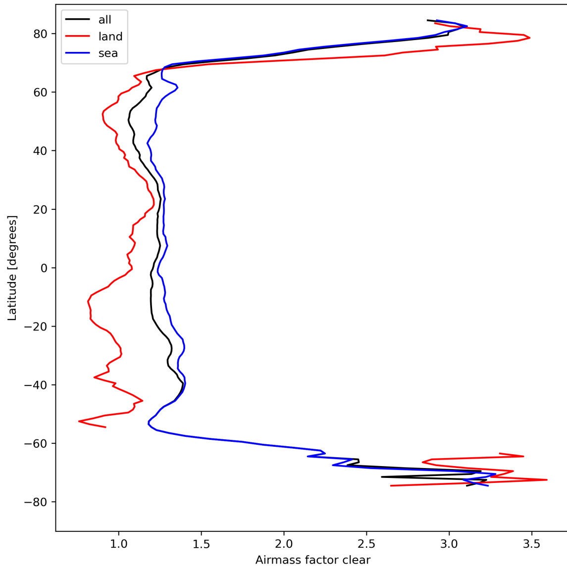
Figure 28: Zonal average of “Airmass factor clear” for 2024-08-24 to 2024-08-26.
