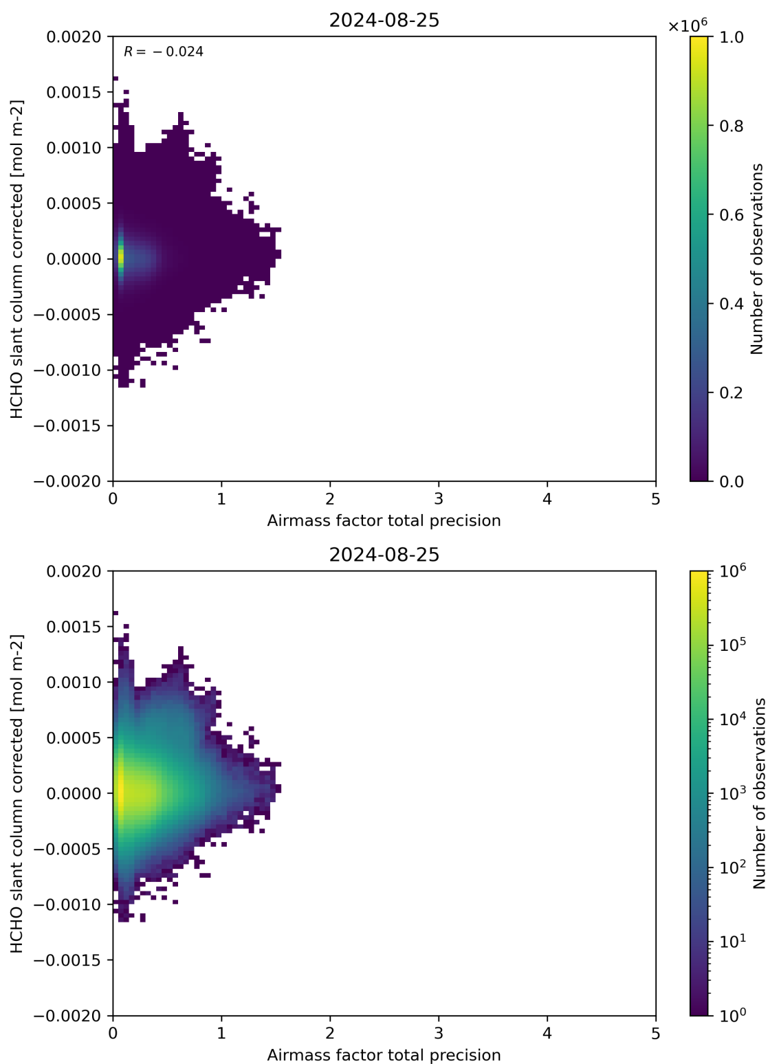
Figure 109: Scatter density plot of “Airmass factor total precision” against “HCHO slant column corrected” for 2024-08-24 to 2024-08-26.
