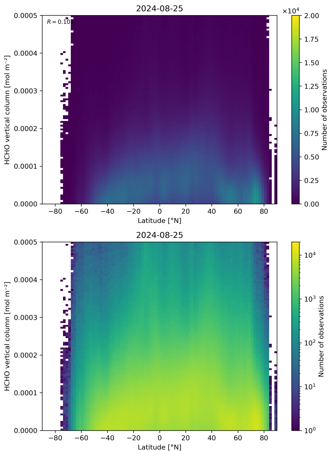
Figure 163: Scatter density plot of “Latitude” against “HCHO vertical column” for 2024-08-24 to 2024-08-26.
