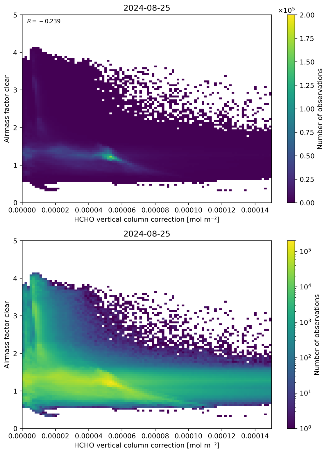
Figure 115: Scatter density plot of “HCHO vertical column correction” against “Airmass factor clear” for 2024-08-24 to 2024-08-26.
