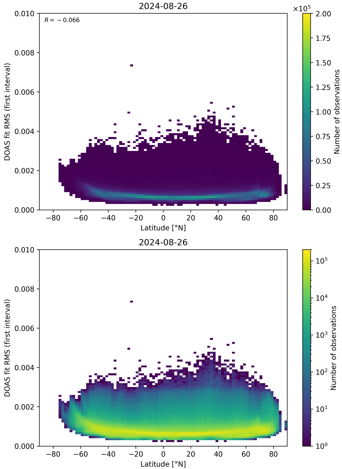
Figure 153: Scatter density plot of “Latitude” against “DOAS fit RMS (first interval)” for 2024-08-25 to 2024-08-27.
