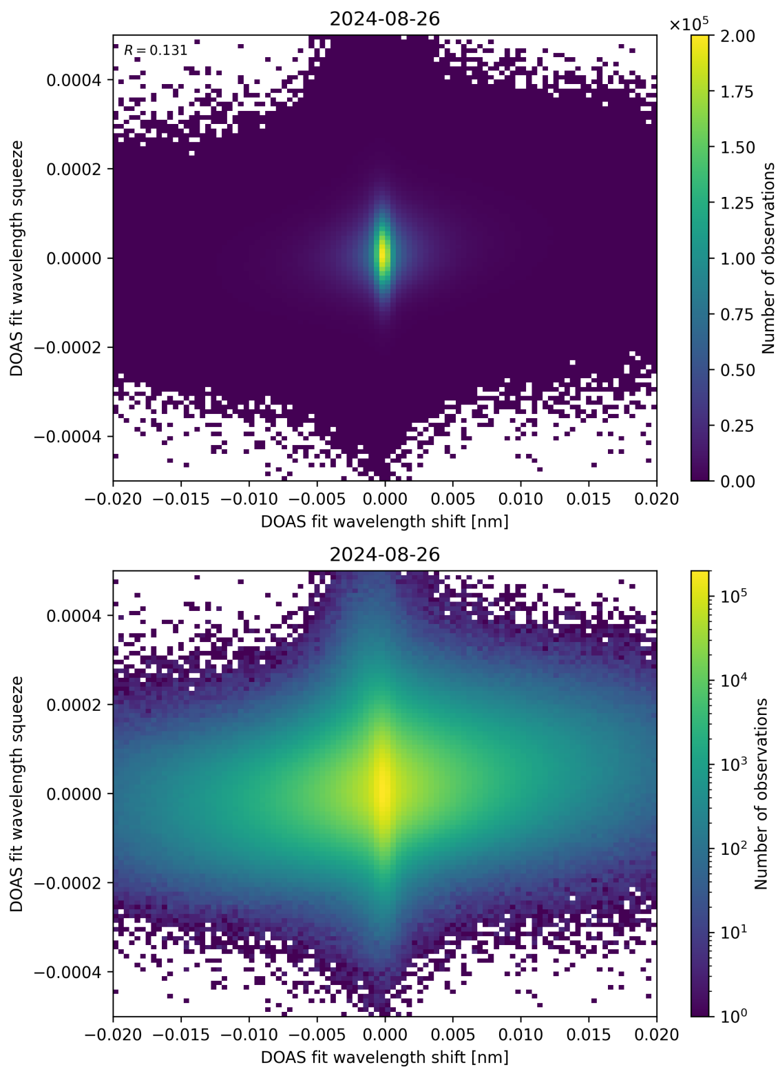
Figure 65: Scatter density plot of “DOAS fit wavelength shift” against “DOAS fit wavelength squeeze” for 2024-08-25 to 2024-08-27.
