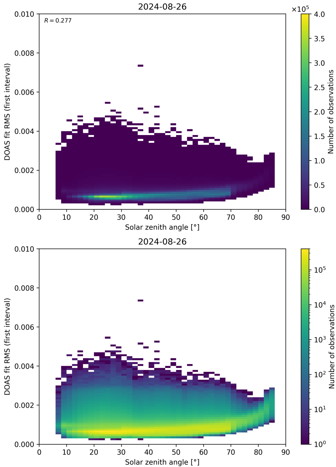
Figure 167: Scatter density plot of “Solar zenith angle” against “DOAS fit RMS (first interval)” for 2024-08-25 to 2024-08-27.
