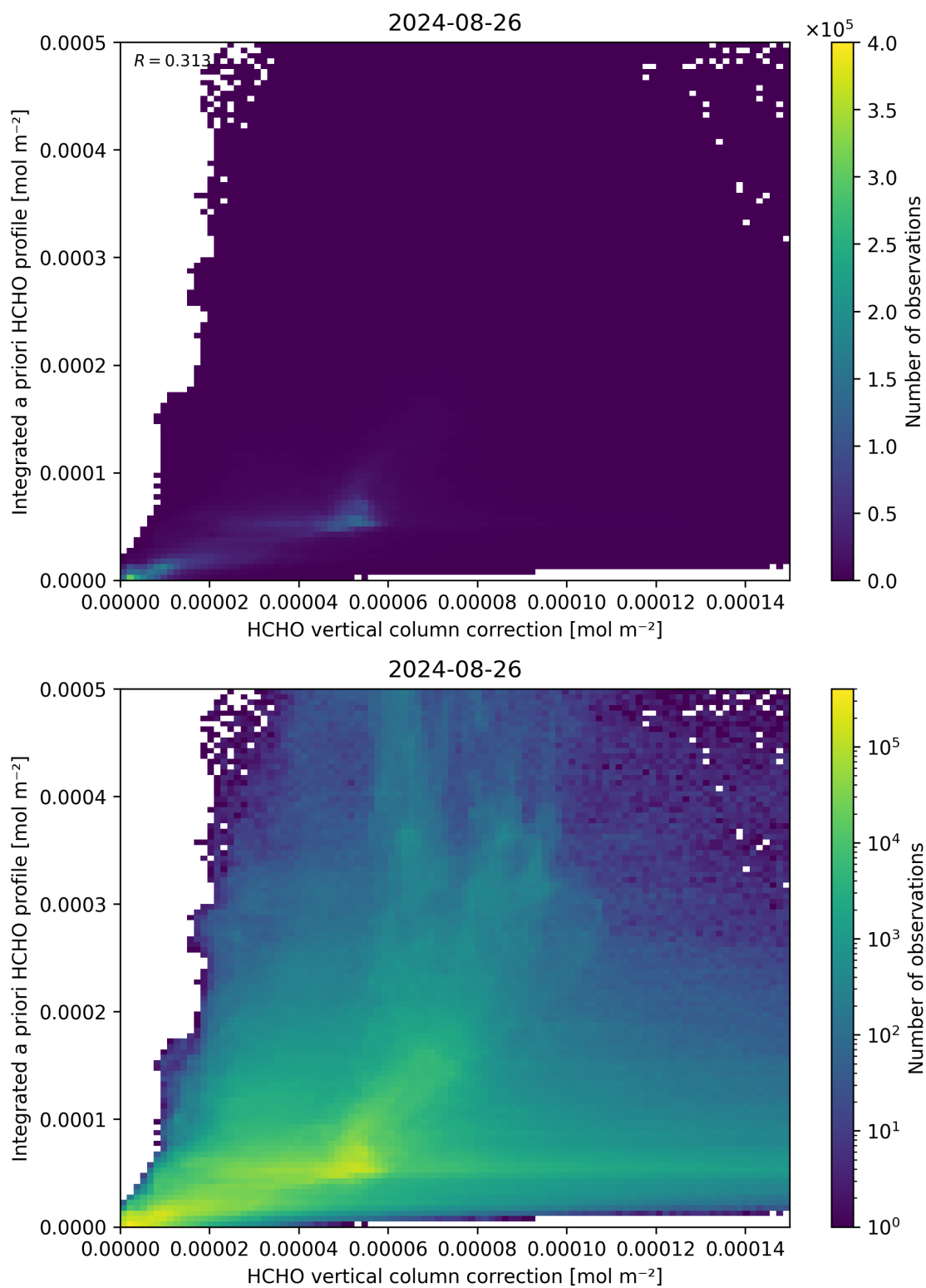
Figure 122: Scatter density plot of “HCHO vertical column correction” against “Integrated a priori HCHO profile” for 2024-08-25 to 2024-08-27.
