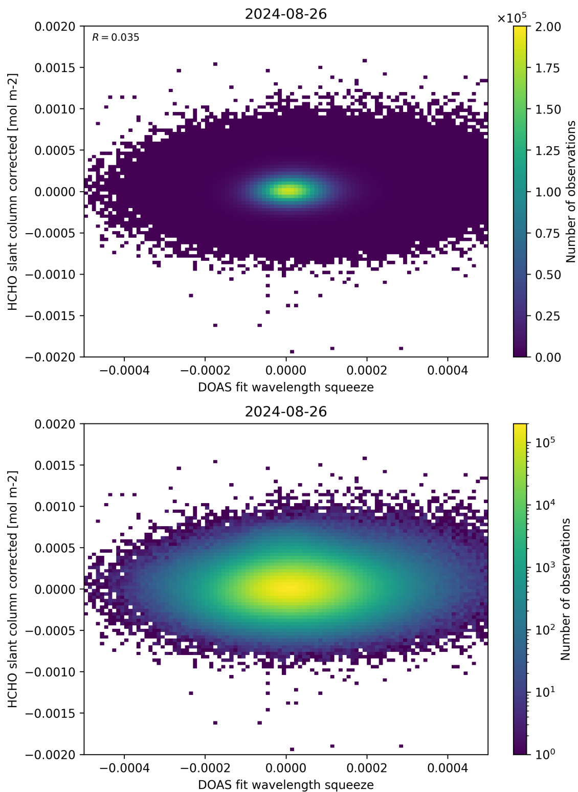
Figure 69: Scatter density plot of “DOAS fit wavelength squeeze” against “HCHO slant column corrected” for 2024-08-25 to 2024-08-27.
