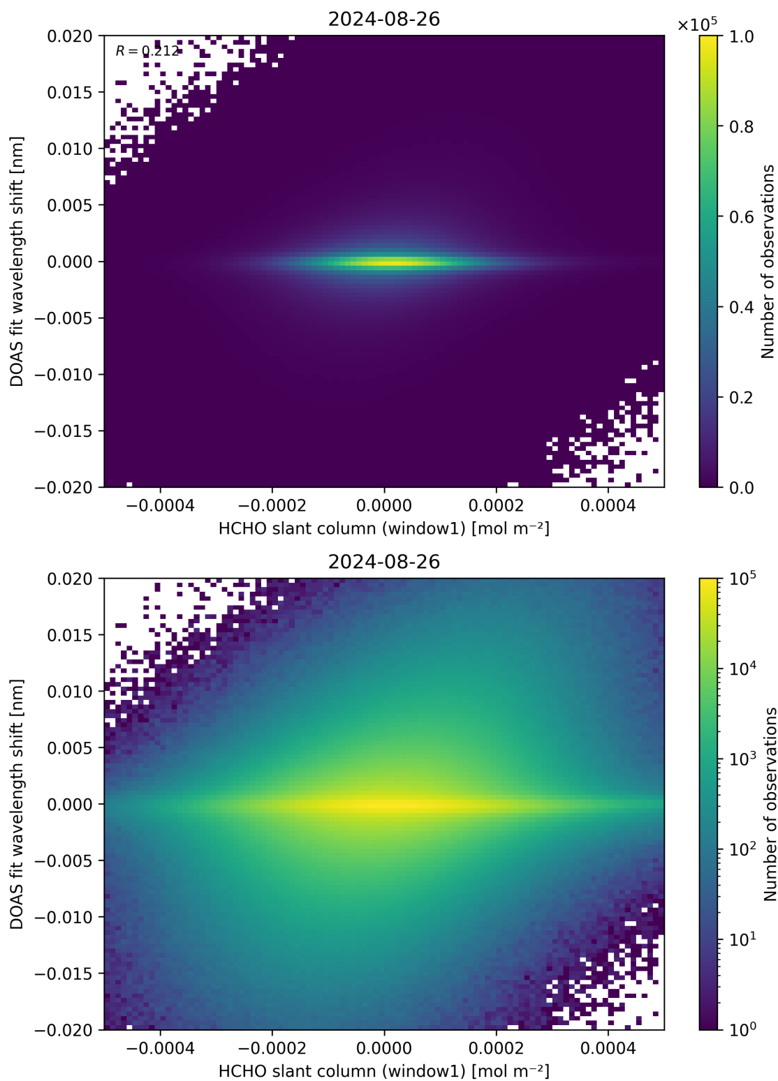
Figure 79: Scatter density plot of “HCHO slant column (window1)” against “DOAS fit wavelength shift” for 2024-08-25 to 2024-08-27.
