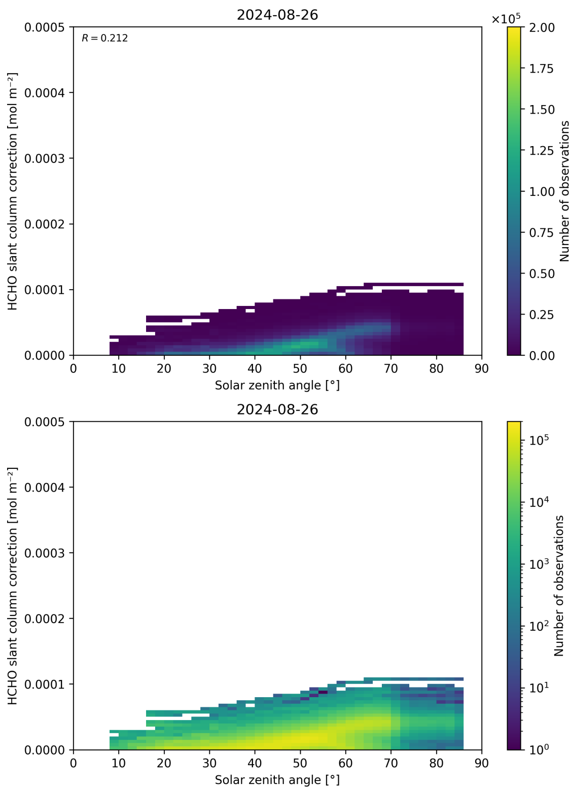
Figure 172: Scatter density plot of “Solar zenith angle” against “HCHO slant column correction” for 2024-08-25 to 2024-08-27.
