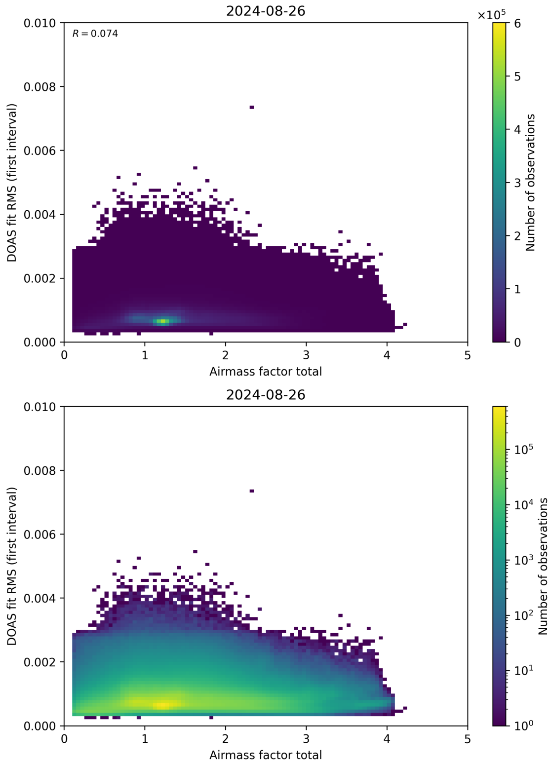
Figure 97: Scatter density plot of “Airmass factor total” against “DOAS fit RMS (first interval)” for 2024-08-25 to 2024-08-27.
