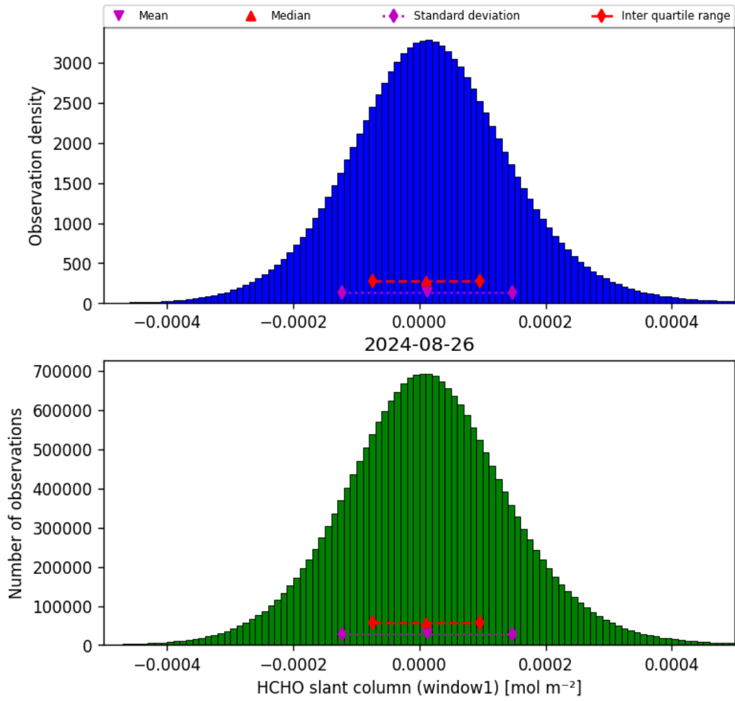
Figure 38: Histogram of “HCHO slant column (window1)” for 2024-08-25 to 2024-08-27
