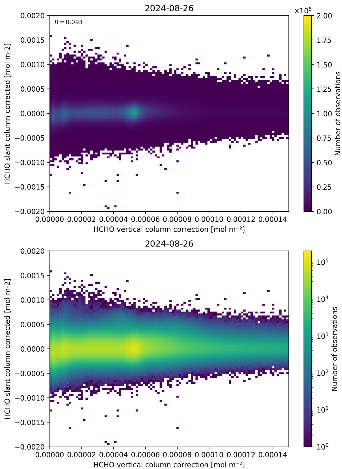
Figure 116: Scatter density plot of “HCHO vertical column correction” against “HCHO slant column corrected” for 2024-08-25 to 2024-08-27.
