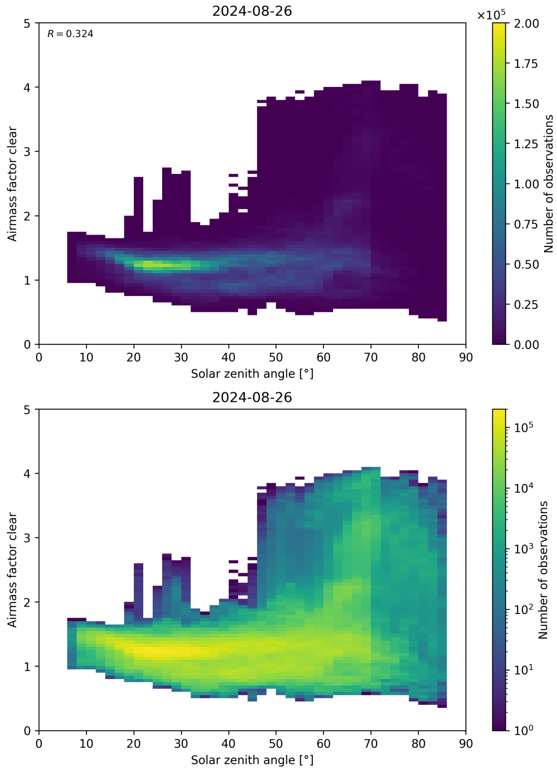
Figure 170: Scatter density plot of “Solar zenith angle” against “Airmass factor clear” for 2024-08-25 to 2024-08-27.
