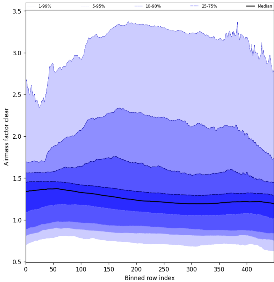
Figure 56: Along track statistics of “Airmass factor clear” for 2024-08-25 to 2024-08-27
