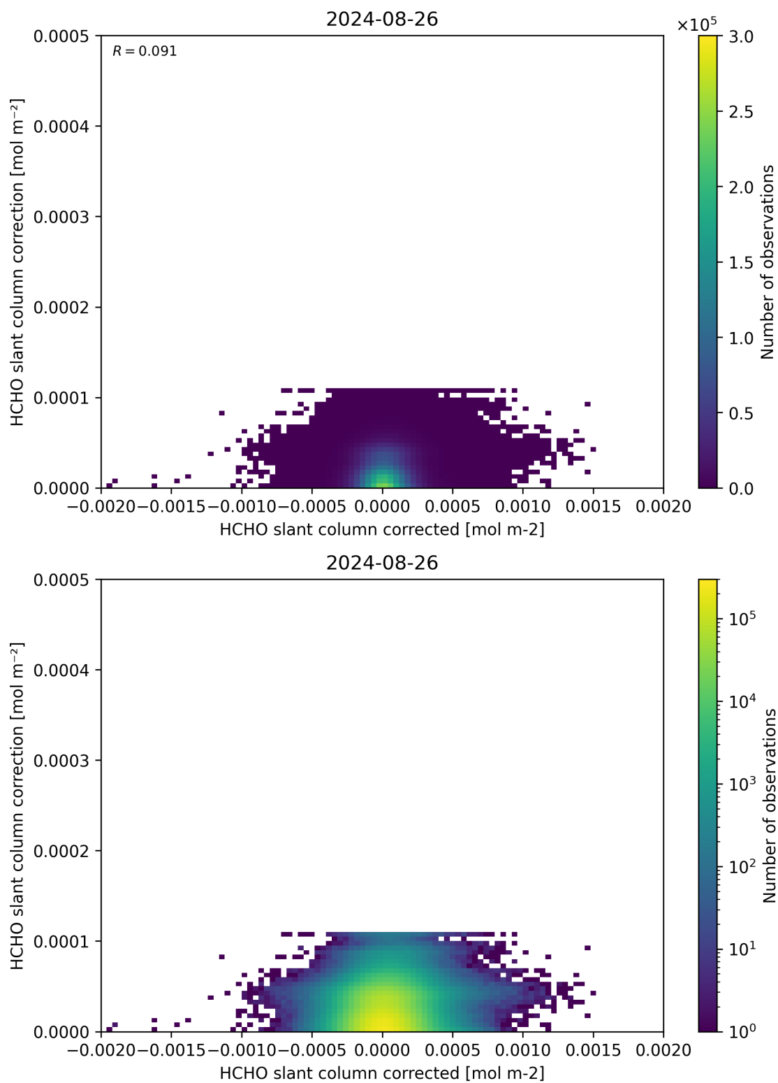
Figure 77: Scatter density plot of “HCHO slant column corrected” against “HCHO slant column correction” for 2024-08-25 to 2024-08-27.
