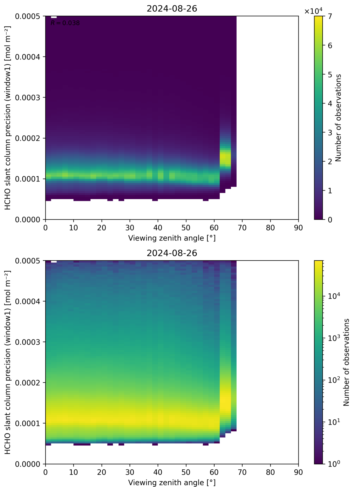
Figure 189: Scatter density plot of “Viewing zenith angle” against “HCHO slant column precision (window1)” for 2024-08-25 to 2024-08-27.
