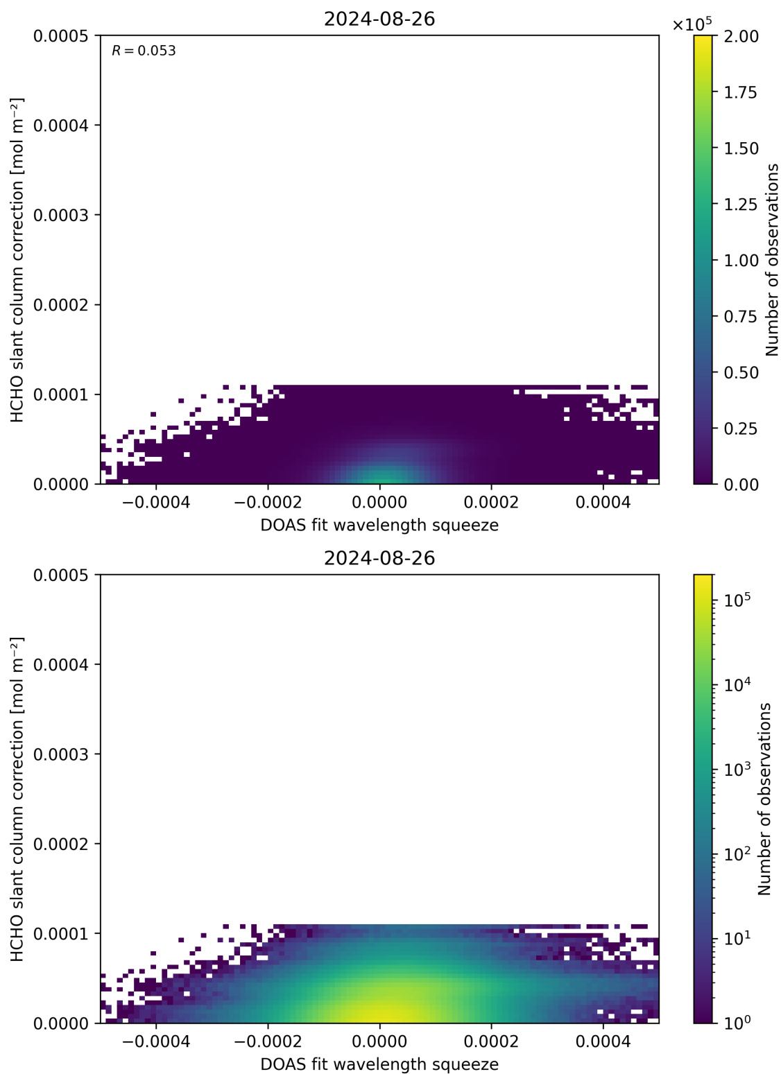
Figure 70: Scatter density plot of “DOAS fit wavelength squeeze” against “HCHO slant column correction” for 2024-08-25 to 2024-08-27.
