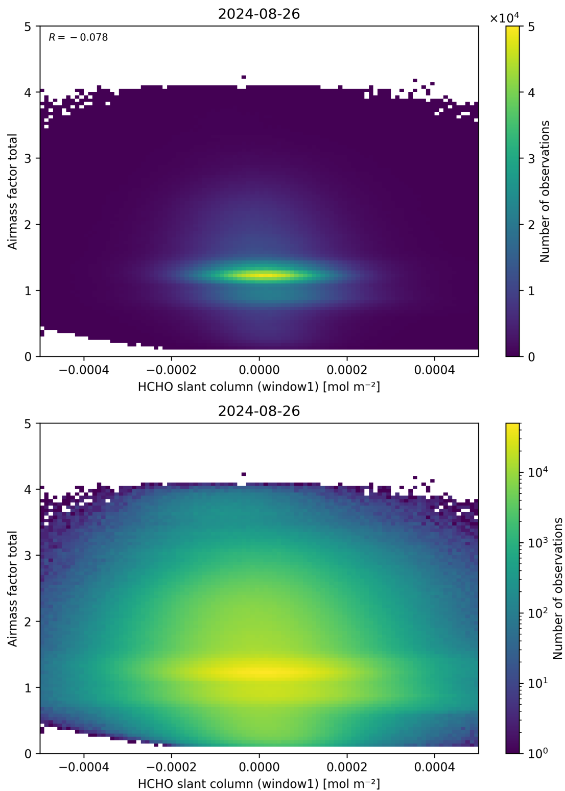
Figure 85: Scatter density plot of “HCHO slant column (window1)” against “Airmass factor total” for 2024-08-25 to 2024-08-27.
