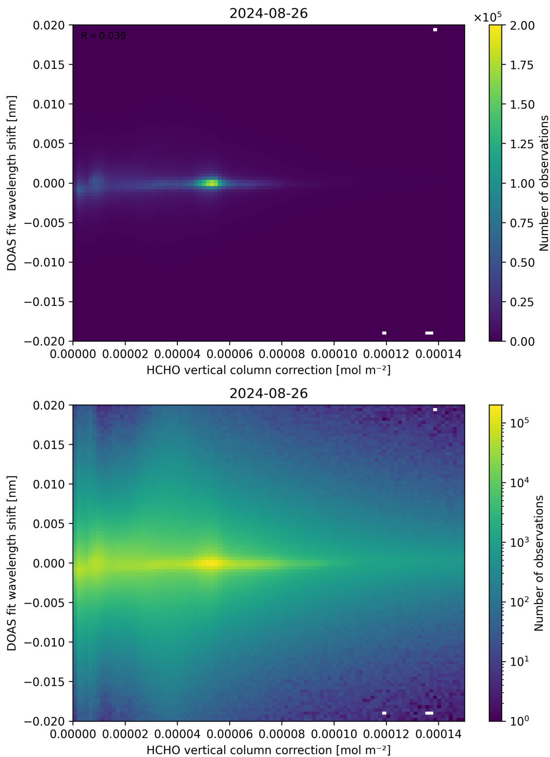
Figure 113: Scatter density plot of “HCHO vertical column correction” against “DOAS fit wavelength shift” for 2024-08-25 to 2024-08-27.
