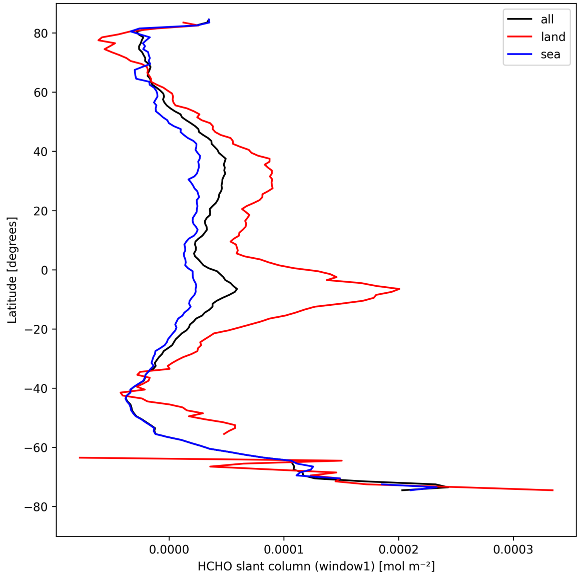
Figure 24: Zonal average of “HCHO slant column (window1)” for 2024-08-25 to 2024-08-27.
