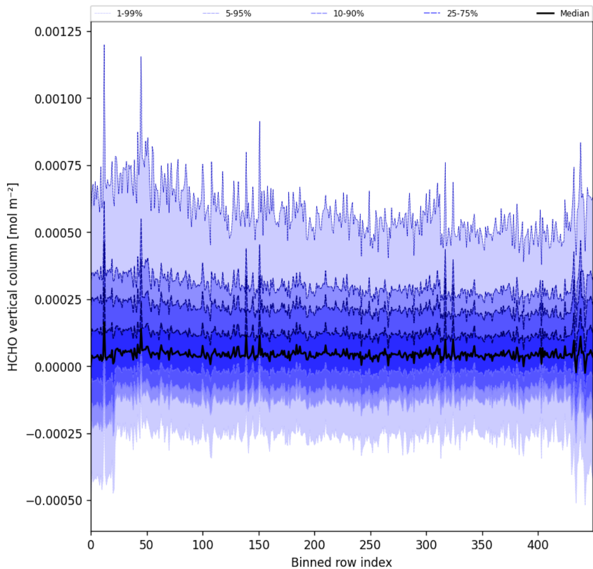
Figure 49: Along track statistics of “HCHO vertical column” for 2024-08-25 to 2024-08-27
