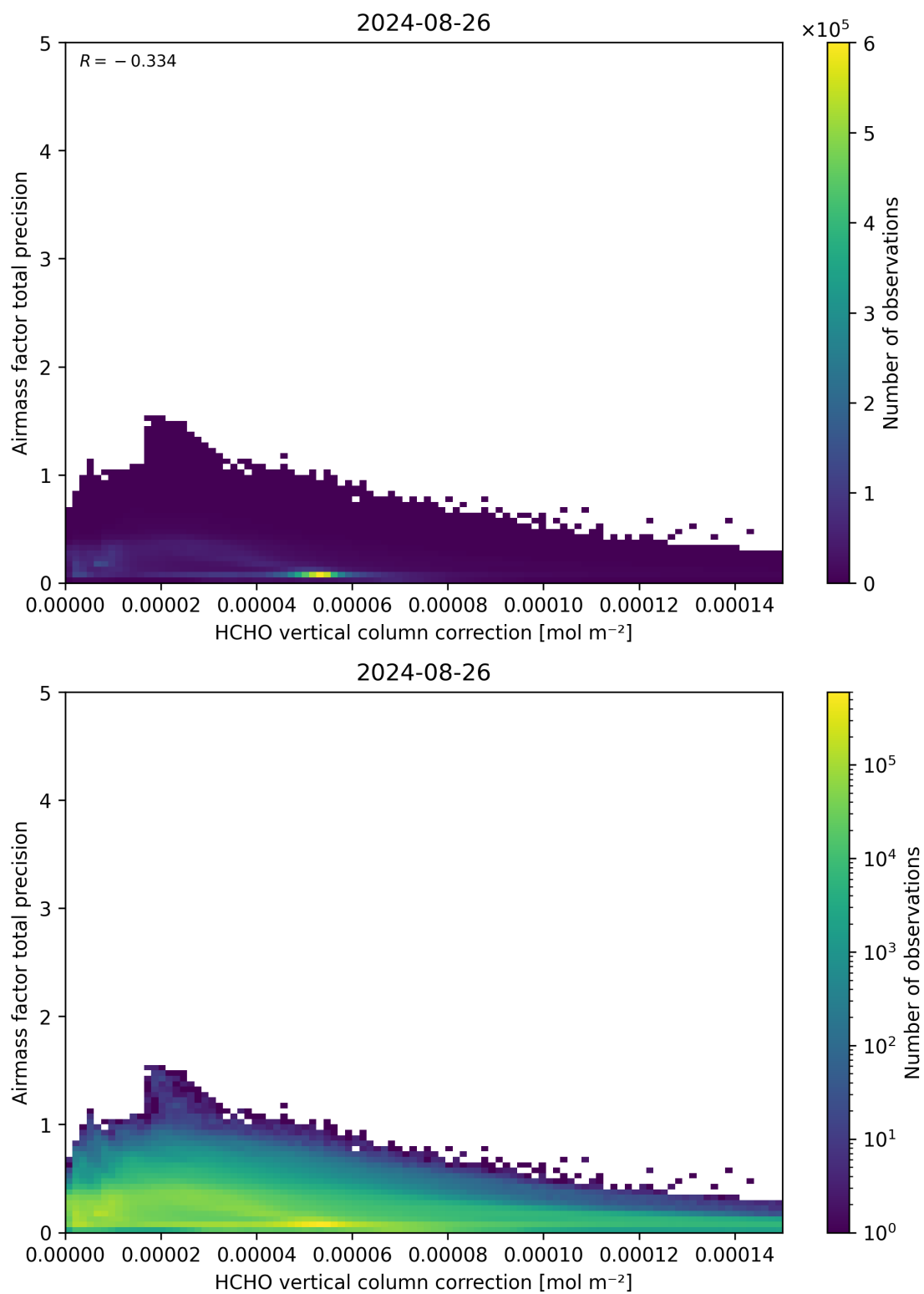
Figure 121: Scatter density plot of “HCHO vertical column correction” against “Airmass factor total precision” for 2024-08-25 to 2024-08-27.
