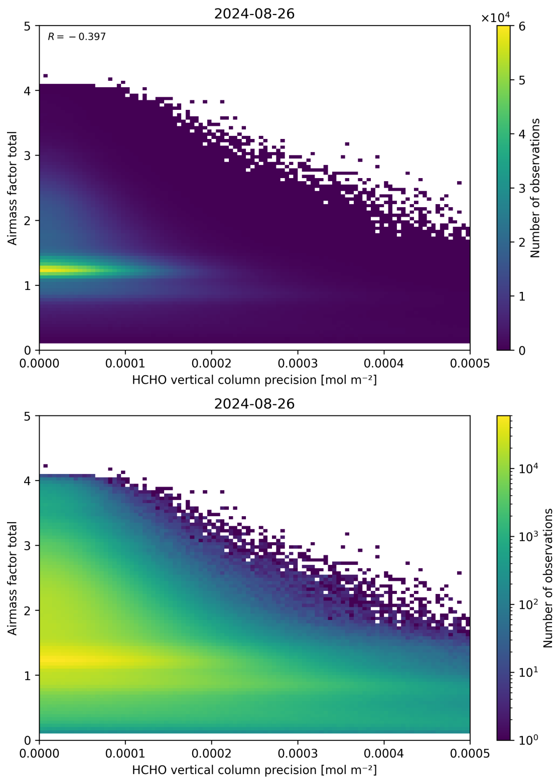
Figure 144: Scatter density plot of “HCHO vertical column precision” against “Airmass factor total” for 2024-08-25 to 2024-08-27.
