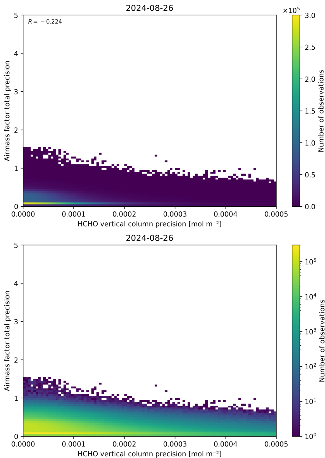
Figure 145: Scatter density plot of “HCHO vertical column precision” against “Airmass factor total precision” for 2024-08-25 to 2024-08-27.
