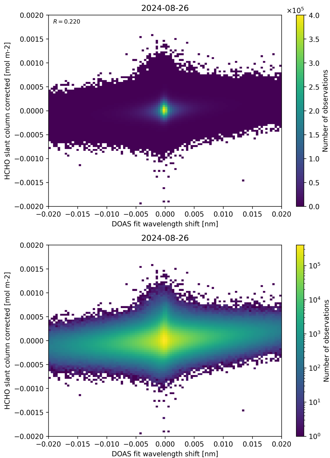
Figure 66: Scatter density plot of “DOAS fit wavelength shift” against “HCHO slant column corrected” for 2024-08-25 to 2024-08-27.
