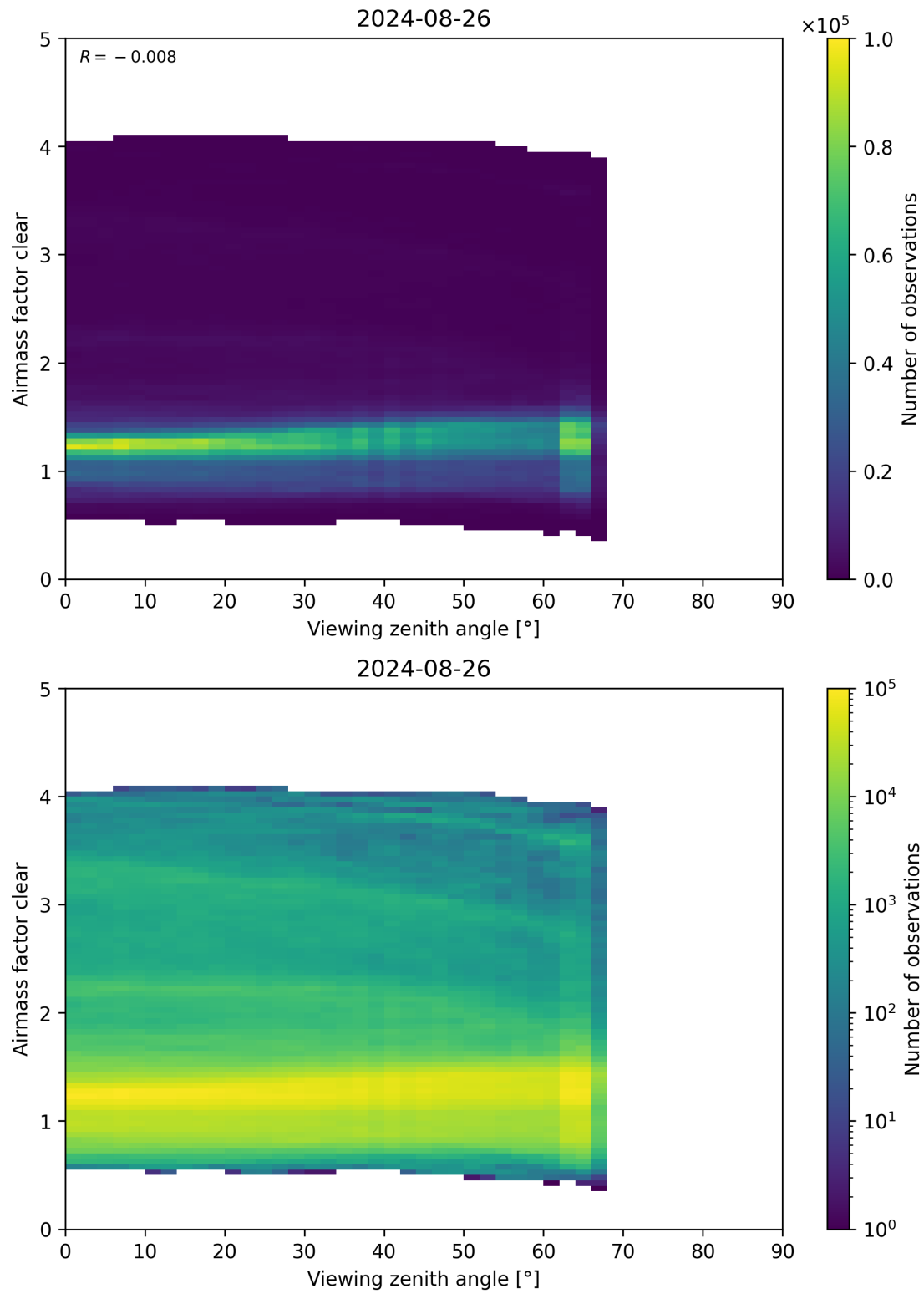
Figure 185: Scatter density plot of “Viewing zenith angle” against “Airmass factor clear” for 2024-08-25 to 2024-08-27.
