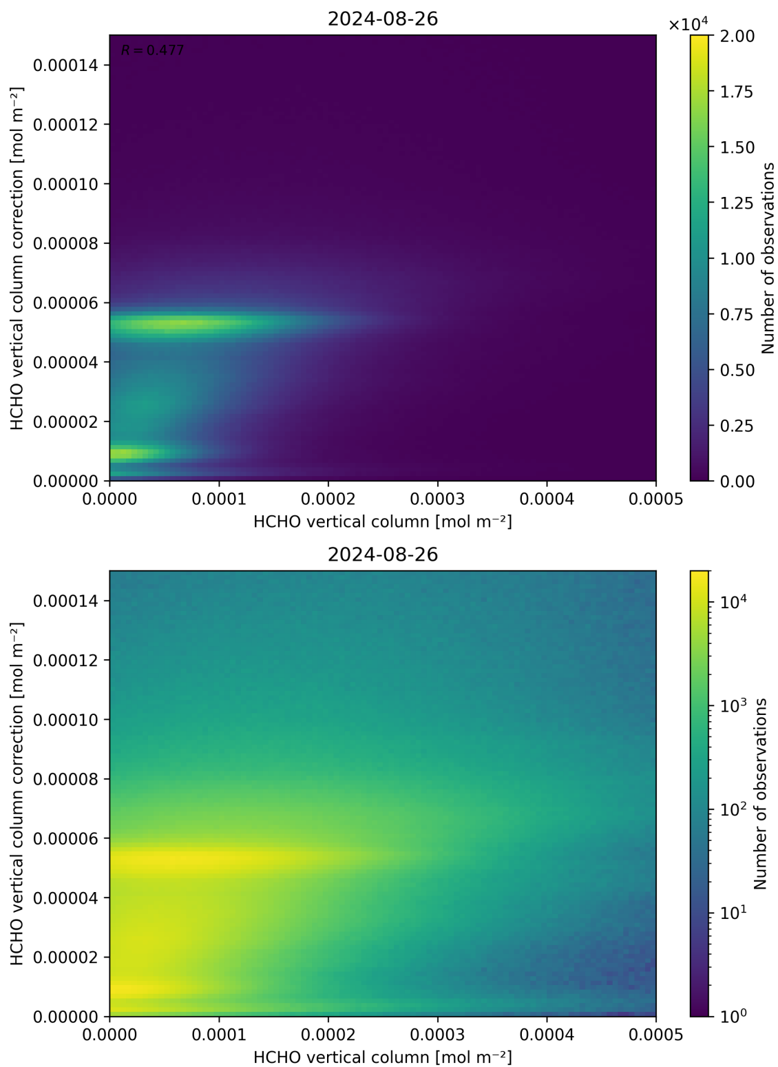
Figure 133: Scatter density plot of “HCHO vertical column” against “HCHO vertical column correction” for 2024-08-25 to 2024-08-27.
