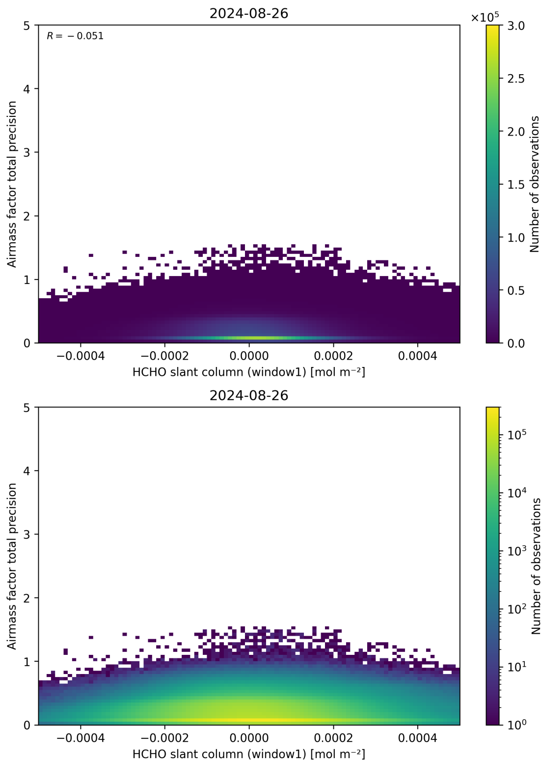
Figure 86: Scatter density plot of “HCHO slant column (window1)” against “Airmass factor total precision” for 2024-08-25 to 2024-08-27.
