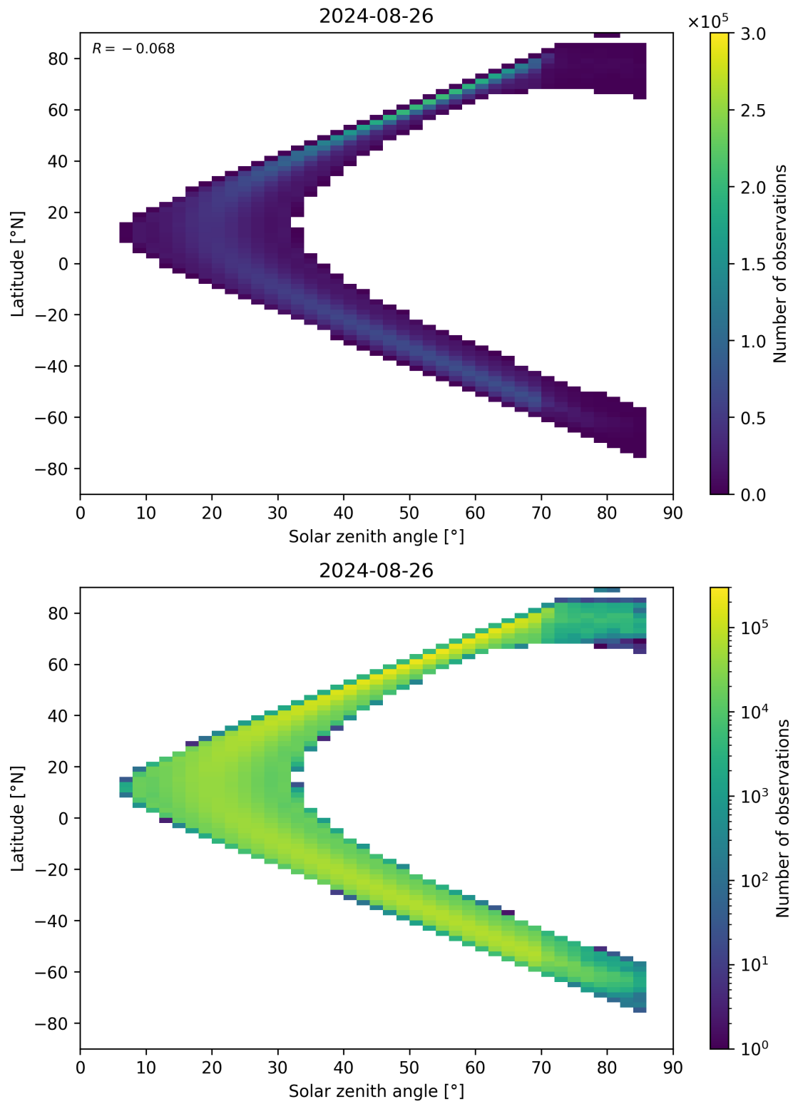
Figure 181: Scatter density plot of “Solar zenith angle” against “Latitude” for 2024-08-25 to 2024-08-27.
