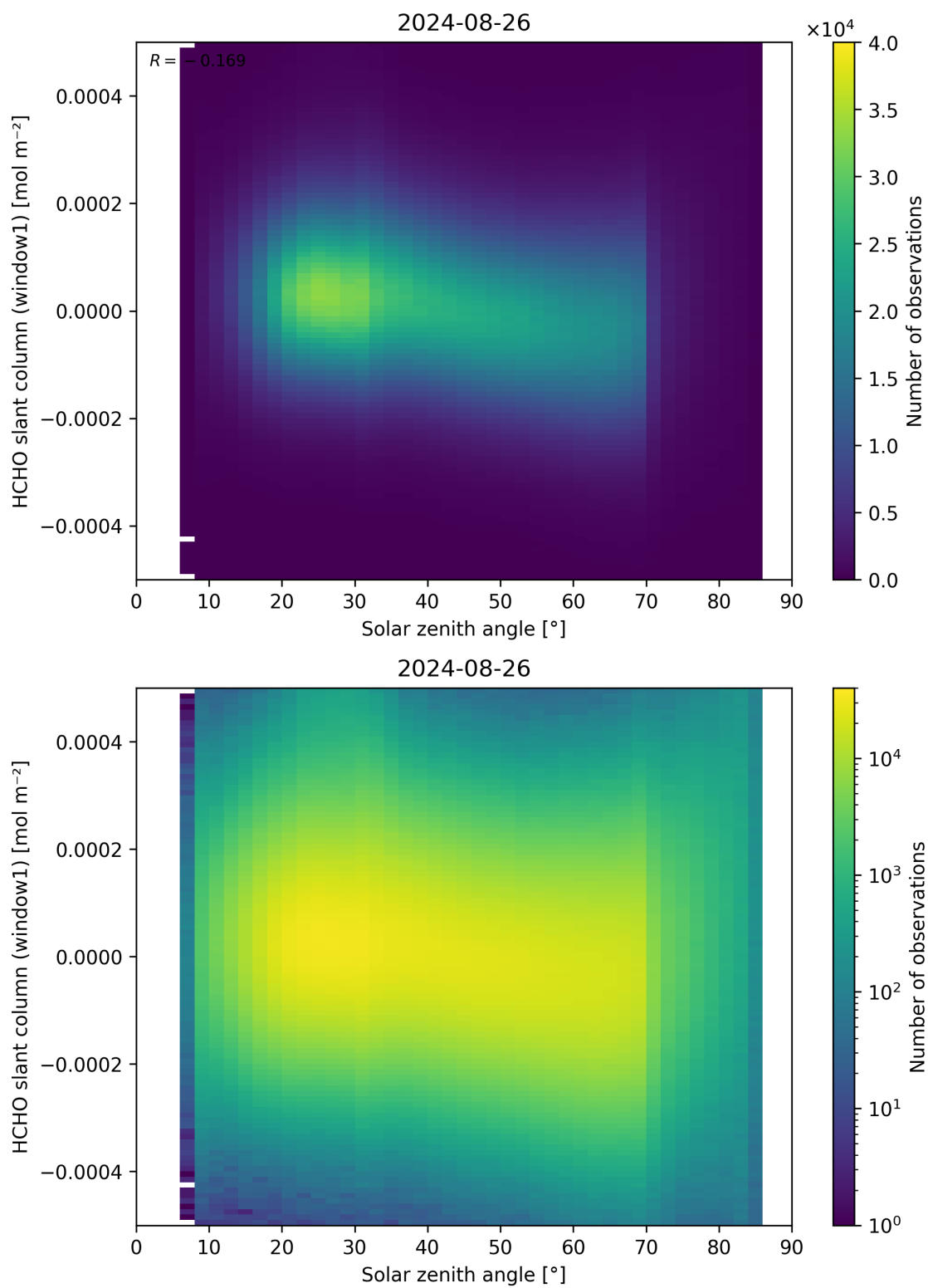
Figure 173: Scatter density plot of “Solar zenith angle” against “HCHO slant column (window1)” for 2024-08-25 to 2024-08-27.
