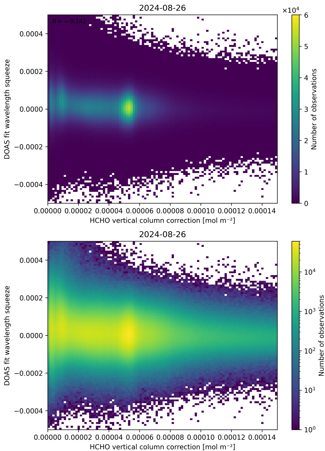
Figure 114: Scatter density plot of “HCHO vertical column correction” against “DOAS fit wavelength squeeze” for 2024-08-25 to 2024-08-27.
