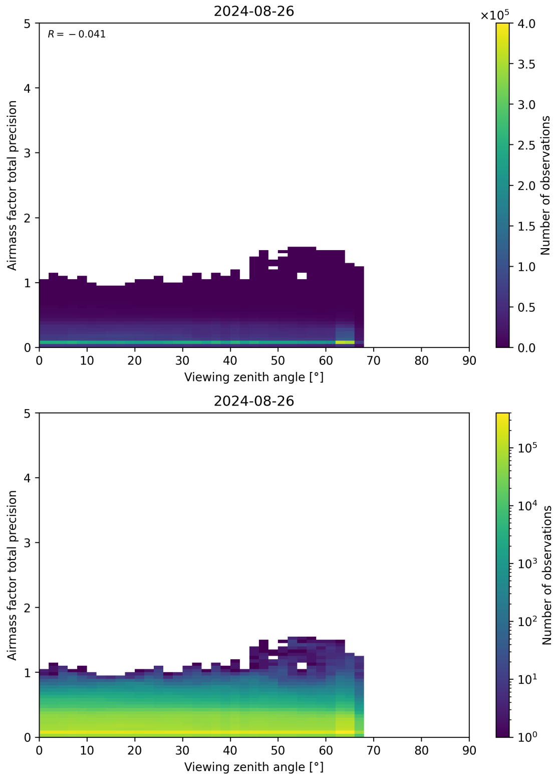
Figure 191: Scatter density plot of “Viewing zenith angle” against “Airmass factor total precision” for 2024-08-25 to 2024-08-27.
