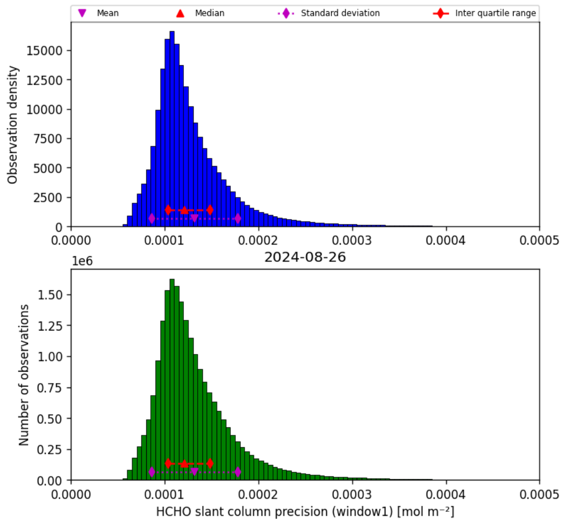
Figure 39: Histogram of “HCHO slant column precision (window1)” for 2024-08-25 to 2024-08-27
