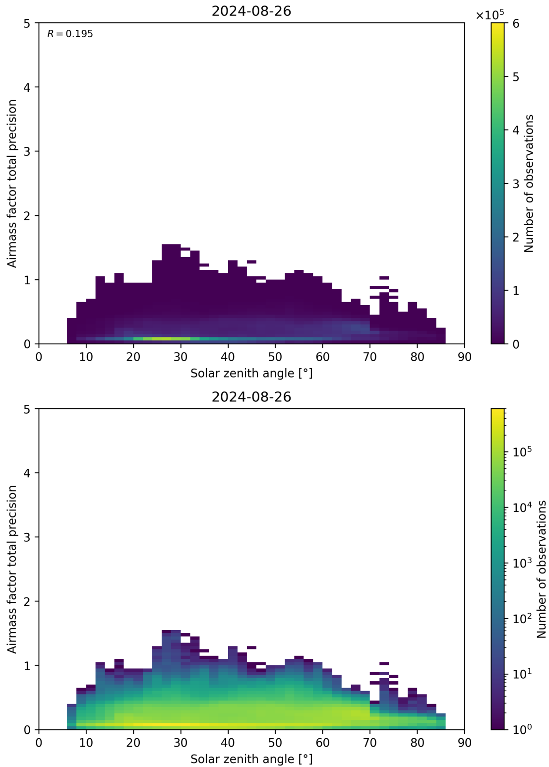
Figure 176: Scatter density plot of “Solar zenith angle” against “Airmass factor total precision” for 2024-08-25 to 2024-08-27.
