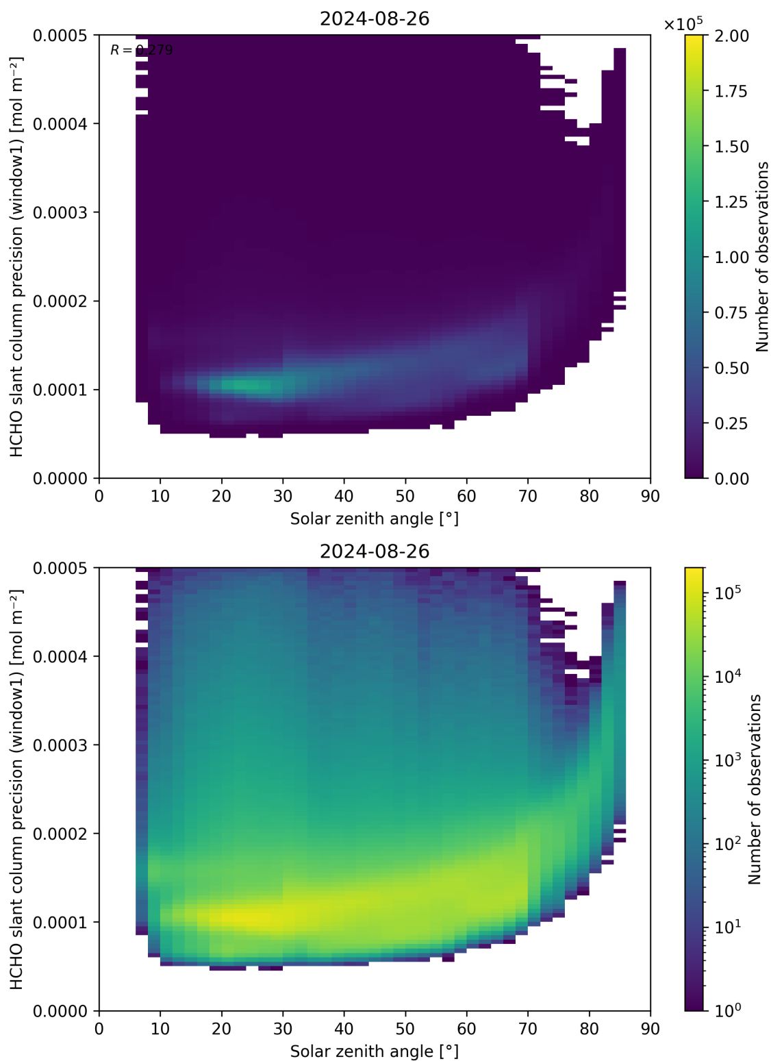
Figure 174: Scatter density plot of “Solar zenith angle” against “HCHO slant column precision (window1)” for 2024-08-25 to 2024-08-27.
