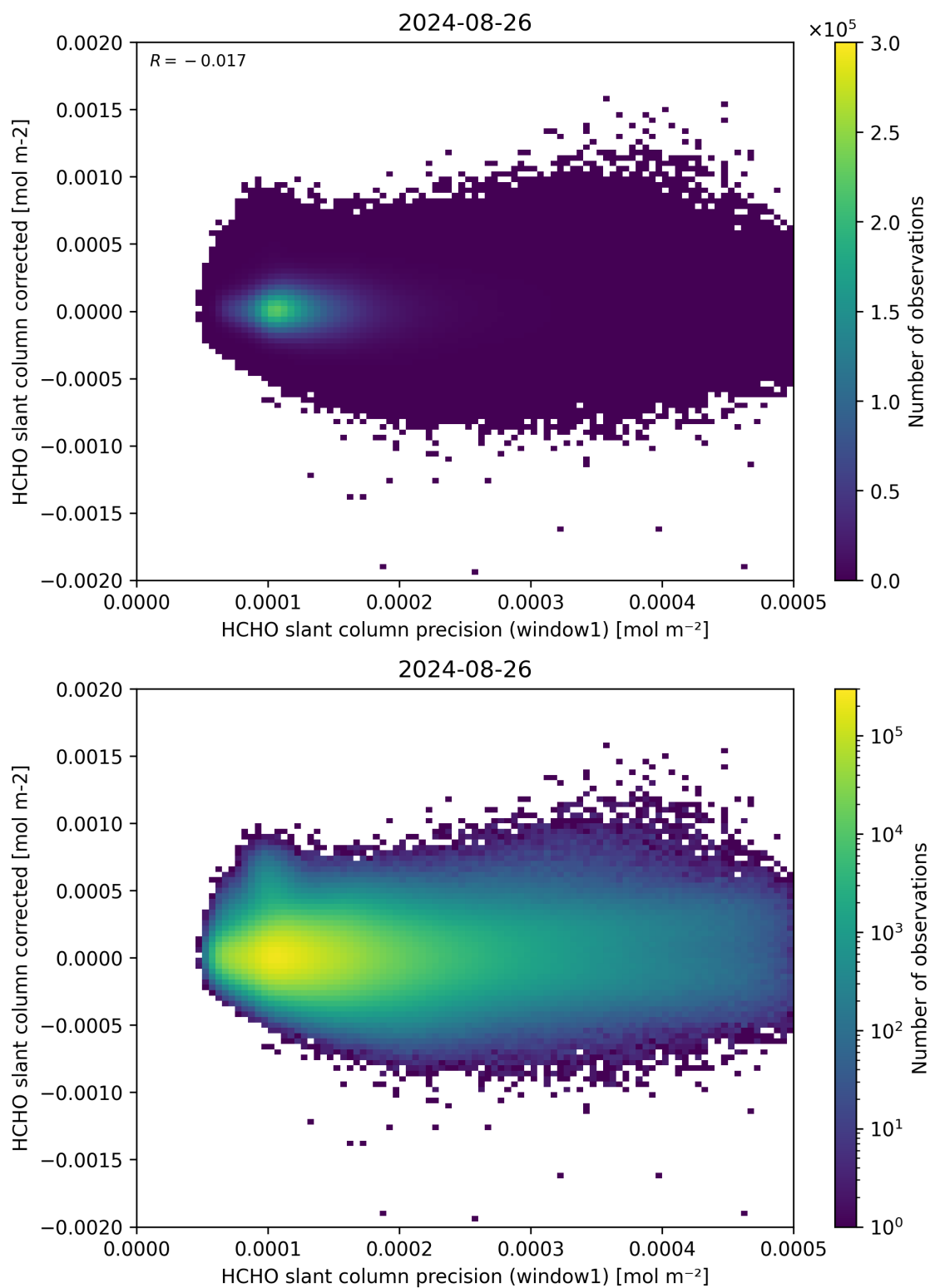
Figure 92: Scatter density plot of “HCHO slant column precision (window1)” against “HCHO slant column corrected” for 2024-08-25 to 2024-08-27.
