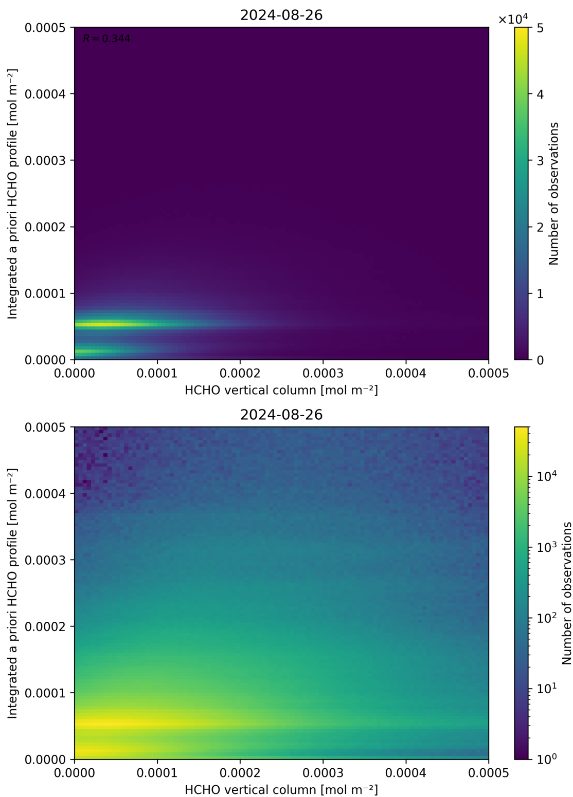
Figure 135: Scatter density plot of “HCHO vertical column” against “Integrated a priori HCHO profile” for 2024-08-25 to 2024-08-27.
