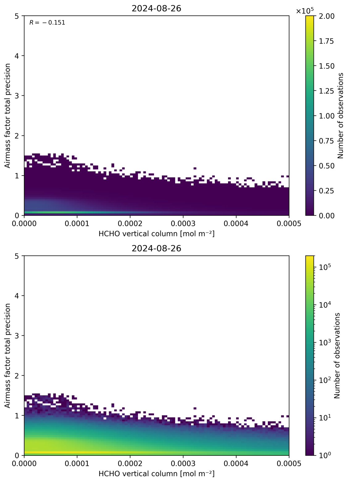
Figure 132: Scatter density plot of “HCHO vertical column” against “Airmass factor total precision” for 2024-08-25 to 2024-08-27.
