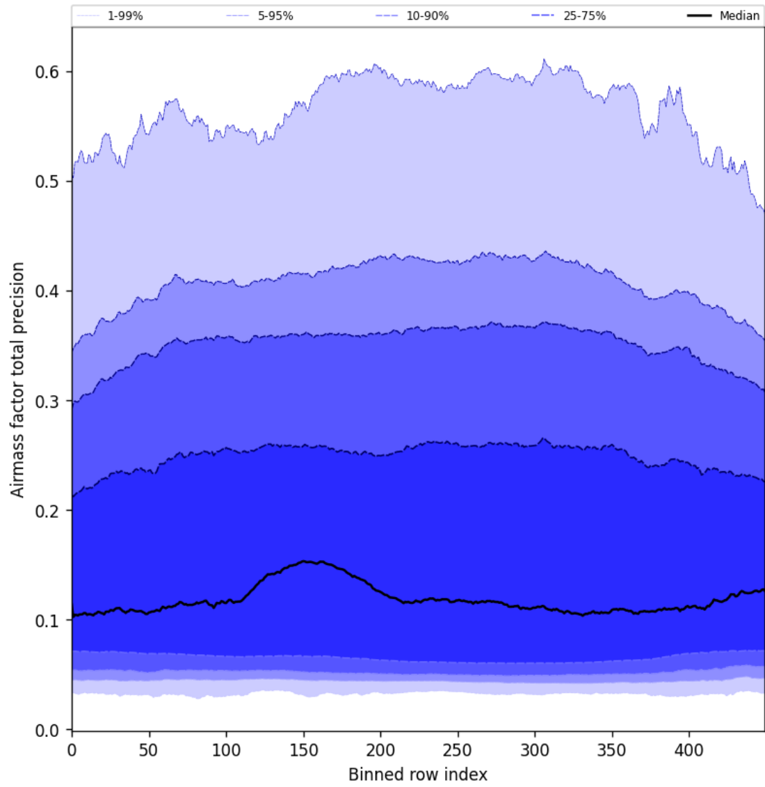
Figure 55: Along track statistics of “Airmass factor total precision” for 2024-08-25 to 2024-08-27
