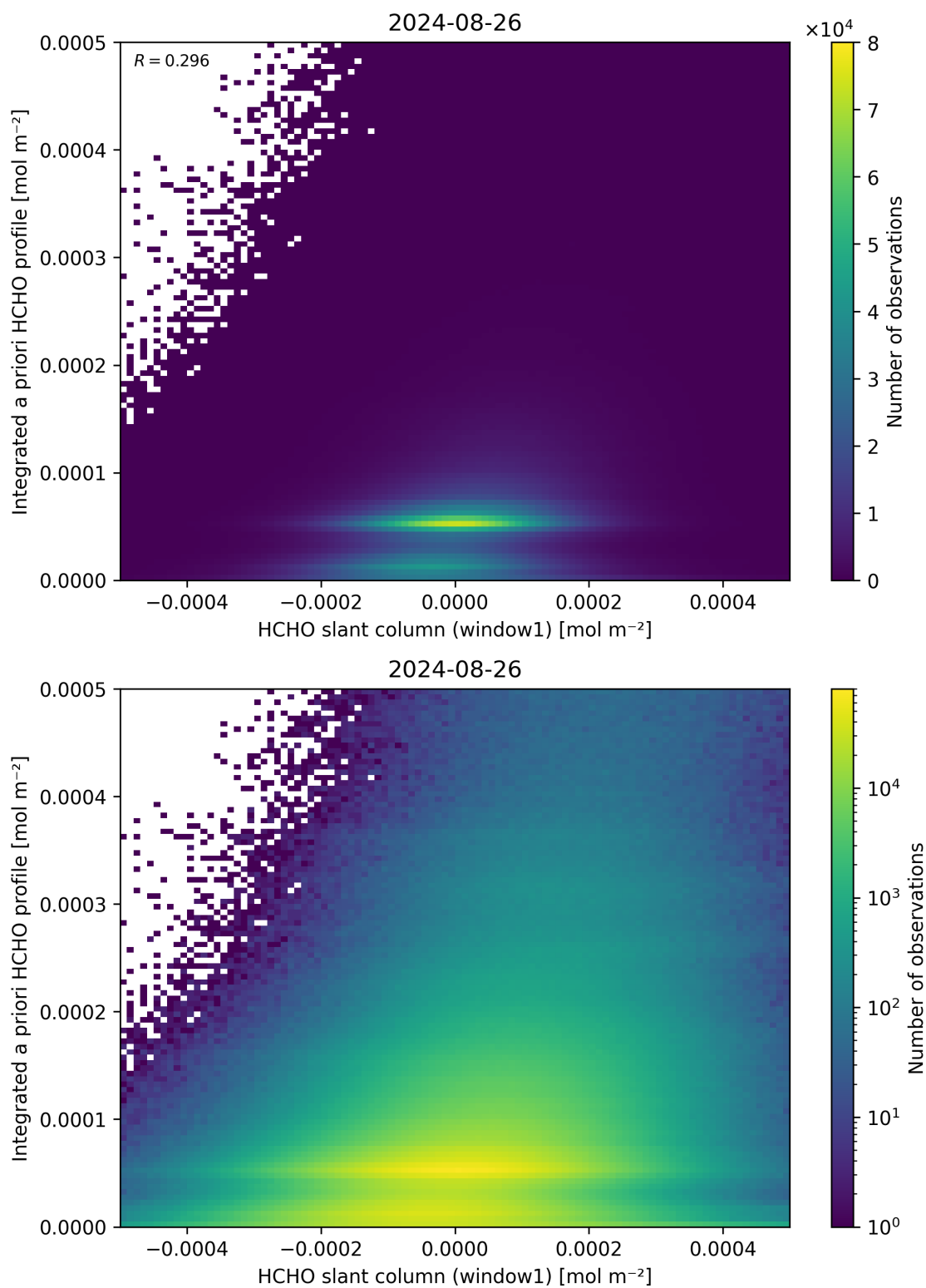
Figure 87: Scatter density plot of “HCHO slant column (window1)” against “Integrated a priori HCHO profile” for 2024-08-25 to 2024-08-27.
