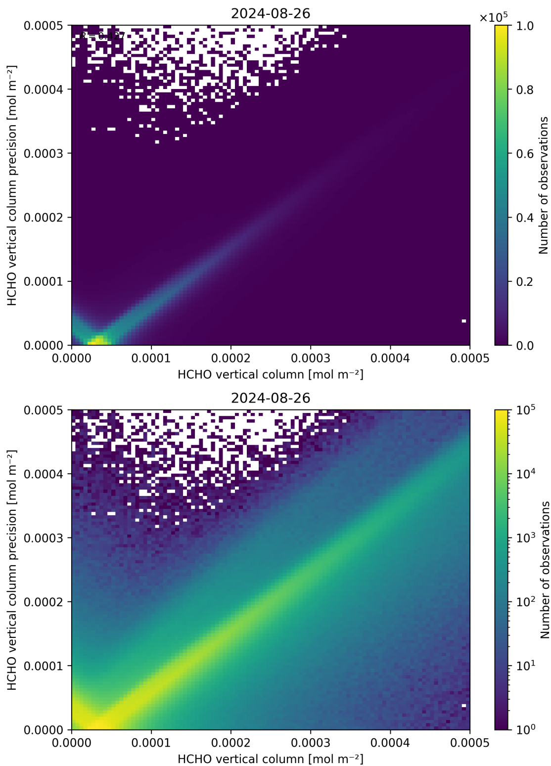
Figure 134: Scatter density plot of “HCHO vertical column” against “HCHO vertical column precision” for 2024-08-25 to 2024-08-27.
