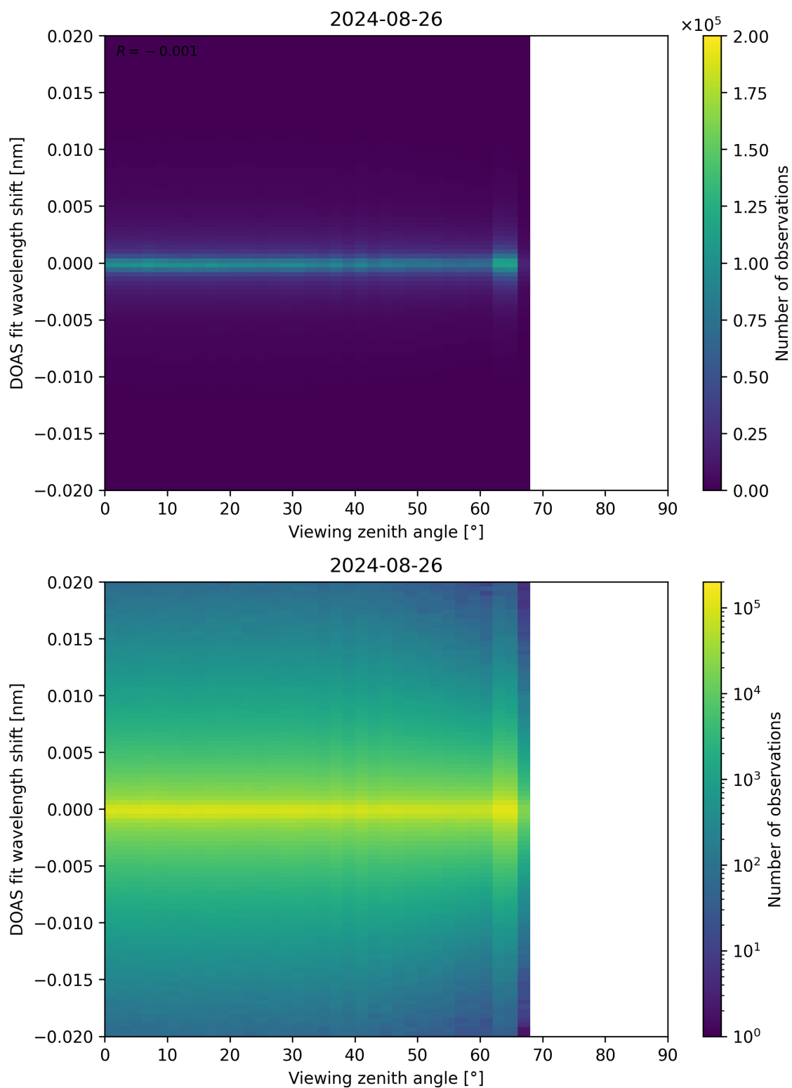
Figure 183: Scatter density plot of “Viewing zenith angle” against “DOAS fit wavelength shift” for 2024-08-25 to 2024-08-27.
