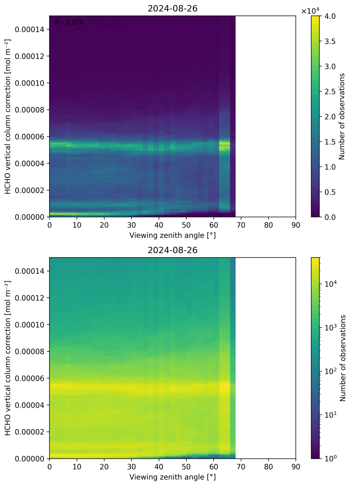
Figure 193: Scatter density plot of “Viewing zenith angle” against “HCHO vertical column correction” for 2024-08-25 to 2024-08-27.
