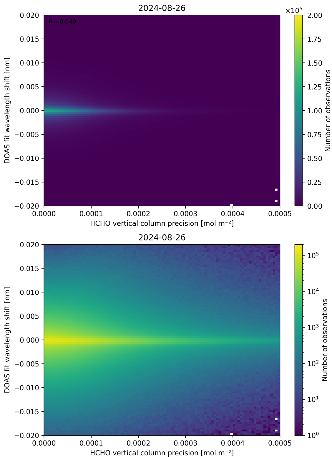
Figure 137: Scatter density plot of “HCHO vertical column precision” against “DOAS fit wavelength shift” for 2024-08-25 to 2024-08-27.
