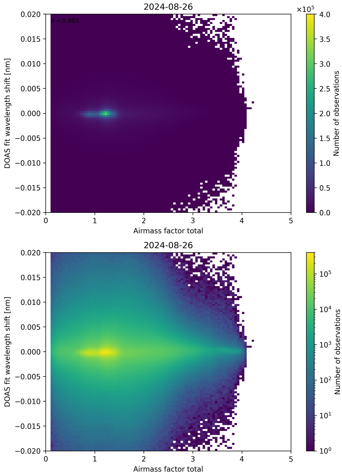
Figure 98: Scatter density plot of “Airmass factor total” against “DOAS fit wavelength shift” for 2024-08-25 to 2024-08-27.
