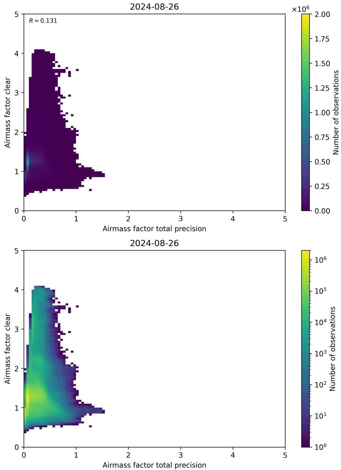
Figure 108: Scatter density plot of “Airmass factor total precision” against “Airmass factor clear” for 2024-08-25 to 2024-08-27.
