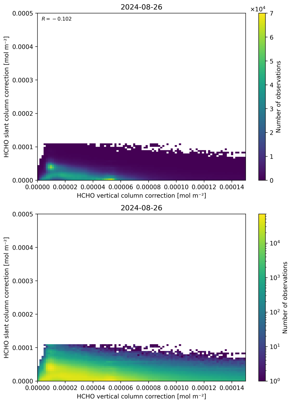
Figure 117: Scatter density plot of “HCHO vertical column correction” against “HCHO slant column correction” for 2024-08-25 to 2024-08-27.
