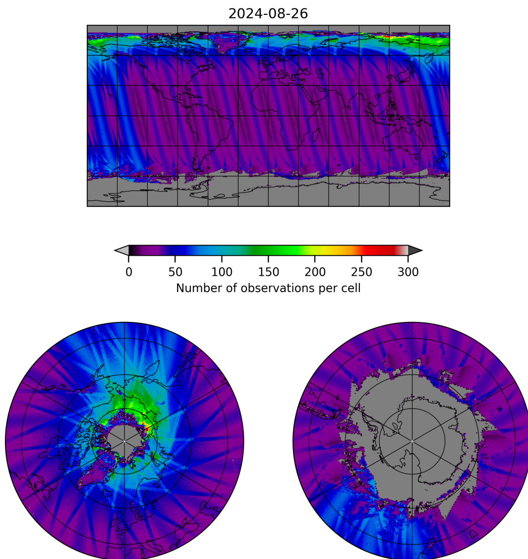
Figure 19: Map of the number of observations for 2024-08-25 to 2024-08-27
