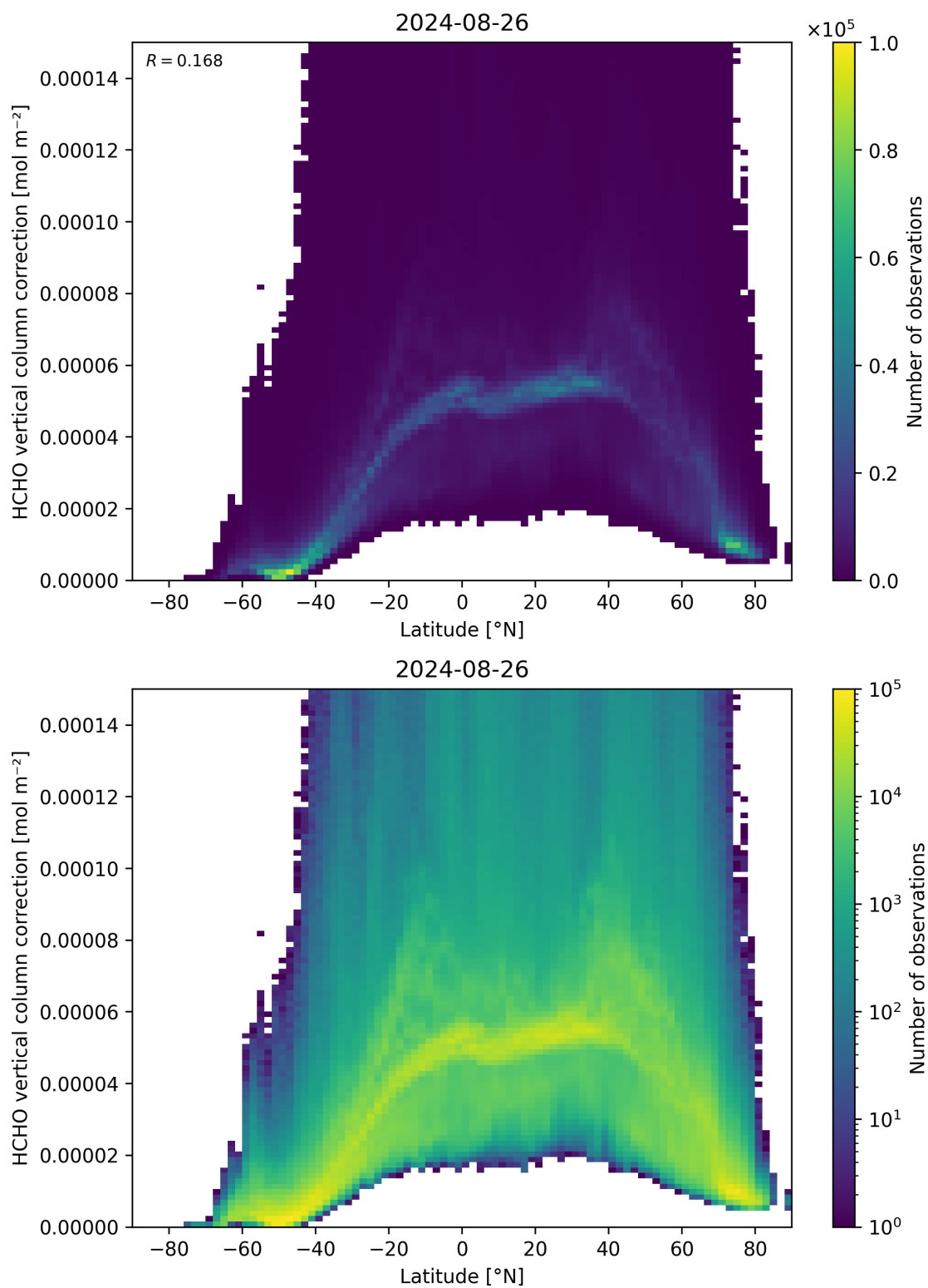
Figure 164: Scatter density plot of “Latitude” against “HCHO vertical column correction” for 2024-08-25 to 2024-08-27.
