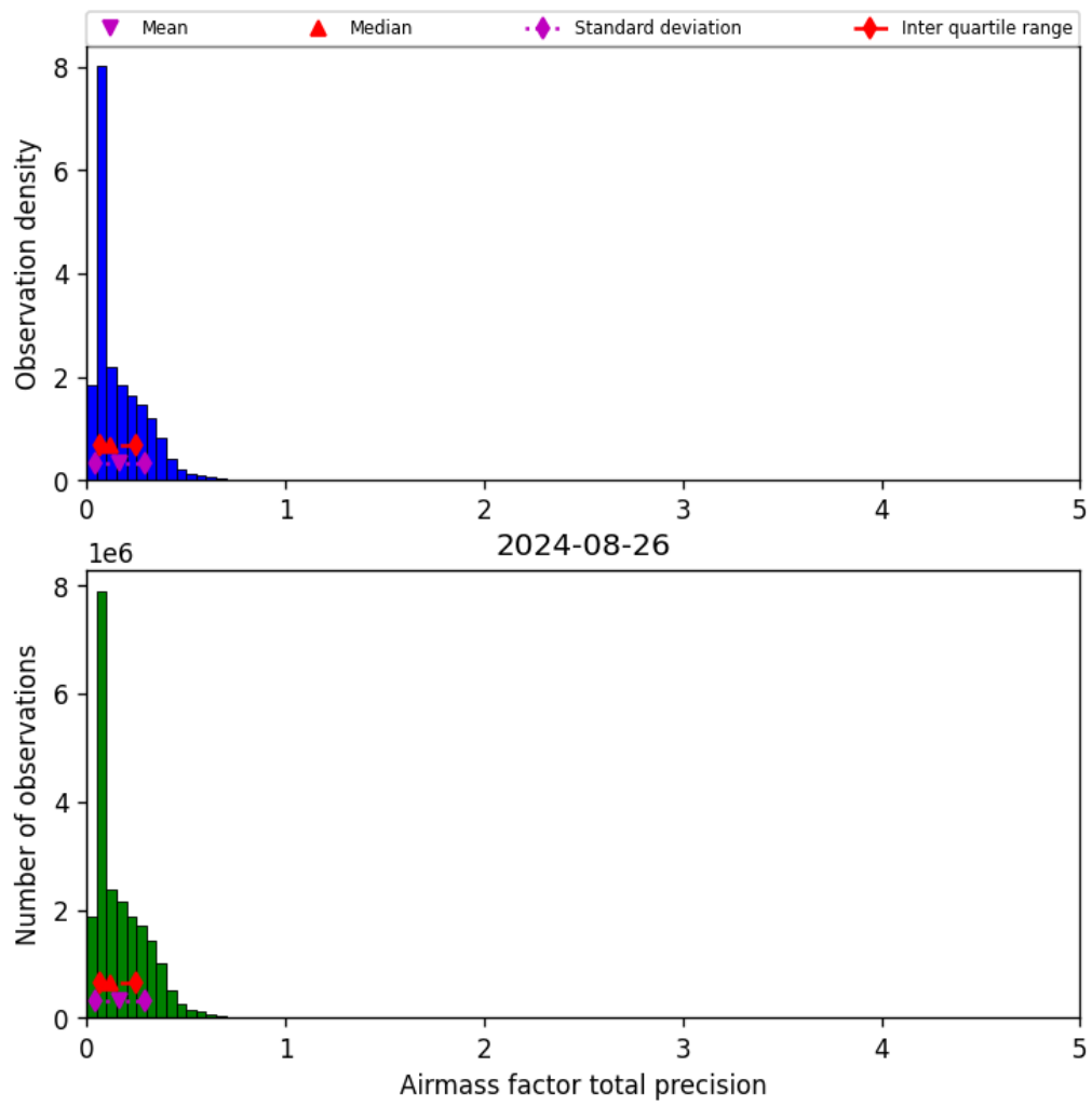
Figure 41: Histogram of “Airmass factor total precision” for 2024-08-25 to 2024-08-27
