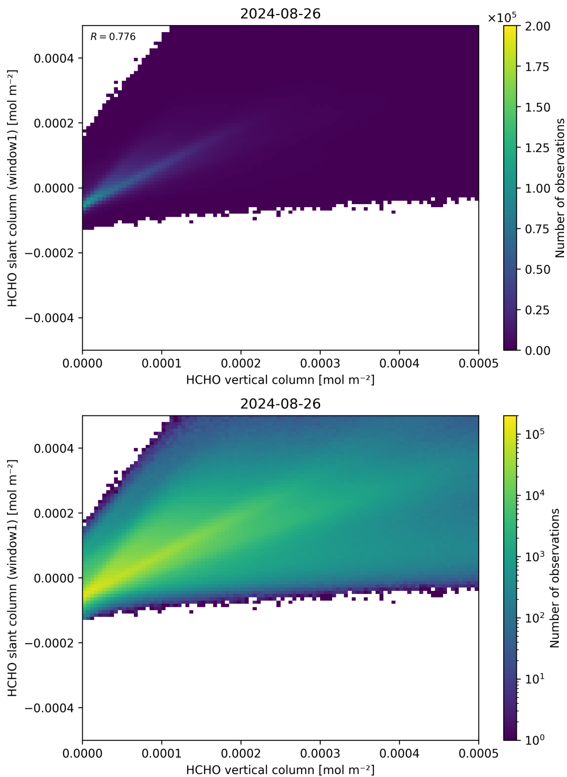
Figure 129: Scatter density plot of “HCHO vertical column” against “HCHO slant column (window1)” for 2024-08-25 to 2024-08-27.
