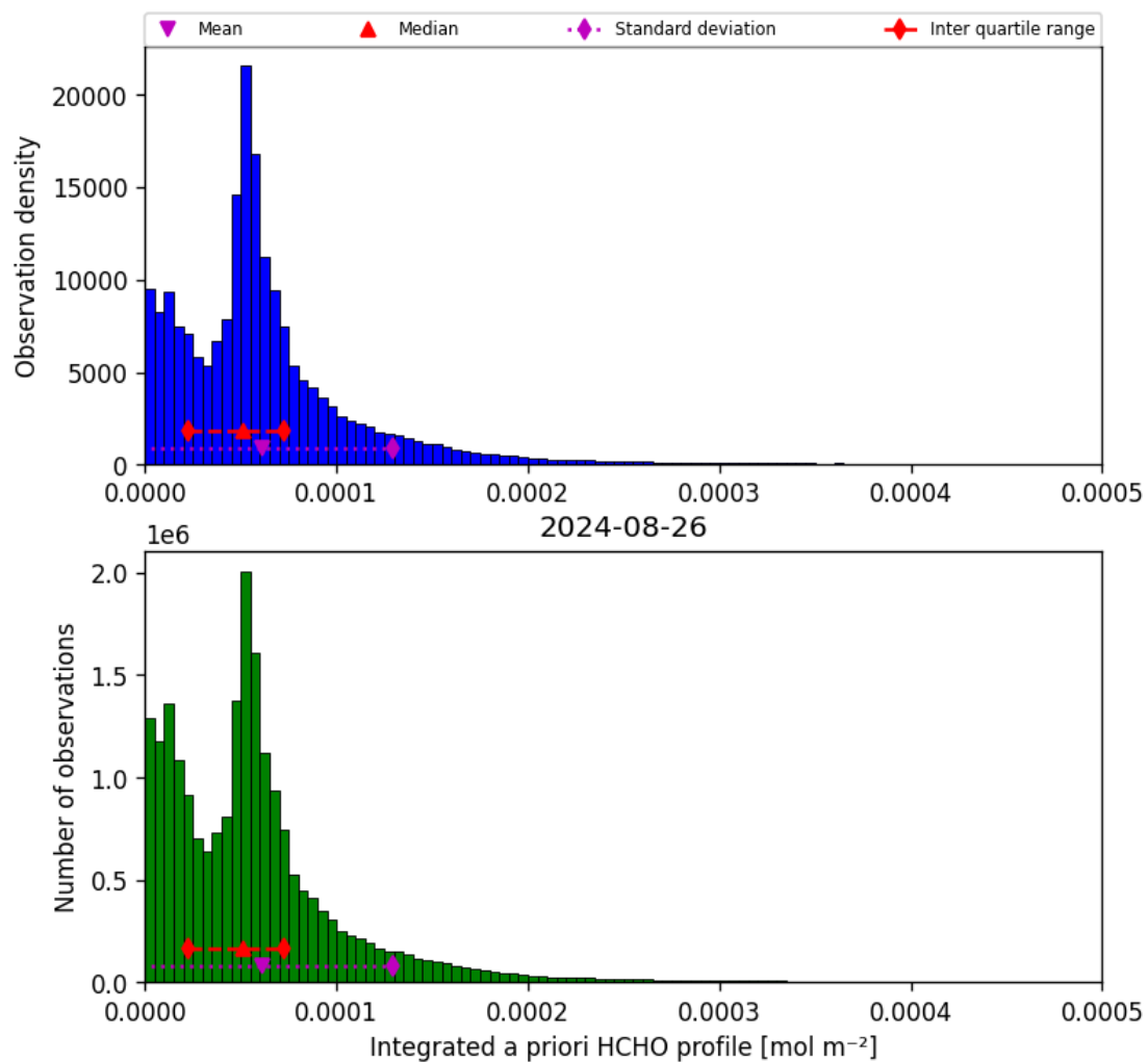
Figure 43: Histogram of “Integrated a priori HCHO profile” for 2024-08-25 to 2024-08-27
