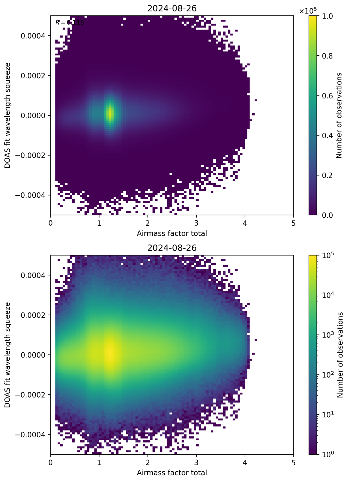
Figure 99: Scatter density plot of “Airmass factor total” against “DOAS fit wavelength squeeze” for 2024-08-25 to 2024-08-27.
