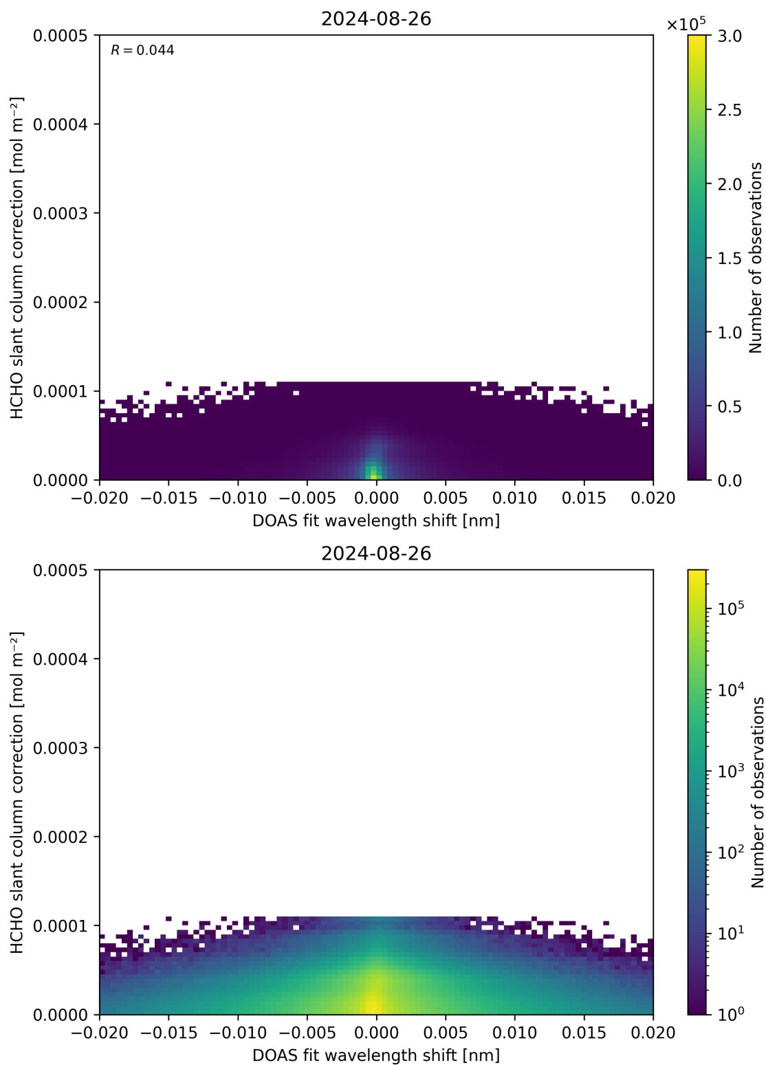
Figure 67: Scatter density plot of “DOAS fit wavelength shift” against “HCHO slant column correction” for 2024-08-25 to 2024-08-27.
