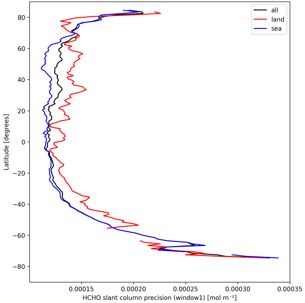
Figure 25: Zonal average of “HCHO slant column precision (window1)” for 2024-08-25 to 2024-08-27.
