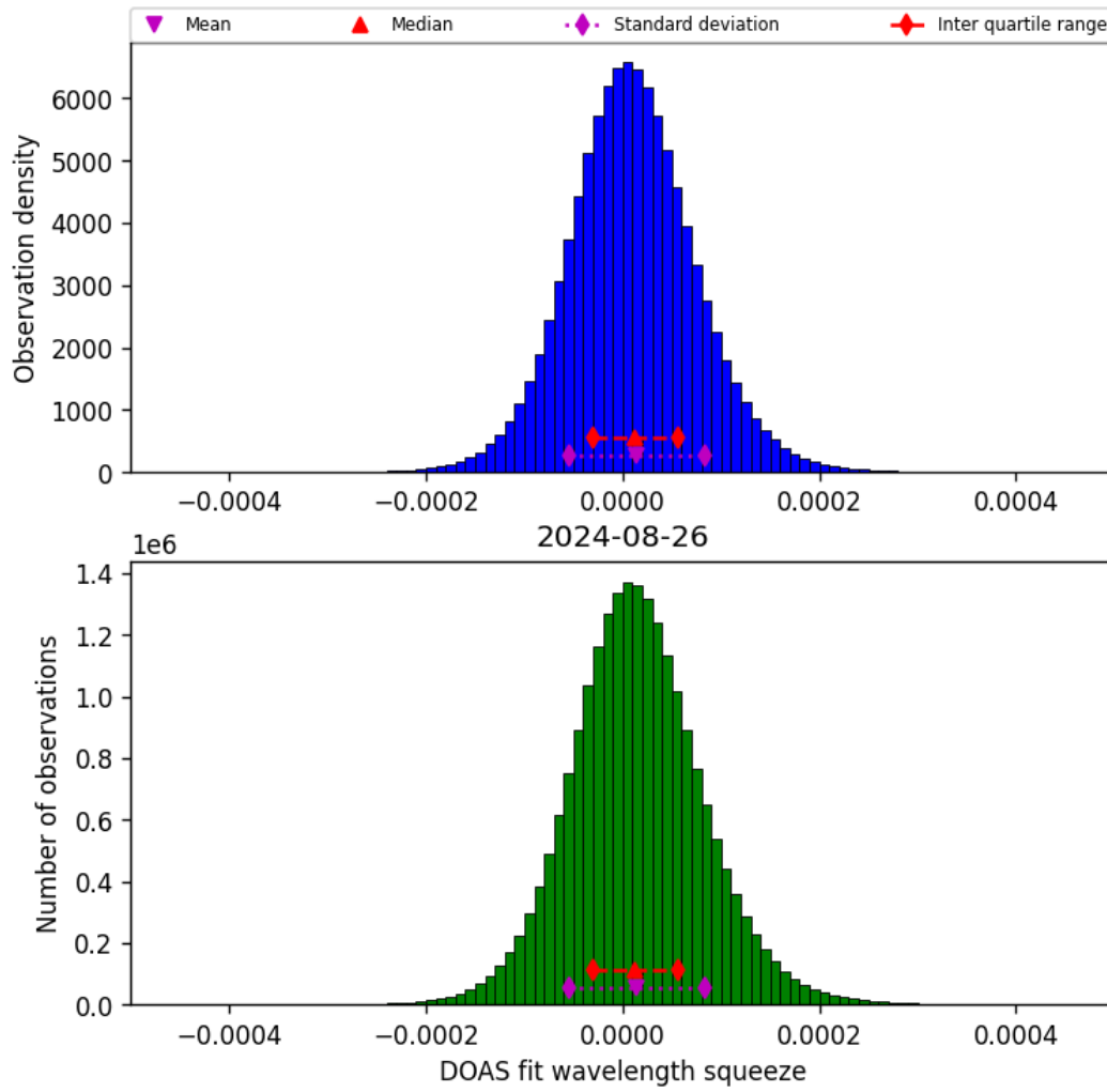
Figure 45: Histogram of “DOAS fit wavelength squeeze” for 2024-08-25 to 2024-08-27
