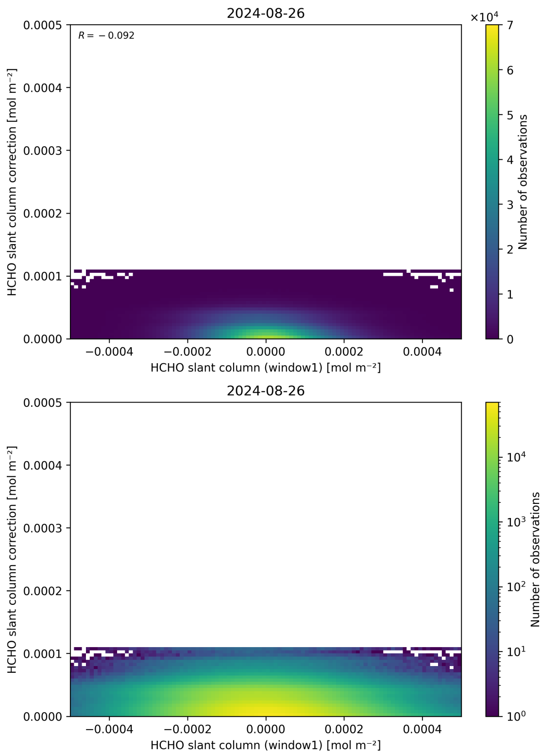
Figure 83: Scatter density plot of “HCHO slant column (window1)” against “HCHO slant column correction” for 2024-08-25 to 2024-08-27.
