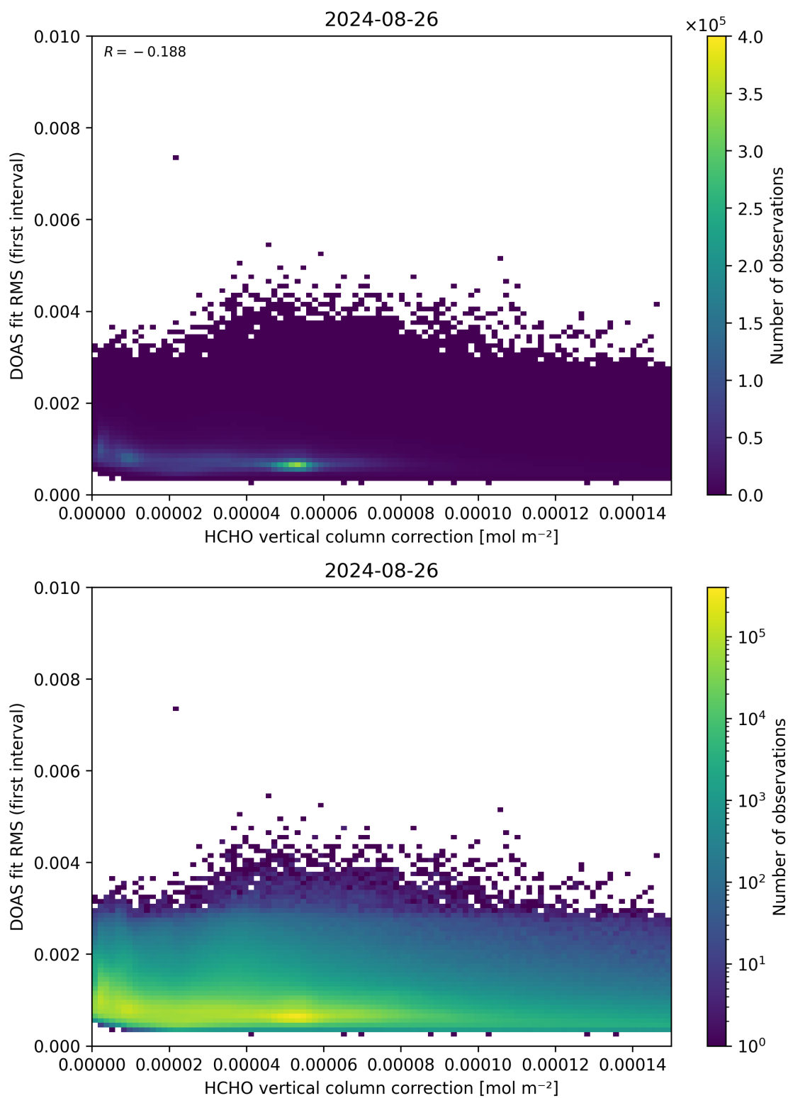
Figure 112: Scatter density plot of “HCHO vertical column correction” against “DOAS fit RMS (first interval)” for 2024-08-25 to 2024-08-27.
