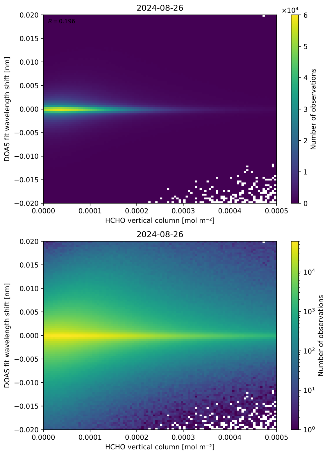
Figure 124: Scatter density plot of “HCHO vertical column” against “DOAS fit wavelength shift” for 2024-08-25 to 2024-08-27.
