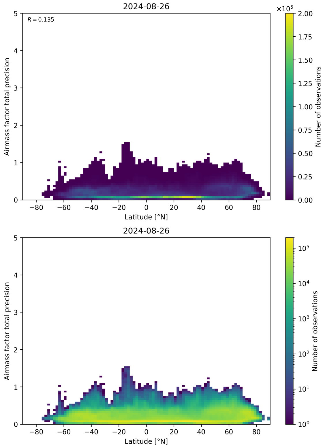
Figure 162: Scatter density plot of “Latitude” against “Airmass factor total precision” for 2024-08-25 to 2024-08-27.
