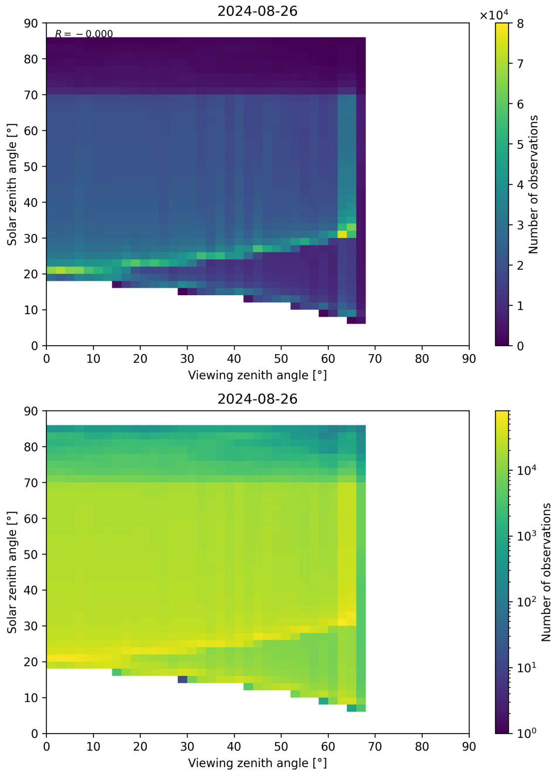
Figure 197: Scatter density plot of “Viewing zenith angle” against “Solar zenith angle” for 2024-08-25 to 2024-08-27.
