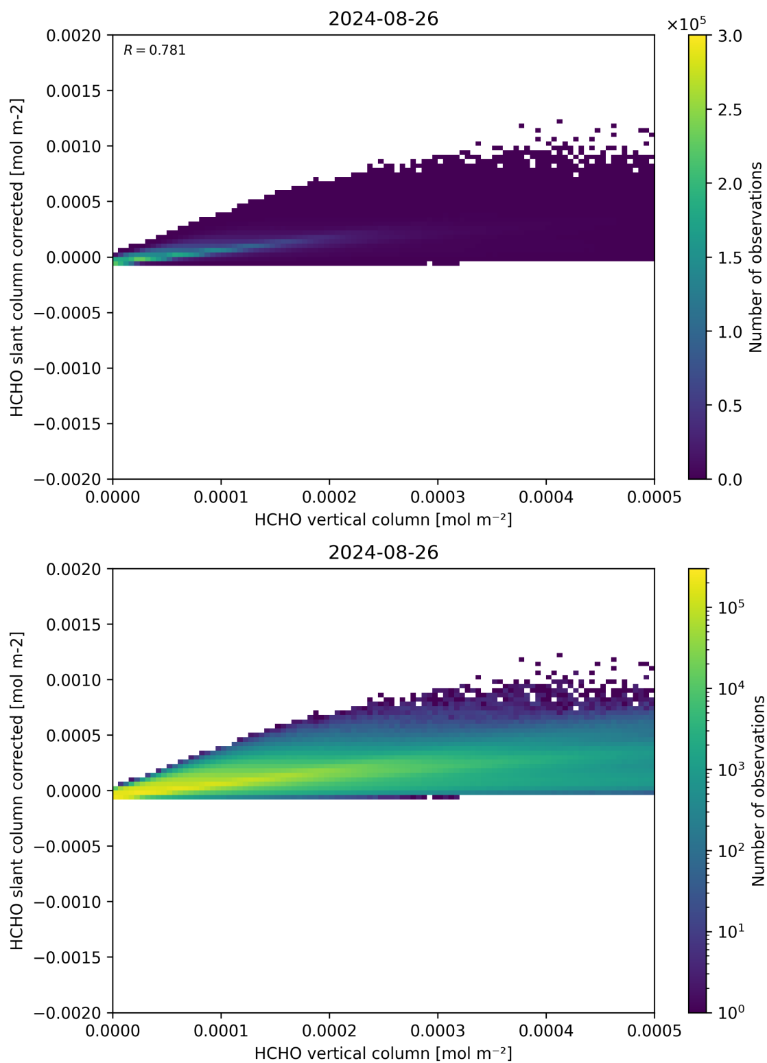
Figure 127: Scatter density plot of “HCHO vertical column” against “HCHO slant column corrected” for 2024-08-25 to 2024-08-27.
