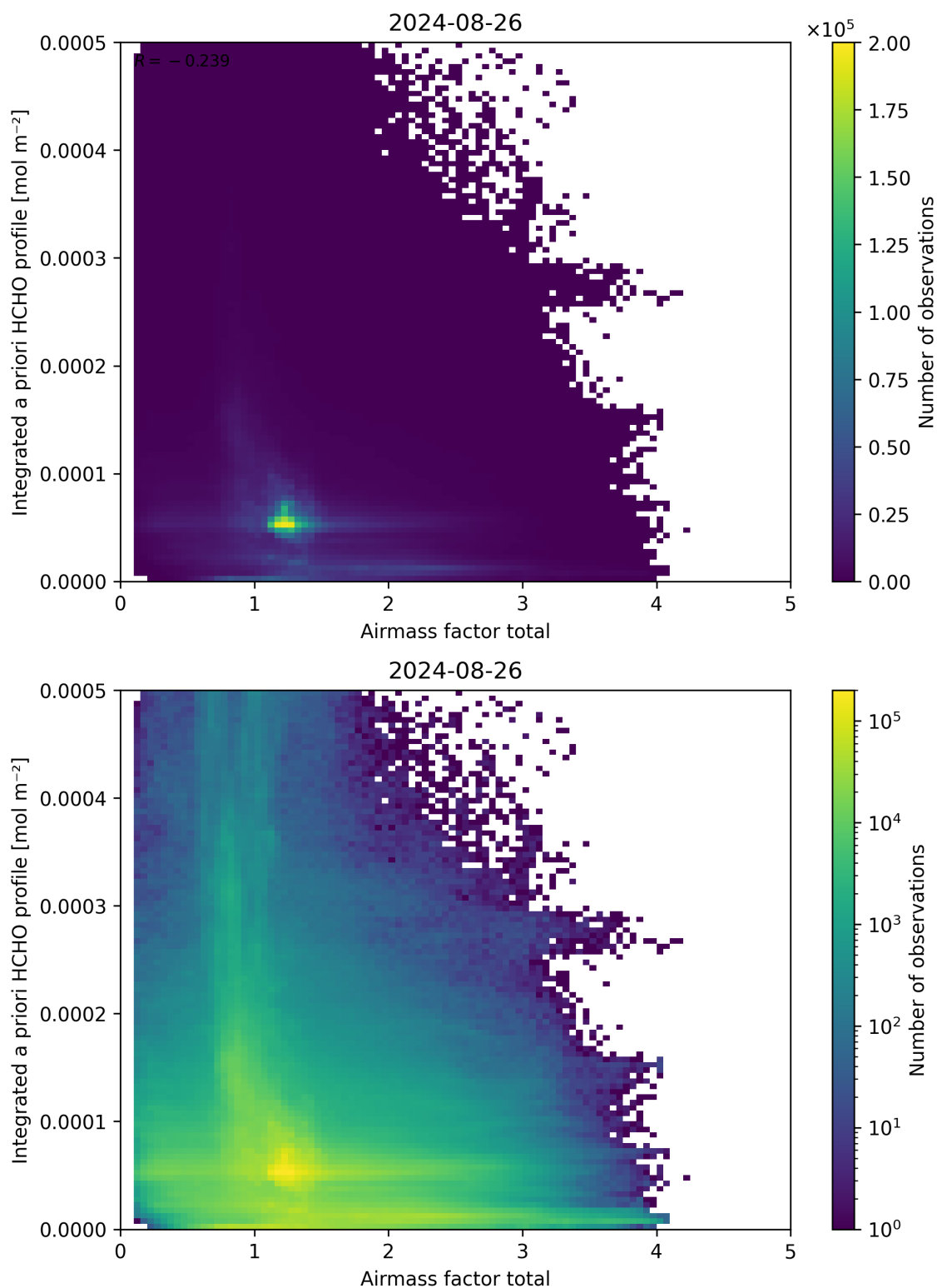
Figure 104: Scatter density plot of “Airmass factor total” against “Integrated a priori HCHO profile” for 2024-08-25 to 2024-08-27.
