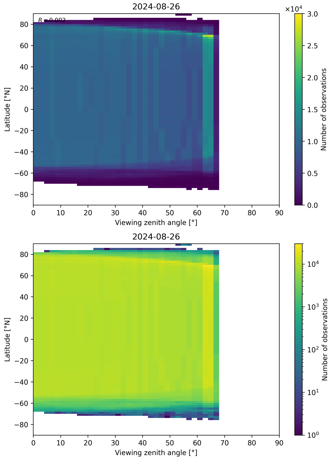
Figure 196: Scatter density plot of “Viewing zenith angle” against “Latitude” for 2024-08-25 to 2024-08-27.
