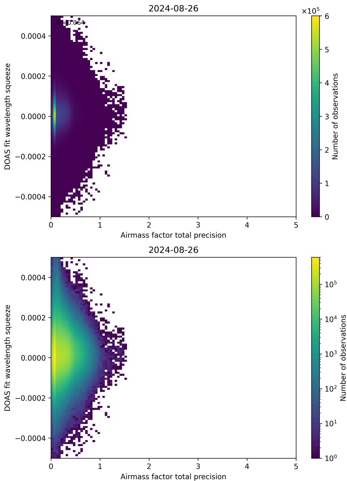
Figure 107: Scatter density plot of “Airmass factor total precision” against “DOAS fit wavelength squeeze” for 2024-08-25 to 2024-08-27.
