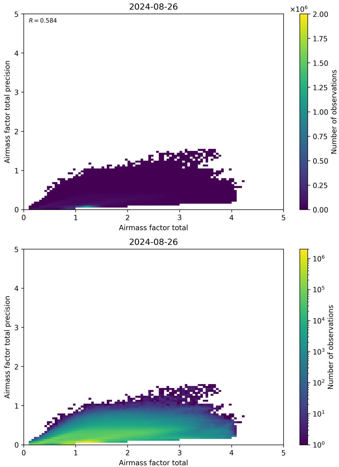
Figure 103: Scatter density plot of “Airmass factor total” against “Airmass factor total precision” for 2024-08-25 to 2024-08-27.
