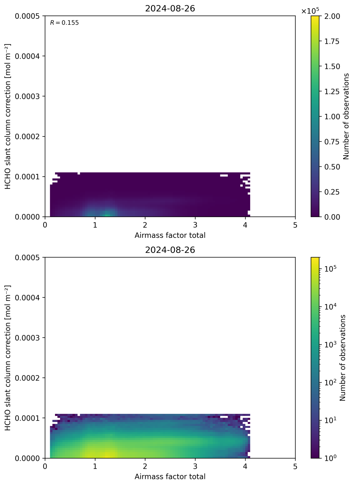
Figure 102: Scatter density plot of “Airmass factor total” against “HCHO slant column correction” for 2024-08-25 to 2024-08-27.
