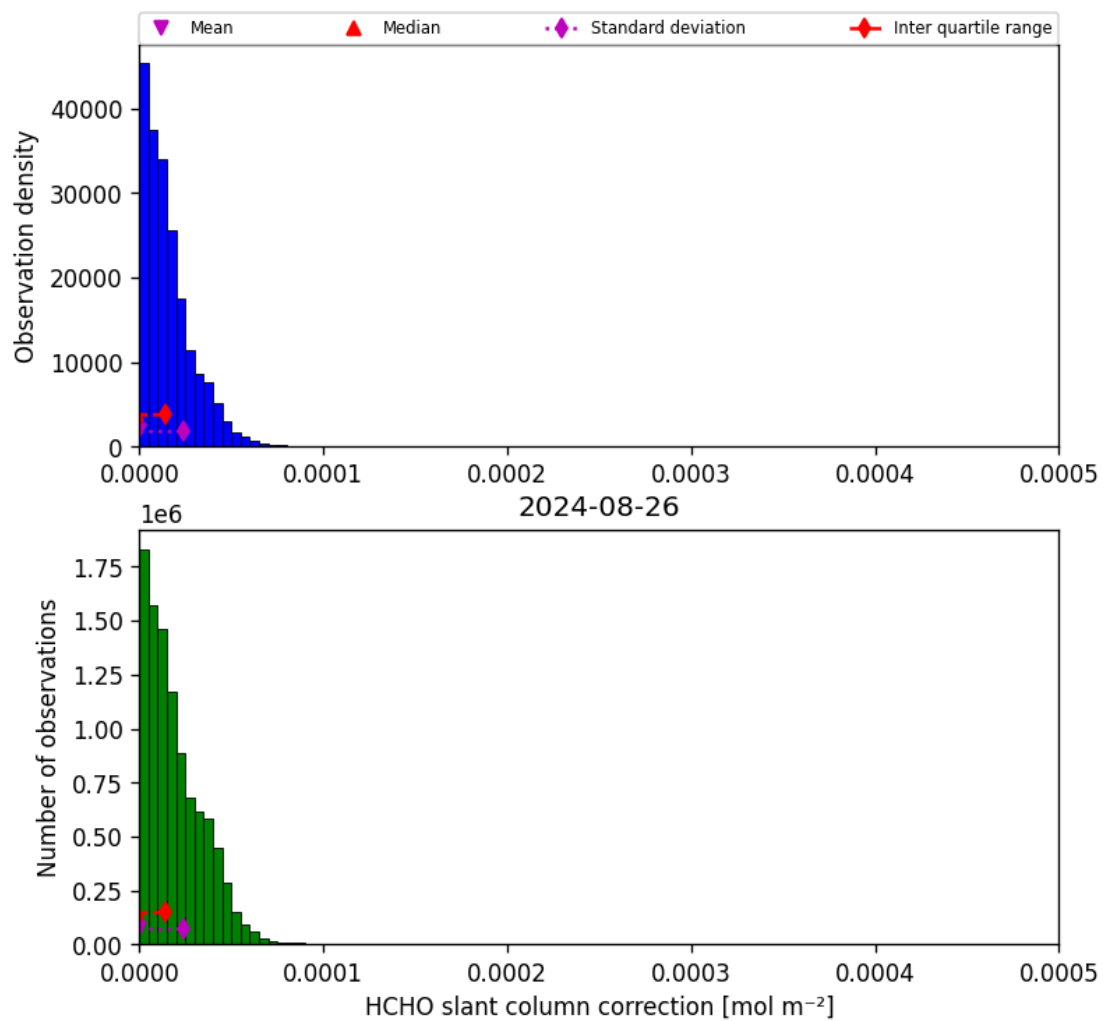
Figure 47: Histogram of “HCHO slant column correction” for 2024-08-25 to 2024-08-27
