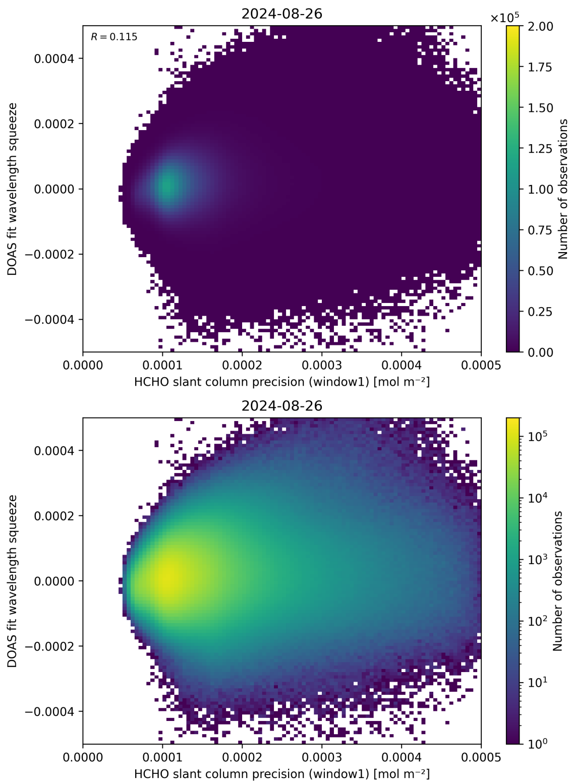
Figure 90: Scatter density plot of “HCHO slant column precision (window1)” against “DOAS fit wavelength squeeze” for 2024-08-25 to 2024-08-27.
