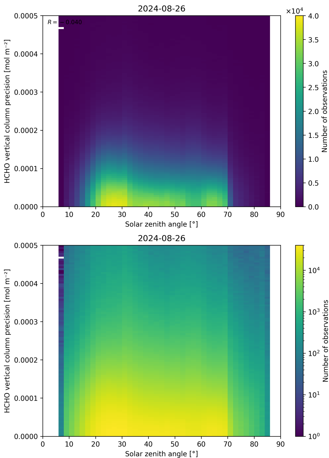
Figure 179: Scatter density plot of “Solar zenith angle” against “HCHO vertical column precision” for 2024-08-25 to 2024-08-27.
