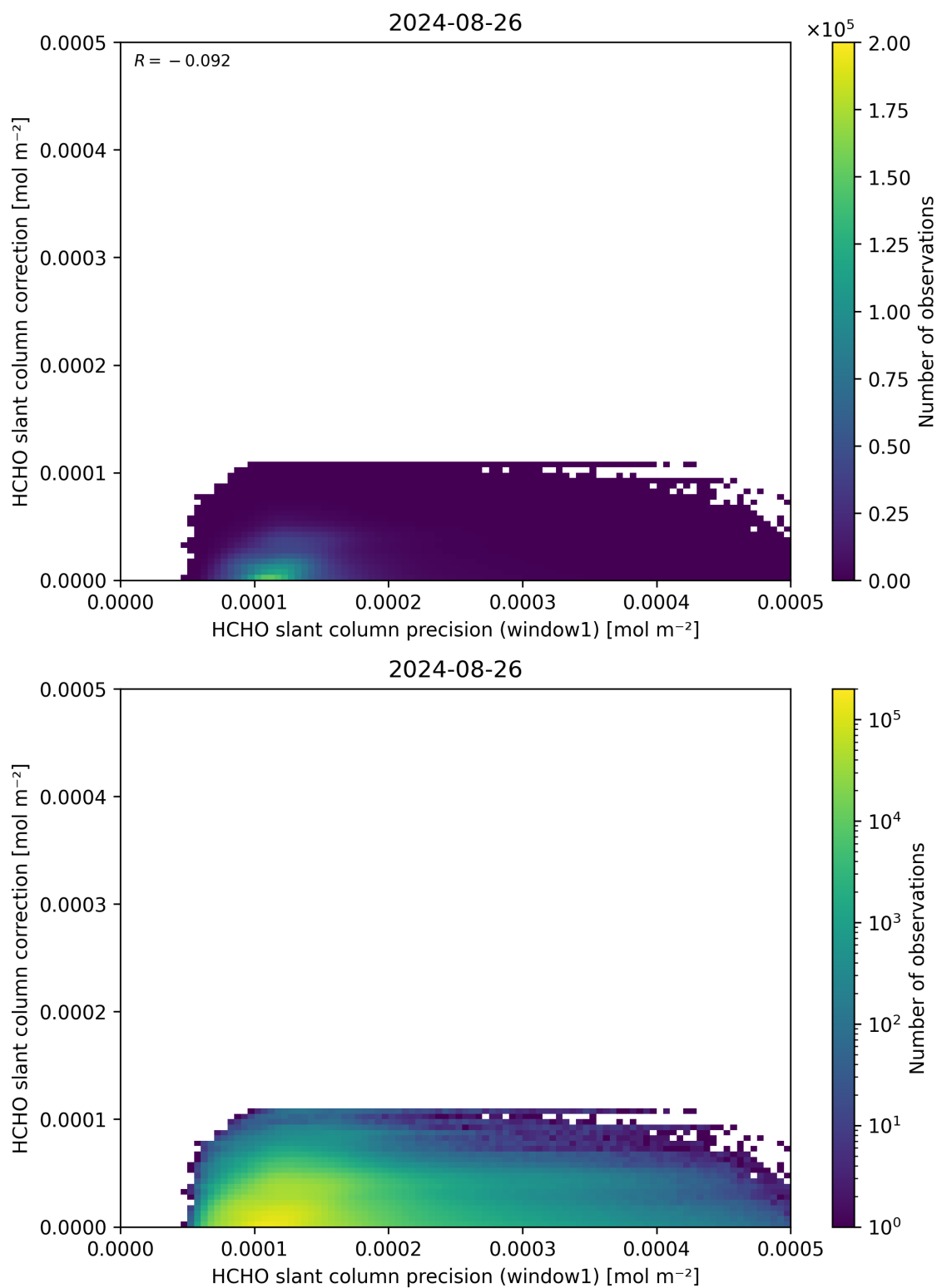
Figure 93: Scatter density plot of “HCHO slant column precision (window1)” against “HCHO slant column correction” for 2024-08-25 to 2024-08-27.
