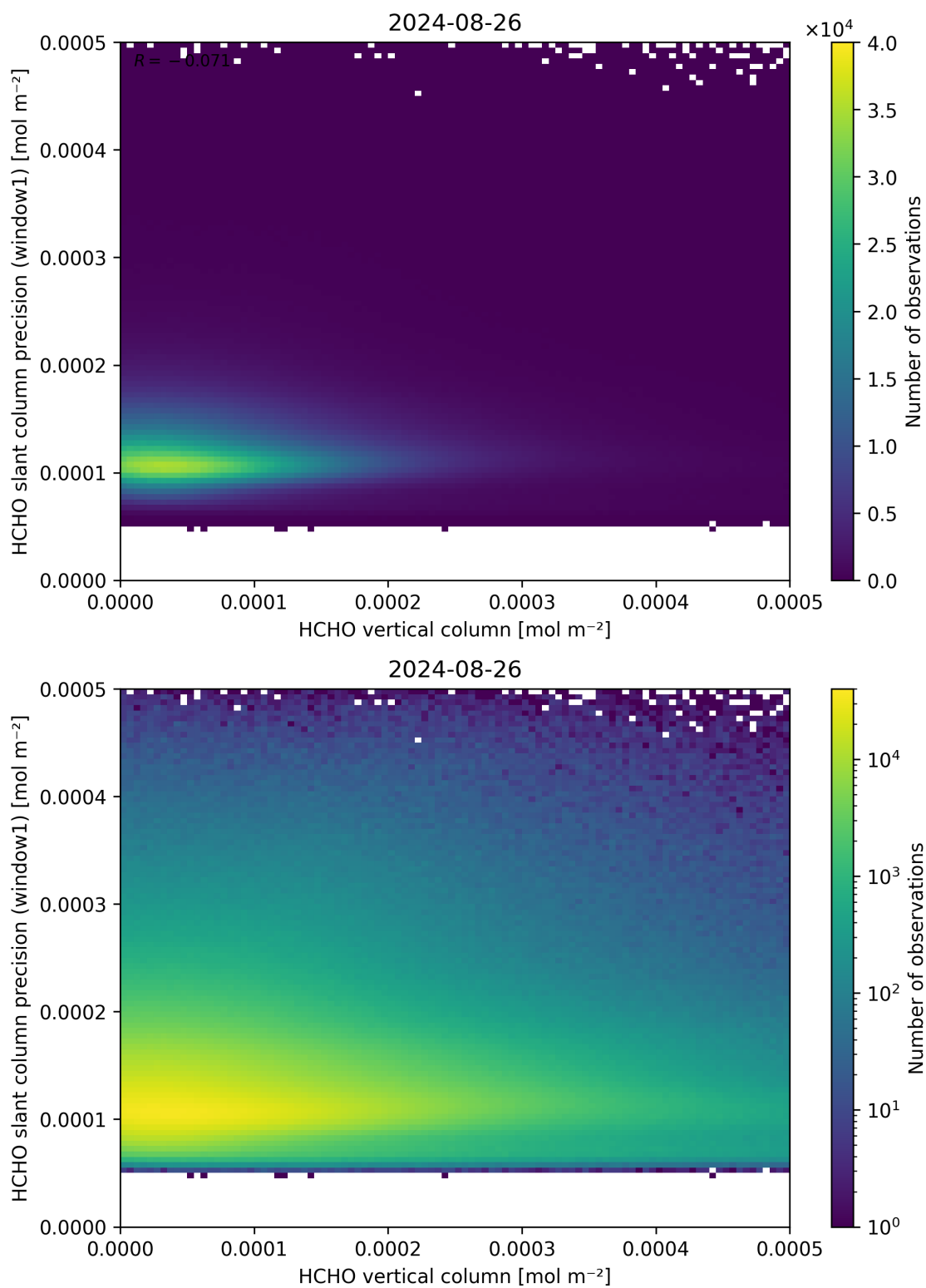
Figure 130: Scatter density plot of “HCHO vertical column” against “HCHO slant column precision (window1)” for 2024-08-25 to 2024-08-27.
