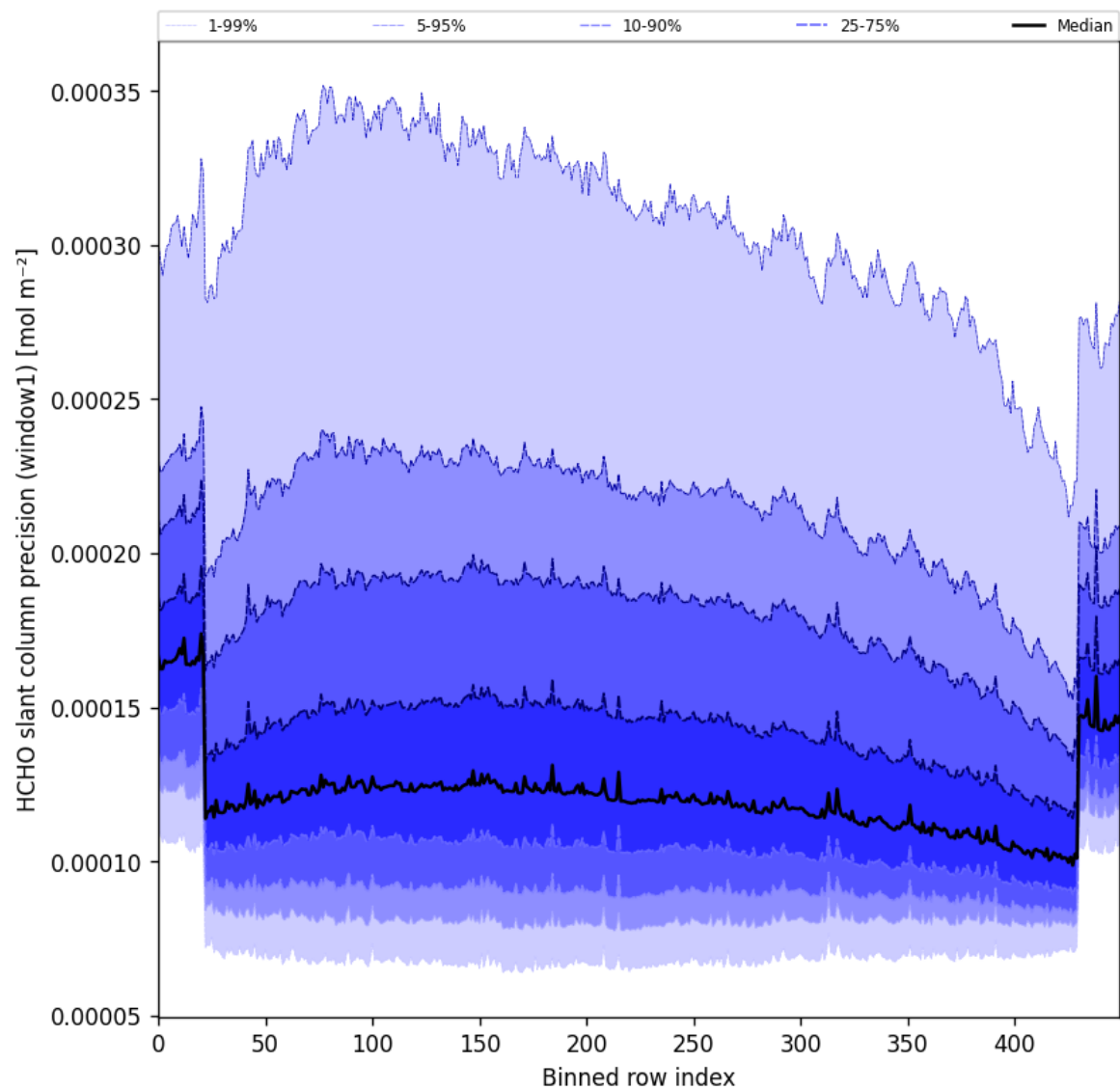
Figure 53: Along track statistics of “HCHO slant column precision (window1)” for 2024-08-25 to 2024-08-27
