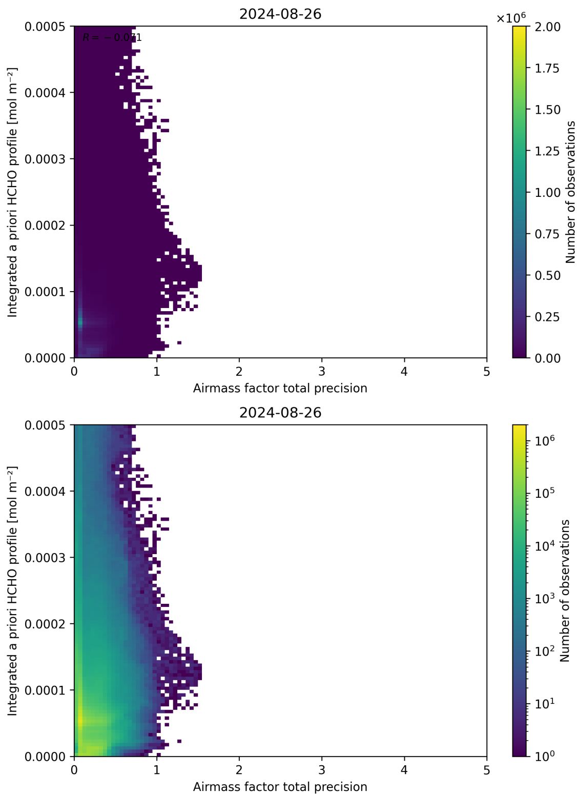
Figure 111: Scatter density plot of “Airmass factor total precision” against “Integrated a priori HCHO profile” for 2024-08-25 to 2024-08-27.
