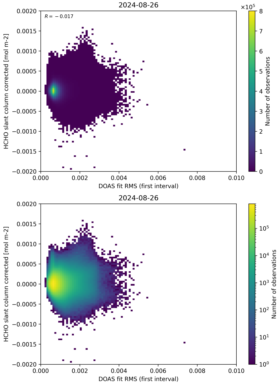
Figure 62: Scatter density plot of “DOAS fit RMS (first interval)” against “HCHO slant column corrected” for 2024-08-25 to 2024-08-27.
