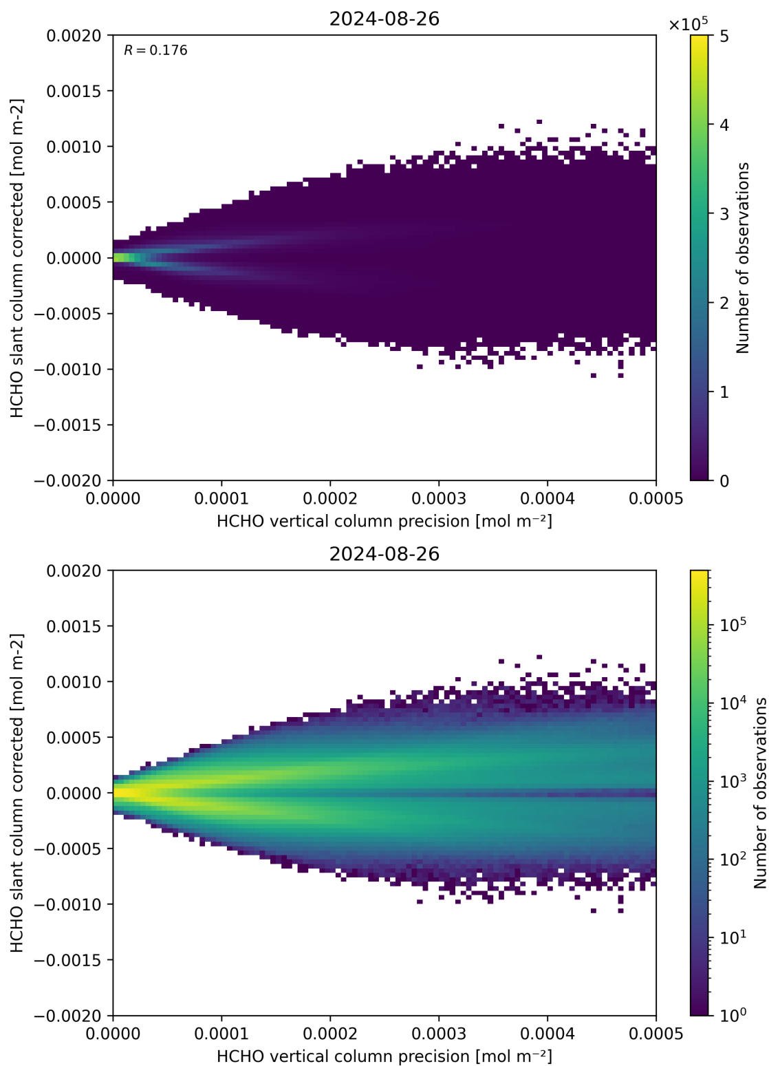
Figure 140: Scatter density plot of “HCHO vertical column precision” against “HCHO slant column corrected” for 2024-08-25 to 2024-08-27.
