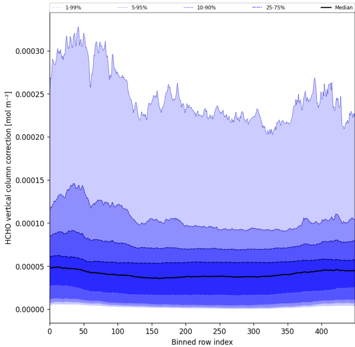
Figure 51: Along track statistics of “HCHO vertical column correction” for 2024-08-25 to 2024-08-27
