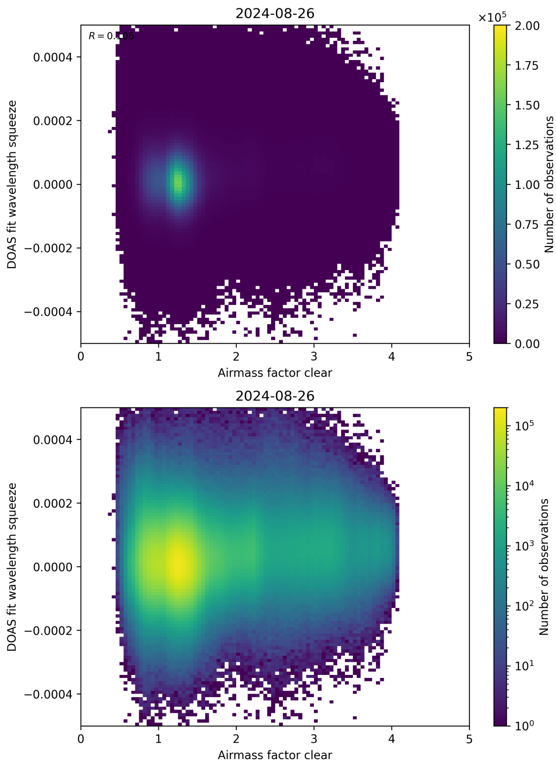
Figure 73: Scatter density plot of “Airmass factor clear” against “DOAS fit wavelength squeeze” for 2024-08-25 to 2024-08-27.
