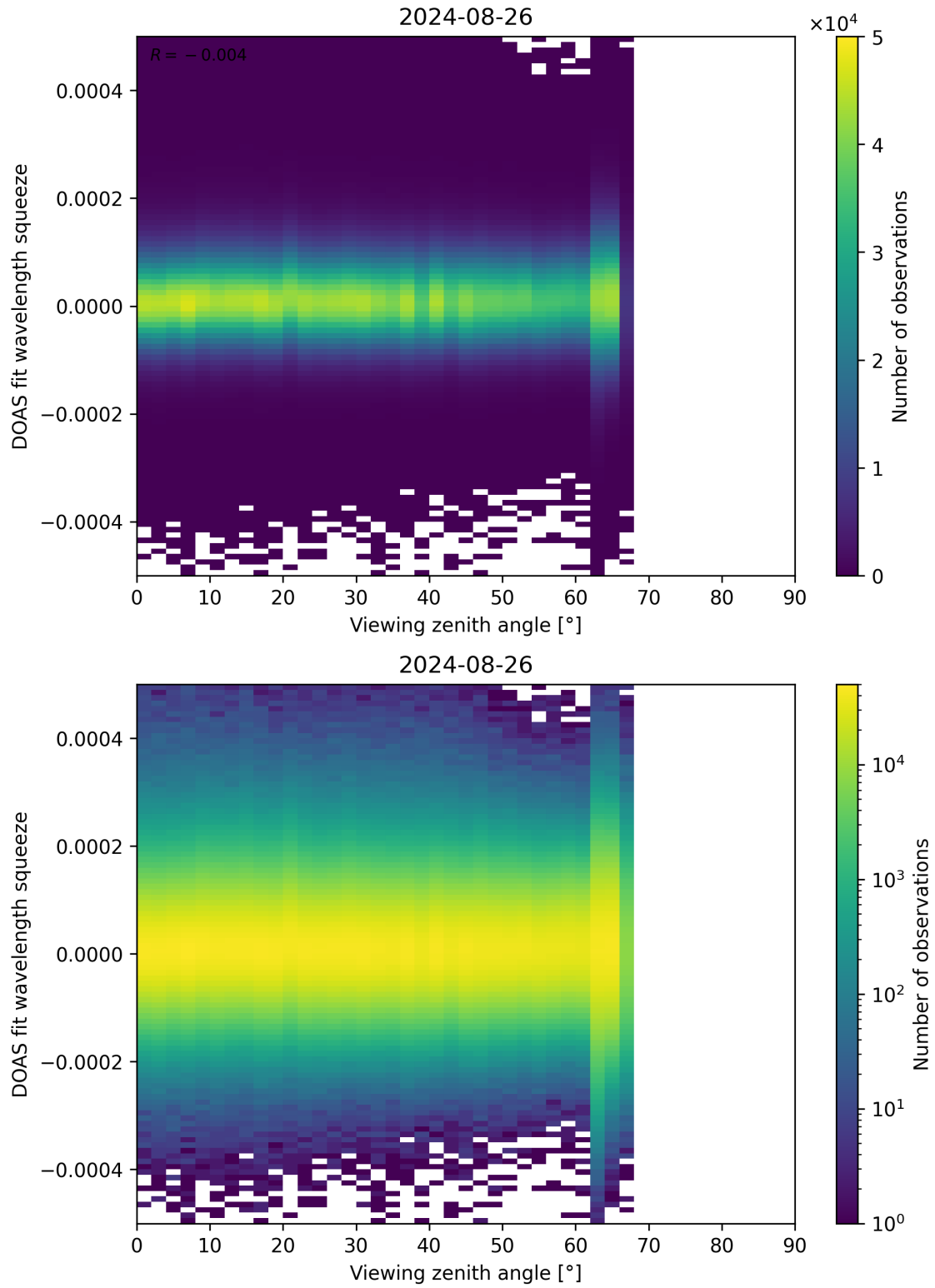
Figure 184: Scatter density plot of “Viewing zenith angle” against “DOAS fit wavelength squeeze” for 2024-08-25 to 2024-08-27.
