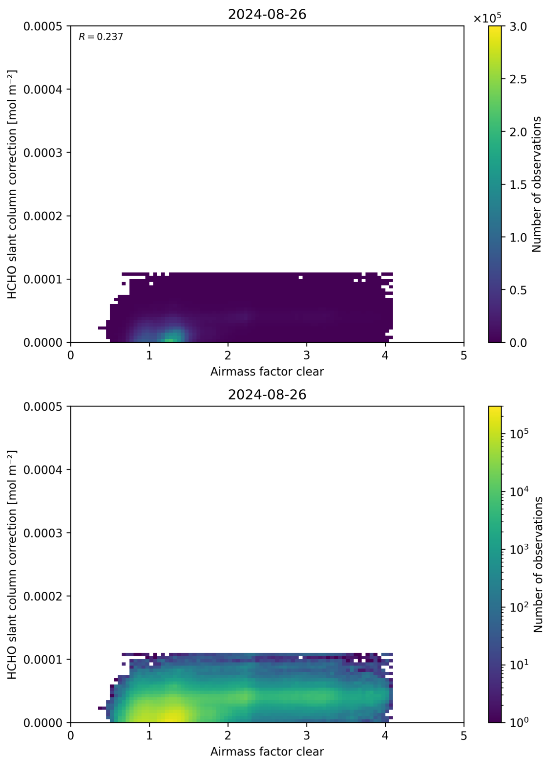
Figure 75: Scatter density plot of “Airmass factor clear” against “HCHO slant column correction” for 2024-08-25 to 2024-08-27.
