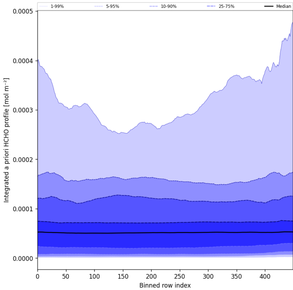
Figure 57: Along track statistics of “Integrated a priori HCHO profile” for 2024-08-25 to 2024-08-27
