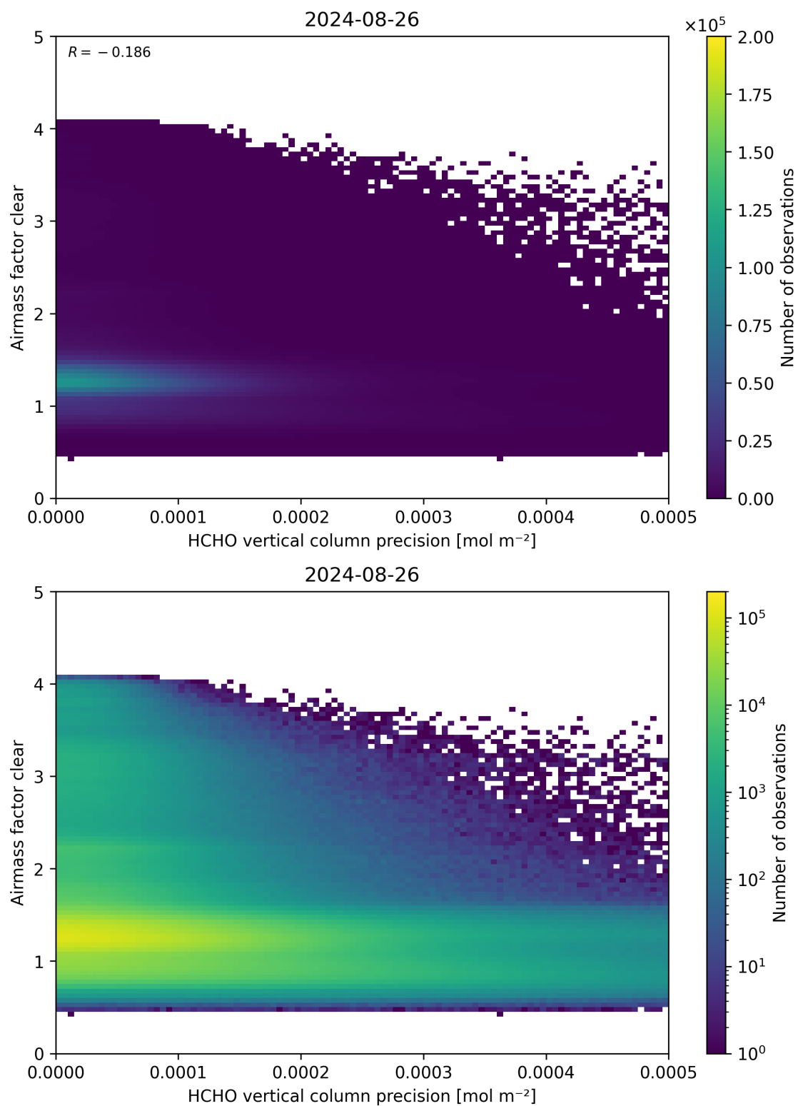
Figure 139: Scatter density plot of “HCHO vertical column precision” against “Airmass factor clear” for 2024-08-25 to 2024-08-27.
