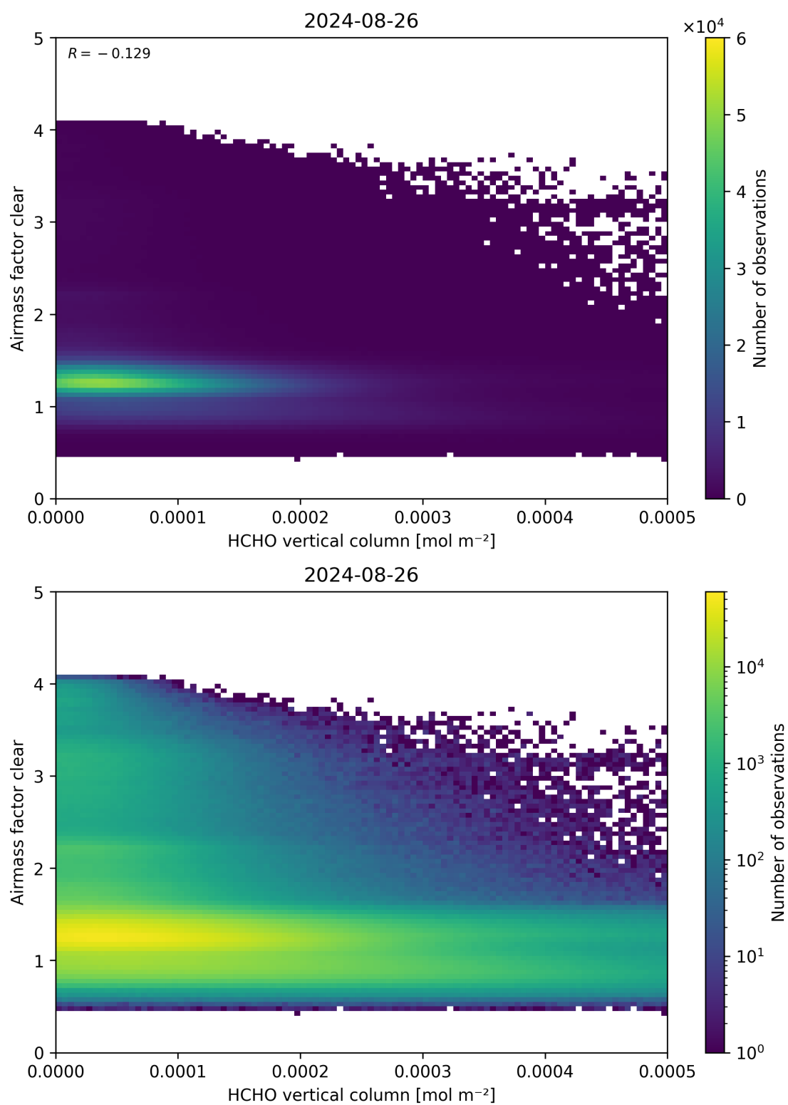
Figure 126: Scatter density plot of “HCHO vertical column” against “Airmass factor clear” for 2024-08-25 to 2024-08-27.
