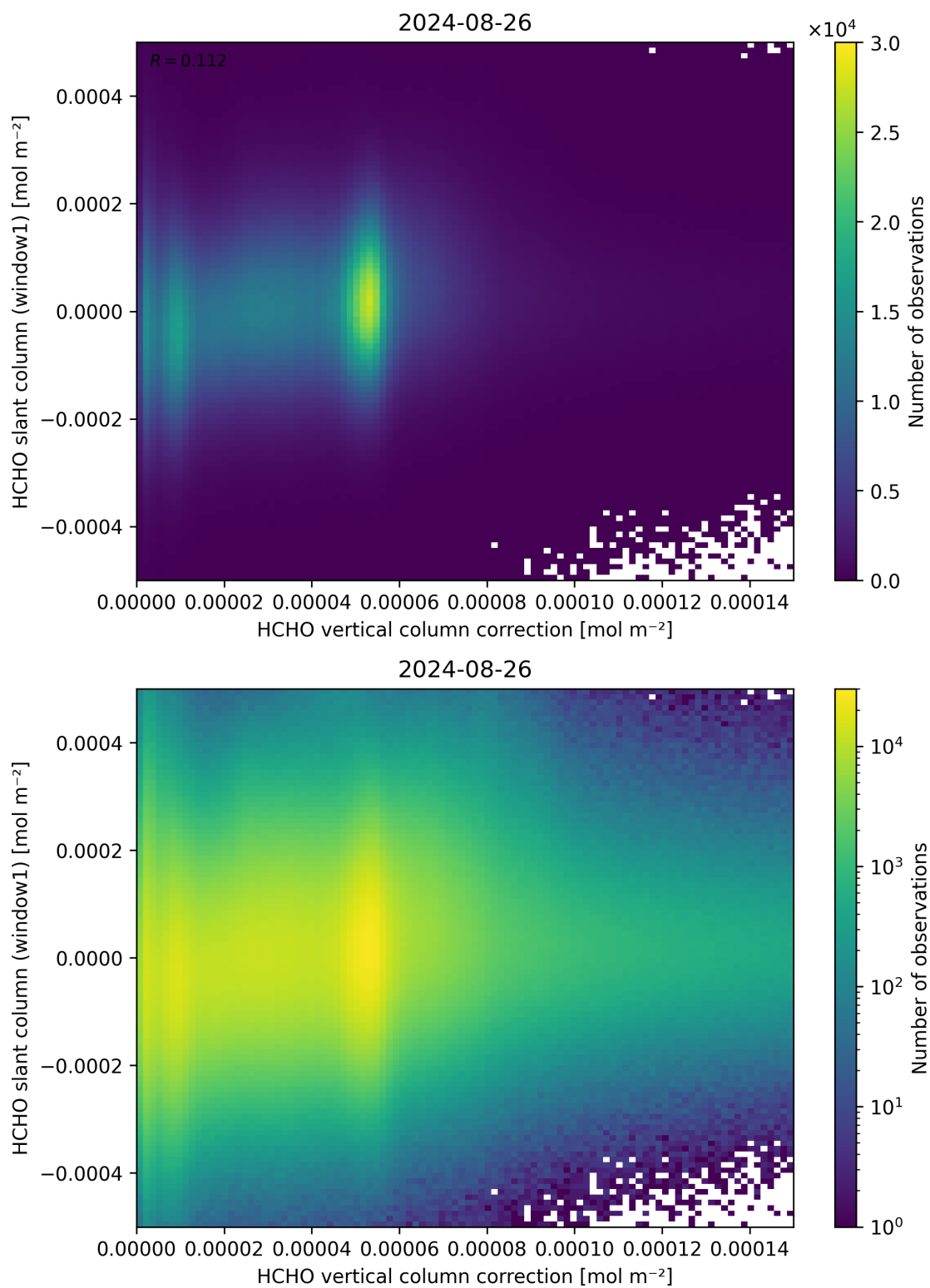
Figure 118: Scatter density plot of “HCHO vertical column correction” against “HCHO slant column (window1)” for 2024-08-25 to 2024-08-27.
