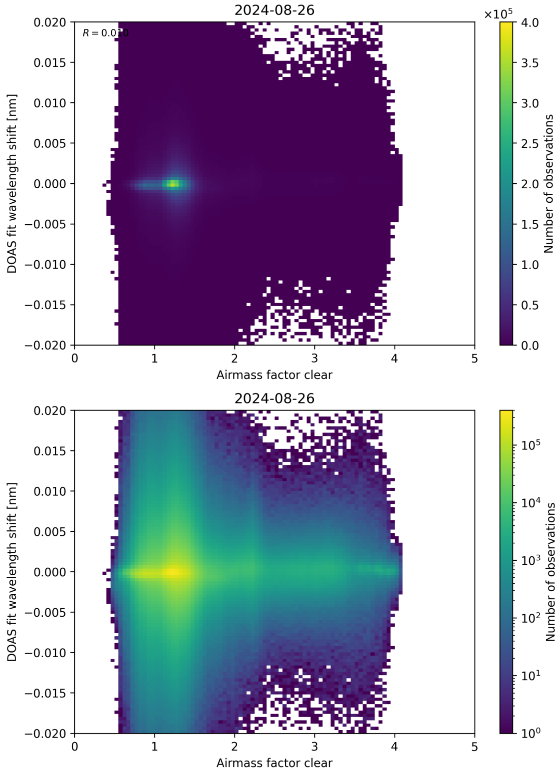
Figure 72: Scatter density plot of “Airmass factor clear” against “DOAS fit wavelength shift” for 2024-08-25 to 2024-08-27.
