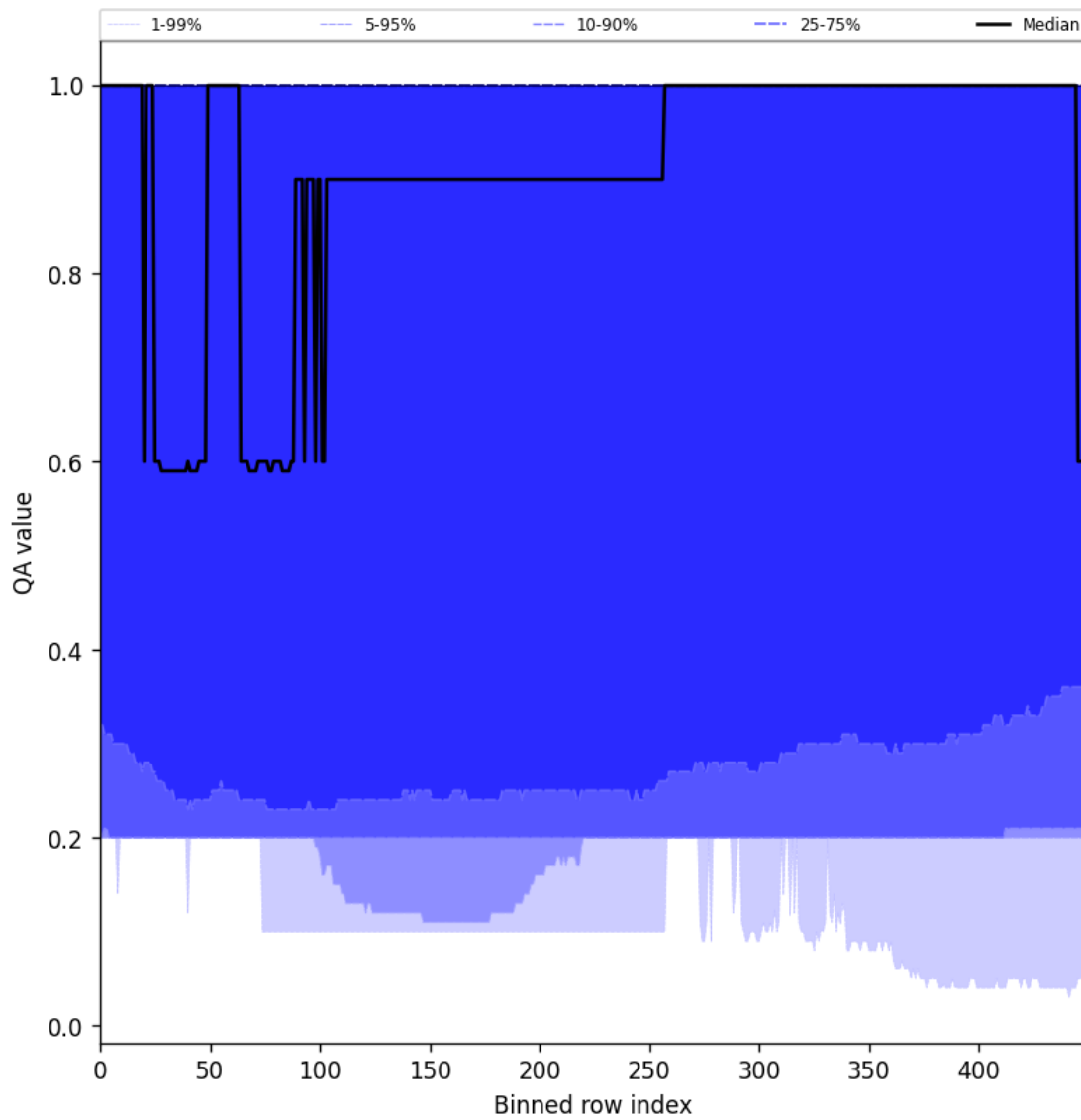
Figure 48: Along track statistics of “QA value” for 2024-08-25 to 2024-08-27
