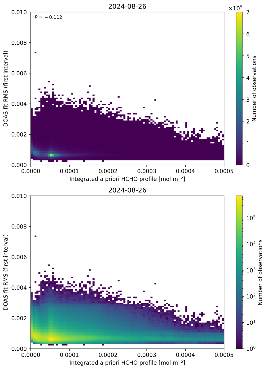
Figure 148: Scatter density plot of “Integrated a priori HCHO profile” against “DOAS fit RMS (first interval)” for 2024-08-25 to 2024-08-27.
