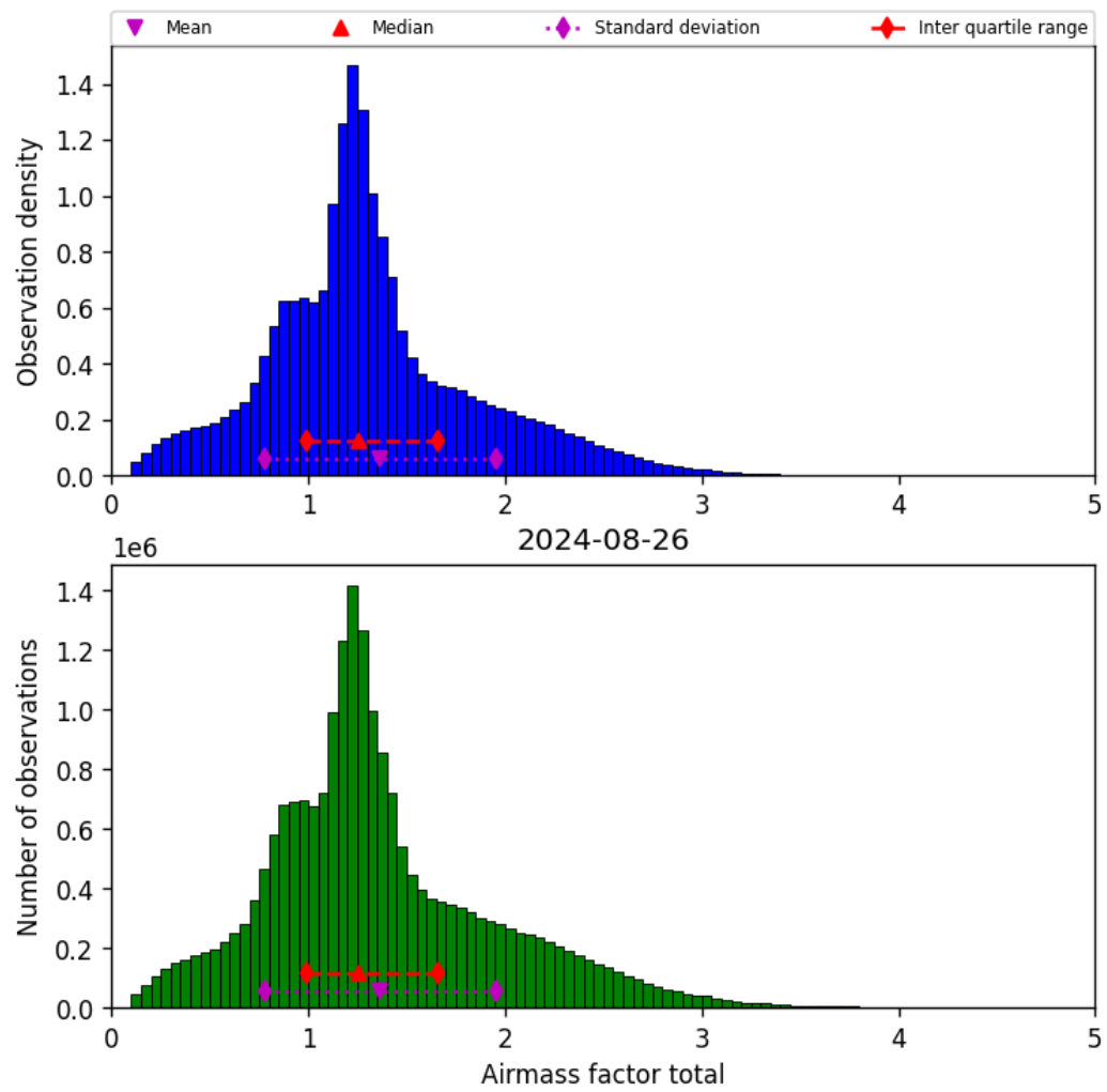
Figure 40: Histogram of “Airmass factor total” for 2024-08-25 to 2024-08-27
