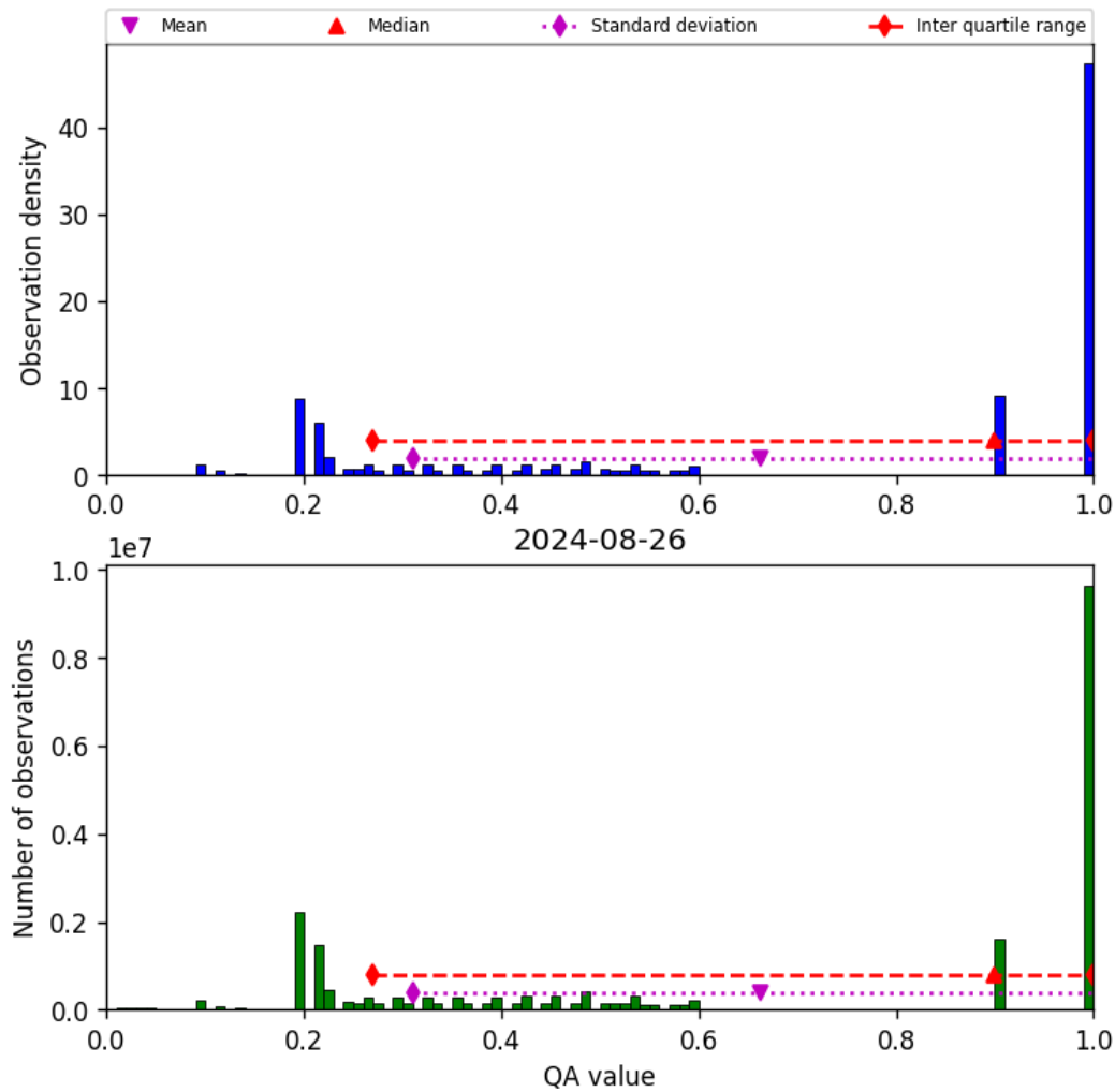
Figure 34: Histogram of “QA value” for 2024-08-25 to 2024-08-27
