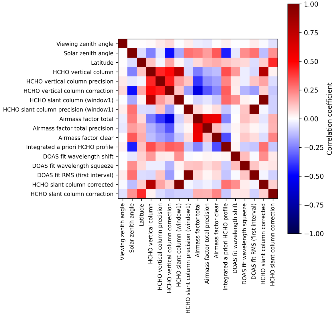
Figure 2: Map of correlation matrix for 2024-08-25 to 2024-08-27.
