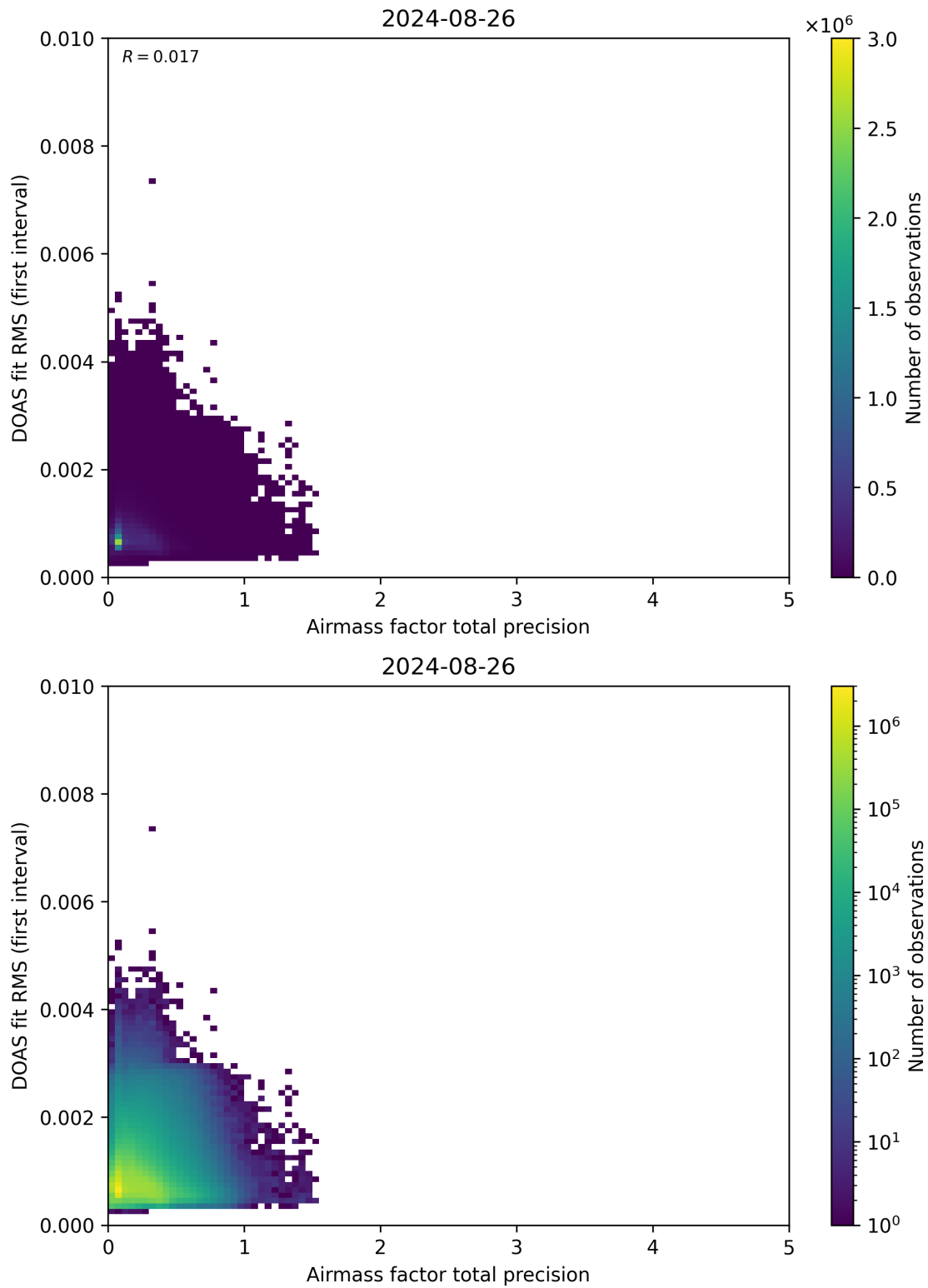
Figure 105: Scatter density plot of “Airmass factor total precision” against “DOAS fit RMS (first interval)” for 2024-08-25 to 2024-08-27.
