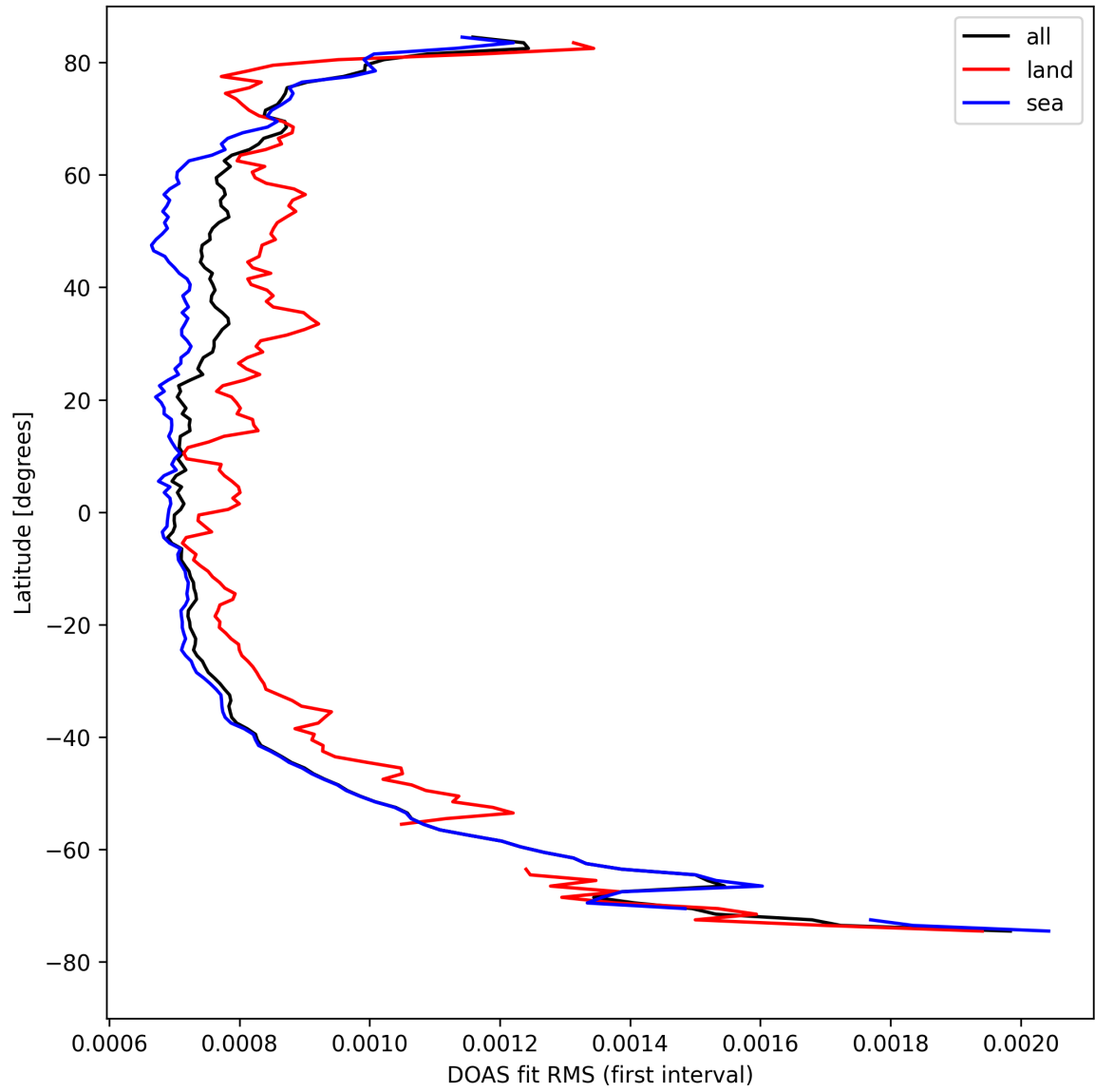
Figure 32: Zonal average of “DOAS fit RMS (first interval)” for 2024-08-25 to 2024-08-27.
