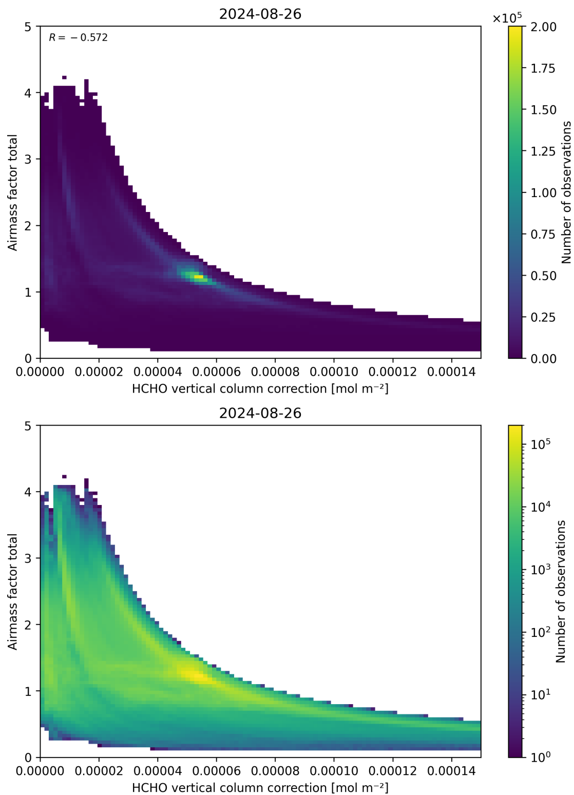
Figure 120: Scatter density plot of “HCHO vertical column correction” against “Airmass factor total” for 2024-08-25 to 2024-08-27.
