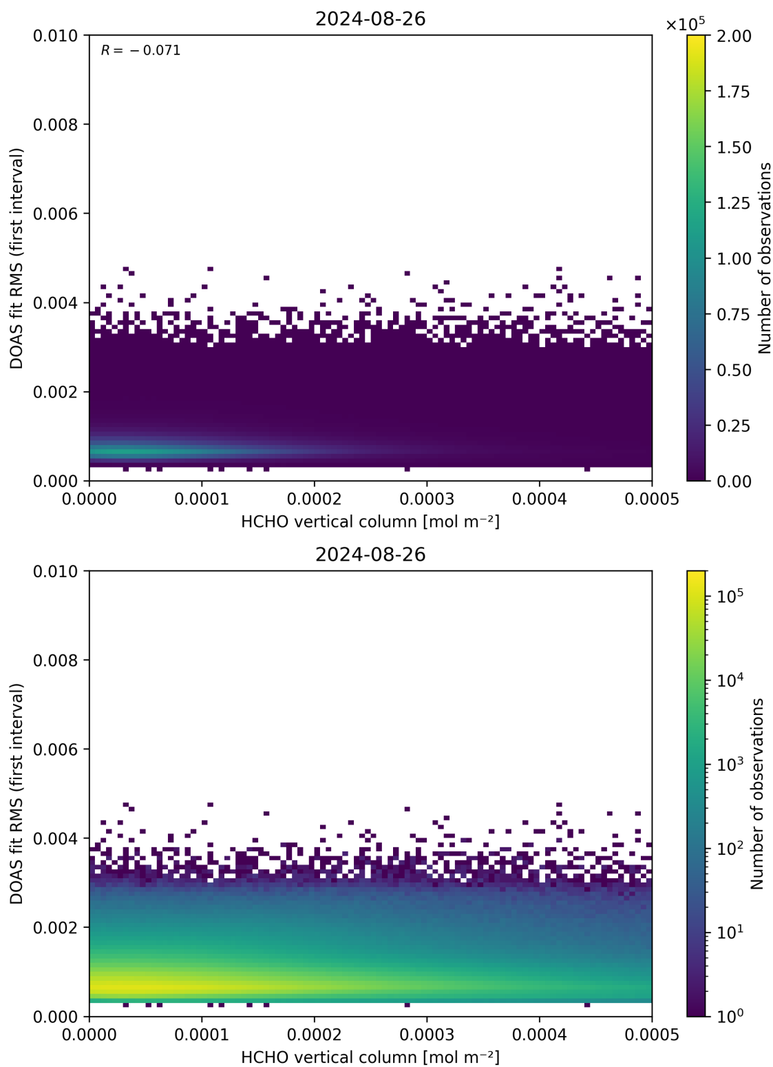
Figure 123: Scatter density plot of “HCHO vertical column” against “DOAS fit RMS (first interval)” for 2024-08-25 to 2024-08-27.
