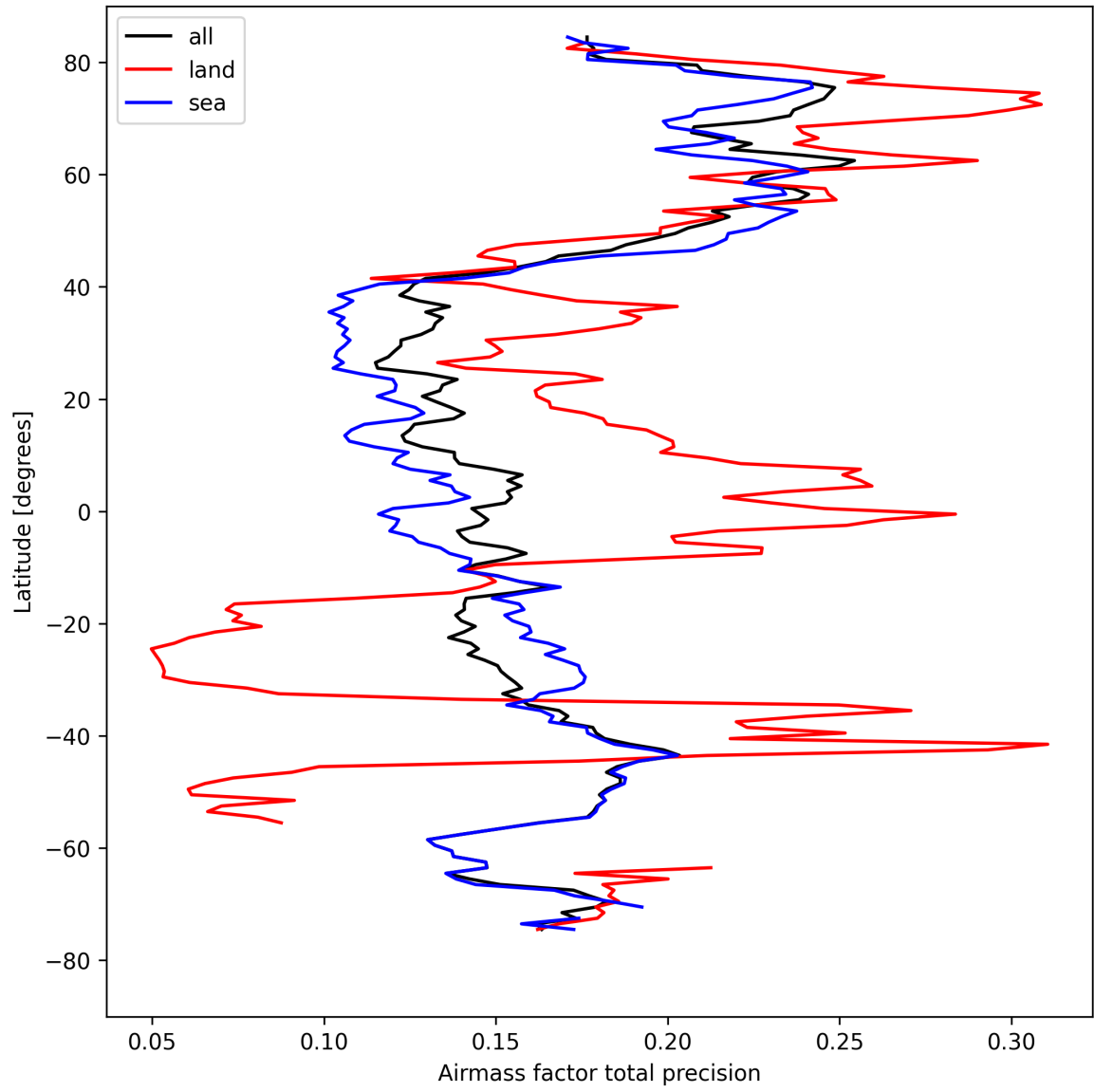
Figure 27: Zonal average of “Airmass factor total precision” for 2024-08-25 to 2024-08-27.
