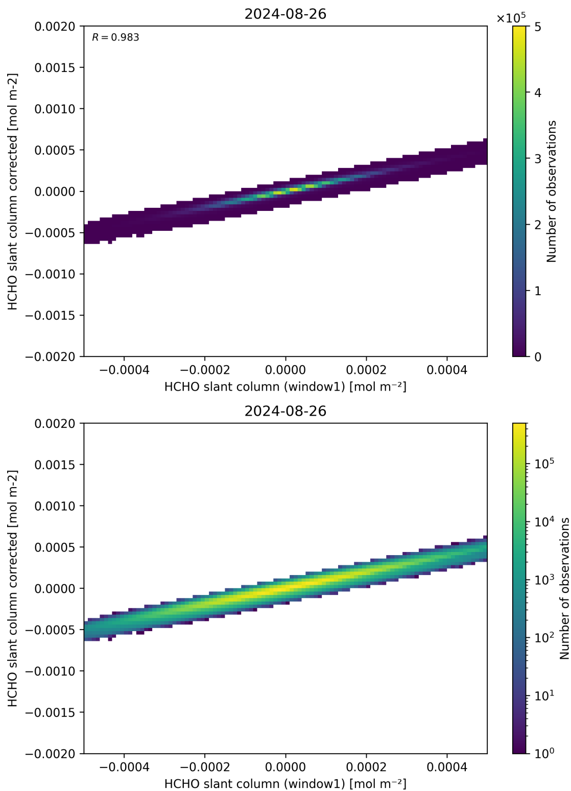
Figure 82: Scatter density plot of “HCHO slant column (window1)” against “HCHO slant column corrected” for 2024-08-25 to 2024-08-27.
