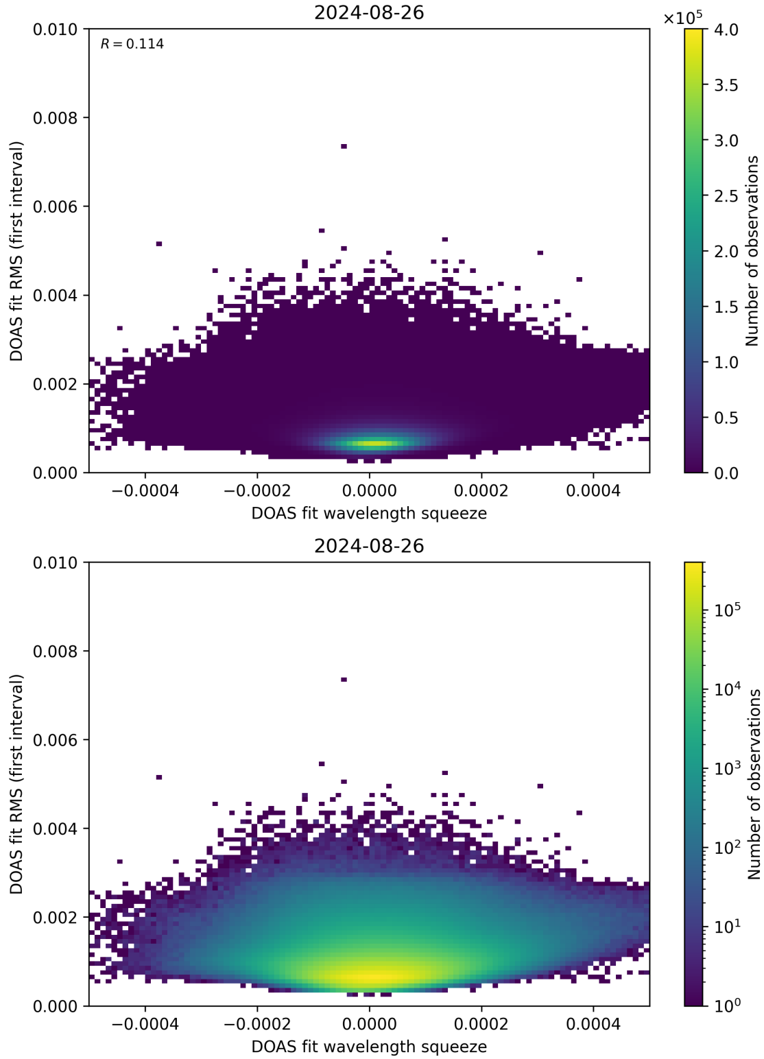
Figure 68: Scatter density plot of “DOAS fit wavelength squeeze” against “DOAS fit RMS (first interval)” for 2024-08-25 to 2024-08-27.
