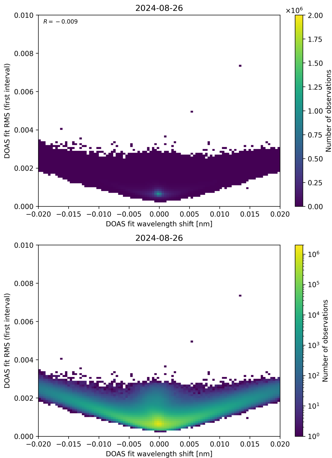
Figure 64: Scatter density plot of “DOAS fit wavelength shift” against “DOAS fit RMS (first interval)” for 2024-08-25 to 2024-08-27.
