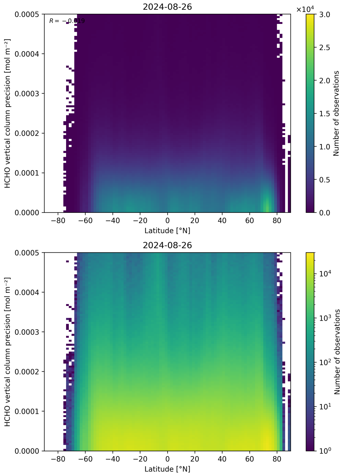
Figure 165: Scatter density plot of “Latitude” against “HCHO vertical column precision” for 2024-08-25 to 2024-08-27.
