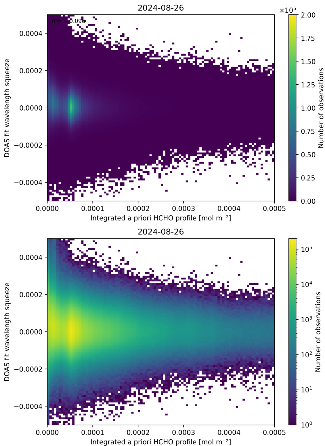
Figure 150: Scatter density plot of “Integrated a priori HCHO profile” against “DOAS fit wavelength squeeze” for 2024-08-25 to 2024-08-27.
