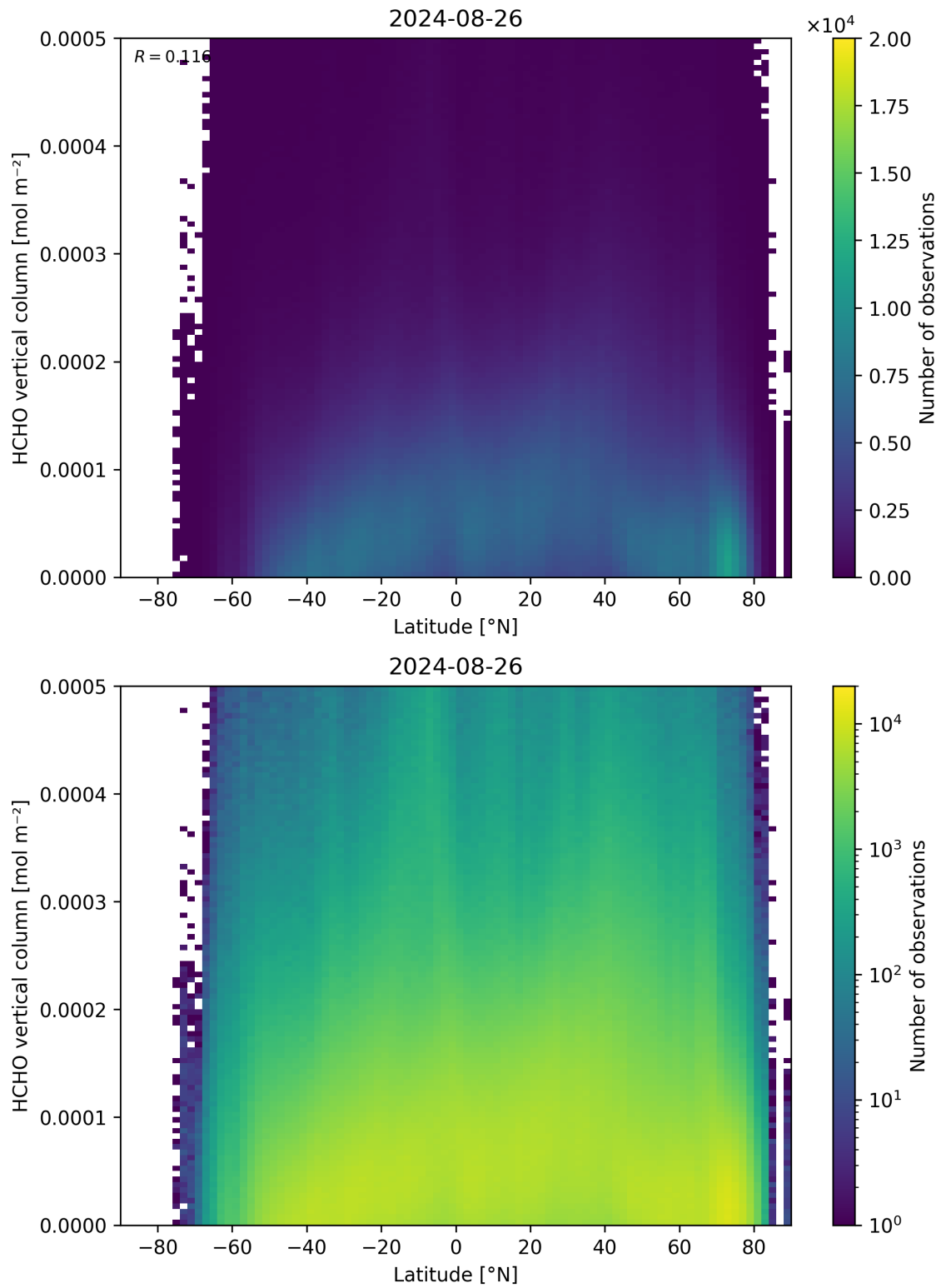
Figure 163: Scatter density plot of “Latitude” against “HCHO vertical column” for 2024-08-25 to 2024-08-27.
