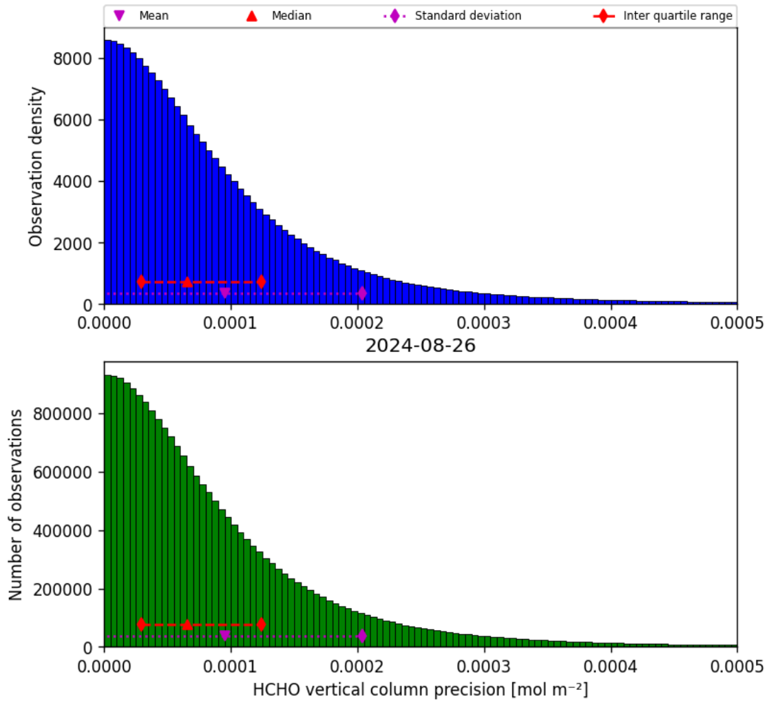
Figure 36: Histogram of “HCHO vertical column precision” for 2024-08-25 to 2024-08-27
