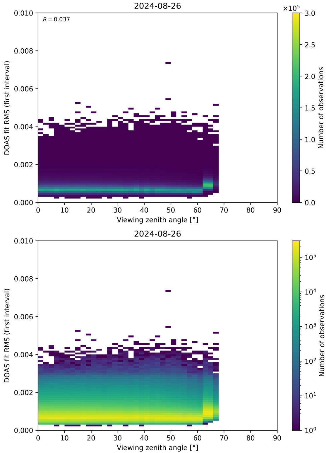
Figure 182: Scatter density plot of “Viewing zenith angle” against “DOAS fit RMS (first interval)” for 2024-08-25 to 2024-08-27.
