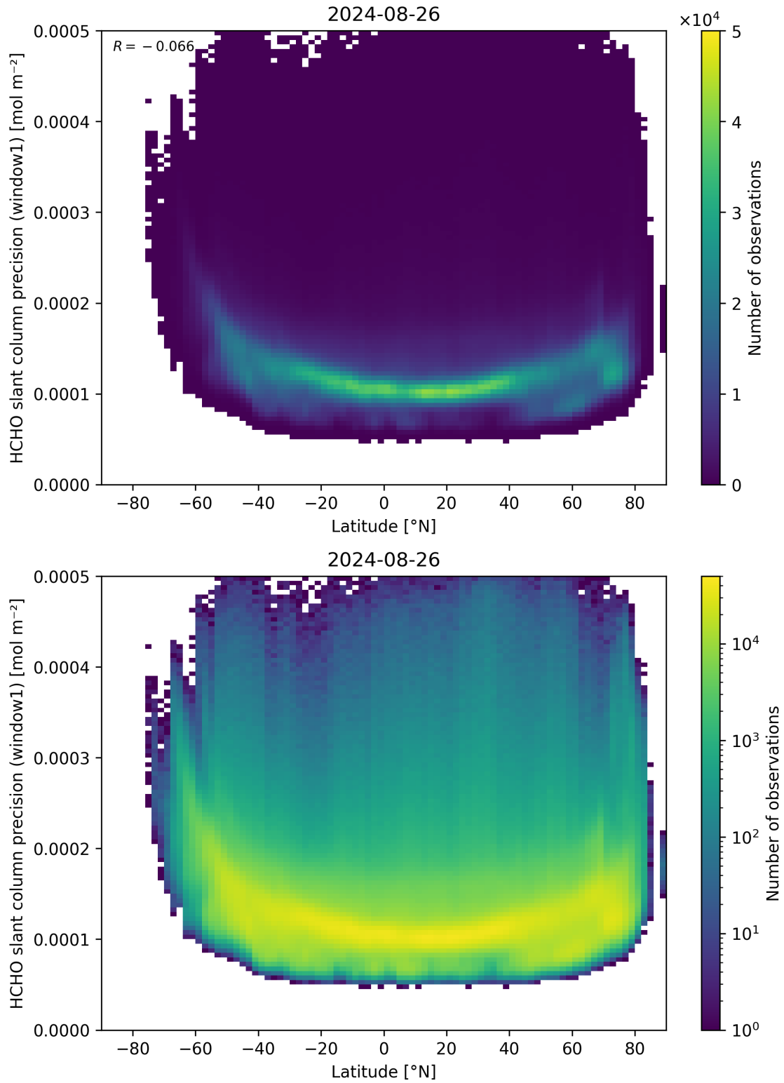
Figure 160: Scatter density plot of “Latitude” against “HCHO slant column precision (window1)” for 2024-08-25 to 2024-08-27.
