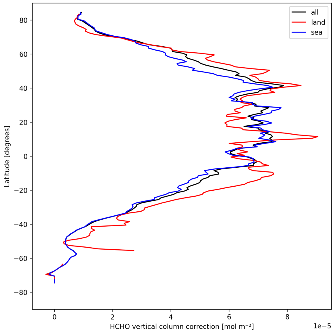
Figure 23: Zonal average of “HCHO vertical column correction” for 2024-08-25 to 2024-08-27.
