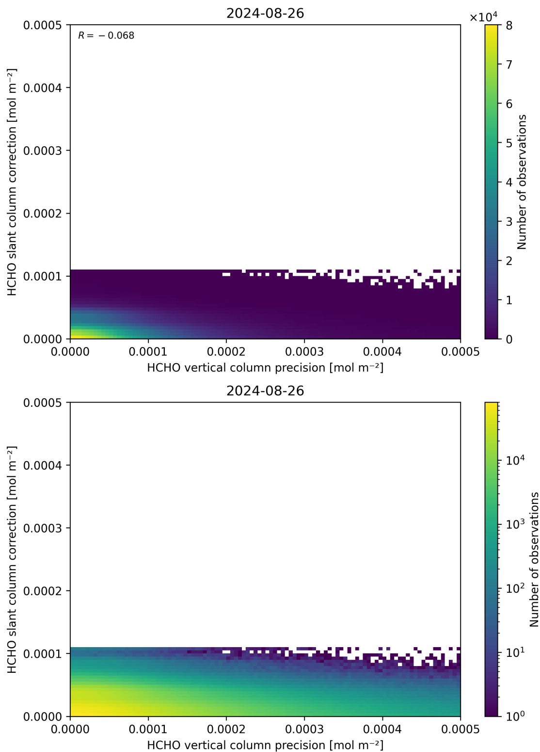
Figure 141: Scatter density plot of “HCHO vertical column precision” against “HCHO slant column correction” for 2024-08-25 to 2024-08-27.
