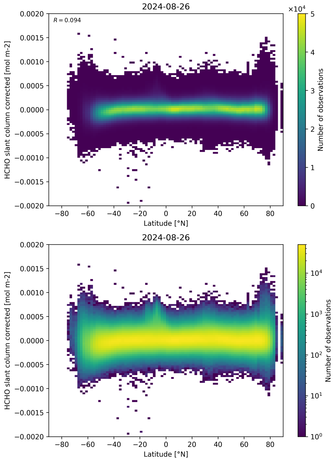
Figure 157: Scatter density plot of “Latitude” against “HCHO slant column corrected” for 2024-08-25 to 2024-08-27.
