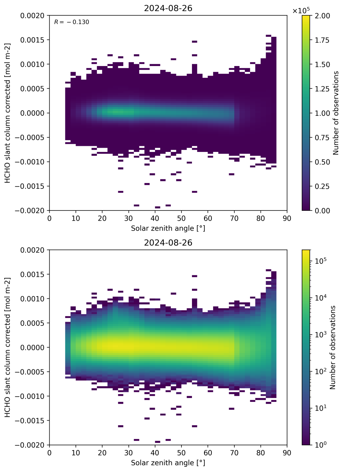
Figure 171: Scatter density plot of “Solar zenith angle” against “HCHO slant column corrected” for 2024-08-25 to 2024-08-27.
