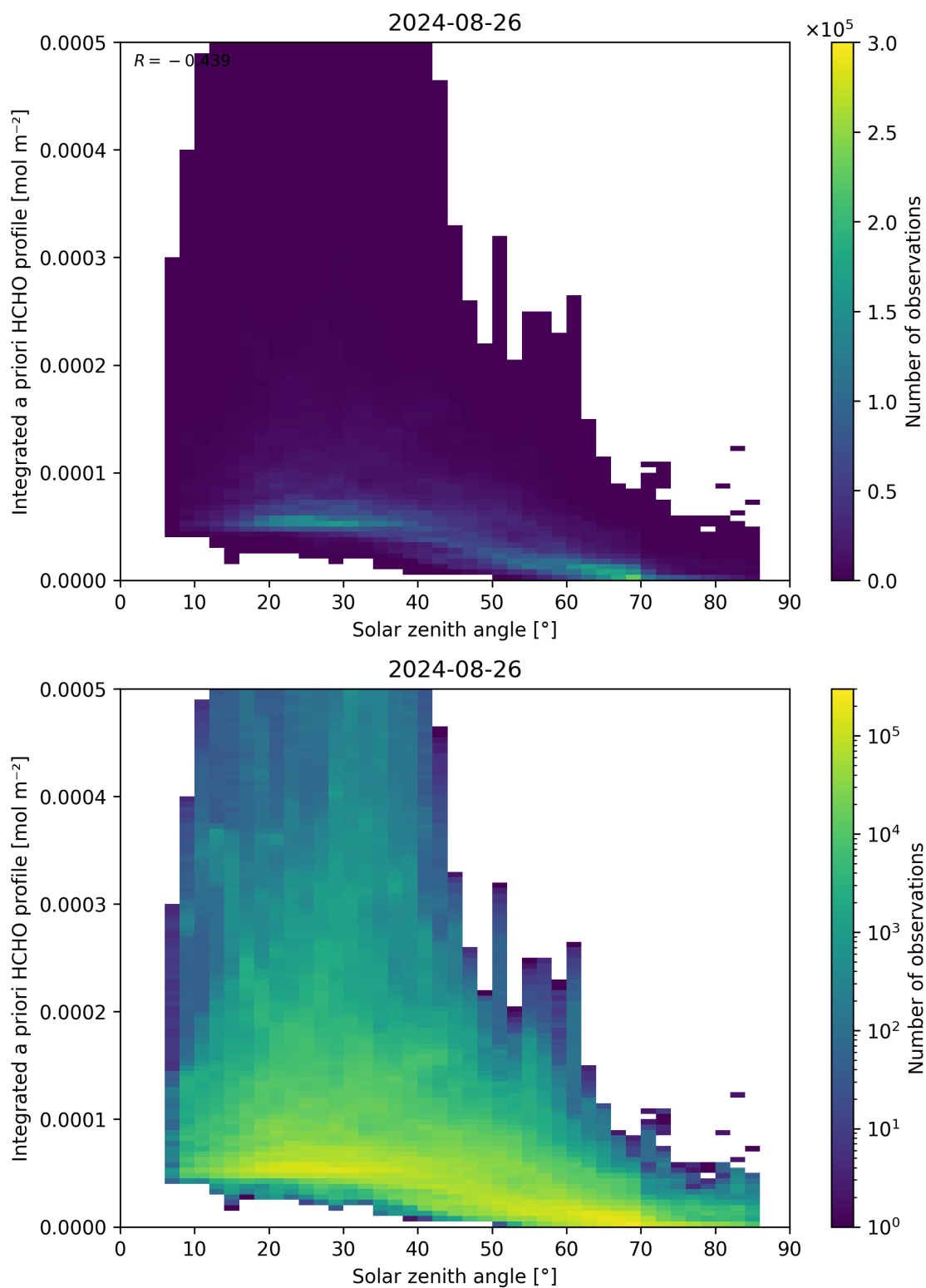
Figure 180: Scatter density plot of “Solar zenith angle” against “Integrated a priori HCHO profile” for 2024-08-25 to 2024-08-27.
