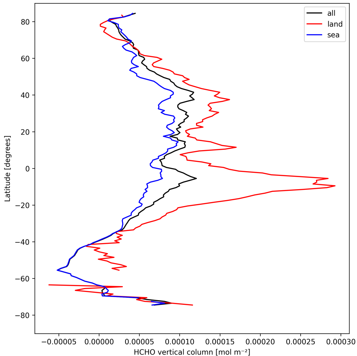
Figure 21: Zonal average of “HCHO vertical column” for 2024-08-25 to 2024-08-27.
