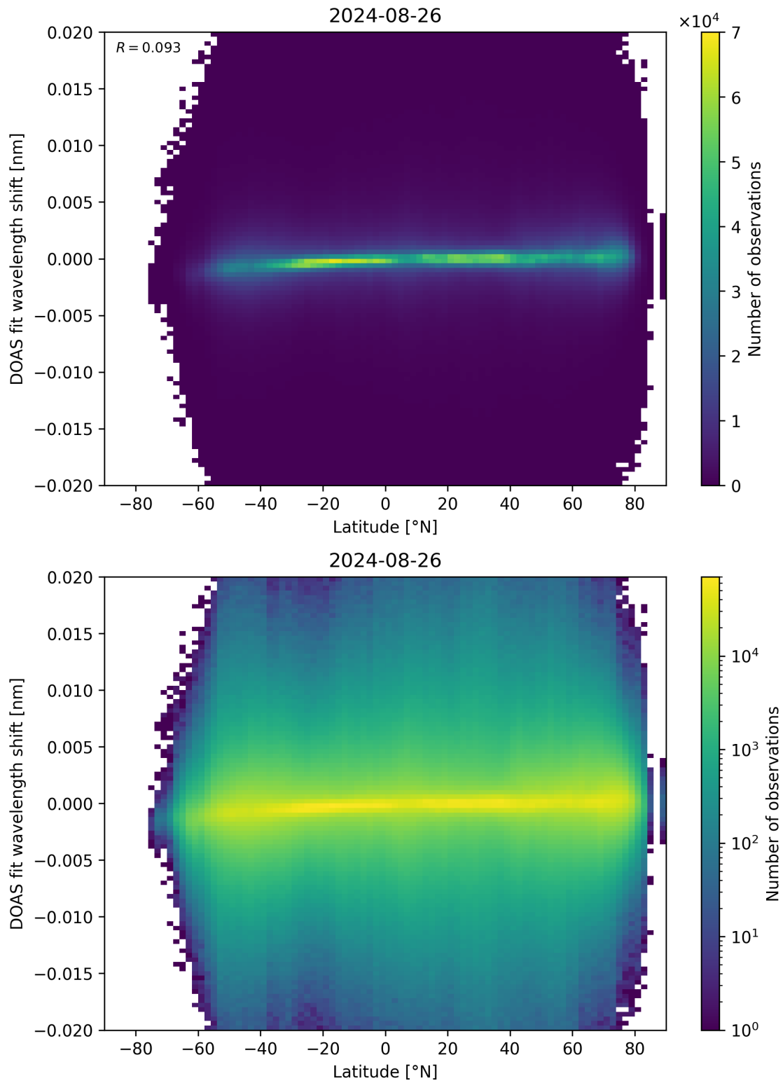
Figure 154: Scatter density plot of “Latitude” against “DOAS fit wavelength shift” for 2024-08-25 to 2024-08-27.
