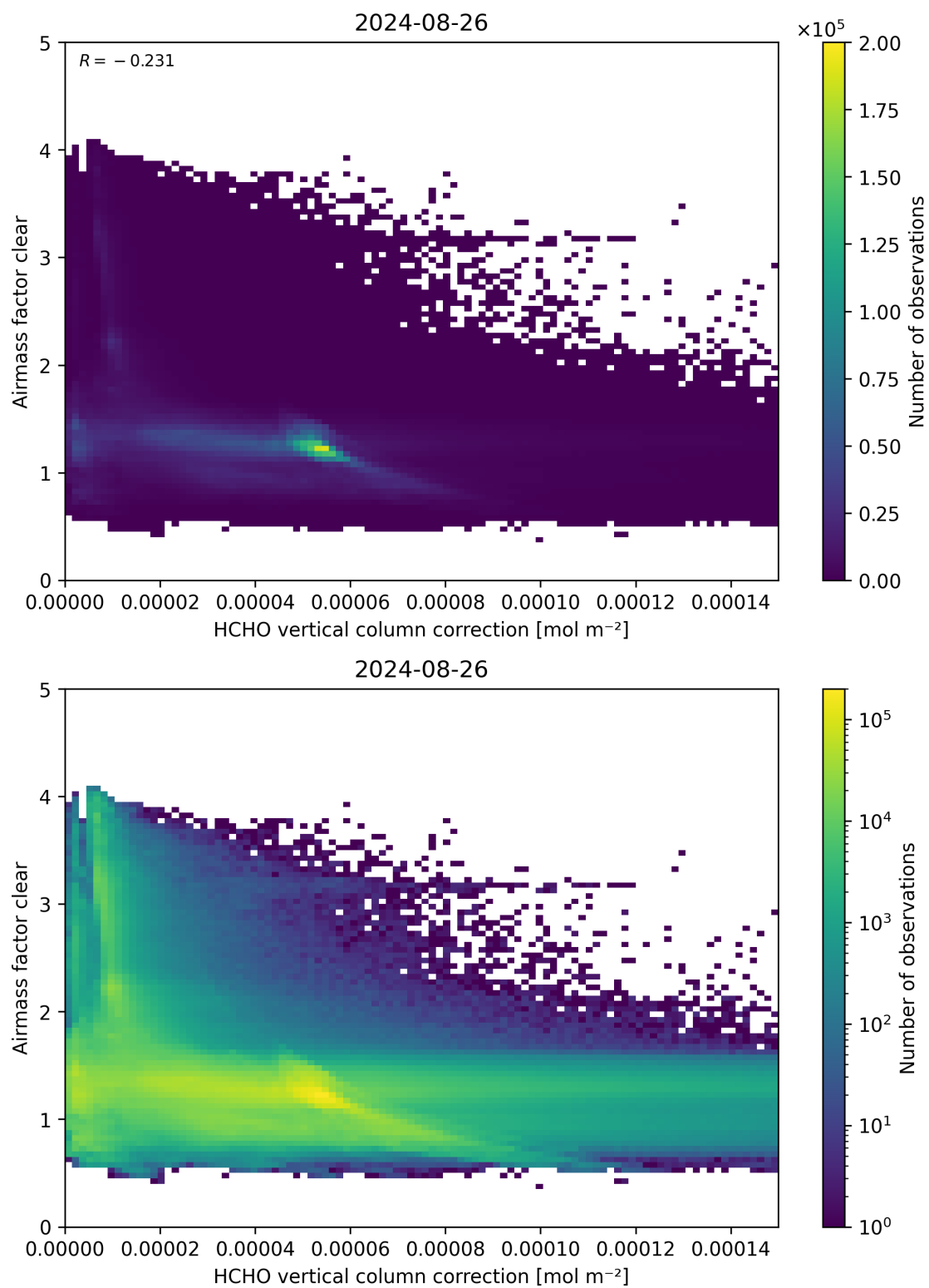
Figure 115: Scatter density plot of “HCHO vertical column correction” against “Airmass factor clear” for 2024-08-25 to 2024-08-27.
