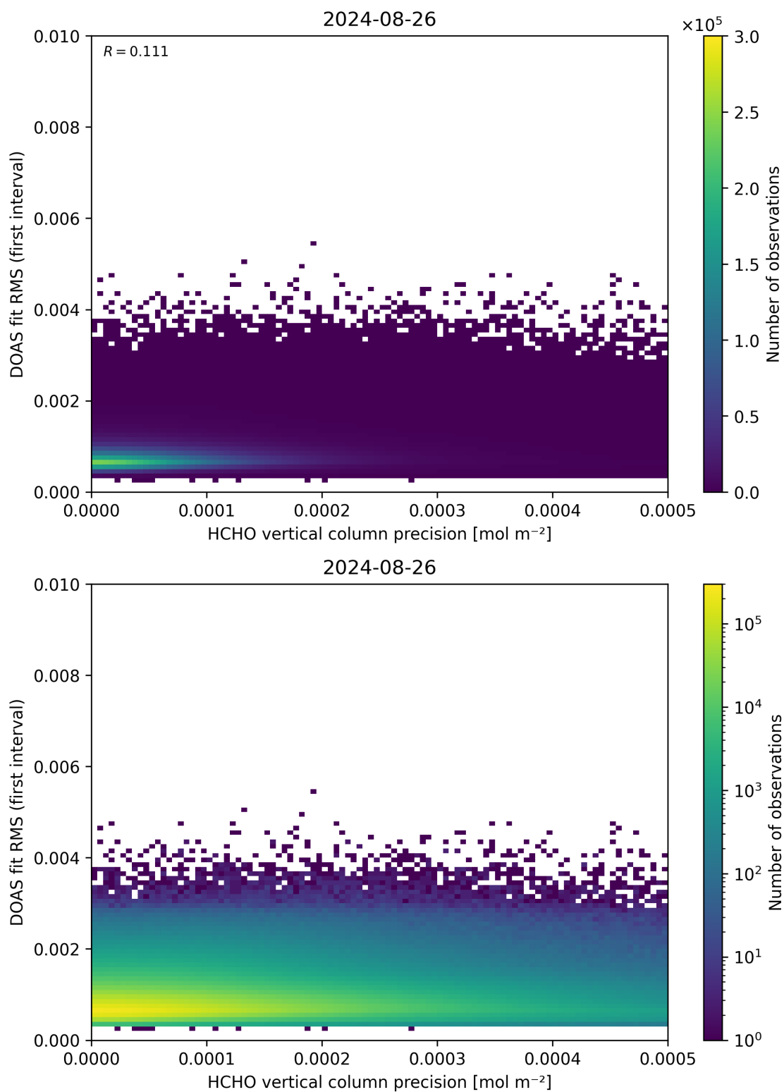
Figure 136: Scatter density plot of “HCHO vertical column precision” against “DOAS fit RMS (first interval)” for 2024-08-25 to 2024-08-27.
