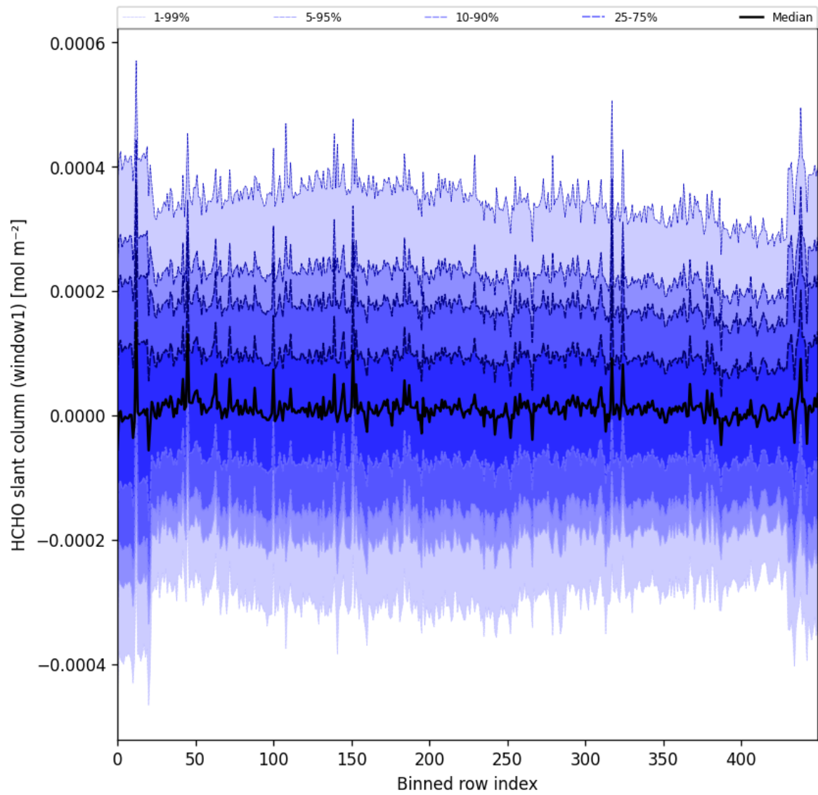
Figure 52: Along track statistics of “HCHO slant column (window1)” for 2024-08-25 to 2024-08-27
