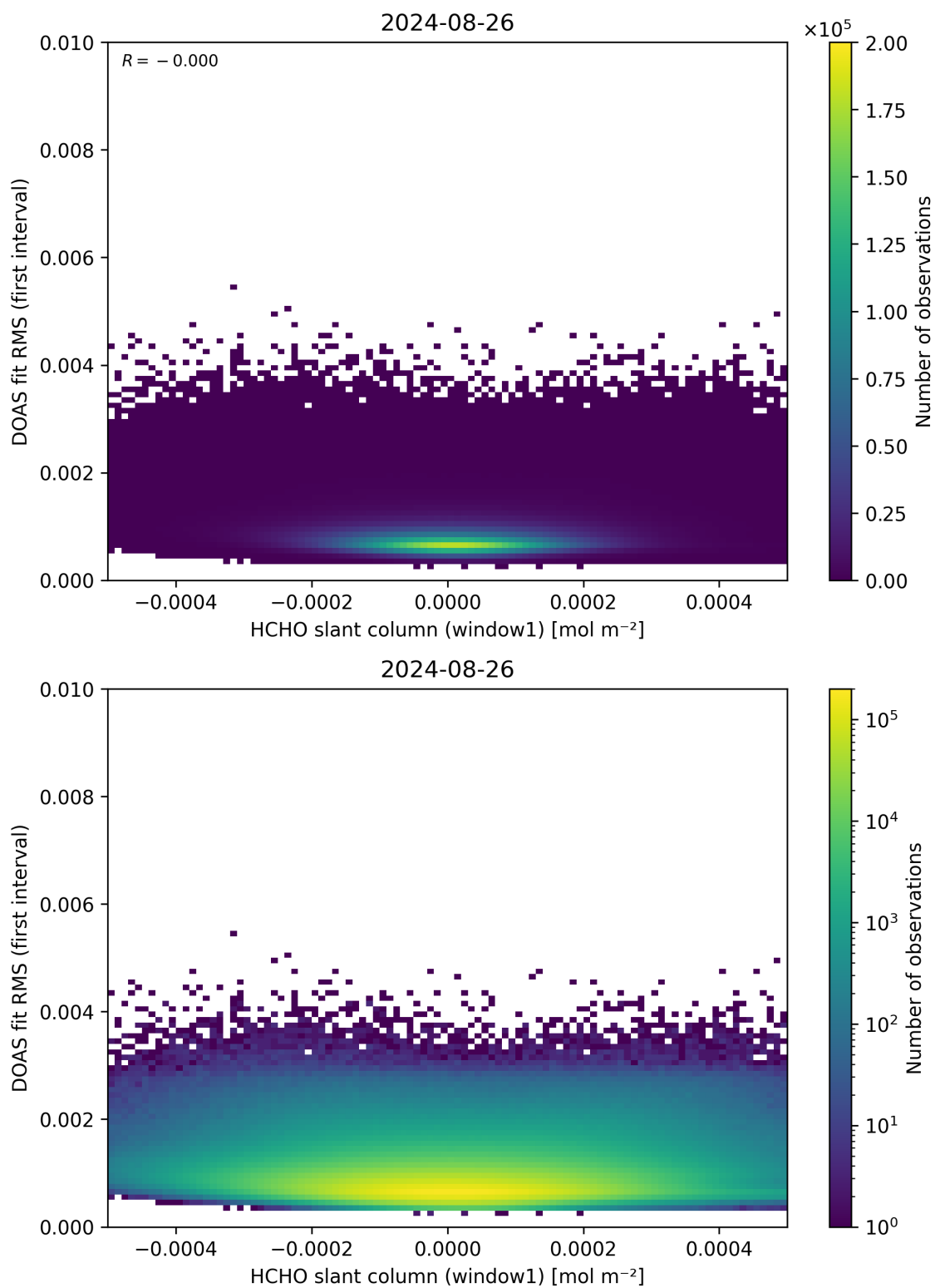
Figure 78: Scatter density plot of “HCHO slant column (window1)” against “DOAS fit RMS (first interval)” for 2024-08-25 to 2024-08-27.
