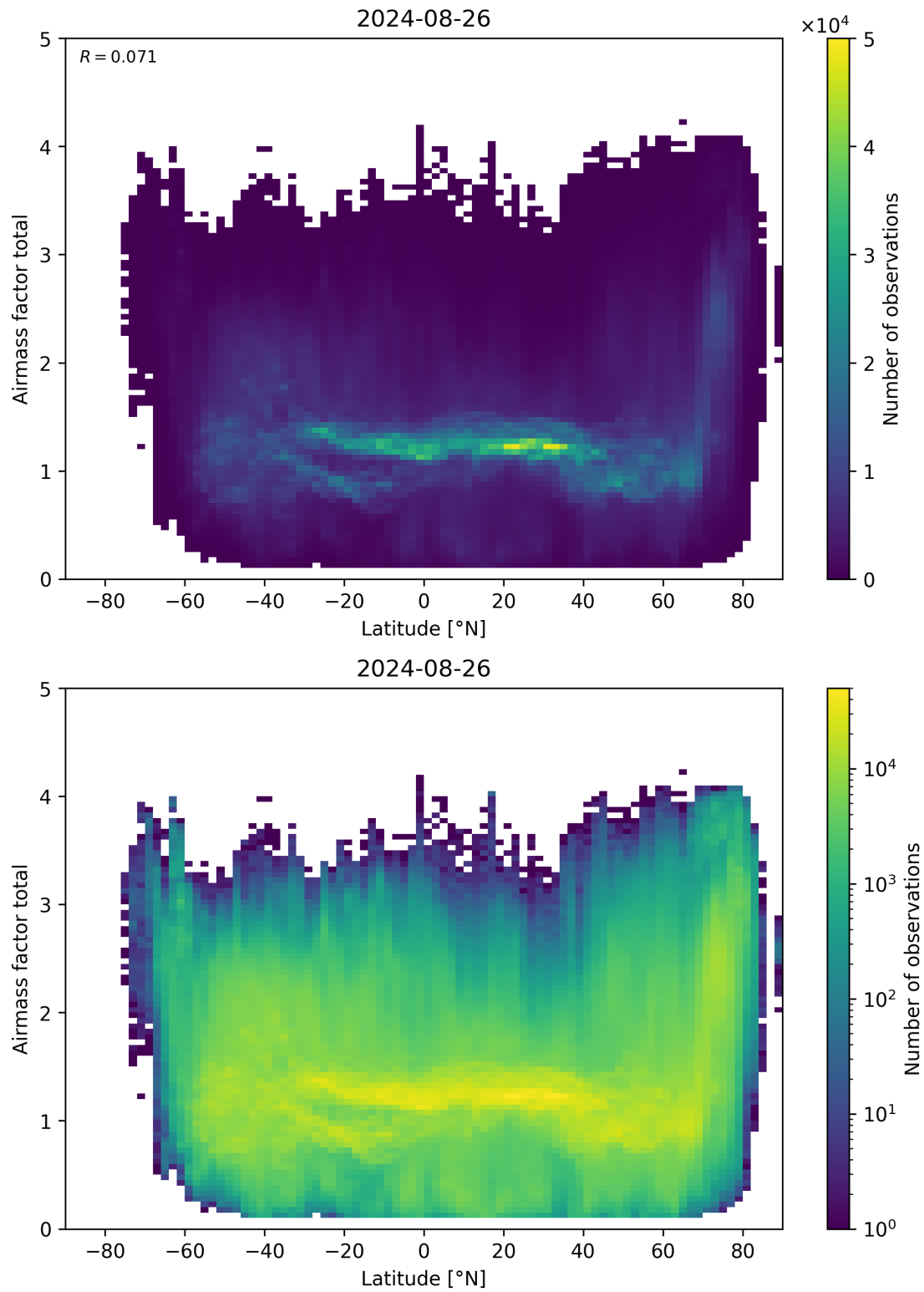
Figure 161: Scatter density plot of “Latitude” against “Airmass factor total” for 2024-08-25 to 2024-08-27.
