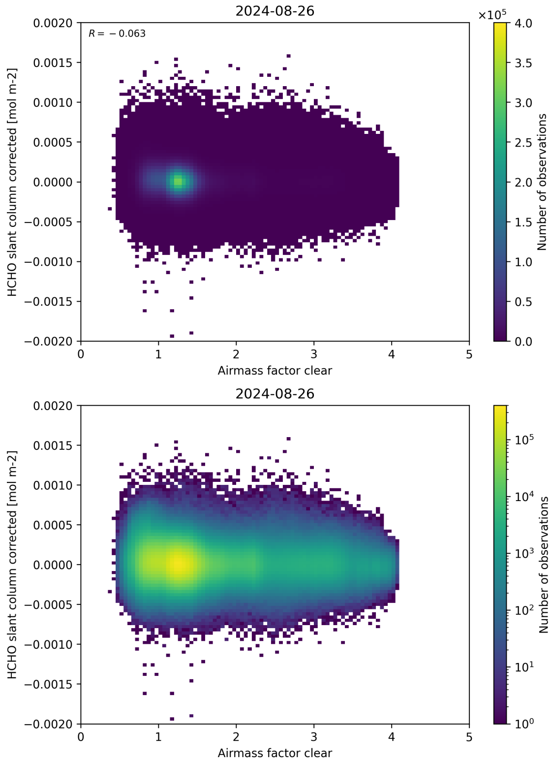
Figure 74: Scatter density plot of “Airmass factor clear” against “HCHO slant column corrected” for 2024-08-25 to 2024-08-27.
