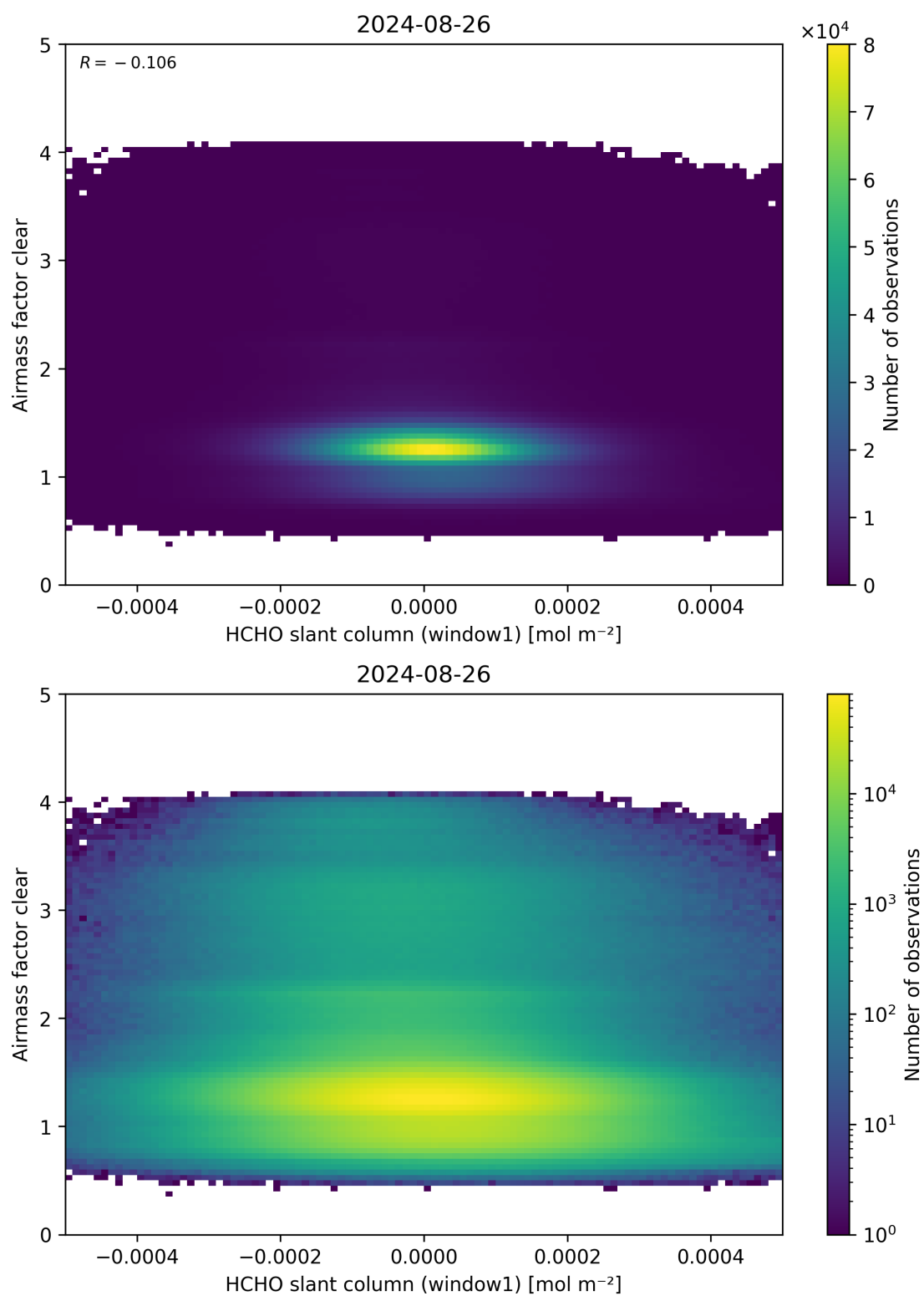
Figure 81: Scatter density plot of “HCHO slant column (window1)” against “Airmass factor clear” for 2024-08-25 to 2024-08-27.
