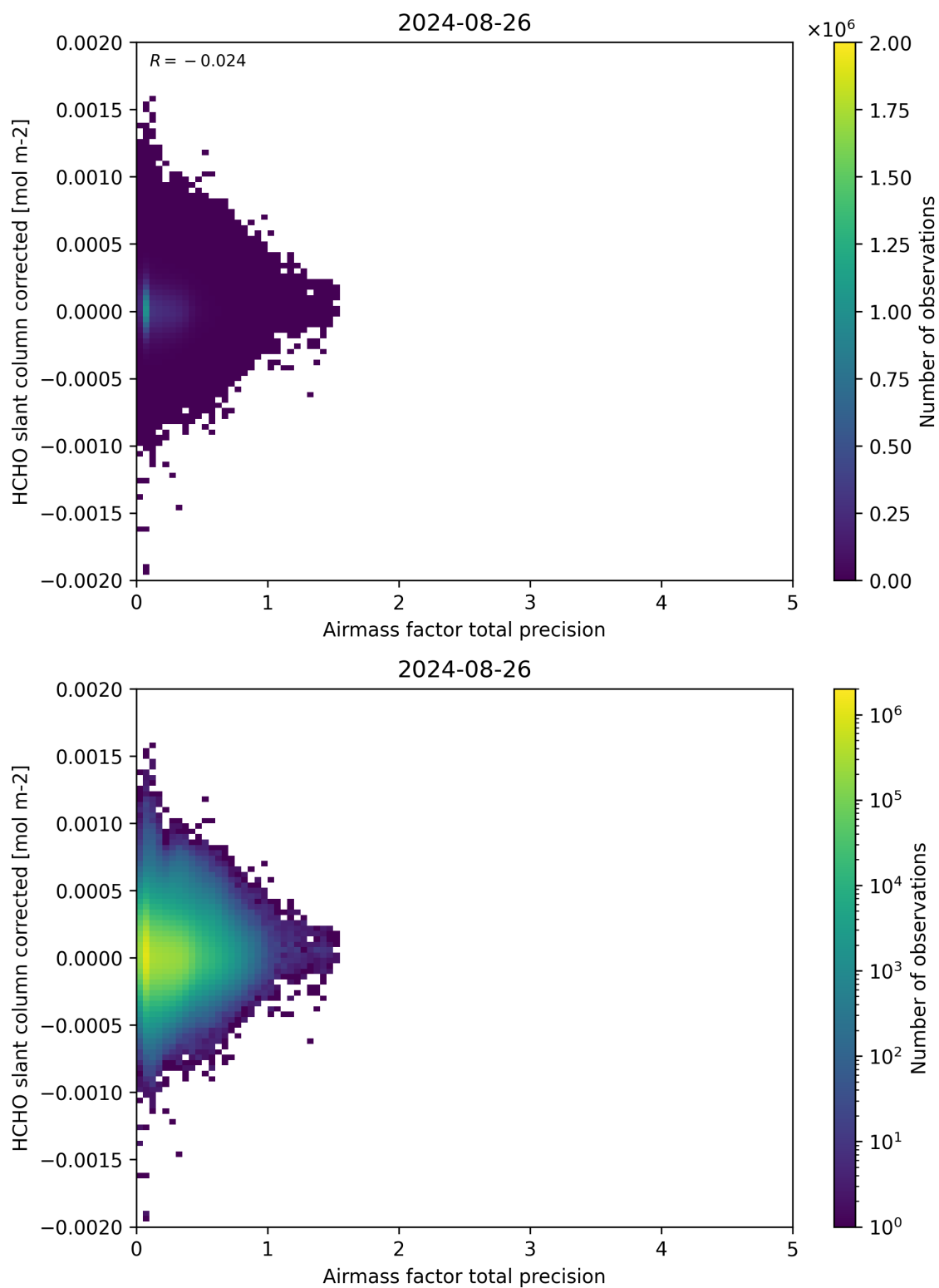
Figure 109: Scatter density plot of “Airmass factor total precision” against “HCHO slant column corrected” for 2024-08-25 to 2024-08-27.
