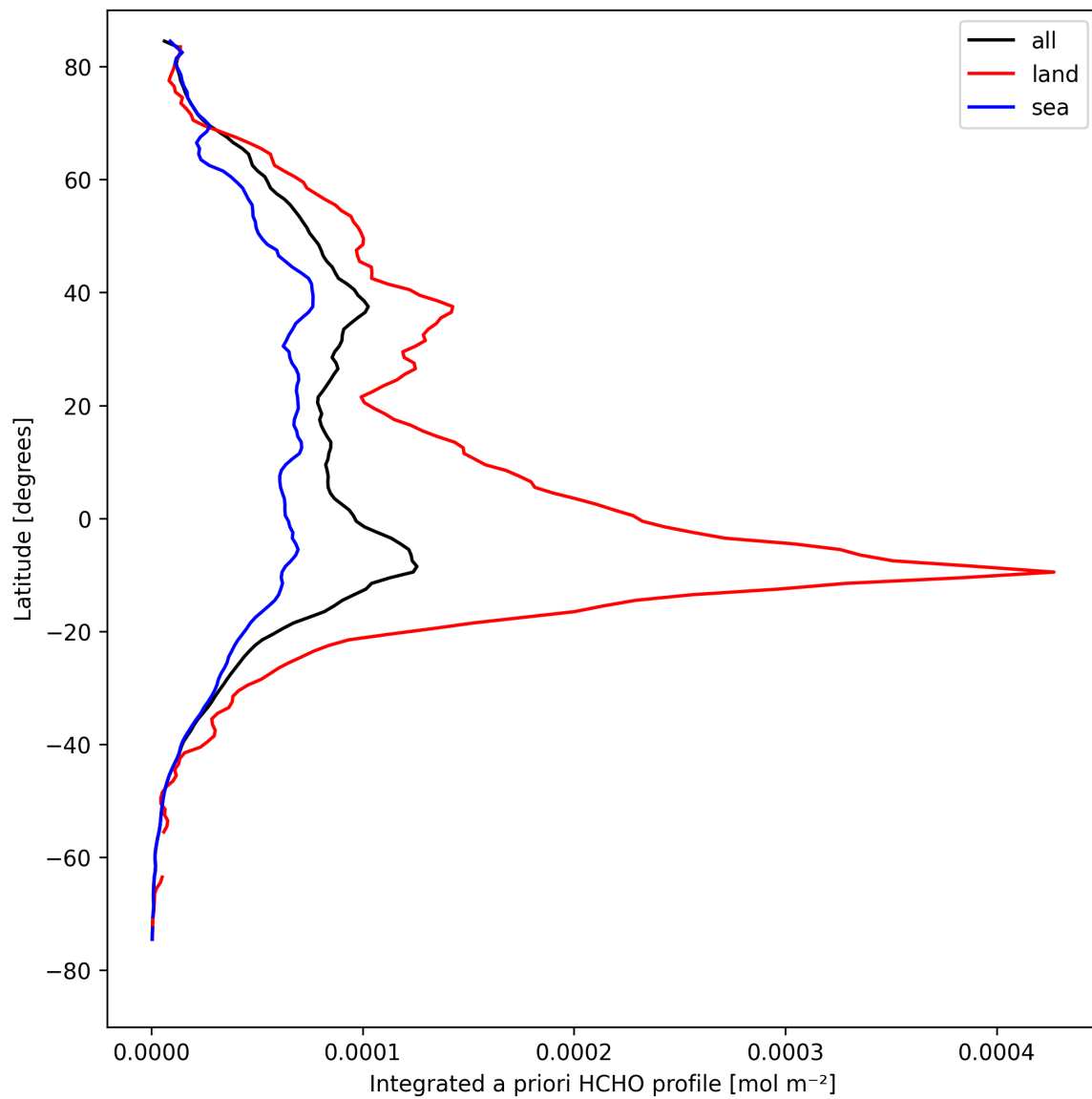
Figure 29: Zonal average of “Integrated a priori HCHO profile” for 2024-08-25 to 2024-08-27.
