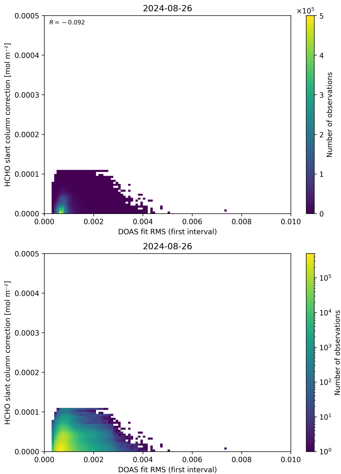
Figure 63: Scatter density plot of “DOAS fit RMS (first interval)” against “HCHO slant column correction” for 2024-08-25 to 2024-08-27.
