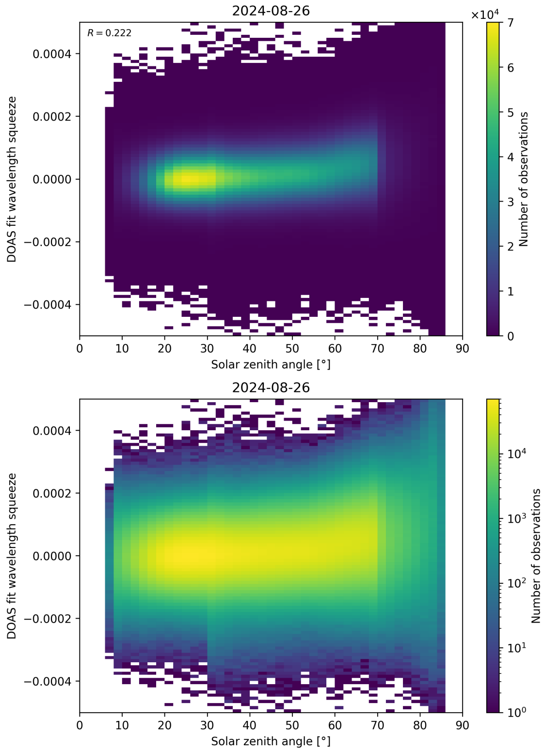
Figure 169: Scatter density plot of “Solar zenith angle” against “DOAS fit wavelength squeeze” for 2024-08-25 to 2024-08-27.
