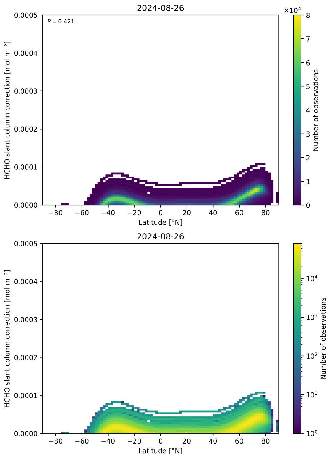
Figure 158: Scatter density plot of “Latitude” against “HCHO slant column correction” for 2024-08-25 to 2024-08-27.
