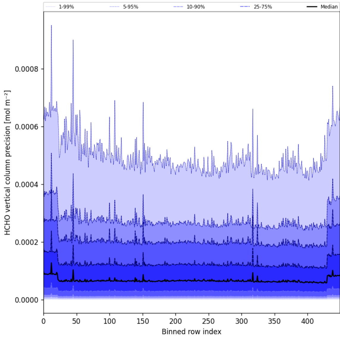
Figure 50: Along track statistics of “HCHO vertical column precision” for 2024-08-25 to 2024-08-27
