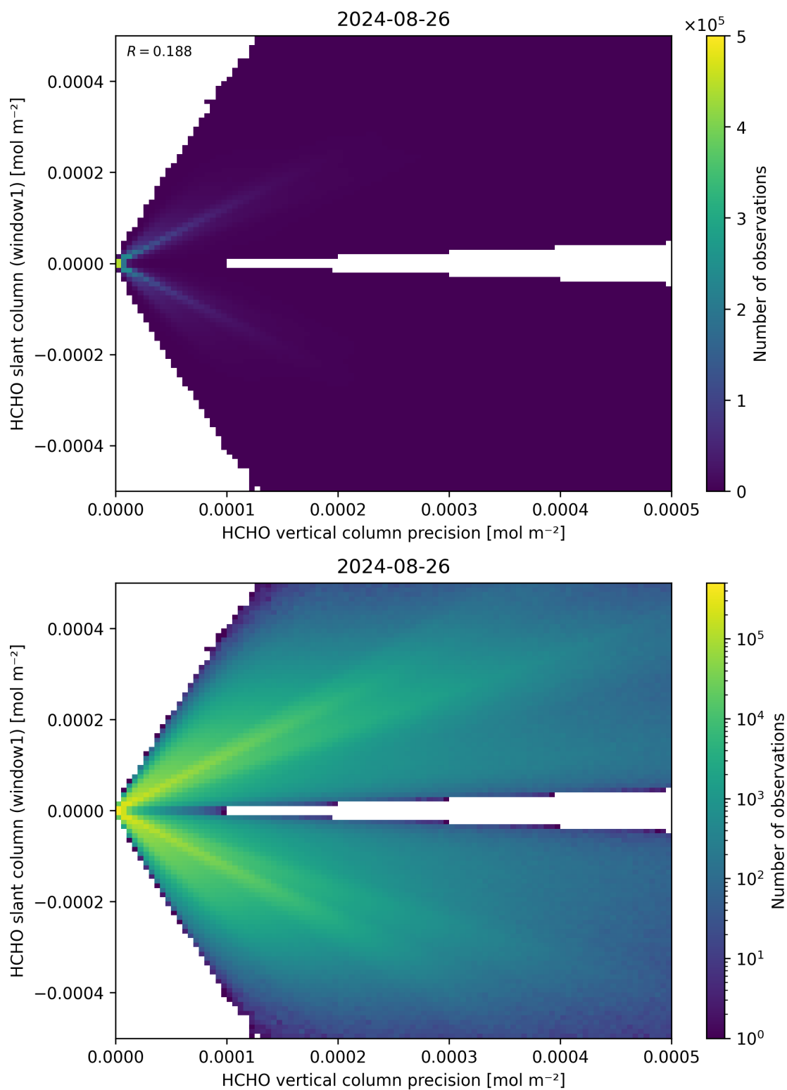
Figure 142: Scatter density plot of “HCHO vertical column precision” against “HCHO slant column (window1)” for 2024-08-25 to 2024-08-27.
