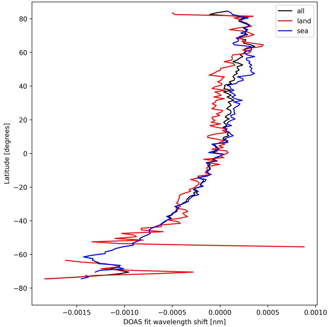
Figure 30: Zonal average of “DOAS fit wavelength shift” for 2024-08-25 to 2024-08-27.
