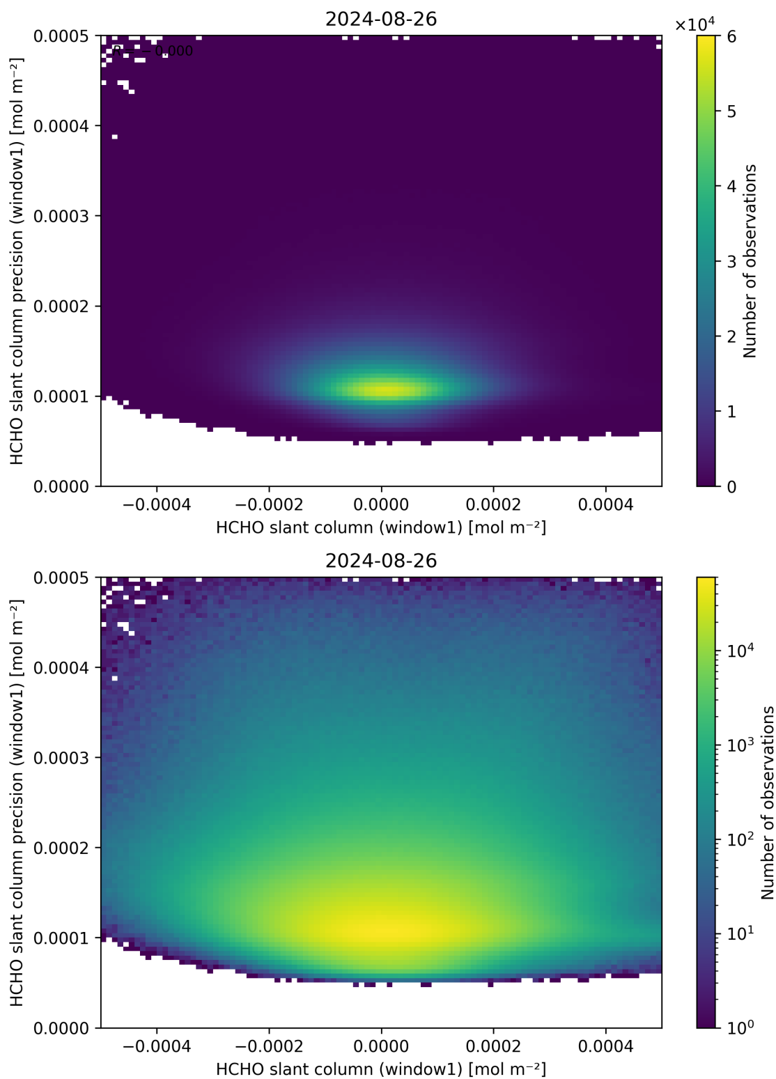
Figure 84: Scatter density plot of “HCHO slant column (window1)” against “HCHO slant column precision (window1)” for 2024-08-25 to 2024-08-27.
