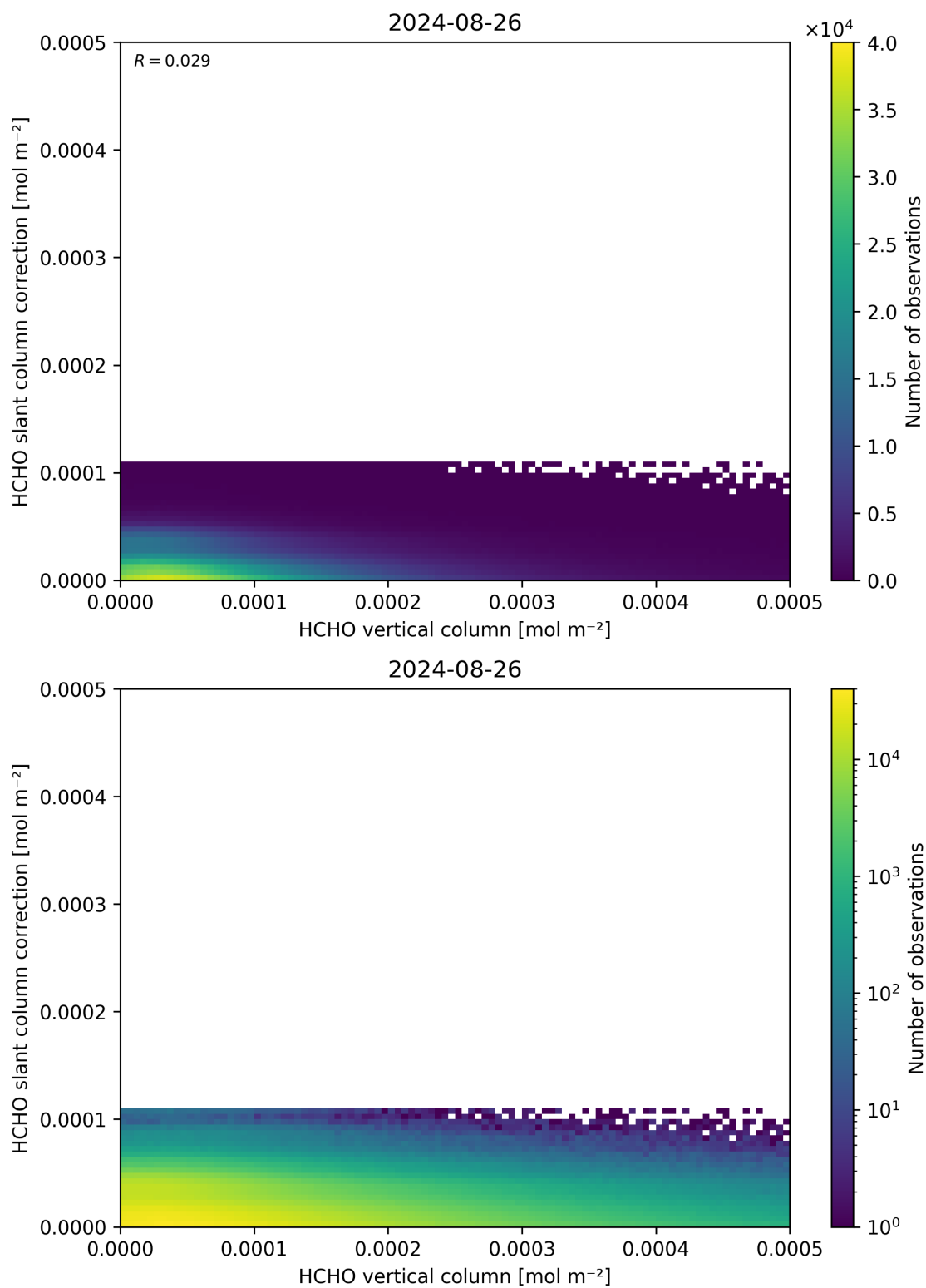
Figure 128: Scatter density plot of “HCHO vertical column” against “HCHO slant column correction” for 2024-08-25 to 2024-08-27.
