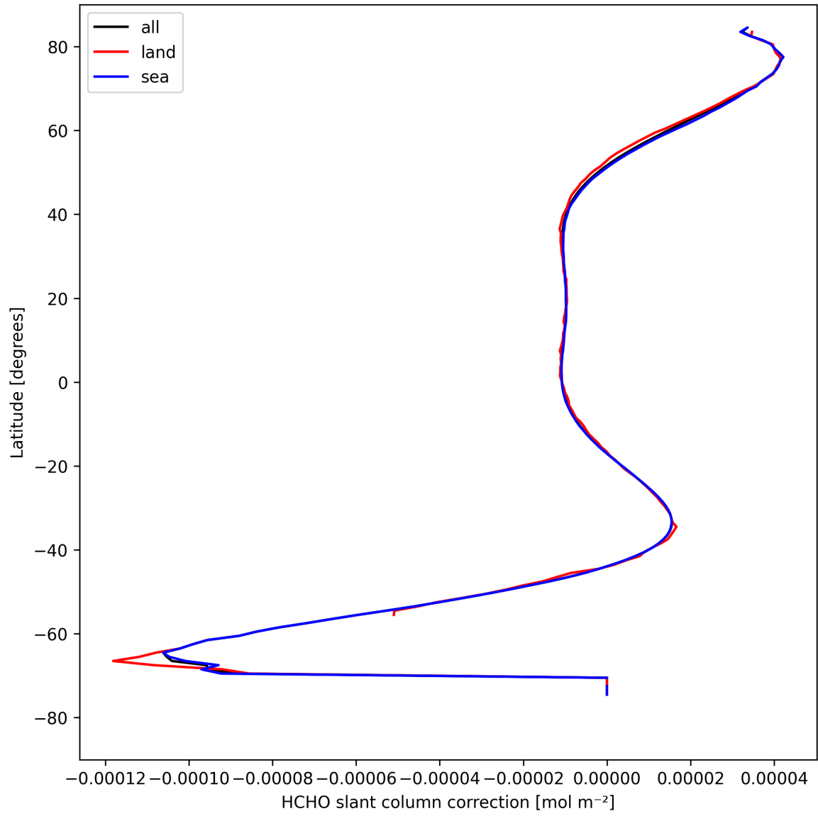
Figure 33: Zonal average of “HCHO slant column correction” for 2024-08-25 to 2024-08-27.
