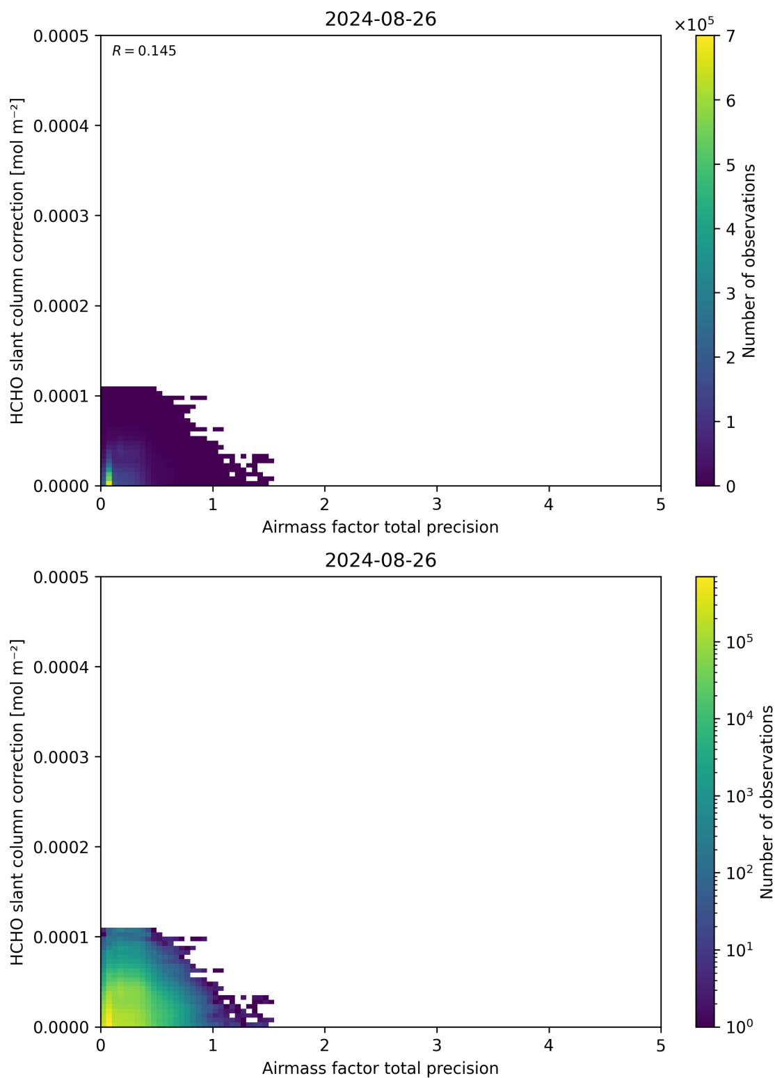
Figure 110: Scatter density plot of “Airmass factor total precision” against “HCHO slant column correction” for 2024-08-25 to 2024-08-27.
