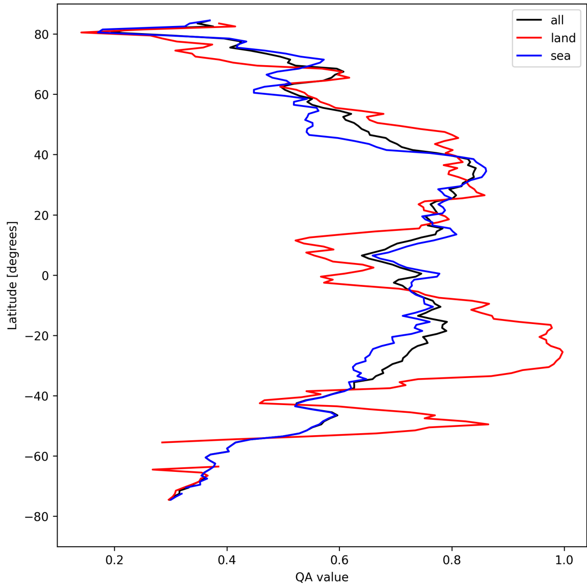
Figure 20: Zonal average of “QA value” for 2024-08-25 to 2024-08-27.
