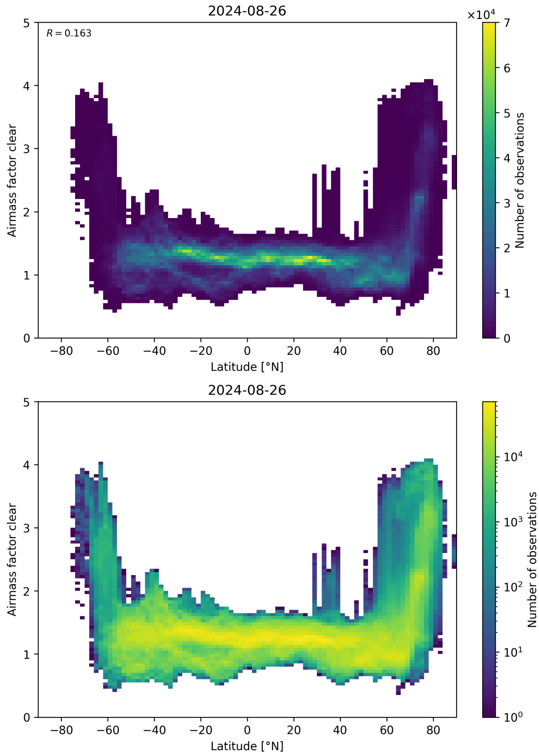
Figure 156: Scatter density plot of “Latitude” against “Airmass factor clear” for 2024-08-25 to 2024-08-27.
