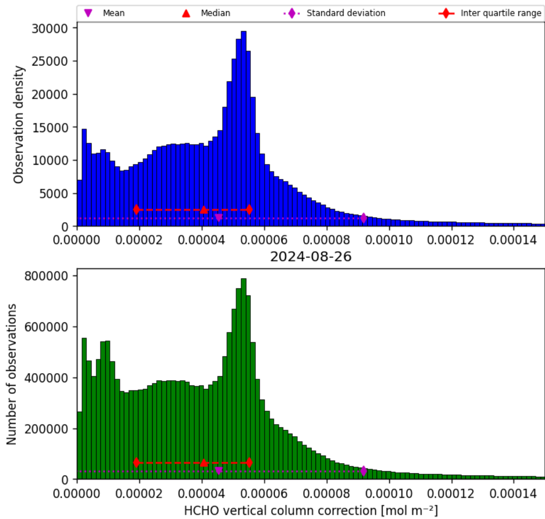
Figure 37: Histogram of “HCHO vertical column correction” for 2024-08-25 to 2024-08-27
