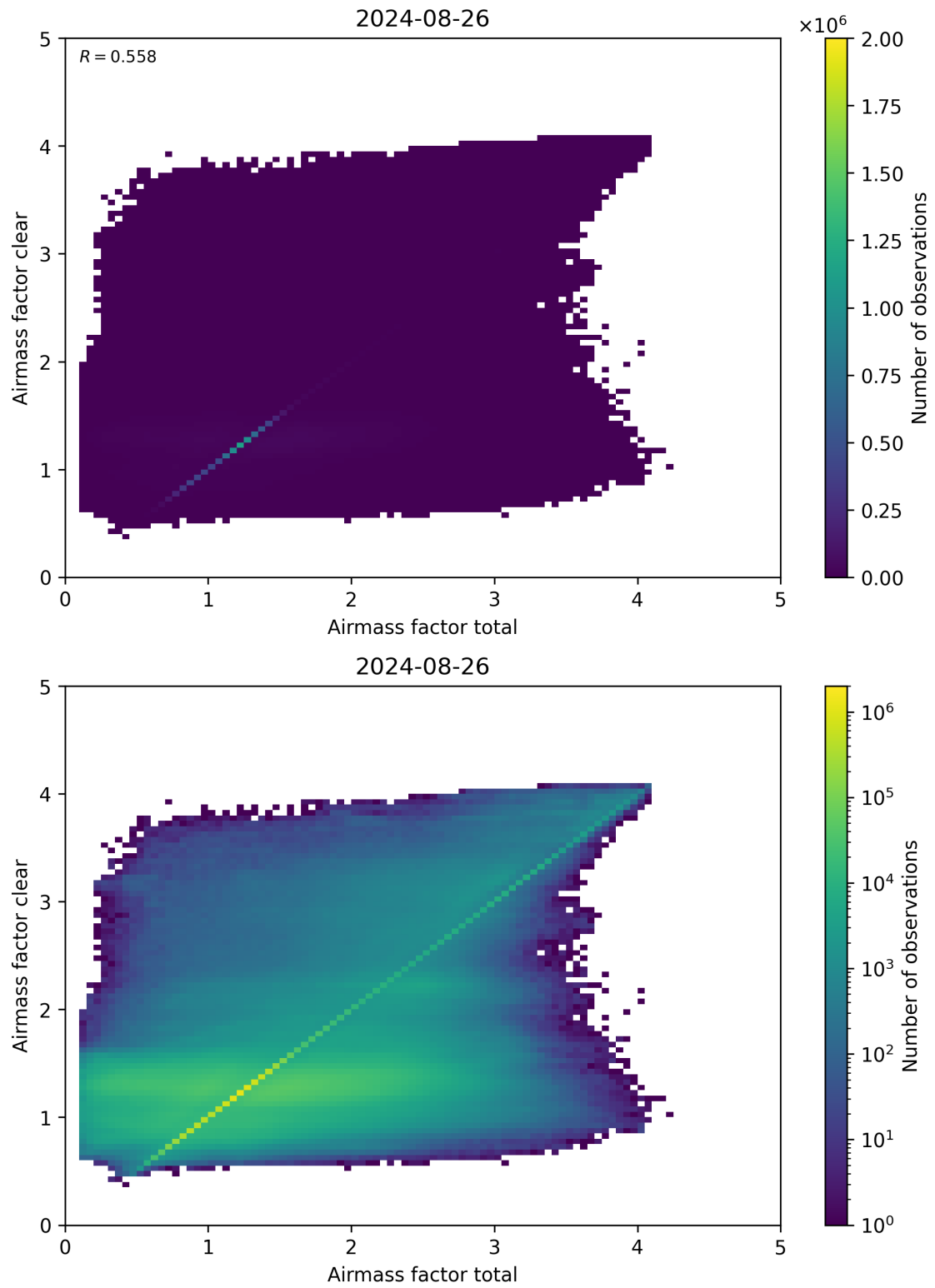
Figure 100: Scatter density plot of “Airmass factor total” against “Airmass factor clear” for 2024-08-25 to 2024-08-27.
