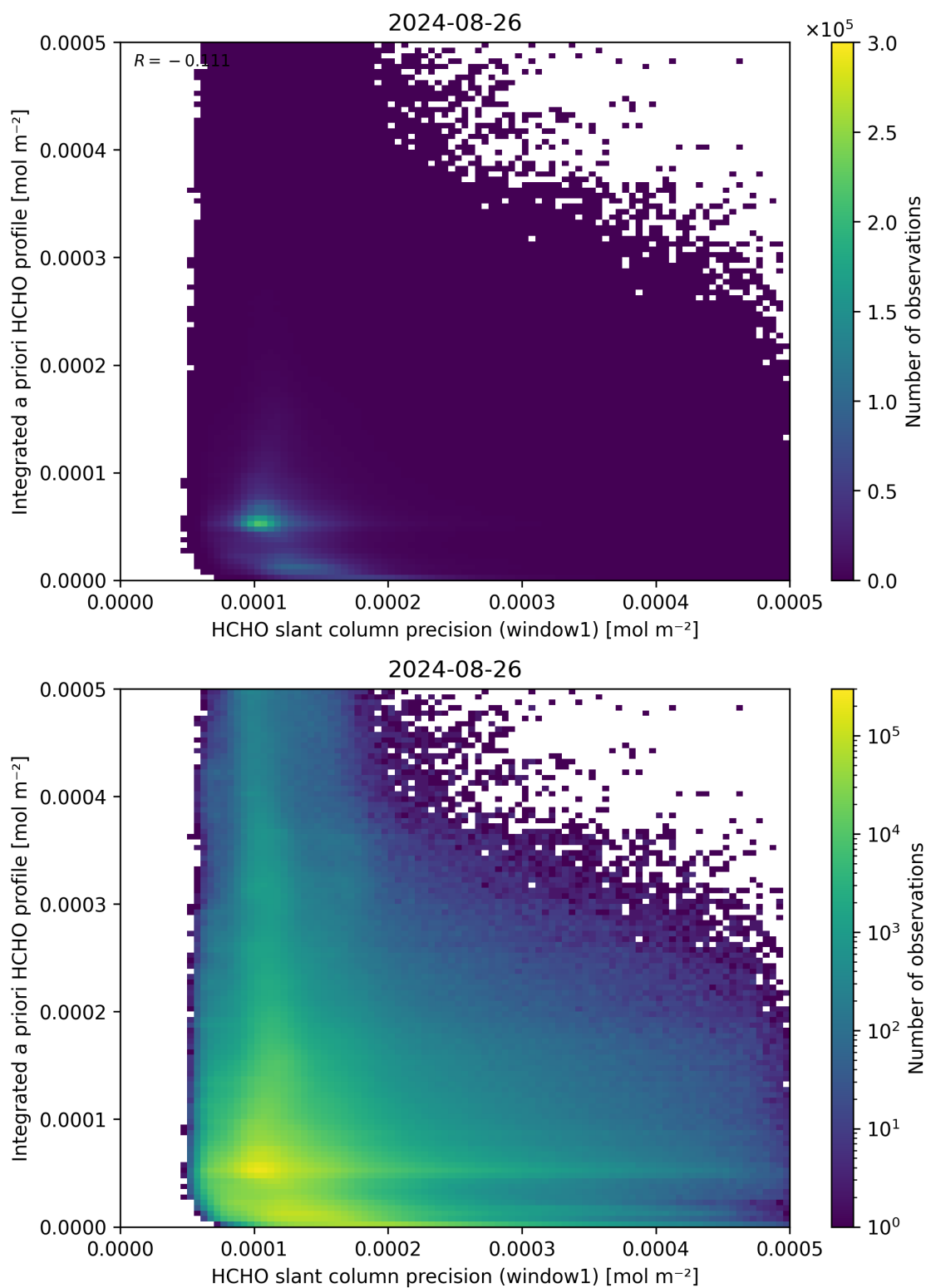
Figure 96: Scatter density plot of “HCHO slant column precision (window1)” against “Integrated a priori HCHO profile” for 2024-08-25 to 2024-08-27.
