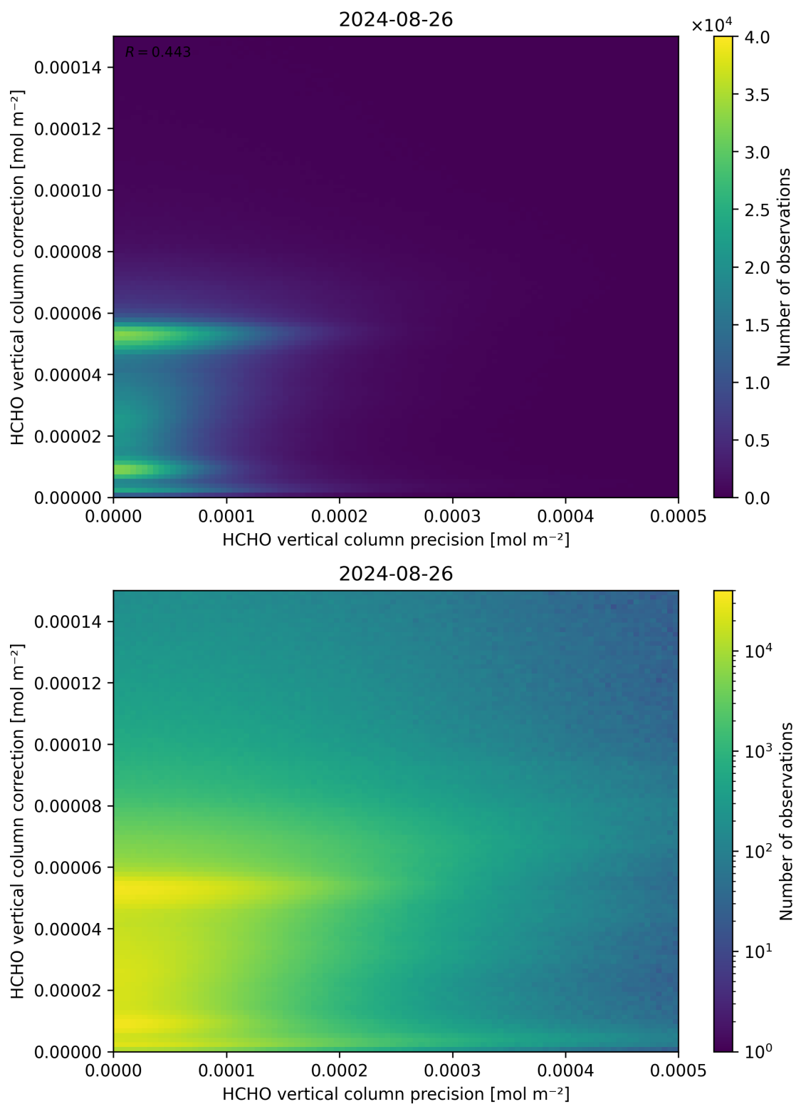
Figure 146: Scatter density plot of “HCHO vertical column precision” against “HCHO vertical column correction” for 2024-08-25 to 2024-08-27.
