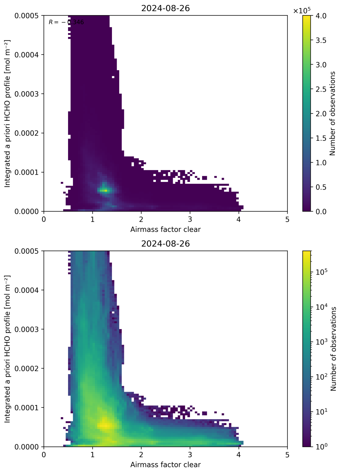
Figure 76: Scatter density plot of “Airmass factor clear” against “Integrated a priori HCHO profile” for 2024-08-25 to 2024-08-27.
