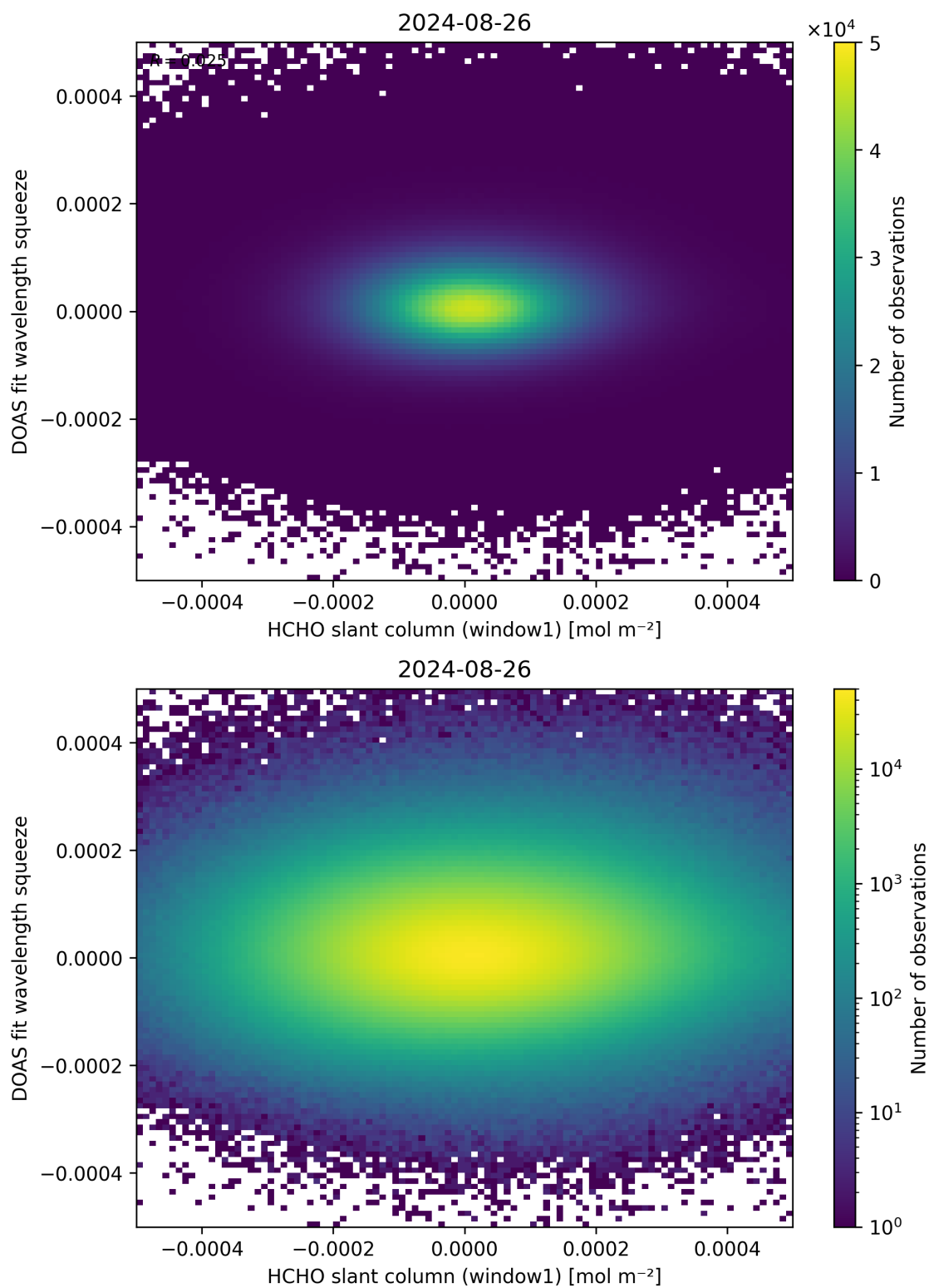
Figure 80: Scatter density plot of “HCHO slant column (window1)” against “DOAS fit wavelength squeeze” for 2024-08-25 to 2024-08-27.
