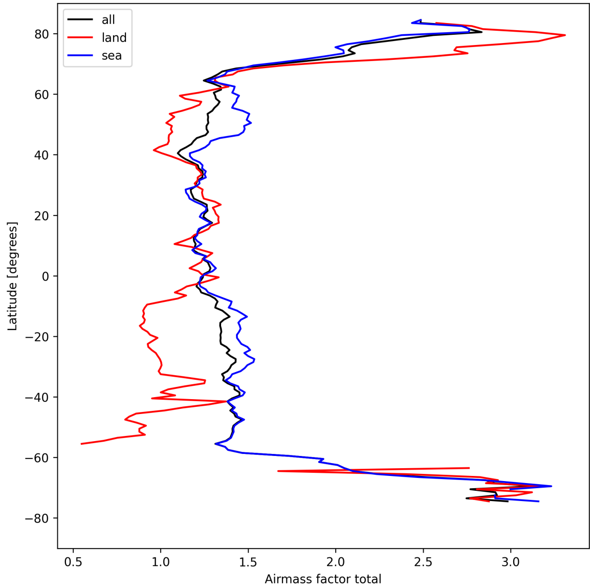
Figure 26: Zonal average of “Airmass factor total” for 2024-08-25 to 2024-08-27.
