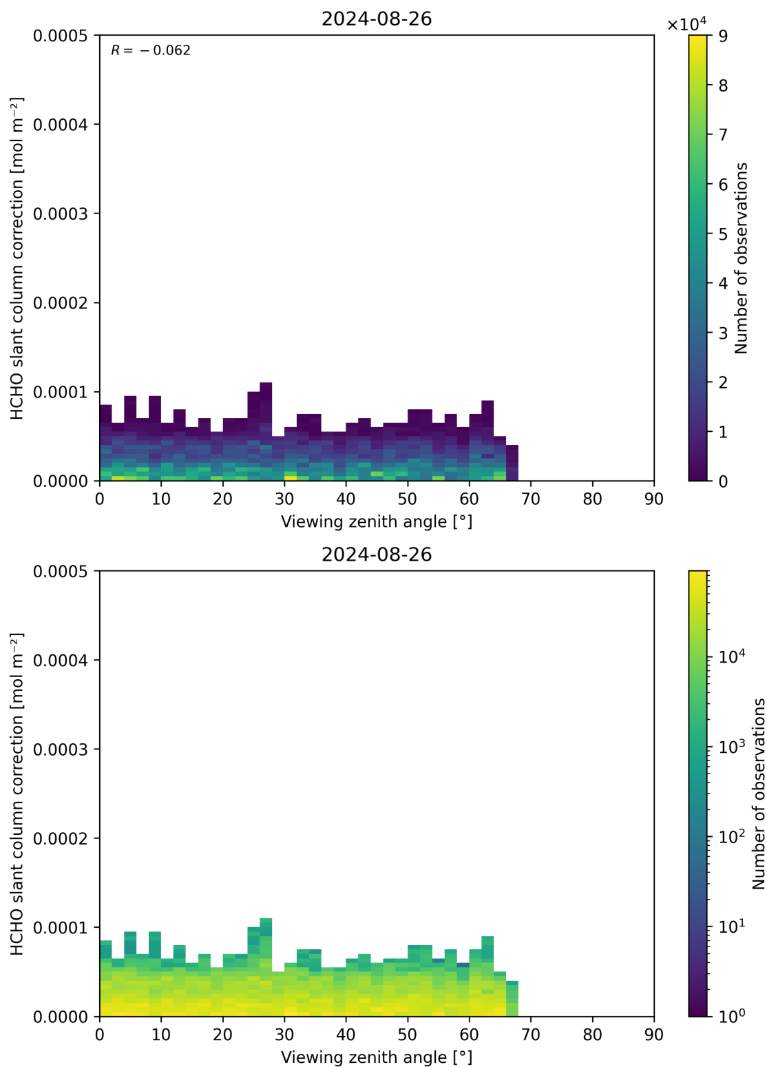
Figure 187: Scatter density plot of “Viewing zenith angle” against “HCHO slant column correction” for 2024-08-25 to 2024-08-27.
