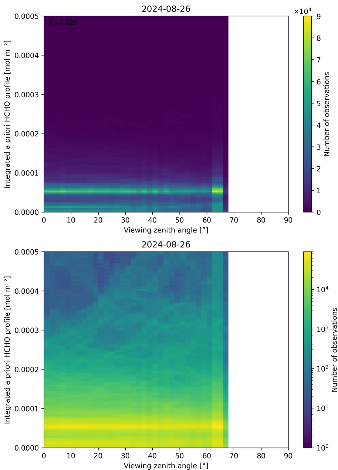
Figure 195: Scatter density plot of “Viewing zenith angle” against “Integrated a priori HCHO profile” for 2024-08-25 to 2024-08-27.
