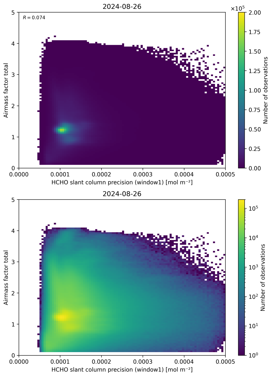
Figure 94: Scatter density plot of “HCHO slant column precision (window1)” against “Airmass factor total” for 2024-08-25 to 2024-08-27.
