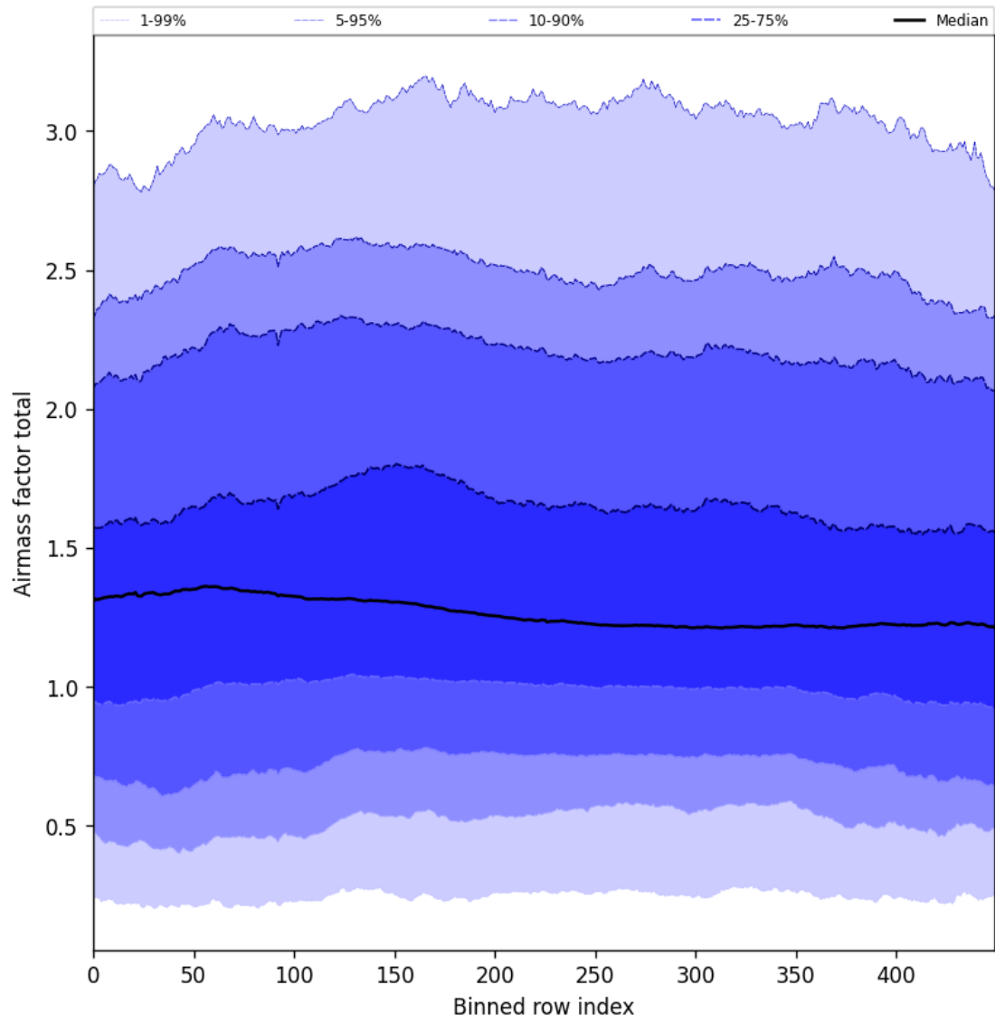
Figure 54: Along track statistics of “Airmass factor total” for 2024-08-25 to 2024-08-27
