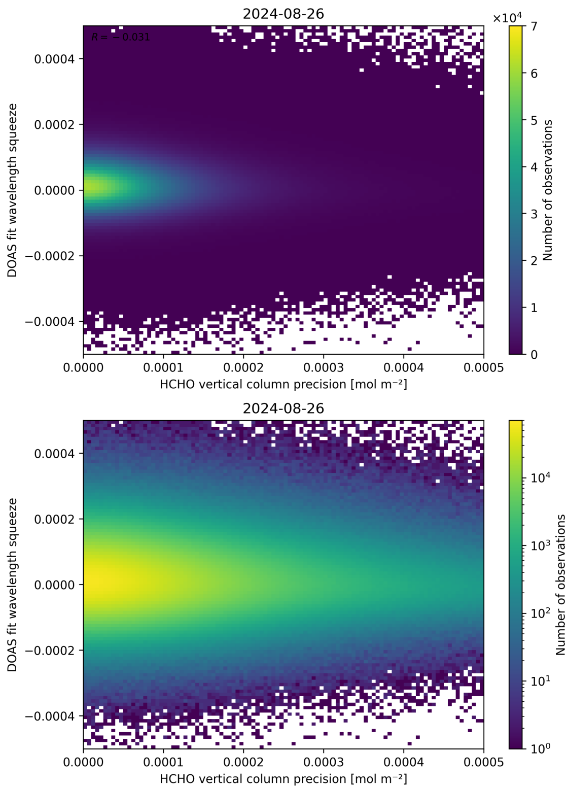
Figure 138: Scatter density plot of “HCHO vertical column precision” against “DOAS fit wavelength squeeze” for 2024-08-25 to 2024-08-27.
