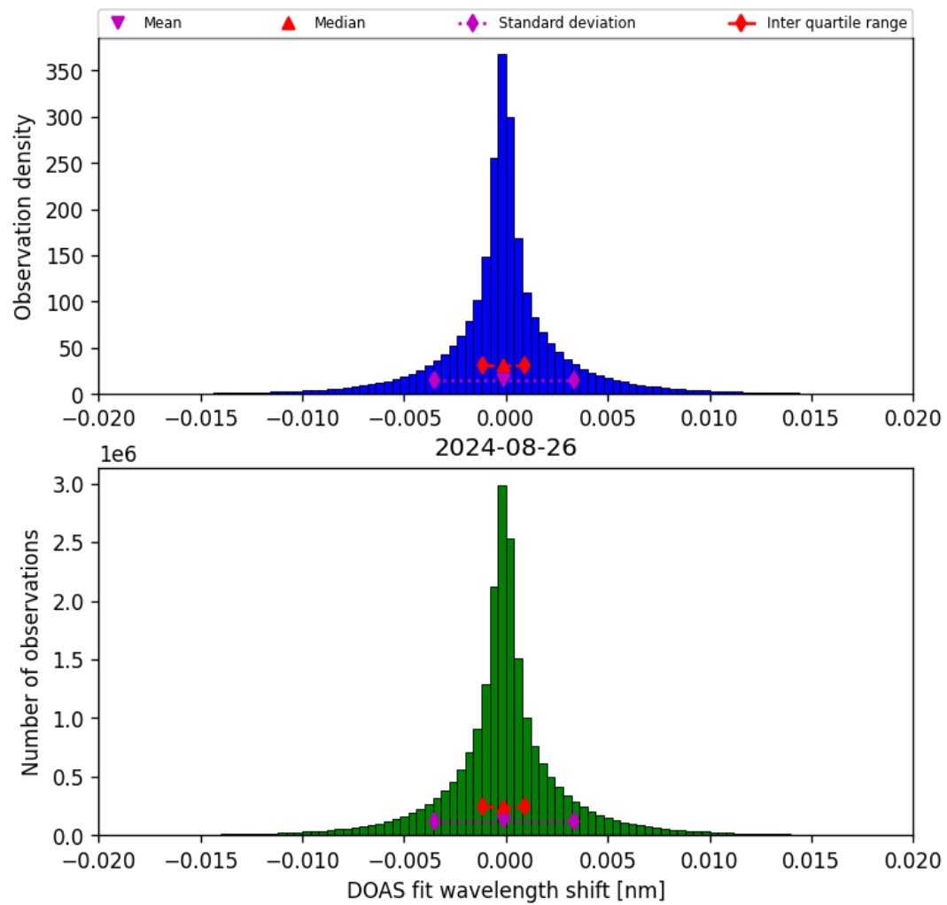
Figure 44: Histogram of “DOAS fit wavelength shift” for 2024-08-25 to 2024-08-27
