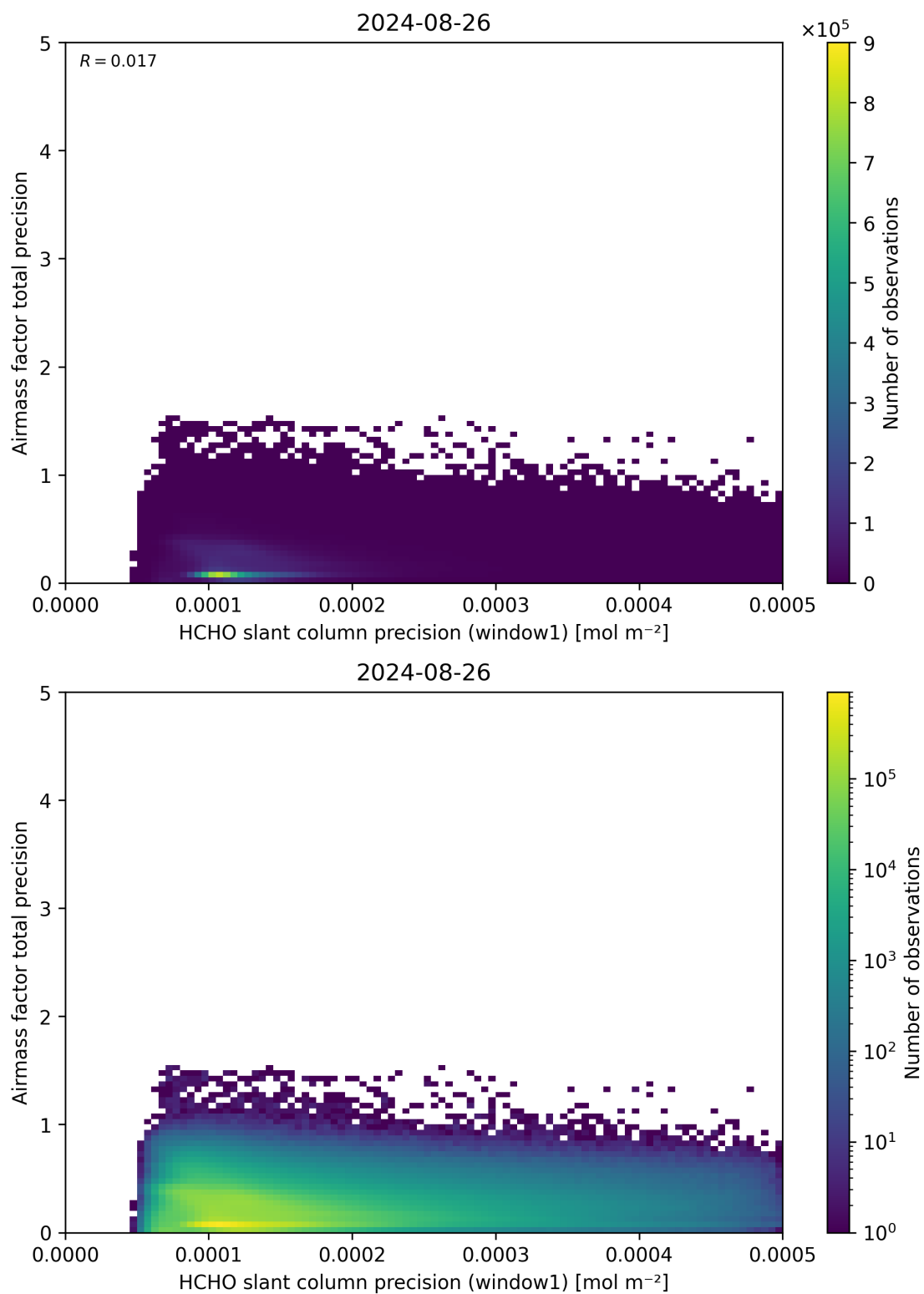
Figure 95: Scatter density plot of “HCHO slant column precision (window1)” against “Airmass factor total precision” for 2024-08-25 to 2024-08-27.
