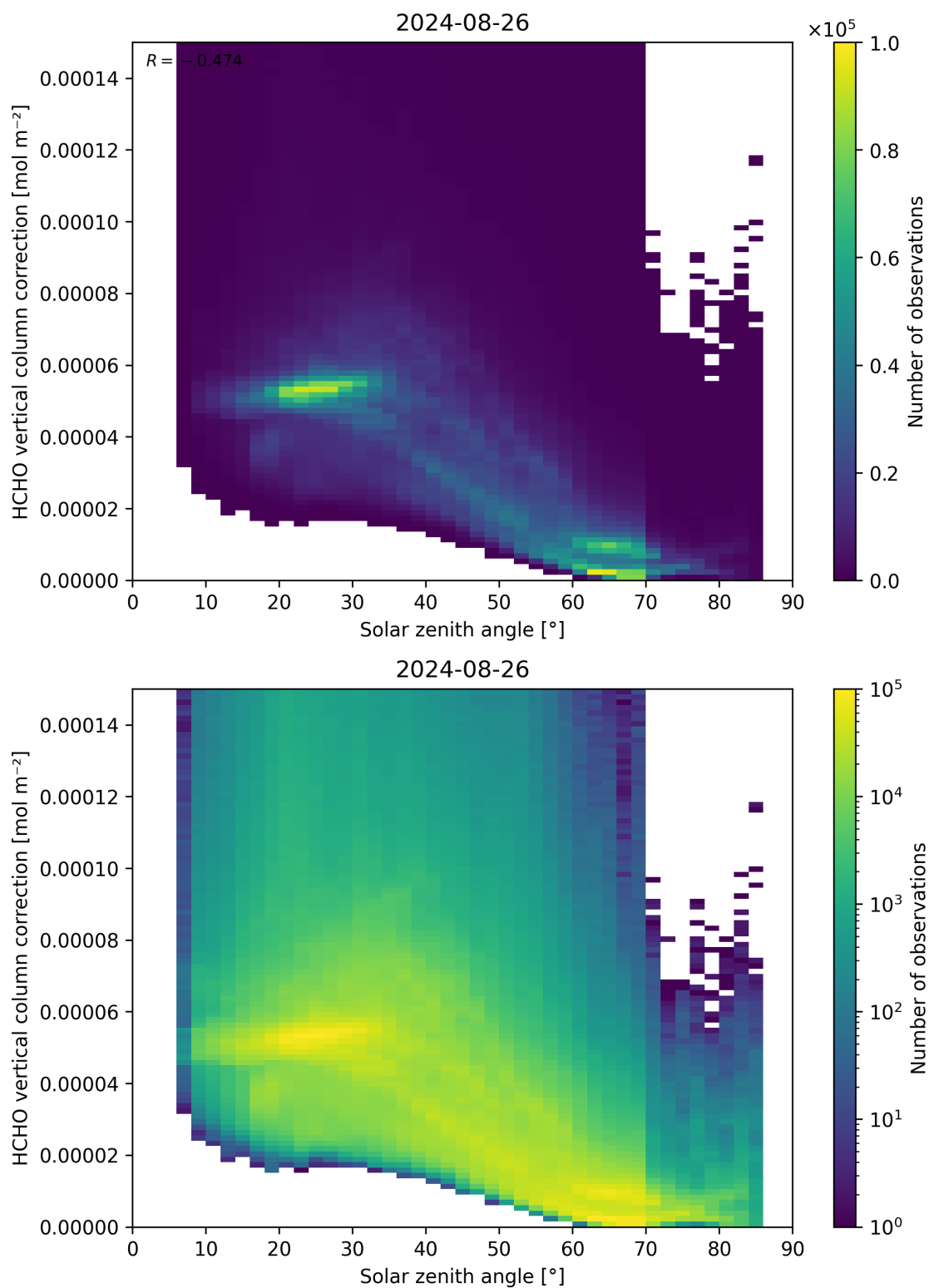
Figure 178: Scatter density plot of “Solar zenith angle” against “HCHO vertical column correction” for 2024-08-25 to 2024-08-27.
