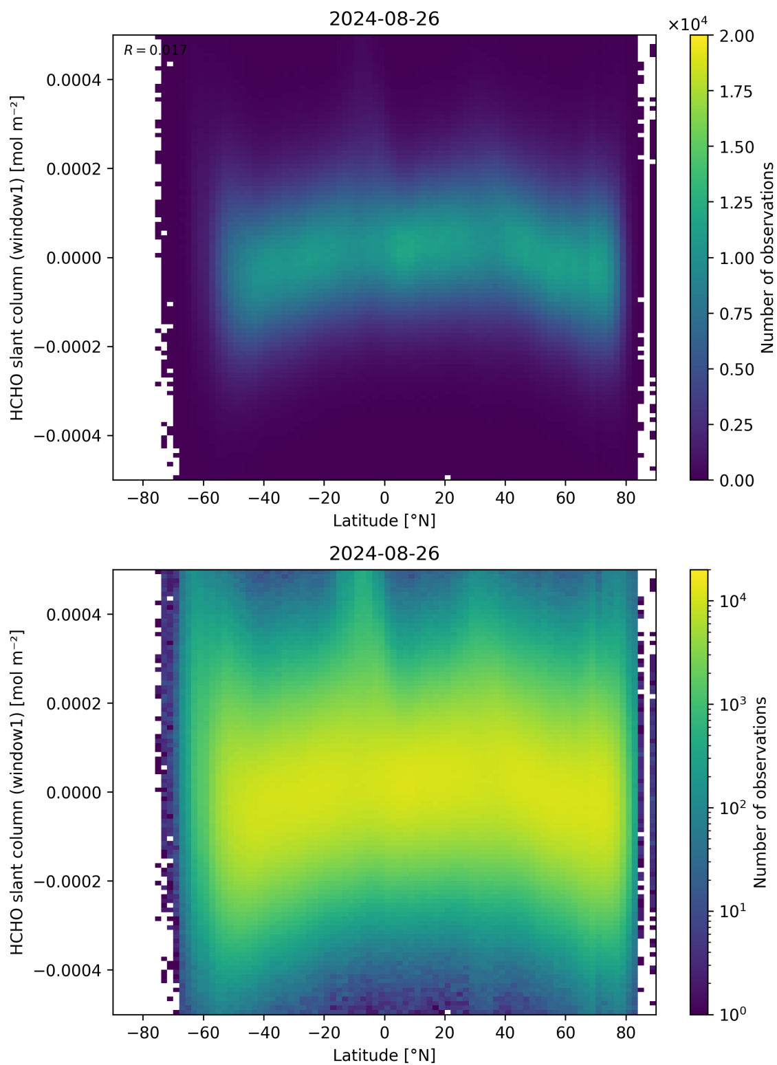
Figure 159: Scatter density plot of “Latitude” against “HCHO slant column (window1)” for 2024-08-25 to 2024-08-27.
