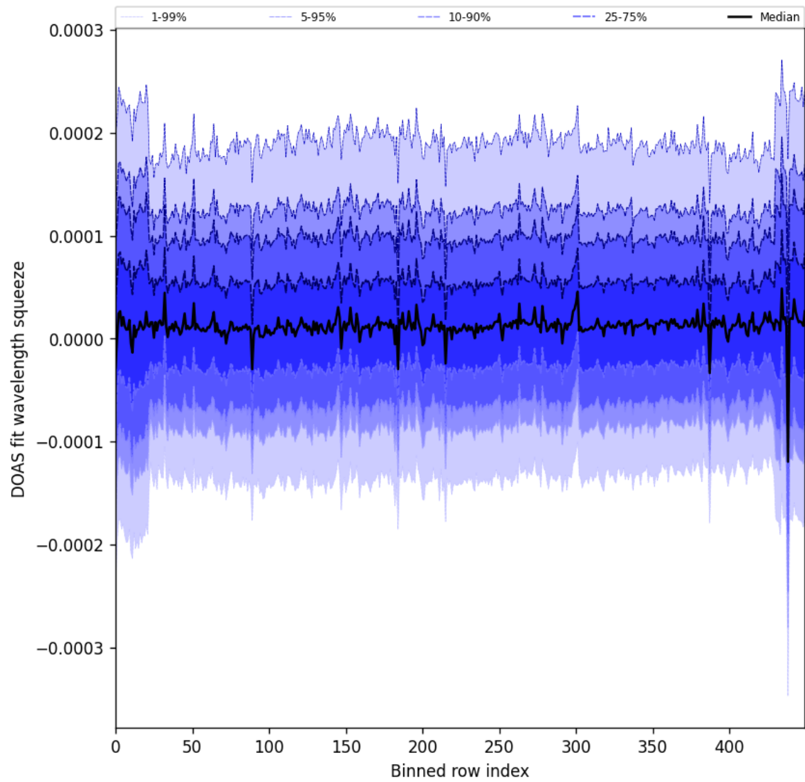
Figure 59: Along track statistics of “DOAS fit wavelength squeeze” for 2024-08-25 to 2024-08-27
