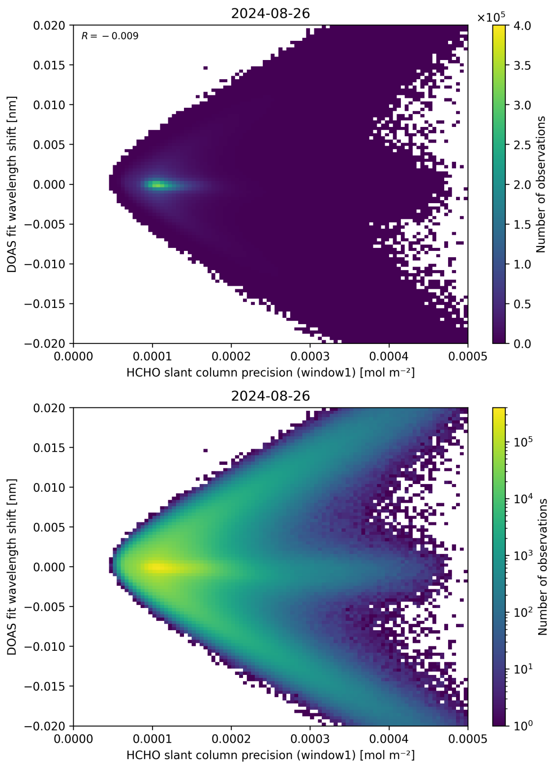
Figure 89: Scatter density plot of “HCHO slant column precision (window1)” against “DOAS fit wavelength shift” for 2024-08-25 to 2024-08-27.
