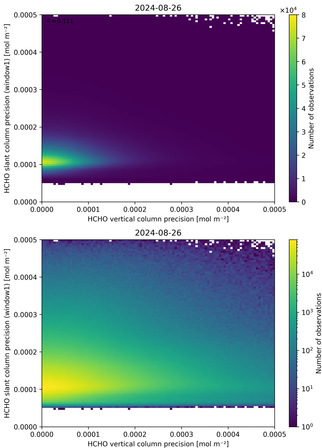
Figure 143: Scatter density plot of “HCHO vertical column precision” against “HCHO slant column precision (window1)” for 2024-08-25 to 2024-08-27.
