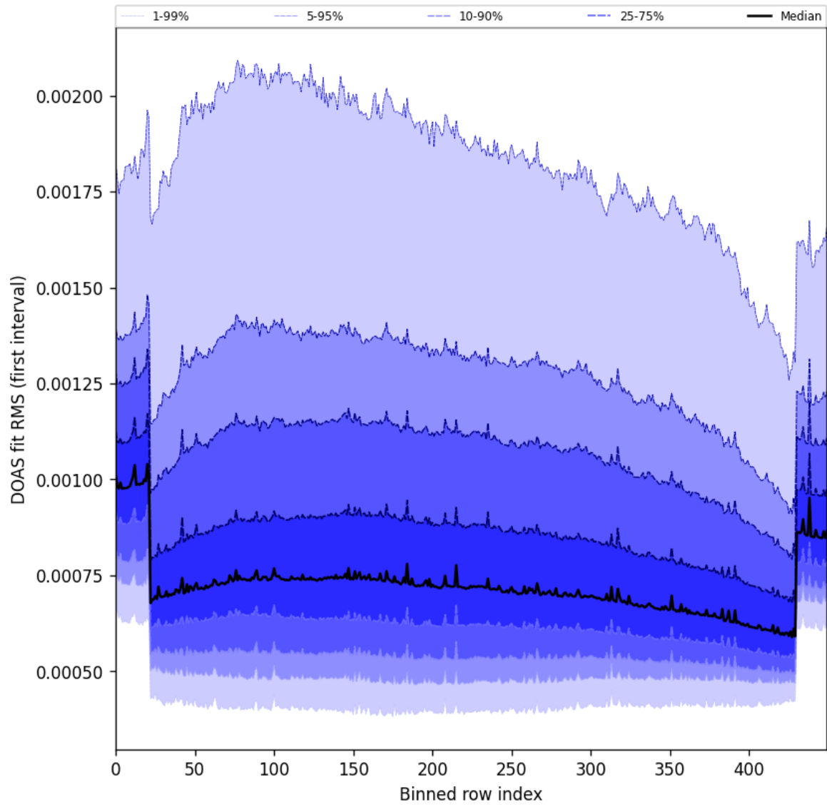
Figure 60: Along track statistics of “DOAS fit RMS (first interval)” for 2024-08-25 to 2024-08-27
