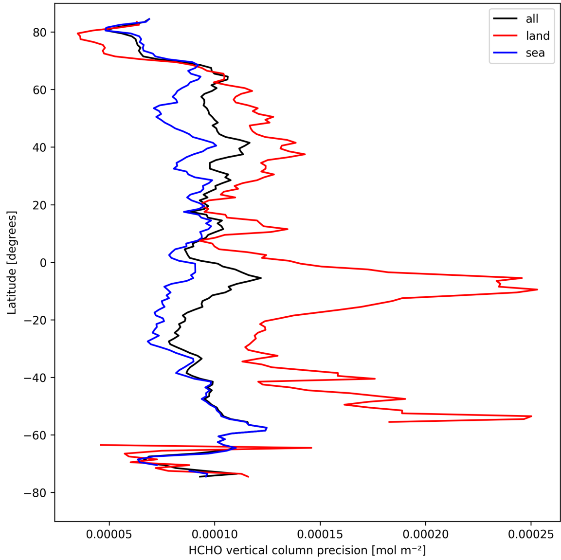
Figure 22: Zonal average of “HCHO vertical column precision” for 2024-08-25 to 2024-08-27.
