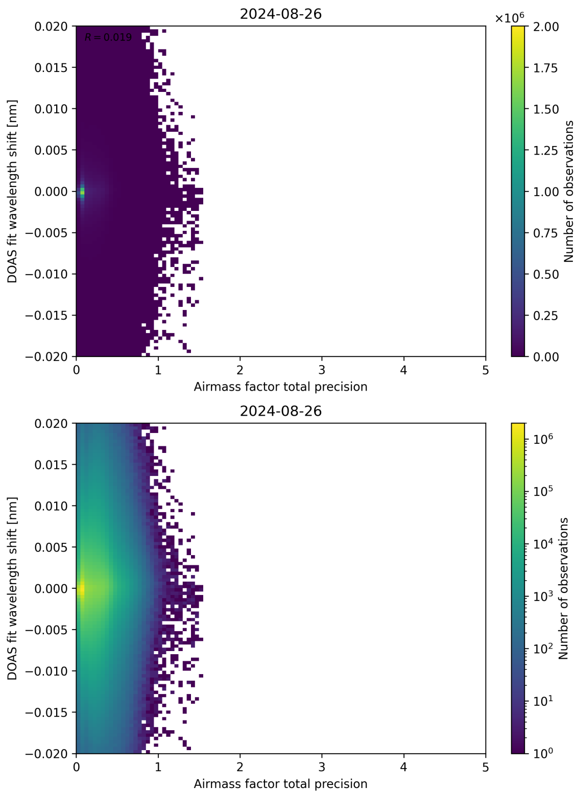
Figure 106: Scatter density plot of “Airmass factor total precision” against “DOAS fit wavelength shift” for 2024-08-25 to 2024-08-27.
