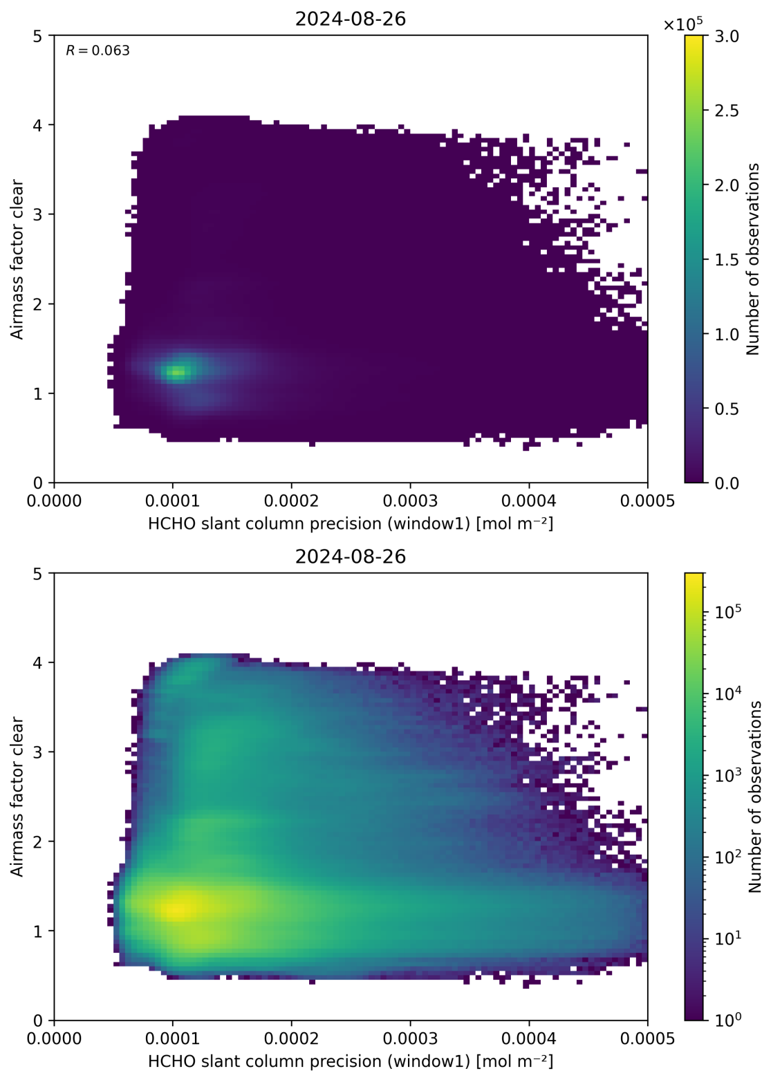
Figure 91: Scatter density plot of “HCHO slant column precision (window1)” against “Airmass factor clear” for 2024-08-25 to 2024-08-27.
