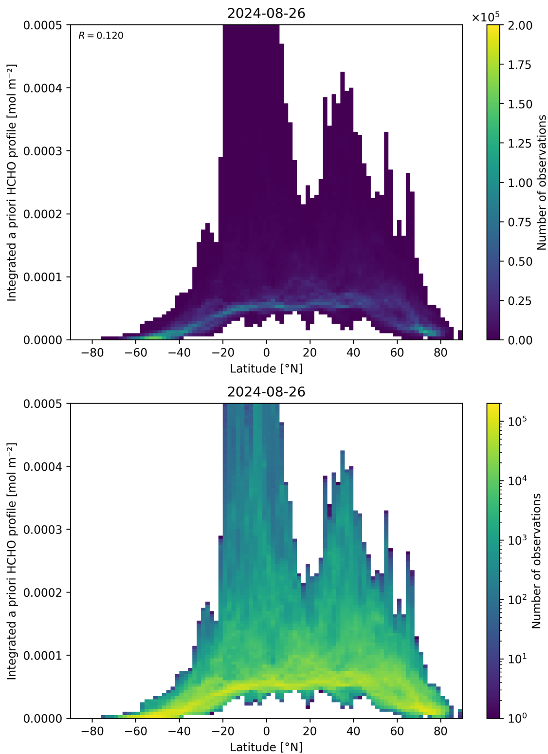
Figure 166: Scatter density plot of “Latitude” against “Integrated a priori HCHO profile” for 2024-08-25 to 2024-08-27.
