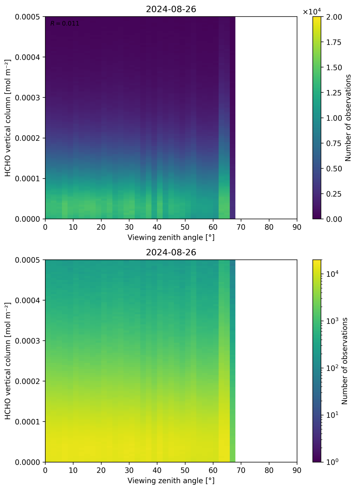
Figure 192: Scatter density plot of “Viewing zenith angle” against “HCHO vertical column” for 2024-08-25 to 2024-08-27.
