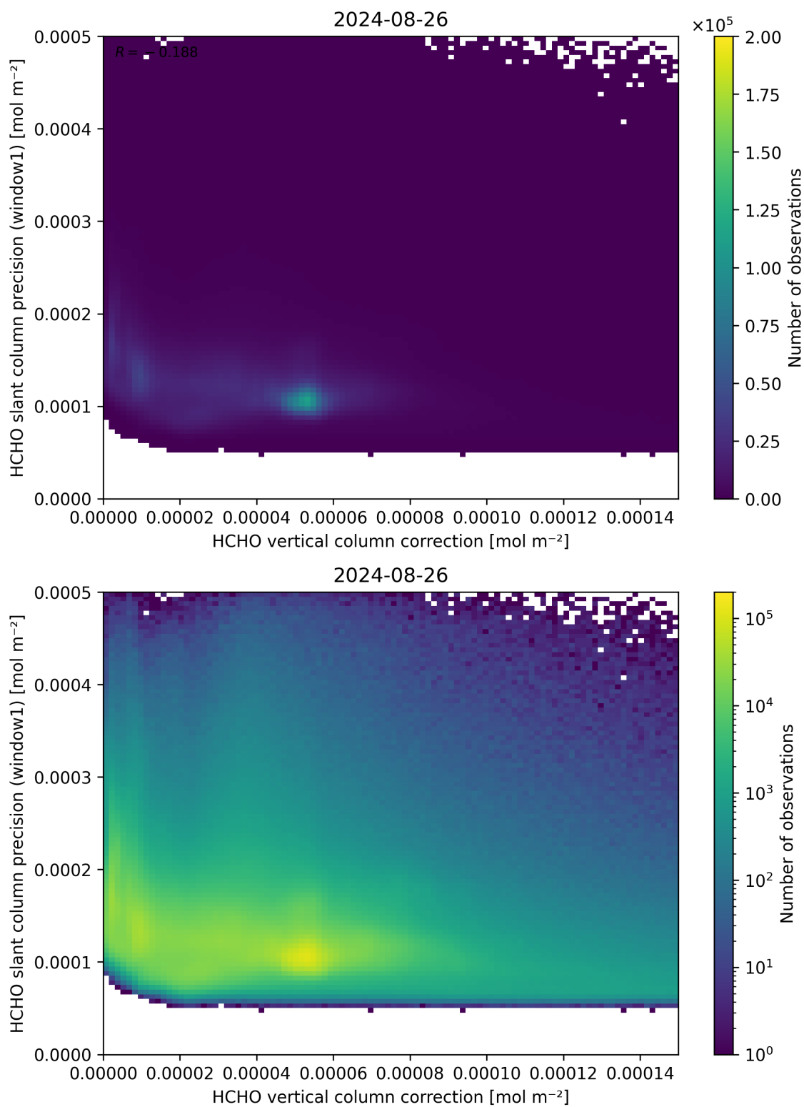
Figure 119: Scatter density plot of “HCHO vertical column correction” against “HCHO slant column precision (window1)” for 2024-08-25 to 2024-08-27.
