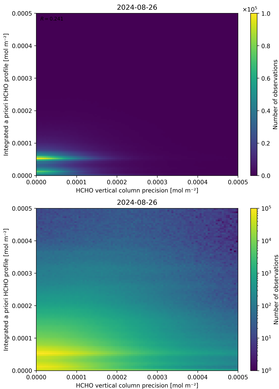
Figure 147: Scatter density plot of “HCHO vertical column precision” against “Integrated a priori HCHO profile” for 2024-08-25 to 2024-08-27.
