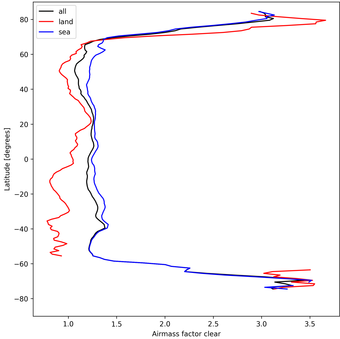
Figure 28: Zonal average of “Airmass factor clear” for 2024-08-25 to 2024-08-27.
