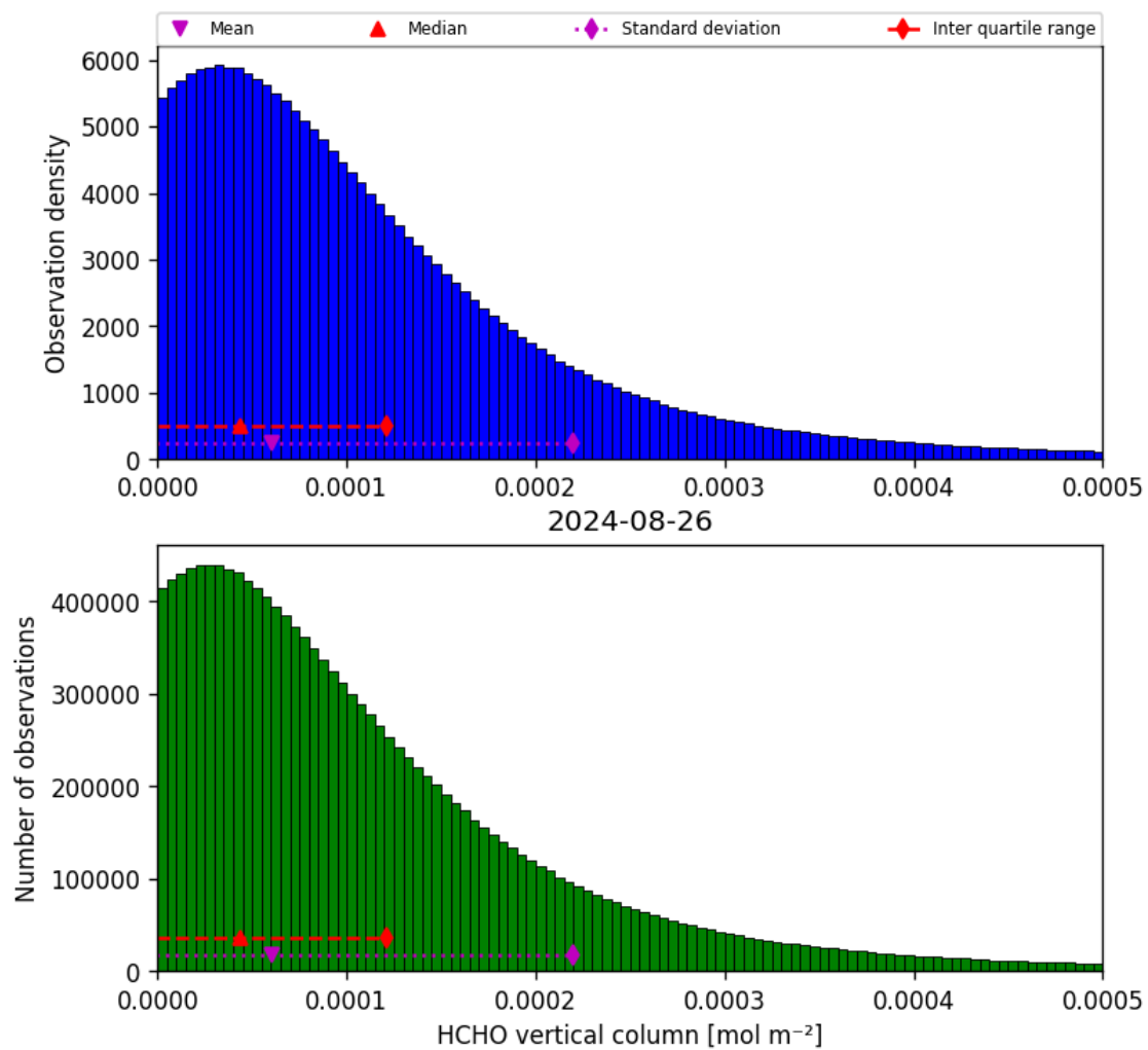
Figure 35: Histogram of “HCHO vertical column” for 2024-08-25 to 2024-08-27
