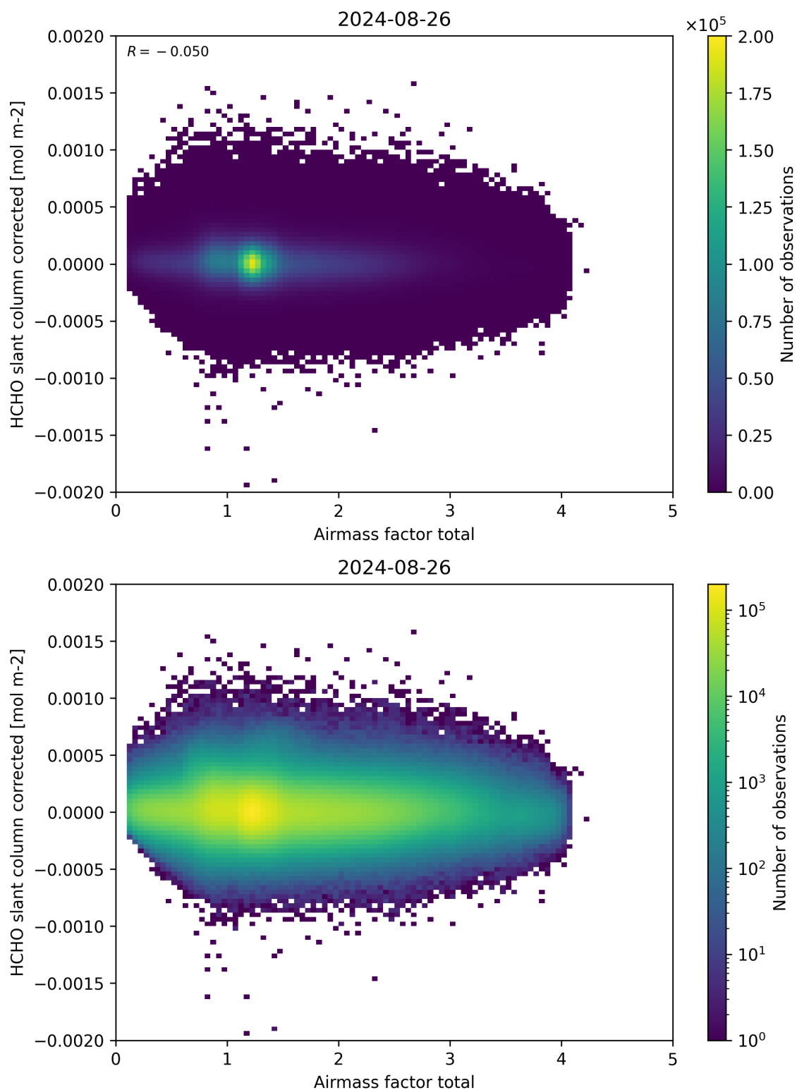
Figure 101: Scatter density plot of “Airmass factor total” against “HCHO slant column corrected” for 2024-08-25 to 2024-08-27.
