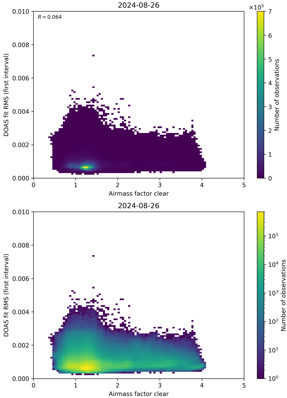
Figure 71: Scatter density plot of “Airmass factor clear” against “DOAS fit RMS (first interval)” for 2024-08-25 to 2024-08-27.
