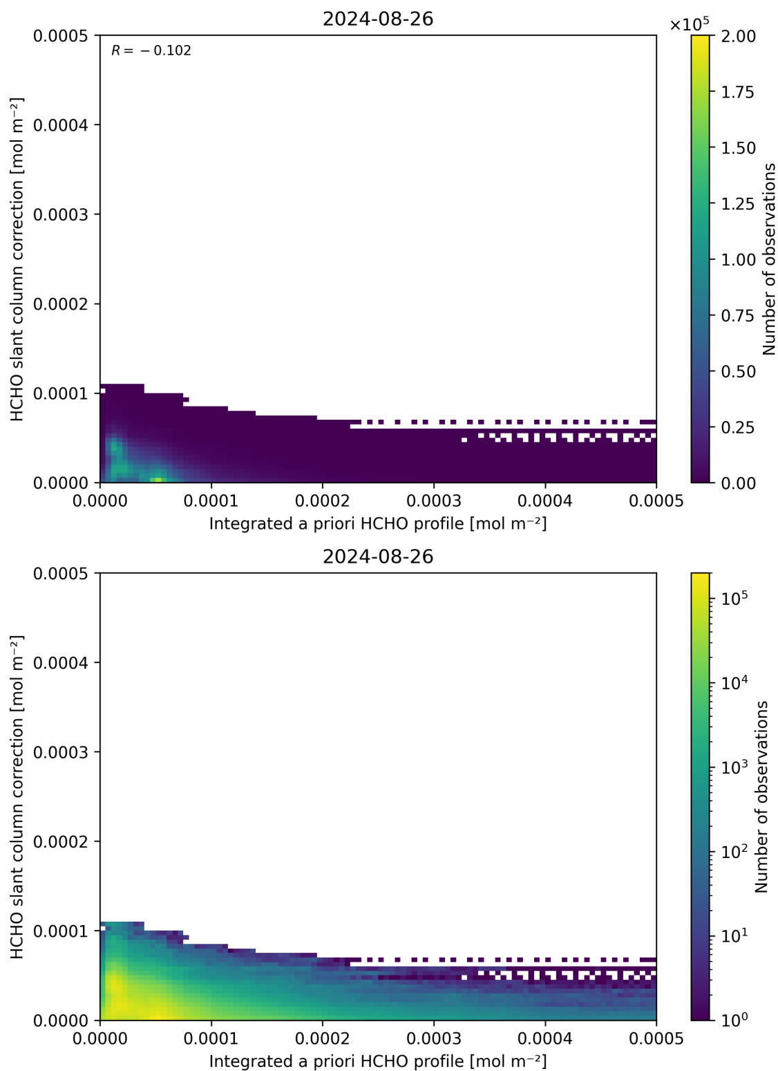
Figure 152: Scatter density plot of “Integrated a priori HCHO profile” against “HCHO slant column correction” for 2024-08-25 to 2024-08-27.
