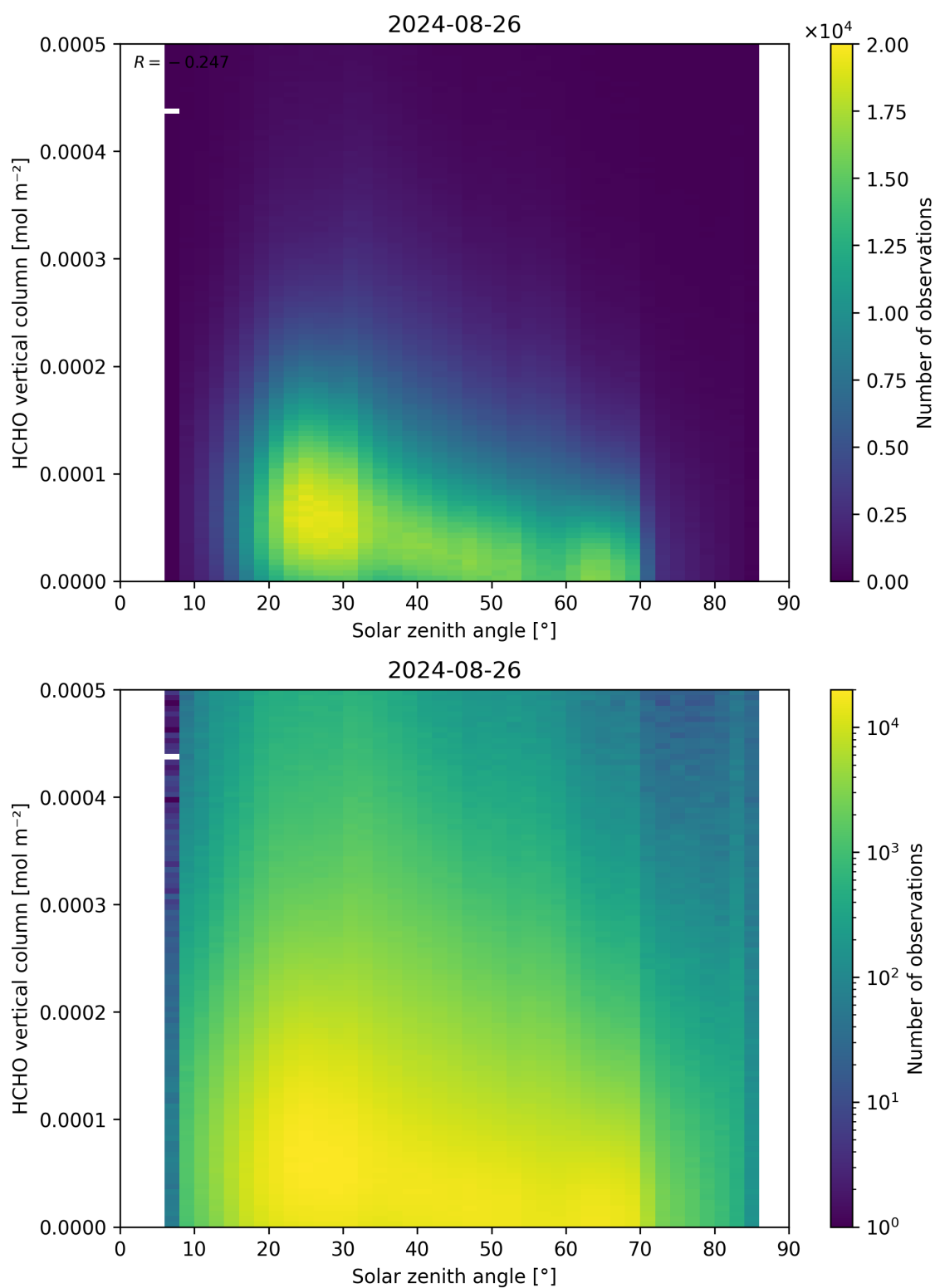
Figure 177: Scatter density plot of “Solar zenith angle” against “HCHO vertical column” for 2024-08-25 to 2024-08-27.
