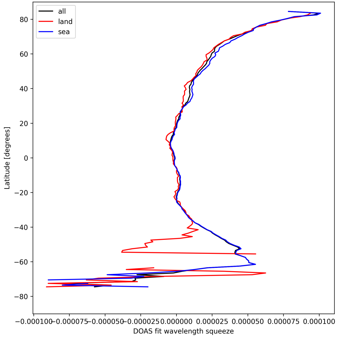
Figure 31: Zonal average of "DOAS fit wavelength squeeze" for 2024-08-25 to 2024-08-27.
