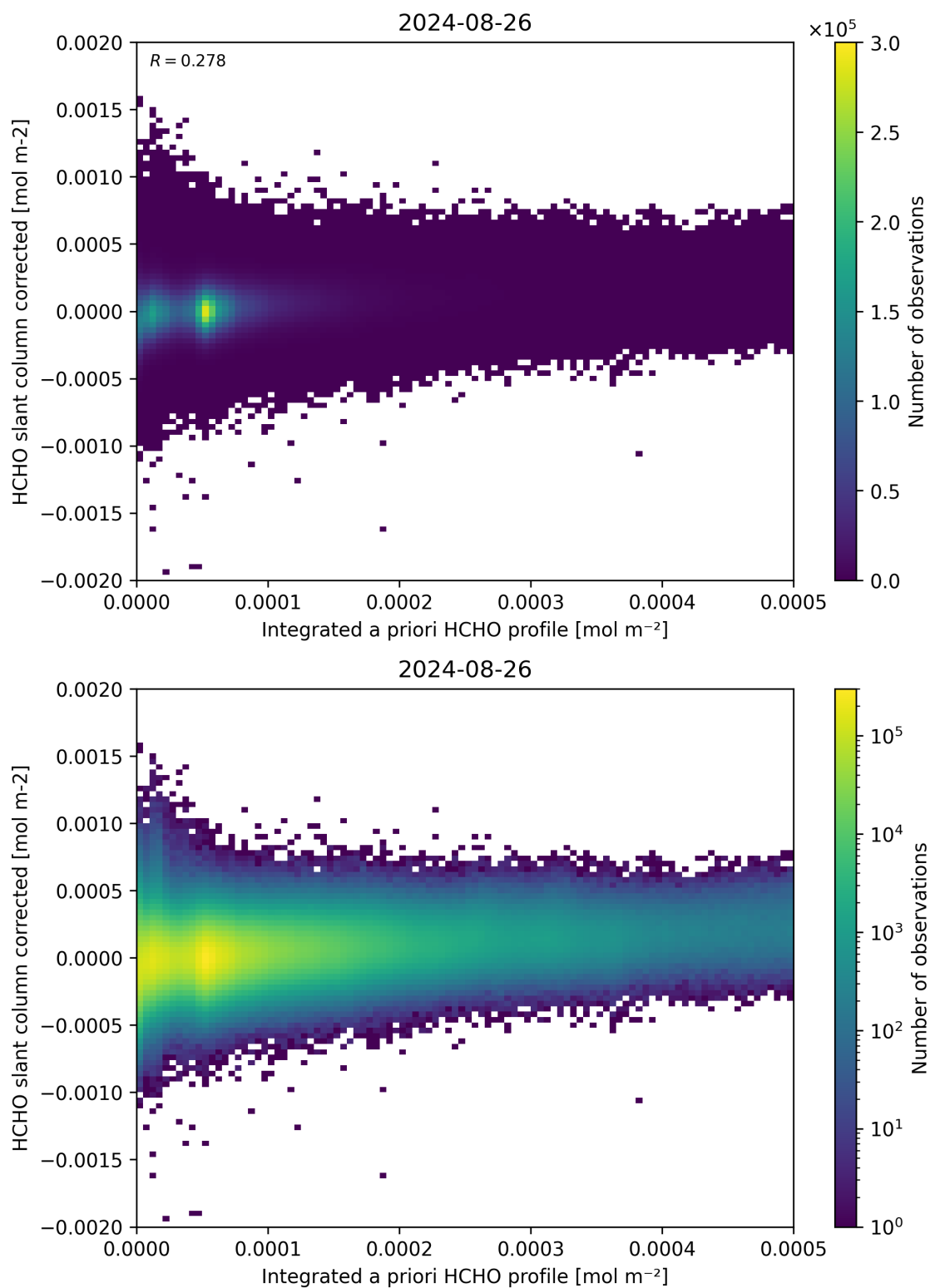
Figure 151: Scatter density plot of “Integrated a priori HCHO profile” against “HCHO slant column corrected” for 2024-08-25 to 2024-08-27.
