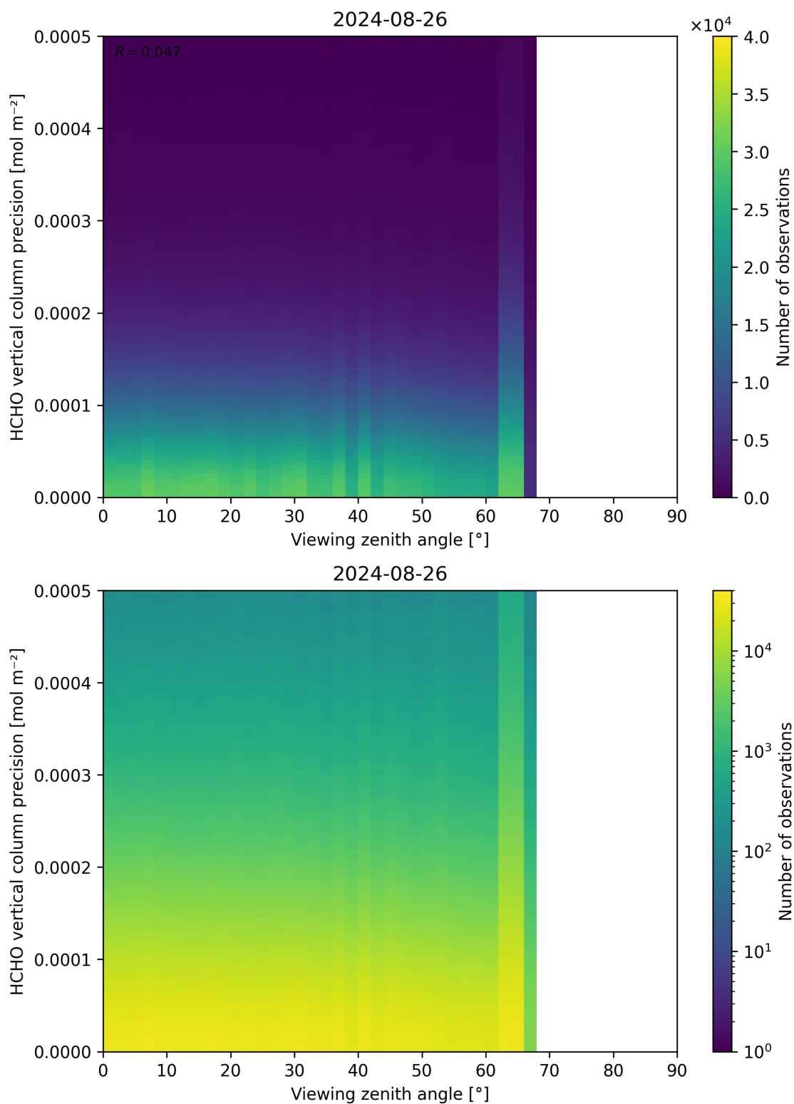
Figure 194: Scatter density plot of “Viewing zenith angle” against “HCHO vertical column precision” for 2024-08-25 to 2024-08-27.
