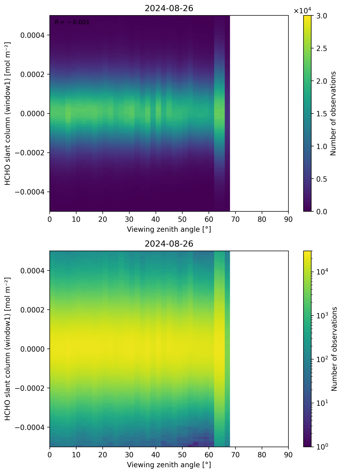
Figure 188: Scatter density plot of “Viewing zenith angle” against “HCHO slant column (window1)” for 2024-08-25 to 2024-08-27.
