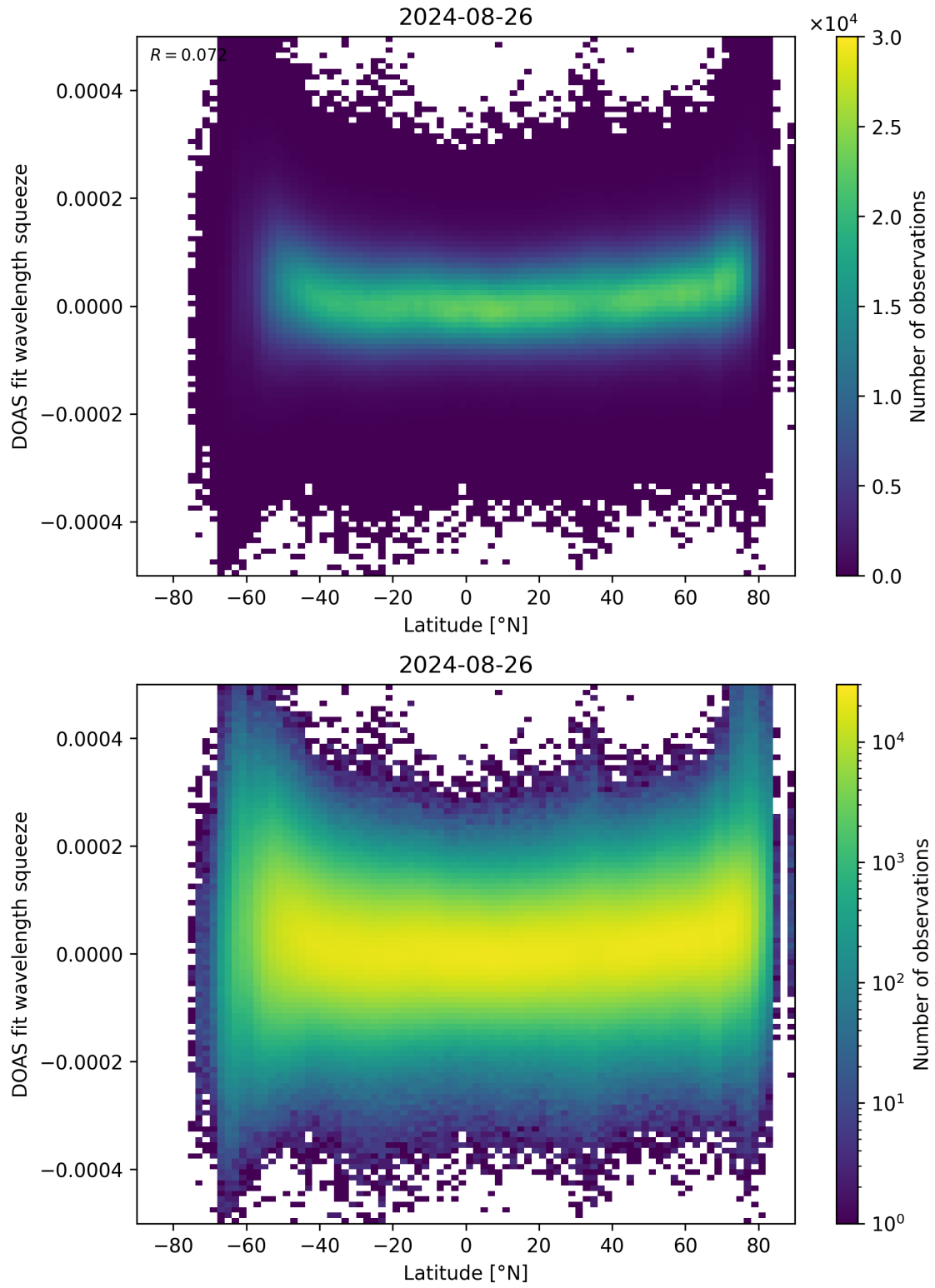
Figure 155: Scatter density plot of “Latitude” against “DOAS fit wavelength squeeze” for 2024-08-25 to 2024-08-27.
