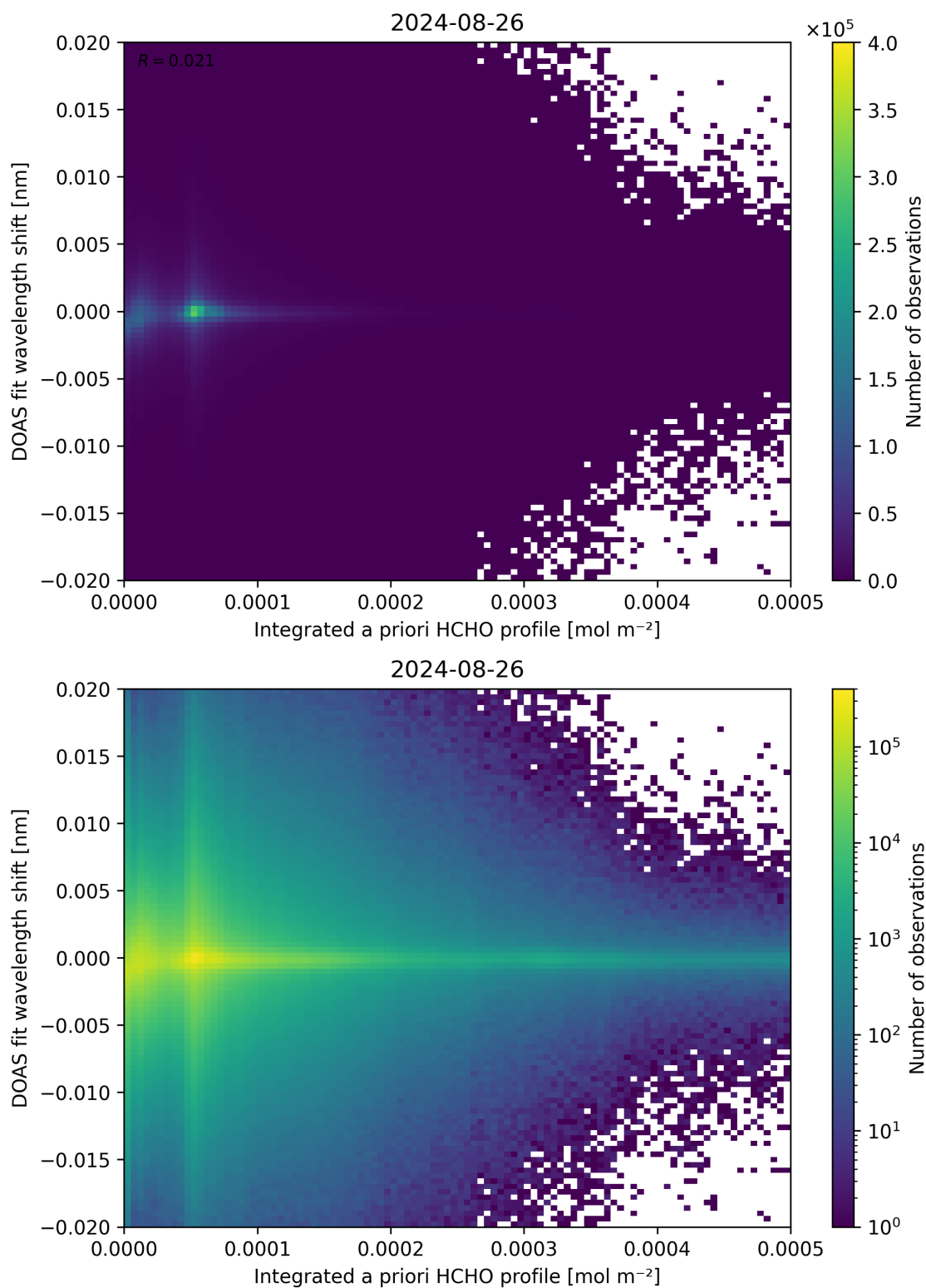
Figure 149: Scatter density plot of “Integrated a priori HCHO profile” against “DOAS fit wavelength shift” for 2024-08-25 to 2024-08-27.
