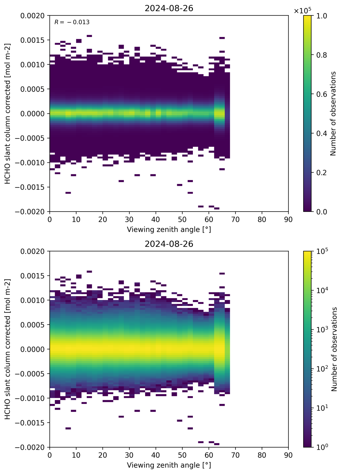
Figure 186: Scatter density plot of “Viewing zenith angle” against “HCHO slant column corrected” for 2024-08-25 to 2024-08-27.
