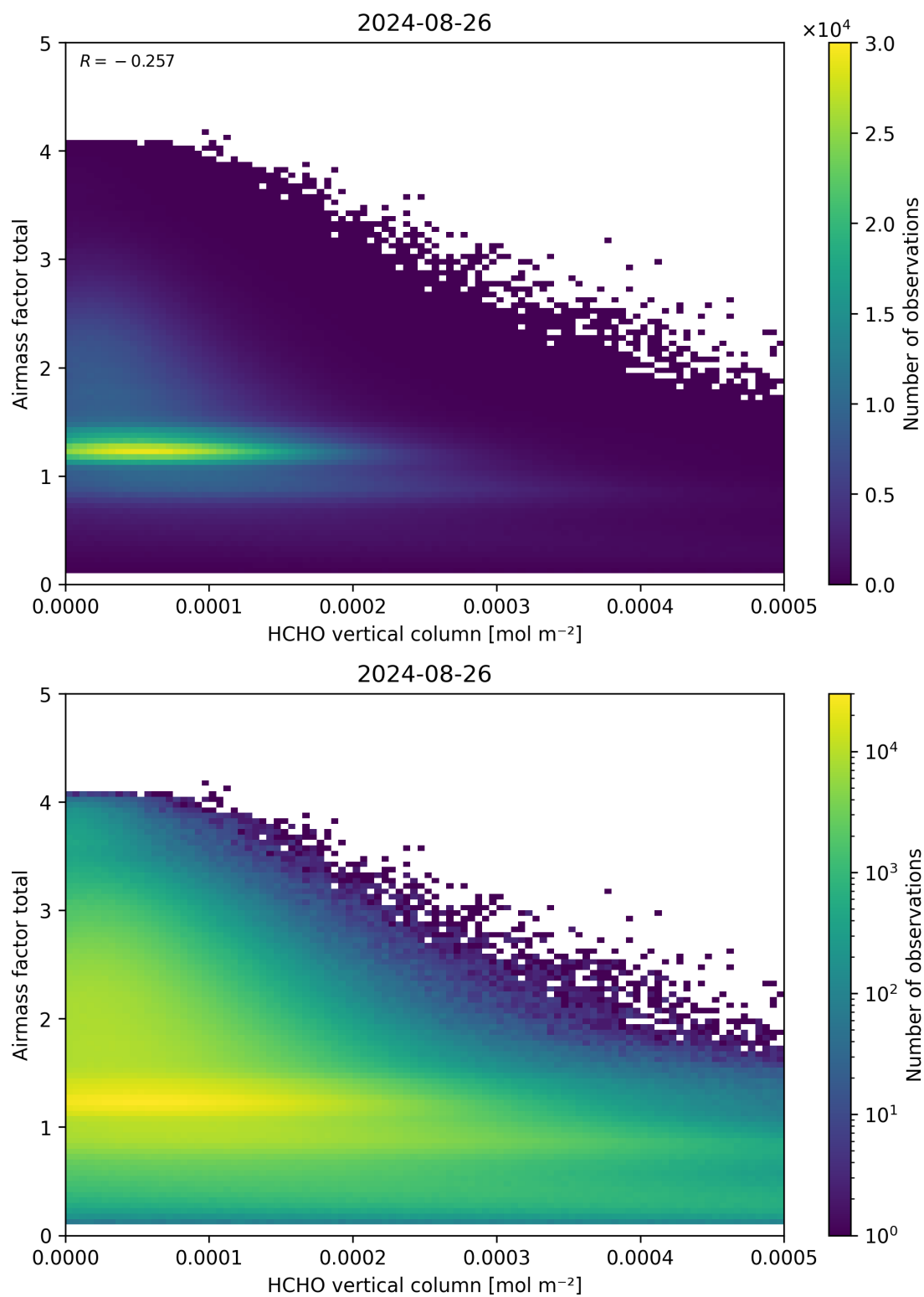
Figure 131: Scatter density plot of “HCHO vertical column” against “Airmass factor total” for 2024-08-25 to 2024-08-27.
