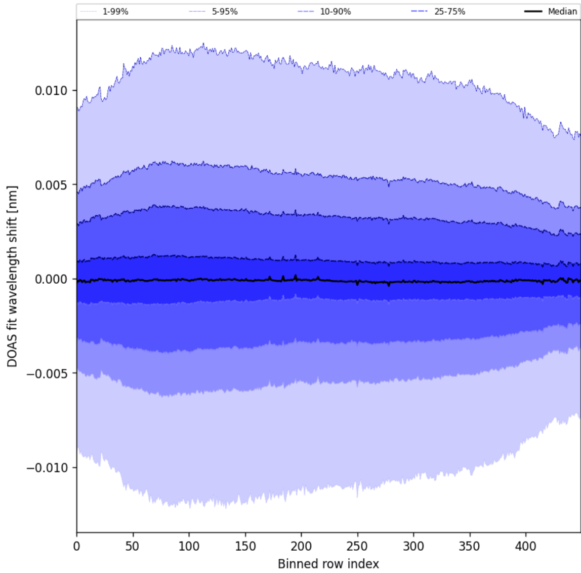
Figure 58: Along track statistics of “DOAS fit wavelength shift” for 2024-08-25 to 2024-08-27
