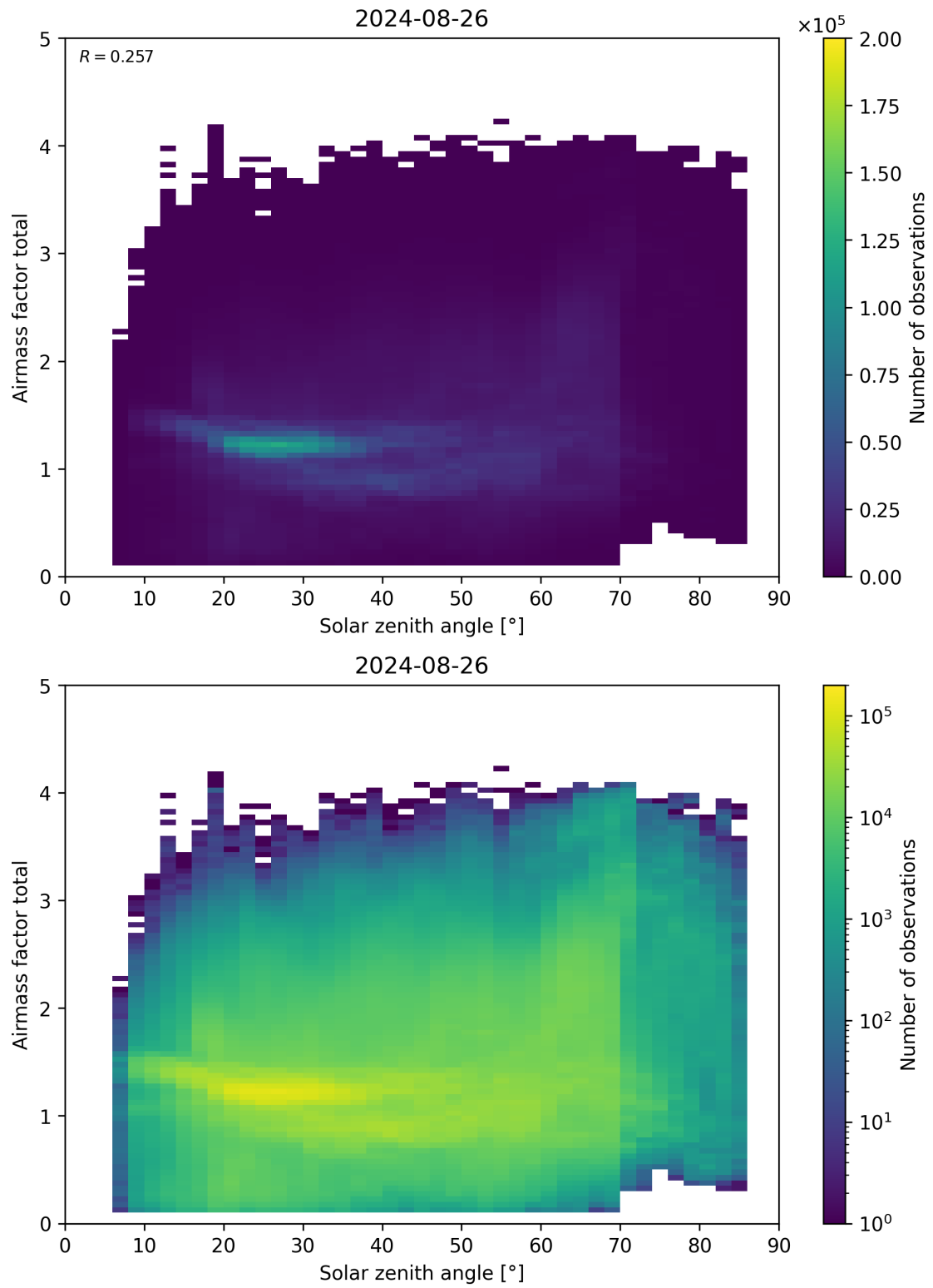
Figure 175: Scatter density plot of “Solar zenith angle” against “Airmass factor total” for 2024-08-25 to 2024-08-27.
