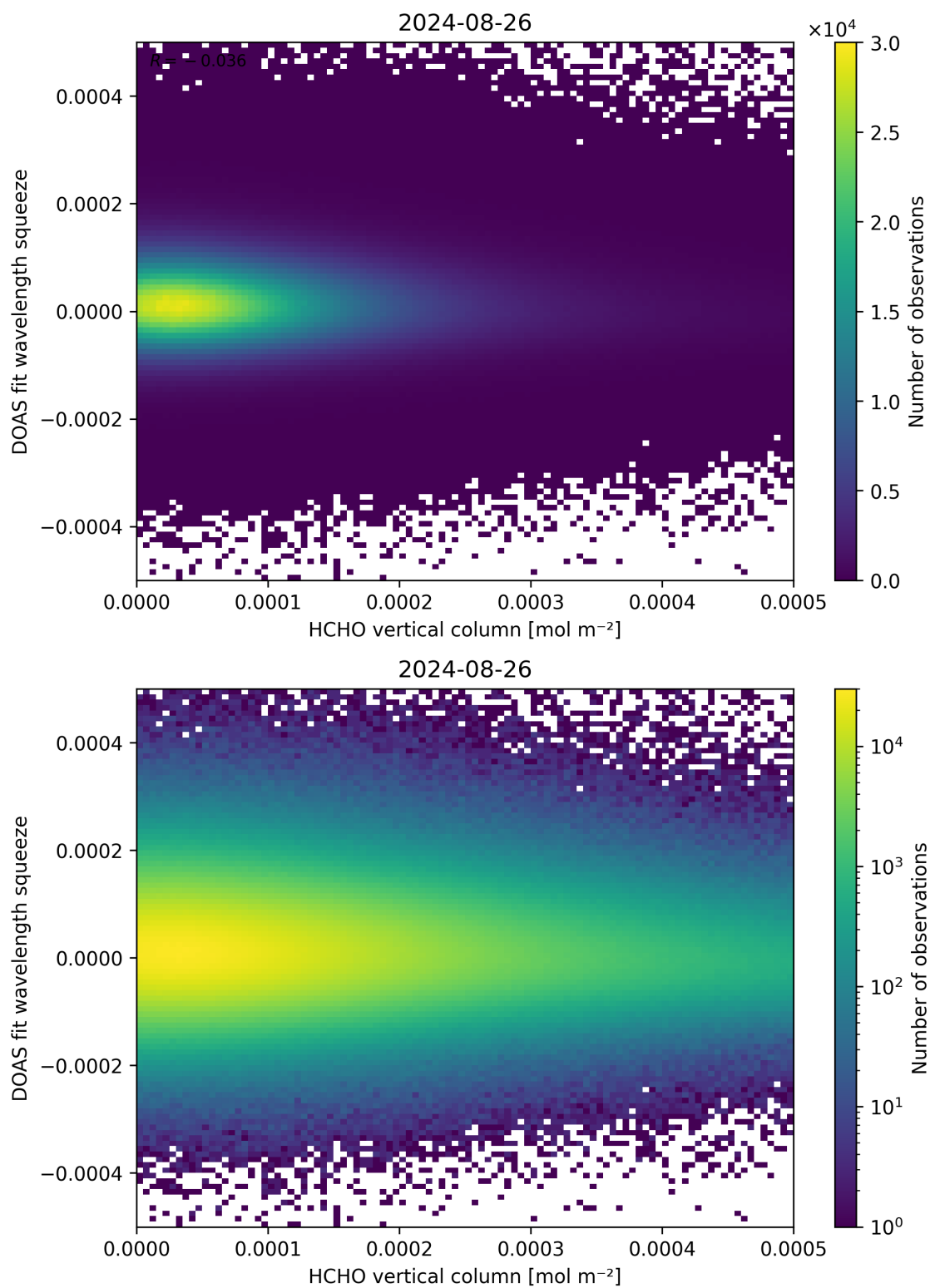
Figure 125: Scatter density plot of “HCHO vertical column” against “DOAS fit wavelength squeeze” for 2024-08-25 to 2024-08-27.
