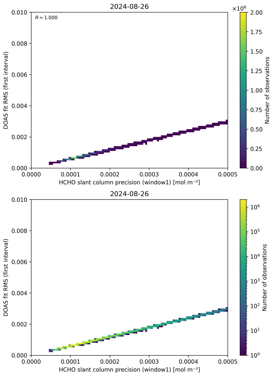
Figure 88: Scatter density plot of “HCHO slant column precision (window1)” against “DOAS fit RMS (first interval)” for 2024-08-25 to 2024-08-27.
