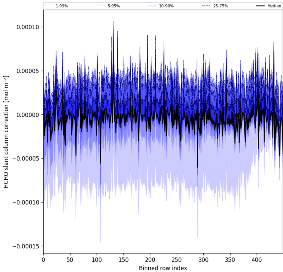
Figure 61: Along track statistics of "HCHO slant column correction" for 2024-08-25 to 2024-08-27
