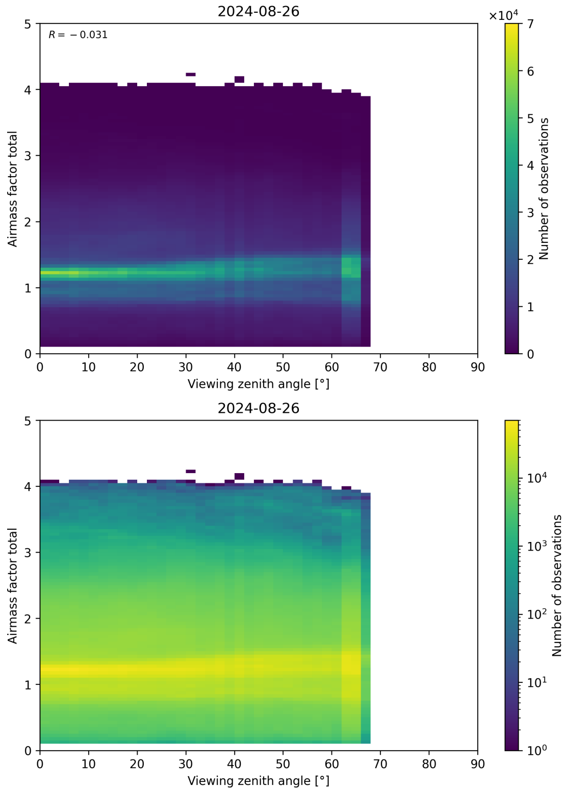
Figure 190: Scatter density plot of “Viewing zenith angle” against “Airmass factor total” for 2024-08-25 to 2024-08-27.
