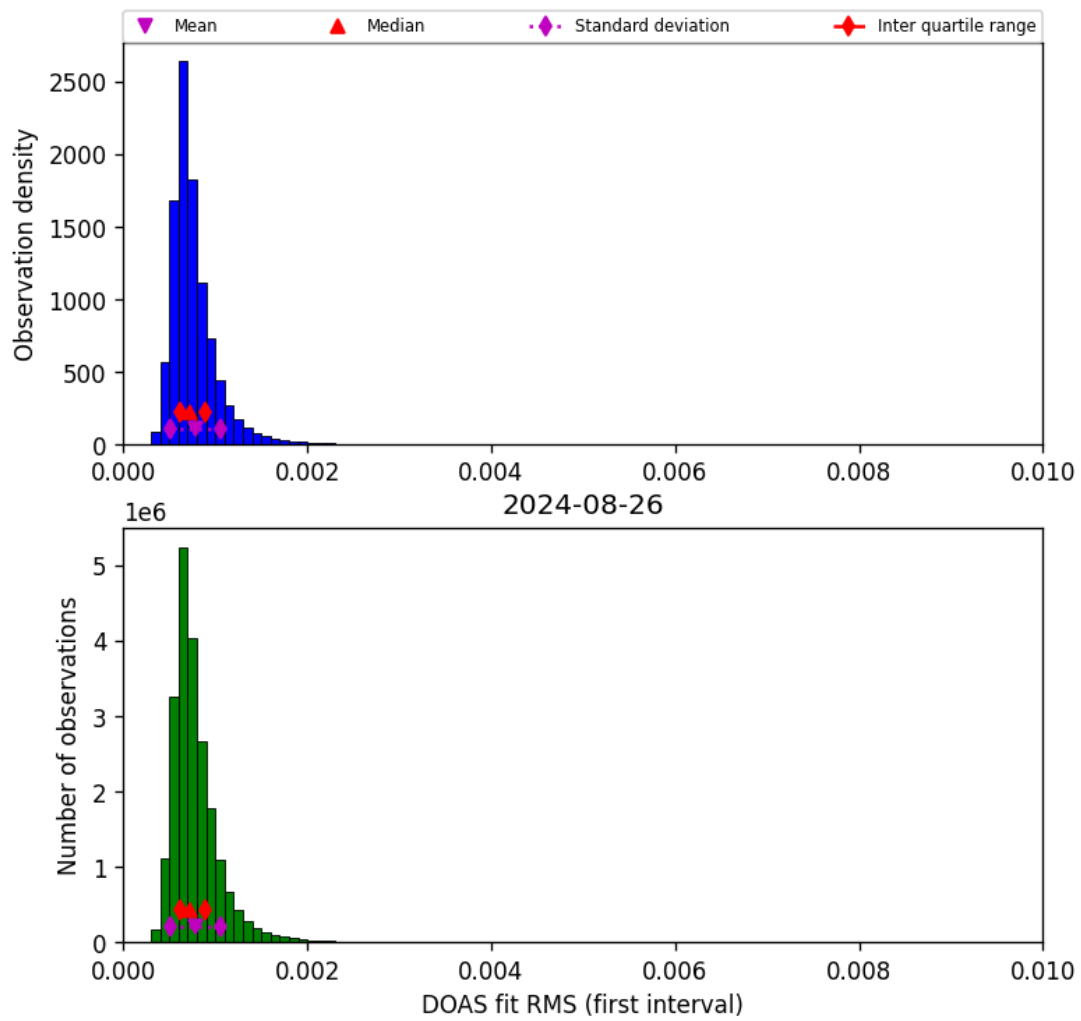
Figure 46: Histogram of “DOAS fit RMS (first interval)” for 2024-08-25 to 2024-08-27
