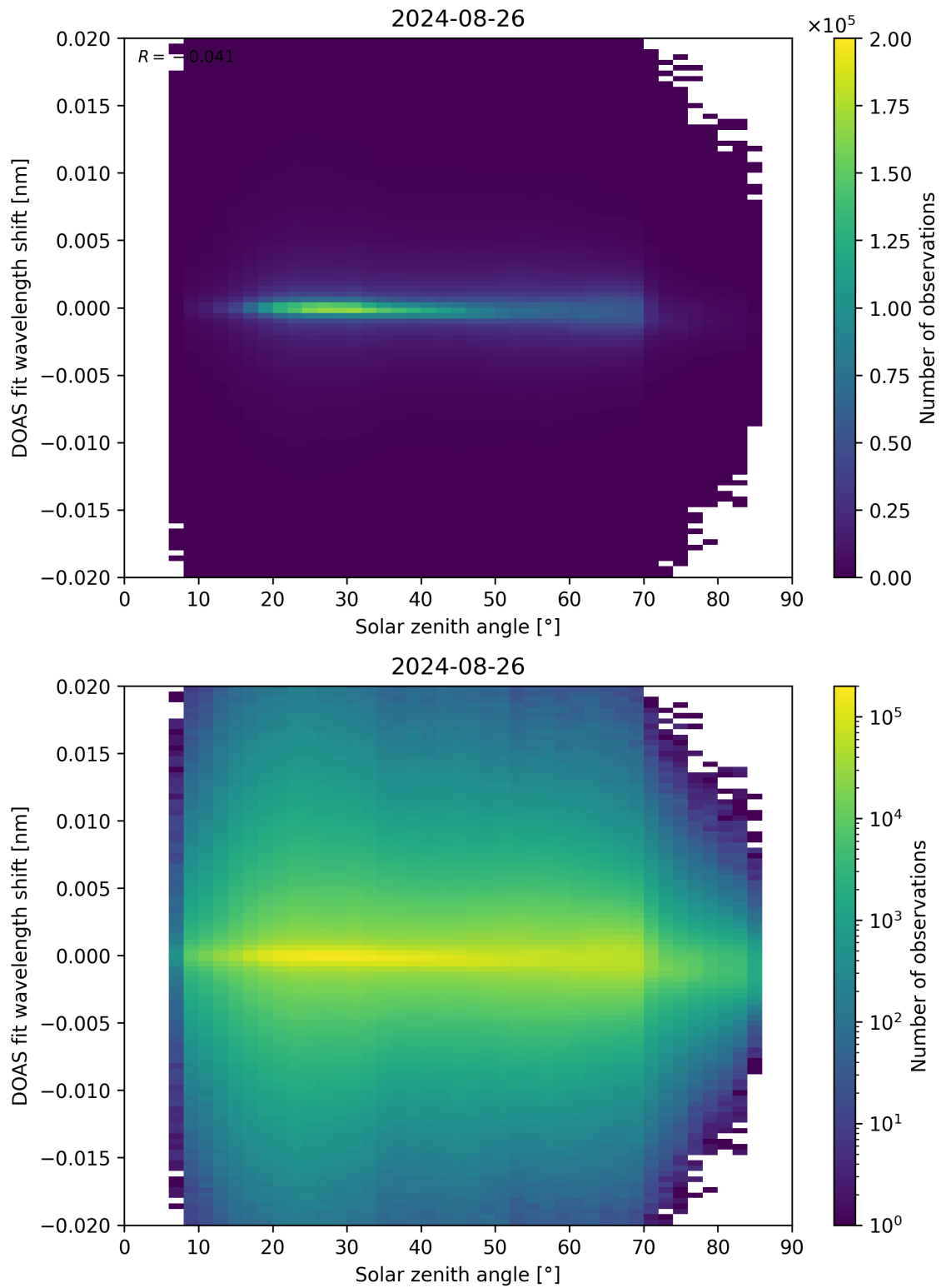
Figure 168: Scatter density plot of “Solar zenith angle” against “DOAS fit wavelength shift” for 2024-08-25 to 2024-08-27.
