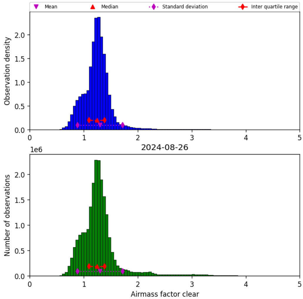
Figure 42: Histogram of “Airmass factor clear” for 2024-08-25 to 2024-08-27
