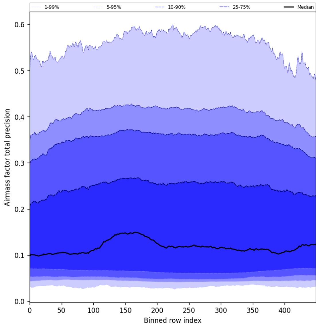
Figure 55: Along track statistics of “Airmass factor total precision” for 2024-08-27 to 2024-08-28
