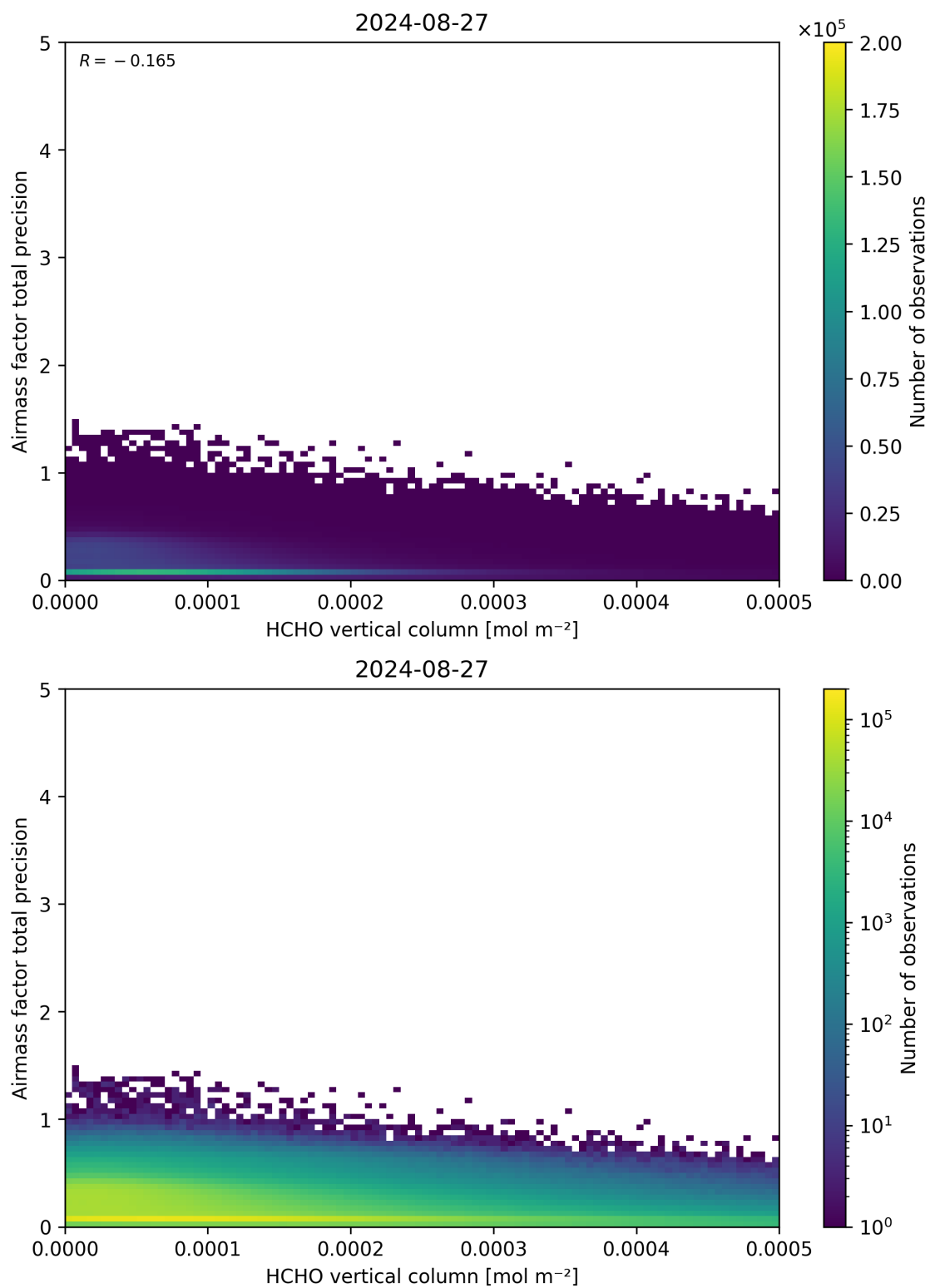
Figure 132: Scatter density plot of “HCHO vertical column” against “Airmass factor total precision” for 2024-08-27 to 2024-08-28.
