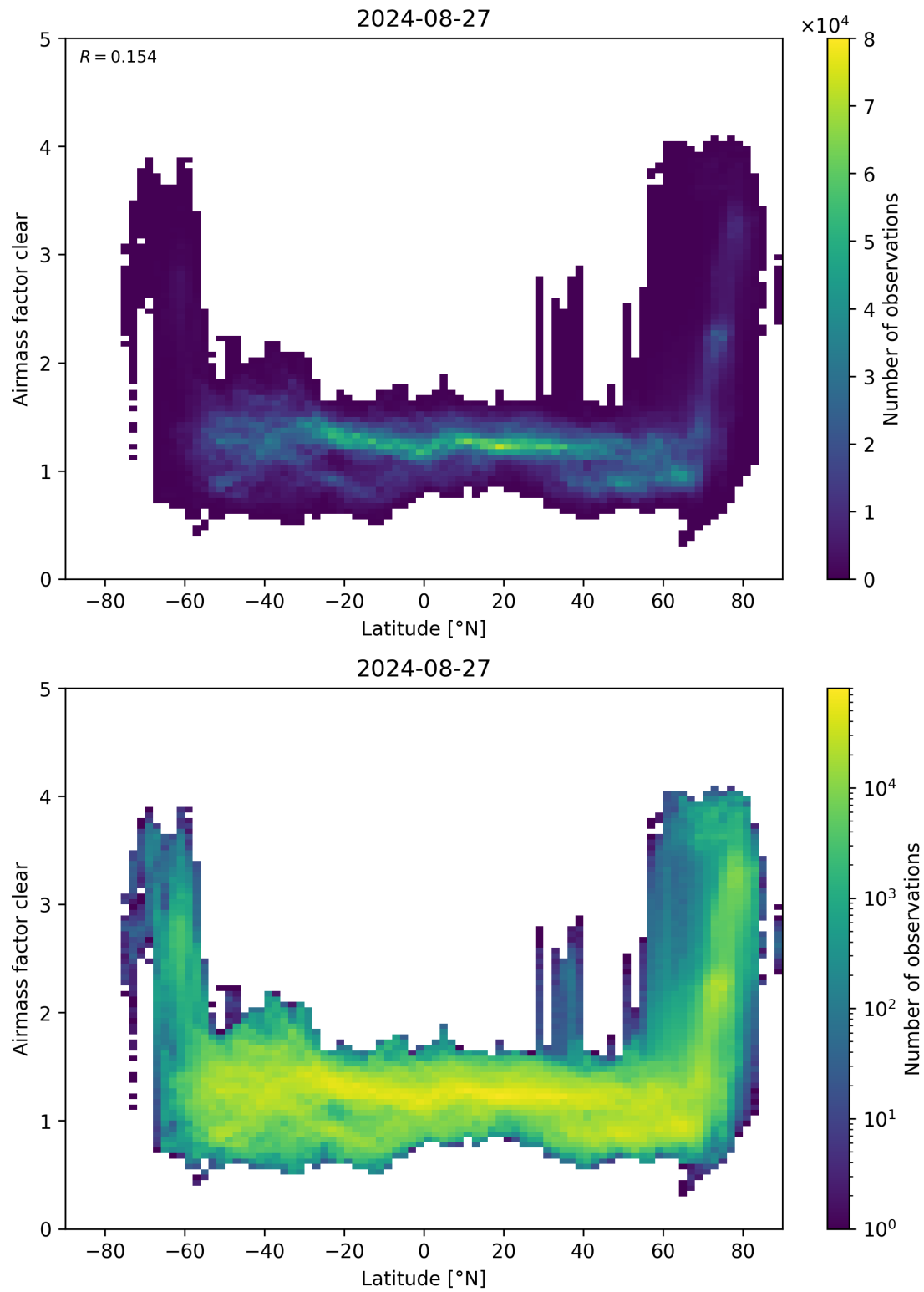
Figure 156: Scatter density plot of “Latitude” against “Airmass factor clear” for 2024-08-27 to 2024-08-28.
