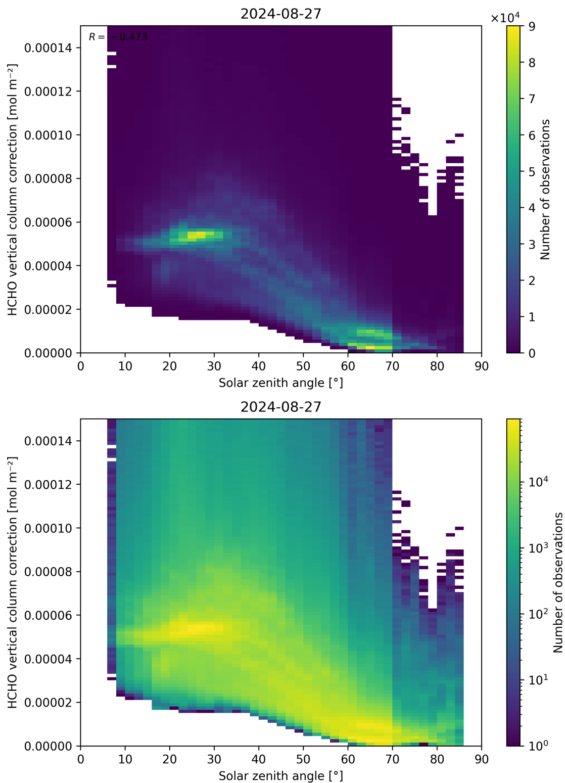
Figure 178: Scatter density plot of “Solar zenith angle” against “HCHO vertical column correction” for 2024-08-27 to 2024-08-28.
