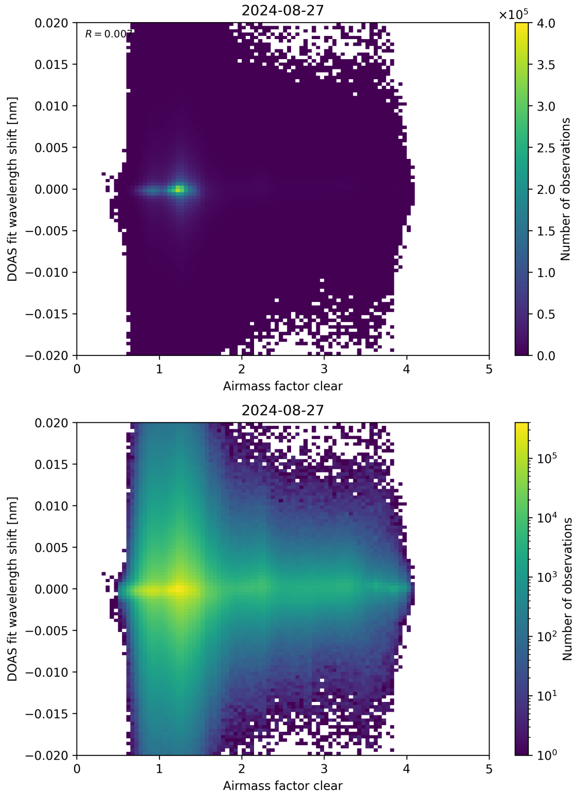
Figure 72: Scatter density plot of “Airmass factor clear” against “DOAS fit wavelength shift” for 2024-08-27 to 2024-08-28.
