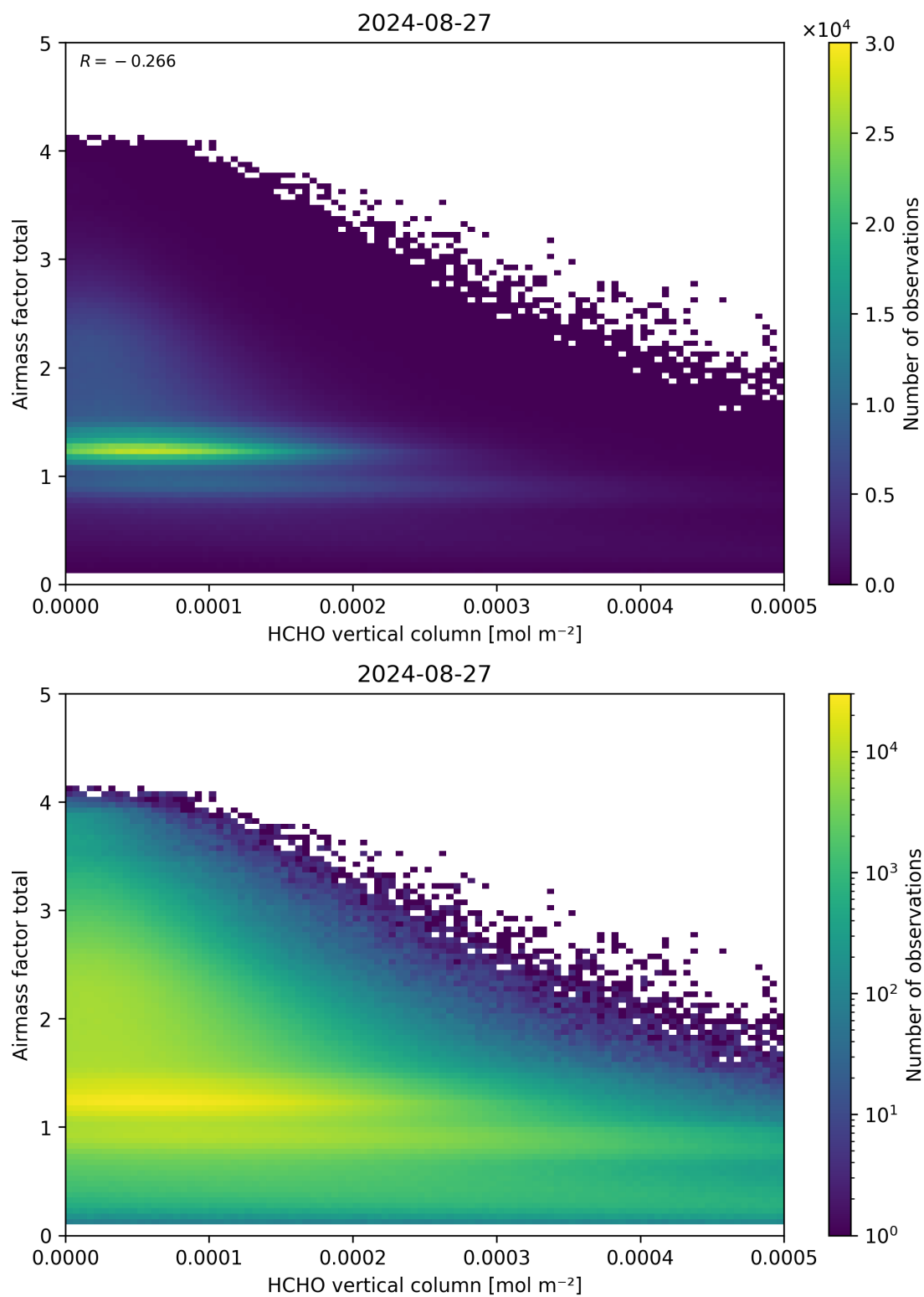
Figure 131: Scatter density plot of “HCHO vertical column” against “Airmass factor total” for 2024-08-27 to 2024-08-28.
