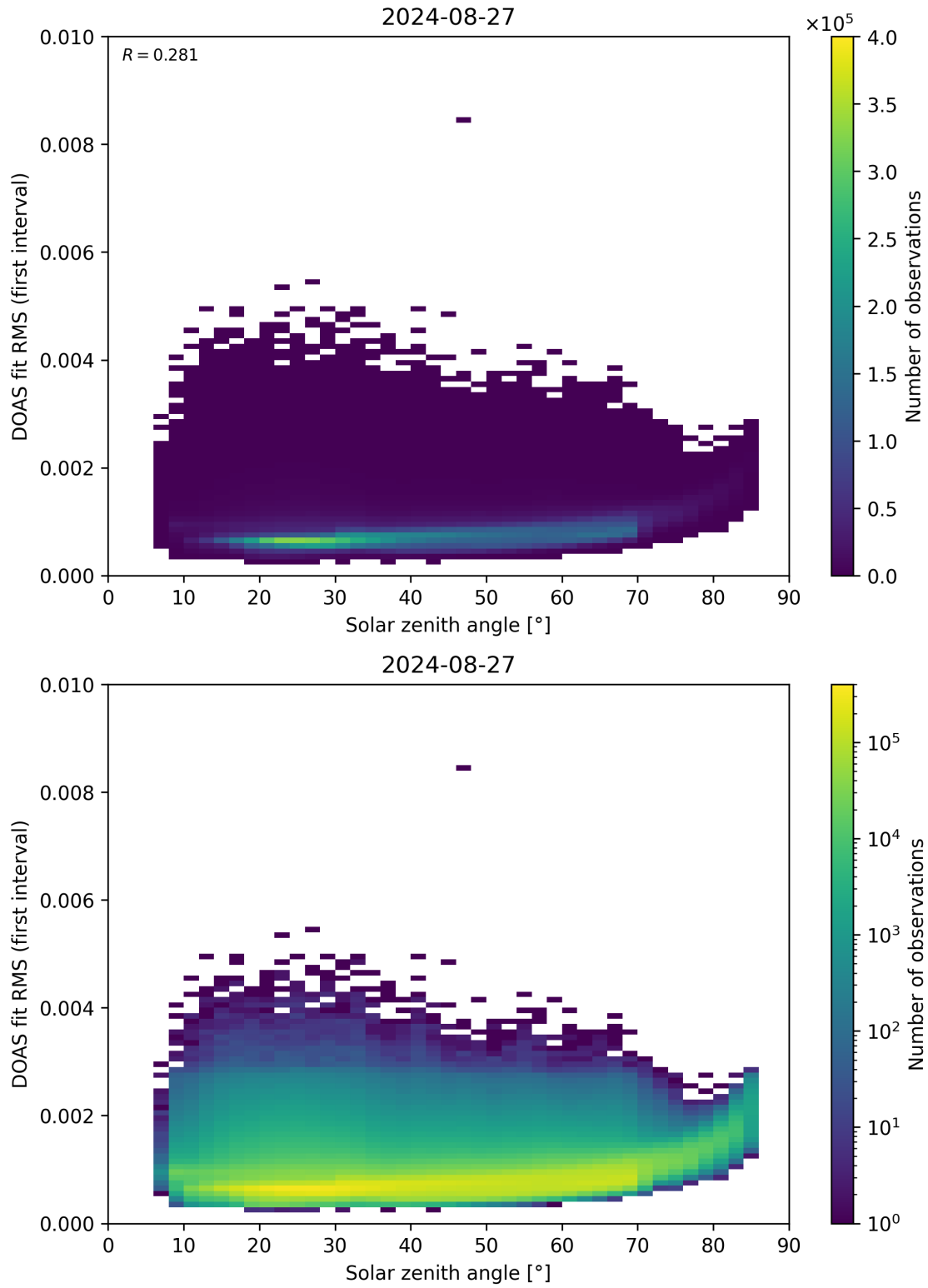
Figure 167: Scatter density plot of “Solar zenith angle” against “DOAS fit RMS (first interval)” for 2024-08-27 to 2024-08-28.
