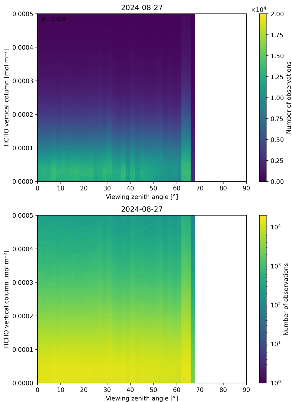
Figure 192: Scatter density plot of “Viewing zenith angle” against “HCHO vertical column” for 2024-08-27 to 2024-08-28.
