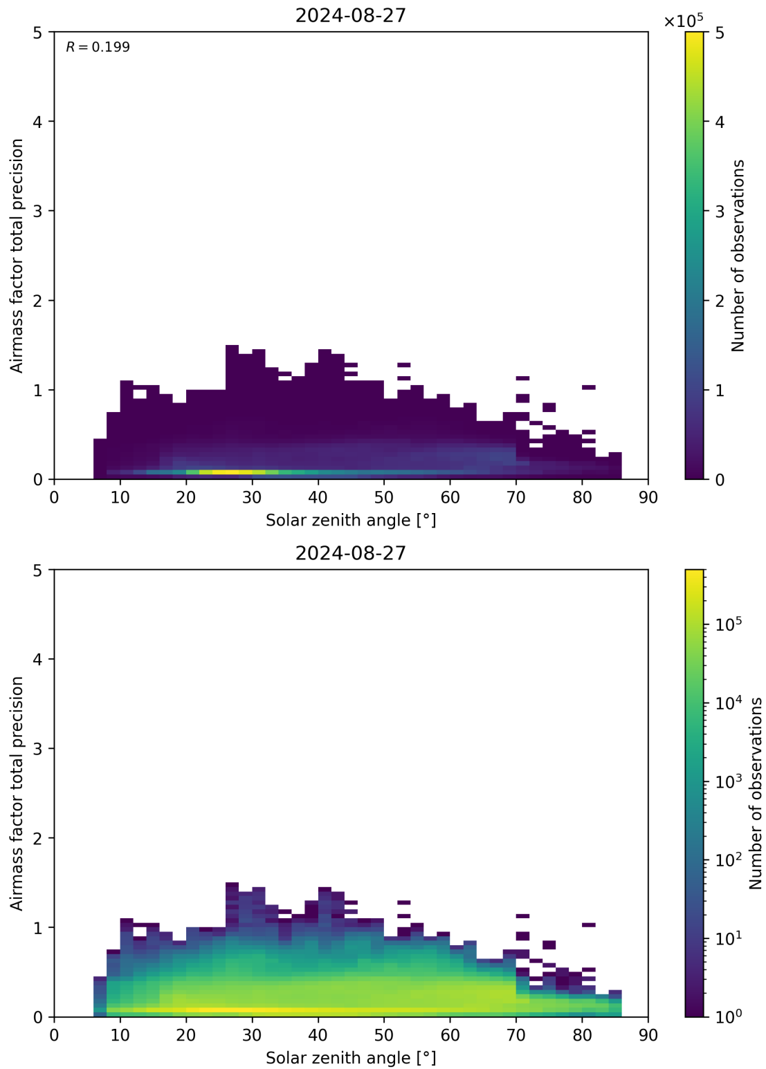
Figure 176: Scatter density plot of “Solar zenith angle” against “Airmass factor total precision” for 2024-08-27 to 2024-08-28.
