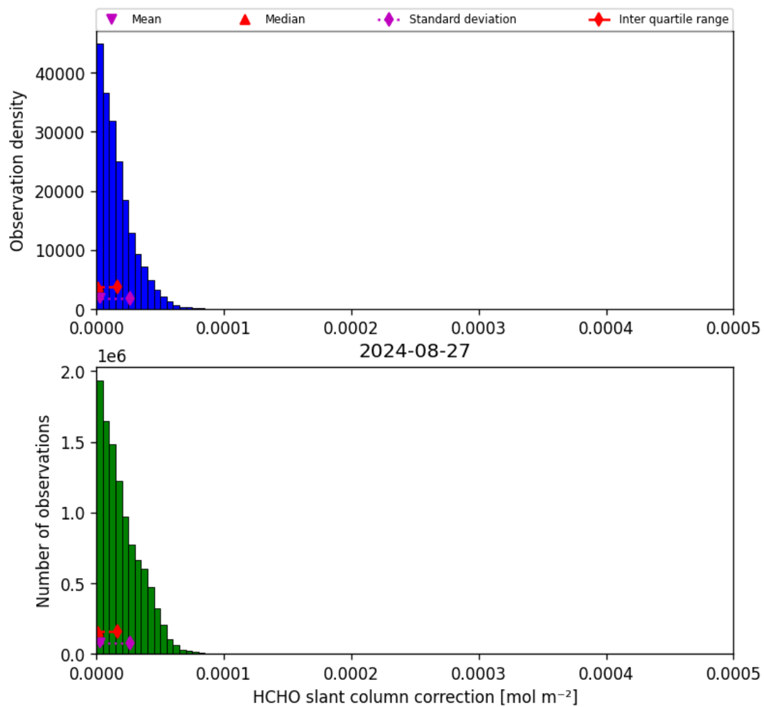
Figure 47: Histogram of “HCHO slant column correction” for 2024-08-27 to 2024-08-28
