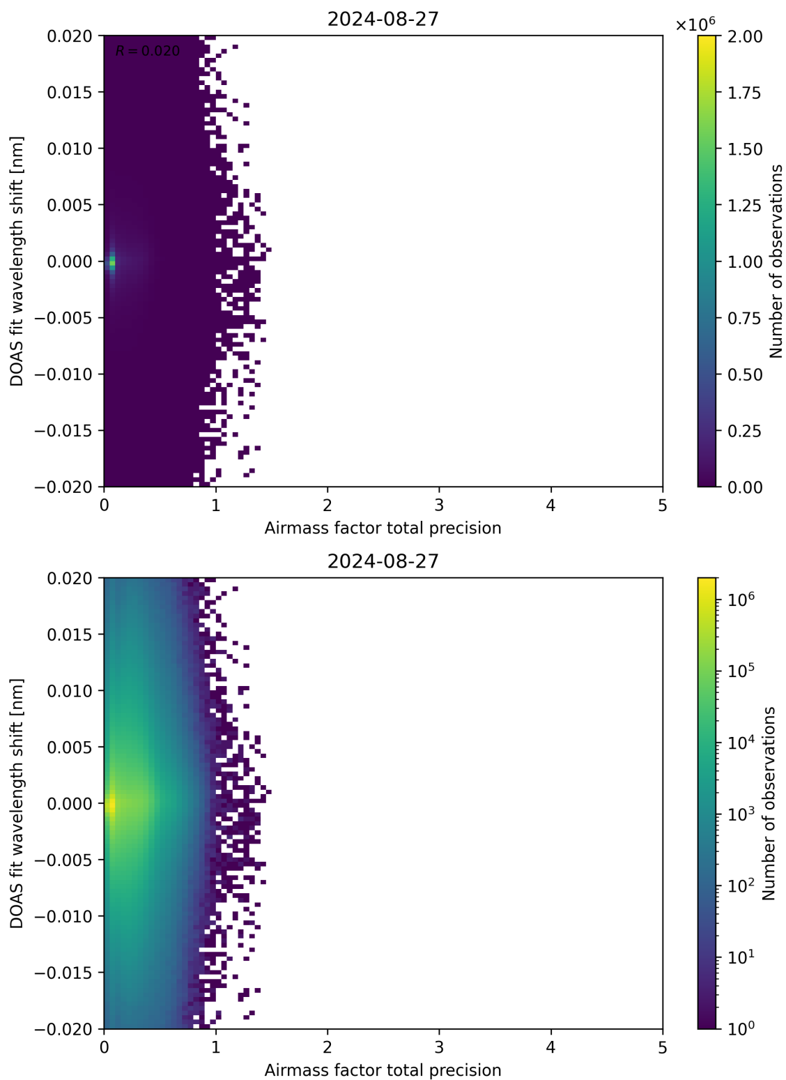
Figure 106: Scatter density plot of “Airmass factor total precision” against “DOAS fit wavelength shift” for 2024-08-27 to 2024-08-28.
