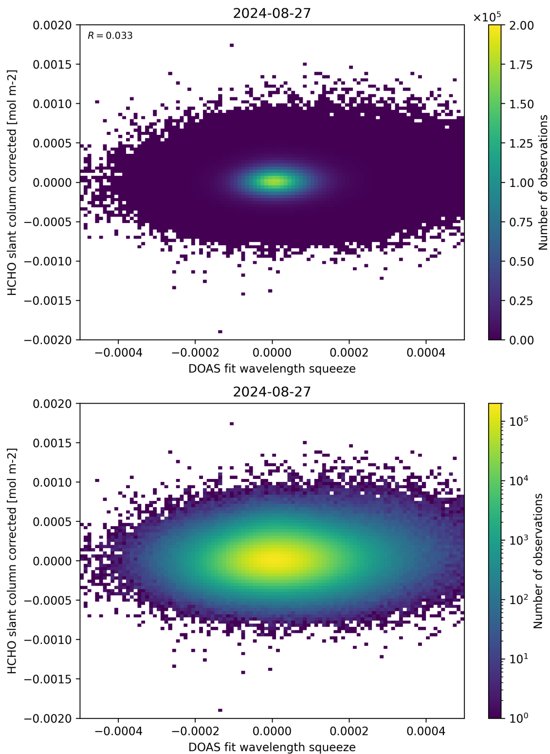
Figure 69: Scatter density plot of “DOAS fit wavelength squeeze” against “HCHO slant column corrected” for 2024-08-27 to 2024-08-28.
