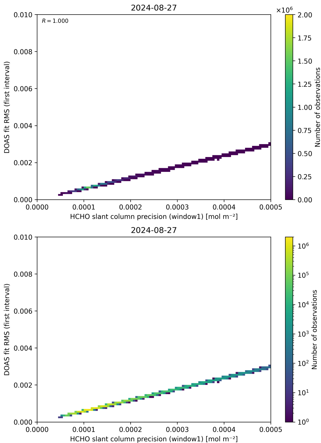
Figure 88: Scatter density plot of “HCHO slant column precision (window1)” against “DOAS fit RMS (first interval)” for 2024-08-27 to 2024-08-28.
