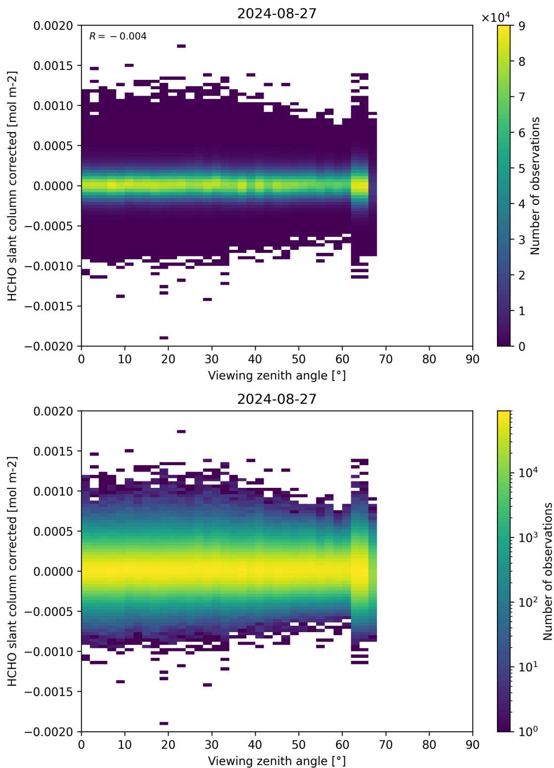
Figure 186: Scatter density plot of “Viewing zenith angle” against “HCHO slant column corrected” for 2024-08-27 to 2024-08-28.
