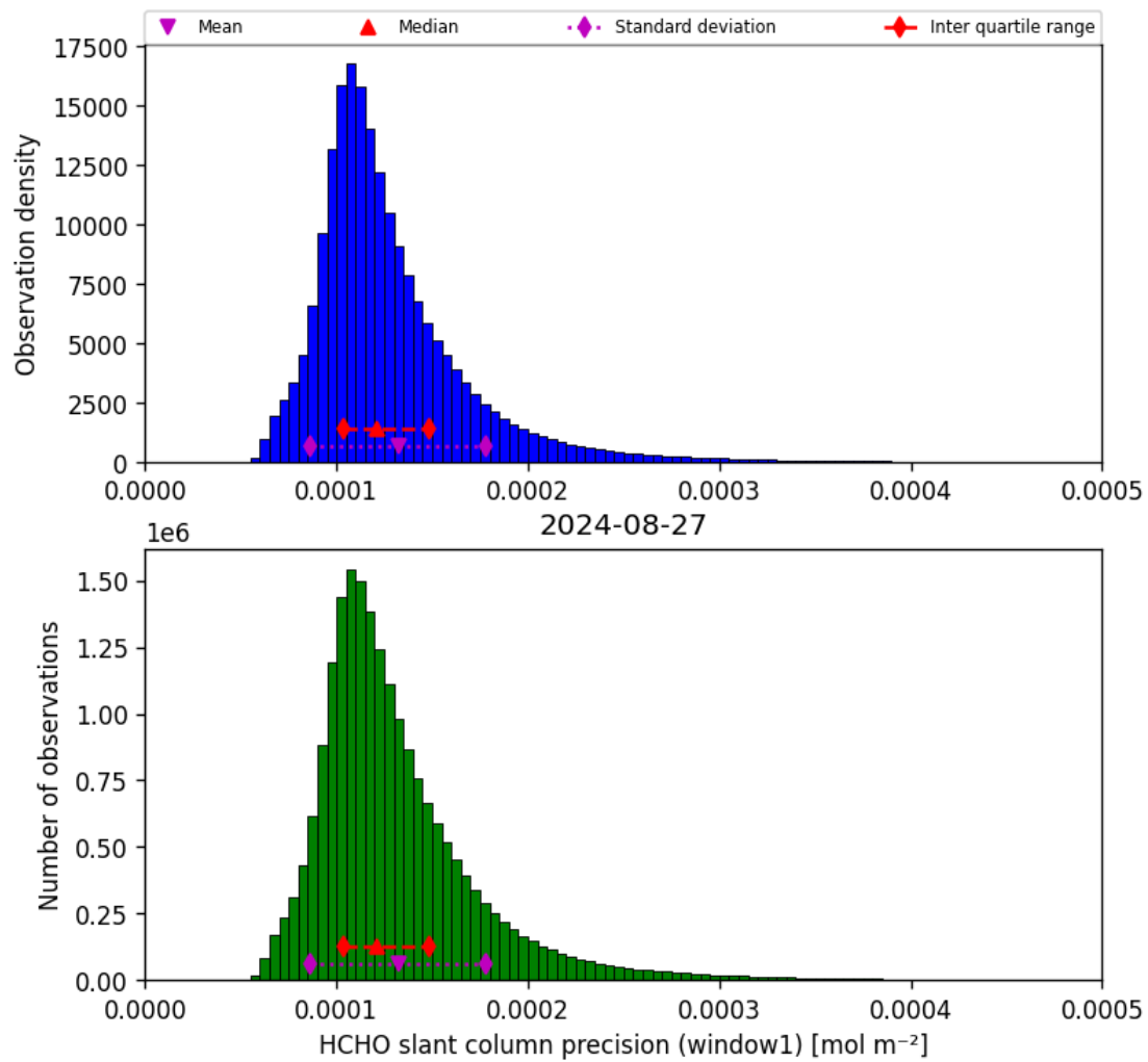
Figure 39: Histogram of “HCHO slant column precision (window1)” for 2024-08-27 to 2024-08-28
