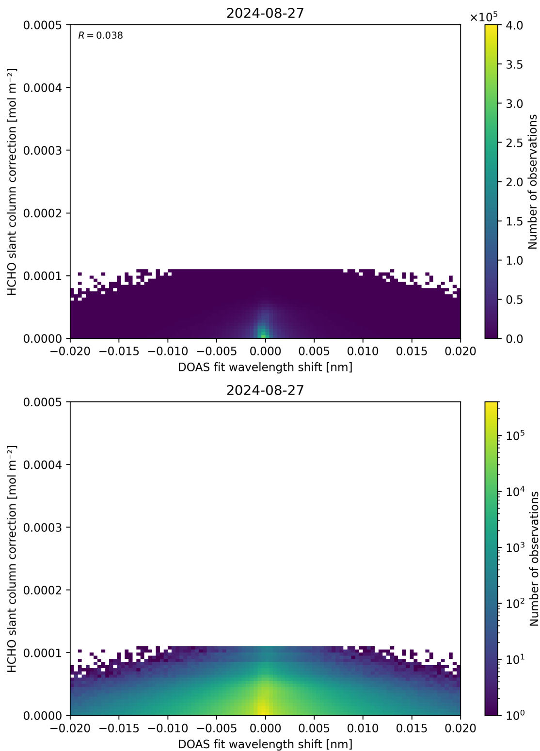
Figure 67: Scatter density plot of “DOAS fit wavelength shift” against “HCHO slant column correction” for 2024-08-27 to 2024-08-28.
