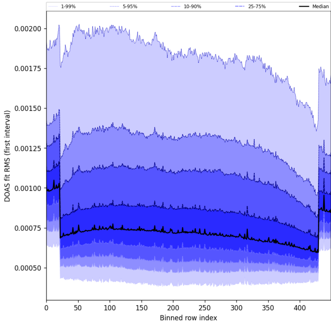
Figure 60: Along track statistics of “DOAS fit RMS (first interval)” for 2024-08-27 to 2024-08-28
