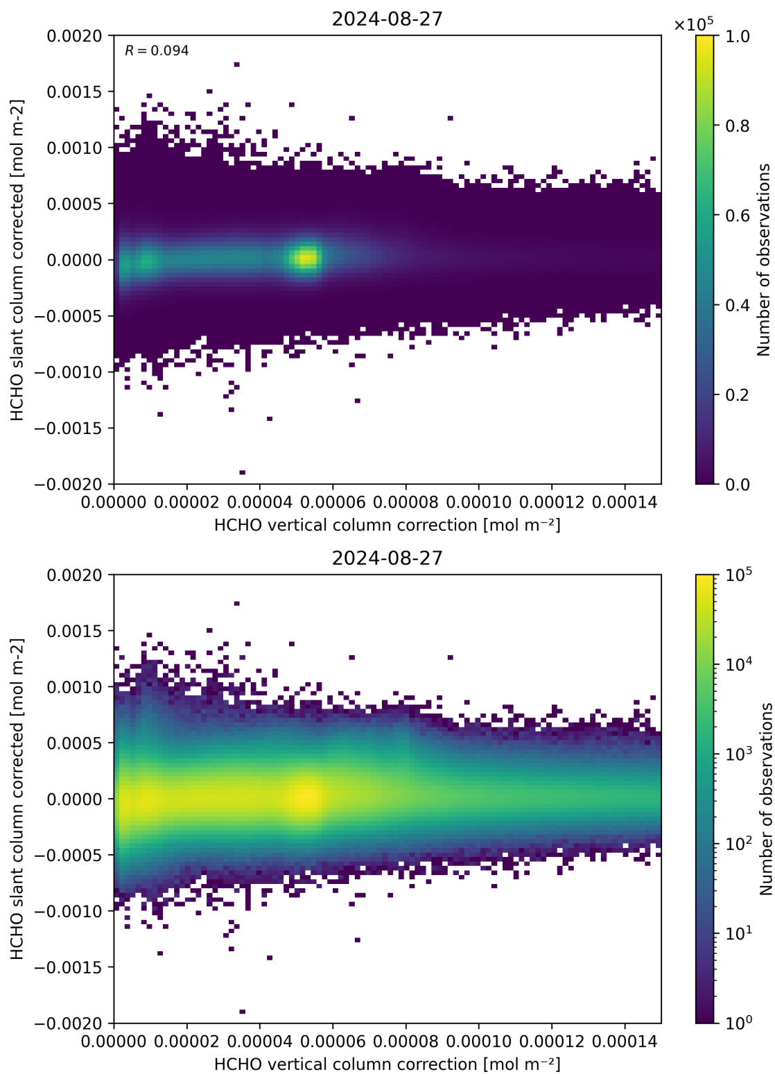
Figure 116: Scatter density plot of “HCHO vertical column correction” against “HCHO slant column corrected” for 2024-08-27 to 2024-08-28.
