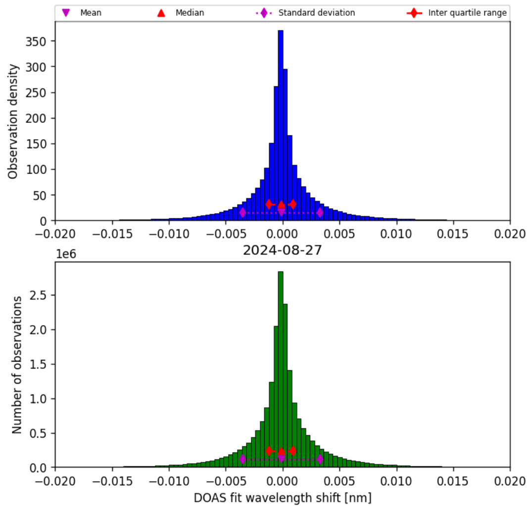
Figure 44: Histogram of “DOAS fit wavelength shift” for 2024-08-27 to 2024-08-28
