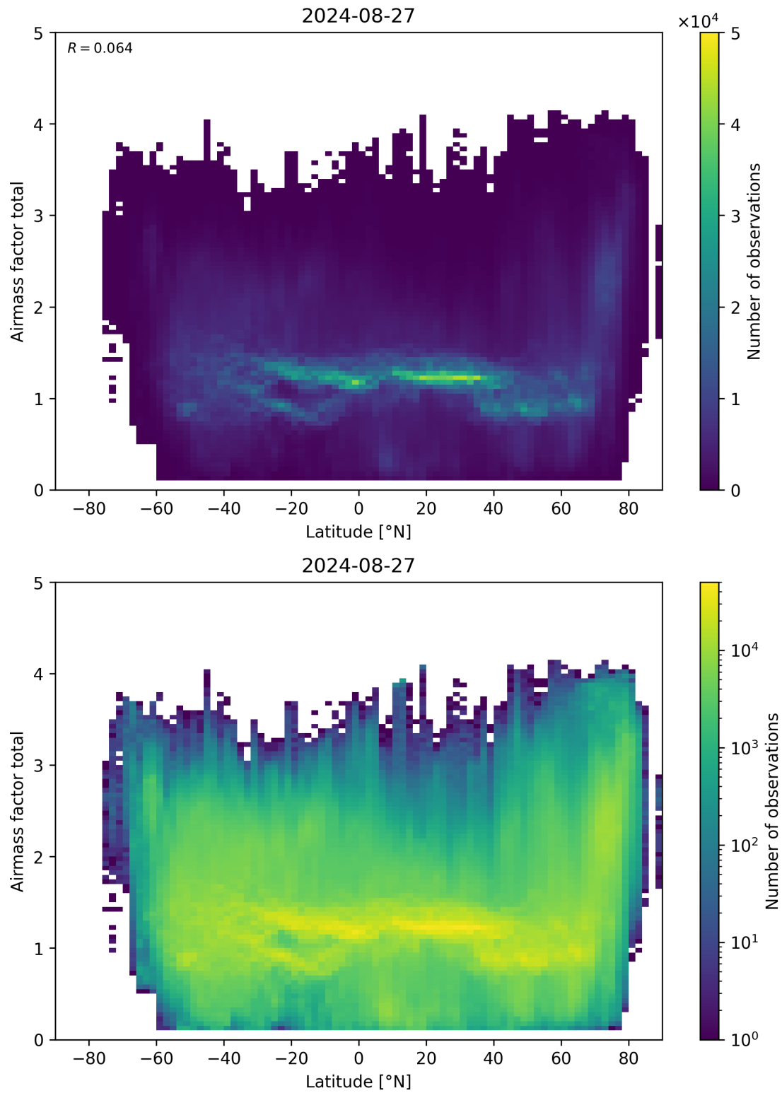
Figure 161: Scatter density plot of “Latitude” against “Airmass factor total” for 2024-08-27 to 2024-08-28.
