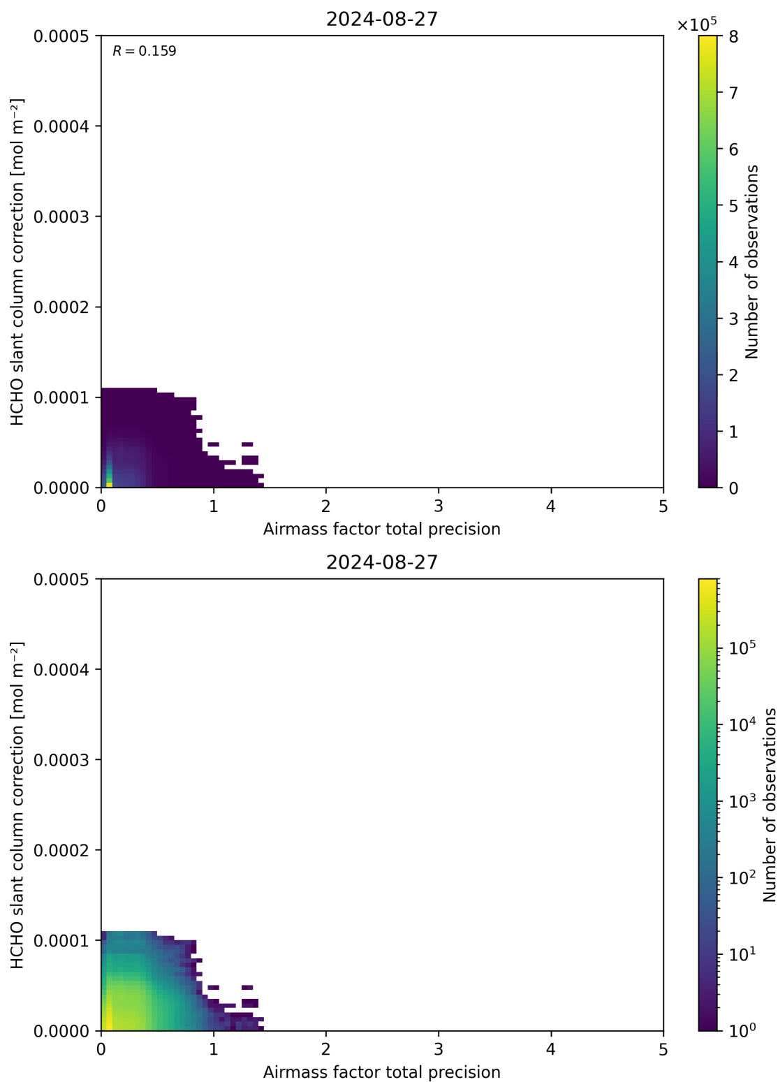
Figure 110: Scatter density plot of “Airmass factor total precision” against “HCHO slant column correction” for 2024-08-27 to 2024-08-28.
