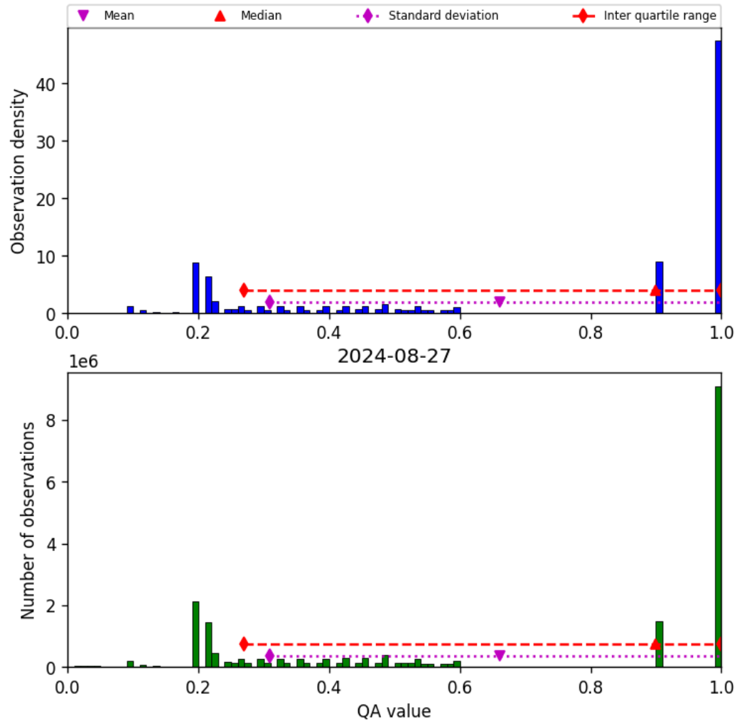
Figure 34: Histogram of “QA value” for 2024-08-27 to 2024-08-28
