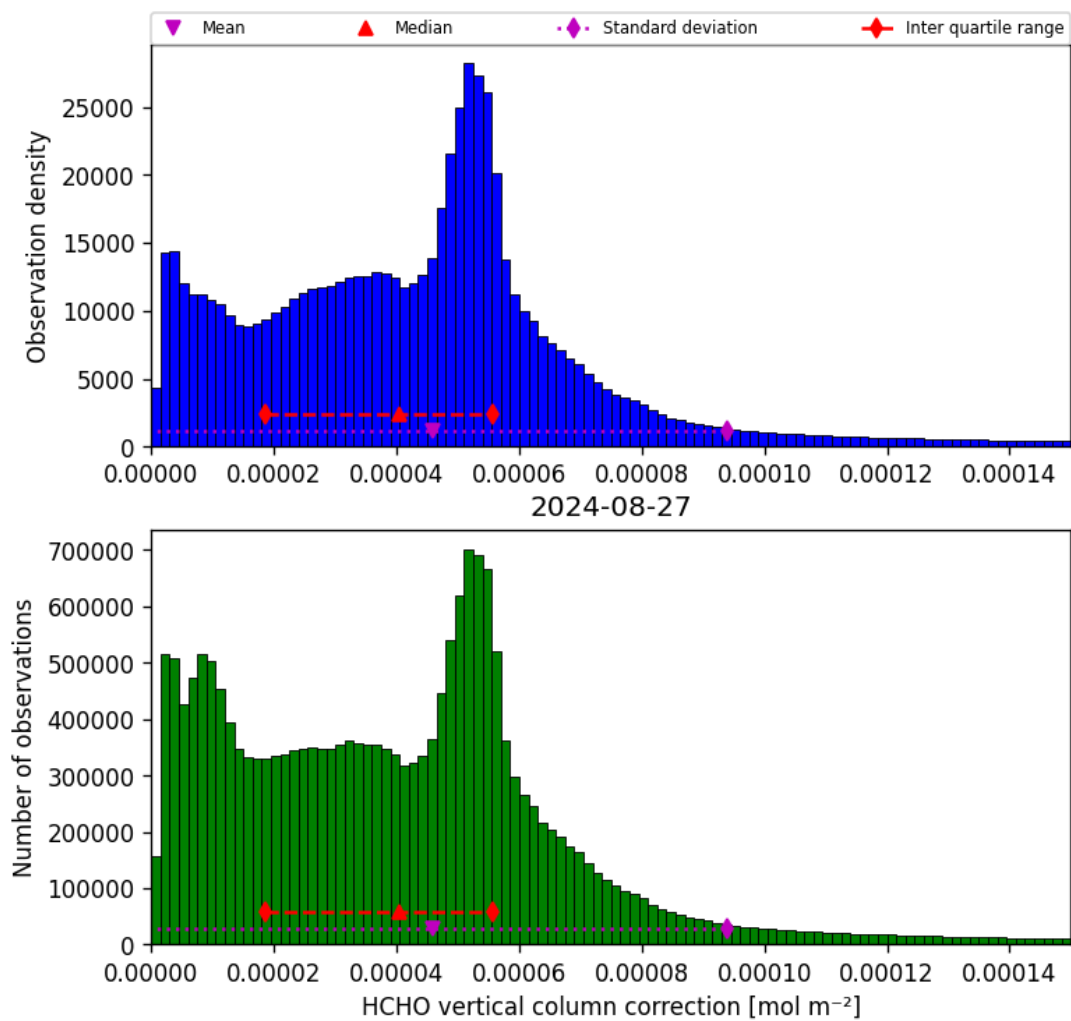
Figure 37: Histogram of “HCHO vertical column correction” for 2024-08-27 to 2024-08-28
