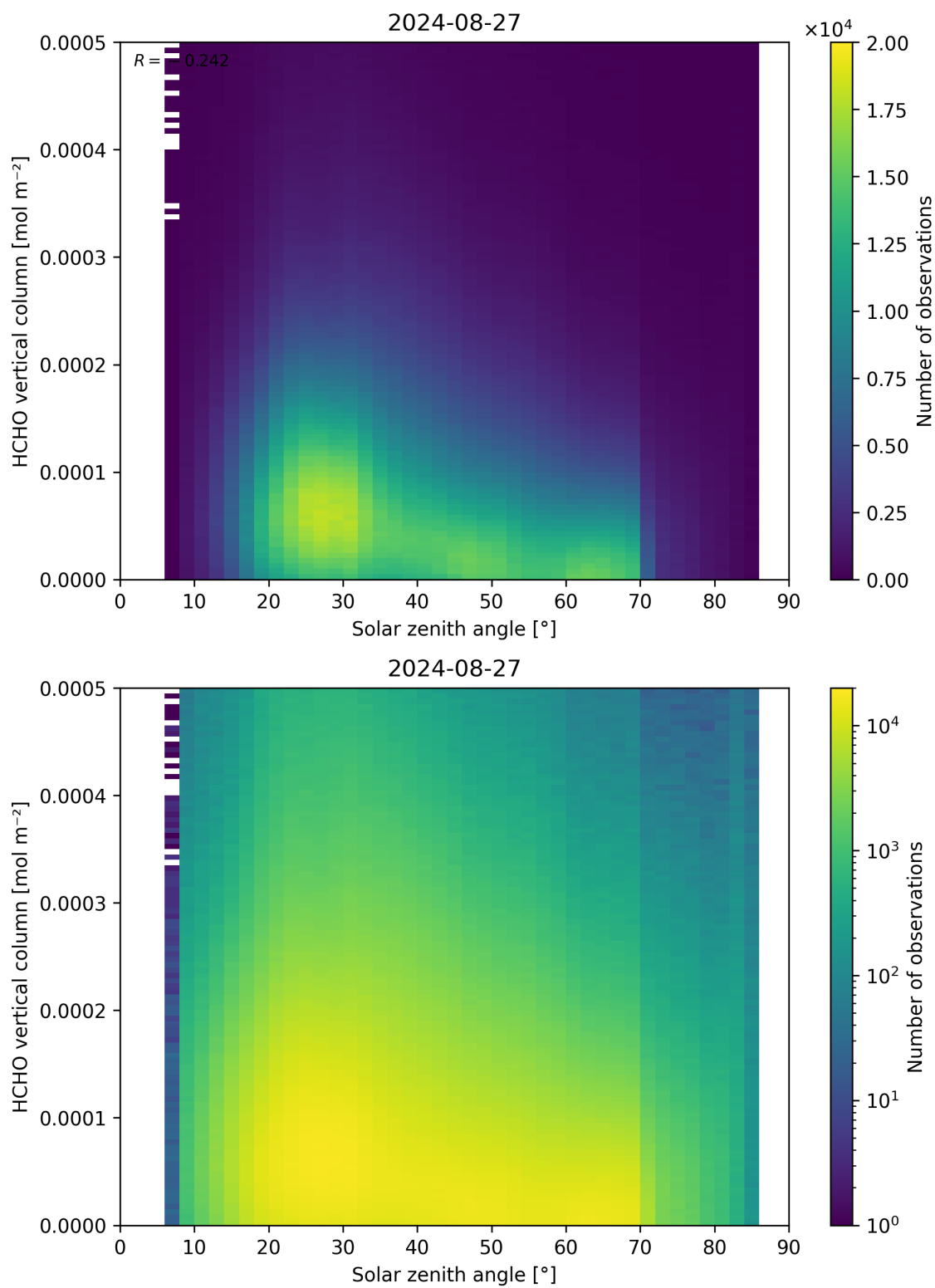
Figure 177: Scatter density plot of “Solar zenith angle” against “HCHO vertical column” for 2024-08-27 to 2024-08-28.
