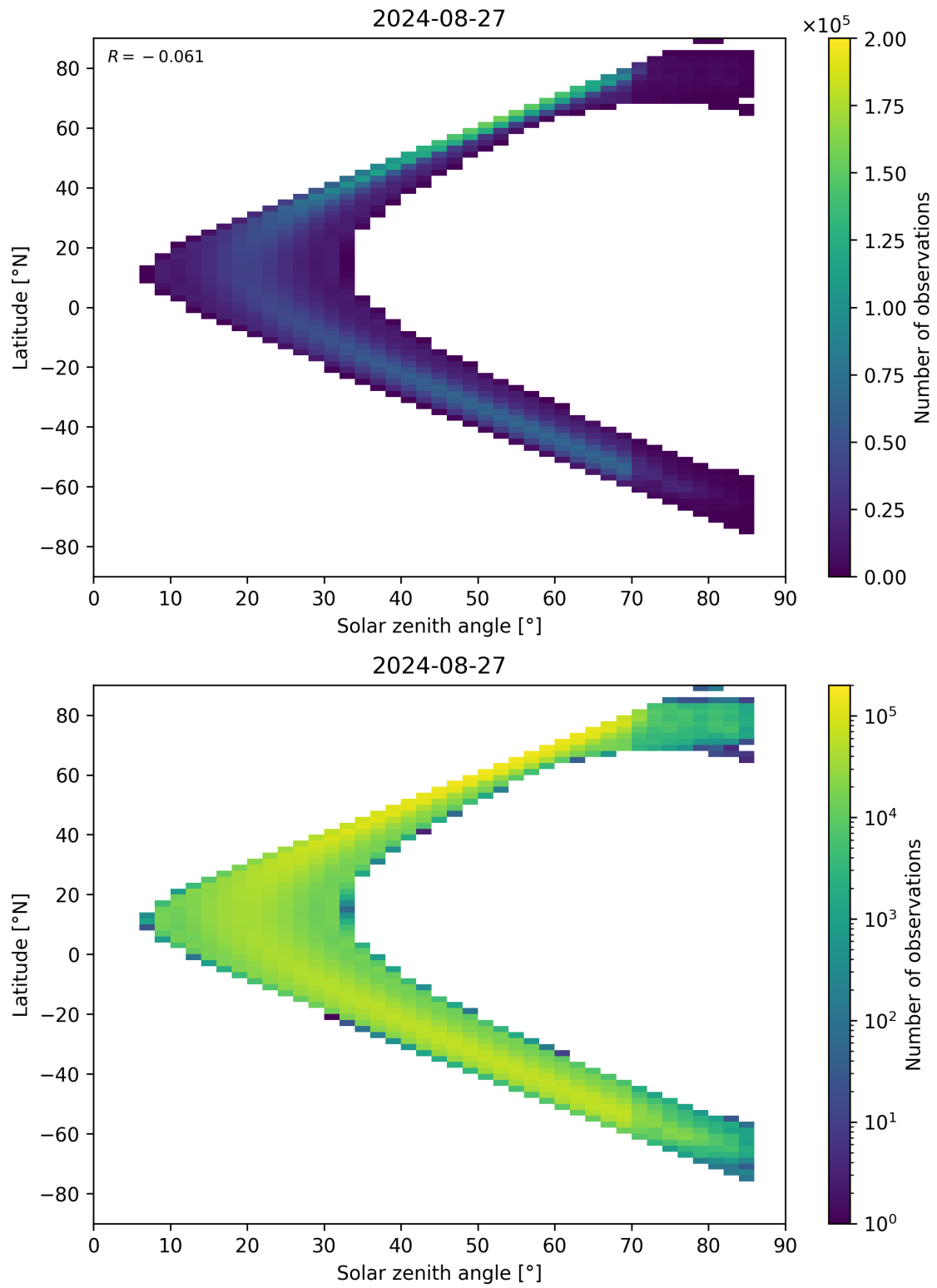
Figure 181: Scatter density plot of “Solar zenith angle” against “Latitude” for 2024-08-27 to 2024-08-28.
