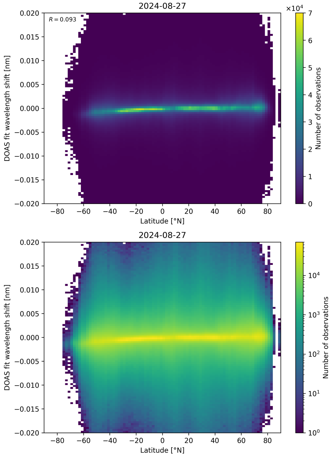
Figure 154: Scatter density plot of “Latitude” against “DOAS fit wavelength shift” for 2024-08-27 to 2024-08-28.
