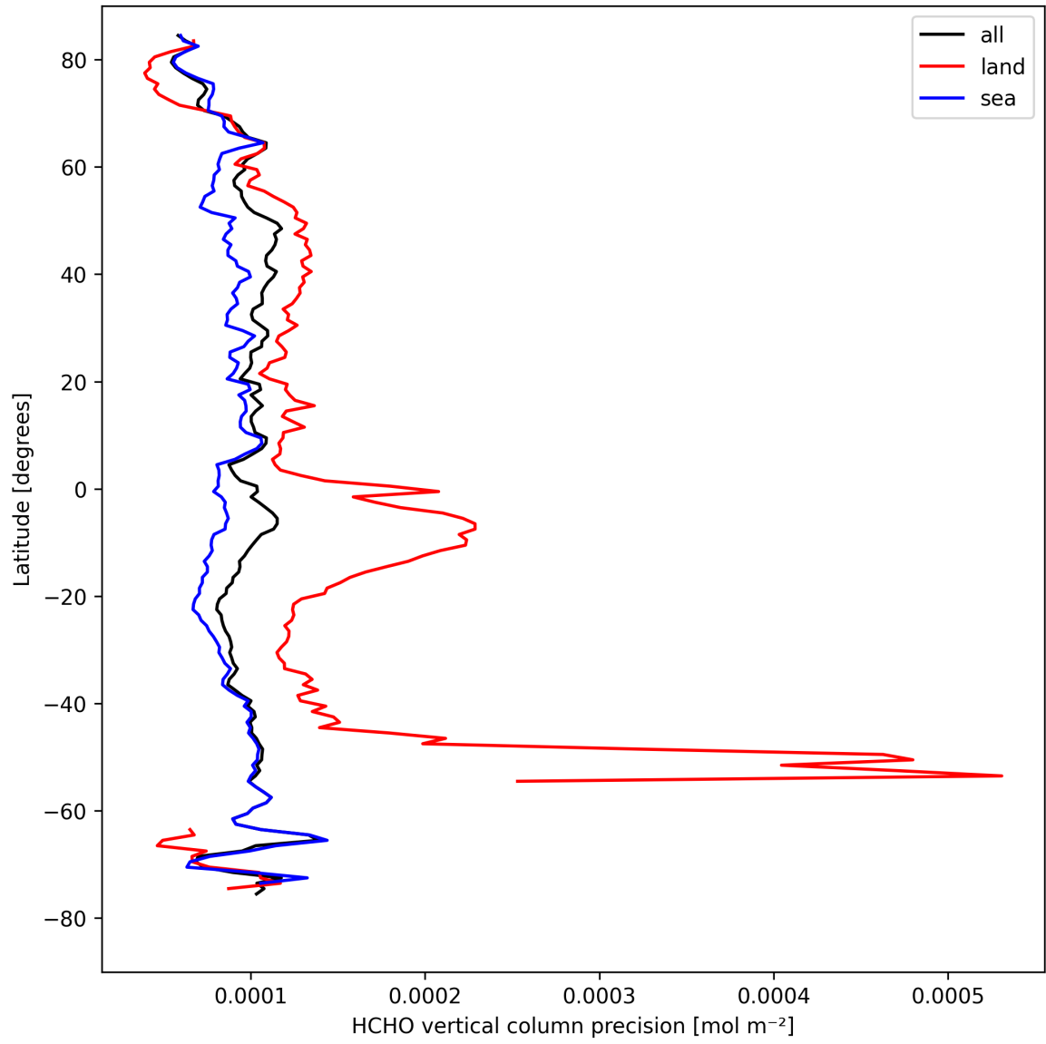
Figure 22: Zonal average of “HCHO vertical column precision” for 2024-08-27 to 2024-08-28.
