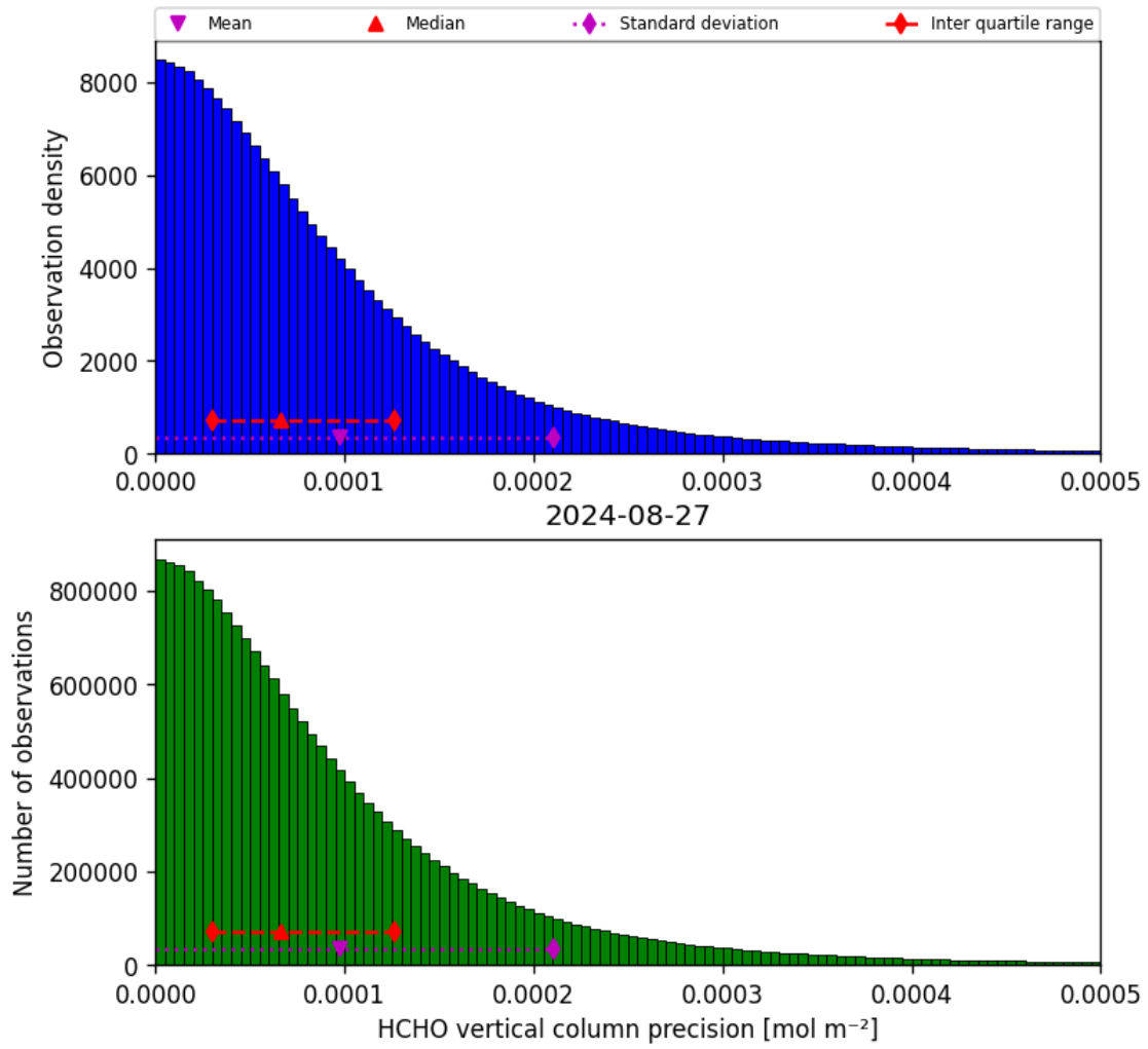
Figure 36: Histogram of “HCHO vertical column precision” for 2024-08-27 to 2024-08-28
