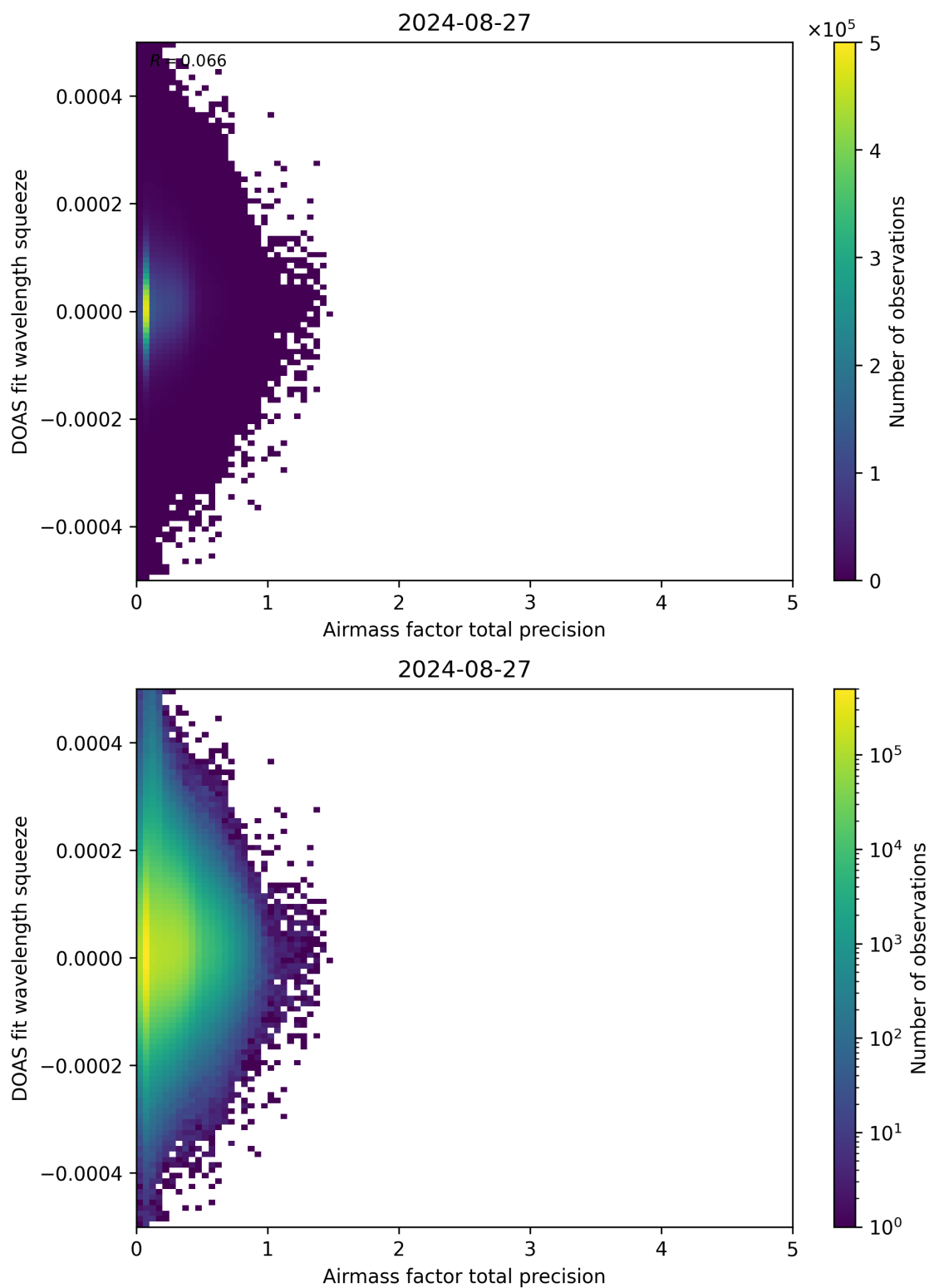
Figure 107: Scatter density plot of “Airmass factor total precision” against “DOAS fit wavelength squeeze” for 2024-08-27 to 2024-08-28.
