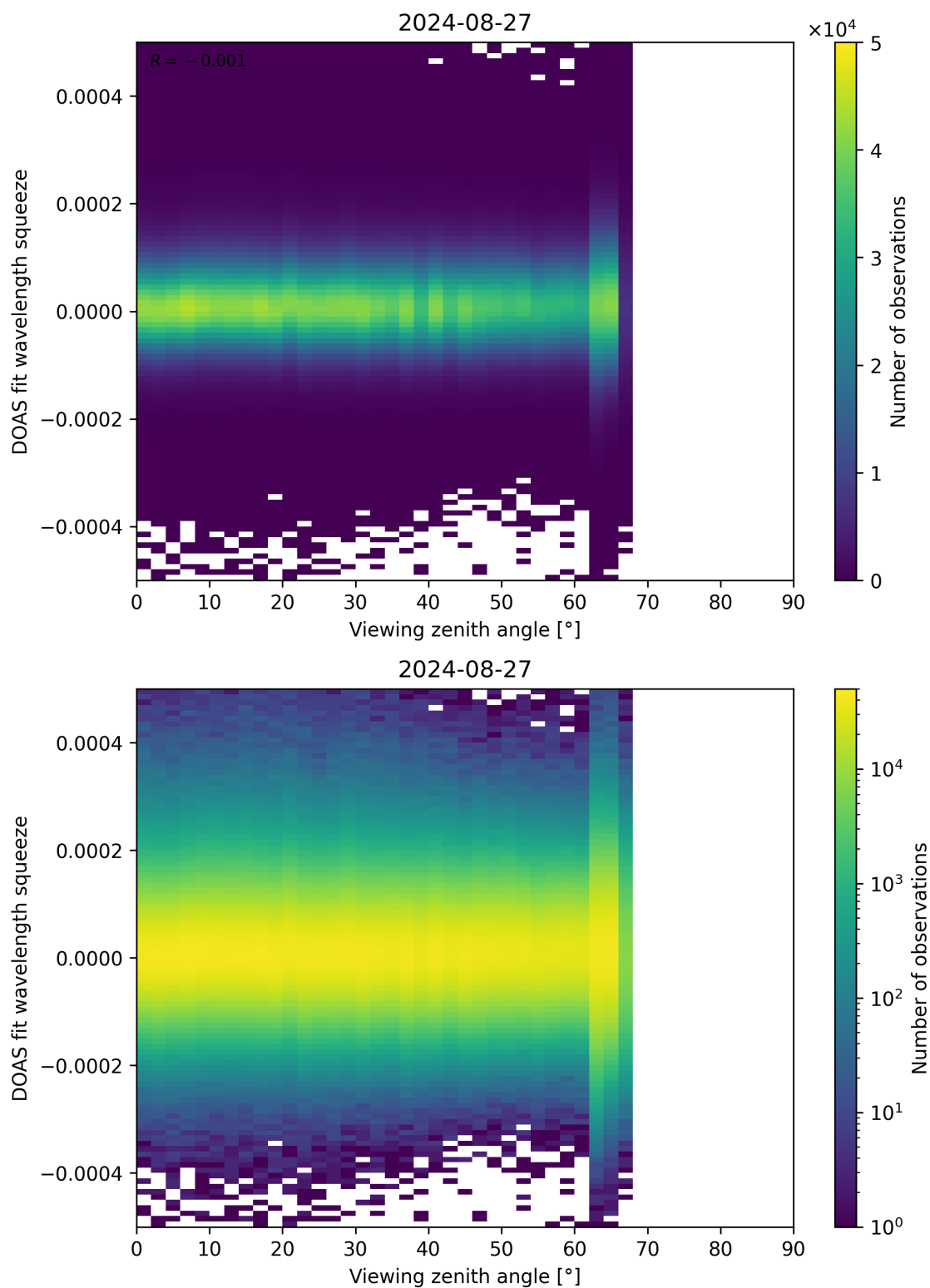
Figure 184: Scatter density plot of “Viewing zenith angle” against “DOAS fit wavelength squeeze” for 2024-08-27 to 2024-08-28.
