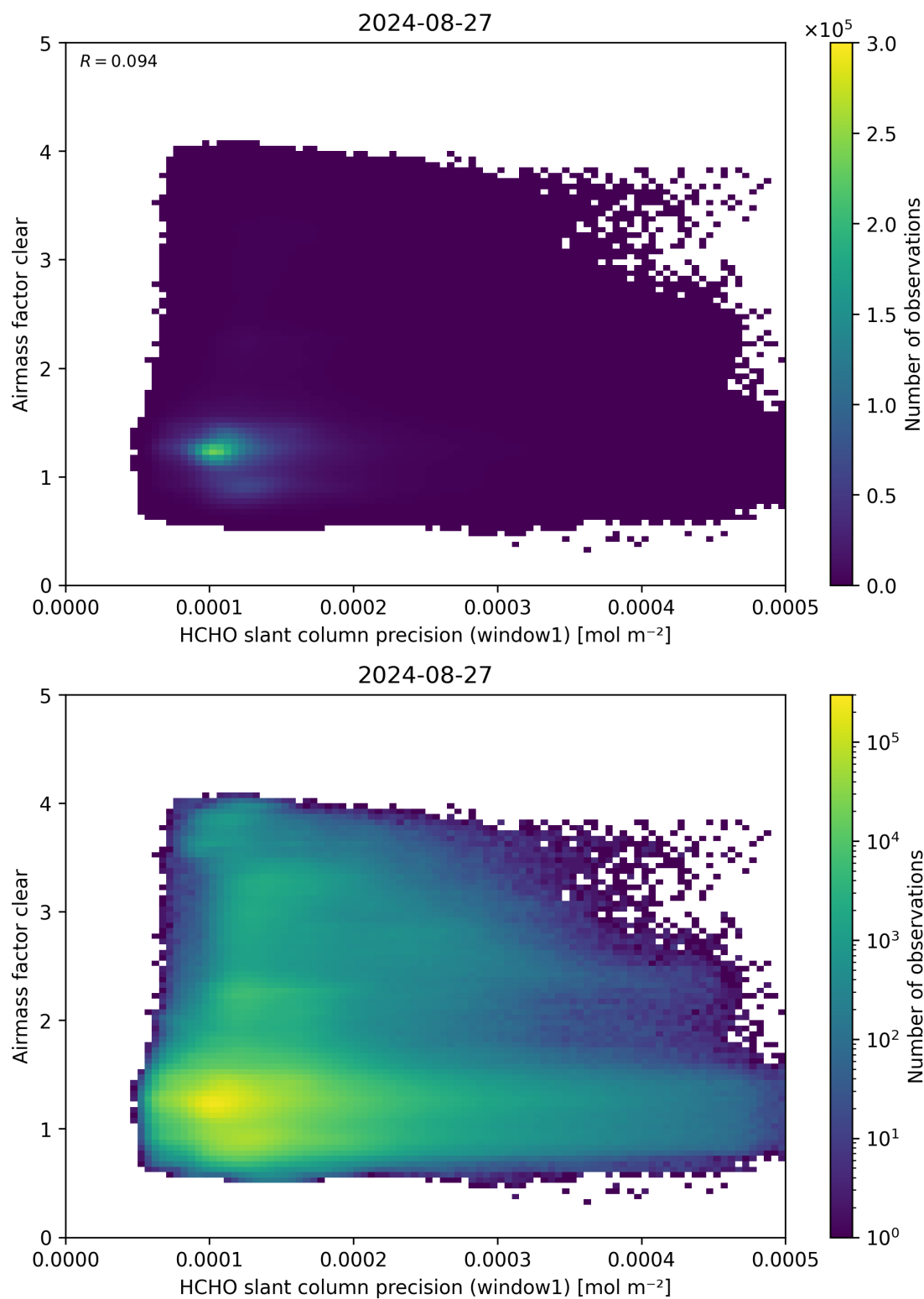
Figure 91: Scatter density plot of “HCHO slant column precision (window1)” against “Airmass factor clear” for 2024-08-27 to 2024-08-28.
