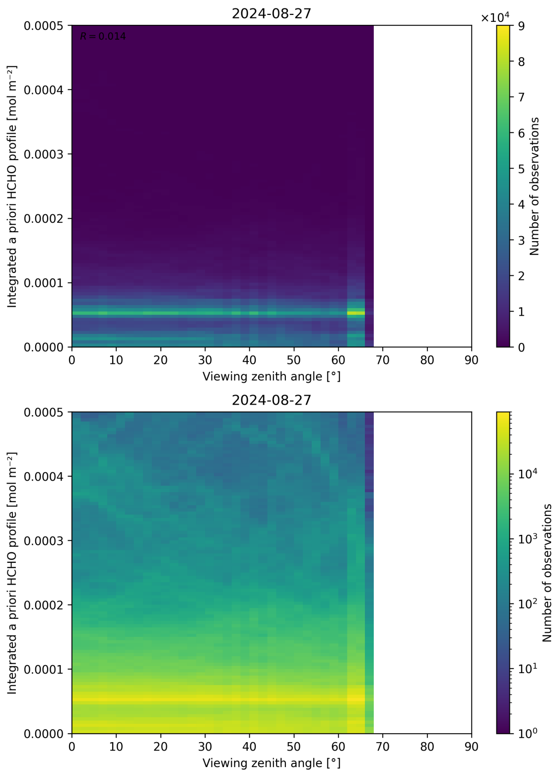
Figure 195: Scatter density plot of “Viewing zenith angle” against “Integrated a priori HCHO profile” for 2024-08-27 to 2024-08-28.
