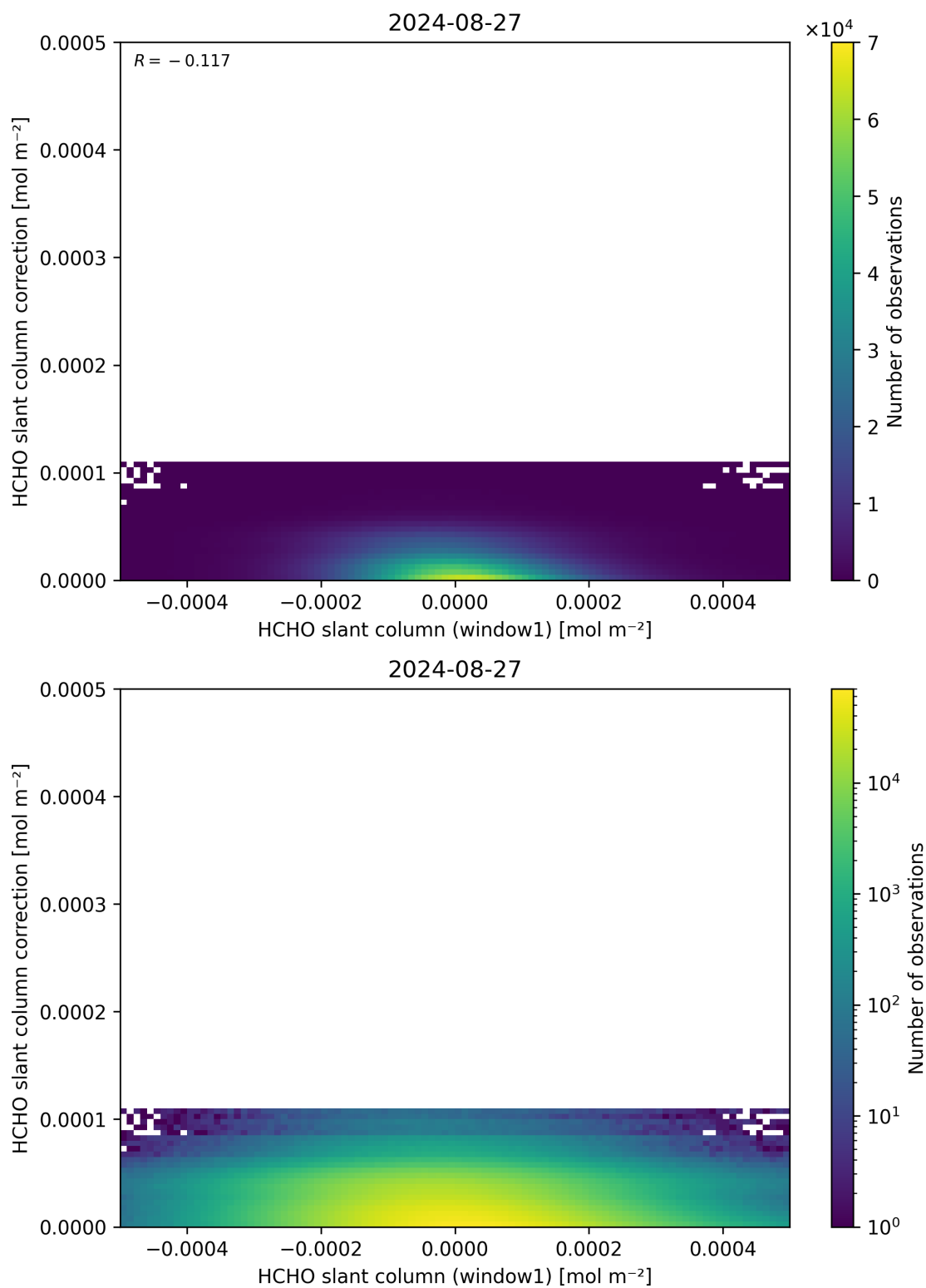
Figure 83: Scatter density plot of “HCHO slant column (window1)” against “HCHO slant column correction” for 2024-08-27 to 2024-08-28.
