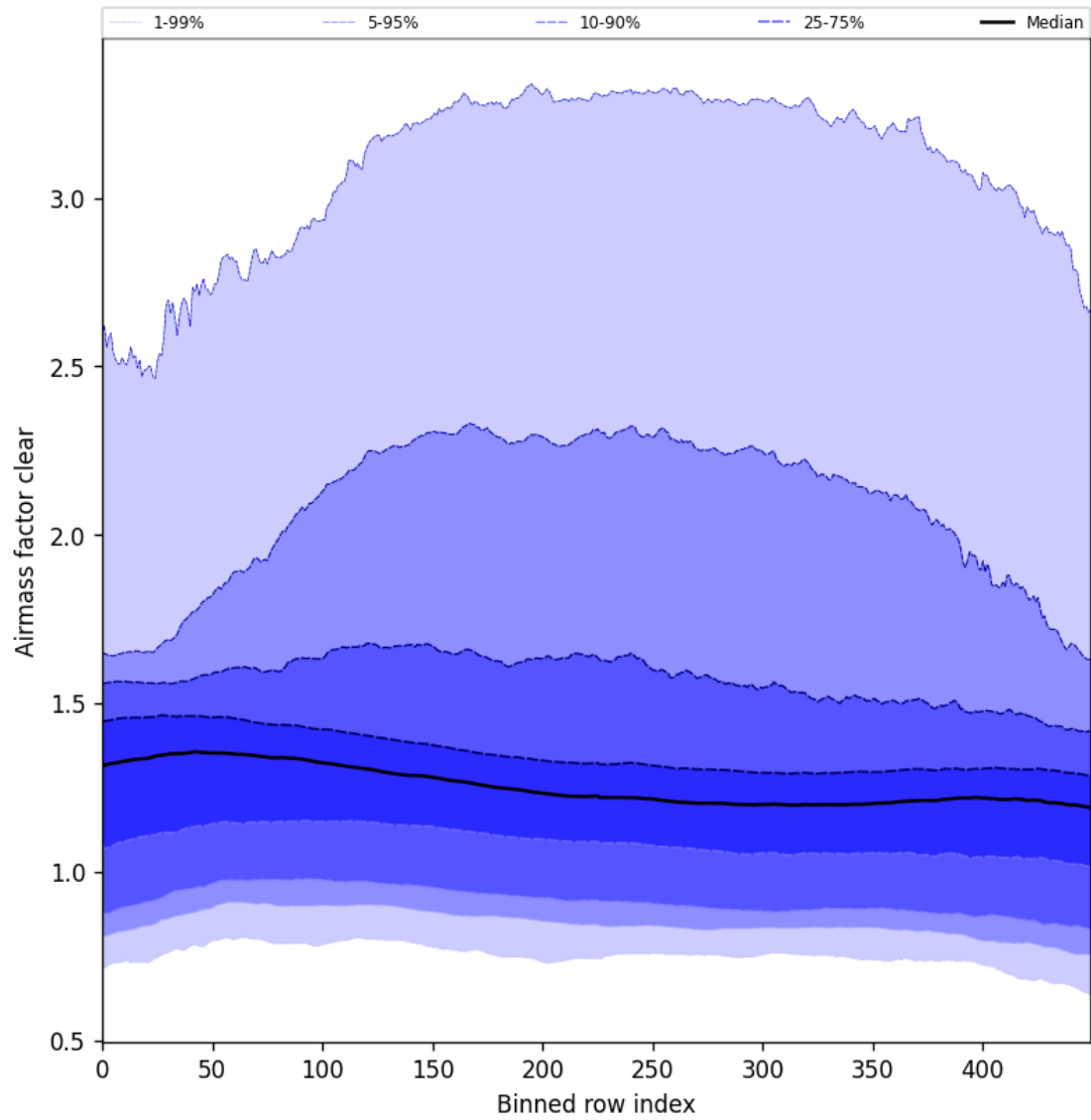
Figure 56: Along track statistics of “Airmass factor clear” for 2024-08-27 to 2024-08-28
