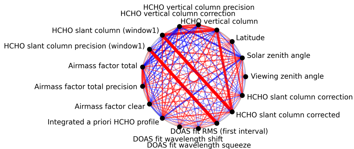
Figure 1: Map of correlation graph for 2024-08-27 to 2024-08-28.
