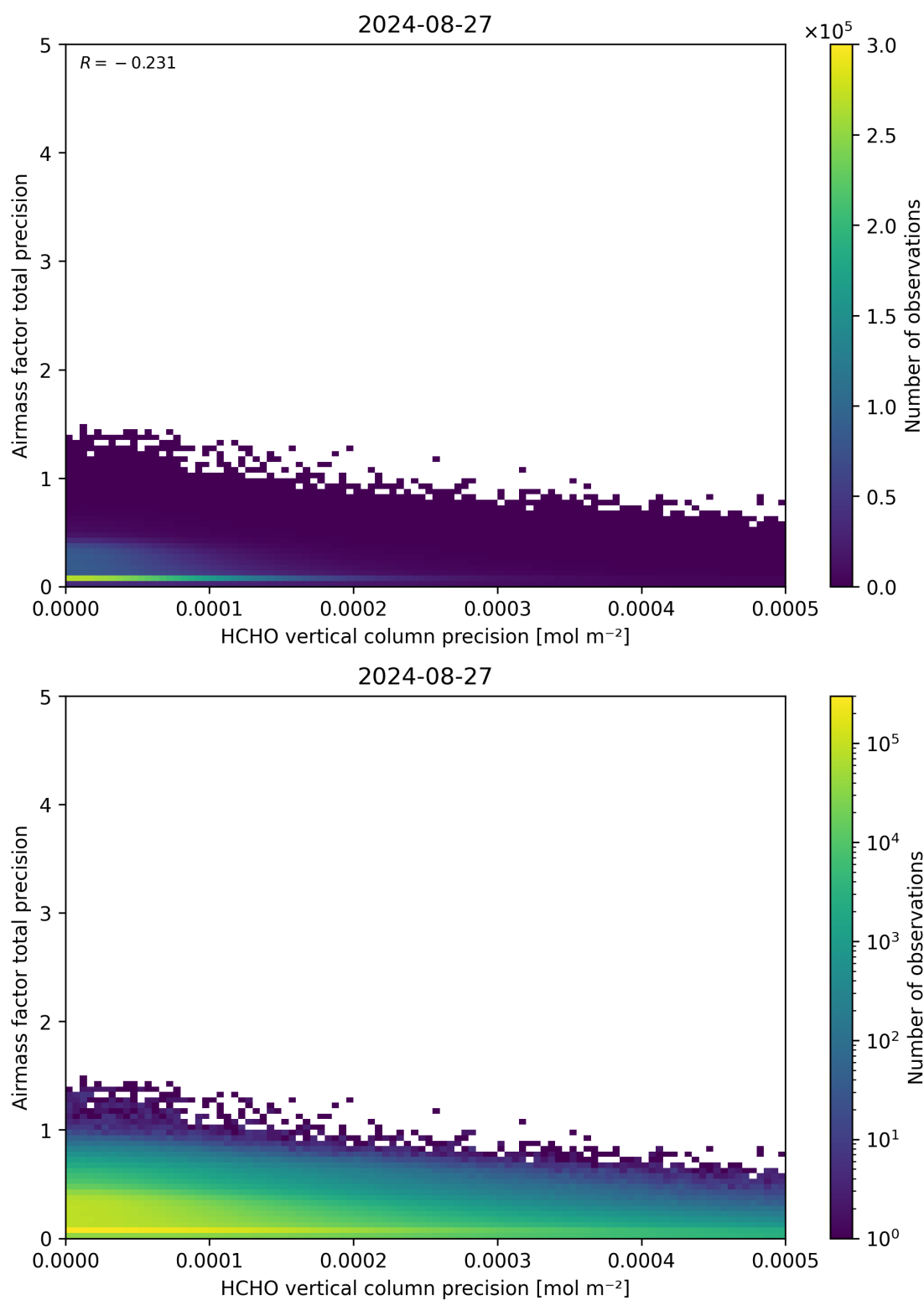
Figure 145: Scatter density plot of “HCHO vertical column precision” against “Airmass factor total precision” for 2024-08-27 to 2024-08-28.
