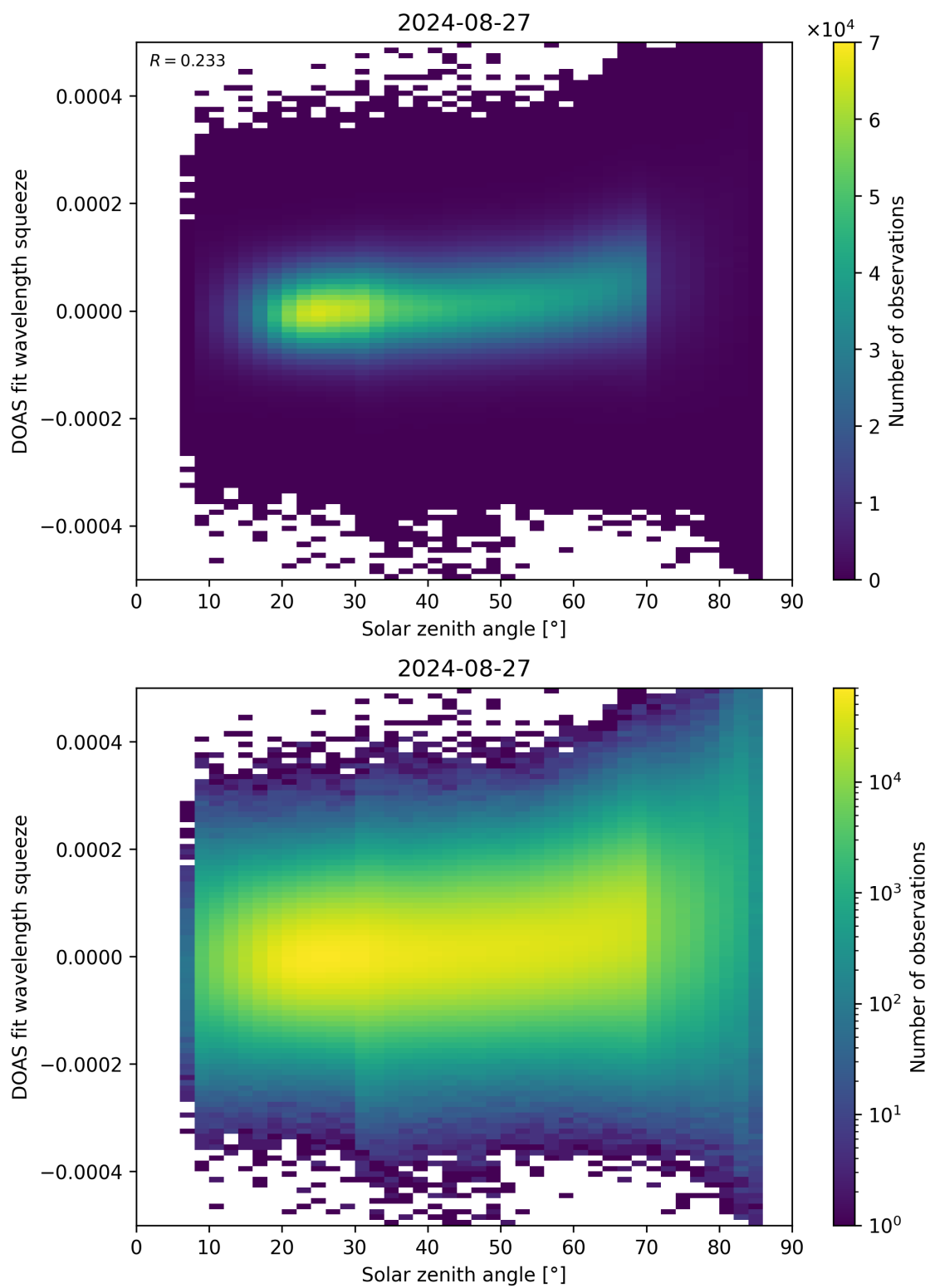
Figure 169: Scatter density plot of “Solar zenith angle” against “DOAS fit wavelength squeeze” for 2024-08-27 to 2024-08-28.
