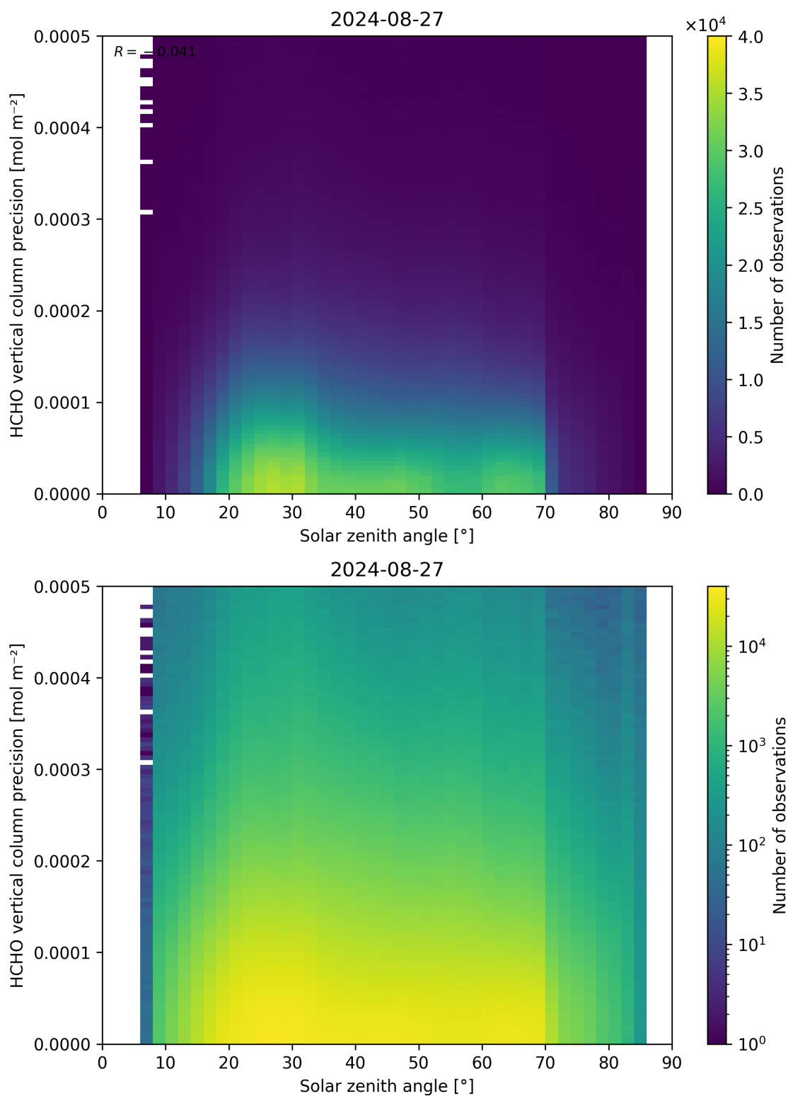
Figure 179: Scatter density plot of “Solar zenith angle” against “HCHO vertical column precision” for 2024-08-27 to 2024-08-28.
