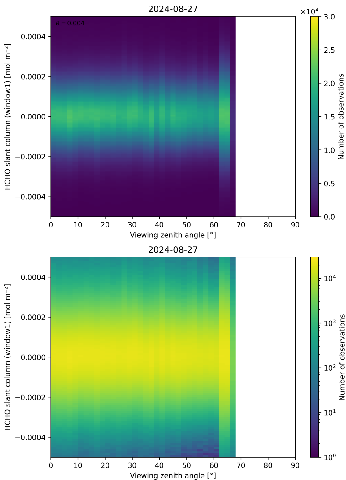
Figure 188: Scatter density plot of “Viewing zenith angle” against “HCHO slant column (window1)” for 2024-08-27 to 2024-08-28.
