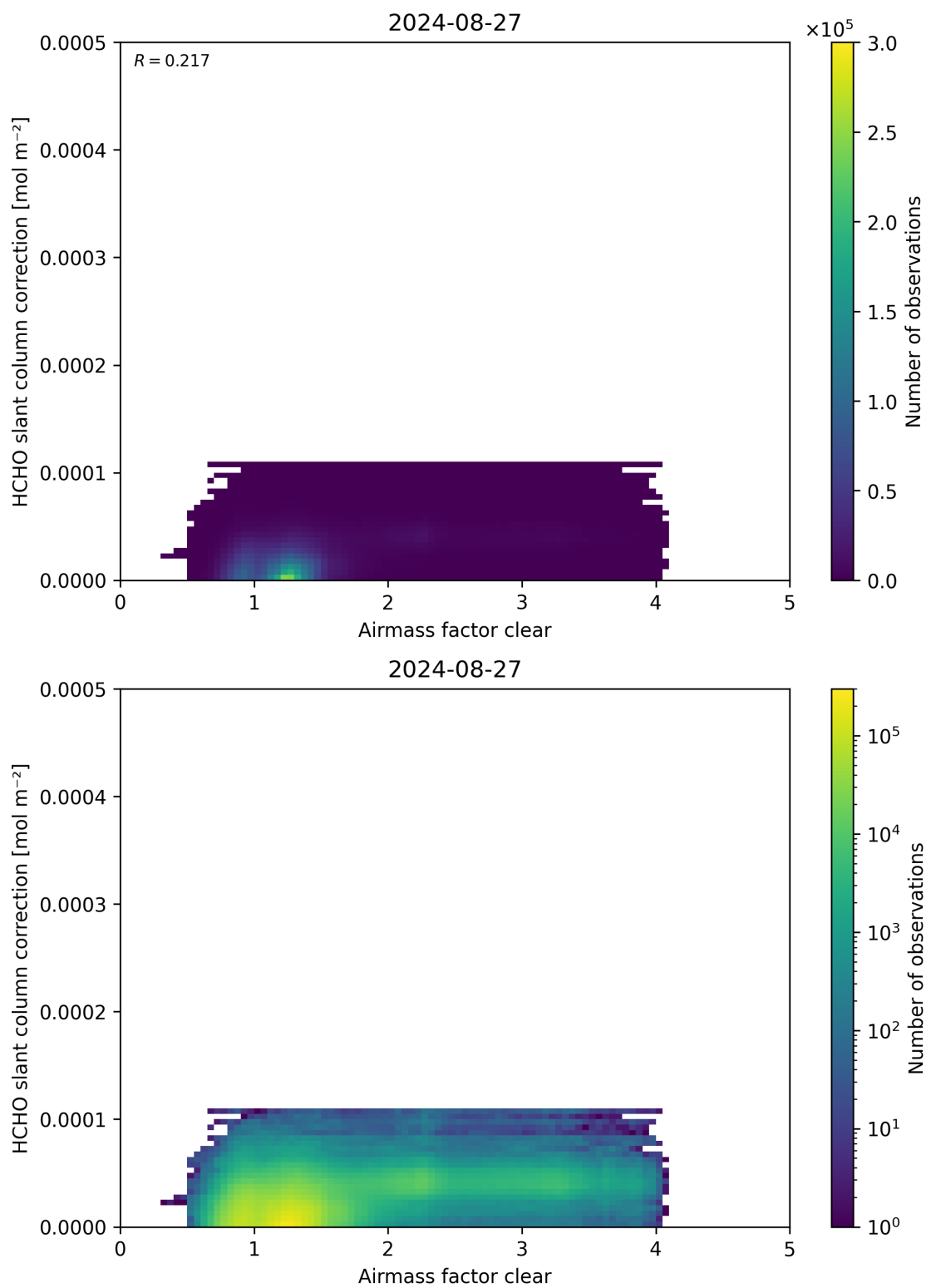
Figure 75: Scatter density plot of “Airmass factor clear” against “HCHO slant column correction” for 2024-08-27 to 2024-08-28.
