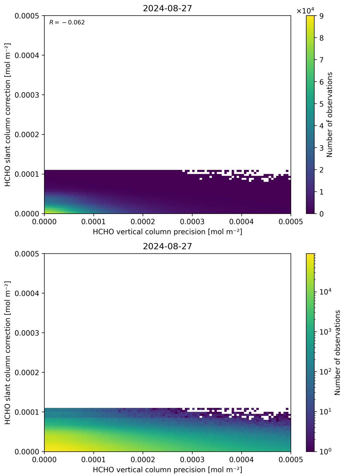
Figure 141: Scatter density plot of “HCHO vertical column precision” against “HCHO slant column correction” for 2024-08-27 to 2024-08-28.
