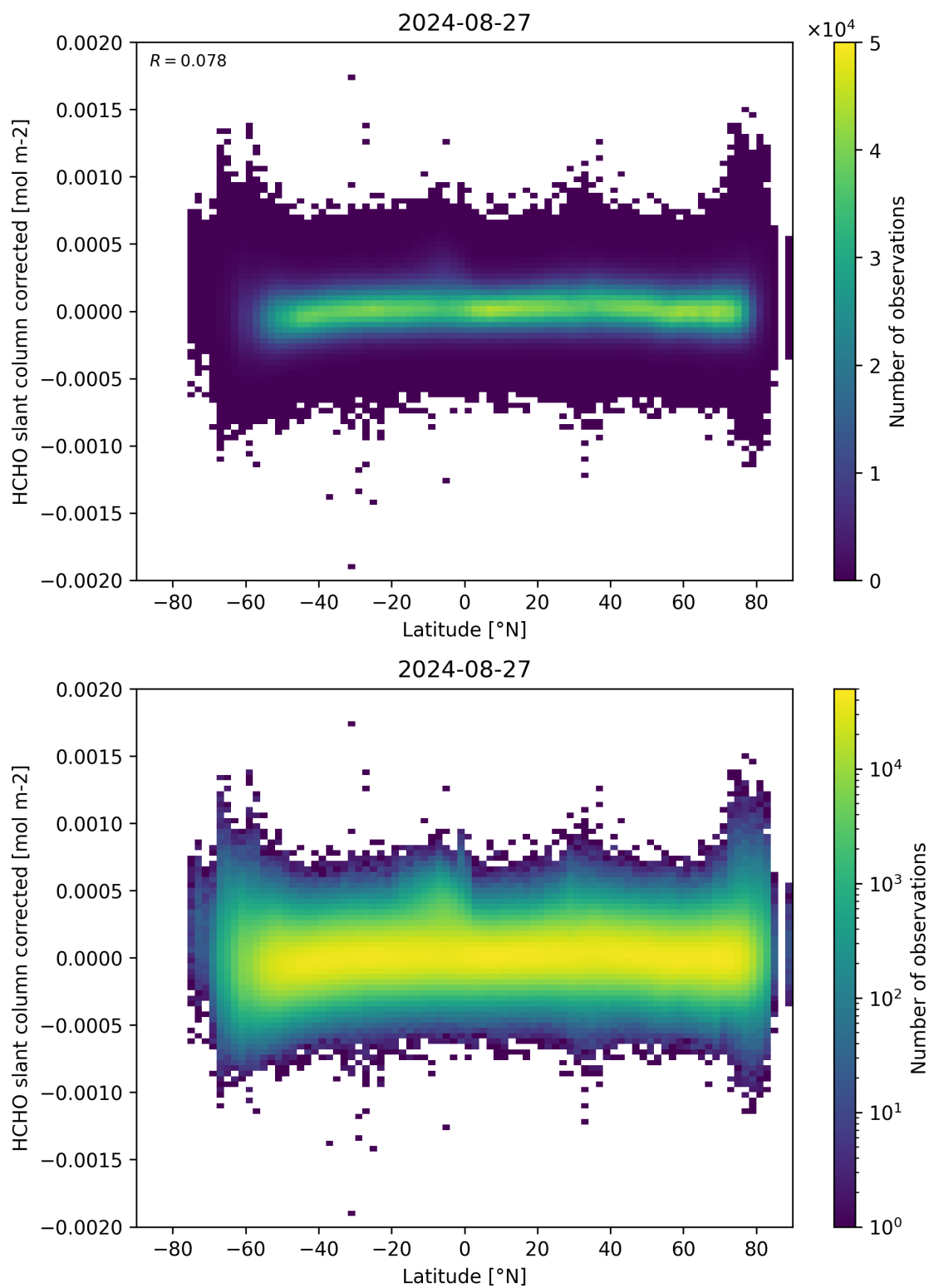
Figure 157: Scatter density plot of “Latitude” against “HCHO slant column corrected” for 2024-08-27 to 2024-08-28.
