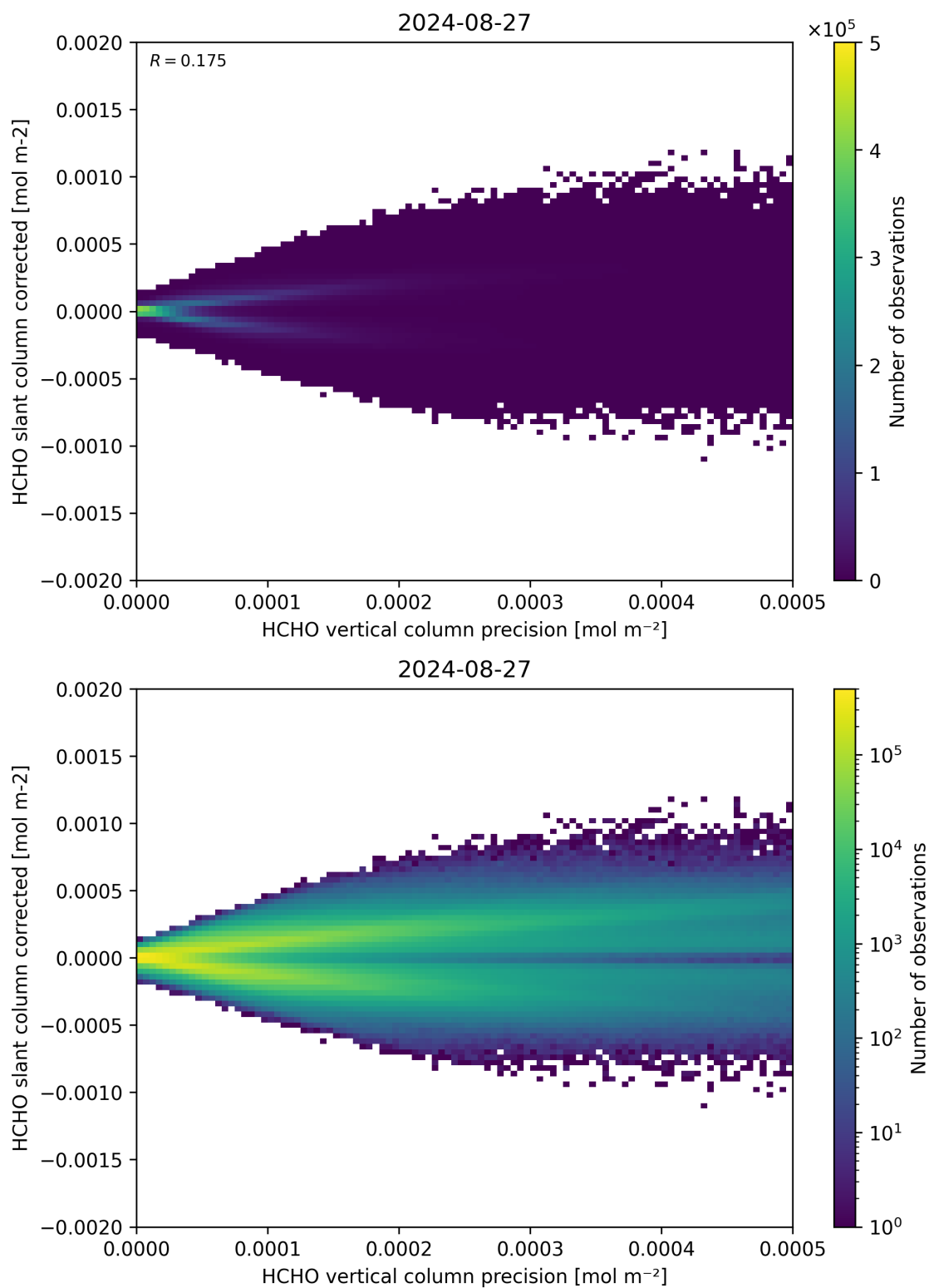
Figure 140: Scatter density plot of “HCHO vertical column precision” against “HCHO slant column corrected” for 2024-08-27 to 2024-08-28.
