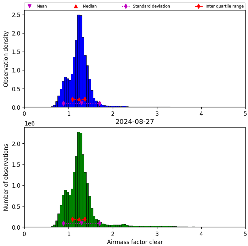
Figure 42: Histogram of “Airmass factor clear” for 2024-08-27 to 2024-08-28
