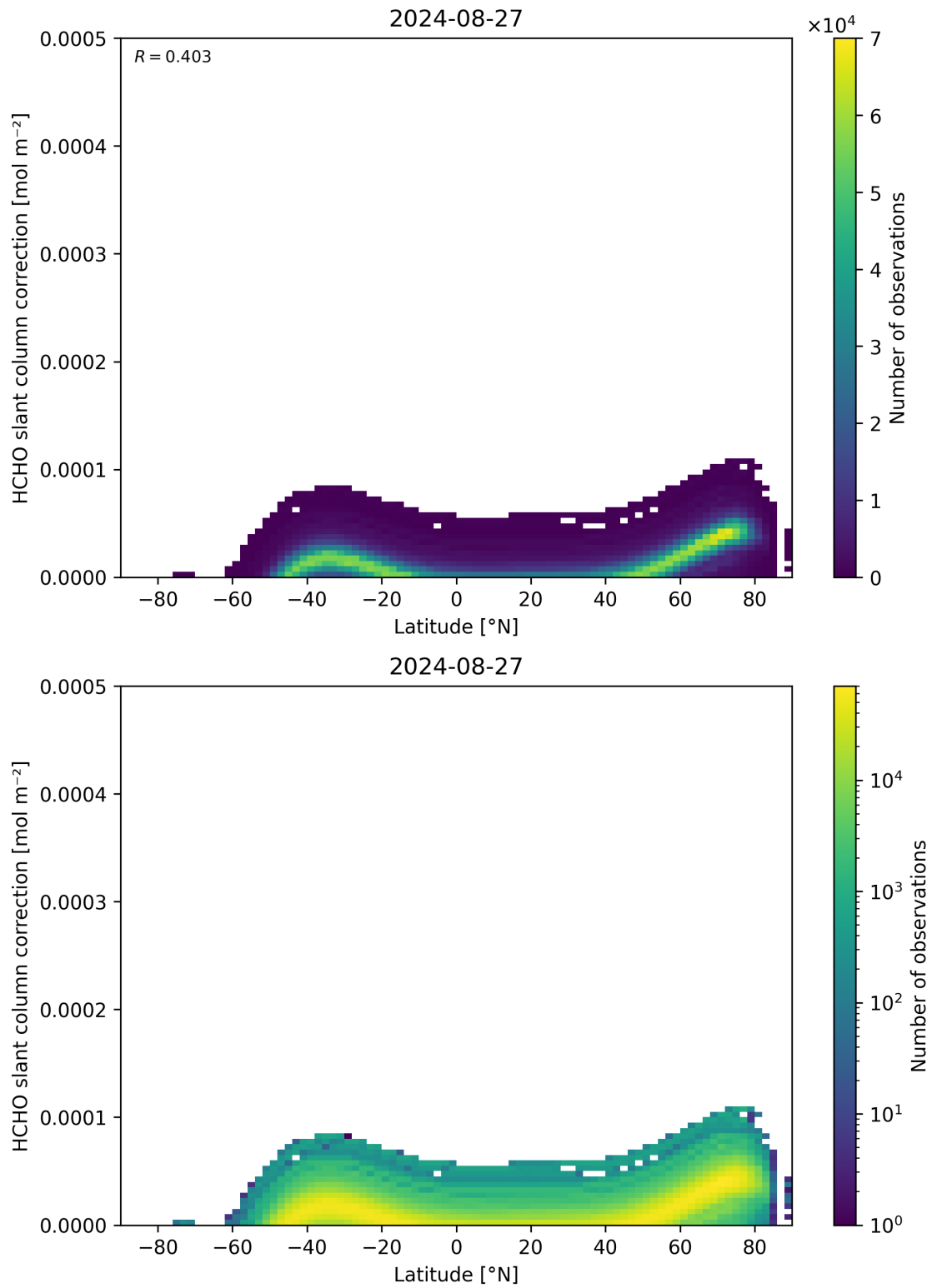
Figure 158: Scatter density plot of “Latitude” against “HCHO slant column correction” for 2024-08-27 to 2024-08-28.
