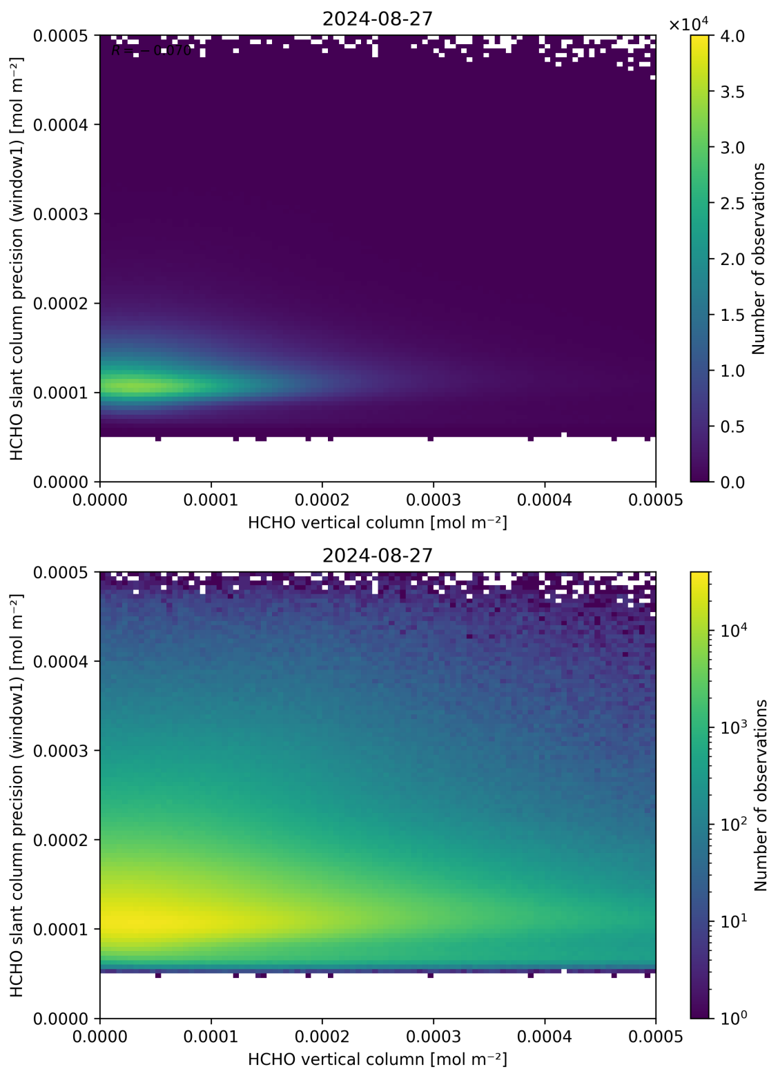
Figure 130: Scatter density plot of “HCHO vertical column” against “HCHO slant column precision (window1)” for 2024-08-27 to 2024-08-28.
