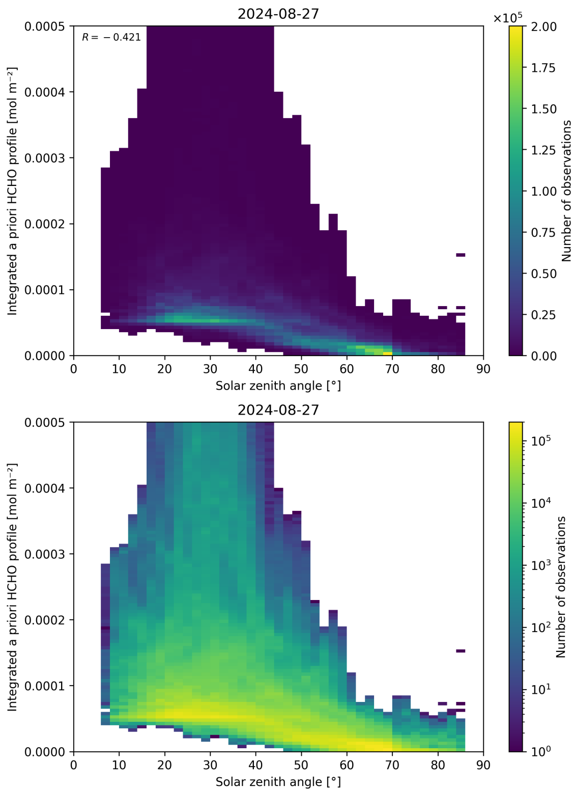
Figure 180: Scatter density plot of “Solar zenith angle” against “Integrated a priori HCHO profile” for 2024-08-27 to 2024-08-28.
