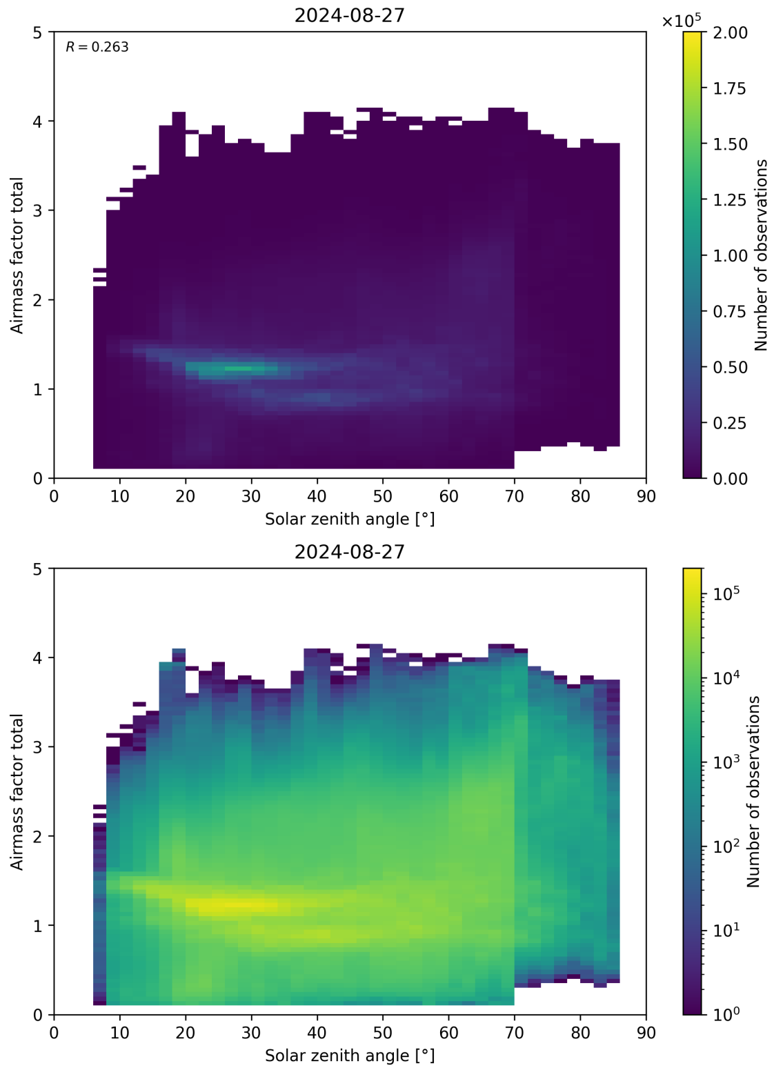
Figure 175: Scatter density plot of “Solar zenith angle” against “Airmass factor total” for 2024-08-27 to 2024-08-28.
