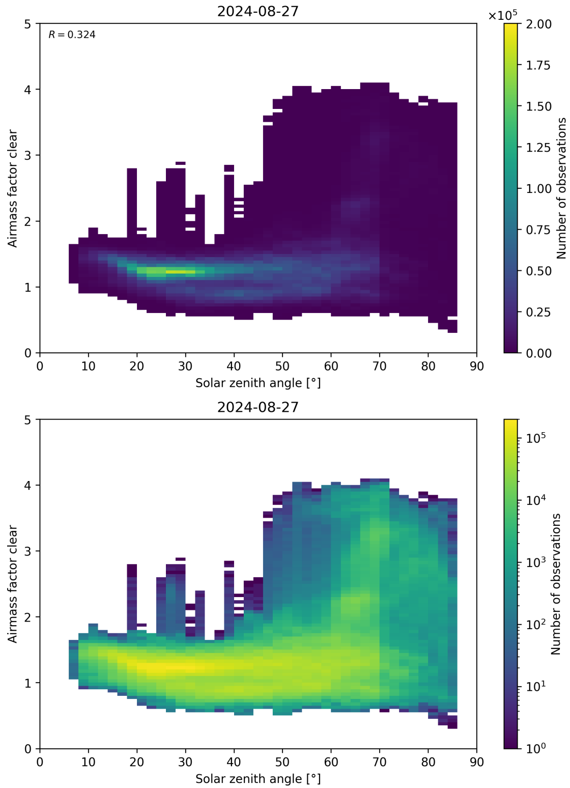
Figure 170: Scatter density plot of “Solar zenith angle” against “Airmass factor clear” for 2024-08-27 to 2024-08-28.
