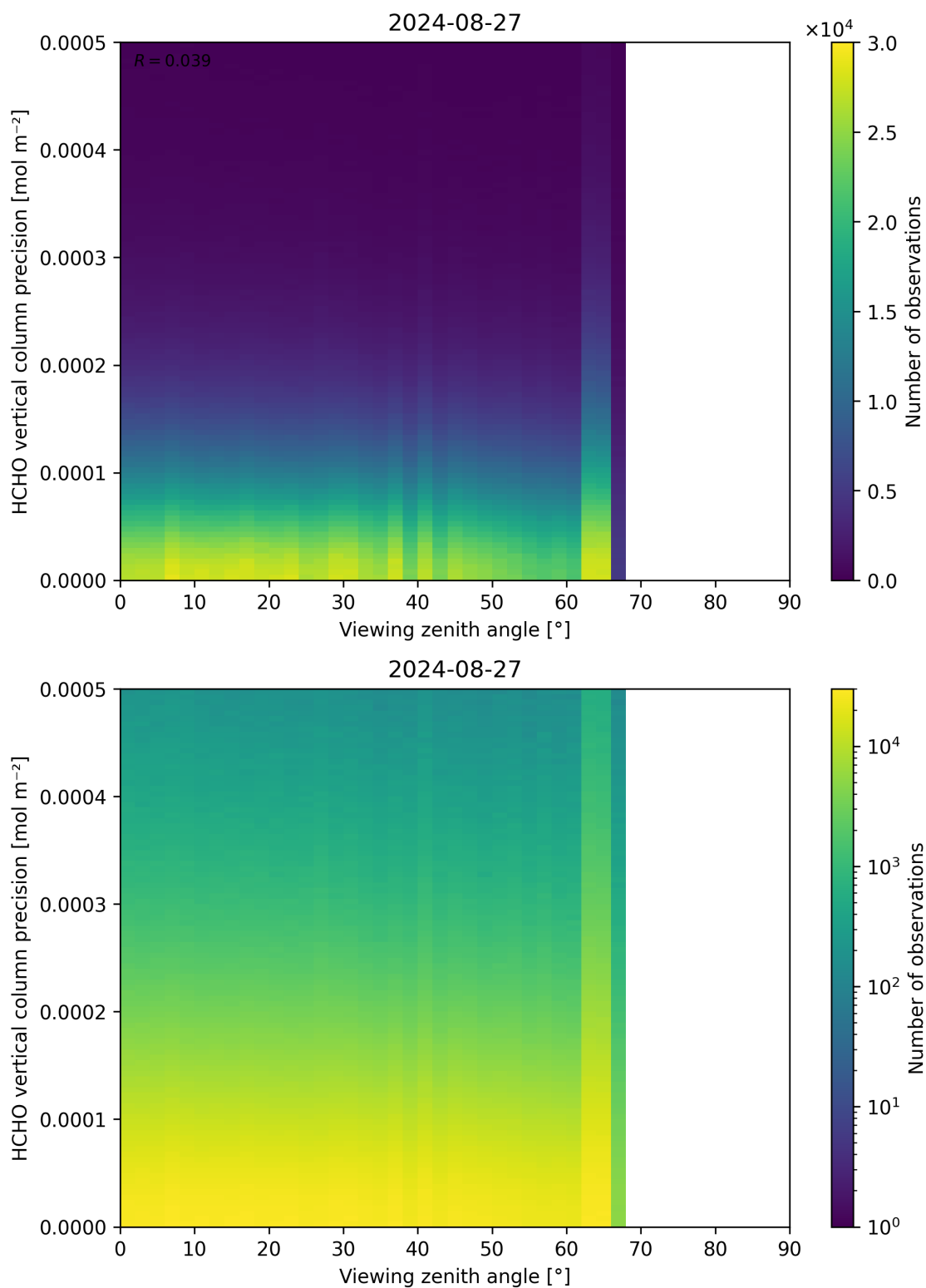
Figure 194: Scatter density plot of “Viewing zenith angle” against “HCHO vertical column precision” for 2024-08-27 to 2024-08-28.
