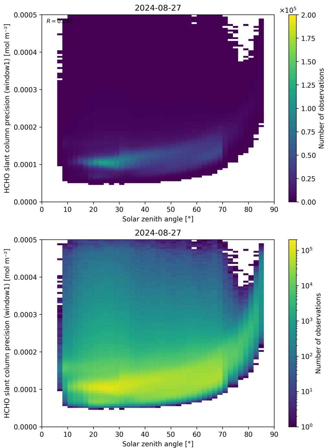
Figure 174: Scatter density plot of “Solar zenith angle” against “HCHO slant column precision (window1)” for 2024-08-27 to 2024-08-28.
