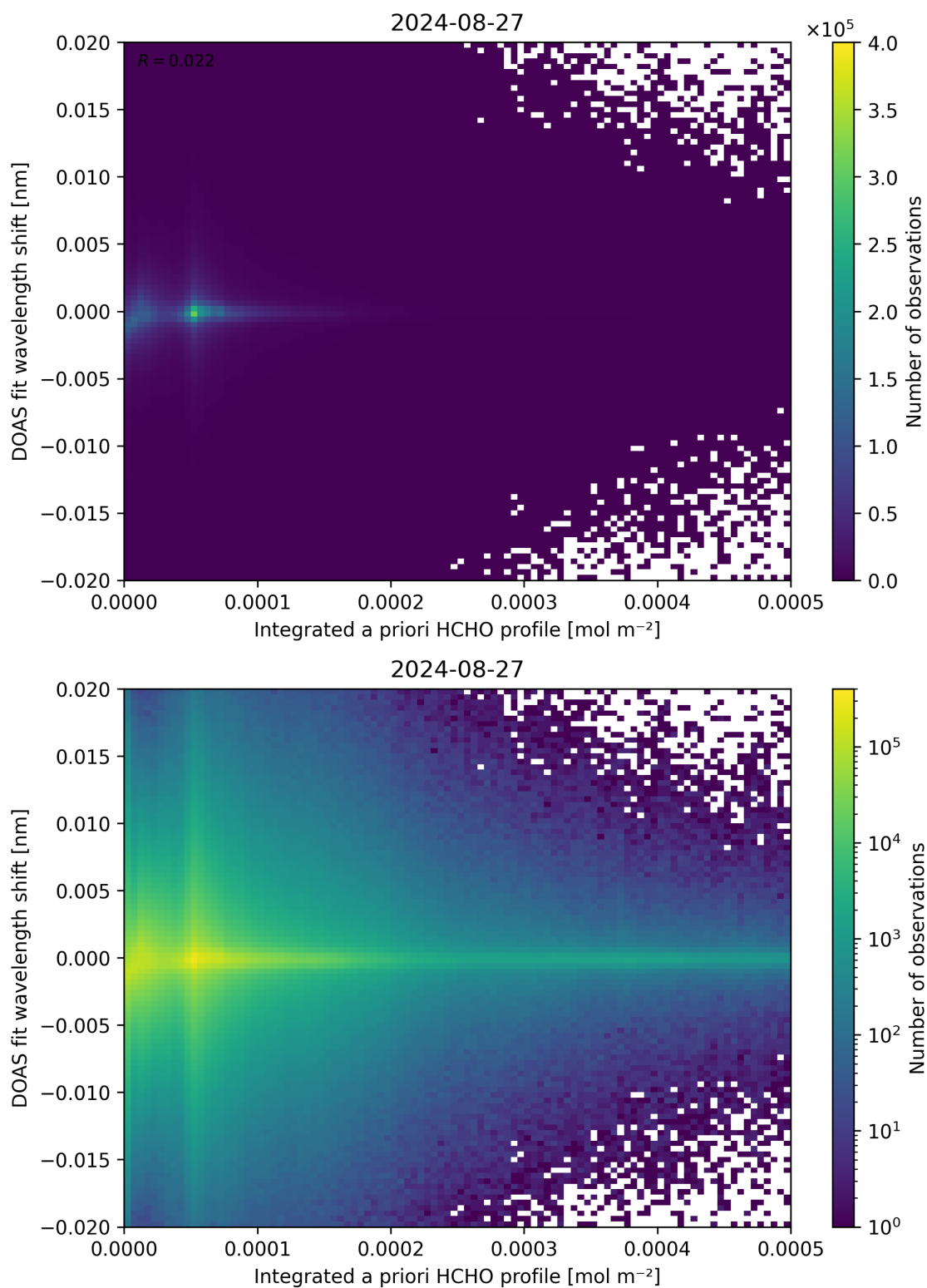
Figure 149: Scatter density plot of “Integrated a priori HCHO profile” against “DOAS fit wavelength shift” for 2024-08-27 to 2024-08-28.
