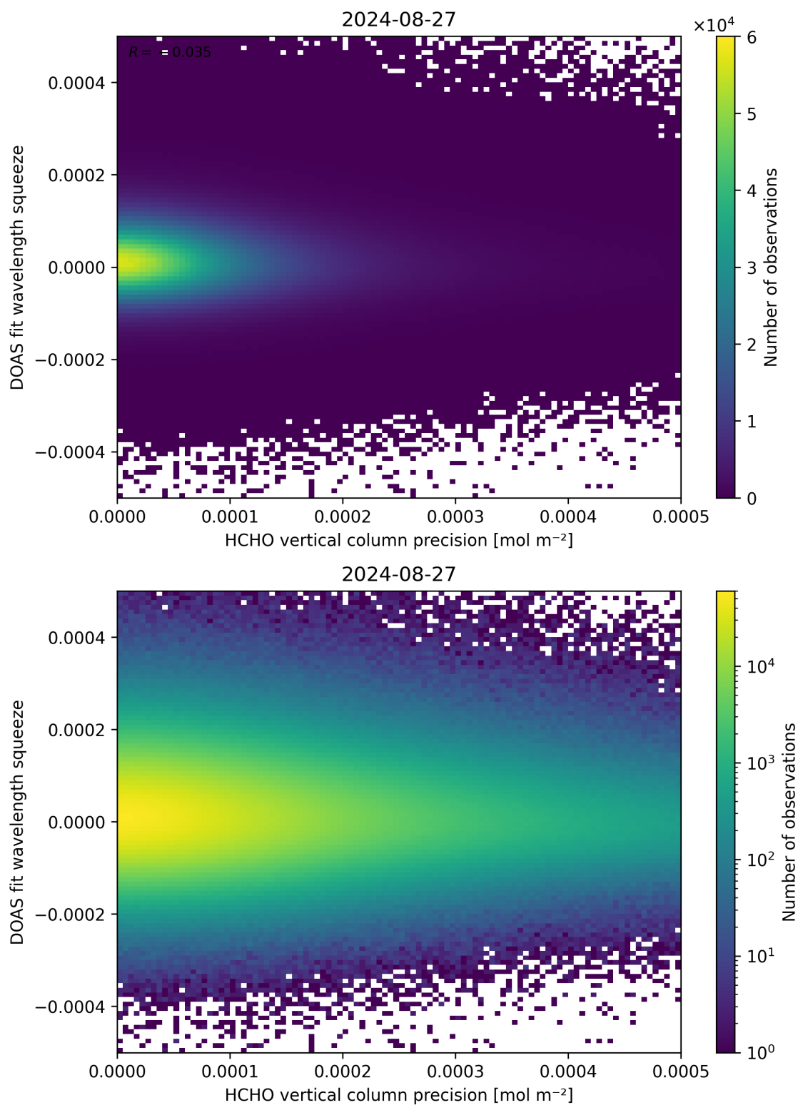
Figure 138: Scatter density plot of “HCHO vertical column precision” against “DOAS fit wavelength squeeze” for 2024-08-27 to 2024-08-28.
