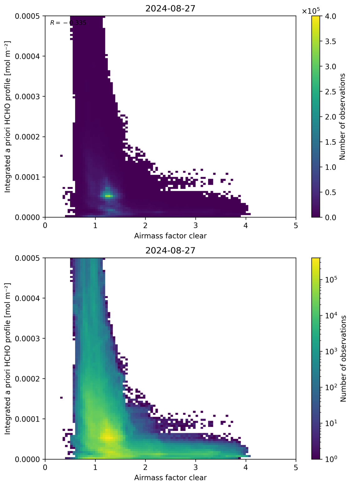
Figure 76: Scatter density plot of “Airmass factor clear” against “Integrated a priori HCHO profile” for 2024-08-27 to 2024-08-28.
