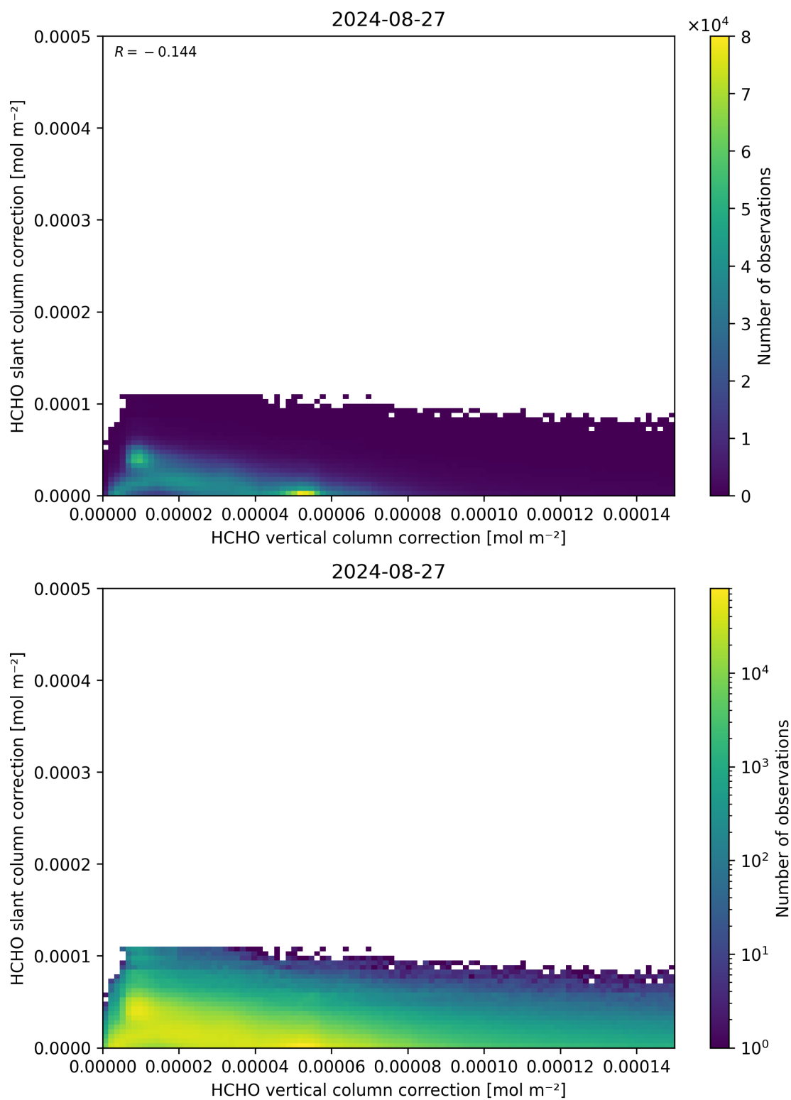
Figure 117: Scatter density plot of “HCHO vertical column correction” against “HCHO slant column correction” for 2024-08-27 to 2024-08-28.
