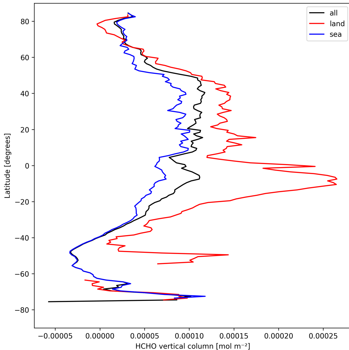
Figure 21: Zonal average of “HCHO vertical column” for 2024-08-27 to 2024-08-28.
