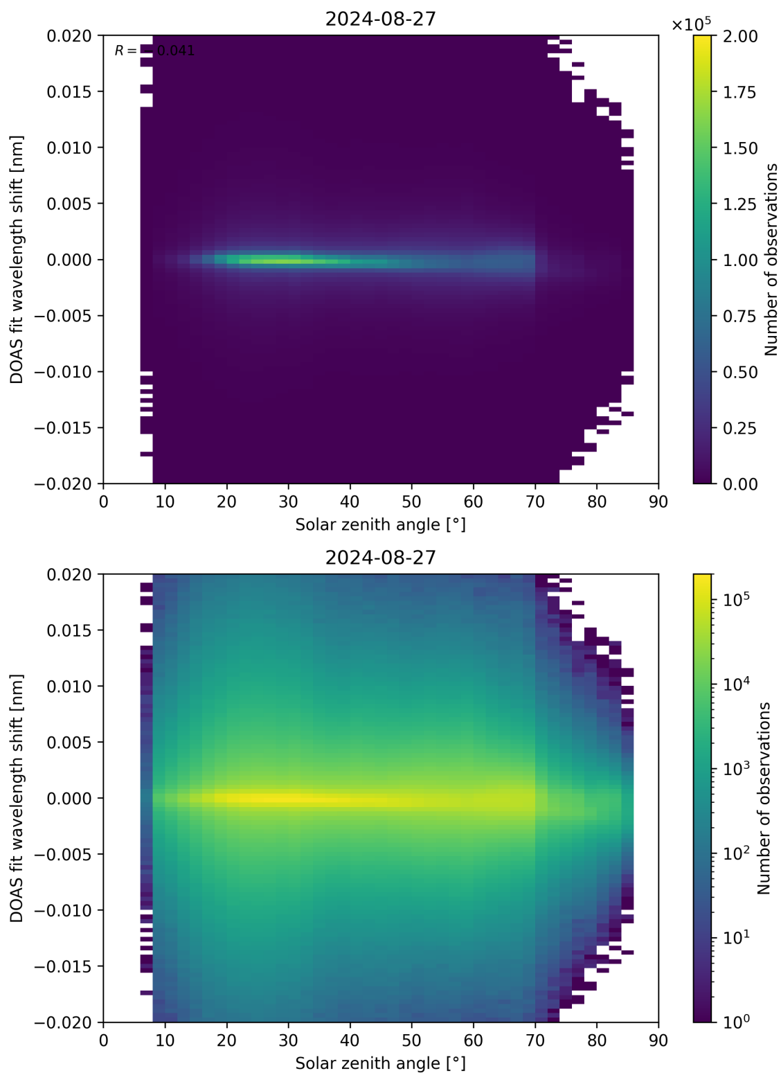
Figure 168: Scatter density plot of “Solar zenith angle” against “DOAS fit wavelength shift” for 2024-08-27 to 2024-08-28.
