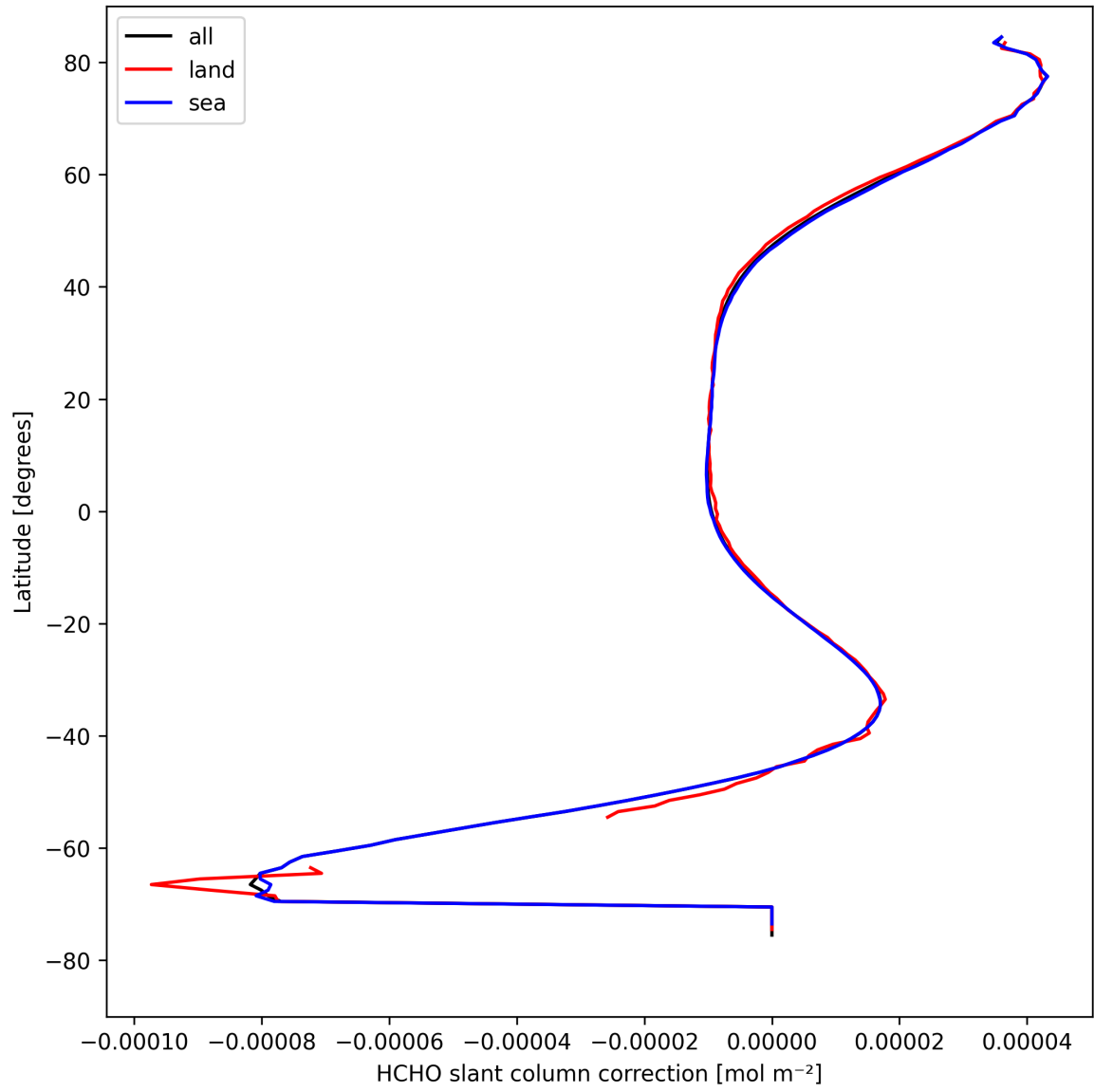
Figure 33: Zonal average of "HCHO slant column correction" for 2024-08-27 to 2024-08-28.
