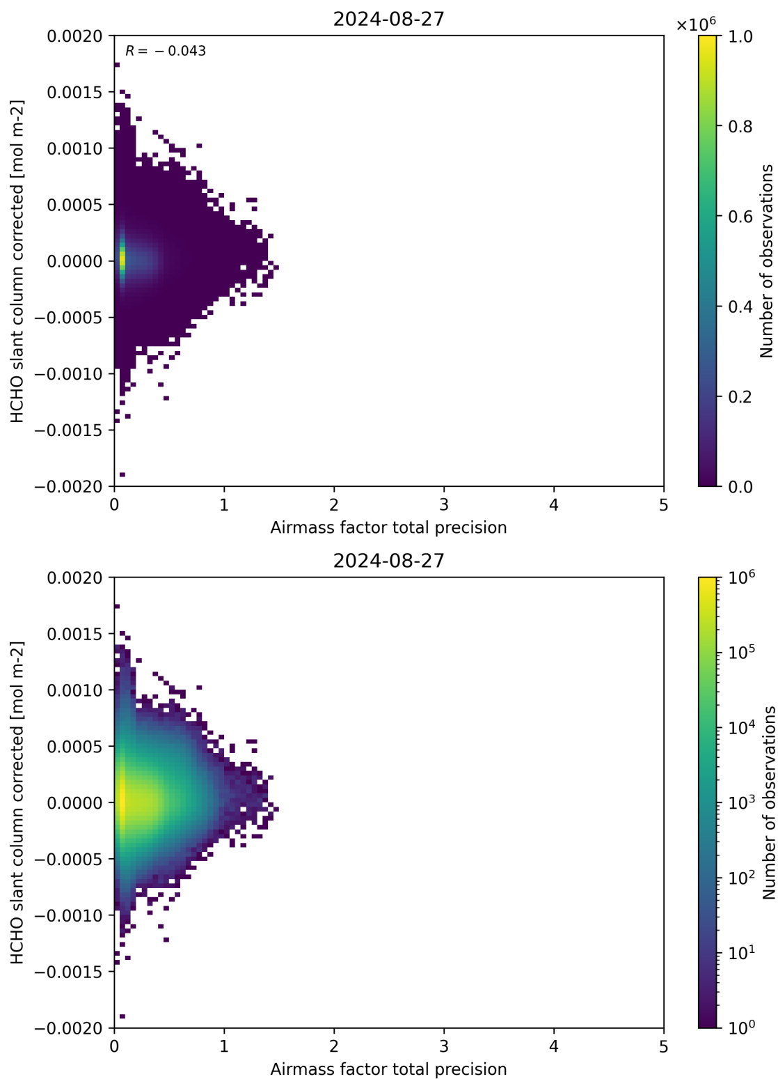
Figure 109: Scatter density plot of “Airmass factor total precision” against “HCHO slant column corrected” for 2024-08-27 to 2024-08-28.
