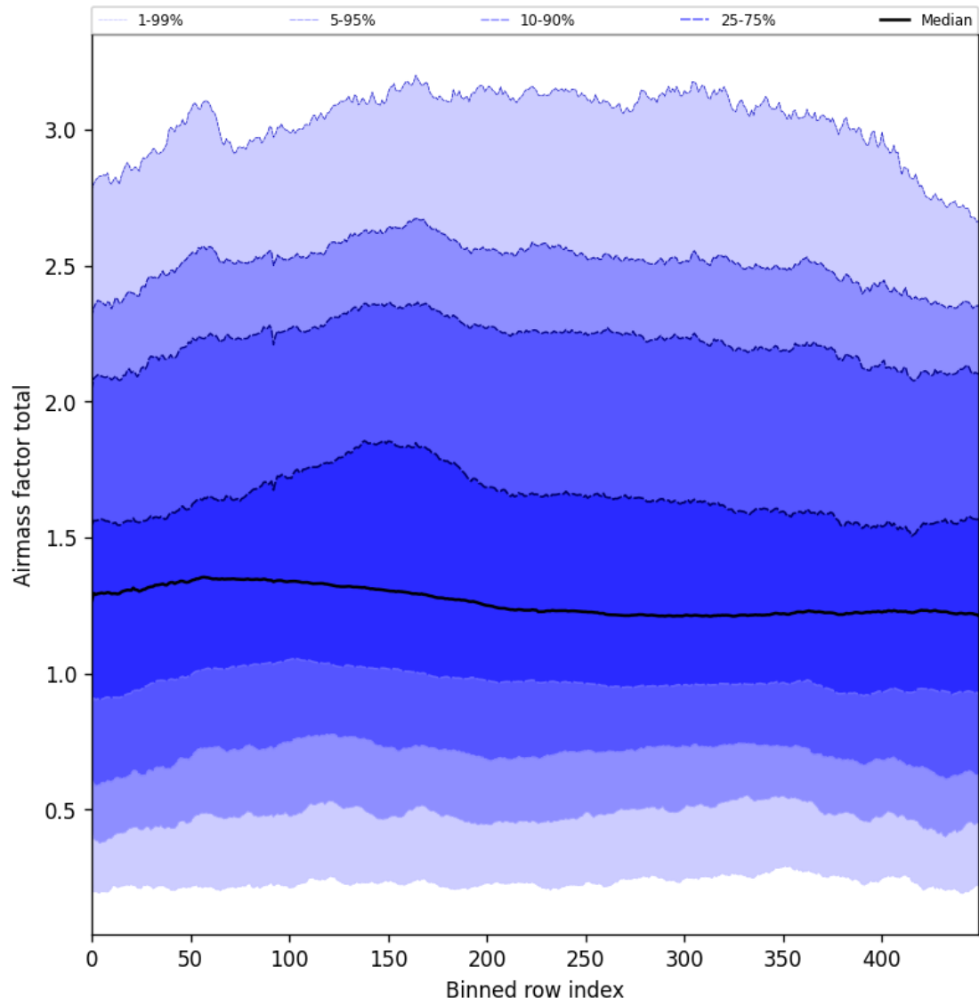
Figure 54: Along track statistics of “Airmass factor total” for 2024-08-27 to 2024-08-28
