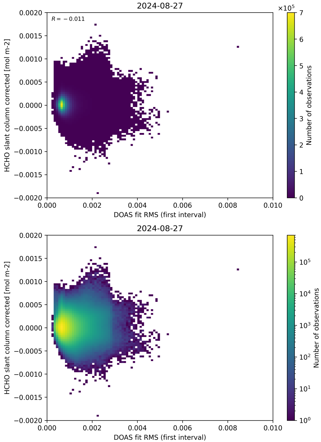
Figure 62: Scatter density plot of “DOAS fit RMS (first interval)” against “HCHO slant column corrected” for 2024-08-27 to 2024-08-28.
