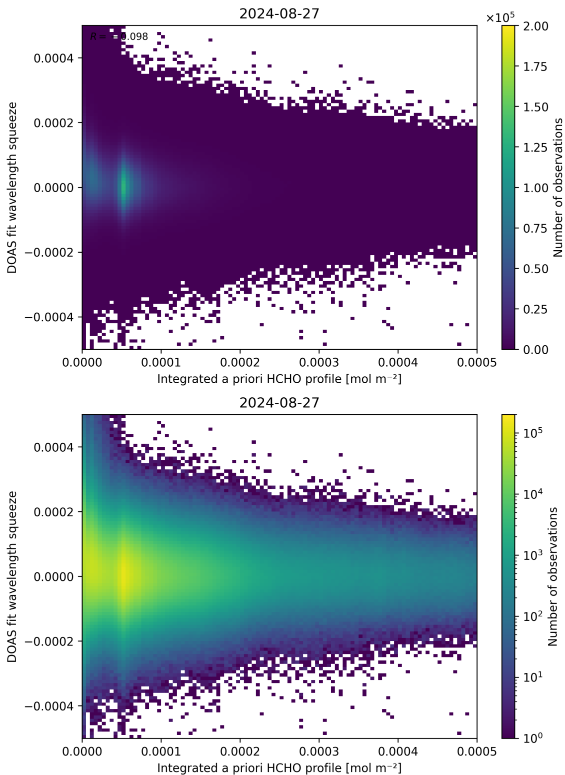
Figure 150: Scatter density plot of “Integrated a priori HCHO profile” against “DOAS fit wavelength squeeze” for 2024-08-27 to 2024-08-28.
