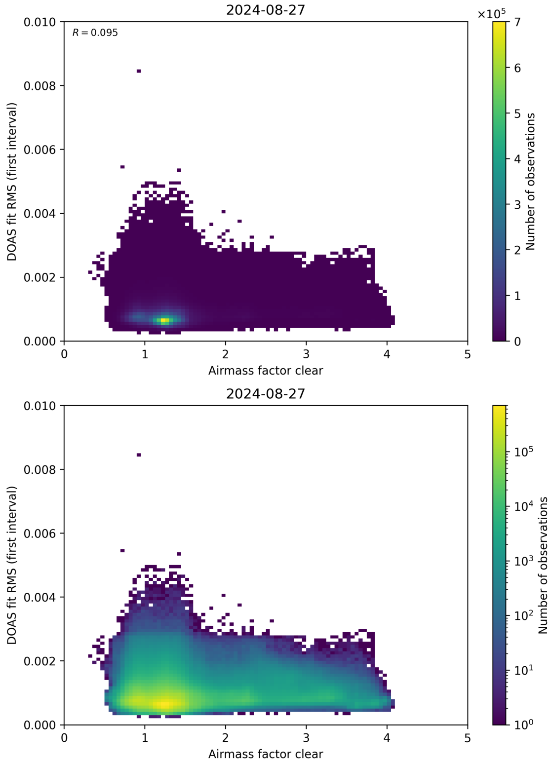
Figure 71: Scatter density plot of “Airmass factor clear” against “DOAS fit RMS (first interval)” for 2024-08-27 to 2024-08-28.
