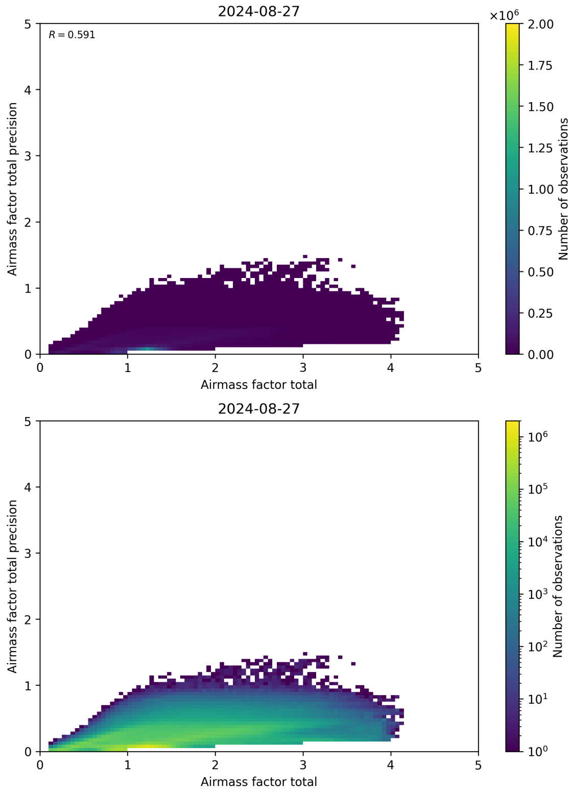
Figure 103: Scatter density plot of “Airmass factor total” against “Airmass factor total precision” for 2024-08-27 to 2024-08-28.
