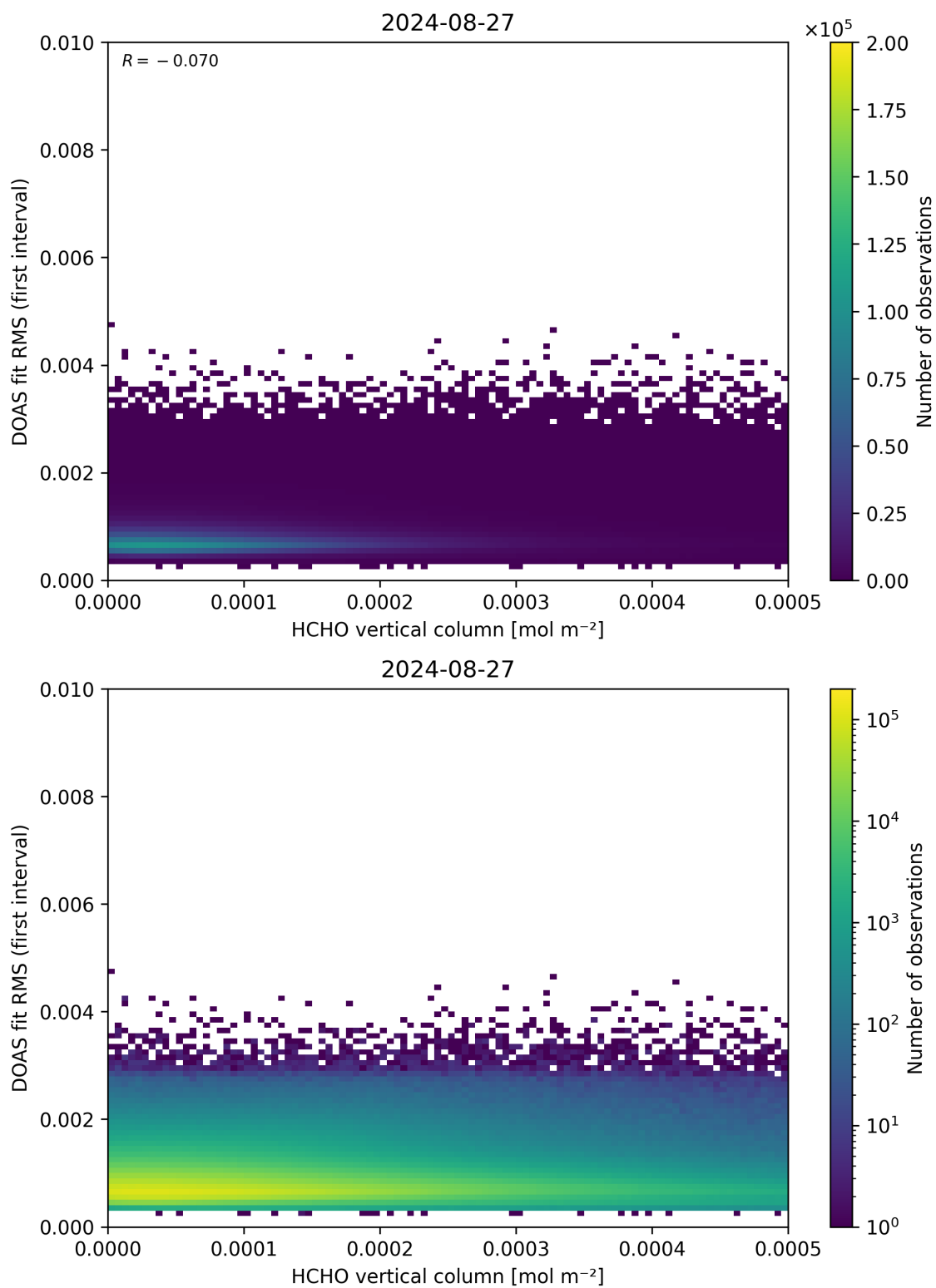
Figure 123: Scatter density plot of “HCHO vertical column” against “DOAS fit RMS (first interval)” for 2024-08-27 to 2024-08-28.
