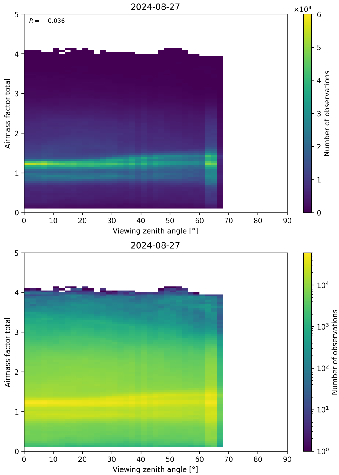
Figure 190: Scatter density plot of “Viewing zenith angle” against “Airmass factor total” for 2024-08-27 to 2024-08-28.
