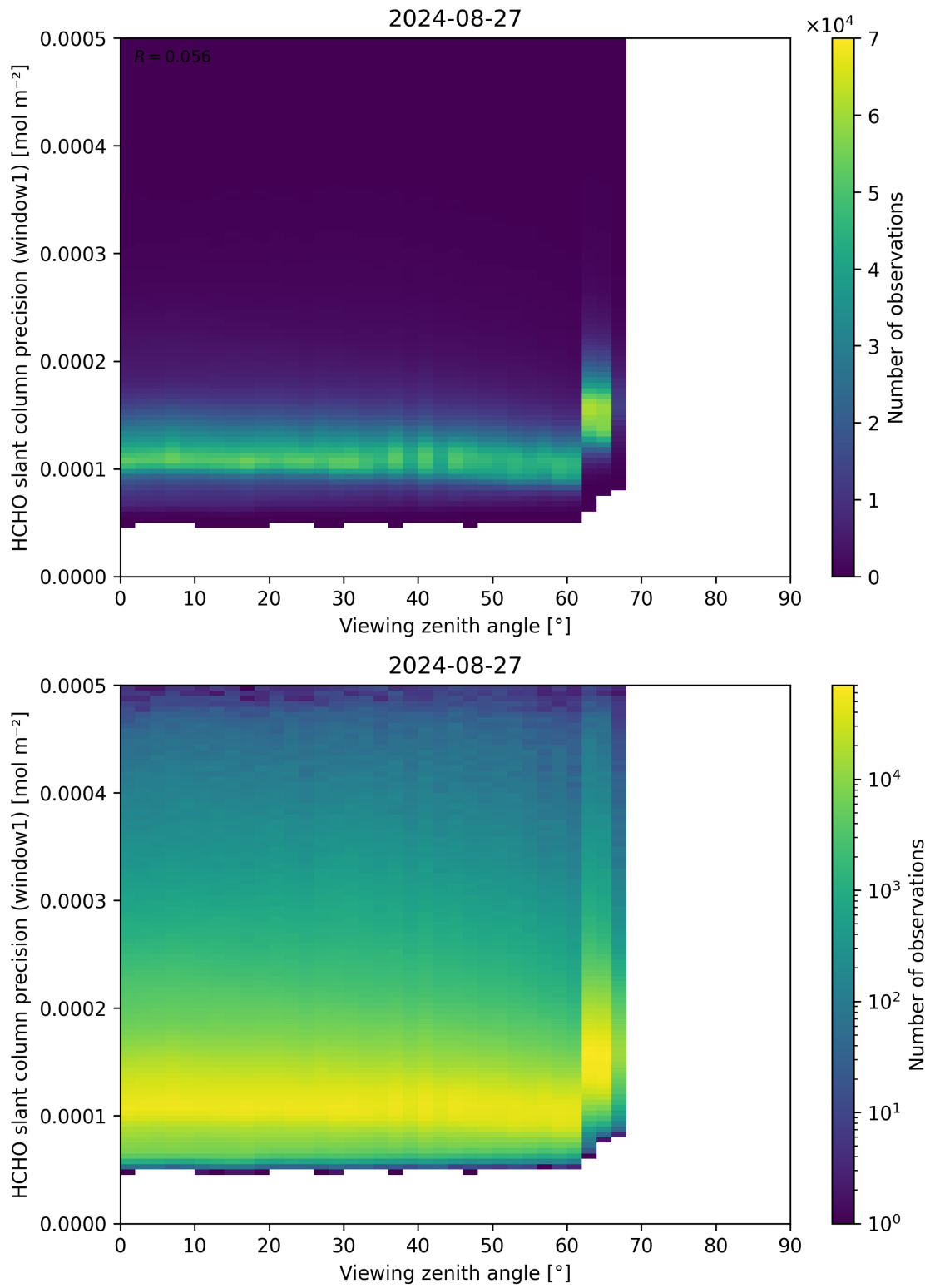
Figure 189: Scatter density plot of “Viewing zenith angle” against “HCHO slant column precision (window1)” for 2024-08-27 to 2024-08-28.
