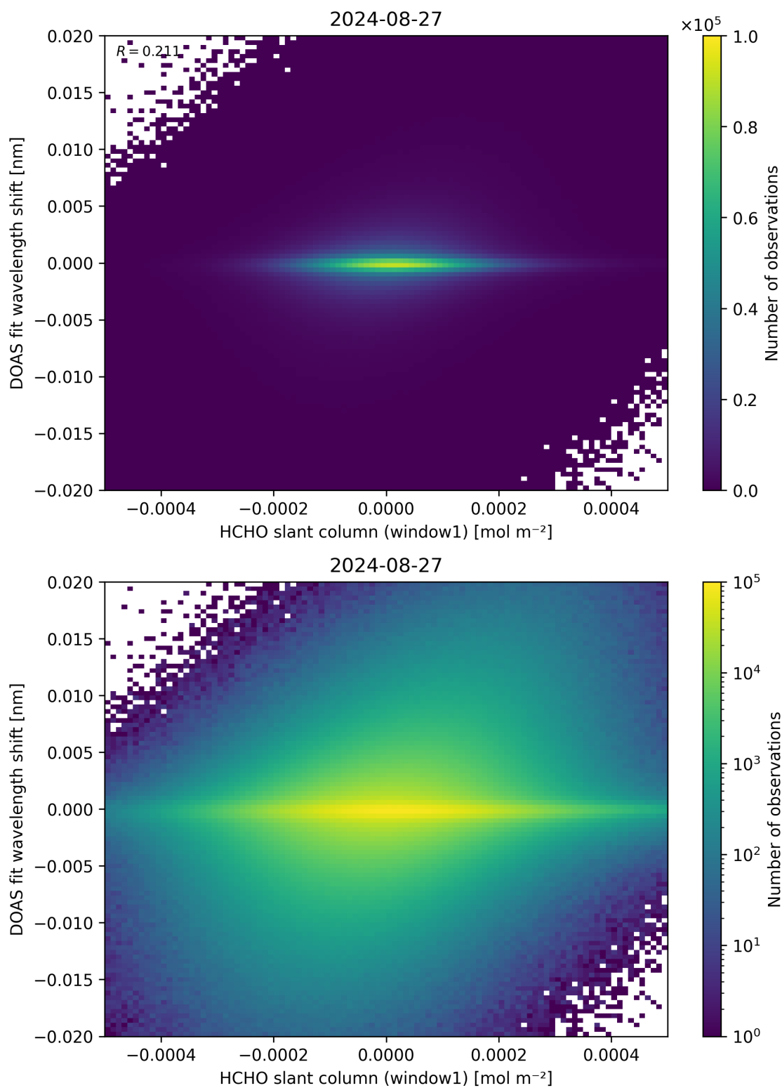
Figure 79: Scatter density plot of “HCHO slant column (window1)” against “DOAS fit wavelength shift” for 2024-08-27 to 2024-08-28.
