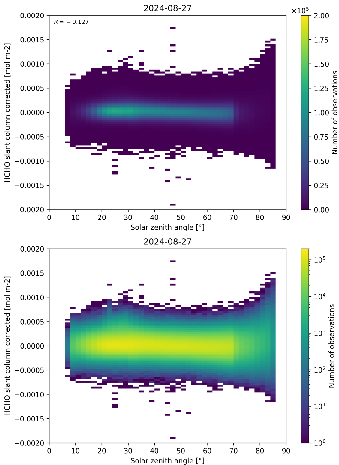
Figure 171: Scatter density plot of “Solar zenith angle” against “HCHO slant column corrected” for 2024-08-27 to 2024-08-28.
