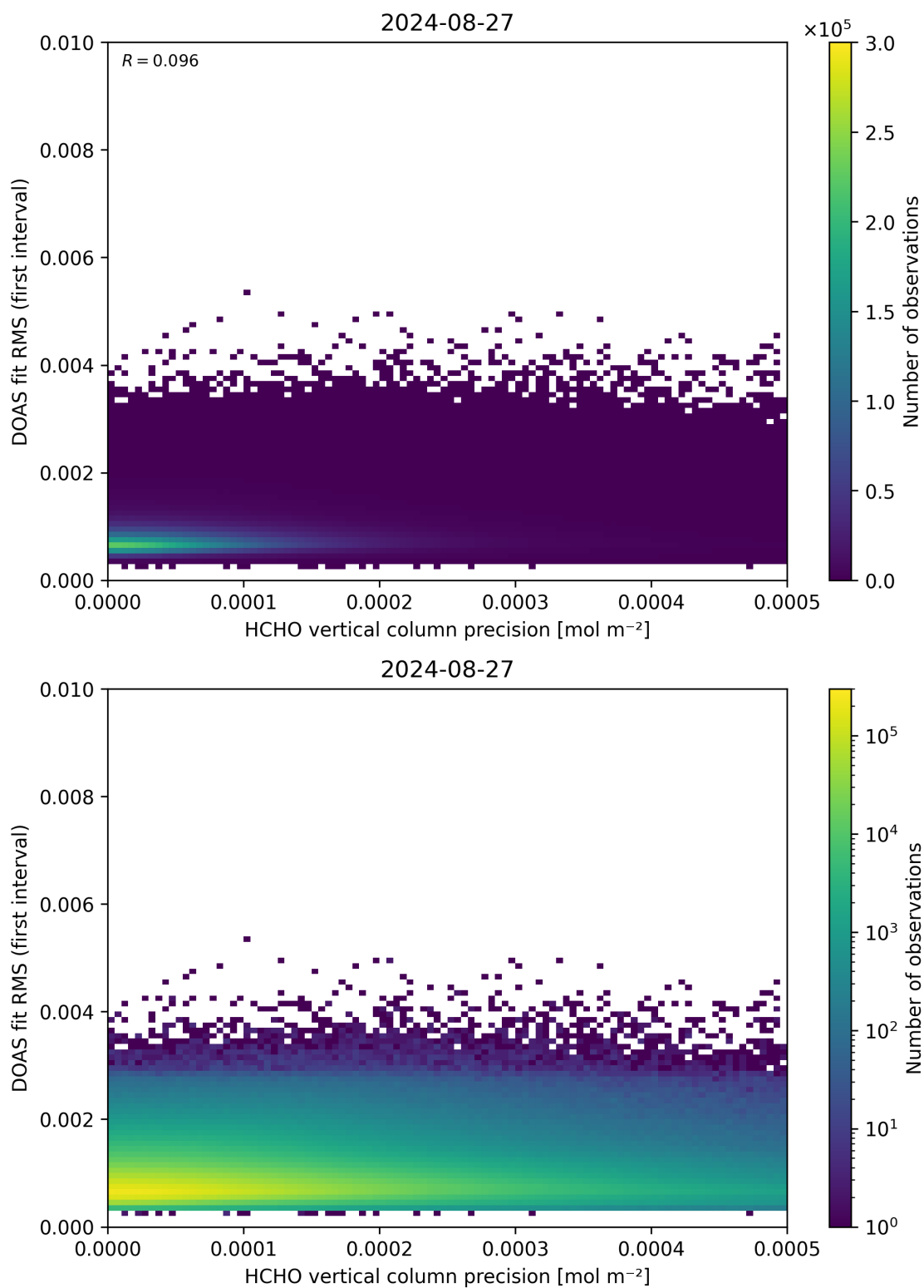
Figure 136: Scatter density plot of “HCHO vertical column precision” against “DOAS fit RMS (first interval)” for 2024-08-27 to 2024-08-28.
