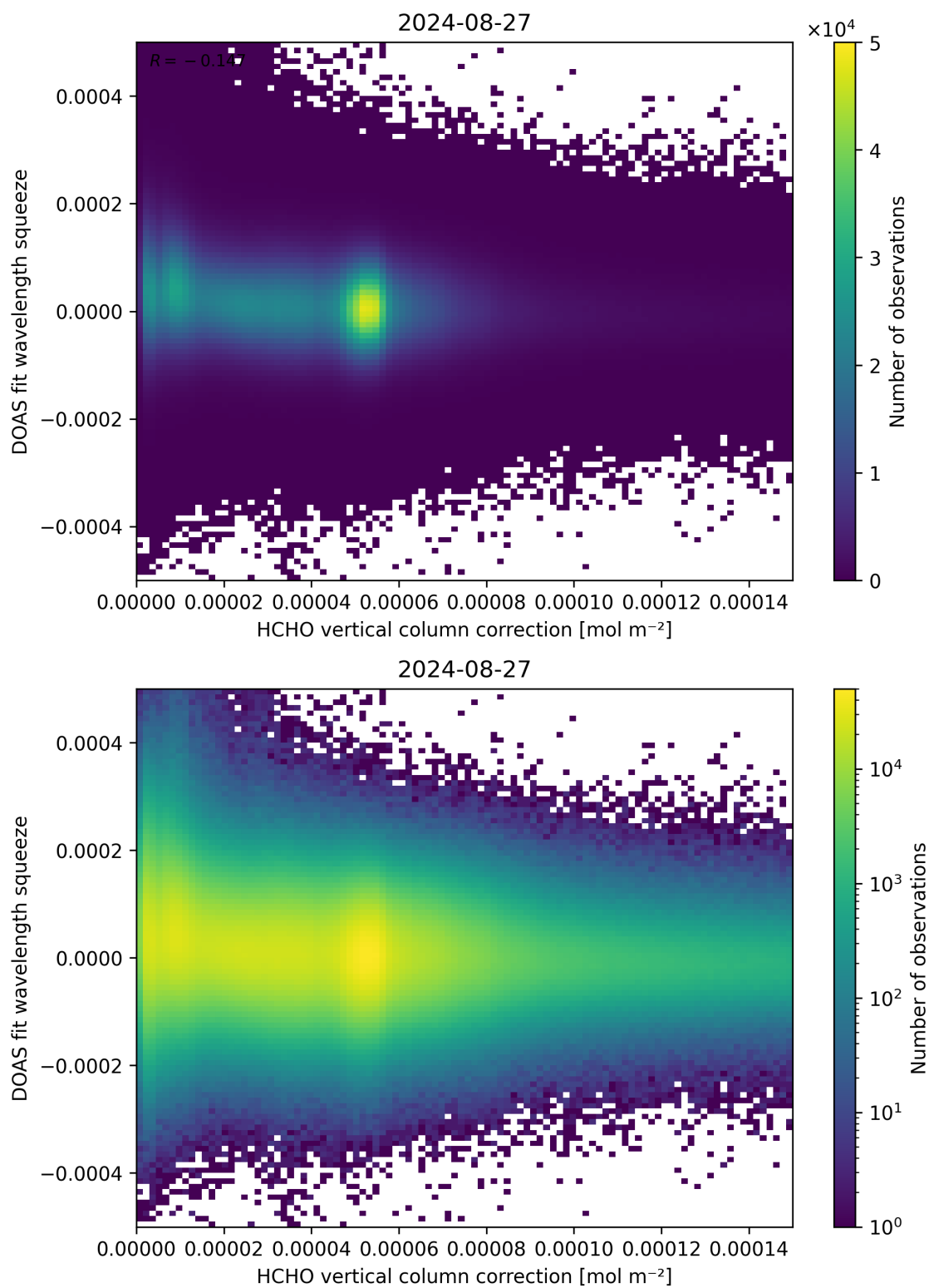
Figure 114: Scatter density plot of “HCHO vertical column correction” against “DOAS fit wavelength squeeze” for 2024-08-27 to 2024-08-28.
