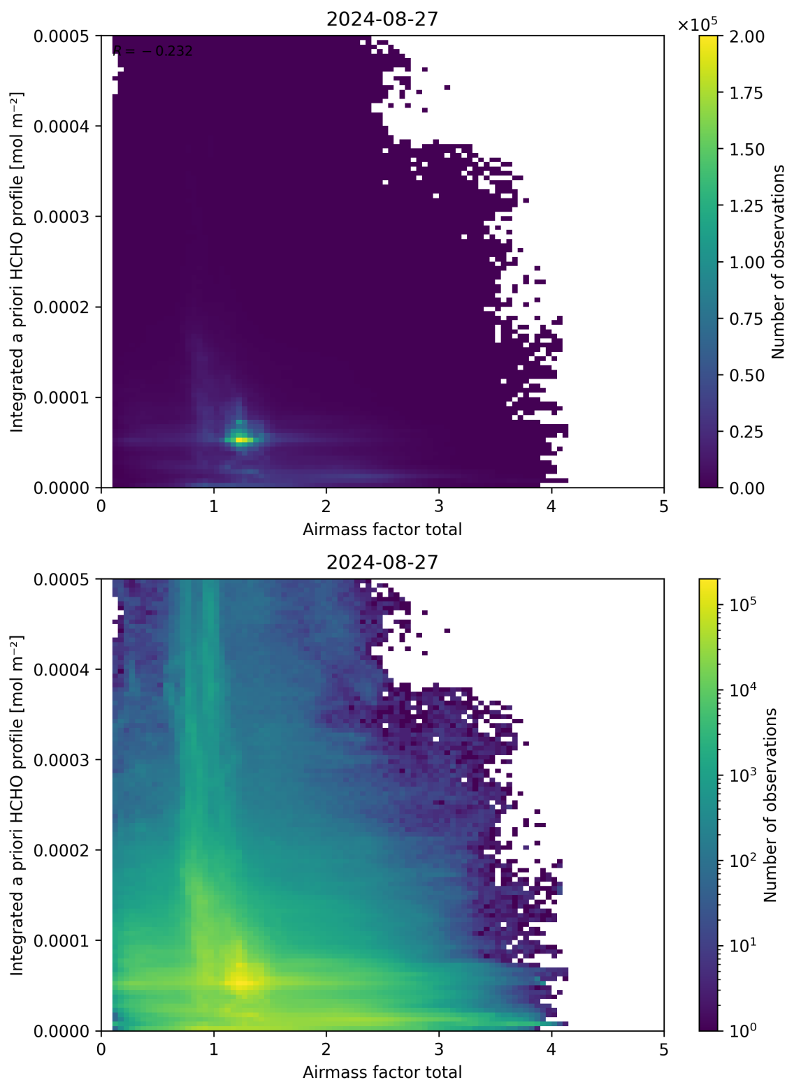
Figure 104: Scatter density plot of “Airmass factor total” against “Integrated a priori HCHO profile” for 2024-08-27 to 2024-08-28.
