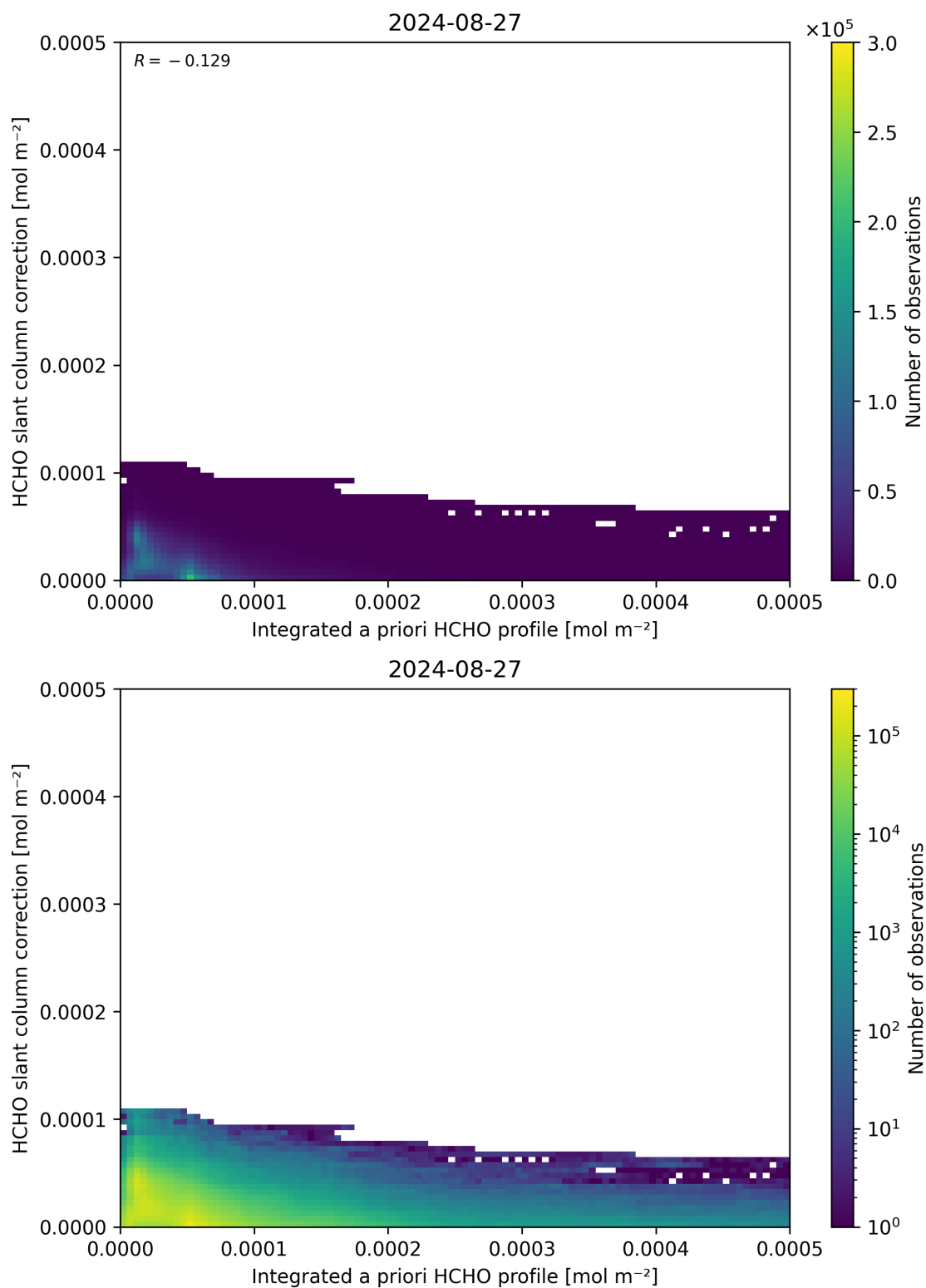
Figure 152: Scatter density plot of “Integrated a priori HCHO profile” against “HCHO slant column correction” for 2024-08-27 to 2024-08-28.
