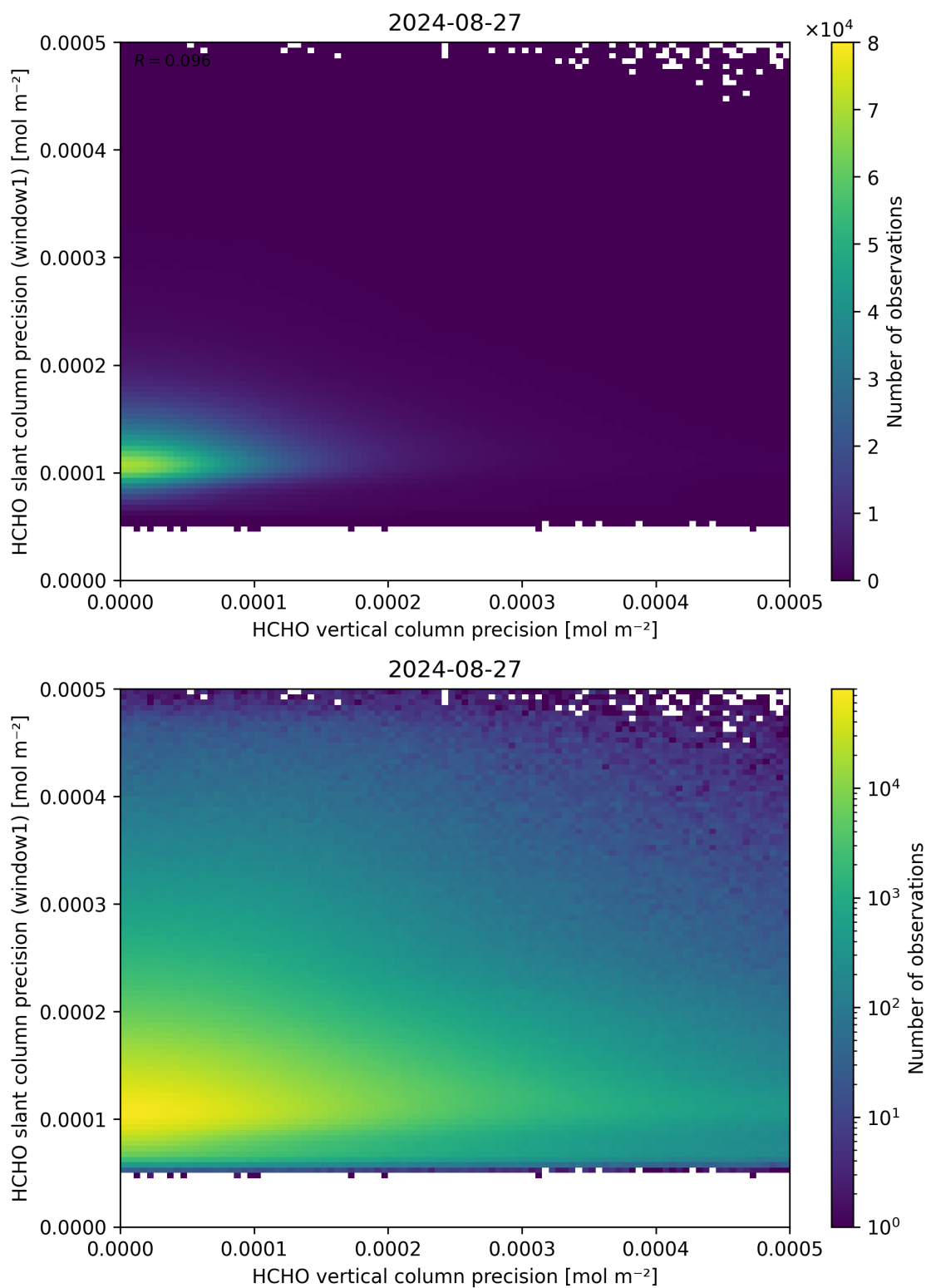
Figure 143: Scatter density plot of “HCHO vertical column precision” against “HCHO slant column precision (window1)” for 2024-08-27 to 2024-08-28.
