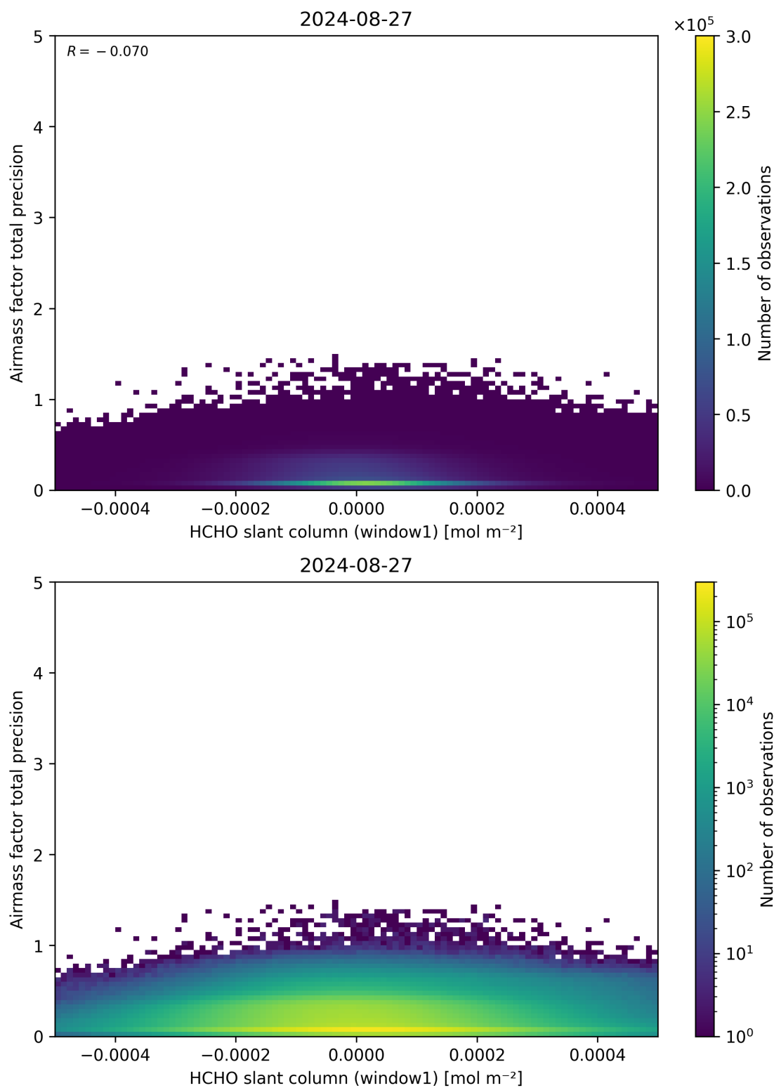
Figure 86: Scatter density plot of “HCHO slant column (window1)” against “Airmass factor total precision” for 2024-08-27 to 2024-08-28.
