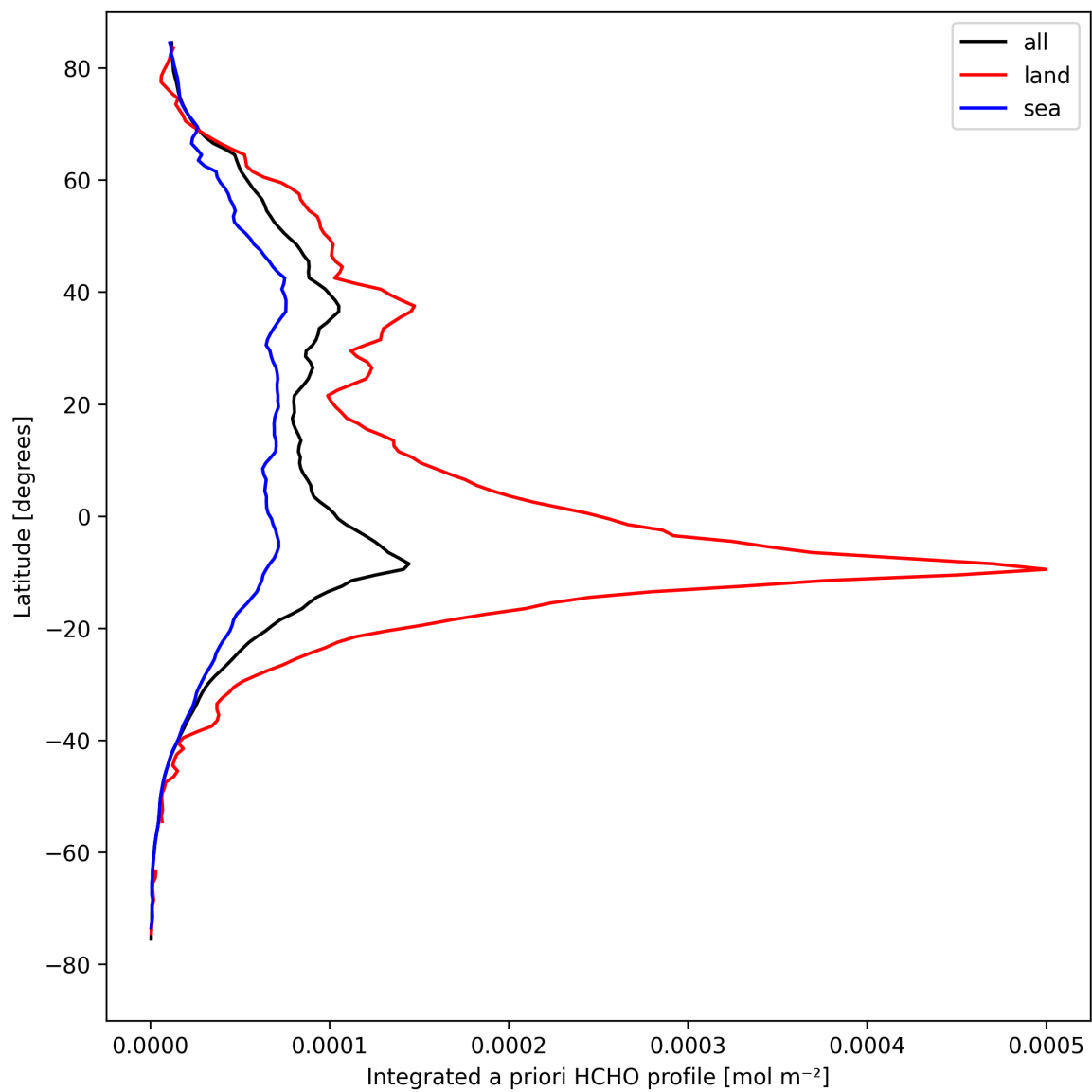
Figure 29: Zonal average of “Integrated a priori HCHO profile” for 2024-08-27 to 2024-08-28.
