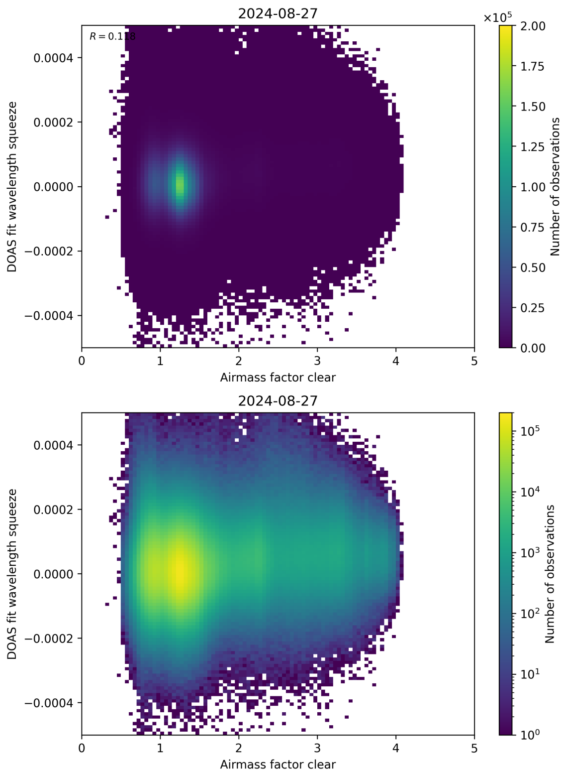
Figure 73: Scatter density plot of “Airmass factor clear” against “DOAS fit wavelength squeeze” for 2024-08-27 to 2024-08-28.
