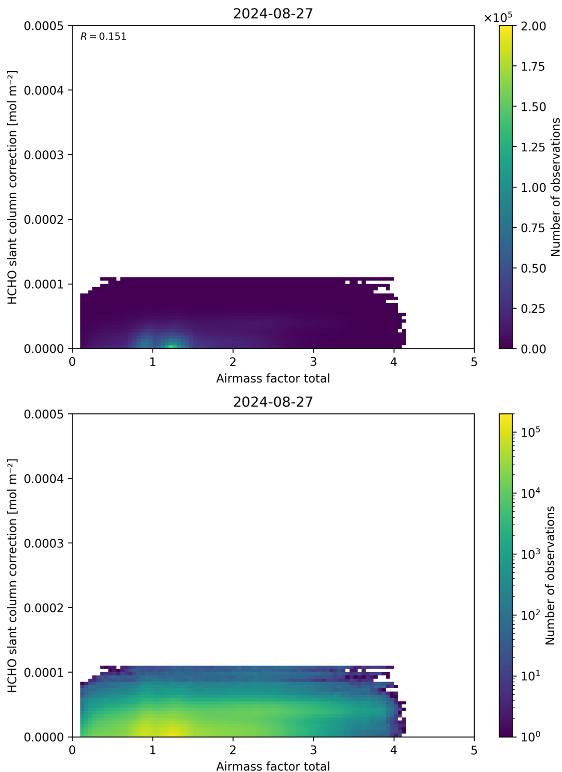
Figure 102: Scatter density plot of “Airmass factor total” against “HCHO slant column correction” for 2024-08-27 to 2024-08-28.
