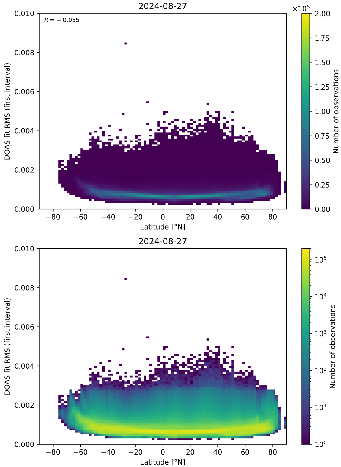
Figure 153: Scatter density plot of “Latitude” against “DOAS fit RMS (first interval)” for 2024-08-27 to 2024-08-28.
