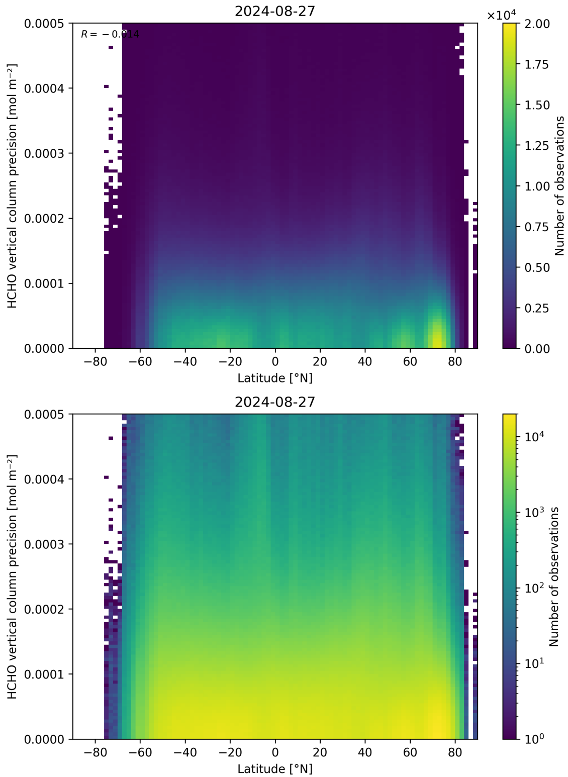
Figure 165: Scatter density plot of “Latitude” against “HCHO vertical column precision” for 2024-08-27 to 2024-08-28.
