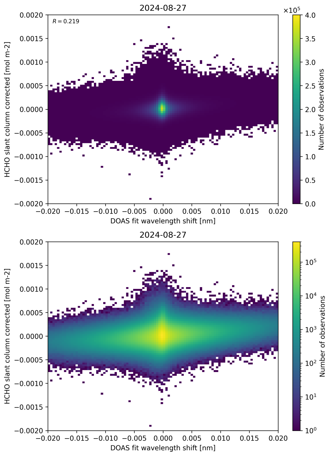
Figure 66: Scatter density plot of “DOAS fit wavelength shift” against “HCHO slant column corrected” for 2024-08-27 to 2024-08-28.
