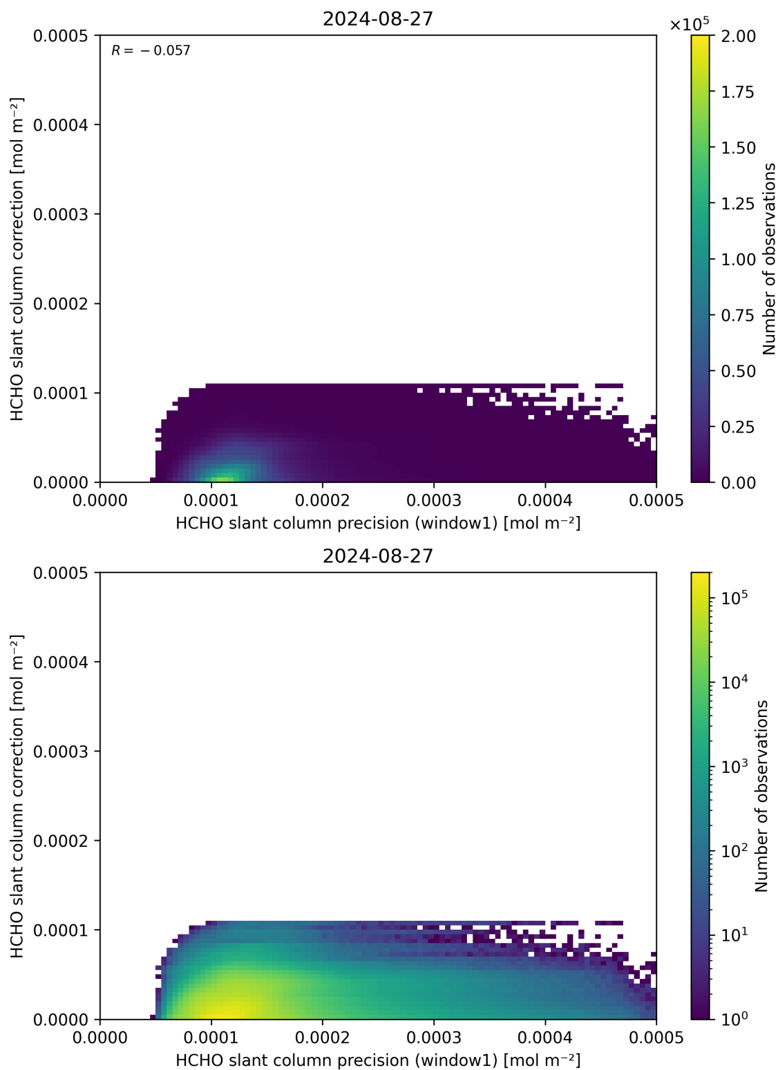
Figure 93: Scatter density plot of “HCHO slant column precision (window1)” against “HCHO slant column correction” for 2024-08-27 to 2024-08-28.
