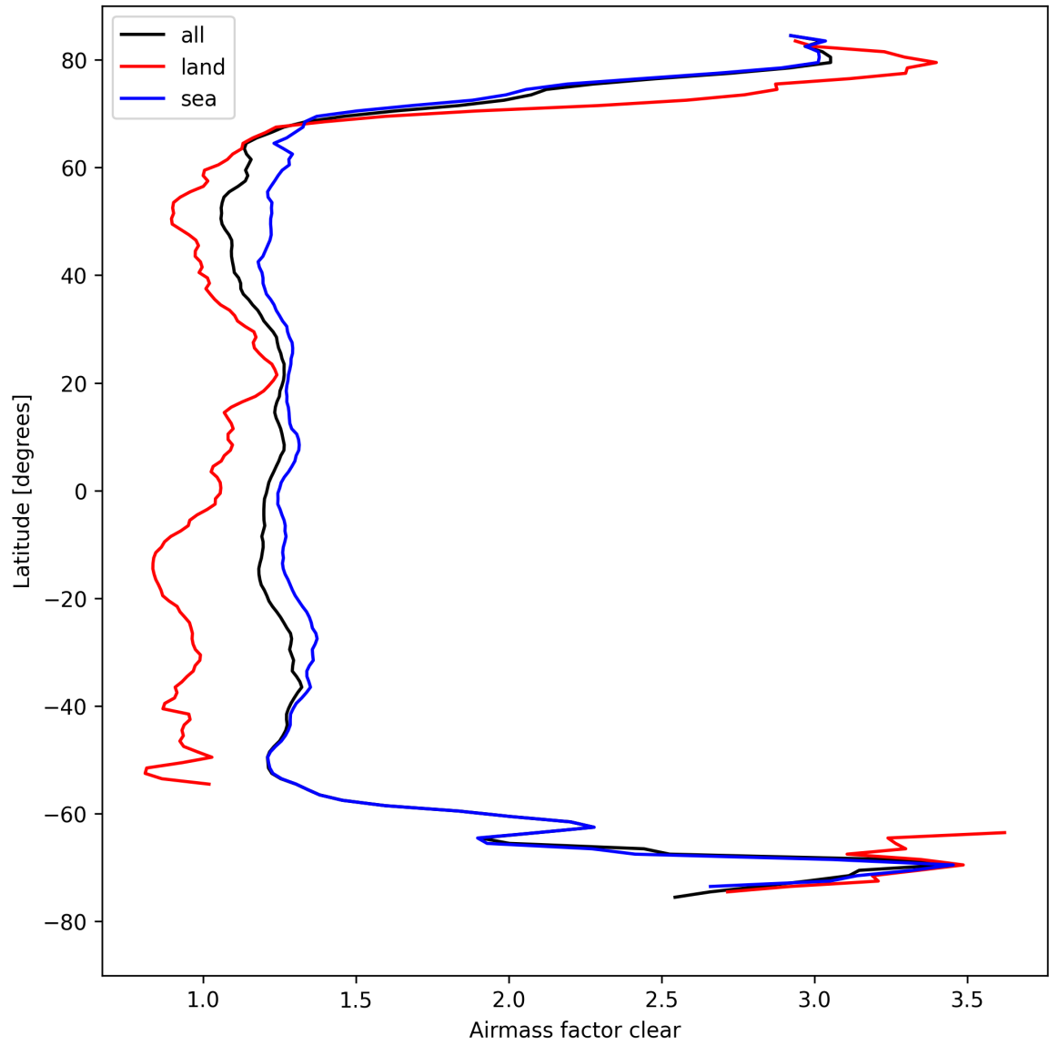
Figure 28: Zonal average of “Airmass factor clear” for 2024-08-27 to 2024-08-28.
