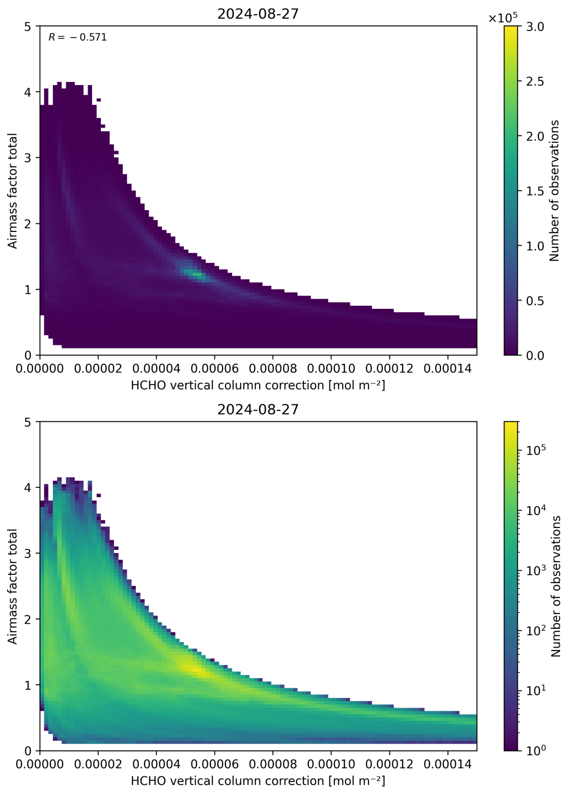
Figure 120: Scatter density plot of “HCHO vertical column correction” against “Airmass factor total” for 2024-08-27 to 2024-08-28.
