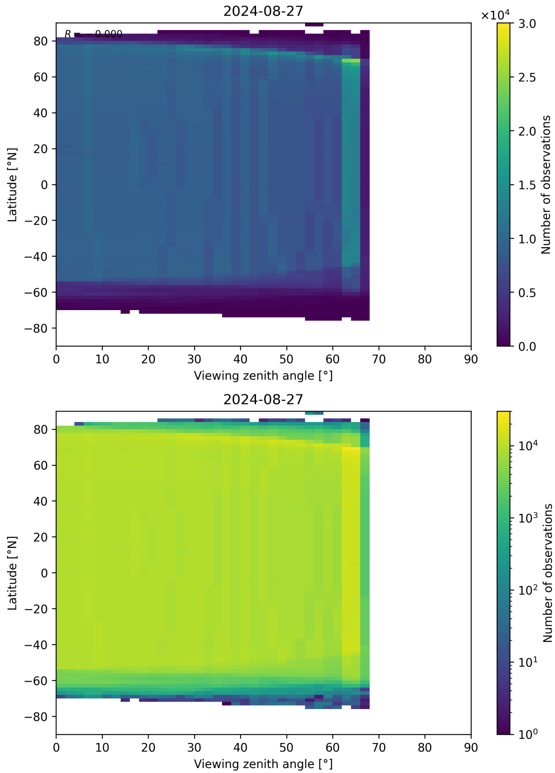
Figure 196: Scatter density plot of “Viewing zenith angle” against “Latitude” for 2024-08-27 to 2024-08-28.
