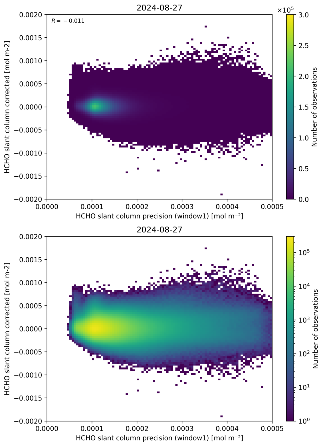
Figure 92: Scatter density plot of “HCHO slant column precision (window1)” against “HCHO slant column corrected” for 2024-08-27 to 2024-08-28.
