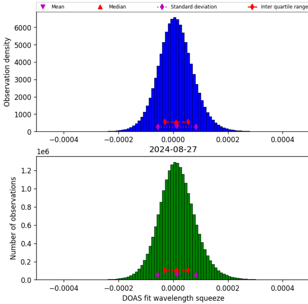
Figure 45: Histogram of “DOAS fit wavelength squeeze” for 2024-08-27 to 2024-08-28
