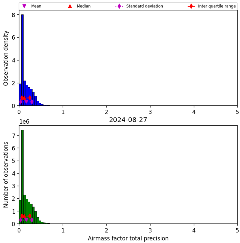
Figure 41: Histogram of “Airmass factor total precision” for 2024-08-27 to 2024-08-28
