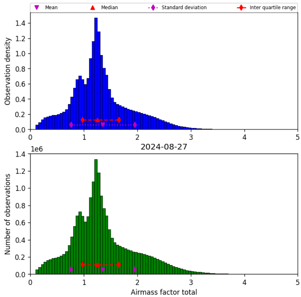
Figure 40: Histogram of “Airmass factor total” for 2024-08-27 to 2024-08-28
