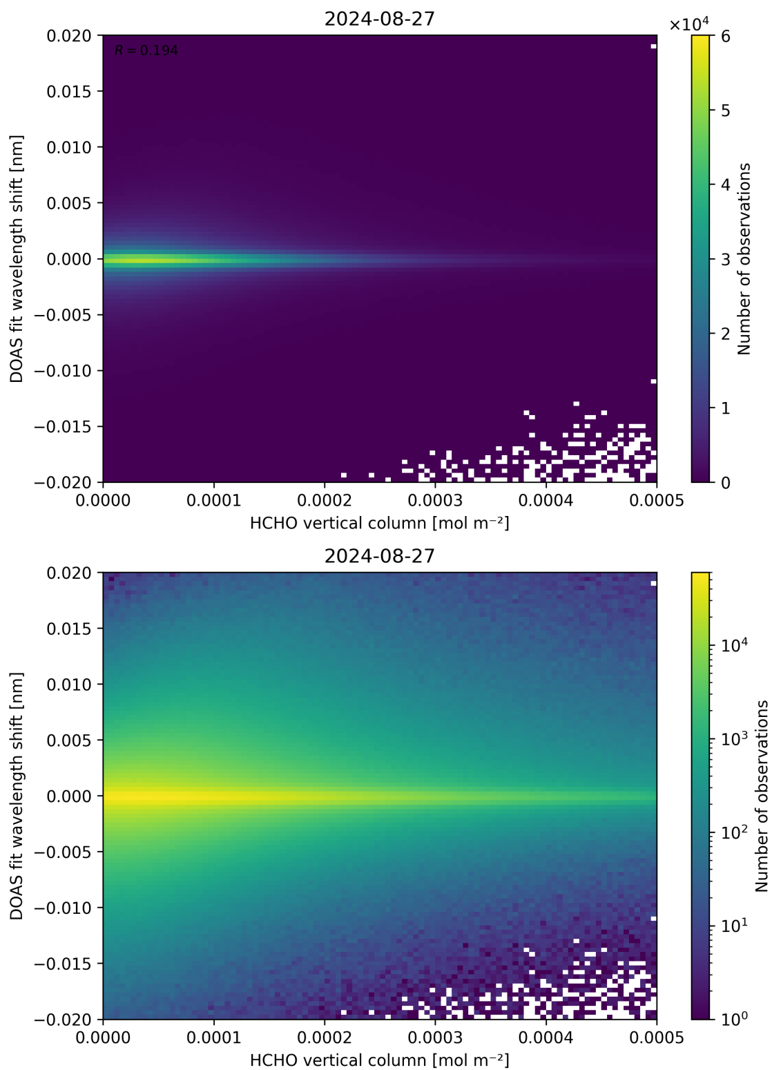
Figure 124: Scatter density plot of “HCHO vertical column” against “DOAS fit wavelength shift” for 2024-08-27 to 2024-08-28.
