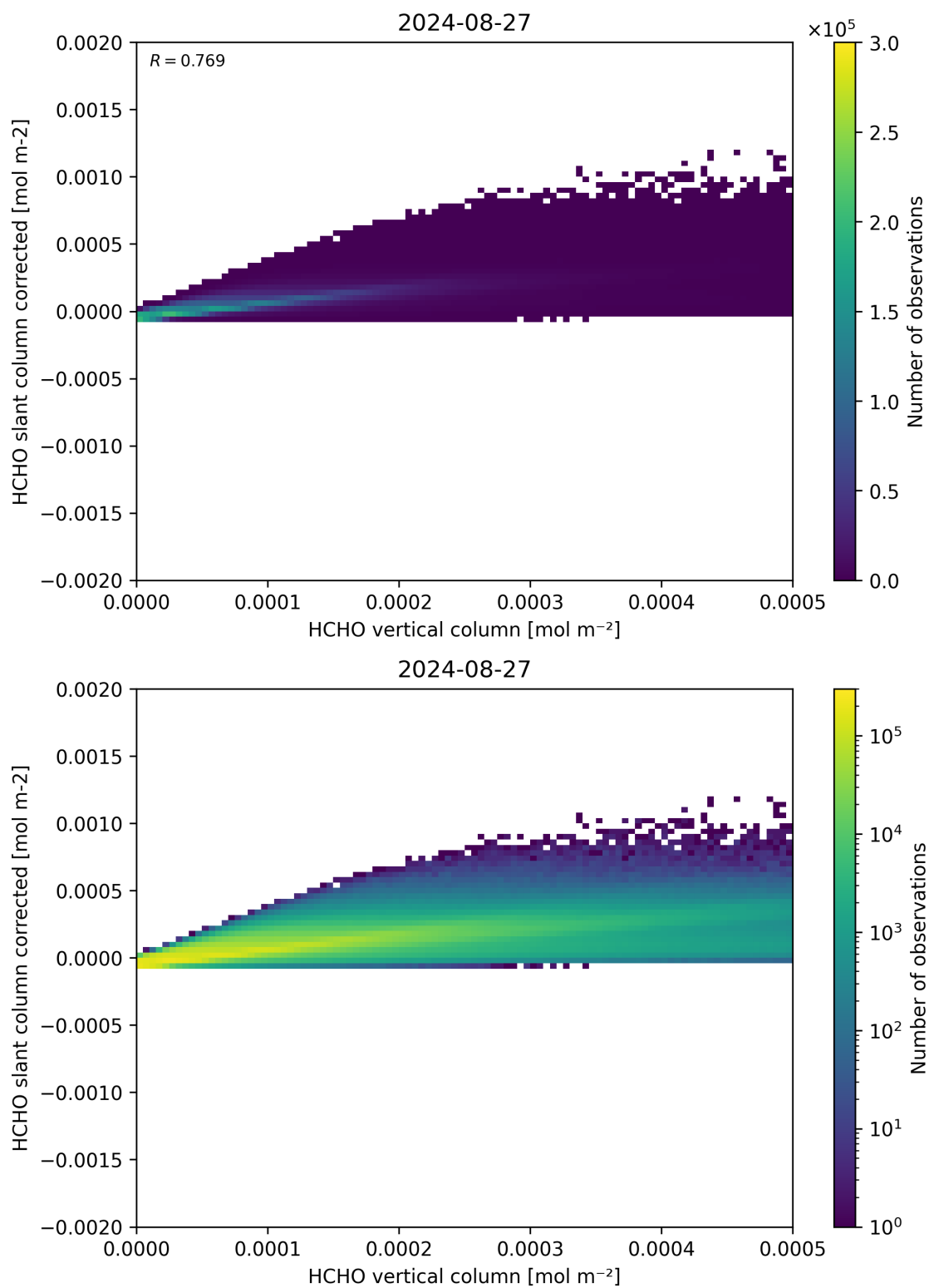
Figure 127: Scatter density plot of “HCHO vertical column” against “HCHO slant column corrected” for 2024-08-27 to 2024-08-28.
