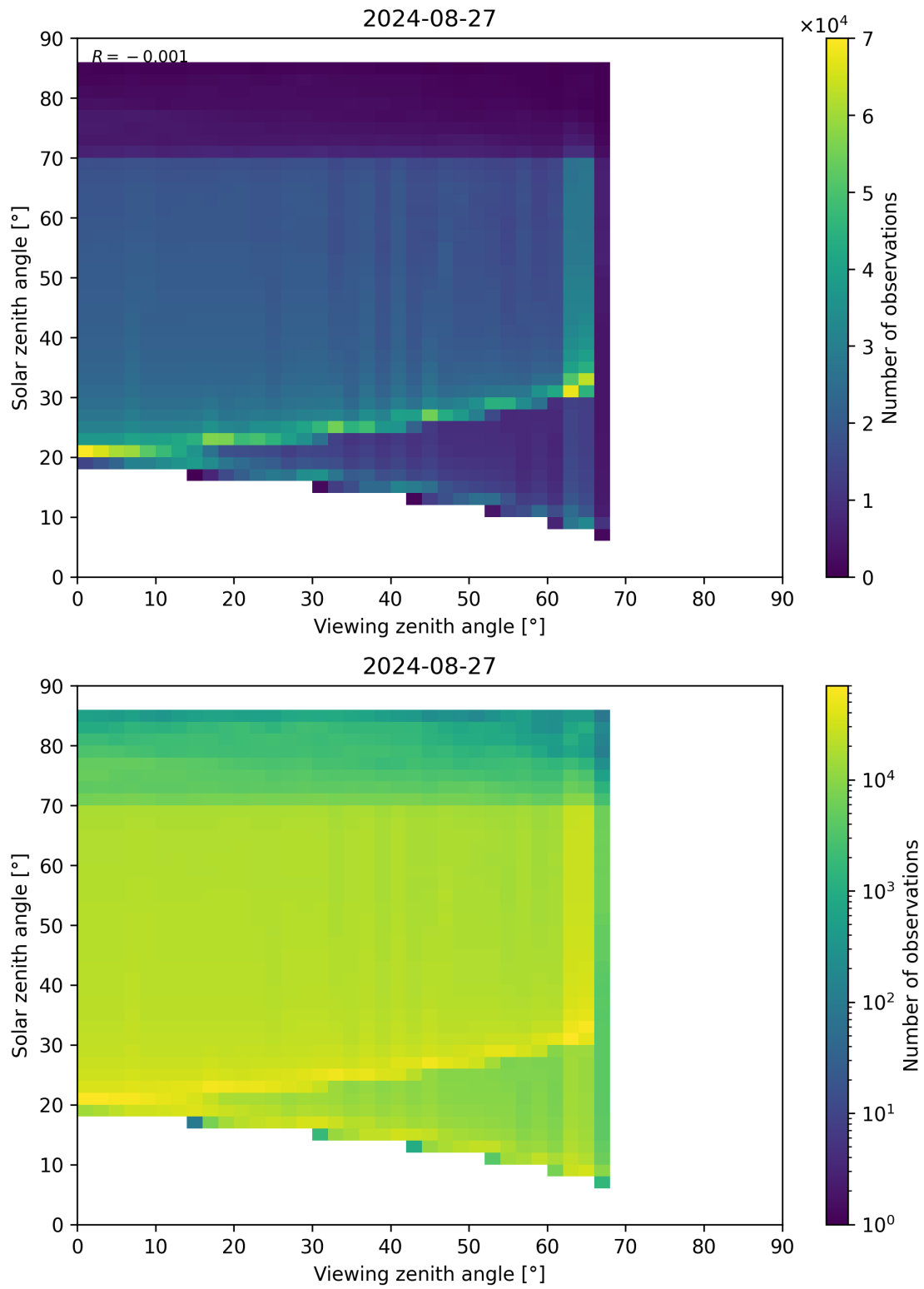
Figure 197: Scatter density plot of “Viewing zenith angle” against “Solar zenith angle” for 2024-08-27 to 2024-08-28.
