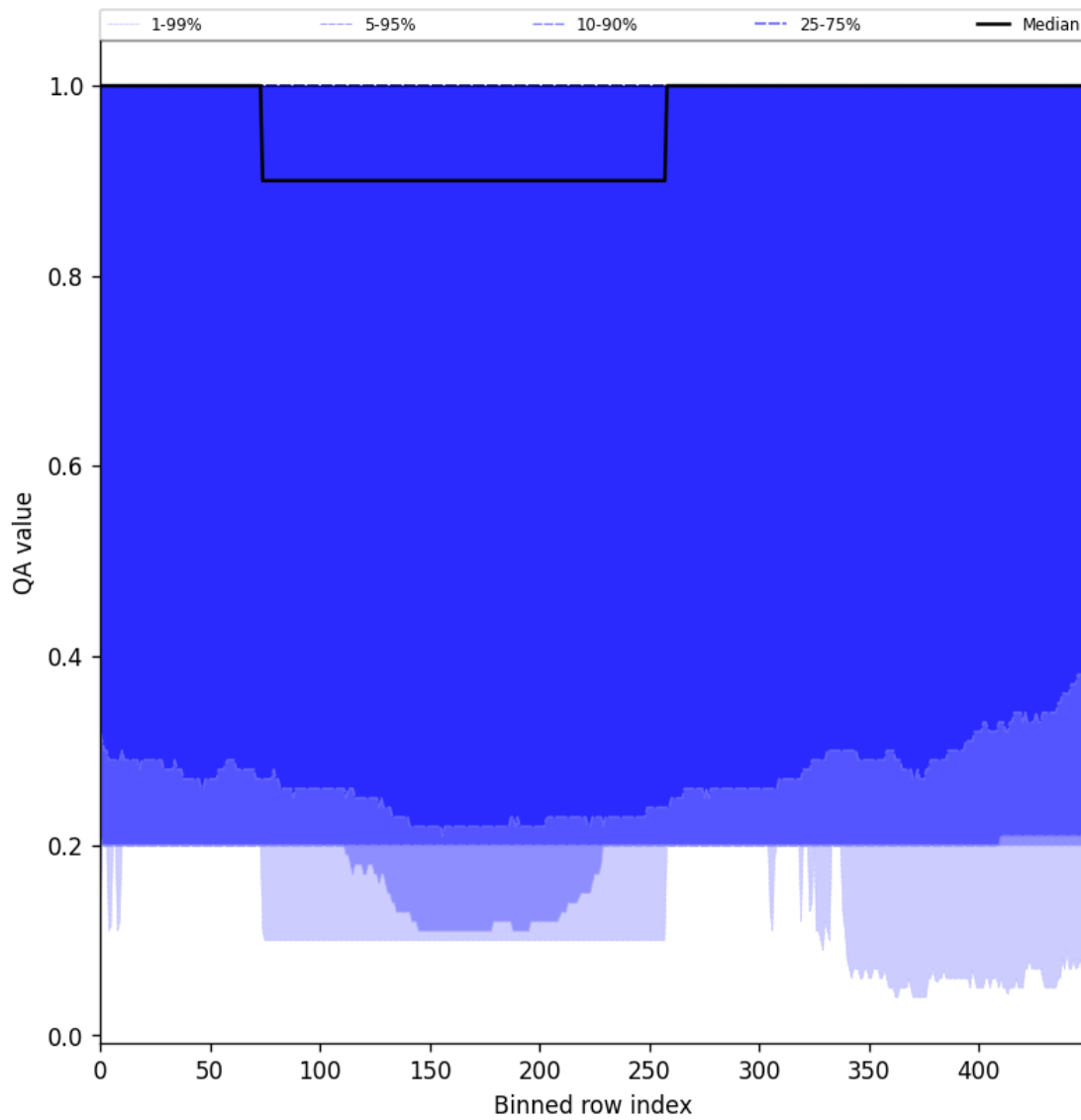
Figure 48: Along track statistics of “QA value” for 2024-08-27 to 2024-08-28
