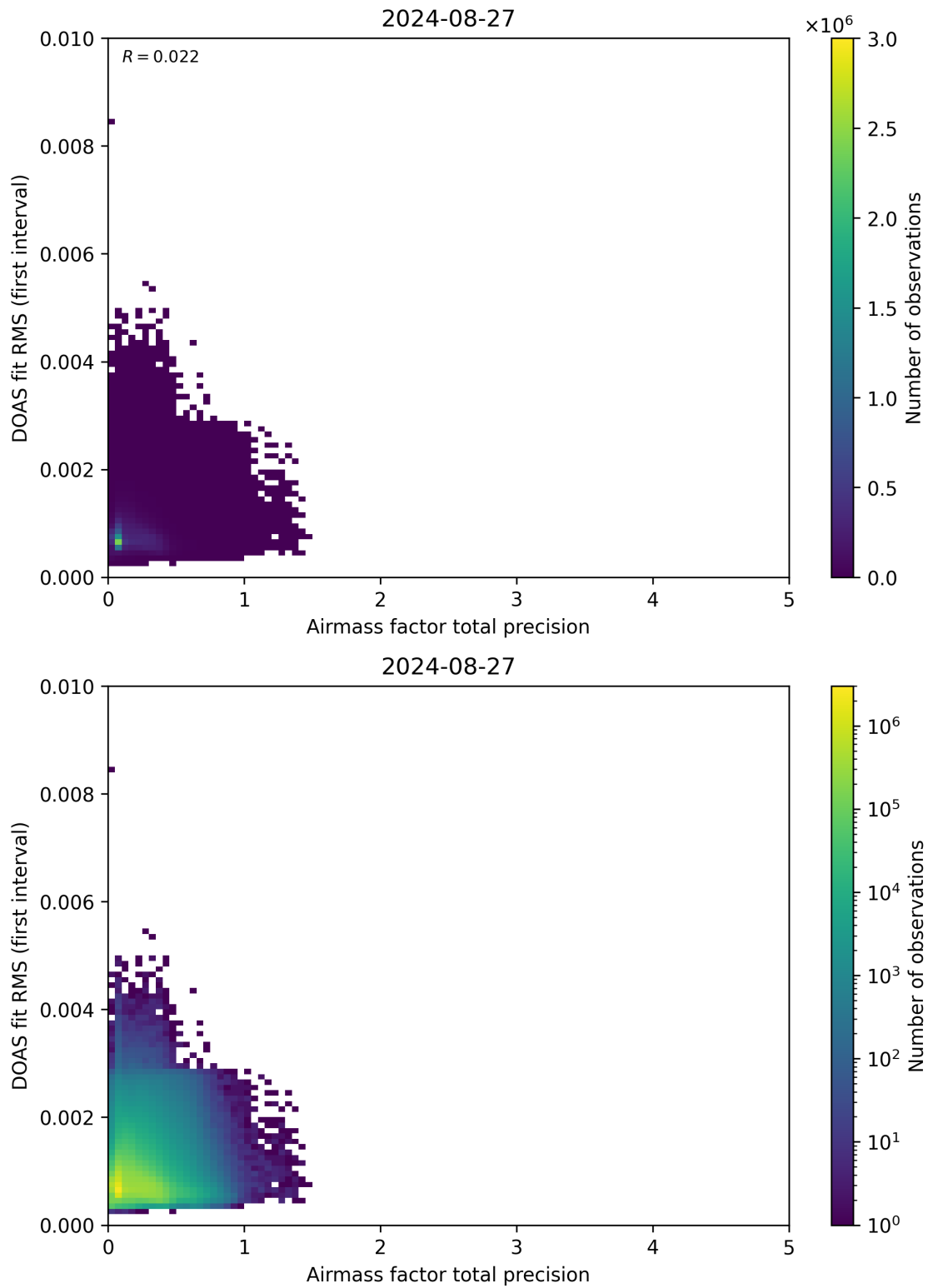
Figure 105: Scatter density plot of “Airmass factor total precision” against “DOAS fit RMS (first interval)” for 2024-08-27 to 2024-08-28.
