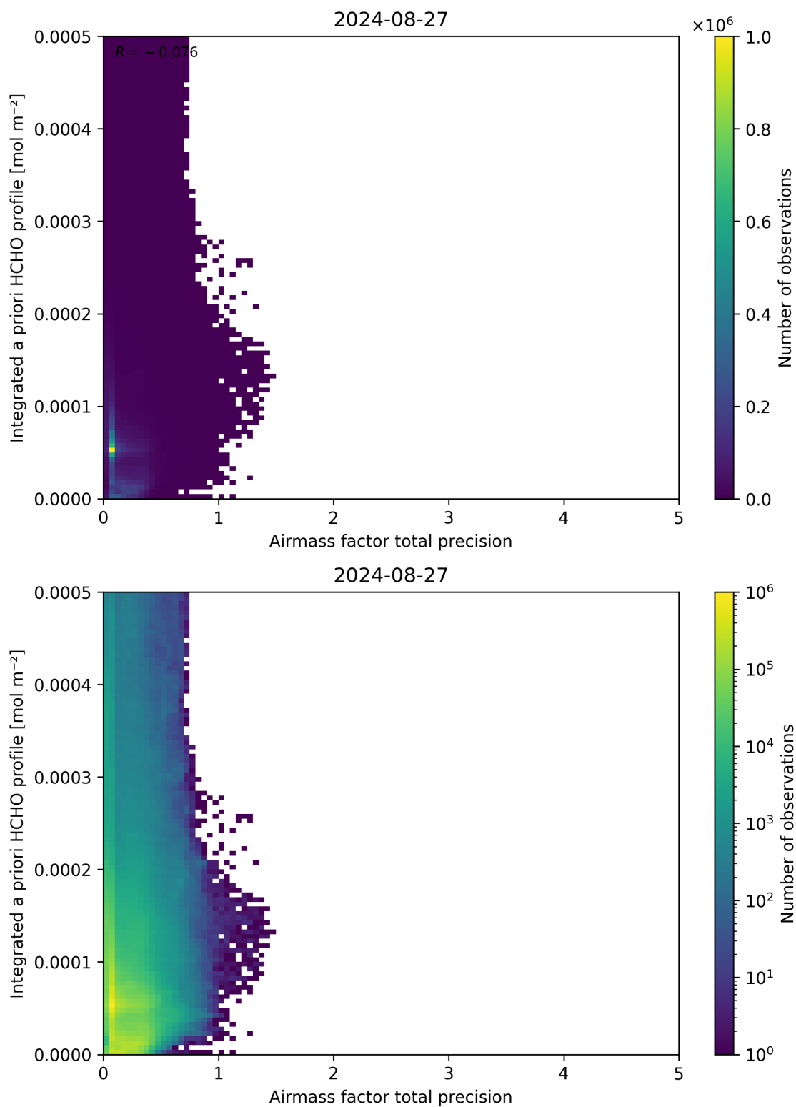
Figure 111: Scatter density plot of “Airmass factor total precision” against “Integrated a priori HCHO profile” for 2024-08-27 to 2024-08-28.
