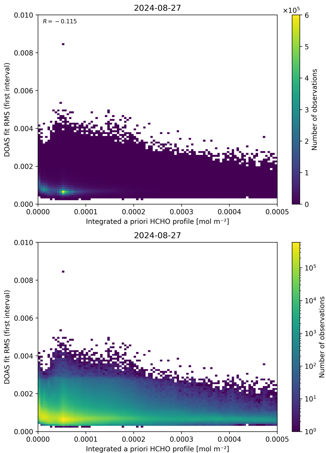
Figure 148: Scatter density plot of “Integrated a priori HCHO profile” against “DOAS fit RMS (first interval)” for 2024-08-27 to 2024-08-28.
