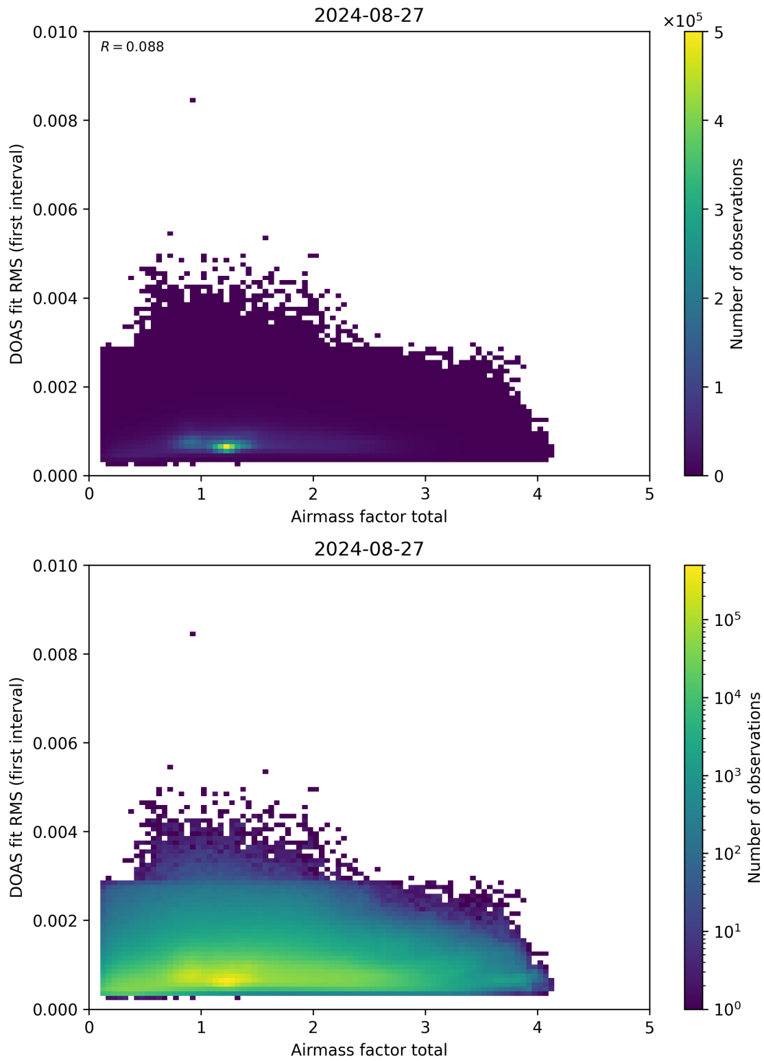
Figure 97: Scatter density plot of “Airmass factor total” against “DOAS fit RMS (first interval)” for 2024-08-27 to 2024-08-28.
