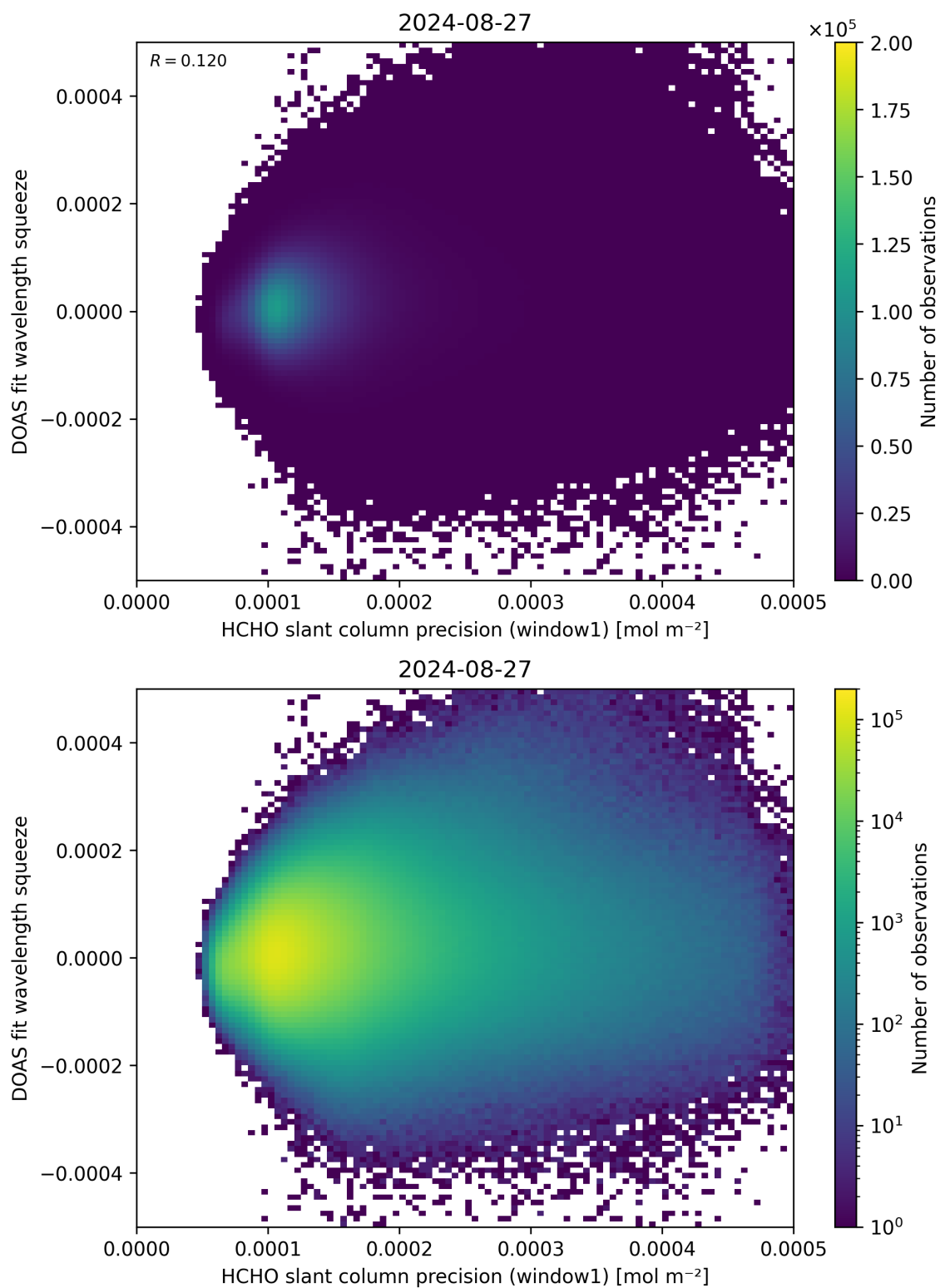
Figure 90: Scatter density plot of “HCHO slant column precision (window1)” against “DOAS fit wavelength squeeze” for 2024-08-27 to 2024-08-28.
