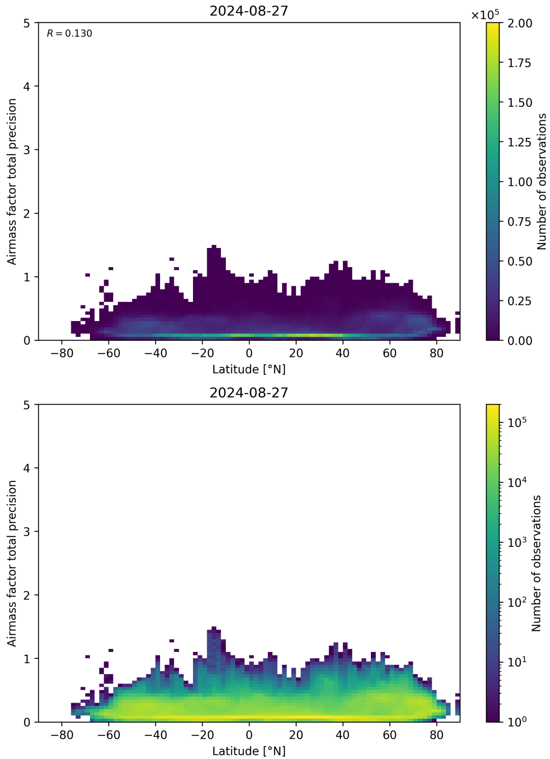
Figure 162: Scatter density plot of “Latitude” against “Airmass factor total precision” for 2024-08-27 to 2024-08-28.
