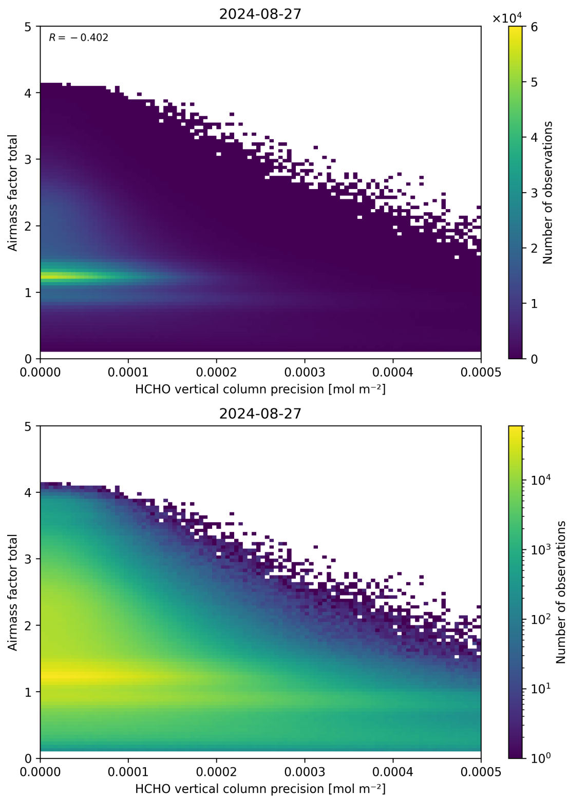
Figure 144: Scatter density plot of “HCHO vertical column precision” against “Airmass factor total” for 2024-08-27 to 2024-08-28.
