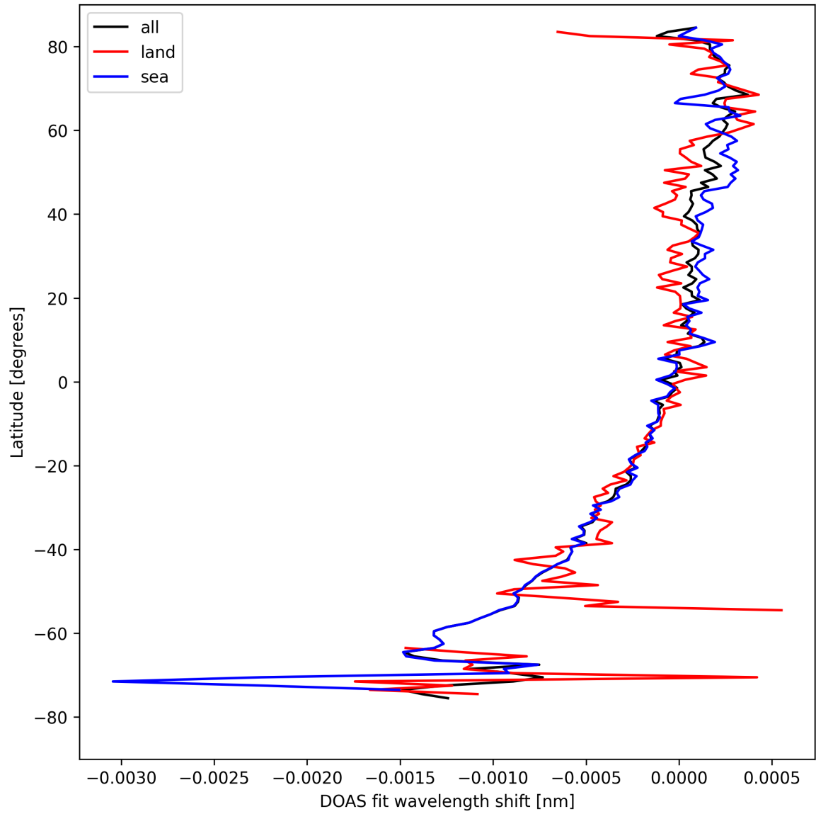
Figure 30: Zonal average of “DOAS fit wavelength shift” for 2024-08-27 to 2024-08-28.
