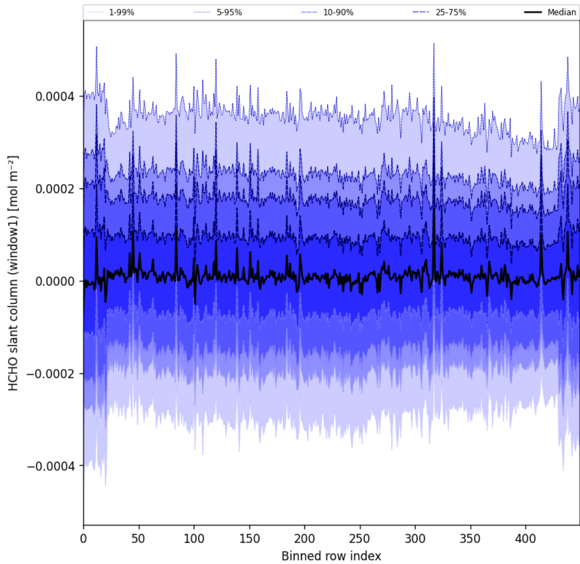
Figure 52: Along track statistics of "HCHO slant column (window1)" for 2024-08-27 to 2024-08-28
