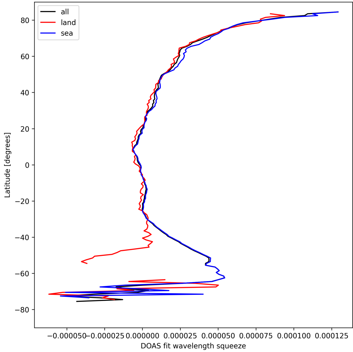
Figure 31: Zonal average of “DOAS fit wavelength squeeze” for 2024-08-27 to 2024-08-28.
