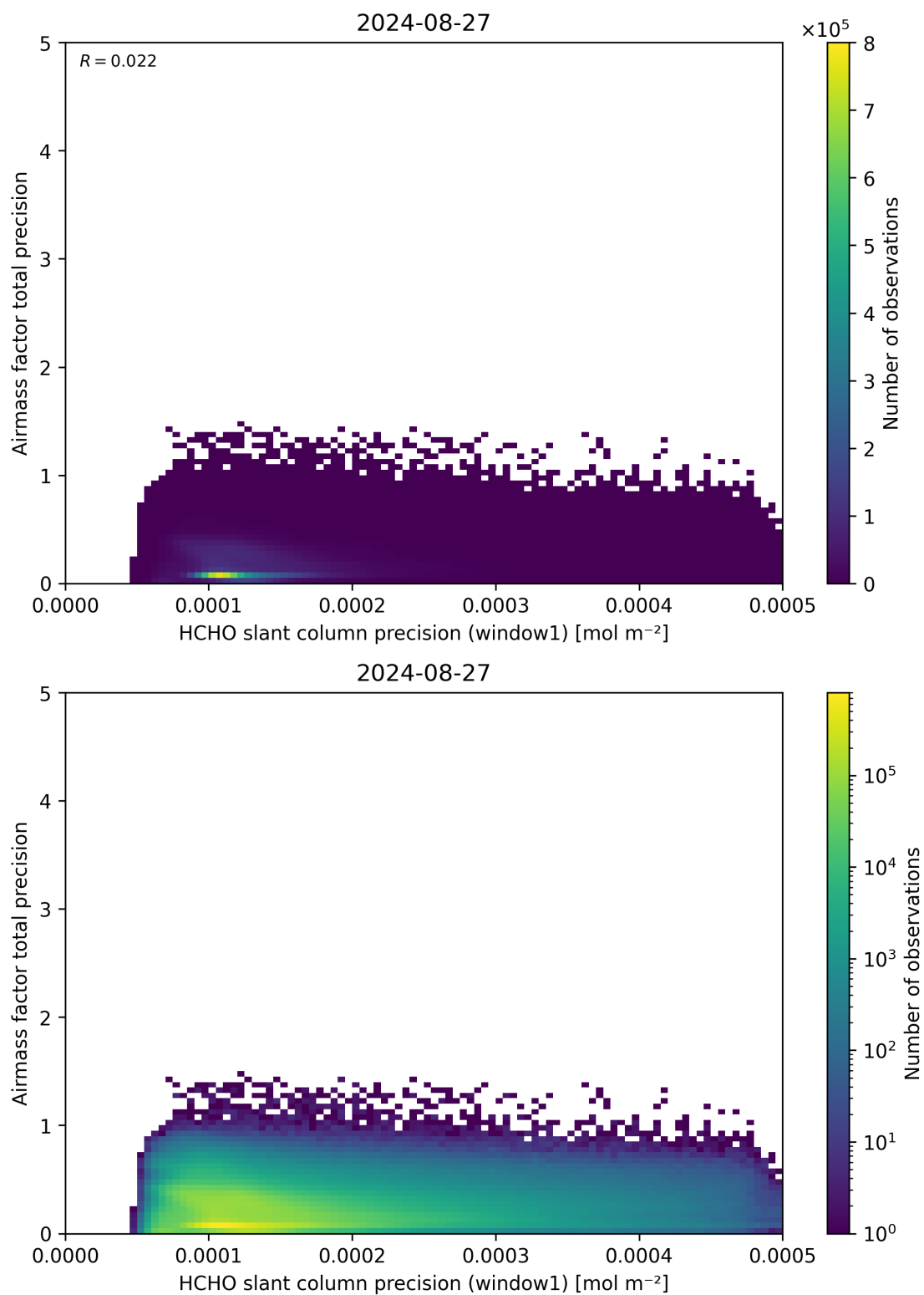
Figure 95: Scatter density plot of “HCHO slant column precision (window1)” against “Airmass factor total precision” for 2024-08-27 to 2024-08-28.
