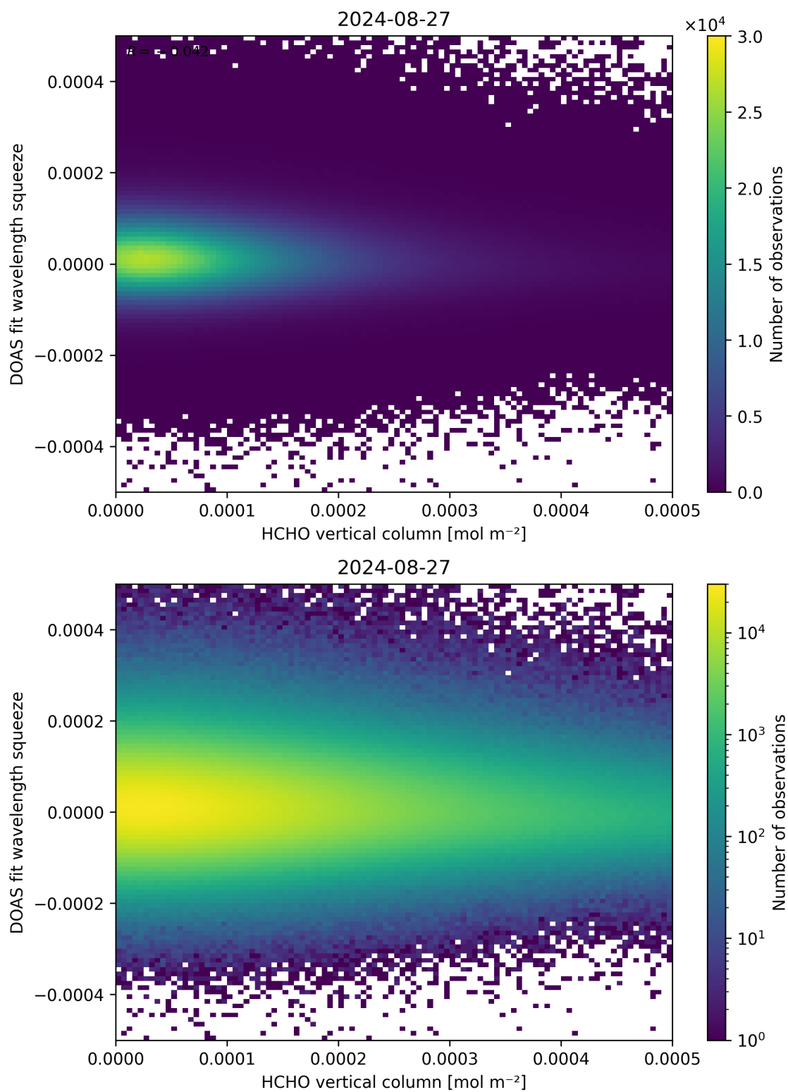
Figure 125: Scatter density plot of “HCHO vertical column” against “DOAS fit wavelength squeeze” for 2024-08-27 to 2024-08-28.
