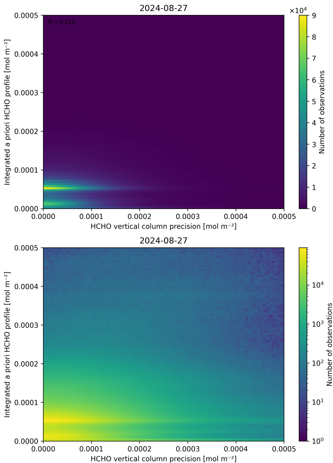
Figure 147: Scatter density plot of “HCHO vertical column precision” against “Integrated a priori HCHO profile” for 2024-08-27 to 2024-08-28.
