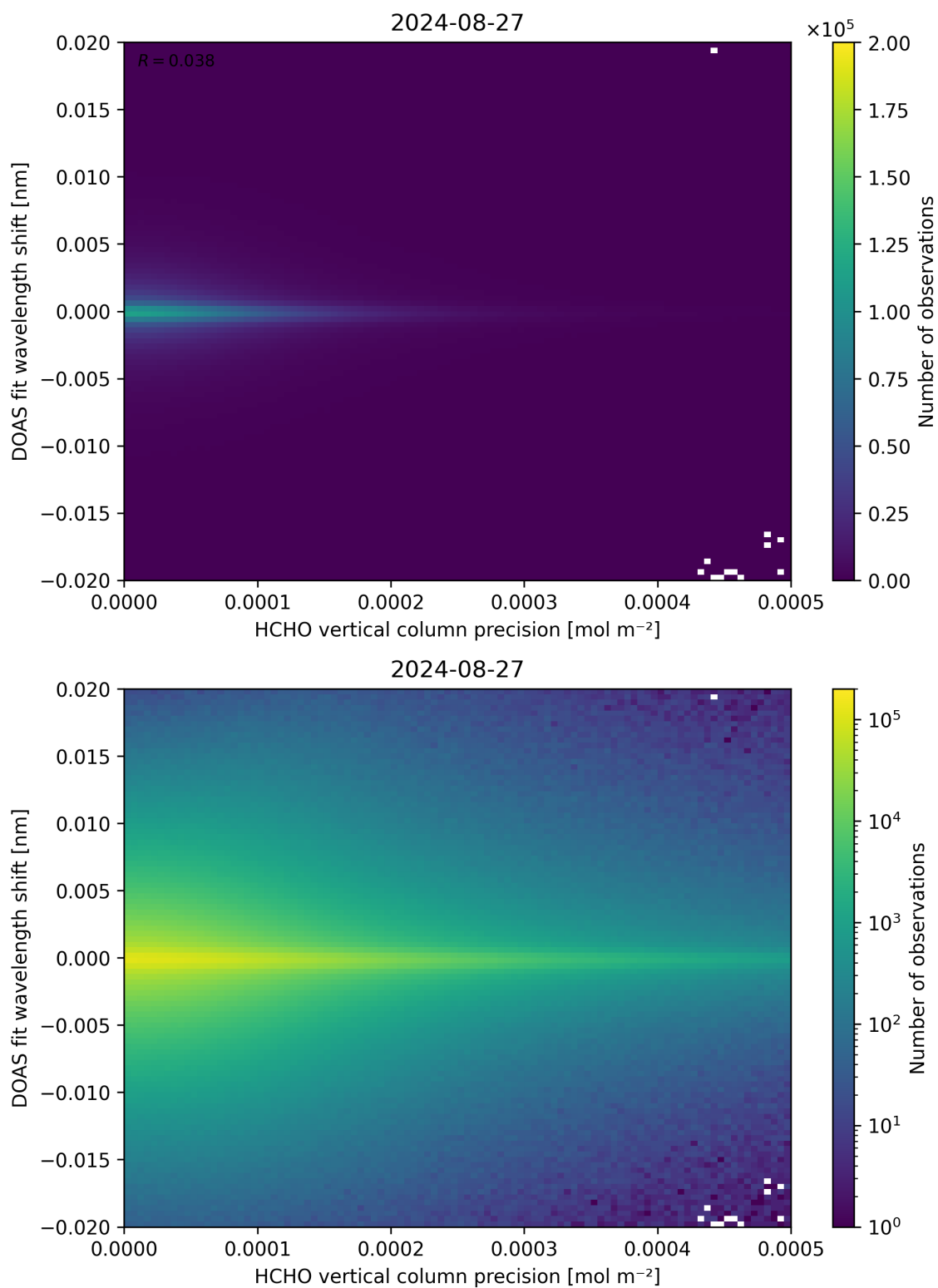
Figure 137: Scatter density plot of “HCHO vertical column precision” against “DOAS fit wavelength shift” for 2024-08-27 to 2024-08-28.
