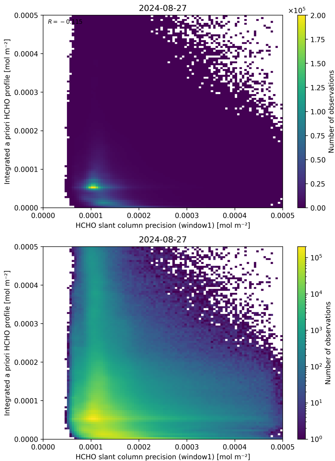
Figure 96: Scatter density plot of “HCHO slant column precision (window1)” against “Integrated a priori HCHO profile” for 2024-08-27 to 2024-08-28.
