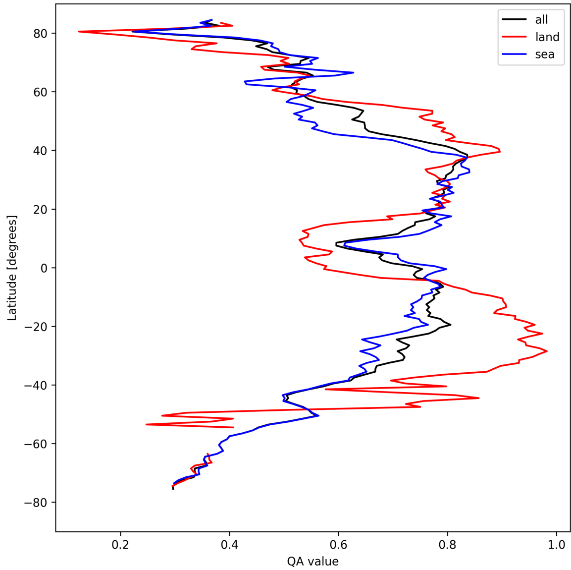
Figure 20: Zonal average of “QA value” for 2024-08-27 to 2024-08-28.
