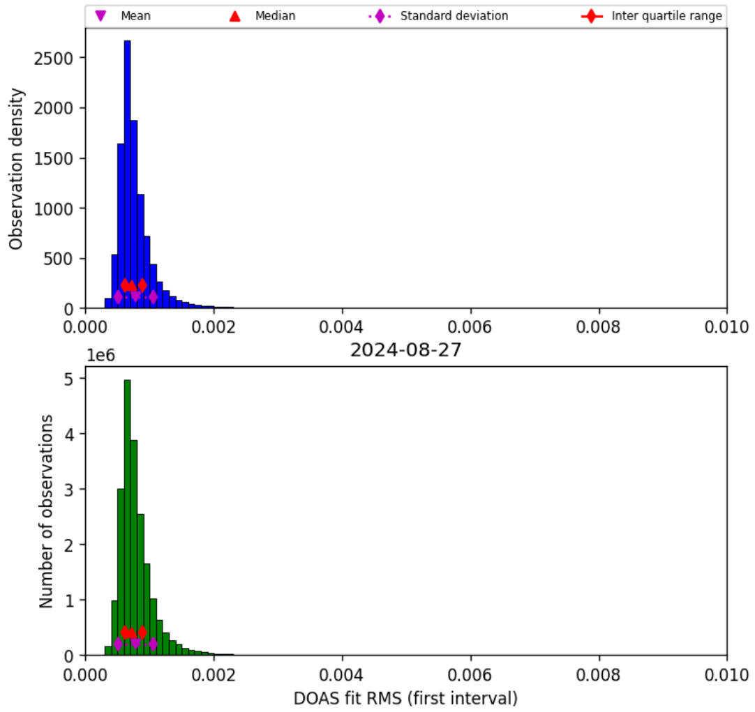
Figure 46: Histogram of “DOAS fit RMS (first interval)” for 2024-08-27 to 2024-08-28
