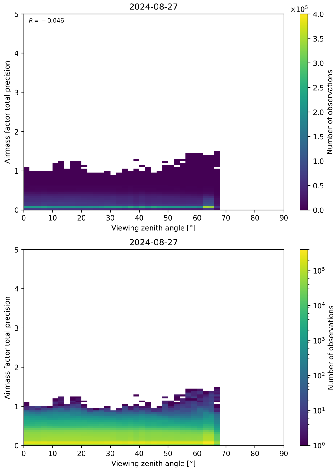
Figure 191: Scatter density plot of “Viewing zenith angle” against “Airmass factor total precision” for 2024-08-27 to 2024-08-28.
