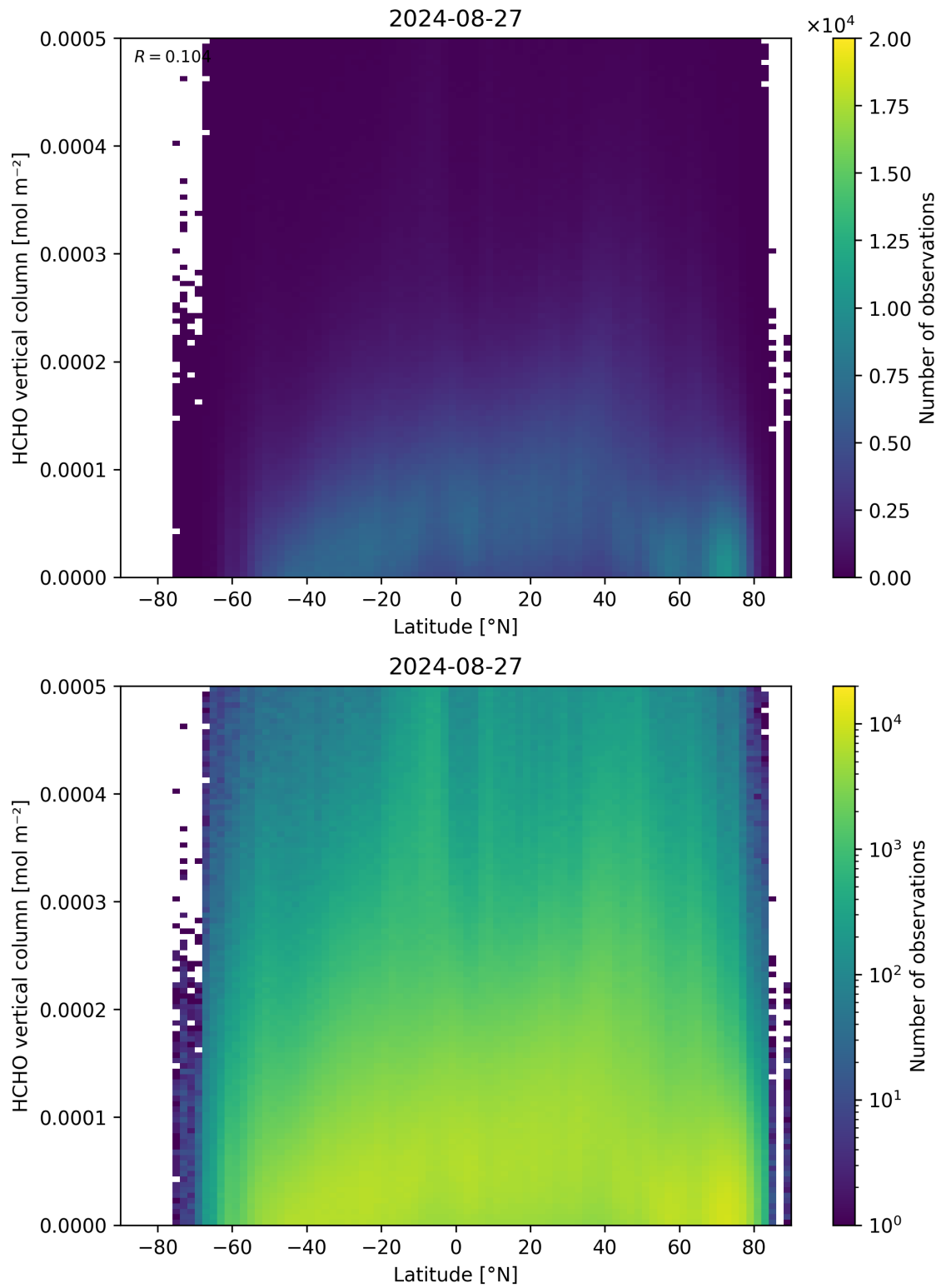
Figure 163: Scatter density plot of “Latitude” against “HCHO vertical column” for 2024-08-27 to 2024-08-28.
