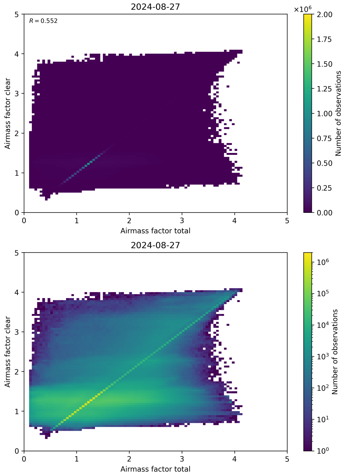
Figure 100: Scatter density plot of “Airmass factor total” against “Airmass factor clear” for 2024-08-27 to 2024-08-28.
