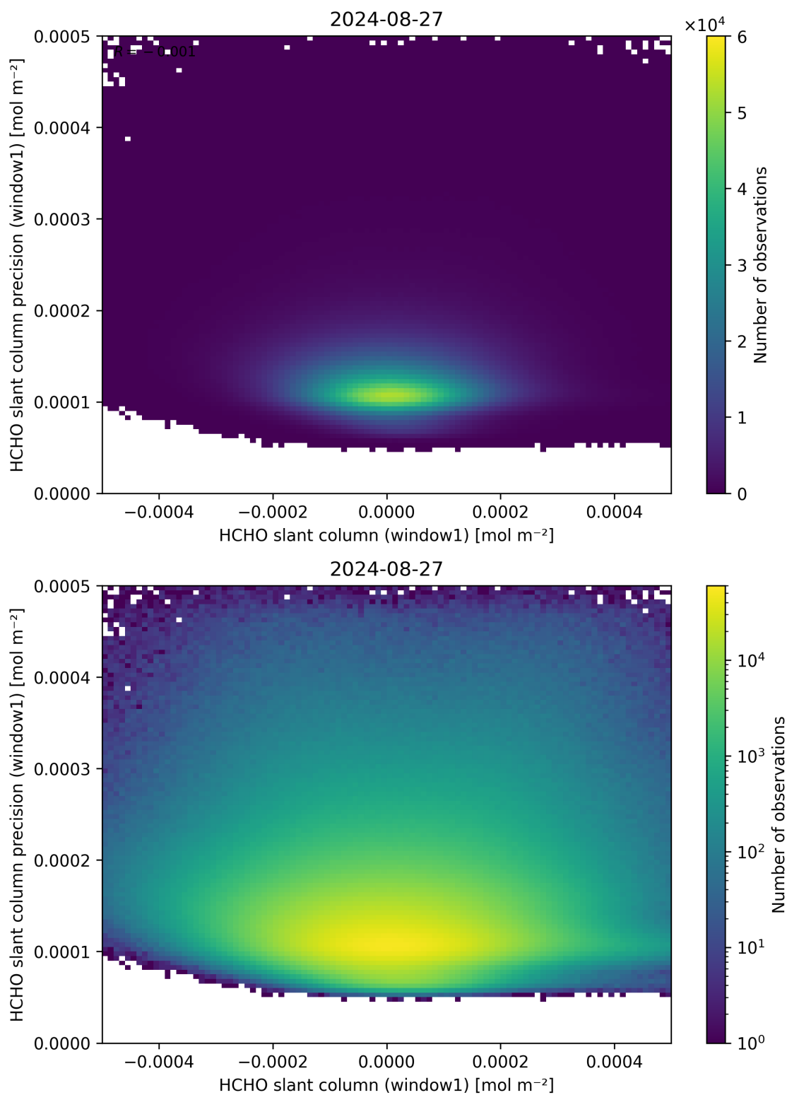
Figure 84: Scatter density plot of “HCHO slant column (window1)” against “HCHO slant column precision (window1)” for 2024-08-27 to 2024-08-28.
