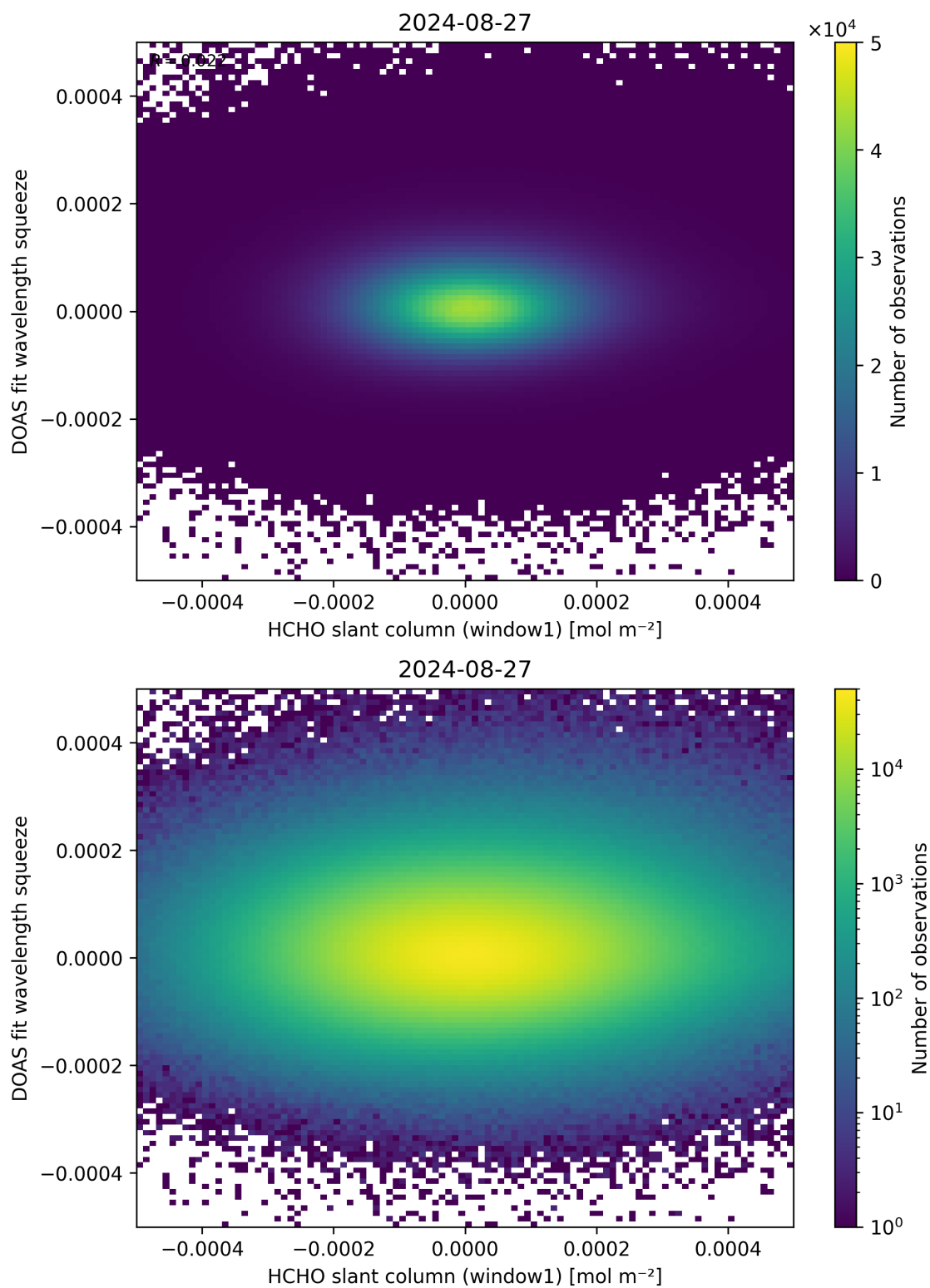
Figure 80: Scatter density plot of “HCHO slant column (window1)” against “DOAS fit wavelength squeeze” for 2024-08-27 to 2024-08-28.
