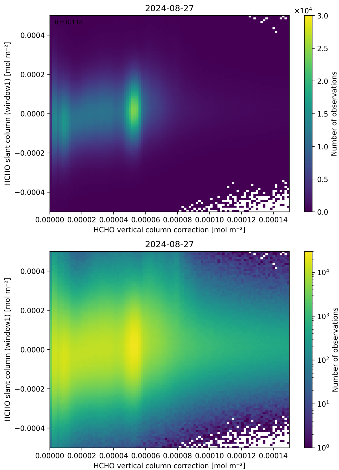
Figure 118: Scatter density plot of “HCHO vertical column correction” against “HCHO slant column (window1)” for 2024-08-27 to 2024-08-28.
