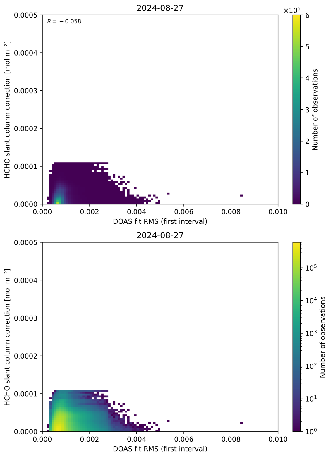
Figure 63: Scatter density plot of “DOAS fit RMS (first interval)” against “HCHO slant column correction” for 2024-08-27 to 2024-08-28.
