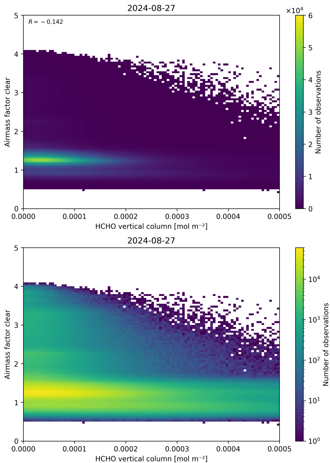
Figure 126: Scatter density plot of “HCHO vertical column” against “Airmass factor clear” for 2024-08-27 to 2024-08-28.
