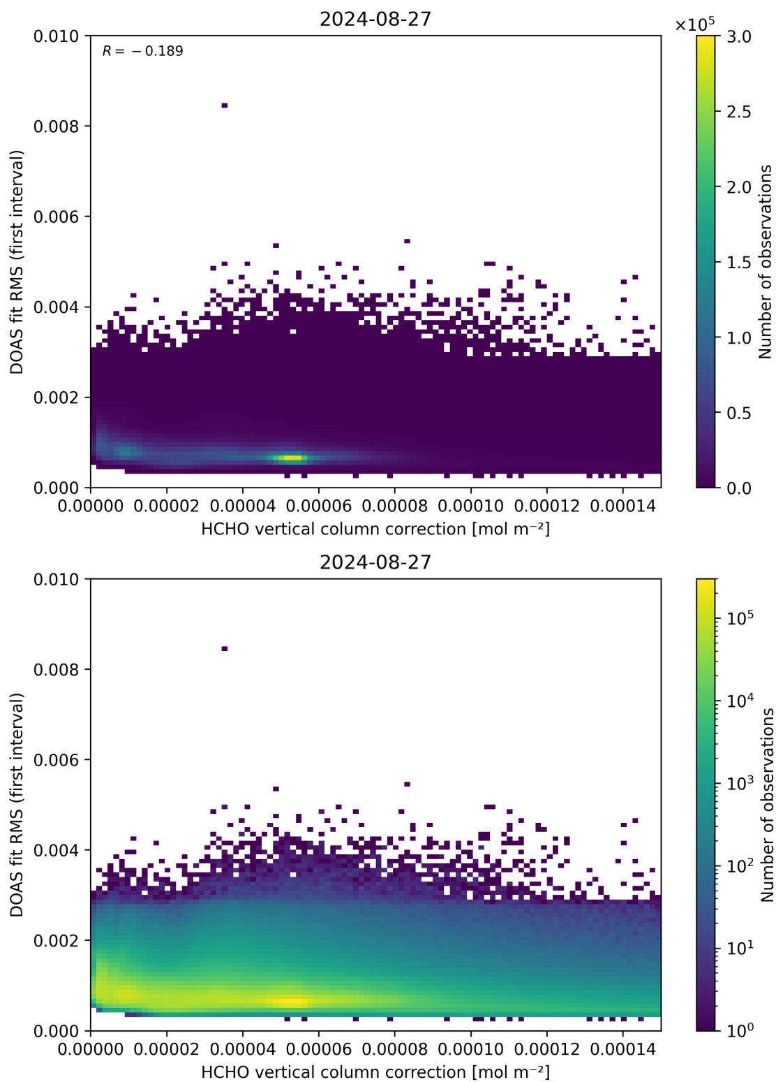
Figure 112: Scatter density plot of “HCHO vertical column correction” against “DOAS fit RMS (first interval)” for 2024-08-27 to 2024-08-28.
