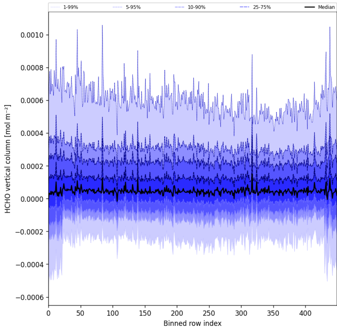
Figure 49: Along track statistics of “HCHO vertical column” for 2024-08-27 to 2024-08-28
