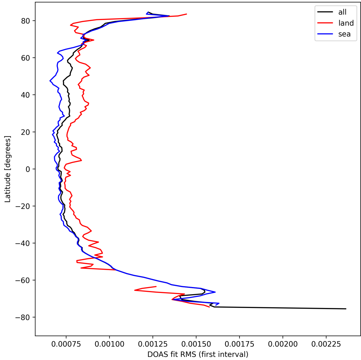
Figure 32: Zonal average of “DOAS fit RMS (first interval)” for 2024-08-27 to 2024-08-28.
