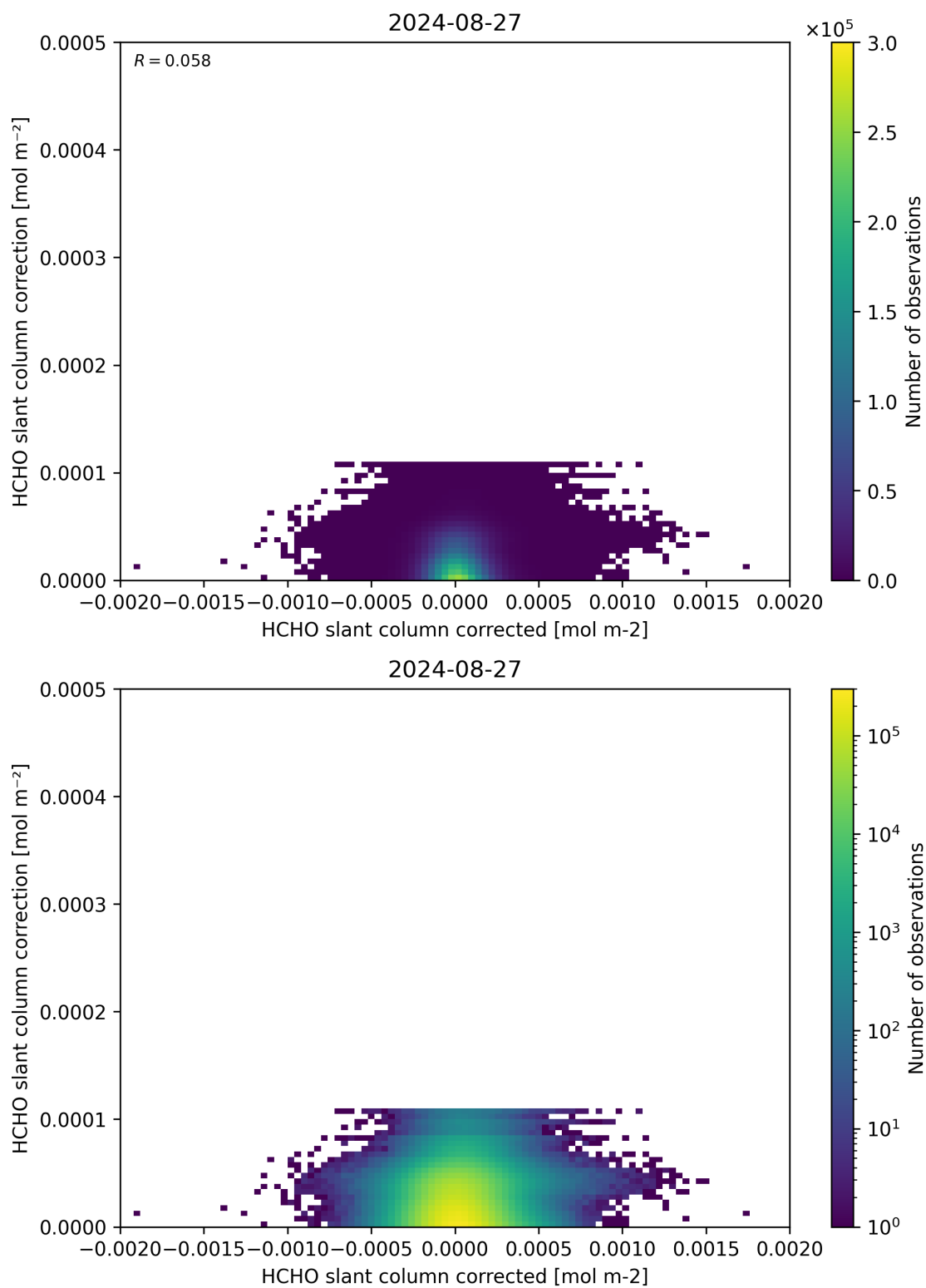
Figure 77: Scatter density plot of “HCHO slant column corrected” against “HCHO slant column correction” for 2024-08-27 to 2024-08-28.
