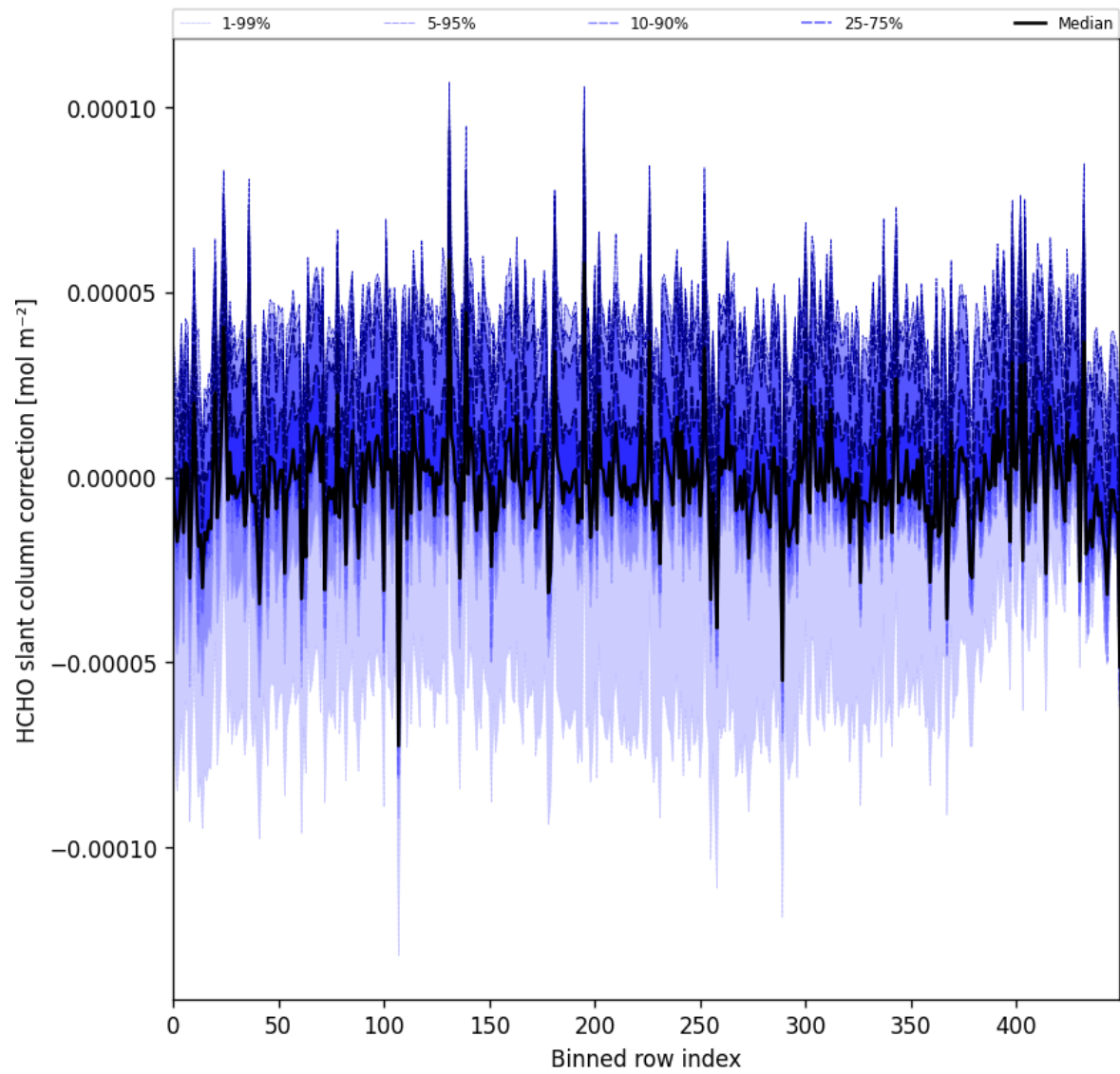
Figure 61: Along track statistics of “HCHO slant column correction” for 2024-08-27 to 2024-08-28
