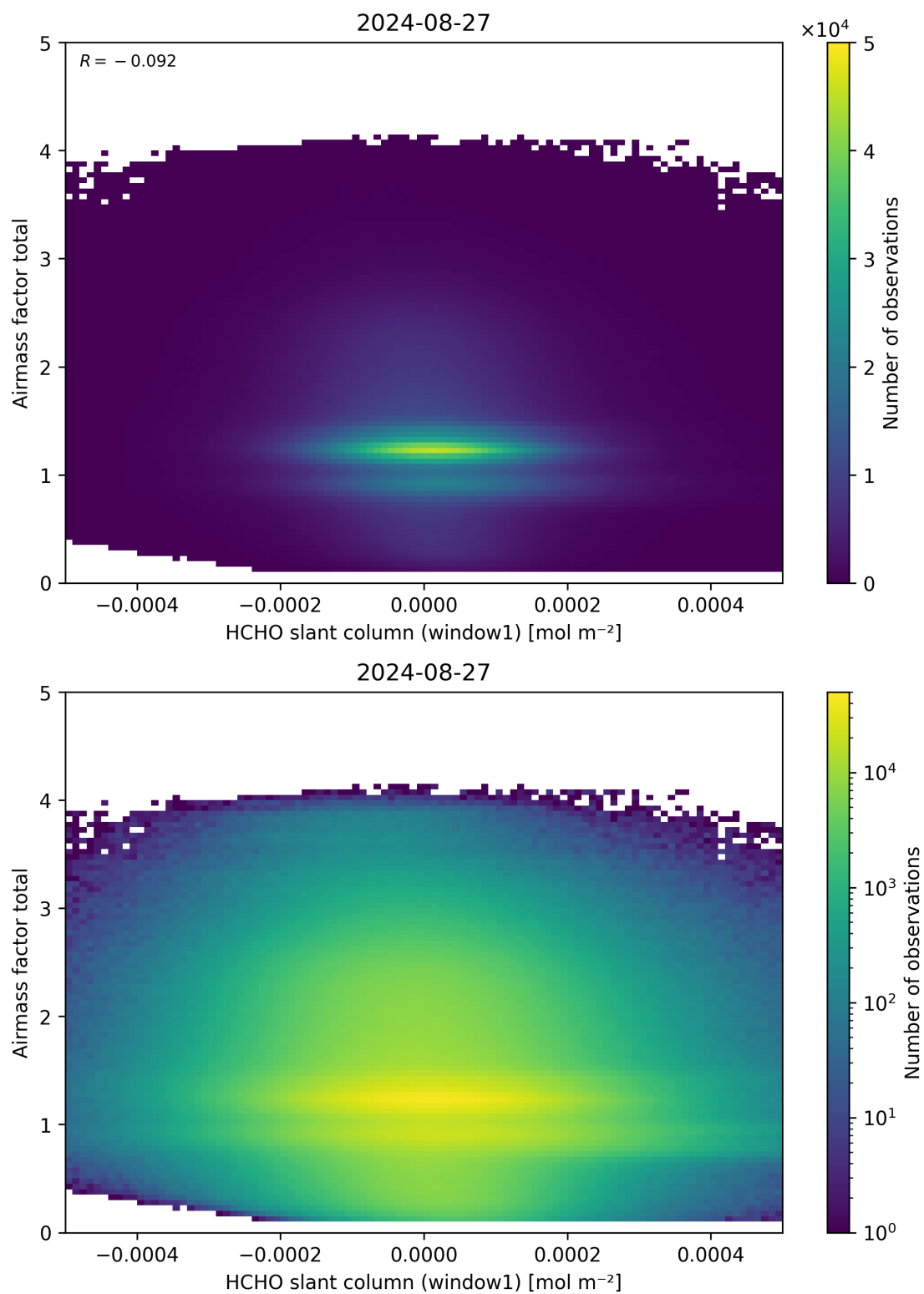
Figure 85: Scatter density plot of “HCHO slant column (window1)” against “Airmass factor total” for 2024-08-27 to 2024-08-28.
