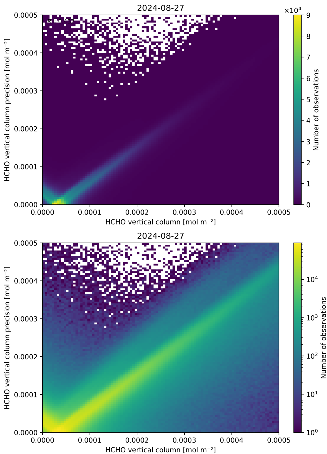
Figure 134: Scatter density plot of “HCHO vertical column” against “HCHO vertical column precision” for 2024-08-27 to 2024-08-28.
