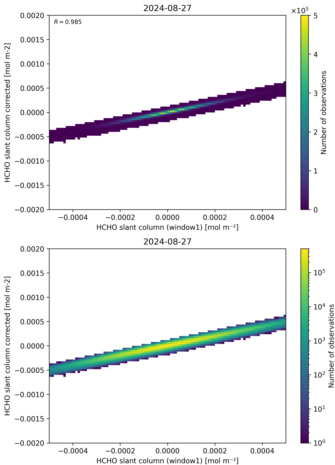
Figure 82: Scatter density plot of “HCHO slant column (window1)” against “HCHO slant column corrected” for 2024-08-27 to 2024-08-28.
