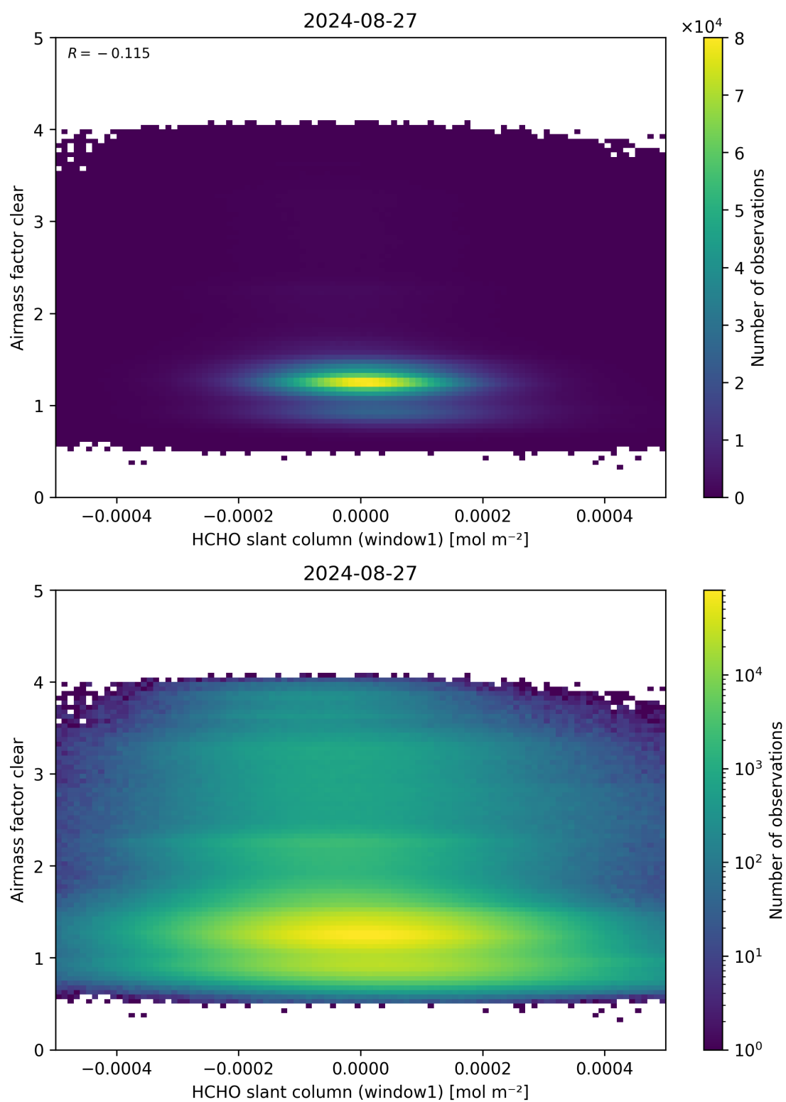
Figure 81: Scatter density plot of “HCHO slant column (window1)” against “Airmass factor clear” for 2024-08-27 to 2024-08-28.
