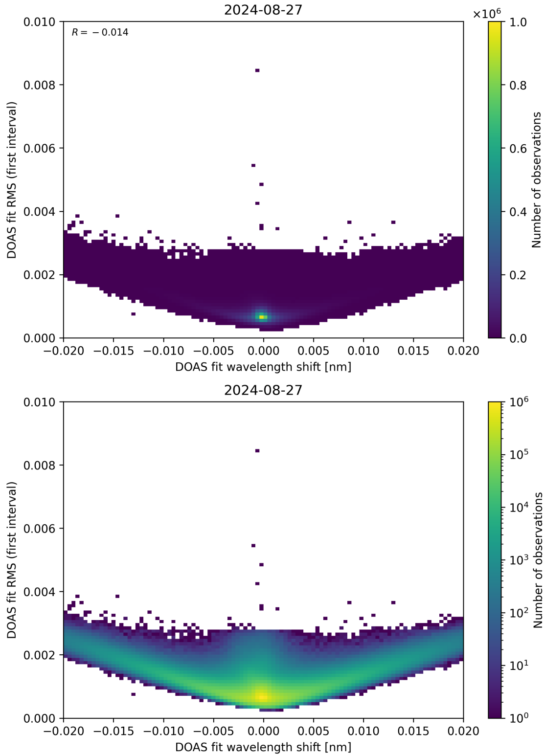
Figure 64: Scatter density plot of “DOAS fit wavelength shift” against “DOAS fit RMS (first interval)” for 2024-08-27 to 2024-08-28.
