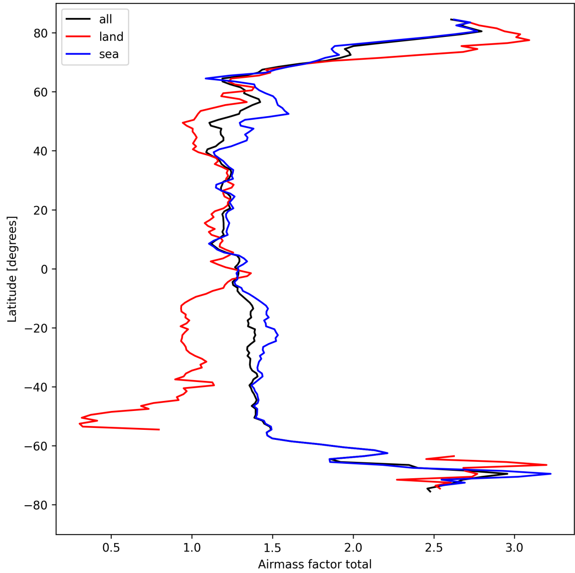
Figure 26: Zonal average of “Airmass factor total” for 2024-08-27 to 2024-08-28.
