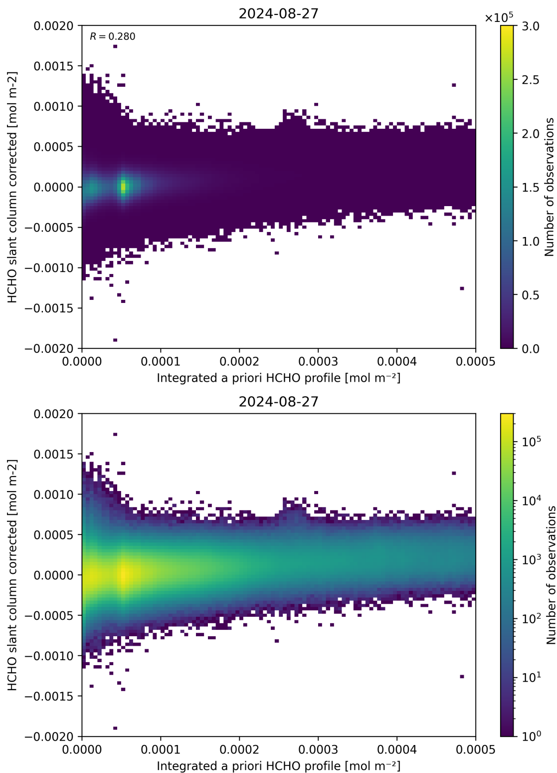
Figure 151: Scatter density plot of “Integrated a priori HCHO profile” against “HCHO slant column corrected” for 2024-08-27 to 2024-08-28.
