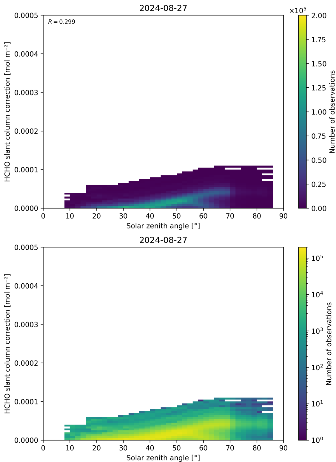
Figure 172: Scatter density plot of “Solar zenith angle” against “HCHO slant column correction” for 2024-08-27 to 2024-08-28.
