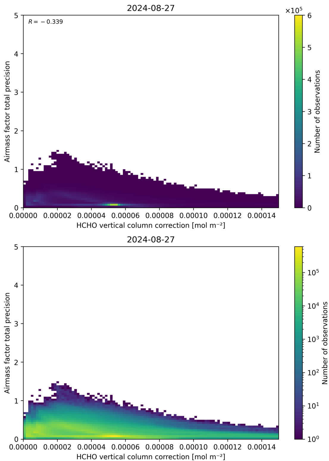
Figure 121: Scatter density plot of “HCHO vertical column correction” against “Airmass factor total precision” for 2024-08-27 to 2024-08-28.
