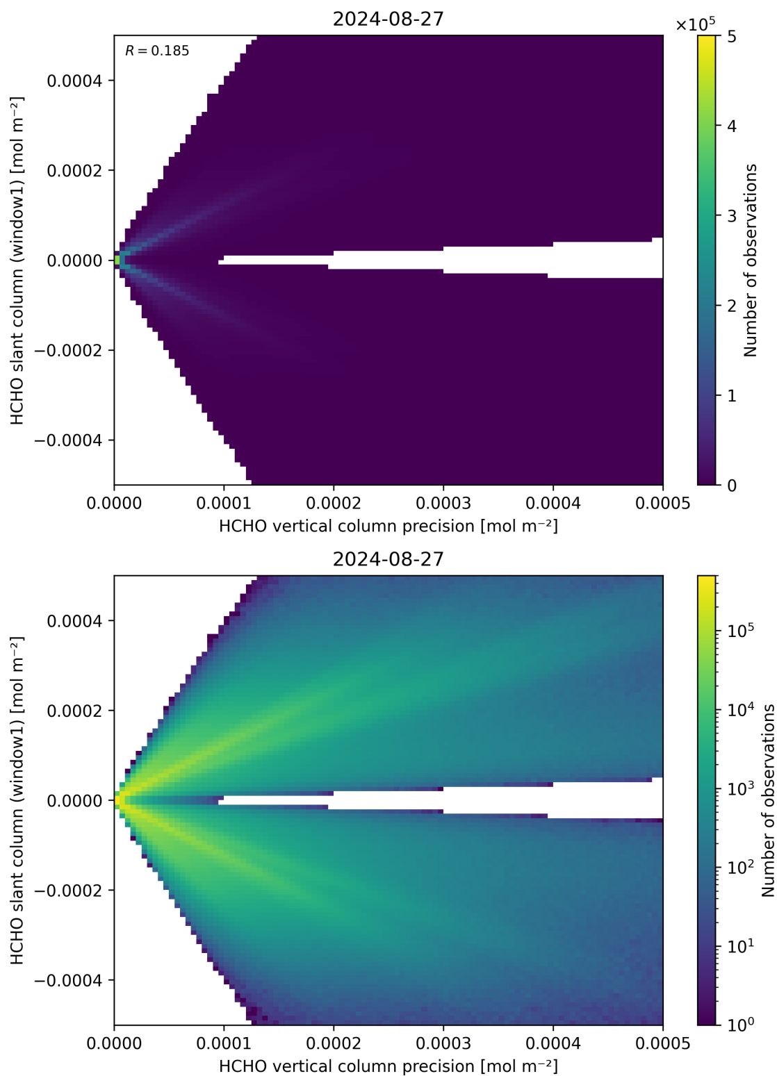
Figure 142: Scatter density plot of “HCHO vertical column precision” against “HCHO slant column (window1)” for 2024-08-27 to 2024-08-28.
