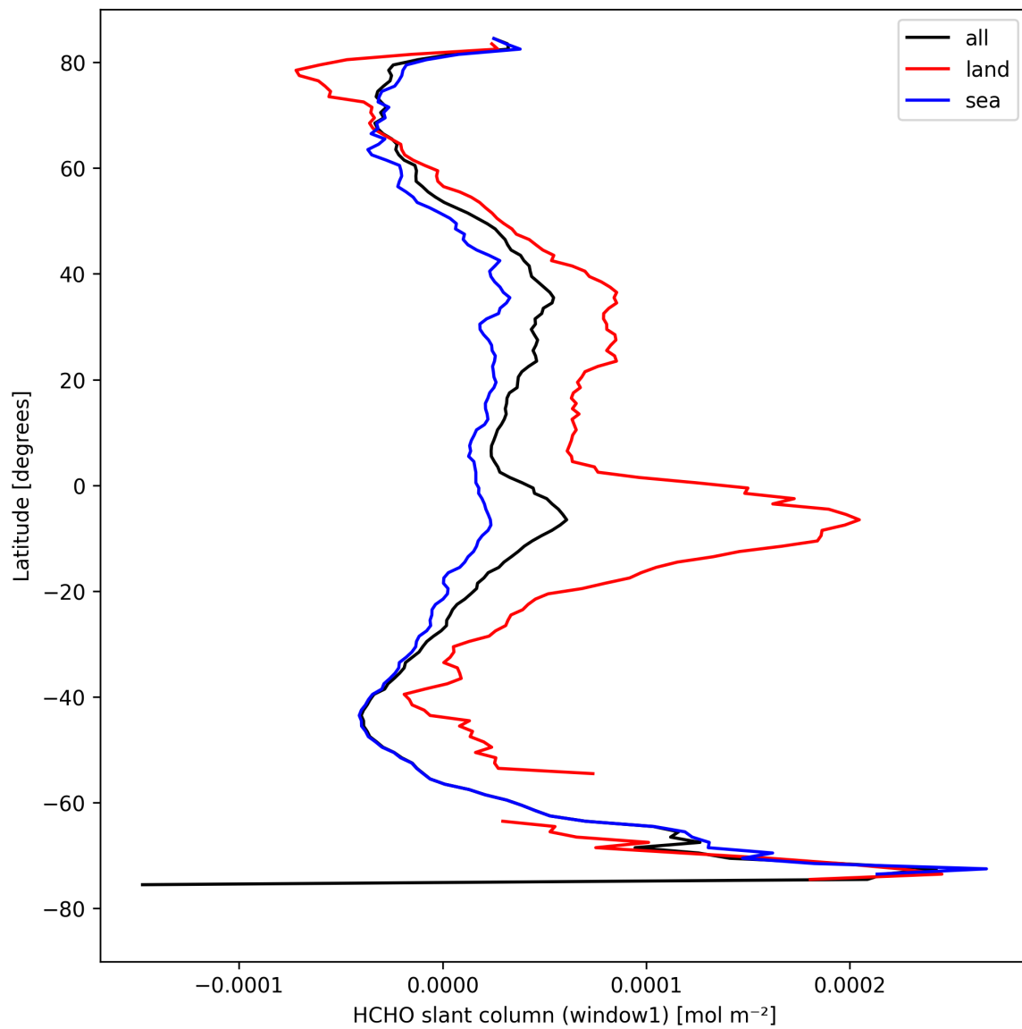
Figure 24: Zonal average of “HCHO slant column (window1)” for 2024-08-27 to 2024-08-28.
