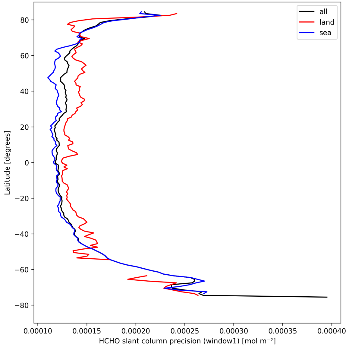
Figure 25: Zonal average of “HCHO slant column precision (window1)” for 2024-08-27 to 2024-08-28.
