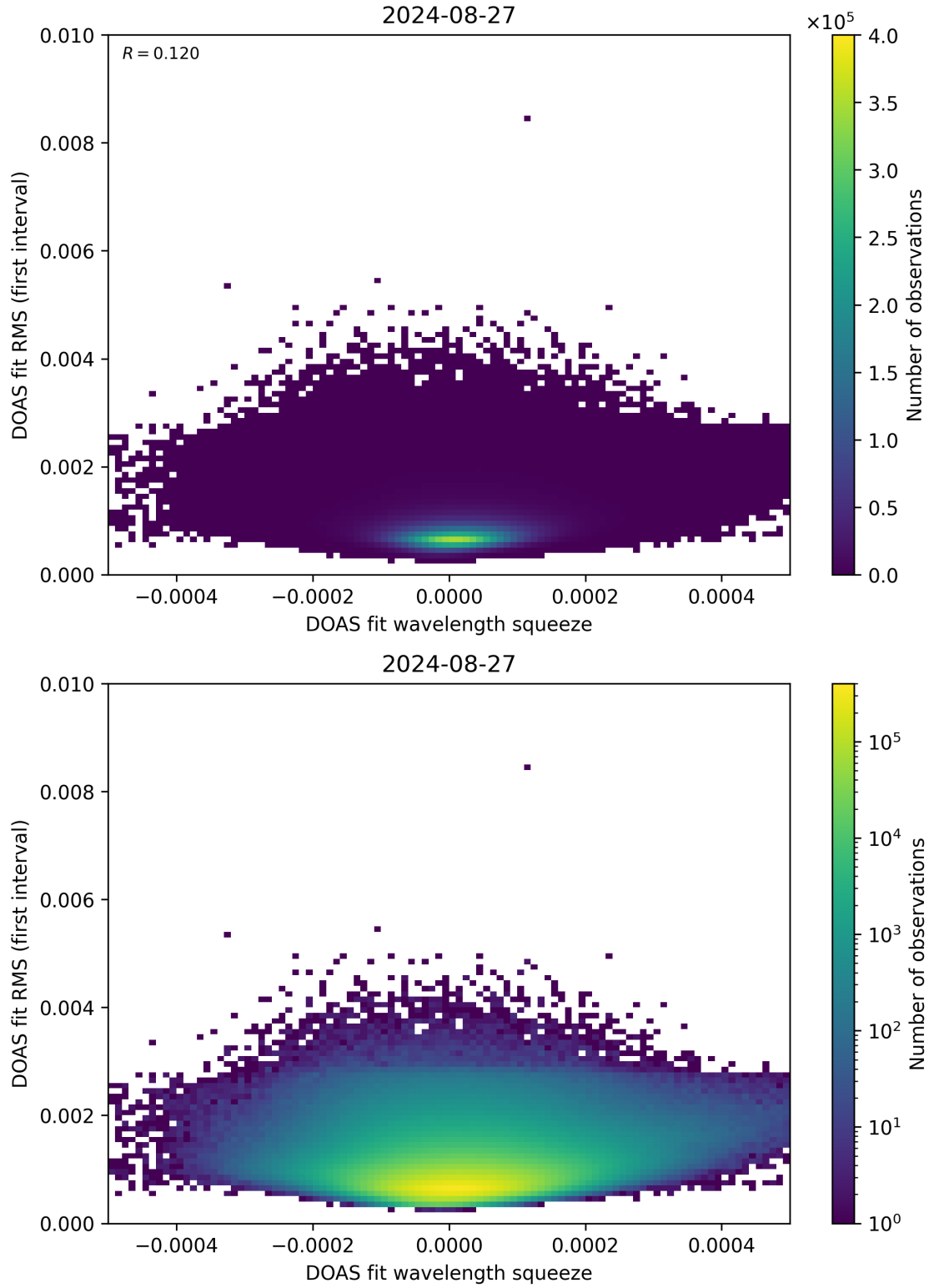
Figure 68: Scatter density plot of “DOAS fit wavelength squeeze” against “DOAS fit RMS (first interval)” for 2024-08-27 to 2024-08-28.
