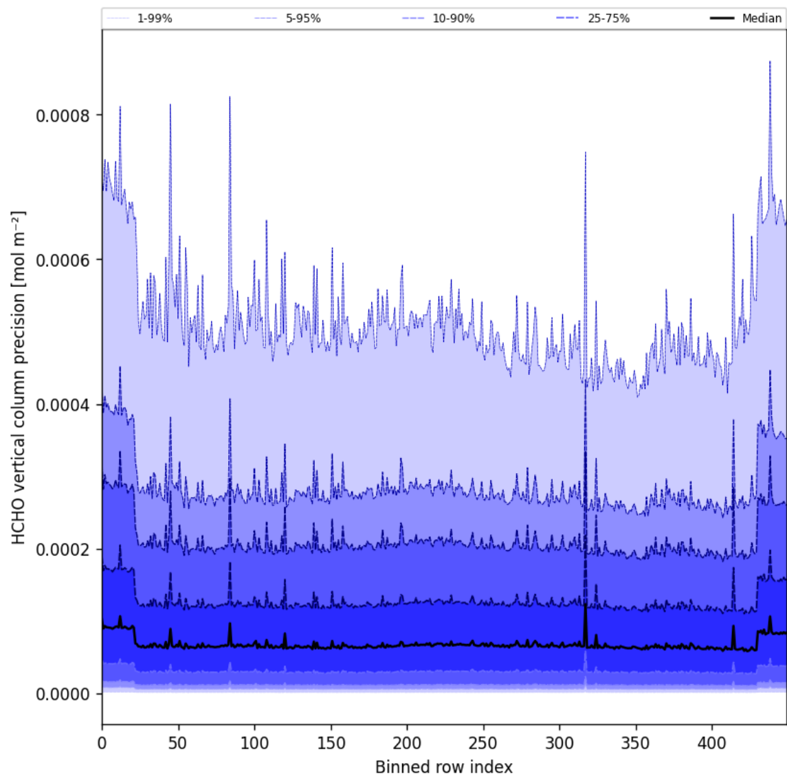
Figure 50: Along track statistics of “HCHO vertical column precision” for 2024-08-27 to 2024-08-28
