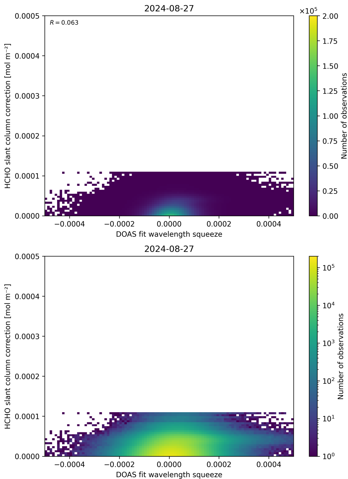
Figure 70: Scatter density plot of “DOAS fit wavelength squeeze” against “HCHO slant column correction” for 2024-08-27 to 2024-08-28.
