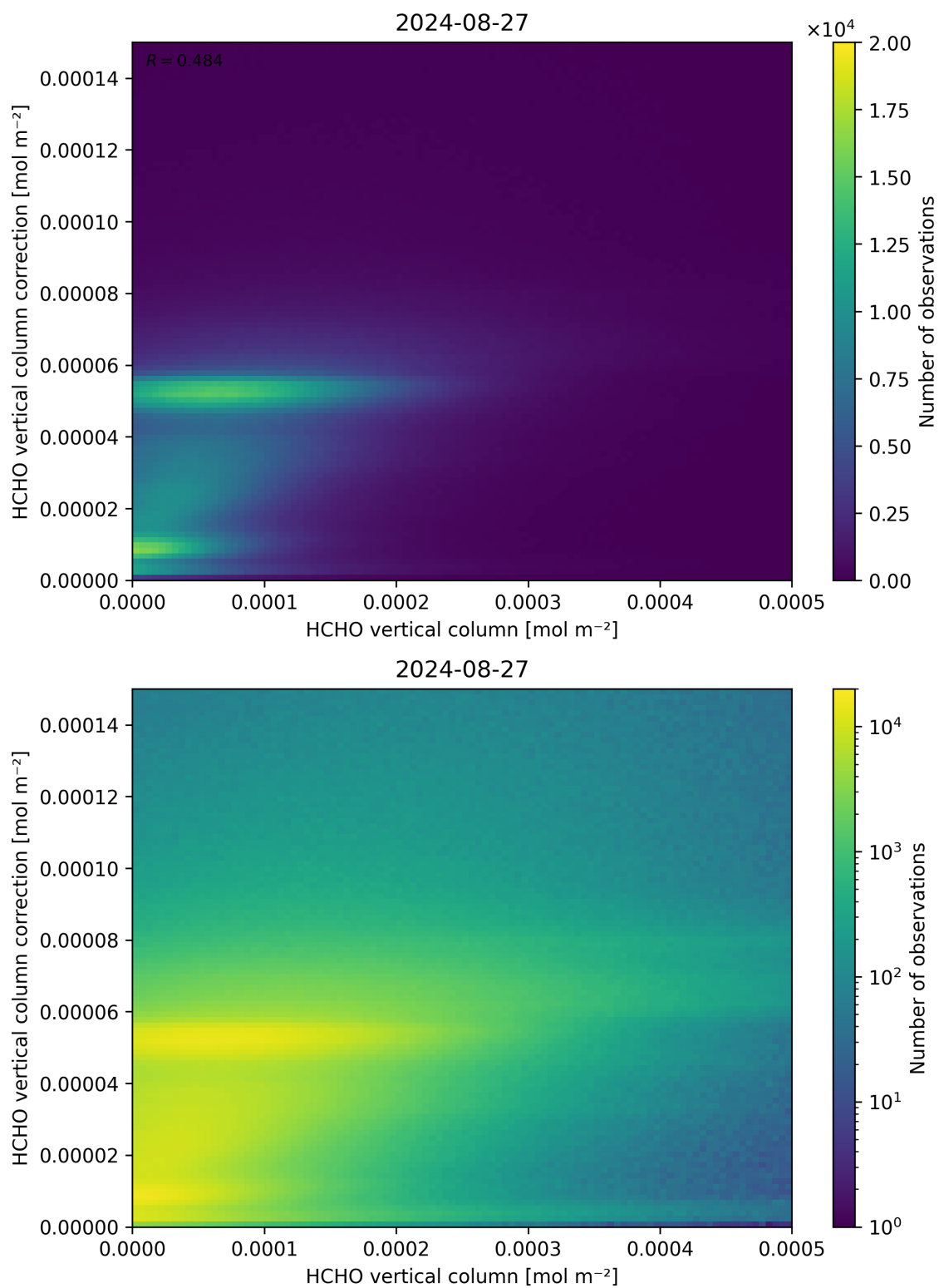
Figure 133: Scatter density plot of “HCHO vertical column” against “HCHO vertical column correction” for 2024-08-27 to 2024-08-28.
