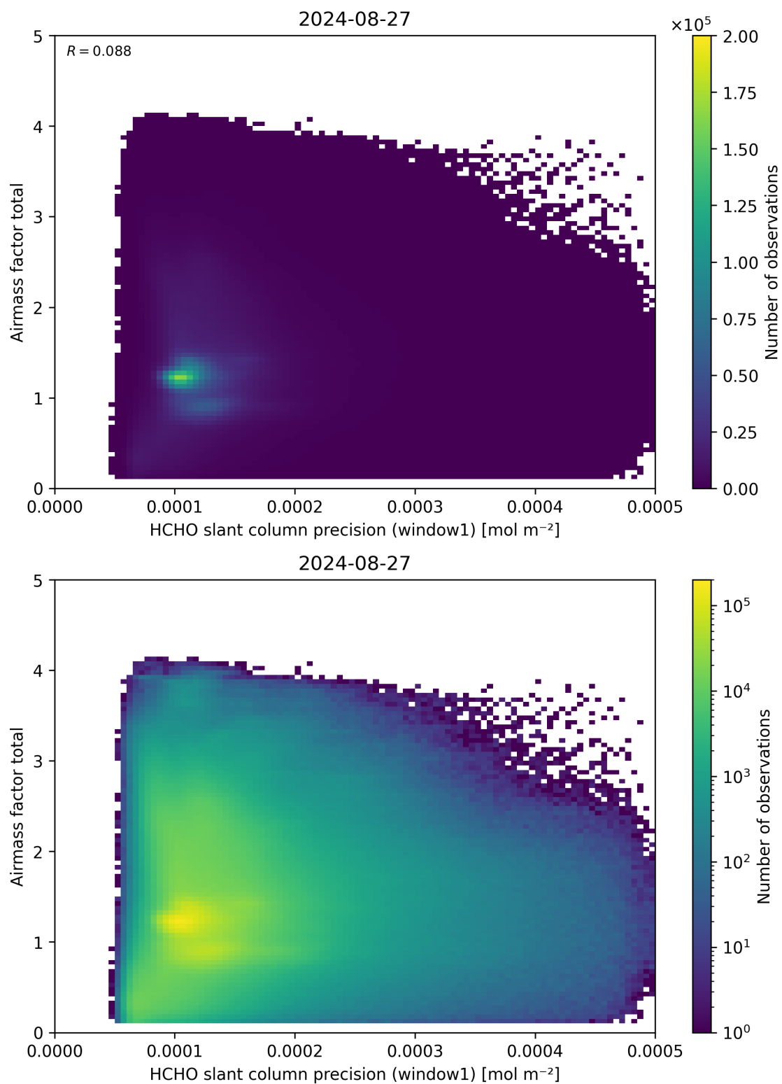
Figure 94: Scatter density plot of “HCHO slant column precision (window1)” against “Airmass factor total” for 2024-08-27 to 2024-08-28.
