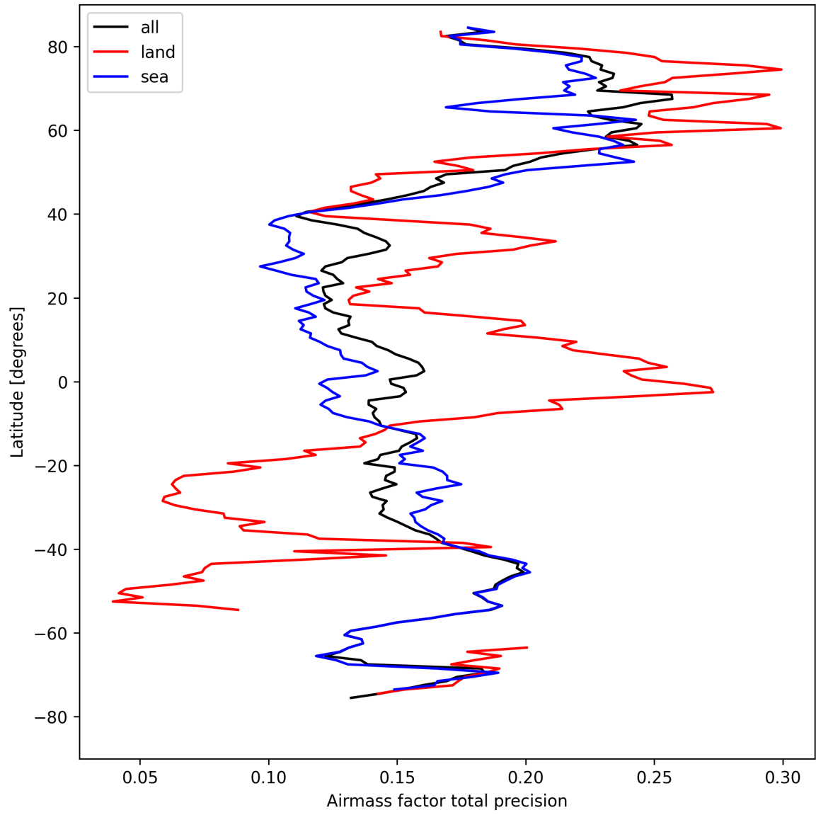
Figure 27: Zonal average of “Airmass factor total precision” for 2024-08-27 to 2024-08-28.
