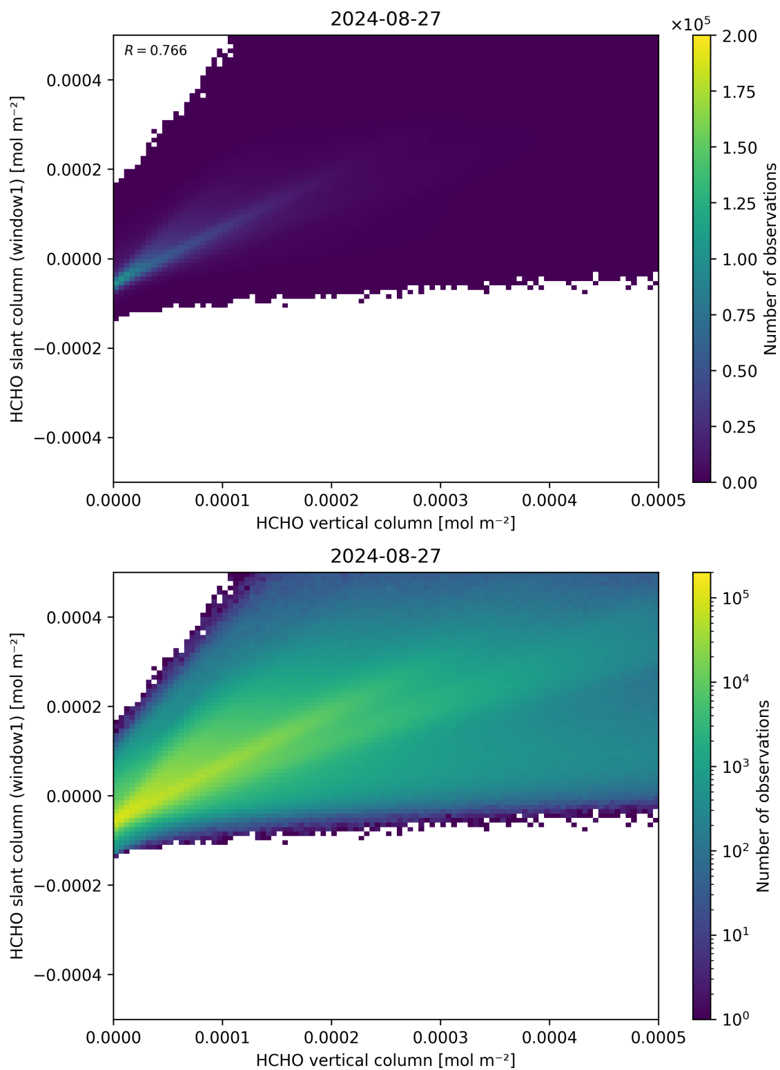
Figure 129: Scatter density plot of “HCHO vertical column” against “HCHO slant column (window1)” for 2024-08-27 to 2024-08-28.
