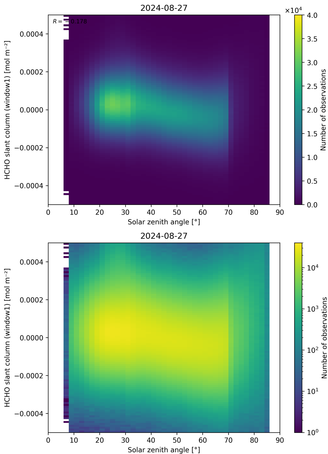
Figure 173: Scatter density plot of “Solar zenith angle” against “HCHO slant column (window1)” for 2024-08-27 to 2024-08-28.
