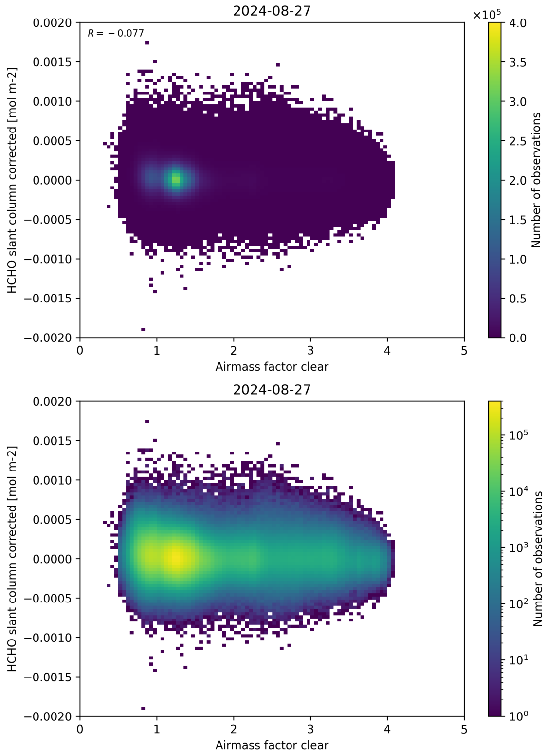
Figure 74: Scatter density plot of “Airmass factor clear” against “HCHO slant column corrected” for 2024-08-27 to 2024-08-28.
