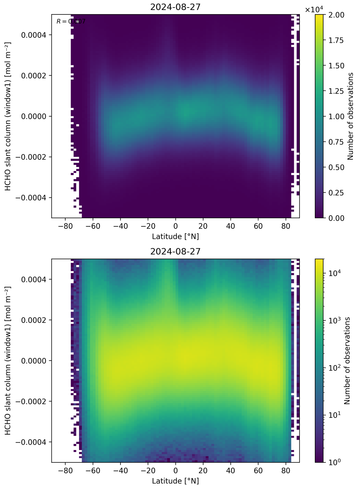
Figure 159: Scatter density plot of “Latitude” against “HCHO slant column (window1)” for 2024-08-27 to 2024-08-28.
