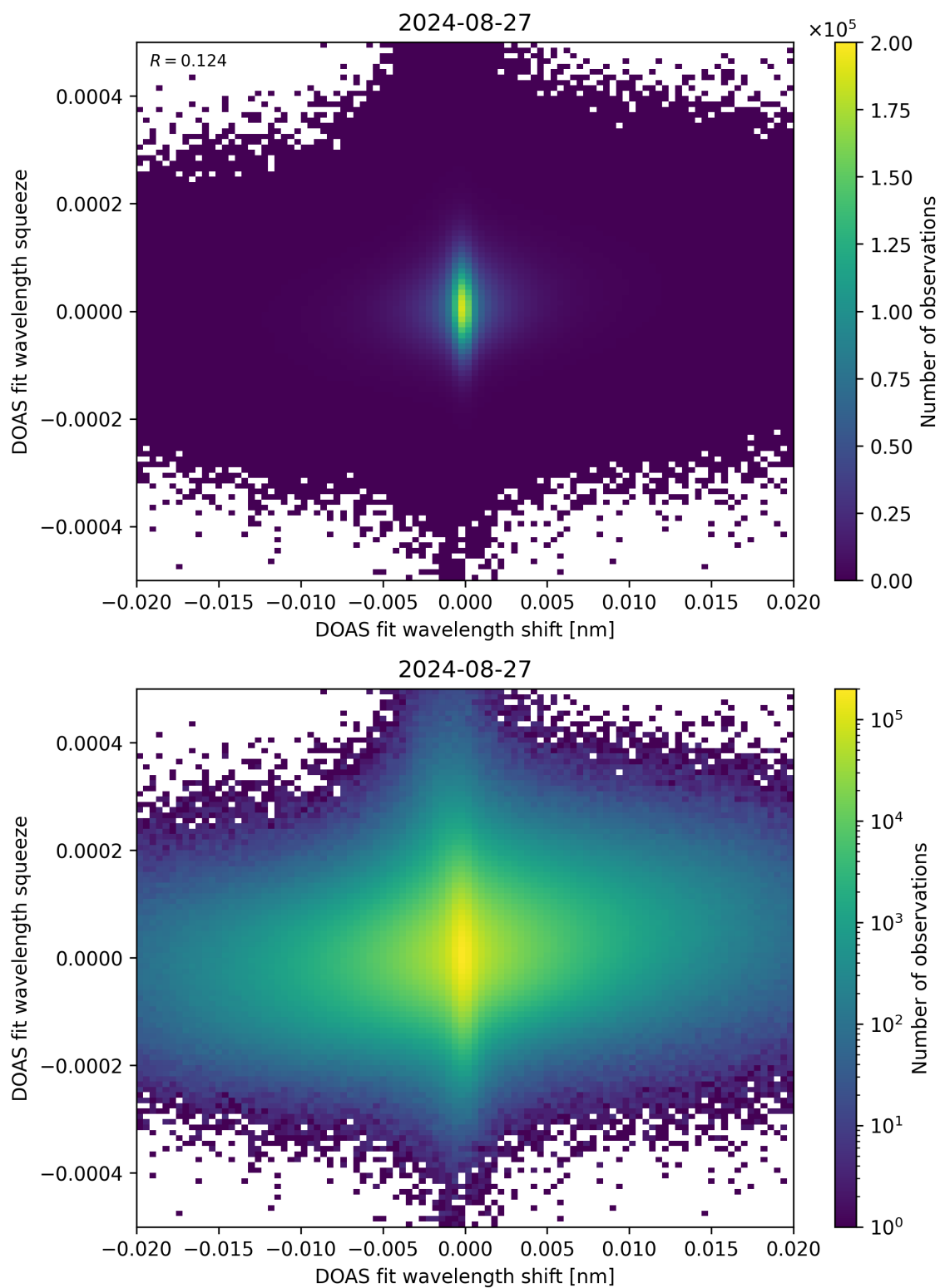
Figure 65: Scatter density plot of “DOAS fit wavelength shift” against “DOAS fit wavelength squeeze” for 2024-08-27 to 2024-08-28.
