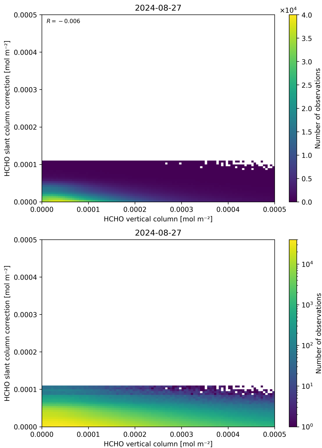
Figure 128: Scatter density plot of “HCHO vertical column” against “HCHO slant column correction” for 2024-08-27 to 2024-08-28.
