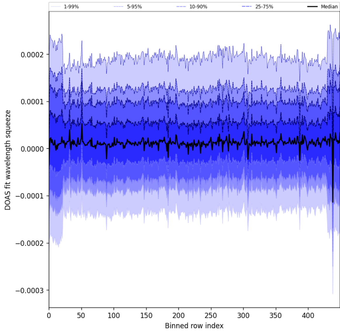
Figure 59: Along track statistics of “DOAS fit wavelength squeeze” for 2024-08-27 to 2024-08-28
