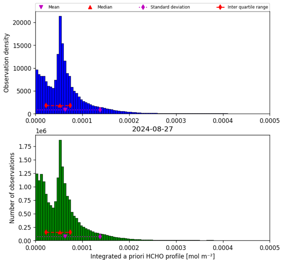
Figure 43: Histogram of “Integrated a priori HCHO profile” for 2024-08-27 to 2024-08-28
