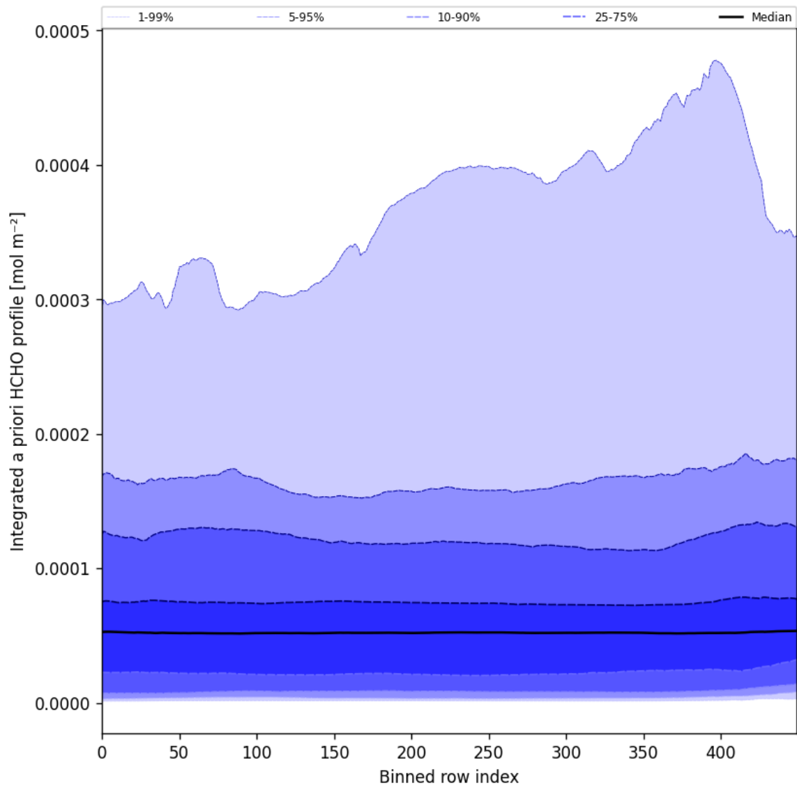
Figure 57: Along track statistics of “Integrated a priori HCHO profile” for 2024-08-27 to 2024-08-28
