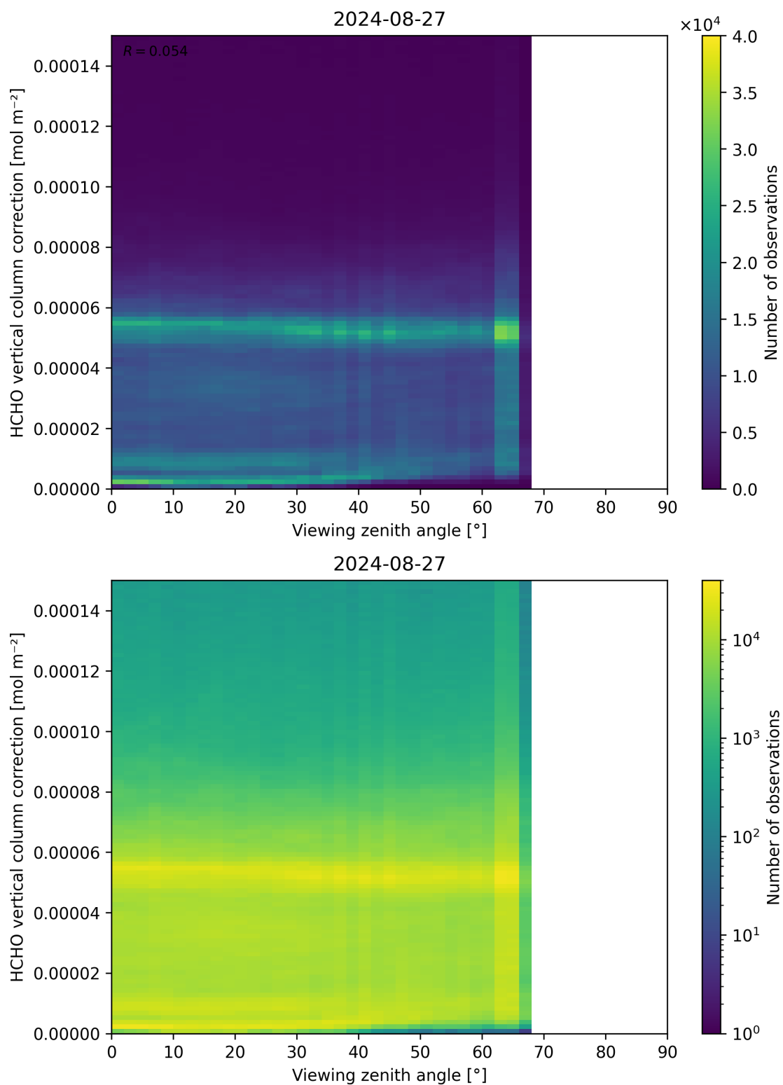
Figure 193: Scatter density plot of “Viewing zenith angle” against “HCHO vertical column correction” for 2024-08-27 to 2024-08-28.
