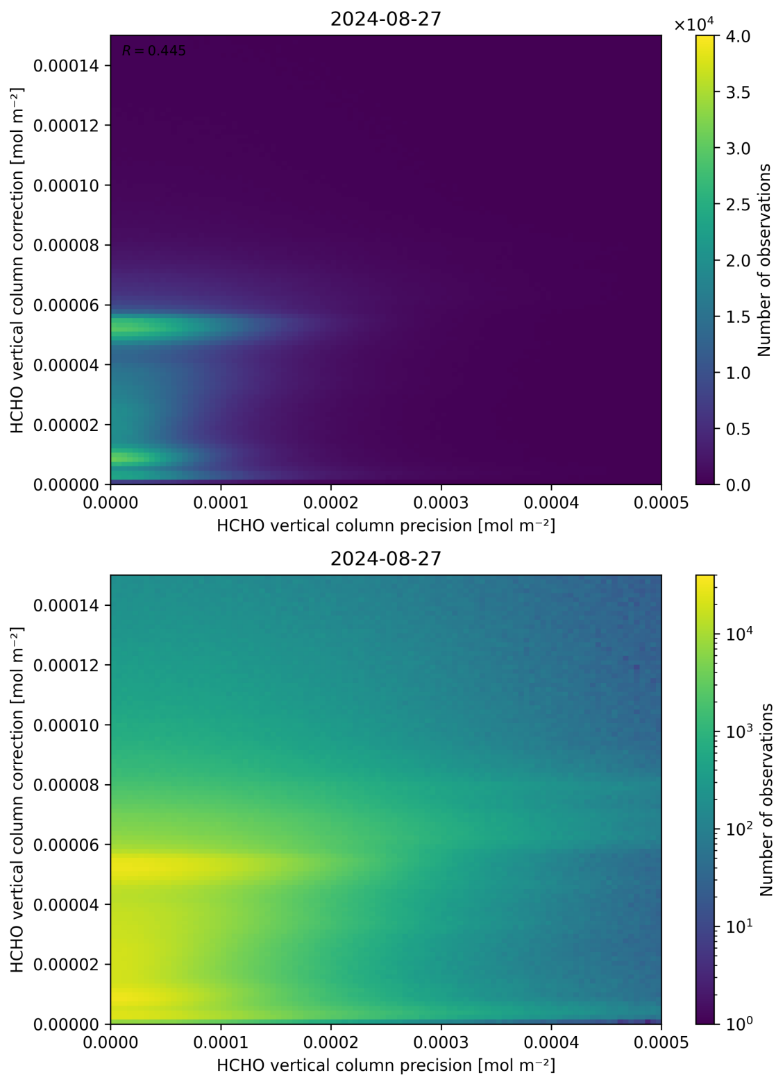
Figure 146: Scatter density plot of “HCHO vertical column precision” against “HCHO vertical column correction” for 2024-08-27 to 2024-08-28.
