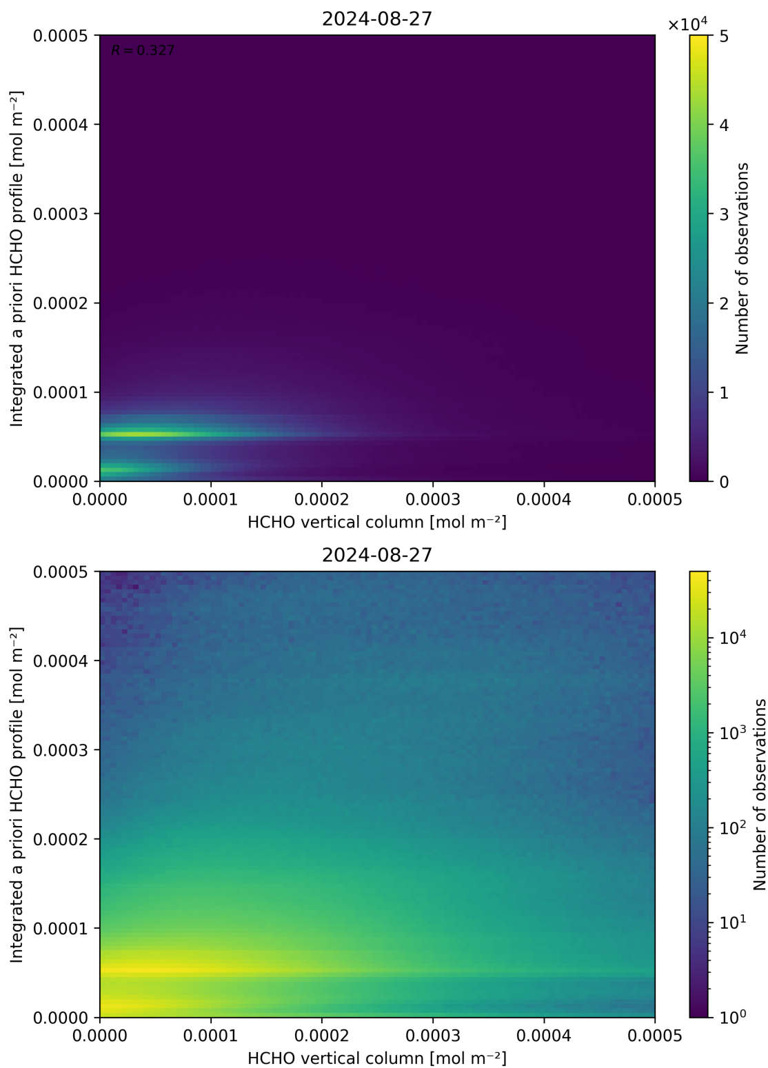
Figure 135: Scatter density plot of “HCHO vertical column” against “Integrated a priori HCHO profile” for 2024-08-27 to 2024-08-28.
