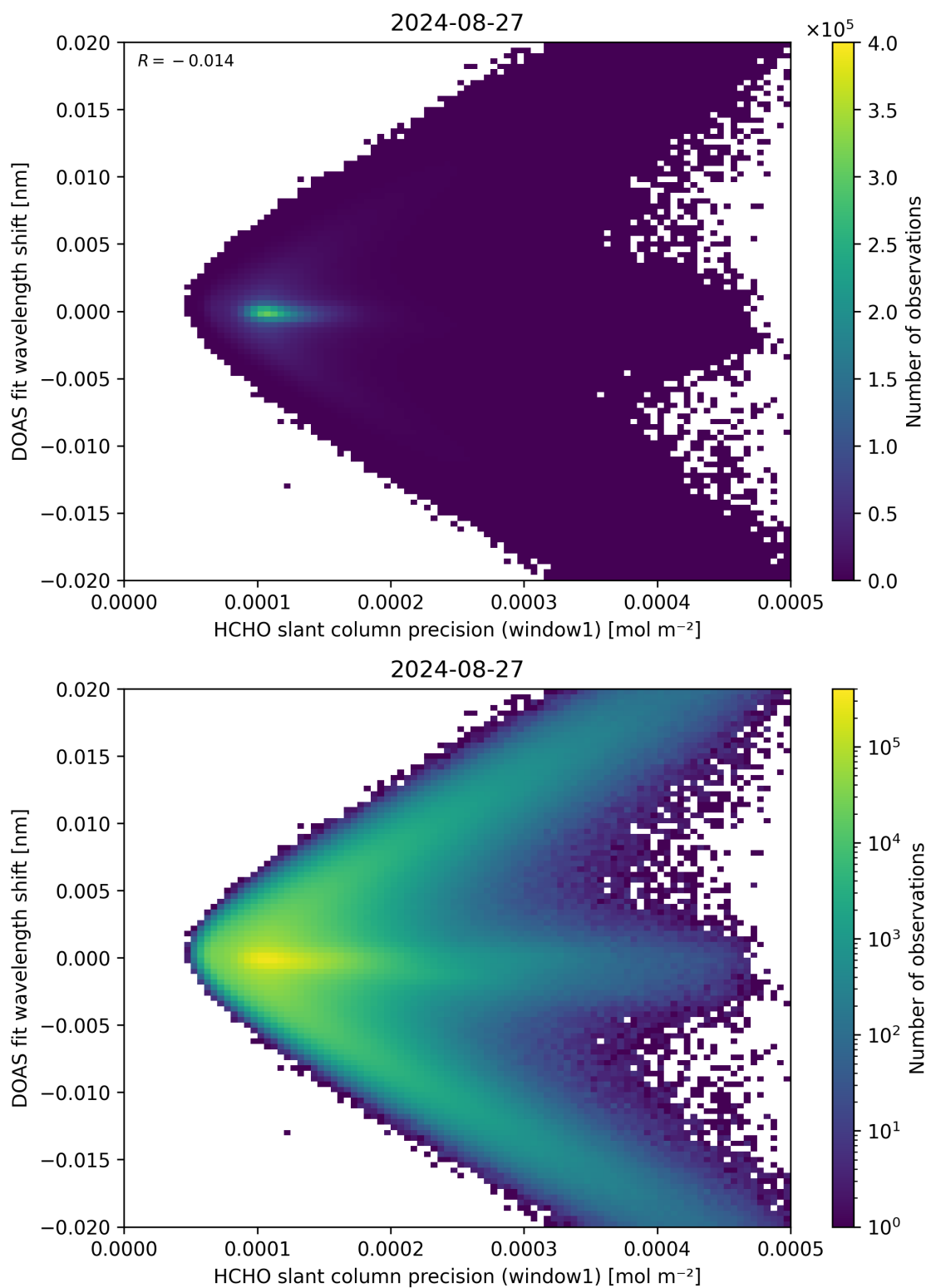
Figure 89: Scatter density plot of “HCHO slant column precision (window1)” against “DOAS fit wavelength shift” for 2024-08-27 to 2024-08-28.
