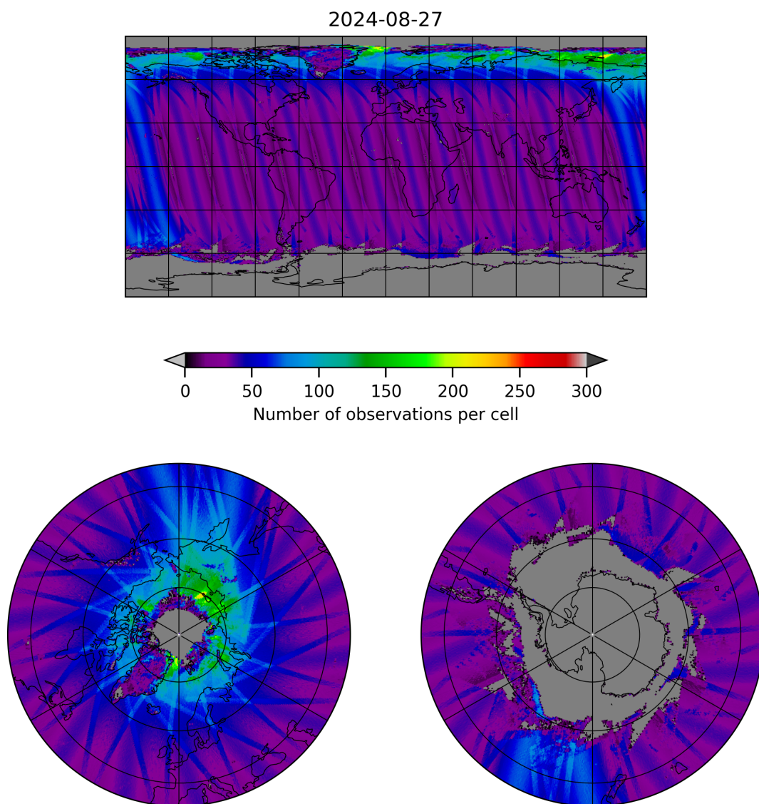
Figure 19: Map of the number of observations for 2024-08-27 to 2024-08-28
