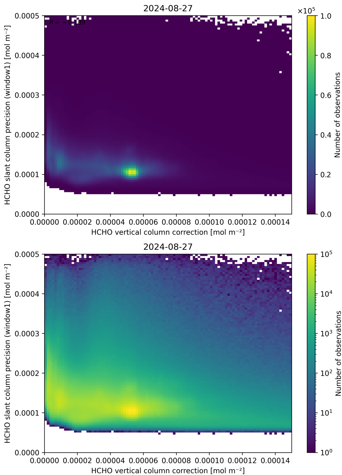
Figure 119: Scatter density plot of “HCHO vertical column correction” against “HCHO slant column precision (window1)” for 2024-08-27 to 2024-08-28.
