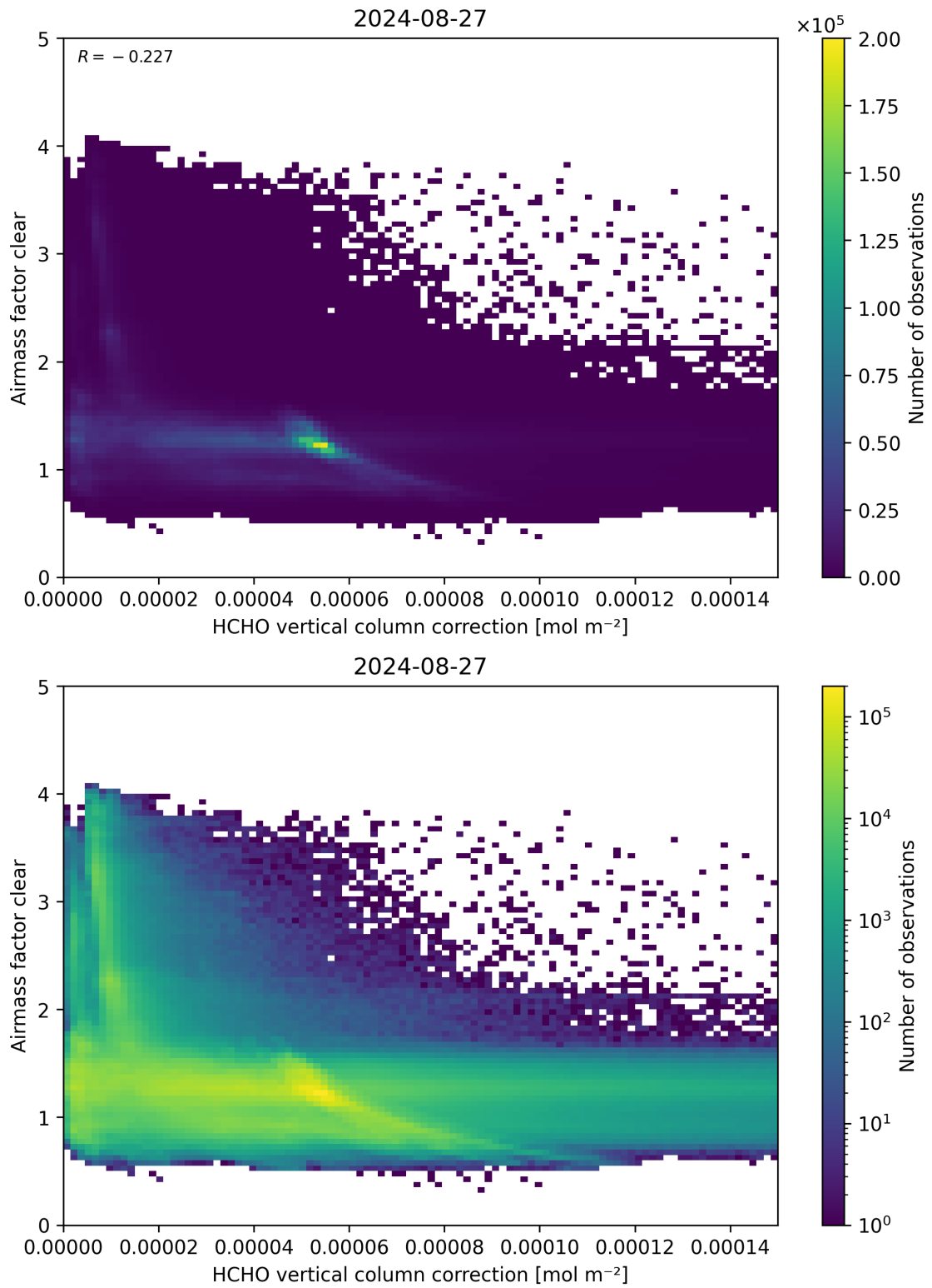
Figure 115: Scatter density plot of “HCHO vertical column correction” against “Airmass factor clear” for 2024-08-27 to 2024-08-28.
