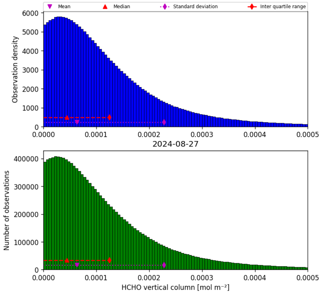
Figure 35: Histogram of “HCHO vertical column” for 2024-08-27 to 2024-08-28
