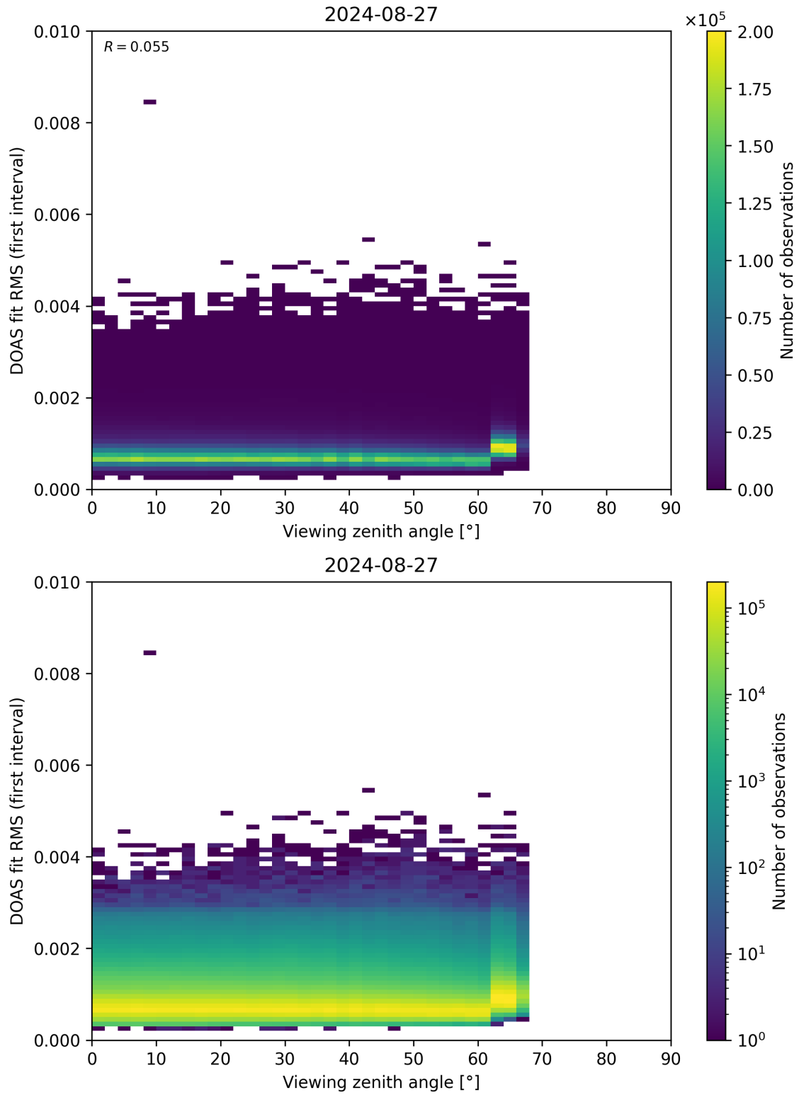
Figure 182: Scatter density plot of “Viewing zenith angle” against “DOAS fit RMS (first interval)” for 2024-08-27 to 2024-08-28.
