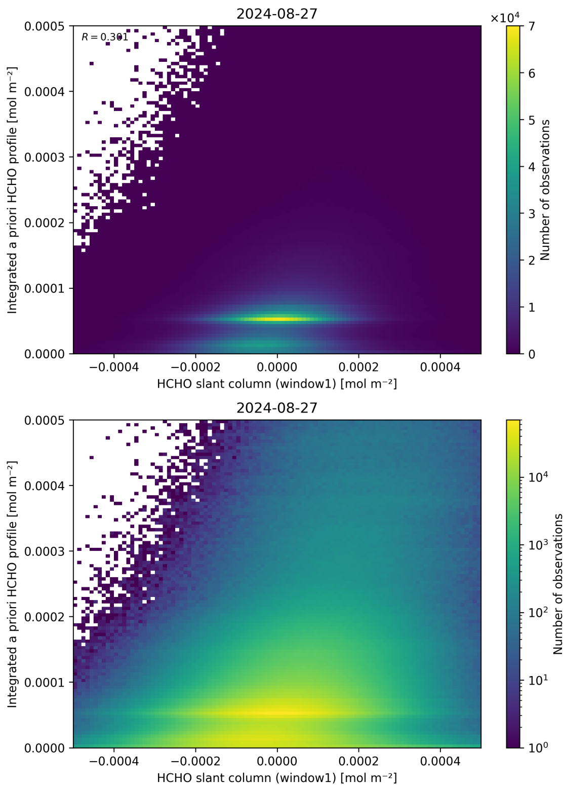
Figure 87: Scatter density plot of “HCHO slant column (window1)” against “Integrated a priori HCHO profile” for 2024-08-27 to 2024-08-28.
