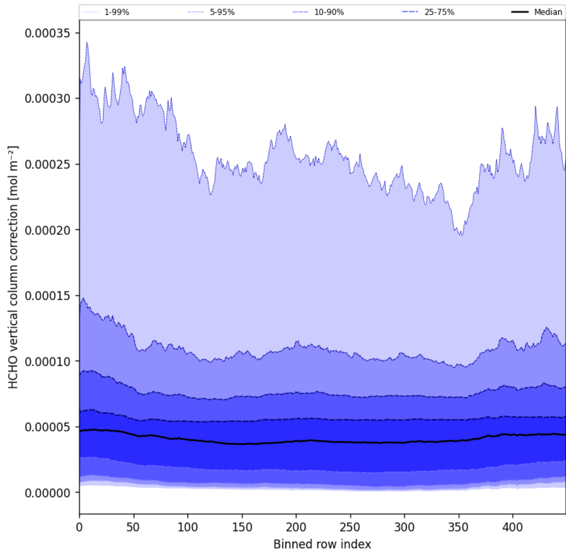
Figure 51: Along track statistics of “HCHO vertical column correction” for 2024-08-27 to 2024-08-28
