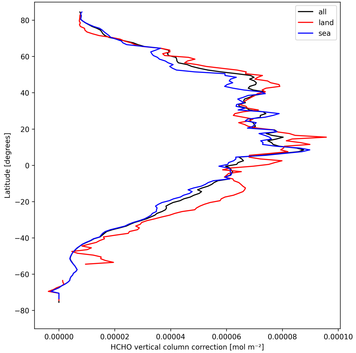
Figure 23: Zonal average of “HCHO vertical column correction” for 2024-08-27 to 2024-08-28.
