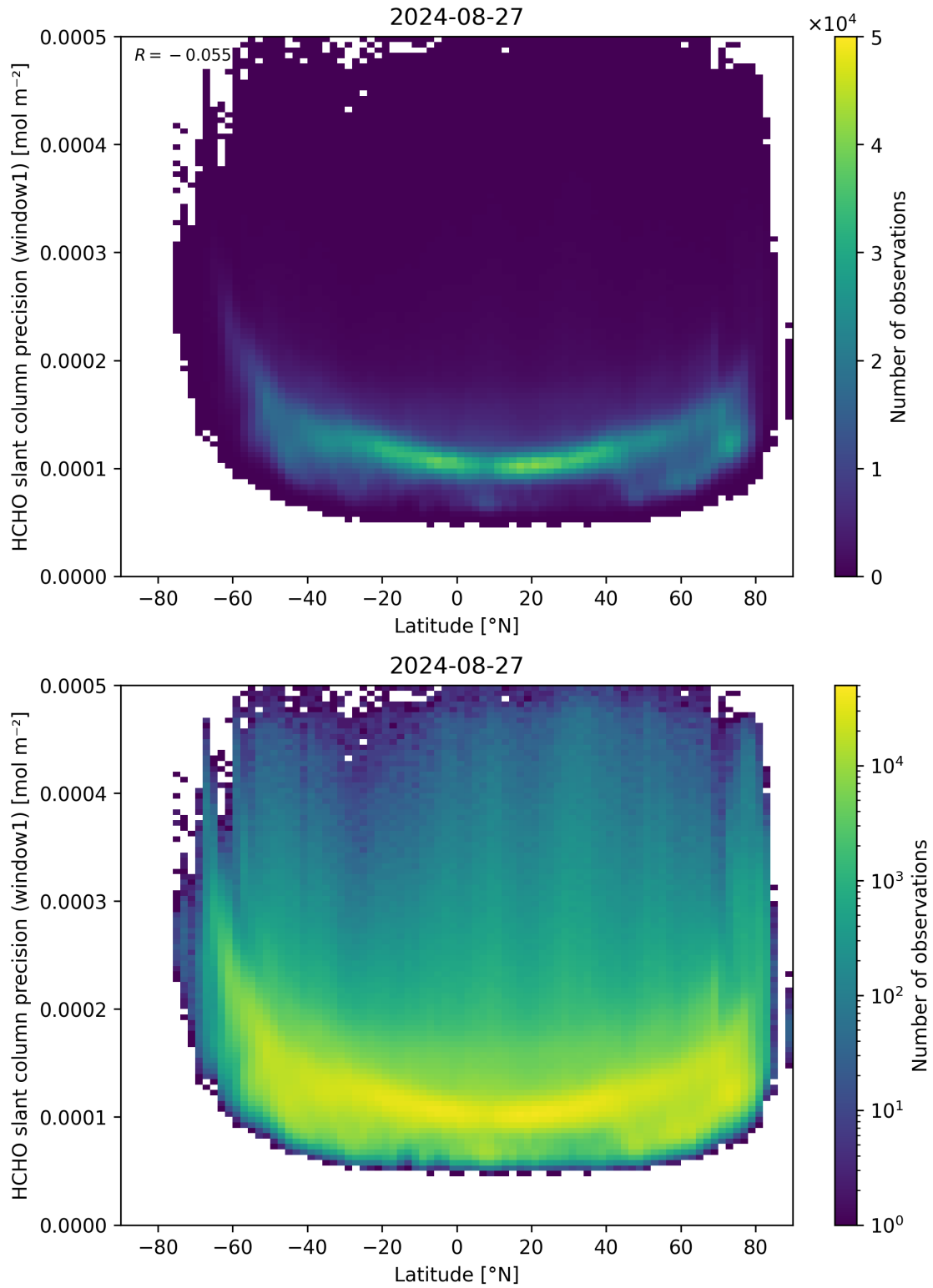
Figure 160: Scatter density plot of “Latitude” against “HCHO slant column precision (window1)” for 2024-08-27 to 2024-08-28.
