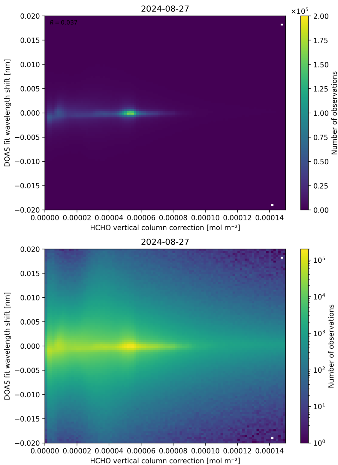
Figure 113: Scatter density plot of “HCHO vertical column correction” against “DOAS fit wavelength shift” for 2024-08-27 to 2024-08-28.
