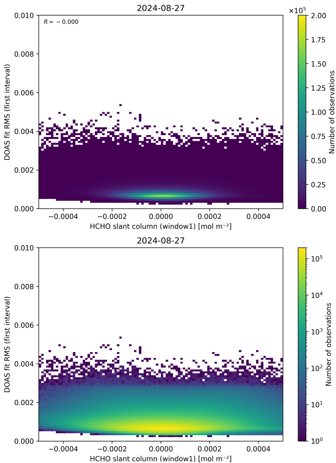
Figure 78: Scatter density plot of “HCHO slant column (window1)” against “DOAS fit RMS (first interval)” for 2024-08-27 to 2024-08-28.
