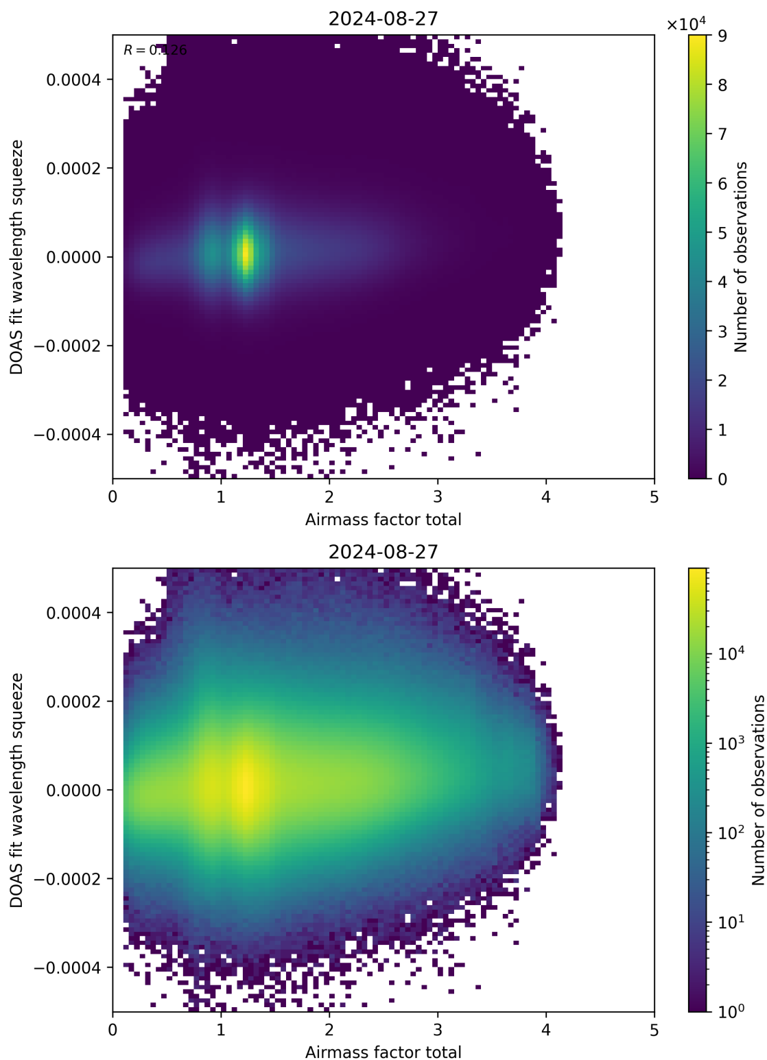
Figure 99: Scatter density plot of “Airmass factor total” against “DOAS fit wavelength squeeze” for 2024-08-27 to 2024-08-28.
