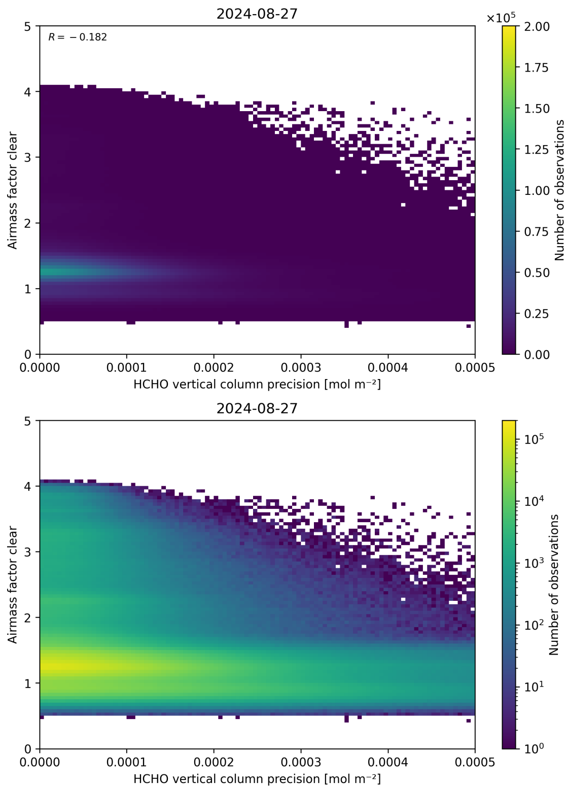
Figure 139: Scatter density plot of “HCHO vertical column precision” against “Airmass factor clear” for 2024-08-27 to 2024-08-28.
