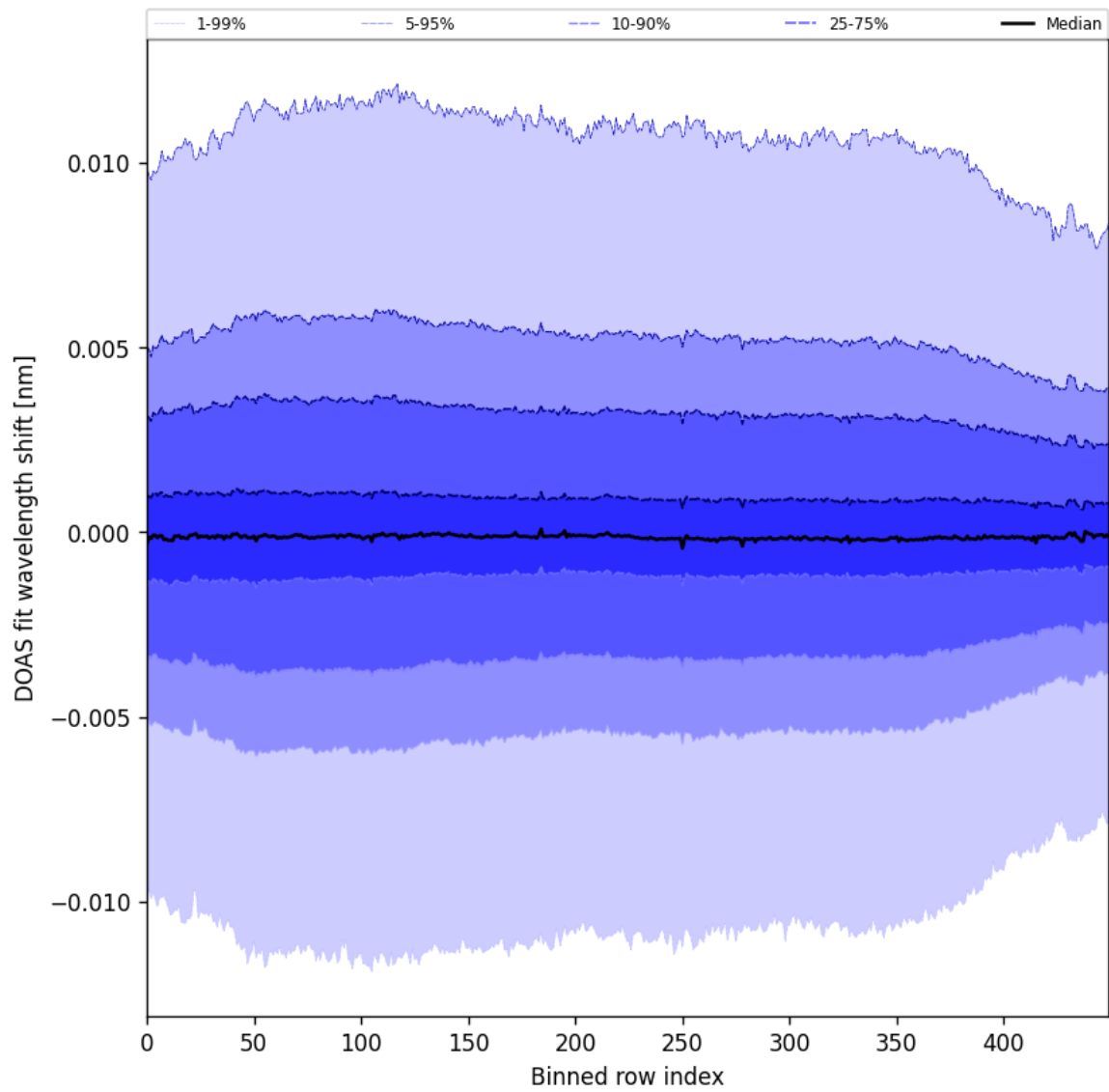
Figure 58: Along track statistics of “DOAS fit wavelength shift” for 2024-08-27 to 2024-08-28
