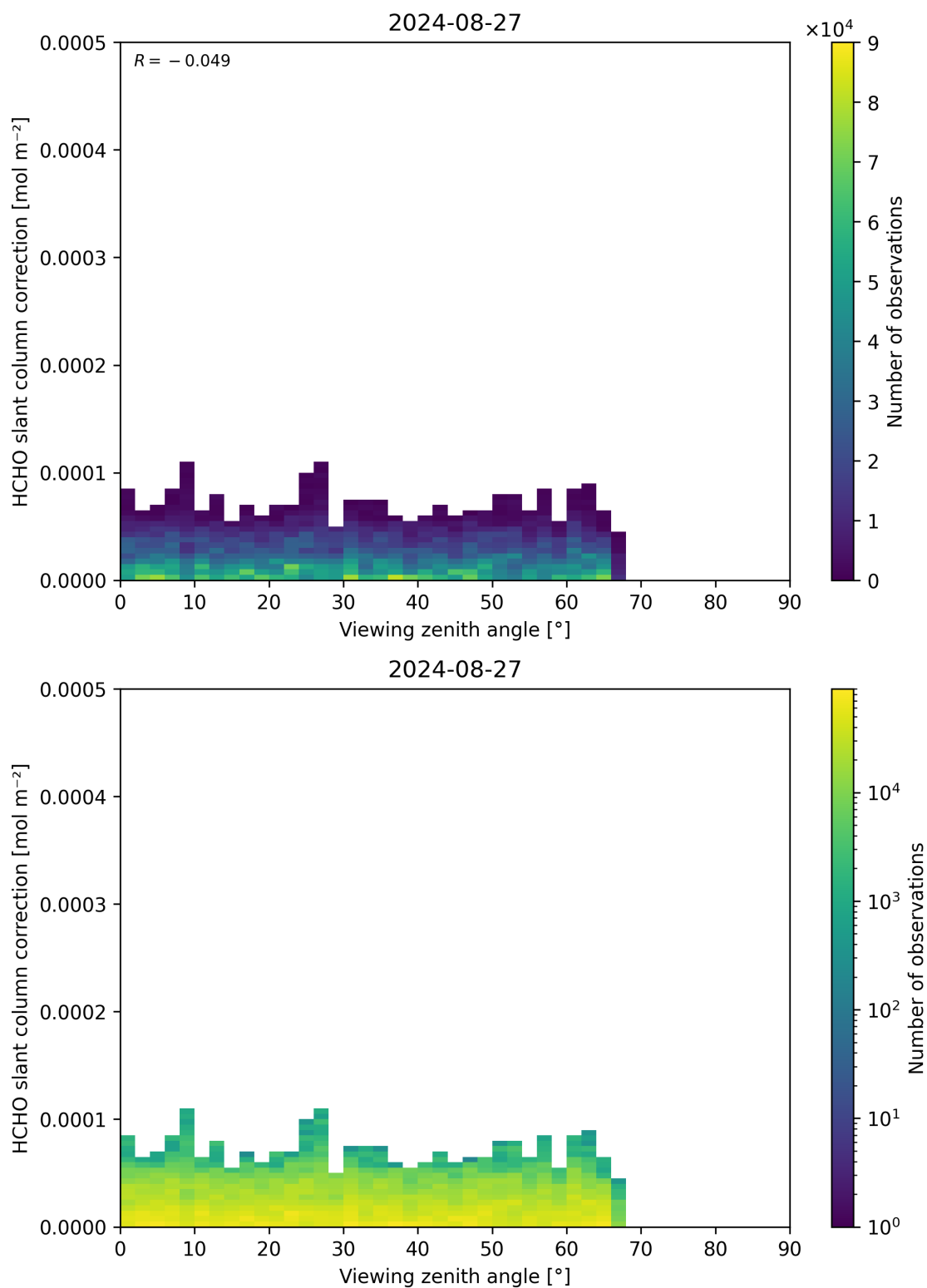
Figure 187: Scatter density plot of “Viewing zenith angle” against “HCHO slant column correction” for 2024-08-27 to 2024-08-28.
