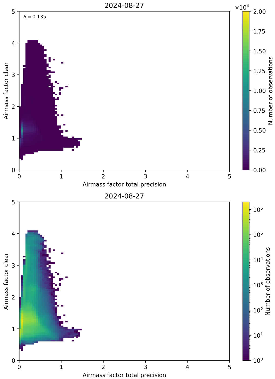
Figure 108: Scatter density plot of “Airmass factor total precision” against “Airmass factor clear” for 2024-08-27 to 2024-08-28.
