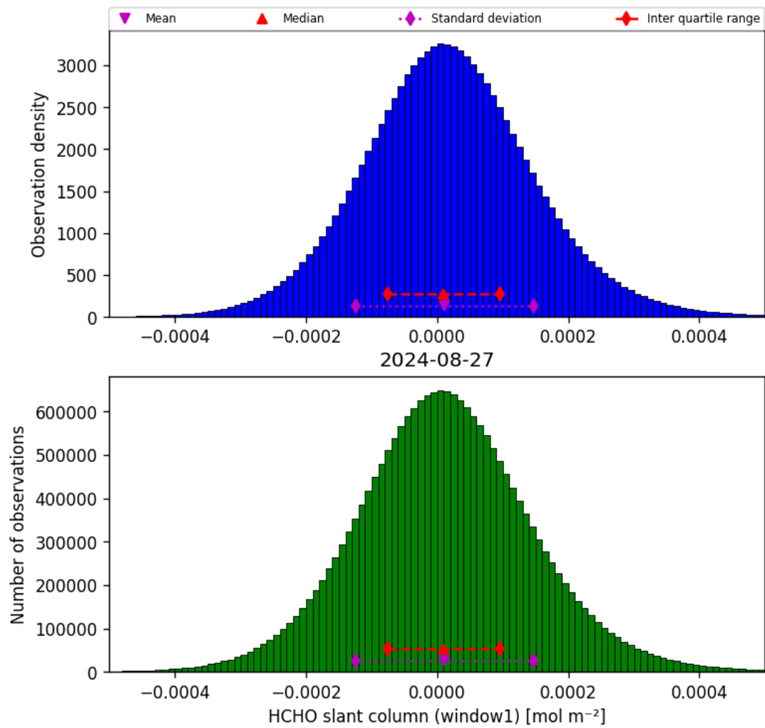
Figure 38: Histogram of “HCHO slant column (window1)” for 2024-08-27 to 2024-08-28
