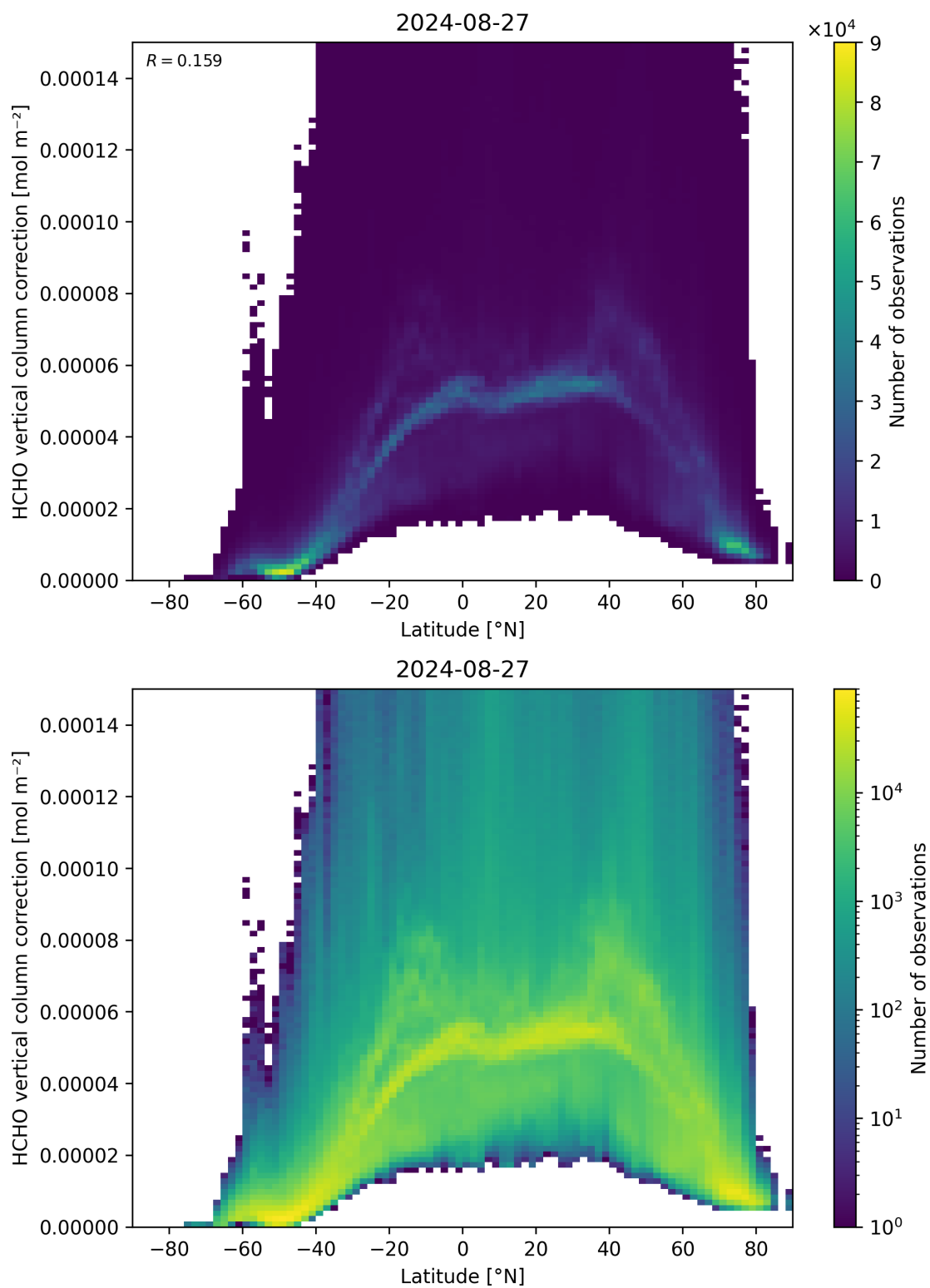
Figure 164: Scatter density plot of “Latitude” against “HCHO vertical column correction” for 2024-08-27 to 2024-08-28.
