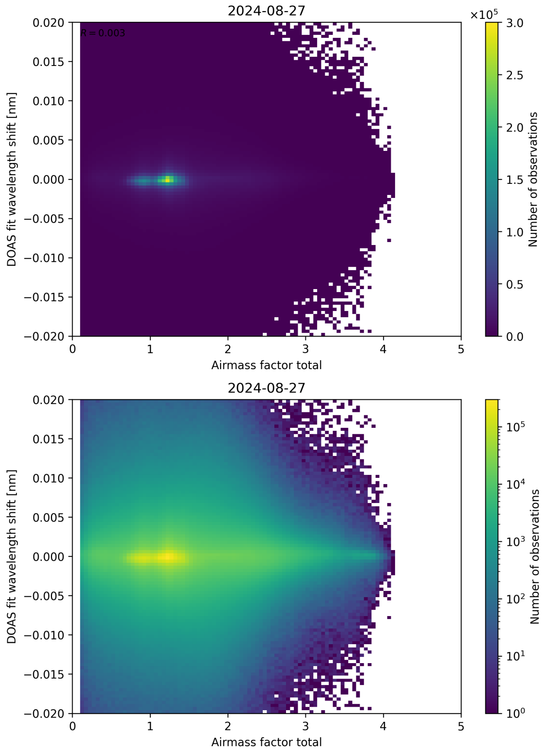
Figure 98: Scatter density plot of “Airmass factor total” against “DOAS fit wavelength shift” for 2024-08-27 to 2024-08-28.
