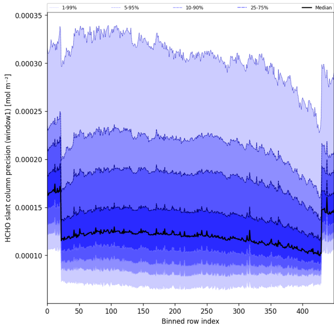
Figure 53: Along track statistics of “HCHO slant column precision (window1)” for 2024-08-27 to 2024-08-28
