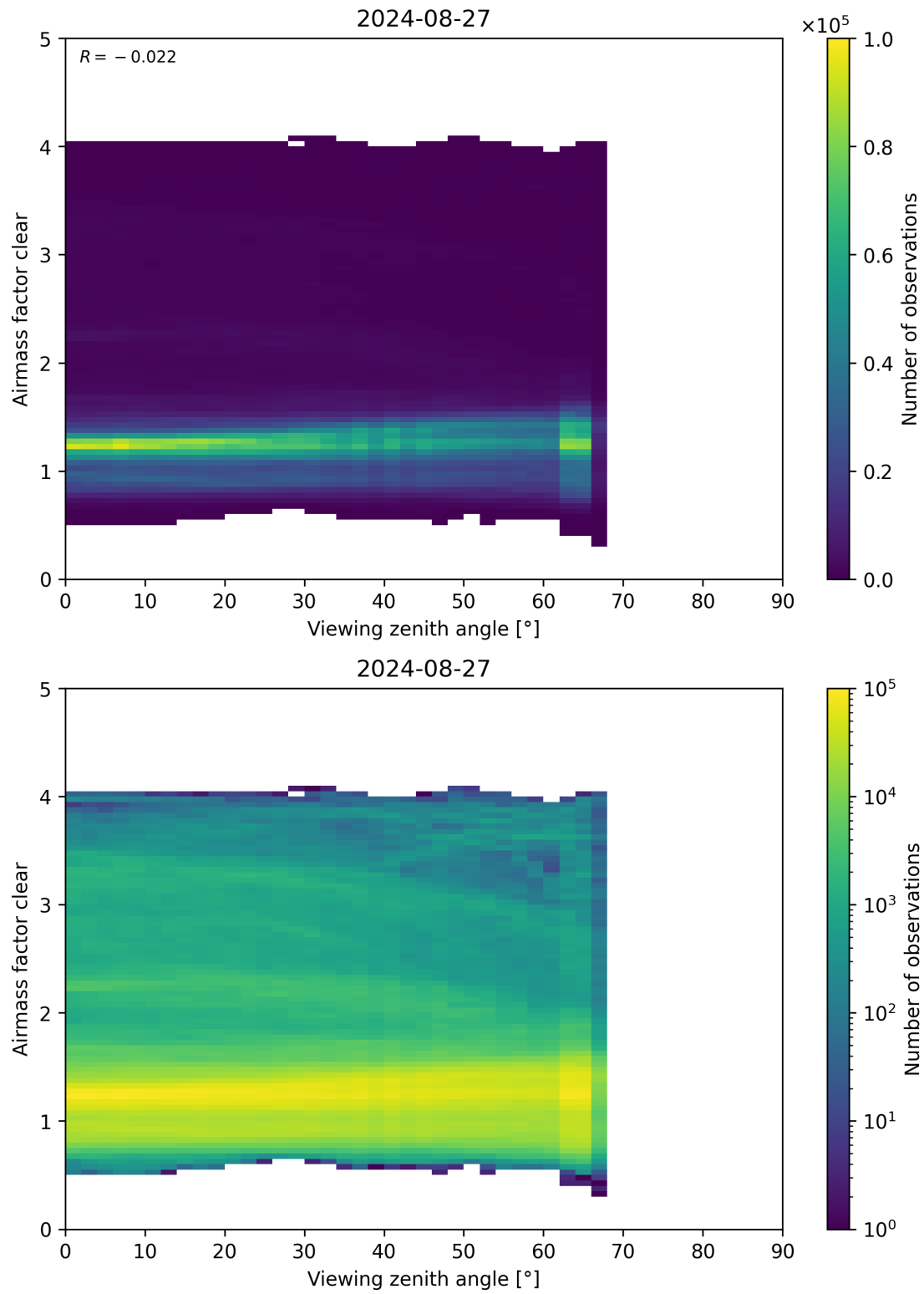
Figure 185: Scatter density plot of “Viewing zenith angle” against “Airmass factor clear” for 2024-08-27 to 2024-08-28.
