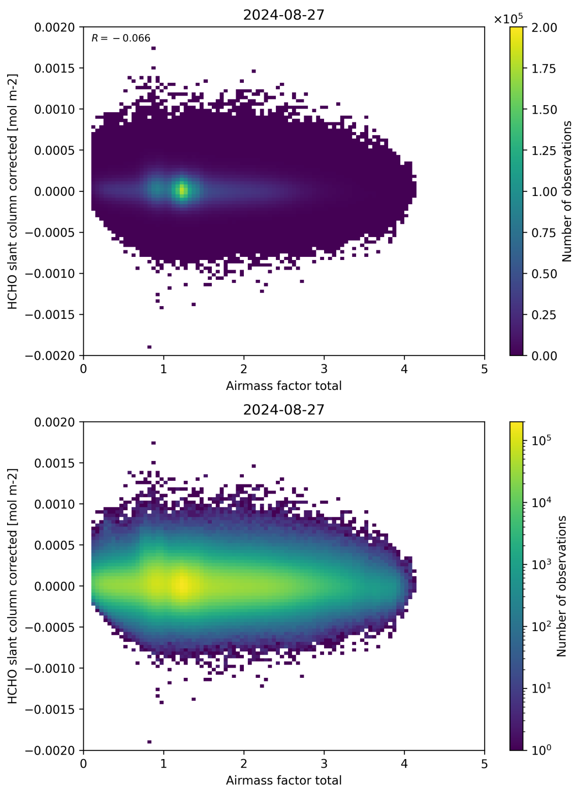
Figure 101: Scatter density plot of “Airmass factor total” against “HCHO slant column corrected” for 2024-08-27 to 2024-08-28.
