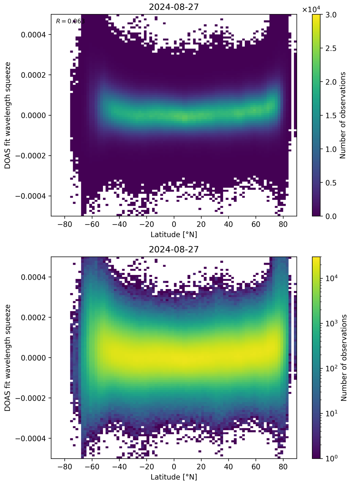
Figure 155: Scatter density plot of “Latitude” against “DOAS fit wavelength squeeze” for 2024-08-27 to 2024-08-28.
