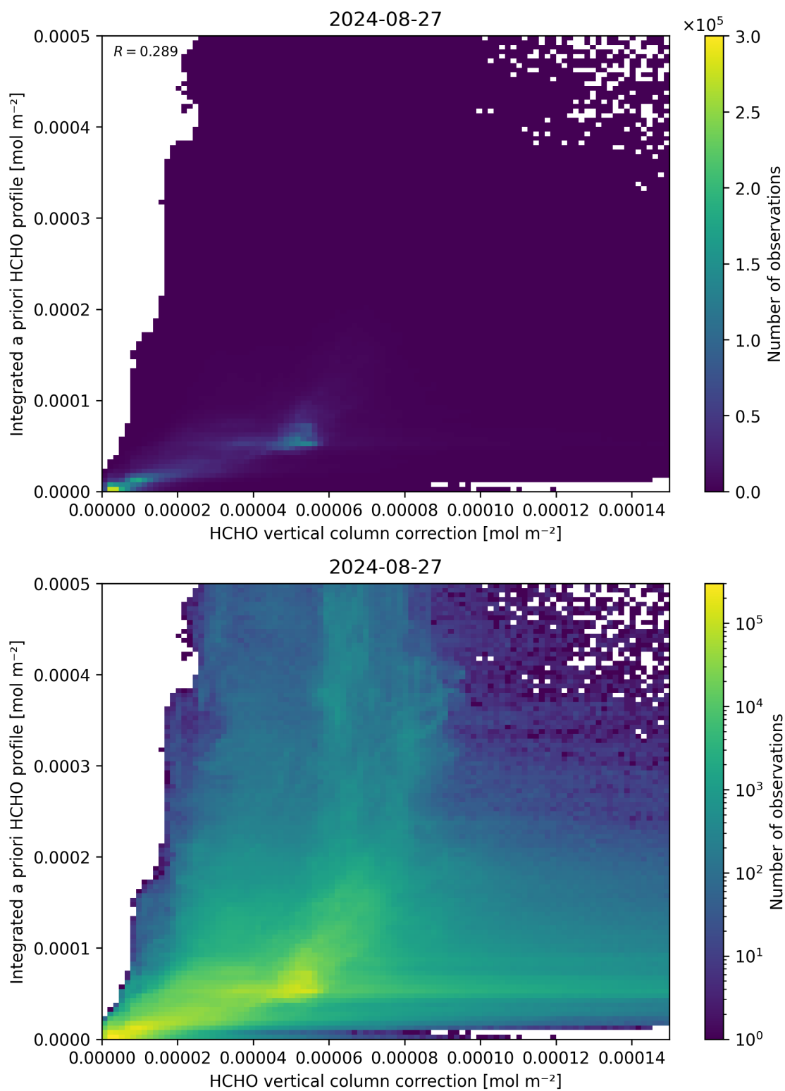
Figure 122: Scatter density plot of “HCHO vertical column correction” against “Integrated a priori HCHO profile” for 2024-08-27 to 2024-08-28.
