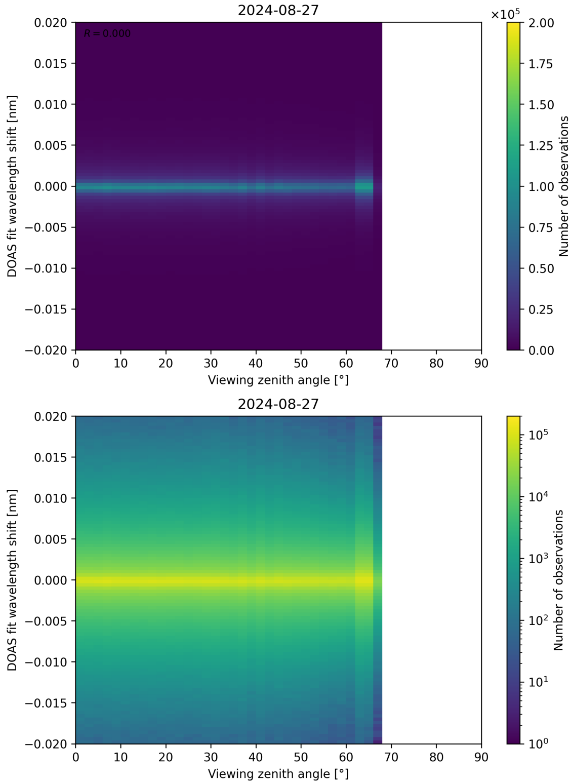
Figure 183: Scatter density plot of “Viewing zenith angle” against “DOAS fit wavelength shift” for 2024-08-27 to 2024-08-28.
