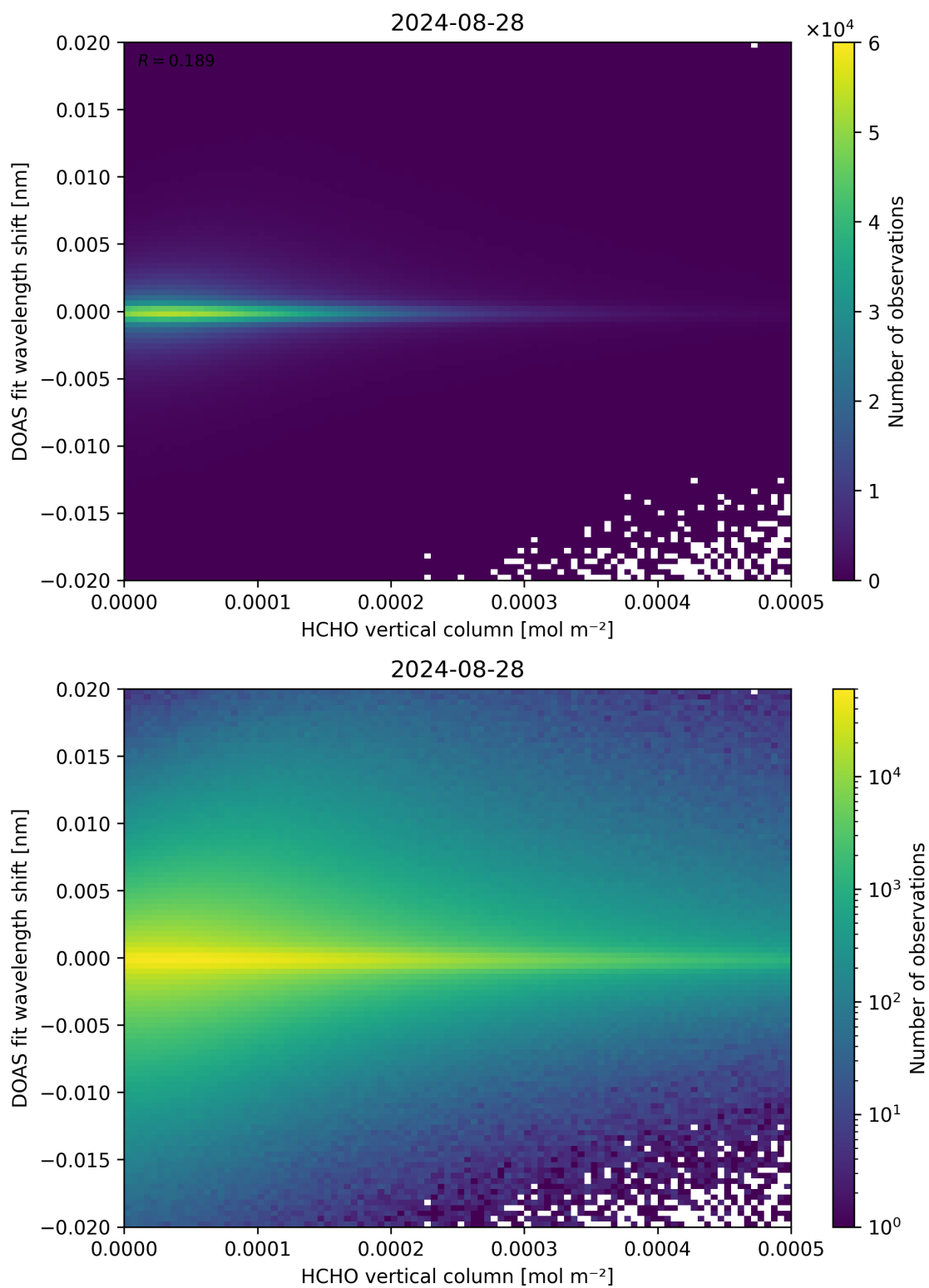
Figure 124: Scatter density plot of “HCHO vertical column” against “DOAS fit wavelength shift” for 2024-08-27 to 2024-08-29.
