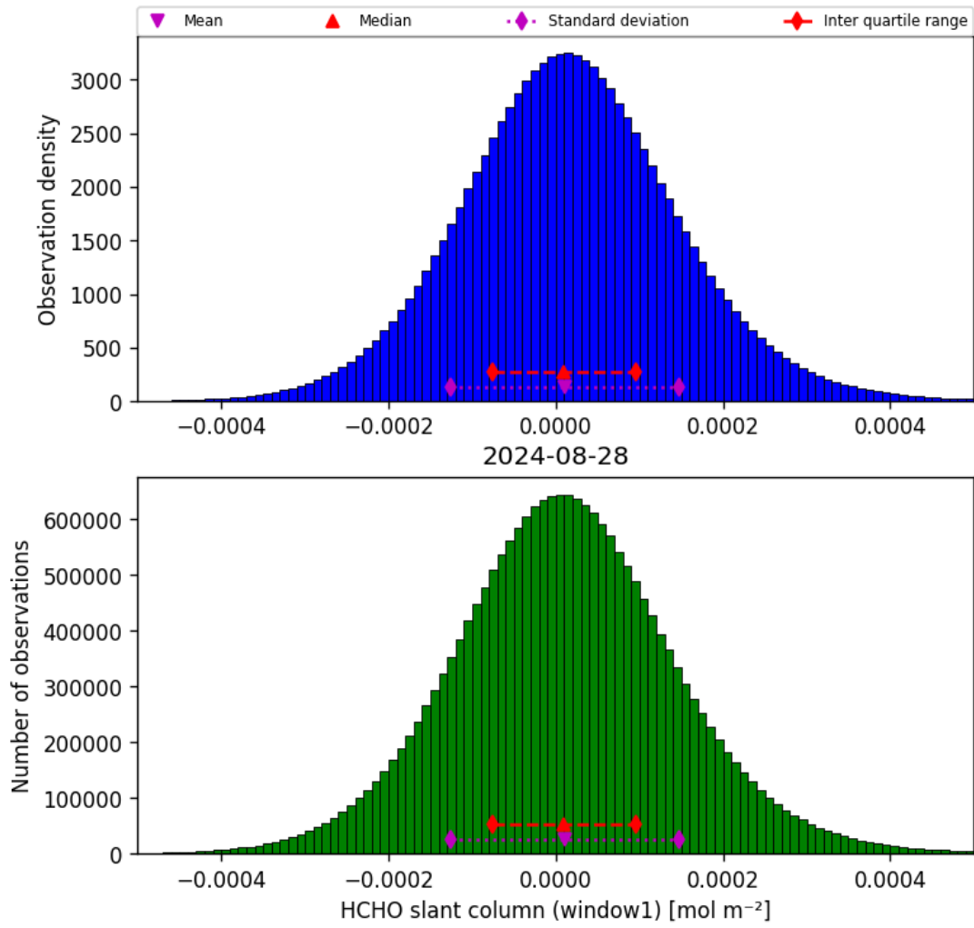
Figure 38: Histogram of “HCHO slant column (window1)” for 2024-08-27 to 2024-08-29
