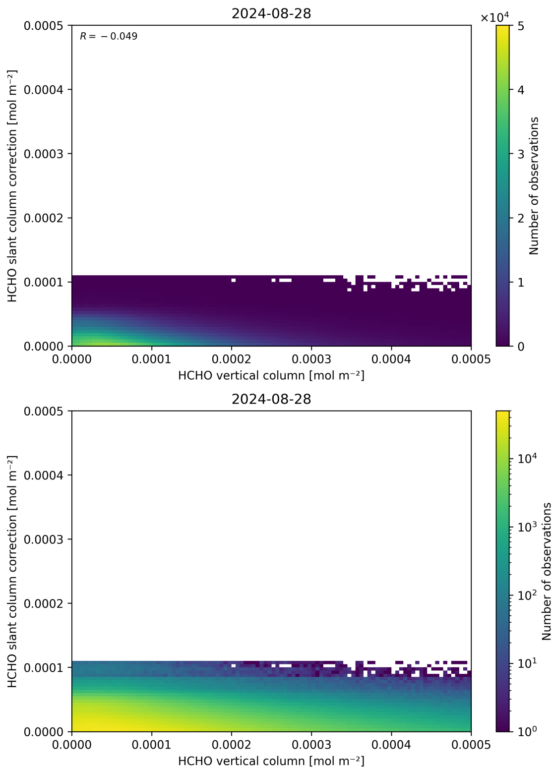
Figure 128: Scatter density plot of “HCHO vertical column” against “HCHO slant column correction” for 2024-08-27 to 2024-08-29.
