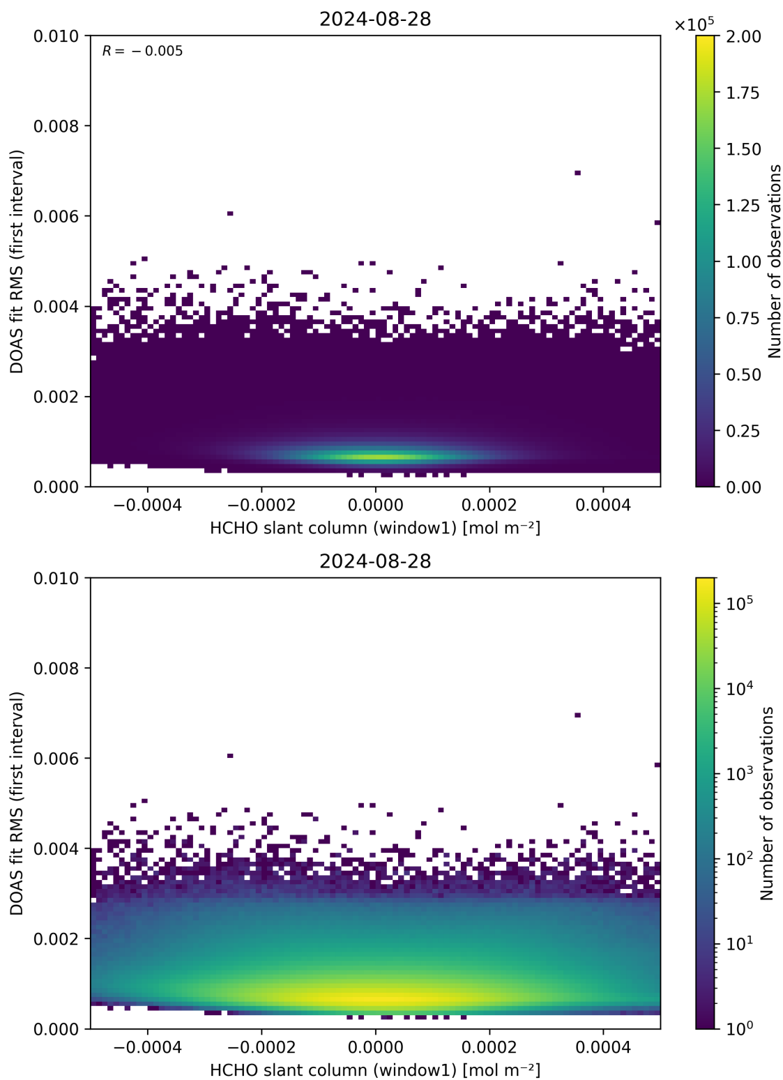
Figure 78: Scatter density plot of “HCHO slant column (window1)” against “DOAS fit RMS (first interval)” for 2024-08-27 to 2024-08-29.
