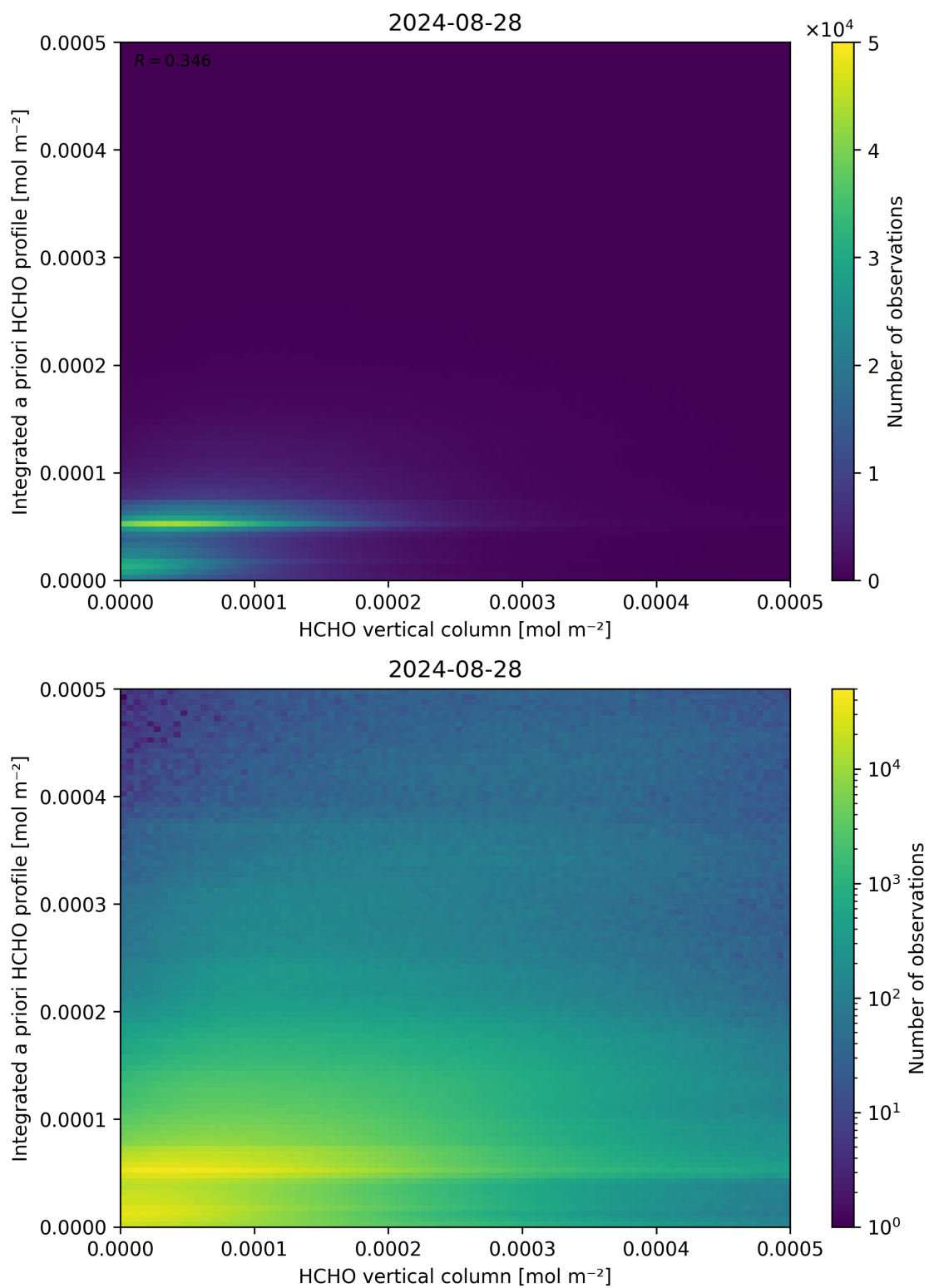
Figure 135: Scatter density plot of “HCHO vertical column” against “Integrated a priori HCHO profile” for 2024-08-27 to 2024-08-29.
