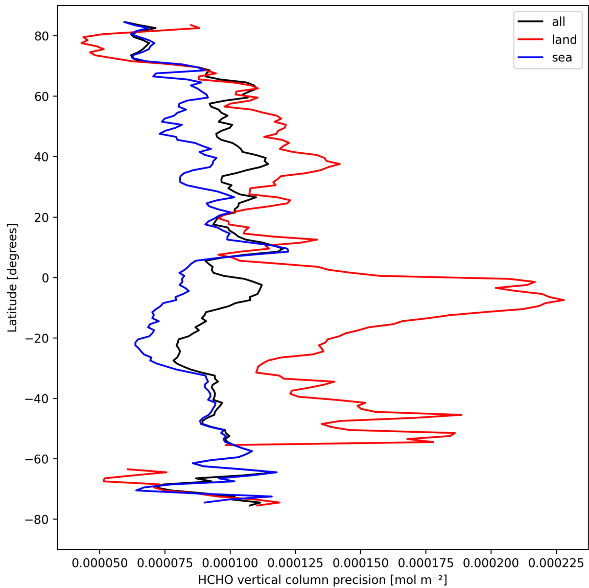
Figure 22: Zonal average of “HCHO vertical column precision” for 2024-08-27 to 2024-08-29.
