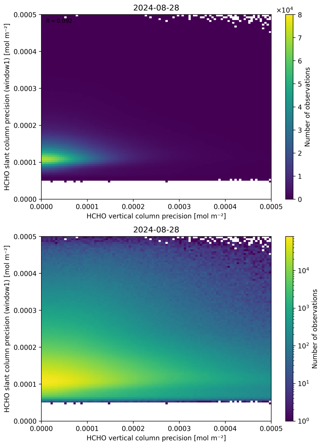
Figure 143: Scatter density plot of “HCHO vertical column precision” against “HCHO slant column precision (window1)” for 2024-08-27 to 2024-08-29.
