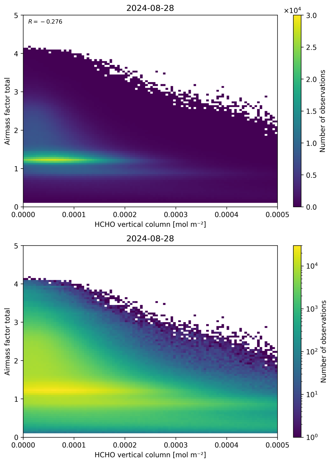
Figure 131: Scatter density plot of “HCHO vertical column” against “Airmass factor total” for 2024-08-27 to 2024-08-29.
