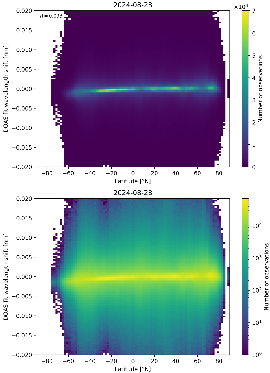
Figure 154: Scatter density plot of “Latitude” against “DOAS fit wavelength shift” for 2024-08-27 to 2024-08-29.
