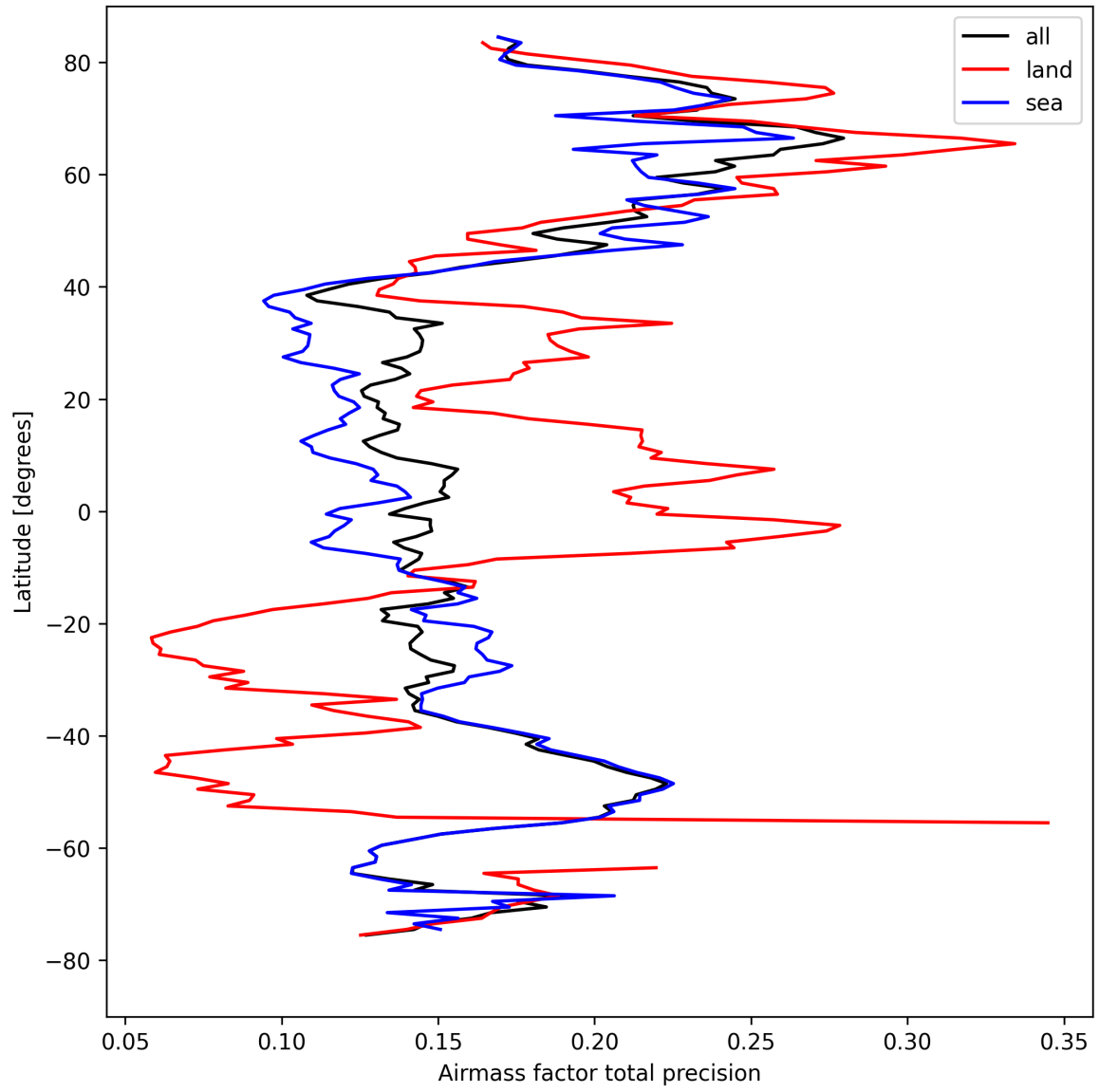
Figure 27: Zonal average of “Airmass factor total precision” for 2024-08-27 to 2024-08-29.
