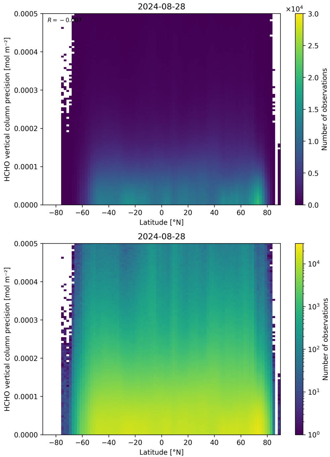
Figure 165: Scatter density plot of “Latitude” against “HCHO vertical column precision” for 2024-08-27 to 2024-08-29.
