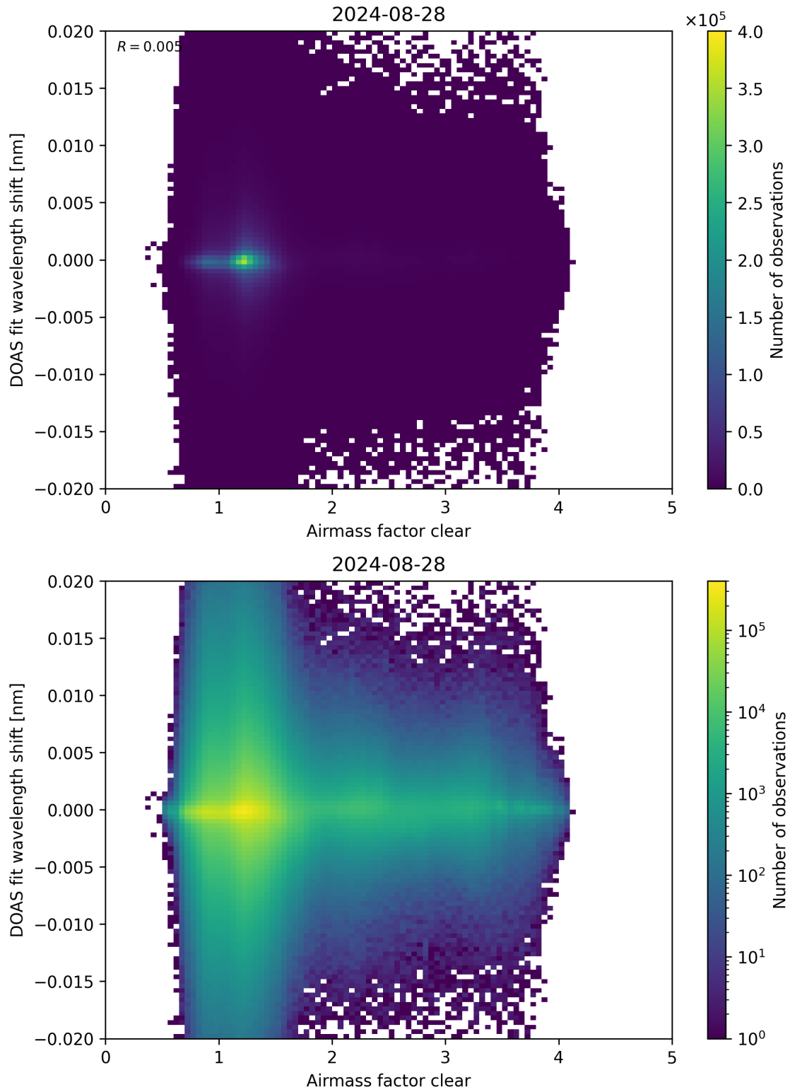
Figure 72: Scatter density plot of “Airmass factor clear” against “DOAS fit wavelength shift” for 2024-08-27 to 2024-08-29.
