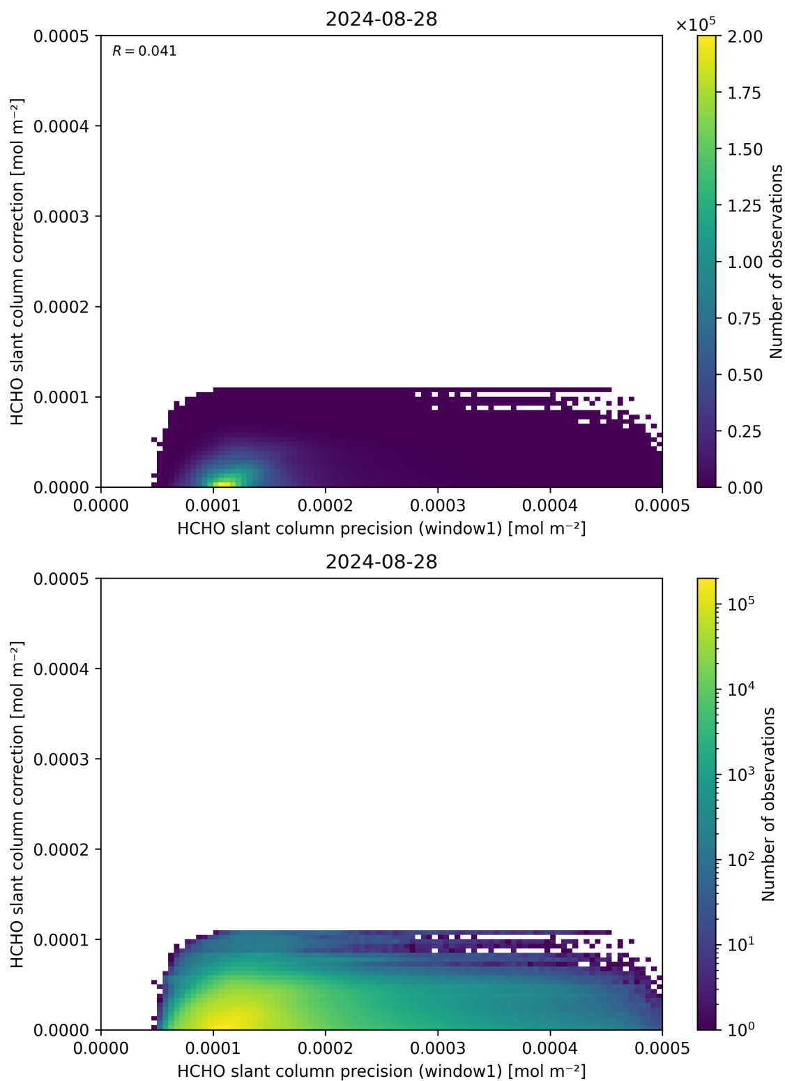
Figure 93: Scatter density plot of “HCHO slant column precision (window1)” against “HCHO slant column correction” for 2024-08-27 to 2024-08-29.
