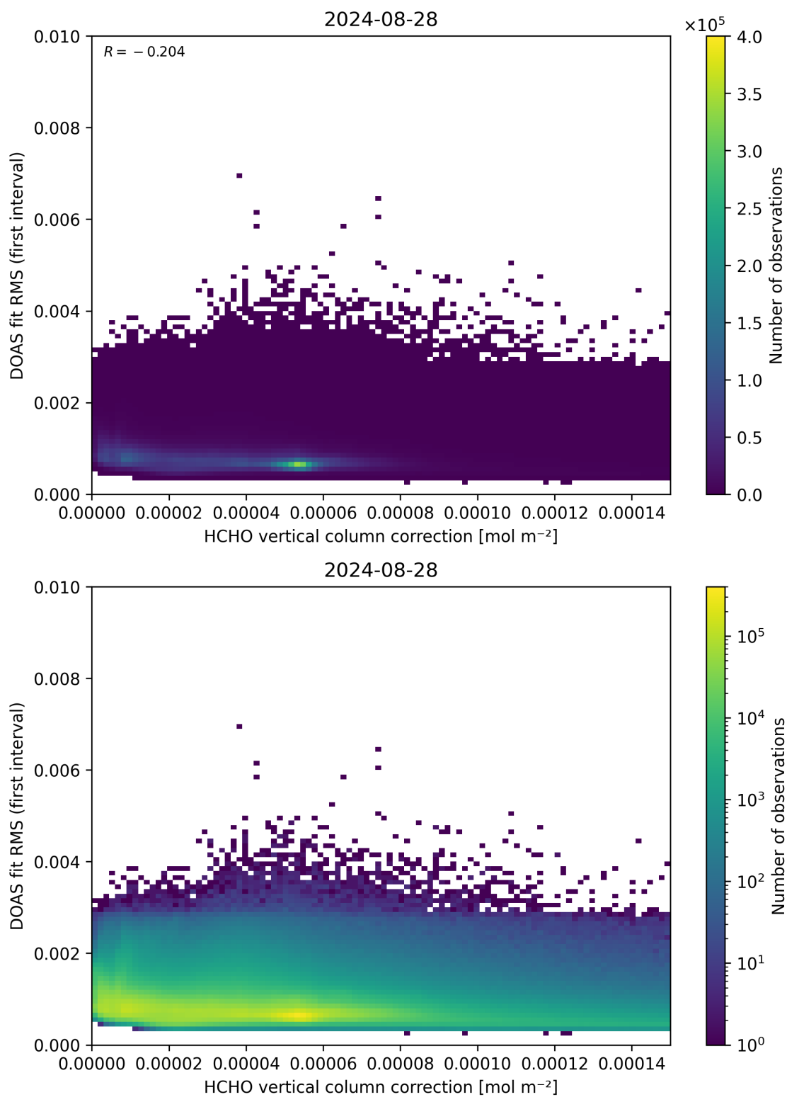
Figure 112: Scatter density plot of “HCHO vertical column correction” against “DOAS fit RMS (first interval)” for 2024-08-27 to 2024-08-29.
