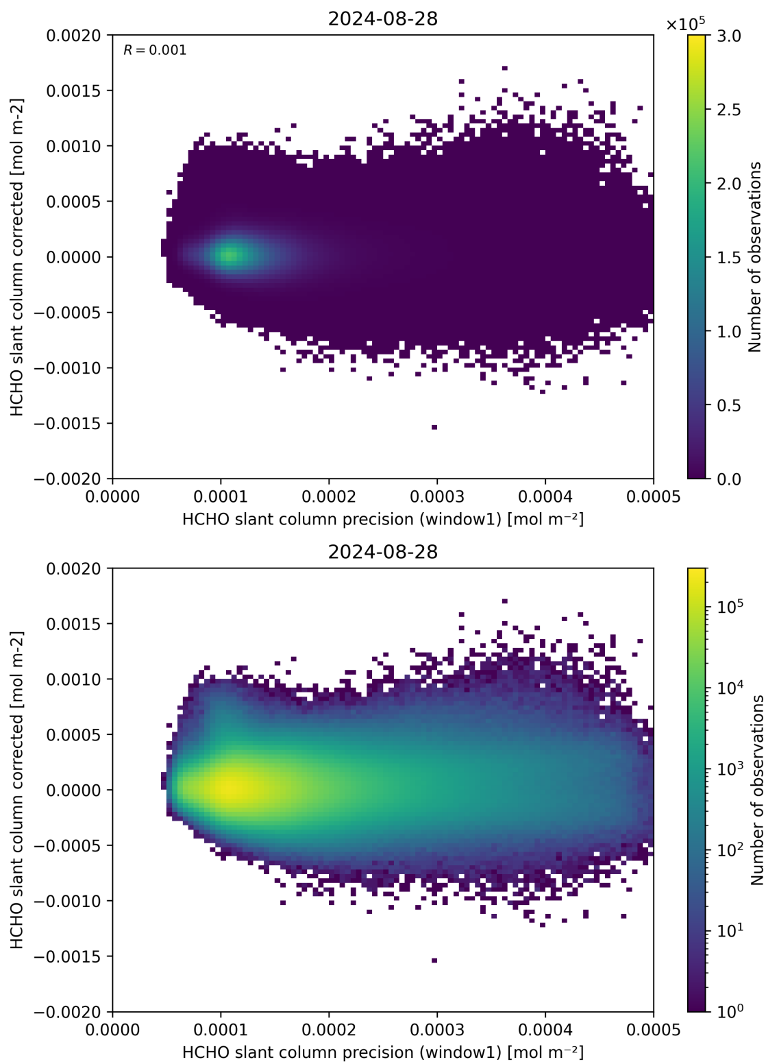
Figure 92: Scatter density plot of “HCHO slant column precision (window1)” against “HCHO slant column corrected” for 2024-08-27 to 2024-08-29.
