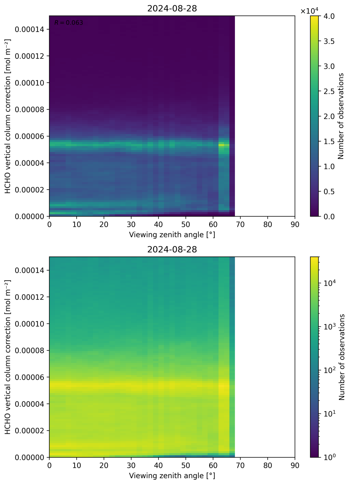
Figure 193: Scatter density plot of “Viewing zenith angle” against “HCHO vertical column correction” for 2024-08-27 to 2024-08-29.
