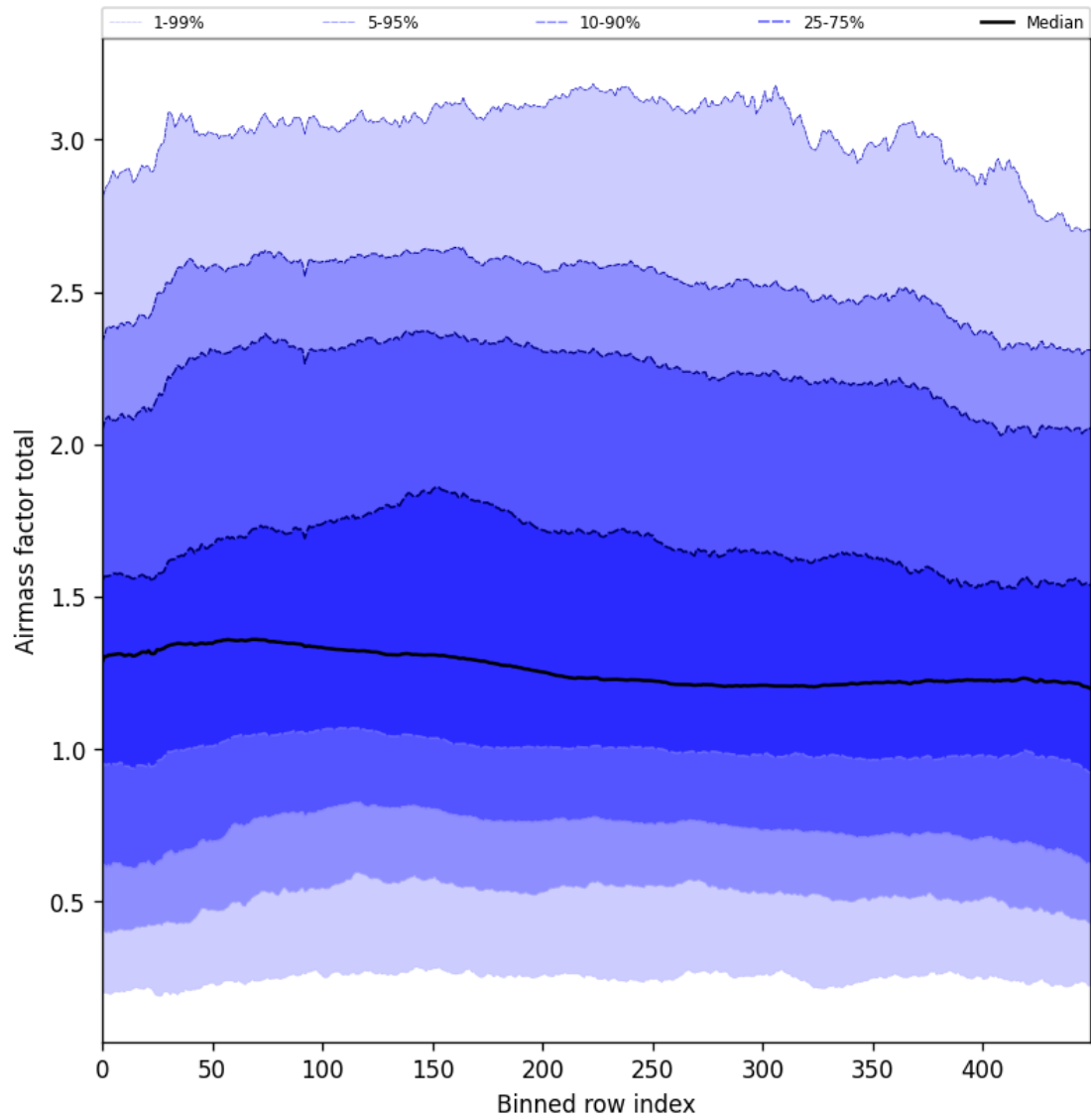
Figure 54: Along track statistics of “Airmass factor total” for 2024-08-27 to 2024-08-29
