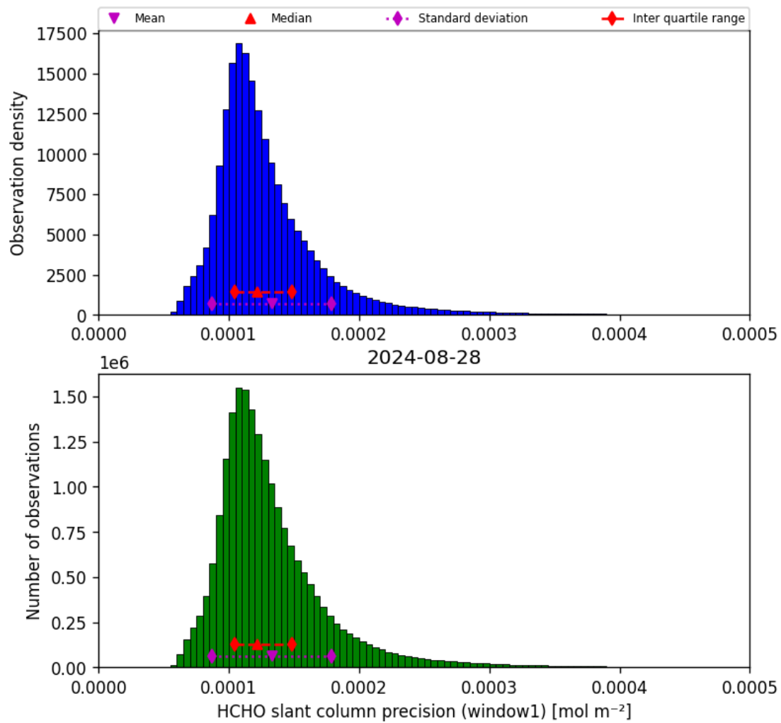
Figure 39: Histogram of “HCHO slant column precision (window1)” for 2024-08-27 to 2024-08-29
