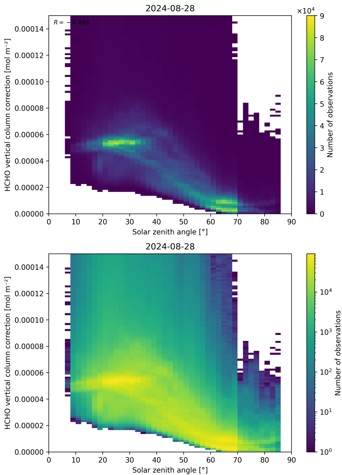
Figure 178: Scatter density plot of “Solar zenith angle” against “HCHO vertical column correction” for 2024-08-27 to 2024-08-29.
