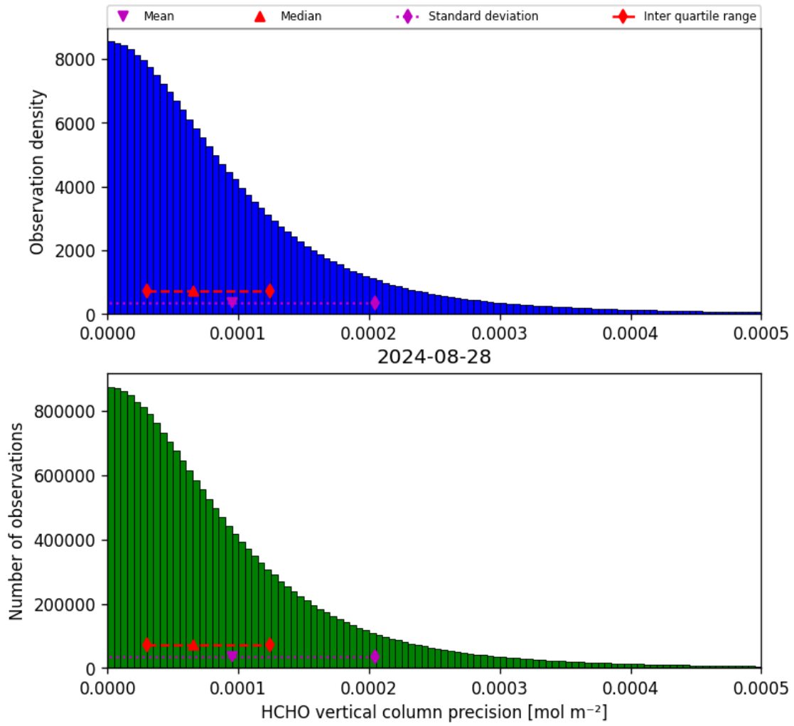
Figure 36: Histogram of “HCHO vertical column precision” for 2024-08-27 to 2024-08-29
