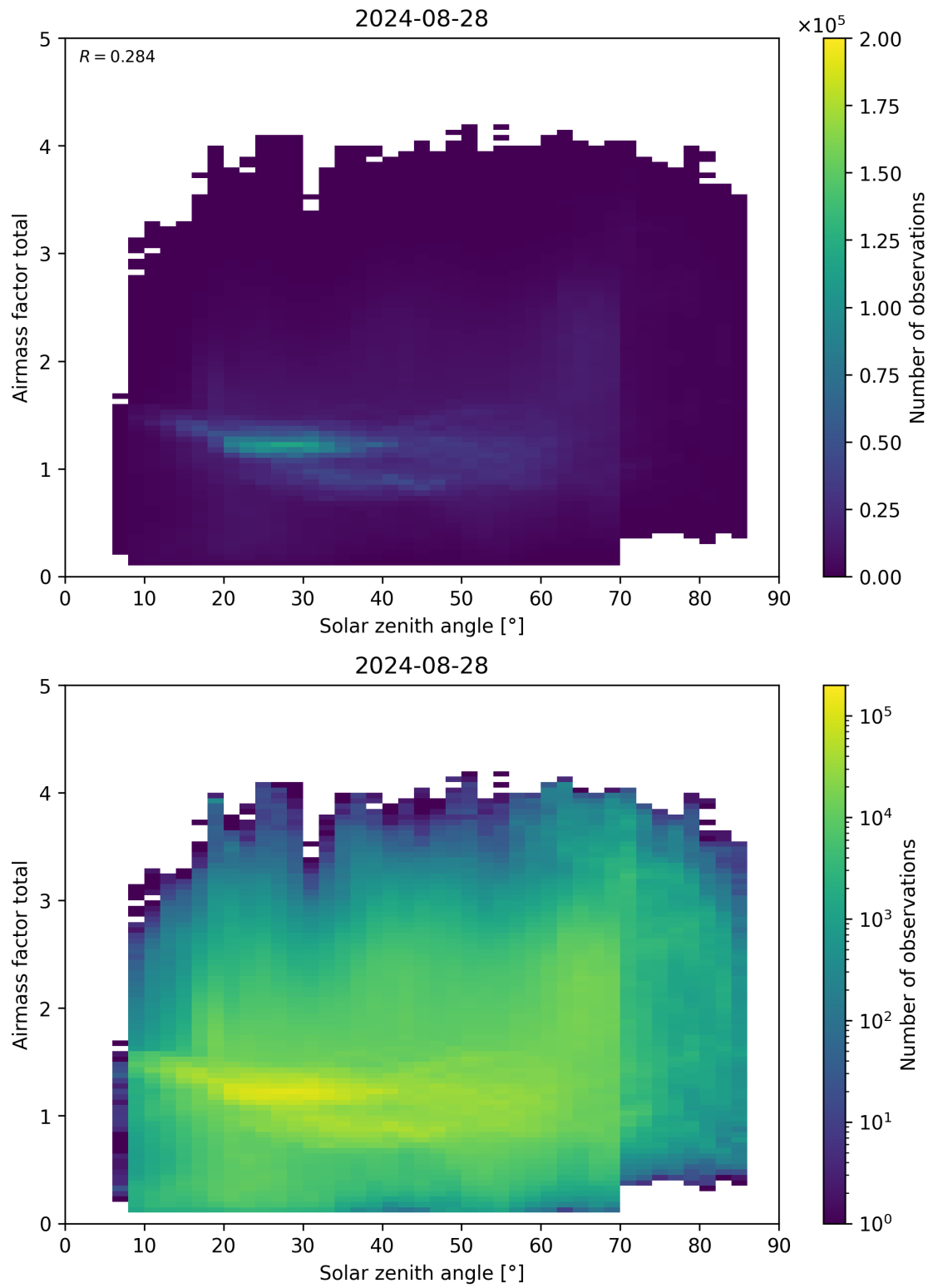
Figure 175: Scatter density plot of “Solar zenith angle” against “Airmass factor total” for 2024-08-27 to 2024-08-29.
