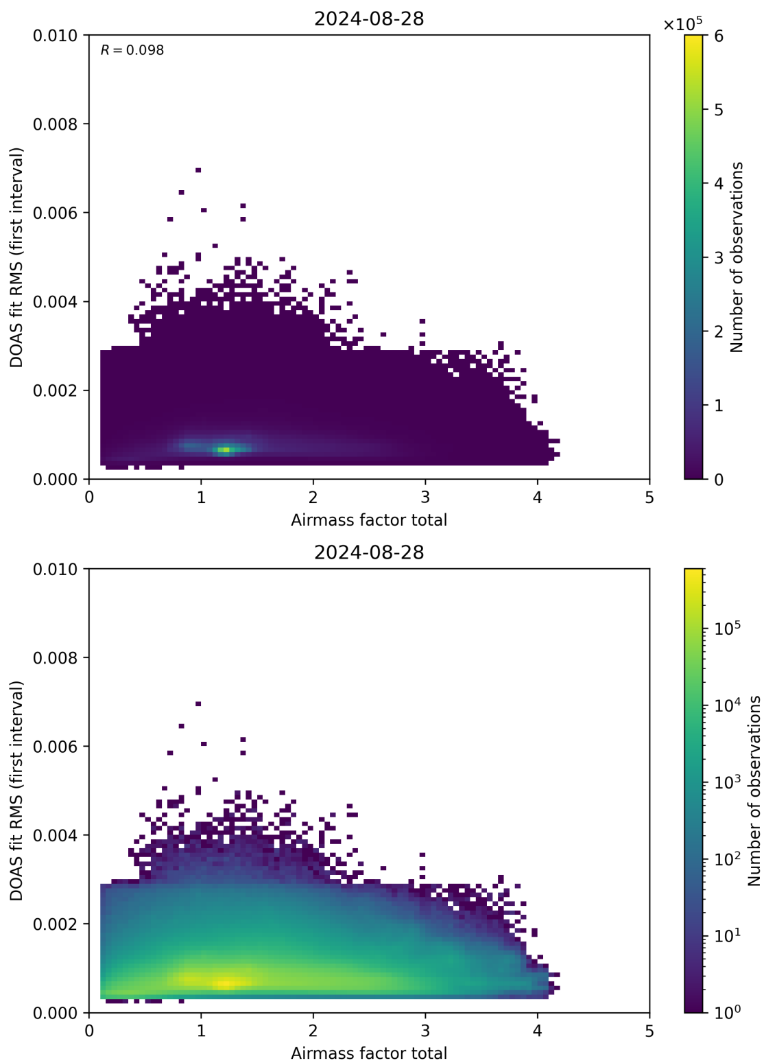
Figure 97: Scatter density plot of “Airmass factor total” against “DOAS fit RMS (first interval)” for 2024-08-27 to 2024-08-29.
