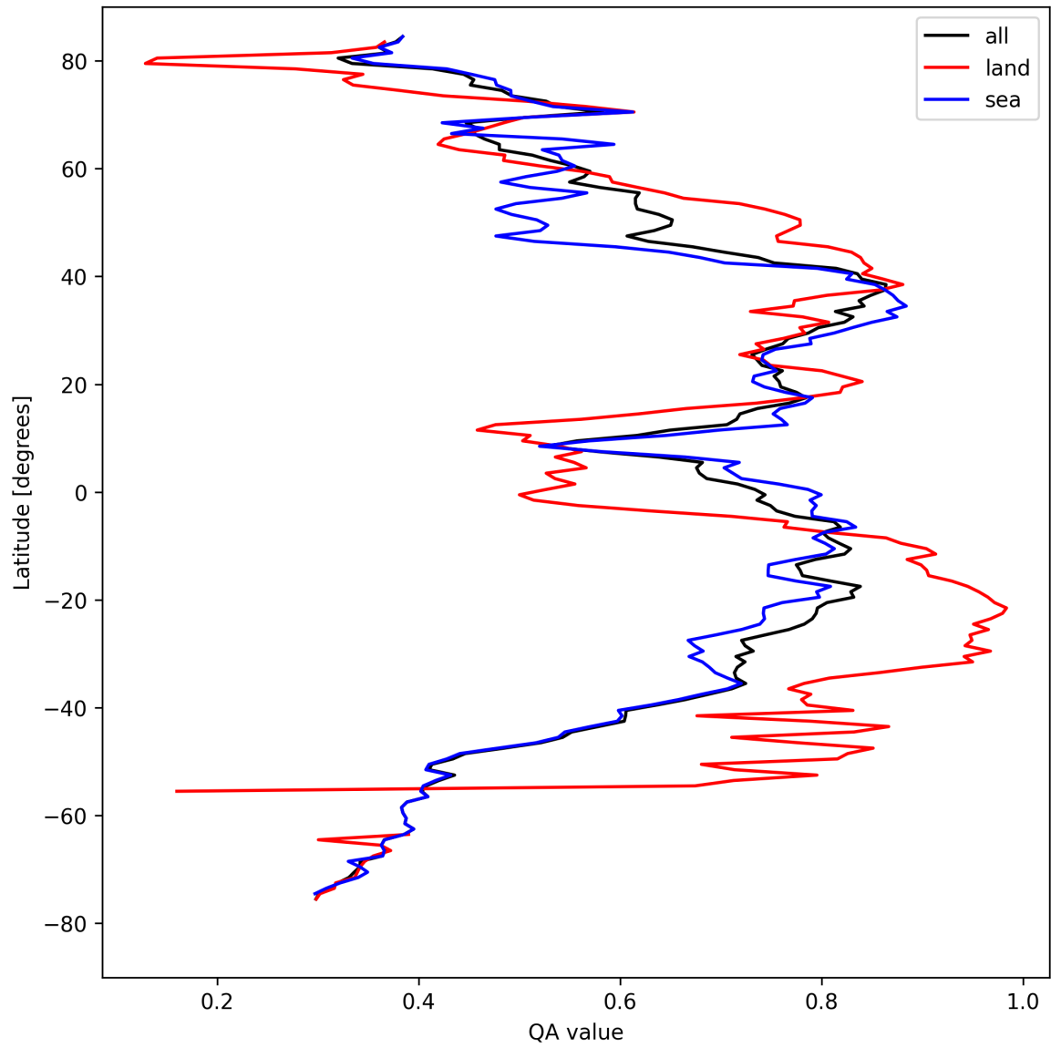
Figure 20: Zonal average of “QA value” for 2024-08-27 to 2024-08-29.
