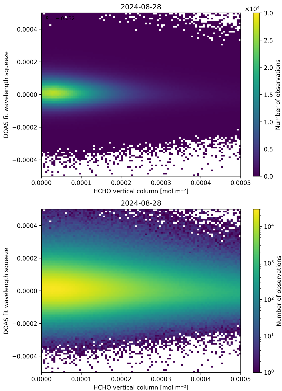
Figure 125: Scatter density plot of “HCHO vertical column” against “DOAS fit wavelength squeeze” for 2024-08-27 to 2024-08-29.
