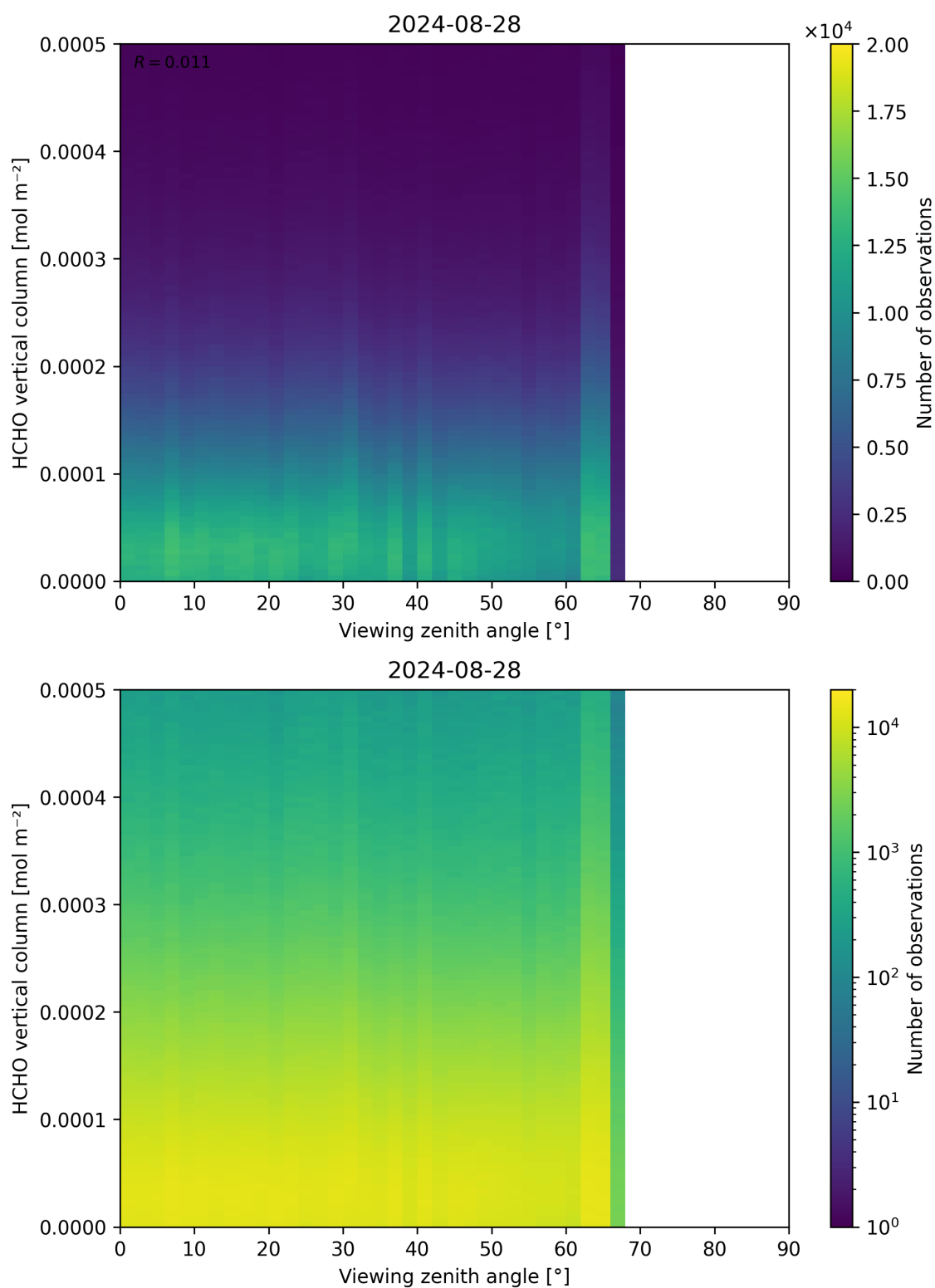
Figure 192: Scatter density plot of “Viewing zenith angle” against “HCHO vertical column” for 2024-08-27 to 2024-08-29.
