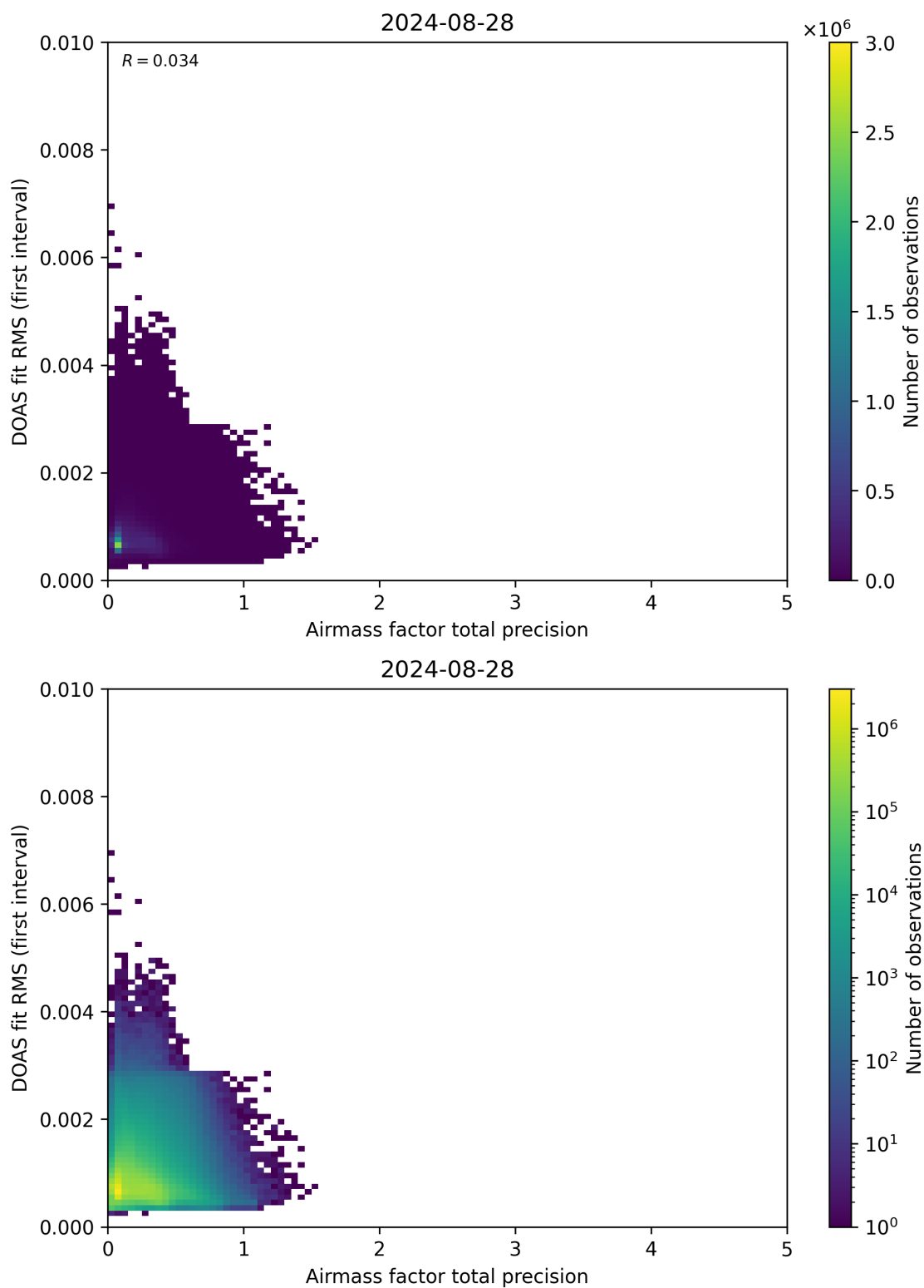
Figure 105: Scatter density plot of “Airmass factor total precision” against “DOAS fit RMS (first interval)” for 2024-08-27 to 2024-08-29.
