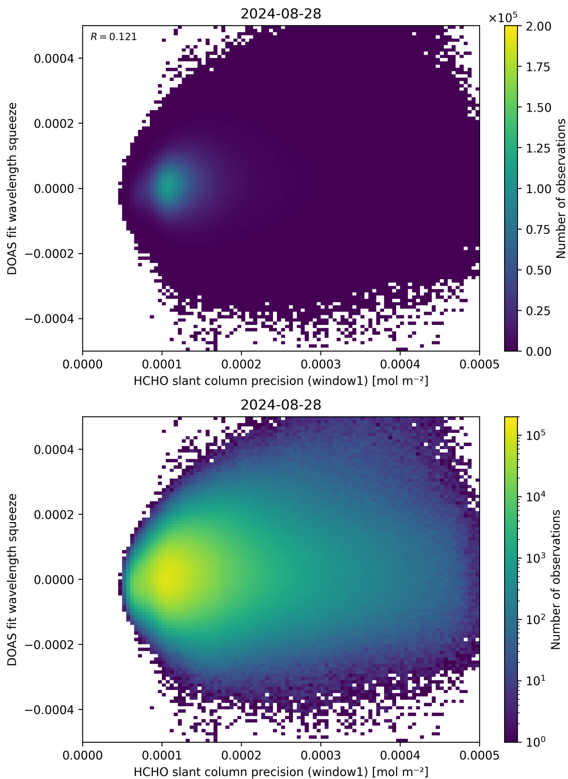
Figure 90: Scatter density plot of “HCHO slant column precision (window1)” against “DOAS fit wavelength squeeze” for 2024-08-27 to 2024-08-29.
