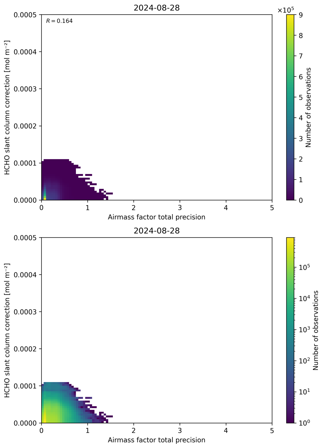
Figure 110: Scatter density plot of “Airmass factor total precision” against “HCHO slant column correction” for 2024-08-27 to 2024-08-29.
