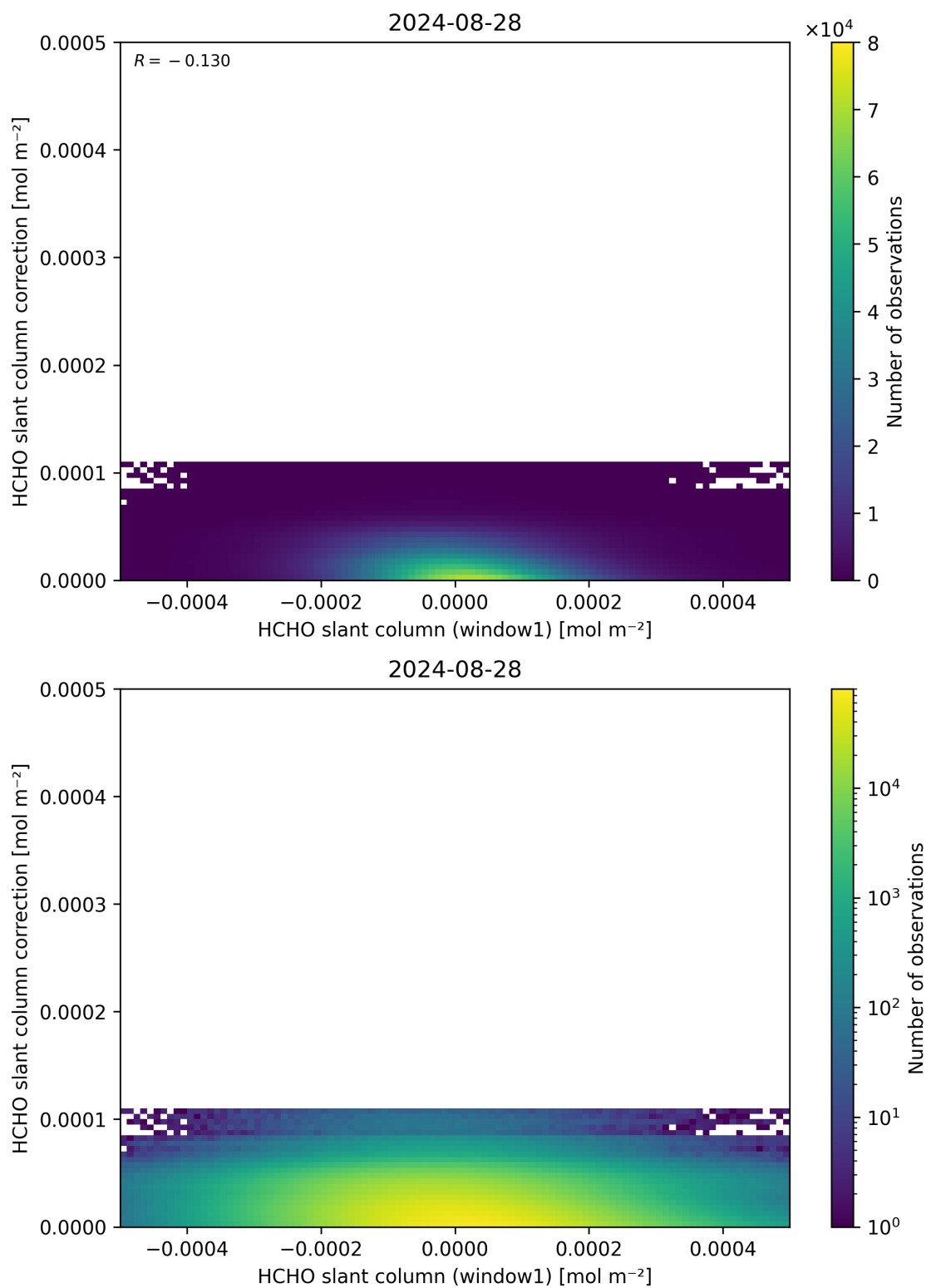
Figure 83: Scatter density plot of “HCHO slant column (window1)” against “HCHO slant column correction” for 2024-08-27 to 2024-08-29.
