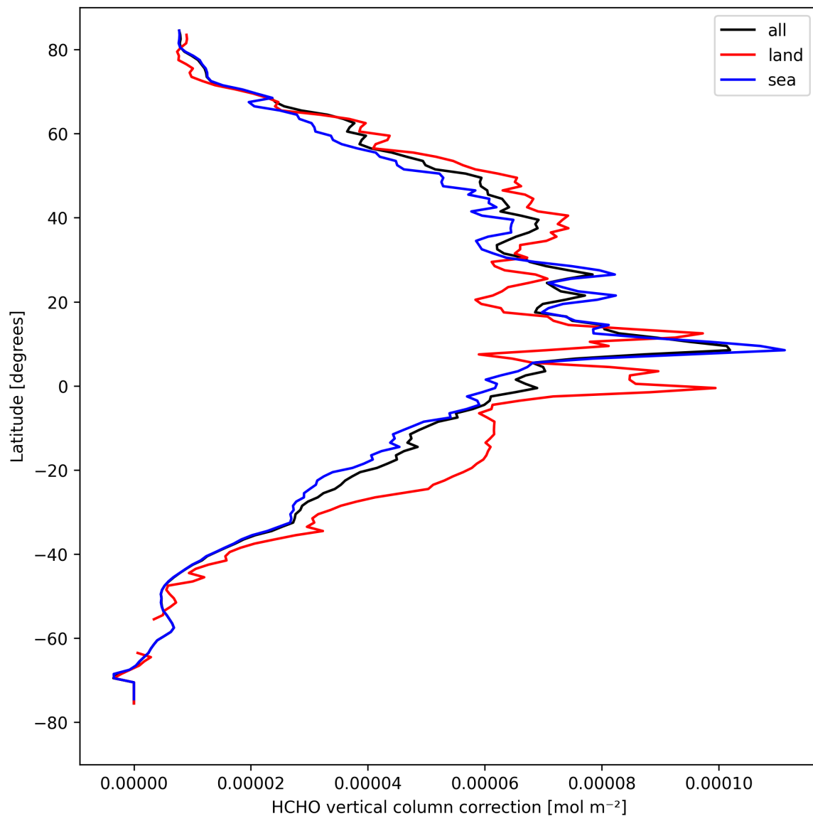
Figure 23: Zonal average of “HCHO vertical column correction” for 2024-08-27 to 2024-08-29.
