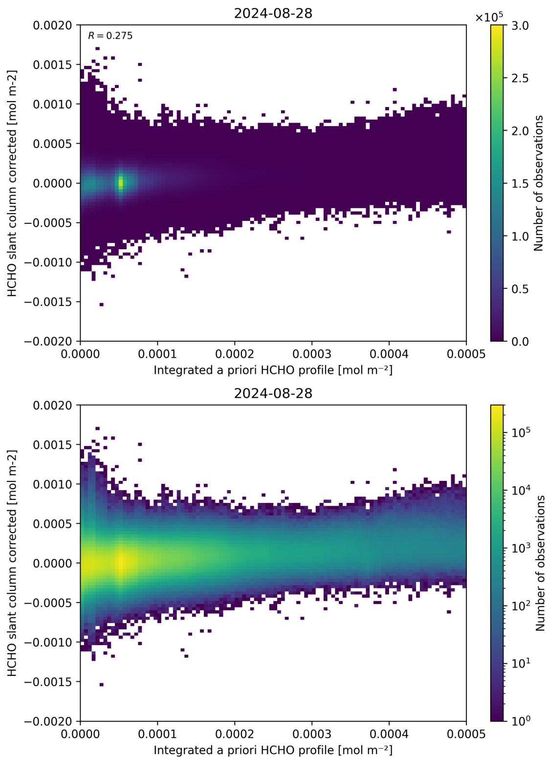
Figure 151: Scatter density plot of “Integrated a priori HCHO profile” against “HCHO slant column corrected” for 2024-08-27 to 2024-08-29.
