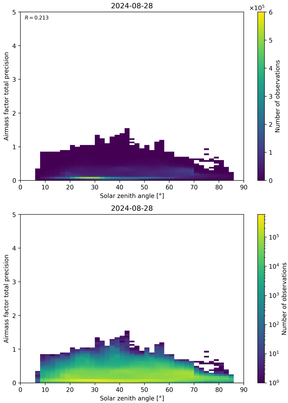
Figure 176: Scatter density plot of “Solar zenith angle” against “Airmass factor total precision” for 2024-08-27 to 2024-08-29.
