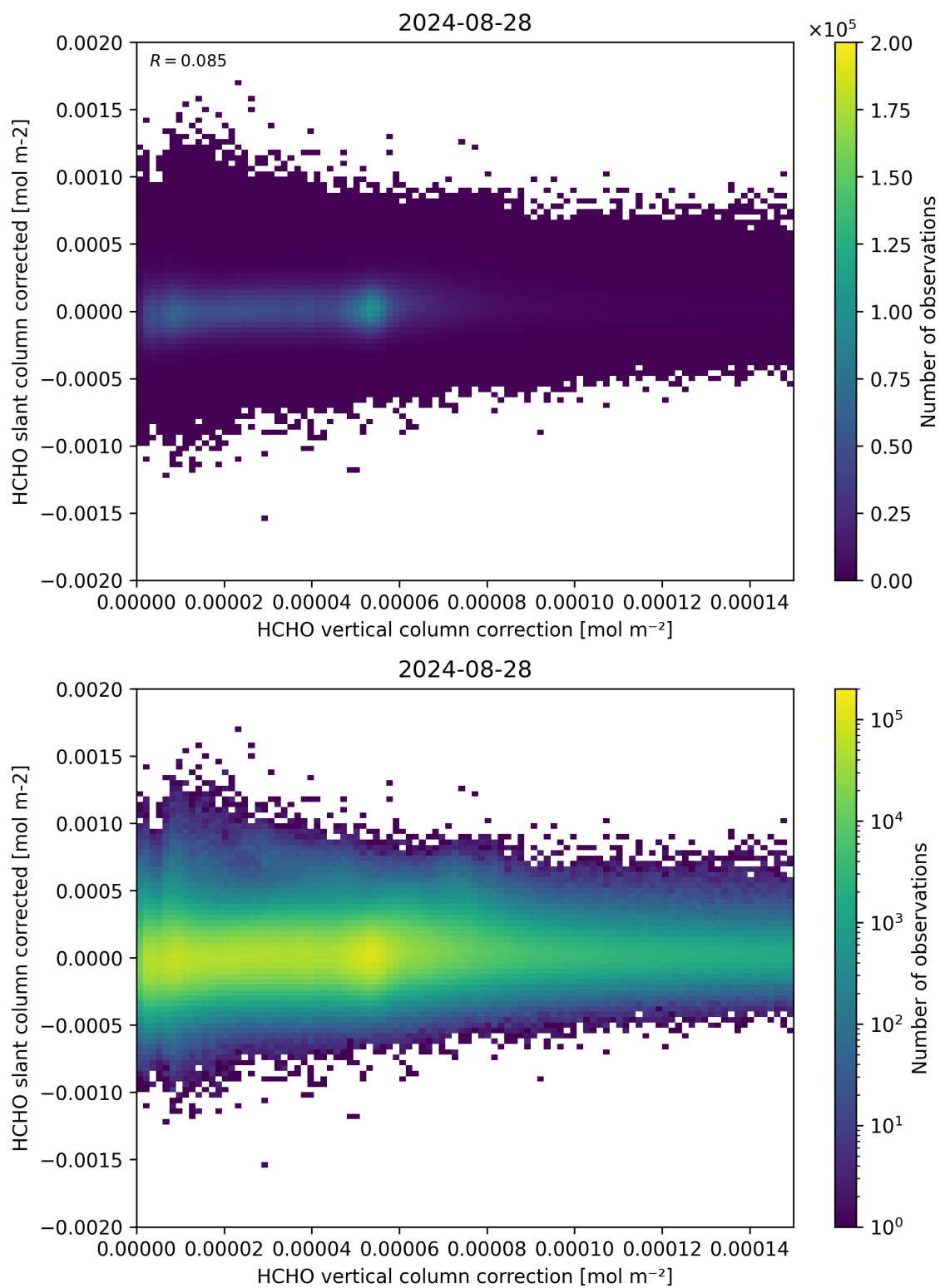
Figure 116: Scatter density plot of “HCHO vertical column correction” against “HCHO slant column corrected” for 2024-08-27 to 2024-08-29.
