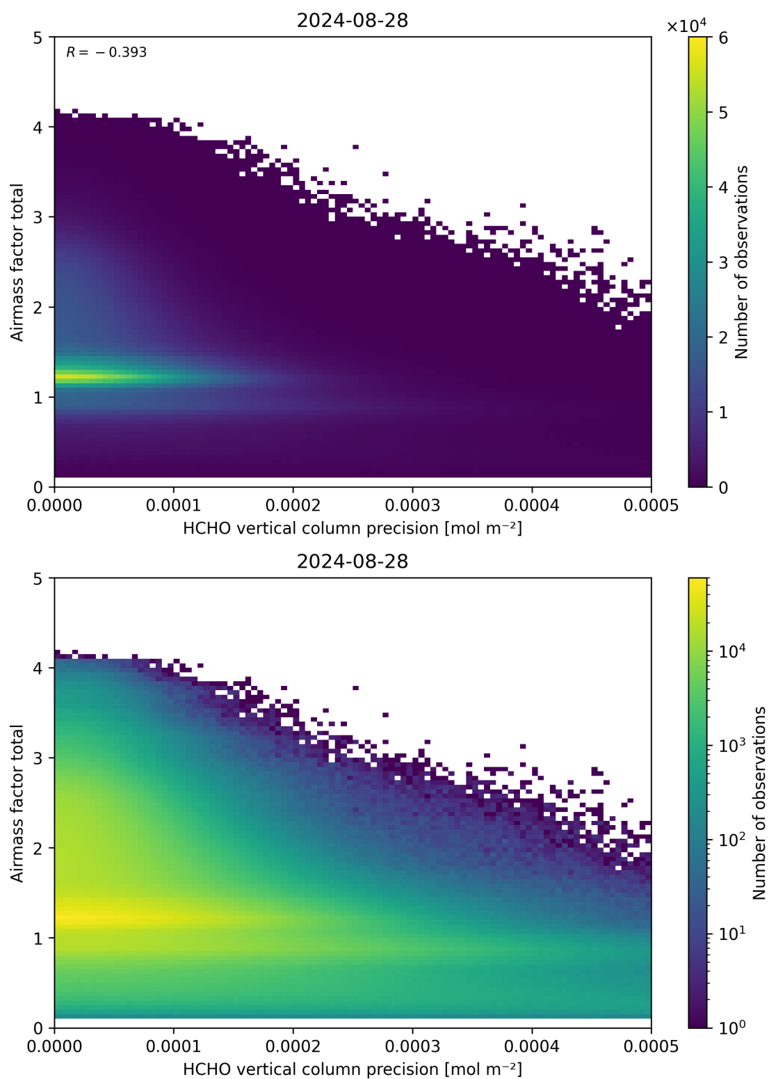
Figure 144: Scatter density plot of “HCHO vertical column precision” against “Airmass factor total” for 2024-08-27 to 2024-08-29.
