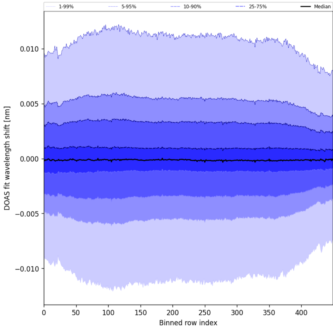
Figure 58: Along track statistics of “DOAS fit wavelength shift” for 2024-08-27 to 2024-08-29
