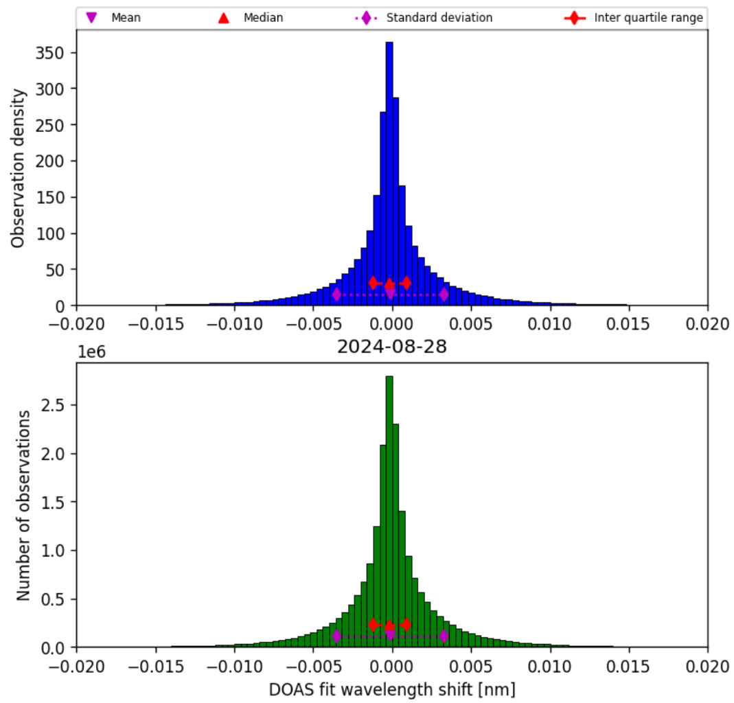
Figure 44: Histogram of “DOAS fit wavelength shift” for 2024-08-27 to 2024-08-29
