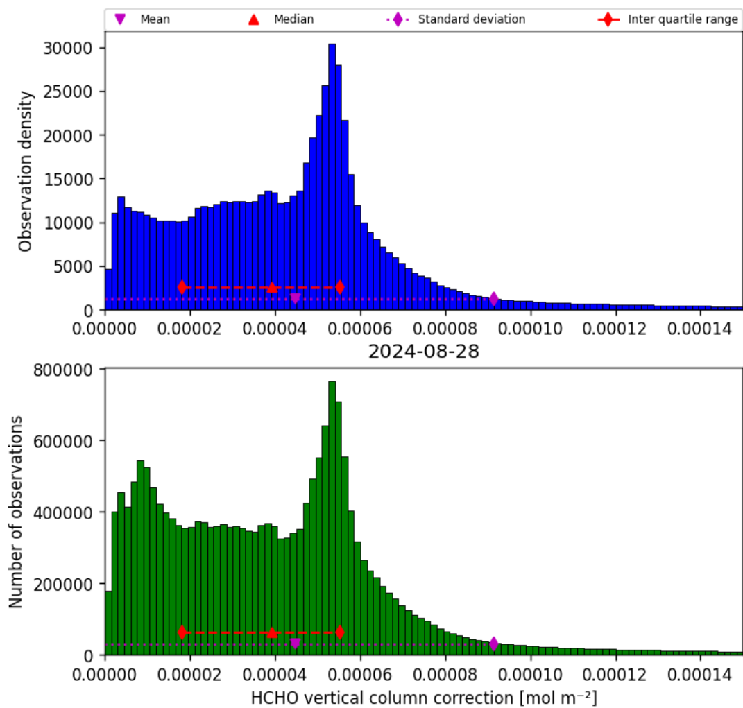
Figure 37: Histogram of “HCHO vertical column correction” for 2024-08-27 to 2024-08-29
