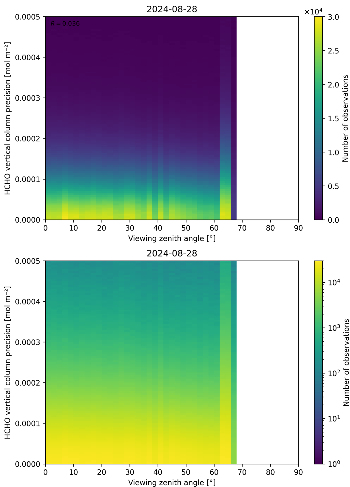
Figure 194: Scatter density plot of “Viewing zenith angle” against “HCHO vertical column precision” for 2024-08-27 to 2024-08-29.
