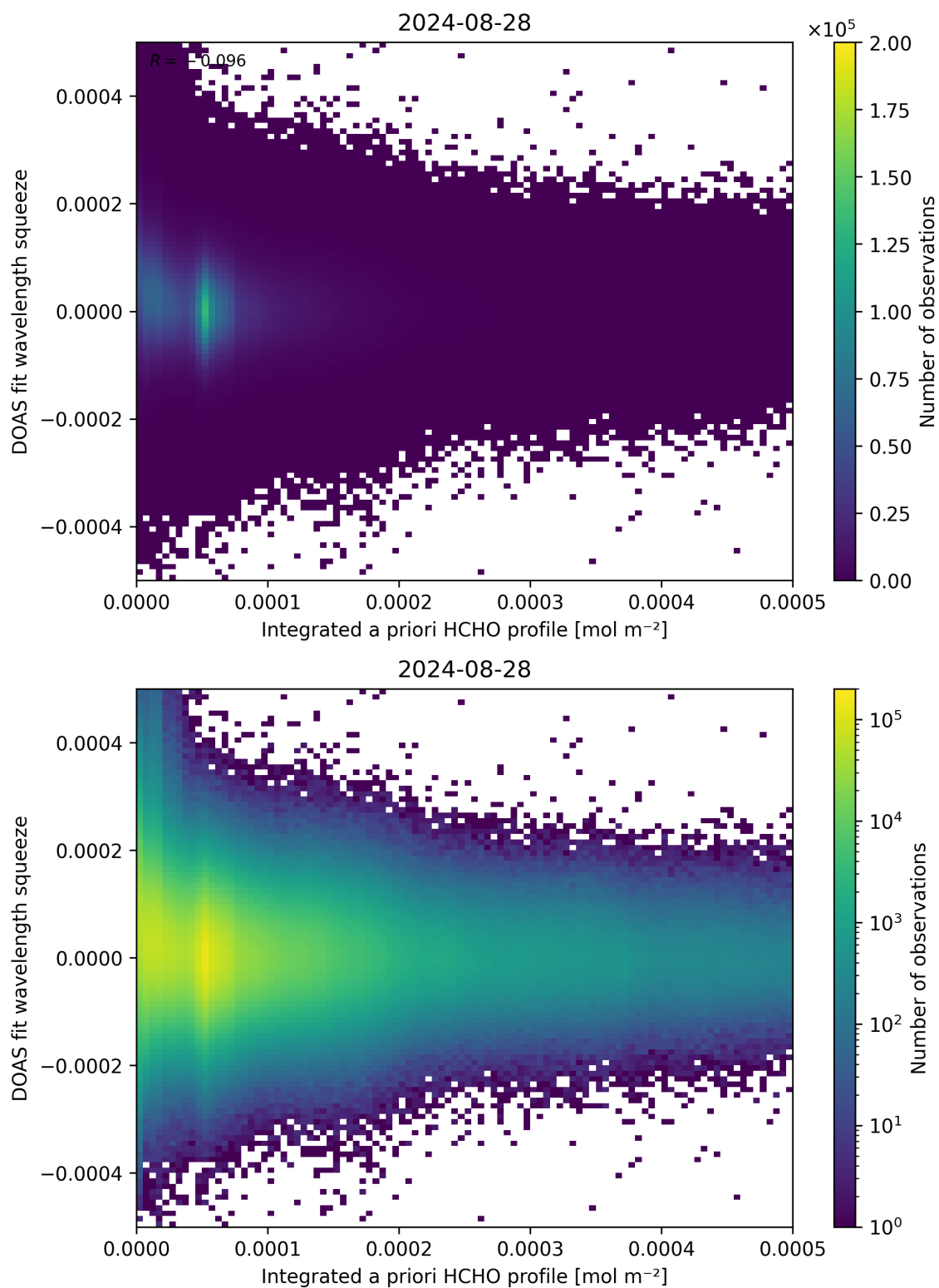
Figure 150: Scatter density plot of “Integrated a priori HCHO profile” against “DOAS fit wavelength squeeze” for 2024-08-27 to 2024-08-29.
