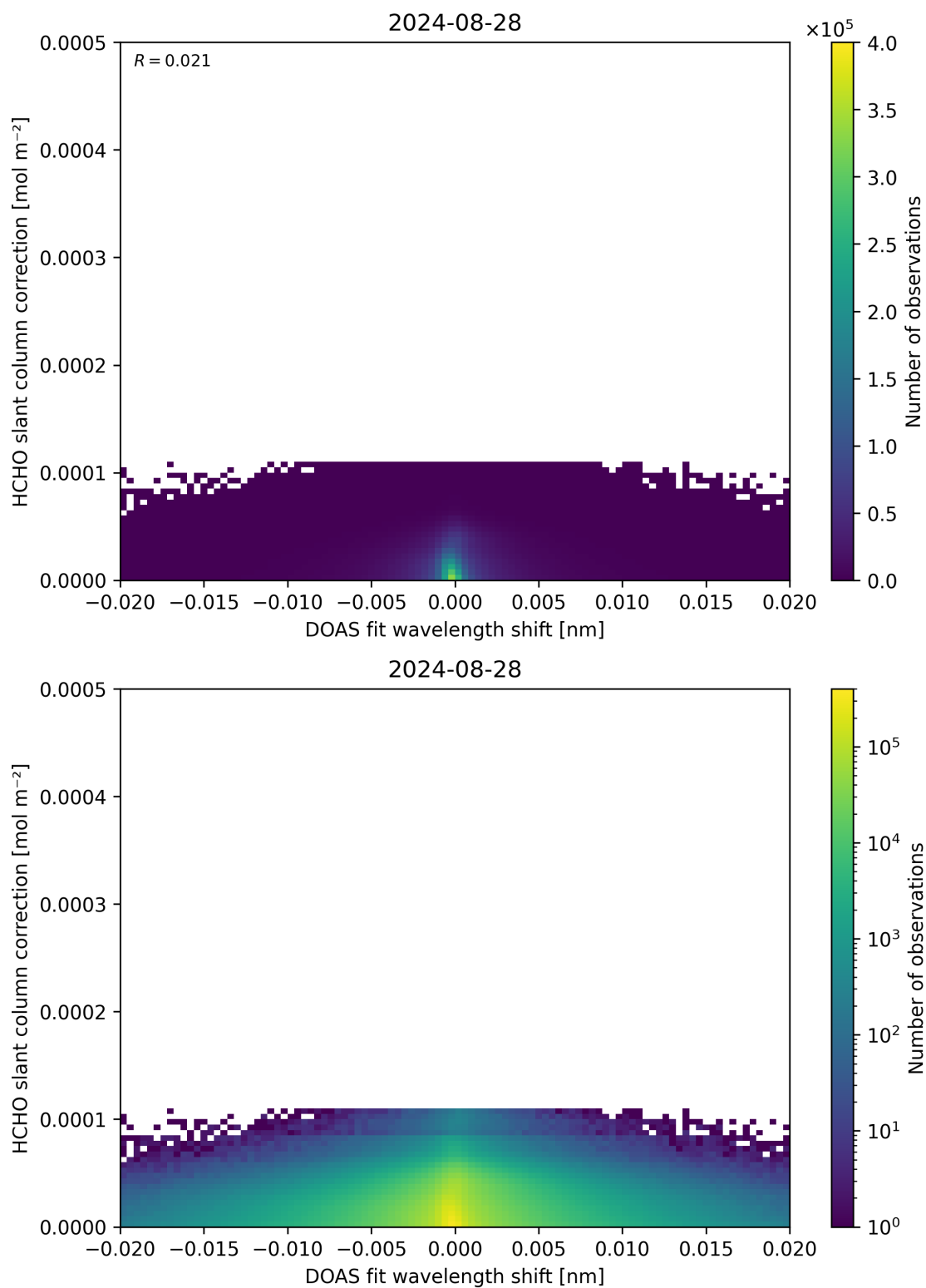
Figure 67: Scatter density plot of “DOAS fit wavelength shift” against “HCHO slant column correction” for 2024-08-27 to 2024-08-29.
