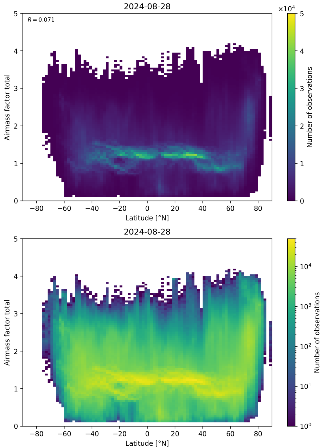
Figure 161: Scatter density plot of “Latitude” against “Airmass factor total” for 2024-08-27 to 2024-08-29.
