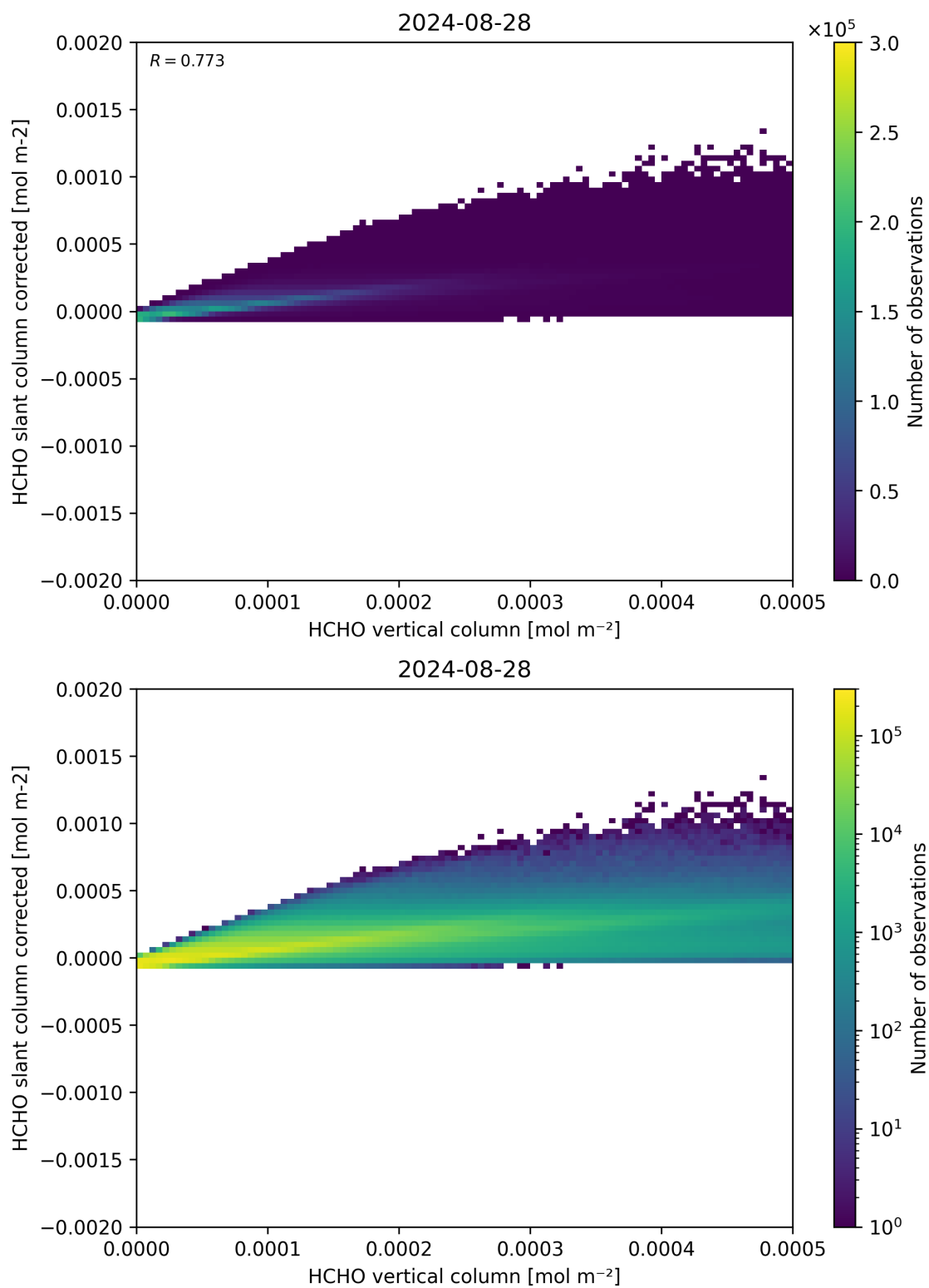
Figure 127: Scatter density plot of “HCHO vertical column” against “HCHO slant column corrected” for 2024-08-27 to 2024-08-29.
