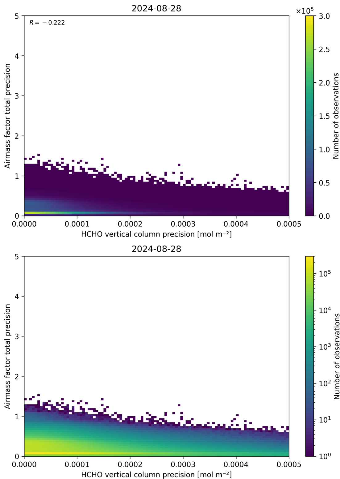
Figure 145: Scatter density plot of “HCHO vertical column precision” against “Airmass factor total precision” for 2024-08-27 to 2024-08-29.
