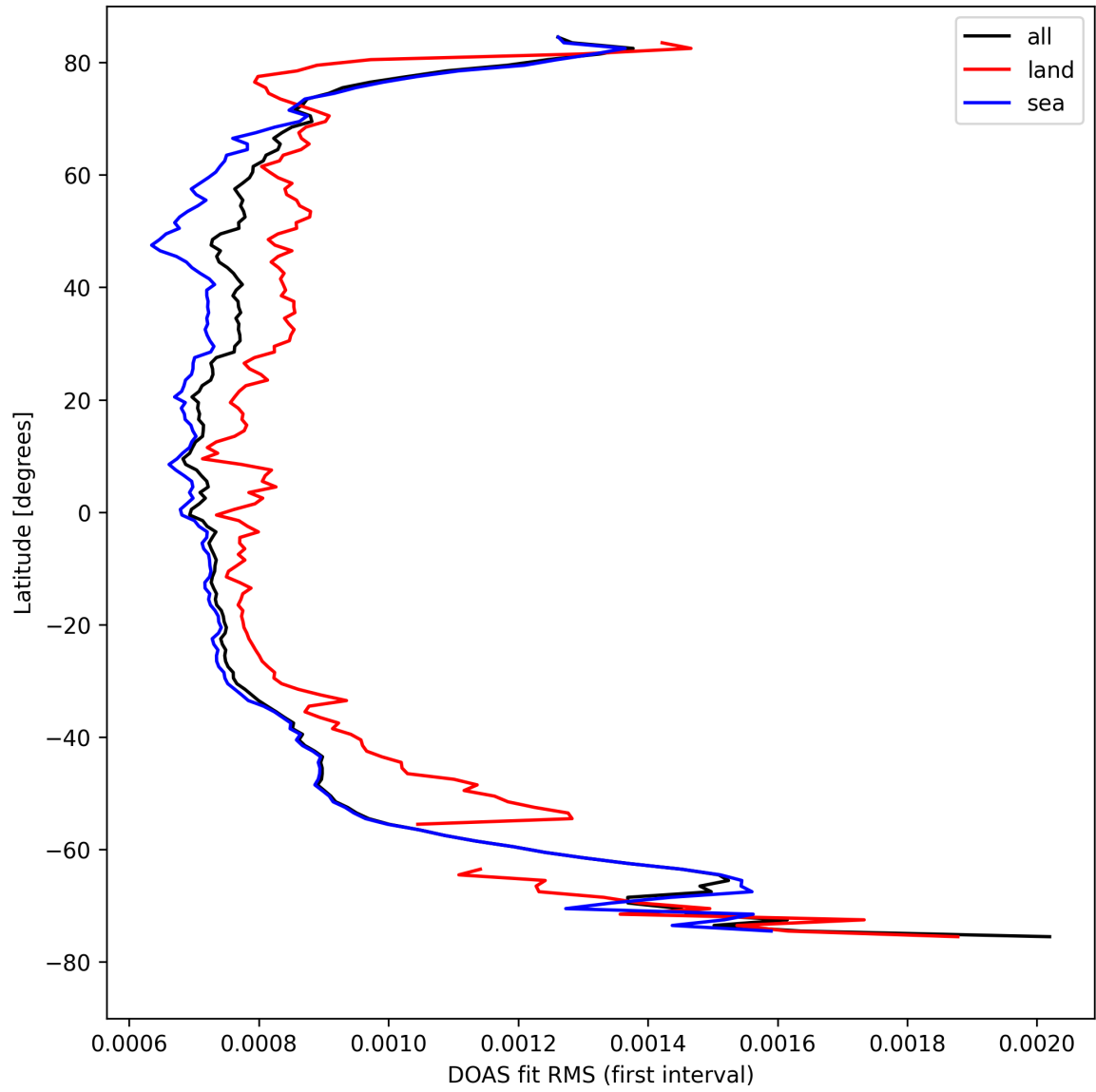
Figure 32: Zonal average of "DOAS fit RMS (first interval)" for 2024-08-27 to 2024-08-29.
