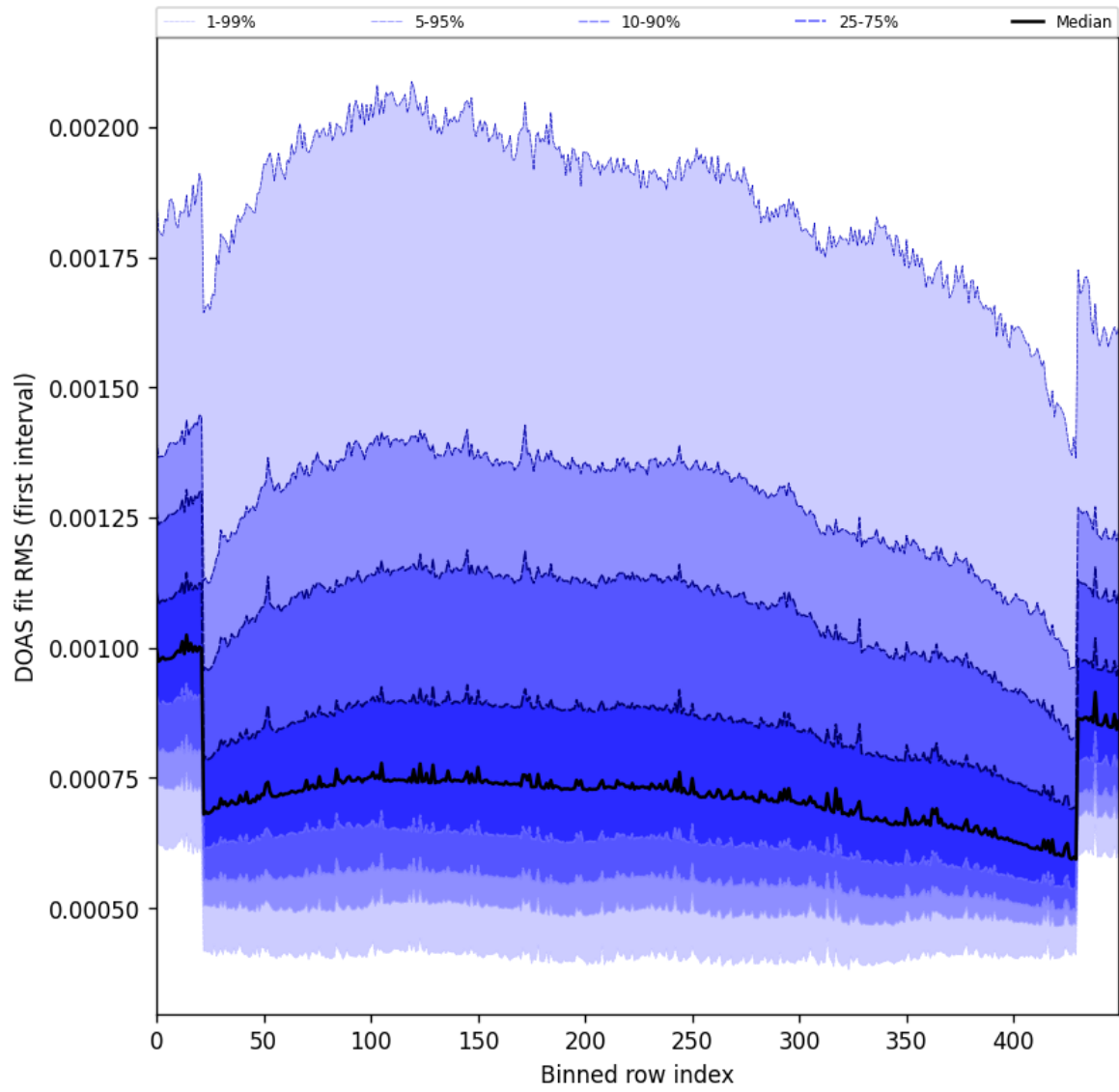
Figure 60: Along track statistics of “DOAS fit RMS (first interval)” for 2024-08-27 to 2024-08-29
