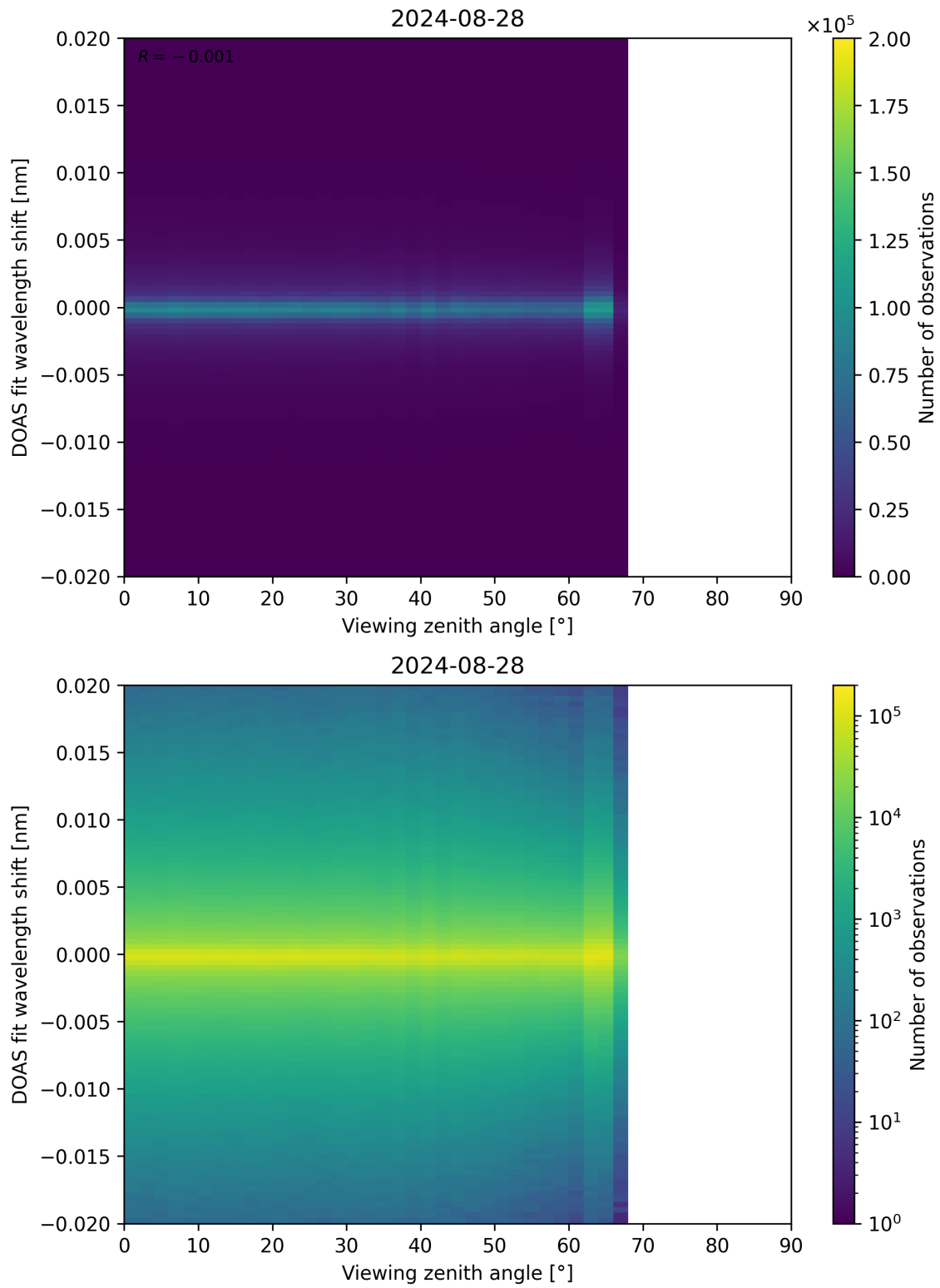
Figure 183: Scatter density plot of “Viewing zenith angle” against “DOAS fit wavelength shift” for 2024-08-27 to 2024-08-29.
