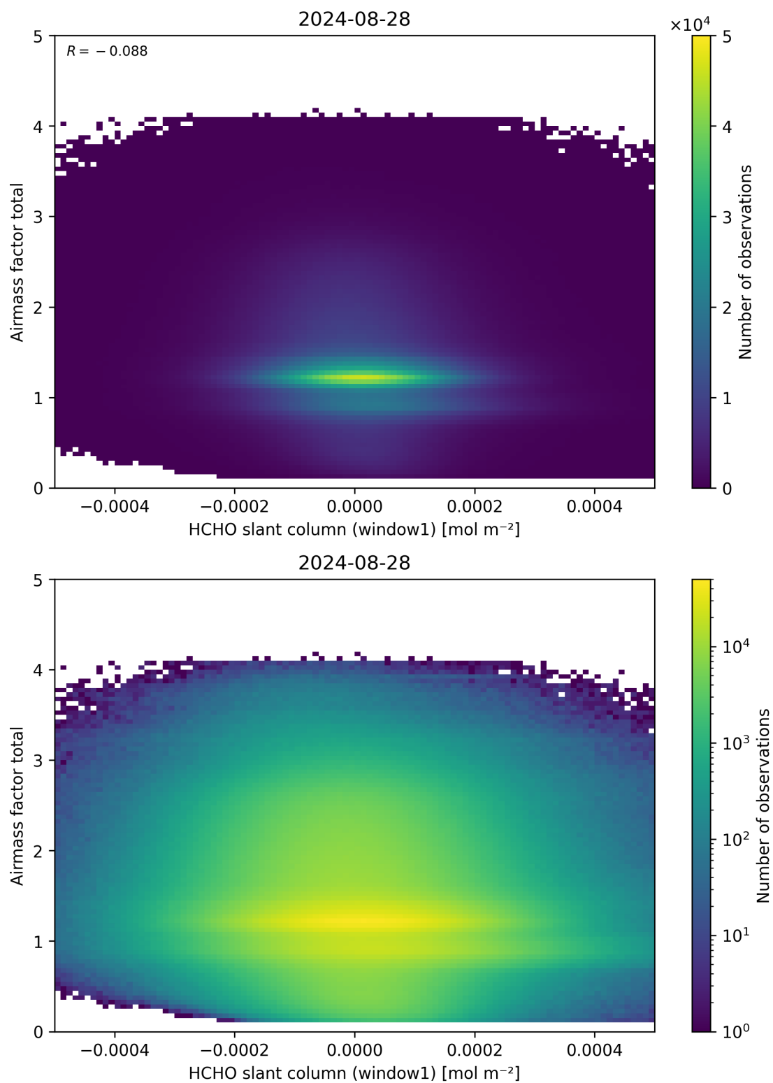
Figure 85: Scatter density plot of “HCHO slant column (window1)” against “Airmass factor total” for 2024-08-27 to 2024-08-29.
