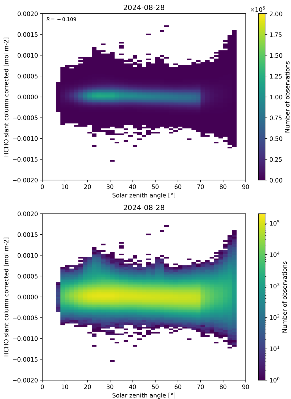
Figure 171: Scatter density plot of “Solar zenith angle” against “HCHO slant column corrected” for 2024-08-27 to 2024-08-29.
