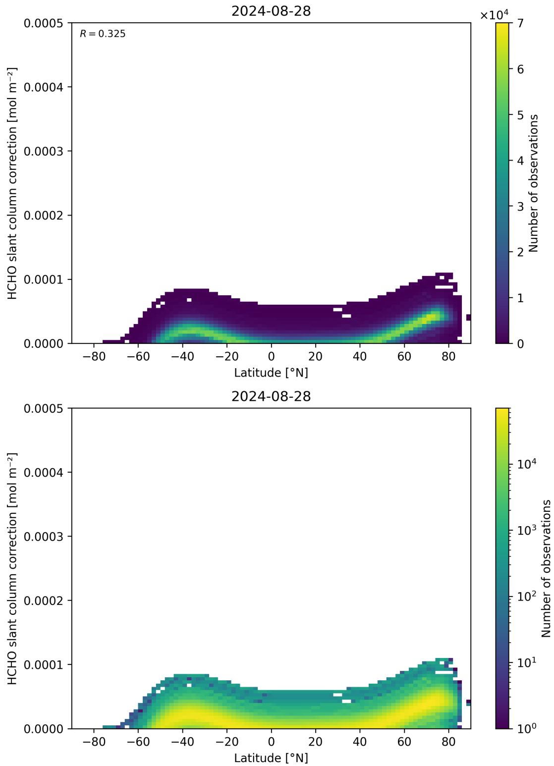
Figure 158: Scatter density plot of “Latitude” against “HCHO slant column correction” for 2024-08-27 to 2024-08-29.
