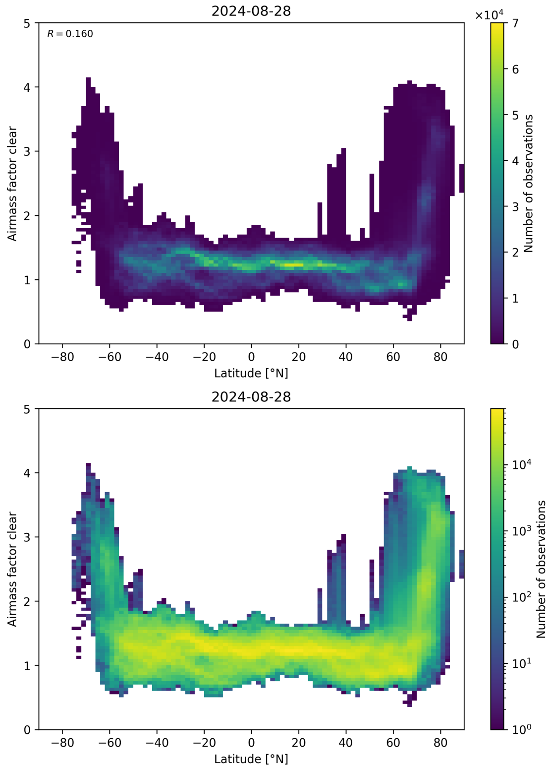
Figure 156: Scatter density plot of “Latitude” against “Airmass factor clear” for 2024-08-27 to 2024-08-29.
