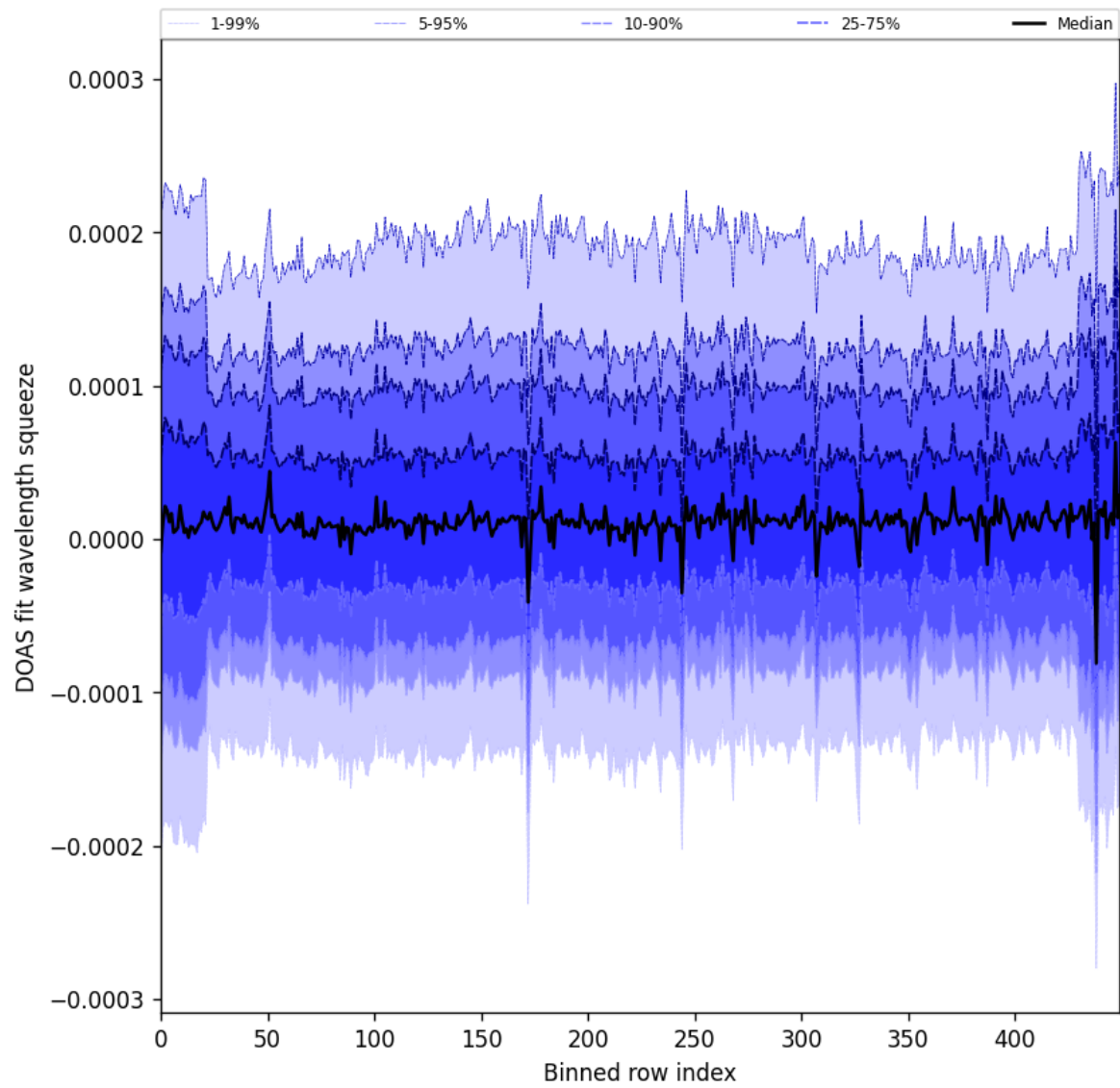
Figure 59: Along track statistics of “DOAS fit wavelength squeeze” for 2024-08-27 to 2024-08-29
