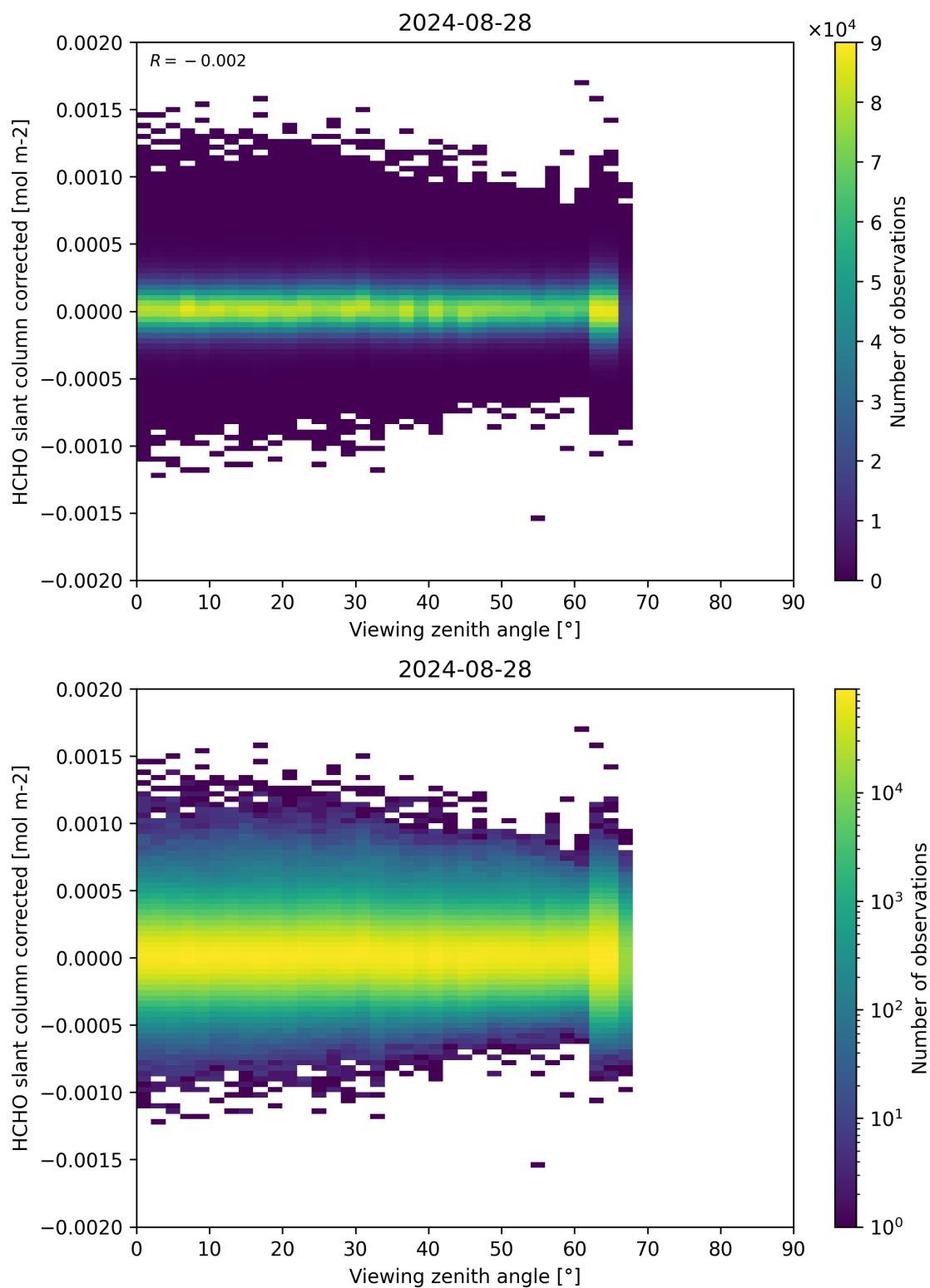
Figure 186: Scatter density plot of “Viewing zenith angle” against “HCHO slant column corrected” for 2024-08-27 to 2024-08-29.
