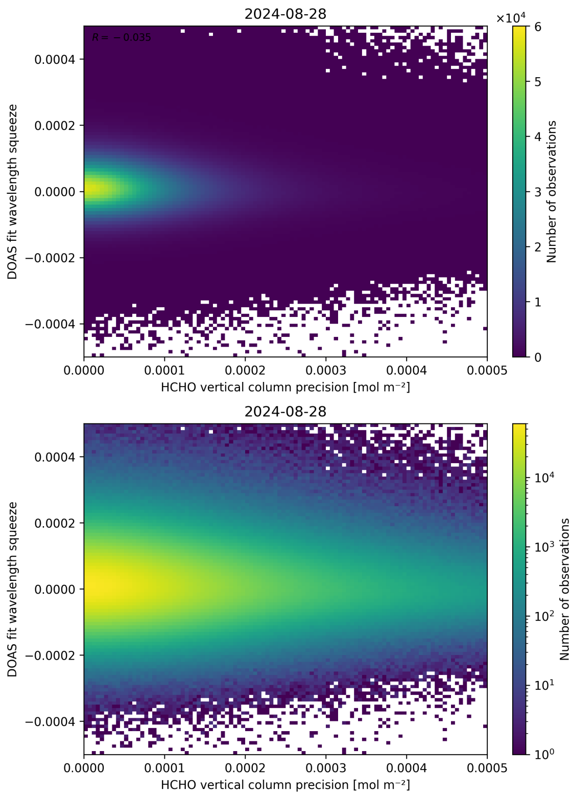
Figure 138: Scatter density plot of “HCHO vertical column precision” against “DOAS fit wavelength squeeze” for 2024-08-27 to 2024-08-29.
