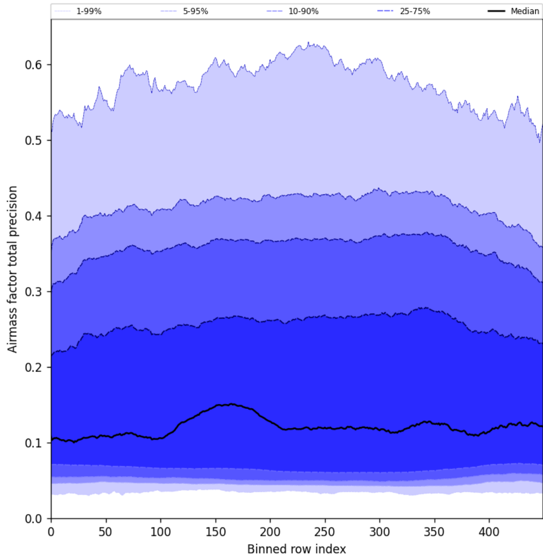
Figure 55: Along track statistics of “Airmass factor total precision” for 2024-08-27 to 2024-08-29
