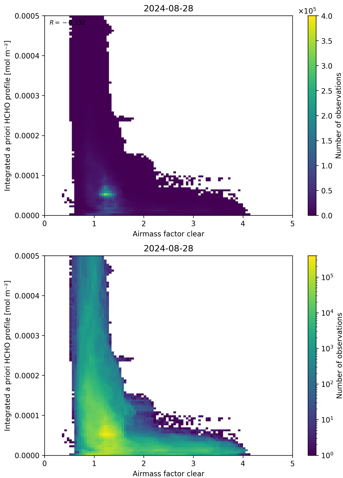
Figure 76: Scatter density plot of “Airmass factor clear” against “Integrated a priori HCHO profile” for 2024-08-27 to 2024-08-29.
