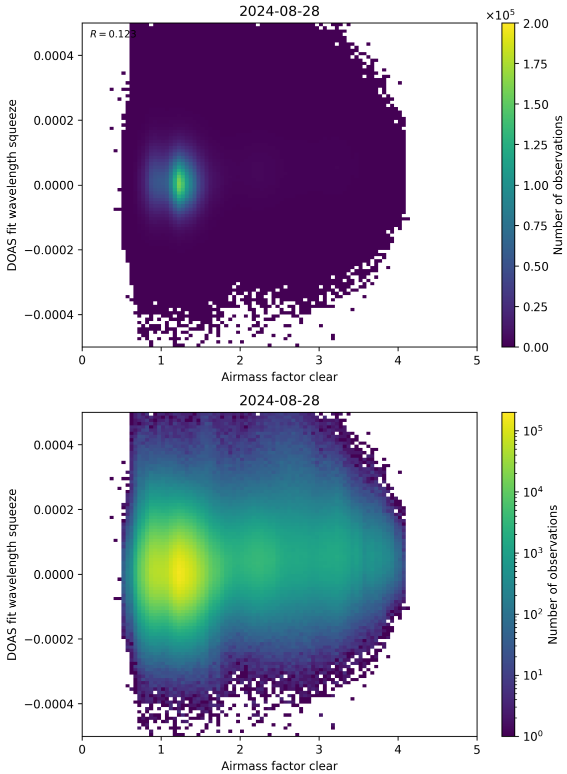
Figure 73: Scatter density plot of “Airmass factor clear” against “DOAS fit wavelength squeeze” for 2024-08-27 to 2024-08-29.
