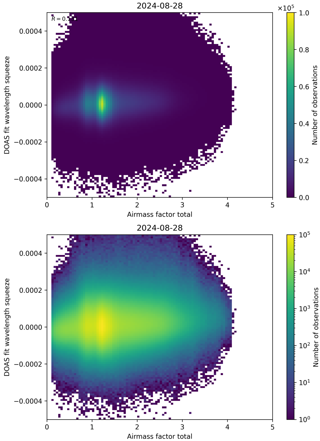
Figure 99: Scatter density plot of “Airmass factor total” against “DOAS fit wavelength squeeze” for 2024-08-27 to 2024-08-29.
