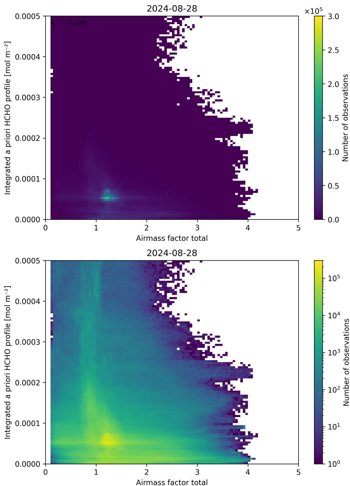
Figure 104: Scatter density plot of “Airmass factor total” against “Integrated a priori HCHO profile” for 2024-08-27 to 2024-08-29.
