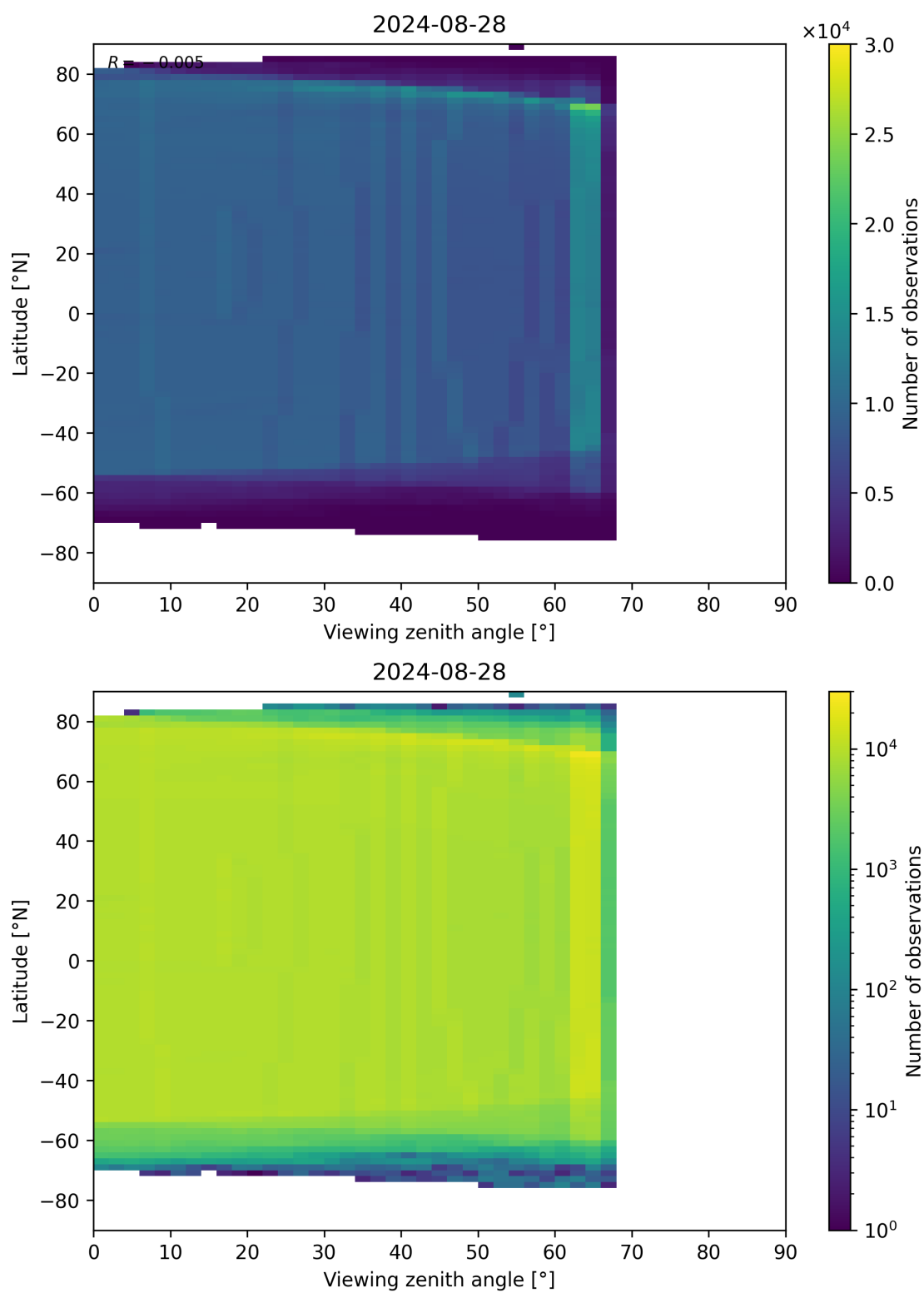
Figure 196: Scatter density plot of “Viewing zenith angle” against “Latitude” for 2024-08-27 to 2024-08-29.
