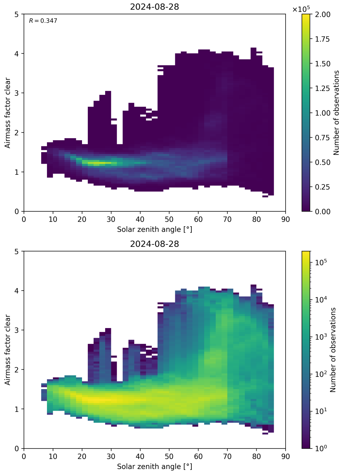
Figure 170: Scatter density plot of “Solar zenith angle” against “Airmass factor clear” for 2024-08-27 to 2024-08-29.
