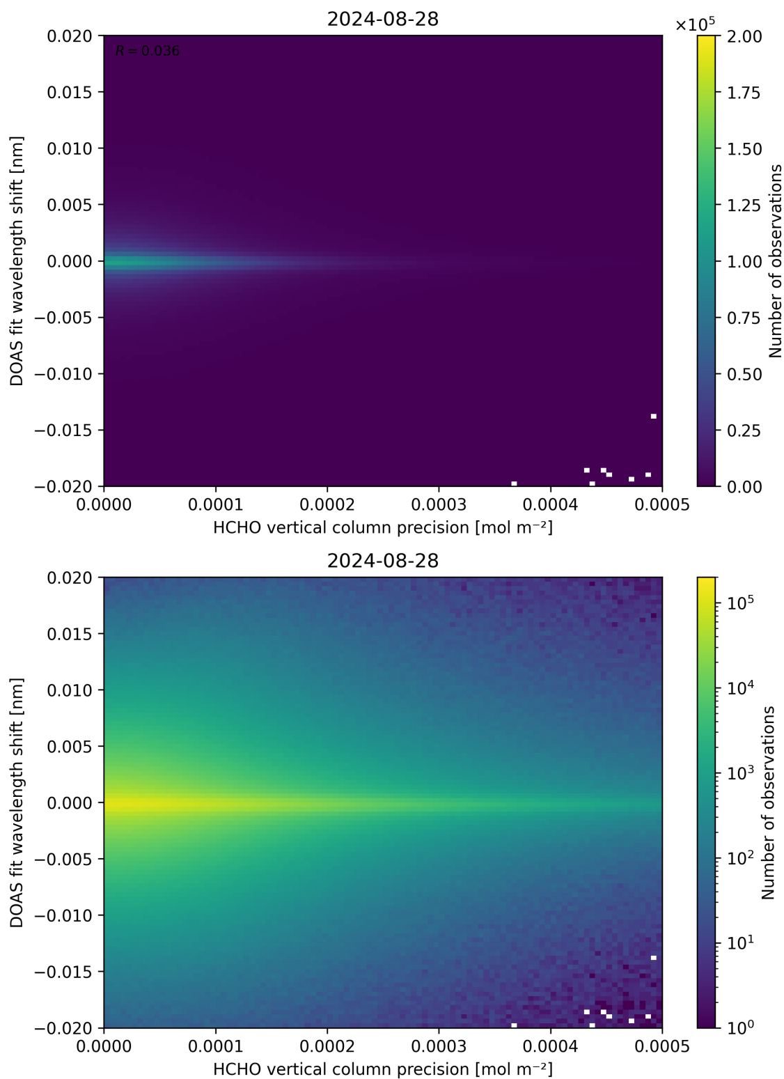
Figure 137: Scatter density plot of “HCHO vertical column precision” against “DOAS fit wavelength shift” for 2024-08-27 to 2024-08-29.
