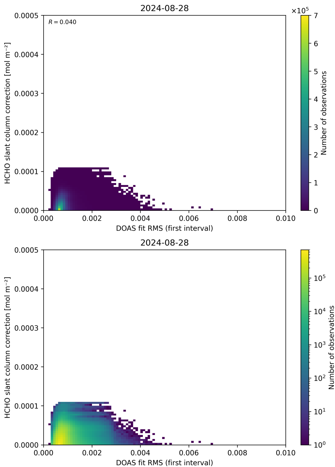
Figure 63: Scatter density plot of “DOAS fit RMS (first interval)” against “HCHO slant column correction” for 2024-08-27 to 2024-08-29.
