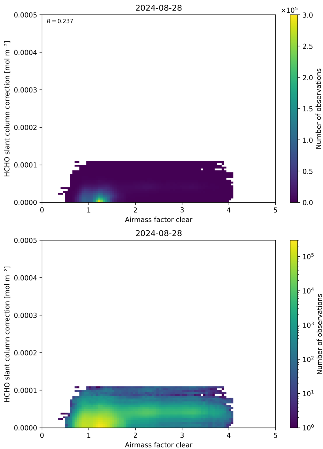
Figure 75: Scatter density plot of “Airmass factor clear” against “HCHO slant column correction” for 2024-08-27 to 2024-08-29.
