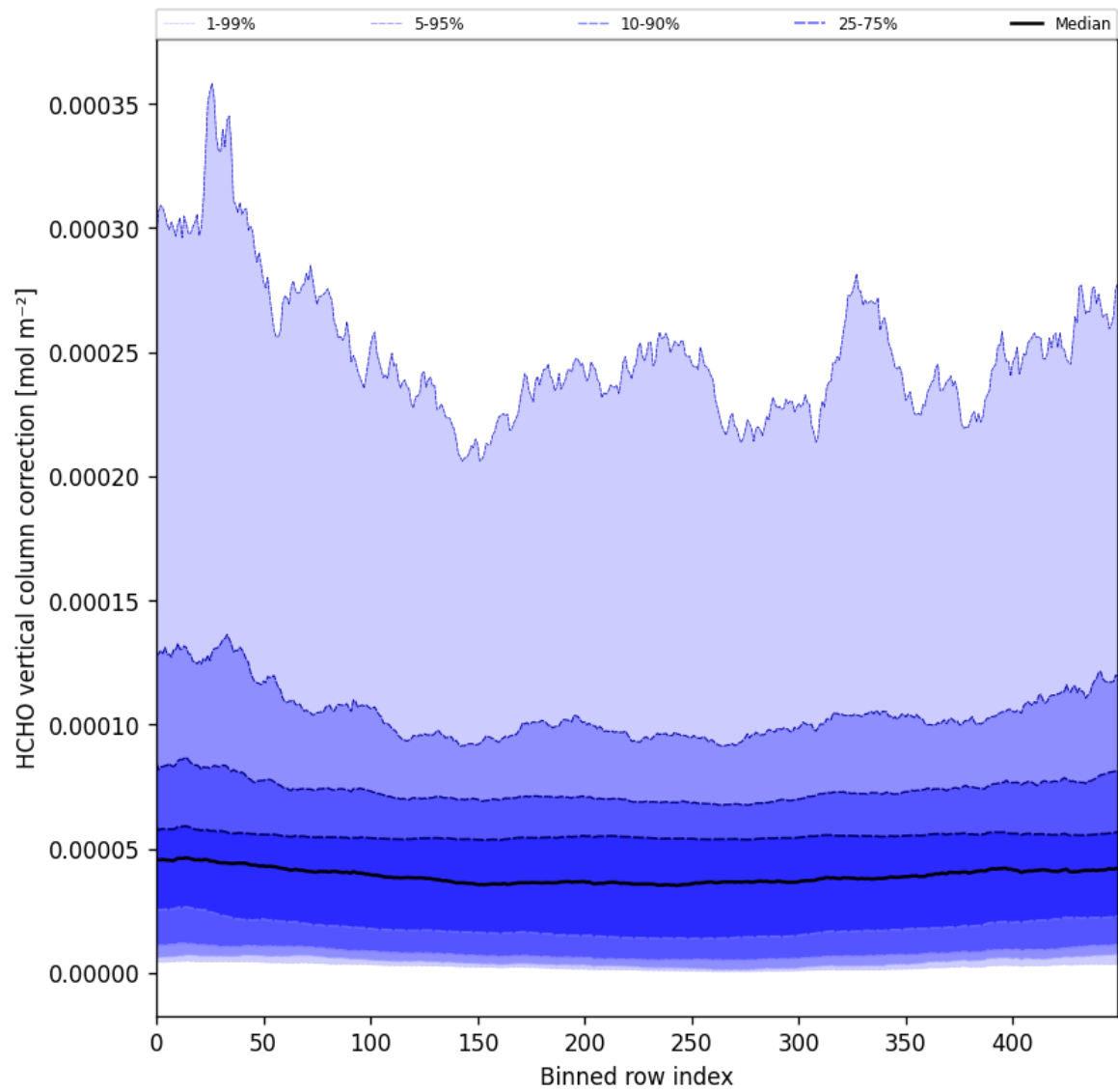
Figure 51: Along track statistics of “HCHO vertical column correction” for 2024-08-27 to 2024-08-29
