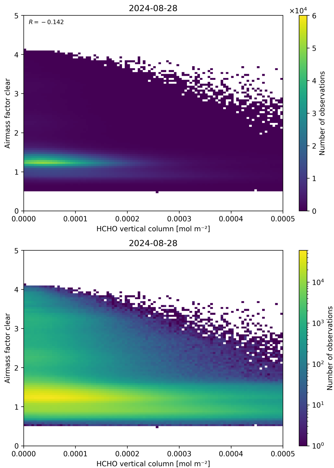
Figure 126: Scatter density plot of “HCHO vertical column” against “Airmass factor clear” for 2024-08-27 to 2024-08-29.
