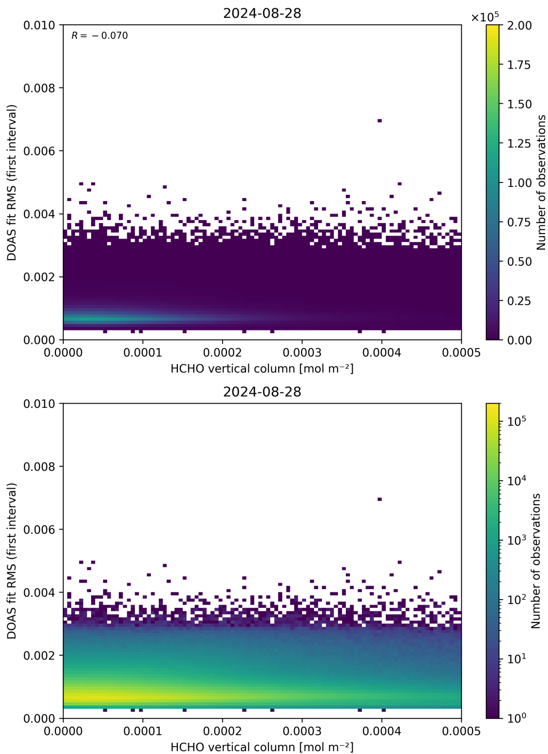
Figure 123: Scatter density plot of “HCHO vertical column” against “DOAS fit RMS (first interval)” for 2024-08-27 to 2024-08-29.
