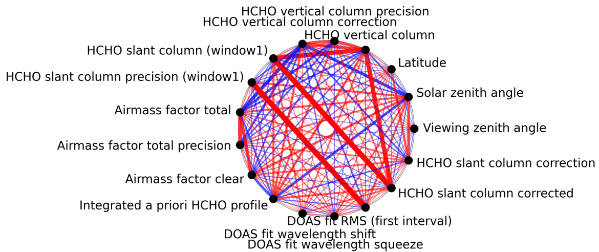
Figure 1: Map of correlation graph for 2024-08-27 to 2024-08-29.
