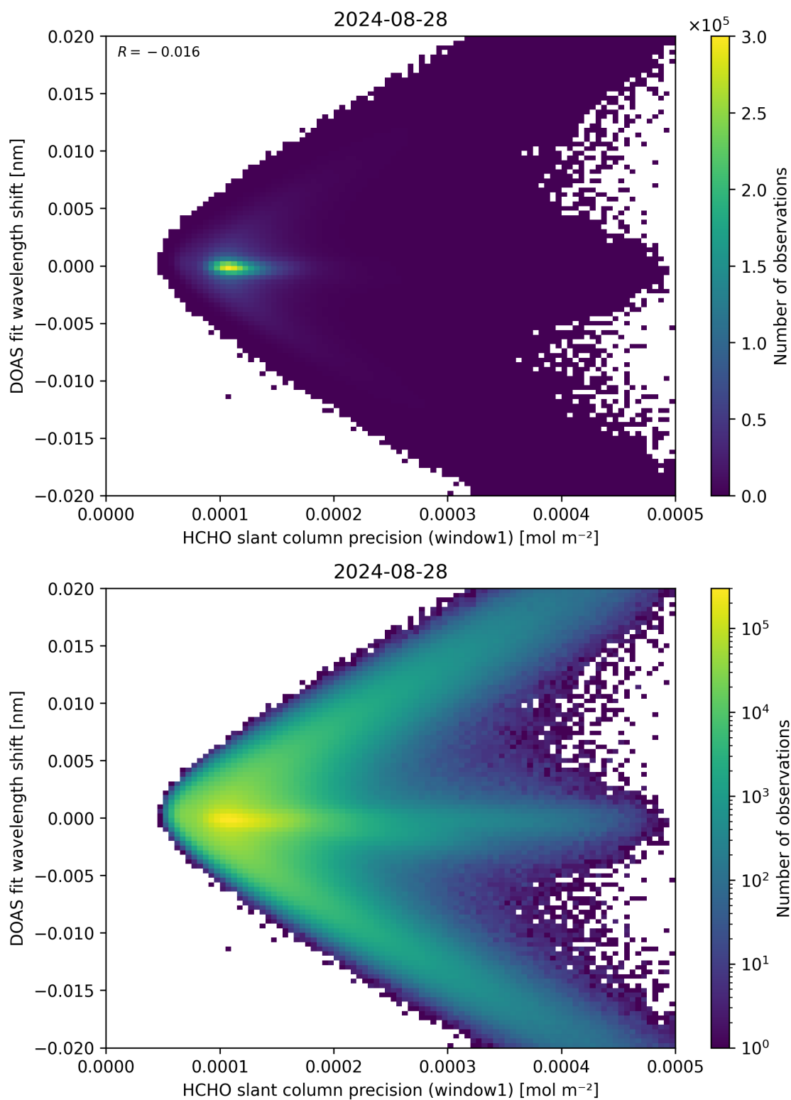
Figure 89: Scatter density plot of “HCHO slant column precision (window1)” against “DOAS fit wavelength shift” for 2024-08-27 to 2024-08-29.
