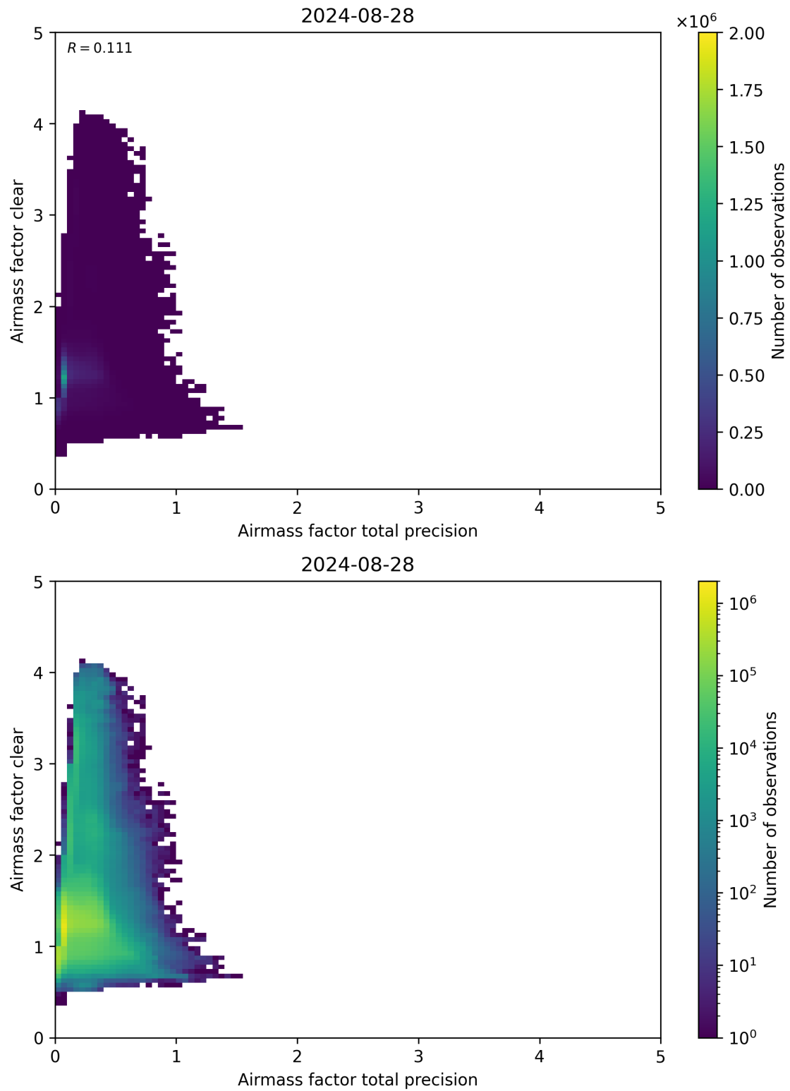
Figure 108: Scatter density plot of “Airmass factor total precision” against “Airmass factor clear” for 2024-08-27 to 2024-08-29.
