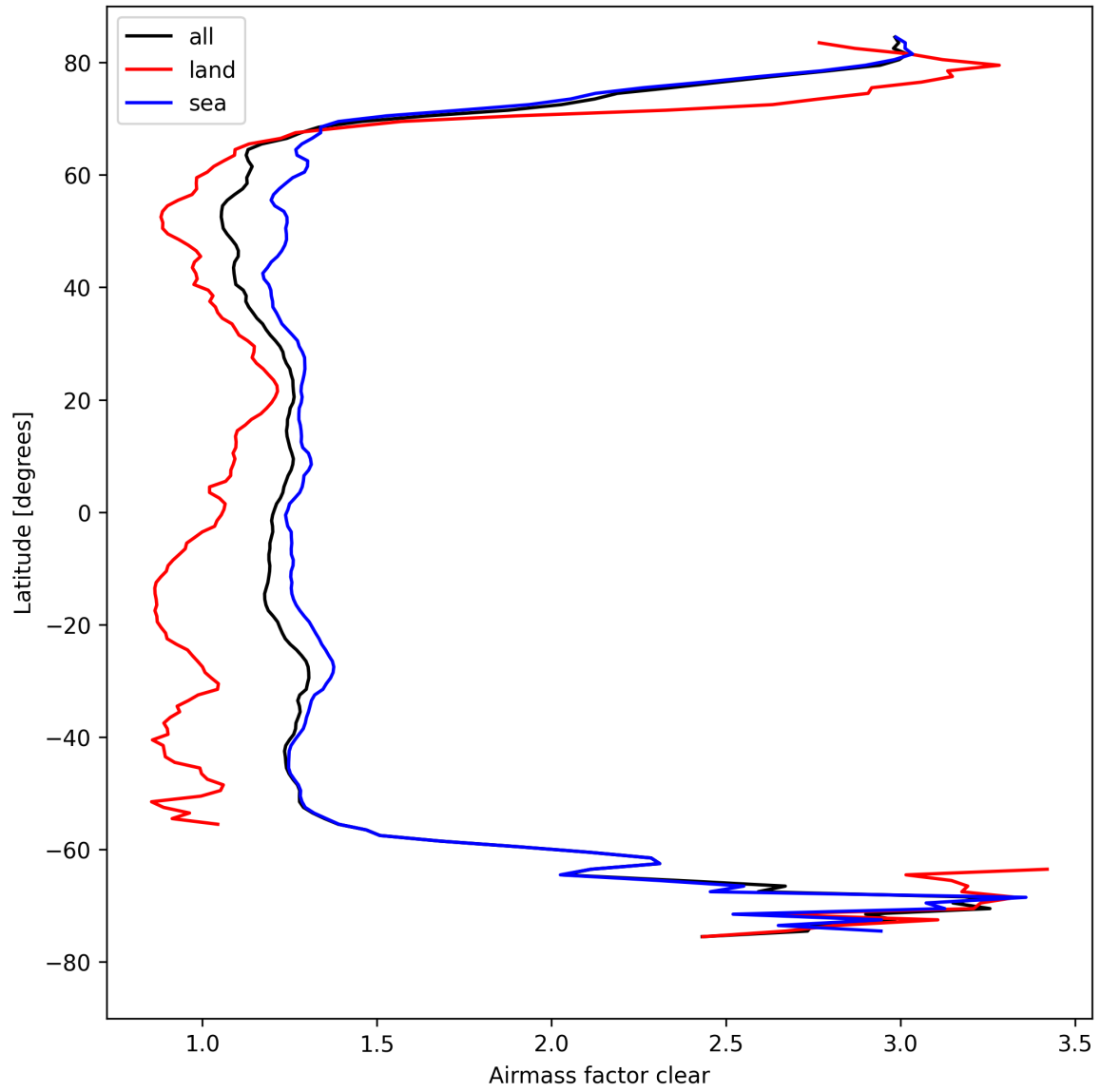
Figure 28: Zonal average of “Airmass factor clear” for 2024-08-27 to 2024-08-29.
