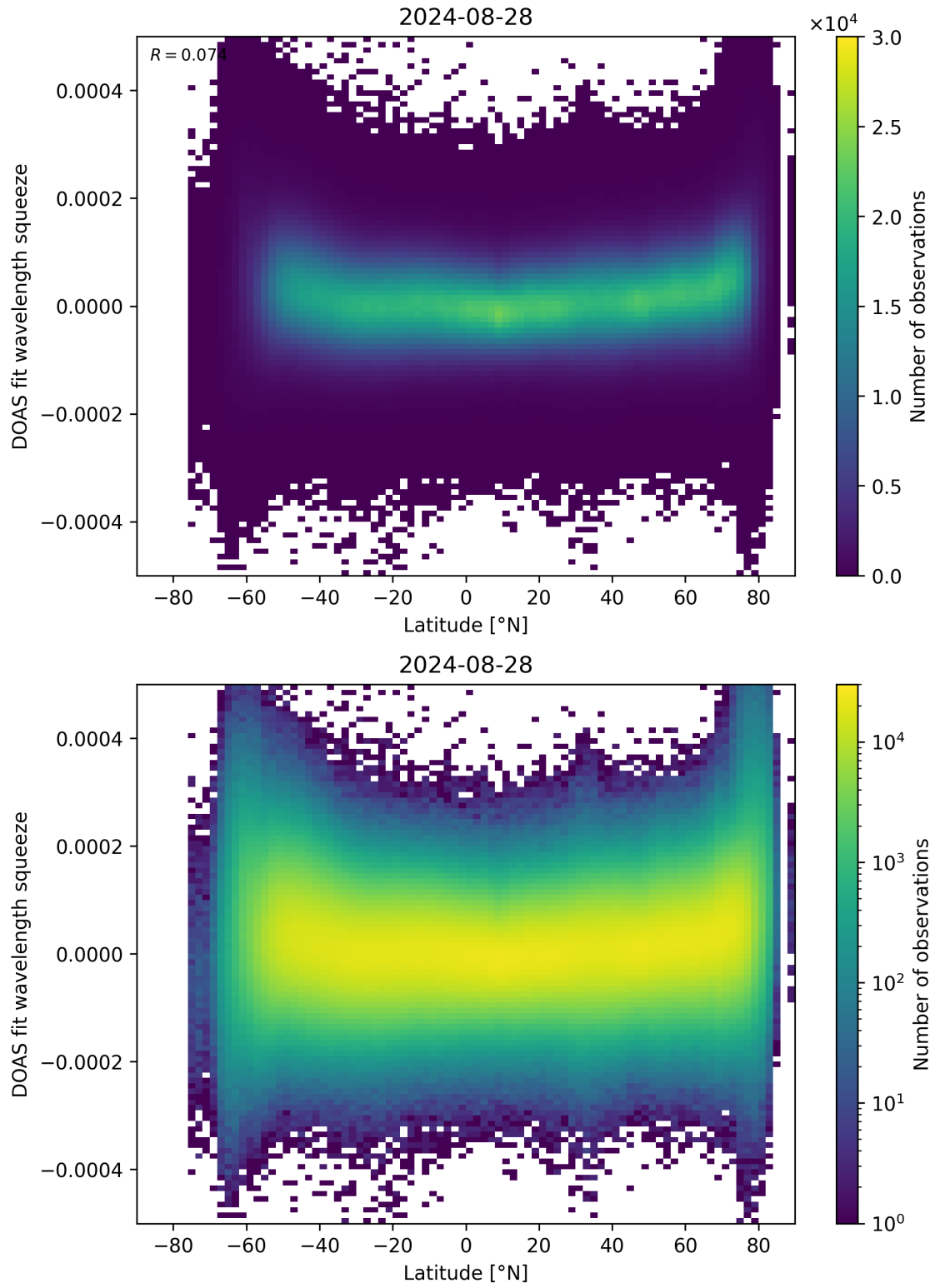
Figure 155: Scatter density plot of “Latitude” against “DOAS fit wavelength squeeze” for 2024-08-27 to 2024-08-29.
