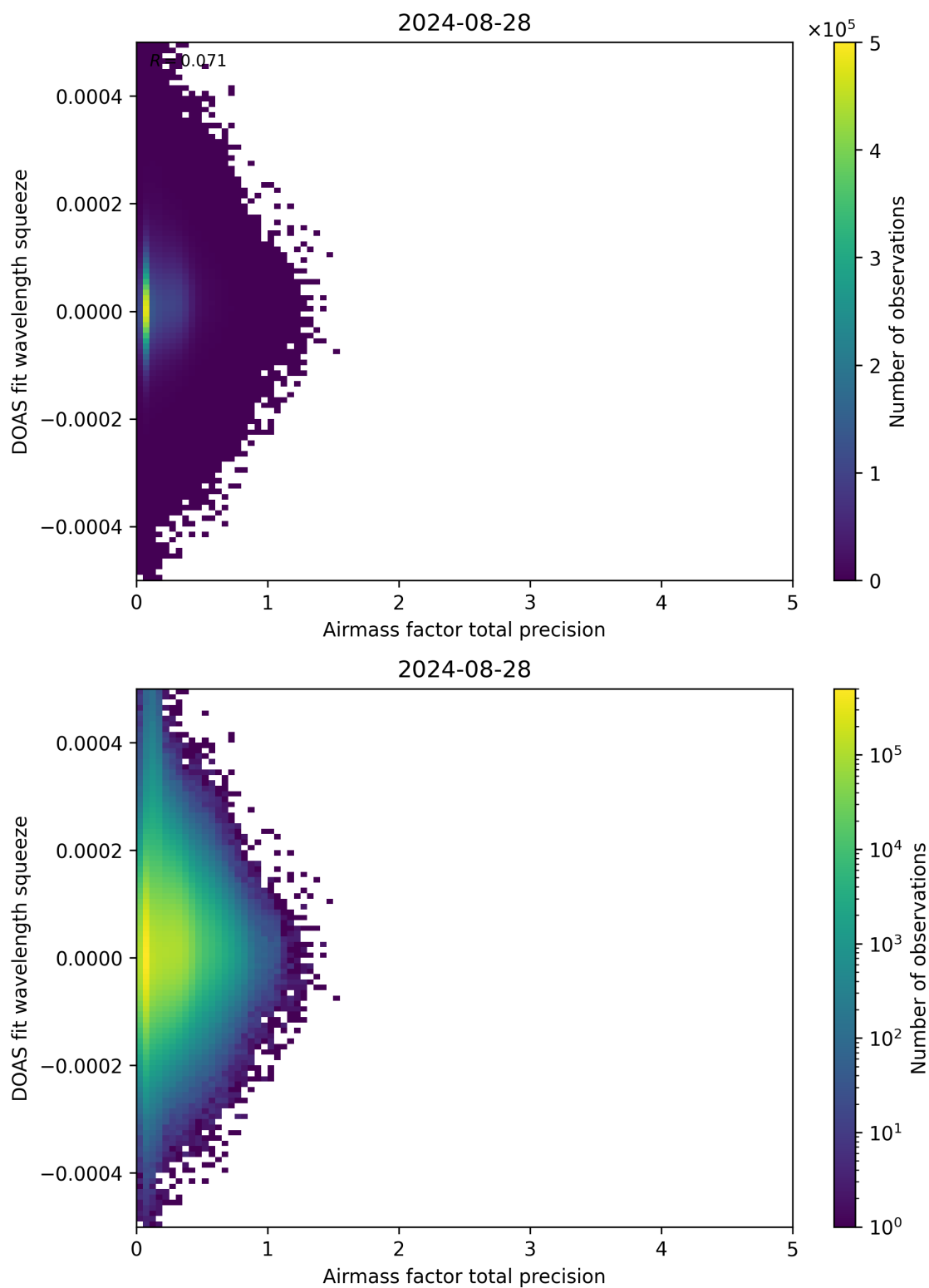
Figure 107: Scatter density plot of “Airmass factor total precision” against “DOAS fit wavelength squeeze” for 2024-08-27 to 2024-08-29.
