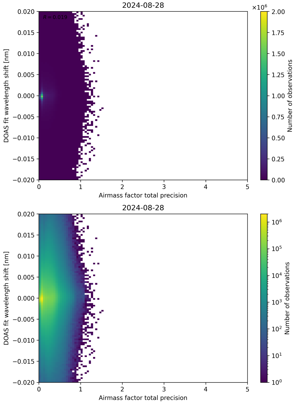
Figure 106: Scatter density plot of “Airmass factor total precision” against “DOAS fit wavelength shift” for 2024-08-27 to 2024-08-29.
