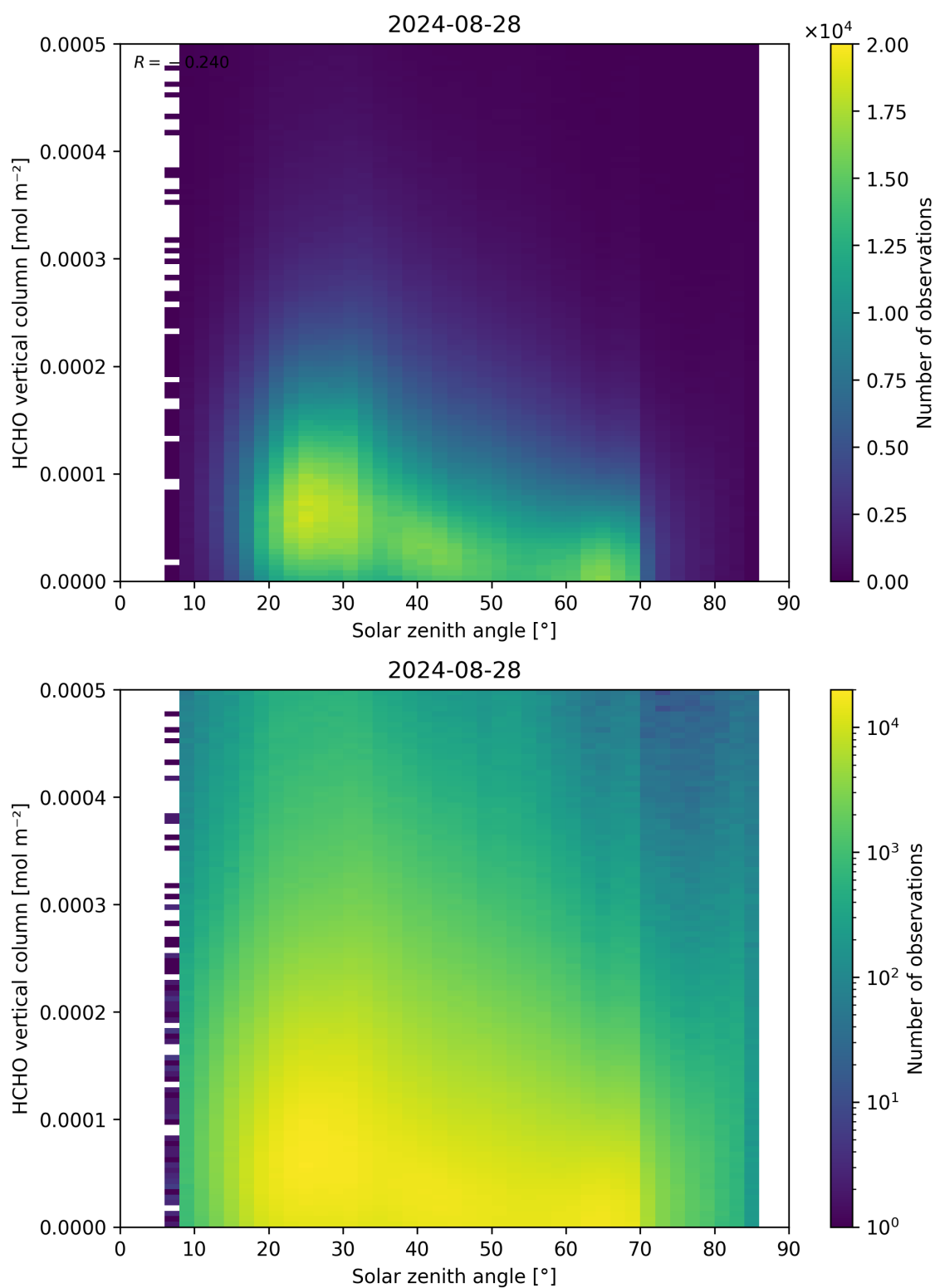
Figure 177: Scatter density plot of “Solar zenith angle” against “HCHO vertical column” for 2024-08-27 to 2024-08-29.
