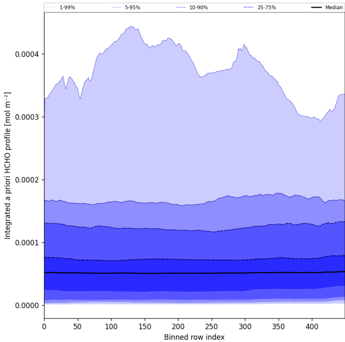
Figure 57: Along track statistics of “Integrated a priori HCHO profile” for 2024-08-27 to 2024-08-29
