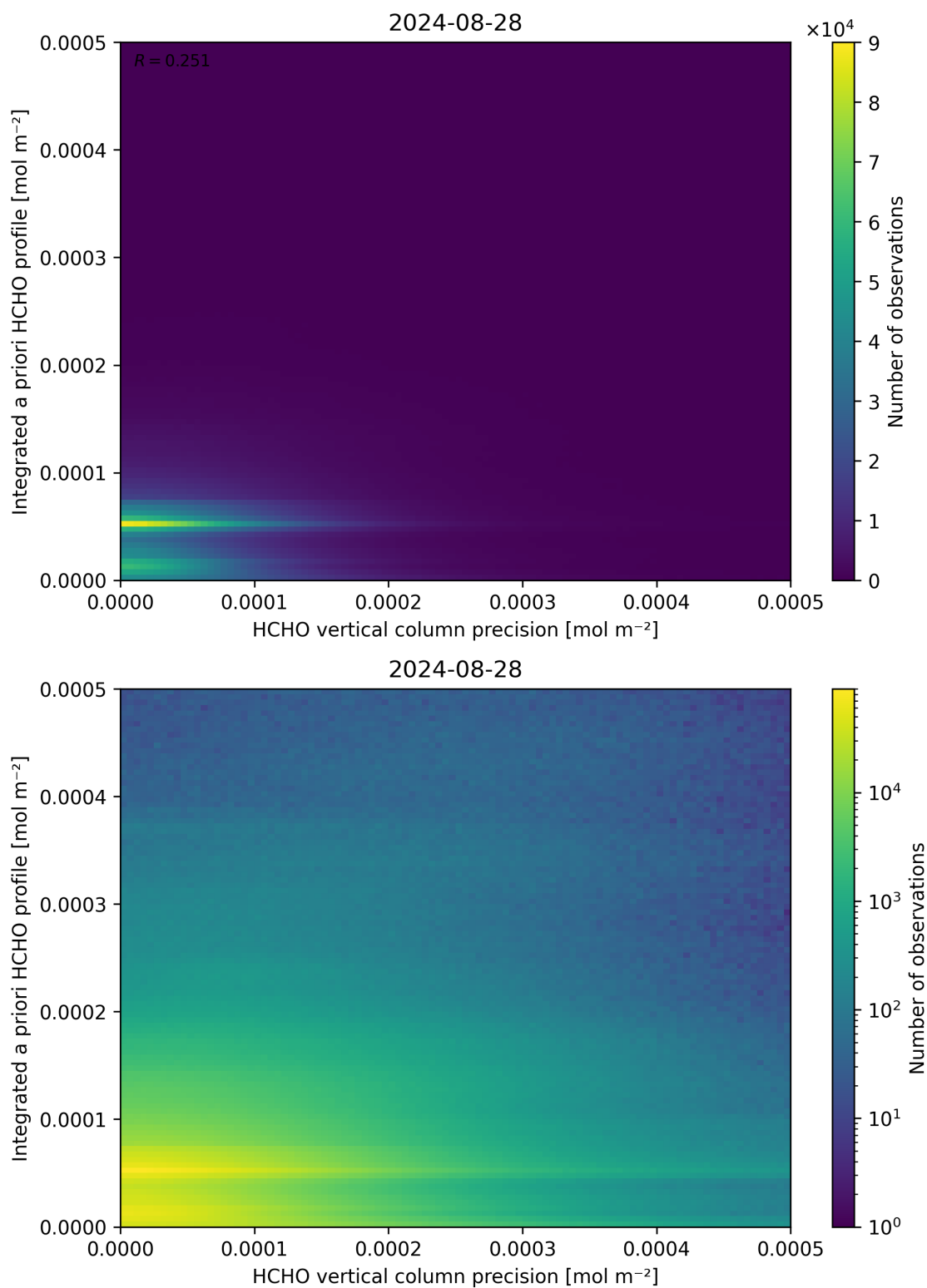
Figure 147: Scatter density plot of “HCHO vertical column precision” against “Integrated a priori HCHO profile” for 2024-08-27 to 2024-08-29.
