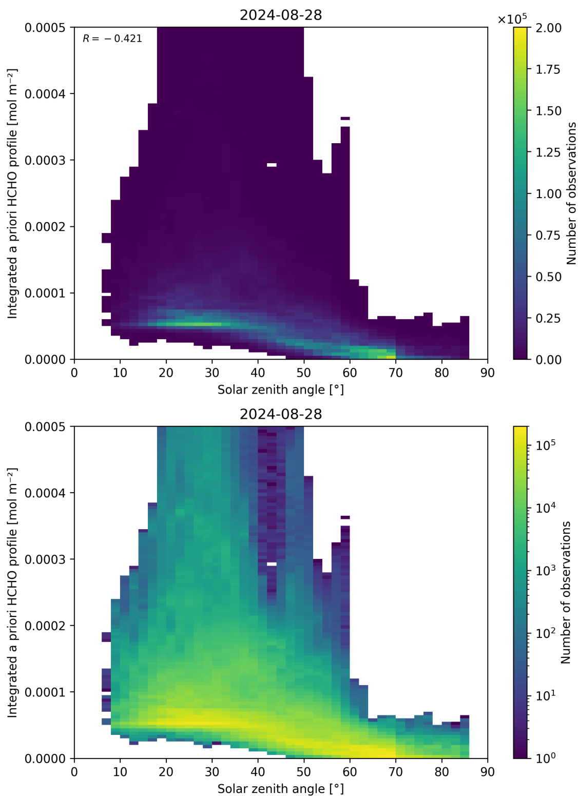
Figure 180: Scatter density plot of “Solar zenith angle” against “Integrated a priori HCHO profile” for 2024-08-27 to 2024-08-29.
