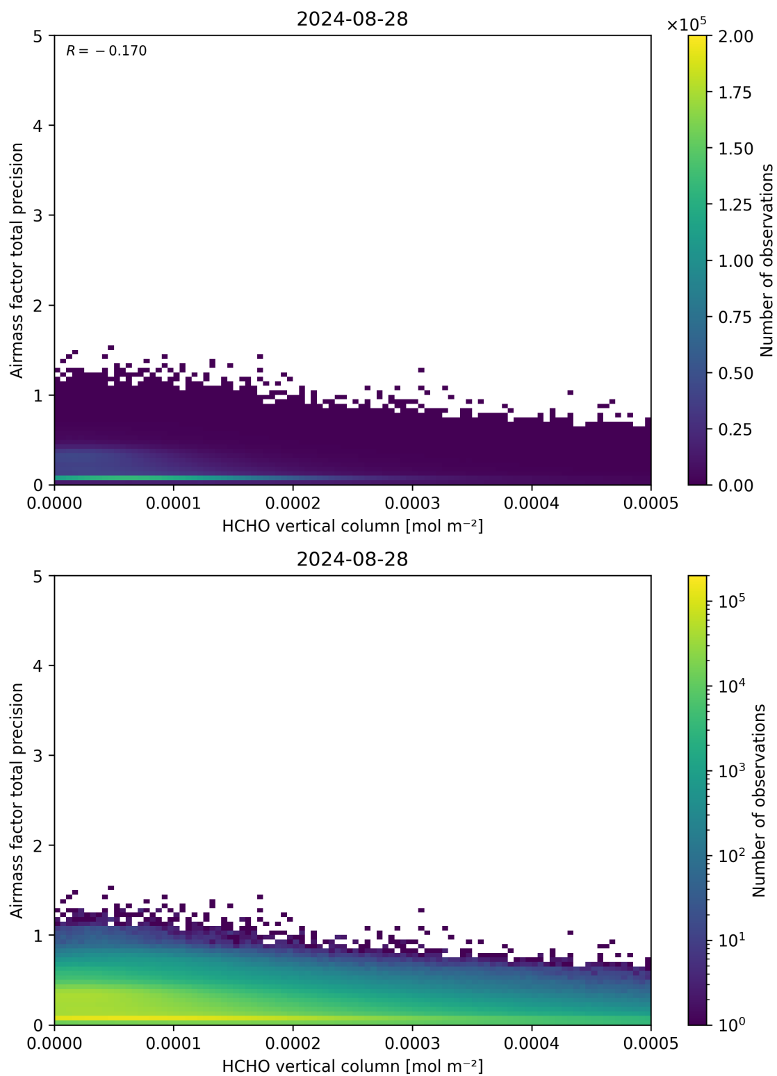
Figure 132: Scatter density plot of “HCHO vertical column” against “Airmass factor total precision” for 2024-08-27 to 2024-08-29.
