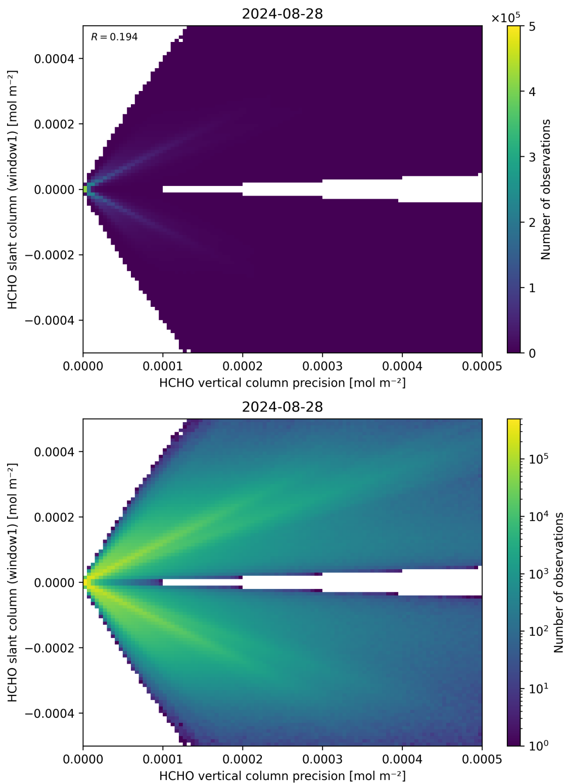
Figure 142: Scatter density plot of “HCHO vertical column precision” against “HCHO slant column (window1)” for 2024-08-27 to 2024-08-29.
