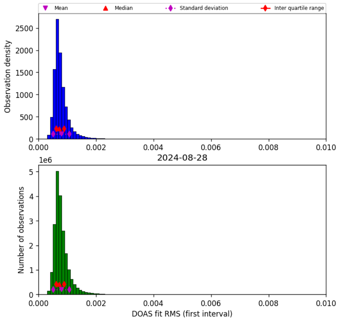
Figure 46: Histogram of “DOAS fit RMS (first interval)” for 2024-08-27 to 2024-08-29
