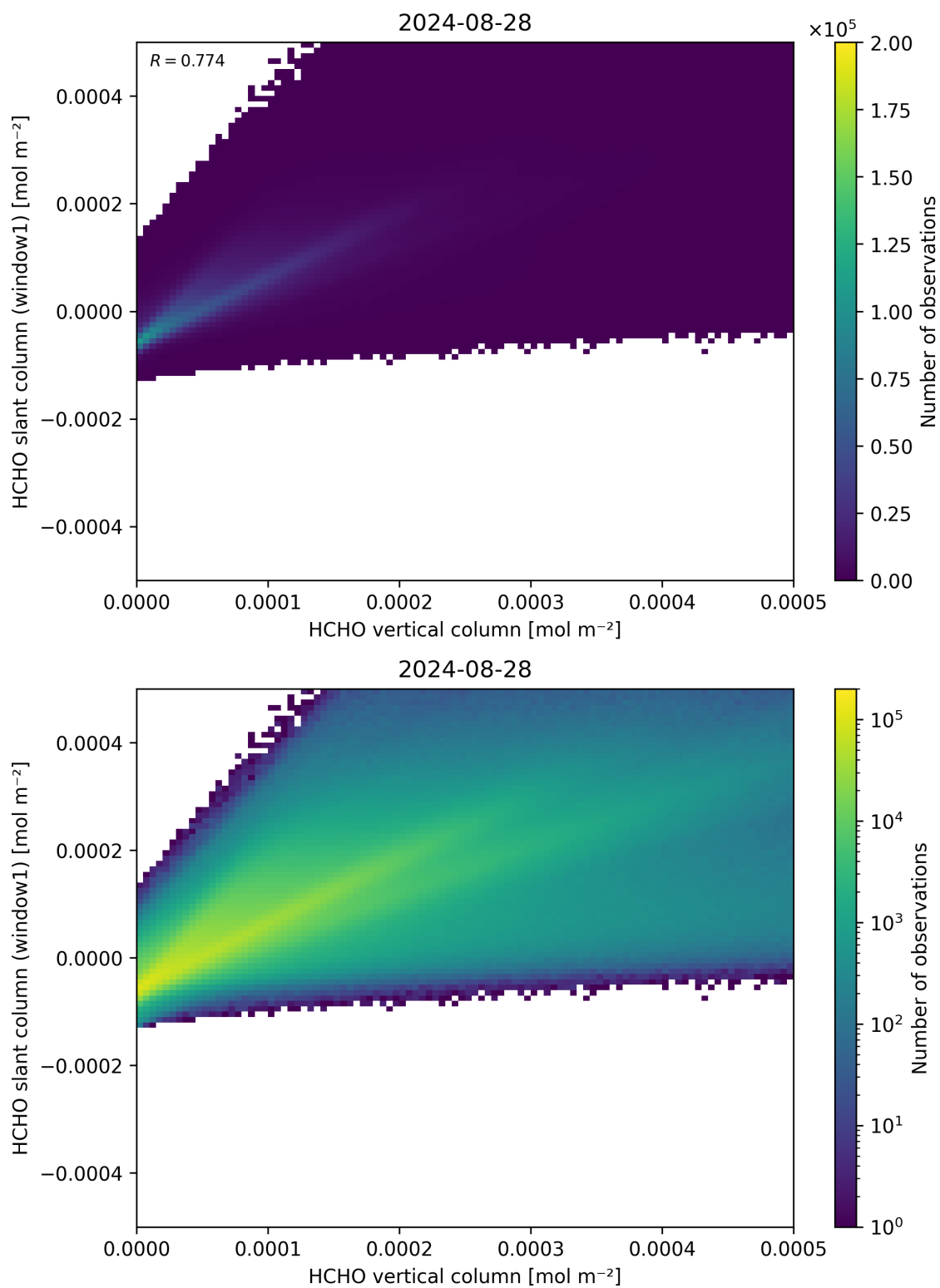
Figure 129: Scatter density plot of “HCHO vertical column” against “HCHO slant column (window1)” for 2024-08-27 to 2024-08-29.
