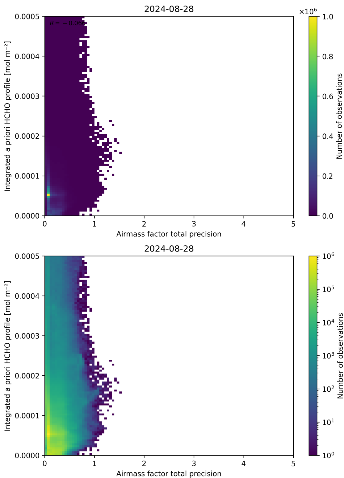
Figure 111: Scatter density plot of “Airmass factor total precision” against “Integrated a priori HCHO profile” for 2024-08-27 to 2024-08-29.
