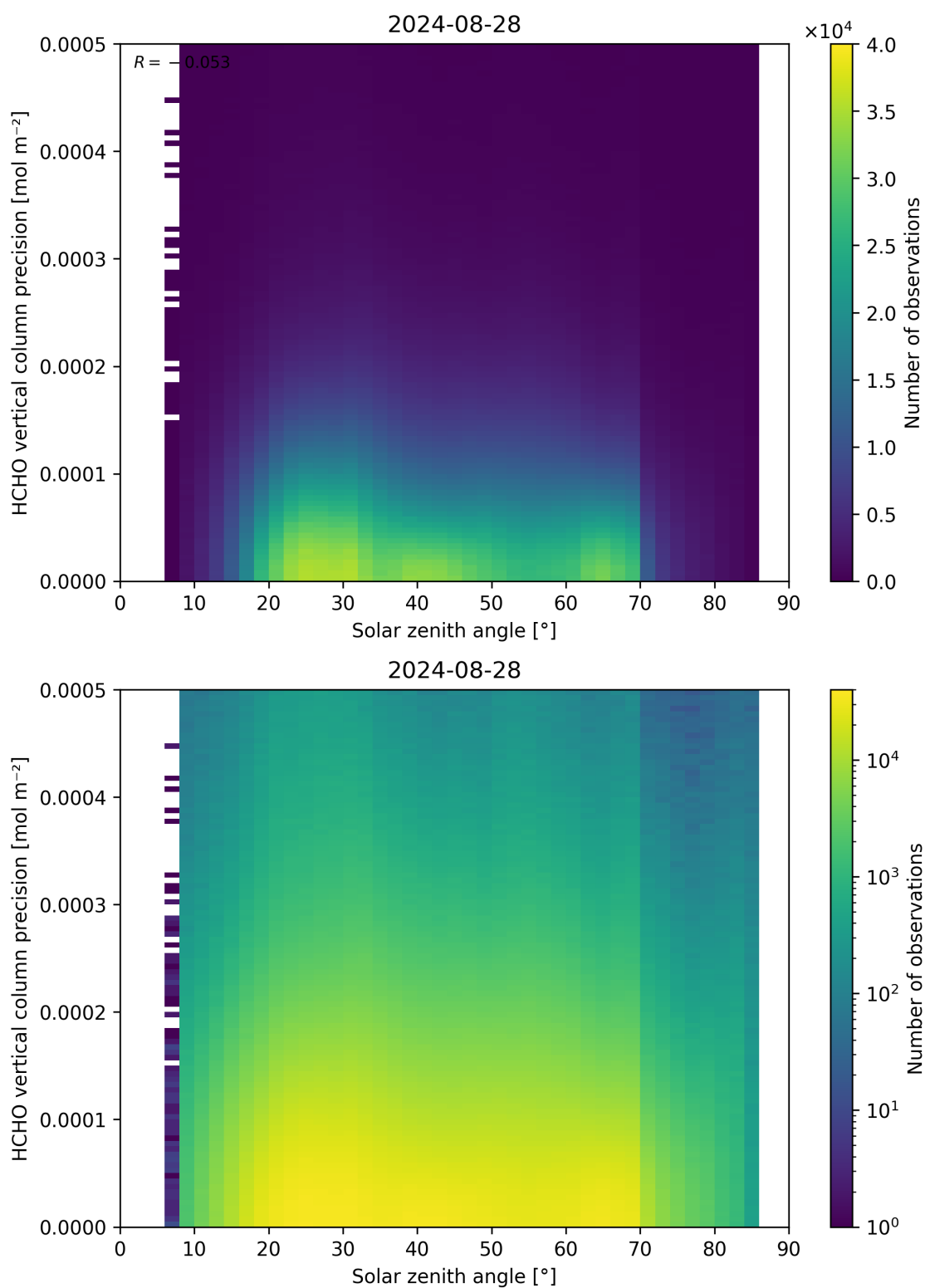
Figure 179: Scatter density plot of “Solar zenith angle” against “HCHO vertical column precision” for 2024-08-27 to 2024-08-29.
