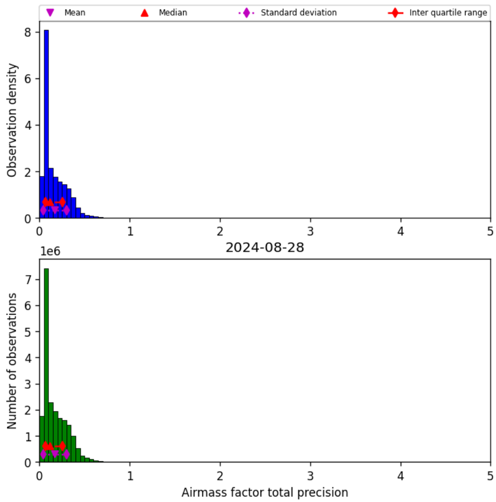
Figure 41: Histogram of “Airmass factor total precision” for 2024-08-27 to 2024-08-29
