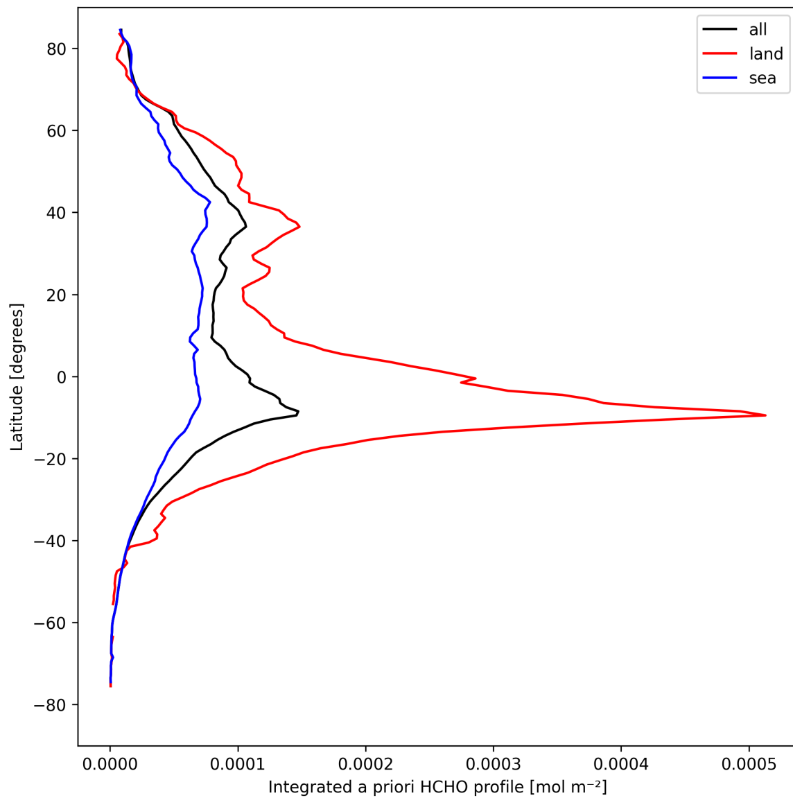
Figure 29: Zonal average of “Integrated a priori HCHO profile” for 2024-08-27 to 2024-08-29.
