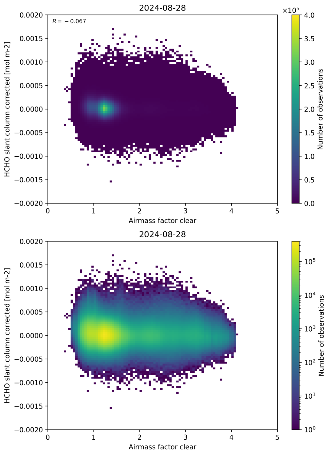
Figure 74: Scatter density plot of “Airmass factor clear” against “HCHO slant column corrected” for 2024-08-27 to 2024-08-29.
