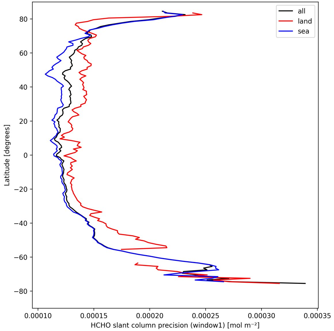
Figure 25: Zonal average of “HCHO slant column precision (window1)” for 2024-08-27 to 2024-08-29.
