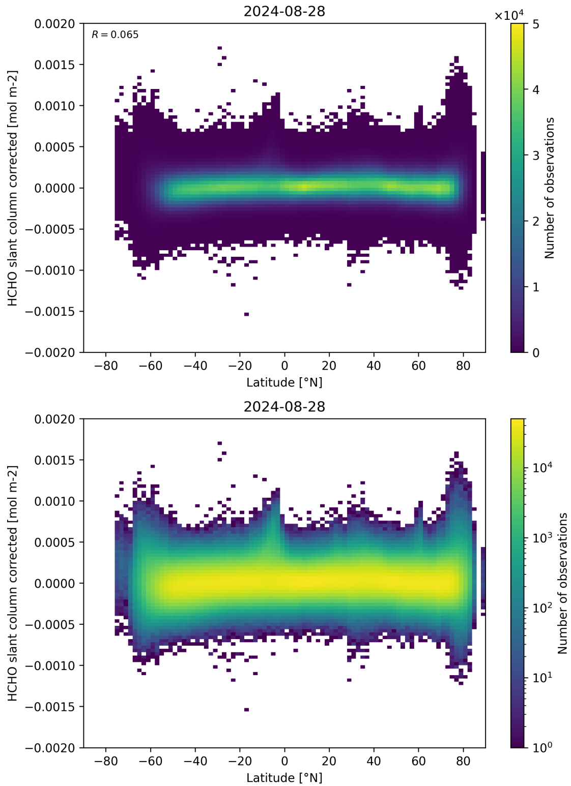
Figure 157: Scatter density plot of “Latitude” against “HCHO slant column corrected” for 2024-08-27 to 2024-08-29.
