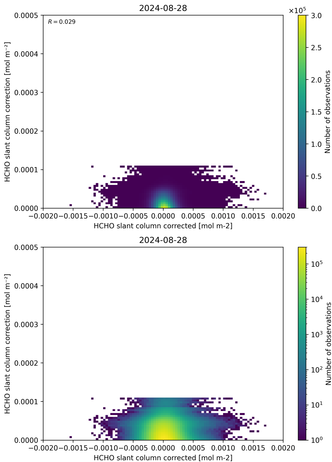
Figure 77: Scatter density plot of “HCHO slant column corrected” against “HCHO slant column correction” for 2024-08-27 to 2024-08-29.
