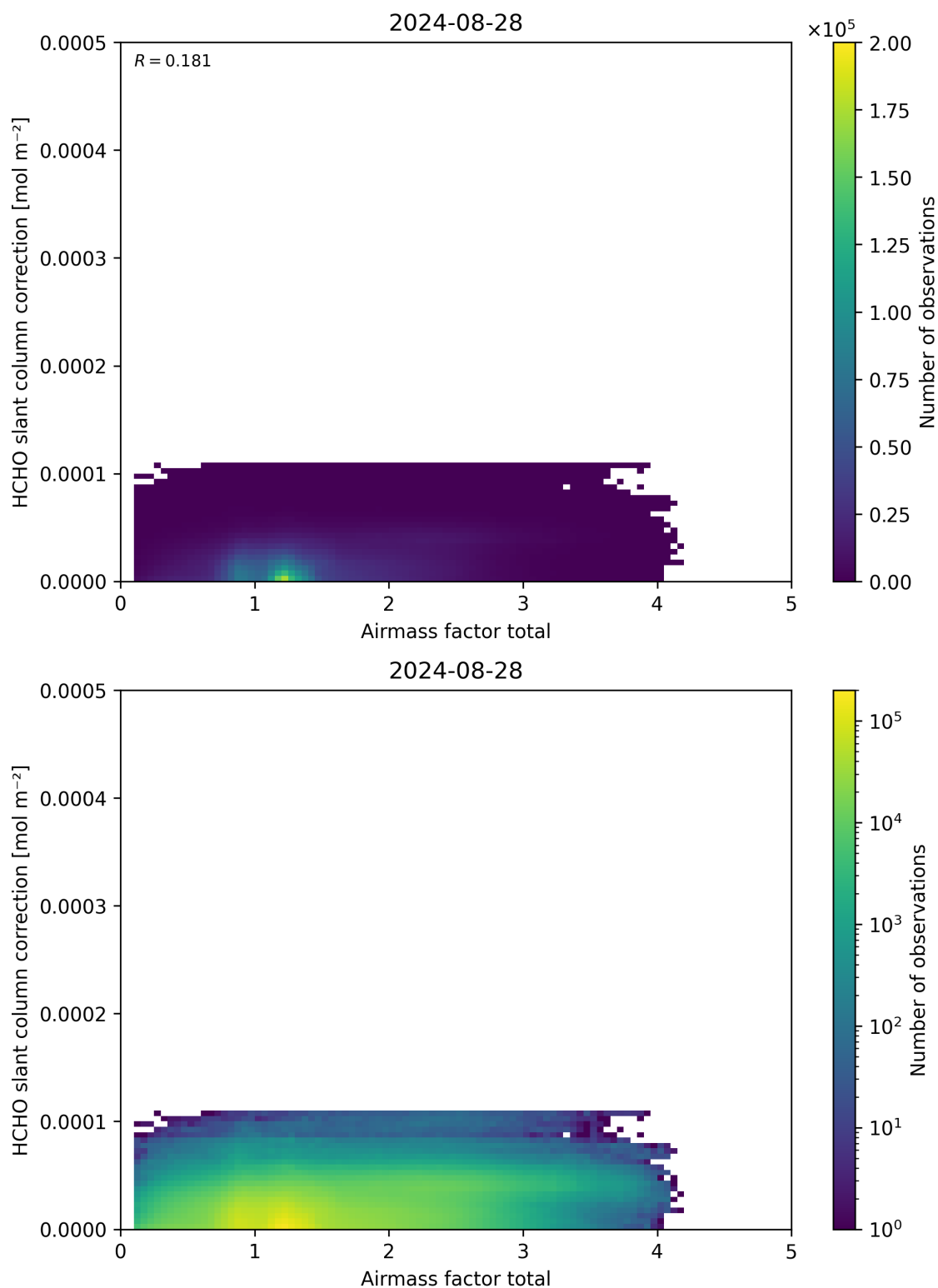
Figure 102: Scatter density plot of “Airmass factor total” against “HCHO slant column correction” for 2024-08-27 to 2024-08-29.
