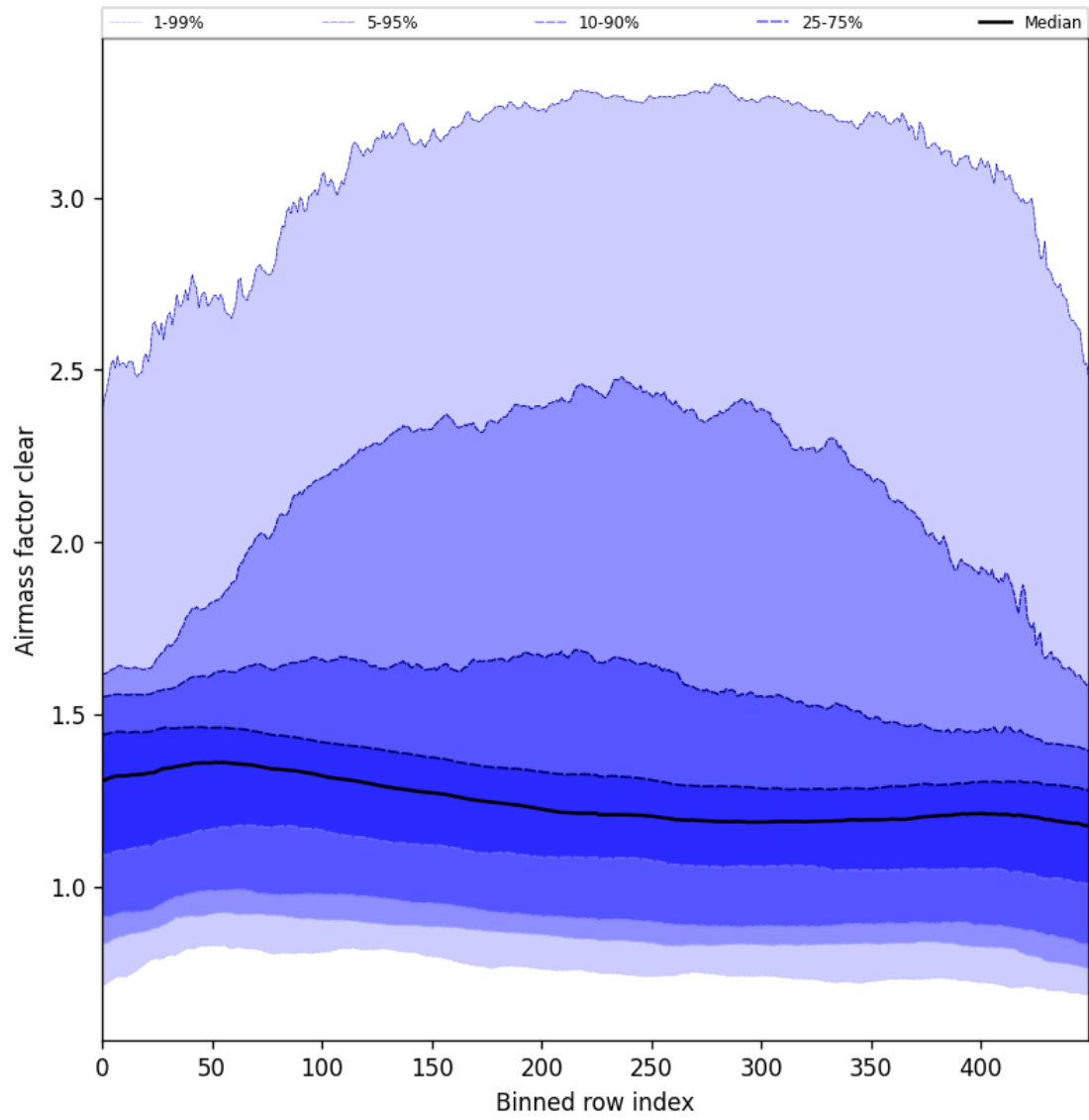
Figure 56: Along track statistics of “Airmass factor clear” for 2024-08-27 to 2024-08-29
