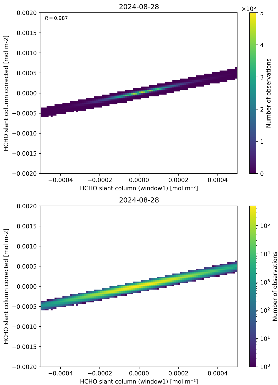
Figure 82: Scatter density plot of “HCHO slant column (window1)” against “HCHO slant column corrected” for 2024-08-27 to 2024-08-29.
