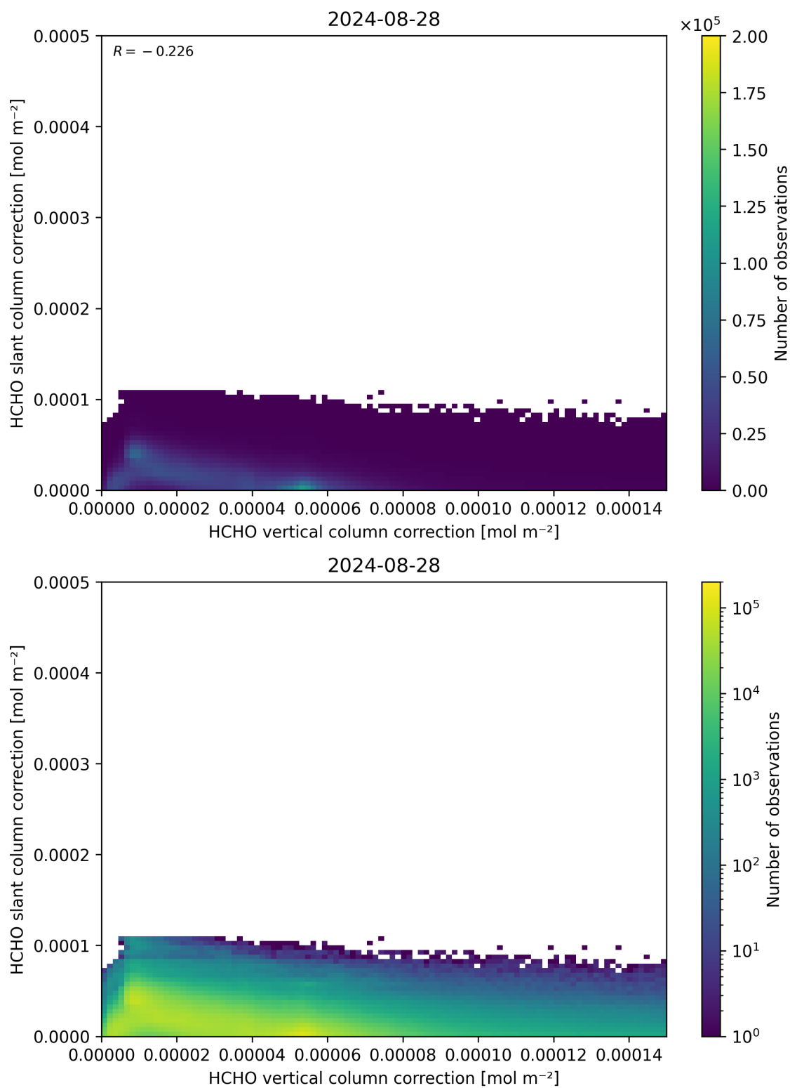
Figure 117: Scatter density plot of “HCHO vertical column correction” against “HCHO slant column correction” for 2024-08-27 to 2024-08-29.
