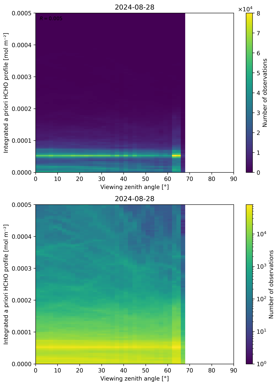
Figure 195: Scatter density plot of “Viewing zenith angle” against “Integrated a priori HCHO profile” for 2024-08-27 to 2024-08-29.
