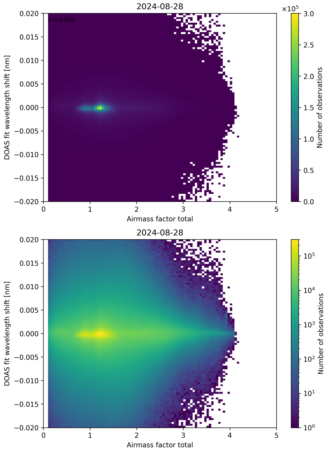
Figure 98: Scatter density plot of “Airmass factor total” against “DOAS fit wavelength shift” for 2024-08-27 to 2024-08-29.
