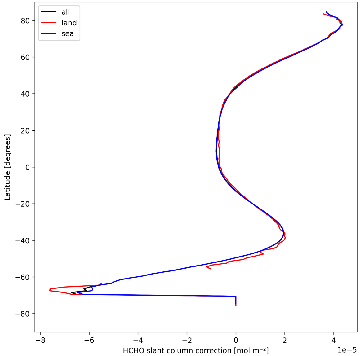
Figure 33: Zonal average of “HCHO slant column correction” for 2024-08-27 to 2024-08-29.
