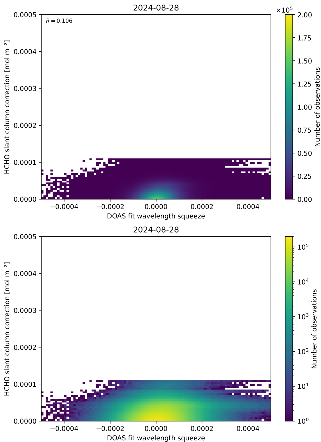
Figure 70: Scatter density plot of “DOAS fit wavelength squeeze” against “HCHO slant column correction” for 2024-08-27 to 2024-08-29.
