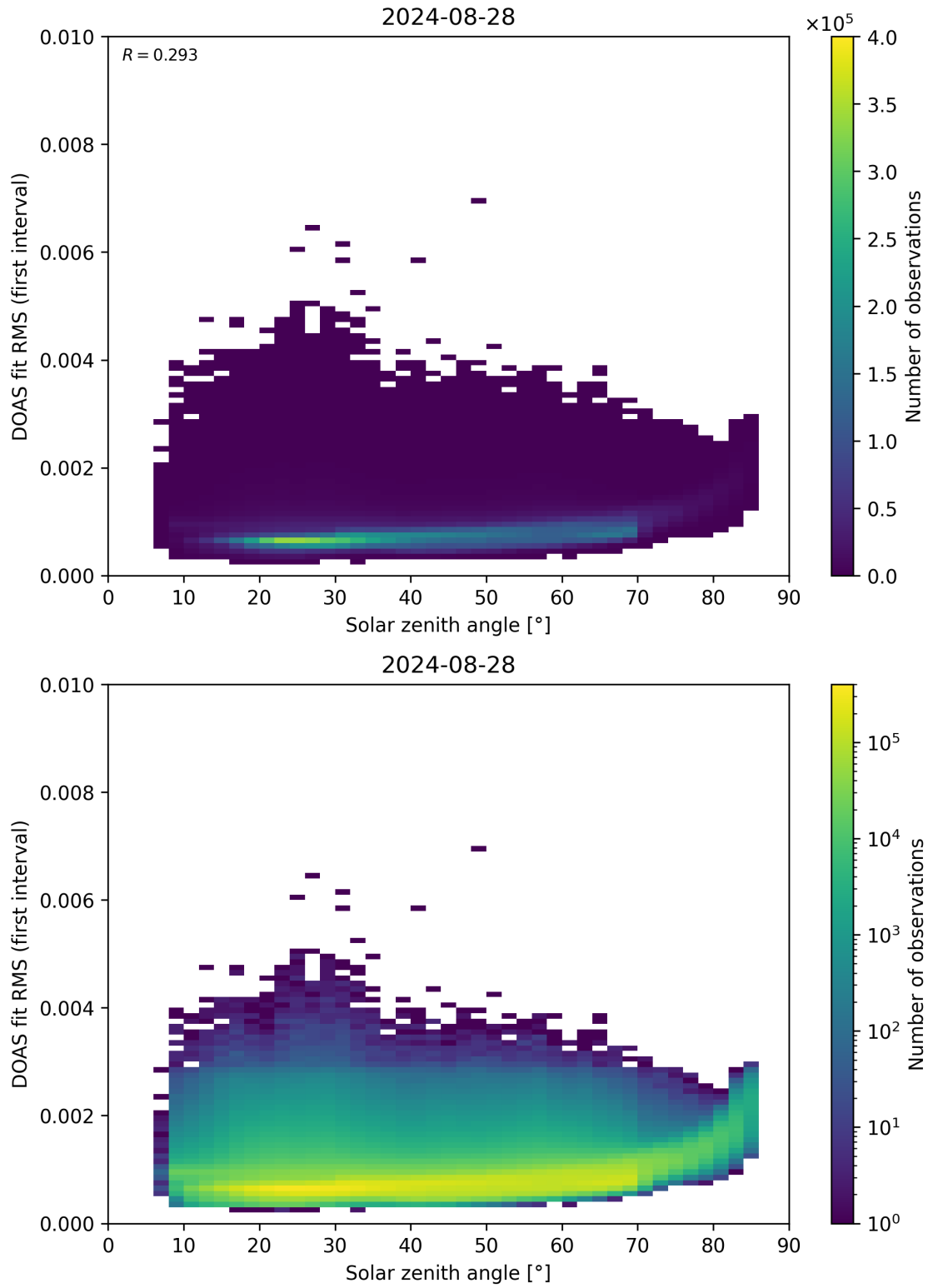
Figure 167: Scatter density plot of “Solar zenith angle” against “DOAS fit RMS (first interval)” for 2024-08-27 to 2024-08-29.
