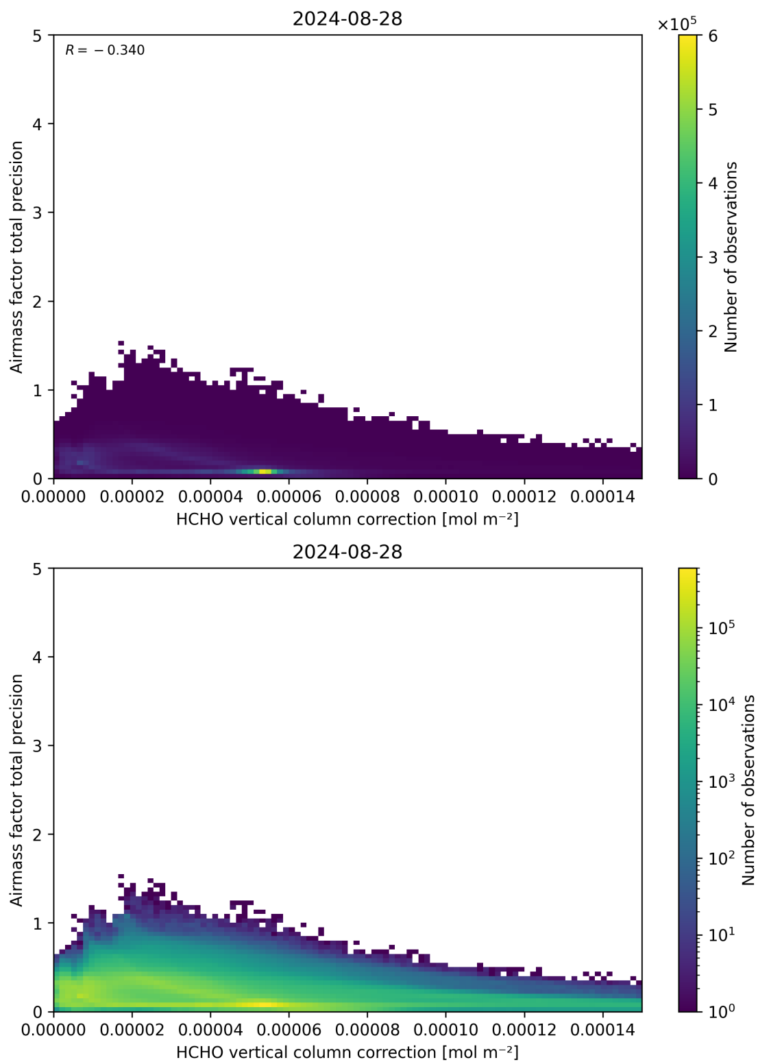
Figure 121: Scatter density plot of “HCHO vertical column correction” against “Airmass factor total precision” for 2024-08-27 to 2024-08-29.
