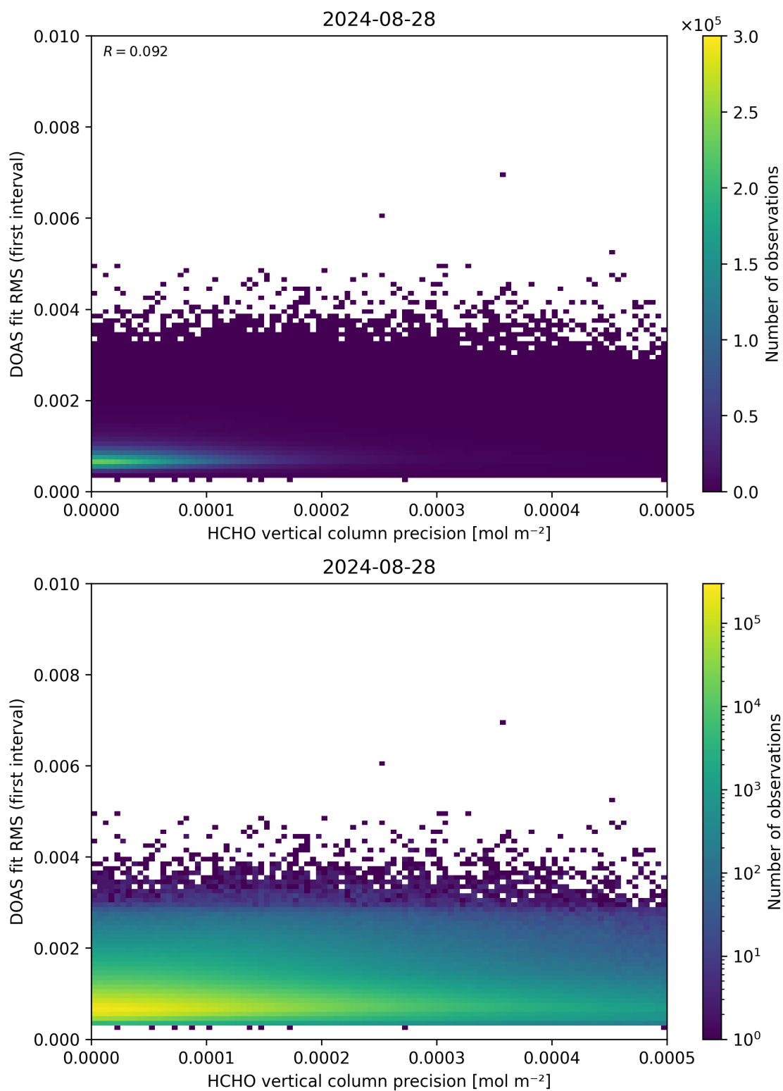
Figure 136: Scatter density plot of “HCHO vertical column precision” against “DOAS fit RMS (first interval)” for 2024-08-27 to 2024-08-29.
