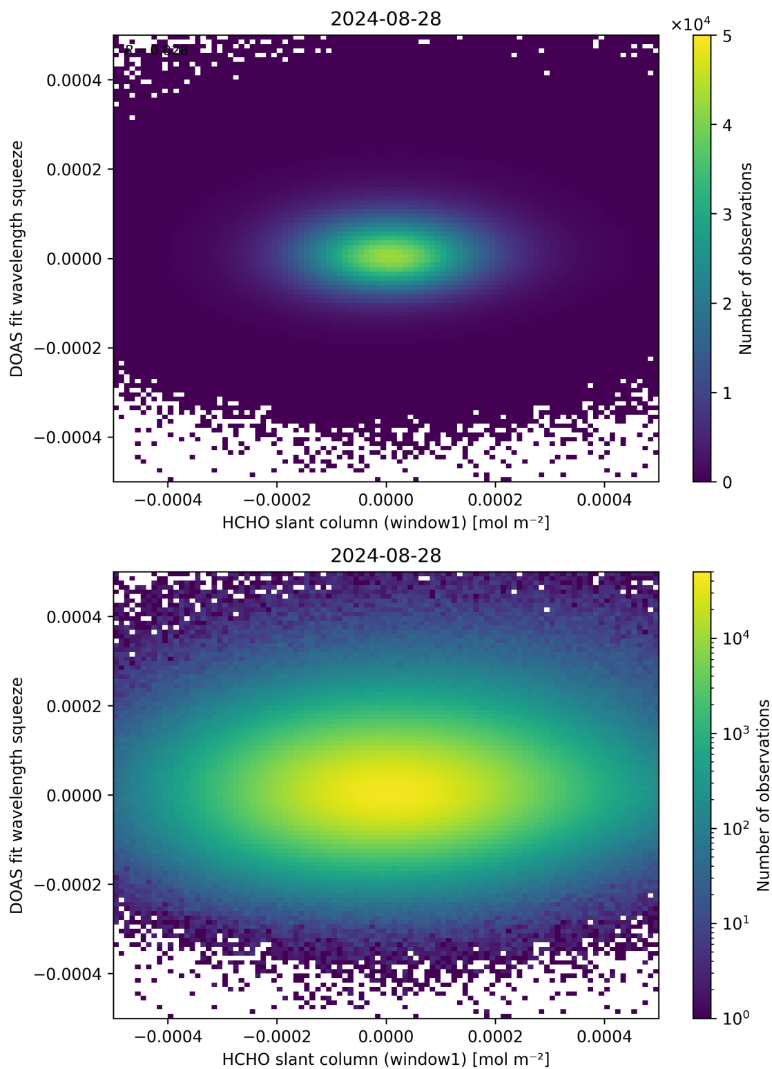
Figure 80: Scatter density plot of “HCHO slant column (window1)” against “DOAS fit wavelength squeeze” for 2024-08-27 to 2024-08-29.
