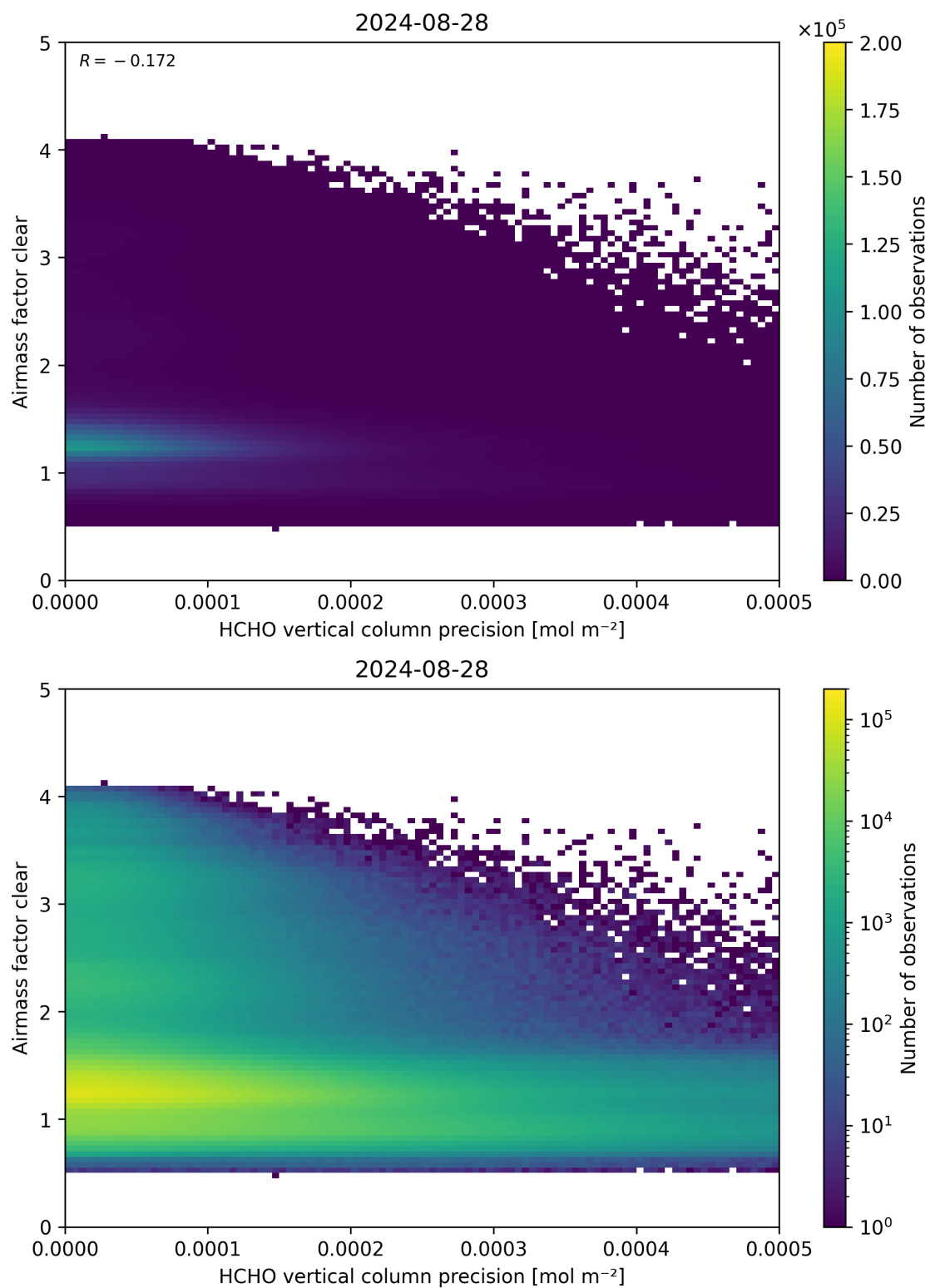
Figure 139: Scatter density plot of “HCHO vertical column precision” against “Airmass factor clear” for 2024-08-27 to 2024-08-29.
