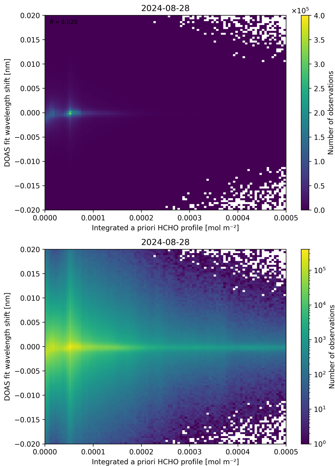
Figure 149: Scatter density plot of “Integrated a priori HCHO profile” against “DOAS fit wavelength shift” for 2024-08-27 to 2024-08-29.
