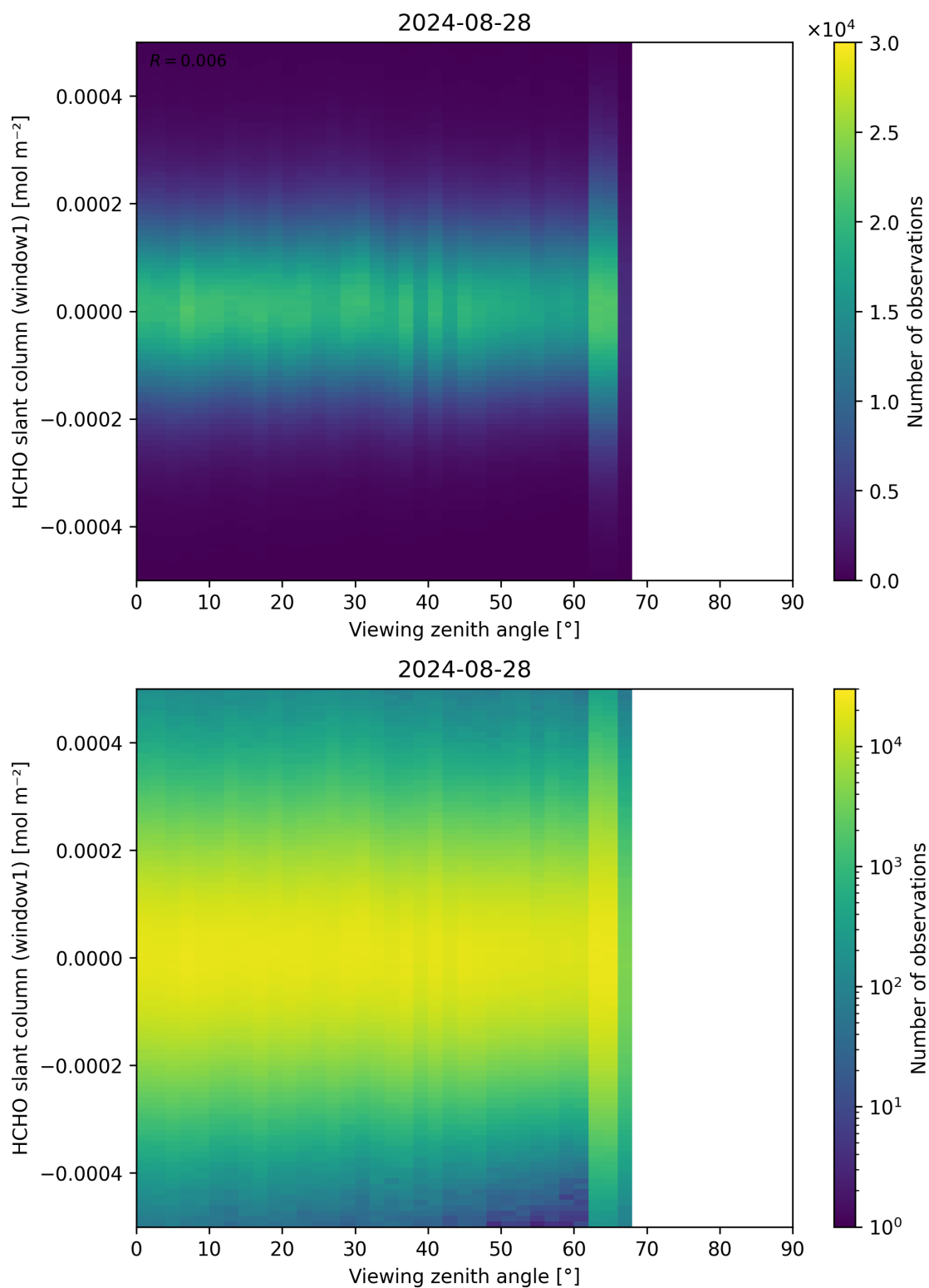
Figure 188: Scatter density plot of “Viewing zenith angle” against “HCHO slant column (window1)” for 2024-08-27 to 2024-08-29.
