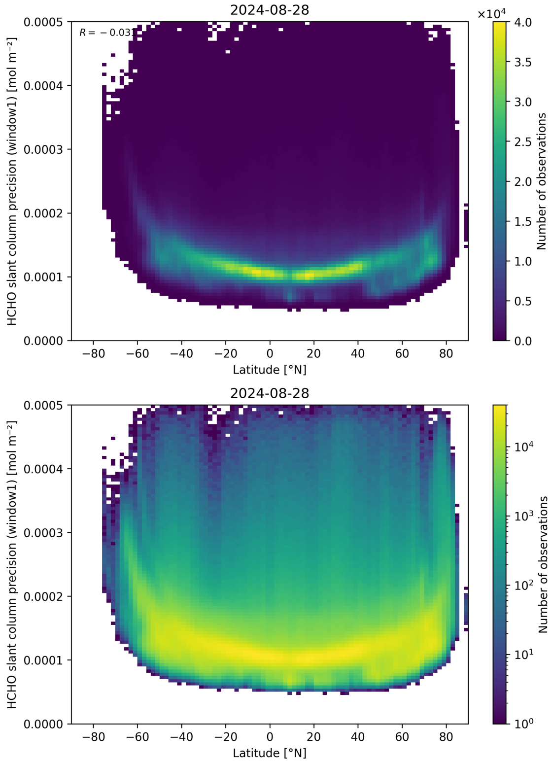
Figure 160: Scatter density plot of “Latitude” against “HCHO slant column precision (window1)” for 2024-08-27 to 2024-08-29.
