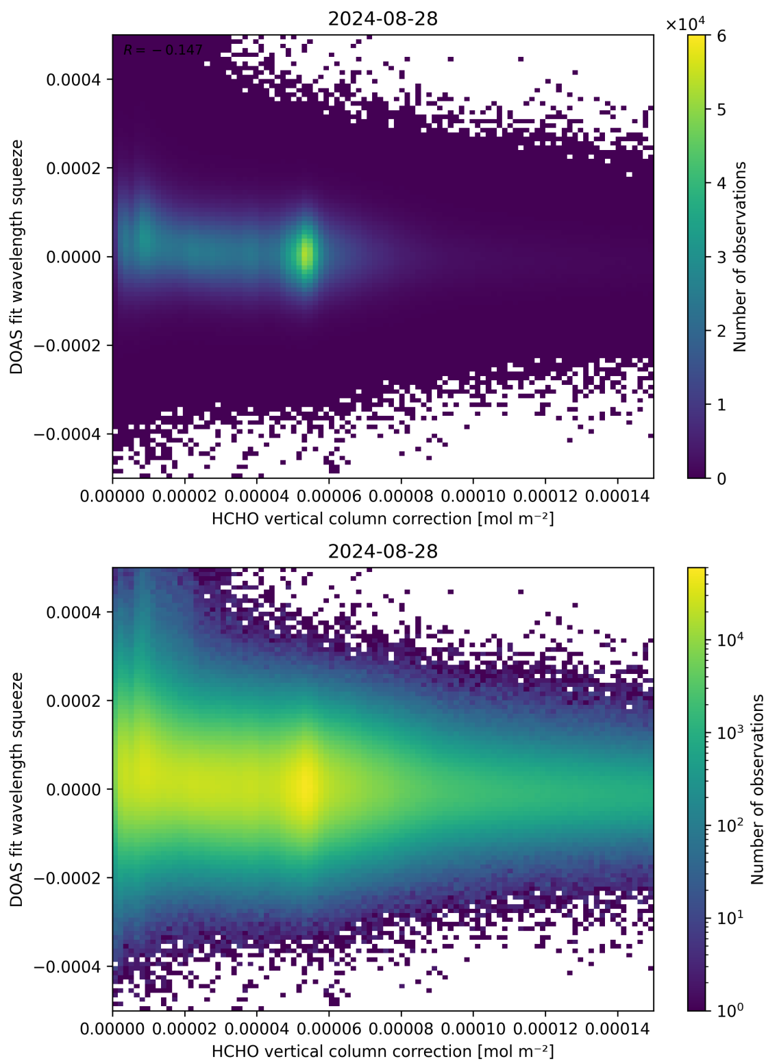
Figure 114: Scatter density plot of “HCHO vertical column correction” against “DOAS fit wavelength squeeze” for 2024-08-27 to 2024-08-29.
