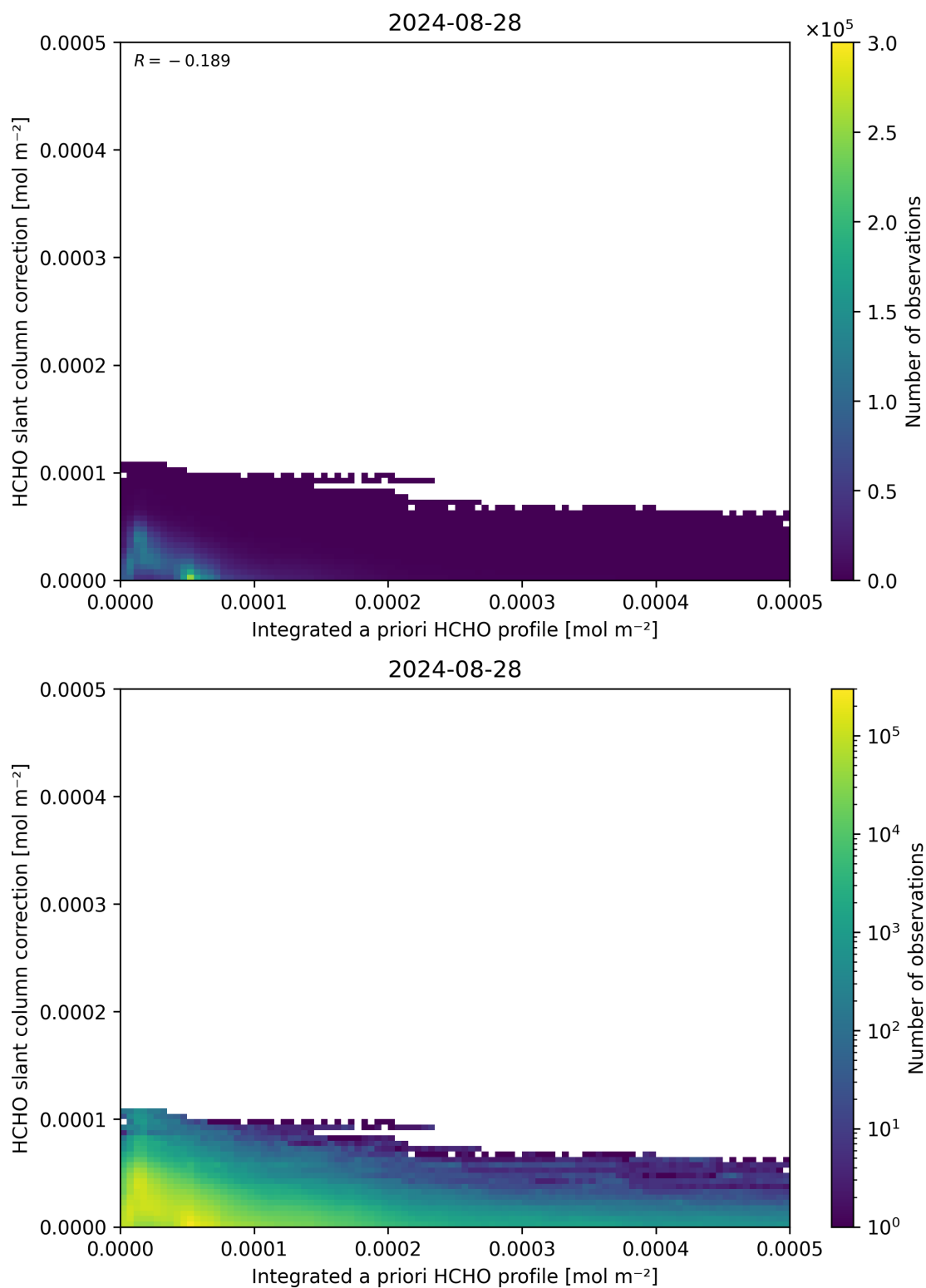
Figure 152: Scatter density plot of “Integrated a priori HCHO profile” against “HCHO slant column correction” for 2024-08-27 to 2024-08-29.
