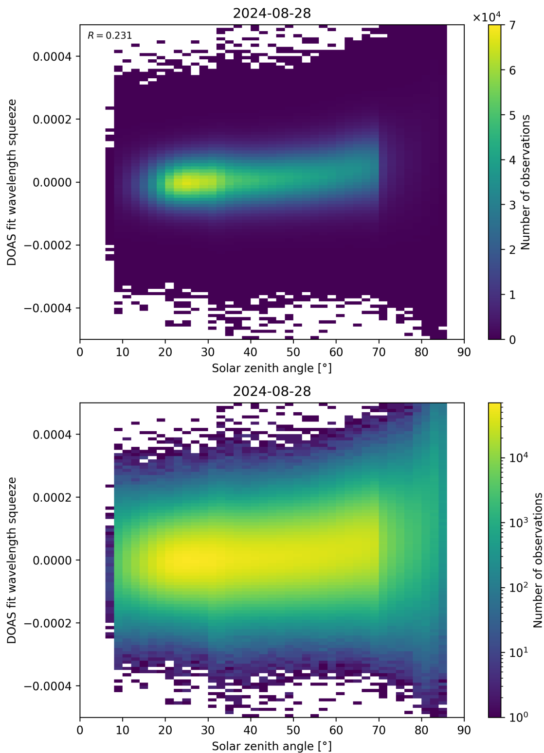
Figure 169: Scatter density plot of “Solar zenith angle” against “DOAS fit wavelength squeeze” for 2024-08-27 to 2024-08-29.
