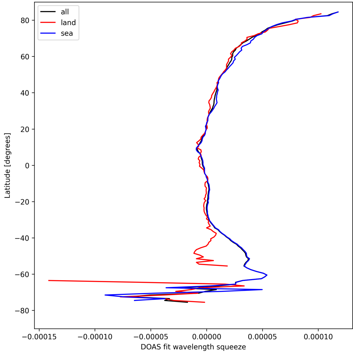
Figure 31: Zonal average of “DOAS fit wavelength squeeze” for 2024-08-27 to 2024-08-29.
