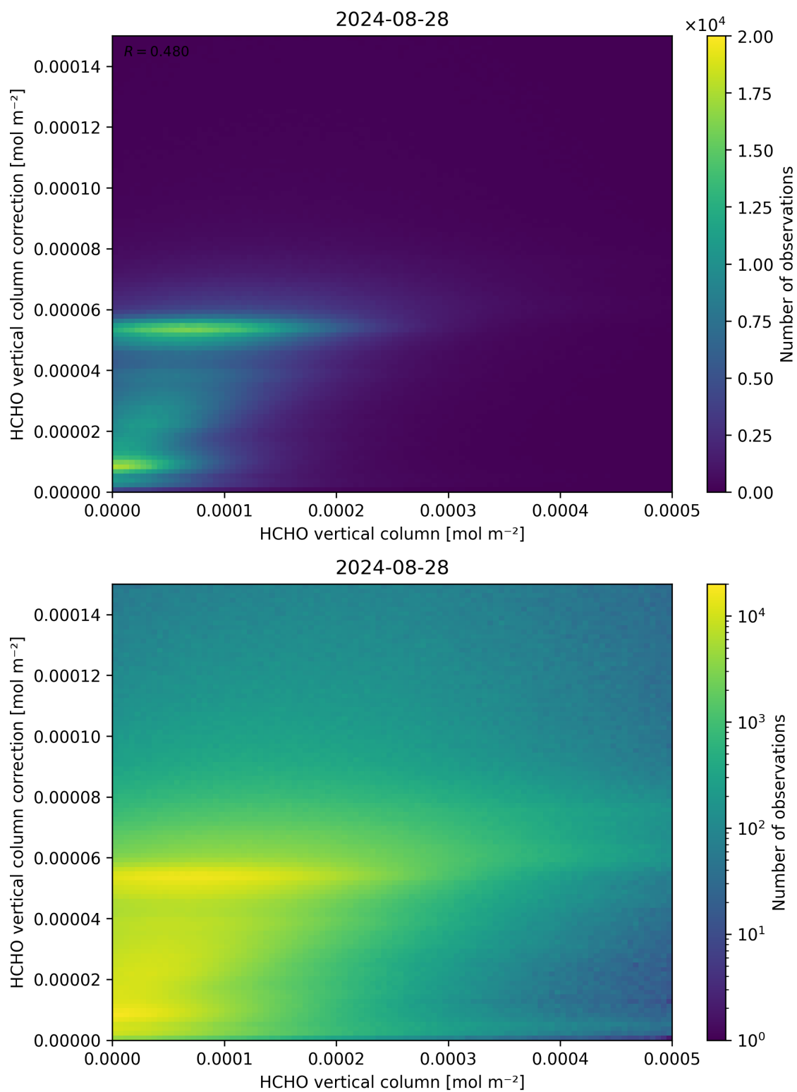
Figure 133: Scatter density plot of “HCHO vertical column” against “HCHO vertical column correction” for 2024-08-27 to 2024-08-29.
