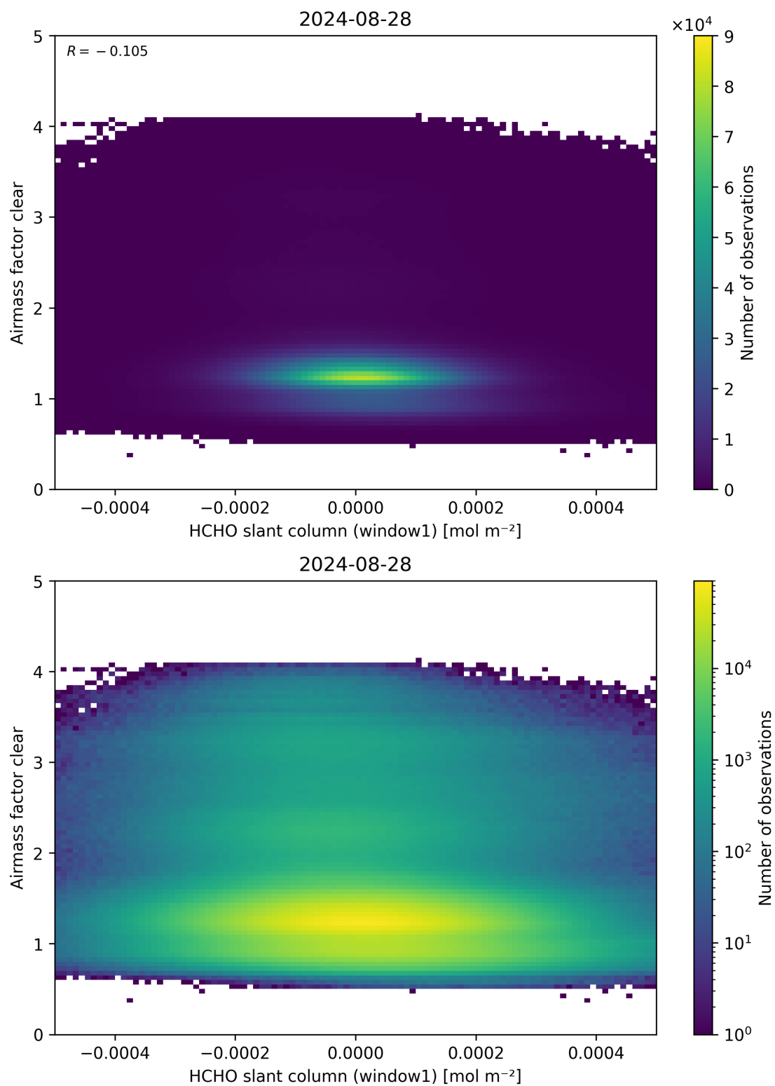
Figure 81: Scatter density plot of “HCHO slant column (window1)” against “Airmass factor clear” for 2024-08-27 to 2024-08-29.
