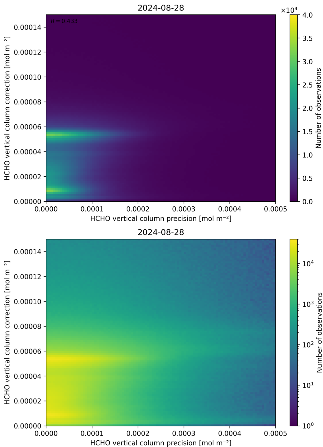
Figure 146: Scatter density plot of “HCHO vertical column precision” against “HCHO vertical column correction” for 2024-08-27 to 2024-08-29.
