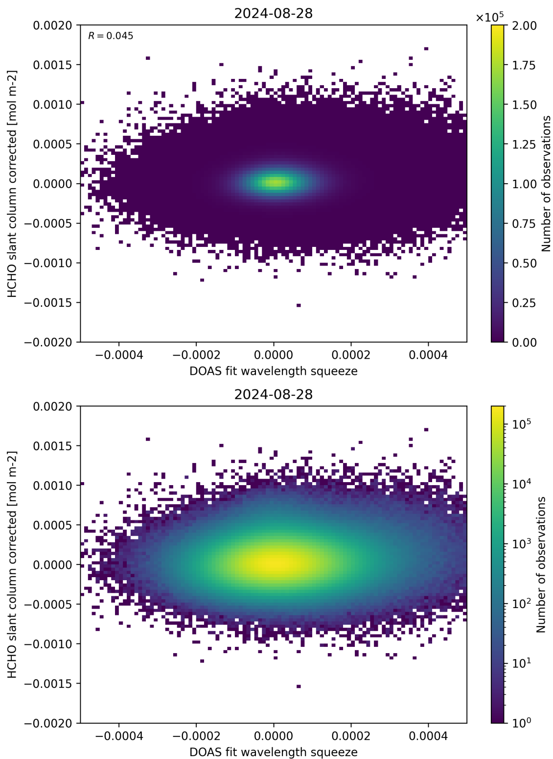
Figure 69: Scatter density plot of “DOAS fit wavelength squeeze” against “HCHO slant column corrected” for 2024-08-27 to 2024-08-29.
