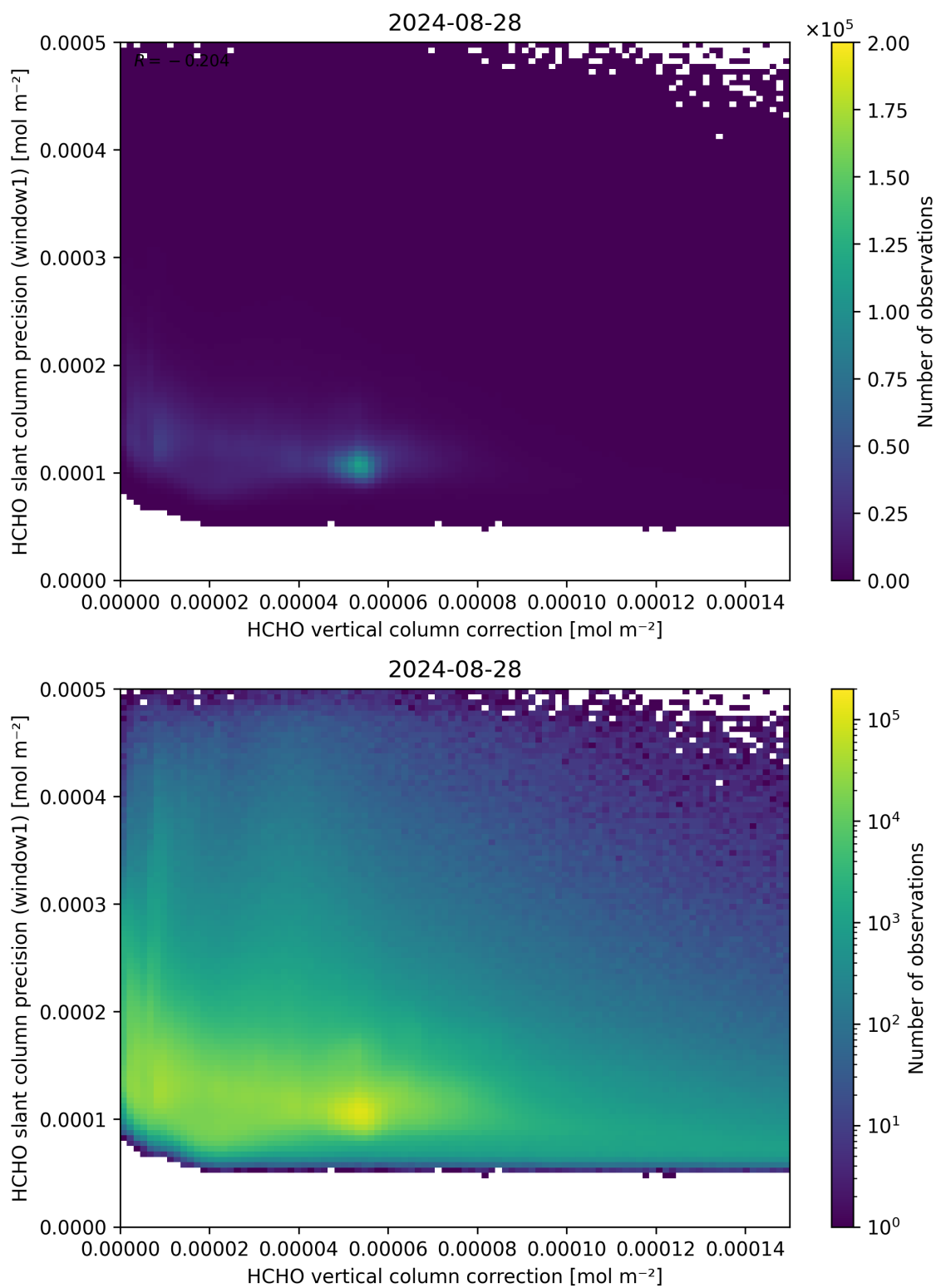
Figure 119: Scatter density plot of “HCHO vertical column correction” against “HCHO slant column precision (window1)” for 2024-08-27 to 2024-08-29.
