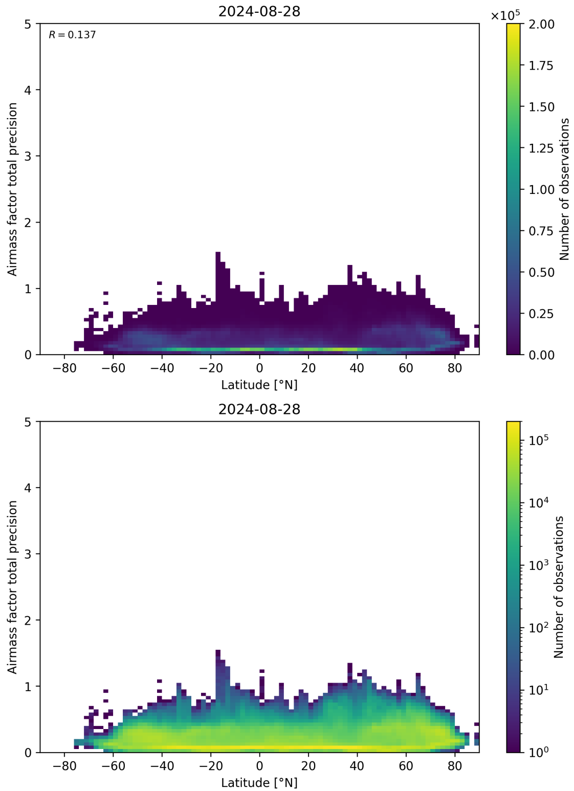
Figure 162: Scatter density plot of “Latitude” against “Airmass factor total precision” for 2024-08-27 to 2024-08-29.
