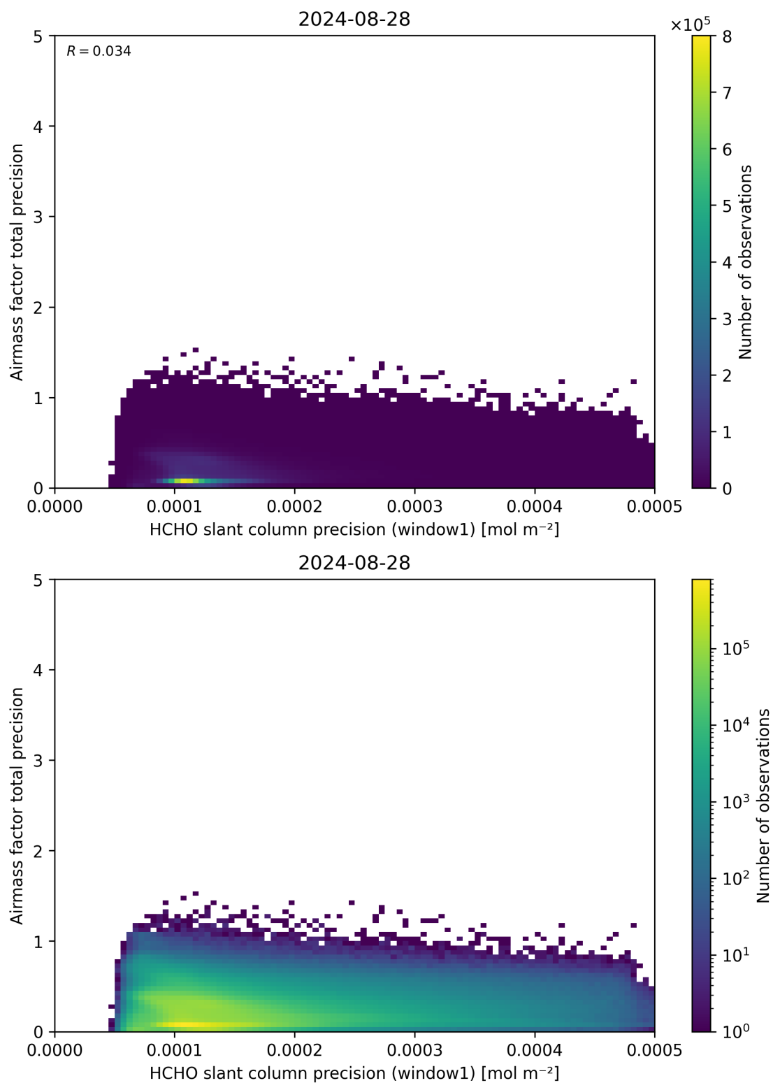
Figure 95: Scatter density plot of “HCHO slant column precision (window1)” against “Airmass factor total precision” for 2024-08-27 to 2024-08-29.
