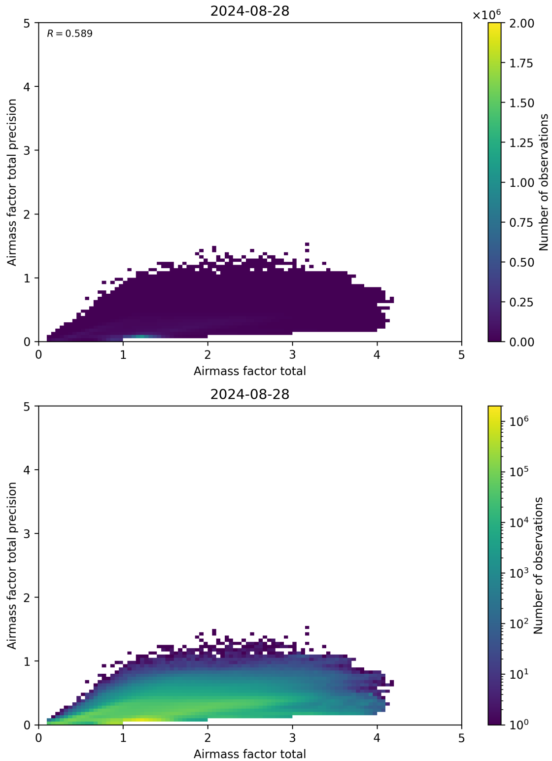
Figure 103: Scatter density plot of “Airmass factor total” against “Airmass factor total precision” for 2024-08-27 to 2024-08-29.
