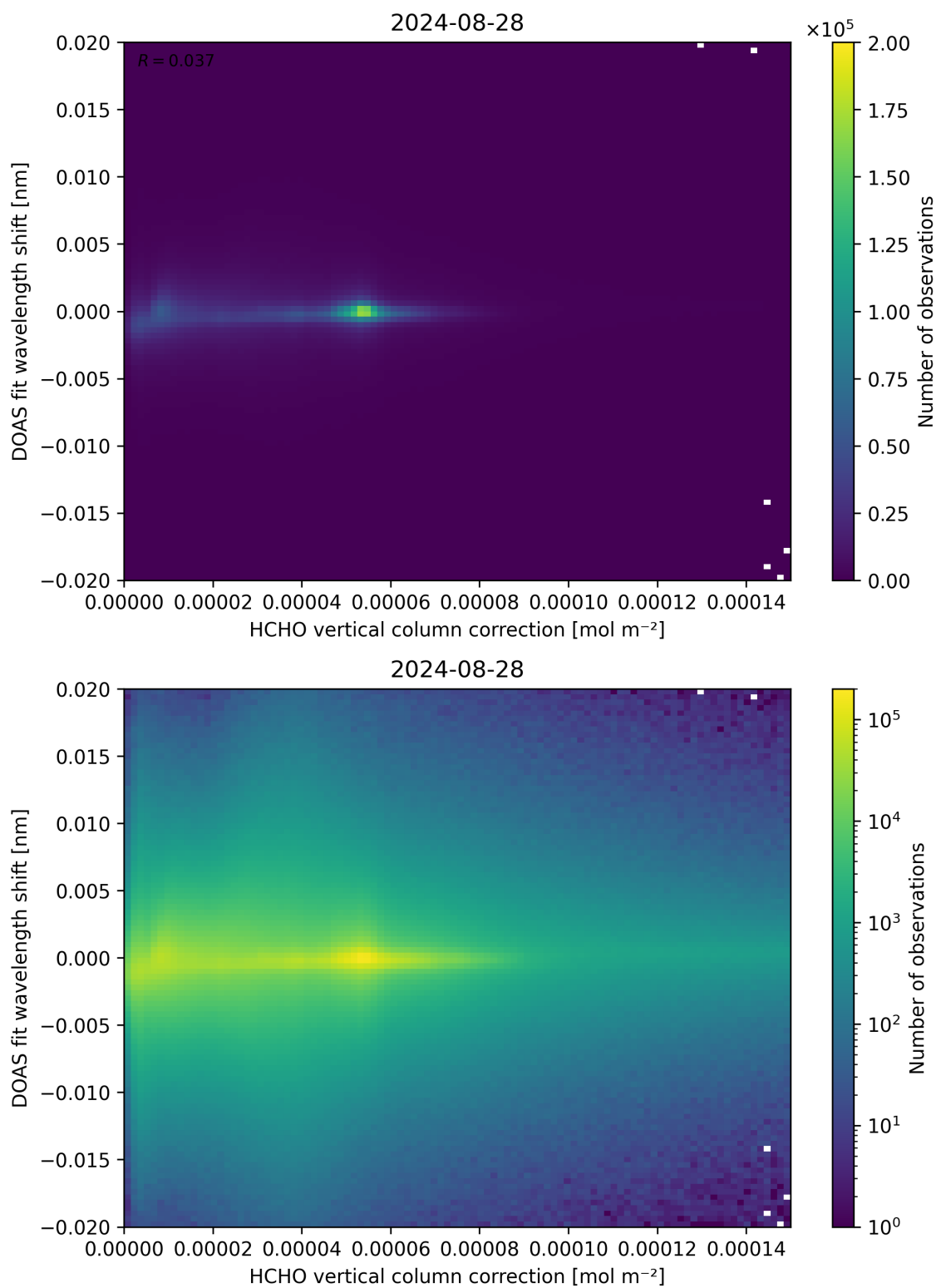
Figure 113: Scatter density plot of “HCHO vertical column correction” against “DOAS fit wavelength shift” for 2024-08-27 to 2024-08-29.
