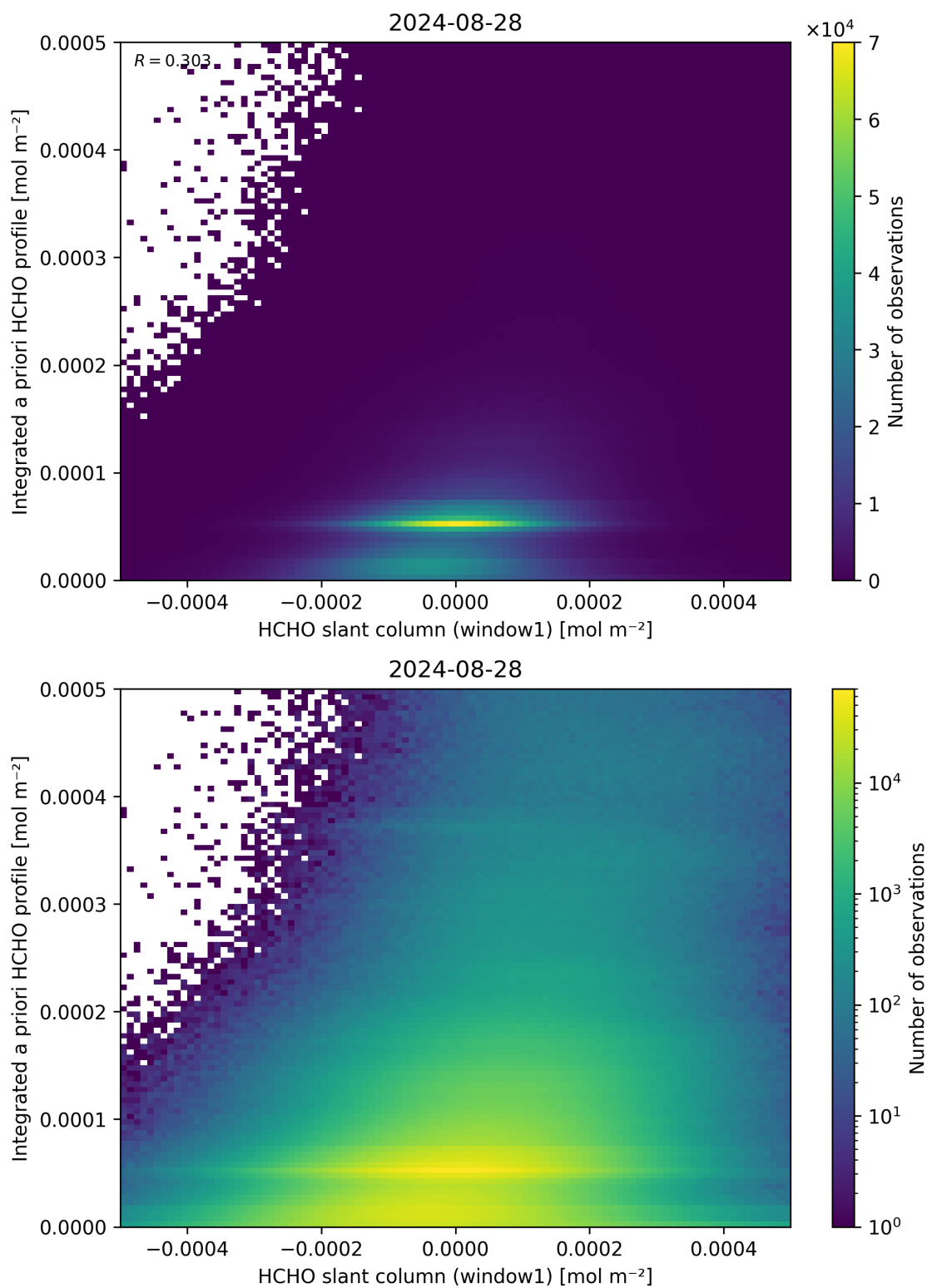
Figure 87: Scatter density plot of “HCHO slant column (window1)” against “Integrated a priori HCHO profile” for 2024-08-27 to 2024-08-29.
