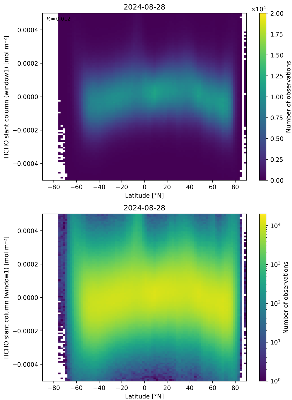
Figure 159: Scatter density plot of “Latitude” against “HCHO slant column (window1)” for 2024-08-27 to 2024-08-29.
