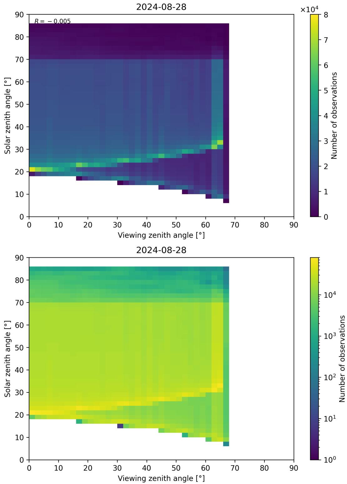
Figure 197: Scatter density plot of “Viewing zenith angle” against “Solar zenith angle” for 2024-08-27 to 2024-08-29.
