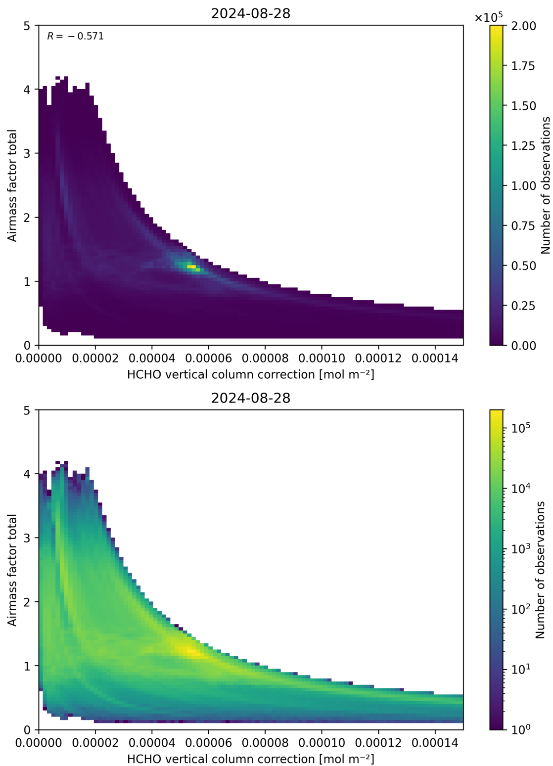
Figure 120: Scatter density plot of “HCHO vertical column correction” against “Airmass factor total” for 2024-08-27 to 2024-08-29.
