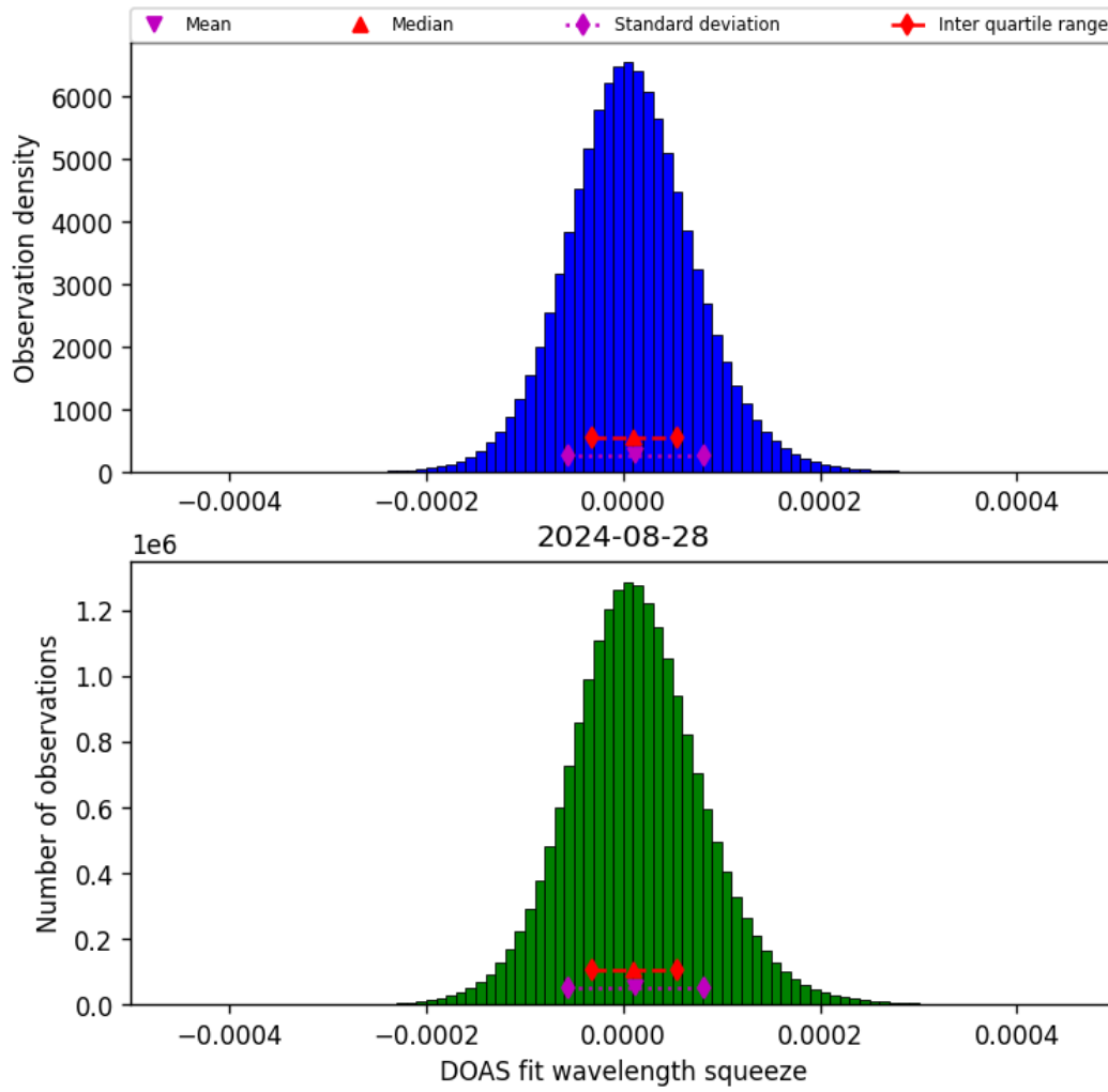
Figure 45: Histogram of “DOAS fit wavelength squeeze” for 2024-08-27 to 2024-08-29
