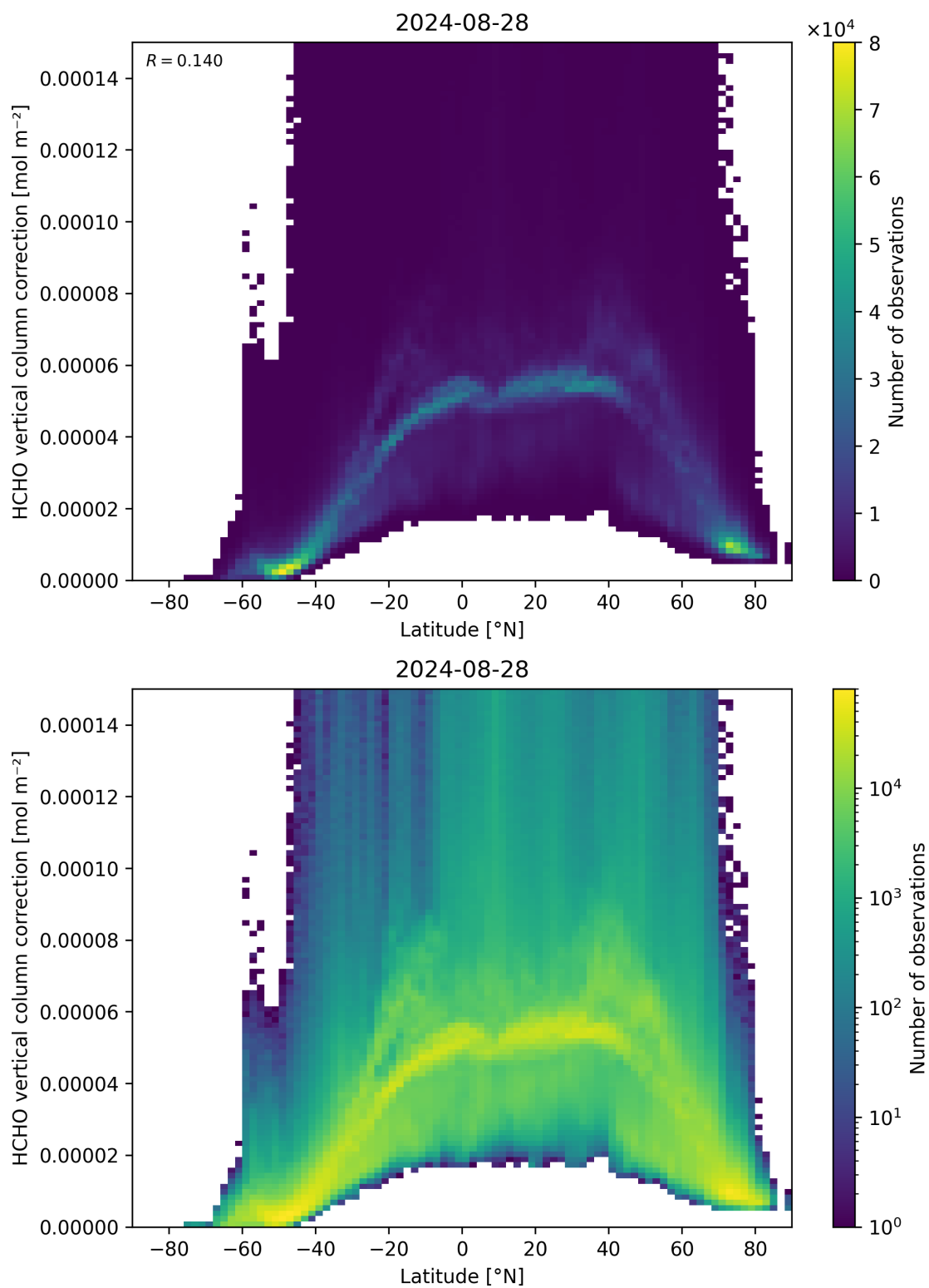
Figure 164: Scatter density plot of “Latitude” against “HCHO vertical column correction” for 2024-08-27 to 2024-08-29.
