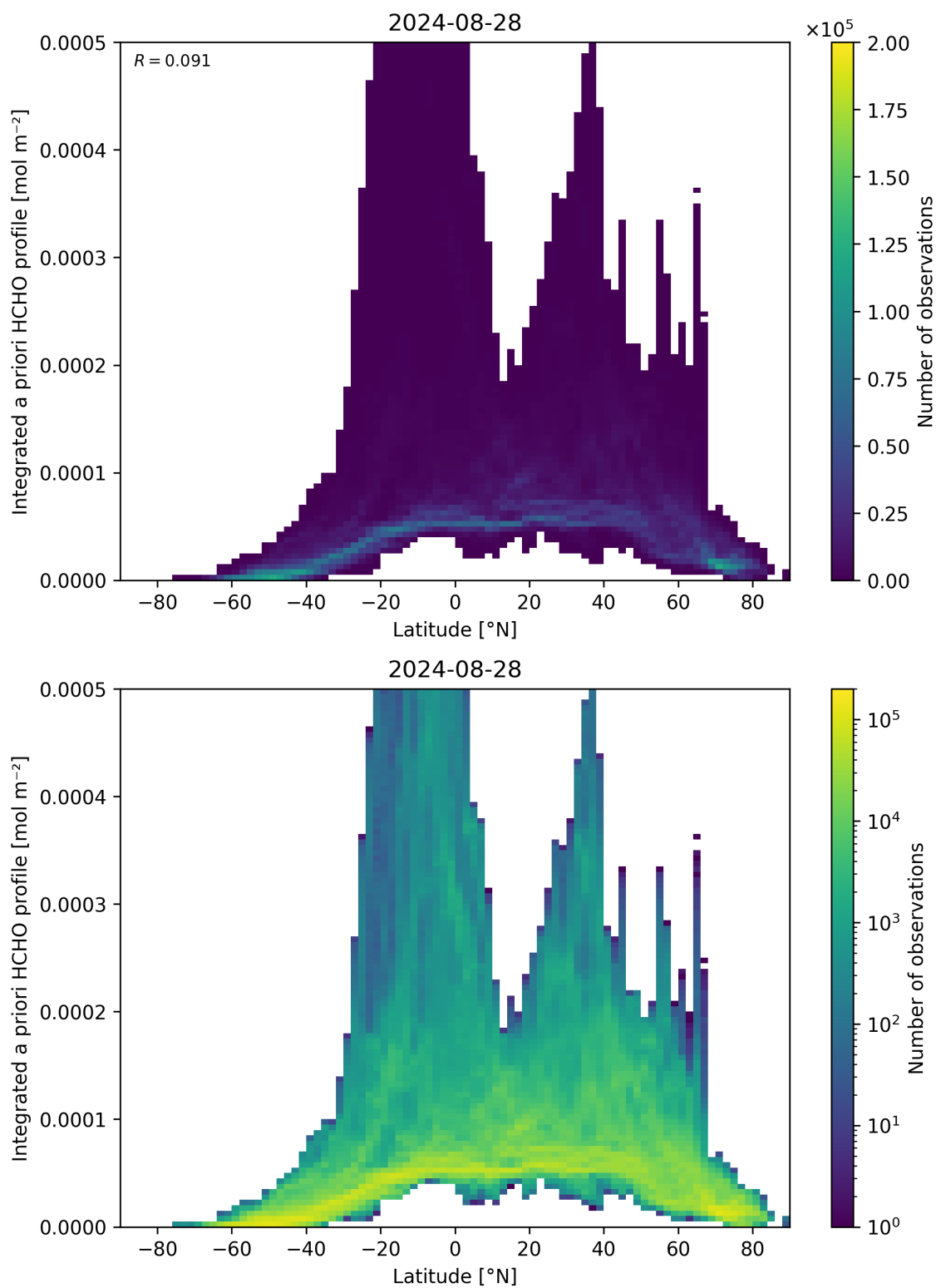
Figure 166: Scatter density plot of “Latitude” against “Integrated a priori HCHO profile” for 2024-08-27 to 2024-08-29.
