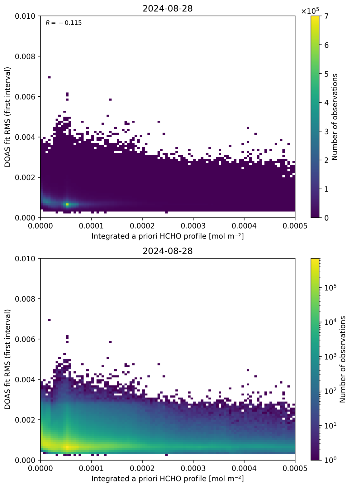
Figure 148: Scatter density plot of “Integrated a priori HCHO profile” against “DOAS fit RMS (first interval)” for 2024-08-27 to 2024-08-29.
