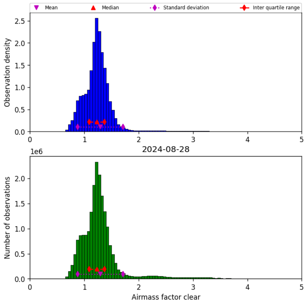
Figure 42: Histogram of “Airmass factor clear” for 2024-08-27 to 2024-08-29
