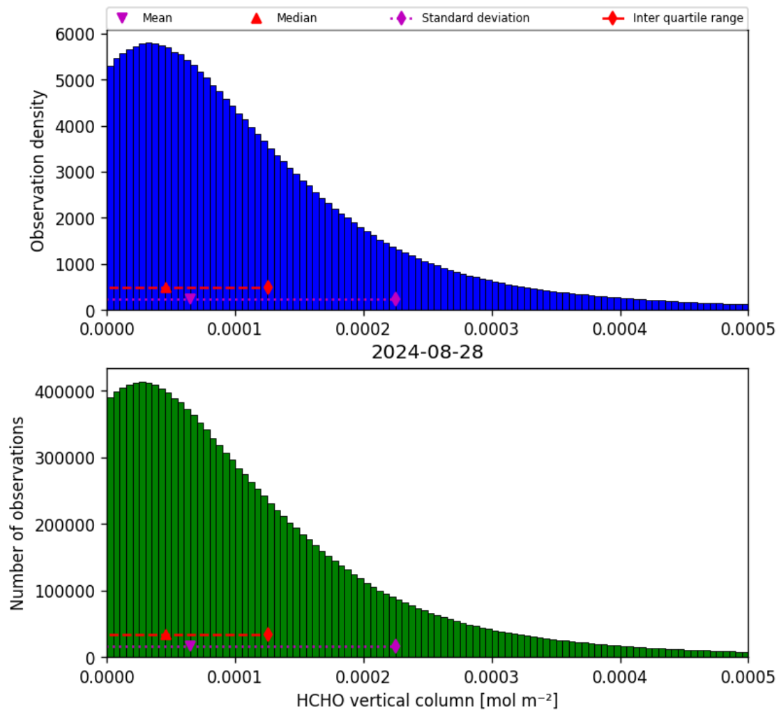
Figure 35: Histogram of “HCHO vertical column” for 2024-08-27 to 2024-08-29
