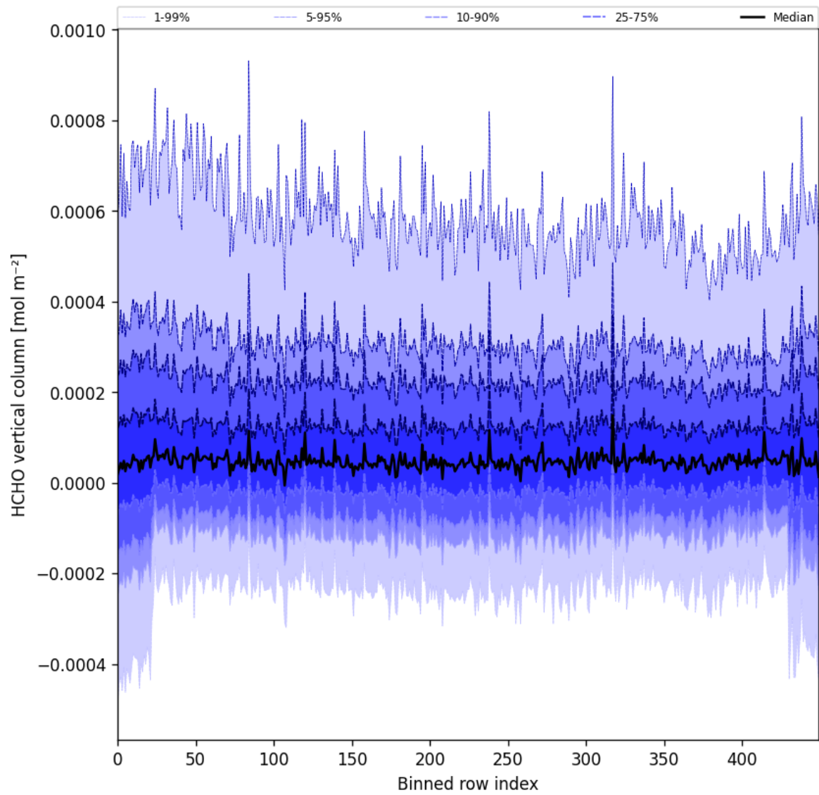
Figure 49: Along track statistics of “HCHO vertical column” for 2024-08-27 to 2024-08-29
