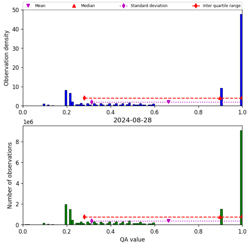
Figure 34: Histogram of “QA value” for 2024-08-27 to 2024-08-29
