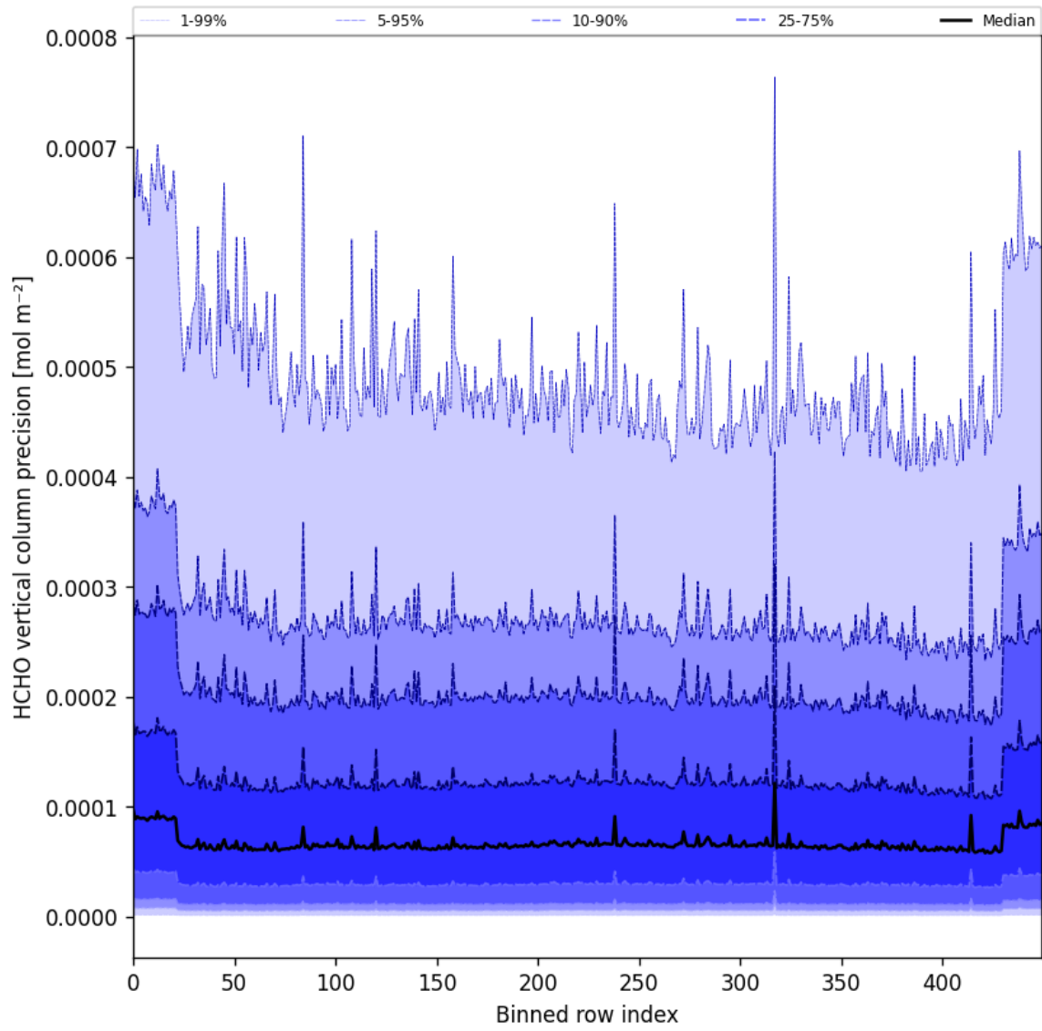
Figure 50: Along track statistics of “HCHO vertical column precision” for 2024-08-27 to 2024-08-29
