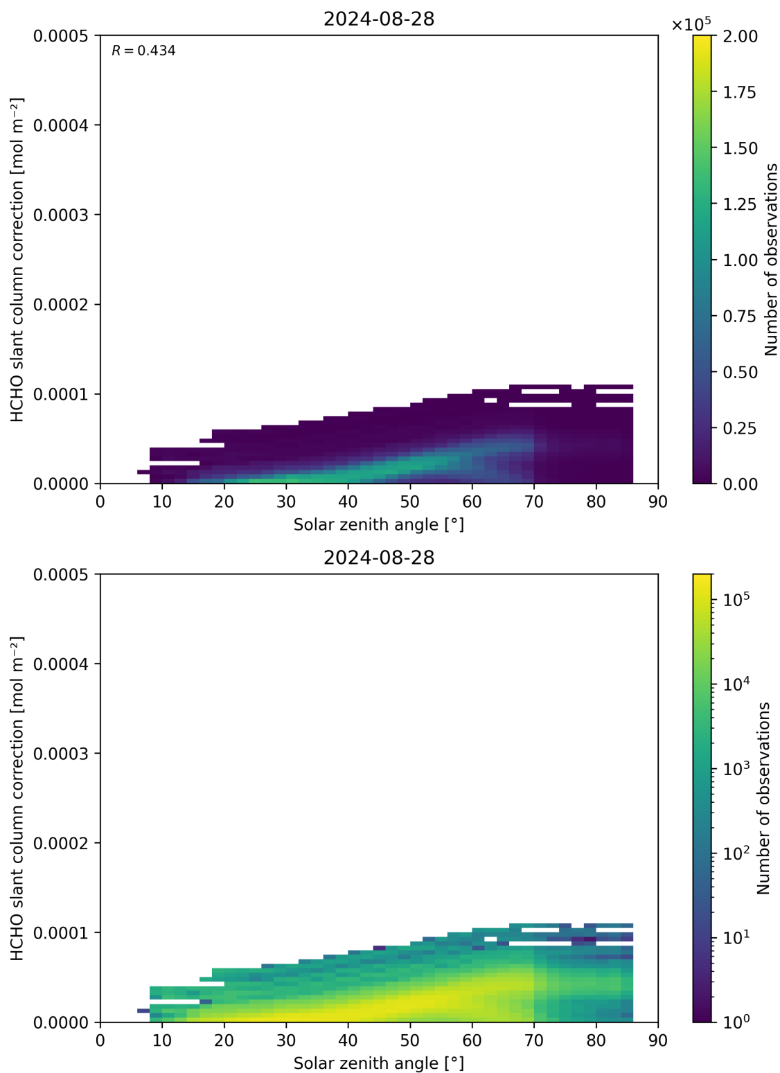
Figure 172: Scatter density plot of “Solar zenith angle” against “HCHO slant column correction” for 2024-08-27 to 2024-08-29.
