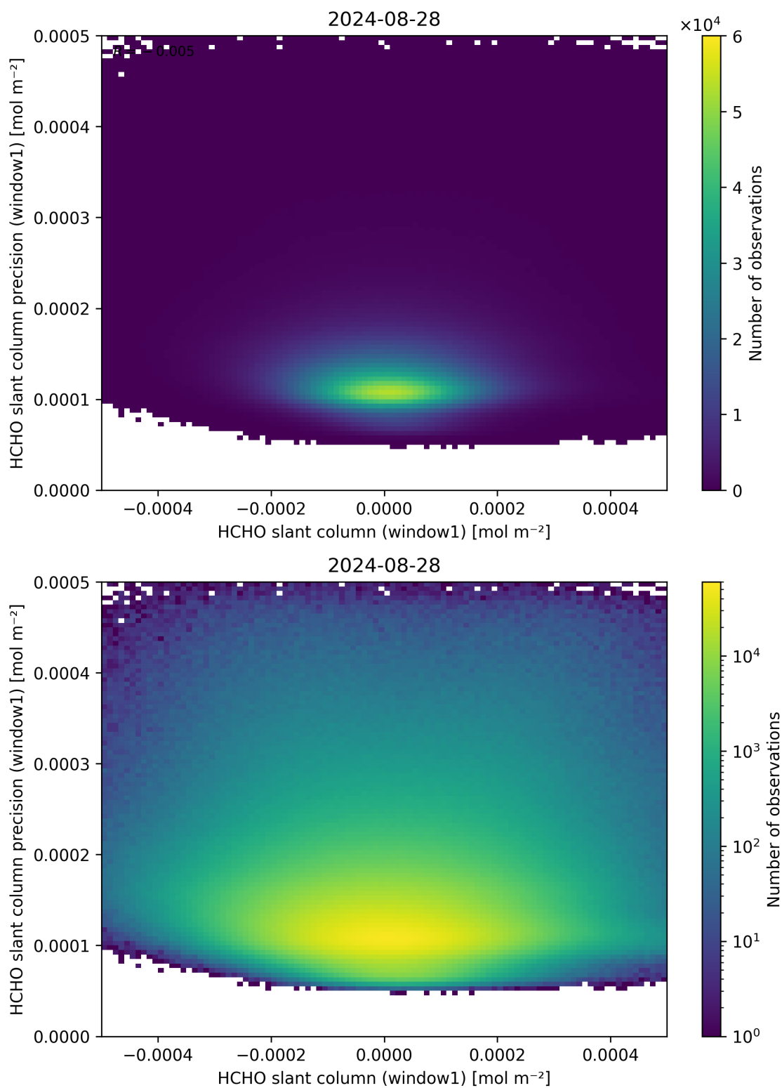
Figure 84: Scatter density plot of “HCHO slant column (window1)” against “HCHO slant column precision (window1)” for 2024-08-27 to 2024-08-29.
