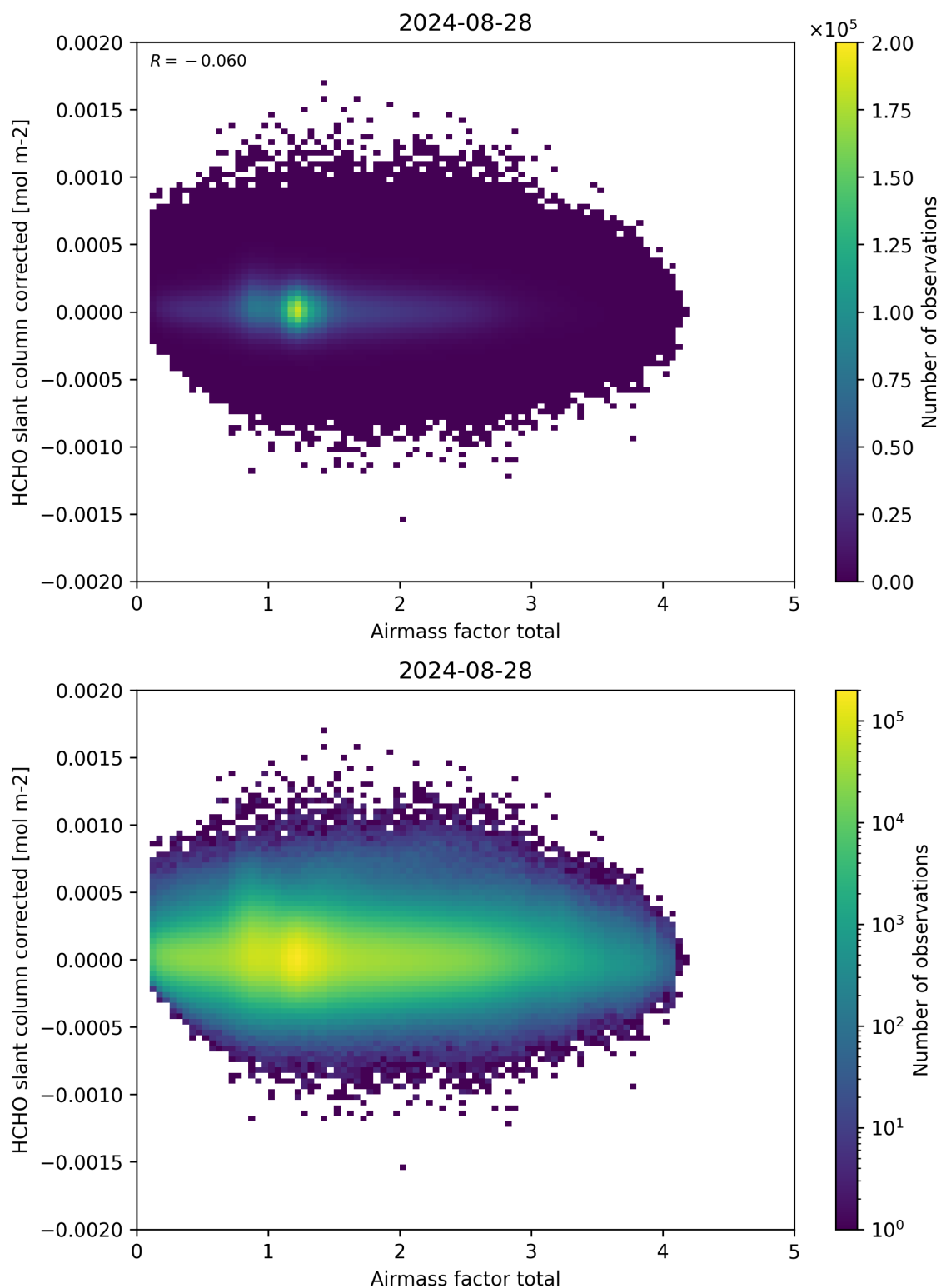
Figure 101: Scatter density plot of “Airmass factor total” against “HCHO slant column corrected” for 2024-08-27 to 2024-08-29.
