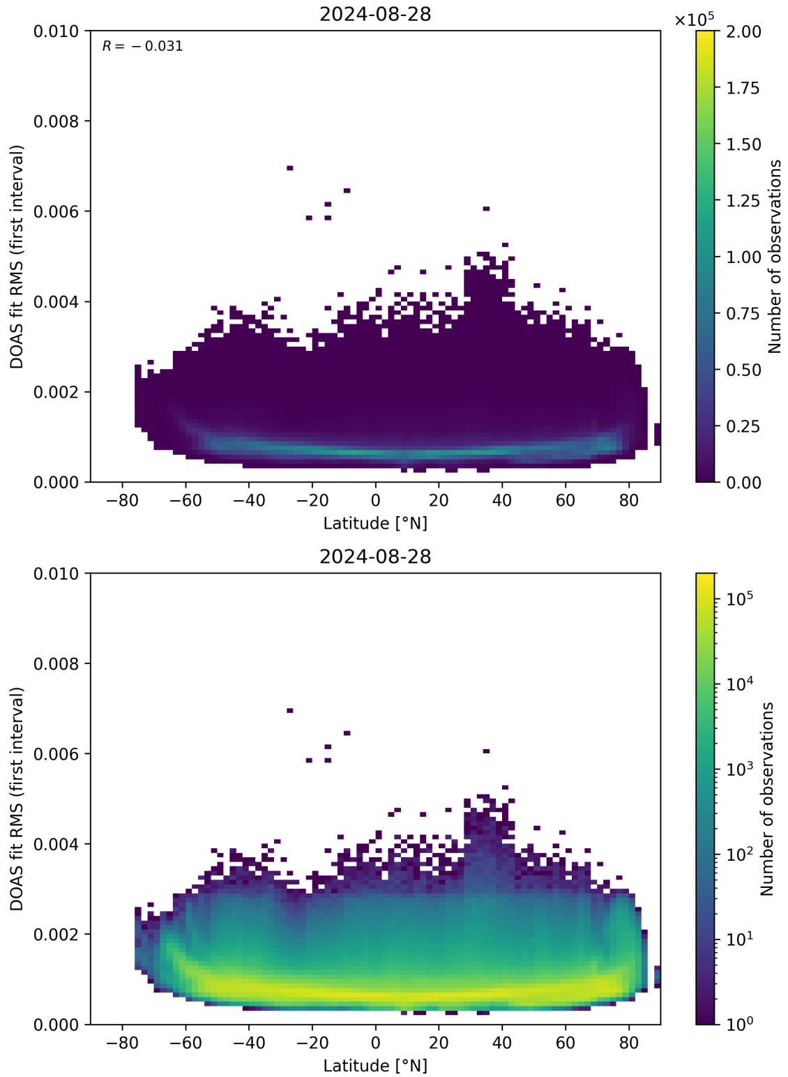
Figure 153: Scatter density plot of “Latitude” against “DOAS fit RMS (first interval)” for 2024-08-27 to 2024-08-29.
