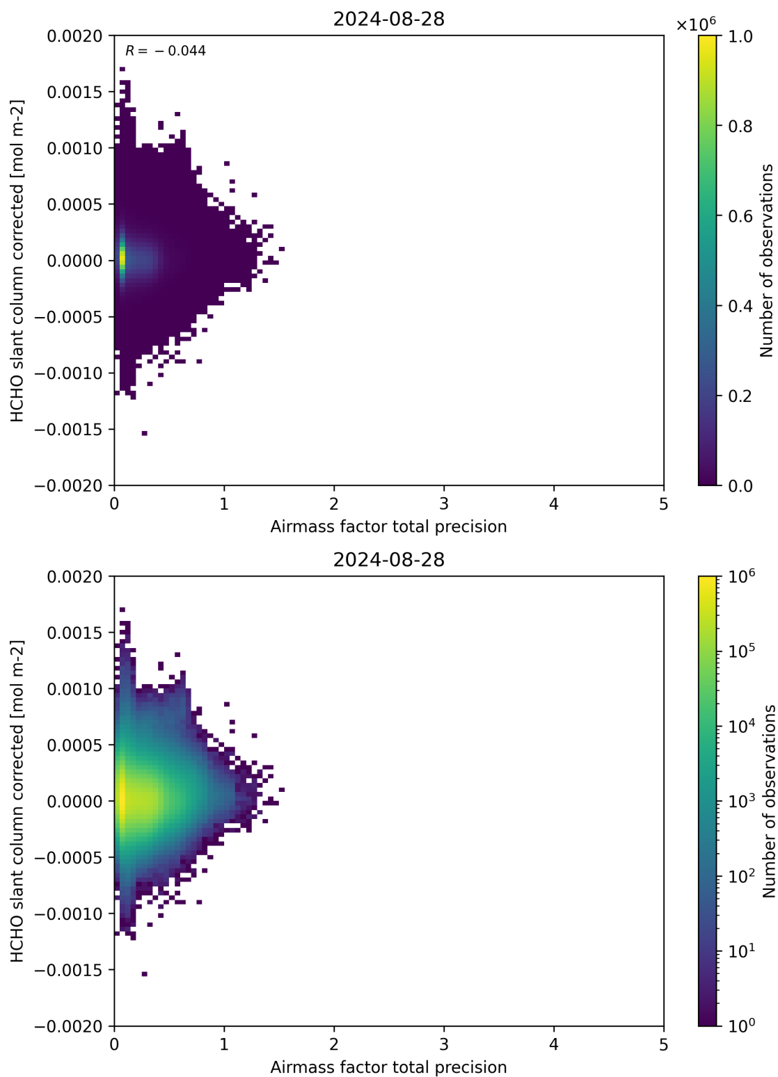
Figure 109: Scatter density plot of “Airmass factor total precision” against “HCHO slant column corrected” for 2024-08-27 to 2024-08-29.
