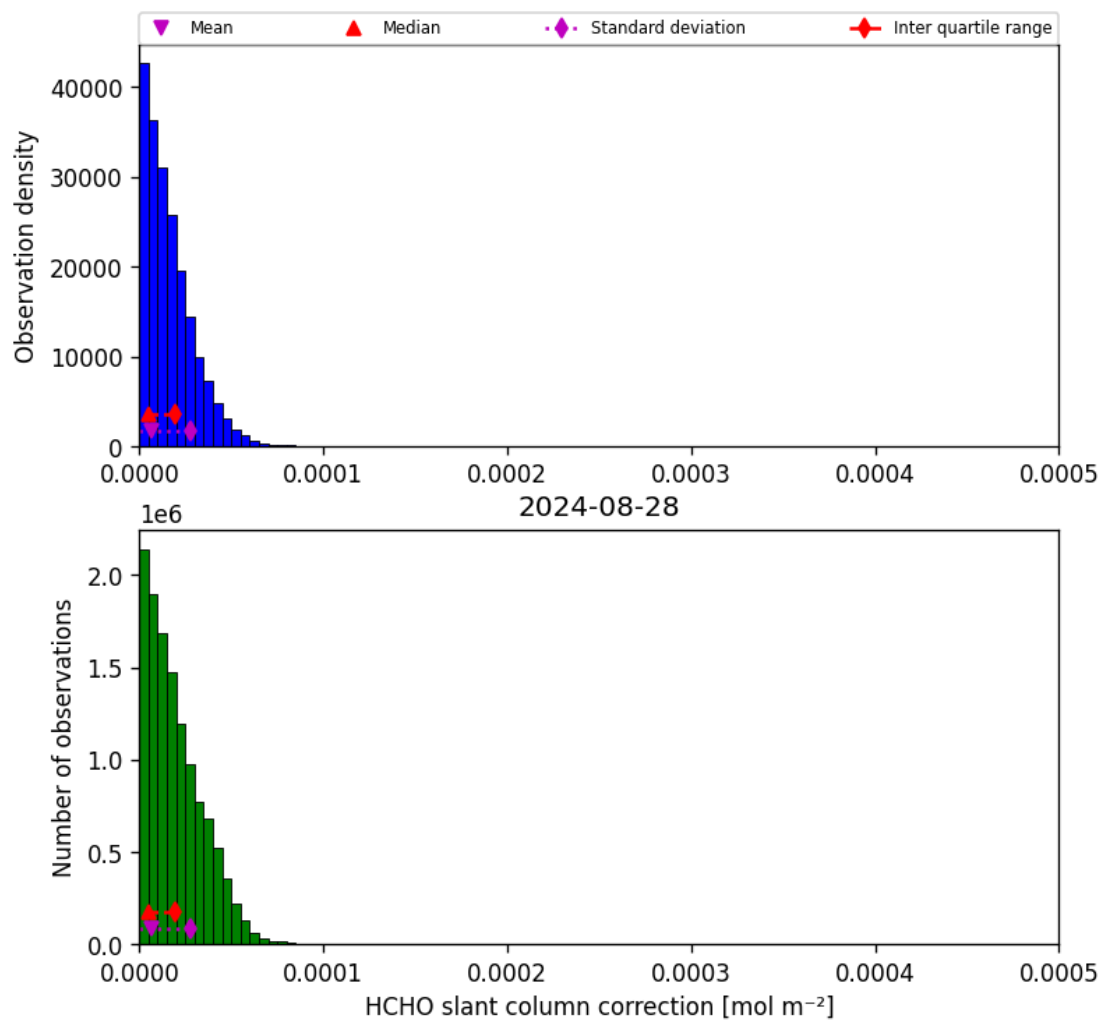
Figure 47: Histogram of “HCHO slant column correction” for 2024-08-27 to 2024-08-29
