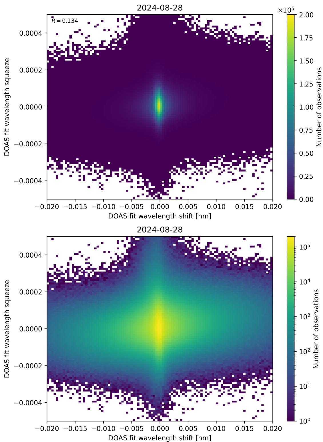
Figure 65: Scatter density plot of “DOAS fit wavelength shift” against “DOAS fit wavelength squeeze” for 2024-08-27 to 2024-08-29.
