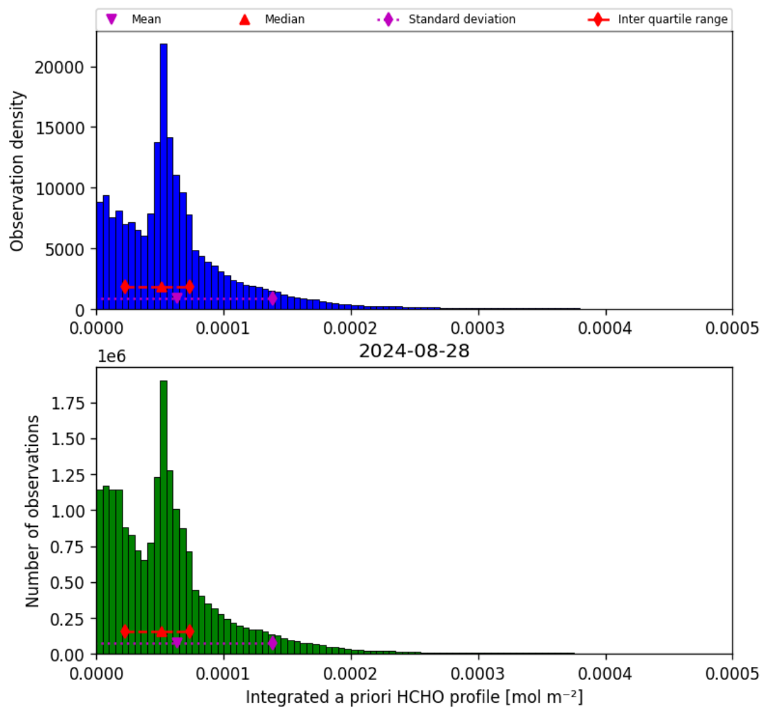
Figure 43: Histogram of “Integrated a priori HCHO profile” for 2024-08-27 to 2024-08-29
