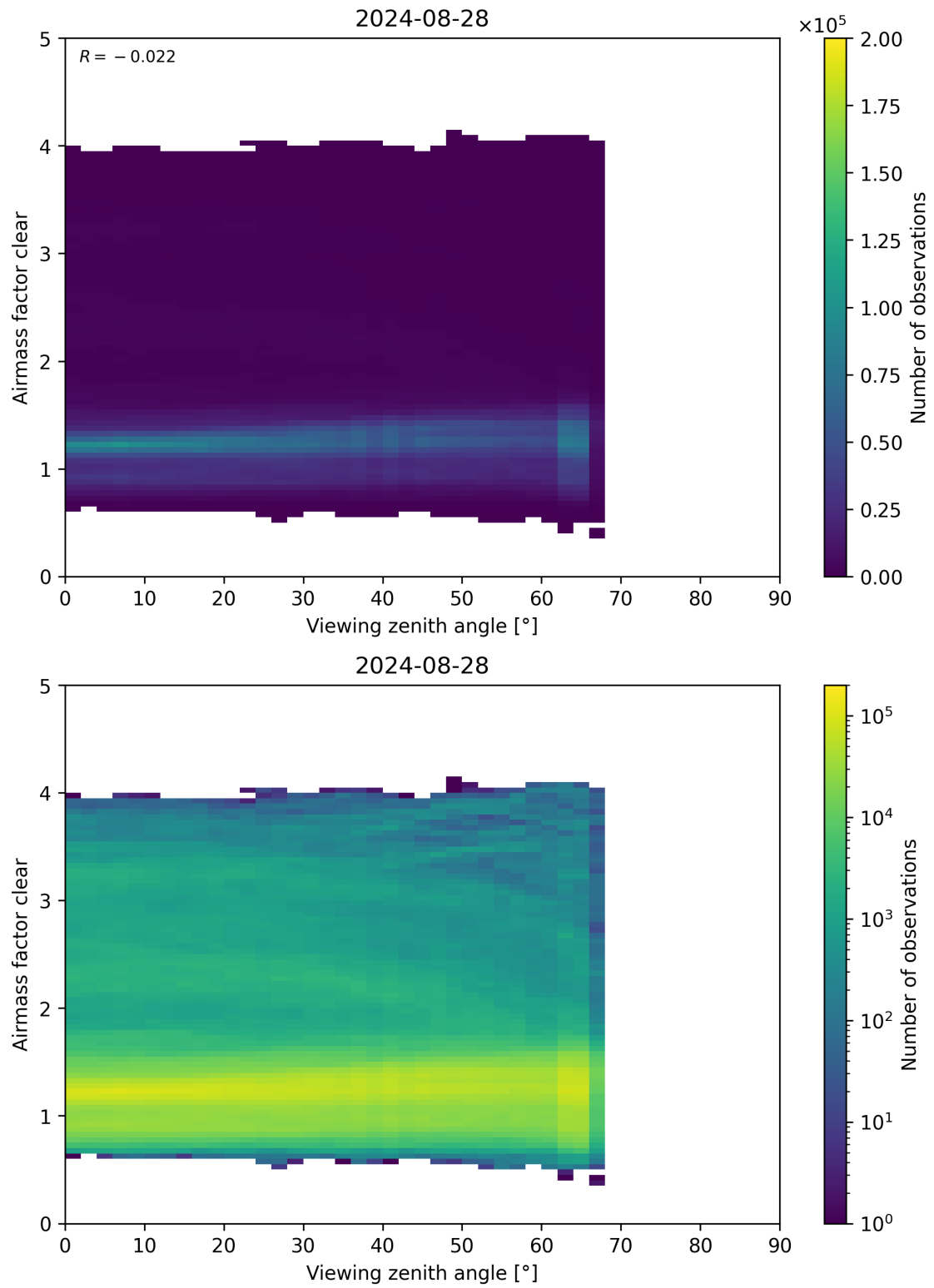
Figure 185: Scatter density plot of “Viewing zenith angle” against “Airmass factor clear” for 2024-08-27 to 2024-08-29.
