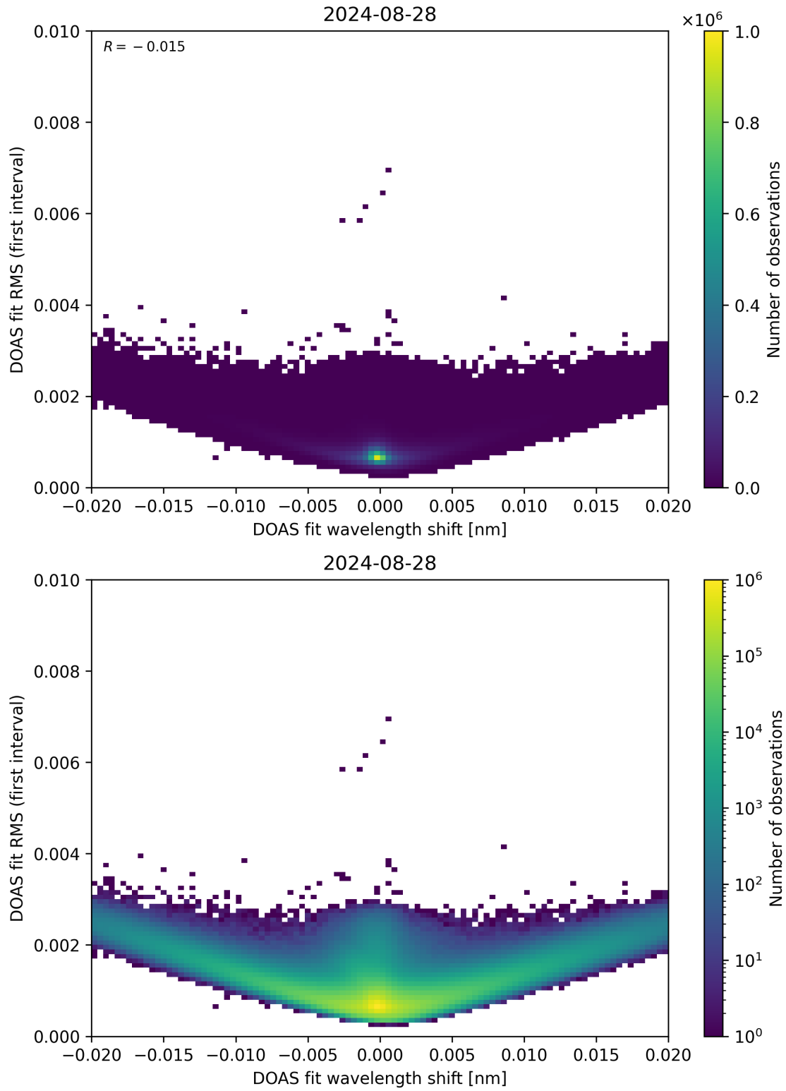
Figure 64: Scatter density plot of “DOAS fit wavelength shift” against “DOAS fit RMS (first interval)” for 2024-08-27 to 2024-08-29.
