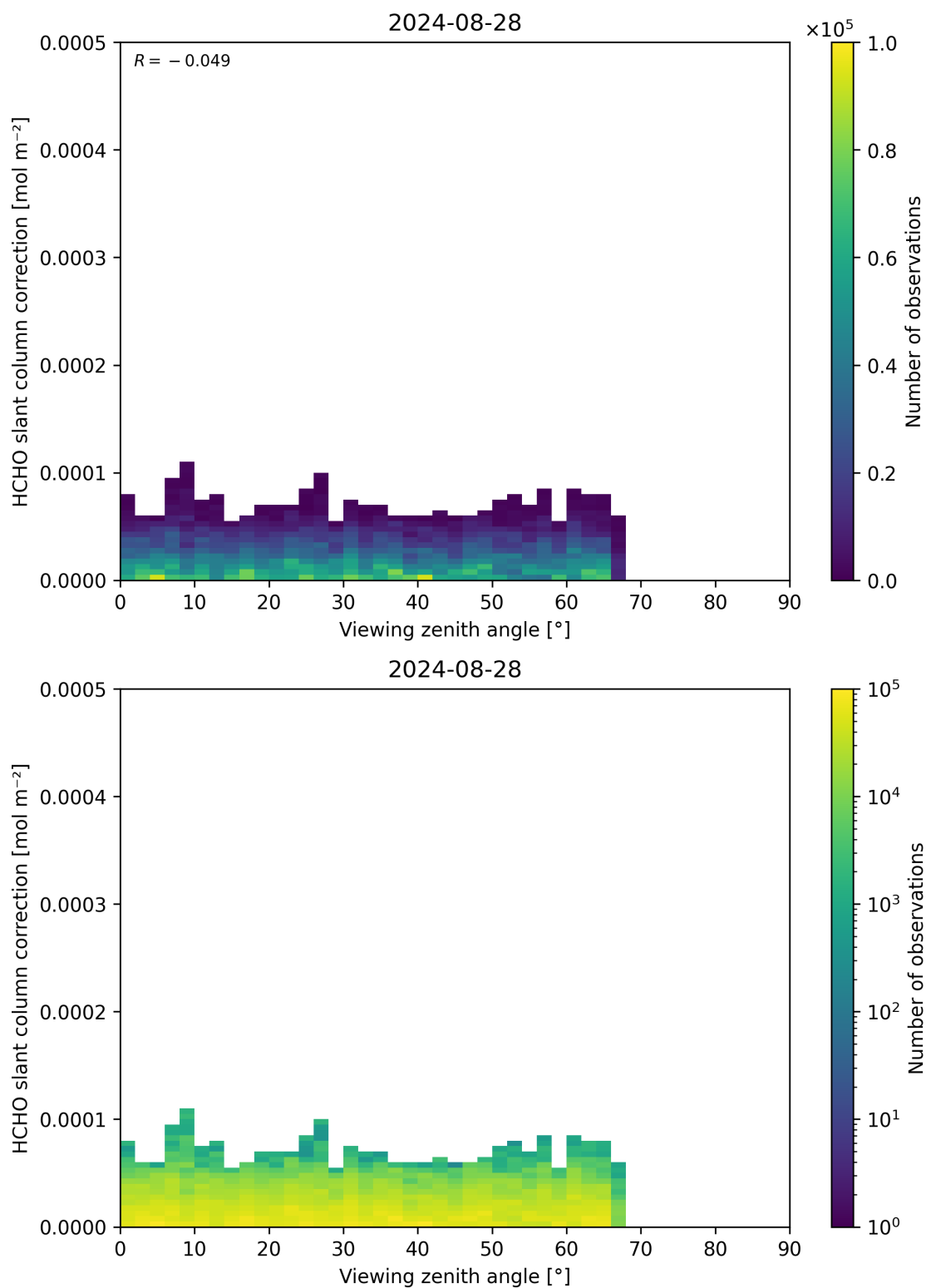
Figure 187: Scatter density plot of “Viewing zenith angle” against “HCHO slant column correction” for 2024-08-27 to 2024-08-29.
