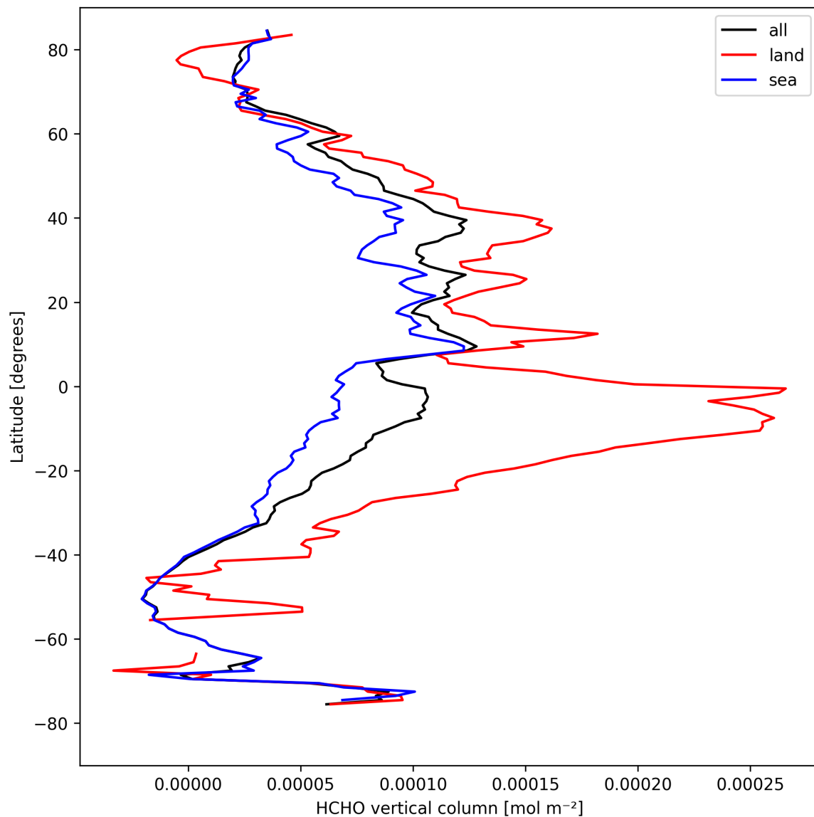
Figure 21: Zonal average of “HCHO vertical column” for 2024-08-27 to 2024-08-29.
