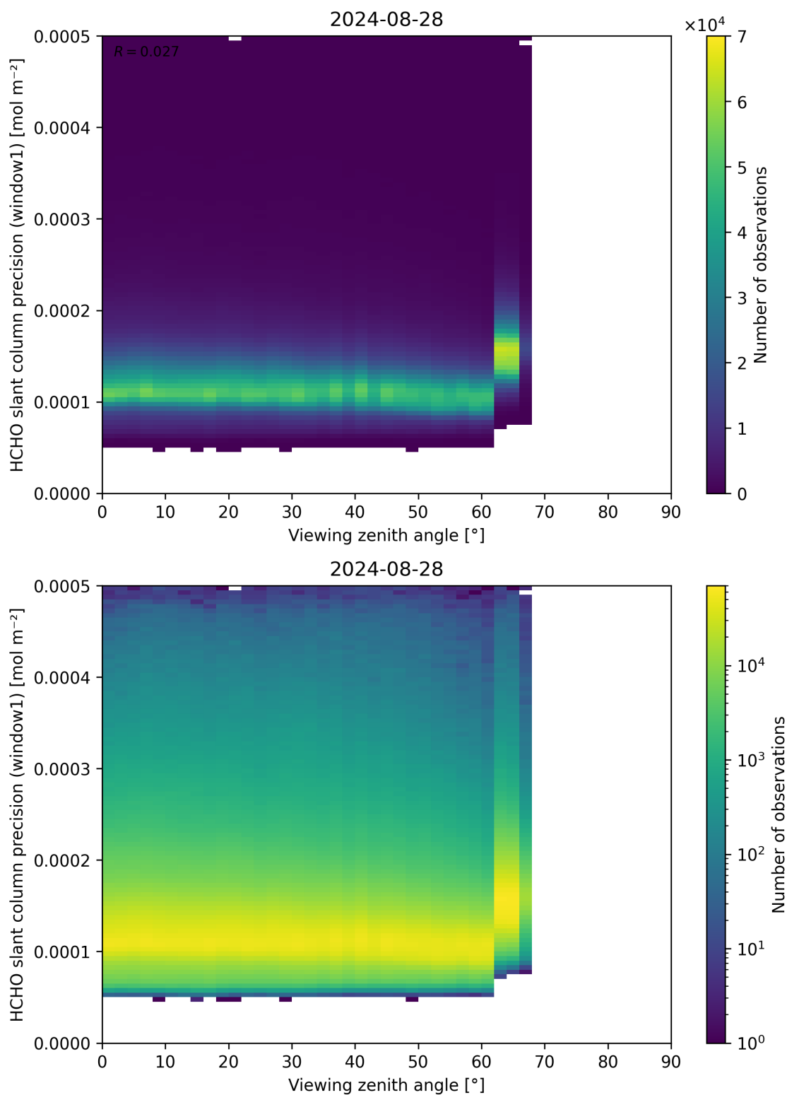
Figure 189: Scatter density plot of “Viewing zenith angle” against “HCHO slant column precision (window1)” for 2024-08-27 to 2024-08-29.
