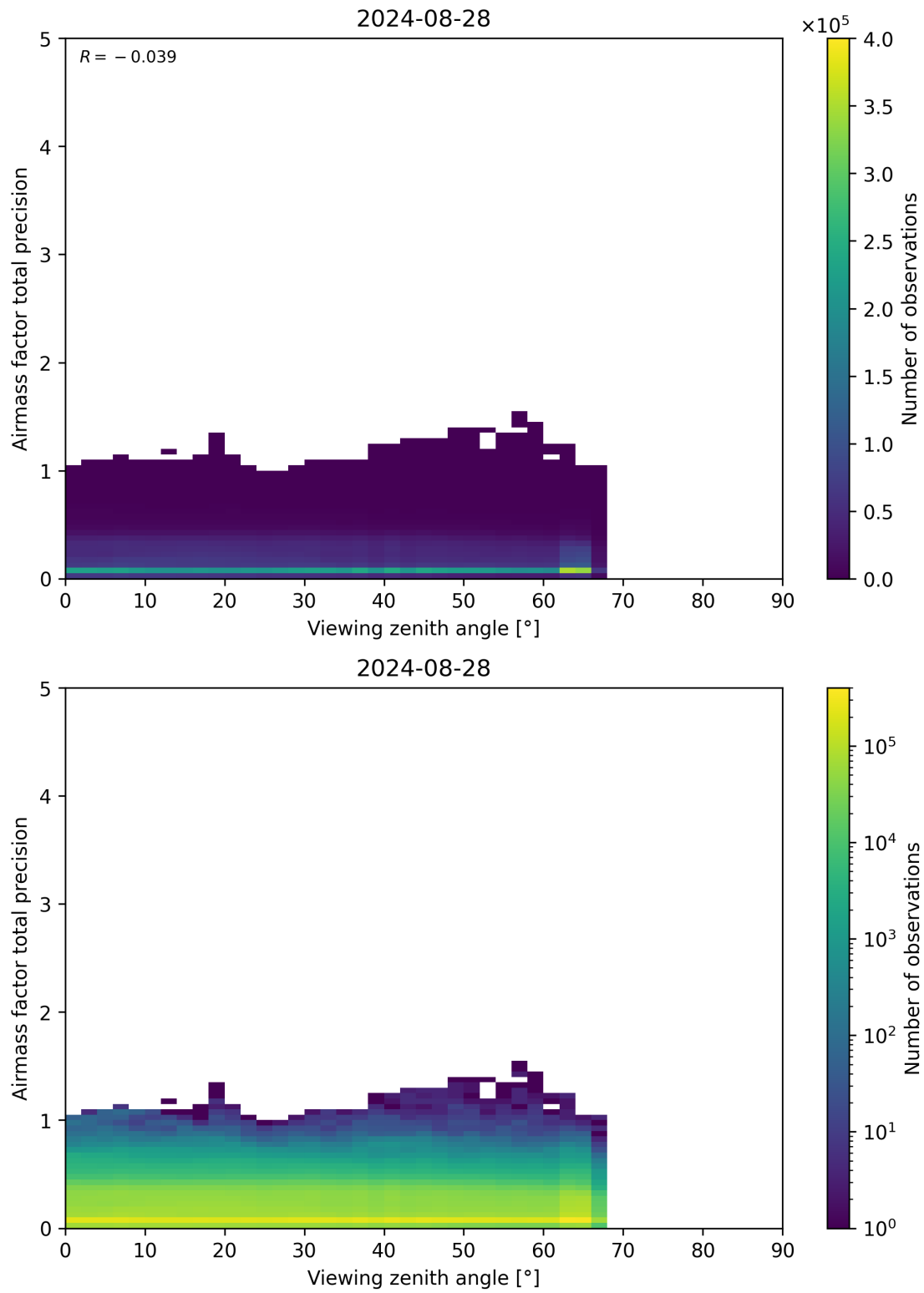
Figure 191: Scatter density plot of “Viewing zenith angle” against “Airmass factor total precision” for 2024-08-27 to 2024-08-29.
