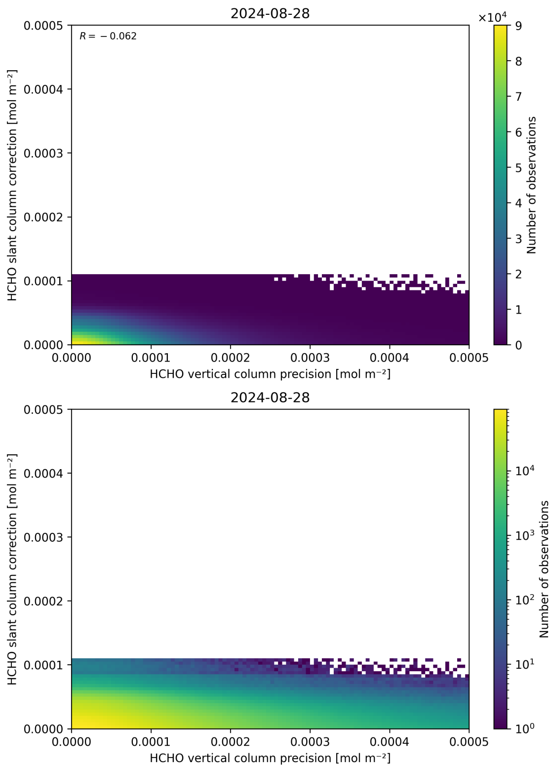
Figure 141: Scatter density plot of “HCHO vertical column precision” against “HCHO slant column correction” for 2024-08-27 to 2024-08-29.
