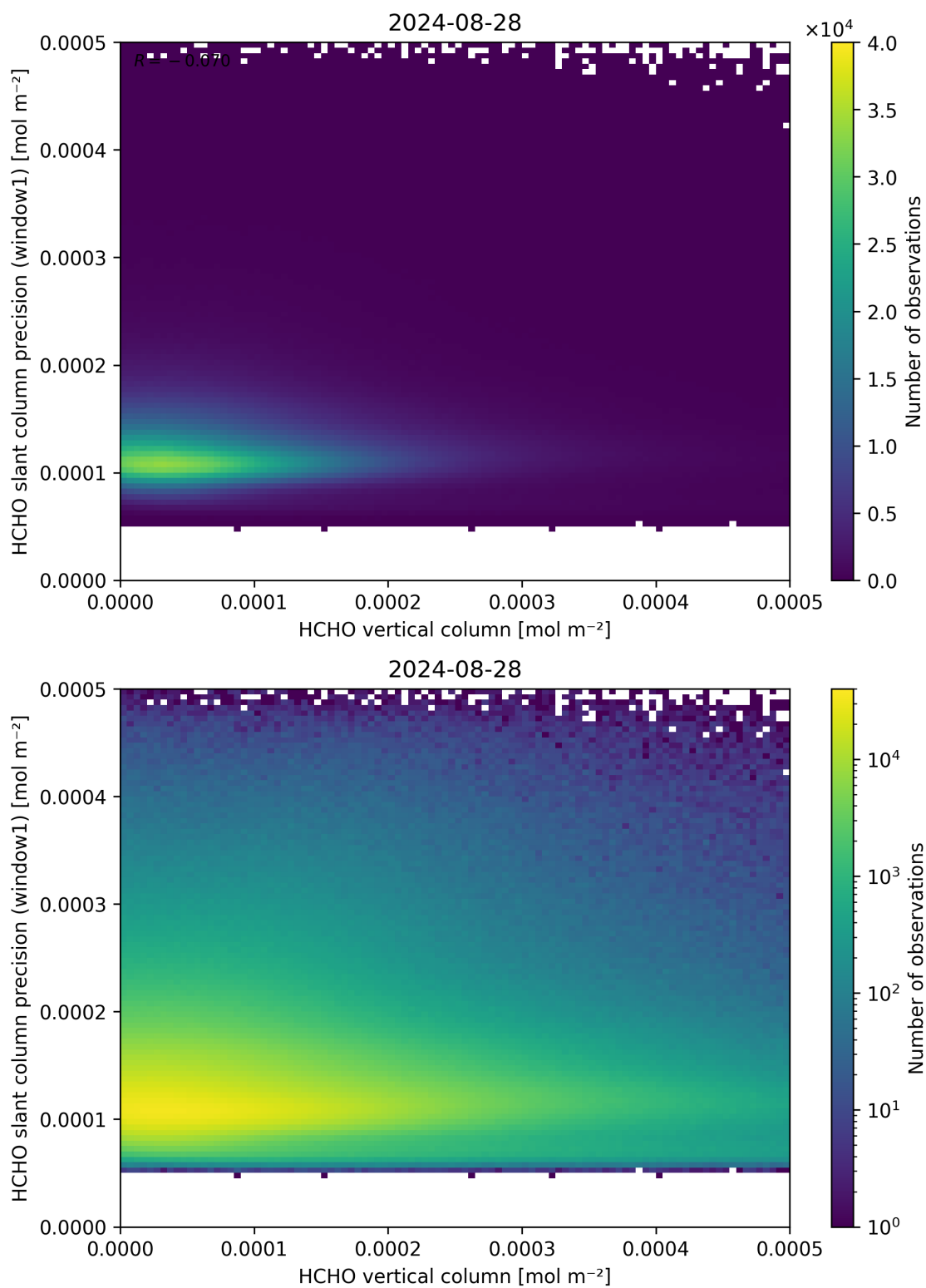
Figure 130: Scatter density plot of “HCHO vertical column” against “HCHO slant column precision (window1)” for 2024-08-27 to 2024-08-29.
