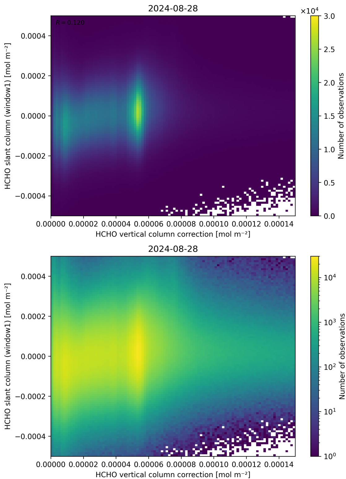
Figure 118: Scatter density plot of “HCHO vertical column correction” against “HCHO slant column (window1)” for 2024-08-27 to 2024-08-29.
