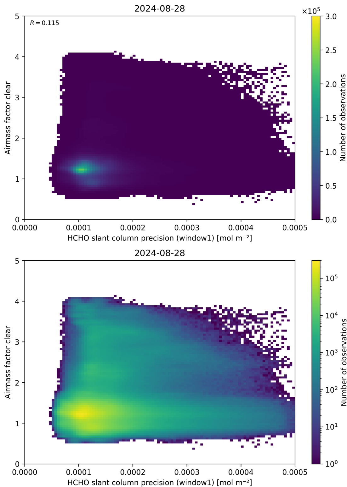
Figure 91: Scatter density plot of “HCHO slant column precision (window1)” against “Airmass factor clear” for 2024-08-27 to 2024-08-29.
