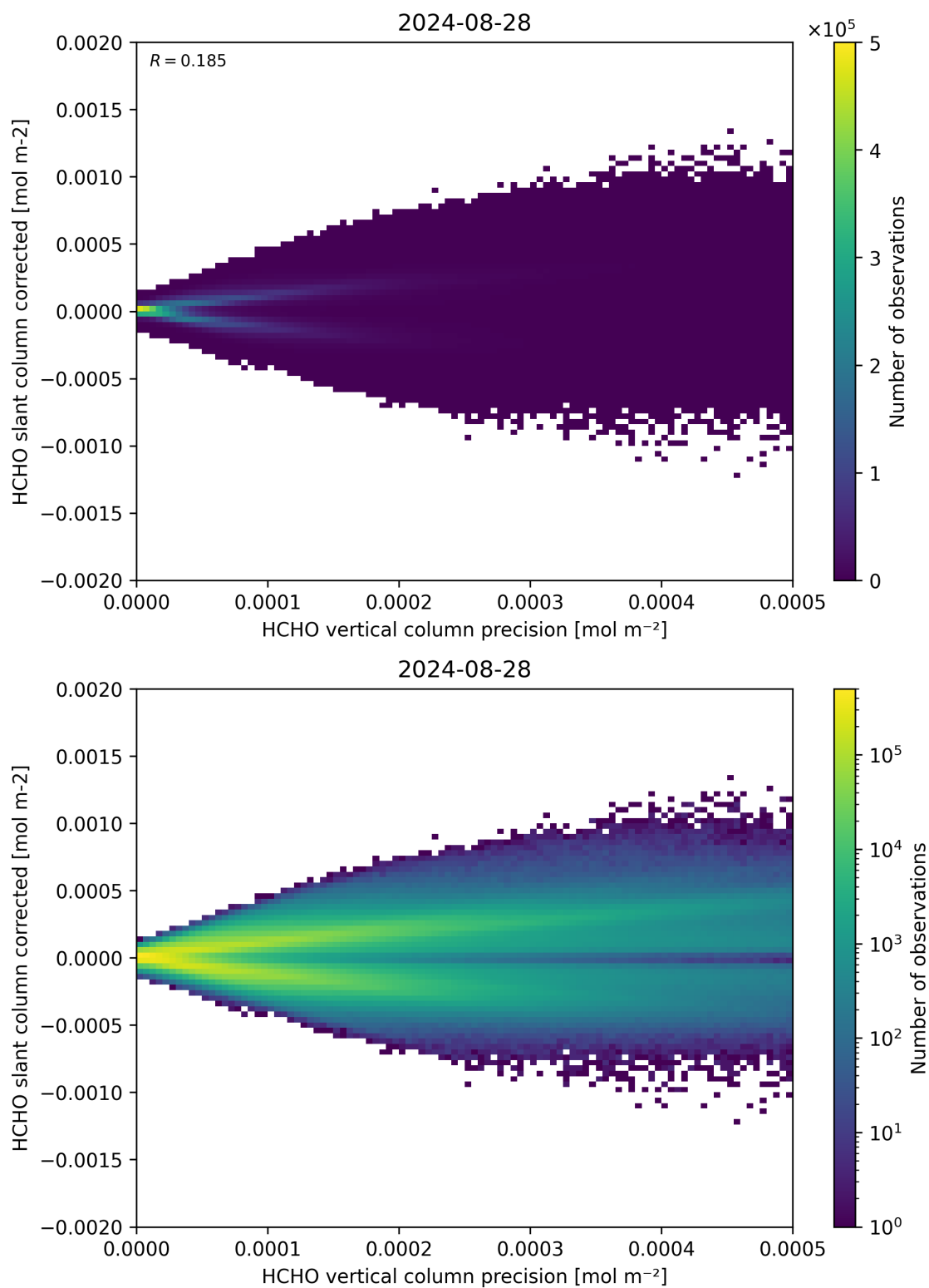
Figure 140: Scatter density plot of “HCHO vertical column precision” against “HCHO slant column corrected” for 2024-08-27 to 2024-08-29.
