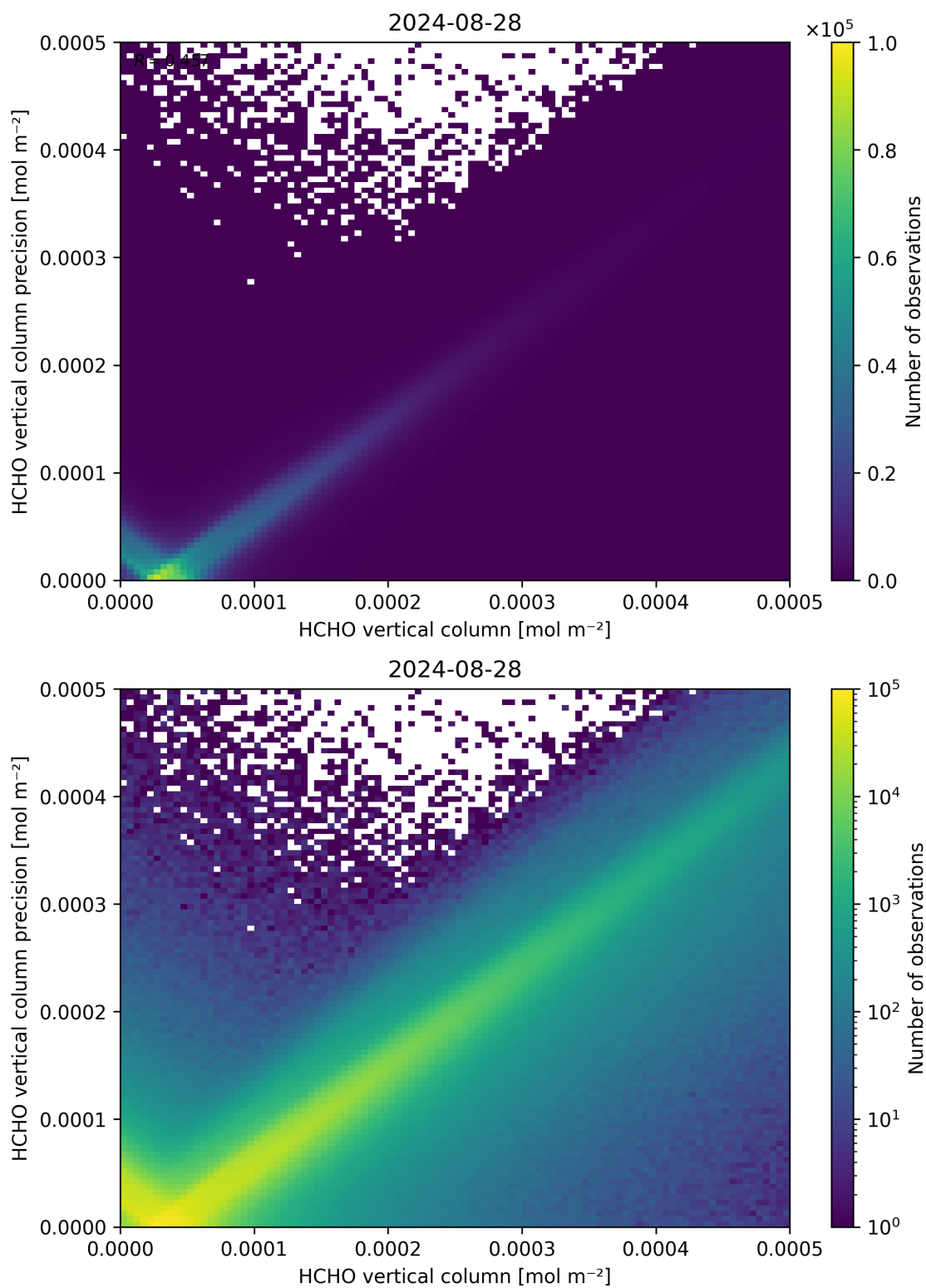
Figure 134: Scatter density plot of “HCHO vertical column” against “HCHO vertical column precision” for 2024-08-27 to 2024-08-29.
