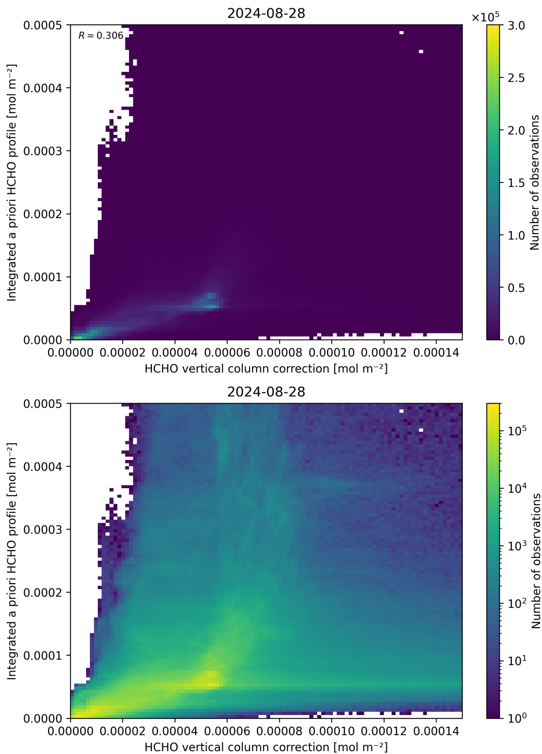
Figure 122: Scatter density plot of “HCHO vertical column correction” against “Integrated a priori HCHO profile” for 2024-08-27 to 2024-08-29.
