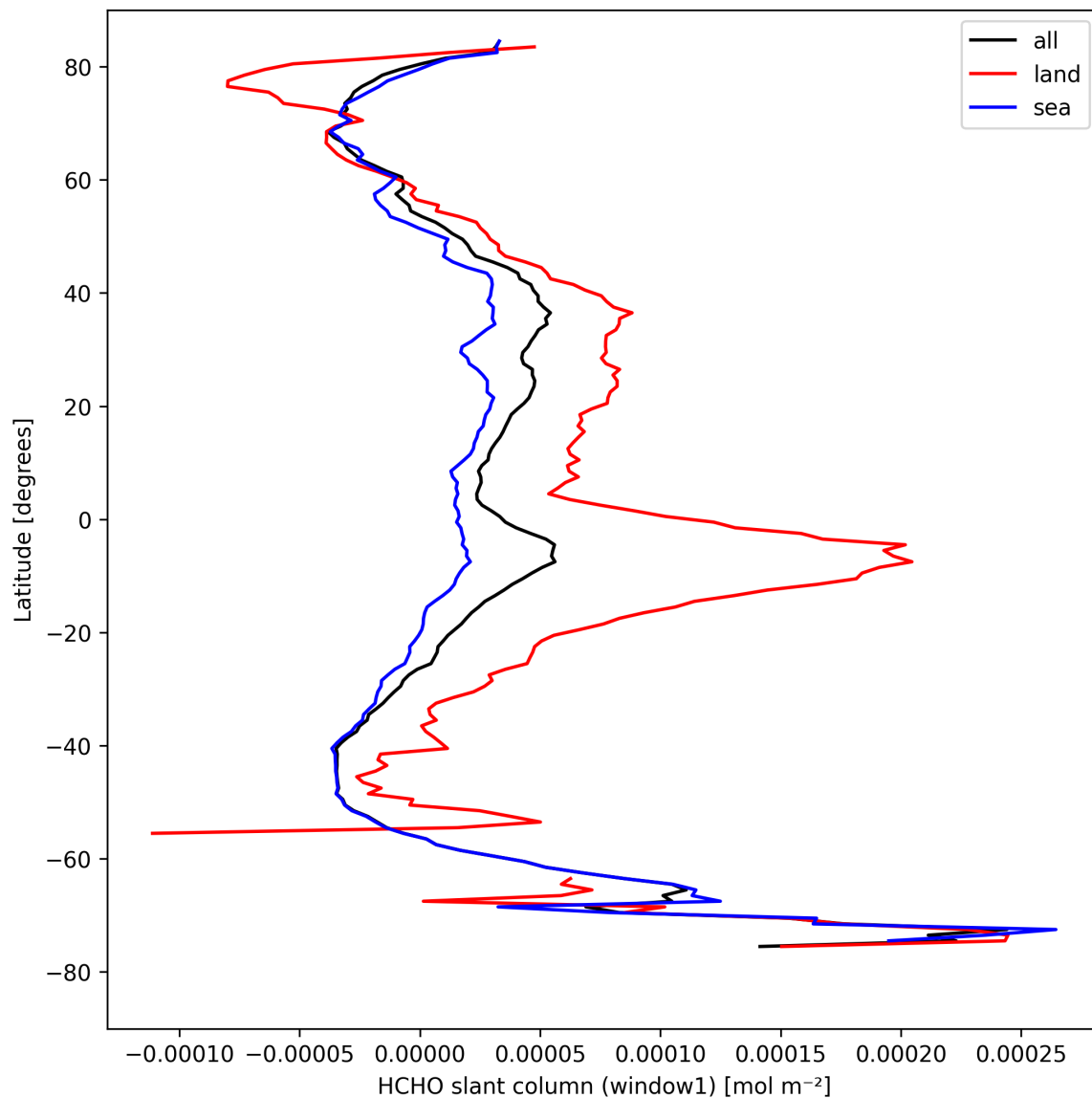
Figure 24: Zonal average of “HCHO slant column (window1)” for 2024-08-27 to 2024-08-29.
