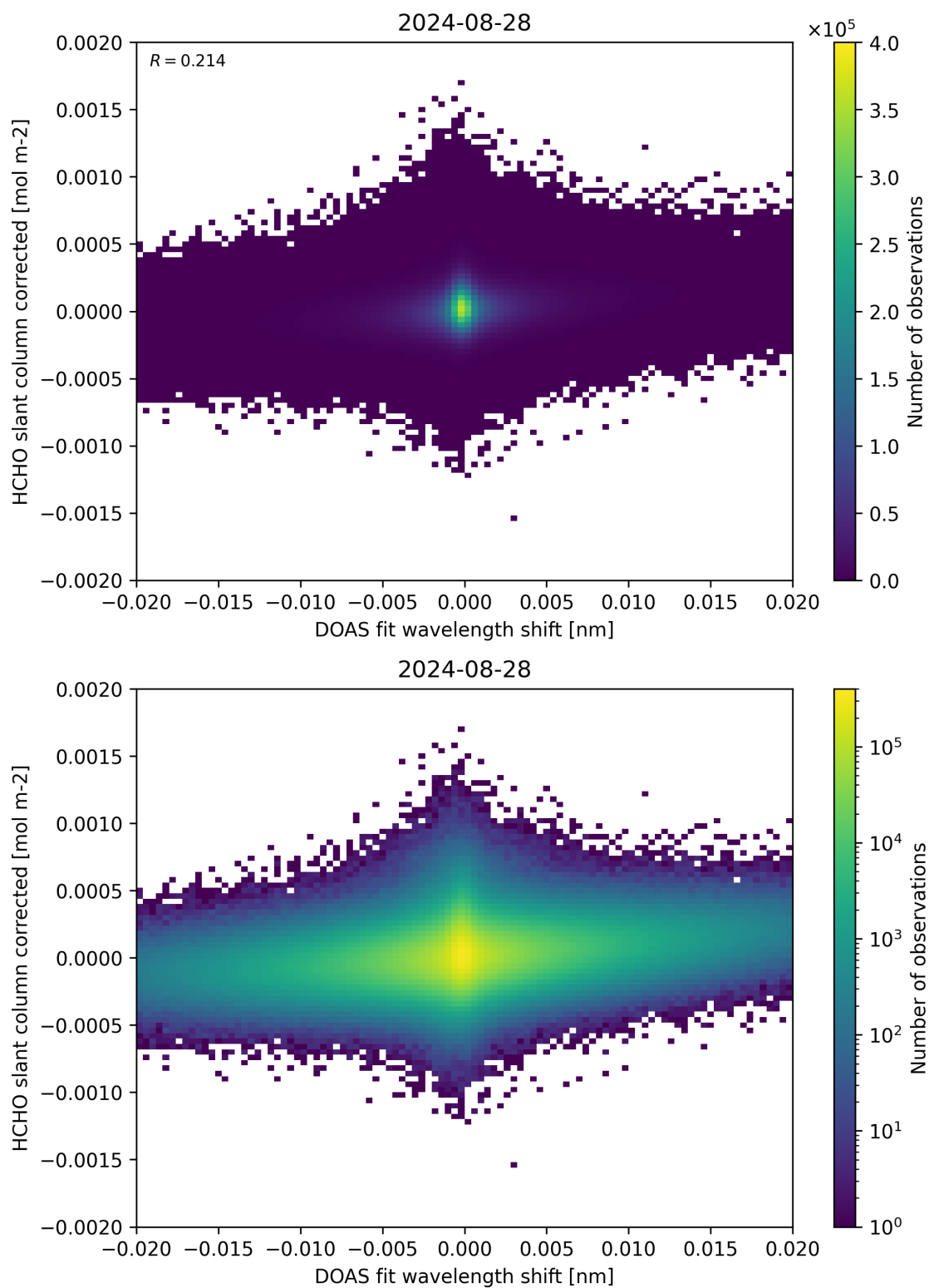
Figure 66: Scatter density plot of “DOAS fit wavelength shift” against “HCHO slant column corrected” for 2024-08-27 to 2024-08-29.
