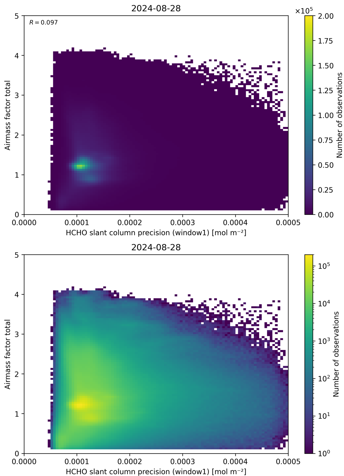
Figure 94: Scatter density plot of “HCHO slant column precision (window1)” against “Airmass factor total” for 2024-08-27 to 2024-08-29.
