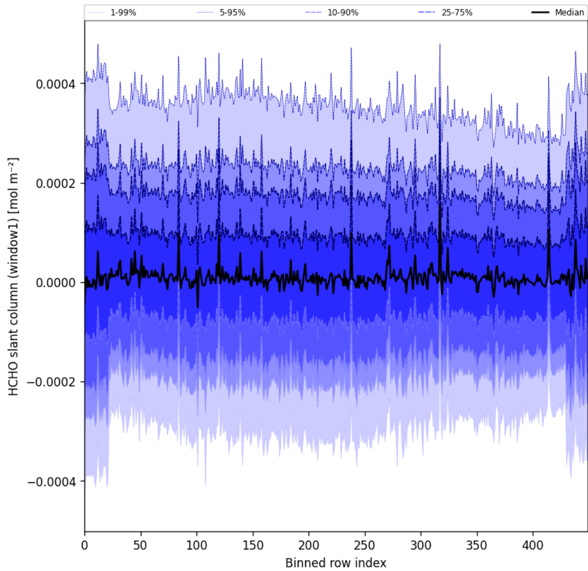
Figure 52: Along track statistics of “HCHO slant column (window1)” for 2024-08-27 to 2024-08-29
