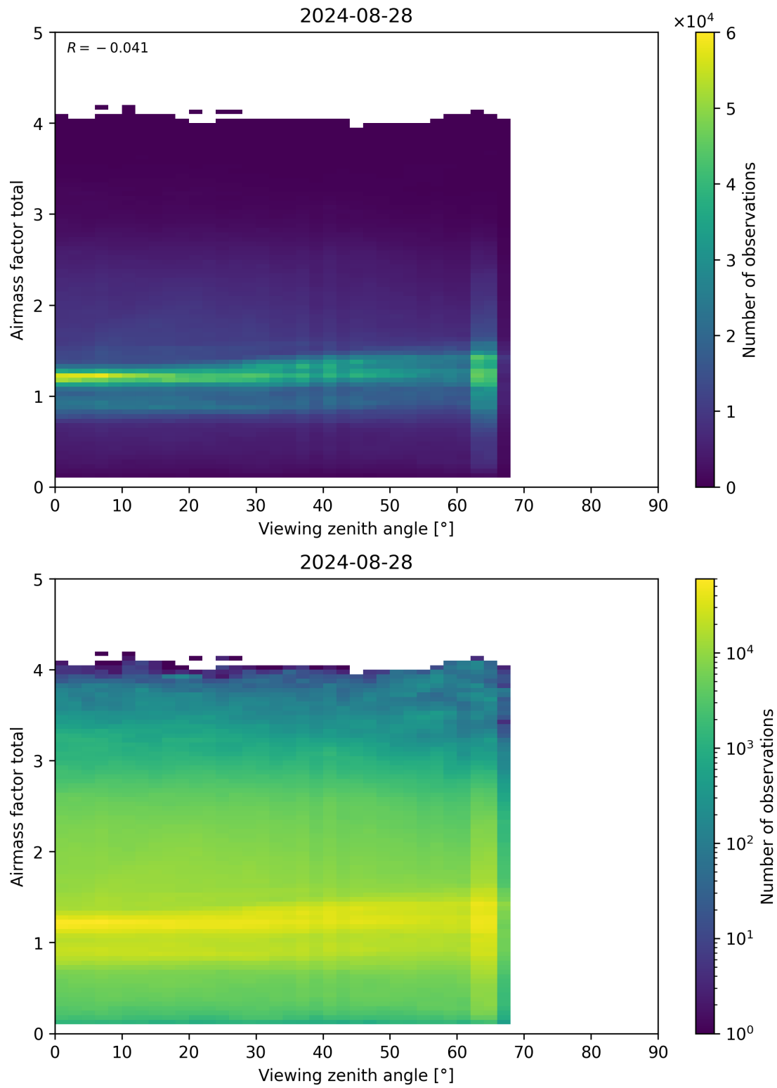
Figure 190: Scatter density plot of “Viewing zenith angle” against “Airmass factor total” for 2024-08-27 to 2024-08-29.
