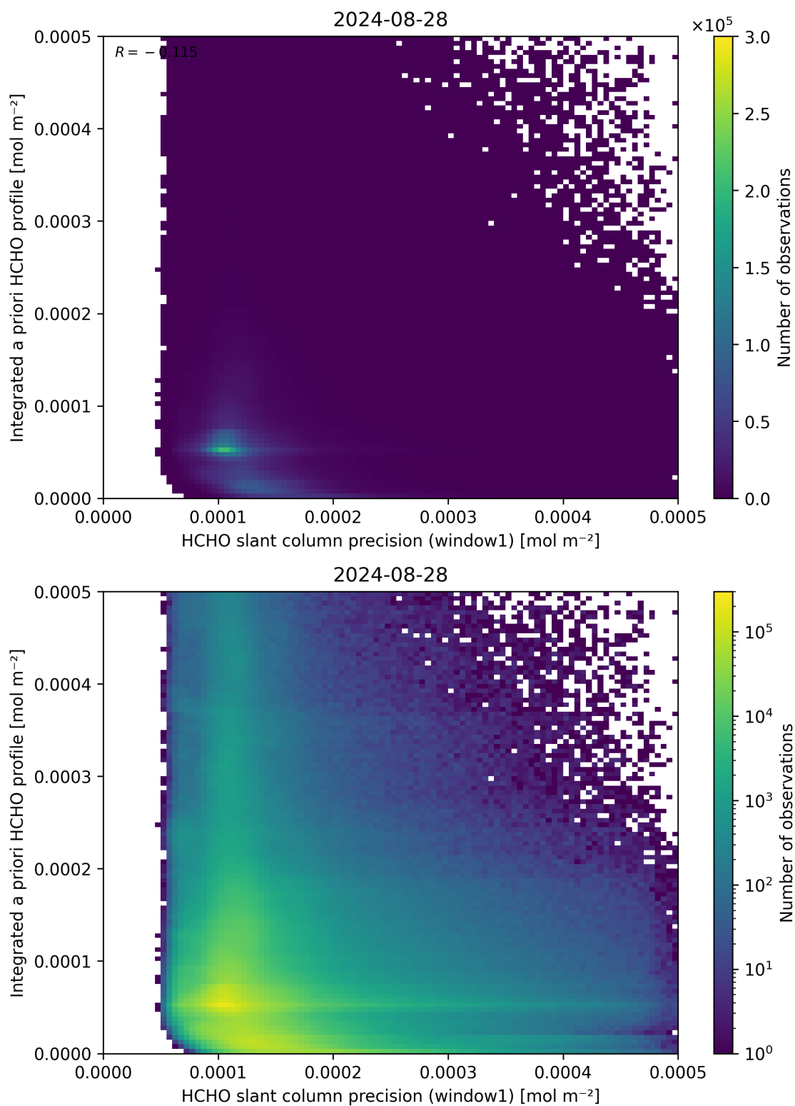
Figure 96: Scatter density plot of “HCHO slant column precision (window1)” against “Integrated a priori HCHO profile” for 2024-08-27 to 2024-08-29.
