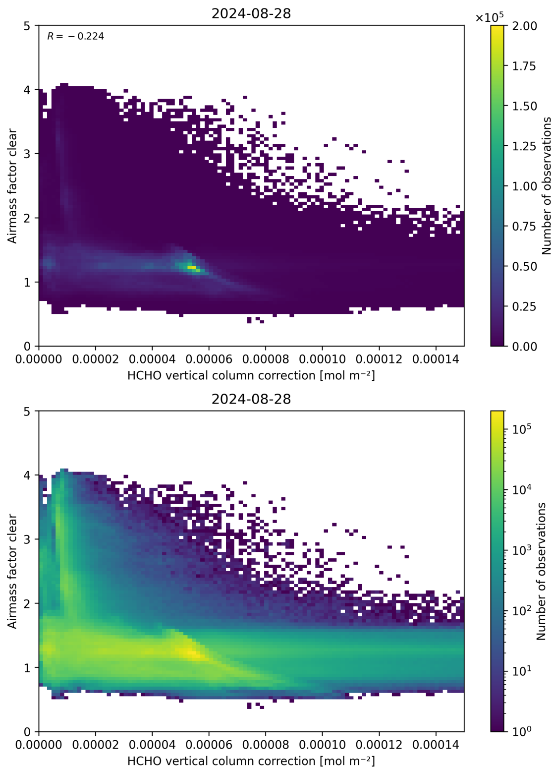
Figure 115: Scatter density plot of “HCHO vertical column correction” against “Airmass factor clear” for 2024-08-27 to 2024-08-29.
