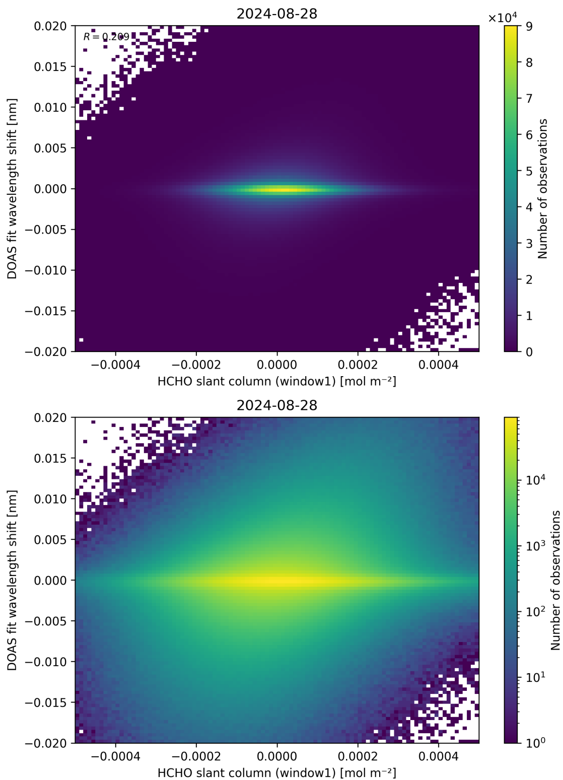
Figure 79: Scatter density plot of “HCHO slant column (window1)” against “DOAS fit wavelength shift” for 2024-08-27 to 2024-08-29.
