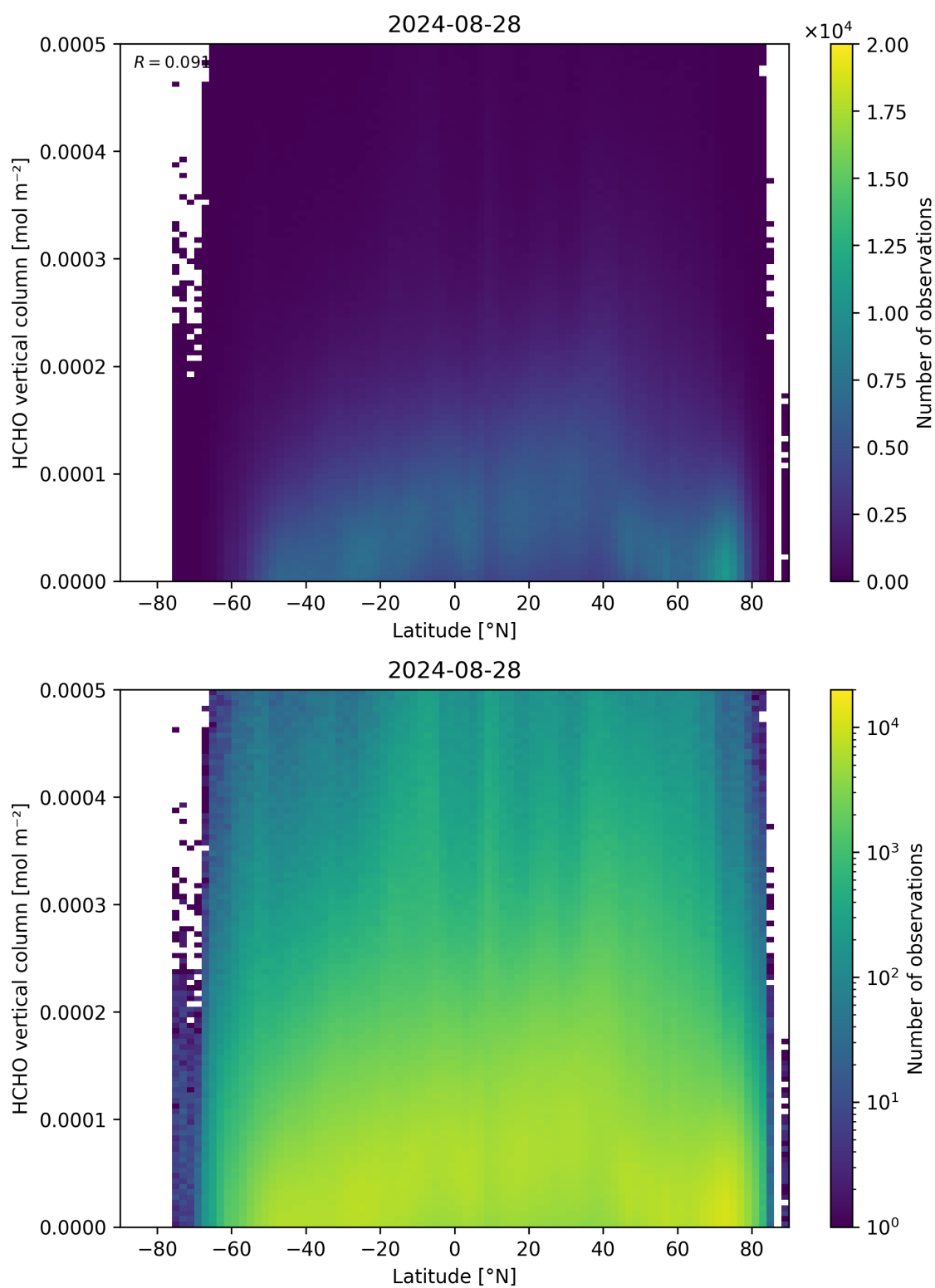
Figure 163: Scatter density plot of “Latitude” against “HCHO vertical column” for 2024-08-27 to 2024-08-29.
