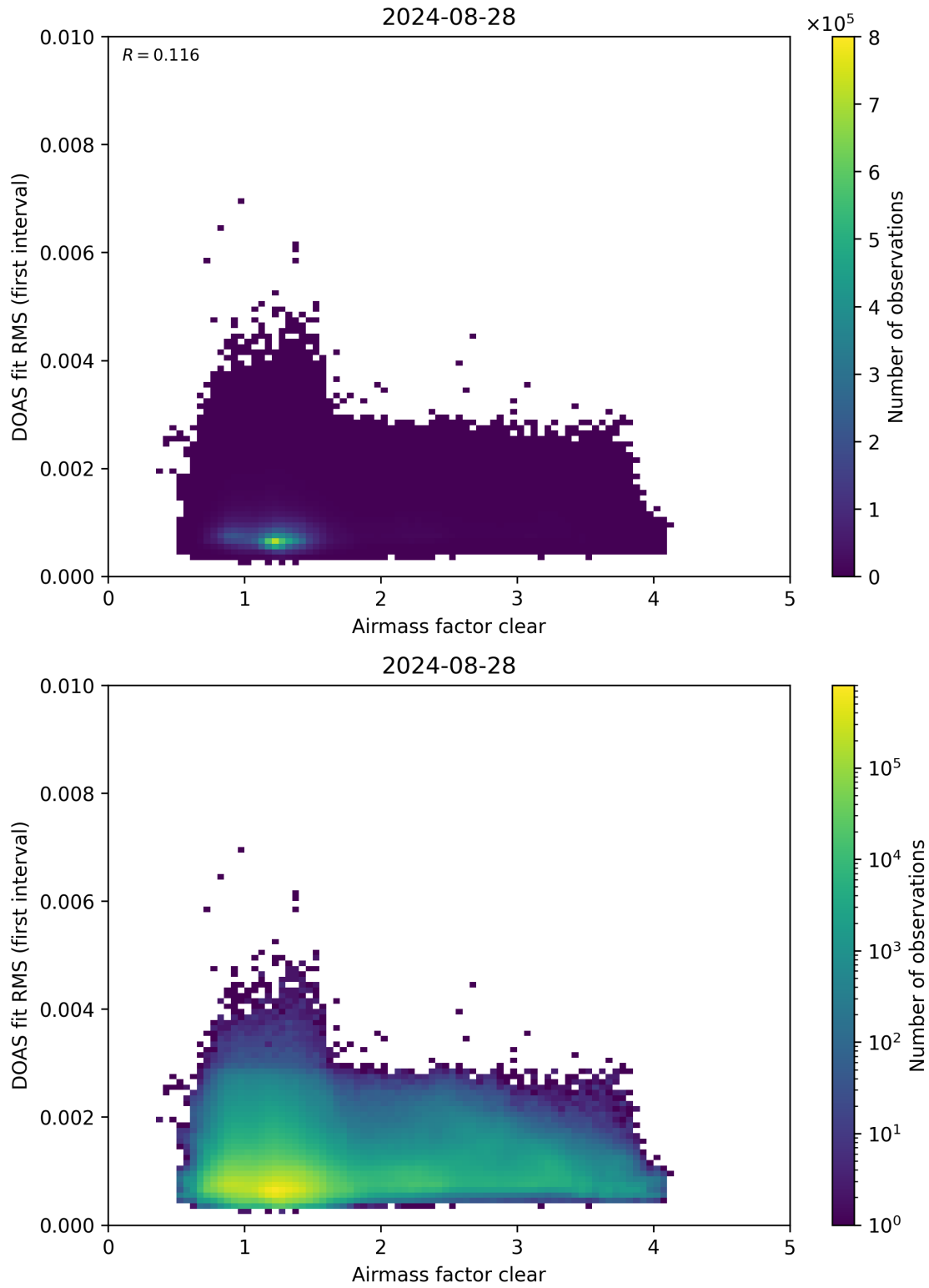
Figure 71: Scatter density plot of “Airmass factor clear” against “DOAS fit RMS (first interval)” for 2024-08-27 to 2024-08-29.
