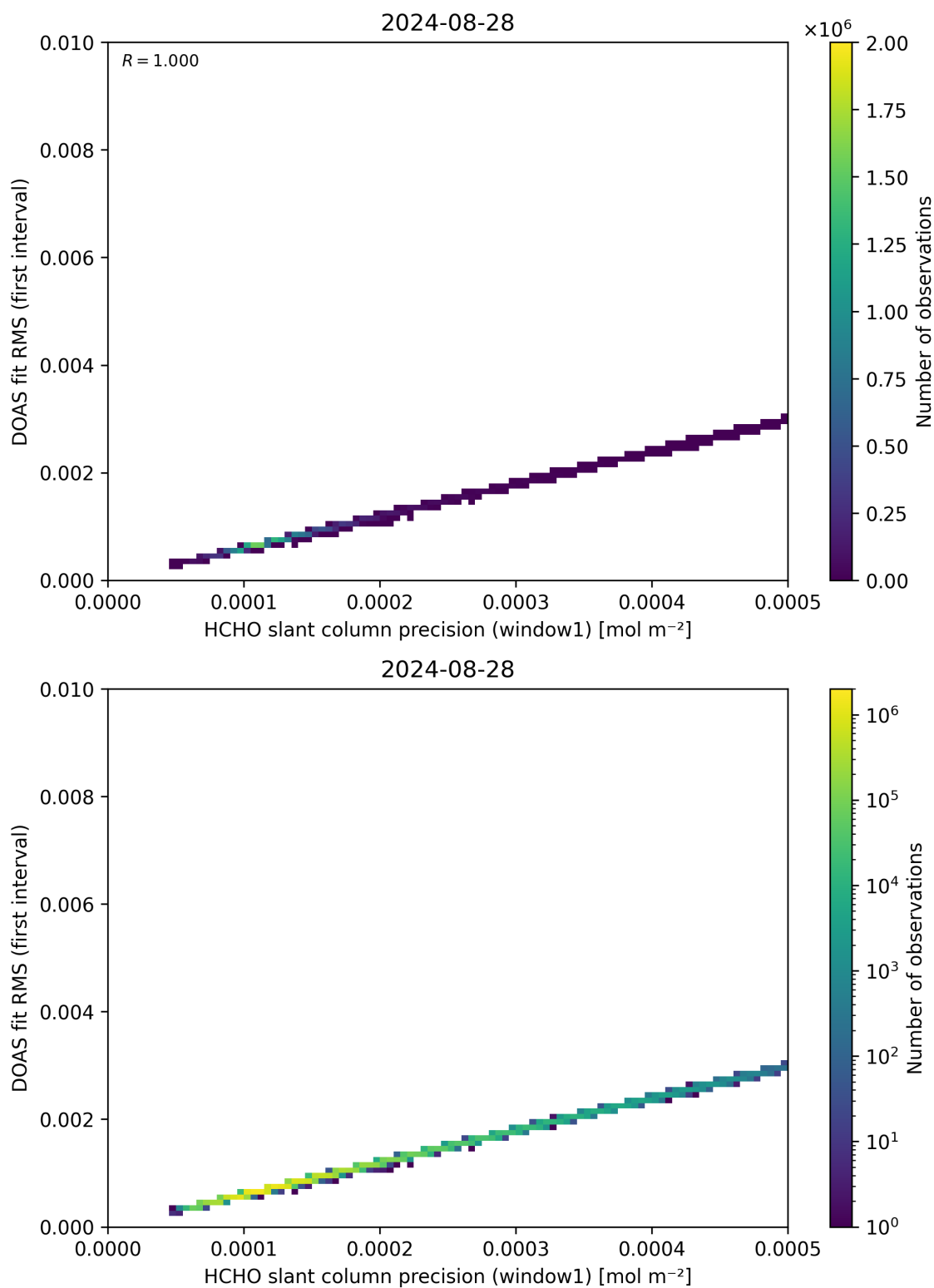
Figure 88: Scatter density plot of “HCHO slant column precision (window1)” against “DOAS fit RMS (first interval)” for 2024-08-27 to 2024-08-29.
