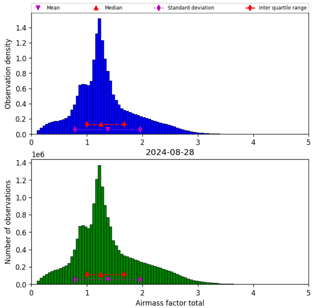
Figure 40: Histogram of “Airmass factor total” for 2024-08-27 to 2024-08-29
