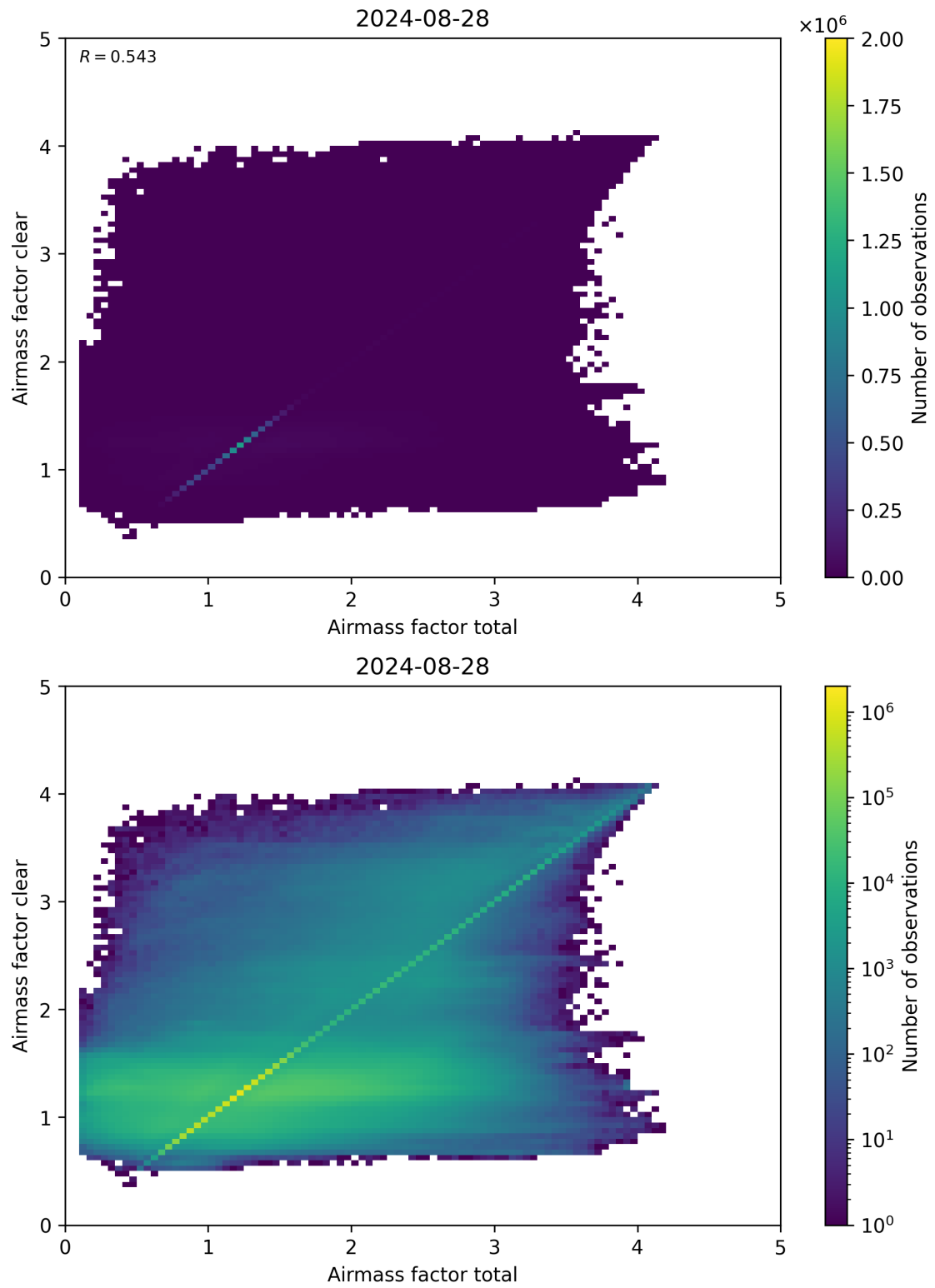
Figure 100: Scatter density plot of “Airmass factor total” against “Airmass factor clear” for 2024-08-27 to 2024-08-29.
