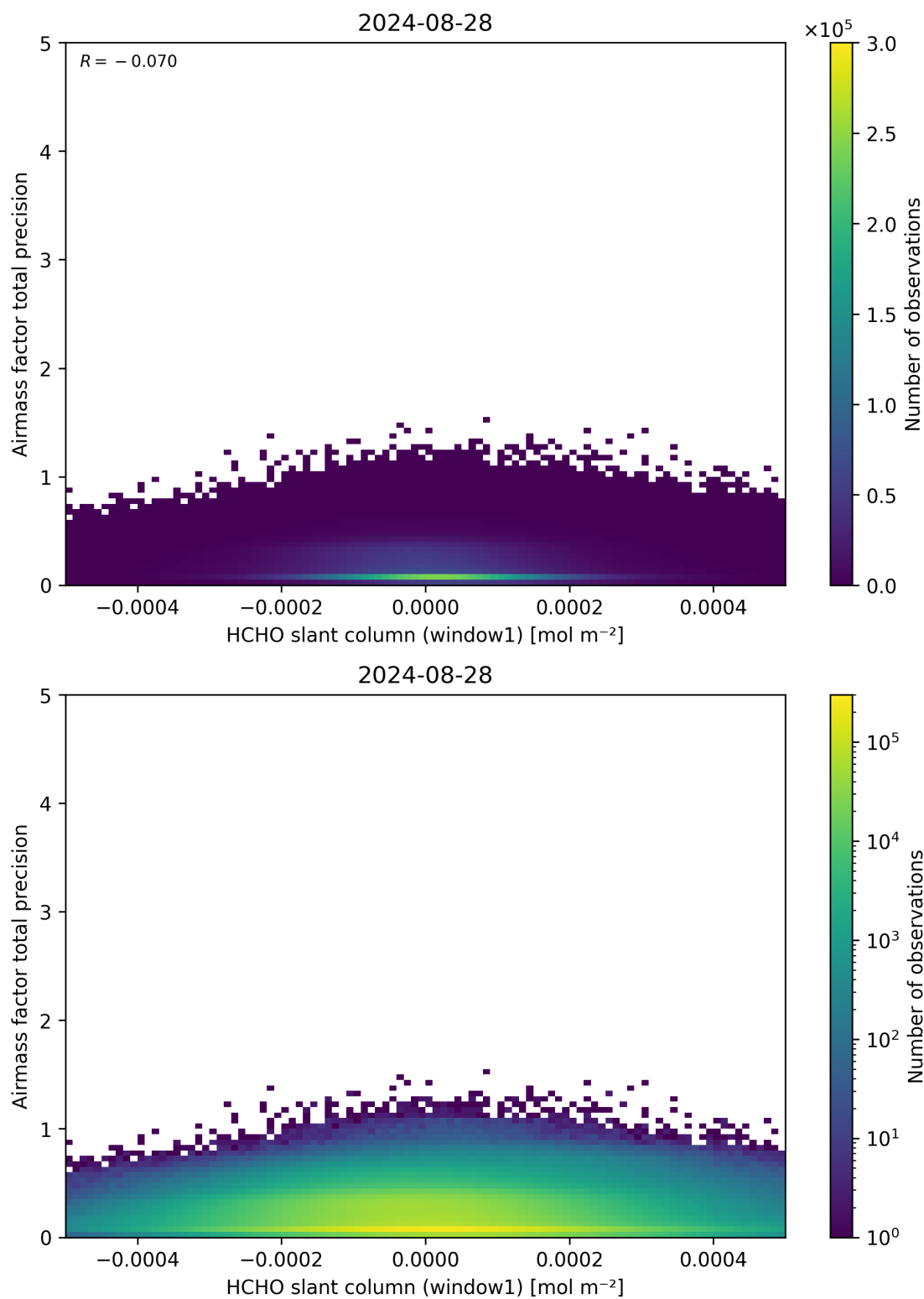
Figure 86: Scatter density plot of “HCHO slant column (window1)” against “Airmass factor total precision” for 2024-08-27 to 2024-08-29.
