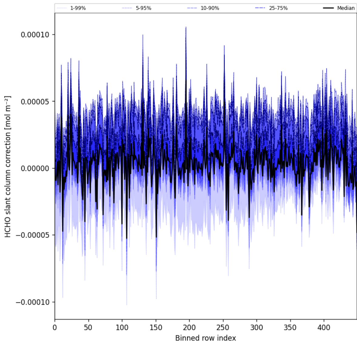
Figure 61: Along track statistics of “HCHO slant column correction” for 2024-08-27 to 2024-08-29
