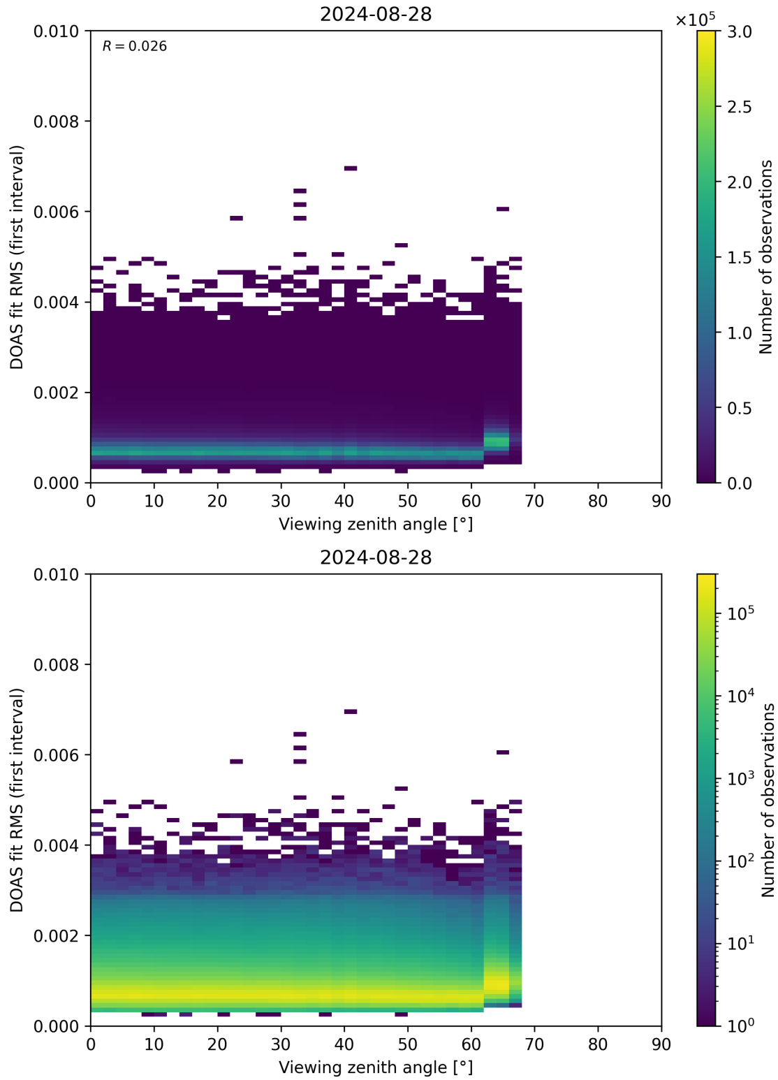
Figure 182: Scatter density plot of “Viewing zenith angle” against “DOAS fit RMS (first interval)” for 2024-08-27 to 2024-08-29.
