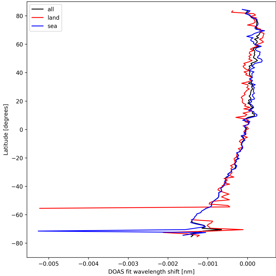
Figure 30: Zonal average of “DOAS fit wavelength shift” for 2024-08-27 to 2024-08-29.
