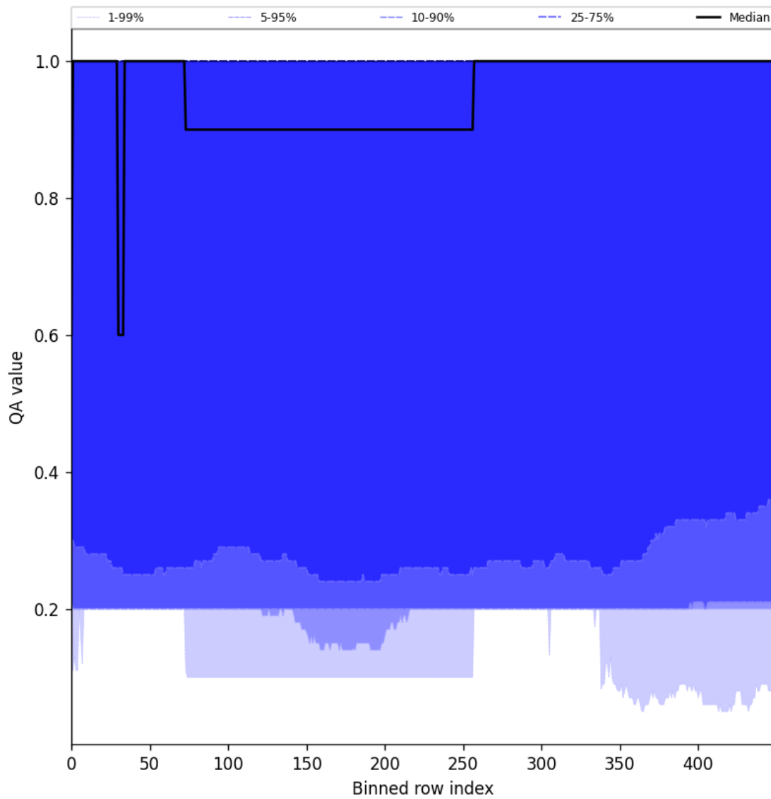
Figure 48: Along track statistics of “QA value” for 2024-08-27 to 2024-08-29
