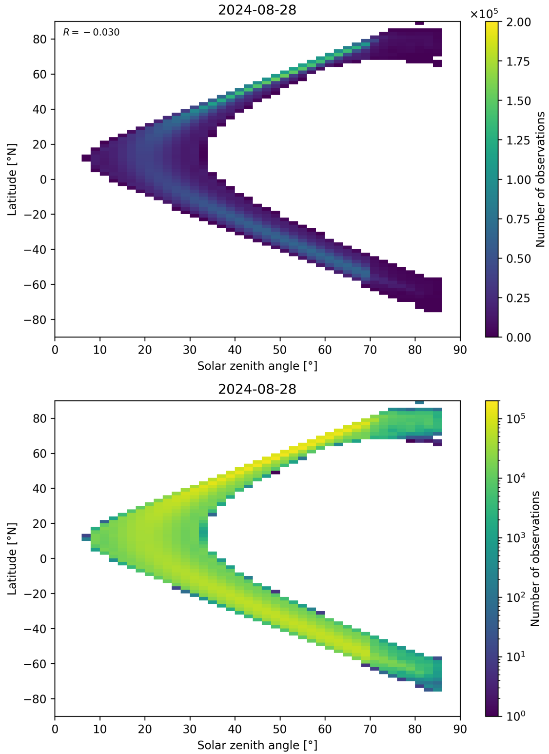
Figure 181: Scatter density plot of “Solar zenith angle” against “Latitude” for 2024-08-27 to 2024-08-29.
