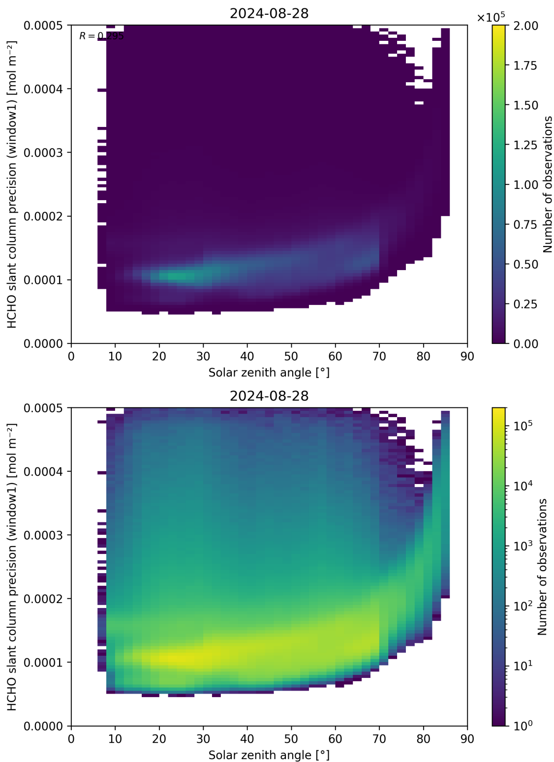
Figure 174: Scatter density plot of “Solar zenith angle” against “HCHO slant column precision (window1)” for 2024-08-27 to 2024-08-29.
