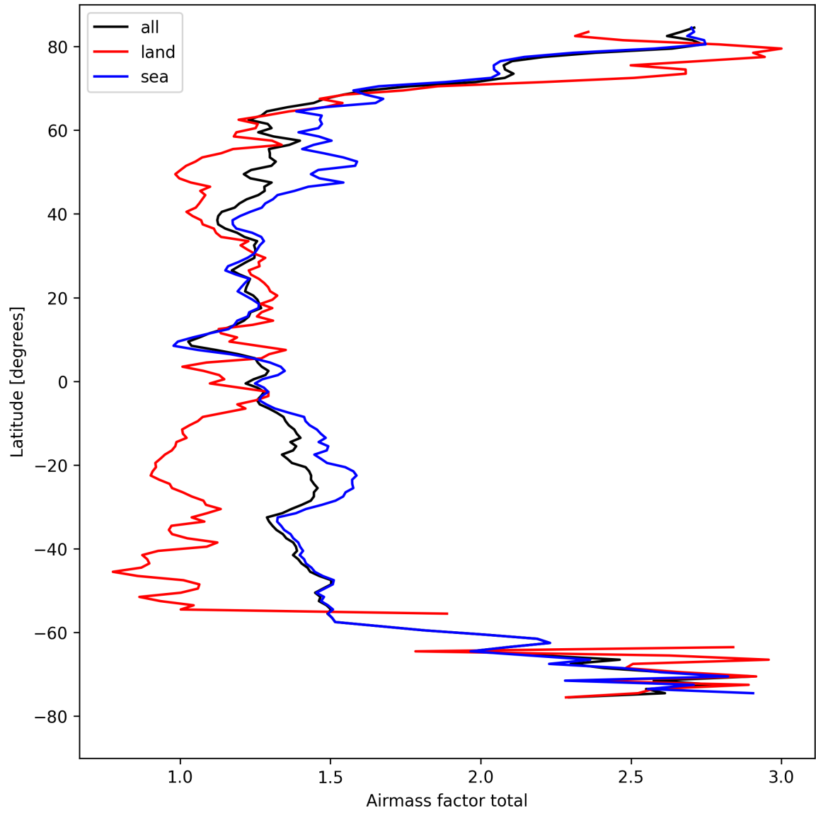
Figure 26: Zonal average of “Airmass factor total” for 2024-08-27 to 2024-08-29.
