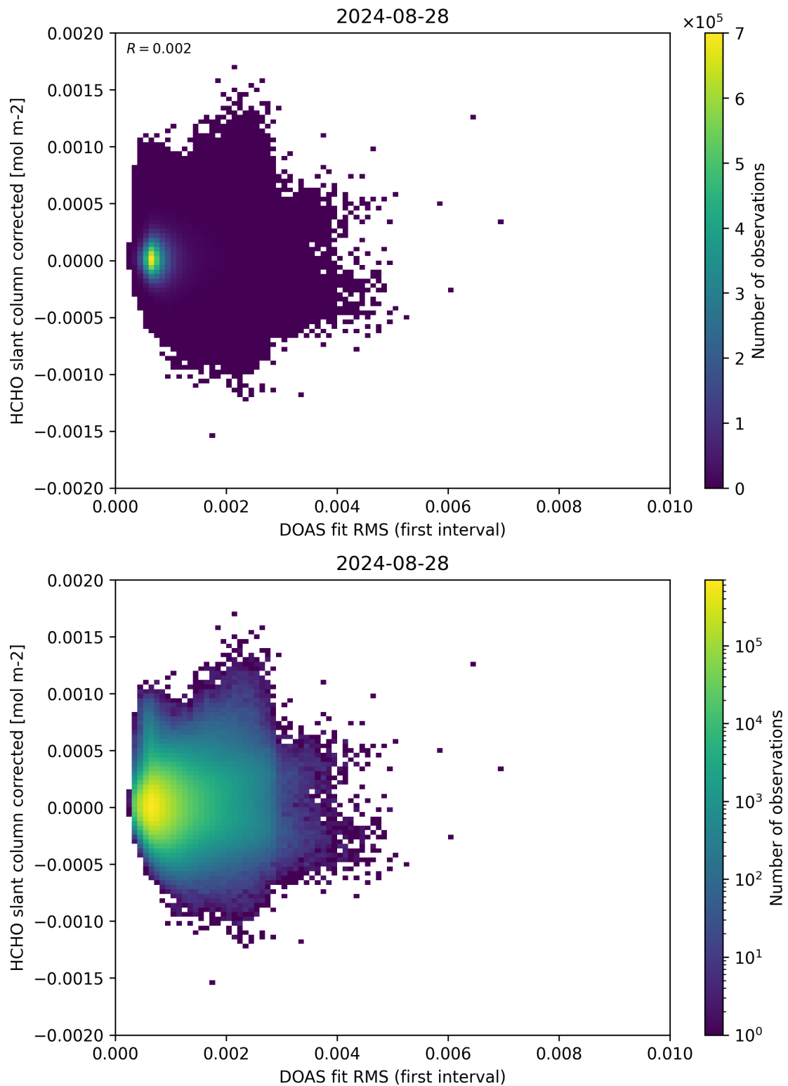
Figure 62: Scatter density plot of “DOAS fit RMS (first interval)” against “HCHO slant column corrected” for 2024-08-27 to 2024-08-29.
