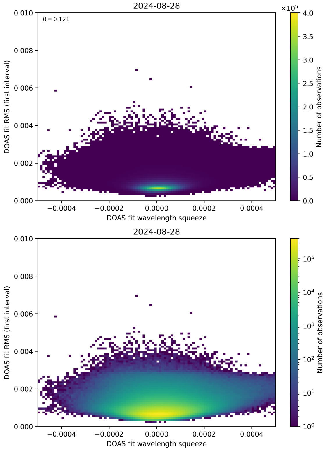
Figure 68: Scatter density plot of “DOAS fit wavelength squeeze” against “DOAS fit RMS (first interval)” for 2024-08-27 to 2024-08-29.
