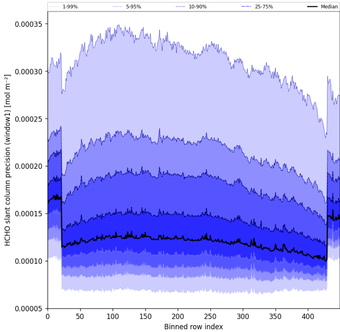
Figure 53: Along track statistics of “HCHO slant column precision (window1)” for 2024-08-27 to 2024-08-29
