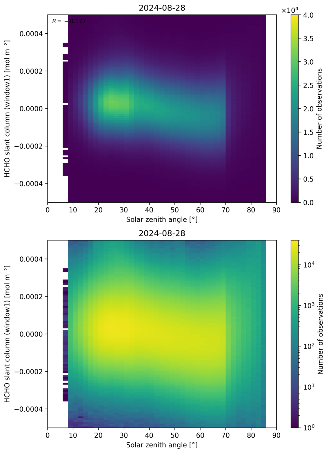
Figure 173: Scatter density plot of “Solar zenith angle” against “HCHO slant column (window1)” for 2024-08-27 to 2024-08-29.
