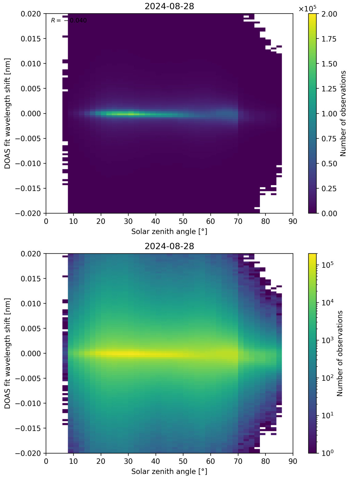
Figure 168: Scatter density plot of “Solar zenith angle” against “DOAS fit wavelength shift” for 2024-08-27 to 2024-08-29.
