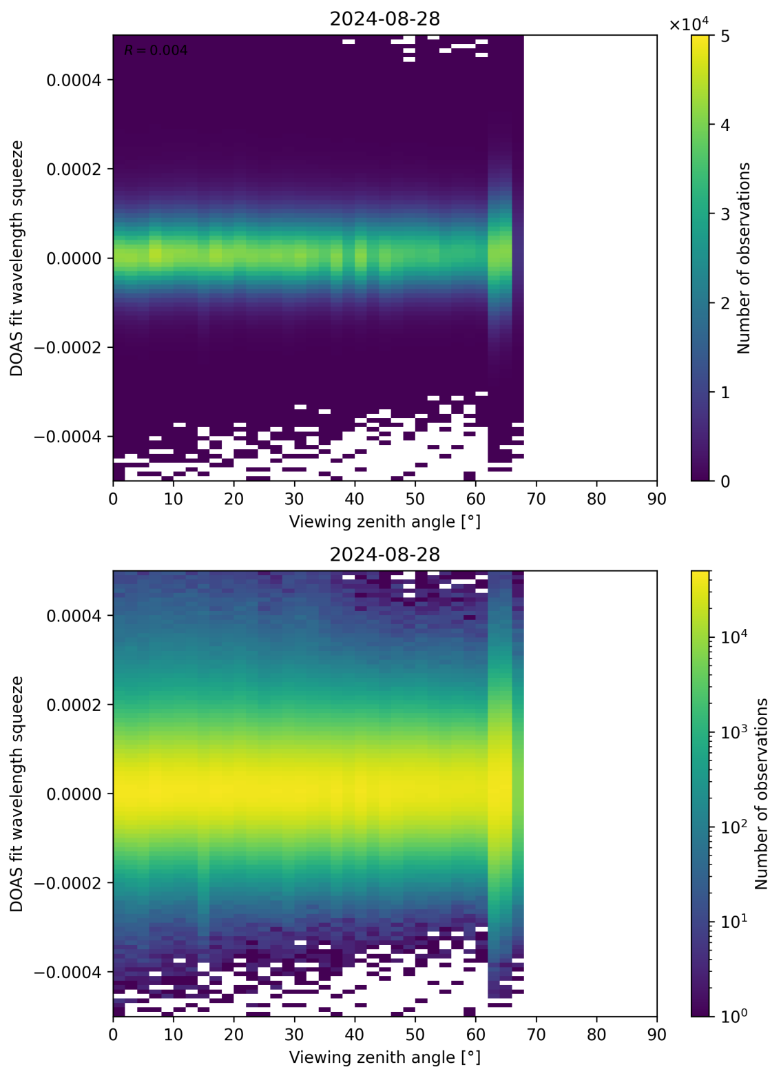
Figure 184: Scatter density plot of “Viewing zenith angle” against “DOAS fit wavelength squeeze” for 2024-08-27 to 2024-08-29.
