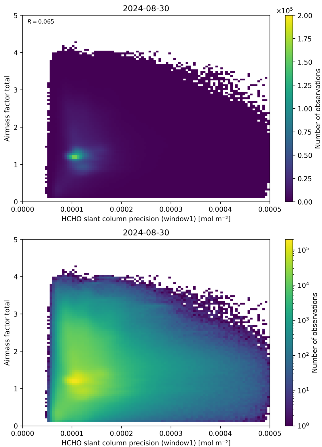
Figure 94: Scatter density plot of “HCHO slant column precision (window1)” against “Airmass factor total” for 2024-08-29 to 2024-08-31.
