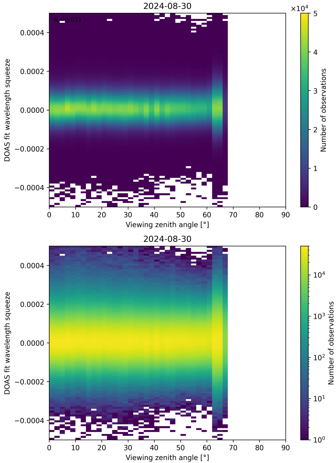
Figure 184: Scatter density plot of “Viewing zenith angle” against “DOAS fit wavelength squeeze” for 2024-08-29 to 2024-08-31.
