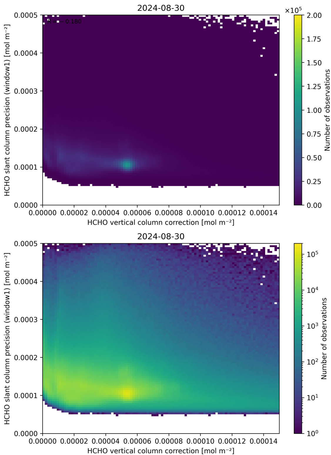
Figure 119: Scatter density plot of “HCHO vertical column correction” against “HCHO slant column precision (window1)” for 2024-08-29 to 2024-08-31.
