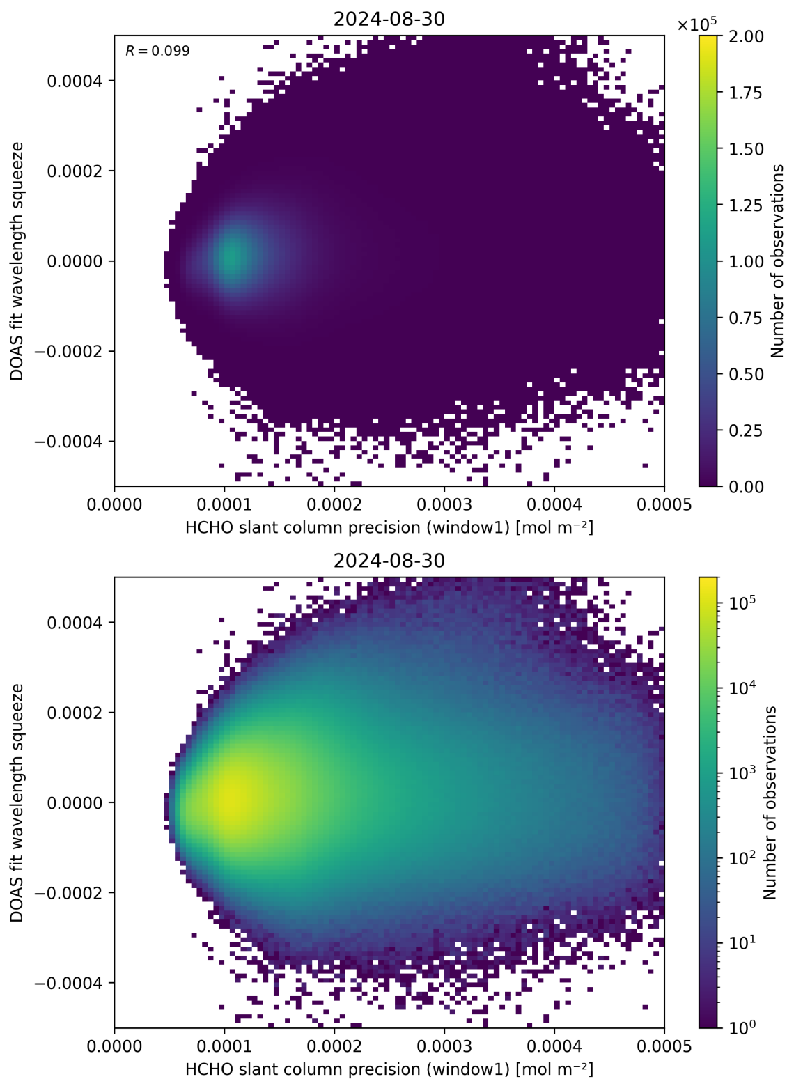
Figure 90: Scatter density plot of “HCHO slant column precision (window1)” against “DOAS fit wavelength squeeze” for 2024-08-29 to 2024-08-31.
