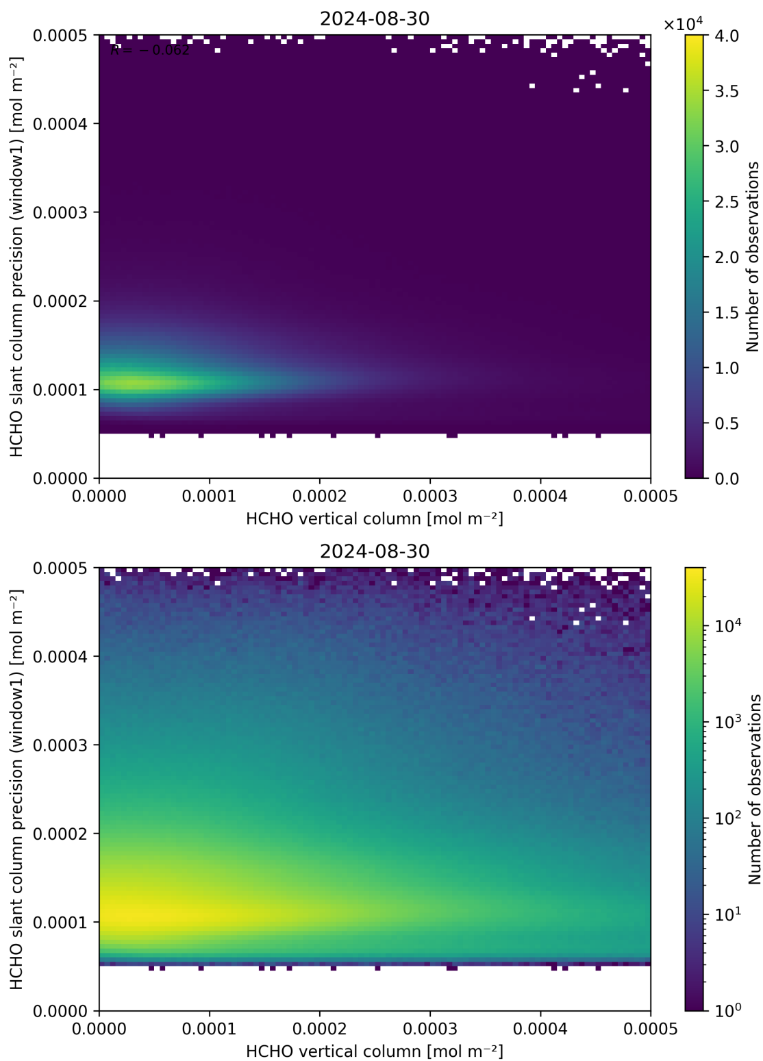
Figure 130: Scatter density plot of “HCHO vertical column” against “HCHO slant column precision (window1)” for 2024-08-29 to 2024-08-31.
