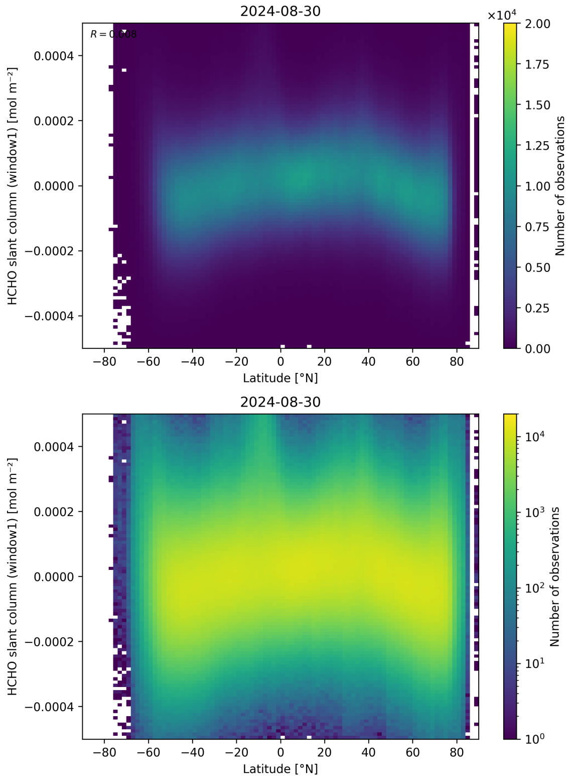
Figure 159: Scatter density plot of “Latitude” against “HCHO slant column (window1)” for 2024-08-29 to 2024-08-31.
