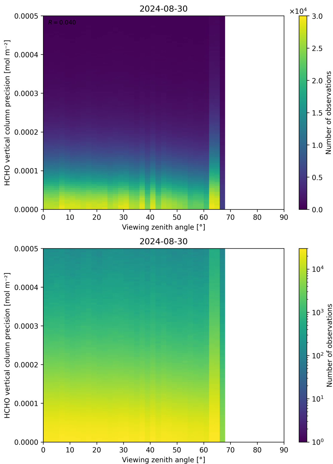
Figure 194: Scatter density plot of “Viewing zenith angle” against “HCHO vertical column precision” for 2024-08-29 to 2024-08-31.
