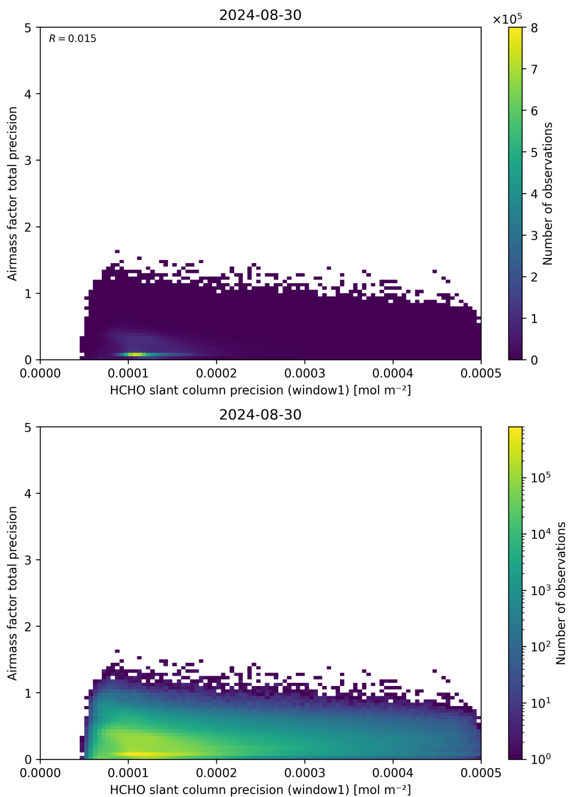
Figure 95: Scatter density plot of “HCHO slant column precision (window1)” against “Airmass factor total precision” for 2024-08-29 to 2024-08-31.
