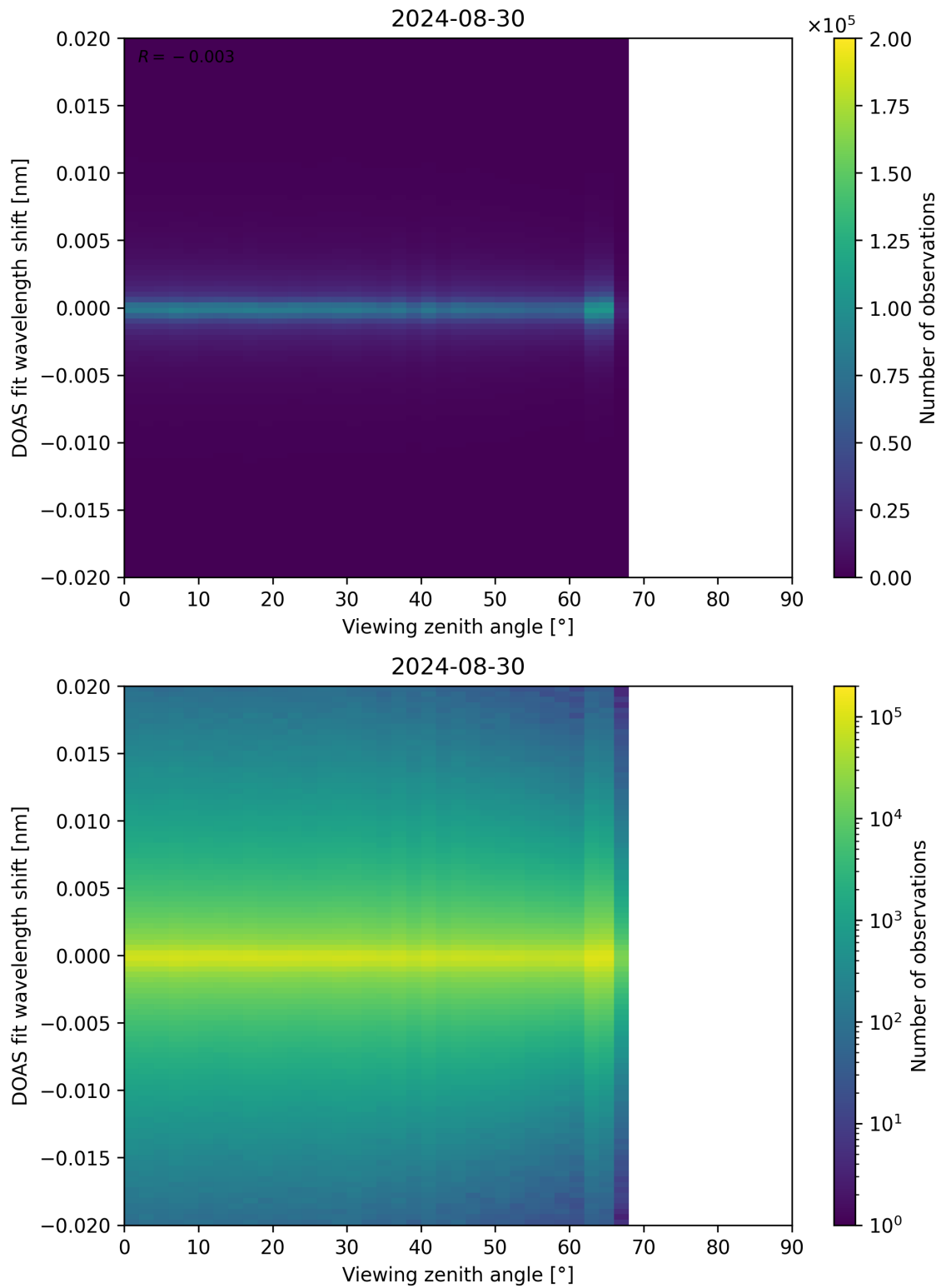
Figure 183: Scatter density plot of “Viewing zenith angle” against “DOAS fit wavelength shift” for 2024-08-29 to 2024-08-31.
