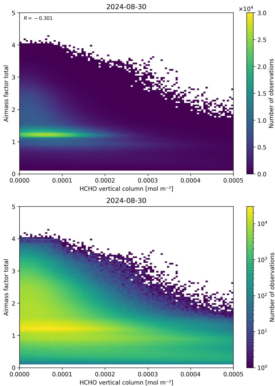
Figure 131: Scatter density plot of “HCHO vertical column” against “Airmass factor total” for 2024-08-29 to 2024-08-31.
