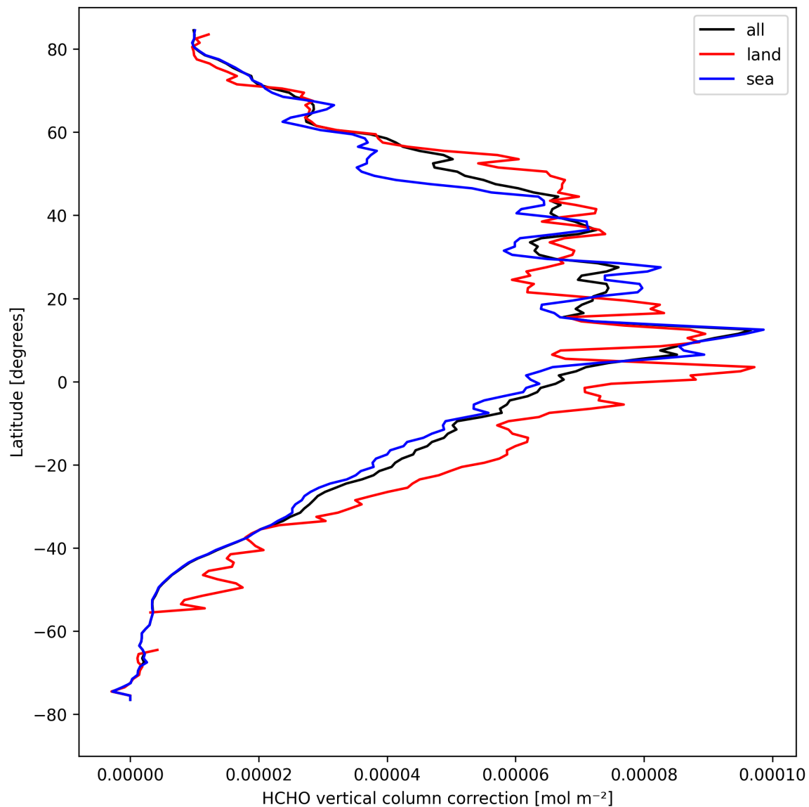
Figure 23: Zonal average of “HCHO vertical column correction” for 2024-08-29 to 2024-08-31.
