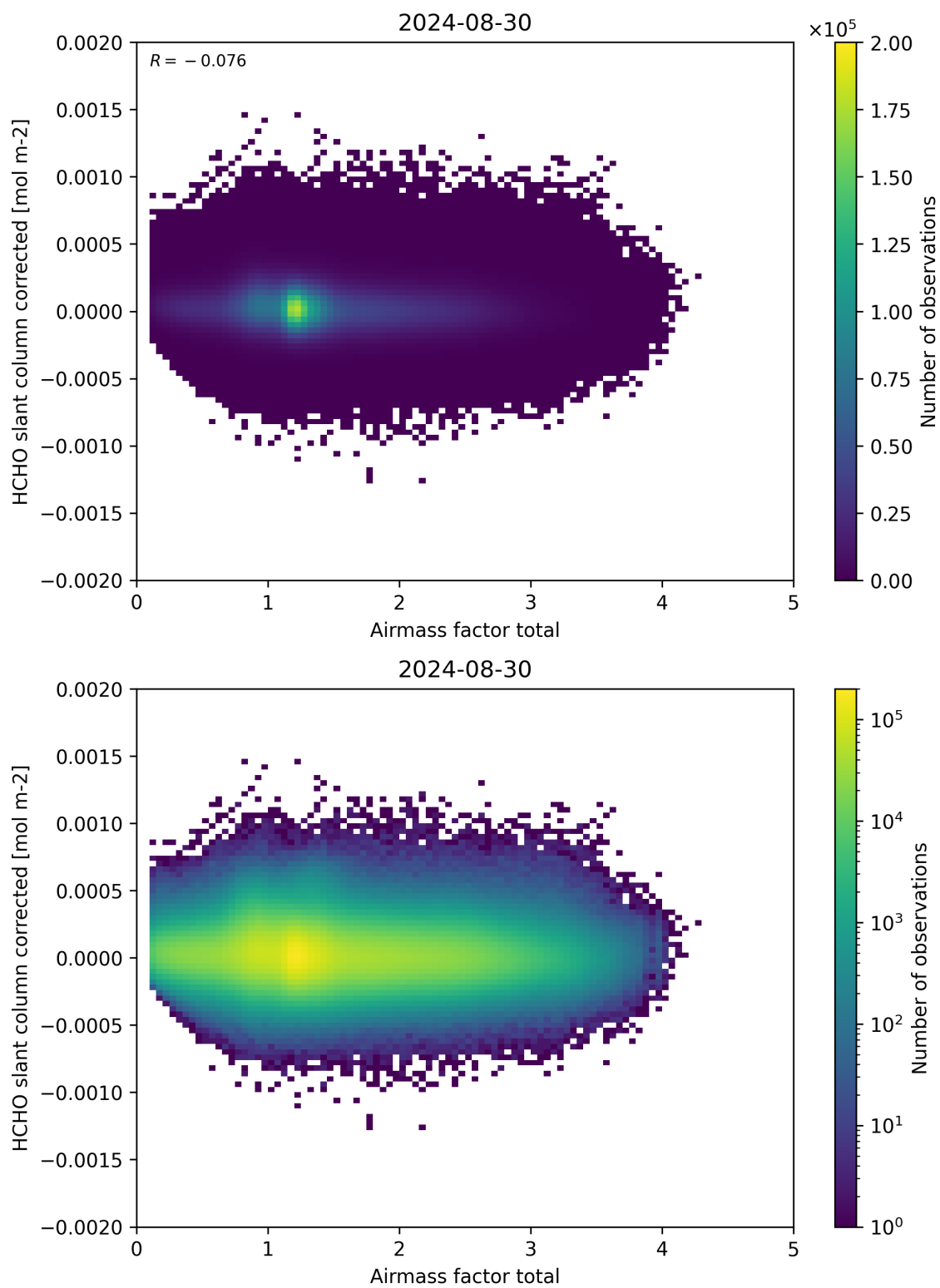
Figure 101: Scatter density plot of “Airmass factor total” against “HCHO slant column corrected” for 2024-08-29 to 2024-08-31.
