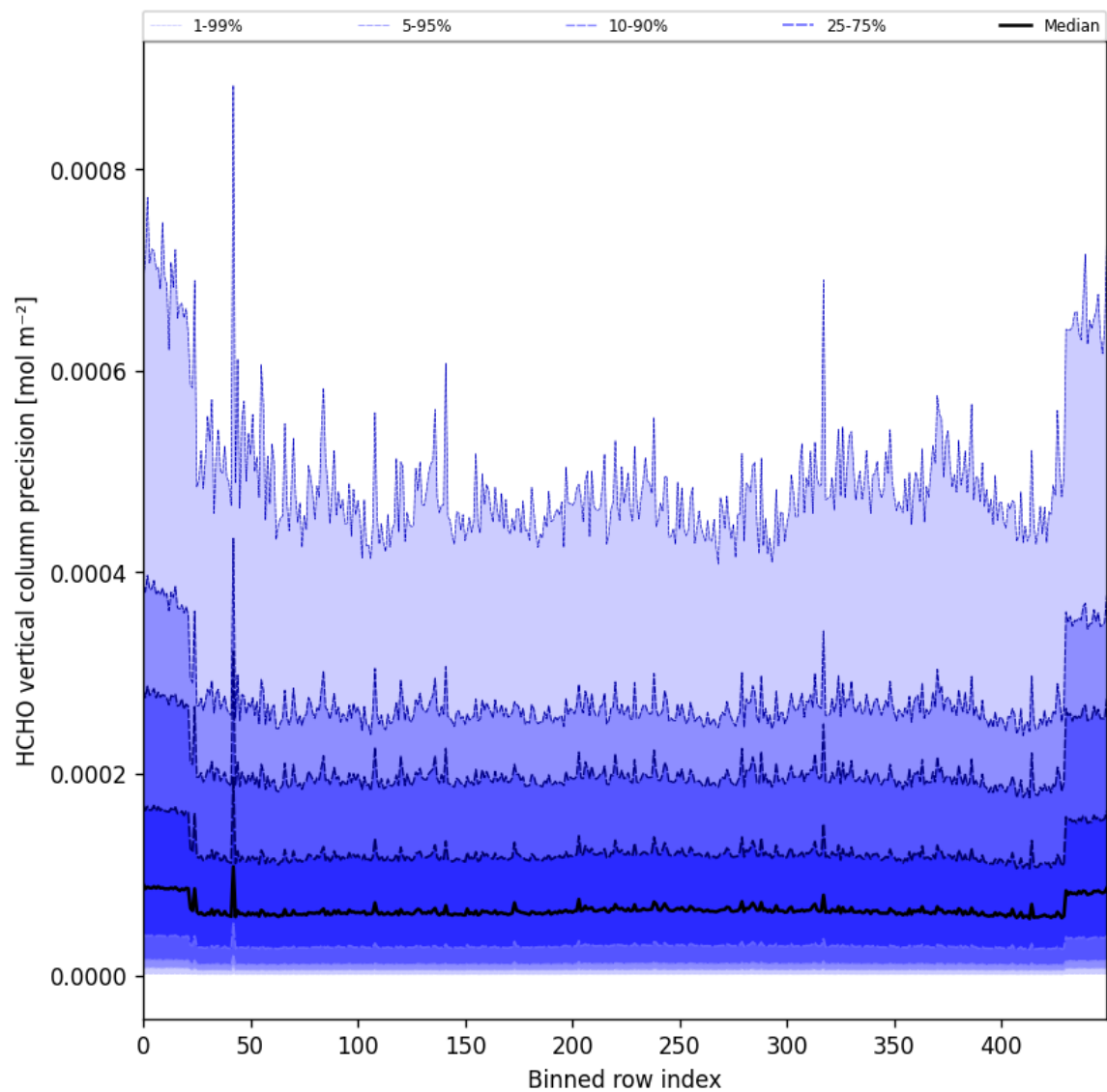
Figure 50: Along track statistics of “HCHO vertical column precision” for 2024-08-29 to 2024-08-31
