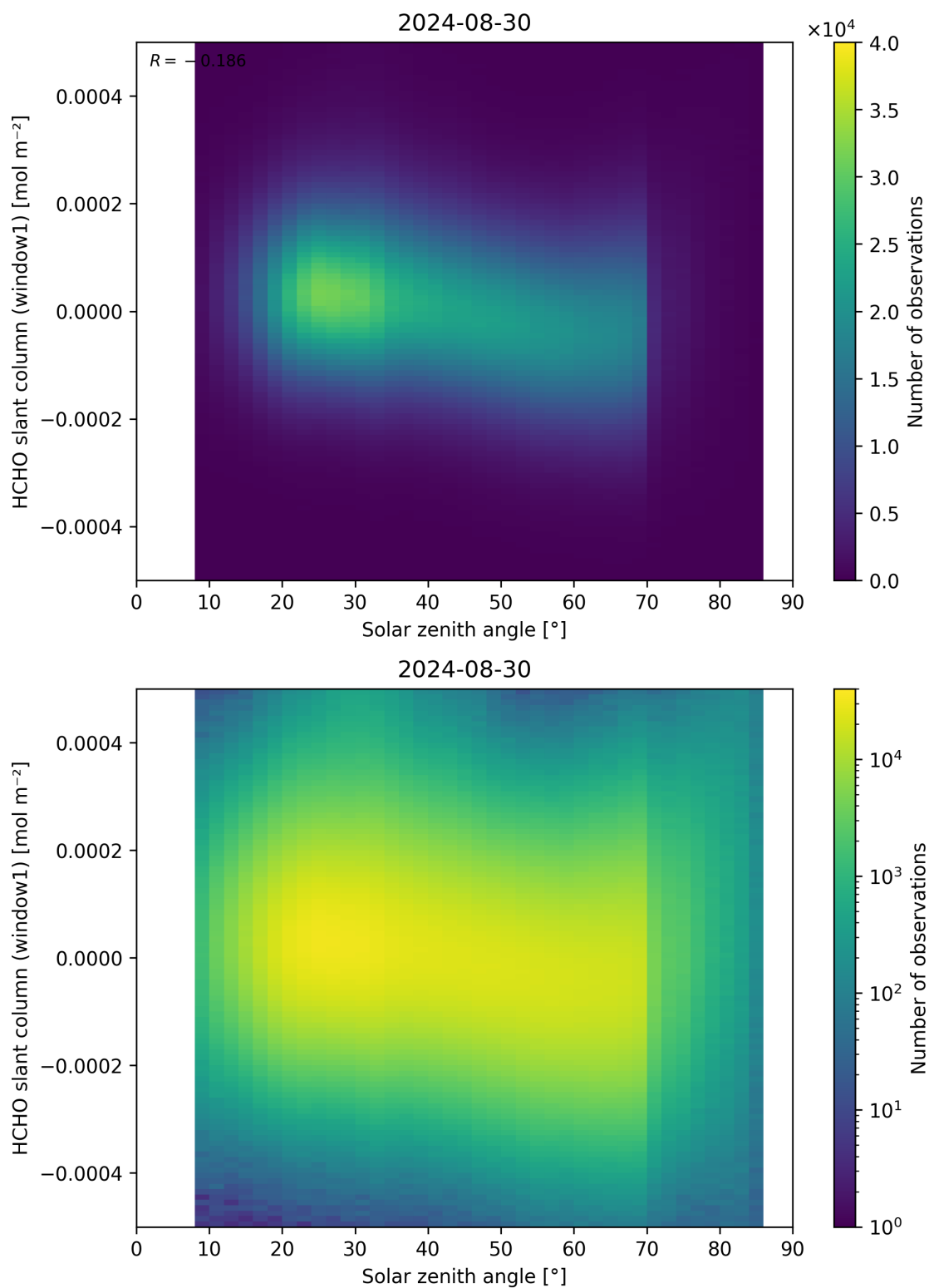
Figure 173: Scatter density plot of “Solar zenith angle” against “HCHO slant column (window1)” for 2024-08-29 to 2024-08-31.
