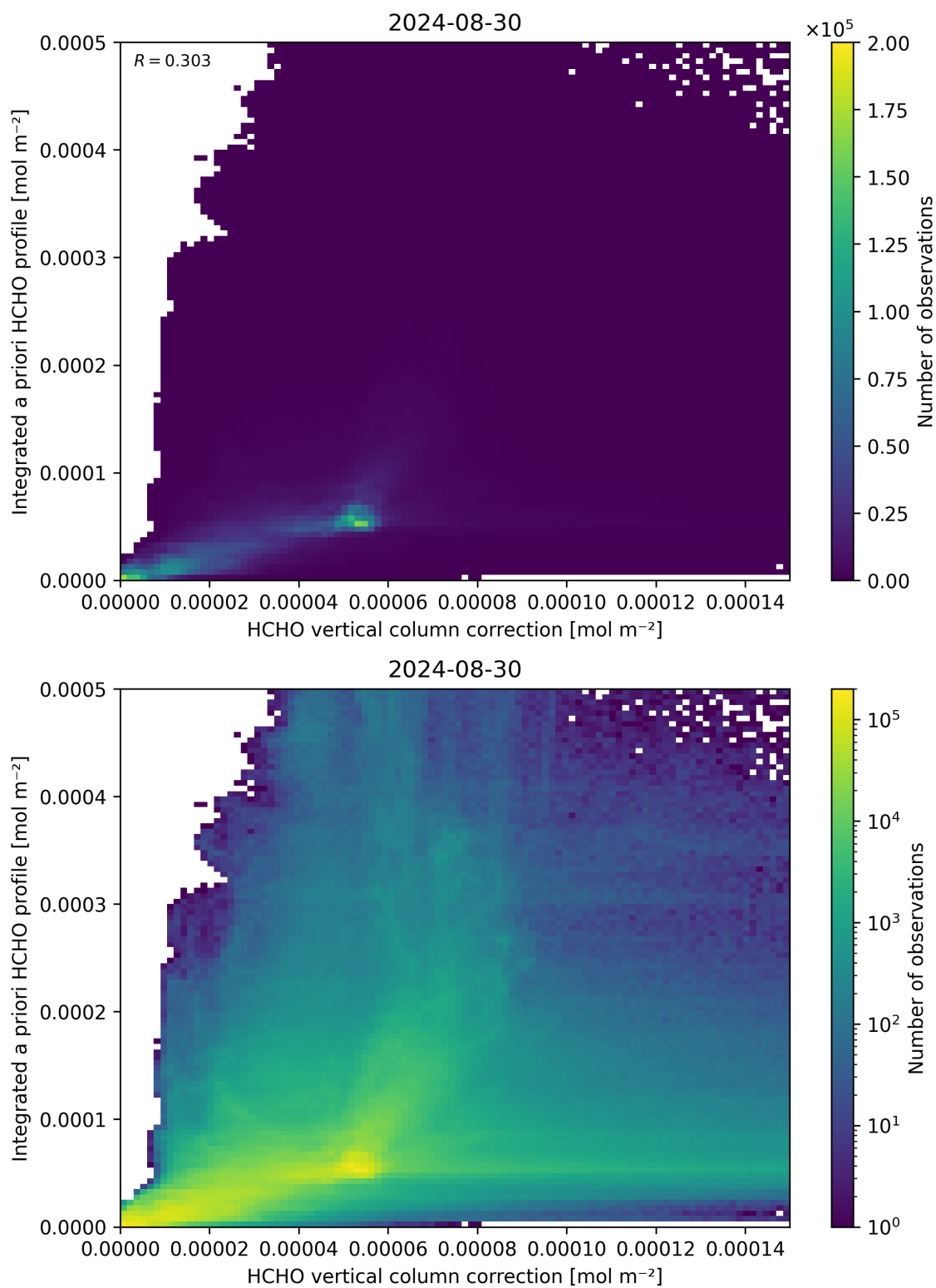
Figure 122: Scatter density plot of “HCHO vertical column correction” against “Integrated a priori HCHO profile” for 2024-08-29 to 2024-08-31.
