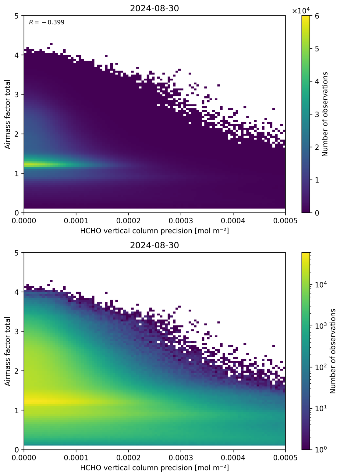
Figure 144: Scatter density plot of “HCHO vertical column precision” against “Airmass factor total” for 2024-08-29 to 2024-08-31.
