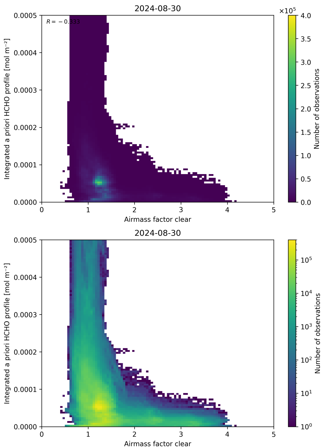
Figure 76: Scatter density plot of “Airmass factor clear” against “Integrated a priori HCHO profile” for 2024-08-29 to 2024-08-31.
