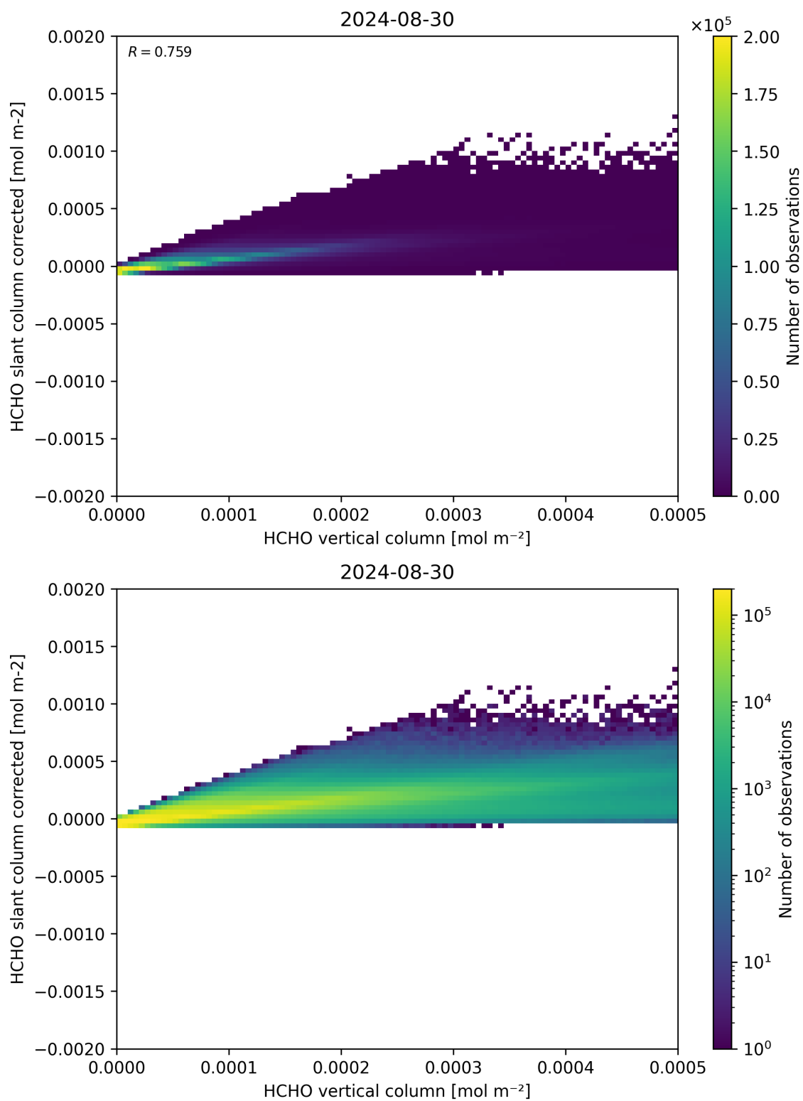
Figure 127: Scatter density plot of “HCHO vertical column” against “HCHO slant column corrected” for 2024-08-29 to 2024-08-31.
