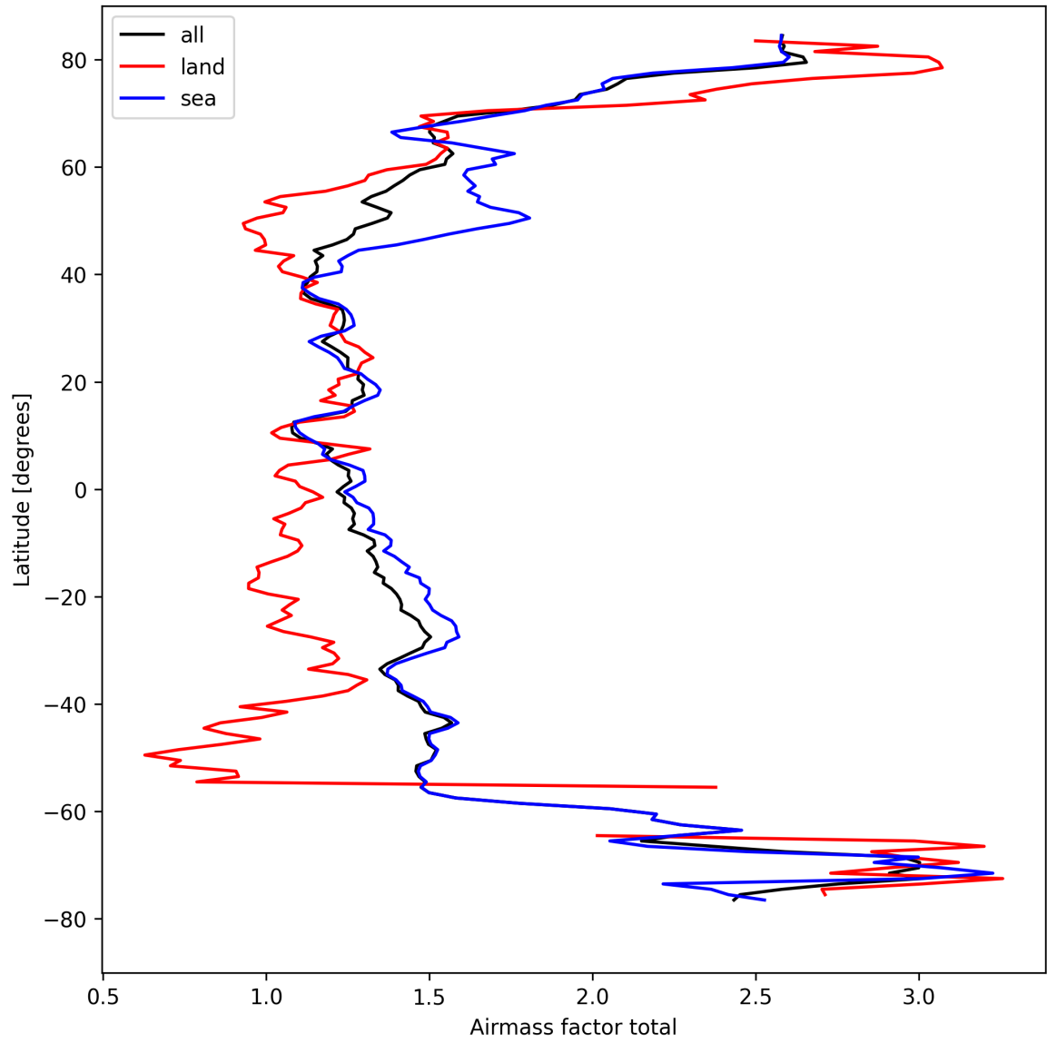
Figure 26: Zonal average of “Airmass factor total” for 2024-08-29 to 2024-08-31.
