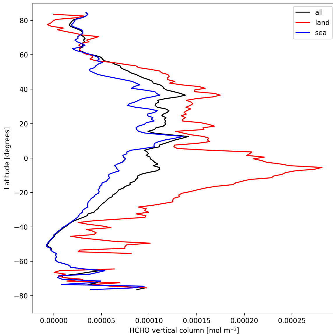
Figure 21: Zonal average of “HCHO vertical column” for 2024-08-29 to 2024-08-31.
