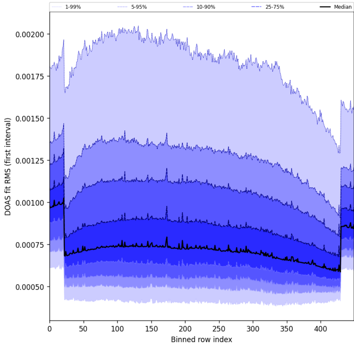
Figure 60: Along track statistics of “DOAS fit RMS (first interval)” for 2024-08-29 to 2024-08-31
