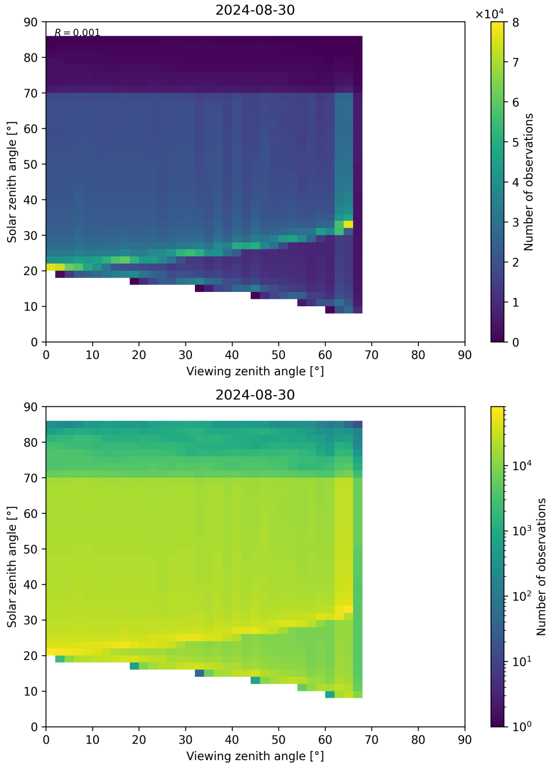
Figure 197: Scatter density plot of “Viewing zenith angle” against “Solar zenith angle” for 2024-08-29 to 2024-08-31.
