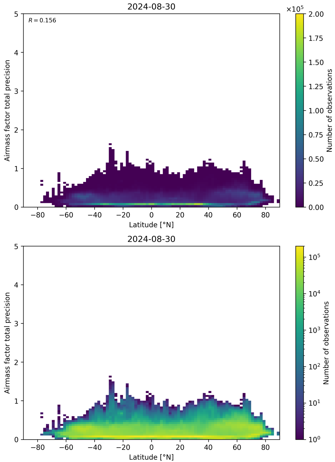
Figure 162: Scatter density plot of “Latitude” against “Airmass factor total precision” for 2024-08-29 to 2024-08-31.
