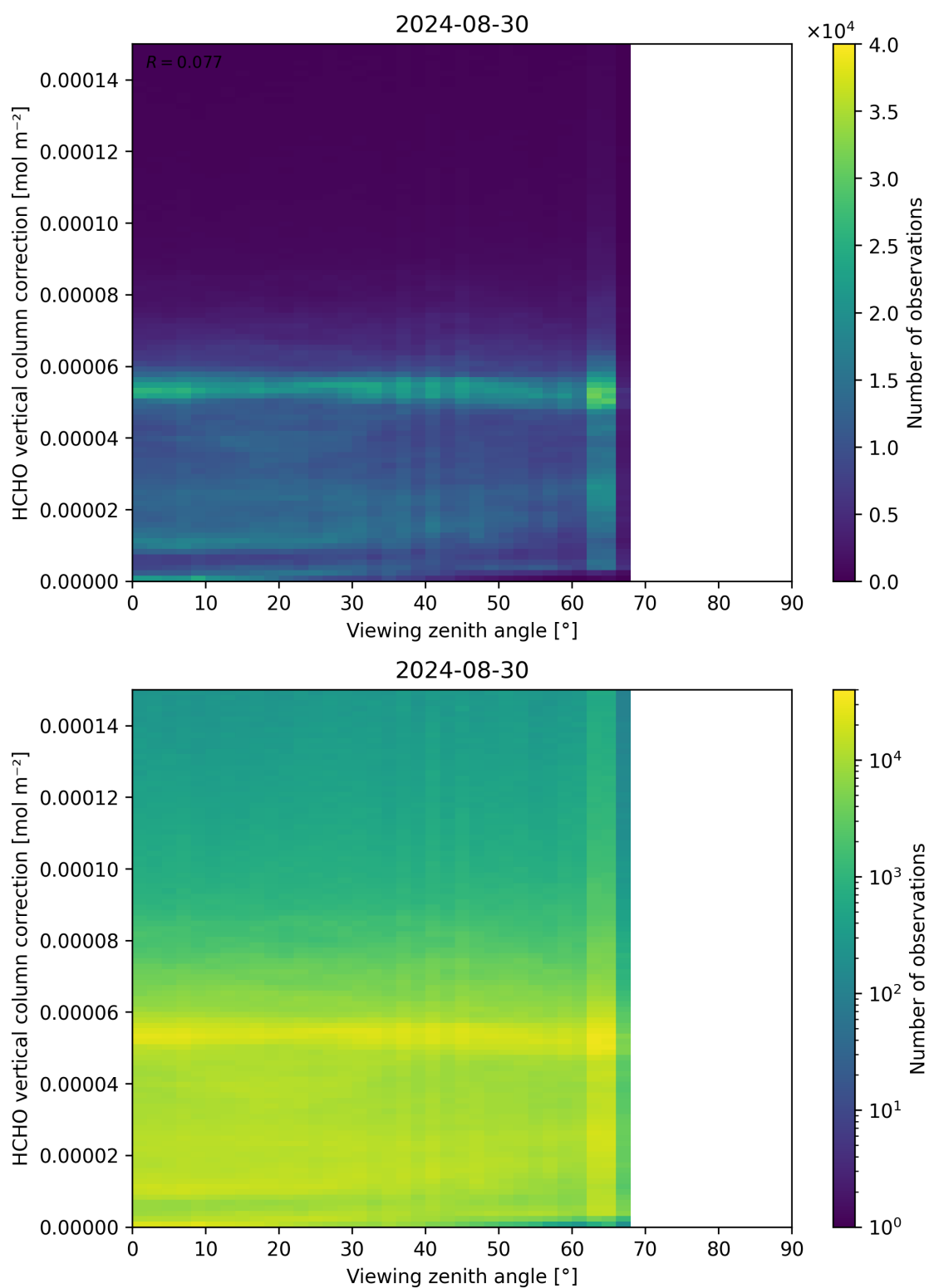
Figure 193: Scatter density plot of “Viewing zenith angle” against “HCHO vertical column correction” for 2024-08-29 to 2024-08-31.
