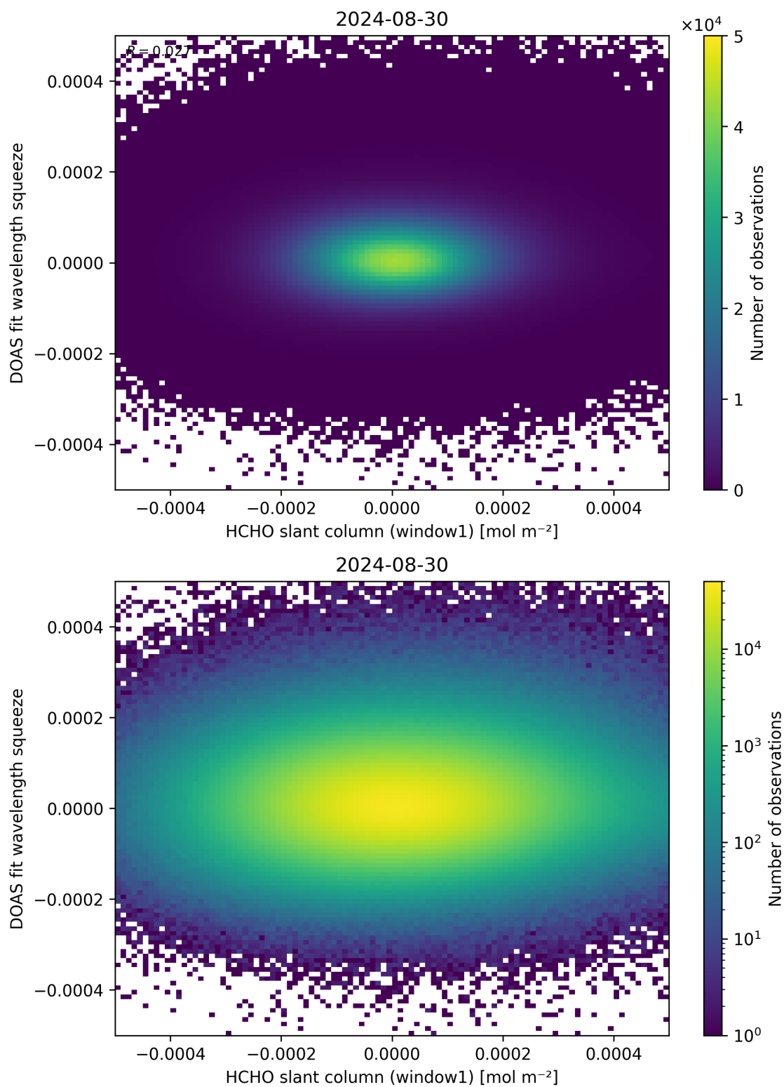
Figure 80: Scatter density plot of “HCHO slant column (window1)” against “DOAS fit wavelength squeeze” for 2024-08-29 to 2024-08-31.
