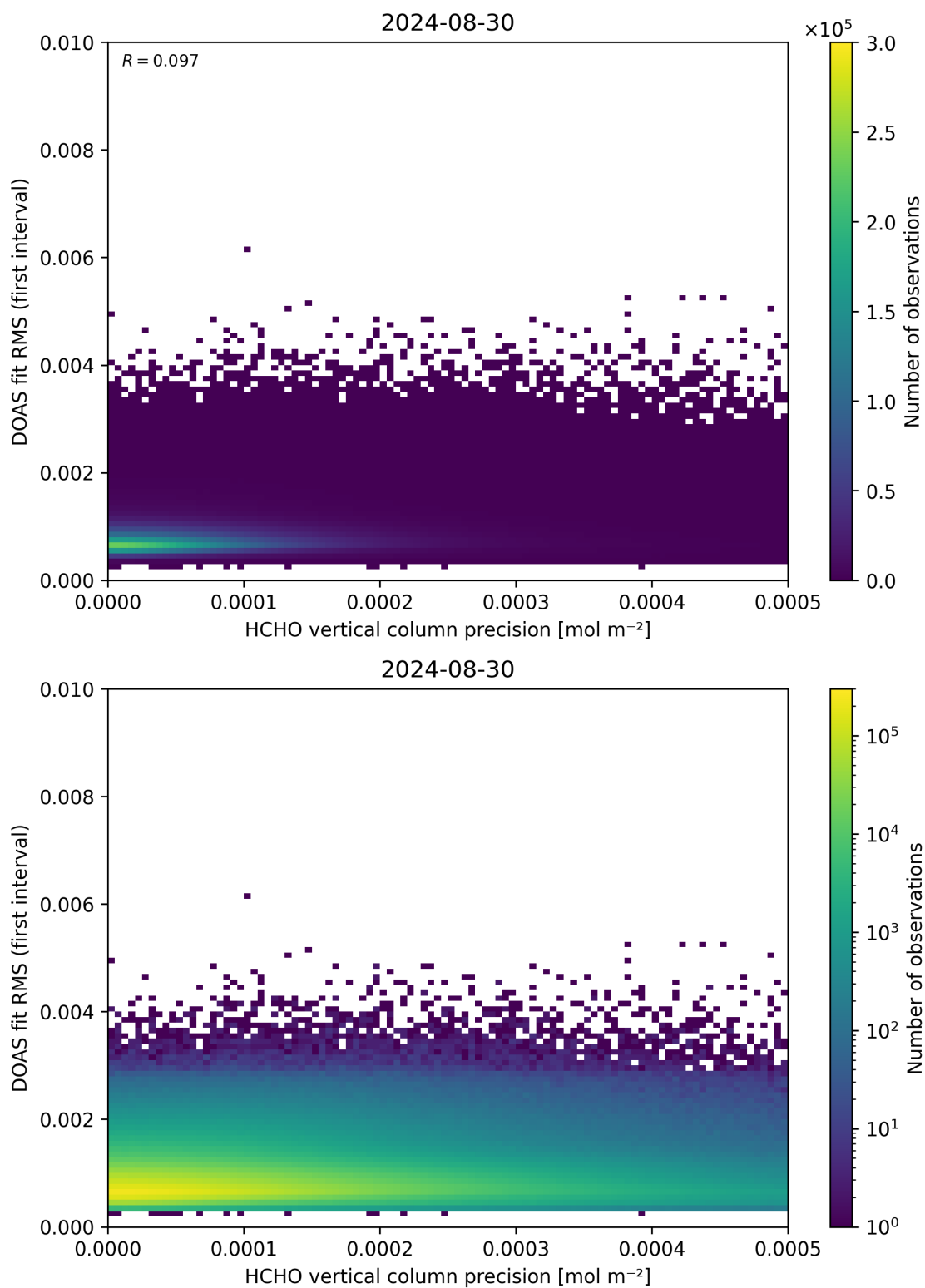
Figure 136: Scatter density plot of “HCHO vertical column precision” against “DOAS fit RMS (first interval)” for 2024-08-29 to 2024-08-31.
