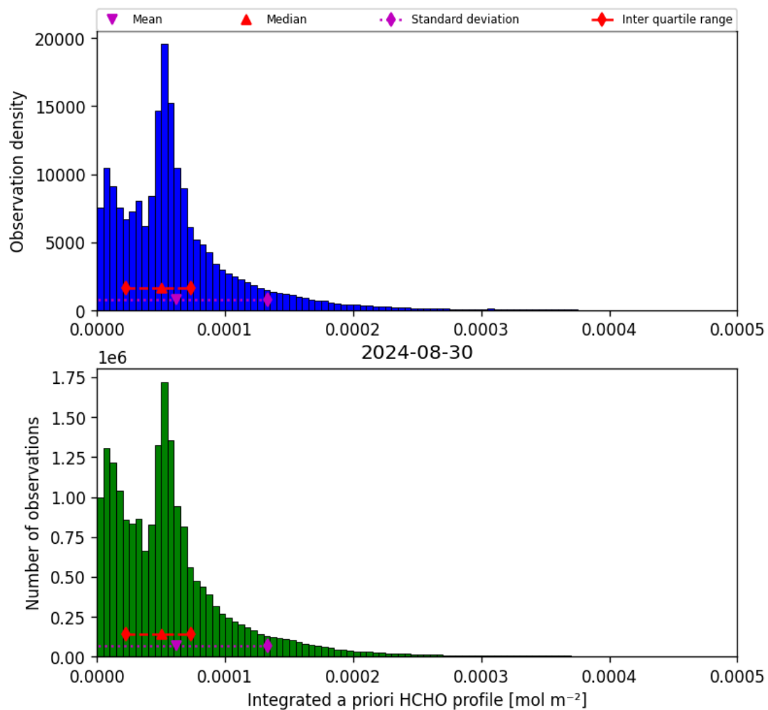
Figure 43: Histogram of “Integrated a priori HCHO profile” for 2024-08-29 to 2024-08-31
