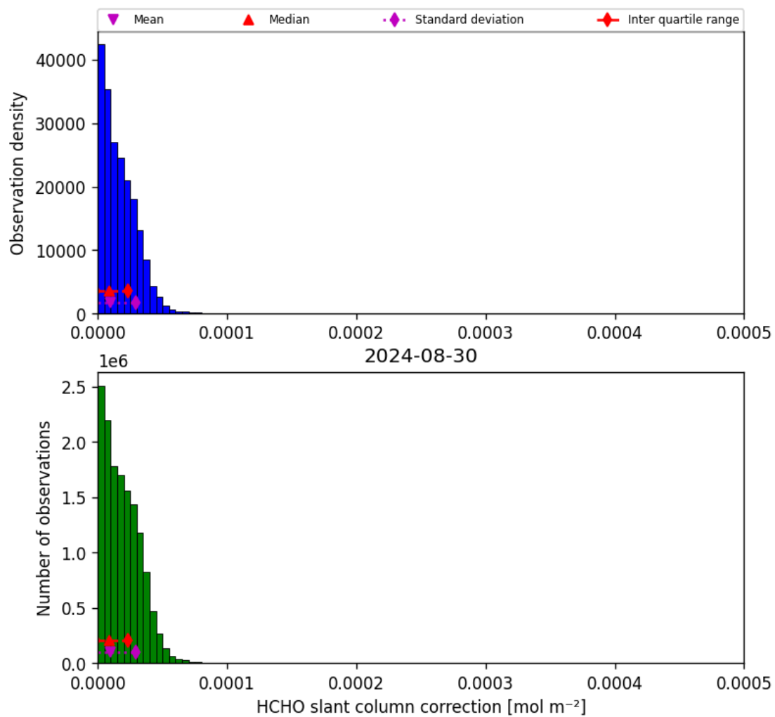
Figure 47: Histogram of “HCHO slant column correction” for 2024-08-29 to 2024-08-31
