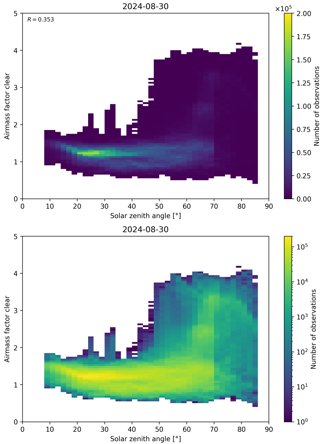
Figure 170: Scatter density plot of “Solar zenith angle” against “Airmass factor clear” for 2024-08-29 to 2024-08-31.
