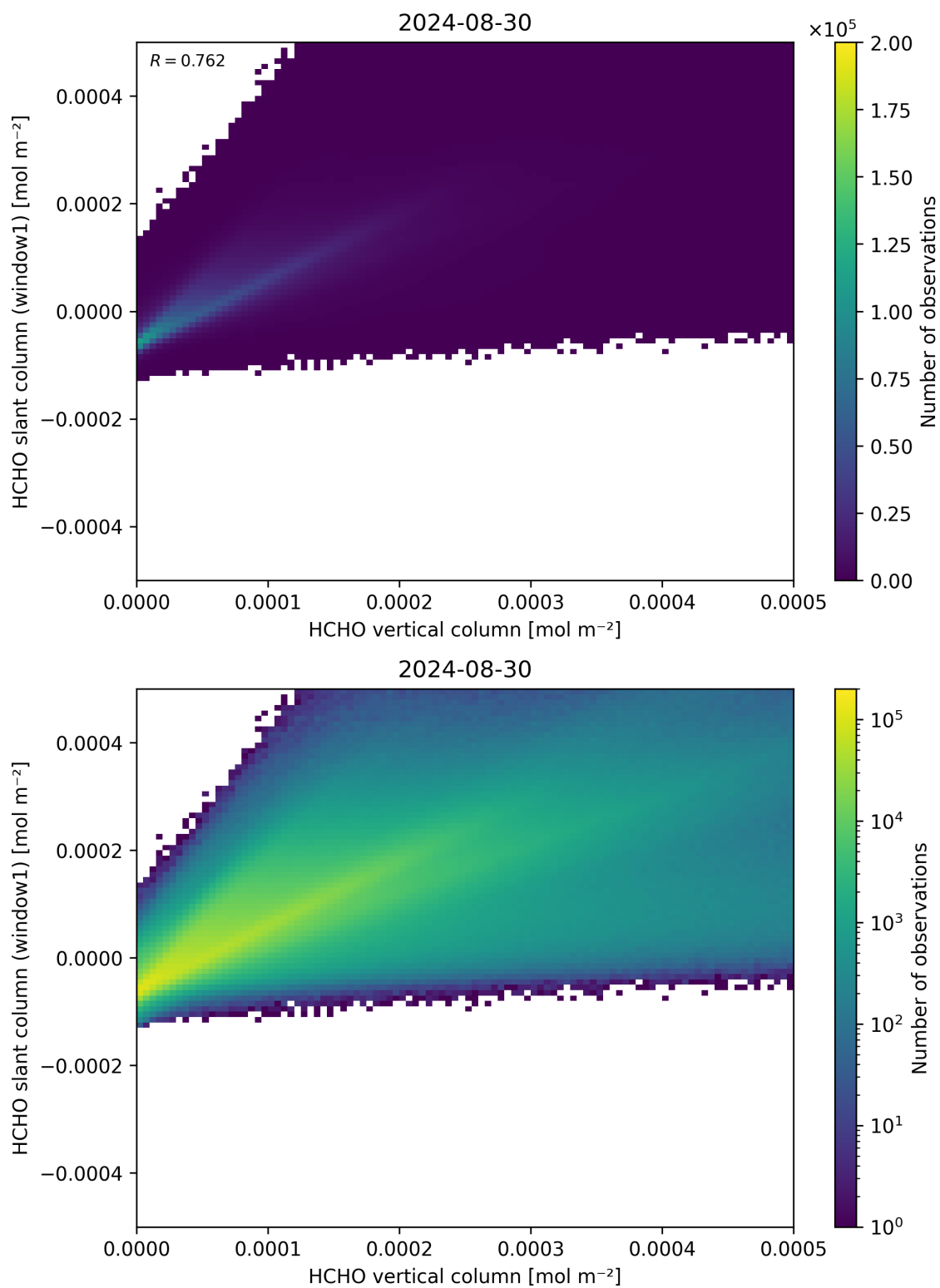
Figure 129: Scatter density plot of “HCHO vertical column” against “HCHO slant column (window1)” for 2024-08-29 to 2024-08-31.
