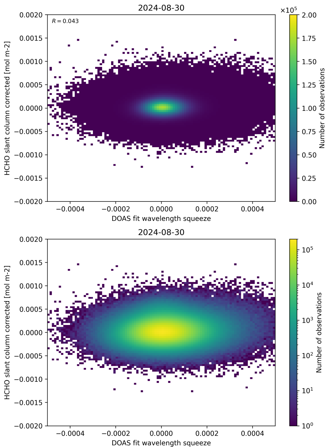
Figure 69: Scatter density plot of “DOAS fit wavelength squeeze” against “HCHO slant column corrected” for 2024-08-29 to 2024-08-31.
