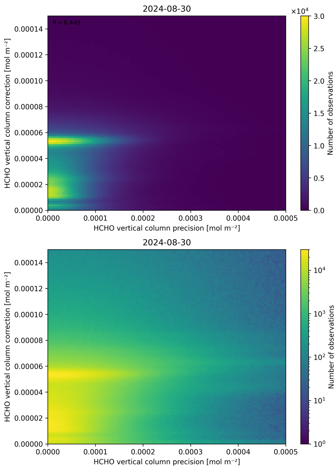
Figure 146: Scatter density plot of “HCHO vertical column precision” against “HCHO vertical column correction” for 2024-08-29 to 2024-08-31.
