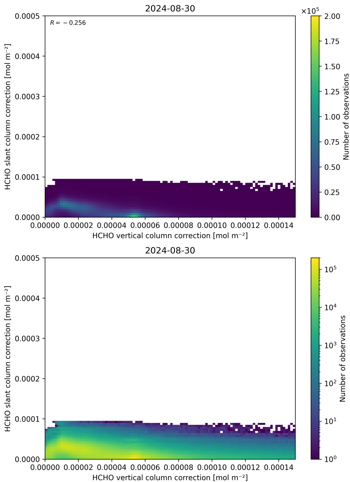
Figure 117: Scatter density plot of “HCHO vertical column correction” against “HCHO slant column correction” for 2024-08-29 to 2024-08-31.
