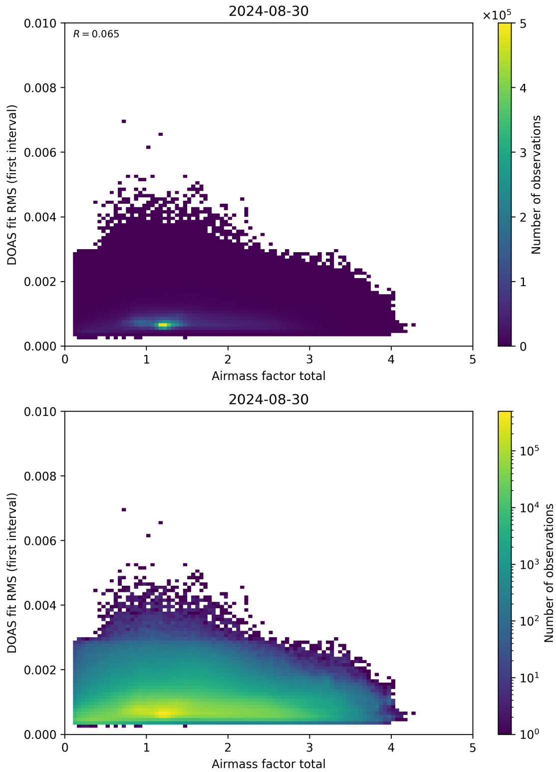
Figure 97: Scatter density plot of “Airmass factor total” against “DOAS fit RMS (first interval)” for 2024-08-29 to 2024-08-31.
