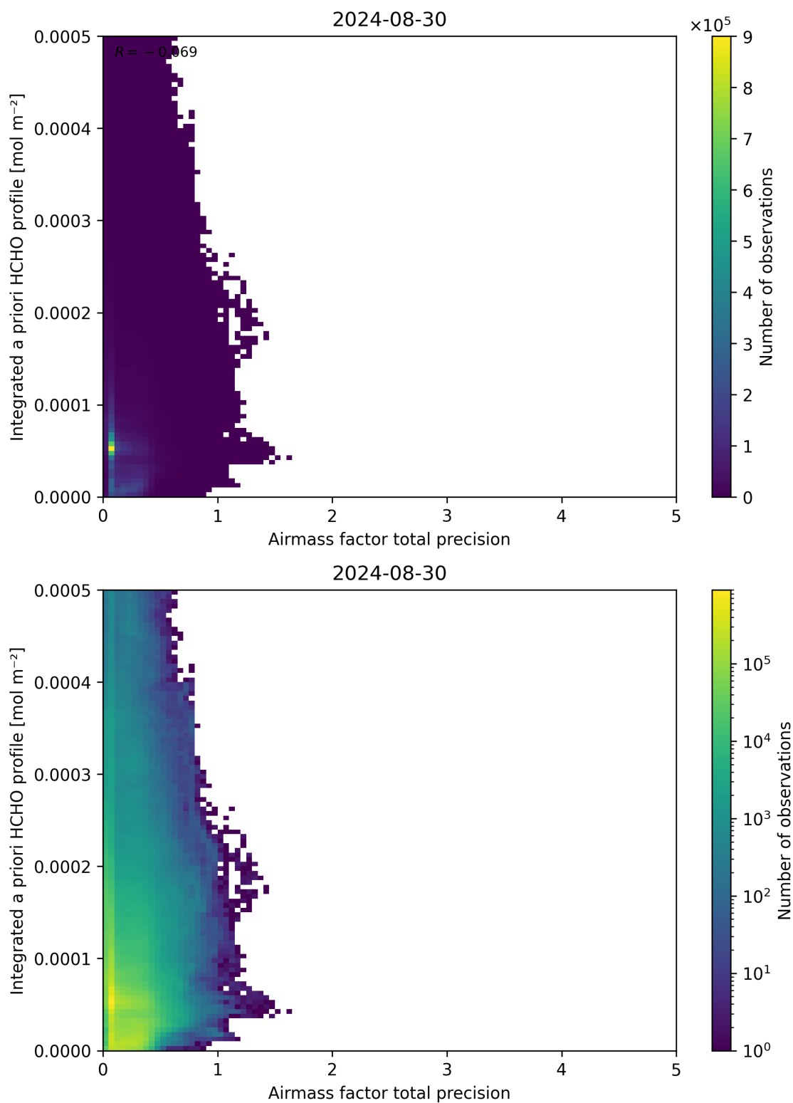
Figure 111: Scatter density plot of “Airmass factor total precision” against “Integrated a priori HCHO profile” for 2024-08-29 to 2024-08-31.
