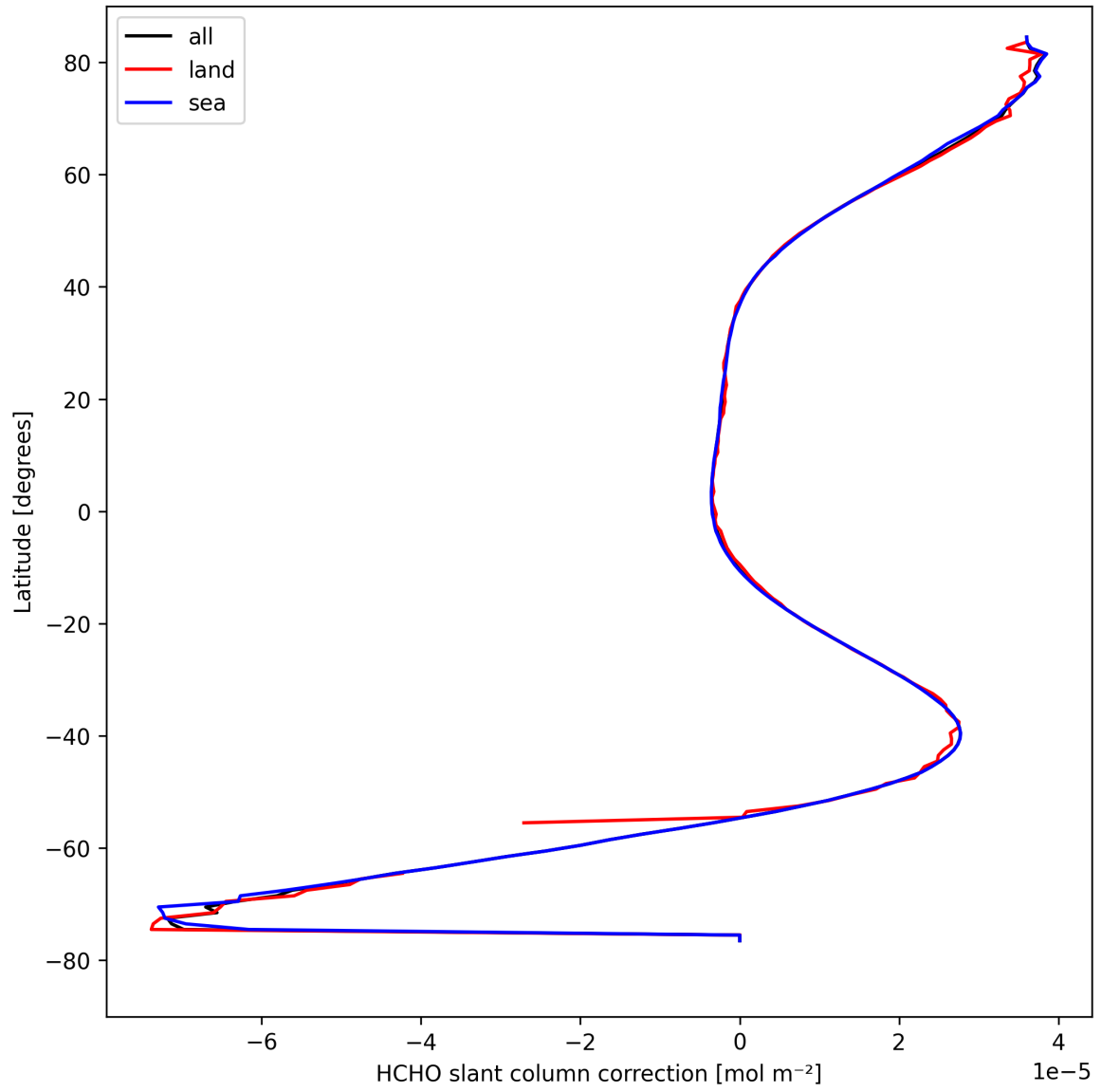
Figure 33: Zonal average of "HCHO slant column correction" for 2024-08-29 to 2024-08-31.
