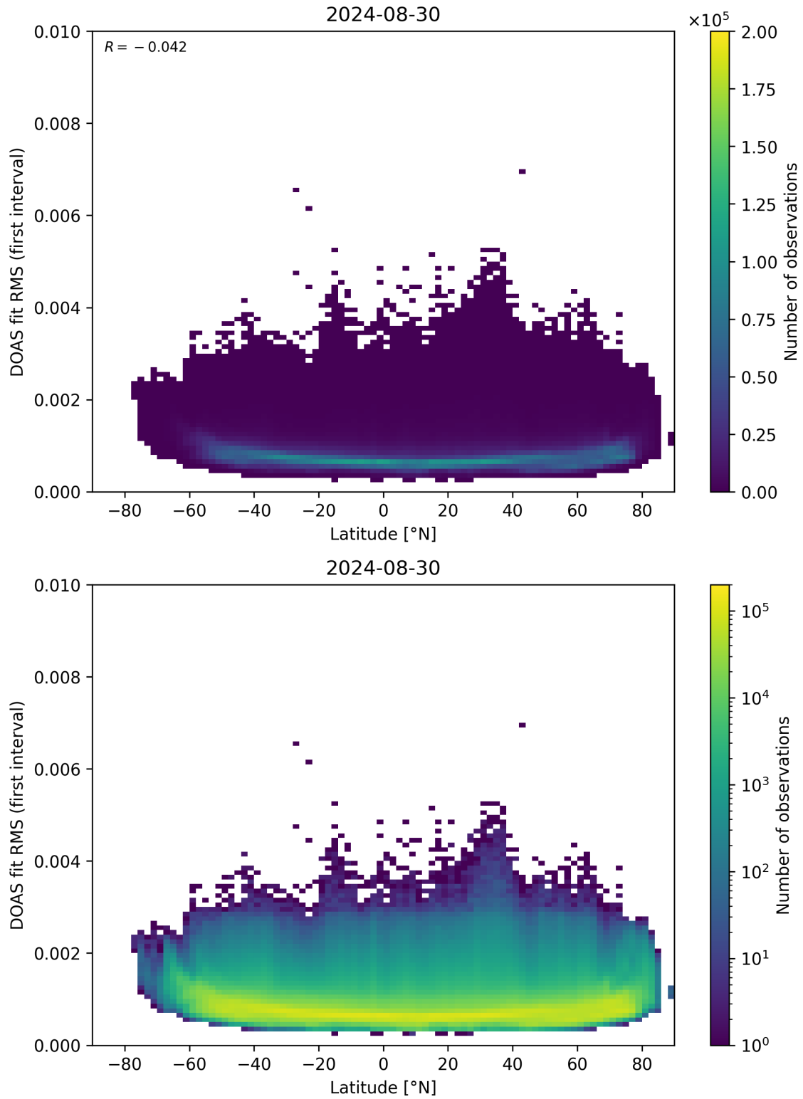
Figure 153: Scatter density plot of “Latitude” against “DOAS fit RMS (first interval)” for 2024-08-29 to 2024-08-31.
