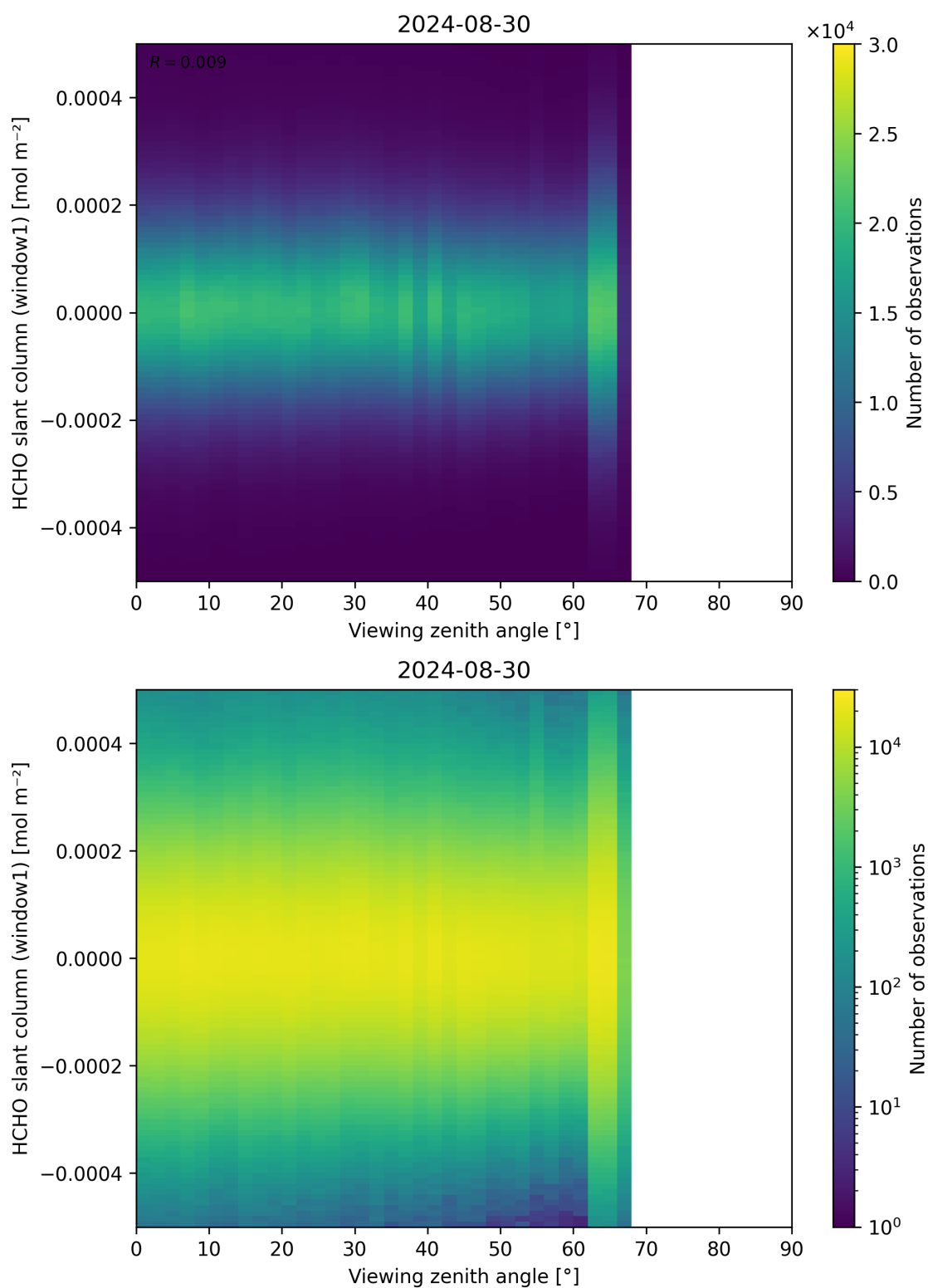
Figure 188: Scatter density plot of “Viewing zenith angle” against “HCHO slant column (window1)” for 2024-08-29 to 2024-08-31.
