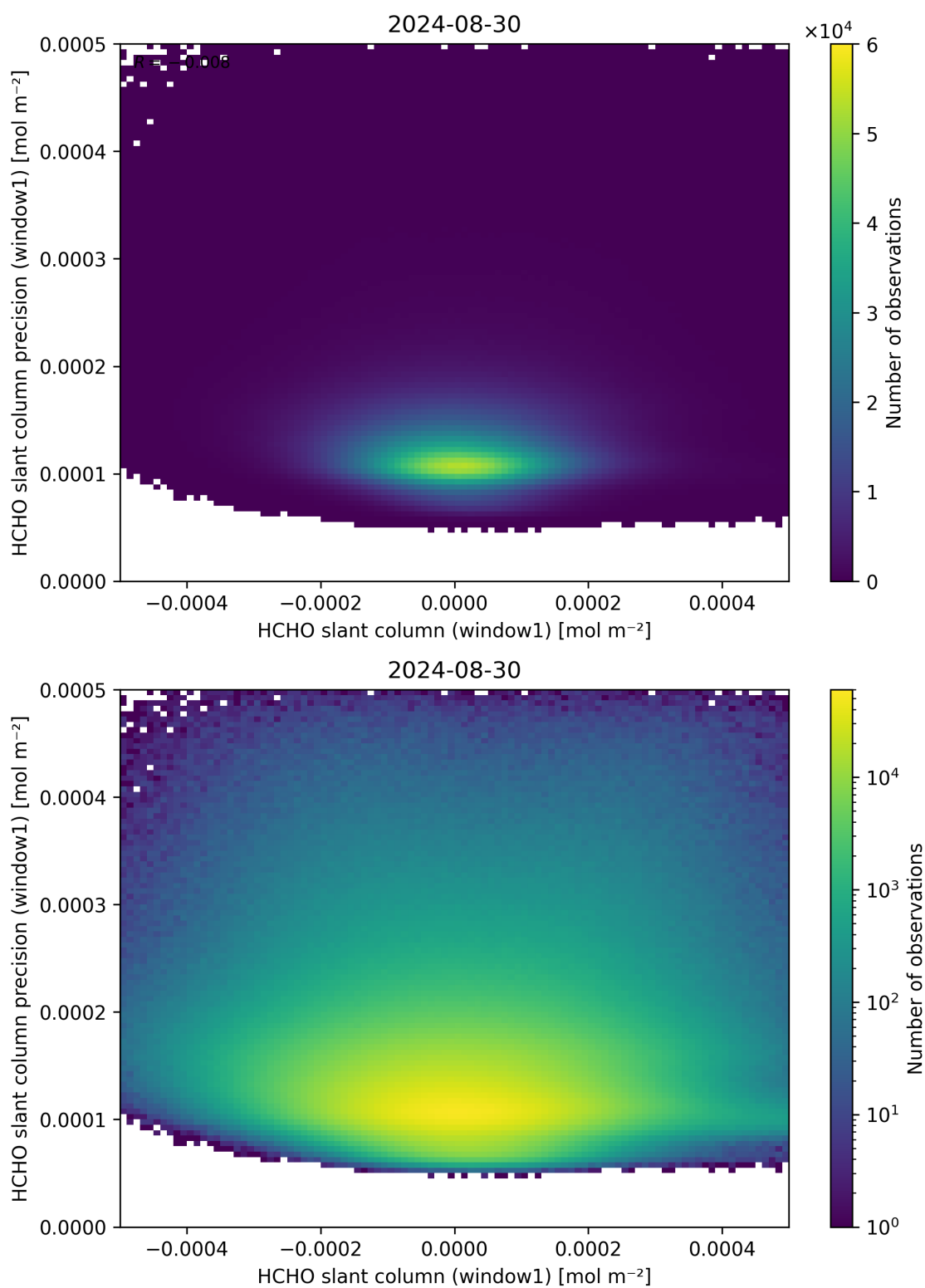
Figure 84: Scatter density plot of “HCHO slant column (window1)” against “HCHO slant column precision (window1)” for 2024-08-29 to 2024-08-31.
