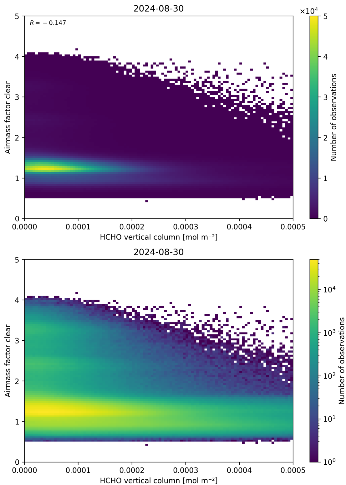
Figure 126: Scatter density plot of “HCHO vertical column” against “Airmass factor clear” for 2024-08-29 to 2024-08-31.
