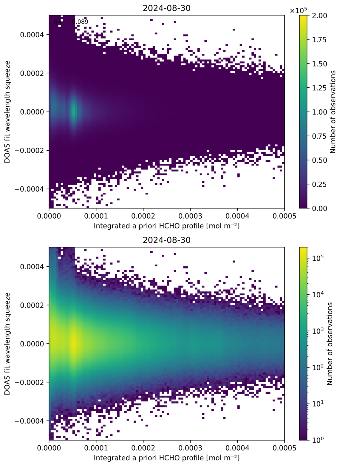
Figure 150: Scatter density plot of “Integrated a priori HCHO profile” against “DOAS fit wavelength squeeze” for 2024-08-29 to 2024-08-31.
