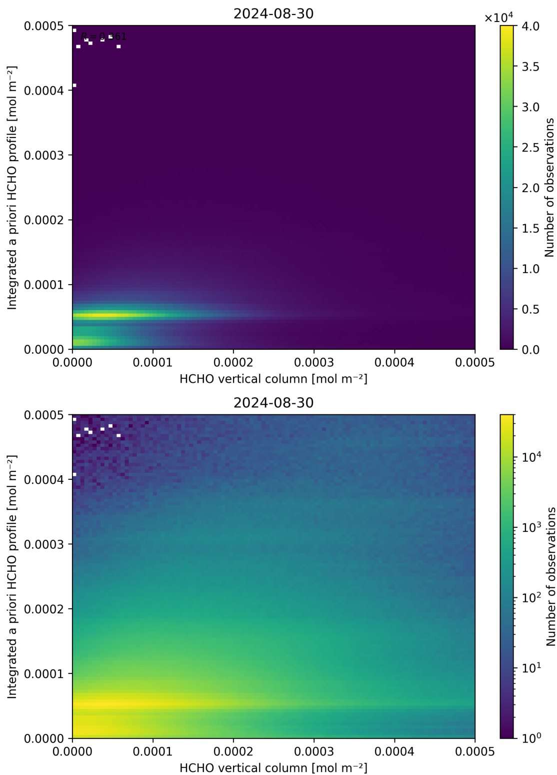
Figure 135: Scatter density plot of “HCHO vertical column” against “Integrated a priori HCHO profile” for 2024-08-29 to 2024-08-31.
