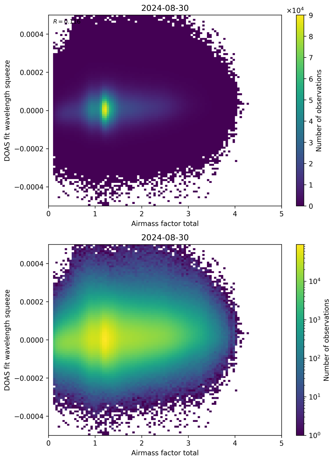
Figure 99: Scatter density plot of “Airmass factor total” against “DOAS fit wavelength squeeze” for 2024-08-29 to 2024-08-31.
