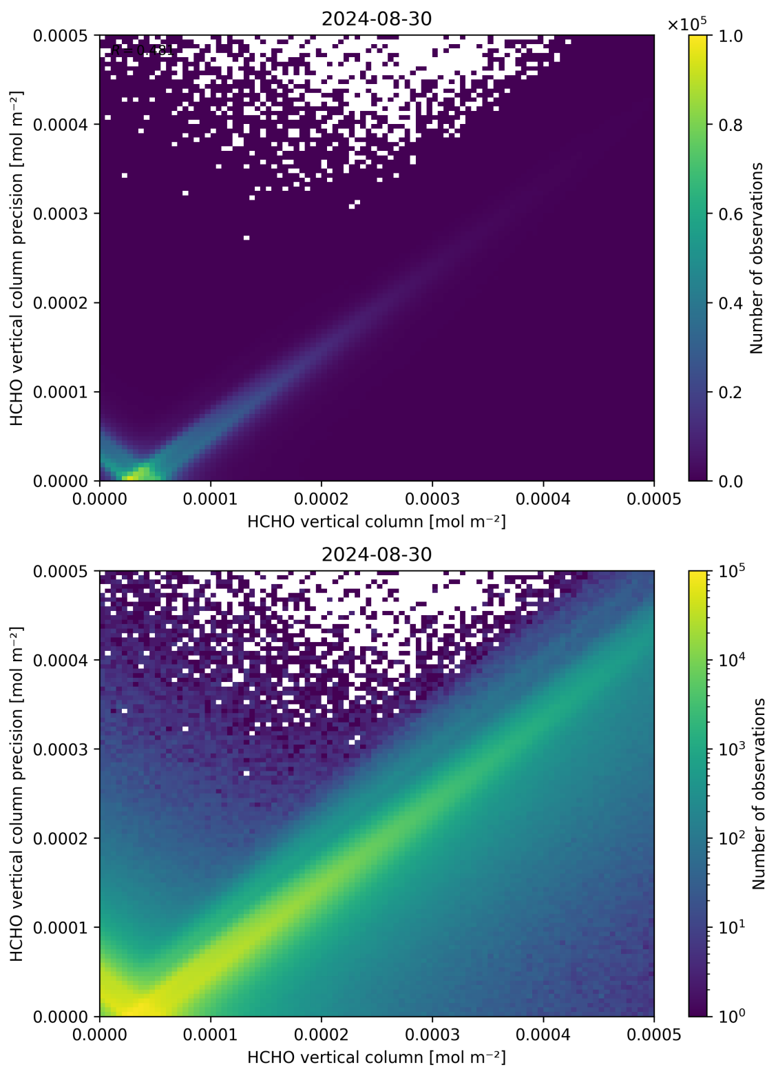
Figure 134: Scatter density plot of “HCHO vertical column” against “HCHO vertical column precision” for 2024-08-29 to 2024-08-31.
