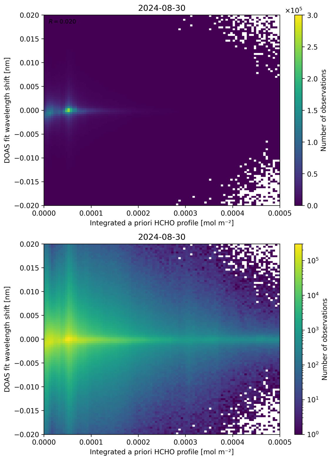
Figure 149: Scatter density plot of “Integrated a priori HCHO profile” against “DOAS fit wavelength shift” for 2024-08-29 to 2024-08-31.
