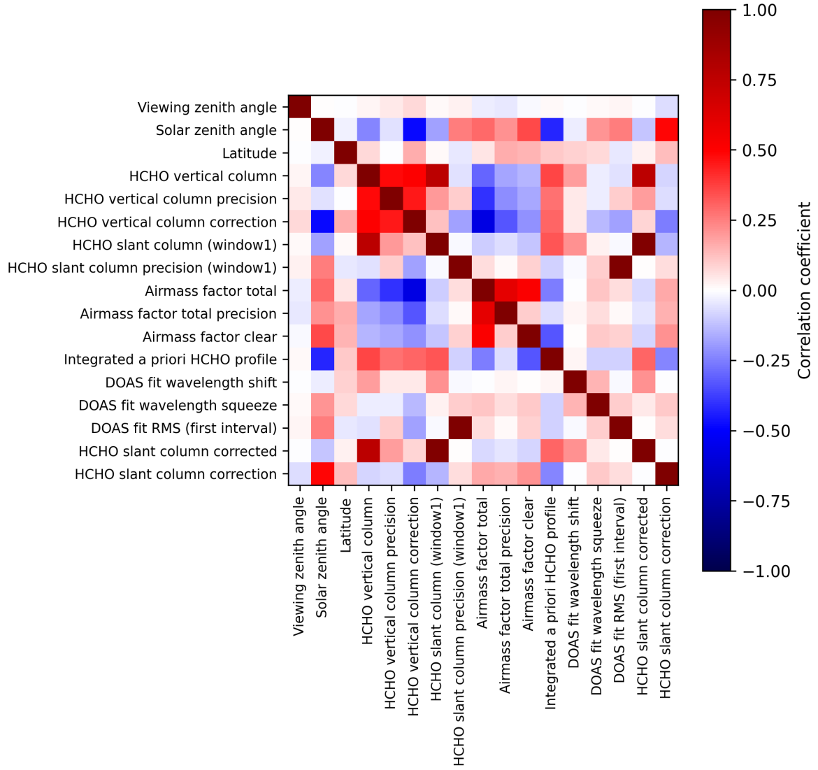
Figure 2: Map of correlation matrix for 2024-08-29 to 2024-08-31.
