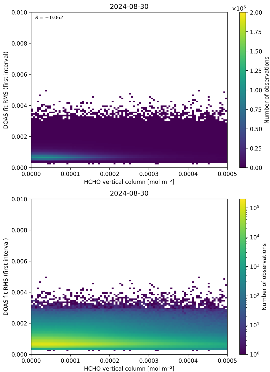
Figure 123: Scatter density plot of “HCHO vertical column” against “DOAS fit RMS (first interval)” for 2024-08-29 to 2024-08-31.
