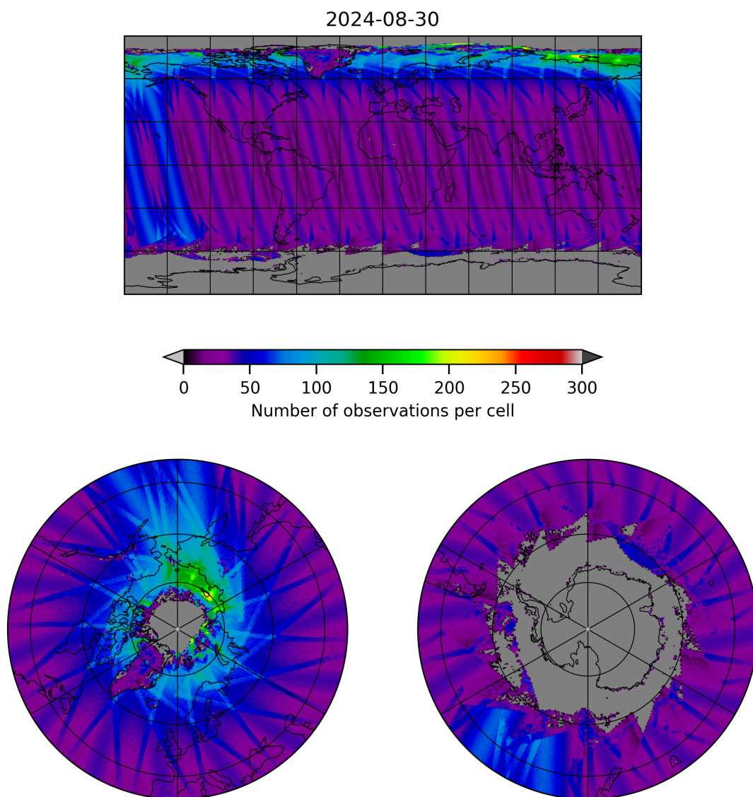
Figure 19: Map of the number of observations for 2024-08-29 to 2024-08-31
