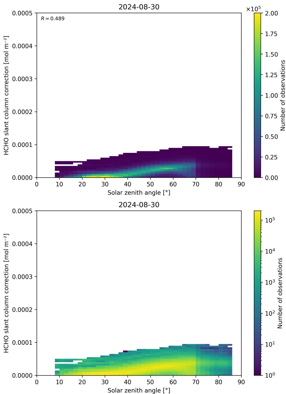
Figure 172: Scatter density plot of “Solar zenith angle” against “HCHO slant column correction” for 2024-08-29 to 2024-08-31.
