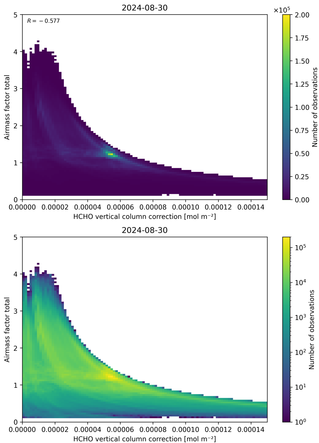
Figure 120: Scatter density plot of “HCHO vertical column correction” against “Airmass factor total” for 2024-08-29 to 2024-08-31.
