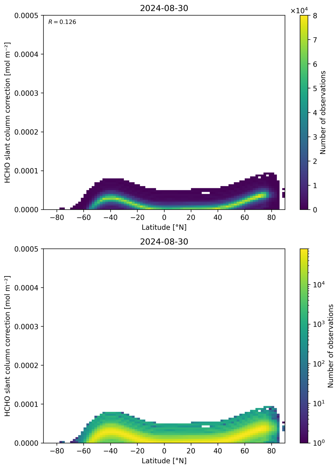
Figure 158: Scatter density plot of “Latitude” against “HCHO slant column correction” for 2024-08-29 to 2024-08-31.
