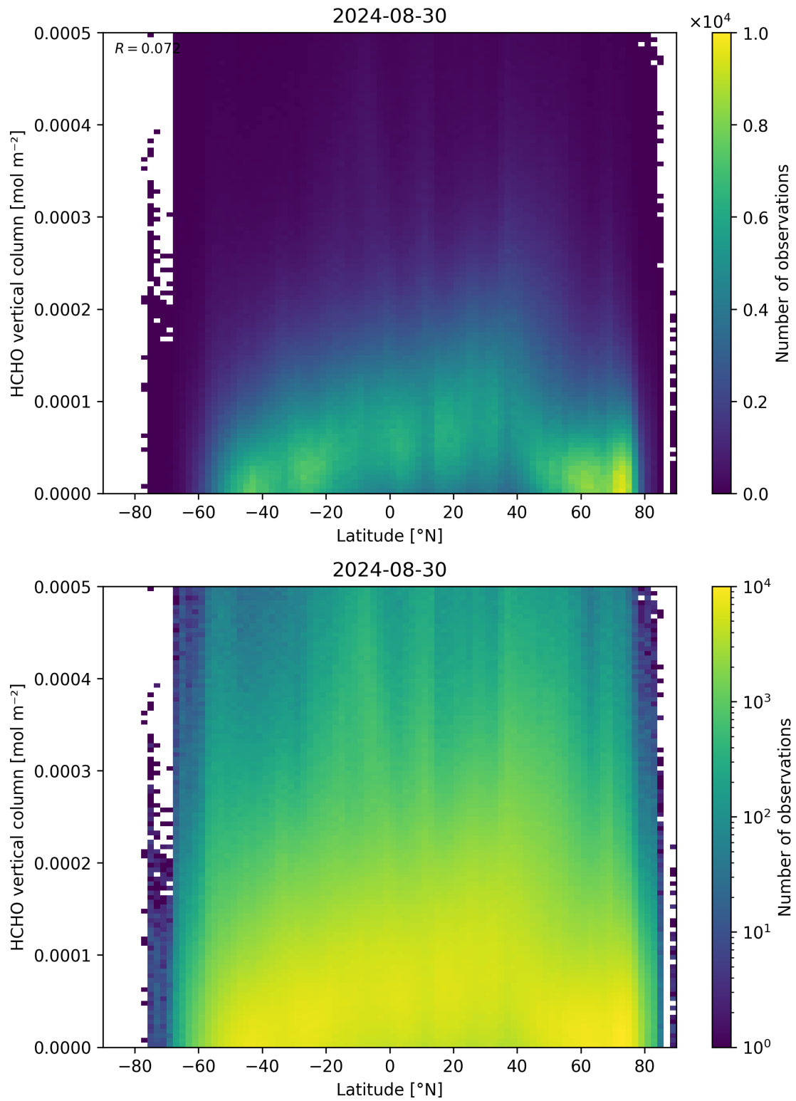
Figure 163: Scatter density plot of “Latitude” against “HCHO vertical column” for 2024-08-29 to 2024-08-31.
