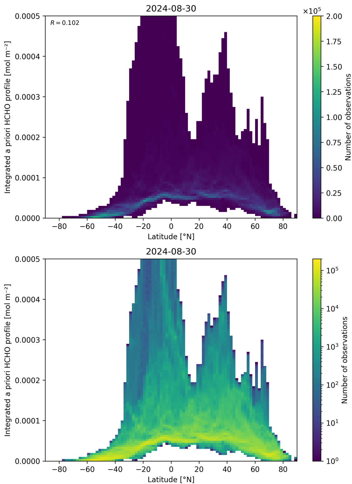
Figure 166: Scatter density plot of “Latitude” against “Integrated a priori HCHO profile” for 2024-08-29 to 2024-08-31.
