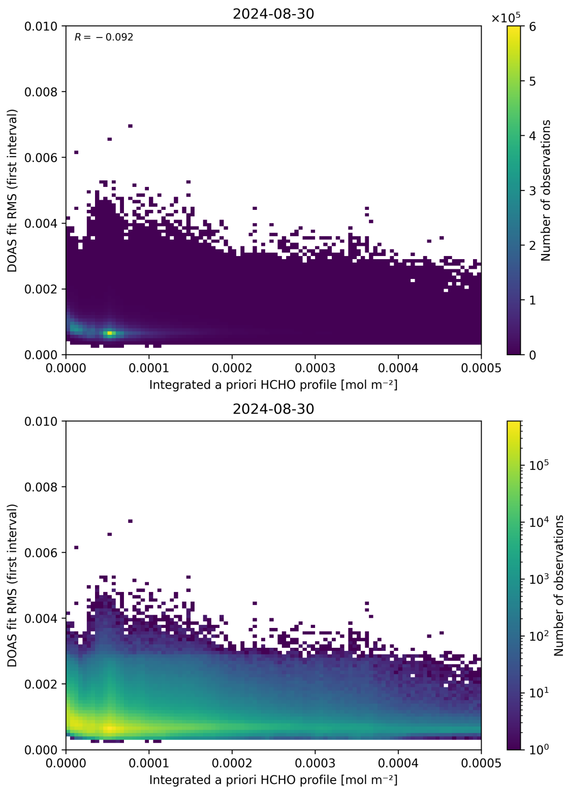
Figure 148: Scatter density plot of “Integrated a priori HCHO profile” against “DOAS fit RMS (first interval)” for 2024-08-29 to 2024-08-31.
