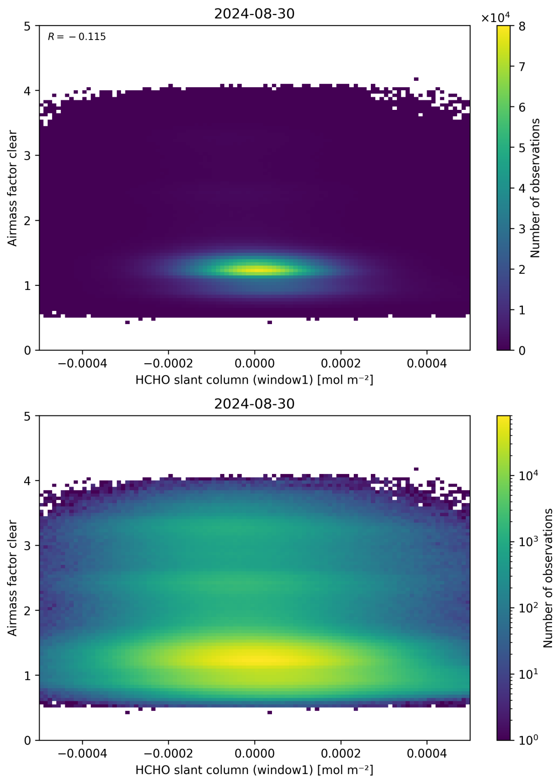
Figure 81: Scatter density plot of “HCHO slant column (window1)” against “Airmass factor clear” for 2024-08-29 to 2024-08-31.
