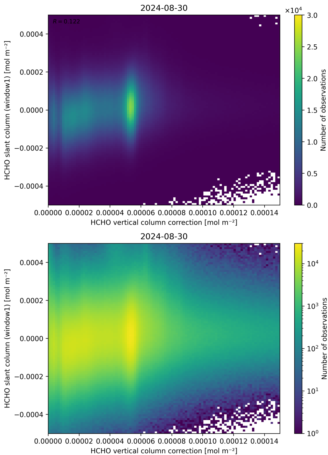
Figure 118: Scatter density plot of “HCHO vertical column correction” against “HCHO slant column (window1)” for 2024-08-29 to 2024-08-31.
