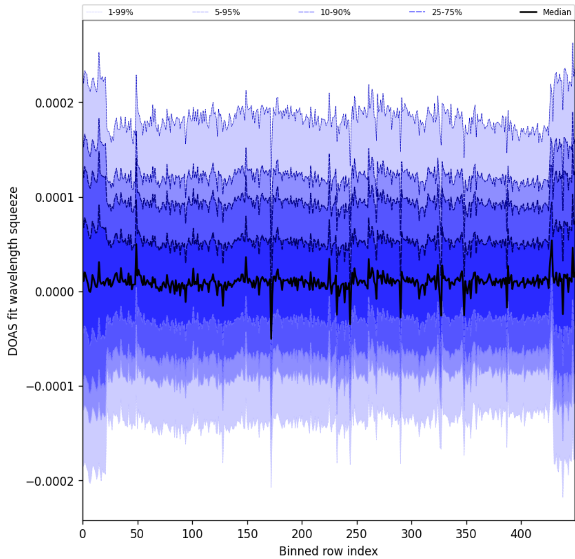
Figure 59: Along track statistics of “DOAS fit wavelength squeeze” for 2024-08-29 to 2024-08-31
