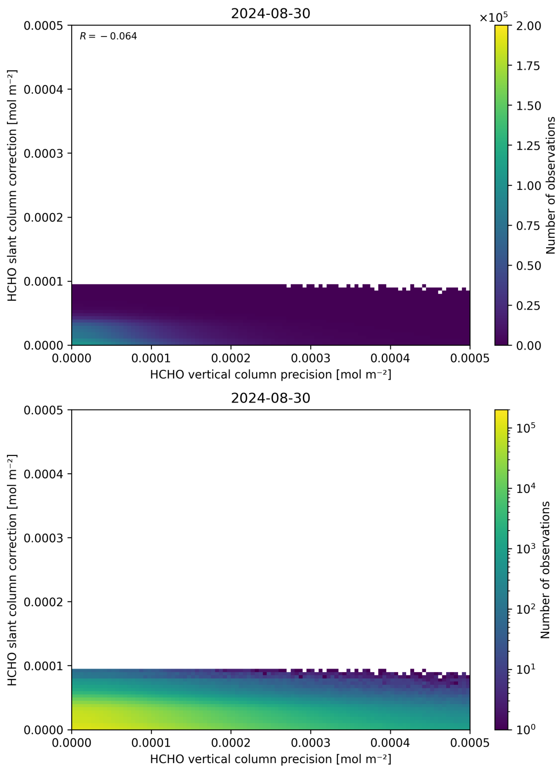
Figure 141: Scatter density plot of “HCHO vertical column precision” against “HCHO slant column correction” for 2024-08-29 to 2024-08-31.
