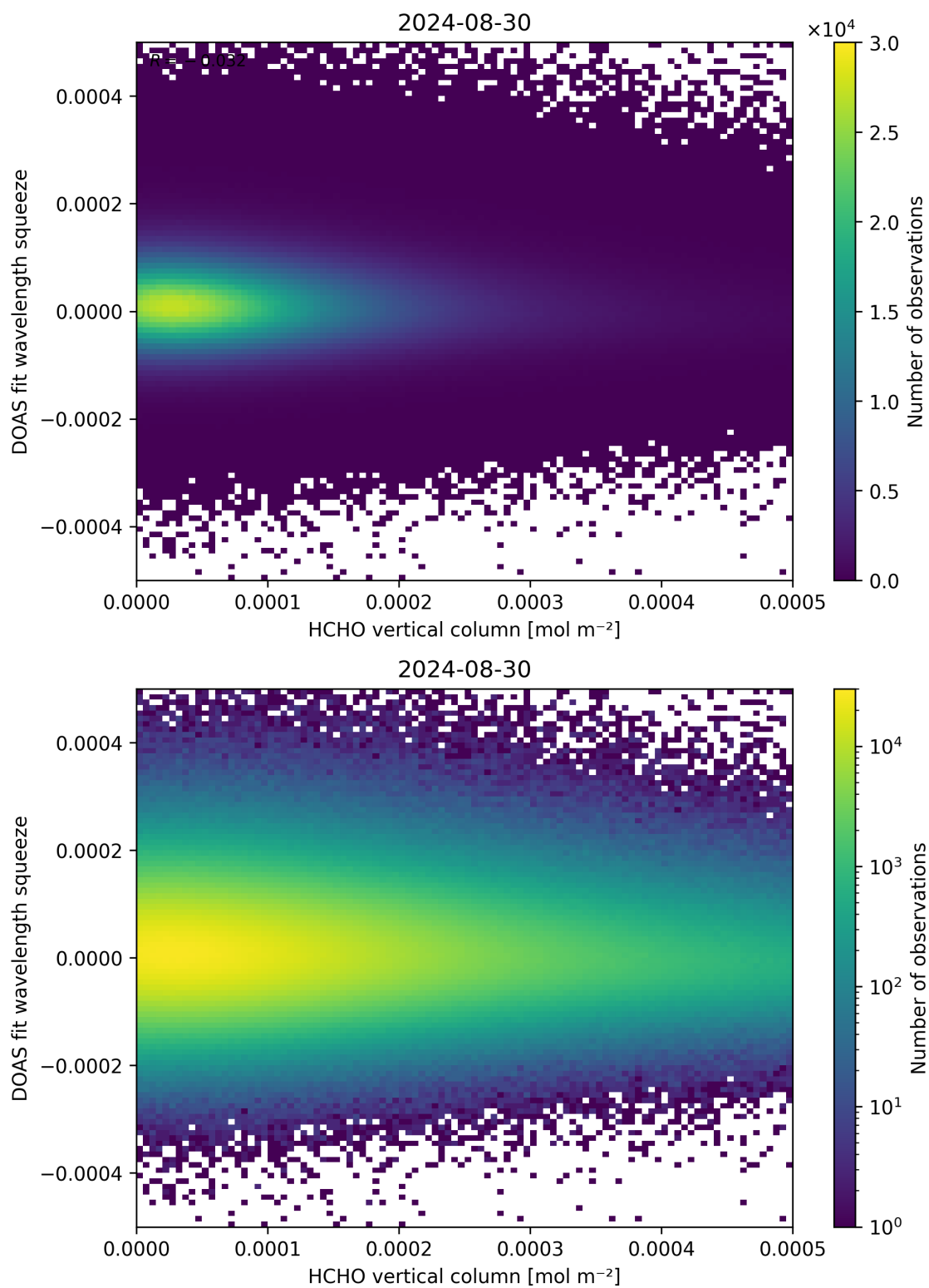
Figure 125: Scatter density plot of “HCHO vertical column” against “DOAS fit wavelength squeeze” for 2024-08-29 to 2024-08-31.
