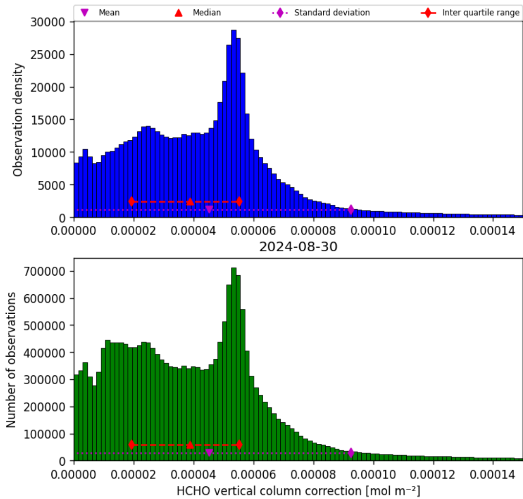
Figure 37: Histogram of “HCHO vertical column correction” for 2024-08-29 to 2024-08-31
