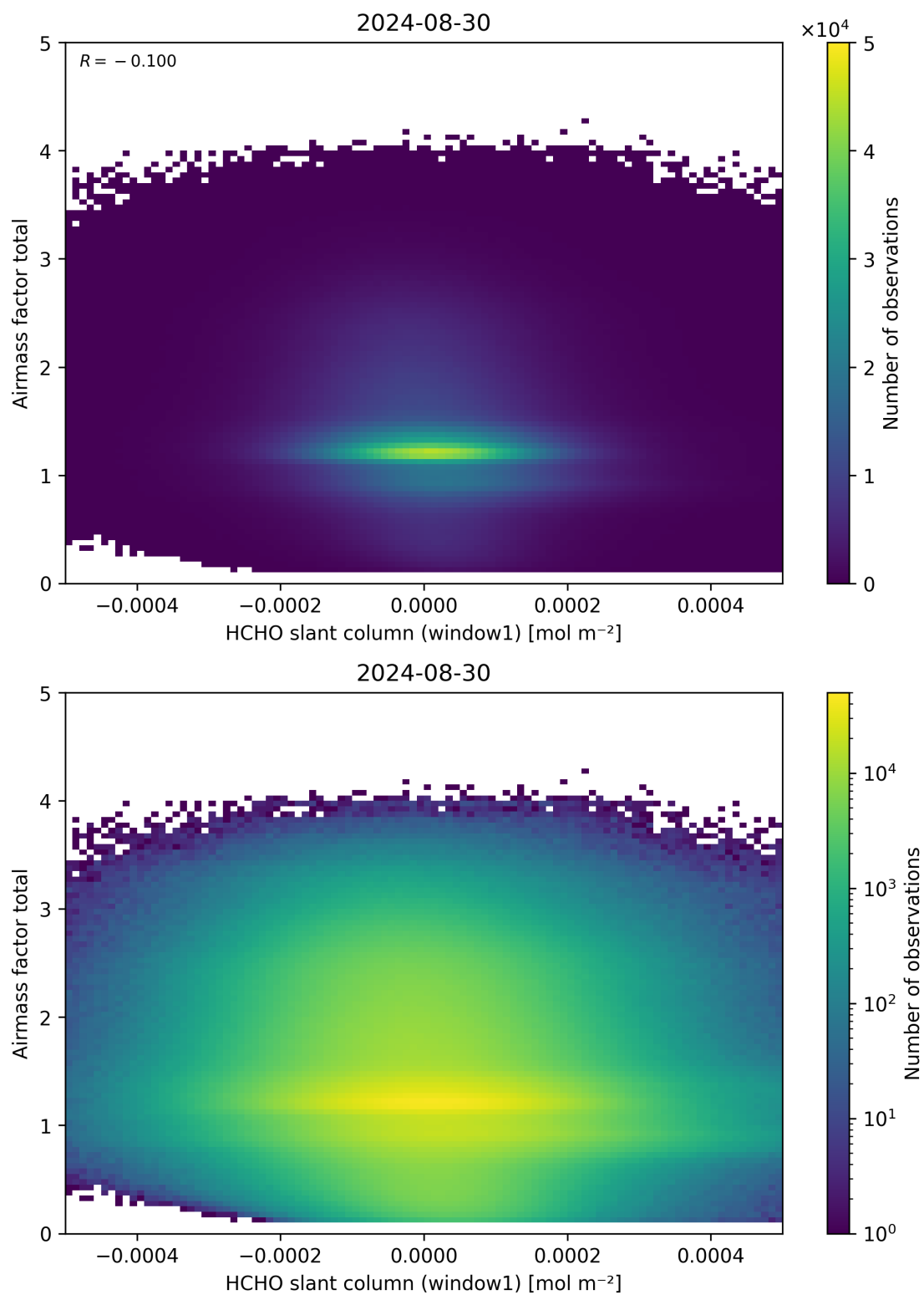
Figure 85: Scatter density plot of “HCHO slant column (window1)” against “Airmass factor total” for 2024-08-29 to 2024-08-31.
