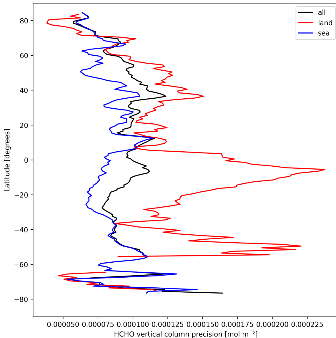
Figure 22: Zonal average of “HCHO vertical column precision” for 2024-08-29 to 2024-08-31.
