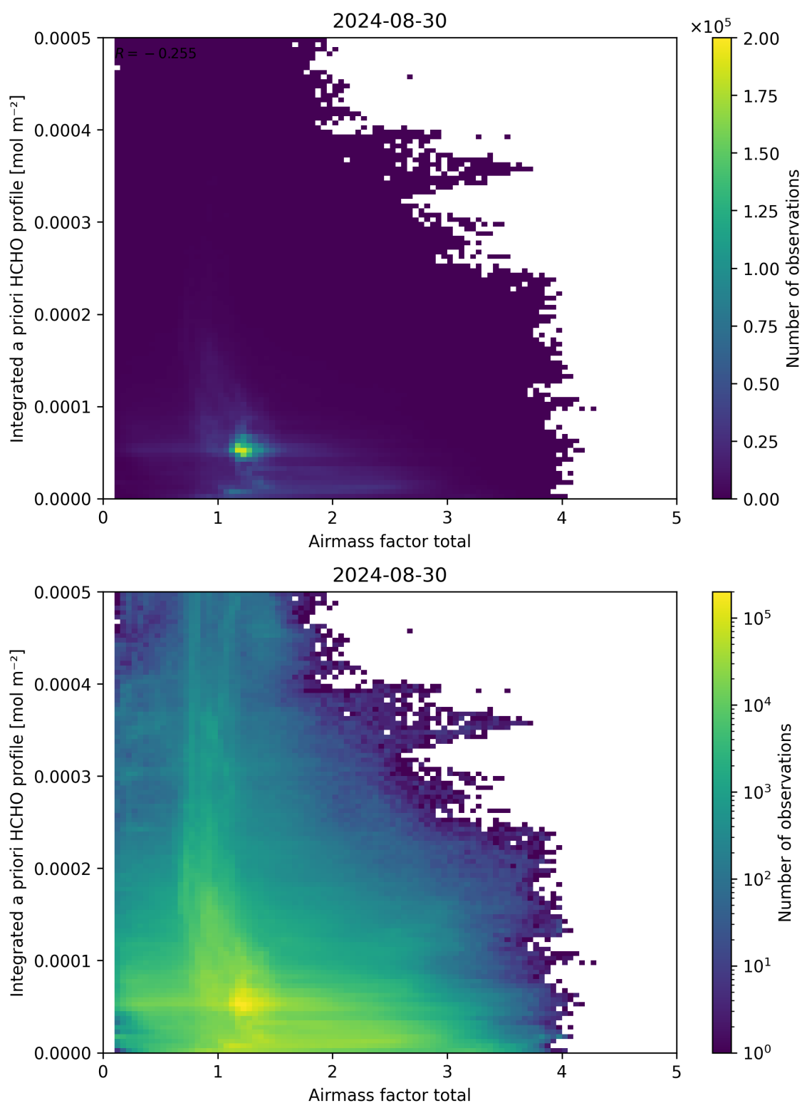
Figure 104: Scatter density plot of “Airmass factor total” against “Integrated a priori HCHO profile” for 2024-08-29 to 2024-08-31.
