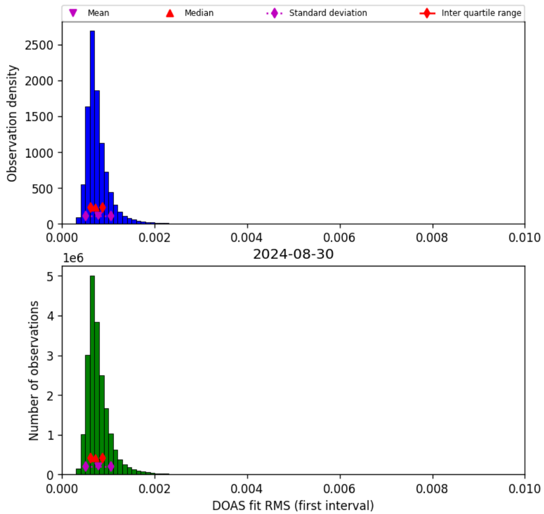
Figure 46: Histogram of “DOAS fit RMS (first interval)” for 2024-08-29 to 2024-08-31
