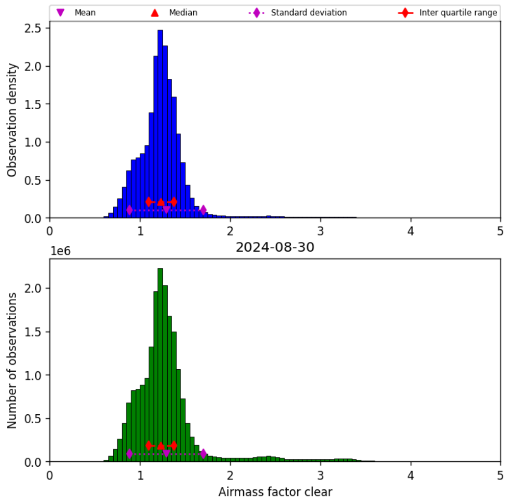
Figure 42: Histogram of “Airmass factor clear” for 2024-08-29 to 2024-08-31
