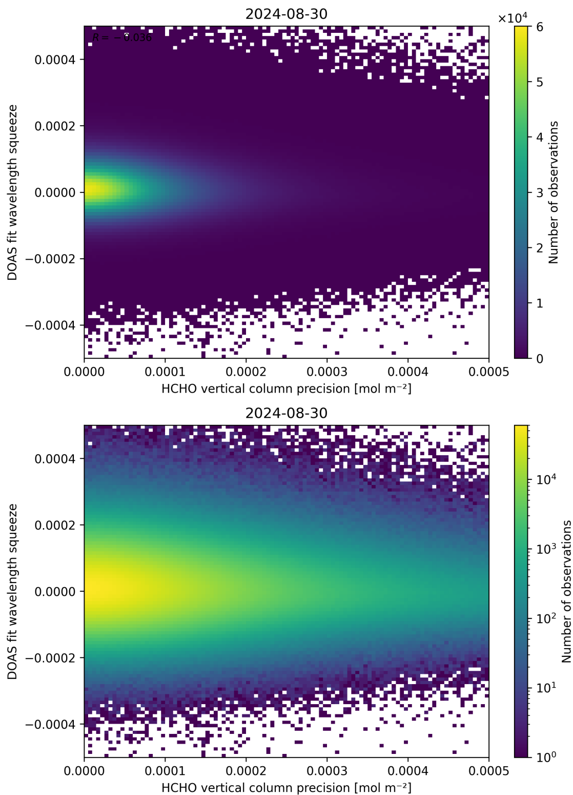
Figure 138: Scatter density plot of “HCHO vertical column precision” against “DOAS fit wavelength squeeze” for 2024-08-29 to 2024-08-31.
