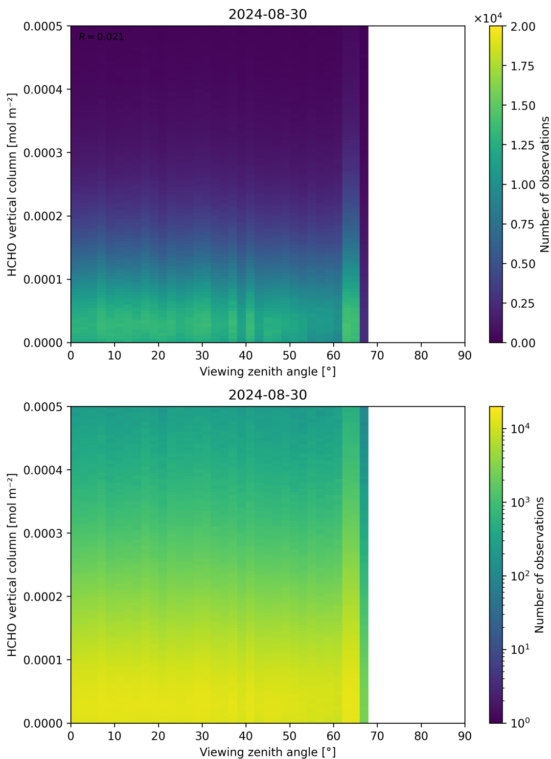
Figure 192: Scatter density plot of “Viewing zenith angle” against “HCHO vertical column” for 2024-08-29 to 2024-08-31.
