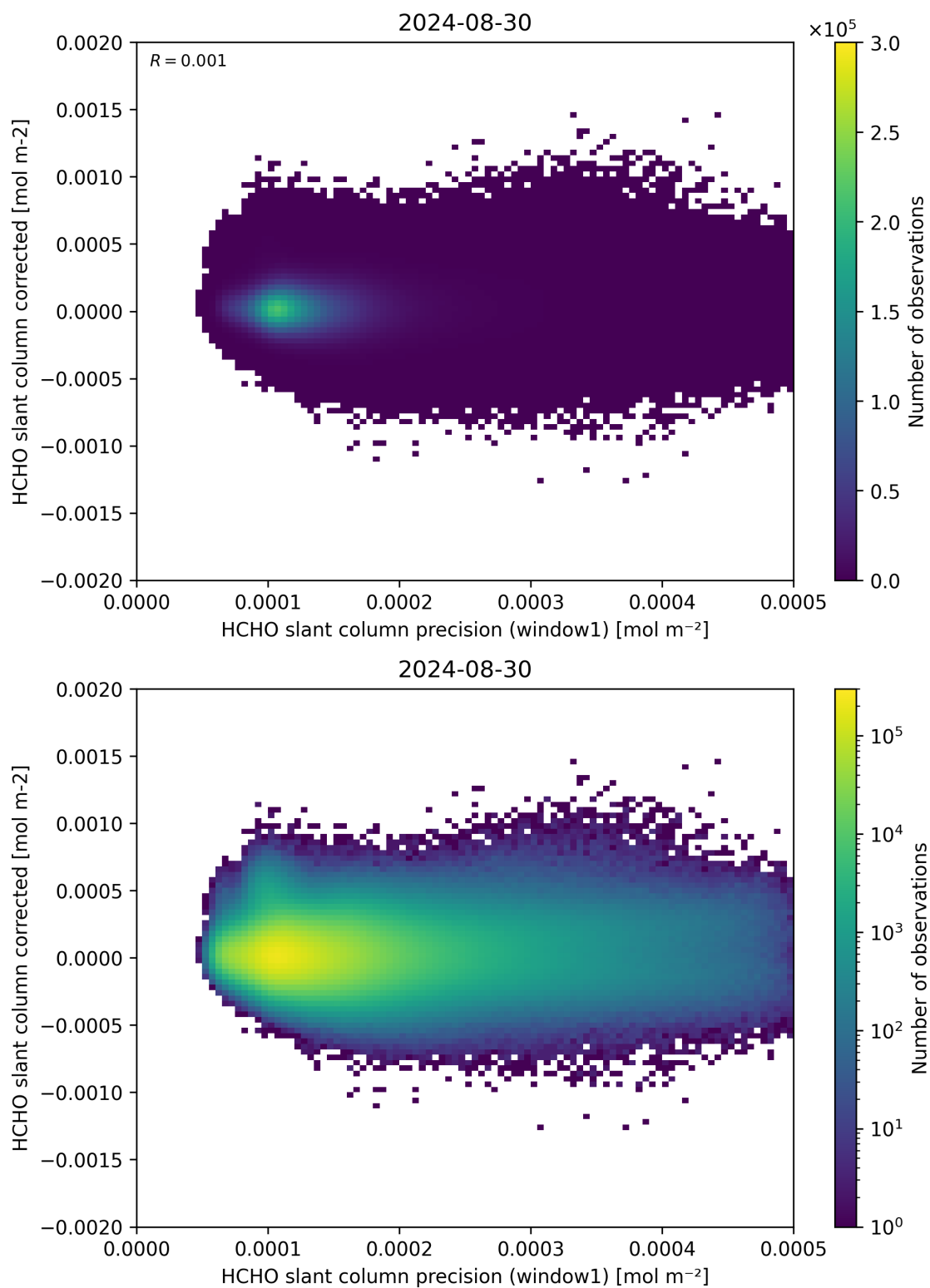
Figure 92: Scatter density plot of “HCHO slant column precision (window1)” against “HCHO slant column corrected” for 2024-08-29 to 2024-08-31.
