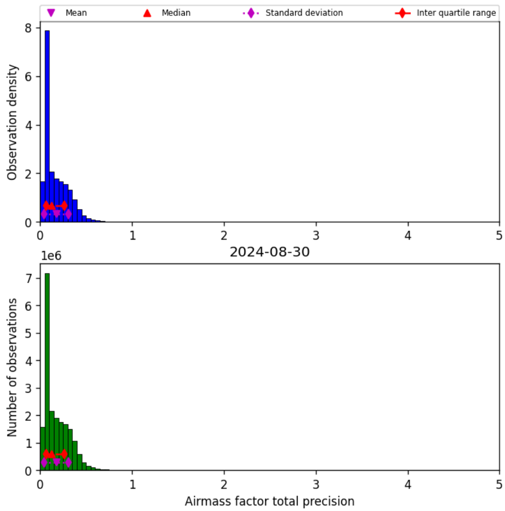
Figure 41: Histogram of “Airmass factor total precision” for 2024-08-29 to 2024-08-31
