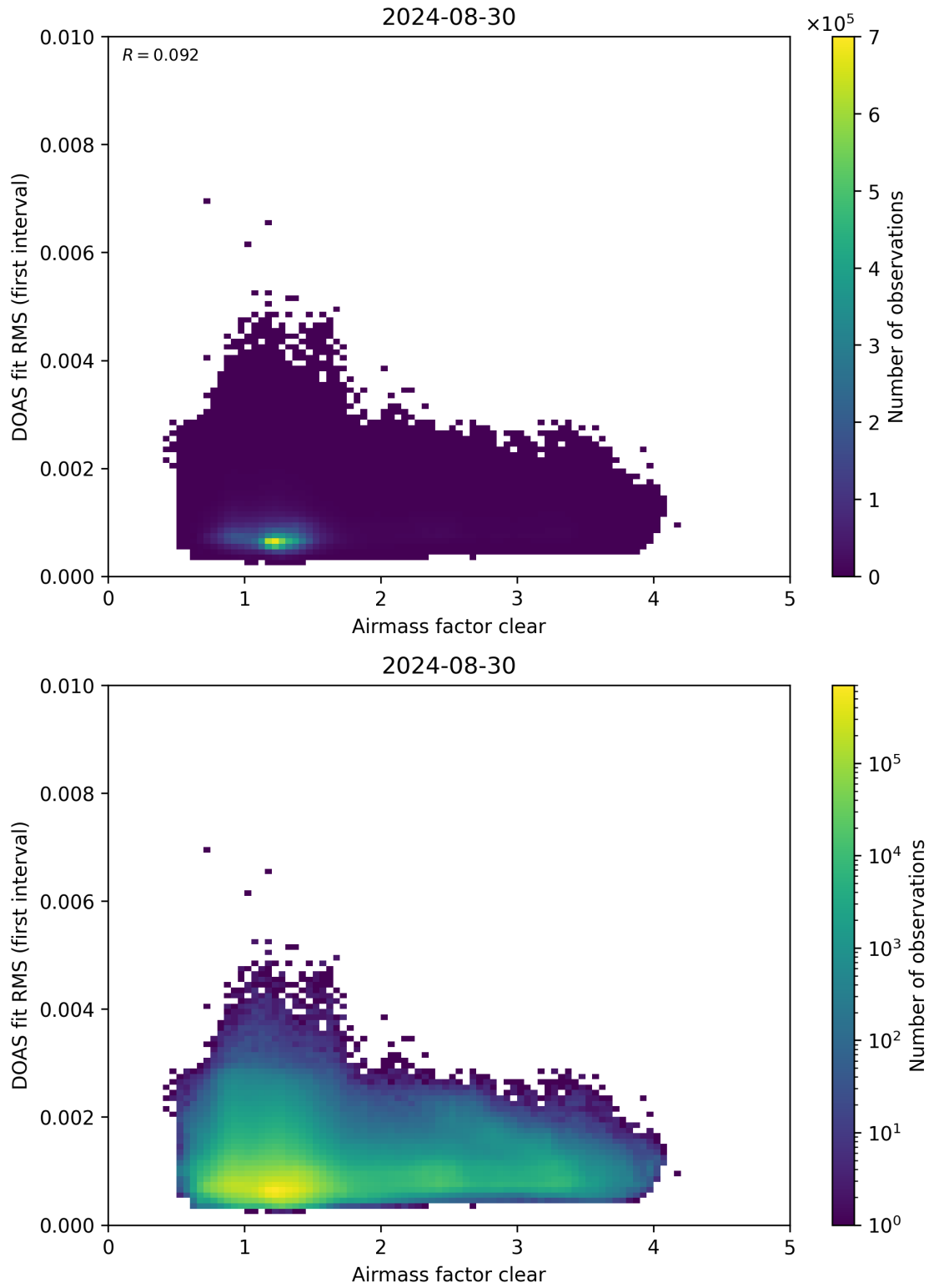
Figure 71: Scatter density plot of “Airmass factor clear” against “DOAS fit RMS (first interval)” for 2024-08-29 to 2024-08-31.
