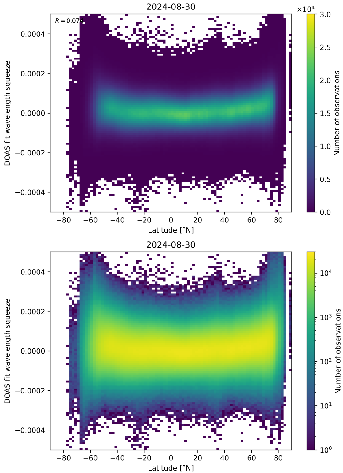
Figure 155: Scatter density plot of “Latitude” against “DOAS fit wavelength squeeze” for 2024-08-29 to 2024-08-31.
