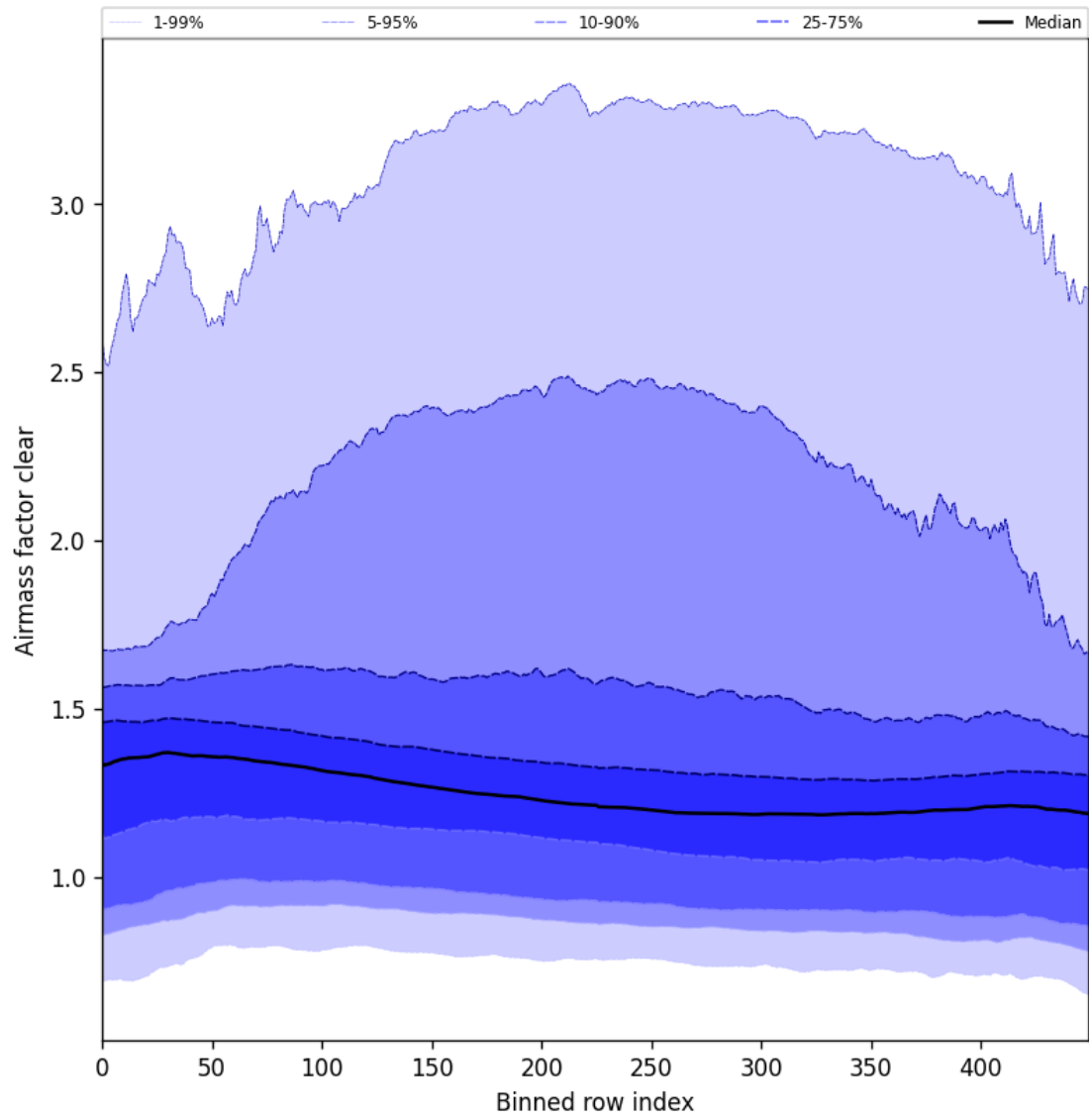
Figure 56: Along track statistics of “Air mass factor clear” for 2024-08-29 to 2024-08-31
