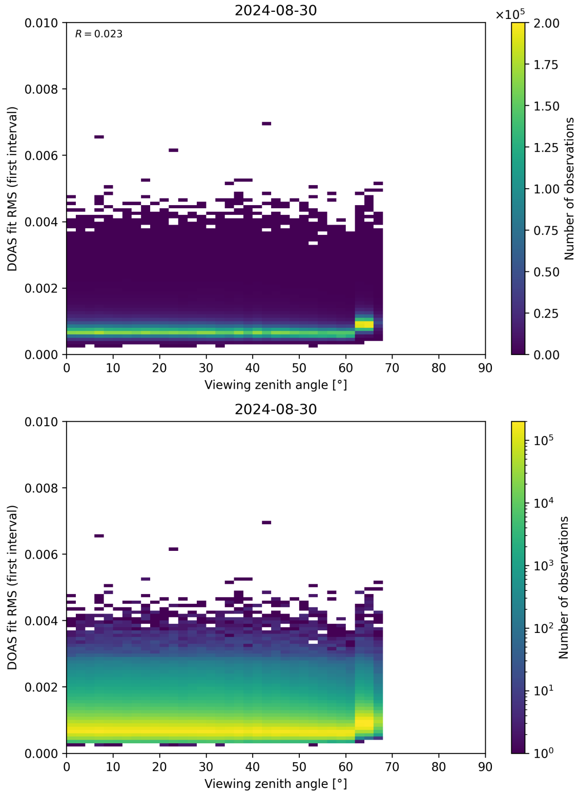
Figure 182: Scatter density plot of “Viewing zenith angle” against “DOAS fit RMS (first interval)” for 2024-08-29 to 2024-08-31.
