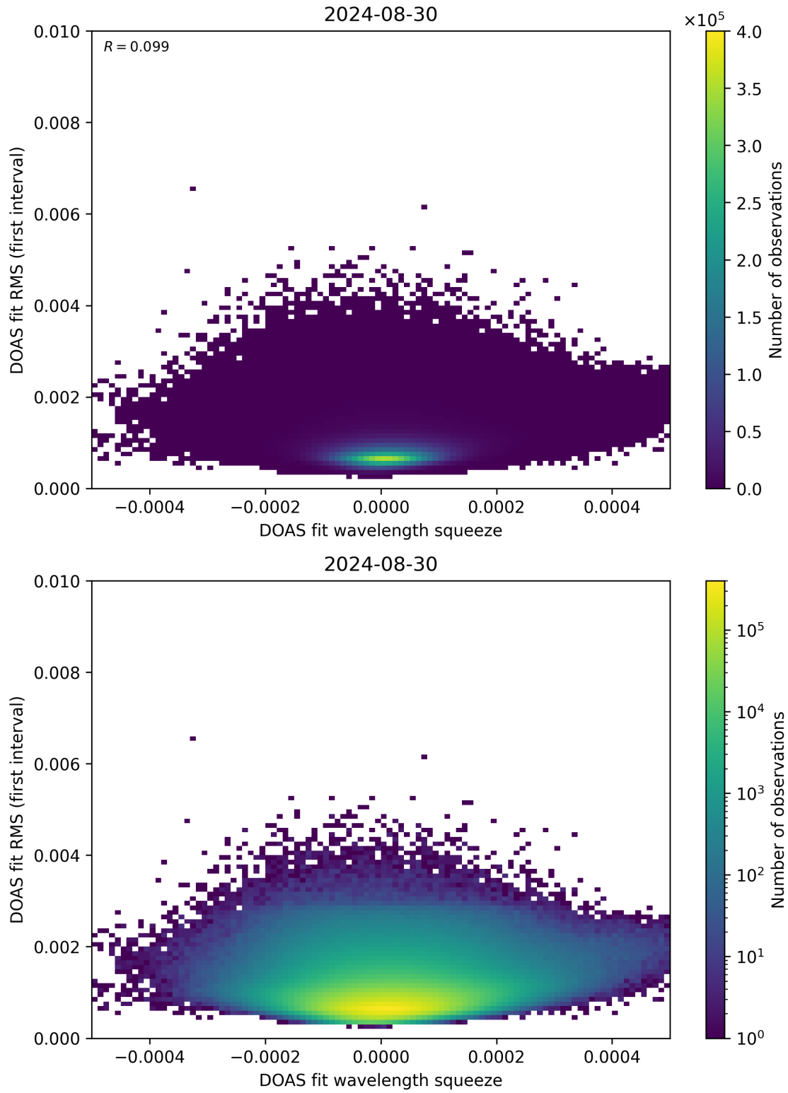
Figure 68: Scatter density plot of “DOAS fit wavelength squeeze” against “DOAS fit RMS (first interval)” for 2024-08-29 to 2024-08-31.
