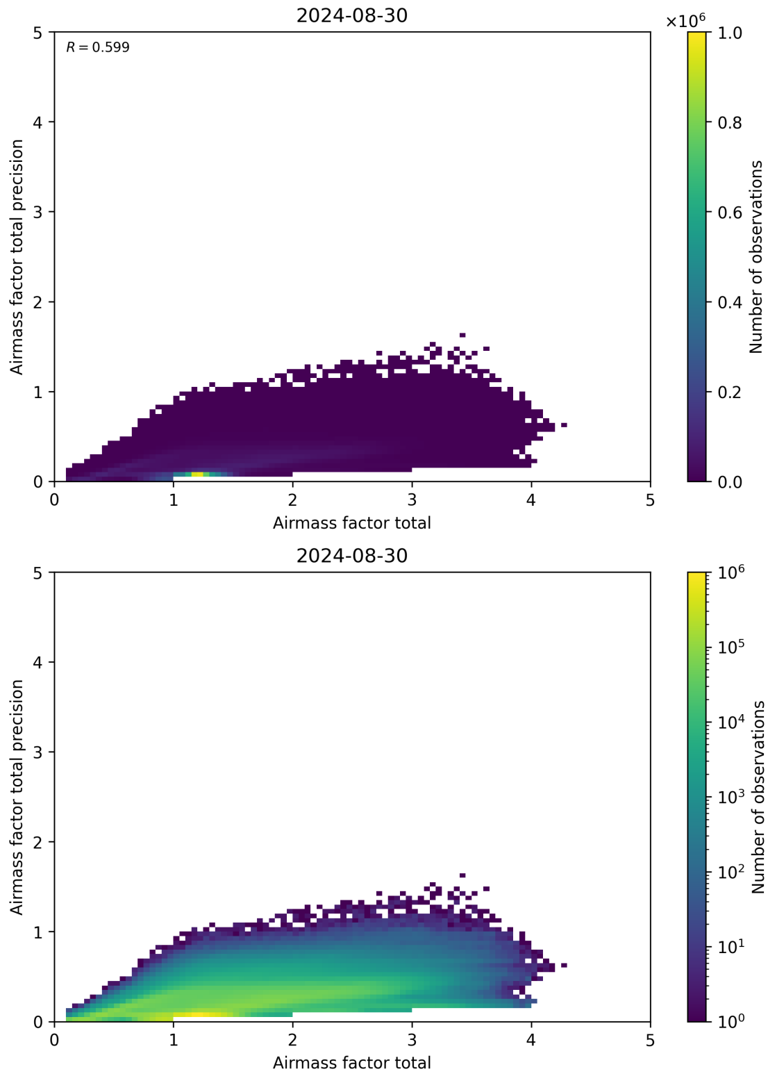
Figure 103: Scatter density plot of “Airmass factor total” against “Airmass factor total precision” for 2024-08-29 to 2024-08-31.
