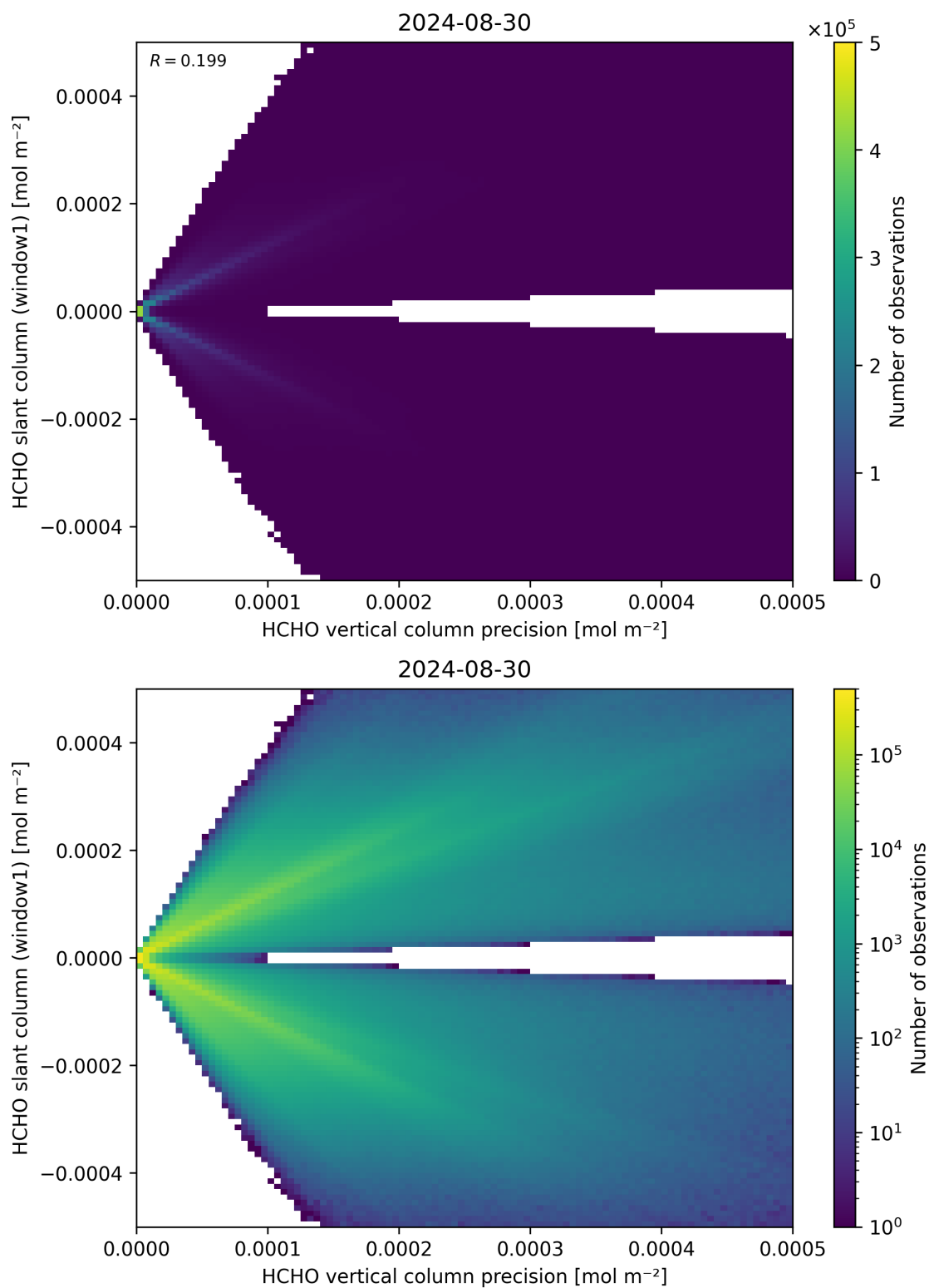
Figure 142: Scatter density plot of “HCHO vertical column precision” against “HCHO slant column (window1)” for 2024-08-29 to 2024-08-31.
