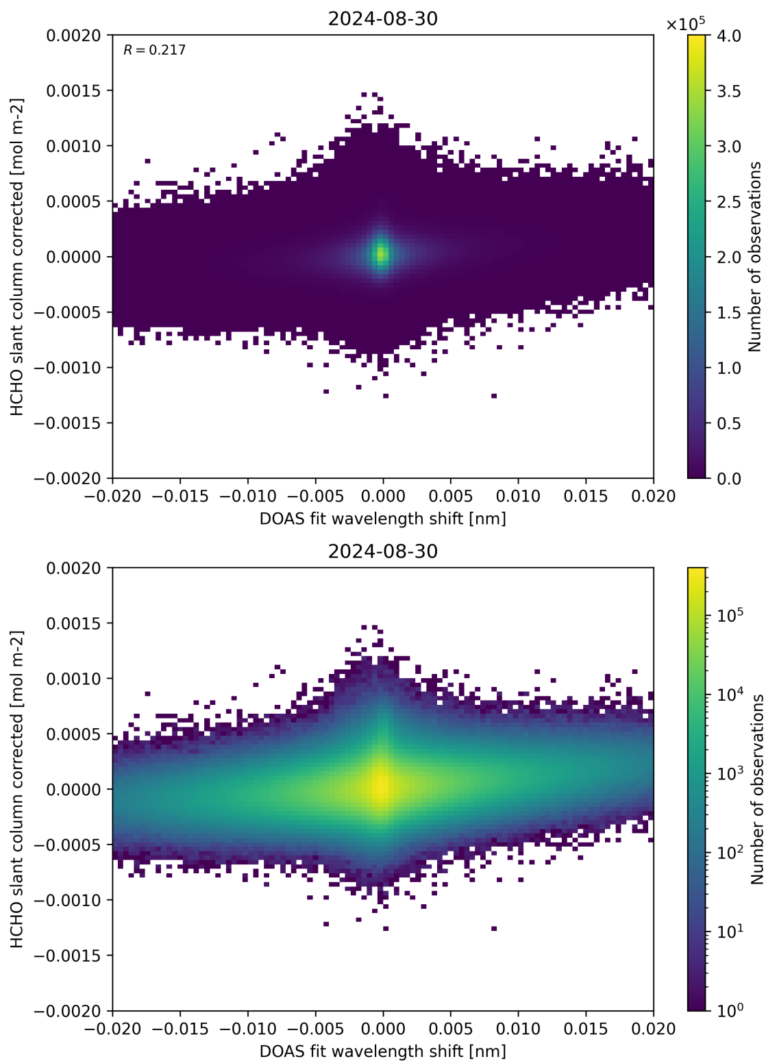
Figure 66: Scatter density plot of “DOAS fit wavelength shift” against “HCHO slant column corrected” for 2024-08-29 to 2024-08-31.
