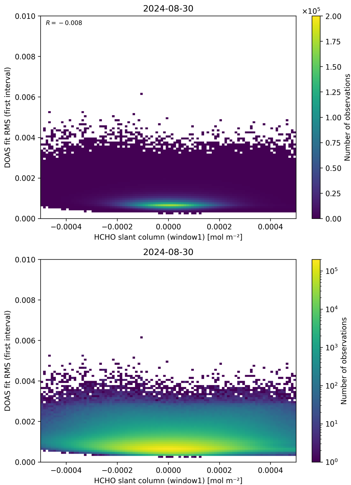
Figure 78: Scatter density plot of “HCHO slant column (window1)” against “DOAS fit RMS (first interval)” for 2024-08-29 to 2024-08-31.
