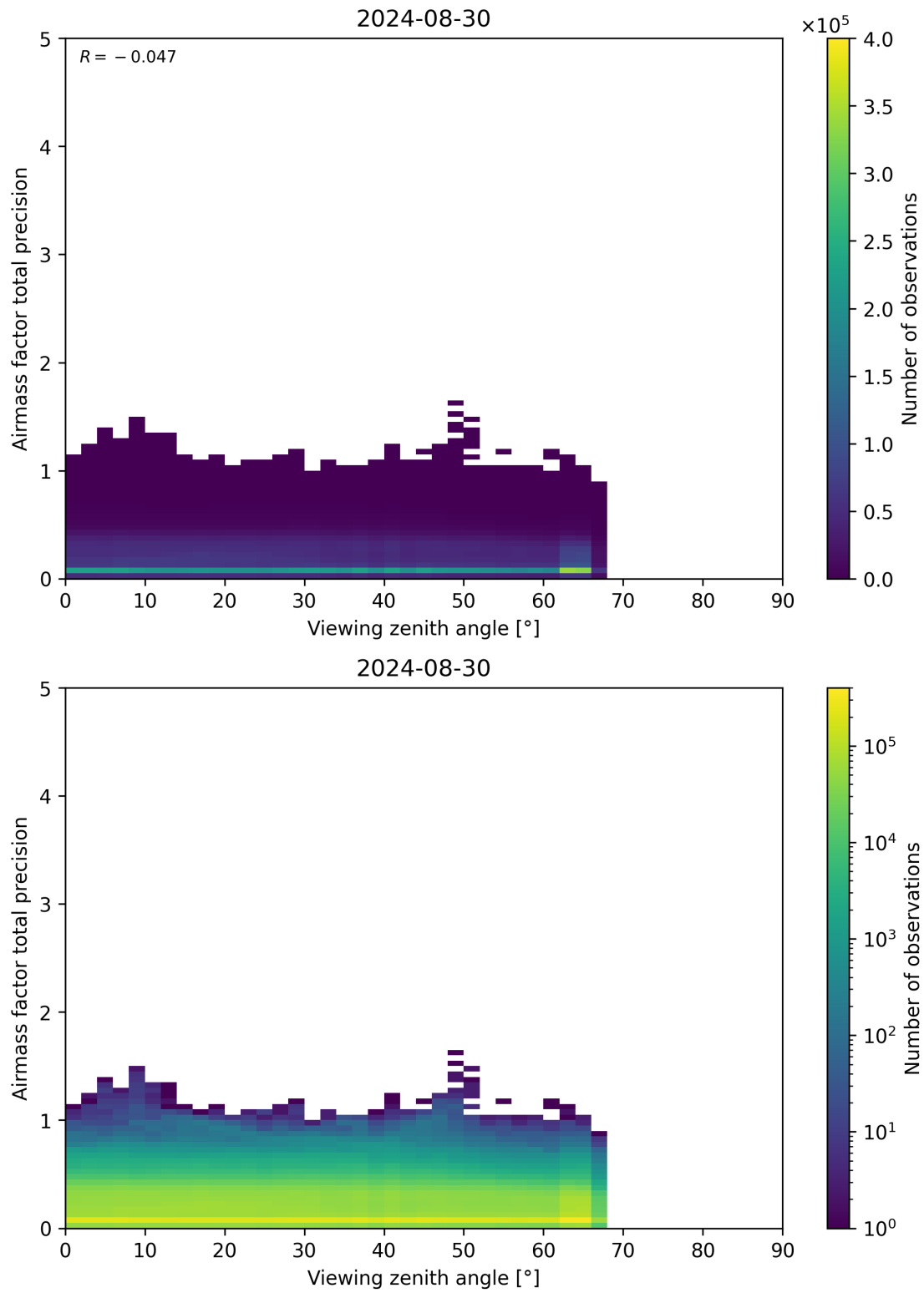
Figure 191: Scatter density plot of “Viewing zenith angle” against “Airmass factor total precision” for 2024-08-29 to 2024-08-31.
