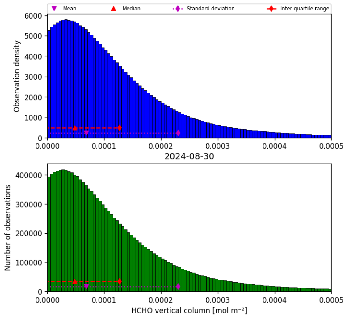
Figure 35: Histogram of “HCHO vertical column” for 2024-08-29 to 2024-08-31
