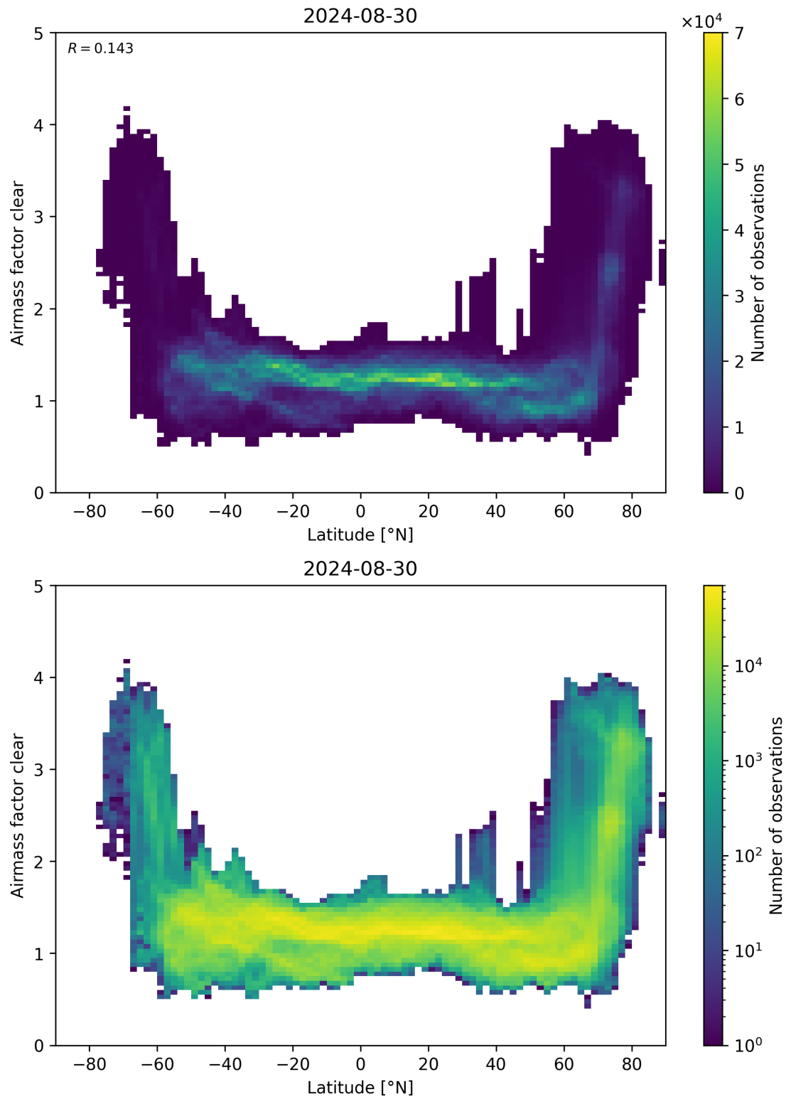
Figure 156: Scatter density plot of “Latitude” against “Airmass factor clear” for 2024-08-29 to 2024-08-31.
