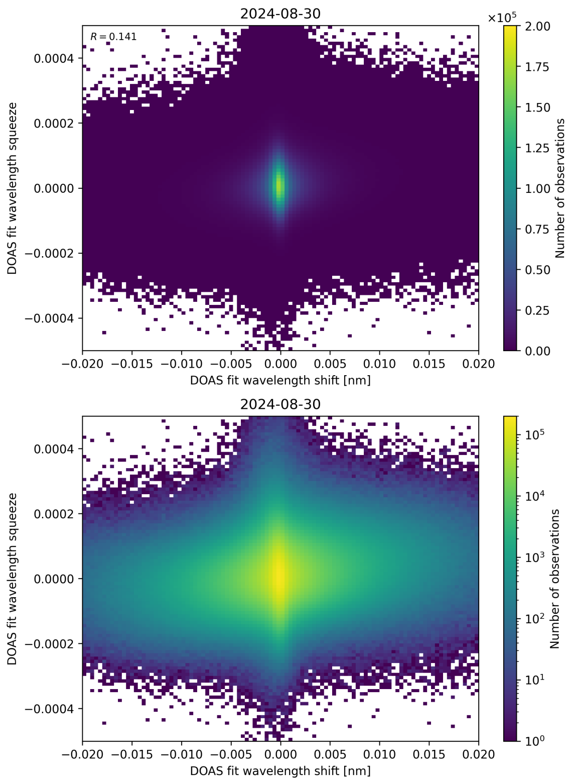
Figure 65: Scatter density plot of “DOAS fit wavelength shift” against “DOAS fit wavelength squeeze” for 2024-08-29 to 2024-08-31.
