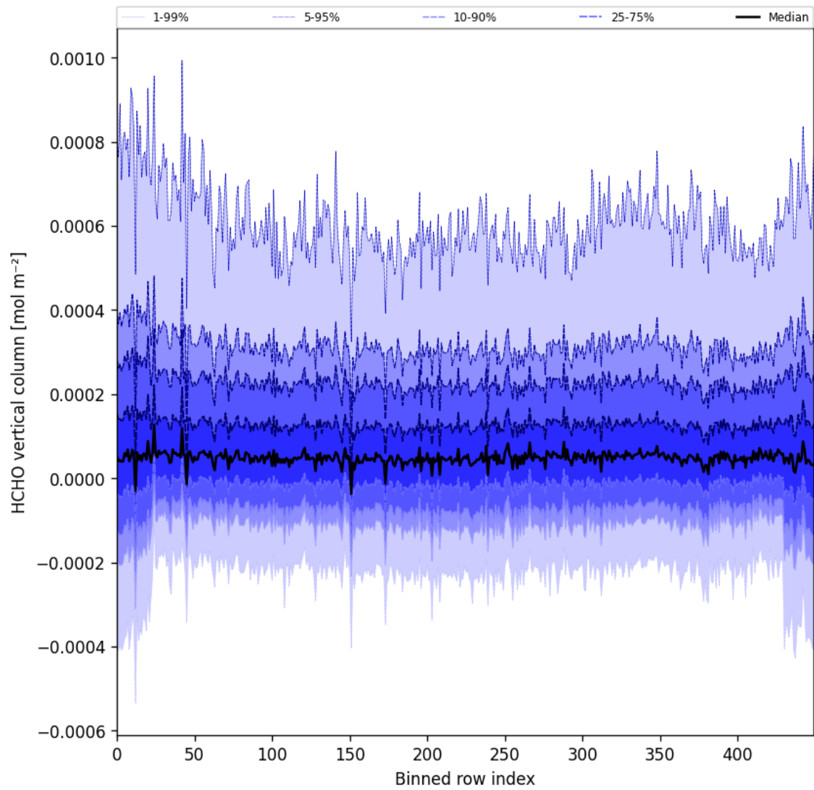
Figure 49: Along track statistics of “HCHO vertical column” for 2024-08-29 to 2024-08-31
