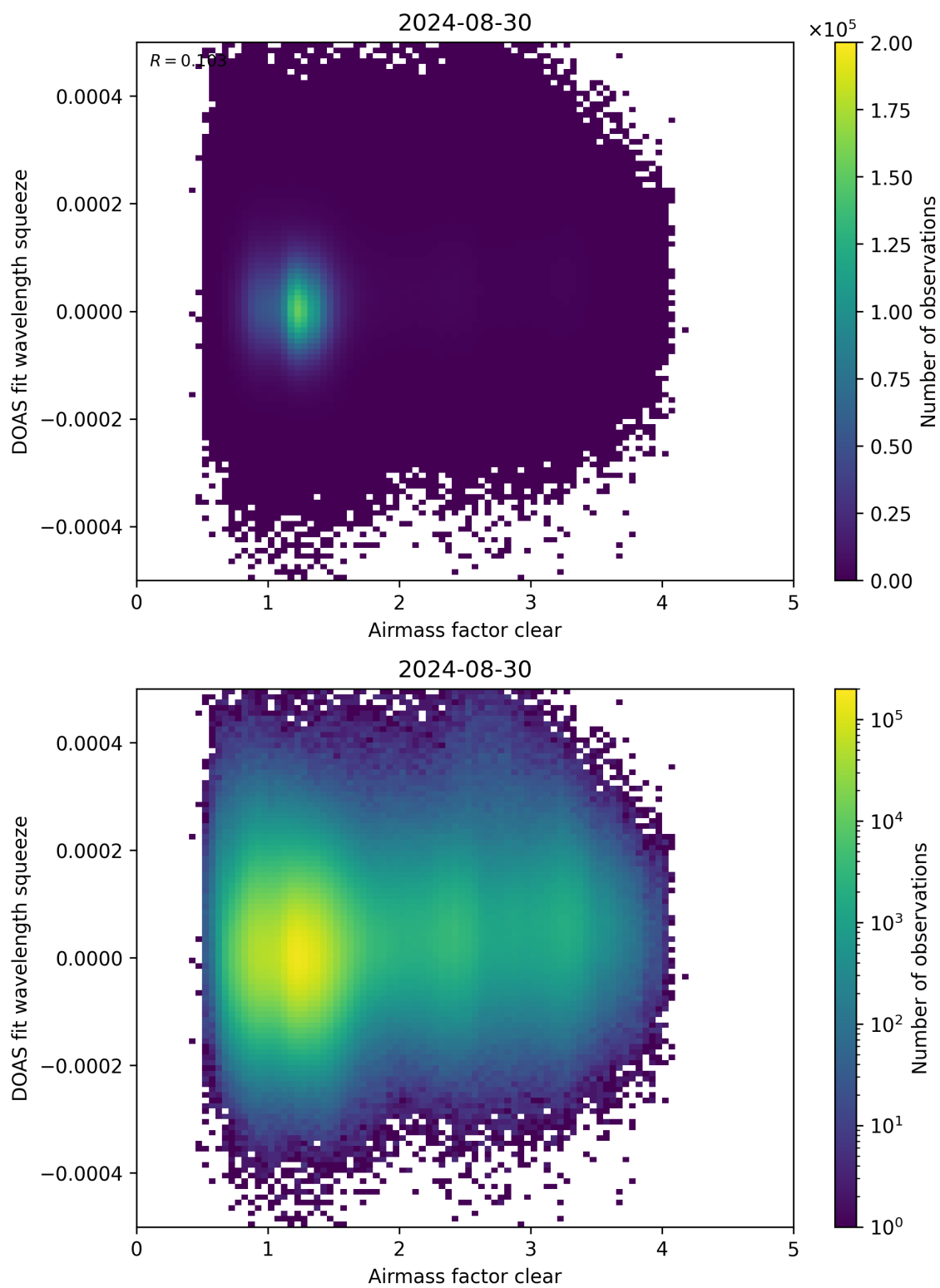
Figure 73: Scatter density plot of “Airmass factor clear” against “DOAS fit wavelength squeeze” for 2024-08-29 to 2024-08-31.
