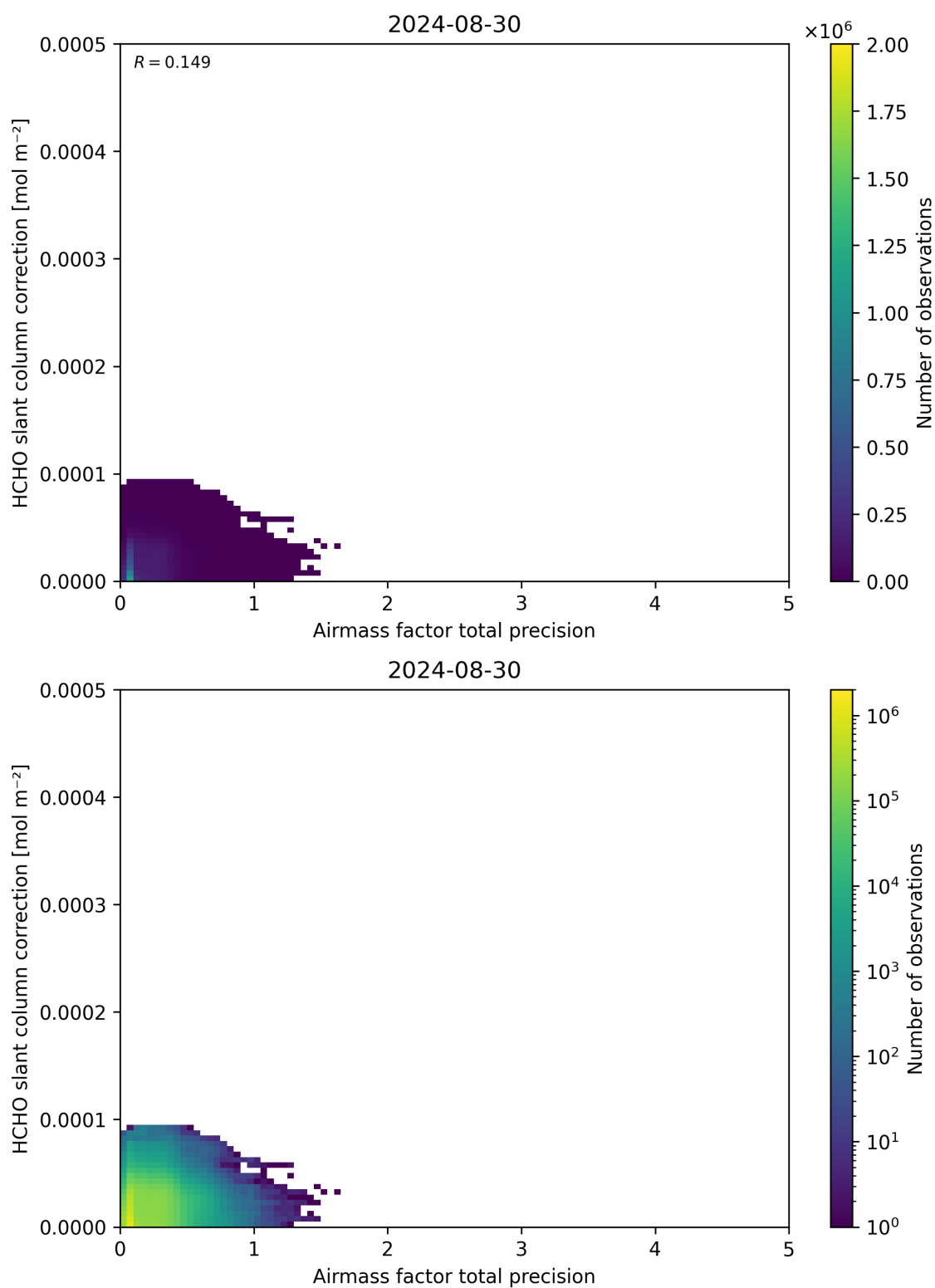
Figure 110: Scatter density plot of “Airmass factor total precision” against “HCHO slant column correction” for 2024-08-29 to 2024-08-31.
