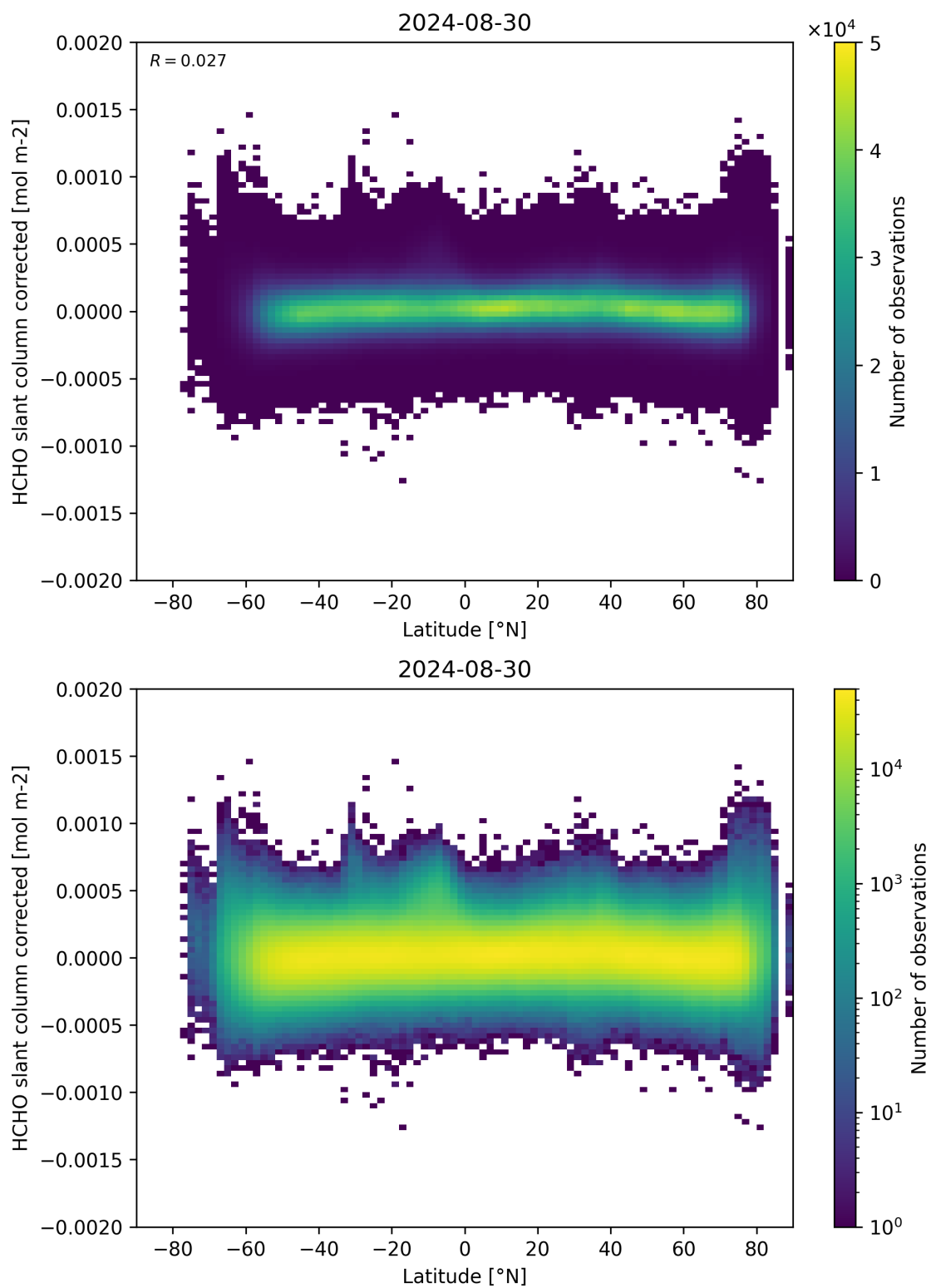
Figure 157: Scatter density plot of “Latitude” against “HCHO slant column corrected” for 2024-08-29 to 2024-08-31.
