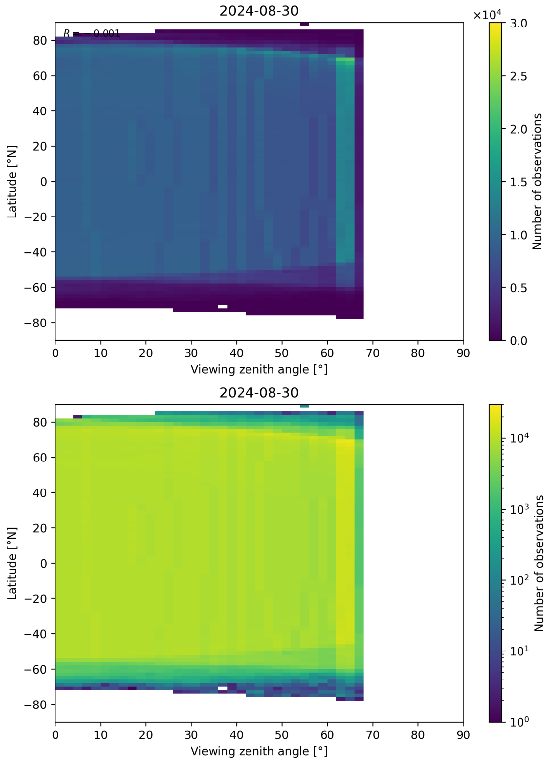
Figure 196: Scatter density plot of “Viewing zenith angle” against “Latitude” for 2024-08-29 to 2024-08-31.
