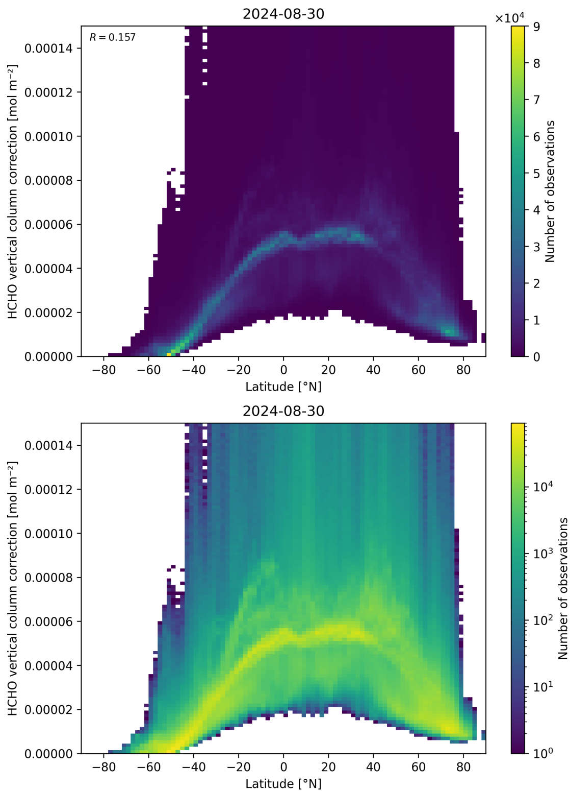
Figure 164: Scatter density plot of “Latitude” against “HCHO vertical column correction” for 2024-08-29 to 2024-08-31.
