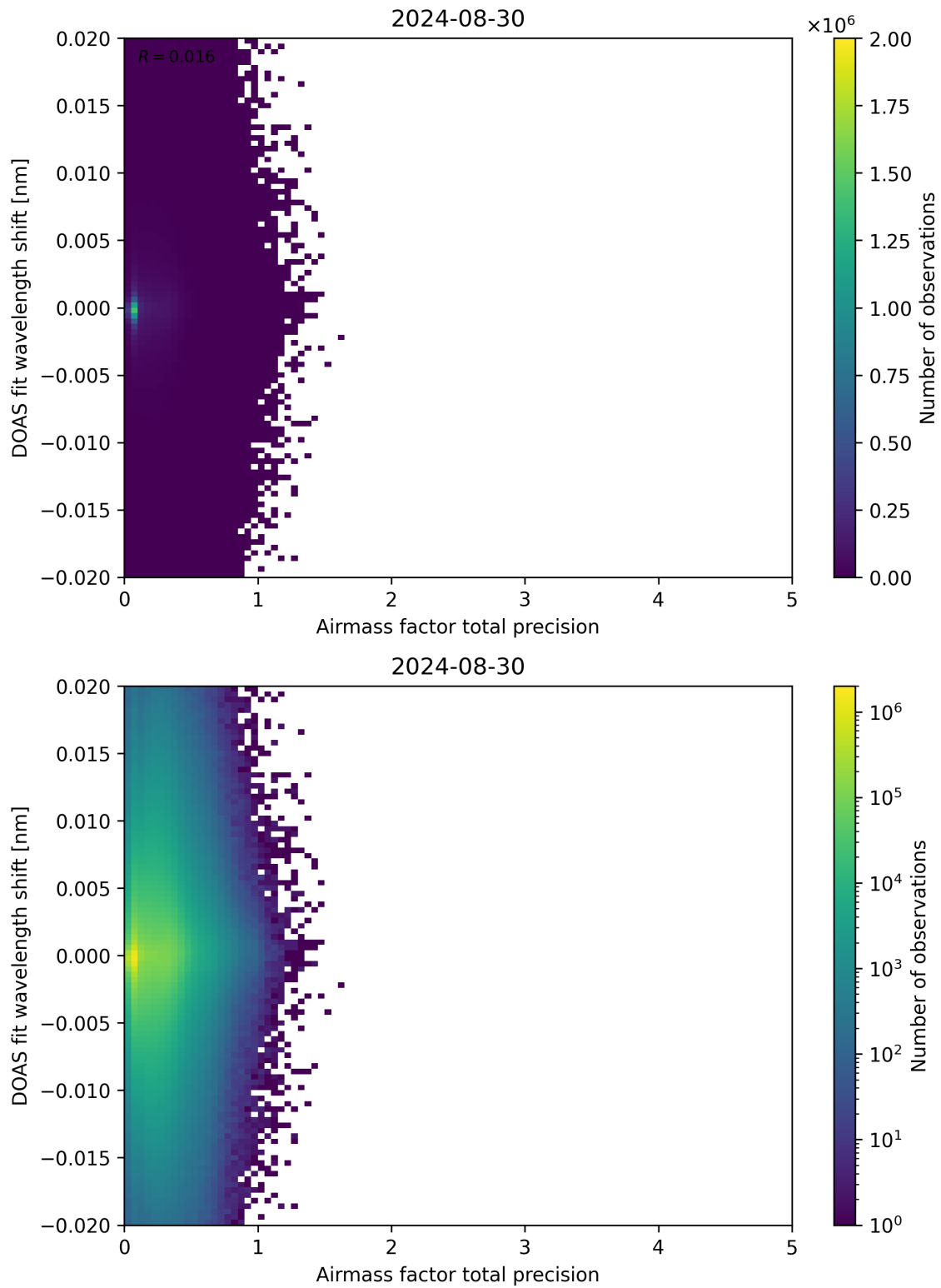
Figure 106: Scatter density plot of “Airmass factor total precision” against “DOAS fit wavelength shift” for 2024-08-29 to 2024-08-31.
