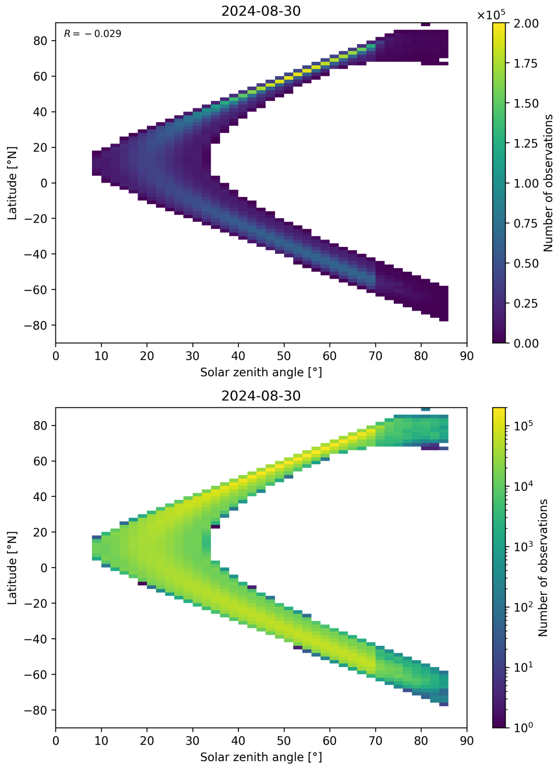
Figure 181: Scatter density plot of “Solar zenith angle” against “Latitude” for 2024-08-29 to 2024-08-31.
