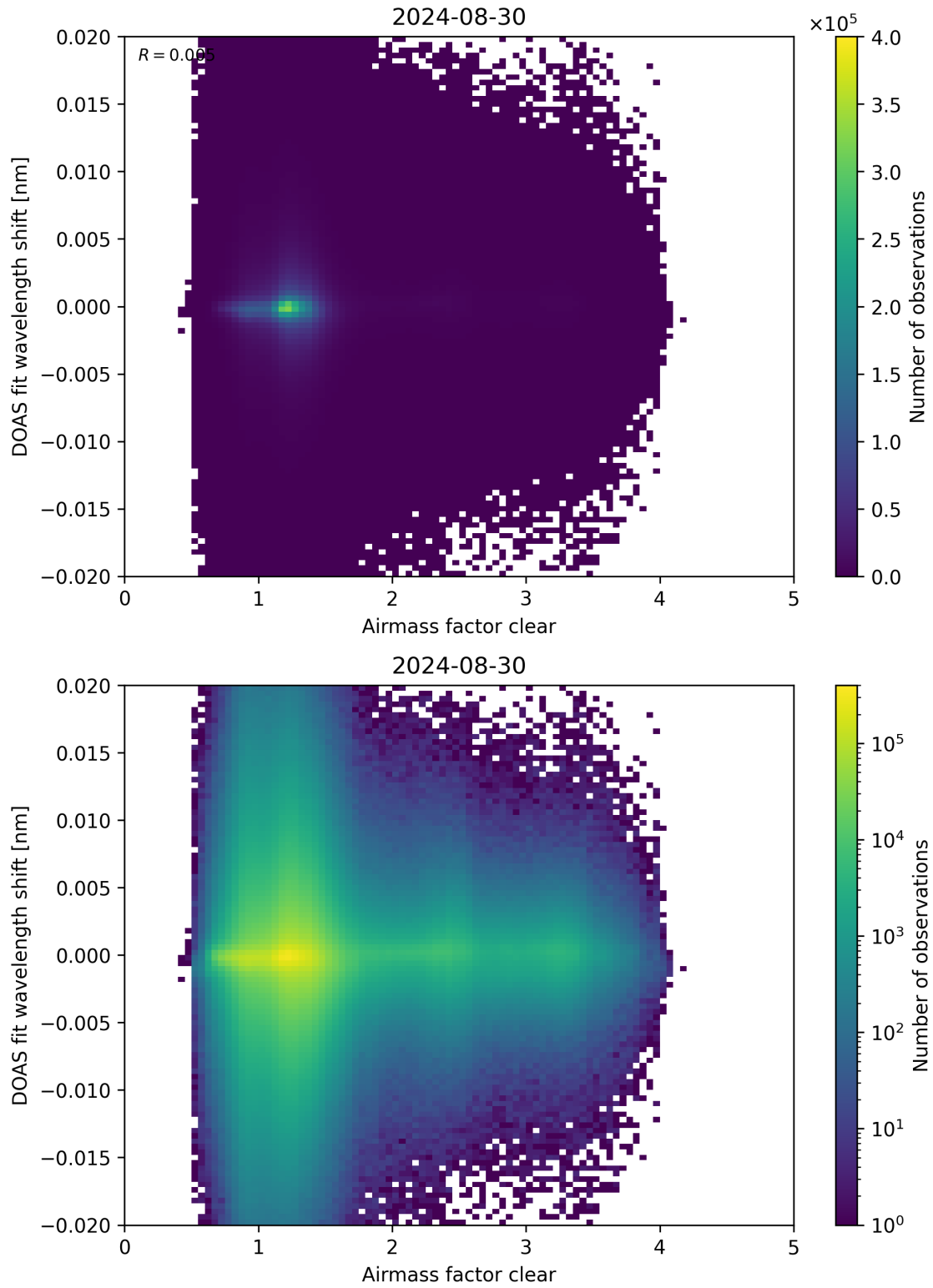
Figure 72: Scatter density plot of “Airmass factor clear” against “DOAS fit wavelength shift” for 2024-08-29 to 2024-08-31.
