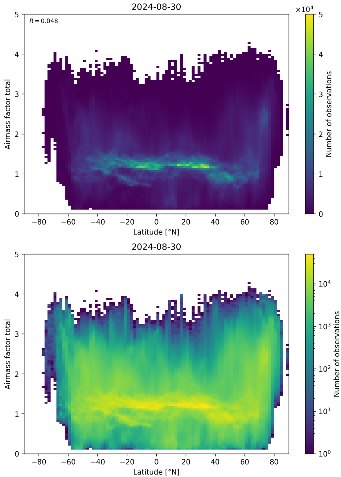
Figure 161: Scatter density plot of “Latitude” against “Airmass factor total” for 2024-08-29 to 2024-08-31.
