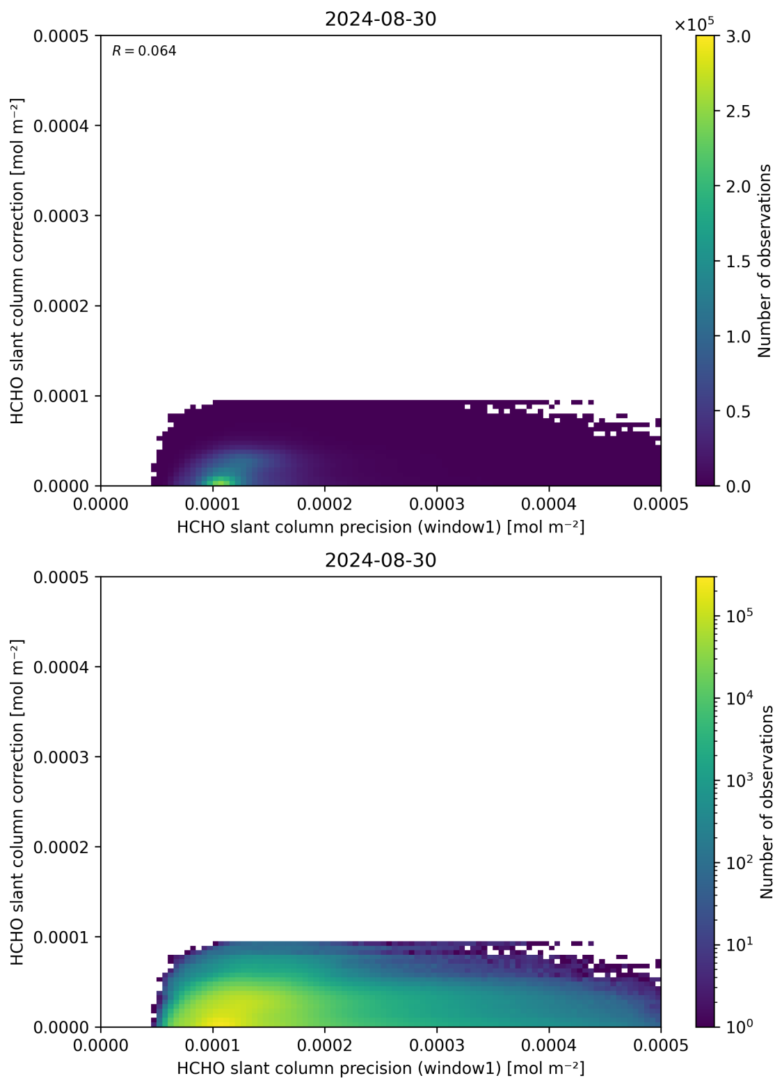
Figure 93: Scatter density plot of “HCHO slant column precision (window1)” against “HCHO slant column correction” for 2024-08-29 to 2024-08-31.
