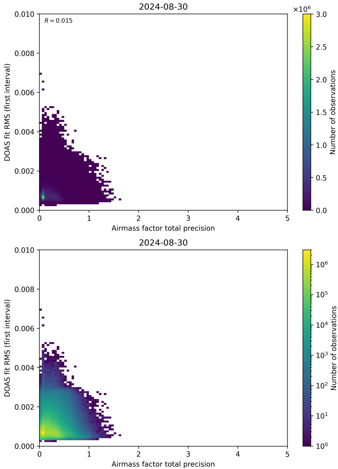
Figure 105: Scatter density plot of “Airmass factor total precision” against “DOAS fit RMS (first interval)” for 2024-08-29 to 2024-08-31.
