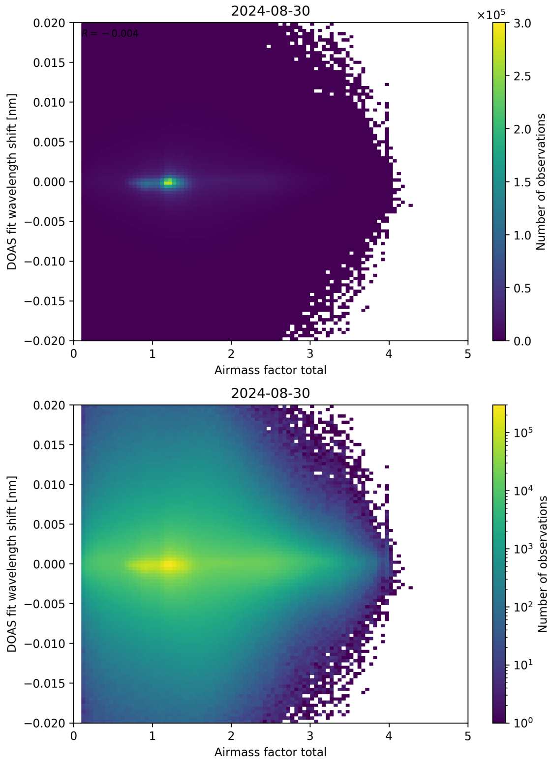
Figure 98: Scatter density plot of “Airmass factor total” against “DOAS fit wavelength shift” for 2024-08-29 to 2024-08-31.
