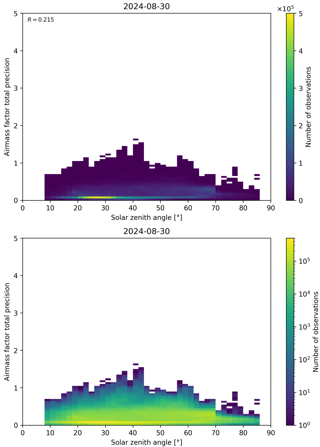
Figure 176: Scatter density plot of “Solar zenith angle” against “Airmass factor total precision” for 2024-08-29 to 2024-08-31.
