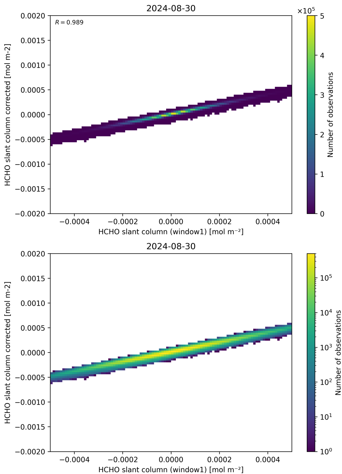
Figure 82: Scatter density plot of “HCHO slant column (window1)” against “HCHO slant column corrected” for 2024-08-29 to 2024-08-31.
