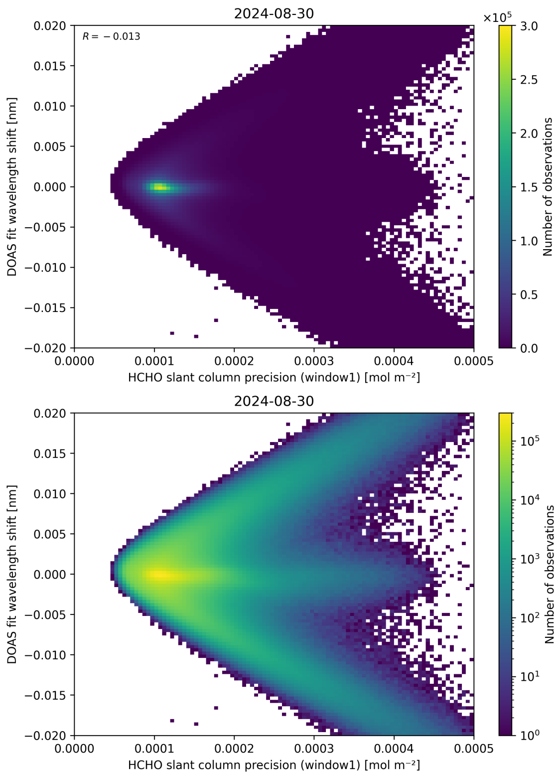
Figure 89: Scatter density plot of “HCHO slant column precision (window1)” against “DOAS fit wavelength shift” for 2024-08-29 to 2024-08-31.
