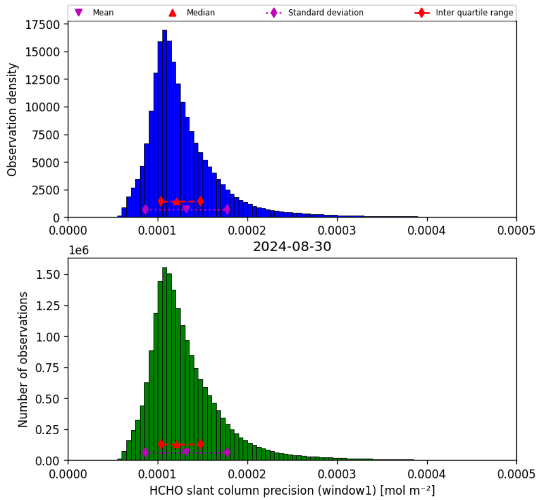
Figure 39: Histogram of “HCHO slant column precision (window1)” for 2024-08-29 to 2024-08-31
