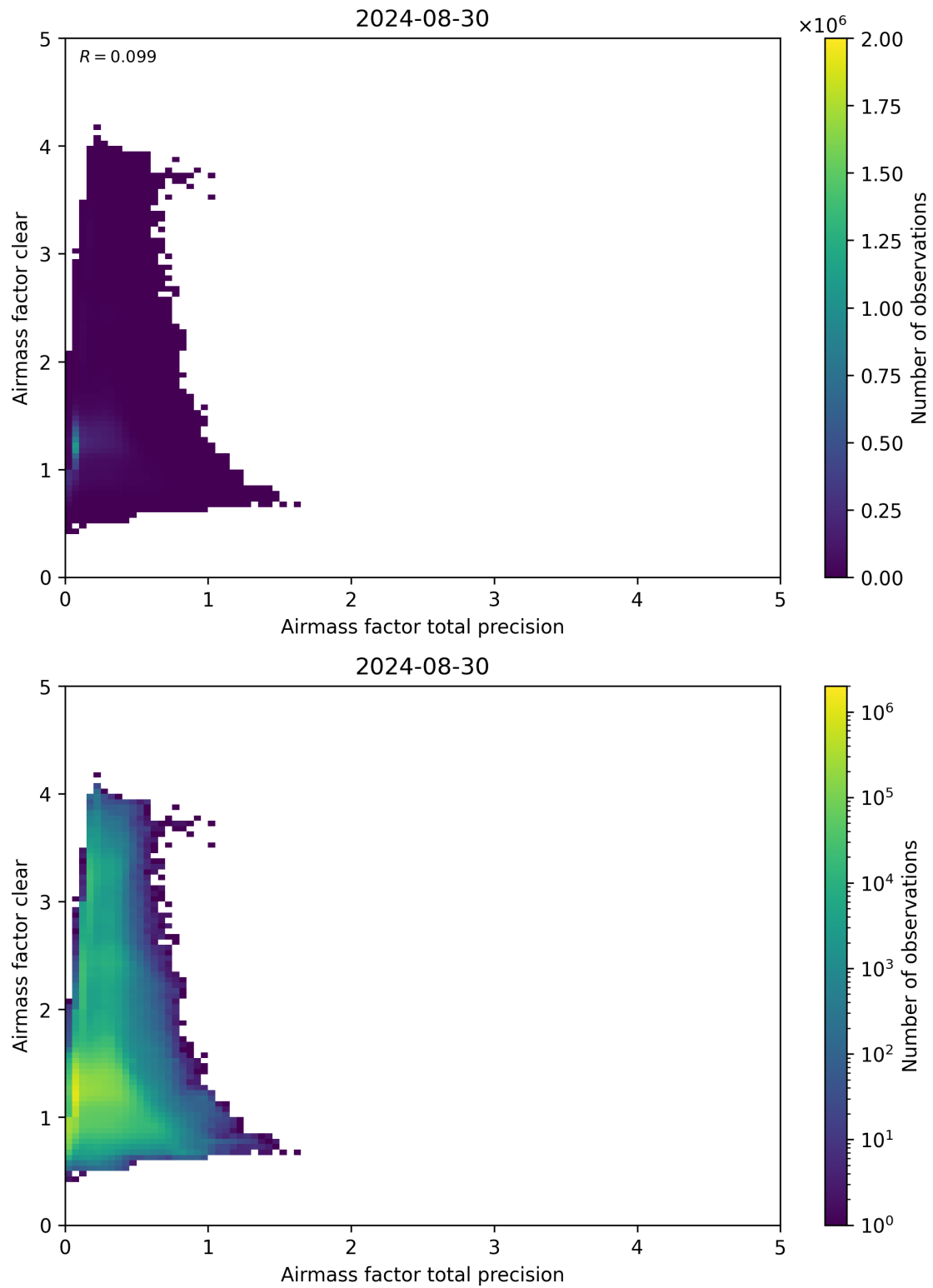
Figure 108: Scatter density plot of “Airmass factor total precision” against “Airmass factor clear” for 2024-08-29 to 2024-08-31.
