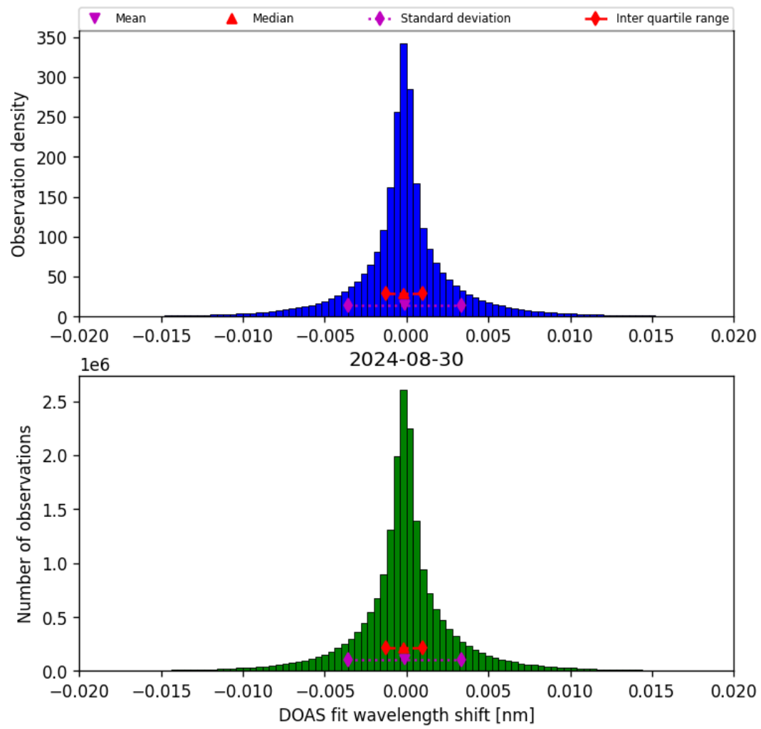
Figure 44: Histogram of “DOAS fit wavelength shift” for 2024-08-29 to 2024-08-31
