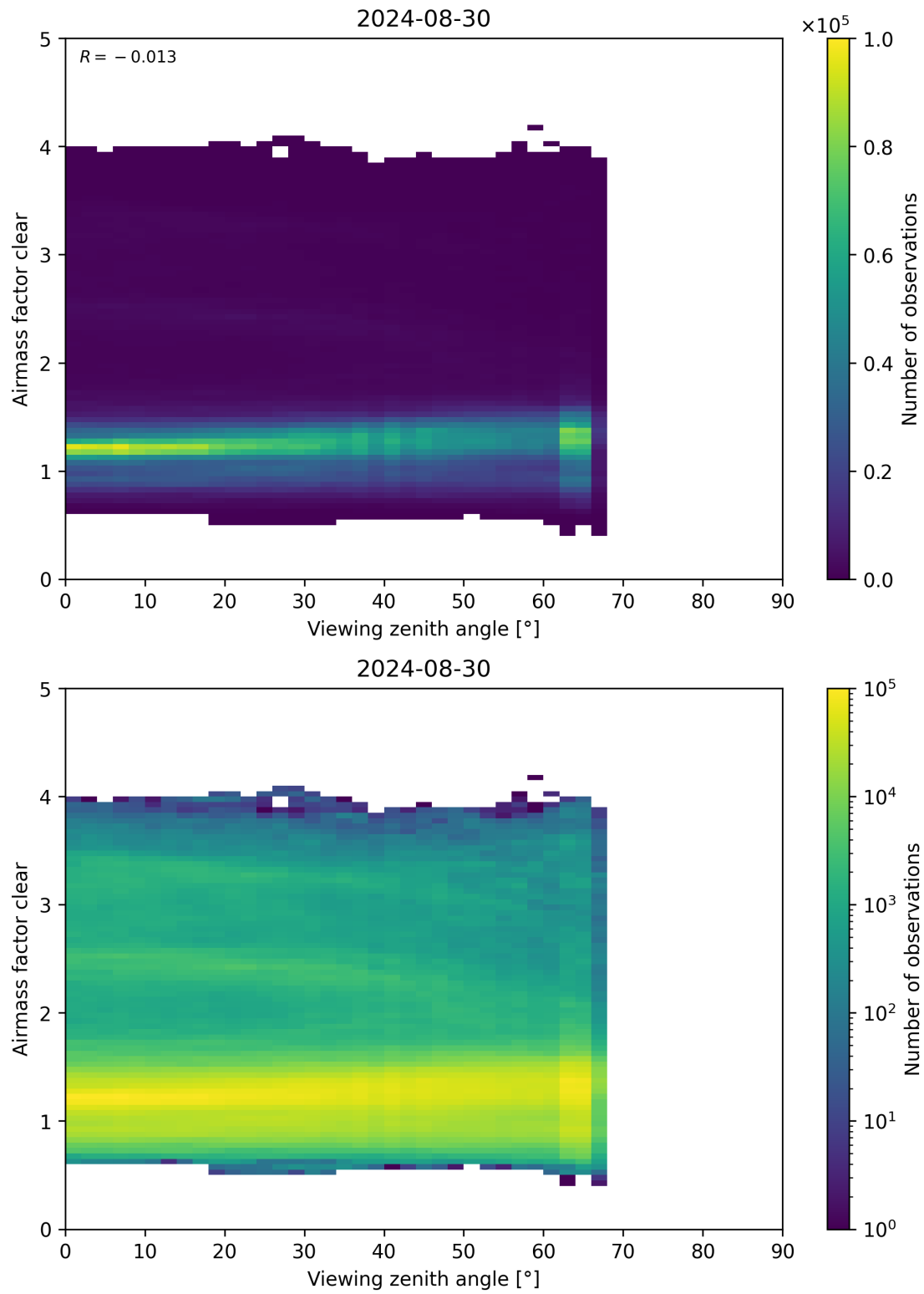
Figure 185: Scatter density plot of “Viewing zenith angle” against “Airmass factor clear” for 2024-08-29 to 2024-08-31.
