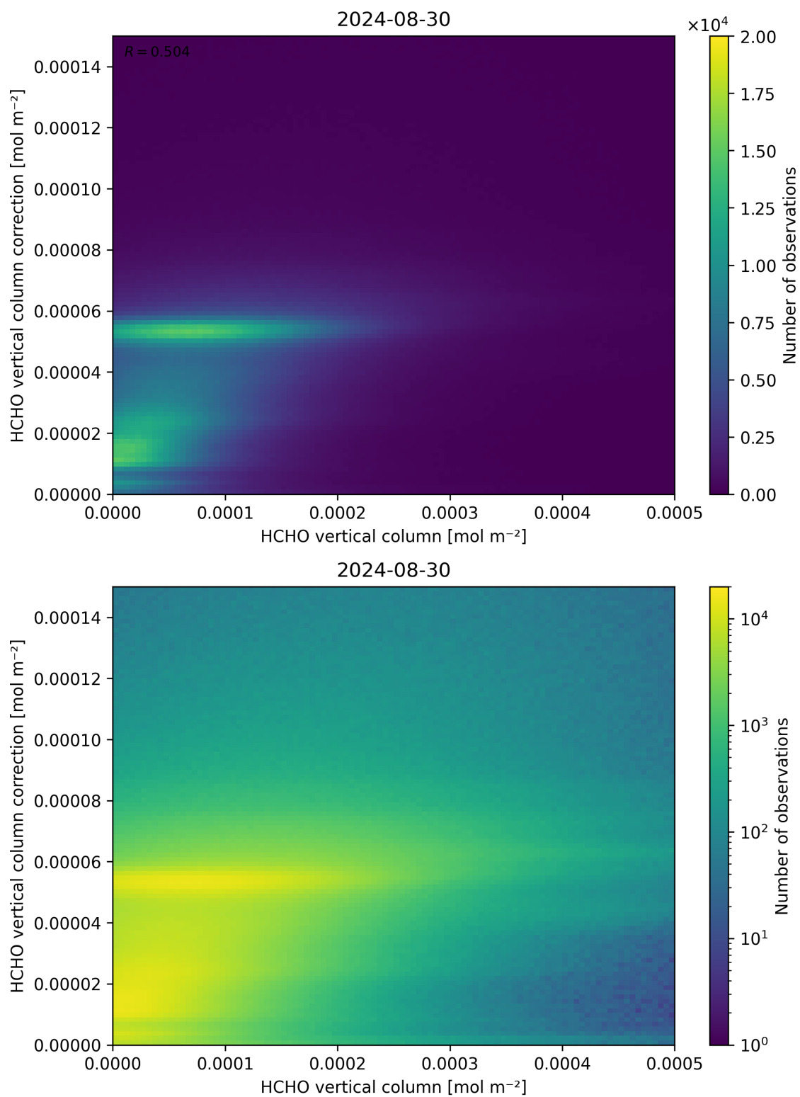
Figure 133: Scatter density plot of “HCHO vertical column” against “HCHO vertical column correction” for 2024-08-29 to 2024-08-31.
