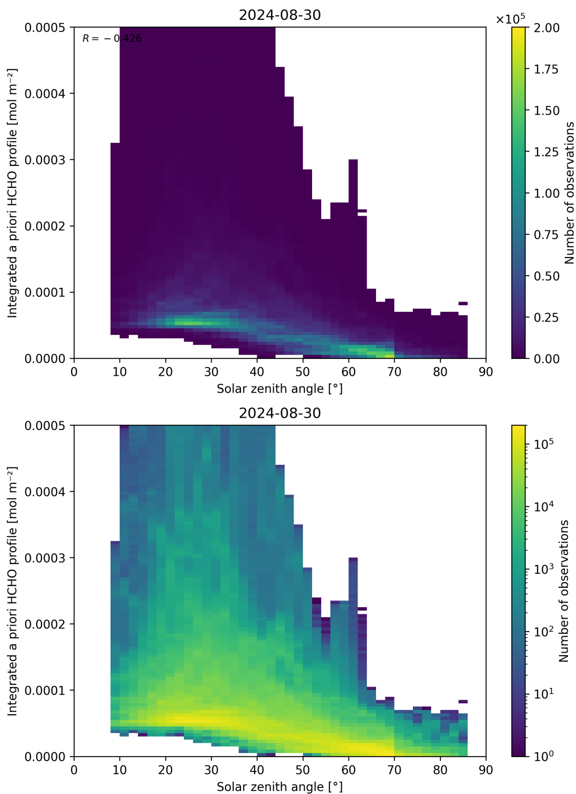
Figure 180: Scatter density plot of “Solar zenith angle” against “Integrated a priori HCHO profile” for 2024-08-29 to 2024-08-31.
