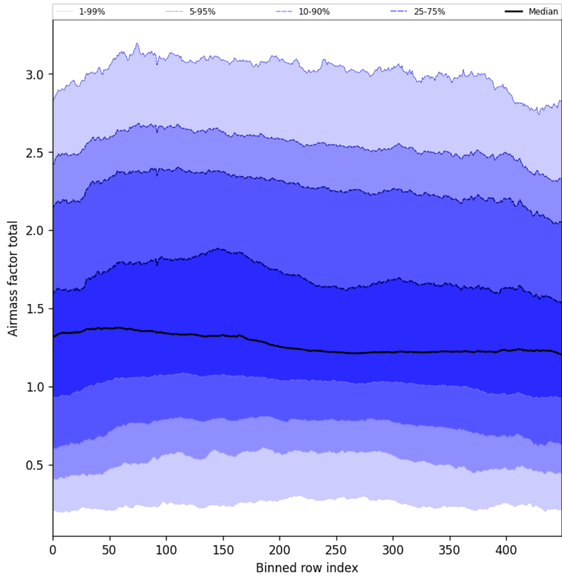
Figure 54: Along track statistics of “Airmass factor total” for 2024-08-29 to 2024-08-31
