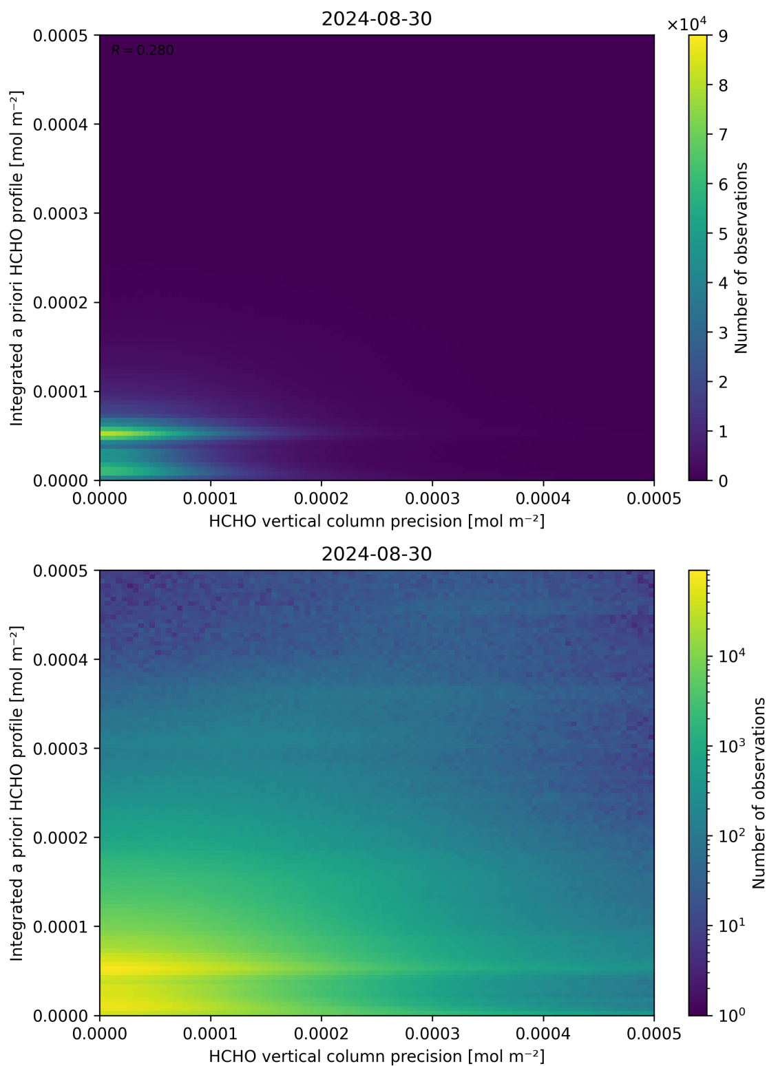
Figure 147: Scatter density plot of “HCHO vertical column precision” against “Integrated a priori HCHO profile” for 2024-08-29 to 2024-08-31.
