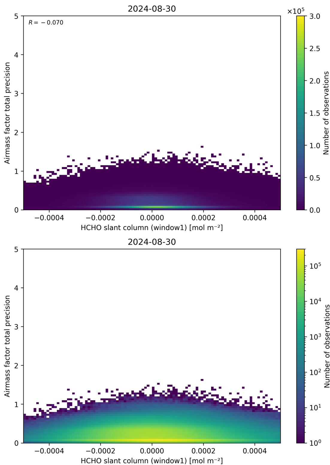
Figure 86: Scatter density plot of “HCHO slant column (window1)” against “Airmass factor total precision” for 2024-08-29 to 2024-08-31.
