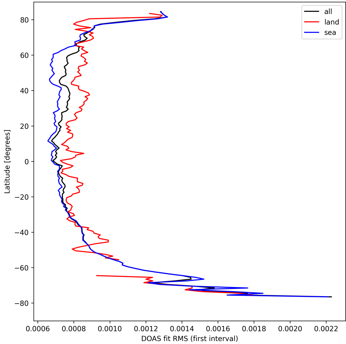
Figure 32: Zonal average of “DOAS fit RMS (first interval)” for 2024-08-29 to 2024-08-31.
