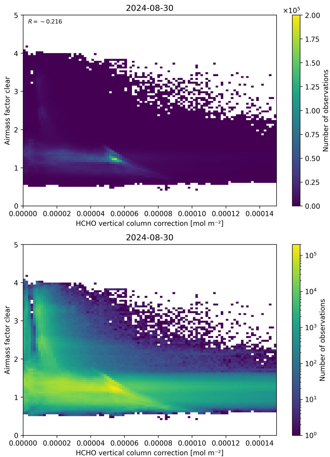
Figure 115: Scatter density plot of “HCHO vertical column correction” against “Airmass factor clear” for 2024-08-29 to 2024-08-31.
