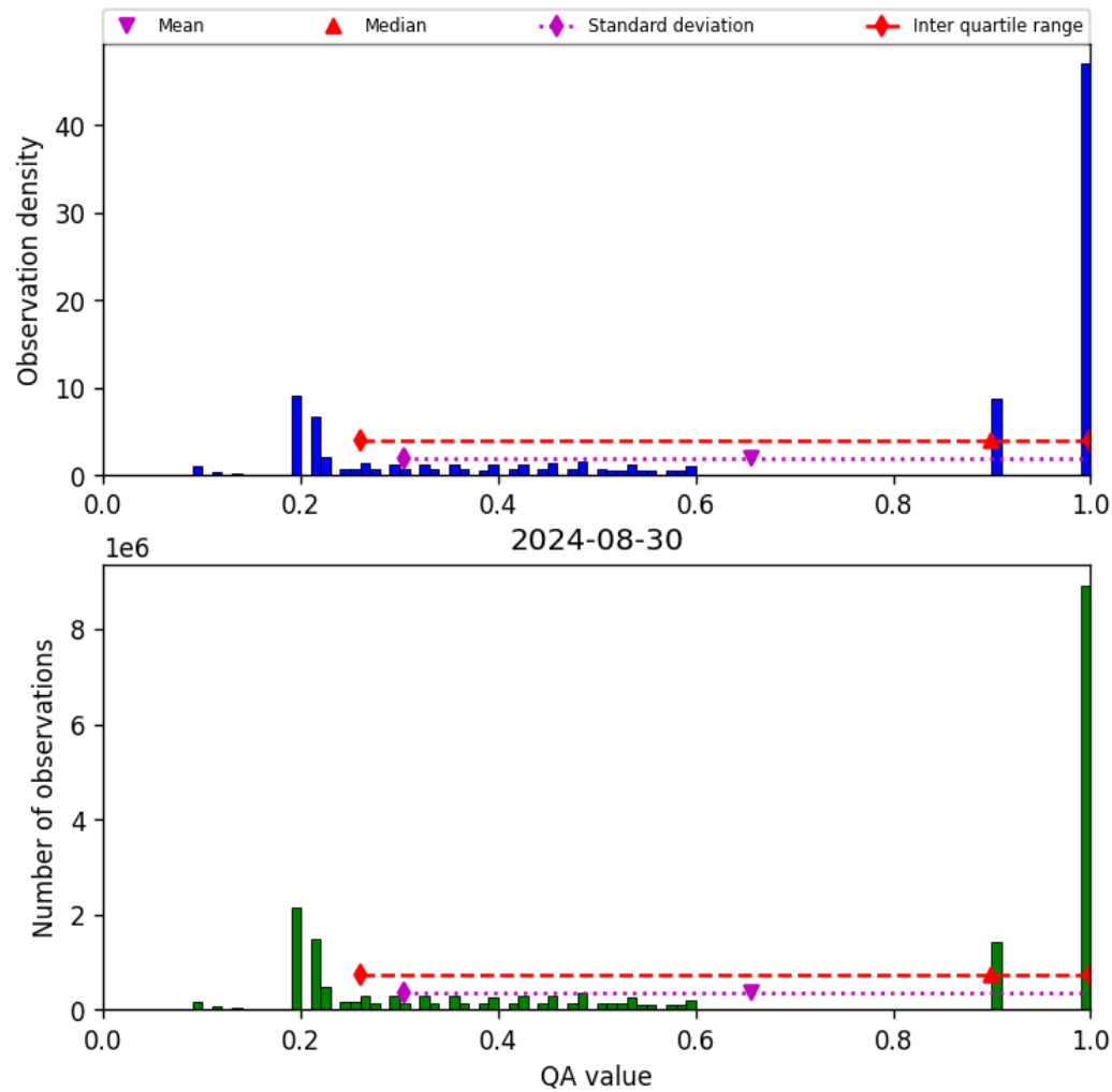
Figure 34: Histogram of “QA value” for 2024-08-29 to 2024-08-31
