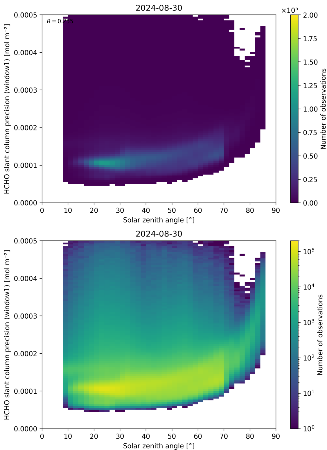
Figure 174: Scatter density plot of “Solar zenith angle” against “HCHO slant column precision (window1)” for 2024-08-29 to 2024-08-31.
