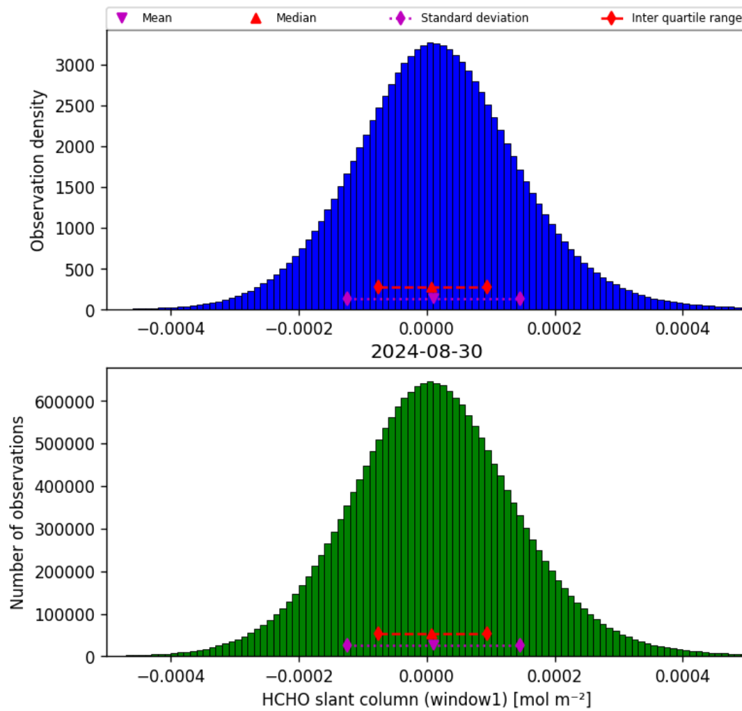
Figure 38: Histogram of “HCHO slant column (window1)” for 2024-08-29 to 2024-08-31
