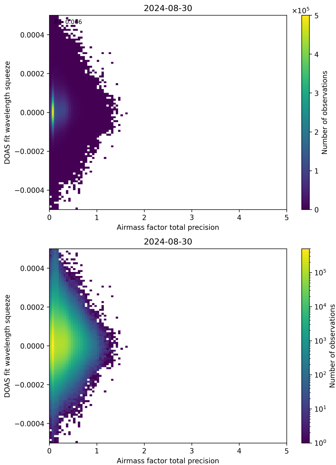
Figure 107: Scatter density plot of “Airmass factor total precision” against “DOAS fit wavelength squeeze” for 2024-08-29 to 2024-08-31.
