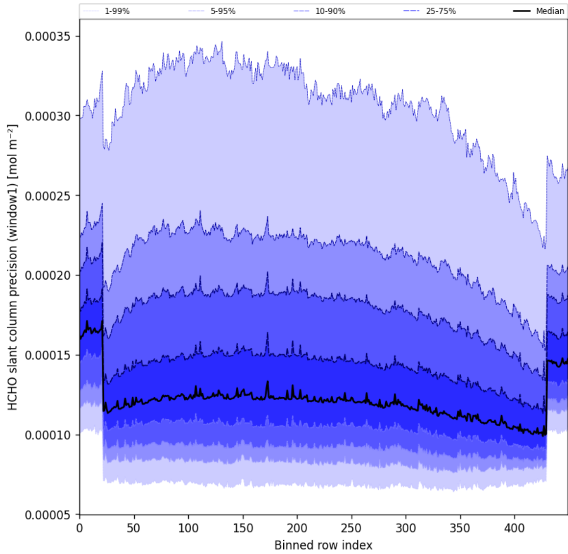
Figure 53: Along track statistics of “HCHO slant column precision (window1)” for 2024-08-29 to 2024-08-31
