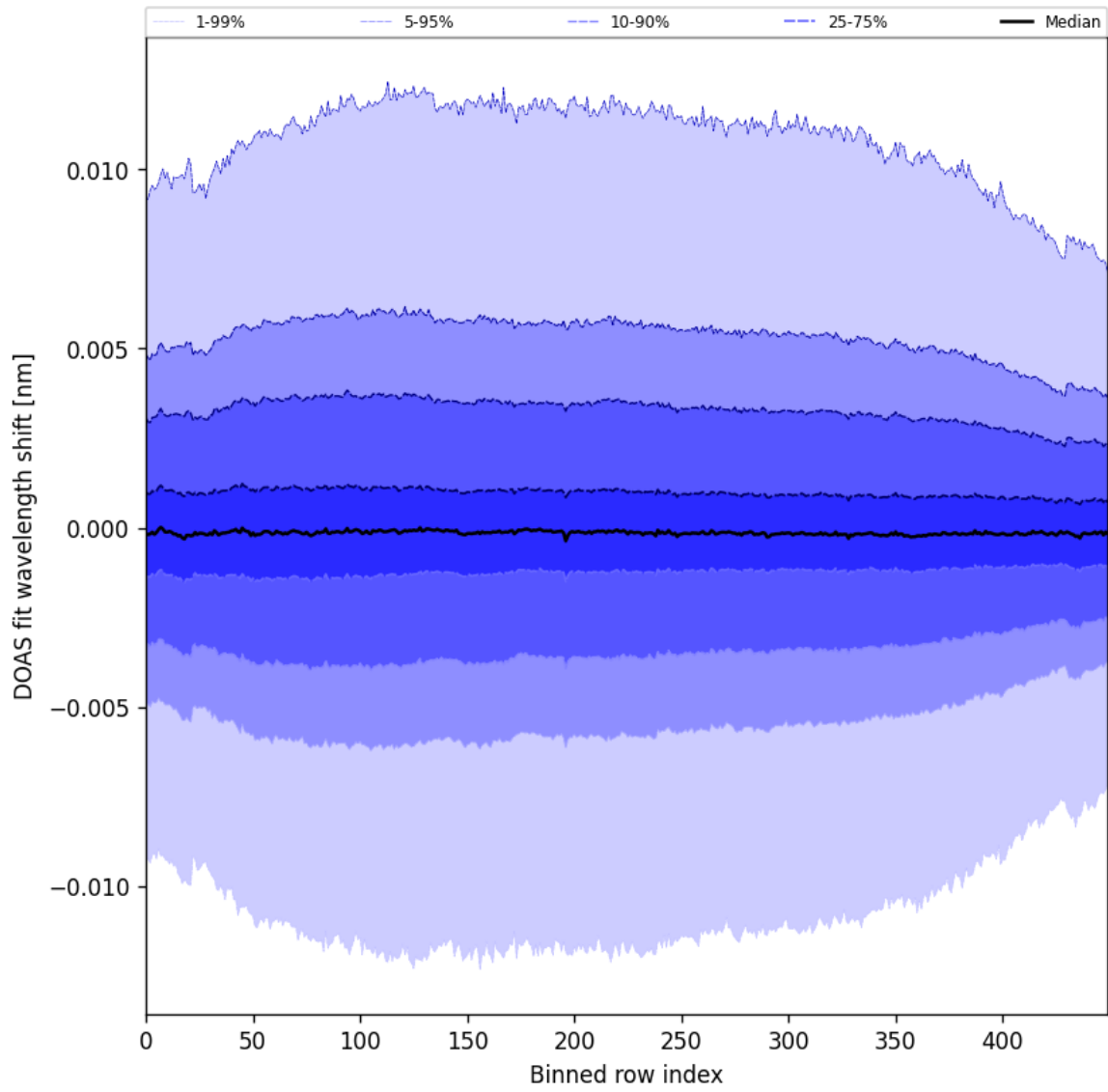
Figure 58: Along track statistics of “DOAS fit wavelength shift” for 2024-08-29 to 2024-08-31
