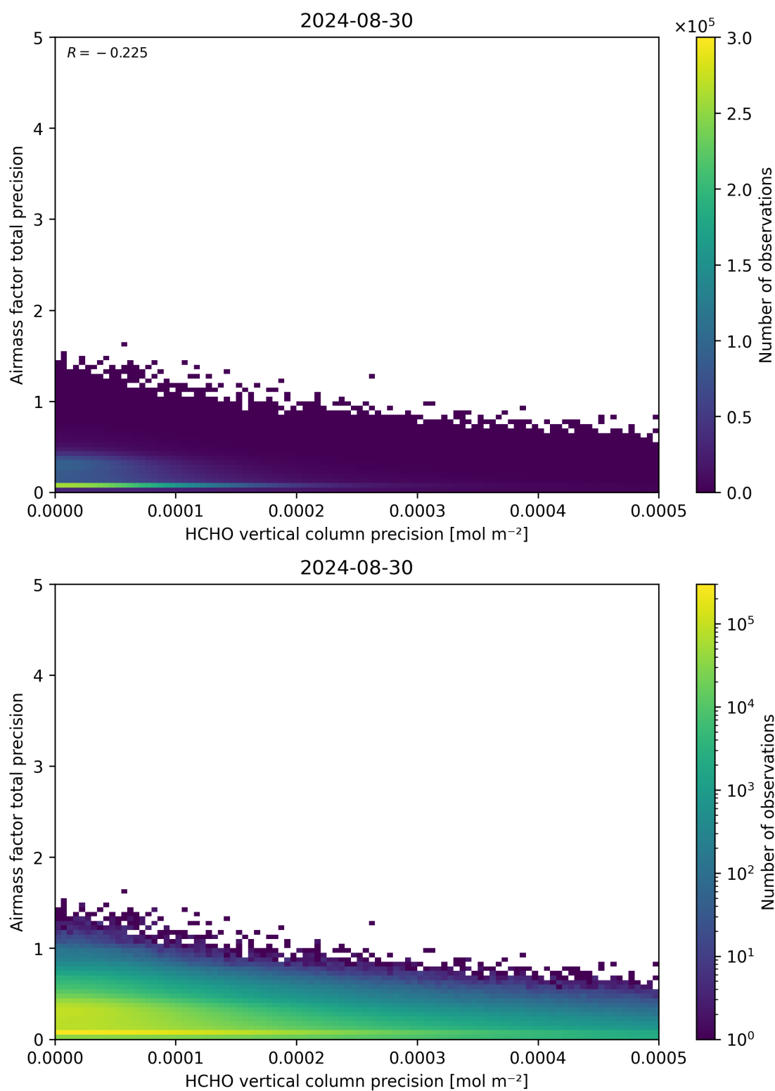
Figure 145: Scatter density plot of “HCHO vertical column precision” against “Airmass factor total precision” for 2024-08-29 to 2024-08-31.
