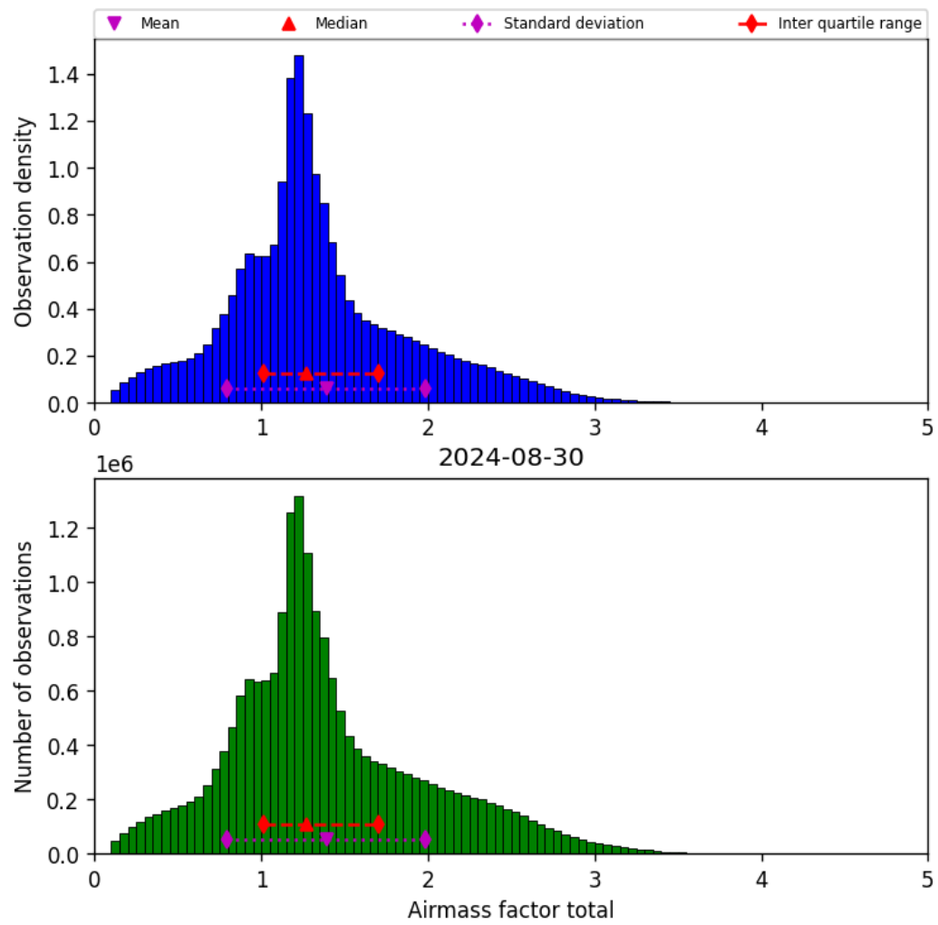
Figure 40: Histogram of “Airmass factor total” for 2024-08-29 to 2024-08-31
