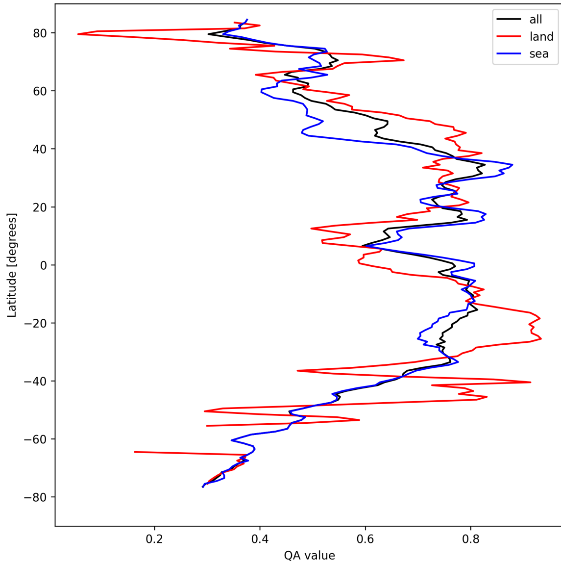
Figure 20: Zonal average of “QA value” for 2024-08-29 to 2024-08-31.
