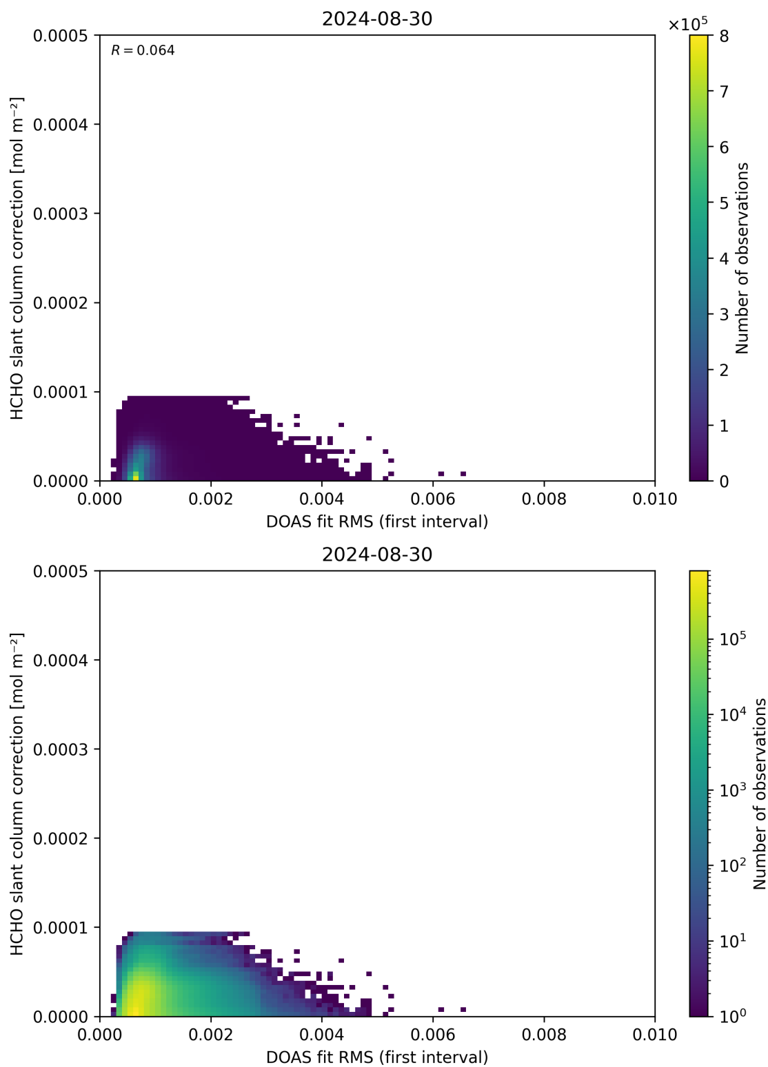
Figure 63: Scatter density plot of “DOAS fit RMS (first interval)” against “HCHO slant column correction” for 2024-08-29 to 2024-08-31.
