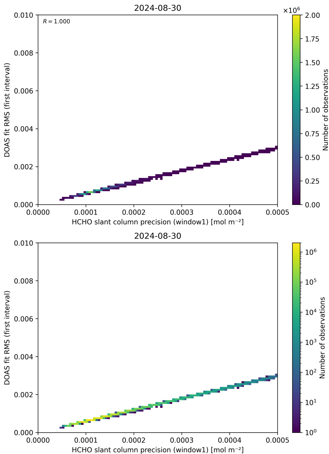
Figure 88: Scatter density plot of “HCHO slant column precision (window1)” against “DOAS fit RMS (first interval)” for 2024-08-29 to 2024-08-31.
