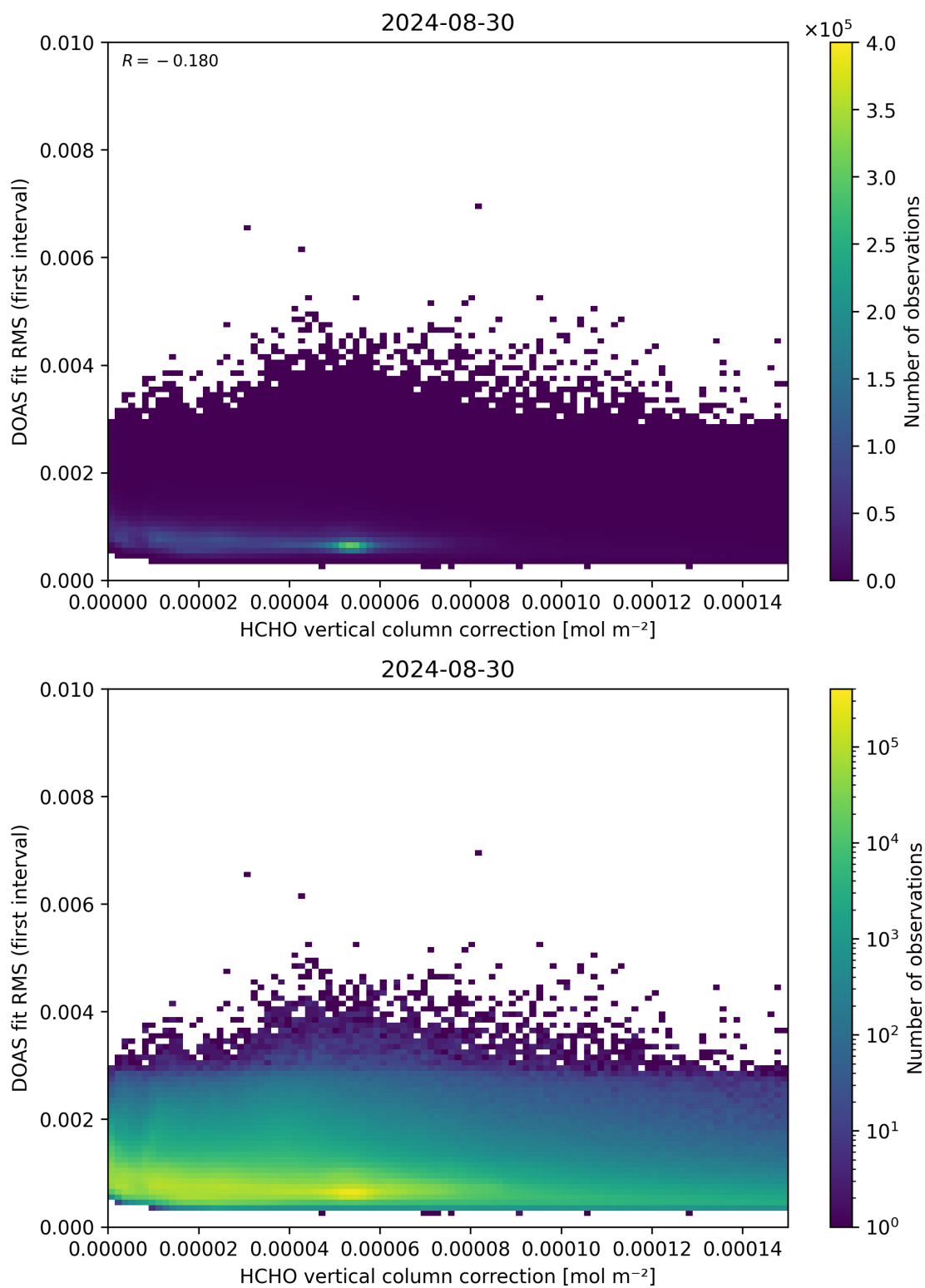
Figure 112: Scatter density plot of “HCHO vertical column correction” against “DOAS fit RMS (first interval)” for 2024-08-29 to 2024-08-31.
