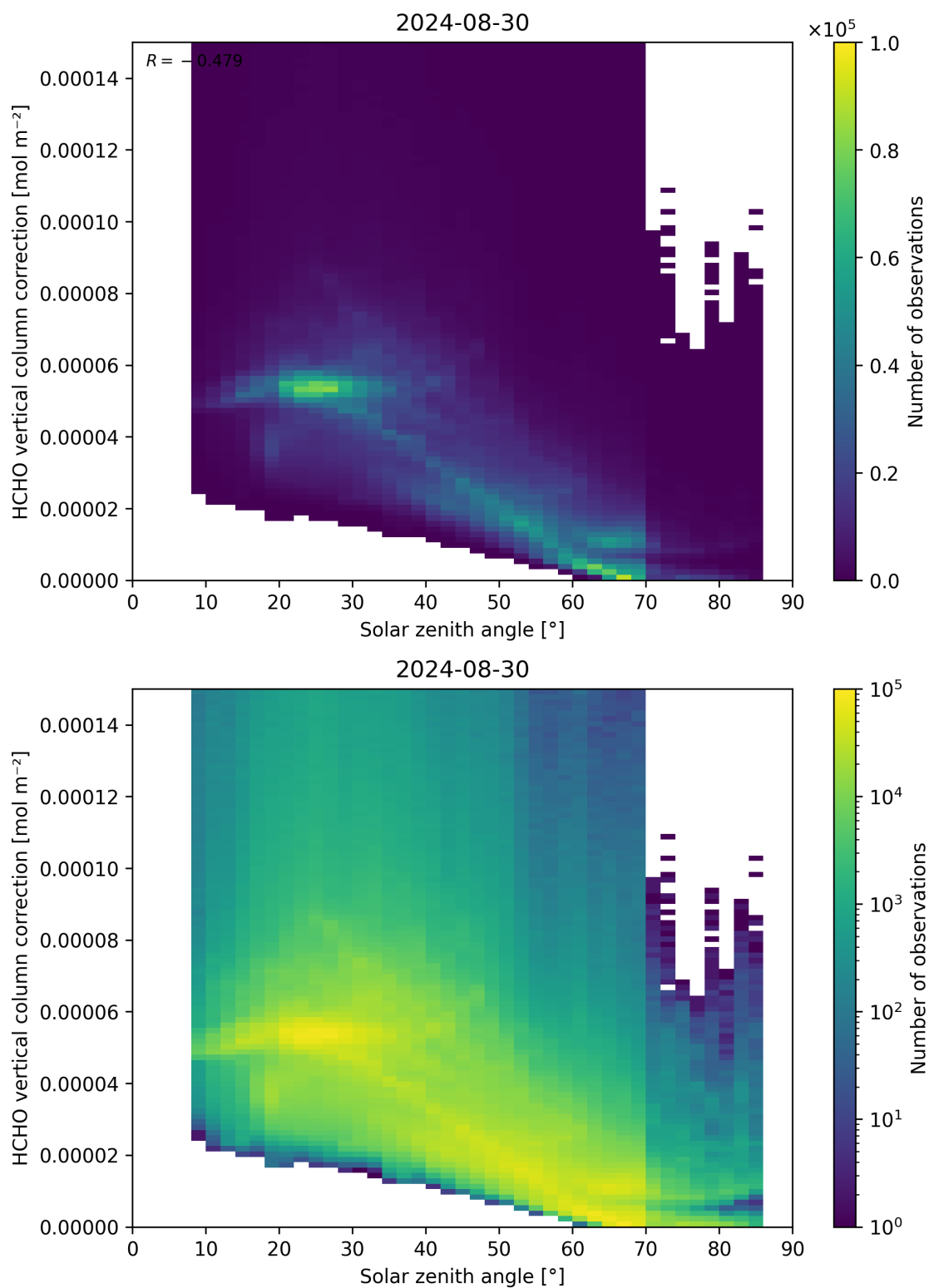
Figure 178: Scatter density plot of “Solar zenith angle” against “HCHO vertical column correction” for 2024-08-29 to 2024-08-31.
