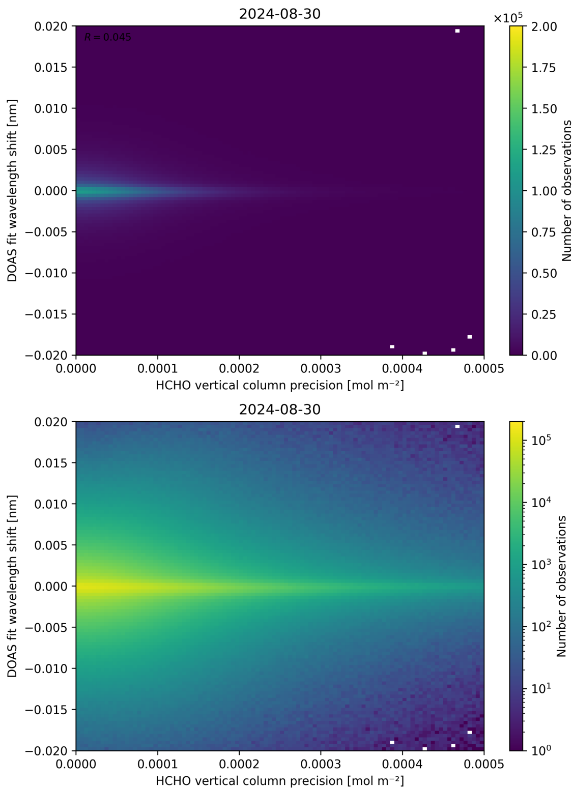
Figure 137: Scatter density plot of “HCHO vertical column precision” against “DOAS fit wavelength shift” for 2024-08-29 to 2024-08-31.
