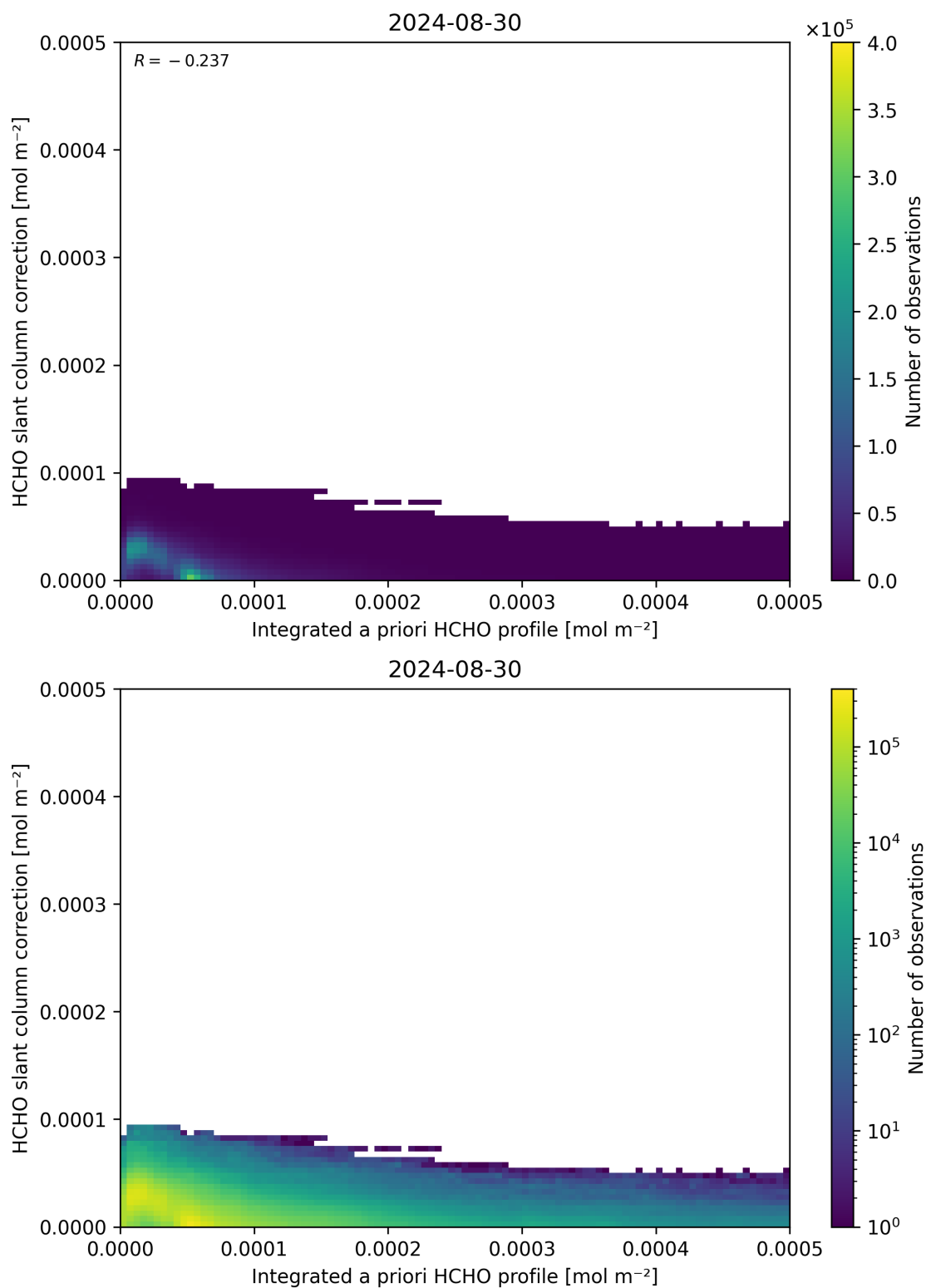
Figure 152: Scatter density plot of “Integrated a priori HCHO profile” against “HCHO slant column correction” for 2024-08-29 to 2024-08-31.
