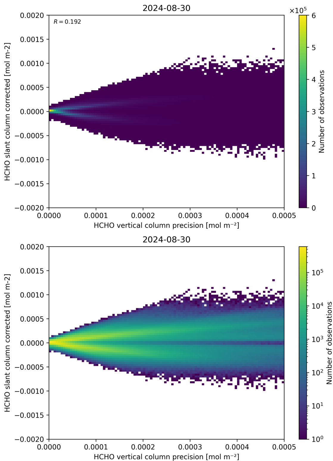
Figure 140: Scatter density plot of “HCHO vertical column precision” against “HCHO slant column corrected” for 2024-08-29 to 2024-08-31.
