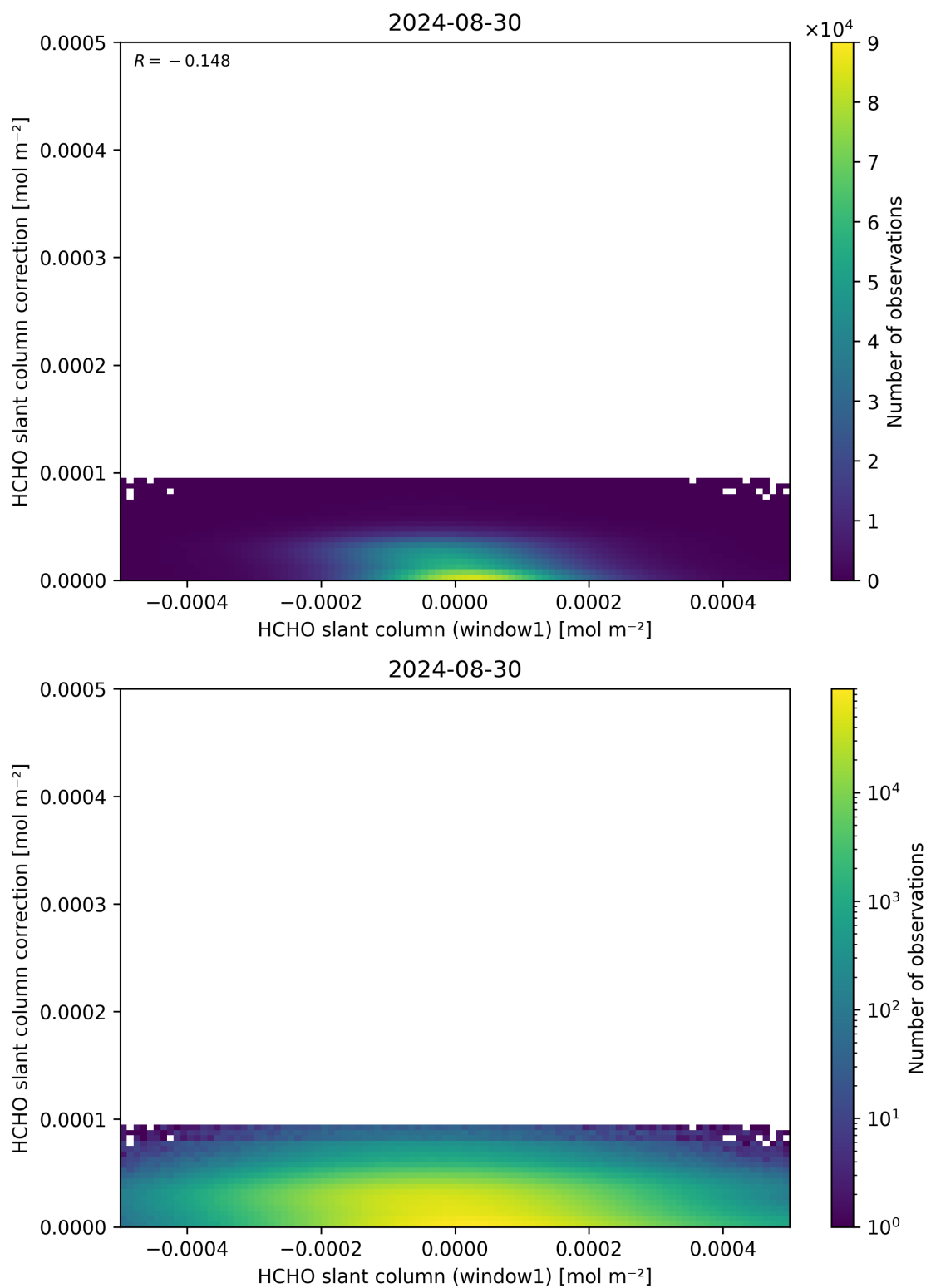
Figure 83: Scatter density plot of “HCHO slant column (window1)” against “HCHO slant column correction” for 2024-08-29 to 2024-08-31.
