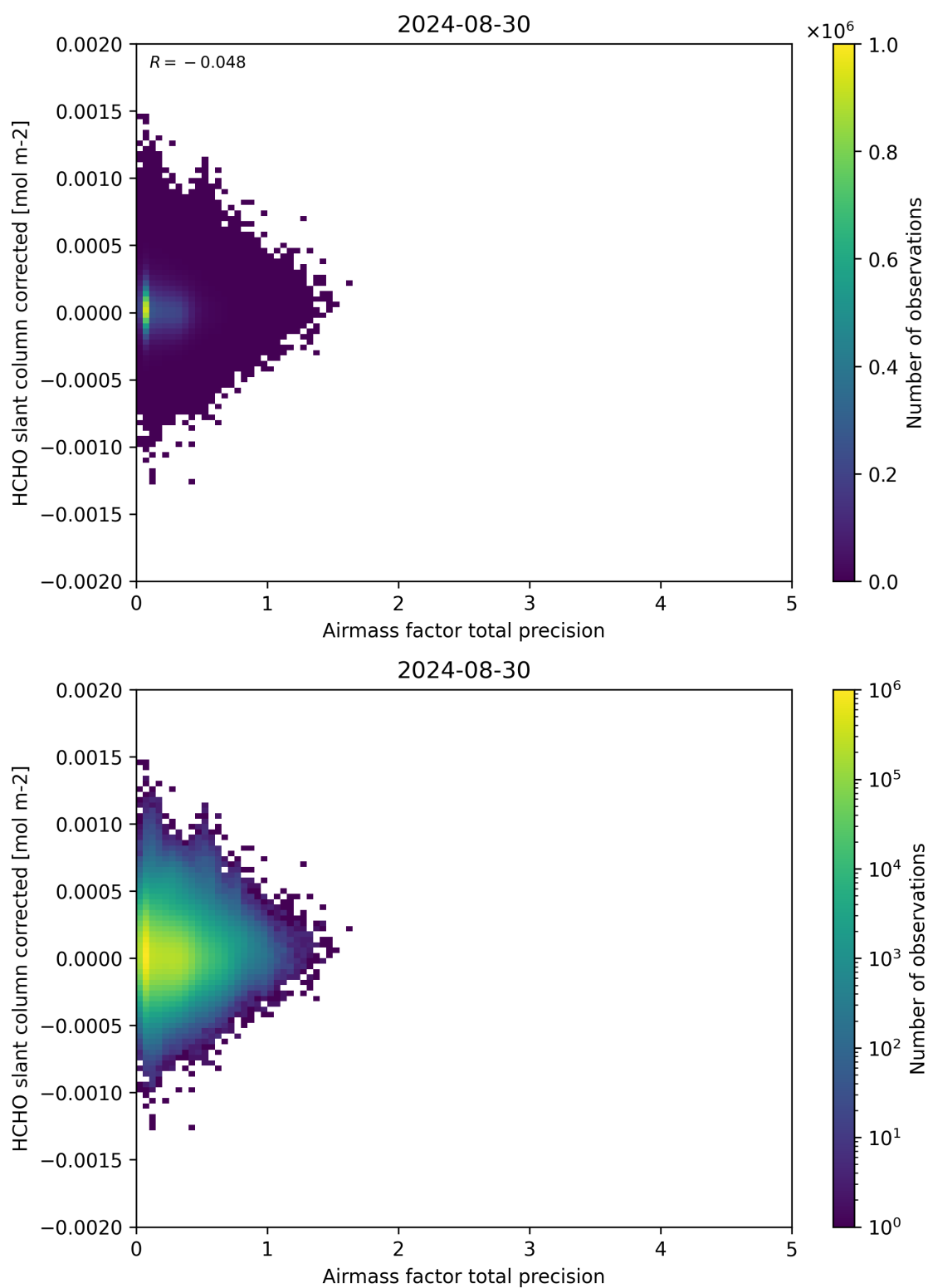
Figure 109: Scatter density plot of “Airmass factor total precision” against “HCHO slant column corrected” for 2024-08-29 to 2024-08-31.
