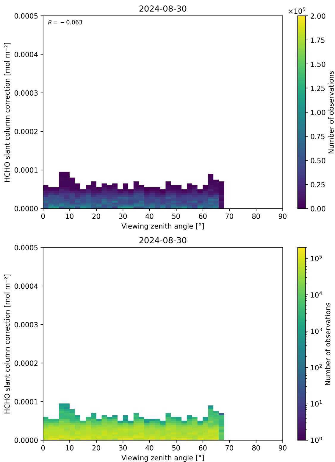
Figure 187: Scatter density plot of “Viewing zenith angle” against “HCHO slant column correction” for 2024-08-29 to 2024-08-31.
