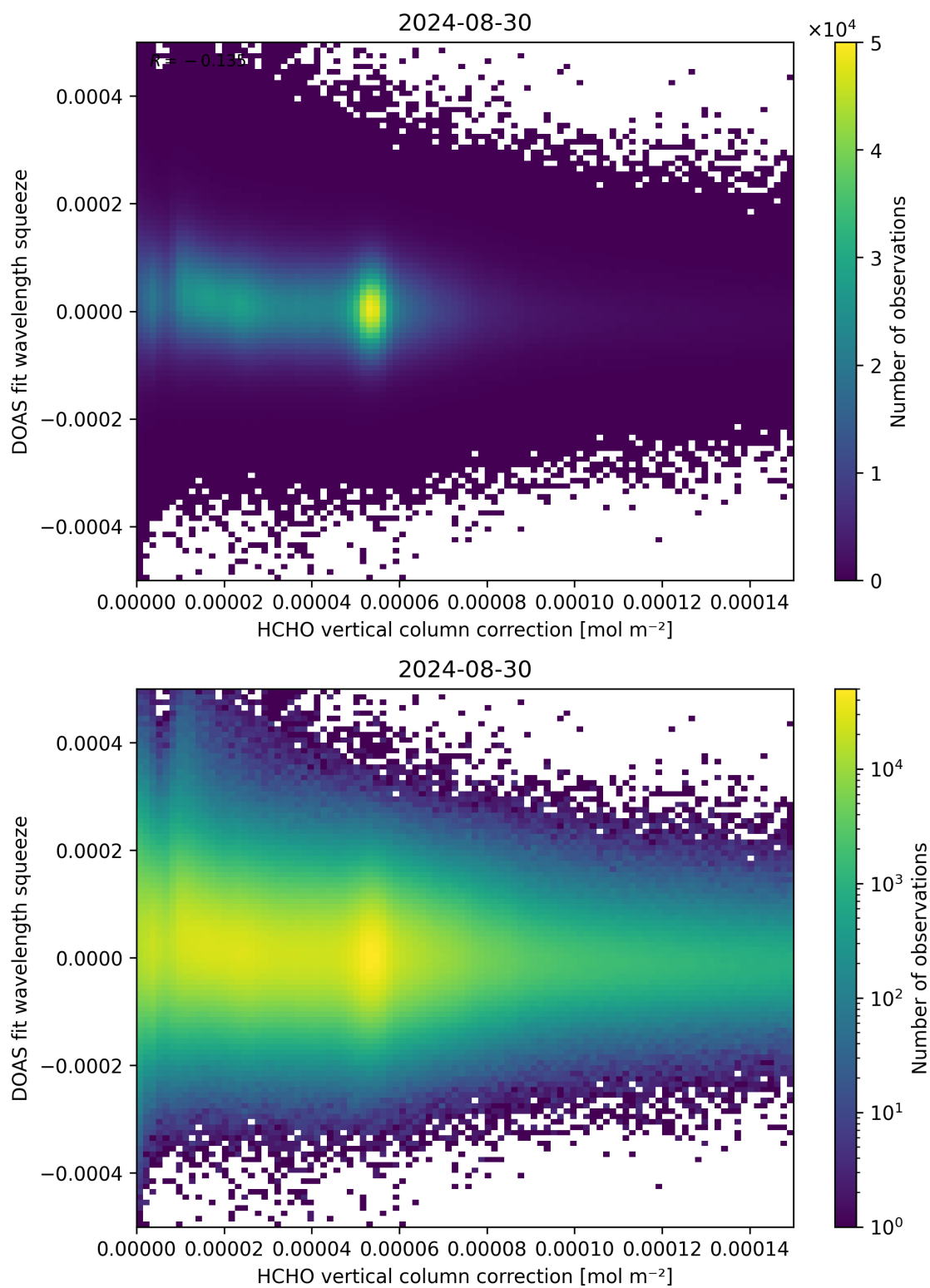
Figure 114: Scatter density plot of “HCHO vertical column correction” against “DOAS fit wavelength squeeze” for 2024-08-29 to 2024-08-31.
