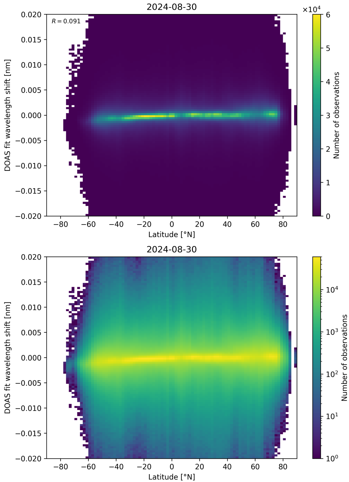
Figure 154: Scatter density plot of “Latitude” against “DOAS fit wavelength shift” for 2024-08-29 to 2024-08-31.
