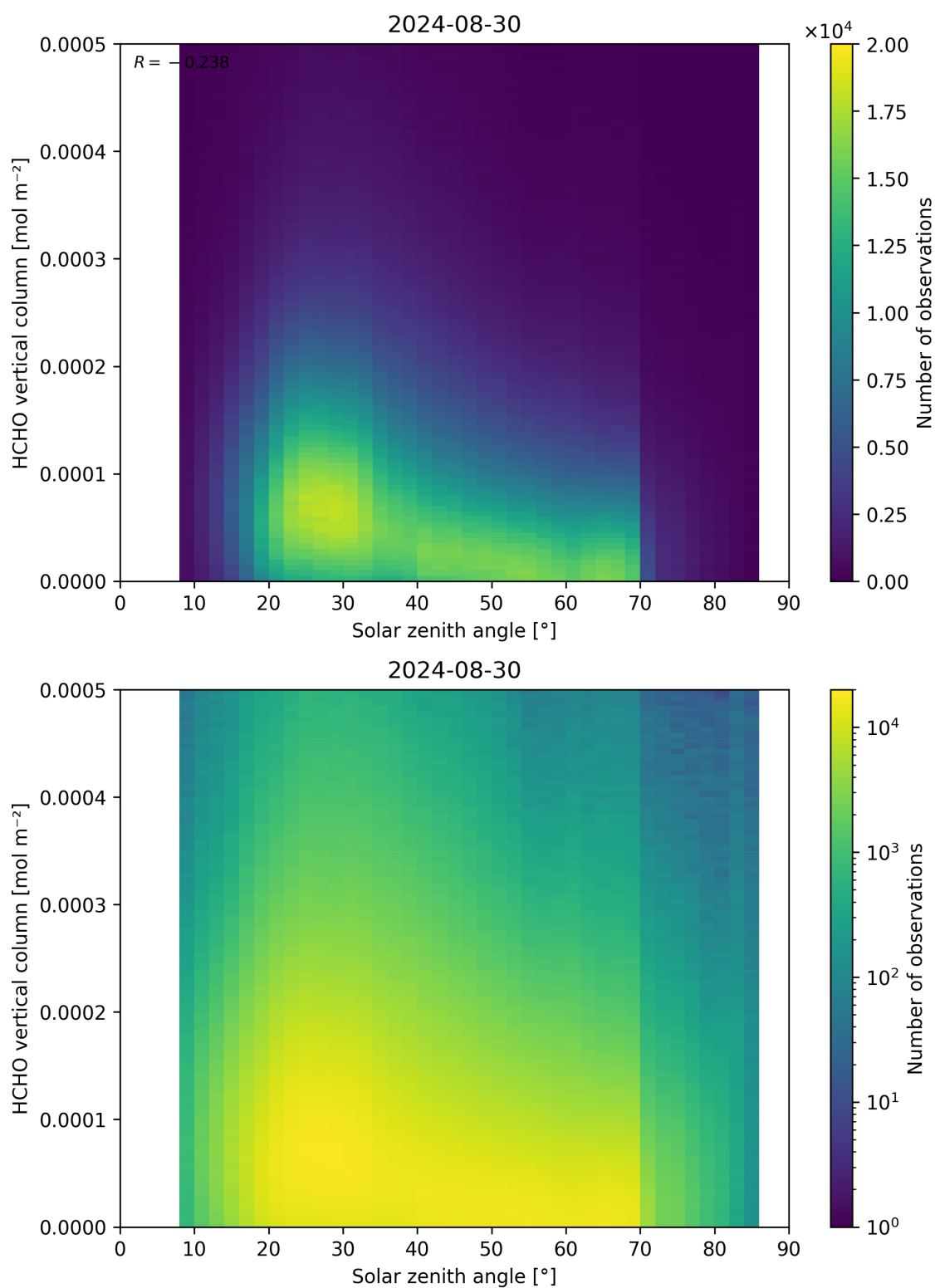
Figure 177: Scatter density plot of “Solar zenith angle” against “HCHO vertical column” for 2024-08-29 to 2024-08-31.
