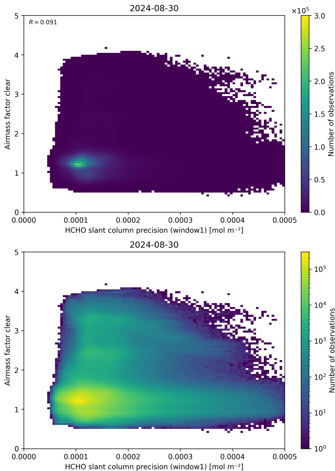
Figure 91: Scatter density plot of “HCHO slant column precision (window1)” against “Airmass factor clear” for 2024-08-29 to 2024-08-31.
