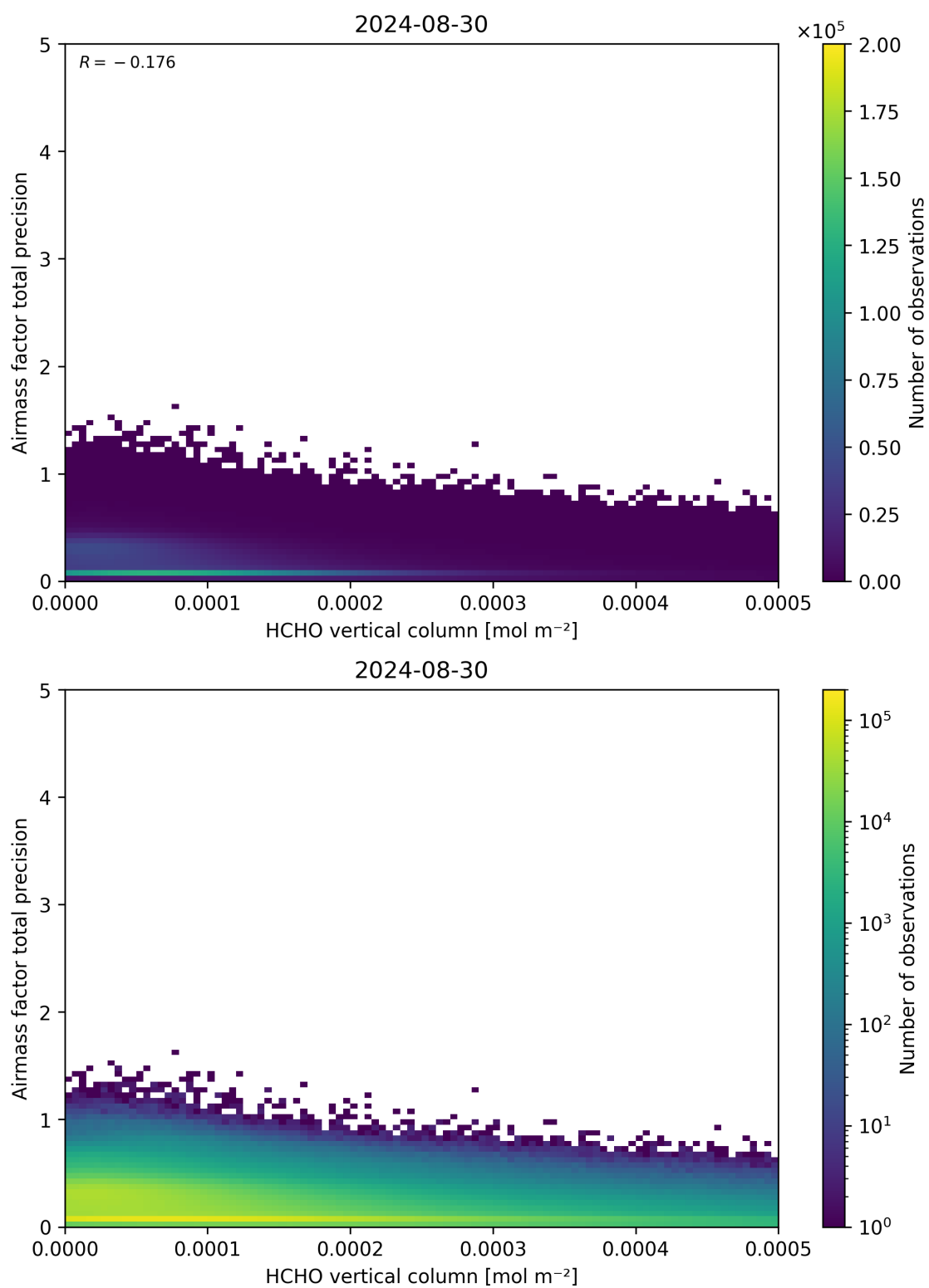
Figure 132: Scatter density plot of “HCHO vertical column” against “Airmass factor total precision” for 2024-08-29 to 2024-08-31.
