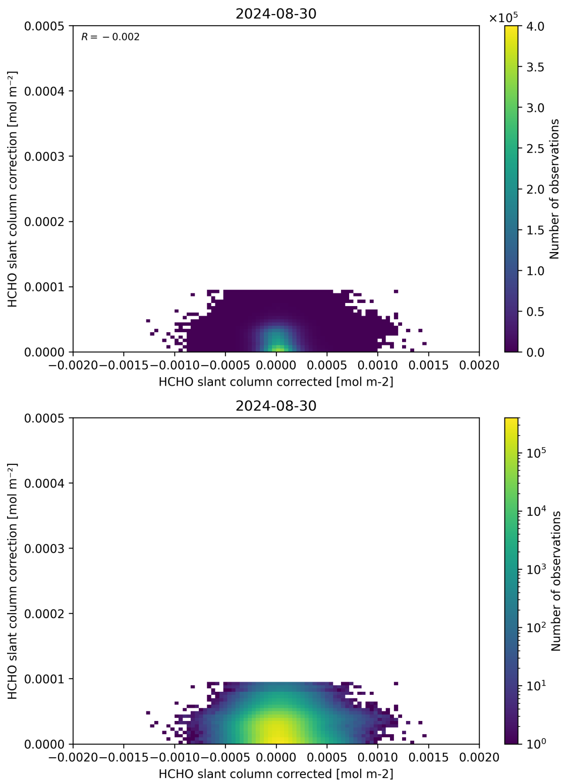
Figure 77: Scatter density plot of “HCHO slant column corrected” against “HCHO slant column correction” for 2024-08-29 to 2024-08-31.
