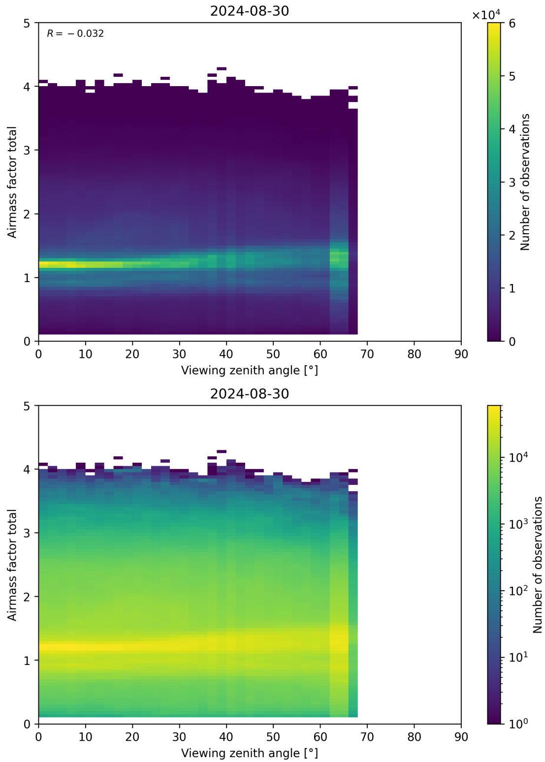
Figure 190: Scatter density plot of “Viewing zenith angle” against “Airmass factor total” for 2024-08-29 to 2024-08-31.
