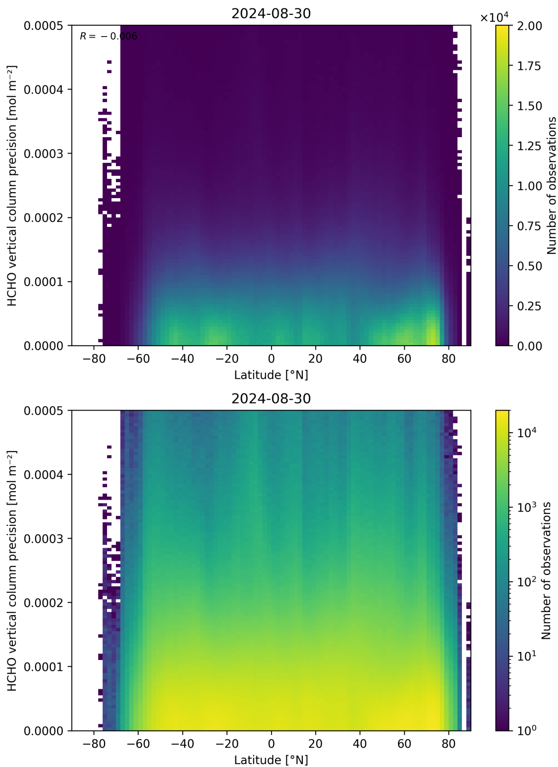
Figure 165: Scatter density plot of “Latitude” against “HCHO vertical column precision” for 2024-08-29 to 2024-08-31.
