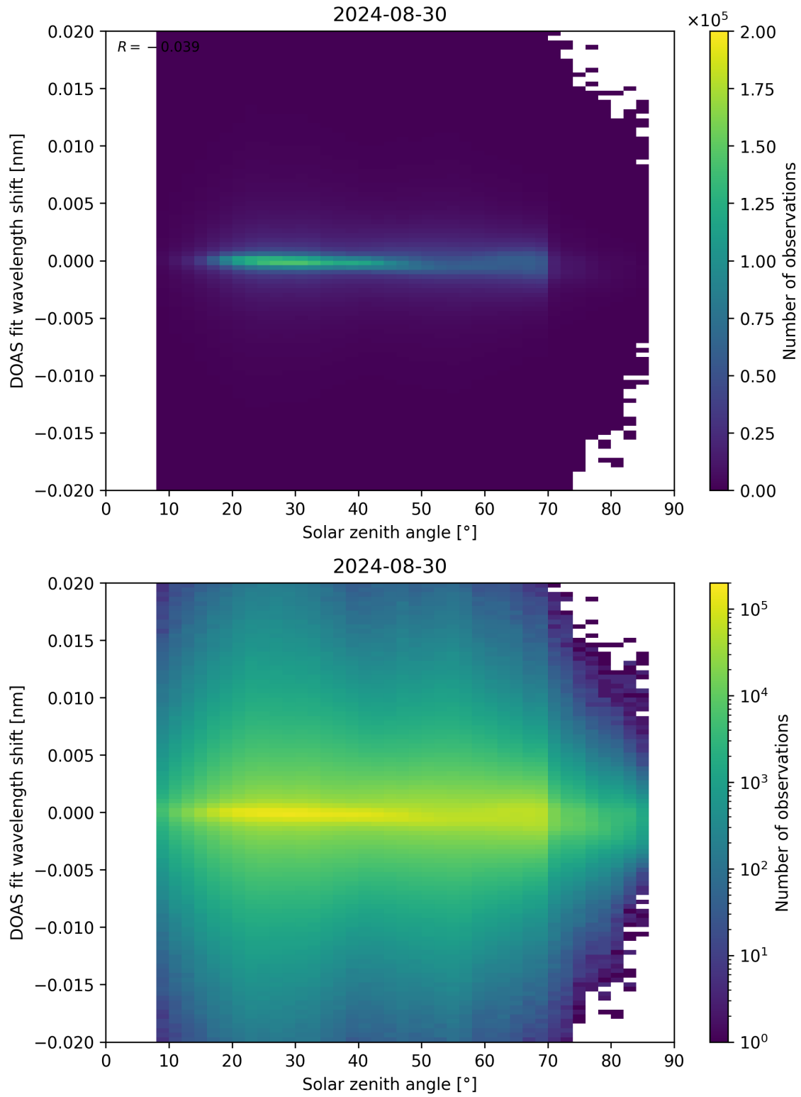
Figure 168: Scatter density plot of “Solar zenith angle” against “DOAS fit wavelength shift” for 2024-08-29 to 2024-08-31.
