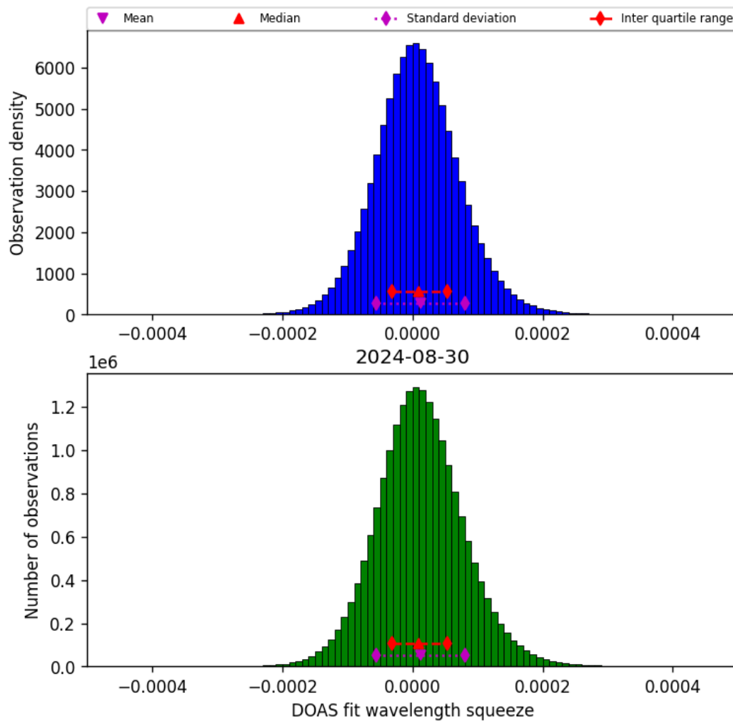
Figure 45: Histogram of “DOAS fit wavelength squeeze” for 2024-08-29 to 2024-08-31
