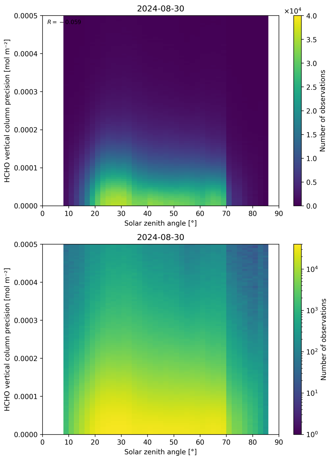
Figure 179: Scatter density plot of “Solar zenith angle” against “HCHO vertical column precision” for 2024-08-29 to 2024-08-31.
