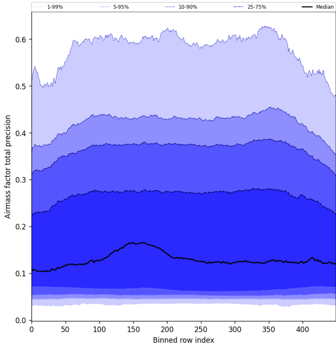
Figure 55: Along track statistics of “Airmass factor total precision” for 2024-08-29 to 2024-08-31
