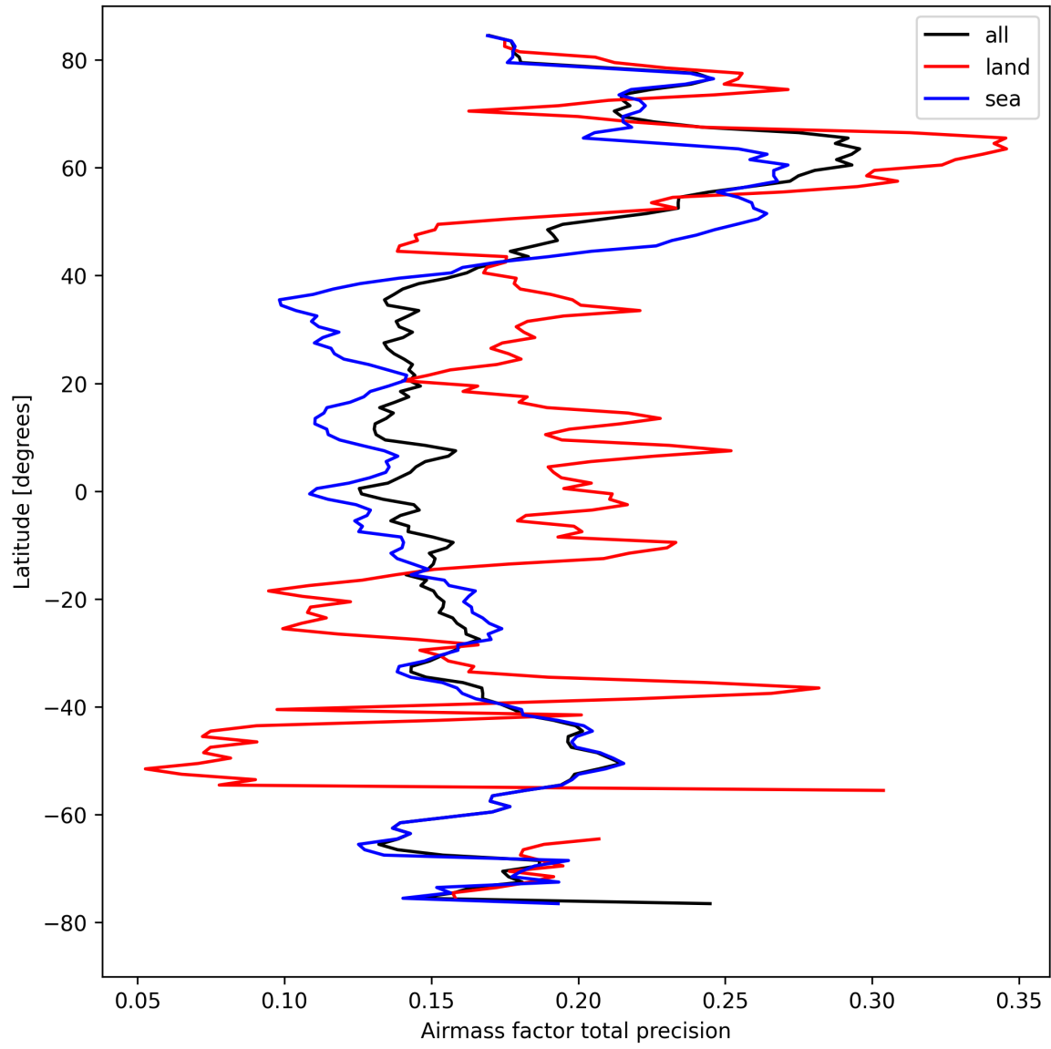
Figure 27: Zonal average of “Airmass factor total precision” for 2024-08-29 to 2024-08-31.
