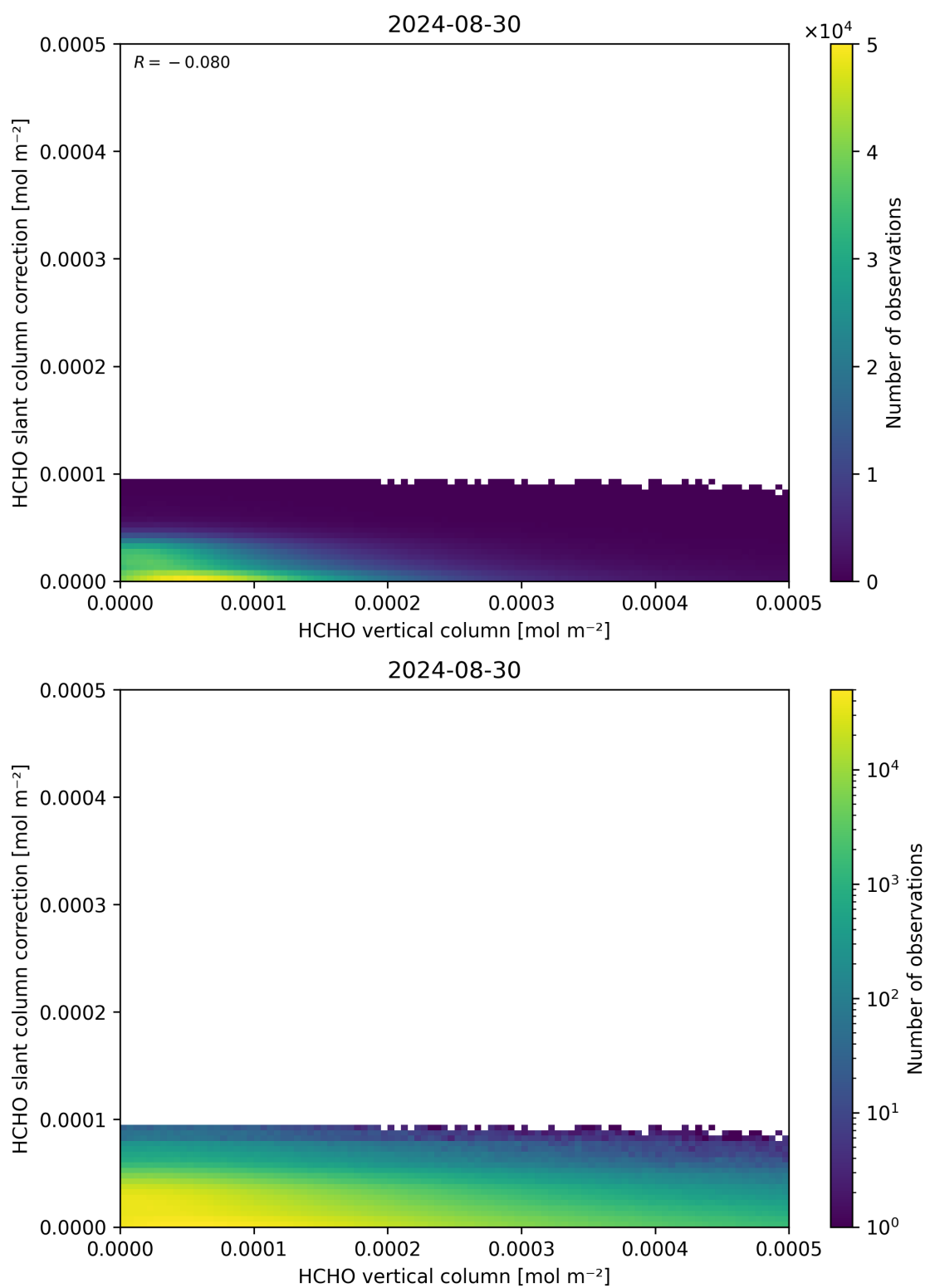
Figure 128: Scatter density plot of “HCHO vertical column” against “HCHO slant column correction” for 2024-08-29 to 2024-08-31.
