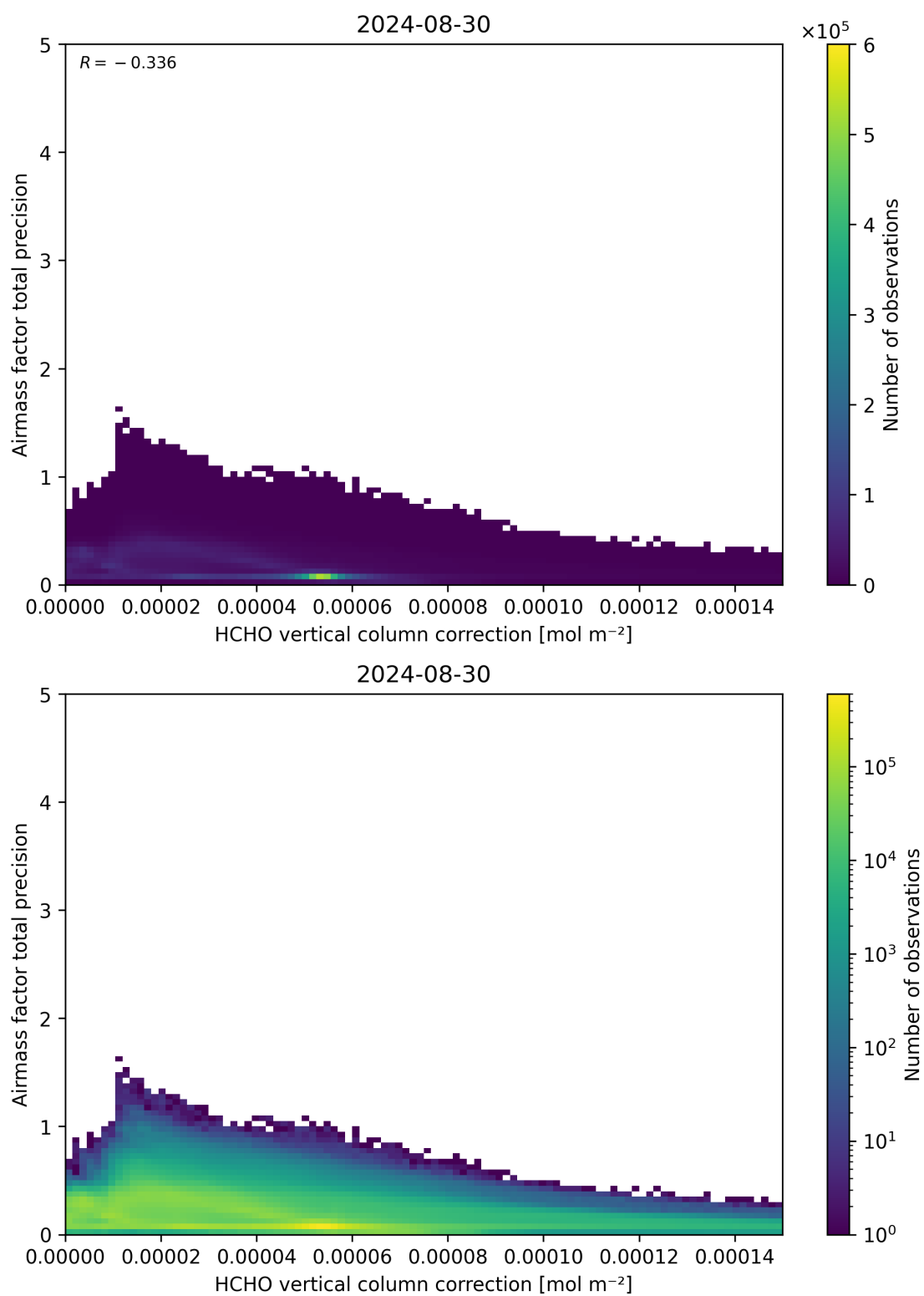
Figure 121: Scatter density plot of “HCHO vertical column correction” against “Airmass factor total precision” for 2024-08-29 to 2024-08-31.
