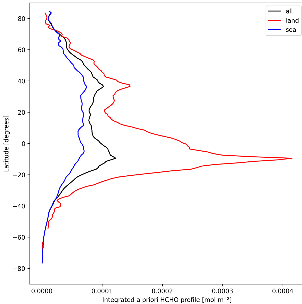
Figure 29: Zonal average of “Integrated a priori HCHO profile” for 2024-08-30 to 2024-09-01.
