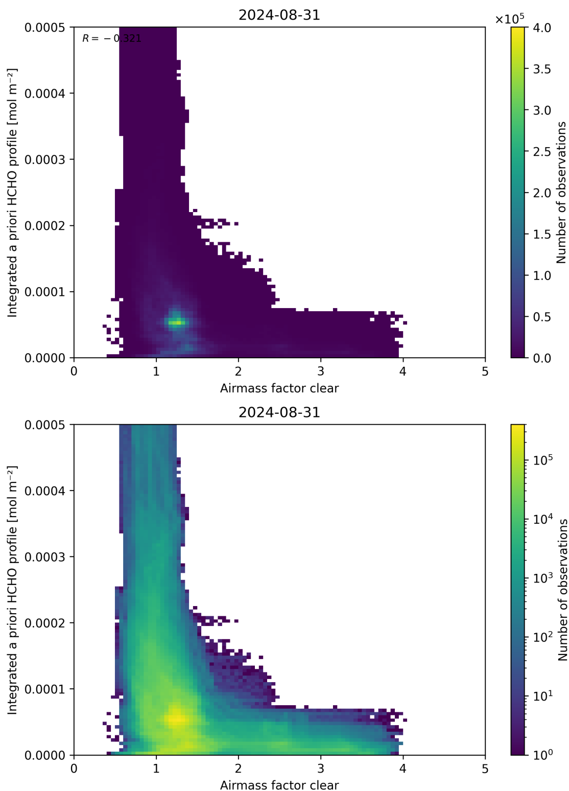
Figure 76: Scatter density plot of “Airmass factor clear” against “Integrated a priori HCHO profile” for 2024-08-30 to 2024-09-01.
