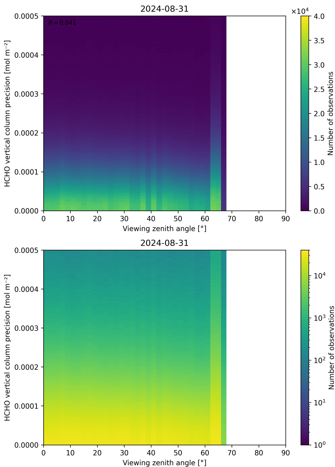
Figure 194: Scatter density plot of “Viewing zenith angle” against “HCHO vertical column precision” for 2024-08-30 to 2024-09-01.
