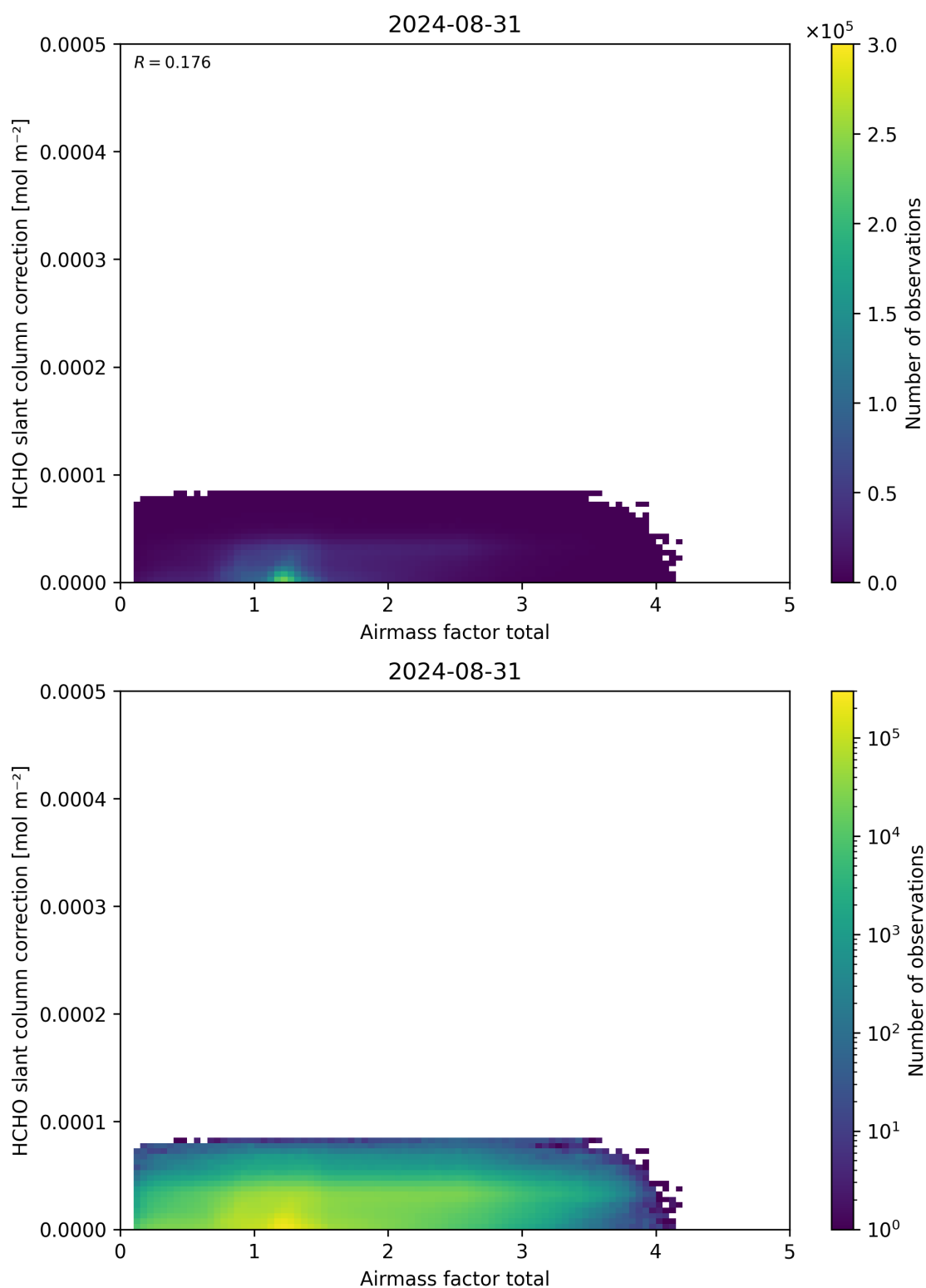
Figure 102: Scatter density plot of “Airmass factor total” against “HCHO slant column correction” for 2024-08-30 to 2024-09-01.
