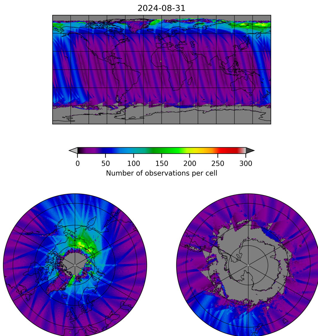
Figure 19: Map of the number of observations for 2024-08-30 to 2024-09-01
