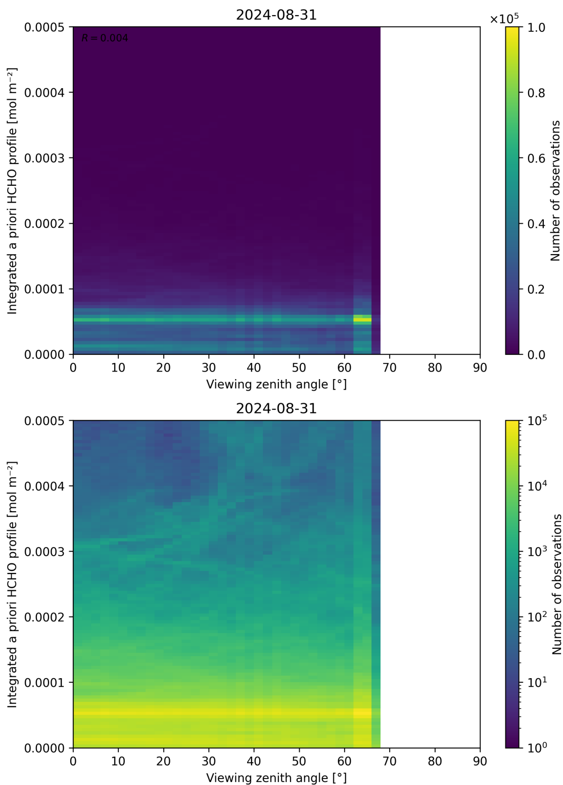
Figure 195: Scatter density plot of “Viewing zenith angle” against “Integrated a priori HCHO profile” for 2024-08-30 to 2024-09-01.
