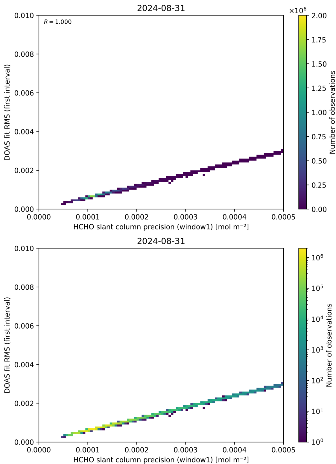
Figure 88: Scatter density plot of “HCHO slant column precision (window1)” against “DOAS fit RMS (first interval)” for 2024-08-30 to 2024-09-01.
