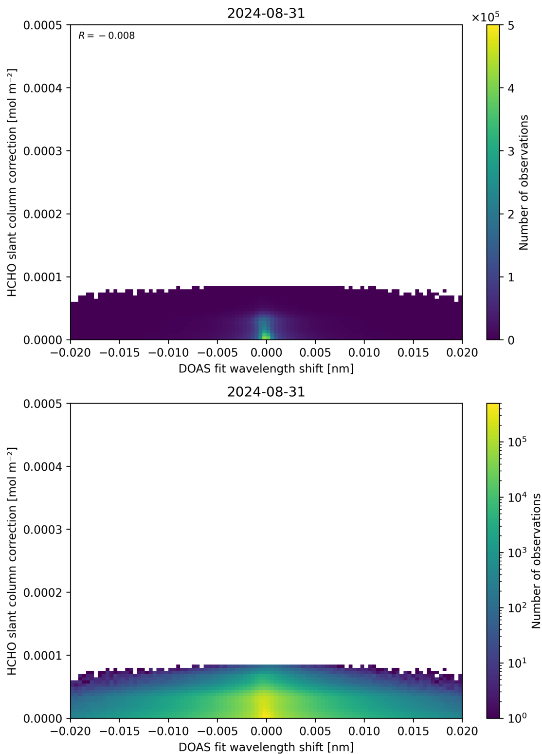
Figure 67: Scatter density plot of “DOAS fit wavelength shift” against “HCHO slant column correction” for 2024-08-30 to 2024-09-01.
