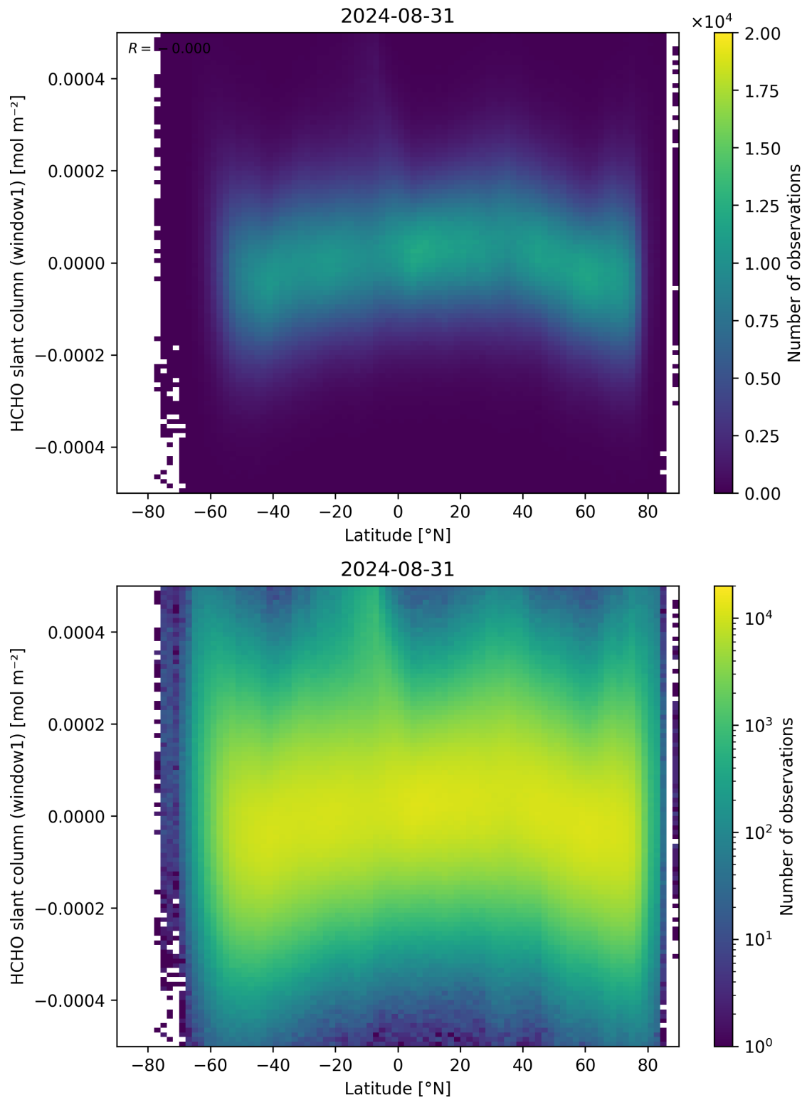
Figure 159: Scatter density plot of “Latitude” against “HCHO slant column (window1)” for 2024-08-30 to 2024-09-01.
