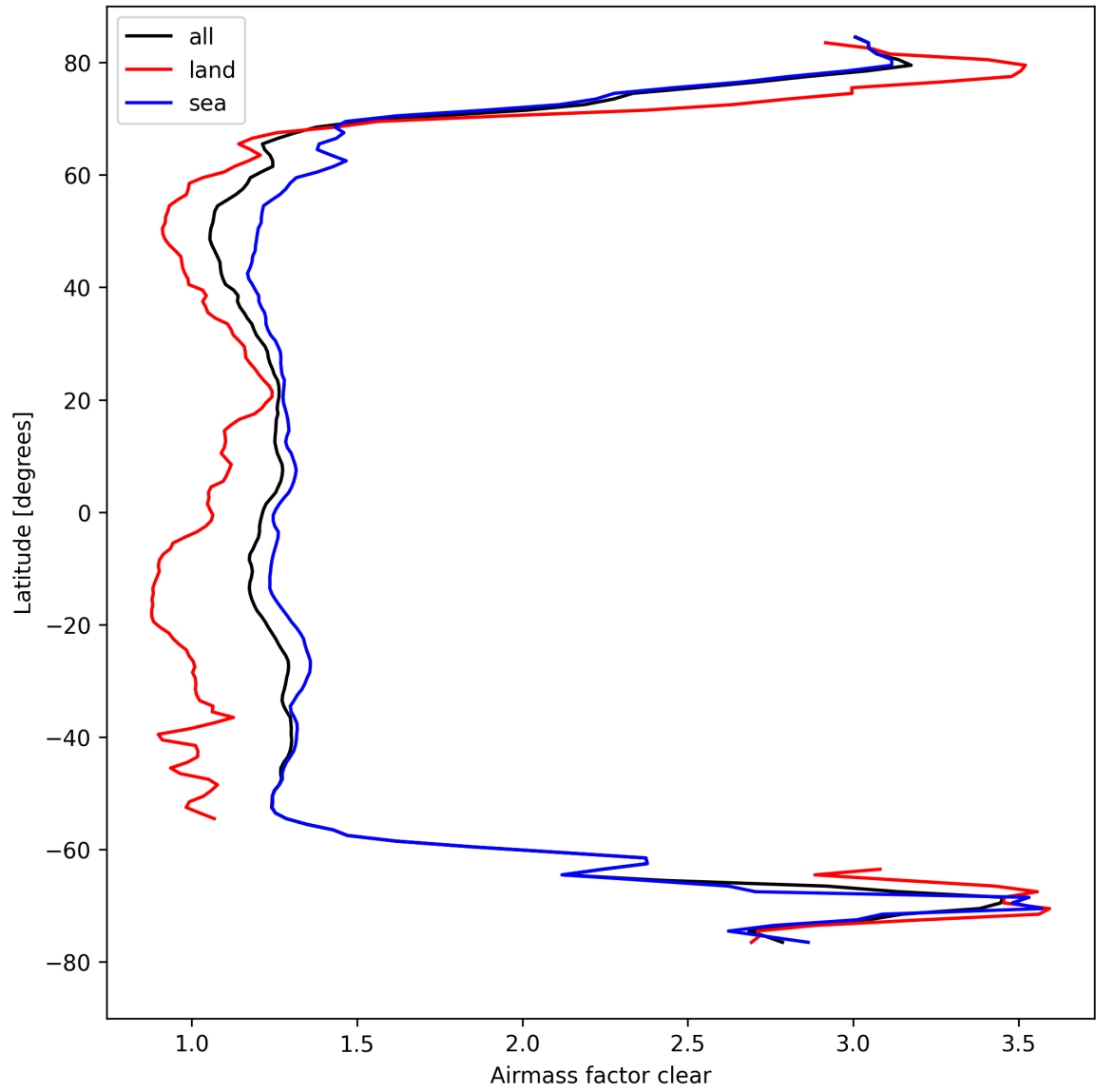
Figure 28: Zonal average of “Airmass factor clear” for 2024-08-30 to 2024-09-01.
