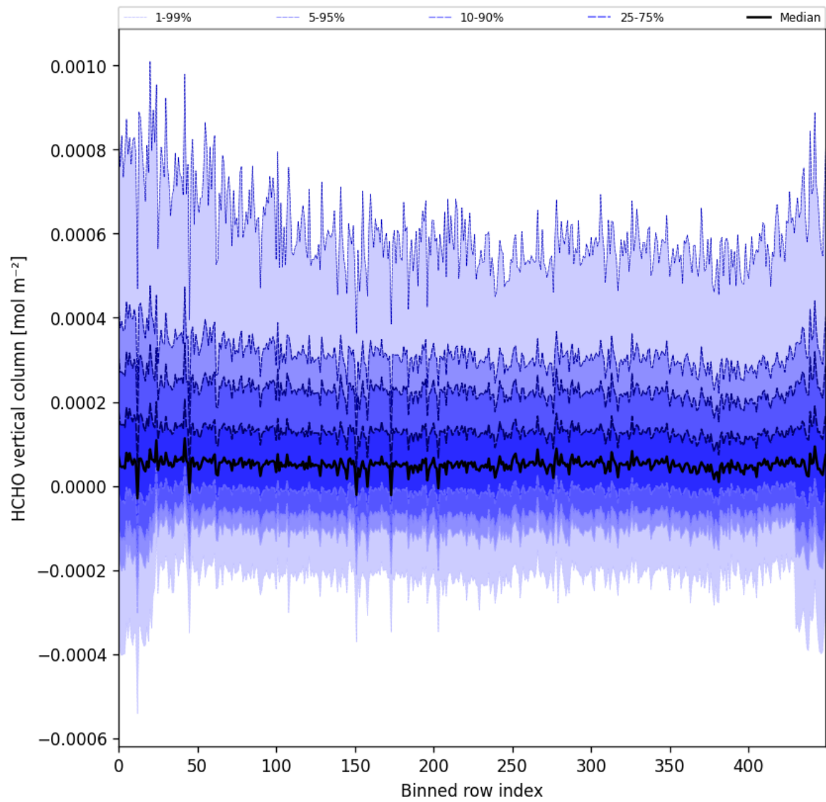
Figure 49: Along track statistics of “HCHO vertical column” for 2024-08-30 to 2024-09-01
