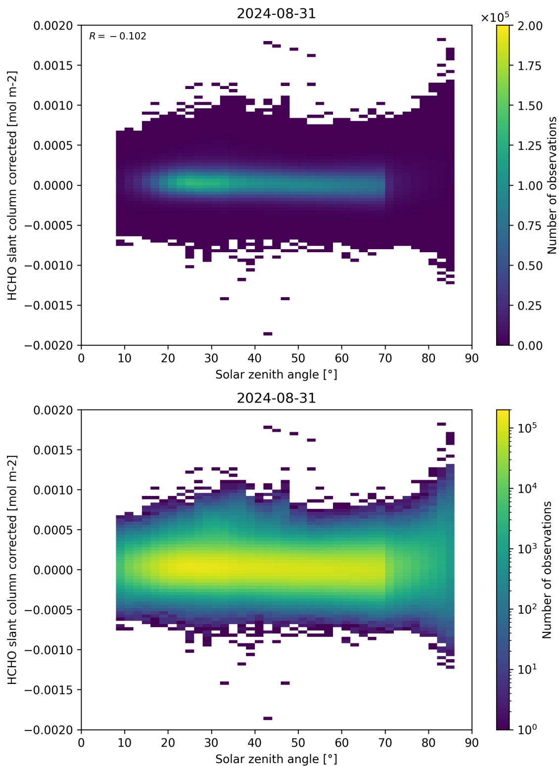
Figure 171: Scatter density plot of “Solar zenith angle” against “HCHO slant column corrected” for 2024-08-30 to 2024-09-01.
