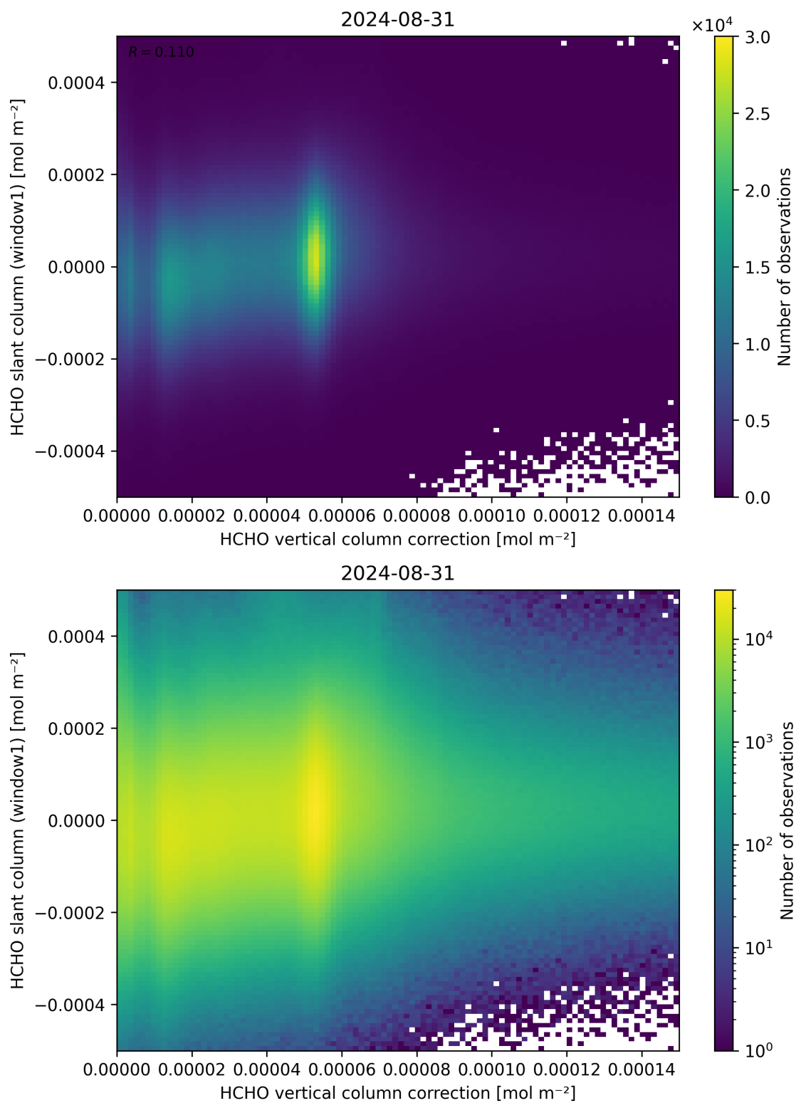
Figure 118: Scatter density plot of “HCHO vertical column correction” against “HCHO slant column (window1)” for 2024-08-30 to 2024-09-01.
