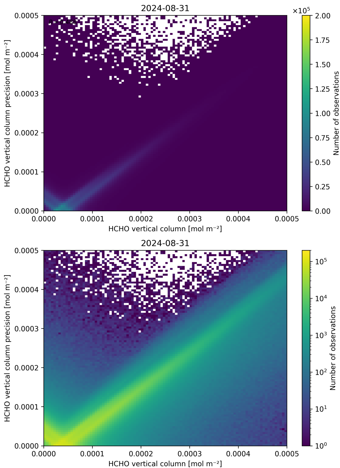
Figure 134: Scatter density plot of “HCHO vertical column” against “HCHO vertical column precision” for 2024-08-30 to 2024-09-01.
