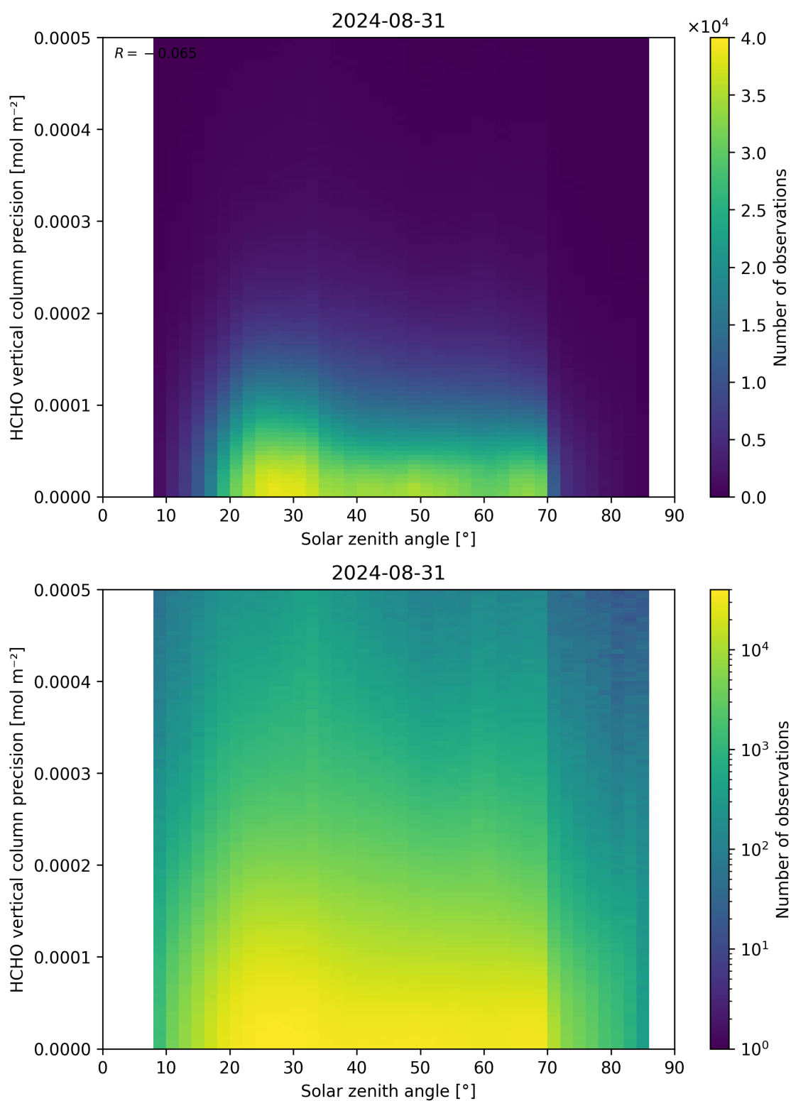
Figure 179: Scatter density plot of “Solar zenith angle” against “HCHO vertical column precision” for 2024-08-30 to 2024-09-01.
