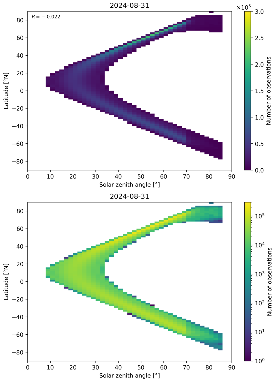
Figure 181: Scatter density plot of “Solar zenith angle” against “Latitude” for 2024-08-30 to 2024-09-01.
