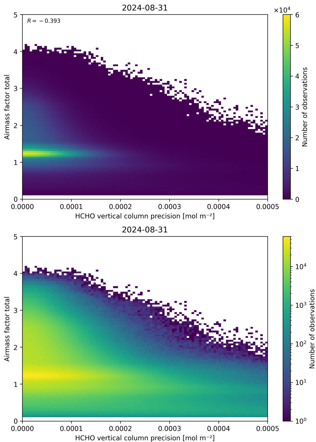
Figure 144: Scatter density plot of “HCHO vertical column precision” against “Airmass factor total” for 2024-08-30 to 2024-09-01.
