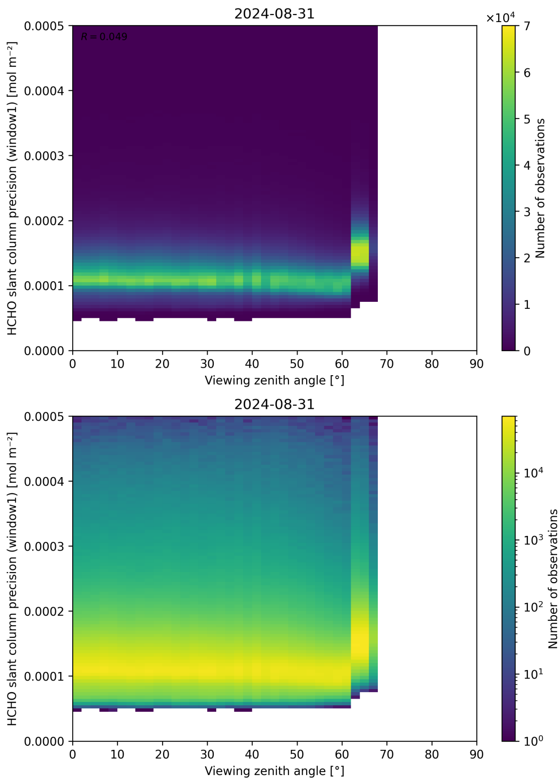
Figure 189: Scatter density plot of “Viewing zenith angle” against “HCHO slant column precision (window1)” for 2024-08-30 to 2024-09-01.
