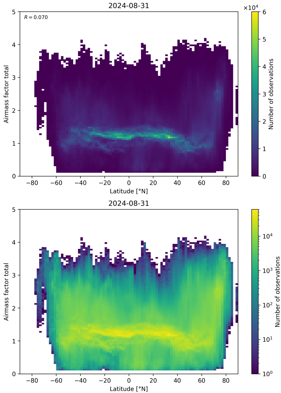
Figure 161: Scatter density plot of “Latitude” against “Airmass factor total” for 2024-08-30 to 2024-09-01.
