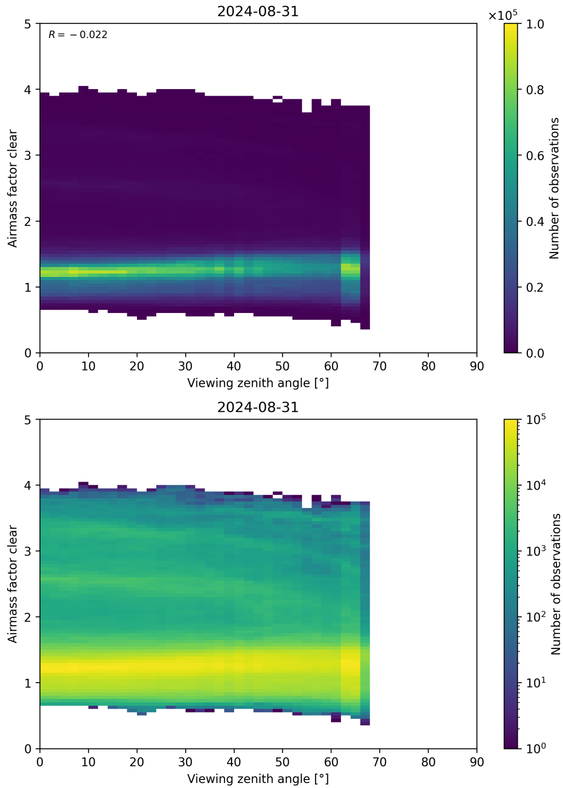
Figure 185: Scatter density plot of “Viewing zenith angle” against “Airmass factor clear” for 2024-08-30 to 2024-09-01.
