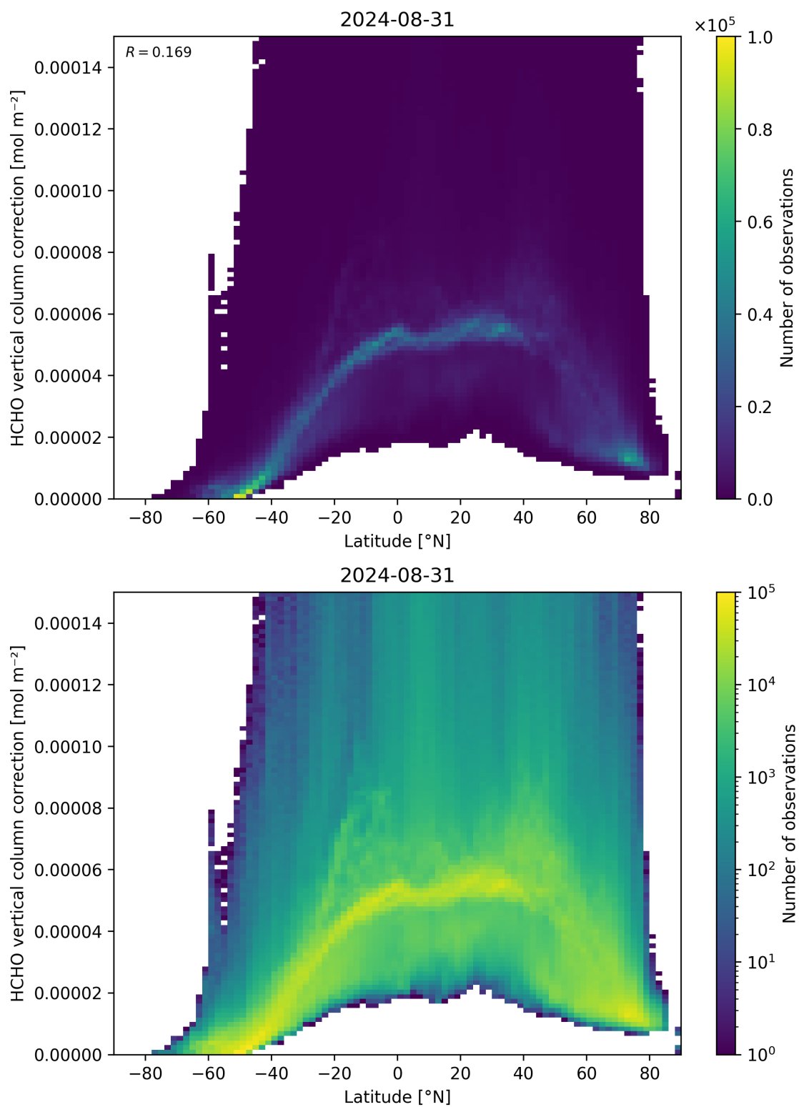
Figure 164: Scatter density plot of “Latitude” against “HCHO vertical column correction” for 2024-08-30 to 2024-09-01.
