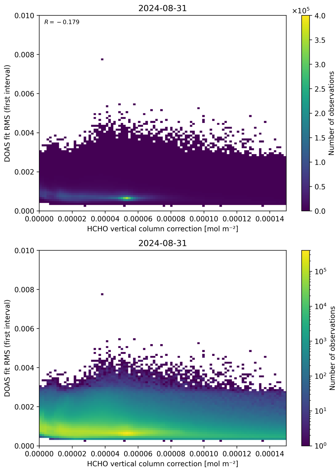
Figure 112: Scatter density plot of “HCHO vertical column correction” against “DOAS fit RMS (first interval)” for 2024-08-30 to 2024-09-01.
