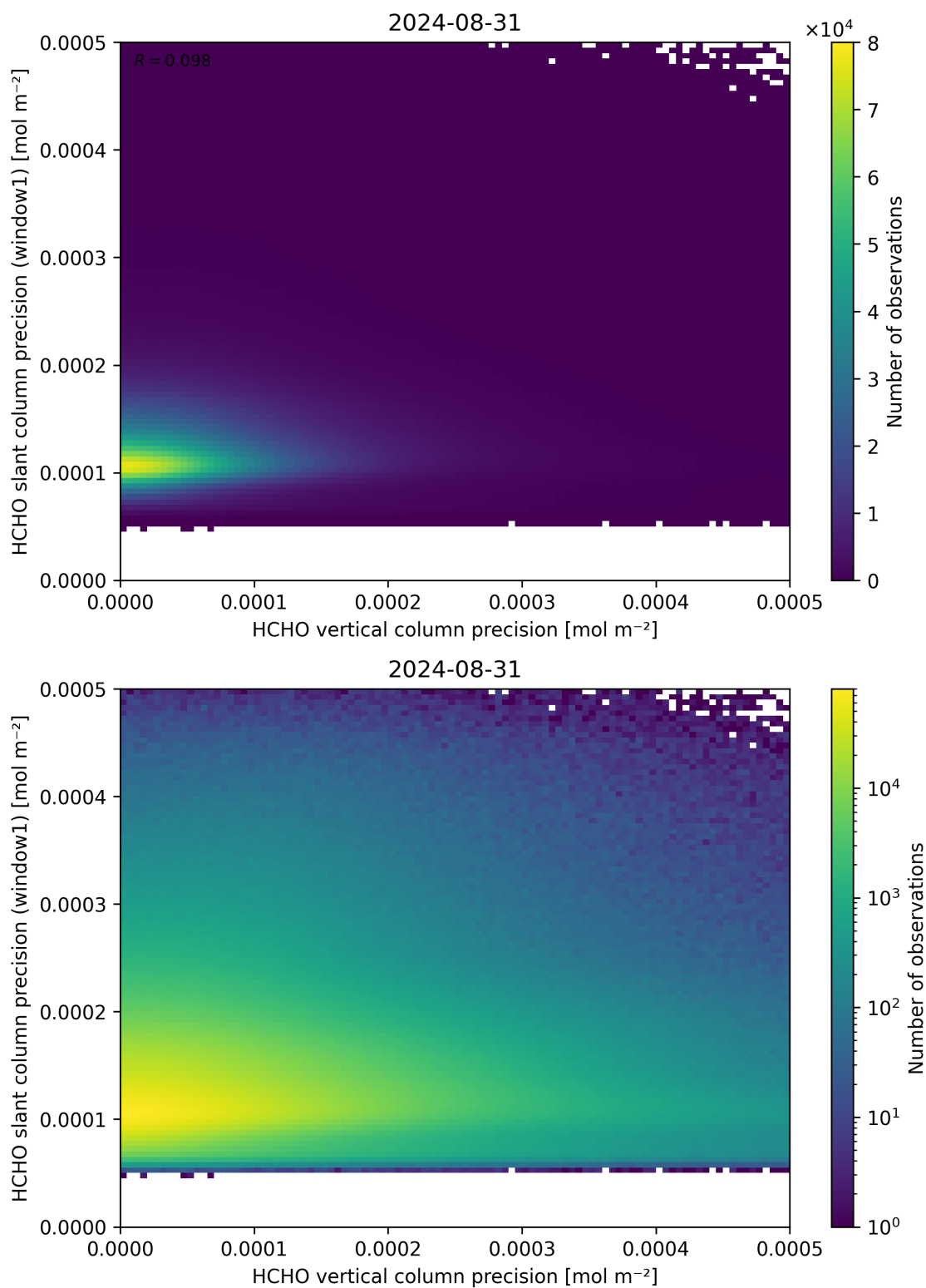
Figure 143: Scatter density plot of “HCHO vertical column precision” against “HCHO slant column precision (window1)” for 2024-08-30 to 2024-09-01.
