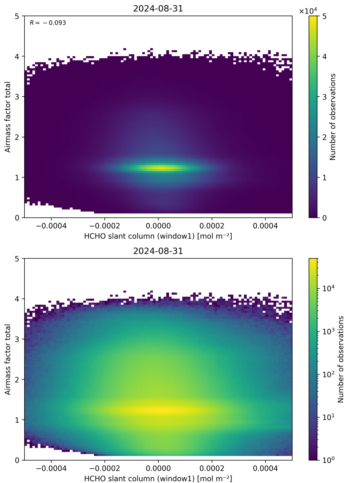
Figure 85: Scatter density plot of “HCHO slant column (window1)” against “Airmass factor total” for 2024-08-30 to 2024-09-01.
