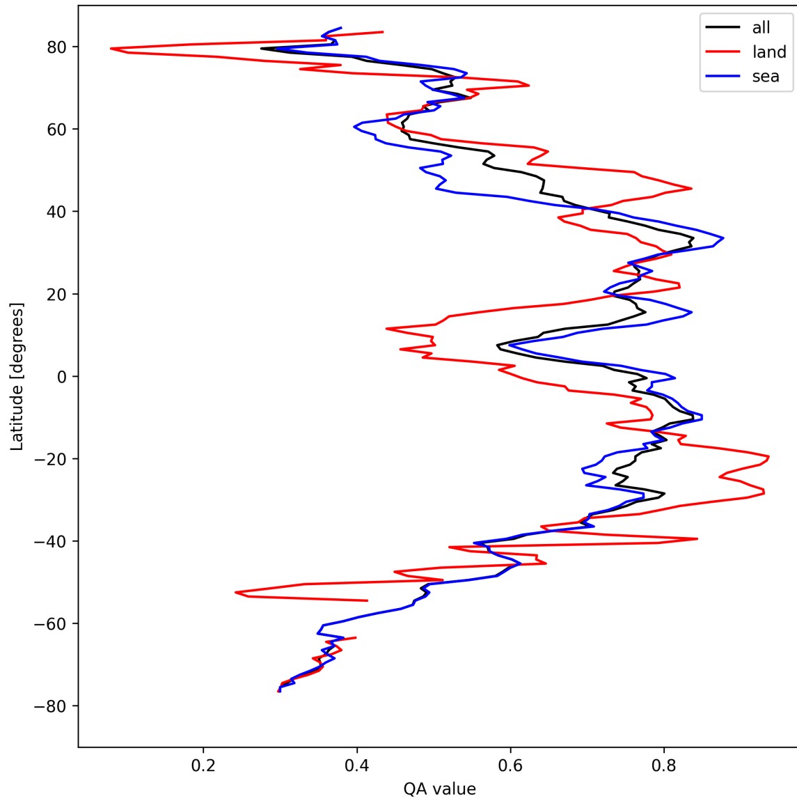
Figure 20: Zonal average of “QA value” for 2024-08-30 to 2024-09-01.
