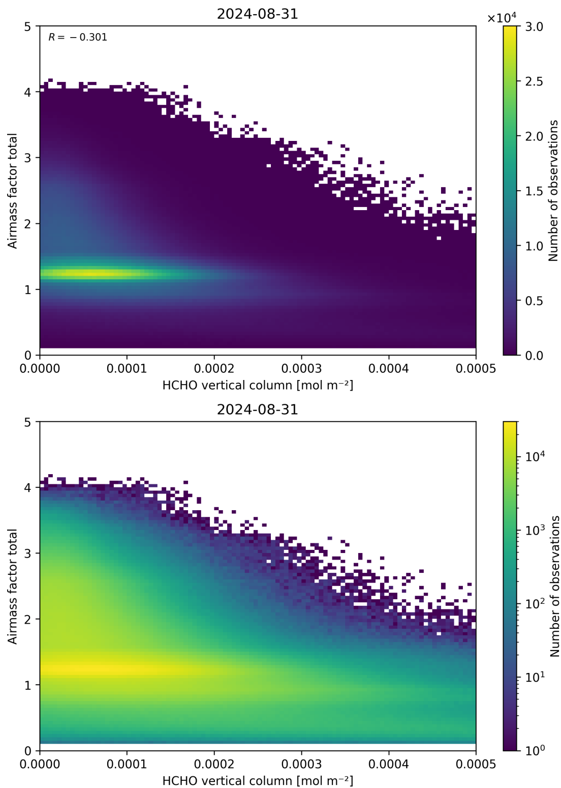
Figure 131: Scatter density plot of “HCHO vertical column” against “Airmass factor total” for 2024-08-30 to 2024-09-01.
