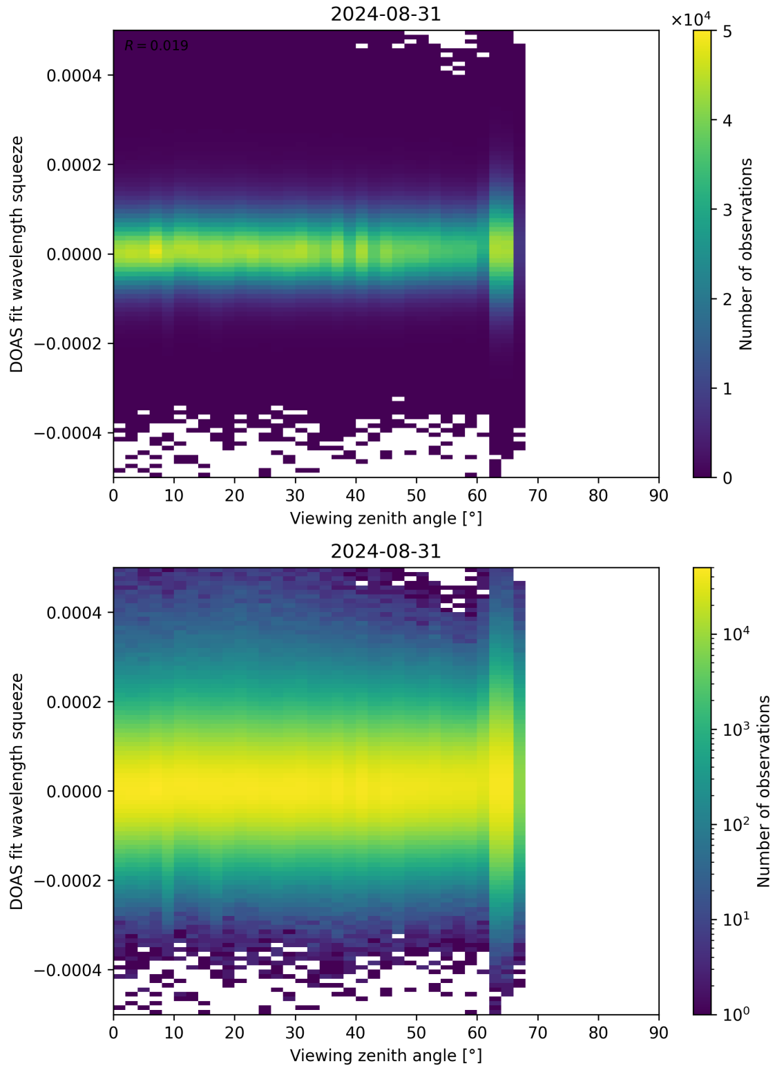
Figure 184: Scatter density plot of “Viewing zenith angle” against “DOAS fit wavelength squeeze” for 2024-08-30 to 2024-09-01.
