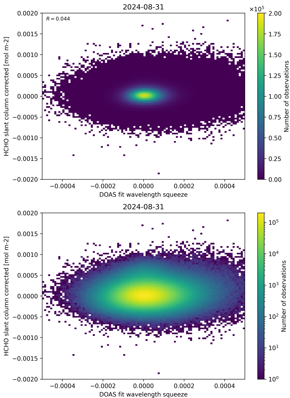
Figure 69: Scatter density plot of “DOAS fit wavelength squeeze” against “HCHO slant column corrected” for 2024-08-30 to 2024-09-01.
