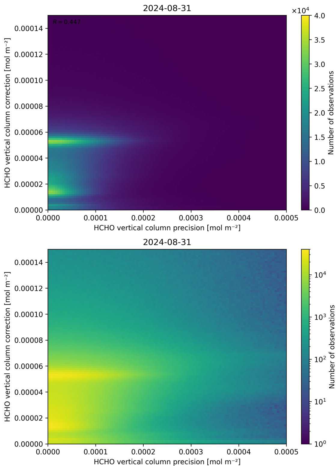
Figure 146: Scatter density plot of “HCHO vertical column precision” against “HCHO vertical column correction” for 2024-08-30 to 2024-09-01.
