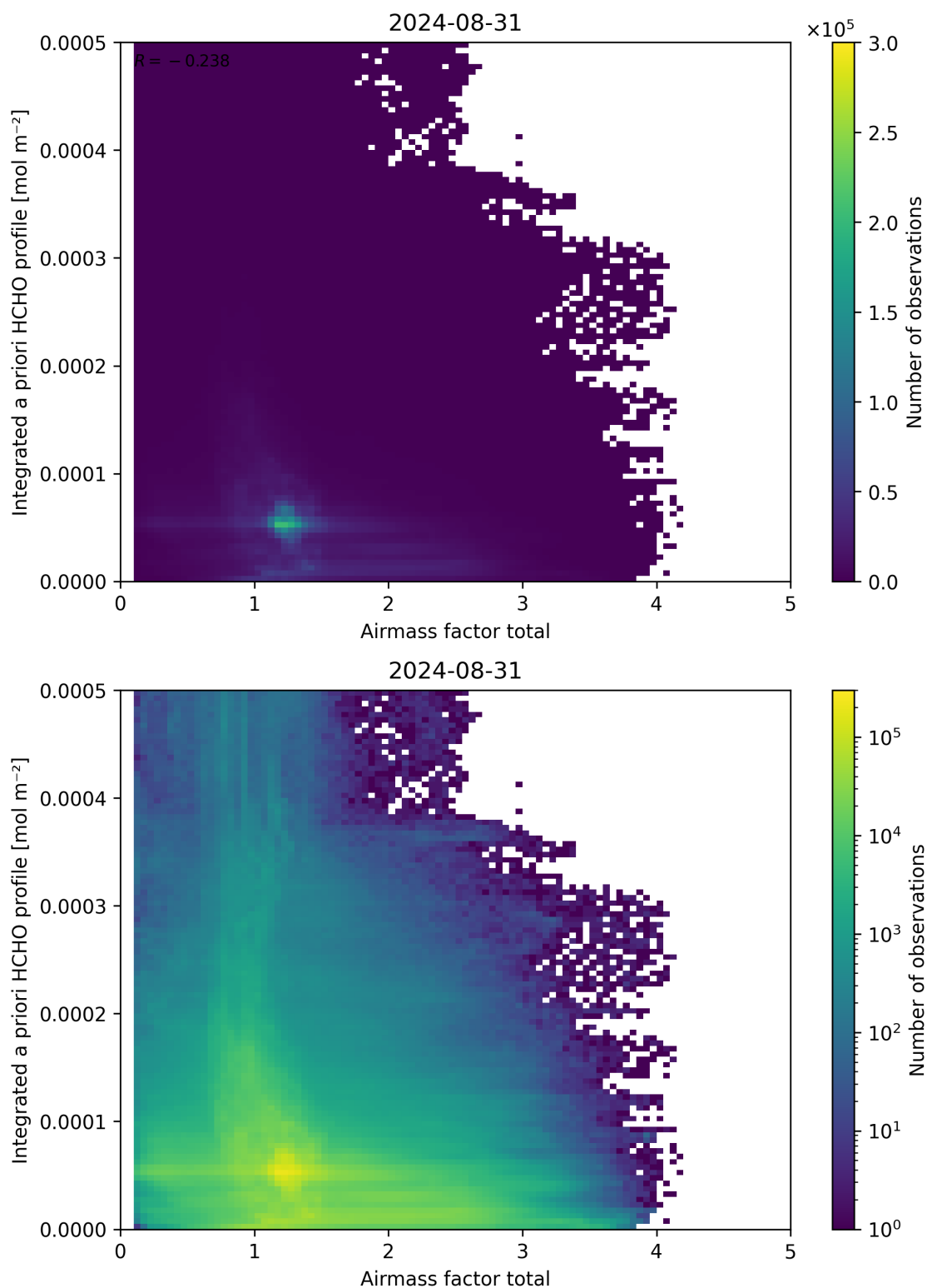
Figure 104: Scatter density plot of “Airmass factor total” against “Integrated a priori HCHO profile” for 2024-08-30 to 2024-09-01.
