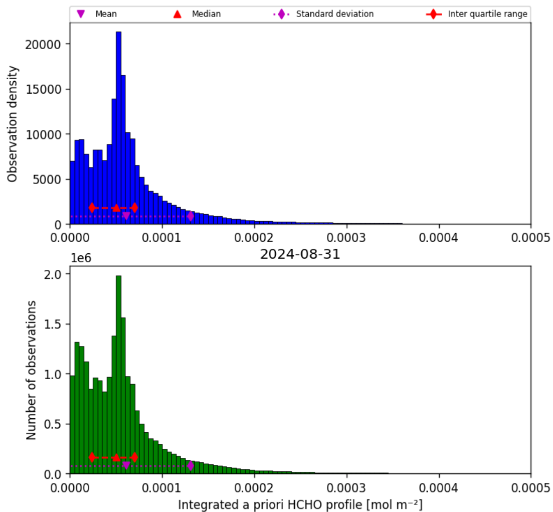
Figure 43: Histogram of “Integrated a priori HCHO profile” for 2024-08-30 to 2024-09-01
