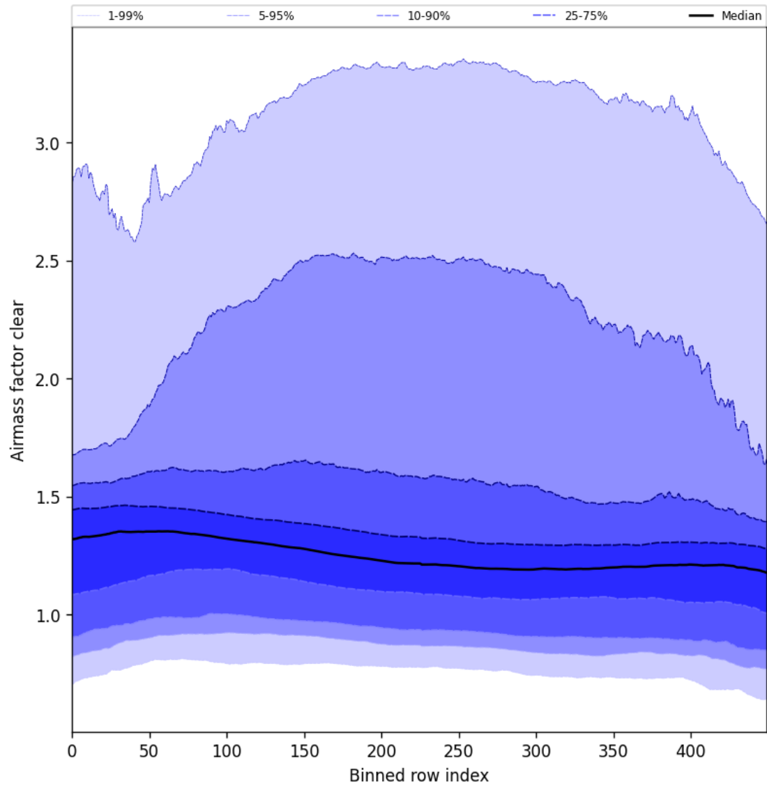
Figure 56: Along track statistics of “Airmass factor clear” for 2024-08-30 to 2024-09-01
