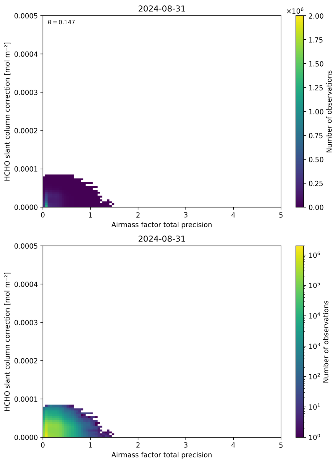
Figure 110: Scatter density plot of “Airmass factor total precision” against “HCHO slant column correction” for 2024-08-30 to 2024-09-01.
