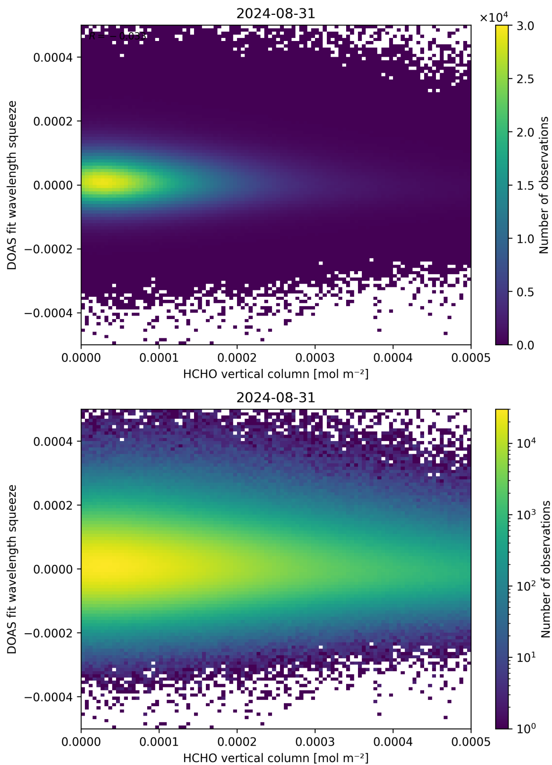
Figure 125: Scatter density plot of “HCHO vertical column” against “DOAS fit wavelength squeeze” for 2024-08-30 to 2024-09-01.
