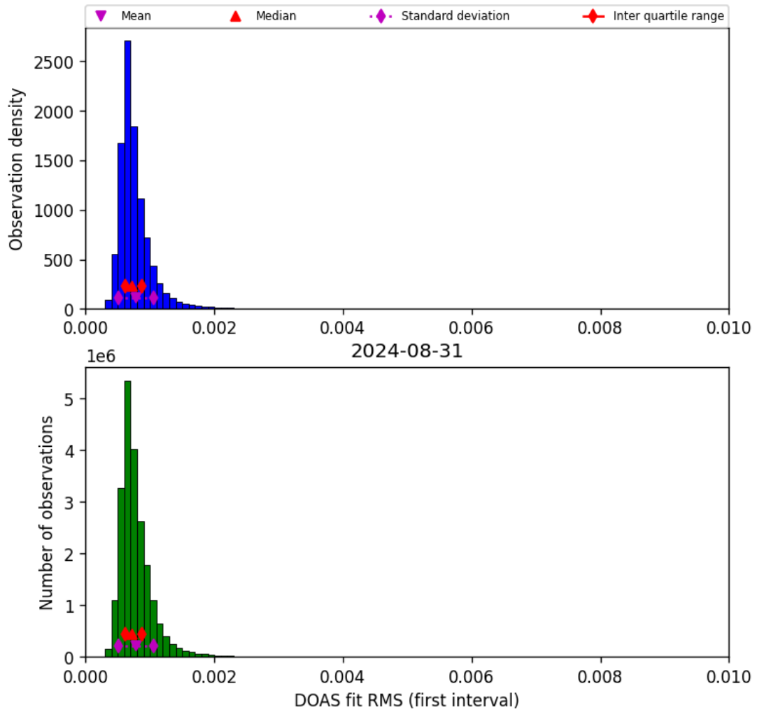
Figure 46: Histogram of “DOAS fit RMS (first interval)” for 2024-08-30 to 2024-09-01
