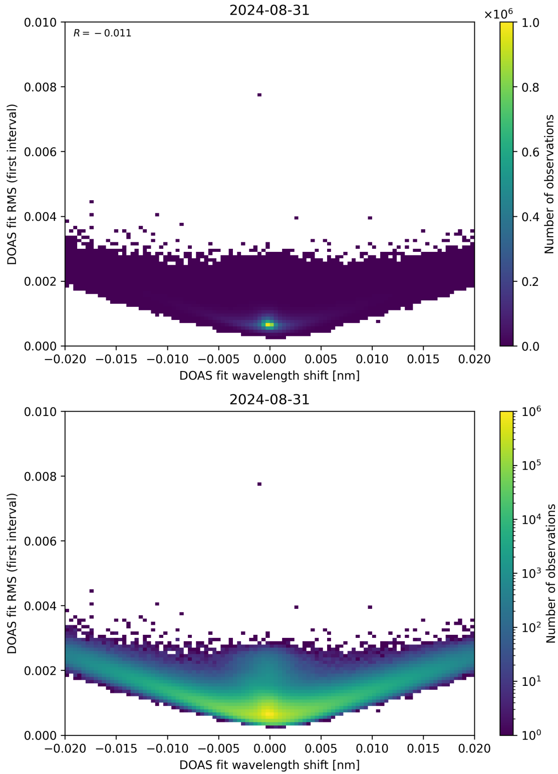
Figure 64: Scatter density plot of “DOAS fit wavelength shift” against “DOAS fit RMS (first interval)” for 2024-08-30 to 2024-09-01.
