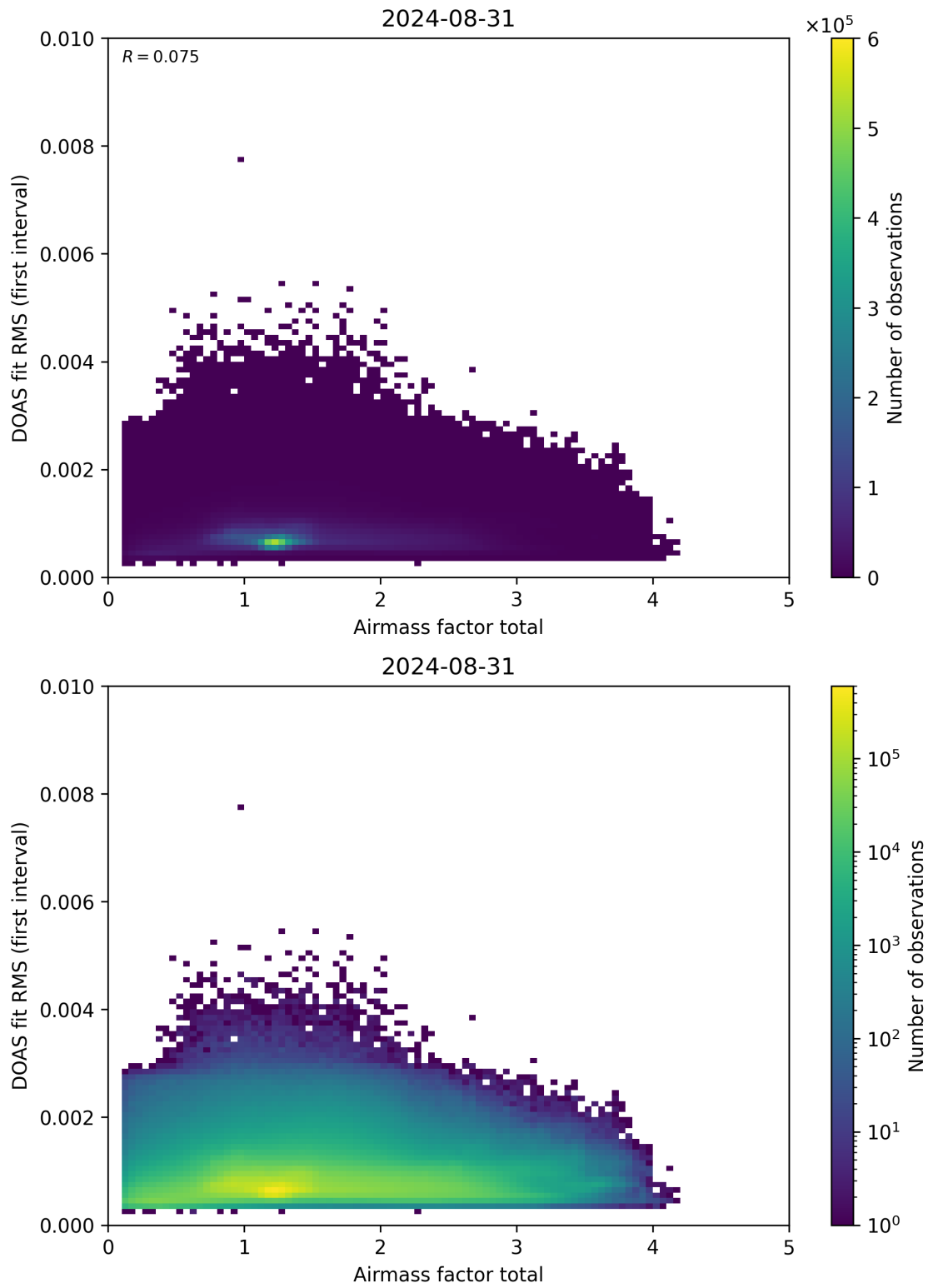
Figure 97: Scatter density plot of “Airmass factor total” against “DOAS fit RMS (first interval)” for 2024-08-30 to 2024-09-01.
