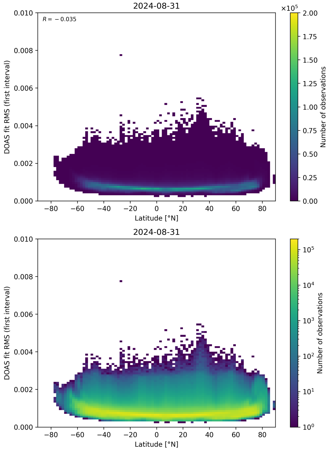
Figure 153: Scatter density plot of “Latitude” against “DOAS fit RMS (first interval)” for 2024-08-30 to 2024-09-01.
