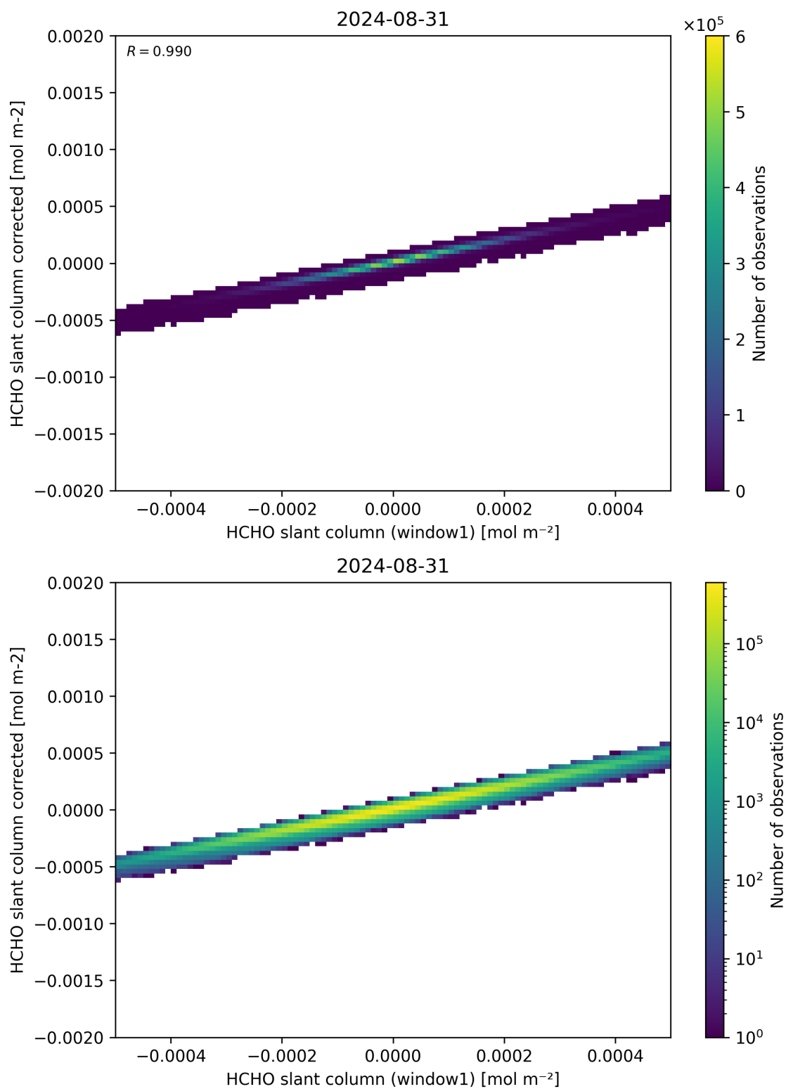
Figure 82: Scatter density plot of “HCHO slant column (window1)” against “HCHO slant column corrected” for 2024-08-30 to 2024-09-01.
