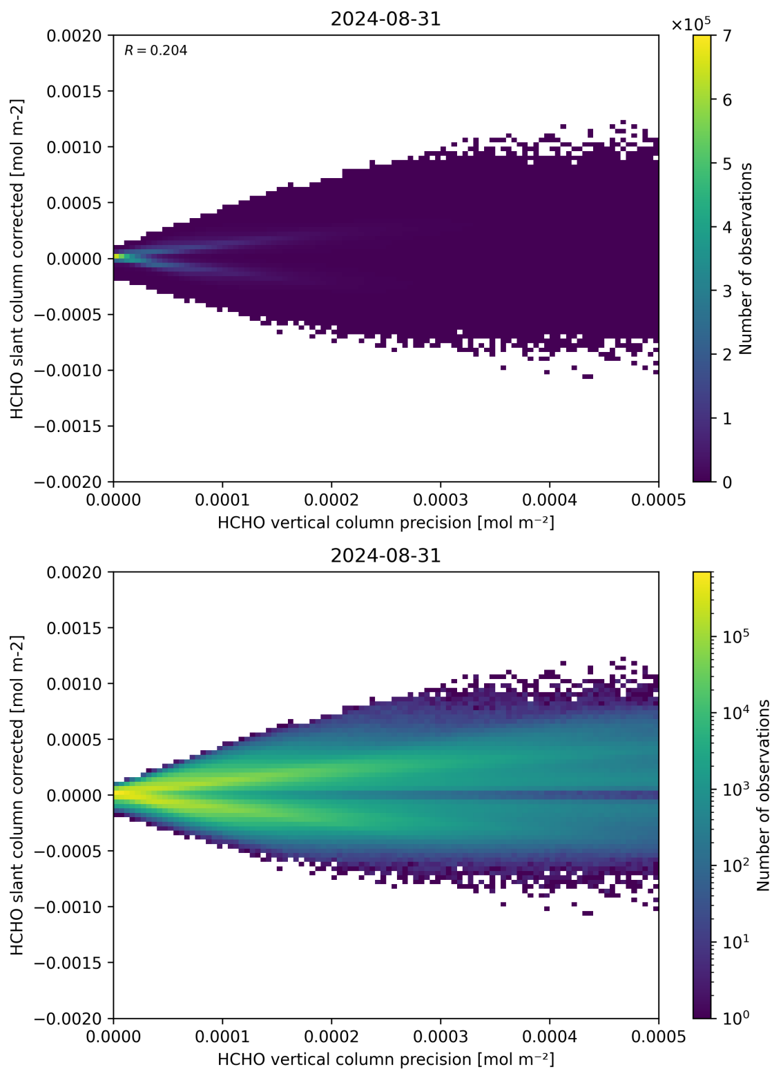
Figure 140: Scatter density plot of “HCHO vertical column precision” against “HCHO slant column corrected” for 2024-08-30 to 2024-09-01.
