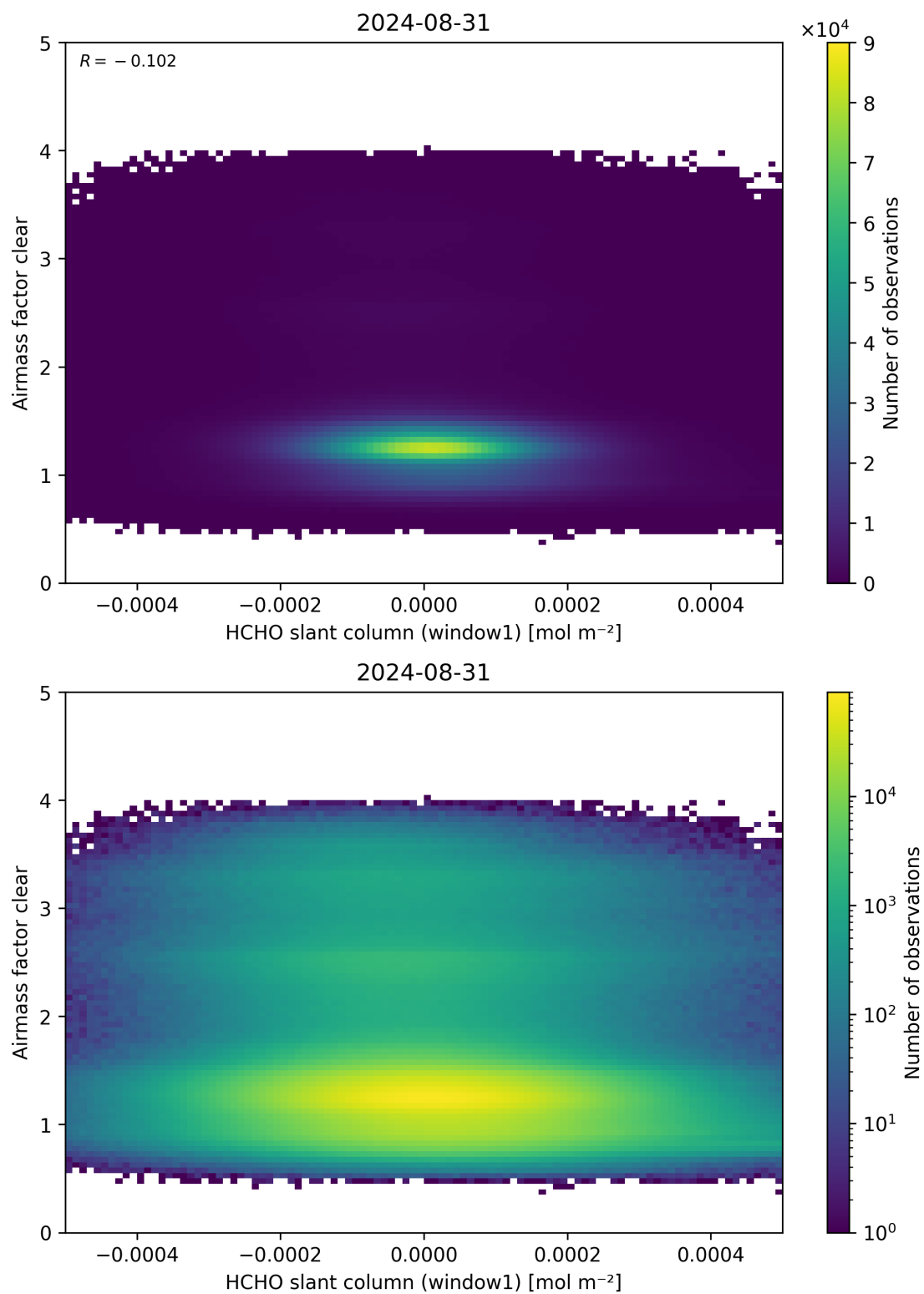
Figure 81: Scatter density plot of “HCHO slant column (window1)” against “Airmass factor clear” for 2024-08-30 to 2024-09-01.
