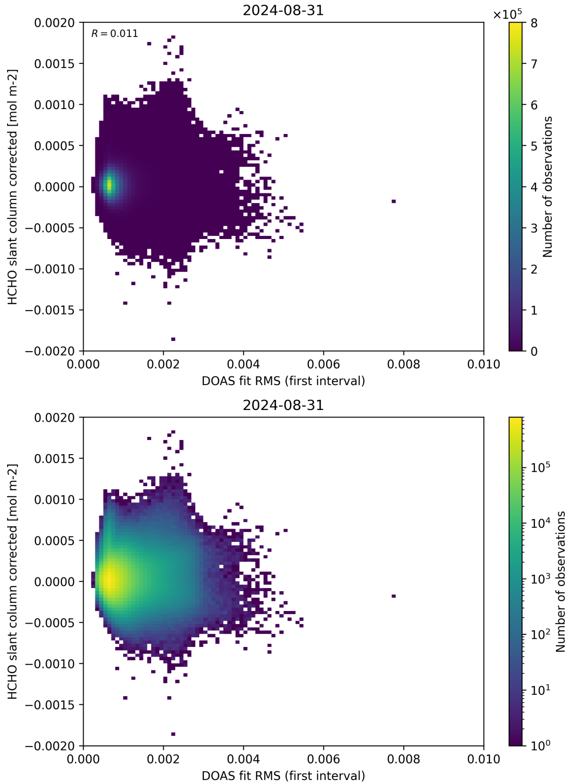
Figure 62: Scatter density plot of “DOAS fit RMS (first interval)” against “HCHO slant column corrected” for 2024-08-30 to 2024-09-01.
