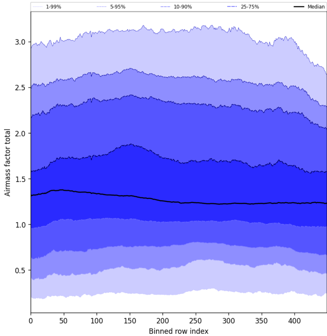
Figure 54: Along track statistics of “Airmass factor total” for 2024-08-30 to 2024-09-01
