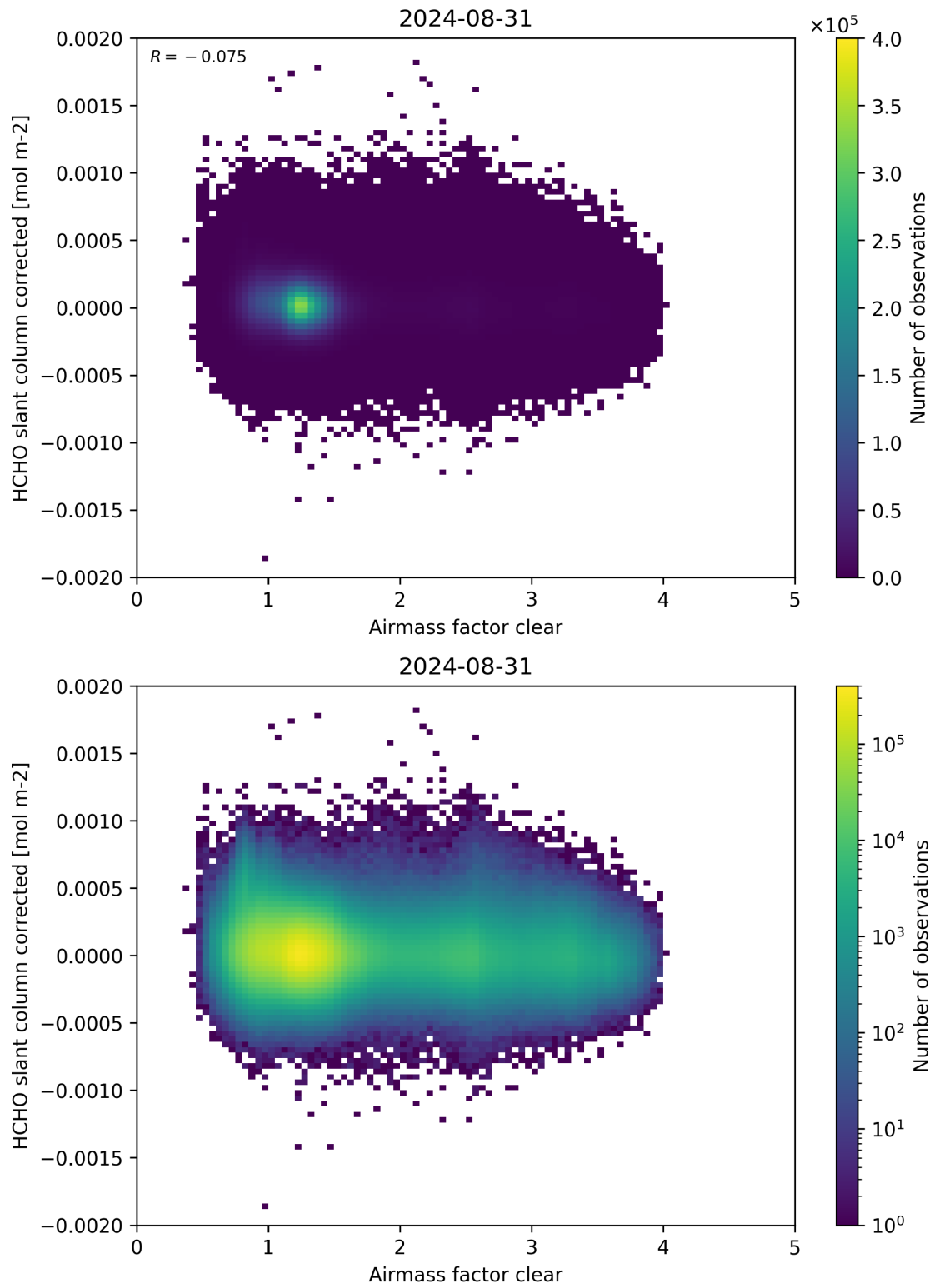
Figure 74: Scatter density plot of “Airmass factor clear” against “HCHO slant column corrected” for 2024-08-30 to 2024-09-01.
