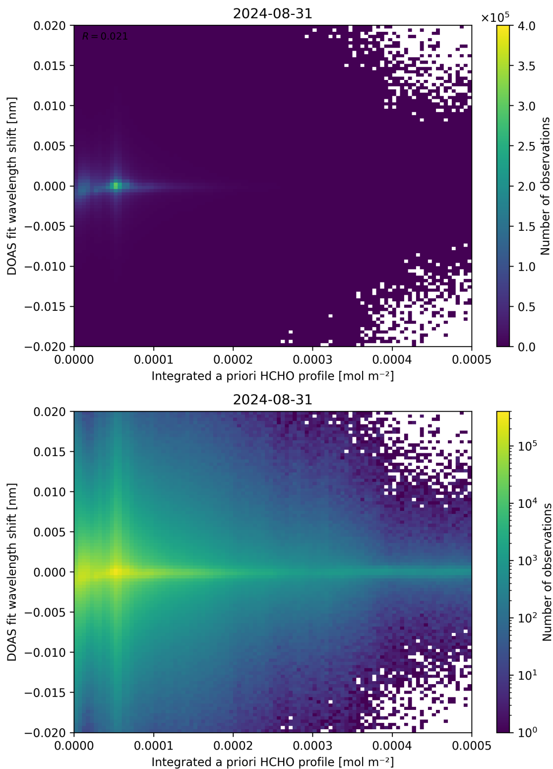
Figure 149: Scatter density plot of “Integrated a priori HCHO profile” against “DOAS fit wavelength shift” for 2024-08-30 to 2024-09-01.
