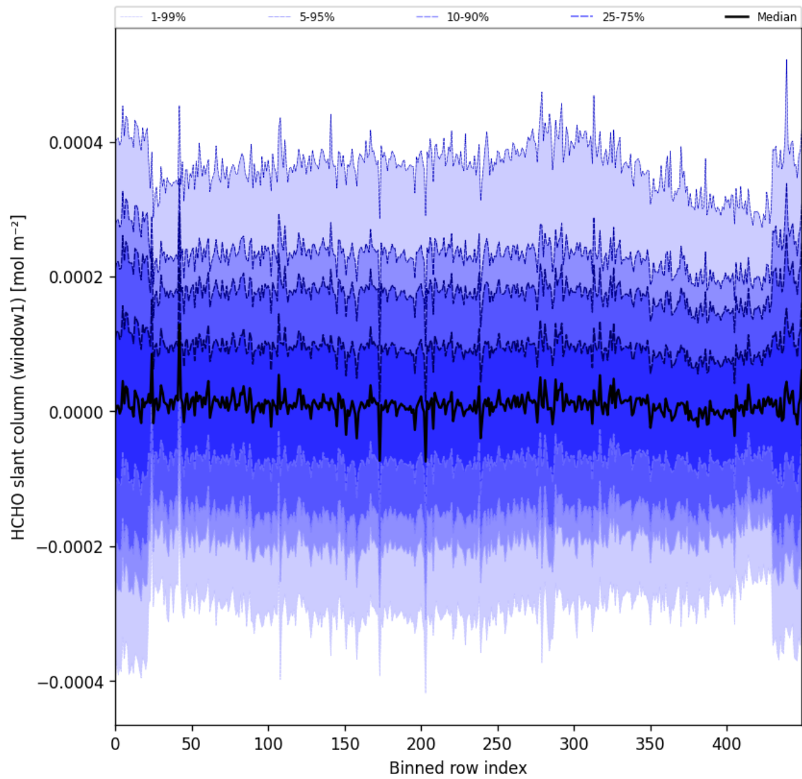
Figure 52: Along track statistics of “HCHO slant column (window1)” for 2024-08-30 to 2024-09-01
