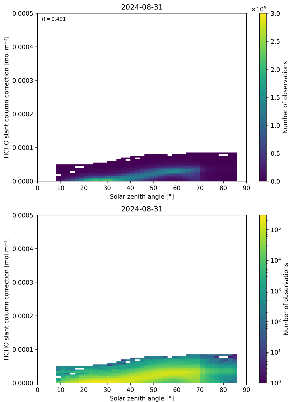
Figure 172: Scatter density plot of “Solar zenith angle” against “HCHO slant column correction” for 2024-08-30 to 2024-09-01.
