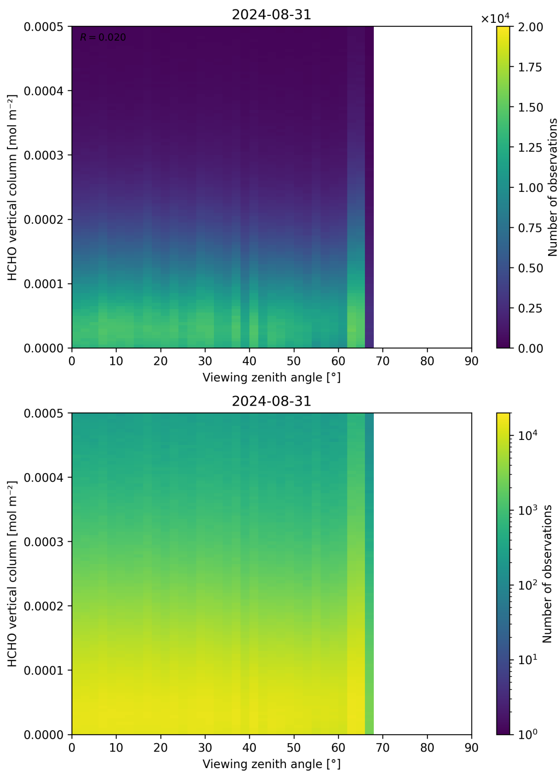
Figure 192: Scatter density plot of “Viewing zenith angle” against “HCHO vertical column” for 2024-08-30 to 2024-09-01.
