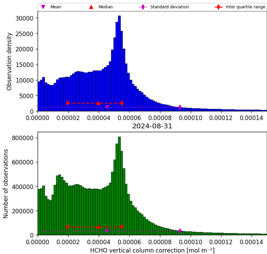
Figure 37: Histogram of “HCHO vertical column correction” for 2024-08-30 to 2024-09-01
