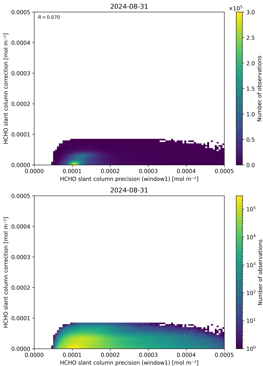
Figure 93: Scatter density plot of “HCHO slant column precision (window1)” against “HCHO slant column correction” for 2024-08-30 to 2024-09-01.
