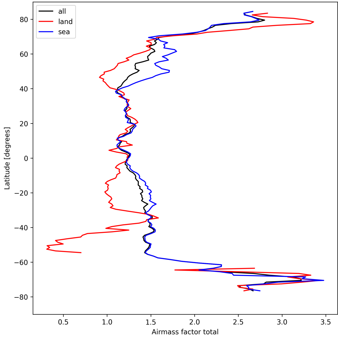
Figure 26: Zonal average of “Airmass factor total” for 2024-08-30 to 2024-09-01.
