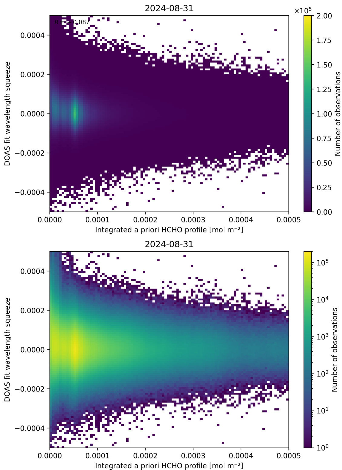
Figure 150: Scatter density plot of “Integrated a priori HCHO profile” against “DOAS fit wavelength squeeze” for 2024-08-30 to 2024-09-01.
