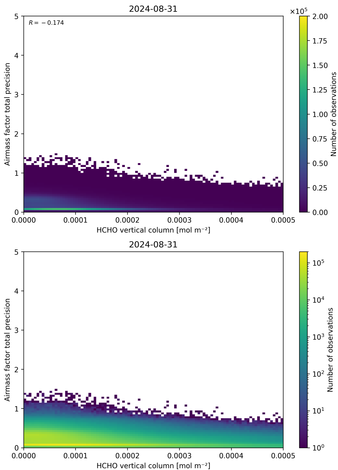
Figure 132: Scatter density plot of “HCHO vertical column” against “Airmass factor total precision” for 2024-08-30 to 2024-09-01.
