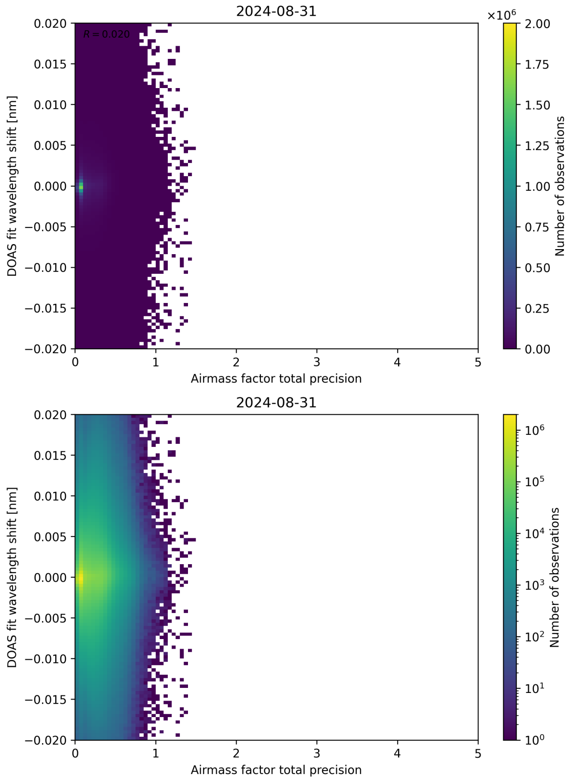
Figure 106: Scatter density plot of “Airmass factor total precision” against “DOAS fit wavelength shift” for 2024-08-30 to 2024-09-01.
