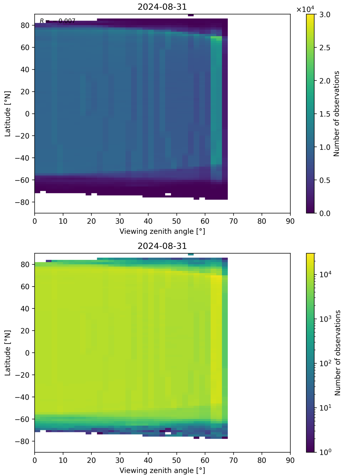
Figure 196: Scatter density plot of “Viewing zenith angle” against “Latitude” for 2024-08-30 to 2024-09-01.
