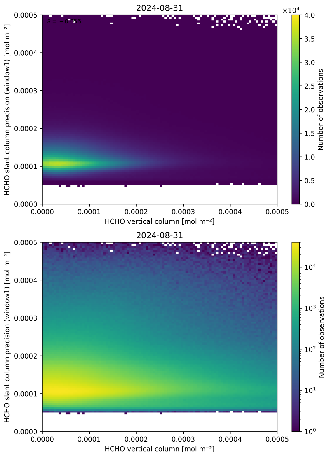
Figure 130: Scatter density plot of “HCHO vertical column” against “HCHO slant column precision (window1)” for 2024-08-30 to 2024-09-01.
