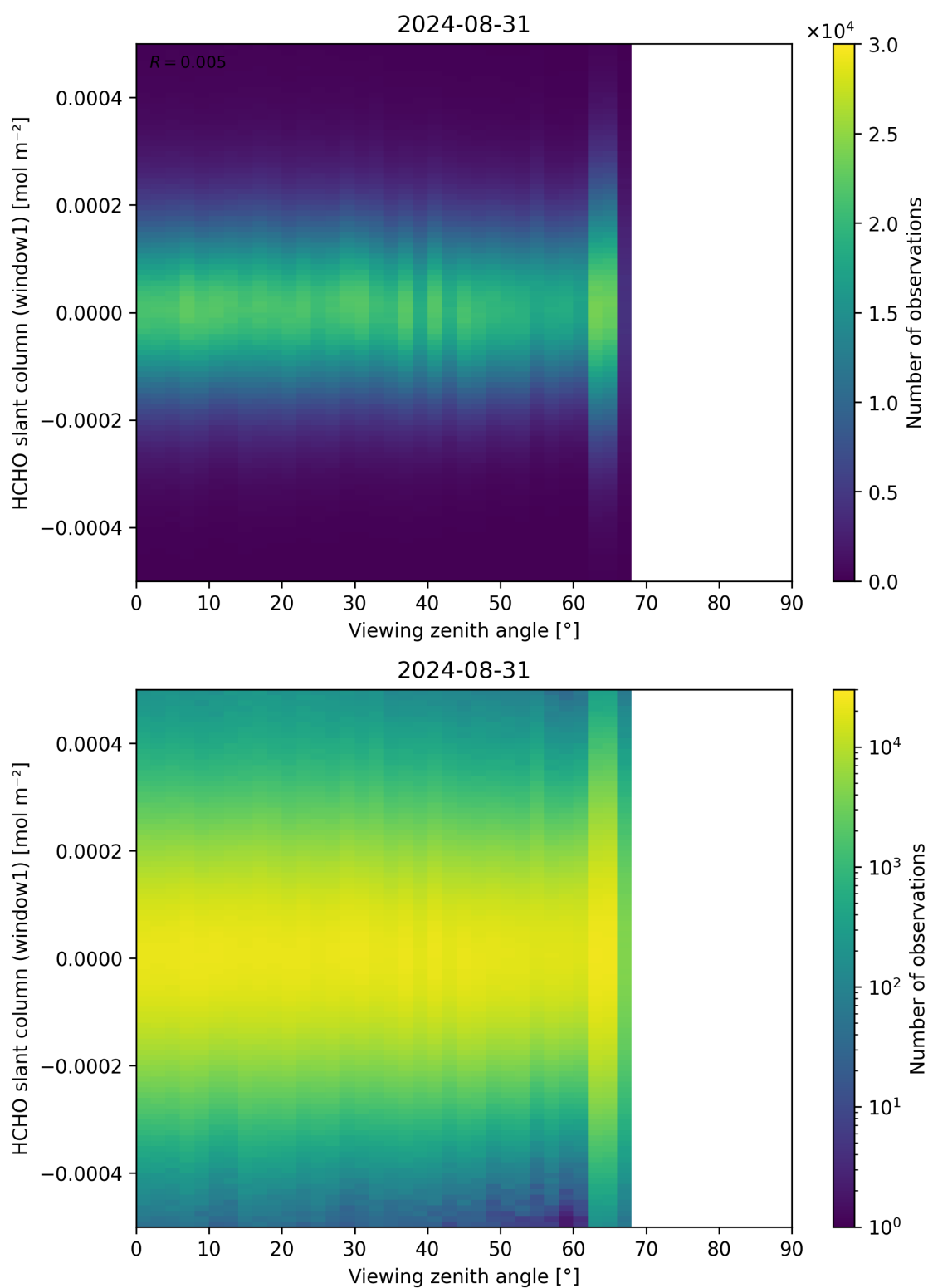
Figure 188: Scatter density plot of “Viewing zenith angle” against “HCHO slant column (window1)” for 2024-08-30 to 2024-09-01.
