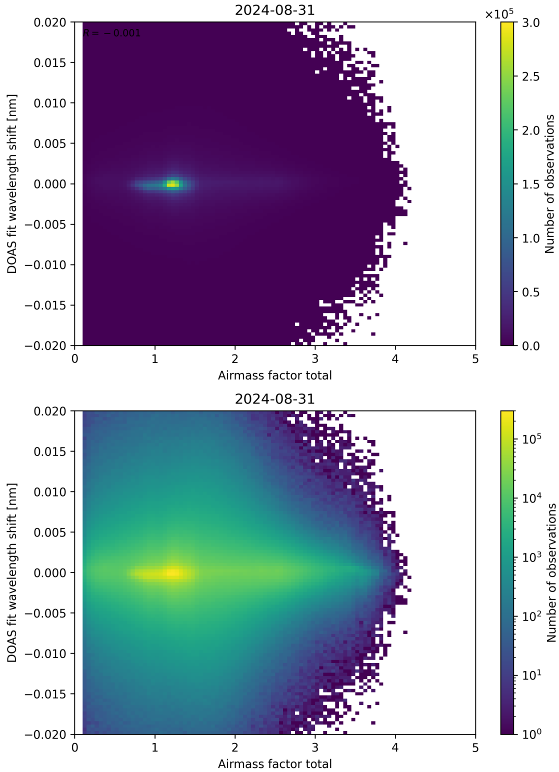
Figure 98: Scatter density plot of “Airmass factor total” against “DOAS fit wavelength shift” for 2024-08-30 to 2024-09-01.
