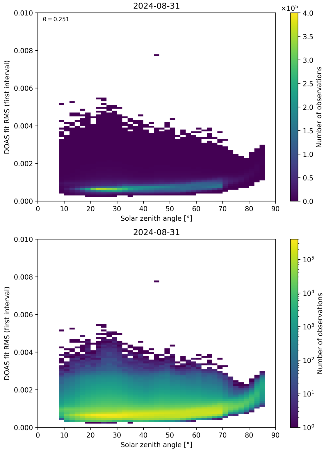
Figure 167: Scatter density plot of “Solar zenith angle” against “DOAS fit RMS (first interval)” for 2024-08-30 to 2024-09-01.
