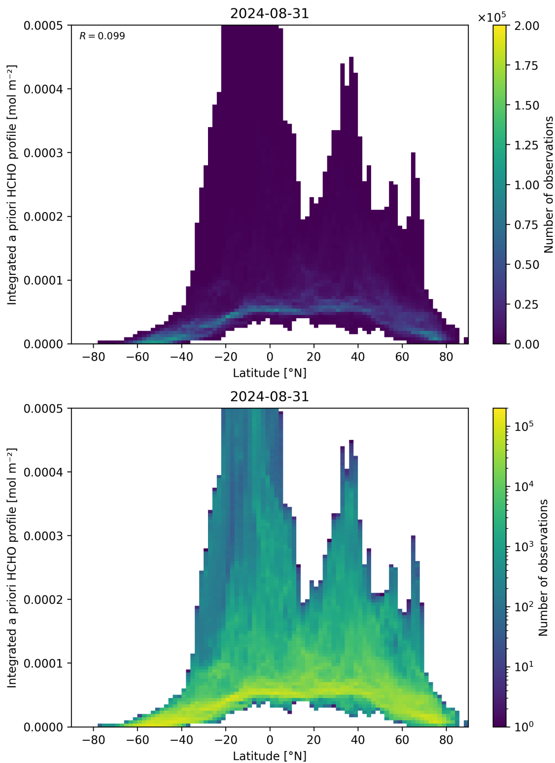
Figure 166: Scatter density plot of “Latitude” against “Integrated a priori HCHO profile” for 2024-08-30 to 2024-09-01.
