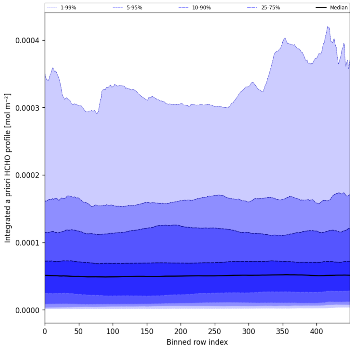
Figure 57: Along track statistics of “Integrated a priori HCHO profile” for 2024-08-30 to 2024-09-01
