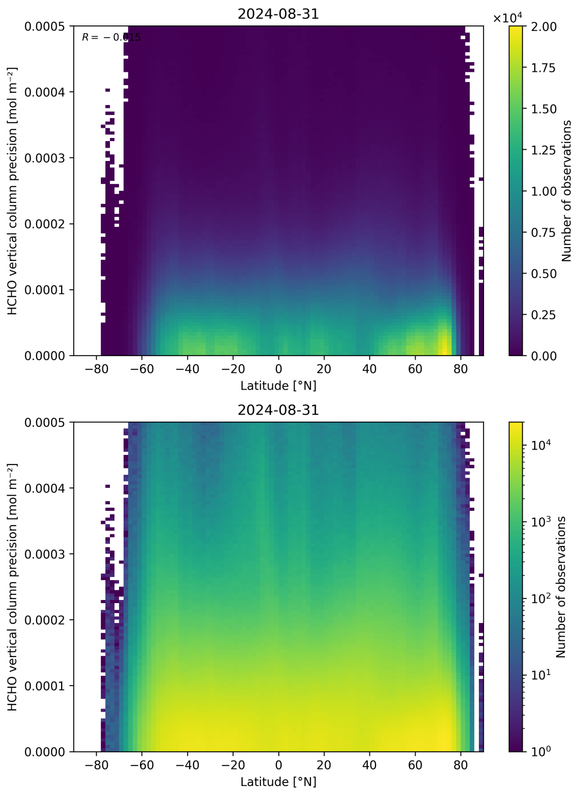
Figure 165: Scatter density plot of “Latitude” against “HCHO vertical column precision” for 2024-08-30 to 2024-09-01.
