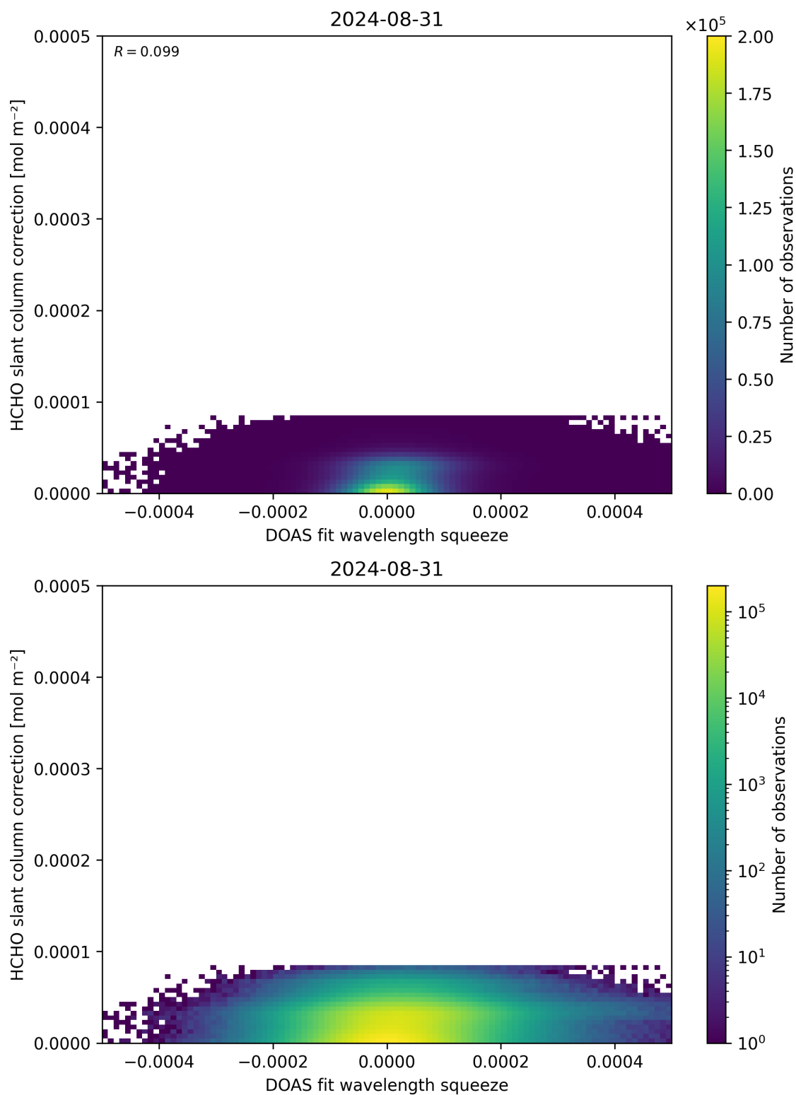
Figure 70: Scatter density plot of “DOAS fit wavelength squeeze” against “HCHO slant column correction” for 2024-08-30 to 2024-09-01.
