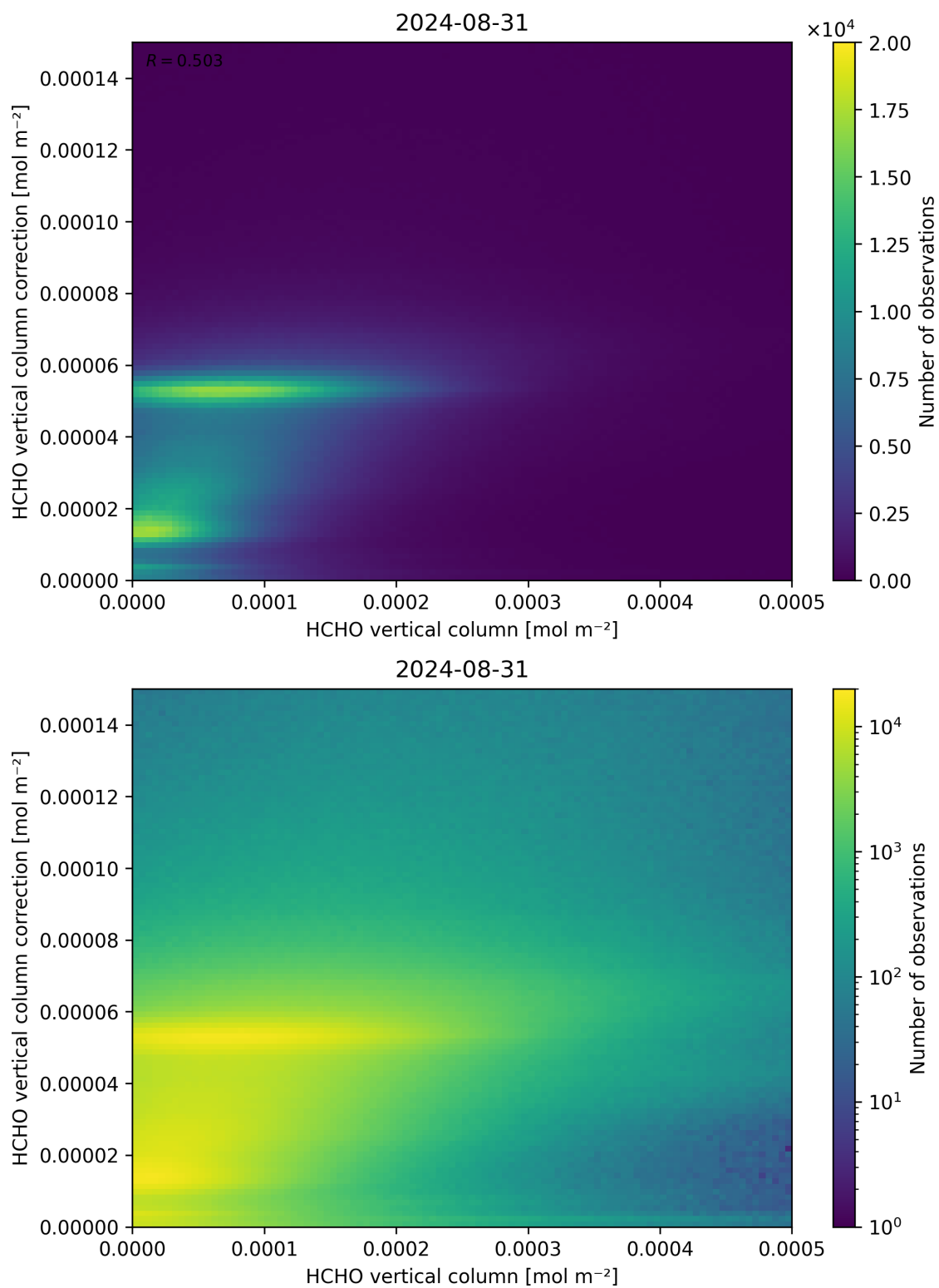
Figure 133: Scatter density plot of “HCHO vertical column” against “HCHO vertical column correction” for 2024-08-30 to 2024-09-01.
