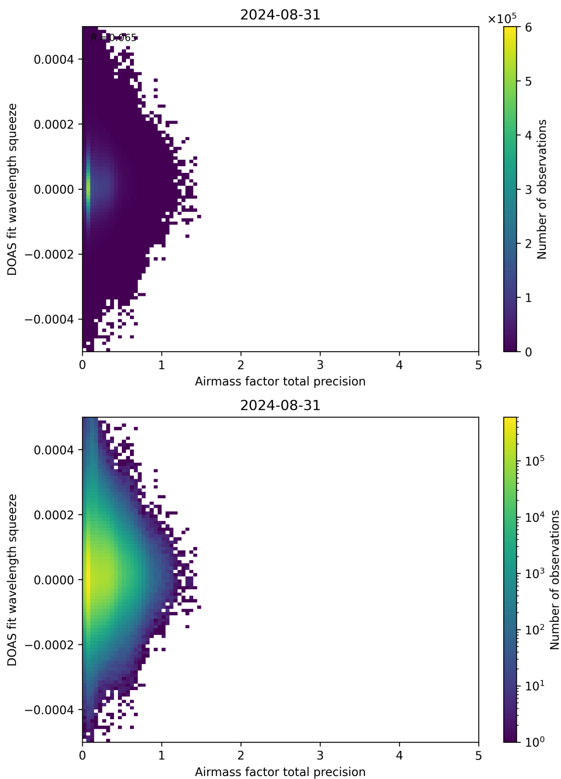
Figure 107: Scatter density plot of “Airmass factor total precision” against “DOAS fit wavelength squeeze” for 2024-08-30 to 2024-09-01.
