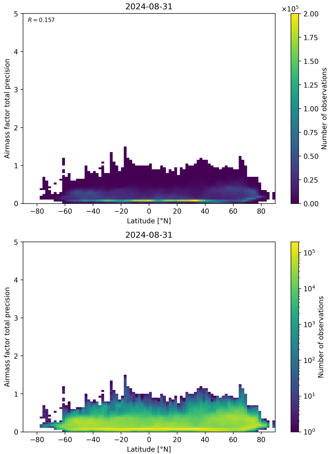
Figure 162: Scatter density plot of “Latitude” against “Airmass factor total precision” for 2024-08-30 to 2024-09-01.
