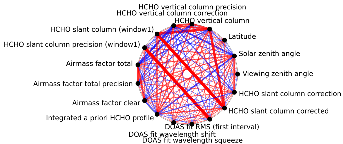
Figure 1: Map of correlation graph for 2024-08-30 to 2024-09-01.
