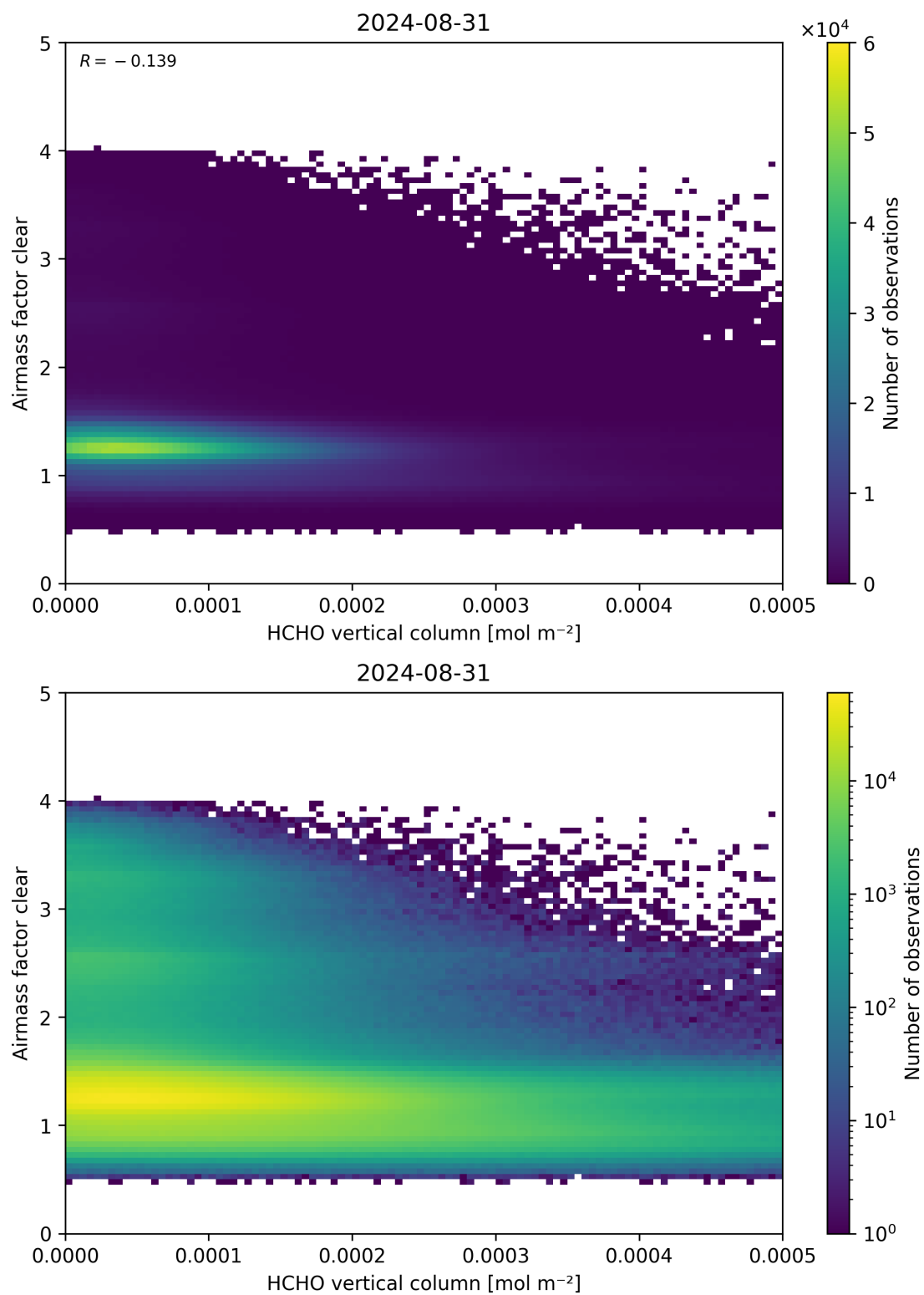
Figure 126: Scatter density plot of “HCHO vertical column” against “Airmass factor clear” for 2024-08-30 to 2024-09-01.
