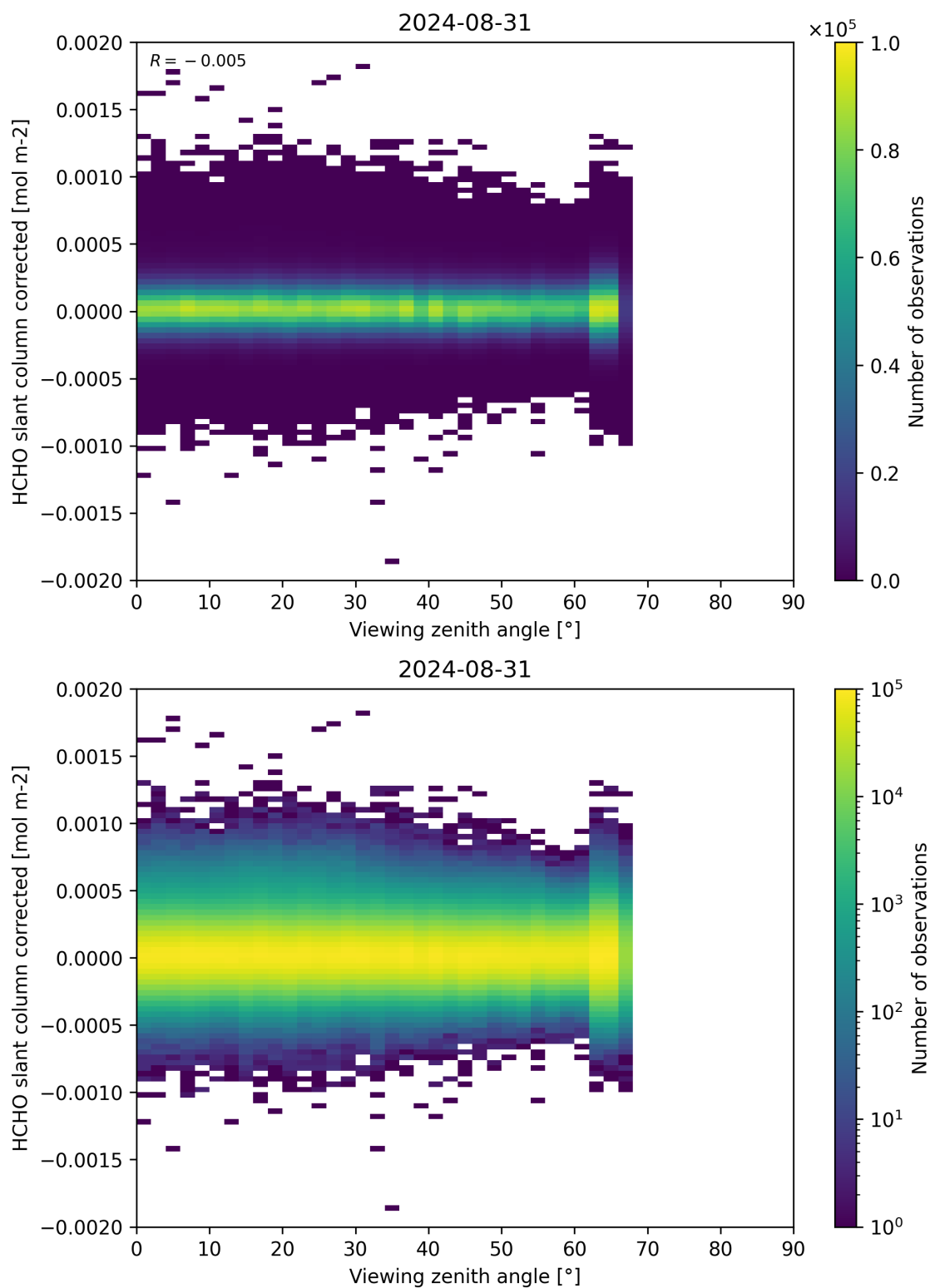
Figure 186: Scatter density plot of “Viewing zenith angle” against “HCHO slant column corrected” for 2024-08-30 to 2024-09-01.
