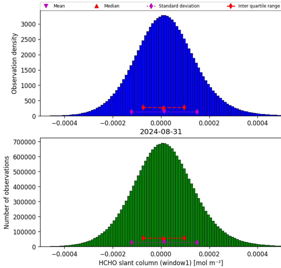
Figure 38: Histogram of “HCHO slant column (window1)” for 2024-08-30 to 2024-09-01
