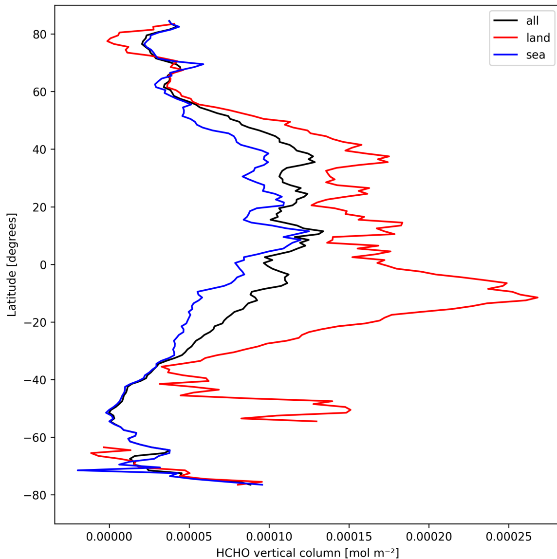
Figure 21: Zonal average of “HCHO vertical column” for 2024-08-30 to 2024-09-01.
