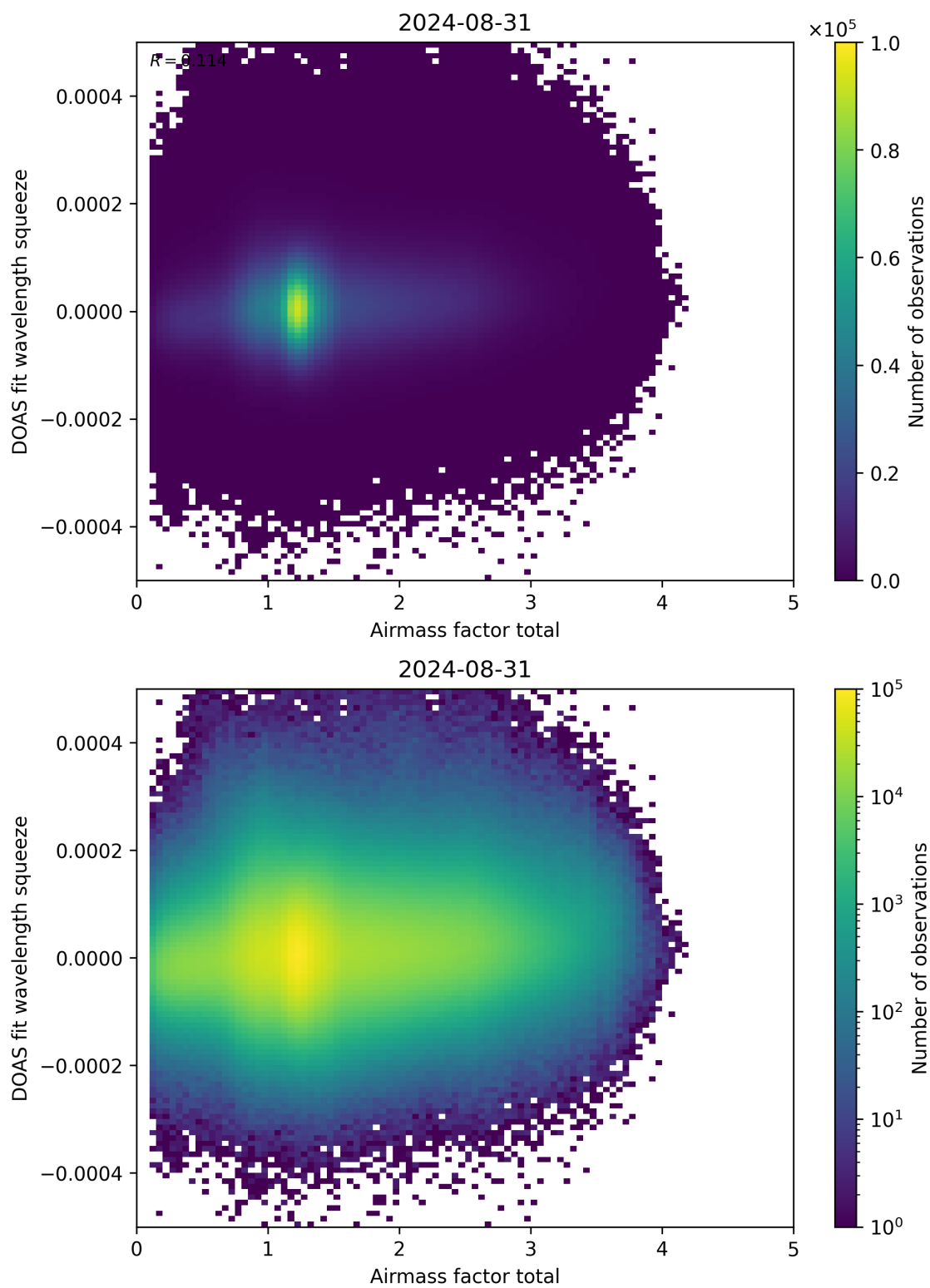
Figure 99: Scatter density plot of “Airmass factor total” against “DOAS fit wavelength squeeze” for 2024-08-30 to 2024-09-01.
