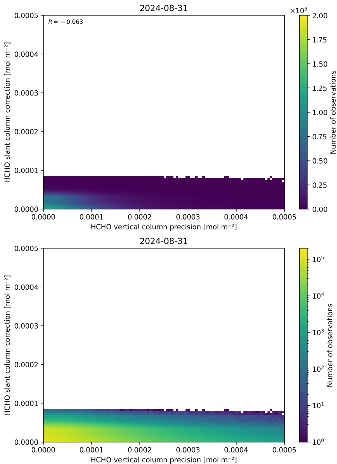
Figure 141: Scatter density plot of “HCHO vertical column precision” against “HCHO slant column correction” for 2024-08-30 to 2024-09-01.
