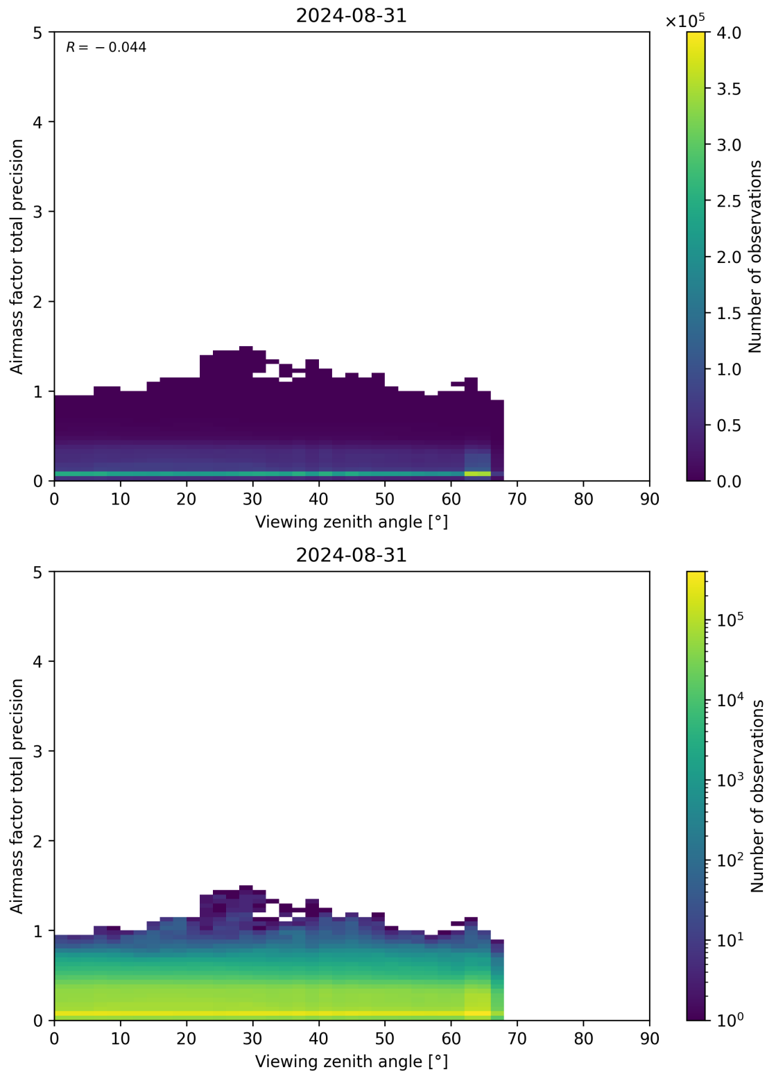
Figure 191: Scatter density plot of “Viewing zenith angle” against “Airmass factor total precision” for 2024-08-30 to 2024-09-01.
