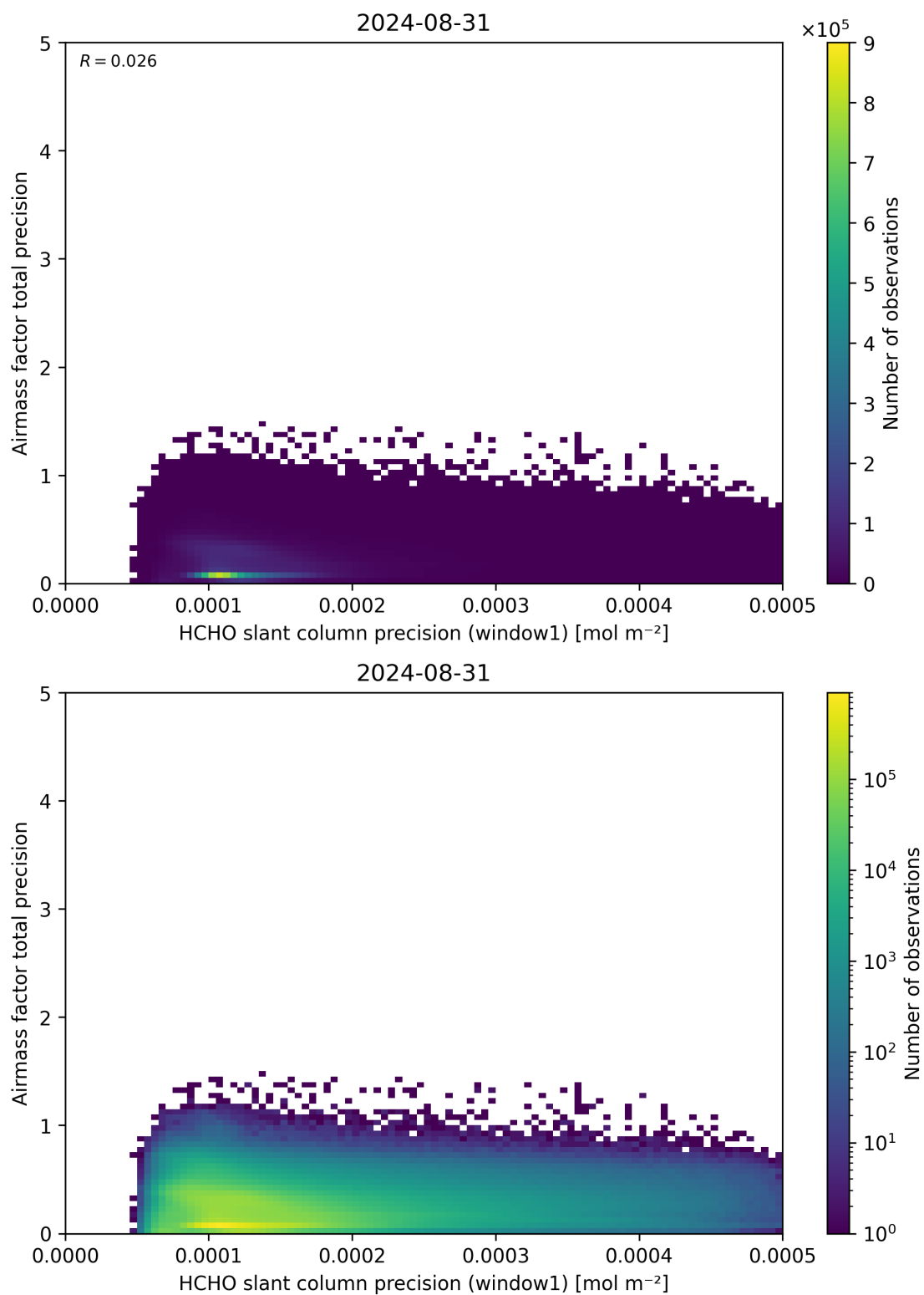
Figure 95: Scatter density plot of “HCHO slant column precision (window1)” against “Airmass factor total precision” for 2024-08-30 to 2024-09-01.
