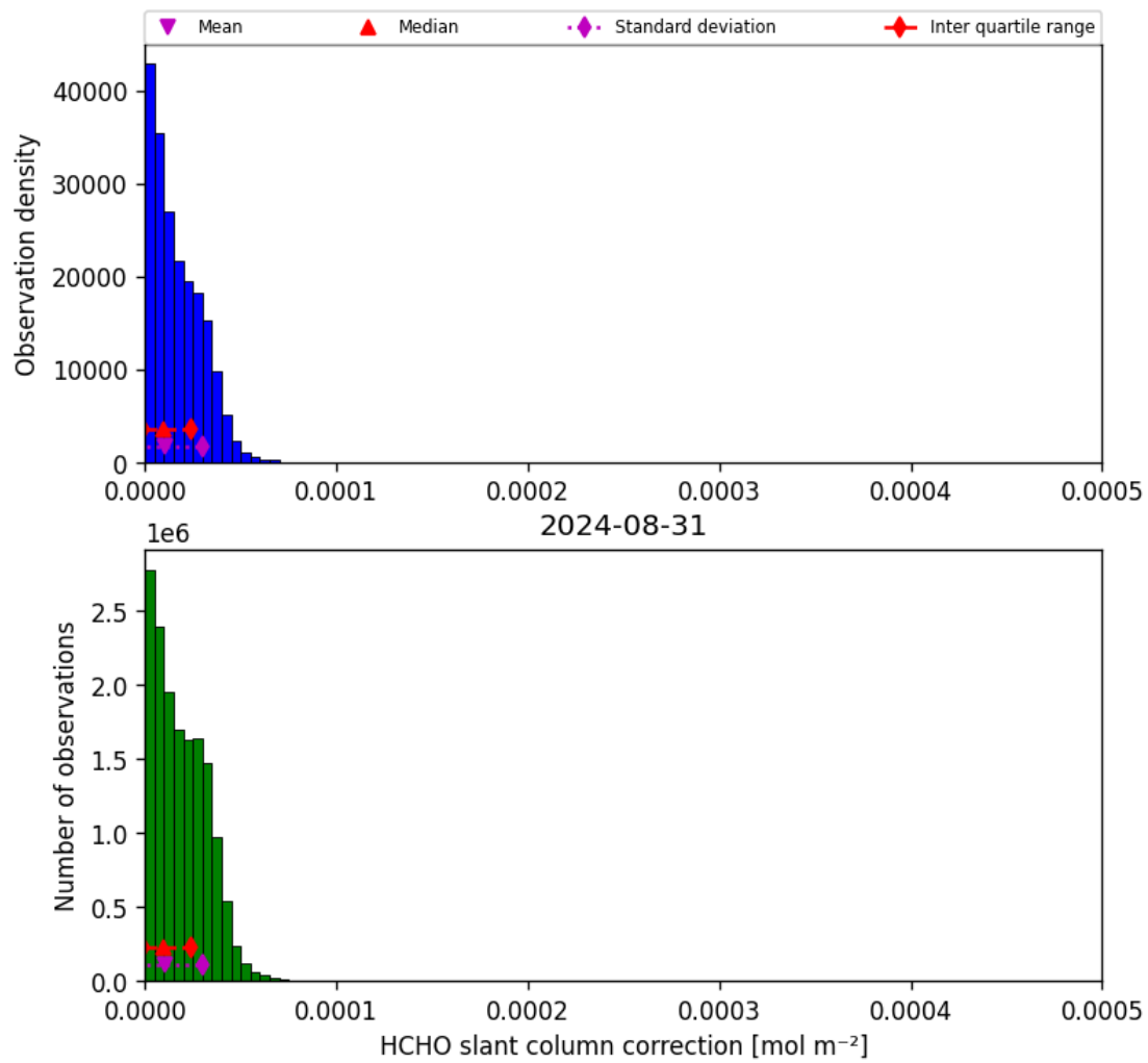
Figure 47: Histogram of “HCHO slant column correction” for 2024-08-30 to 2024-09-01
