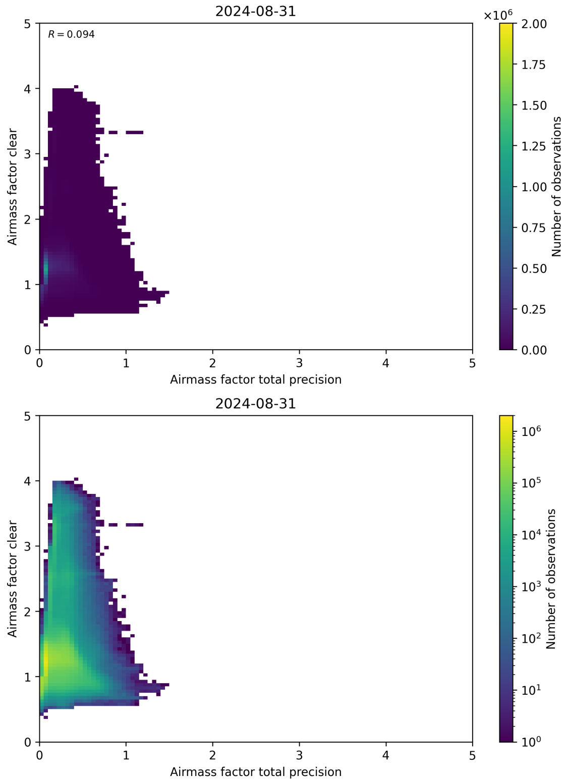
Figure 108: Scatter density plot of “Airmass factor total precision” against “Airmass factor clear” for 2024-08-30 to 2024-09-01.
