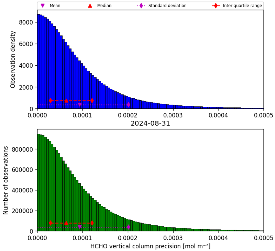
Figure 36: Histogram of “HCHO vertical column precision” for 2024-08-30 to 2024-09-01
