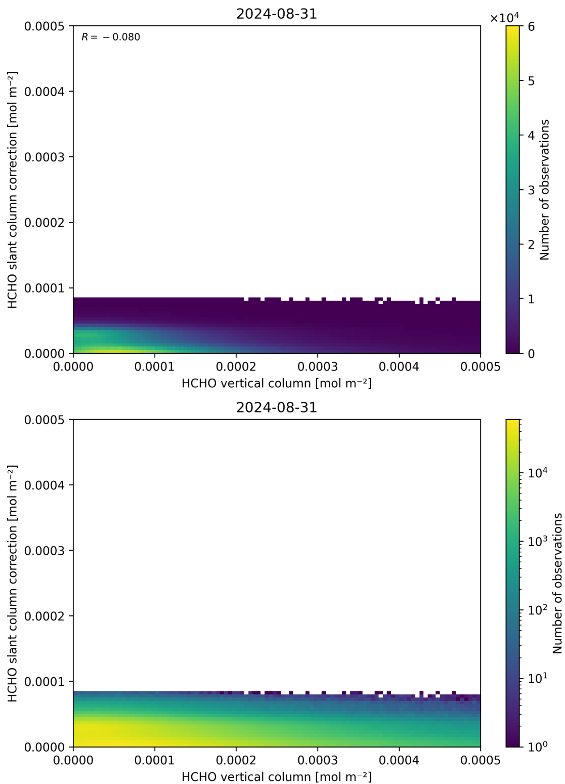
Figure 128: Scatter density plot of “HCHO vertical column” against “HCHO slant column correction” for 2024-08-30 to 2024-09-01.
