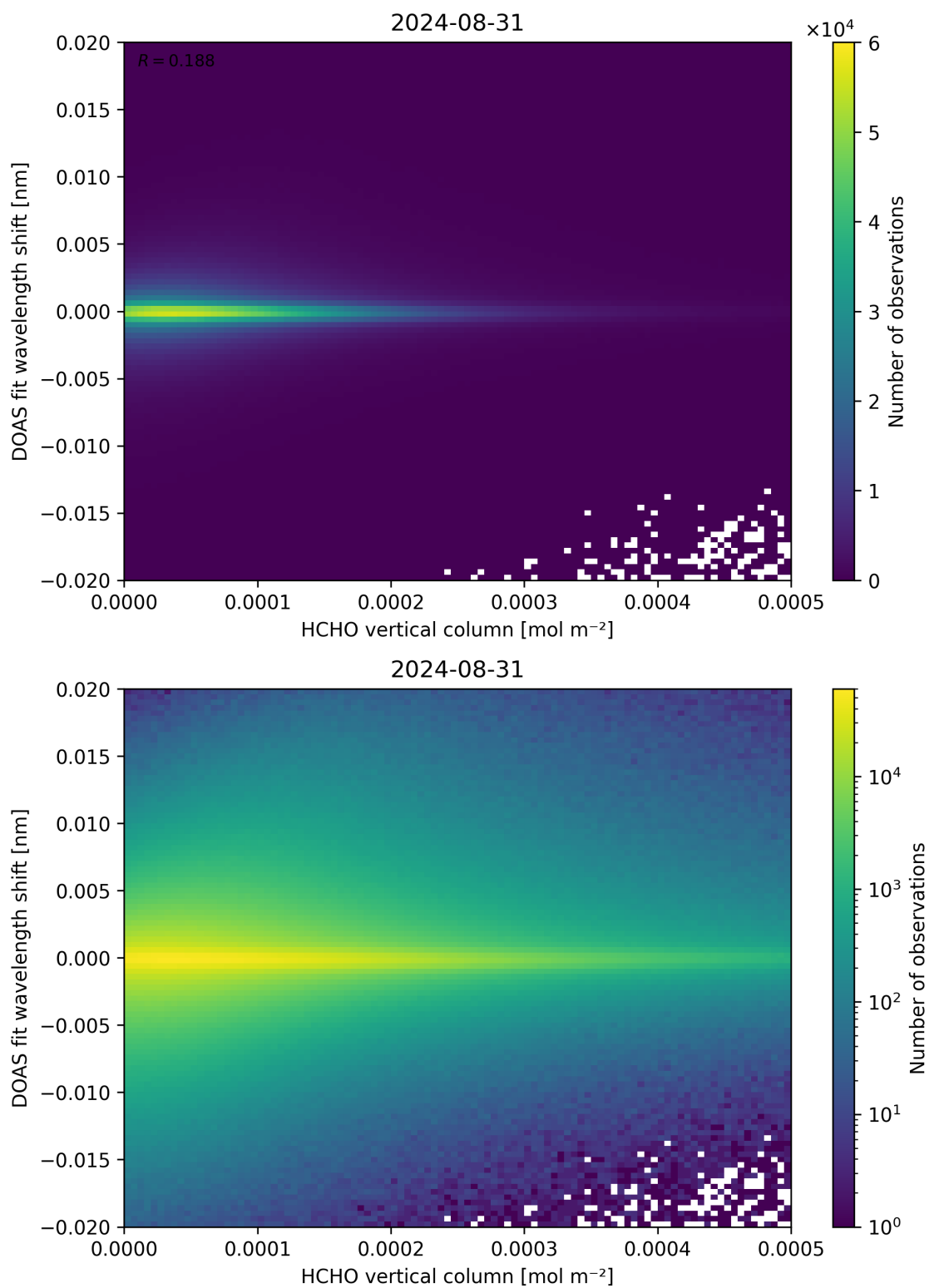
Figure 124: Scatter density plot of “HCHO vertical column” against “DOAS fit wavelength shift” for 2024-08-30 to 2024-09-01.
