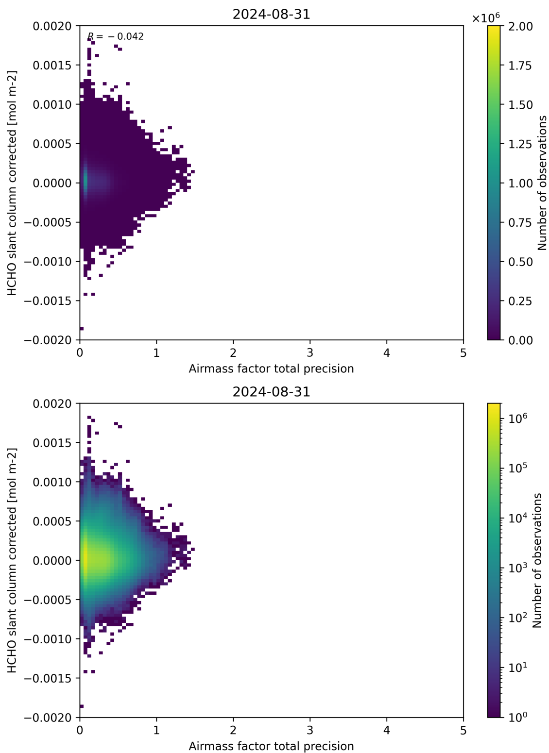
Figure 109: Scatter density plot of “Airmass factor total precision” against “HCHO slant column corrected” for 2024-08-30 to 2024-09-01.
