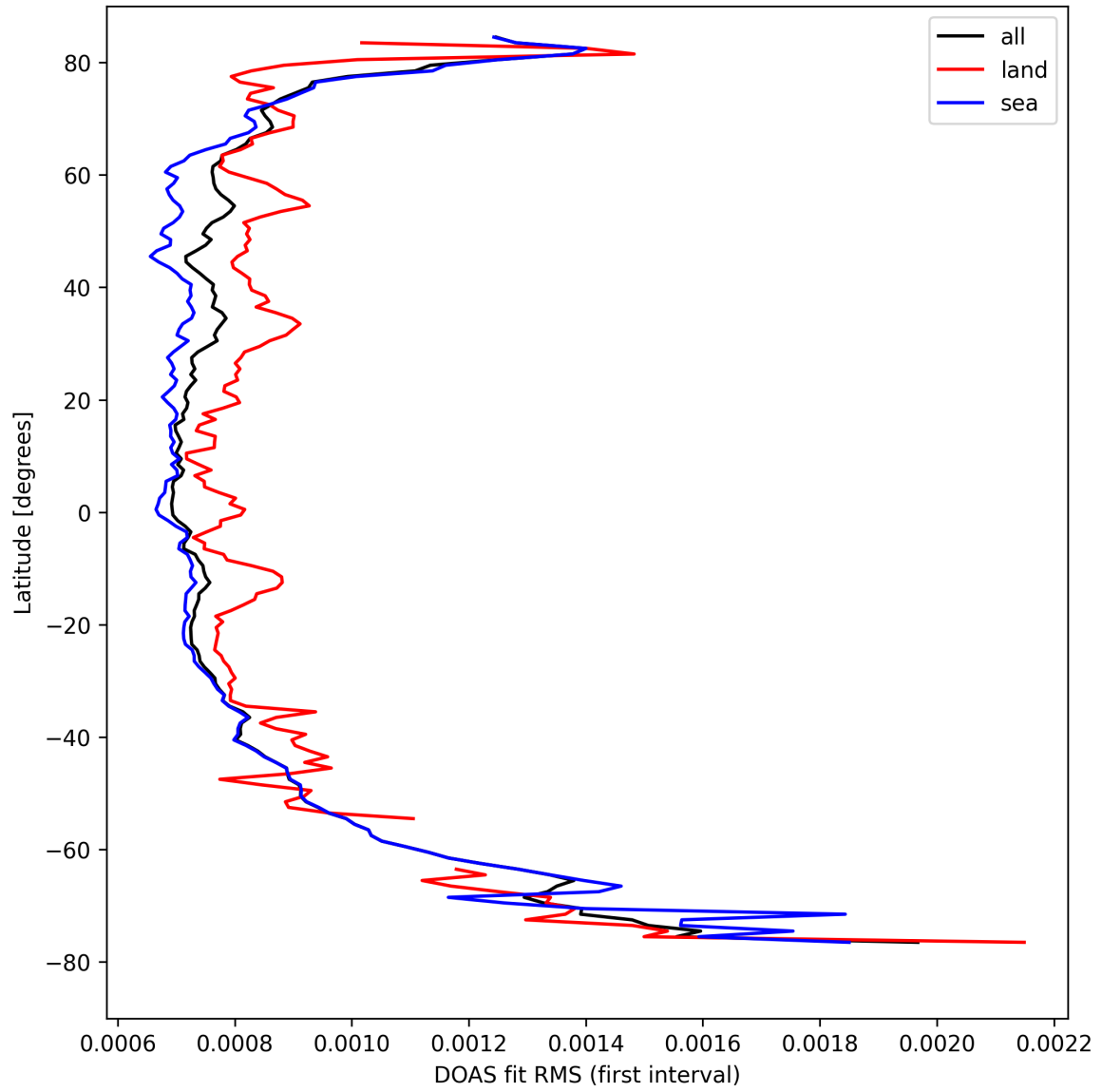
Figure 32: Zonal average of “DOAS fit RMS (first interval)” for 2024-08-30 to 2024-09-01.
