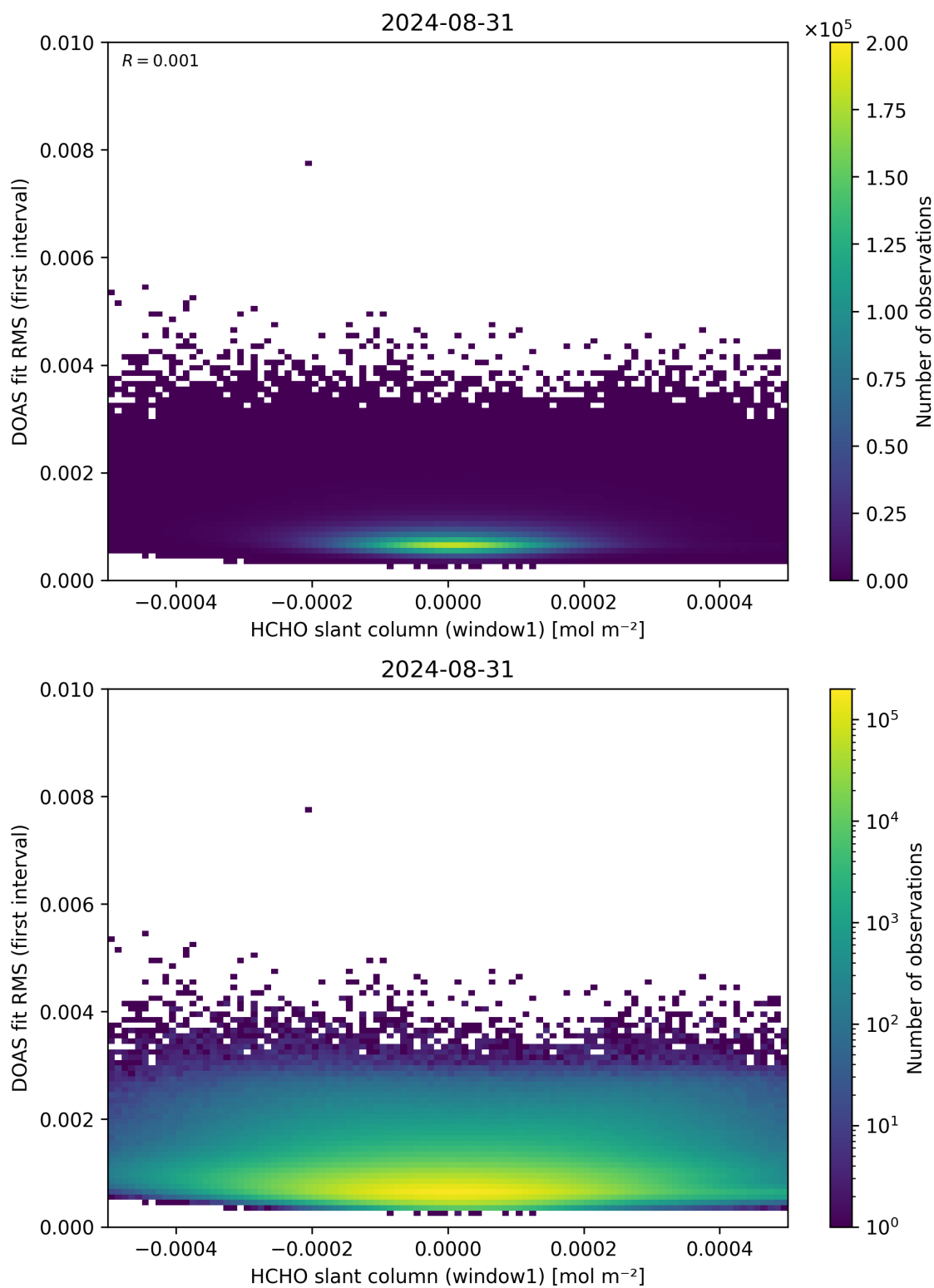
Figure 78: Scatter density plot of “HCHO slant column (window1)” against “DOAS fit RMS (first interval)” for 2024-08-30 to 2024-09-01.
