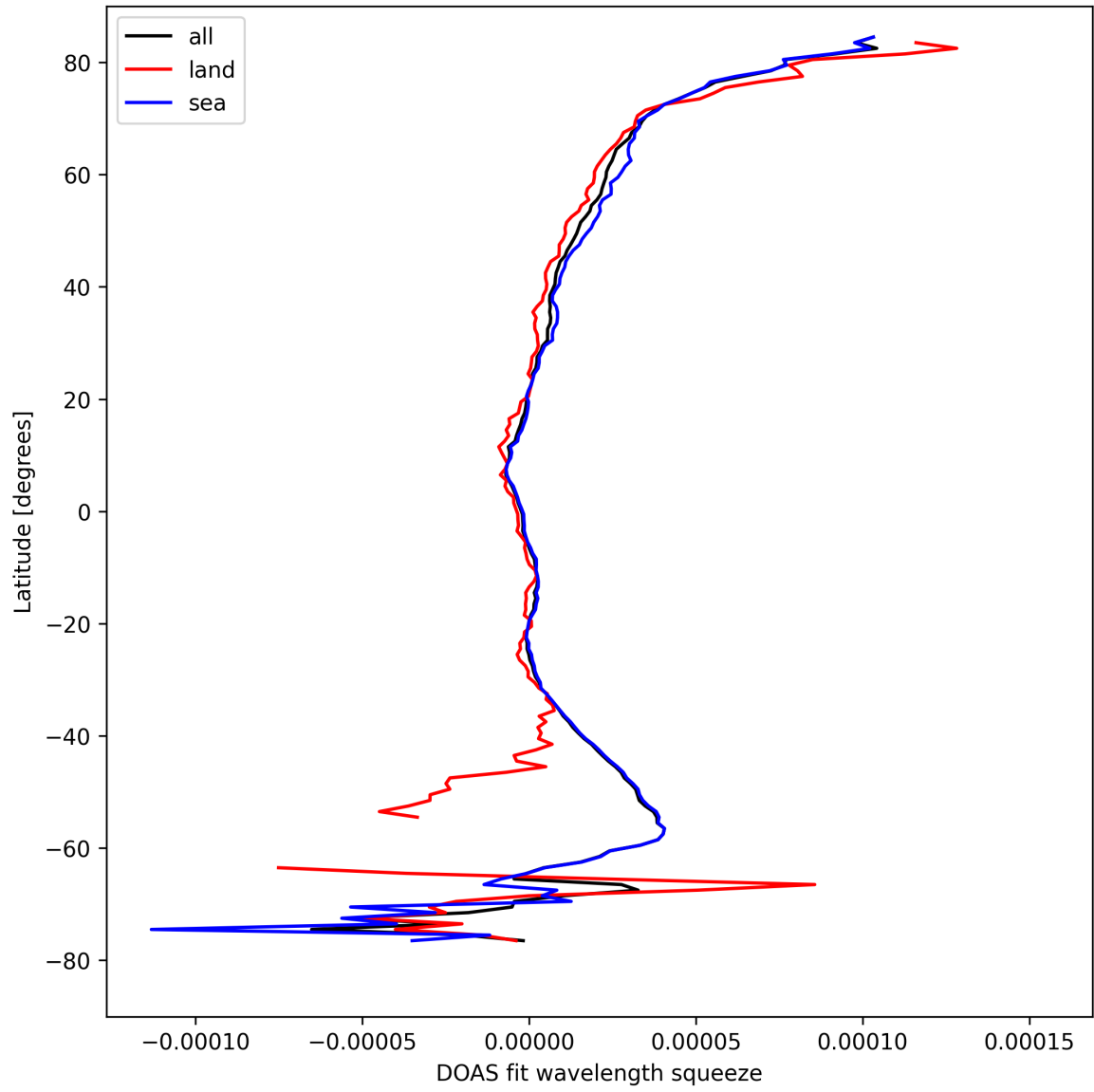
Figure 31: Zonal average of “DOAS fit wavelength squeeze” for 2024-08-30 to 2024-09-01.
