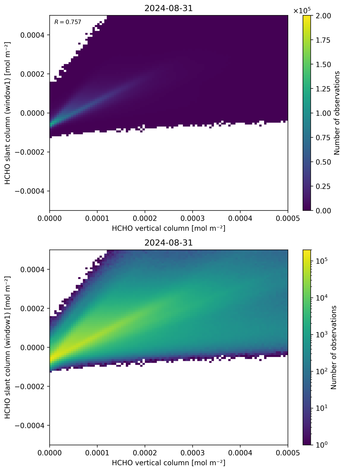
Figure 129: Scatter density plot of “HCHO vertical column” against “HCHO slant column (window1)” for 2024-08-30 to 2024-09-01.
