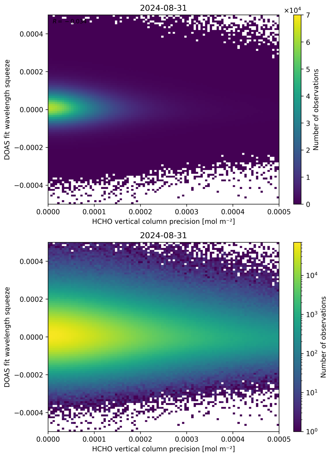
Figure 138: Scatter density plot of “HCHO vertical column precision” against “DOAS fit wavelength squeeze” for 2024-08-30 to 2024-09-01.
