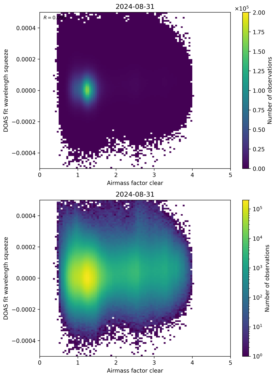
Figure 73: Scatter density plot of “Airmass factor clear” against “DOAS fit wavelength squeeze” for 2024-08-30 to 2024-09-01.
