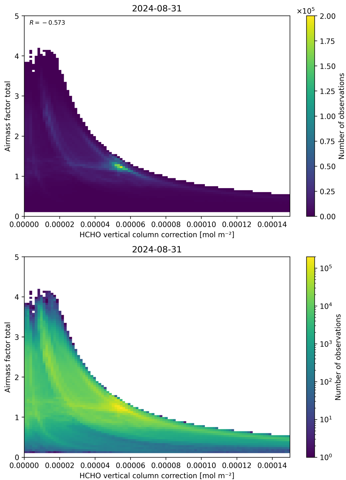
Figure 120: Scatter density plot of “HCHO vertical column correction” against “Airmass factor total” for 2024-08-30 to 2024-09-01.
