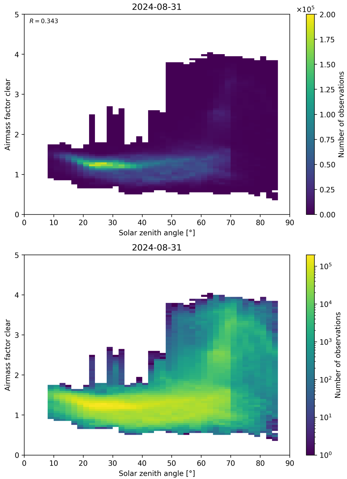
Figure 170: Scatter density plot of “Solar zenith angle” against “Airmass factor clear” for 2024-08-30 to 2024-09-01.
