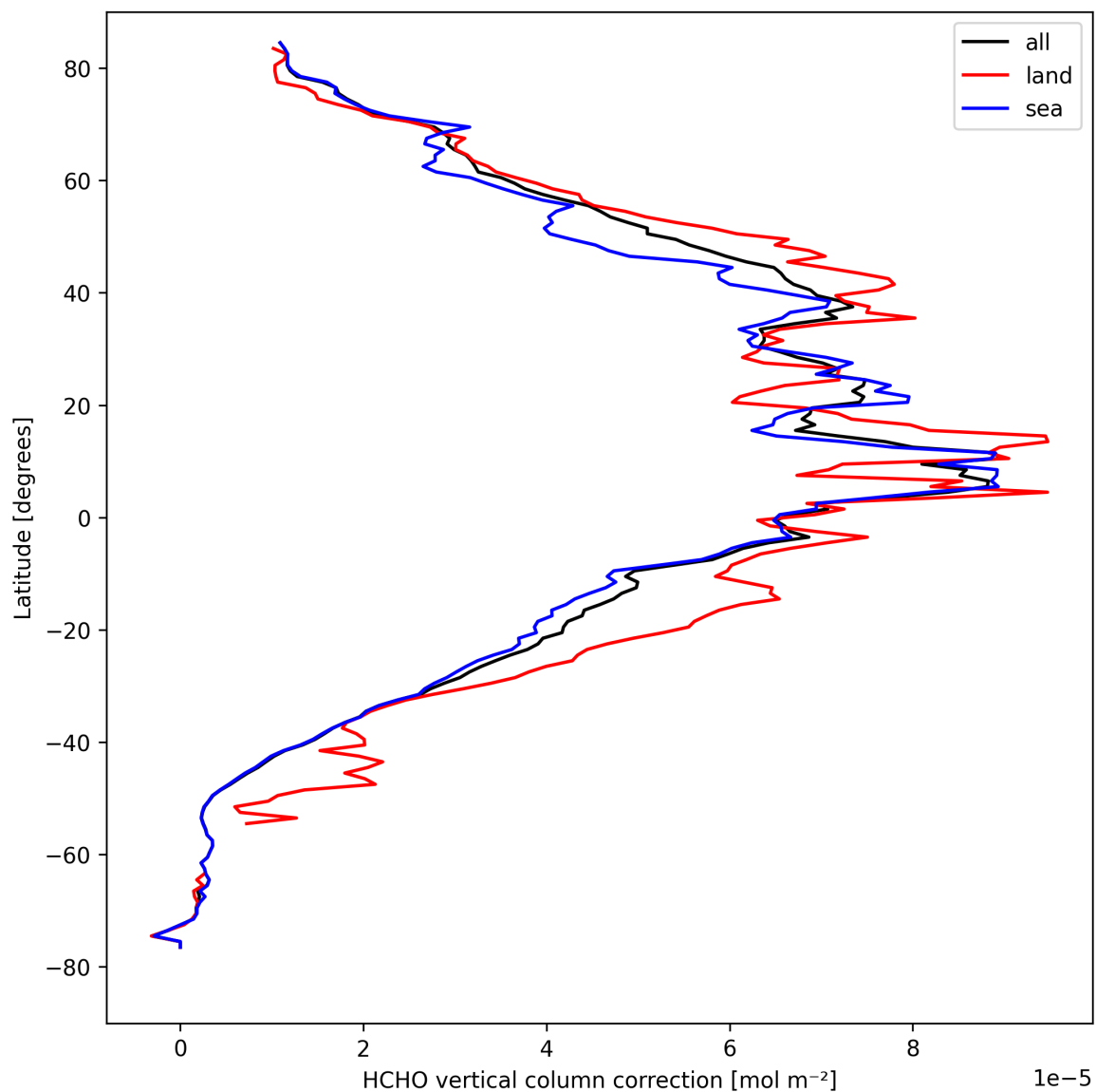
Figure 23: Zonal average of “HCHO vertical column correction” for 2024-08-30 to 2024-09-01.
