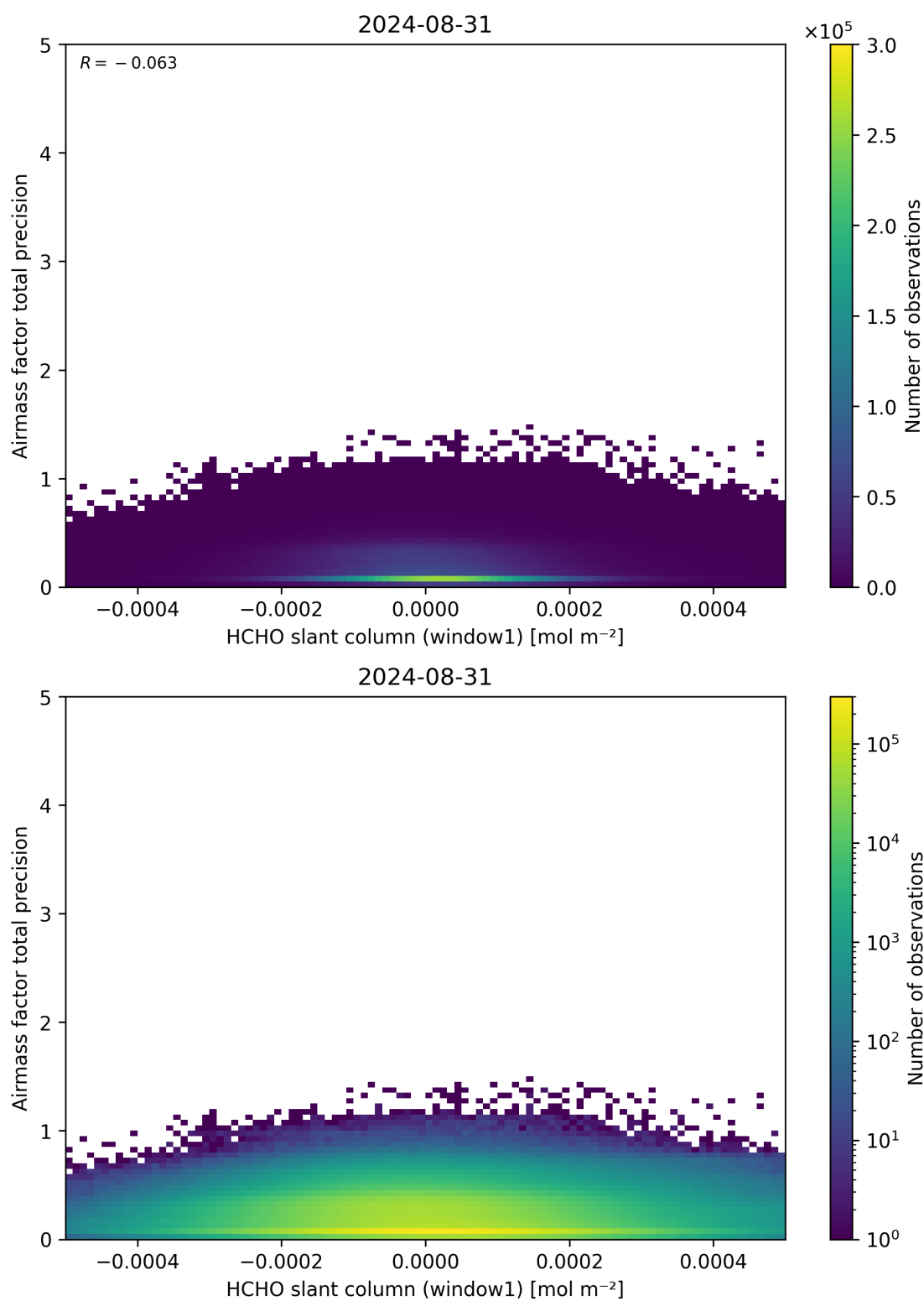
Figure 86: Scatter density plot of “HCHO slant column (window1)” against “Airmass factor total precision” for 2024-08-30 to 2024-09-01.
