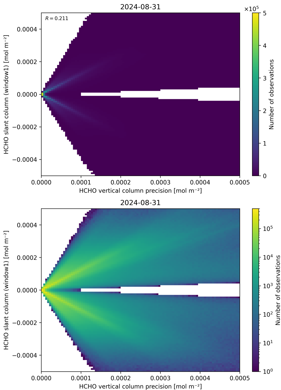
Figure 142: Scatter density plot of “HCHO vertical column precision” against “HCHO slant column (window1)” for 2024-08-30 to 2024-09-01.
