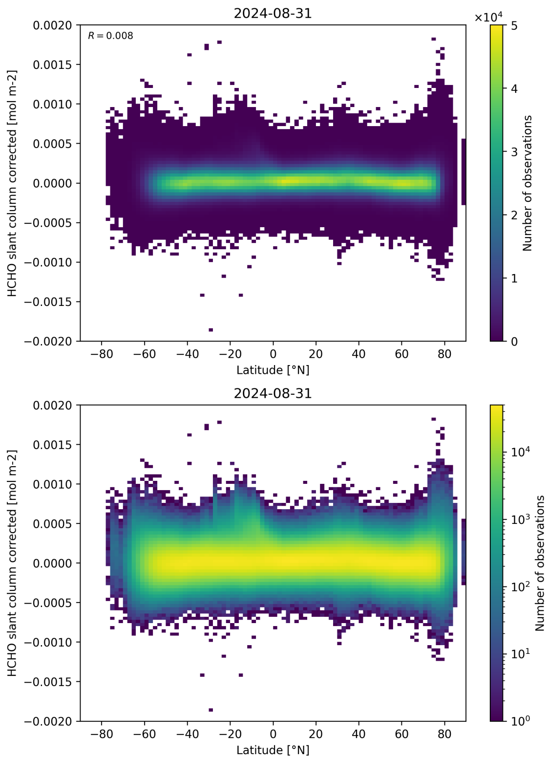
Figure 157: Scatter density plot of “Latitude” against “HCHO slant column corrected” for 2024-08-30 to 2024-09-01.
