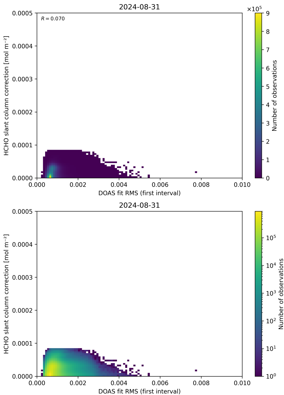
Figure 63: Scatter density plot of “DOAS fit RMS (first interval)” against “HCHO slant column correction” for 2024-08-30 to 2024-09-01.
