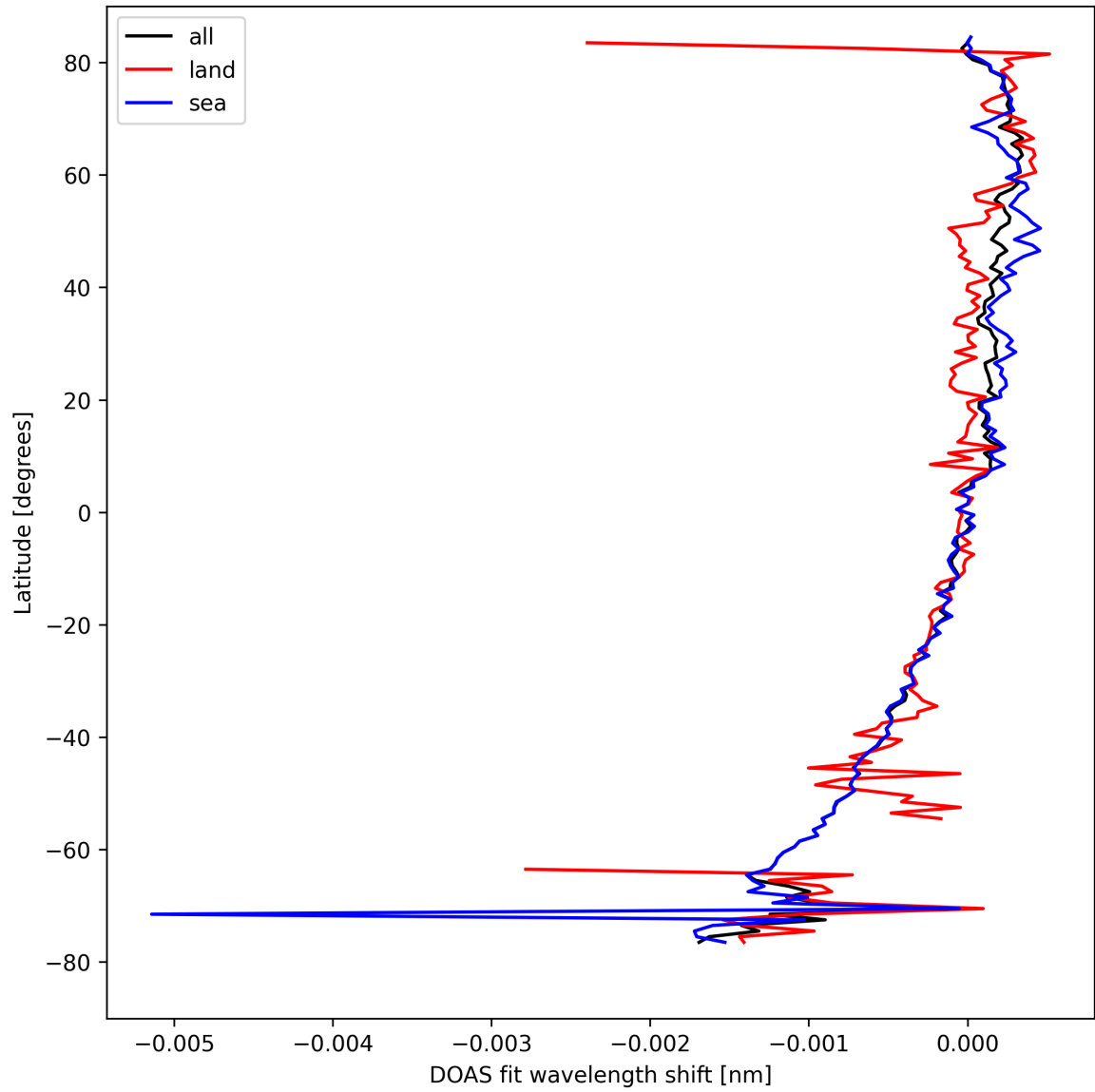
Figure 30: Zonal average of "DOAS fit wavelength shift" for 2024-08-30 to 2024-09-01.
