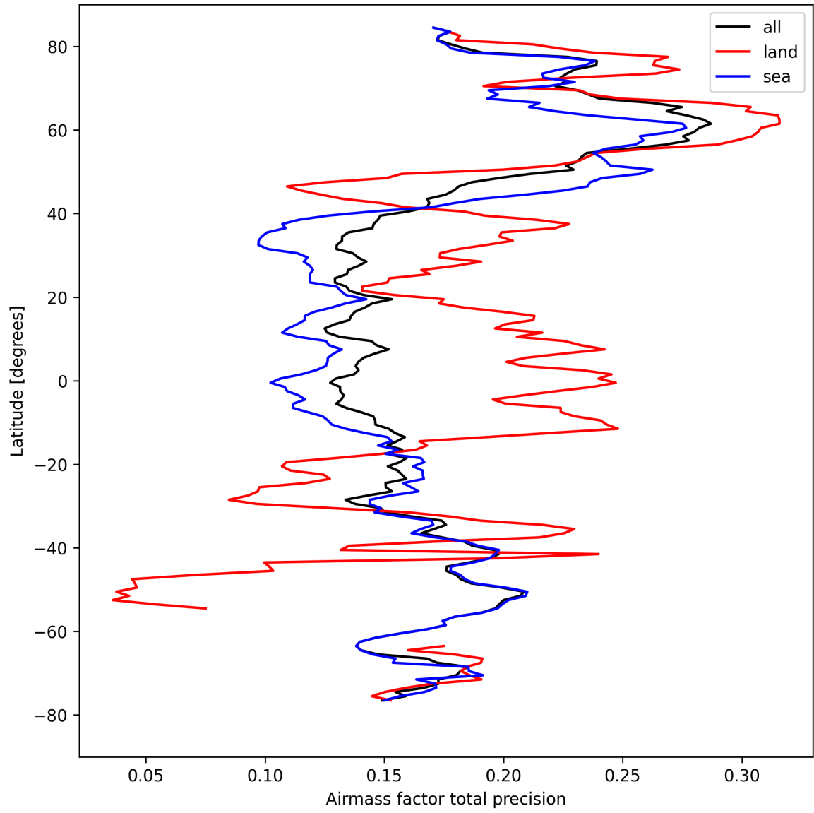
Figure 27: Zonal average of “Airmass factor total precision” for 2024-08-30 to 2024-09-01.
