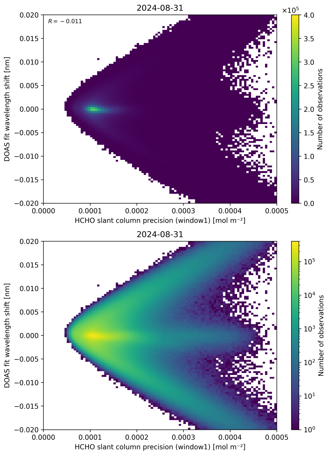
Figure 89: Scatter density plot of “HCHO slant column precision (window1)” against “DOAS fit wavelength shift” for 2024-08-30 to 2024-09-01.
