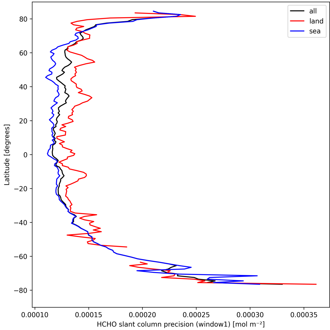
Figure 25: Zonal average of “HCHO slant column precision (window1)” for 2024-08-30 to 2024-09-01.
