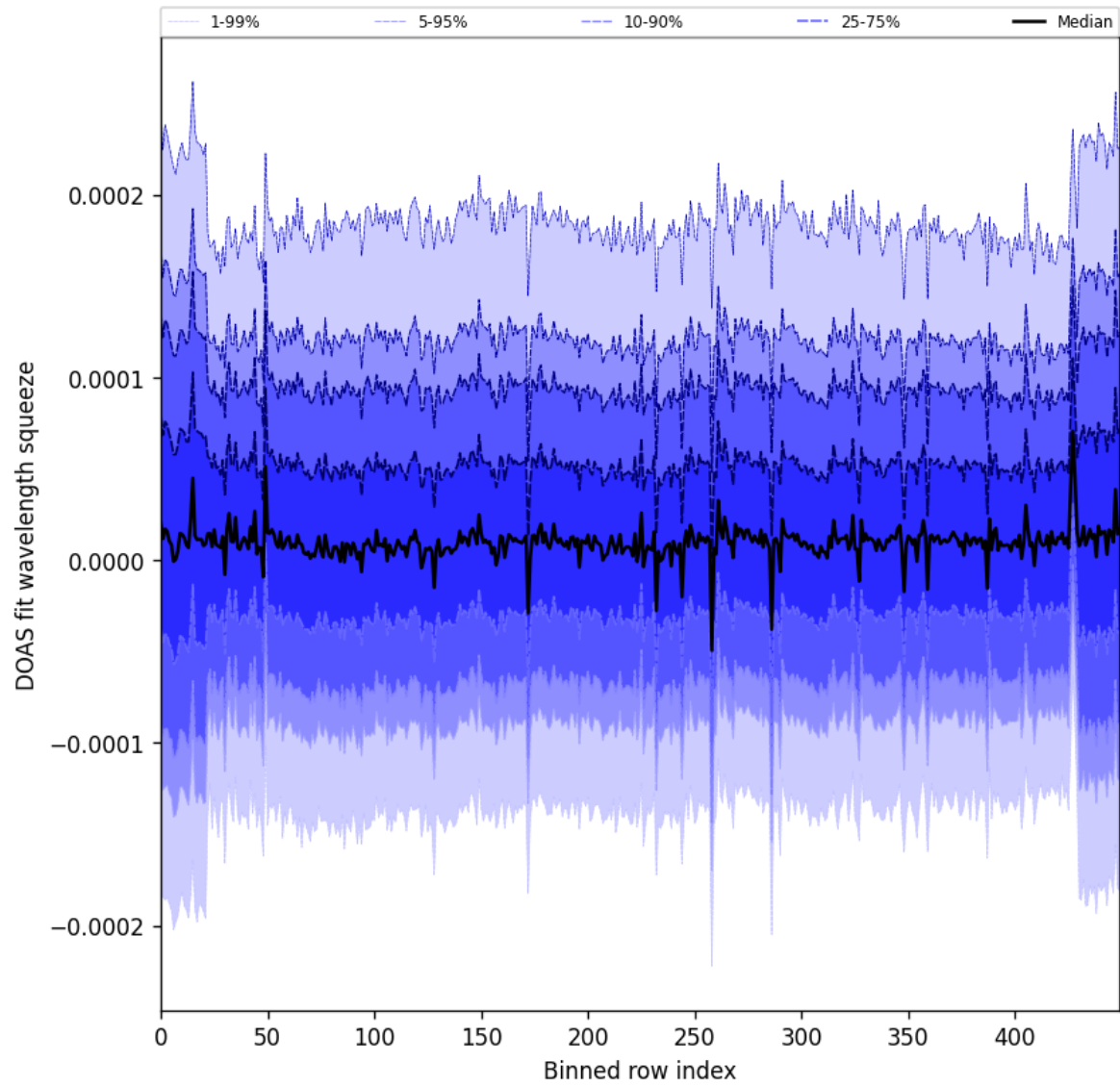
Figure 59: Along track statistics of “DOAS fit wavelength squeeze” for 2024-08-30 to 2024-09-01
