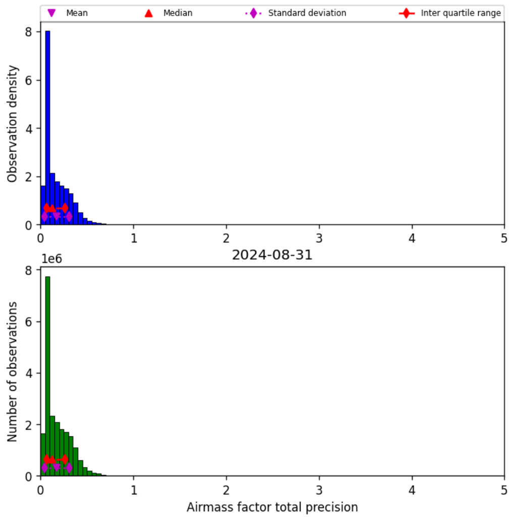
Figure 41: Histogram of “Airmass factor total precision” for 2024-08-30 to 2024-09-01
