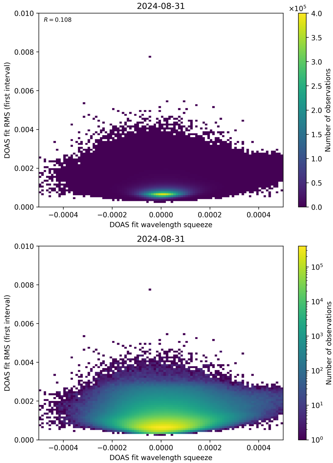
Figure 68: Scatter density plot of “DOAS fit wavelength squeeze” against “DOAS fit RMS (first interval)” for 2024-08-30 to 2024-09-01.
