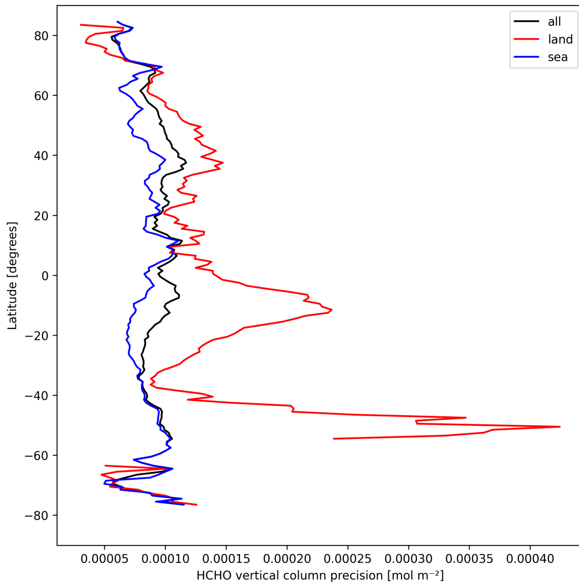
Figure 22: Zonal average of “HCHO vertical column precision” for 2024-08-30 to 2024-09-01.
