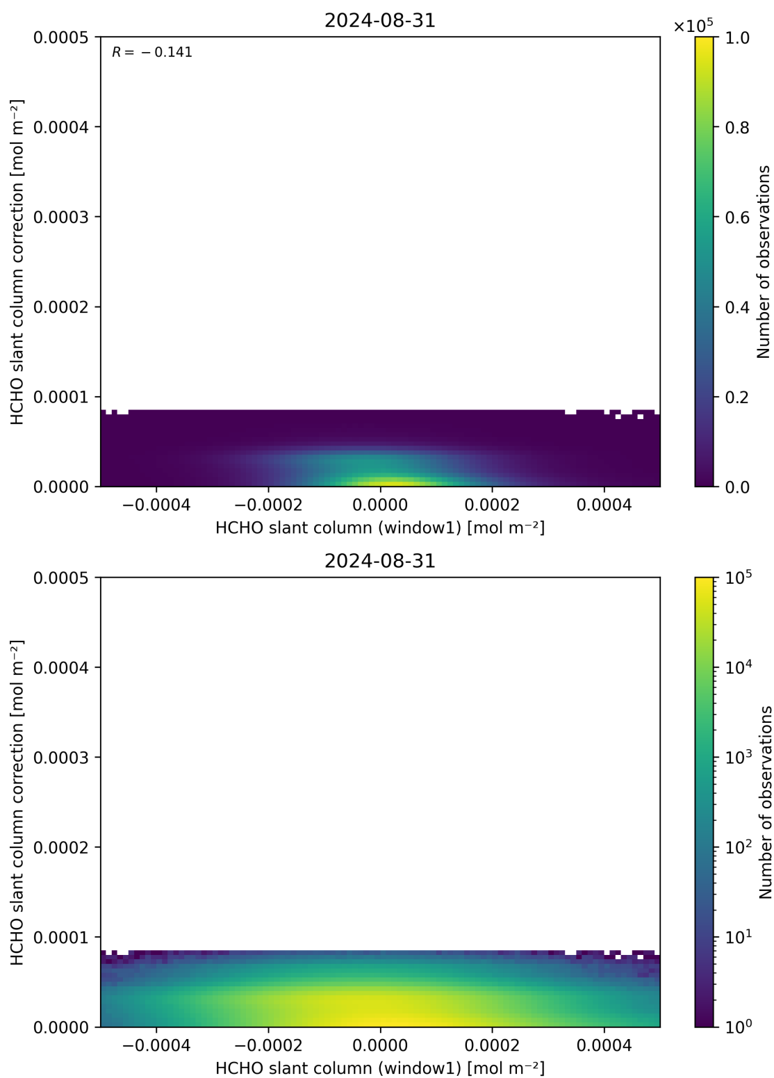
Figure 83: Scatter density plot of “HCHO slant column (window1)” against “HCHO slant column correction” for 2024-08-30 to 2024-09-01.
