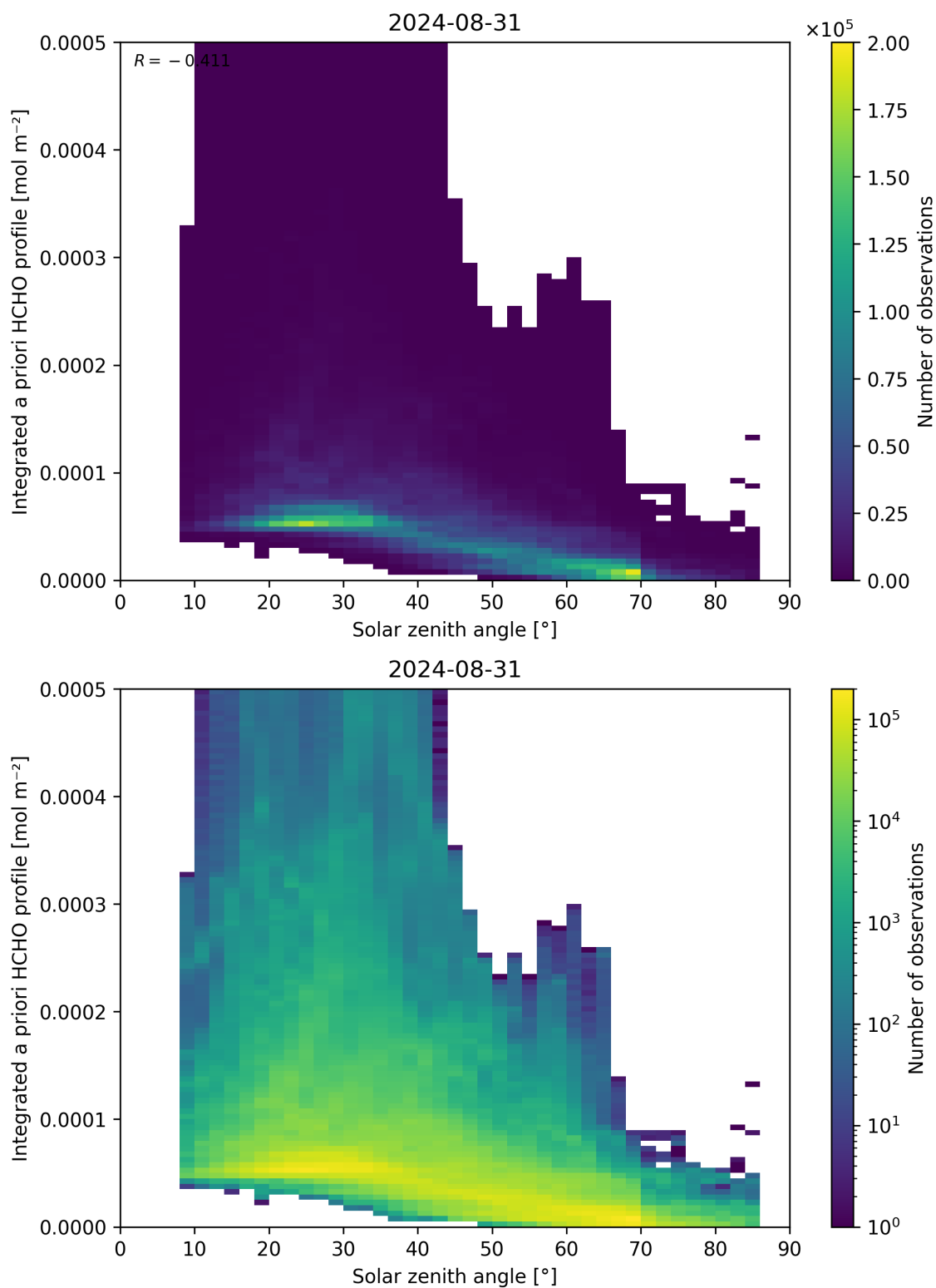
Figure 180: Scatter density plot of “Solar zenith angle” against “Integrated a priori HCHO profile” for 2024-08-30 to 2024-09-01.
