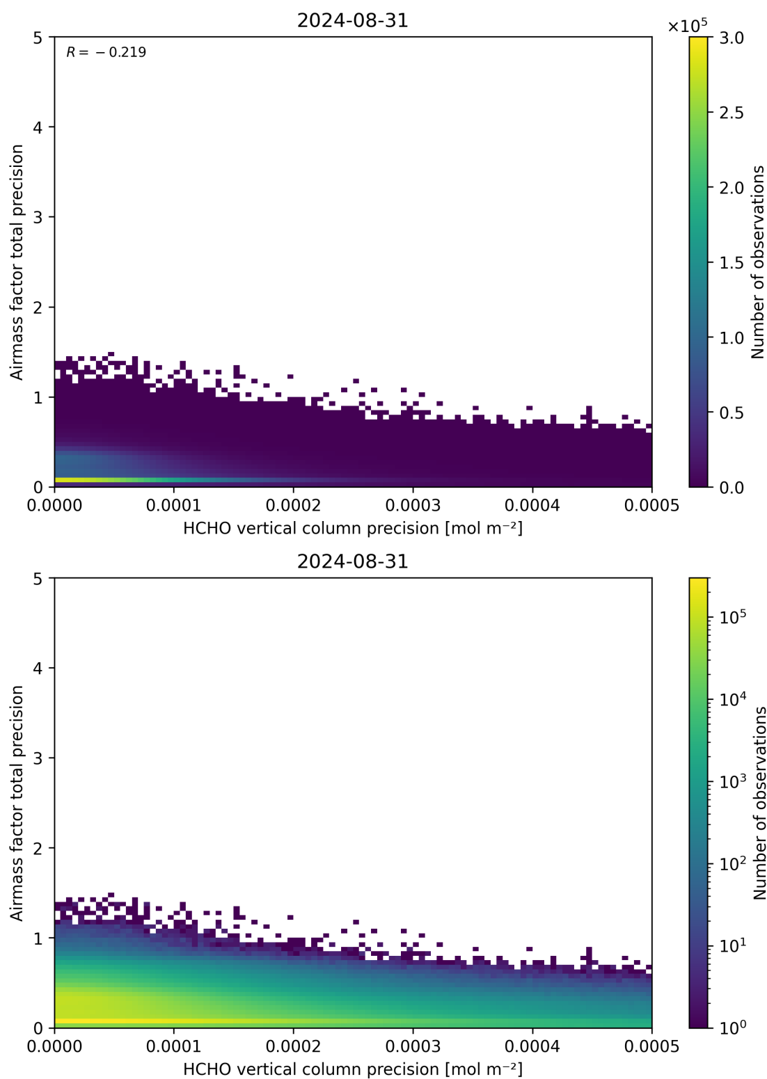
Figure 145: Scatter density plot of “HCHO vertical column precision” against “Airmass factor total precision” for 2024-08-30 to 2024-09-01.
