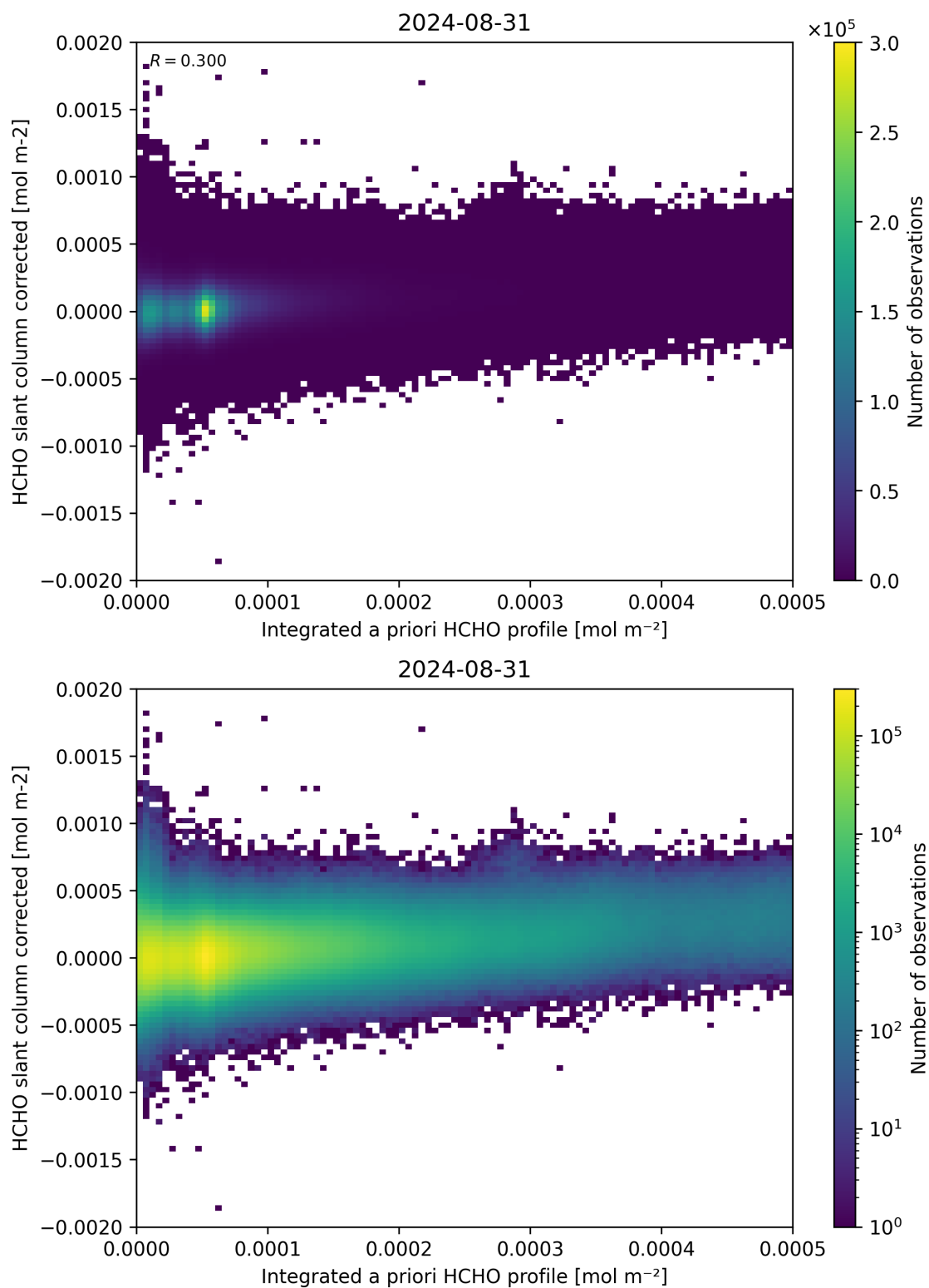
Figure 151: Scatter density plot of “Integrated a priori HCHO profile” against “HCHO slant column corrected” for 2024-08-30 to 2024-09-01.
