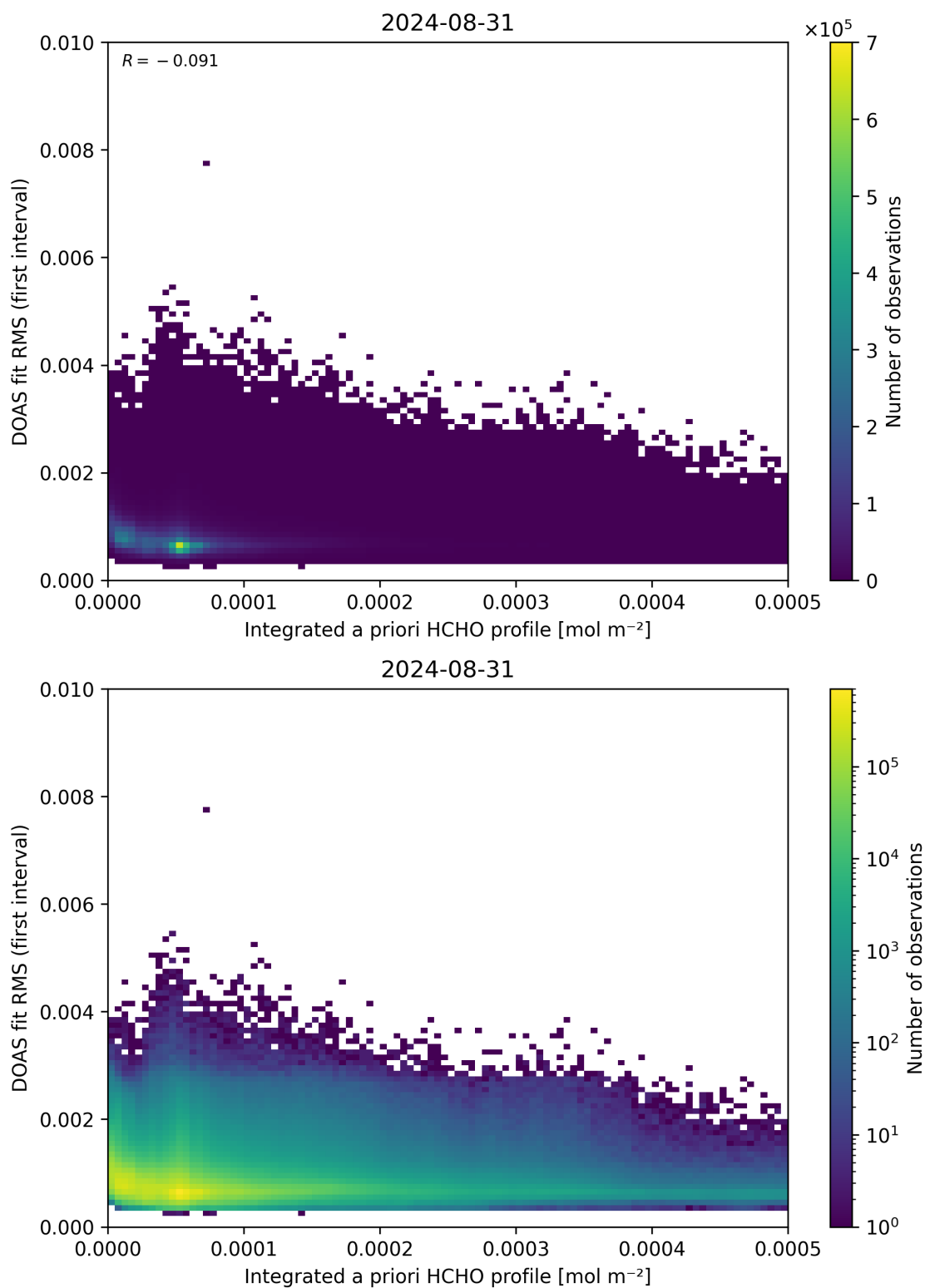
Figure 148: Scatter density plot of “Integrated a priori HCHO profile” against “DOAS fit RMS (first interval)” for 2024-08-30 to 2024-09-01.
