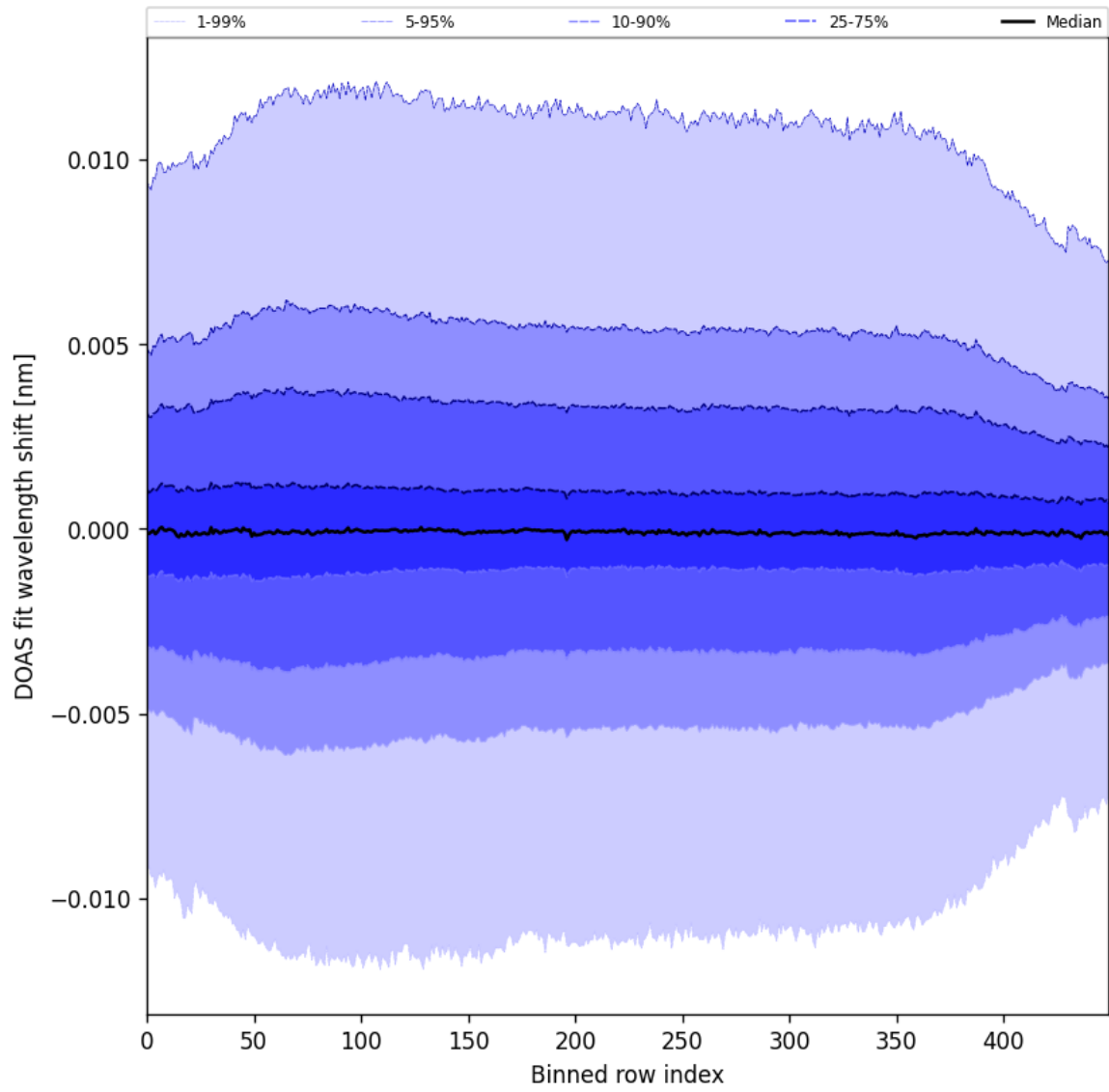
Figure 58: Along track statistics of “DOAS fit wavelength shift” for 2024-08-30 to 2024-09-01
