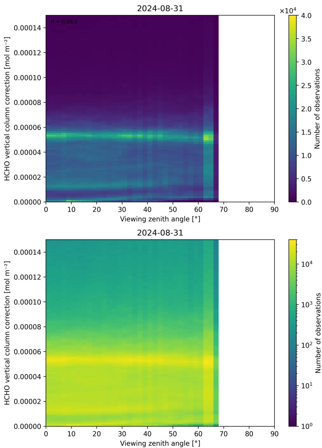
Figure 193: Scatter density plot of “Viewing zenith angle” against “HCHO vertical column correction” for 2024-08-30 to 2024-09-01.
