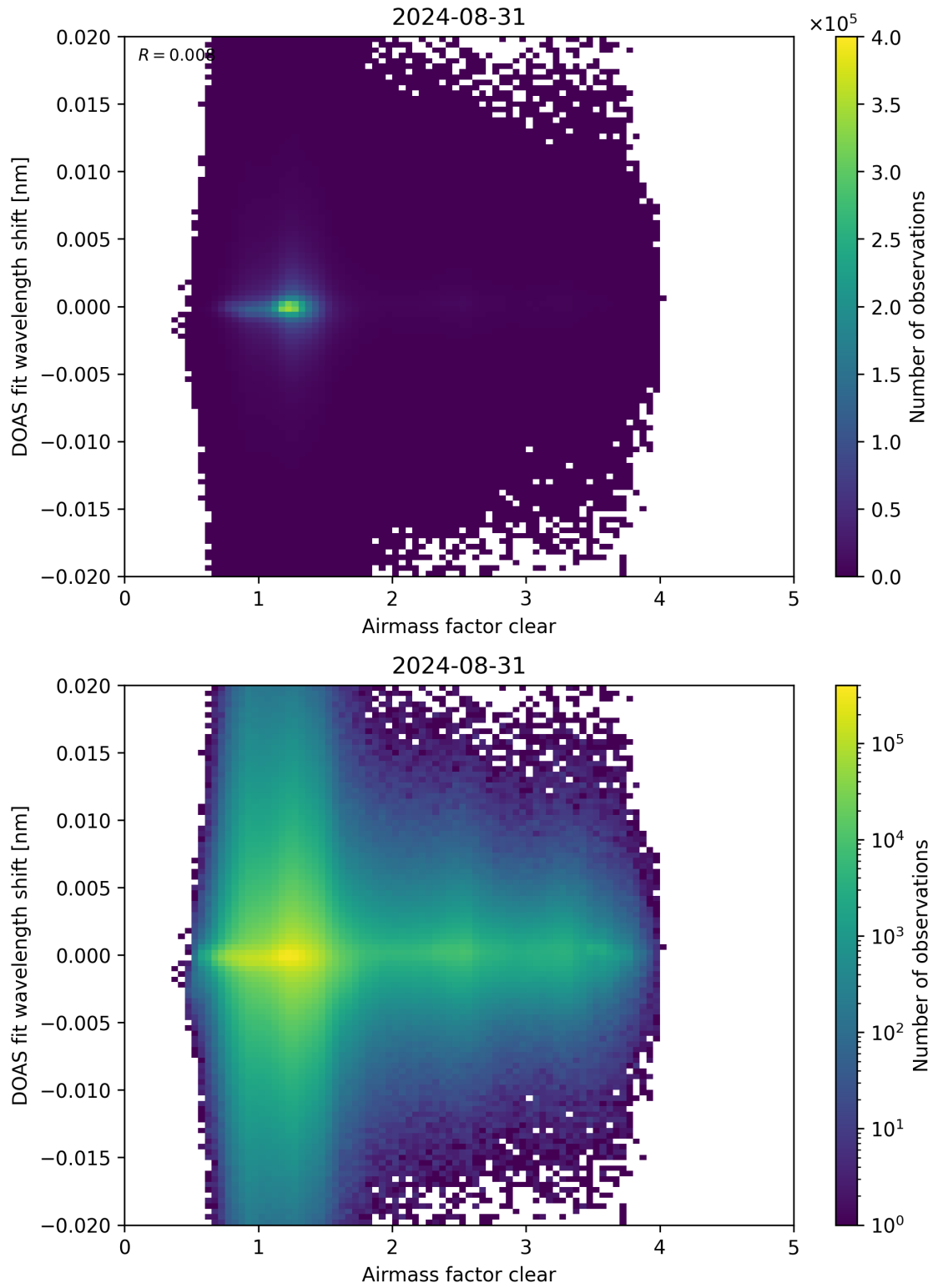
Figure 72: Scatter density plot of “Airmass factor clear” against “DOAS fit wavelength shift” for 2024-08-30 to 2024-09-01.
