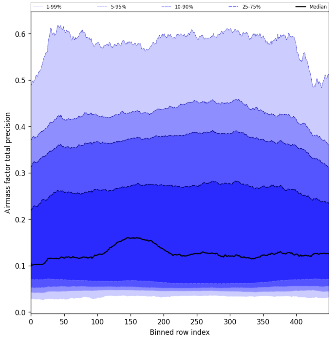
Figure 55: Along track statistics of “Airmass factor total precision” for 2024-08-30 to 2024-09-01
