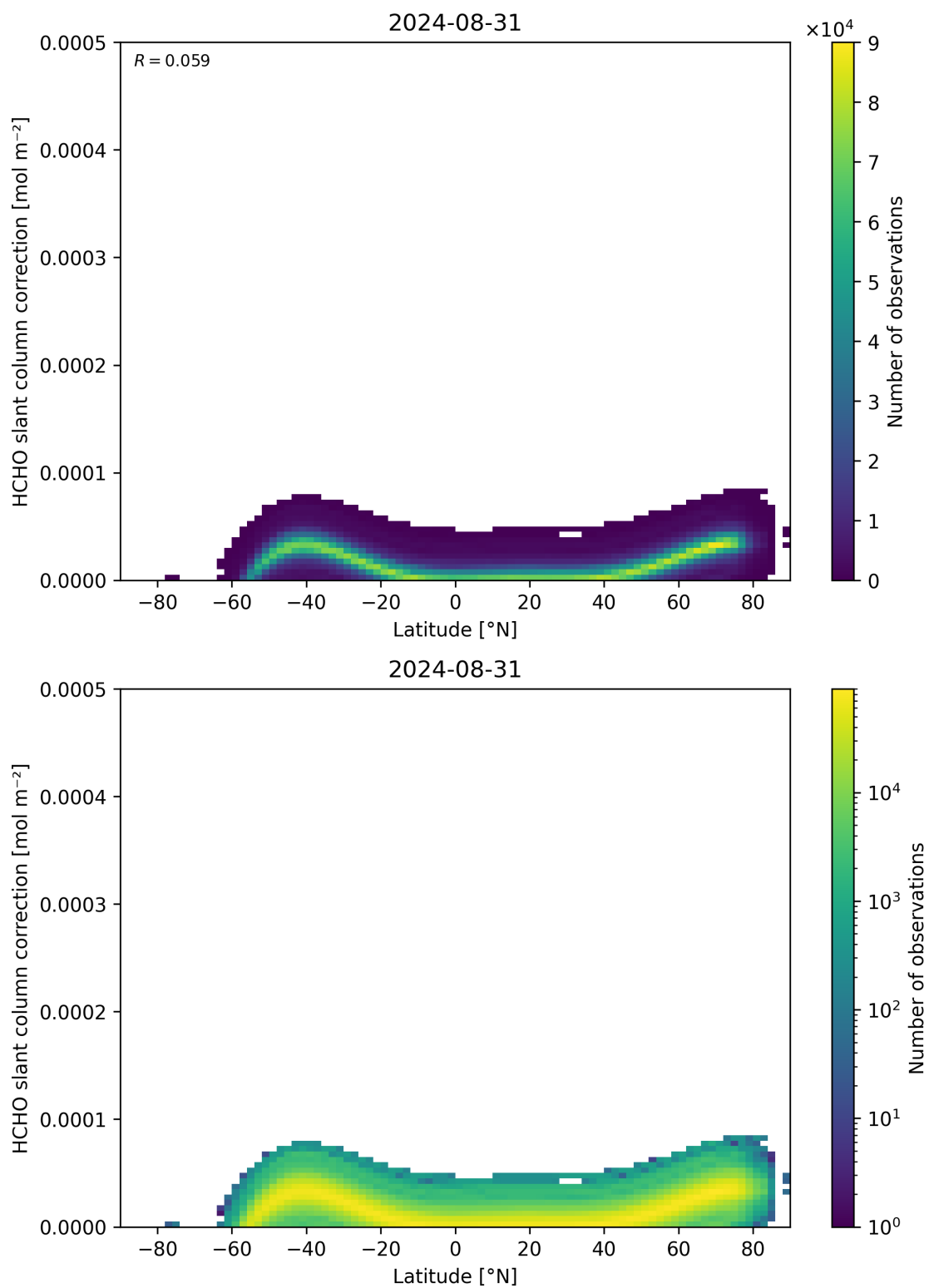
Figure 158: Scatter density plot of “Latitude” against “HCHO slant column correction” for 2024-08-30 to 2024-09-01.
