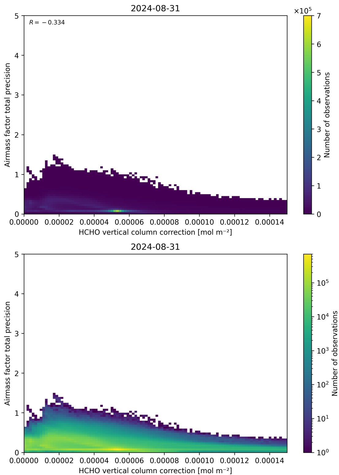
Figure 121: Scatter density plot of “HCHO vertical column correction” against “Airmass factor total precision” for 2024-08-30 to 2024-09-01.
