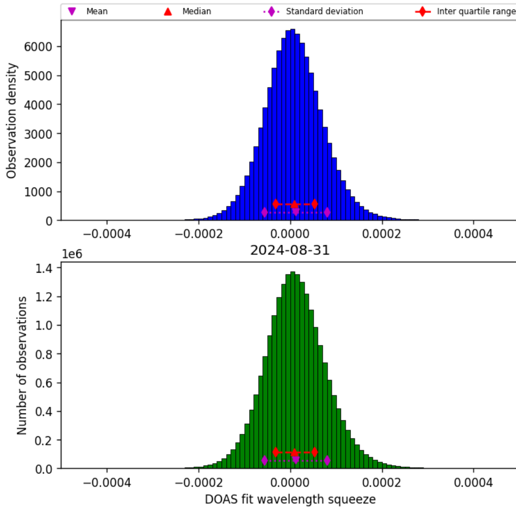
Figure 45: Histogram of “DOAS fit wavelength squeeze” for 2024-08-30 to 2024-09-01
