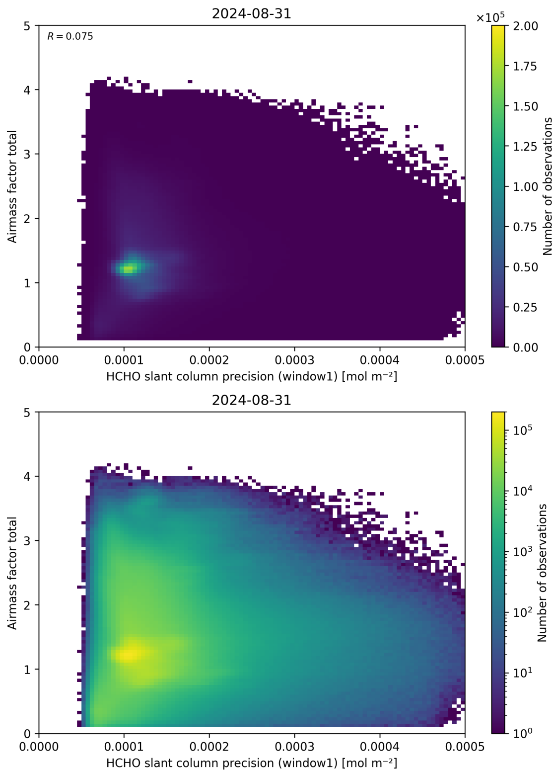
Figure 94: Scatter density plot of “HCHO slant column precision (window1)” against “Airmass factor total” for 2024-08-30 to 2024-09-01.
