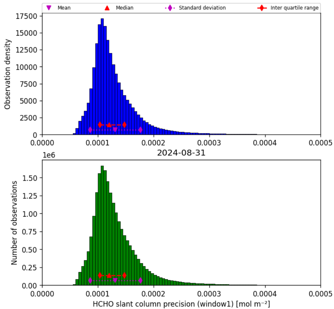
Figure 39: Histogram of “HCHO slant column precision (window1)” for 2024-08-30 to 2024-09-01
