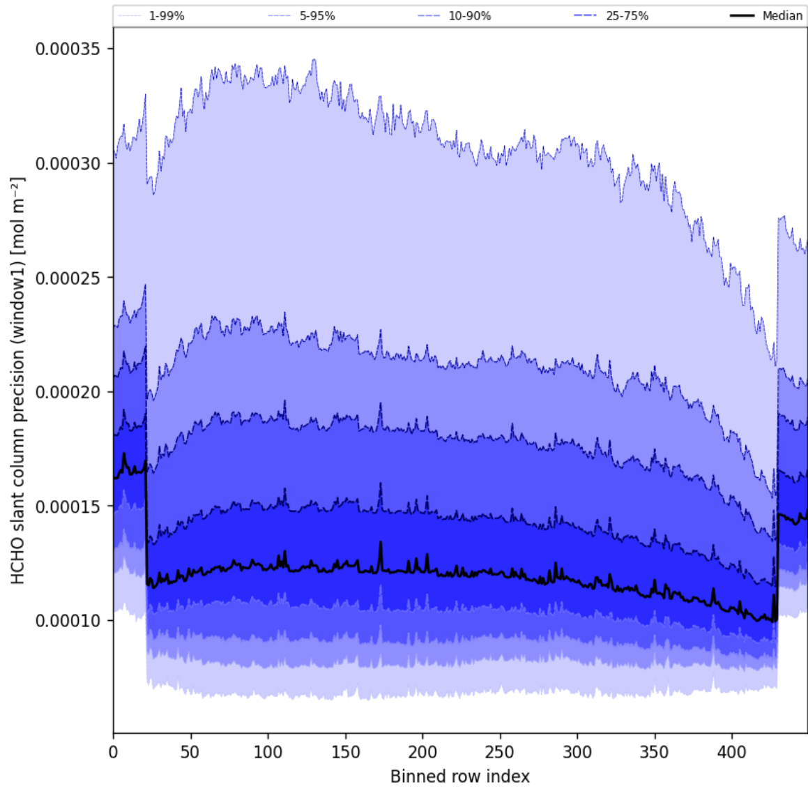
Figure 53: Along track statistics of “HCHO slant column precision (window1)” for 2024-08-30 to 2024-09-01
