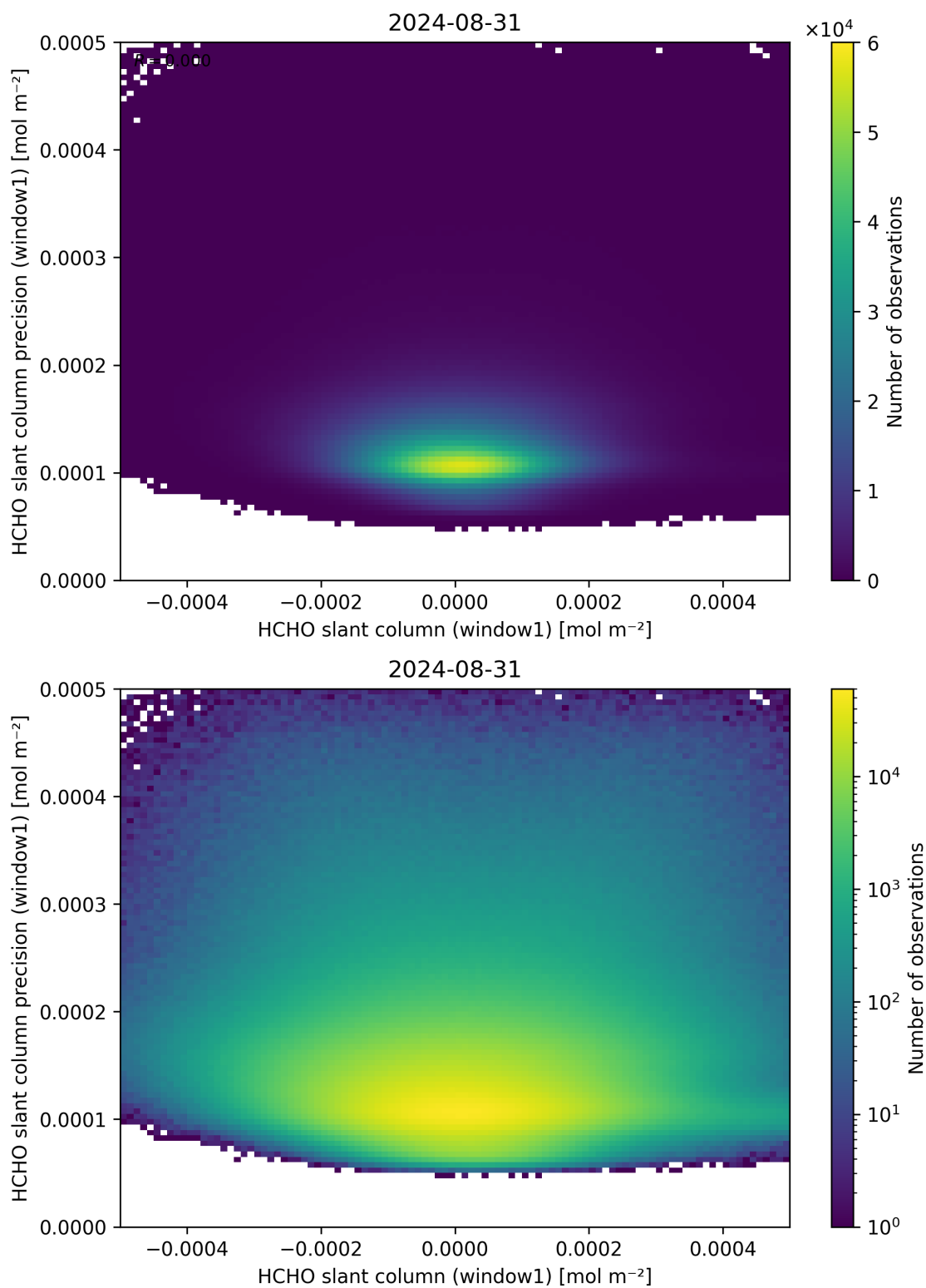
Figure 84: Scatter density plot of “HCHO slant column (window1)” against “HCHO slant column precision (window1)” for 2024-08-30 to 2024-09-01.
