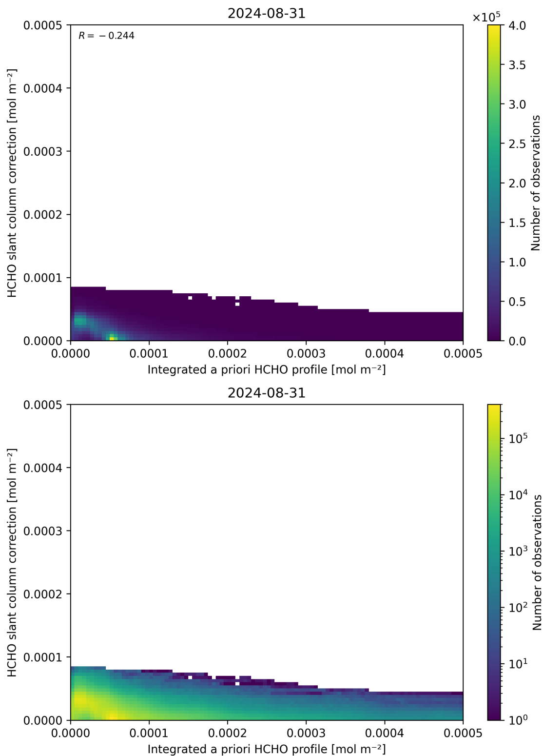
Figure 152: Scatter density plot of “Integrated a priori HCHO profile” against “HCHO slant column correction” for 2024-08-30 to 2024-09-01.
