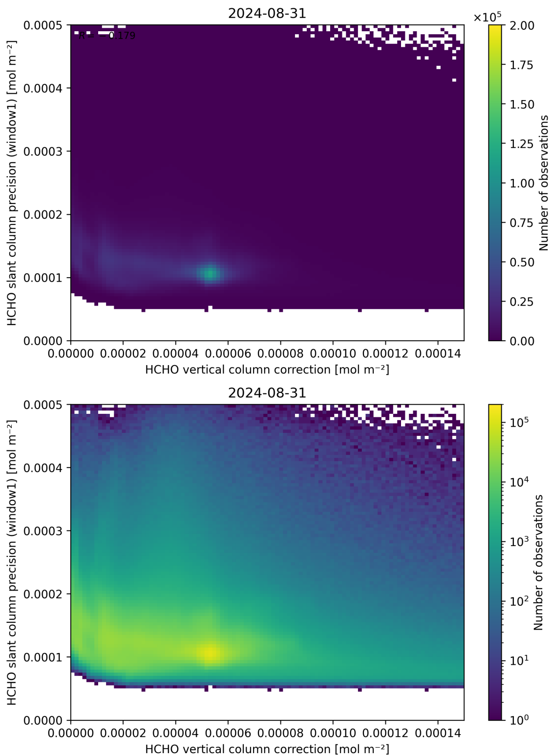
Figure 119: Scatter density plot of “HCHO vertical column correction” against “HCHO slant column precision (window1)” for 2024-08-30 to 2024-09-01.
