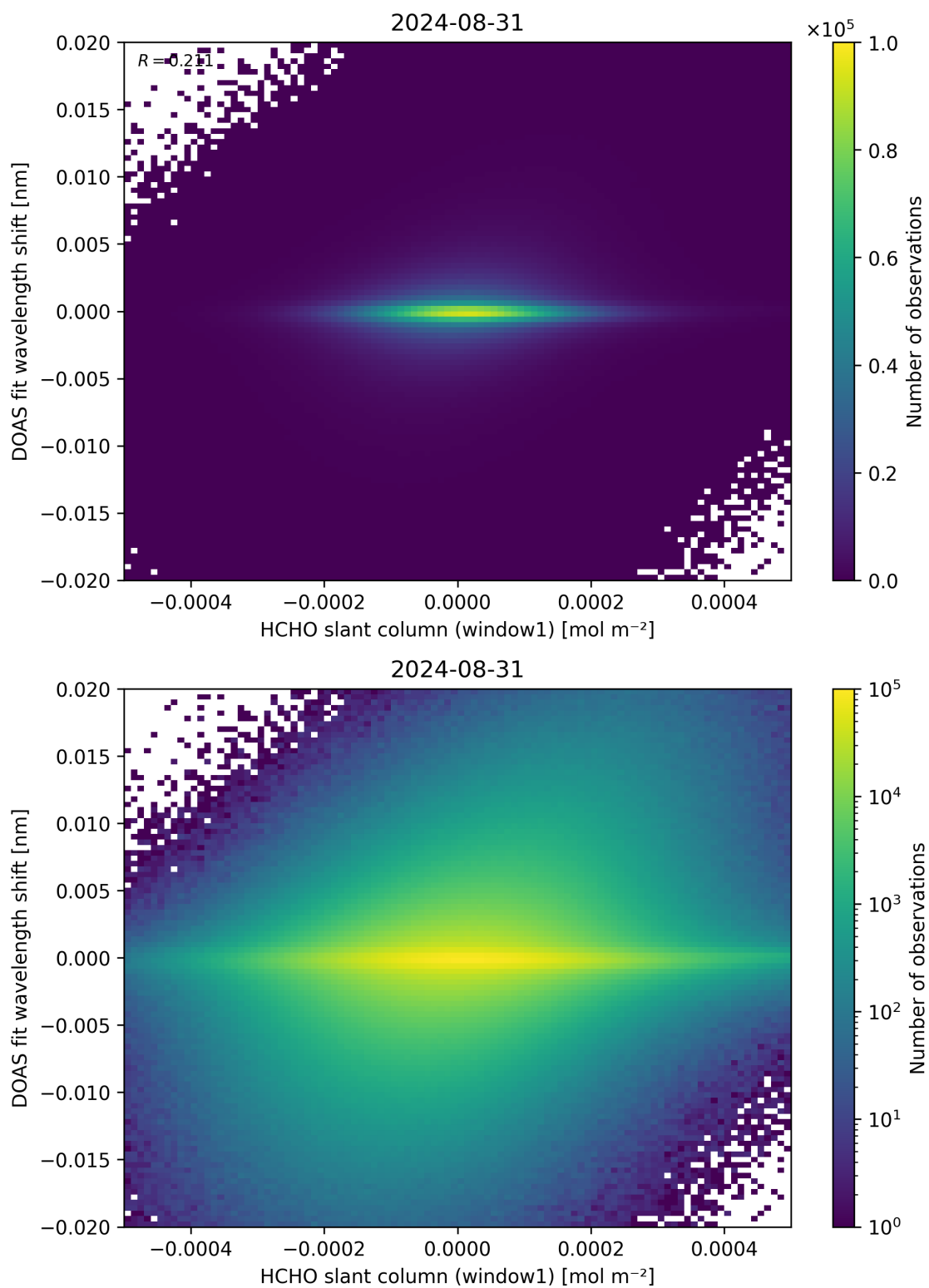
Figure 79: Scatter density plot of “HCHO slant column (window1)” against “DOAS fit wavelength shift” for 2024-08-30 to 2024-09-01.
