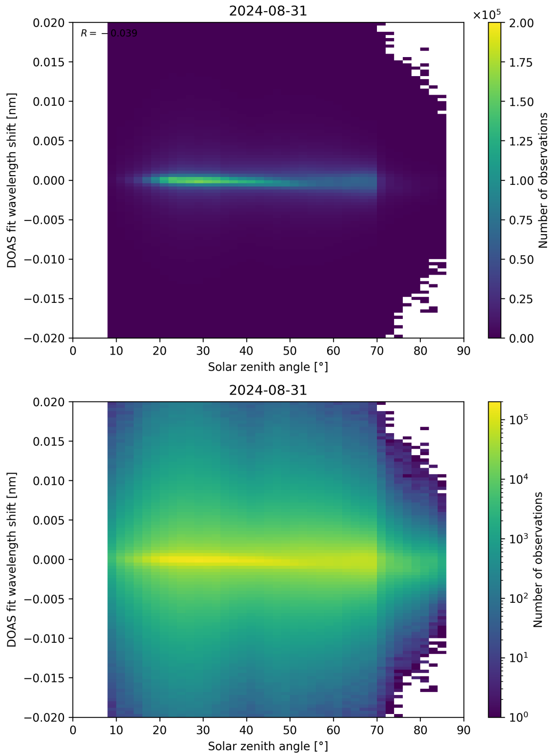
Figure 168: Scatter density plot of “Solar zenith angle” against “DOAS fit wavelength shift” for 2024-08-30 to 2024-09-01.
