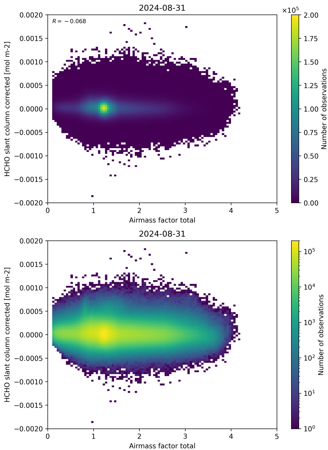
Figure 101: Scatter density plot of “Airmass factor total” against “HCHO slant column corrected” for 2024-08-30 to 2024-09-01.
