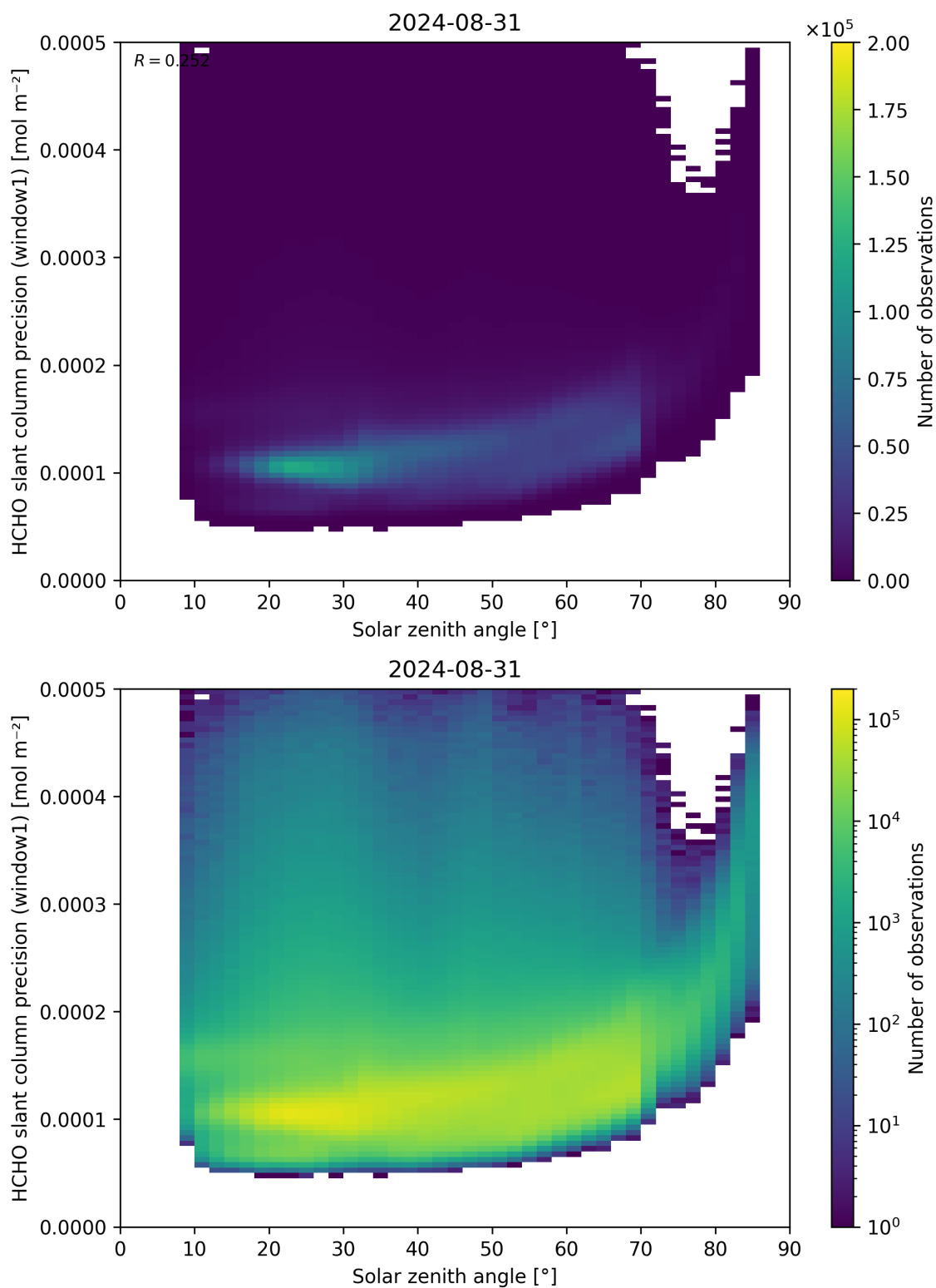
Figure 174: Scatter density plot of “Solar zenith angle” against “HCHO slant column precision (window1)” for 2024-08-30 to 2024-09-01.
