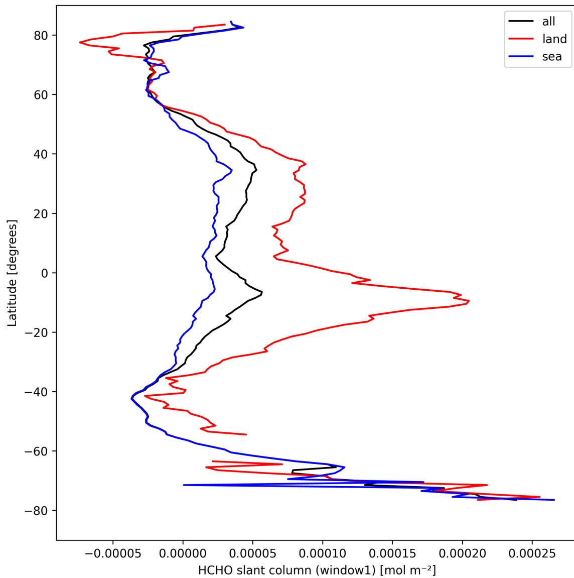
Figure 24: Zonal average of “HCHO slant column (window1)” for 2024-08-30 to 2024-09-01.
