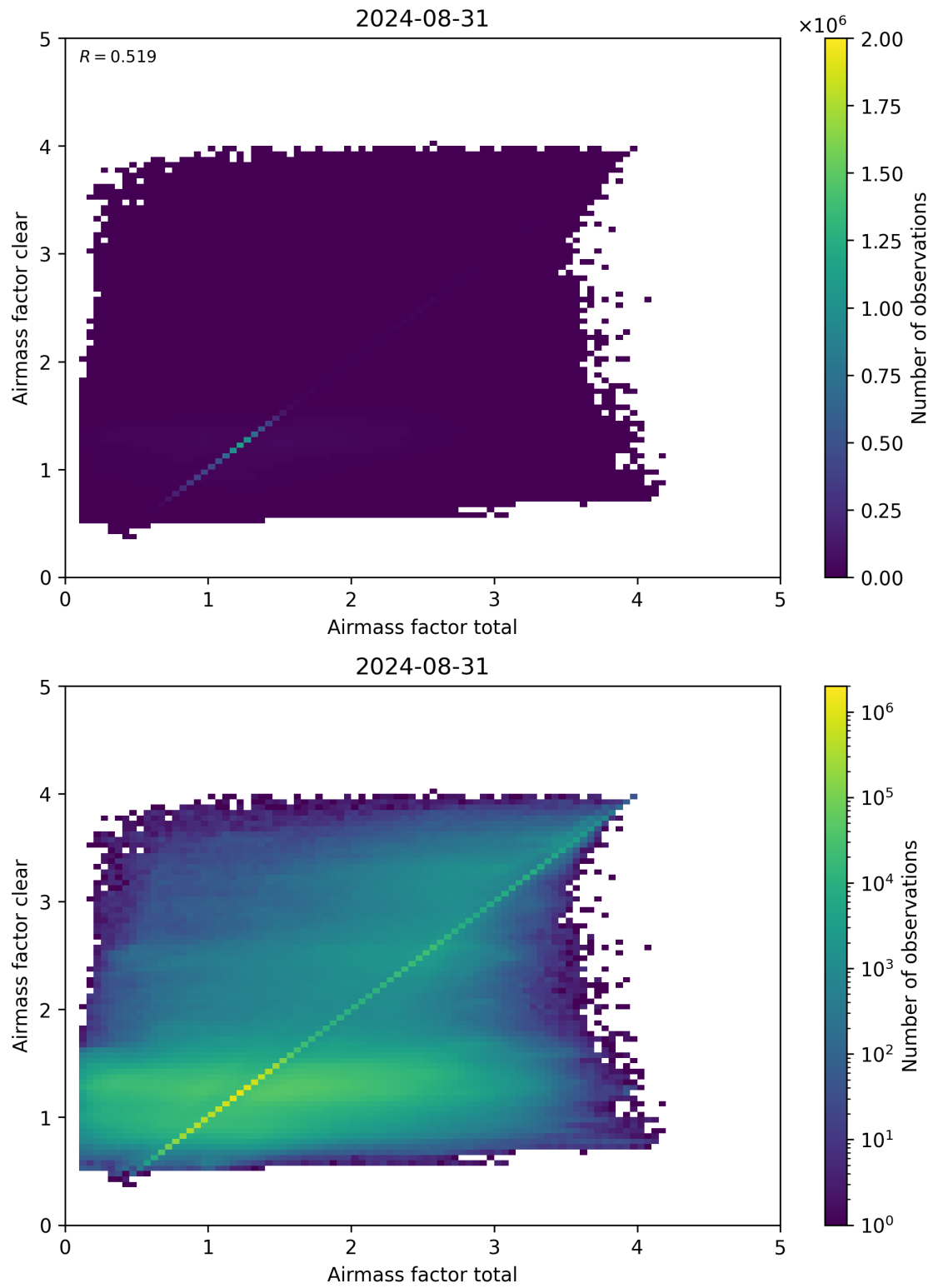
Figure 100: Scatter density plot of “Airmass factor total” against “Airmass factor clear” for 2024-08-30 to 2024-09-01.
