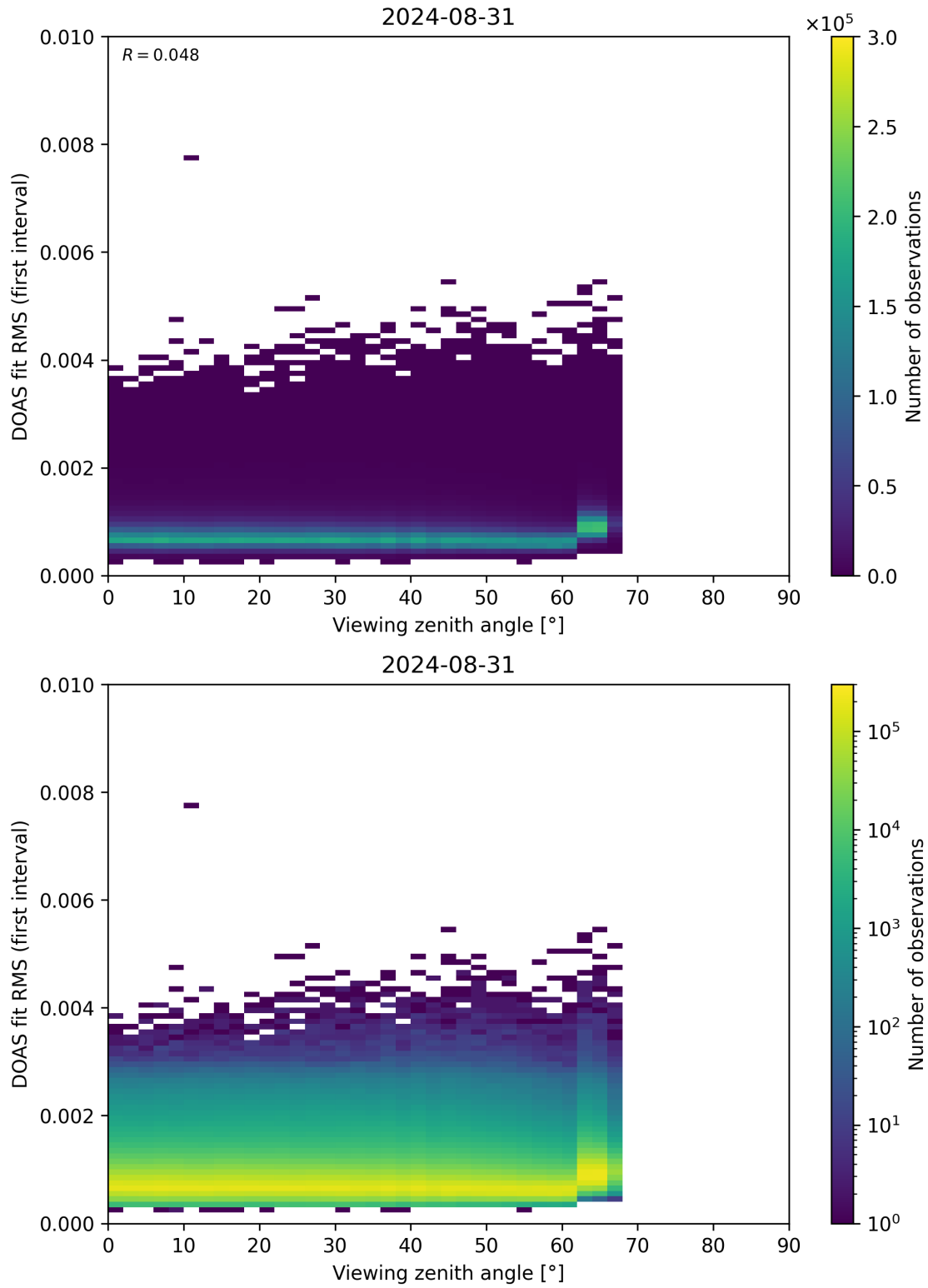
Figure 182: Scatter density plot of “Viewing zenith angle” against “DOAS fit RMS (first interval)” for 2024-08-30 to 2024-09-01.
