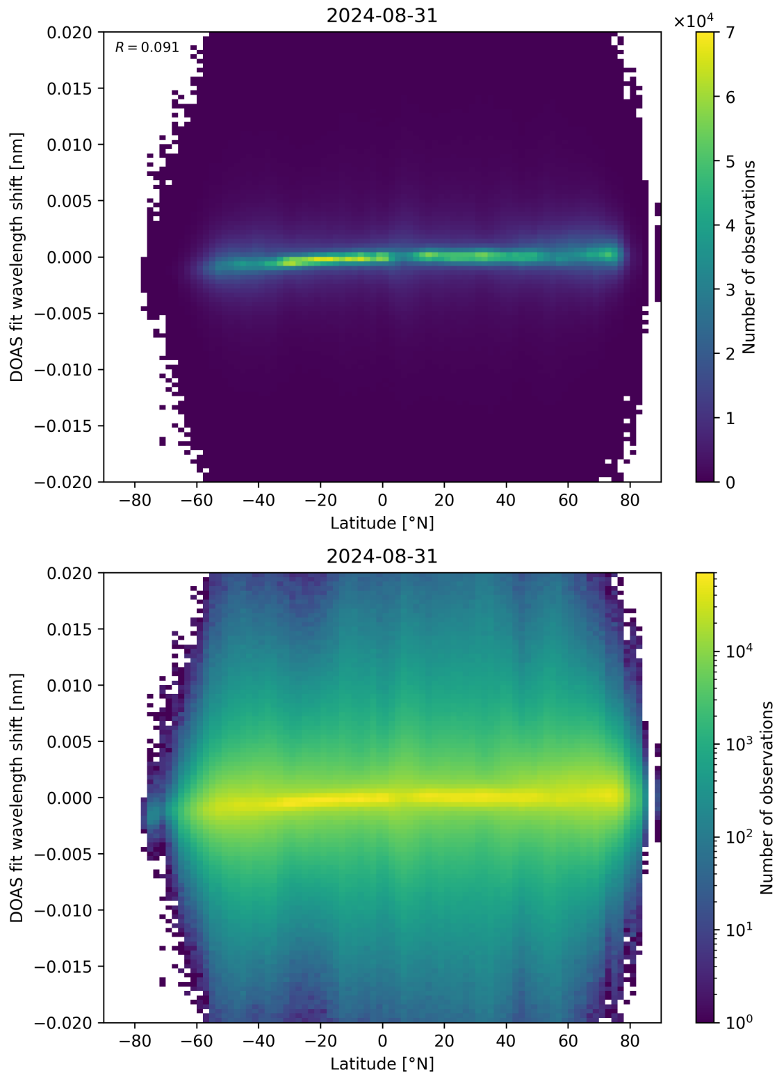
Figure 154: Scatter density plot of “Latitude” against “DOAS fit wavelength shift” for 2024-08-30 to 2024-09-01.
