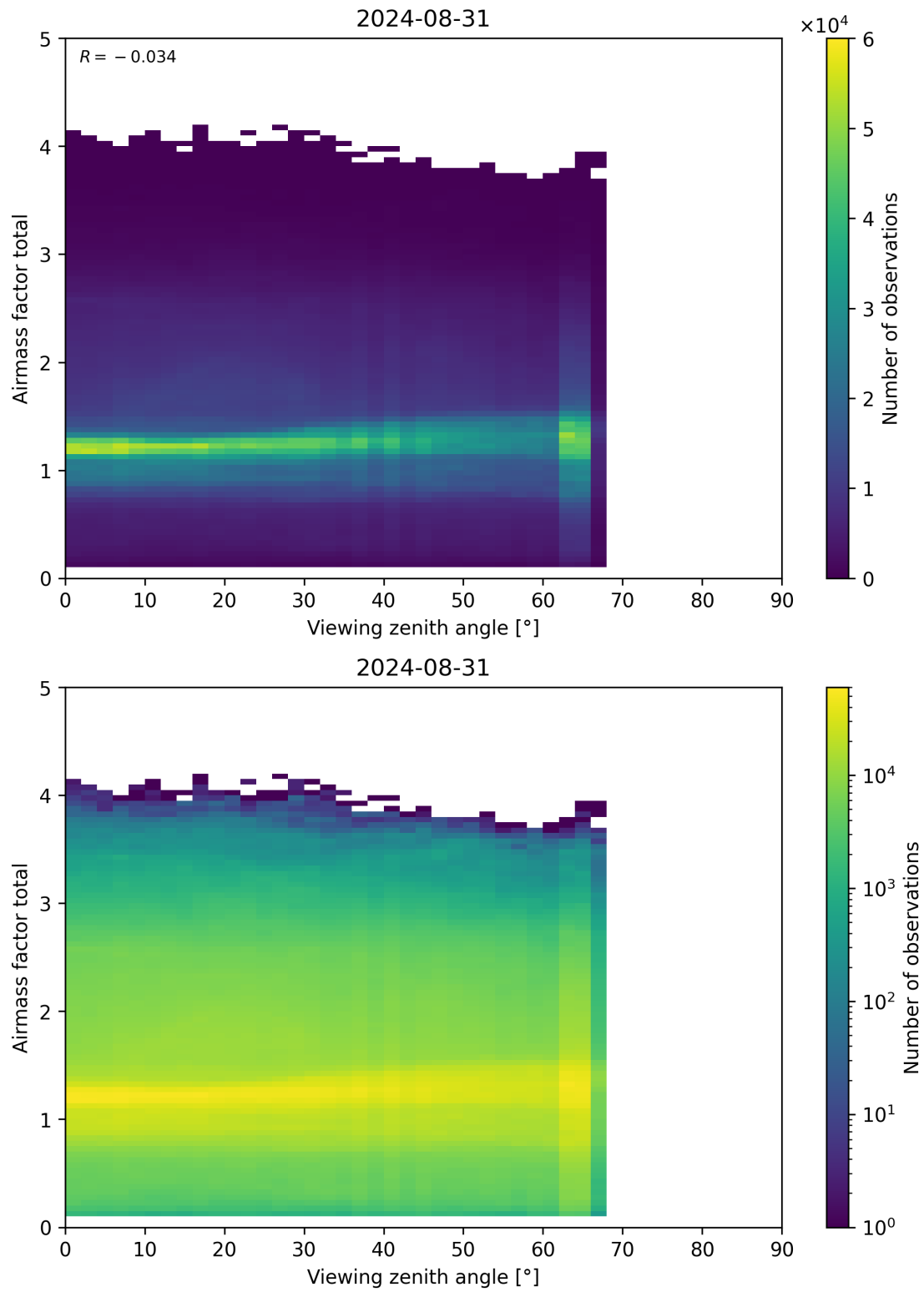
Figure 190: Scatter density plot of “Viewing zenith angle” against “Airmass factor total” for 2024-08-30 to 2024-09-01.
