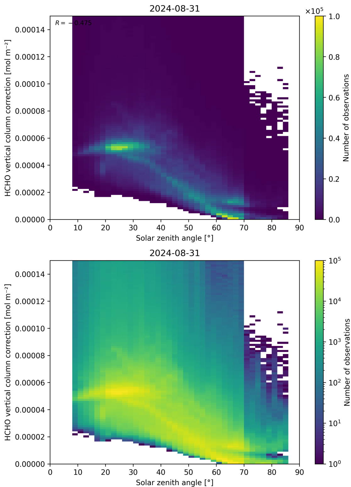
Figure 178: Scatter density plot of “Solar zenith angle” against “HCHO vertical column correction” for 2024-08-30 to 2024-09-01.
