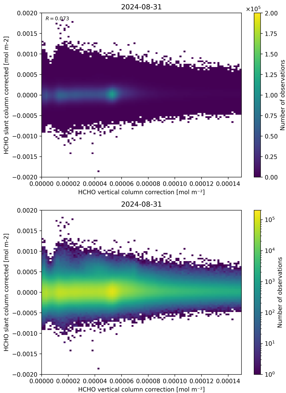
Figure 116: Scatter density plot of “HCHO vertical column correction” against “HCHO slant column corrected” for 2024-08-30 to 2024-09-01.
