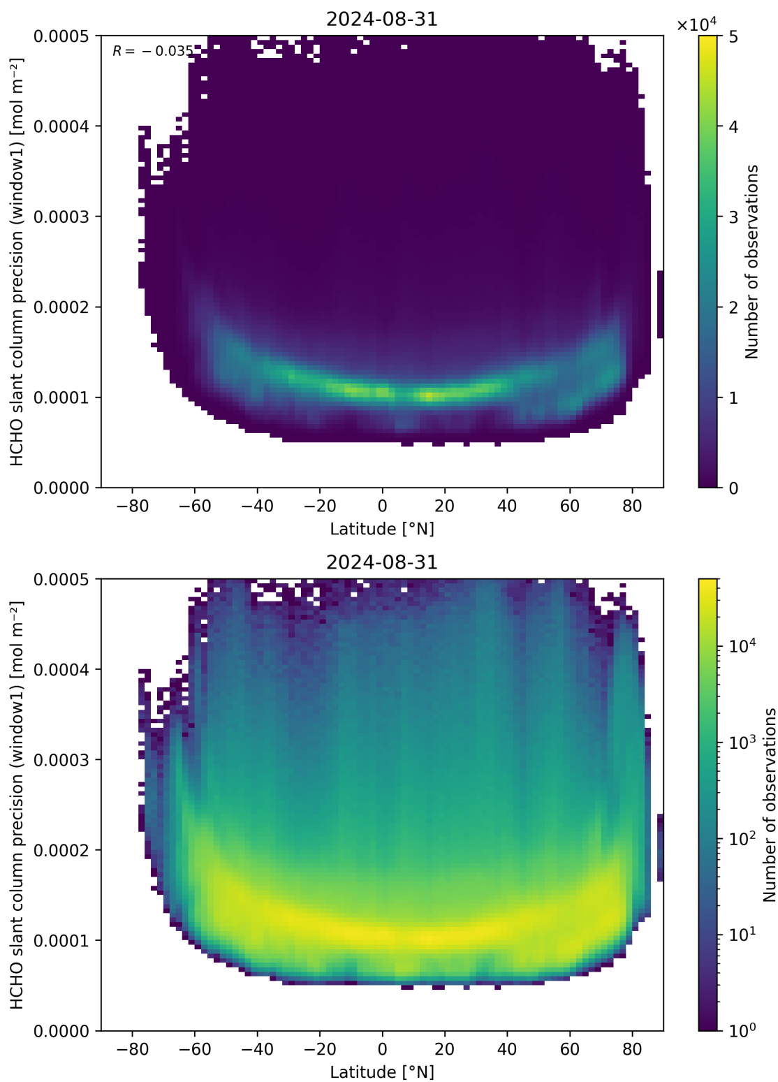
Figure 160: Scatter density plot of “Latitude” against “HCHO slant column precision (window1)” for 2024-08-30 to 2024-09-01.
