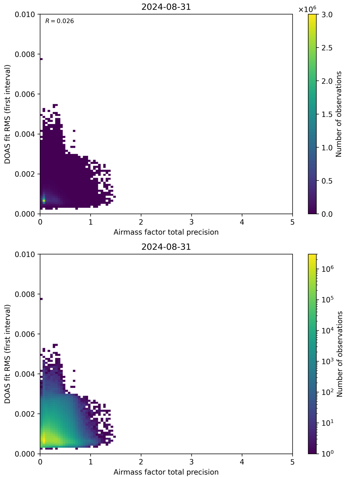
Figure 105: Scatter density plot of “Airmass factor total precision” against “DOAS fit RMS (first interval)” for 2024-08-30 to 2024-09-01.
