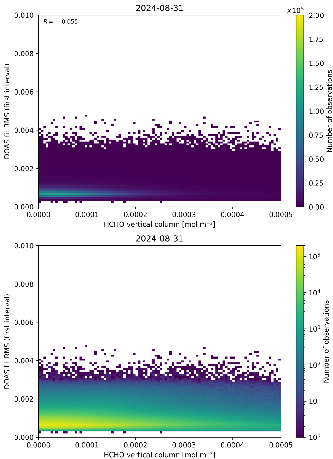
Figure 123: Scatter density plot of “HCHO vertical column” against “DOAS fit RMS (first interval)” for 2024-08-30 to 2024-09-01.
