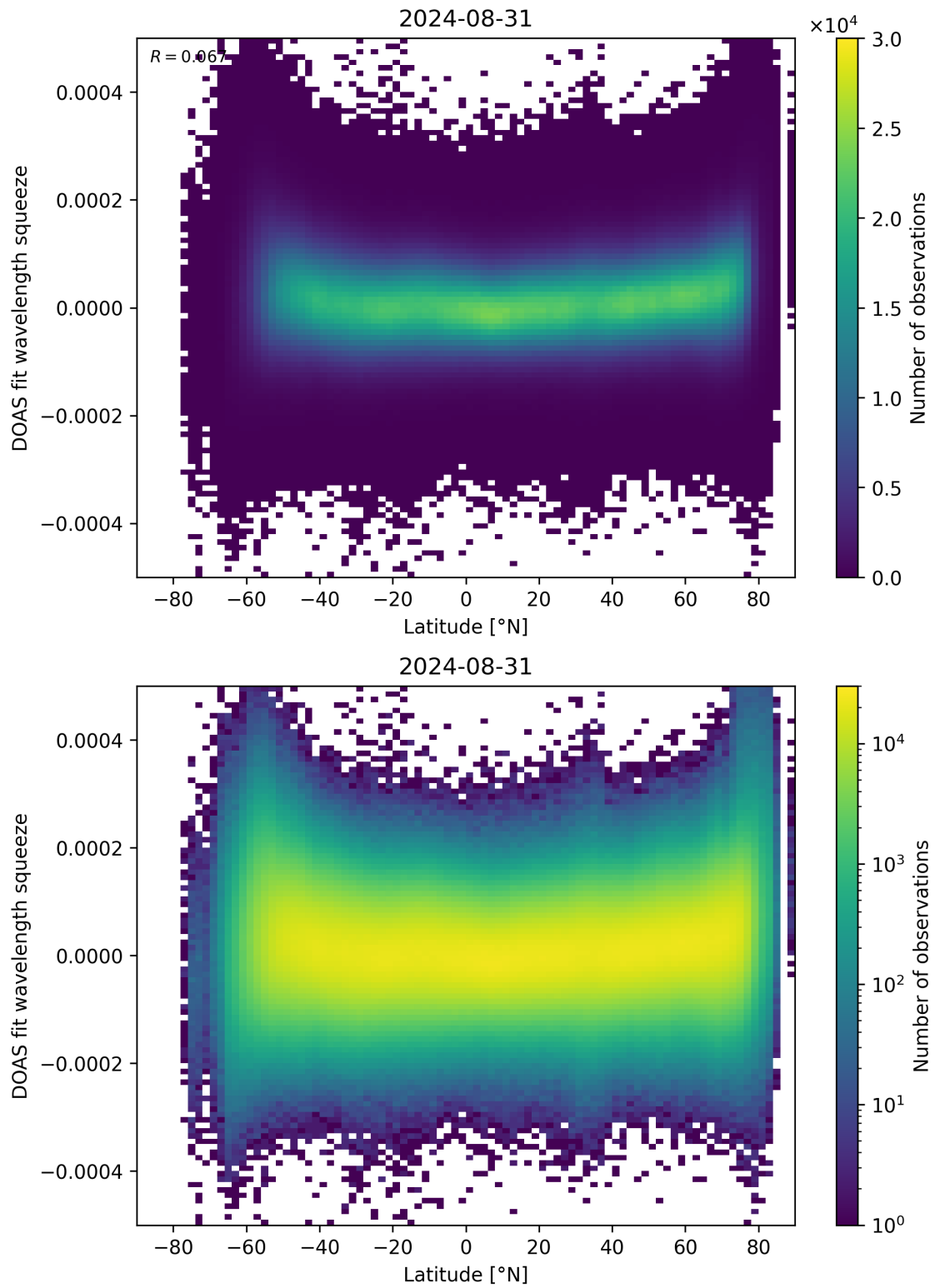
Figure 155: Scatter density plot of “Latitude” against “DOAS fit wavelength squeeze” for 2024-08-30 to 2024-09-01.
