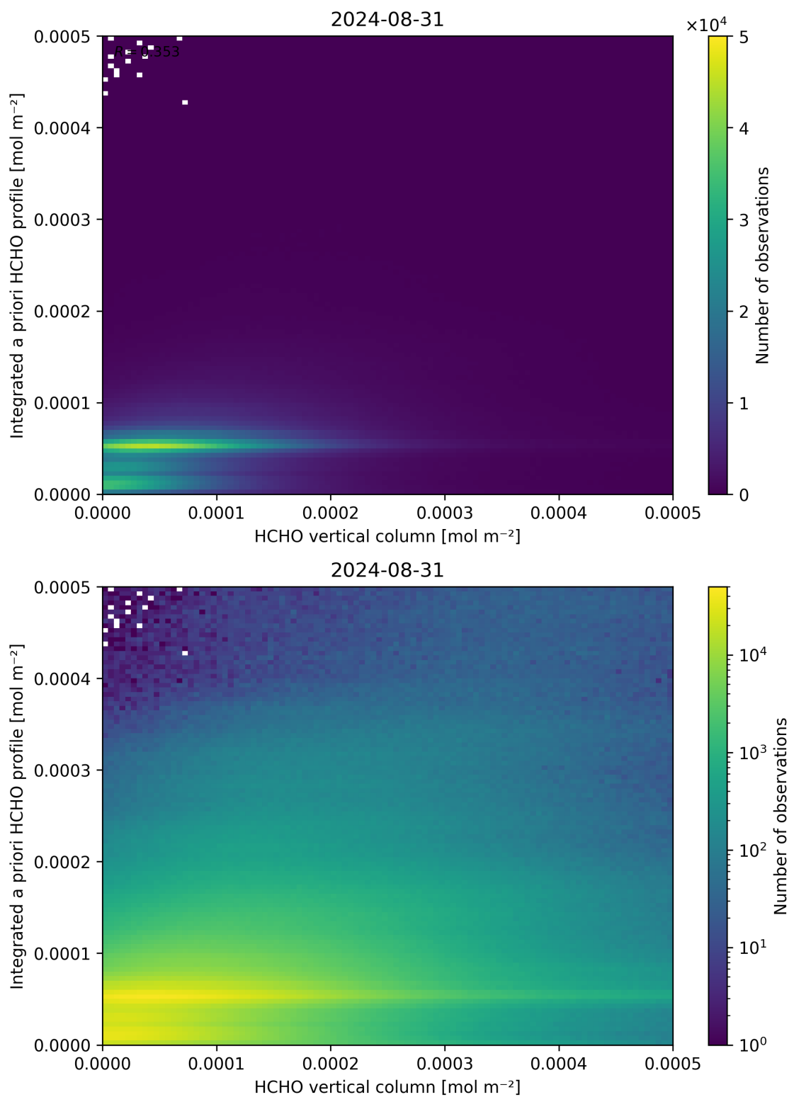
Figure 135: Scatter density plot of “HCHO vertical column” against “Integrated a priori HCHO profile” for 2024-08-30 to 2024-09-01.
