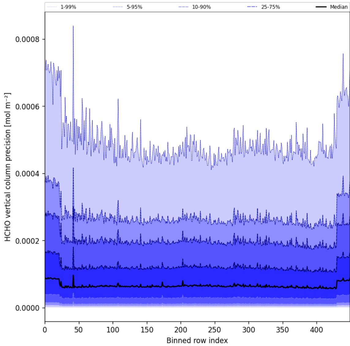
Figure 50: Along track statistics of “HCHO vertical column precision” for 2024-08-30 to 2024-09-01
