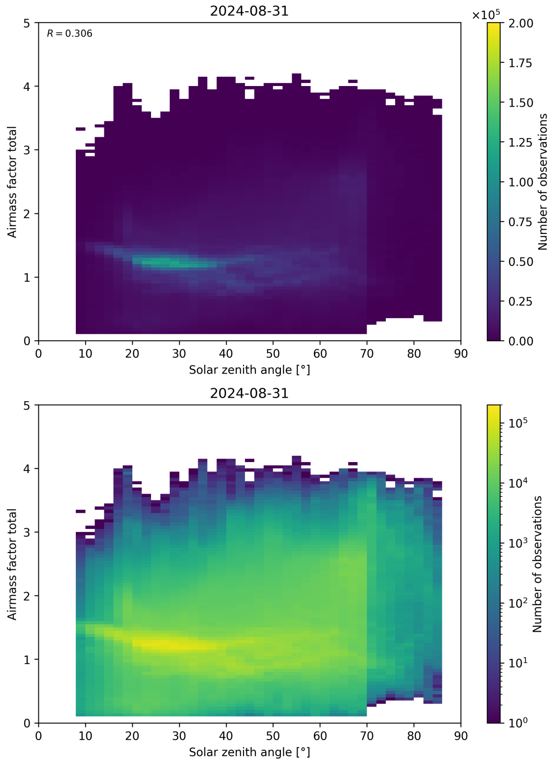
Figure 175: Scatter density plot of “Solar zenith angle” against “Airmass factor total” for 2024-08-30 to 2024-09-01.
