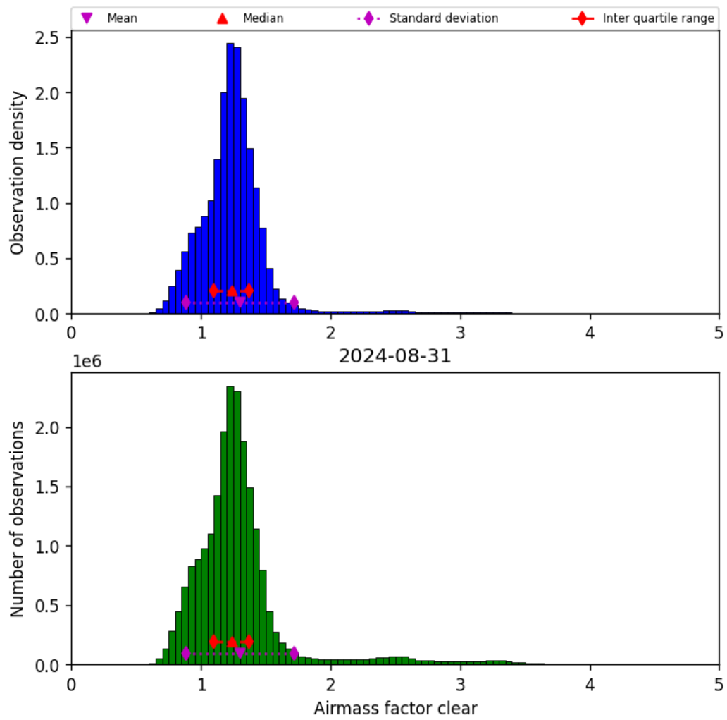
Figure 42: Histogram of “Airmass factor clear” for 2024-08-30 to 2024-09-01
