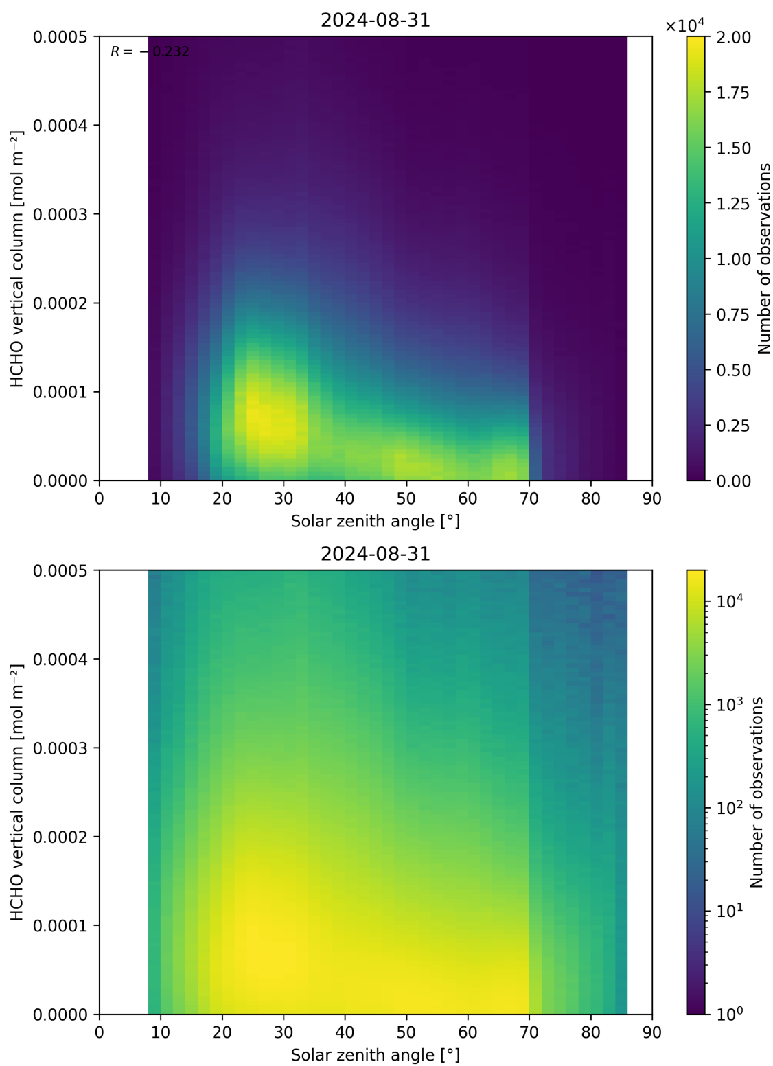
Figure 177: Scatter density plot of “Solar zenith angle” against “HCHO vertical column” for 2024-08-30 to 2024-09-01.
