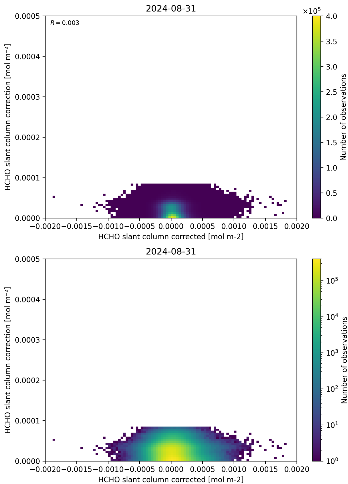
Figure 77: Scatter density plot of “HCHO slant column corrected” against “HCHO slant column correction” for 2024-08-30 to 2024-09-01.
