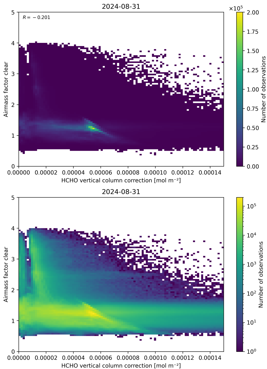
Figure 115: Scatter density plot of “HCHO vertical column correction” against “Airmass factor clear” for 2024-08-30 to 2024-09-01.
