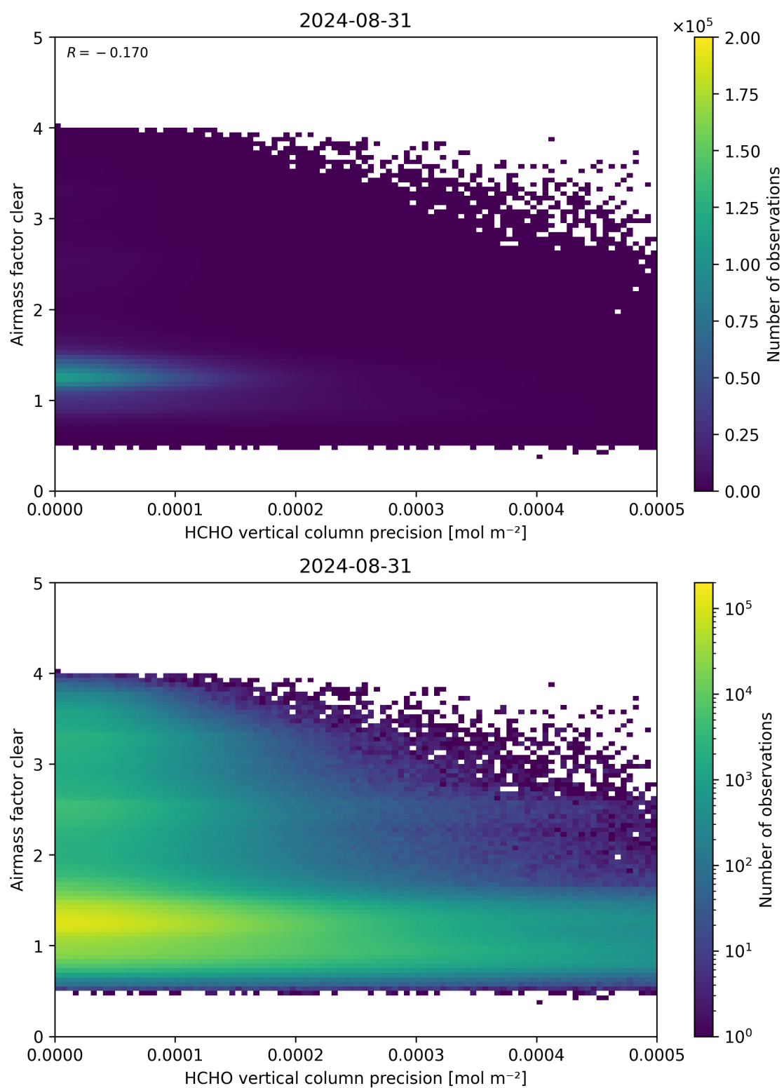
Figure 139: Scatter density plot of “HCHO vertical column precision” against “Airmass factor clear” for 2024-08-30 to 2024-09-01.
