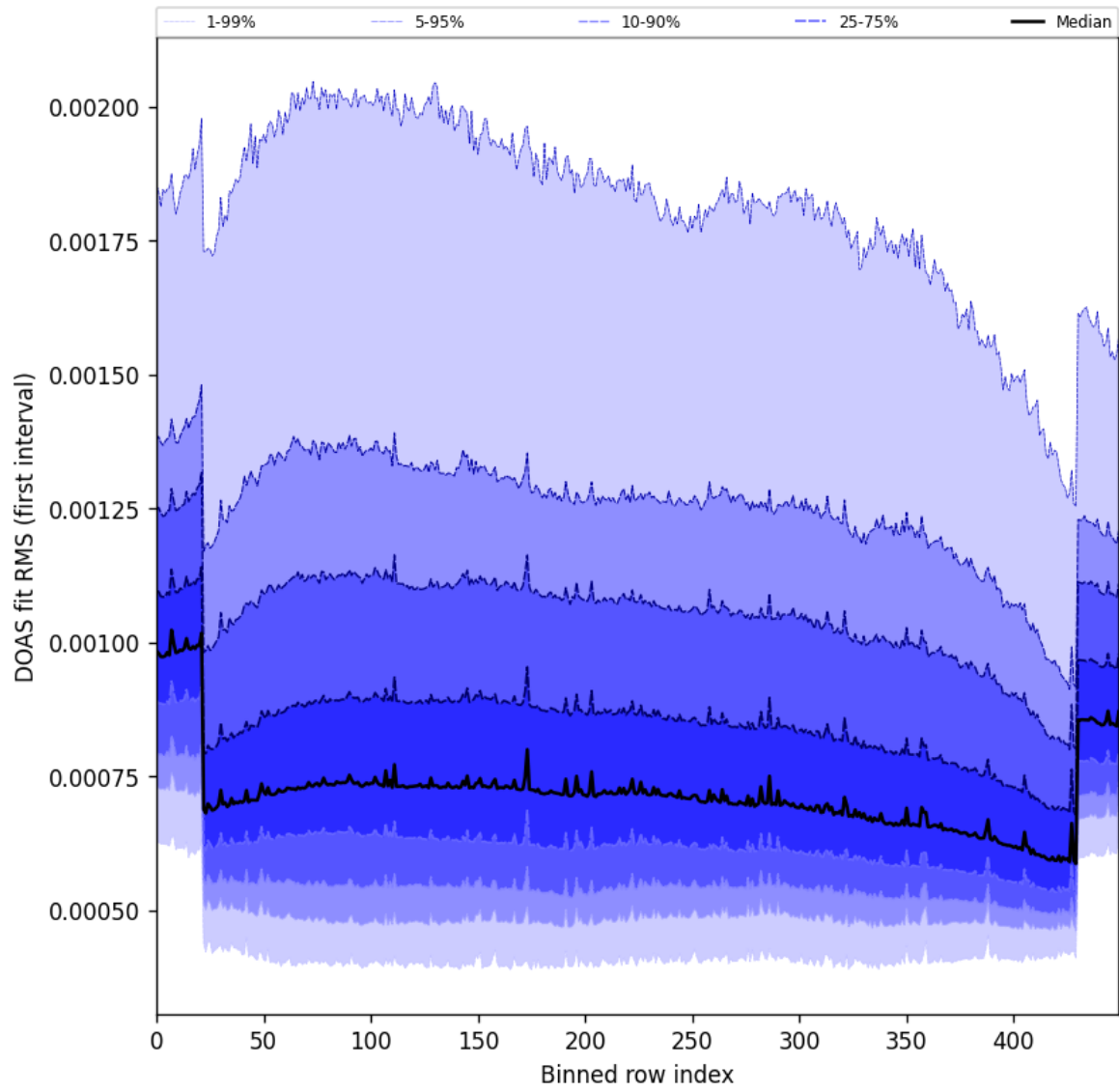
Figure 60: Along track statistics of “DOAS fit RMS (first interval)” for 2024-08-30 to 2024-09-01
