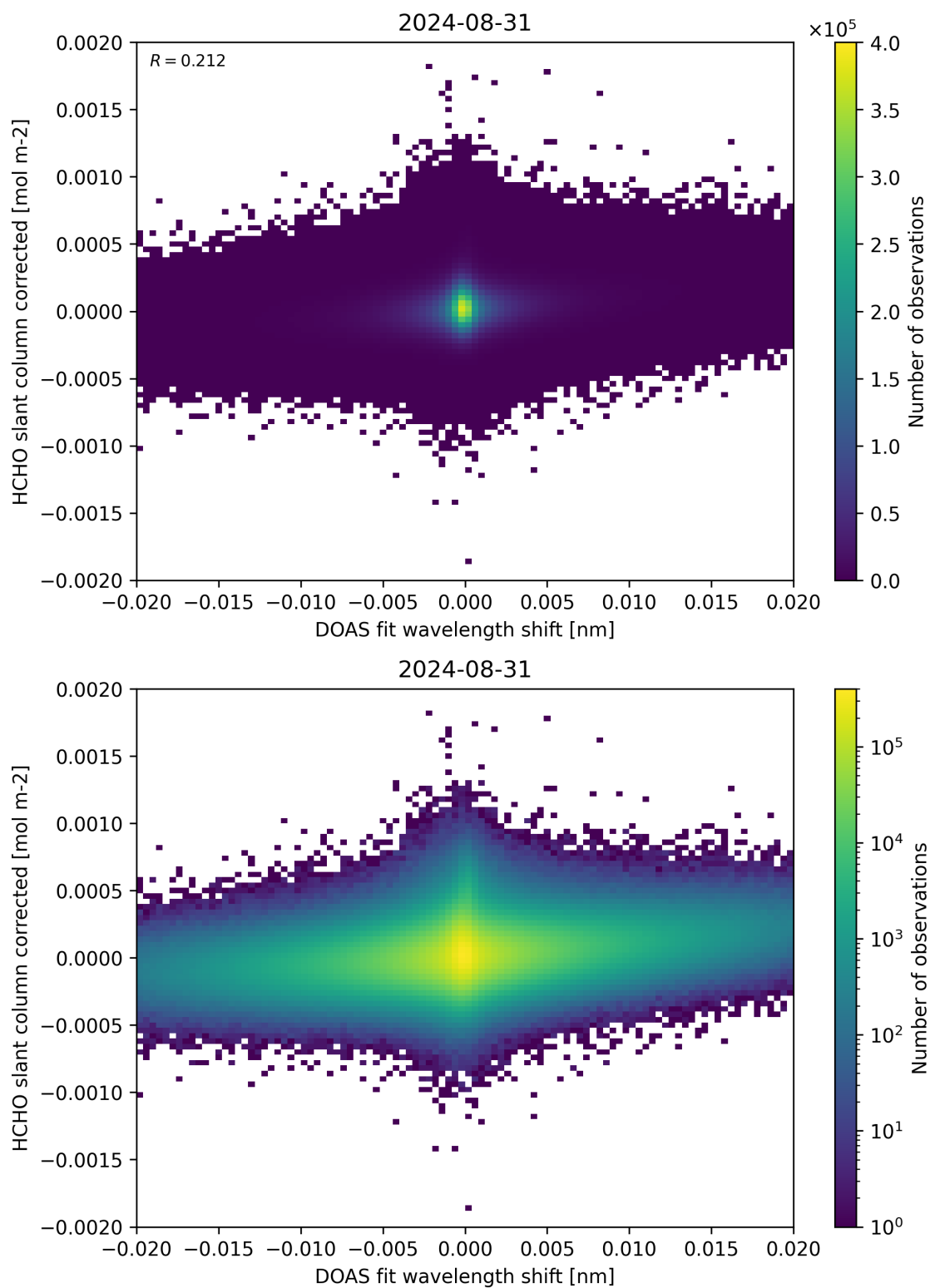
Figure 66: Scatter density plot of “DOAS fit wavelength shift” against “HCHO slant column corrected” for 2024-08-30 to 2024-09-01.
