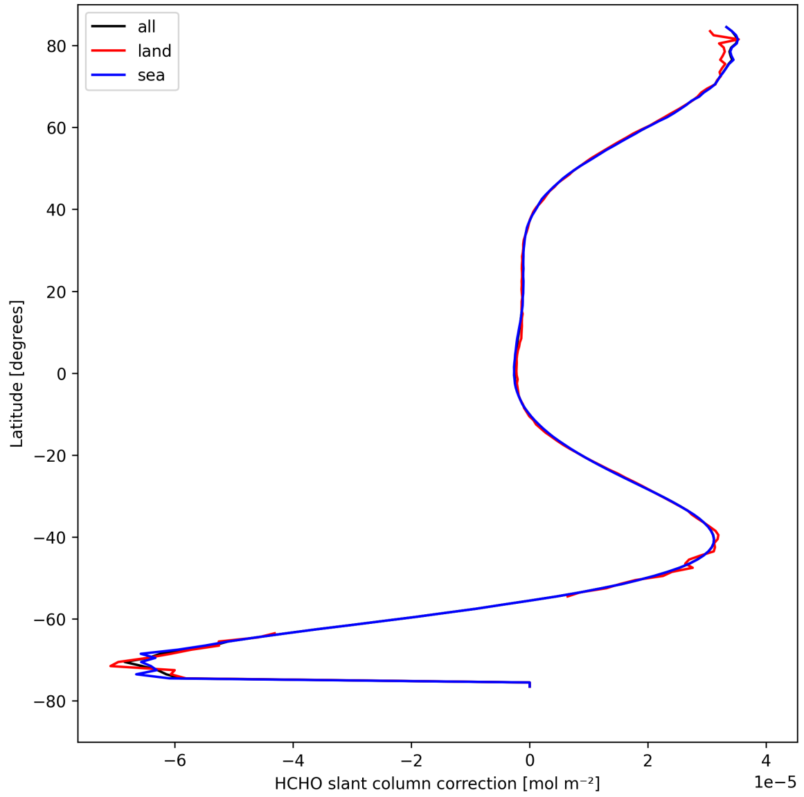
Figure 33: Zonal average of "HCHO slant column correction" for 2024-08-30 to 2024-09-01.
