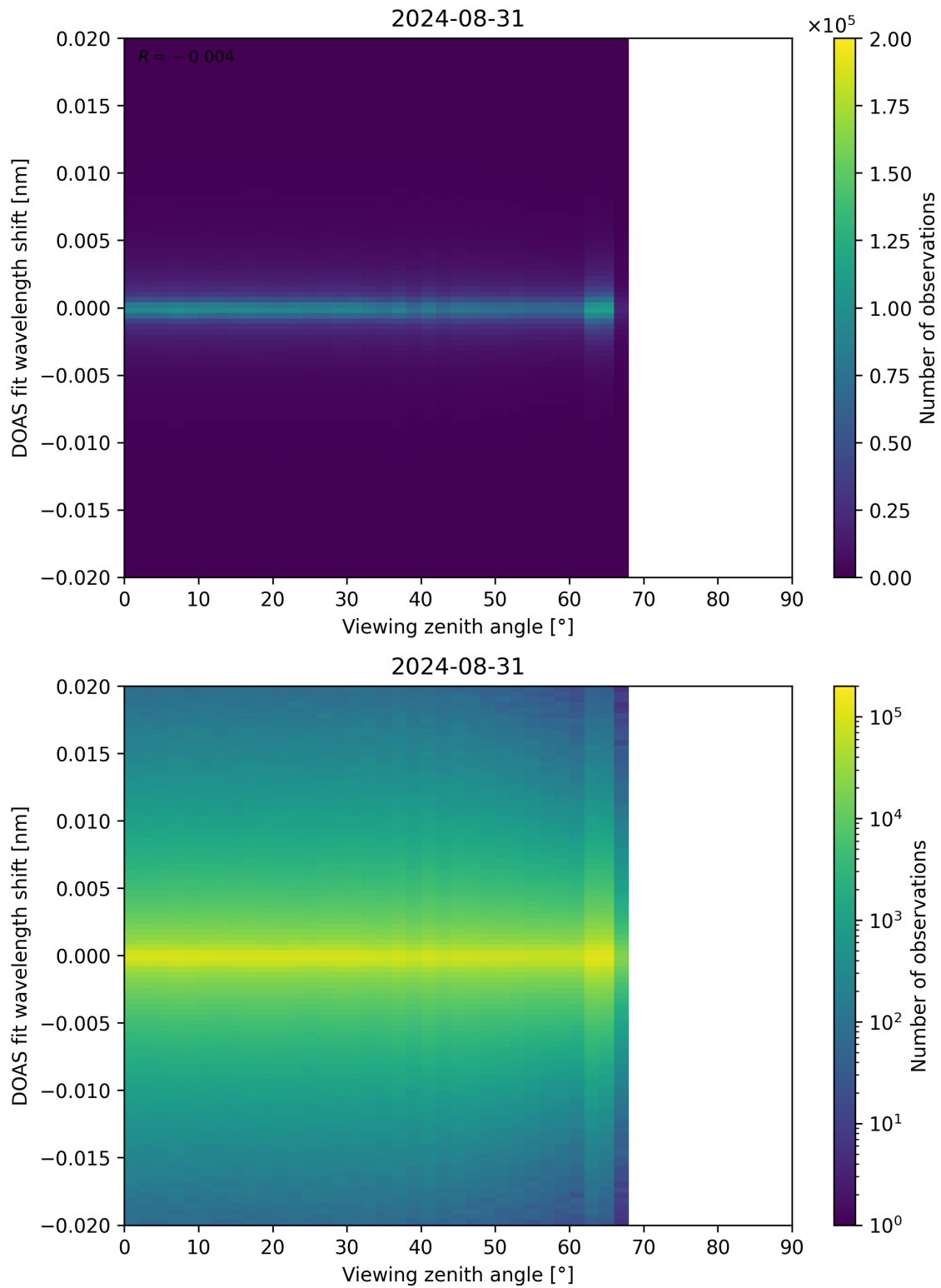
Figure 183: Scatter density plot of “Viewing zenith angle” against “DOAS fit wavelength shift” for 2024-08-30 to 2024-09-01.
