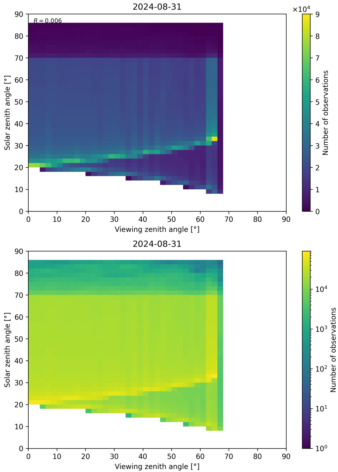
Figure 197: Scatter density plot of “Viewing zenith angle” against “Solar zenith angle” for 2024-08-30 to 2024-09-01.
