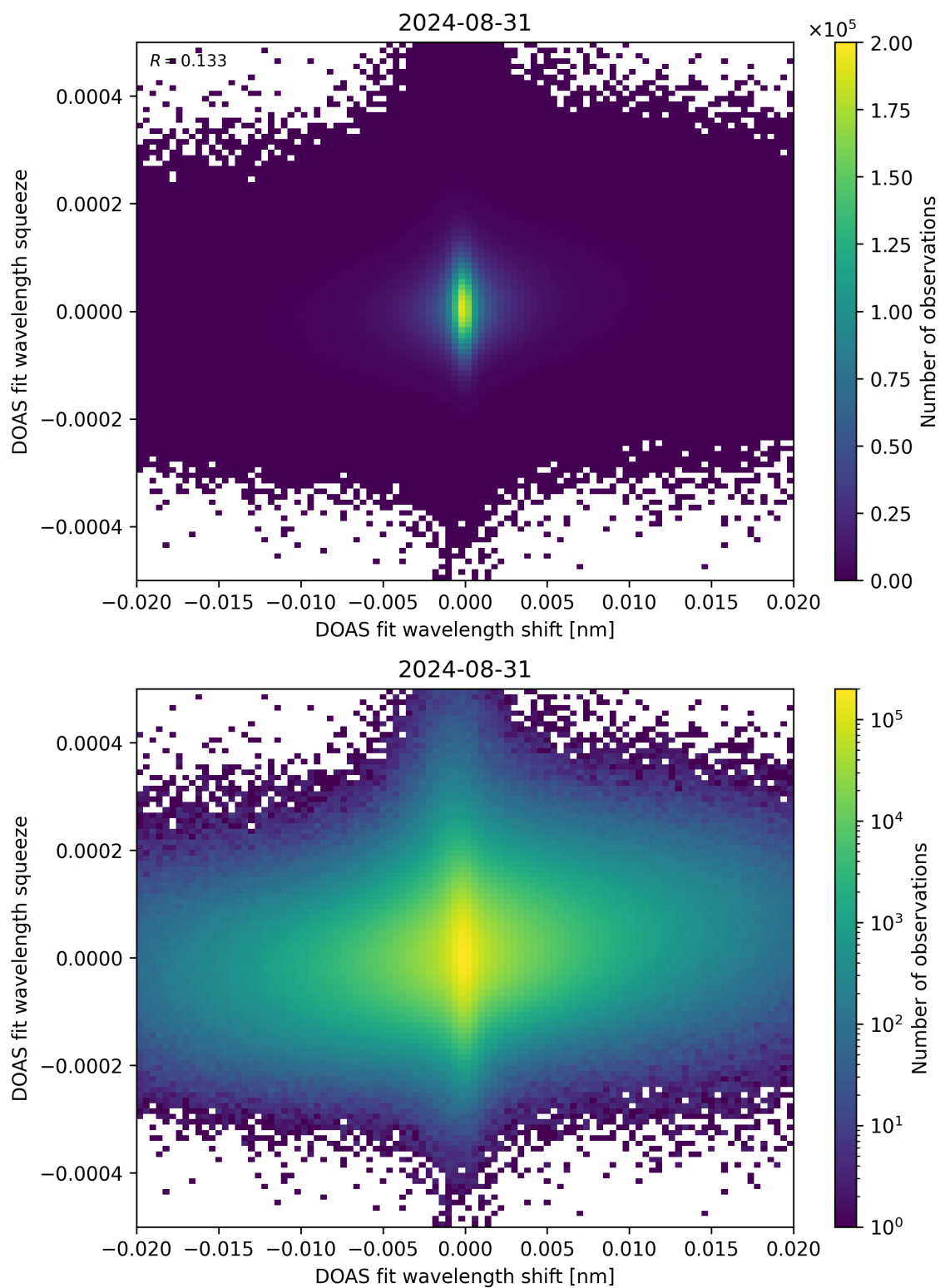
Figure 65: Scatter density plot of “DOAS fit wavelength shift” against “DOAS fit wavelength squeeze” for 2024-08-30 to 2024-09-01.
