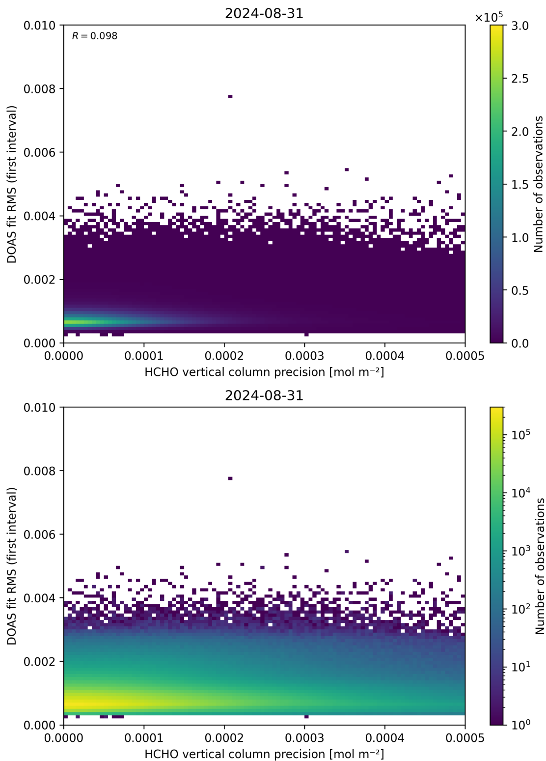
Figure 136: Scatter density plot of “HCHO vertical column precision” against “DOAS fit RMS (first interval)” for 2024-08-30 to 2024-09-01.
