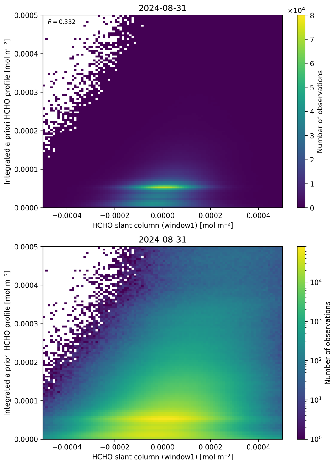
Figure 87: Scatter density plot of “HCHO slant column (window1)” against “Integrated a priori HCHO profile” for 2024-08-30 to 2024-09-01.
