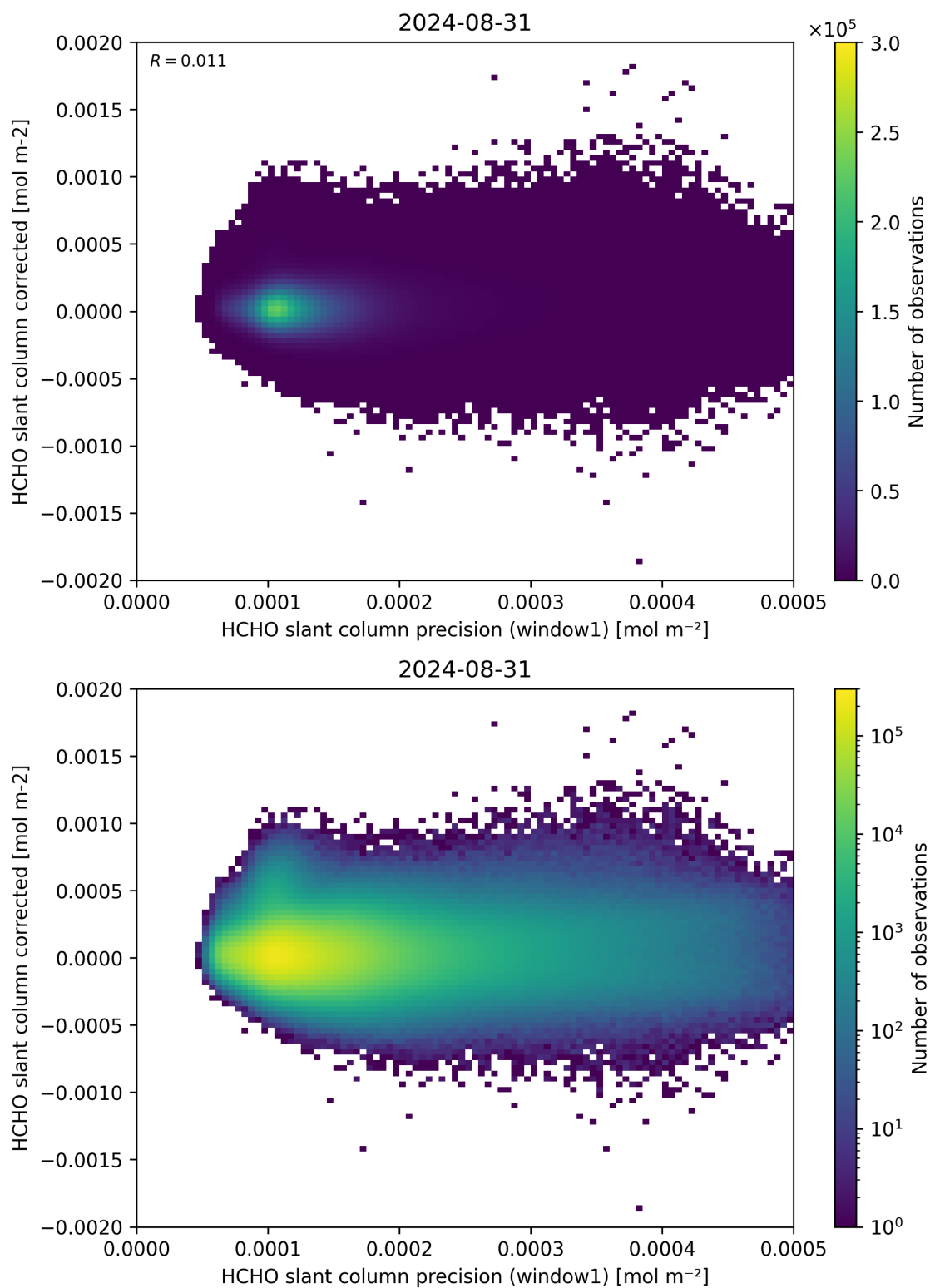
Figure 92: Scatter density plot of “HCHO slant column precision (window1)” against “HCHO slant column corrected” for 2024-08-30 to 2024-09-01.
