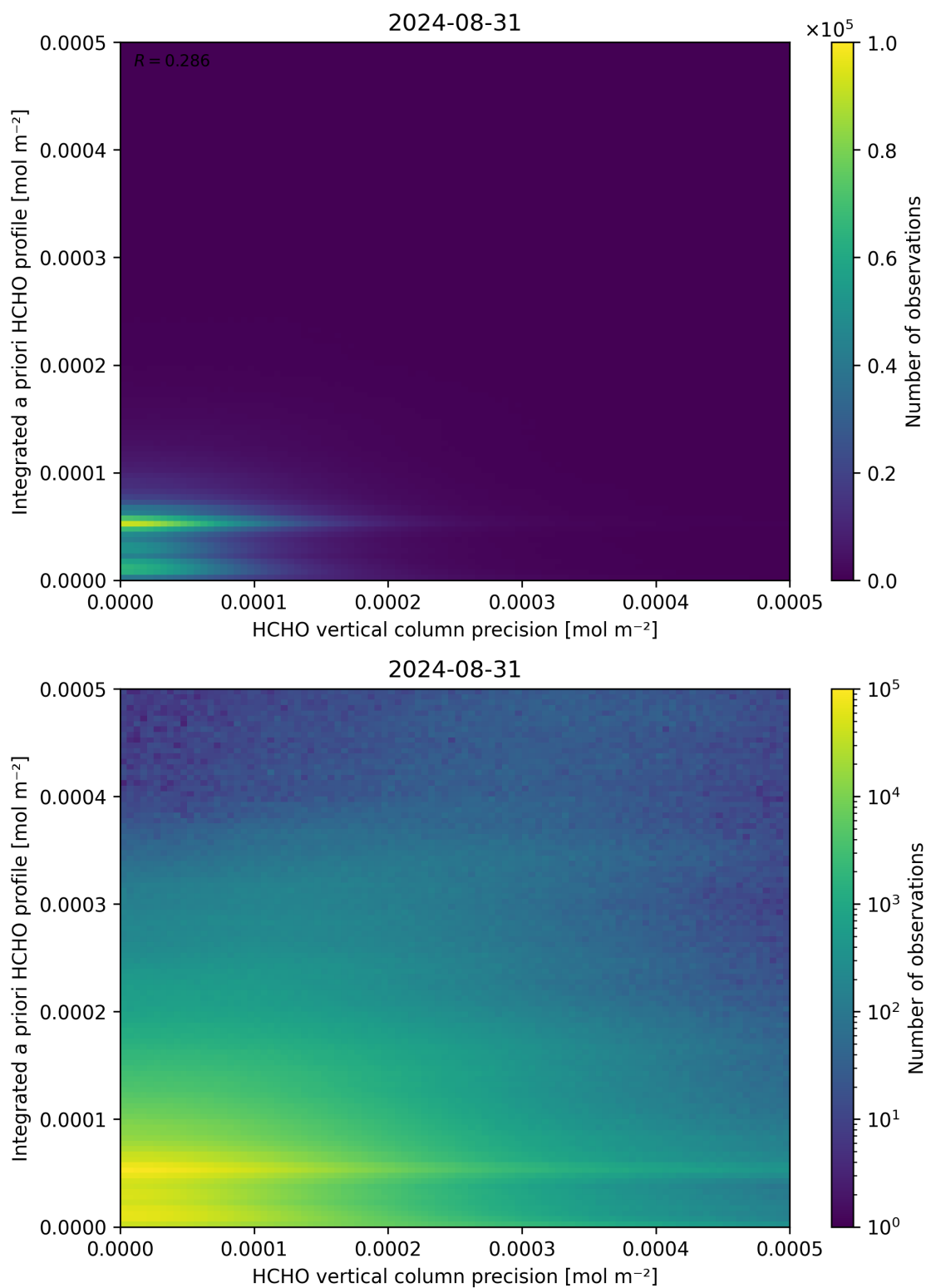
Figure 147: Scatter density plot of “HCHO vertical column precision” against “Integrated a priori HCHO profile” for 2024-08-30 to 2024-09-01.
