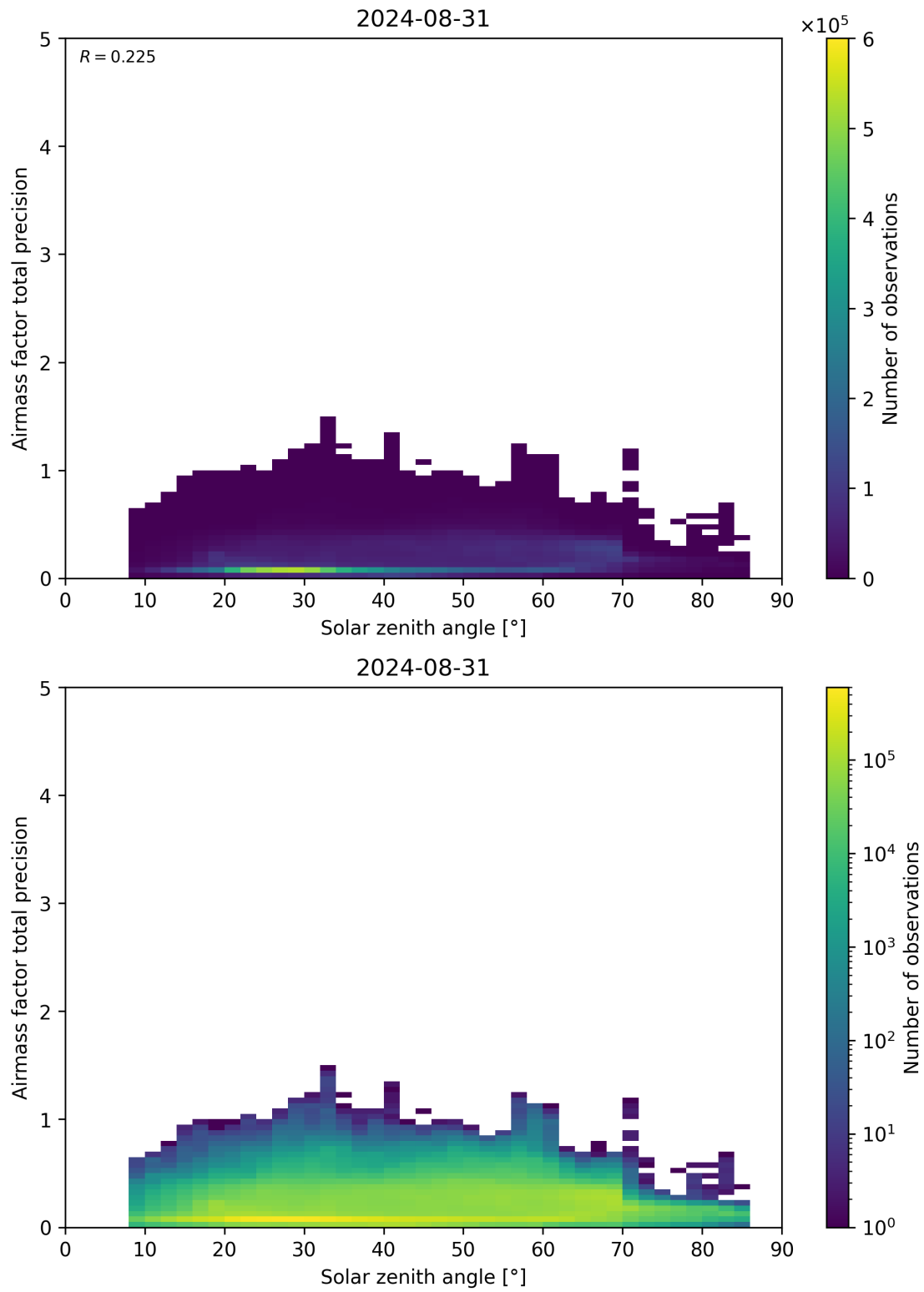
Figure 176: Scatter density plot of “Solar zenith angle” against “Airmass factor total precision” for 2024-08-30 to 2024-09-01.
