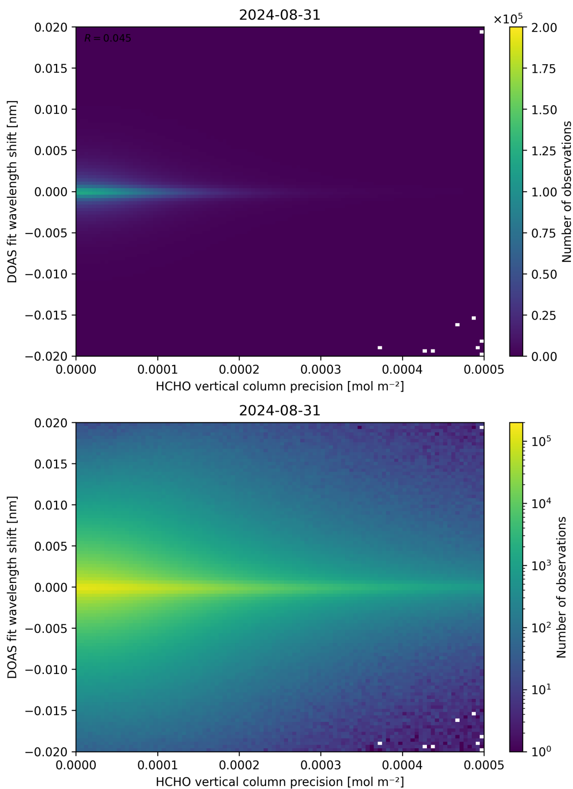
Figure 137: Scatter density plot of “HCHO vertical column precision” against “DOAS fit wavelength shift” for 2024-08-30 to 2024-09-01.
