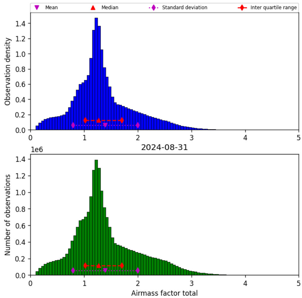
Figure 40: Histogram of “Airmass factor total” for 2024-08-30 to 2024-09-01
