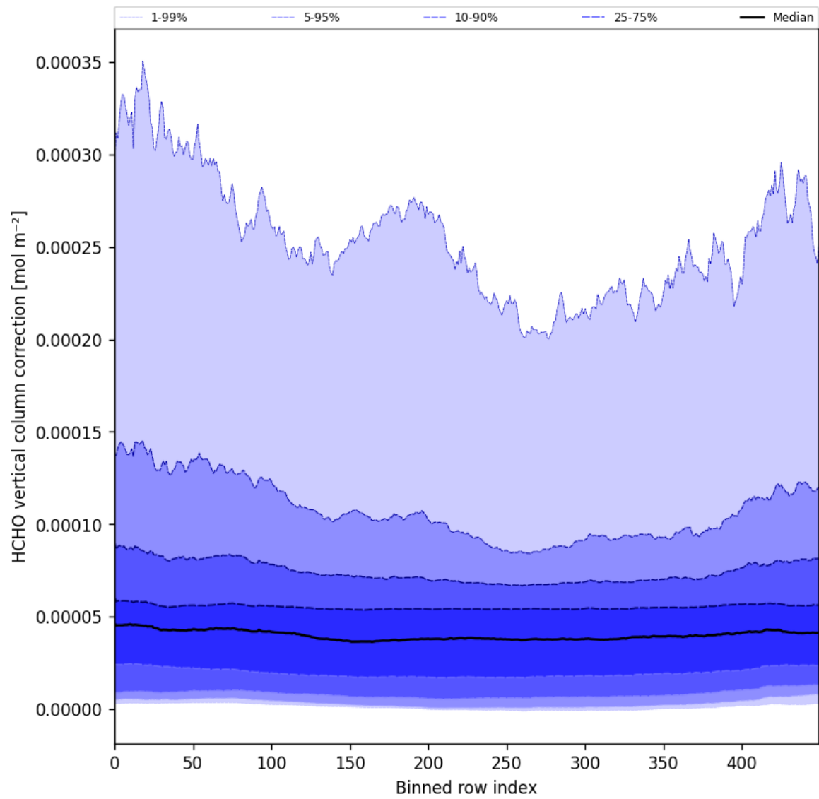
Figure 51: Along track statistics of “HCHO vertical column correction” for 2024-08-30 to 2024-09-01
