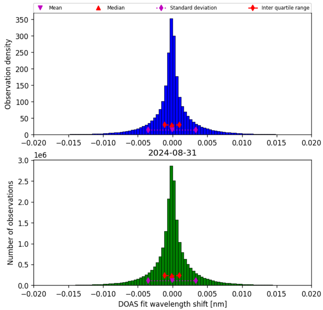
Figure 44: Histogram of “DOAS fit wavelength shift” for 2024-08-30 to 2024-09-01
