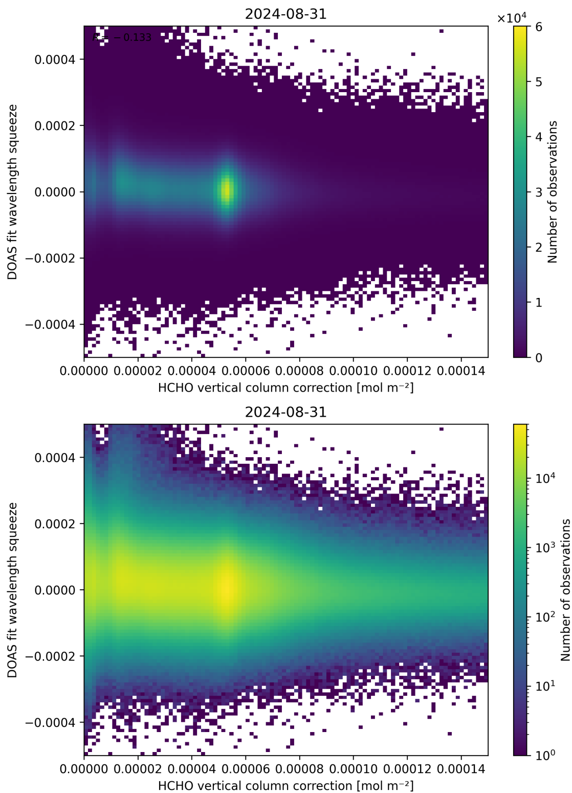
Figure 114: Scatter density plot of “HCHO vertical column correction” against “DOAS fit wavelength squeeze” for 2024-08-30 to 2024-09-01.
