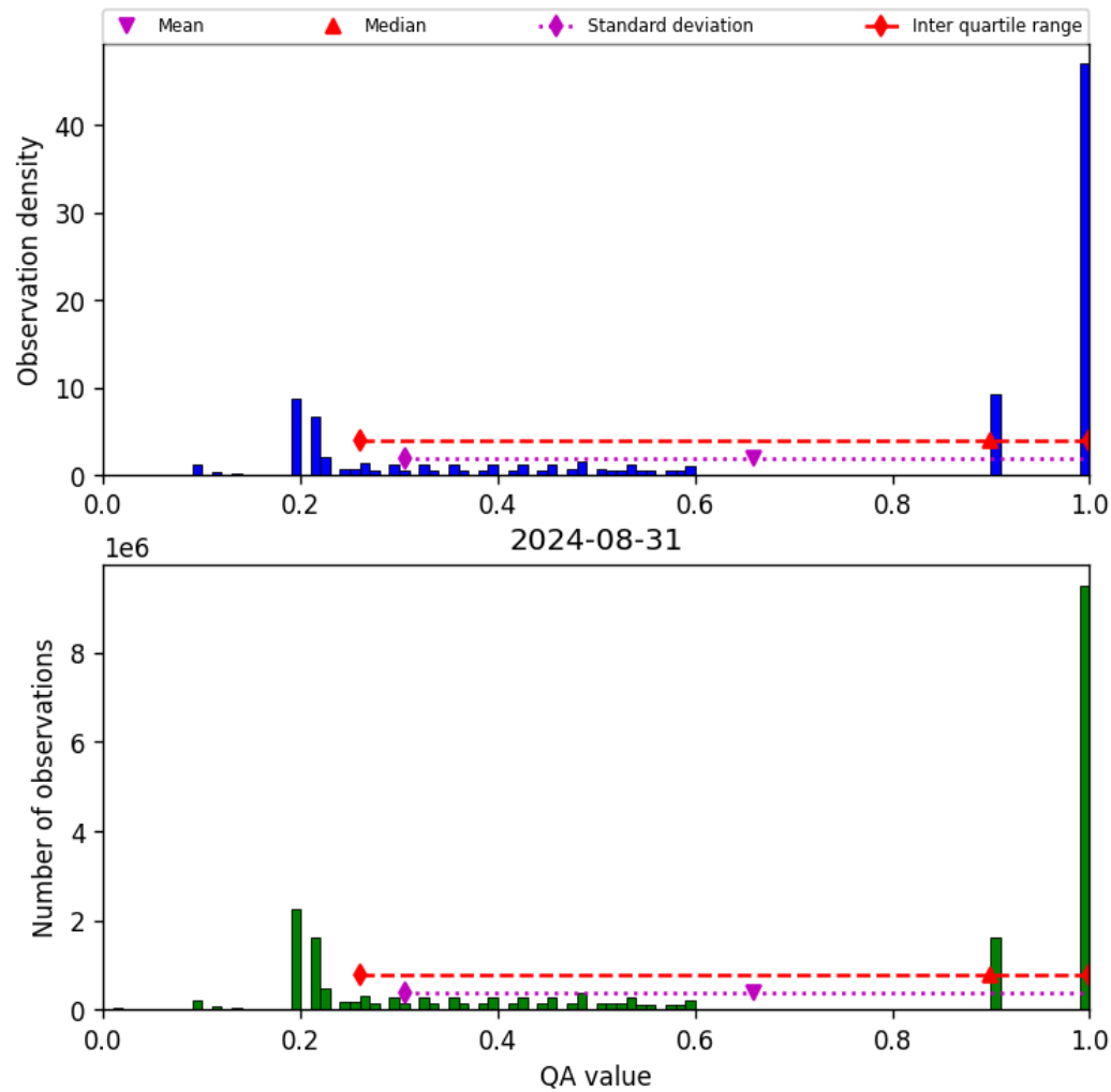
Figure 34: Histogram of “QA value” for 2024-08-30 to 2024-09-01
