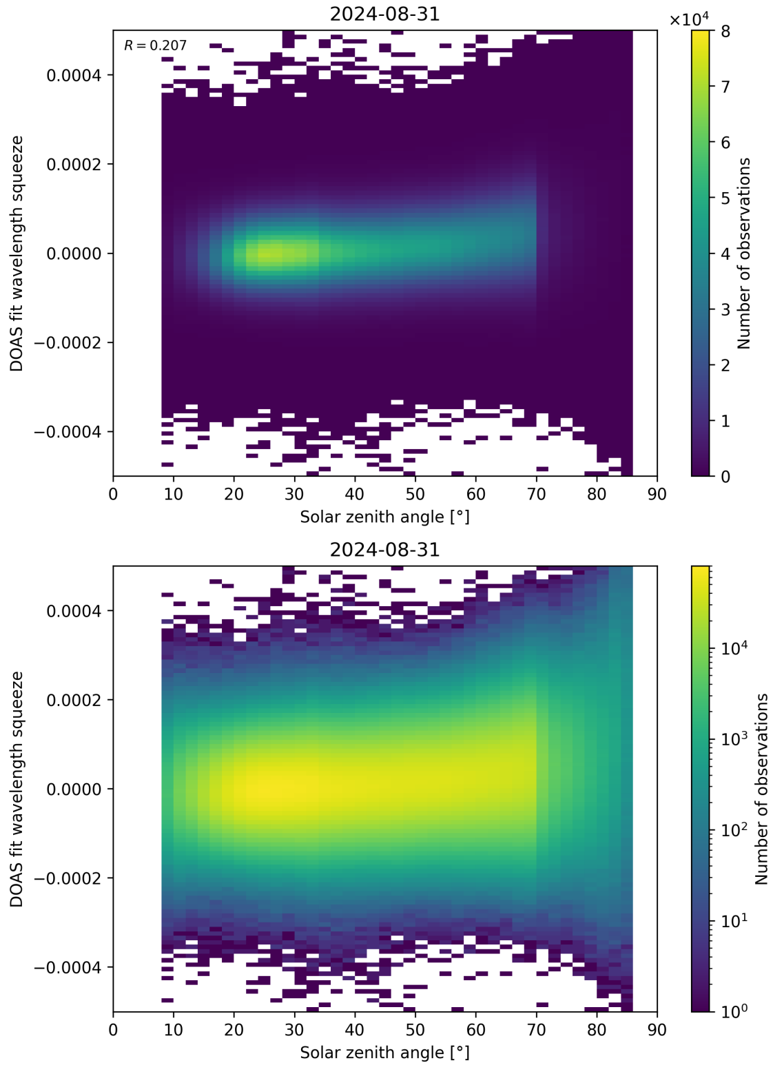
Figure 169: Scatter density plot of “Solar zenith angle” against “DOAS fit wavelength squeeze” for 2024-08-30 to 2024-09-01.
