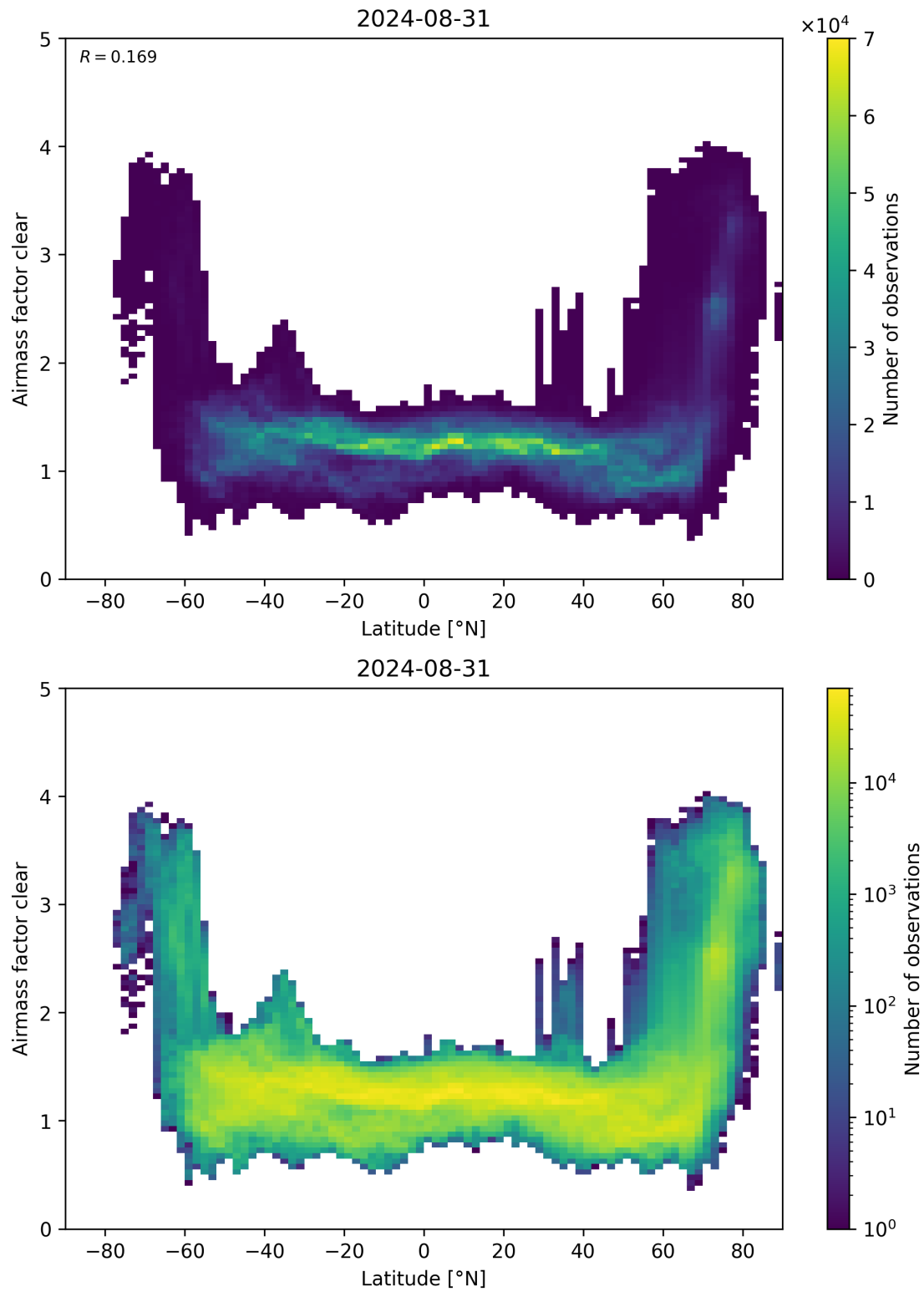
Figure 156: Scatter density plot of “Latitude” against “Airmass factor clear” for 2024-08-30 to 2024-09-01.
