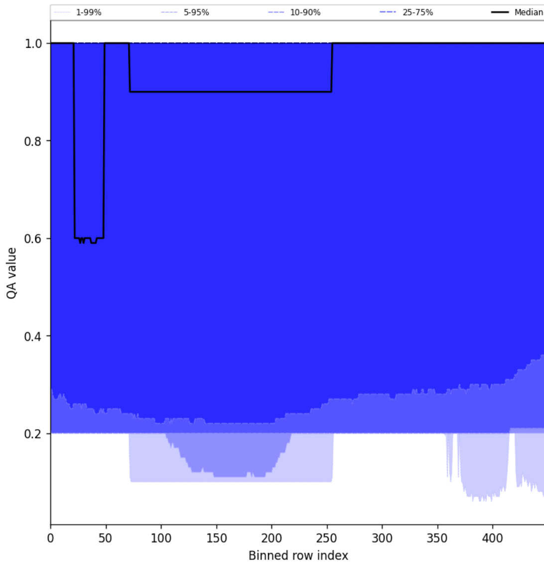
Figure 48: Along track statistics of “QA value” for 2024-08-30 to 2024-09-01
