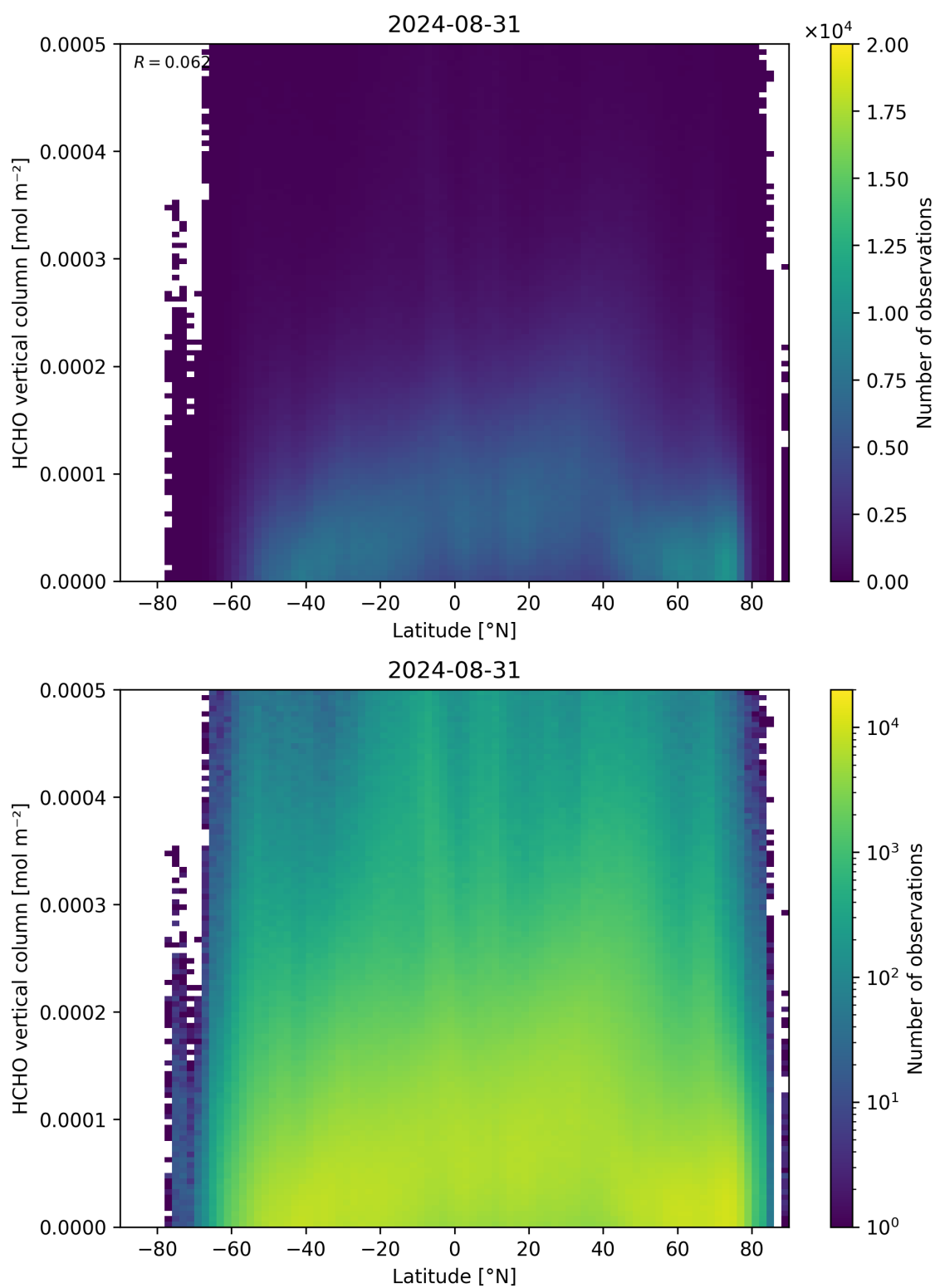
Figure 163: Scatter density plot of “Latitude” against “HCHO vertical column” for 2024-08-30 to 2024-09-01.
