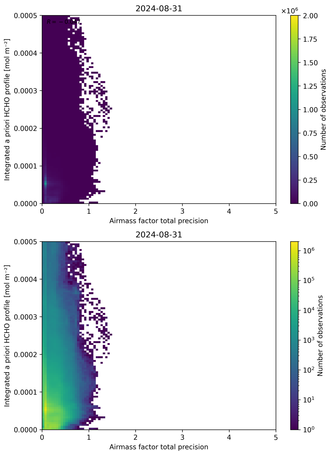
Figure 111: Scatter density plot of “Airmass factor total precision” against “Integrated a priori HCHO profile” for 2024-08-30 to 2024-09-01.
