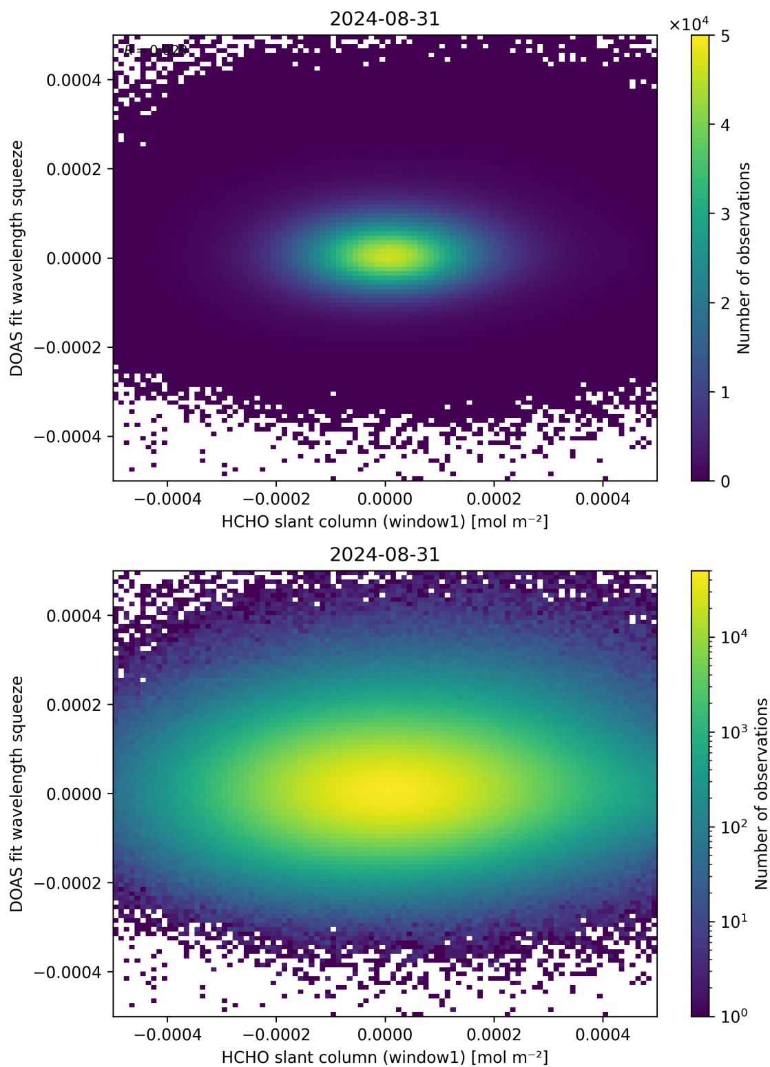
Figure 80: Scatter density plot of “HCHO slant column (window1)” against “DOAS fit wavelength squeeze” for 2024-08-30 to 2024-09-01.
