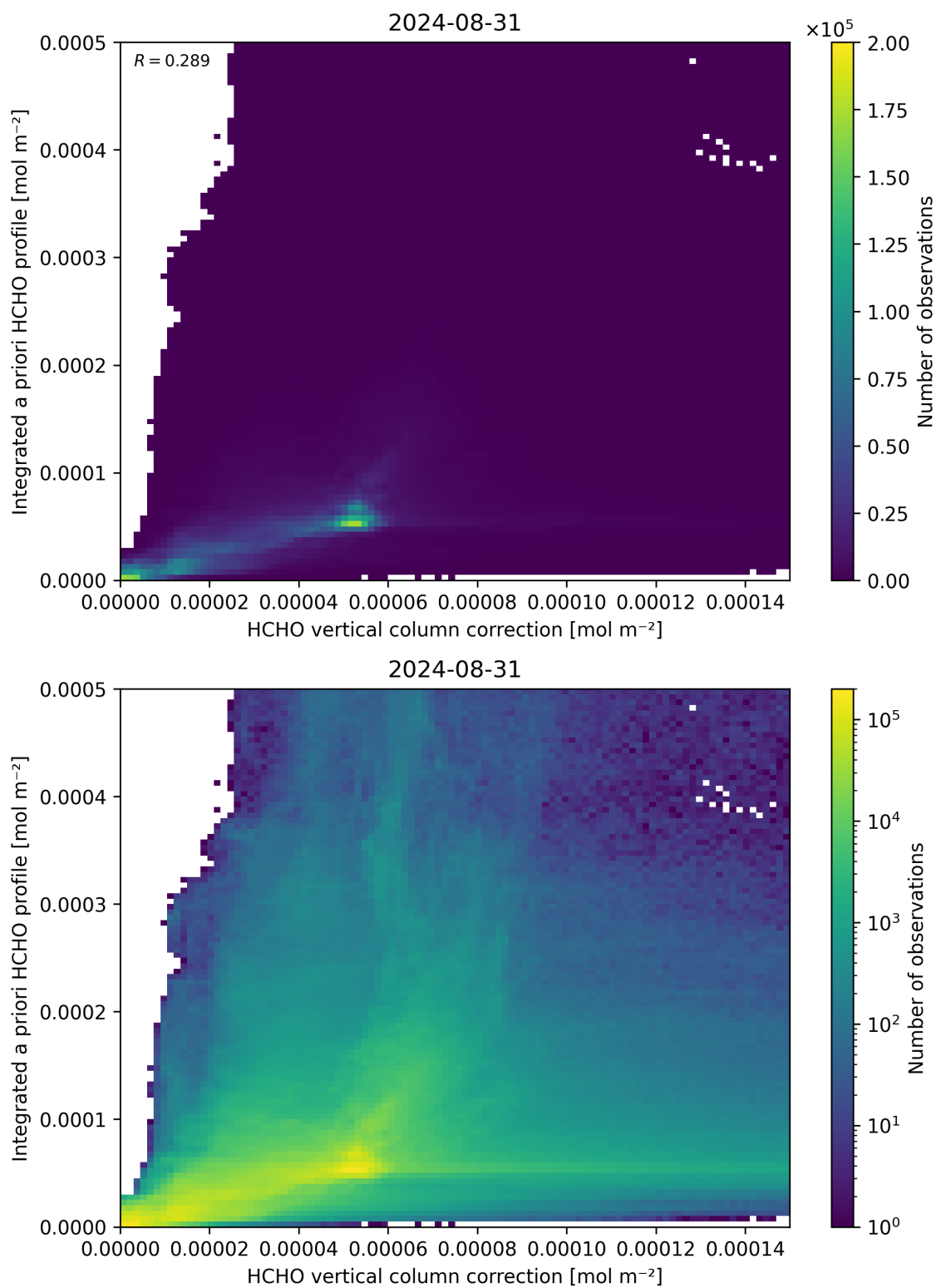
Figure 122: Scatter density plot of “HCHO vertical column correction” against “Integrated a priori HCHO profile” for 2024-08-30 to 2024-09-01.
