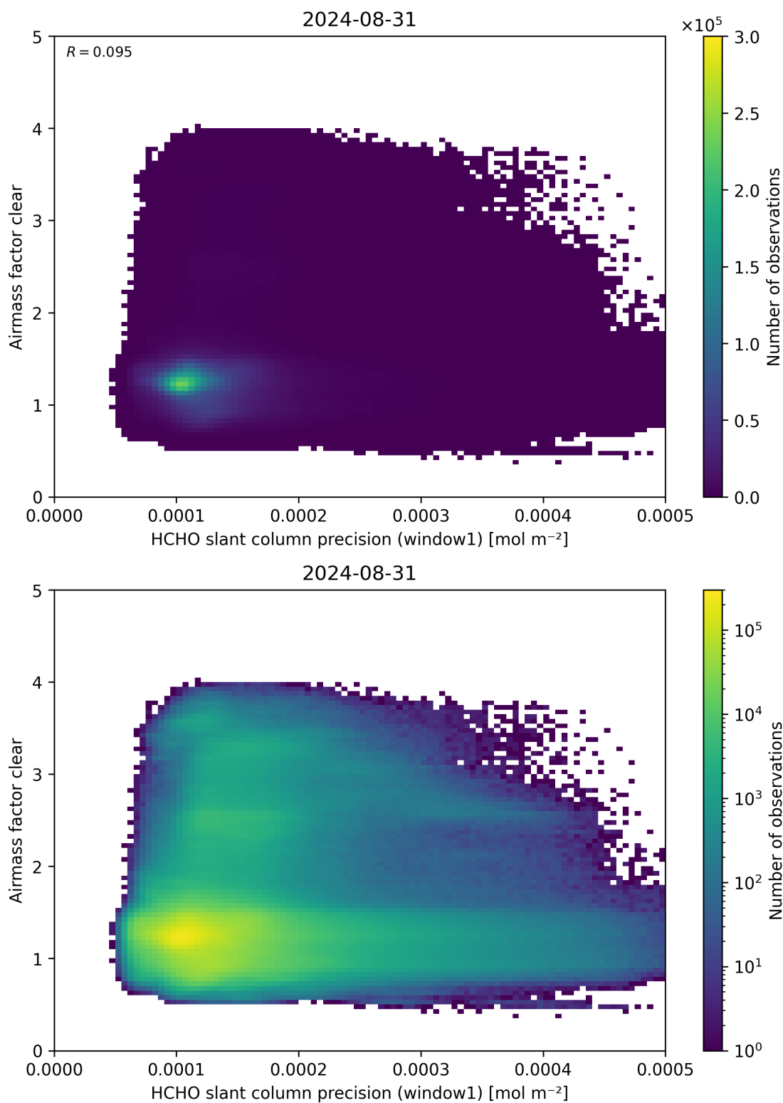
Figure 91: Scatter density plot of “HCHO slant column precision (window1)” against “Airmass factor clear” for 2024-08-30 to 2024-09-01.
