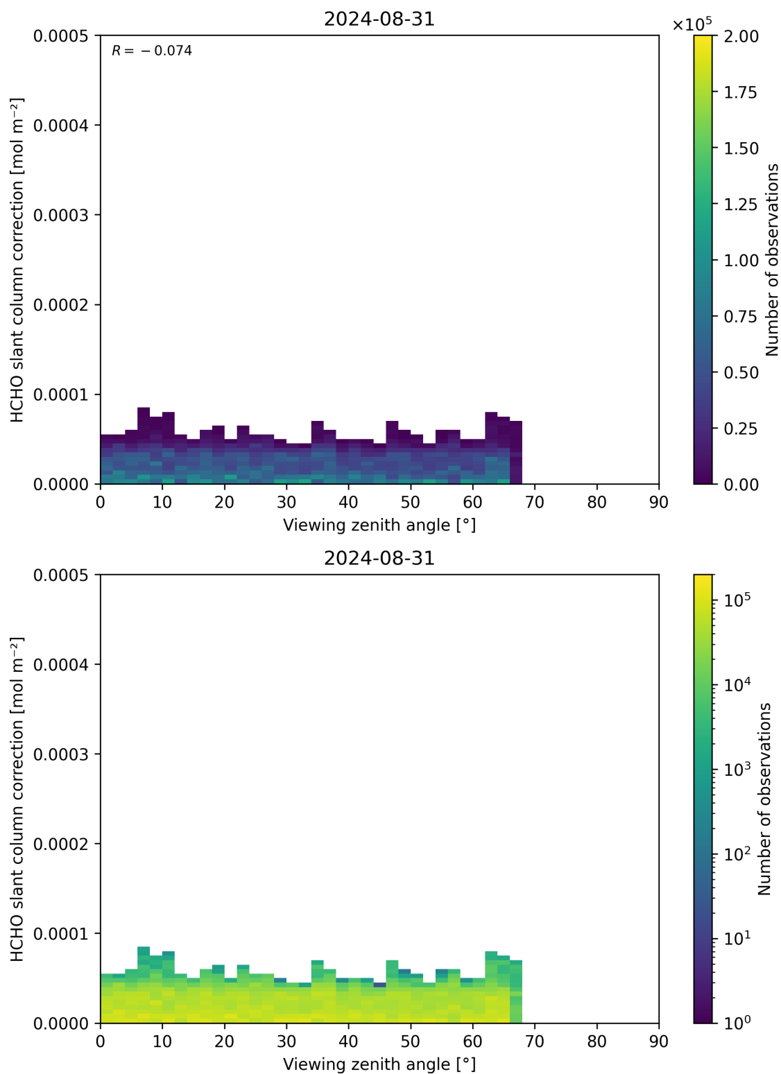
Figure 187: Scatter density plot of “Viewing zenith angle” against “HCHO slant column correction” for 2024-08-30 to 2024-09-01.
