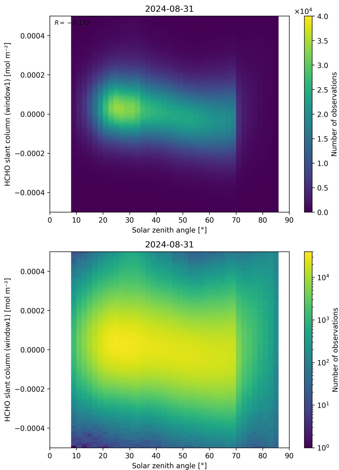
Figure 173: Scatter density plot of “Solar zenith angle” against “HCHO slant column (window1)” for 2024-08-30 to 2024-09-01.
