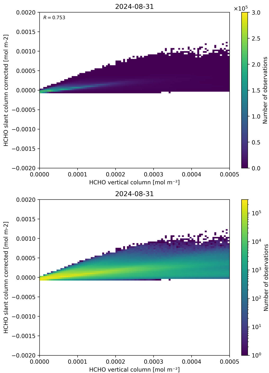
Figure 127: Scatter density plot of “HCHO vertical column” against “HCHO slant column corrected” for 2024-08-30 to 2024-09-01.
