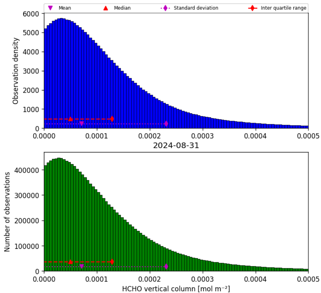
Figure 35: Histogram of “HCHO vertical column” for 2024-08-30 to 2024-09-01
