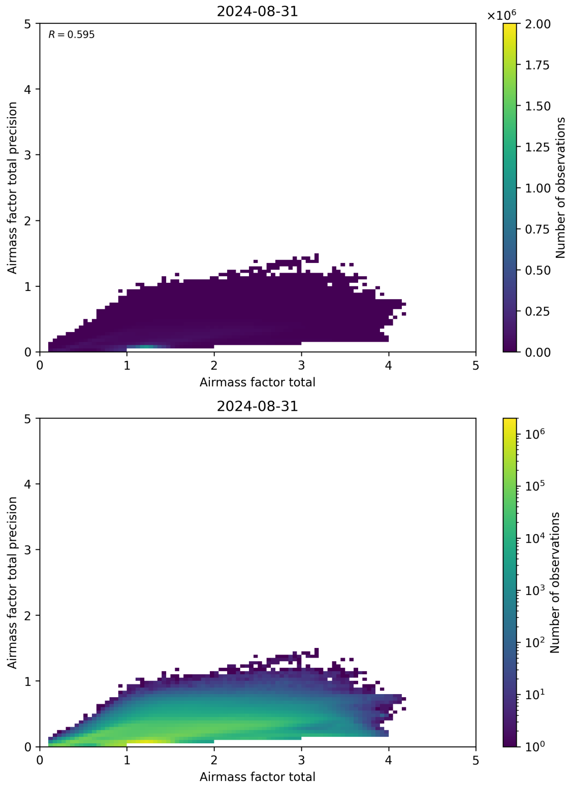
Figure 103: Scatter density plot of “Airmass factor total” against “Airmass factor total precision” for 2024-08-30 to 2024-09-01.
