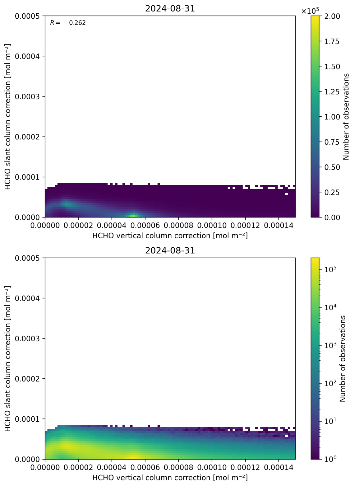
Figure 117: Scatter density plot of “HCHO vertical column correction” against “HCHO slant column correction” for 2024-08-30 to 2024-09-01.
