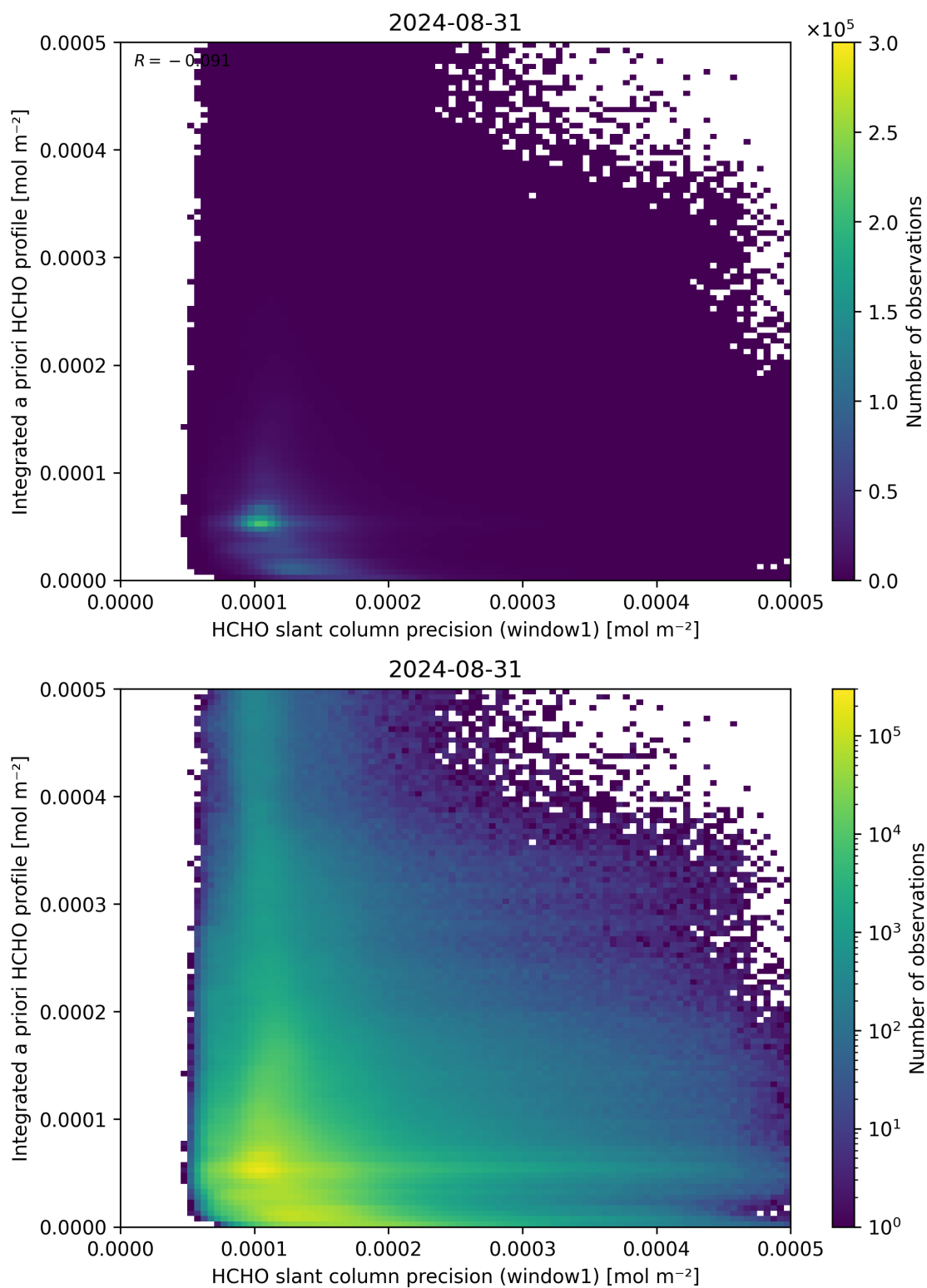
Figure 96: Scatter density plot of “HCHO slant column precision (window1)” against “Integrated a priori HCHO profile” for 2024-08-30 to 2024-09-01.
