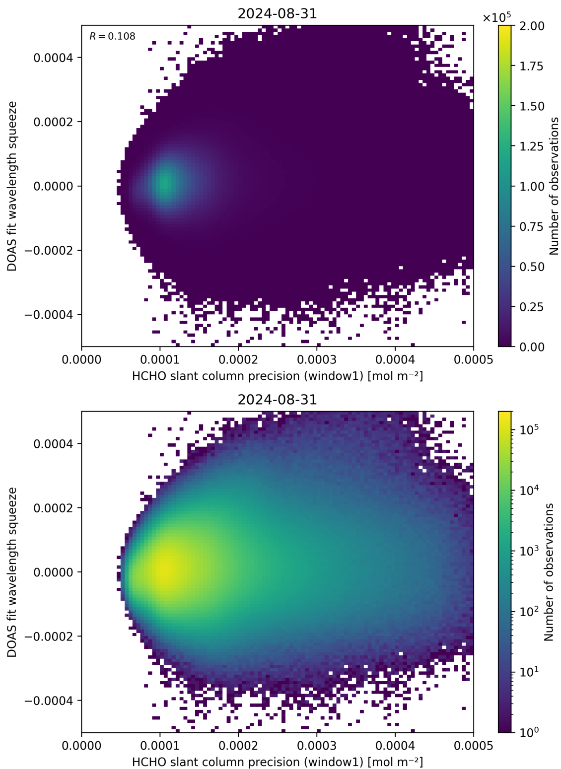
Figure 90: Scatter density plot of “HCHO slant column precision (window1)” against “DOAS fit wavelength squeeze” for 2024-08-30 to 2024-09-01.
