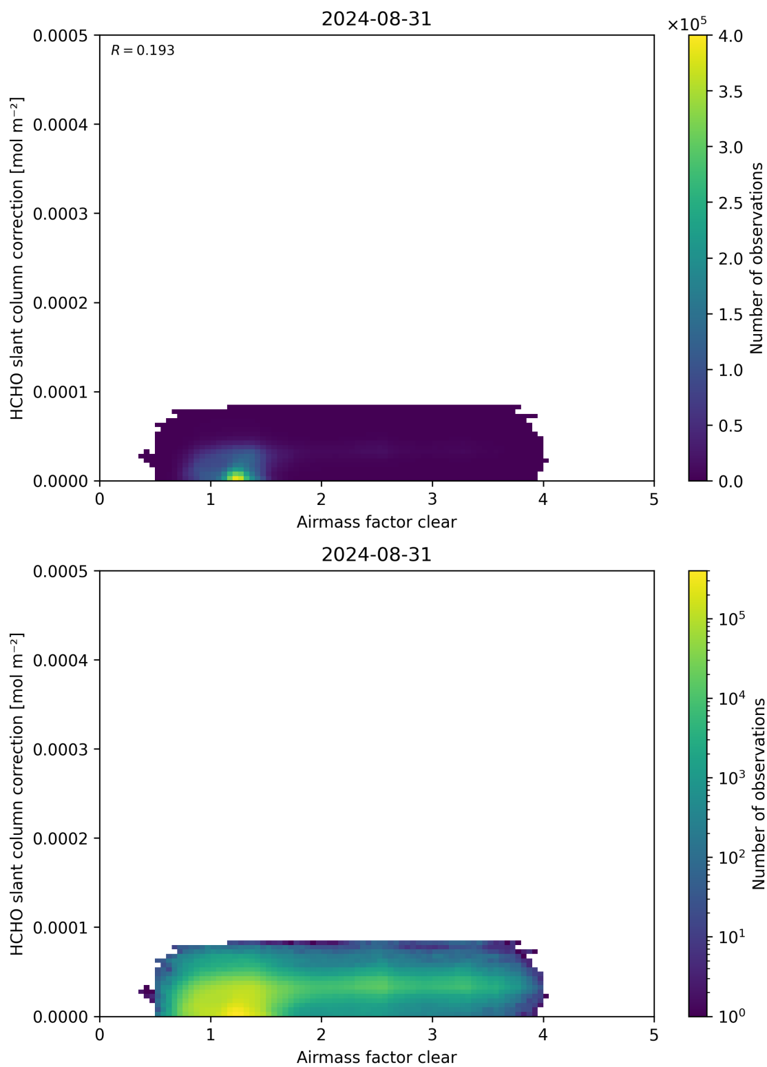
Figure 75: Scatter density plot of “Air mass factor clear” against “HCHO slant column correction” for 2024-08-30 to 2024-09-01.
