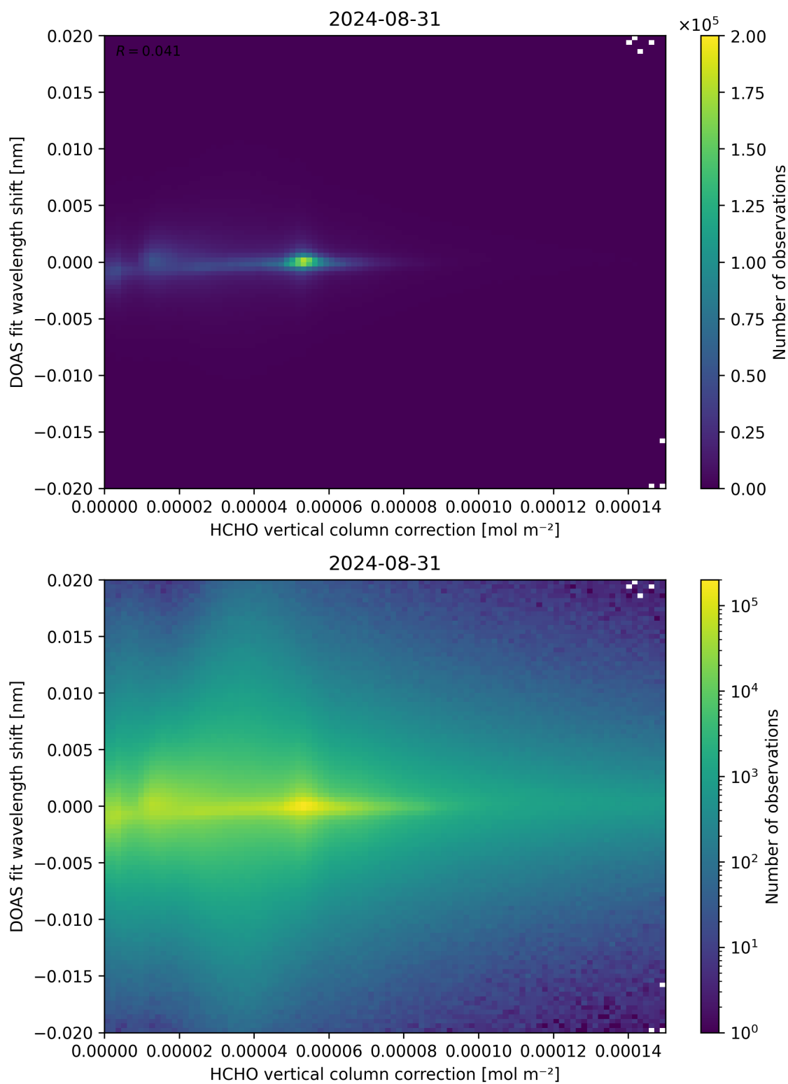
Figure 113: Scatter density plot of “HCHO vertical column correction” against “DOAS fit wavelength shift” for 2024-08-30 to 2024-09-01.
