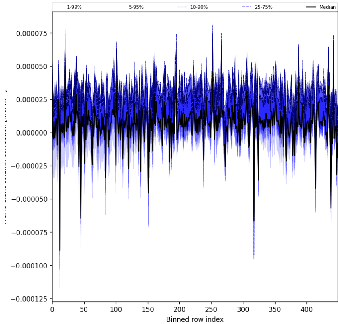
Figure 61: Along track statistics of “HCHO slant column correction” for 2024-08-30 to 2024-09-01
