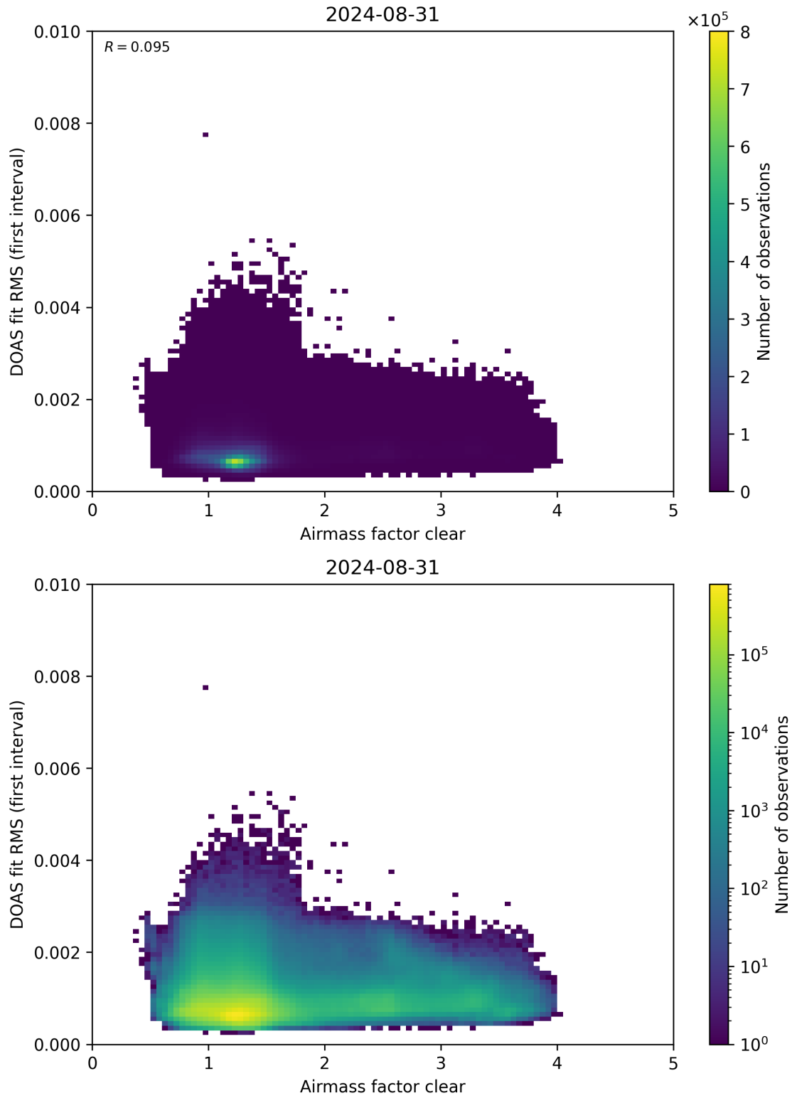
Figure 71: Scatter density plot of “Airmass factor clear” against “DOAS fit RMS (first interval)” for 2024-08-30 to 2024-09-01.
