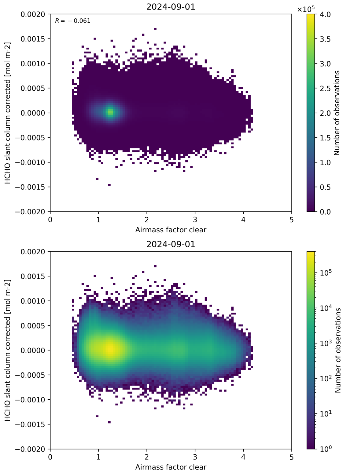
Figure 74: Scatter density plot of “Airmass factor clear” against “HCHO slant column corrected” for 2024-09-01 to 2024-09-02.
