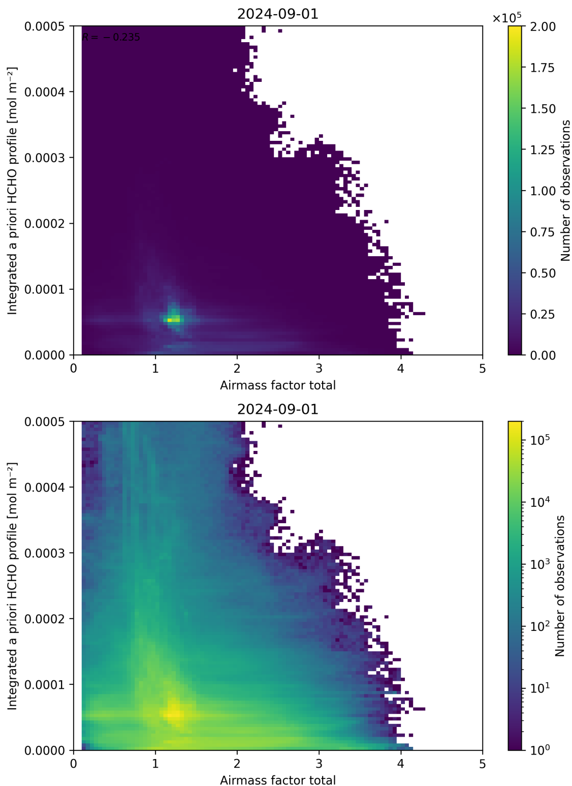
Figure 104: Scatter density plot of “Airmass factor total” against “Integrated a priori HCHO profile” for 2024-09-01 to 2024-09-02.
