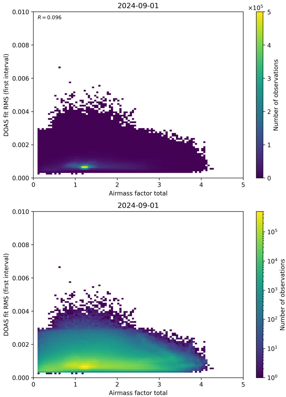
Figure 97: Scatter density plot of “Airmass factor total” against “DOAS fit RMS (first interval)” for 2024-09-01 to 2024-09-02.
