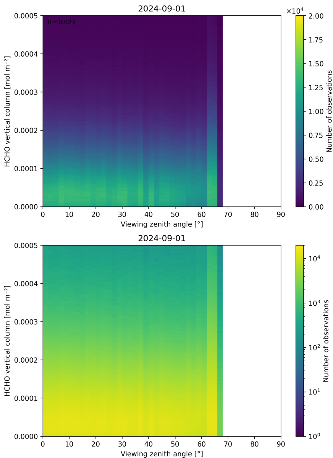
Figure 192: Scatter density plot of “Viewing zenith angle” against “HCHO vertical column” for 2024-09-01 to 2024-09-02.
