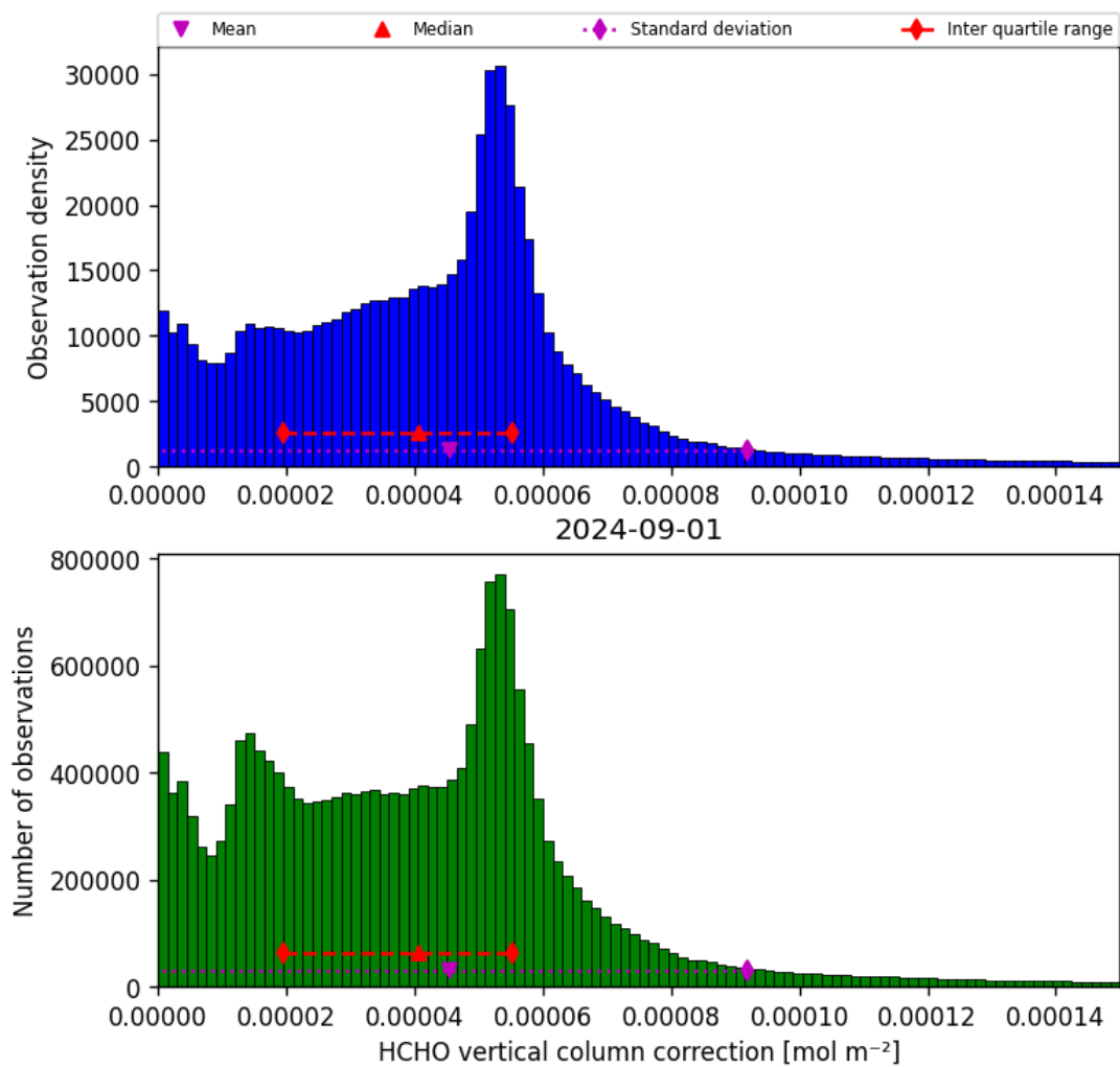
Figure 37: Histogram of “HCHO vertical column correction” for 2024-09-01 to 2024-09-02
