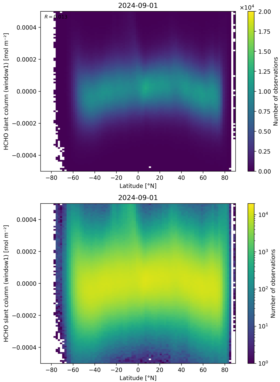
Figure 159: Scatter density plot of “Latitude” against “HCHO slant column (window1)” for 2024-09-01 to 2024-09-02.
