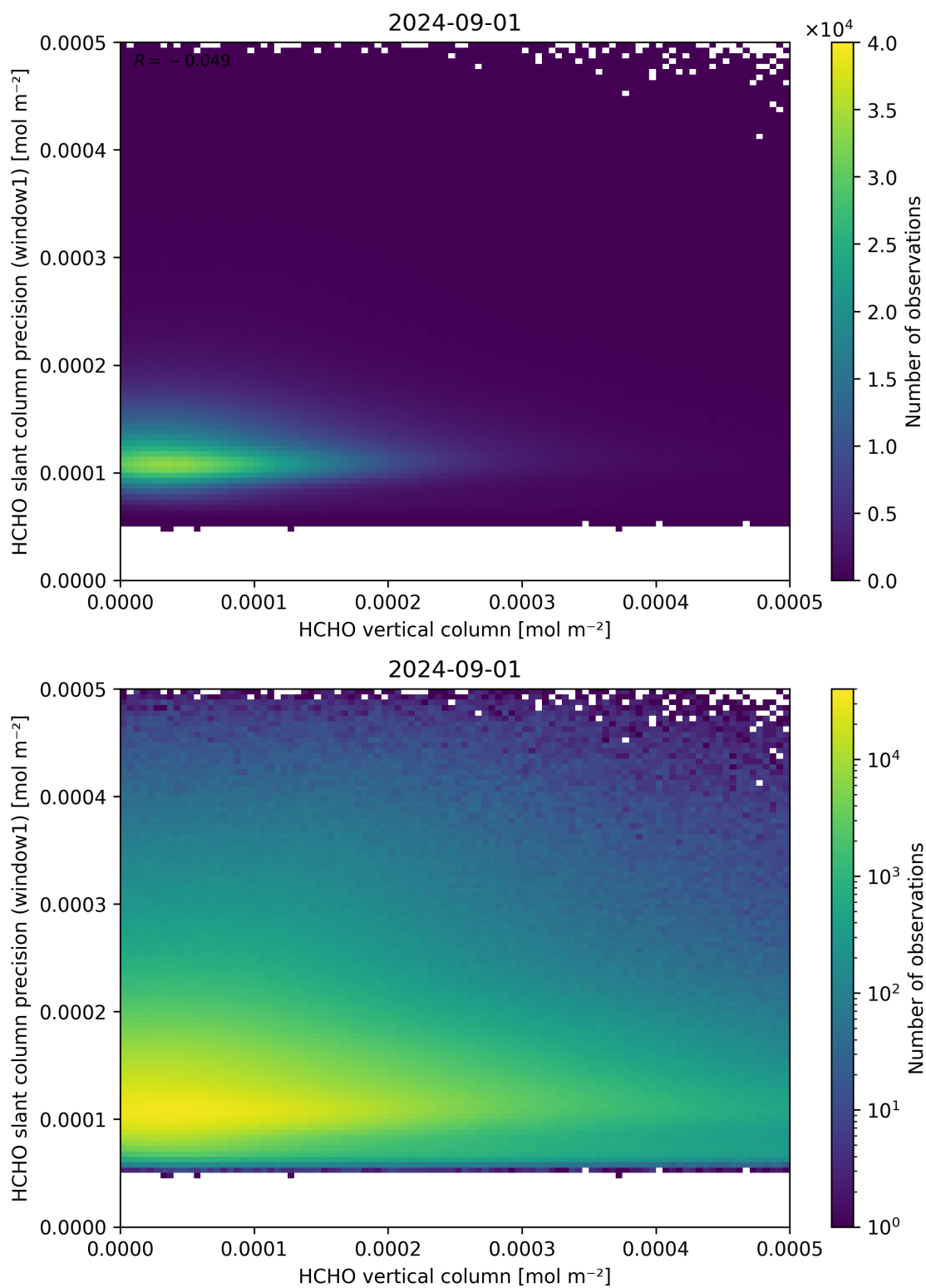
Figure 130: Scatter density plot of “HCHO vertical column” against “HCHO slant column precision (window1)” for 2024-09-01 to 2024-09-02.
