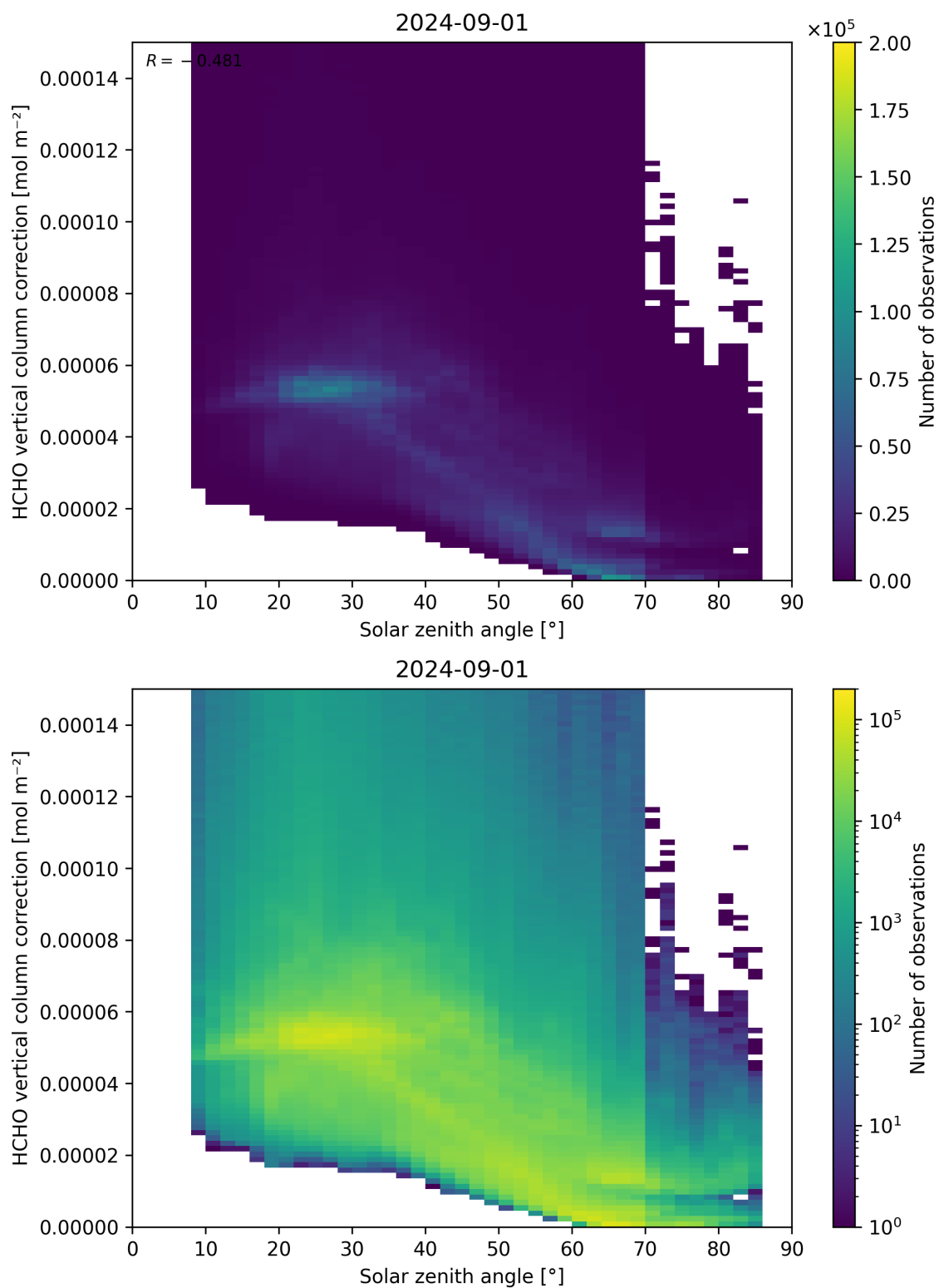
Figure 178: Scatter density plot of “Solar zenith angle” against “HCHO vertical column correction” for 2024-09-01 to 2024-09-02.
