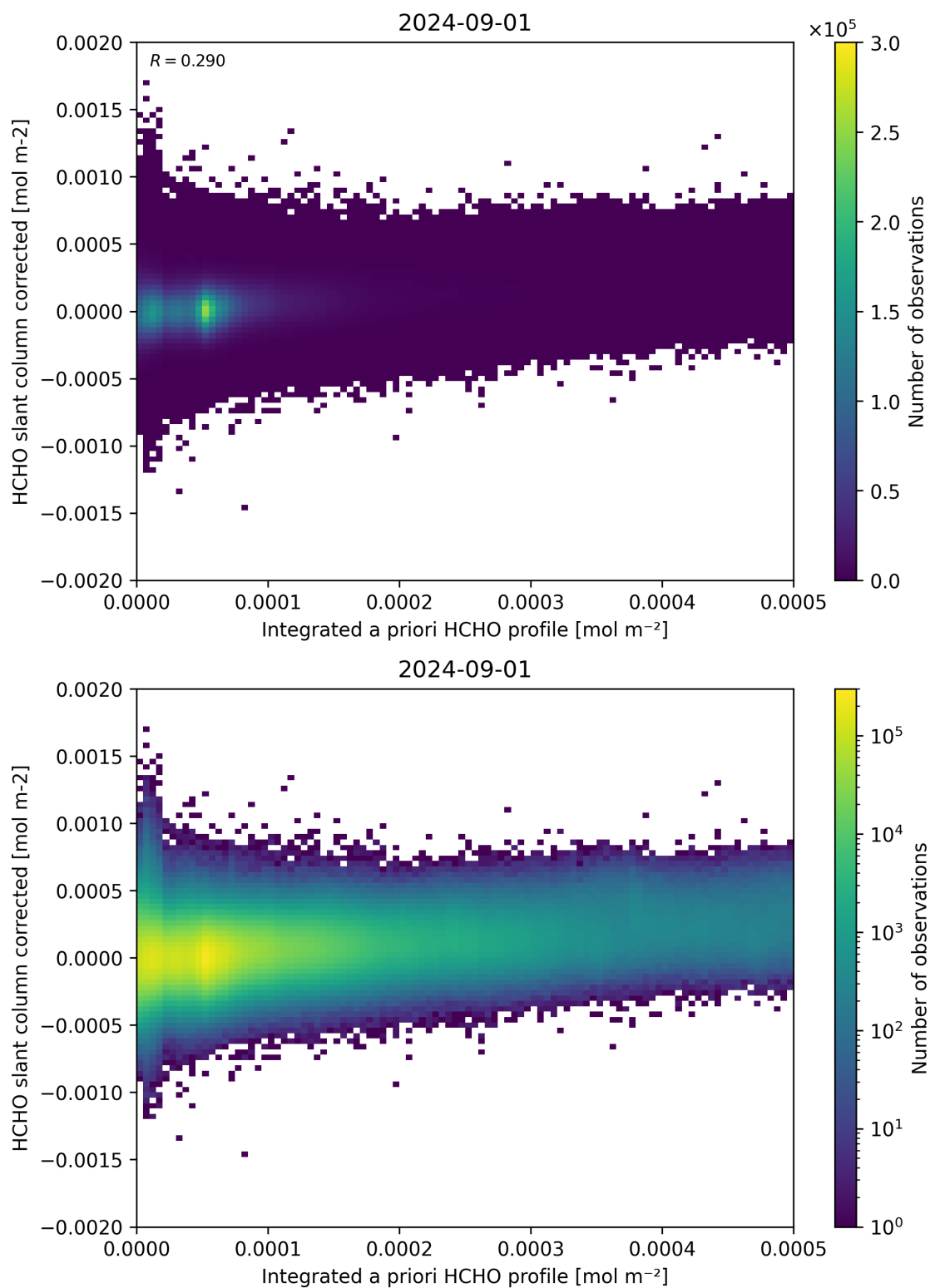
Figure 151: Scatter density plot of “Integrated a priori HCHO profile” against “HCHO slant column corrected” for 2024-09-01 to 2024-09-02.
