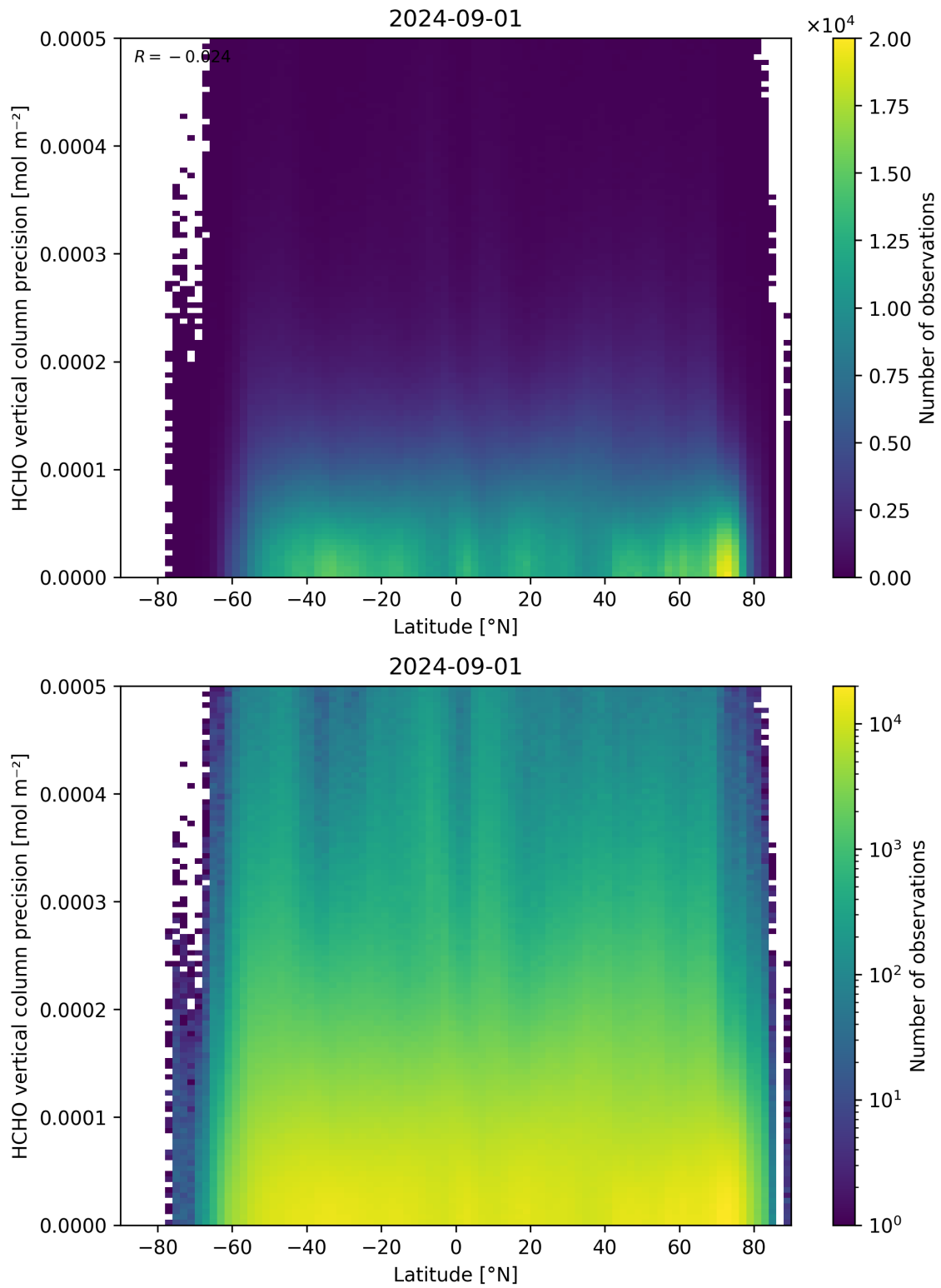
Figure 165: Scatter density plot of “Latitude” against “HCHO vertical column precision” for 2024-09-01 to 2024-09-02.
