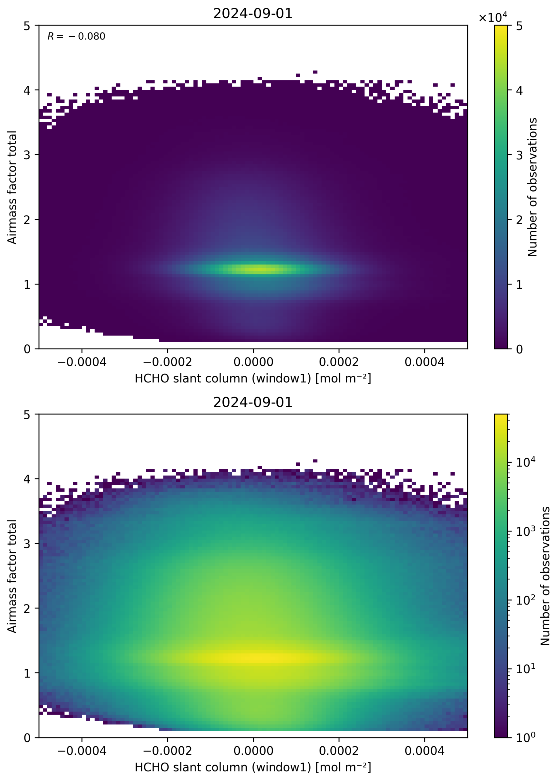
Figure 85: Scatter density plot of “HCHO slant column (window1)” against “Airmass factor total” for 2024-09-01 to 2024-09-02.
