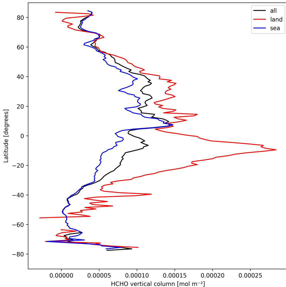
Figure 21: Zonal average of “HCHO vertical column” for 2024-09-01 to 2024-09-02.
