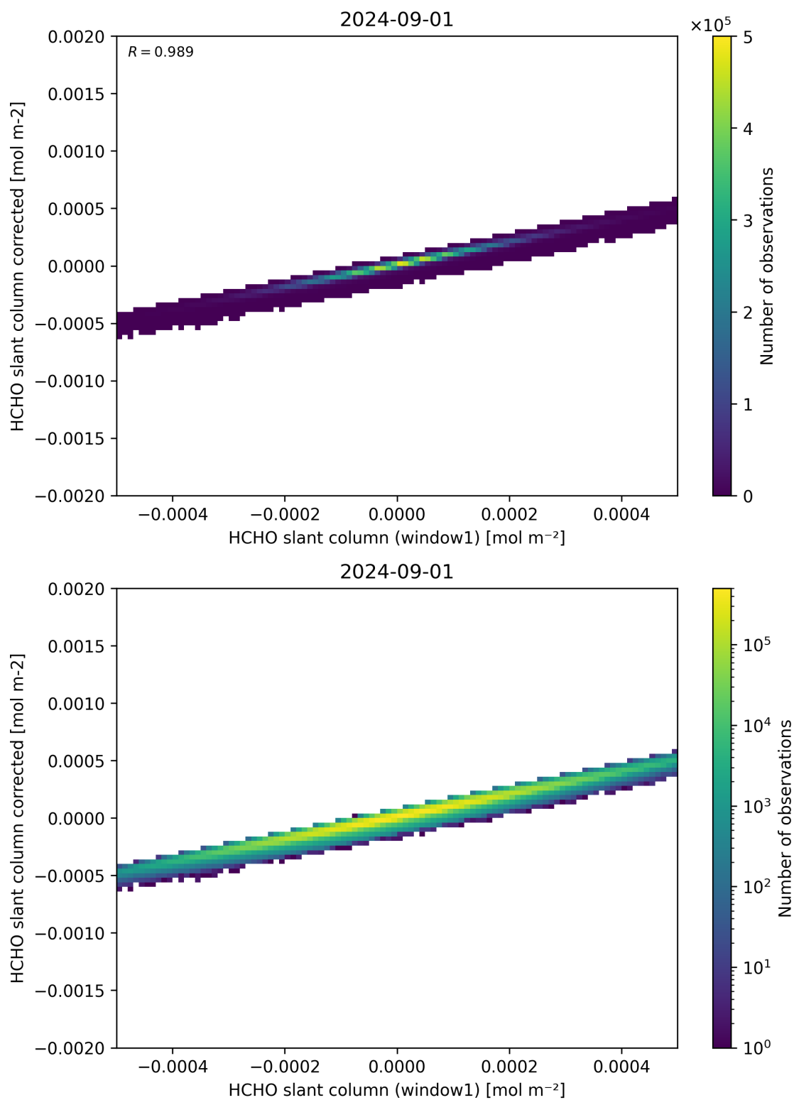
Figure 82: Scatter density plot of “HCHO slant column (window1)” against “HCHO slant column corrected” for 2024-09-01 to 2024-09-02.
