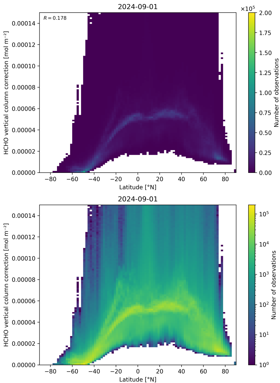
Figure 164: Scatter density plot of “Latitude” against “HCHO vertical column correction” for 2024-09-01 to 2024-09-02.
