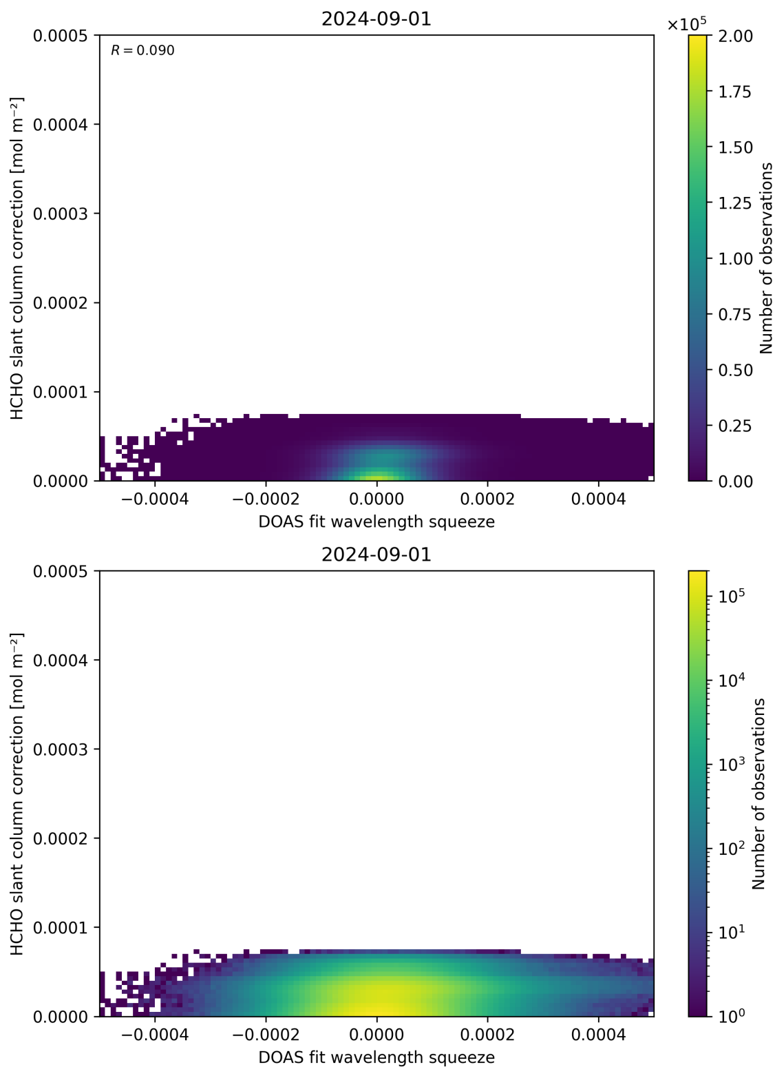
Figure 70: Scatter density plot of “DOAS fit wavelength squeeze” against “HCHO slant column correction” for 2024-09-01 to 2024-09-02.
