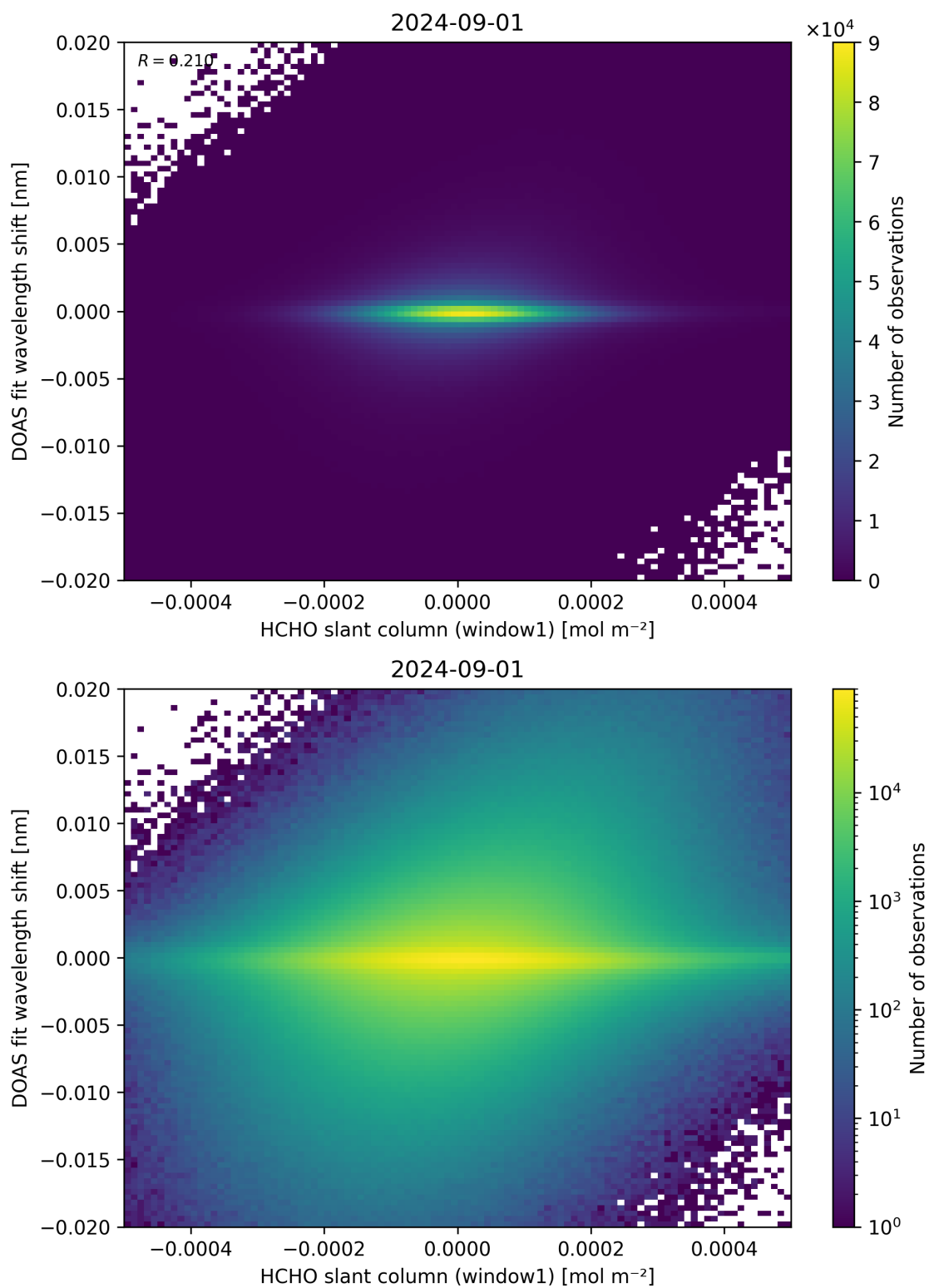
Figure 79: Scatter density plot of “HCHO slant column (window1)” against “DOAS fit wavelength shift” for 2024-09-01 to 2024-09-02.
