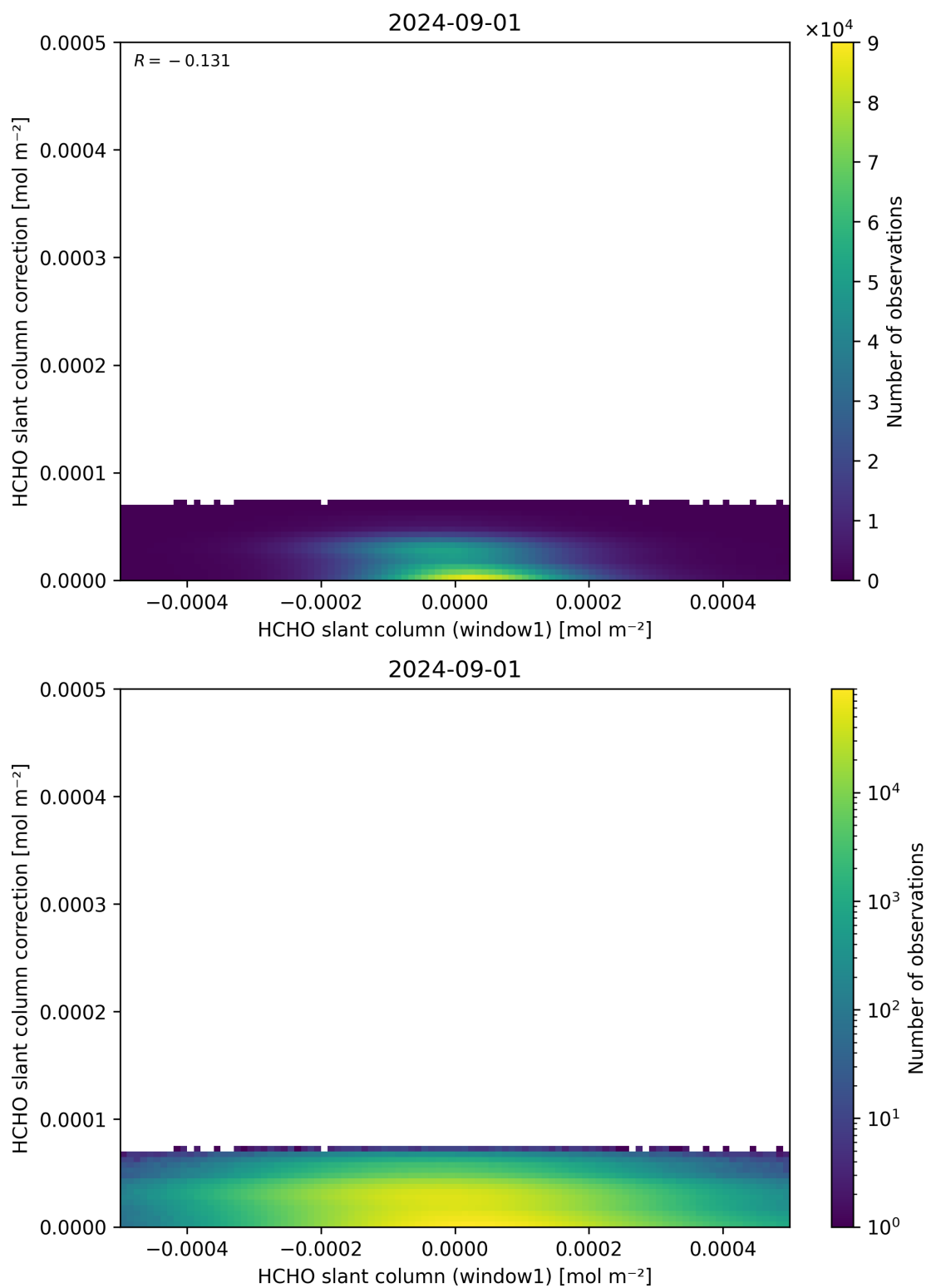
Figure 83: Scatter density plot of “HCHO slant column (window1)” against “HCHO slant column correction” for 2024-09-01 to 2024-09-02.
