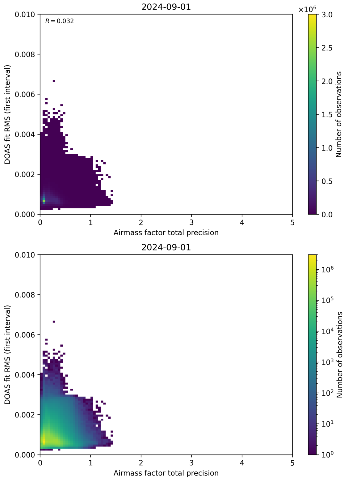
Figure 105: Scatter density plot of “Airmass factor total precision” against “DOAS fit RMS (first interval)” for 2024-09-01 to 2024-09-02.
