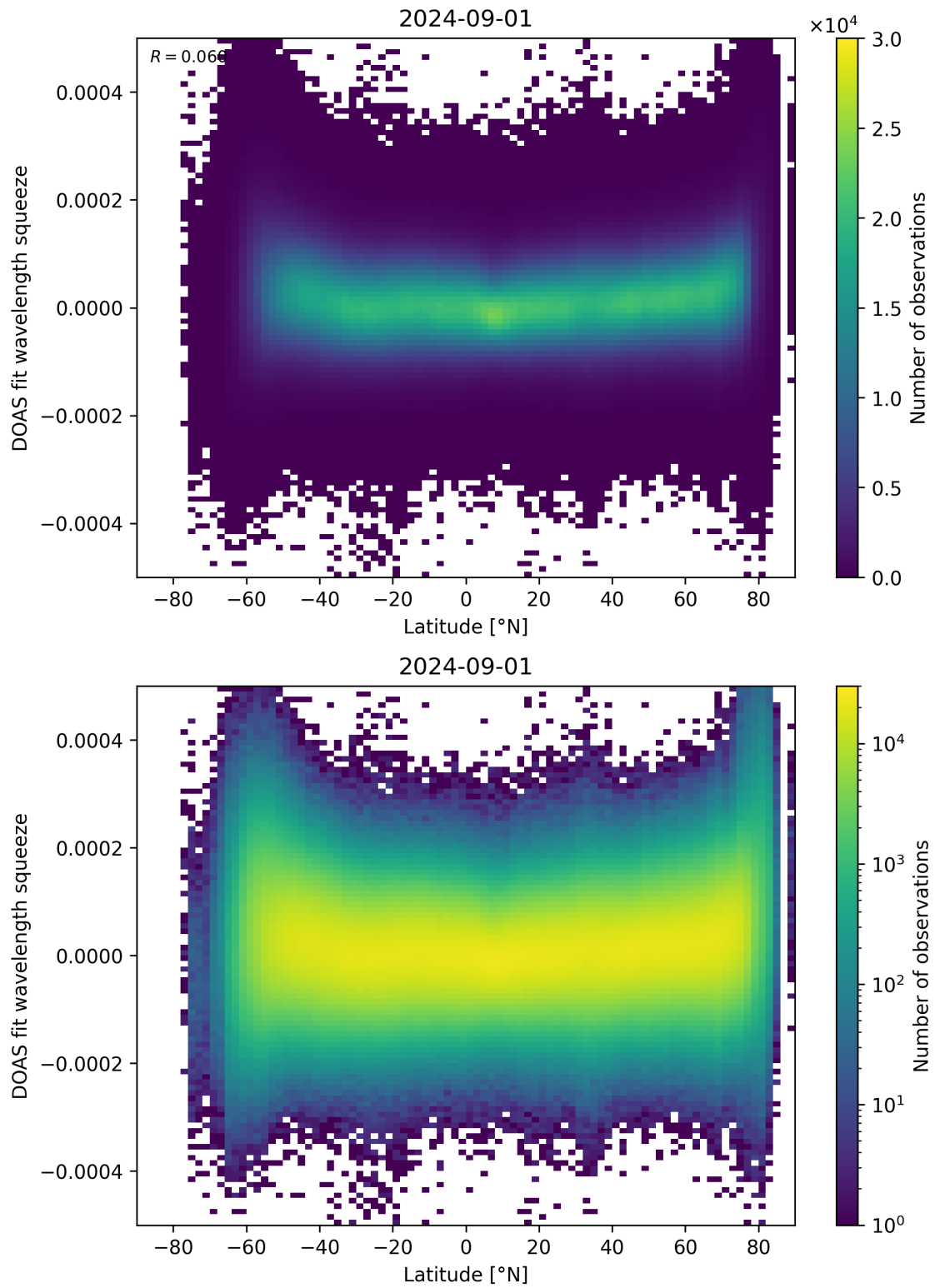
Figure 155: Scatter density plot of “Latitude” against “DOAS fit wavelength squeeze” for 2024-09-01 to 2024-09-02.
