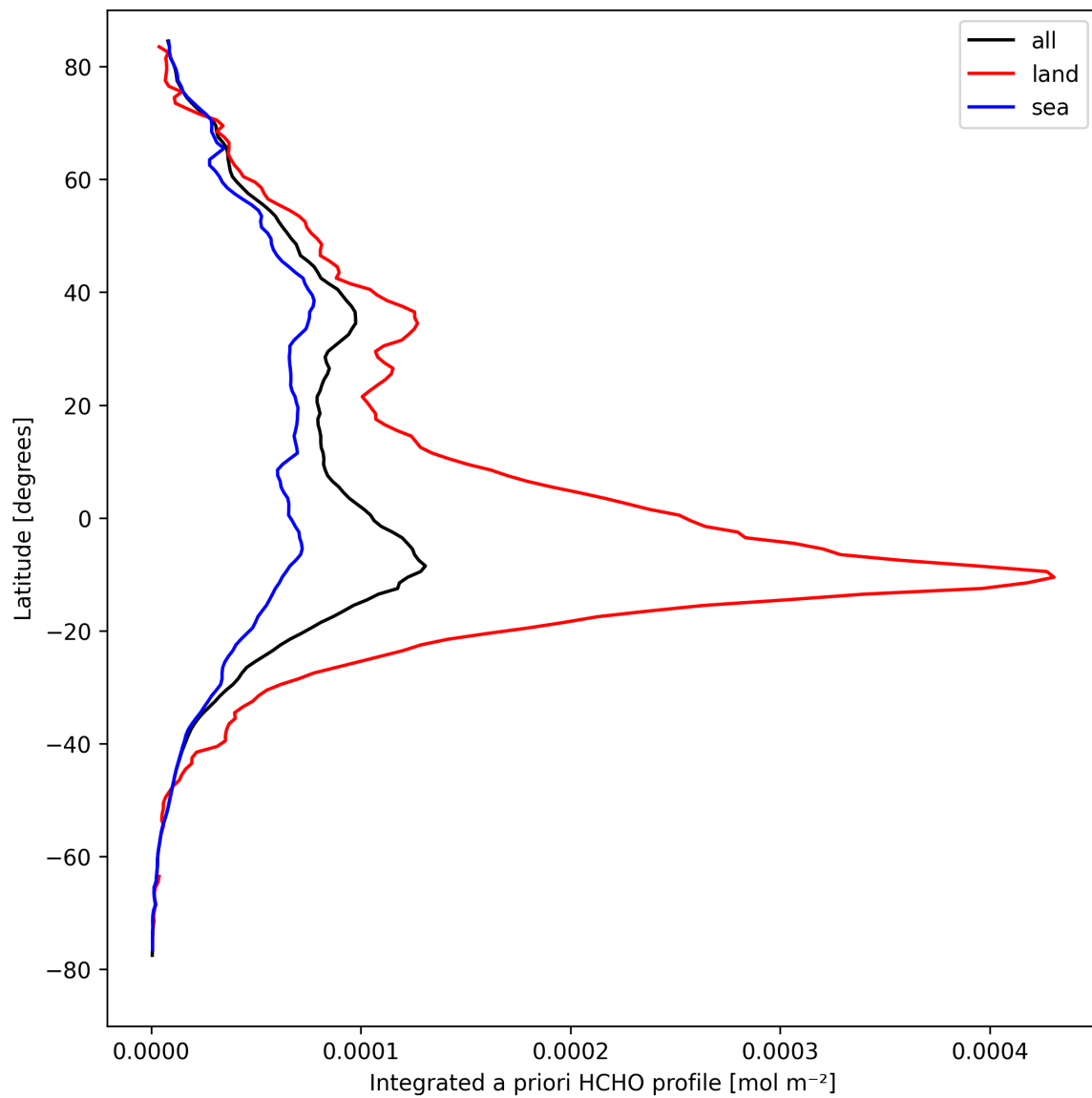
Figure 29: Zonal average of “Integrated a priori HCHO profile” for 2024-09-01 to 2024-09-02.
