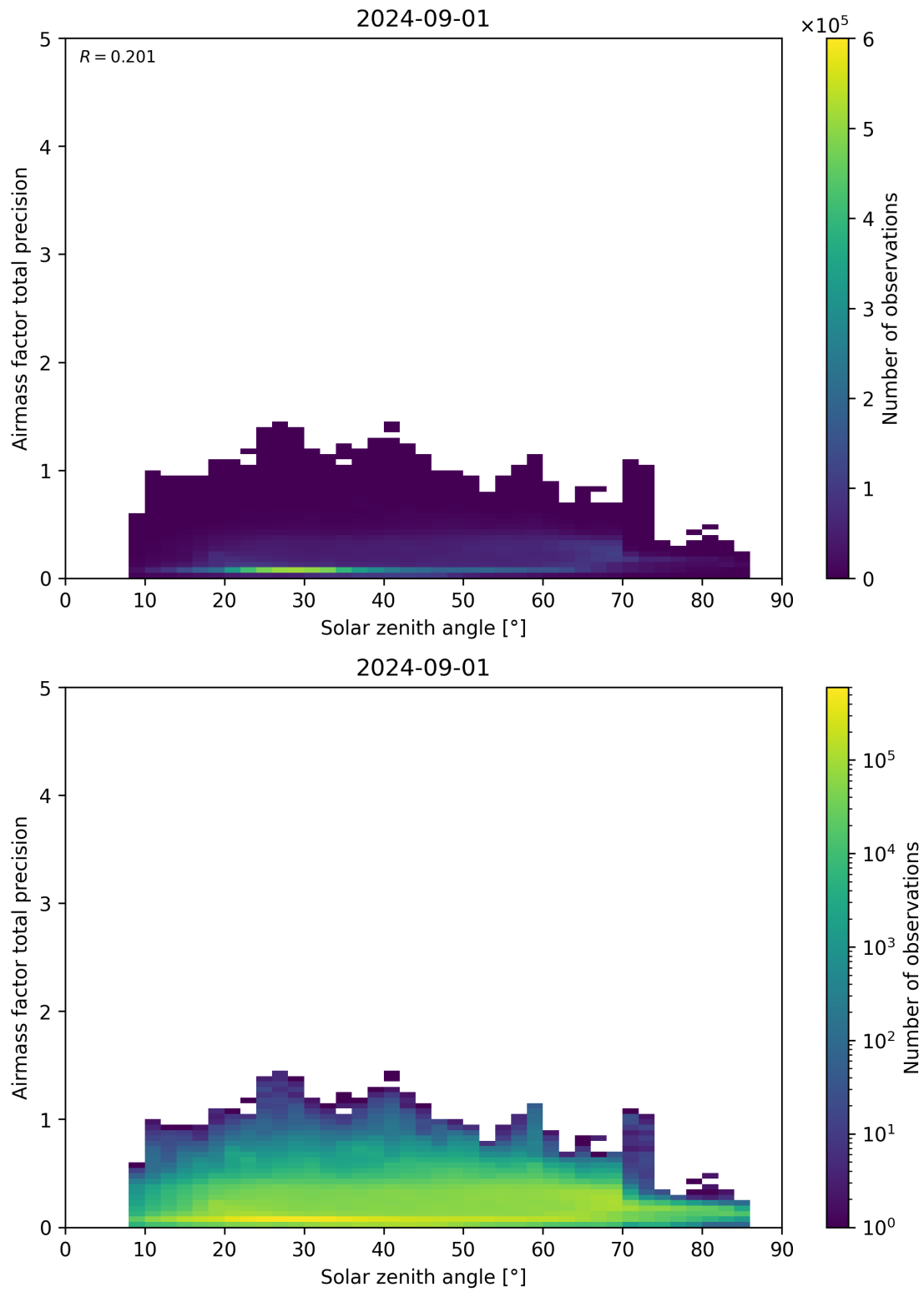
Figure 176: Scatter density plot of “Solar zenith angle” against “Airmass factor total precision” for 2024-09-01 to 2024-09-02.
