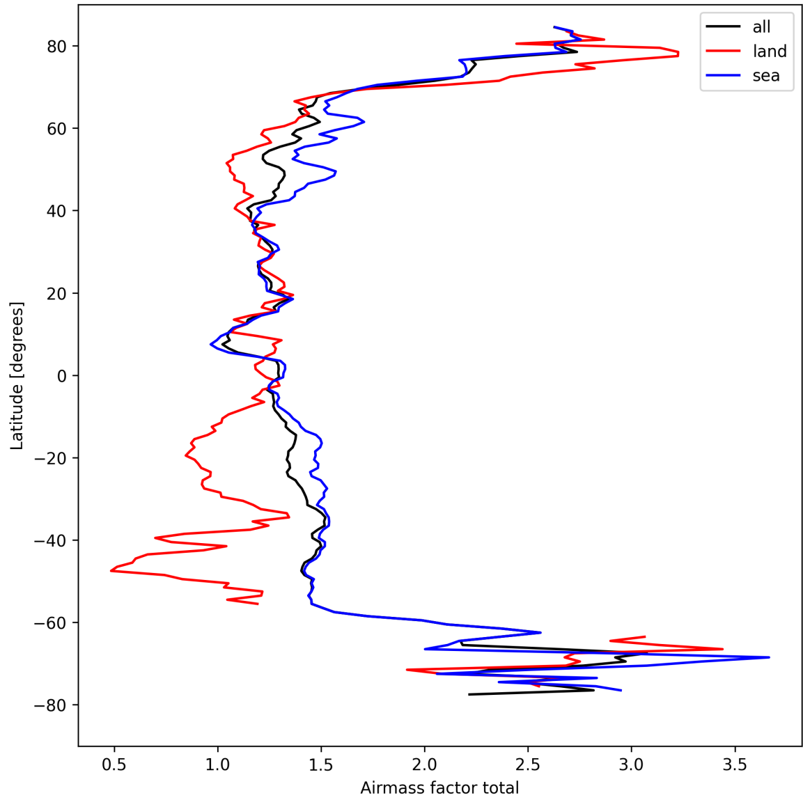
Figure 26: Zonal average of “Airmass factor total” for 2024-09-01 to 2024-09-02.
