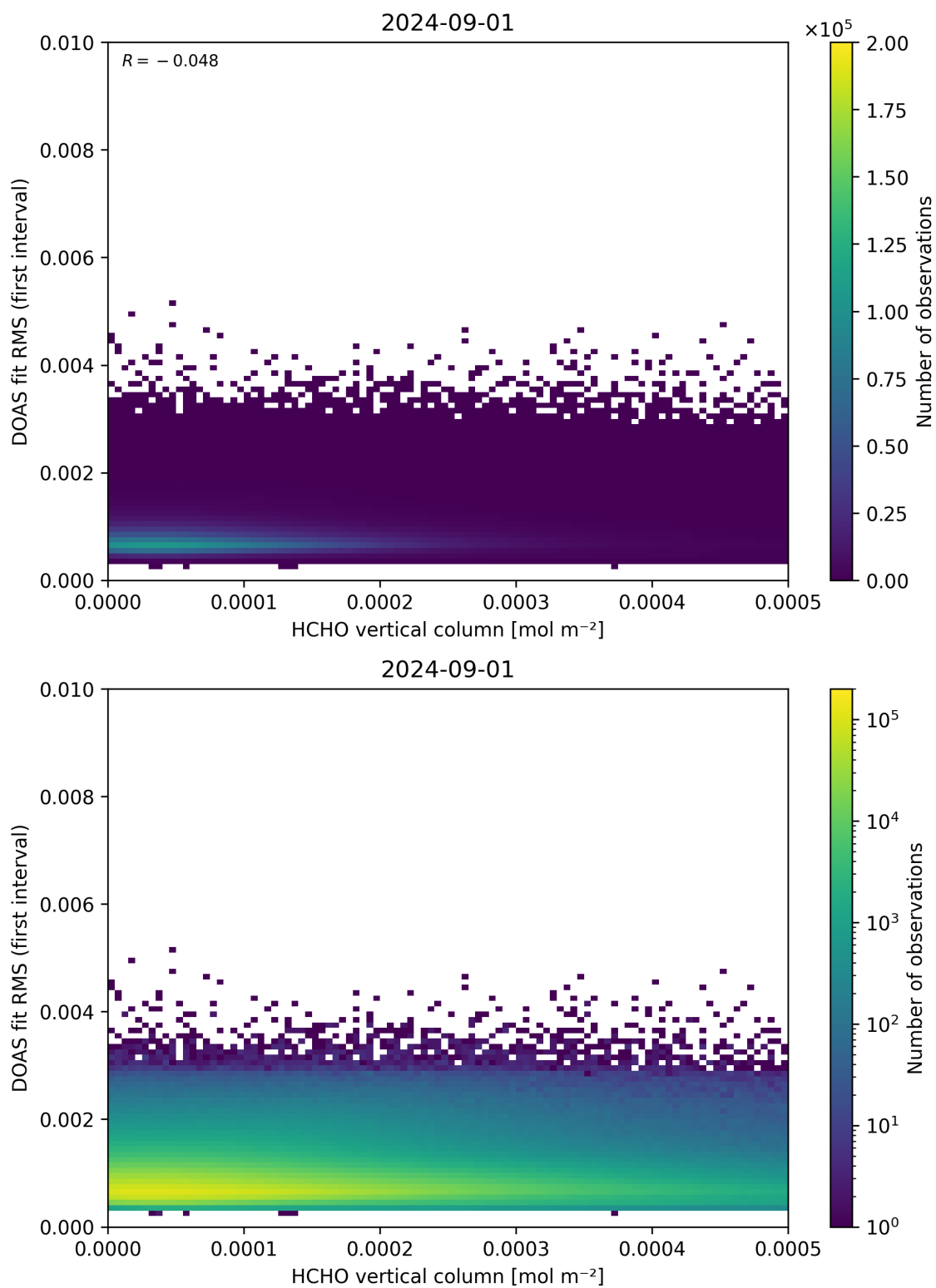
Figure 123: Scatter density plot of “HCHO vertical column” against “DOAS fit RMS (first interval)” for 2024-09-01 to 2024-09-02.
