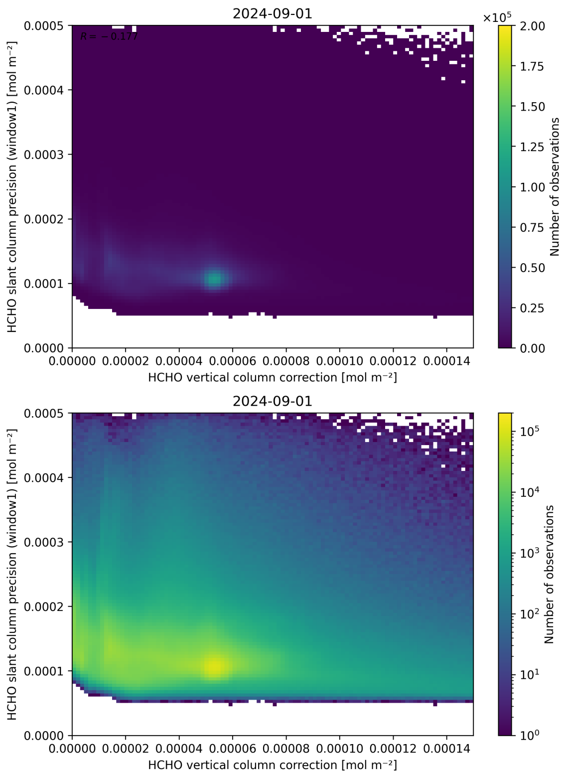
Figure 119: Scatter density plot of “HCHO vertical column correction” against “HCHO slant column precision (window1)” for 2024-09-01 to 2024-09-02.
