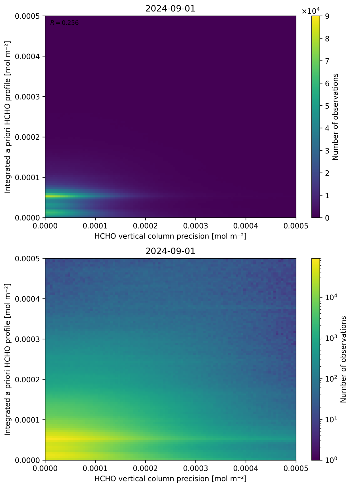
Figure 147: Scatter density plot of “HCHO vertical column precision” against “Integrated a priori HCHO profile” for 2024-09-01 to 2024-09-02.
