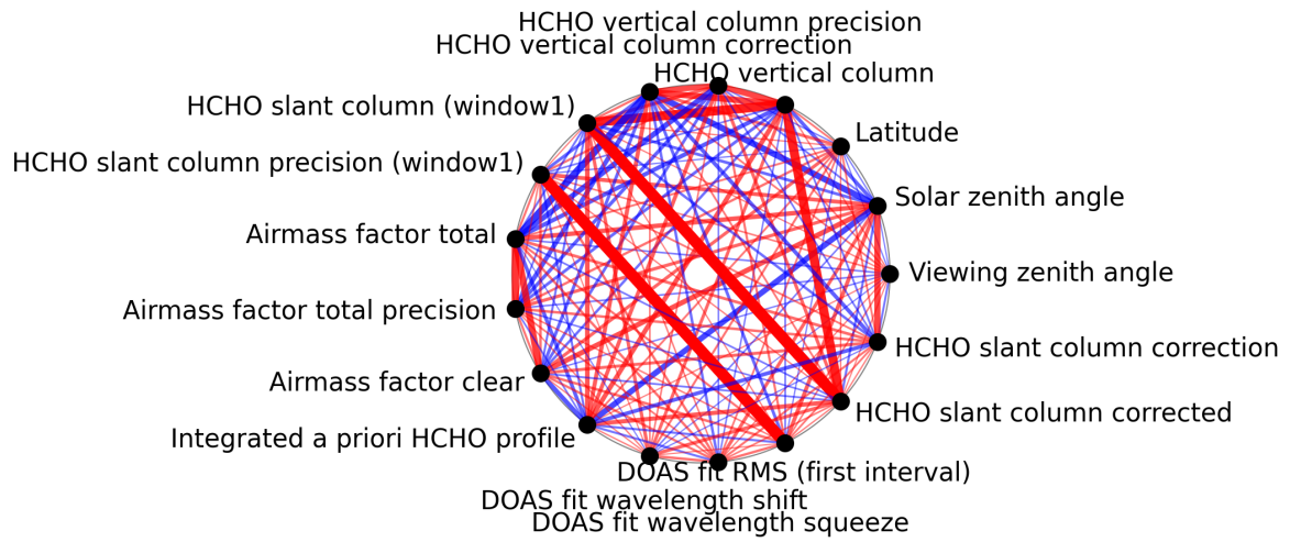
Figure 1: Map of correlation graph for 2024-09-01 to 2024-09-02.
