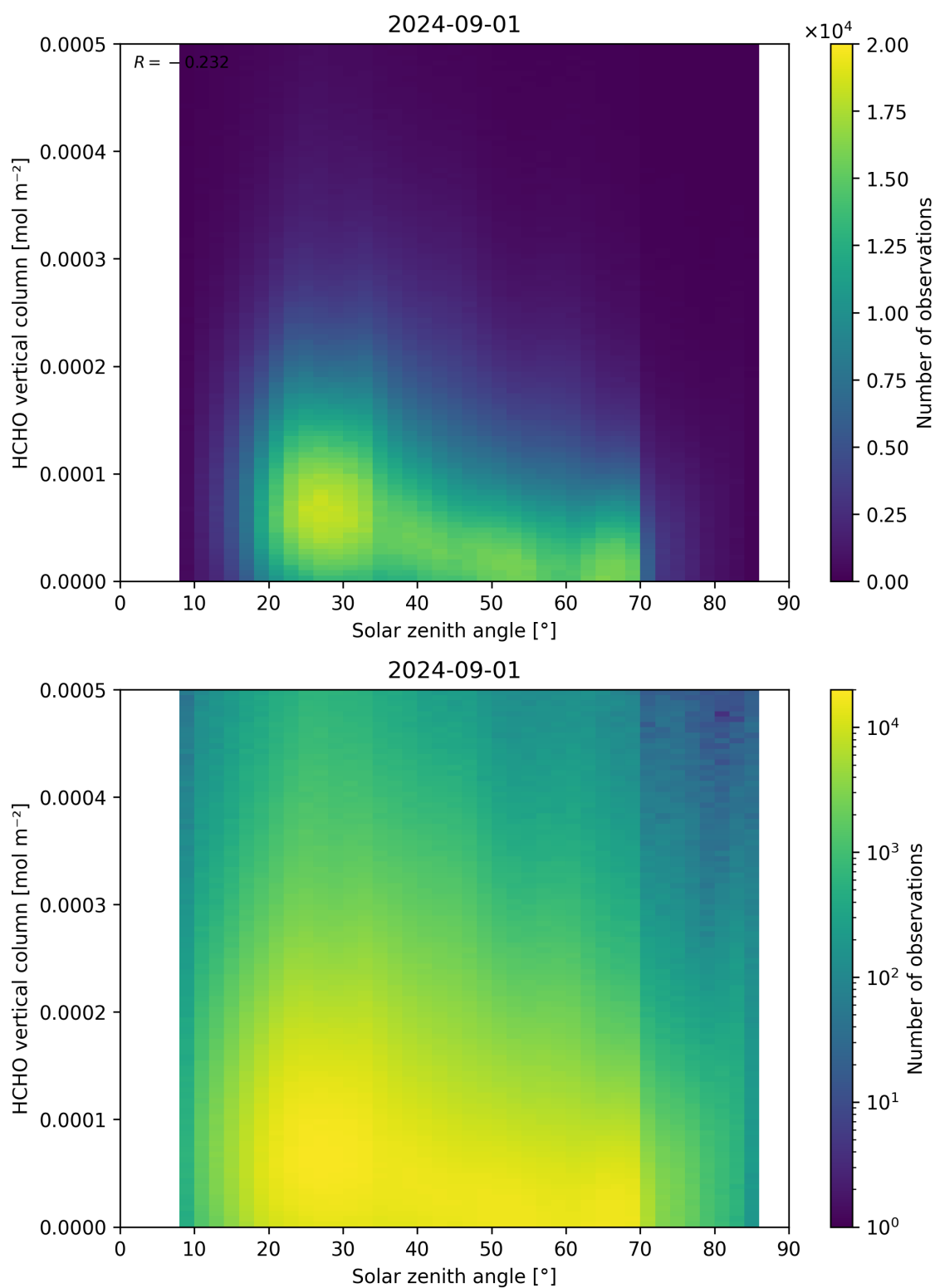
Figure 177: Scatter density plot of “Solar zenith angle” against “HCHO vertical column” for 2024-09-01 to 2024-09-02.
