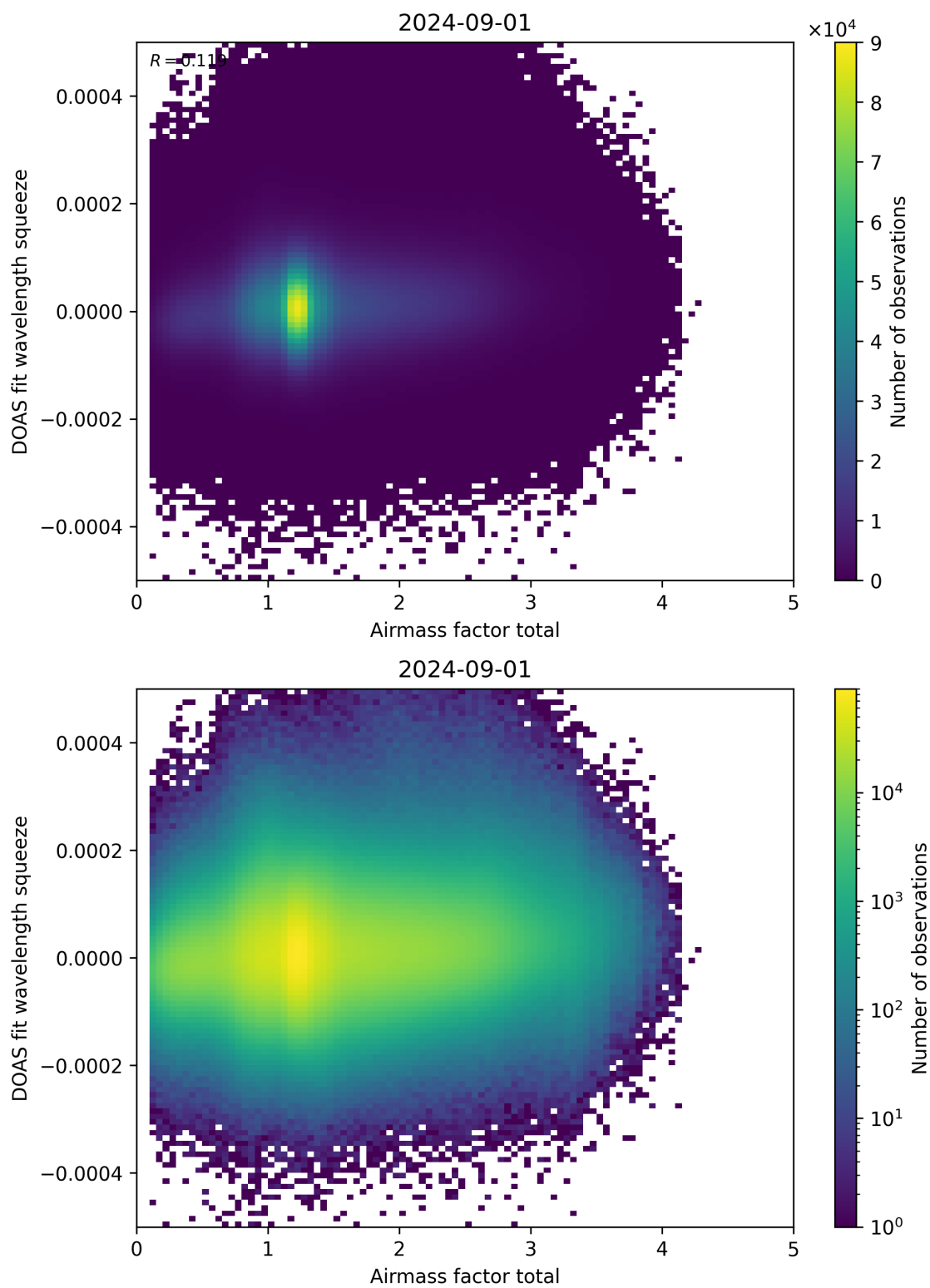
Figure 99: Scatter density plot of “Airmass factor total” against “DOAS fit wavelength squeeze” for 2024-09-01 to 2024-09-02.
