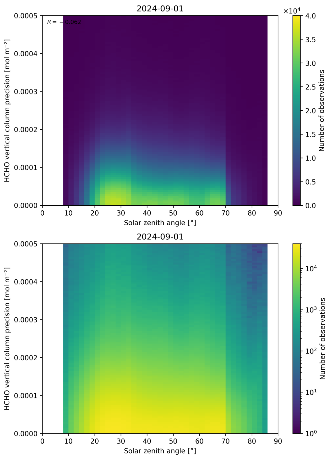
Figure 179: Scatter density plot of “Solar zenith angle” against “HCHO vertical column precision” for 2024-09-01 to 2024-09-02.
