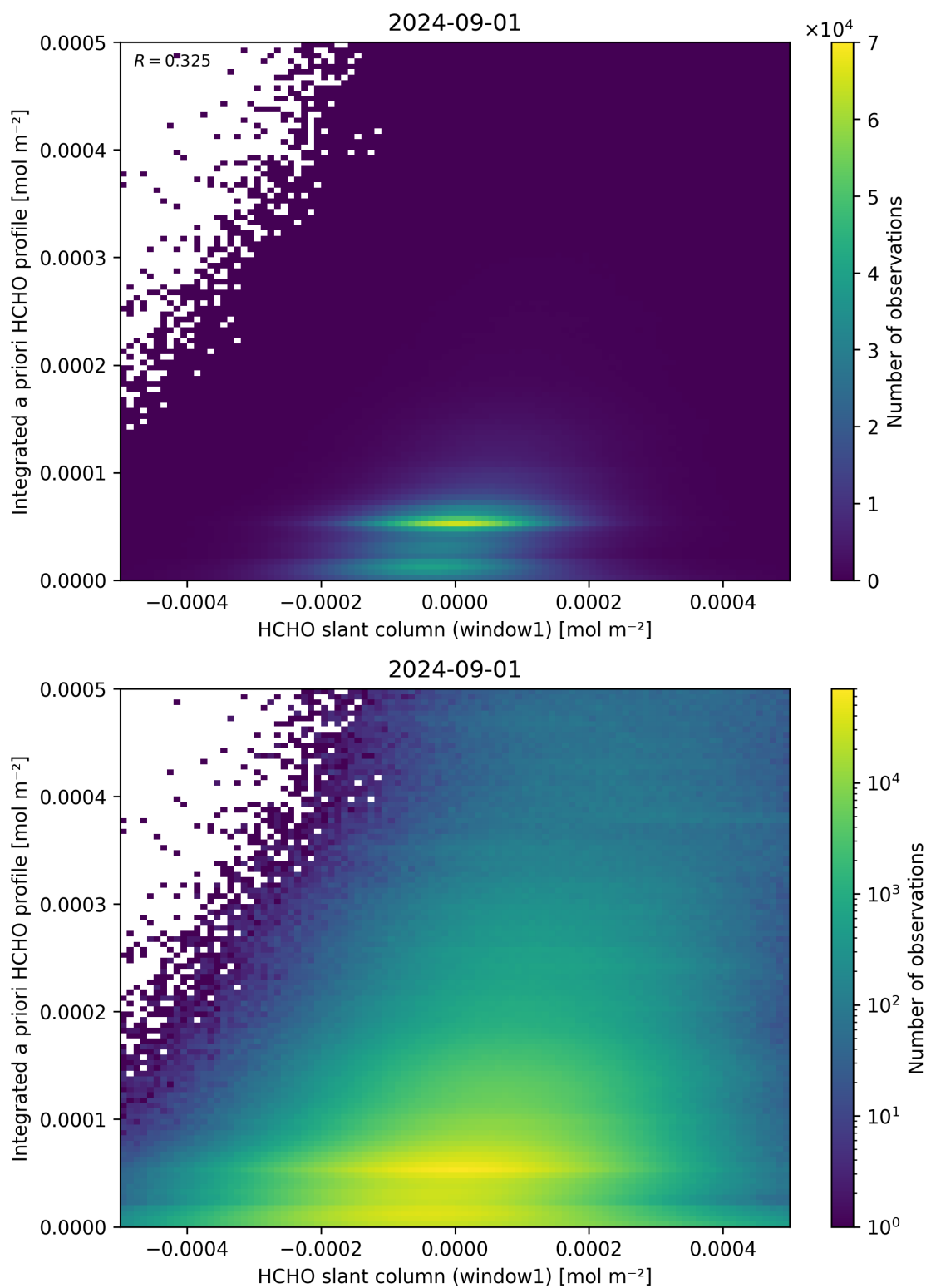
Figure 87: Scatter density plot of “HCHO slant column (window1)” against “Integrated a priori HCHO profile” for 2024-09-01 to 2024-09-02.
