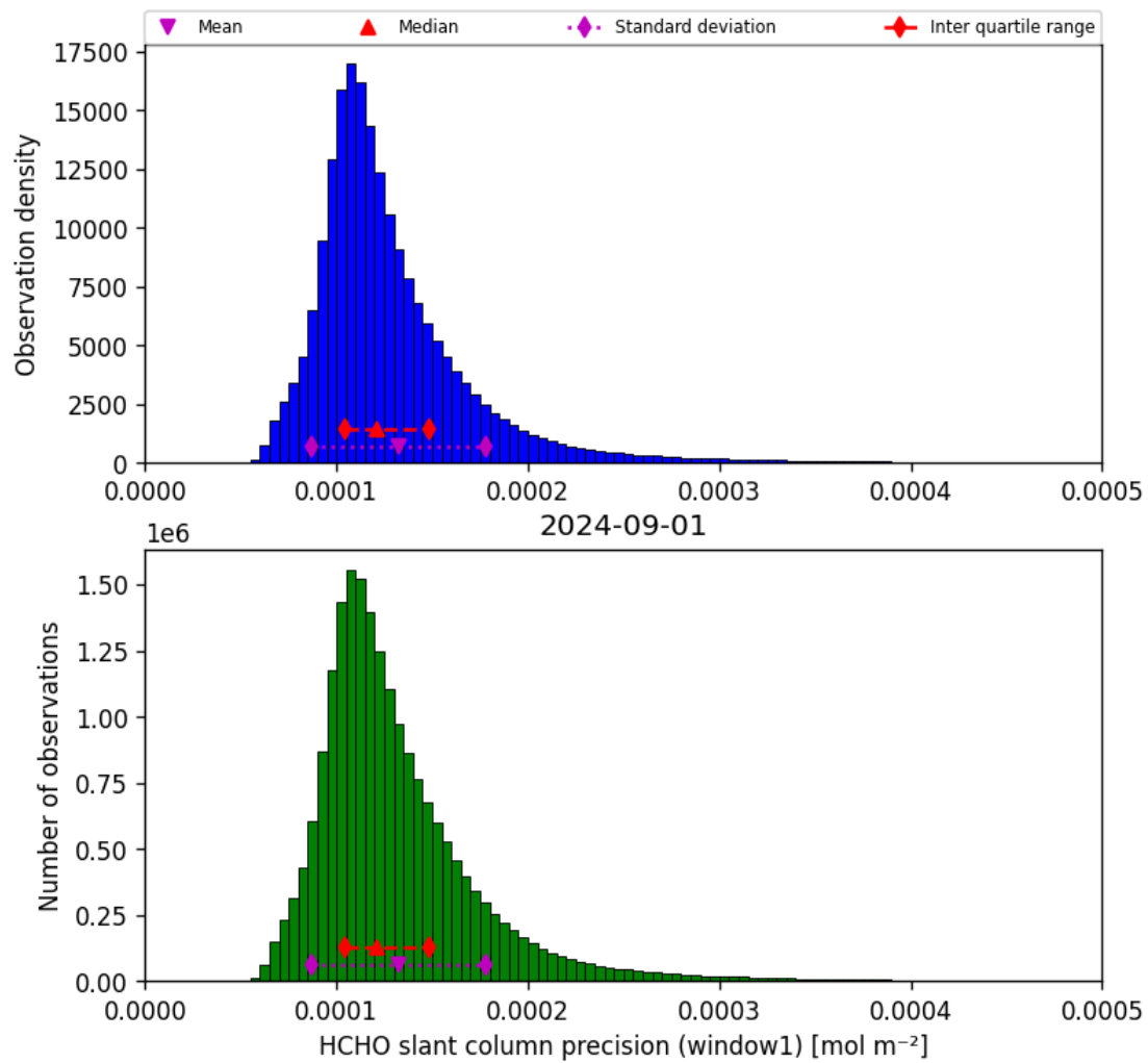
Figure 39: Histogram of “HCHO slant column precision (window1)” for 2024-09-01 to 2024-09-02
