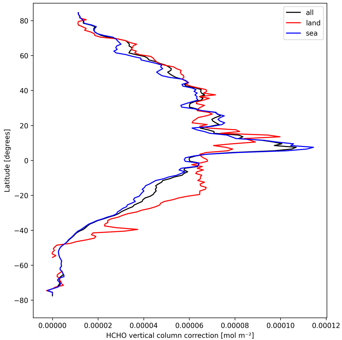
Figure 23: Zonal average of “HCHO vertical column correction” for 2024-09-01 to 2024-09-02.
