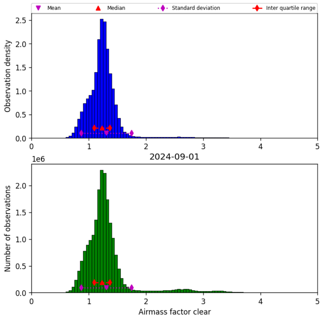
Figure 42: Histogram of “Airmass factor clear” for 2024-09-01 to 2024-09-02
