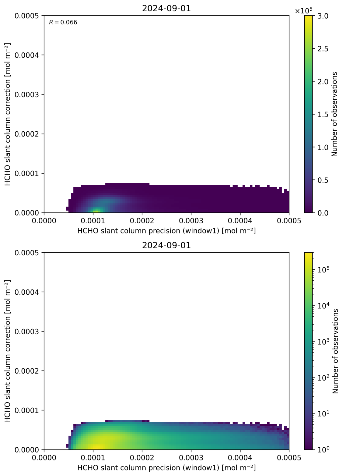
Figure 93: Scatter density plot of “HCHO slant column precision (window1)” against “HCHO slant column correction” for 2024-09-01 to 2024-09-02.
