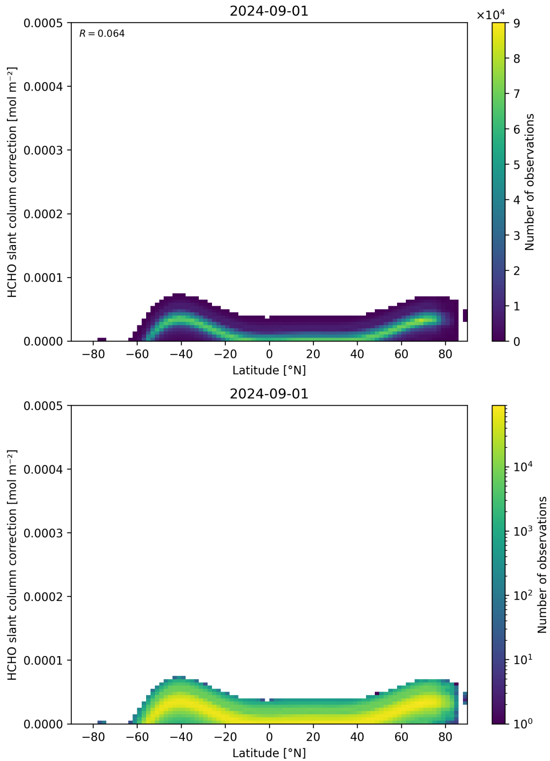
Figure 158: Scatter density plot of “Latitude” against “HCHO slant column correction” for 2024-09-01 to 2024-09-02.
