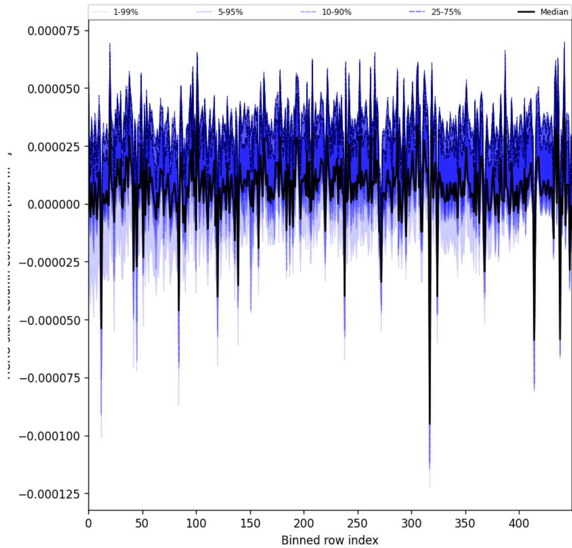
Figure 61: Along track statistics of “HCHO slant column correction” for 2024-09-01 to 2024-09-02
