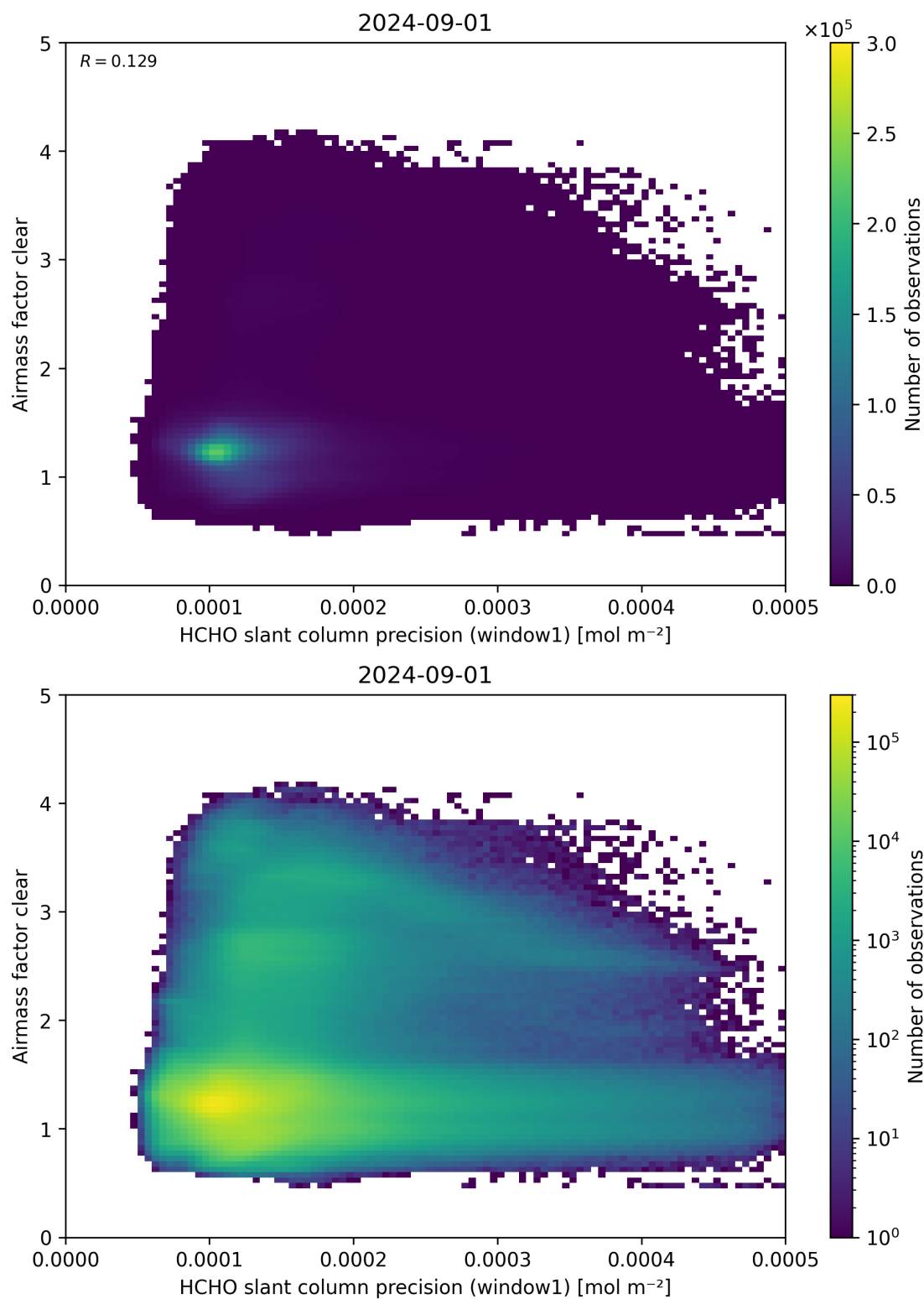
Figure 91: Scatter density plot of “HCHO slant column precision (window1)” against “Airmass factor clear” for 2024-09-01 to 2024-09-02.
