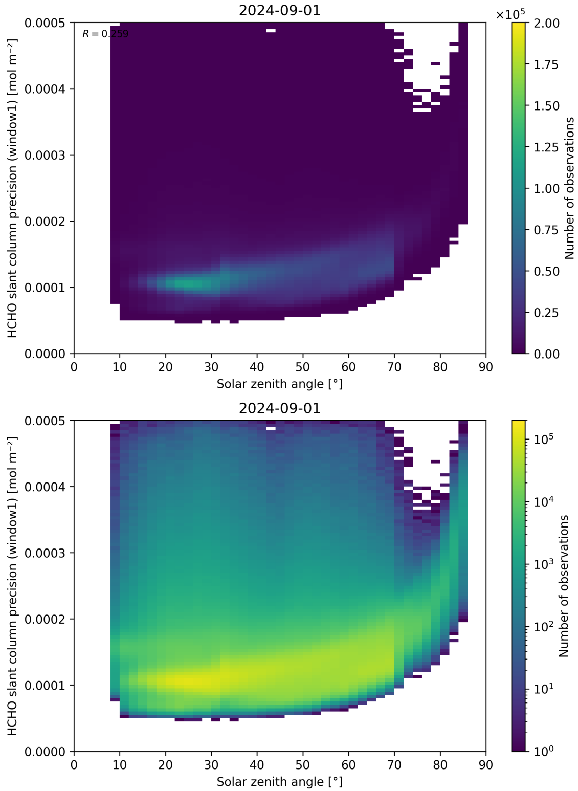
Figure 174: Scatter density plot of “Solar zenith angle” against “HCHO slant column precision (window1)” for 2024-09-01 to 2024-09-02.
