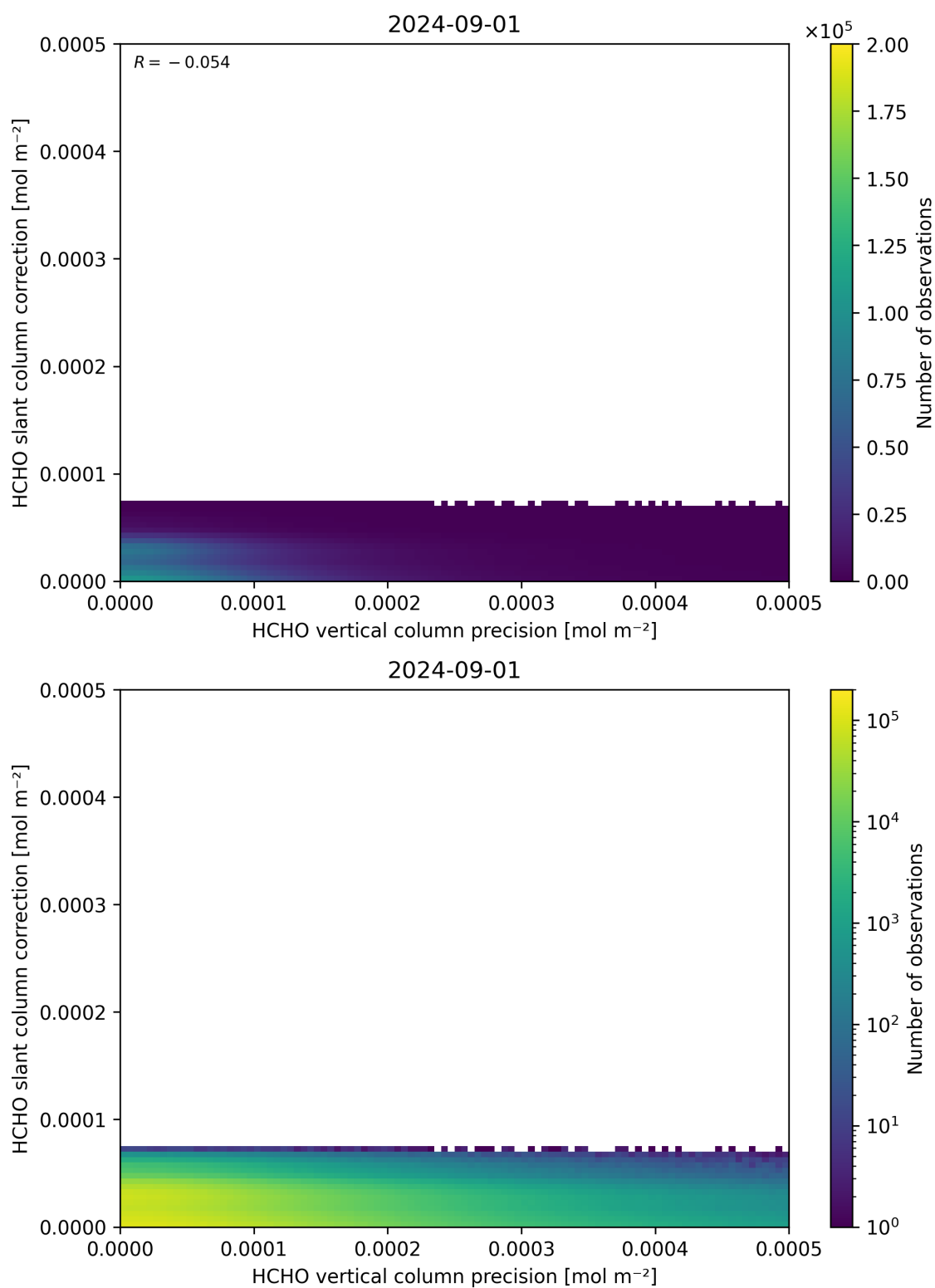
Figure 141: Scatter density plot of “HCHO vertical column precision” against “HCHO slant column correction” for 2024-09-01 to 2024-09-02.
