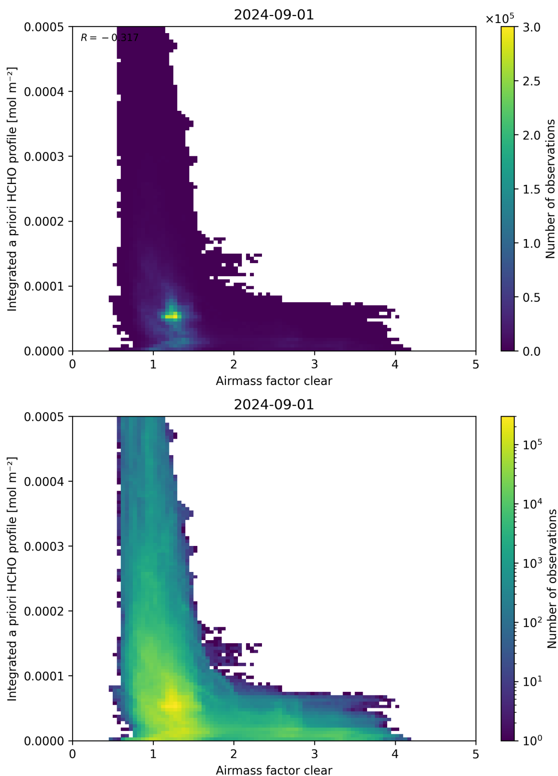
Figure 76: Scatter density plot of “Airmass factor clear” against “Integrated a priori HCHO profile” for 2024-09-01 to 2024-09-02.
