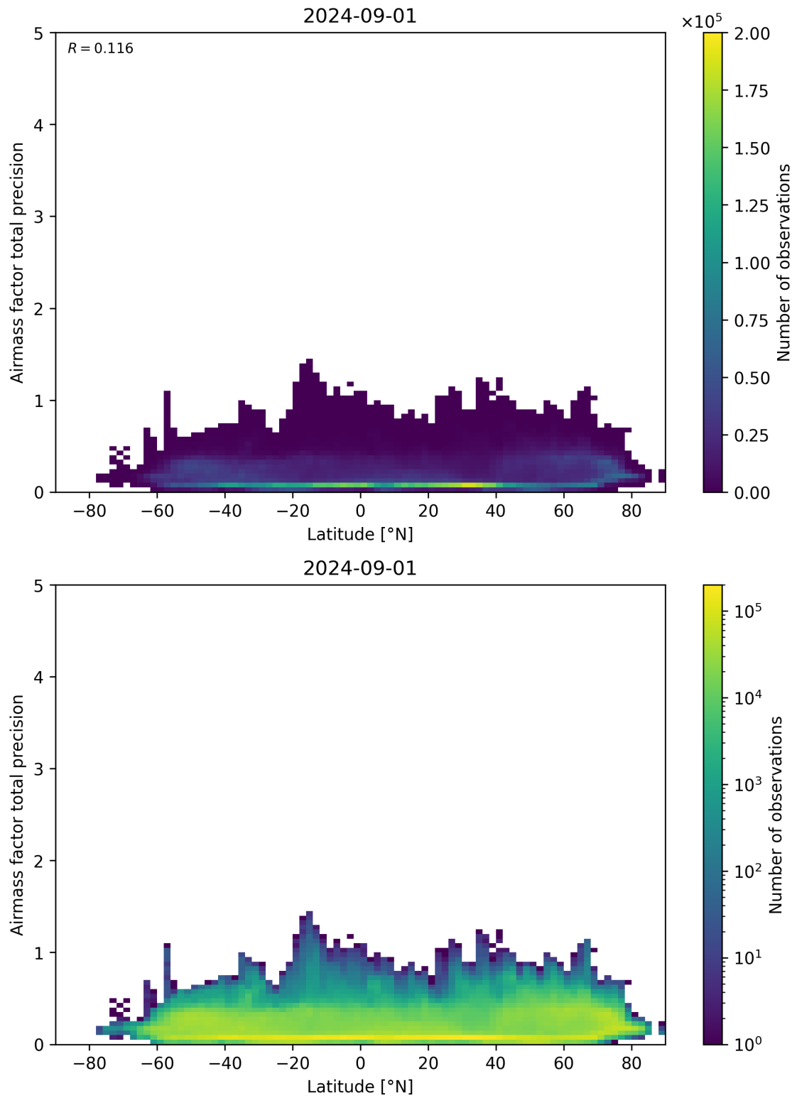
Figure 162: Scatter density plot of “Latitude” against “Airmass factor total precision” for 2024-09-01 to 2024-09-02.
