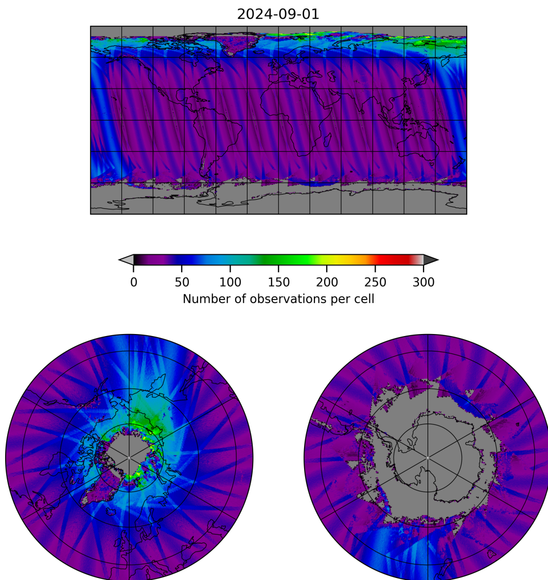
Figure 19: Map of the number of observations for 2024-09-01 to 2024-09-02
