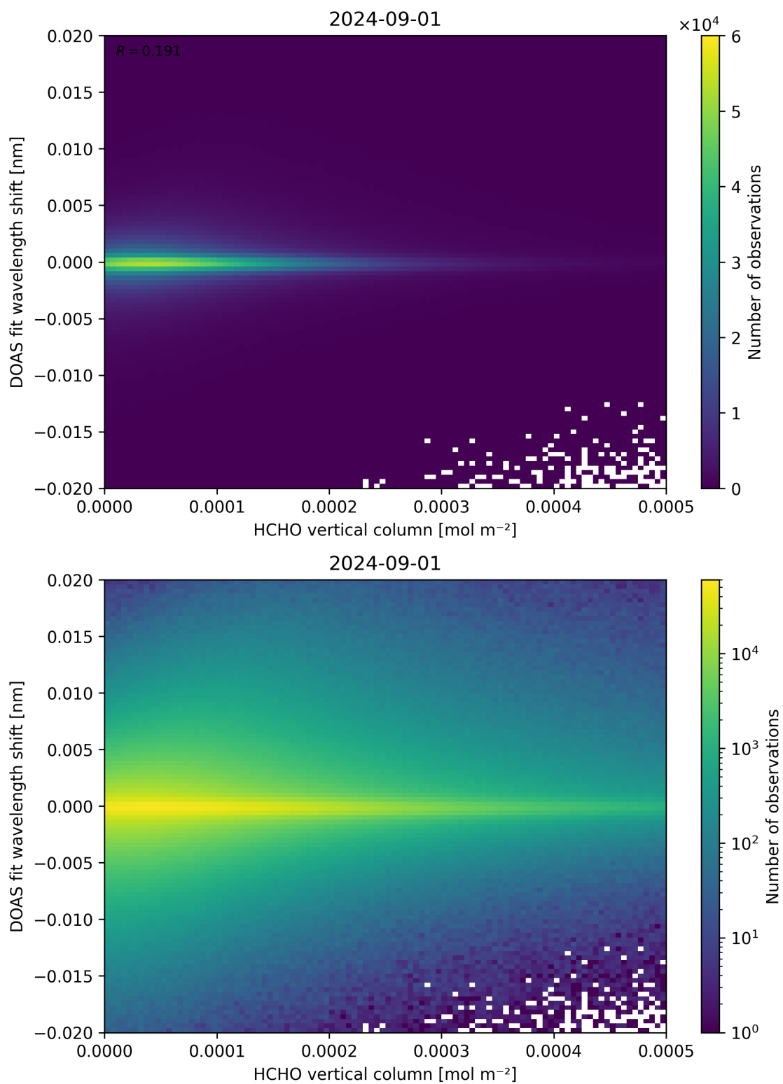
Figure 124: Scatter density plot of “HCHO vertical column” against “DOAS fit wavelength shift” for 2024-09-01 to 2024-09-02.
