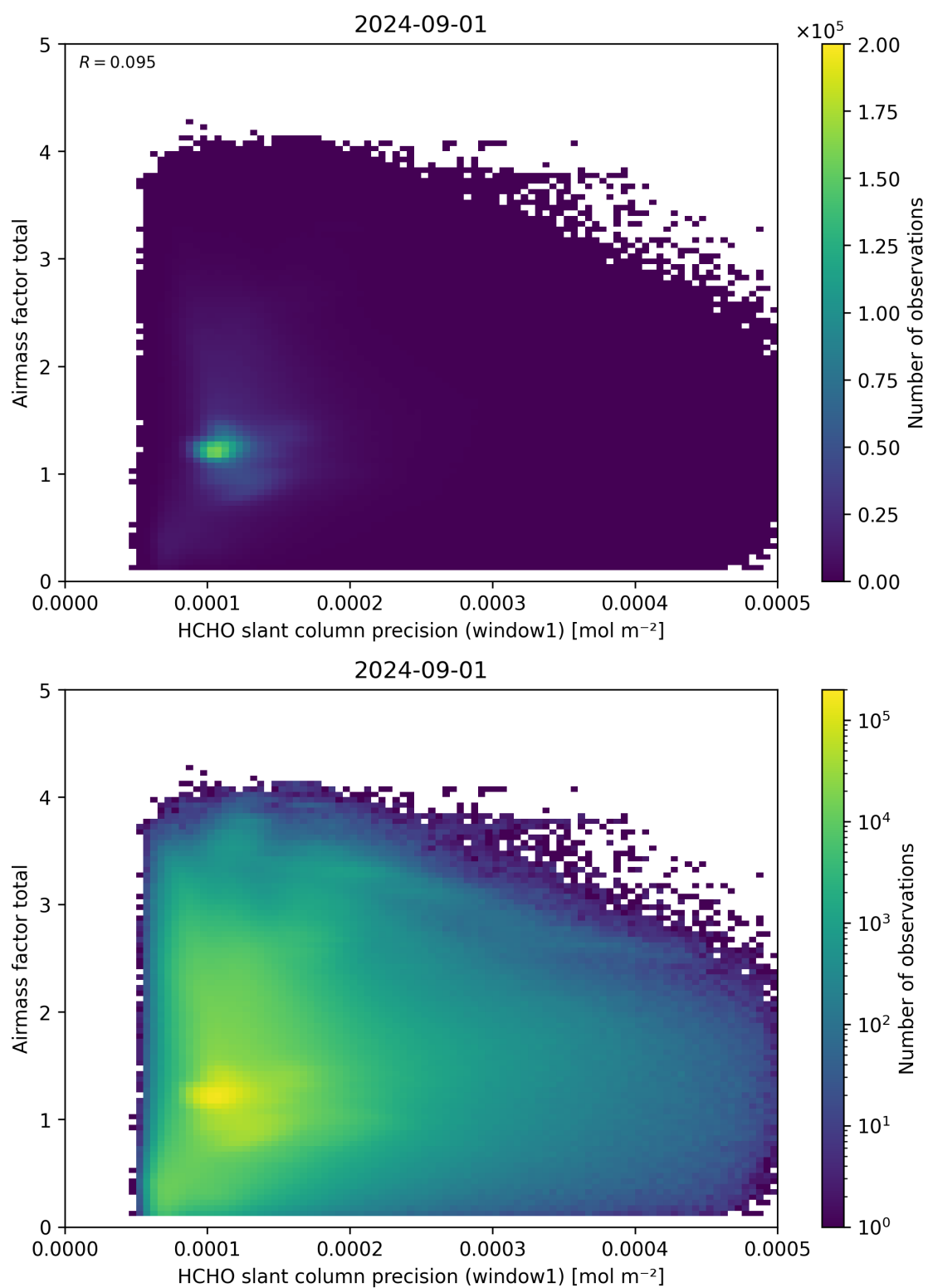
Figure 94: Scatter density plot of “HCHO slant column precision (window1)” against “Airmass factor total” for 2024-09-01 to 2024-09-02.
