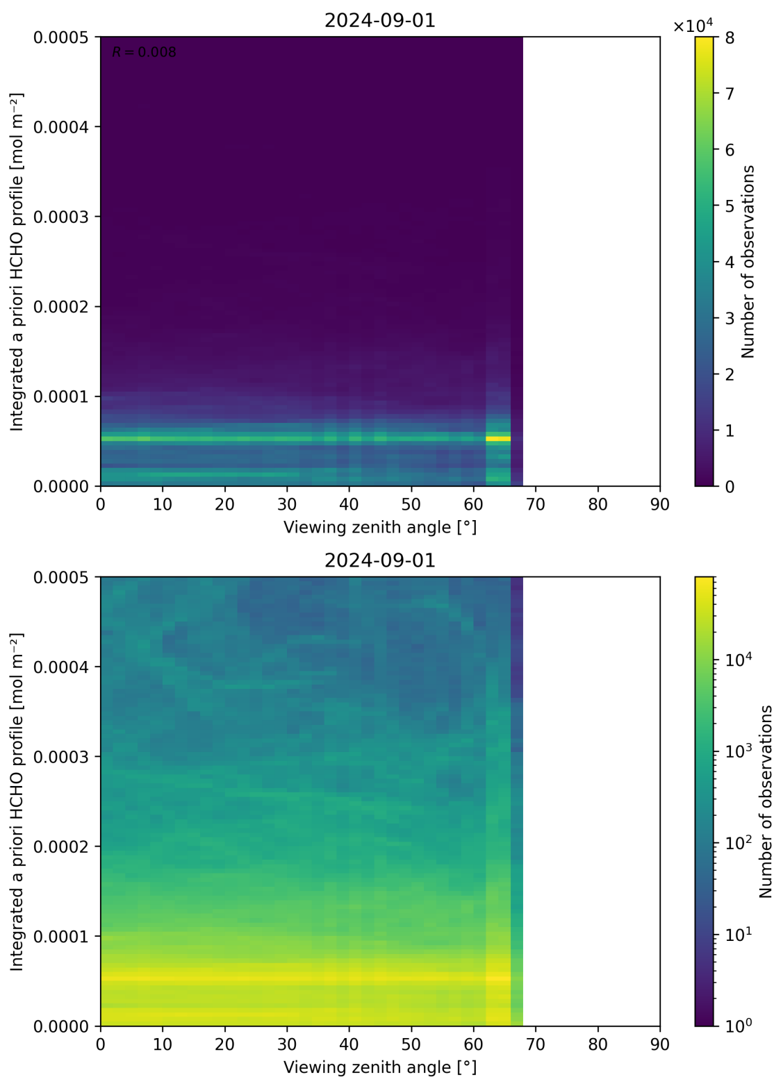
Figure 195: Scatter density plot of “Viewing zenith angle” against “Integrated a priori HCHO profile” for 2024-09-01 to 2024-09-02.
