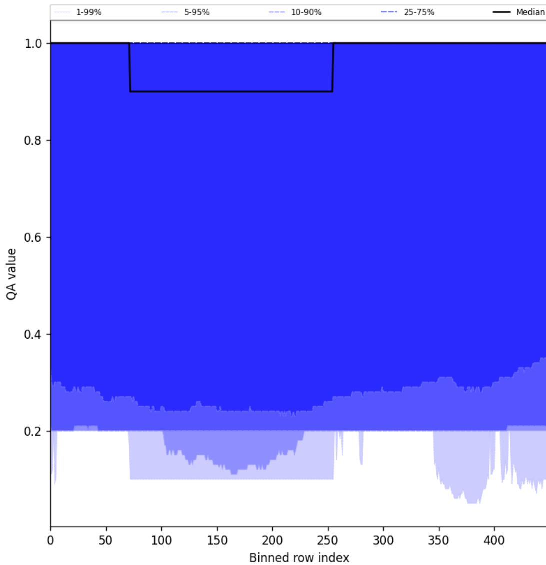
Figure 48: Along track statistics of “QA value” for 2024-09-01 to 2024-09-02
