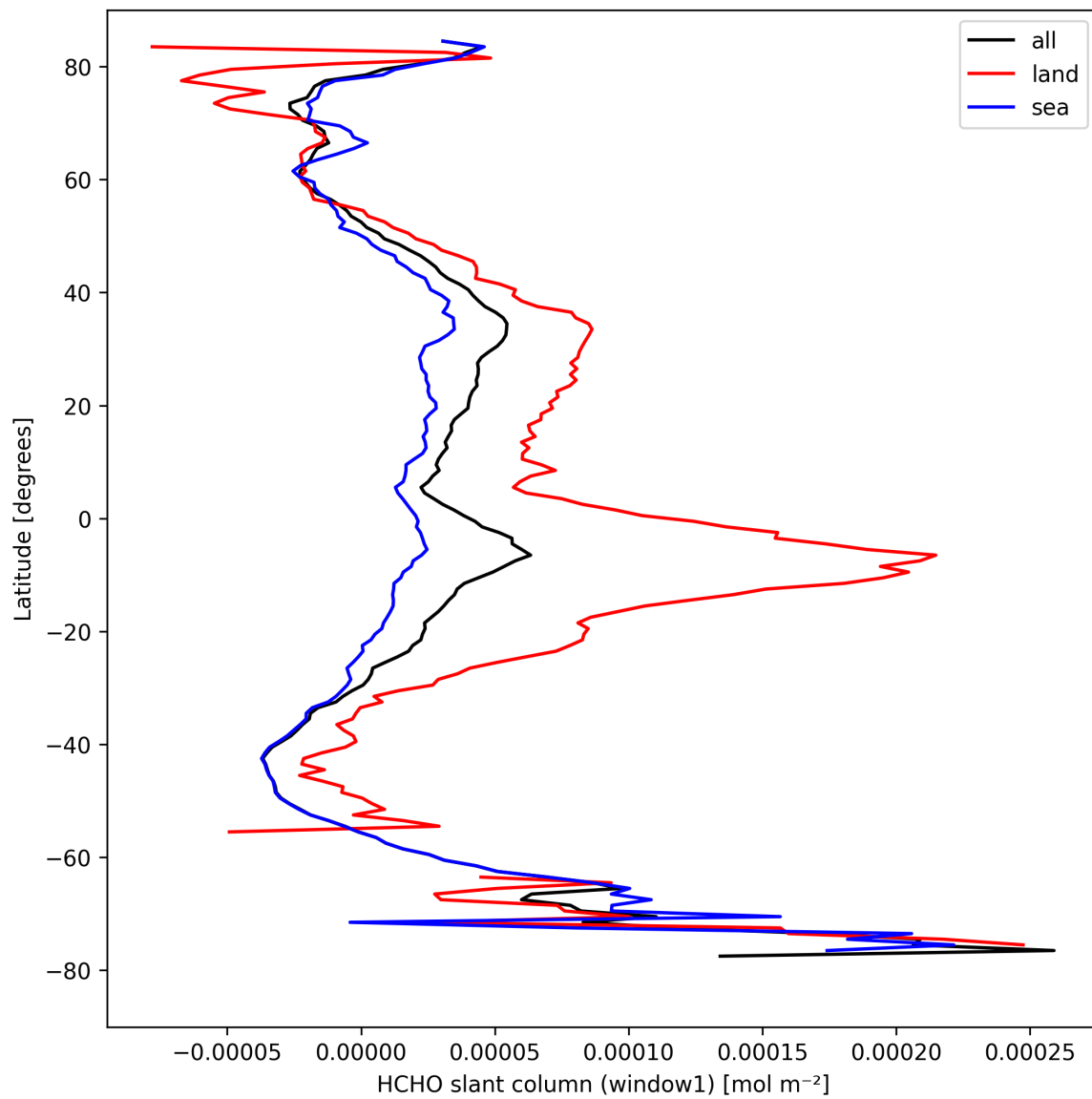
Figure 24: Zonal average of “HCHO slant column (window1)” for 2024-09-01 to 2024-09-02.
