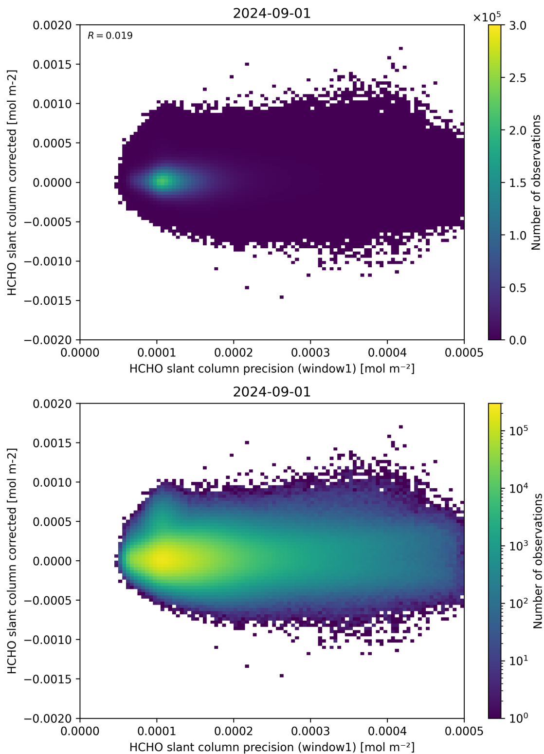
Figure 92: Scatter density plot of “HCHO slant column precision (window1)” against “HCHO slant column corrected” for 2024-09-01 to 2024-09-02.
