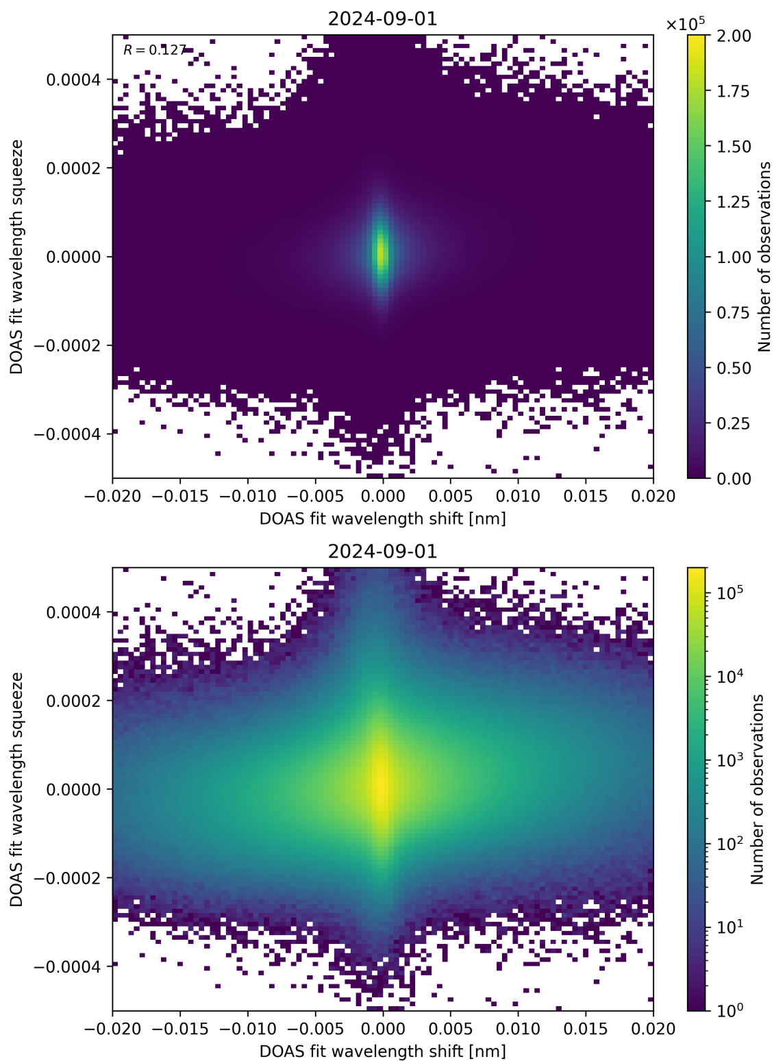
Figure 65: Scatter density plot of “DOAS fit wavelength shift” against “DOAS fit wavelength squeeze” for 2024-09-01 to 2024-09-02.
