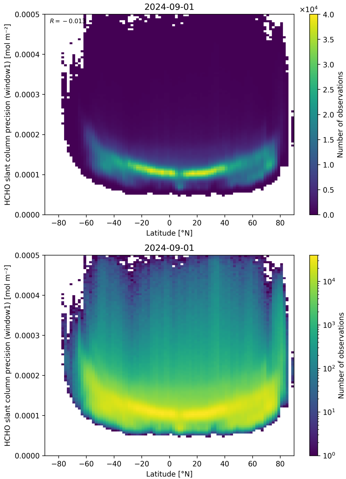
Figure 160: Scatter density plot of “Latitude” against “HCHO slant column precision (window1)” for 2024-09-01 to 2024-09-02.
