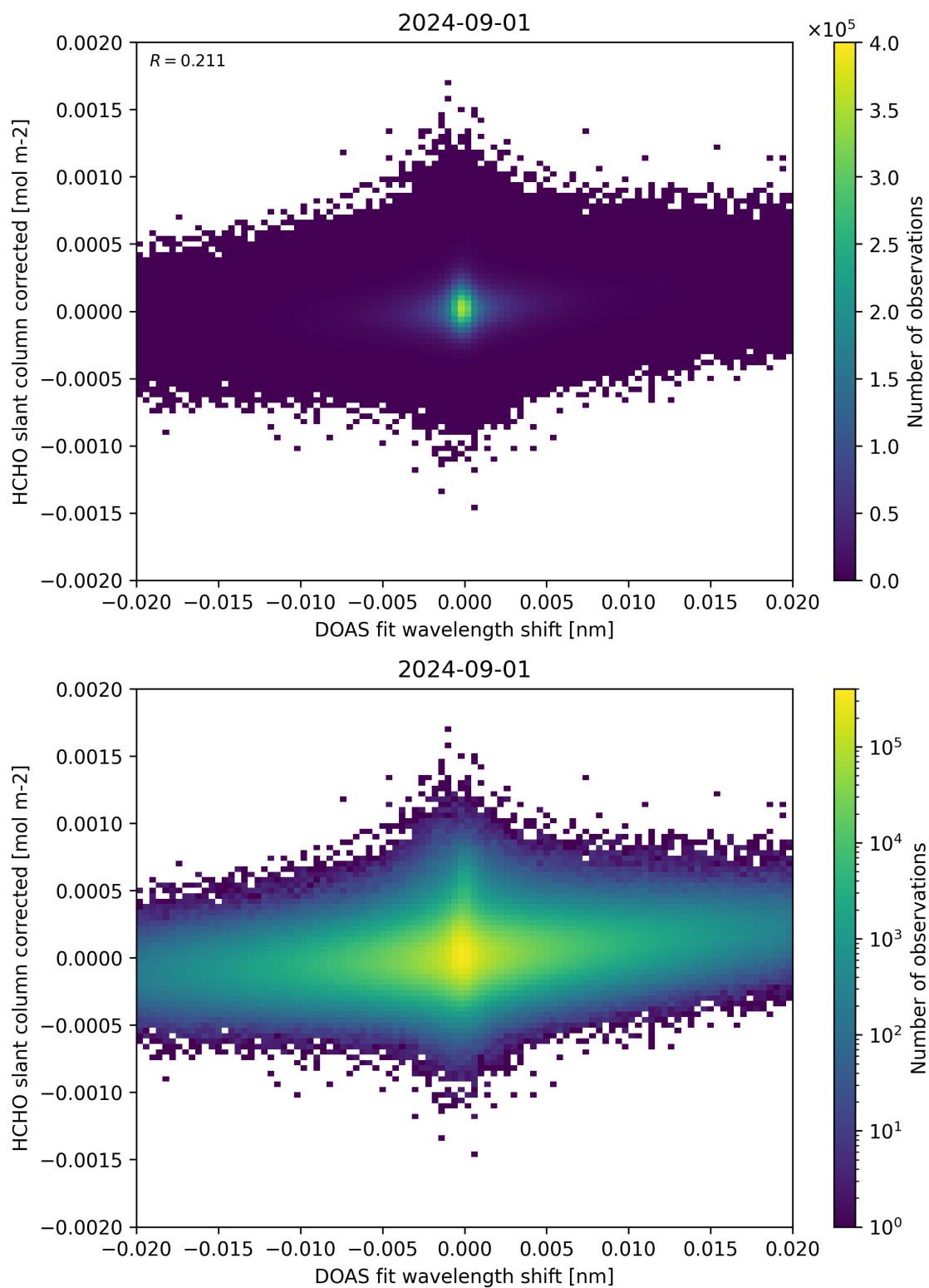
Figure 66: Scatter density plot of “DOAS fit wavelength shift” against “HCHO slant column corrected” for 2024-09-01 to 2024-09-02.
