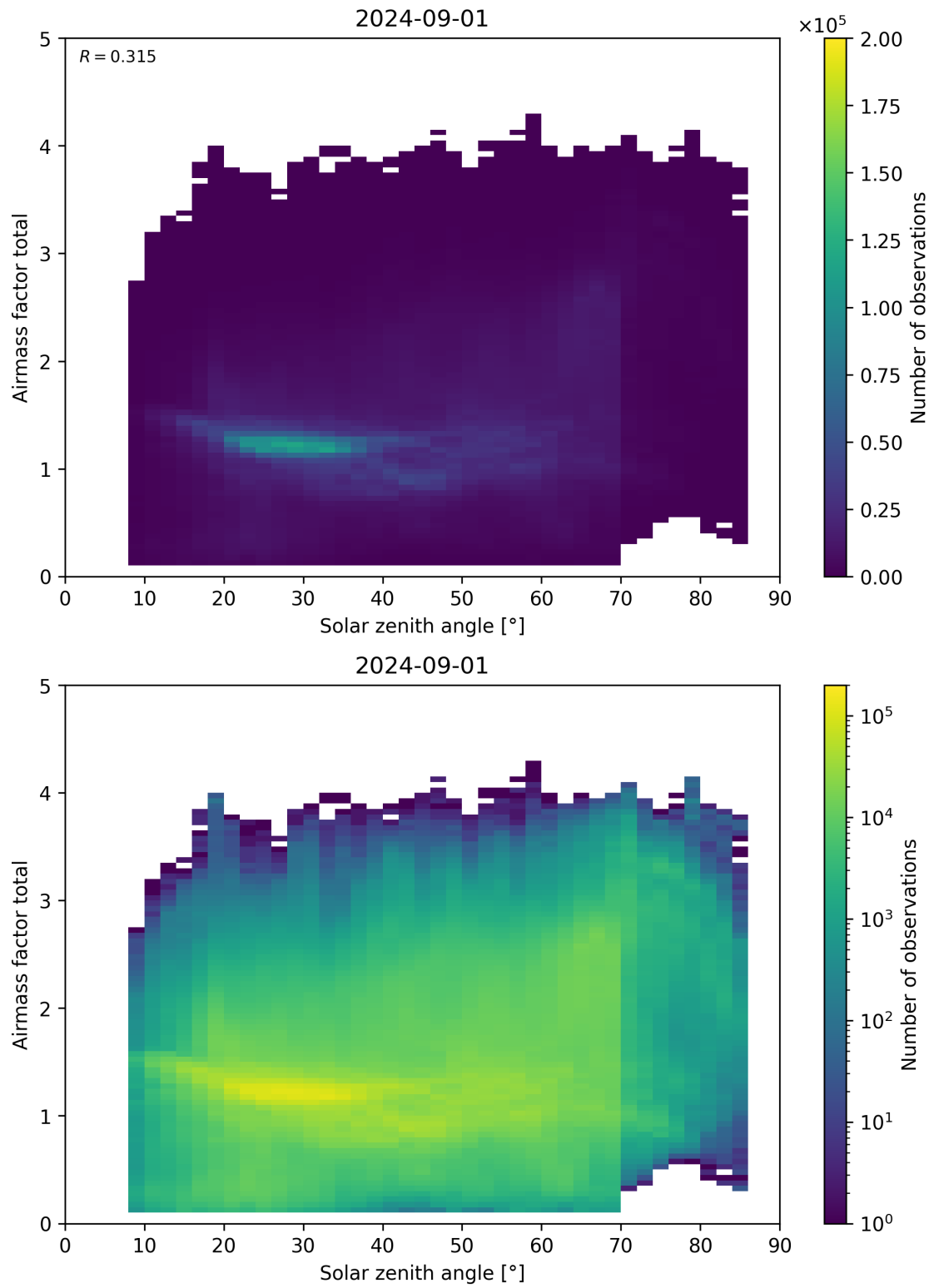
Figure 175: Scatter density plot of “Solar zenith angle” against “Airmass factor total” for 2024-09-01 to 2024-09-02.
