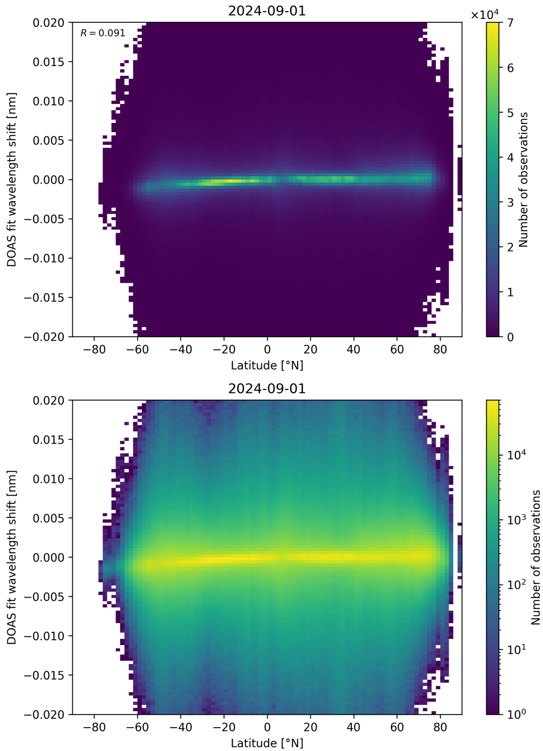
Figure 154: Scatter density plot of “Latitude” against “DOAS fit wavelength shift” for 2024-09-01 to 2024-09-02.
