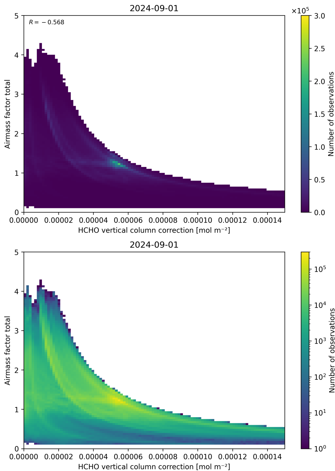
Figure 120: Scatter density plot of “HCHO vertical column correction” against “Airmass factor total” for 2024-09-01 to 2024-09-02.
