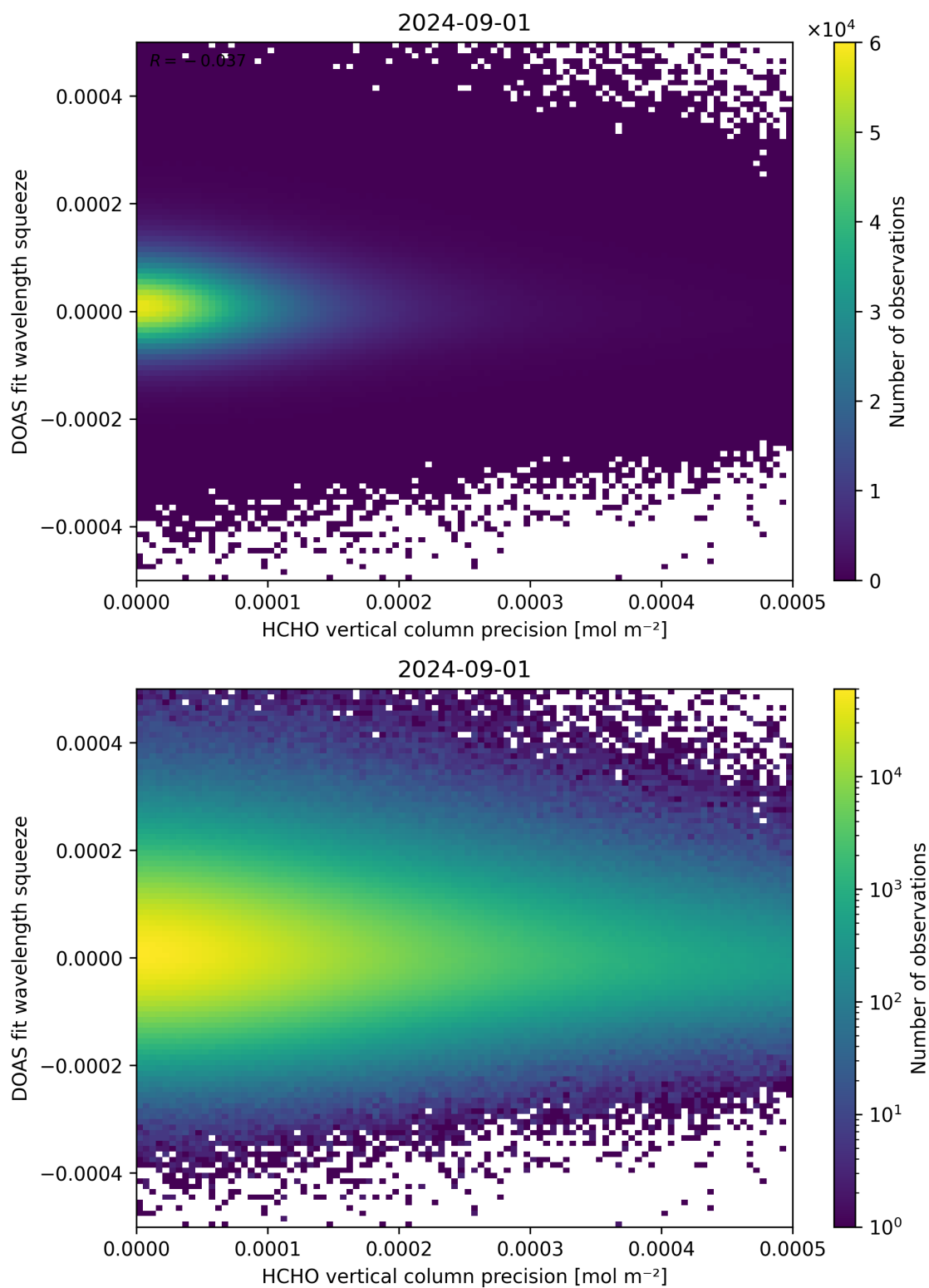
Figure 138: Scatter density plot of “HCHO vertical column precision” against “DOAS fit wavelength squeeze” for 2024-09-01 to 2024-09-02.
