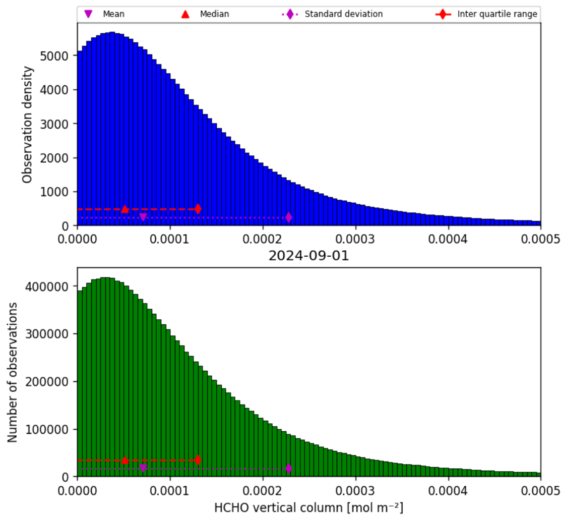
Figure 35: Histogram of “HCHO vertical column” for 2024-09-01 to 2024-09-02
