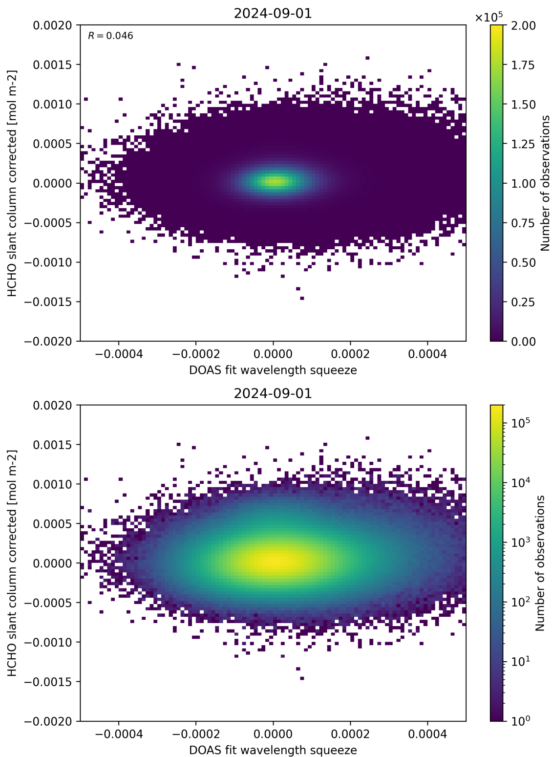
Figure 69: Scatter density plot of “DOAS fit wavelength squeeze” against “HCHO slant column corrected” for 2024-09-01 to 2024-09-02.
