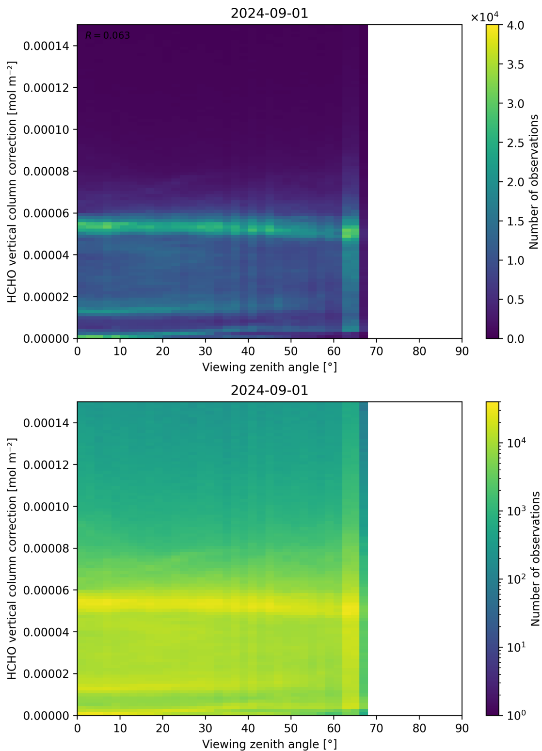
Figure 193: Scatter density plot of “Viewing zenith angle” against “HCHO vertical column correction” for 2024-09-01 to 2024-09-02.
