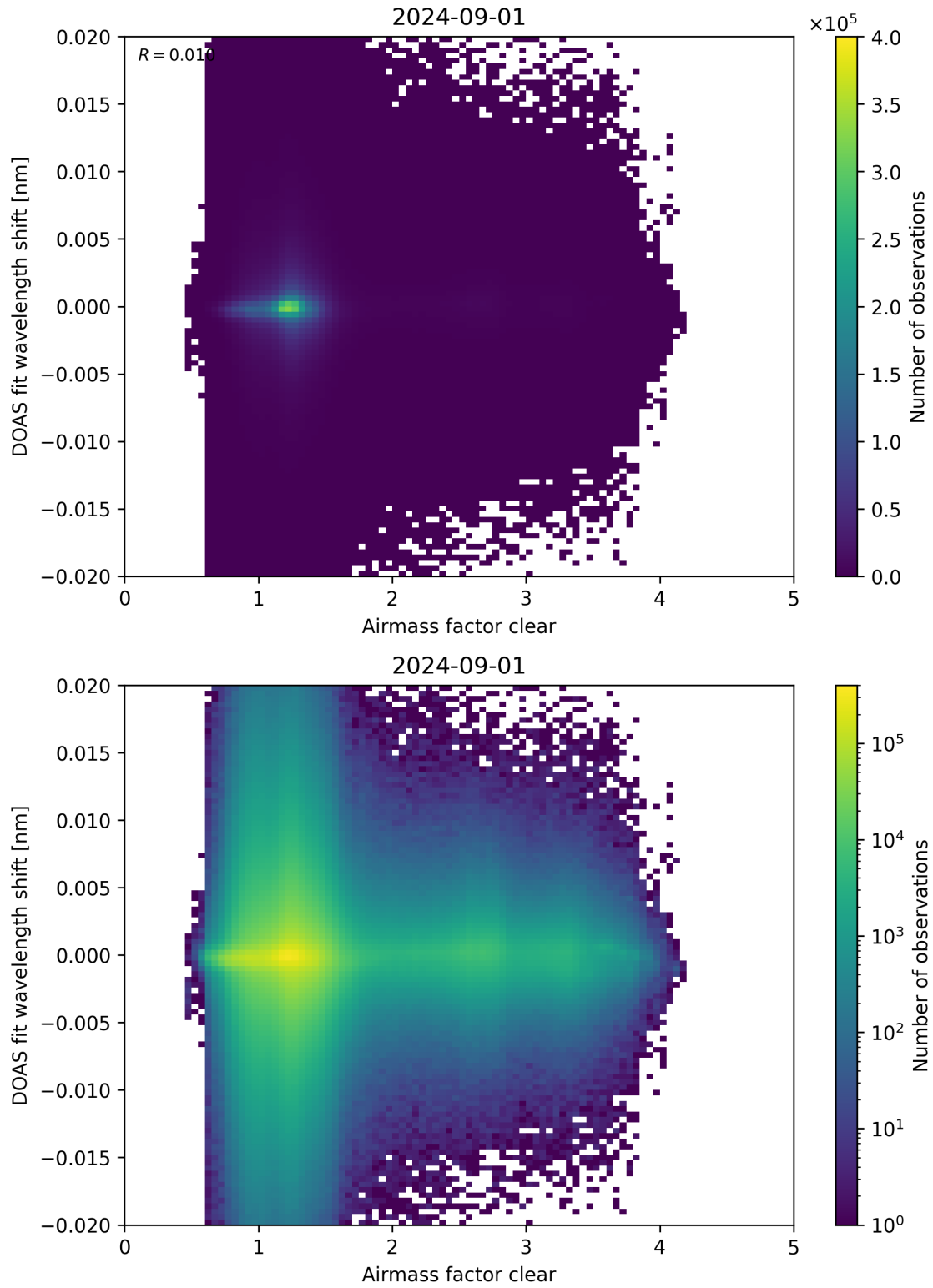
Figure 72: Scatter density plot of “Airmass factor clear” against “DOAS fit wavelength shift” for 2024-09-01 to 2024-09-02.
