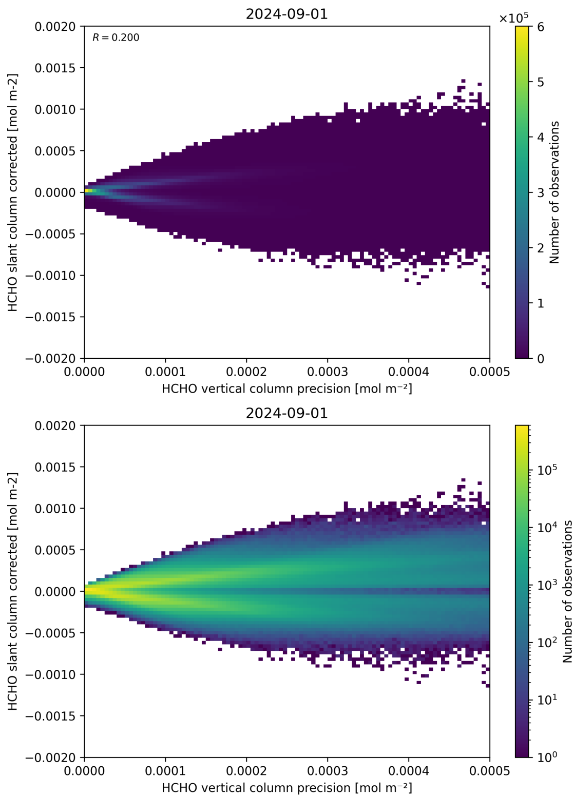
Figure 140: Scatter density plot of “HCHO vertical column precision” against “HCHO slant column corrected” for 2024-09-01 to 2024-09-02.
