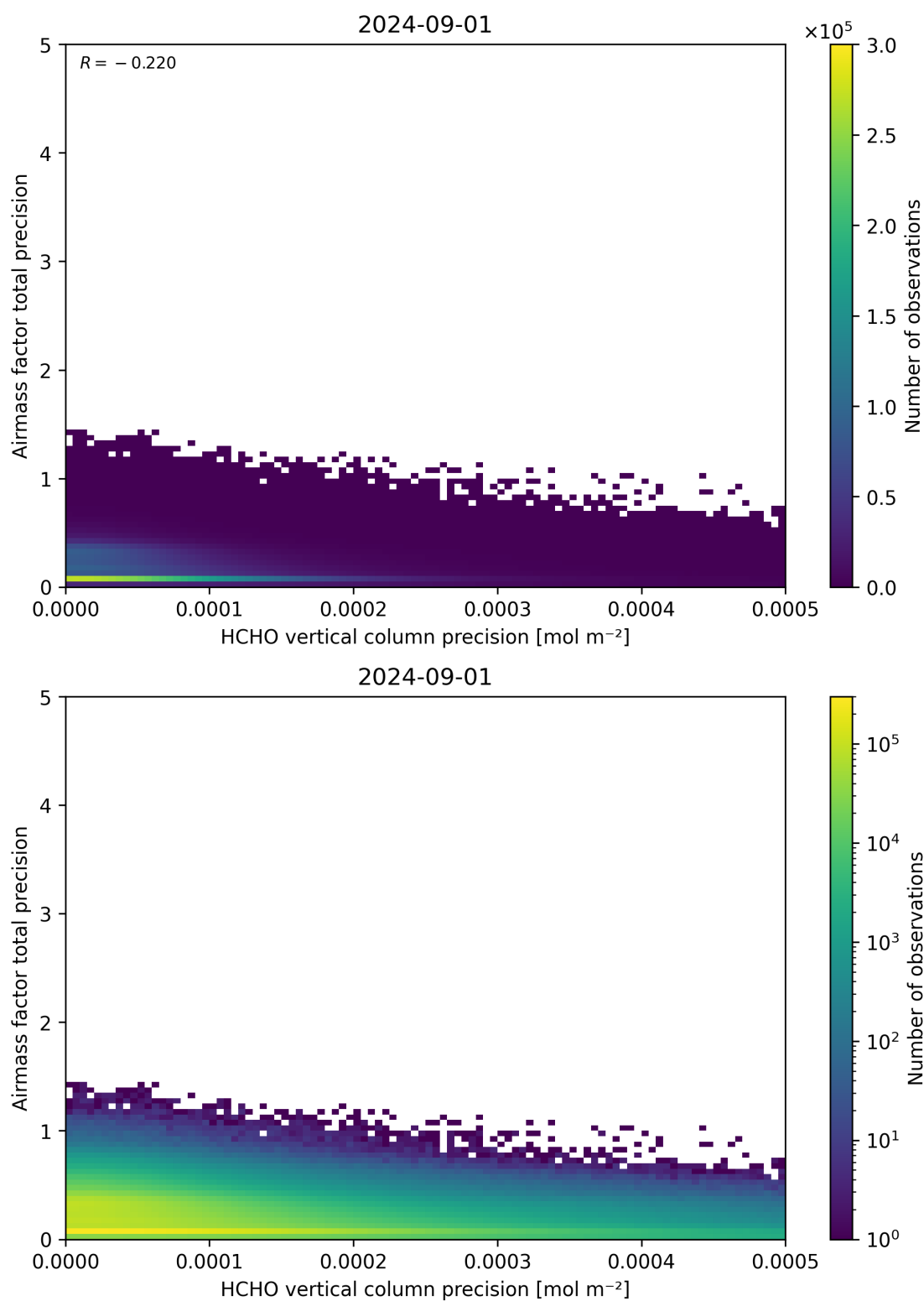
Figure 145: Scatter density plot of “HCHO vertical column precision” against “Airmass factor total precision” for 2024-09-01 to 2024-09-02.
