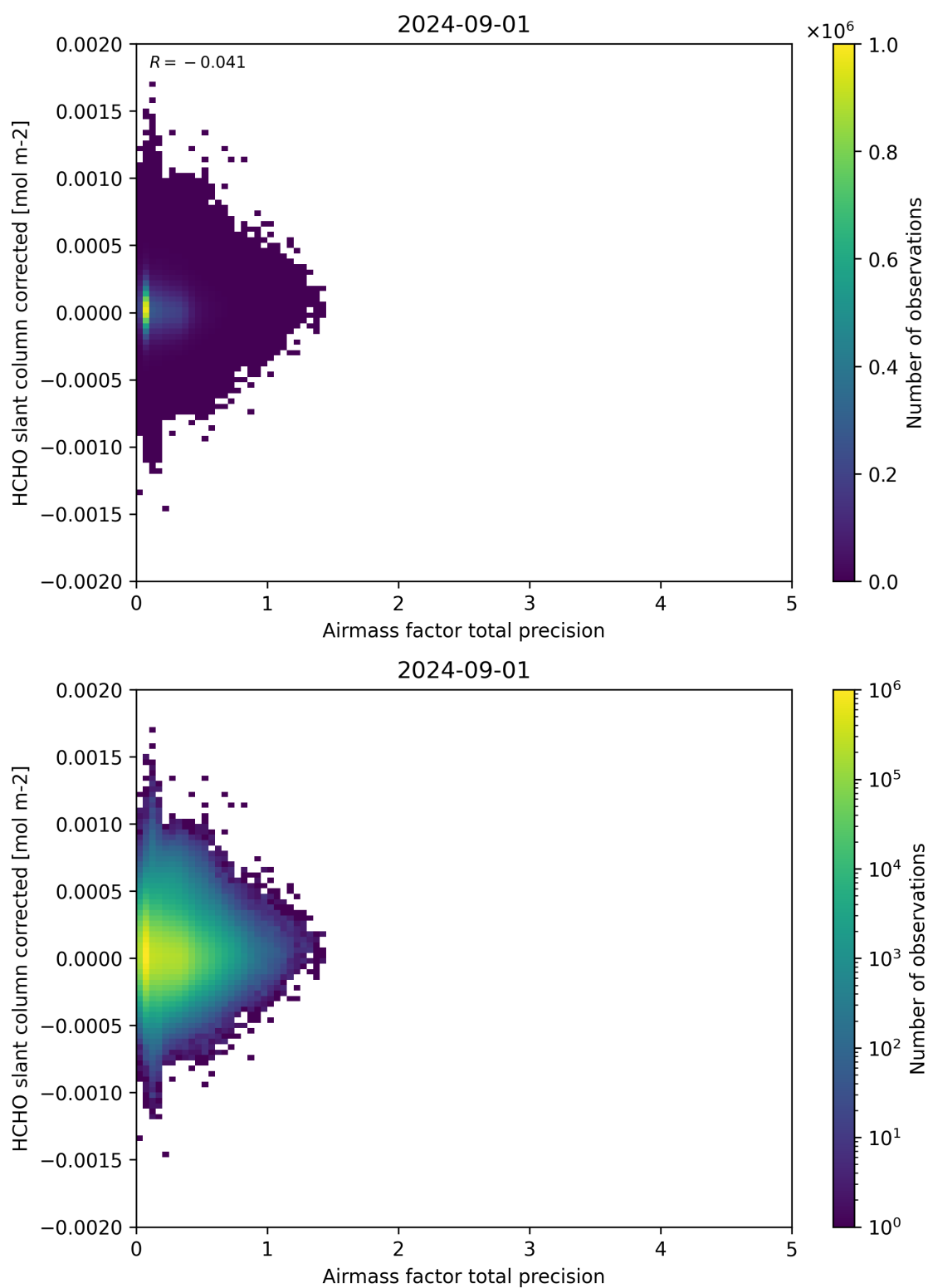
Figure 109: Scatter density plot of “Airmass factor total precision” against “HCHO slant column corrected” for 2024-09-01 to 2024-09-02.
