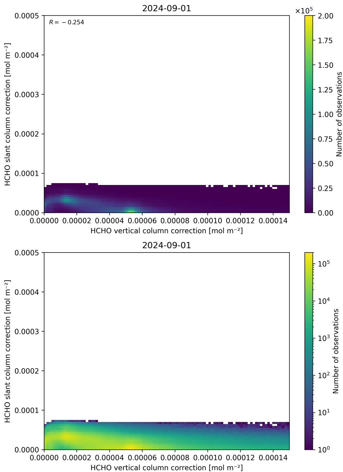
Figure 117: Scatter density plot of “HCHO vertical column correction” against “HCHO slant column correction” for 2024-09-01 to 2024-09-02.
