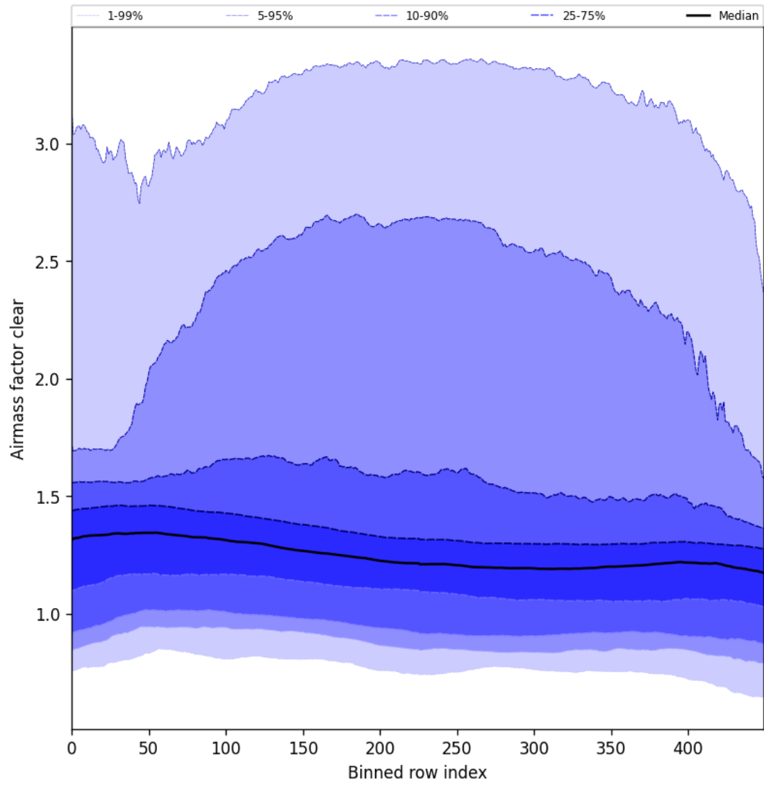
Figure 56: Along track statistics of “Airmass factor clear” for 2024-09-01 to 2024-09-02
