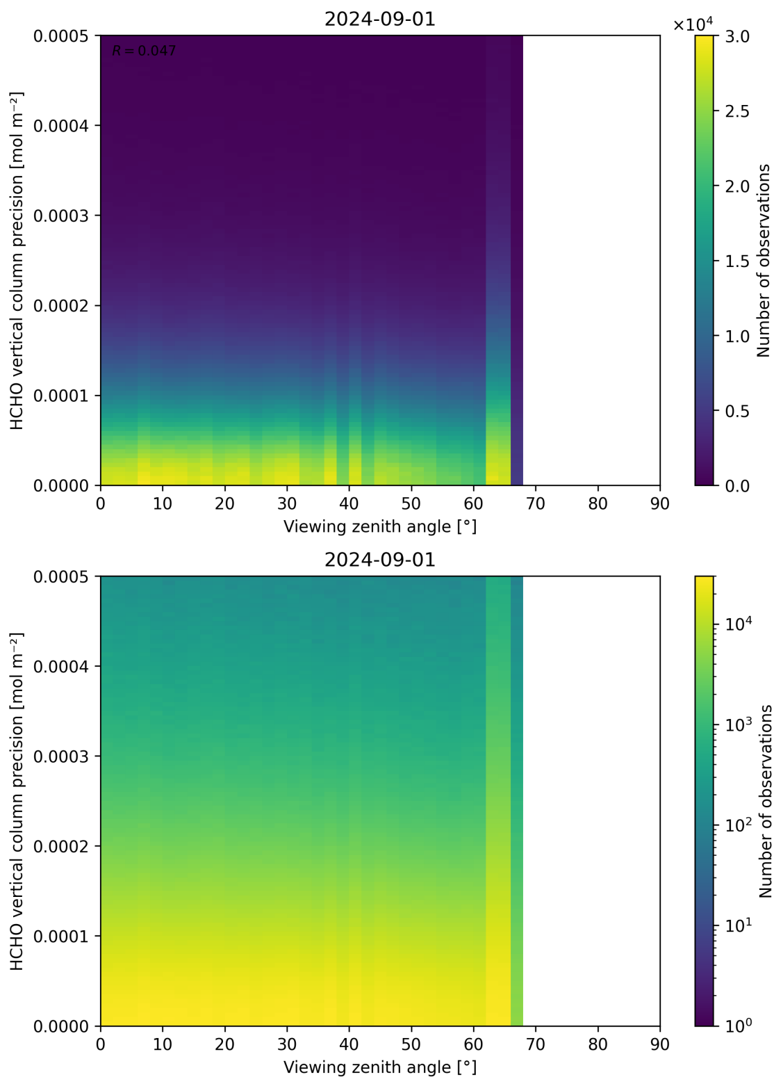
Figure 194: Scatter density plot of “Viewing zenith angle” against “HCHO vertical column precision” for 2024-09-01 to 2024-09-02.
