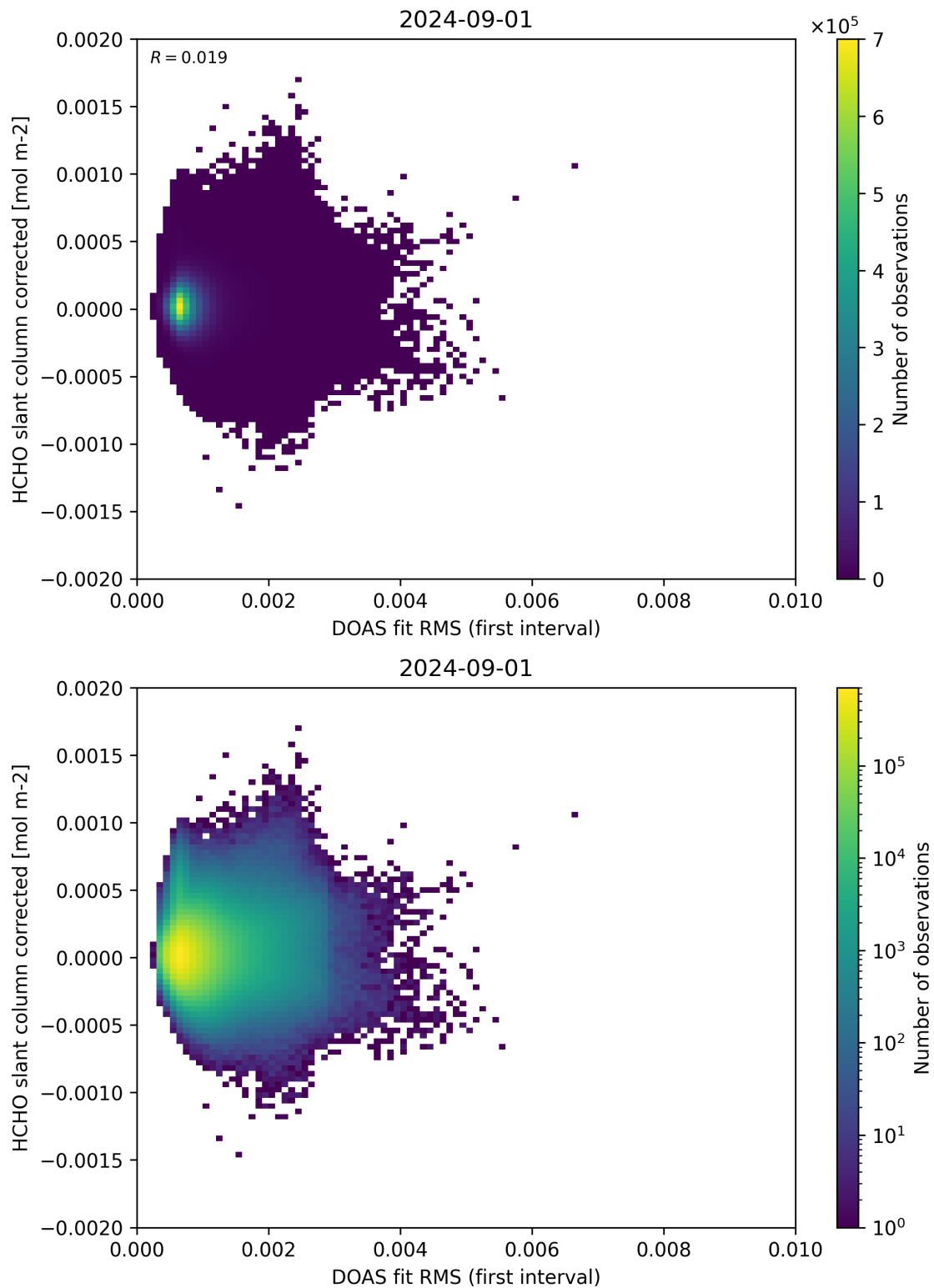
Figure 62: Scatter density plot of “DOAS fit RMS (first interval)” against “HCHO slant column corrected” for 2024-09-01 to 2024-09-02.
