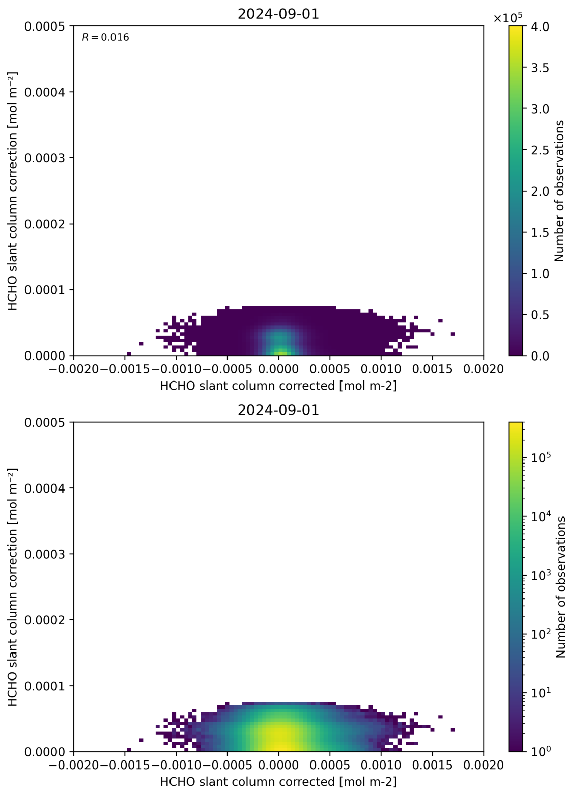
Figure 77: Scatter density plot of “HCHO slant column corrected” against “HCHO slant column correction” for 2024-09-01 to 2024-09-02.
