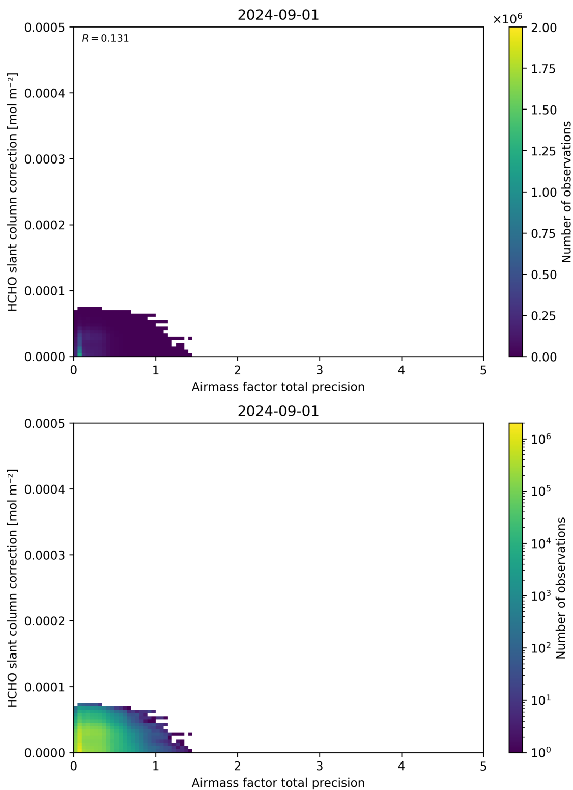
Figure 110: Scatter density plot of “Airmass factor total precision” against “HCHO slant column correction” for 2024-09-01 to 2024-09-02.
