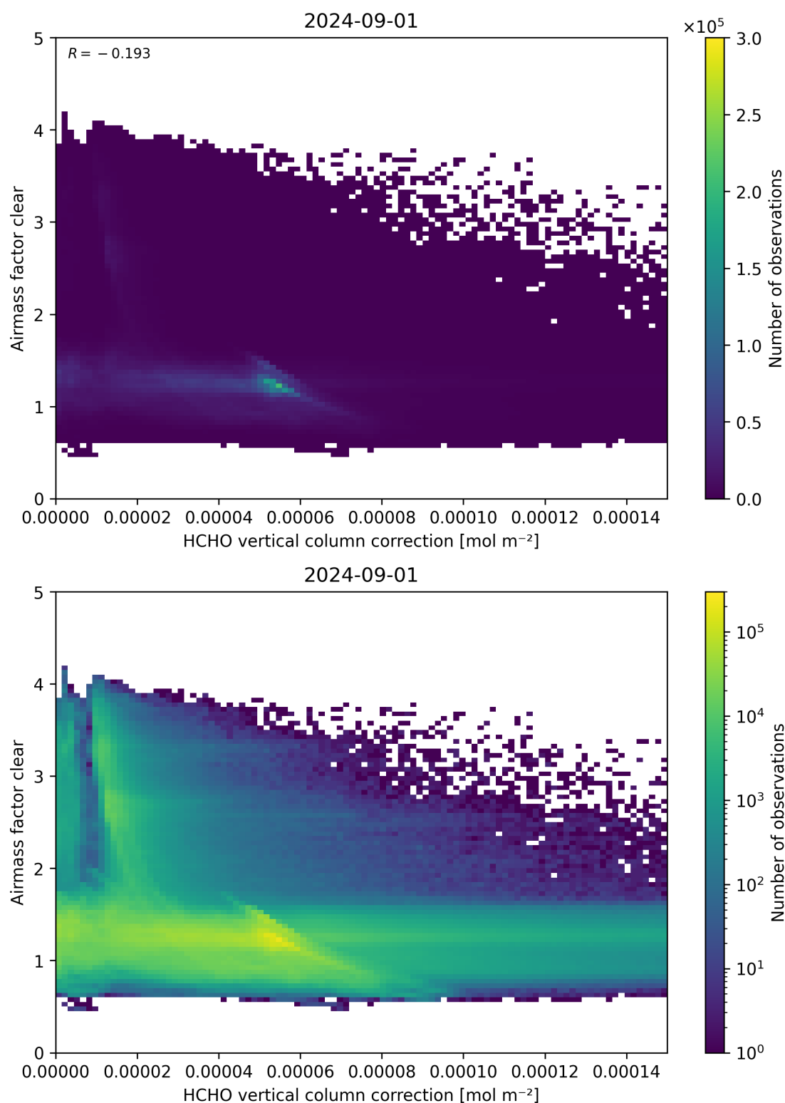
Figure 115: Scatter density plot of “HCHO vertical column correction” against “Airmass factor clear” for 2024-09-01 to 2024-09-02.
