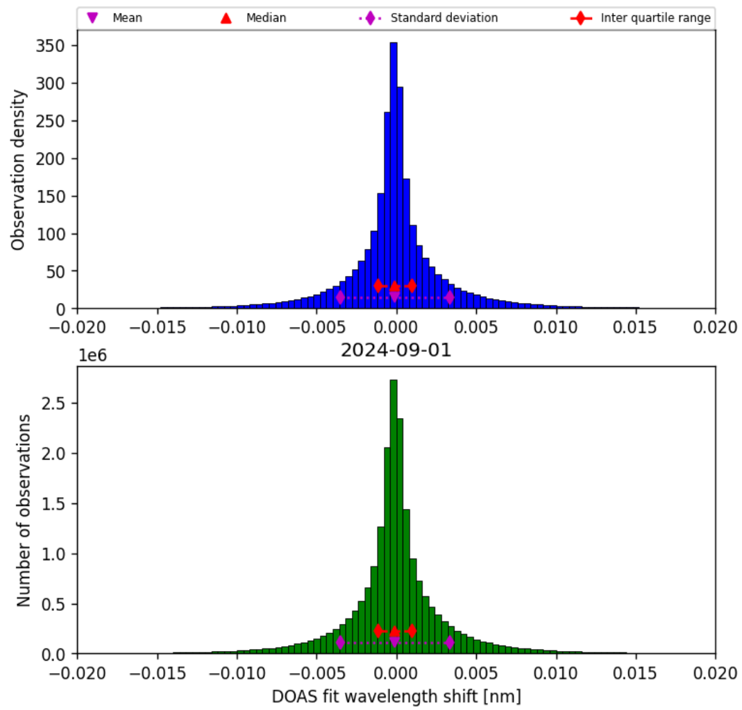
Figure 44: Histogram of “DOAS fit wavelength shift” for 2024-09-01 to 2024-09-02
