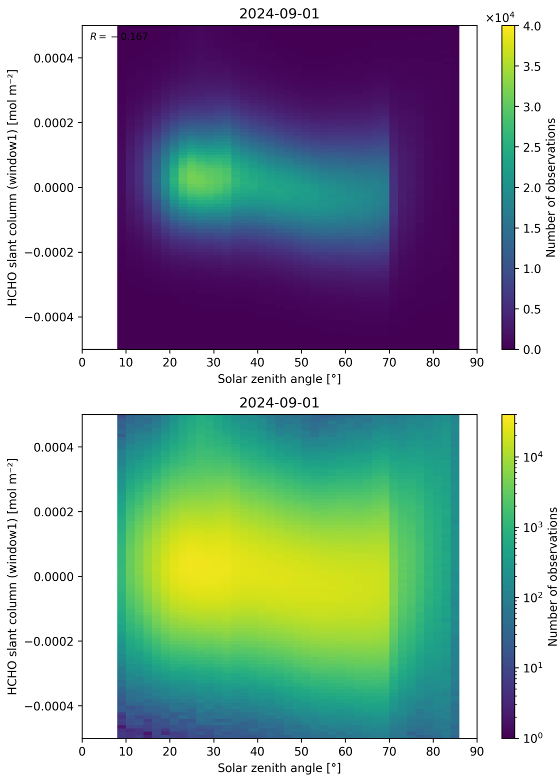
Figure 173: Scatter density plot of “Solar zenith angle” against “HCHO slant column (window1)” for 2024-09-01 to 2024-09-02.
