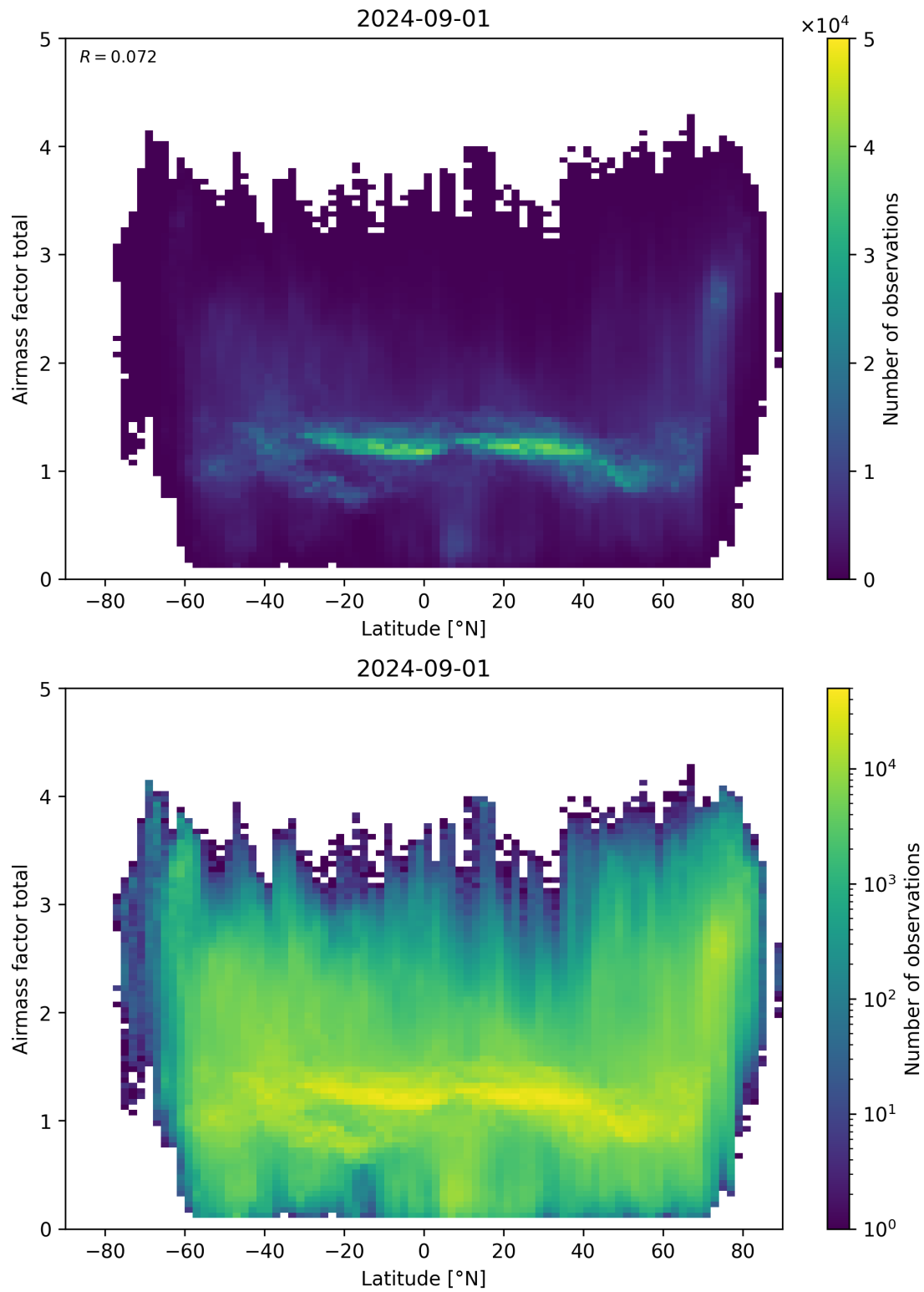
Figure 161: Scatter density plot of “Latitude” against “Airmass factor total” for 2024-09-01 to 2024-09-02.
