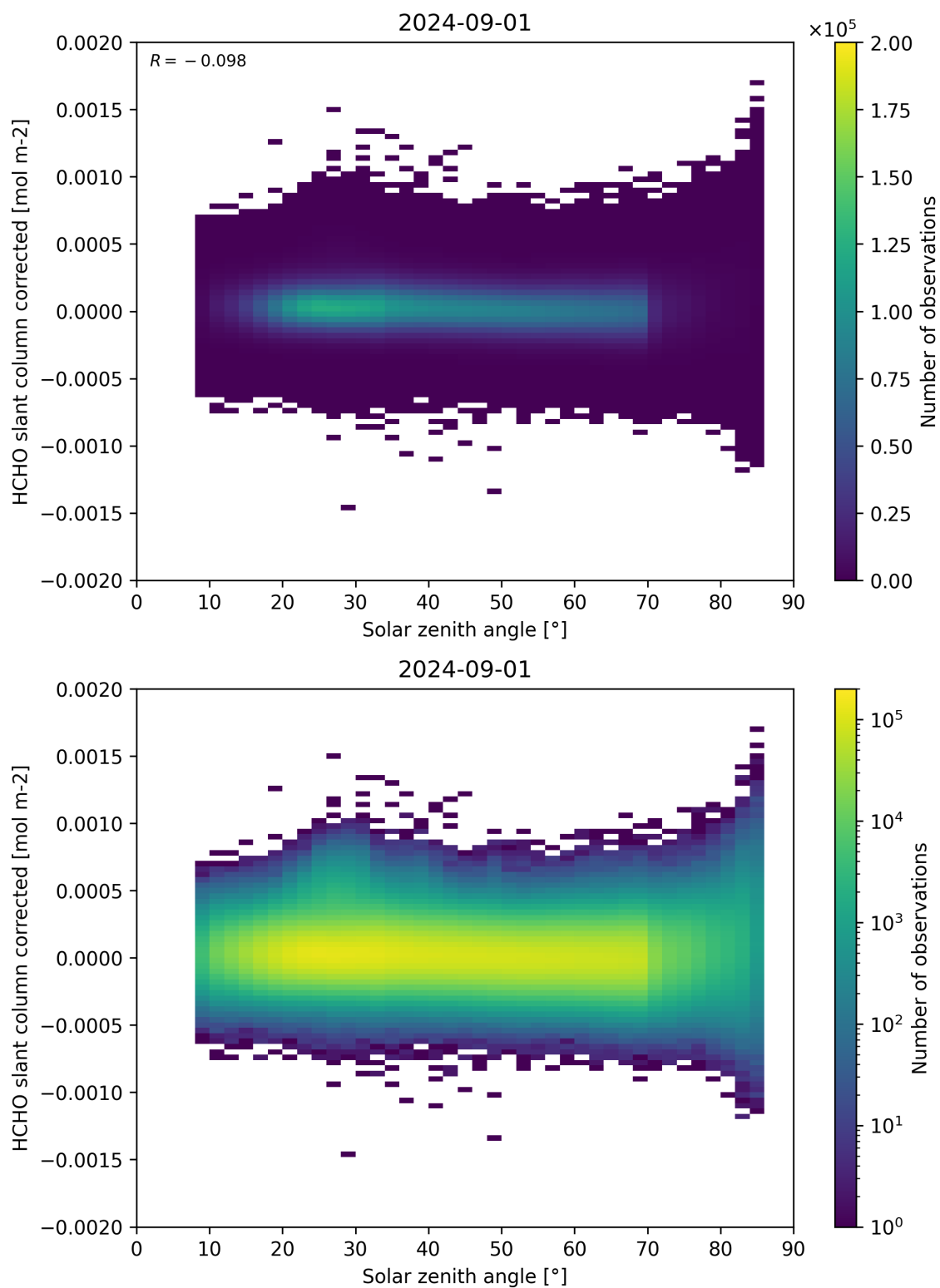
Figure 171: Scatter density plot of “Solar zenith angle” against “HCHO slant column corrected” for 2024-09-01 to 2024-09-02.
