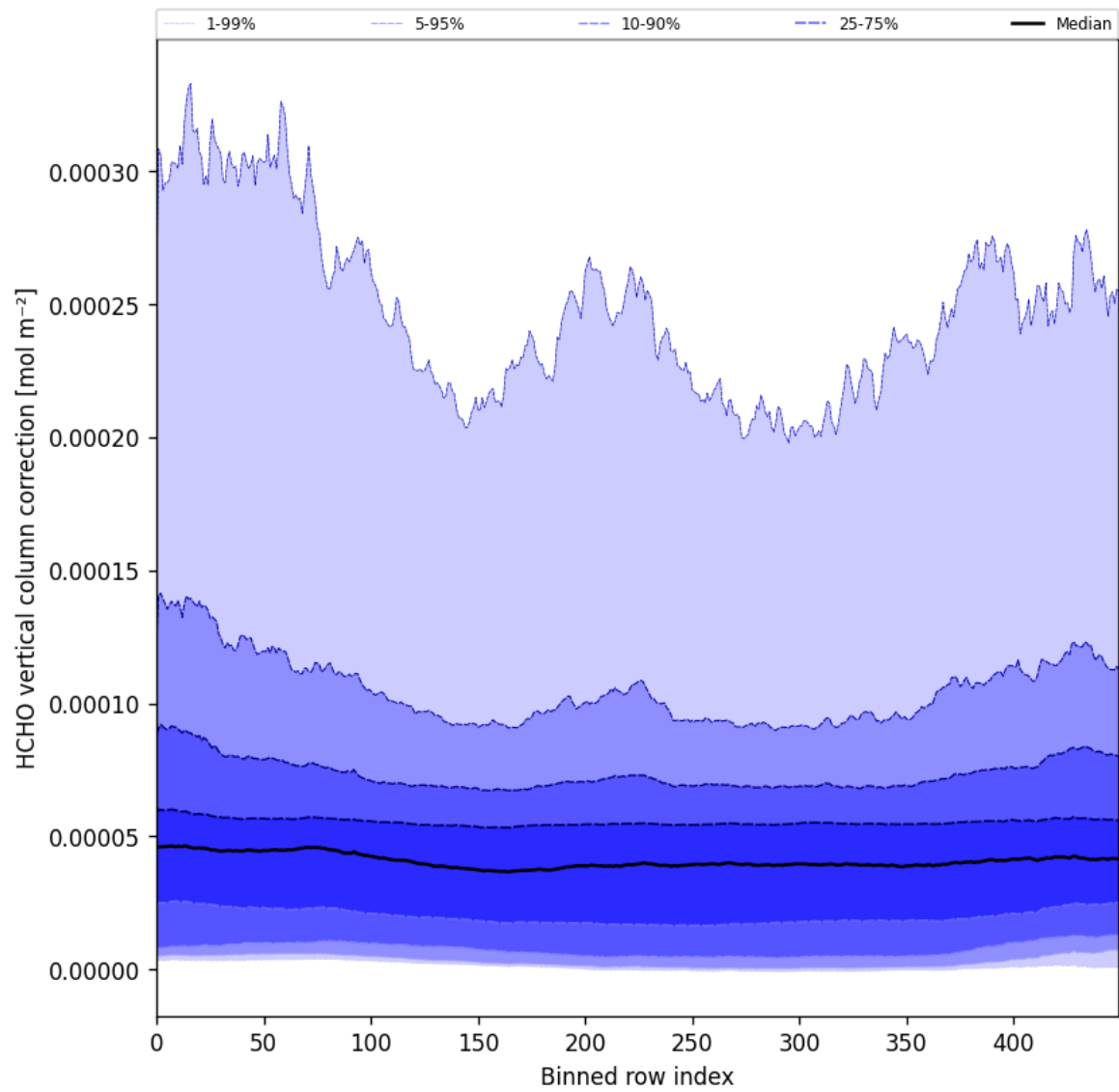
Figure 51: Along track statistics of “HCHO vertical column correction” for 2024-09-01 to 2024-09-02
