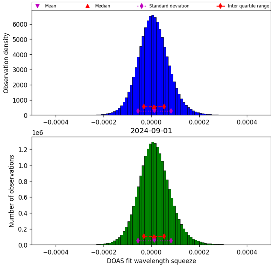
Figure 45: Histogram of “DOAS fit wavelength squeeze” for 2024-09-01 to 2024-09-02
