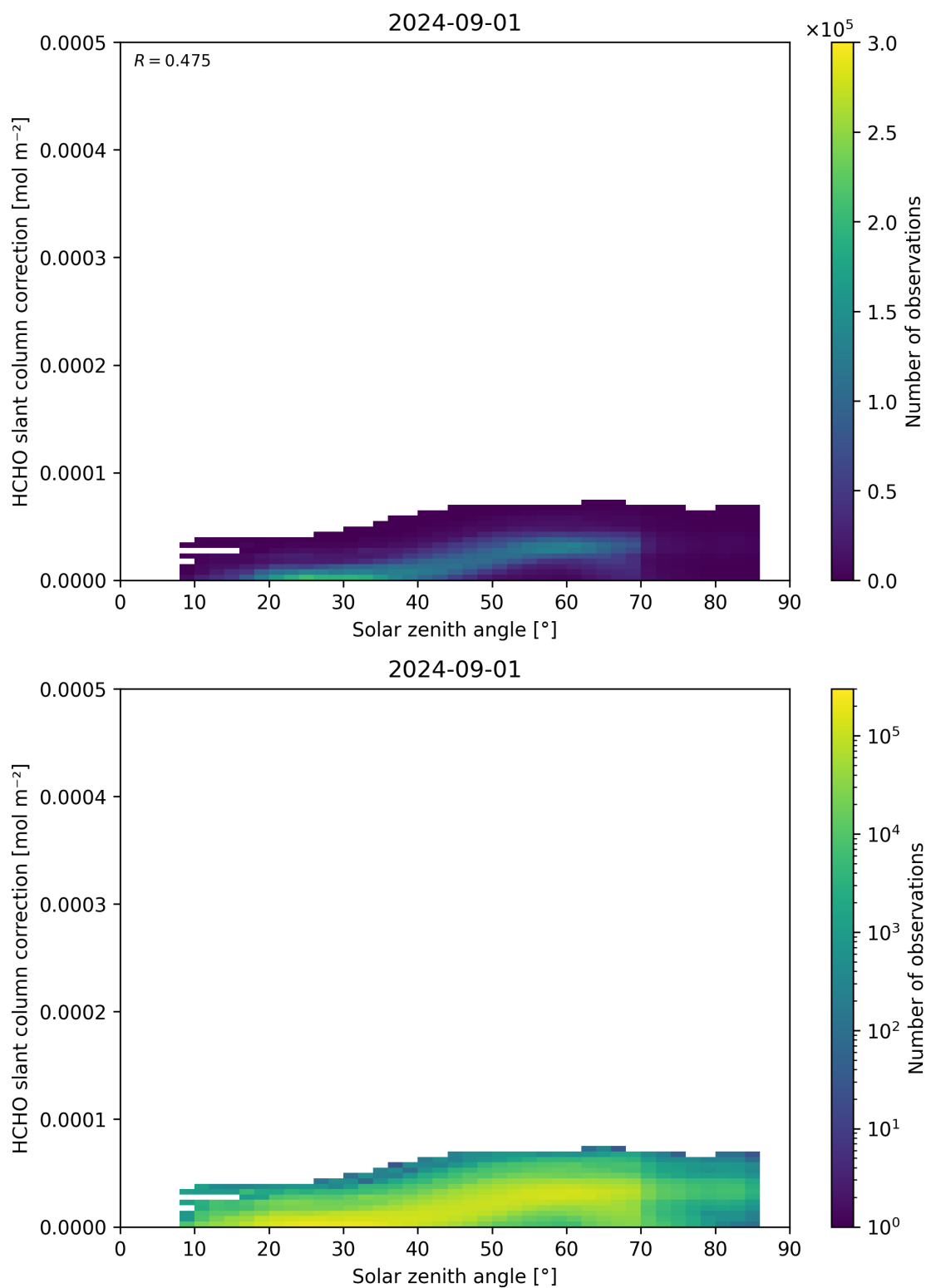
Figure 172: Scatter density plot of “Solar zenith angle” against “HCHO slant column correction” for 2024-09-01 to 2024-09-02.
