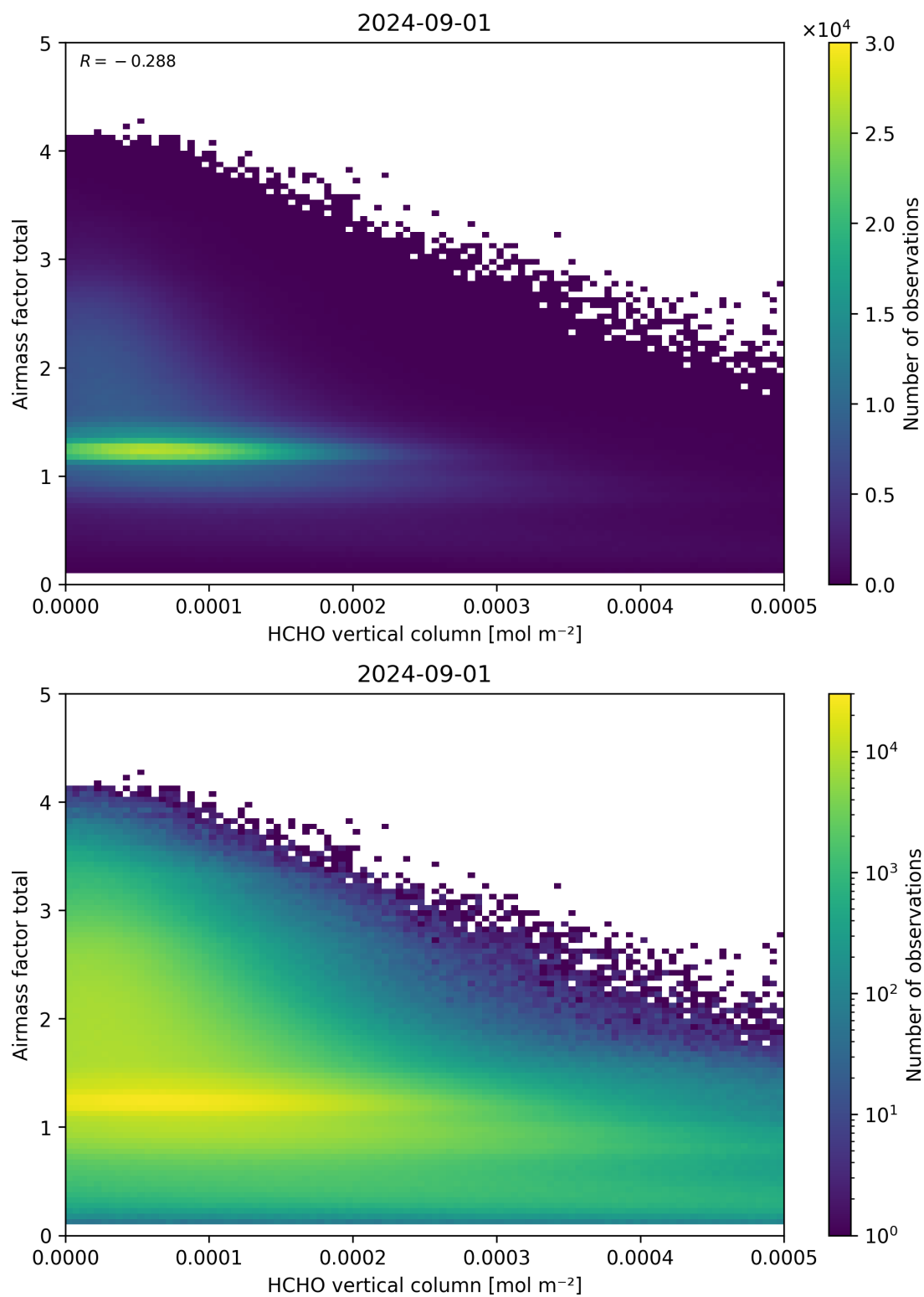
Figure 131: Scatter density plot of “HCHO vertical column” against “Airmass factor total” for 2024-09-01 to 2024-09-02.
