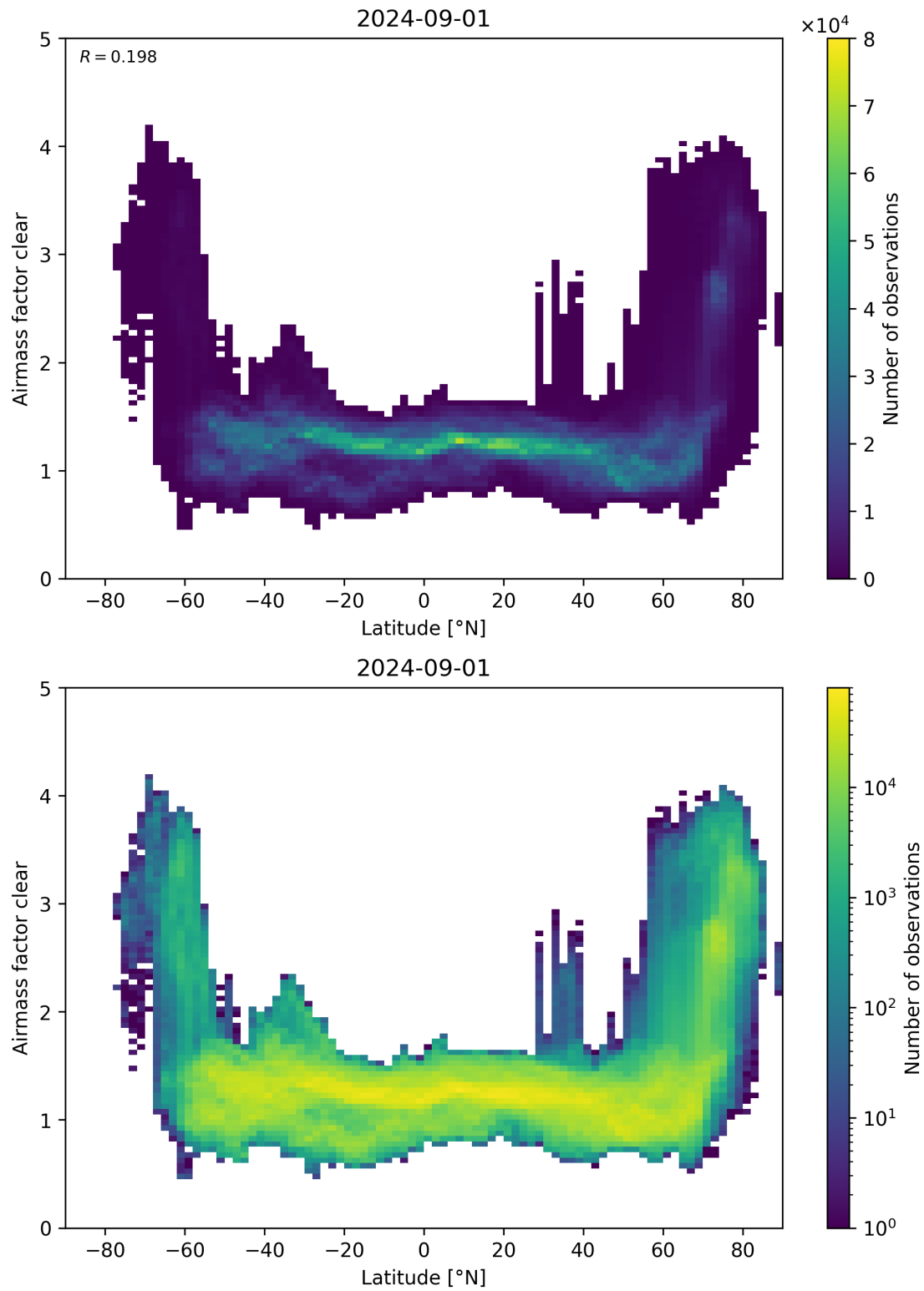
Figure 156: Scatter density plot of “Latitude” against “Airmass factor clear” for 2024-09-01 to 2024-09-02.
