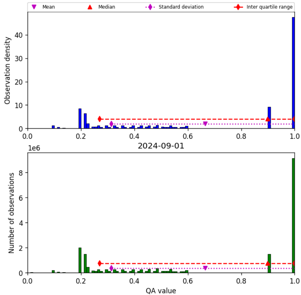
Figure 34: Histogram of “QA value” for 2024-09-01 to 2024-09-02
