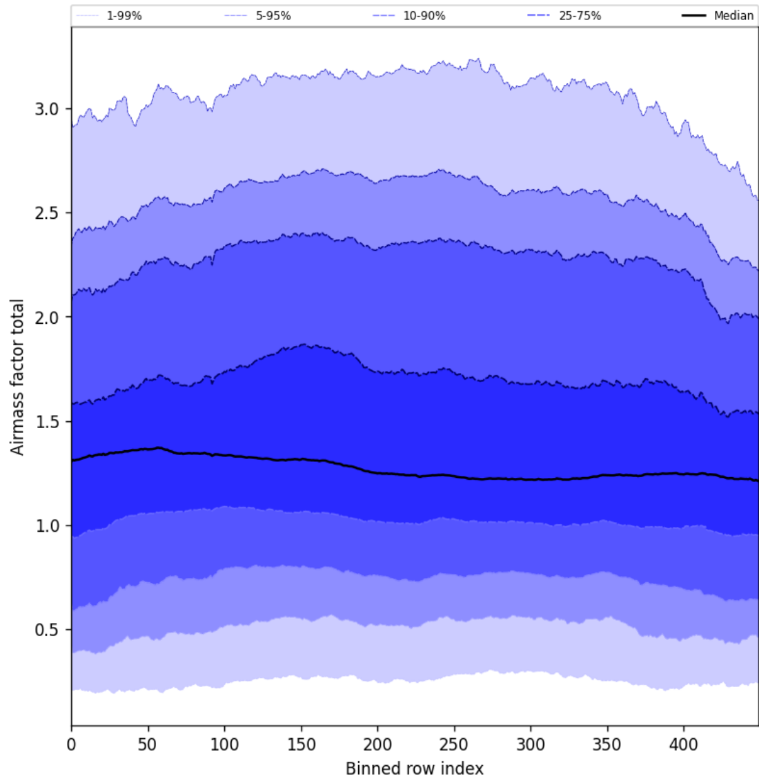
Figure 54: Along track statistics of “Airmass factor total” for 2024-09-01 to 2024-09-02
