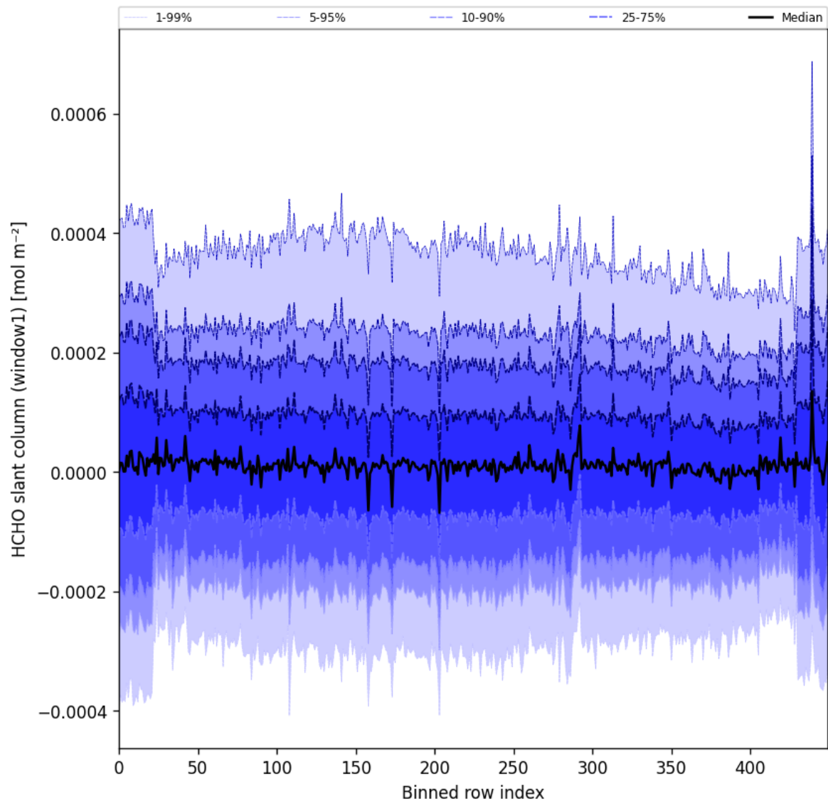
Figure 52: Along track statistics of “HCHO slant column (window1)” for 2024-09-01 to 2024-09-02
