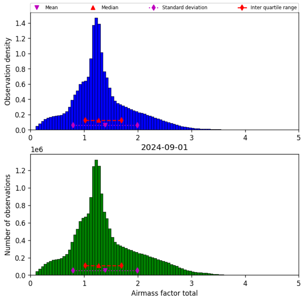
Figure 40: Histogram of “Airmass factor total” for 2024-09-01 to 2024-09-02
