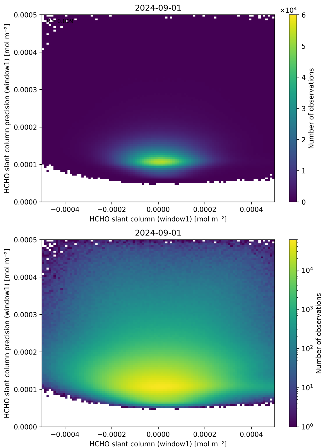
Figure 84: Scatter density plot of “HCHO slant column (window1)” against “HCHO slant column precision (window1)” for 2024-09-01 to 2024-09-02.
