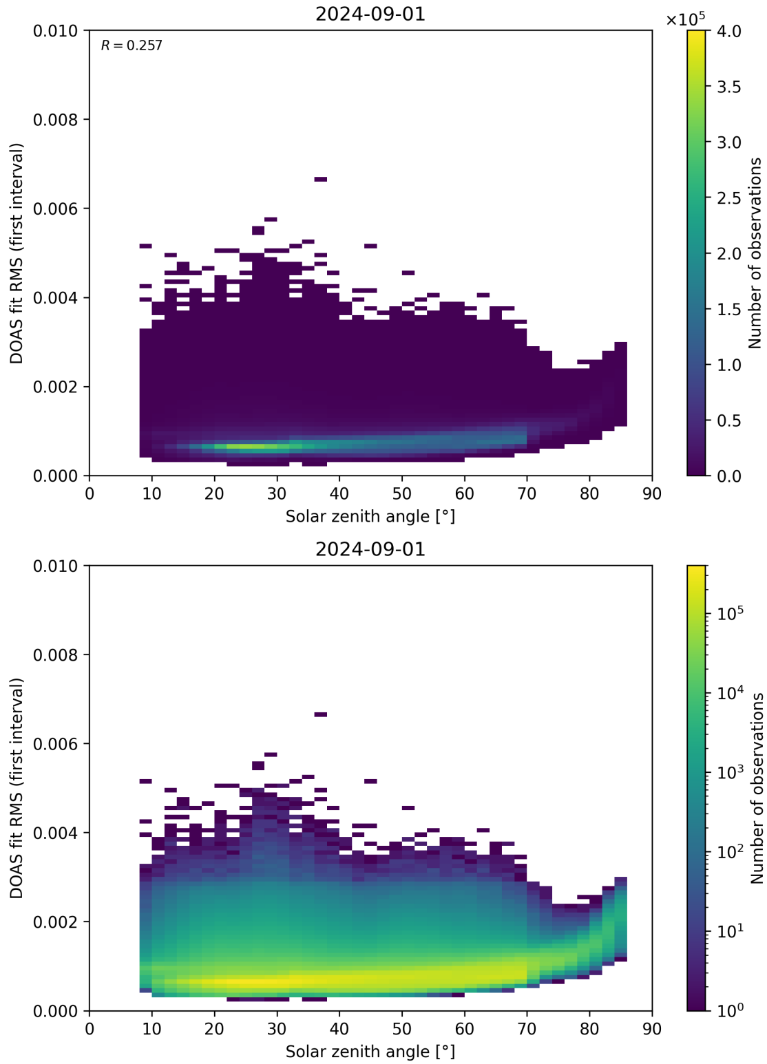
Figure 167: Scatter density plot of “Solar zenith angle” against “DOAS fit RMS (first interval)” for 2024-09-01 to 2024-09-02.
