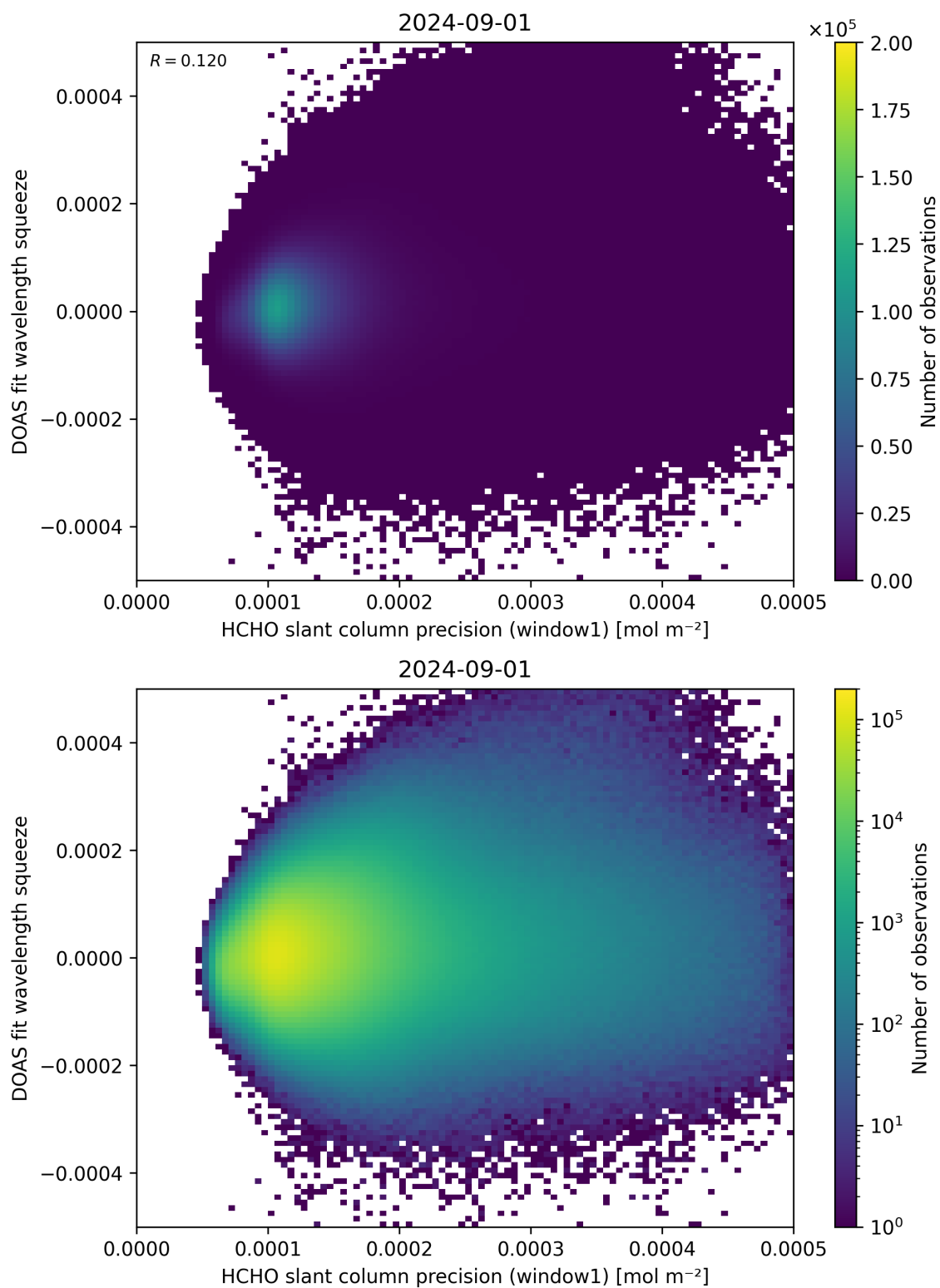
Figure 90: Scatter density plot of “HCHO slant column precision (window1)” against “DOAS fit wavelength squeeze” for 2024-09-01 to 2024-09-02.
