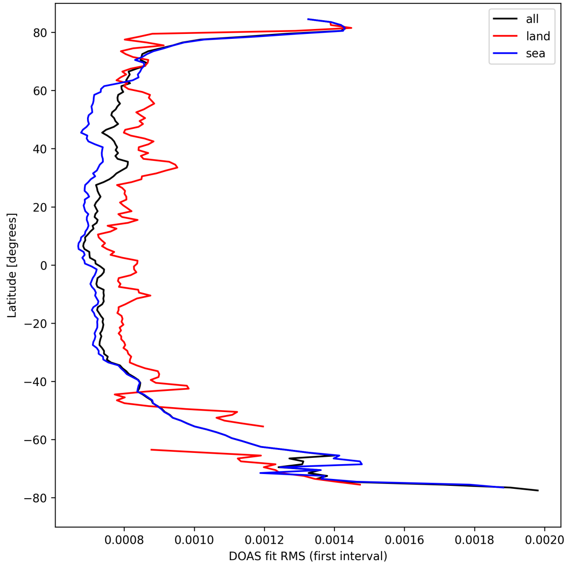
Figure 32: Zonal average of "DOAS fit RMS (first interval)" for 2024-09-01 to 2024-09-02.
