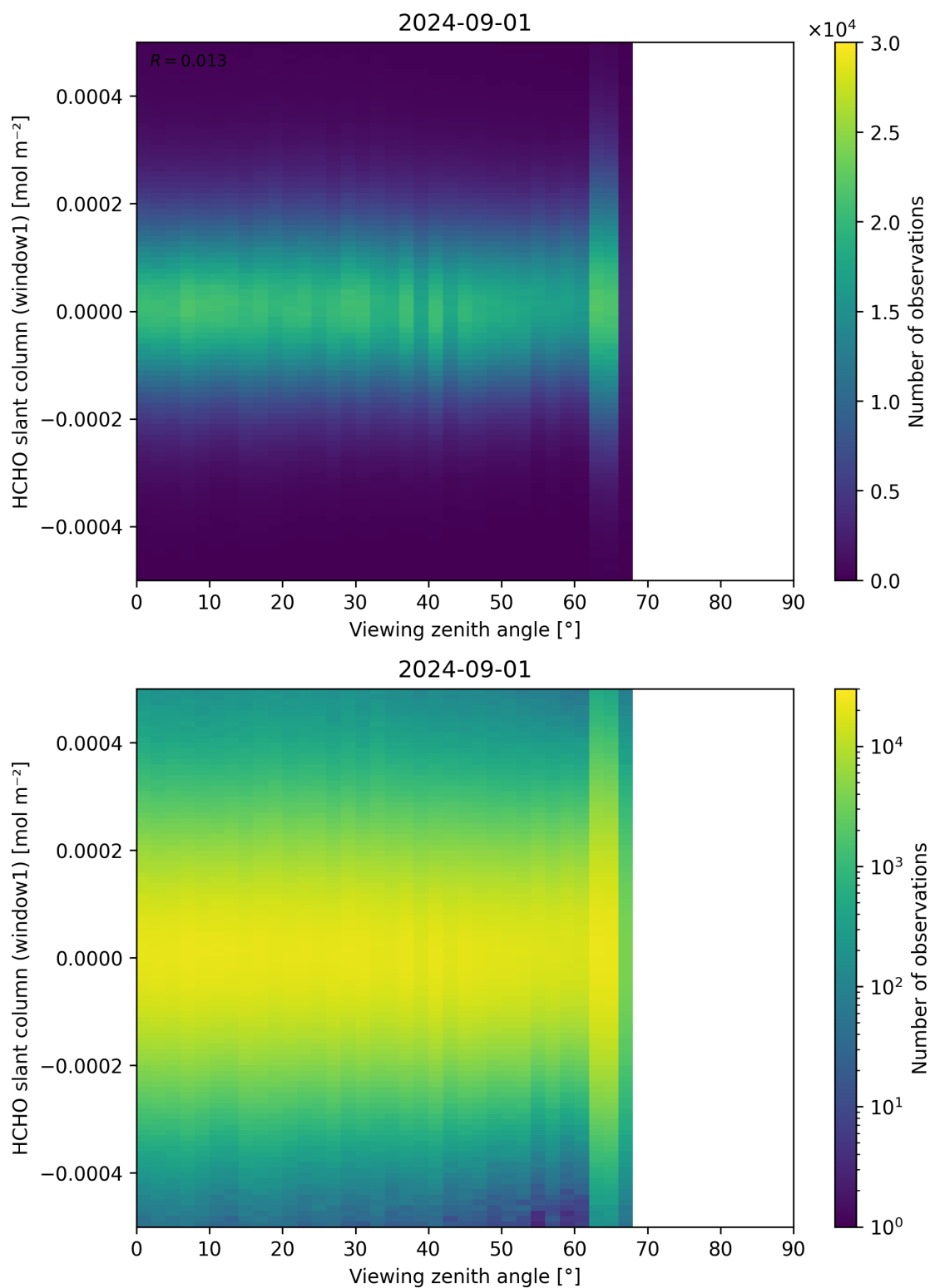
Figure 188: Scatter density plot of “Viewing zenith angle” against “HCHO slant column (window1)” for 2024-09-01 to 2024-09-02.
