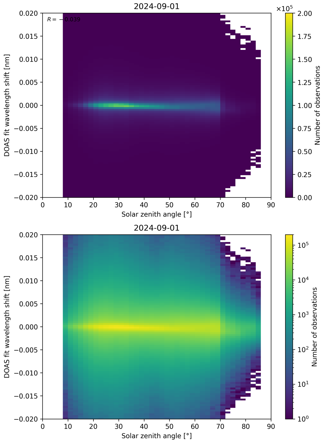
Figure 168: Scatter density plot of “Solar zenith angle” against “DOAS fit wavelength shift” for 2024-09-01 to 2024-09-02.
