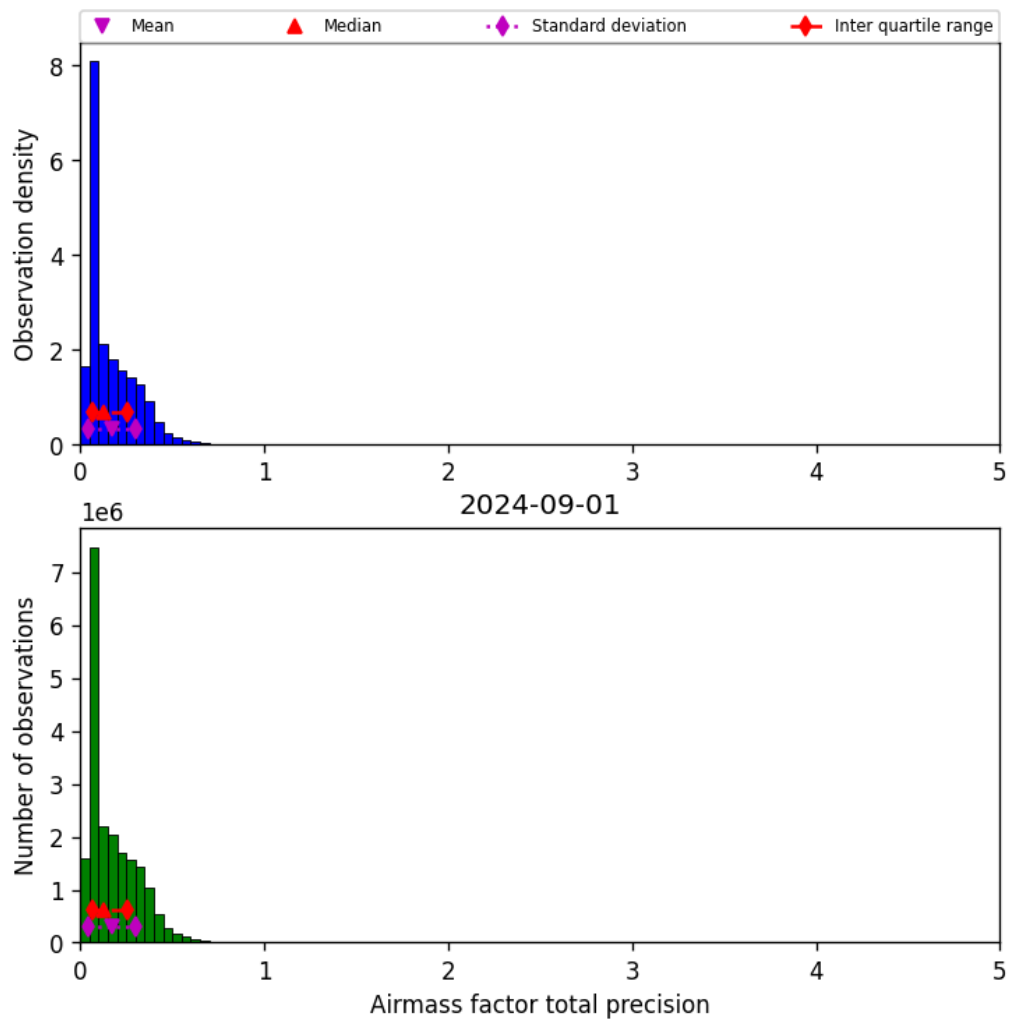
Figure 41: Histogram of “Airmass factor total precision” for 2024-09-01 to 2024-09-02
