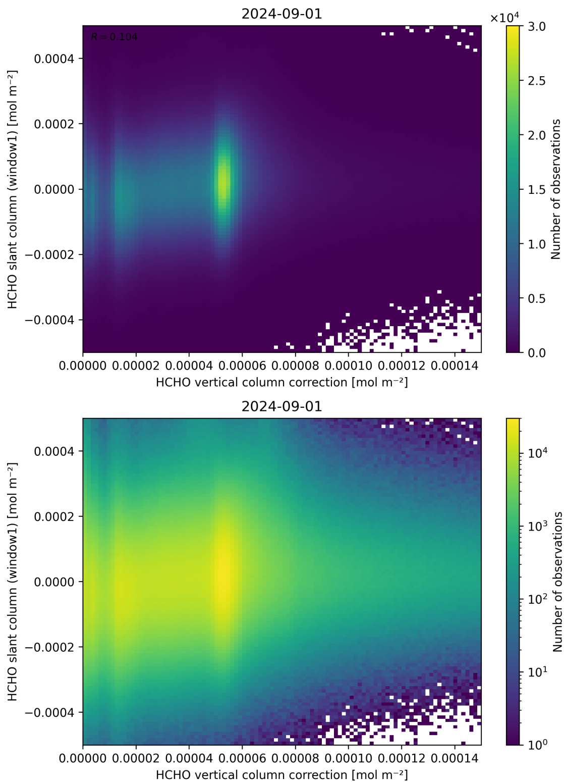
Figure 118: Scatter density plot of “HCHO vertical column correction” against “HCHO slant column (window1)” for 2024-09-01 to 2024-09-02.
