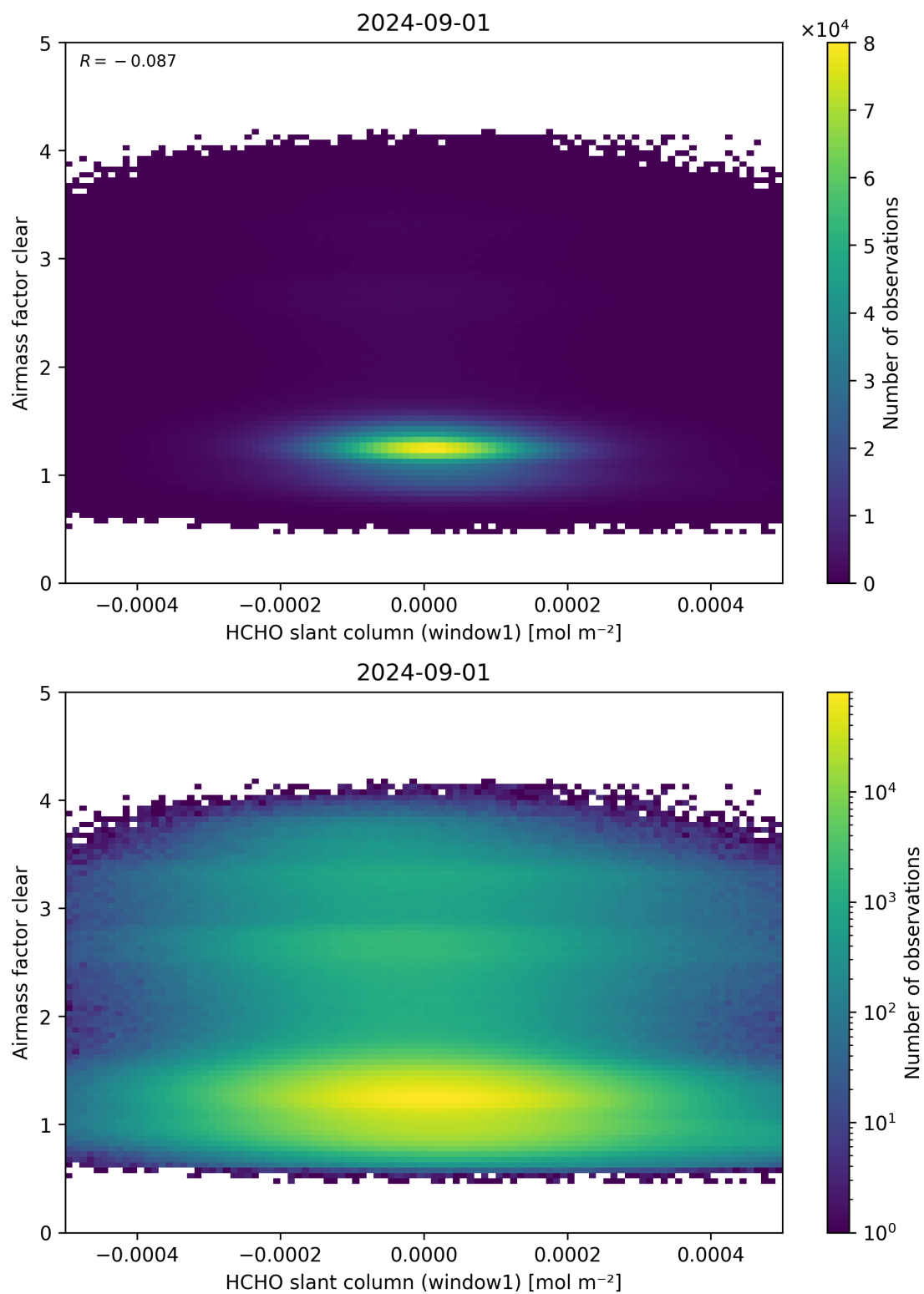
Figure 81: Scatter density plot of “HCHO slant column (window1)” against “Airmass factor clear” for 2024-09-01 to 2024-09-02.
