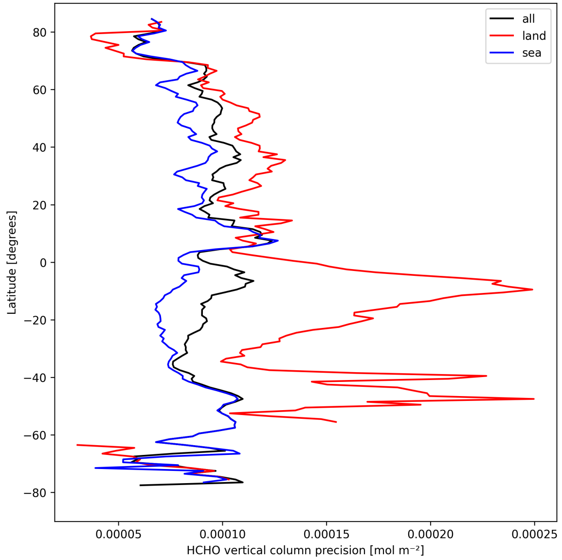
Figure 22: Zonal average of “HCHO vertical column precision” for 2024-09-01 to 2024-09-02.
