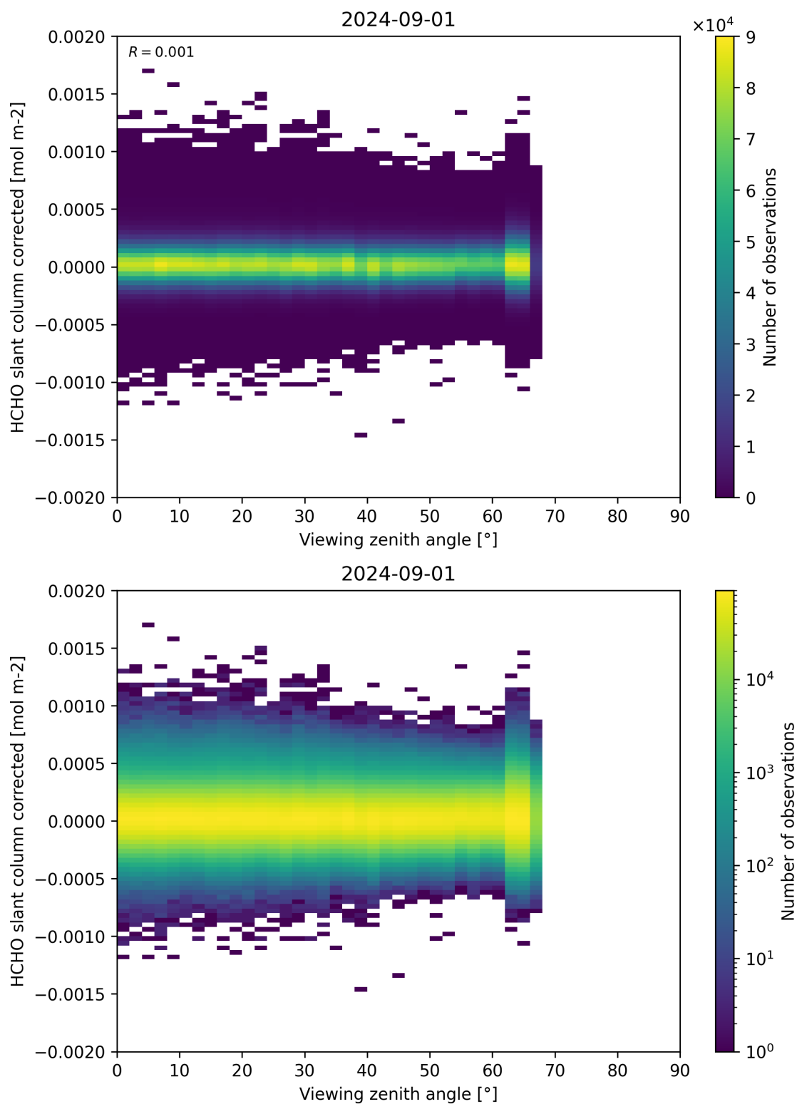
Figure 186: Scatter density plot of “Viewing zenith angle” against “HCHO slant column corrected” for 2024-09-01 to 2024-09-02.
