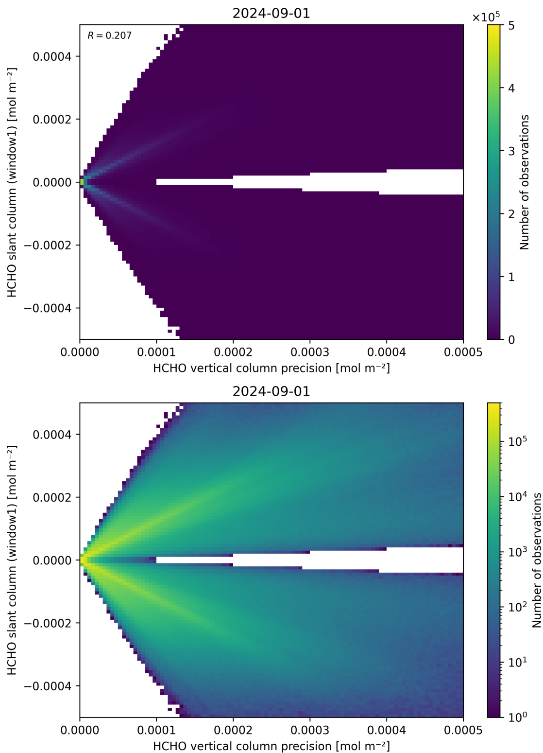
Figure 142: Scatter density plot of “HCHO vertical column precision” against “HCHO slant column (window1)” for 2024-09-01 to 2024-09-02.
