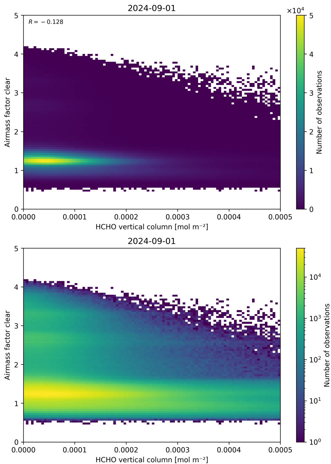
Figure 126: Scatter density plot of “HCHO vertical column” against “Airmass factor clear” for 2024-09-01 to 2024-09-02.
