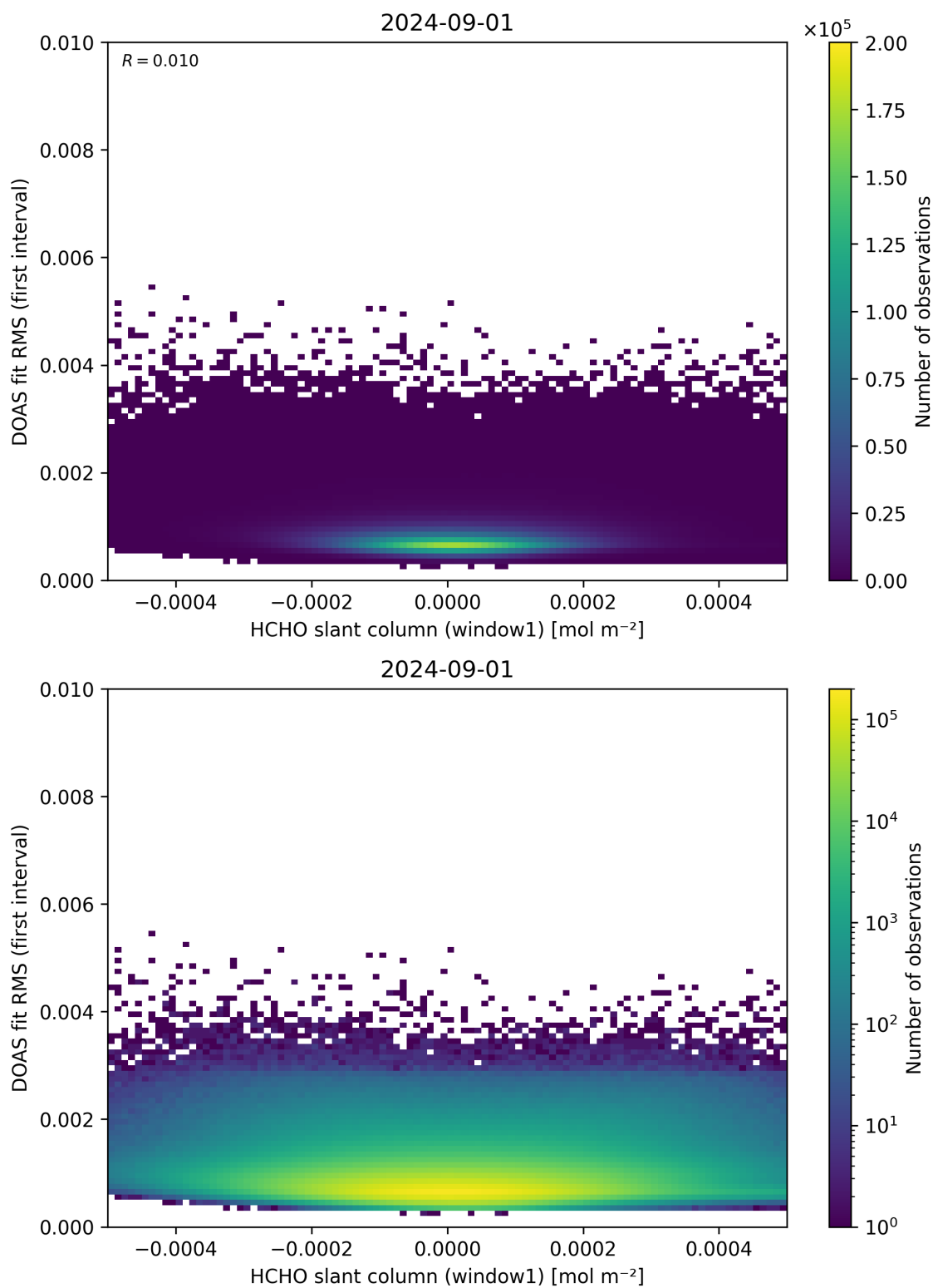
Figure 78: Scatter density plot of “HCHO slant column (window1)” against “DOAS fit RMS (first interval)” for 2024-09-01 to 2024-09-02.
