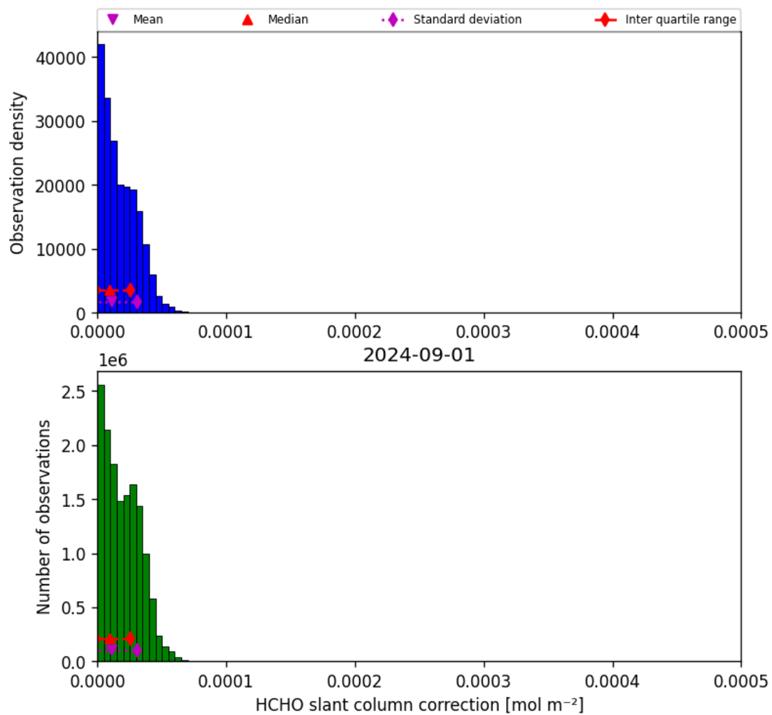
Figure 47: Histogram of “HCHO slant column correction” for 2024-09-01 to 2024-09-02
