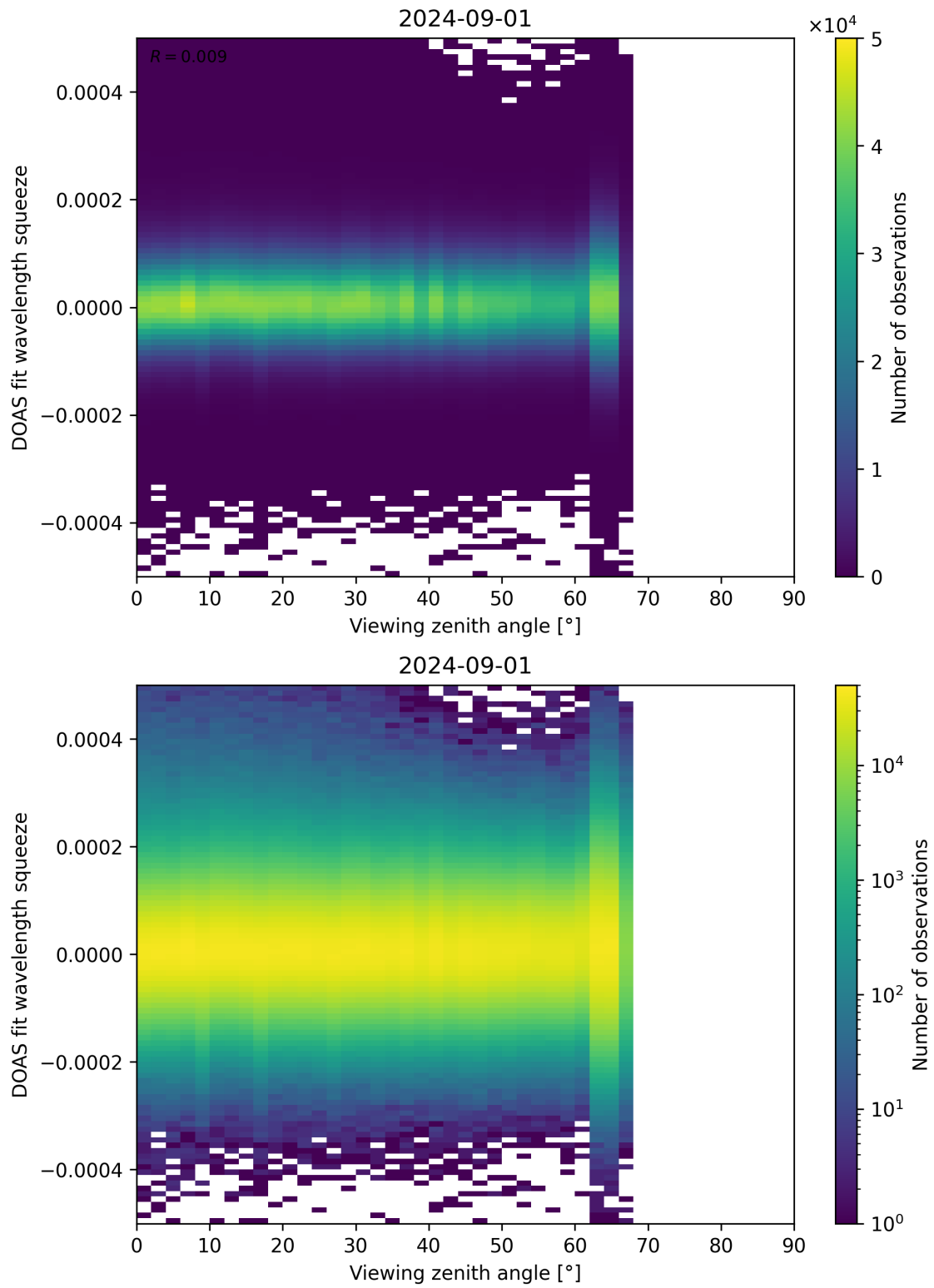
Figure 184: Scatter density plot of “Viewing zenith angle” against “DOAS fit wavelength squeeze” for 2024-09-01 to 2024-09-02.
