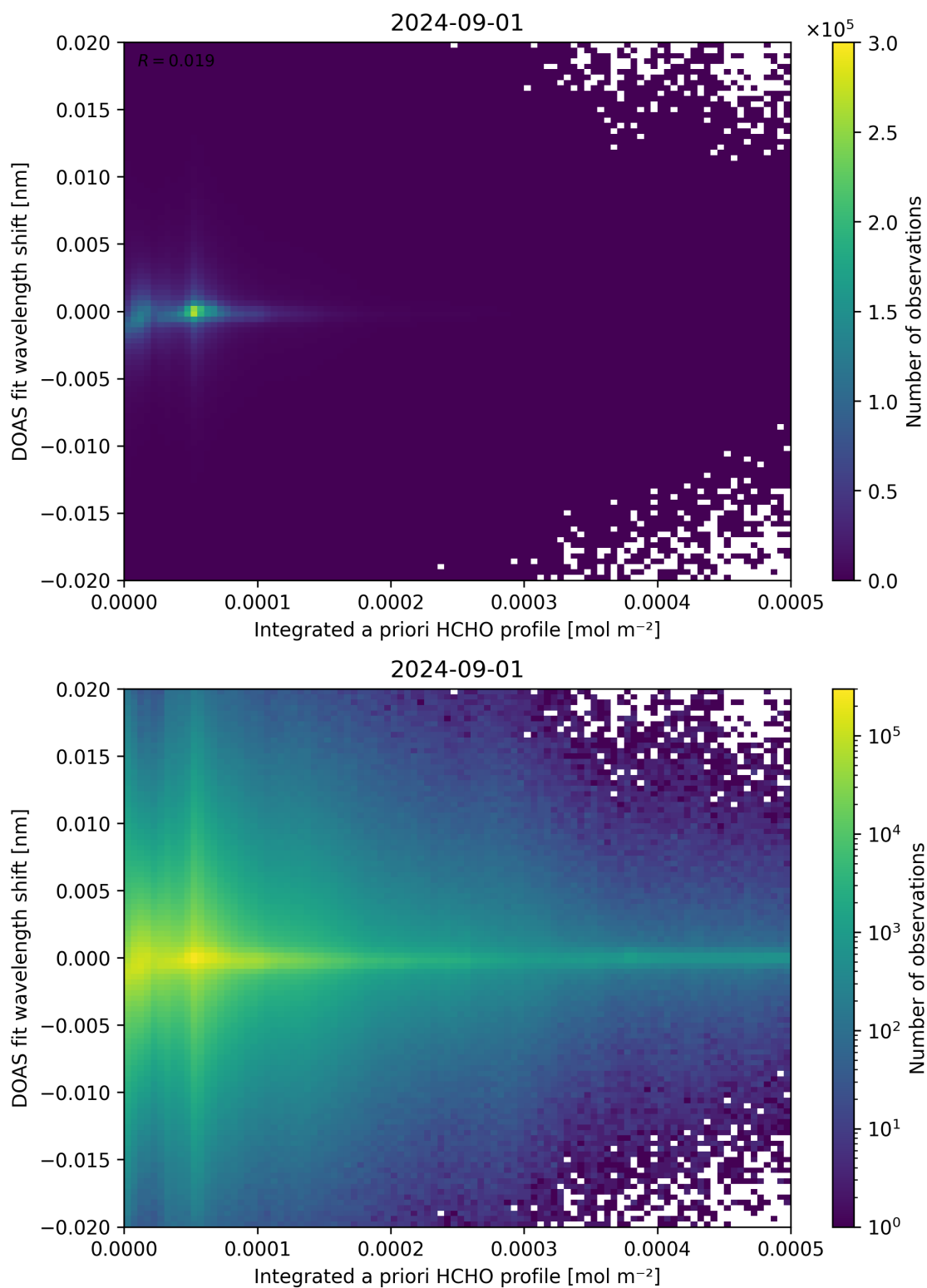
Figure 149: Scatter density plot of “Integrated a priori HCHO profile” against “DOAS fit wavelength shift” for 2024-09-01 to 2024-09-02.
