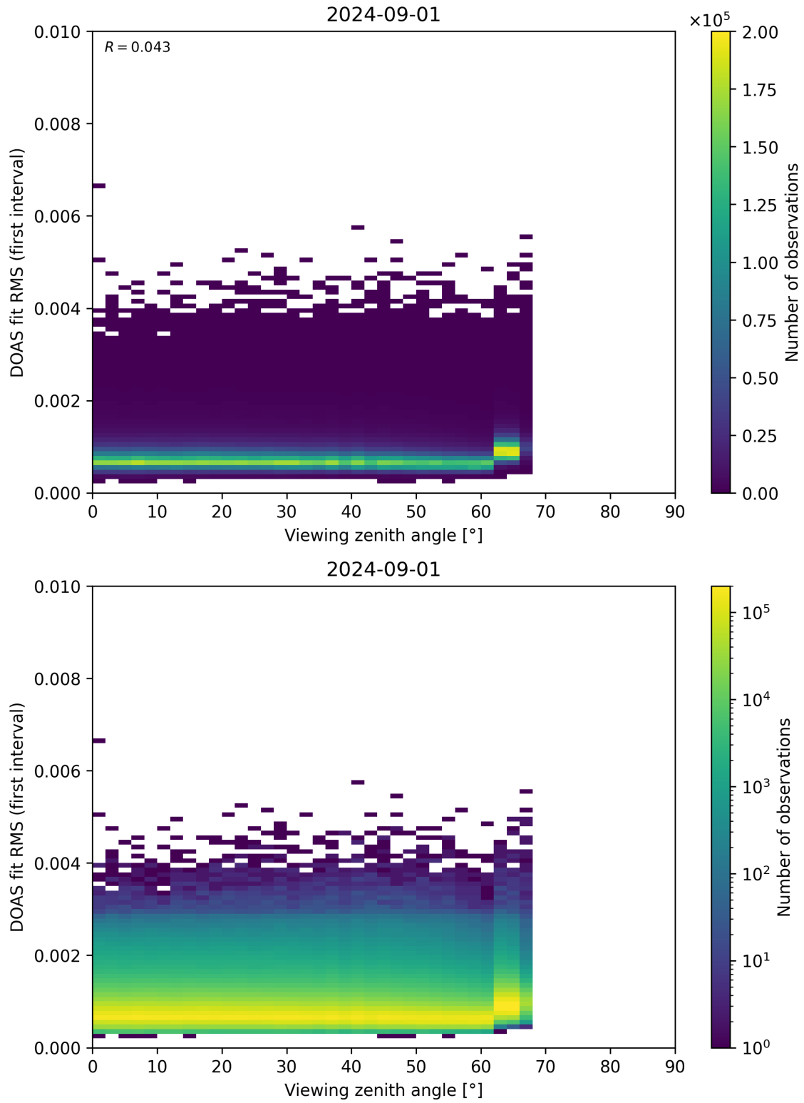
Figure 182: Scatter density plot of “Viewing zenith angle” against “DOAS fit RMS (first interval)” for 2024-09-01 to 2024-09-02.
