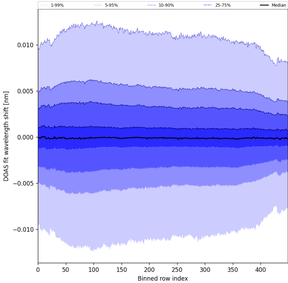
Figure 58: Along track statistics of “DOAS fit wavelength shift” for 2024-09-01 to 2024-09-02
