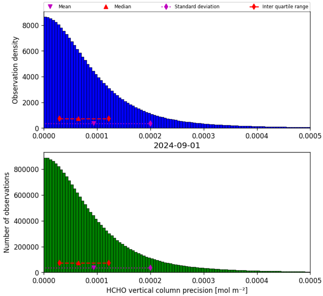
Figure 36: Histogram of “HCHO vertical column precision” for 2024-09-01 to 2024-09-02
