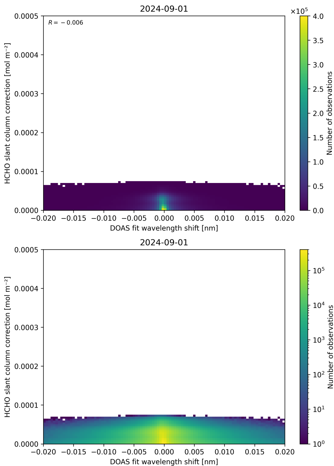
Figure 67: Scatter density plot of “DOAS fit wavelength shift” against “HCHO slant column correction” for 2024-09-01 to 2024-09-02.
