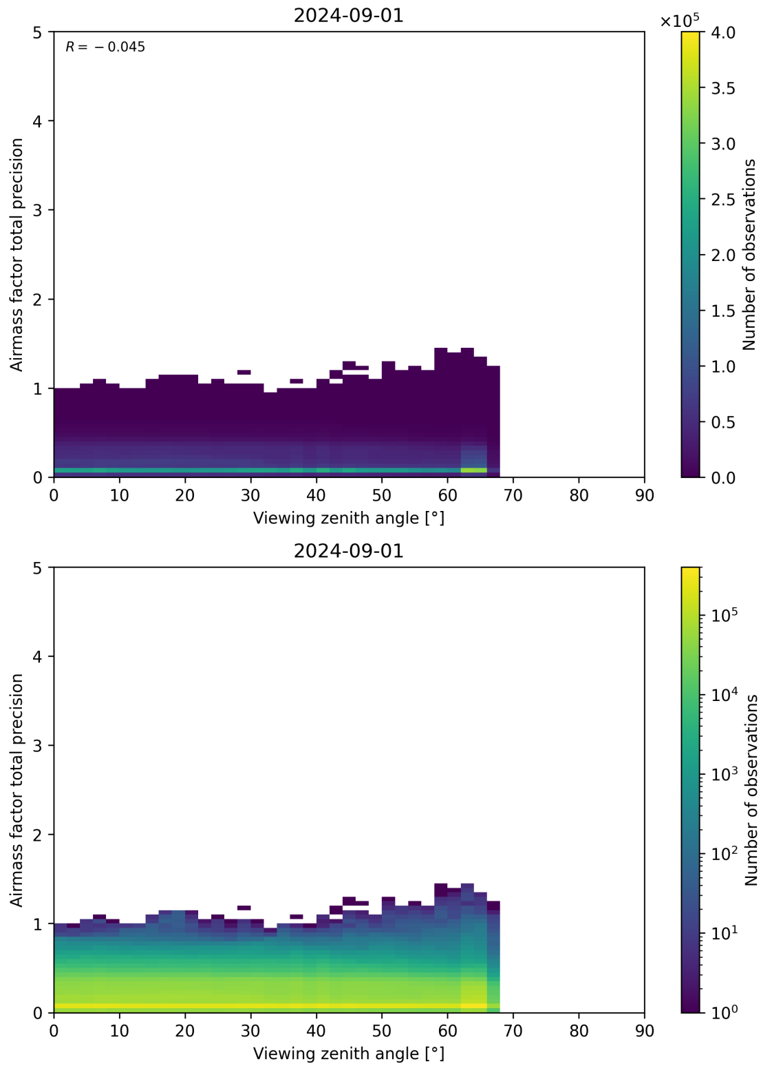
Figure 191: Scatter density plot of “Viewing zenith angle” against “Airmass factor total precision” for 2024-09-01 to 2024-09-02.
