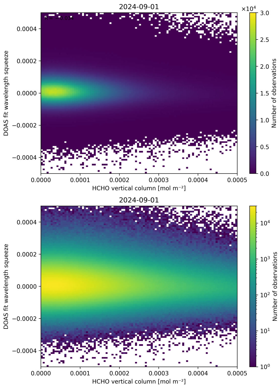
Figure 125: Scatter density plot of “HCHO vertical column” against “DOAS fit wavelength squeeze” for 2024-09-01 to 2024-09-02.
