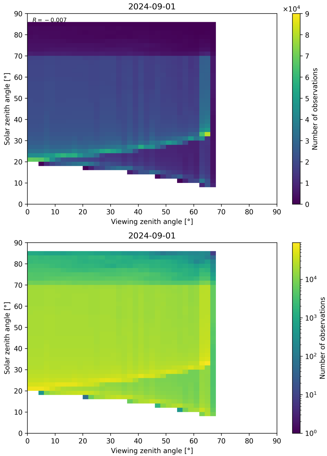
Figure 197: Scatter density plot of “Viewing zenith angle” against “Solar zenith angle” for 2024-09-01 to 2024-09-02.
