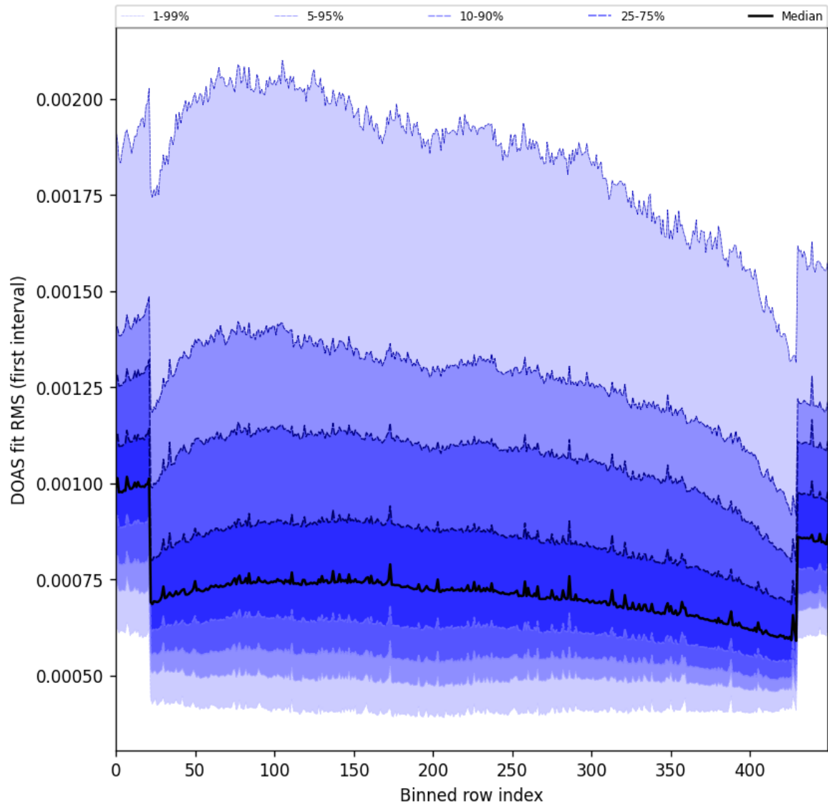
Figure 60: Along track statistics of “DOAS fit RMS (first interval)” for 2024-09-01 to 2024-09-02
