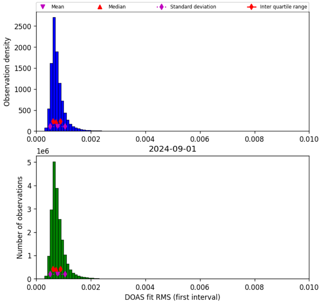
Figure 46: Histogram of “DOAS fit RMS (first interval)” for 2024-09-01 to 2024-09-02
