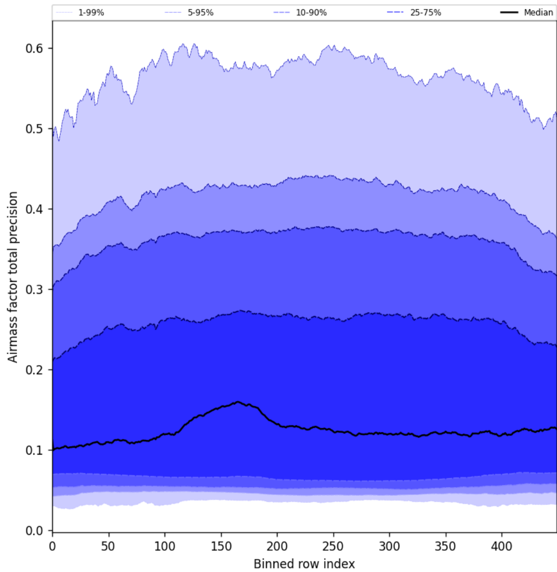
Figure 55: Along track statistics of “Airmass factor total precision” for 2024-09-01 to 2024-09-02
