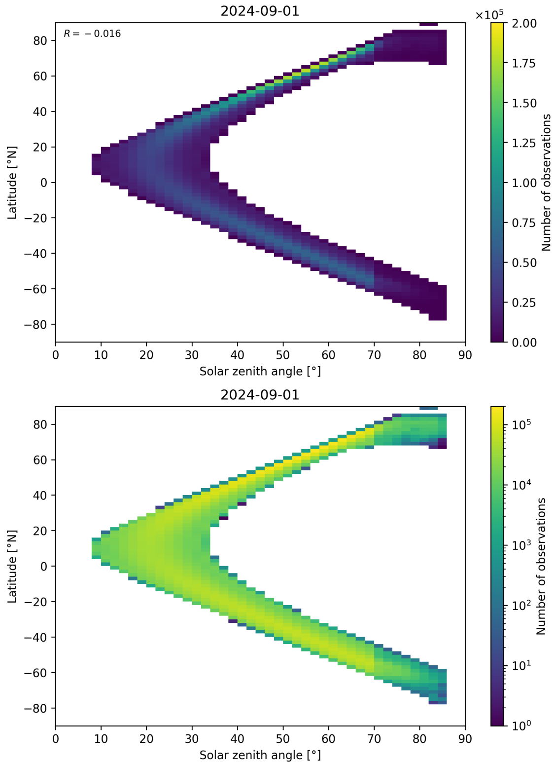
Figure 181: Scatter density plot of “Solar zenith angle” against “Latitude” for 2024-09-01 to 2024-09-02.
