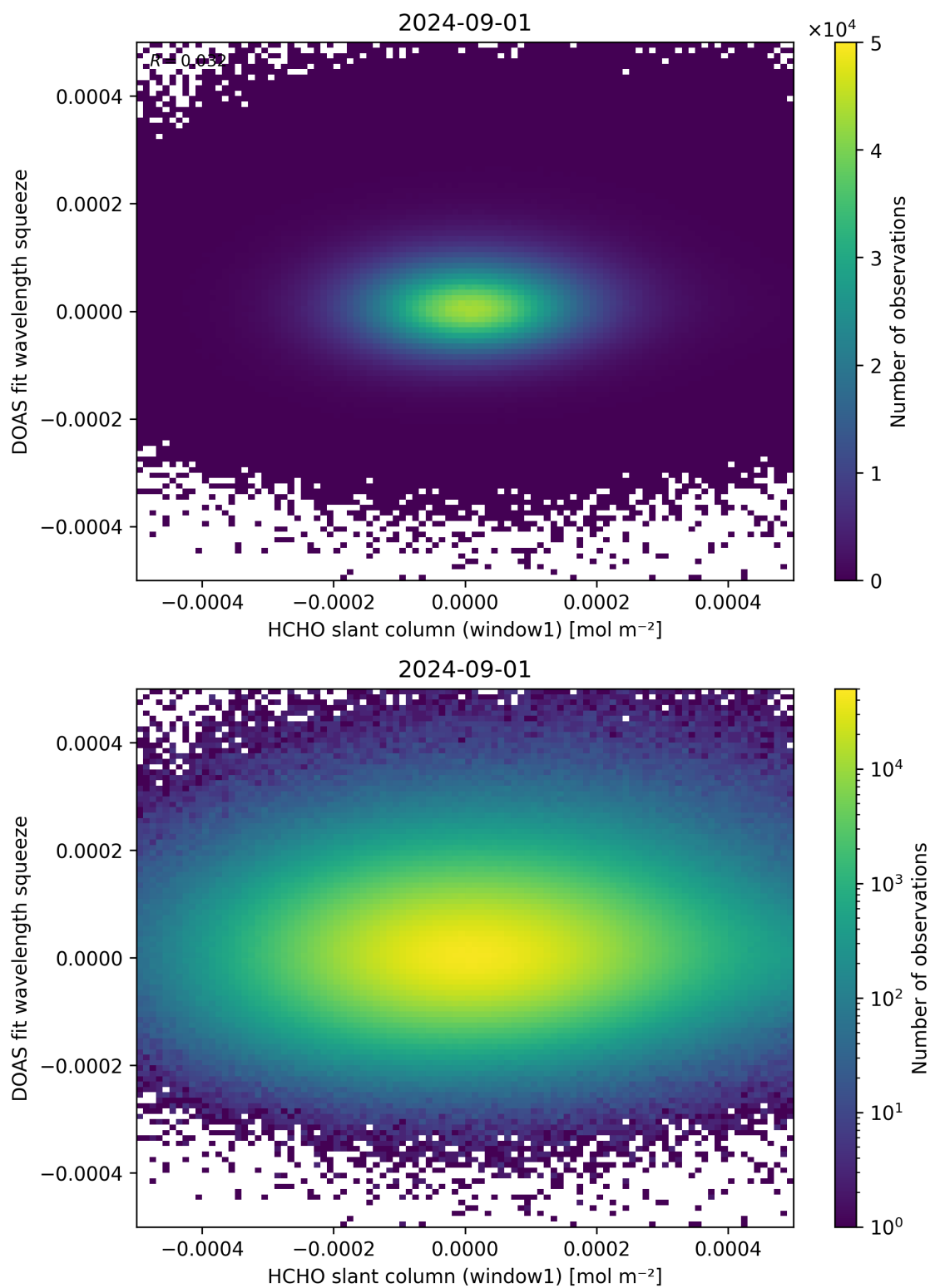
Figure 80: Scatter density plot of “HCHO slant column (window1)” against “DOAS fit wavelength squeeze” for 2024-09-01 to 2024-09-02.
