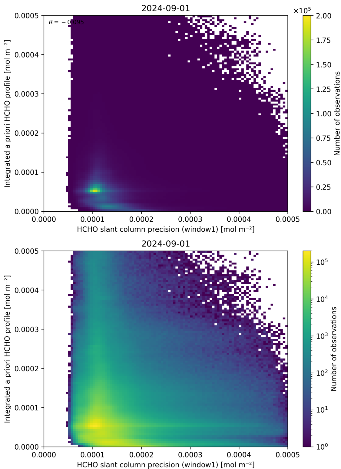
Figure 96: Scatter density plot of “HCHO slant column precision (window1)” against “Integrated a priori HCHO profile” for 2024-09-01 to 2024-09-02.
