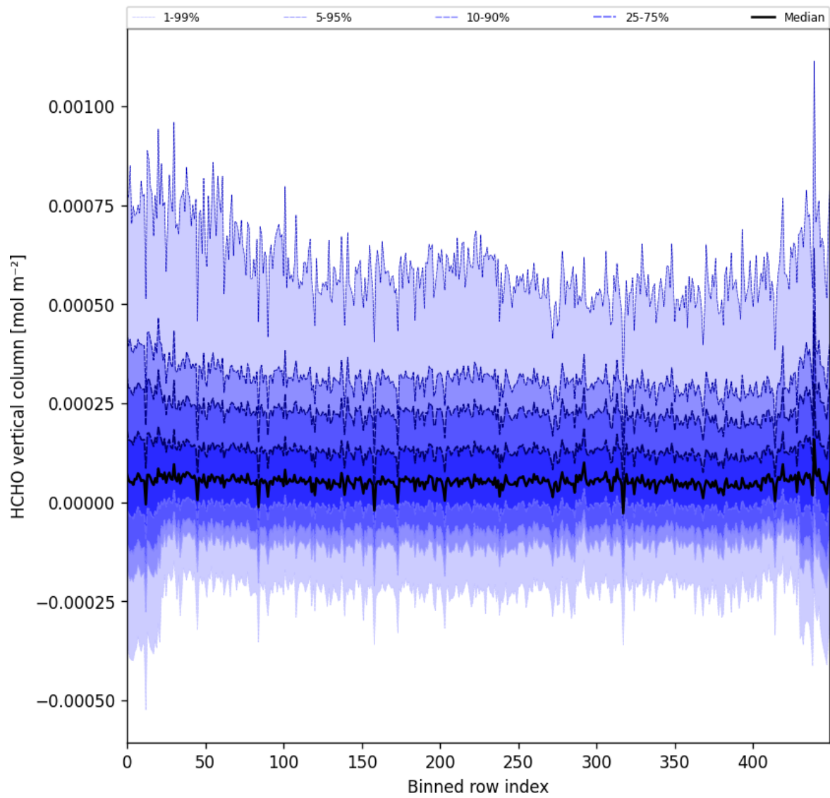
Figure 49: Along track statistics of “HCHO vertical column” for 2024-09-01 to 2024-09-02
