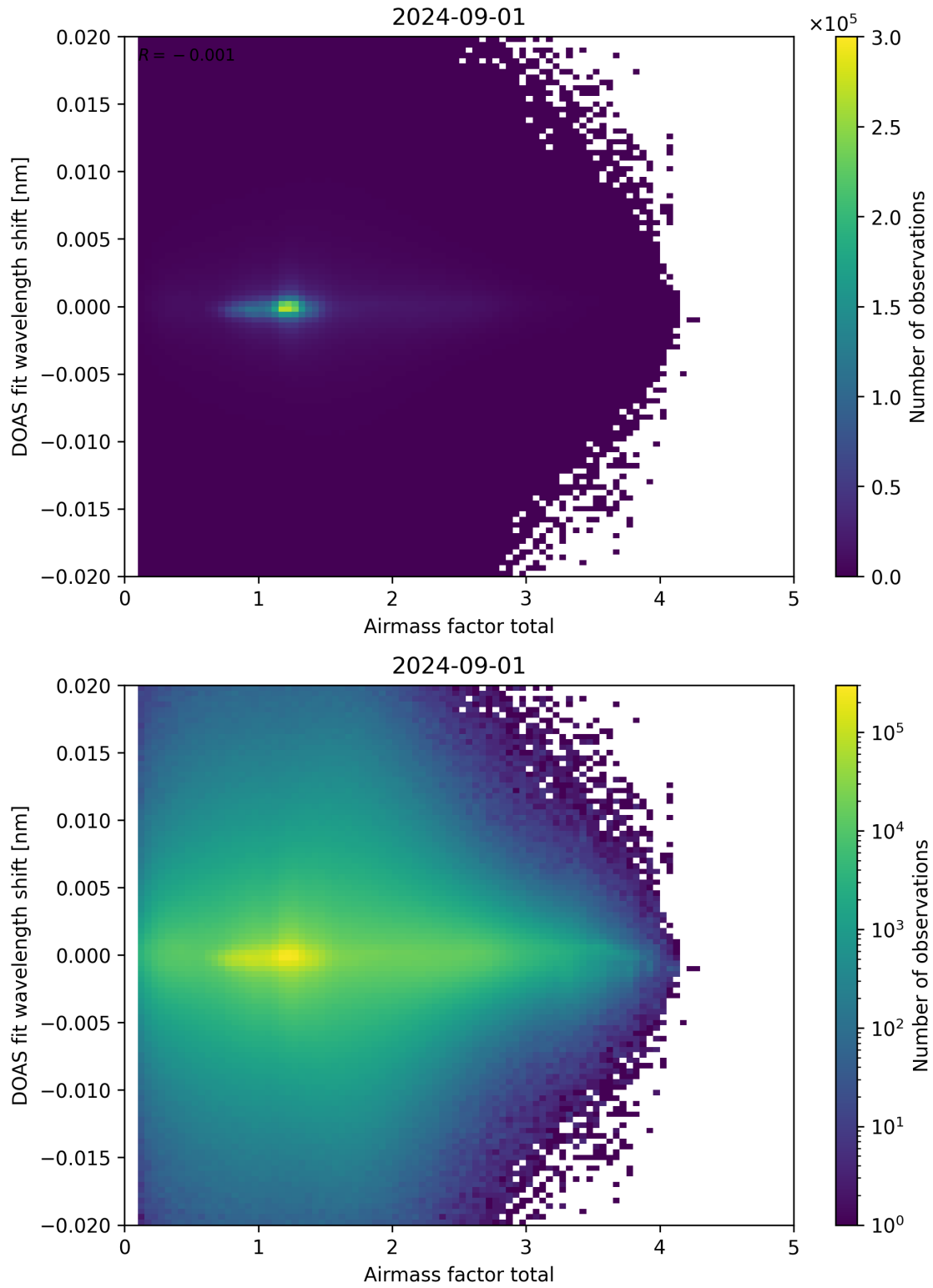
Figure 98: Scatter density plot of “Airmass factor total” against “DOAS fit wavelength shift” for 2024-09-01 to 2024-09-02.
