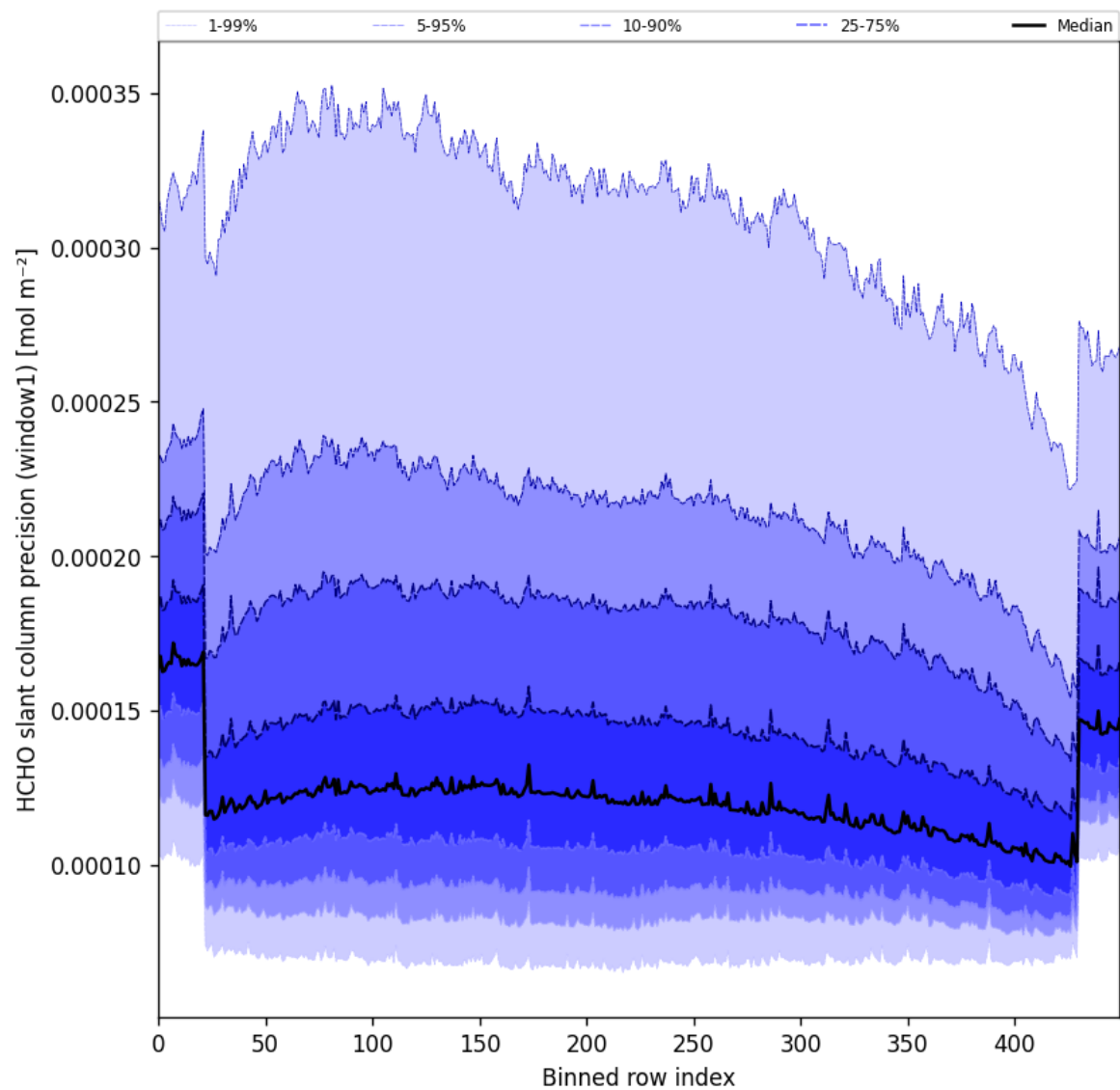
Figure 53: Along track statistics of “HCHO slant column precision (window1)” for 2024-09-01 to 2024-09-02
