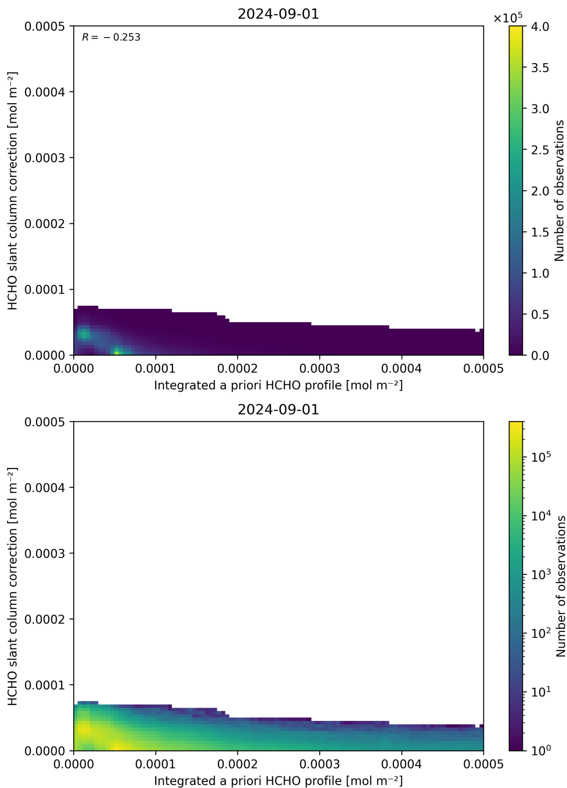
Figure 152: Scatter density plot of “Integrated a priori HCHO profile” against “HCHO slant column correction” for 2024-09-01 to 2024-09-02.
