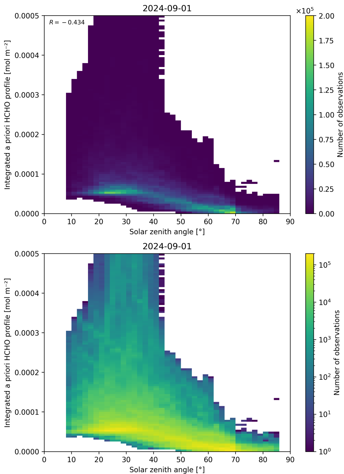
Figure 180: Scatter density plot of “Solar zenith angle” against “Integrated a priori HCHO profile” for 2024-09-01 to 2024-09-02.
