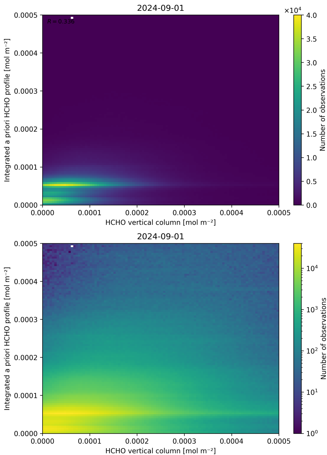
Figure 135: Scatter density plot of “HCHO vertical column” against “Integrated a priori HCHO profile” for 2024-09-01 to 2024-09-02.
