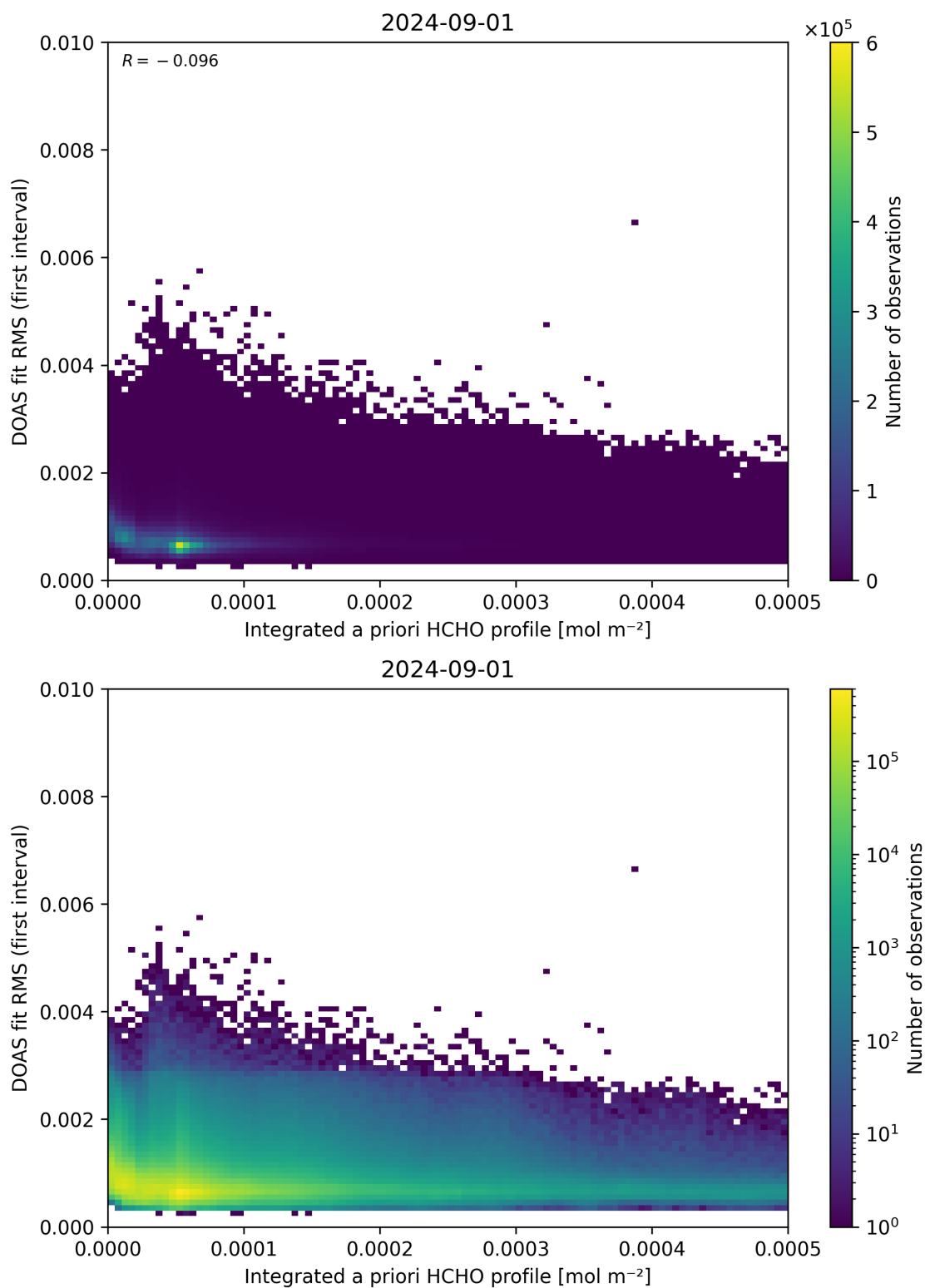
Figure 148: Scatter density plot of “Integrated a priori HCHO profile” against “DOAS fit RMS (first interval)” for 2024-09-01 to 2024-09-02.
