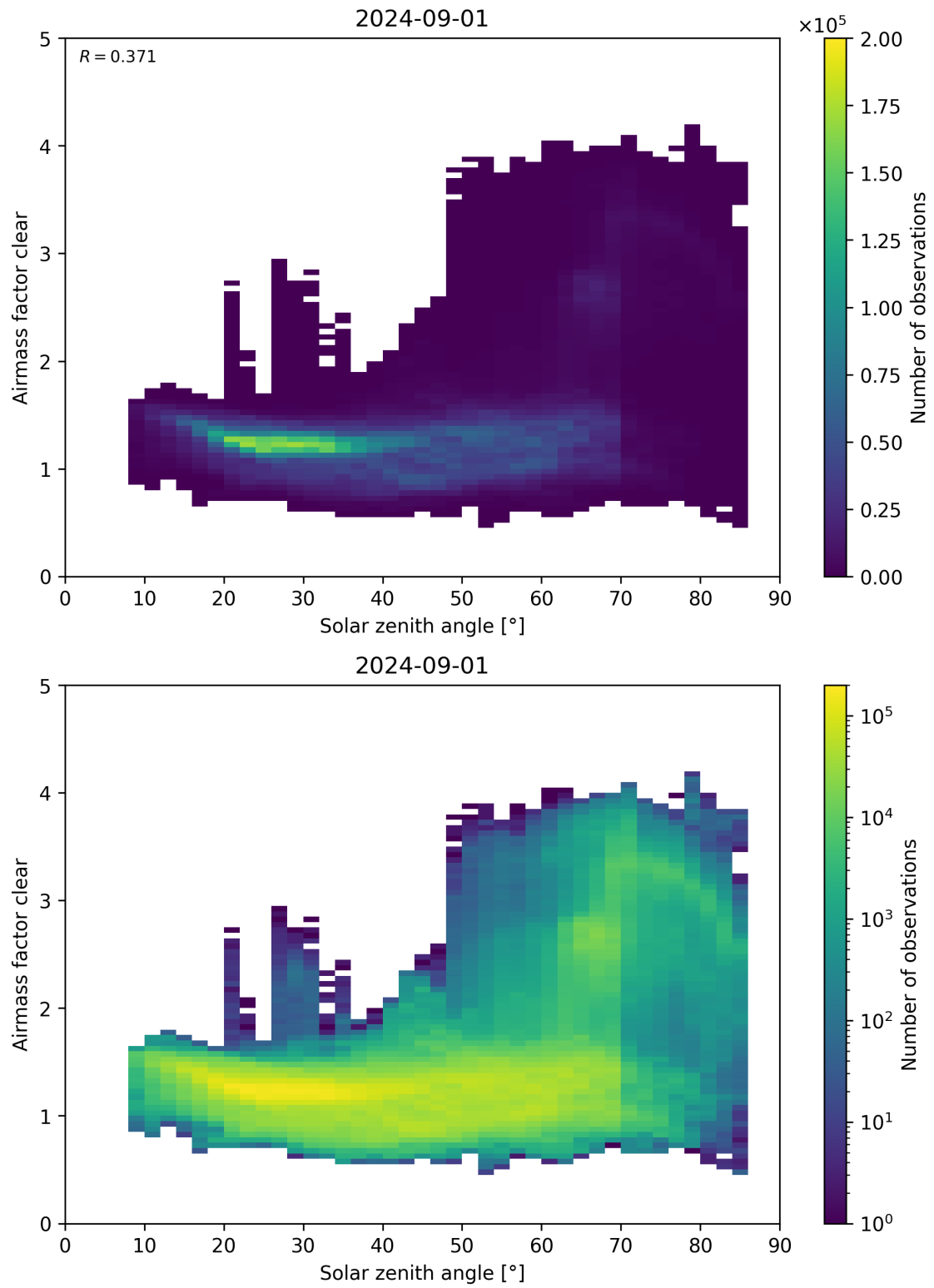
Figure 170: Scatter density plot of “Solar zenith angle” against “Airmass factor clear” for 2024-09-01 to 2024-09-02.
