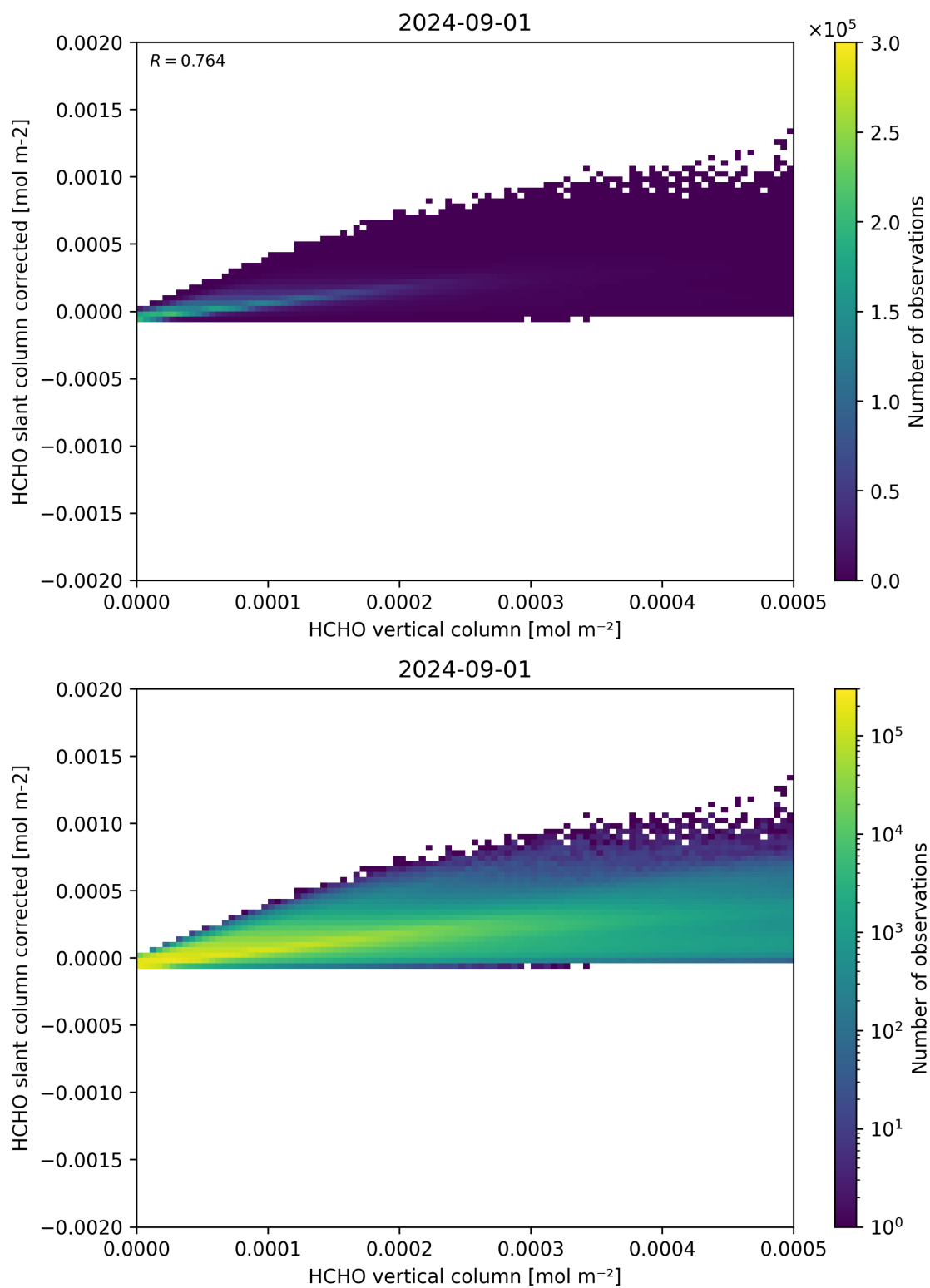
Figure 127: Scatter density plot of “HCHO vertical column” against “HCHO slant column corrected” for 2024-09-01 to 2024-09-02.
