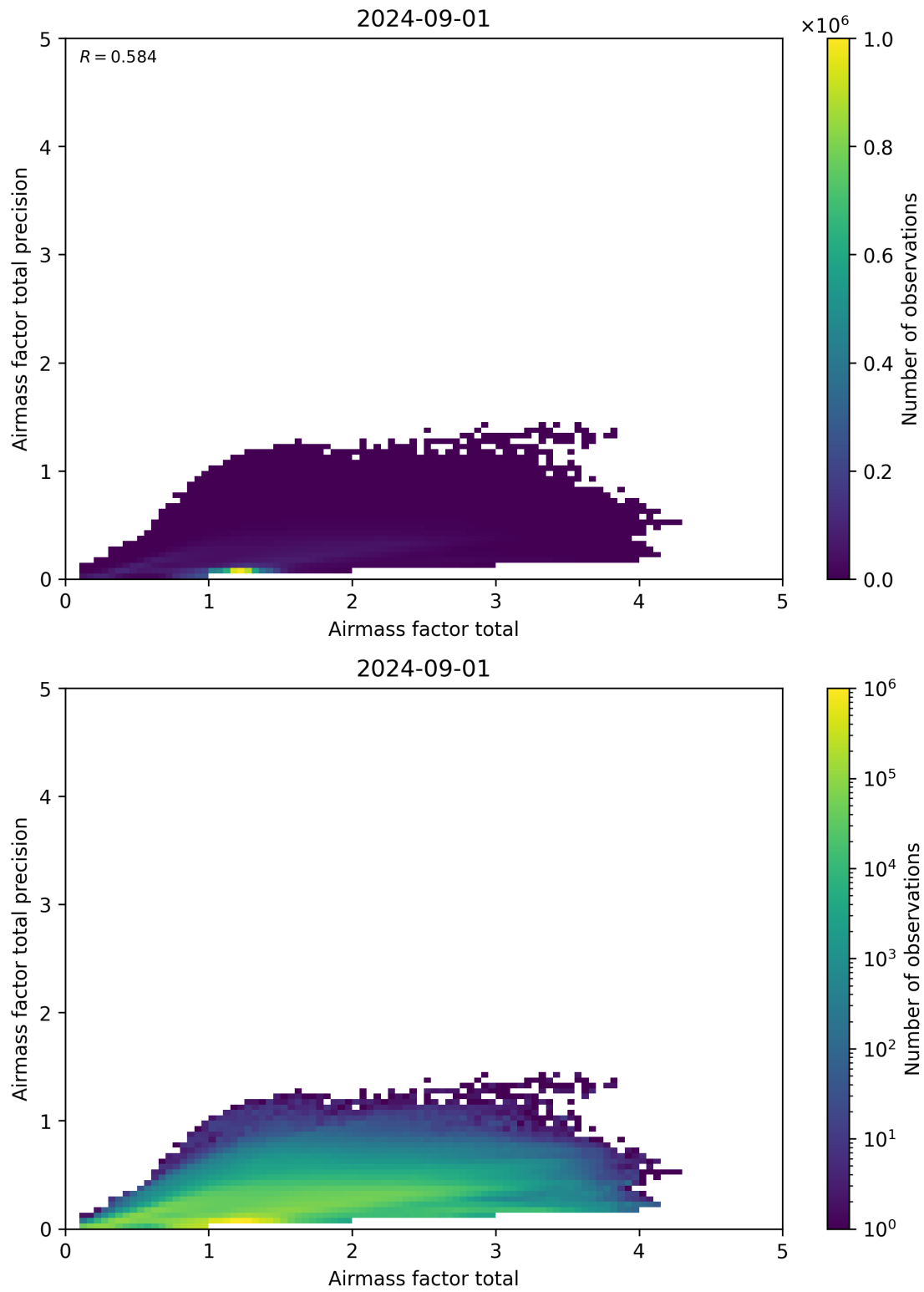
Figure 103: Scatter density plot of “Airmass factor total” against “Airmass factor total precision” for 2024-09-01 to 2024-09-02.
