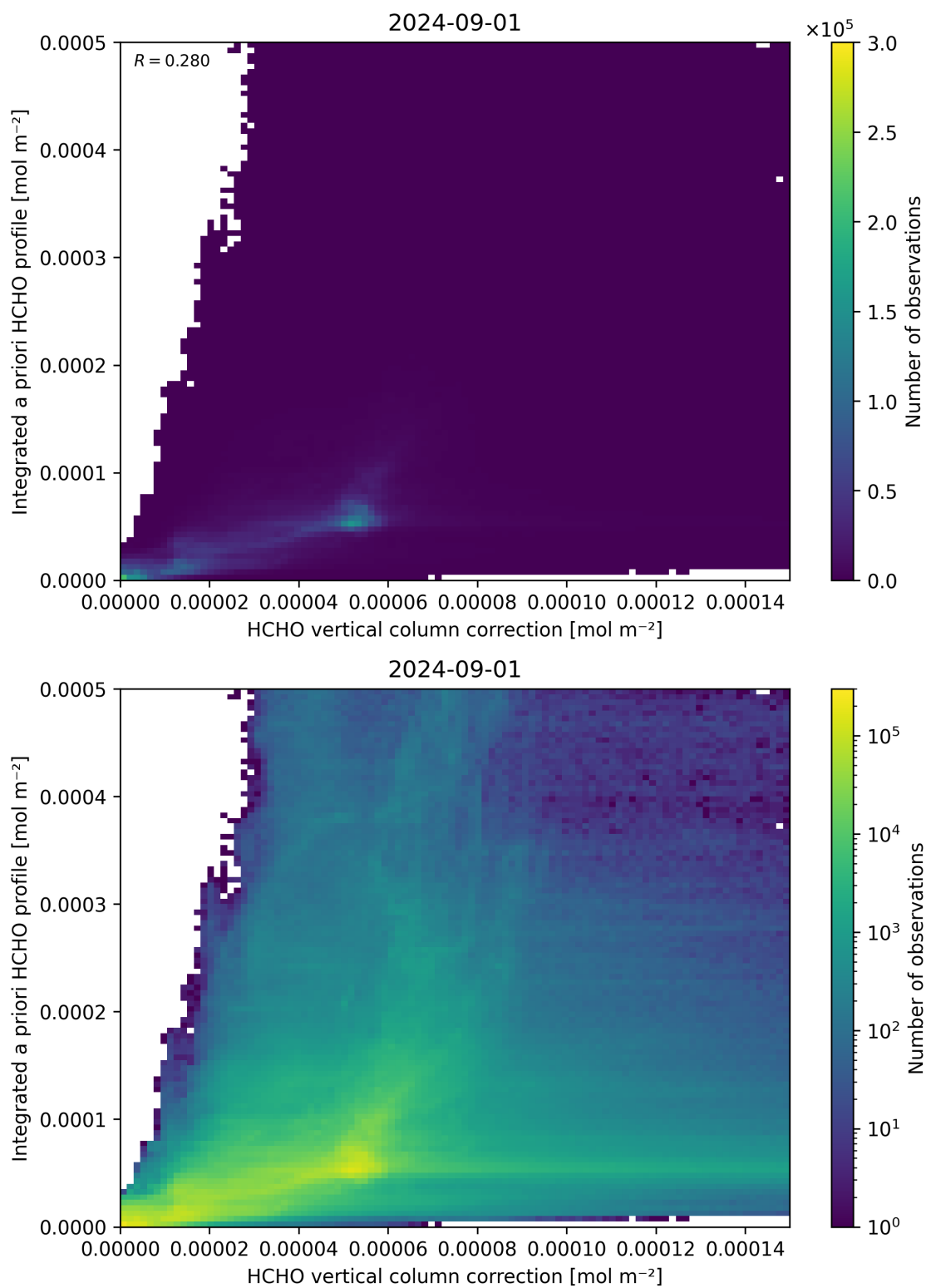
Figure 122: Scatter density plot of “HCHO vertical column correction” against “Integrated a priori HCHO profile” for 2024-09-01 to 2024-09-02.
