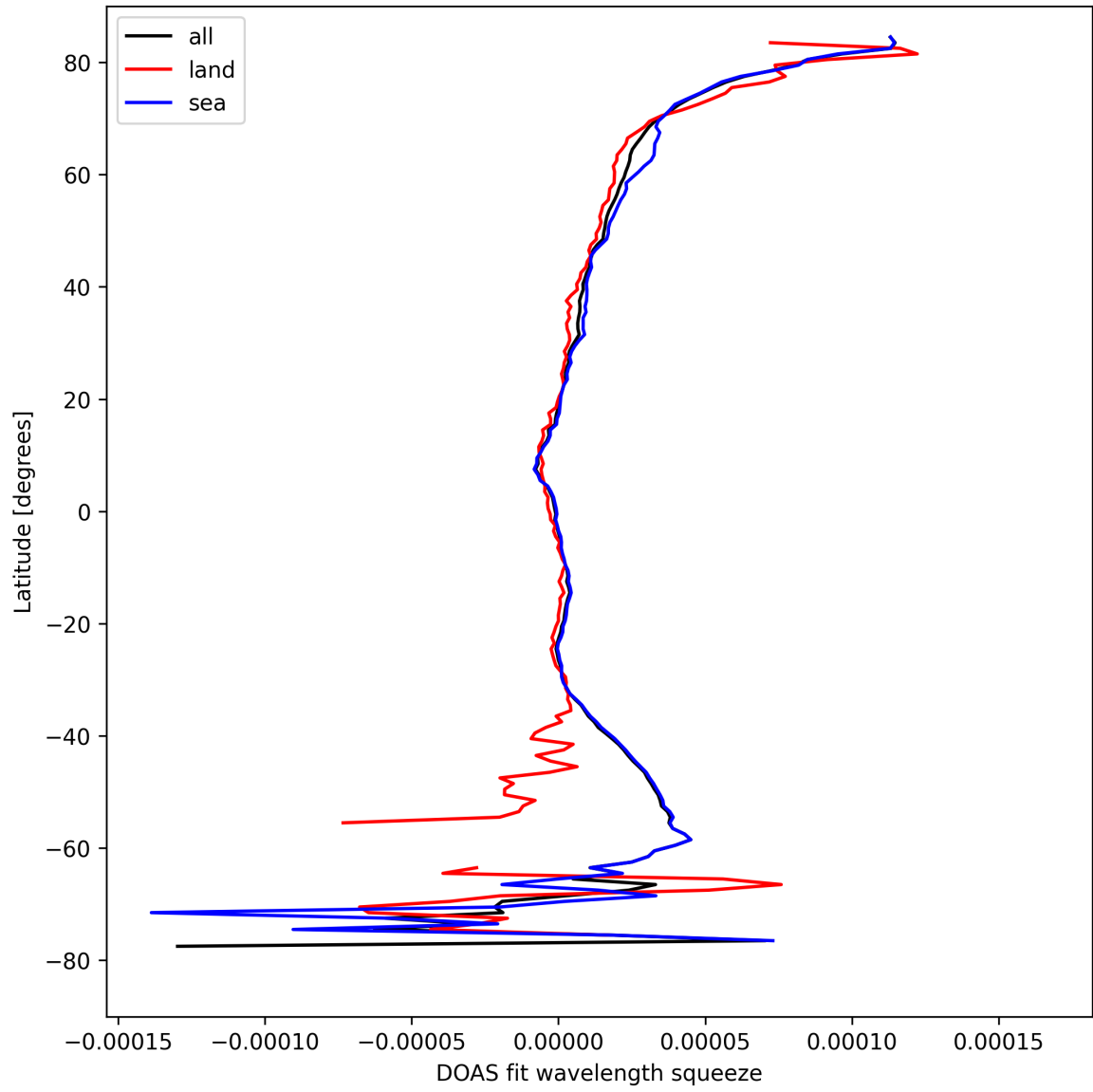
Figure 31: Zonal average of “DOAS fit wavelength squeeze” for 2024-09-01 to 2024-09-02.
