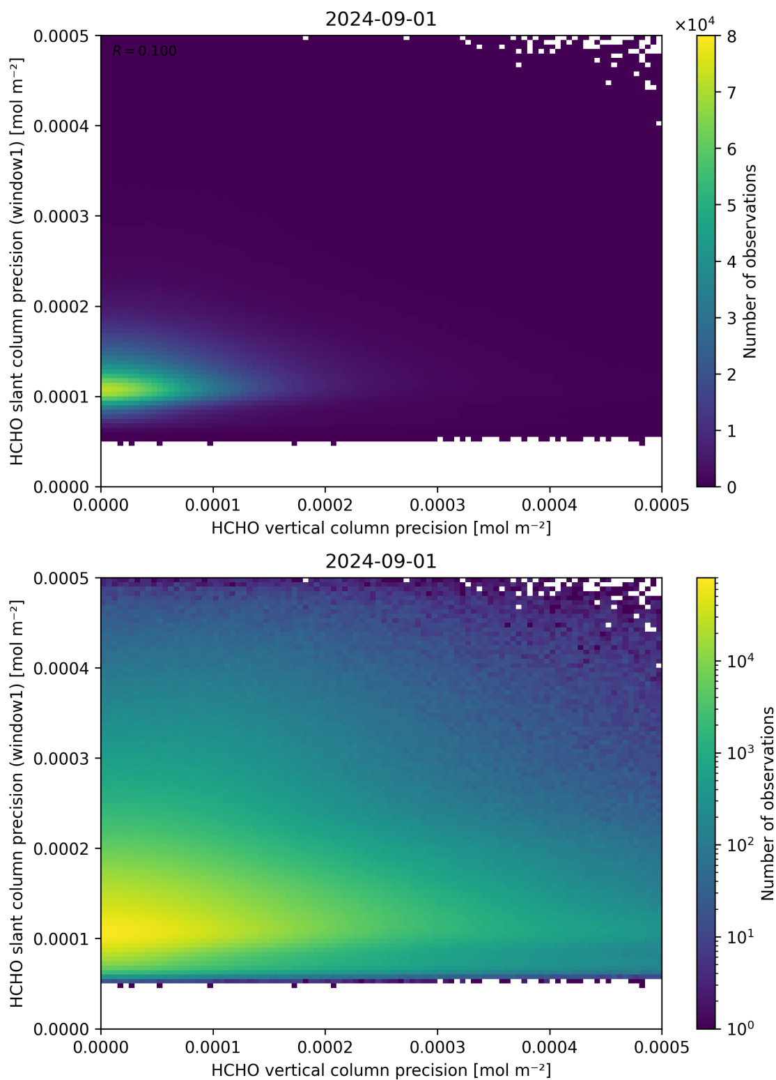
Figure 143: Scatter density plot of “HCHO vertical column precision” against “HCHO slant column precision (window1)” for 2024-09-01 to 2024-09-02.
