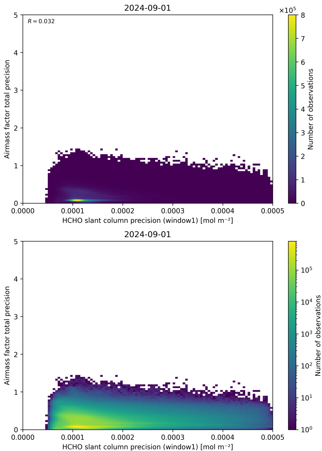
Figure 95: Scatter density plot of “HCHO slant column precision (window1)” against “Airmass factor total precision” for 2024-09-01 to 2024-09-02.
