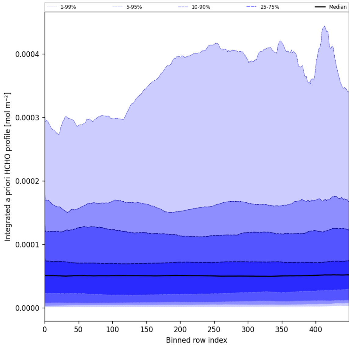
Figure 57: Along track statistics of “Integrated a priori HCHO profile” for 2024-09-01 to 2024-09-02
