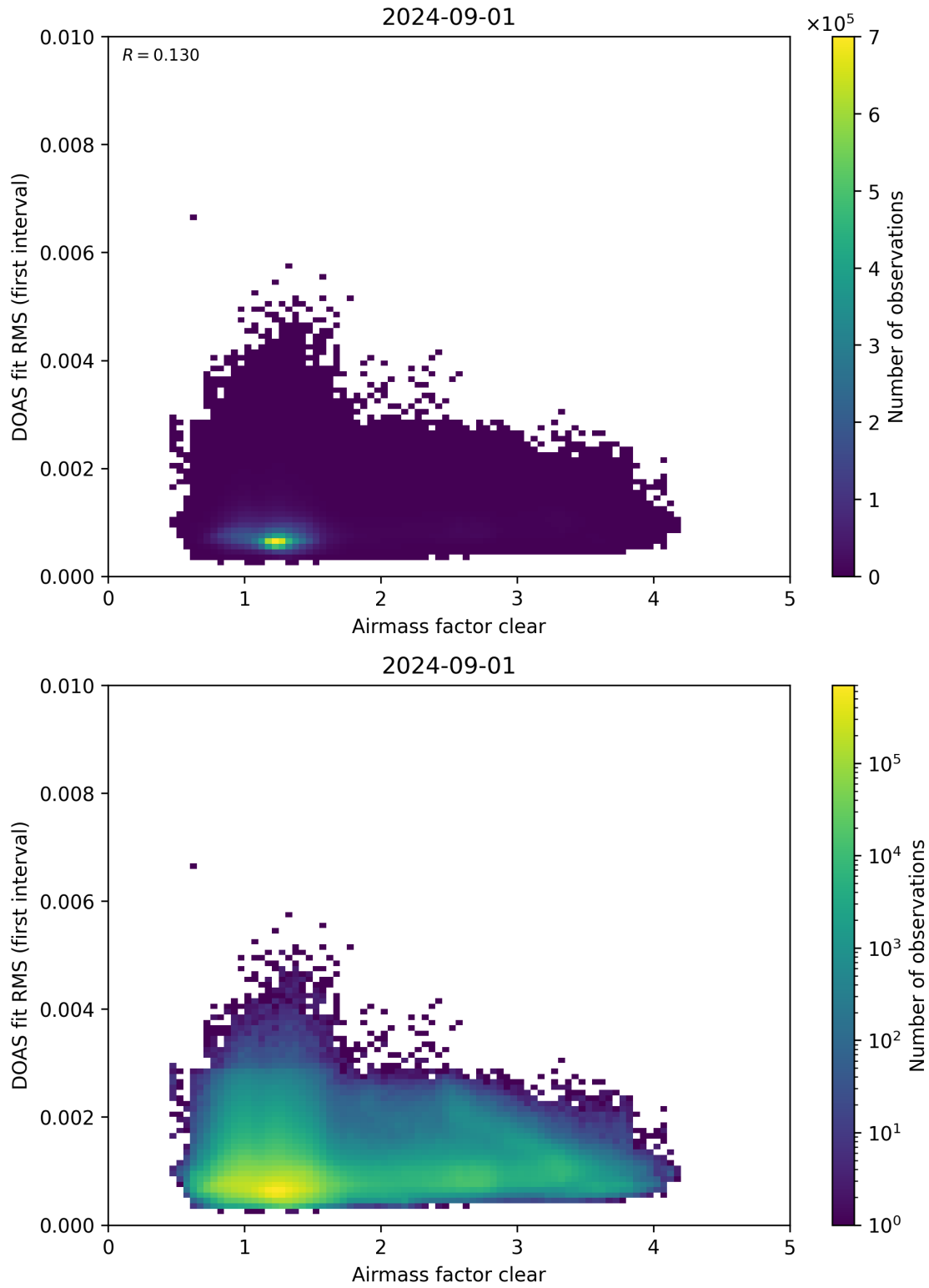
Figure 71: Scatter density plot of “Airmass factor clear” against “DOAS fit RMS (first interval)” for 2024-09-01 to 2024-09-02.
