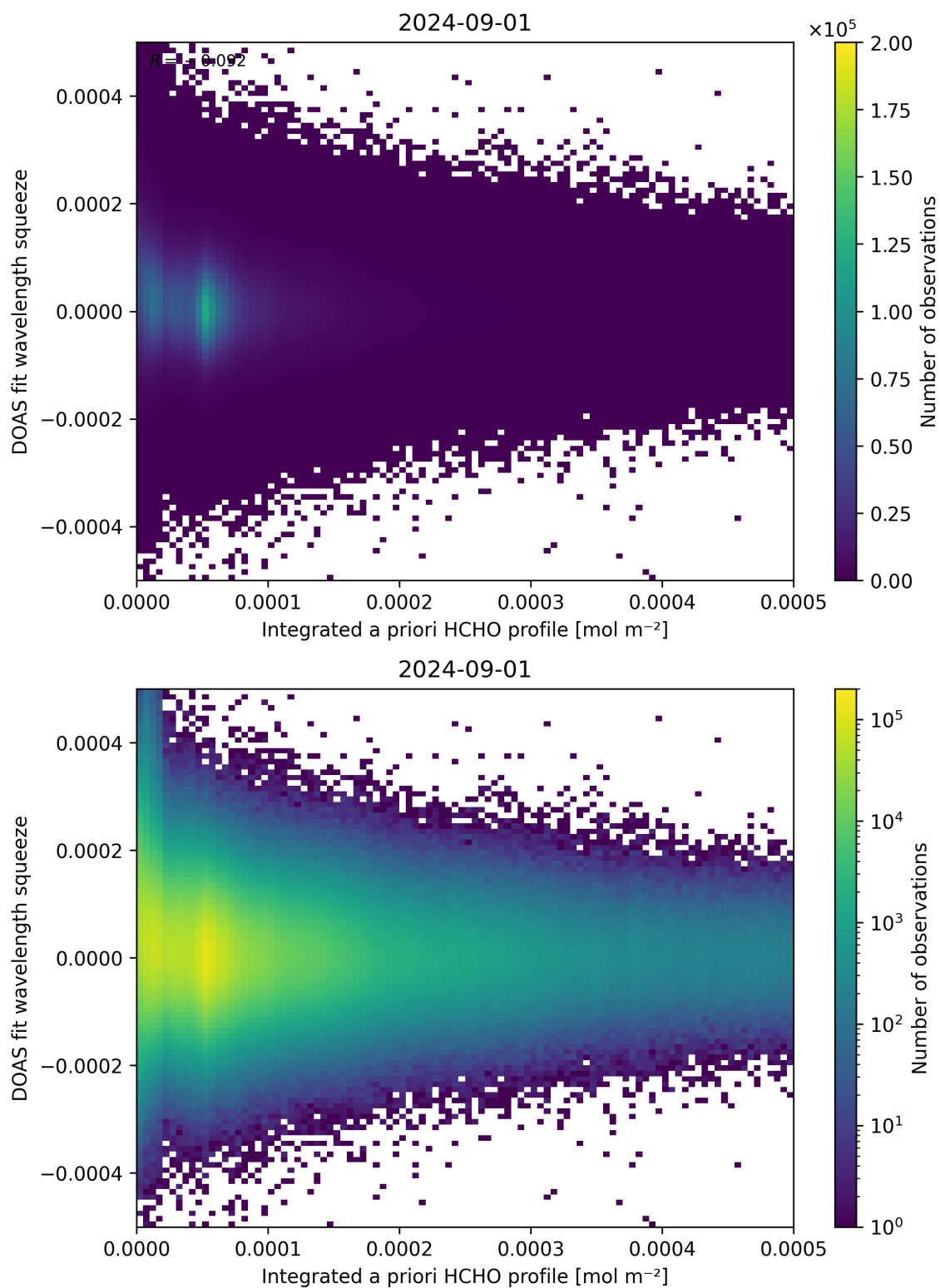
Figure 150: Scatter density plot of “Integrated a priori HCHO profile” against “DOAS fit wavelength squeeze” for 2024-09-01 to 2024-09-02.
