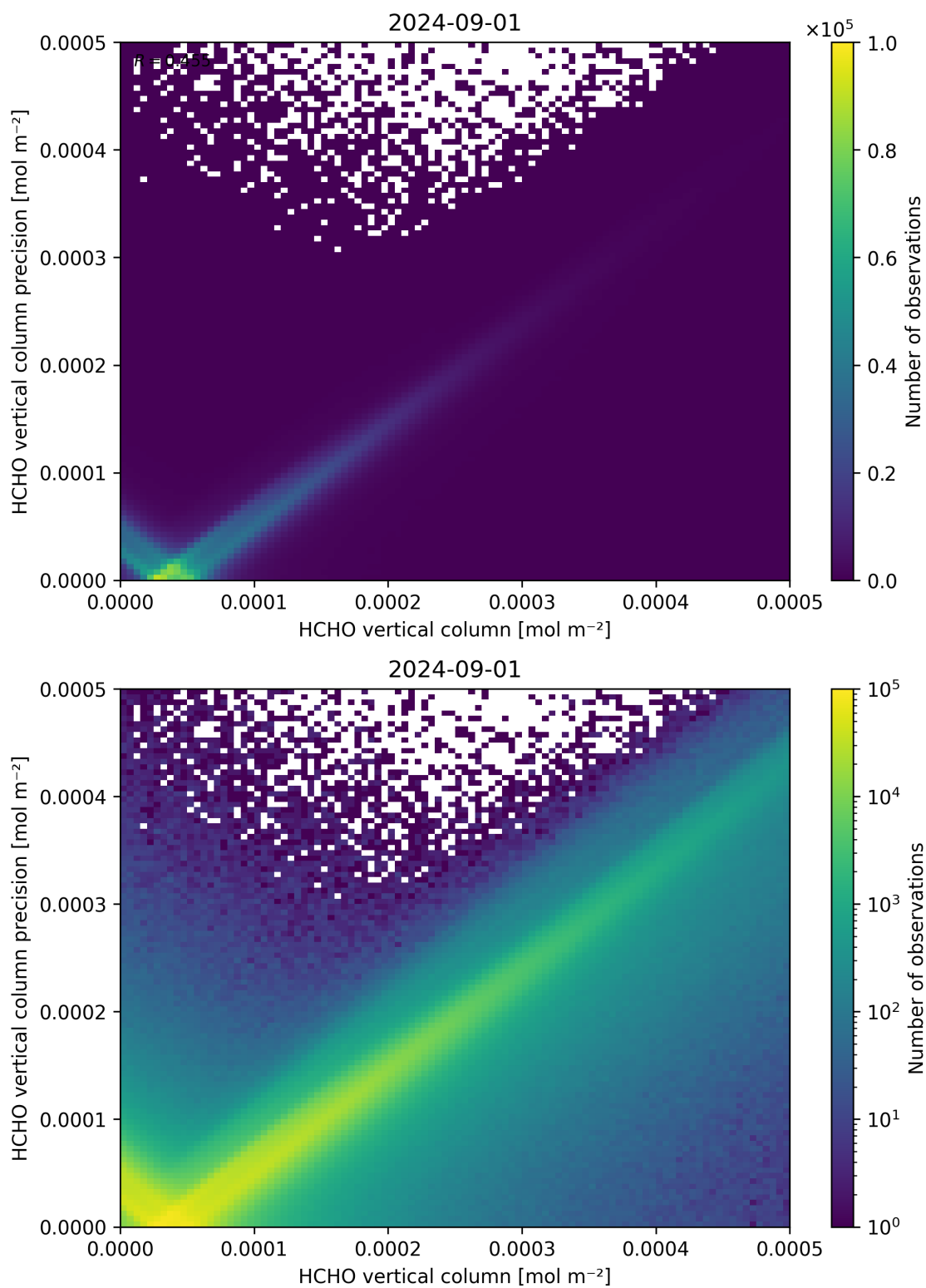
Figure 134: Scatter density plot of “HCHO vertical column” against “HCHO vertical column precision” for 2024-09-01 to 2024-09-02.
