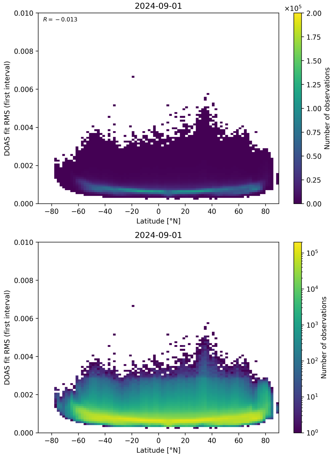
Figure 153: Scatter density plot of “Latitude” against “DOAS fit RMS (first interval)” for 2024-09-01 to 2024-09-02.
