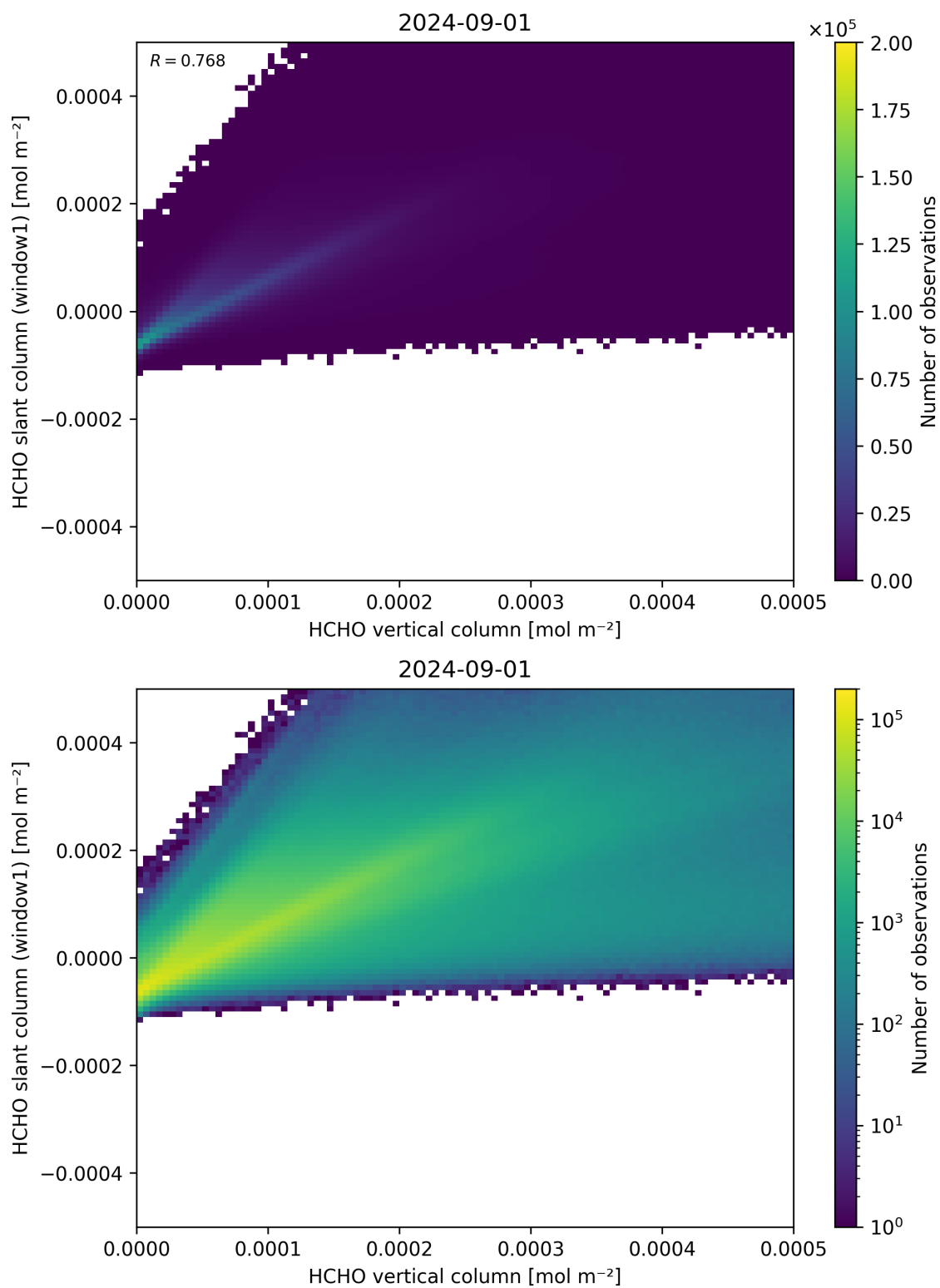
Figure 129: Scatter density plot of “HCHO vertical column” against “HCHO slant column (window1)” for 2024-09-01 to 2024-09-02.
