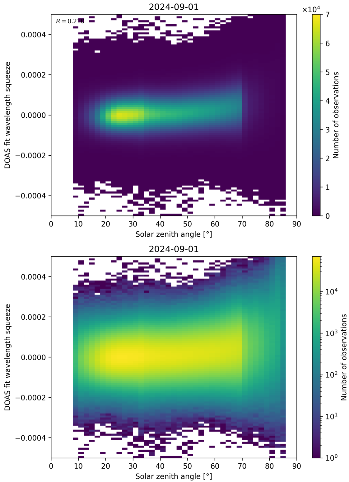
Figure 169: Scatter density plot of “Solar zenith angle” against “DOAS fit wavelength squeeze” for 2024-09-01 to 2024-09-02.
