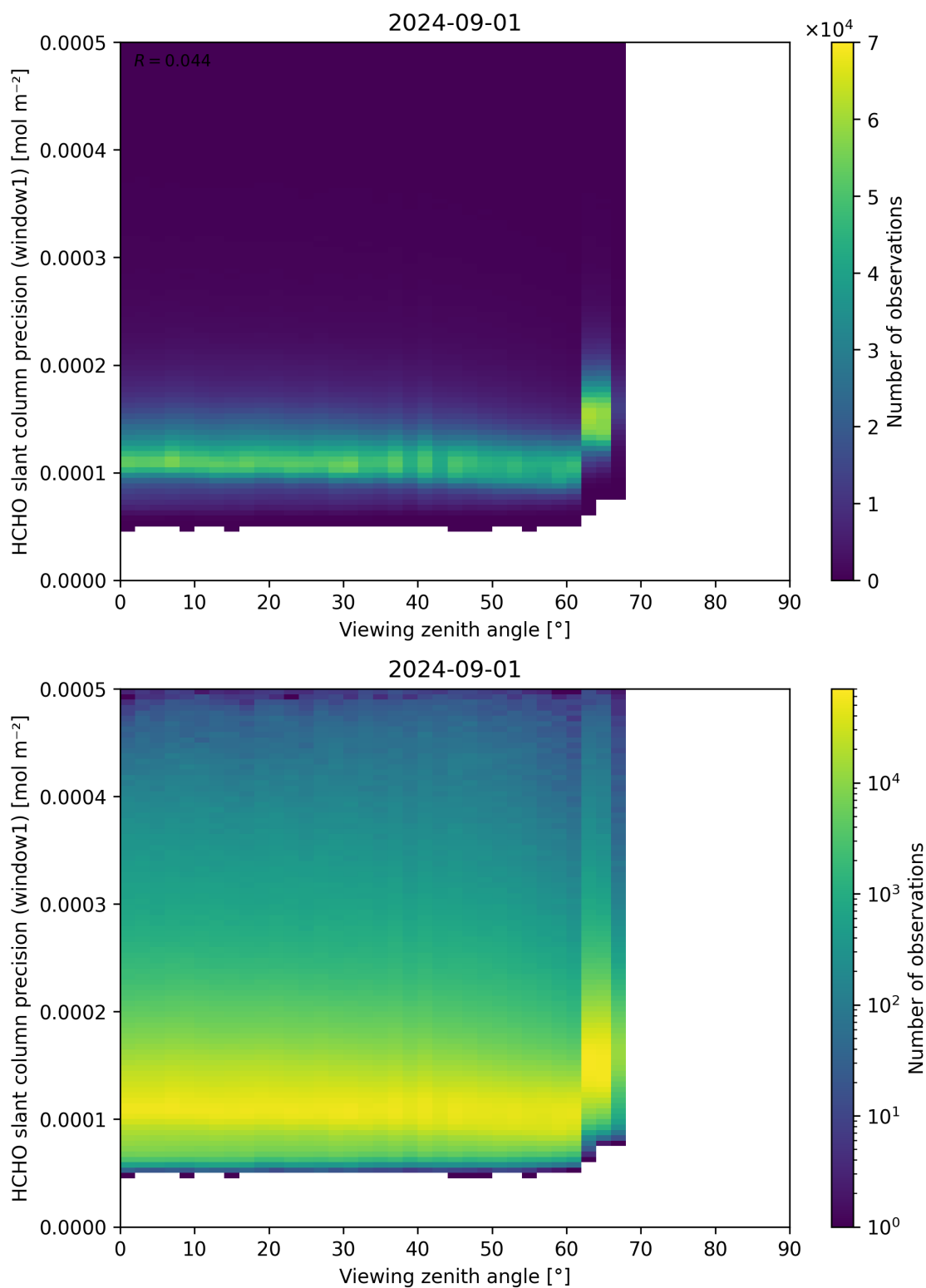
Figure 189: Scatter density plot of “Viewing zenith angle” against “HCHO slant column precision (window1)” for 2024-09-01 to 2024-09-02.
