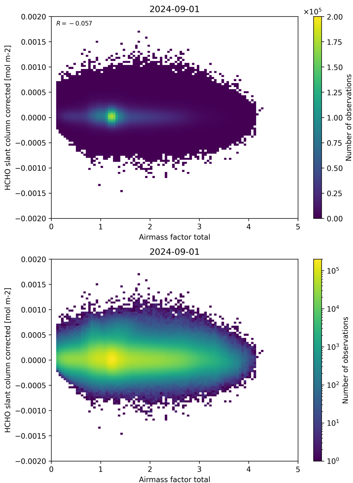
Figure 101: Scatter density plot of “Airmass factor total” against “HCHO slant column corrected” for 2024-09-01 to 2024-09-02.
