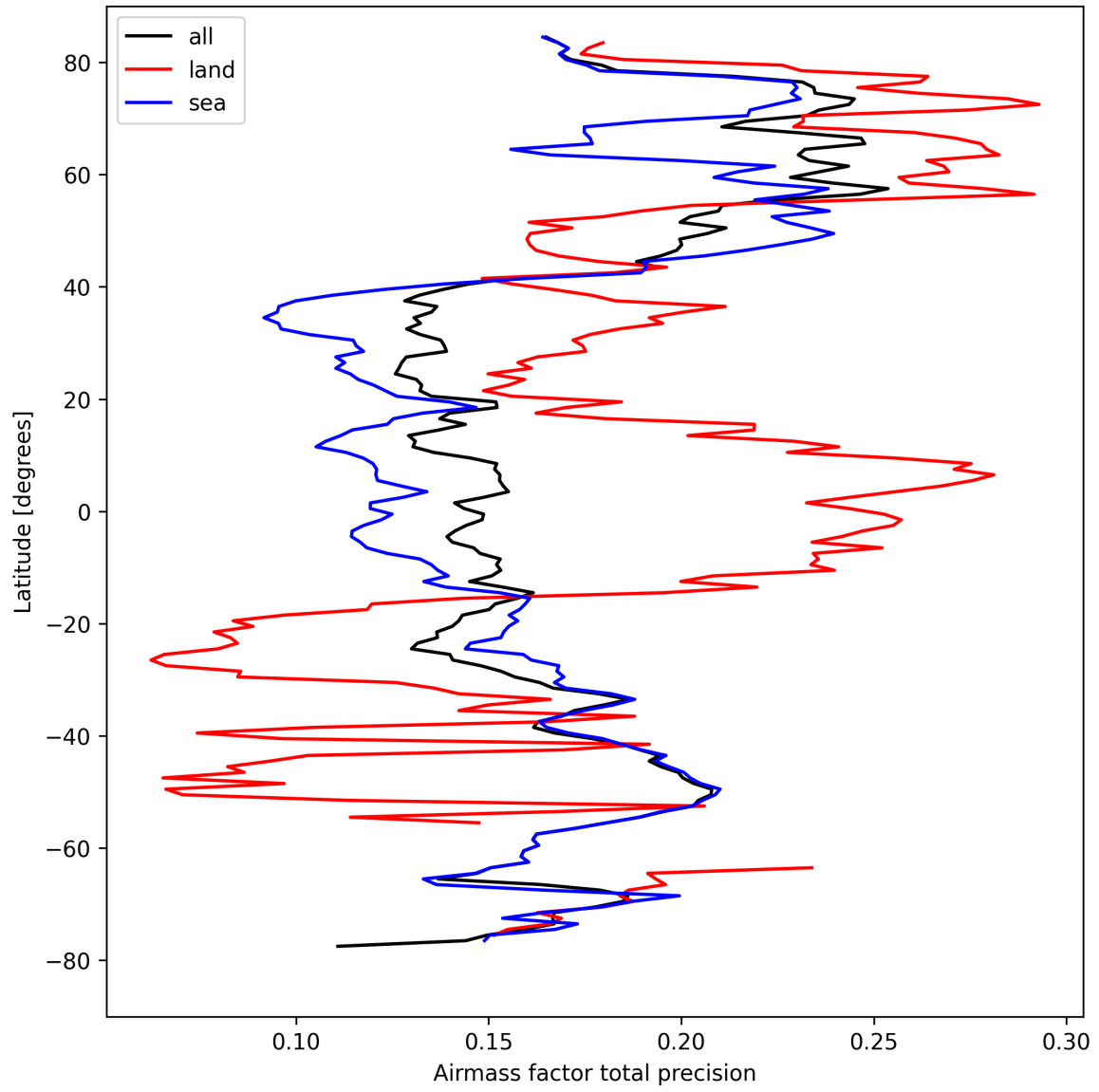
Figure 27: Zonal average of “Airmass factor total precision” for 2024-09-01 to 2024-09-02.
