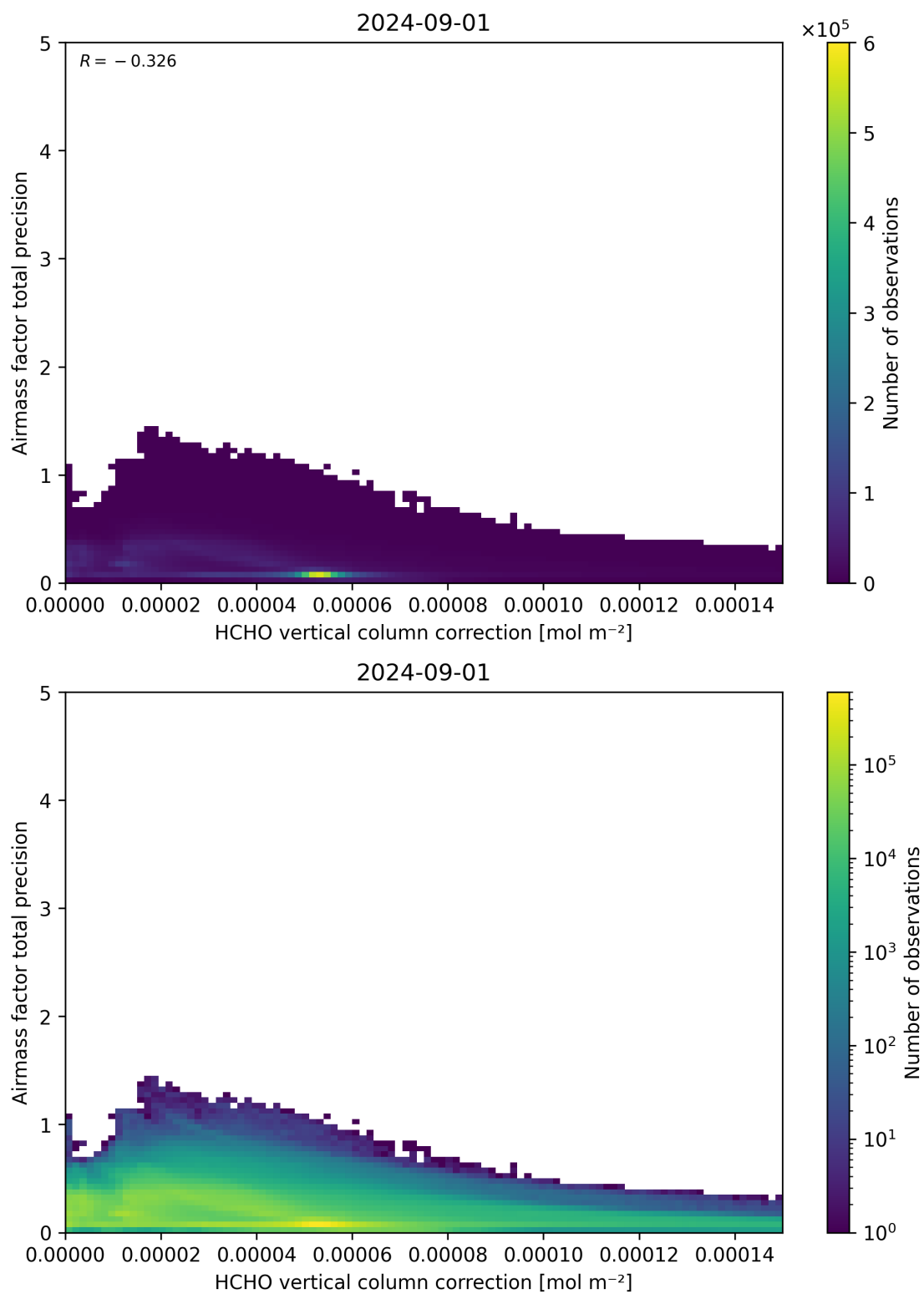
Figure 121: Scatter density plot of “HCHO vertical column correction” against “Airmass factor total precision” for 2024-09-01 to 2024-09-02.
