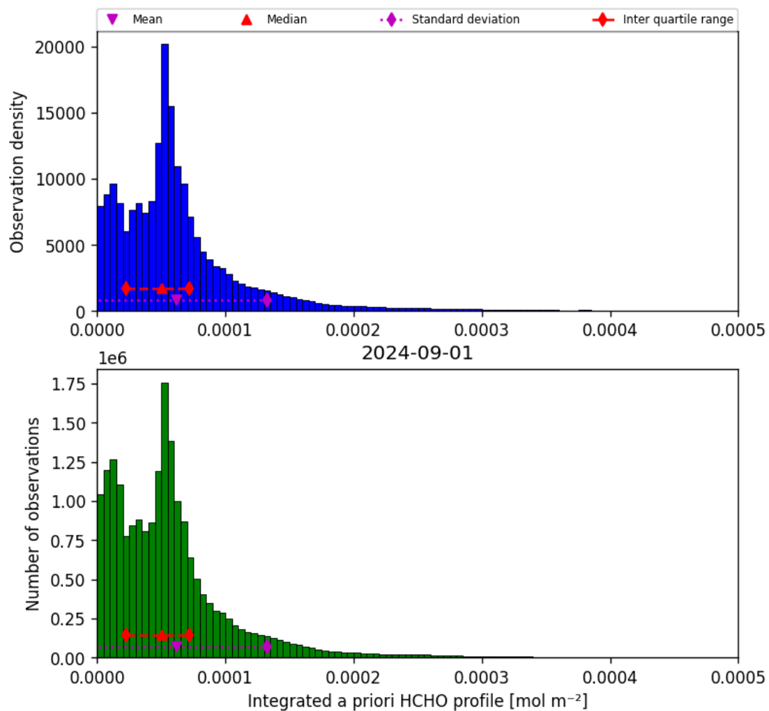
Figure 43: Histogram of “Integrated a priori HCHO profile” for 2024-09-01 to 2024-09-02
