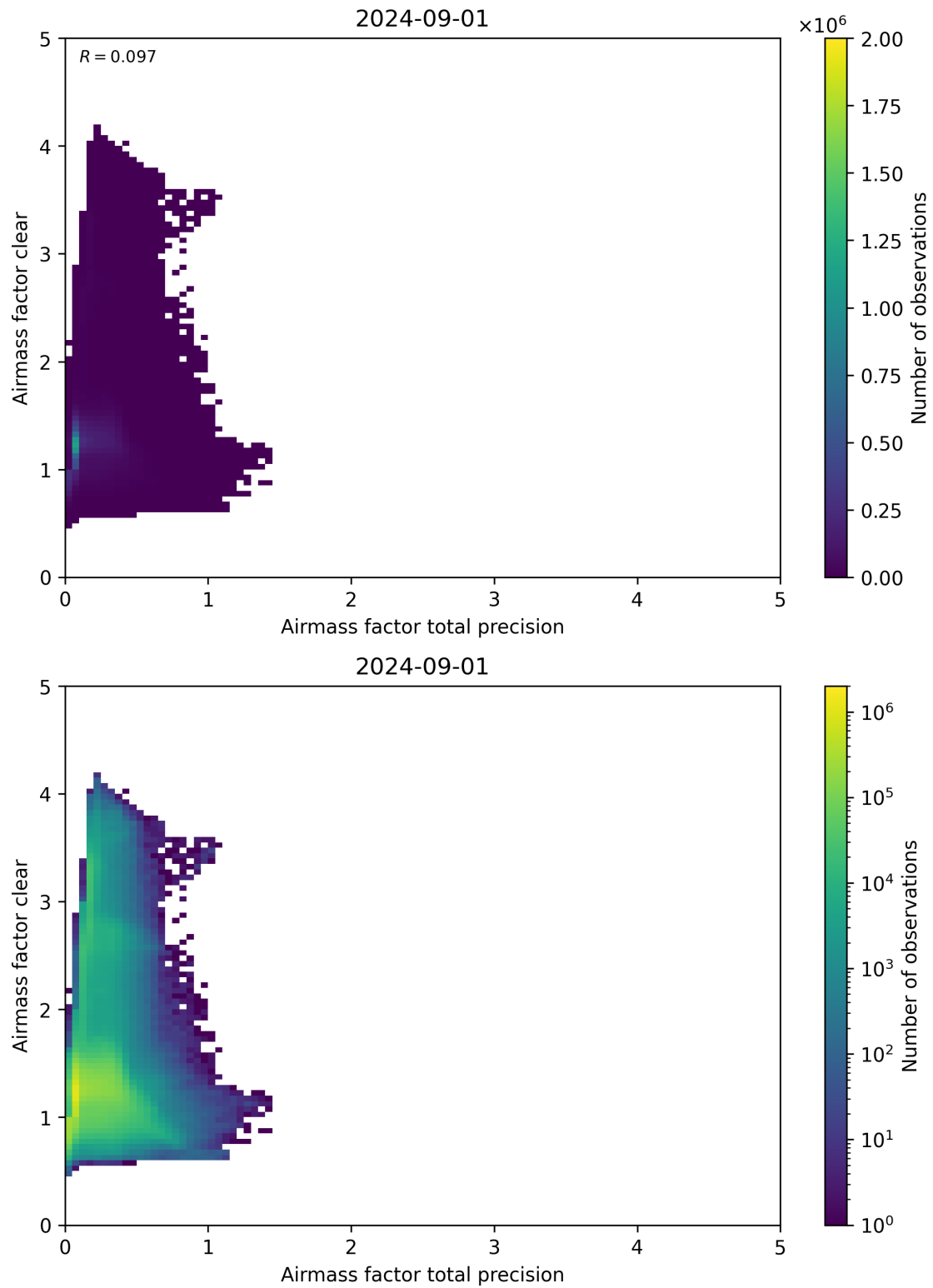
Figure 108: Scatter density plot of “Airmass factor total precision” against “Airmass factor clear” for 2024-09-01 to 2024-09-02.
