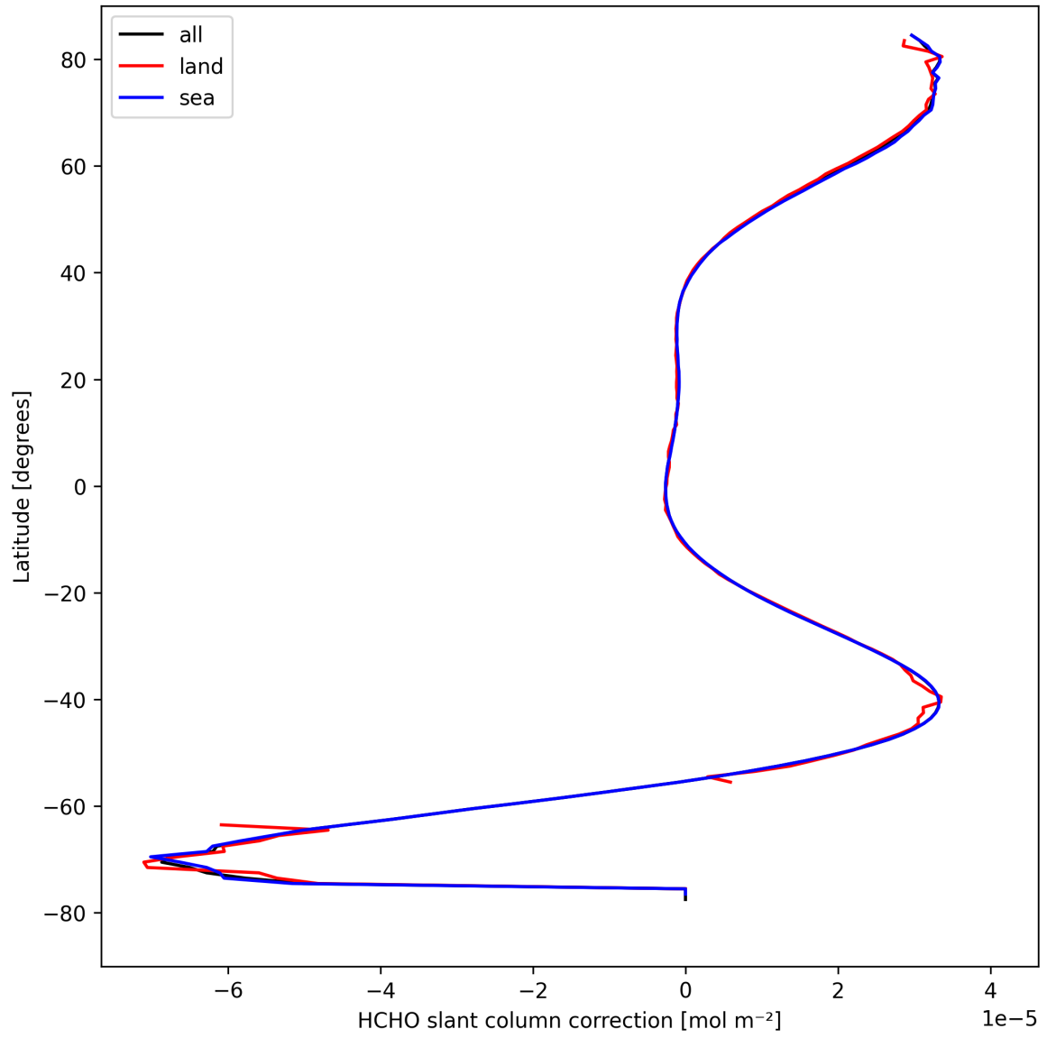
Figure 33: Zonal average of "HCHO slant column correction" for 2024-09-01 to 2024-09-02.
