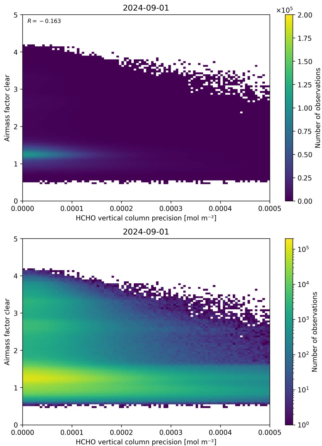
Figure 139: Scatter density plot of “HCHO vertical column precision” against “Airmass factor clear” for 2024-09-01 to 2024-09-02.
