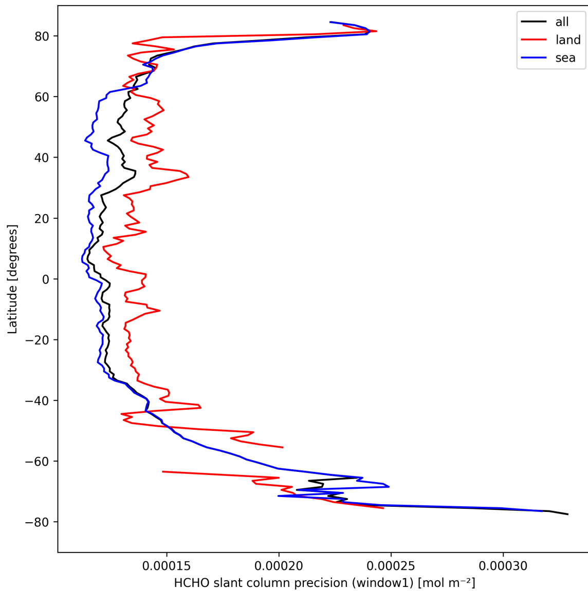
Figure 25: Zonal average of "HCHO slant column precision (window1)" for 2024-09-01 to 2024-09-02.
