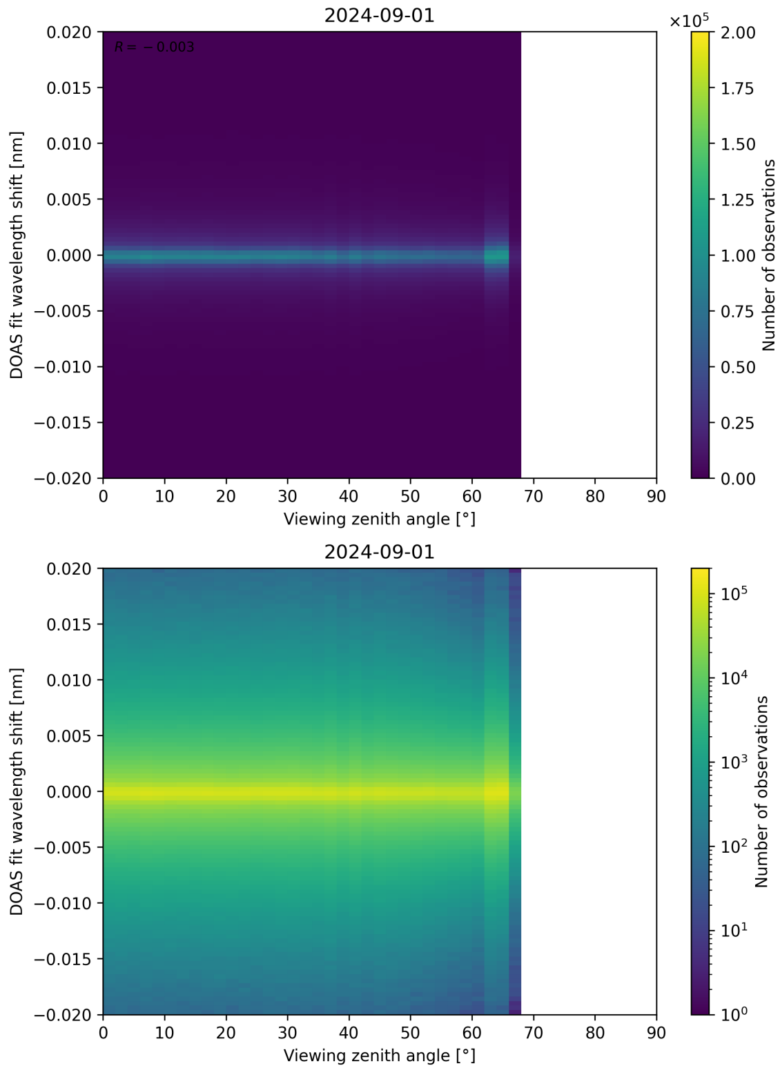
Figure 183: Scatter density plot of “Viewing zenith angle” against “DOAS fit wavelength shift” for 2024-09-01 to 2024-09-02.
