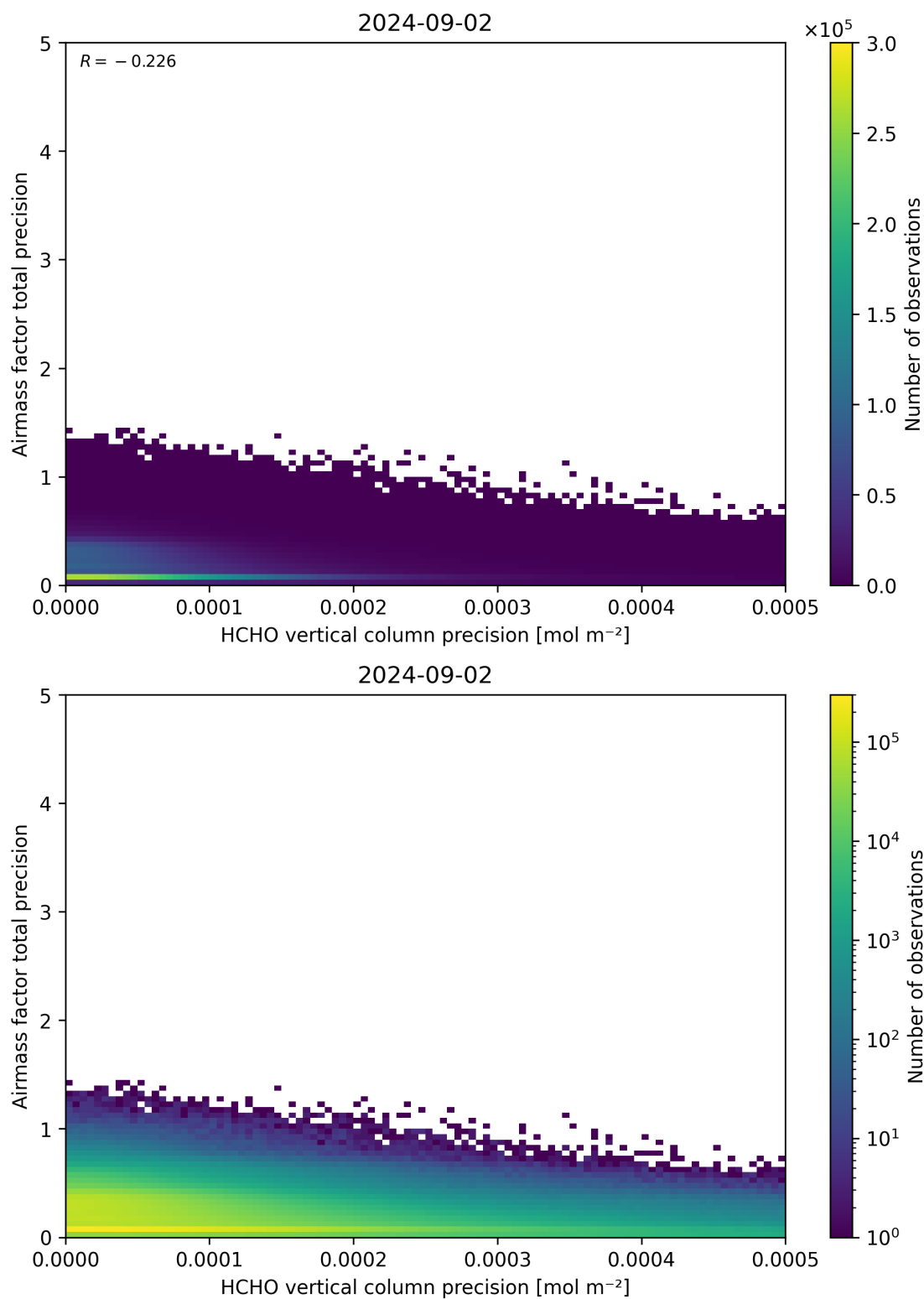
Figure 145: Scatter density plot of “HCHO vertical column precision” against “Airmass factor total precision” for 2024-09-01 to 2024-09-03.
