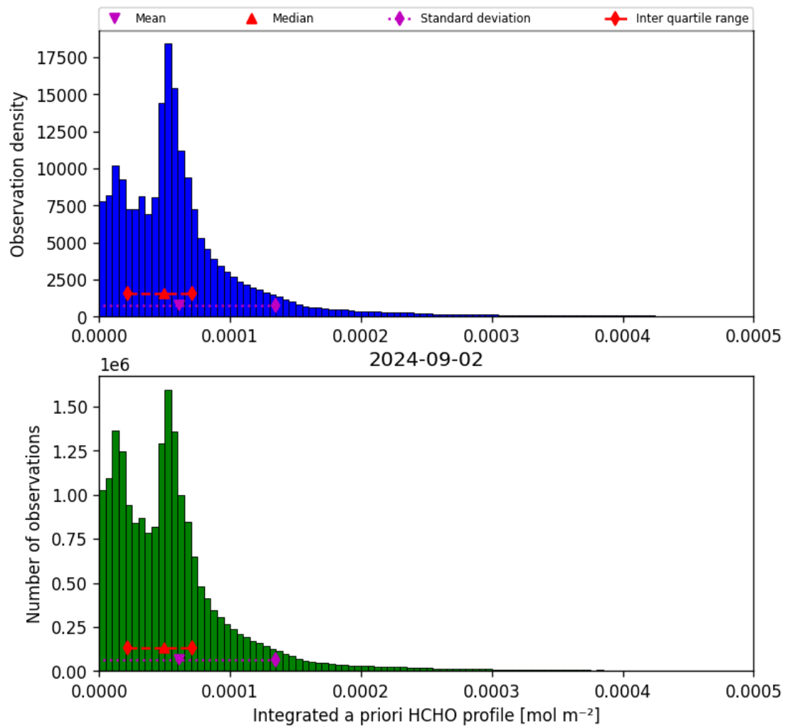
Figure 43: Histogram of “Integrated a priori HCHO profile” for 2024-09-01 to 2024-09-03
