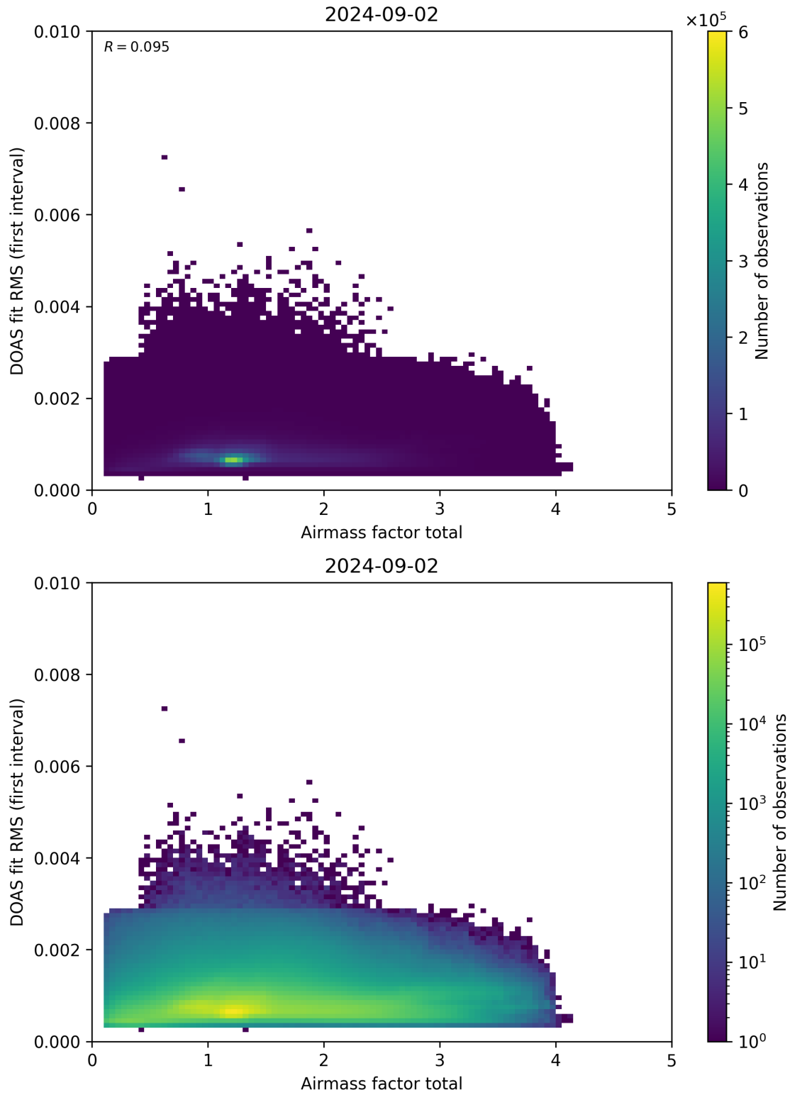
Figure 97: Scatter density plot of “Airmass factor total” against “DOAS fit RMS (first interval)” for 2024-09-01 to 2024-09-03.
