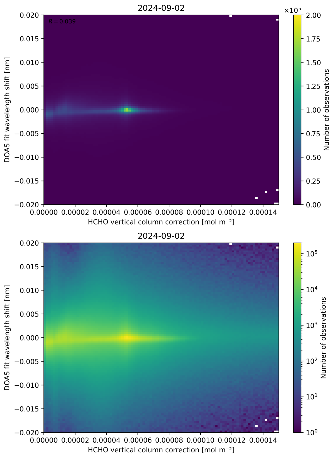
Figure 113: Scatter density plot of “HCHO vertical column correction” against “DOAS fit wavelength shift” for 2024-09-01 to 2024-09-03.
