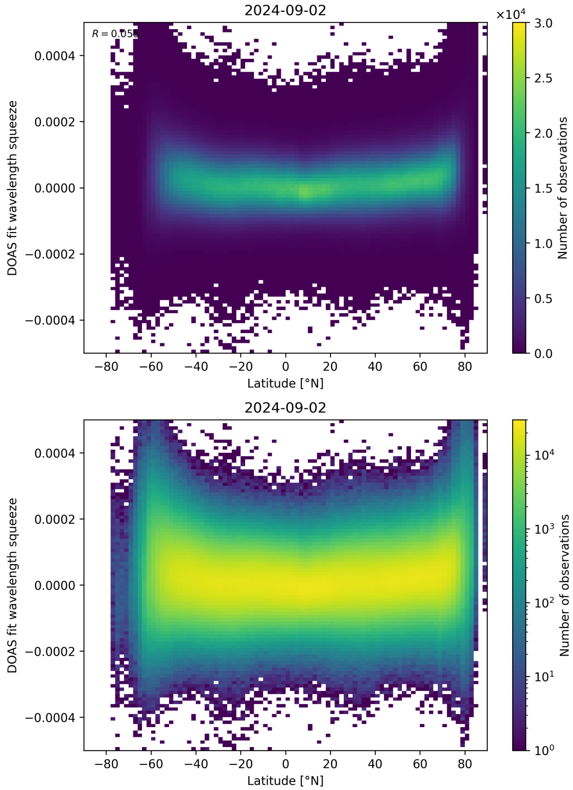
Figure 155: Scatter density plot of “Latitude” against “DOAS fit wavelength squeeze” for 2024-09-01 to 2024-09-03.
