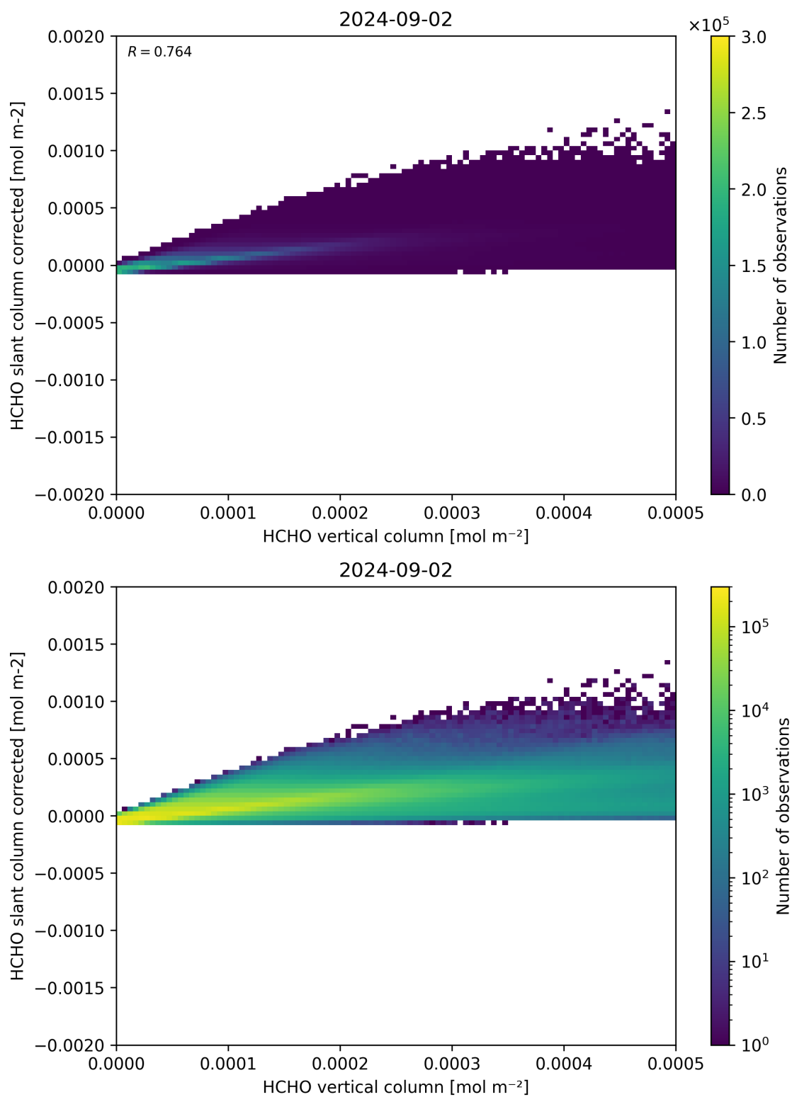
Figure 127: Scatter density plot of “HCHO vertical column” against “HCHO slant column corrected” for 2024-09-01 to 2024-09-03.
