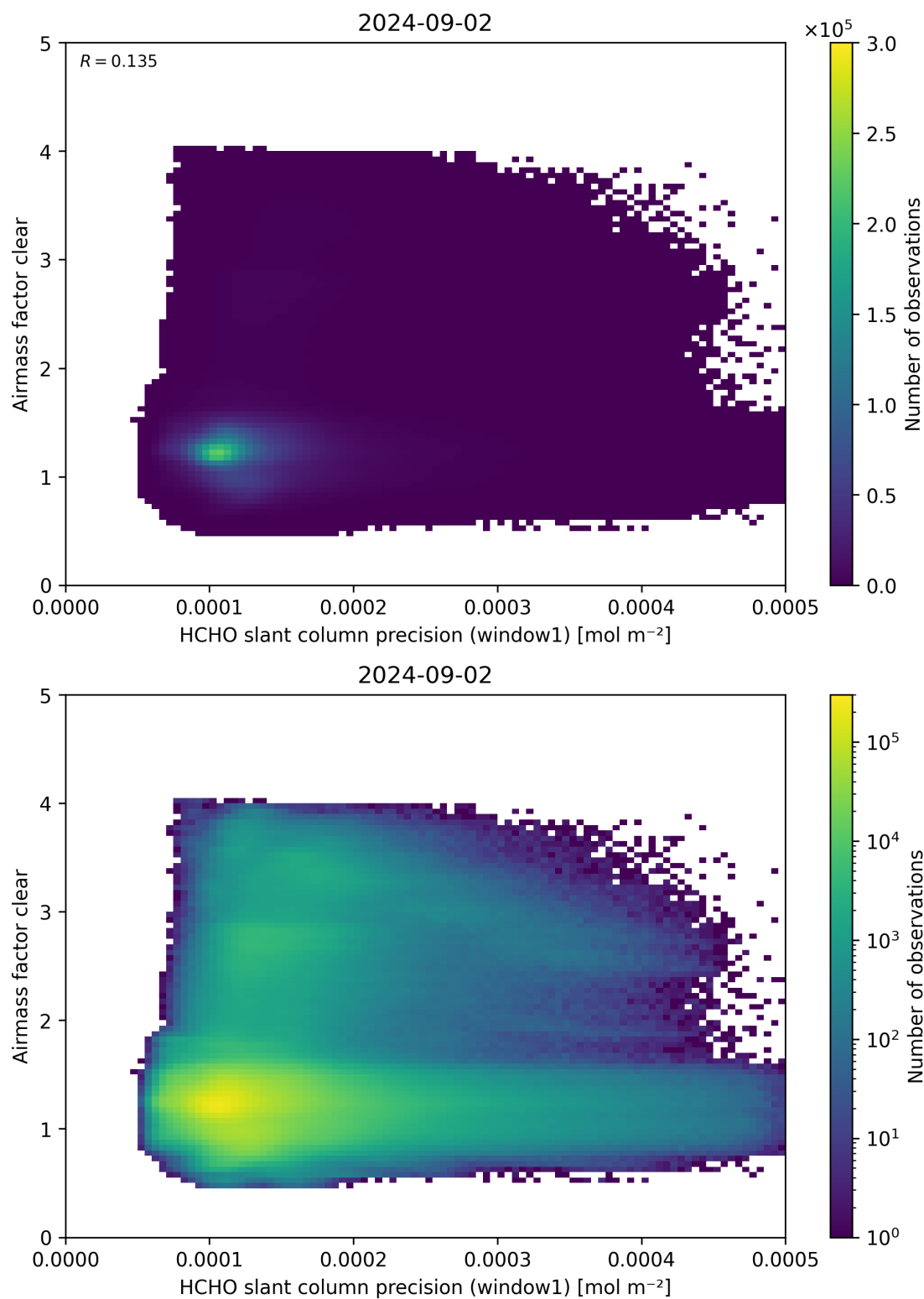
Figure 91: Scatter density plot of “HCHO slant column precision (window1)” against “Airmass factor clear” for 2024-09-01 to 2024-09-03.
