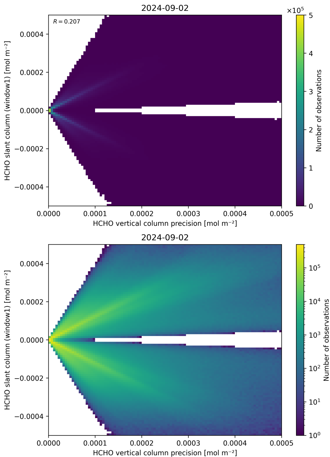
Figure 142: Scatter density plot of “HCHO vertical column precision” against “HCHO slant column (window1)” for 2024-09-01 to 2024-09-03.
