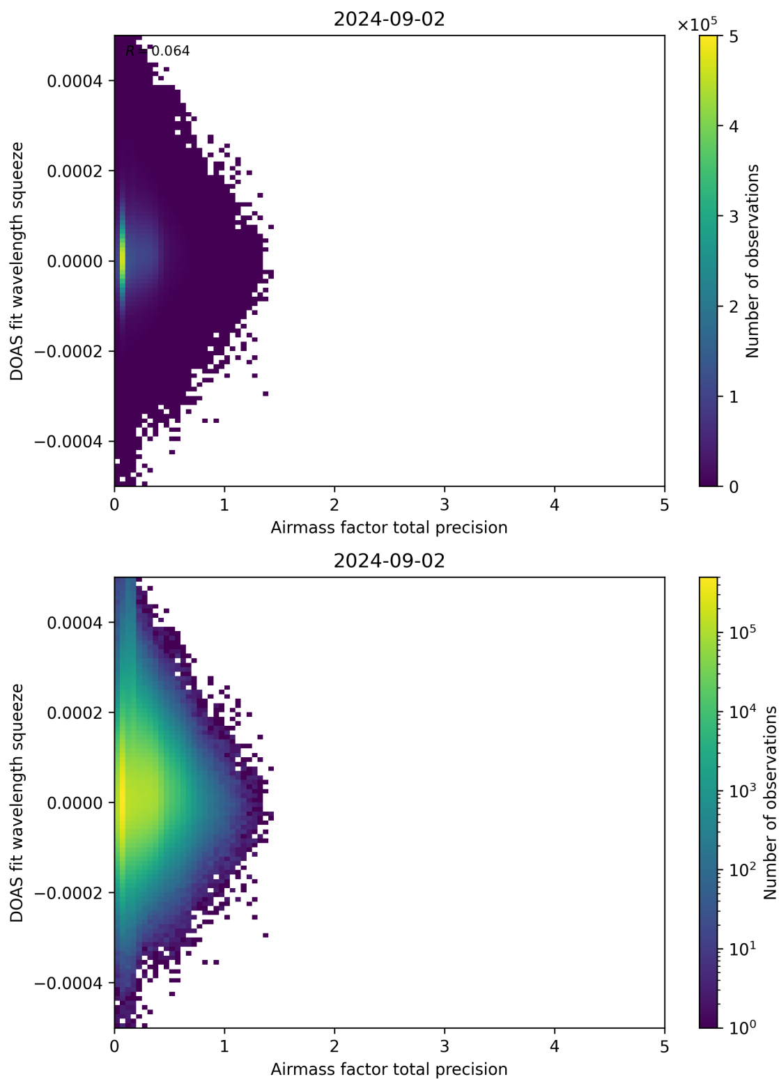
Figure 107: Scatter density plot of “Airmass factor total precision” against “DOAS fit wavelength squeeze” for 2024-09-01 to 2024-09-03.
