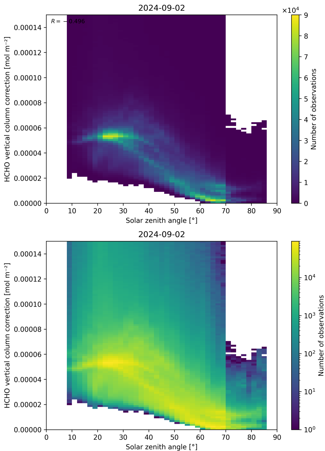
Figure 178: Scatter density plot of “Solar zenith angle” against “HCHO vertical column correction” for 2024-09-01 to 2024-09-03.
