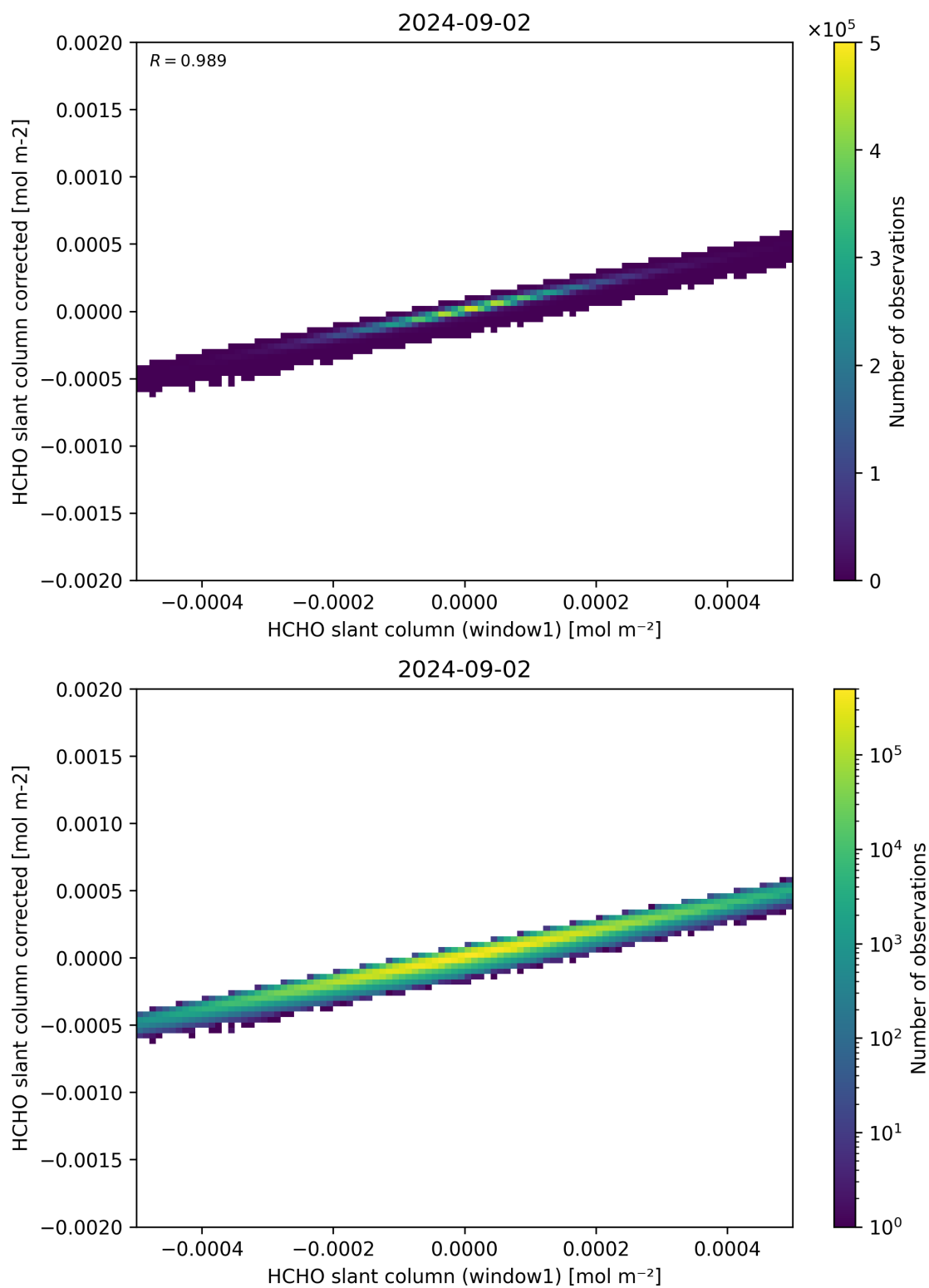
Figure 82: Scatter density plot of “HCHO slant column (window1)” against “HCHO slant column corrected” for 2024-09-01 to 2024-09-03.
