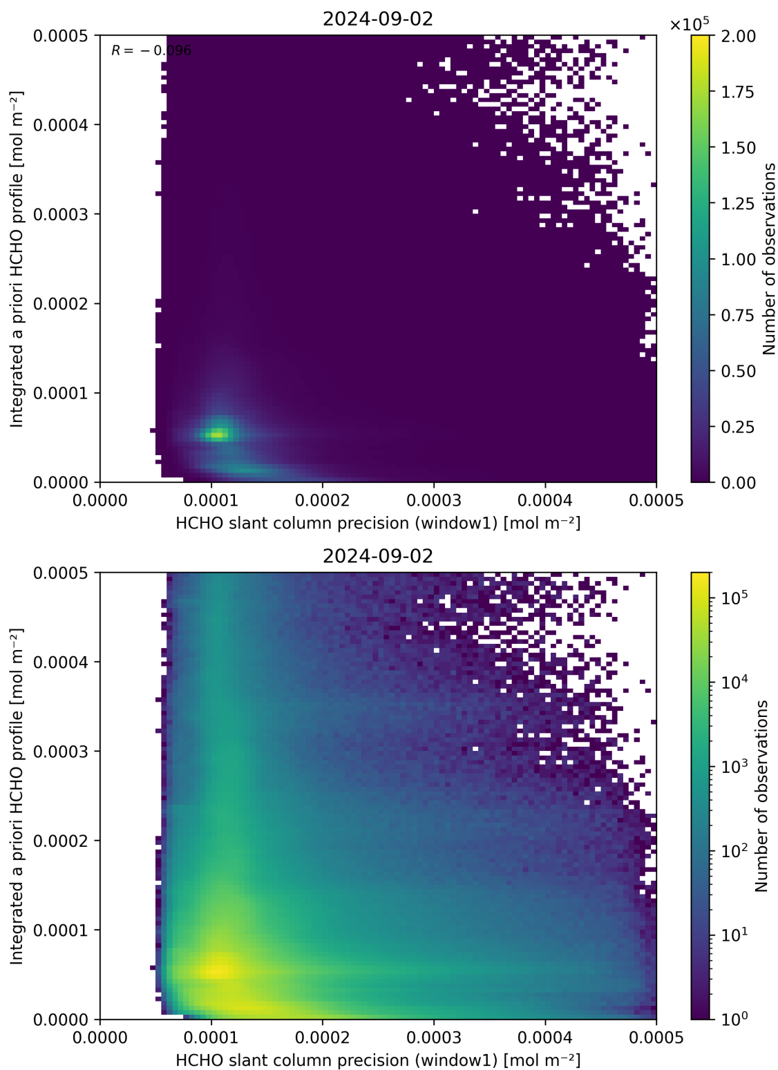
Figure 96: Scatter density plot of “HCHO slant column precision (window1)” against “Integrated a priori HCHO profile” for 2024-09-01 to 2024-09-03.
