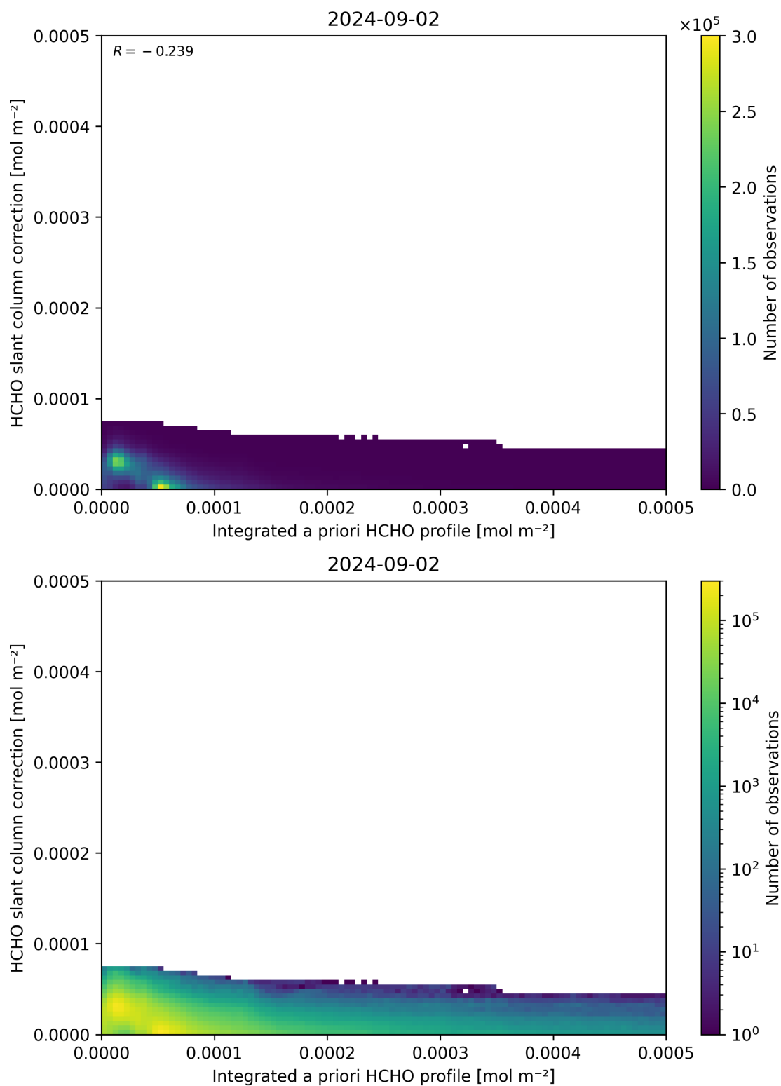
Figure 152: Scatter density plot of “Integrated a priori HCHO profile” against “HCHO slant column correction” for 2024-09-01 to 2024-09-03.
