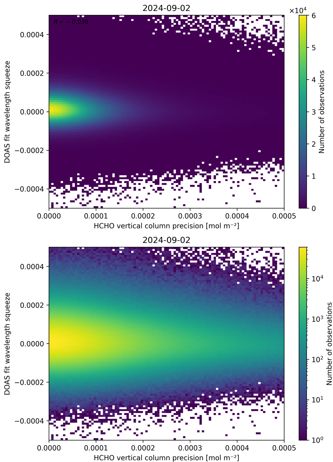
Figure 138: Scatter density plot of “HCHO vertical column precision” against “DOAS fit wavelength squeeze” for 2024-09-01 to 2024-09-03.
