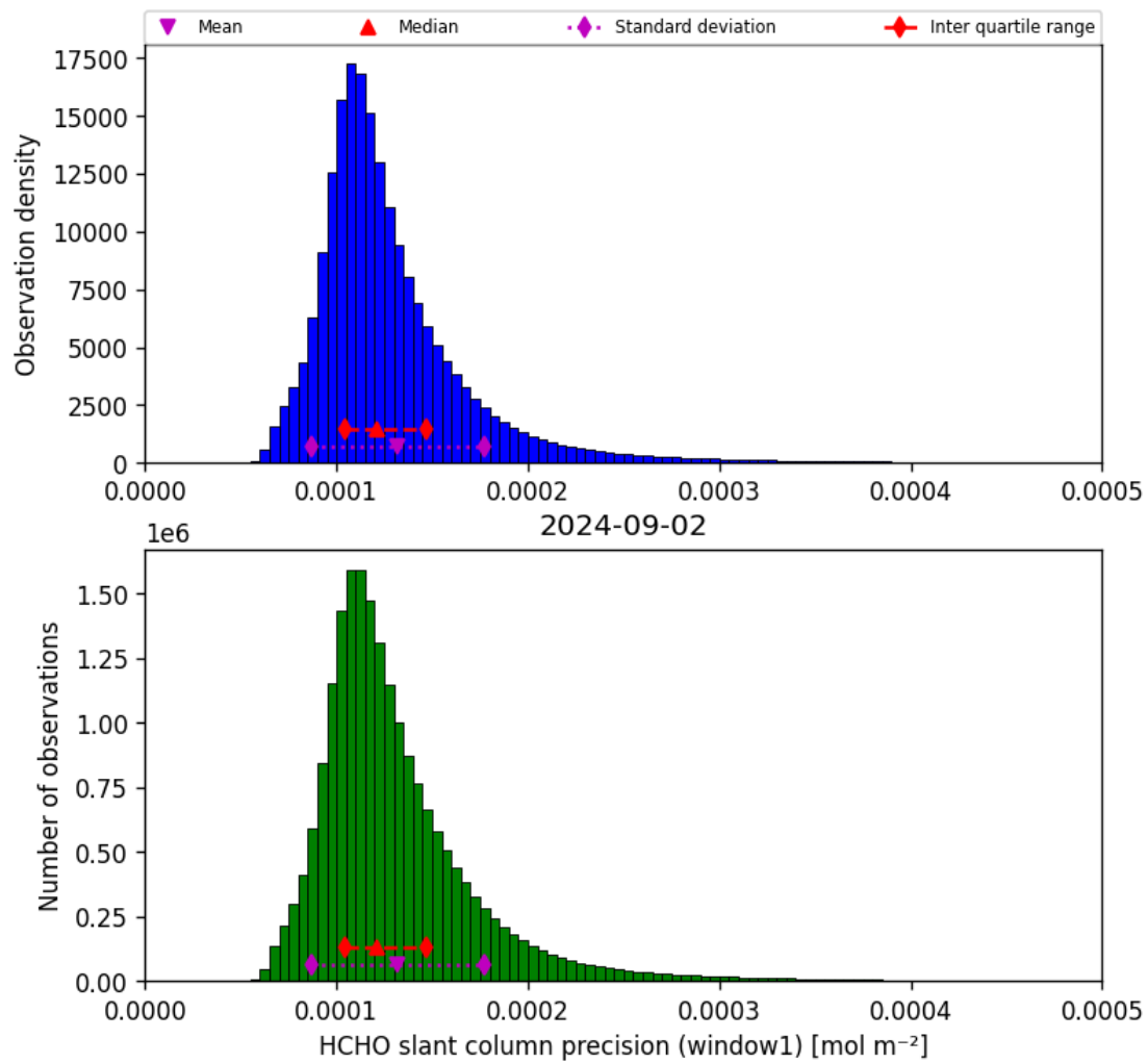
Figure 39: Histogram of “HCHO slant column precision (window1)” for 2024-09-01 to 2024-09-03
