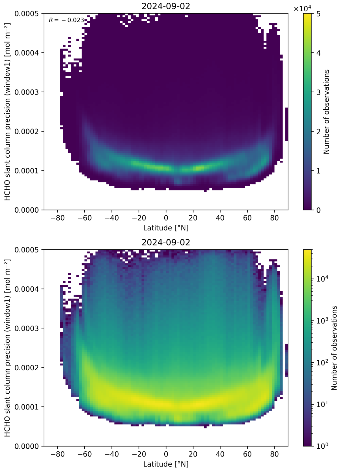
Figure 160: Scatter density plot of “Latitude” against “HCHO slant column precision (window1)” for 2024-09-01 to 2024-09-03.
