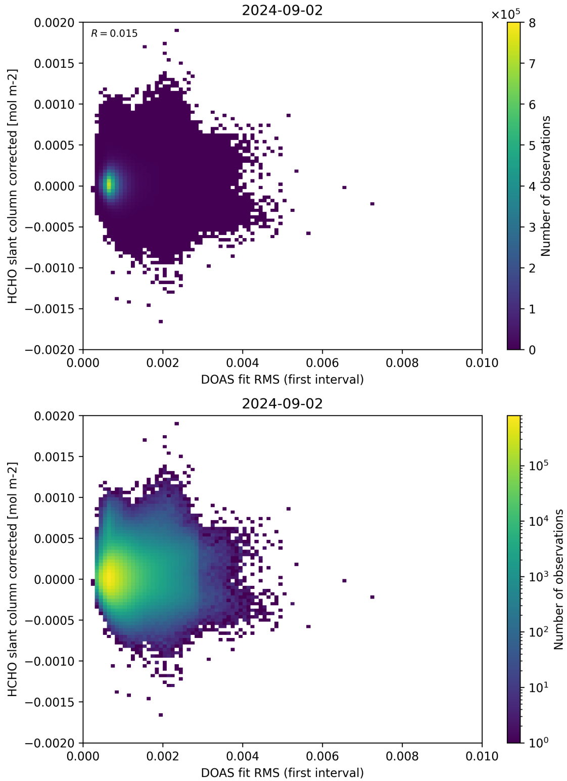
Figure 62: Scatter density plot of “DOAS fit RMS (first interval)” against “HCHO slant column corrected” for 2024-09-01 to 2024-09-03.
