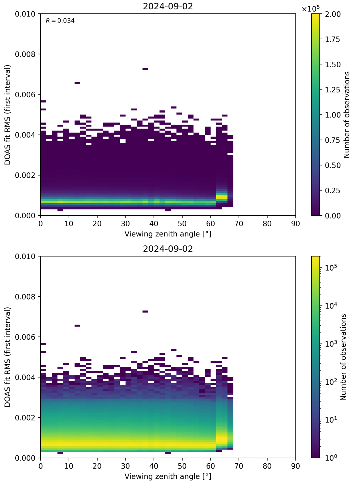
Figure 182: Scatter density plot of “Viewing zenith angle” against “DOAS fit RMS (first interval)” for 2024-09-01 to 2024-09-03.
