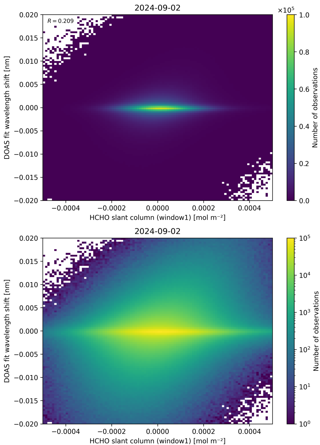
Figure 79: Scatter density plot of “HCHO slant column (window1)” against “DOAS fit wavelength shift” for 2024-09-01 to 2024-09-03.
