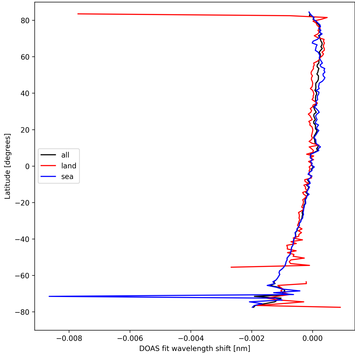
Figure 30: Zonal average of “DOAS fit wavelength shift” for 2024-09-01 to 2024-09-03.
