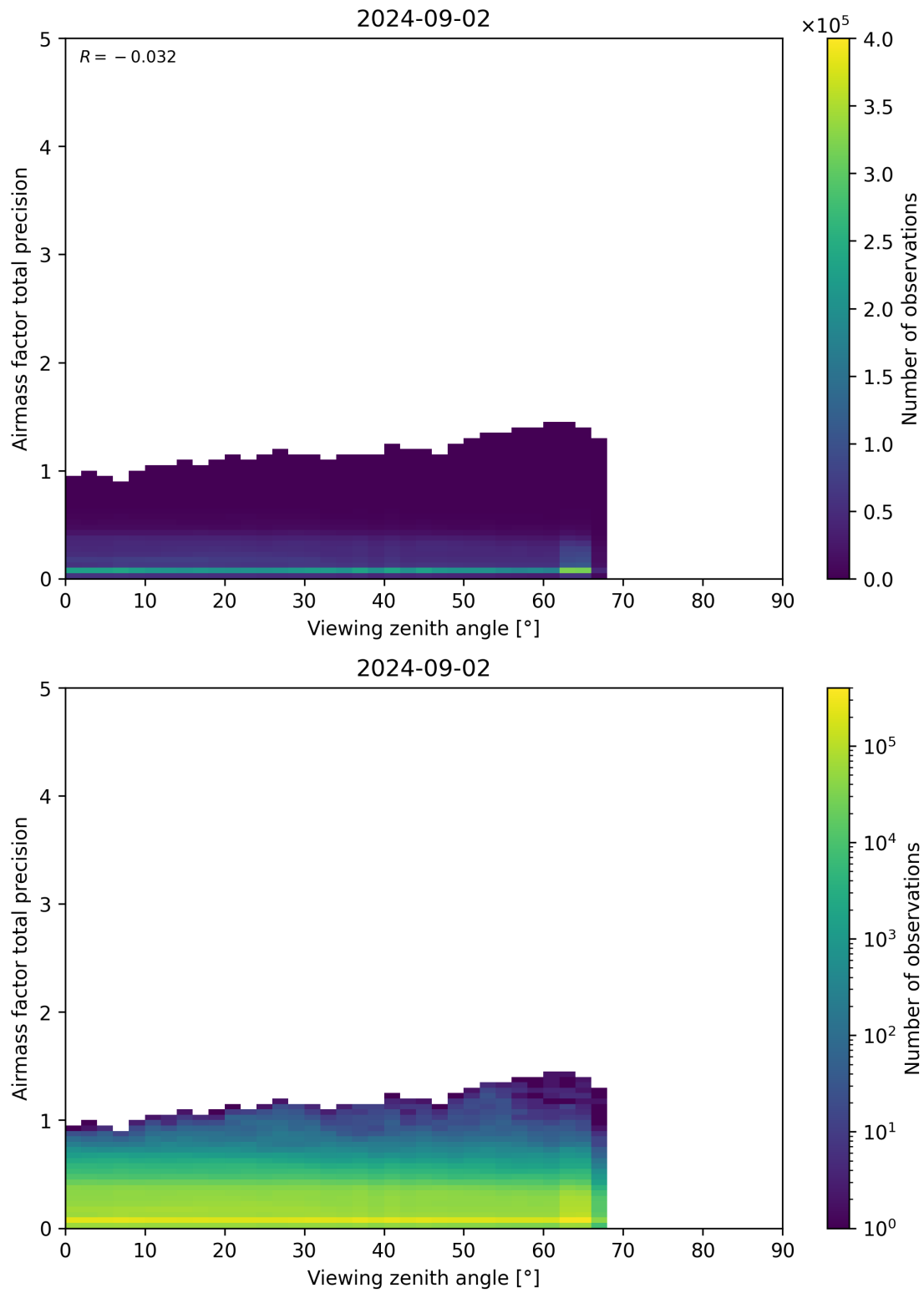
Figure 191: Scatter density plot of “Viewing zenith angle” against “Airmass factor total precision” for 2024-09-01 to 2024-09-03.
