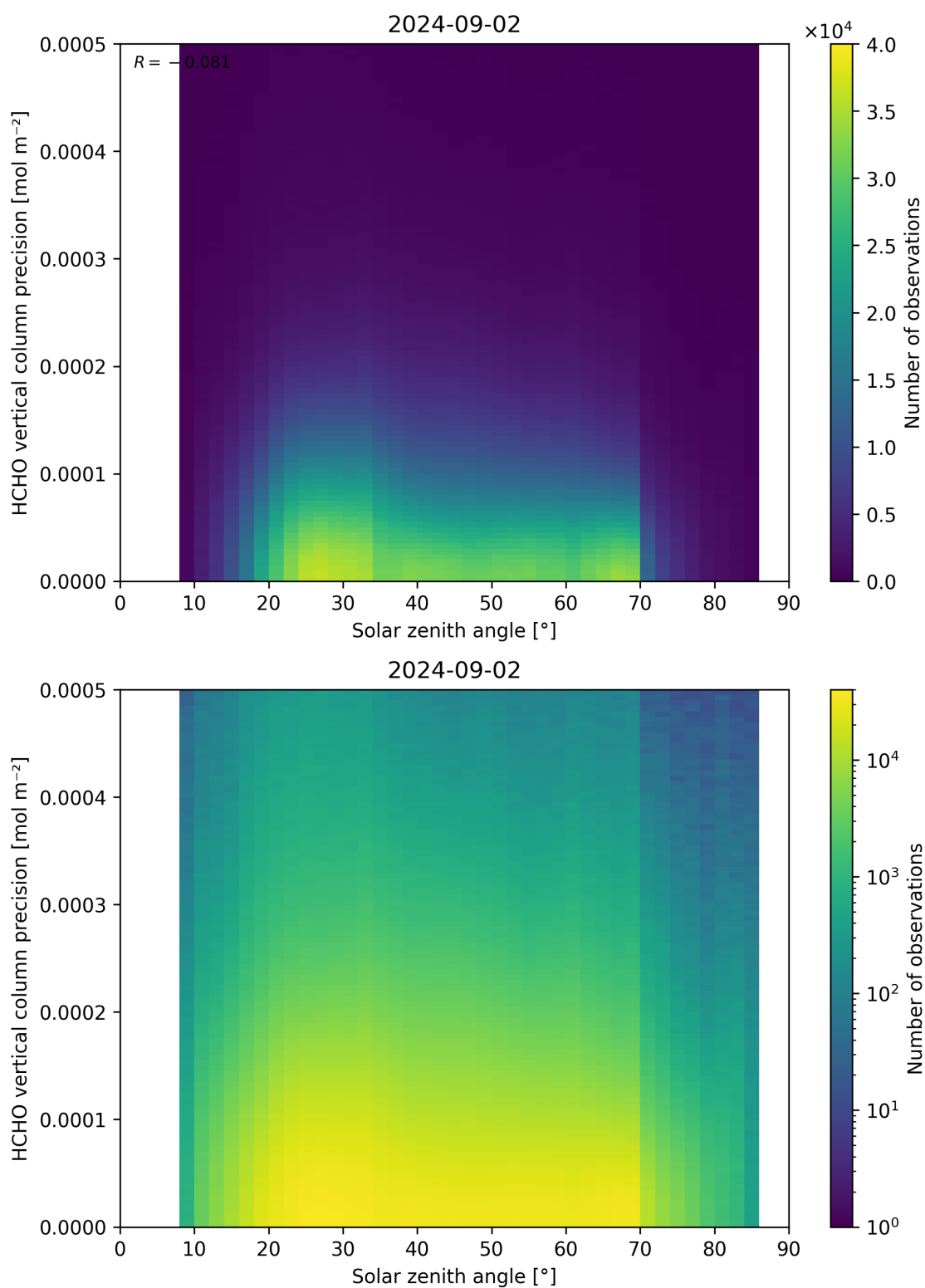
Figure 179: Scatter density plot of “Solar zenith angle” against “HCHO vertical column precision” for 2024-09-01 to 2024-09-03.
