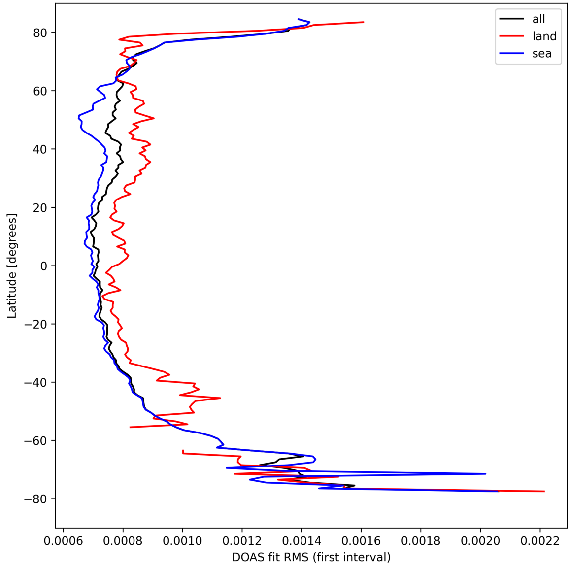
Figure 32: Zonal average of “DOAS fit RMS (first interval)” for 2024-09-01 to 2024-09-03.
