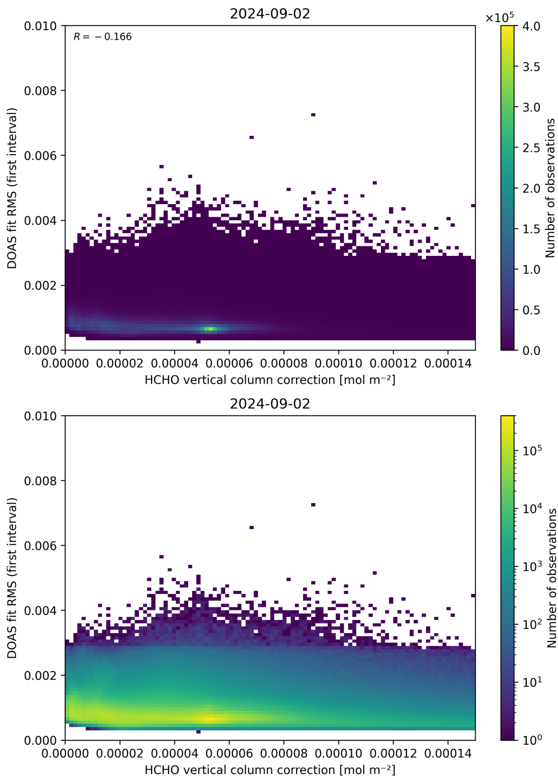
Figure 112: Scatter density plot of “HCHO vertical column correction” against “DOAS fit RMS (first interval)” for 2024-09-01 to 2024-09-03.
