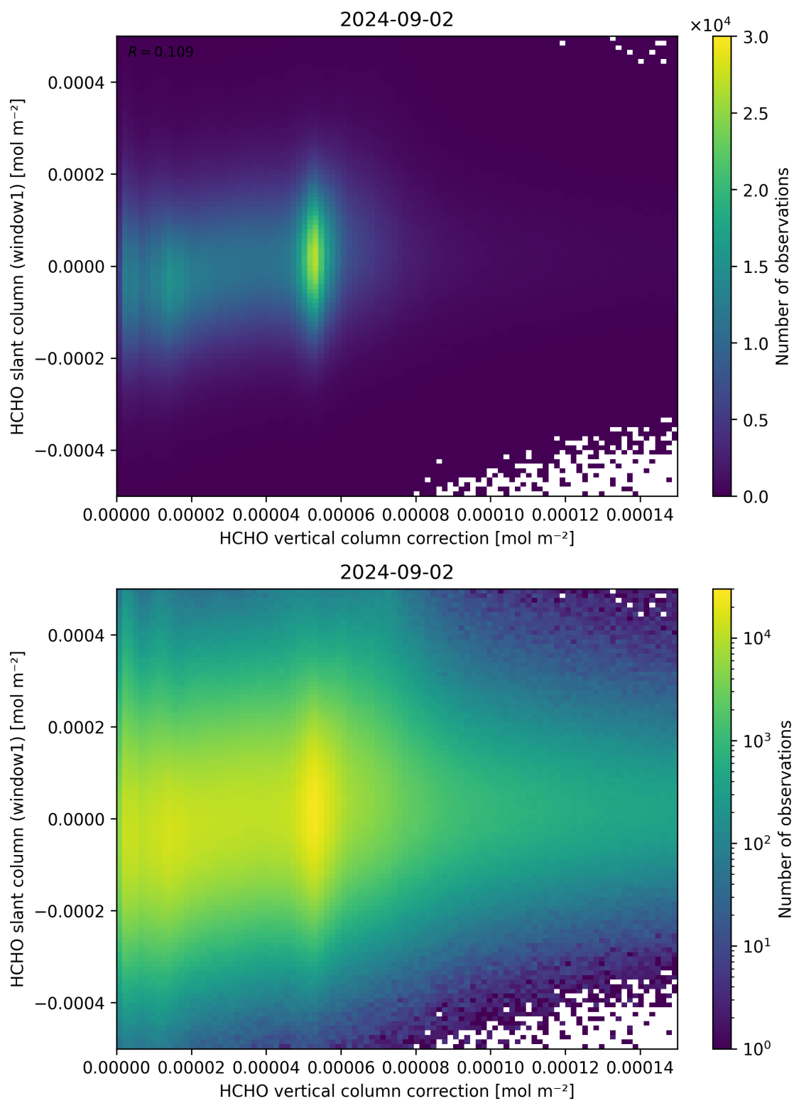
Figure 118: Scatter density plot of “HCHO vertical column correction” against “HCHO slant column (window1)” for 2024-09-01 to 2024-09-03.
