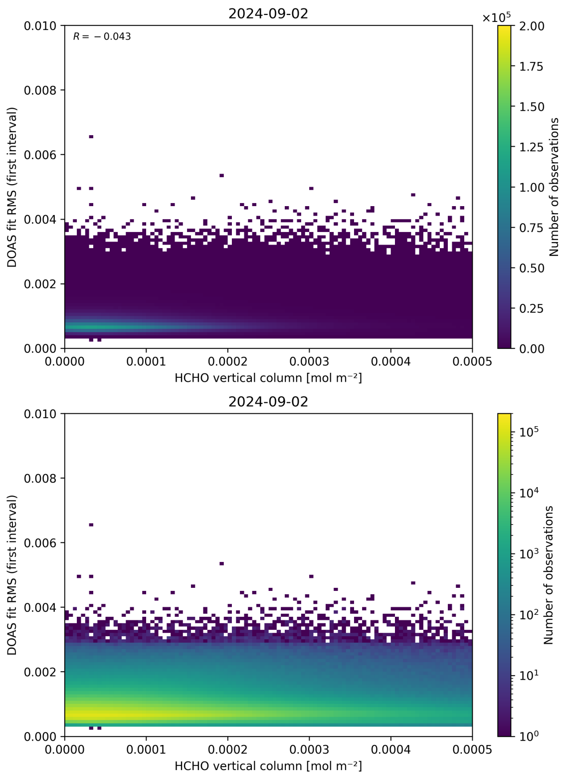
Figure 123: Scatter density plot of “HCHO vertical column” against “DOAS fit RMS (first interval)” for 2024-09-01 to 2024-09-03.
