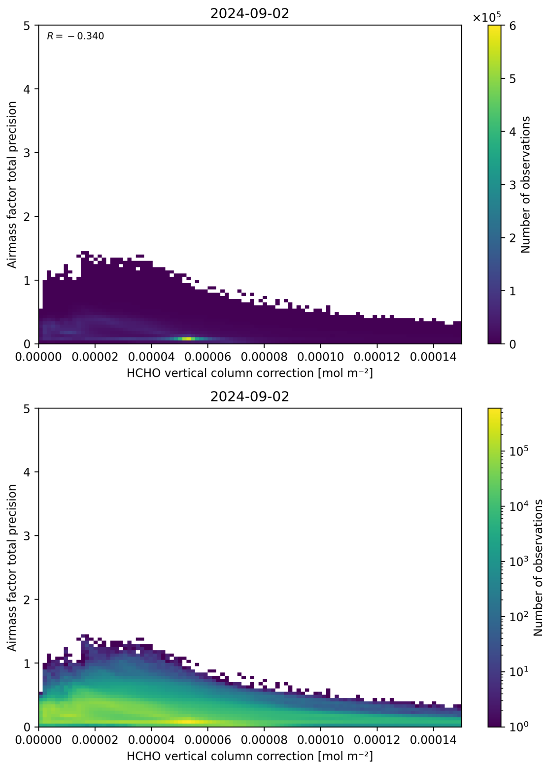
Figure 121: Scatter density plot of “HCHO vertical column correction” against “Airmass factor total precision” for 2024-09-01 to 2024-09-03.
