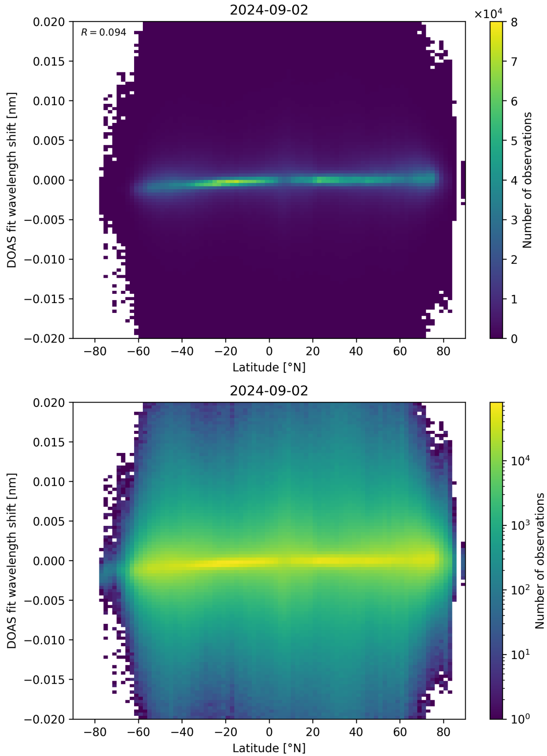
Figure 154: Scatter density plot of “Latitude” against “DOAS fit wavelength shift” for 2024-09-01 to 2024-09-03.
