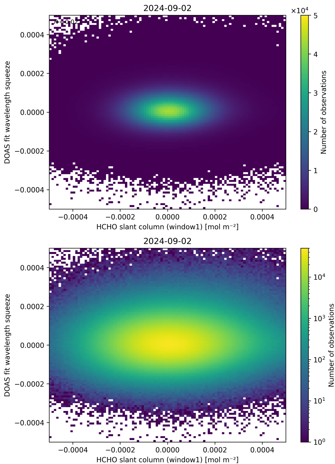
Figure 80: Scatter density plot of “HCHO slant column (window1)” against “DOAS fit wavelength squeeze” for 2024-09-01 to 2024-09-03.
