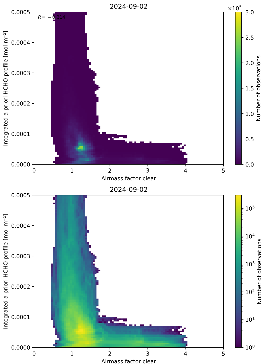
Figure 76: Scatter density plot of “Airmass factor clear” against “Integrated a priori HCHO profile” for 2024-09-01 to 2024-09-03.
