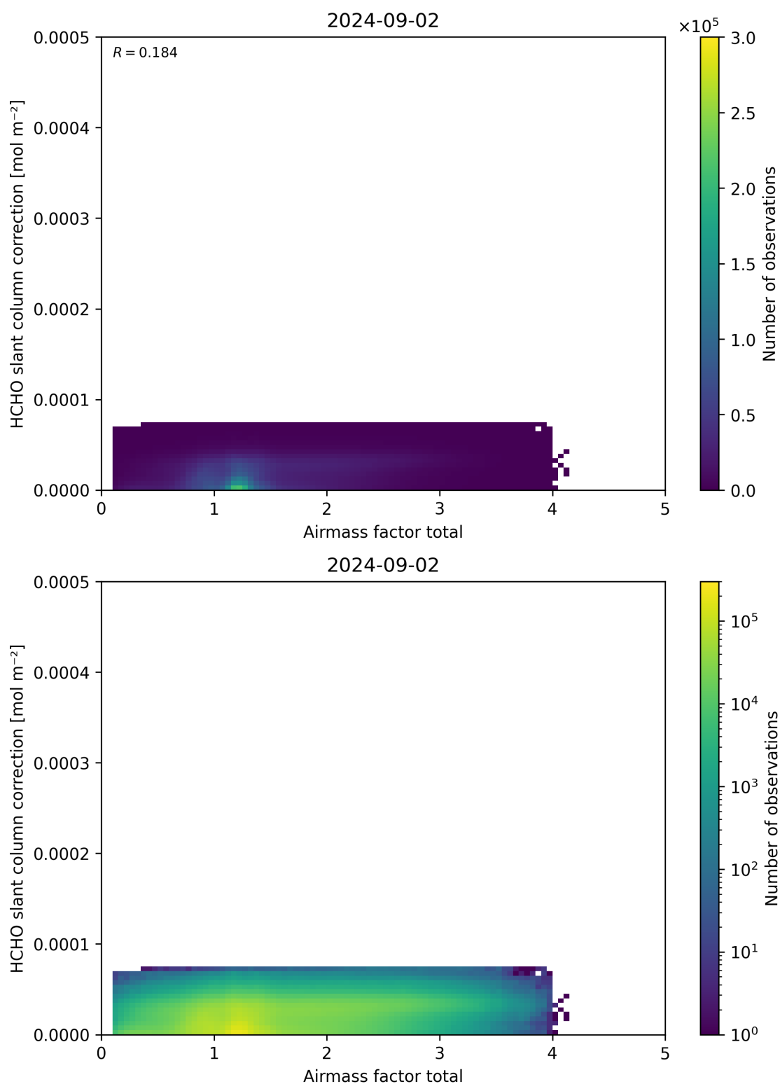
Figure 102: Scatter density plot of “Airmass factor total” against “HCHO slant column correction” for 2024-09-01 to 2024-09-03.
