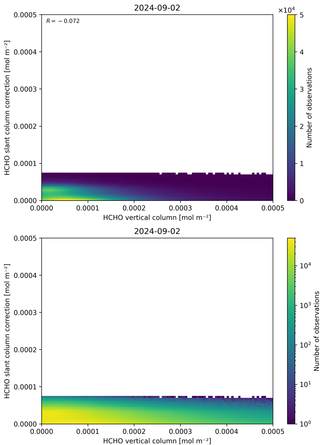
Figure 128: Scatter density plot of “HCHO vertical column” against “HCHO slant column correction” for 2024-09-01 to 2024-09-03.
