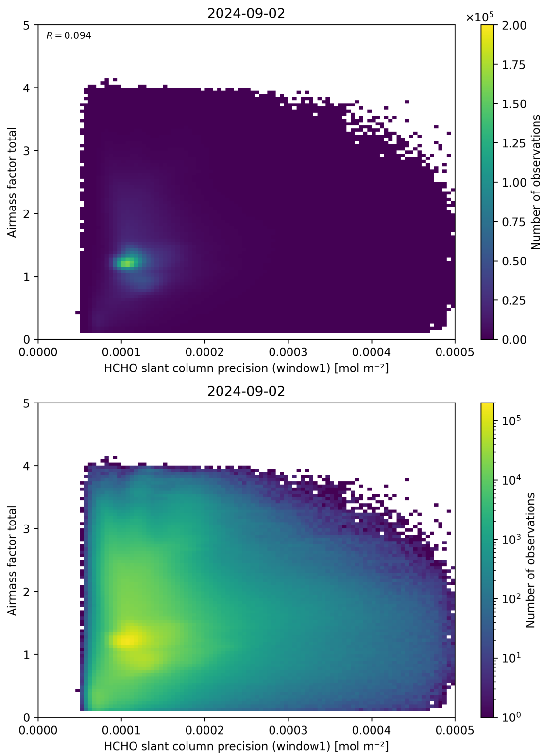
Figure 94: Scatter density plot of “HCHO slant column precision (window1)” against “Airmass factor total” for 2024-09-01 to 2024-09-03.
