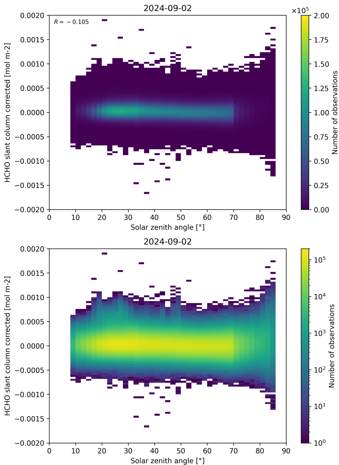
Figure 171: Scatter density plot of “Solar zenith angle” against “HCHO slant column corrected” for 2024-09-01 to 2024-09-03.
