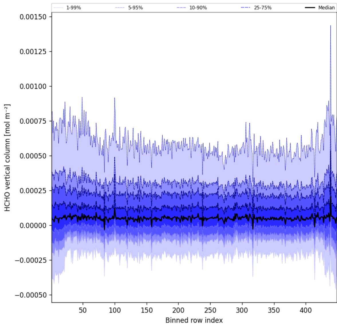
Figure 49: Along track statistics of “HCHO vertical column” for 2024-09-01 to 2024-09-03
