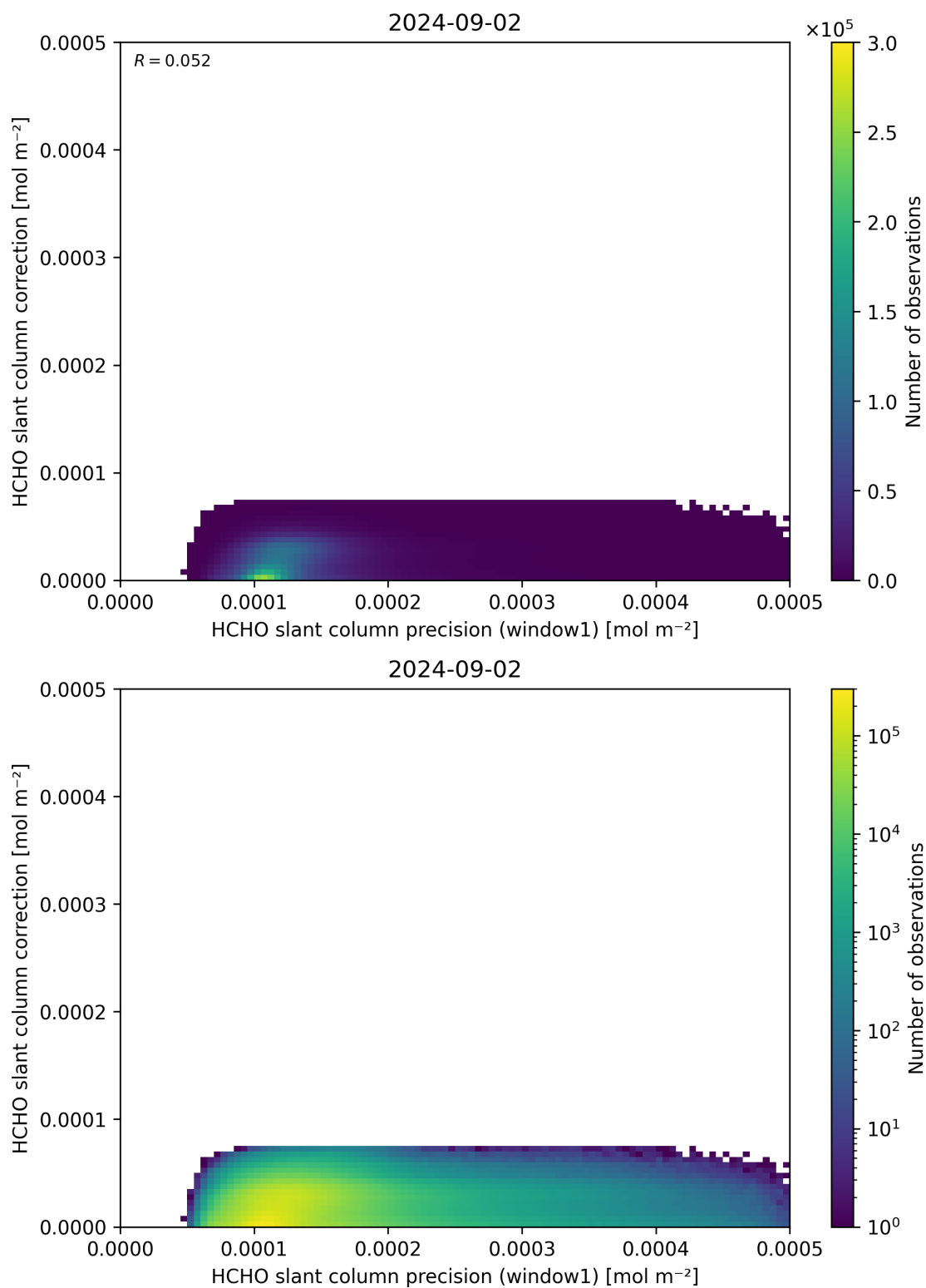
Figure 93: Scatter density plot of “HCHO slant column precision (window1)” against “HCHO slant column correction” for 2024-09-01 to 2024-09-03.
