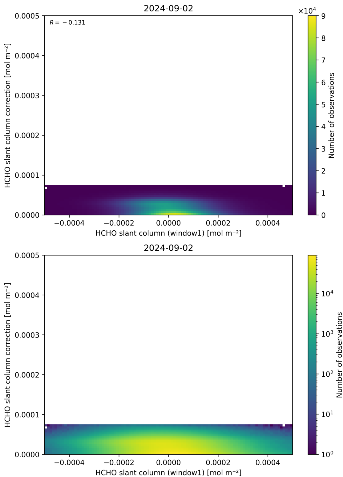
Figure 83: Scatter density plot of “HCHO slant column (window1)” against “HCHO slant column correction” for 2024-09-01 to 2024-09-03.
