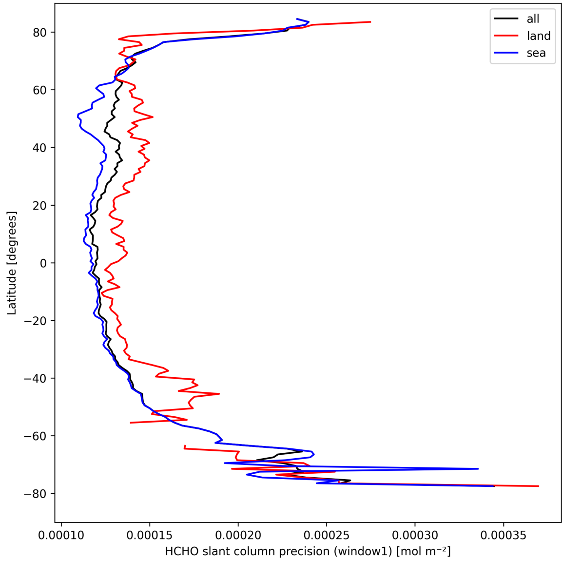
Figure 25: Zonal average of “HCHO slant column precision (window1)” for 2024-09-01 to 2024-09-03.
