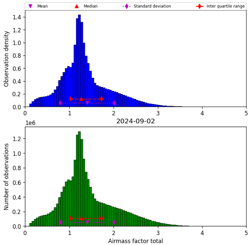
Figure 40: Histogram of “Airmass factor total” for 2024-09-01 to 2024-09-03
