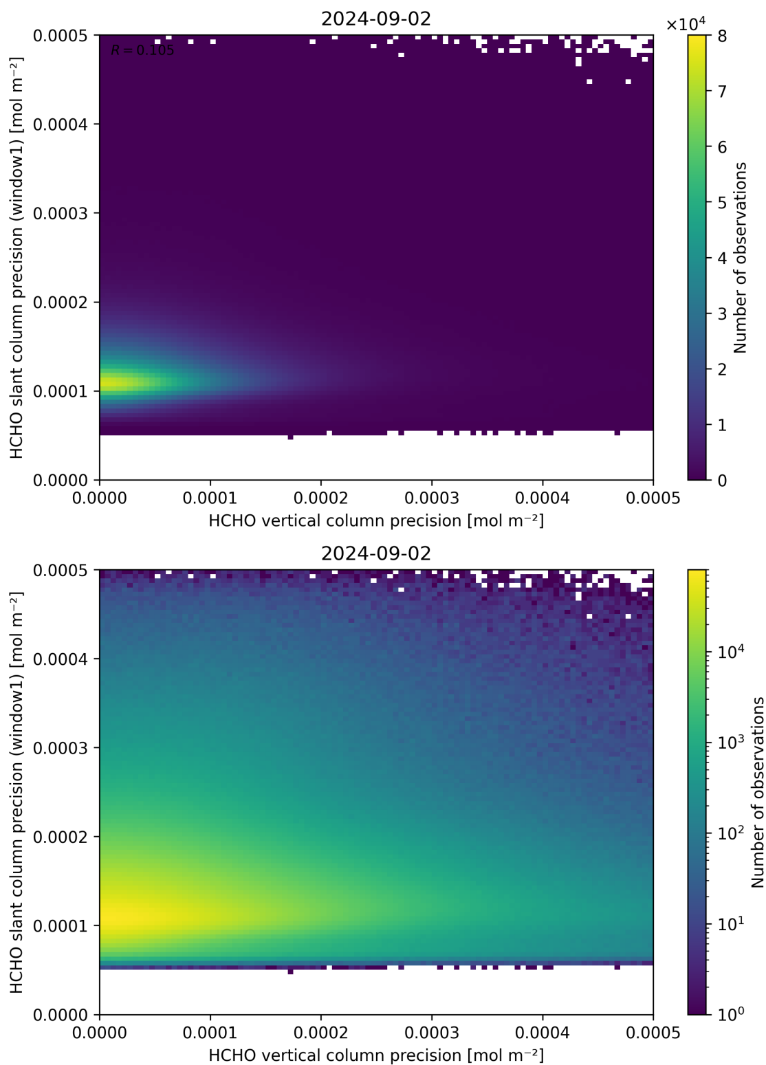
Figure 143: Scatter density plot of “HCHO vertical column precision” against “HCHO slant column precision (window1)” for 2024-09-01 to 2024-09-03.
