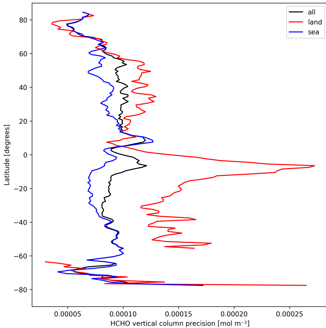
Figure 22: Zonal average of “HCHO vertical column precision” for 2024-09-01 to 2024-09-03.
