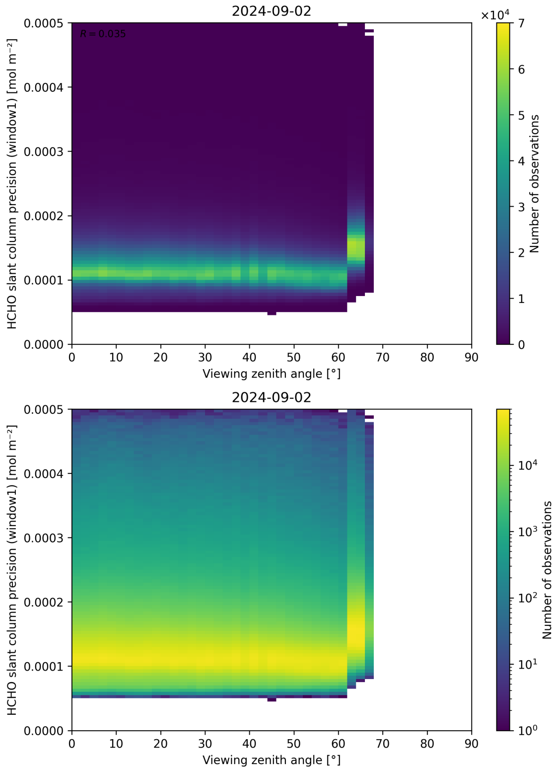
Figure 189: Scatter density plot of “Viewing zenith angle” against “HCHO slant column precision (window1)” for 2024-09-01 to 2024-09-03.
