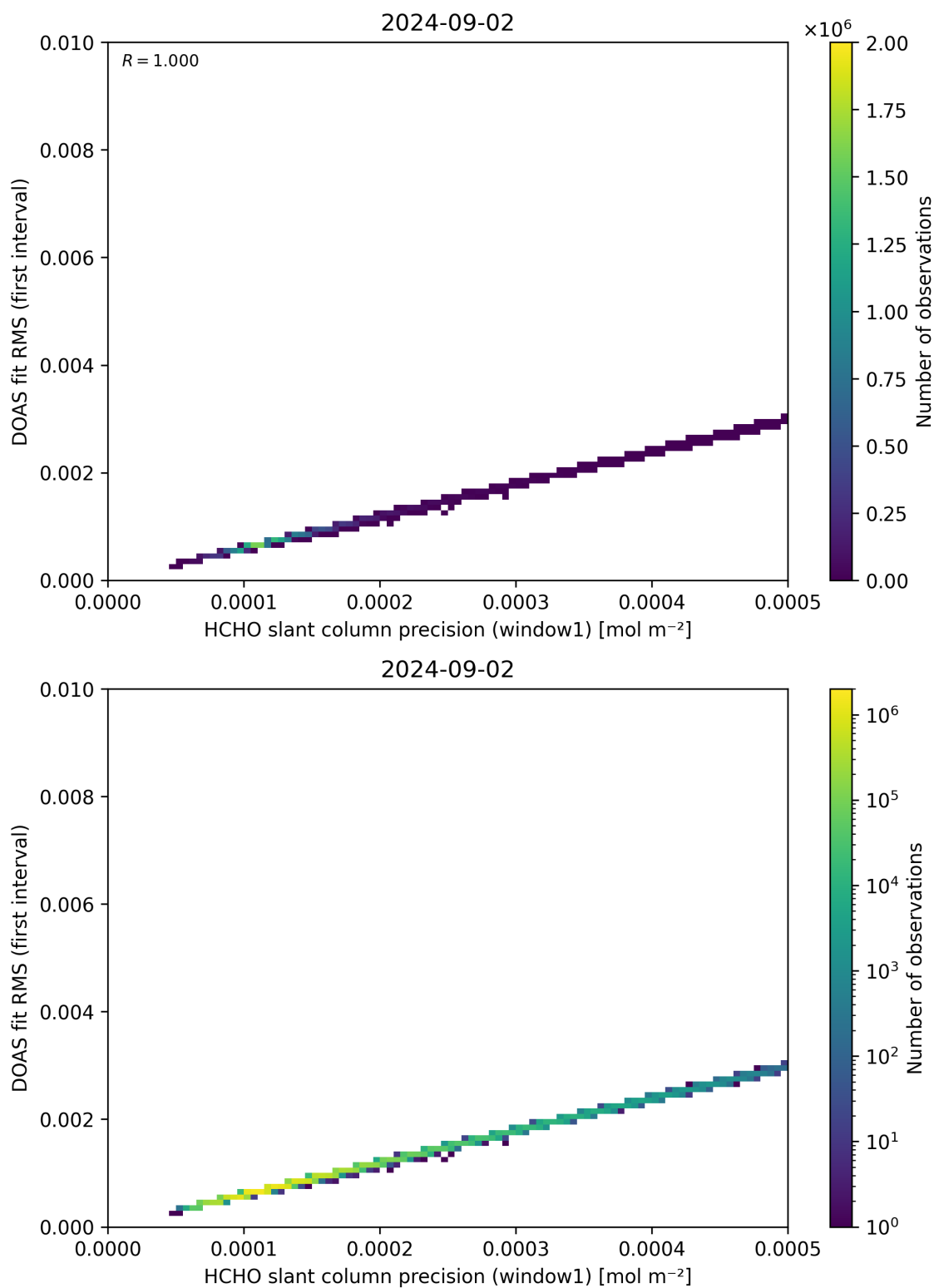
Figure 88: Scatter density plot of “HCHO slant column precision (window1)” against “DOAS fit RMS (first interval)” for 2024-09-01 to 2024-09-03.
