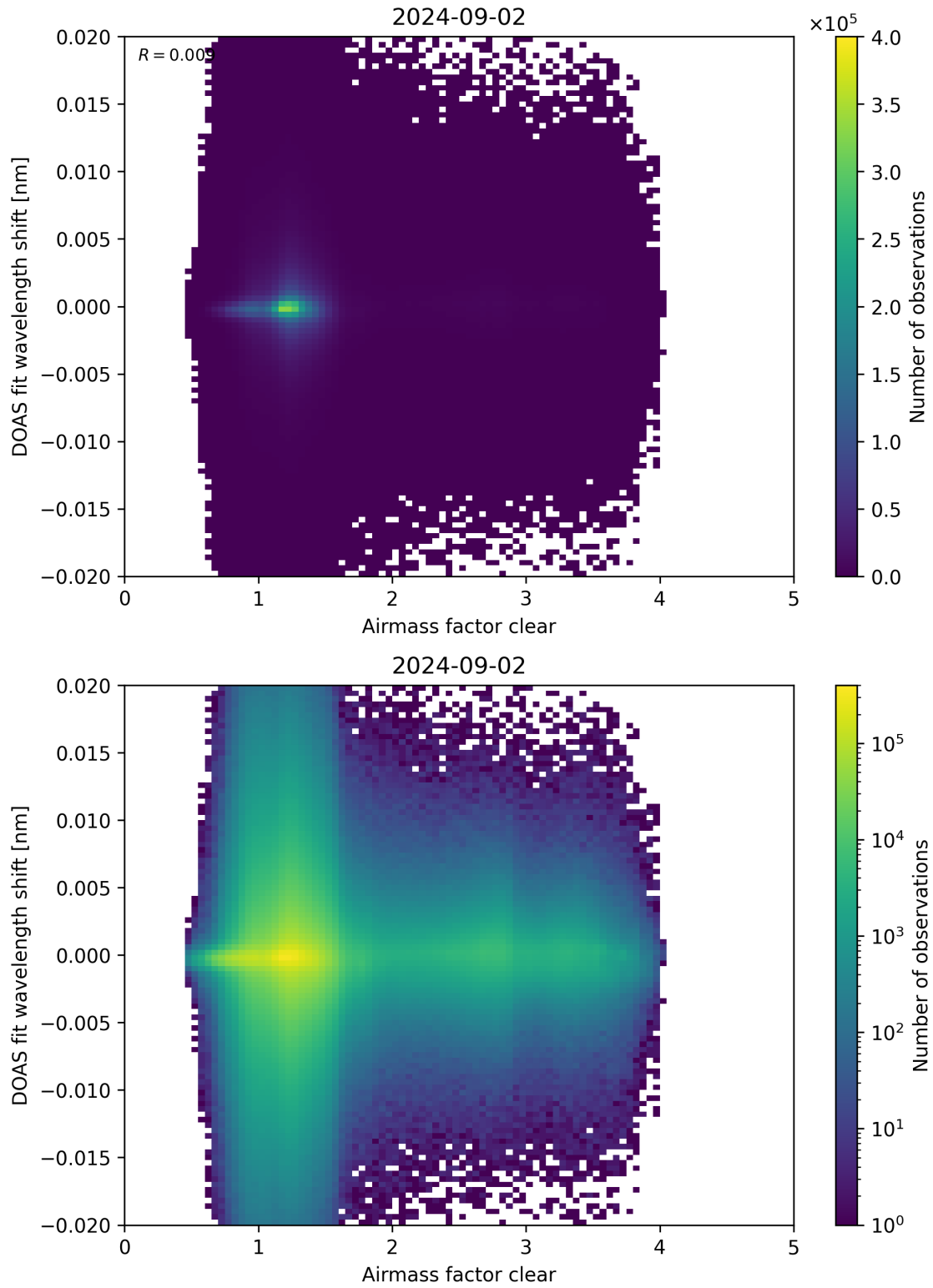
Figure 72: Scatter density plot of “Airmass factor clear” against “DOAS fit wavelength shift” for 2024-09-01 to 2024-09-03.
