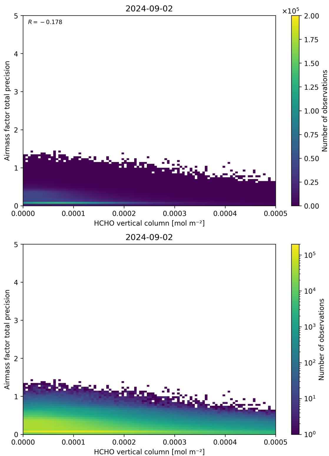
Figure 132: Scatter density plot of “HCHO vertical column” against “Airmass factor total precision” for 2024-09-01 to 2024-09-03.
