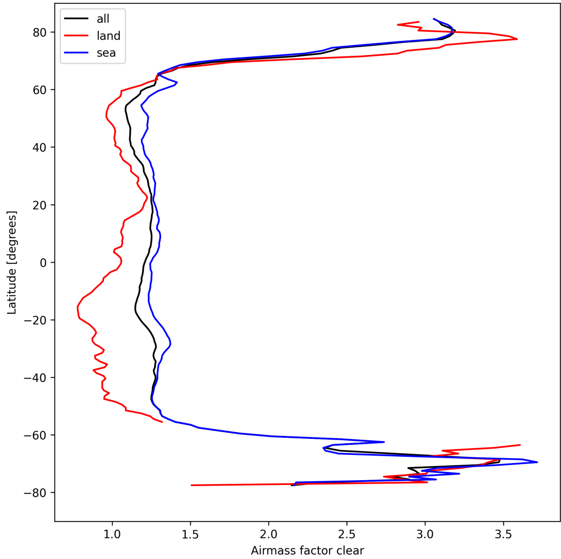
Figure 28: Zonal average of “Airmass factor clear” for 2024-09-01 to 2024-09-03.
