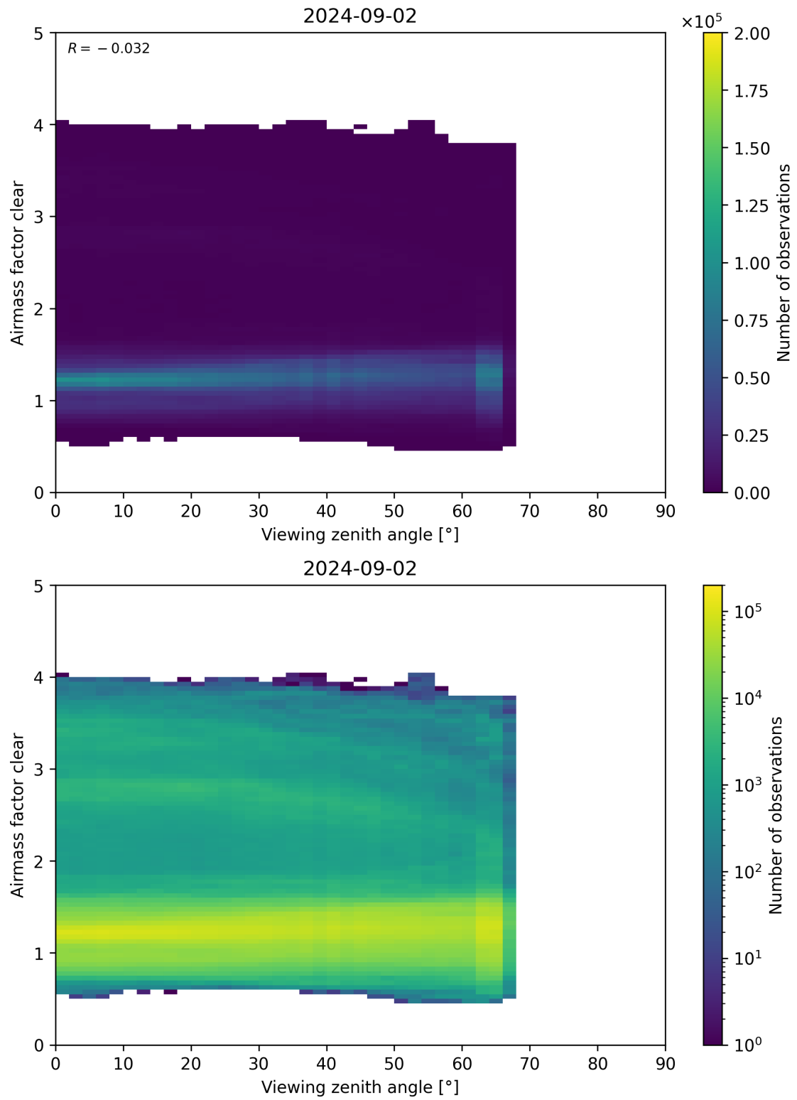
Figure 185: Scatter density plot of “Viewing zenith angle” against “Airmass factor clear” for 2024-09-01 to 2024-09-03.
