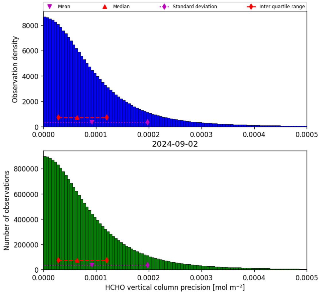
Figure 36: Histogram of “HCHO vertical column precision” for 2024-09-01 to 2024-09-03
