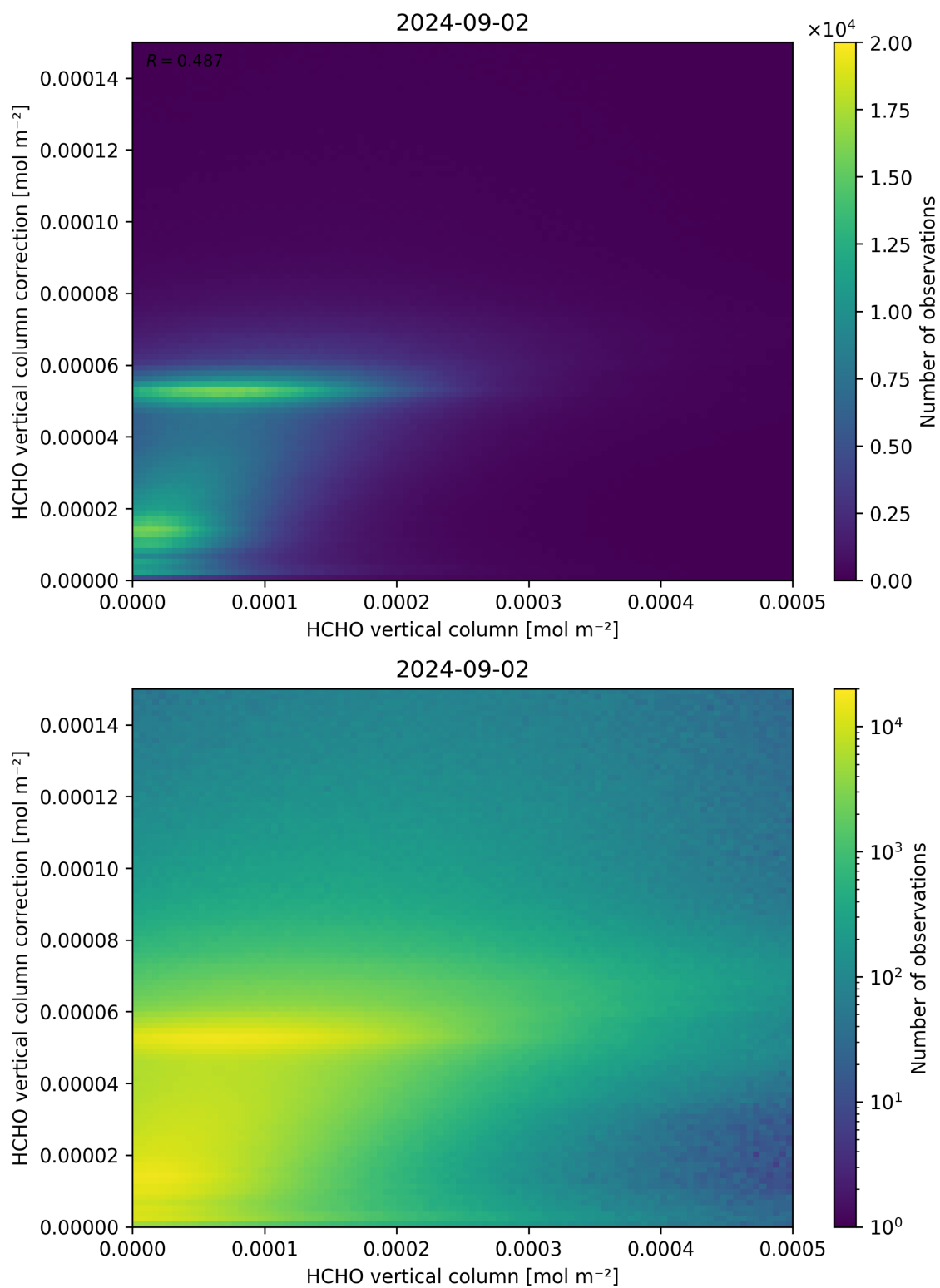
Figure 133: Scatter density plot of “HCHO vertical column” against “HCHO vertical column correction” for 2024-09-01 to 2024-09-03.
