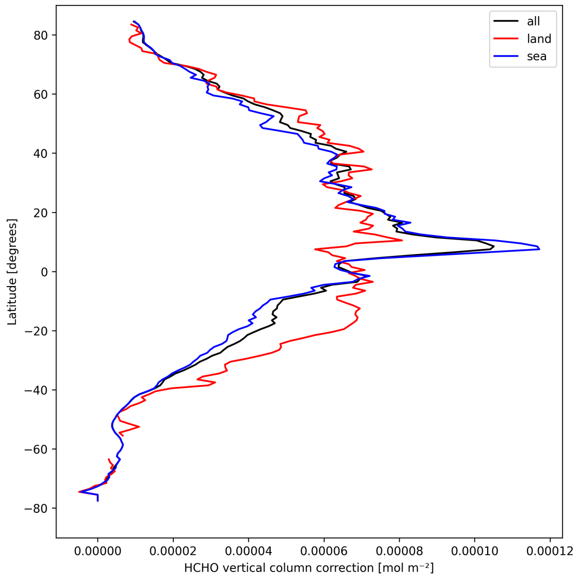
Figure 23: Zonal average of “HCHO vertical column correction” for 2024-09-01 to 2024-09-03.
