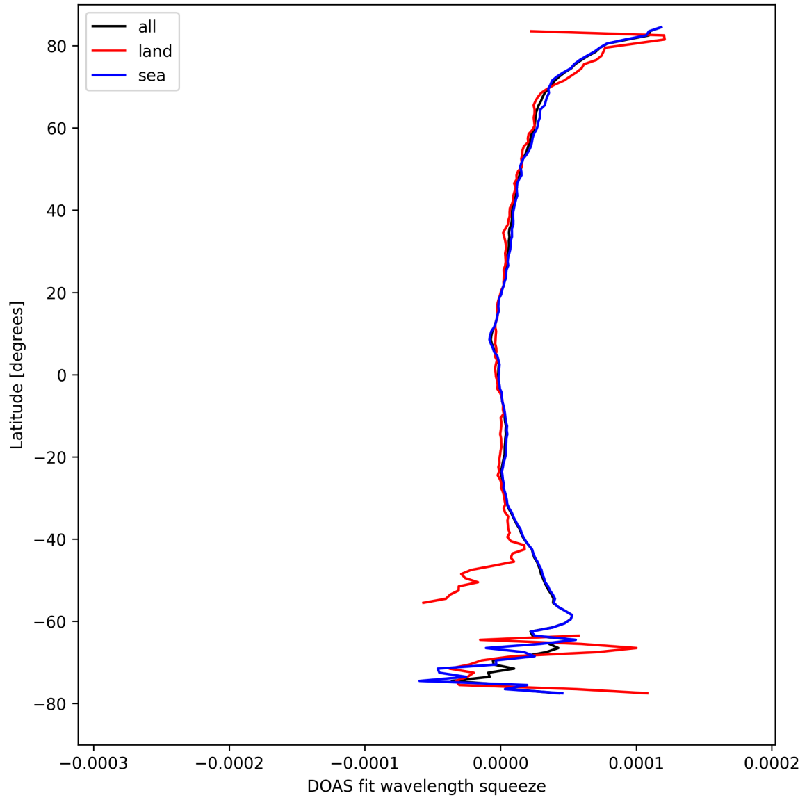
Figure 31: Zonal average of “DOAS fit wavelength squeeze” for 2024-09-01 to 2024-09-03.
