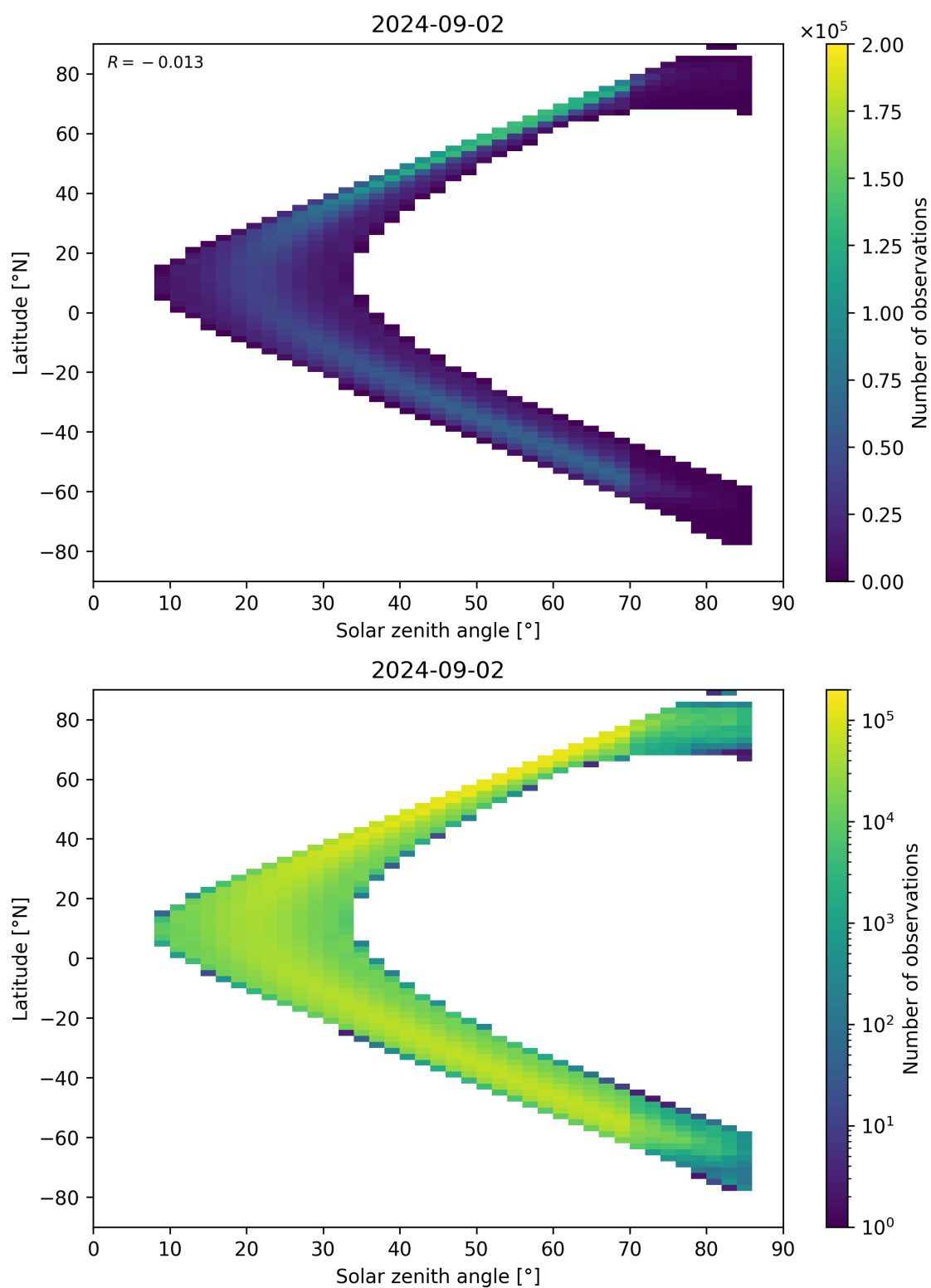
Figure 181: Scatter density plot of “Solar zenith angle” against “Latitude” for 2024-09-01 to 2024-09-03.
