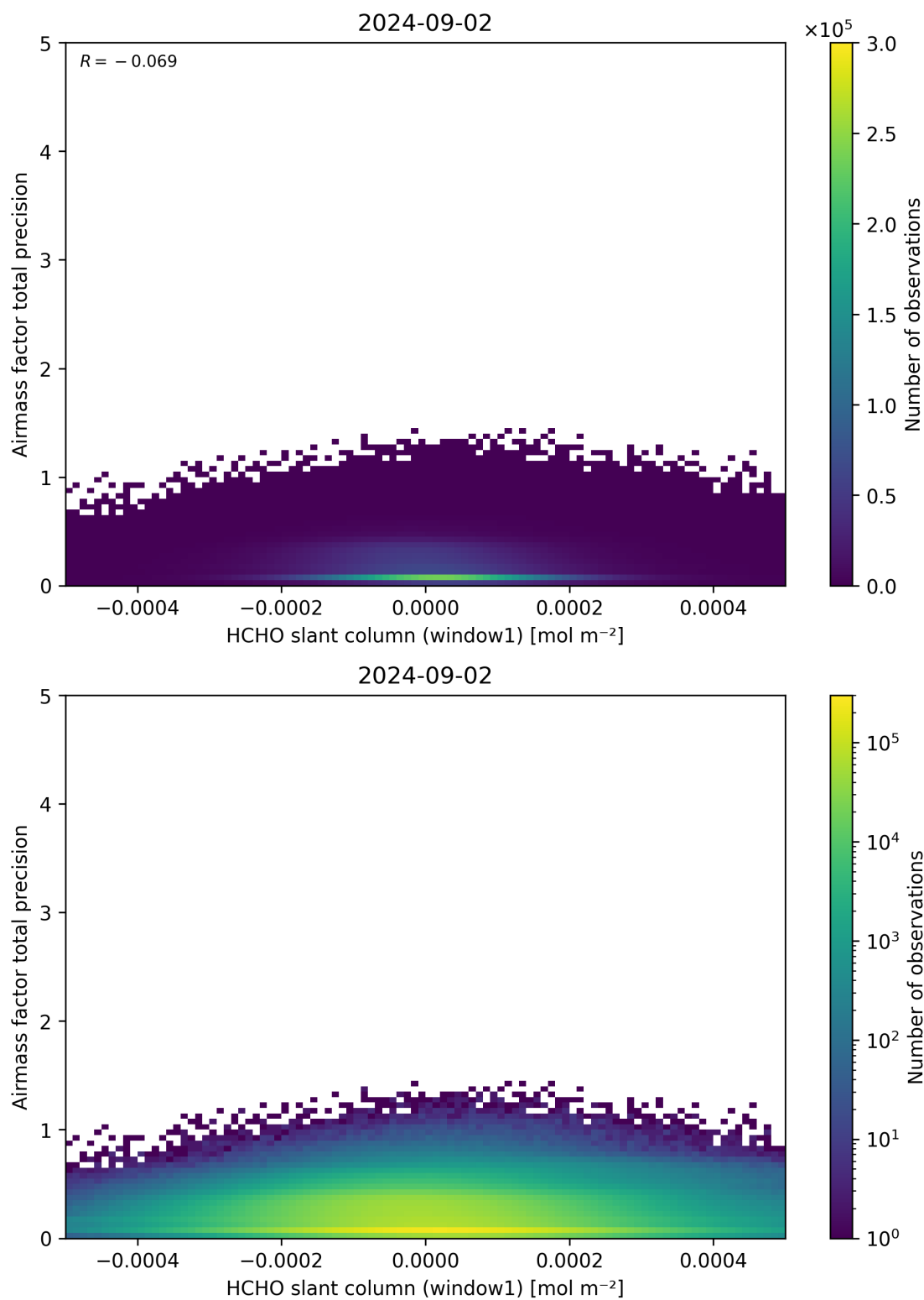
Figure 86: Scatter density plot of “HCHO slant column (window1)” against “Airmass factor total precision” for 2024-09-01 to 2024-09-03.
