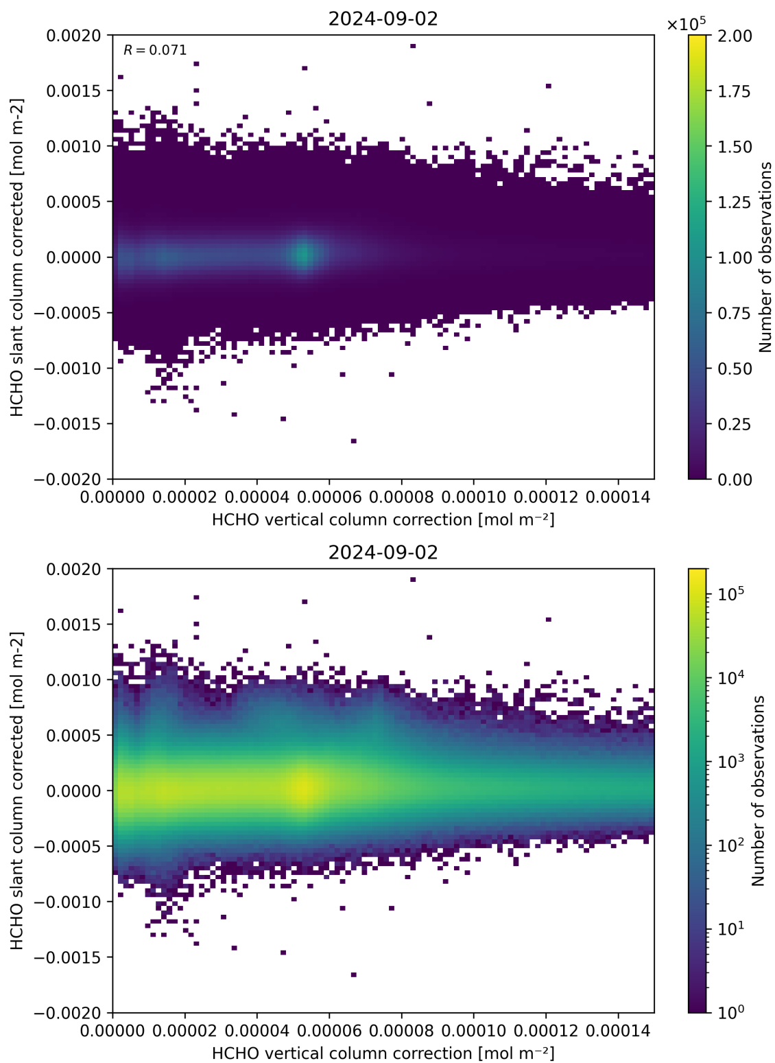
Figure 116: Scatter density plot of “HCHO vertical column correction” against “HCHO slant column corrected” for 2024-09-01 to 2024-09-03.
