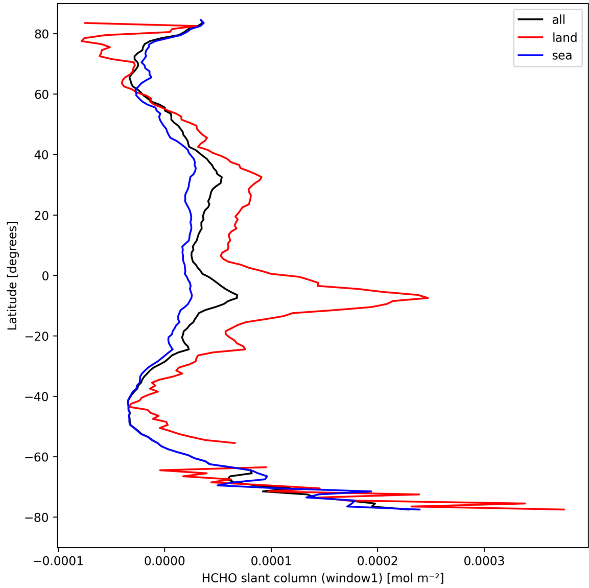
Figure 24: Zonal average of “HCHO slant column (window1)” for 2024-09-01 to 2024-09-03.
