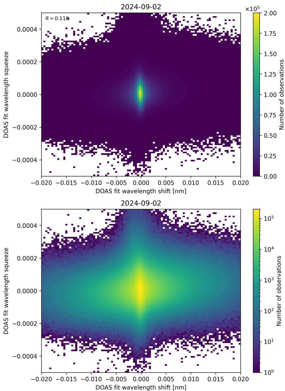
Figure 65: Scatter density plot of “DOAS fit wavelength shift” against “DOAS fit wavelength squeeze” for 2024-09-01 to 2024-09-03.
