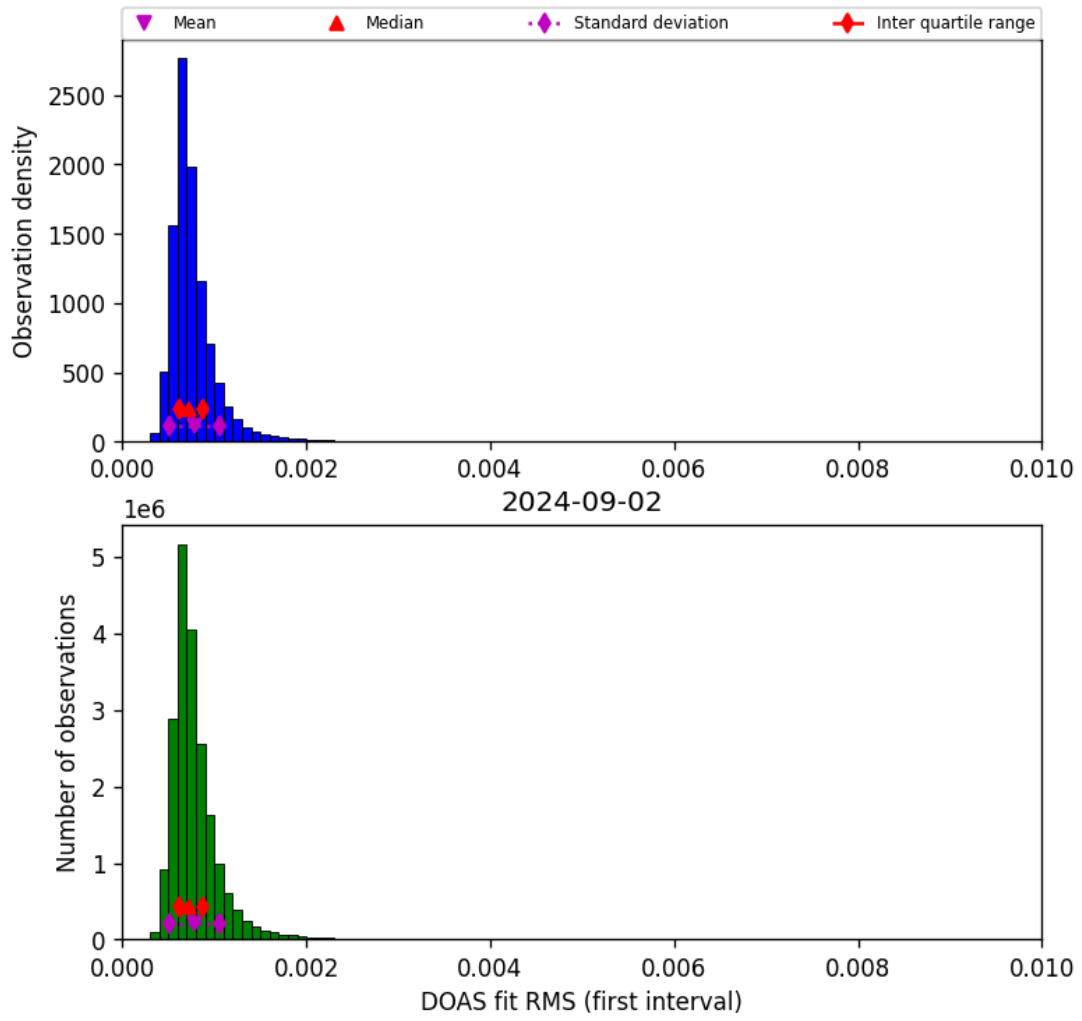
Figure 46: Histogram of “DOAS fit RMS (first interval)” for 2024-09-01 to 2024-09-03
