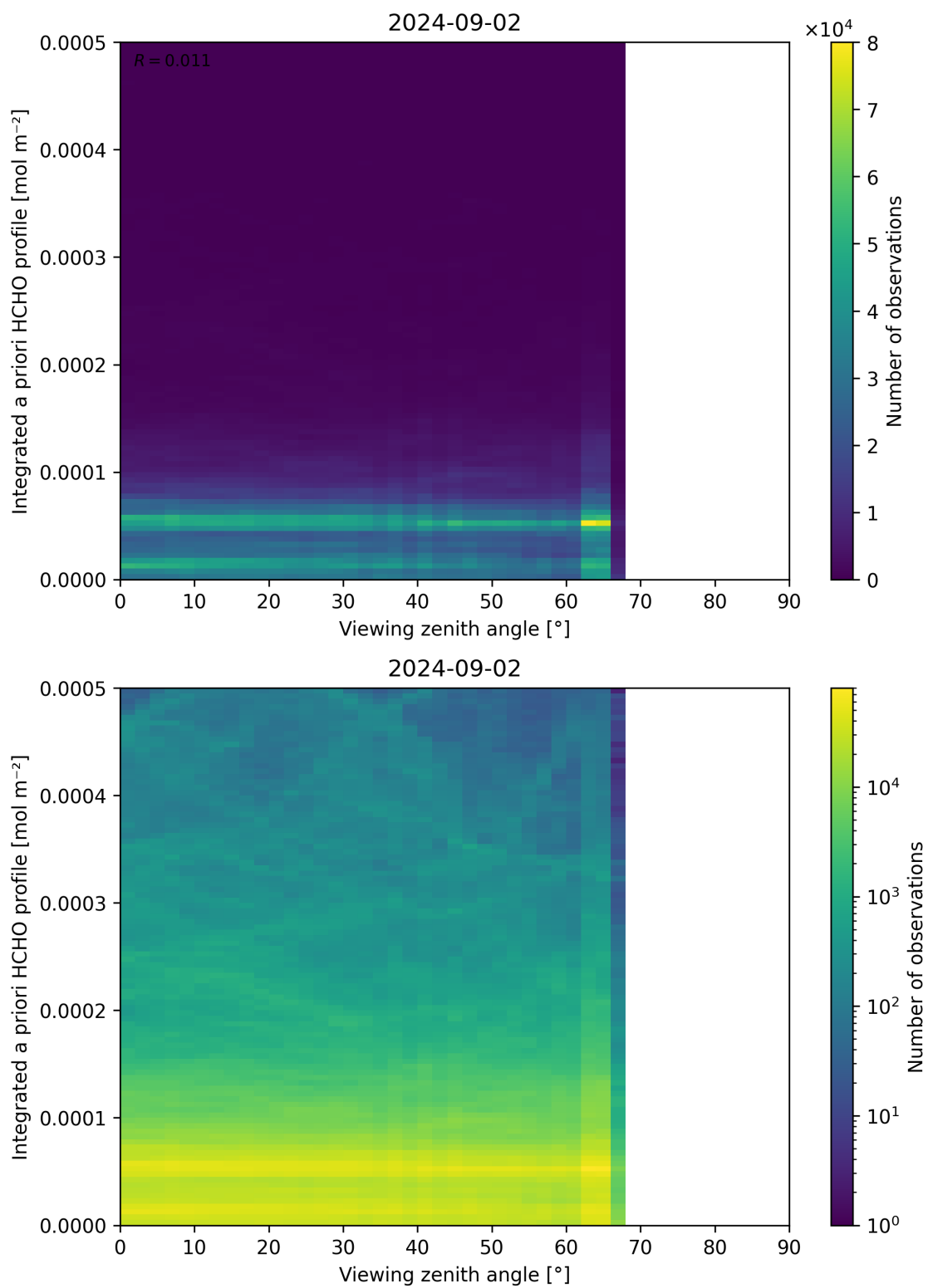
Figure 195: Scatter density plot of “Viewing zenith angle” against “Integrated a priori HCHO profile” for 2024-09-01 to 2024-09-03.
