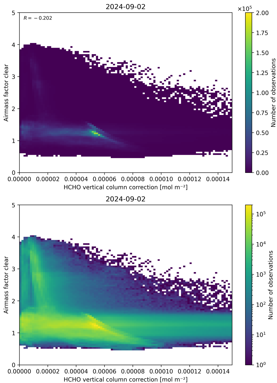
Figure 115: Scatter density plot of “HCHO vertical column correction” against “Airmass factor clear” for 2024-09-01 to 2024-09-03.
