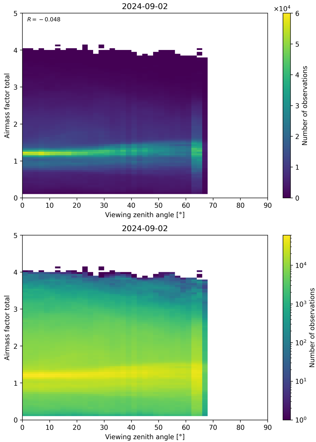
Figure 190: Scatter density plot of “Viewing zenith angle” against “Airmass factor total” for 2024-09-01 to 2024-09-03.
