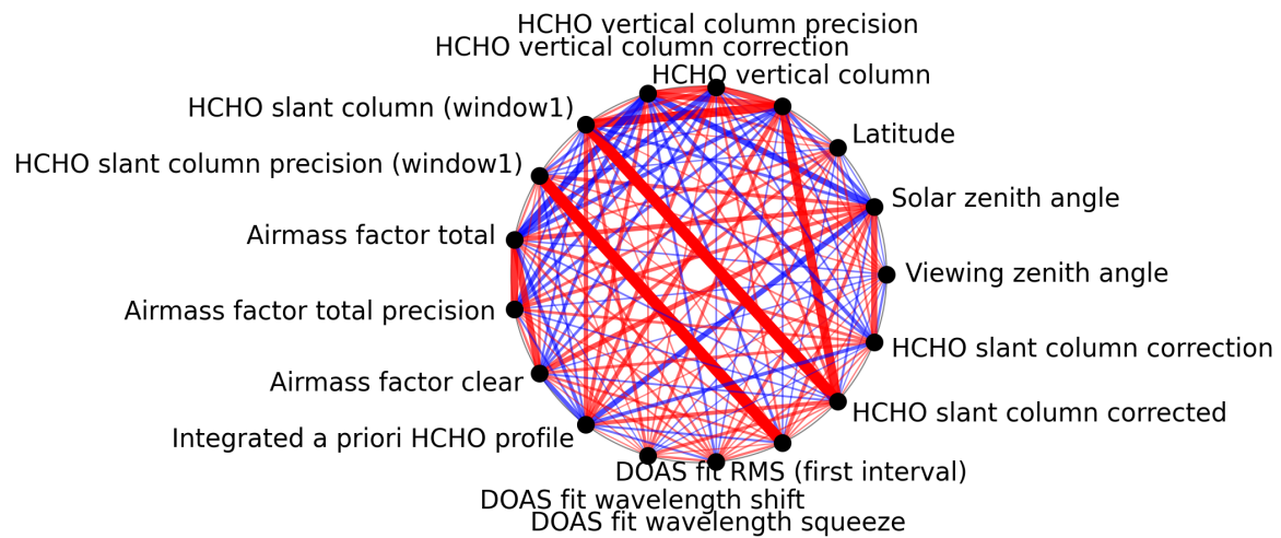
Figure 1: Map of correlation graph for 2024-09-01 to 2024-09-03.
