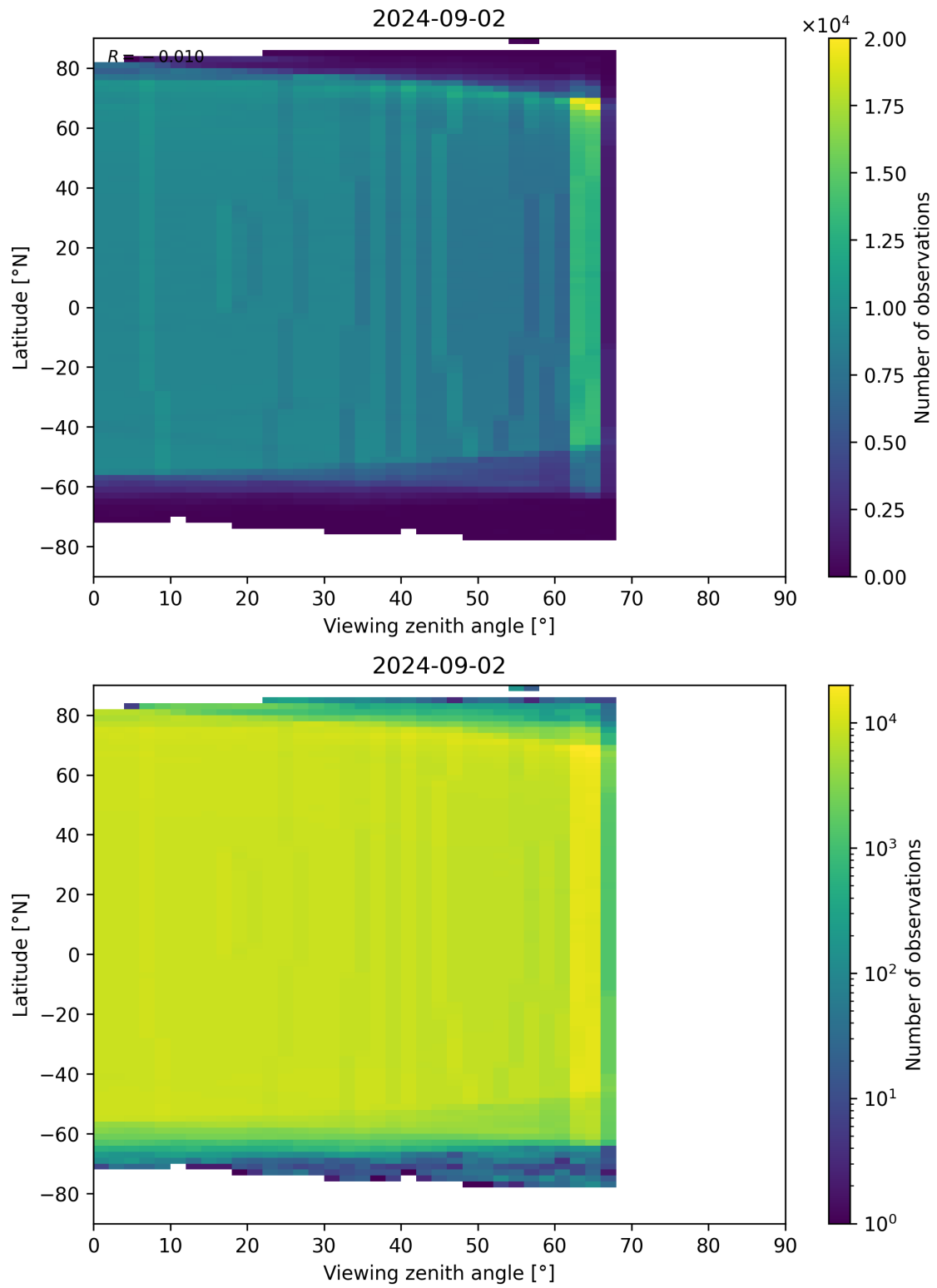
Figure 196: Scatter density plot of “Viewing zenith angle” against “Latitude” for 2024-09-01 to 2024-09-03.
