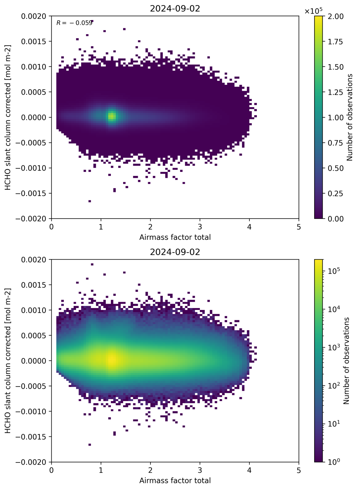
Figure 101: Scatter density plot of “Airmass factor total” against “HCHO slant column corrected” for 2024-09-01 to 2024-09-03.
