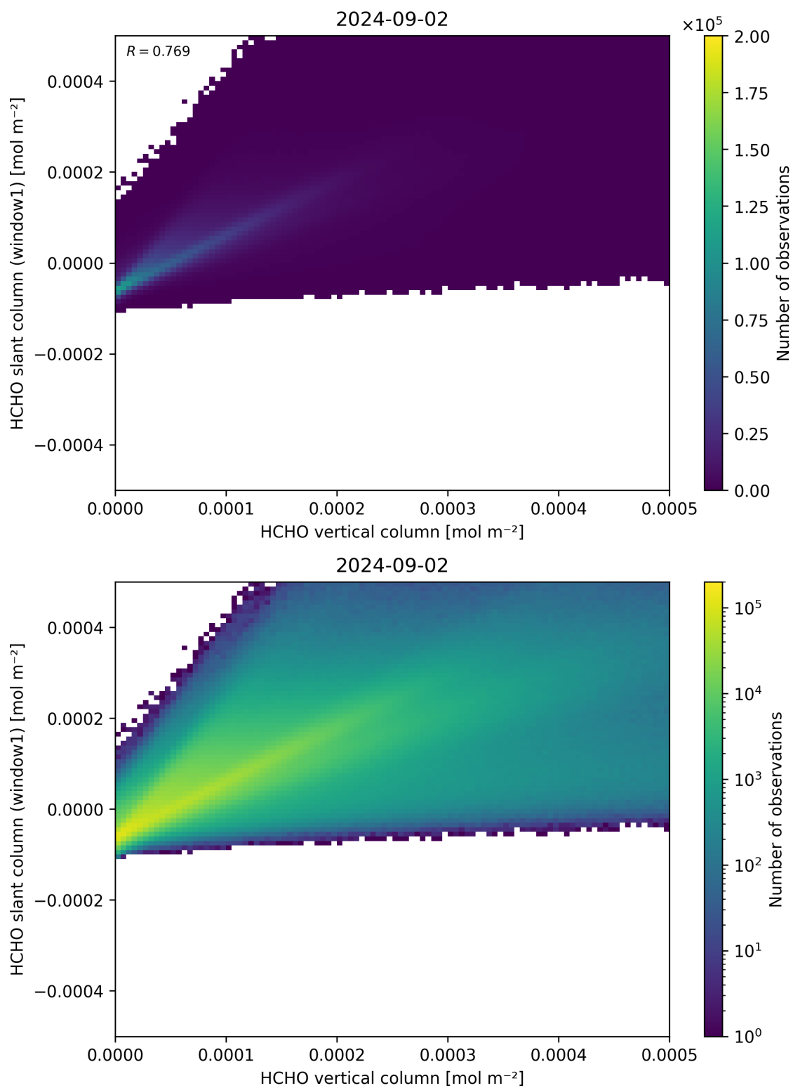
Figure 129: Scatter density plot of “HCHO vertical column” against “HCHO slant column (window1)” for 2024-09-01 to 2024-09-03.
