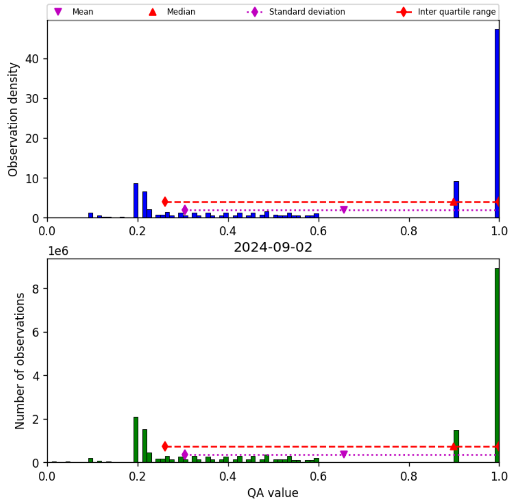
Figure 34: Histogram of “QA value” for 2024-09-01 to 2024-09-03
