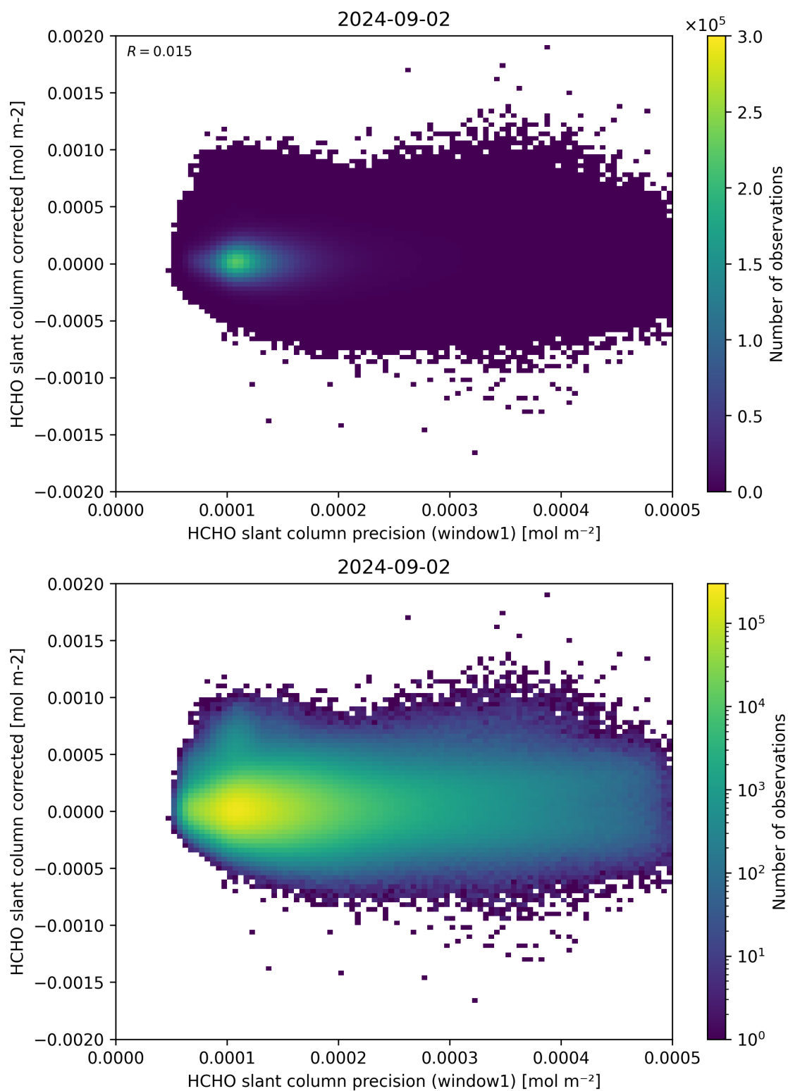
Figure 92: Scatter density plot of “HCHO slant column precision (window1)” against “HCHO slant column corrected” for 2024-09-01 to 2024-09-03.
