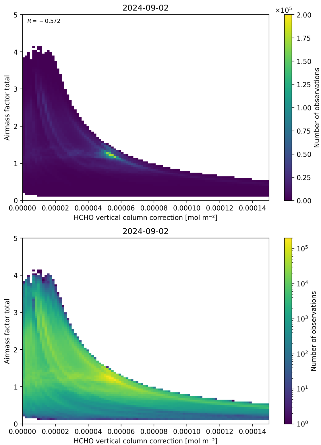
Figure 120: Scatter density plot of “HCHO vertical column correction” against “Airmass factor total” for 2024-09-01 to 2024-09-03.
