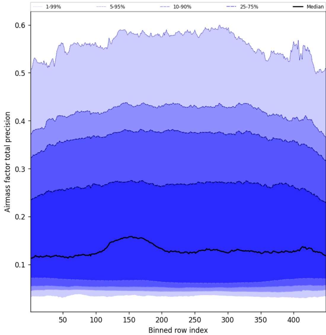
Figure 55: Along track statistics of “Airmass factor total precision” for 2024-09-01 to 2024-09-03
