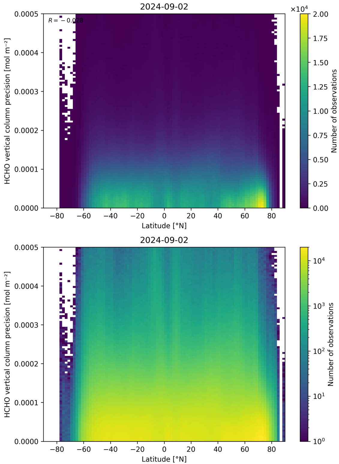
Figure 165: Scatter density plot of “Latitude” against “HCHO vertical column precision” for 2024-09-01 to 2024-09-03.
