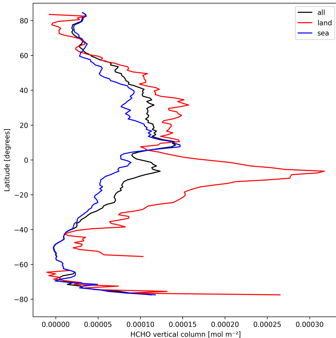
Figure 21: Zonal average of “HCHO vertical column” for 2024-09-01 to 2024-09-03.
