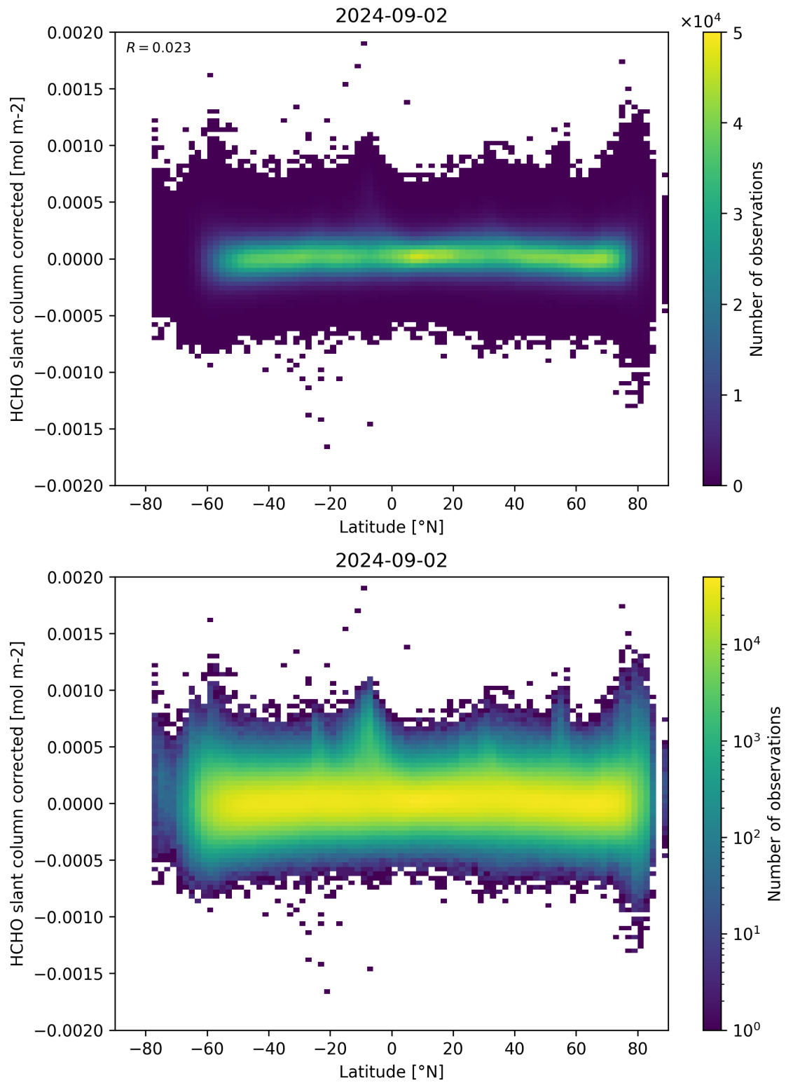
Figure 157: Scatter density plot of “Latitude” against “HCHO slant column corrected” for 2024-09-01 to 2024-09-03.
