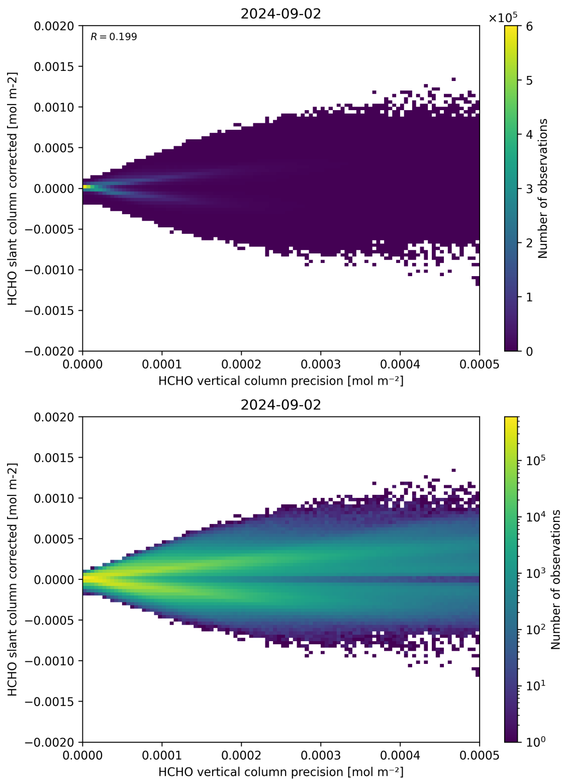
Figure 140: Scatter density plot of “HCHO vertical column precision” against “HCHO slant column corrected” for 2024-09-01 to 2024-09-03.
