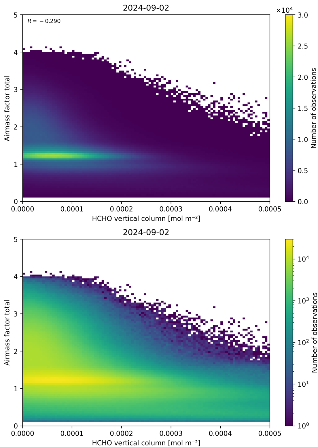
Figure 131: Scatter density plot of “HCHO vertical column” against “Airmass factor total” for 2024-09-01 to 2024-09-03.
