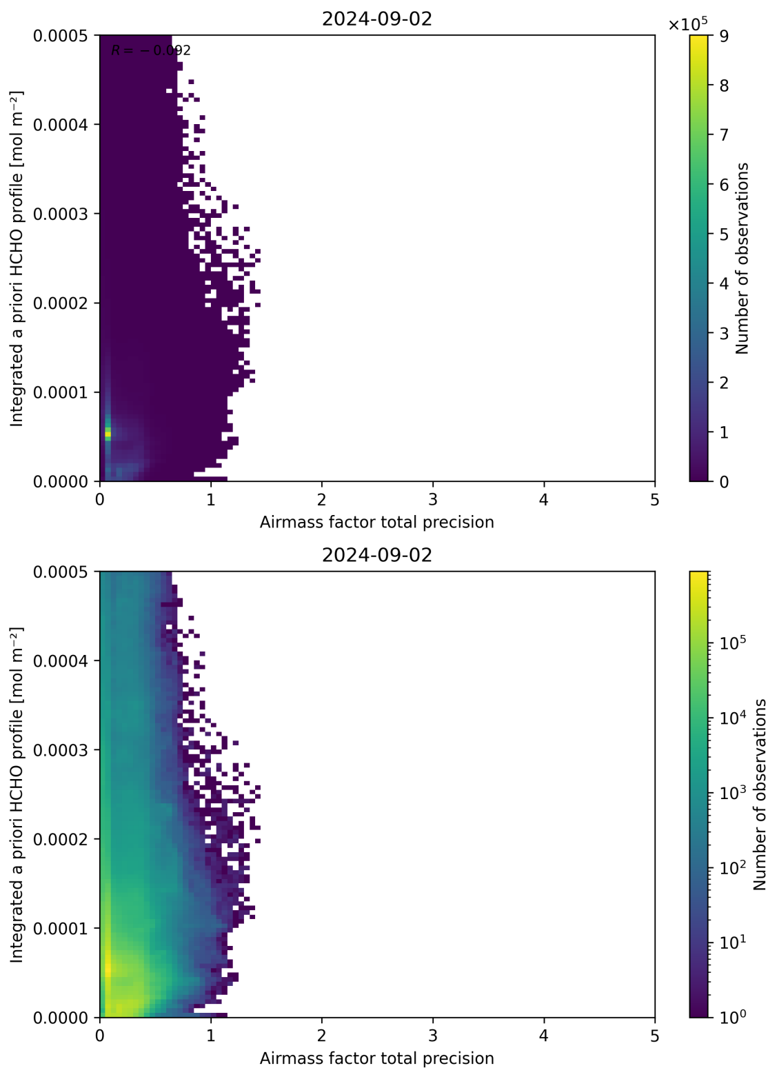
Figure 111: Scatter density plot of “Airmass factor total precision” against “Integrated a priori HCHO profile” for 2024-09-01 to 2024-09-03.
