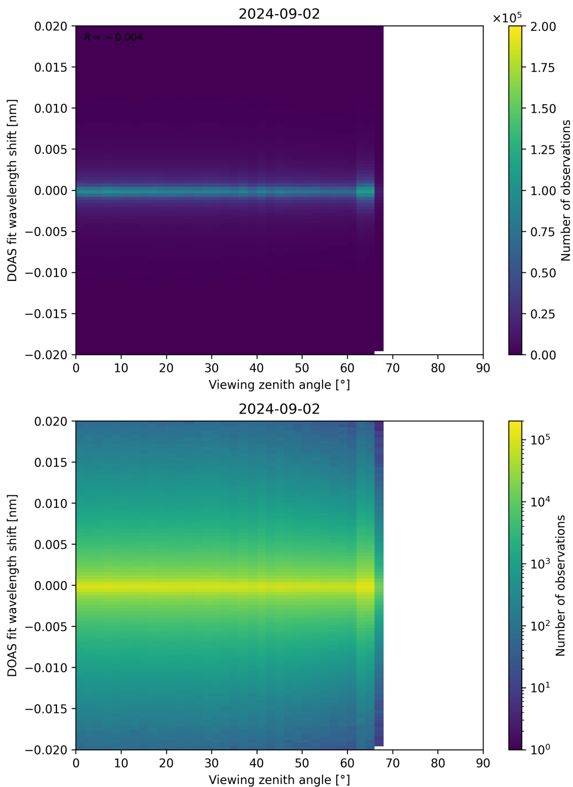
Figure 183: Scatter density plot of “Viewing zenith angle” against “DOAS fit wavelength shift” for 2024-09-01 to 2024-09-03.
