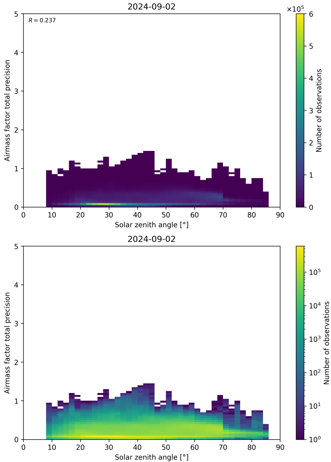
Figure 176: Scatter density plot of “Solar zenith angle” against “Airmass factor total precision” for 2024-09-01 to 2024-09-03.
