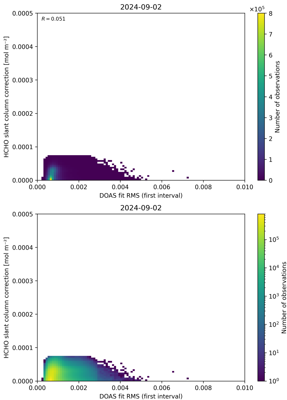
Figure 63: Scatter density plot of “DOAS fit RMS (first interval)” against “HCHO slant column correction” for 2024-09-01 to 2024-09-03.
