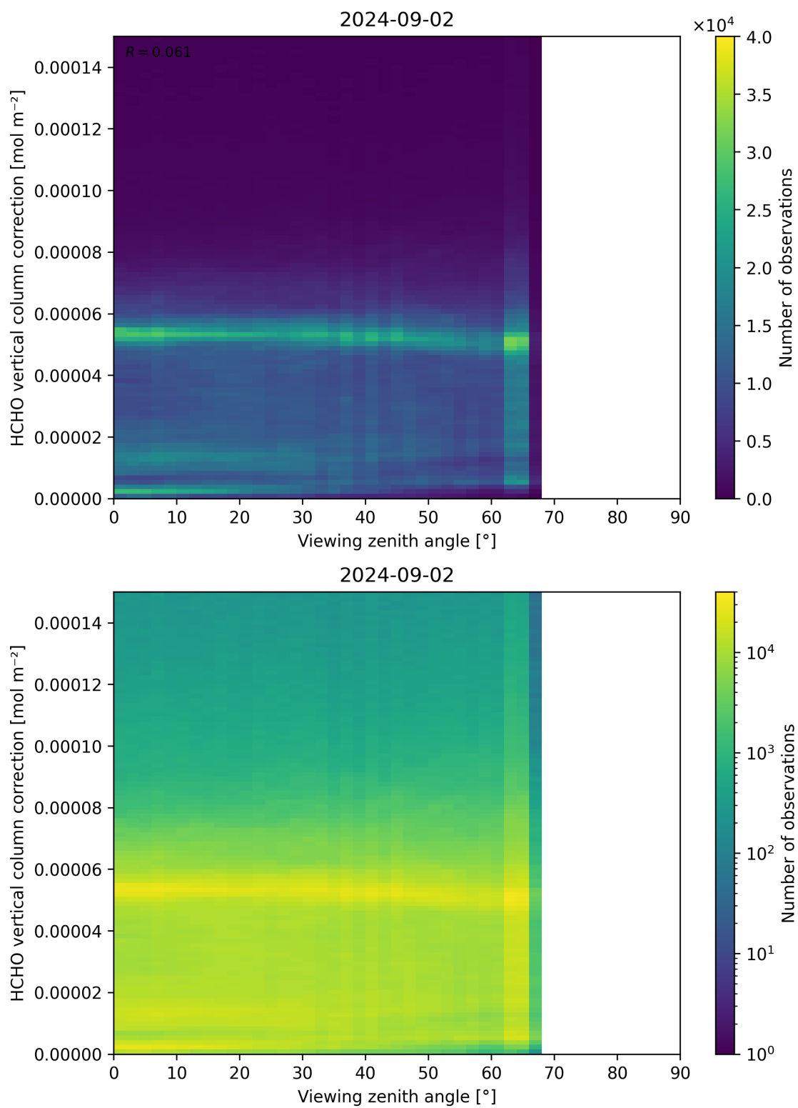
Figure 193: Scatter density plot of “Viewing zenith angle” against “HCHO vertical column correction” for 2024-09-01 to 2024-09-03.
