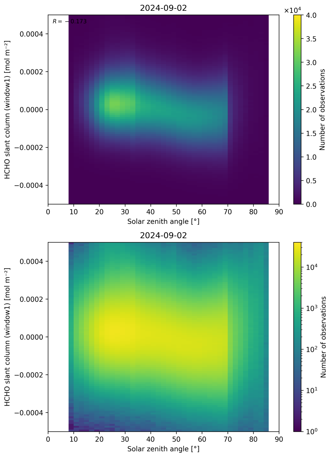
Figure 173: Scatter density plot of “Solar zenith angle” against “HCHO slant column (window1)” for 2024-09-01 to 2024-09-03.
