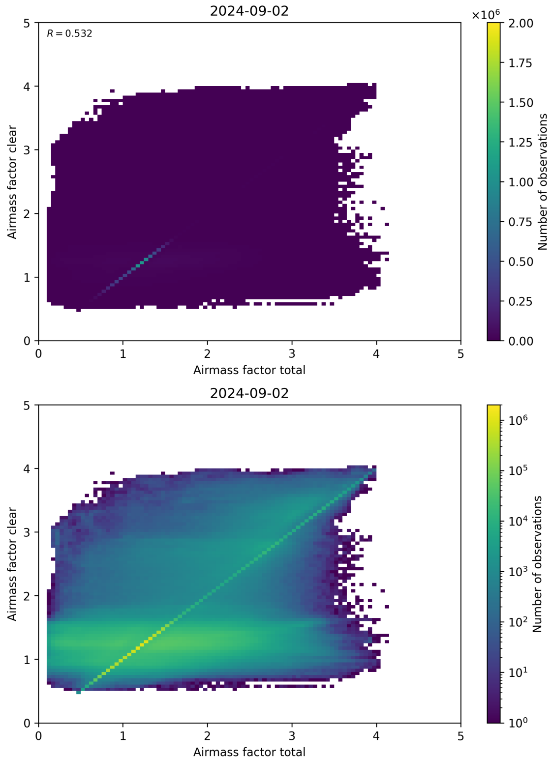
Figure 100: Scatter density plot of “Airmass factor total” against “Airmass factor clear” for 2024-09-01 to 2024-09-03.
