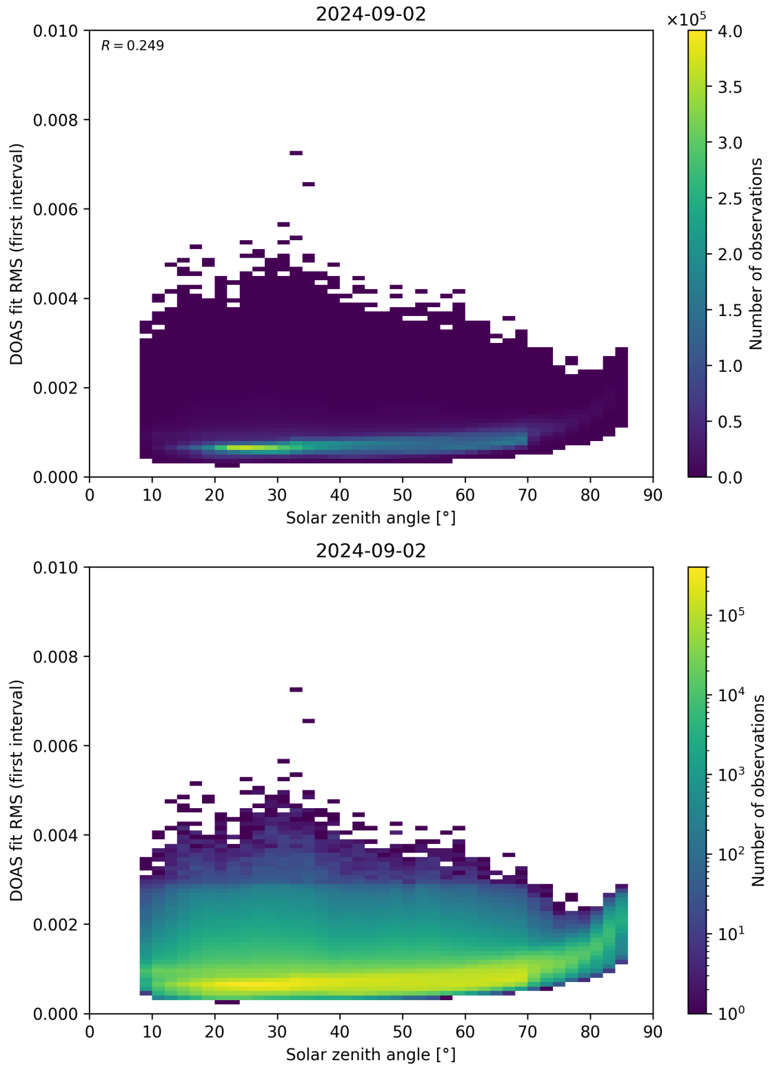
Figure 167: Scatter density plot of “Solar zenith angle” against “DOAS fit RMS (first interval)” for 2024-09-01 to 2024-09-03.
