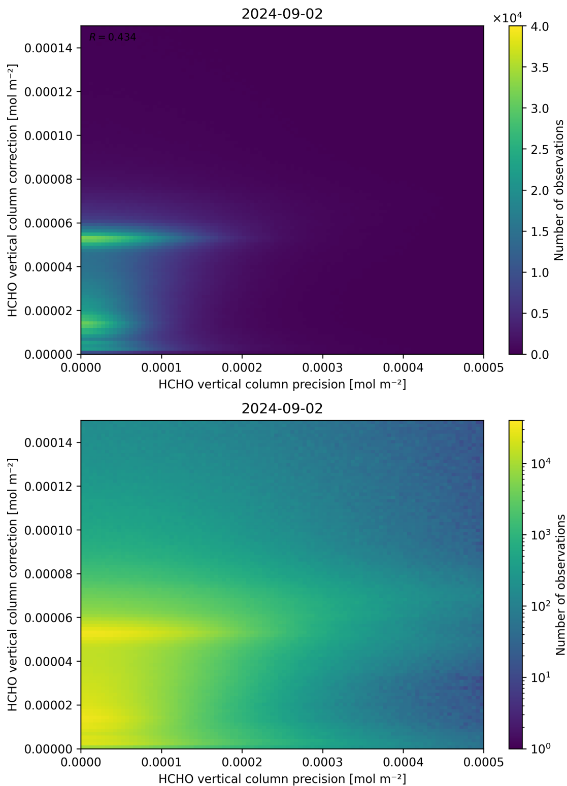
Figure 146: Scatter density plot of “HCHO vertical column precision” against “HCHO vertical column correction” for 2024-09-01 to 2024-09-03.
