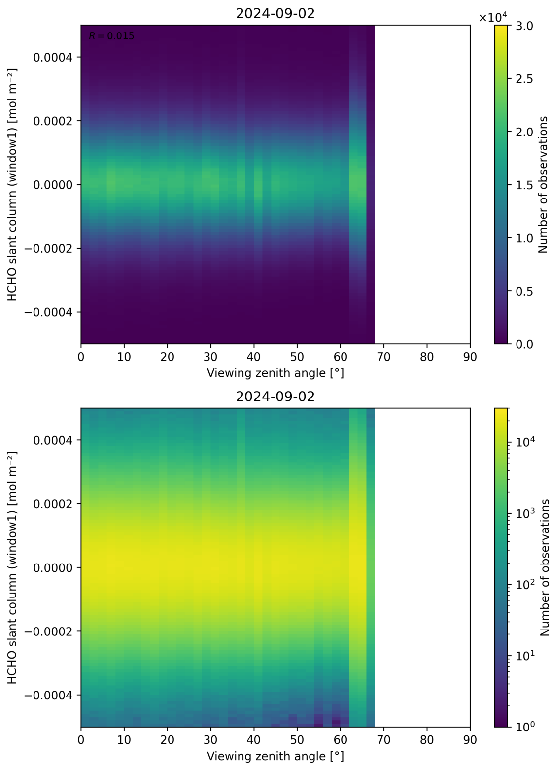
Figure 188: Scatter density plot of “Viewing zenith angle” against “HCHO slant column (window1)” for 2024-09-01 to 2024-09-03.
