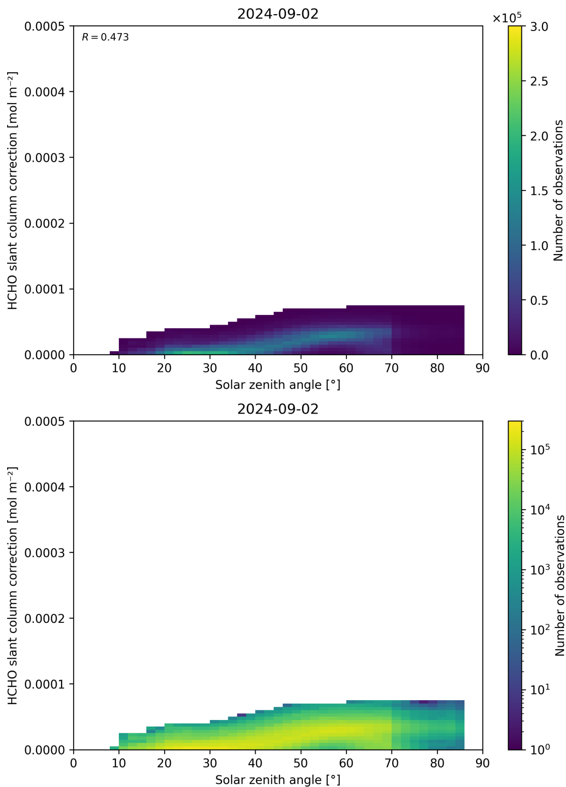
Figure 172: Scatter density plot of “Solar zenith angle” against “HCHO slant column correction” for 2024-09-01 to 2024-09-03.
