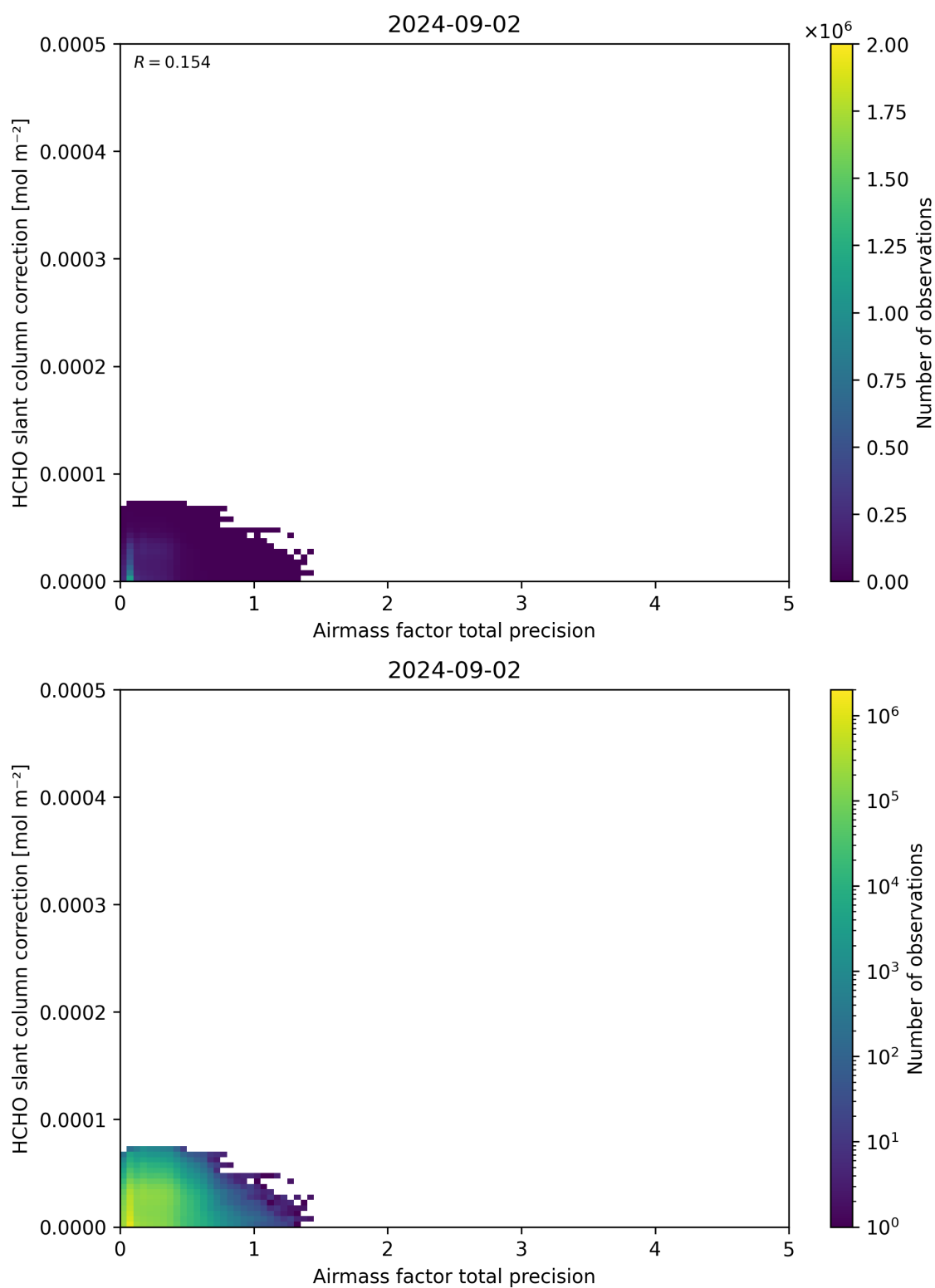
Figure 110: Scatter density plot of “Airmass factor total precision” against “HCHO slant column correction” for 2024-09-01 to 2024-09-03.
