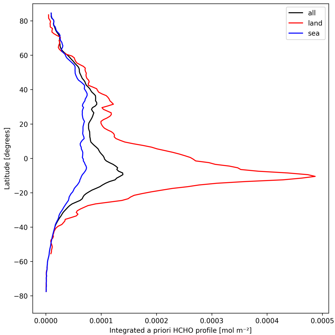
Figure 29: Zonal average of “Integrated a priori HCHO profile” for 2024-09-01 to 2024-09-03.
