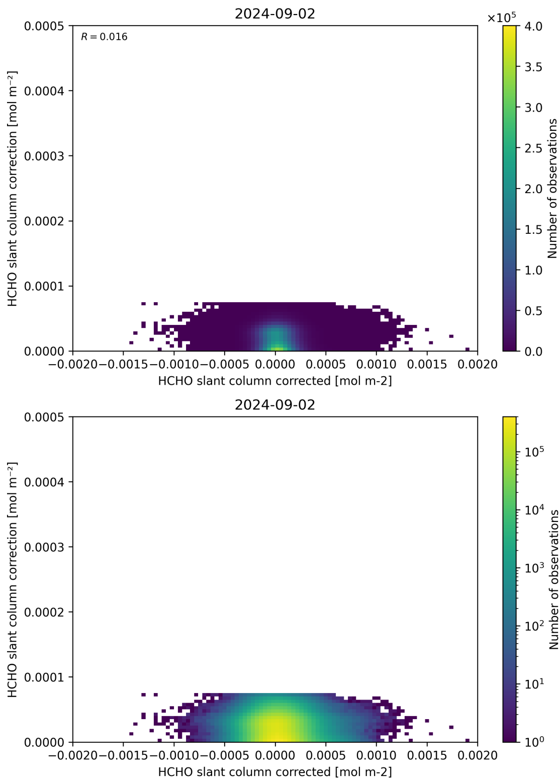
Figure 77: Scatter density plot of “HCHO slant column corrected” against “HCHO slant column correction” for 2024-09-01 to 2024-09-03.
