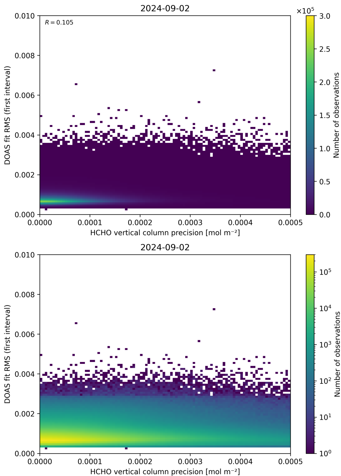
Figure 136: Scatter density plot of “HCHO vertical column precision” against “DOAS fit RMS (first interval)” for 2024-09-01 to 2024-09-03.
