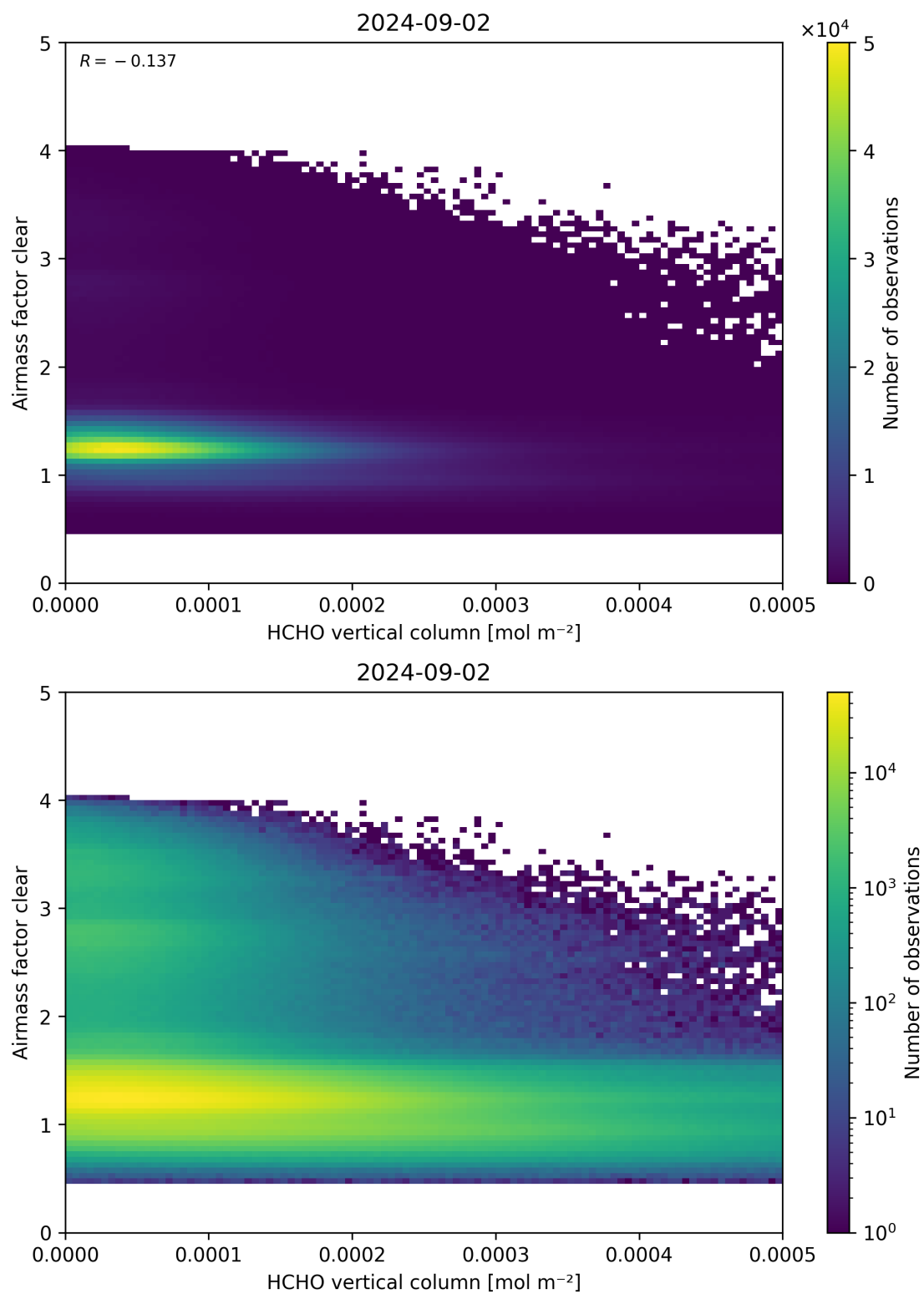
Figure 126: Scatter density plot of “HCHO vertical column” against “Airmass factor clear” for 2024-09-01 to 2024-09-03.
