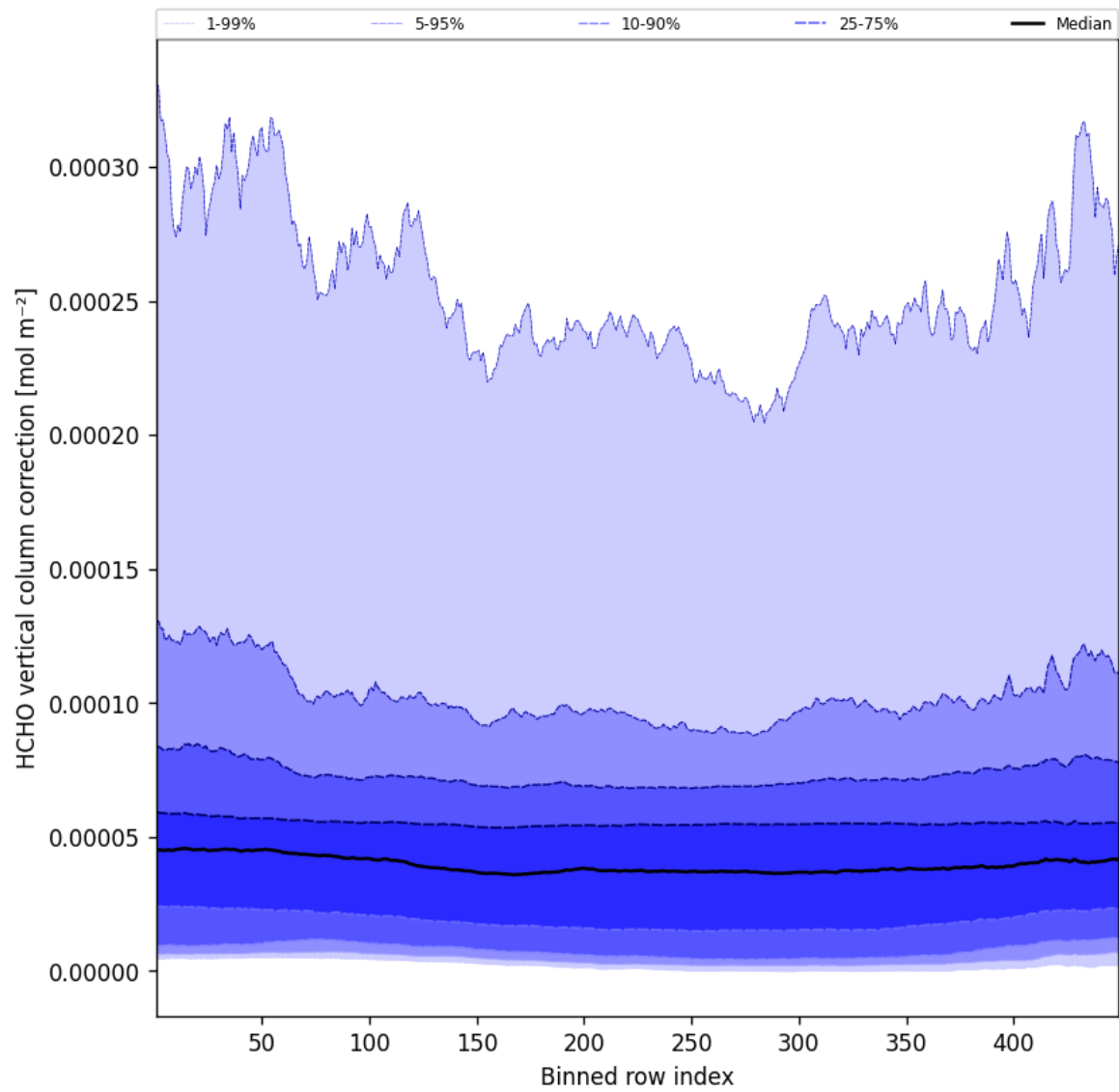
Figure 51: Along track statistics of “HCHO vertical column correction” for 2024-09-01 to 2024-09-03
