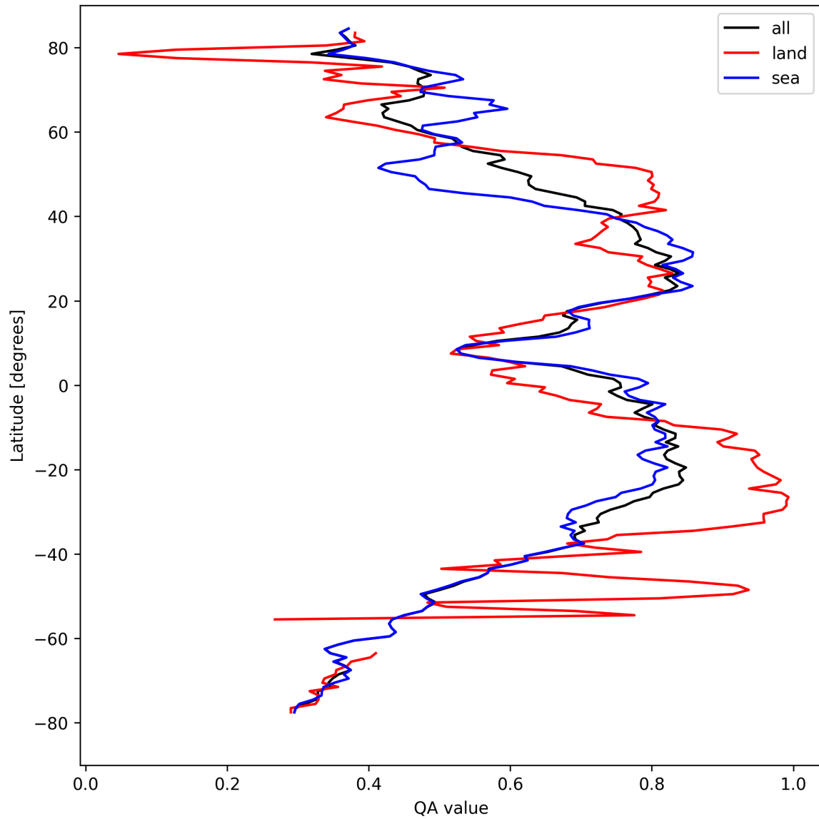
Figure 20: Zonal average of “QA value” for 2024-09-01 to 2024-09-03.
