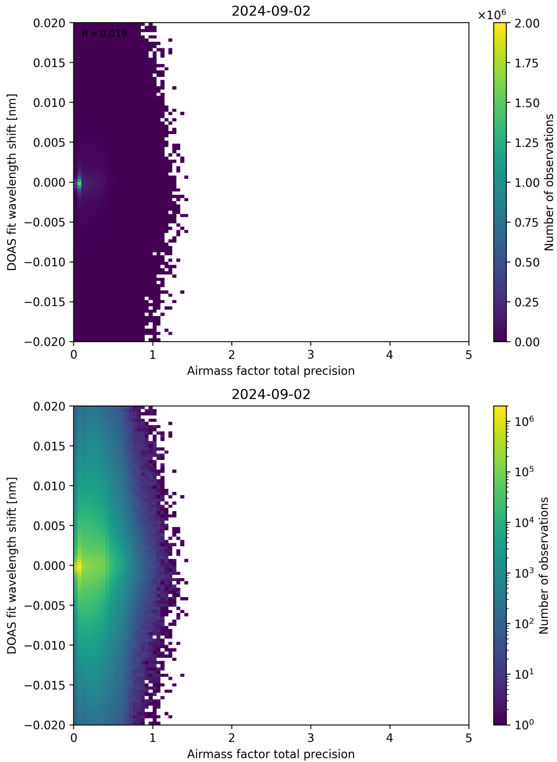
Figure 106: Scatter density plot of “Airmass factor total precision” against “DOAS fit wavelength shift” for 2024-09-01 to 2024-09-03.
