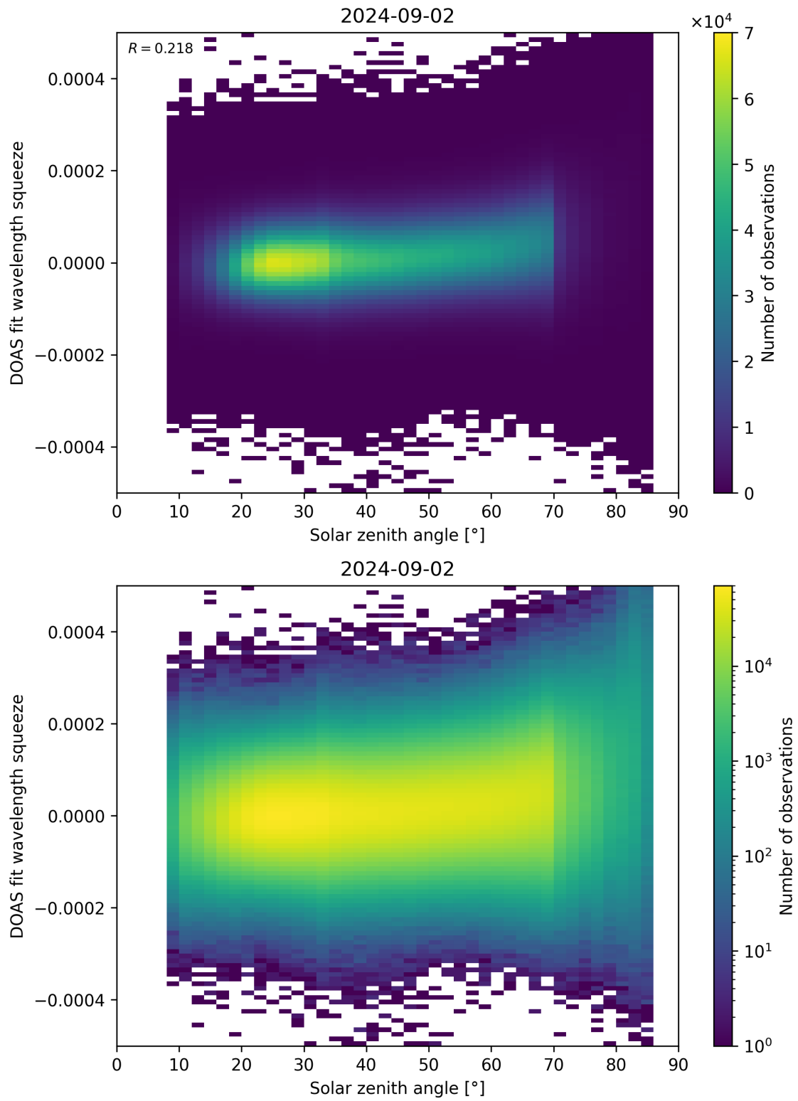
Figure 169: Scatter density plot of “Solar zenith angle” against “DOAS fit wavelength squeeze” for 2024-09-01 to 2024-09-03.
