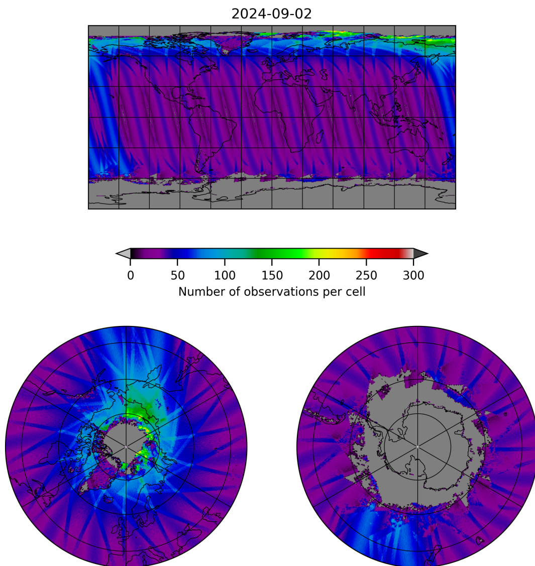
Figure 19: Map of the number of observations for 2024-09-01 to 2024-09-03
