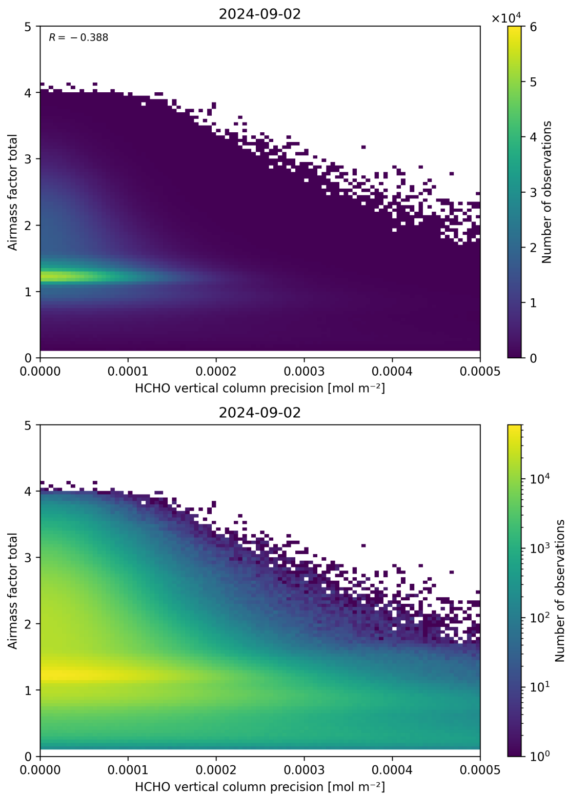
Figure 144: Scatter density plot of “HCHO vertical column precision” against “Airmass factor total” for 2024-09-01 to 2024-09-03.
