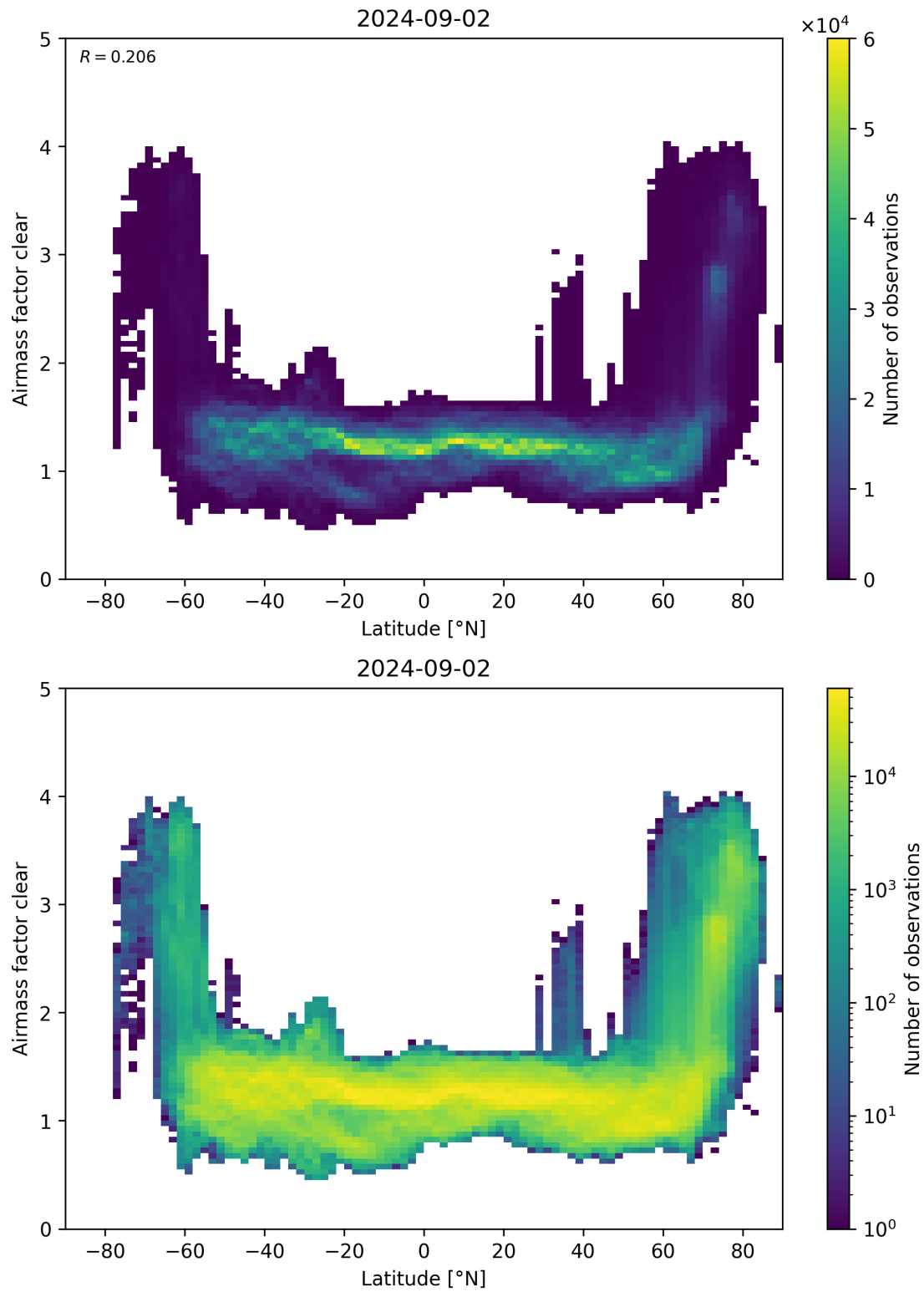
Figure 156: Scatter density plot of “Latitude” against “Airmass factor clear” for 2024-09-01 to 2024-09-03.
