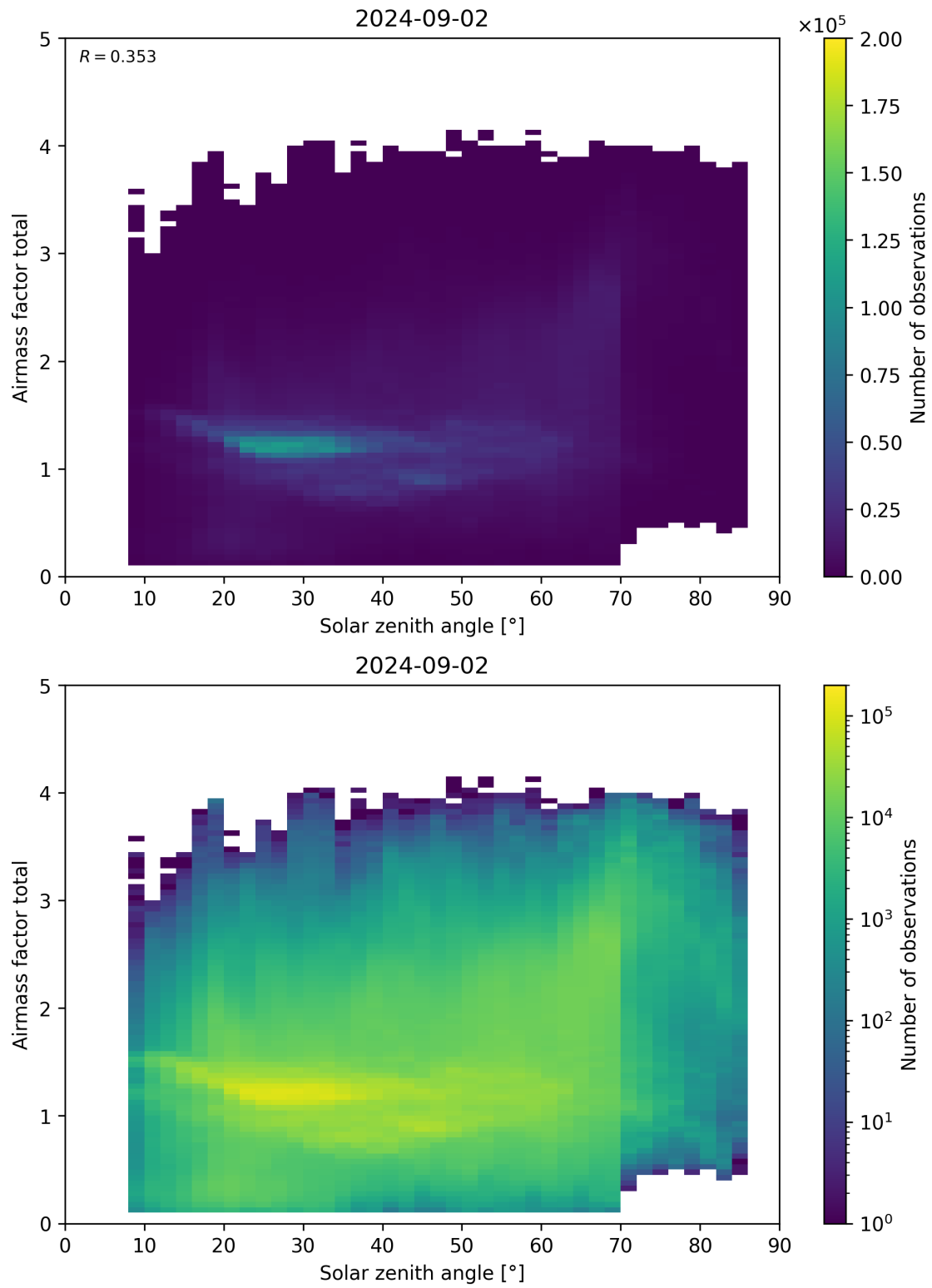
Figure 175: Scatter density plot of “Solar zenith angle” against “Airmass factor total” for 2024-09-01 to 2024-09-03.
