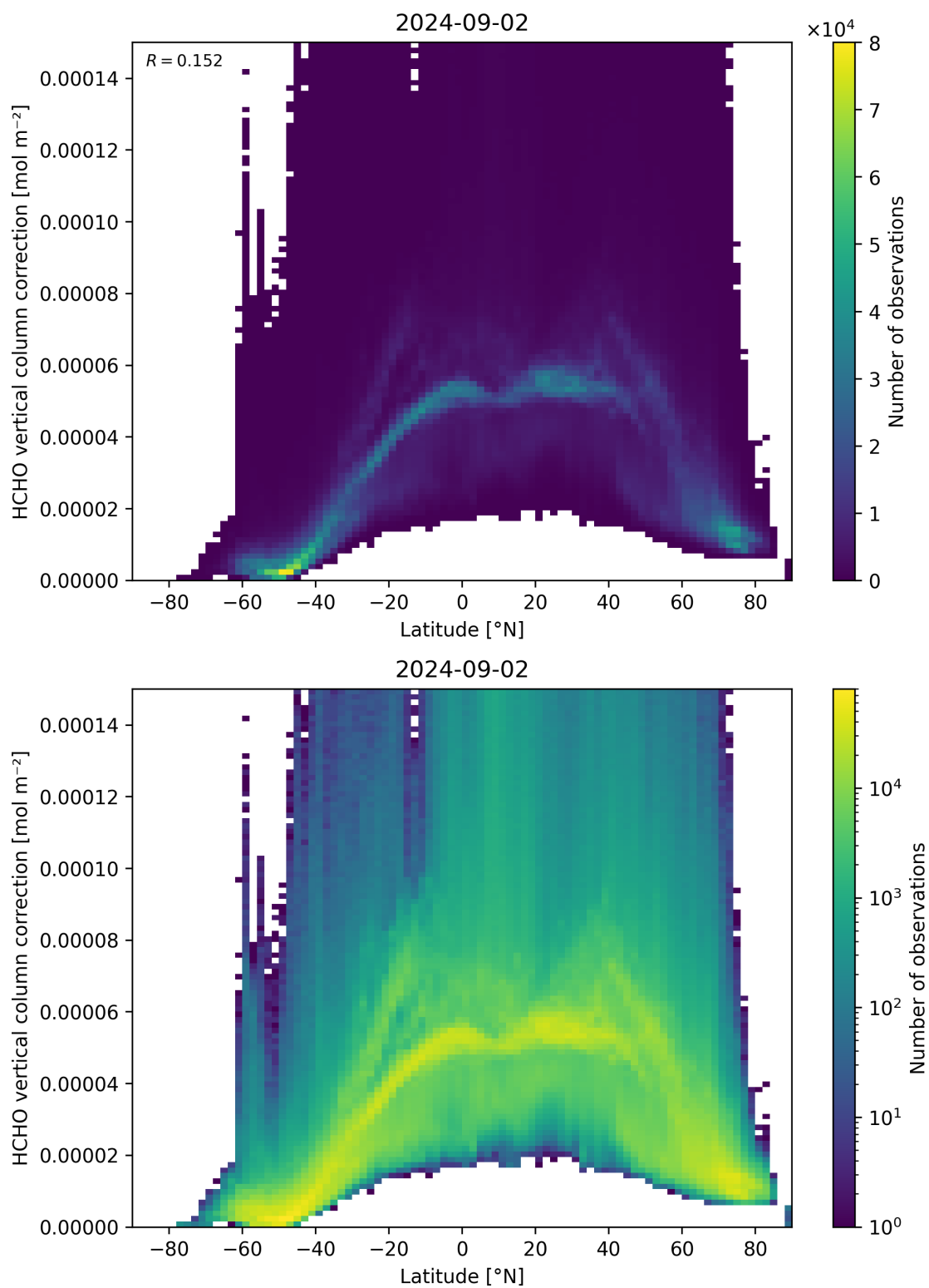
Figure 164: Scatter density plot of “Latitude” against “HCHO vertical column correction” for 2024-09-01 to 2024-09-03.
