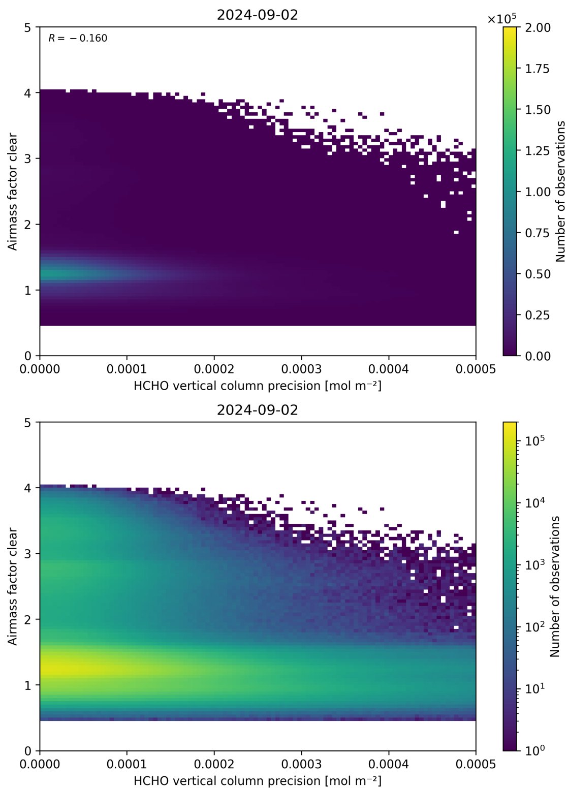
Figure 139: Scatter density plot of “HCHO vertical column precision” against “Airmass factor clear” for 2024-09-01 to 2024-09-03.
