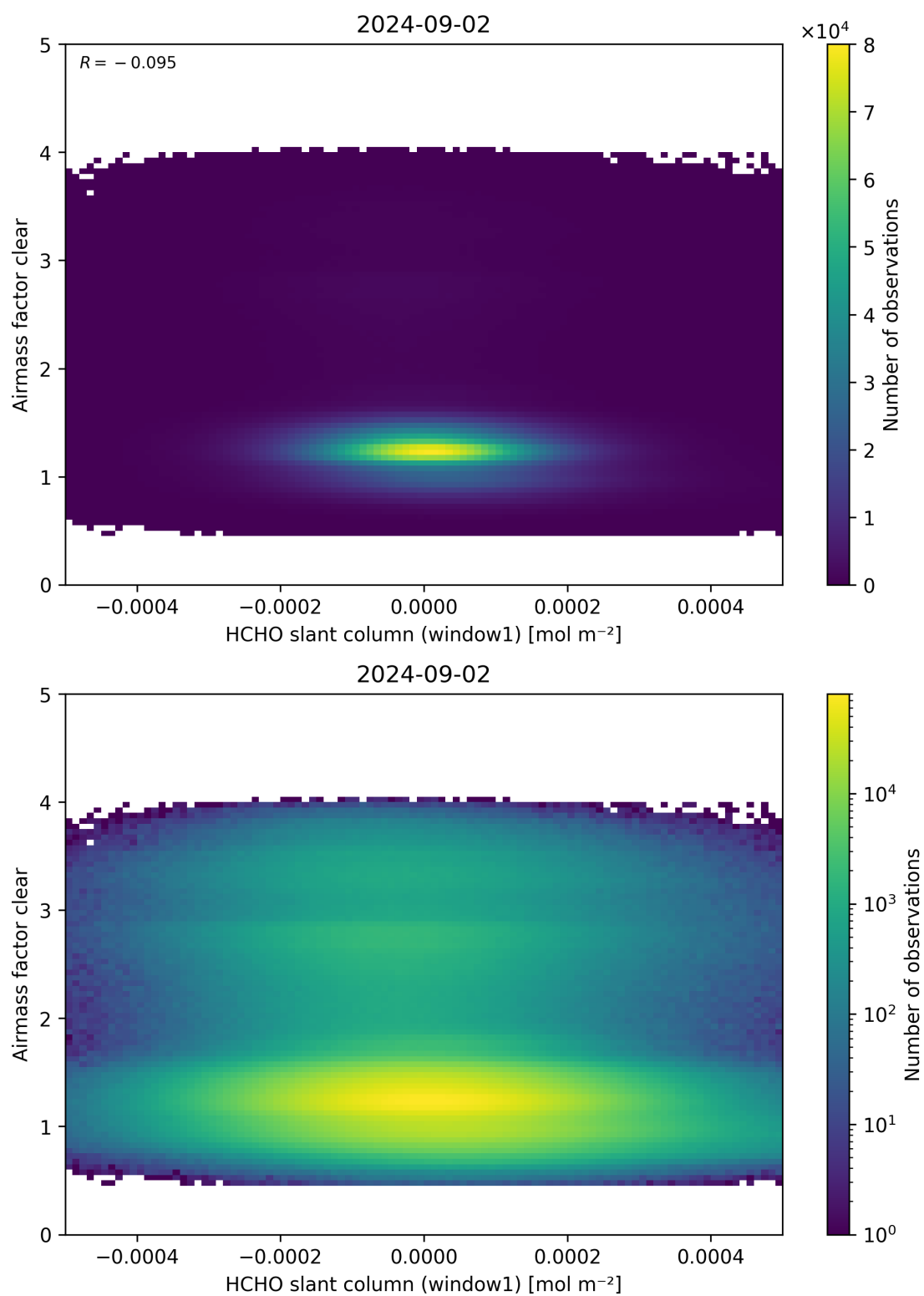
Figure 81: Scatter density plot of “HCHO slant column (window1)” against “Airmass factor clear” for 2024-09-01 to 2024-09-03.
