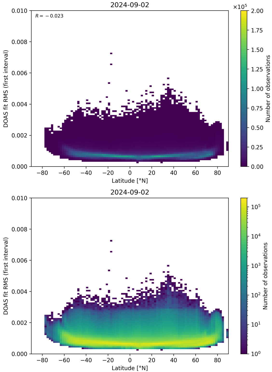
Figure 153: Scatter density plot of “Latitude” against “DOAS fit RMS (first interval)” for 2024-09-01 to 2024-09-03.
