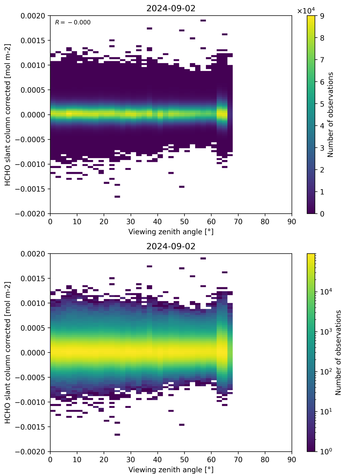
Figure 186: Scatter density plot of “Viewing zenith angle” against “HCHO slant column corrected” for 2024-09-01 to 2024-09-03.
