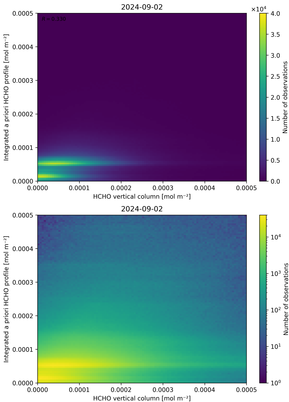
Figure 135: Scatter density plot of “HCHO vertical column” against “Integrated a priori HCHO profile” for 2024-09-01 to 2024-09-03.
