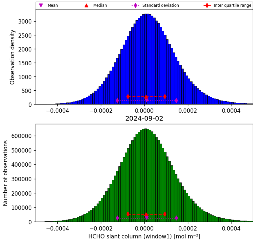
Figure 38: Histogram of “HCHO slant column (window1)” for 2024-09-01 to 2024-09-03
