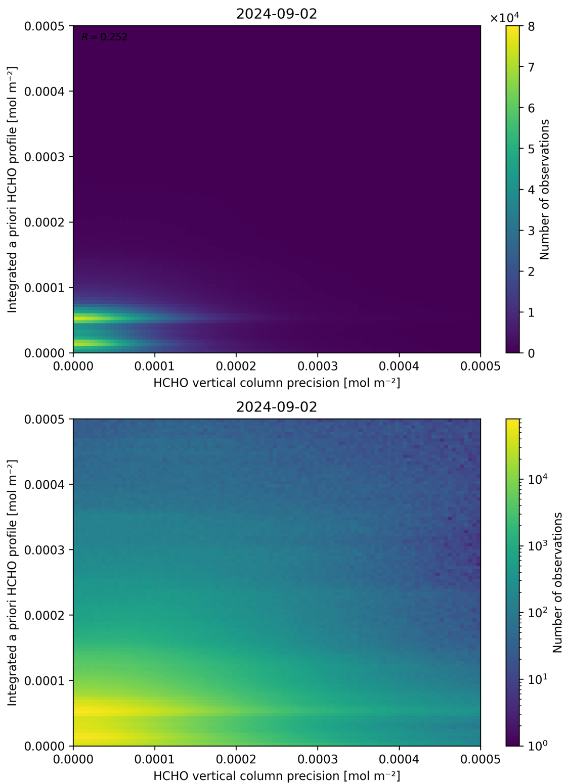
Figure 147: Scatter density plot of “HCHO vertical column precision” against “Integrated a priori HCHO profile” for 2024-09-01 to 2024-09-03.
