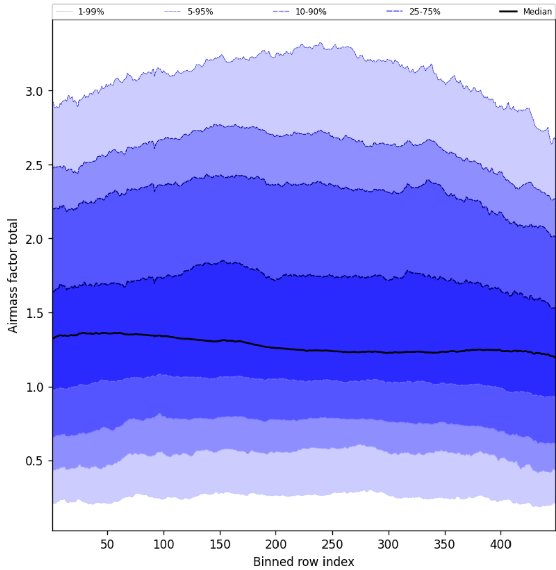
Figure 54: Along track statistics of “Airmass factor total” for 2024-09-01 to 2024-09-03
