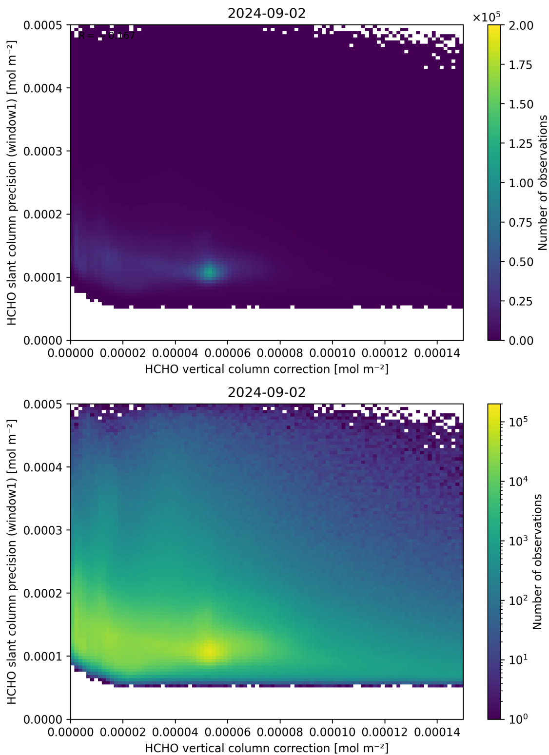
Figure 119: Scatter density plot of “HCHO vertical column correction” against “HCHO slant column precision (window1)” for 2024-09-01 to 2024-09-03.
