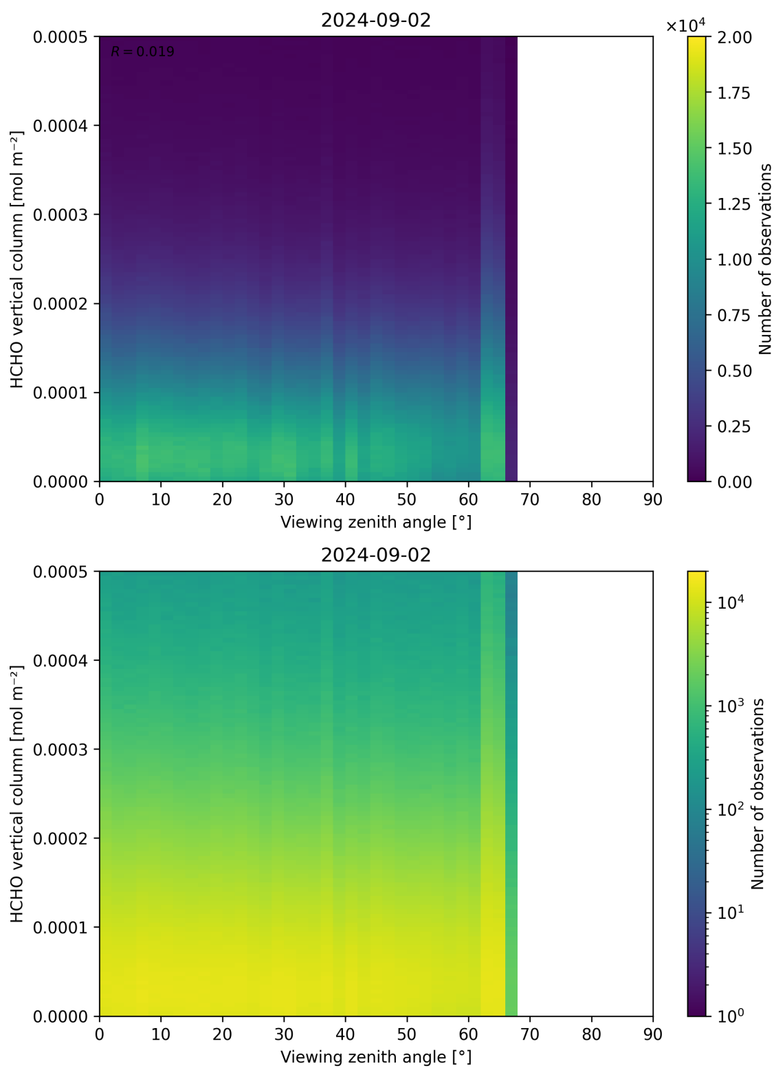
Figure 192: Scatter density plot of “Viewing zenith angle” against “HCHO vertical column” for 2024-09-01 to 2024-09-03.
