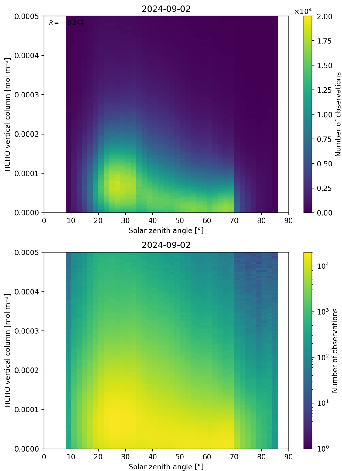
Figure 177: Scatter density plot of “Solar zenith angle” against “HCHO vertical column” for 2024-09-01 to 2024-09-03.
