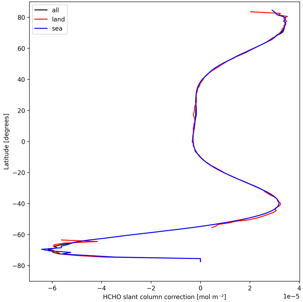
Figure 33: Zonal average of “HCHO slant column correction” for 2024-09-01 to 2024-09-03.
