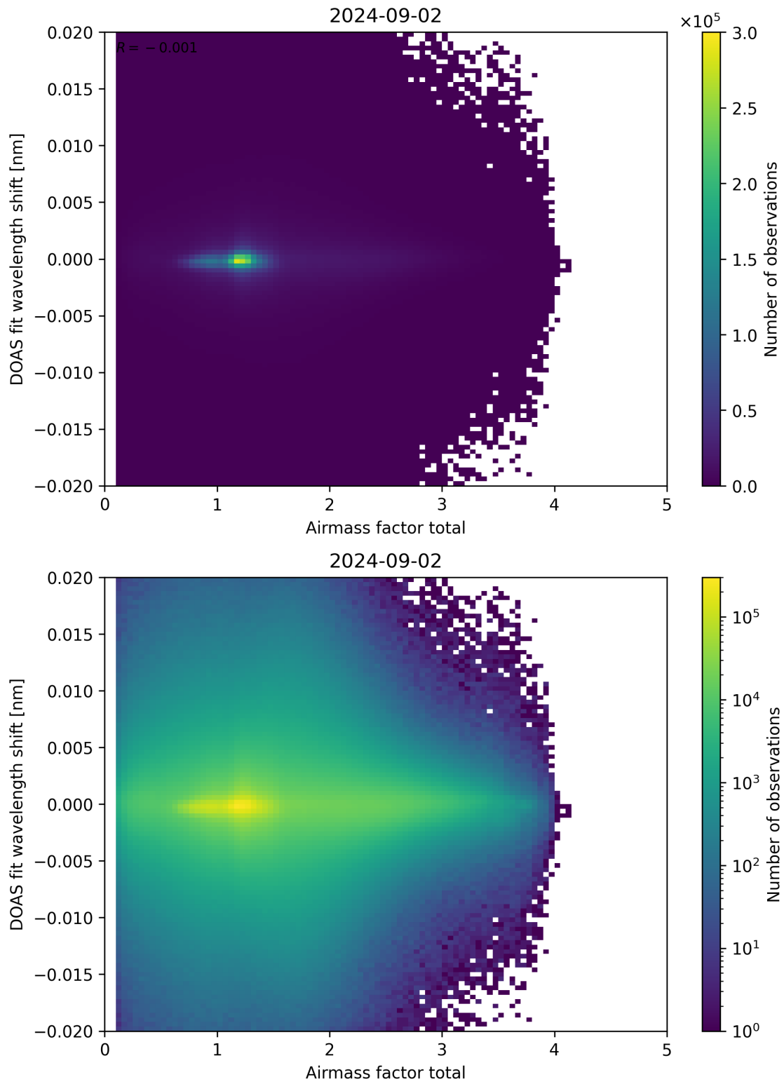
Figure 98: Scatter density plot of “Airmass factor total” against “DOAS fit wavelength shift” for 2024-09-01 to 2024-09-03.
