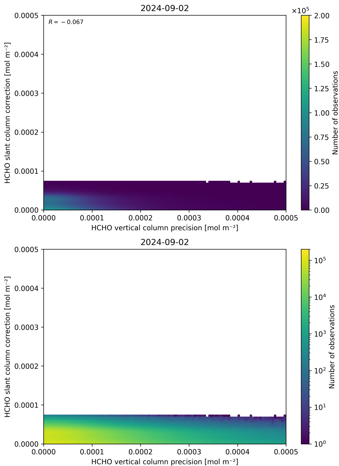
Figure 141: Scatter density plot of “HCHO vertical column precision” against “HCHO slant column correction” for 2024-09-01 to 2024-09-03.
