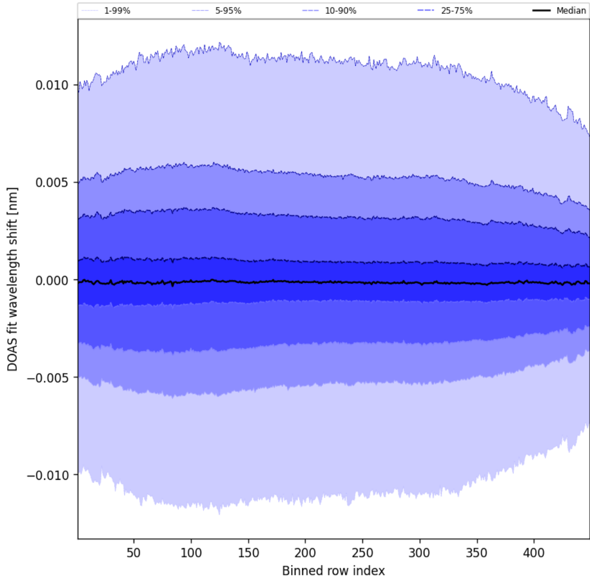
Figure 58: Along track statistics of “DOAS fit wavelength shift” for 2024-09-01 to 2024-09-03
