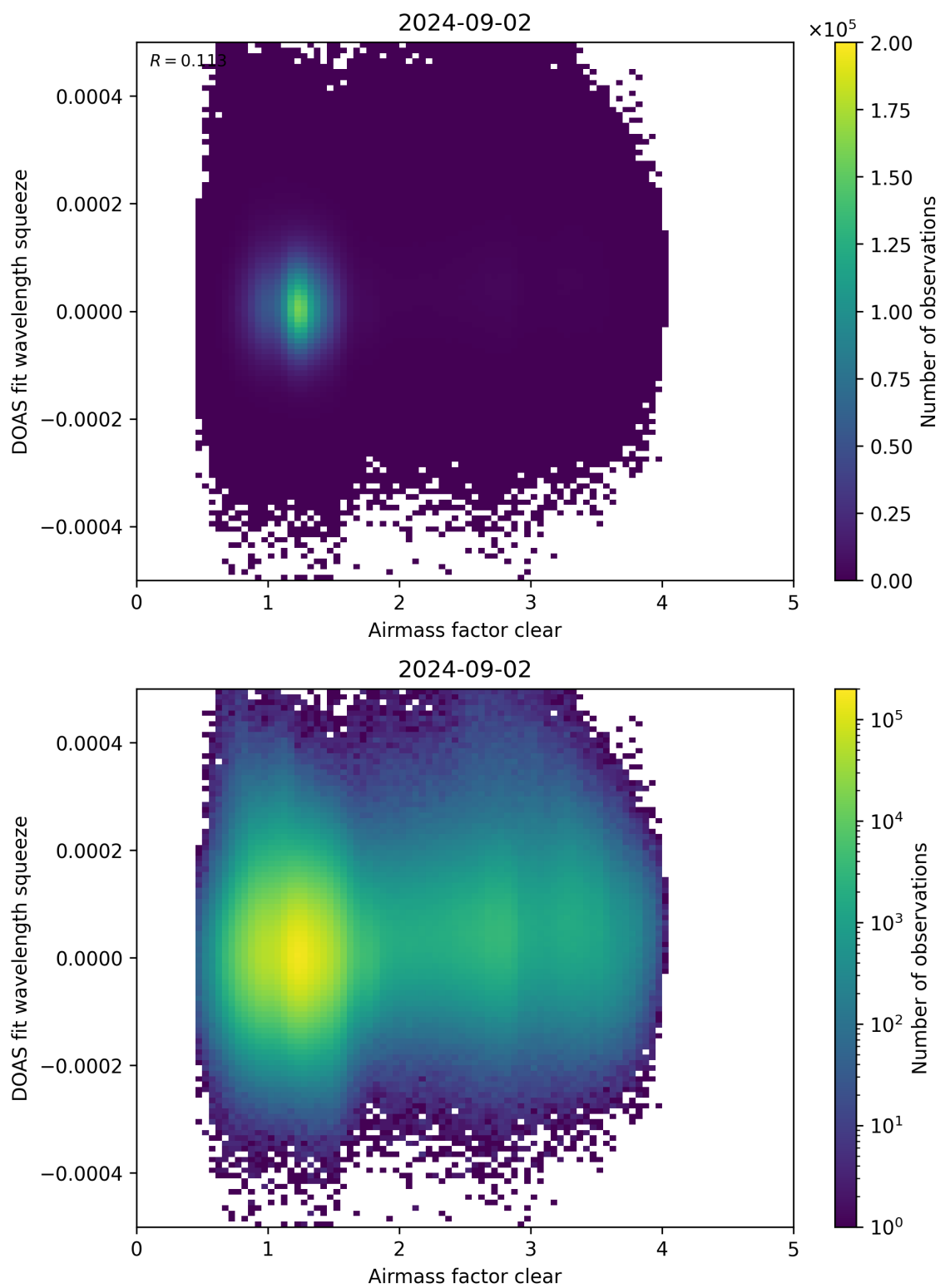
Figure 73: Scatter density plot of “Airmass factor clear” against “DOAS fit wavelength squeeze” for 2024-09-01 to 2024-09-03.
