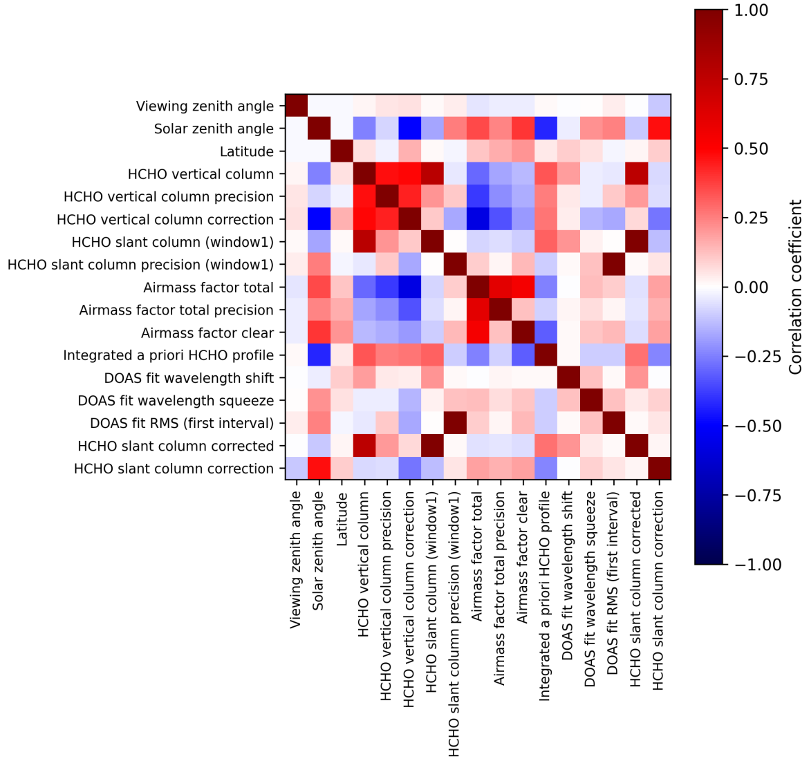
Figure 2: Map of correlation matrix for 2024-09-01 to 2024-09-03.
