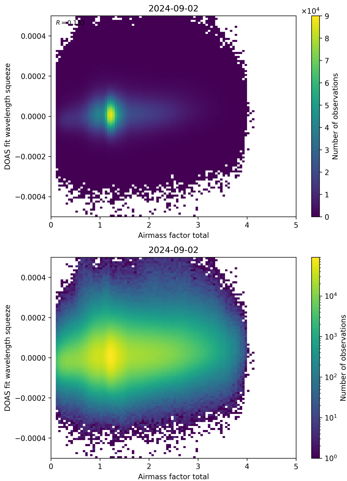
Figure 99: Scatter density plot of “Airmass factor total” against “DOAS fit wavelength squeeze” for 2024-09-01 to 2024-09-03.
