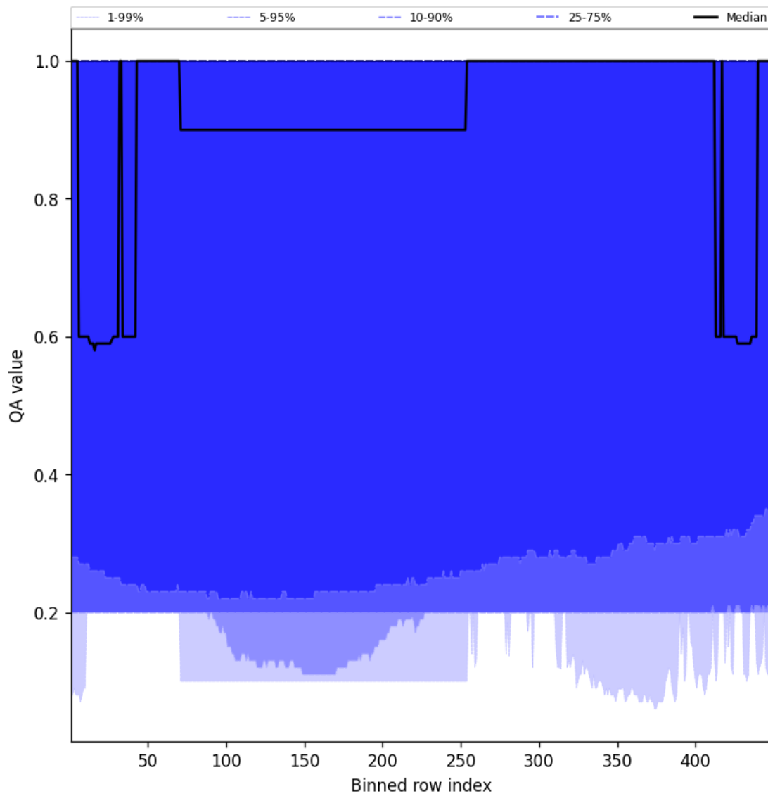
Figure 48: Along track statistics of “QA value” for 2024-09-01 to 2024-09-03
