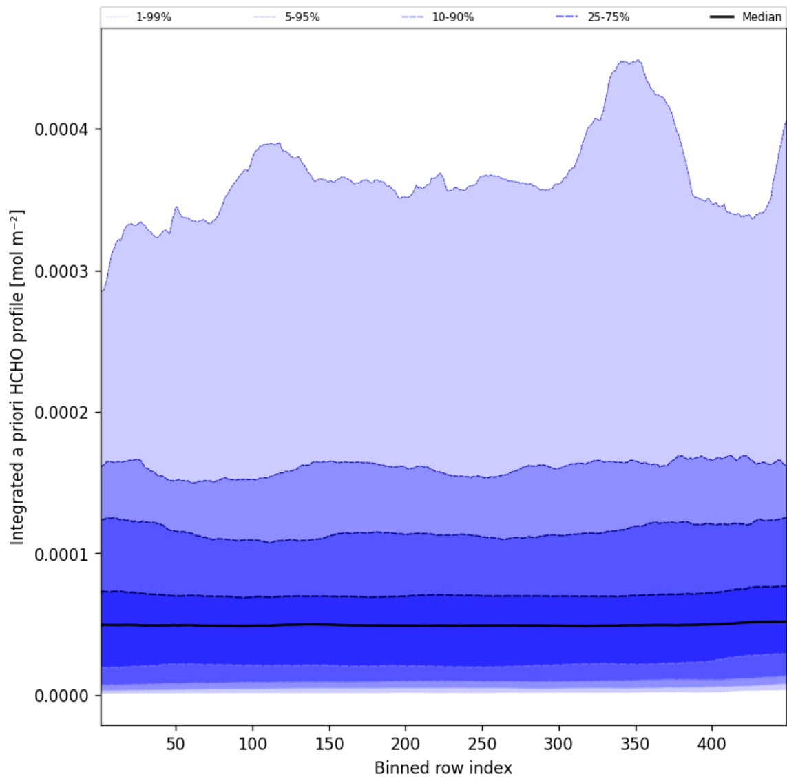
Figure 57: Along track statistics of “Integrated a priori HCHO profile” for 2024-09-01 to 2024-09-03
