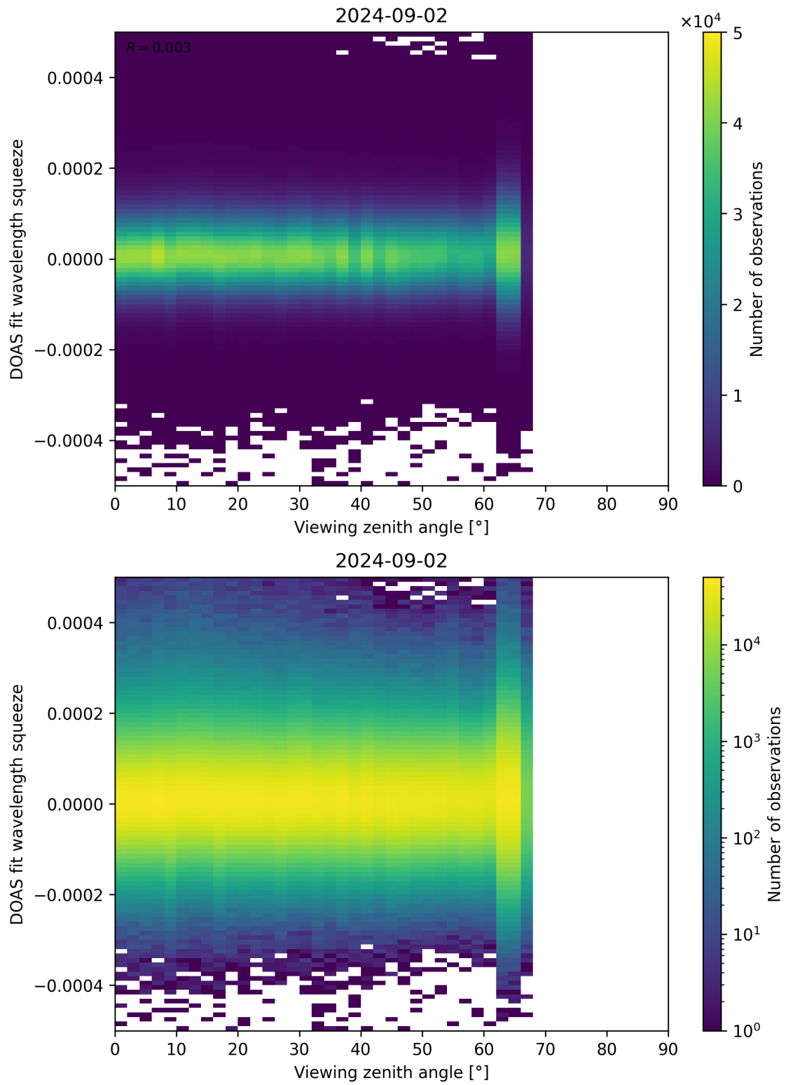
Figure 184: Scatter density plot of “Viewing zenith angle” against “DOAS fit wavelength squeeze” for 2024-09-01 to 2024-09-03.
