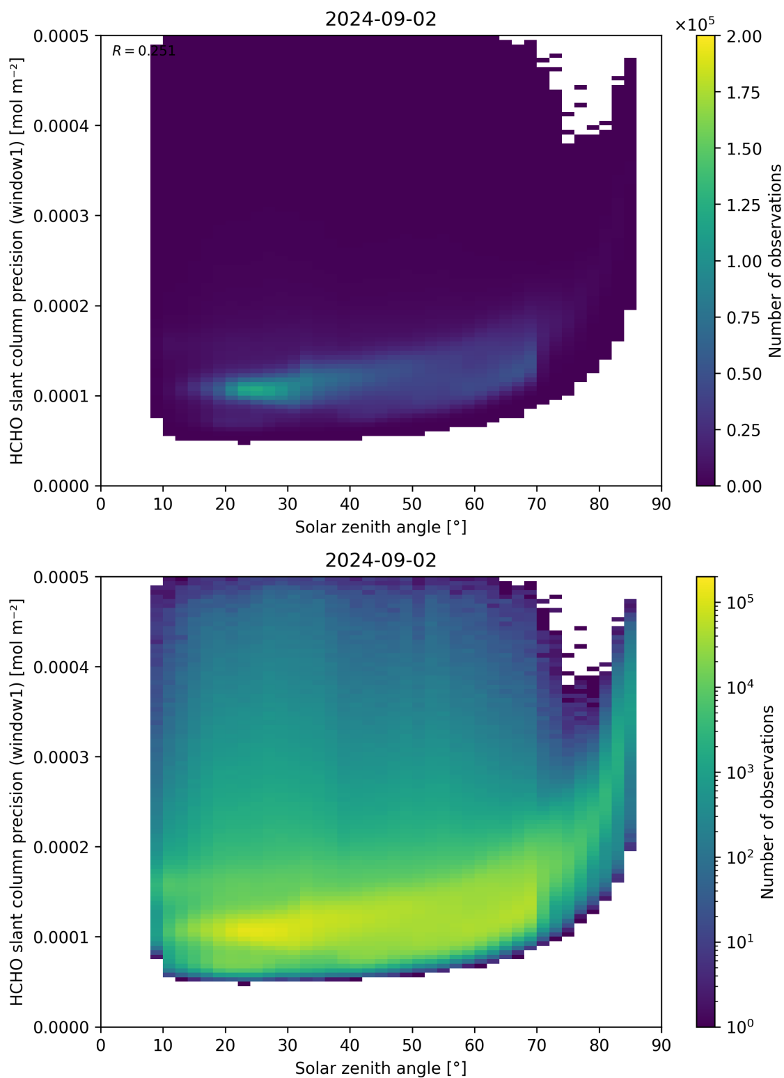
Figure 174: Scatter density plot of “Solar zenith angle” against “HCHO slant column precision (window1)” for 2024-09-01 to 2024-09-03.
