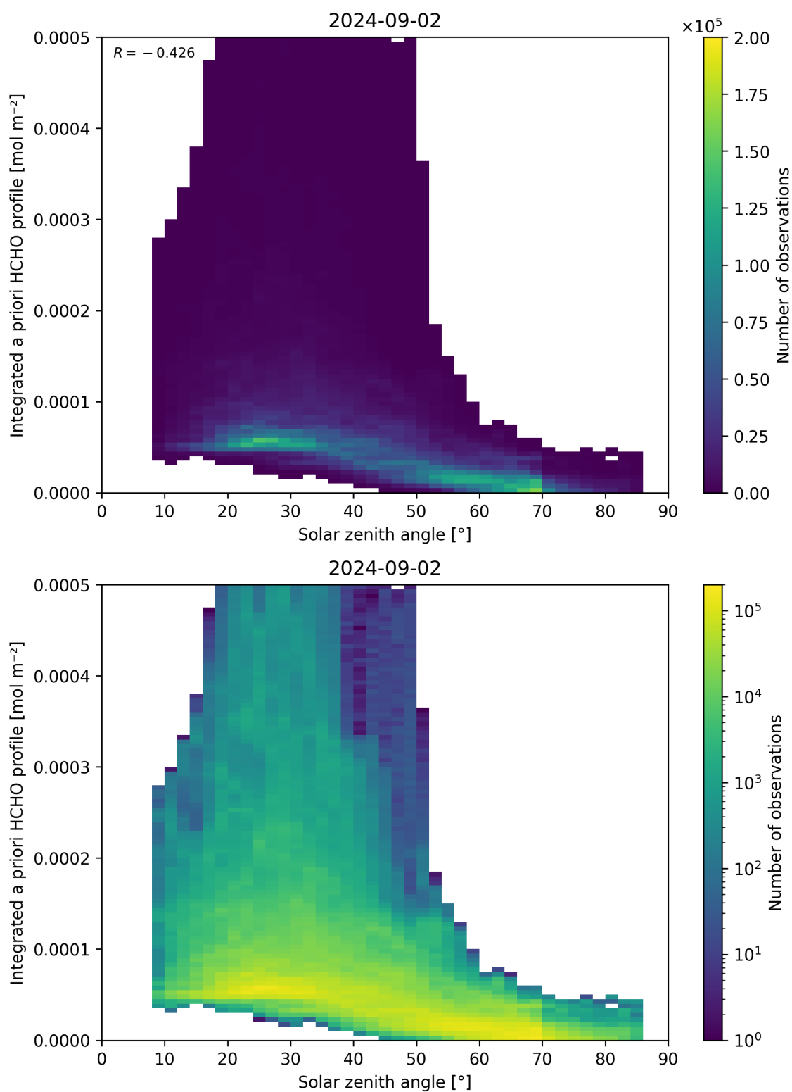
Figure 180: Scatter density plot of “Solar zenith angle” against “Integrated a priori HCHO profile” for 2024-09-01 to 2024-09-03.
