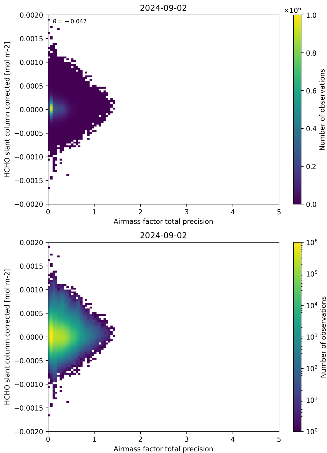
Figure 109: Scatter density plot of “Airmass factor total precision” against “HCHO slant column corrected” for 2024-09-01 to 2024-09-03.
