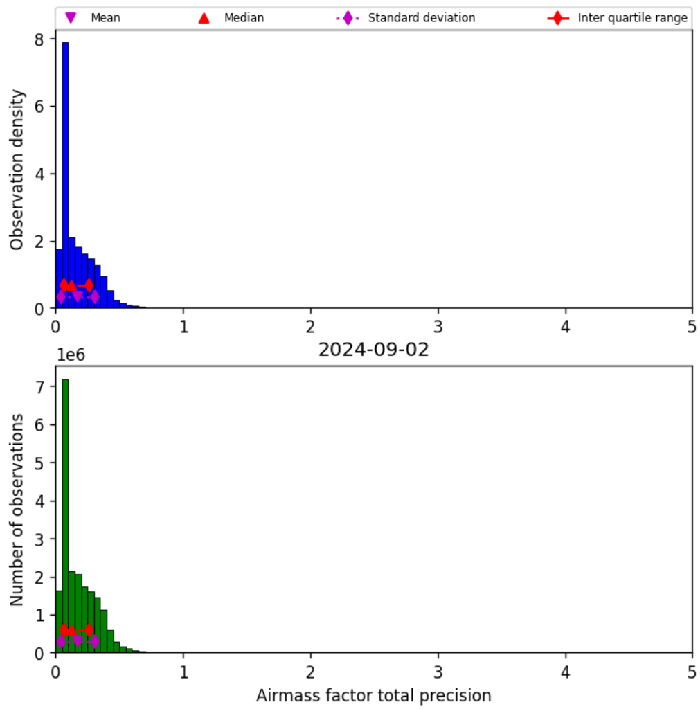
Figure 41: Histogram of “Airmass factor total precision” for 2024-09-01 to 2024-09-03
