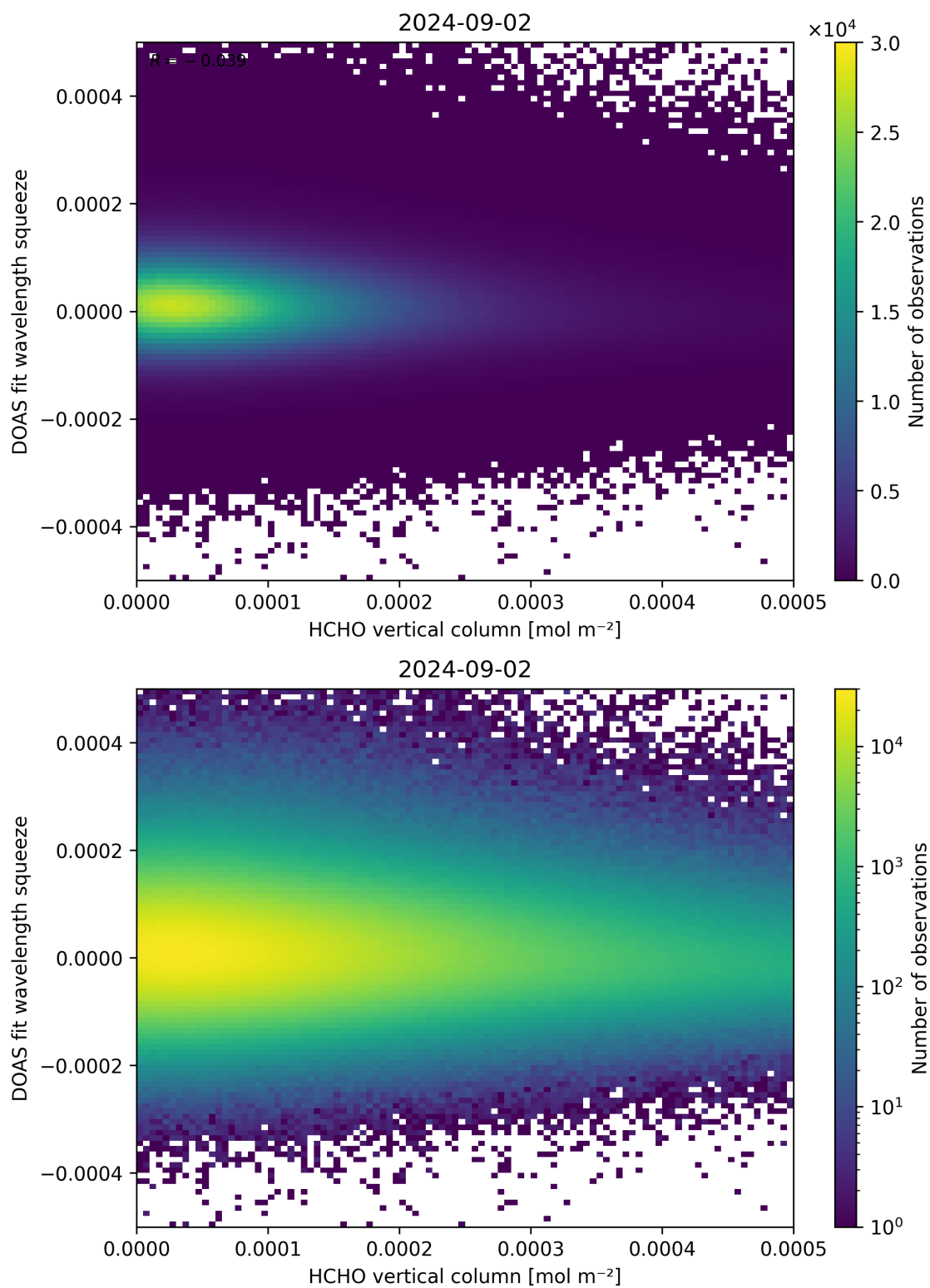
Figure 125: Scatter density plot of “HCHO vertical column” against “DOAS fit wavelength squeeze” for 2024-09-01 to 2024-09-03.
