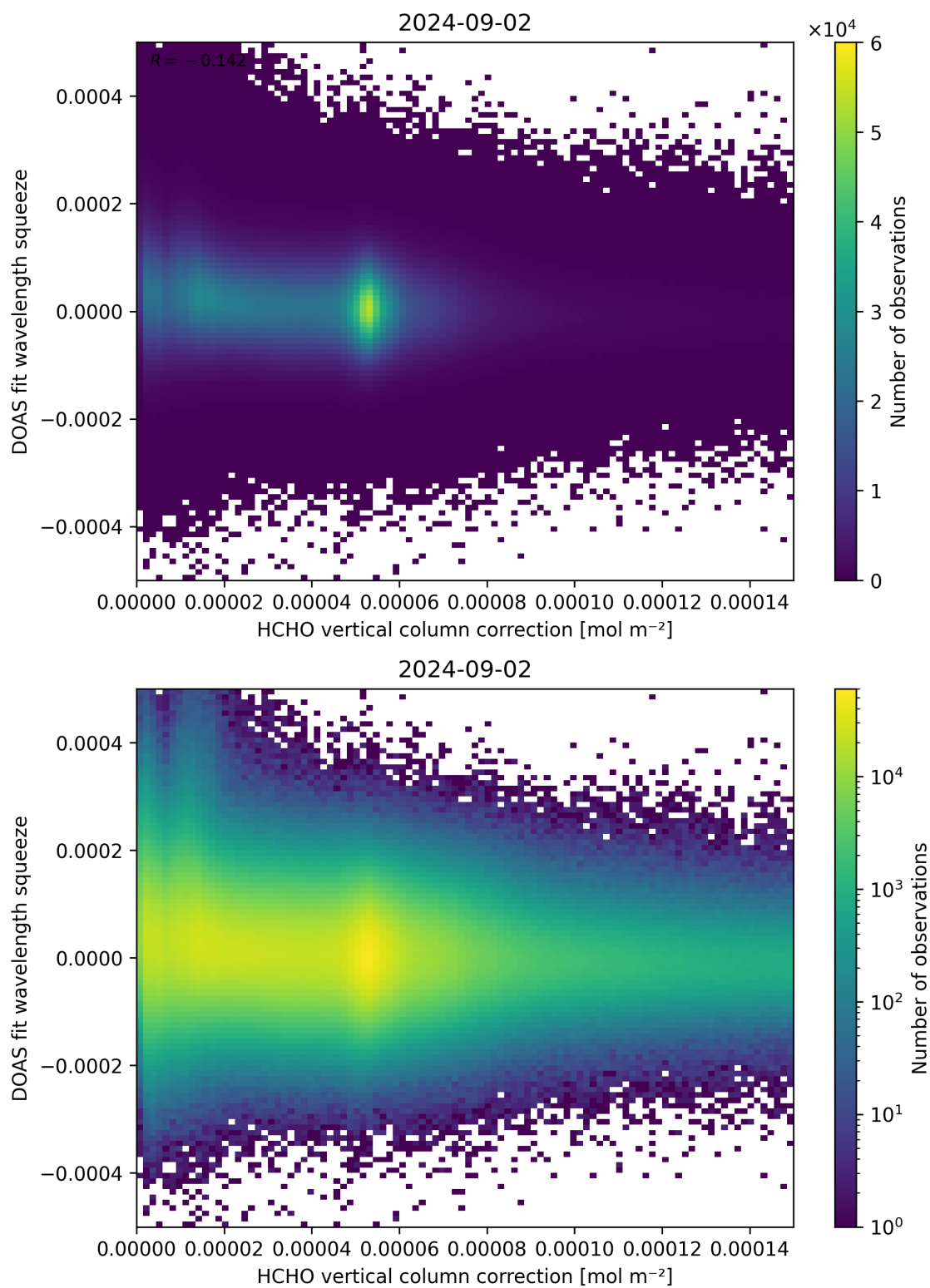
Figure 114: Scatter density plot of “HCHO vertical column correction” against “DOAS fit wavelength squeeze” for 2024-09-01 to 2024-09-03.
