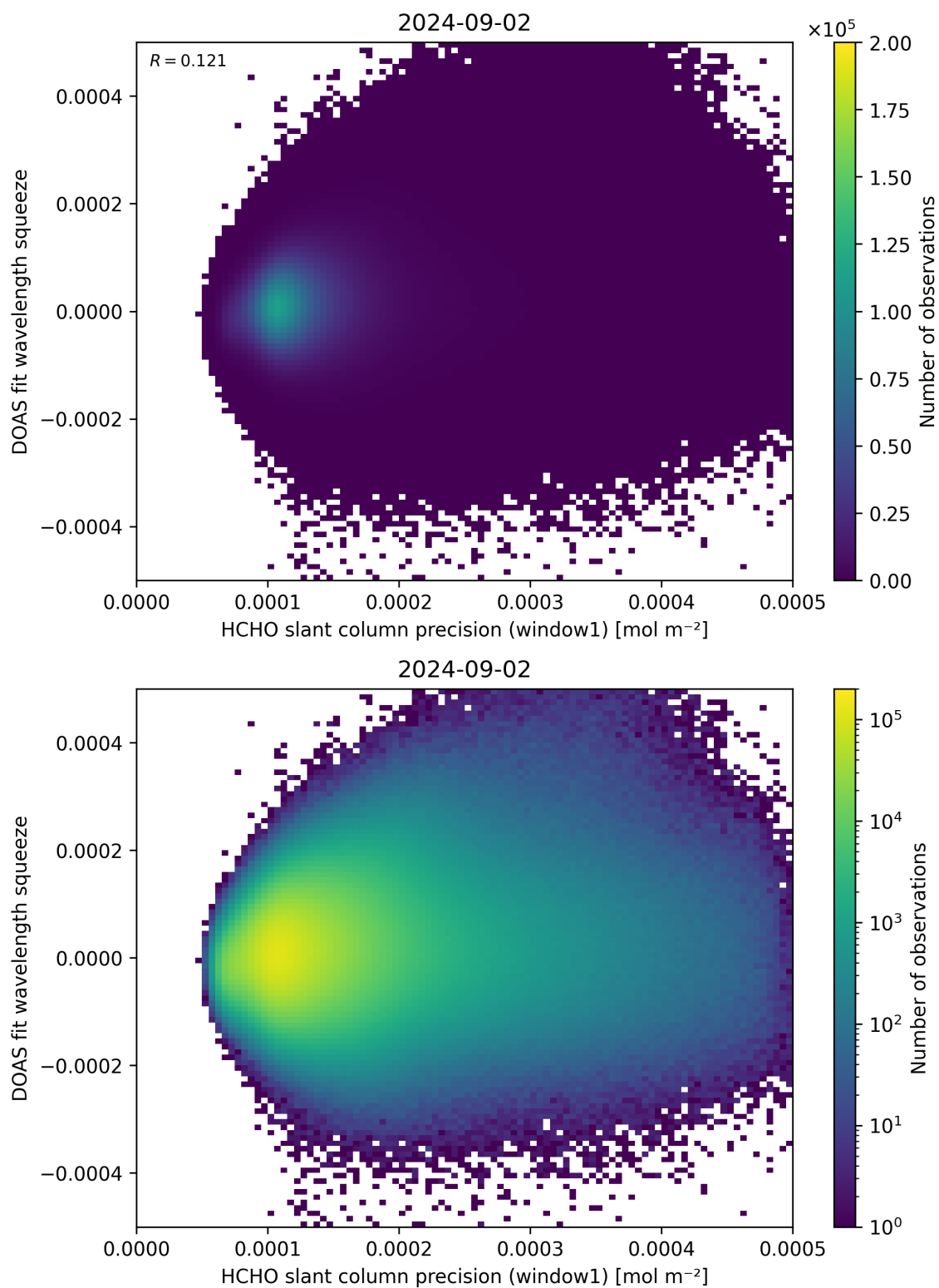
Figure 90: Scatter density plot of “HCHO slant column precision (window1)” against “DOAS fit wavelength squeeze” for 2024-09-01 to 2024-09-03.
