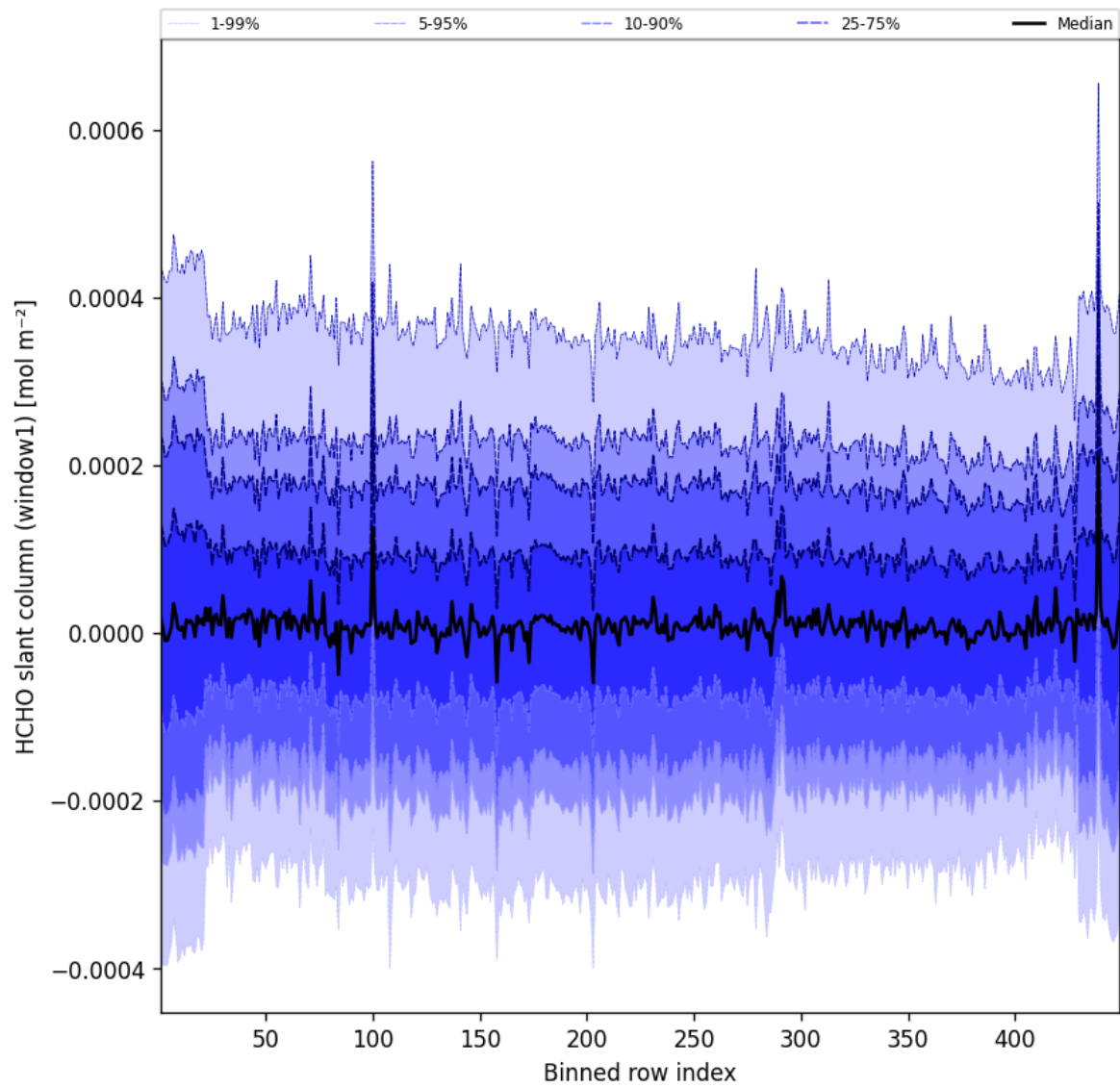
Figure 52: Along track statistics of “HCHO slant column (window1)” for 2024-09-01 to 2024-09-03
