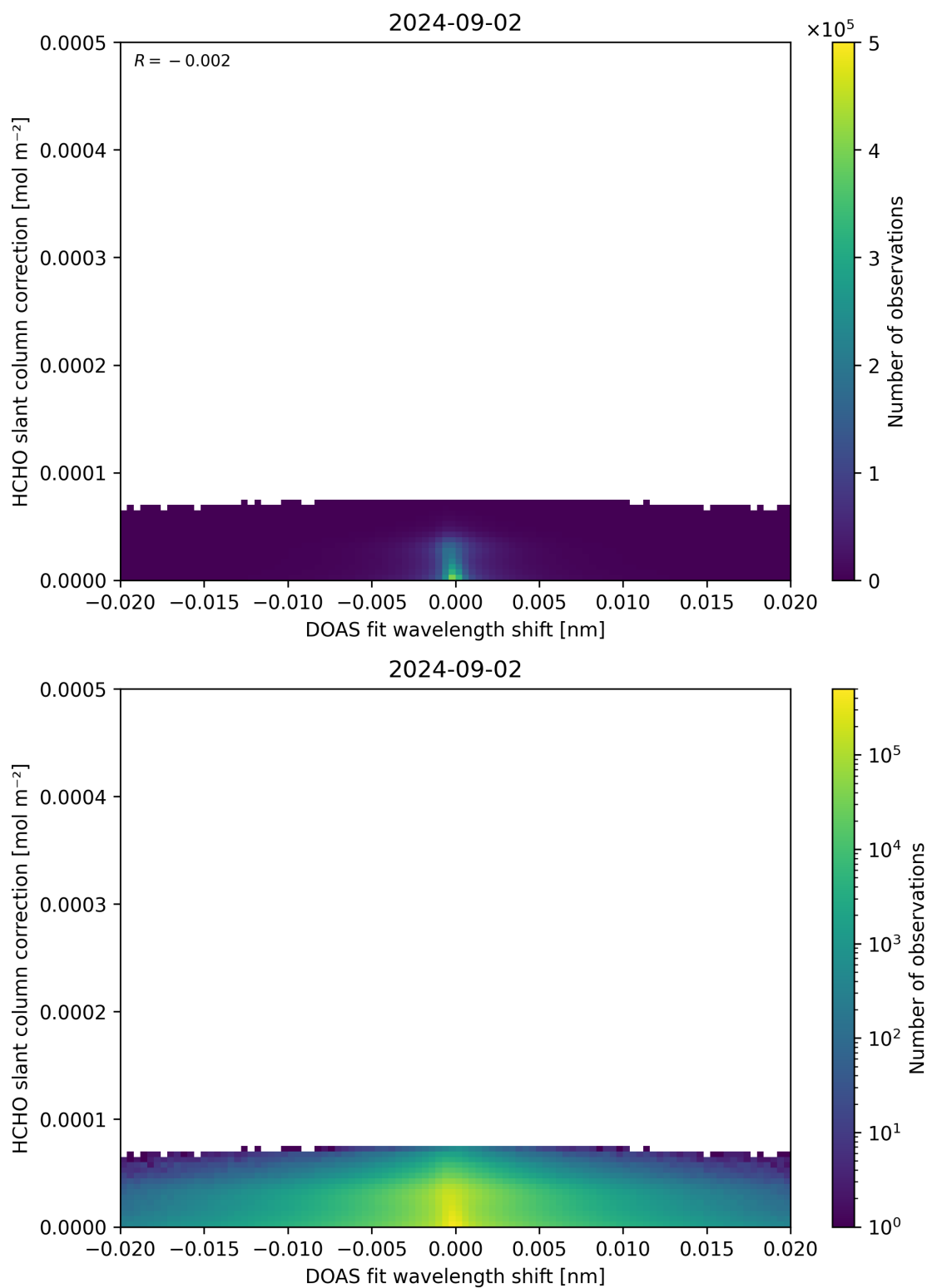
Figure 67: Scatter density plot of “DOAS fit wavelength shift” against “HCHO slant column correction” for 2024-09-01 to 2024-09-03.
