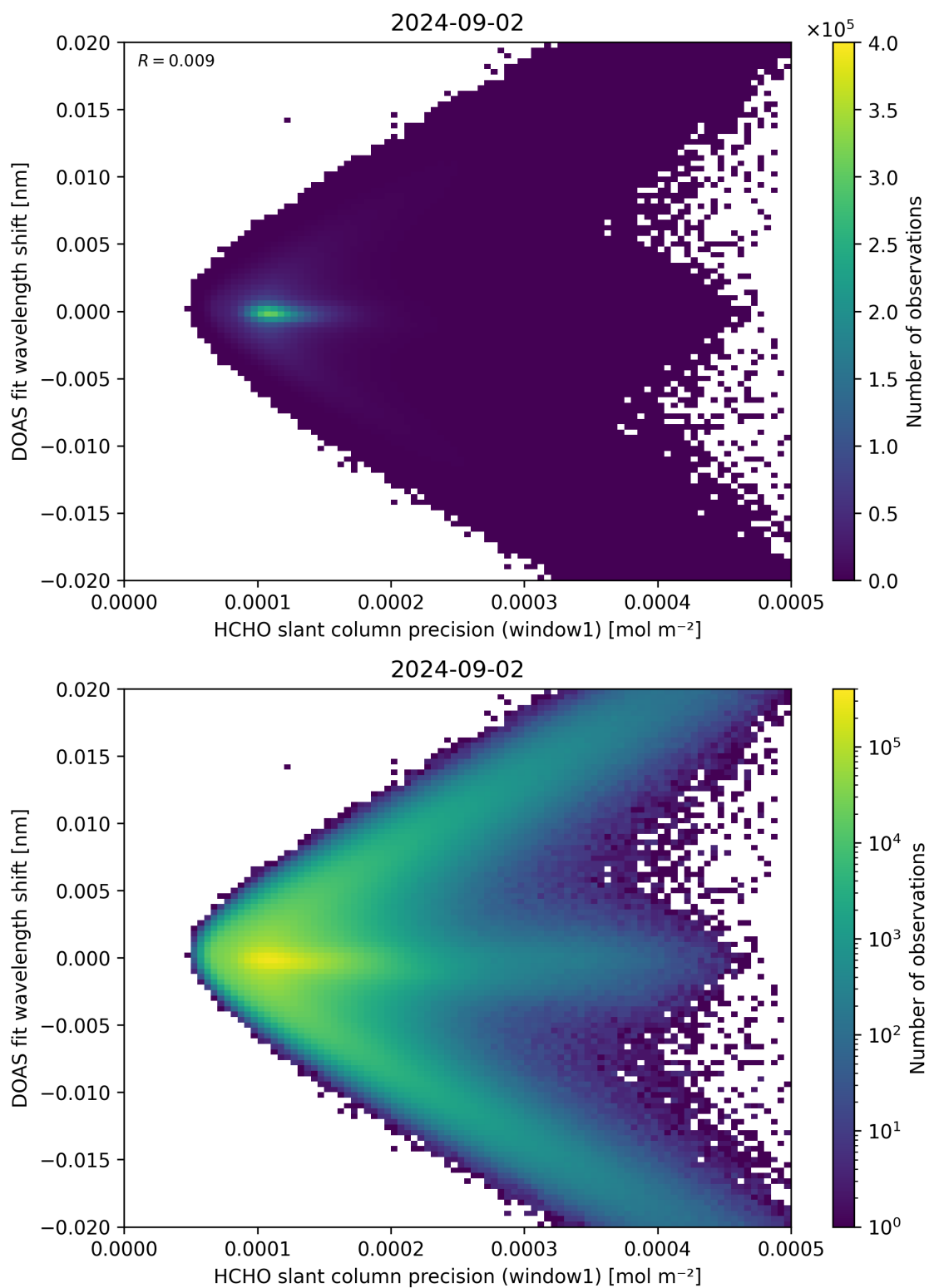
Figure 89: Scatter density plot of “HCHO slant column precision (window1)” against “DOAS fit wavelength shift” for 2024-09-01 to 2024-09-03.
