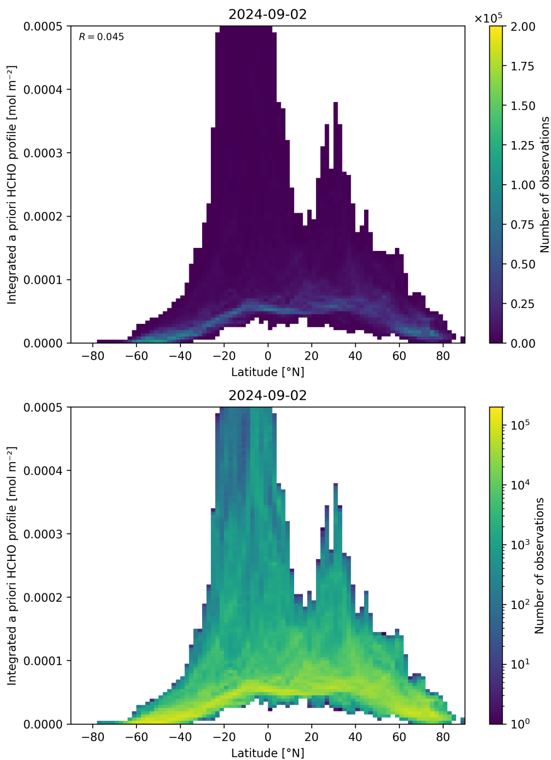
Figure 166: Scatter density plot of “Latitude” against “Integrated a priori HCHO profile” for 2024-09-01 to 2024-09-03.
