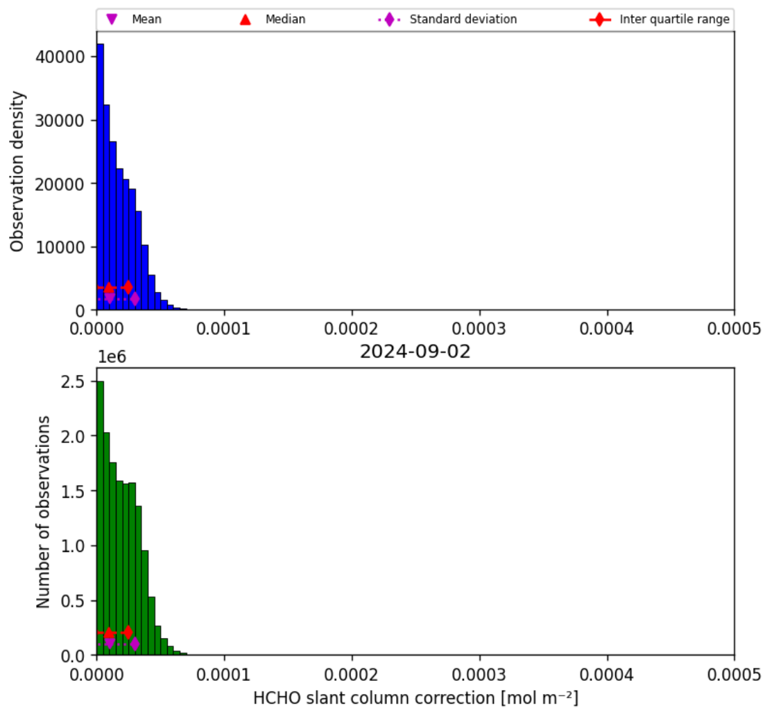
Figure 47: Histogram of “HCHO slant column correction” for 2024-09-01 to 2024-09-03
