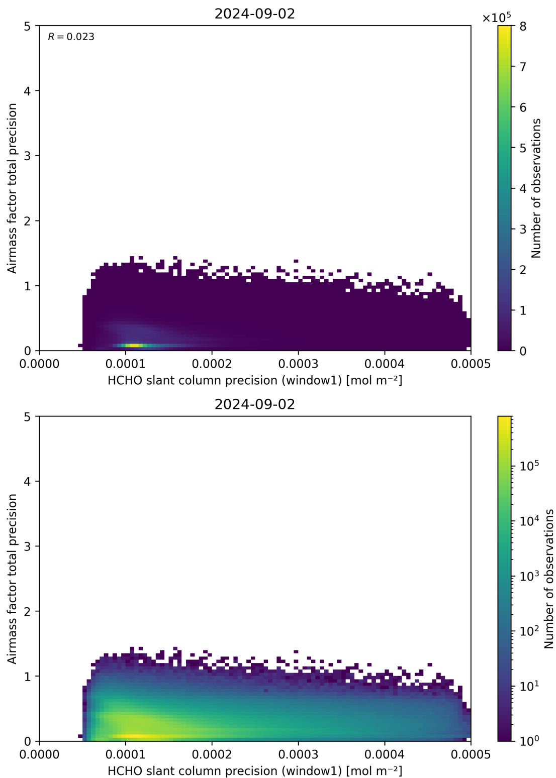
Figure 95: Scatter density plot of “HCHO slant column precision (window1)” against “Airmass factor total precision” for 2024-09-01 to 2024-09-03.
