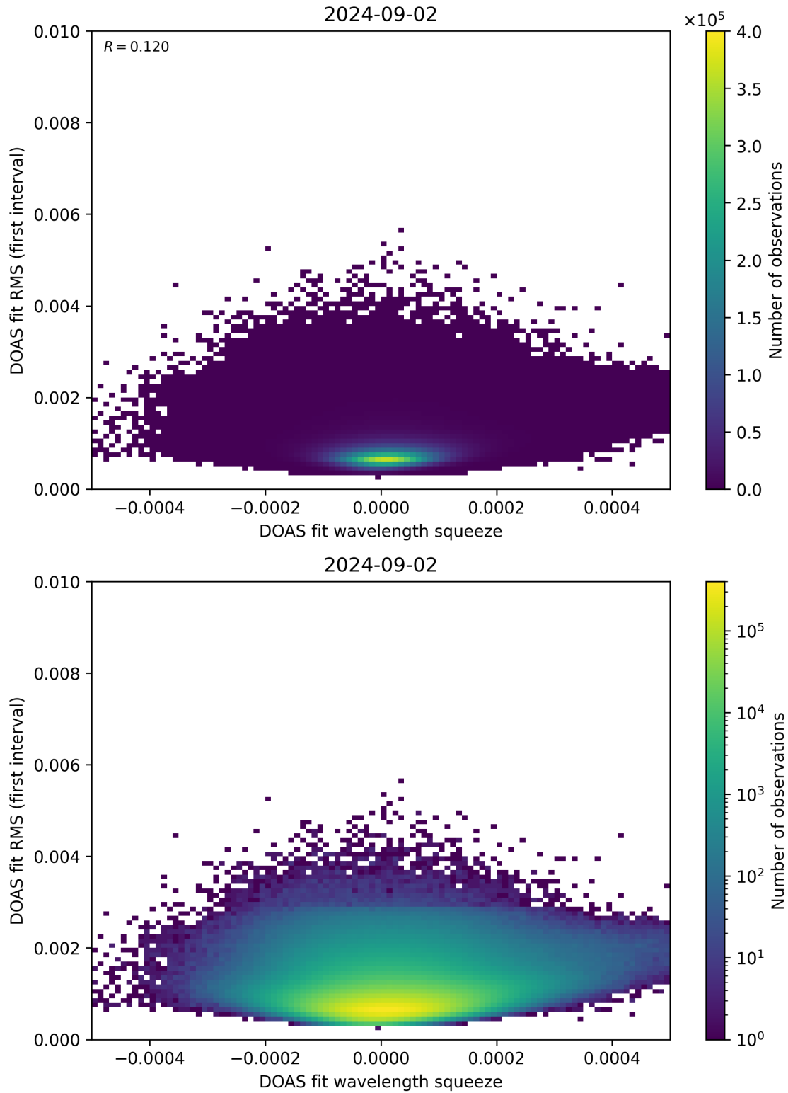
Figure 68: Scatter density plot of “DOAS fit wavelength squeeze” against “DOAS fit RMS (first interval)” for 2024-09-01 to 2024-09-03.
