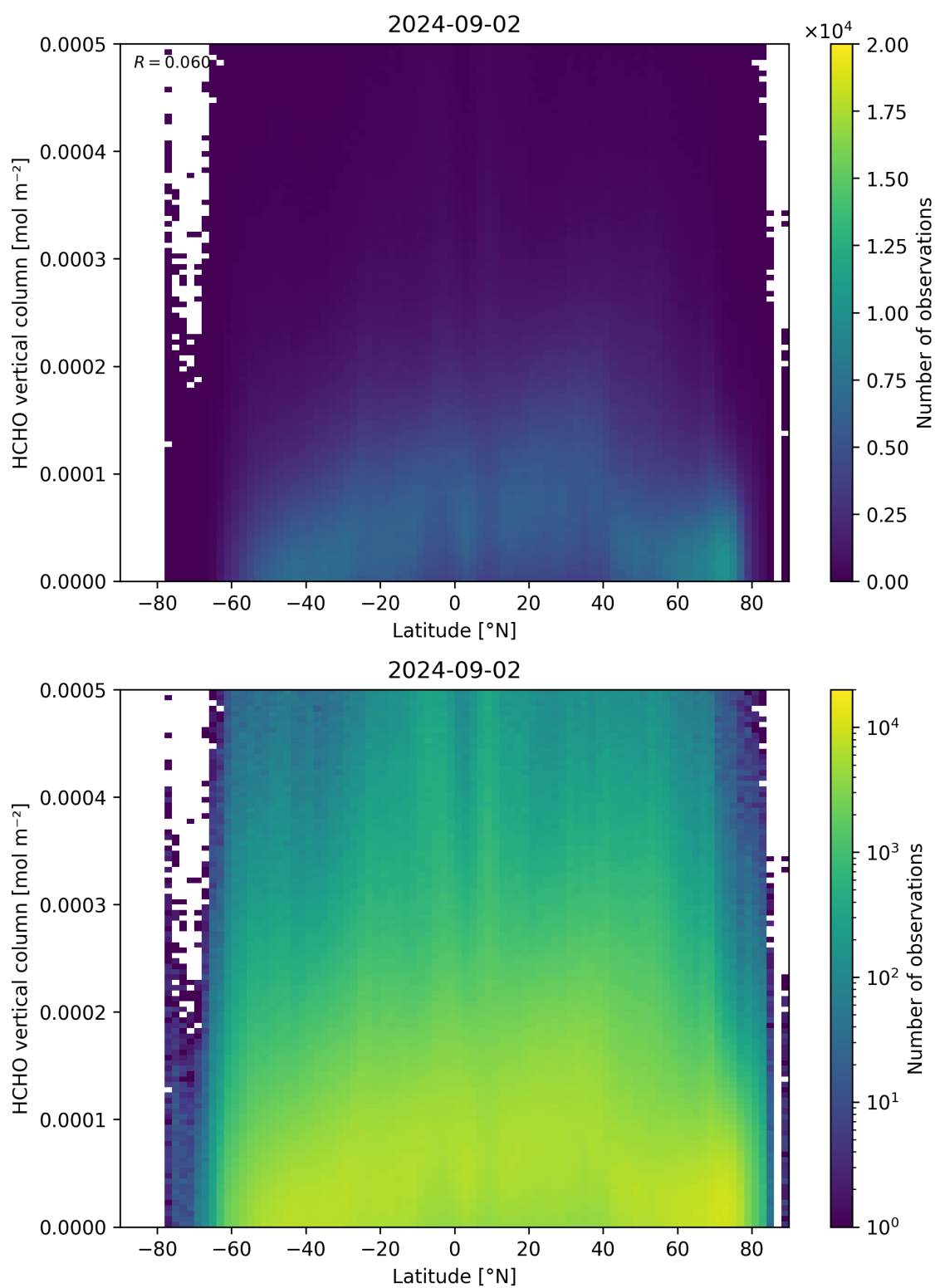
Figure 163: Scatter density plot of “Latitude” against “HCHO vertical column” for 2024-09-01 to 2024-09-03.
