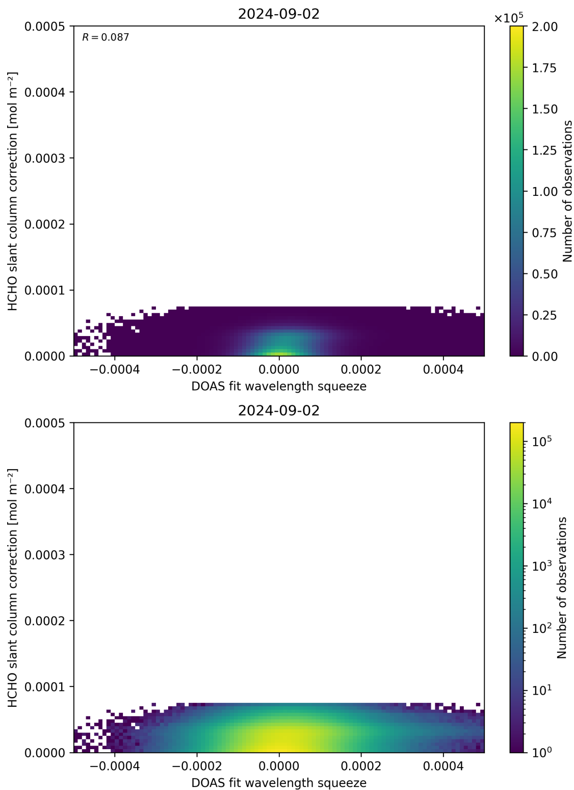
Figure 70: Scatter density plot of “DOAS fit wavelength squeeze” against “HCHO slant column correction” for 2024-09-01 to 2024-09-03.
