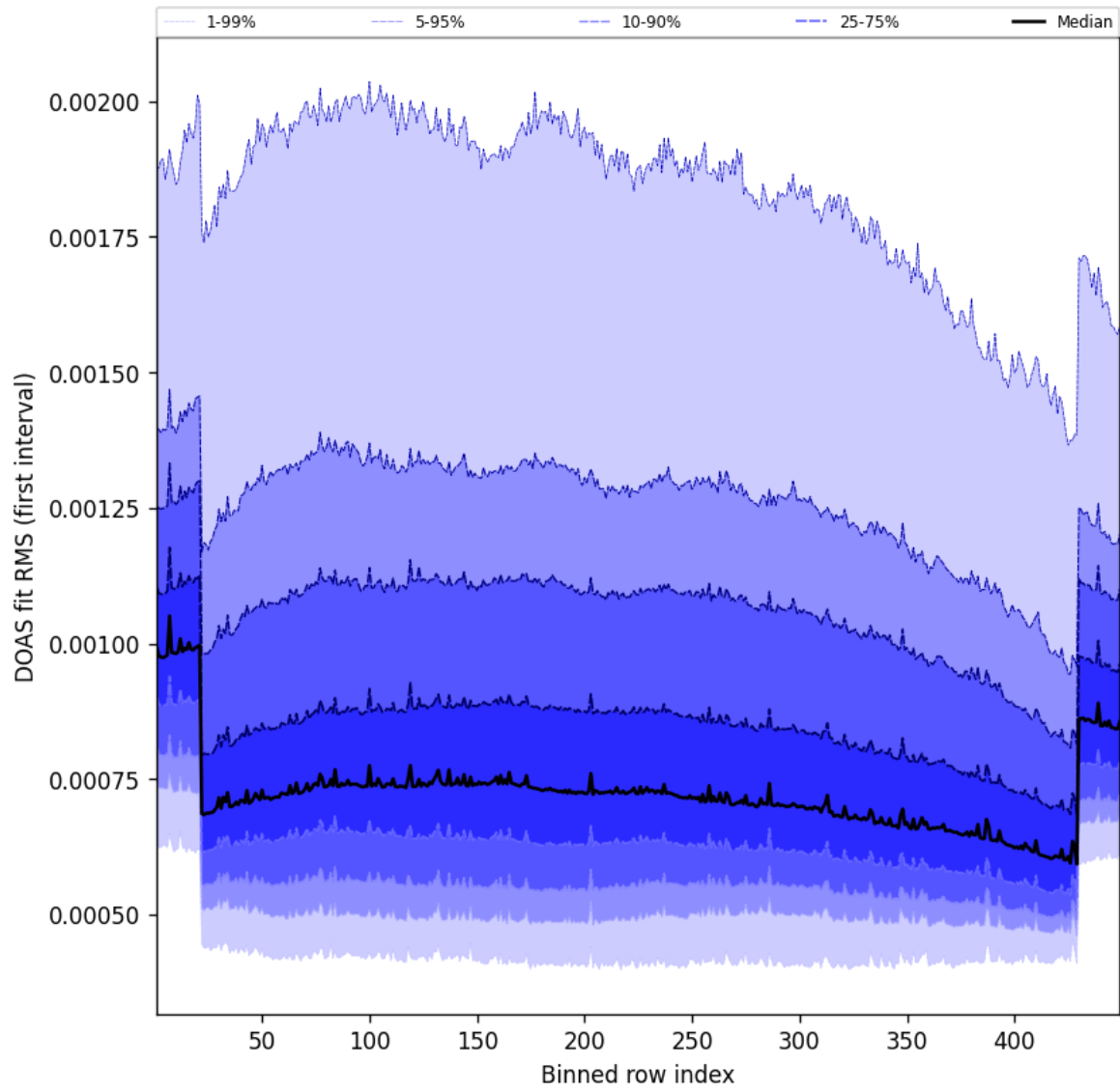
Figure 60: Along track statistics of “DOAS fit RMS (first interval)” for 2024-09-01 to 2024-09-03
