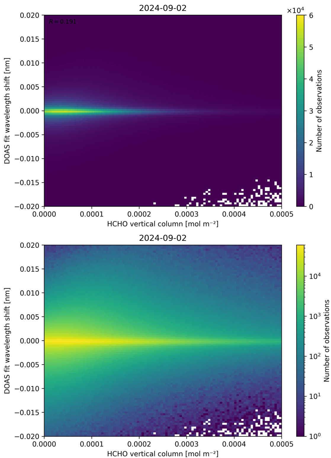
Figure 124: Scatter density plot of “HCHO vertical column” against “DOAS fit wavelength shift” for 2024-09-01 to 2024-09-03.
