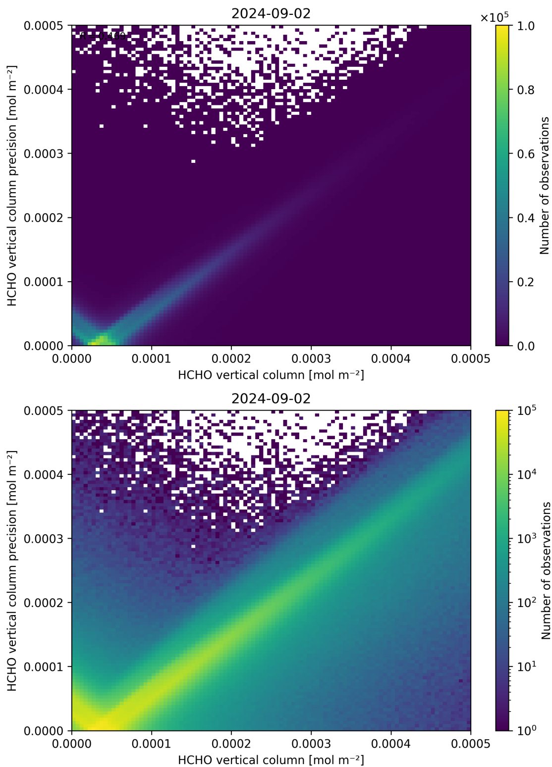
Figure 134: Scatter density plot of “HCHO vertical column” against “HCHO vertical column precision” for 2024-09-01 to 2024-09-03.
