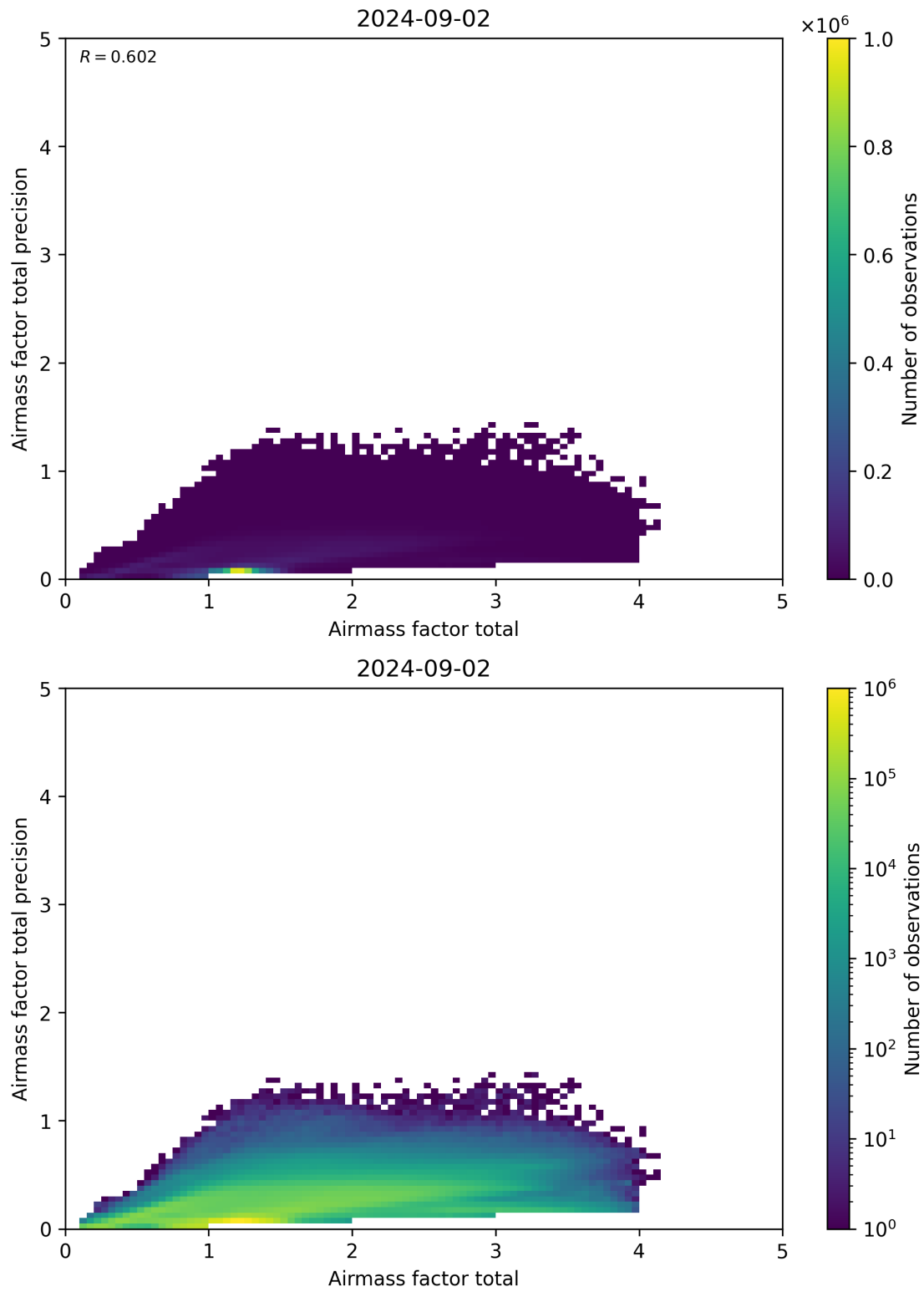
Figure 103: Scatter density plot of “Airmass factor total” against “Airmass factor total precision” for 2024-09-01 to 2024-09-03.
