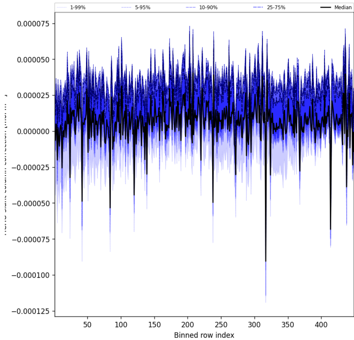
Figure 61: Along track statistics of “HCHO slant column correction” for 2024-09-01 to 2024-09-03
