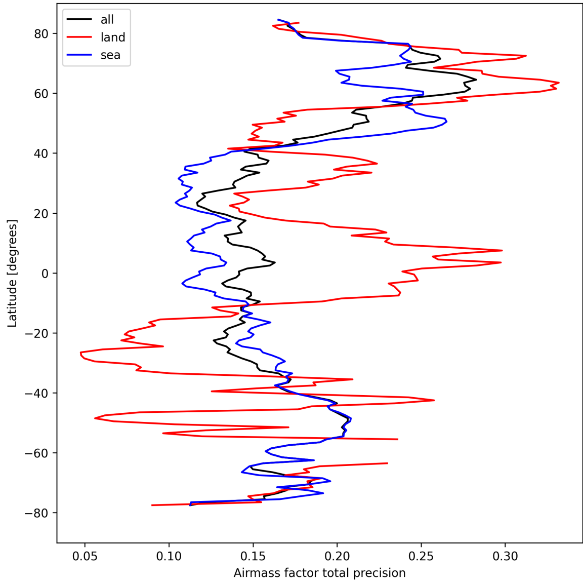
Figure 27: Zonal average of “Airmass factor total precision” for 2024-09-01 to 2024-09-03.
