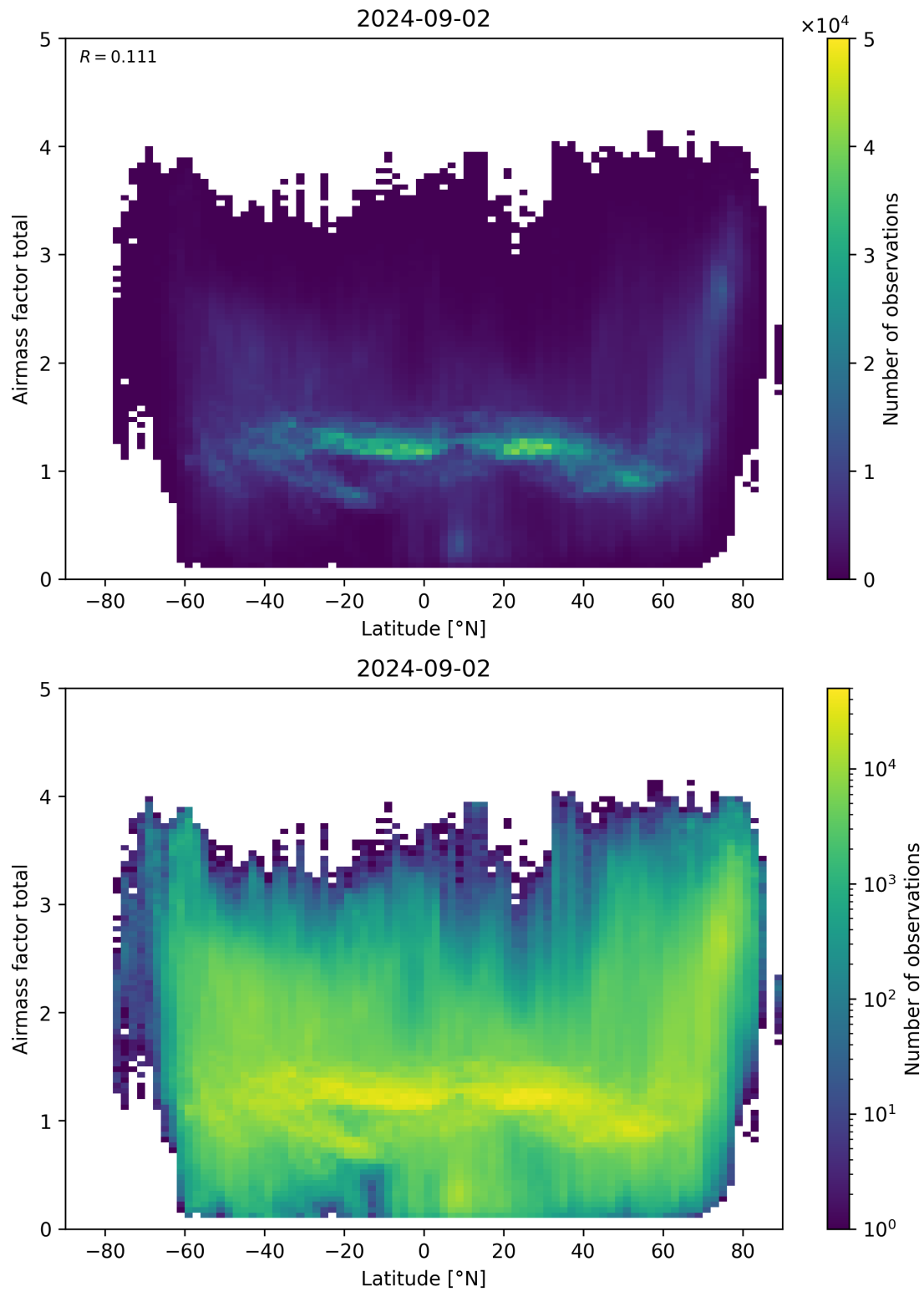
Figure 161: Scatter density plot of “Latitude” against “Airmass factor total” for 2024-09-01 to 2024-09-03.
