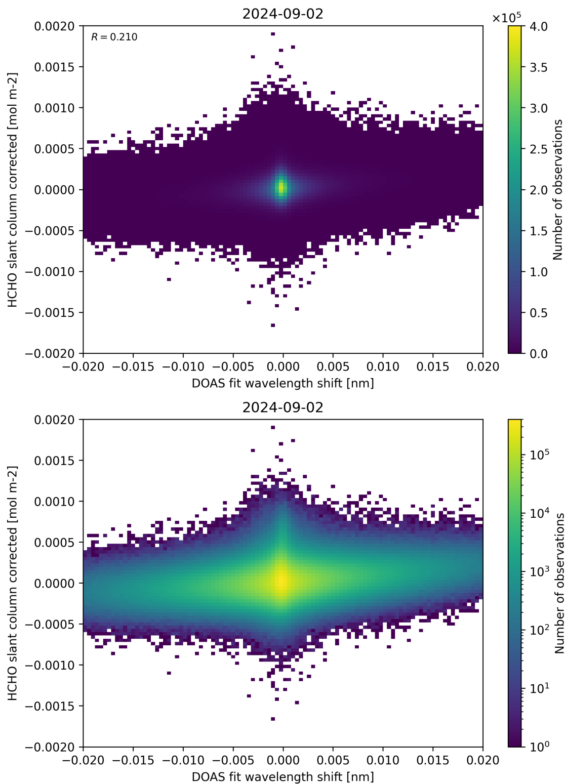
Figure 66: Scatter density plot of “DOAS fit wavelength shift” against “HCHO slant column corrected” for 2024-09-01 to 2024-09-03.
