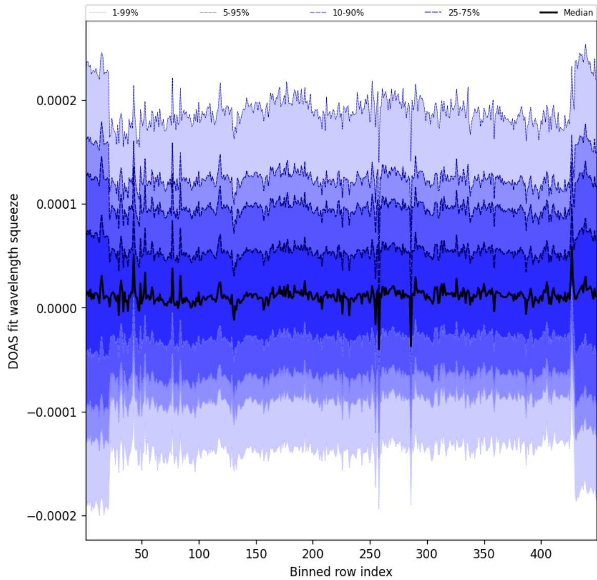
Figure 59: Along track statistics of “DOAS fit wavelength squeeze” for 2024-09-01 to 2024-09-03
