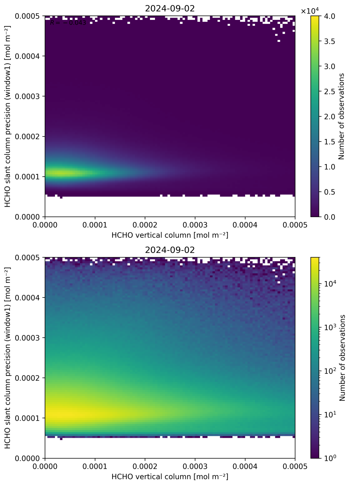
Figure 130: Scatter density plot of “HCHO vertical column” against “HCHO slant column precision (window1)” for 2024-09-01 to 2024-09-03.
