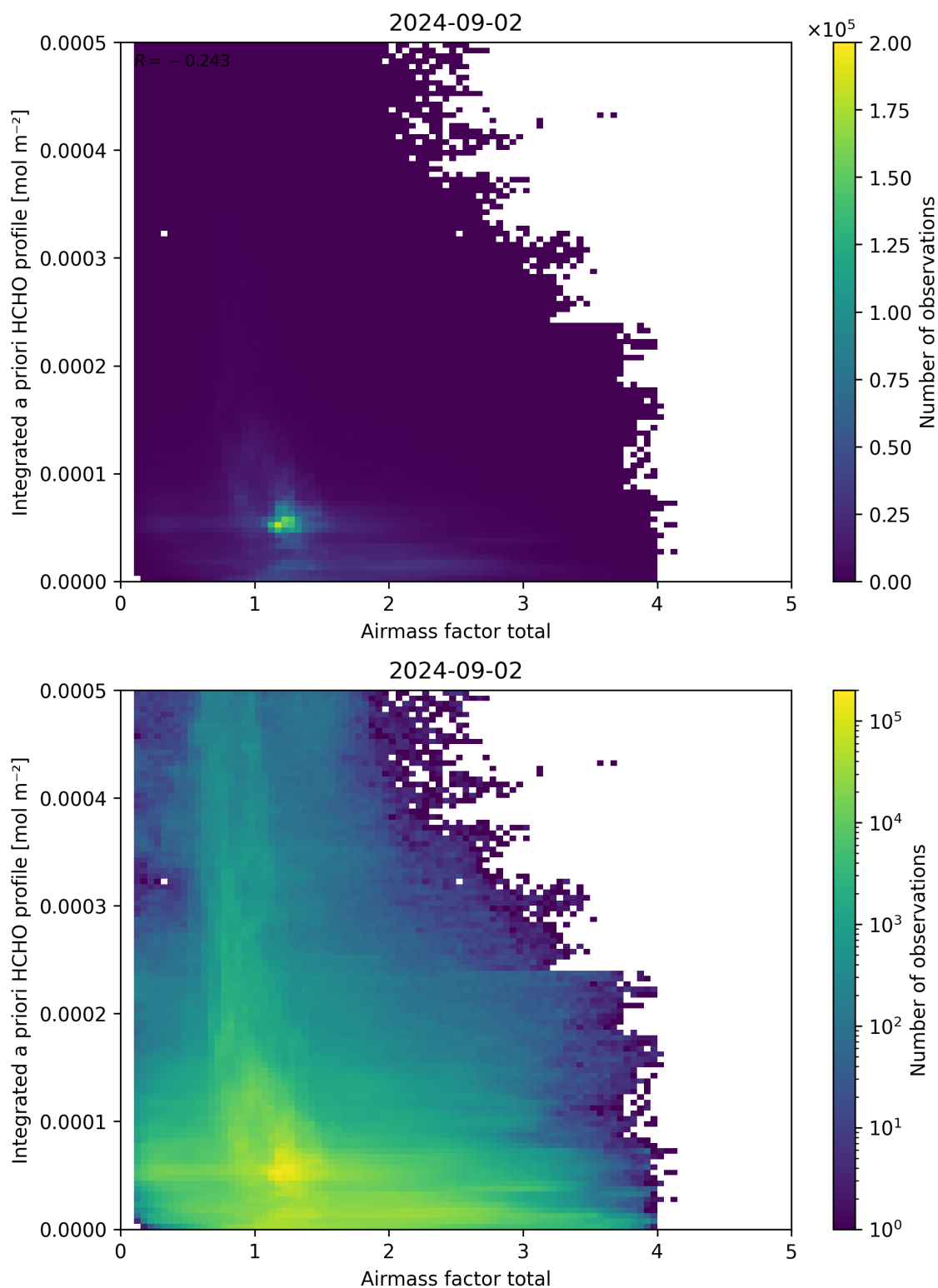
Figure 104: Scatter density plot of “Airmass factor total” against “Integrated a priori HCHO profile” for 2024-09-01 to 2024-09-03.
