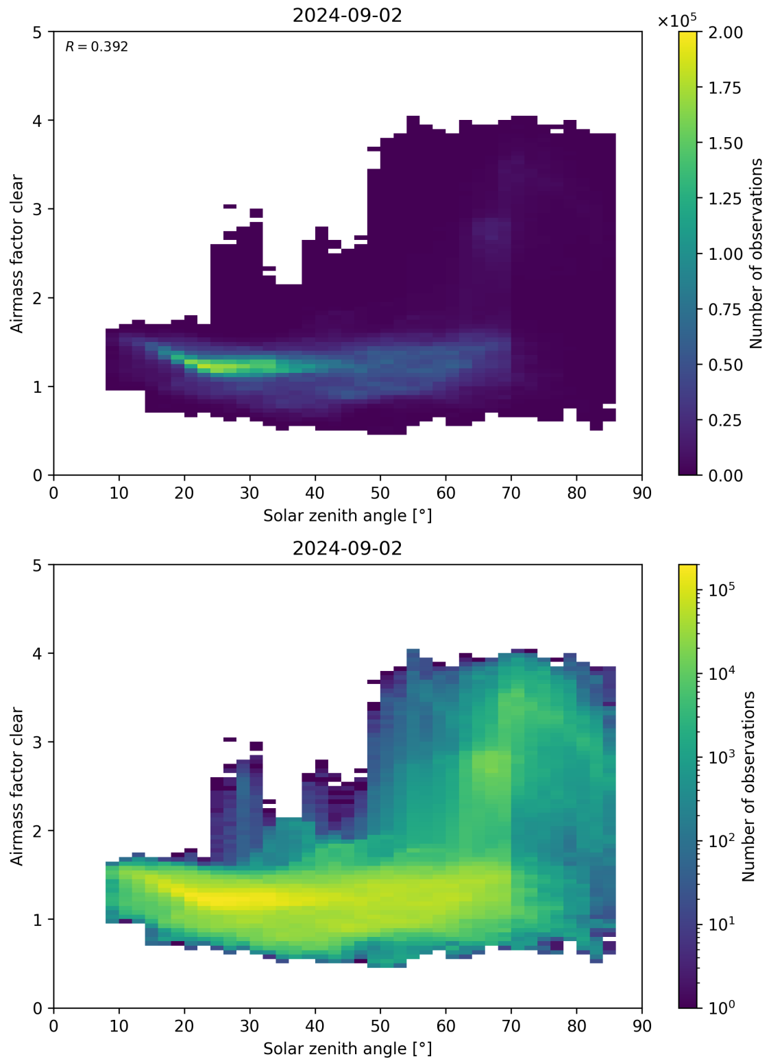
Figure 170: Scatter density plot of “Solar zenith angle” against “Airmass factor clear” for 2024-09-01 to 2024-09-03.
