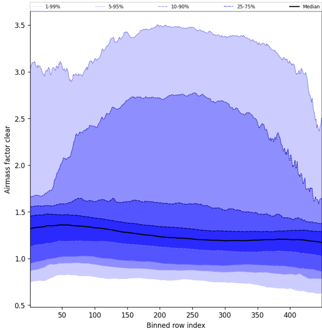
Figure 56: Along track statistics of “Airmass factor clear” for 2024-09-01 to 2024-09-03
