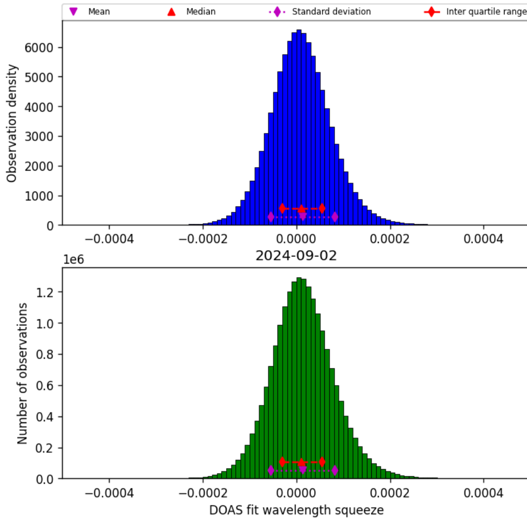
Figure 45: Histogram of “DOAS fit wavelength squeeze” for 2024-09-01 to 2024-09-03
