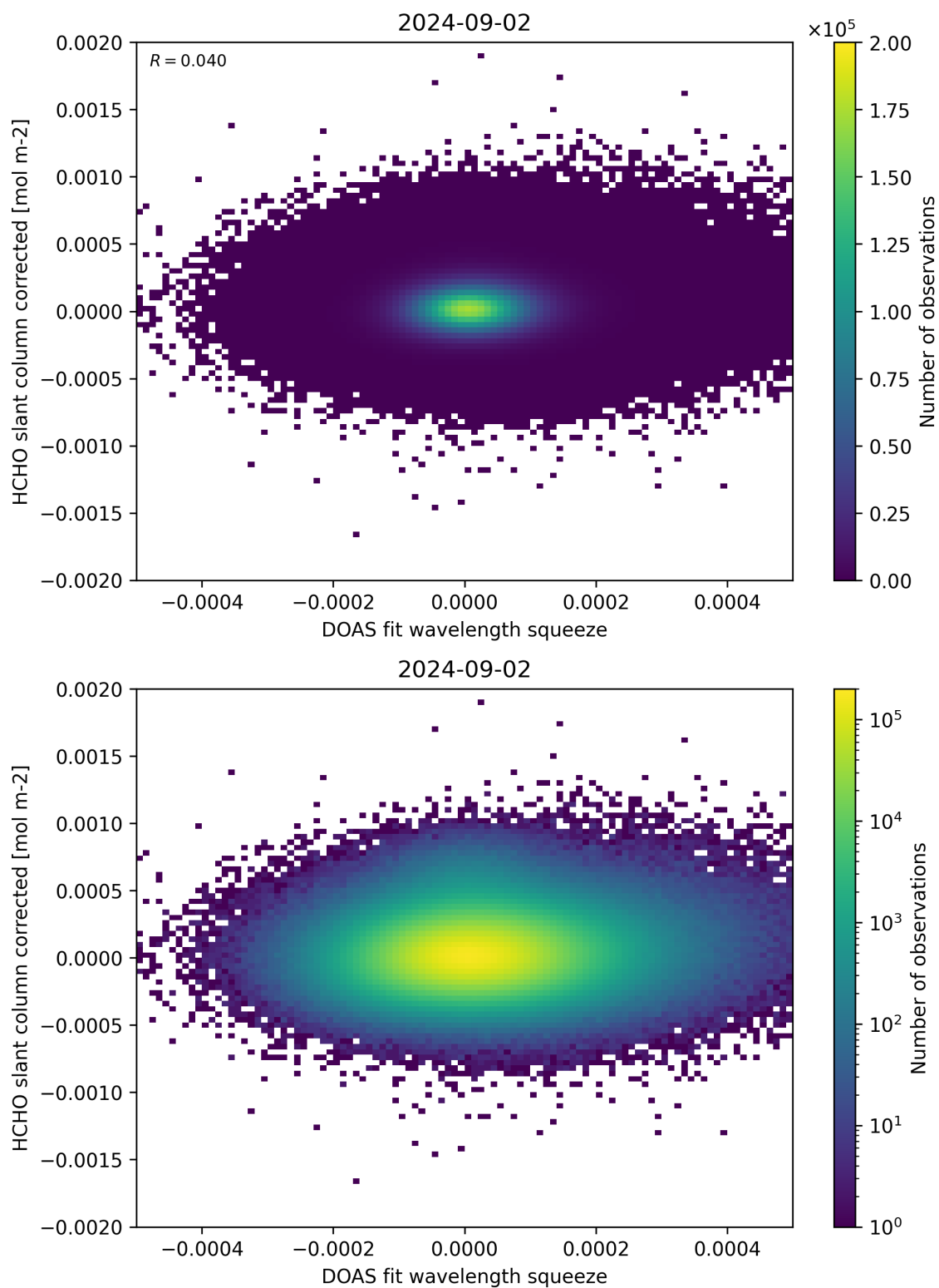
Figure 69: Scatter density plot of “DOAS fit wavelength squeeze” against “HCHO slant column corrected” for 2024-09-01 to 2024-09-03.
