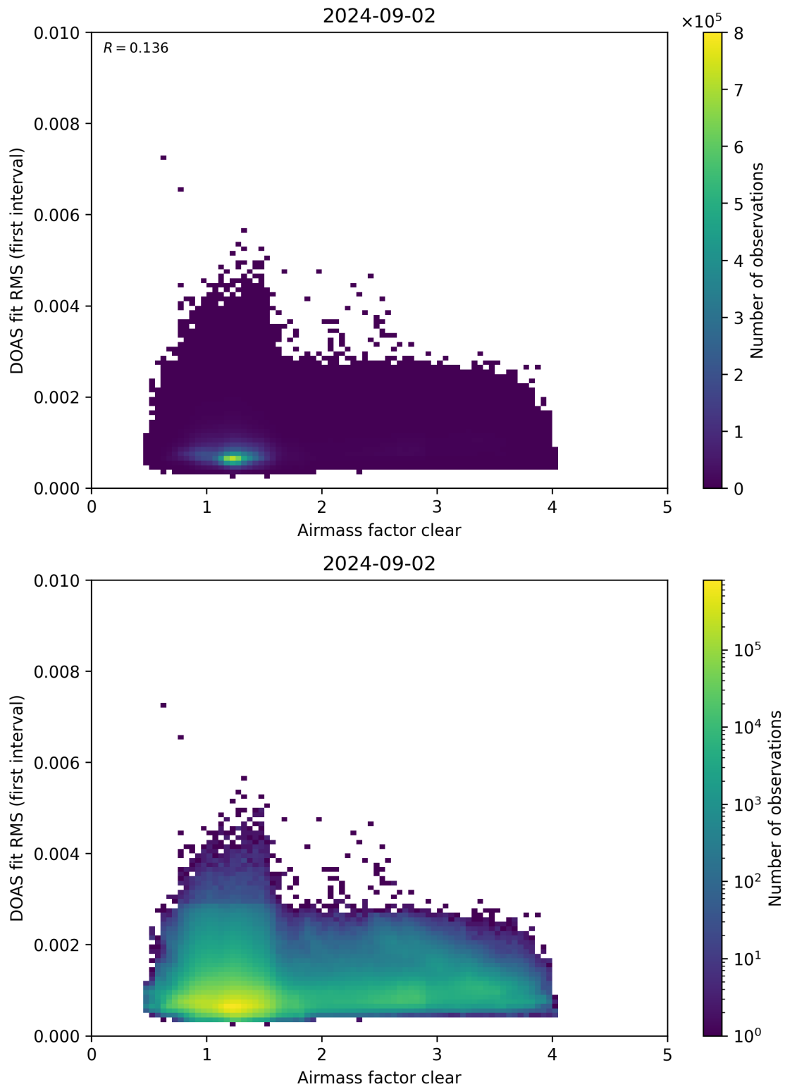
Figure 71: Scatter density plot of “Airmass factor clear” against “DOAS fit RMS (first interval)” for 2024-09-01 to 2024-09-03.
