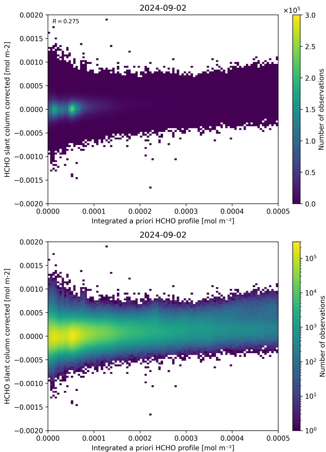
Figure 151: Scatter density plot of “Integrated a priori HCHO profile” against “HCHO slant column corrected” for 2024-09-01 to 2024-09-03.
