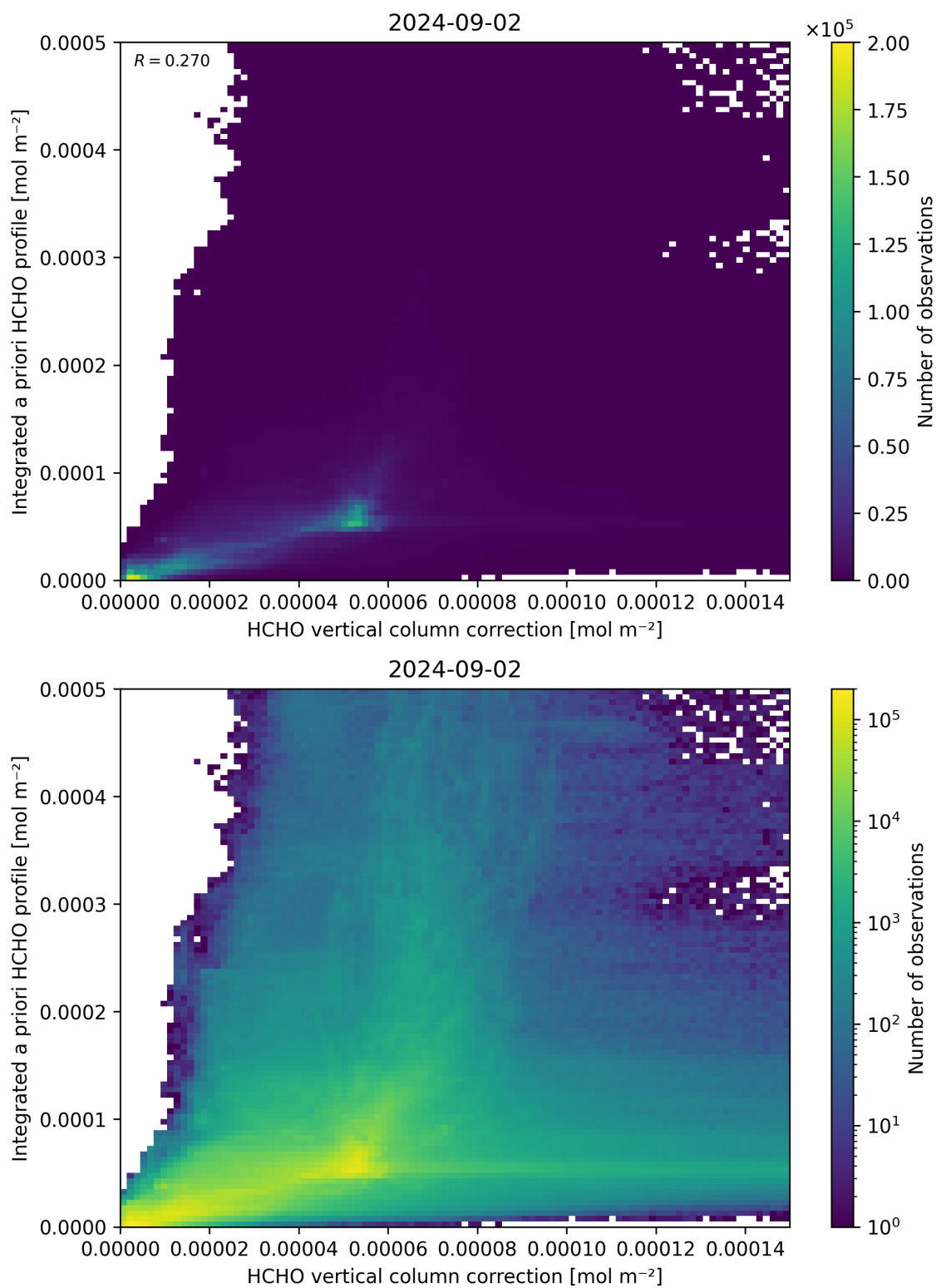
Figure 122: Scatter density plot of “HCHO vertical column correction” against “Integrated a priori HCHO profile” for 2024-09-01 to 2024-09-03.
