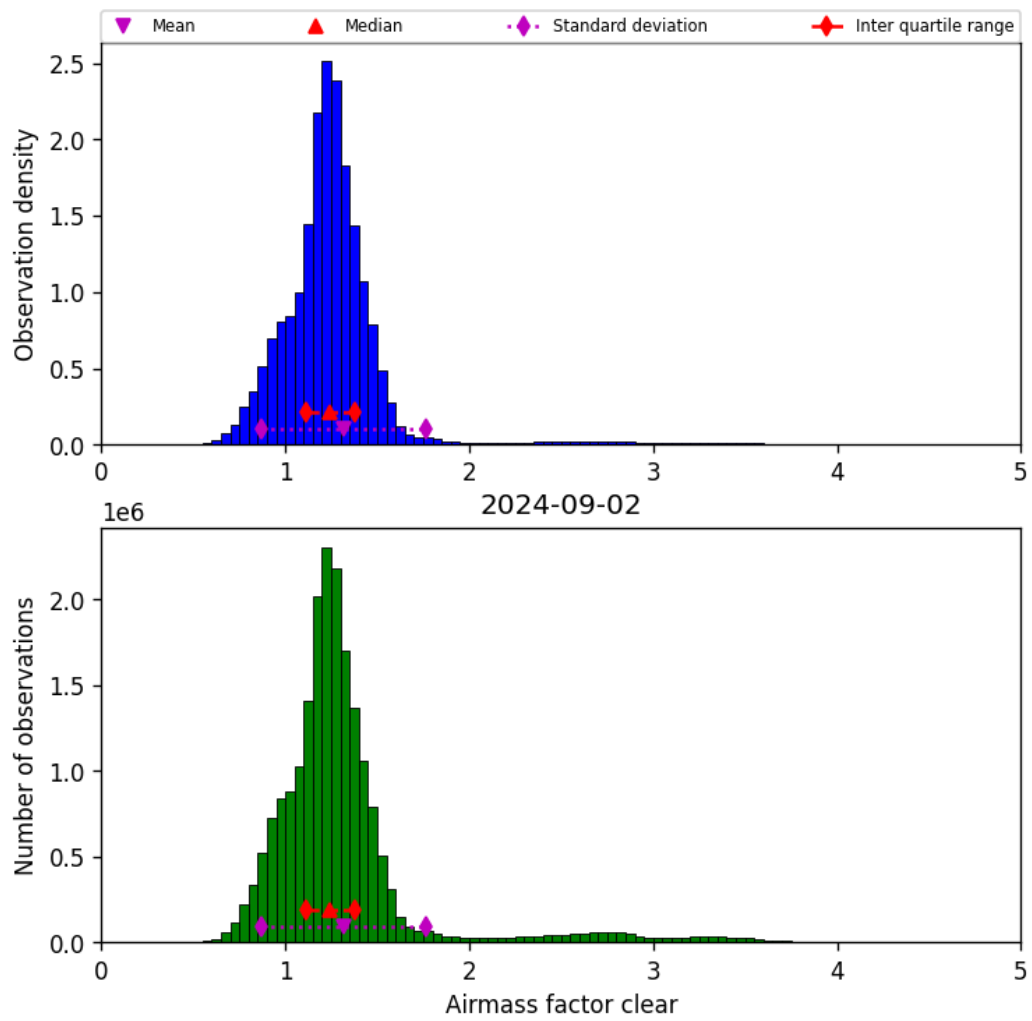
Figure 42: Histogram of “Airmass factor clear” for 2024-09-01 to 2024-09-03
