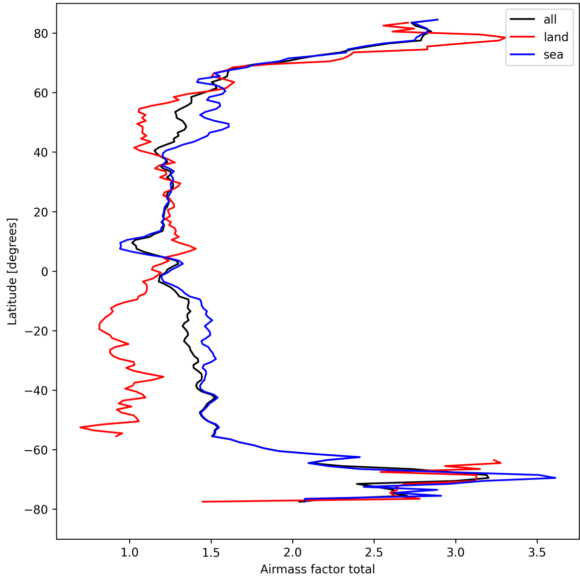
Figure 26: Zonal average of “Airmass factor total” for 2024-09-01 to 2024-09-03.
