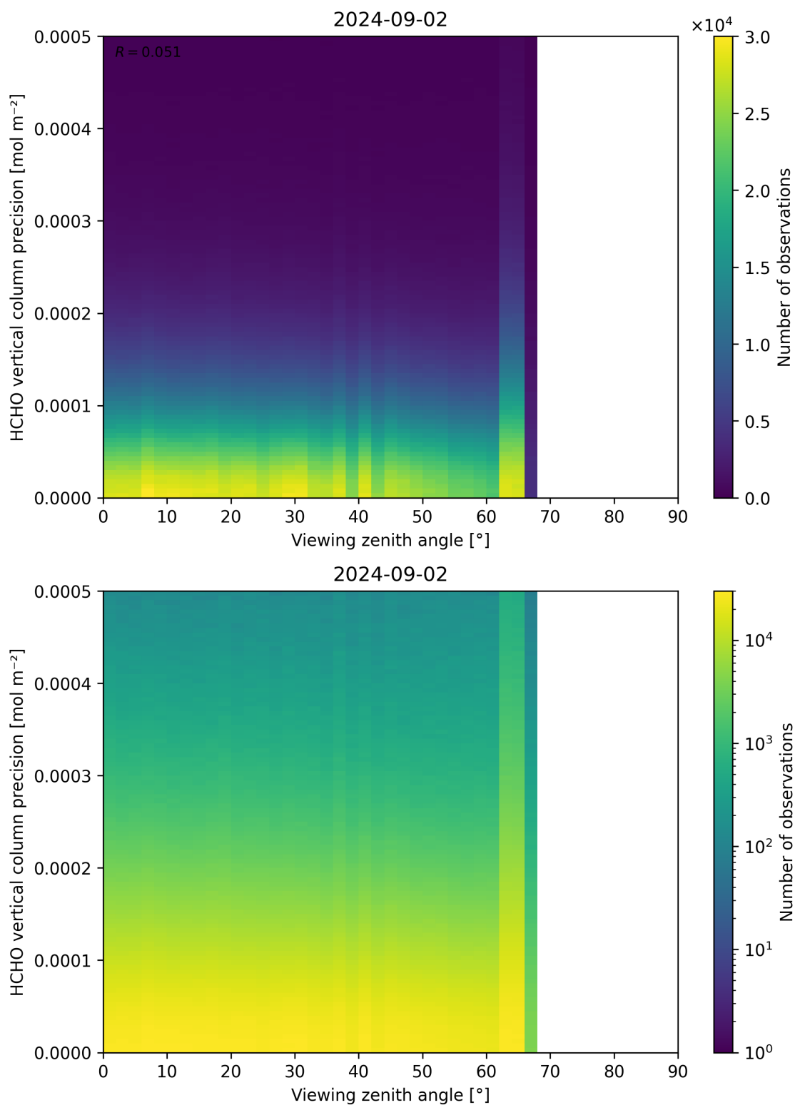
Figure 194: Scatter density plot of “Viewing zenith angle” against “HCHO vertical column precision” for 2024-09-01 to 2024-09-03.
