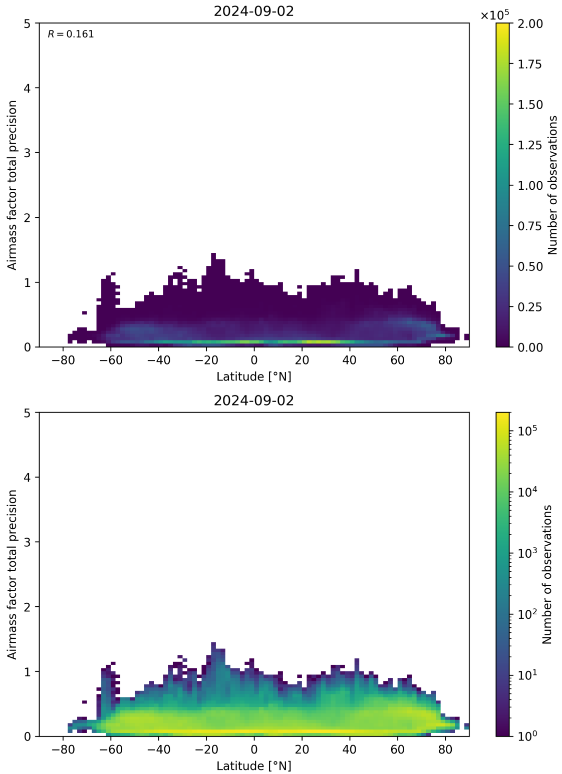
Figure 162: Scatter density plot of “Latitude” against “Airmass factor total precision” for 2024-09-01 to 2024-09-03.
