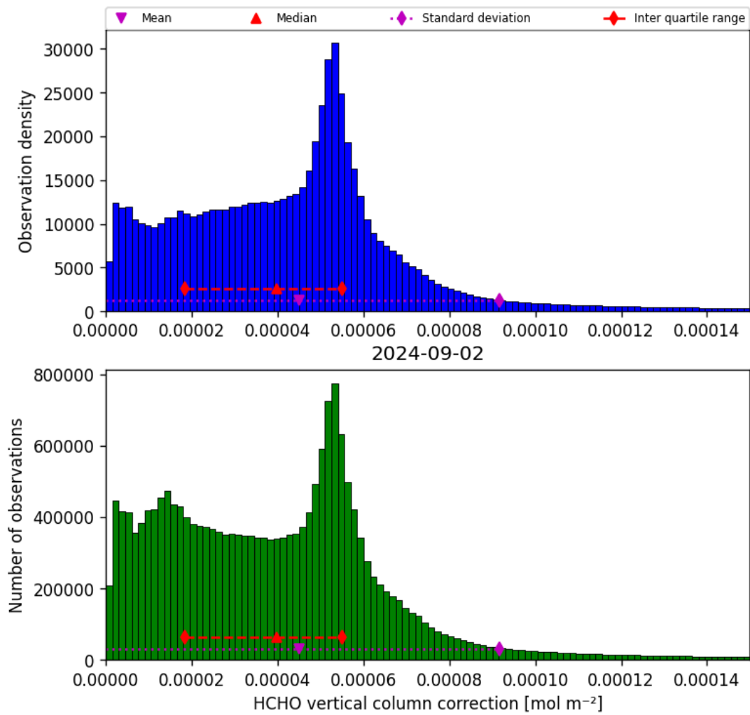
Figure 37: Histogram of “HCHO vertical column correction” for 2024-09-01 to 2024-09-03
