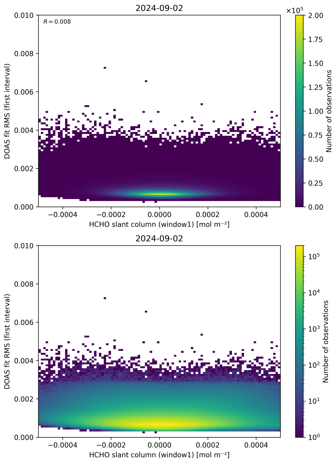
Figure 78: Scatter density plot of “HCHO slant column (window1)” against “DOAS fit RMS (first interval)” for 2024-09-01 to 2024-09-03.
