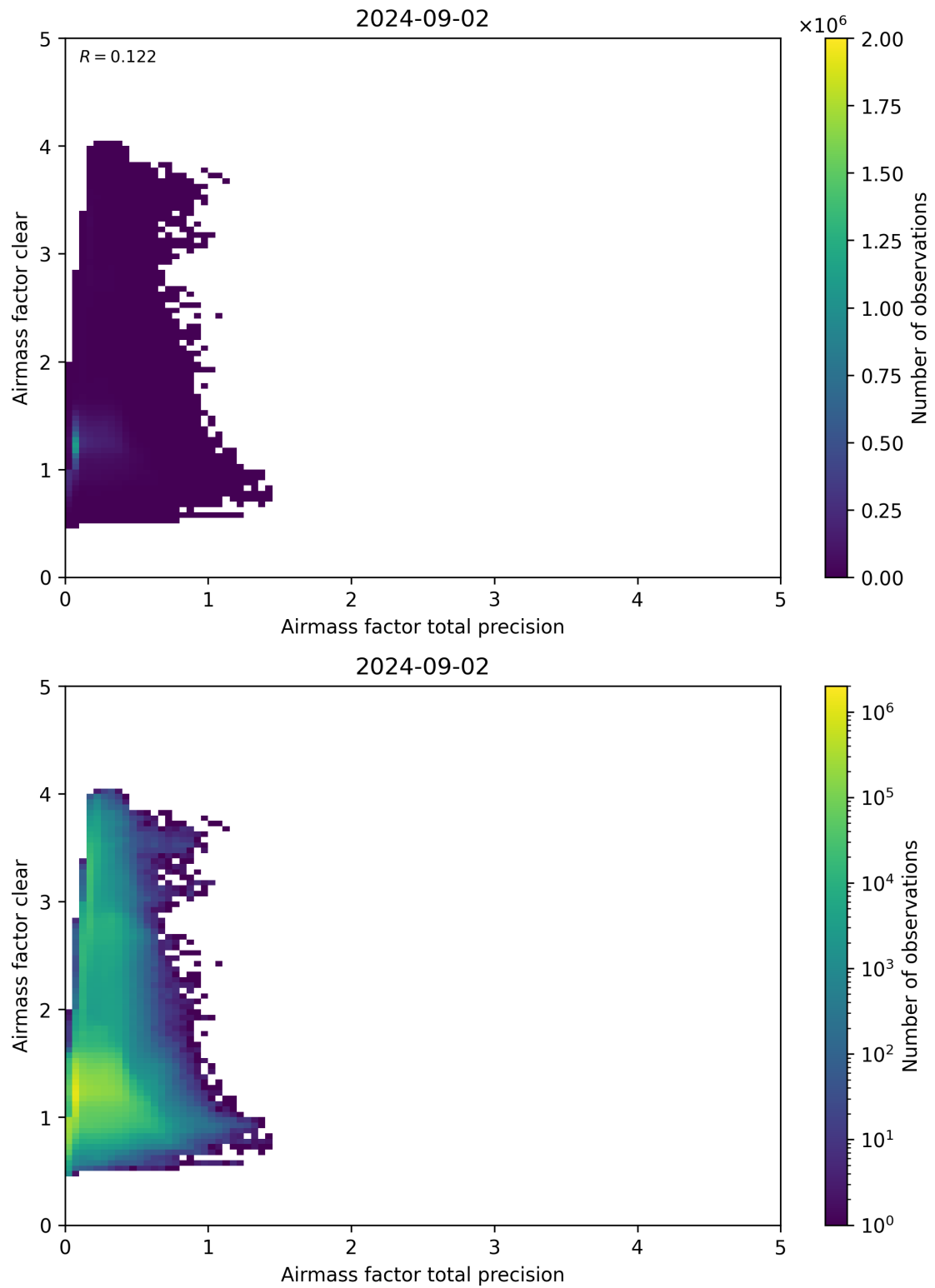
Figure 108: Scatter density plot of “Airmass factor total precision” against “Airmass factor clear” for 2024-09-01 to 2024-09-03.
