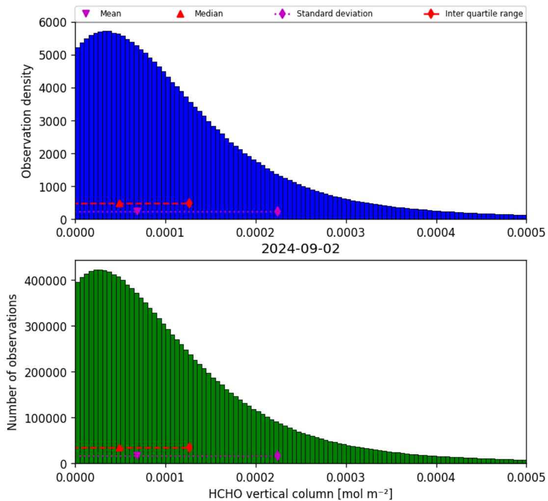
Figure 35: Histogram of “HCHO vertical column” for 2024-09-01 to 2024-09-03
