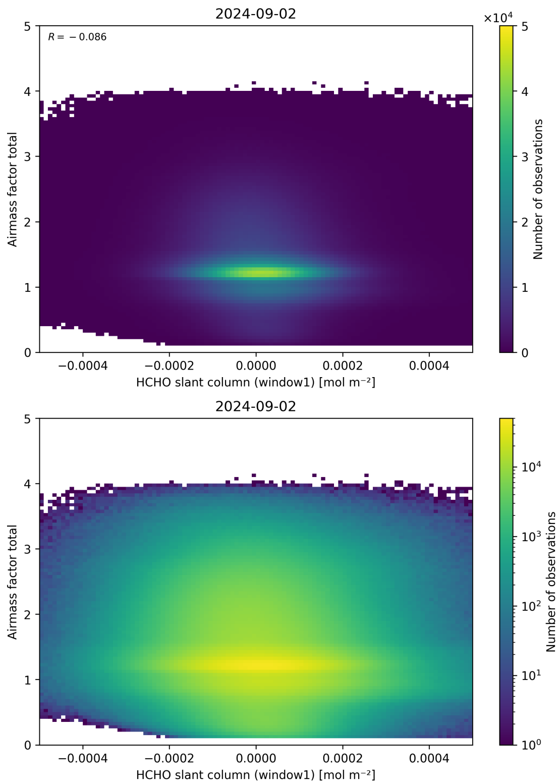
Figure 85: Scatter density plot of “HCHO slant column (window1)” against “Airmass factor total” for 2024-09-01 to 2024-09-03.
