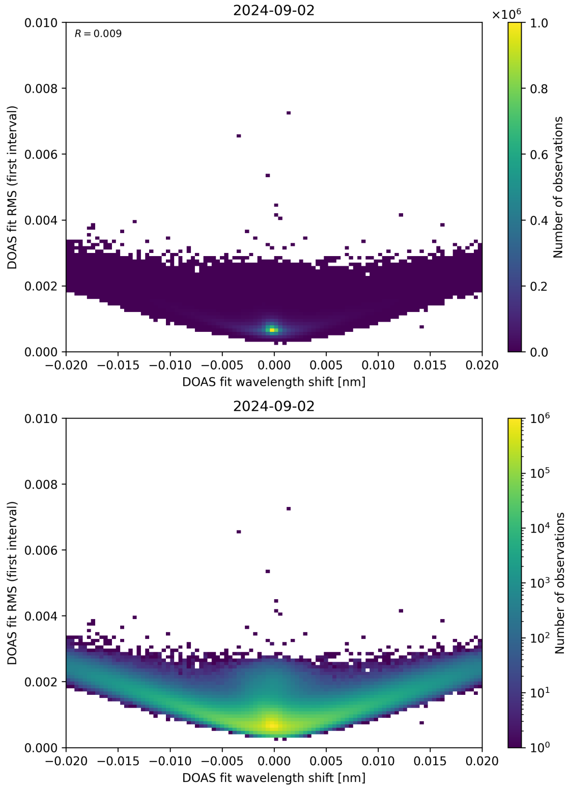
Figure 64: Scatter density plot of “DOAS fit wavelength shift” against “DOAS fit RMS (first interval)” for 2024-09-01 to 2024-09-03.
