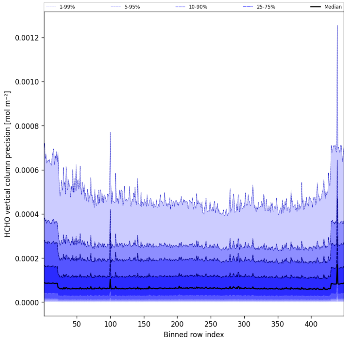
Figure 50: Along track statistics of “HCHO vertical column precision” for 2024-09-01 to 2024-09-03
