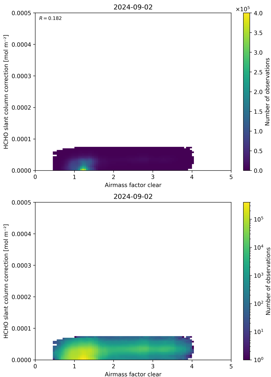
Figure 75: Scatter density plot of “Airmass factor clear” against “HCHO slant column correction” for 2024-09-01 to 2024-09-03.
