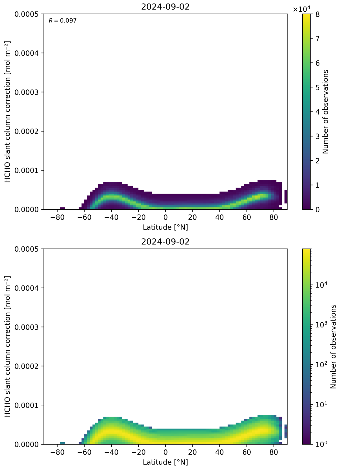
Figure 158: Scatter density plot of “Latitude” against “HCHO slant column correction” for 2024-09-01 to 2024-09-03.
