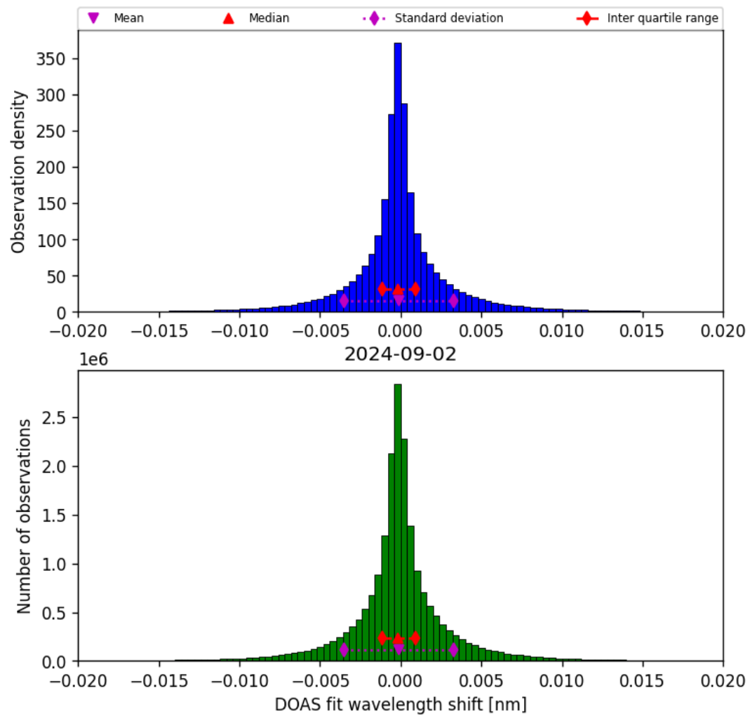
Figure 44: Histogram of “DOAS fit wavelength shift” for 2024-09-01 to 2024-09-03
