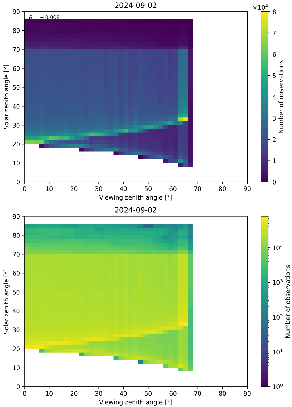
Figure 197: Scatter density plot of “Viewing zenith angle” against “Solar zenith angle” for 2024-09-01 to 2024-09-03.
