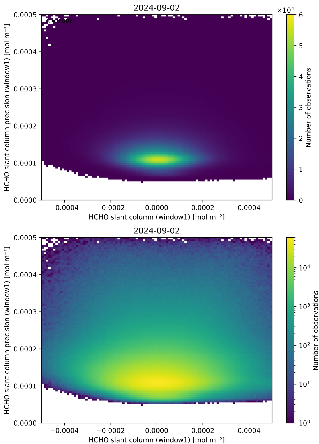
Figure 84: Scatter density plot of “HCHO slant column (window1)” against “HCHO slant column precision (window1)” for 2024-09-01 to 2024-09-03.
