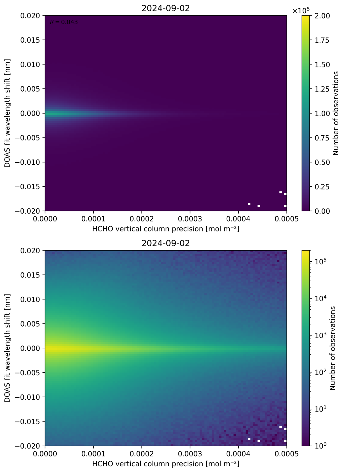
Figure 137: Scatter density plot of “HCHO vertical column precision” against “DOAS fit wavelength shift” for 2024-09-01 to 2024-09-03.
