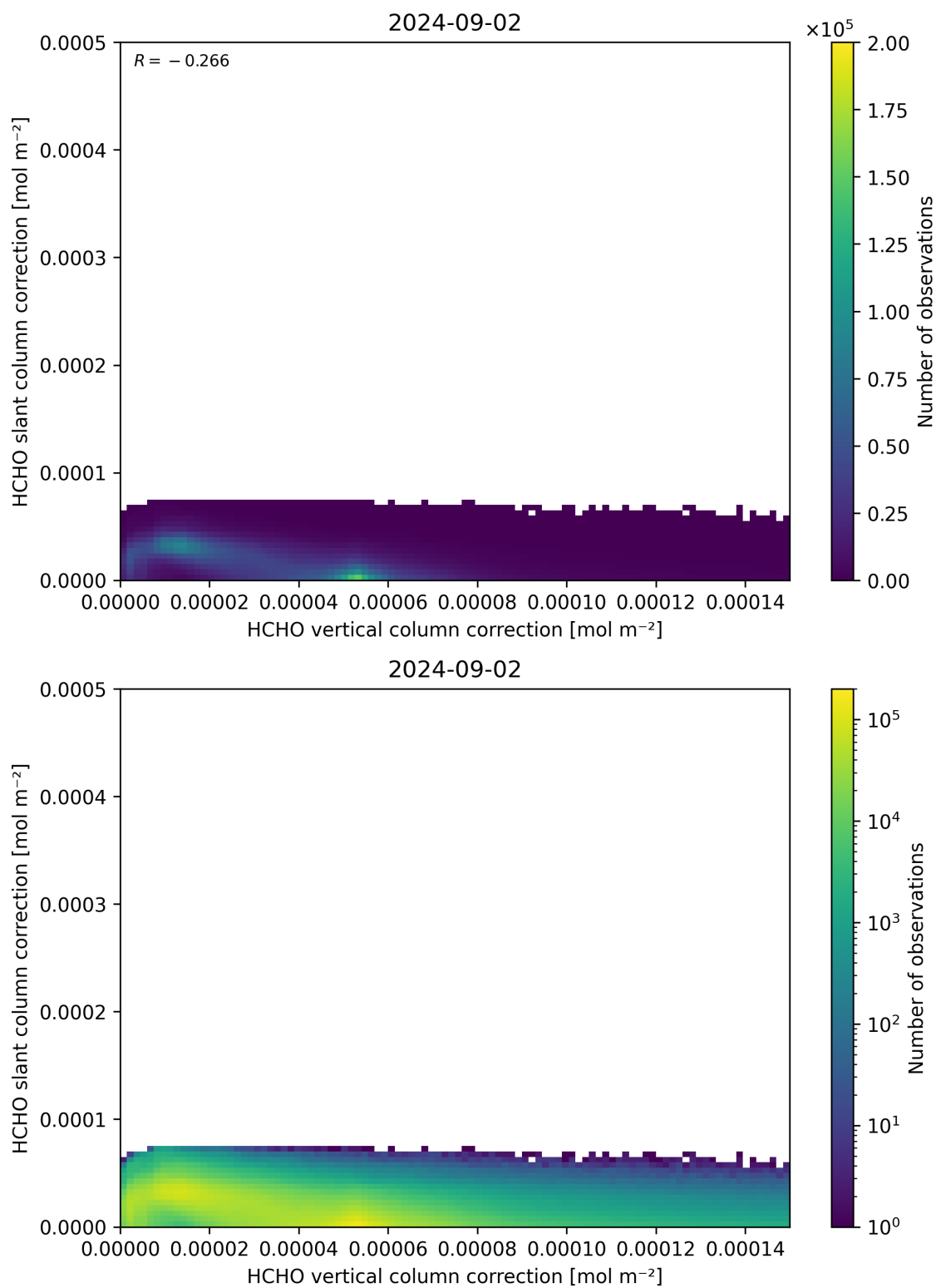
Figure 117: Scatter density plot of “HCHO vertical column correction” against “HCHO slant column correction” for 2024-09-01 to 2024-09-03.
