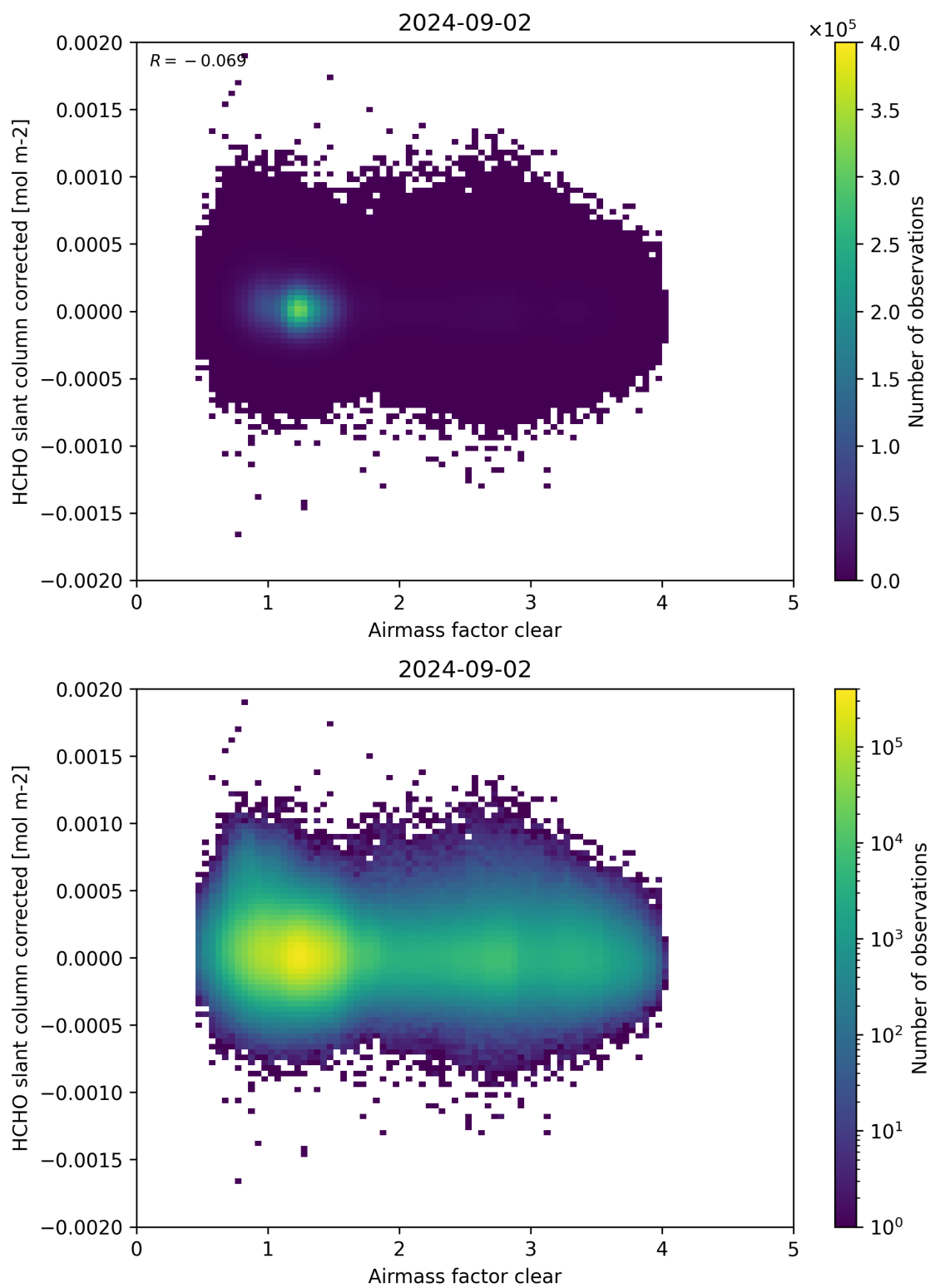
Figure 74: Scatter density plot of “Airmass factor clear” against “HCHO slant column corrected” for 2024-09-01 to 2024-09-03.
