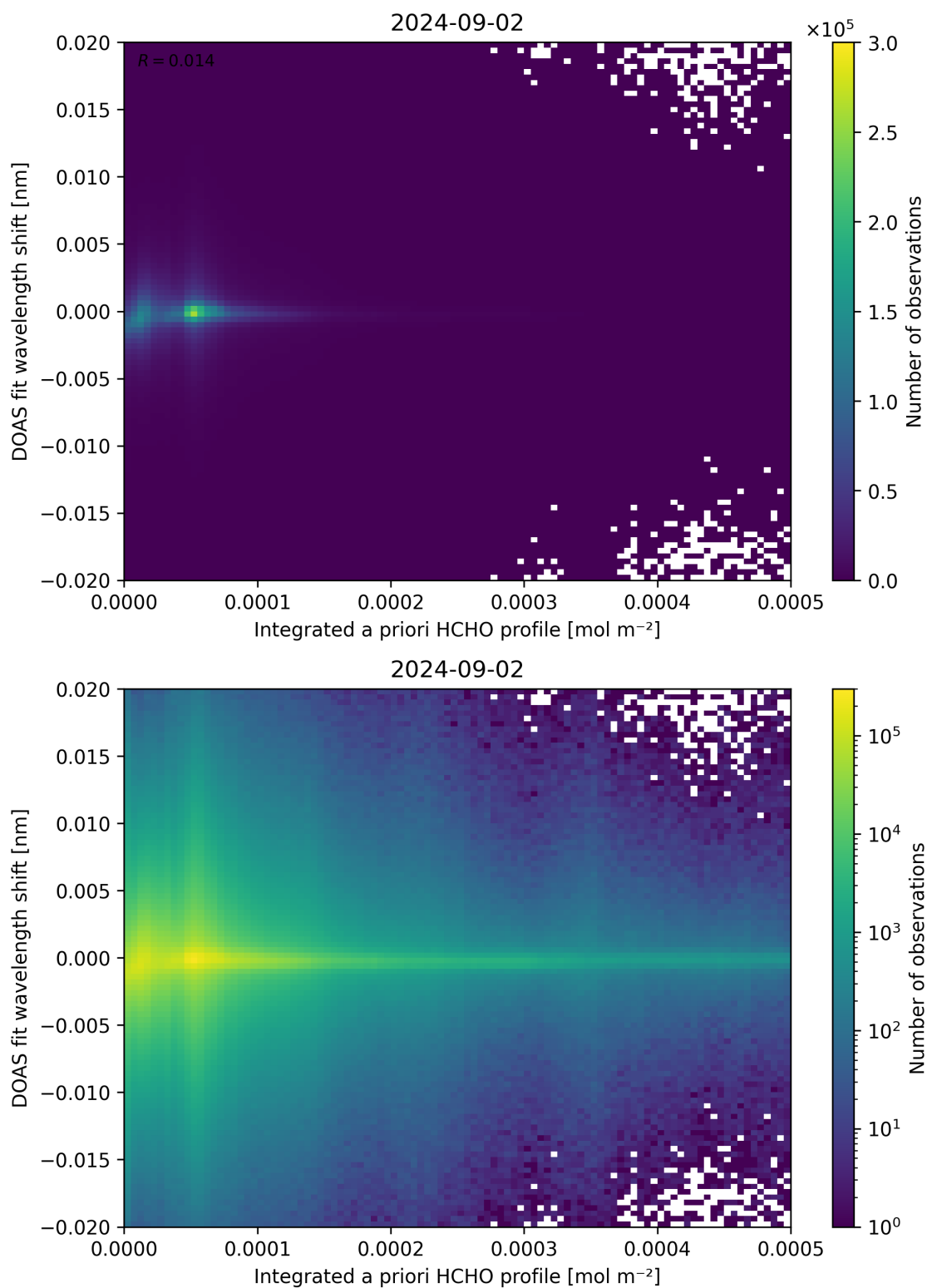
Figure 149: Scatter density plot of “Integrated a priori HCHO profile” against “DOAS fit wavelength shift” for 2024-09-01 to 2024-09-03.
