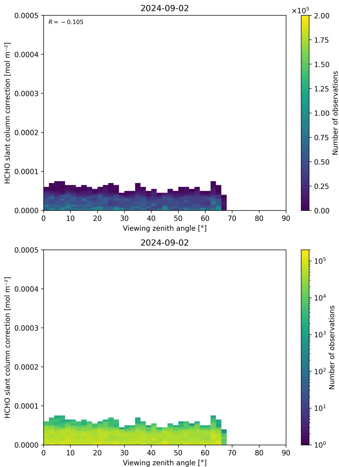
Figure 187: Scatter density plot of “Viewing zenith angle” against “HCHO slant column correction” for 2024-09-01 to 2024-09-03.
