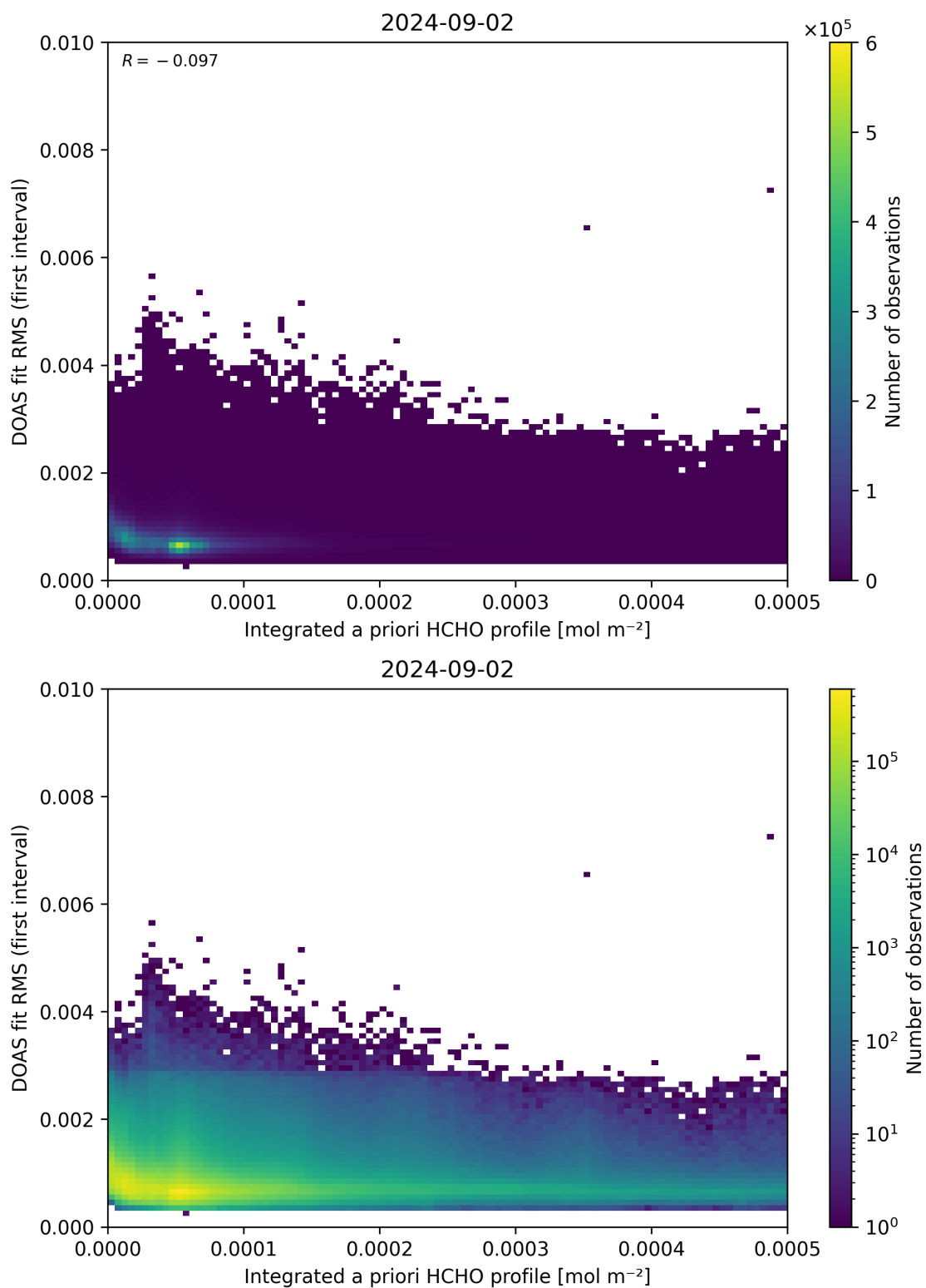
Figure 148: Scatter density plot of “Integrated a priori HCHO profile” against “DOAS fit RMS (first interval)” for 2024-09-01 to 2024-09-03.
