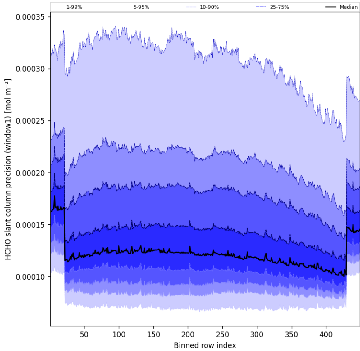
Figure 53: Along track statistics of “HCHO slant column precision (window1)” for 2024-09-01 to 2024-09-03
