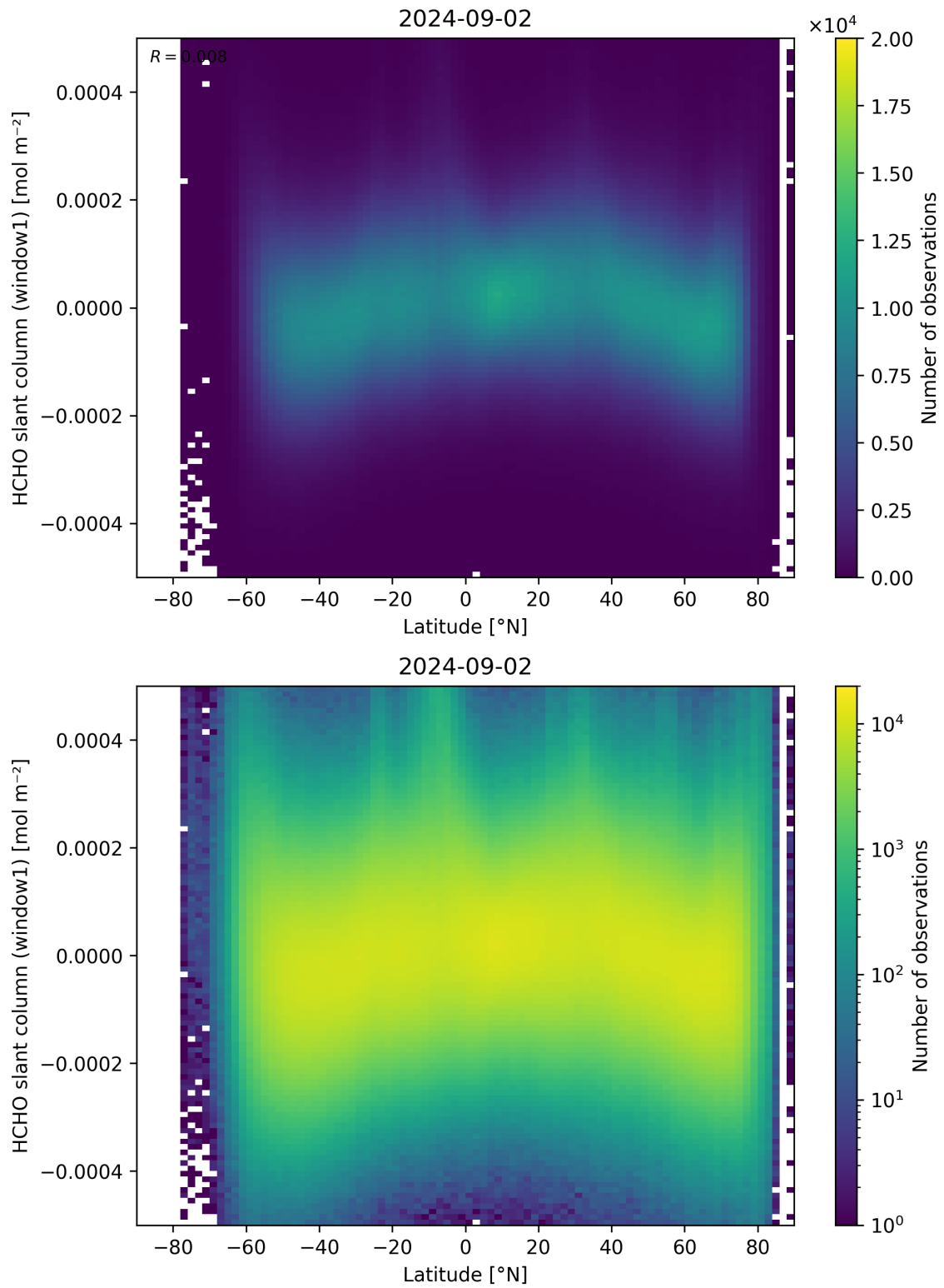
Figure 159: Scatter density plot of “Latitude” against “HCHO slant column (window1)” for 2024-09-01 to 2024-09-03.
