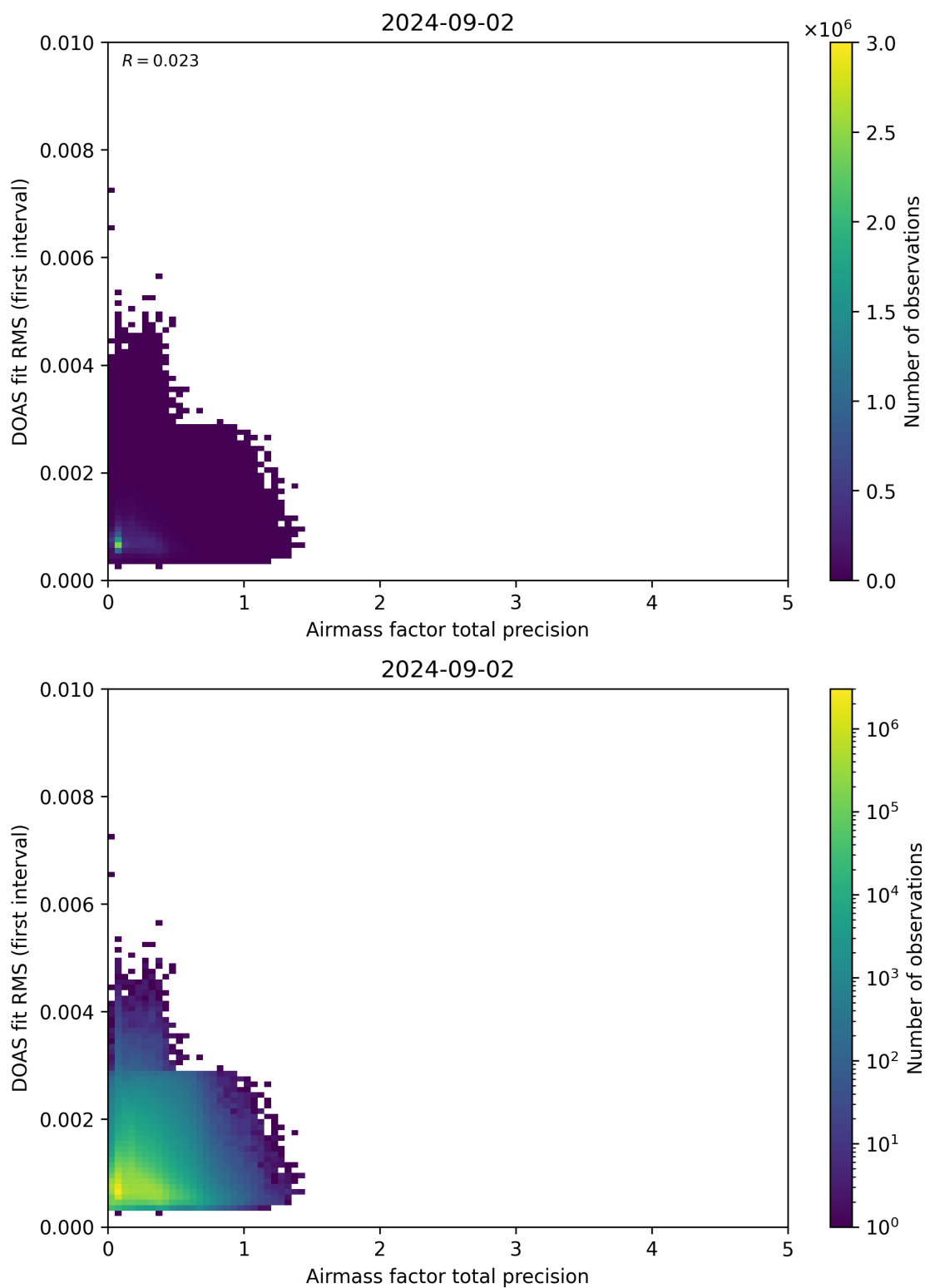
Figure 105: Scatter density plot of “Airmass factor total precision” against “DOAS fit RMS (first interval)” for 2024-09-01 to 2024-09-03.
