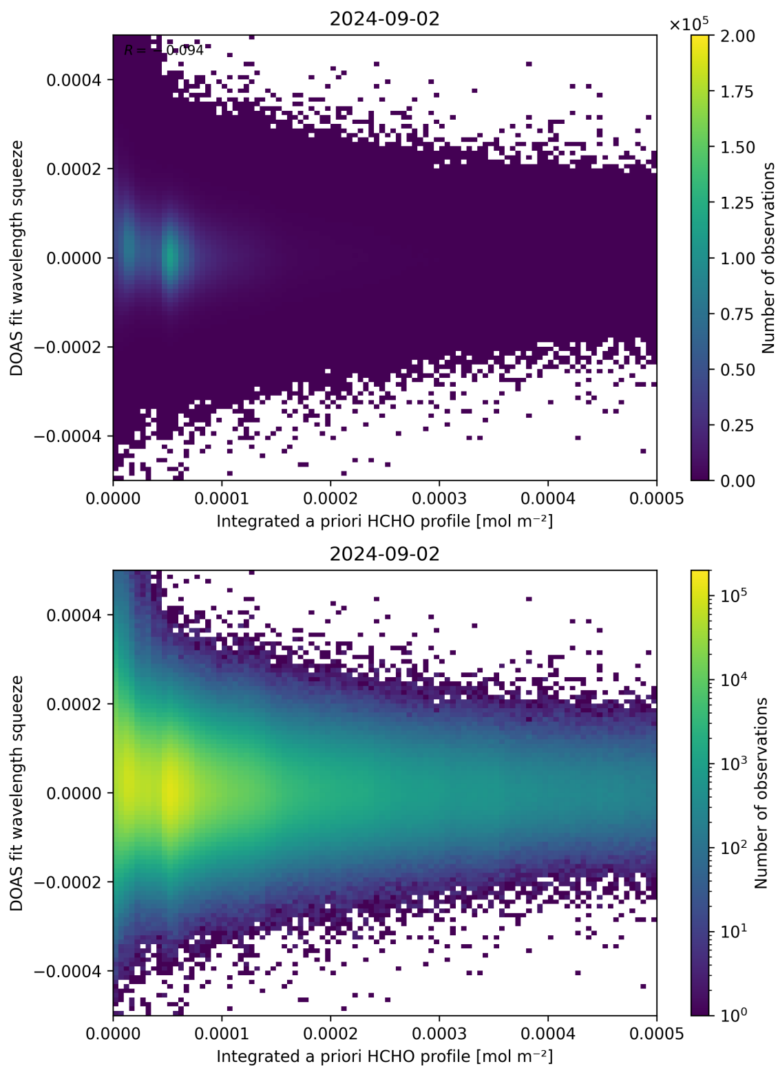
Figure 150: Scatter density plot of “Integrated a priori HCHO profile” against “DOAS fit wavelength squeeze” for 2024-09-01 to 2024-09-03.
