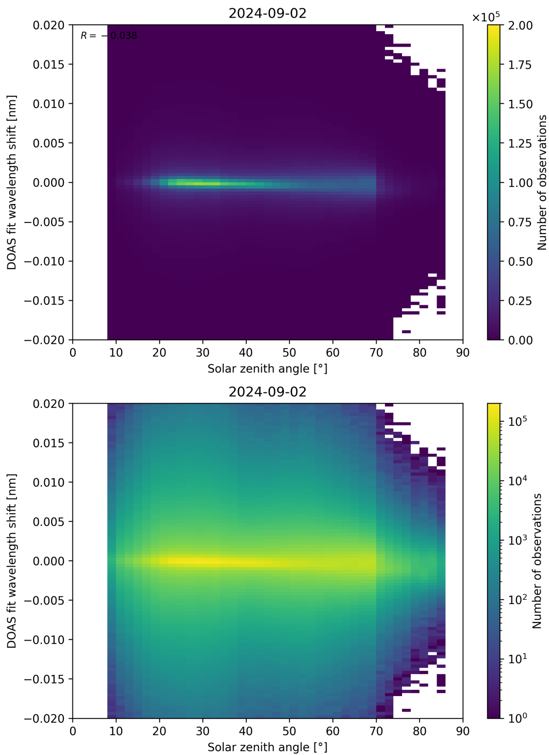
Figure 168: Scatter density plot of “Solar zenith angle” against “DOAS fit wavelength shift” for 2024-09-01 to 2024-09-03.
