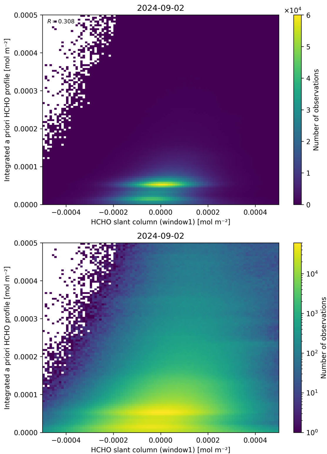
Figure 87: Scatter density plot of “HCHO slant column (window1)” against “Integrated a priori HCHO profile” for 2024-09-01 to 2024-09-03.
