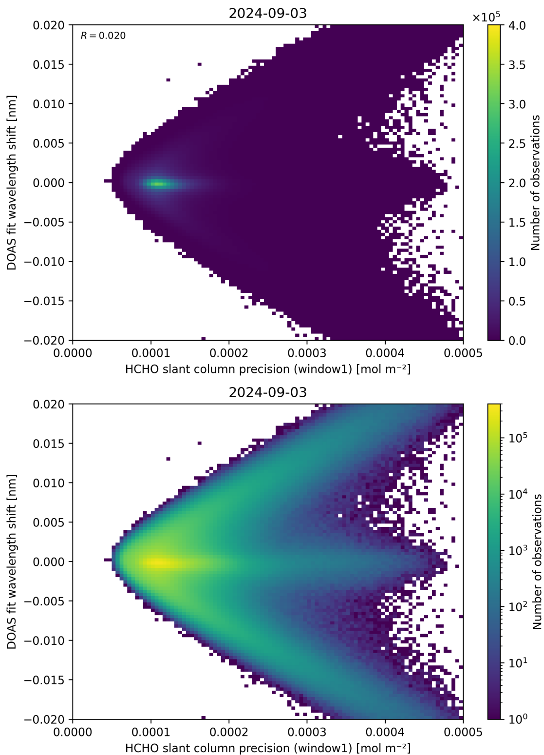
Figure 89: Scatter density plot of “HCHO slant column precision (window1)” against “DOAS fit wavelength shift” for 2024-09-02 to 2024-09-04.
