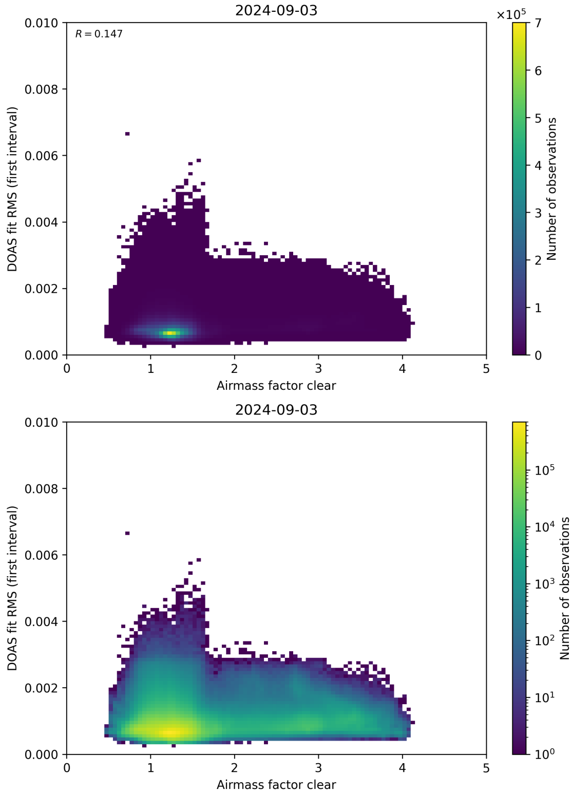
Figure 71: Scatter density plot of “Airmass factor clear” against “DOAS fit RMS (first interval)” for 2024-09-02 to 2024-09-04.
