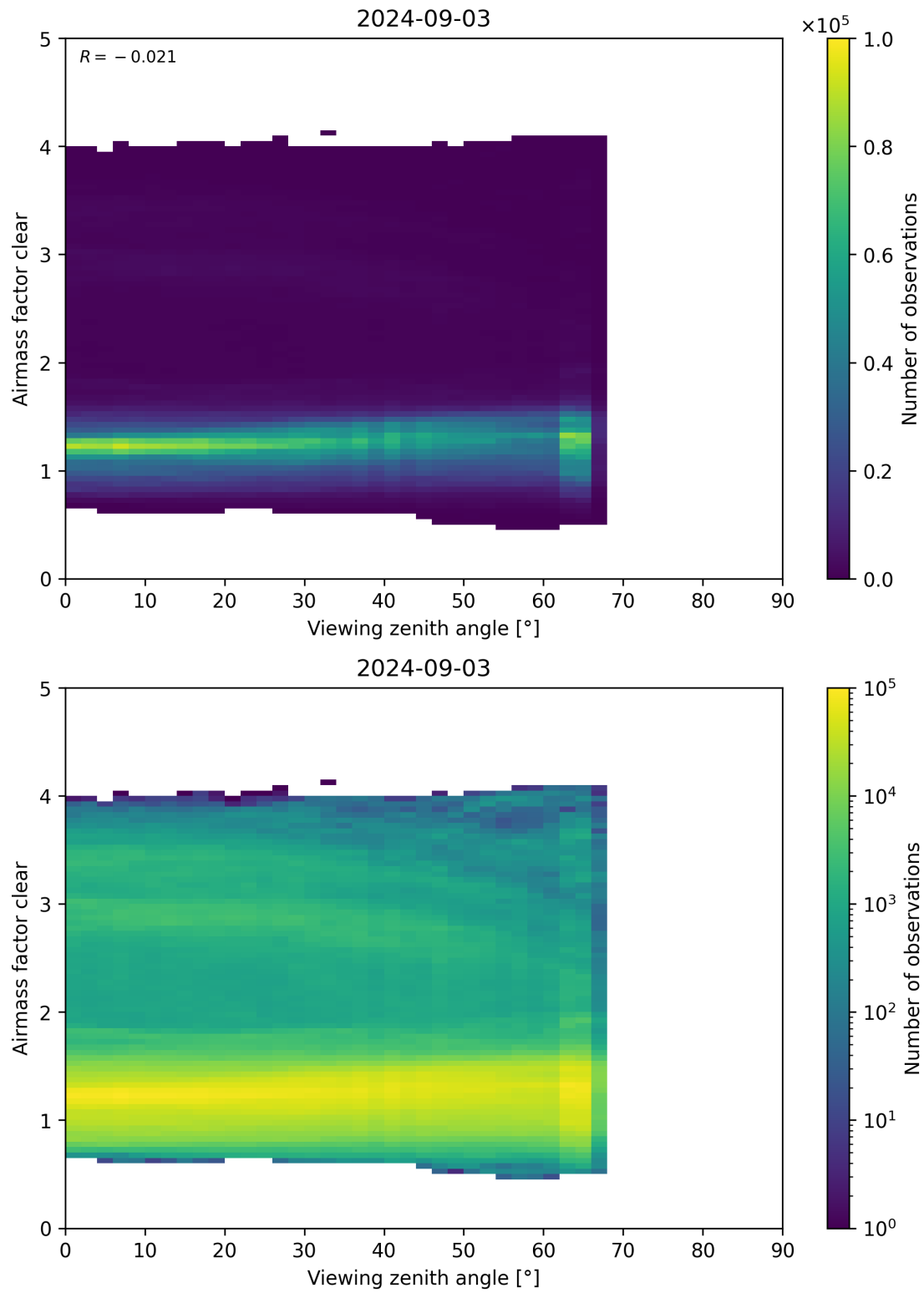
Figure 185: Scatter density plot of “Viewing zenith angle” against “Airmass factor clear” for 2024-09-02 to 2024-09-04.
