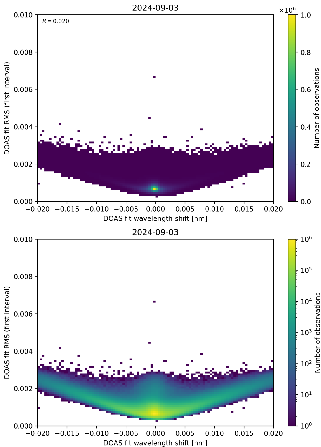
Figure 64: Scatter density plot of “DOAS fit wavelength shift” against “DOAS fit RMS (first interval)” for 2024-09-02 to 2024-09-04.
