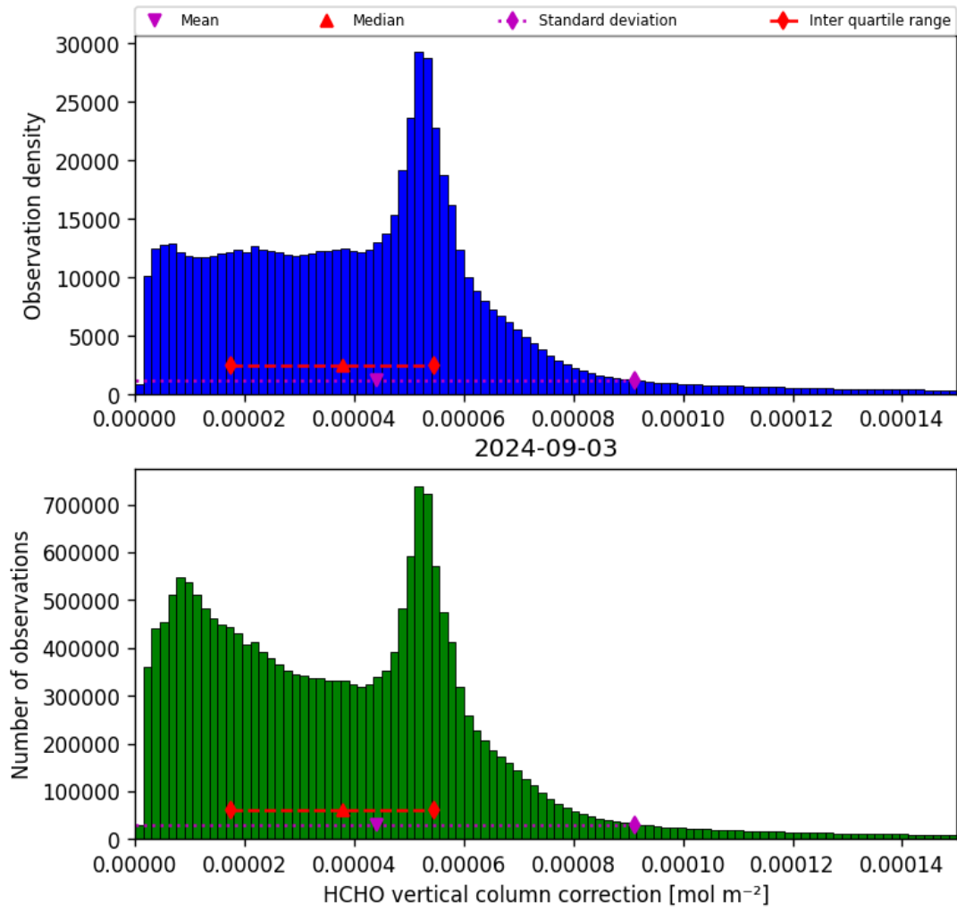
Figure 37: Histogram of “HCHO vertical column correction” for 2024-09-02 to 2024-09-04
