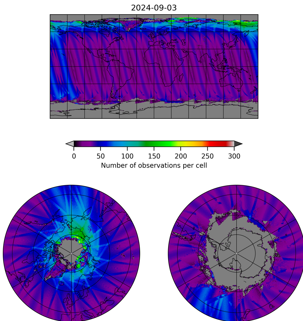
Figure 19: Map of the number of observations for 2024-09-02 to 2024-09-04
