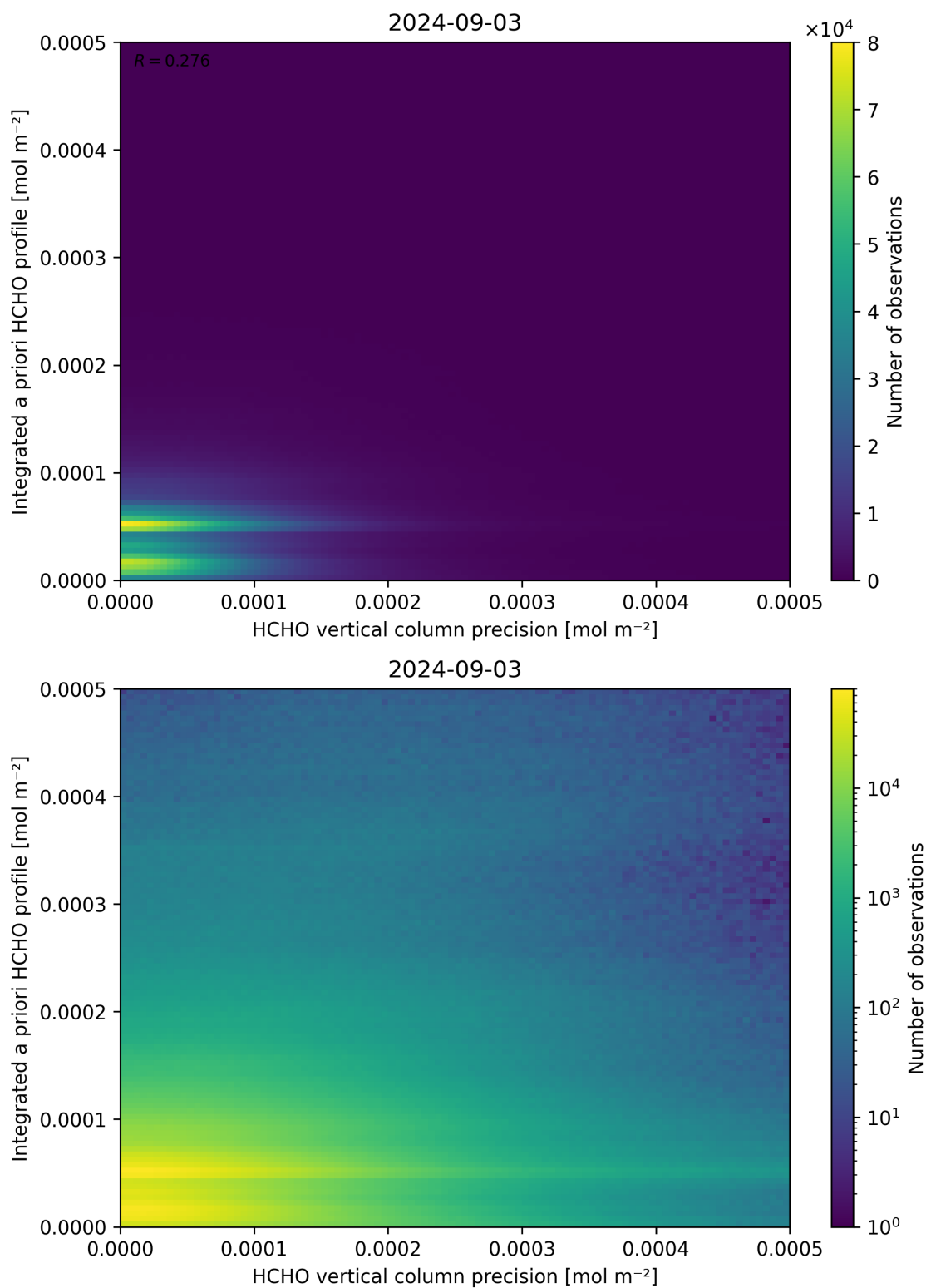
Figure 147: Scatter density plot of “HCHO vertical column precision” against “Integrated a priori HCHO profile” for 2024-09-02 to 2024-09-04.
