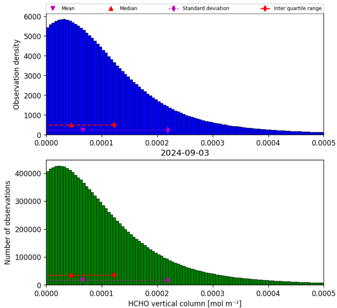
Figure 35: Histogram of “HCHO vertical column” for 2024-09-02 to 2024-09-04
