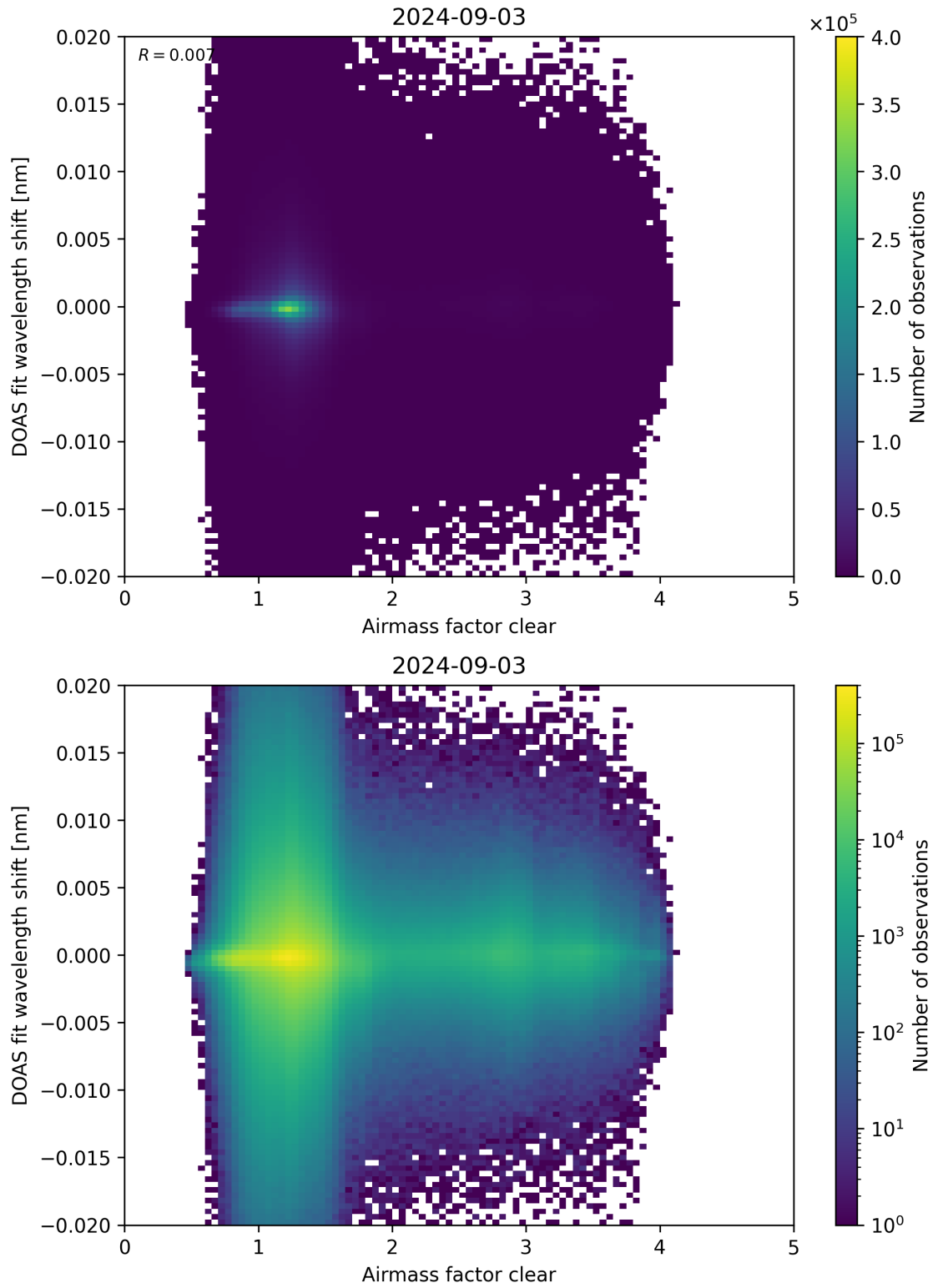
Figure 72: Scatter density plot of “Airmass factor clear” against “DOAS fit wavelength shift” for 2024-09-02 to 2024-09-04.
