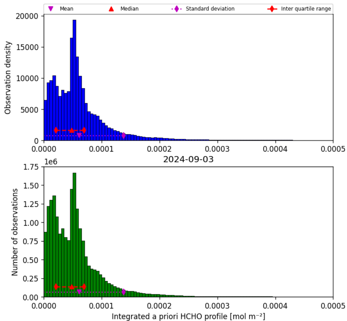
Figure 43: Histogram of “Integrated a priori HCHO profile” for 2024-09-02 to 2024-09-04
