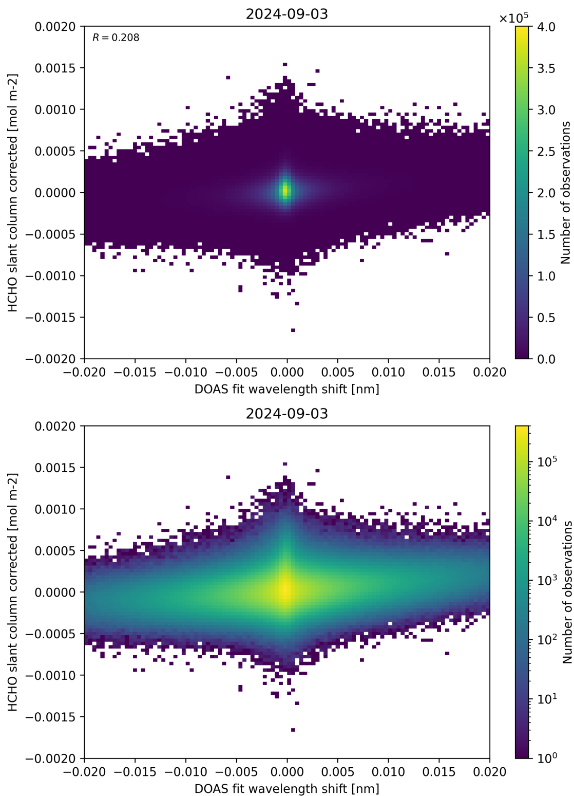
Figure 66: Scatter density plot of “DOAS fit wavelength shift” against “HCHO slant column corrected” for 2024-09-02 to 2024-09-04.
