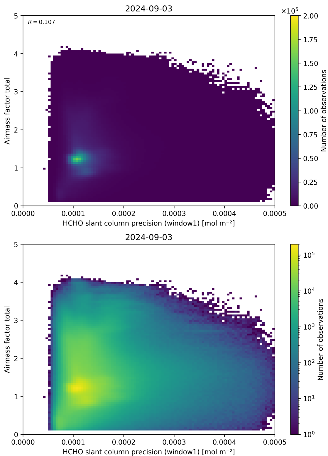
Figure 94: Scatter density plot of “HCHO slant column precision (window1)” against “Airmass factor total” for 2024-09-02 to 2024-09-04.
