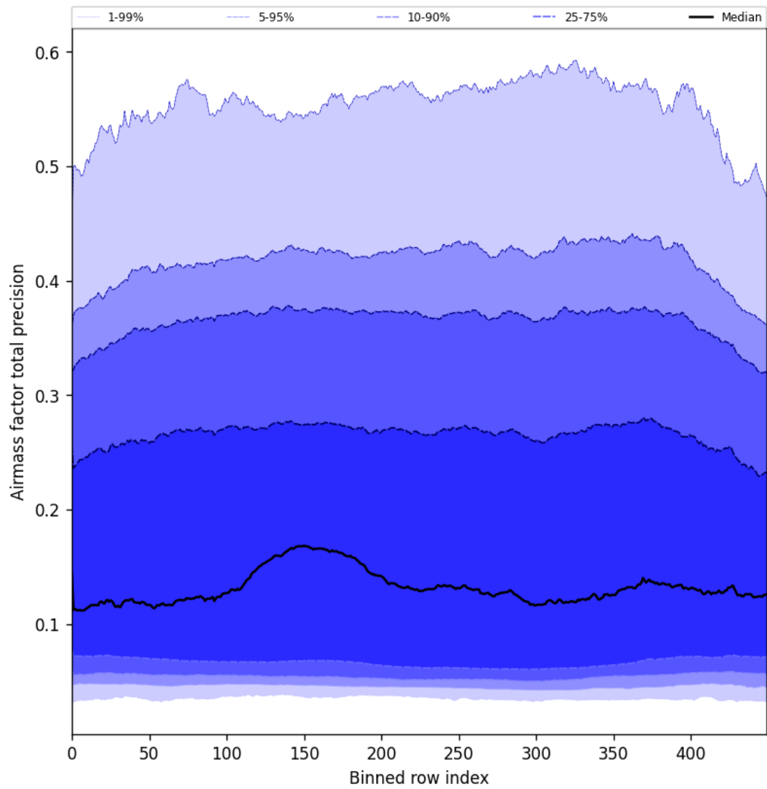
Figure 55: Along track statistics of “Airmass factor total precision” for 2024-09-02 to 2024-09-04
