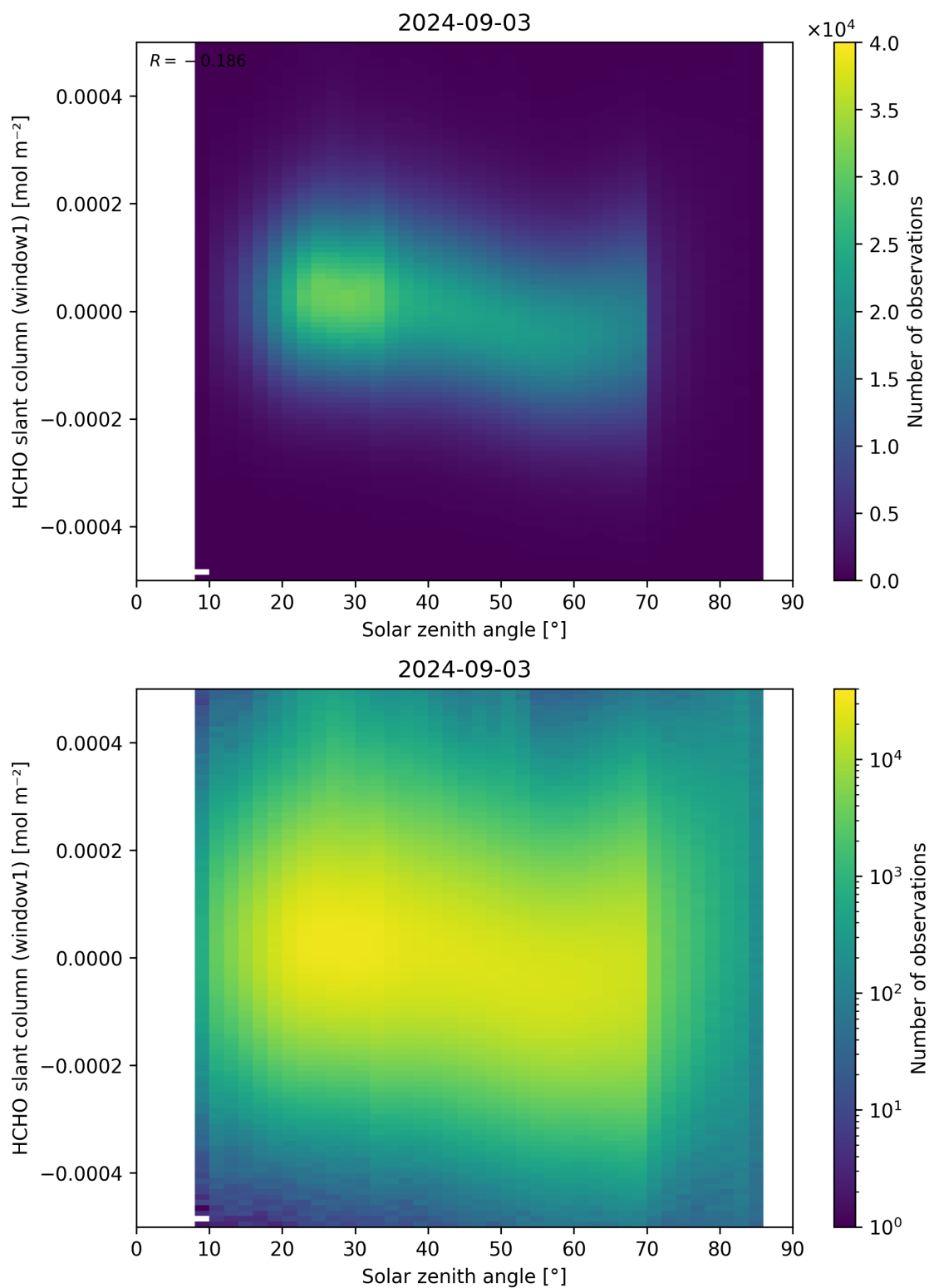
Figure 173: Scatter density plot of “Solar zenith angle” against “HCHO slant column (window1)” for 2024-09-02 to 2024-09-04.
