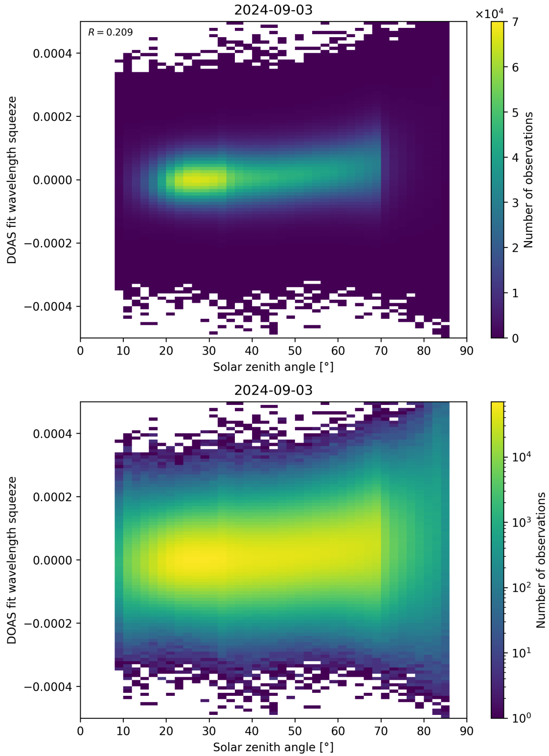
Figure 169: Scatter density plot of “Solar zenith angle” against “DOAS fit wavelength squeeze” for 2024-09-02 to 2024-09-04.
