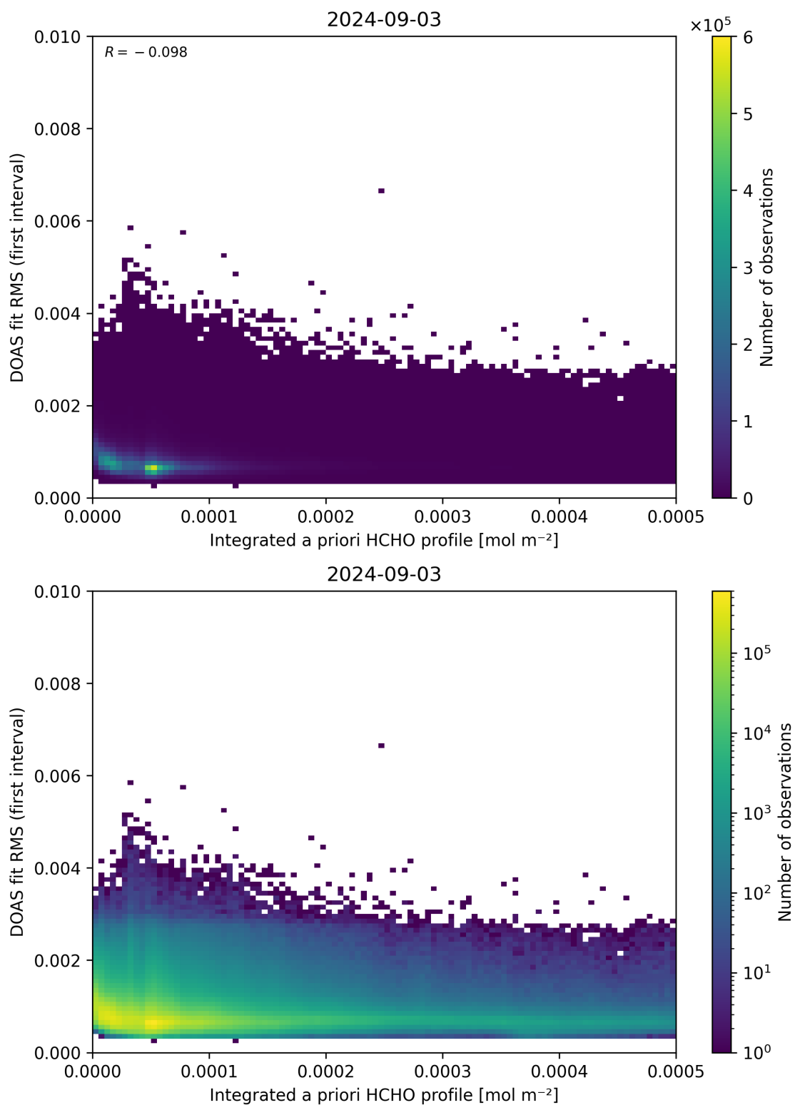
Figure 148: Scatter density plot of “Integrated a priori HCHO profile” against “DOAS fit RMS (first interval)” for 2024-09-02 to 2024-09-04.
