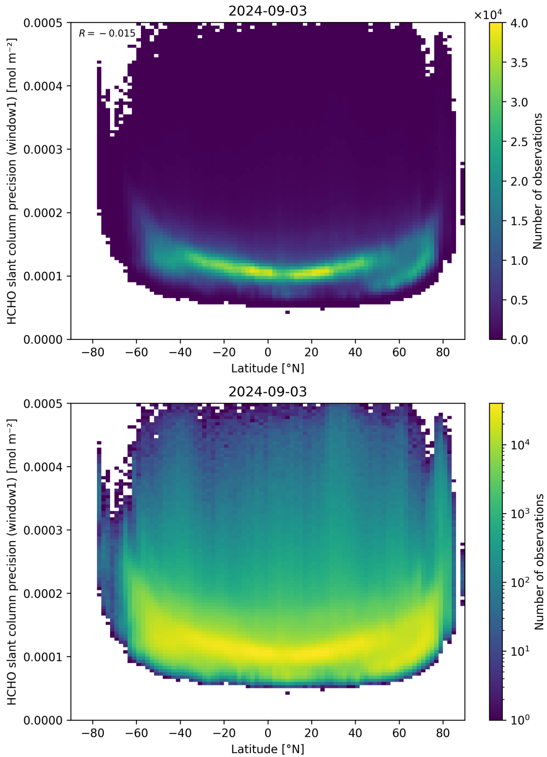
Figure 160: Scatter density plot of “Latitude” against “HCHO slant column precision (window1)” for 2024-09-02 to 2024-09-04.
