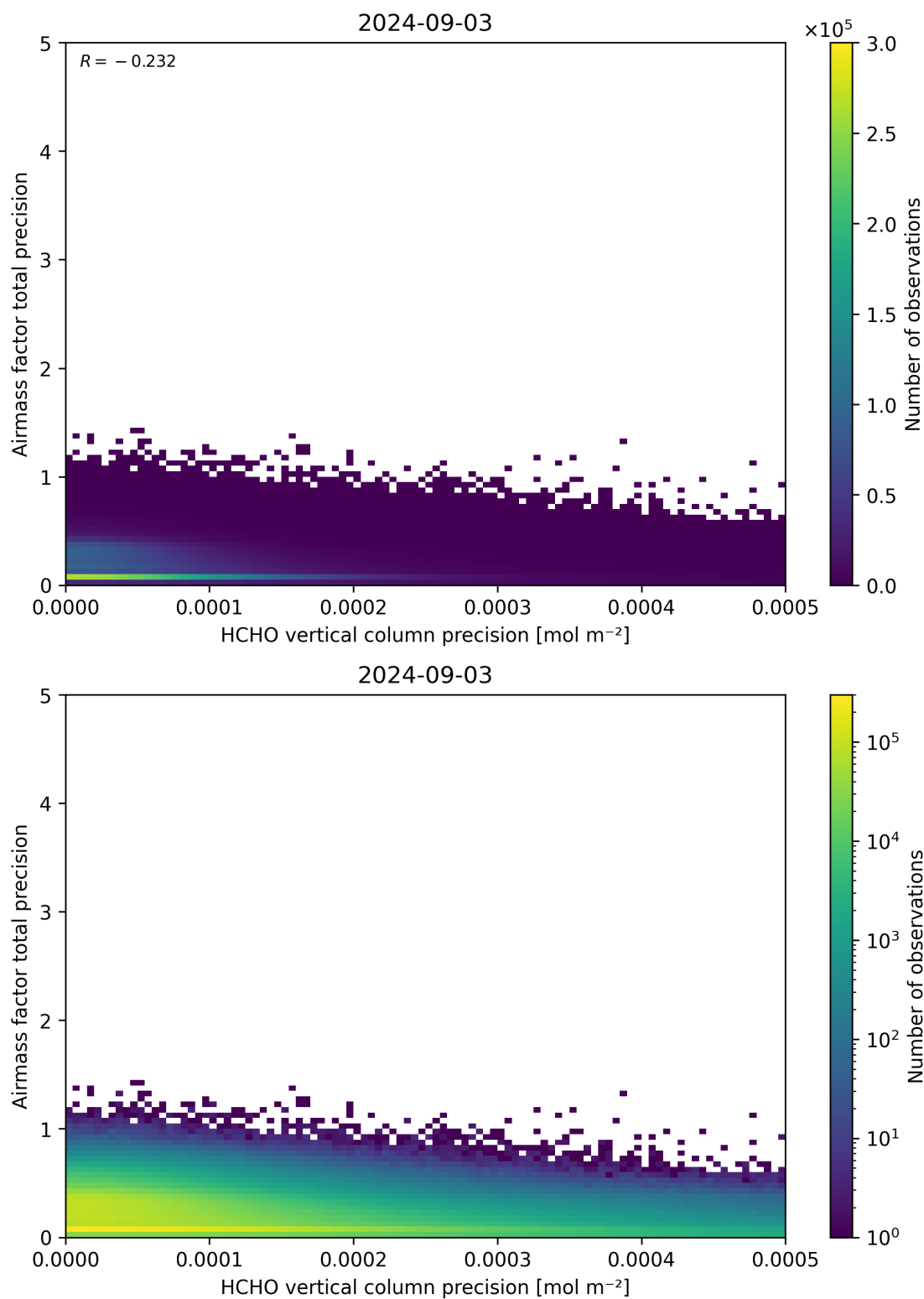
Figure 145: Scatter density plot of “HCHO vertical column precision” against “Airmass factor total precision” for 2024-09-02 to 2024-09-04.
