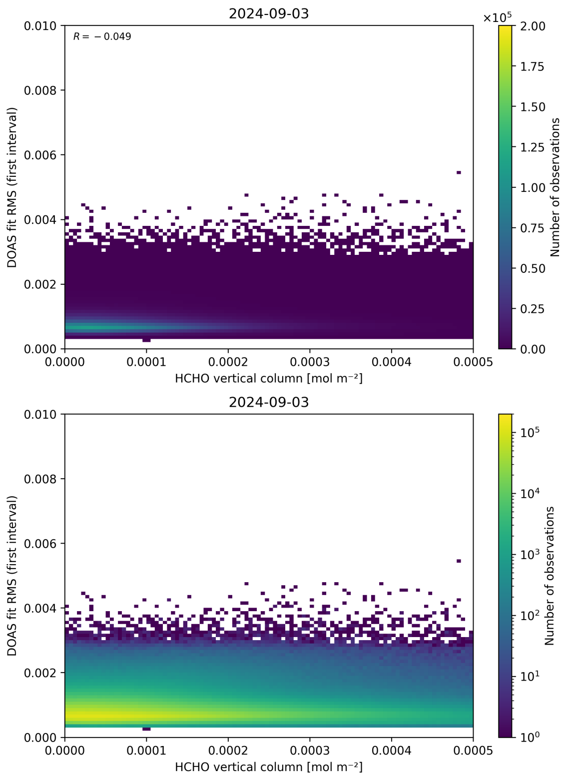
Figure 123: Scatter density plot of “HCHO vertical column” against “DOAS fit RMS (first interval)” for 2024-09-02 to 2024-09-04.
