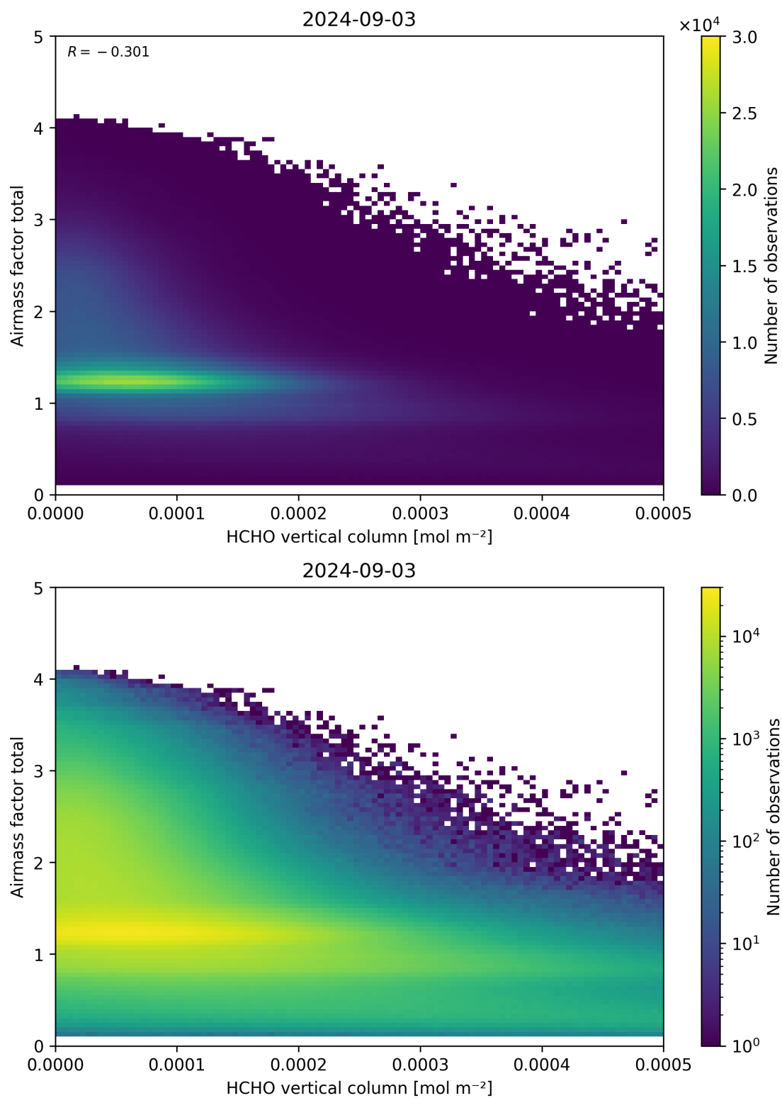
Figure 131: Scatter density plot of “HCHO vertical column” against “Airmass factor total” for 2024-09-02 to 2024-09-04.
