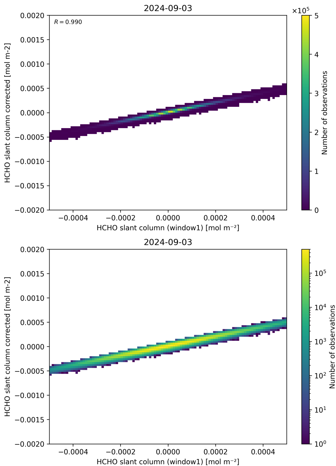
Figure 82: Scatter density plot of “HCHO slant column (window1)” against “HCHO slant column corrected” for 2024-09-02 to 2024-09-04.
