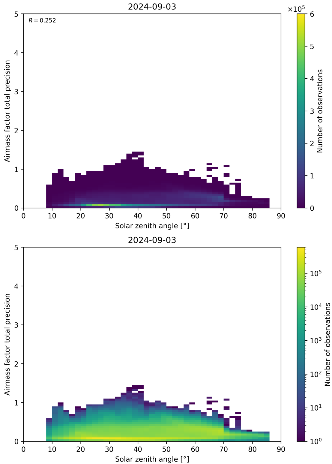
Figure 176: Scatter density plot of “Solar zenith angle” against “Airmass factor total precision” for 2024-09-02 to 2024-09-04.
