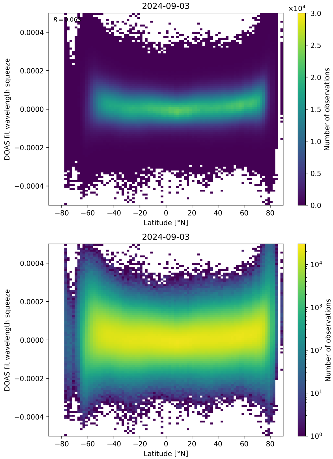
Figure 155: Scatter density plot of “Latitude” against “DOAS fit wavelength squeeze” for 2024-09-02 to 2024-09-04.
