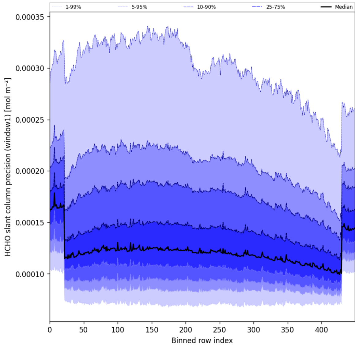
Figure 53: Along track statistics of “HCHO slant column precision (window1)” for 2024-09-02 to 2024-09-04
