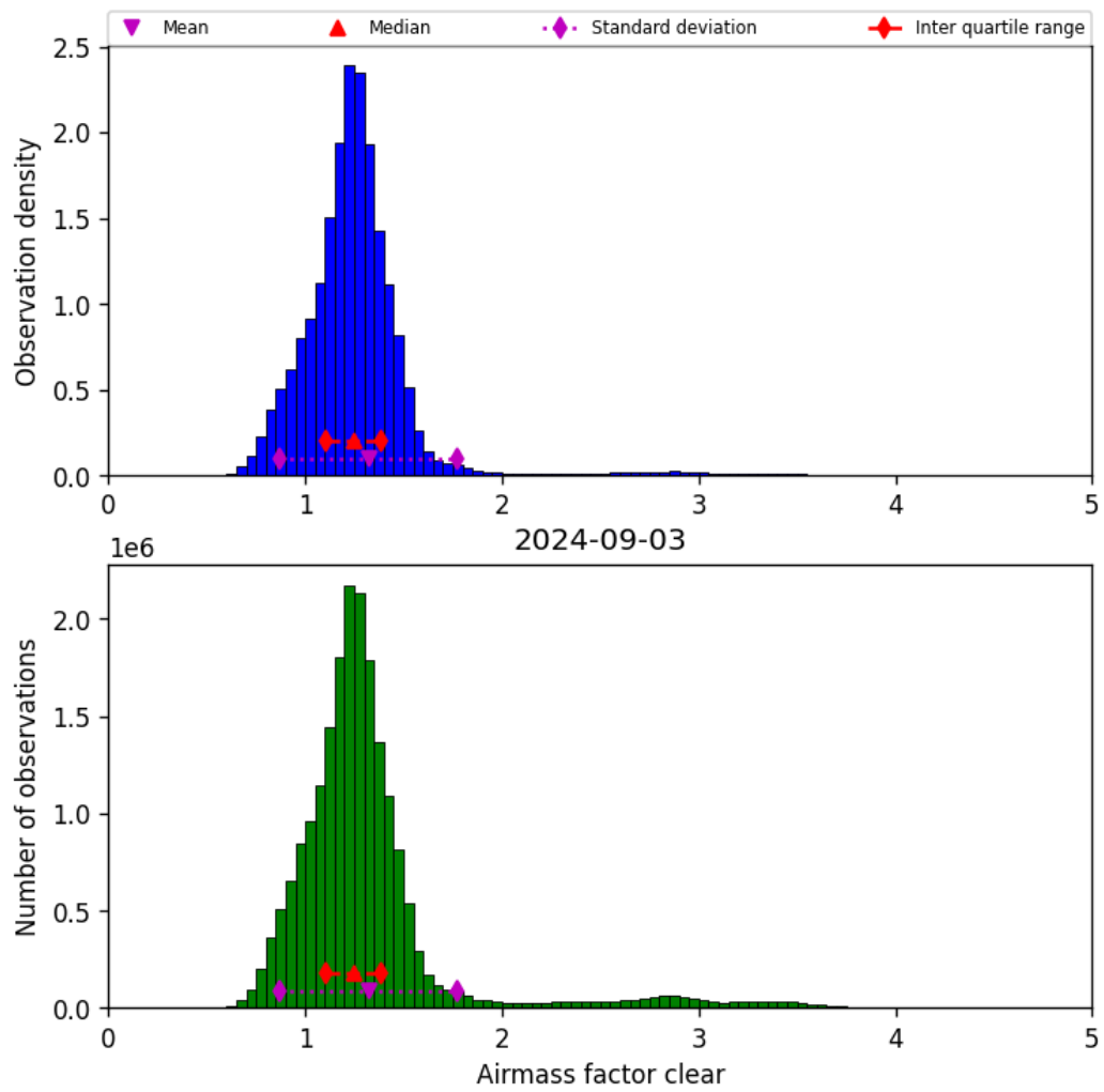
Figure 42: Histogram of “Airmass factor clear” for 2024-09-02 to 2024-09-04
