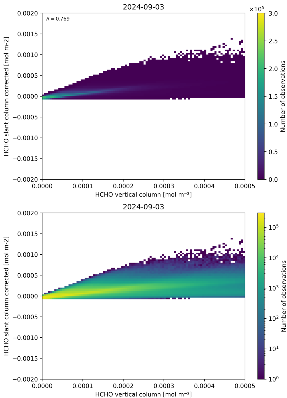
Figure 127: Scatter density plot of “HCHO vertical column” against “HCHO slant column corrected” for 2024-09-02 to 2024-09-04.
