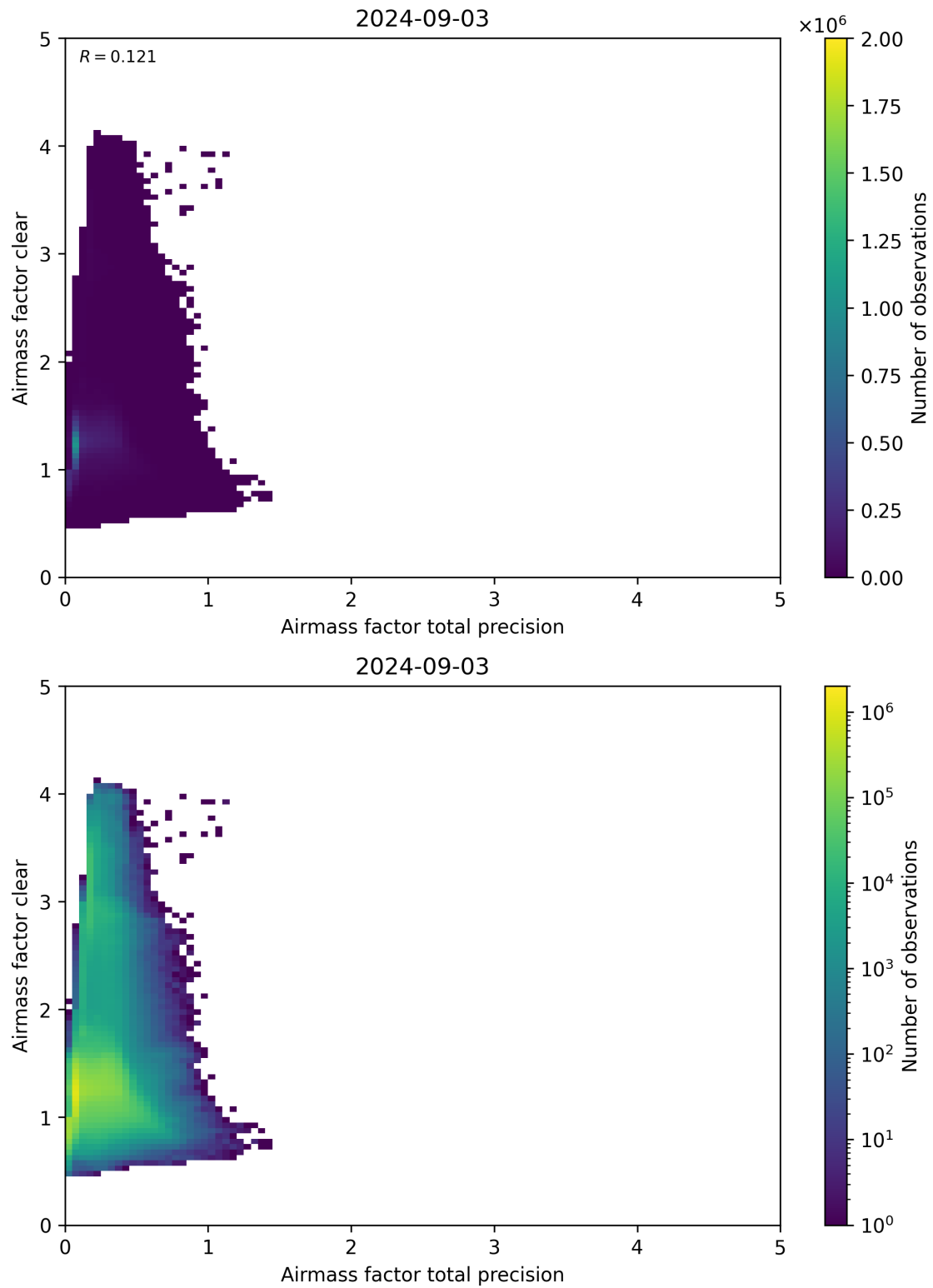
Figure 108: Scatter density plot of “Airmass factor total precision” against “Airmass factor clear” for 2024-09-02 to 2024-09-04.
