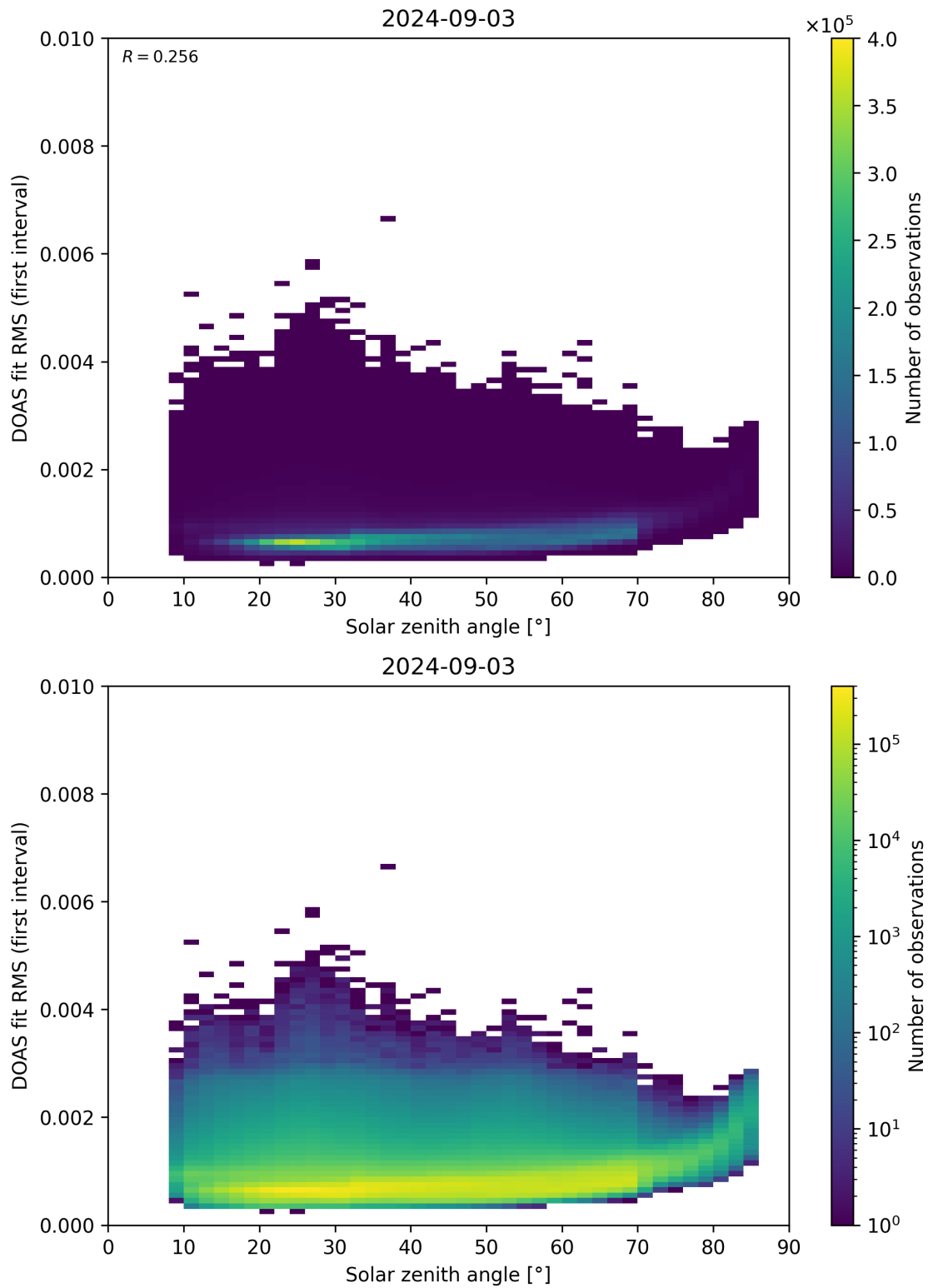
Figure 167: Scatter density plot of “Solar zenith angle” against “DOAS fit RMS (first interval)” for 2024-09-02 to 2024-09-04.
