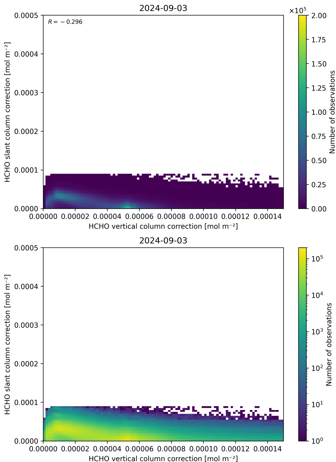
Figure 117: Scatter density plot of “HCHO vertical column correction” against “HCHO slant column correction” for 2024-09-02 to 2024-09-04.
