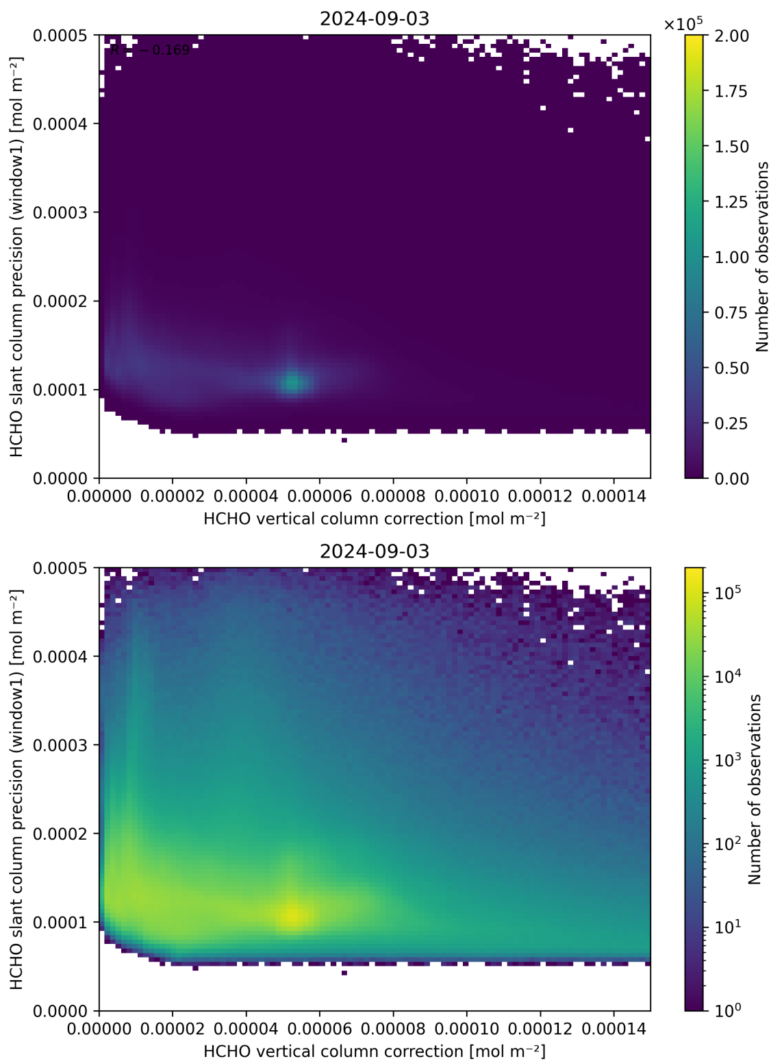
Figure 119: Scatter density plot of “HCHO vertical column correction” against “HCHO slant column precision (window1)” for 2024-09-02 to 2024-09-04.
