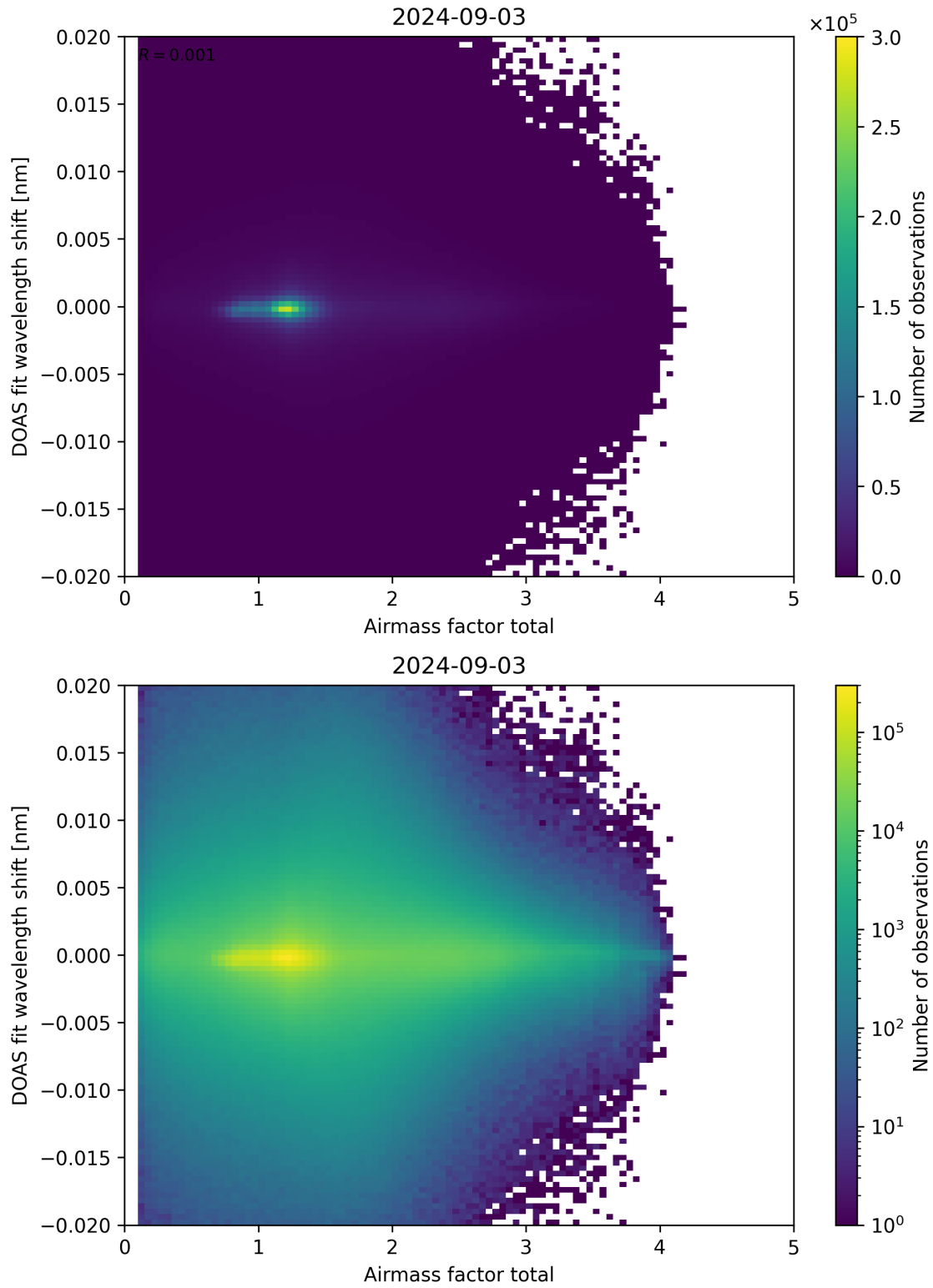
Figure 98: Scatter density plot of “Airmass factor total” against “DOAS fit wavelength shift” for 2024-09-02 to 2024-09-04.
