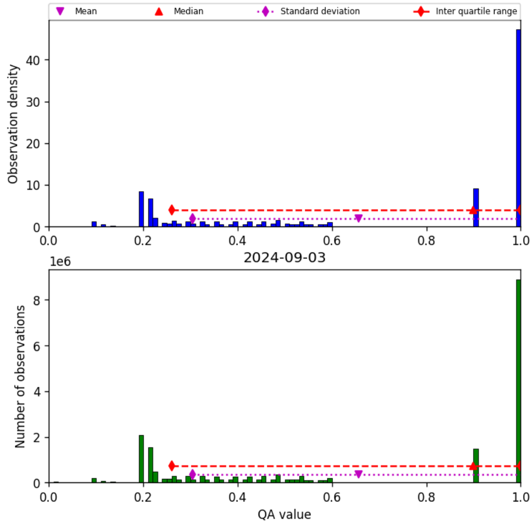
Figure 34: Histogram of “QA value” for 2024-09-02 to 2024-09-04
