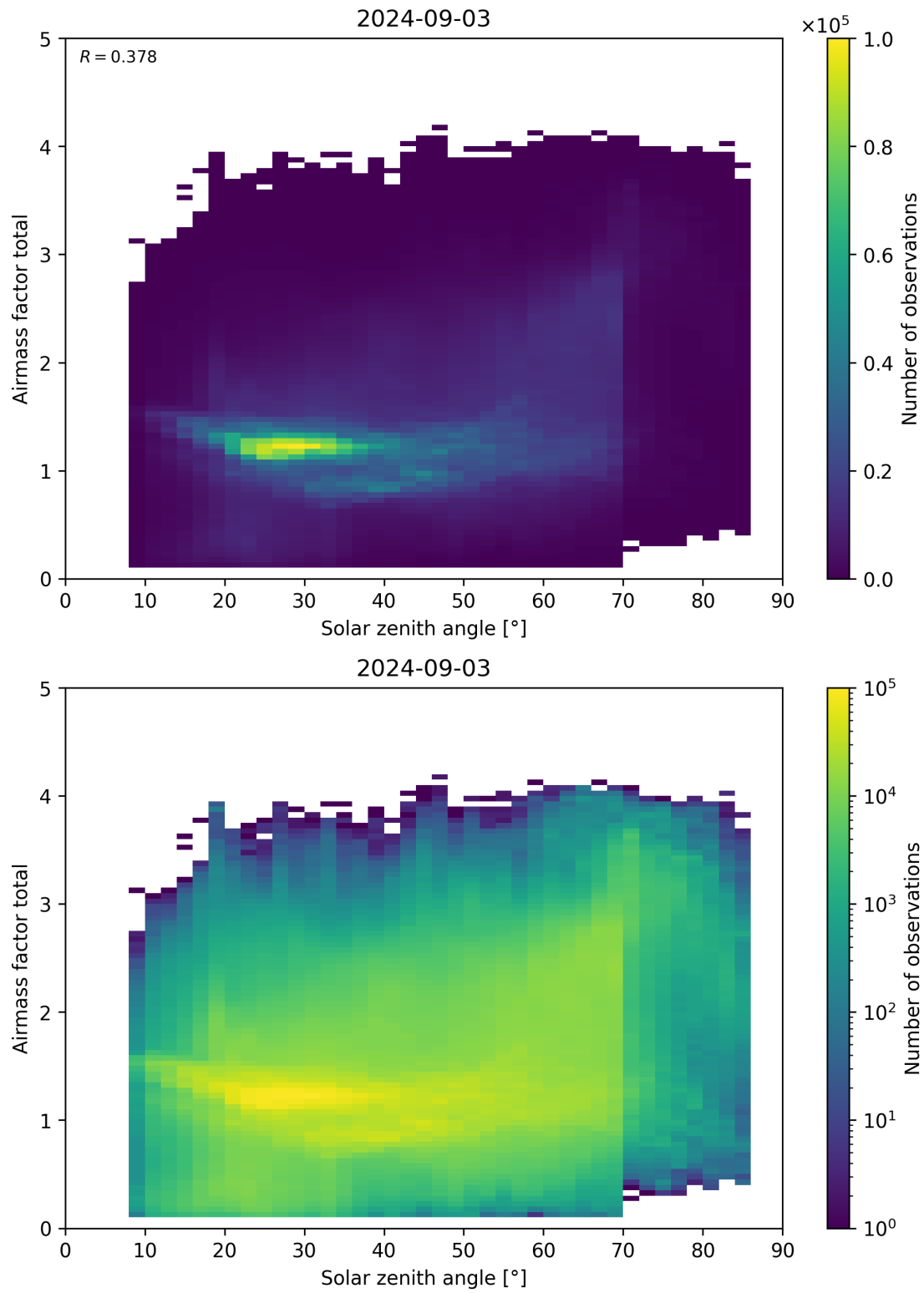
Figure 175: Scatter density plot of “Solar zenith angle” against “Airmass factor total” for 2024-09-02 to 2024-09-04.
