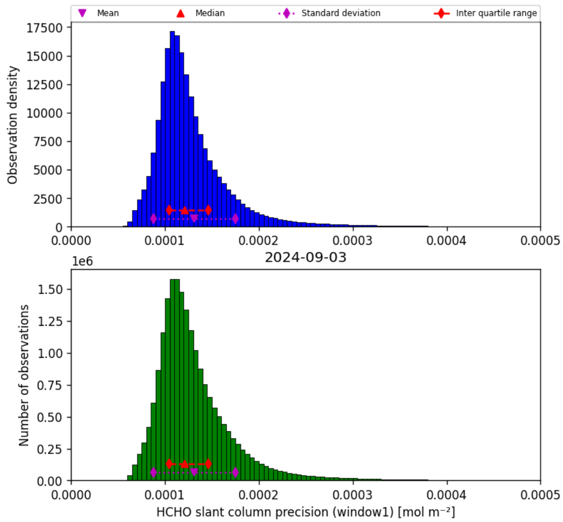
Figure 39: Histogram of “HCHO slant column precision (window1)” for 2024-09-02 to 2024-09-04
