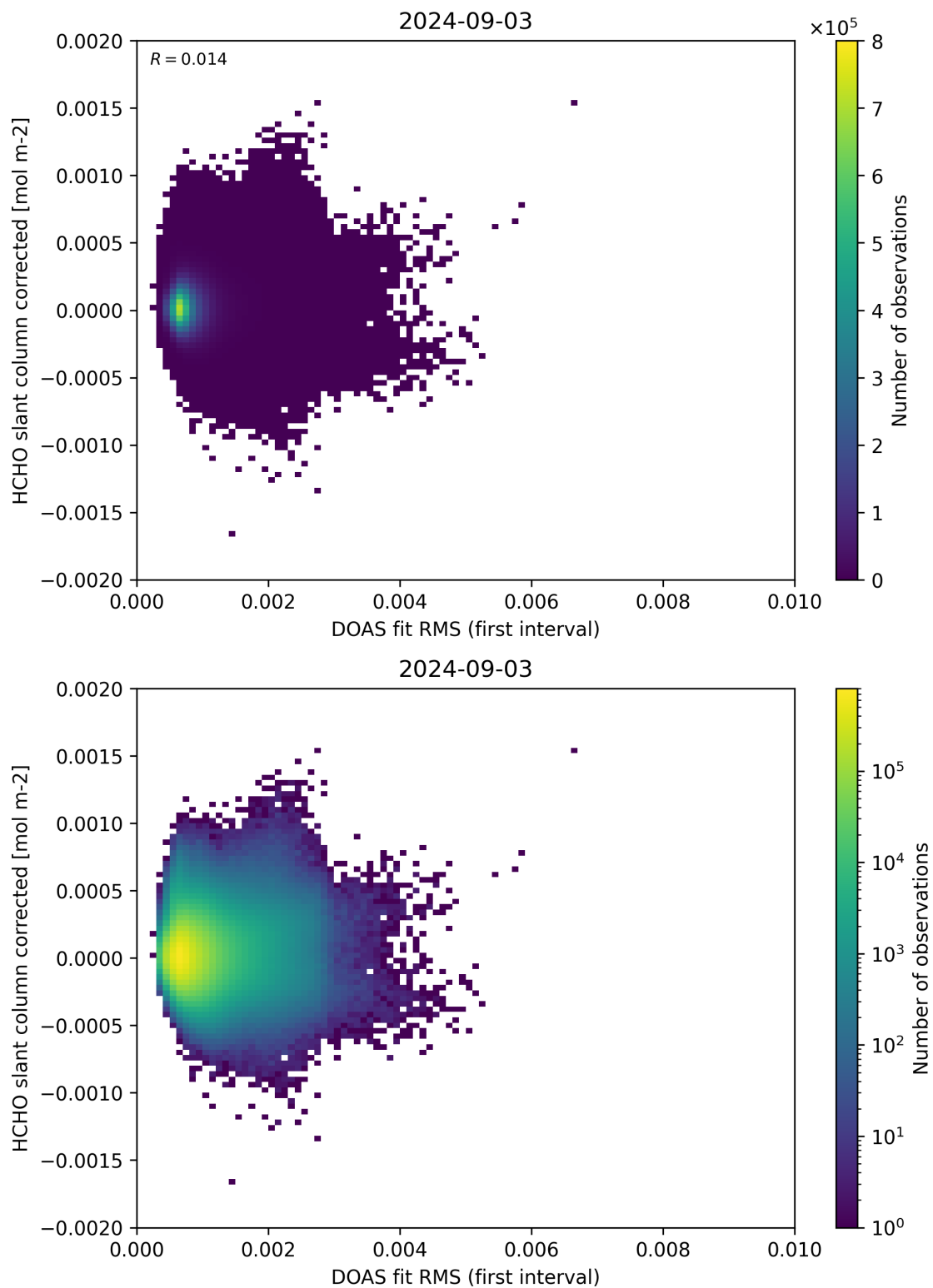
Figure 62: Scatter density plot of “DOAS fit RMS (first interval)” against “HCHO slant column corrected” for 2024-09-02 to 2024-09-04.
