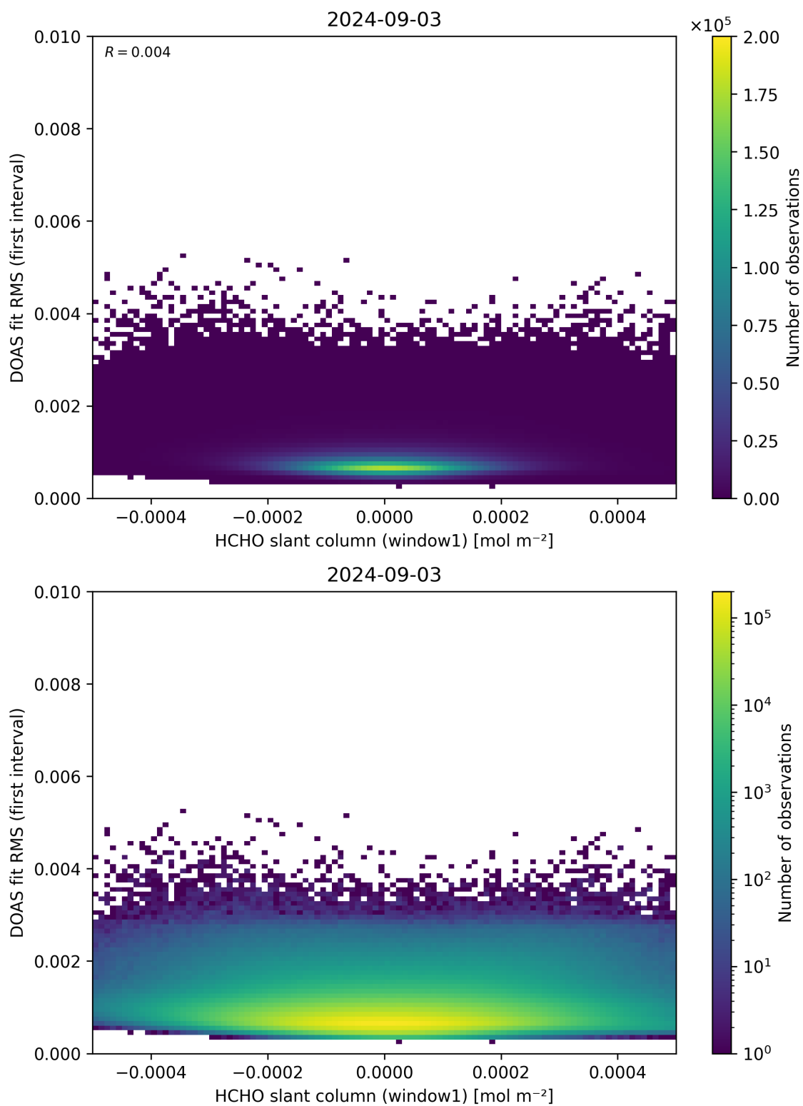
Figure 78: Scatter density plot of “HCHO slant column (window1)” against “DOAS fit RMS (first interval)” for 2024-09-02 to 2024-09-04.
