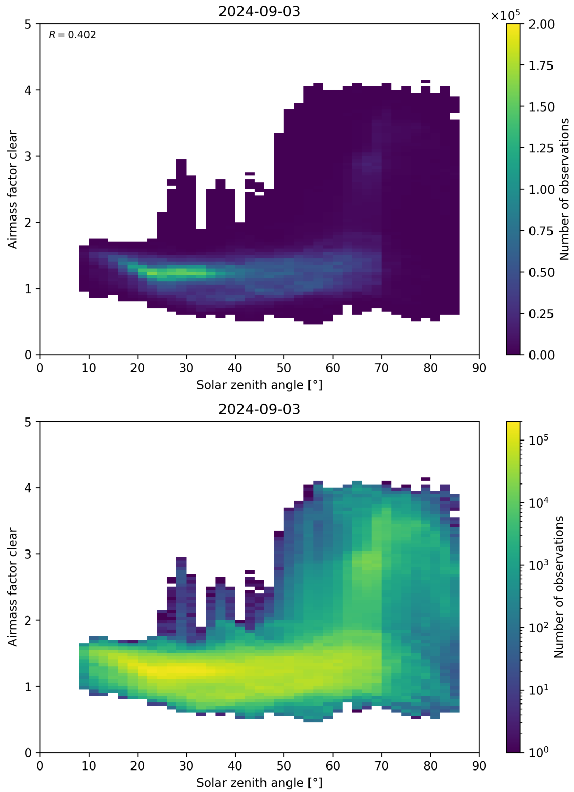
Figure 170: Scatter density plot of “Solar zenith angle” against “Airmass factor clear” for 2024-09-02 to 2024-09-04.
