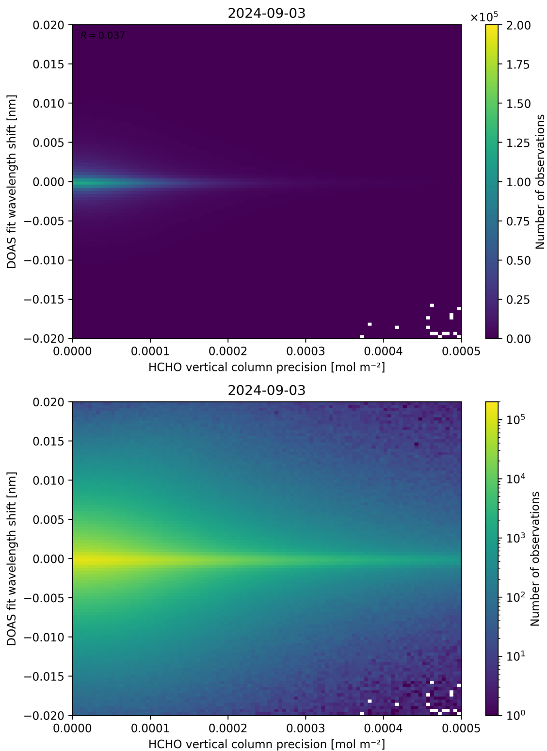
Figure 137: Scatter density plot of “HCHO vertical column precision” against “DOAS fit wavelength shift” for 2024-09-02 to 2024-09-04.
