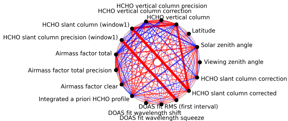
Figure 1: Map of correlation graph for 2024-09-02 to 2024-09-04.
