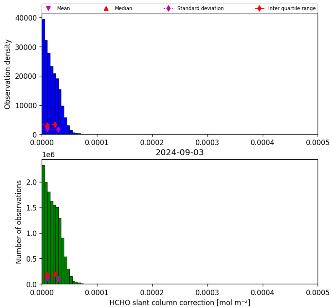
Figure 47: Histogram of “HCHO slant column correction” for 2024-09-02 to 2024-09-04
