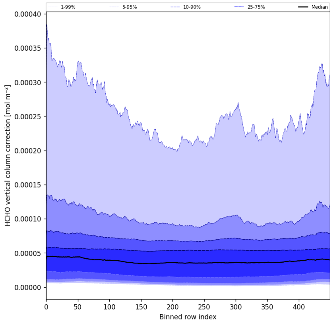
Figure 51: Along track statistics of “HCHO vertical column correction” for 2024-09-02 to 2024-09-04
