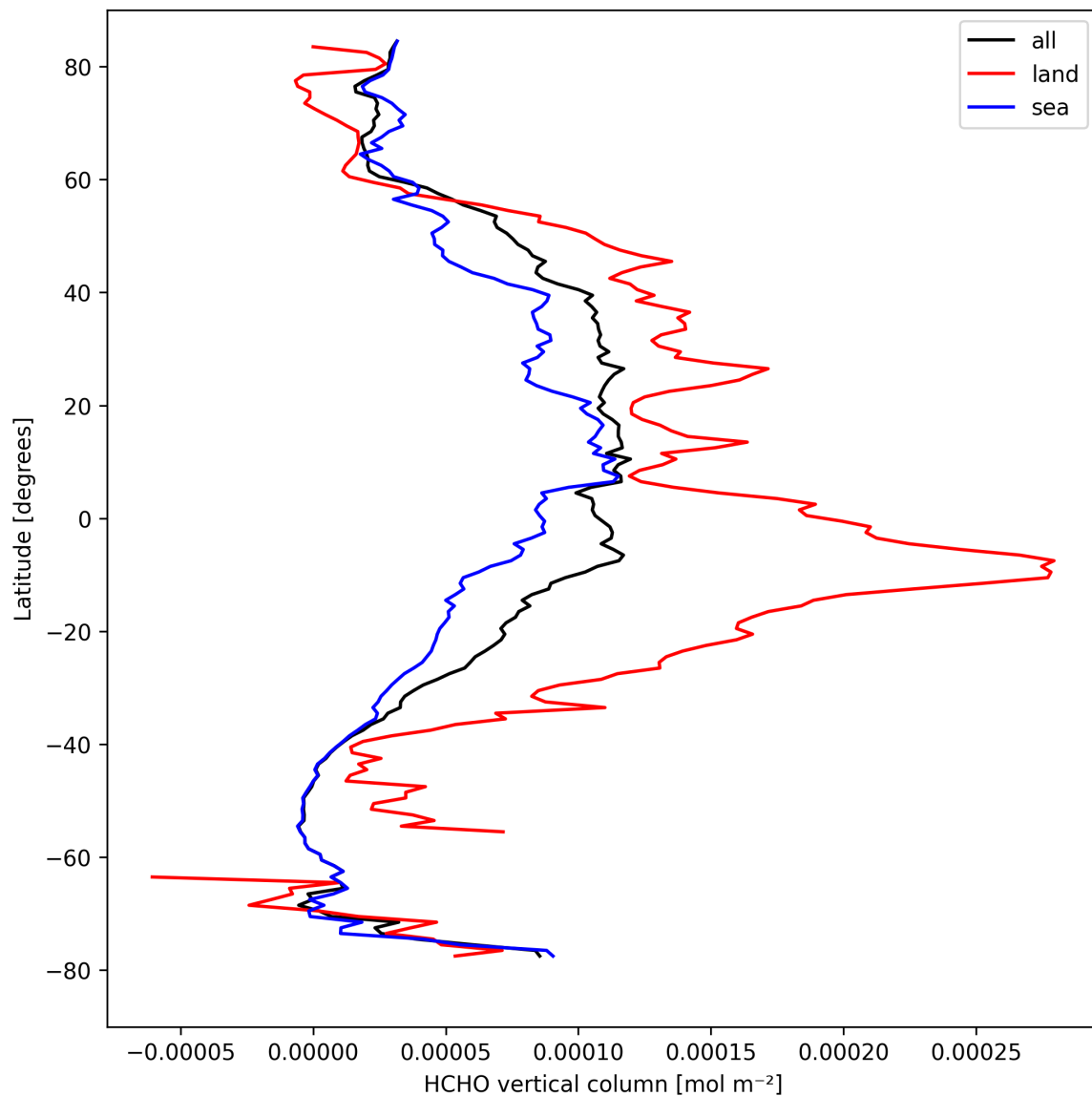
Figure 21: Zonal average of “HCHO vertical column” for 2024-09-02 to 2024-09-04.
