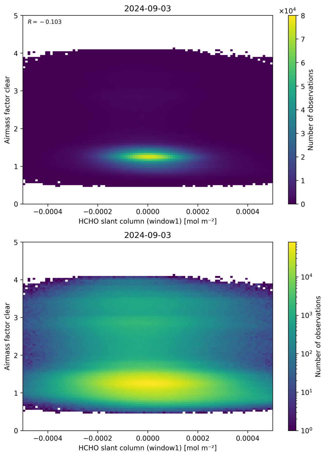
Figure 81: Scatter density plot of “HCHO slant column (window1)” against “Airmass factor clear” for 2024-09-02 to 2024-09-04.
