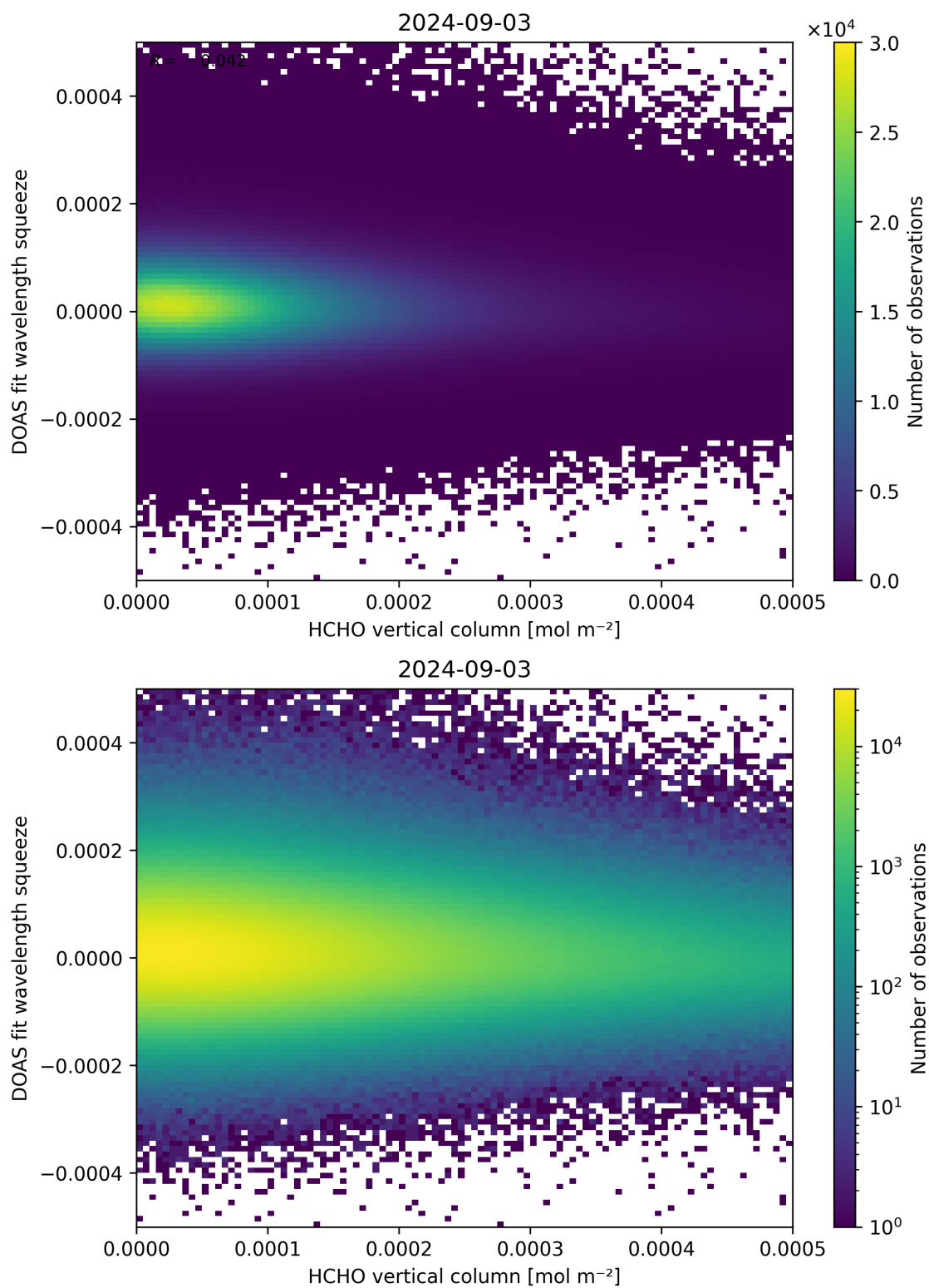
Figure 125: Scatter density plot of “HCHO vertical column” against “DOAS fit wavelength squeeze” for 2024-09-02 to 2024-09-04.
