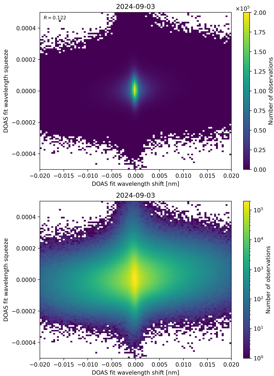
Figure 65: Scatter density plot of “DOAS fit wavelength shift” against “DOAS fit wavelength squeeze” for 2024-09-02 to 2024-09-04.
