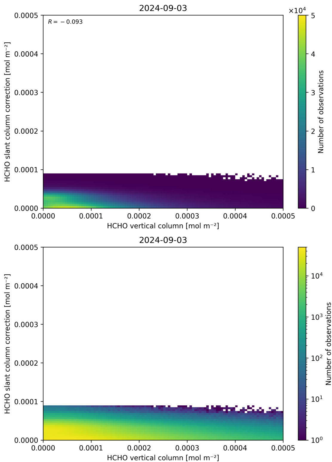
Figure 128: Scatter density plot of “HCHO vertical column” against “HCHO slant column correction” for 2024-09-02 to 2024-09-04.
