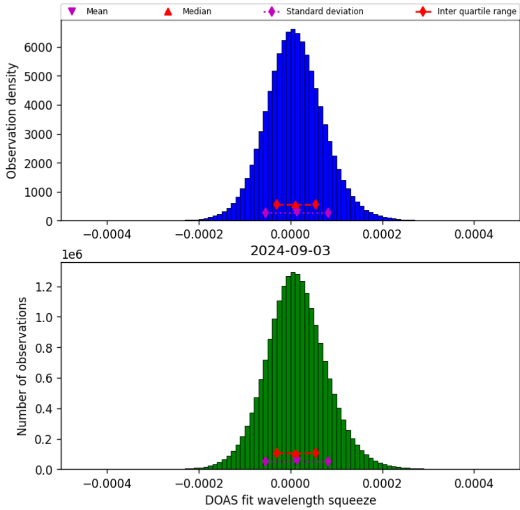
Figure 45: Histogram of “DOAS fit wavelength squeeze” for 2024-09-02 to 2024-09-04
