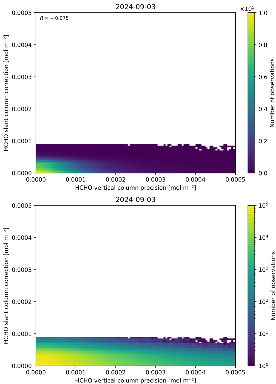
Figure 141: Scatter density plot of “HCHO vertical column precision” against “HCHO slant column correction” for 2024-09-02 to 2024-09-04.
