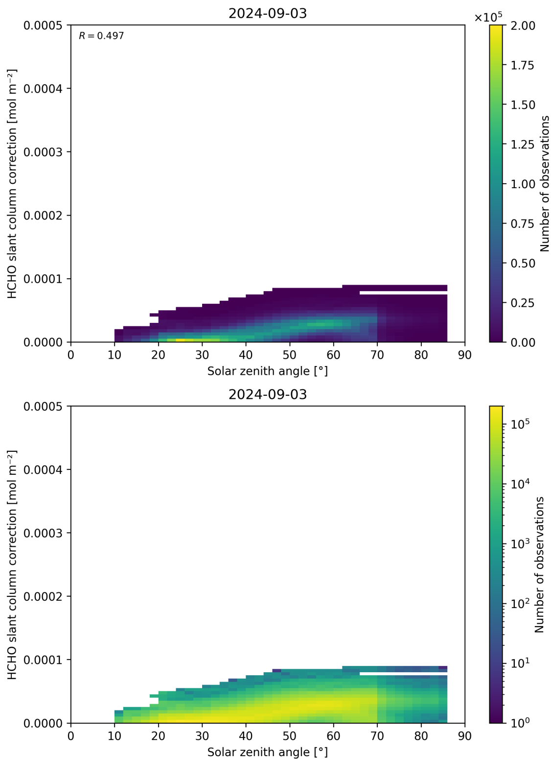
Figure 172: Scatter density plot of “Solar zenith angle” against “HCHO slant column correction” for 2024-09-02 to 2024-09-04.
