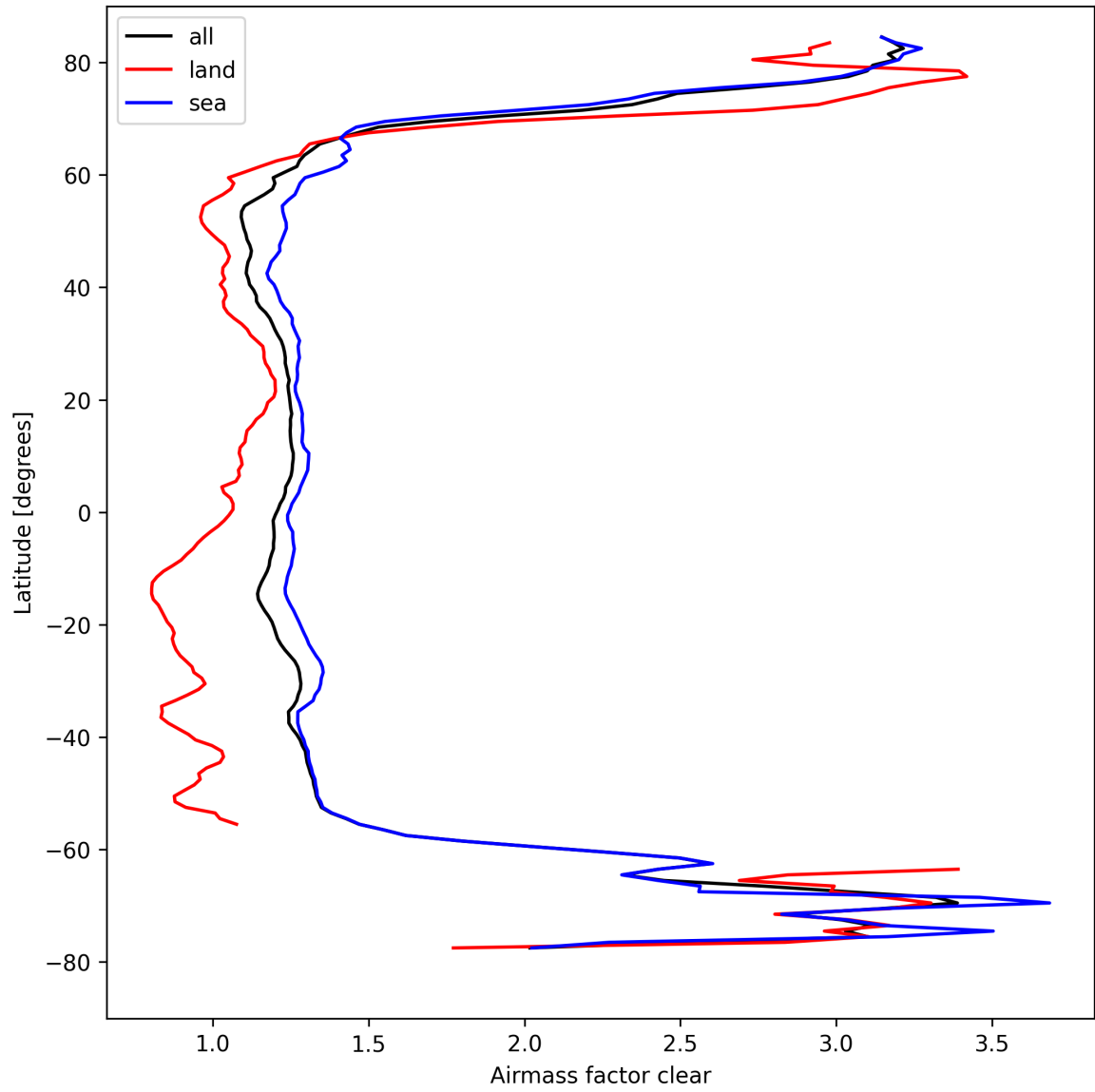
Figure 28: Zonal average of “Airmass factor clear” for 2024-09-02 to 2024-09-04.
