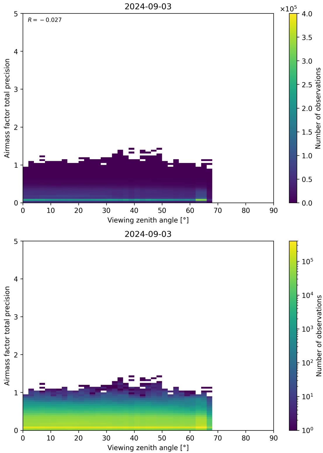
Figure 191: Scatter density plot of “Viewing zenith angle” against “Airmass factor total precision” for 2024-09-02 to 2024-09-04.
