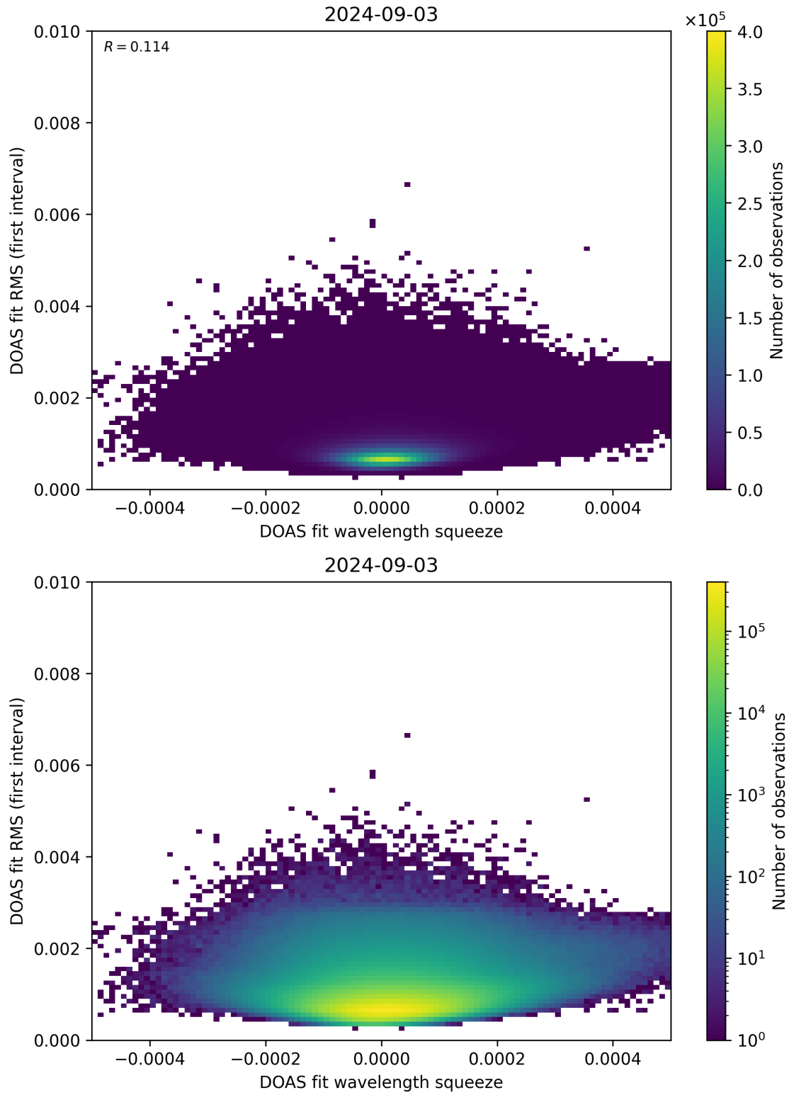
Figure 68: Scatter density plot of “DOAS fit wavelength squeeze” against “DOAS fit RMS (first interval)” for 2024-09-02 to 2024-09-04.
