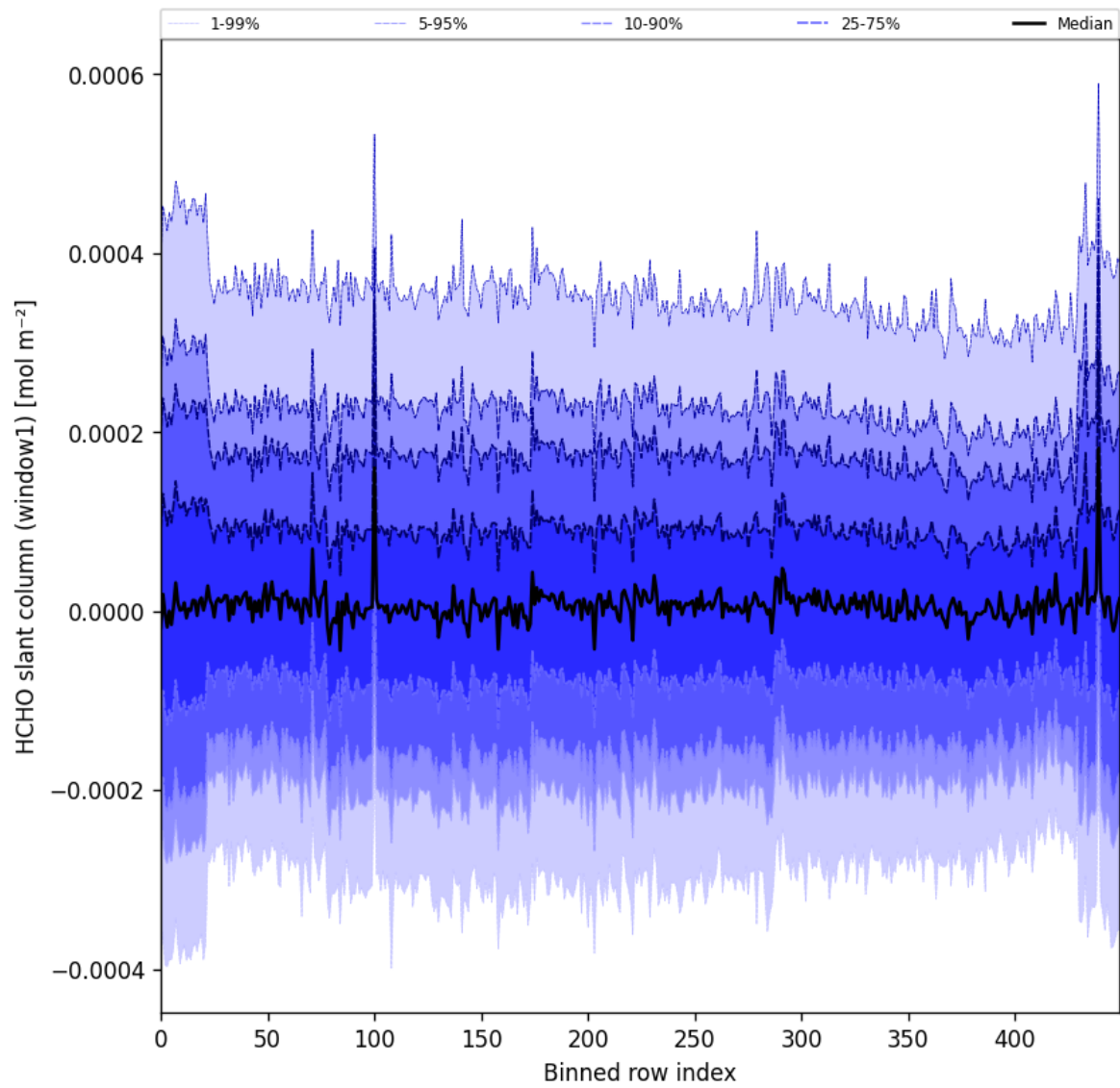
Figure 52: Along track statistics of “HCHO slant column (window1)” for 2024-09-02 to 2024-09-04
