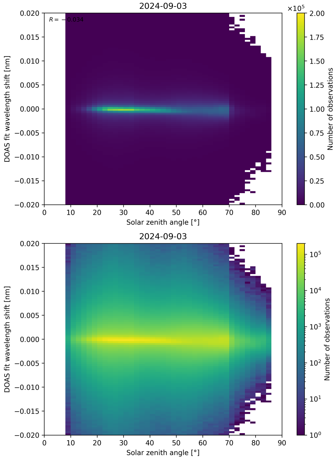
Figure 168: Scatter density plot of “Solar zenith angle” against “DOAS fit wavelength shift” for 2024-09-02 to 2024-09-04.
