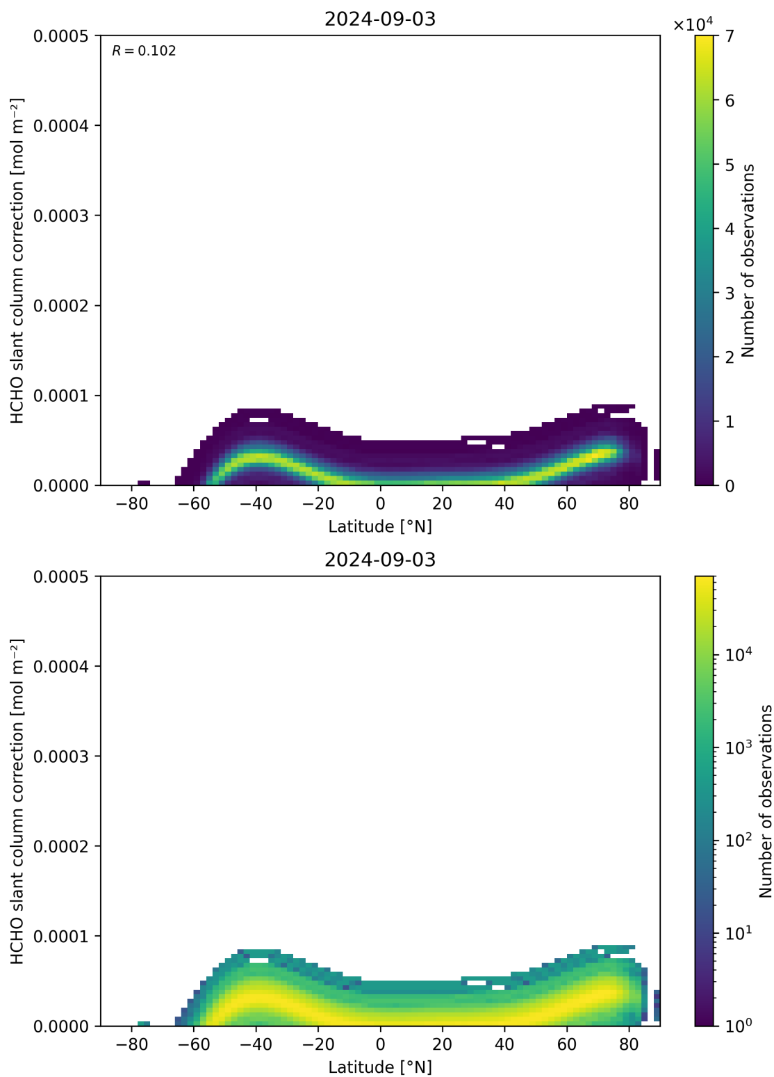
Figure 158: Scatter density plot of “Latitude” against “HCHO slant column correction” for 2024-09-02 to 2024-09-04.
