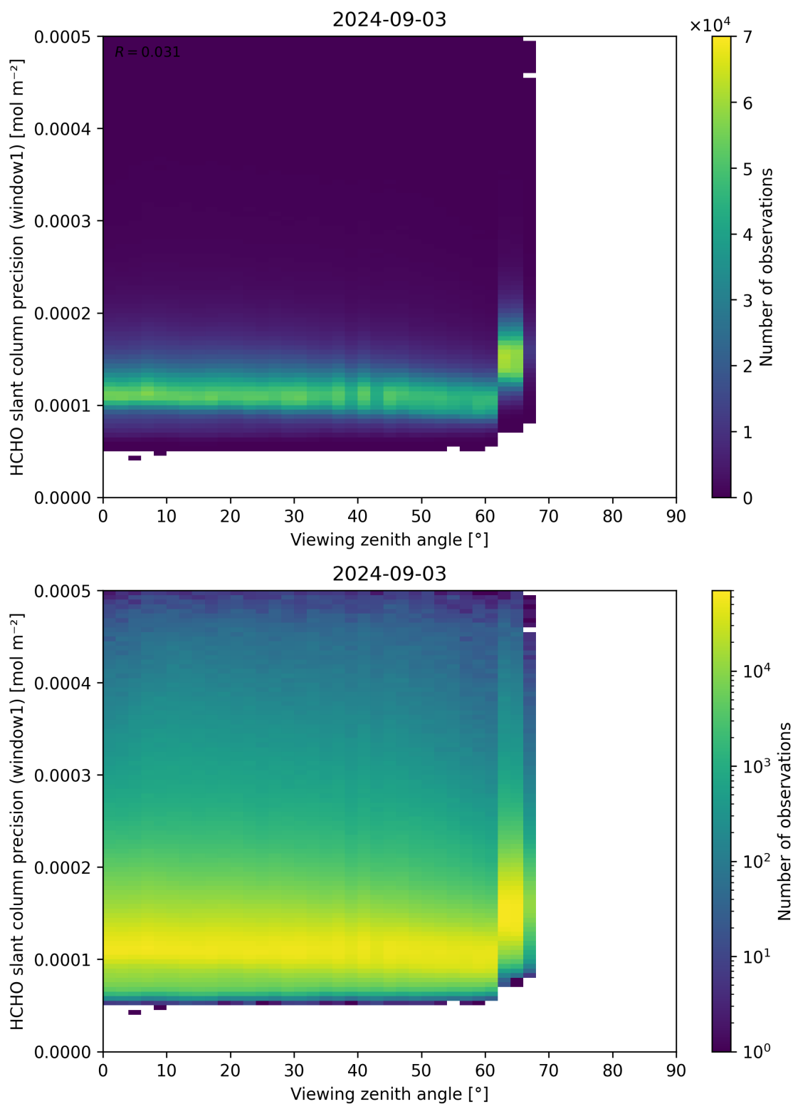
Figure 189: Scatter density plot of “Viewing zenith angle” against “HCHO slant column precision (window1)” for 2024-09-02 to 2024-09-04.
