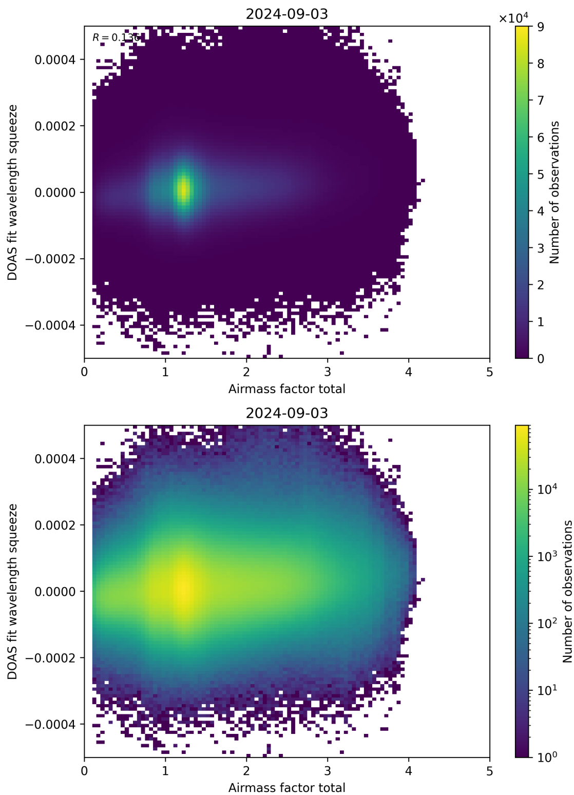
Figure 99: Scatter density plot of “Airmass factor total” against “DOAS fit wavelength squeeze” for 2024-09-02 to 2024-09-04.
