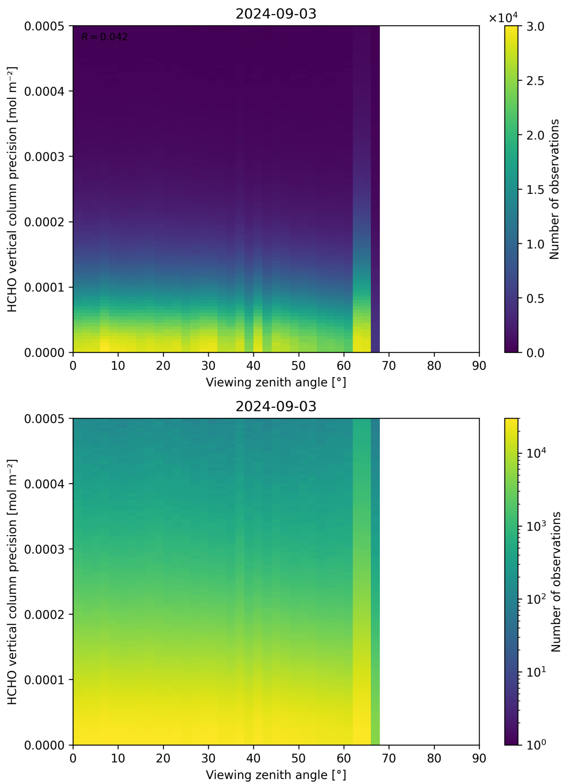
Figure 194: Scatter density plot of “Viewing zenith angle” against “HCHO vertical column precision” for 2024-09-02 to 2024-09-04.
