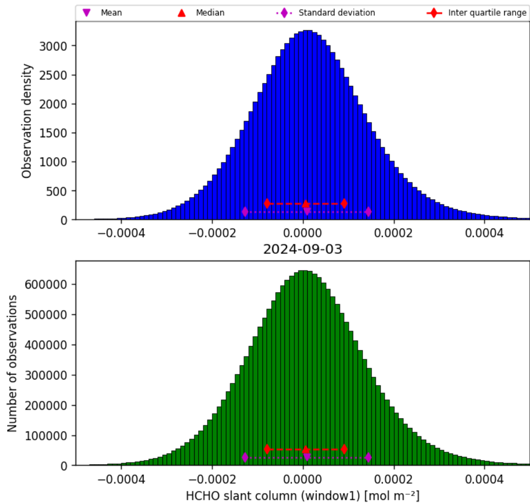
Figure 38: Histogram of “HCHO slant column (window1)” for 2024-09-02 to 2024-09-04
