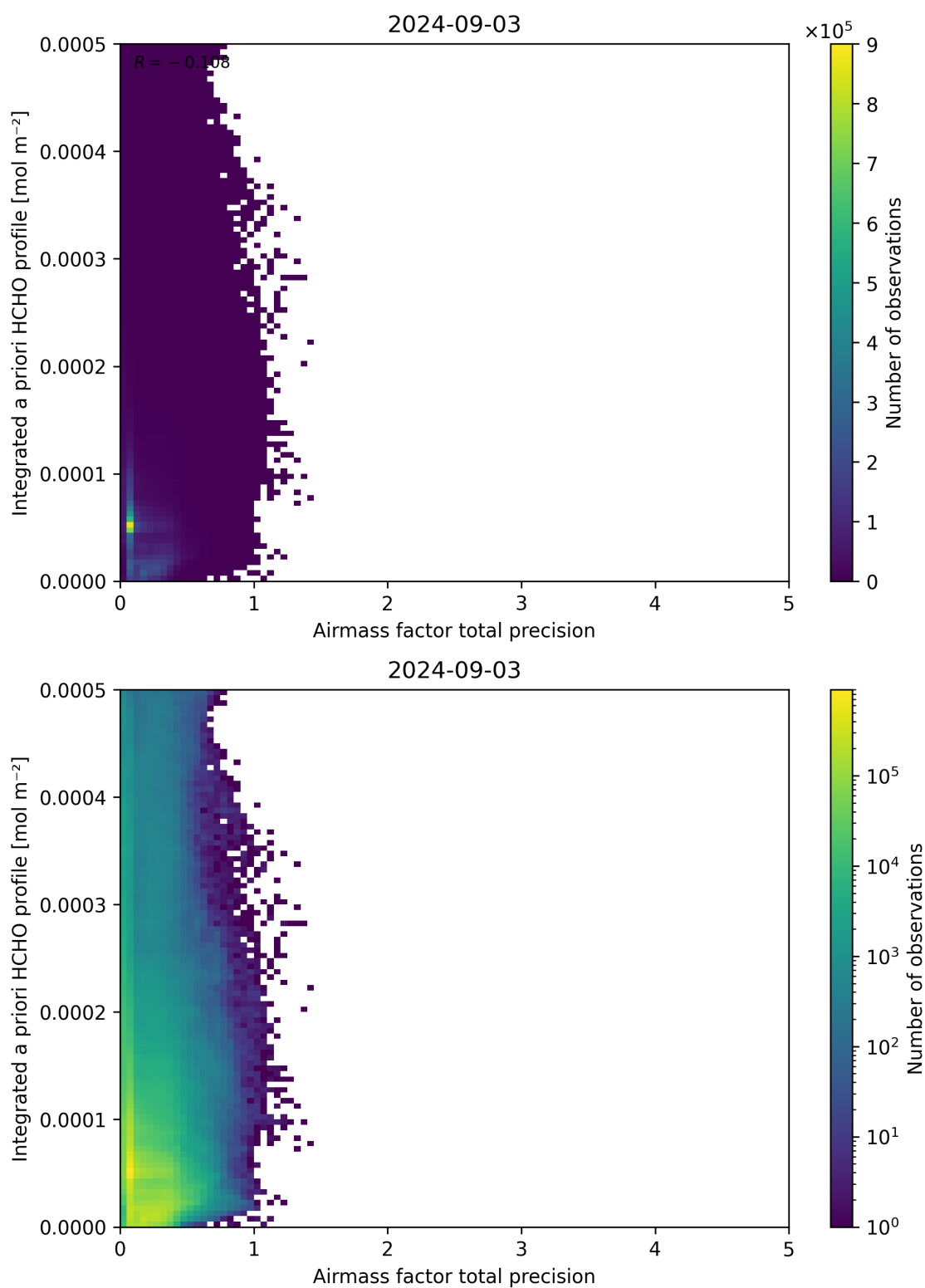
Figure 111: Scatter density plot of “Airmass factor total precision” against “Integrated a priori HCHO profile” for 2024-09-02 to 2024-09-04.
