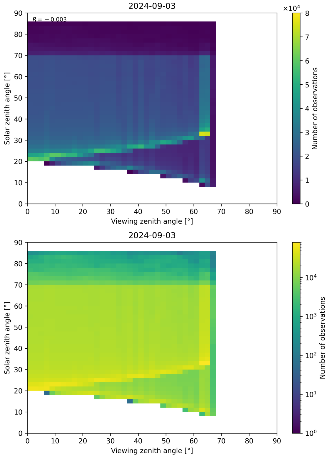
Figure 197: Scatter density plot of “Viewing zenith angle” against “Solar zenith angle” for 2024-09-02 to 2024-09-04.
