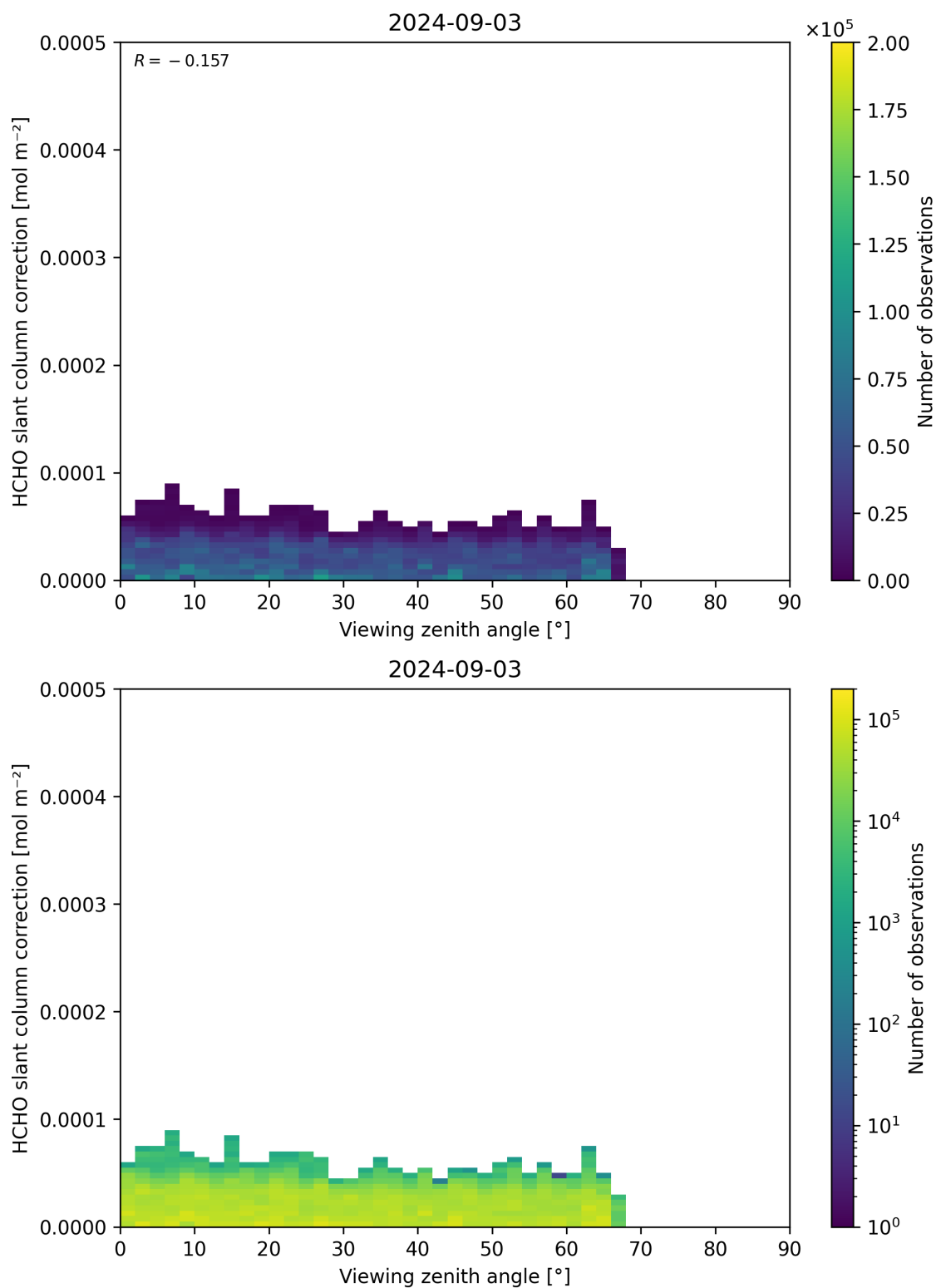
Figure 187: Scatter density plot of “Viewing zenith angle” against “HCHO slant column correction” for 2024-09-02 to 2024-09-04.
