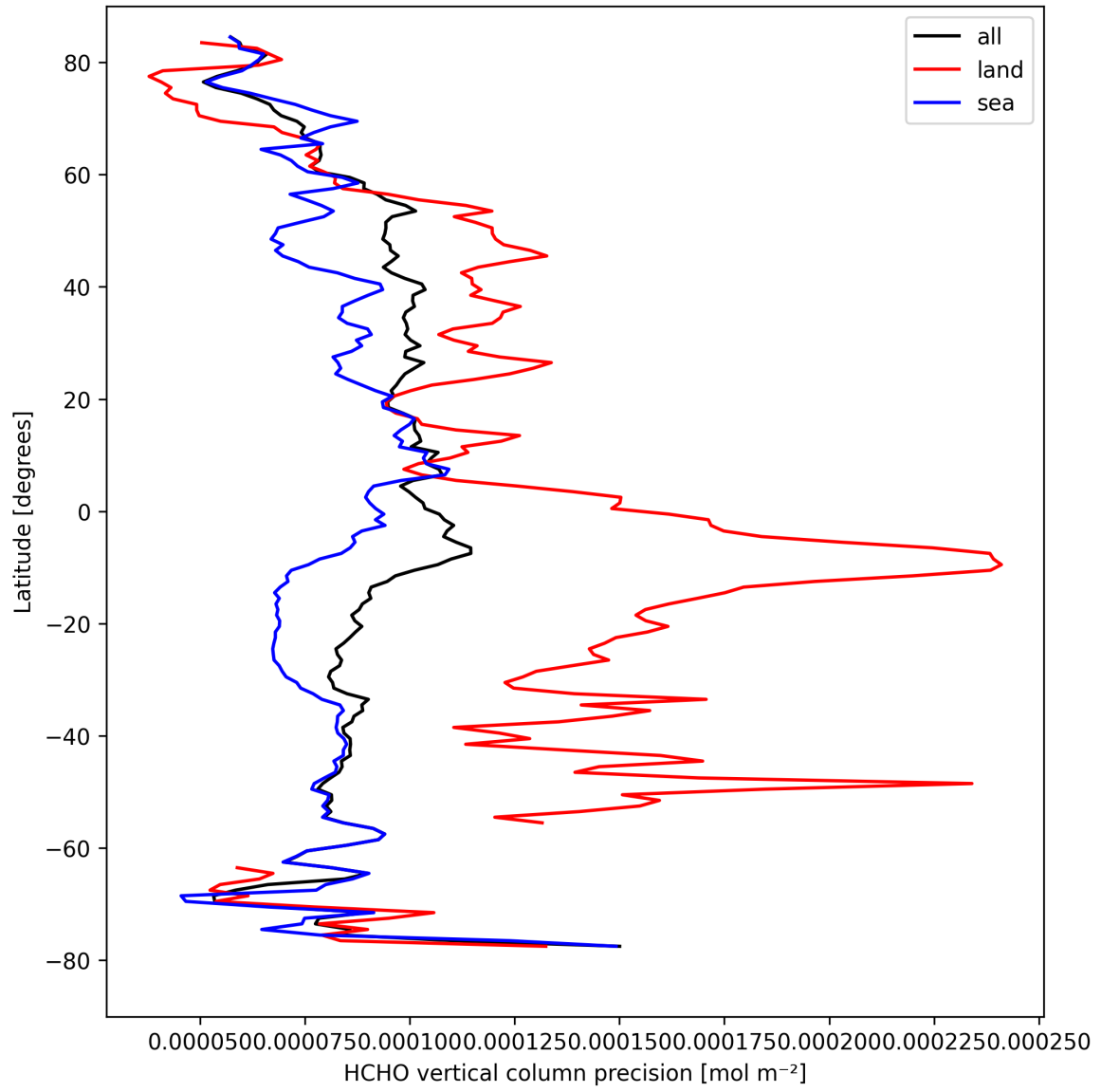
Figure 22: Zonal average of "HCHO vertical column precision" for 2024-09-02 to 2024-09-04.
