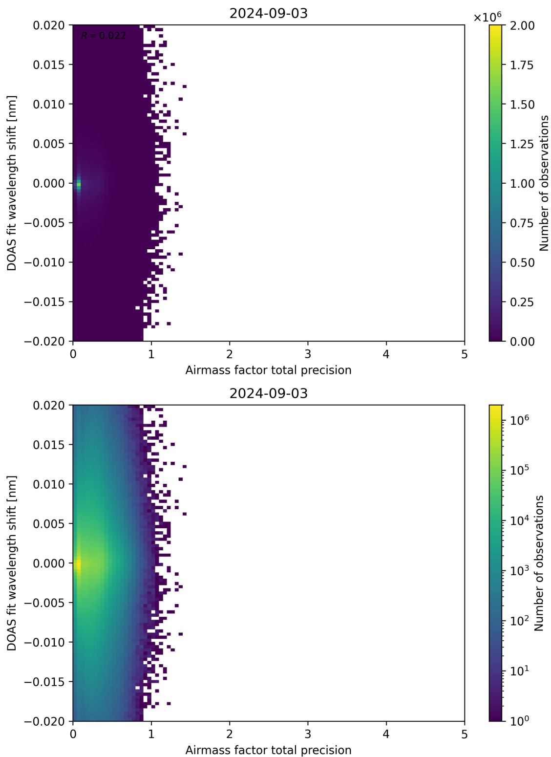
Figure 106: Scatter density plot of “Airmass factor total precision” against “DOAS fit wavelength shift” for 2024-09-02 to 2024-09-04.
