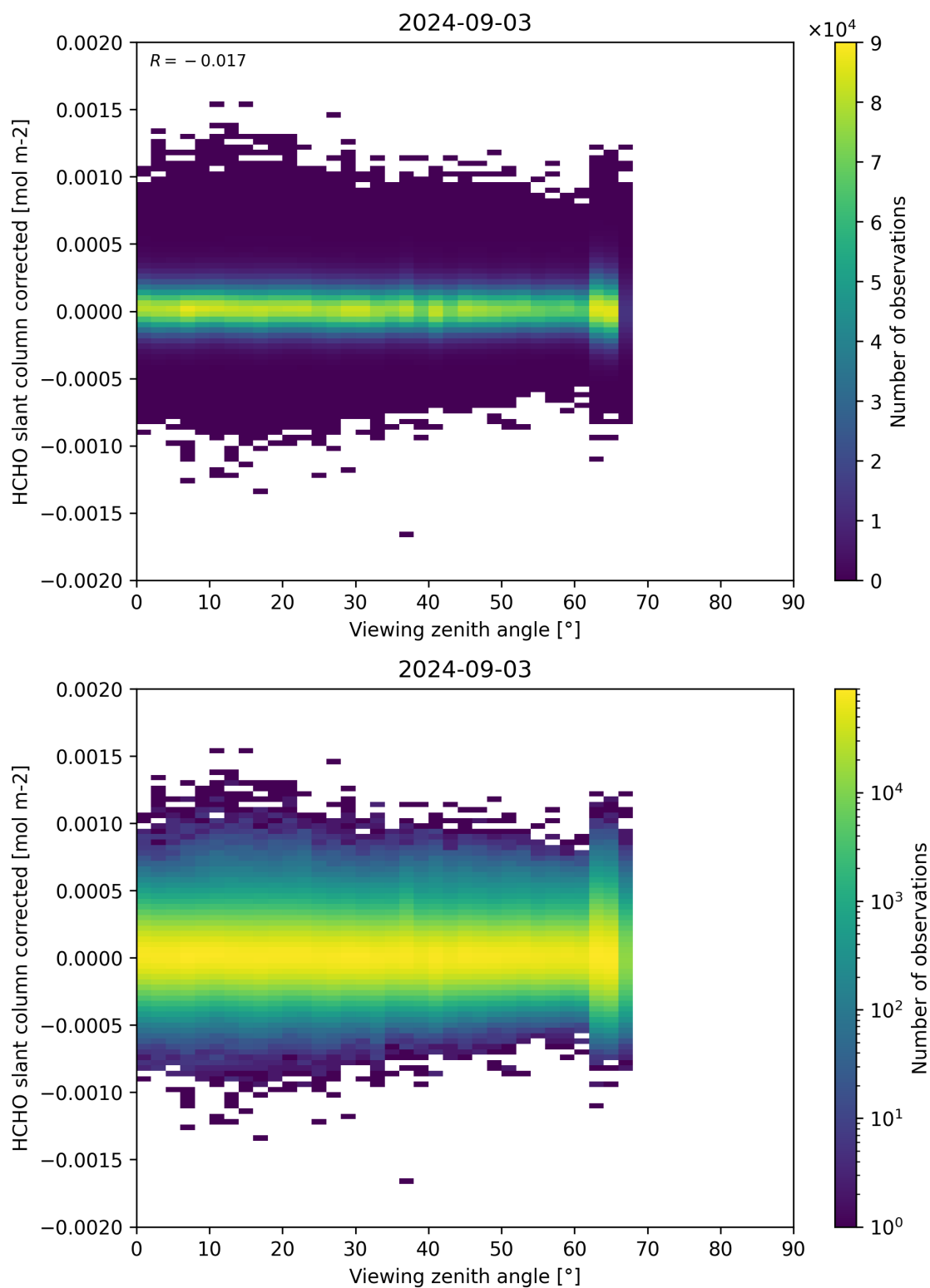
Figure 186: Scatter density plot of “Viewing zenith angle” against “HCHO slant column corrected” for 2024-09-02 to 2024-09-04.
