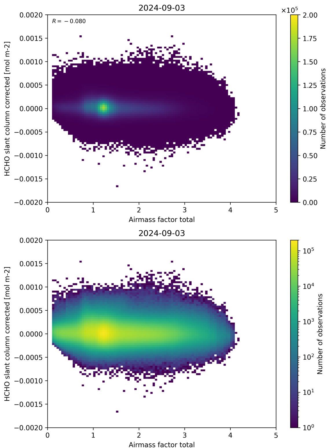
Figure 101: Scatter density plot of “Airmass factor total” against “HCHO slant column corrected” for 2024-09-02 to 2024-09-04.
