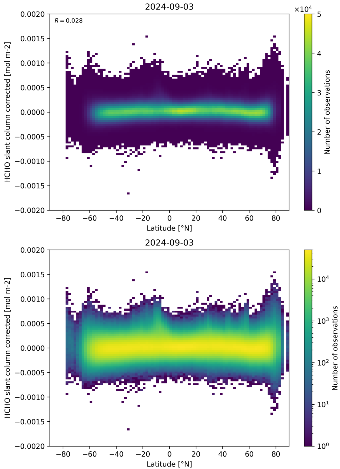
Figure 157: Scatter density plot of “Latitude” against “HCHO slant column corrected” for 2024-09-02 to 2024-09-04.
