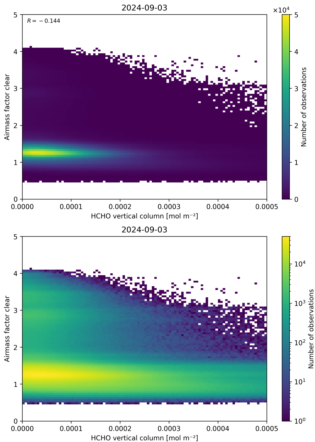
Figure 126: Scatter density plot of “HCHO vertical column” against “Airmass factor clear” for 2024-09-02 to 2024-09-04.
