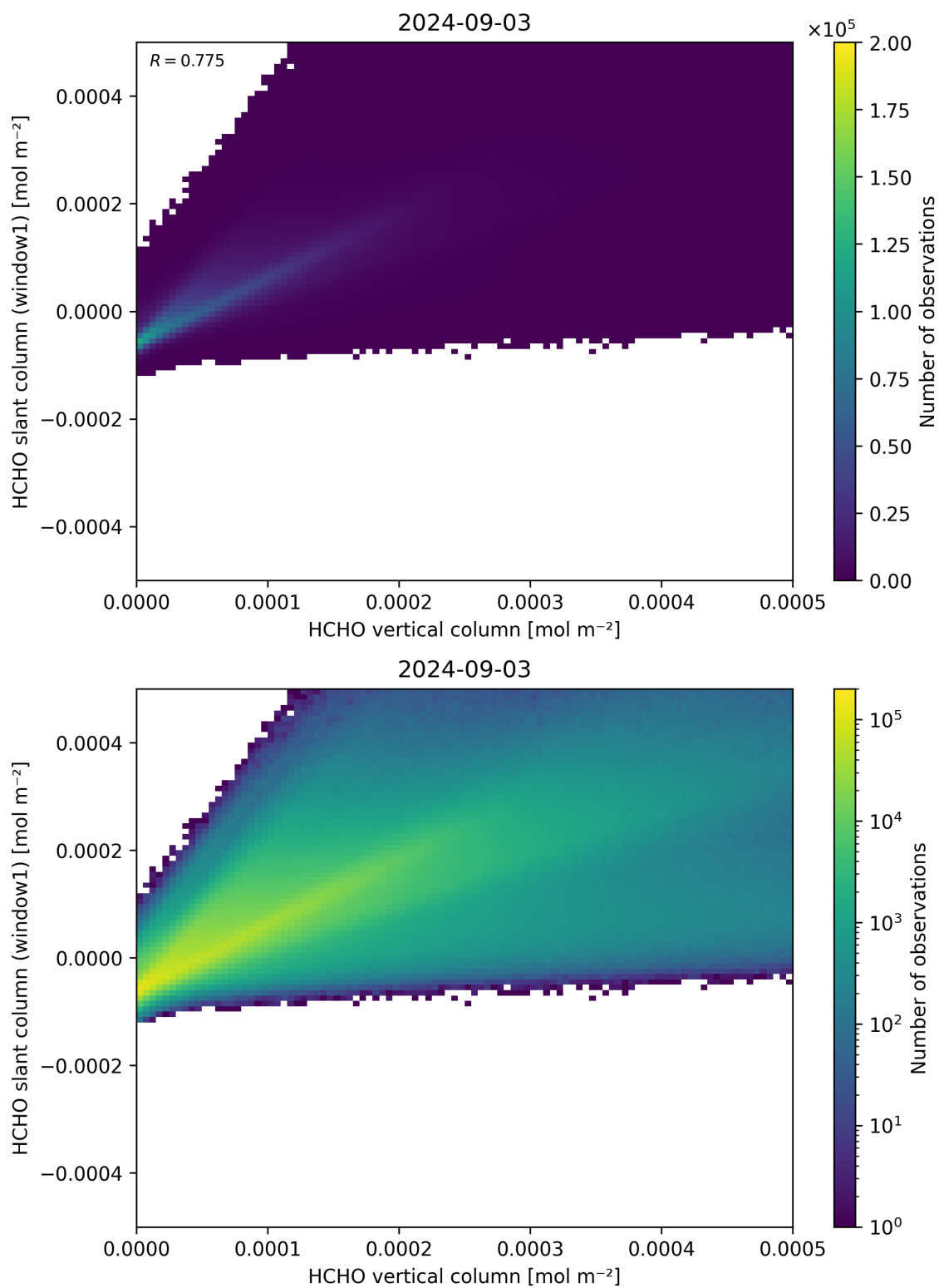
Figure 129: Scatter density plot of “HCHO vertical column” against “HCHO slant column (window1)” for 2024-09-02 to 2024-09-04.
