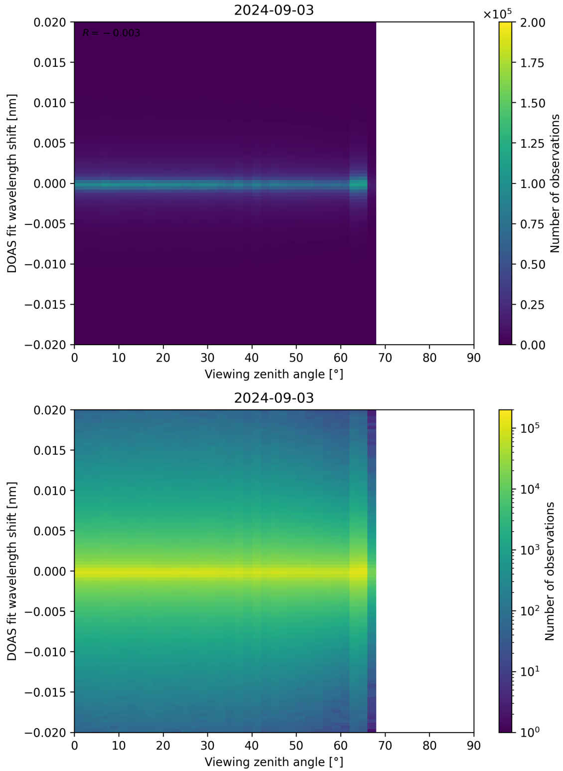
Figure 183: Scatter density plot of “Viewing zenith angle” against “DOAS fit wavelength shift” for 2024-09-02 to 2024-09-04.
