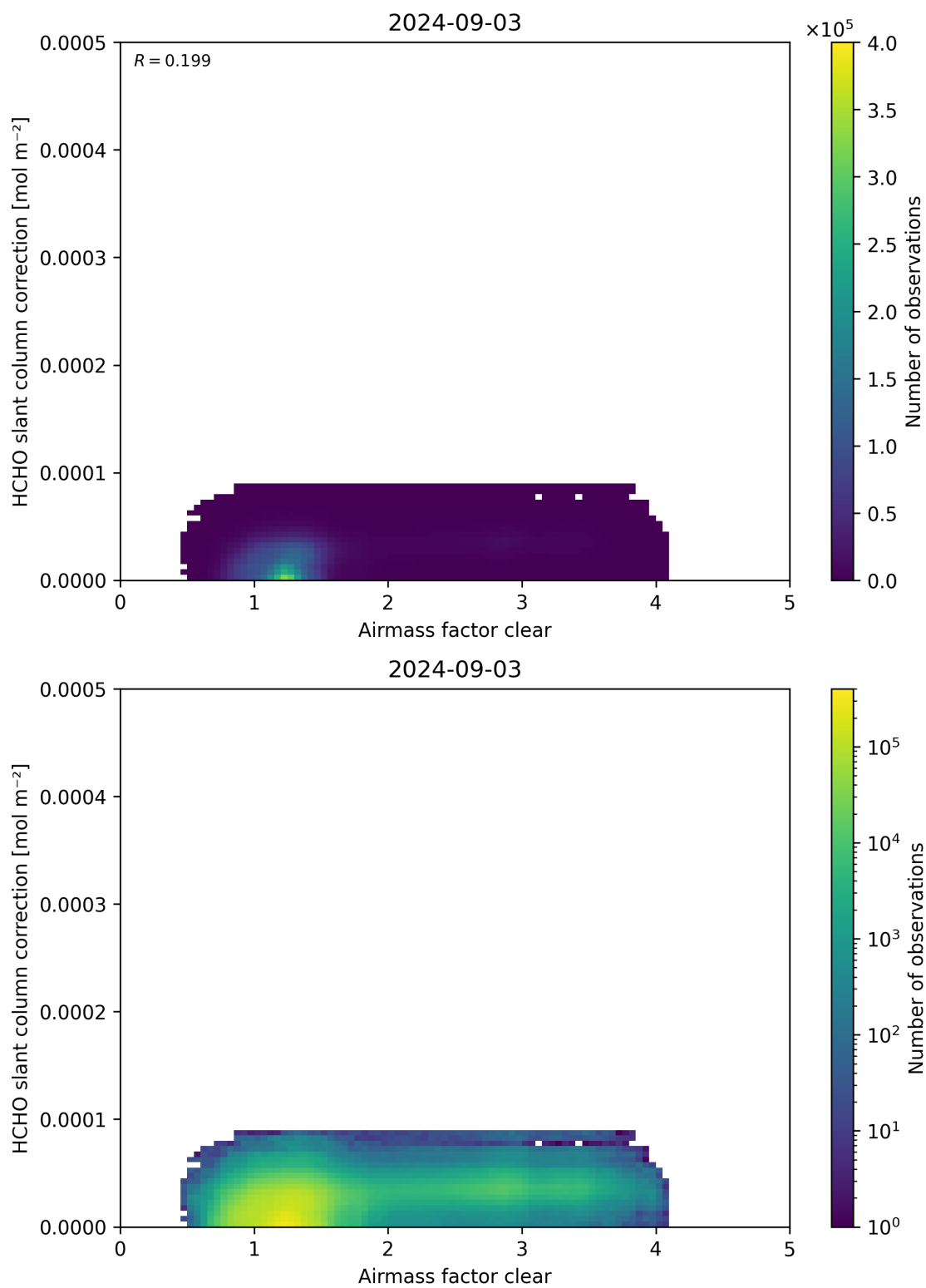
Figure 75: Scatter density plot of “Airmass factor clear” against “HCHO slant column correction” for 2024-09-02 to 2024-09-04.
