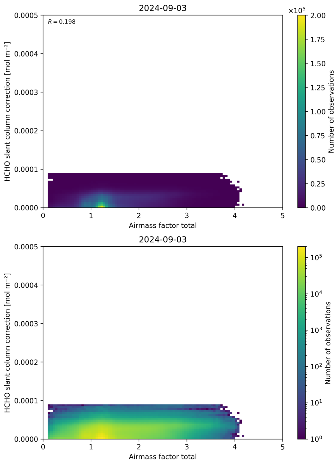
Figure 102: Scatter density plot of “Airmass factor total” against “HCHO slant column correction” for 2024-09-02 to 2024-09-04.
