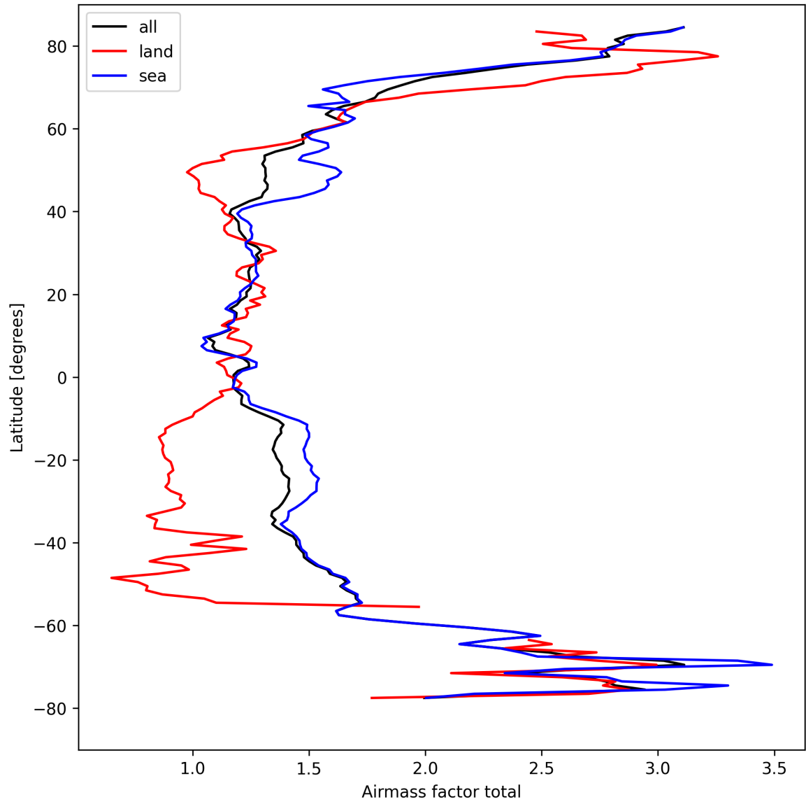
Figure 26: Zonal average of “Airmass factor total” for 2024-09-02 to 2024-09-04.
