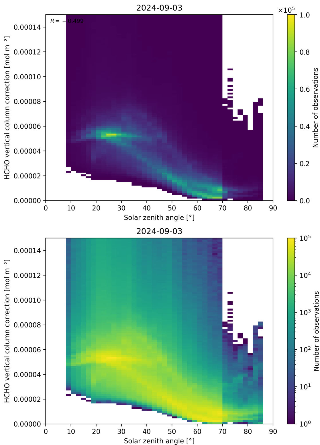
Figure 178: Scatter density plot of “Solar zenith angle” against “HCHO vertical column correction” for 2024-09-02 to 2024-09-04.
