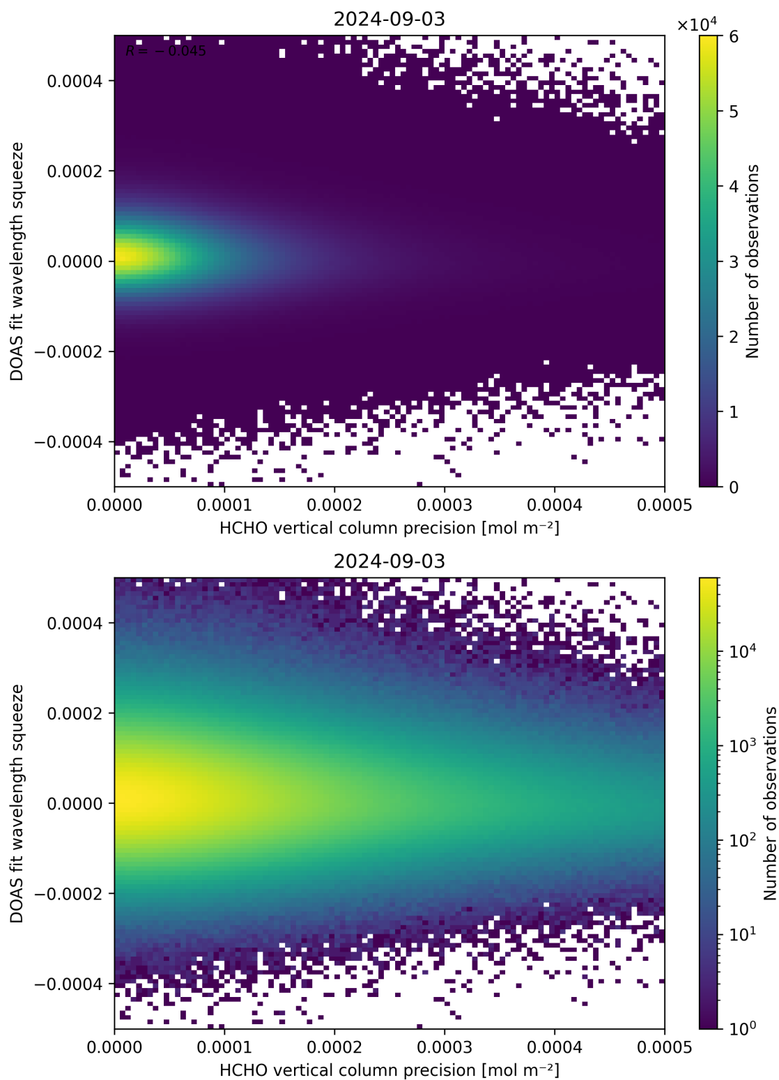
Figure 138: Scatter density plot of “HCHO vertical column precision” against “DOAS fit wavelength squeeze” for 2024-09-02 to 2024-09-04.
