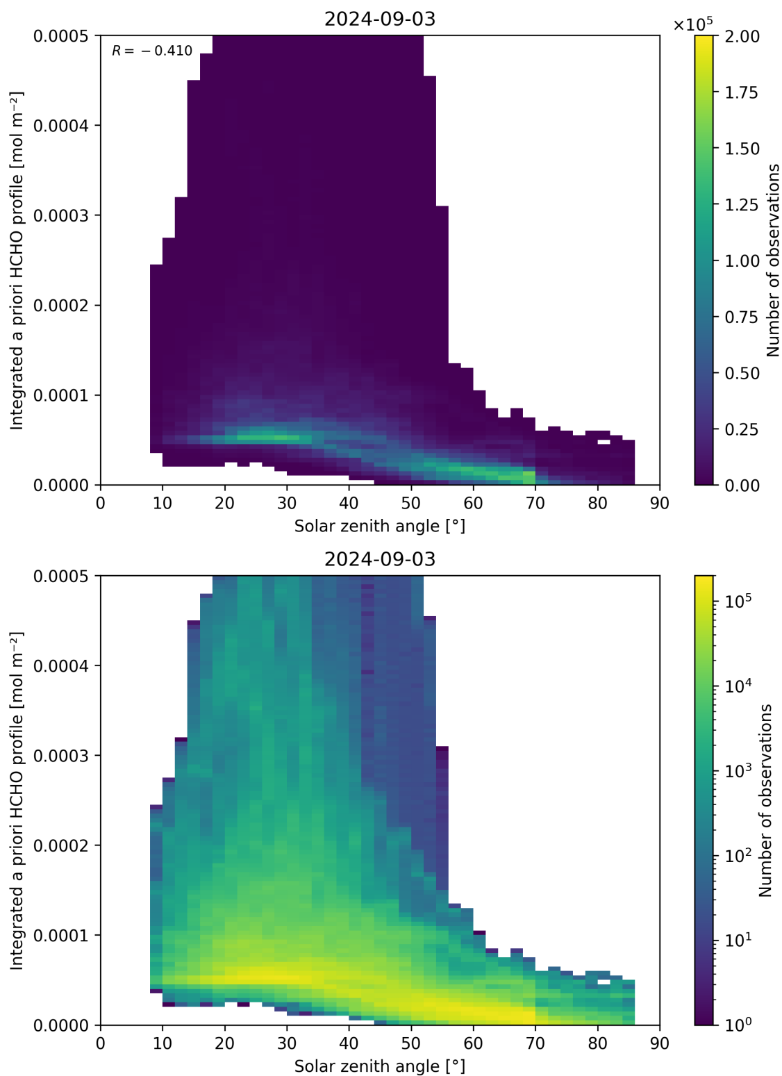
Figure 180: Scatter density plot of “Solar zenith angle” against “Integrated a priori HCHO profile” for 2024-09-02 to 2024-09-04.
