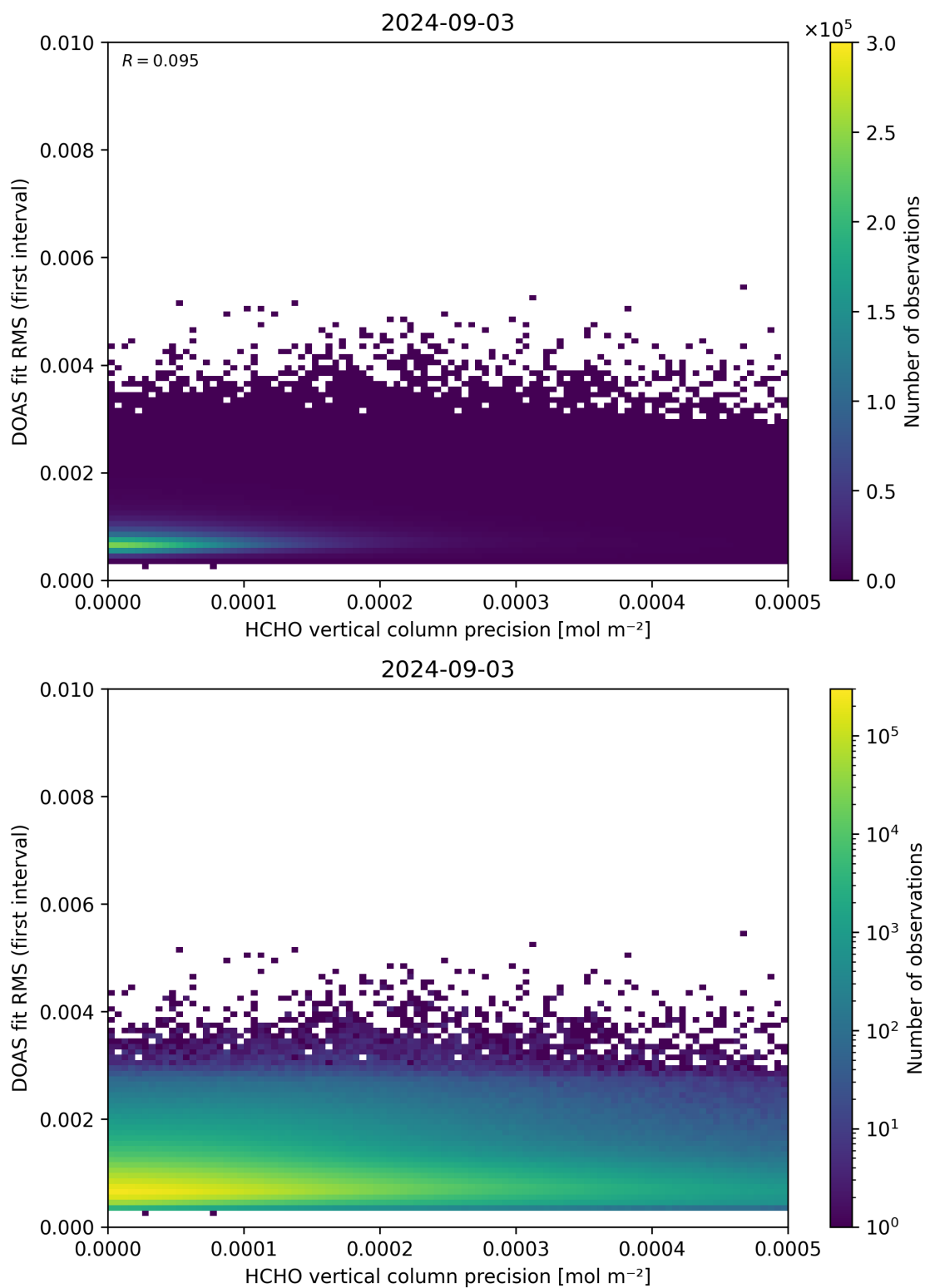
Figure 136: Scatter density plot of “HCHO vertical column precision” against “DOAS fit RMS (first interval)” for 2024-09-02 to 2024-09-04.
