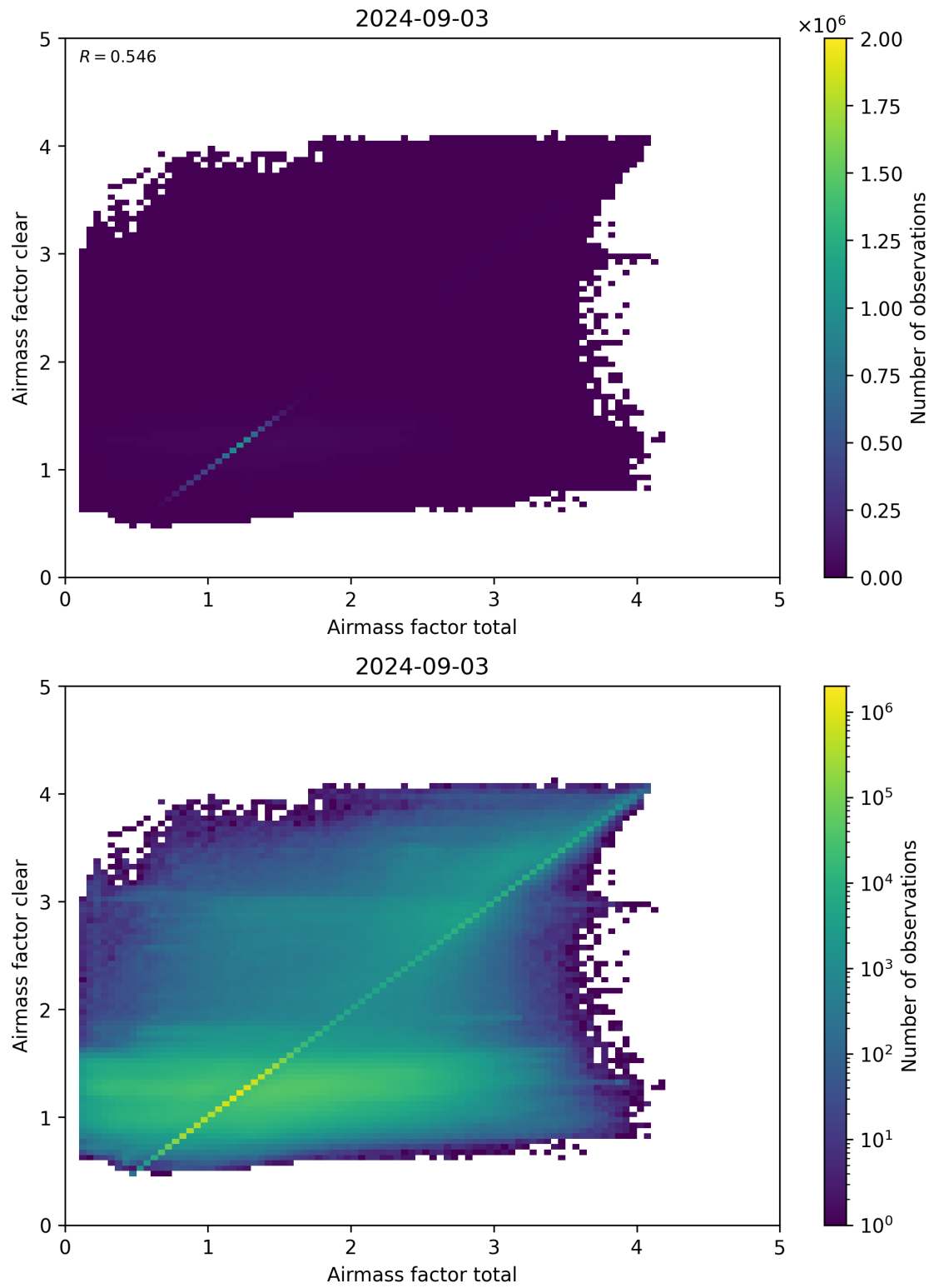
Figure 100: Scatter density plot of “Airmass factor total” against “Airmass factor clear” for 2024-09-02 to 2024-09-04.
