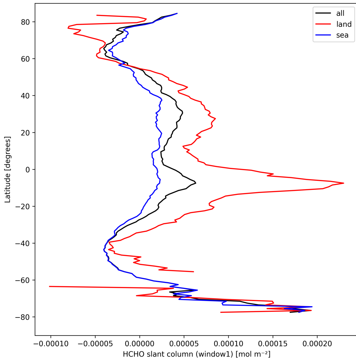
Figure 24: Zonal average of “HCHO slant column (window1)” for 2024-09-02 to 2024-09-04.
