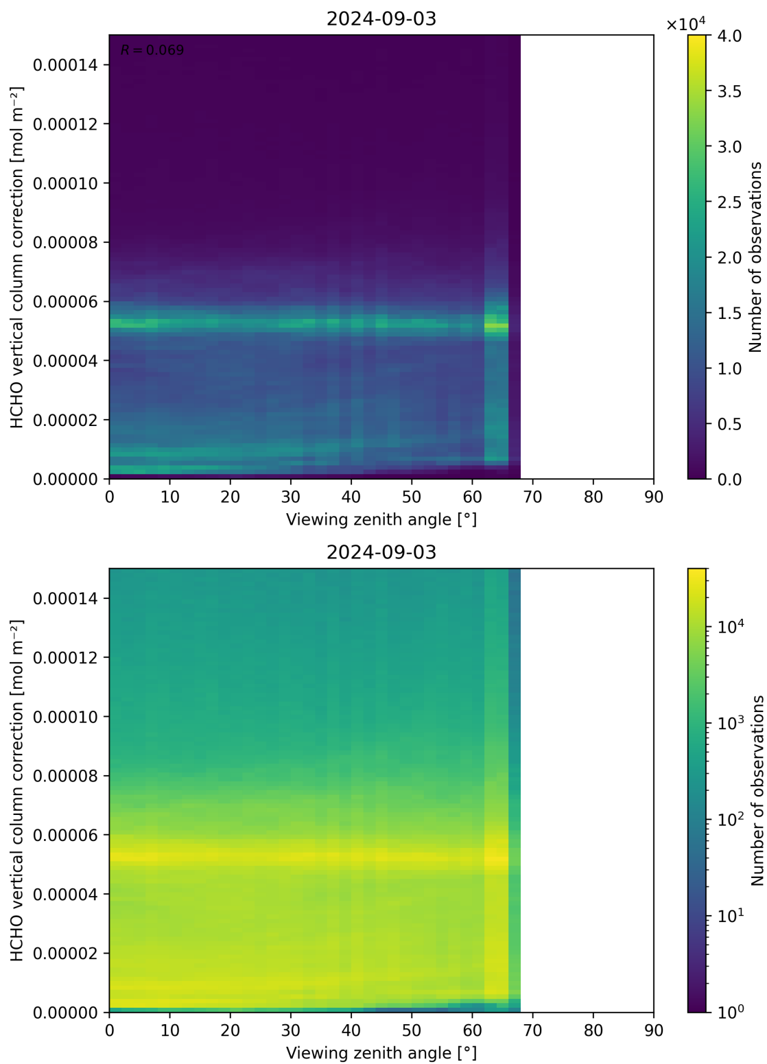
Figure 193: Scatter density plot of “Viewing zenith angle” against “HCHO vertical column correction” for 2024-09-02 to 2024-09-04.
