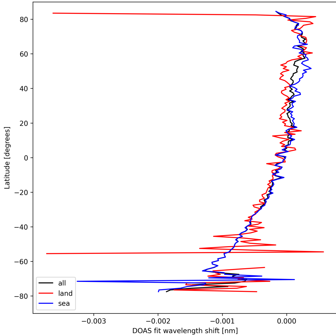
Figure 30: Zonal average of "DOAS fit wavelength shift" for 2024-09-02 to 2024-09-04.
