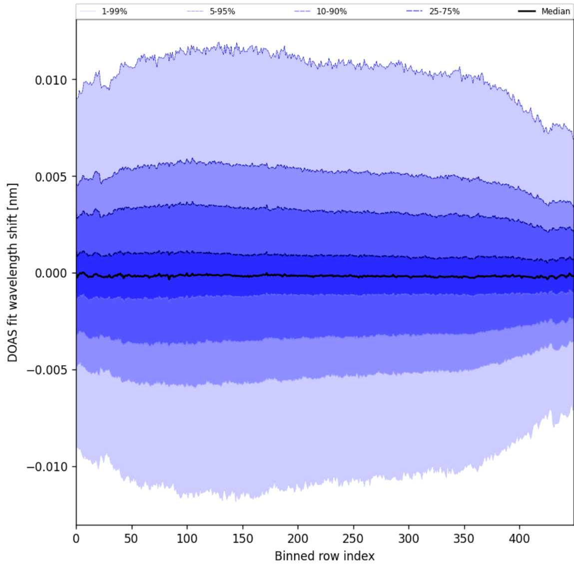
Figure 58: Along track statistics of “DOAS fit wavelength shift” for 2024-09-02 to 2024-09-04
