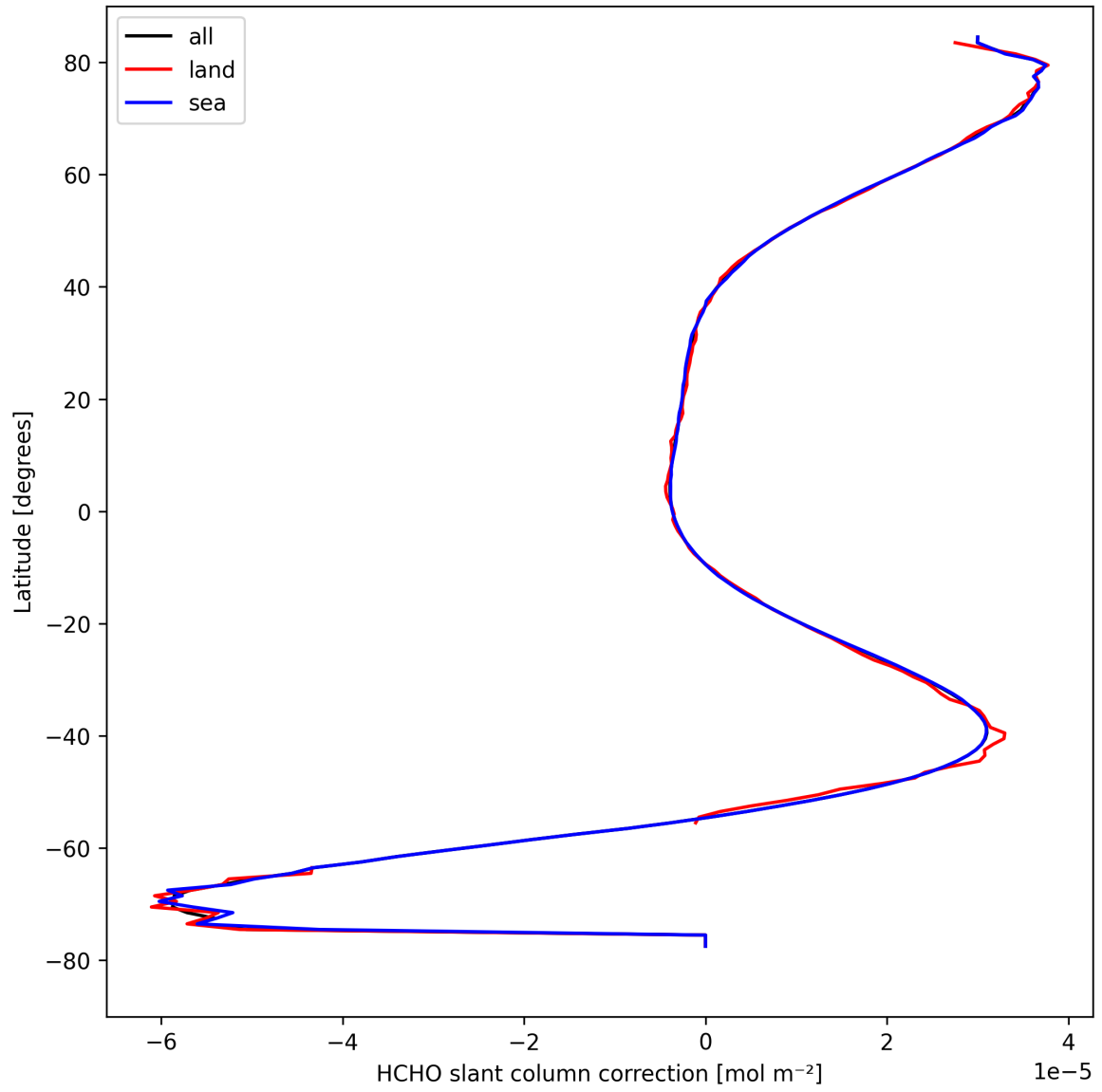
Figure 33: Zonal average of “HCHO slant column correction” for 2024-09-02 to 2024-09-04.
