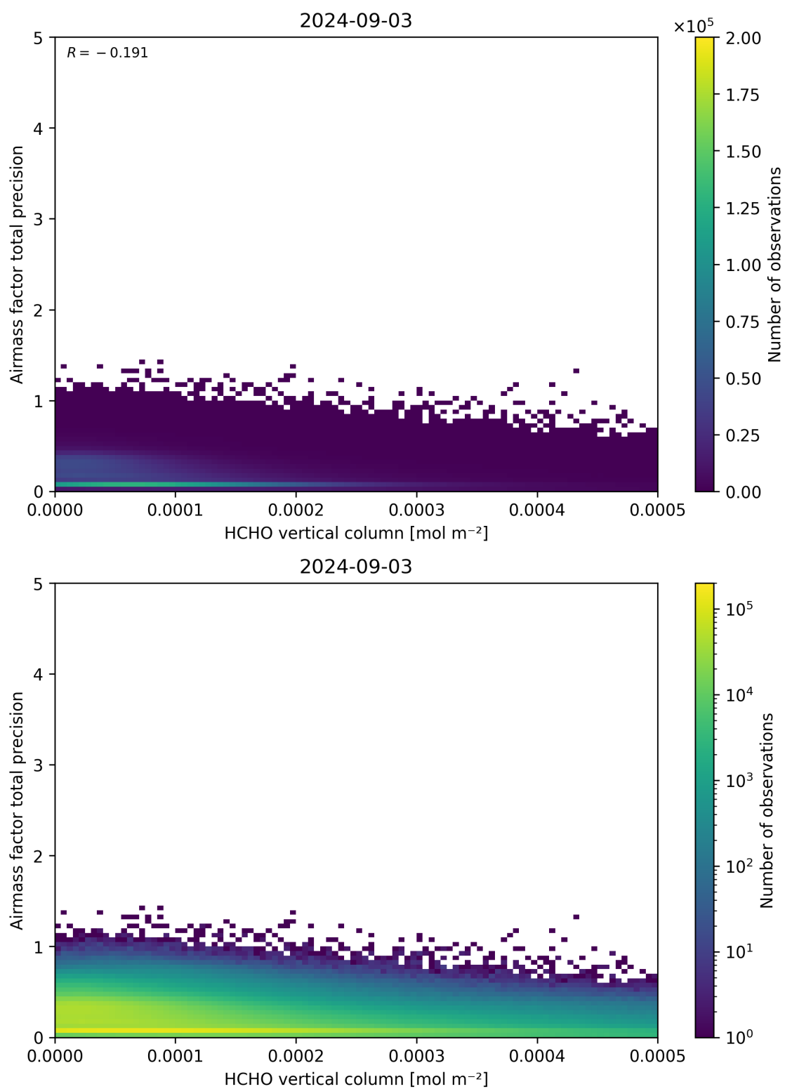
Figure 132: Scatter density plot of “HCHO vertical column” against “Airmass factor total precision” for 2024-09-02 to 2024-09-04.
