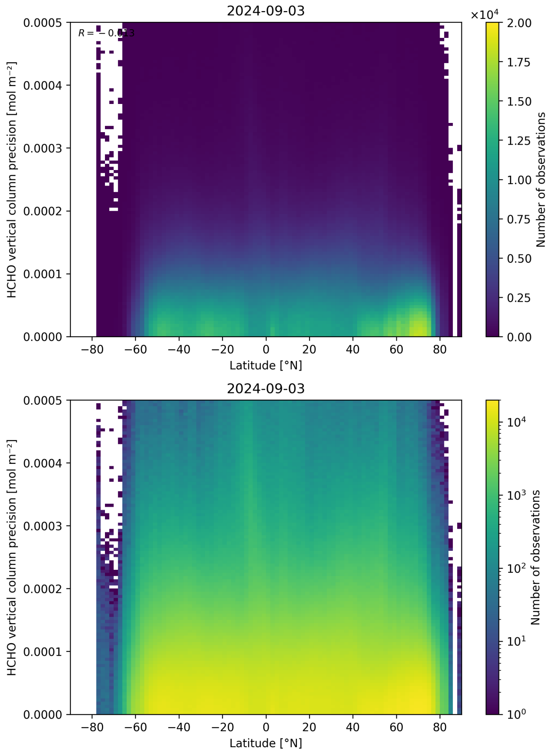
Figure 165: Scatter density plot of “Latitude” against “HCHO vertical column precision” for 2024-09-02 to 2024-09-04.
