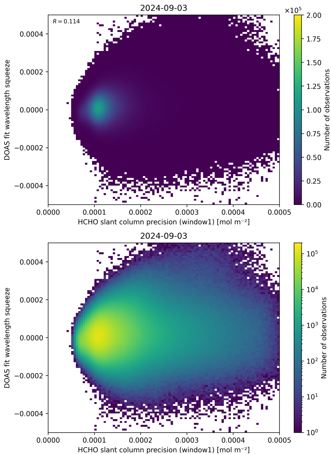
Figure 90: Scatter density plot of “HCHO slant column precision (window1)” against “DOAS fit wavelength squeeze” for 2024-09-02 to 2024-09-04.
