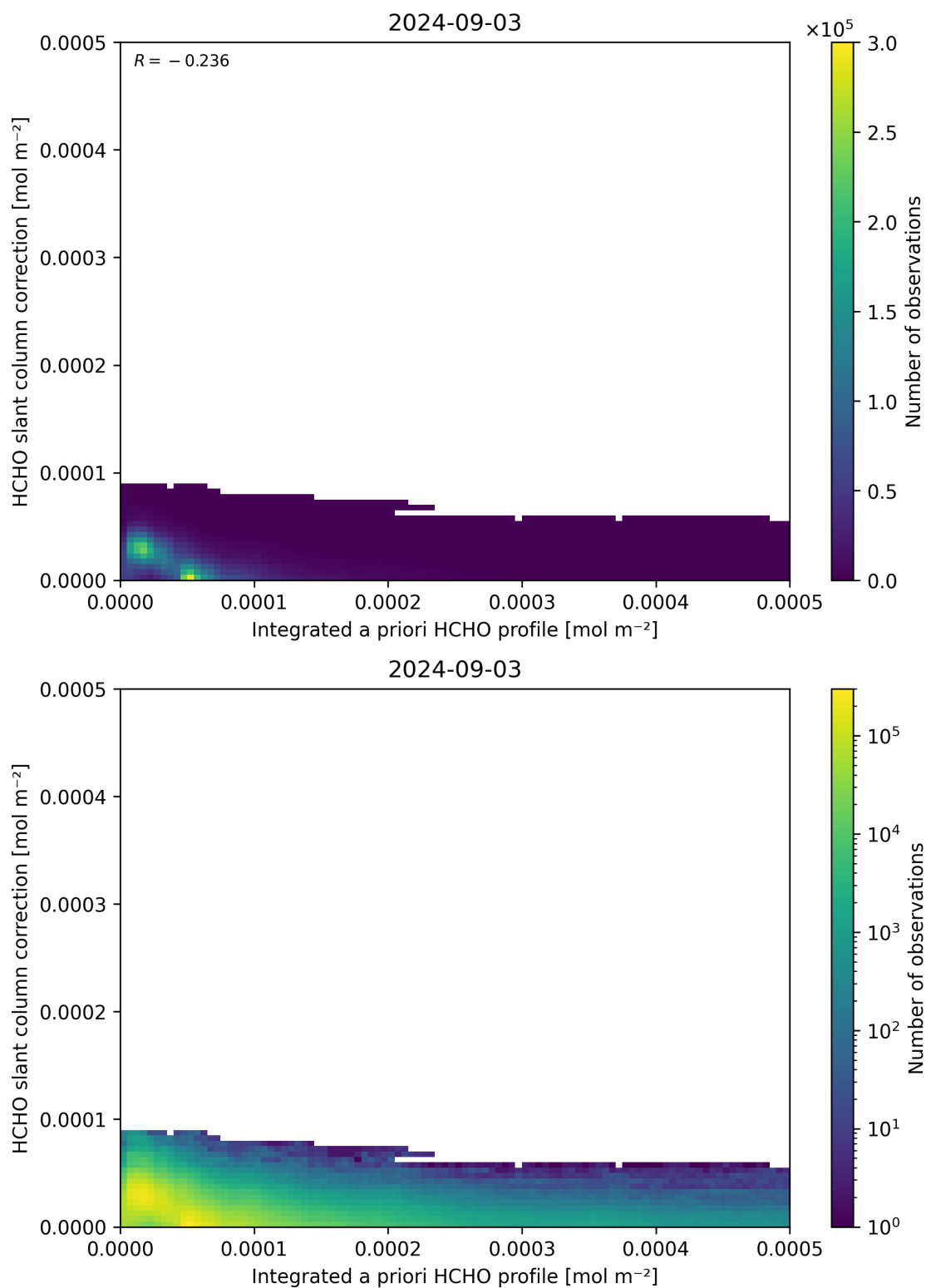
Figure 152: Scatter density plot of “Integrated a priori HCHO profile” against “HCHO slant column correction” for 2024-09-02 to 2024-09-04.
