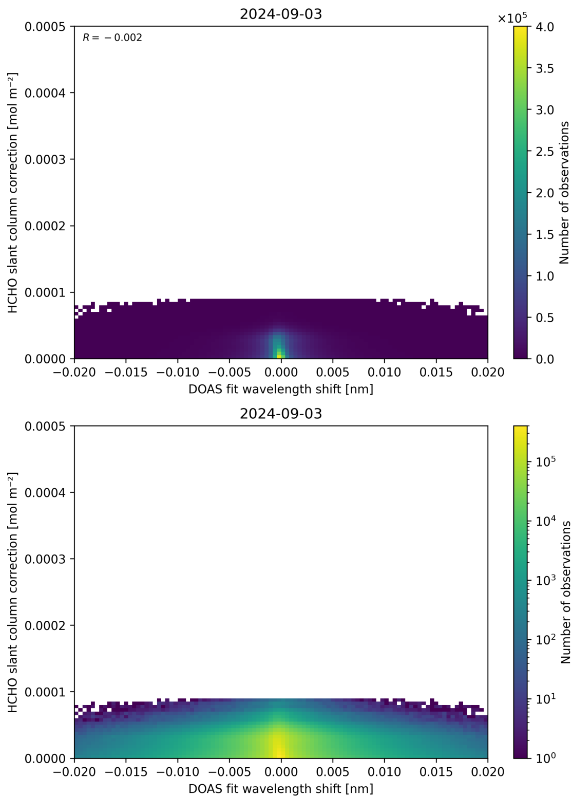
Figure 67: Scatter density plot of “DOAS fit wavelength shift” against “HCHO slant column correction” for 2024-09-02 to 2024-09-04.
