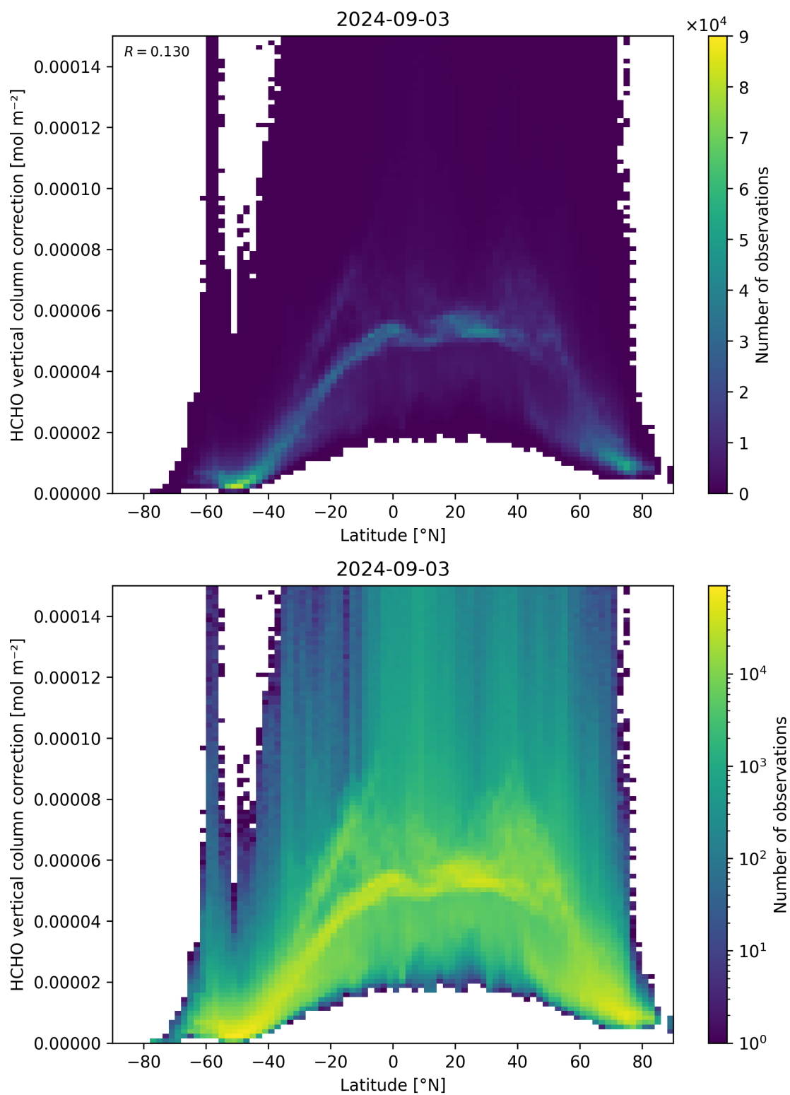
Figure 164: Scatter density plot of “Latitude” against “HCHO vertical column correction” for 2024-09-02 to 2024-09-04.
