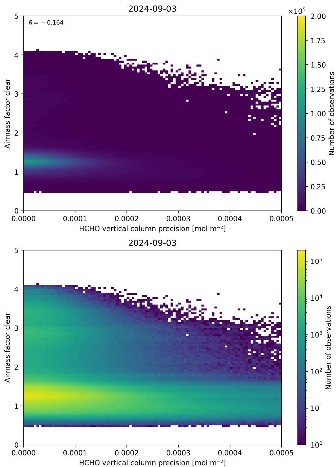
Figure 139: Scatter density plot of “HCHO vertical column precision” against “Airmass factor clear” for 2024-09-02 to 2024-09-04.
