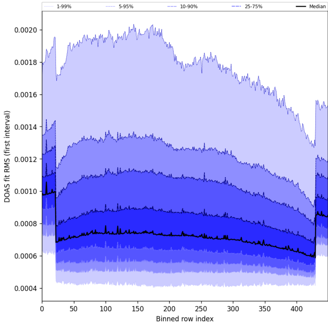
Figure 60: Along track statistics of “DOAS fit RMS (first interval)” for 2024-09-02 to 2024-09-04
