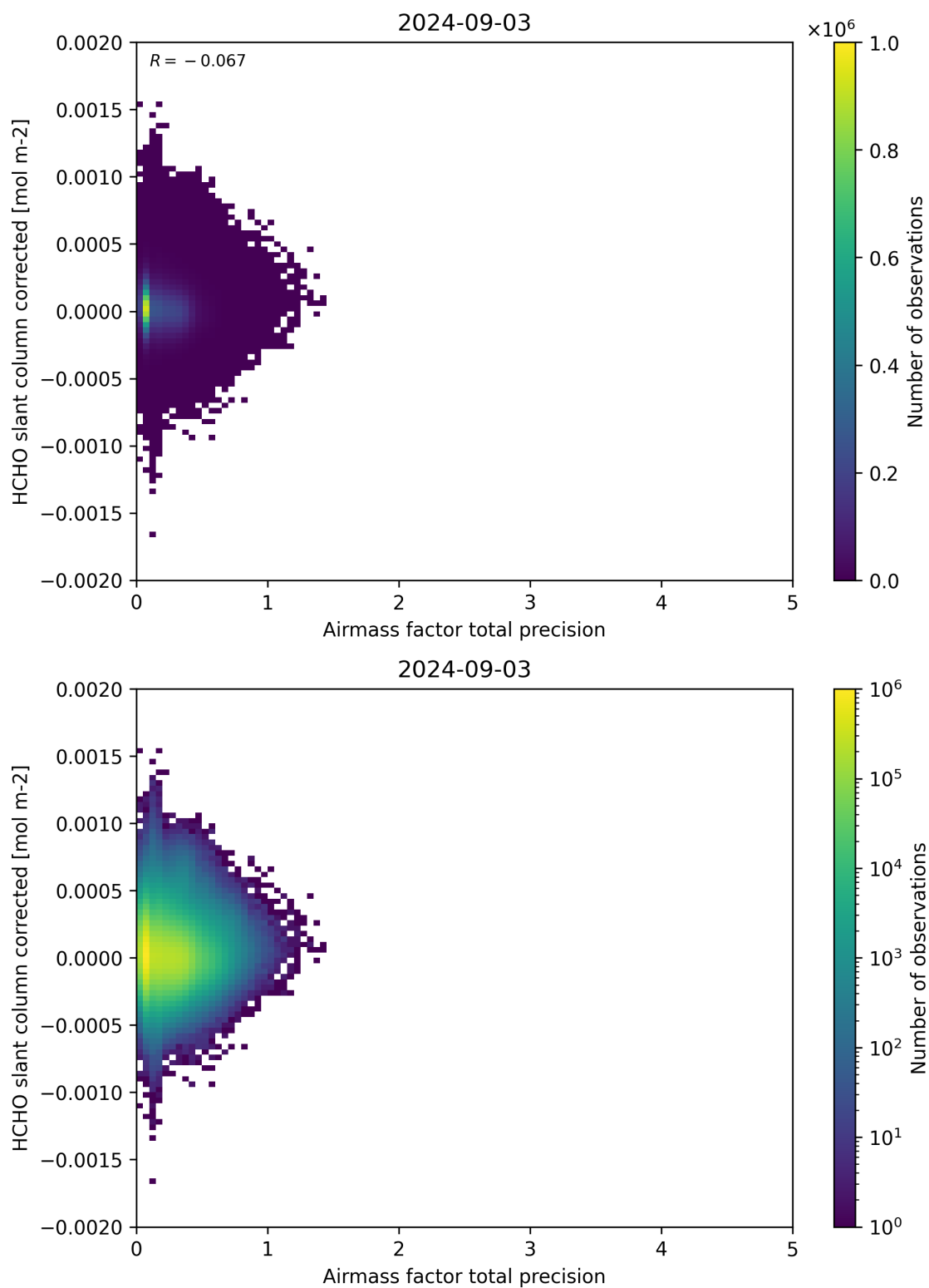
Figure 109: Scatter density plot of “Airmass factor total precision” against “HCHO slant column corrected” for 2024-09-02 to 2024-09-04.
