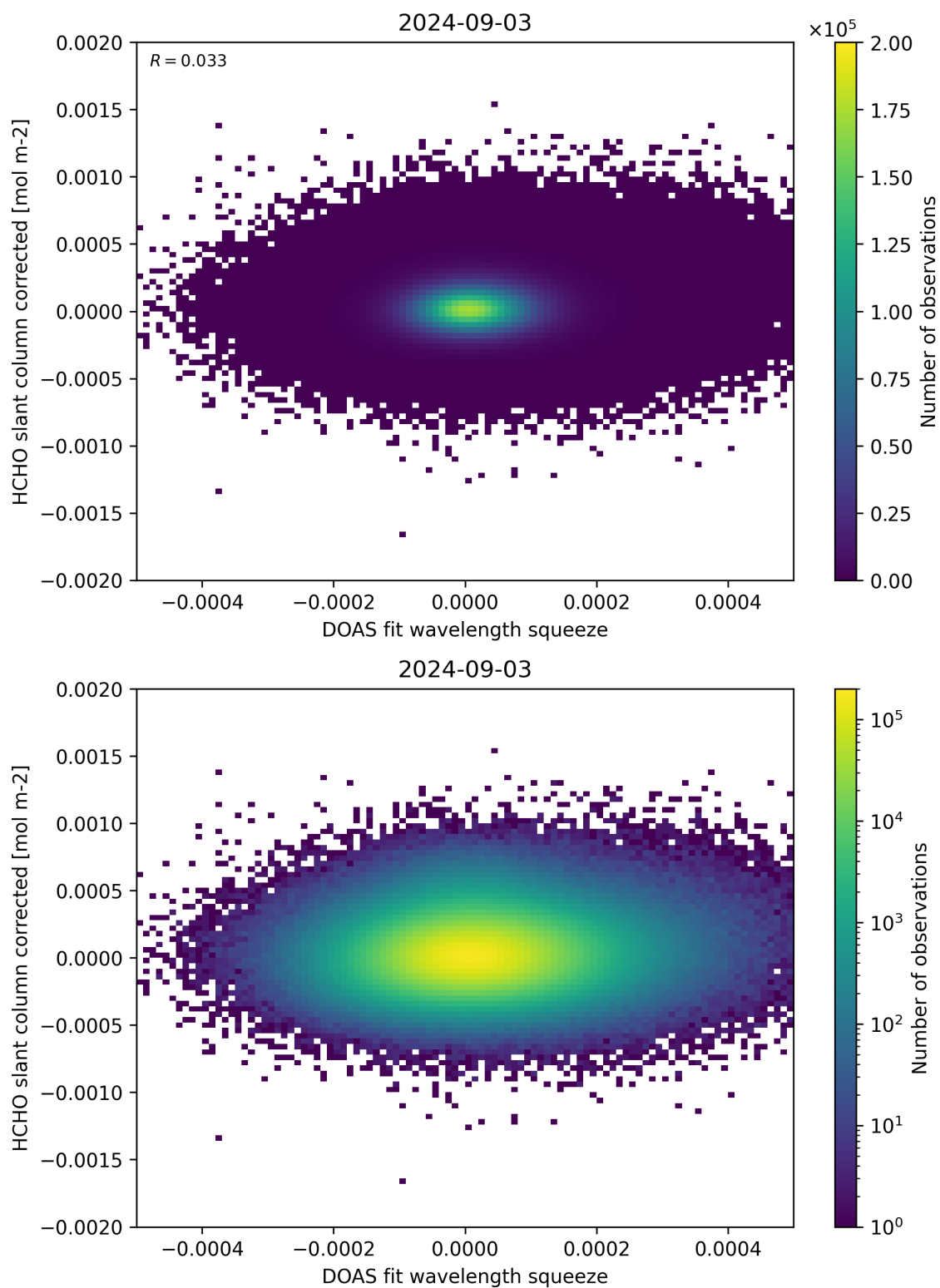
Figure 69: Scatter density plot of “DOAS fit wavelength squeeze” against “HCHO slant column corrected” for 2024-09-02 to 2024-09-04.
