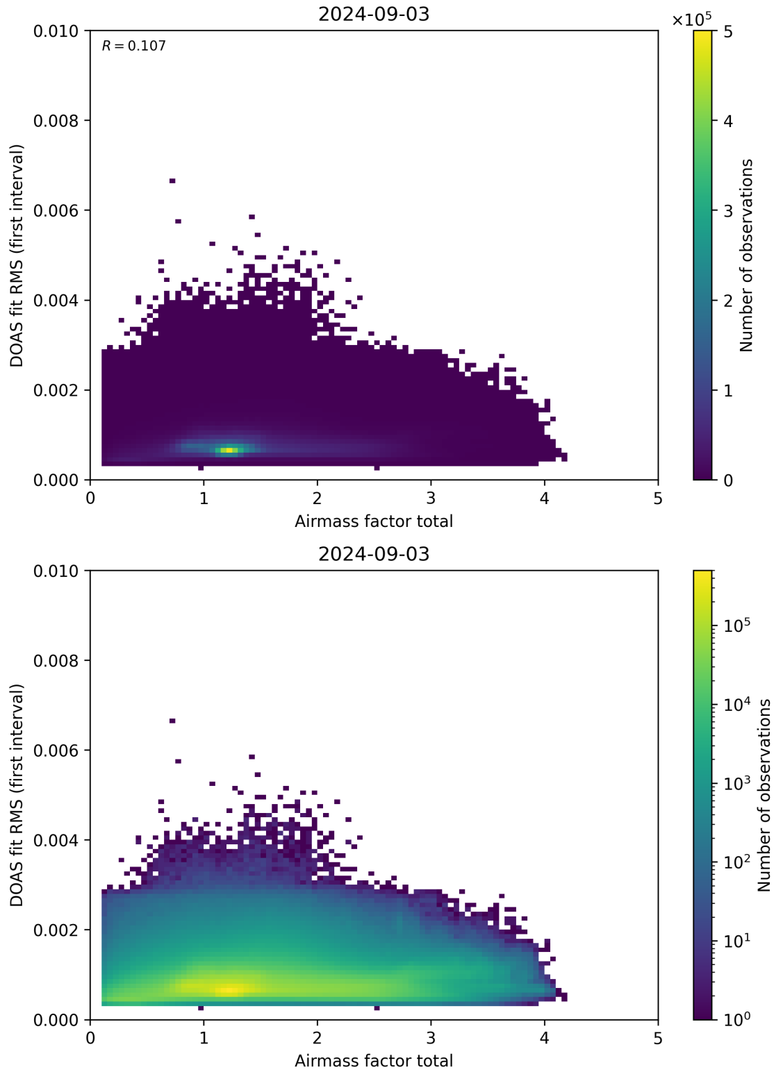
Figure 97: Scatter density plot of “Airmass factor total” against “DOAS fit RMS (first interval)” for 2024-09-02 to 2024-09-04.
