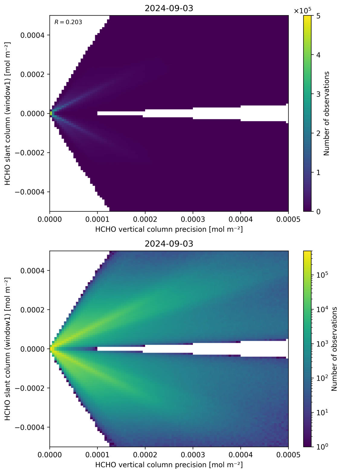
Figure 142: Scatter density plot of “HCHO vertical column precision” against “HCHO slant column (window1)” for 2024-09-02 to 2024-09-04.
