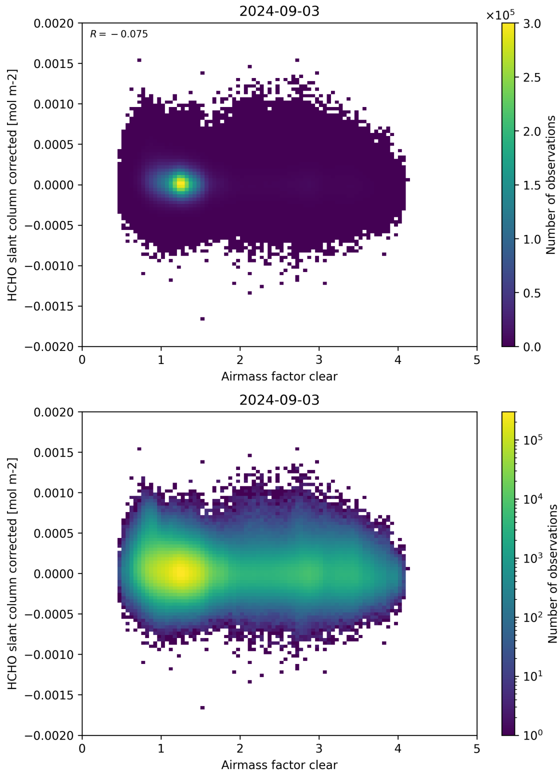
Figure 74: Scatter density plot of “Airmass factor clear” against “HCHO slant column corrected” for 2024-09-02 to 2024-09-04.
