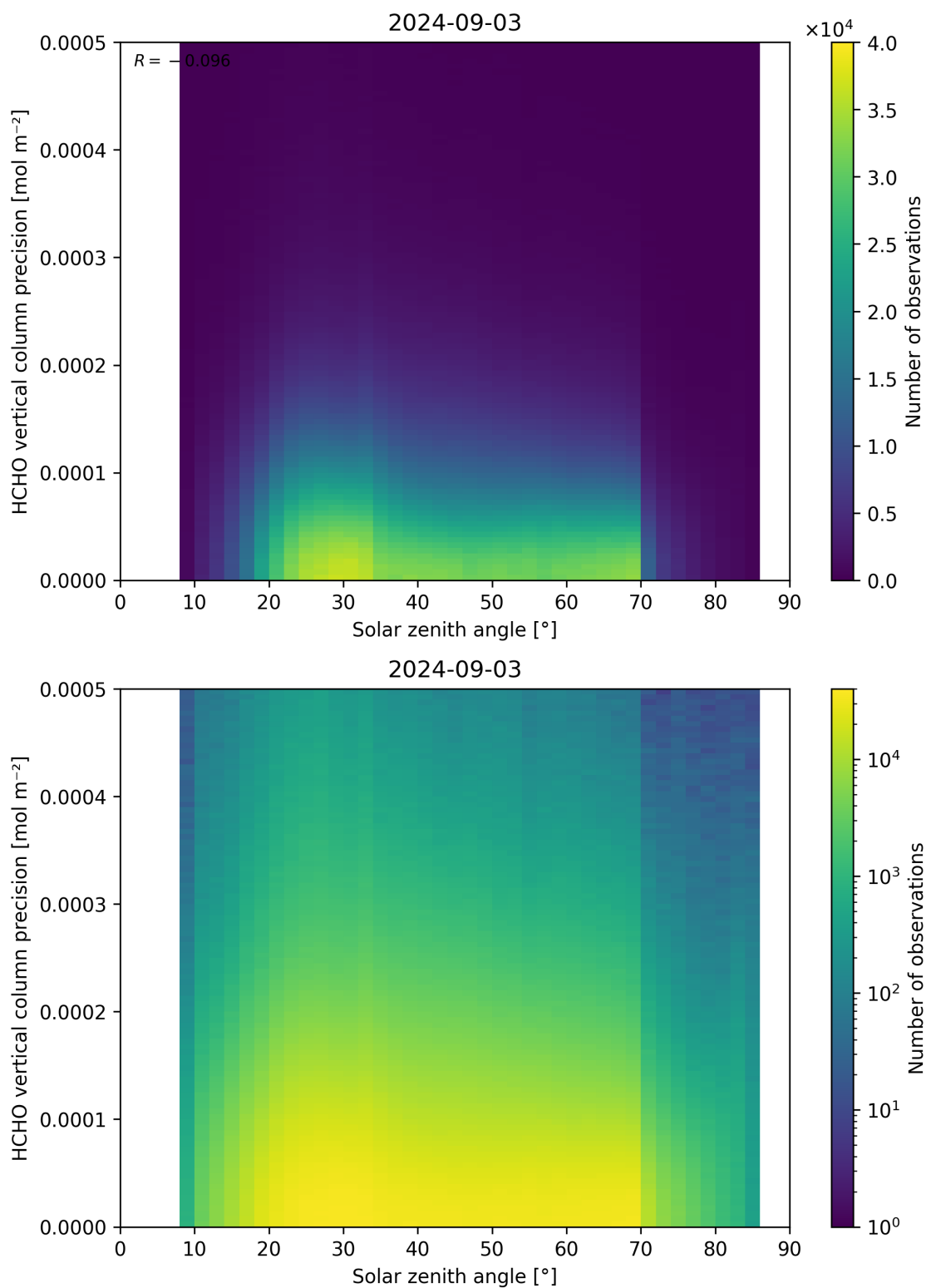
Figure 179: Scatter density plot of “Solar zenith angle” against “HCHO vertical column precision” for 2024-09-02 to 2024-09-04.
