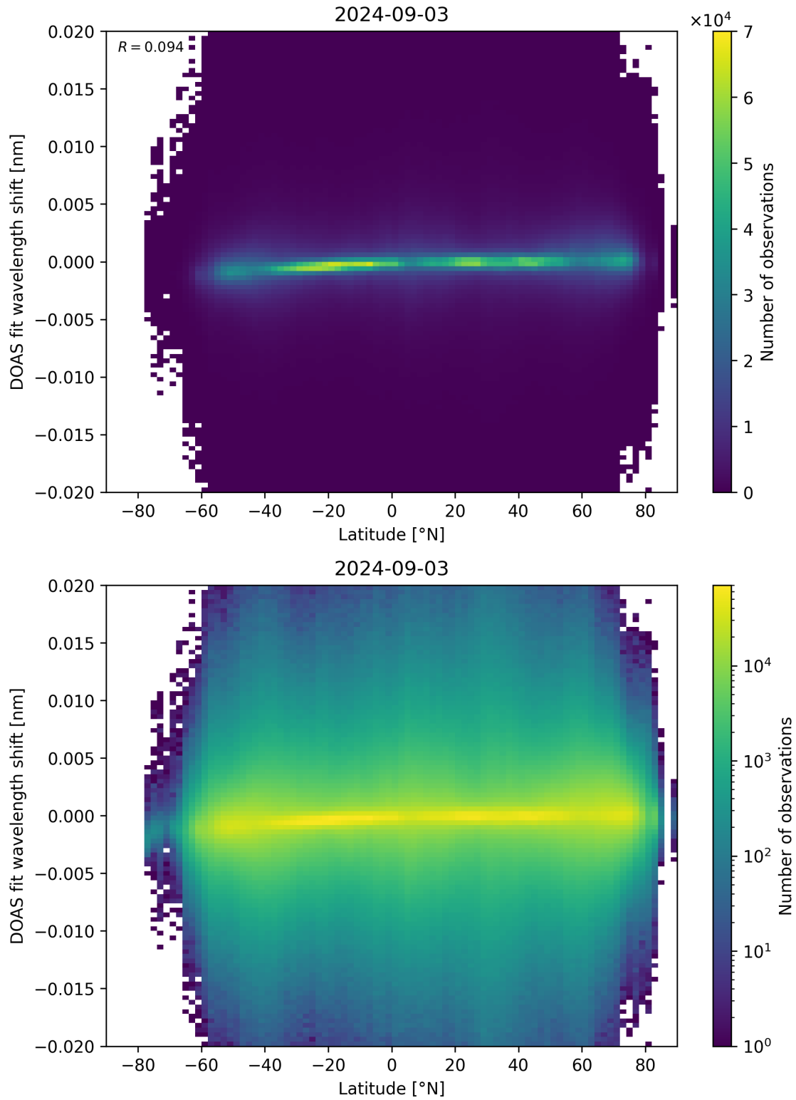
Figure 154: Scatter density plot of “Latitude” against “DOAS fit wavelength shift” for 2024-09-02 to 2024-09-04.
