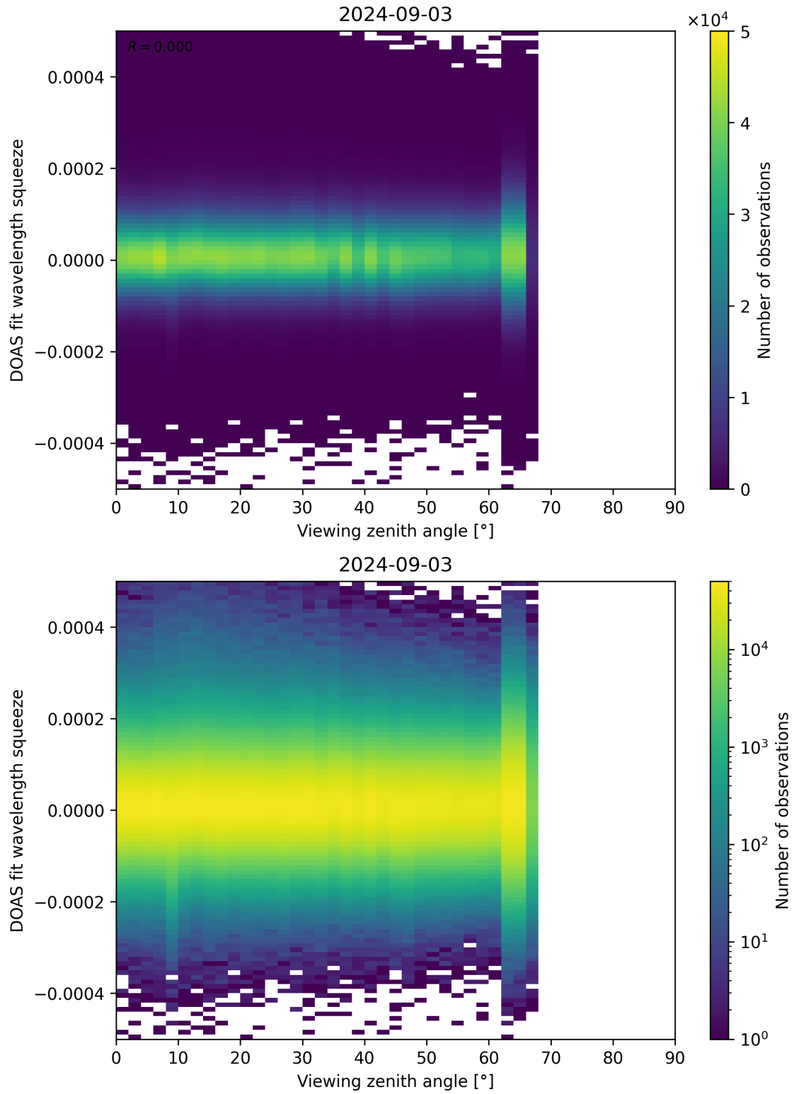
Figure 184: Scatter density plot of “Viewing zenith angle” against “DOAS fit wavelength squeeze” for 2024-09-02 to 2024-09-04.
