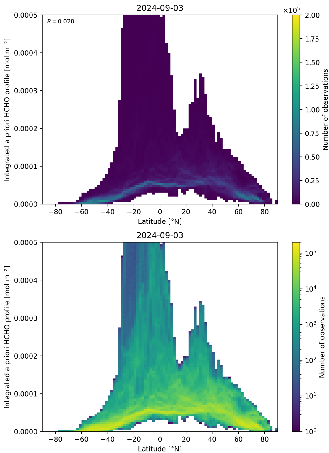
Figure 166: Scatter density plot of “Latitude” against “Integrated a priori HCHO profile” for 2024-09-02 to 2024-09-04.
