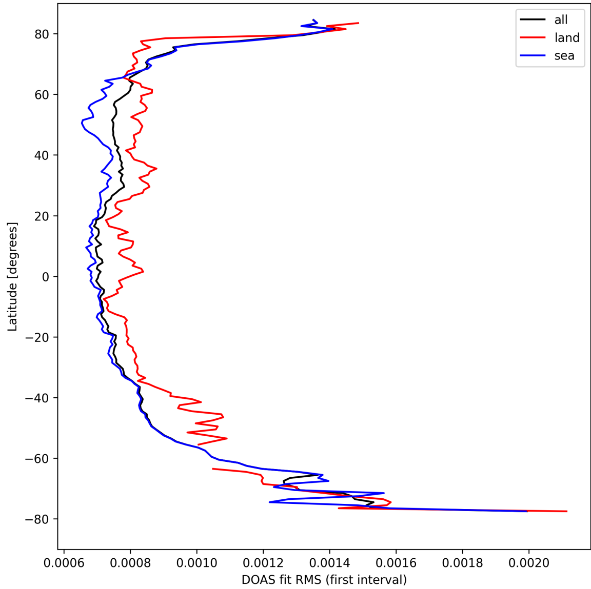
Figure 32: Zonal average of “DOAS fit RMS (first interval)” for 2024-09-02 to 2024-09-04.
