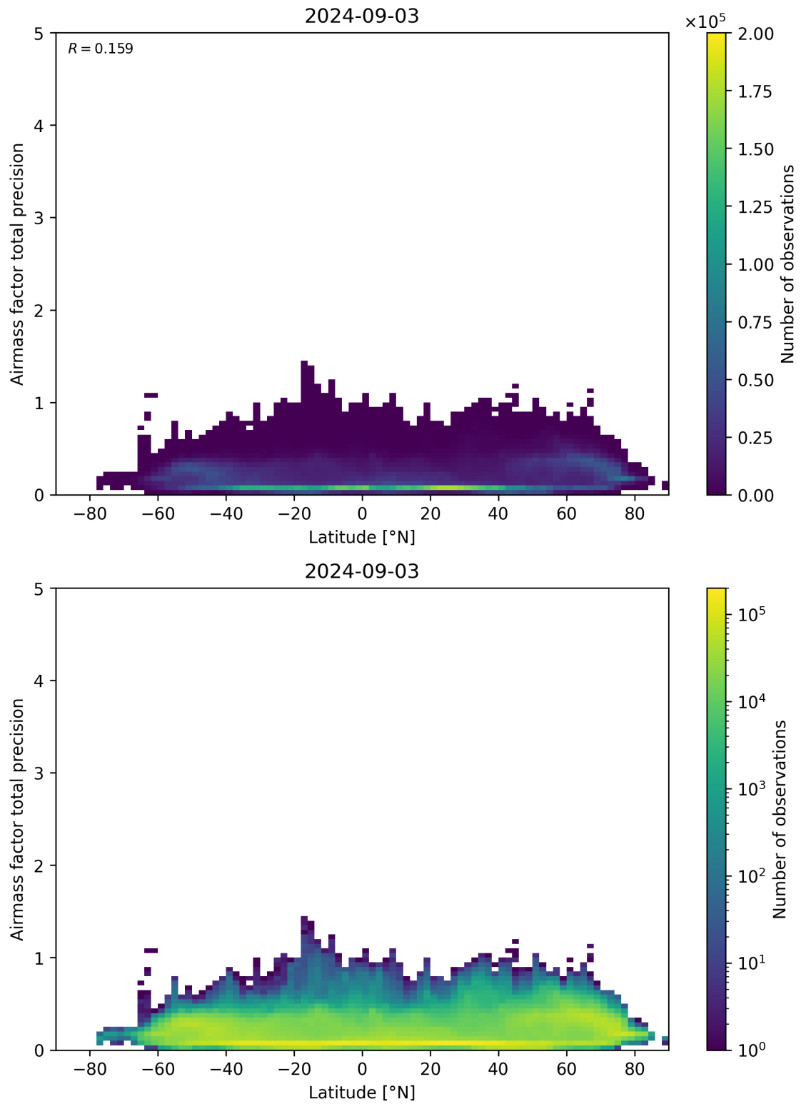
Figure 162: Scatter density plot of “Latitude” against “Airmass factor total precision” for 2024-09-02 to 2024-09-04.
