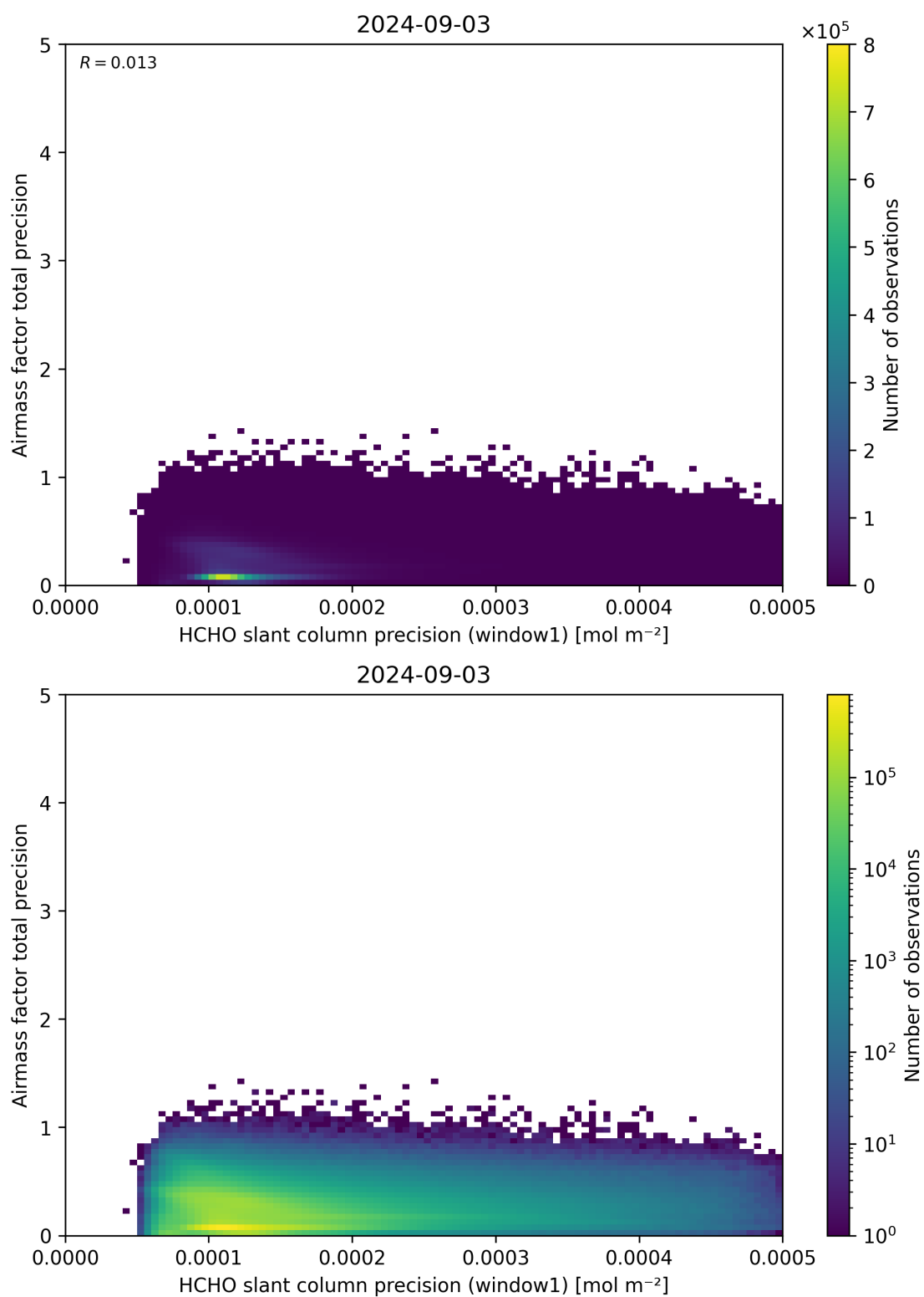
Figure 95: Scatter density plot of “HCHO slant column precision (window1)” against “Airmass factor total precision” for 2024-09-02 to 2024-09-04.
