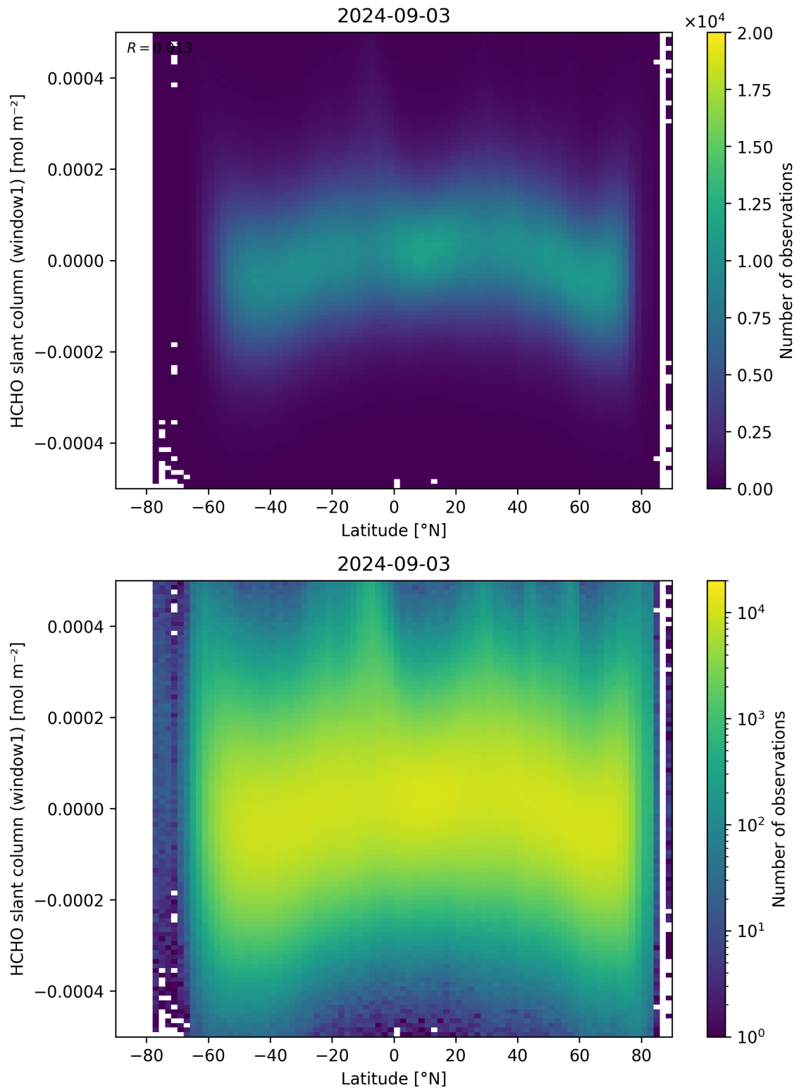
Figure 159: Scatter density plot of “Latitude” against “HCHO slant column (window1)” for 2024-09-02 to 2024-09-04.
