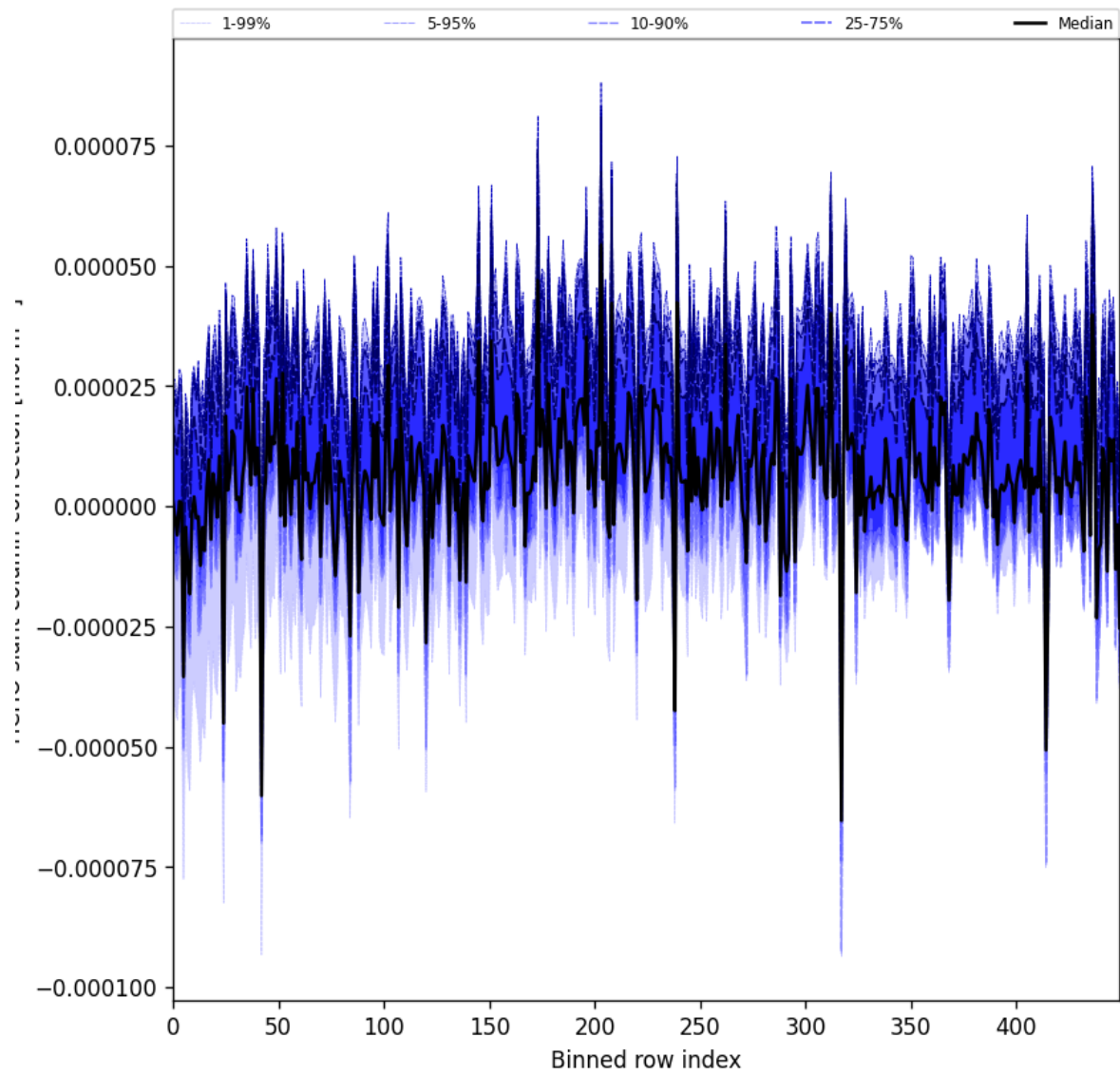
Figure 61: Along track statistics of “HCHO slant column correction” for 2024-09-02 to 2024-09-04
