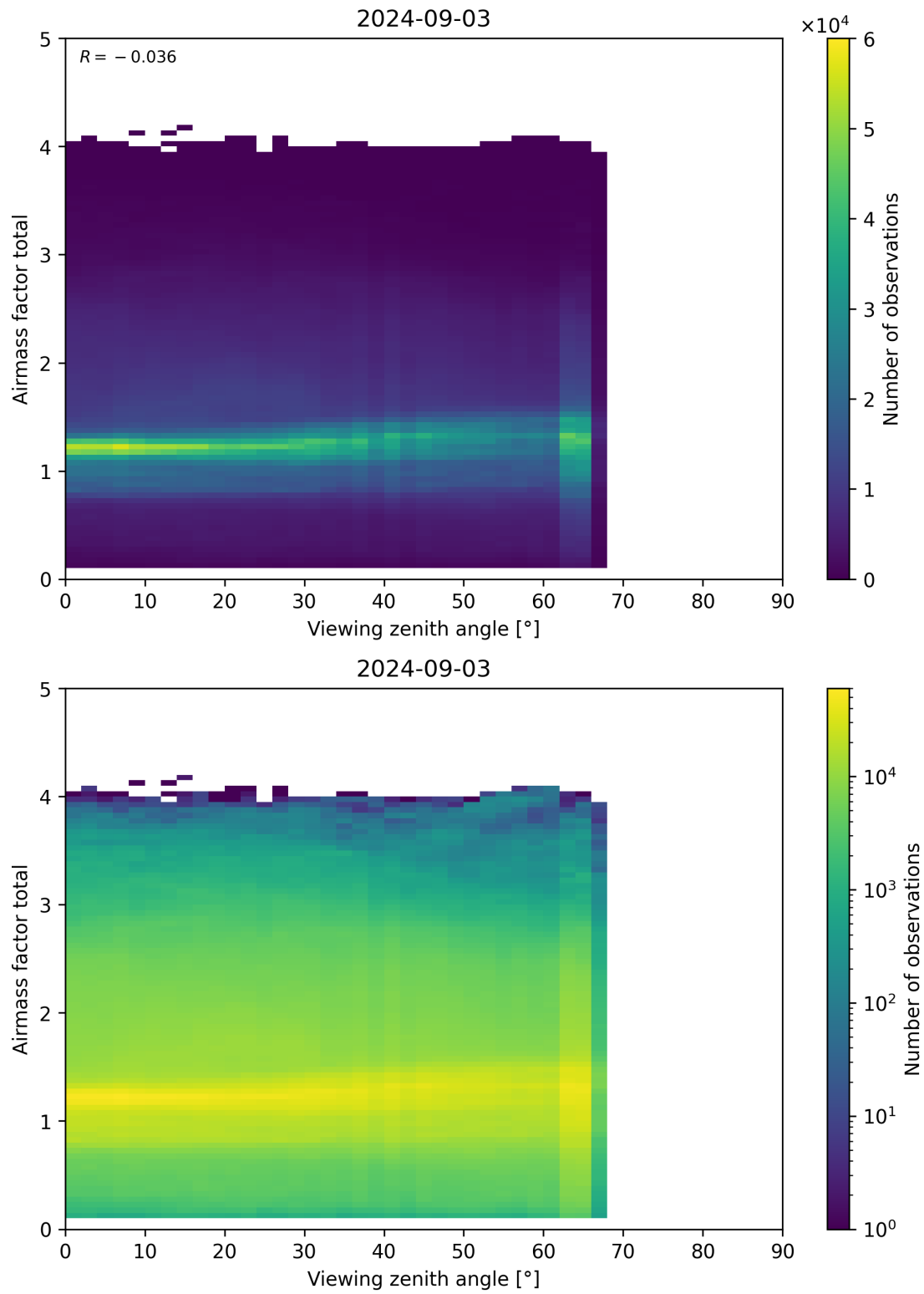
Figure 190: Scatter density plot of “Viewing zenith angle” against “Airmass factor total” for 2024-09-02 to 2024-09-04.
