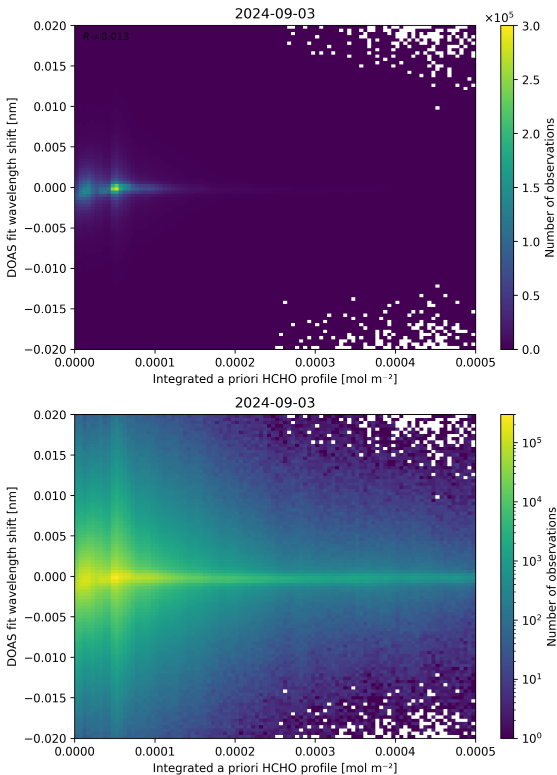
Figure 149: Scatter density plot of “Integrated a priori HCHO profile” against “DOAS fit wavelength shift” for 2024-09-02 to 2024-09-04.
