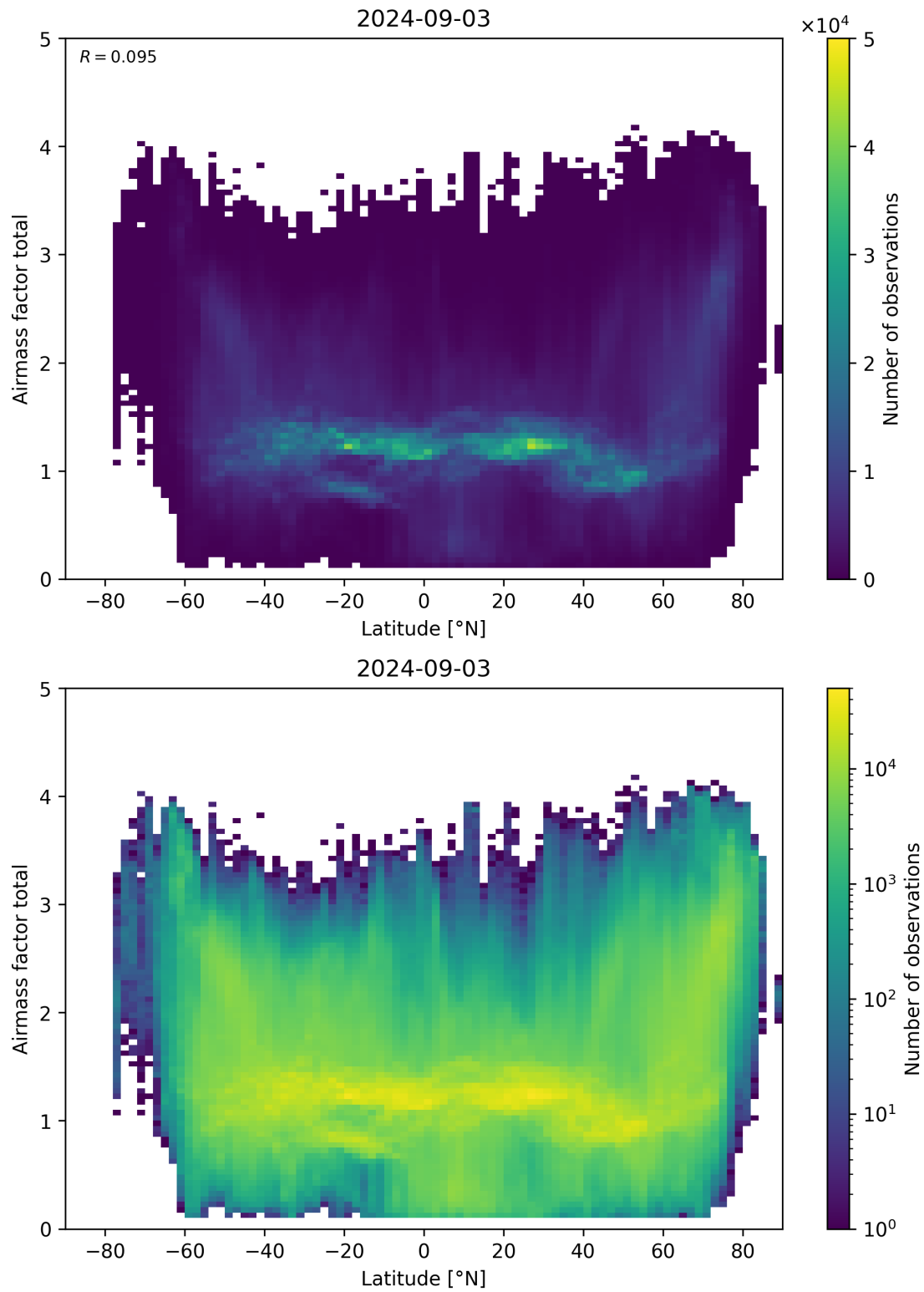
Figure 161: Scatter density plot of “Latitude” against “Airmass factor total” for 2024-09-02 to 2024-09-04.
