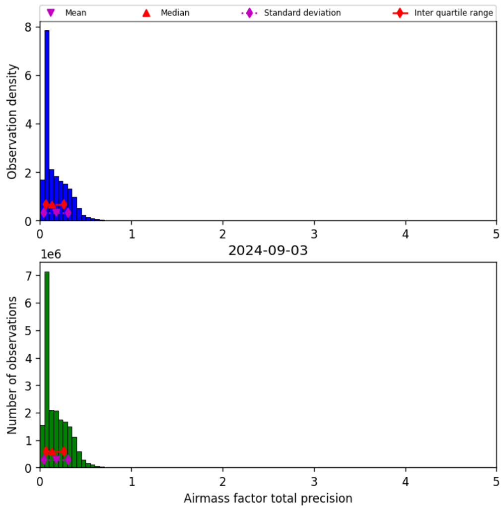
Figure 41: Histogram of “Airmass factor total precision” for 2024-09-02 to 2024-09-04
