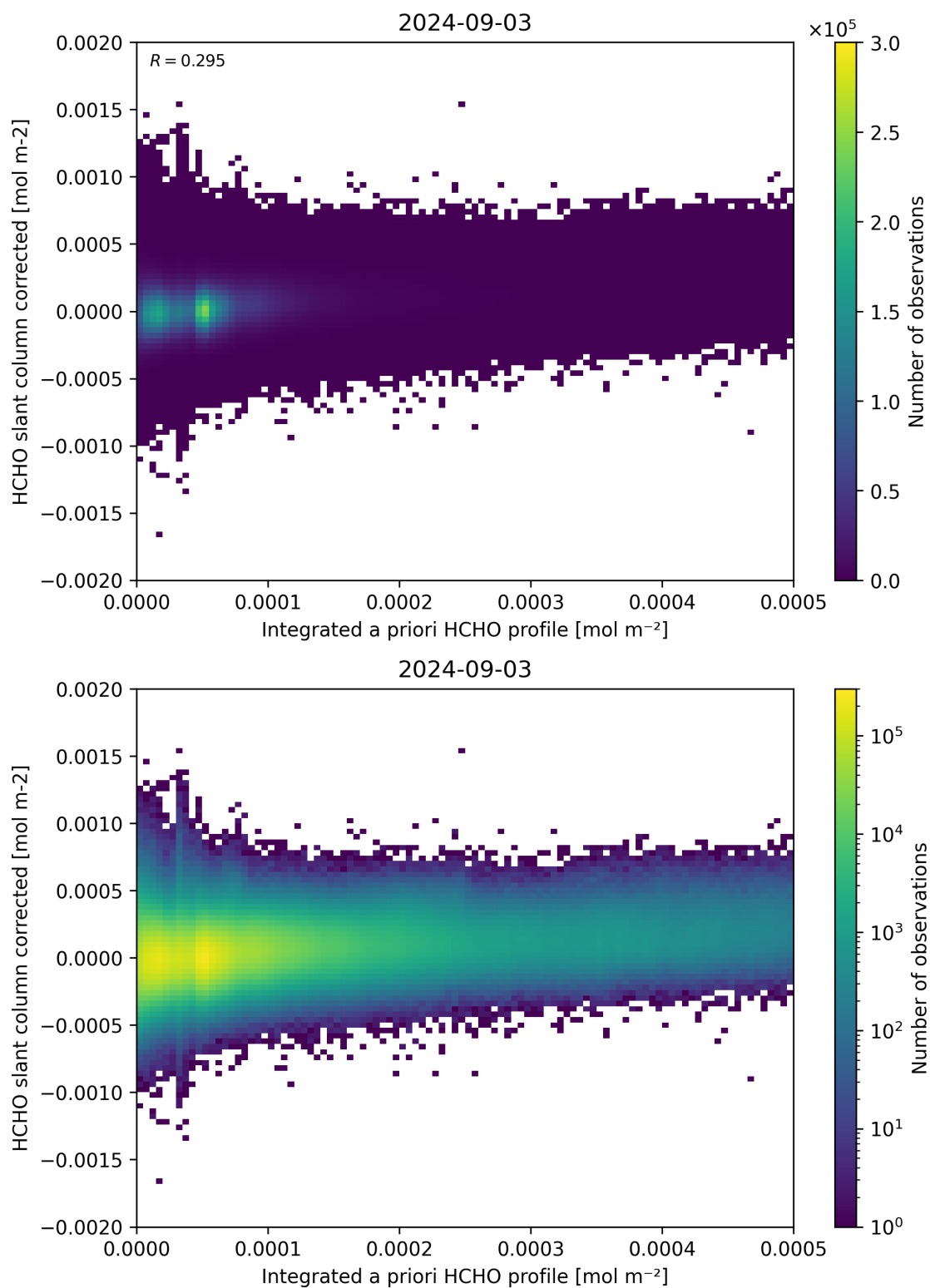
Figure 151: Scatter density plot of “Integrated a priori HCHO profile” against “HCHO slant column corrected” for 2024-09-02 to 2024-09-04.
