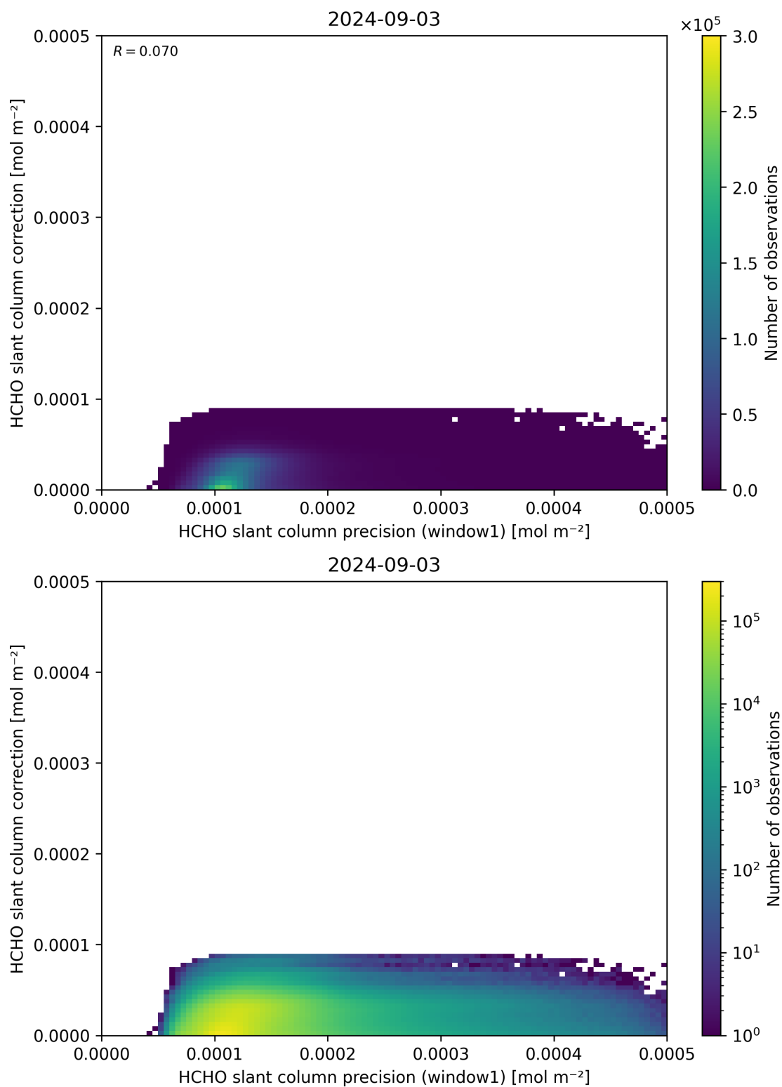
Figure 93: Scatter density plot of “HCHO slant column precision (window1)” against “HCHO slant column correction” for 2024-09-02 to 2024-09-04.
