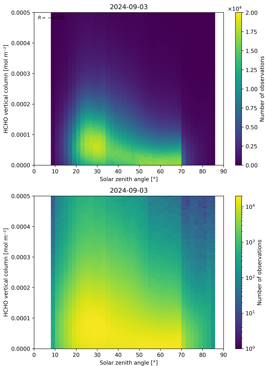
Figure 177: Scatter density plot of “Solar zenith angle” against “HCHO vertical column” for 2024-09-02 to 2024-09-04.
