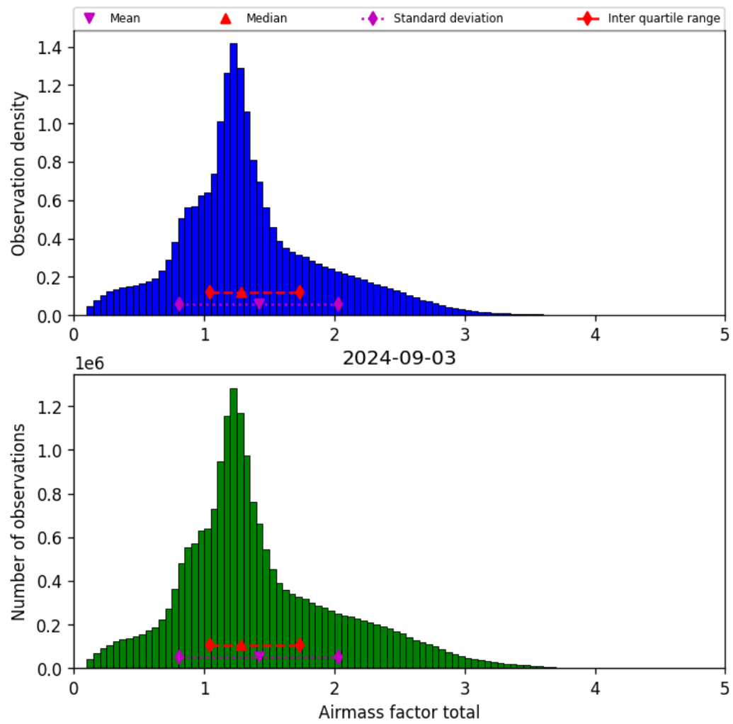
Figure 40: Histogram of “Airmass factor total” for 2024-09-02 to 2024-09-04
