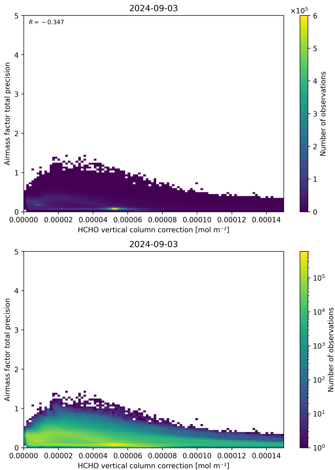
Figure 121: Scatter density plot of “HCHO vertical column correction” against “Airmass factor total precision” for 2024-09-02 to 2024-09-04.
