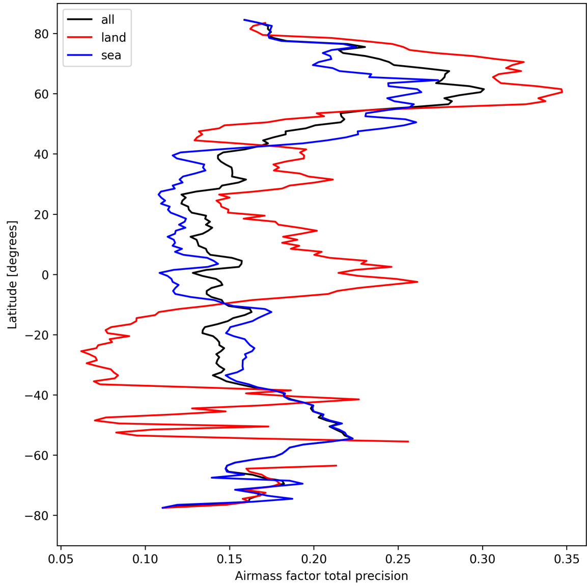
Figure 27: Zonal average of “Airmass factor total precision” for 2024-09-02 to 2024-09-04.
