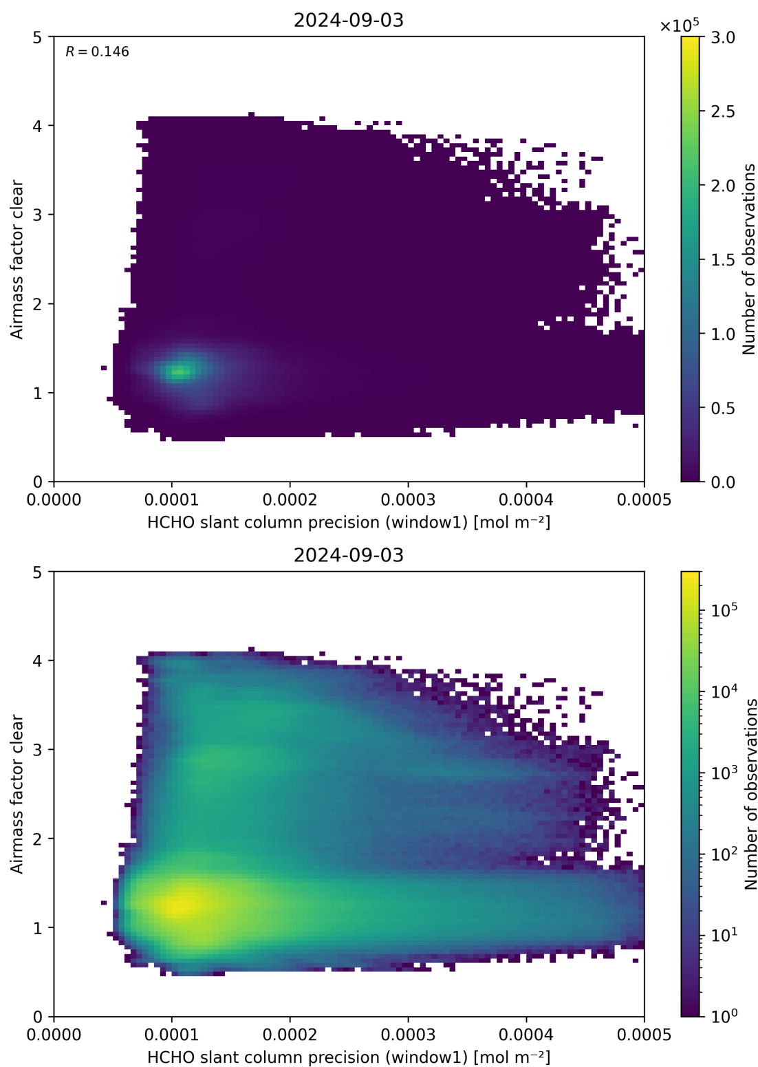
Figure 91: Scatter density plot of “HCHO slant column precision (window1)” against “Airmass factor clear” for 2024-09-02 to 2024-09-04.
