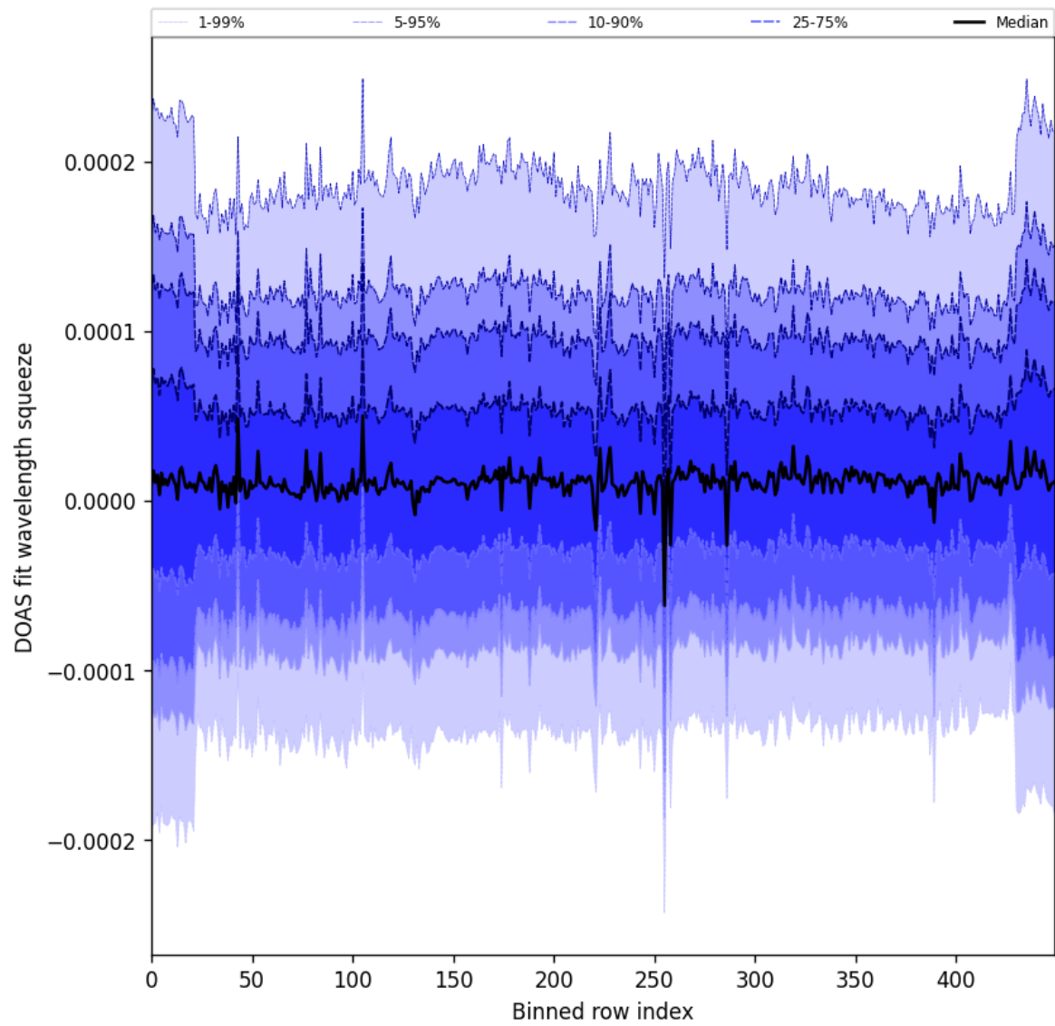
Figure 59: Along track statistics of “DOAS fit wavelength squeeze” for 2024-09-02 to 2024-09-04
