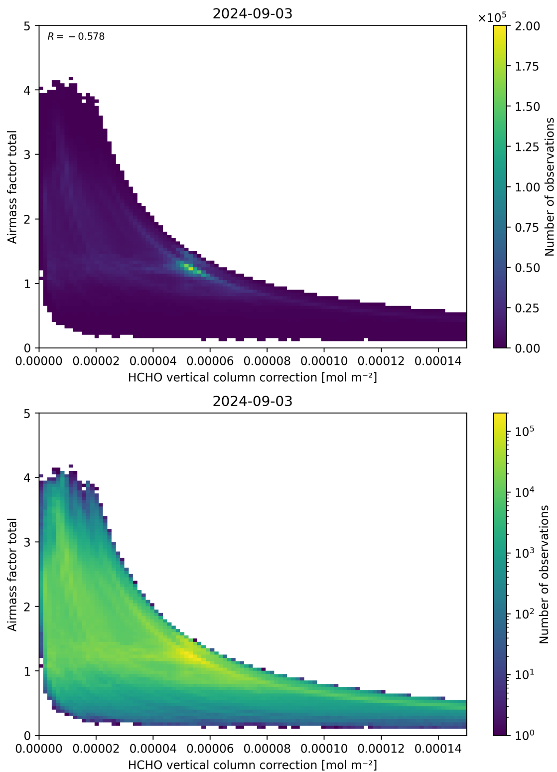
Figure 120: Scatter density plot of “HCHO vertical column correction” against “Airmass factor total” for 2024-09-02 to 2024-09-04.
