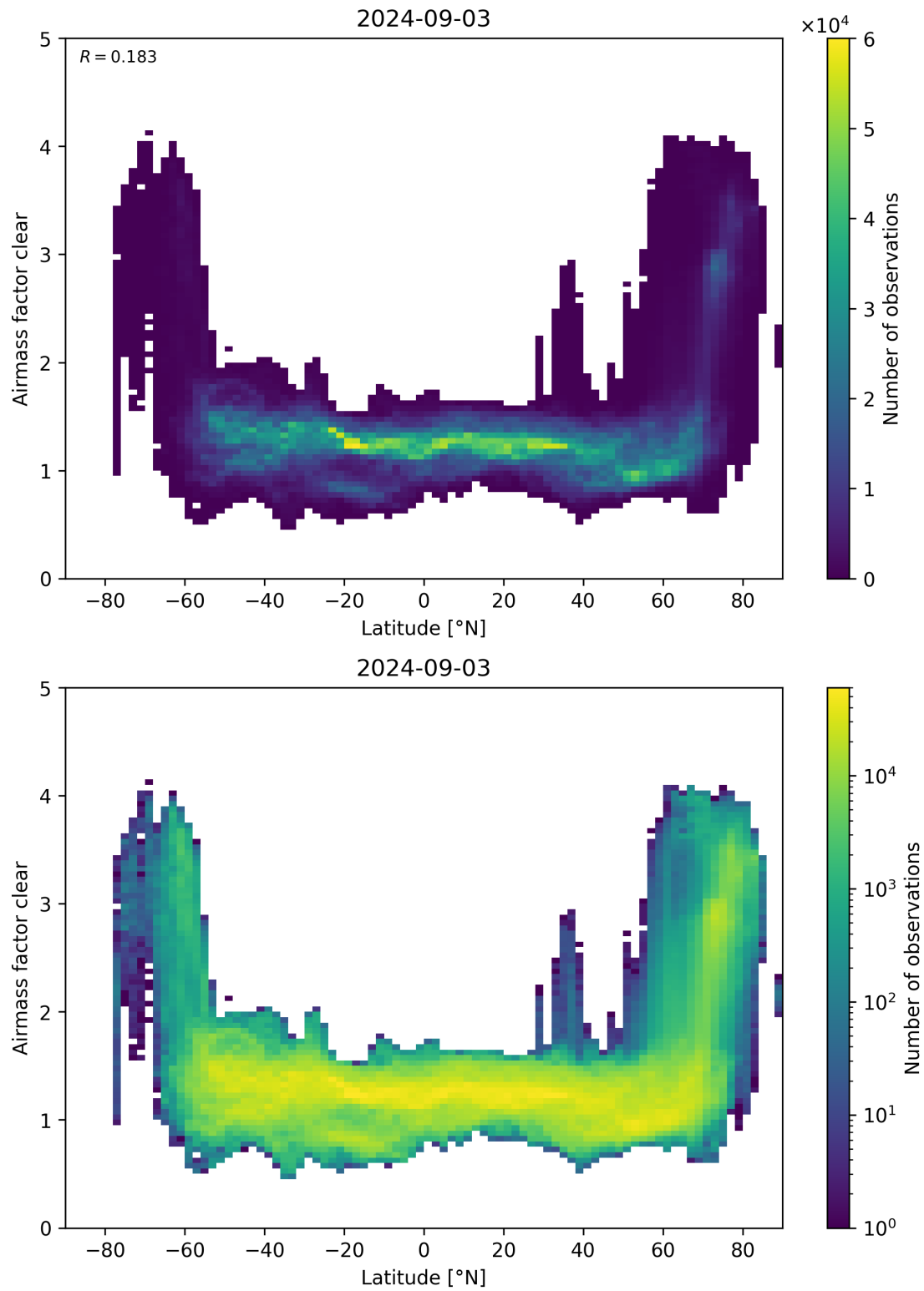
Figure 156: Scatter density plot of “Latitude” against “Airmass factor clear” for 2024-09-02 to 2024-09-04.
