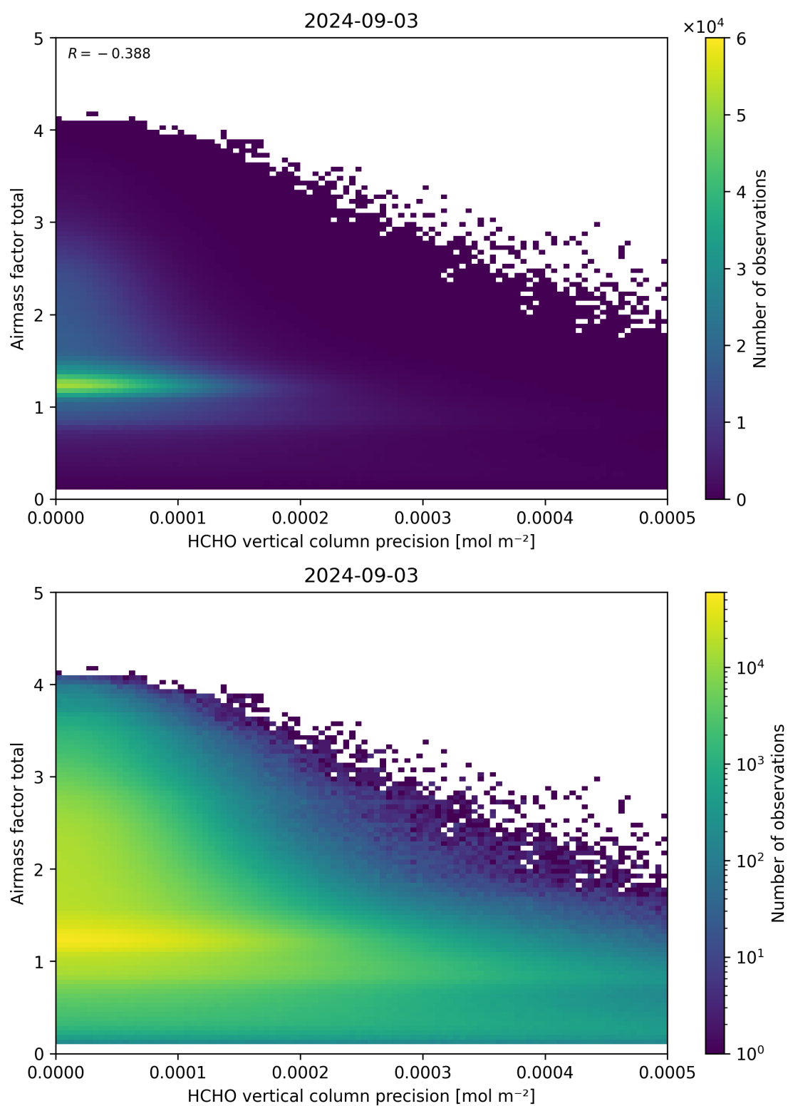
Figure 144: Scatter density plot of “HCHO vertical column precision” against “Airmass factor total” for 2024-09-02 to 2024-09-04.
