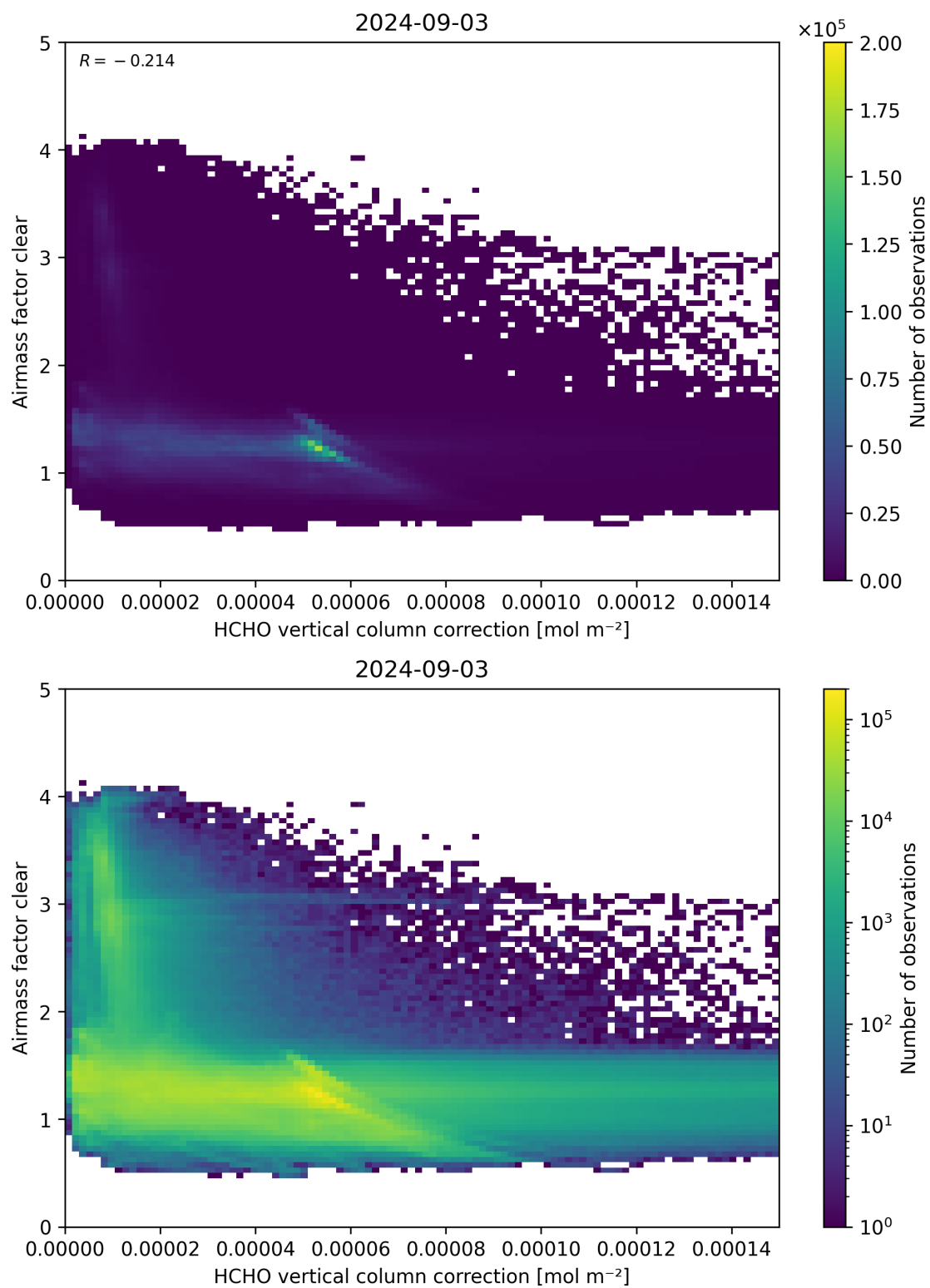
Figure 115: Scatter density plot of “HCHO vertical column correction” against “Airmass factor clear” for 2024-09-02 to 2024-09-04.
