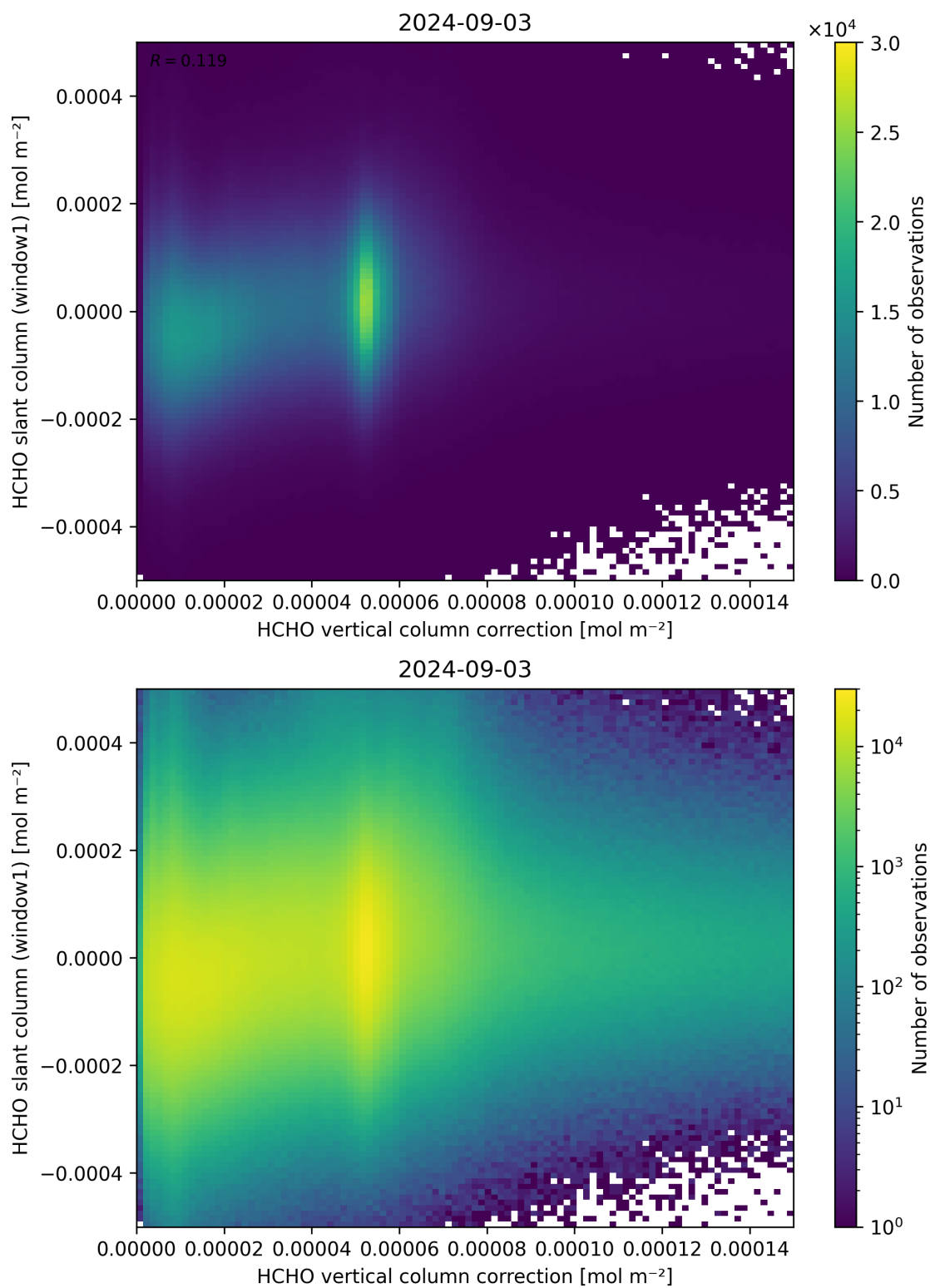
Figure 118: Scatter density plot of “HCHO vertical column correction” against “HCHO slant column (window1)” for 2024-09-02 to 2024-09-04.
