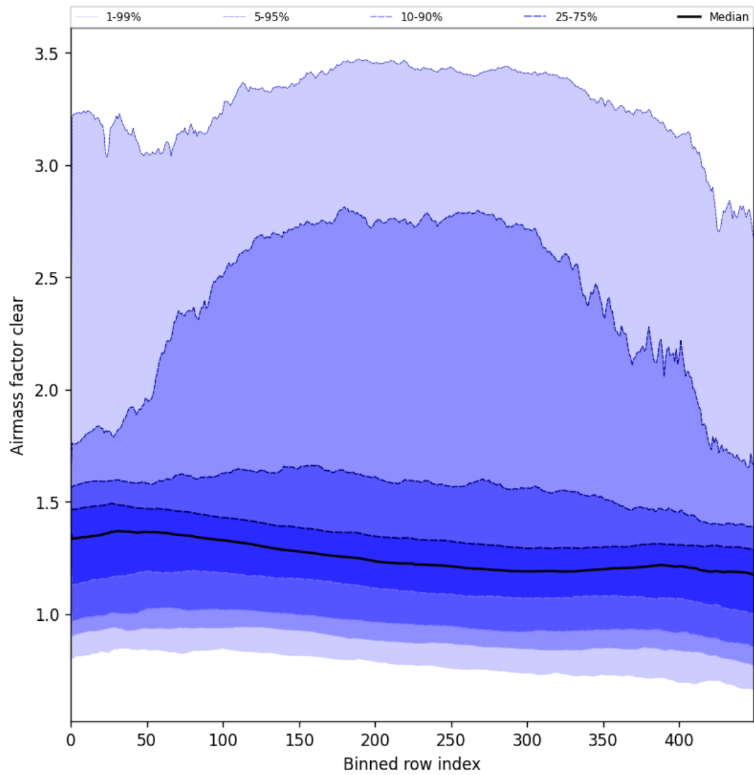
Figure 56: Along track statistics of “Airmass factor clear” for 2024-09-02 to 2024-09-04
