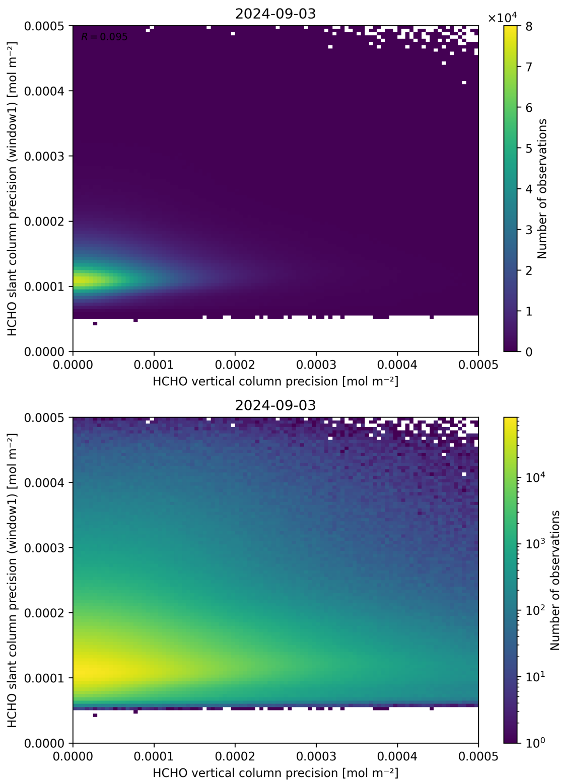
Figure 143: Scatter density plot of “HCHO vertical column precision” against “HCHO slant column precision (window1)” for 2024-09-02 to 2024-09-04.
