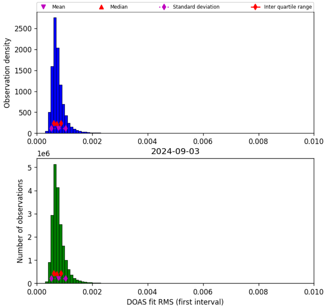
Figure 46: Histogram of “DOAS fit RMS (first interval)” for 2024-09-02 to 2024-09-04
