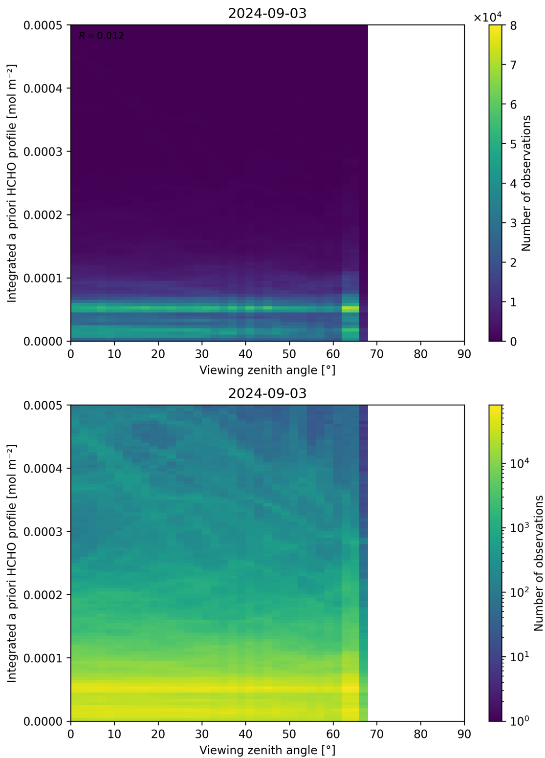
Figure 195: Scatter density plot of “Viewing zenith angle” against “Integrated a priori HCHO profile” for 2024-09-02 to 2024-09-04.
