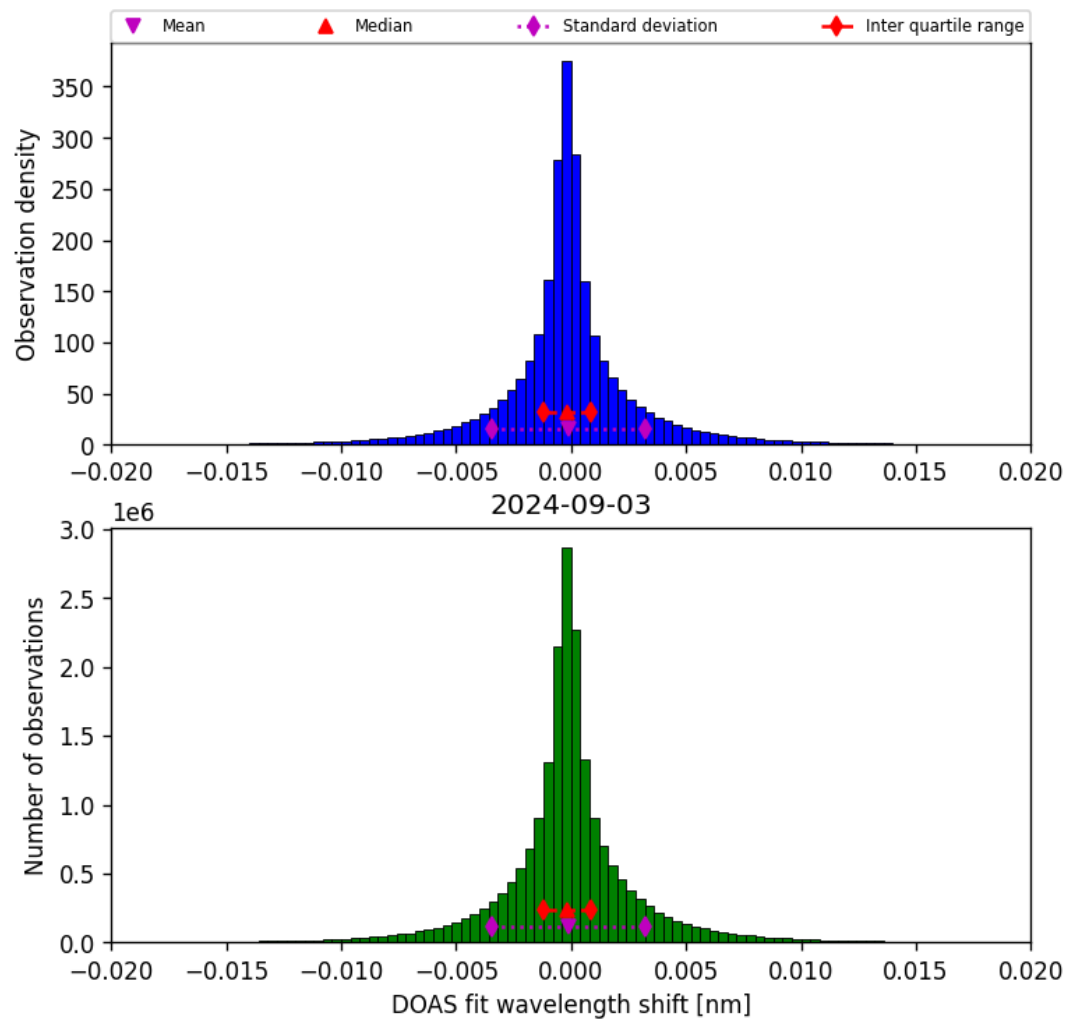
Figure 44: Histogram of “DOAS fit wavelength shift” for 2024-09-02 to 2024-09-04
