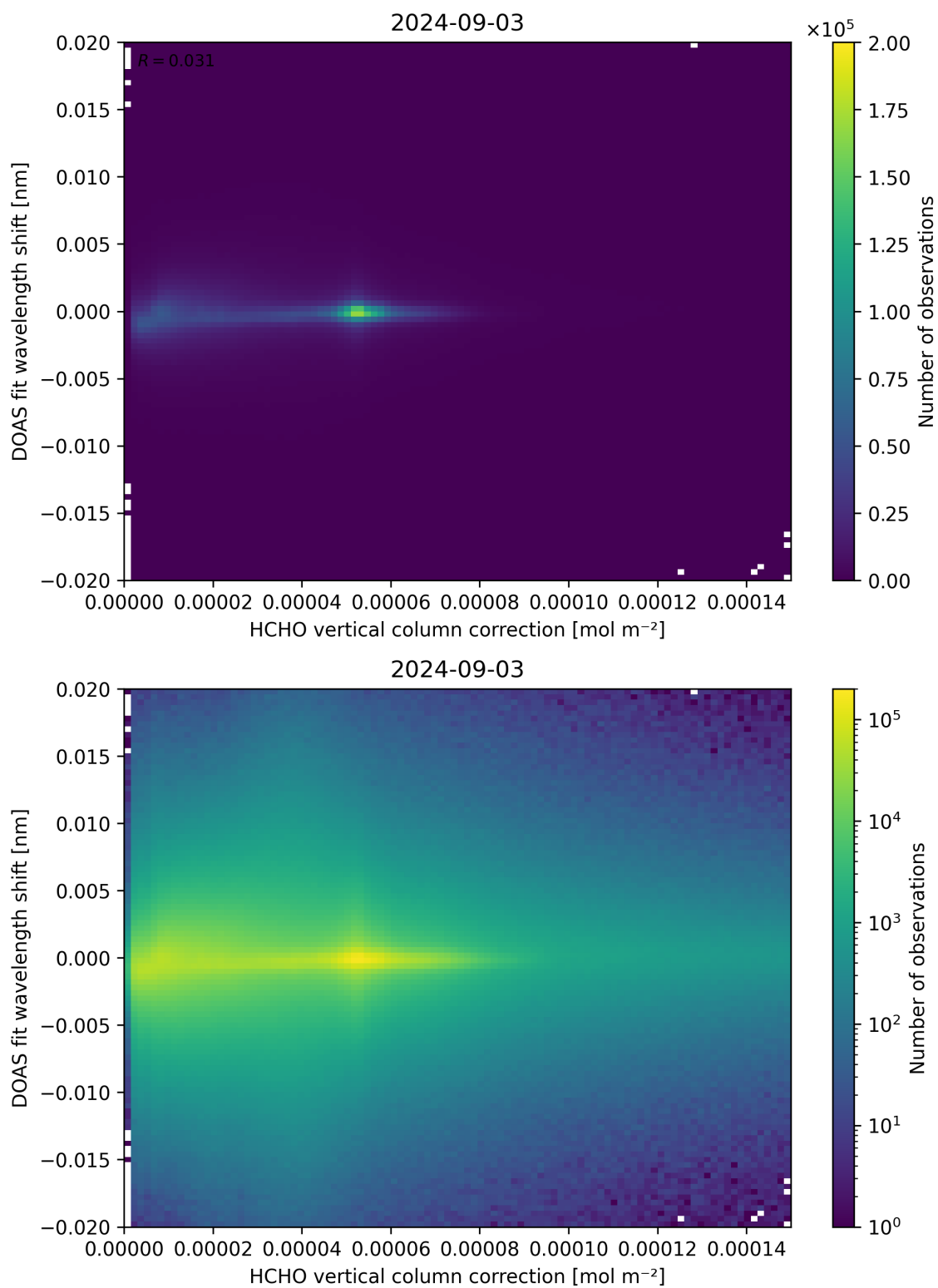
Figure 113: Scatter density plot of “HCHO vertical column correction” against “DOAS fit wavelength shift” for 2024-09-02 to 2024-09-04.
