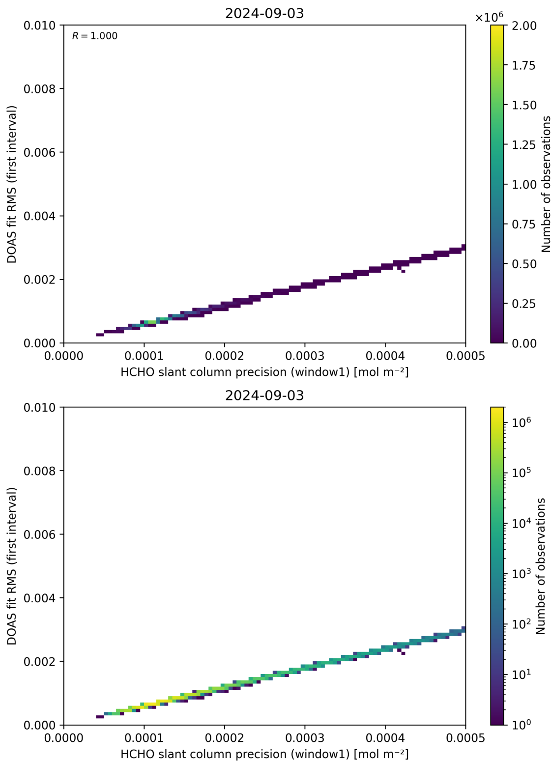
Figure 88: Scatter density plot of “HCHO slant column precision (window1)” against “DOAS fit RMS (first interval)” for 2024-09-02 to 2024-09-04.
