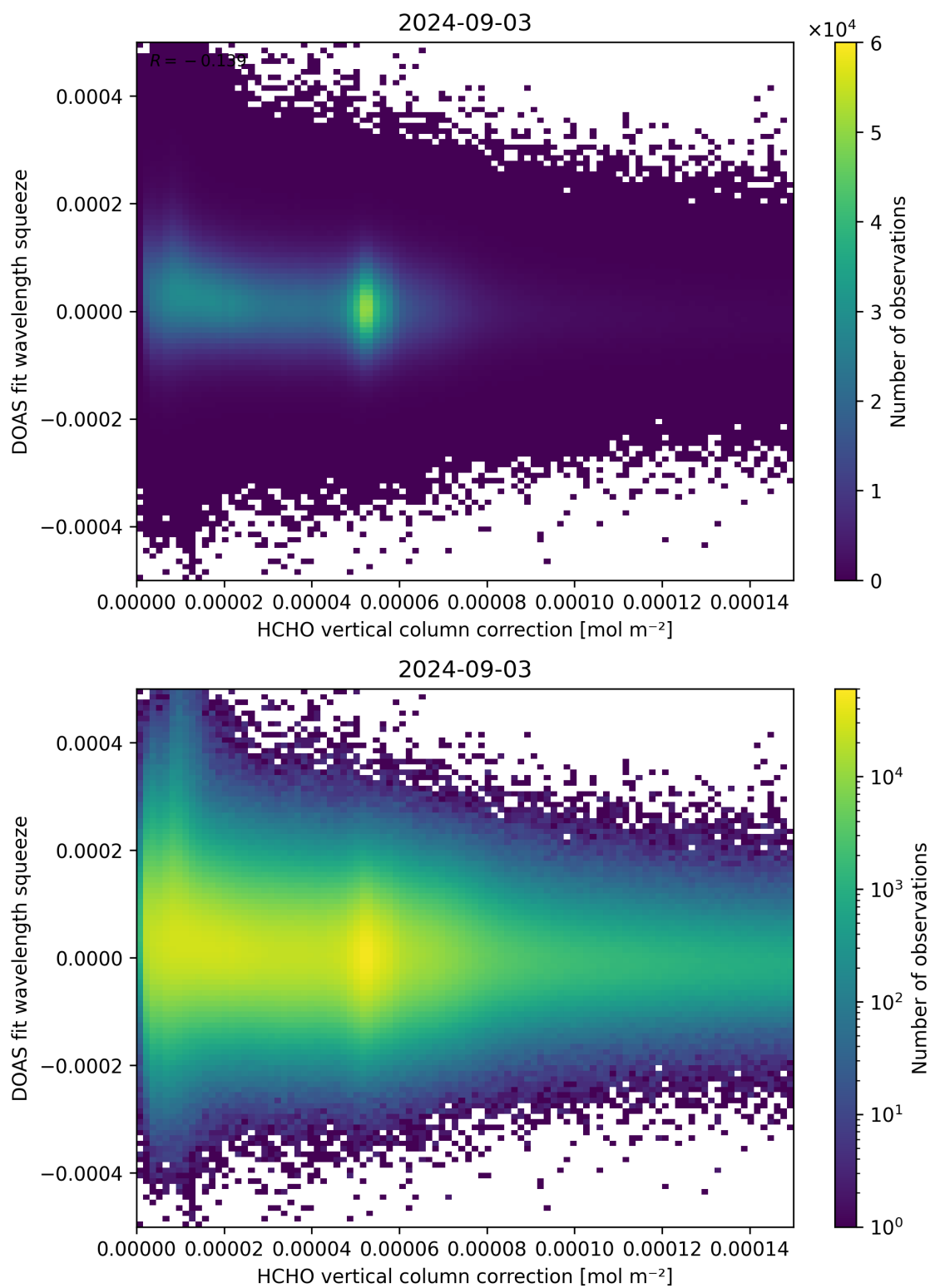
Figure 114: Scatter density plot of “HCHO vertical column correction” against “DOAS fit wavelength squeeze” for 2024-09-02 to 2024-09-04.
