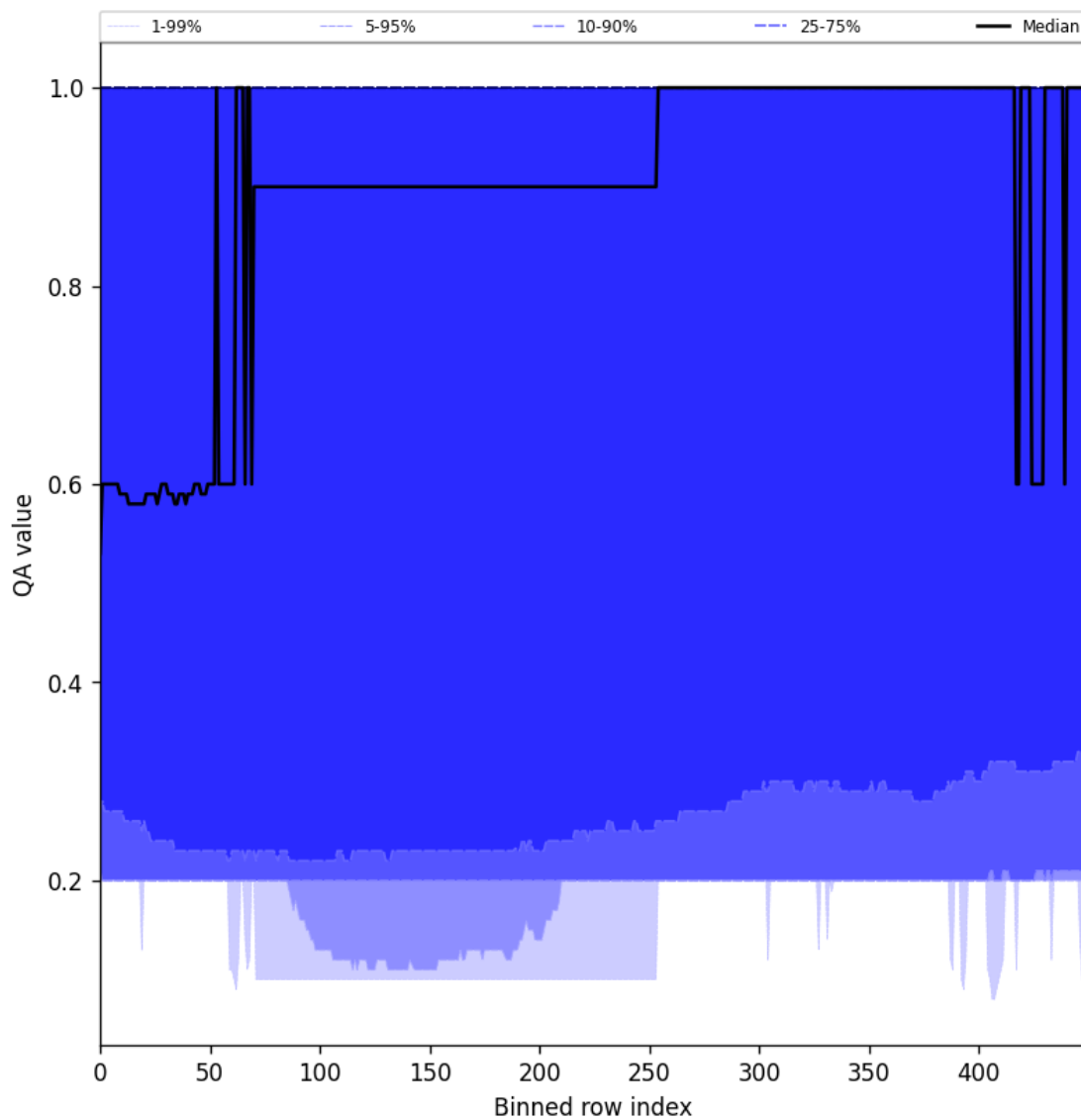
Figure 48: Along track statistics of “QA value” for 2024-09-02 to 2024-09-04
