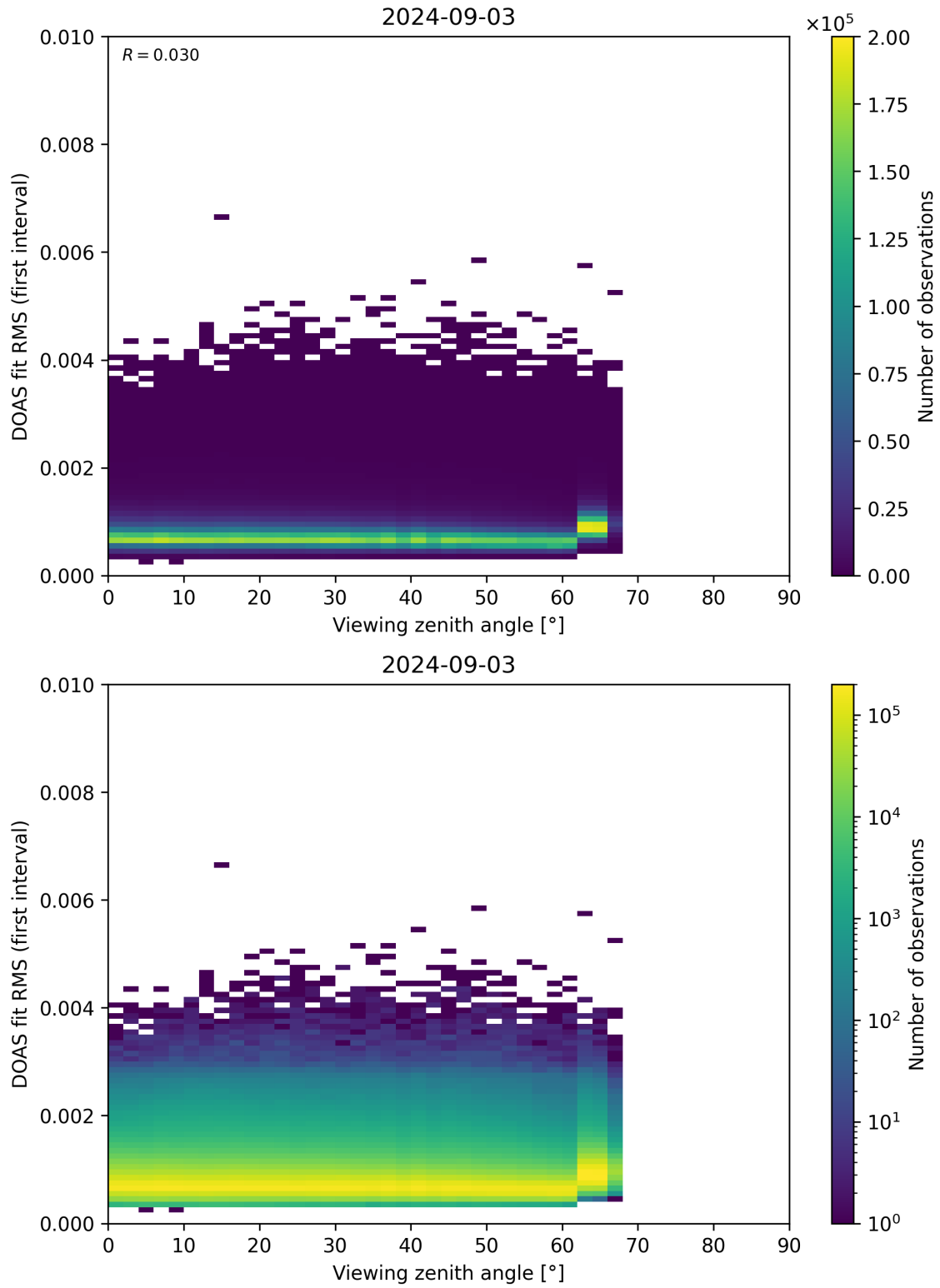
Figure 182: Scatter density plot of “Viewing zenith angle” against “DOAS fit RMS (first interval)” for 2024-09-02 to 2024-09-04.
