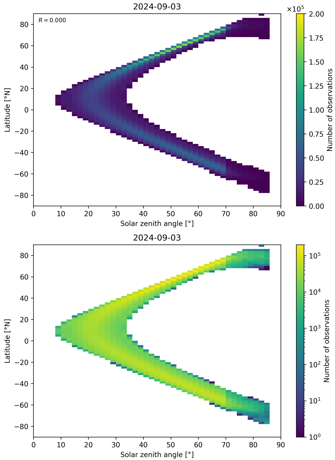
Figure 181: Scatter density plot of “Solar zenith angle” against “Latitude” for 2024-09-02 to 2024-09-04.
