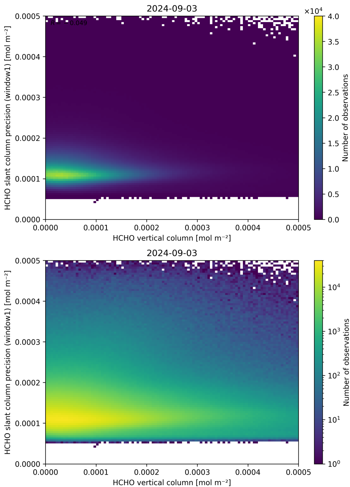
Figure 130: Scatter density plot of “HCHO vertical column” against “HCHO slant column precision (window1)” for 2024-09-02 to 2024-09-04.
