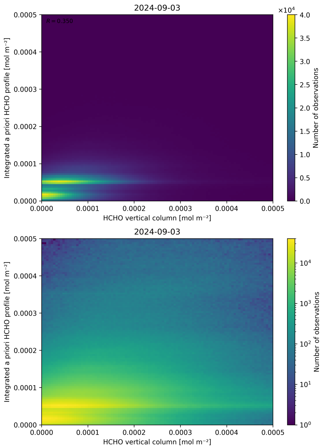
Figure 135: Scatter density plot of “HCHO vertical column” against “Integrated a priori HCHO profile” for 2024-09-02 to 2024-09-04.
