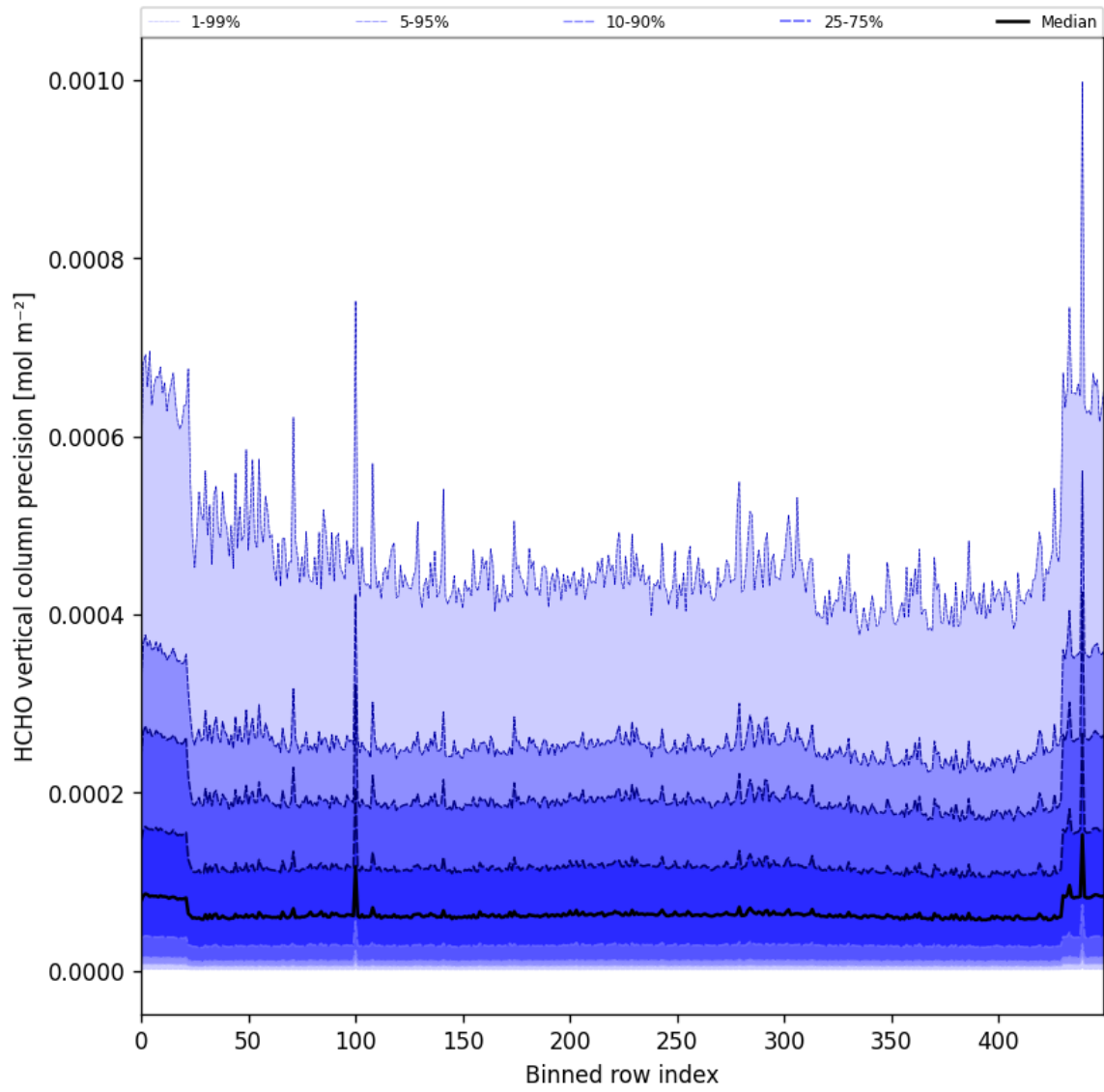
Figure 50: Along track statistics of “HCHO vertical column precision” for 2024-09-02 to 2024-09-04
