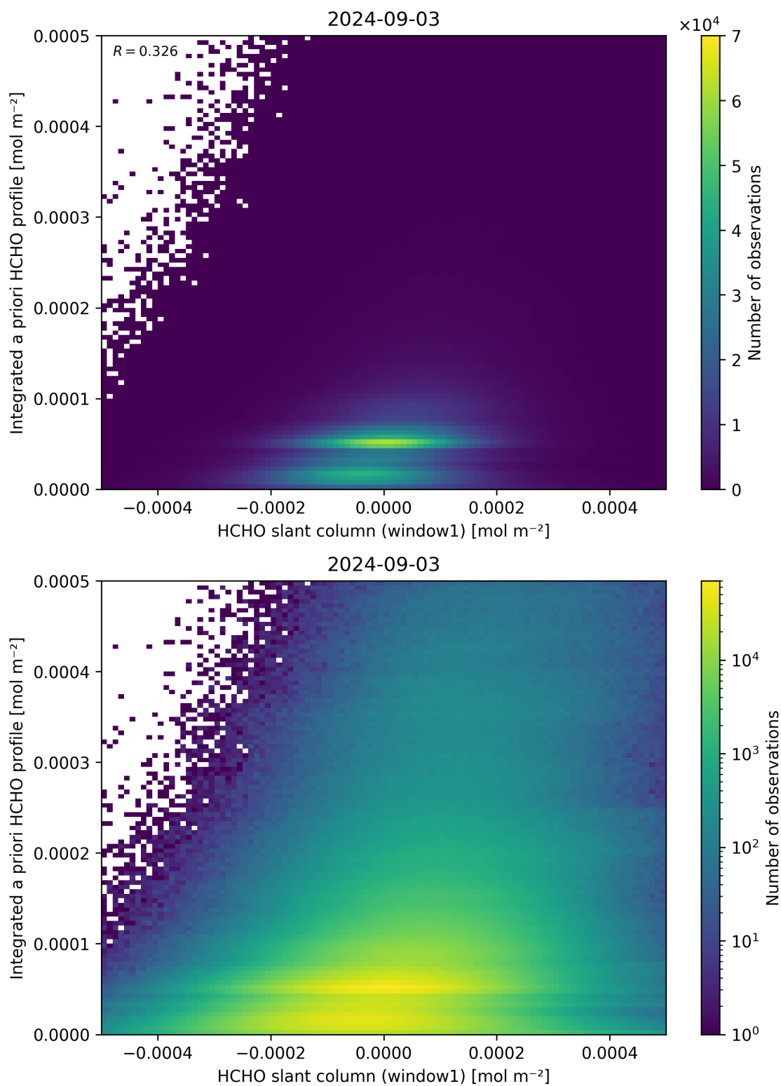
Figure 87: Scatter density plot of “HCHO slant column (window1)” against “Integrated a priori HCHO profile” for 2024-09-02 to 2024-09-04.
