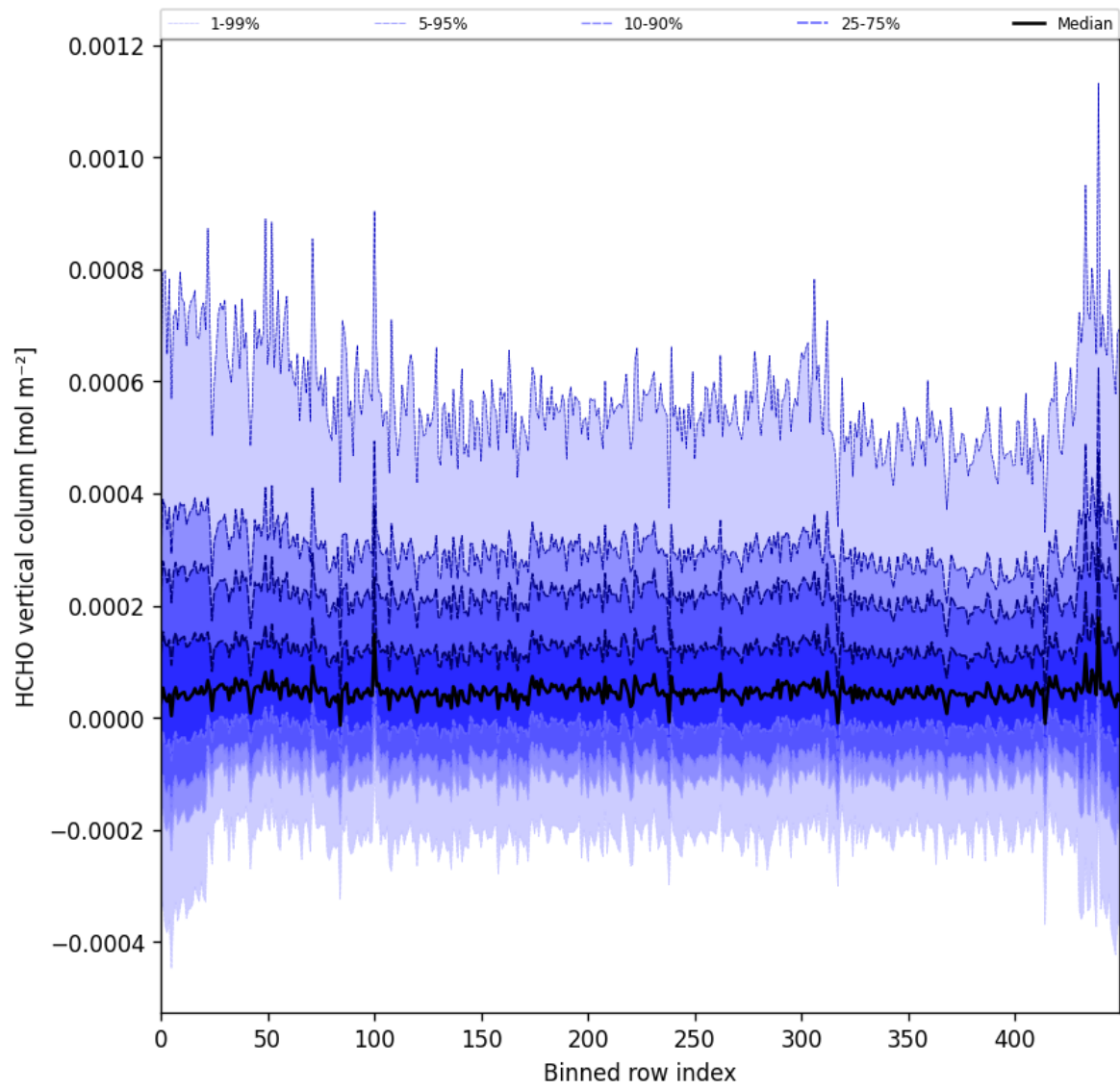
Figure 49: Along track statistics of “HCHO vertical column” for 2024-09-02 to 2024-09-04
