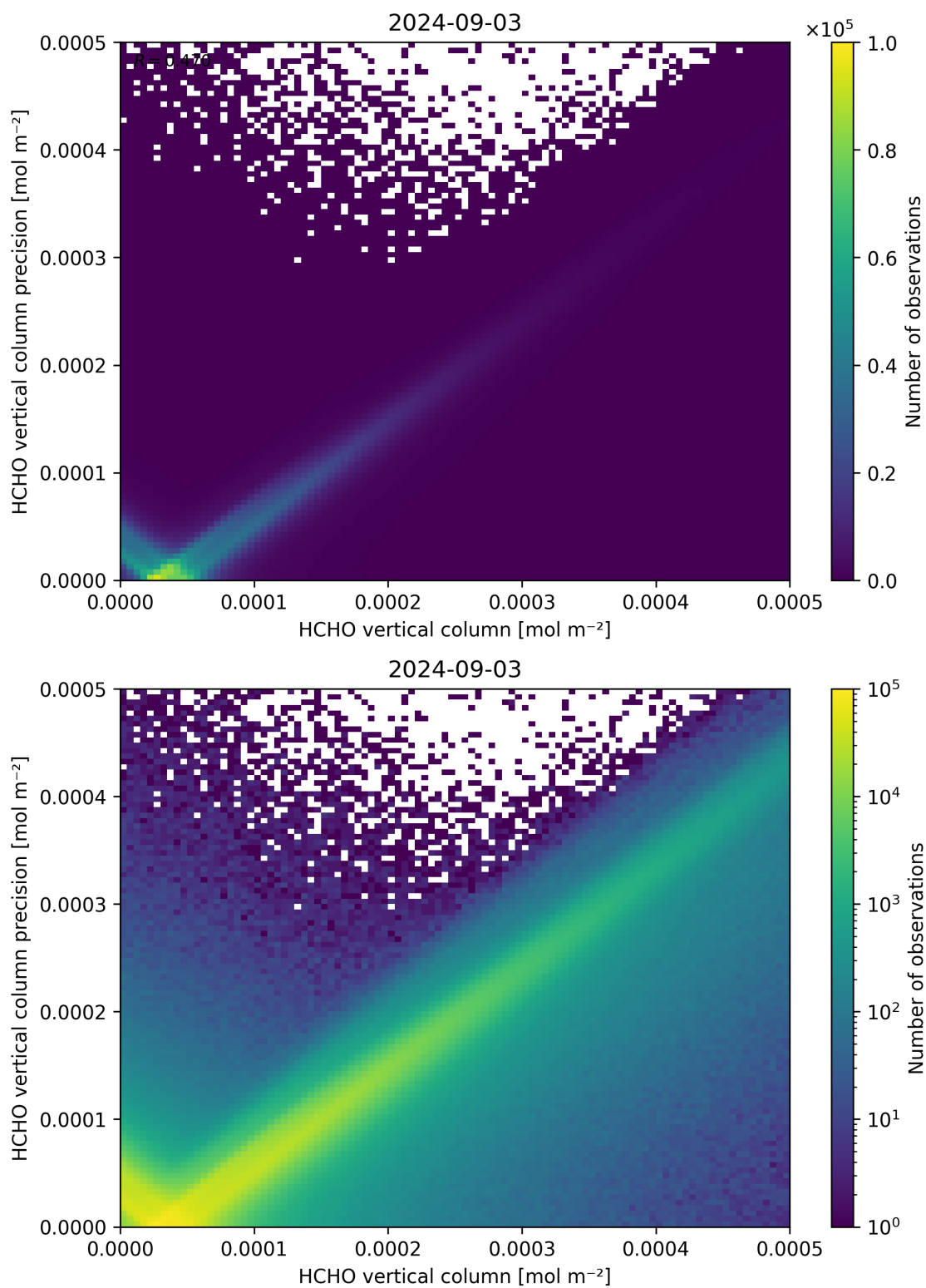
Figure 134: Scatter density plot of “HCHO vertical column” against “HCHO vertical column precision” for 2024-09-02 to 2024-09-04.
