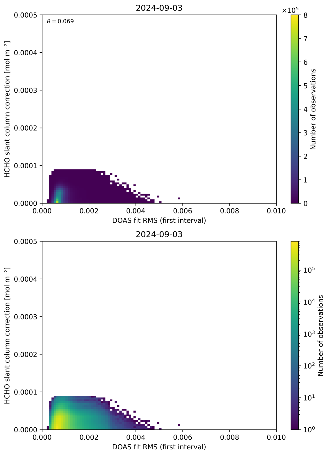
Figure 63: Scatter density plot of “DOAS fit RMS (first interval)” against “HCHO slant column correction” for 2024-09-02 to 2024-09-04.
