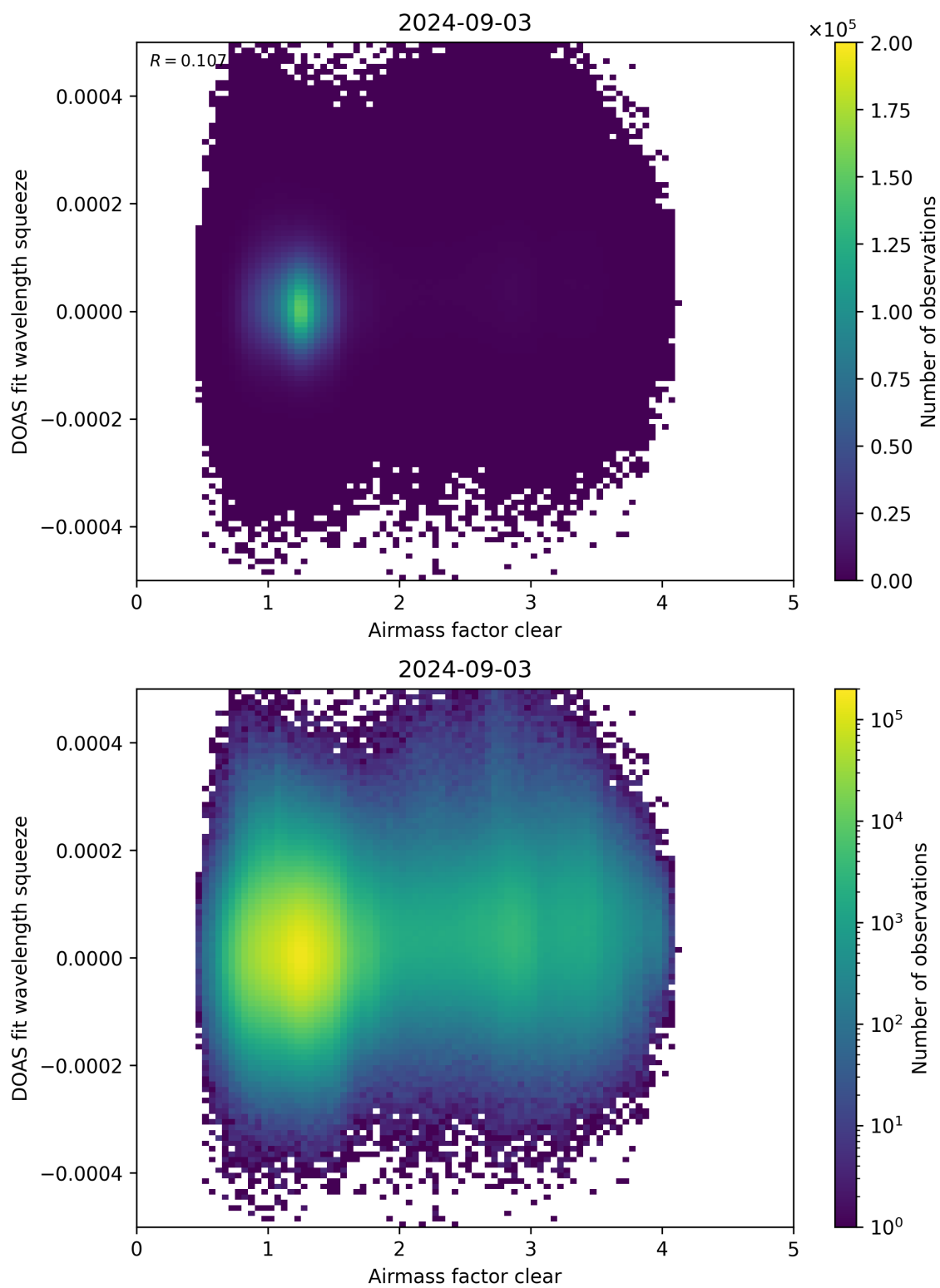
Figure 73: Scatter density plot of “Airmass factor clear” against “DOAS fit wavelength squeeze” for 2024-09-02 to 2024-09-04.
