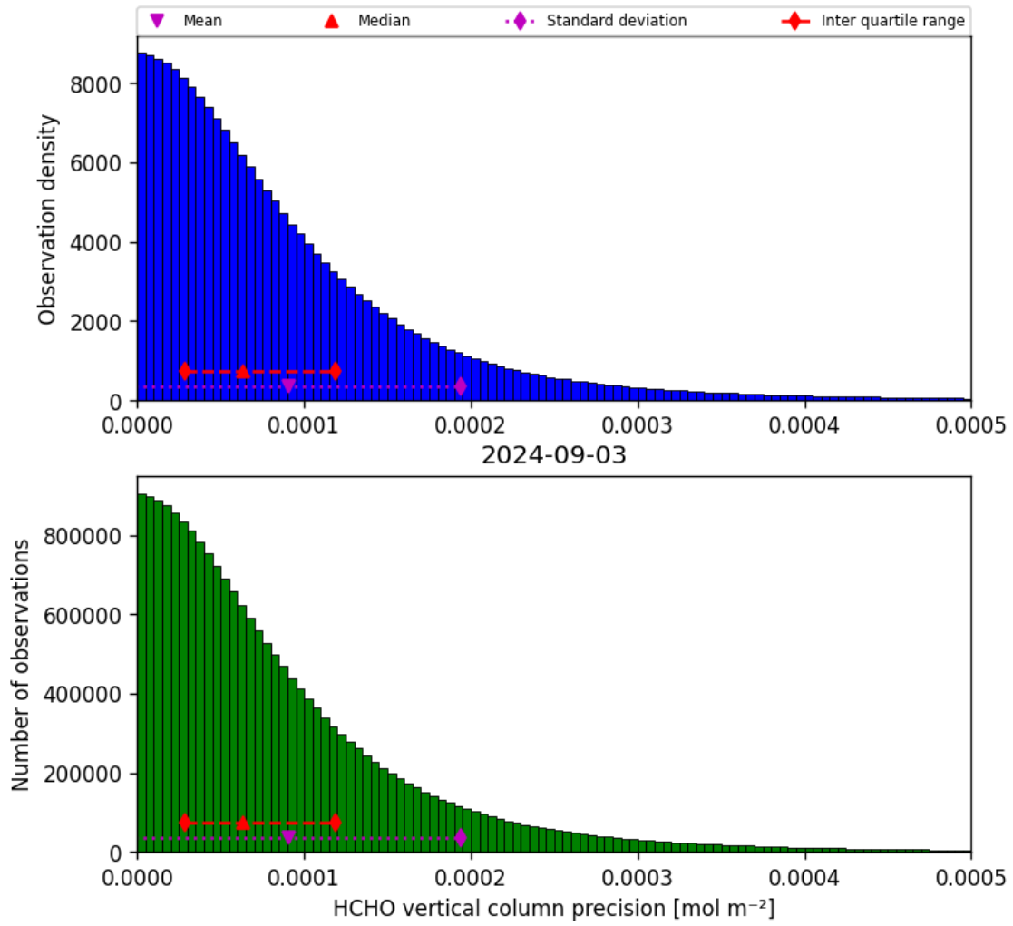
Figure 36: Histogram of “HCHO vertical column precision” for 2024-09-02 to 2024-09-04
