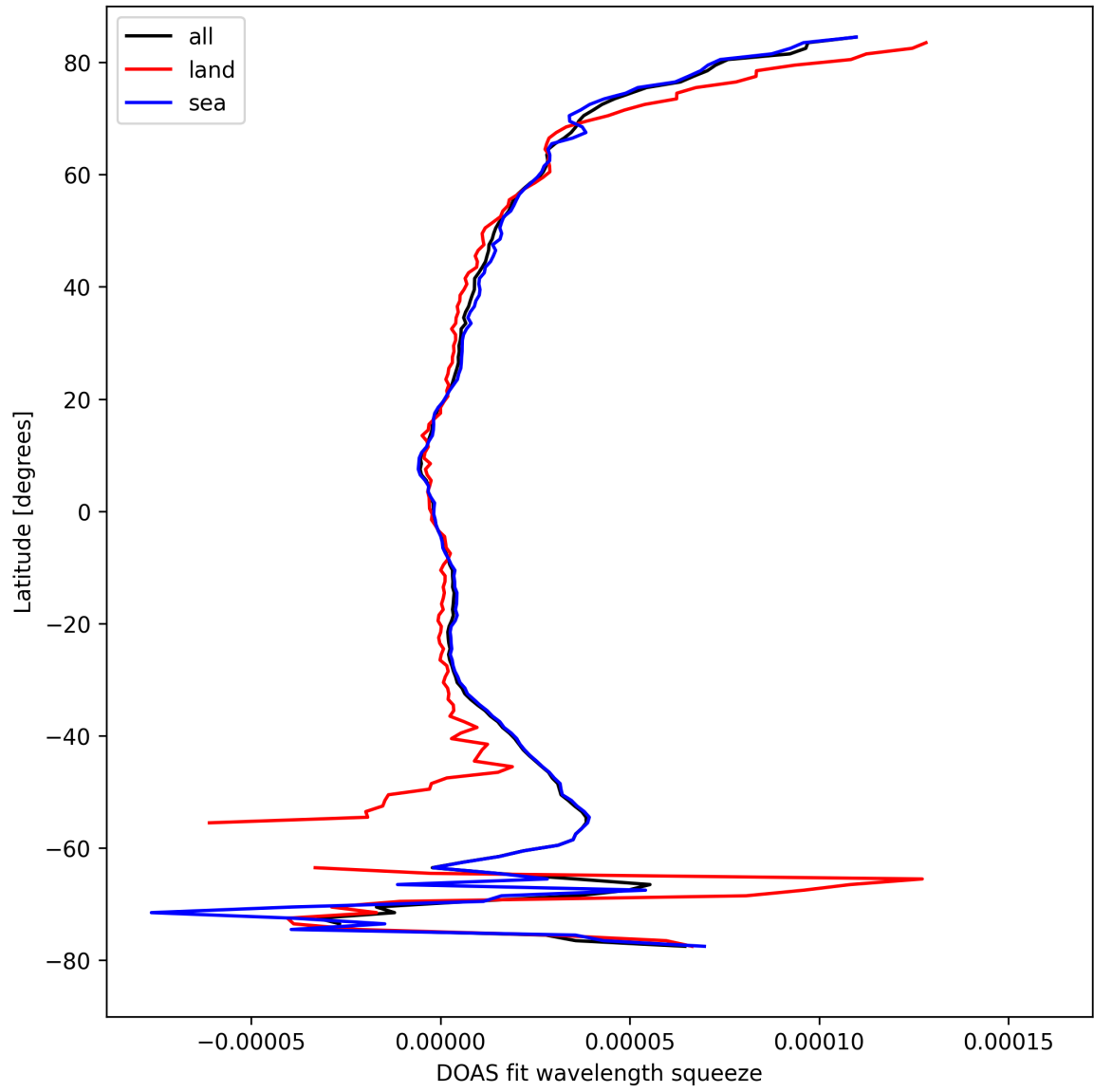
Figure 31: Zonal average of “DOAS fit wavelength squeeze” for 2024-09-02 to 2024-09-04.
