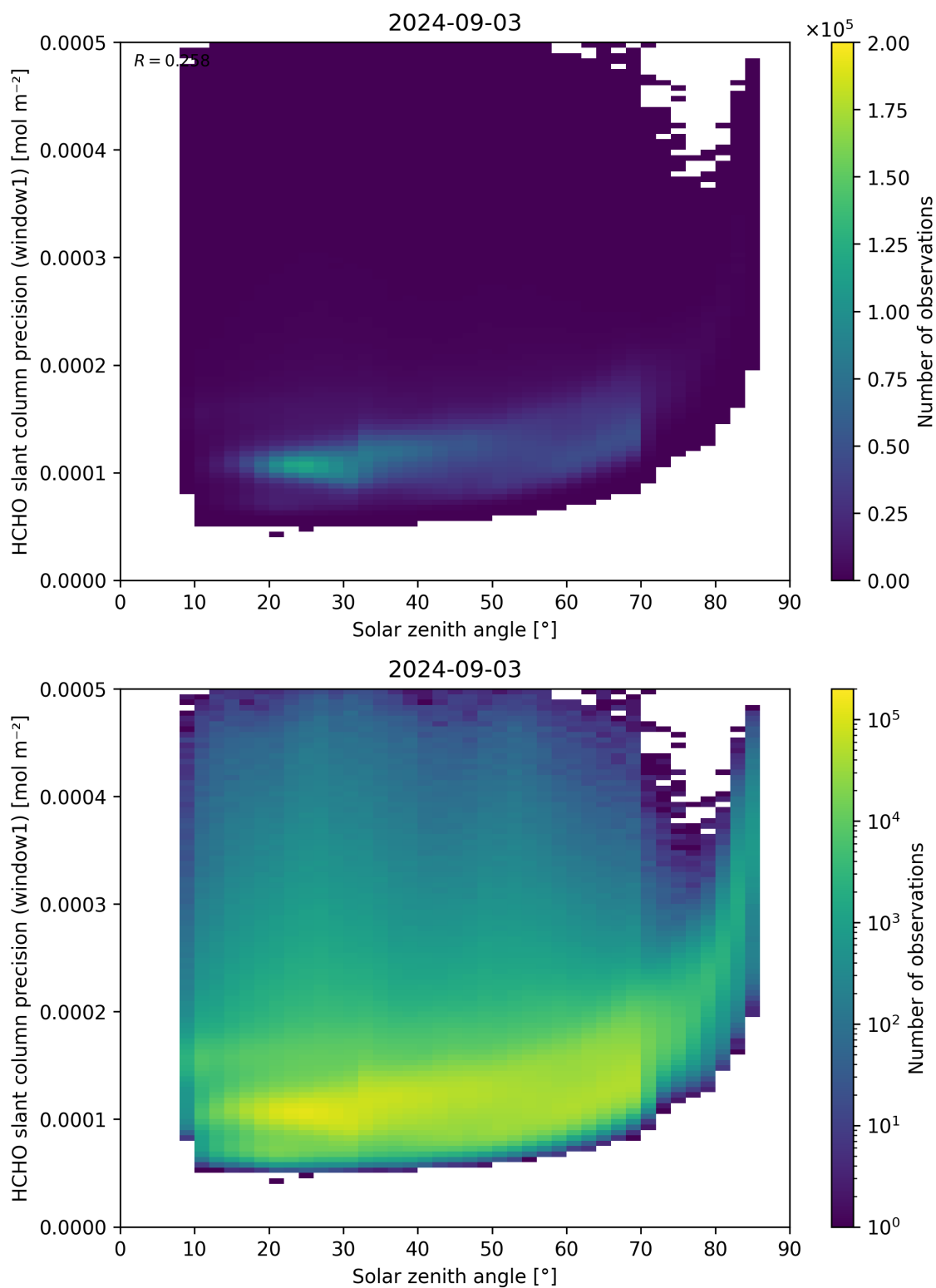
Figure 174: Scatter density plot of “Solar zenith angle” against “HCHO slant column precision (window1)” for 2024-09-02 to 2024-09-04.
