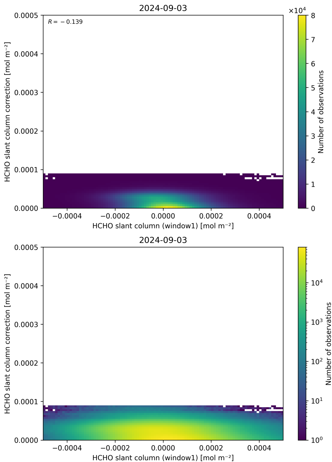
Figure 83: Scatter density plot of “HCHO slant column (window1)” against “HCHO slant column correction” for 2024-09-02 to 2024-09-04.
