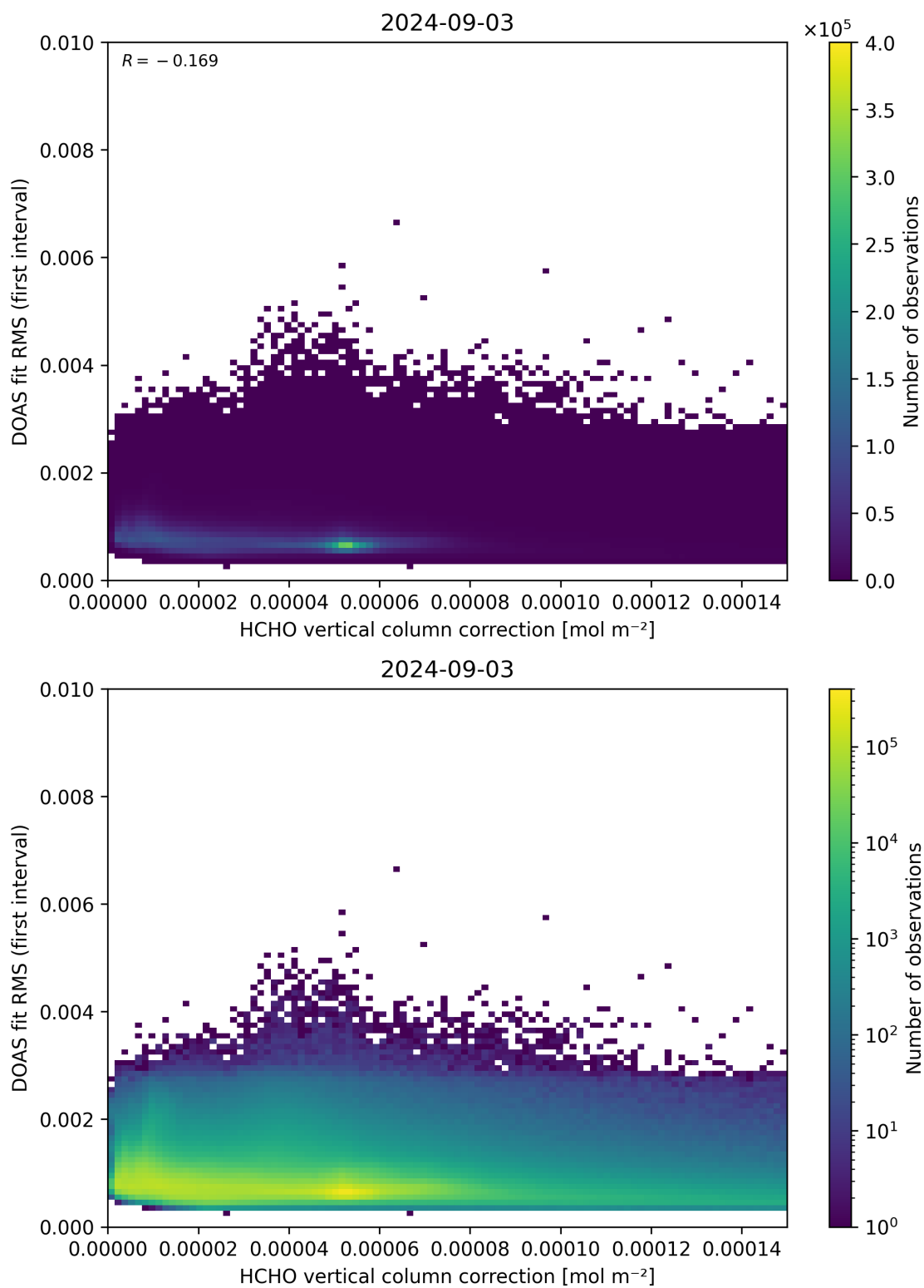
Figure 112: Scatter density plot of “HCHO vertical column correction” against “DOAS fit RMS (first interval)” for 2024-09-02 to 2024-09-04.
