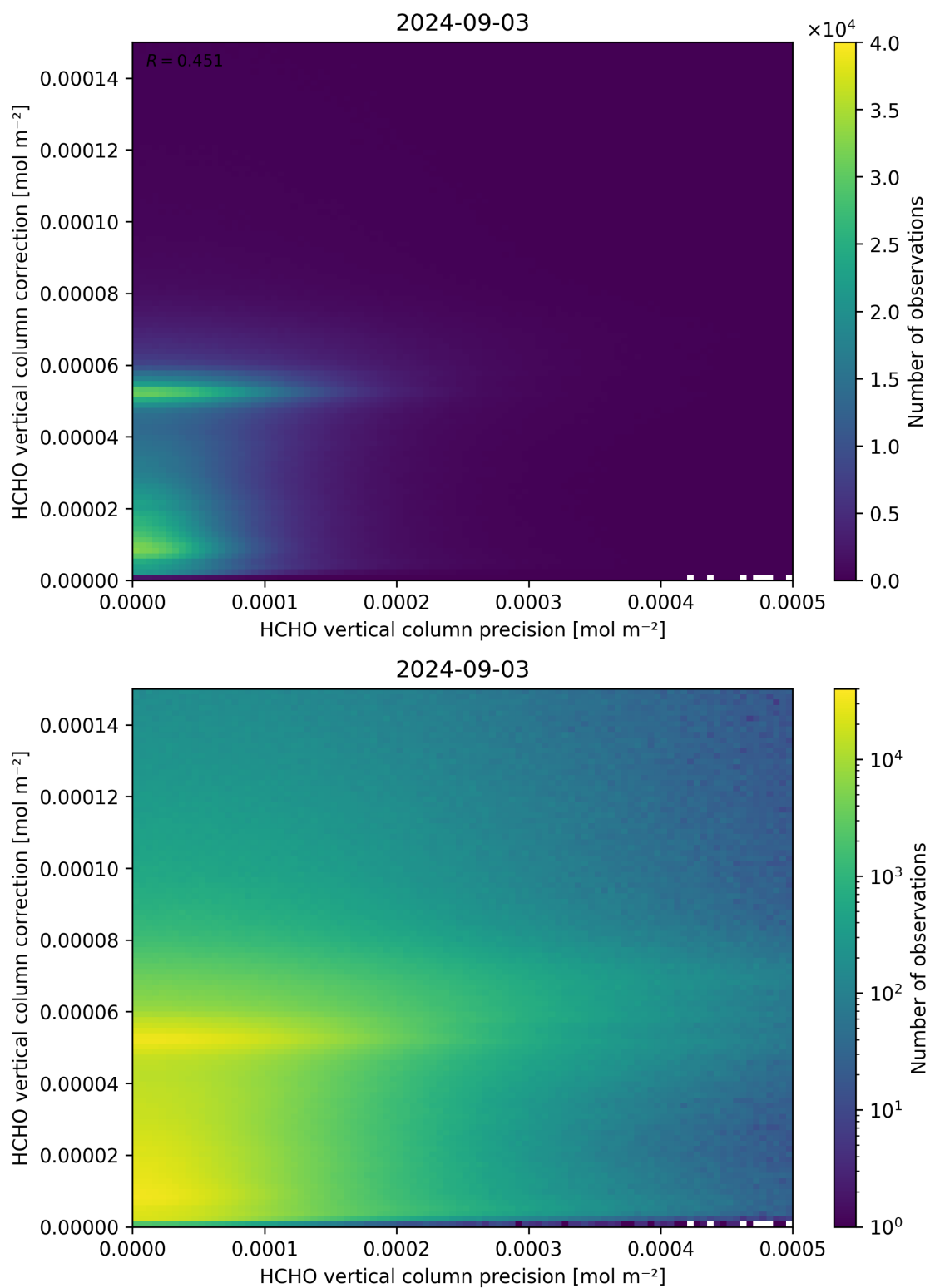
Figure 146: Scatter density plot of “HCHO vertical column precision” against “HCHO vertical column correction” for 2024-09-02 to 2024-09-04.
