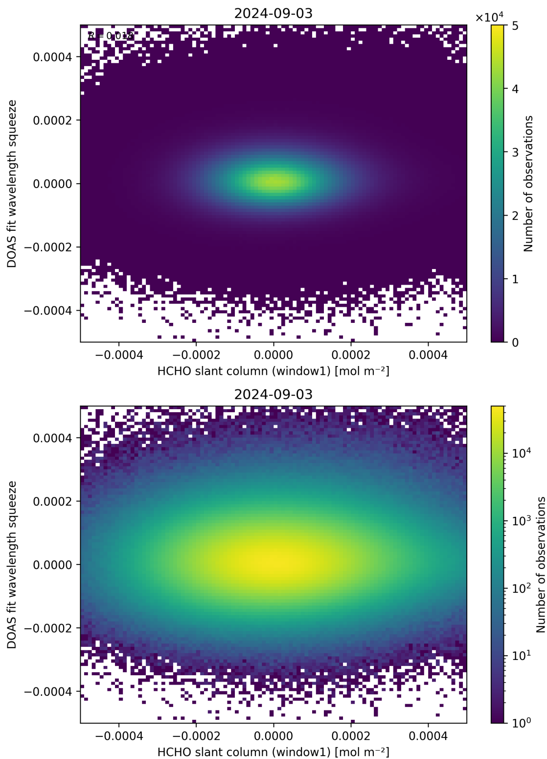
Figure 80: Scatter density plot of “HCHO slant column (window1)” against “DOAS fit wavelength squeeze” for 2024-09-02 to 2024-09-04.
