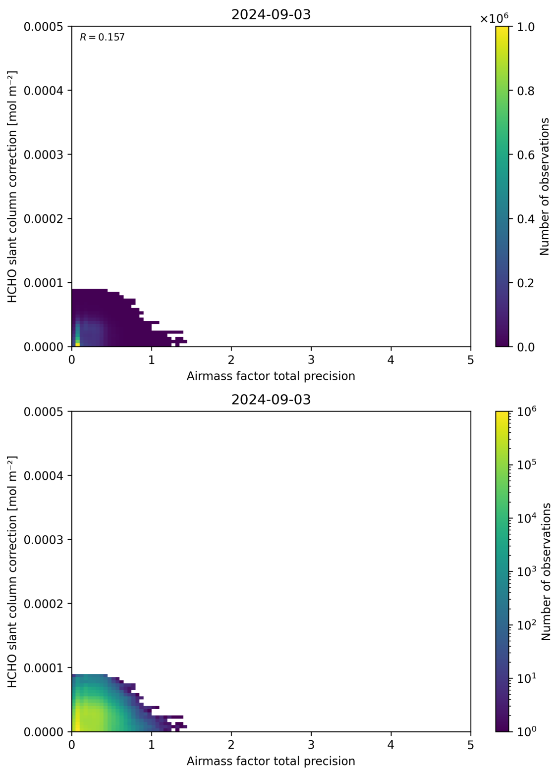
Figure 110: Scatter density plot of “Airmass factor total precision” against “HCHO slant column correction” for 2024-09-02 to 2024-09-04.
