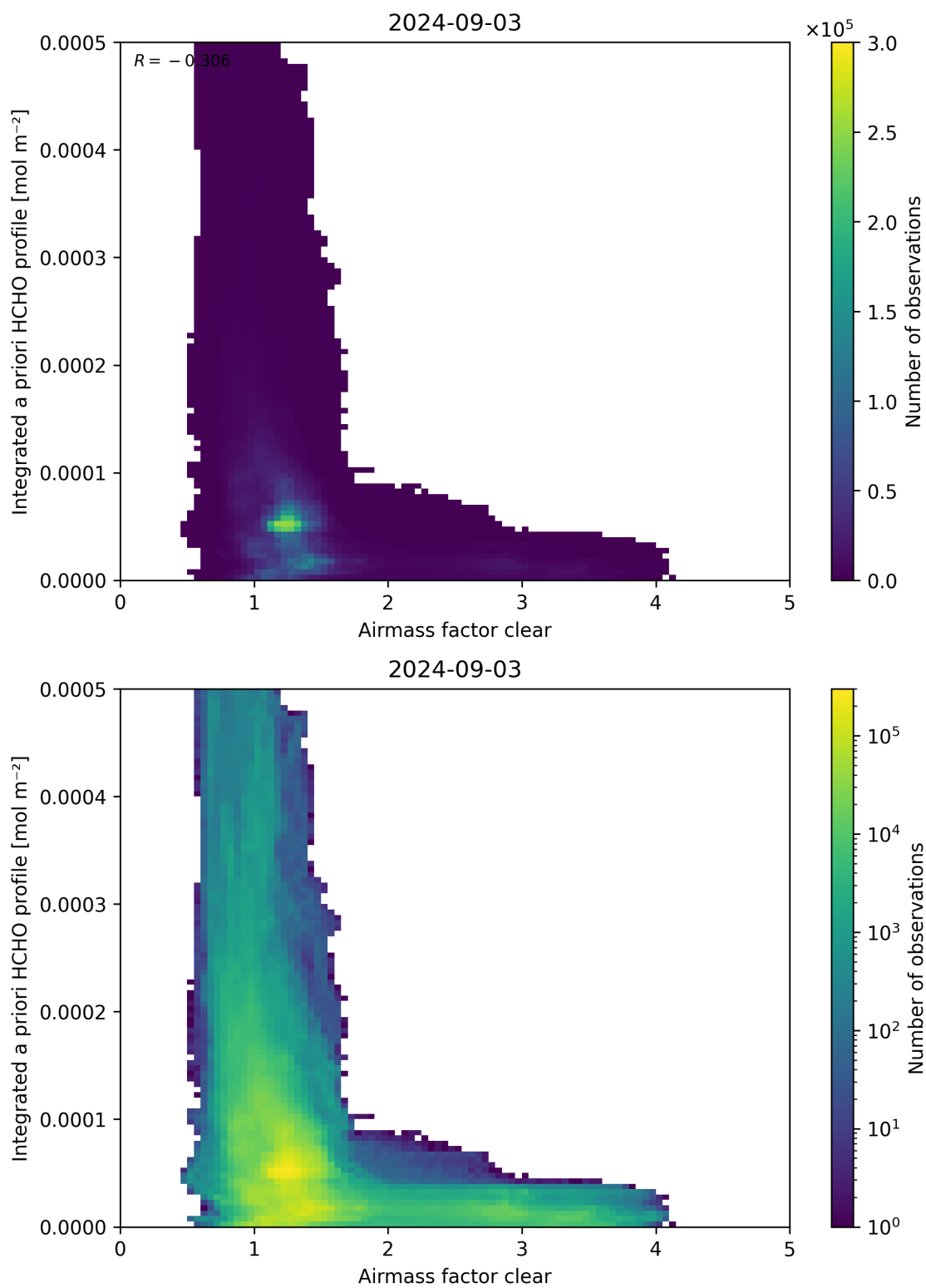
Figure 76: Scatter density plot of “Airmass factor clear” against “Integrated a priori HCHO profile” for 2024-09-02 to 2024-09-04.
