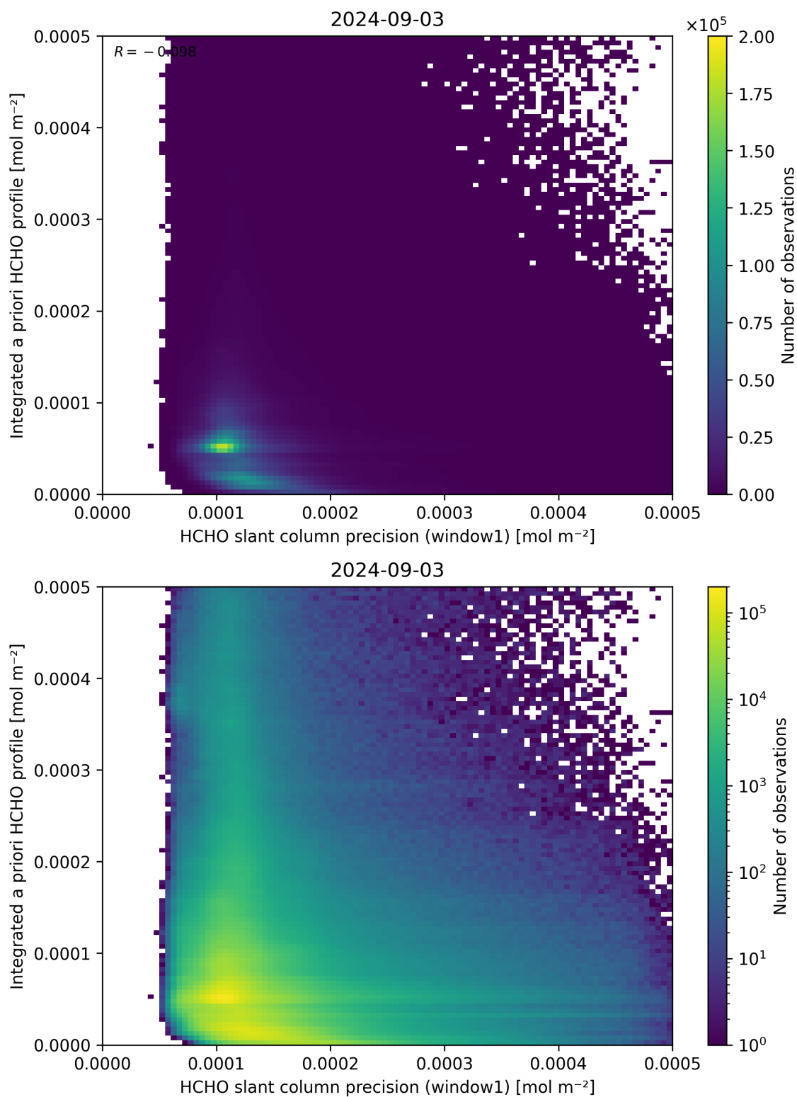
Figure 96: Scatter density plot of “HCHO slant column precision (window1)” against “Integrated a priori HCHO profile” for 2024-09-02 to 2024-09-04.
