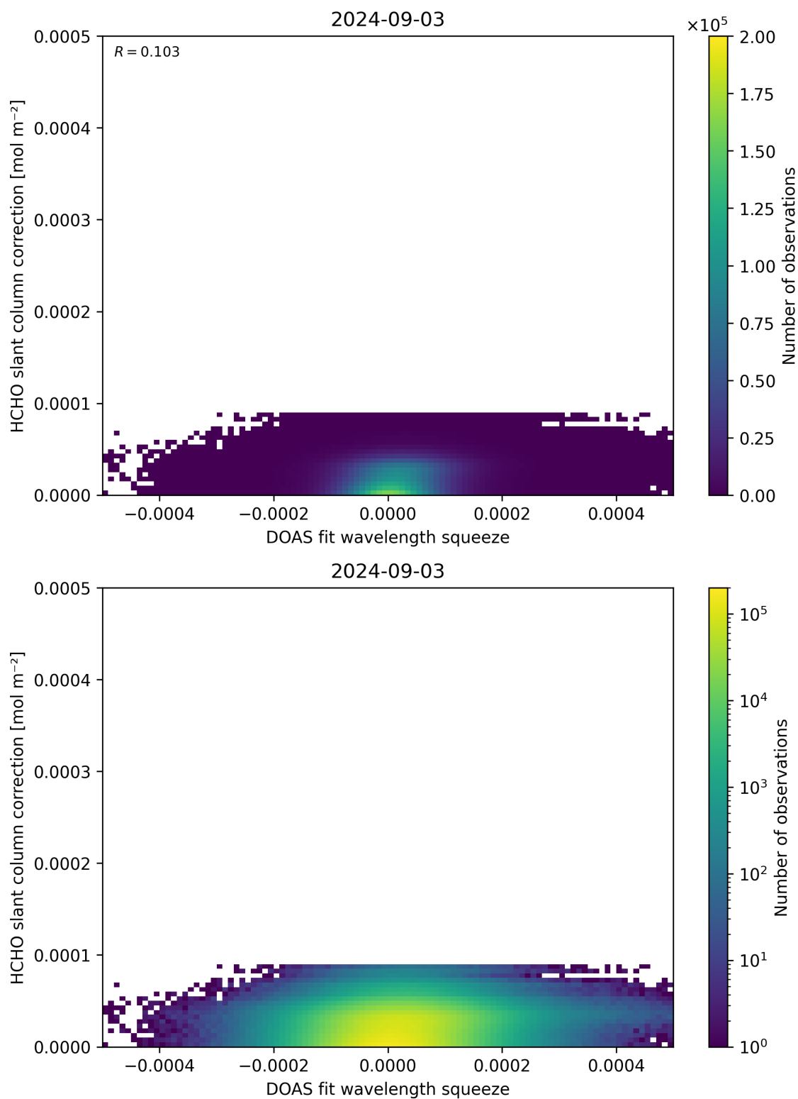
Figure 70: Scatter density plot of “DOAS fit wavelength squeeze” against “HCHO slant column correction” for 2024-09-02 to 2024-09-04.
