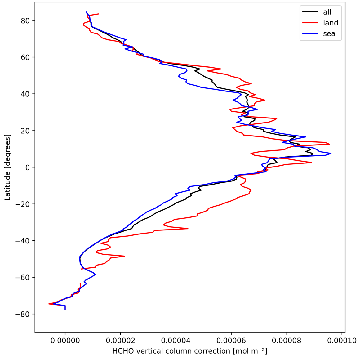
Figure 23: Zonal average of “HCHO vertical column correction” for 2024-09-02 to 2024-09-04.
