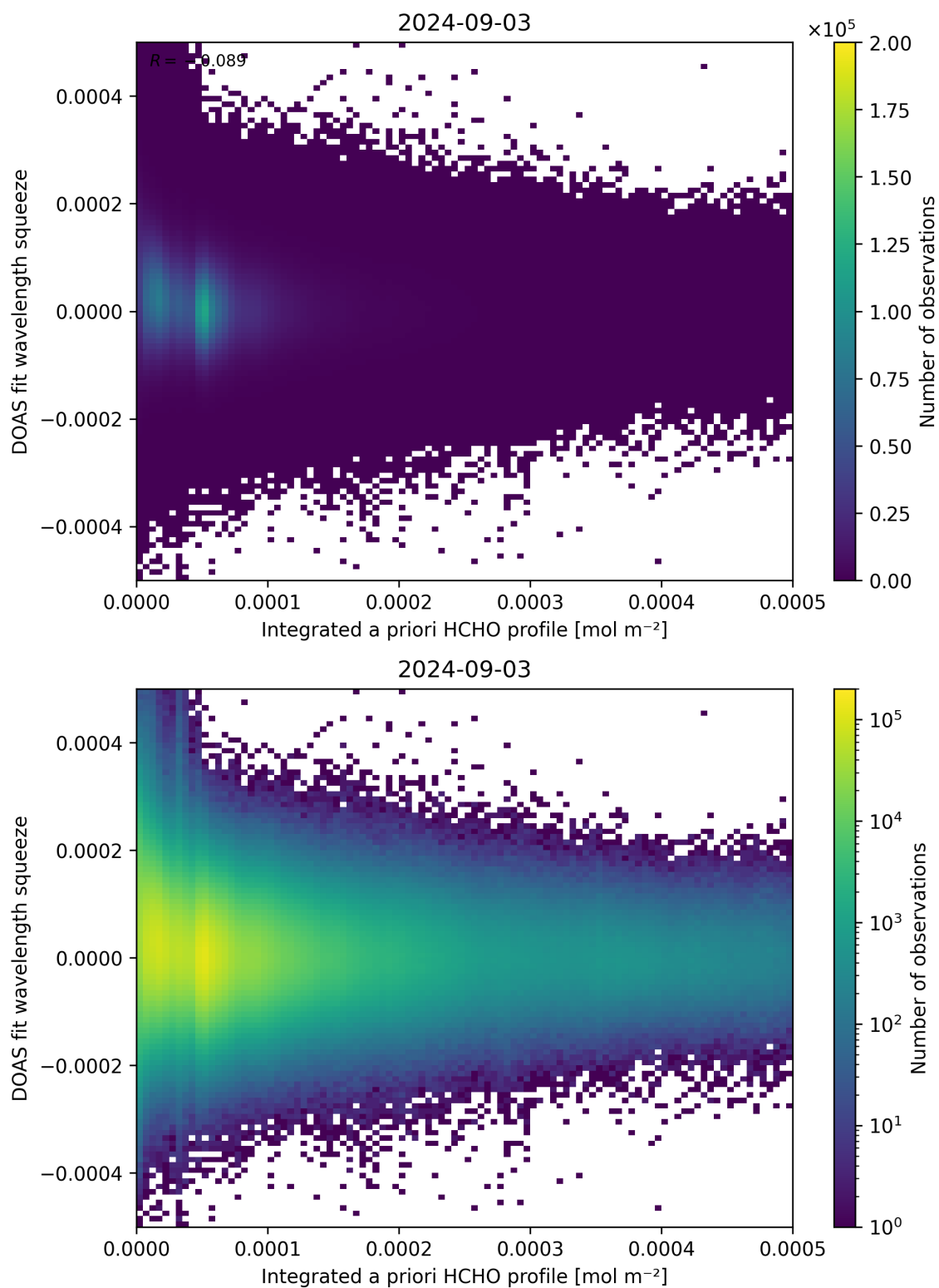
Figure 150: Scatter density plot of “Integrated a priori HCHO profile” against “DOAS fit wavelength squeeze” for 2024-09-02 to 2024-09-04.
