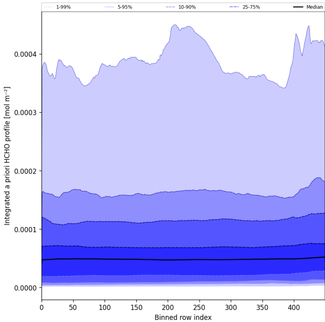
Figure 57: Along track statistics of “Integrated a priori HCHO profile” for 2024-09-02 to 2024-09-04
