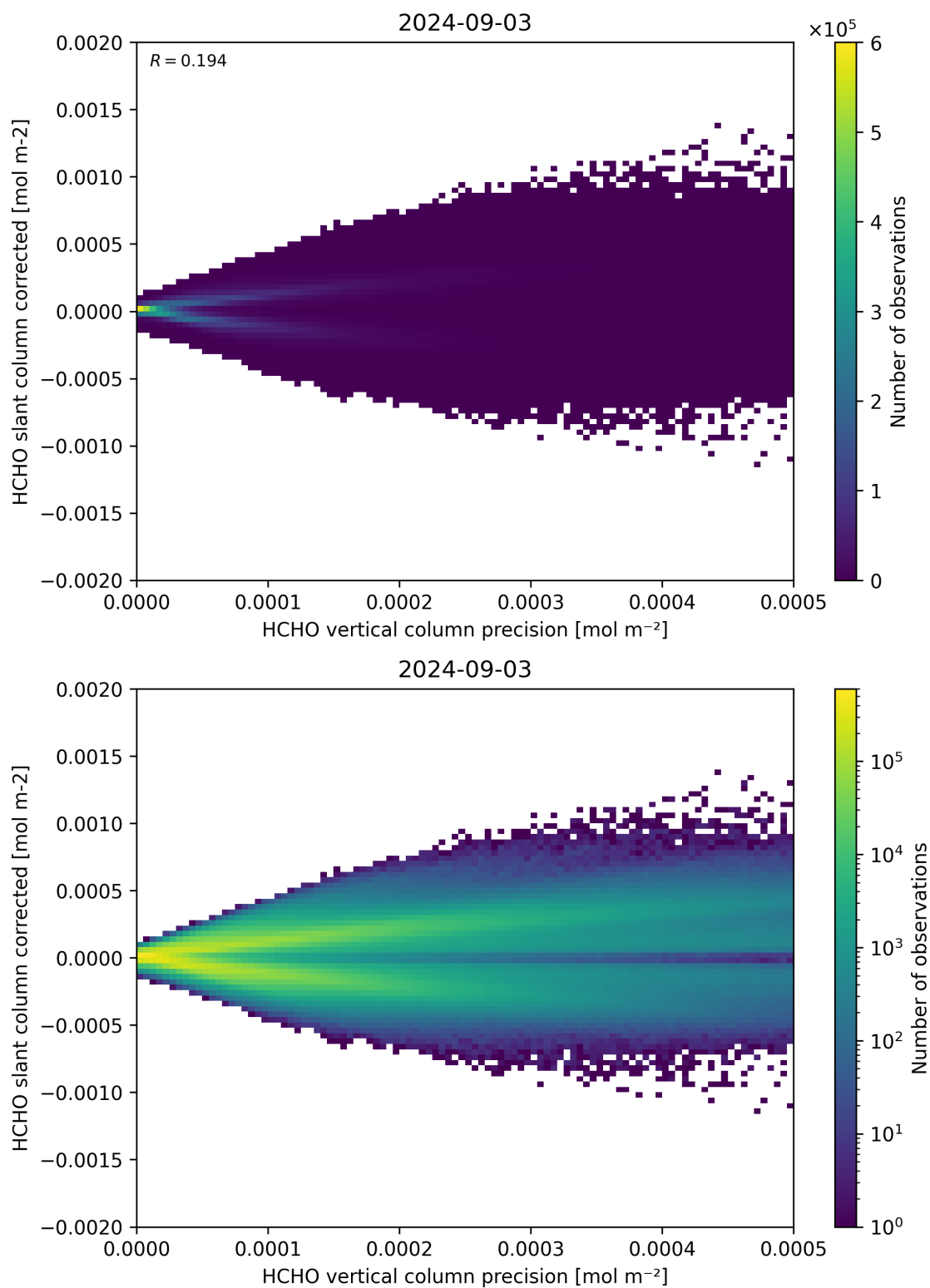
Figure 140: Scatter density plot of “HCHO vertical column precision” against “HCHO slant column corrected” for 2024-09-02 to 2024-09-04.
