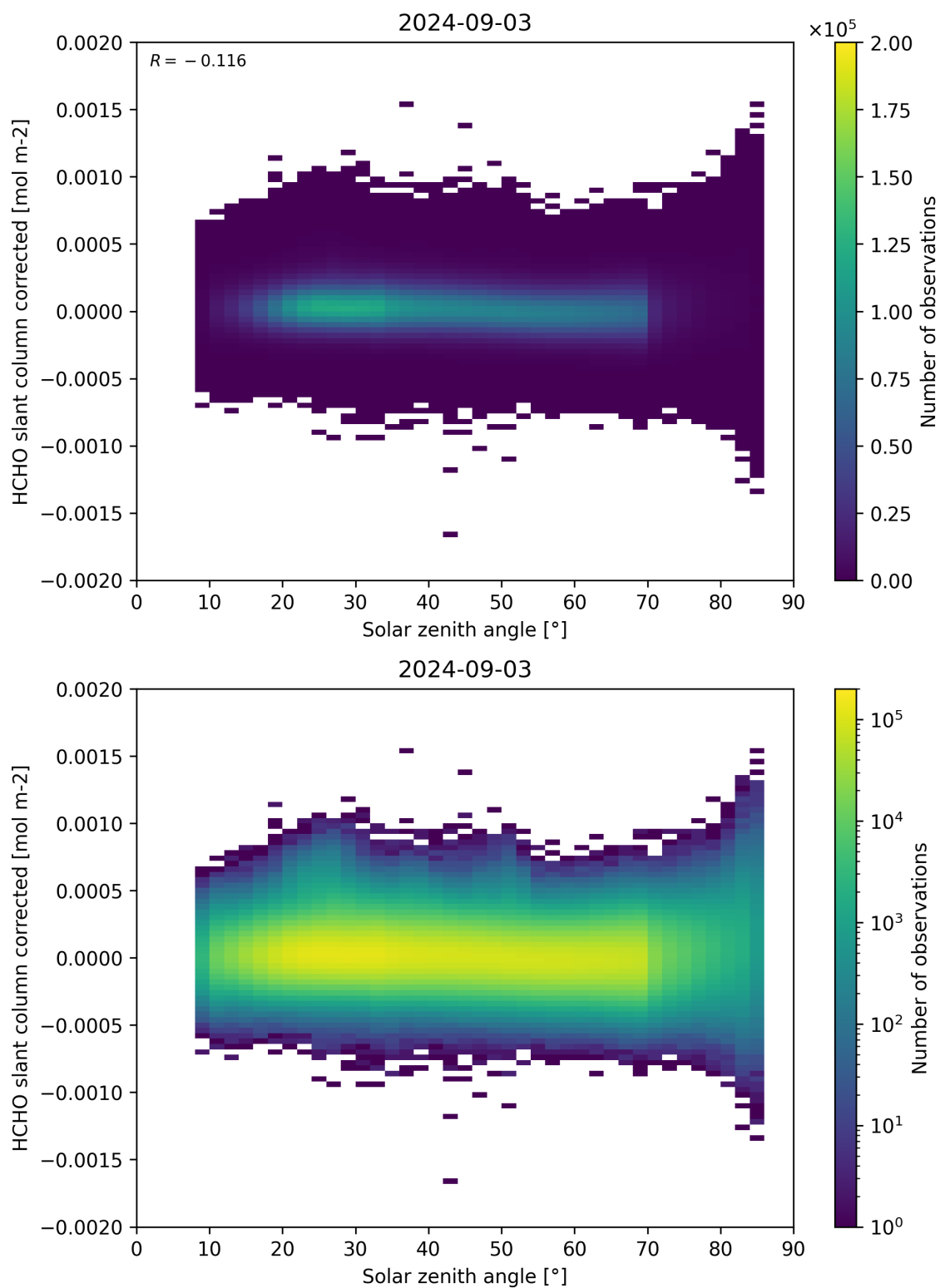
Figure 171: Scatter density plot of “Solar zenith angle” against “HCHO slant column corrected” for 2024-09-02 to 2024-09-04.
