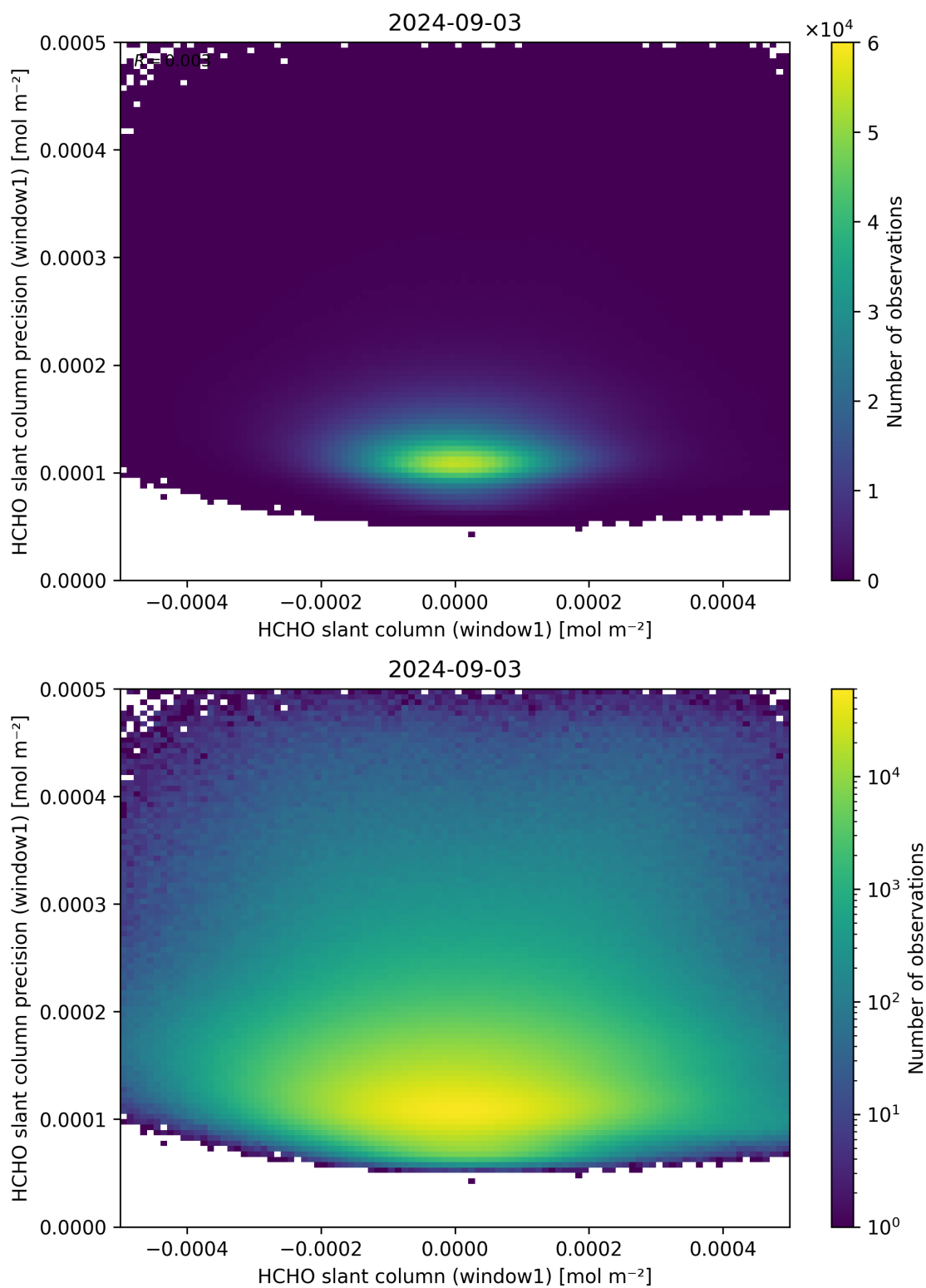
Figure 84: Scatter density plot of “HCHO slant column (window1)” against “HCHO slant column precision (window1)” for 2024-09-02 to 2024-09-04.
