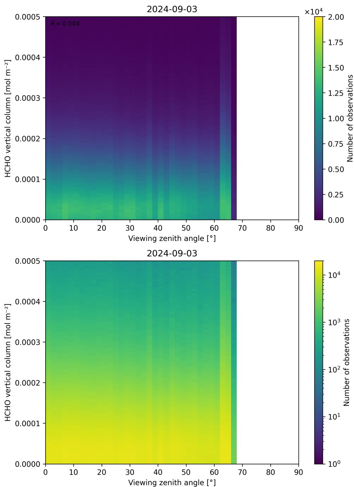
Figure 192: Scatter density plot of “Viewing zenith angle” against “HCHO vertical column” for 2024-09-02 to 2024-09-04.
