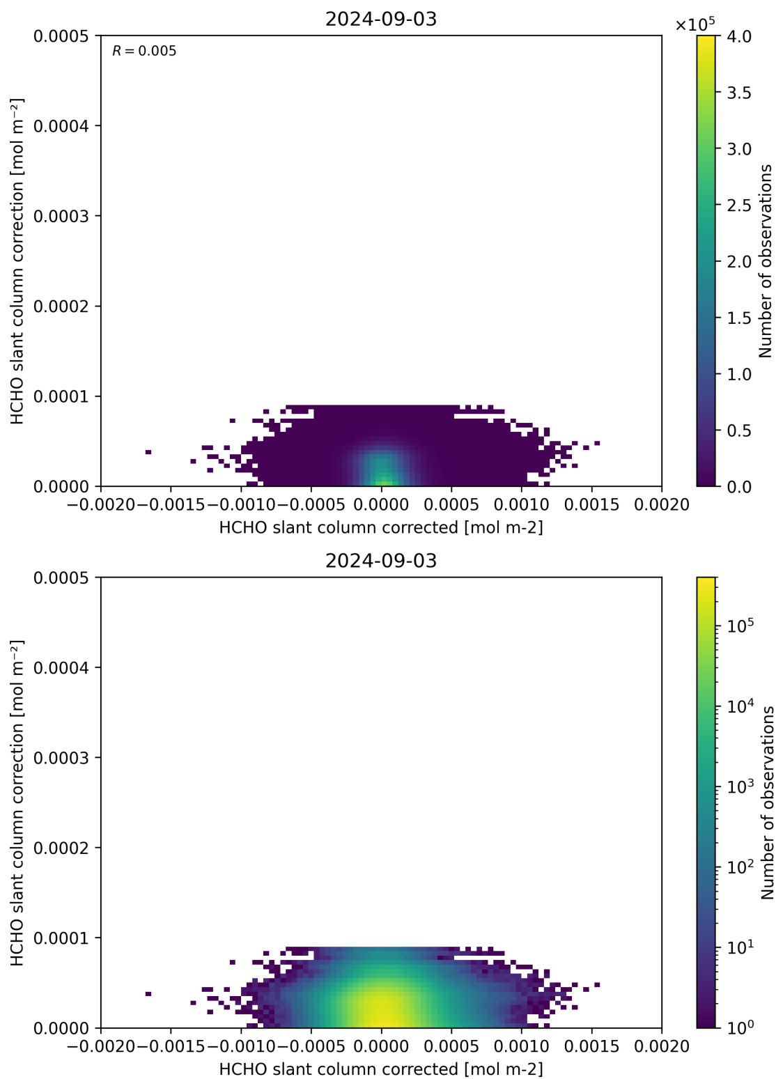
Figure 77: Scatter density plot of “HCHO slant column corrected” against “HCHO slant column correction” for 2024-09-02 to 2024-09-04.
