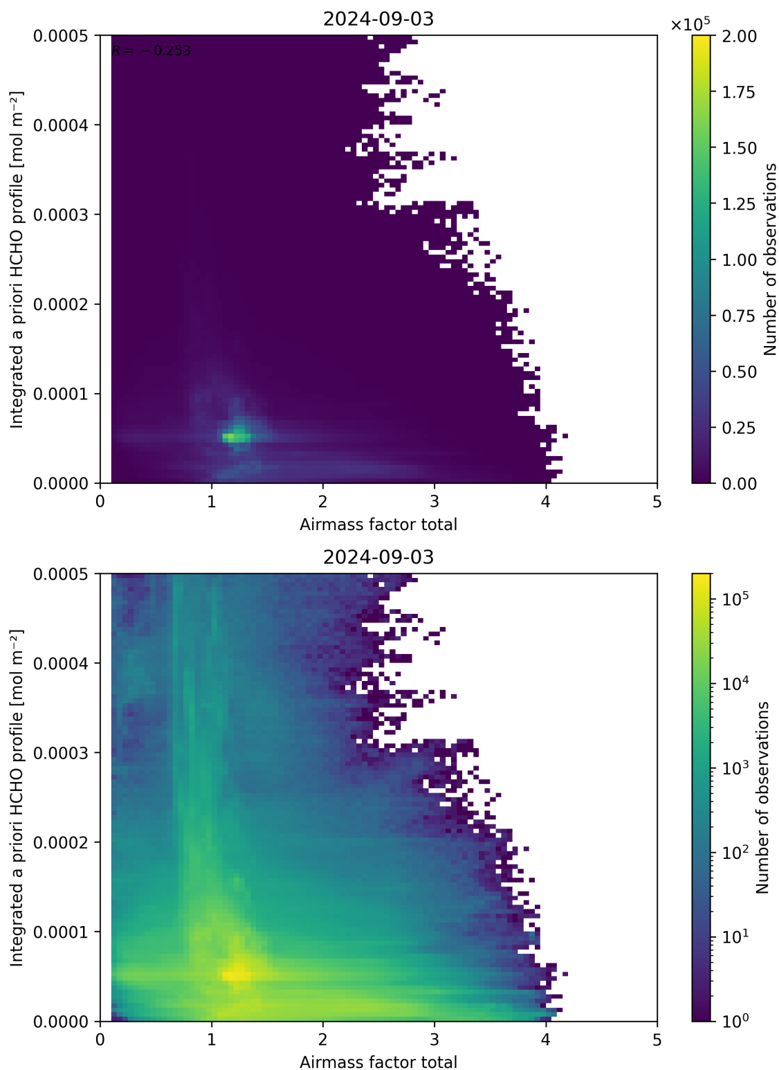
Figure 104: Scatter density plot of “Airmass factor total” against “Integrated a priori HCHO profile” for 2024-09-02 to 2024-09-04.
