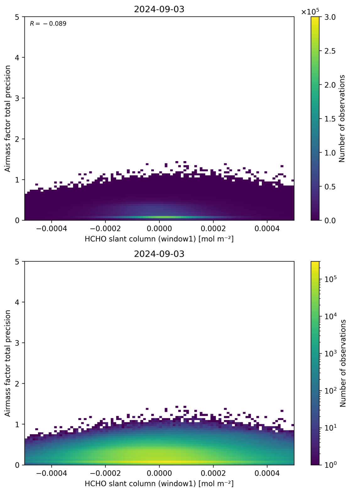
Figure 86: Scatter density plot of “HCHO slant column (window1)” against “Airmass factor total precision” for 2024-09-02 to 2024-09-04.
