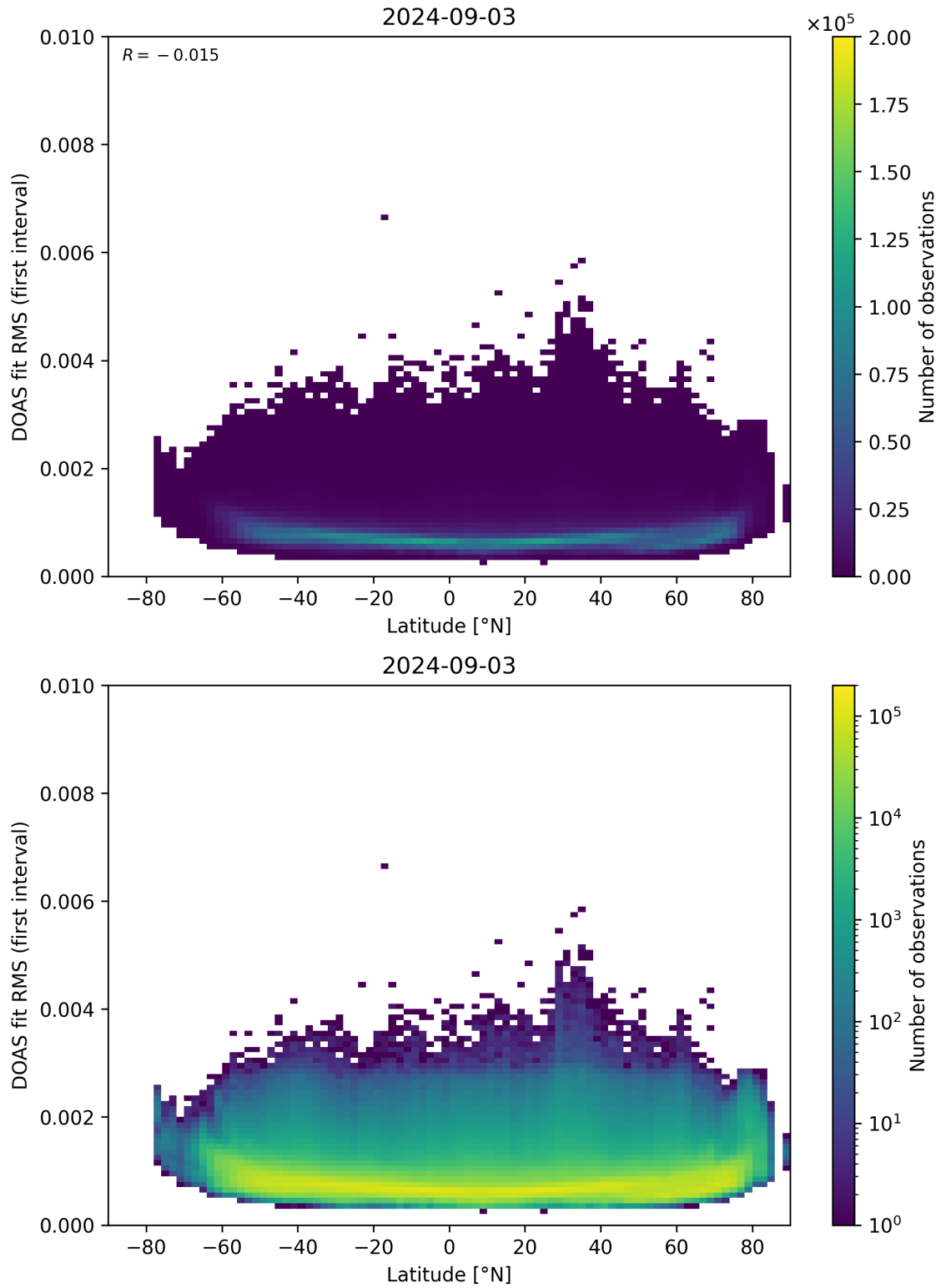
Figure 153: Scatter density plot of “Latitude” against “DOAS fit RMS (first interval)” for 2024-09-02 to 2024-09-04.
