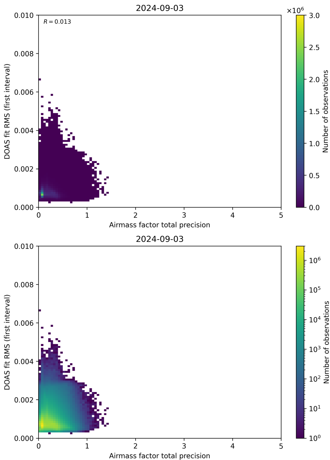
Figure 105: Scatter density plot of “Airmass factor total precision” against “DOAS fit RMS (first interval)” for 2024-09-02 to 2024-09-04.
