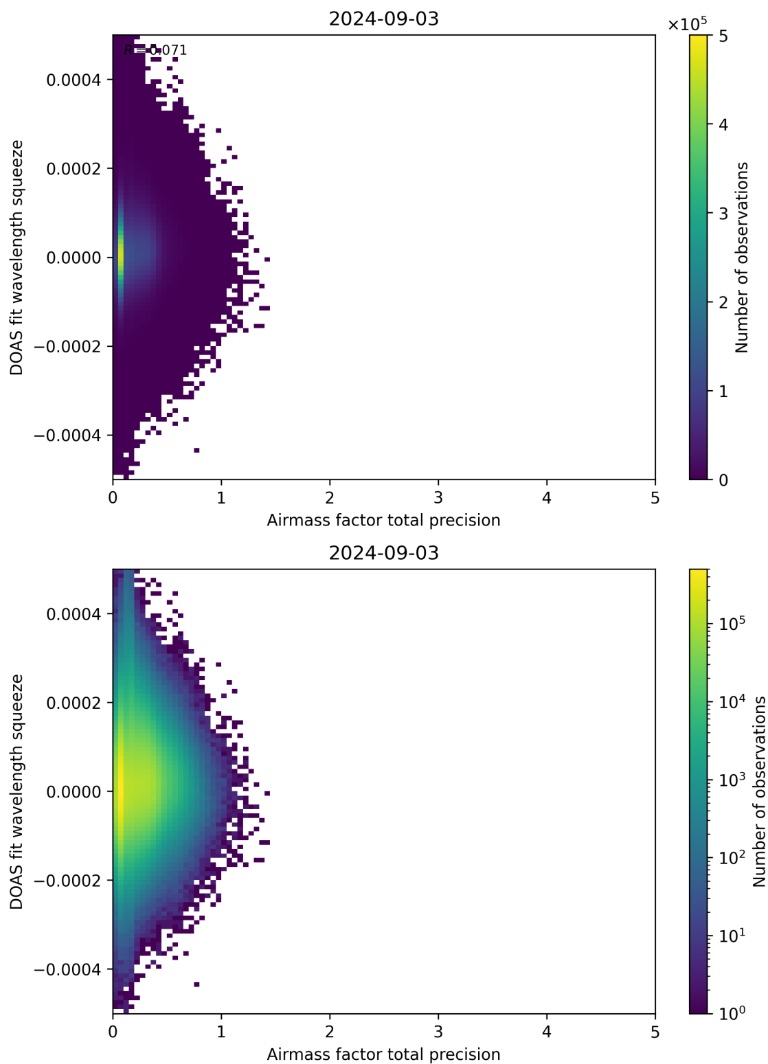
Figure 107: Scatter density plot of “Airmass factor total precision” against “DOAS fit wavelength squeeze” for 2024-09-02 to 2024-09-04.
