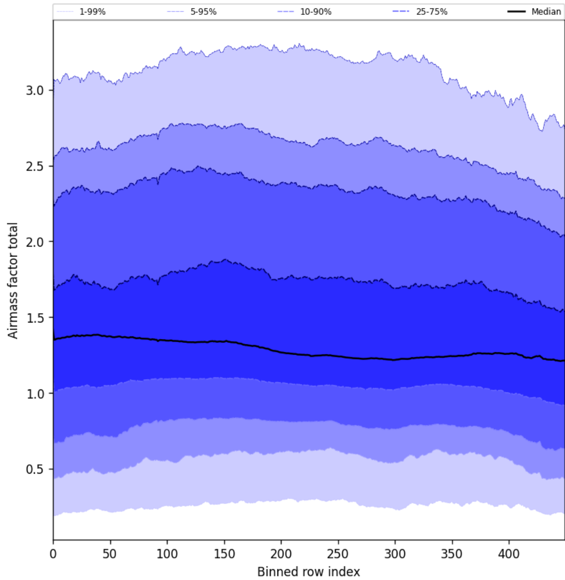
Figure 54: Along track statistics of “Airmass factor total” for 2024-09-02 to 2024-09-04
