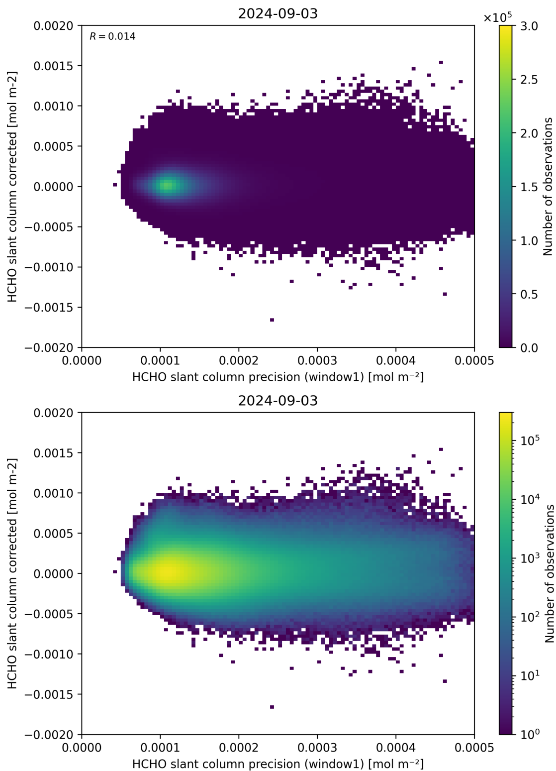
Figure 92: Scatter density plot of “HCHO slant column precision (window1)” against “HCHO slant column corrected” for 2024-09-02 to 2024-09-04.
