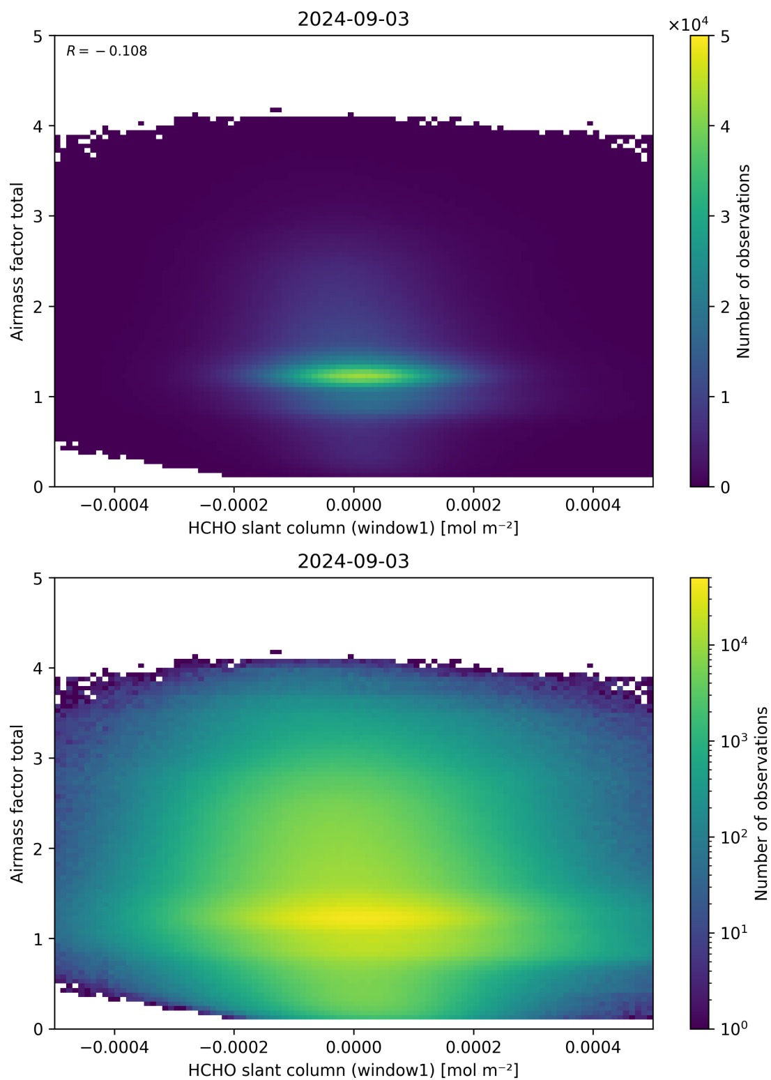
Figure 85: Scatter density plot of “HCHO slant column (window1)” against “Airmass factor total” for 2024-09-02 to 2024-09-04.
