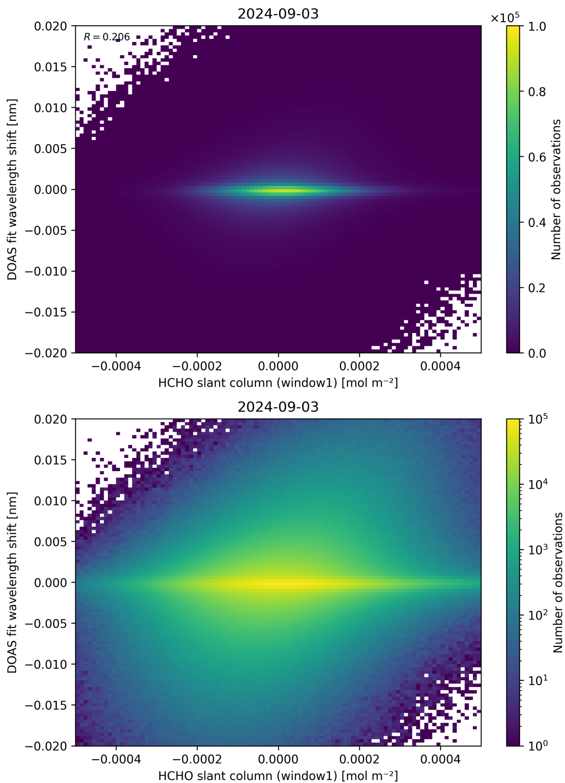
Figure 79: Scatter density plot of “HCHO slant column (window1)” against “DOAS fit wavelength shift” for 2024-09-02 to 2024-09-04.
