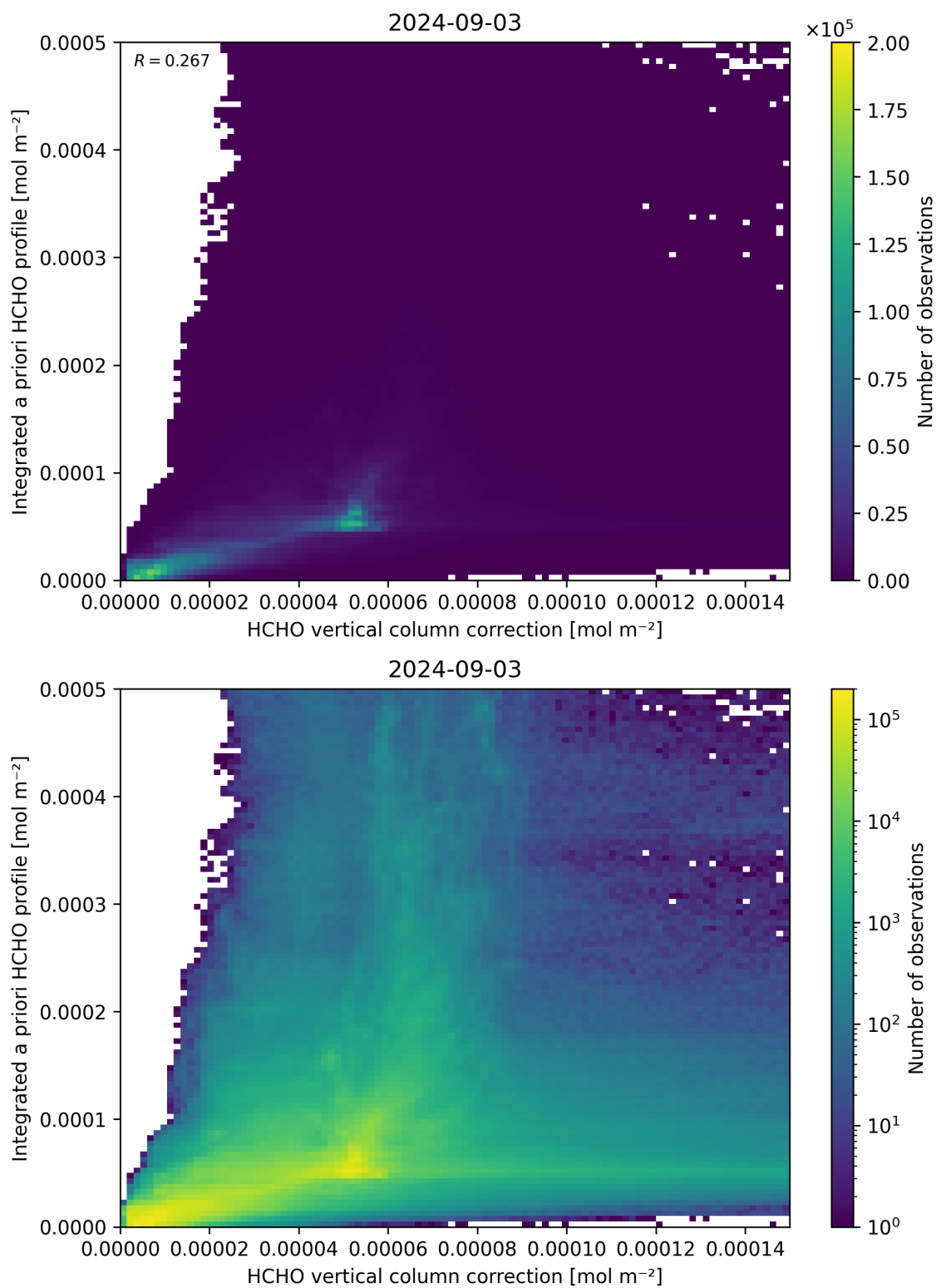
Figure 122: Scatter density plot of “HCHO vertical column correction” against “Integrated a priori HCHO profile” for 2024-09-02 to 2024-09-04.
