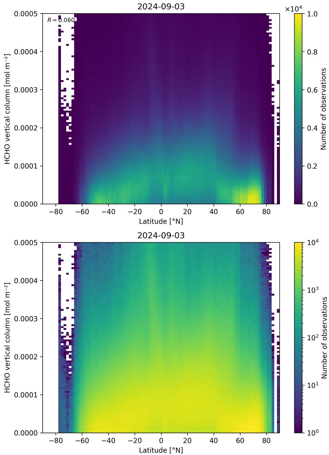
Figure 163: Scatter density plot of “Latitude” against “HCHO vertical column” for 2024-09-02 to 2024-09-04.
