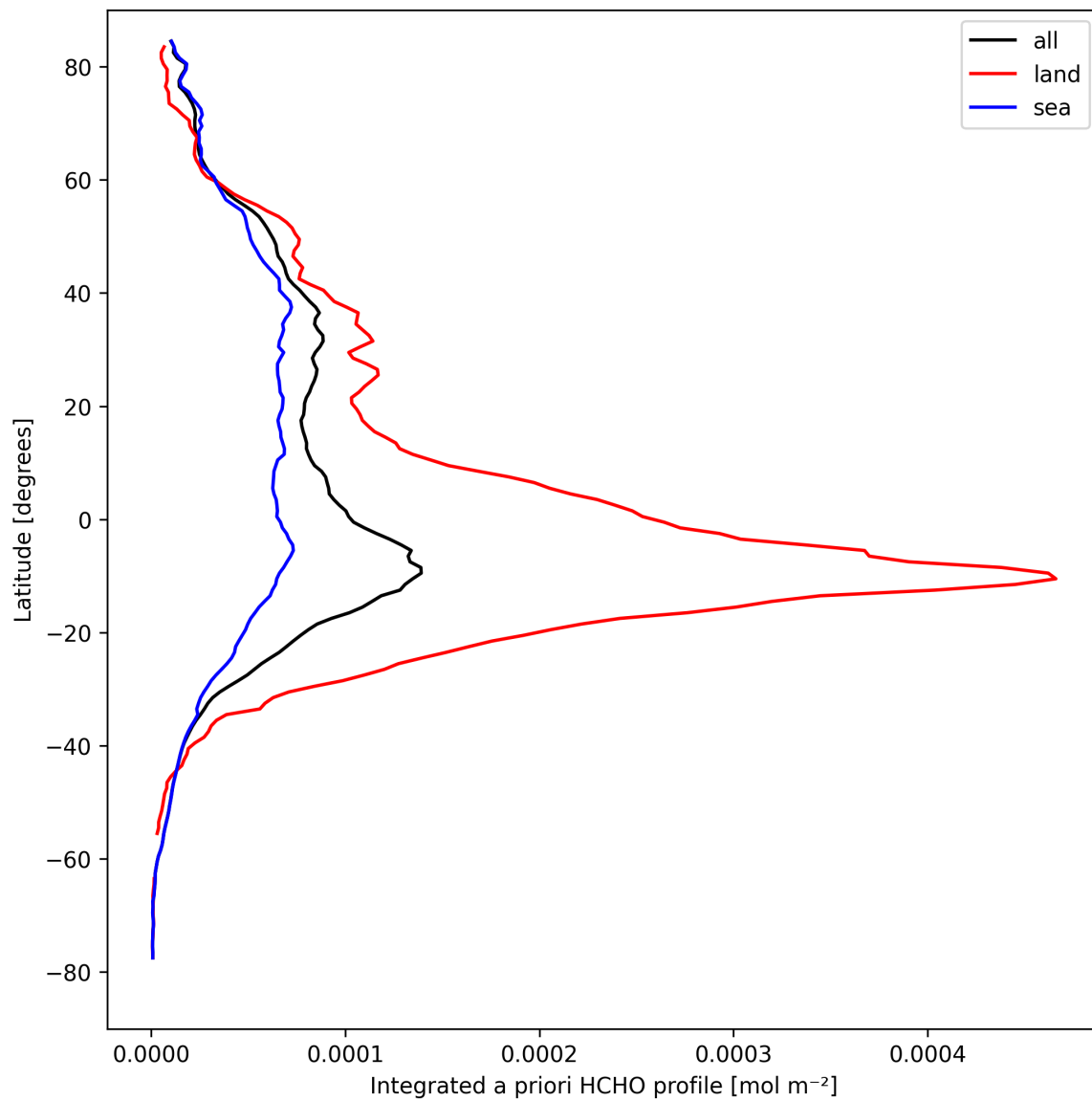
Figure 29: Zonal average of “Integrated a priori HCHO profile” for 2024-09-02 to 2024-09-04.
