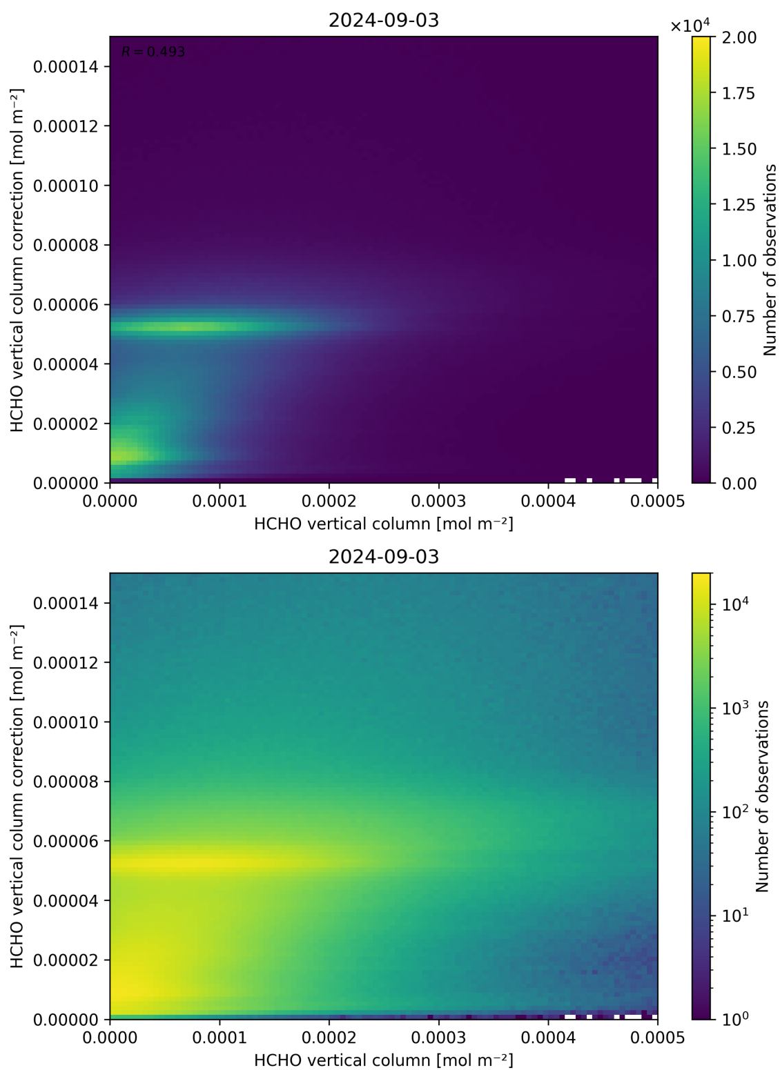
Figure 133: Scatter density plot of “HCHO vertical column” against “HCHO vertical column correction” for 2024-09-02 to 2024-09-04.
