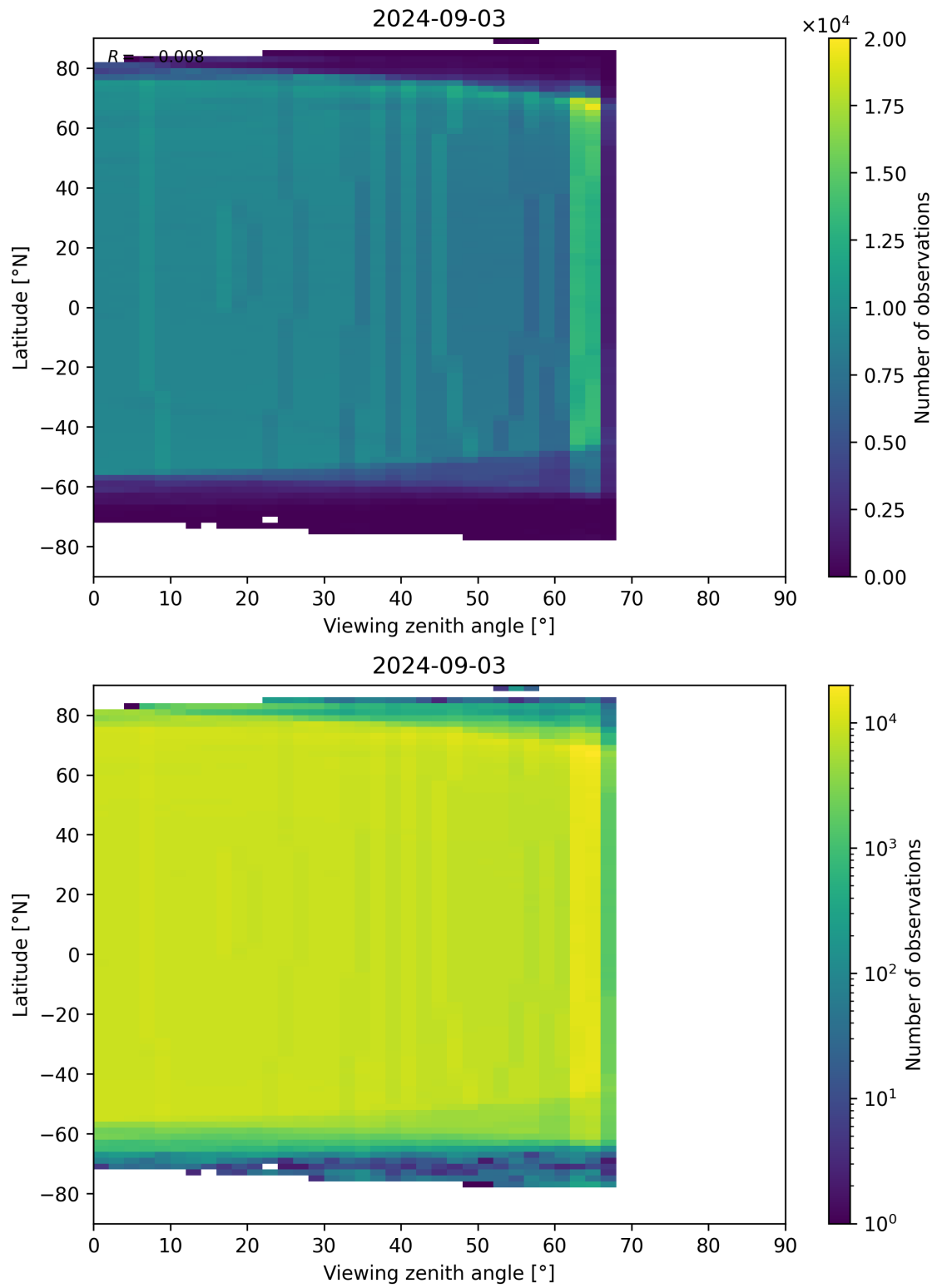
Figure 196: Scatter density plot of “Viewing zenith angle” against “Latitude” for 2024-09-02 to 2024-09-04.
