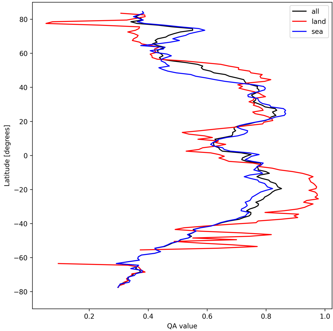
Figure 20: Zonal average of “QA value” for 2024-09-02 to 2024-09-04.
