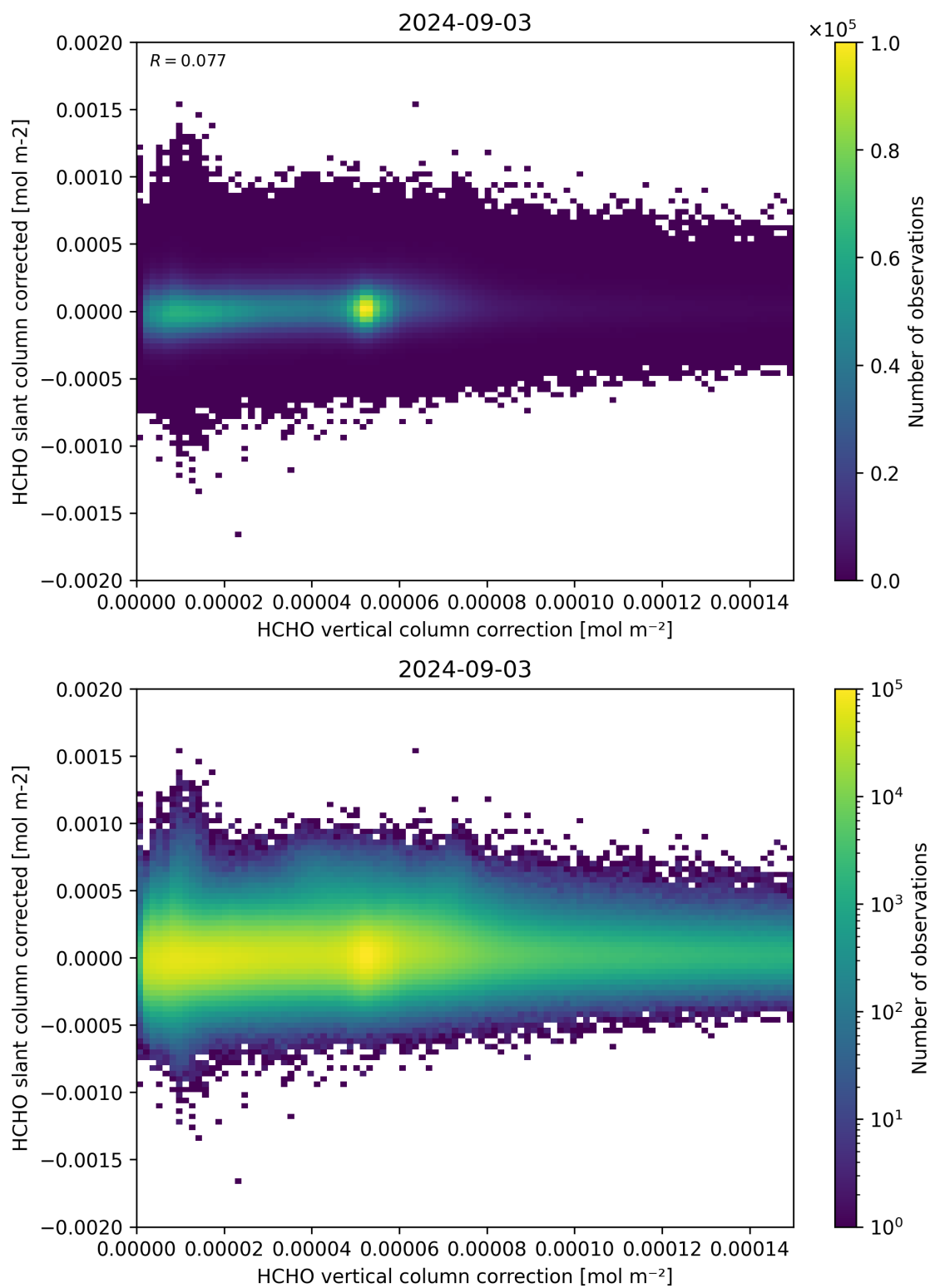
Figure 116: Scatter density plot of “HCHO vertical column correction” against “HCHO slant column corrected” for 2024-09-02 to 2024-09-04.
