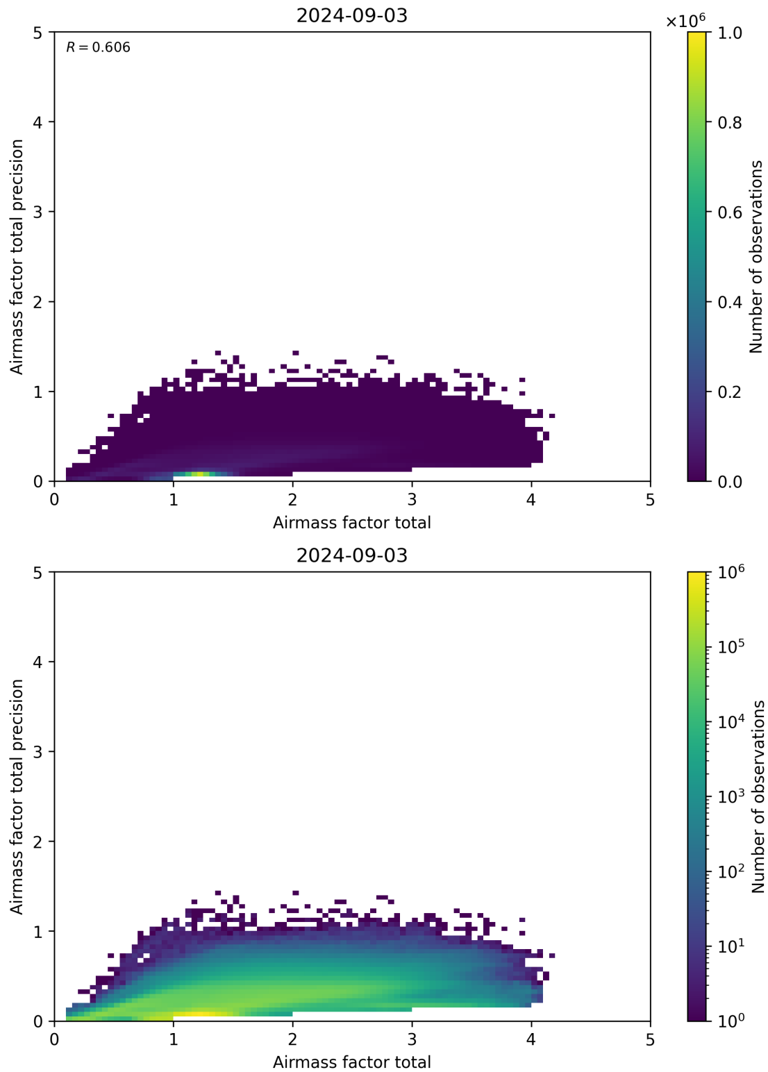
Figure 103: Scatter density plot of “Airmass factor total” against “Airmass factor total precision” for 2024-09-02 to 2024-09-04.
