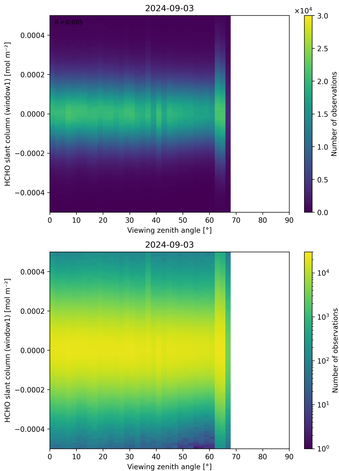
Figure 188: Scatter density plot of “Viewing zenith angle” against “HCHO slant column (window1)” for 2024-09-02 to 2024-09-04.
