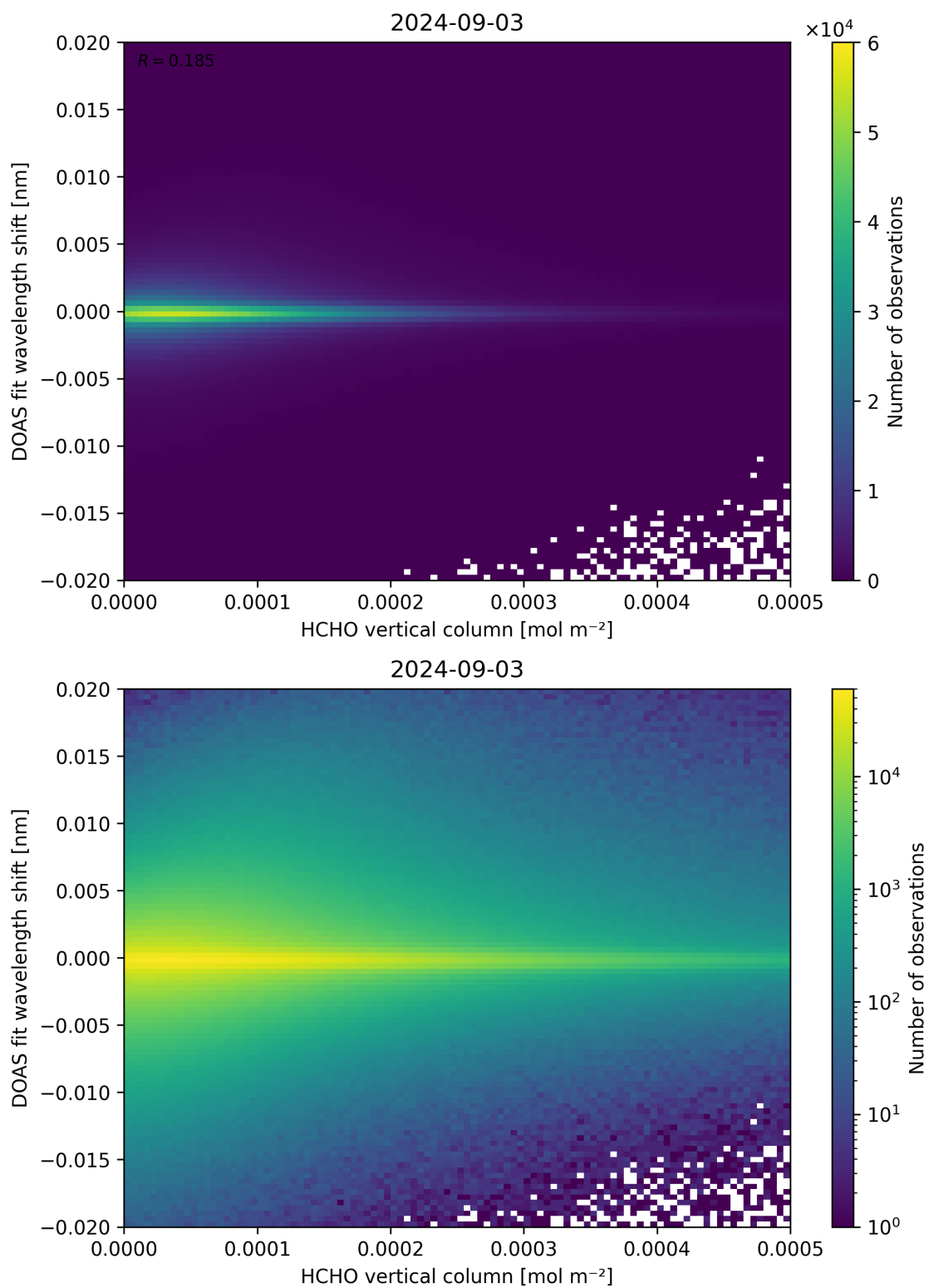
Figure 124: Scatter density plot of “HCHO vertical column” against “DOAS fit wavelength shift” for 2024-09-02 to 2024-09-04.
