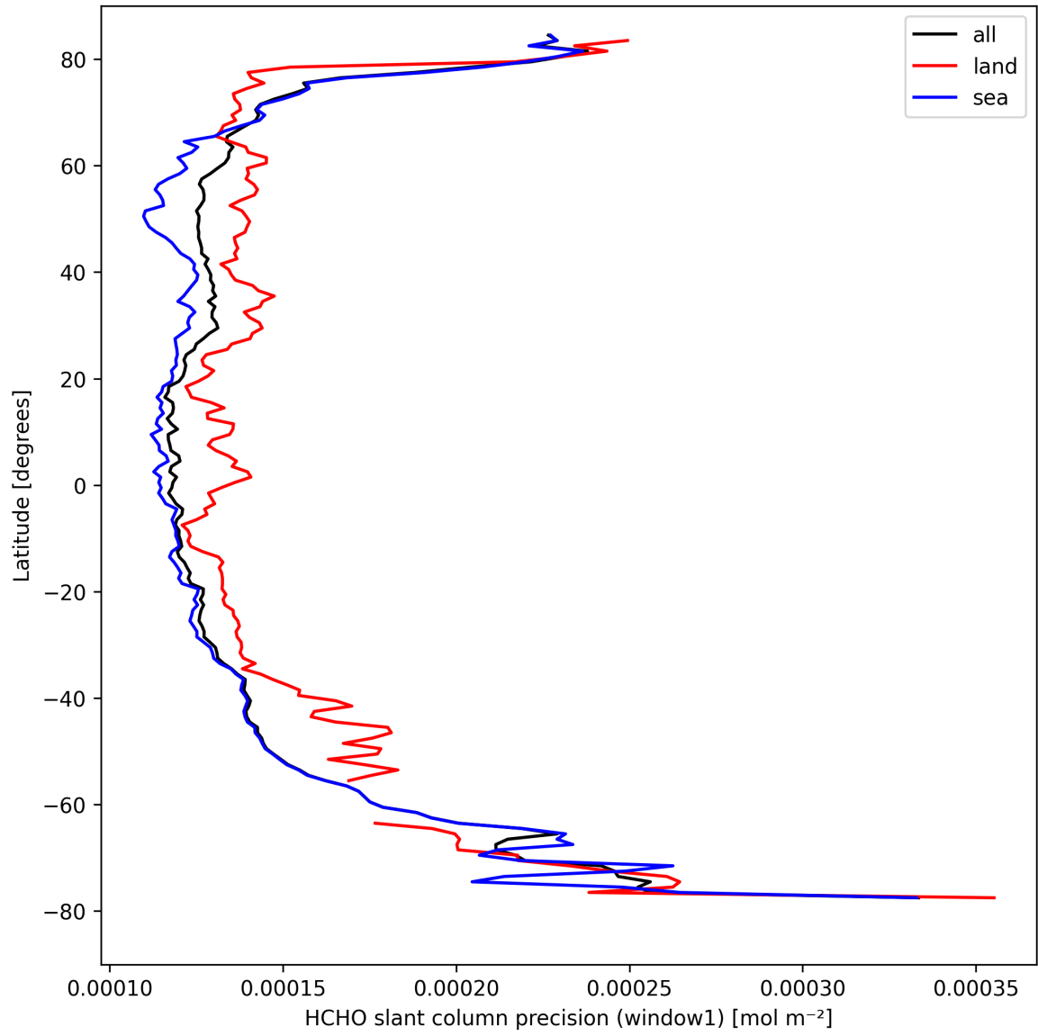
Figure 25: Zonal average of “HCHO slant column precision (window1)” for 2024-09-02 to 2024-09-04.
