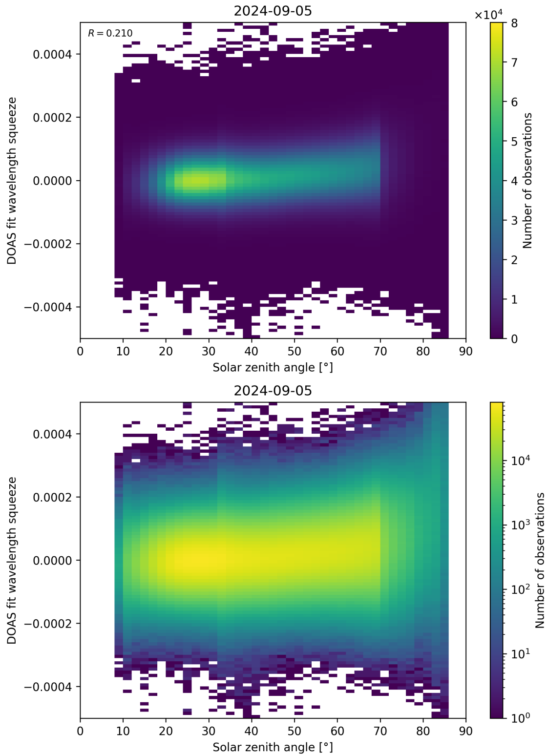
Figure 169: Scatter density plot of “Solar zenith angle” against “DOAS fit wavelength squeeze” for 2024-09-04 to 2024-09-06.
