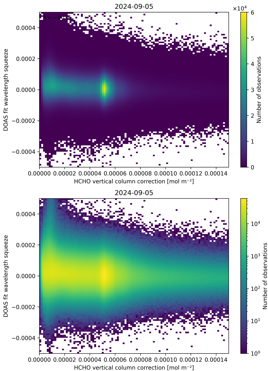
Figure 114: Scatter density plot of “HCHO vertical column correction” against “DOAS fit wavelength squeeze” for 2024-09-04 to 2024-09-06.
