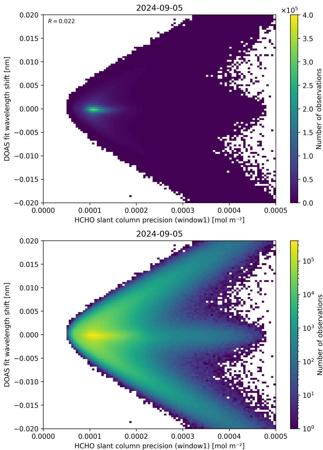
Figure 89: Scatter density plot of “HCHO slant column precision (window1)” against “DOAS fit wavelength shift” for 2024-09-04 to 2024-09-06.
