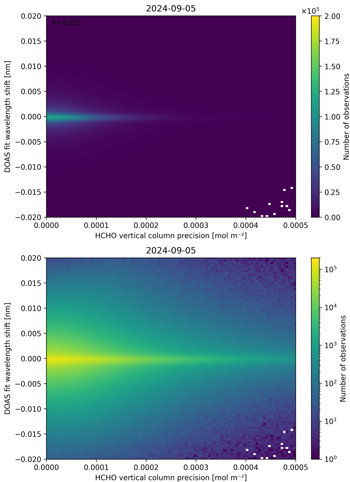
Figure 137: Scatter density plot of “HCHO vertical column precision” against “DOAS fit wavelength shift” for 2024-09-04 to 2024-09-06.
