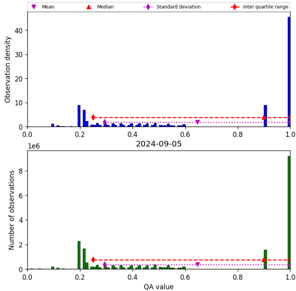
Figure 34: Histogram of “QA value” for 2024-09-04 to 2024-09-06
