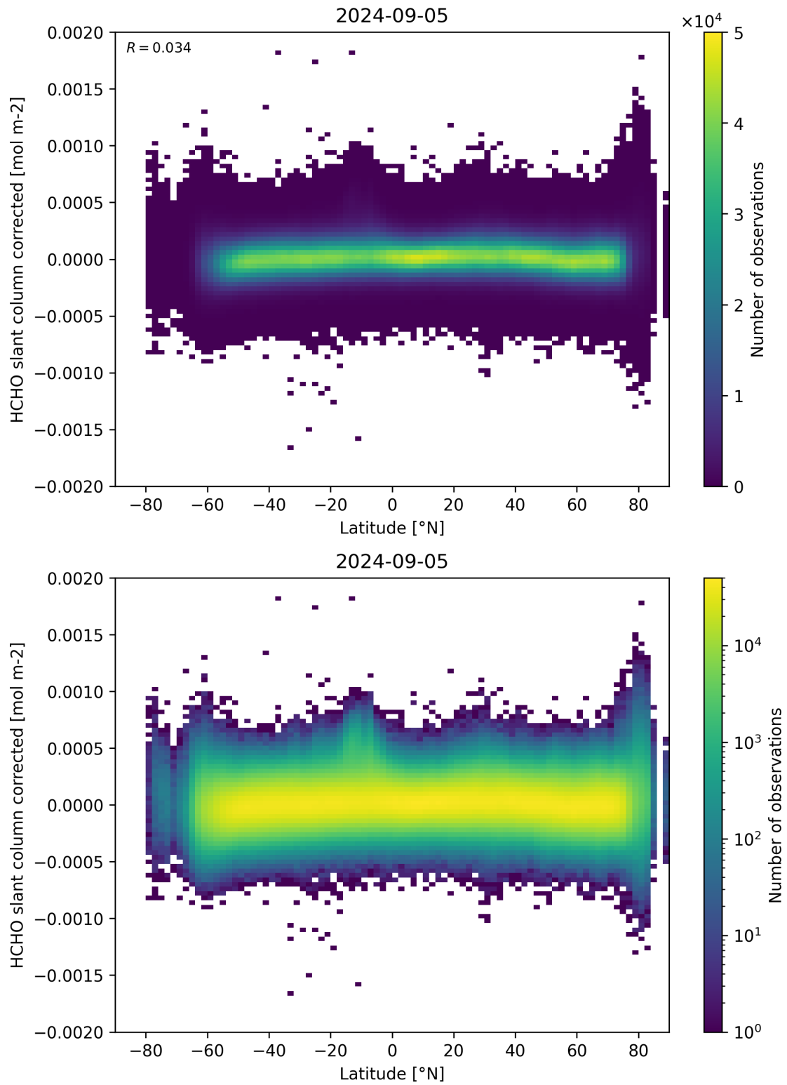
Figure 157: Scatter density plot of “Latitude” against “HCHO slant column corrected” for 2024-09-04 to 2024-09-06.
