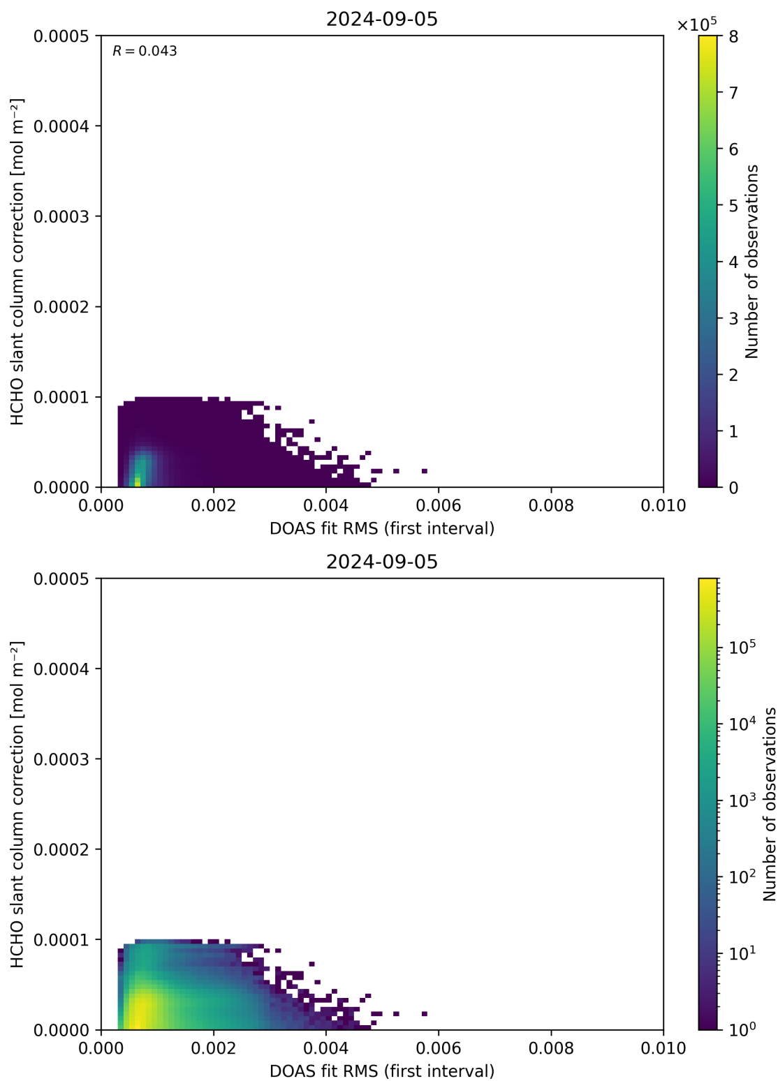
Figure 63: Scatter density plot of “DOAS fit RMS (first interval)” against “HCHO slant column correction” for 2024-09-04 to 2024-09-06.
