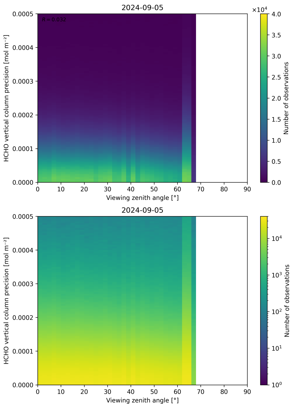
Figure 194: Scatter density plot of “Viewing zenith angle” against “HCHO vertical column precision” for 2024-09-04 to 2024-09-06.
