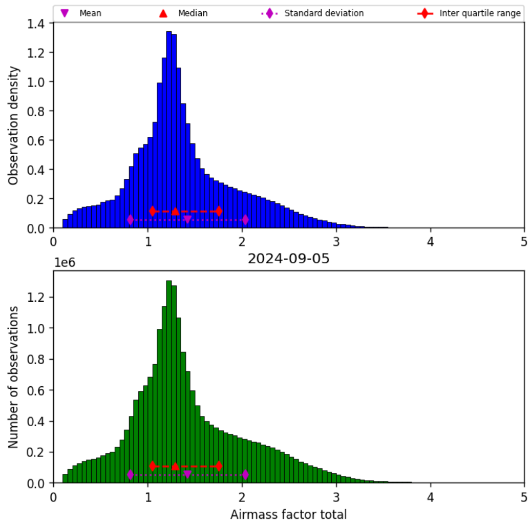
Figure 40: Histogram of “Airmass factor total” for 2024-09-04 to 2024-09-06
