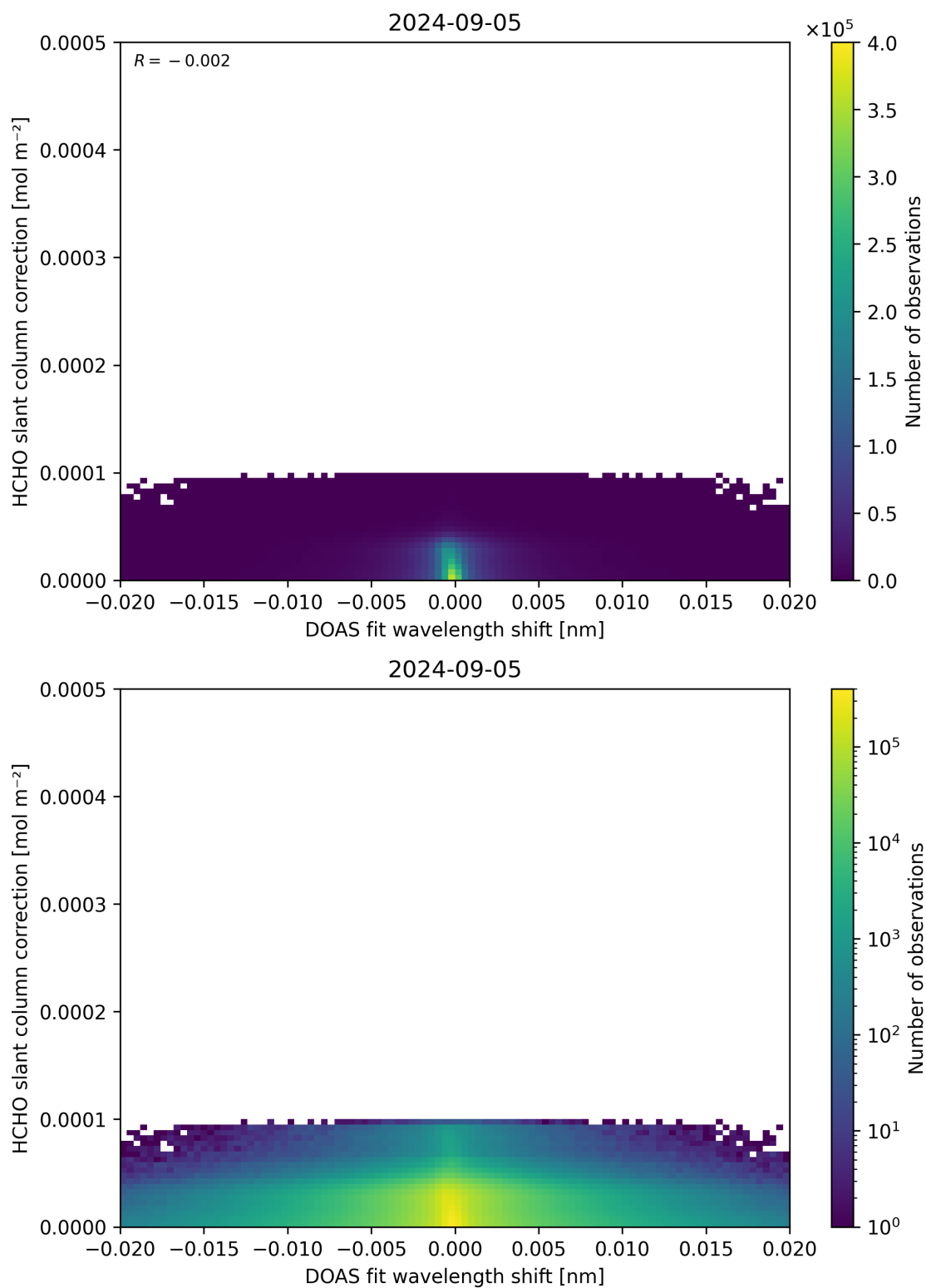
Figure 67: Scatter density plot of “DOAS fit wavelength shift” against “HCHO slant column correction” for 2024-09-04 to 2024-09-06.
