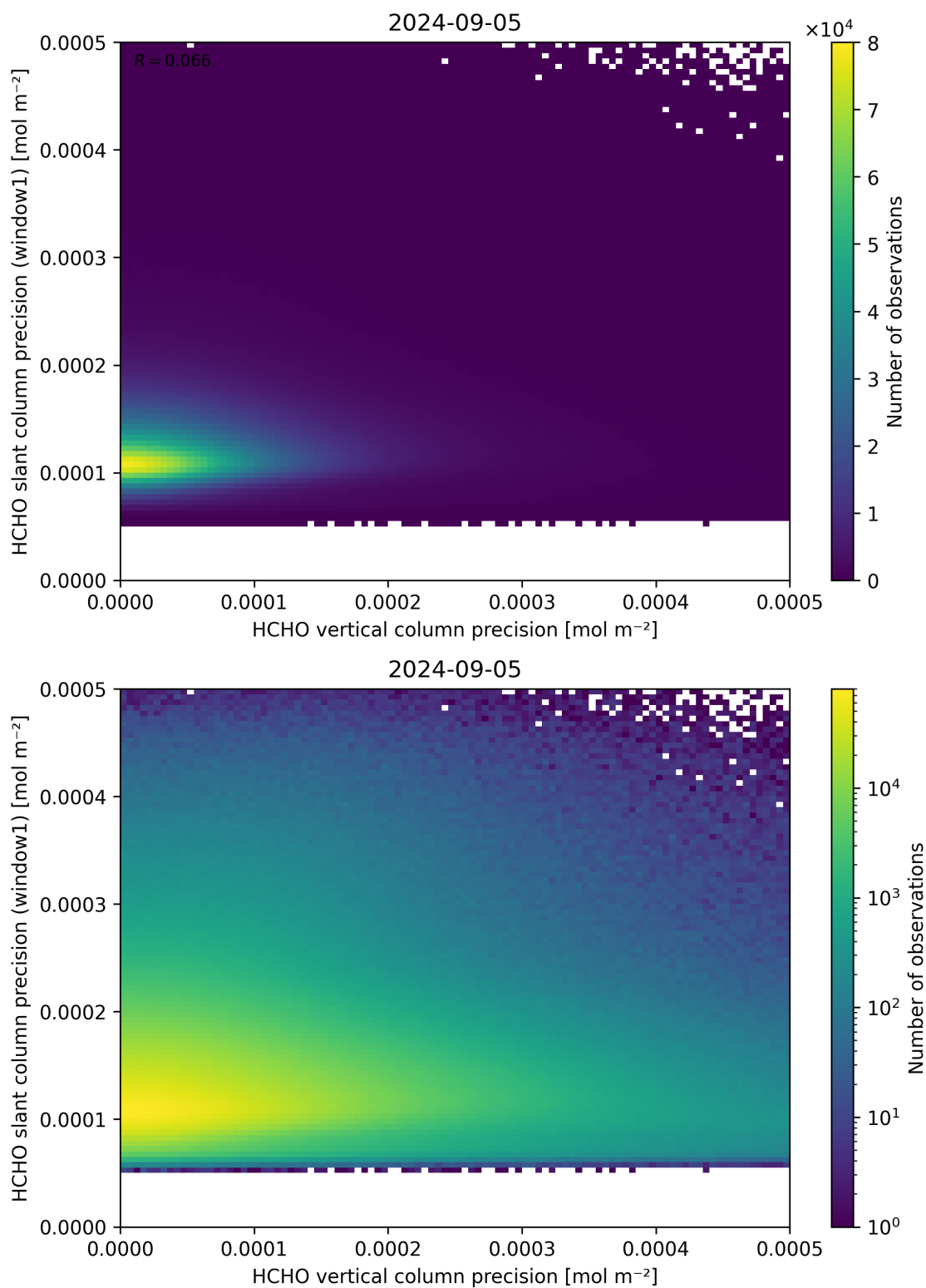
Figure 143: Scatter density plot of “HCHO vertical column precision” against “HCHO slant column precision (window1)” for 2024-09-04 to 2024-09-06.
