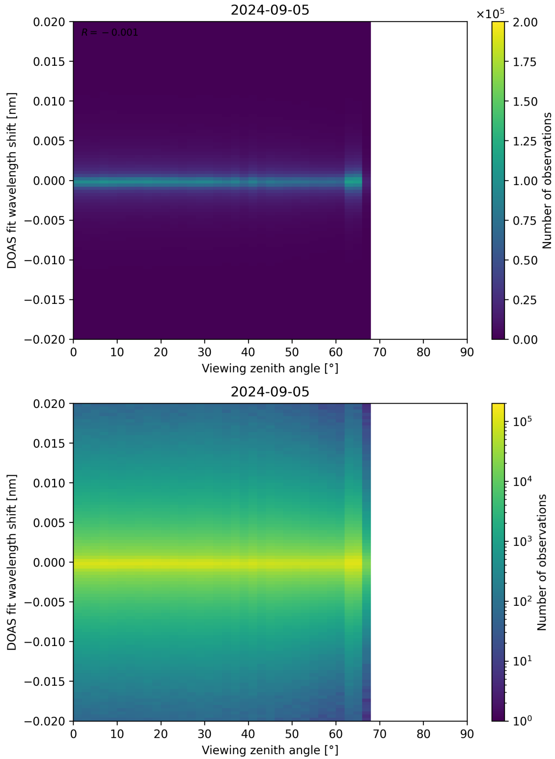
Figure 183: Scatter density plot of “Viewing zenith angle” against “DOAS fit wavelength shift” for 2024-09-04 to 2024-09-06.
