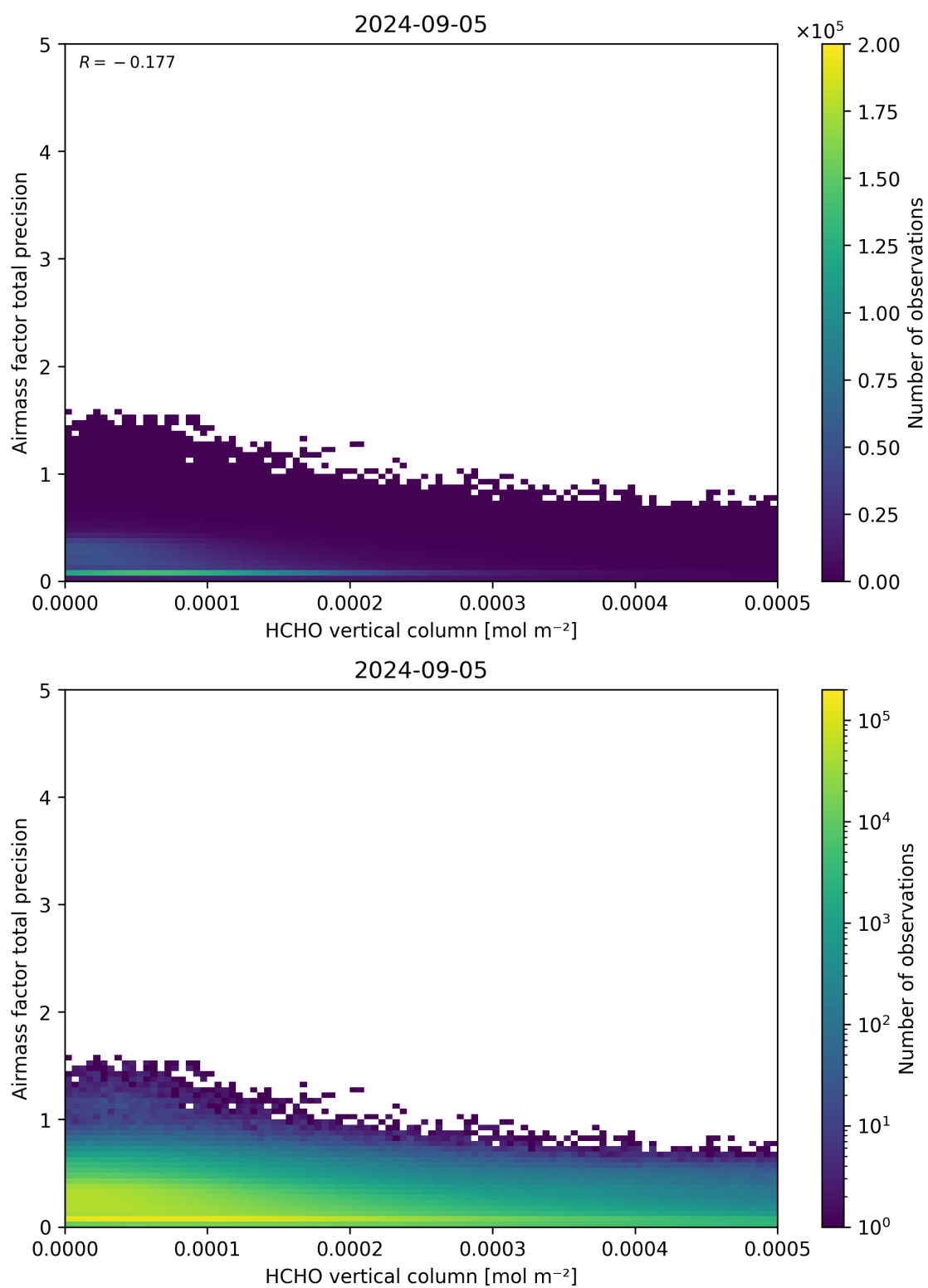
Figure 132: Scatter density plot of “HCHO vertical column” against “Airmass factor total precision” for 2024-09-04 to 2024-09-06.
