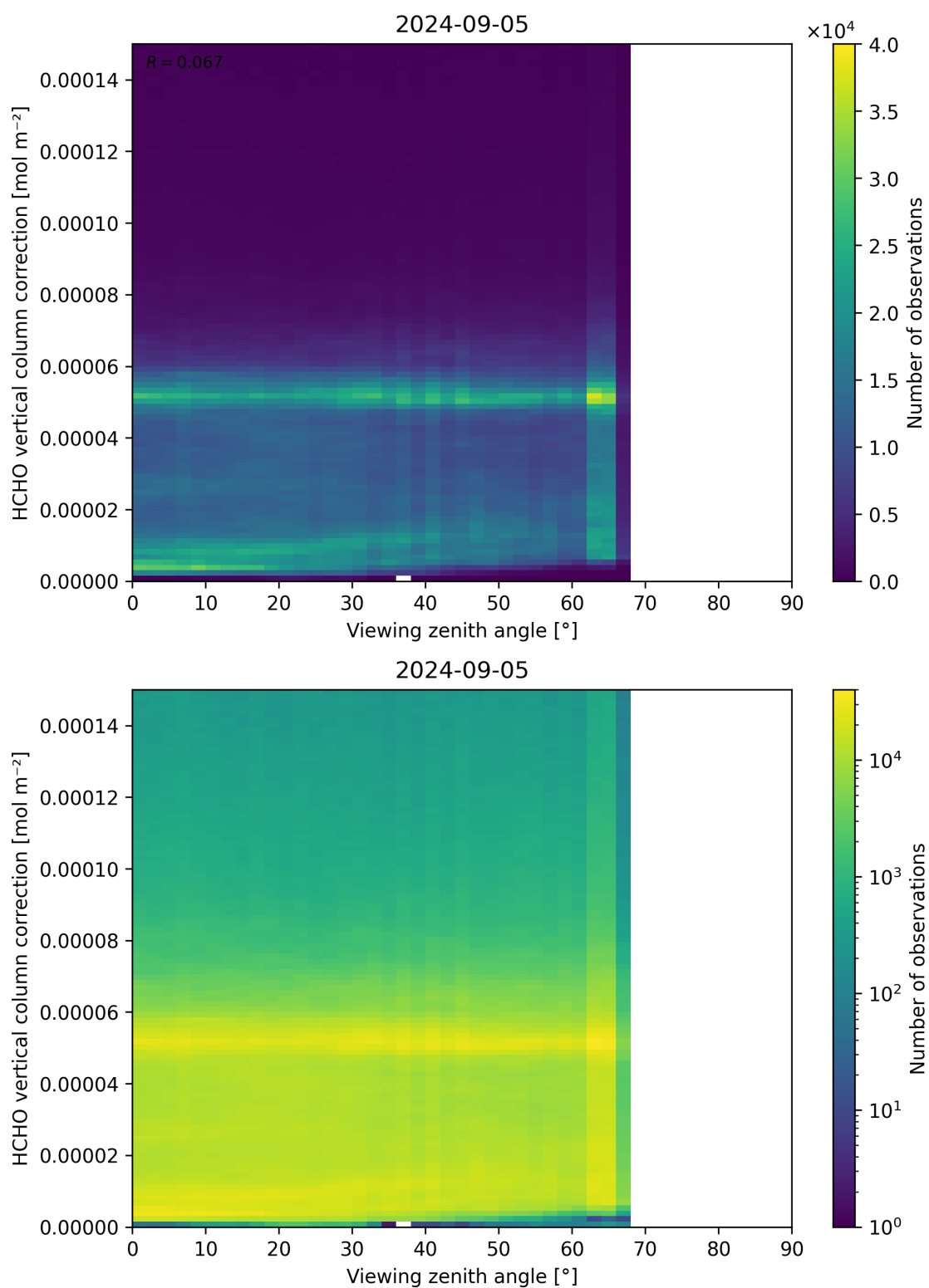
Figure 193: Scatter density plot of “Viewing zenith angle” against “HCHO vertical column correction” for 2024-09-04 to 2024-09-06.
