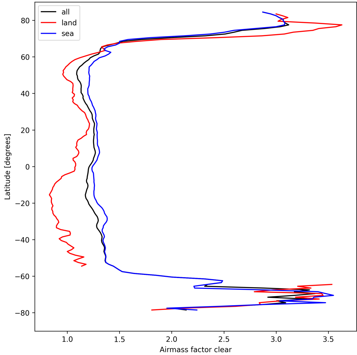
Figure 28: Zonal average of “Airmass factor clear” for 2024-09-04 to 2024-09-06.
