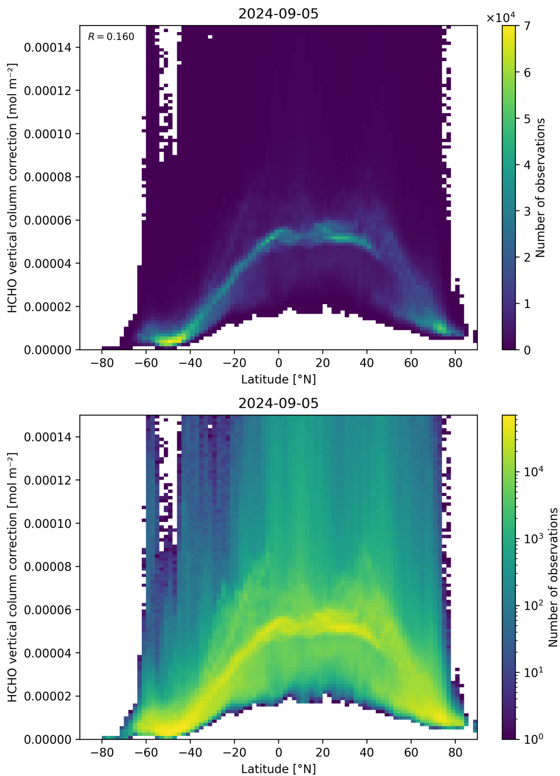
Figure 164: Scatter density plot of “Latitude” against “HCHO vertical column correction” for 2024-09-04 to 2024-09-06.
