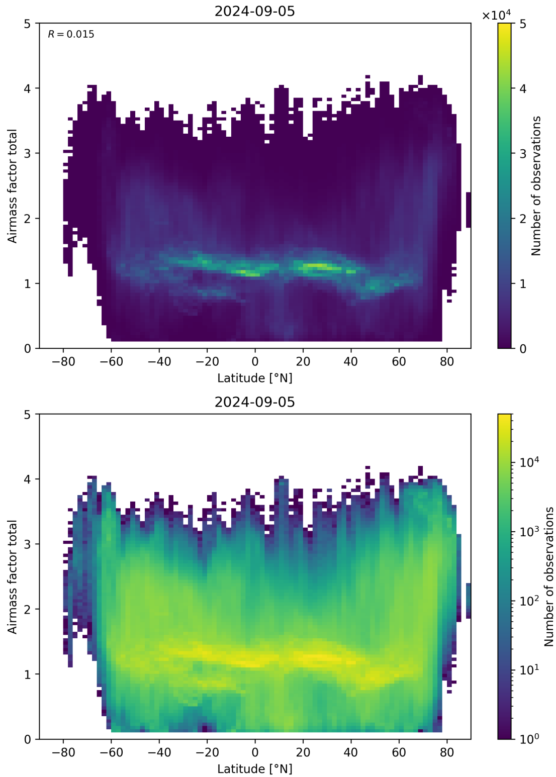
Figure 161: Scatter density plot of “Latitude” against “Airmass factor total” for 2024-09-04 to 2024-09-06.
