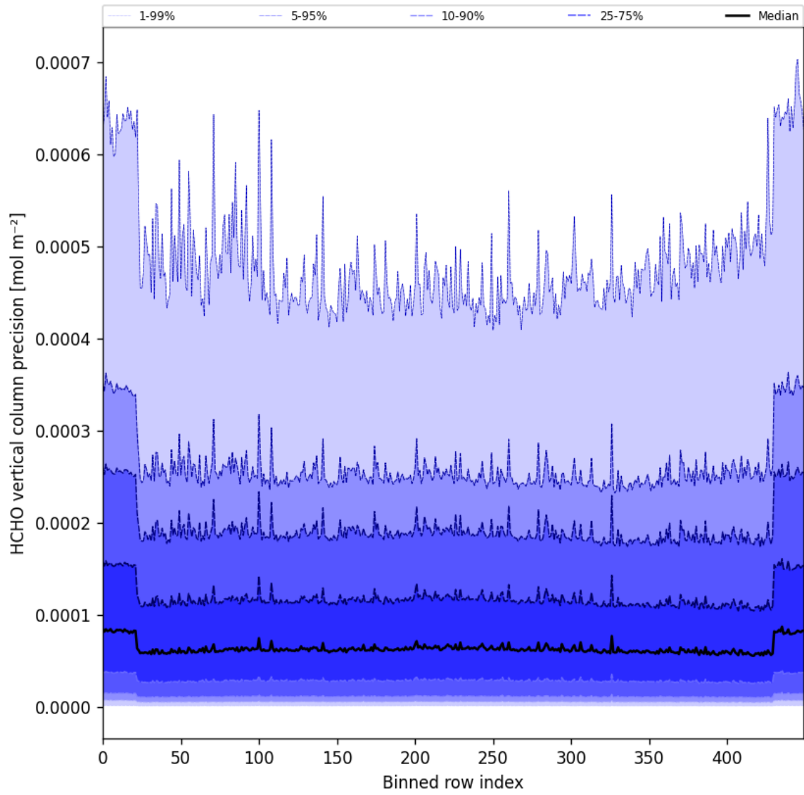
Figure 50: Along track statistics of “HCHO vertical column precision” for 2024-09-04 to 2024-09-06
