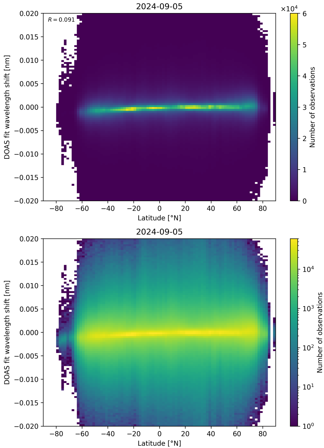
Figure 154: Scatter density plot of “Latitude” against “DOAS fit wavelength shift” for 2024-09-04 to 2024-09-06.
