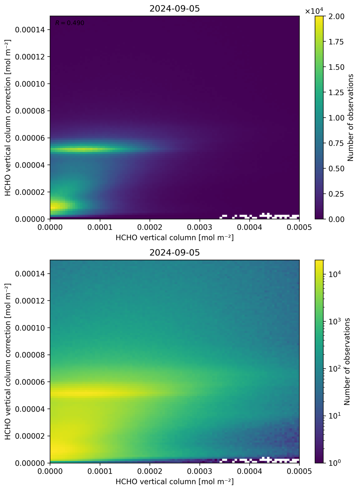
Figure 133: Scatter density plot of “HCHO vertical column” against “HCHO vertical column correction” for 2024-09-04 to 2024-09-06.
