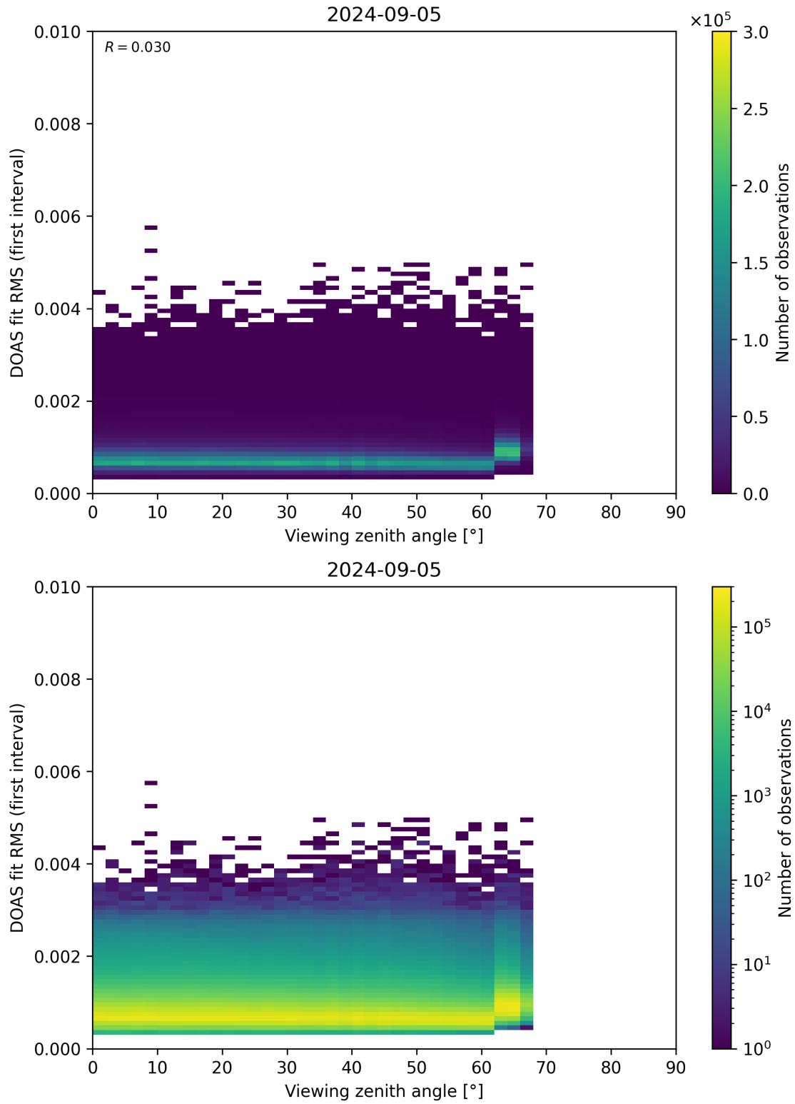
Figure 182: Scatter density plot of “Viewing zenith angle” against “DOAS fit RMS (first interval)” for 2024-09-04 to 2024-09-06.
