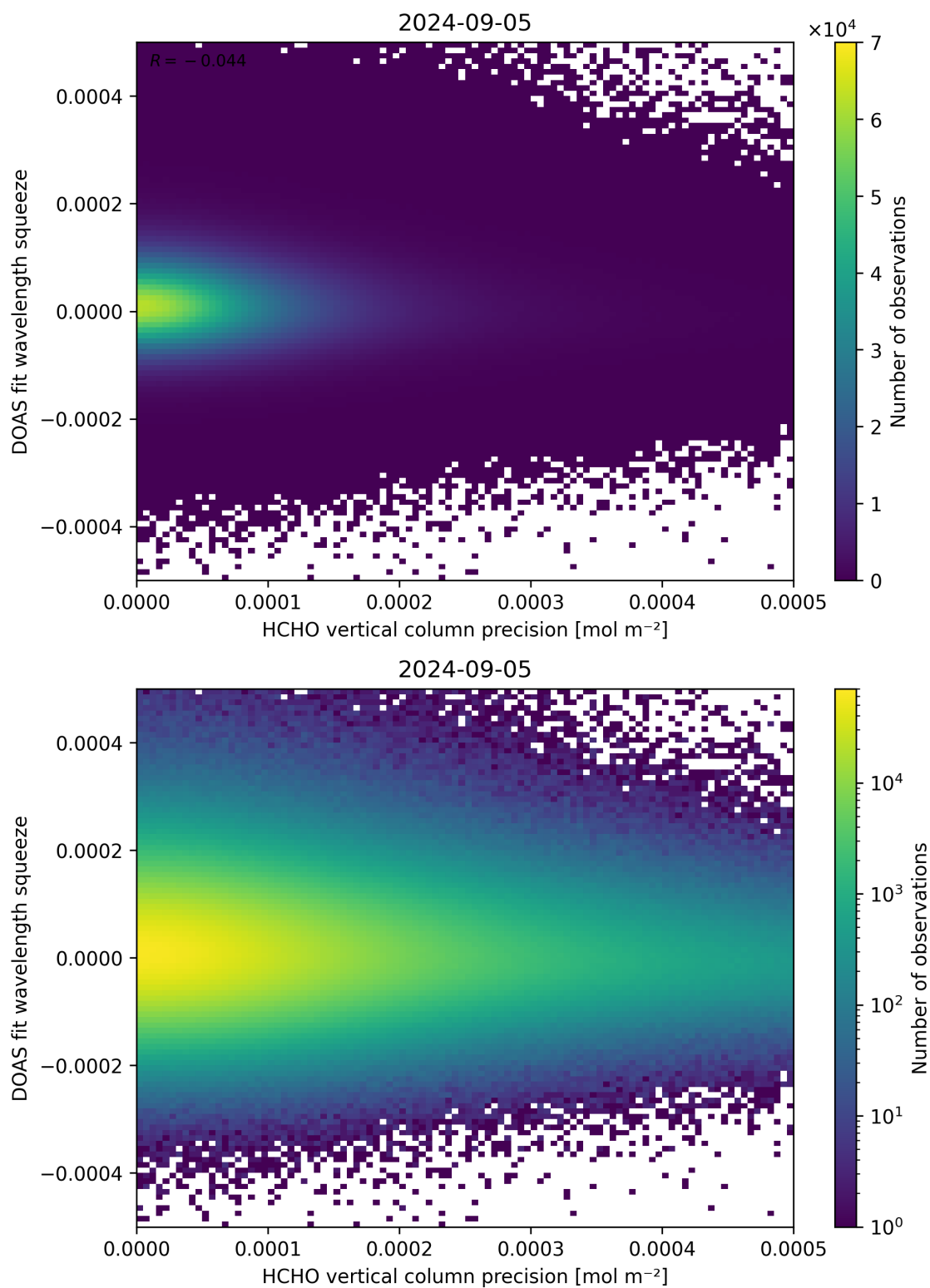
Figure 138: Scatter density plot of “HCHO vertical column precision” against “DOAS fit wavelength squeeze” for 2024-09-04 to 2024-09-06.
