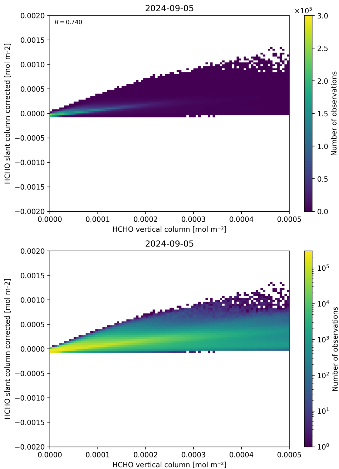
Figure 127: Scatter density plot of “HCHO vertical column” against “HCHO slant column corrected” for 2024-09-04 to 2024-09-06.
