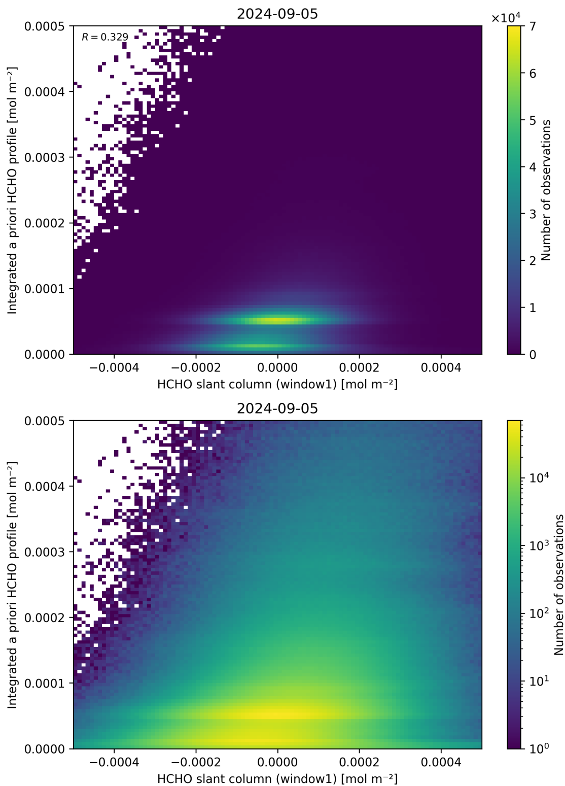
Figure 87: Scatter density plot of “HCHO slant column (window1)” against “Integrated a priori HCHO profile” for 2024-09-04 to 2024-09-06.
