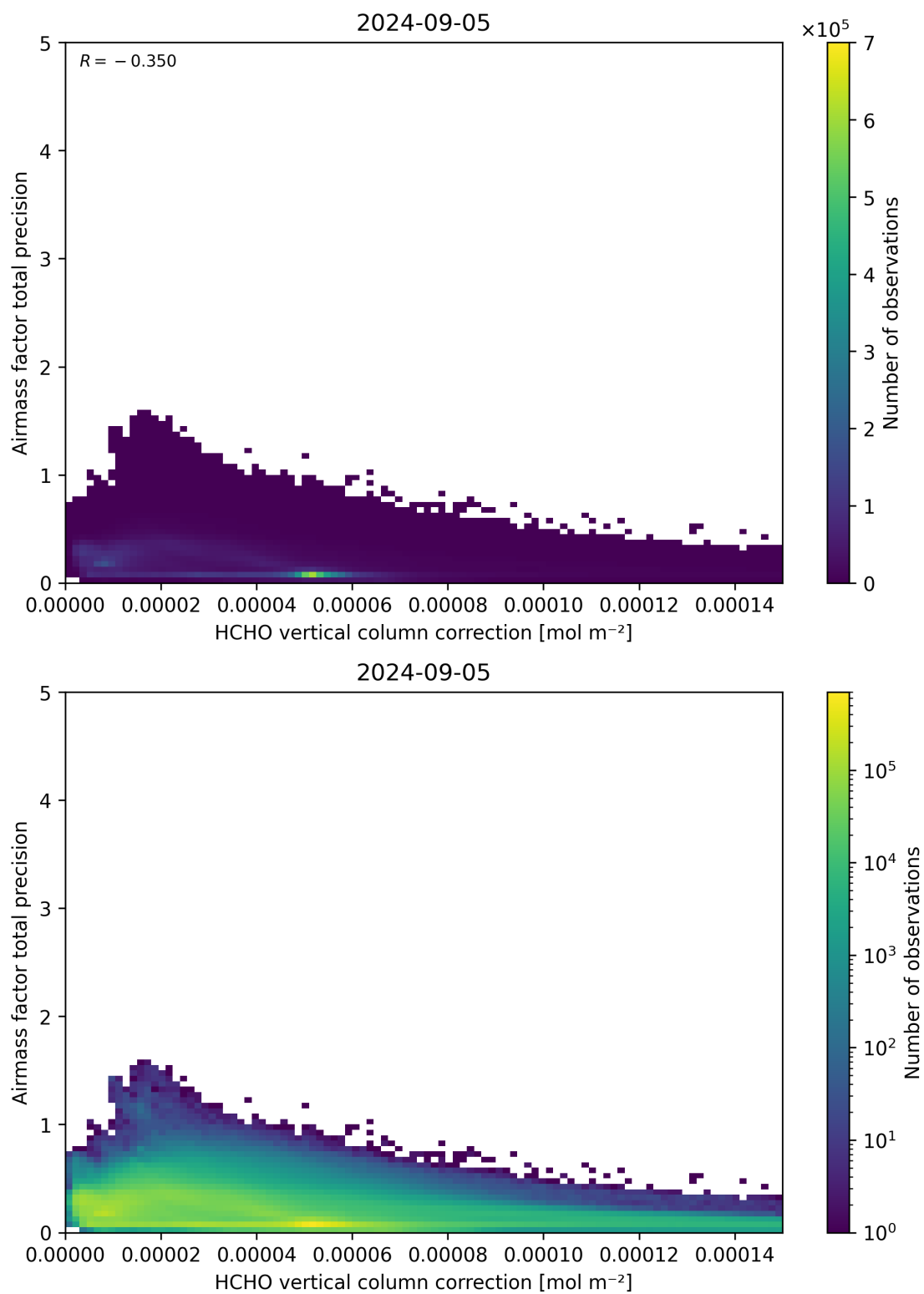
Figure 121: Scatter density plot of “HCHO vertical column correction” against “Airmass factor total precision” for 2024-09-04 to 2024-09-06.
