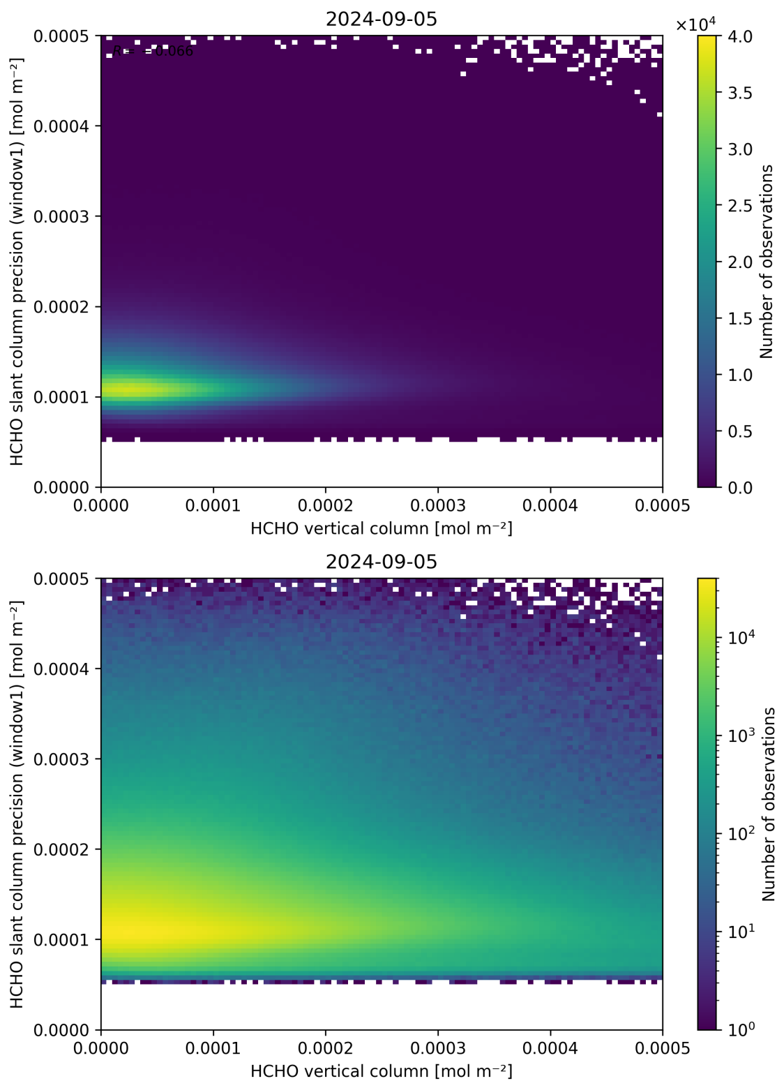
Figure 130: Scatter density plot of “HCHO vertical column” against “HCHO slant column precision (window1)” for 2024-09-04 to 2024-09-06.
