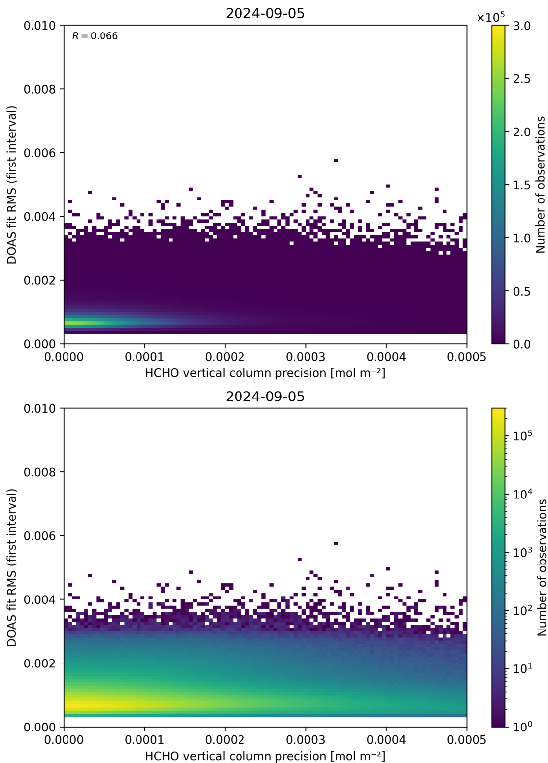
Figure 136: Scatter density plot of “HCHO vertical column precision” against “DOAS fit RMS (first interval)” for 2024-09-04 to 2024-09-06.
