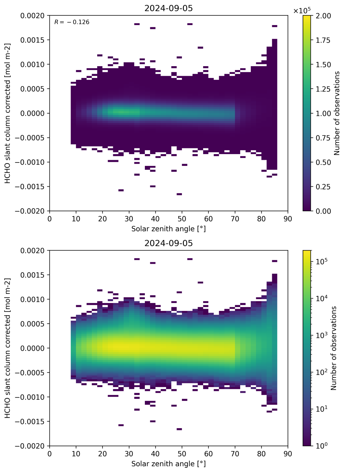
Figure 171: Scatter density plot of “Solar zenith angle” against “HCHO slant column corrected” for 2024-09-04 to 2024-09-06.
