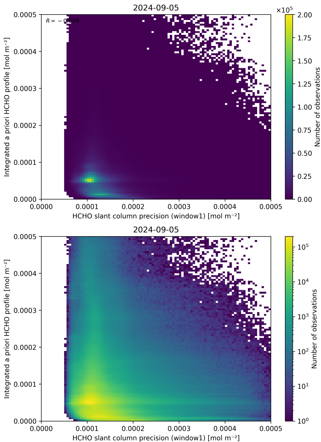
Figure 96: Scatter density plot of “HCHO slant column precision (window1)” against “Integrated a priori HCHO profile” for 2024-09-04 to 2024-09-06.
