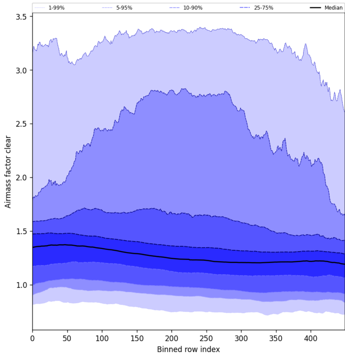
Figure 56: Along track statistics of “Airmass factor clear” for 2024-09-04 to 2024-09-06
