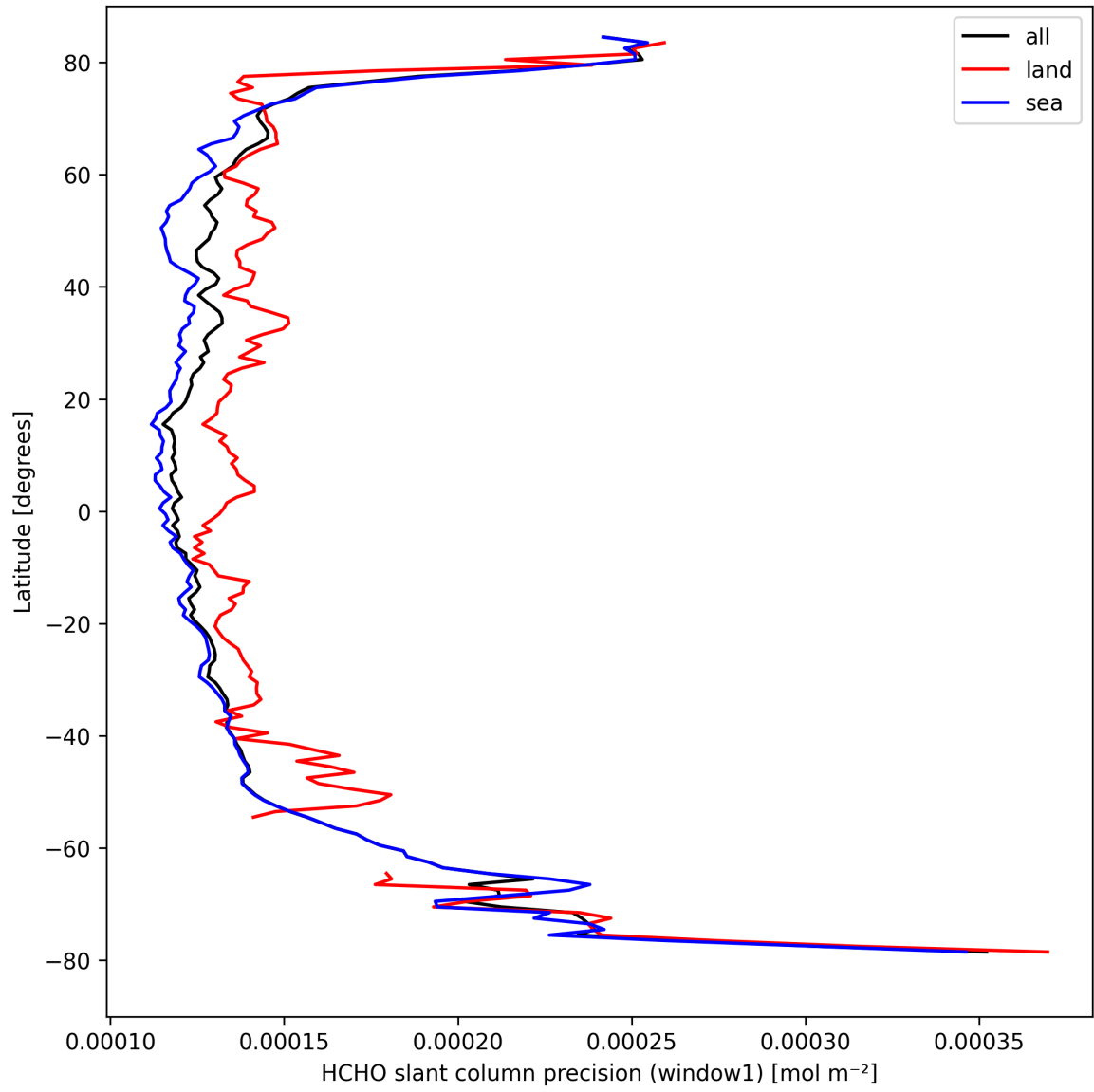
Figure 25: Zonal average of “HCHO slant column precision (window1)” for 2024-09-04 to 2024-09-06.
