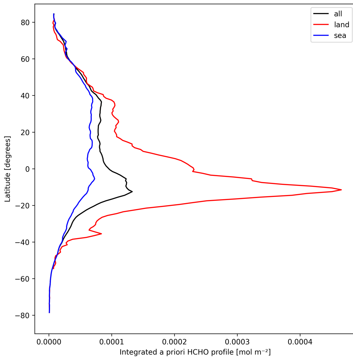
Figure 29: Zonal average of “Integrated a priori HCHO profile” for 2024-09-04 to 2024-09-06.
