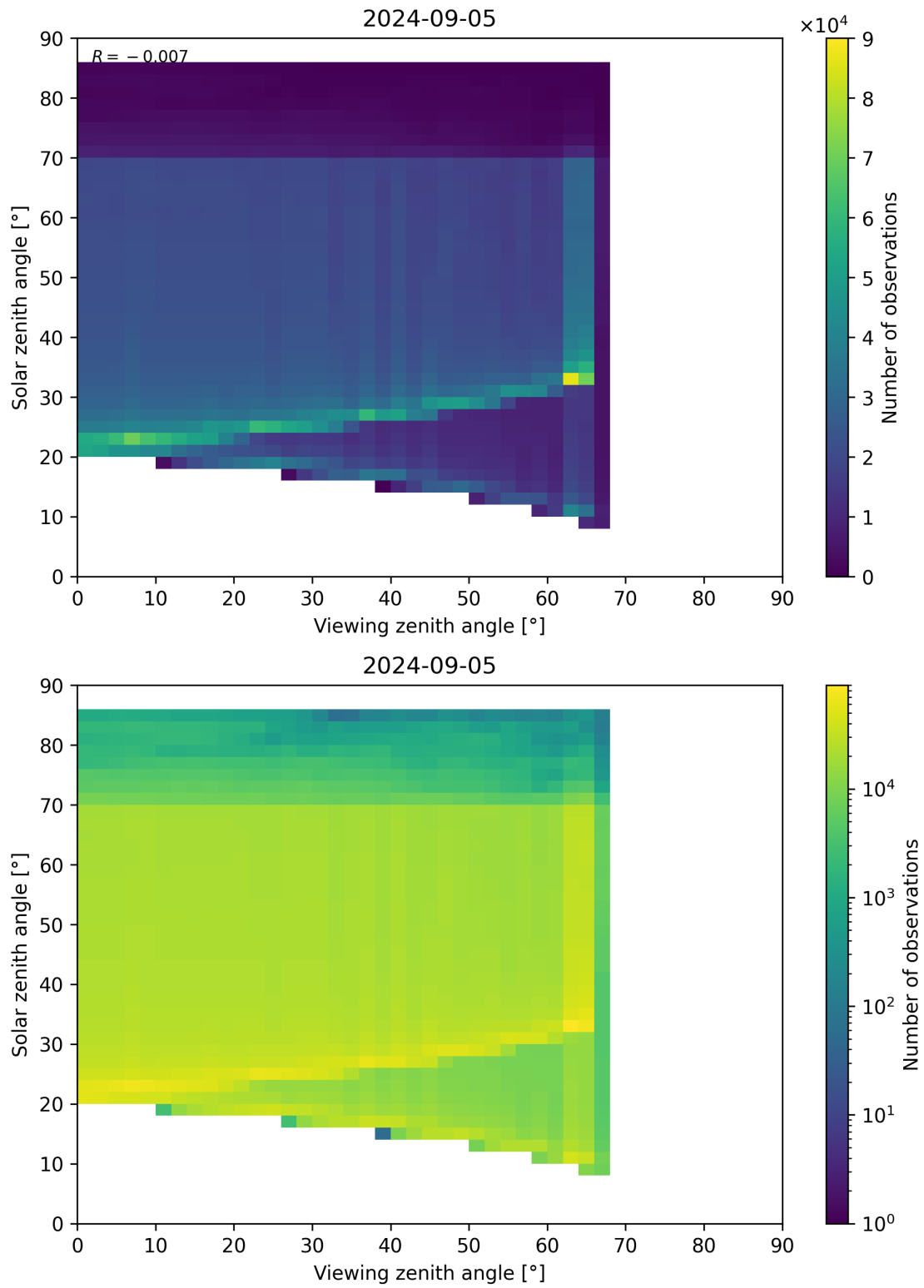
Figure 197: Scatter density plot of “Viewing zenith angle” against “Solar zenith angle” for 2024-09-04 to 2024-09-06.
