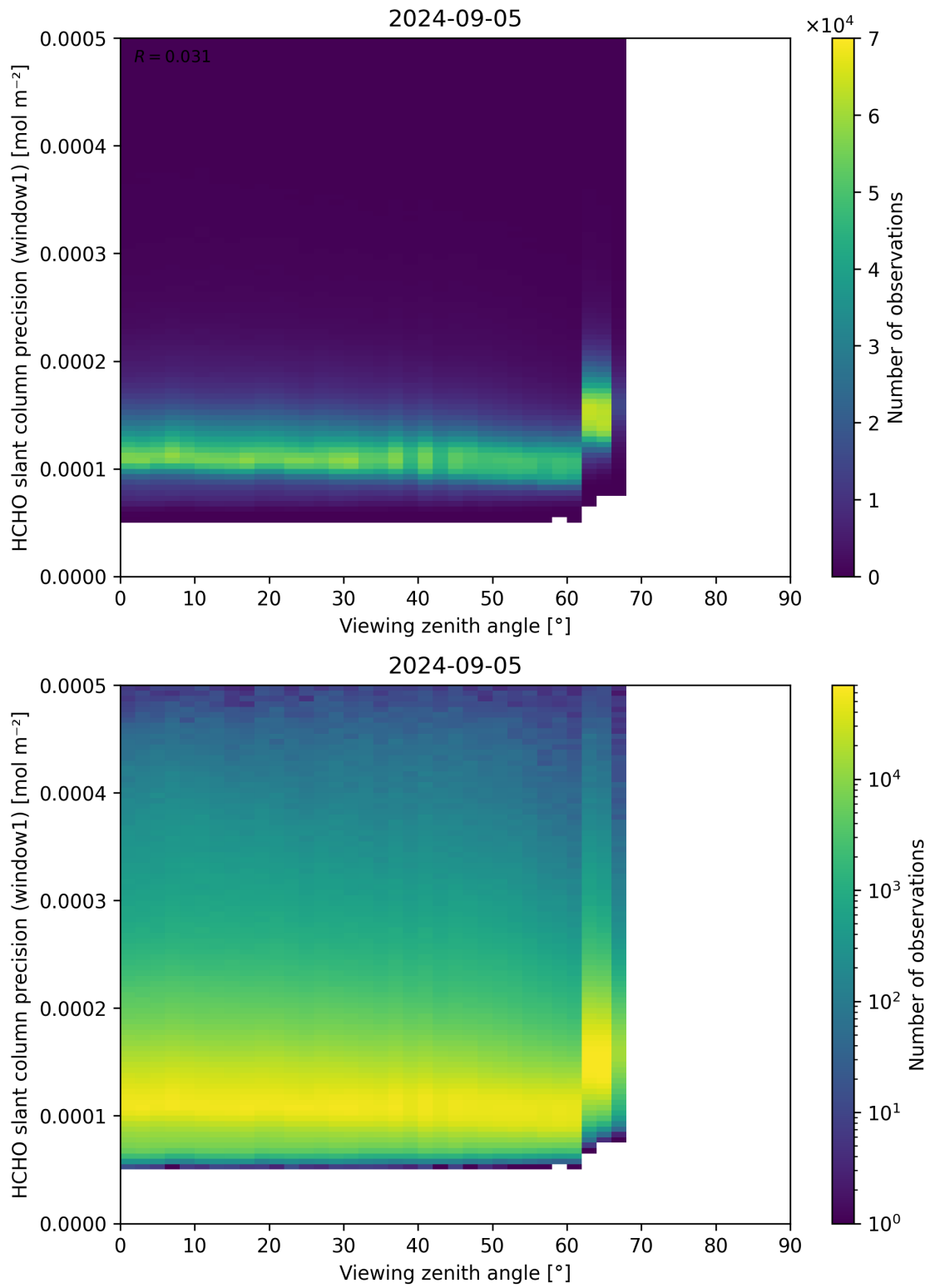
Figure 189: Scatter density plot of “Viewing zenith angle” against “HCHO slant column precision (window1)” for 2024-09-04 to 2024-09-06.
