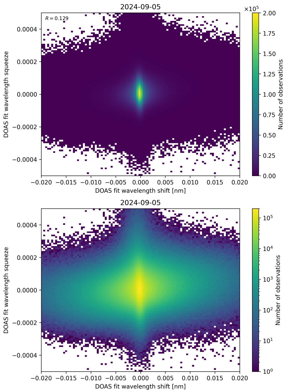
Figure 65: Scatter density plot of “DOAS fit wavelength shift” against “DOAS fit wavelength squeeze” for 2024-09-04 to 2024-09-06.
