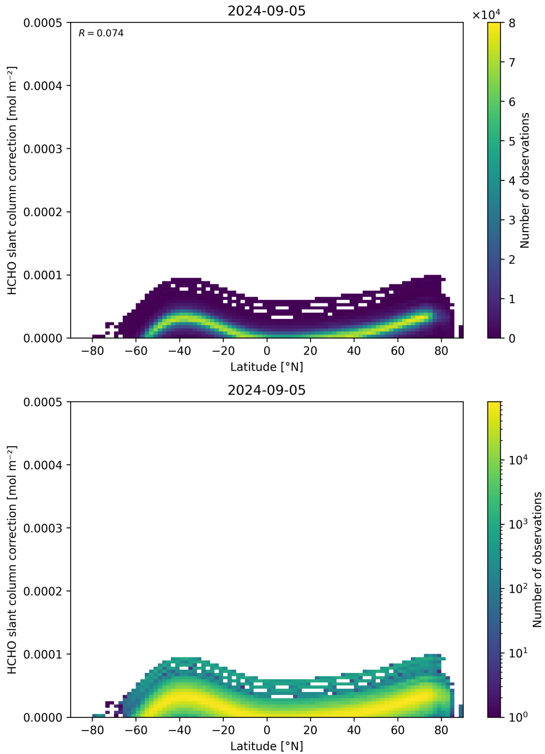
Figure 158: Scatter density plot of “Latitude” against “HCHO slant column correction” for 2024-09-04 to 2024-09-06.
