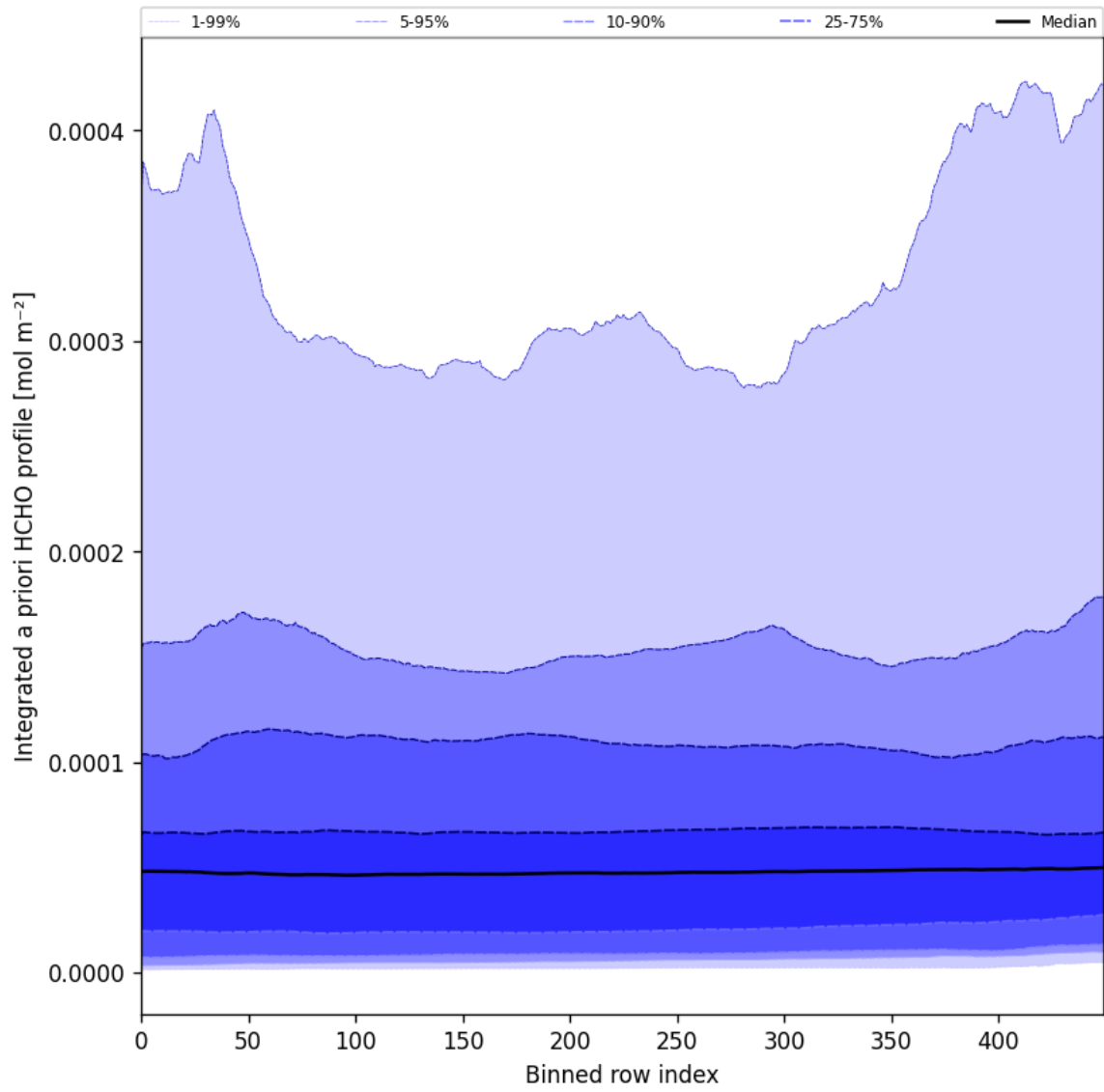
Figure 57: Along track statistics of "Integrated a priori HCHO profile" for 2024-09-04 to 2024-09-06
