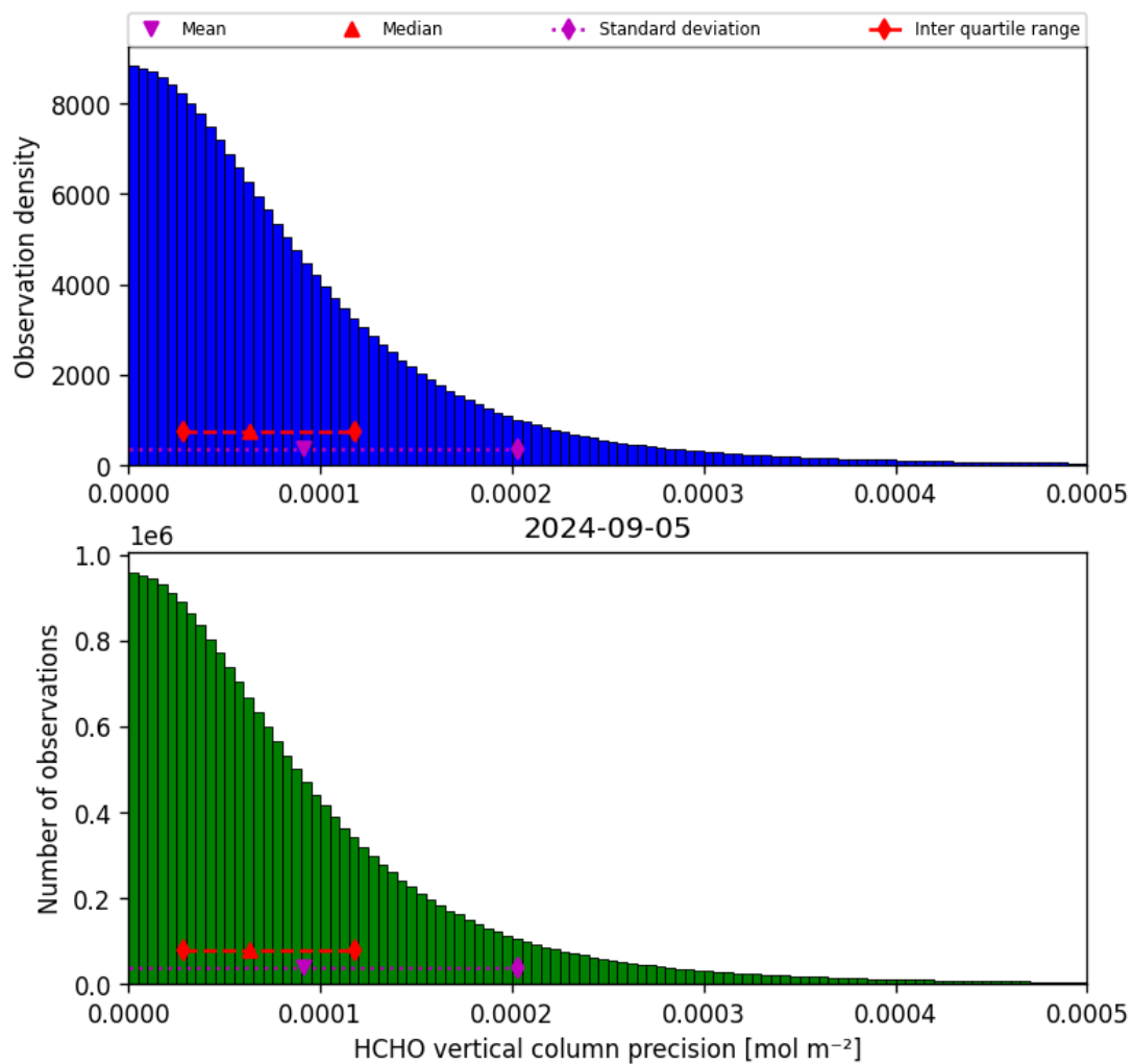
Figure 36: Histogram of “HCHO vertical column precision” for 2024-09-04 to 2024-09-06
