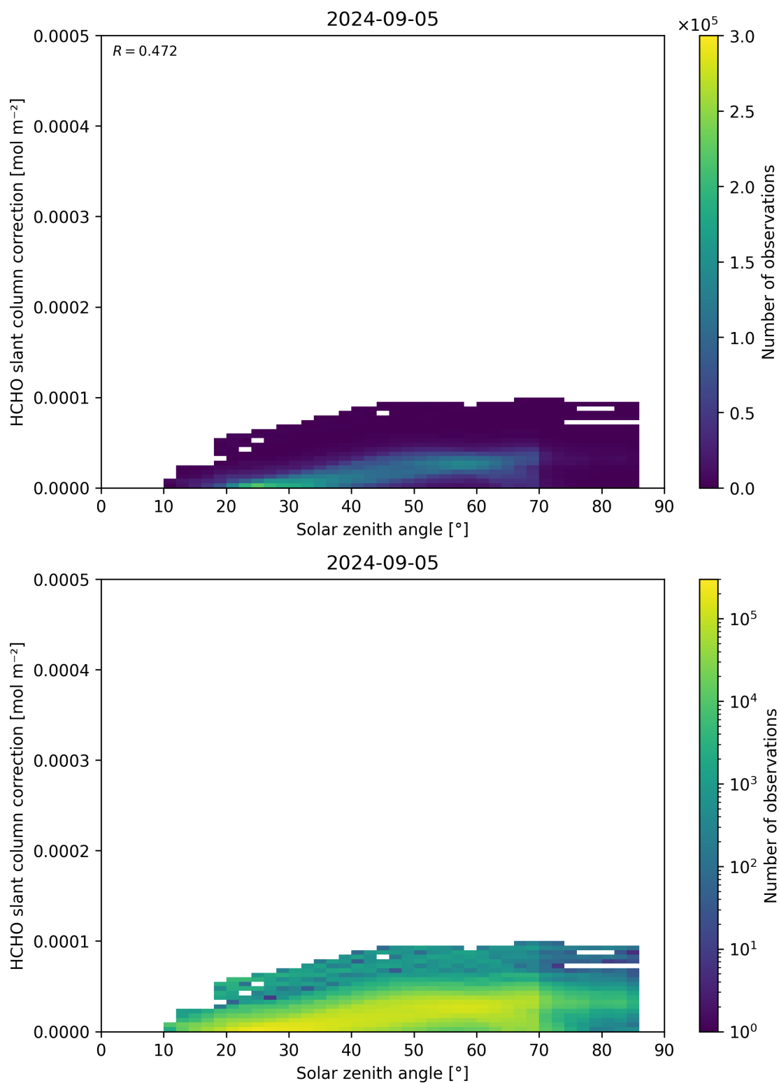
Figure 172: Scatter density plot of “Solar zenith angle” against “HCHO slant column correction” for 2024-09-04 to 2024-09-06.
