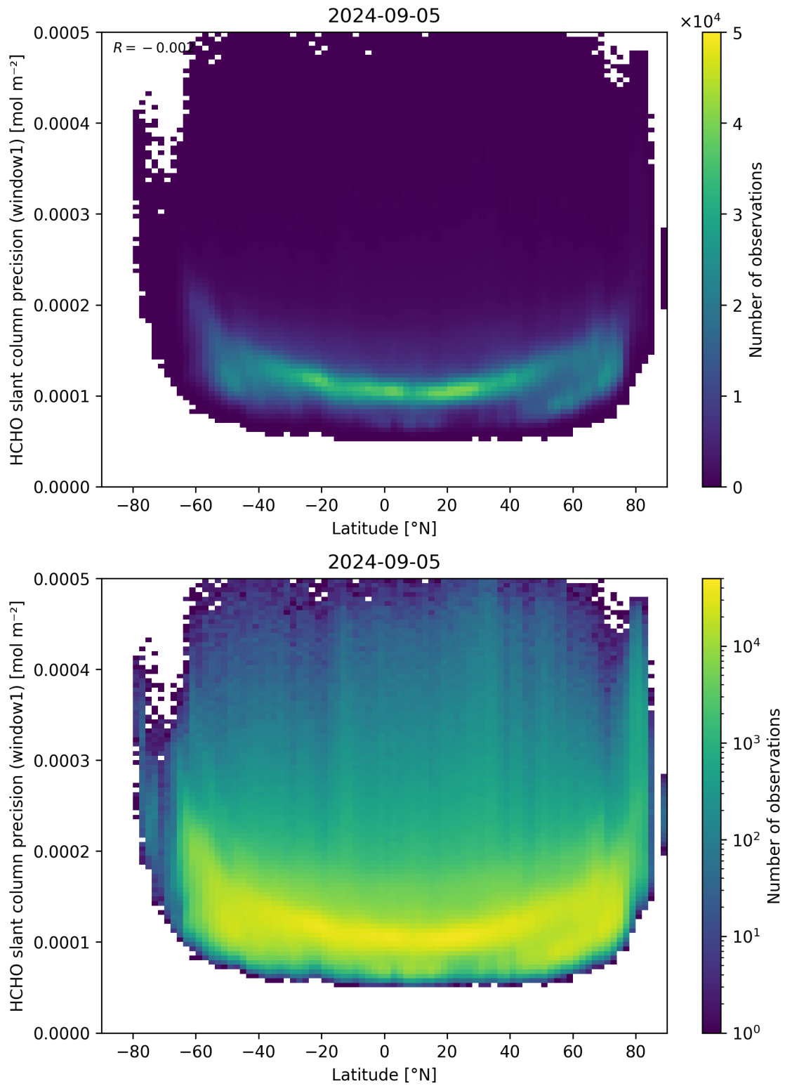
Figure 160: Scatter density plot of “Latitude” against “HCHO slant column precision (window1)” for 2024-09-04 to 2024-09-06.
