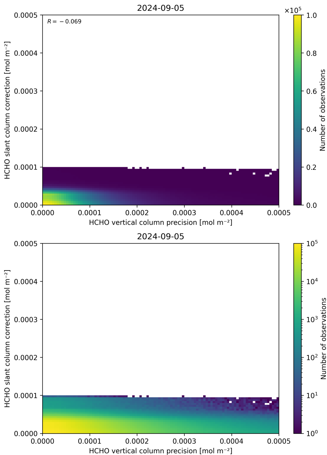
Figure 141: Scatter density plot of “HCHO vertical column precision” against “HCHO slant column correction” for 2024-09-04 to 2024-09-06.
