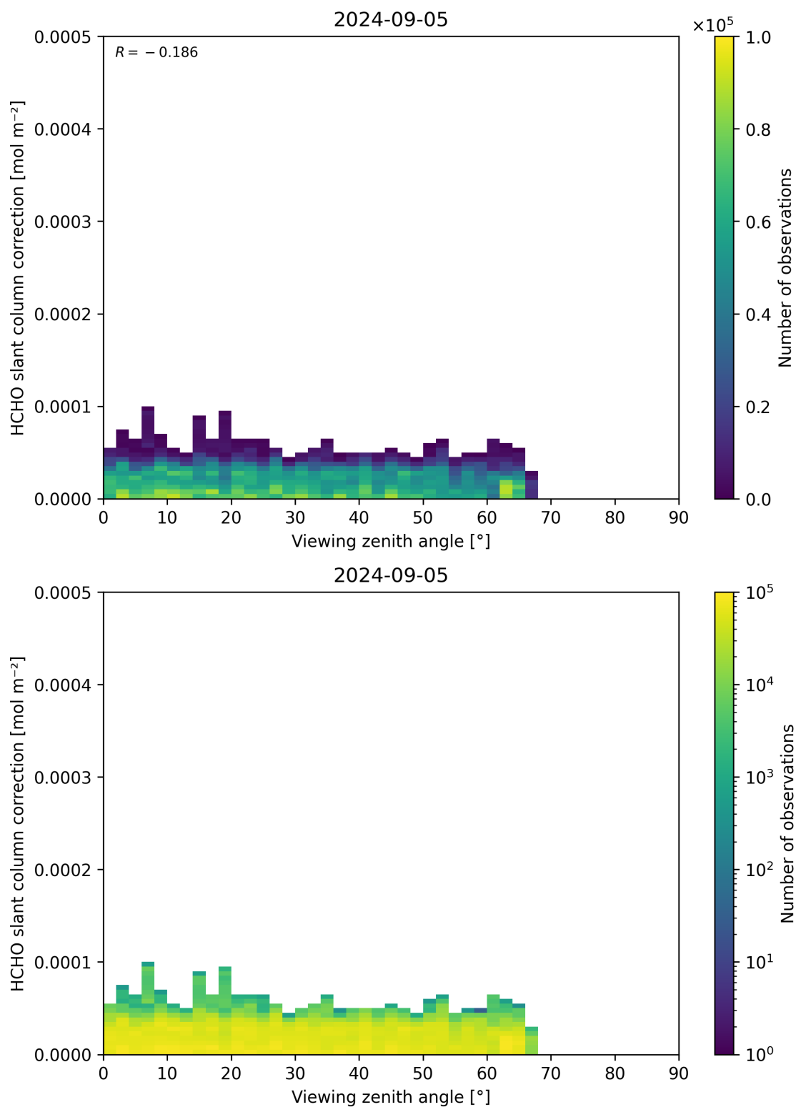
Figure 187: Scatter density plot of “Viewing zenith angle” against “HCHO slant column correction” for 2024-09-04 to 2024-09-06.
