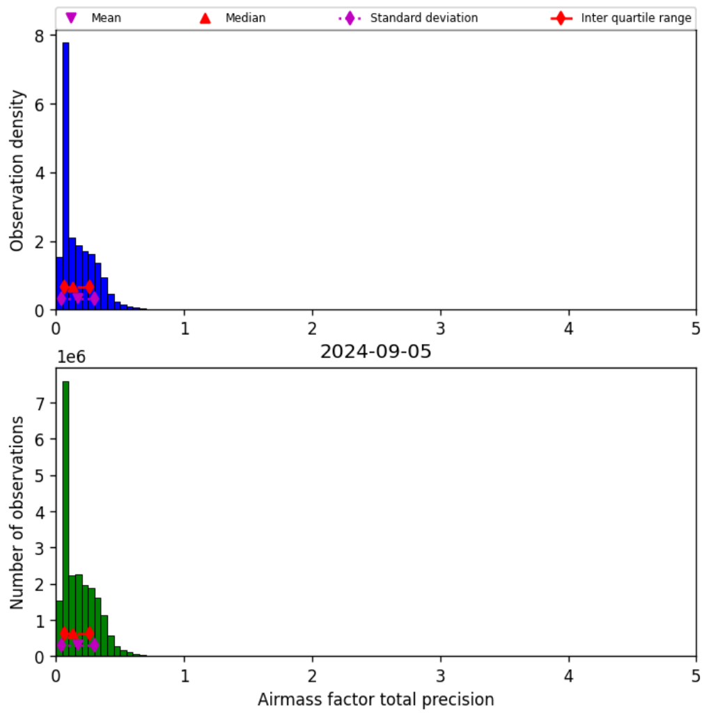
Figure 41: Histogram of “Airmass factor total precision” for 2024-09-04 to 2024-09-06
