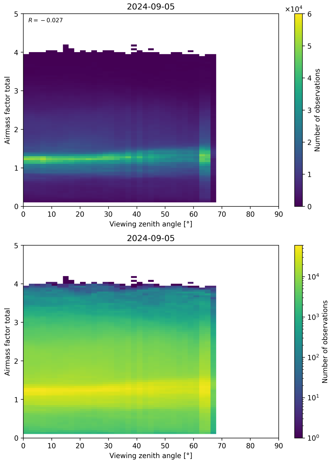
Figure 190: Scatter density plot of “Viewing zenith angle” against “Airmass factor total” for 2024-09-04 to 2024-09-06.
