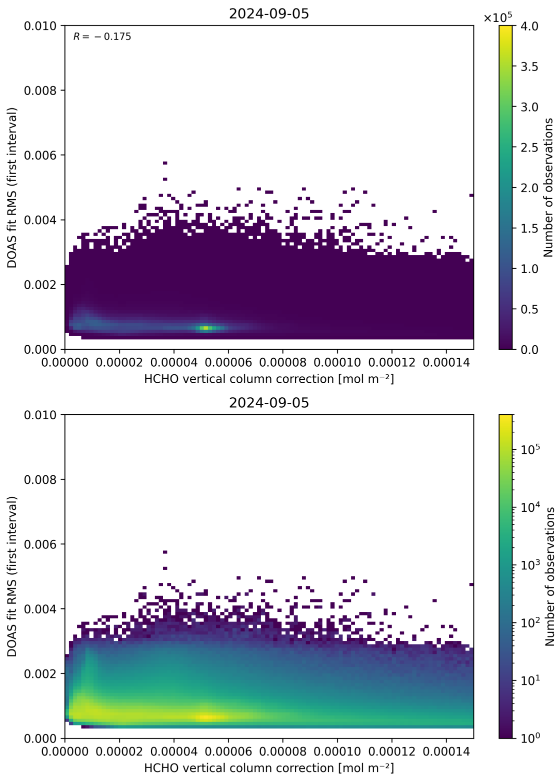
Figure 112: Scatter density plot of “HCHO vertical column correction” against “DOAS fit RMS (first interval)” for 2024-09-04 to 2024-09-06.
