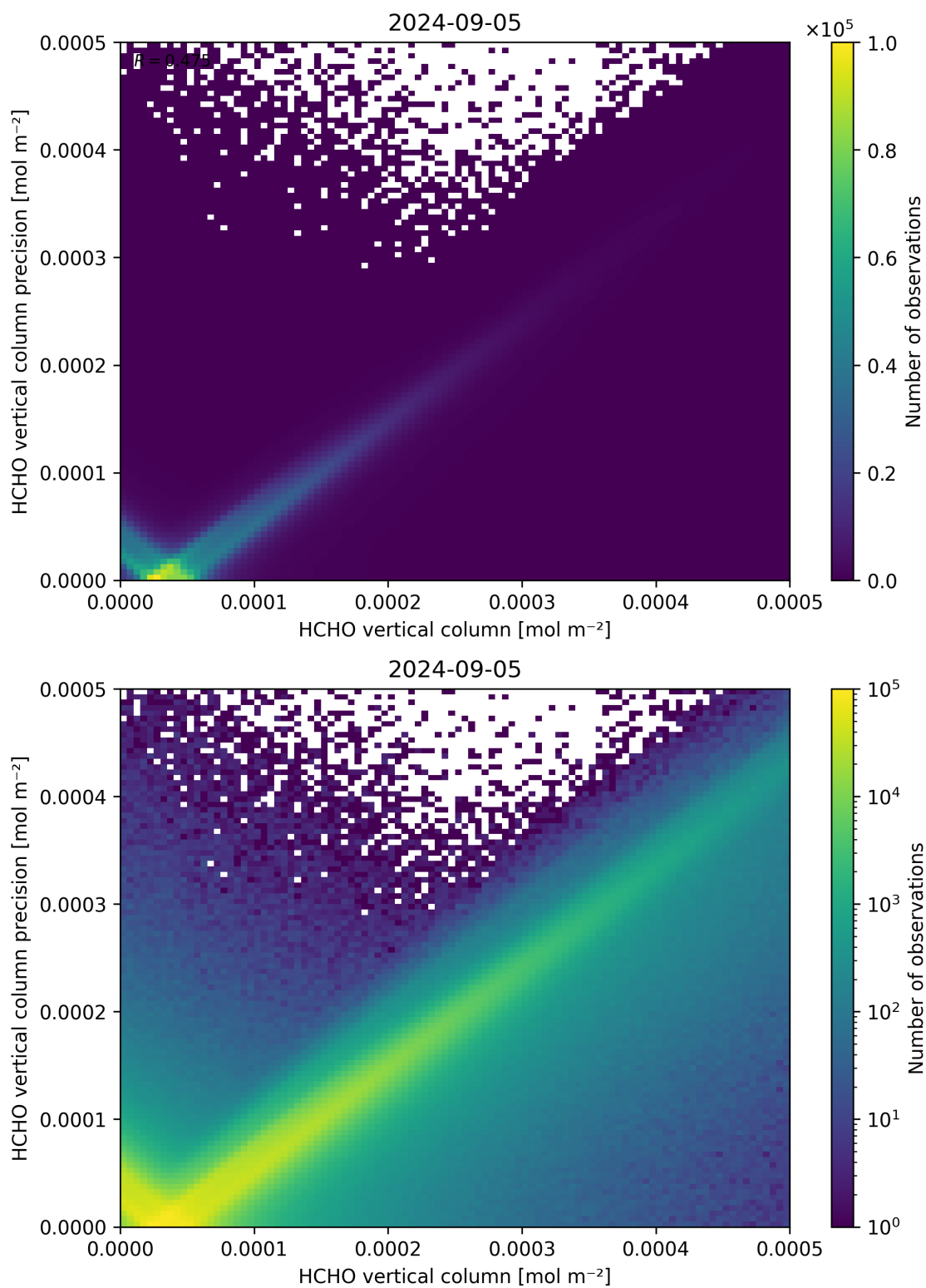
Figure 134: Scatter density plot of “HCHO vertical column” against “HCHO vertical column precision” for 2024-09-04 to 2024-09-06.
