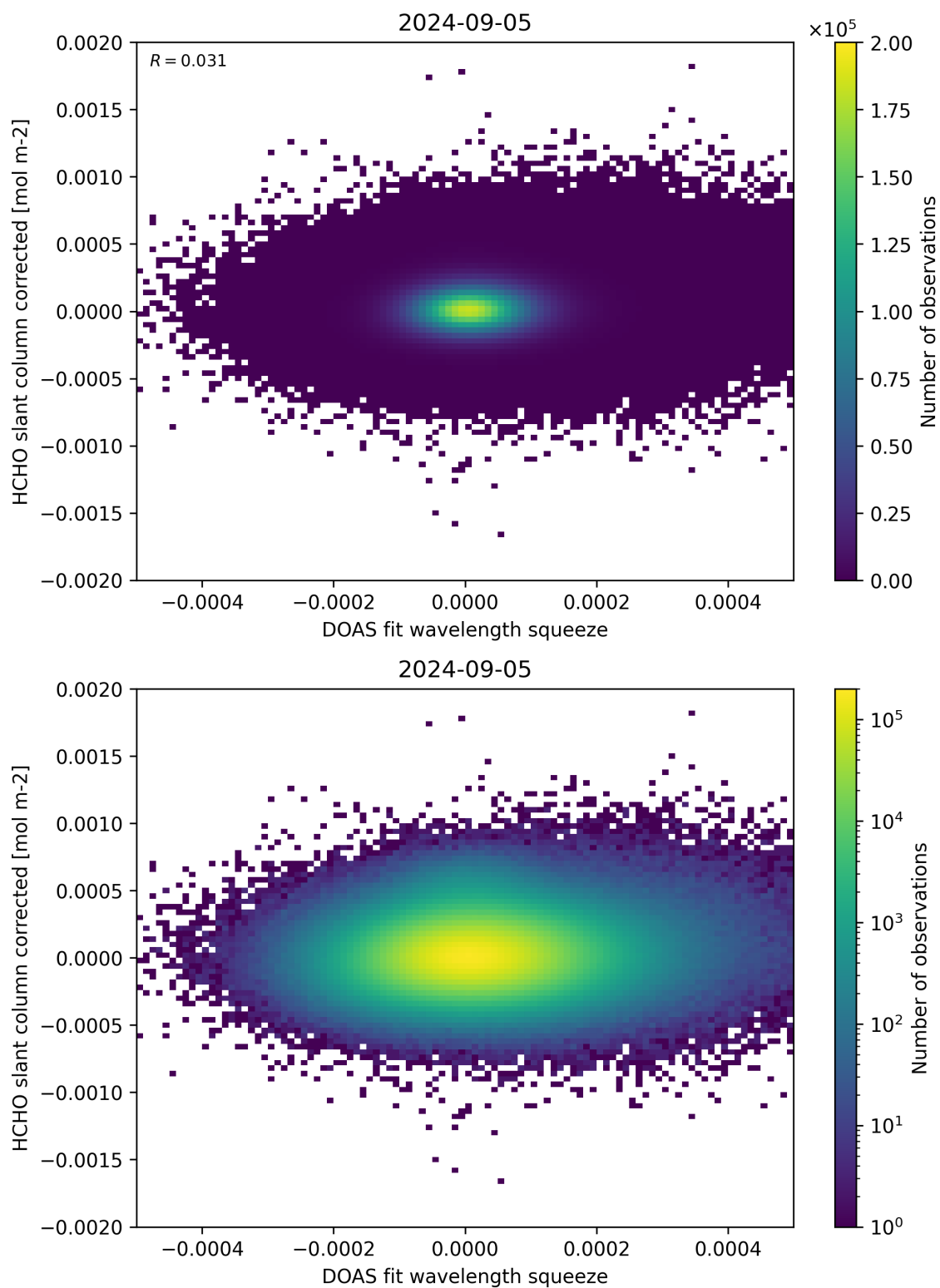
Figure 69: Scatter density plot of “DOAS fit wavelength squeeze” against “HCHO slant column corrected” for 2024-09-04 to 2024-09-06.
