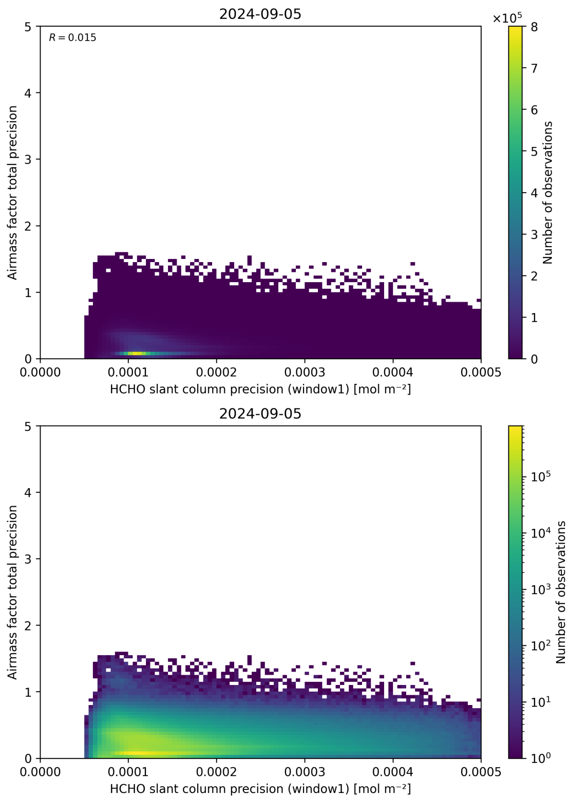
Figure 95: Scatter density plot of “HCHO slant column precision (window1)” against “Airmass factor total precision” for 2024-09-04 to 2024-09-06.
