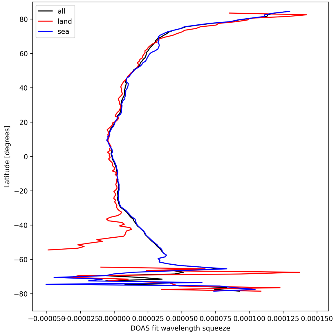
Figure 31: Zonal average of “DOAS fit wavelength squeeze” for 2024-09-04 to 2024-09-06.
