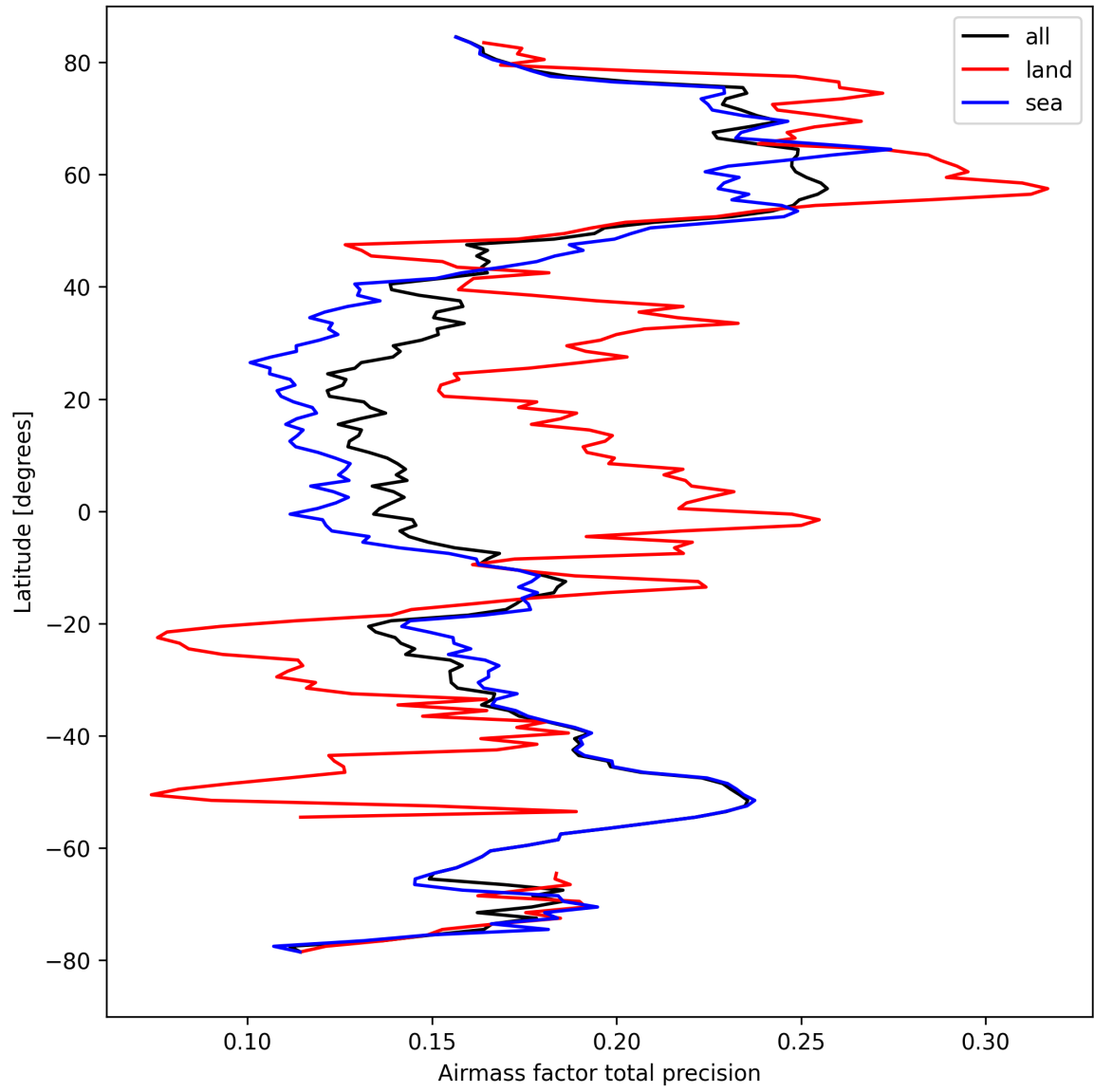
Figure 27: Zonal average of “Airmass factor total precision” for 2024-09-04 to 2024-09-06.
