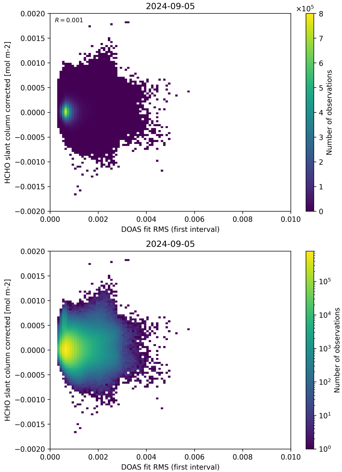
Figure 62: Scatter density plot of “DOAS fit RMS (first interval)” against “HCHO slant column corrected” for 2024-09-04 to 2024-09-06.
