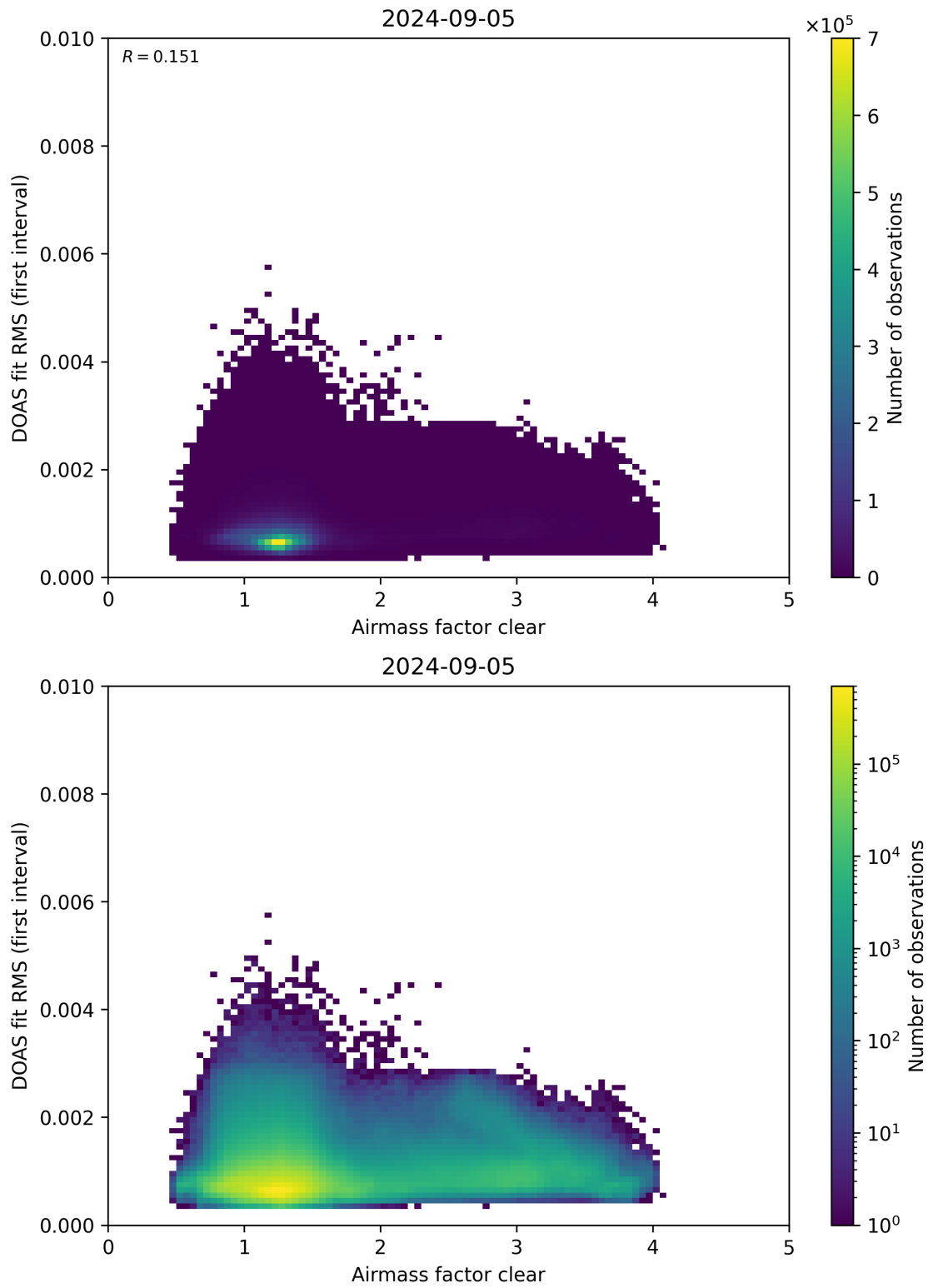
Figure 71: Scatter density plot of “Airmass factor clear” against “DOAS fit RMS (first interval)” for 2024-09-04 to 2024-09-06.
