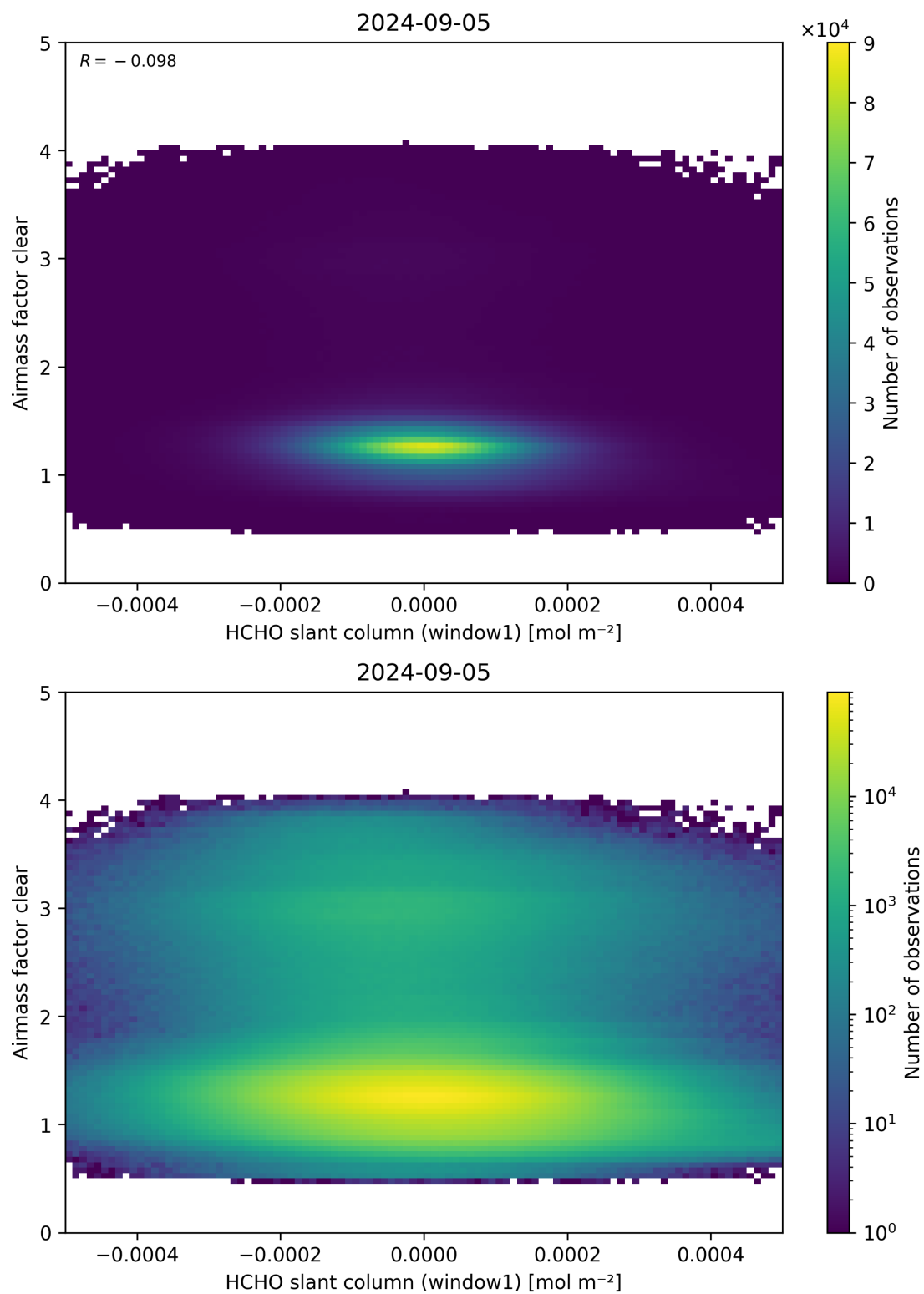
Figure 81: Scatter density plot of “HCHO slant column (window1)” against “Airmass factor clear” for 2024-09-04 to 2024-09-06.
