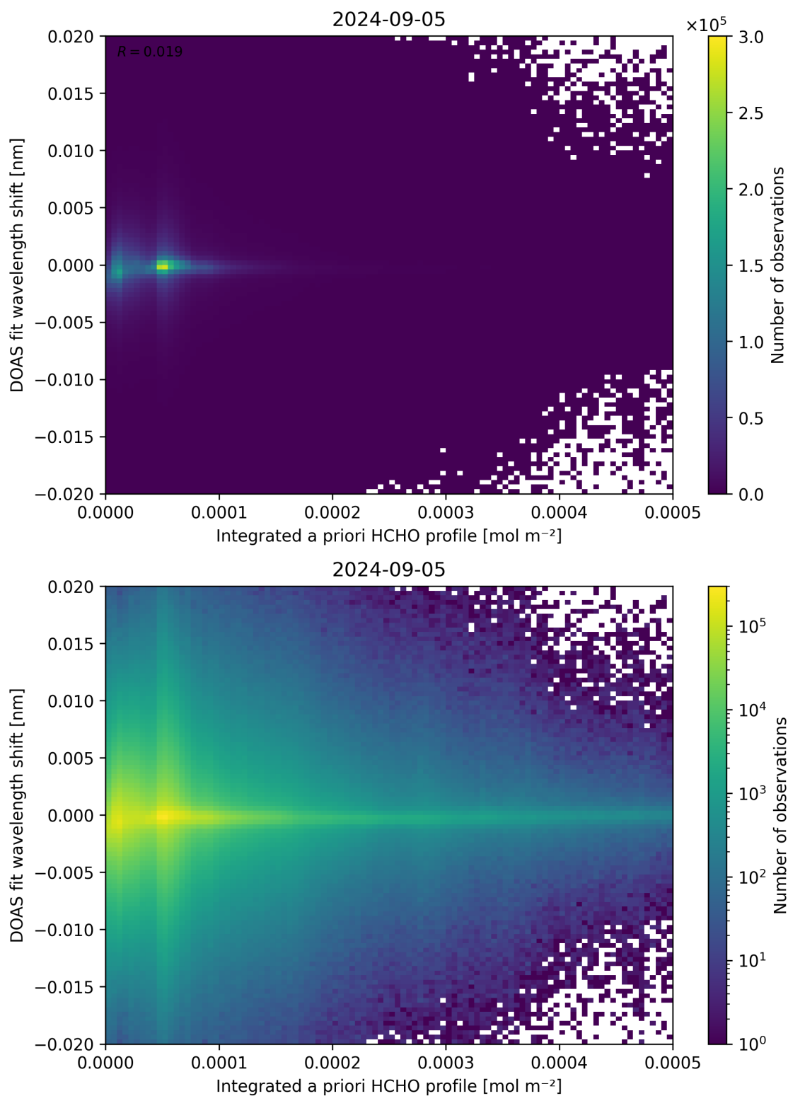
Figure 149: Scatter density plot of “Integrated a priori HCHO profile” against “DOAS fit wavelength shift” for 2024-09-04 to 2024-09-06.
