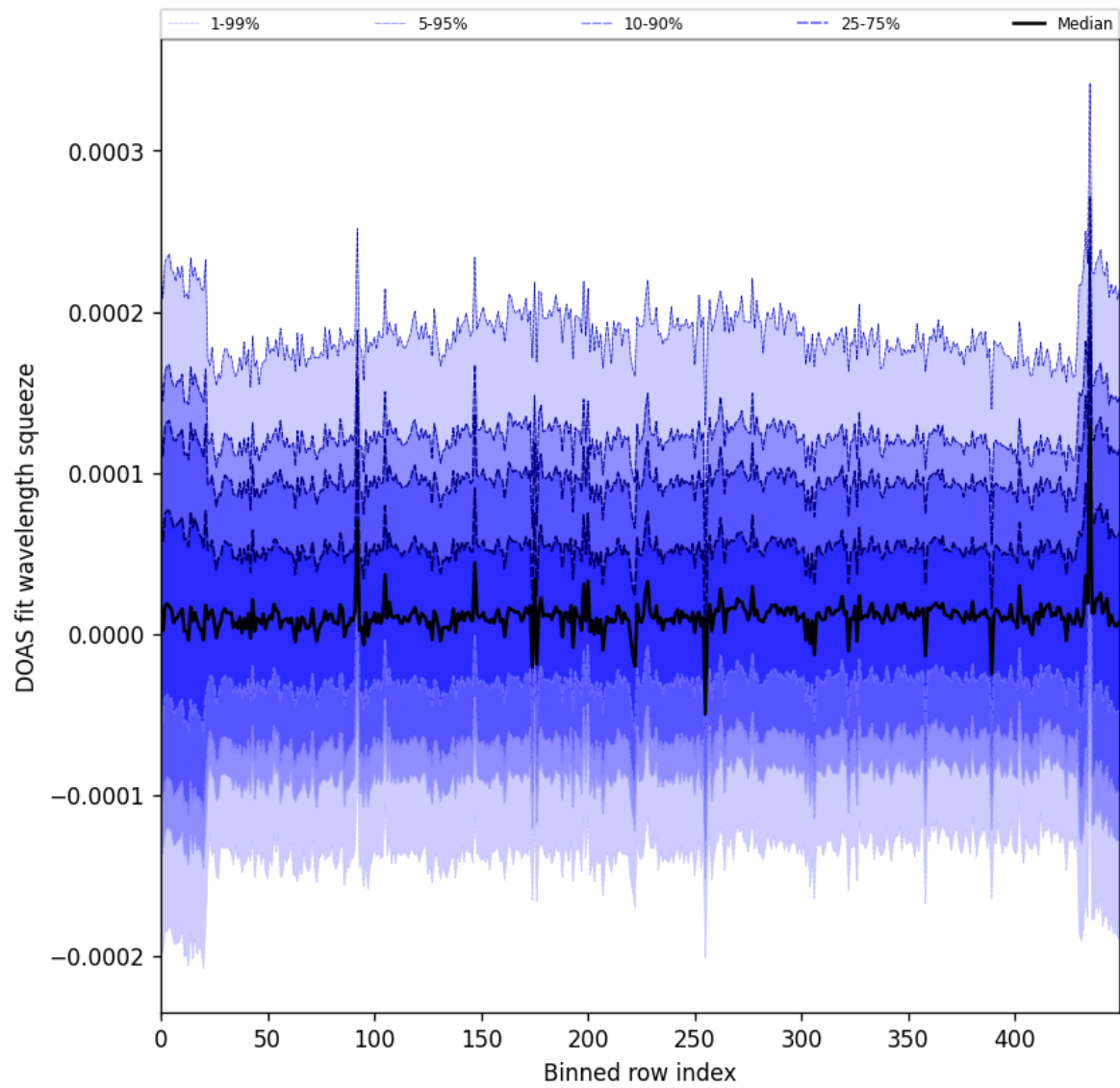
Figure 59: Along track statistics of “DOAS fit wavelength squeeze” for 2024-09-04 to 2024-09-06
