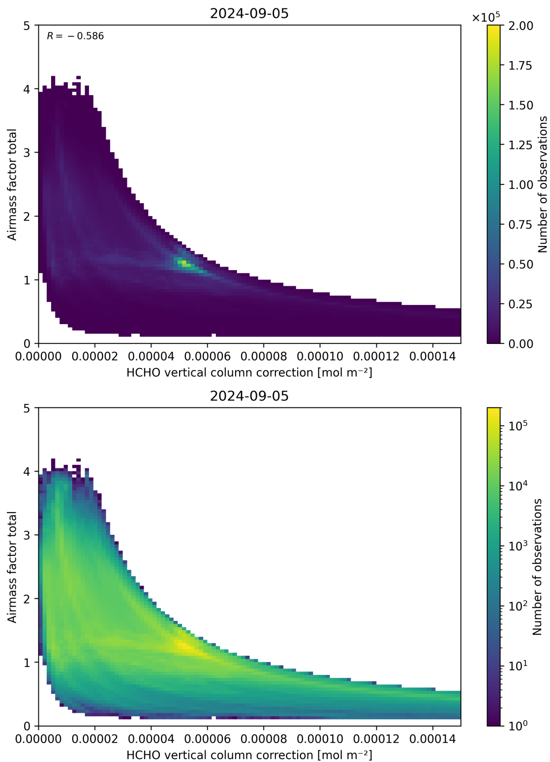
Figure 120: Scatter density plot of “HCHO vertical column correction” against “Airmass factor total” for 2024-09-04 to 2024-09-06.
