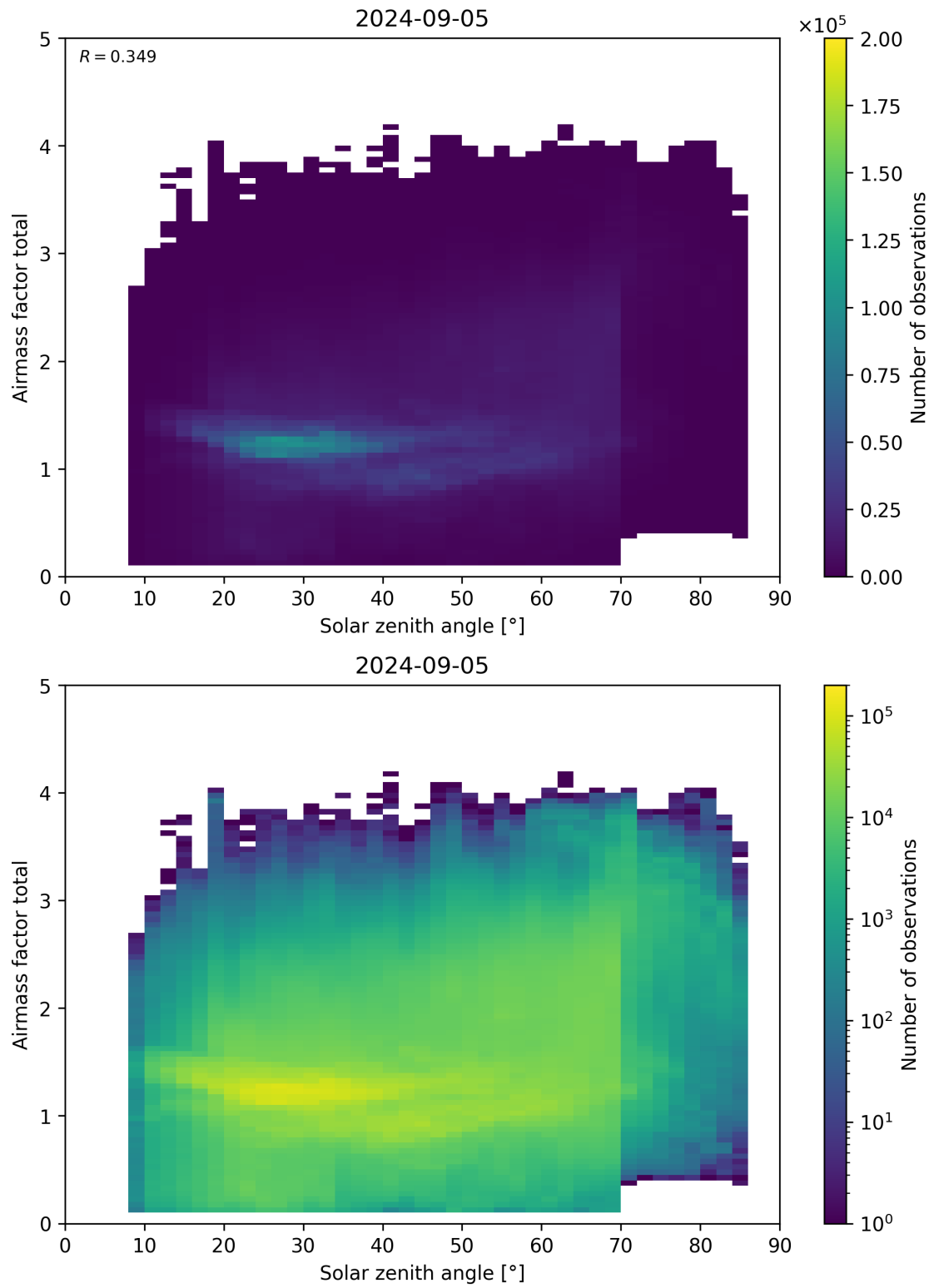
Figure 175: Scatter density plot of “Solar zenith angle” against “Airmass factor total” for 2024-09-04 to 2024-09-06.
