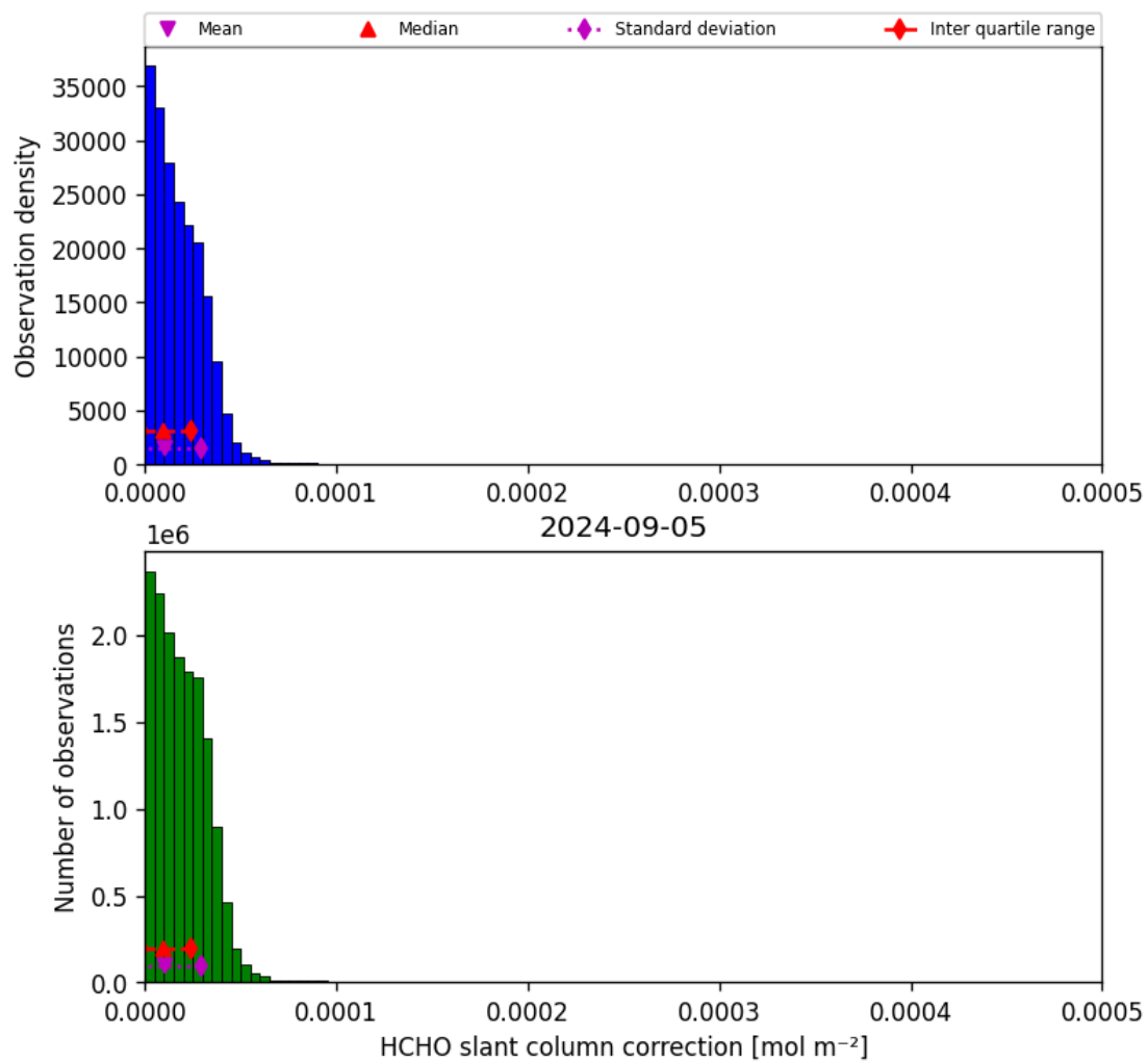
Figure 47: Histogram of “HCHO slant column correction” for 2024-09-04 to 2024-09-06
