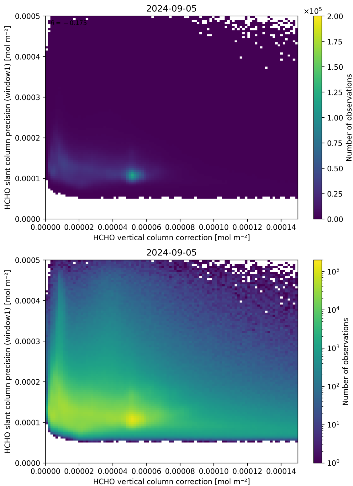
Figure 119: Scatter density plot of “HCHO vertical column correction” against “HCHO slant column precision (window1)” for 2024-09-04 to 2024-09-06.
