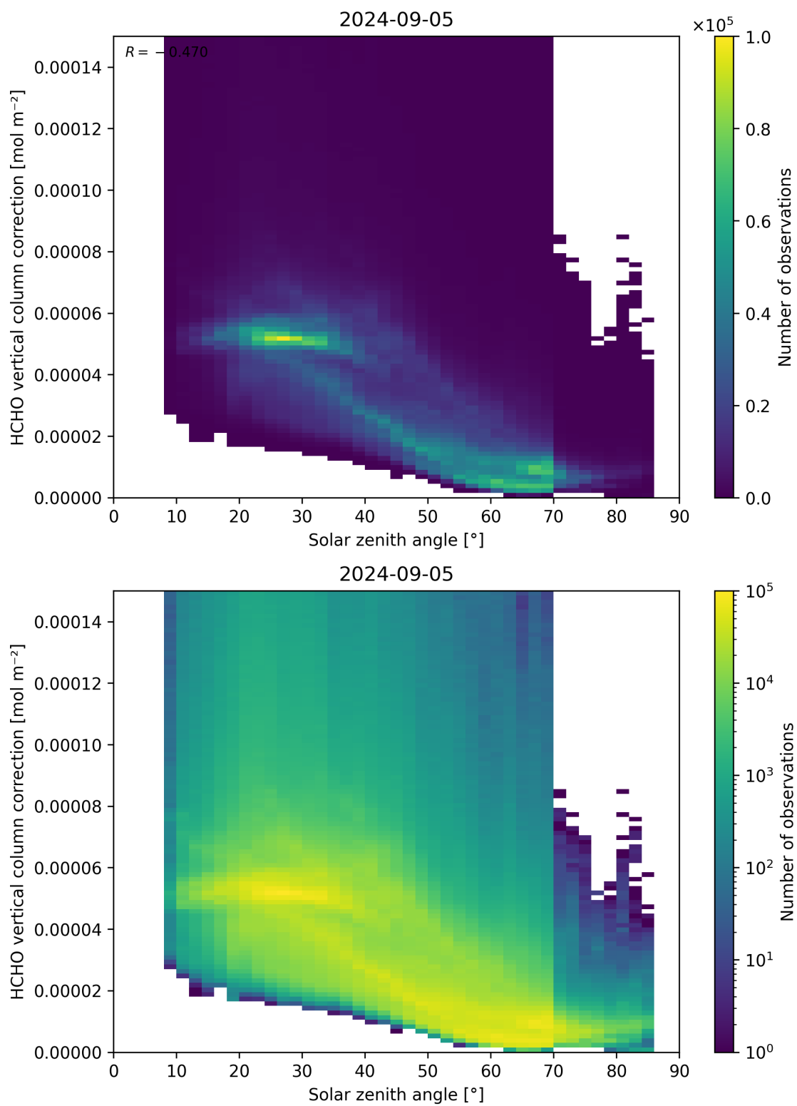
Figure 178: Scatter density plot of “Solar zenith angle” against “HCHO vertical column correction” for 2024-09-04 to 2024-09-06.
