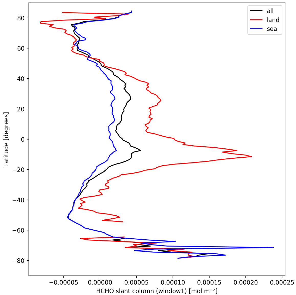
Figure 24: Zonal average of “HCHO slant column (window1)” for 2024-09-04 to 2024-09-06.
