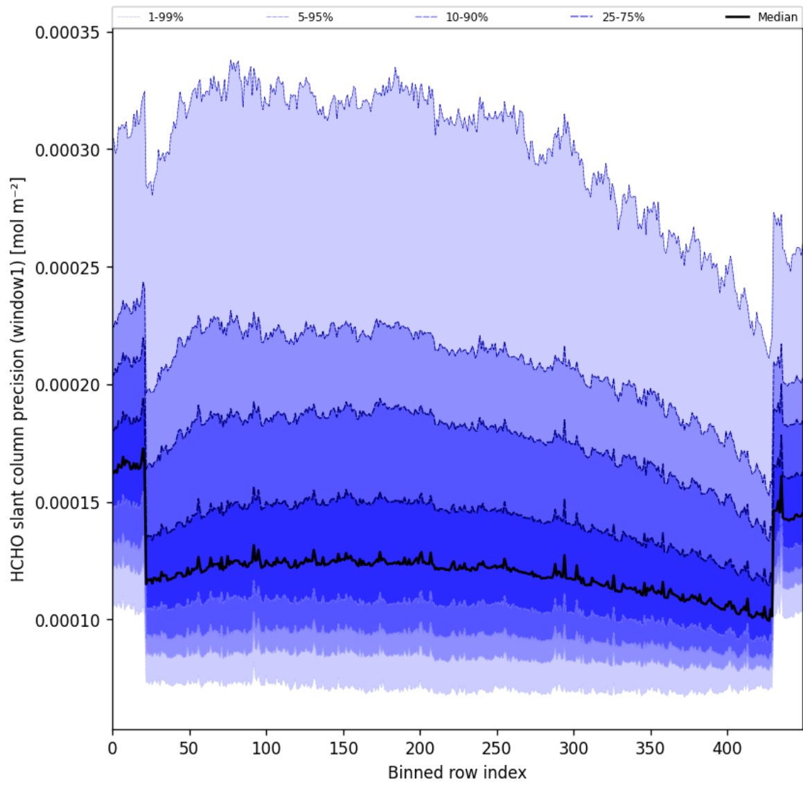
Figure 53: Along track statistics of “HCHO slant column precision (window1)” for 2024-09-04 to 2024-09-06
