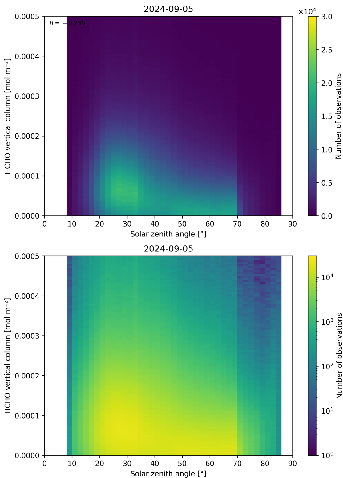
Figure 177: Scatter density plot of “Solar zenith angle” against “HCHO vertical column” for 2024-09-04 to 2024-09-06.
