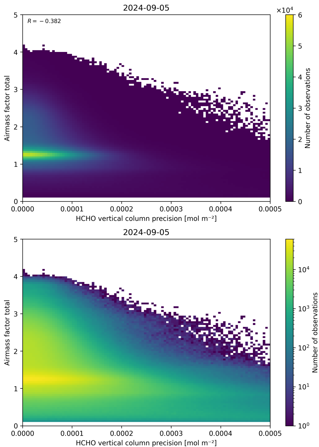
Figure 144: Scatter density plot of “HCHO vertical column precision” against “Airmass factor total” for 2024-09-04 to 2024-09-06.
