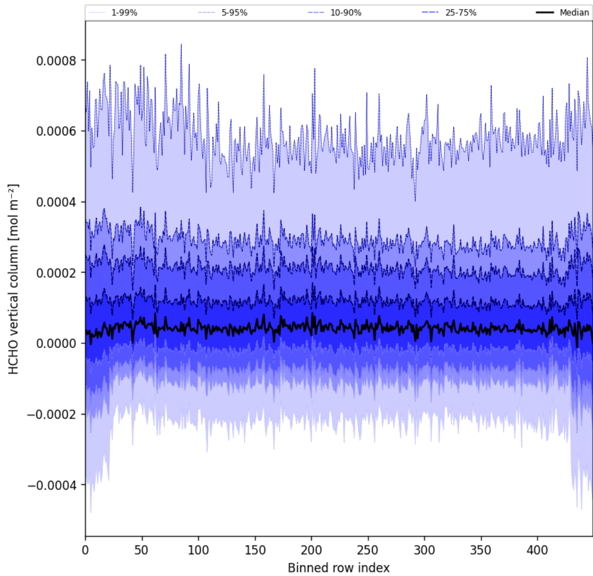
Figure 49: Along track statistics of “HCHO vertical column” for 2024-09-04 to 2024-09-06
