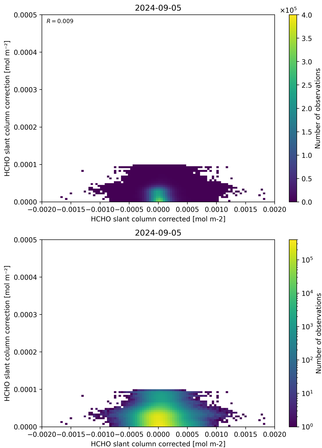
Figure 77: Scatter density plot of “HCHO slant column corrected” against “HCHO slant column correction” for 2024-09-04 to 2024-09-06.
