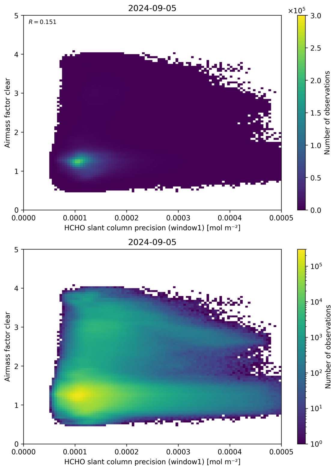
Figure 91: Scatter density plot of “HCHO slant column precision (window1)” against “Airmass factor clear” for 2024-09-04 to 2024-09-06.
