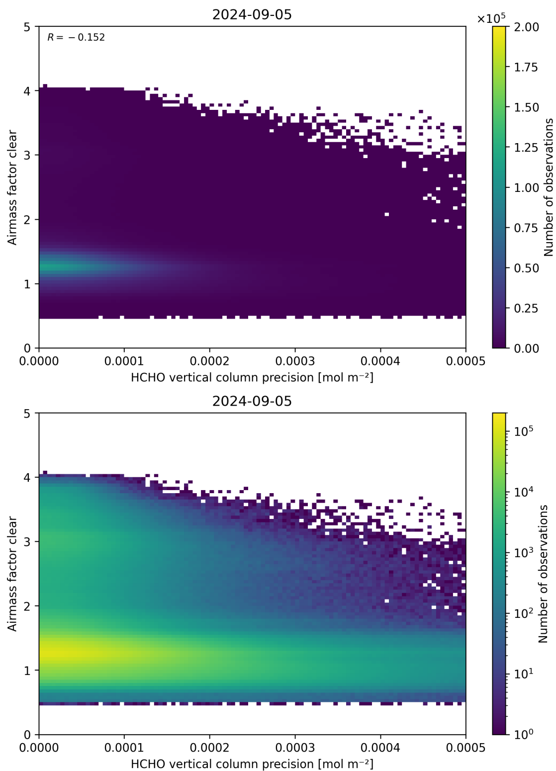
Figure 139: Scatter density plot of “HCHO vertical column precision” against “Airmass factor clear” for 2024-09-04 to 2024-09-06.
