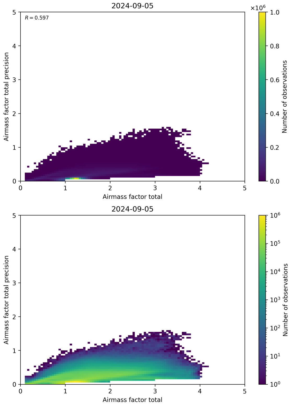
Figure 103: Scatter density plot of “Airmass factor total” against “Airmass factor total precision” for 2024-09-04 to 2024-09-06.
