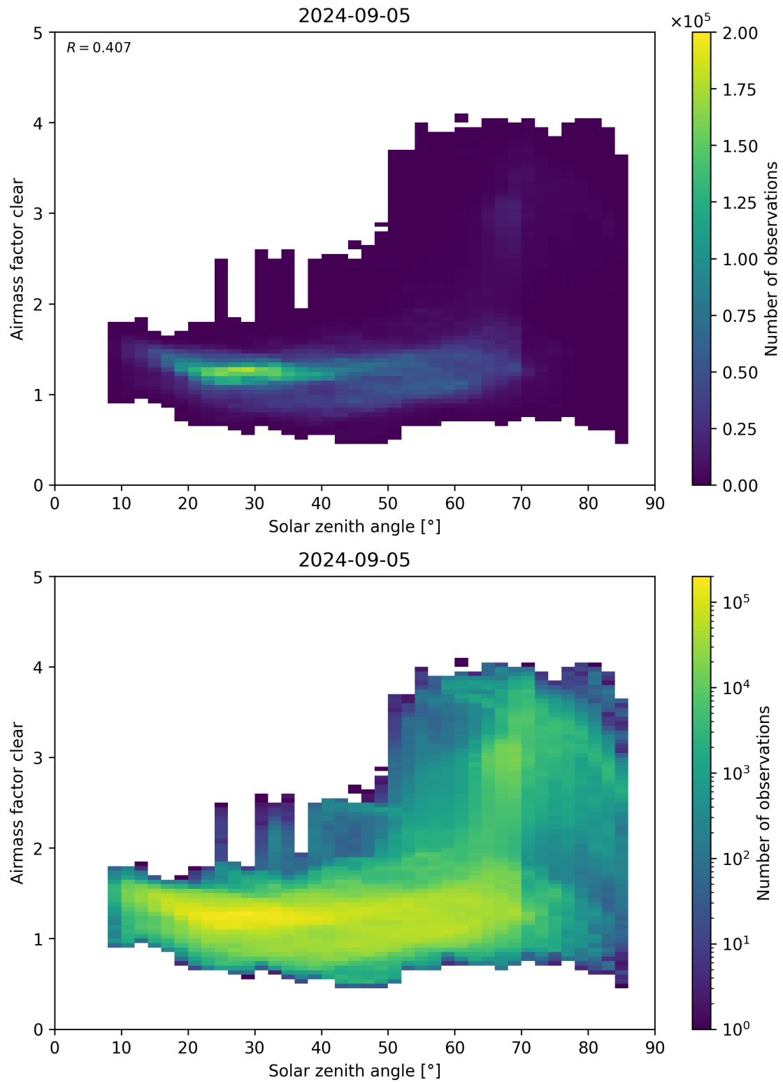
Figure 170: Scatter density plot of “Solar zenith angle” against “Airmass factor clear” for 2024-09-04 to 2024-09-06.
