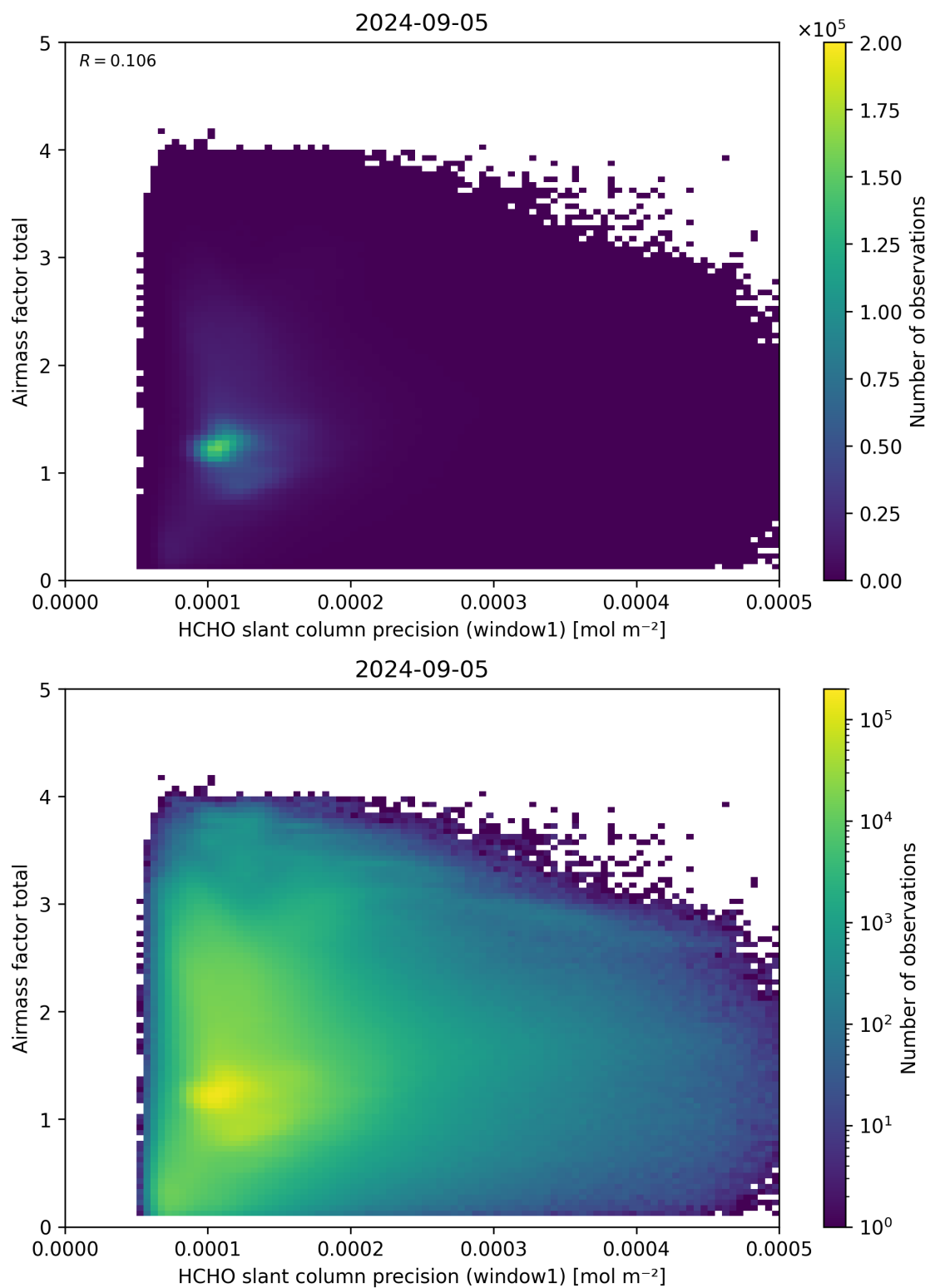
Figure 94: Scatter density plot of “HCHO slant column precision (window1)” against “Airmass factor total” for 2024-09-04 to 2024-09-06.
