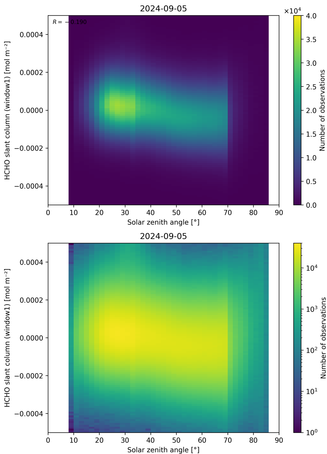
Figure 173: Scatter density plot of “Solar zenith angle” against “HCHO slant column (window1)” for 2024-09-04 to 2024-09-06.
