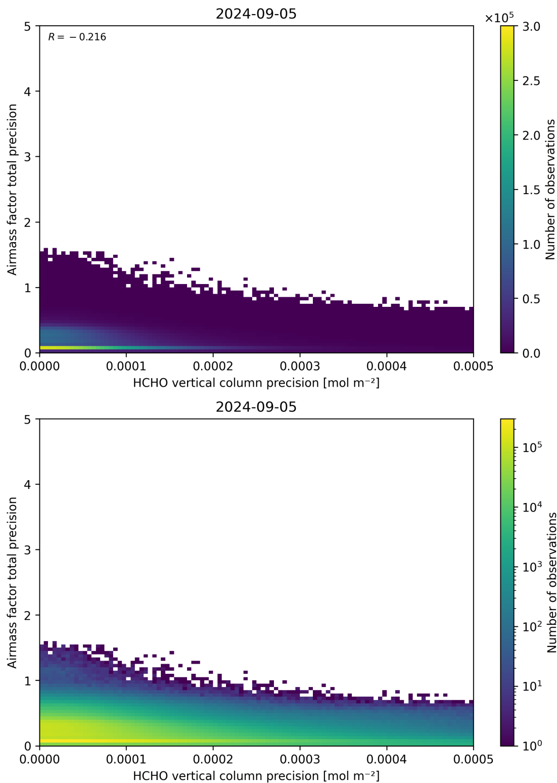
Figure 145: Scatter density plot of “HCHO vertical column precision” against “Airmass factor total precision” for 2024-09-04 to 2024-09-06.
