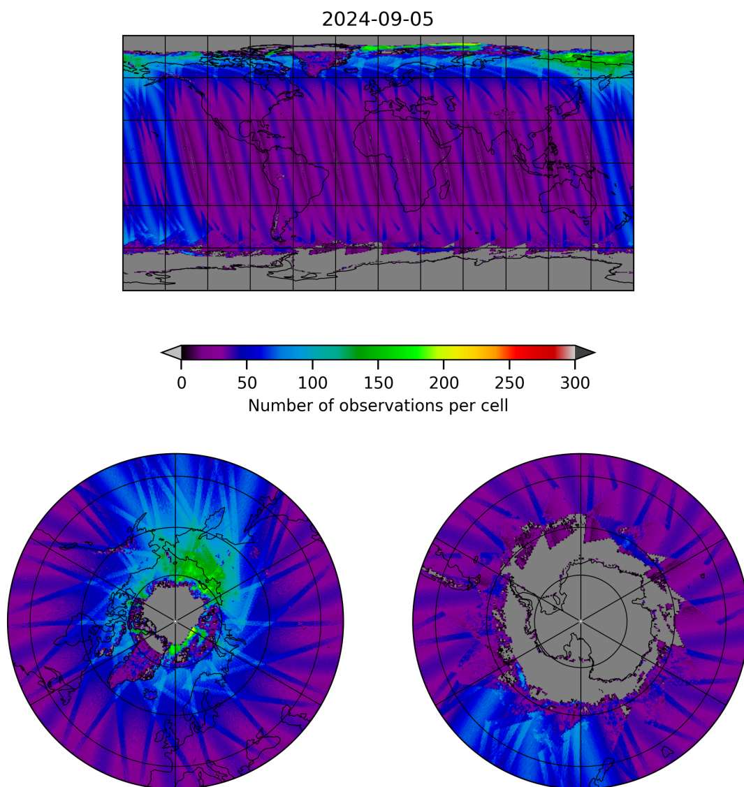
Figure 19: Map of the number of observations for 2024-09-04 to 2024-09-06
