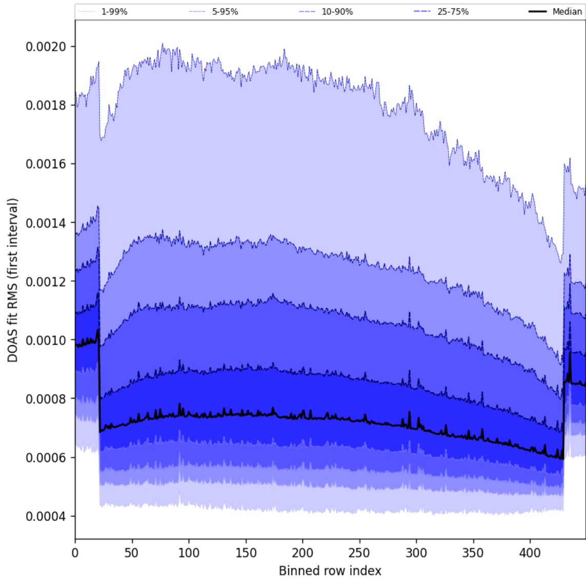
Figure 60: Along track statistics of “DOAS fit RMS (first interval)” for 2024-09-04 to 2024-09-06
