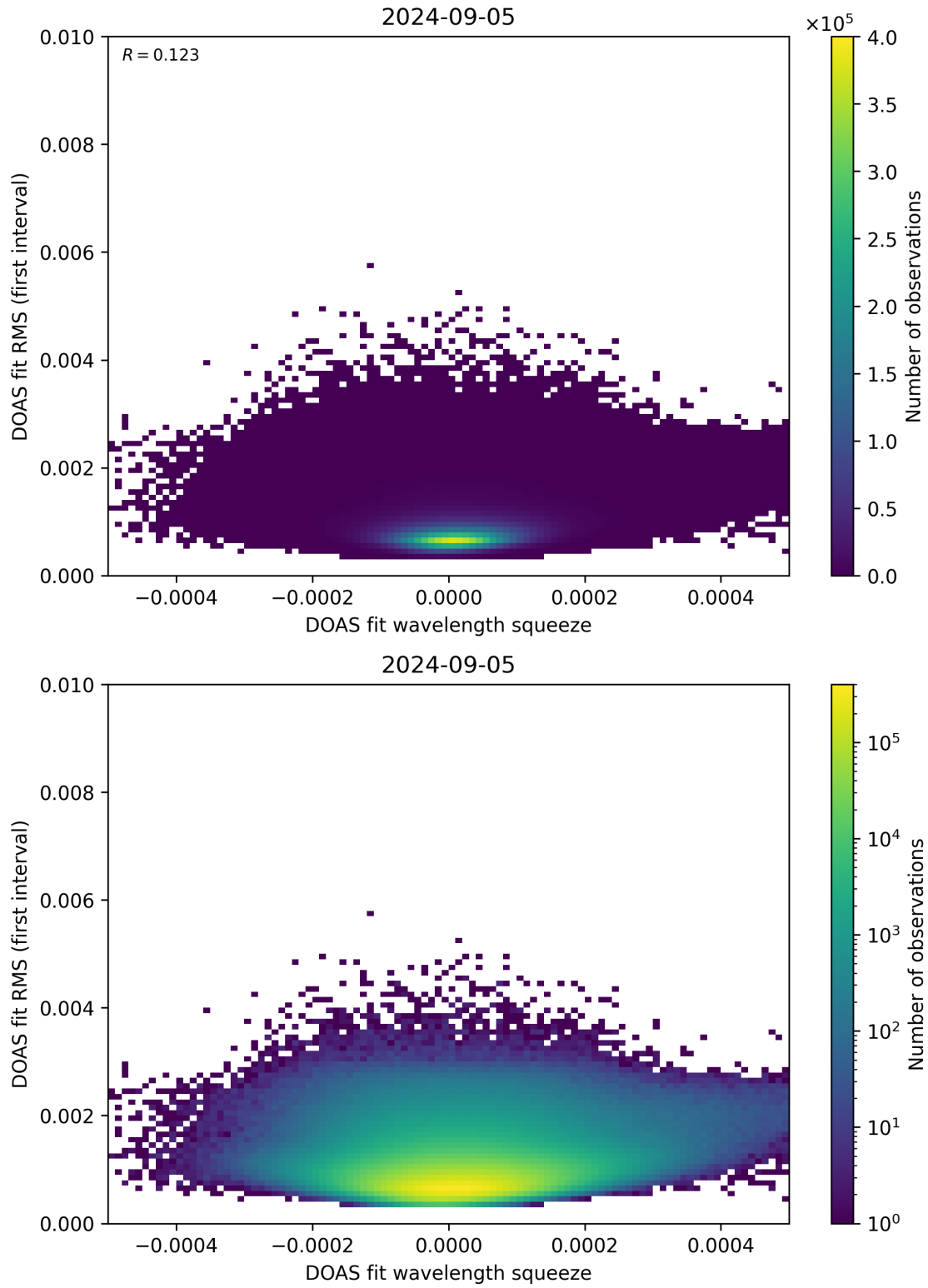
Figure 68: Scatter density plot of “DOAS fit wavelength squeeze” against “DOAS fit RMS (first interval)” for 2024-09-04 to 2024-09-06.
