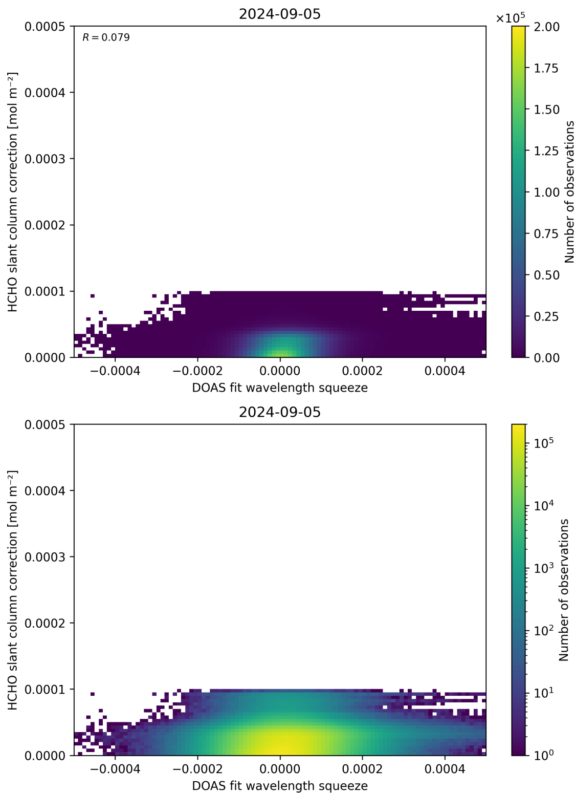
Figure 70: Scatter density plot of “DOAS fit wavelength squeeze” against “HCHO slant column correction” for 2024-09-04 to 2024-09-06.
