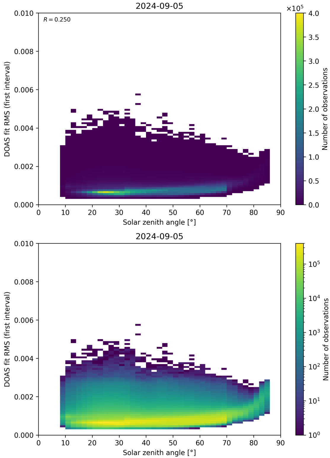
Figure 167: Scatter density plot of “Solar zenith angle” against “DOAS fit RMS (first interval)” for 2024-09-04 to 2024-09-06.
