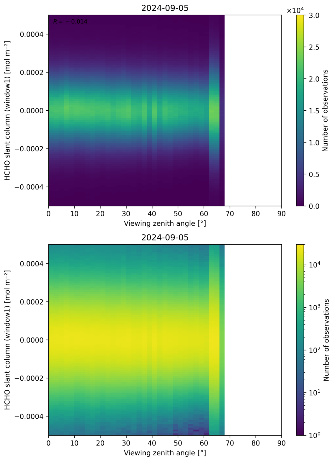
Figure 188: Scatter density plot of “Viewing zenith angle” against “HCHO slant column (window1)” for 2024-09-04 to 2024-09-06.
