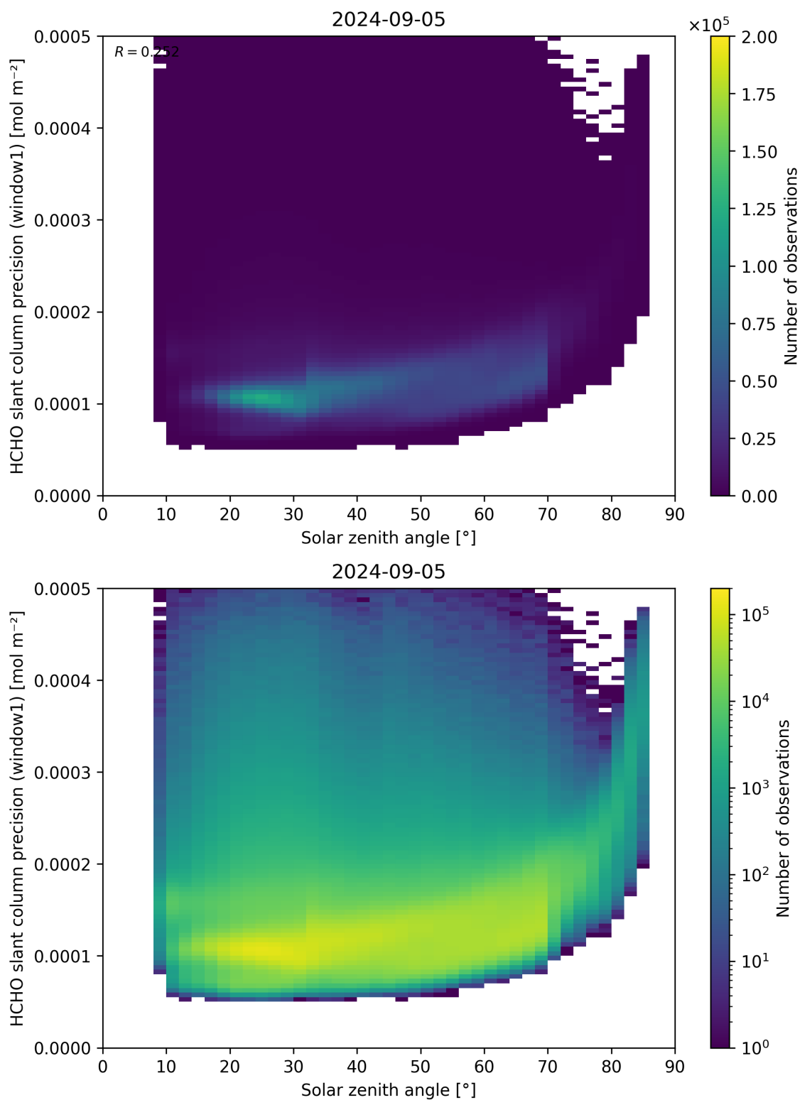
Figure 174: Scatter density plot of “Solar zenith angle” against “HCHO slant column precision (window1)” for 2024-09-04 to 2024-09-06.
