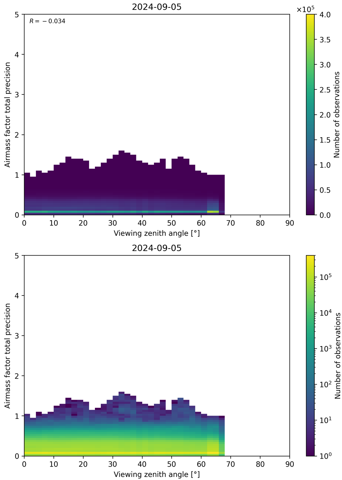
Figure 191: Scatter density plot of “Viewing zenith angle” against “Airmass factor total precision” for 2024-09-04 to 2024-09-06.
