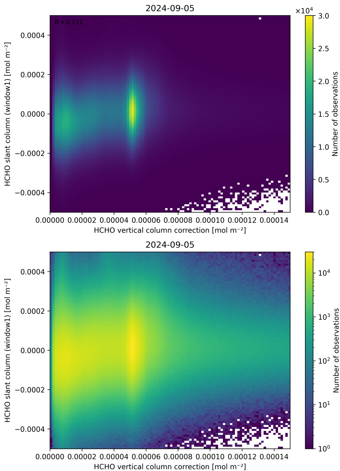
Figure 118: Scatter density plot of “HCHO vertical column correction” against “HCHO slant column (window1)” for 2024-09-04 to 2024-09-06.
