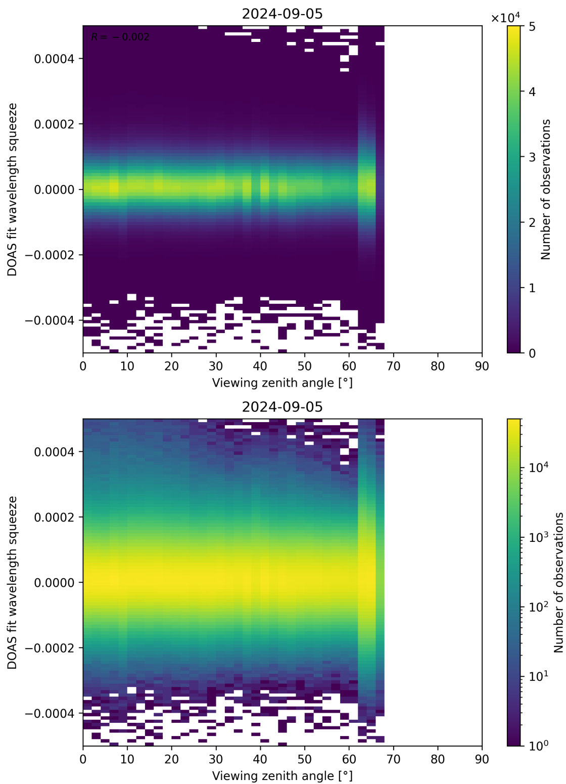
Figure 184: Scatter density plot of “Viewing zenith angle” against “DOAS fit wavelength squeeze” for 2024-09-04 to 2024-09-06.
