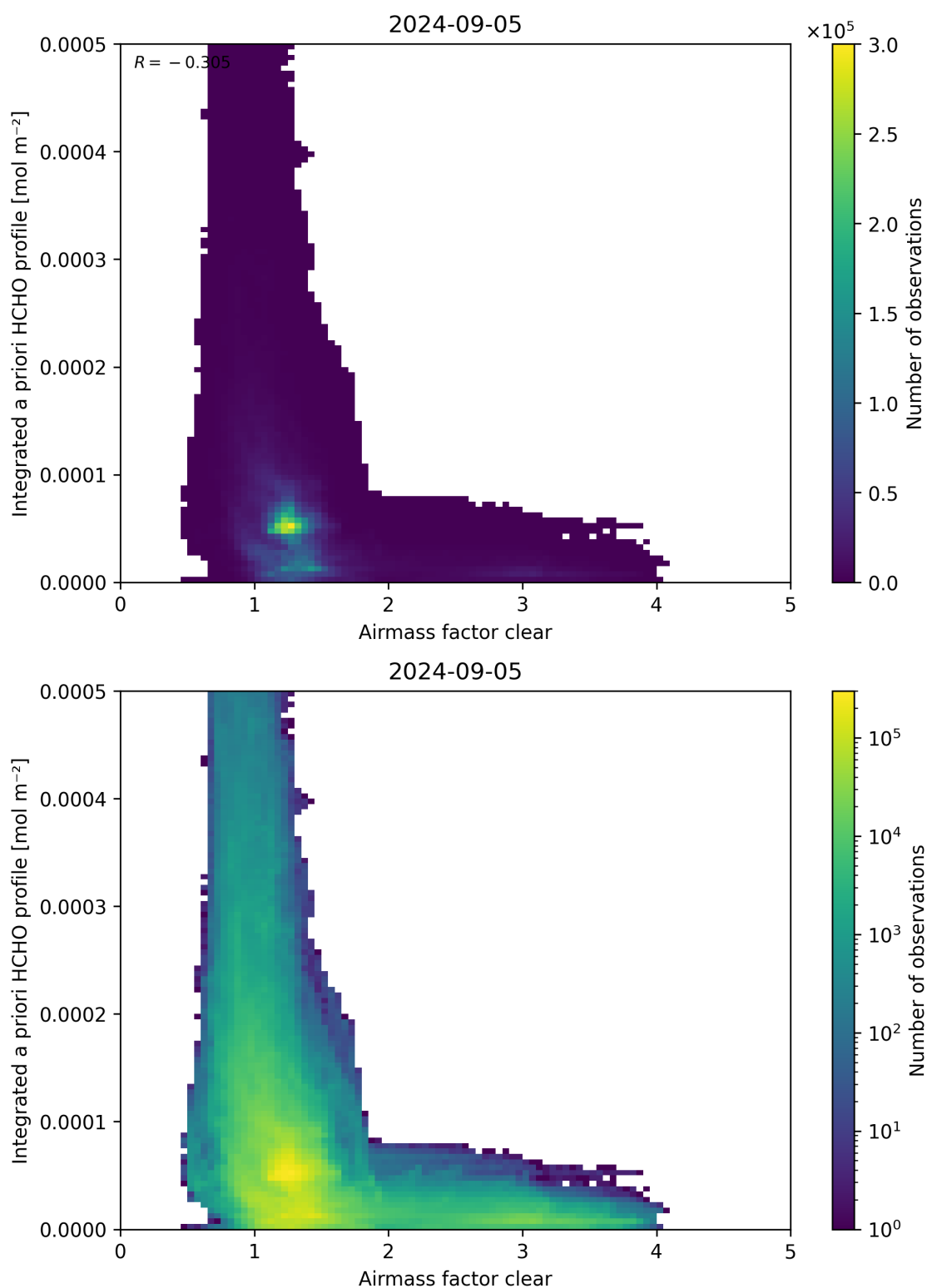
Figure 76: Scatter density plot of “Airmass factor clear” against “Integrated a priori HCHO profile” for 2024-09-04 to 2024-09-06.
