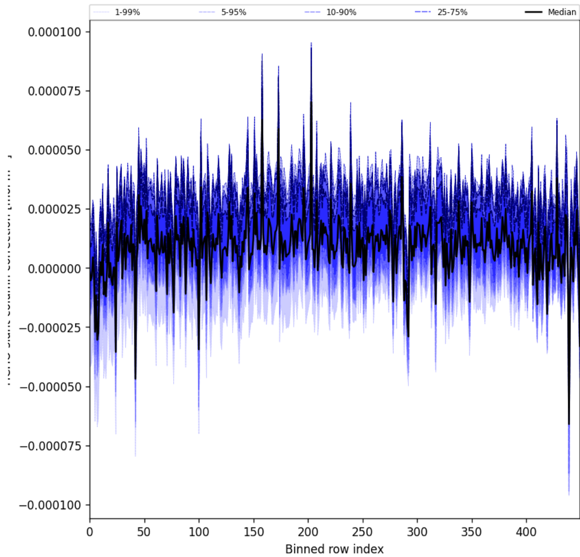
Figure 61: Along track statistics of “HCHO slant column correction” for 2024-09-04 to 2024-09-06
