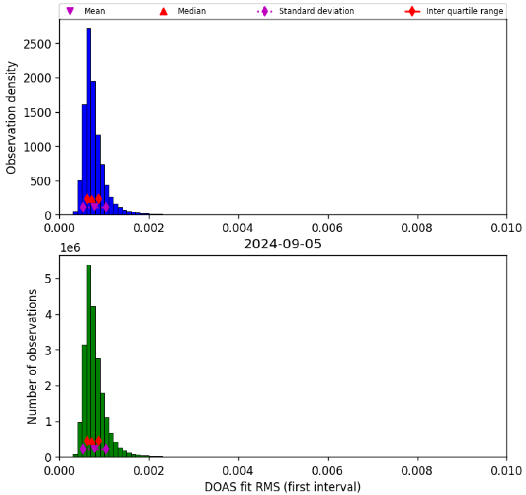
Figure 46: Histogram of “DOAS fit RMS (first interval)” for 2024-09-04 to 2024-09-06
