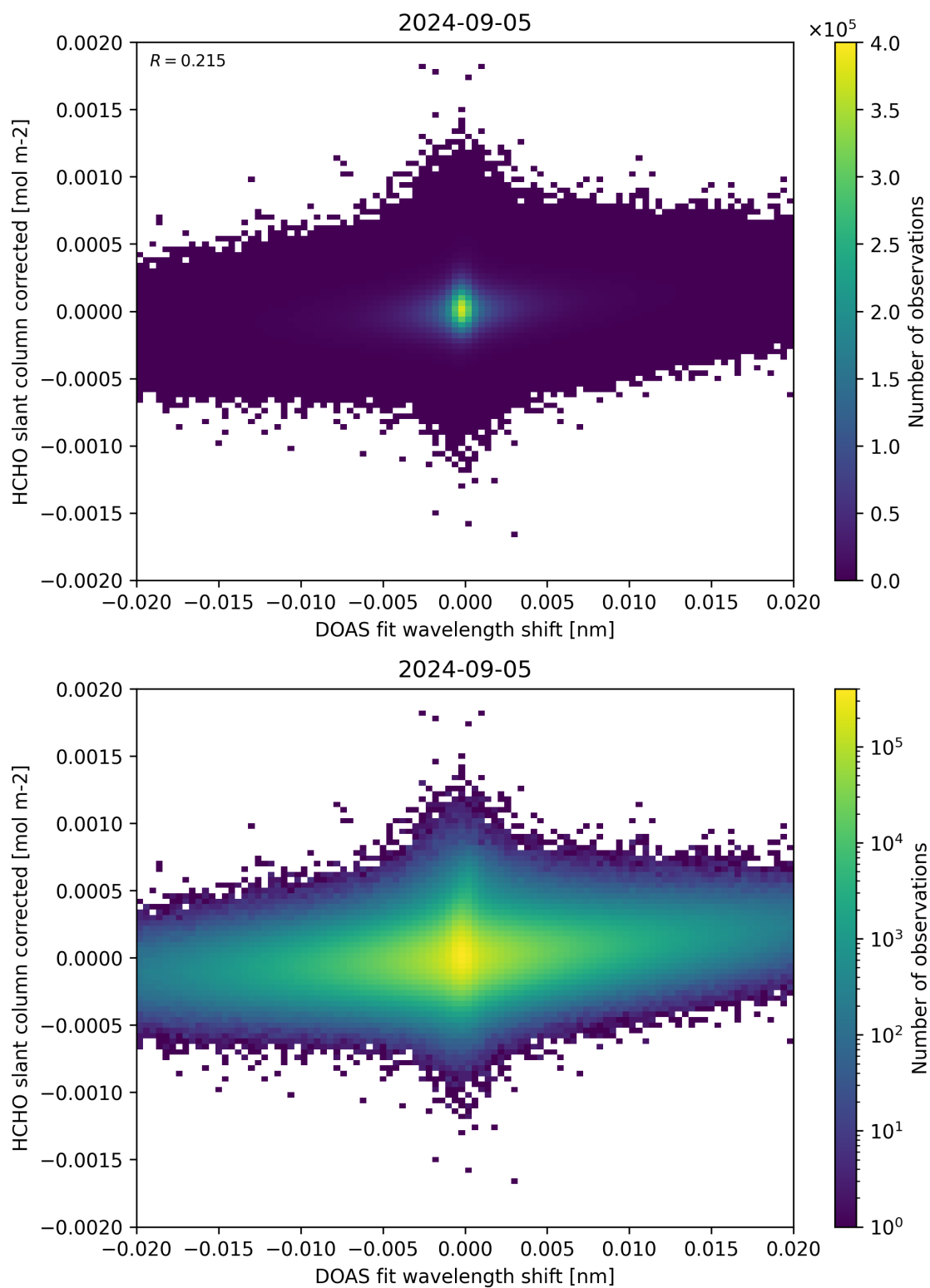
Figure 66: Scatter density plot of “DOAS fit wavelength shift” against “HCHO slant column corrected” for 2024-09-04 to 2024-09-06.
