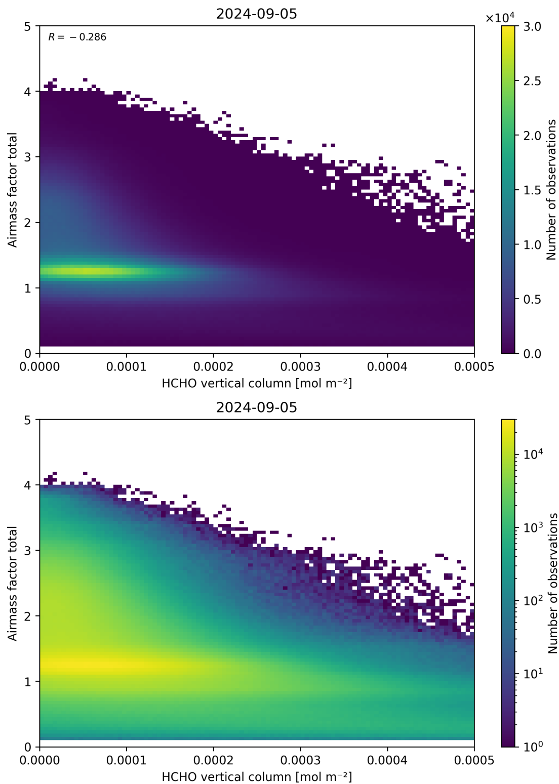
Figure 131: Scatter density plot of “HCHO vertical column” against “Airmass factor total” for 2024-09-04 to 2024-09-06.
