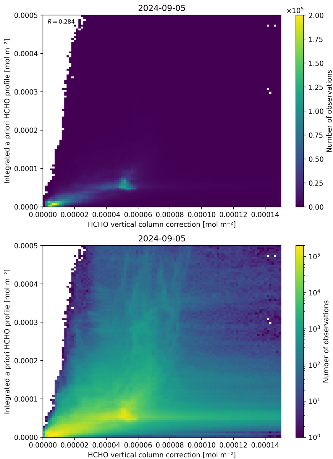
Figure 122: Scatter density plot of “HCHO vertical column correction” against “Integrated a priori HCHO profile” for 2024-09-04 to 2024-09-06.
