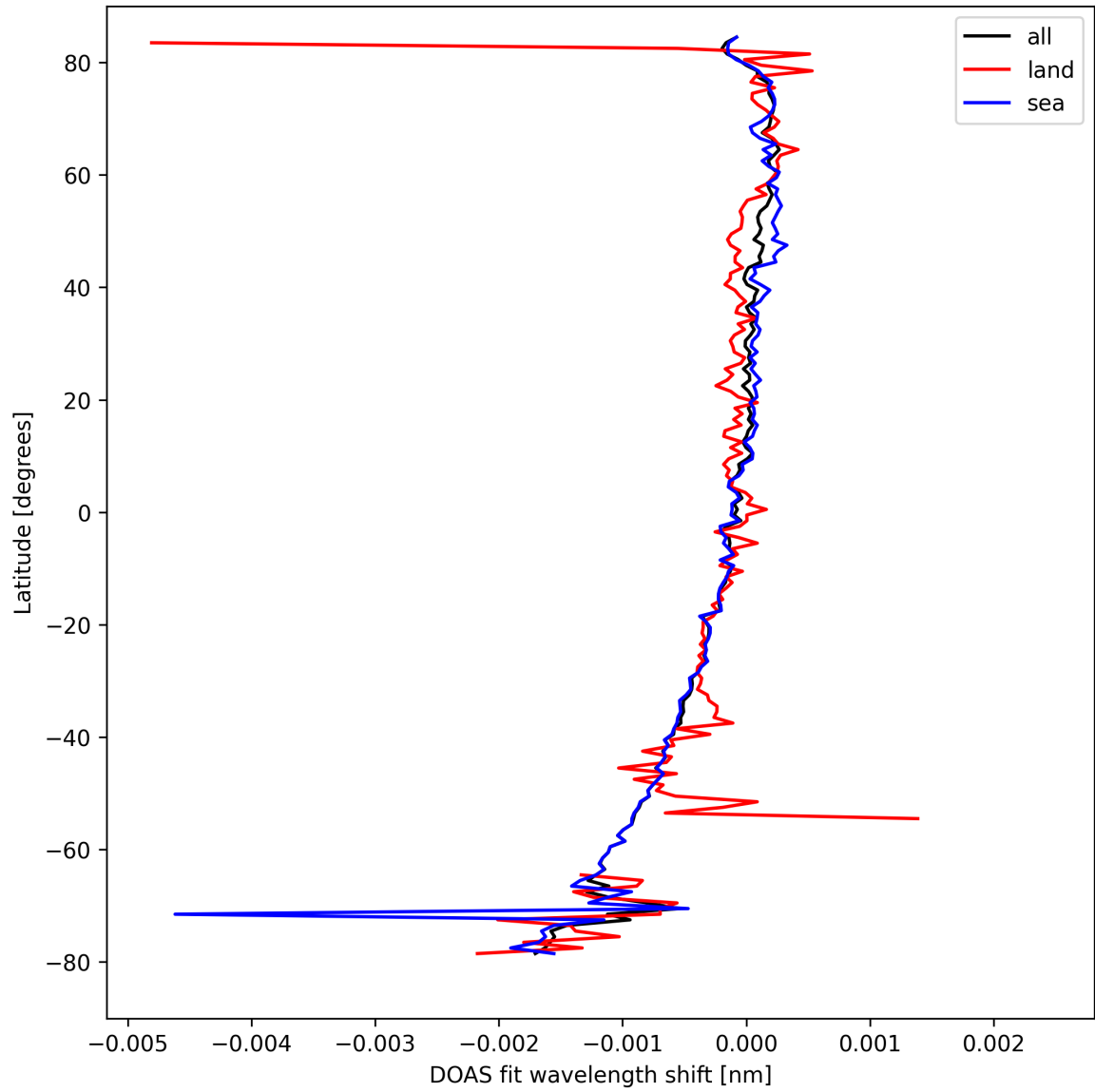
Figure 30: Zonal average of "DOAS fit wavelength shift" for 2024-09-04 to 2024-09-06.
