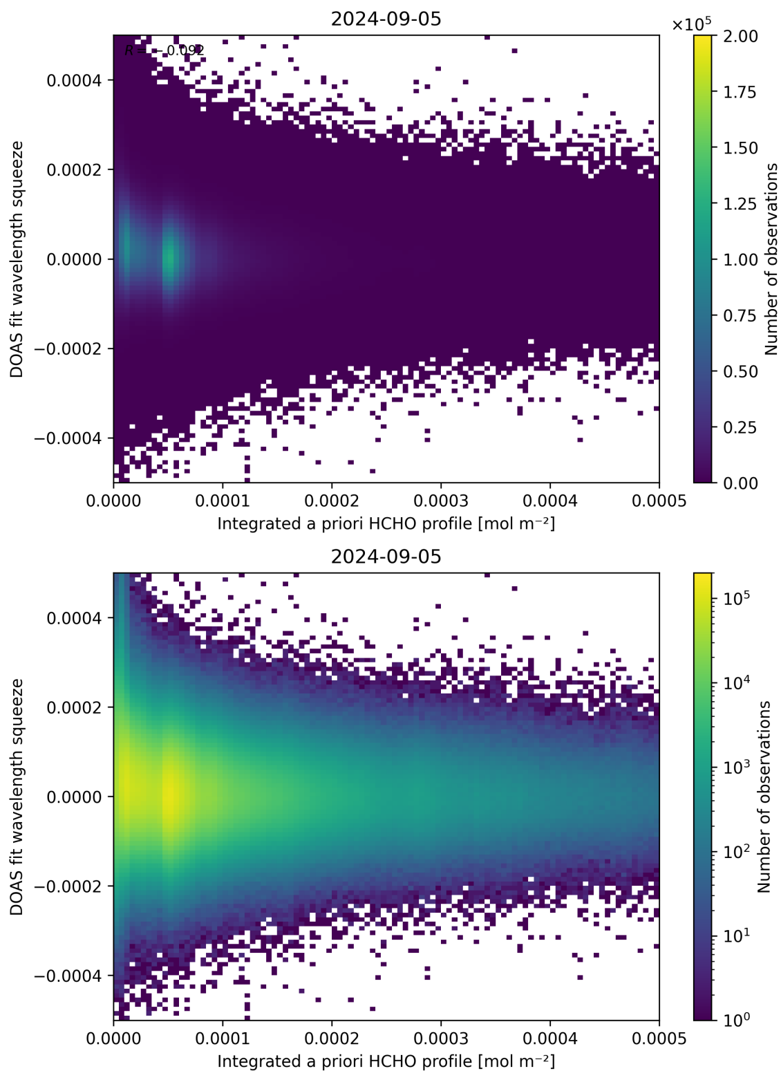
Figure 150: Scatter density plot of “Integrated a priori HCHO profile” against “DOAS fit wavelength squeeze” for 2024-09-04 to 2024-09-06.
