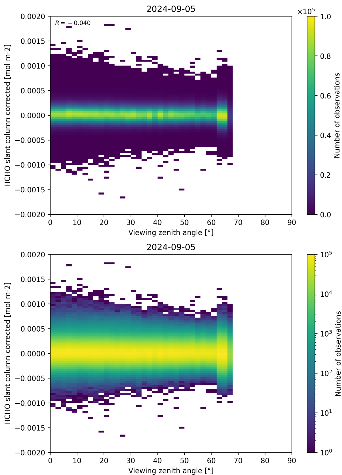
Figure 186: Scatter density plot of “Viewing zenith angle” against “HCHO slant column corrected” for 2024-09-04 to 2024-09-06.
