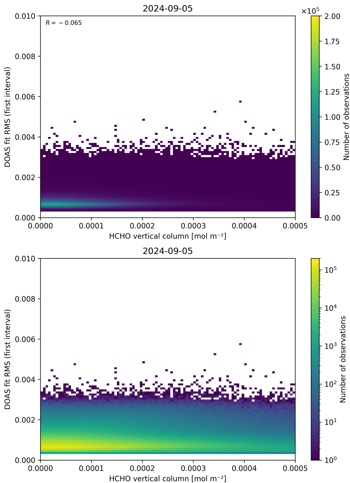
Figure 123: Scatter density plot of “HCHO vertical column” against “DOAS fit RMS (first interval)” for 2024-09-04 to 2024-09-06.
