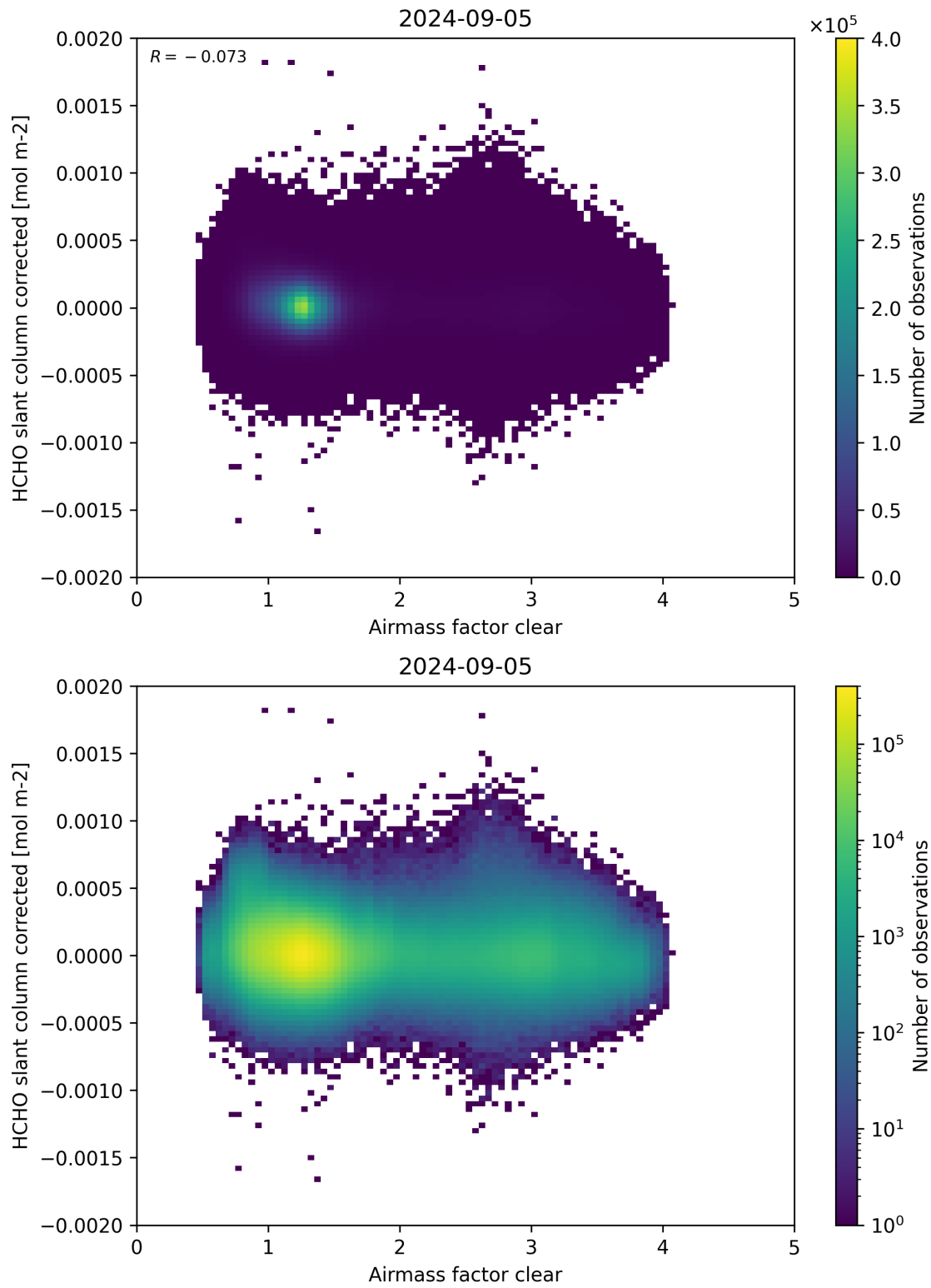
Figure 74: Scatter density plot of “Airmass factor clear” against “HCHO slant column corrected” for 2024-09-04 to 2024-09-06.
