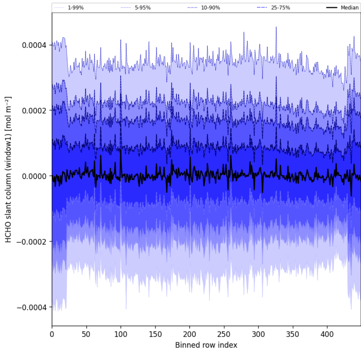
Figure 52: Along track statistics of “HCHO slant column (window1)” for 2024-09-04 to 2024-09-06
