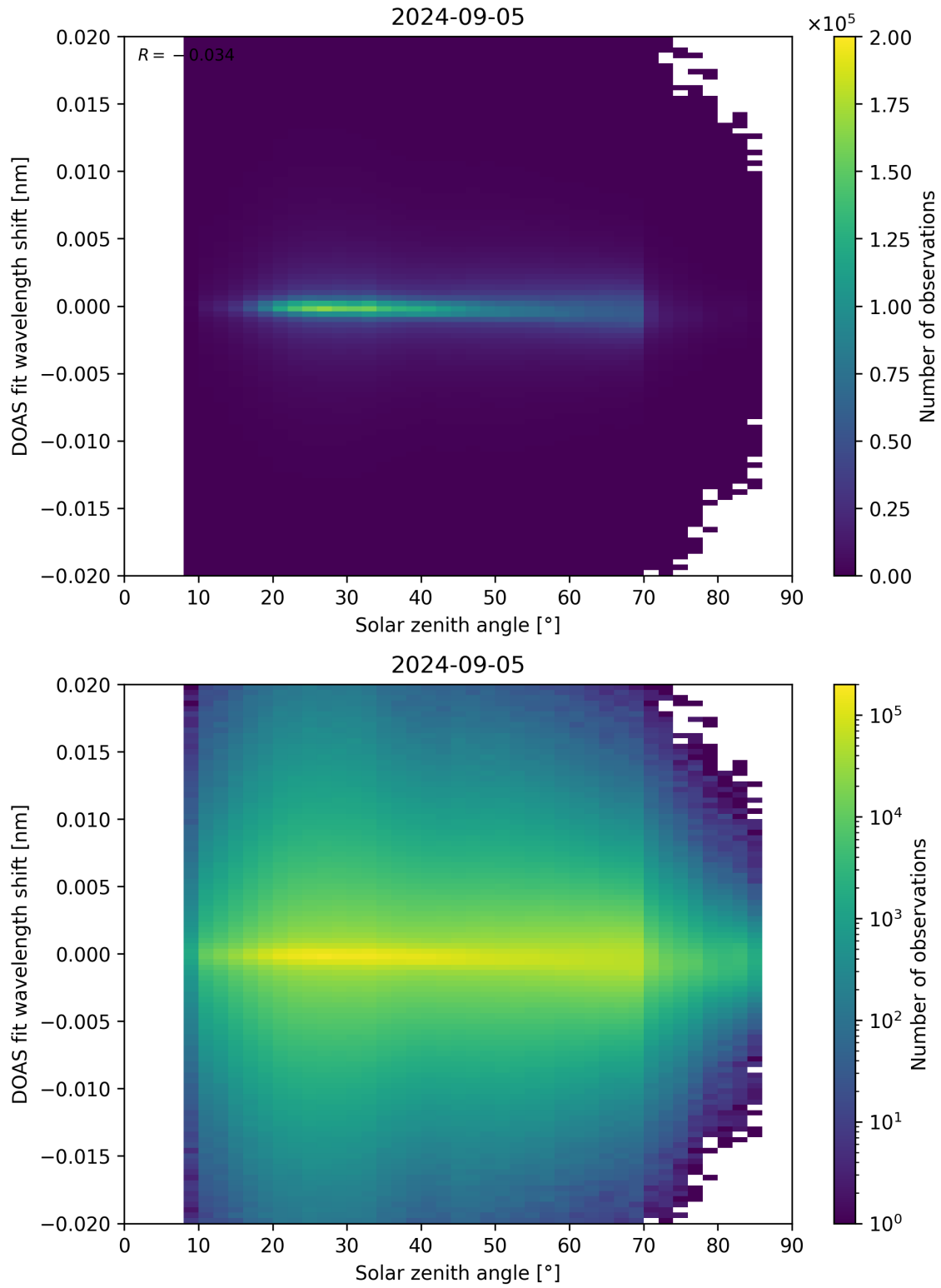
Figure 168: Scatter density plot of “Solar zenith angle” against “DOAS fit wavelength shift” for 2024-09-04 to 2024-09-06.
