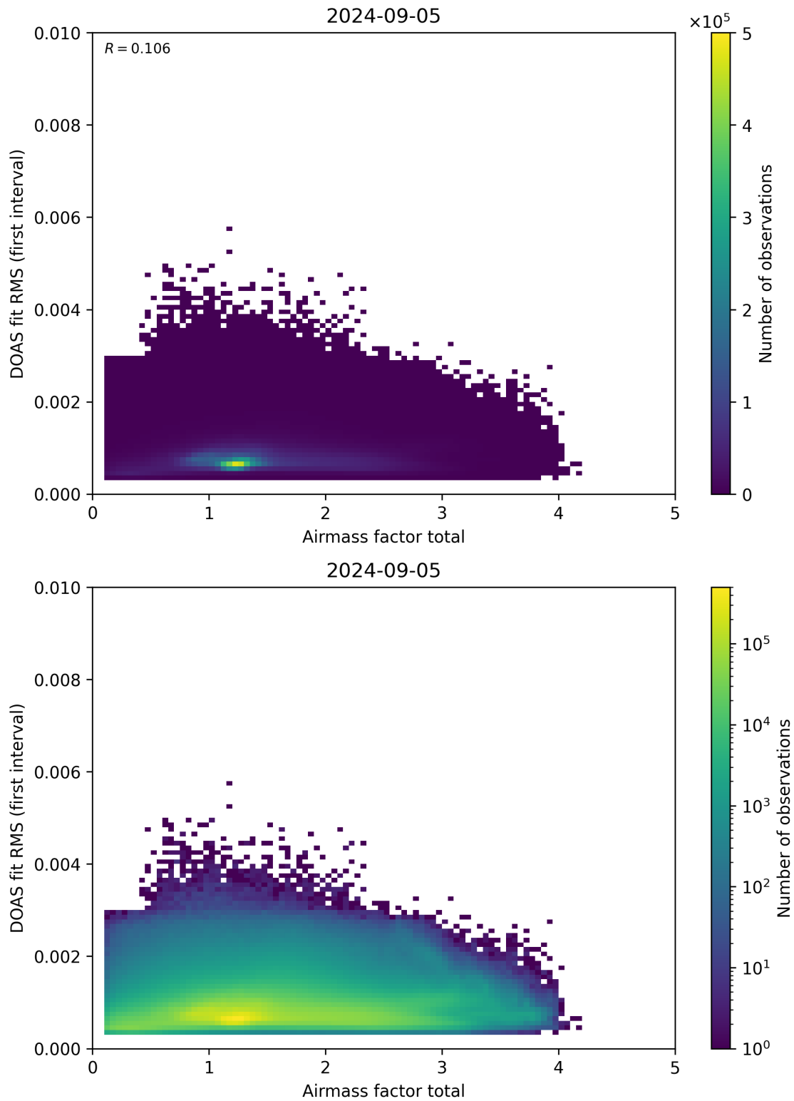
Figure 97: Scatter density plot of “Airmass factor total” against “DOAS fit RMS (first interval)” for 2024-09-04 to 2024-09-06.
