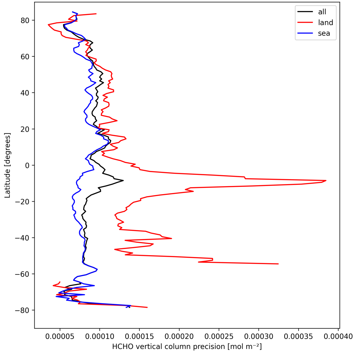
Figure 22: Zonal average of “HCHO vertical column precision” for 2024-09-04 to 2024-09-06.
