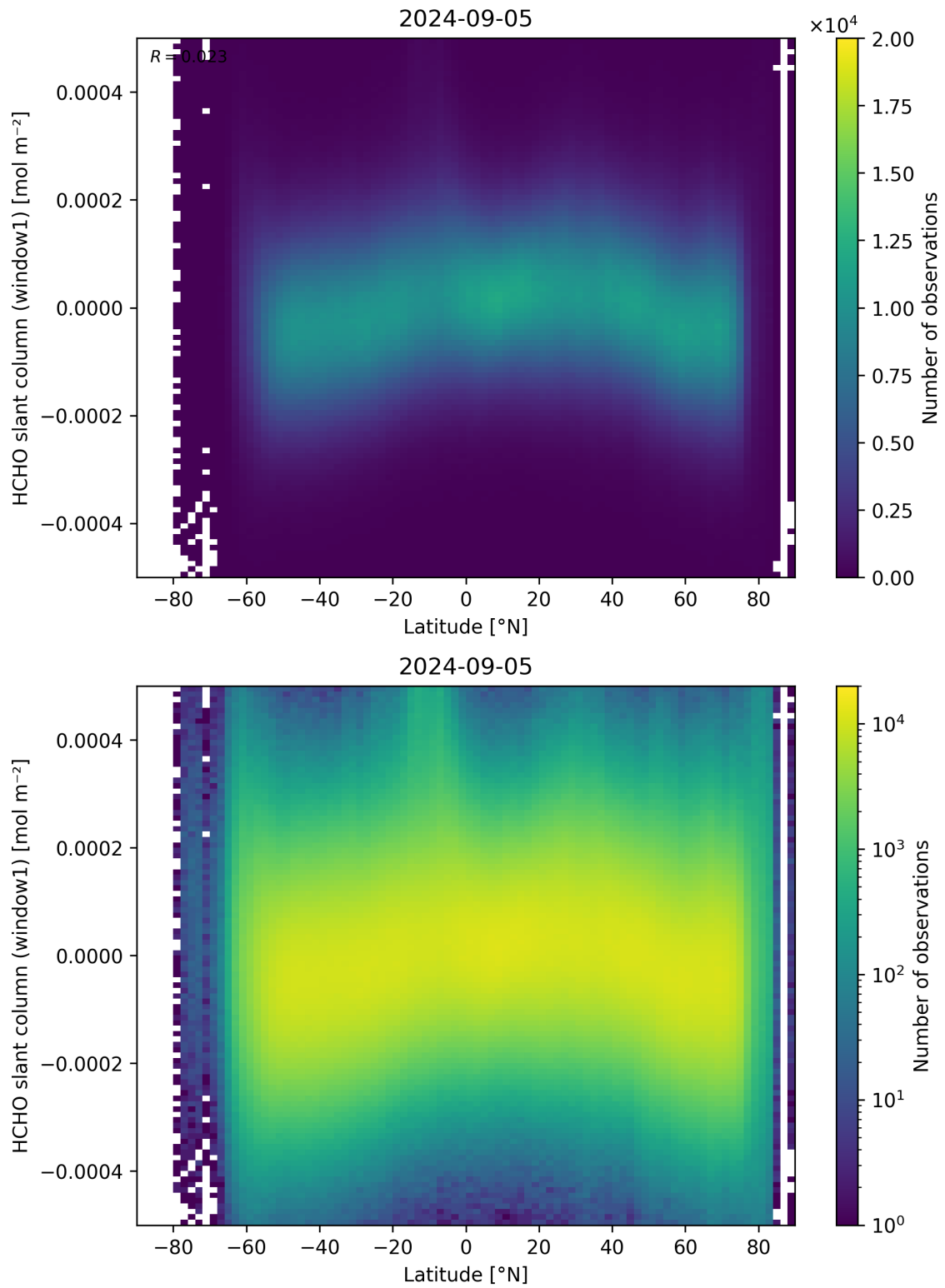
Figure 159: Scatter density plot of “Latitude” against “HCHO slant column (window1)” for 2024-09-04 to 2024-09-06.
