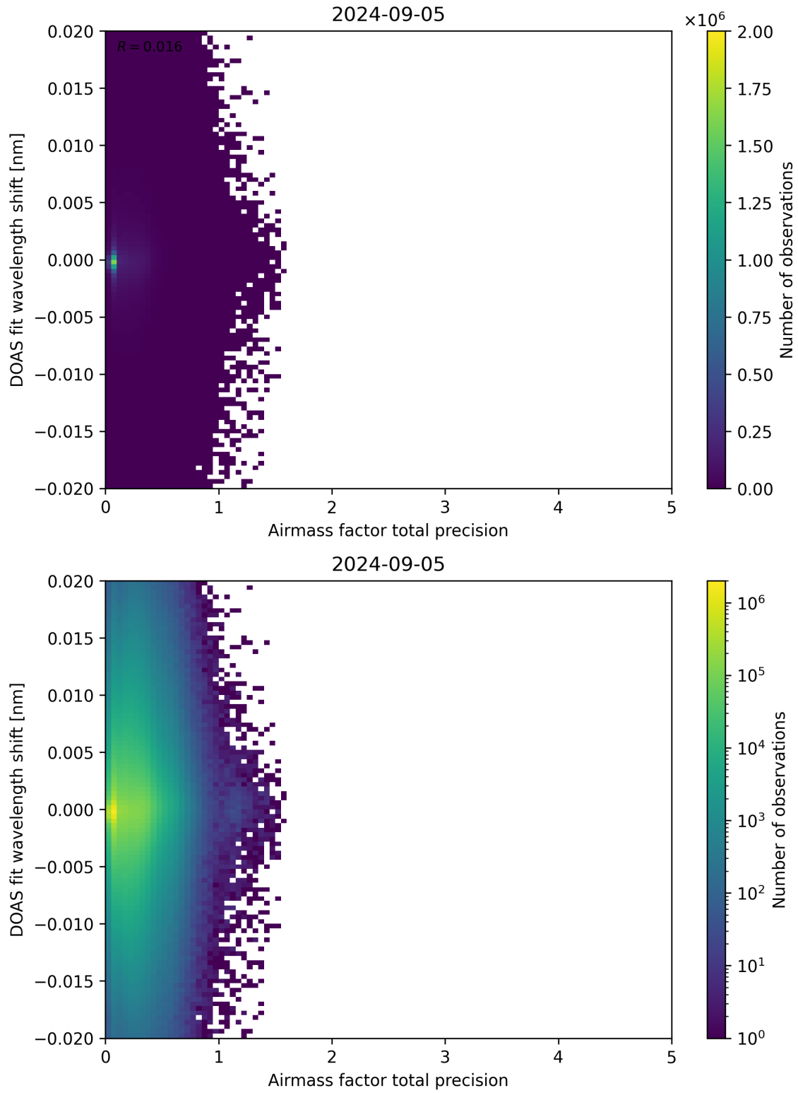
Figure 106: Scatter density plot of “Airmass factor total precision” against “DOAS fit wavelength shift” for 2024-09-04 to 2024-09-06.
