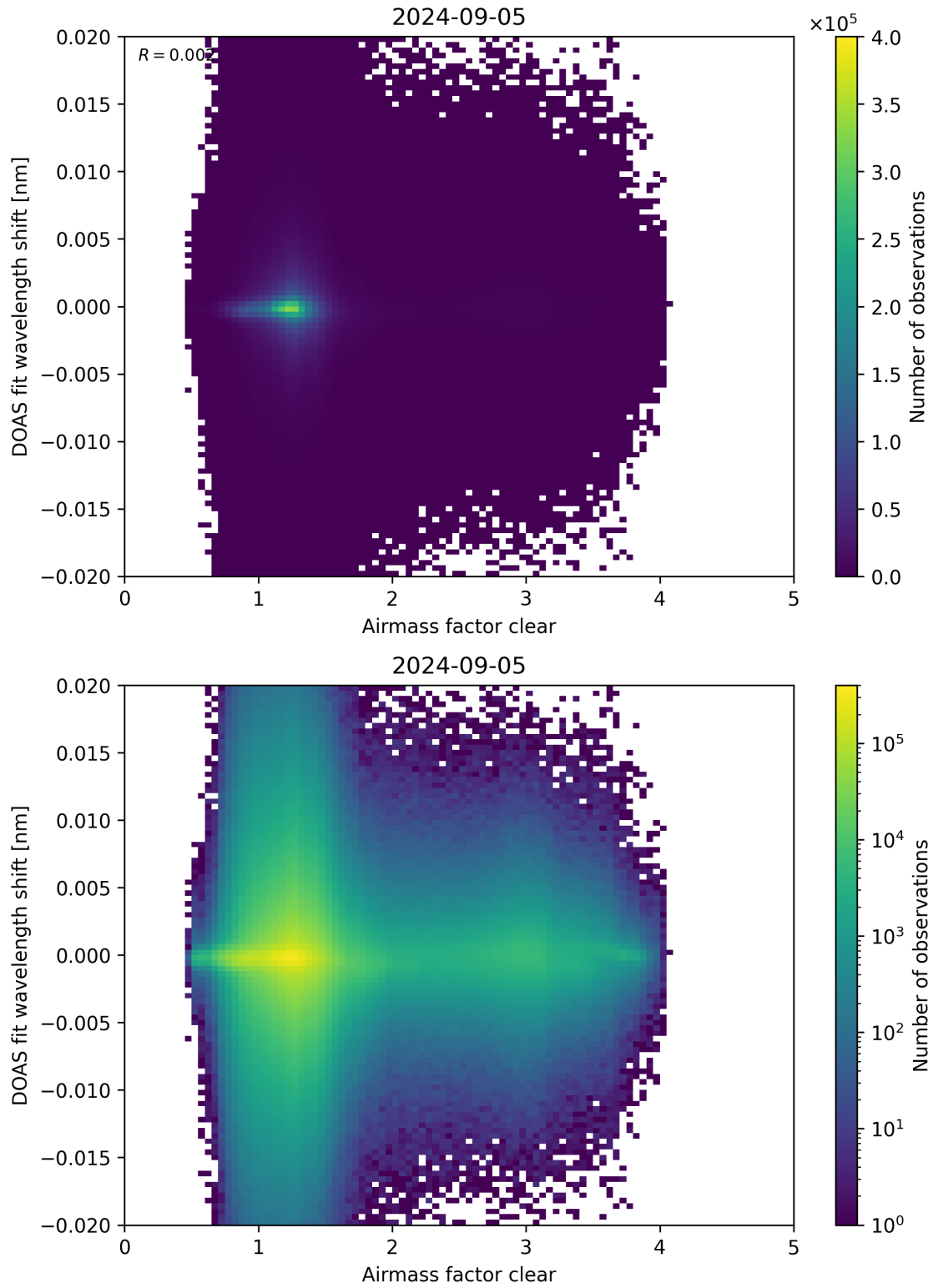
Figure 72: Scatter density plot of “Airmass factor clear” against “DOAS fit wavelength shift” for 2024-09-04 to 2024-09-06.
