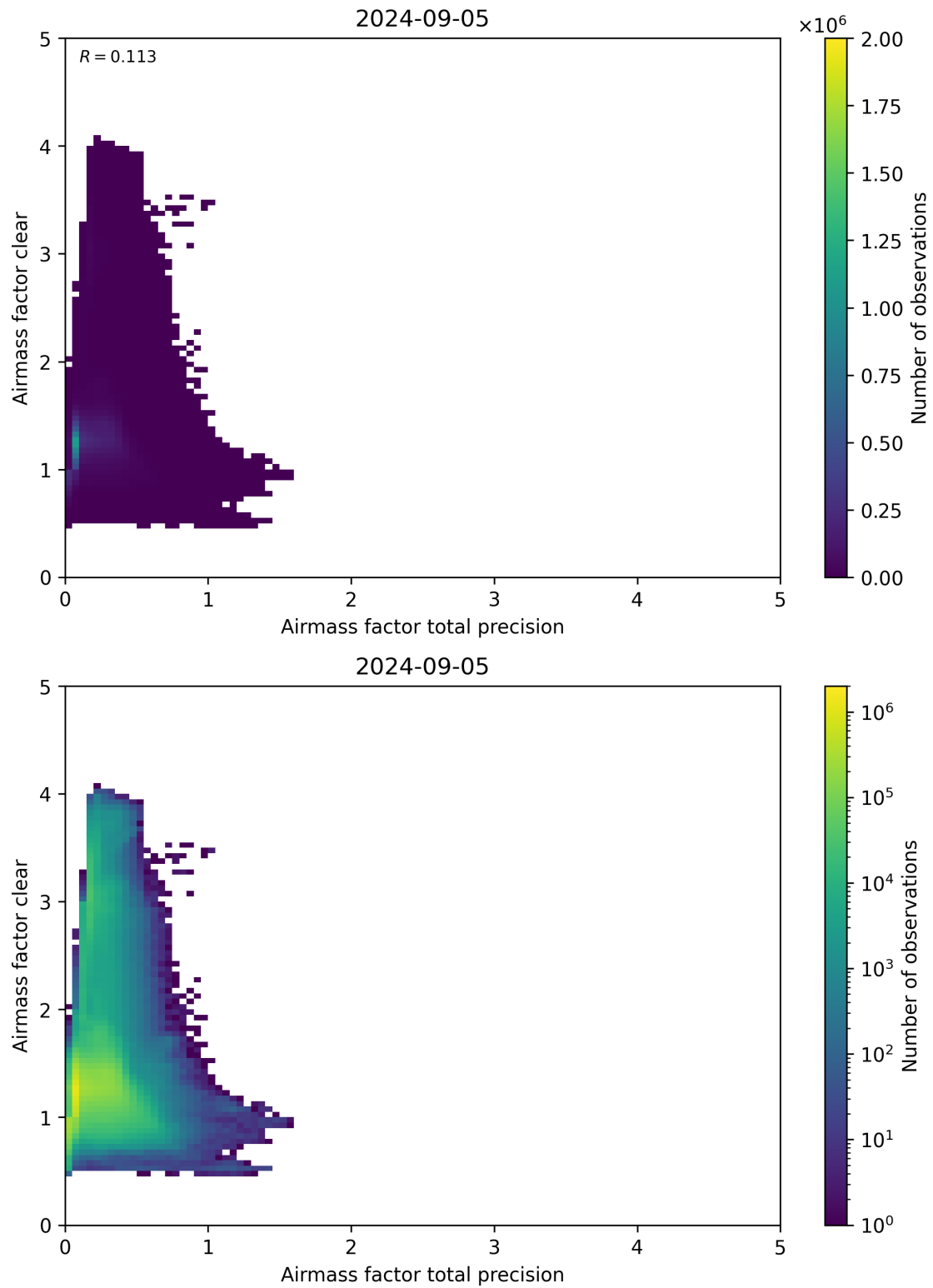
Figure 108: Scatter density plot of “Airmass factor total precision” against “Airmass factor clear” for 2024-09-04 to 2024-09-06.
