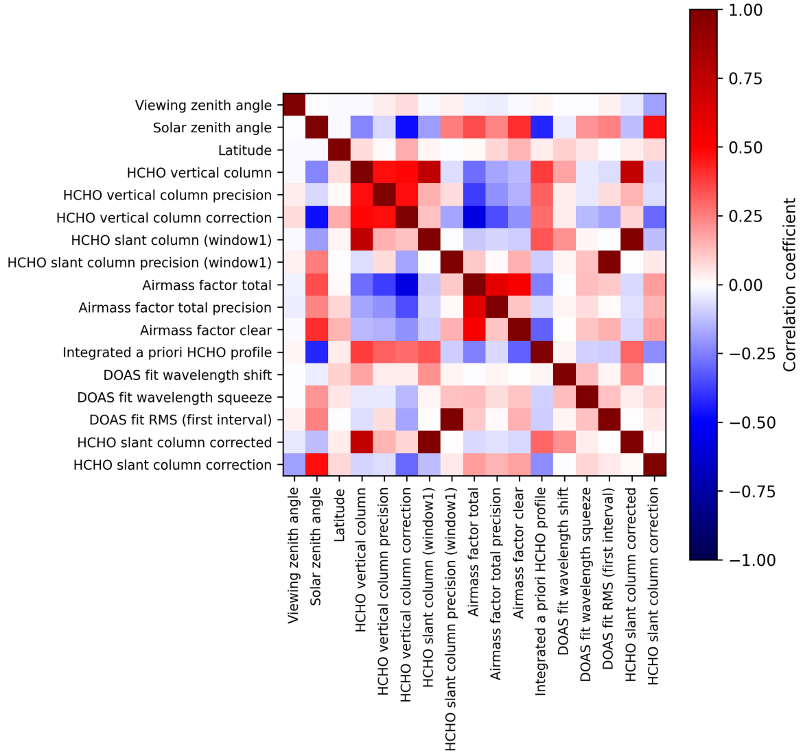
Figure 2: Map of correlation matrix for 2024-09-04 to 2024-09-06.
