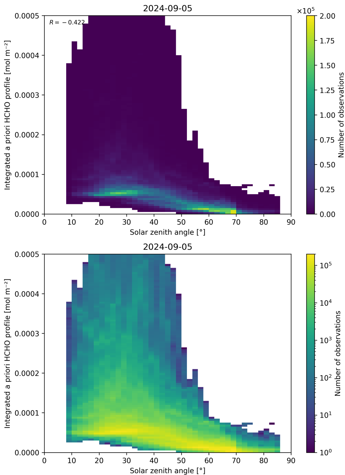
Figure 180: Scatter density plot of “Solar zenith angle” against “Integrated a priori HCHO profile” for 2024-09-04 to 2024-09-06.
