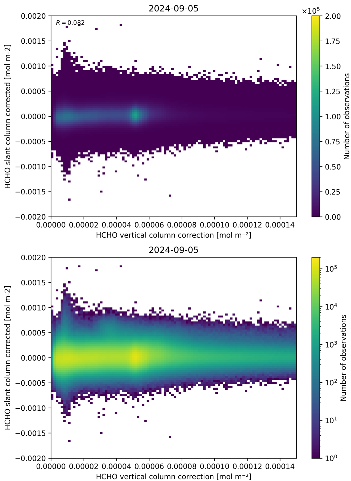
Figure 116: Scatter density plot of “HCHO vertical column correction” against “HCHO slant column corrected” for 2024-09-04 to 2024-09-06.
