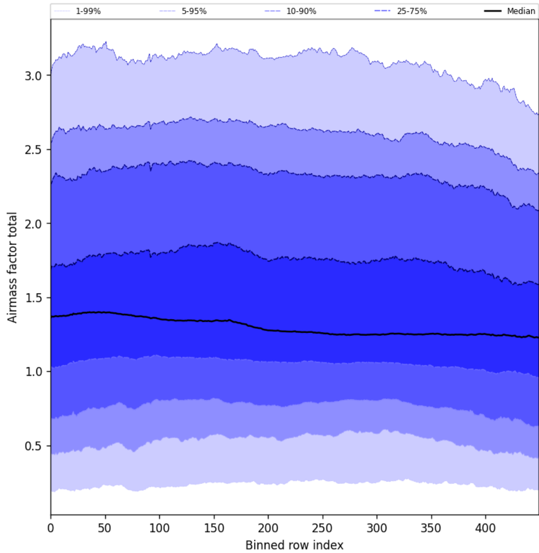
Figure 54: Along track statistics of “Airmass factor total” for 2024-09-04 to 2024-09-06
