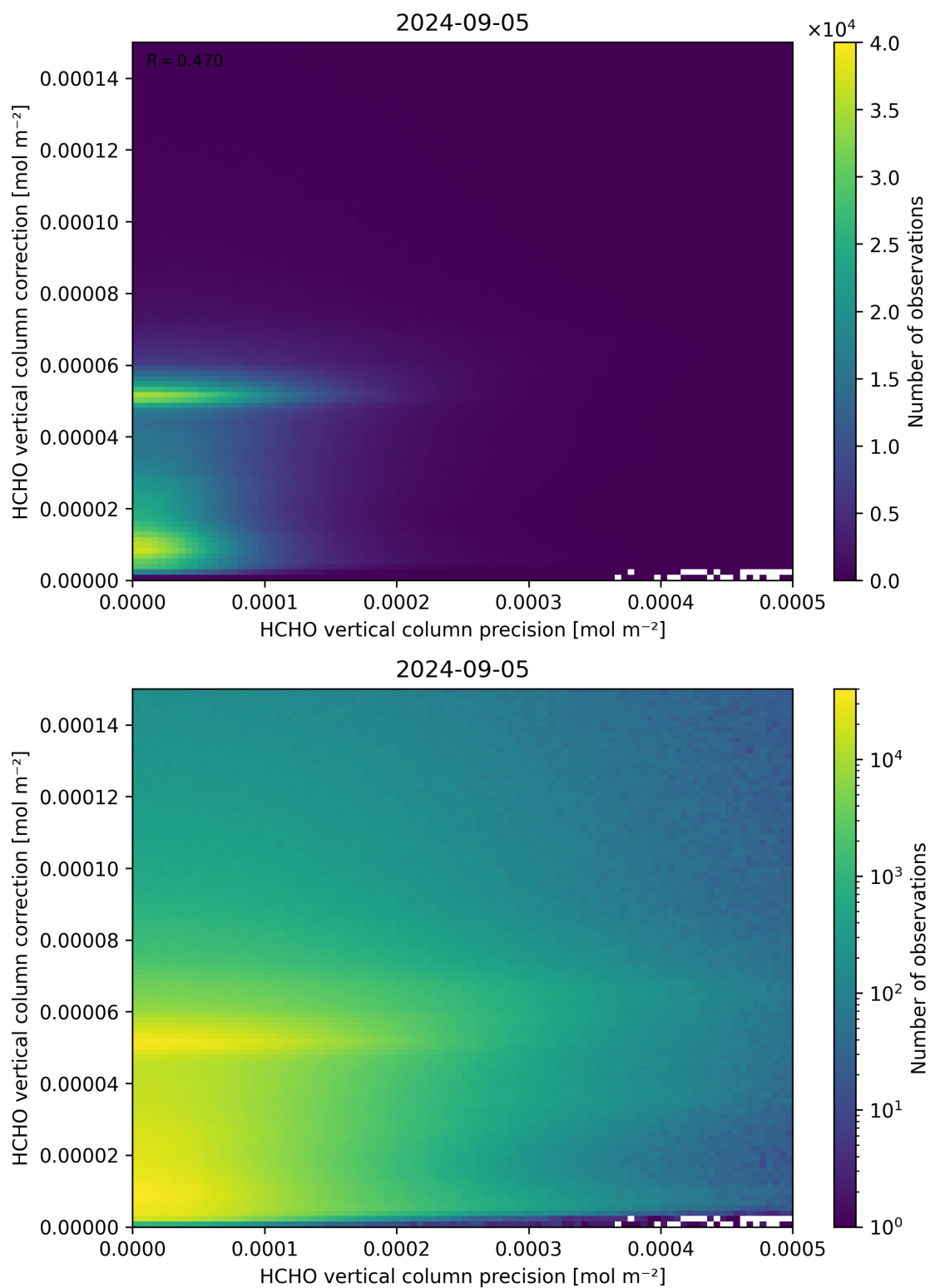
Figure 146: Scatter density plot of “HCHO vertical column precision” against “HCHO vertical column correction” for 2024-09-04 to 2024-09-06.
