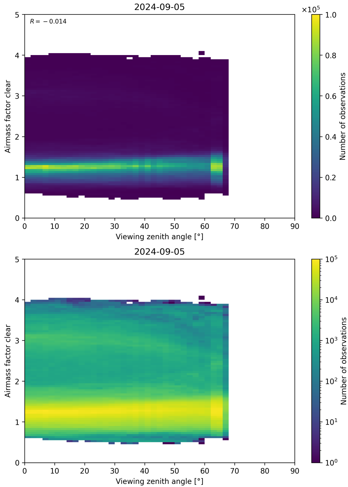
Figure 185: Scatter density plot of “Viewing zenith angle” against “Airmass factor clear” for 2024-09-04 to 2024-09-06.
