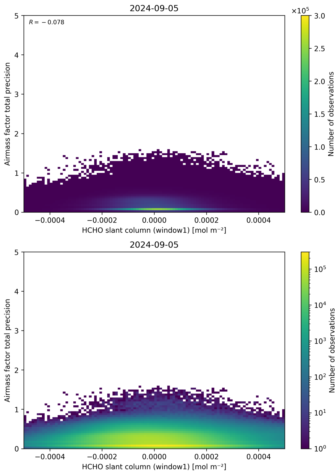
Figure 86: Scatter density plot of “HCHO slant column (window1)” against “Airmass factor total precision” for 2024-09-04 to 2024-09-06.
