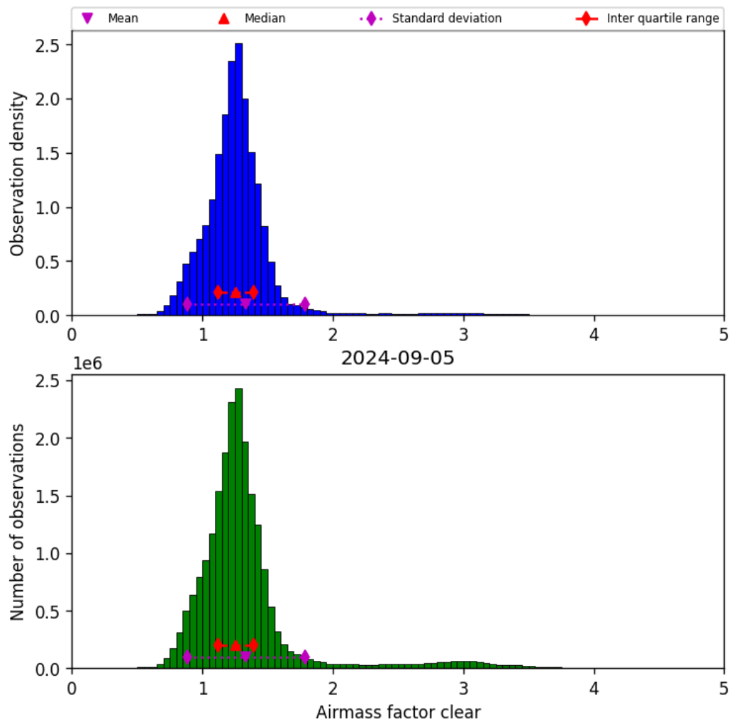
Figure 42: Histogram of “Airmass factor clear” for 2024-09-04 to 2024-09-06
