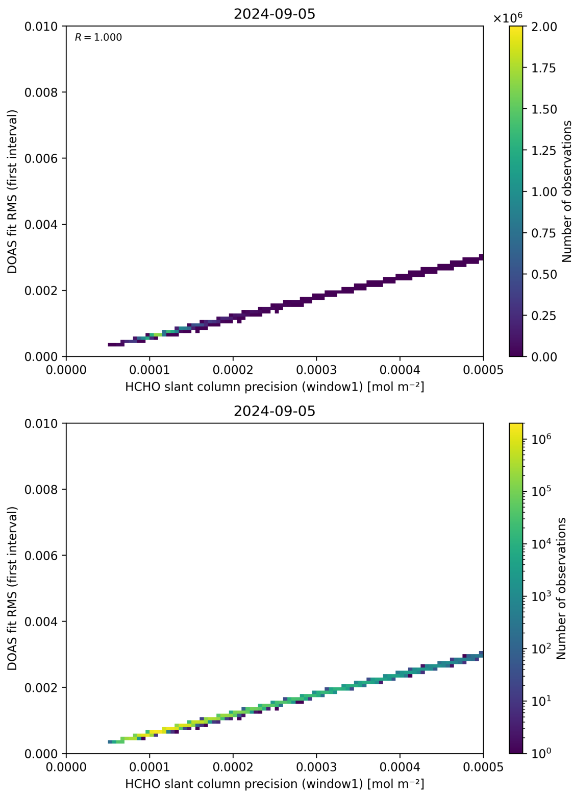
Figure 88: Scatter density plot of “HCHO slant column precision (window1)” against “DOAS fit RMS (first interval)” for 2024-09-04 to 2024-09-06.
