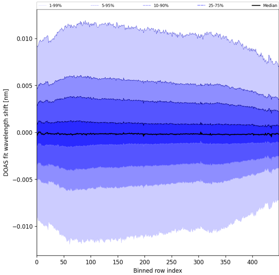
Figure 58: Along track statistics of “DOAS fit wavelength shift” for 2024-09-04 to 2024-09-06
