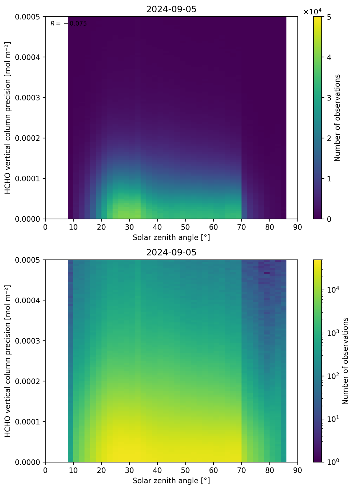
Figure 179: Scatter density plot of “Solar zenith angle” against “HCHO vertical column precision” for 2024-09-04 to 2024-09-06.
