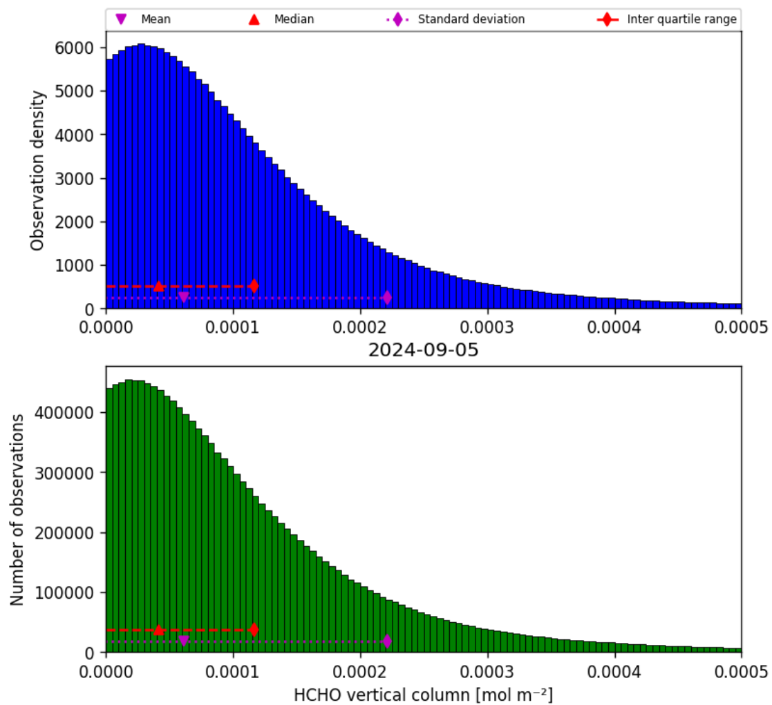
Figure 35: Histogram of “HCHO vertical column” for 2024-09-04 to 2024-09-06
