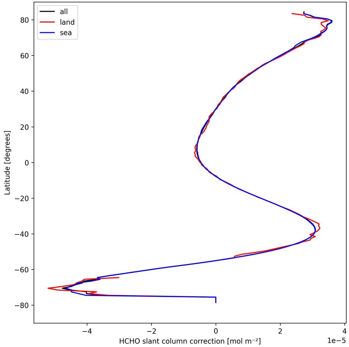
Figure 33: Zonal average of “HCHO slant column correction” for 2024-09-04 to 2024-09-06.
