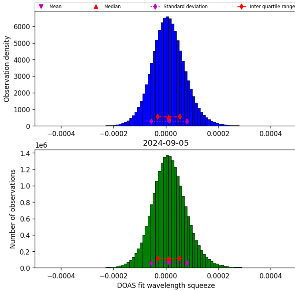
Figure 45: Histogram of “DOAS fit wavelength squeeze” for 2024-09-04 to 2024-09-06
