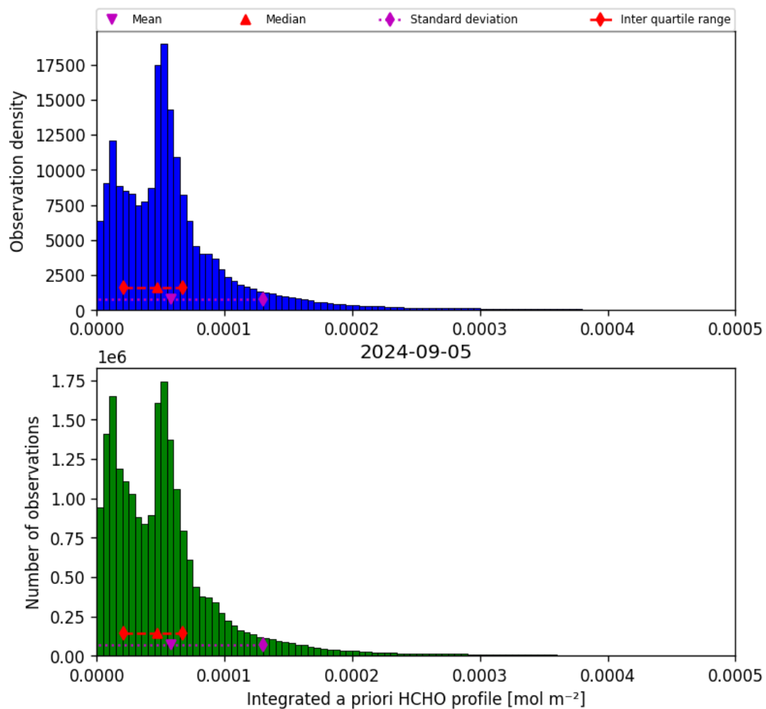
Figure 43: Histogram of “Integrated a priori HCHO profile” for 2024-09-04 to 2024-09-06
