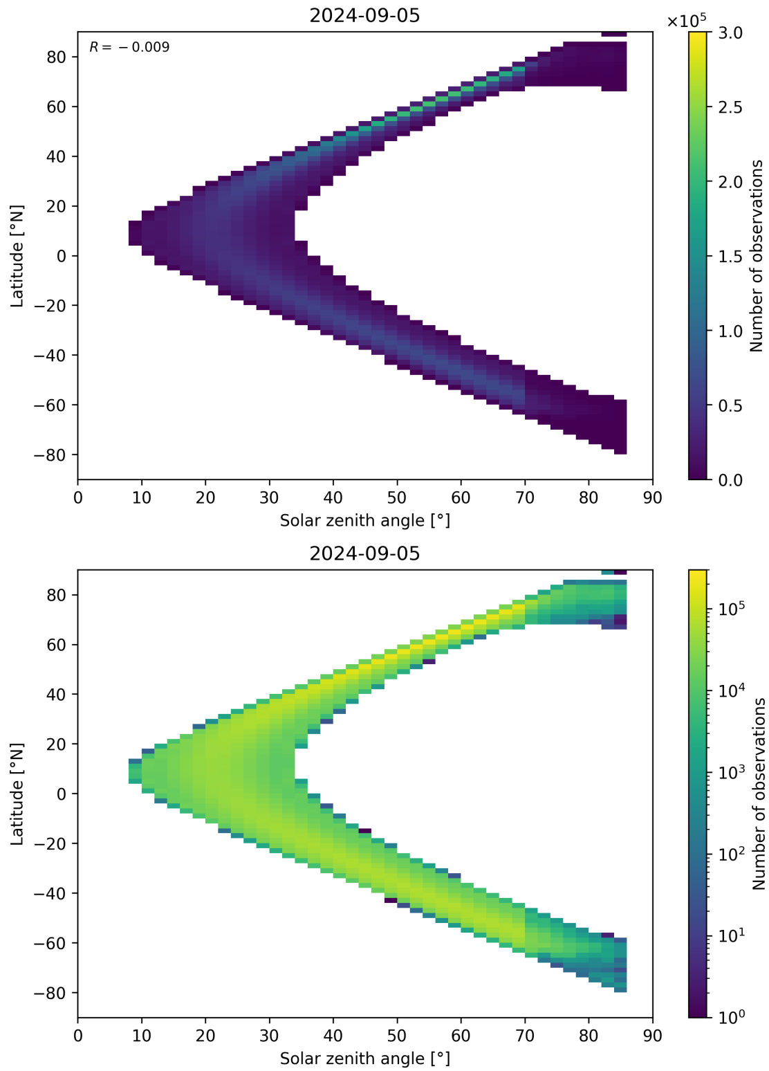
Figure 181: Scatter density plot of “Solar zenith angle” against “Latitude” for 2024-09-04 to 2024-09-06.
