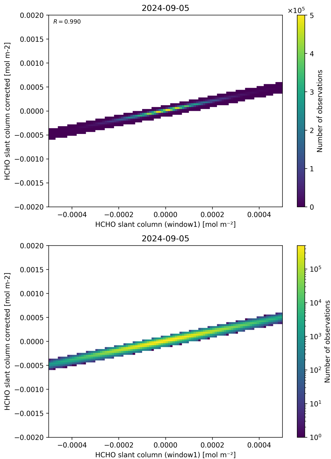
Figure 82: Scatter density plot of “HCHO slant column (window1)” against “HCHO slant column corrected” for 2024-09-04 to 2024-09-06.
