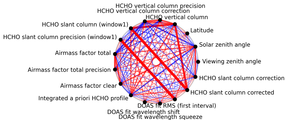
Figure 1: Map of correlation graph for 2024-09-04 to 2024-09-06.
