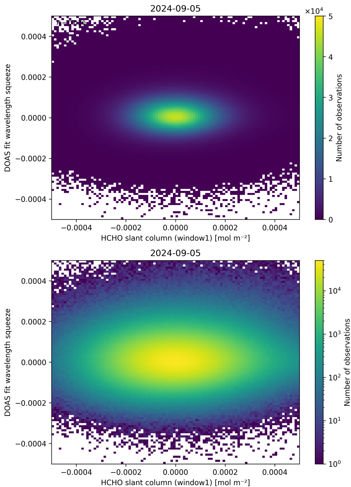
Figure 80: Scatter density plot of “HCHO slant column (window1)” against “DOAS fit wavelength squeeze” for 2024-09-04 to 2024-09-06.
