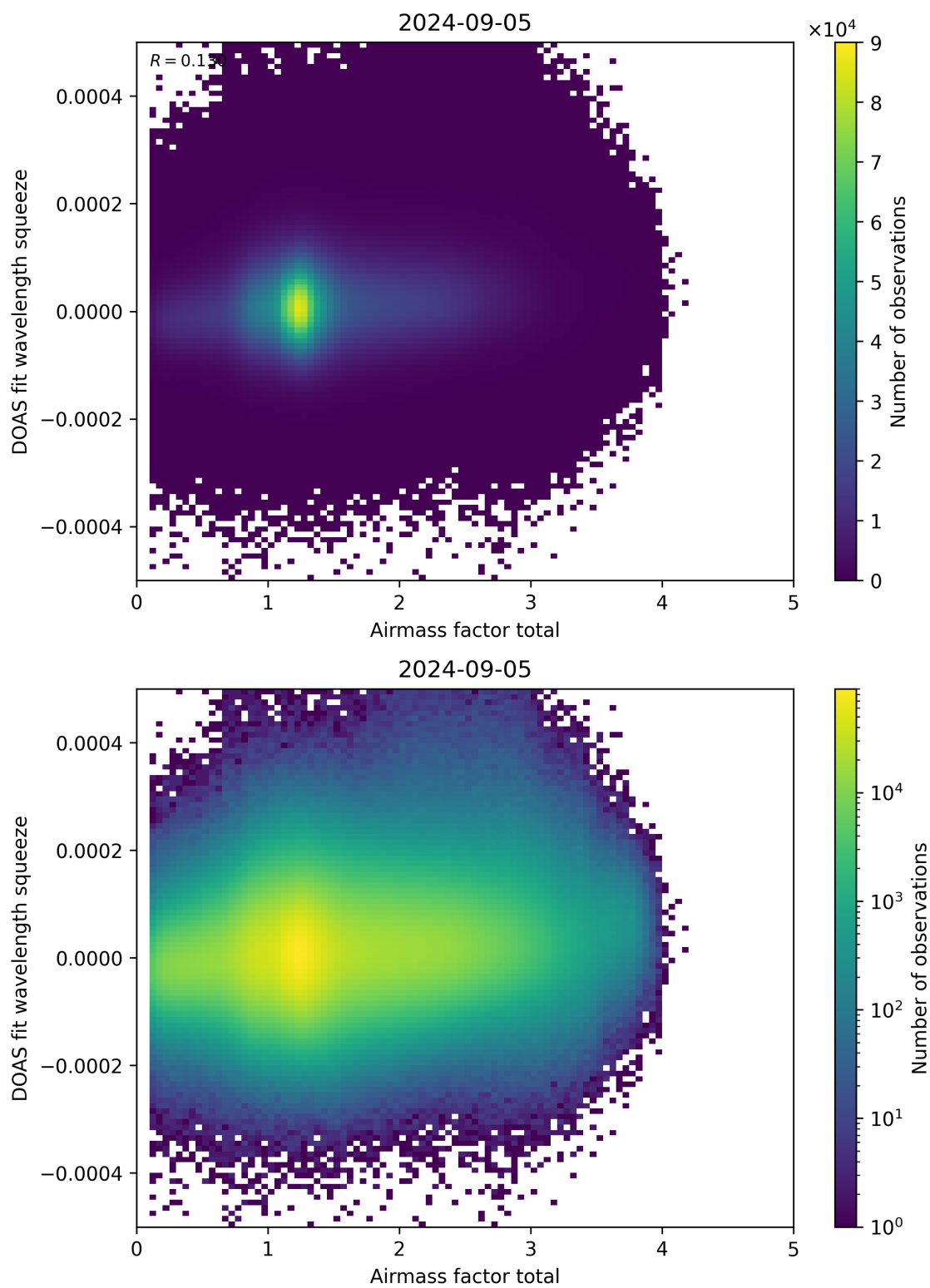
Figure 99: Scatter density plot of “Airmass factor total” against “DOAS fit wavelength squeeze” for 2024-09-04 to 2024-09-06.
