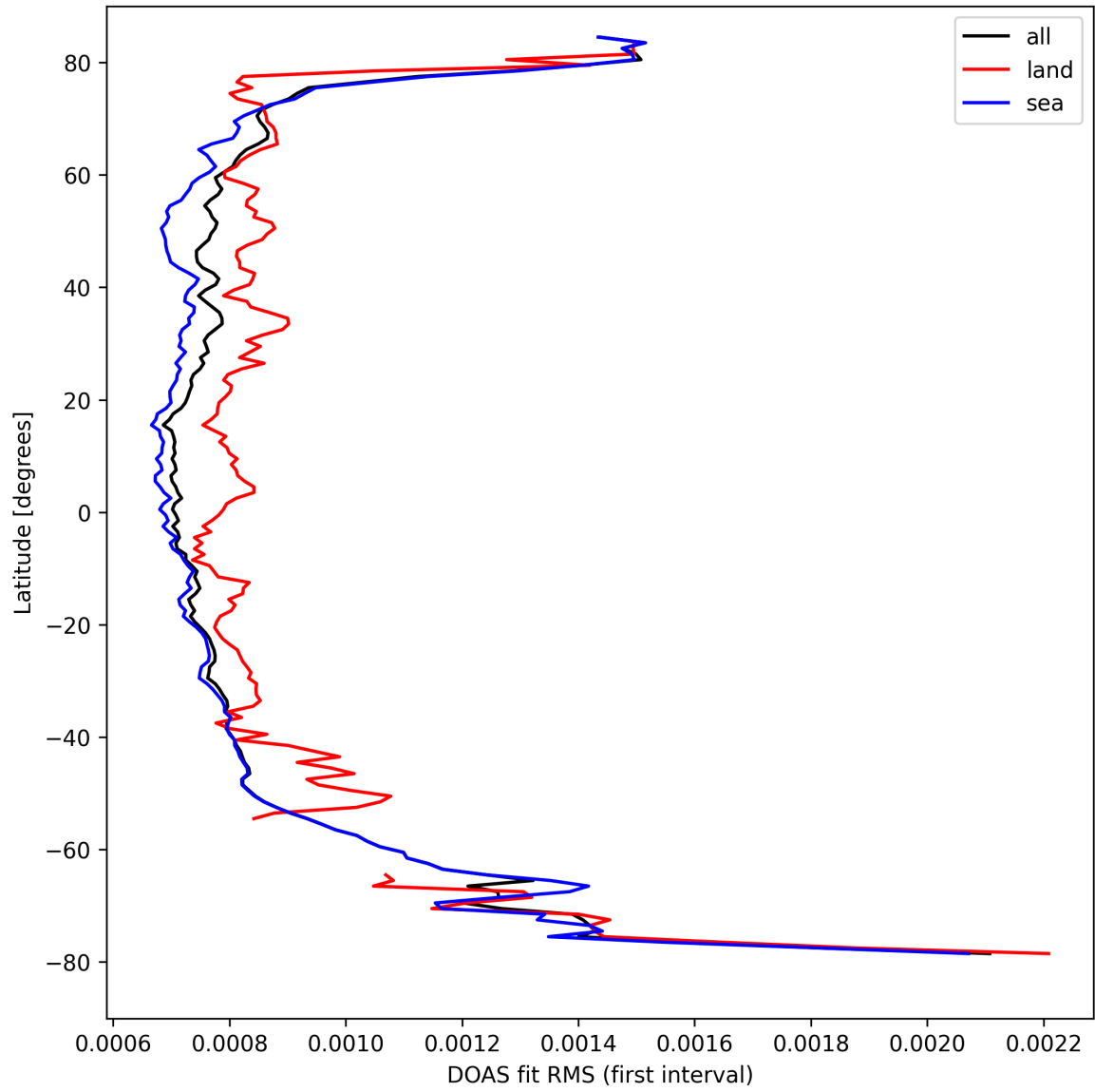
Figure 32: Zonal average of “DOAS fit RMS (first interval)” for 2024-09-04 to 2024-09-06.
