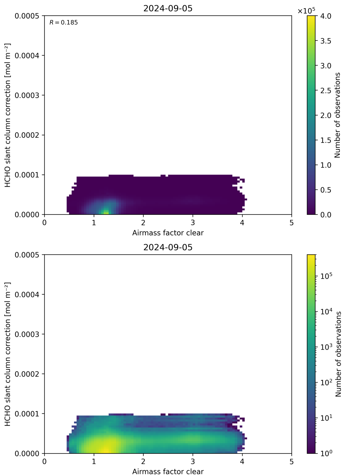
Figure 75: Scatter density plot of “Airmass factor clear” against “HCHO slant column correction” for 2024-09-04 to 2024-09-06.
