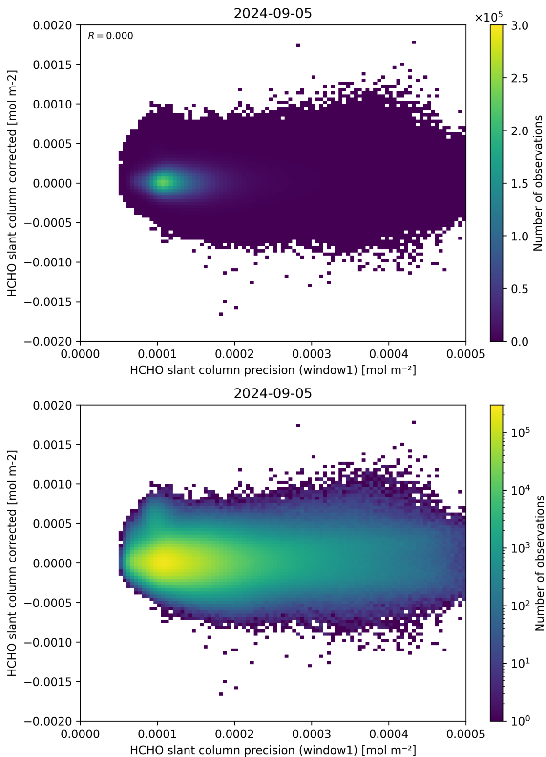
Figure 92: Scatter density plot of “HCHO slant column precision (window1)” against “HCHO slant column corrected” for 2024-09-04 to 2024-09-06.
