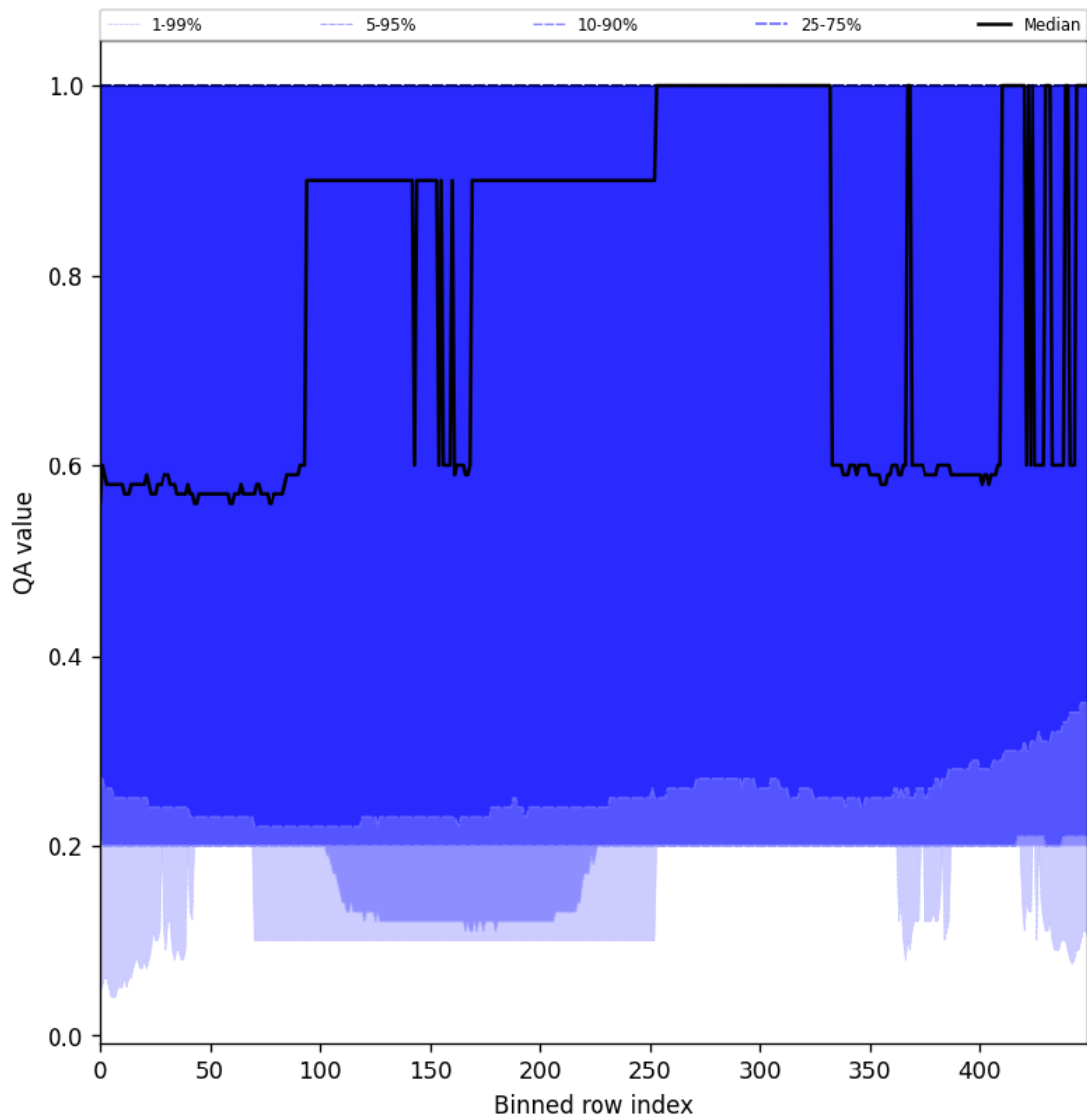
Figure 48: Along track statistics of “QA value” for 2024-09-04 to 2024-09-06
