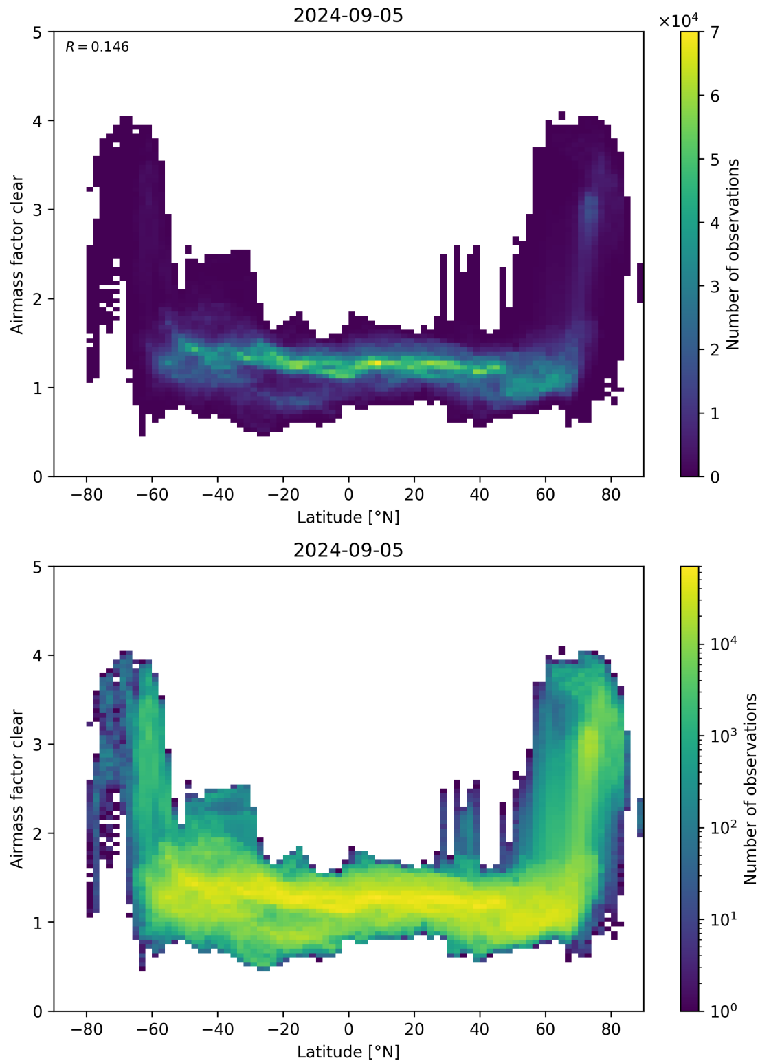
Figure 156: Scatter density plot of “Latitude” against “Airmass factor clear” for 2024-09-04 to 2024-09-06.
