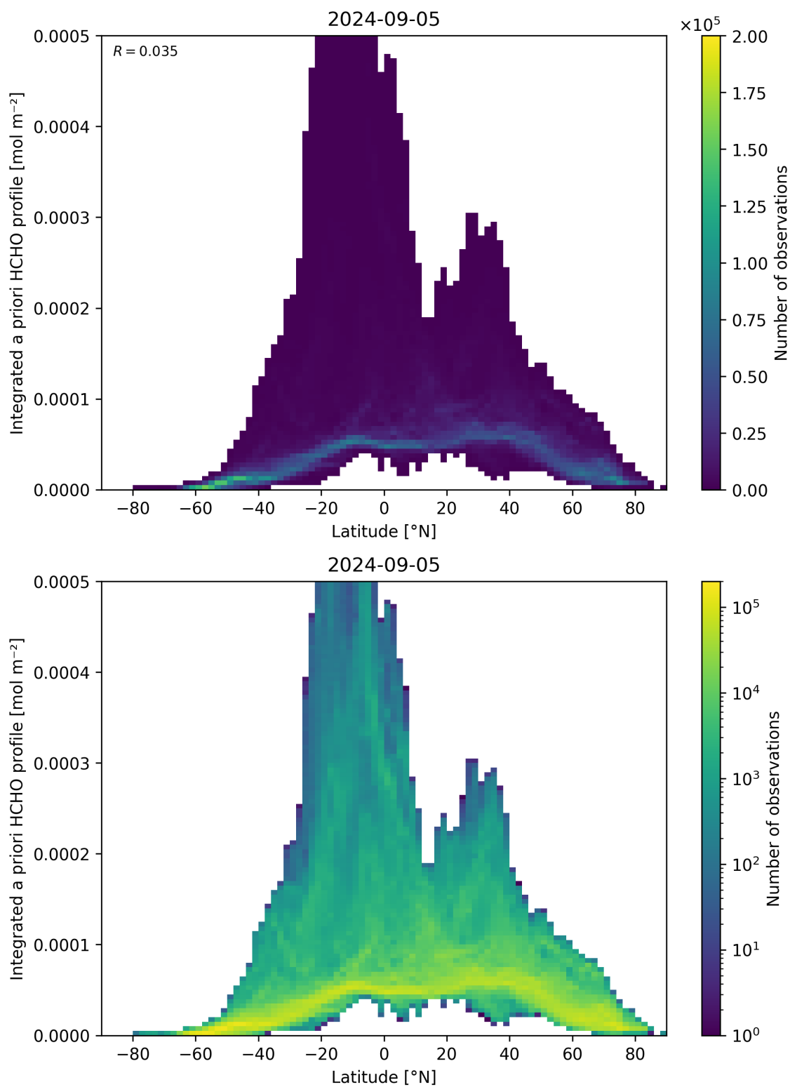
Figure 166: Scatter density plot of “Latitude” against “Integrated a priori HCHO profile” for 2024-09-04 to 2024-09-06.
