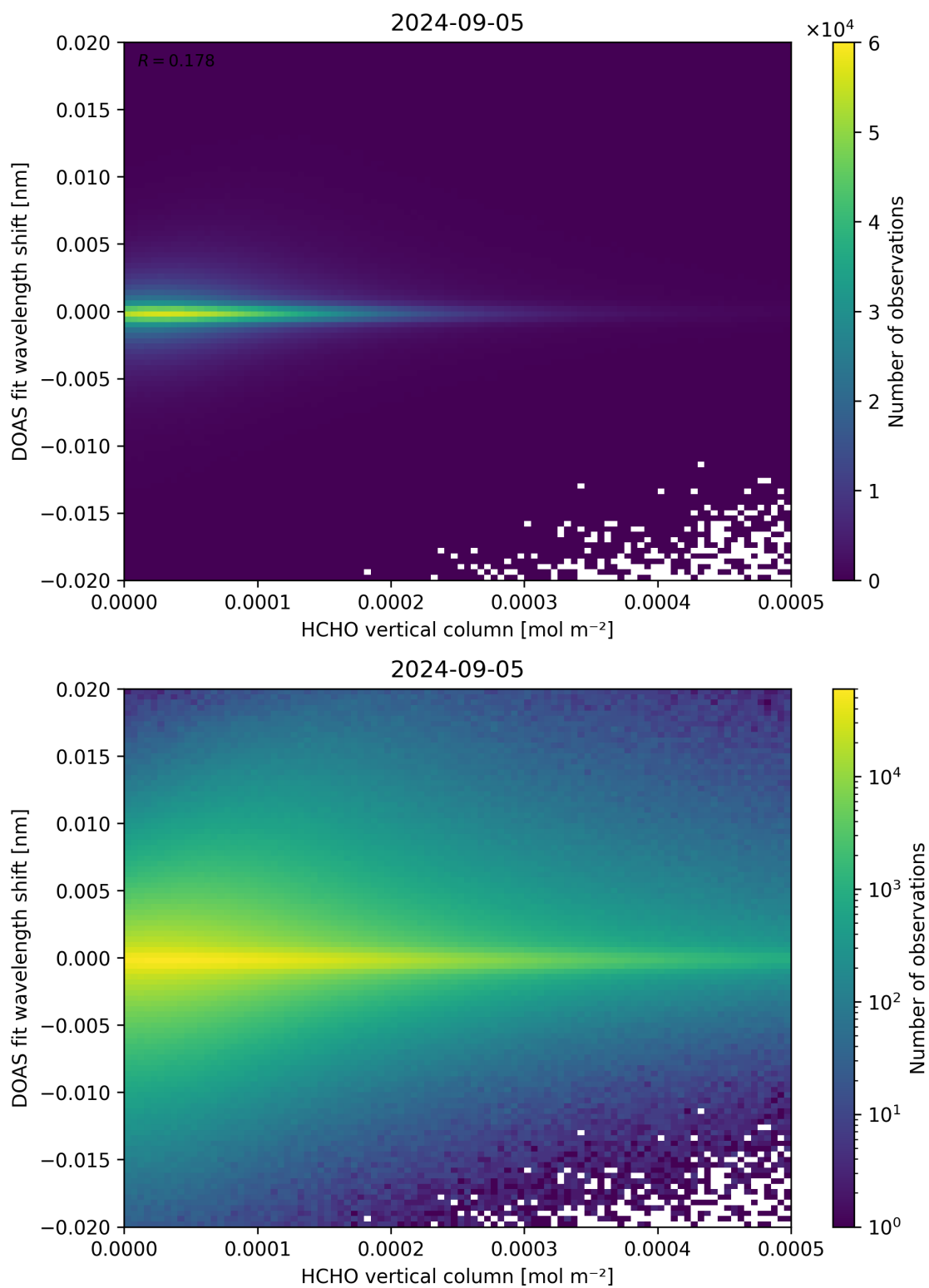
Figure 124: Scatter density plot of “HCHO vertical column” against “DOAS fit wavelength shift” for 2024-09-04 to 2024-09-06.
