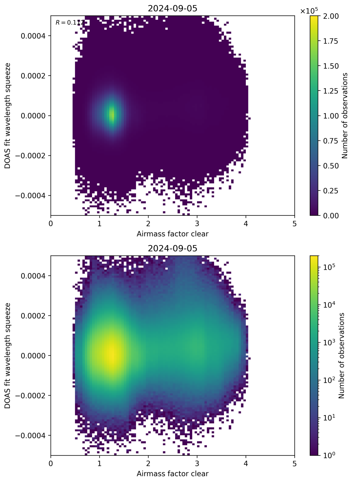
Figure 73: Scatter density plot of “Airmass factor clear” against “DOAS fit wavelength squeeze” for 2024-09-04 to 2024-09-06.
