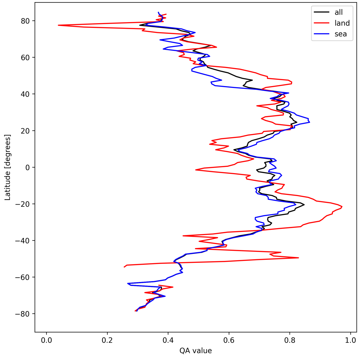
Figure 20: Zonal average of “QA value” for 2024-09-04 to 2024-09-06.
