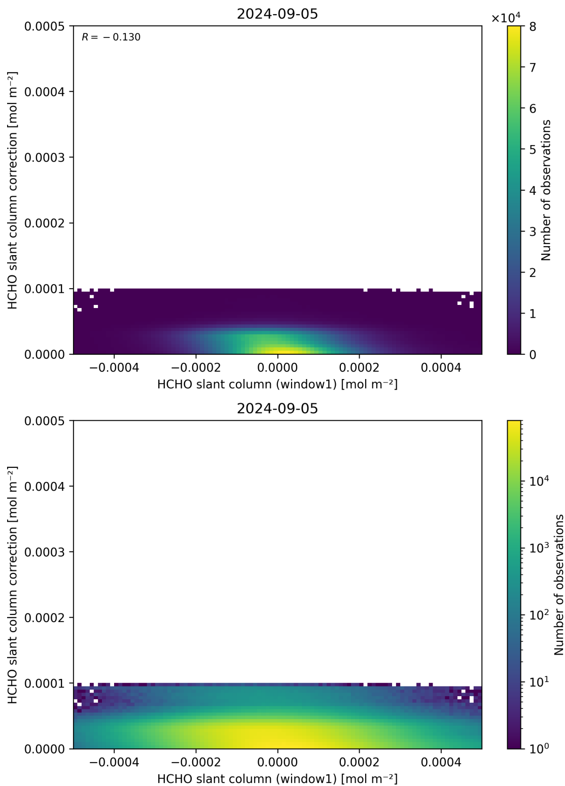
Figure 83: Scatter density plot of “HCHO slant column (window1)” against “HCHO slant column correction” for 2024-09-04 to 2024-09-06.
