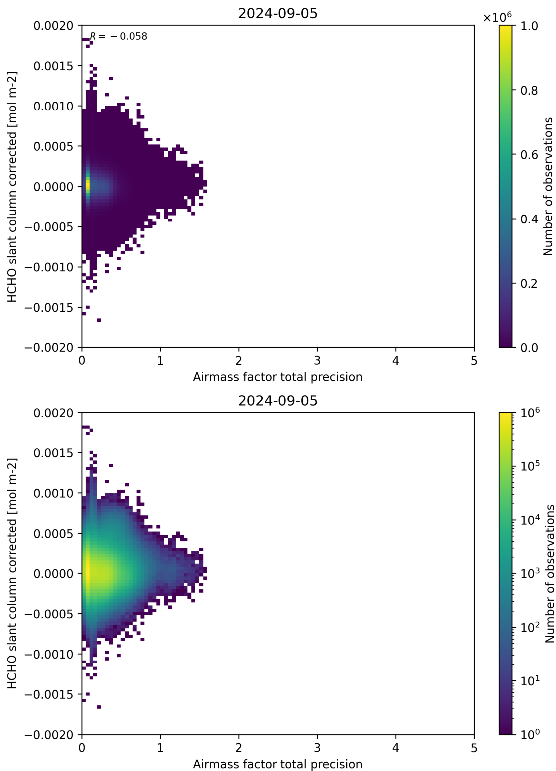
Figure 109: Scatter density plot of “Airmass factor total precision” against “HCHO slant column corrected” for 2024-09-04 to 2024-09-06.
