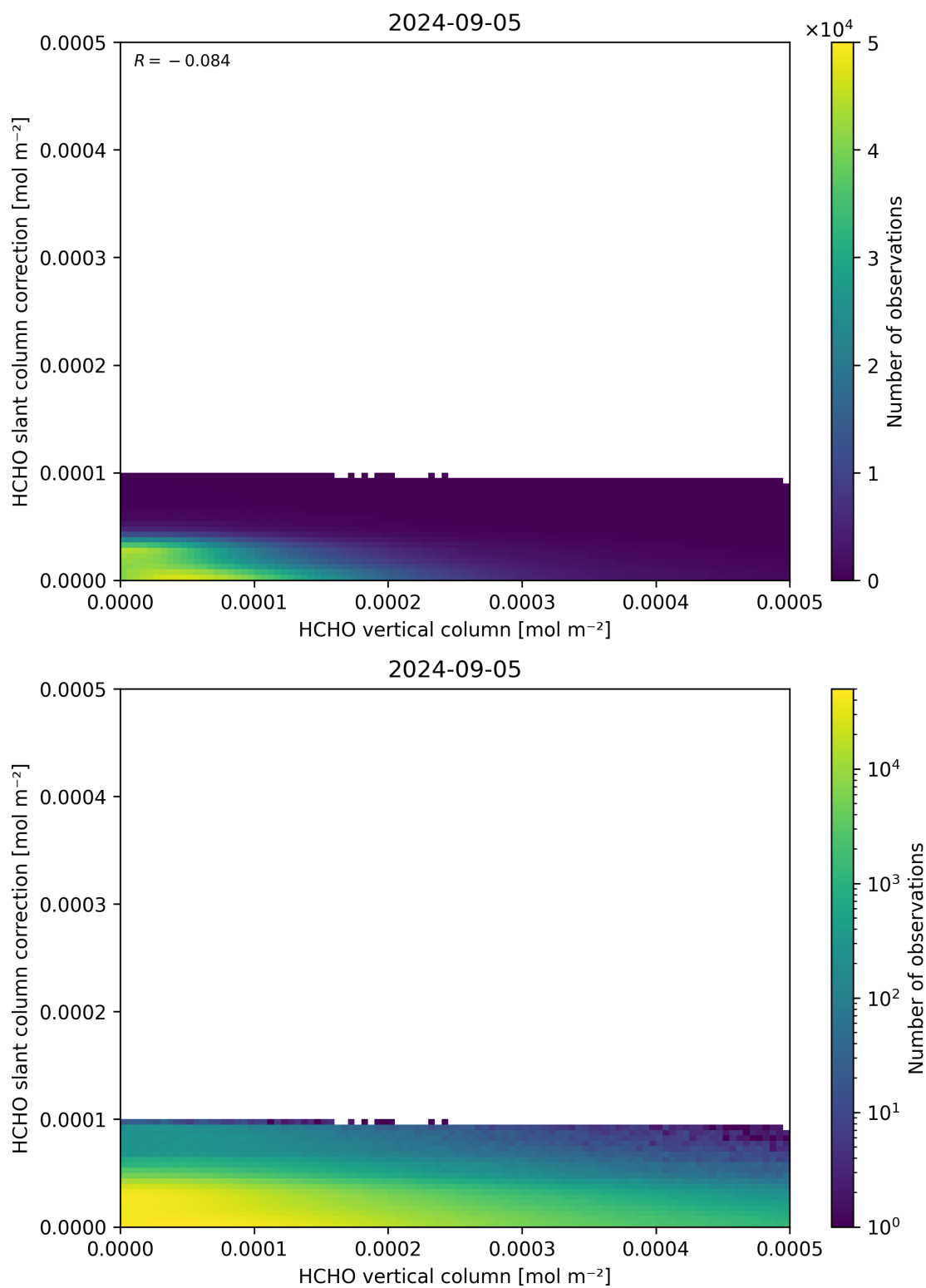
Figure 128: Scatter density plot of “HCHO vertical column” against “HCHO slant column correction” for 2024-09-04 to 2024-09-06.
