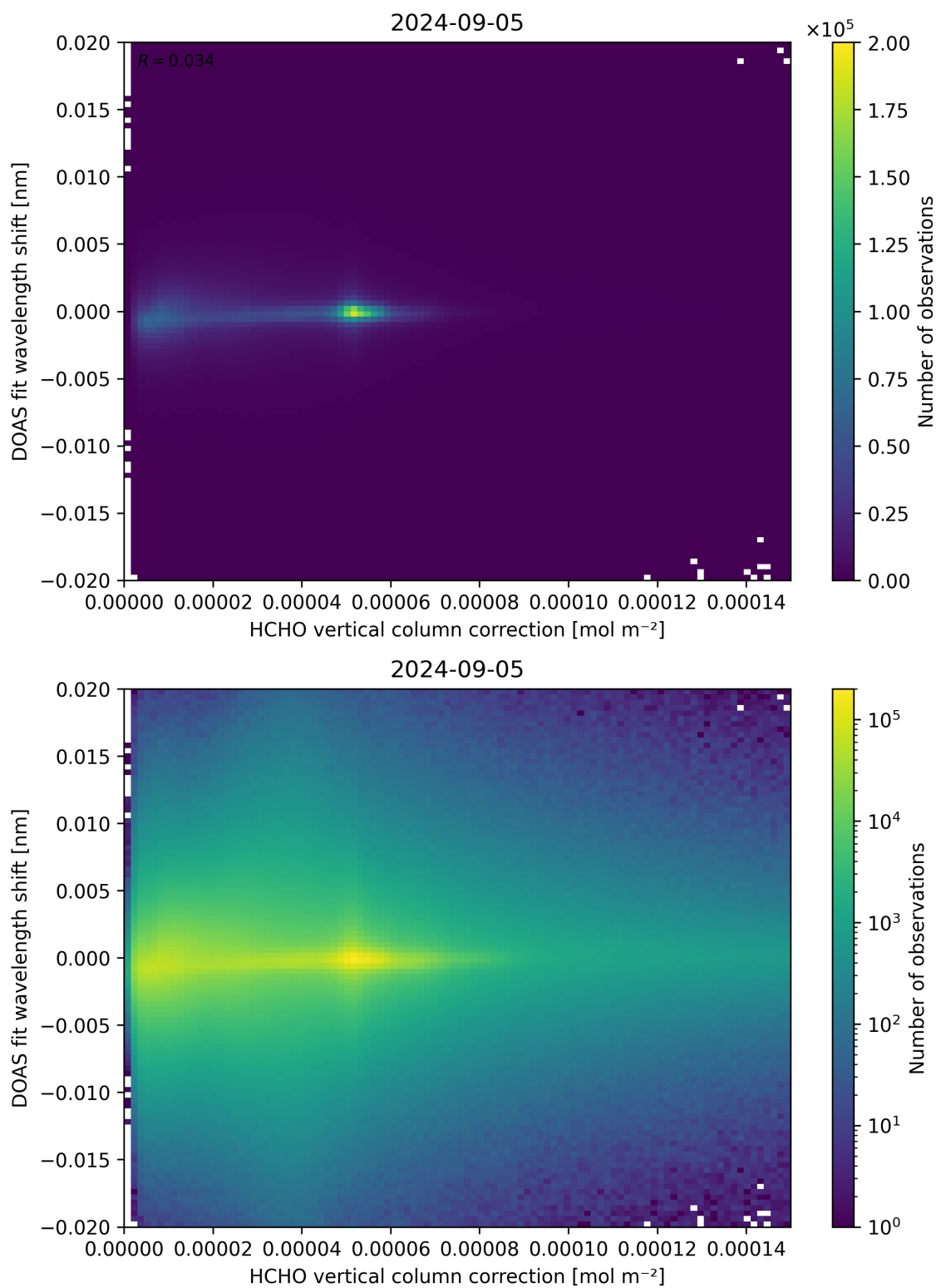
Figure 113: Scatter density plot of “HCHO vertical column correction” against “DOAS fit wavelength shift” for 2024-09-04 to 2024-09-06.
