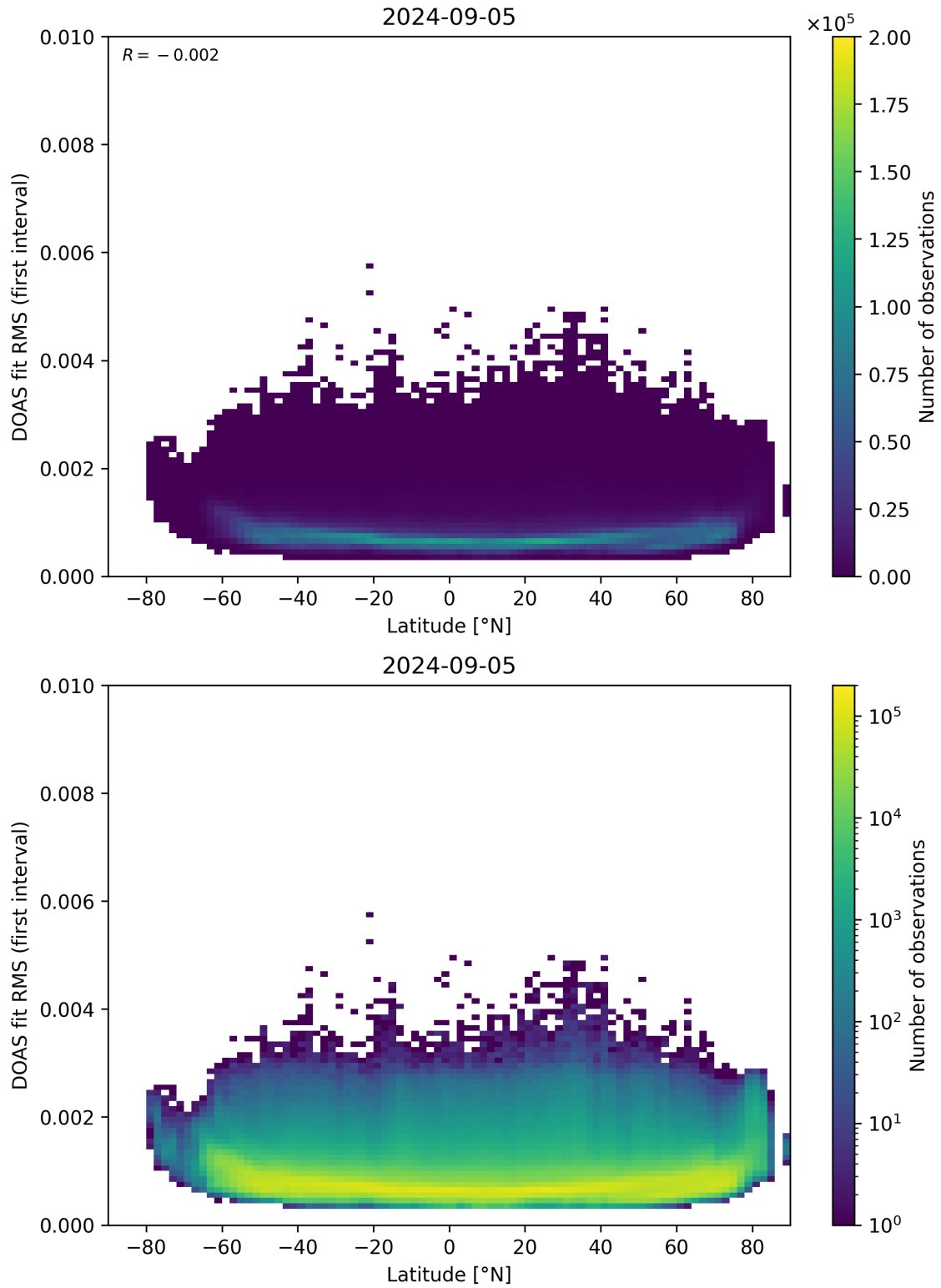
Figure 153: Scatter density plot of “Latitude” against “DOAS fit RMS (first interval)” for 2024-09-04 to 2024-09-06.
