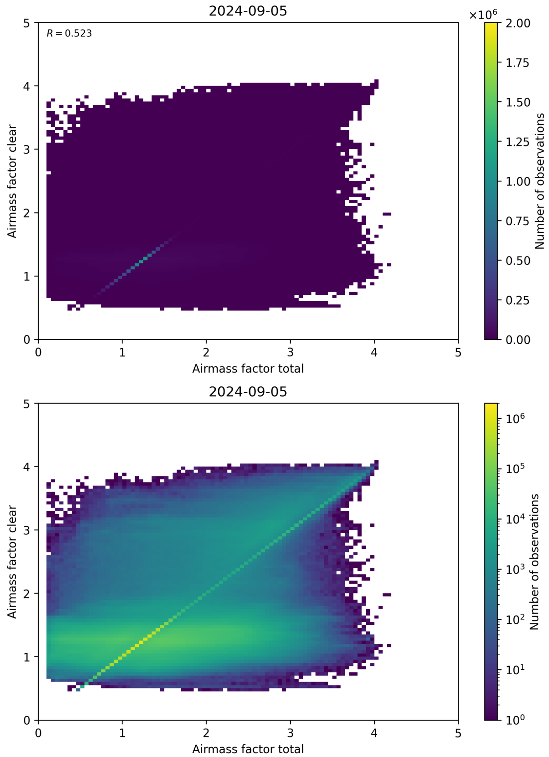
Figure 100: Scatter density plot of “Airmass factor total” against “Airmass factor clear” for 2024-09-04 to 2024-09-06.
