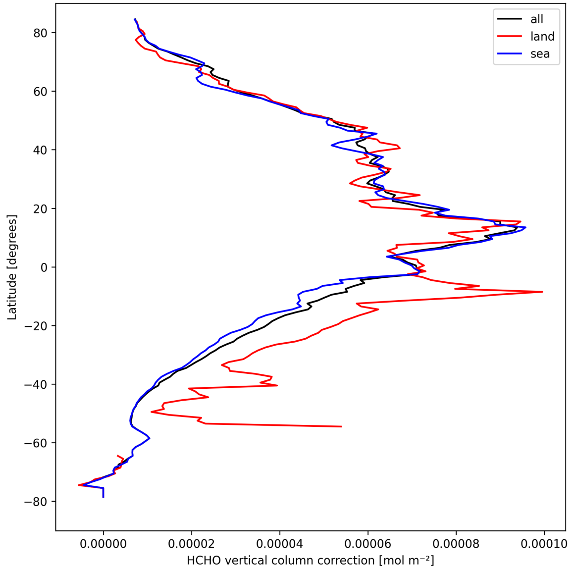
Figure 23: Zonal average of “HCHO vertical column correction” for 2024-09-04 to 2024-09-06.
