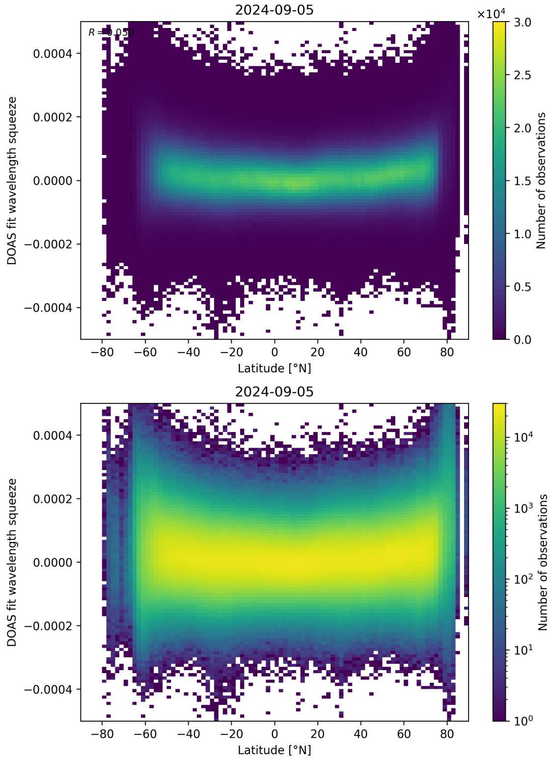
Figure 155: Scatter density plot of “Latitude” against “DOAS fit wavelength squeeze” for 2024-09-04 to 2024-09-06.
