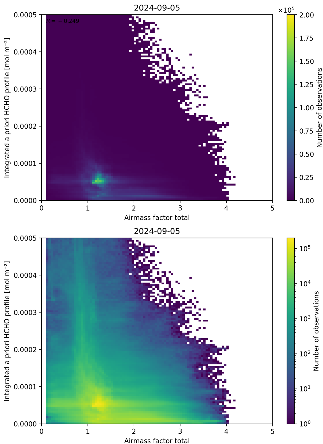
Figure 104: Scatter density plot of “Airmass factor total” against “Integrated a priori HCHO profile” for 2024-09-04 to 2024-09-06.
