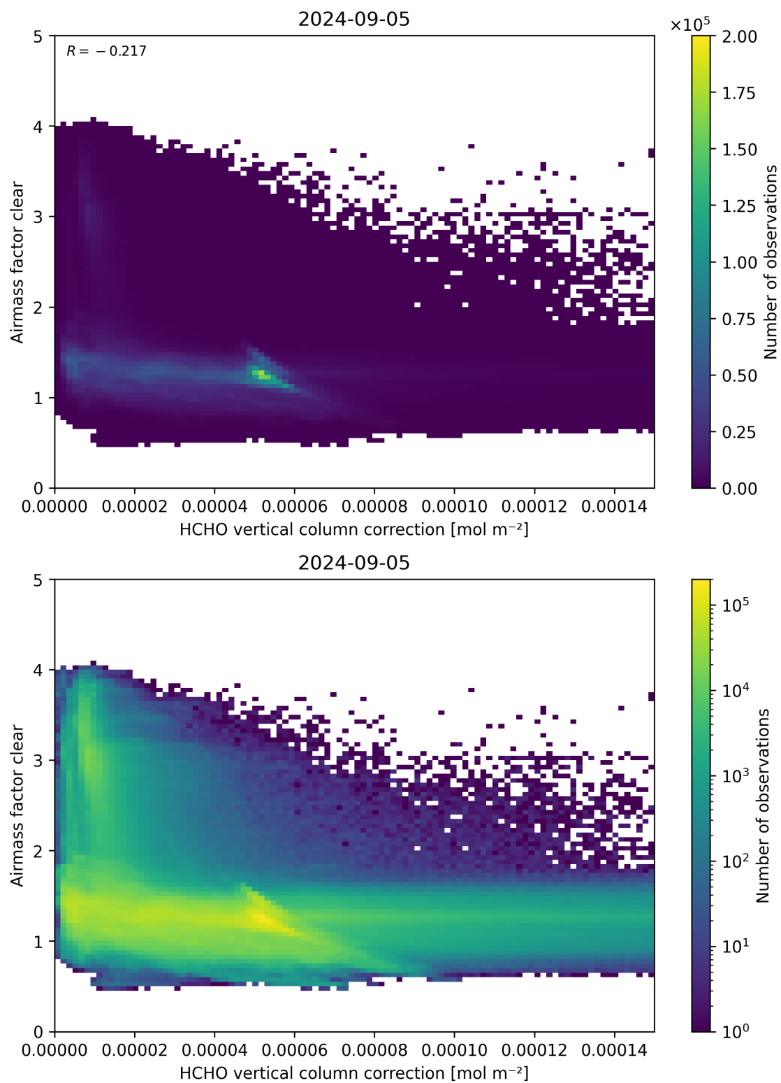
Figure 115: Scatter density plot of “HCHO vertical column correction” against “Airmass factor clear” for 2024-09-04 to 2024-09-06.
