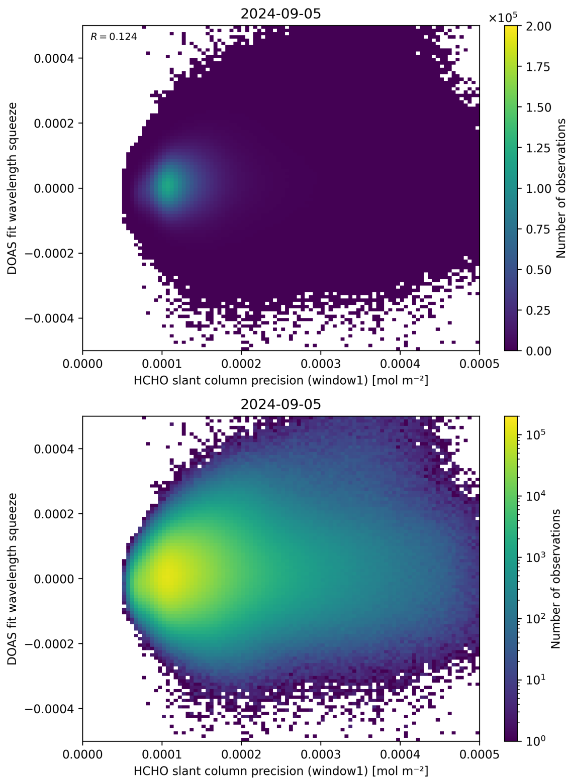
Figure 90: Scatter density plot of “HCHO slant column precision (window1)” against “DOAS fit wavelength squeeze” for 2024-09-04 to 2024-09-06.
