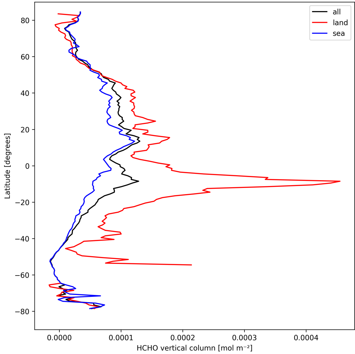
Figure 21: Zonal average of “HCHO vertical column” for 2024-09-04 to 2024-09-06.
