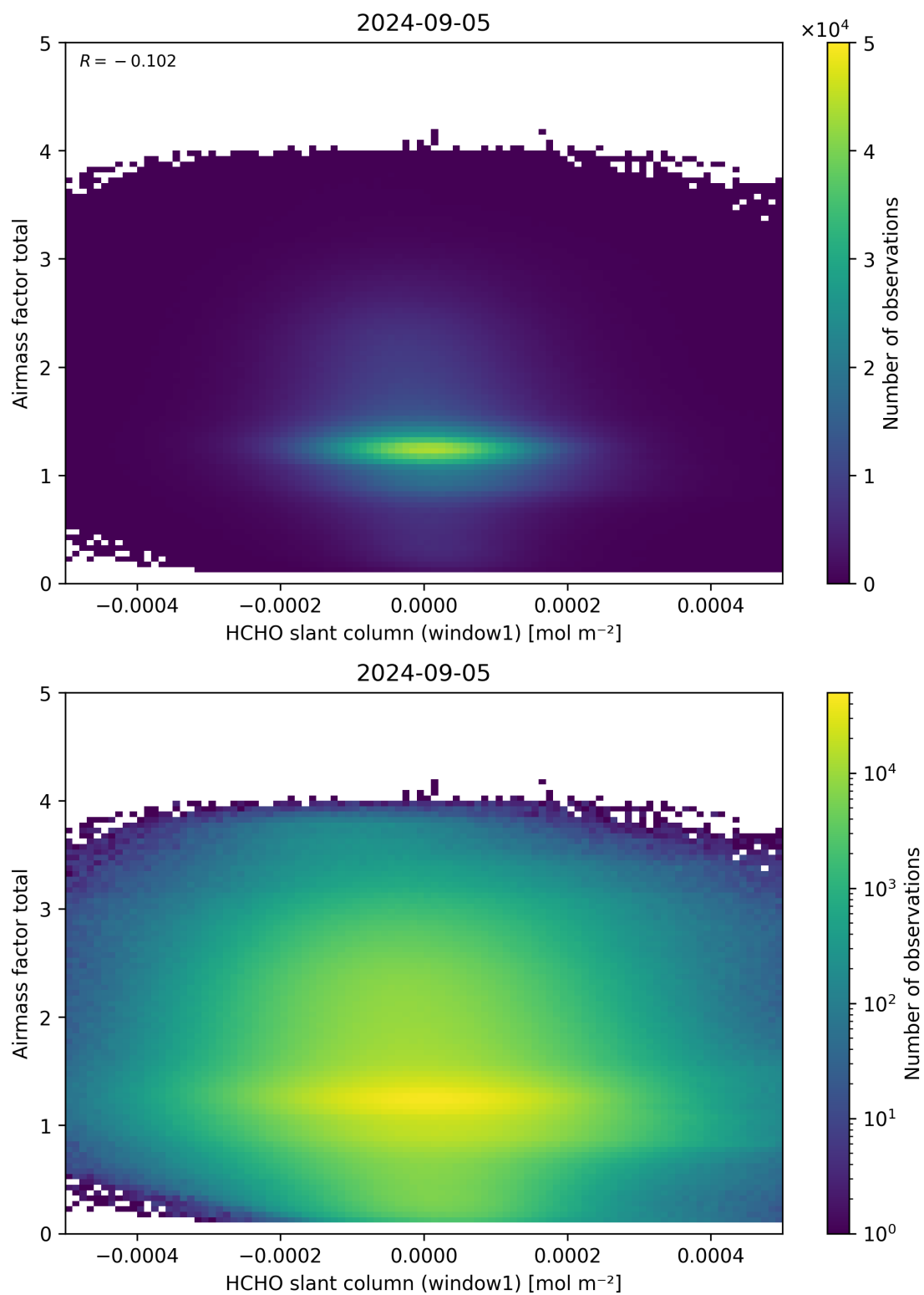
Figure 85: Scatter density plot of “HCHO slant column (window1)” against “Airmass factor total” for 2024-09-04 to 2024-09-06.
