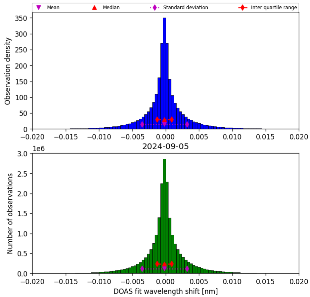
Figure 44: Histogram of “DOAS fit wavelength shift” for 2024-09-04 to 2024-09-06
