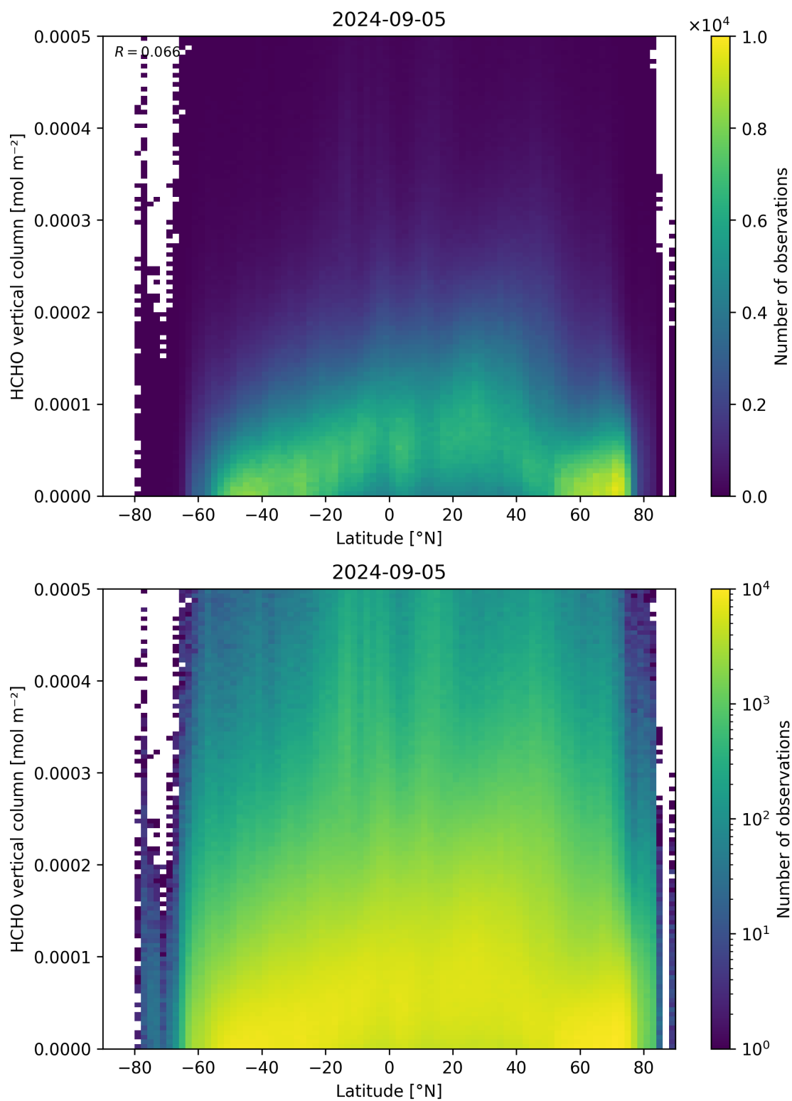
Figure 163: Scatter density plot of “Latitude” against “HCHO vertical column” for 2024-09-04 to 2024-09-06.
