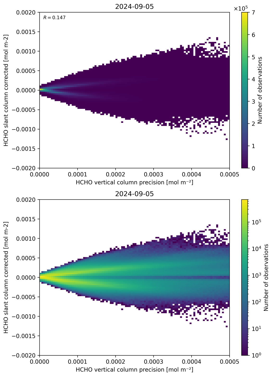
Figure 140: Scatter density plot of “HCHO vertical column precision” against “HCHO slant column corrected” for 2024-09-04 to 2024-09-06.
