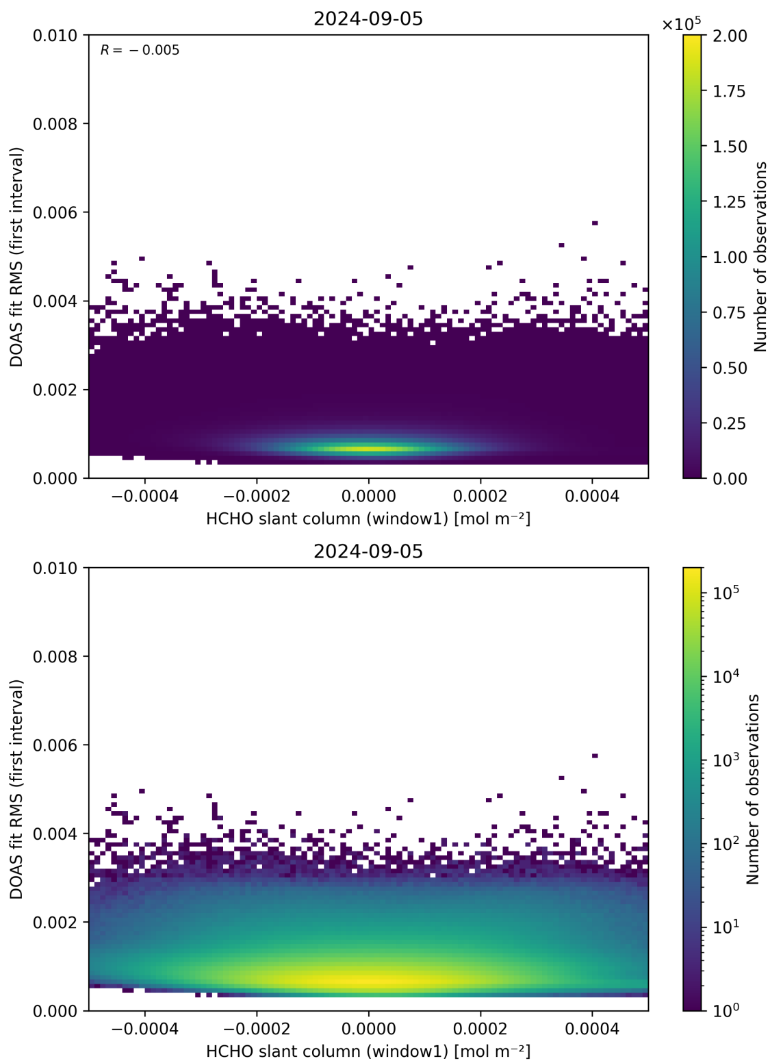
Figure 78: Scatter density plot of “HCHO slant column (window1)” against “DOAS fit RMS (first interval)” for 2024-09-04 to 2024-09-06.
