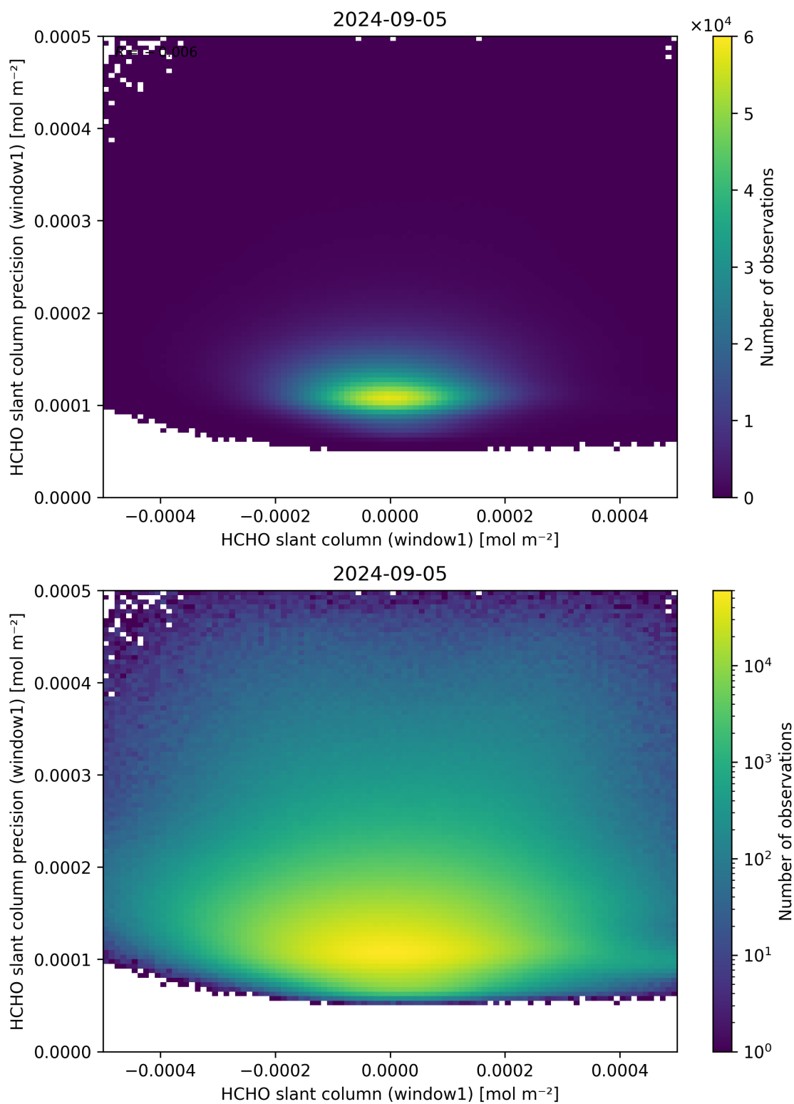
Figure 84: Scatter density plot of “HCHO slant column (window1)” against “HCHO slant column precision (window1)” for 2024-09-04 to 2024-09-06.
