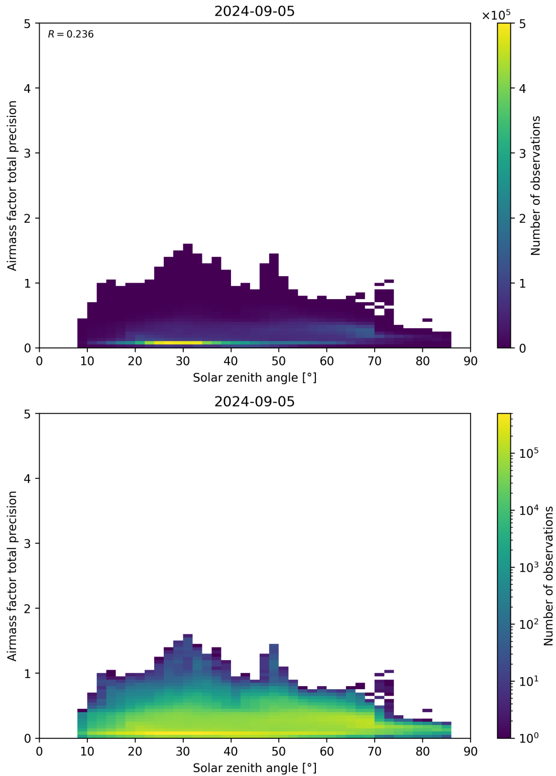
Figure 176: Scatter density plot of “Solar zenith angle” against “Airmass factor total precision” for 2024-09-04 to 2024-09-06.
