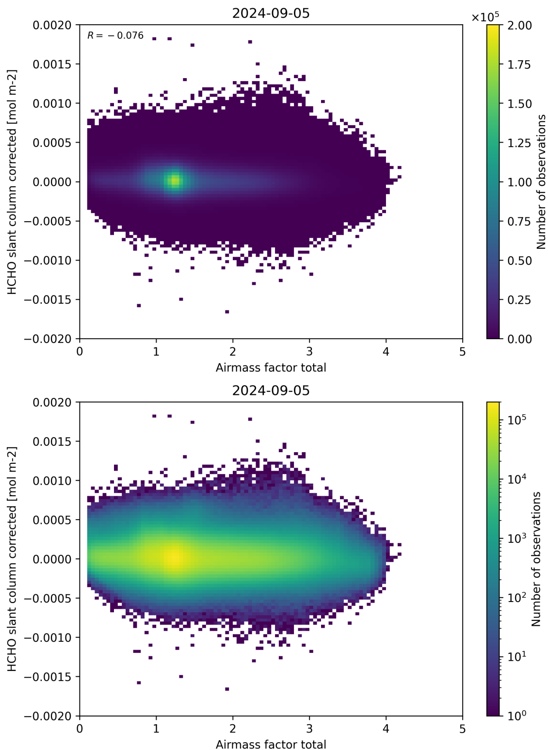
Figure 101: Scatter density plot of “Airmass factor total” against “HCHO slant column corrected” for 2024-09-04 to 2024-09-06.
