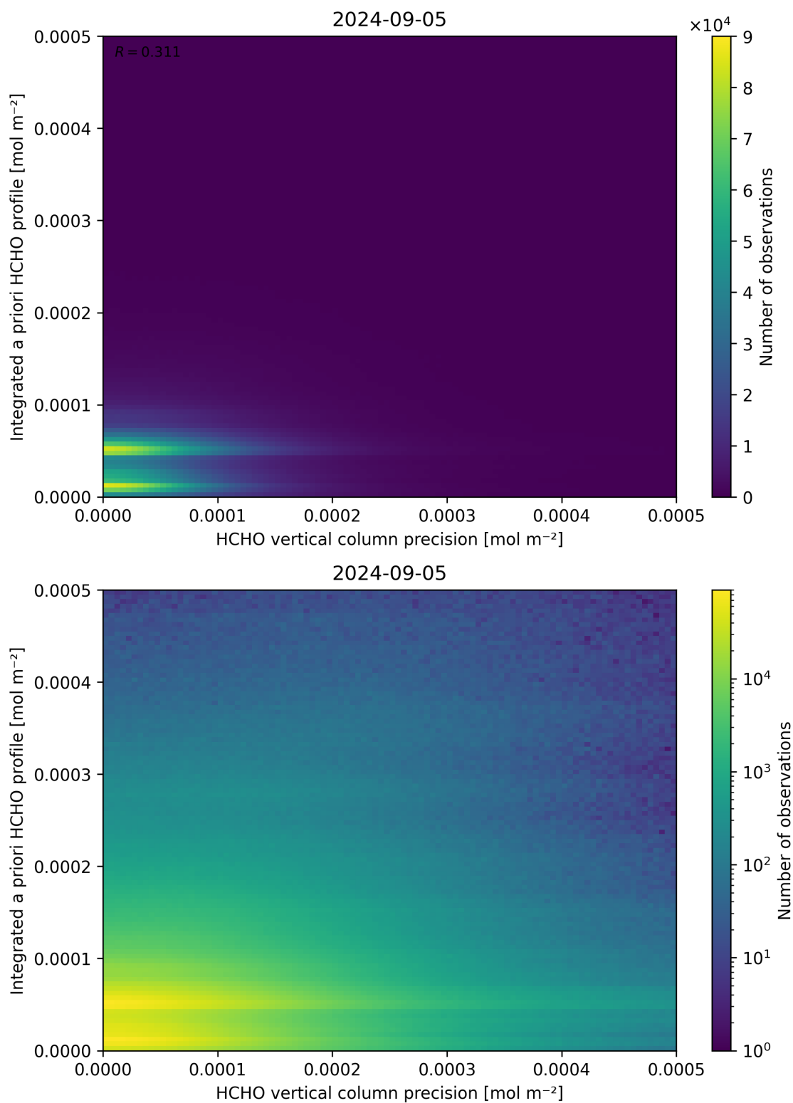
Figure 147: Scatter density plot of “HCHO vertical column precision” against “Integrated a priori HCHO profile” for 2024-09-04 to 2024-09-06.
