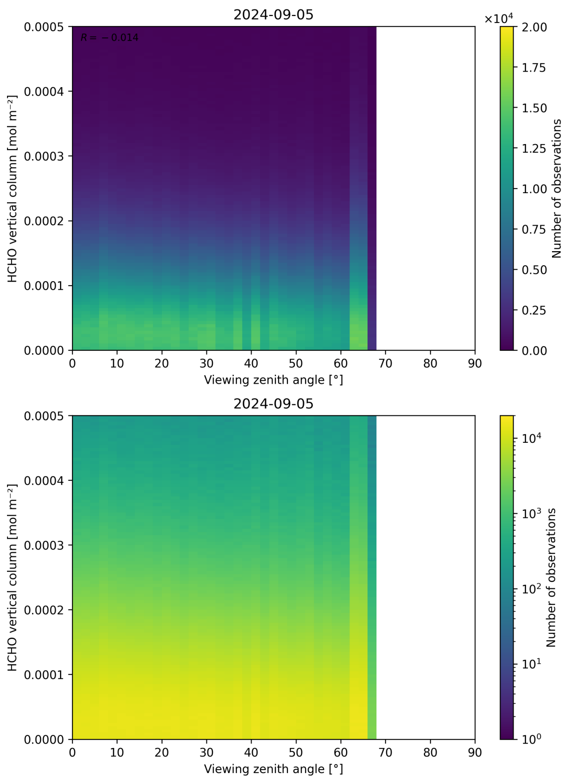
Figure 192: Scatter density plot of “Viewing zenith angle” against “HCHO vertical column” for 2024-09-04 to 2024-09-06.
