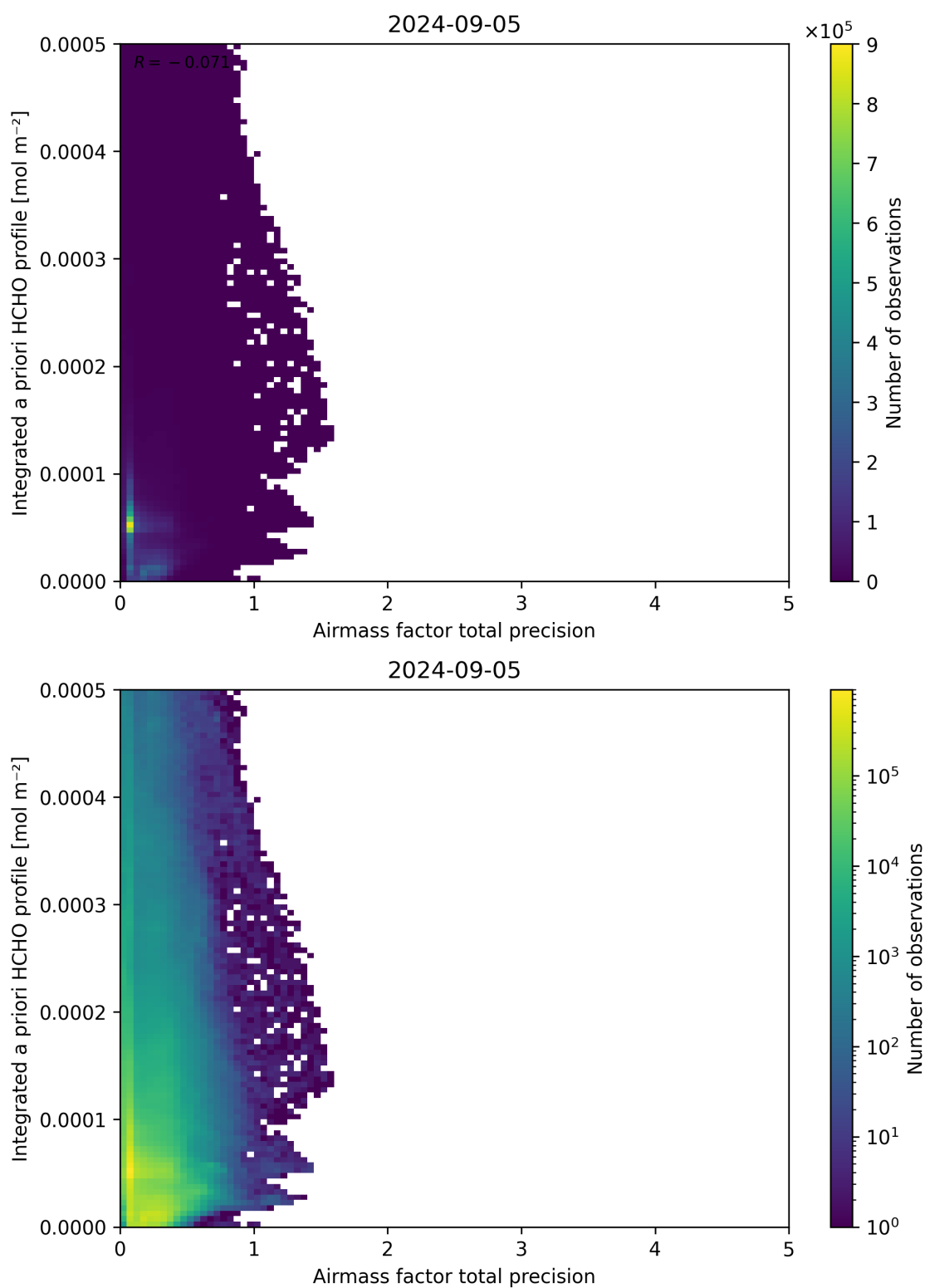
Figure 111: Scatter density plot of “Airmass factor total precision” against “Integrated a priori HCHO profile” for 2024-09-04 to 2024-09-06.
