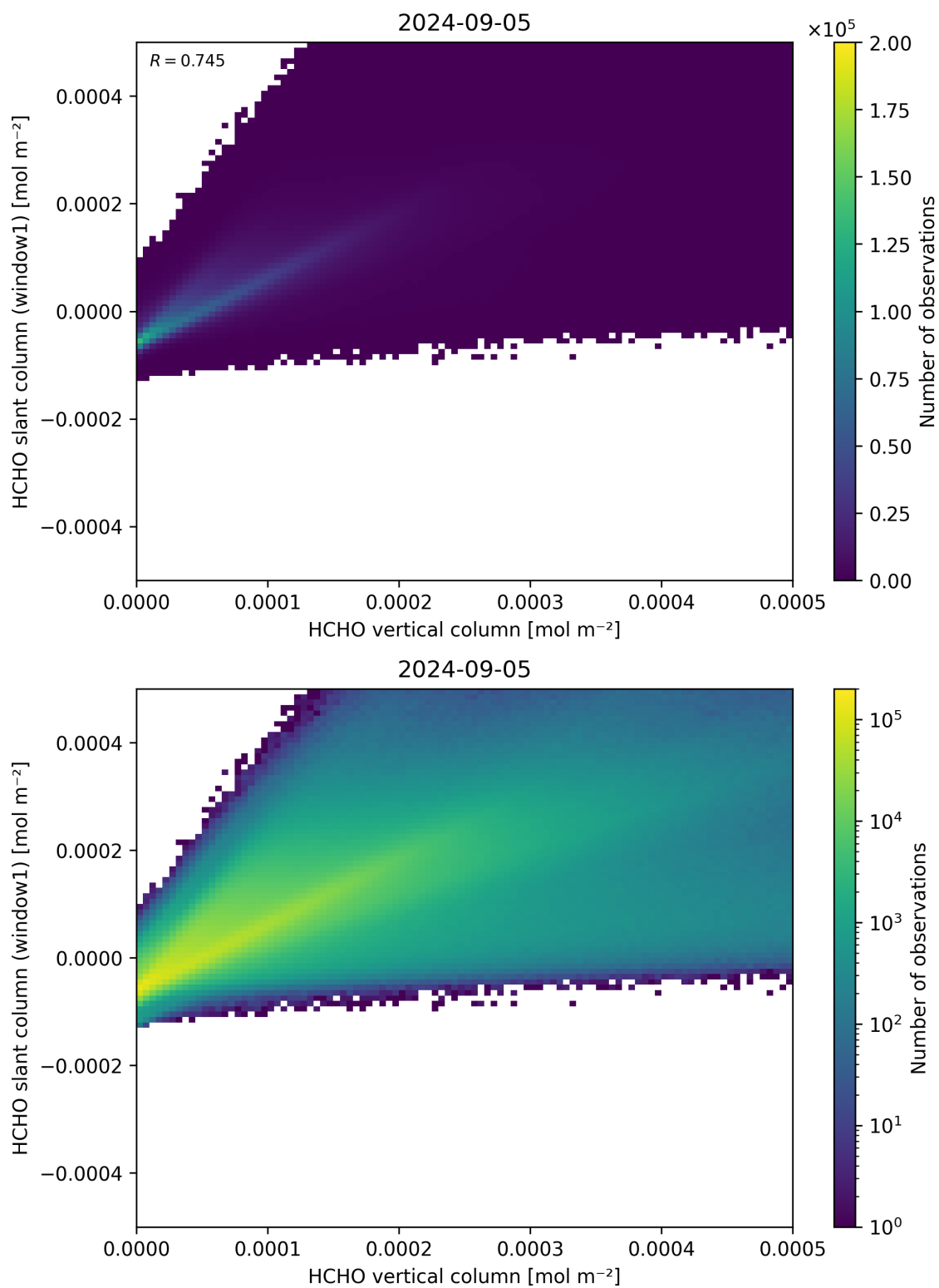
Figure 129: Scatter density plot of “HCHO vertical column” against “HCHO slant column (window1)” for 2024-09-04 to 2024-09-06.
