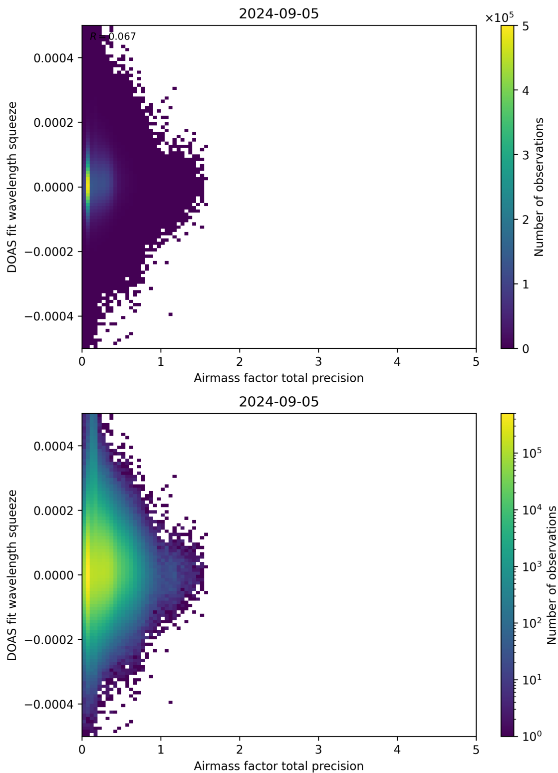
Figure 107: Scatter density plot of “Airmass factor total precision” against “DOAS fit wavelength squeeze” for 2024-09-04 to 2024-09-06.
