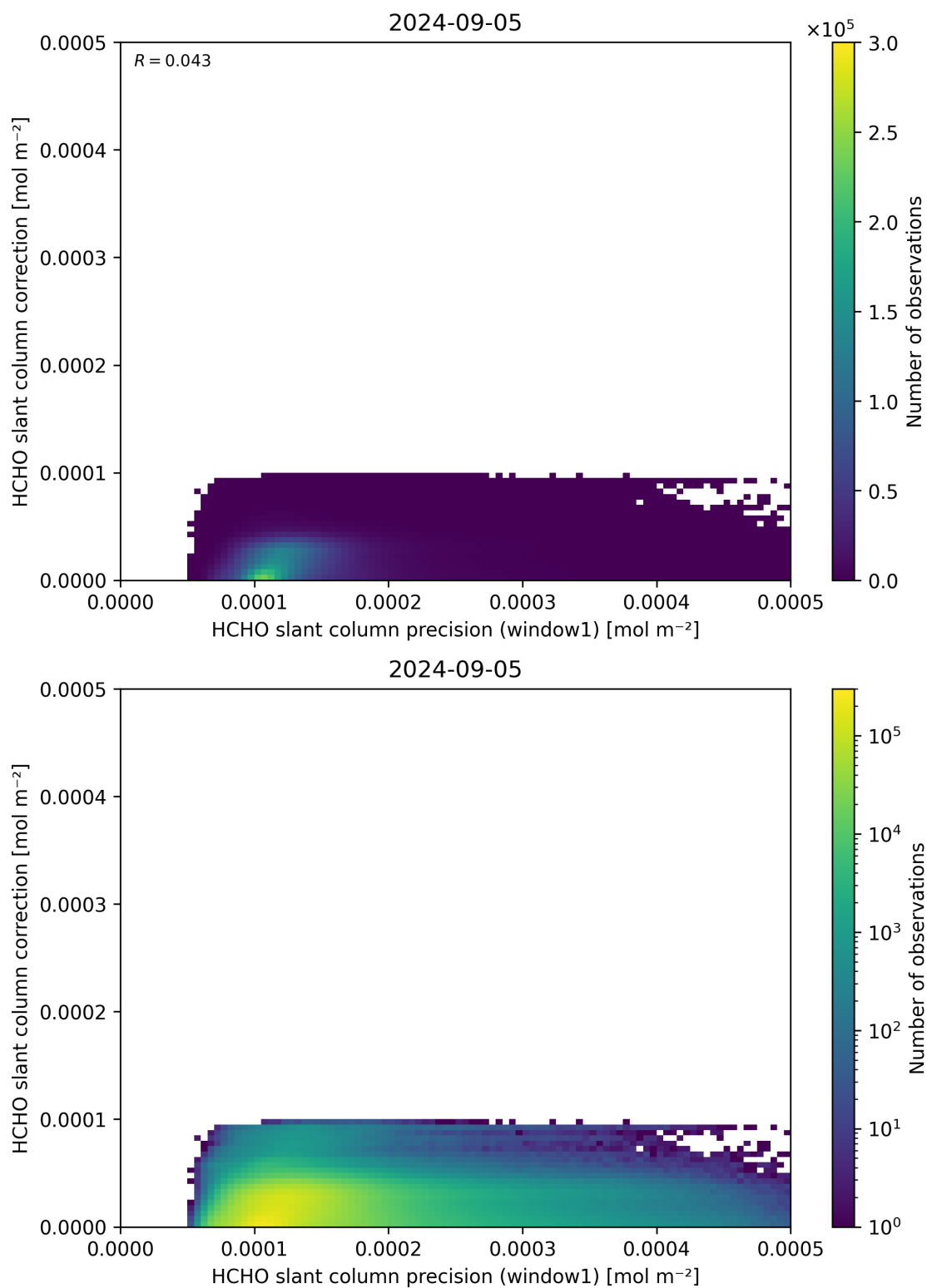
Figure 93: Scatter density plot of “HCHO slant column precision (window1)” against “HCHO slant column correction” for 2024-09-04 to 2024-09-06.
