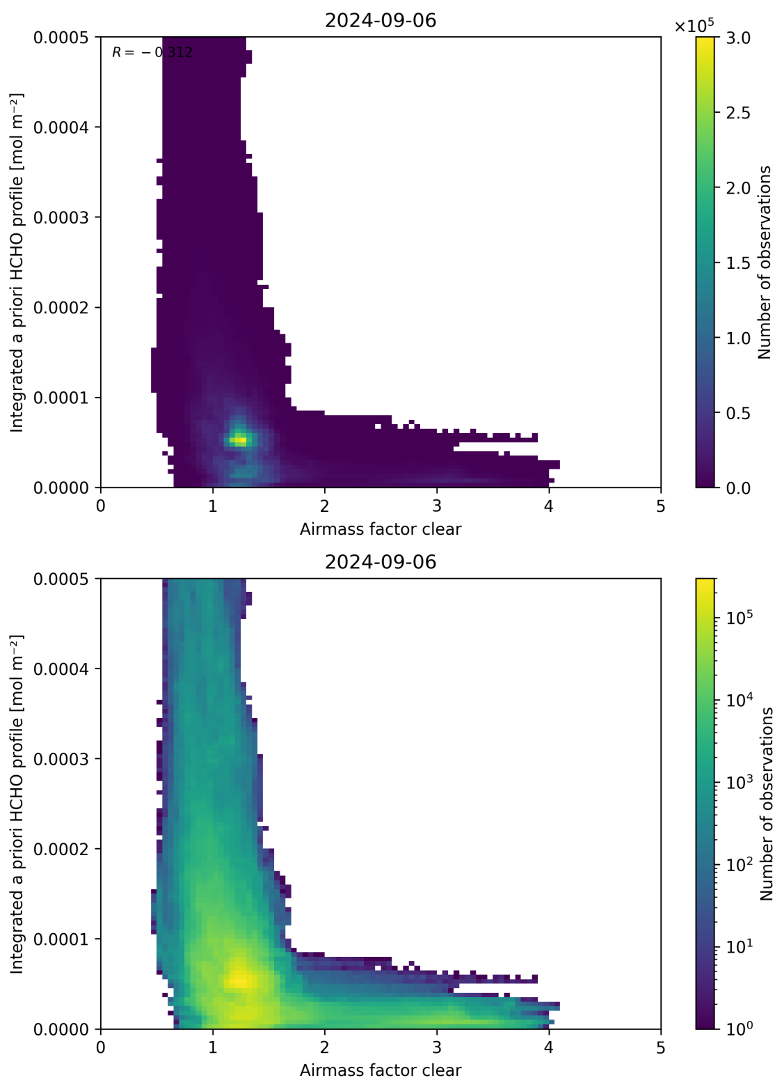
Figure 76: Scatter density plot of “Airmass factor clear” against “Integrated a priori HCHO profile” for 2024-09-06 to 2024-09-07.
