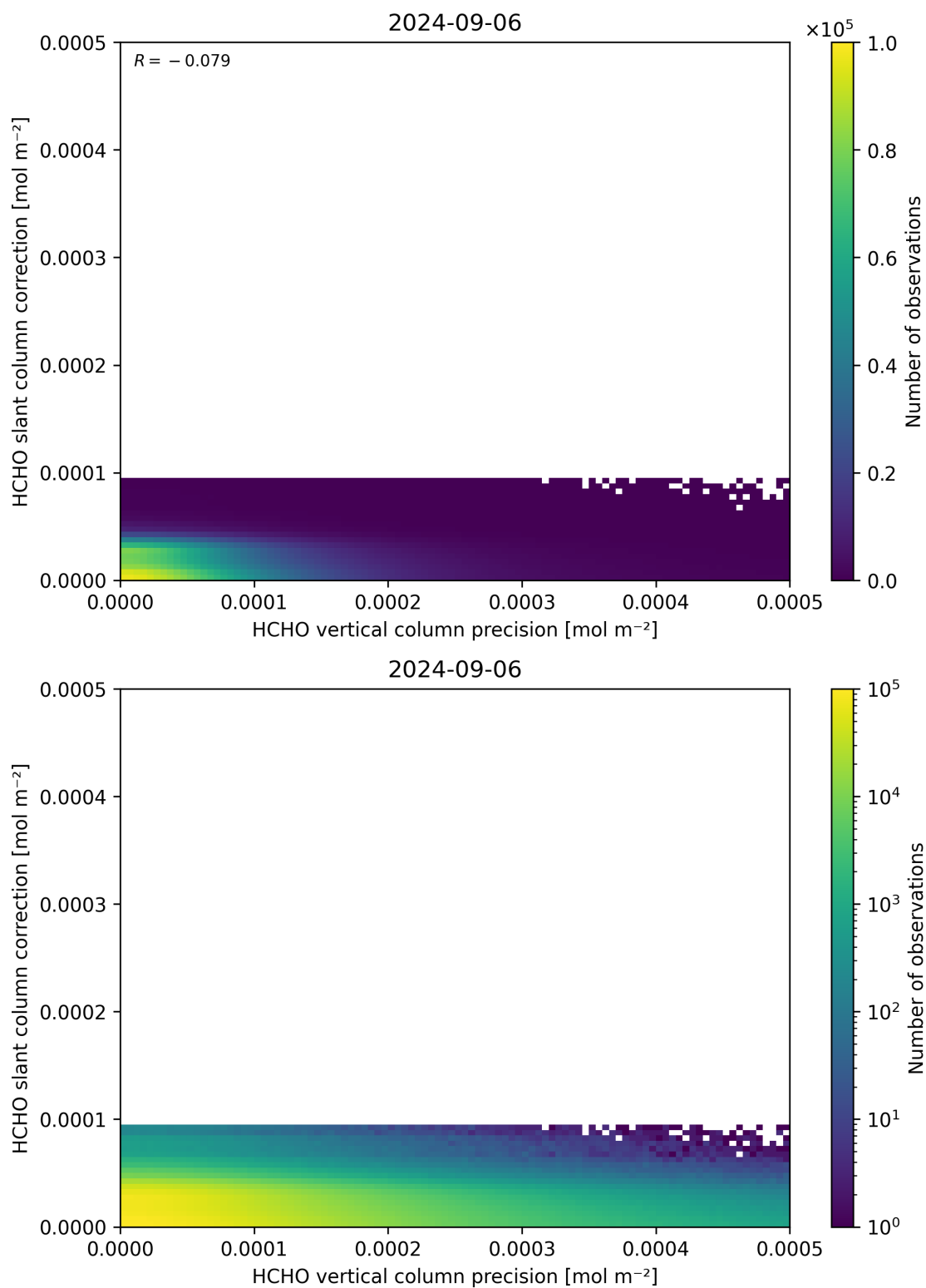
Figure 141: Scatter density plot of “HCHO vertical column precision” against “HCHO slant column correction” for 2024-09-06 to 2024-09-07.
