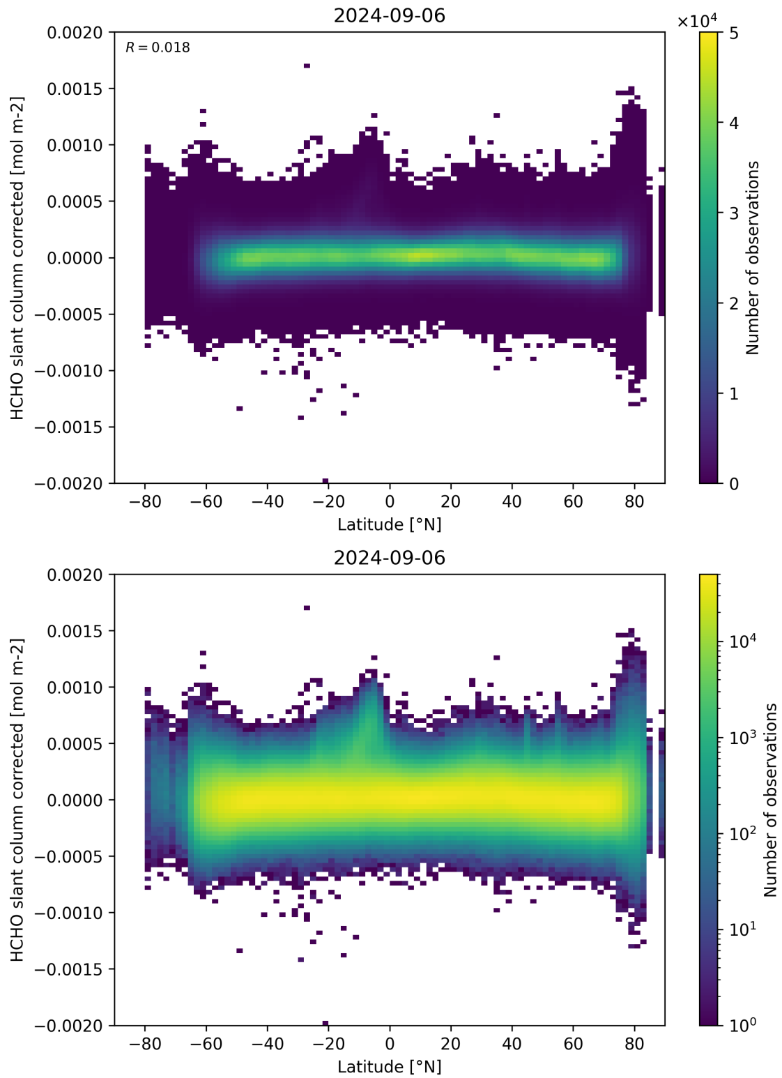
Figure 157: Scatter density plot of “Latitude” against “HCHO slant column corrected” for 2024-09-06 to 2024-09-07.
