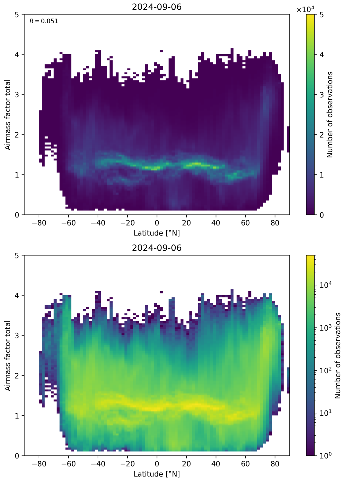
Figure 161: Scatter density plot of “Latitude” against “Airmass factor total” for 2024-09-06 to 2024-09-07.
