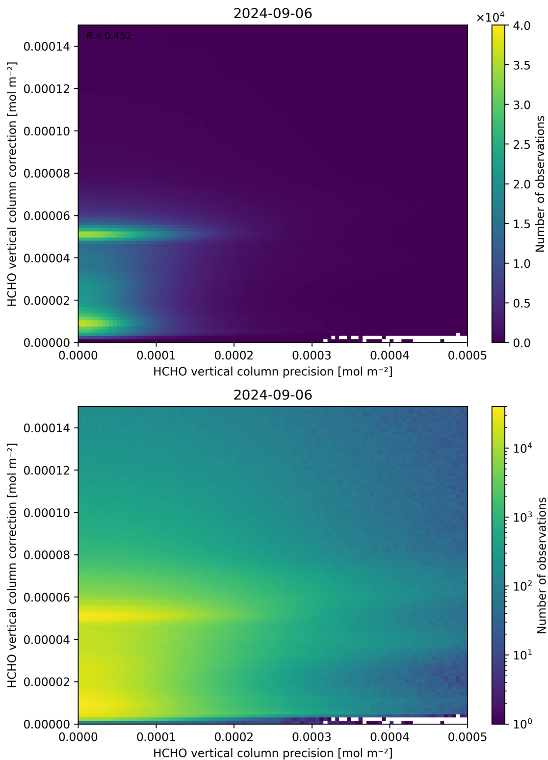
Figure 146: Scatter density plot of “HCHO vertical column precision” against “HCHO vertical column correction” for 2024-09-06 to 2024-09-07.
