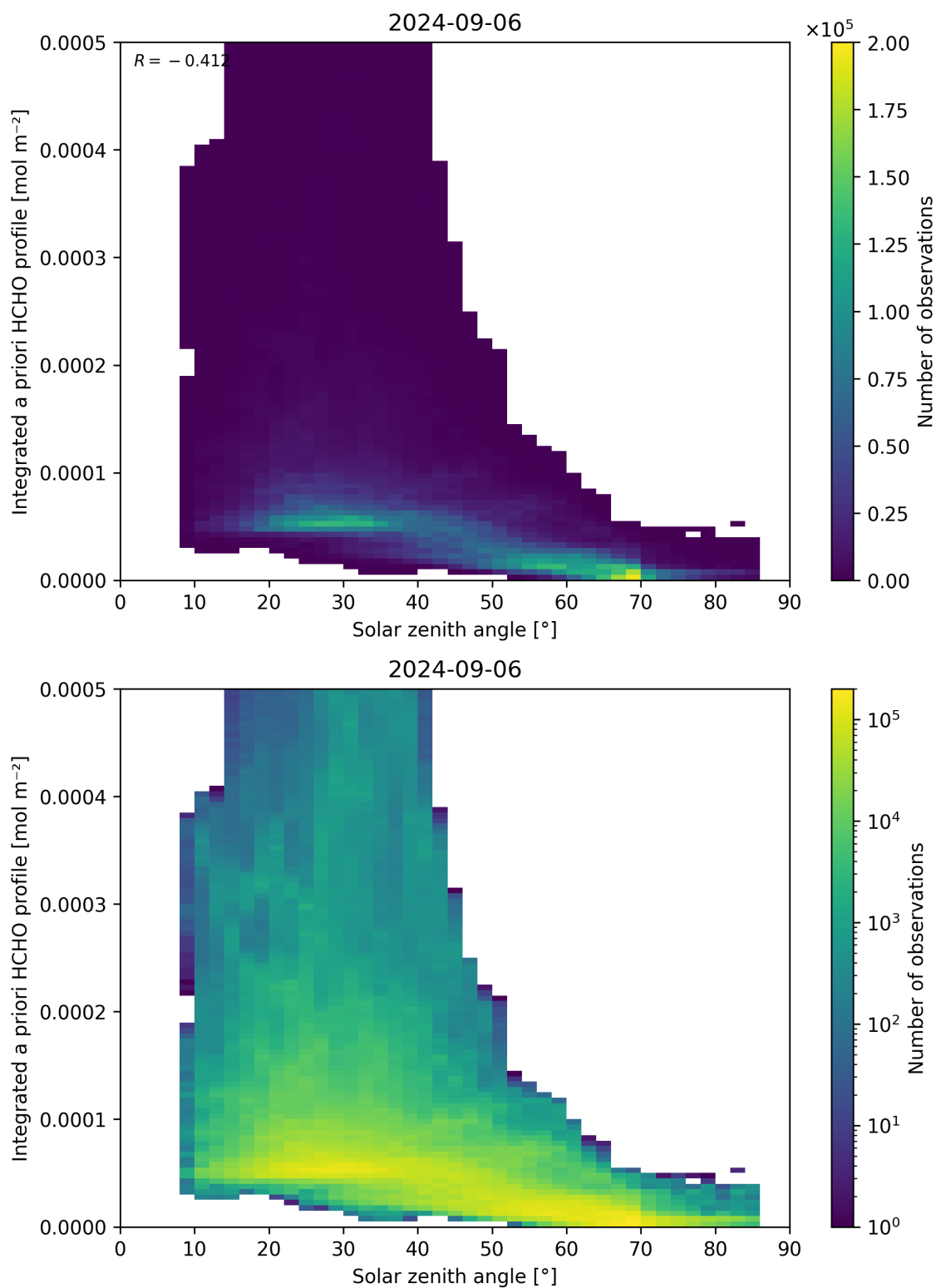
Figure 180: Scatter density plot of “Solar zenith angle” against “Integrated a priori HCHO profile” for 2024-09-06 to 2024-09-07.
