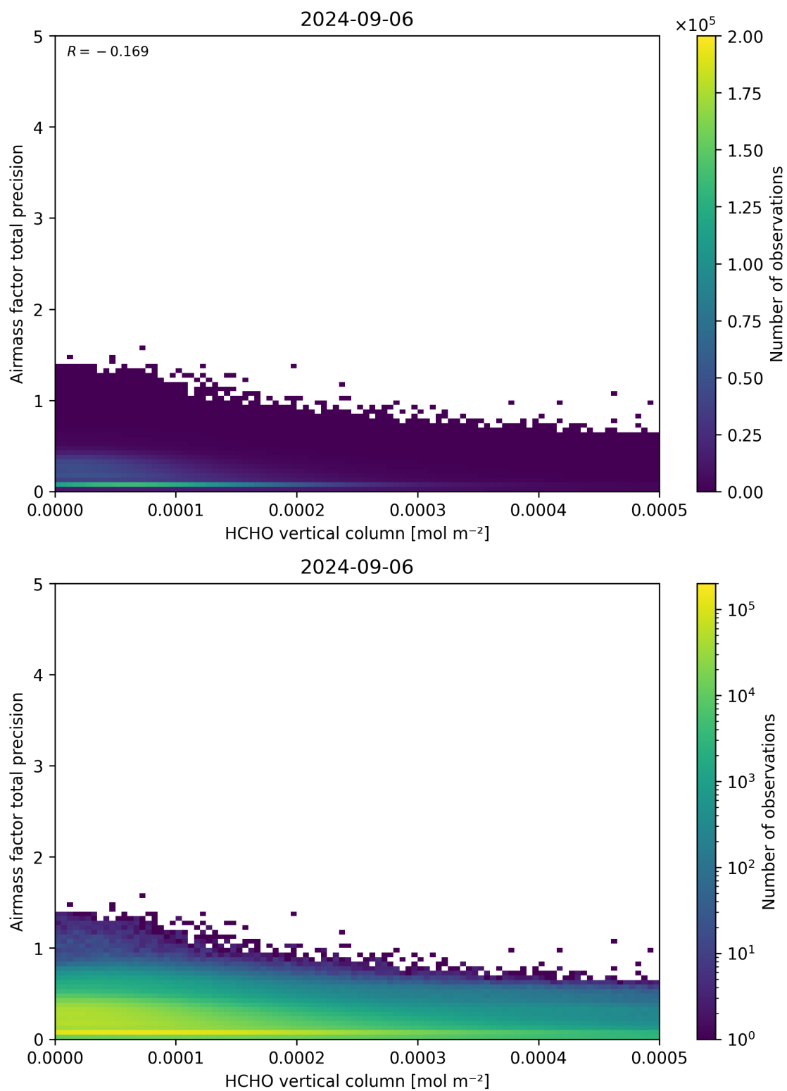
Figure 132: Scatter density plot of “HCHO vertical column” against “Airmass factor total precision” for 2024-09-06 to 2024-09-07.
