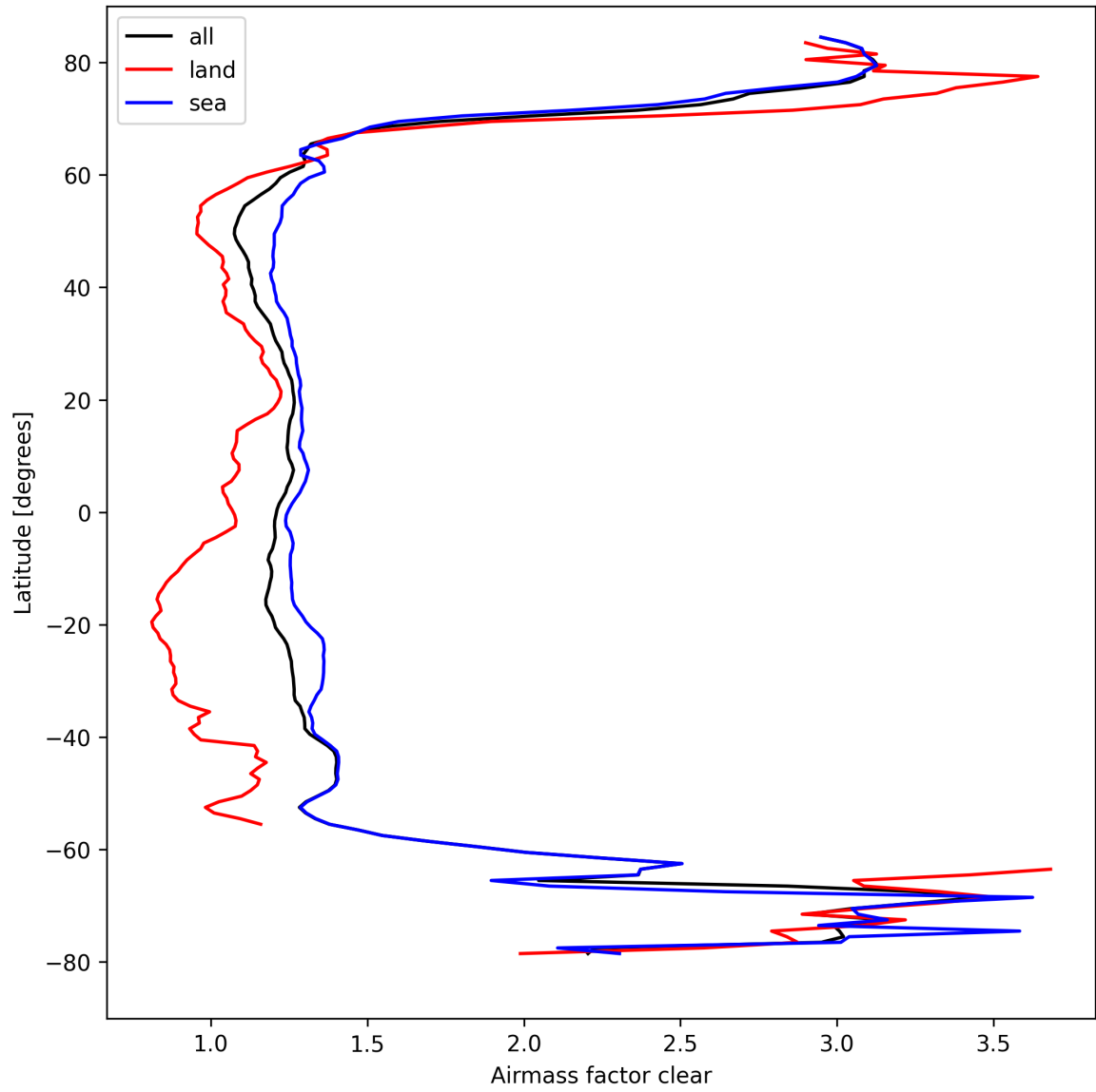
Figure 28: Zonal average of “Airmass factor clear” for 2024-09-06 to 2024-09-07.
