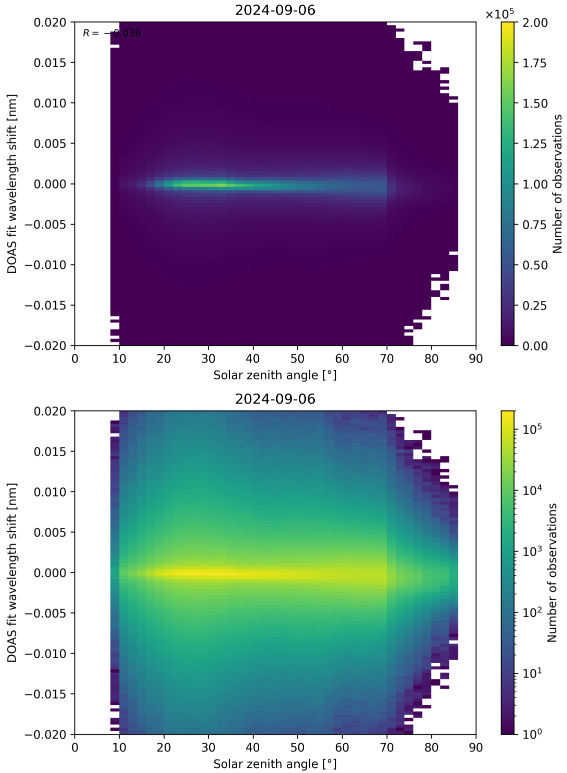
Figure 168: Scatter density plot of “Solar zenith angle” against “DOAS fit wavelength shift” for 2024-09-06 to 2024-09-07.
