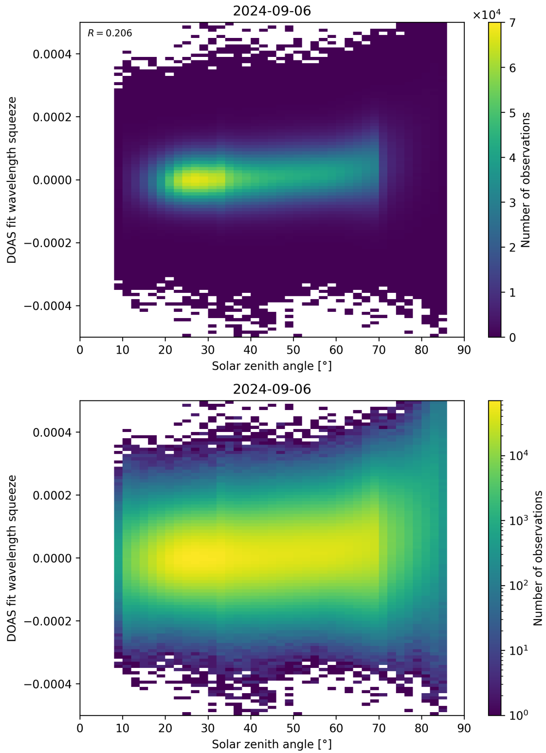
Figure 169: Scatter density plot of “Solar zenith angle” against “DOAS fit wavelength squeeze” for 2024-09-06 to 2024-09-07.
