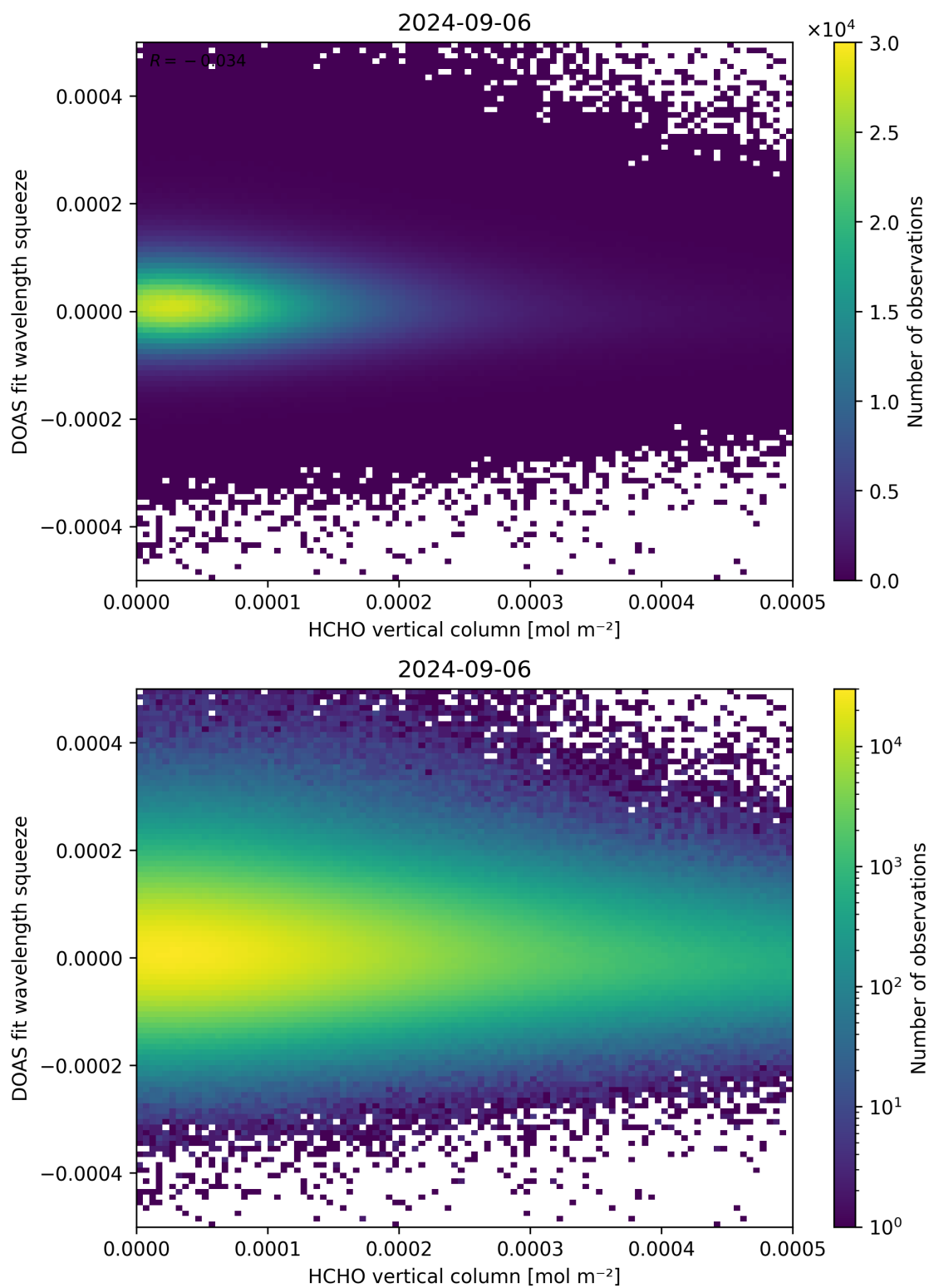
Figure 125: Scatter density plot of “HCHO vertical column” against “DOAS fit wavelength squeeze” for 2024-09-06 to 2024-09-07.
