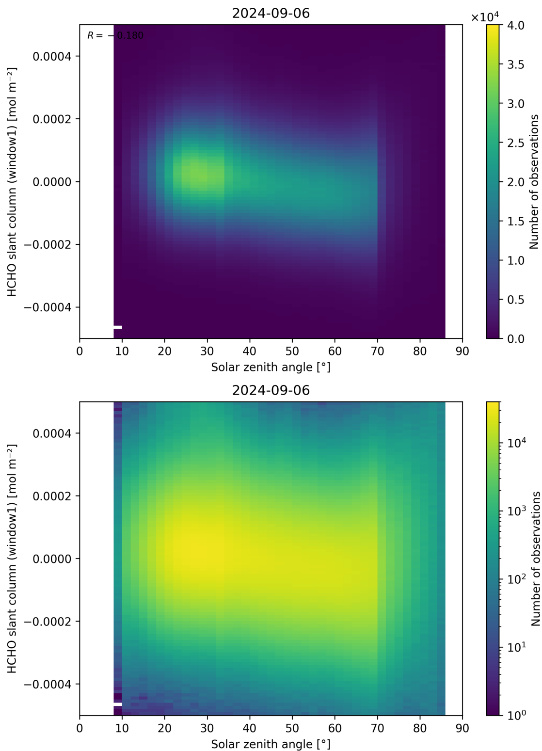
Figure 173: Scatter density plot of “Solar zenith angle” against “HCHO slant column (window1)” for 2024-09-06 to 2024-09-07.
