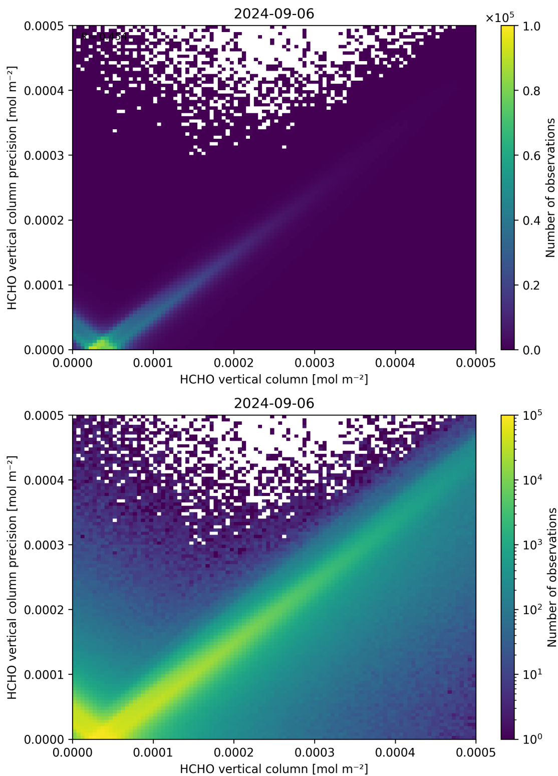
Figure 134: Scatter density plot of “HCHO vertical column” against “HCHO vertical column precision” for 2024-09-06 to 2024-09-07.
