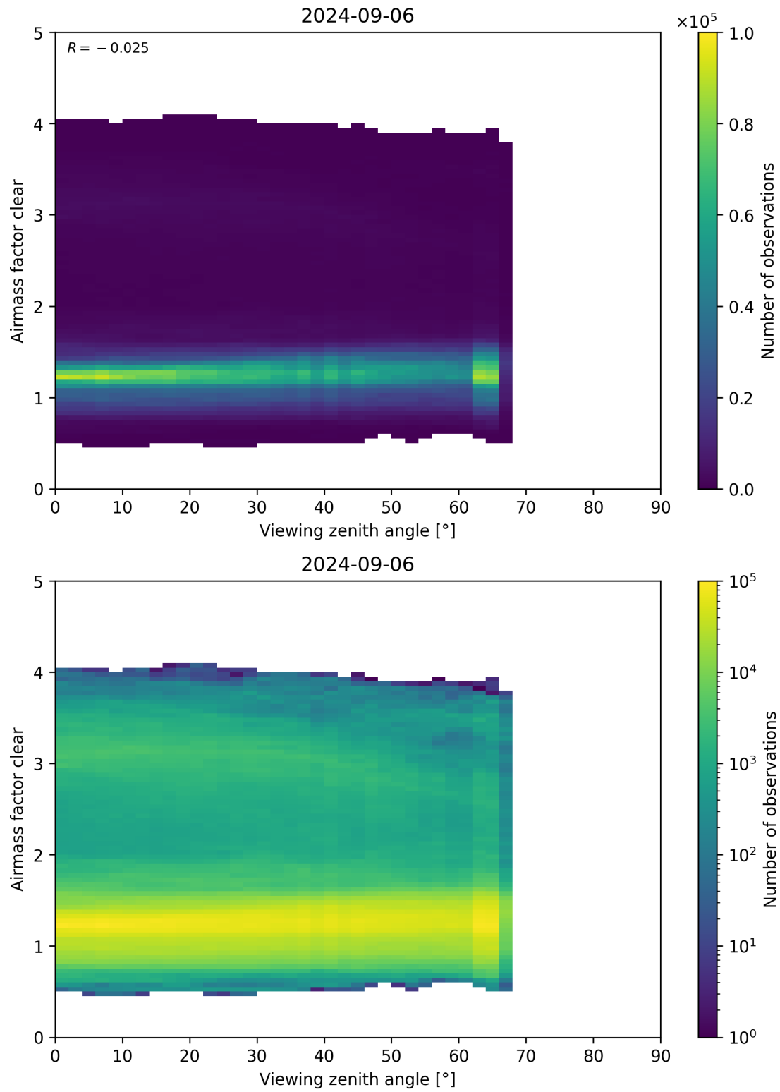
Figure 185: Scatter density plot of “Viewing zenith angle” against “Airmass factor clear” for 2024-09-06 to 2024-09-07.
