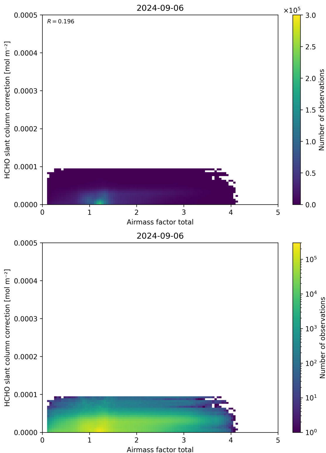
Figure 102: Scatter density plot of “Airmass factor total” against “HCHO slant column correction” for 2024-09-06 to 2024-09-07.
