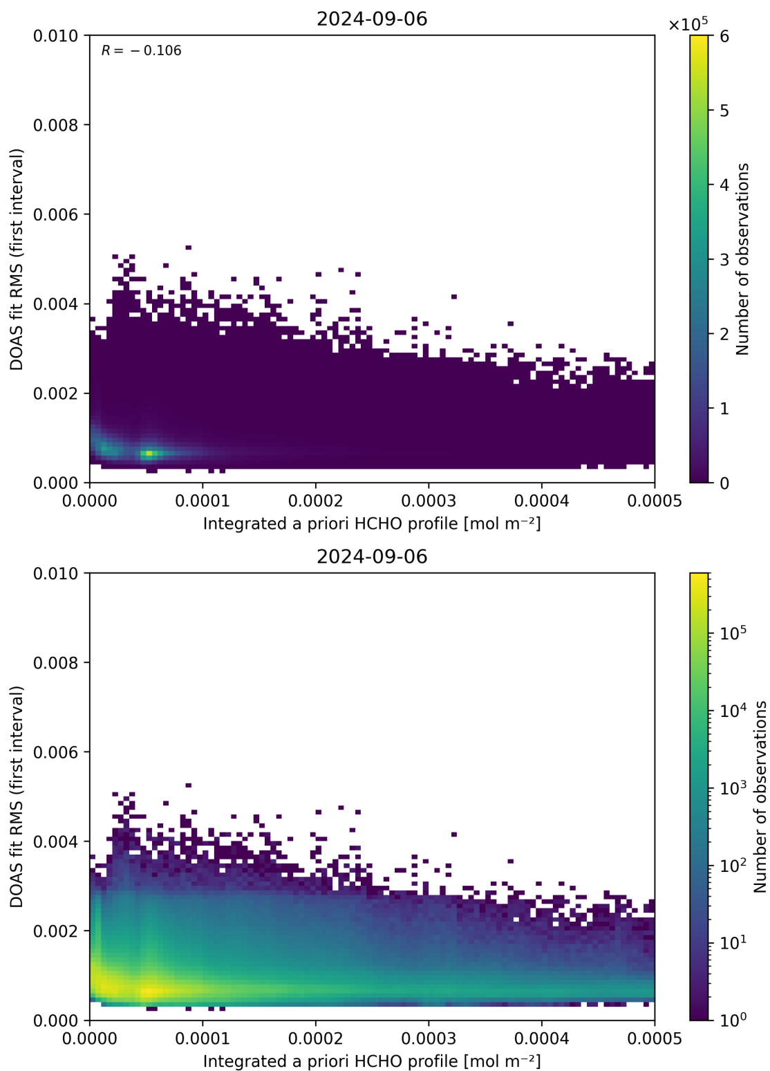
Figure 148: Scatter density plot of “Integrated a priori HCHO profile” against “DOAS fit RMS (first interval)” for 2024-09-06 to 2024-09-07.
