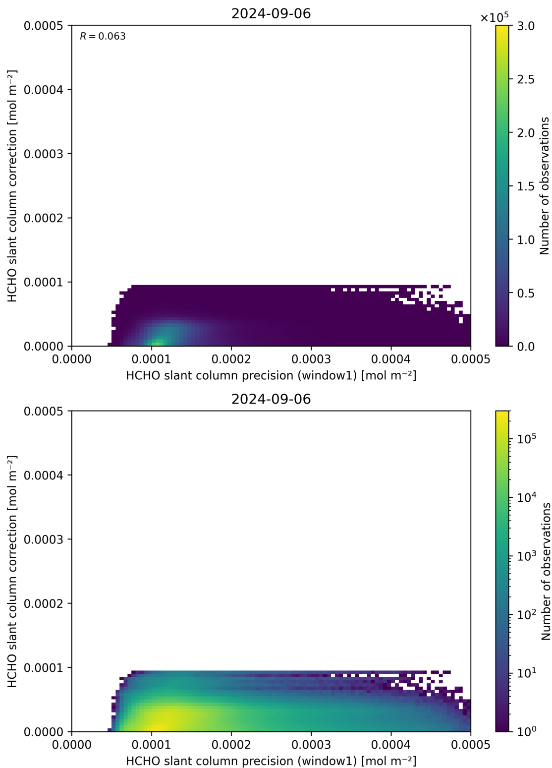
Figure 93: Scatter density plot of “HCHO slant column precision (window1)” against “HCHO slant column correction” for 2024-09-06 to 2024-09-07.
