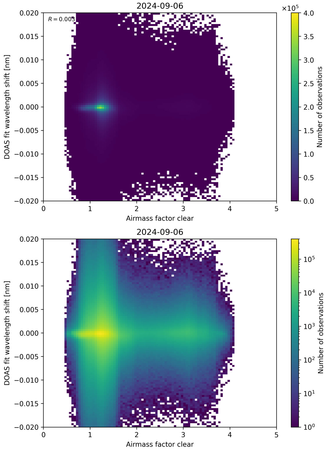
Figure 72: Scatter density plot of “Airmass factor clear” against “DOAS fit wavelength shift” for 2024-09-06 to 2024-09-07.
