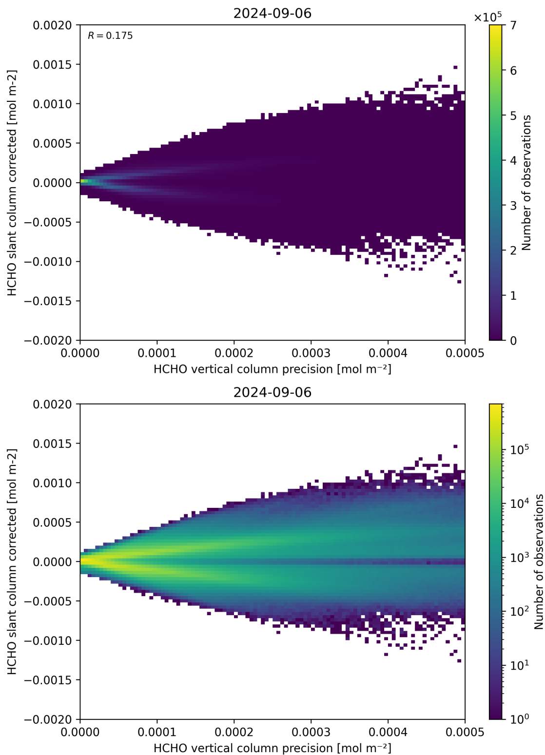
Figure 140: Scatter density plot of “HCHO vertical column precision” against “HCHO slant column corrected” for 2024-09-06 to 2024-09-07.
