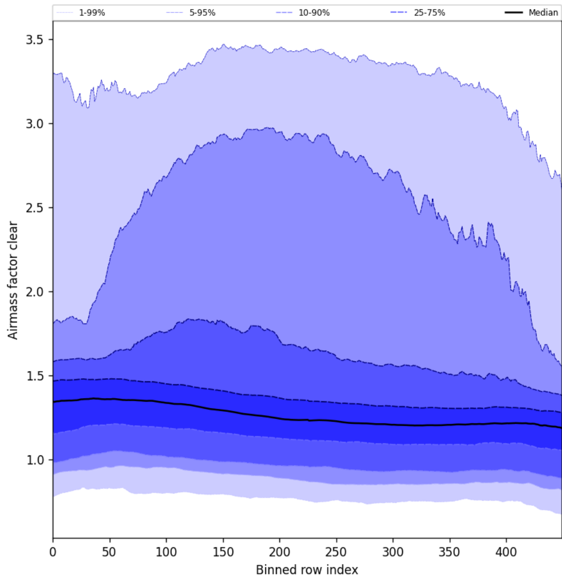
Figure 56: Along track statistics of “Airmass factor clear” for 2024-09-06 to 2024-09-07
