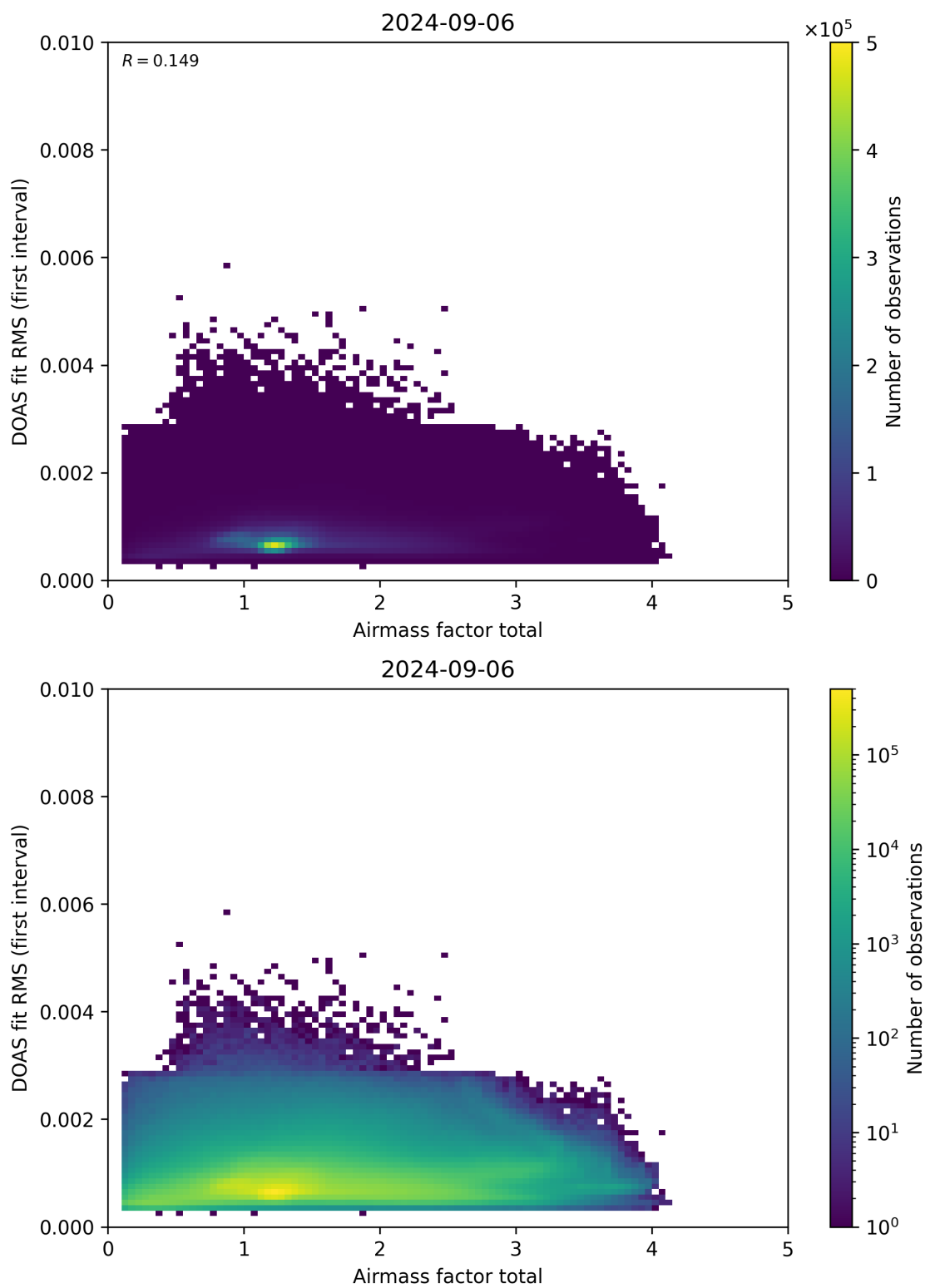
Figure 97: Scatter density plot of “Airmass factor total” against “DOAS fit RMS (first interval)” for 2024-09-06 to 2024-09-07.
