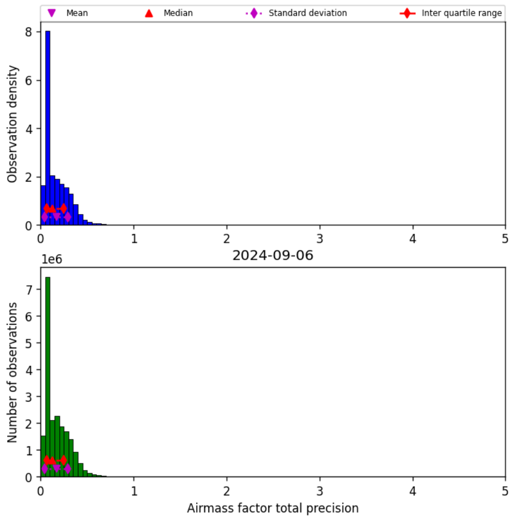
Figure 41: Histogram of “Airmass factor total precision” for 2024-09-06 to 2024-09-07
