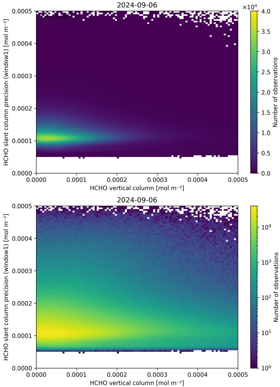
Figure 130: Scatter density plot of “HCHO vertical column” against “HCHO slant column precision (window1)” for 2024-09-06 to 2024-09-07.
