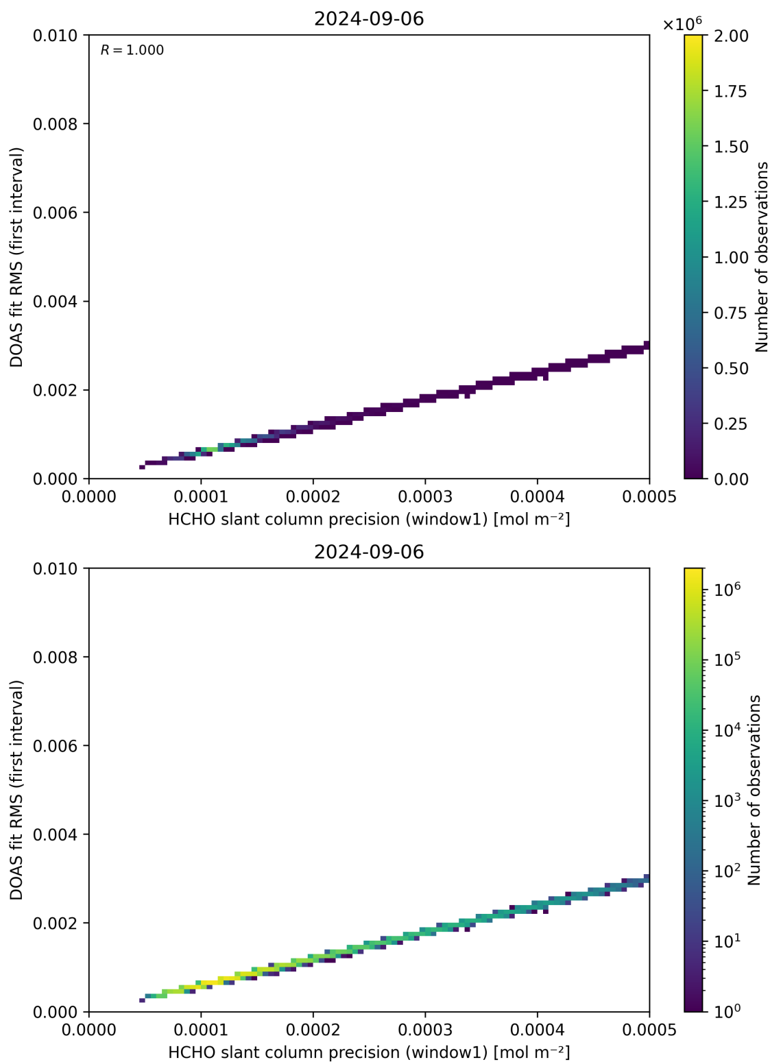
Figure 88: Scatter density plot of “HCHO slant column precision (window1)” against “DOAS fit RMS (first interval)” for 2024-09-06 to 2024-09-07.
