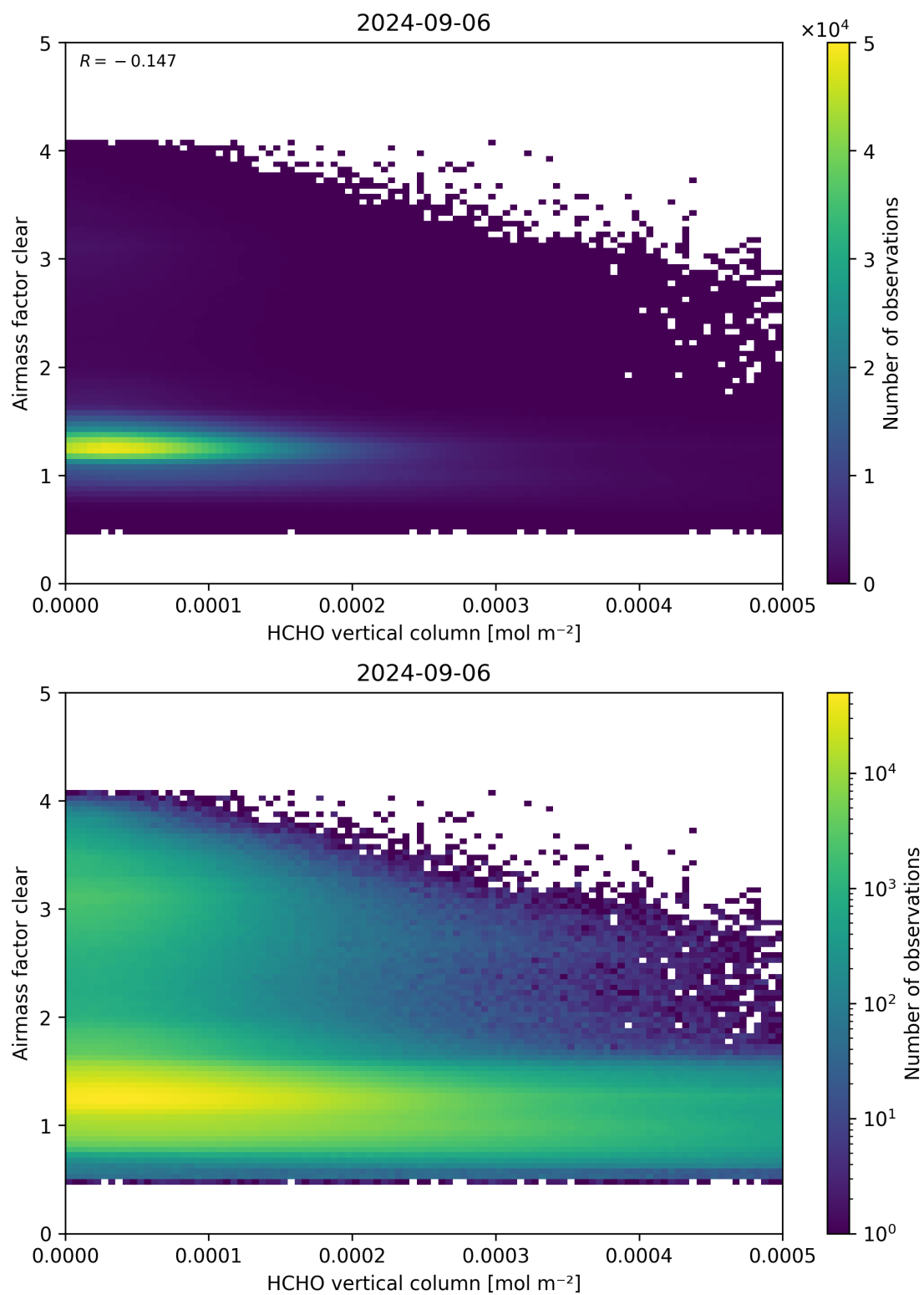
Figure 126: Scatter density plot of “HCHO vertical column” against “Airmass factor clear” for 2024-09-06 to 2024-09-07.
