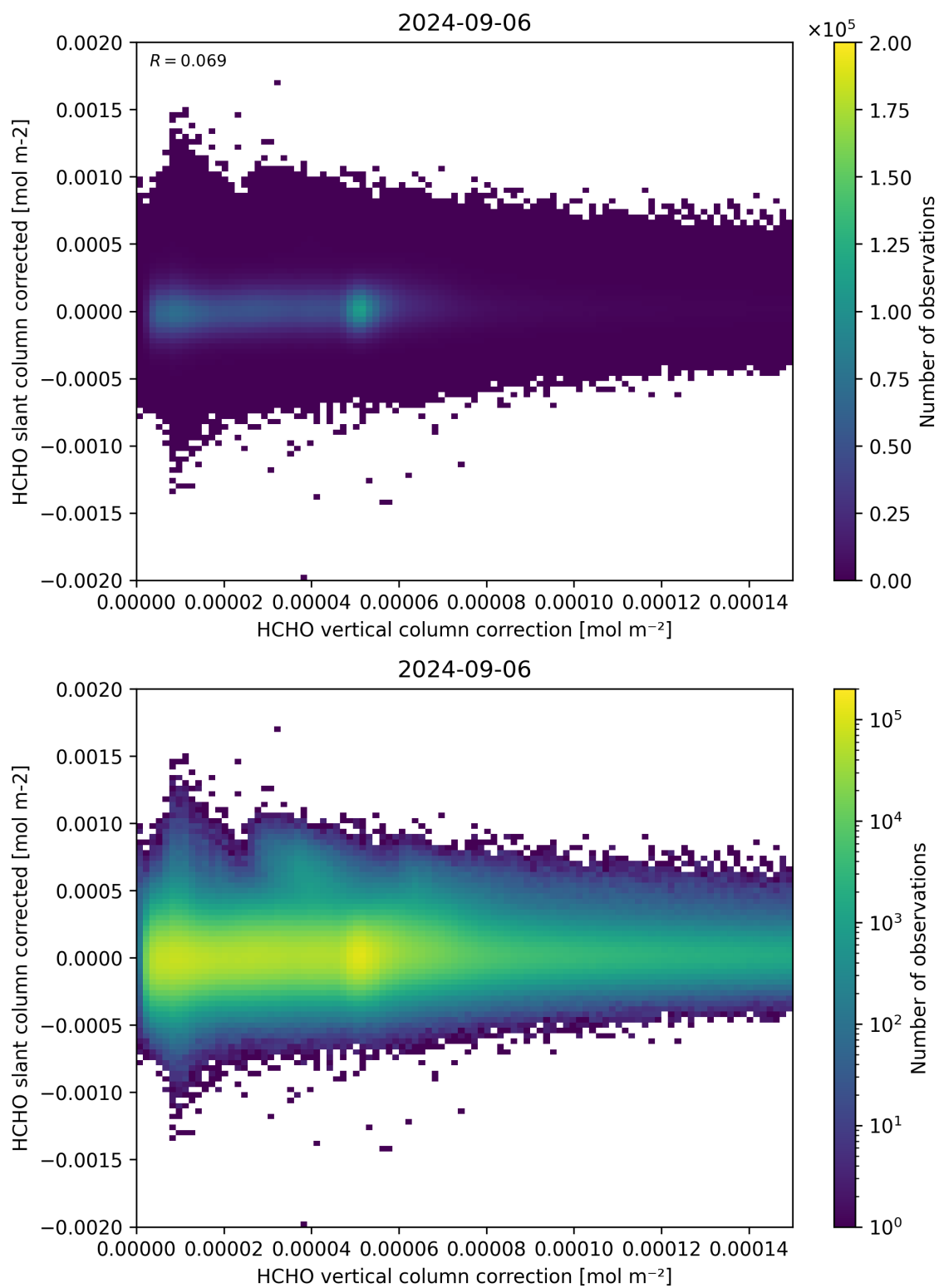
Figure 116: Scatter density plot of “HCHO vertical column correction” against “HCHO slant column corrected” for 2024-09-06 to 2024-09-07.
