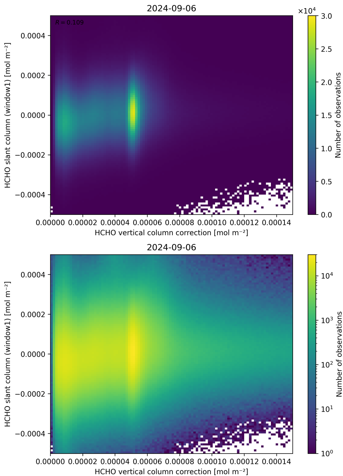
Figure 118: Scatter density plot of “HCHO vertical column correction” against “HCHO slant column (window1)” for 2024-09-06 to 2024-09-07.
