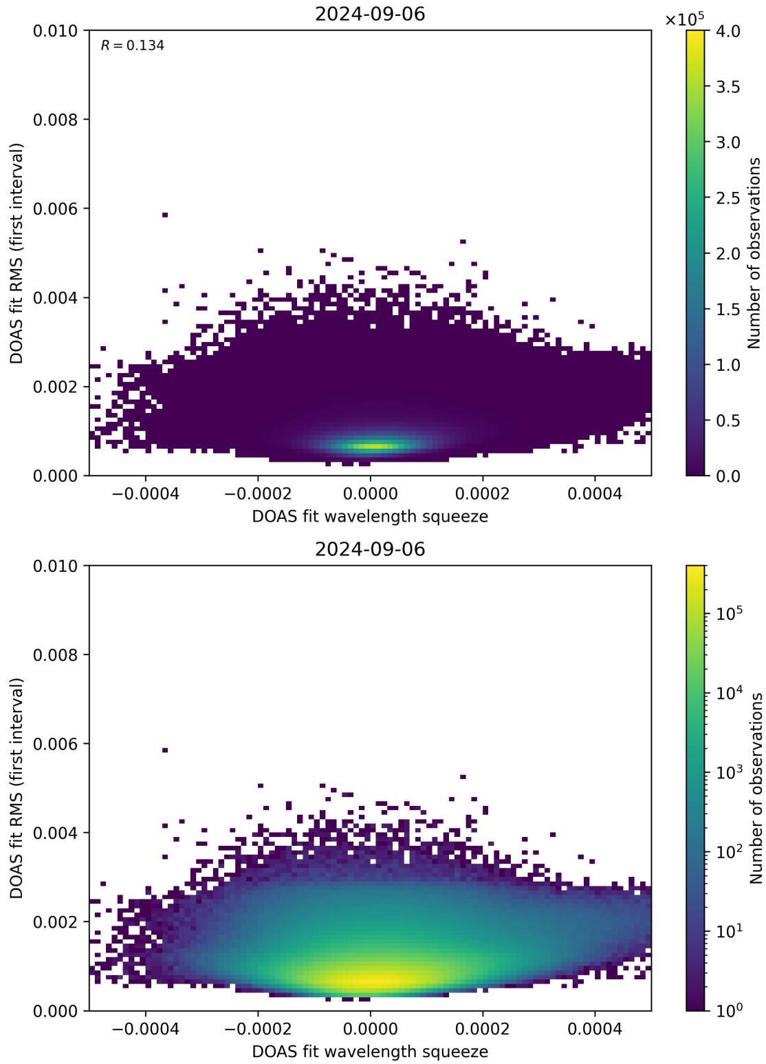
Figure 68: Scatter density plot of “DOAS fit wavelength squeeze” against “DOAS fit RMS (first interval)” for 2024-09-06 to 2024-09-07.
