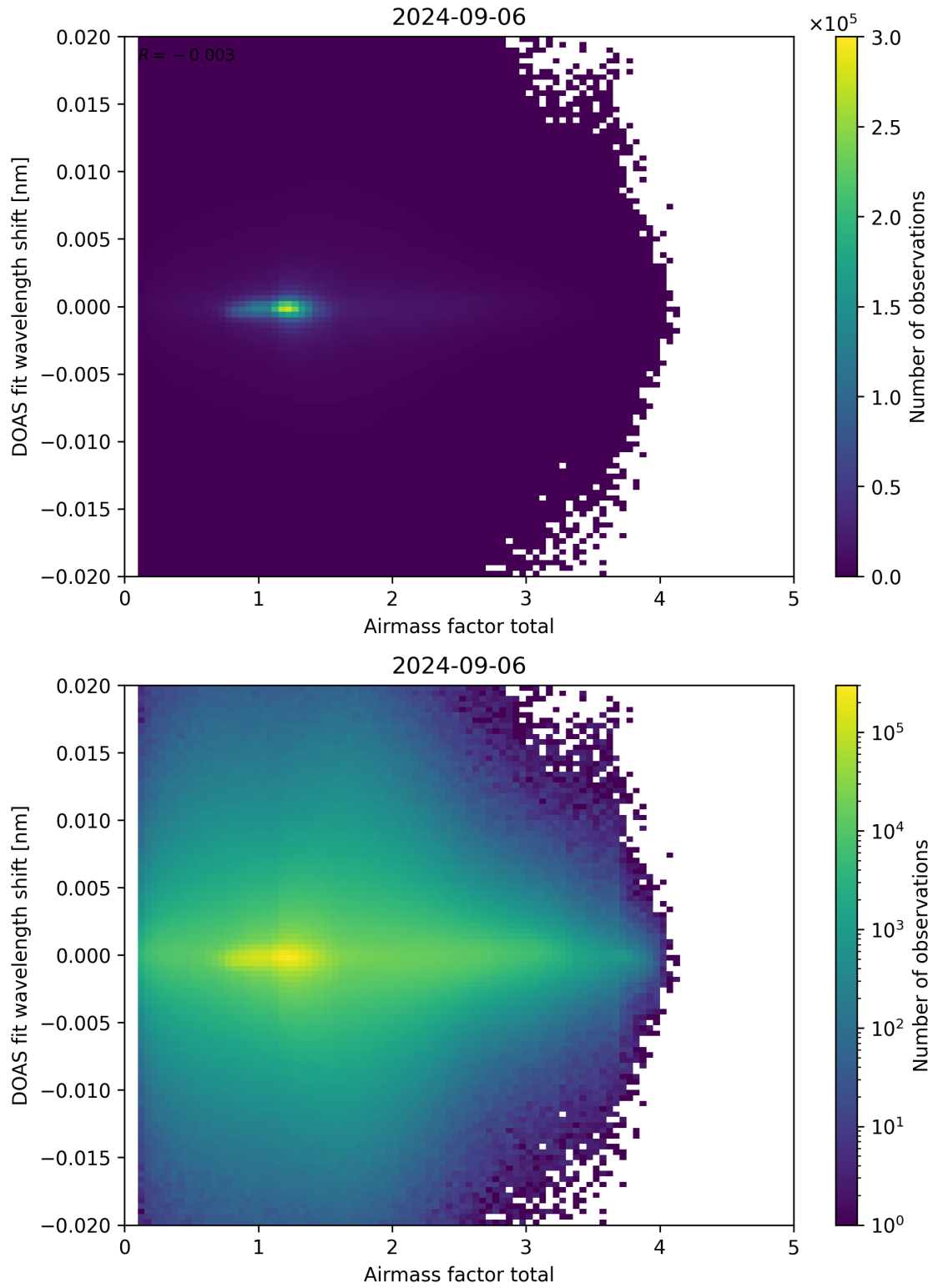
Figure 98: Scatter density plot of “Airmass factor total” against “DOAS fit wavelength shift” for 2024-09-06 to 2024-09-07.
