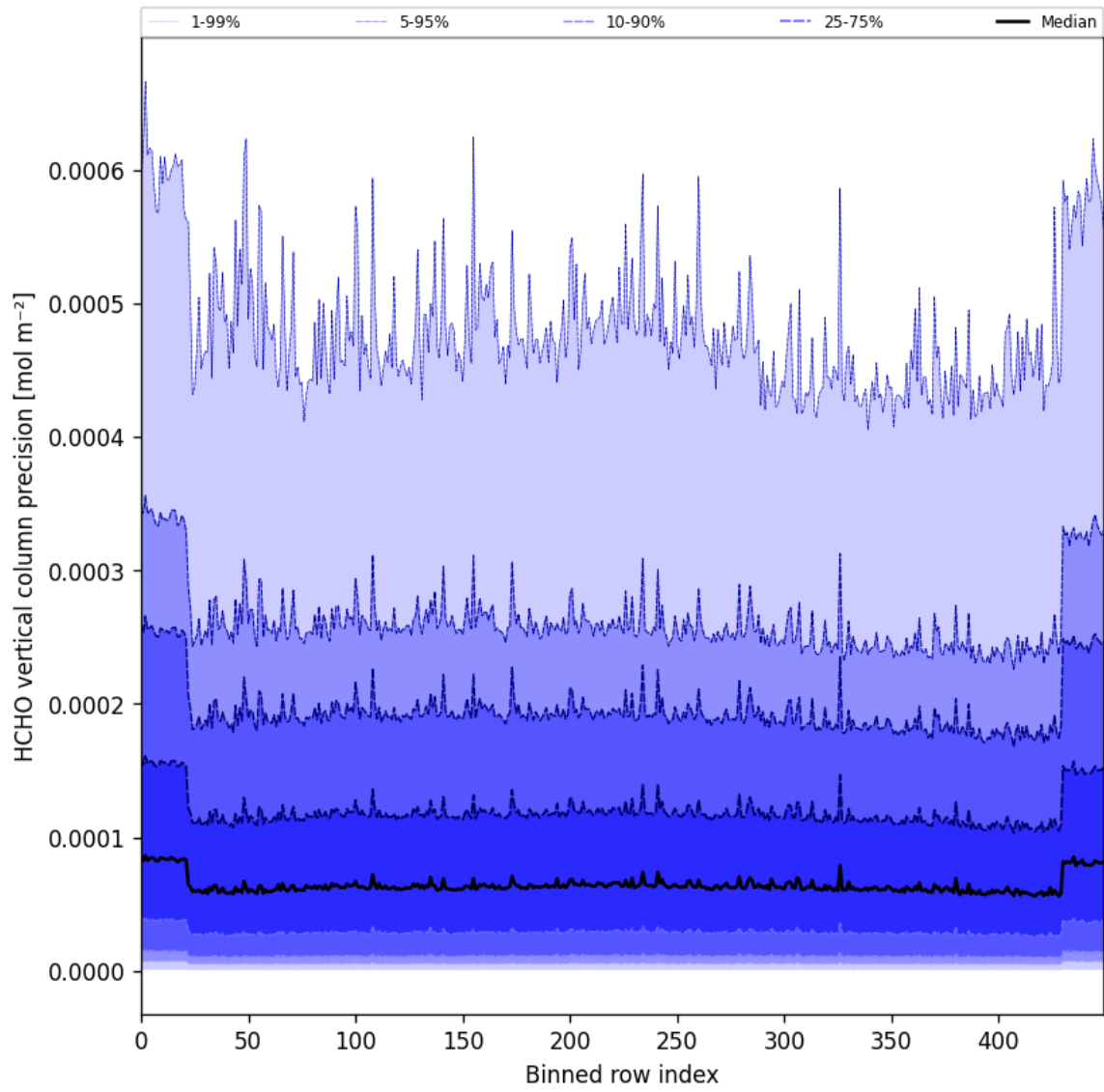
Figure 50: Along track statistics of “HCHO vertical column precision” for 2024-09-06 to 2024-09-07
