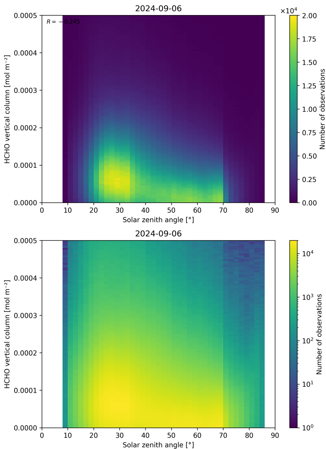
Figure 177: Scatter density plot of “Solar zenith angle” against “HCHO vertical column” for 2024-09-06 to 2024-09-07.
