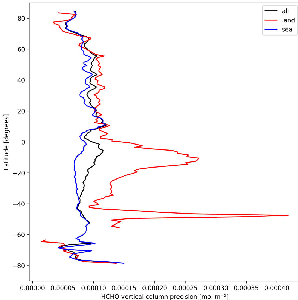
Figure 22: Zonal average of “HCHO vertical column precision” for 2024-09-06 to 2024-09-07.
