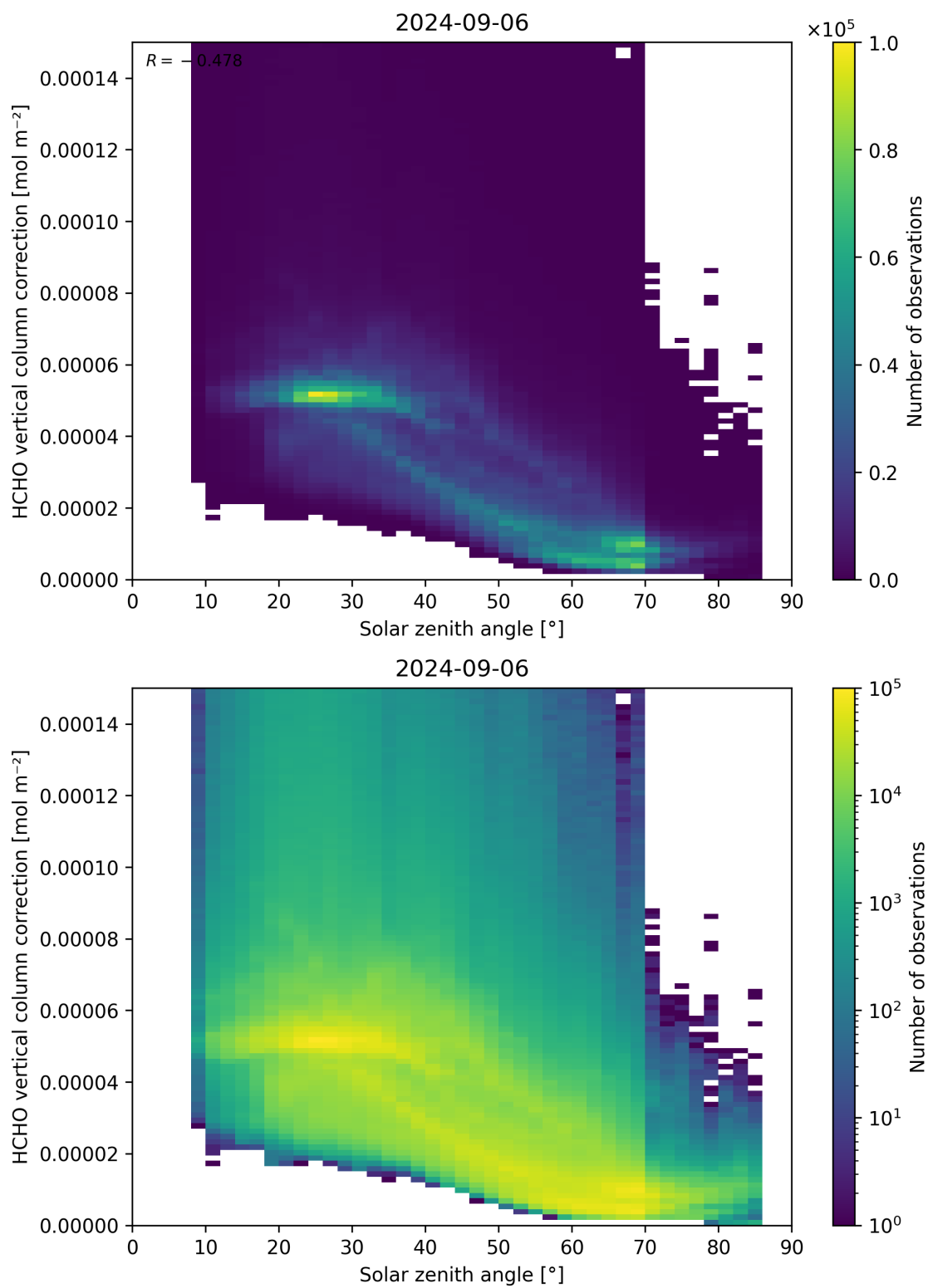
Figure 178: Scatter density plot of “Solar zenith angle” against “HCHO vertical column correction” for 2024-09-06 to 2024-09-07.
