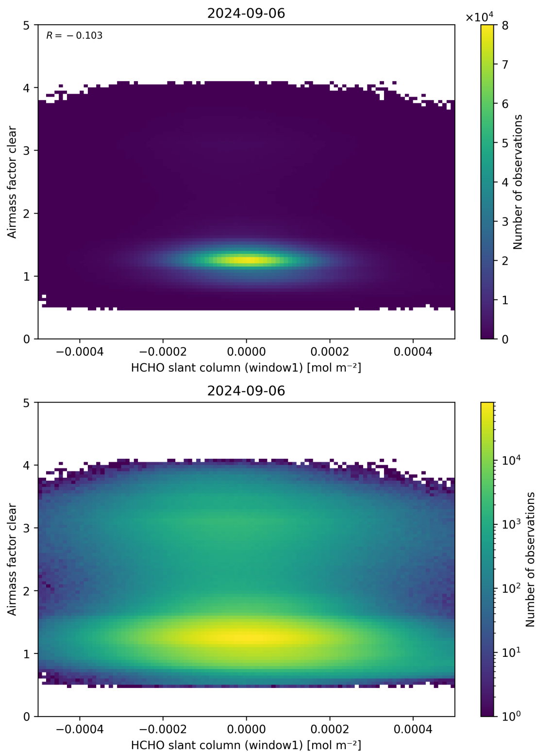
Figure 81: Scatter density plot of “HCHO slant column (window1)” against “Airmass factor clear” for 2024-09-06 to 2024-09-07.
