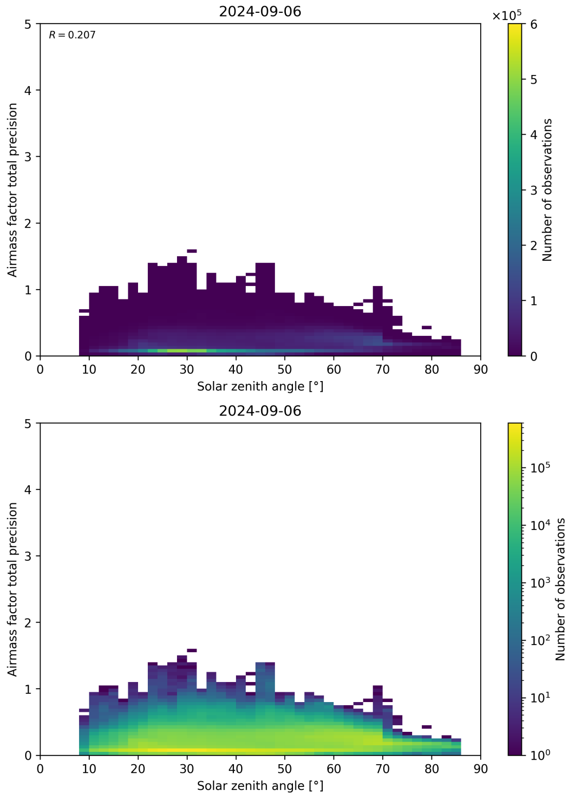
Figure 176: Scatter density plot of “Solar zenith angle” against “Airmass factor total precision” for 2024-09-06 to 2024-09-07.
