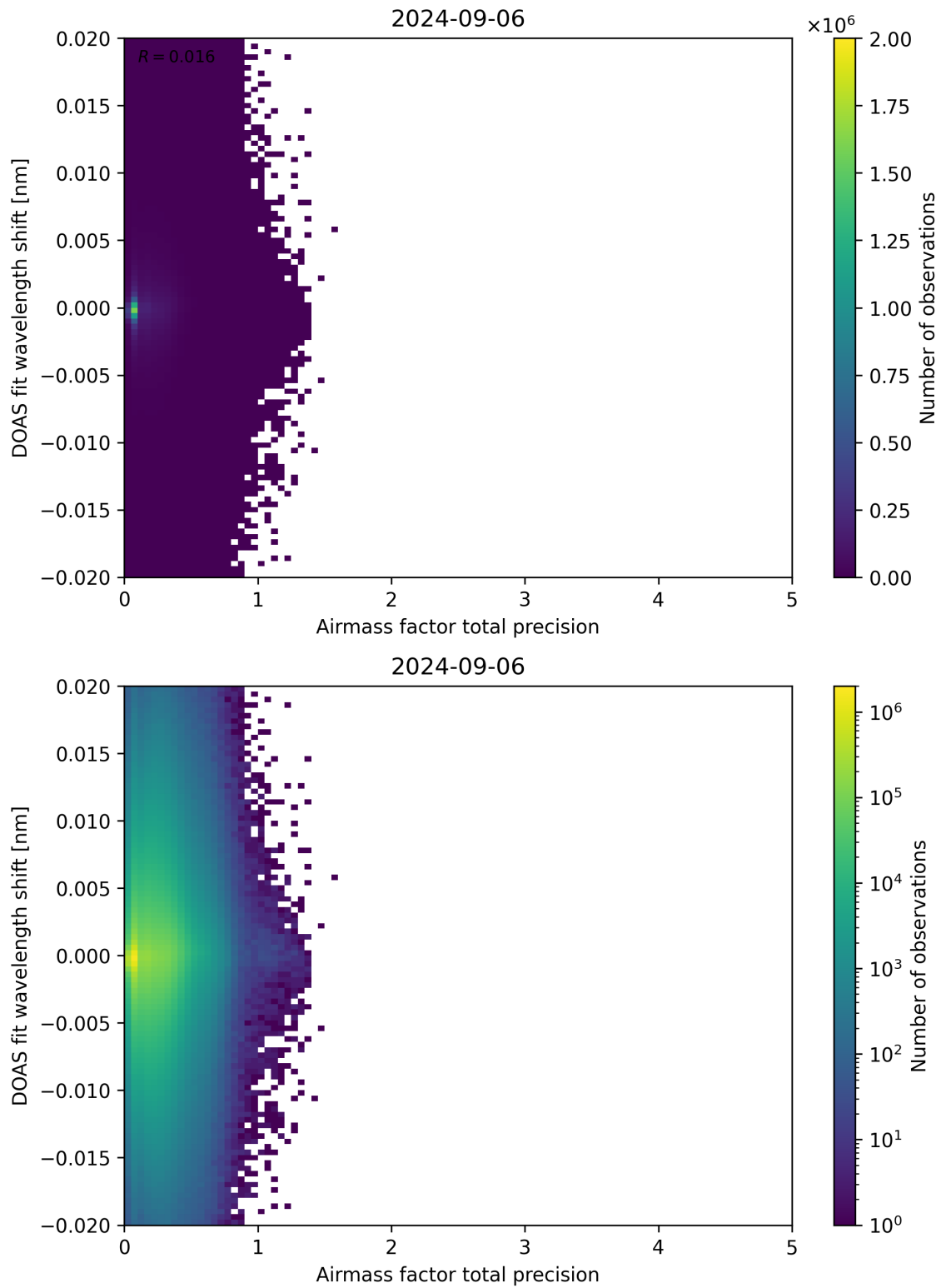
Figure 106: Scatter density plot of “Airmass factor total precision” against “DOAS fit wavelength shift” for 2024-09-06 to 2024-09-07.
