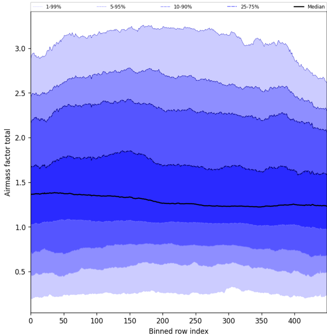
Figure 54: Along track statistics of “Airmass factor total” for 2024-09-06 to 2024-09-07
