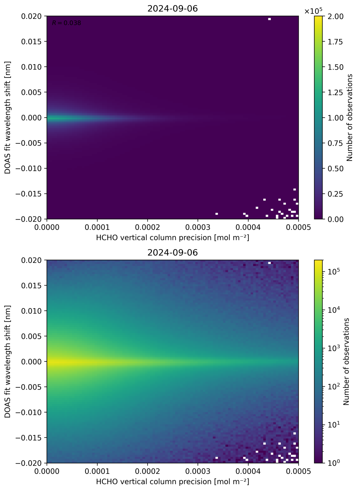
Figure 137: Scatter density plot of “HCHO vertical column precision” against “DOAS fit wavelength shift” for 2024-09-06 to 2024-09-07.
