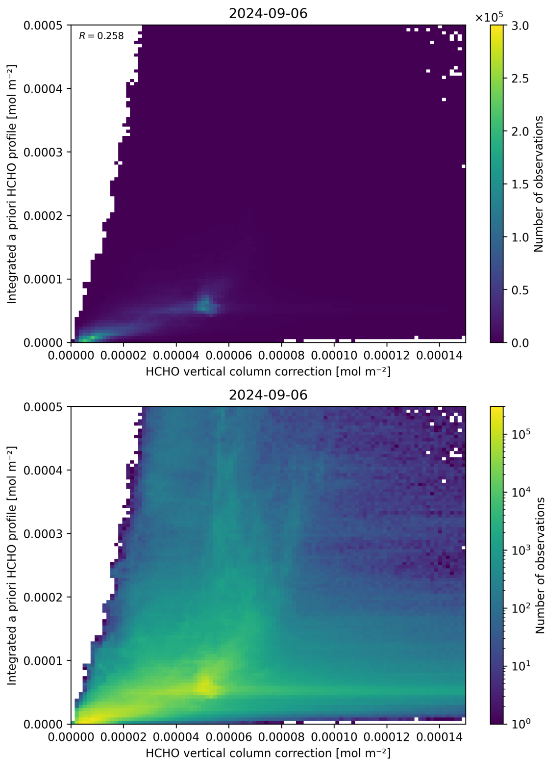
Figure 122: Scatter density plot of “HCHO vertical column correction” against “Integrated a priori HCHO profile” for 2024-09-06 to 2024-09-07.
