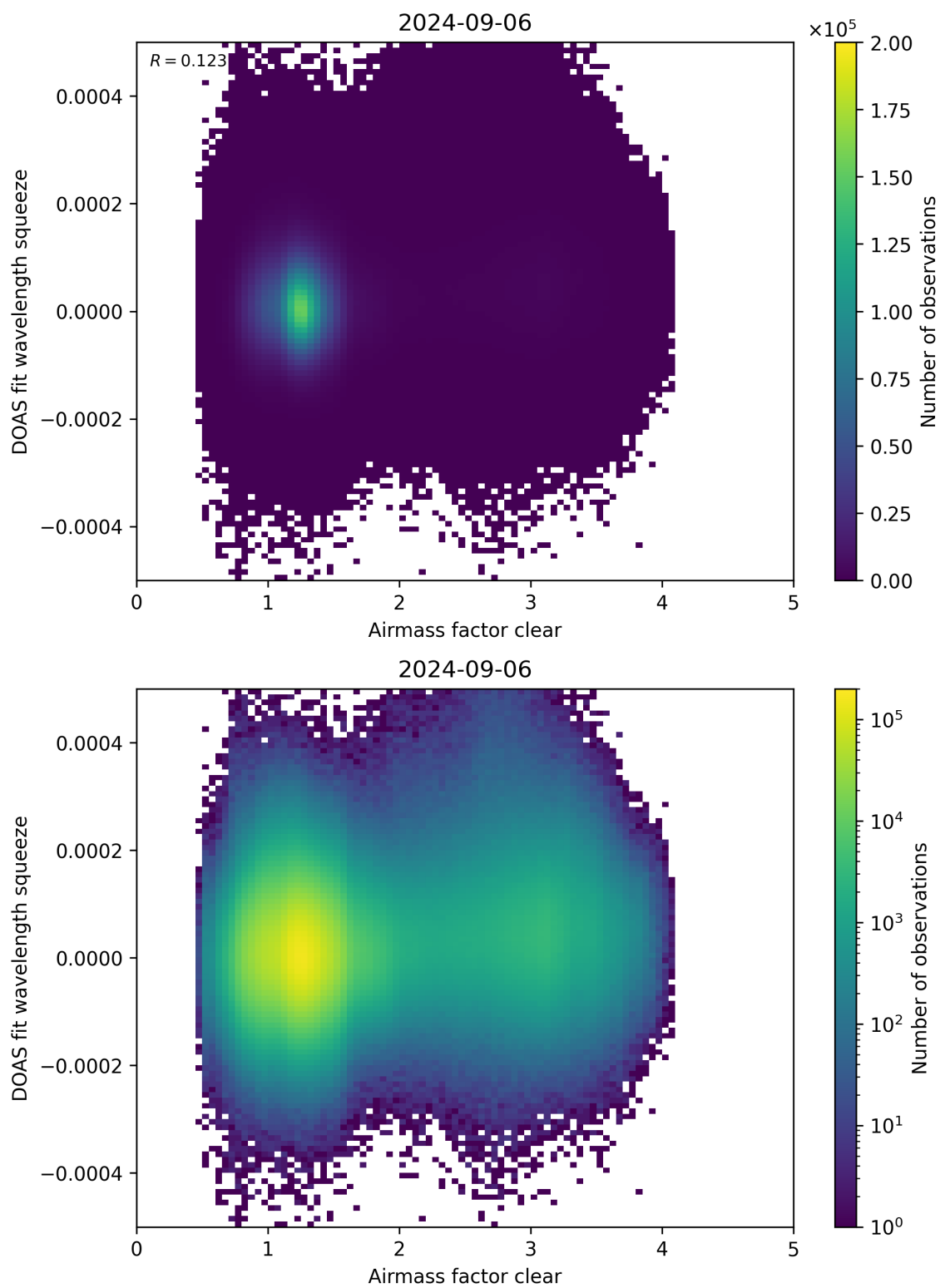
Figure 73: Scatter density plot of “Airmass factor clear” against “DOAS fit wavelength squeeze” for 2024-09-06 to 2024-09-07.
