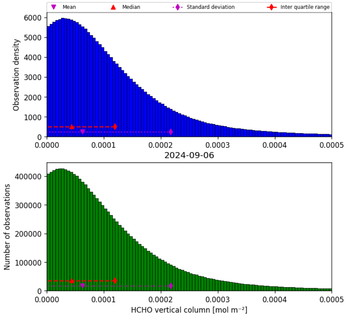
Figure 35: Histogram of “HCHO vertical column” for 2024-09-06 to 2024-09-07
