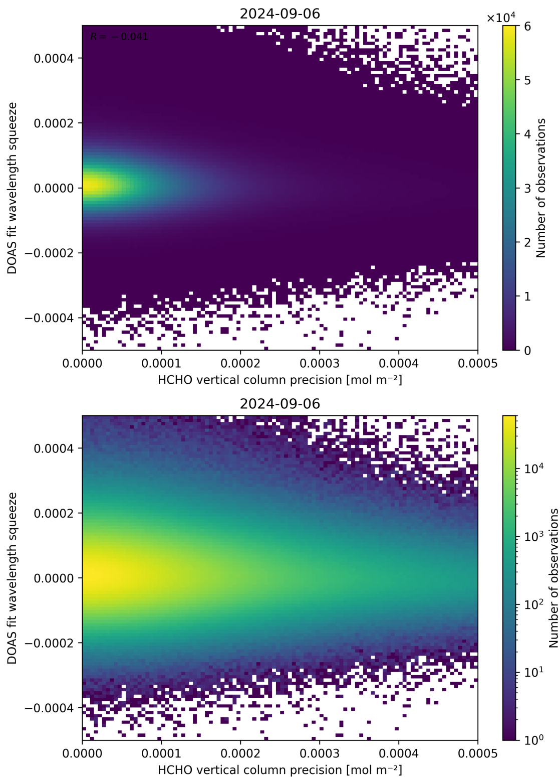
Figure 138: Scatter density plot of “HCHO vertical column precision” against “DOAS fit wavelength squeeze” for 2024-09-06 to 2024-09-07.
