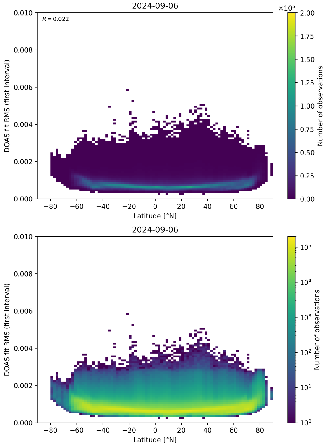
Figure 153: Scatter density plot of “Latitude” against “DOAS fit RMS (first interval)” for 2024-09-06 to 2024-09-07.
