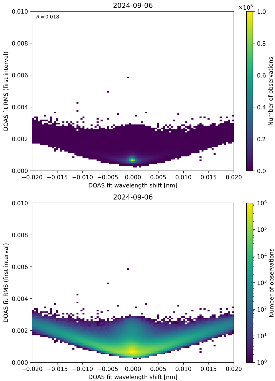
Figure 64: Scatter density plot of “DOAS fit wavelength shift” against “DOAS fit RMS (first interval)” for 2024-09-06 to 2024-09-07.
