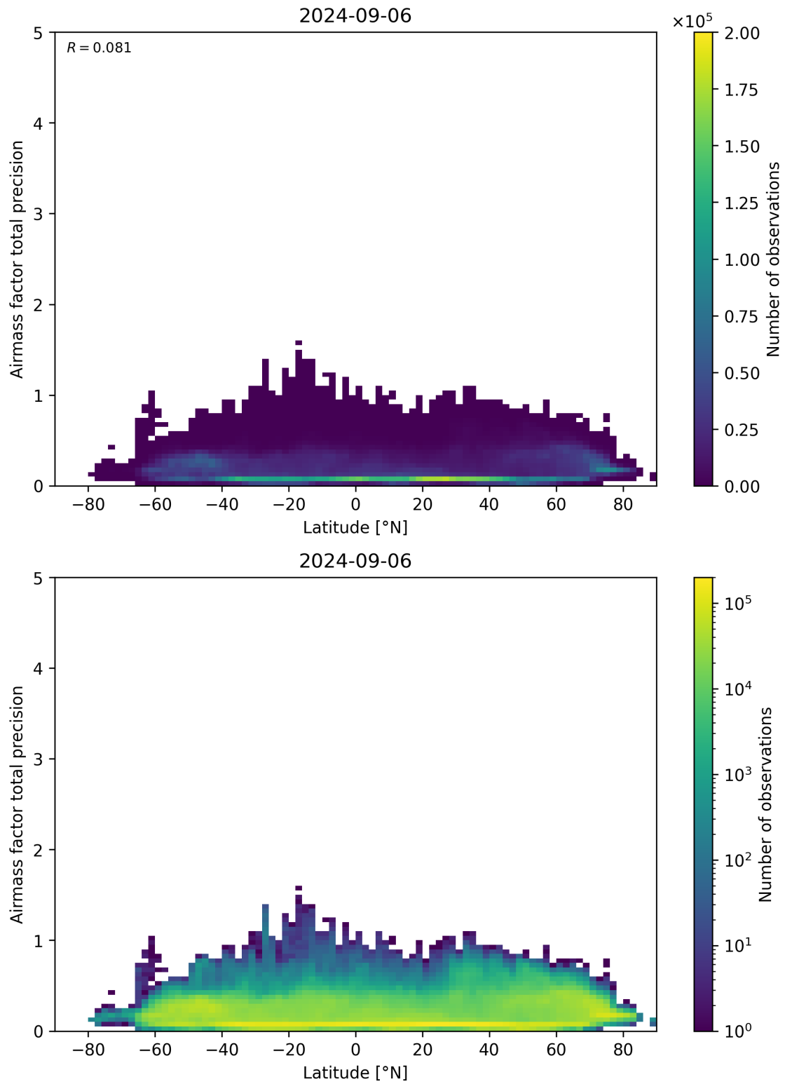
Figure 162: Scatter density plot of “Latitude” against “Airmass factor total precision” for 2024-09-06 to 2024-09-07.
