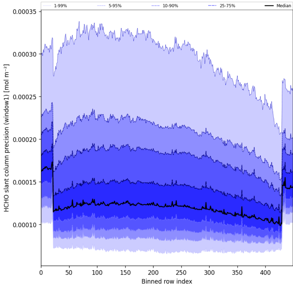
Figure 53: Along track statistics of “HCHO slant column precision (window1)” for 2024-09-06 to 2024-09-07
