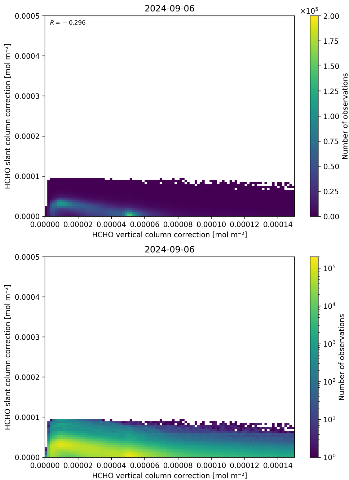
Figure 117: Scatter density plot of “HCHO vertical column correction” against “HCHO slant column correction” for 2024-09-06 to 2024-09-07.
