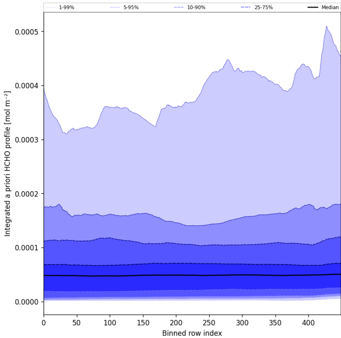
Figure 57: Along track statistics of “Integrated a priori HCHO profile” for 2024-09-06 to 2024-09-07
