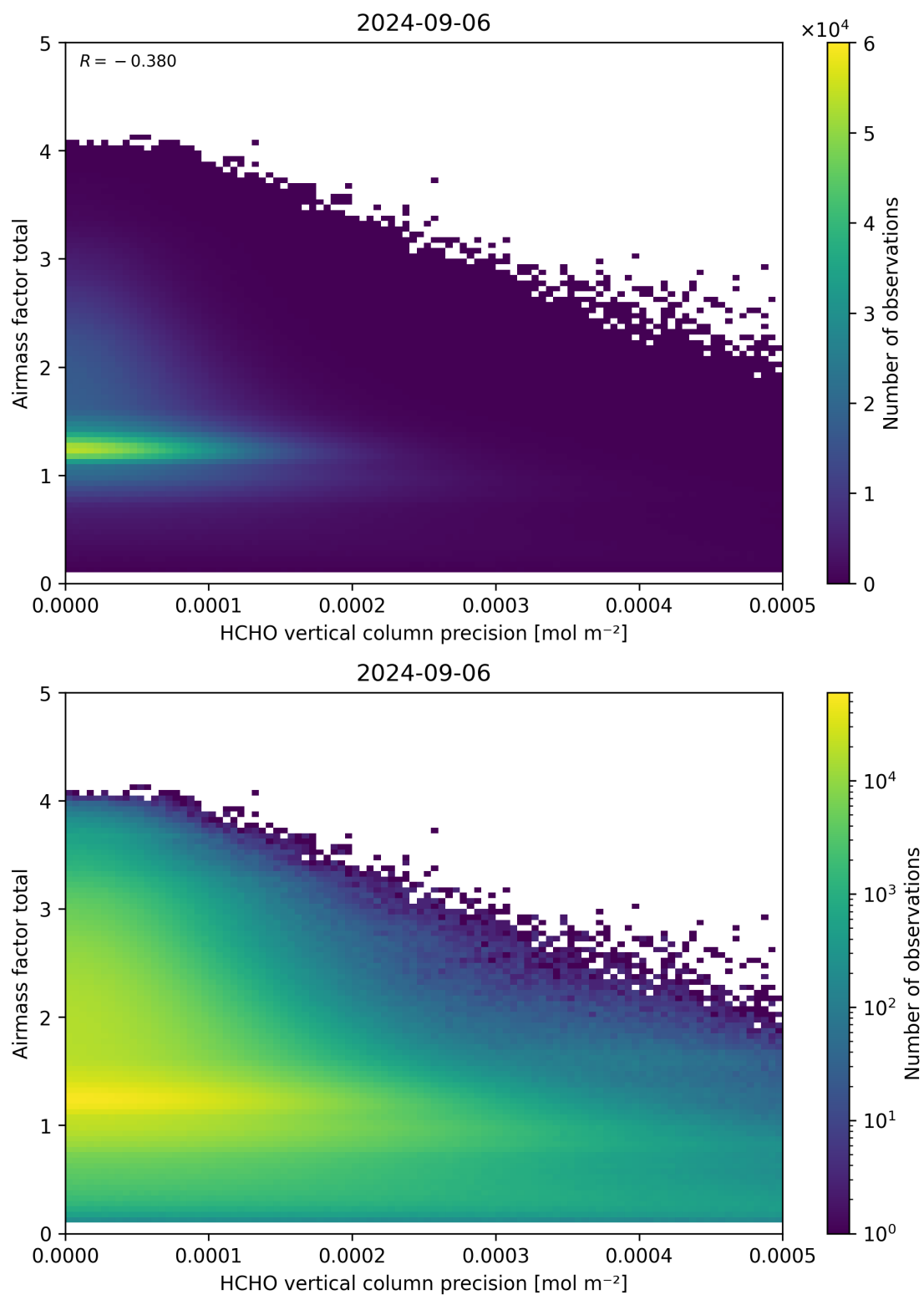
Figure 144: Scatter density plot of “HCHO vertical column precision” against “Airmass factor total” for 2024-09-06 to 2024-09-07.
