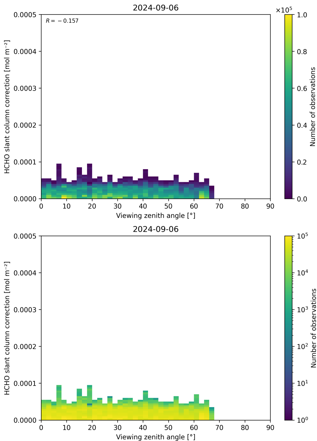
Figure 187: Scatter density plot of “Viewing zenith angle” against “HCHO slant column correction” for 2024-09-06 to 2024-09-07.
