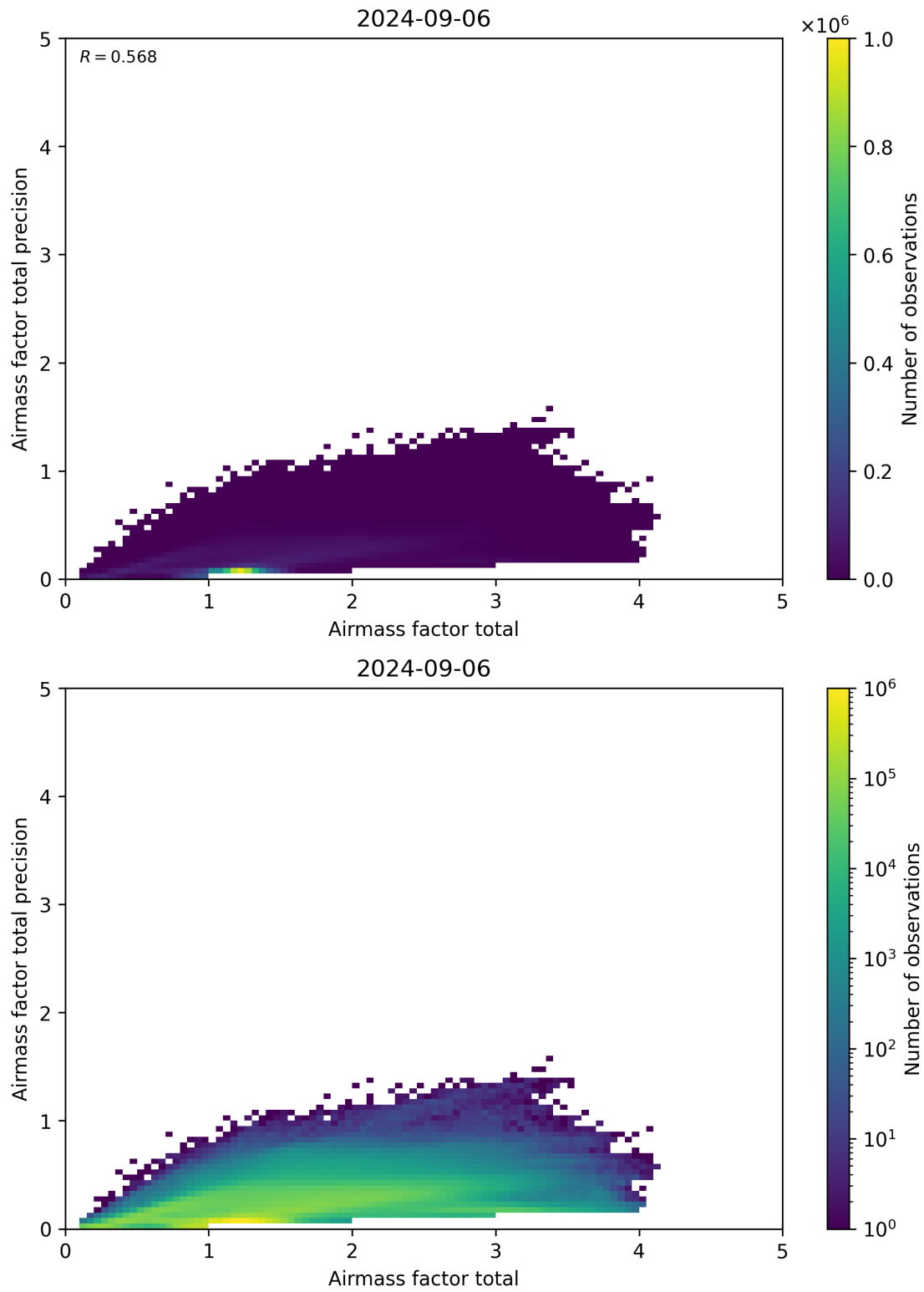
Figure 103: Scatter density plot of “Airmass factor total” against “Airmass factor total precision” for 2024-09-06 to 2024-09-07.
