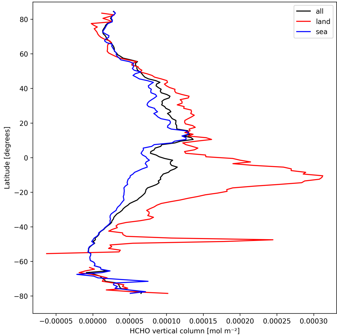
Figure 21: Zonal average of “HCHO vertical column” for 2024-09-06 to 2024-09-07.
