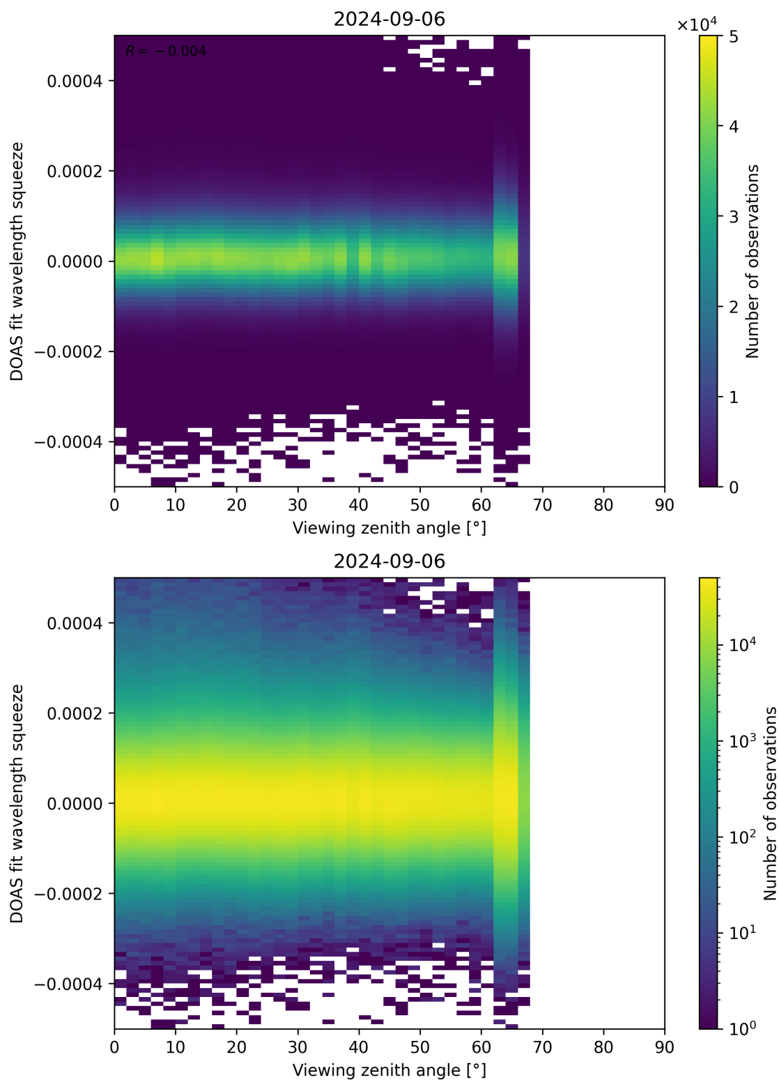
Figure 184: Scatter density plot of “Viewing zenith angle” against “DOAS fit wavelength squeeze” for 2024-09-06 to 2024-09-07.
