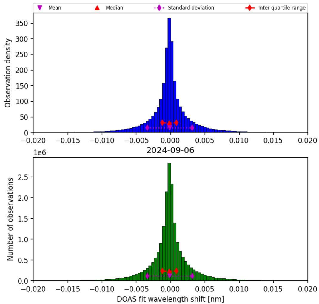
Figure 44: Histogram of “DOAS fit wavelength shift” for 2024-09-06 to 2024-09-07
