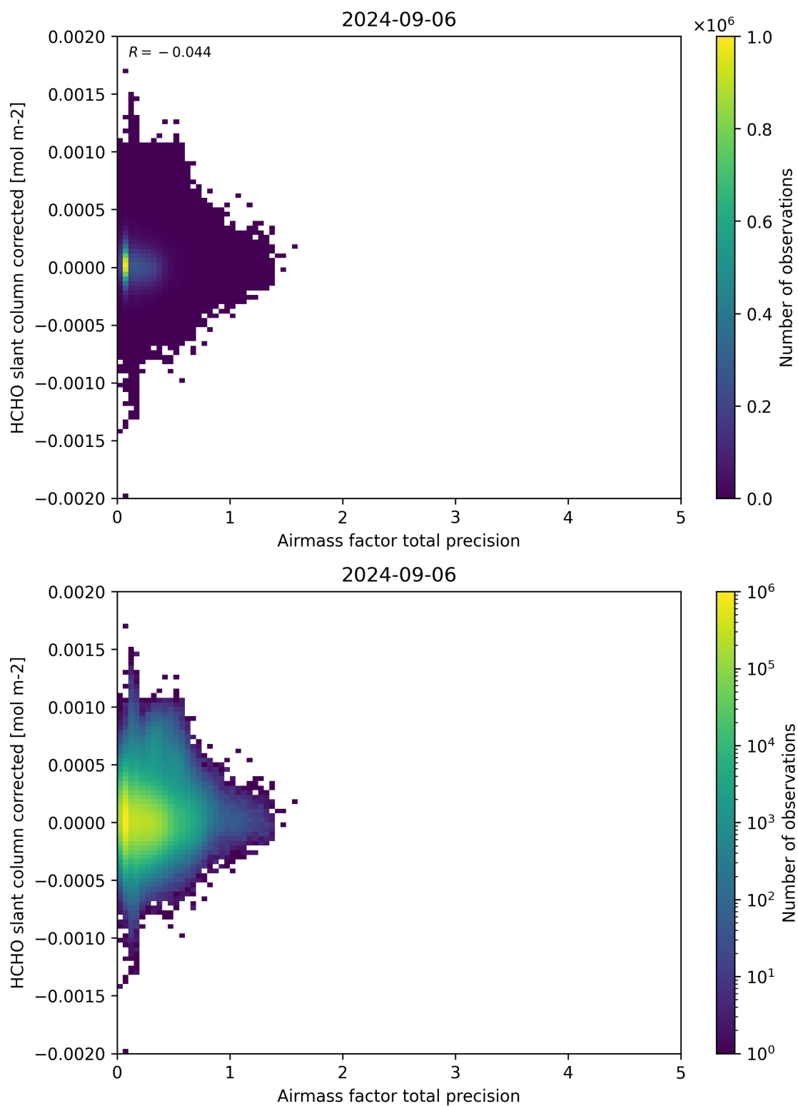
Figure 109: Scatter density plot of “Airmass factor total precision” against “HCHO slant column corrected” for 2024-09-06 to 2024-09-07.
