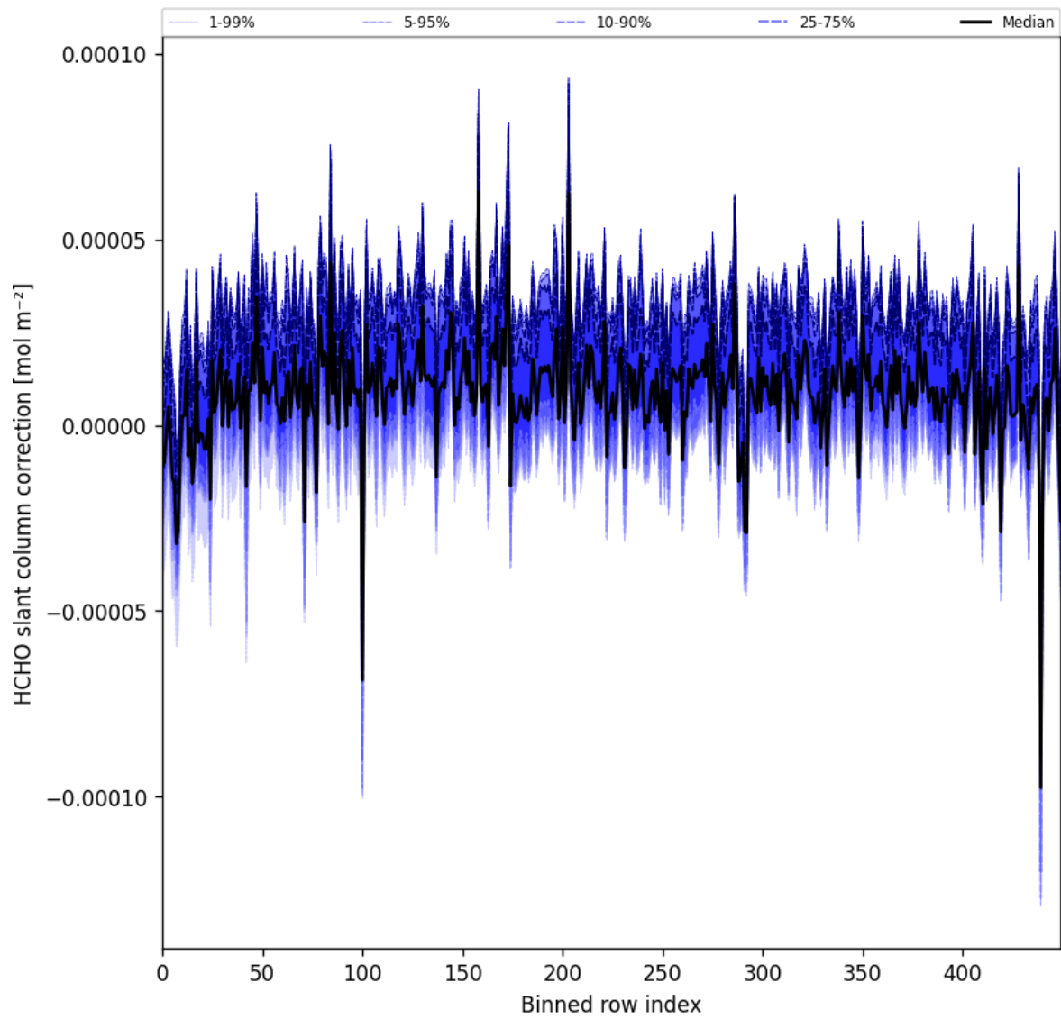
Figure 61: Along track statistics of “HCHO slant column correction” for 2024-09-06 to 2024-09-07
