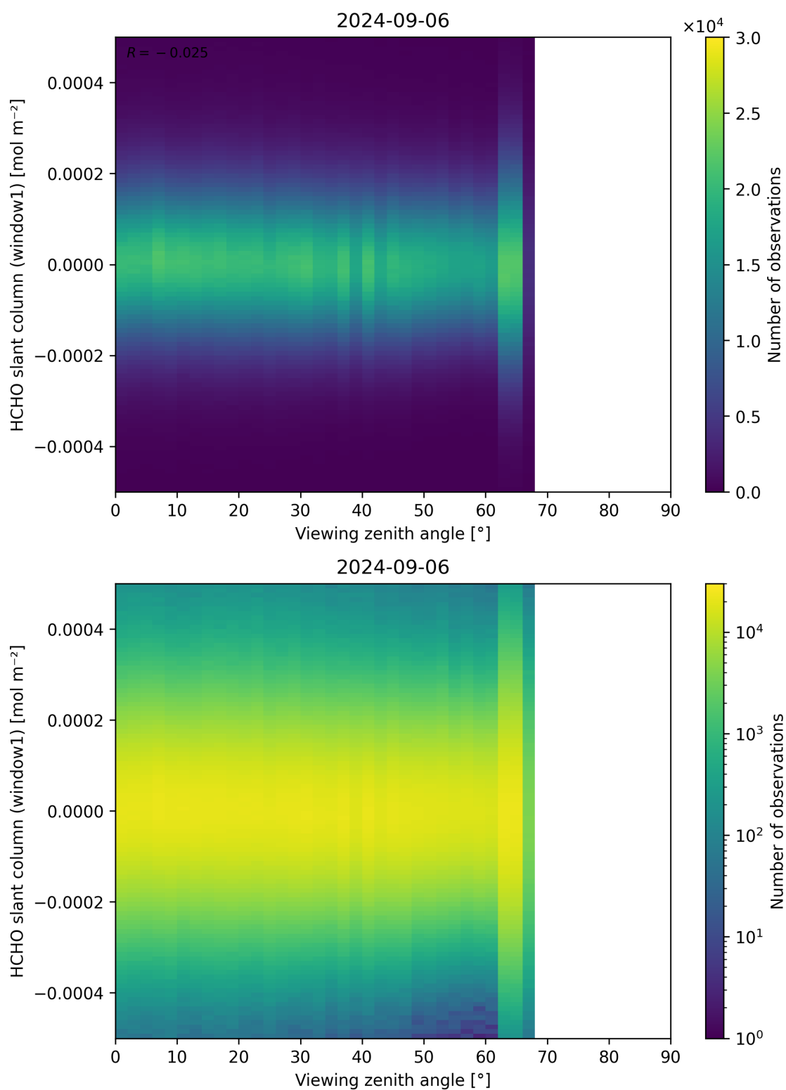
Figure 188: Scatter density plot of “Viewing zenith angle” against “HCHO slant column (window1)” for 2024-09-06 to 2024-09-07.
