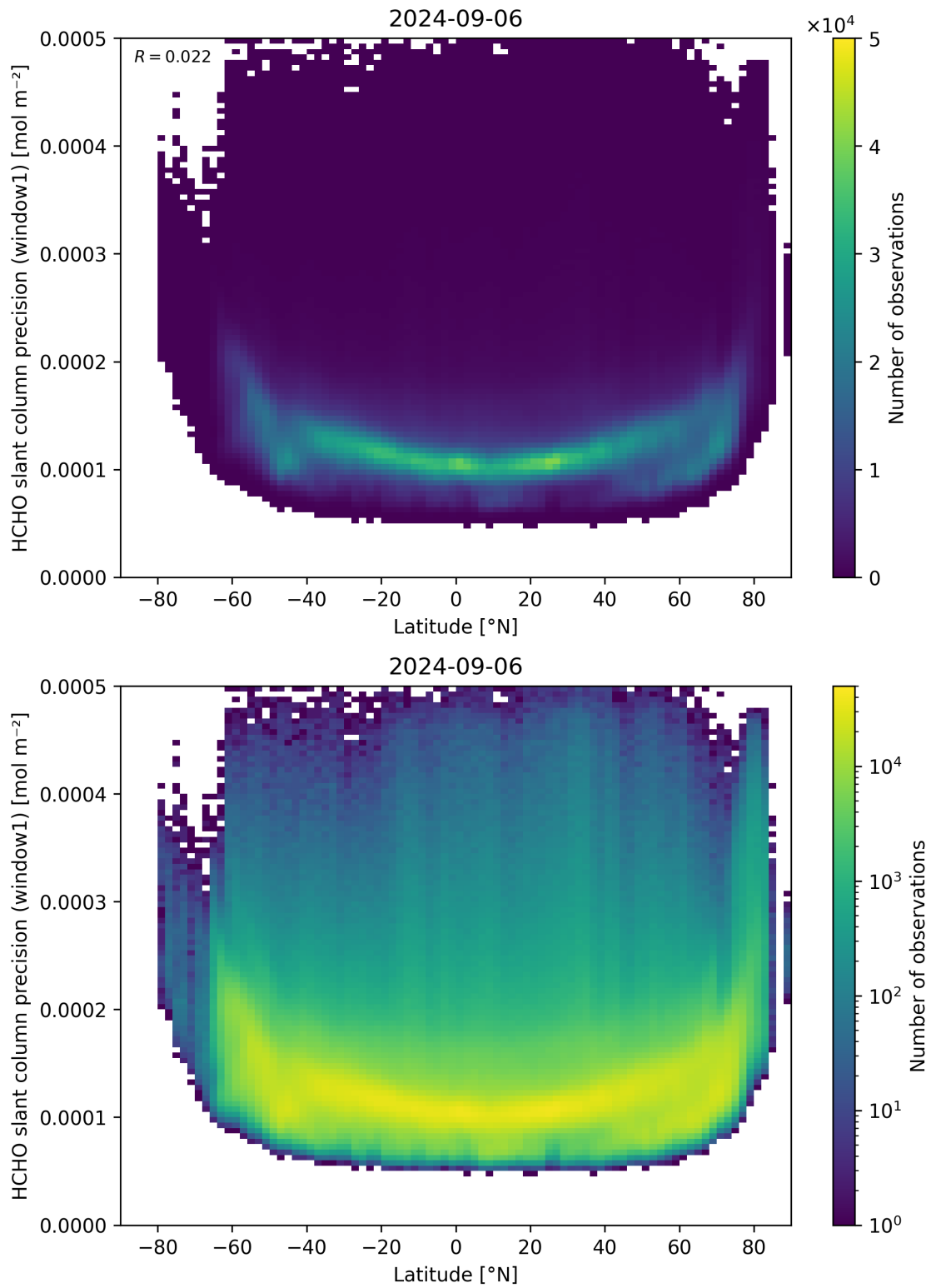
Figure 160: Scatter density plot of “Latitude” against “HCHO slant column precision (window1)” for 2024-09-06 to 2024-09-07.
