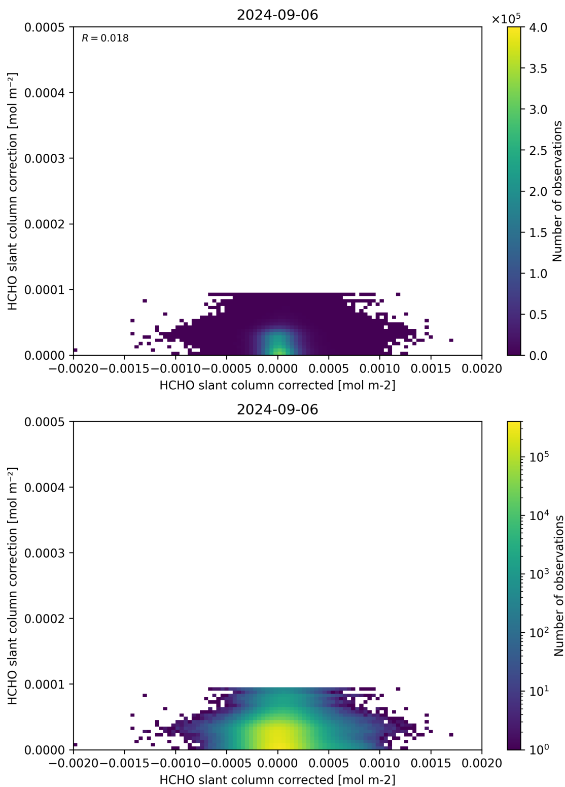
Figure 77: Scatter density plot of “HCHO slant column corrected” against “HCHO slant column correction” for 2024-09-06 to 2024-09-07.
