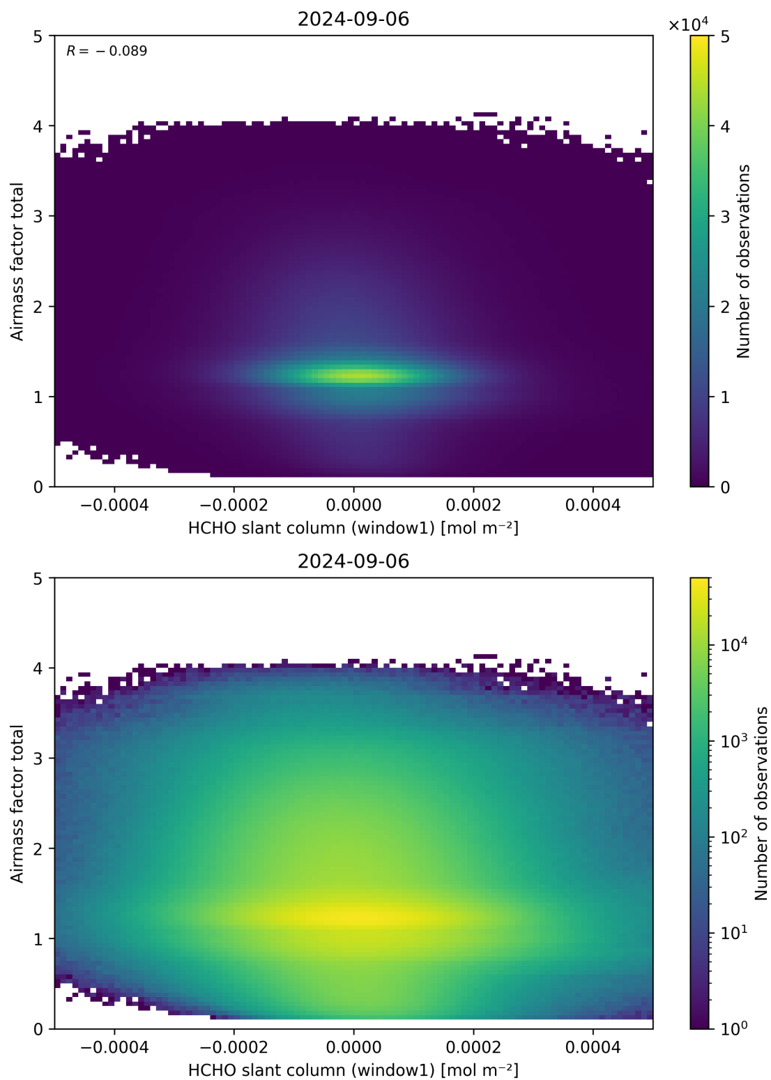
Figure 85: Scatter density plot of “HCHO slant column (window1)” against “Airmass factor total” for 2024-09-06 to 2024-09-07.
