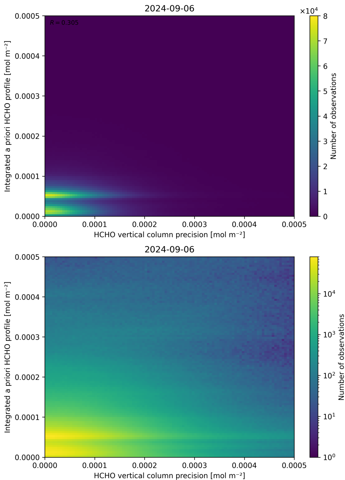
Figure 147: Scatter density plot of “HCHO vertical column precision” against “Integrated a priori HCHO profile” for 2024-09-06 to 2024-09-07.
