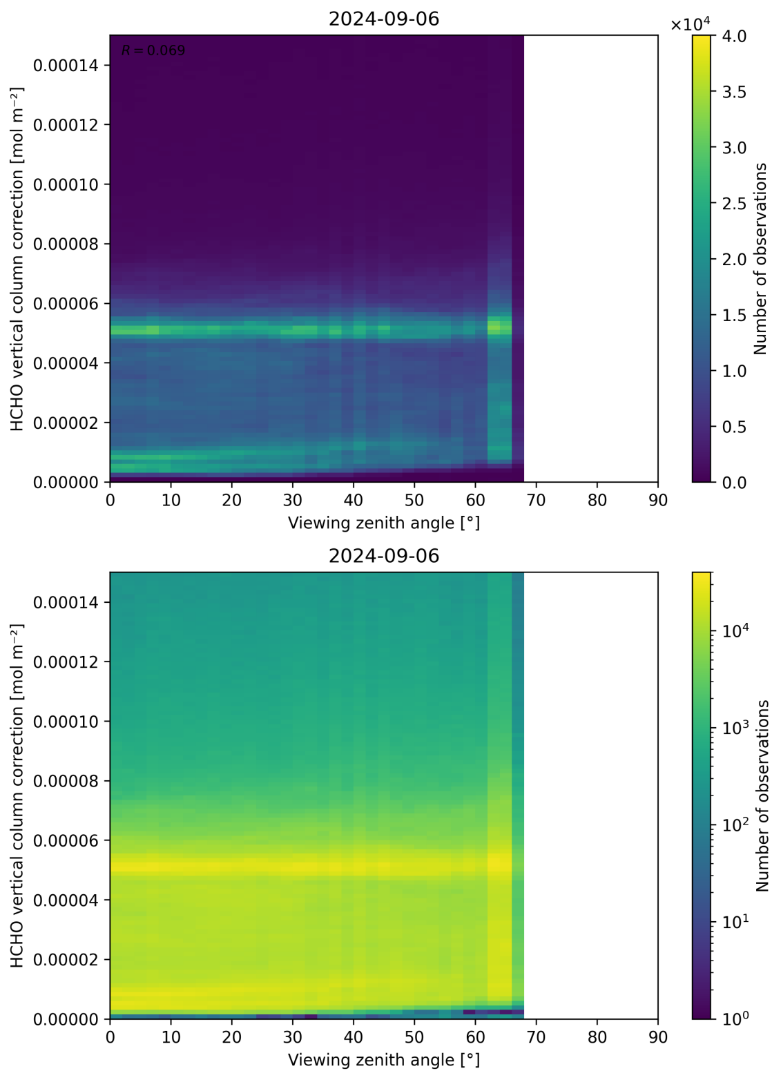
Figure 193: Scatter density plot of “Viewing zenith angle” against “HCHO vertical column correction” for 2024-09-06 to 2024-09-07.
