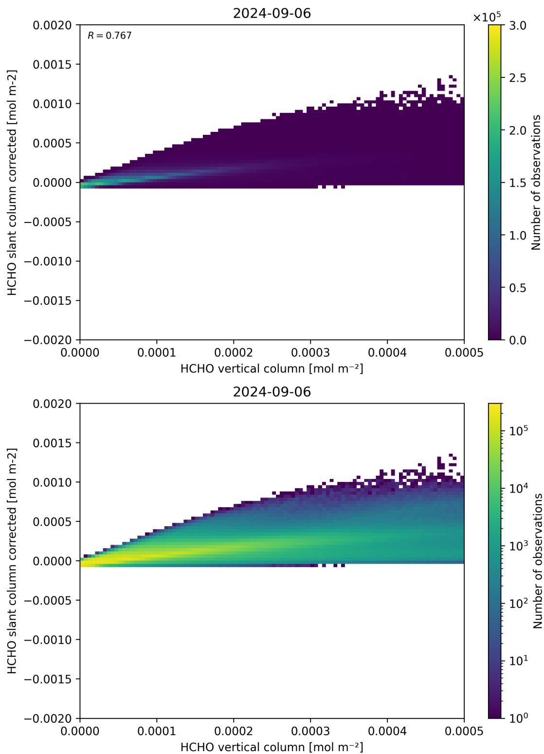
Figure 127: Scatter density plot of “HCHO vertical column” against “HCHO slant column corrected” for 2024-09-06 to 2024-09-07.
