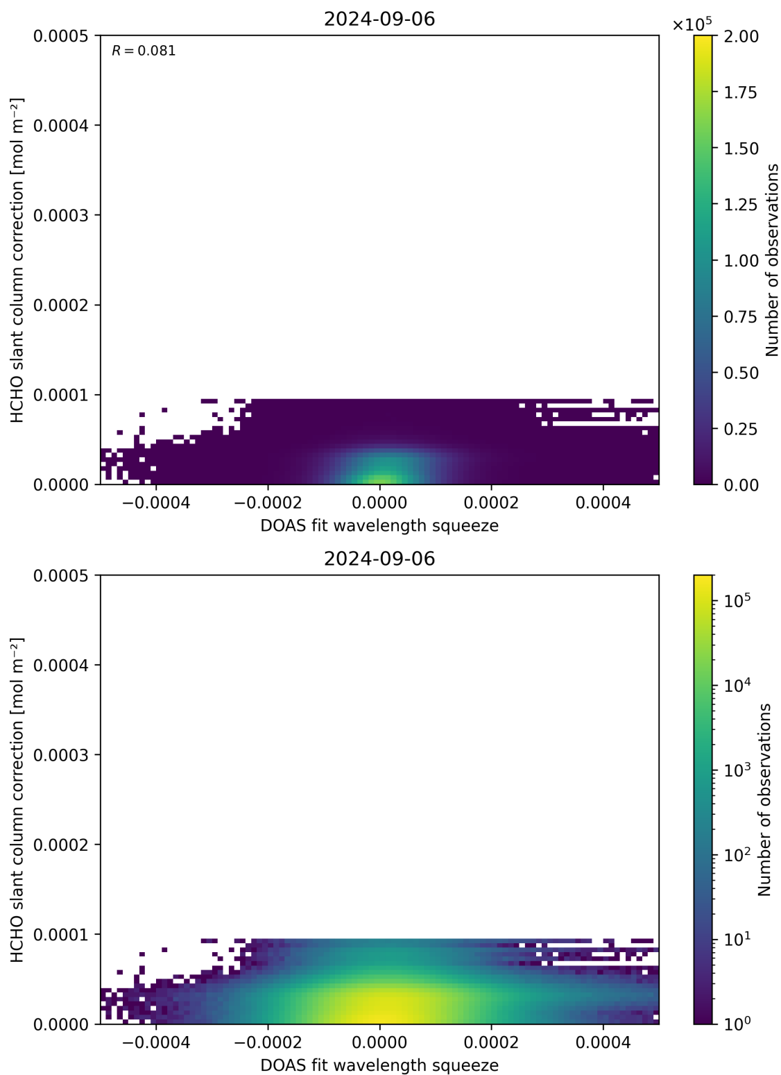
Figure 70: Scatter density plot of “DOAS fit wavelength squeeze” against “HCHO slant column correction” for 2024-09-06 to 2024-09-07.
