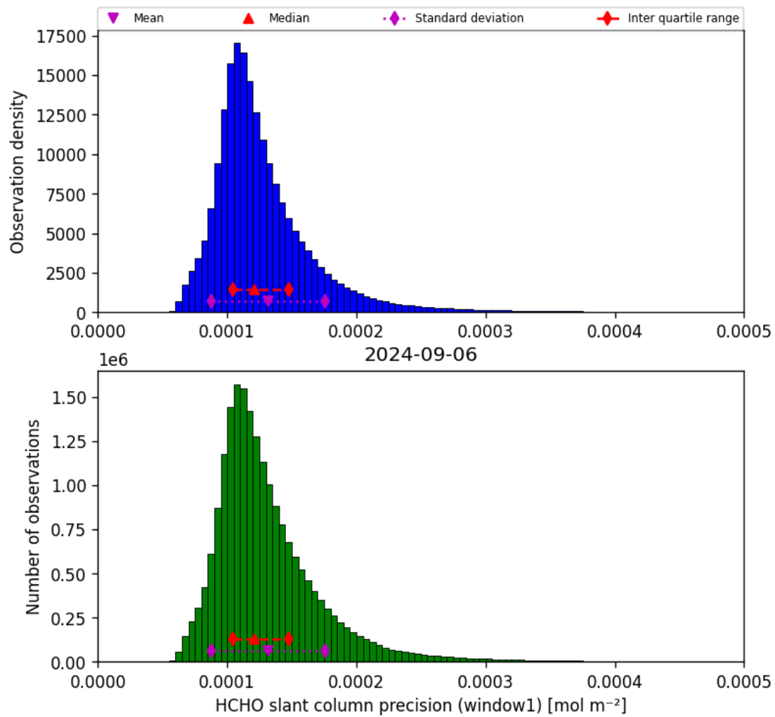
Figure 39: Histogram of “HCHO slant column precision (window1)” for 2024-09-06 to 2024-09-07
