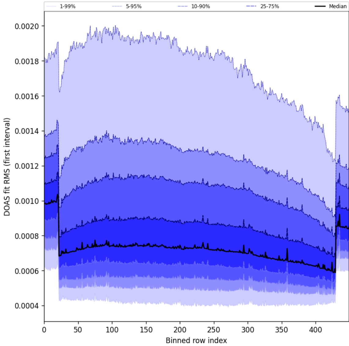
Figure 60: Along track statistics of “DOAS fit RMS (first interval)” for 2024-09-06 to 2024-09-07
