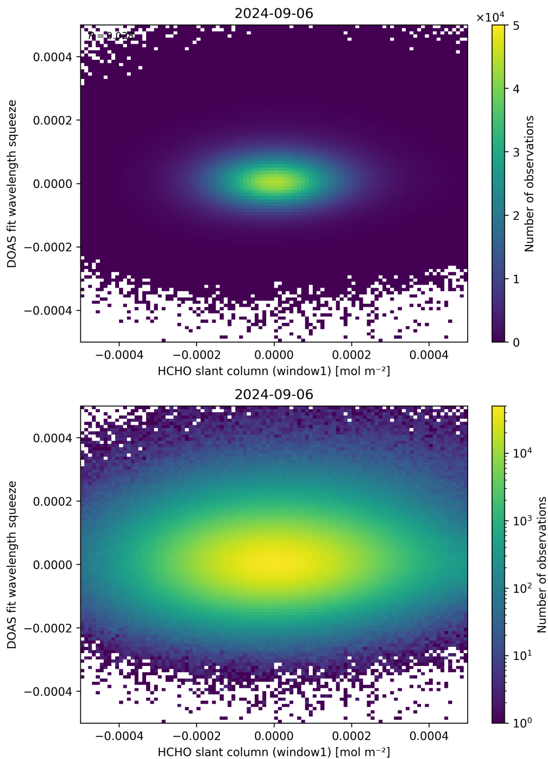
Figure 80: Scatter density plot of “HCHO slant column (window1)” against “DOAS fit wavelength squeeze” for 2024-09-06 to 2024-09-07.
