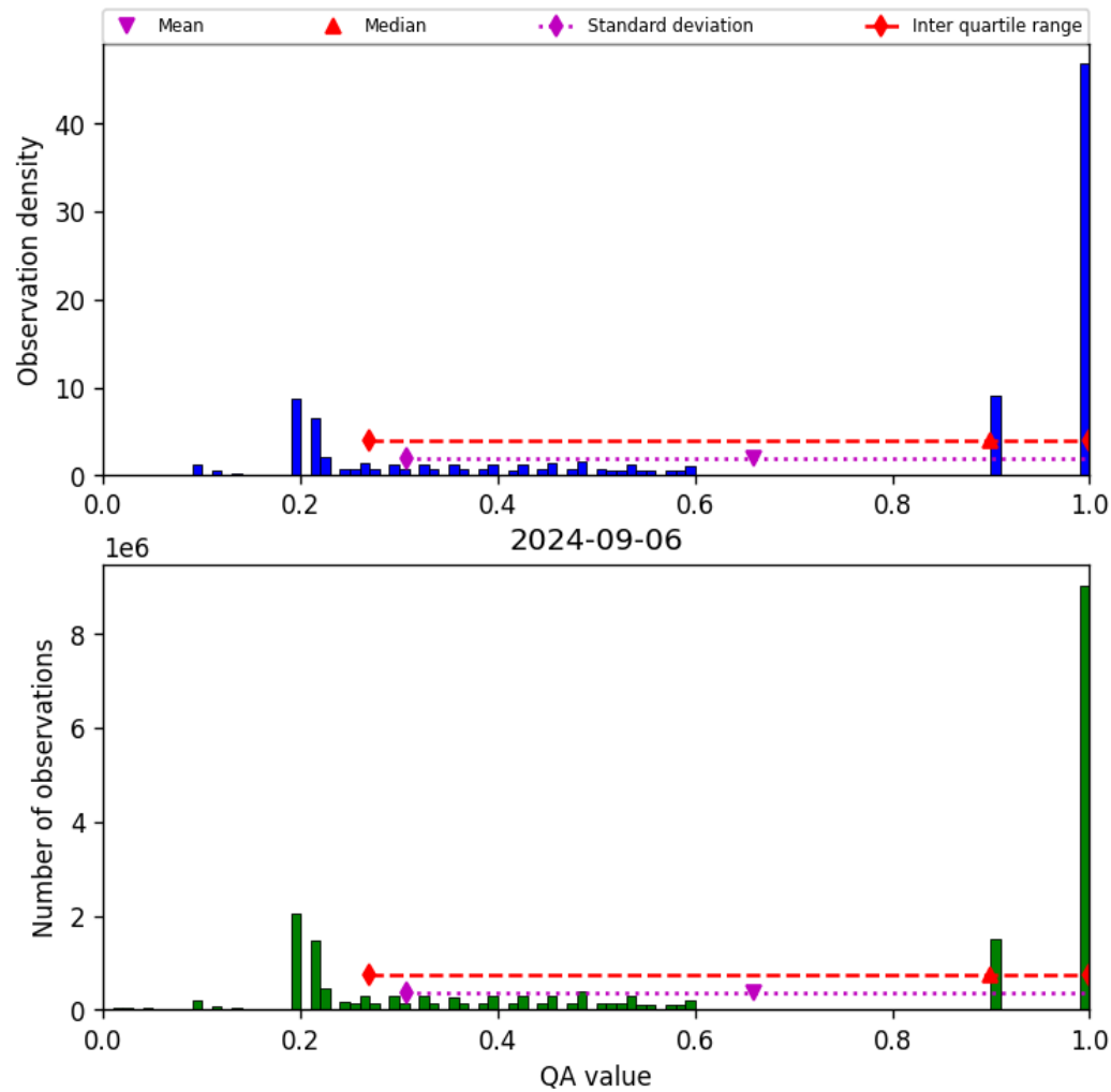
Figure 34: Histogram of “QA value” for 2024-09-06 to 2024-09-07
