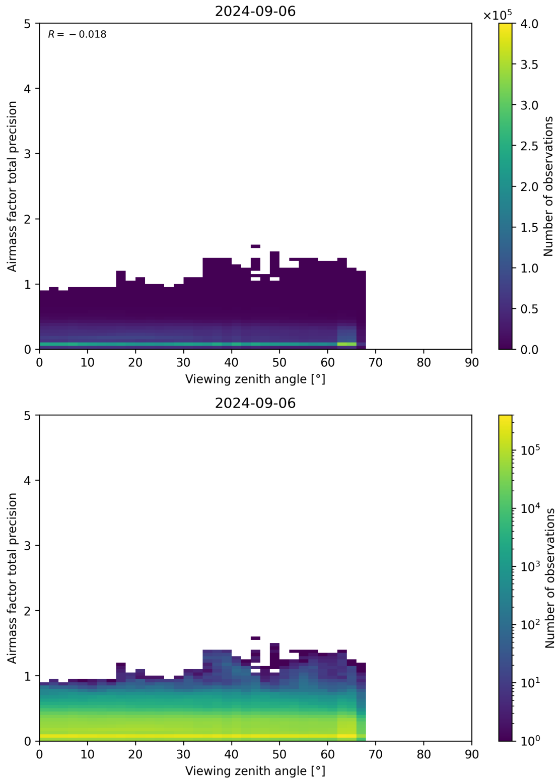
Figure 191: Scatter density plot of “Viewing zenith angle” against “Airmass factor total precision” for 2024-09-06 to 2024-09-07.
