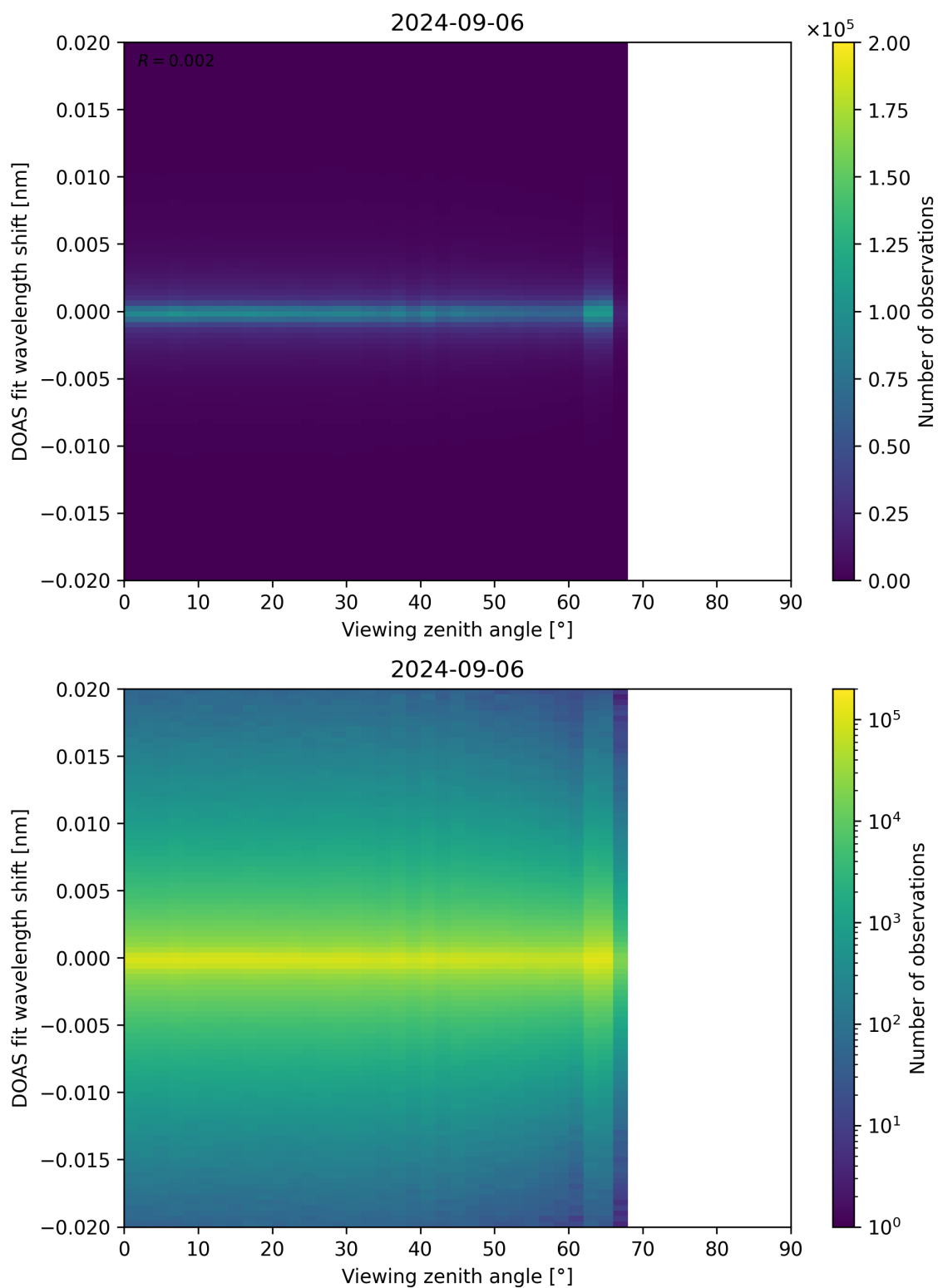
Figure 183: Scatter density plot of “Viewing zenith angle” against “DOAS fit wavelength shift” for 2024-09-06 to 2024-09-07.
