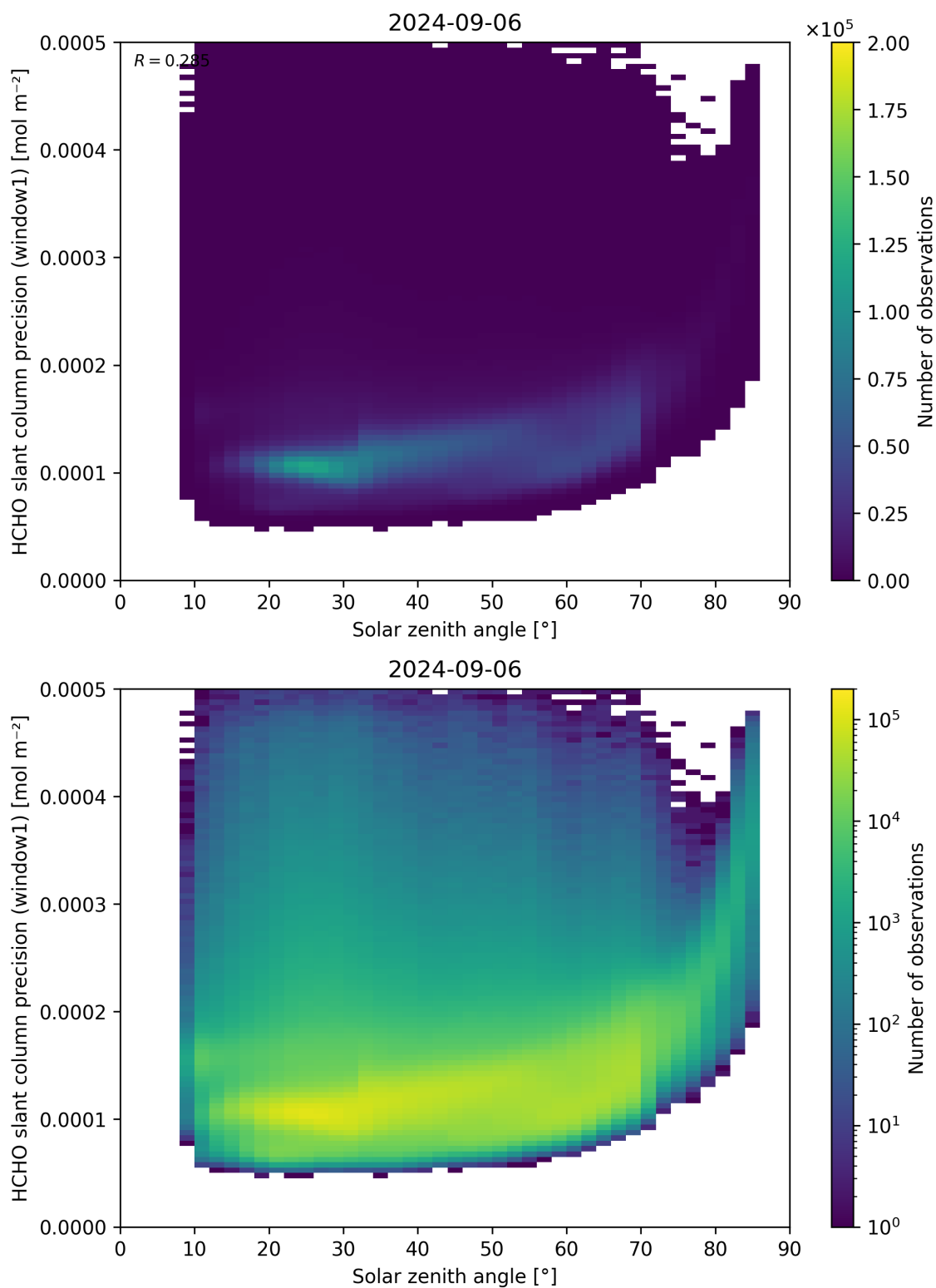
Figure 174: Scatter density plot of “Solar zenith angle” against “HCHO slant column precision (window1)” for 2024-09-06 to 2024-09-07.
