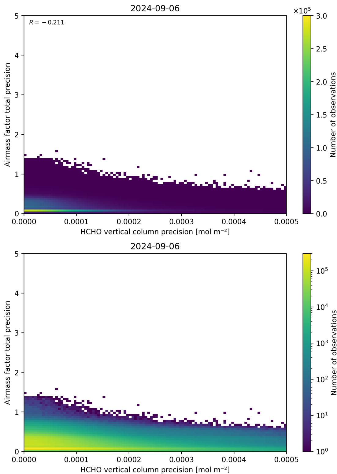
Figure 145: Scatter density plot of “HCHO vertical column precision” against “Airmass factor total precision” for 2024-09-06 to 2024-09-07.
