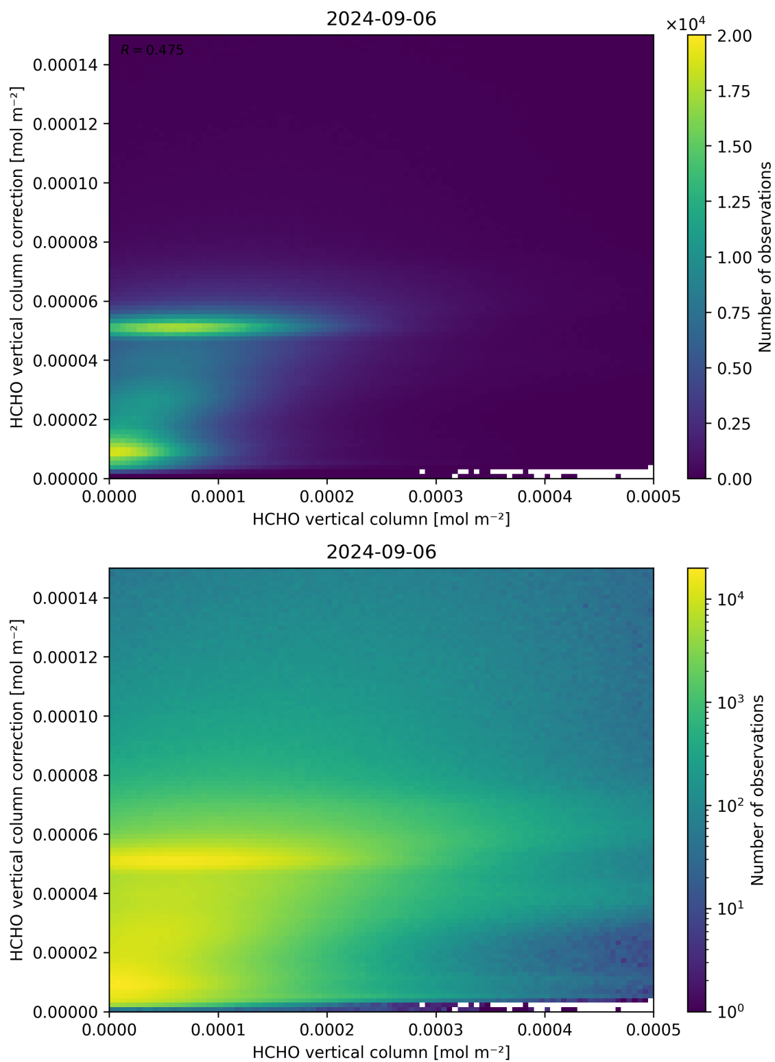
Figure 133: Scatter density plot of “HCHO vertical column” against “HCHO vertical column correction” for 2024-09-06 to 2024-09-07.
