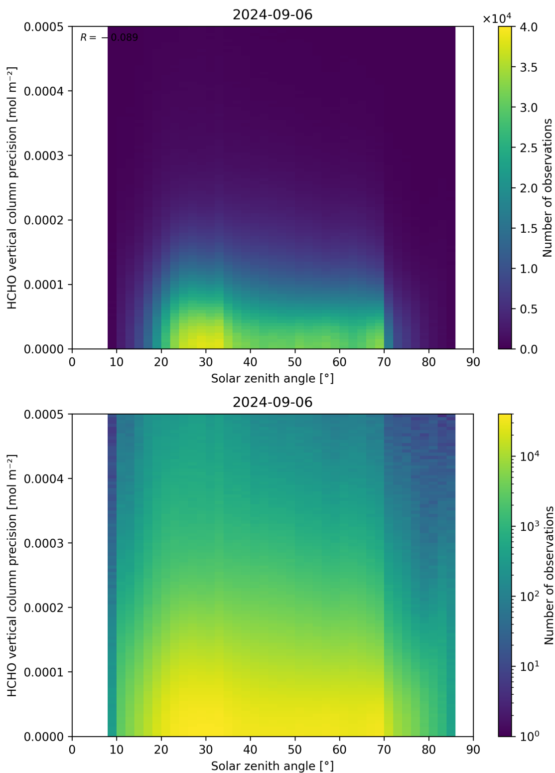
Figure 179: Scatter density plot of “Solar zenith angle” against “HCHO vertical column precision” for 2024-09-06 to 2024-09-07.
