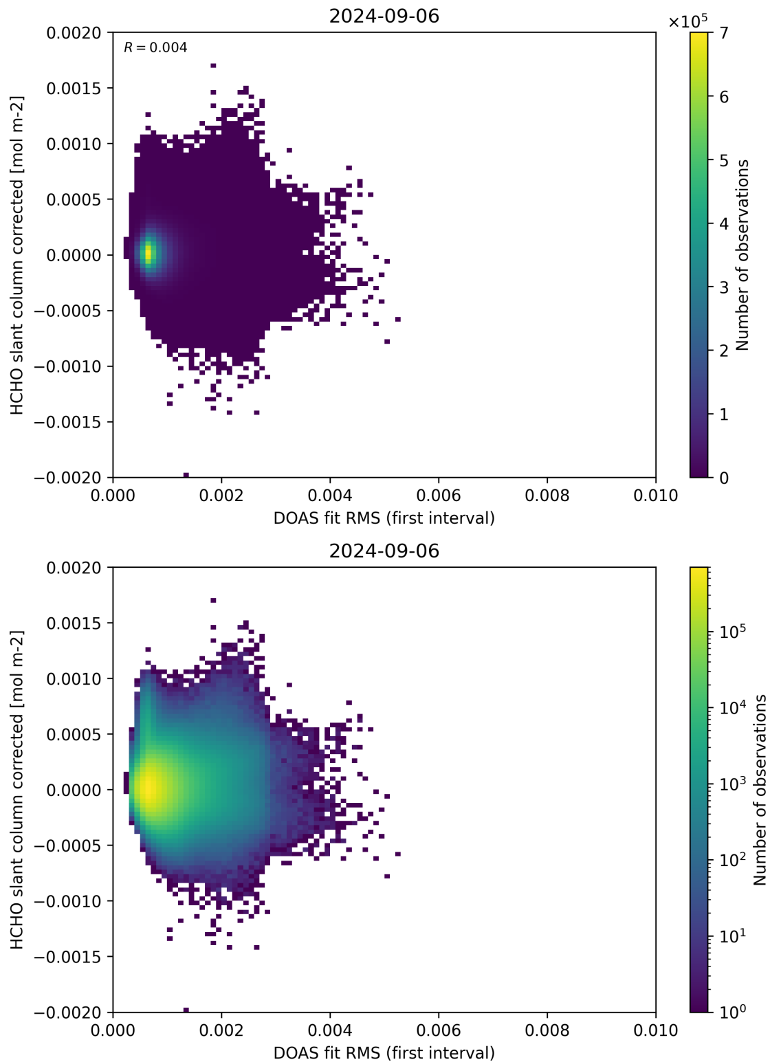
Figure 62: Scatter density plot of “DOAS fit RMS (first interval)” against “HCHO slant column corrected” for 2024-09-06 to 2024-09-07.
