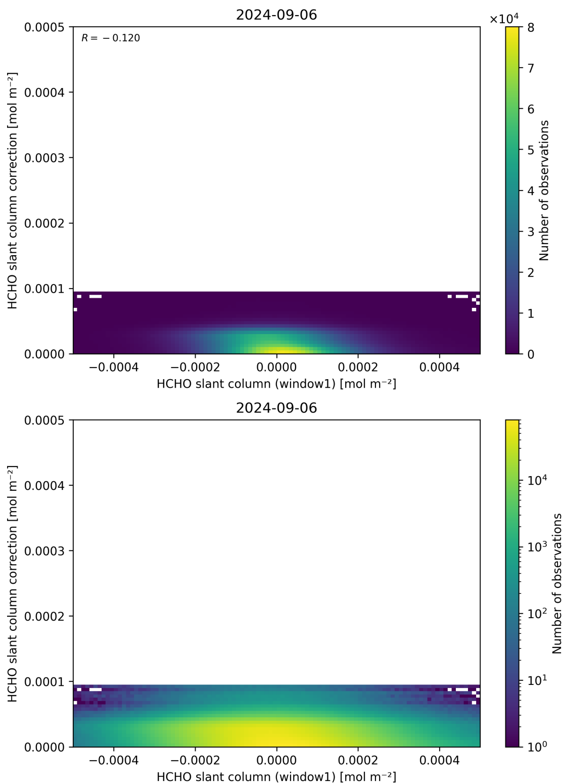
Figure 83: Scatter density plot of “HCHO slant column (window1)” against “HCHO slant column correction” for 2024-09-06 to 2024-09-07.
