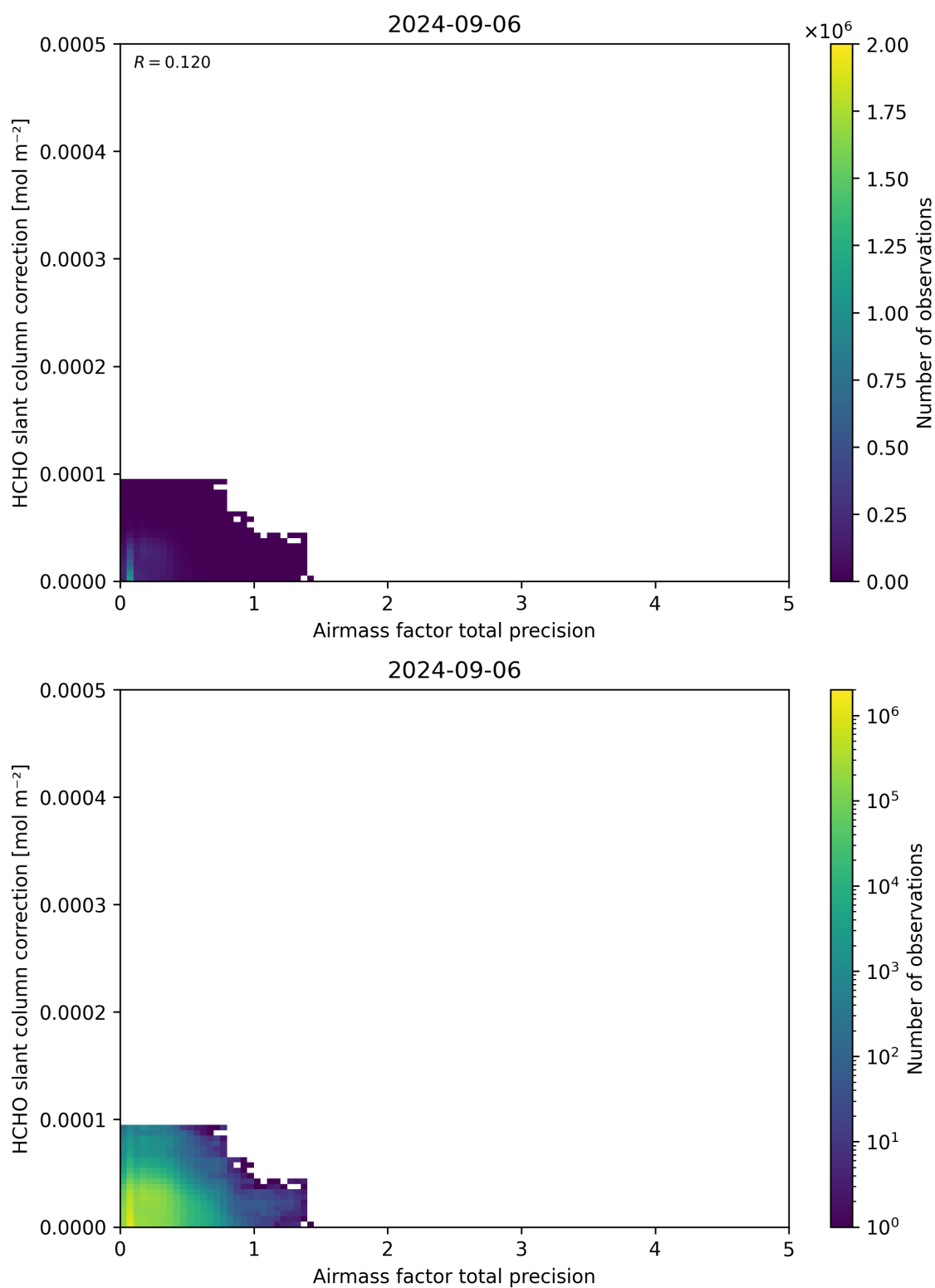
Figure 110: Scatter density plot of “Airmass factor total precision” against “HCHO slant column correction” for 2024-09-06 to 2024-09-07.
