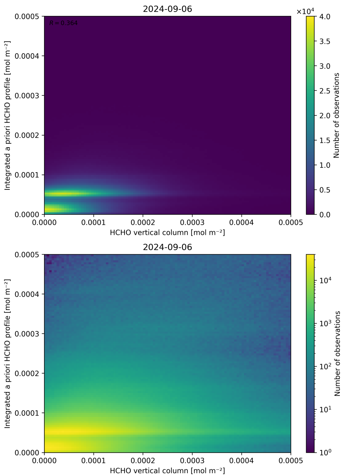
Figure 135: Scatter density plot of “HCHO vertical column” against “Integrated a priori HCHO profile” for 2024-09-06 to 2024-09-07.
