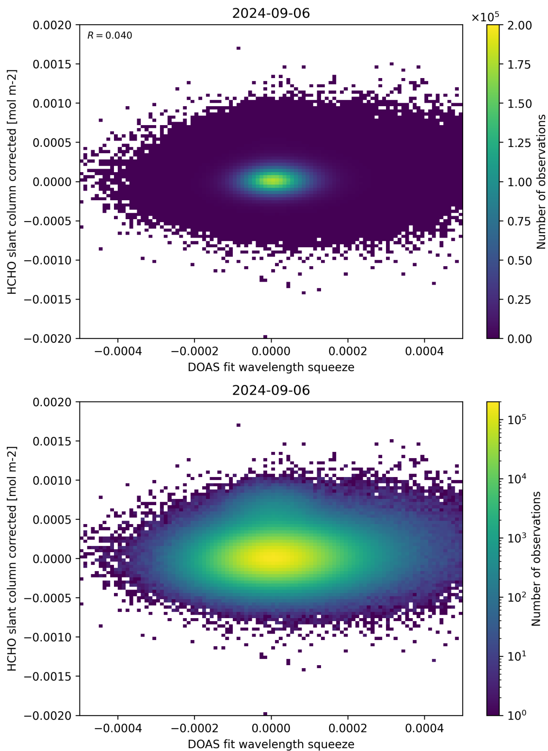
Figure 69: Scatter density plot of “DOAS fit wavelength squeeze” against “HCHO slant column corrected” for 2024-09-06 to 2024-09-07.
