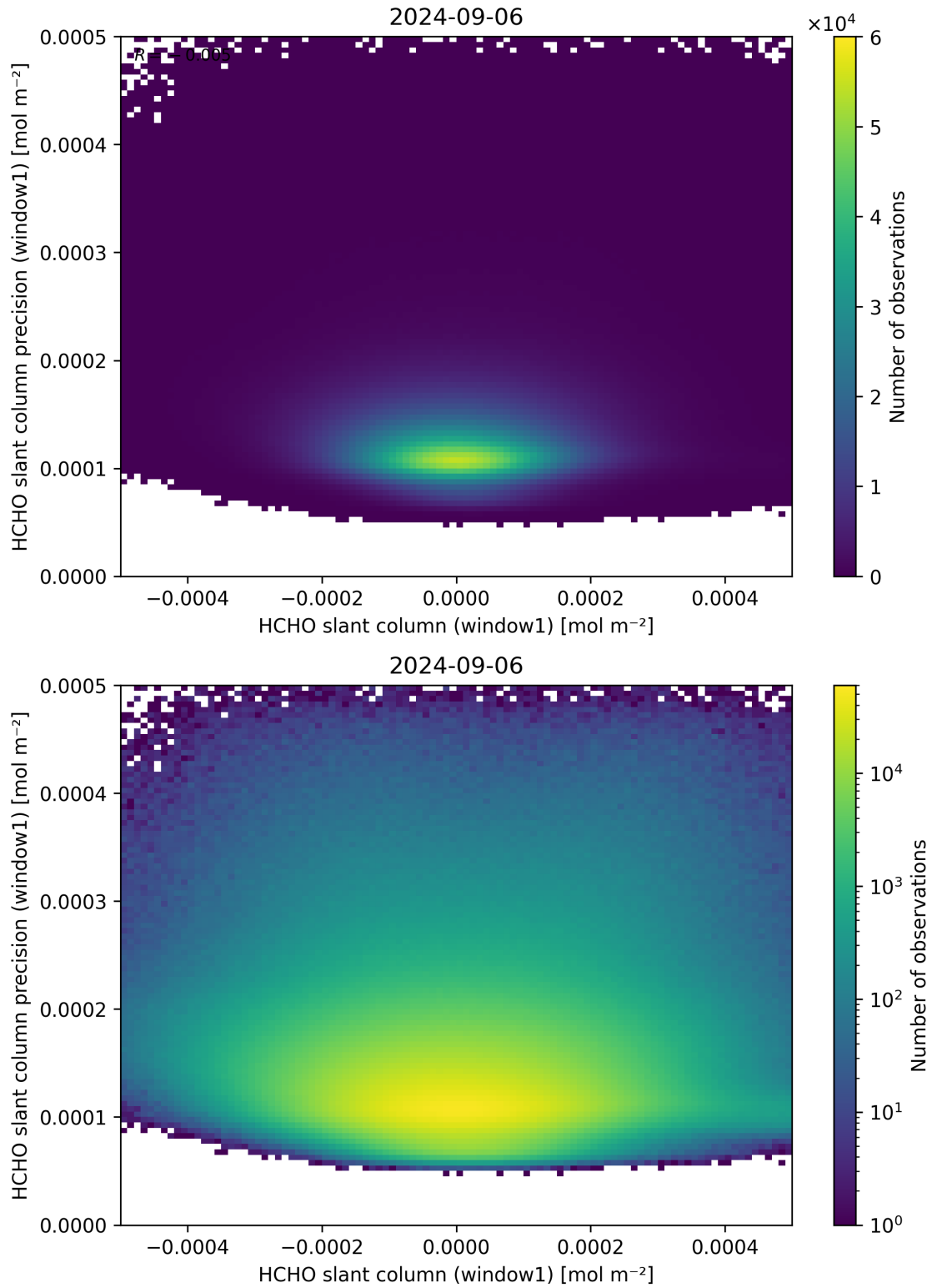
Figure 84: Scatter density plot of “HCHO slant column (window1)” against “HCHO slant column precision (window1)” for 2024-09-06 to 2024-09-07.
