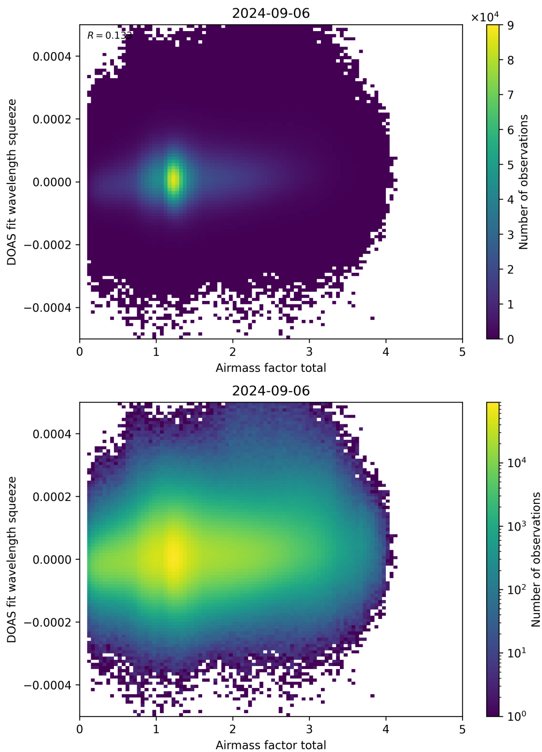
Figure 99: Scatter density plot of “Airmass factor total” against “DOAS fit wavelength squeeze” for 2024-09-06 to 2024-09-07.
