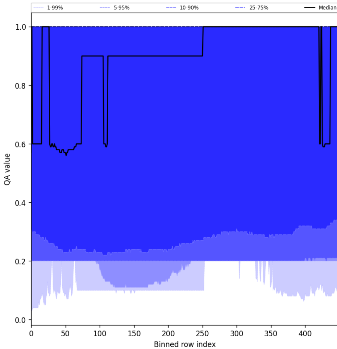
Figure 48: Along track statistics of “QA value” for 2024-09-06 to 2024-09-07
