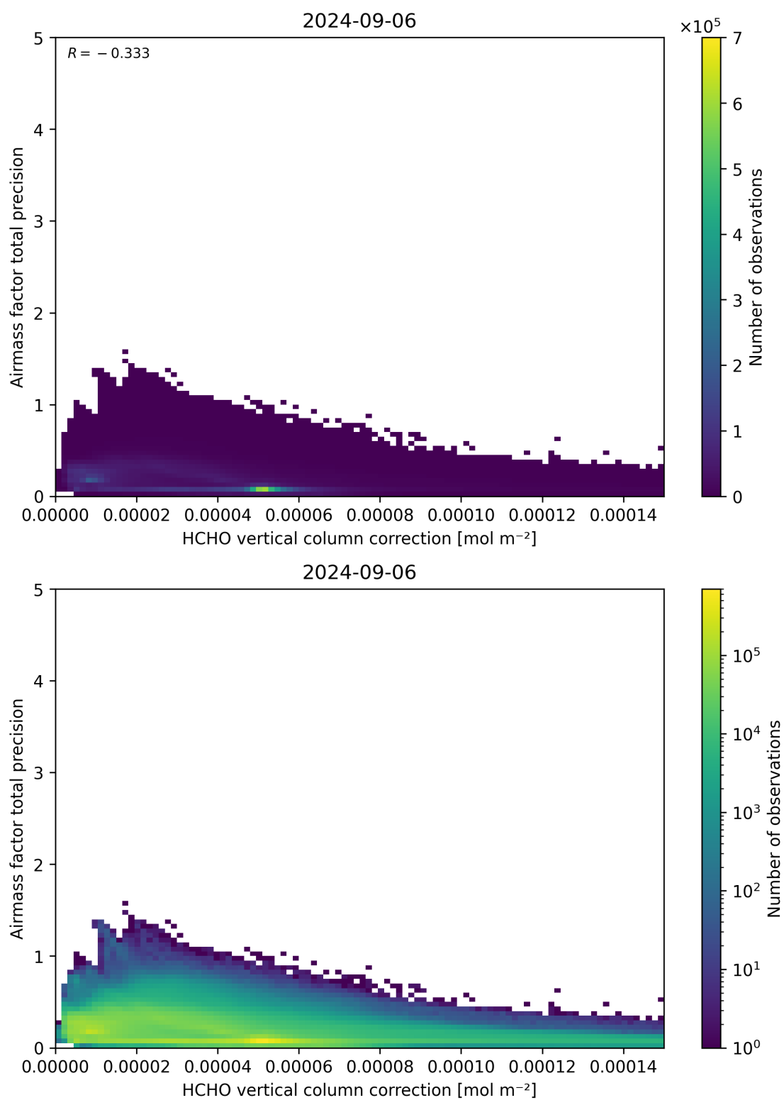
Figure 121: Scatter density plot of “HCHO vertical column correction” against “Airmass factor total precision” for 2024-09-06 to 2024-09-07.
