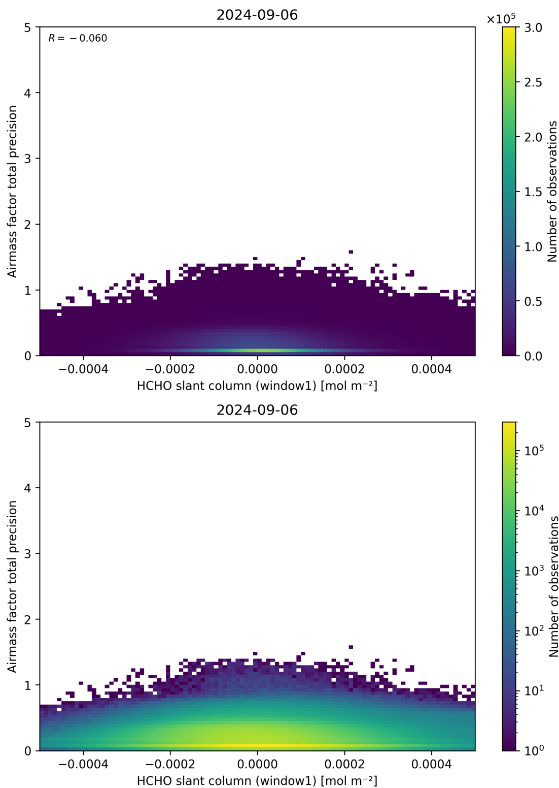
Figure 86: Scatter density plot of “HCHO slant column (window1)” against “Airmass factor total precision” for 2024-09-06 to 2024-09-07.
