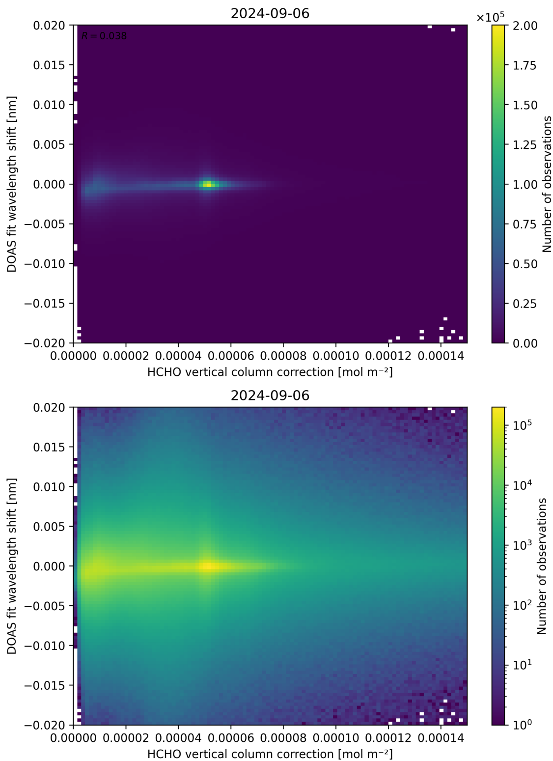
Figure 113: Scatter density plot of “HCHO vertical column correction” against “DOAS fit wavelength shift” for 2024-09-06 to 2024-09-07.
