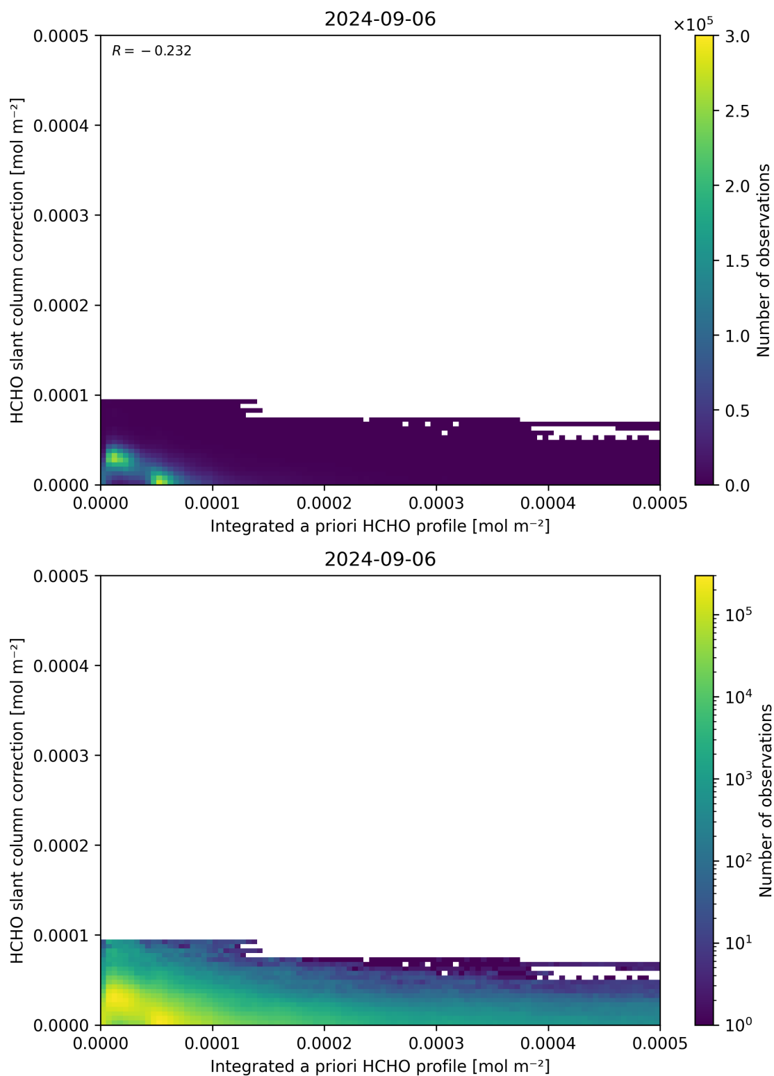
Figure 152: Scatter density plot of “Integrated a priori HCHO profile” against “HCHO slant column correction” for 2024-09-06 to 2024-09-07.
