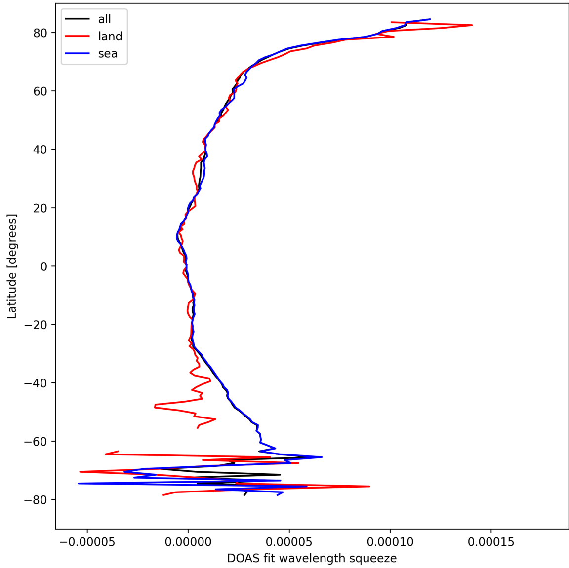
Figure 31: Zonal average of “DOAS fit wavelength squeeze” for 2024-09-06 to 2024-09-07.
