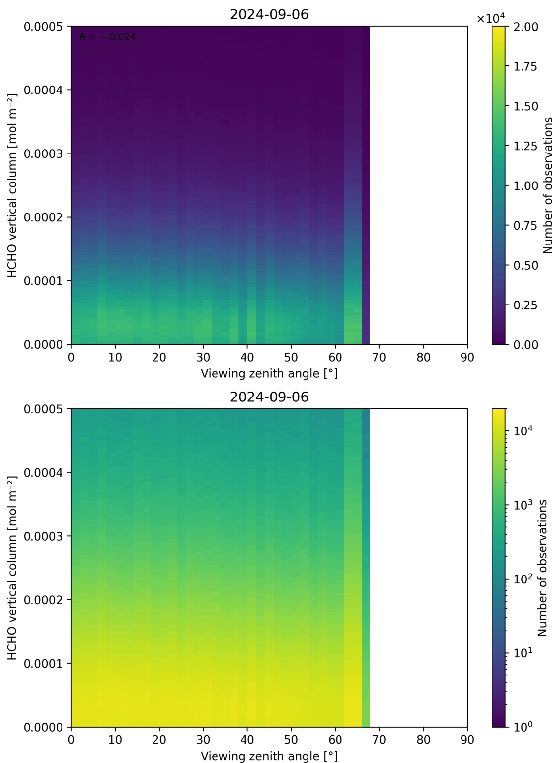
Figure 192: Scatter density plot of “Viewing zenith angle” against “HCHO vertical column” for 2024-09-06 to 2024-09-07.
