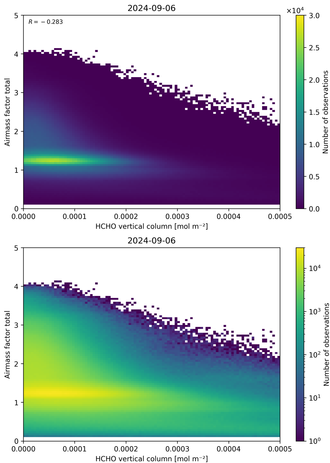
Figure 131: Scatter density plot of “HCHO vertical column” against “Airmass factor total” for 2024-09-06 to 2024-09-07.
