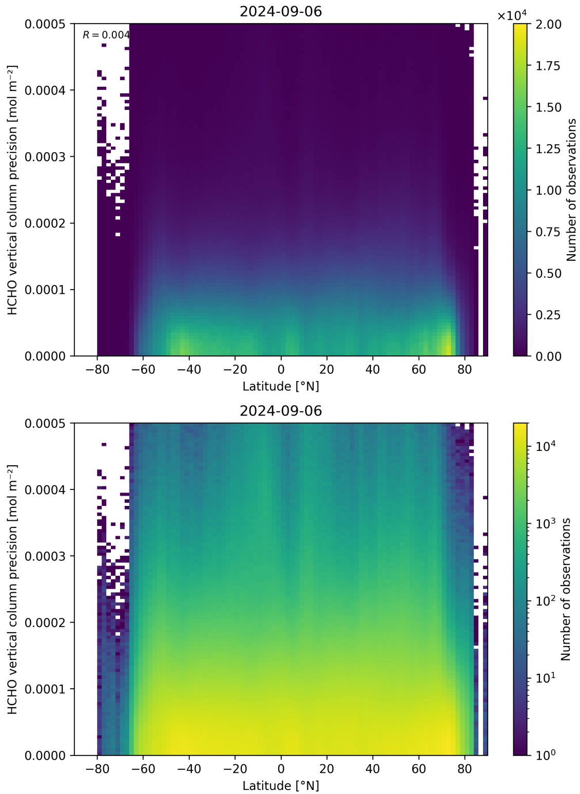
Figure 165: Scatter density plot of “Latitude” against “HCHO vertical column precision” for 2024-09-06 to 2024-09-07.
