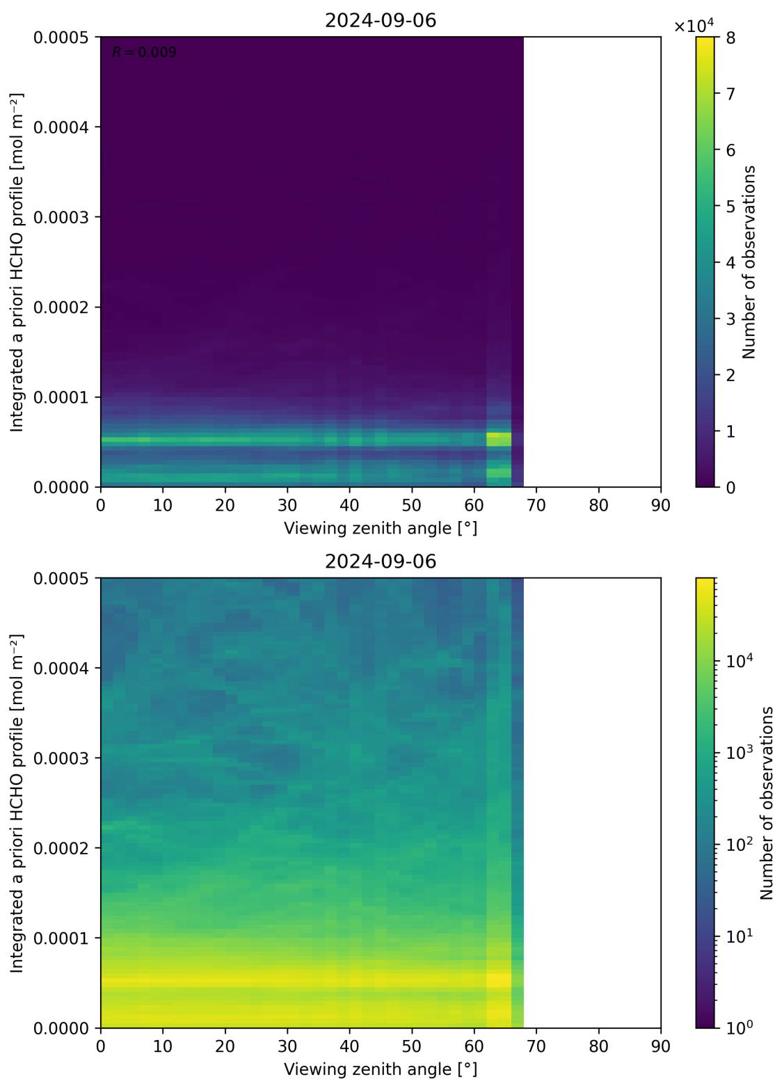
Figure 195: Scatter density plot of “Viewing zenith angle” against “Integrated a priori HCHO profile” for 2024-09-06 to 2024-09-07.
