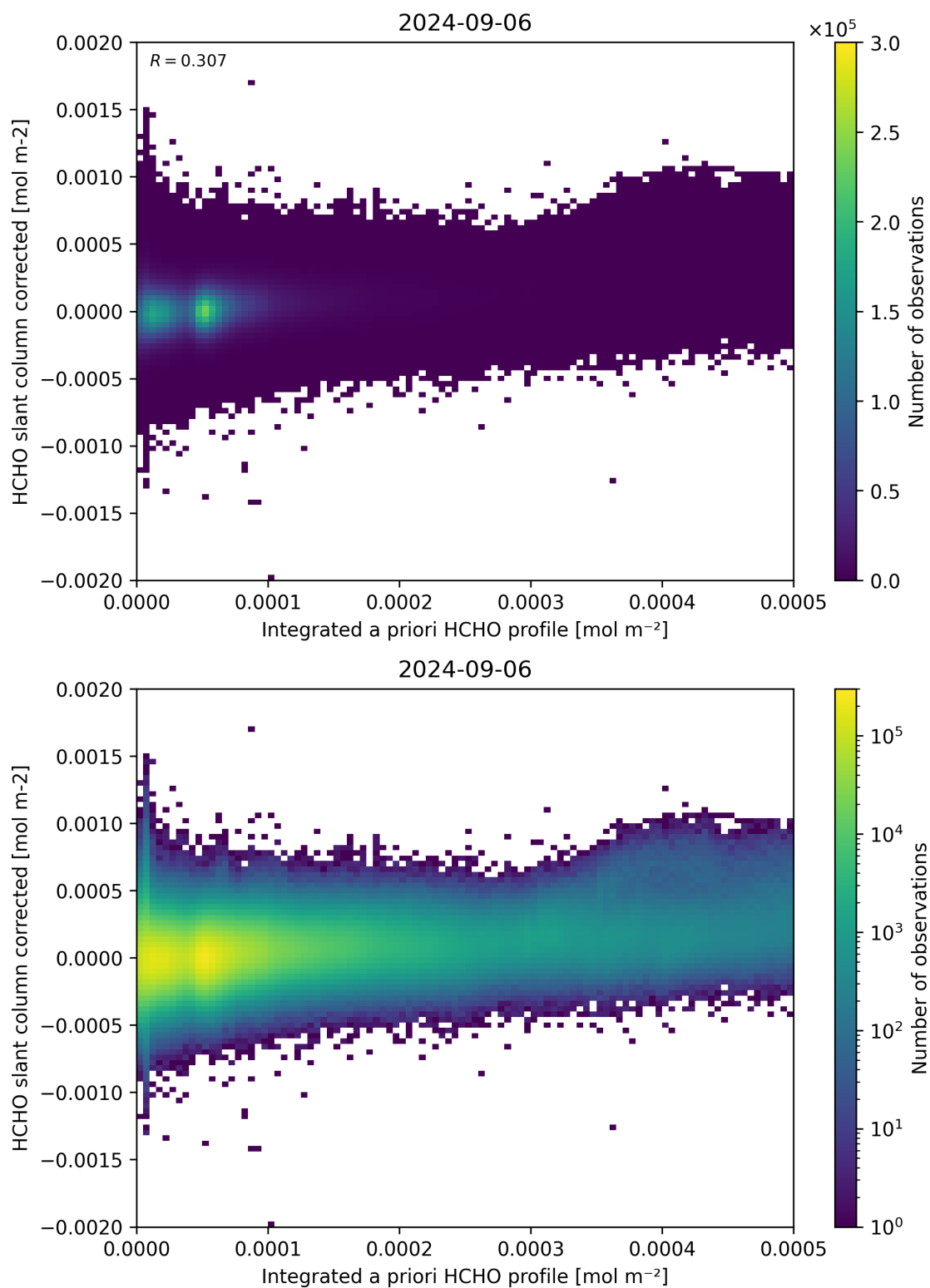
Figure 151: Scatter density plot of “Integrated a priori HCHO profile” against “HCHO slant column corrected” for 2024-09-06 to 2024-09-07.
