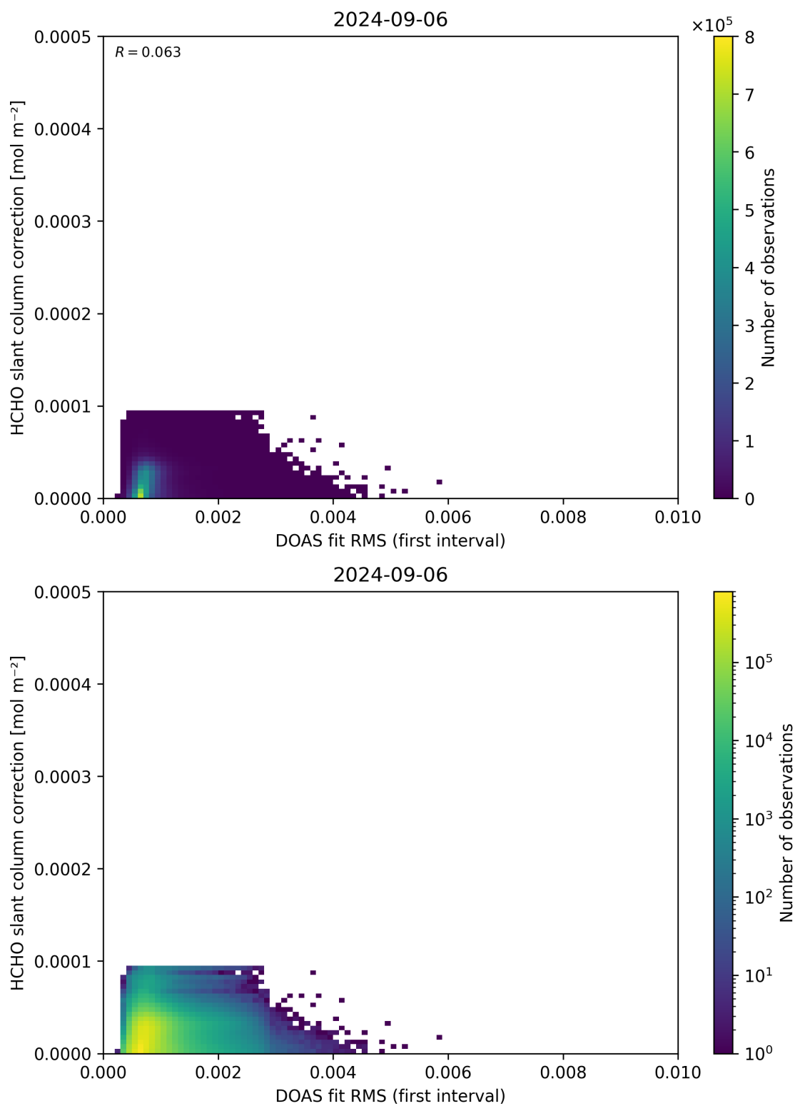
Figure 63: Scatter density plot of “DOAS fit RMS (first interval)” against “HCHO slant column correction” for 2024-09-06 to 2024-09-07.
