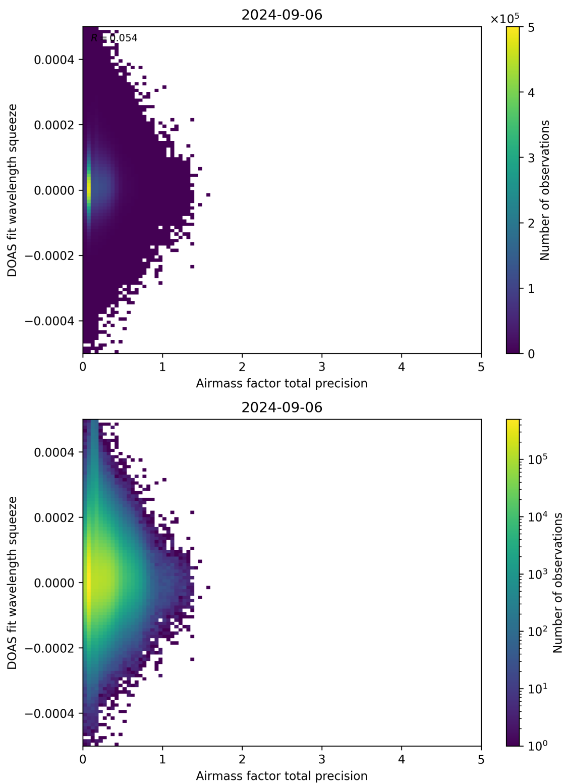
Figure 107: Scatter density plot of “Airmass factor total precision” against “DOAS fit wavelength squeeze” for 2024-09-06 to 2024-09-07.
