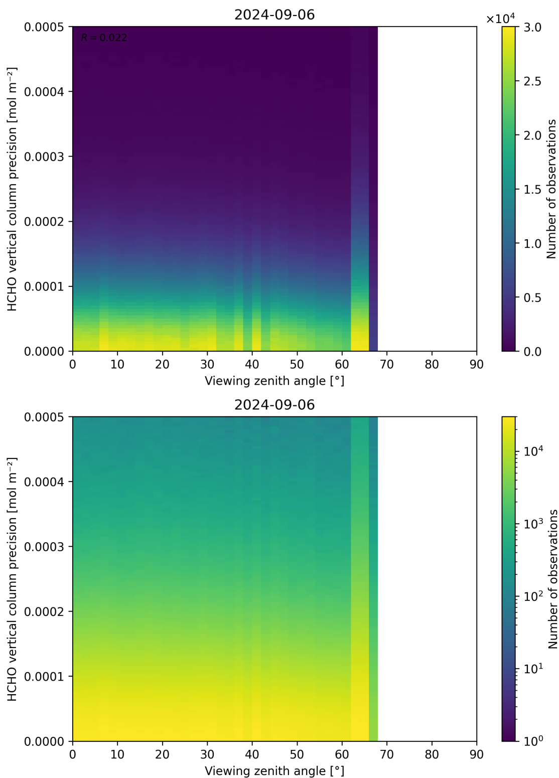
Figure 194: Scatter density plot of “Viewing zenith angle” against “HCHO vertical column precision” for 2024-09-06 to 2024-09-07.
