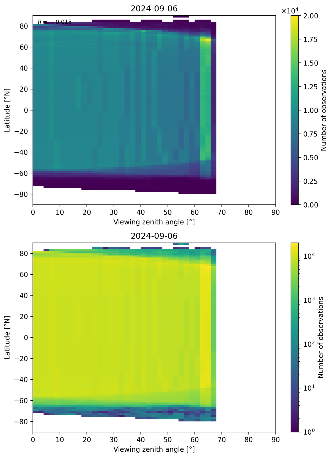
Figure 196: Scatter density plot of “Viewing zenith angle” against “Latitude” for 2024-09-06 to 2024-09-07.
