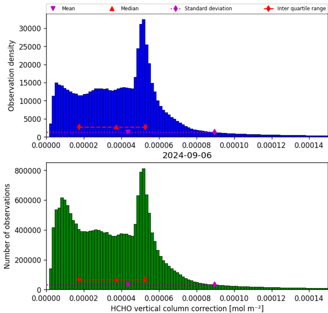
Figure 37: Histogram of “HCHO vertical column correction” for 2024-09-06 to 2024-09-07
