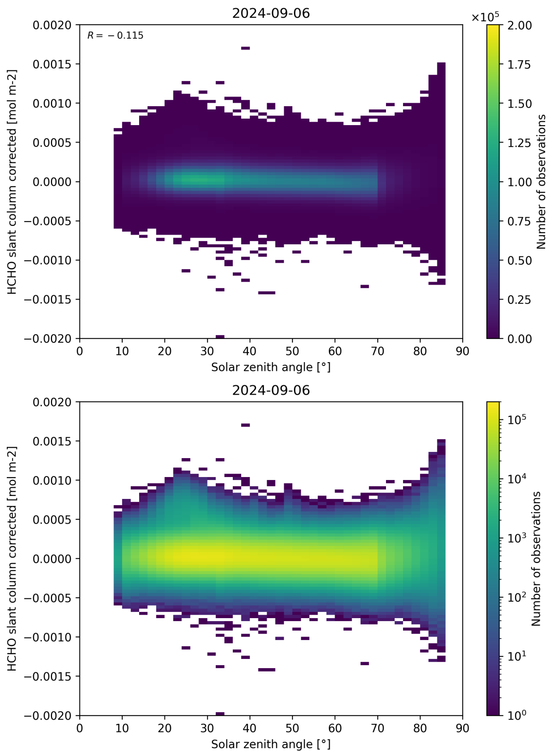
Figure 171: Scatter density plot of “Solar zenith angle” against “HCHO slant column corrected” for 2024-09-06 to 2024-09-07.
