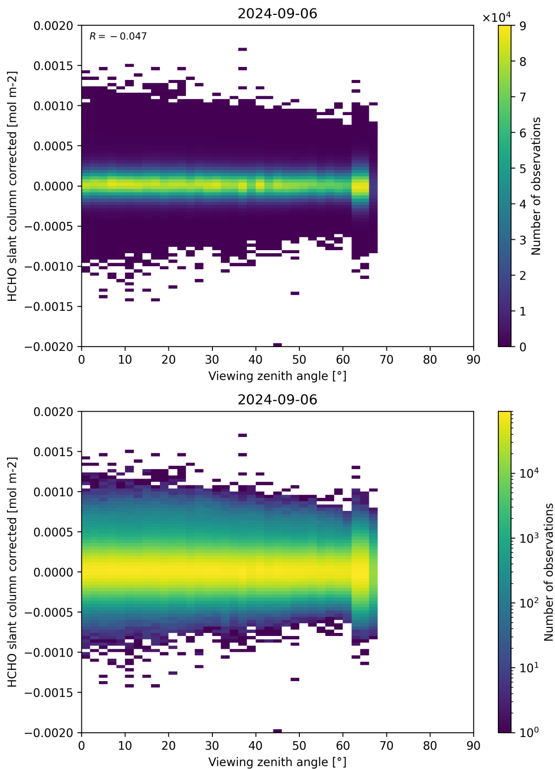
Figure 186: Scatter density plot of “Viewing zenith angle” against “HCHO slant column corrected” for 2024-09-06 to 2024-09-07.
