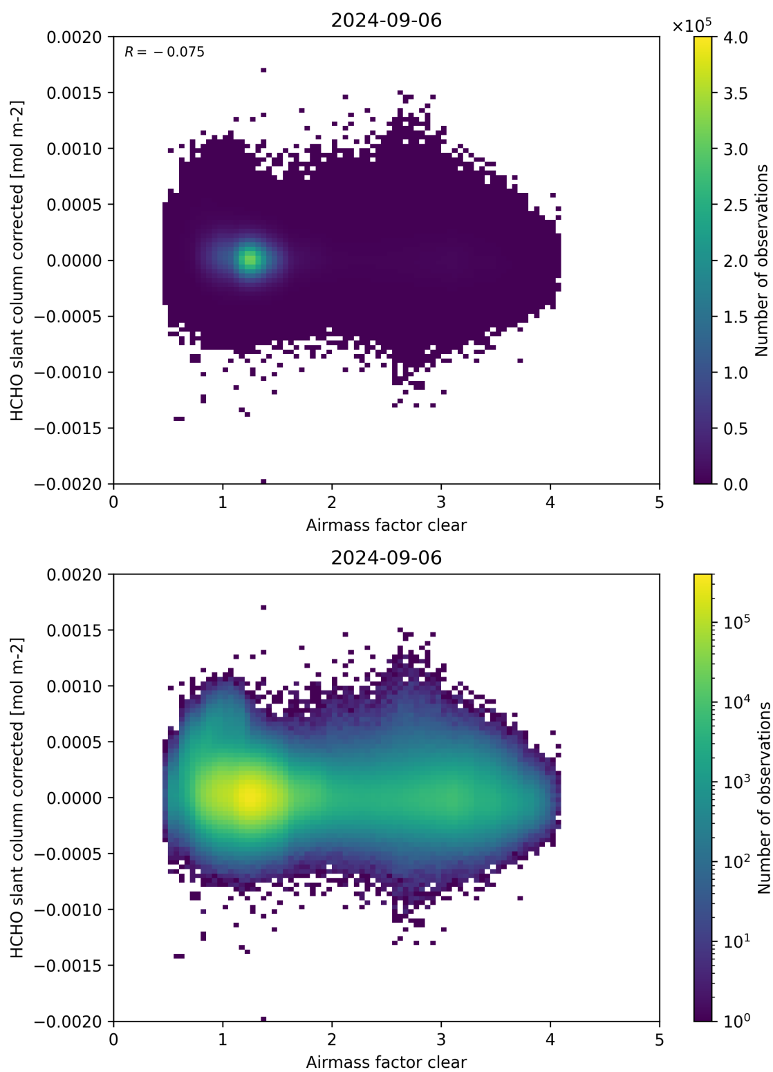
Figure 74: Scatter density plot of “Airmass factor clear” against “HCHO slant column corrected” for 2024-09-06 to 2024-09-07.
