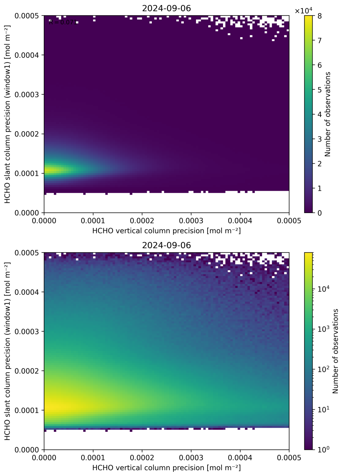
Figure 143: Scatter density plot of “HCHO vertical column precision” against “HCHO slant column precision (window1)” for 2024-09-06 to 2024-09-07.
