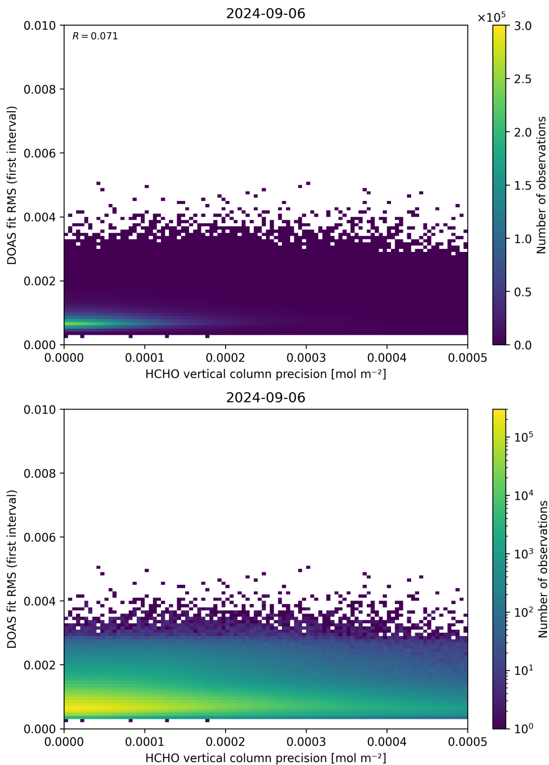
Figure 136: Scatter density plot of “HCHO vertical column precision” against “DOAS fit RMS (first interval)” for 2024-09-06 to 2024-09-07.
