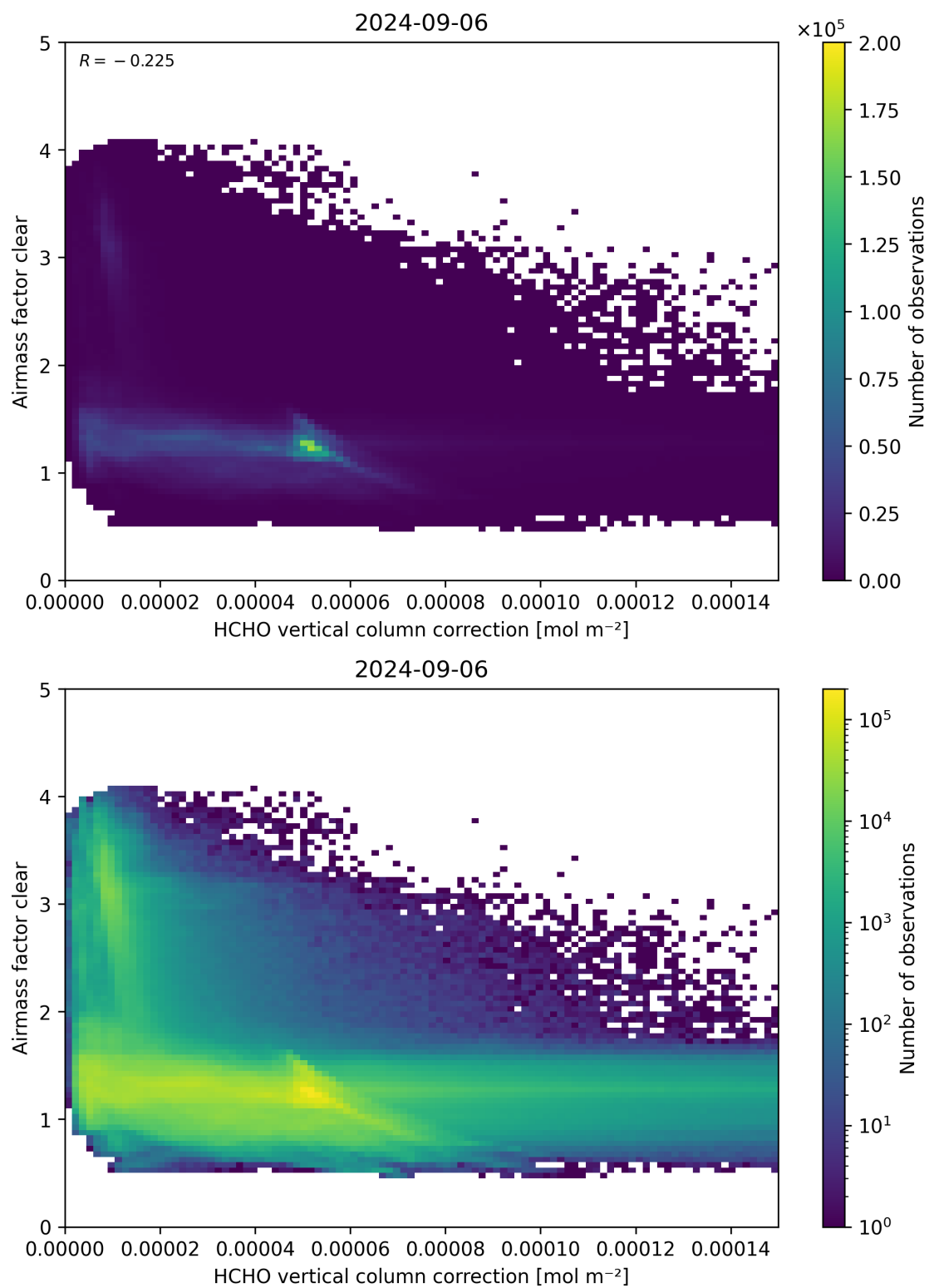
Figure 115: Scatter density plot of “HCHO vertical column correction” against “Airmass factor clear” for 2024-09-06 to 2024-09-07.
