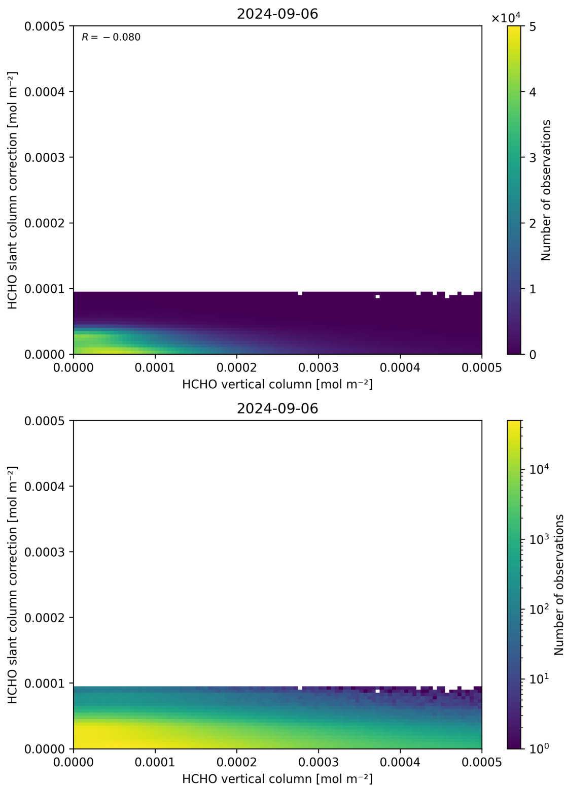
Figure 128: Scatter density plot of “HCHO vertical column” against “HCHO slant column correction” for 2024-09-06 to 2024-09-07.
