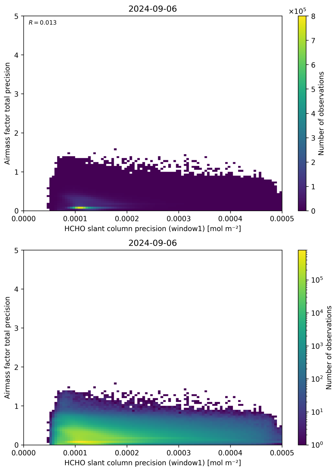
Figure 95: Scatter density plot of “HCHO slant column precision (window1)” against “Airmass factor total precision” for 2024-09-06 to 2024-09-07.
