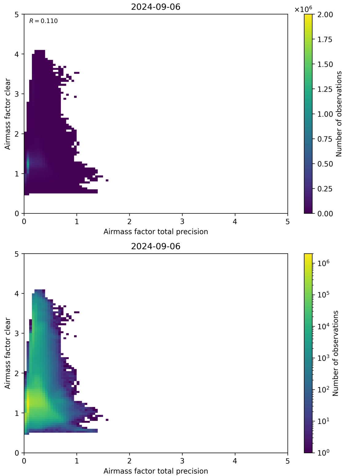
Figure 108: Scatter density plot of “Airmass factor total precision” against “Airmass factor clear” for 2024-09-06 to 2024-09-07.
