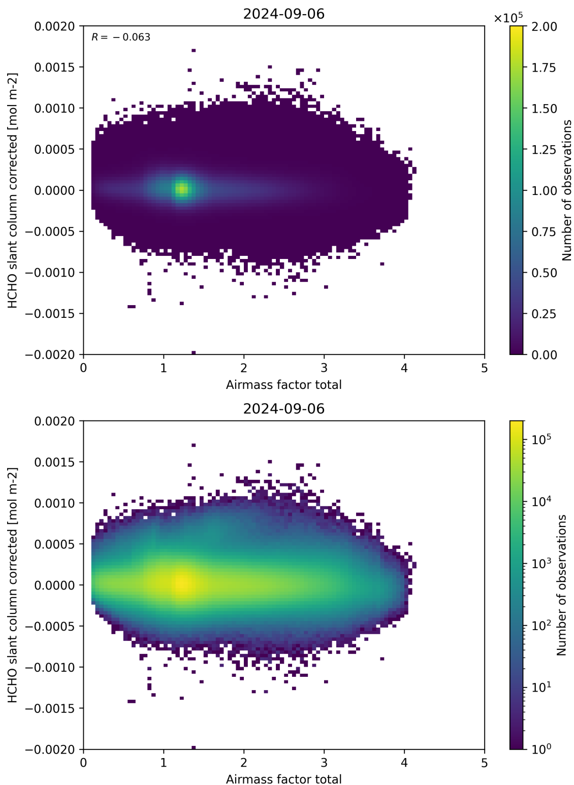
Figure 101: Scatter density plot of “Airmass factor total” against “HCHO slant column corrected” for 2024-09-06 to 2024-09-07.
