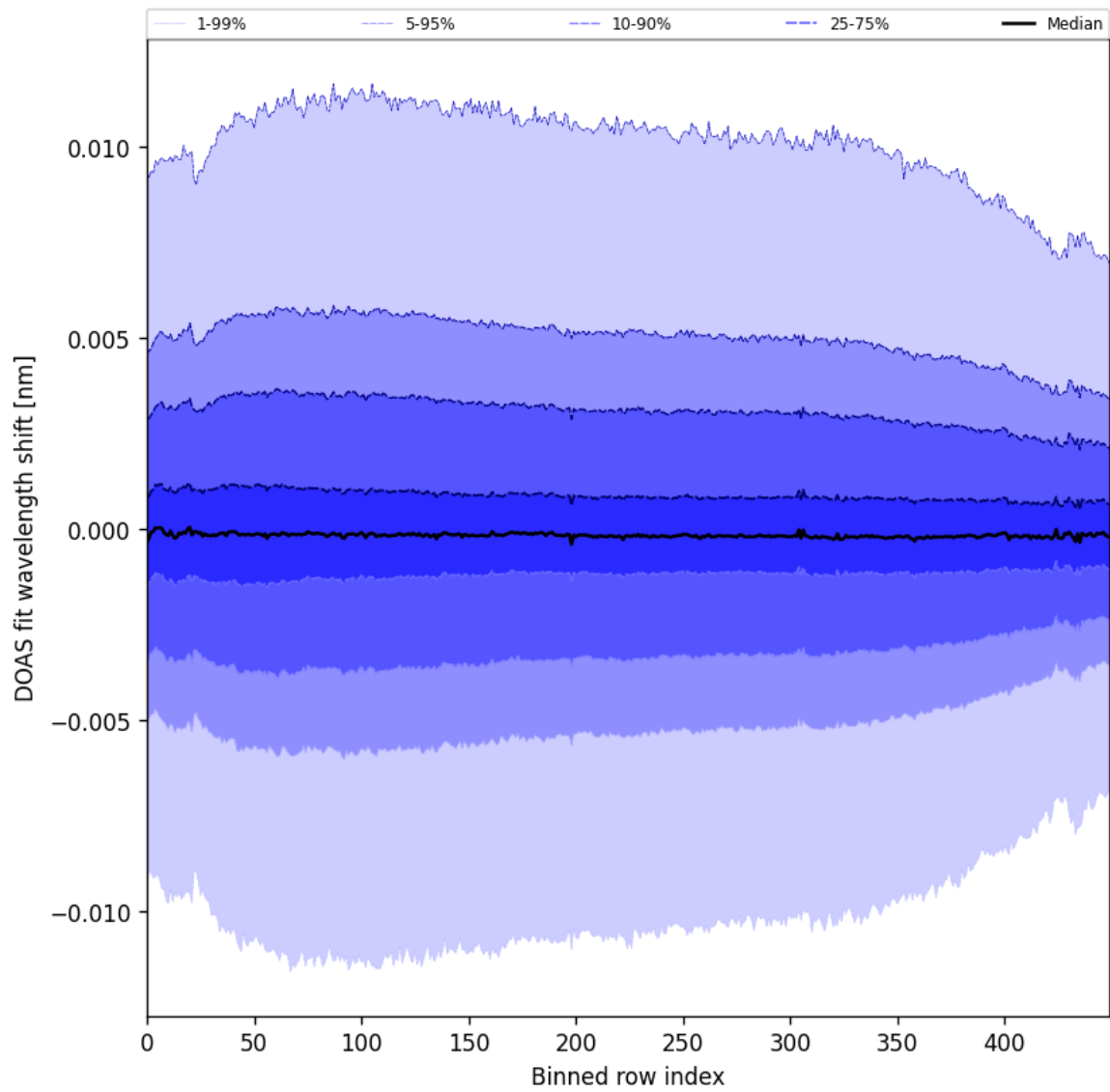
Figure 58: Along track statistics of “DOAS fit wavelength shift” for 2024-09-06 to 2024-09-07
