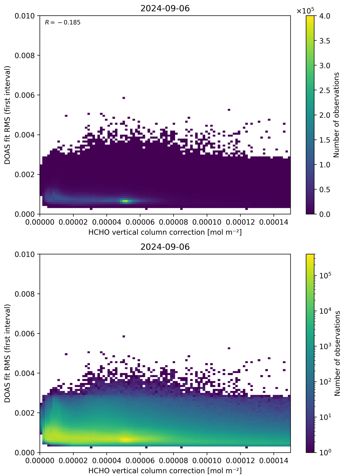
Figure 112: Scatter density plot of “HCHO vertical column correction” against “DOAS fit RMS (first interval)” for 2024-09-06 to 2024-09-07.
