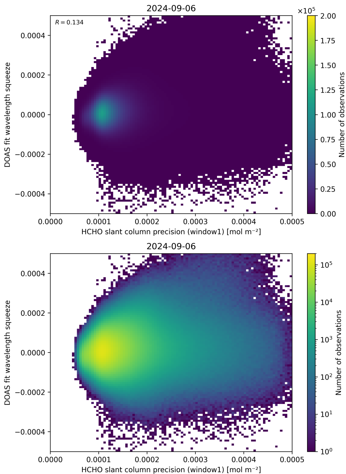
Figure 90: Scatter density plot of “HCHO slant column precision (window1)” against “DOAS fit wavelength squeeze” for 2024-09-06 to 2024-09-07.
