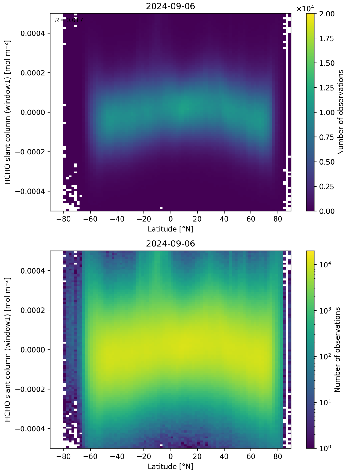
Figure 159: Scatter density plot of “Latitude” against “HCHO slant column (window1)” for 2024-09-06 to 2024-09-07.
