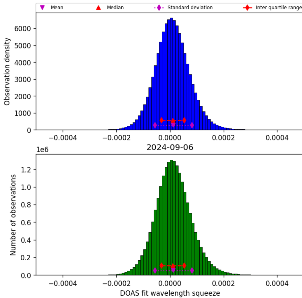
Figure 45: Histogram of “DOAS fit wavelength squeeze” for 2024-09-06 to 2024-09-07
