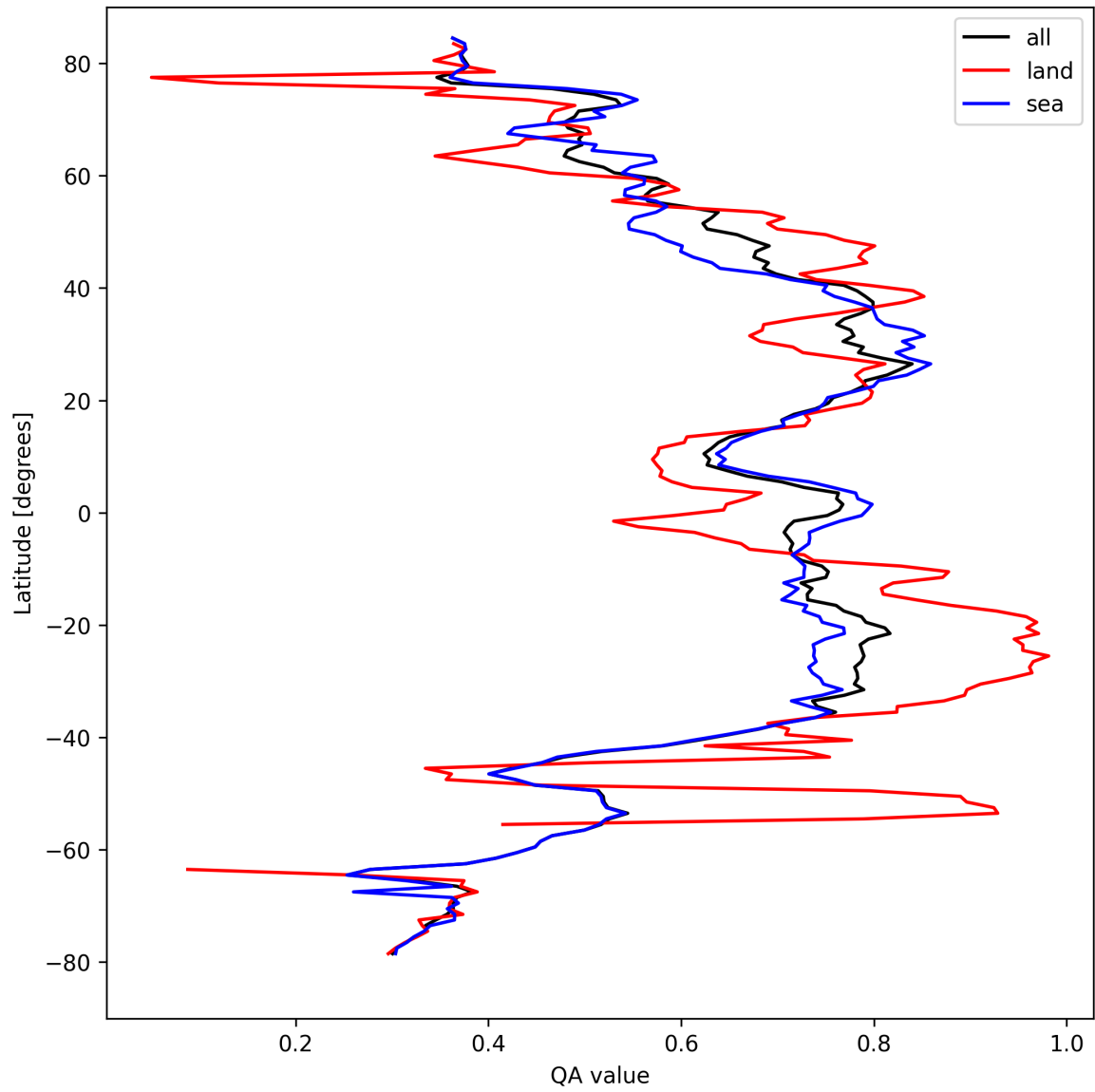
Figure 20: Zonal average of “QA value” for 2024-09-06 to 2024-09-07.
