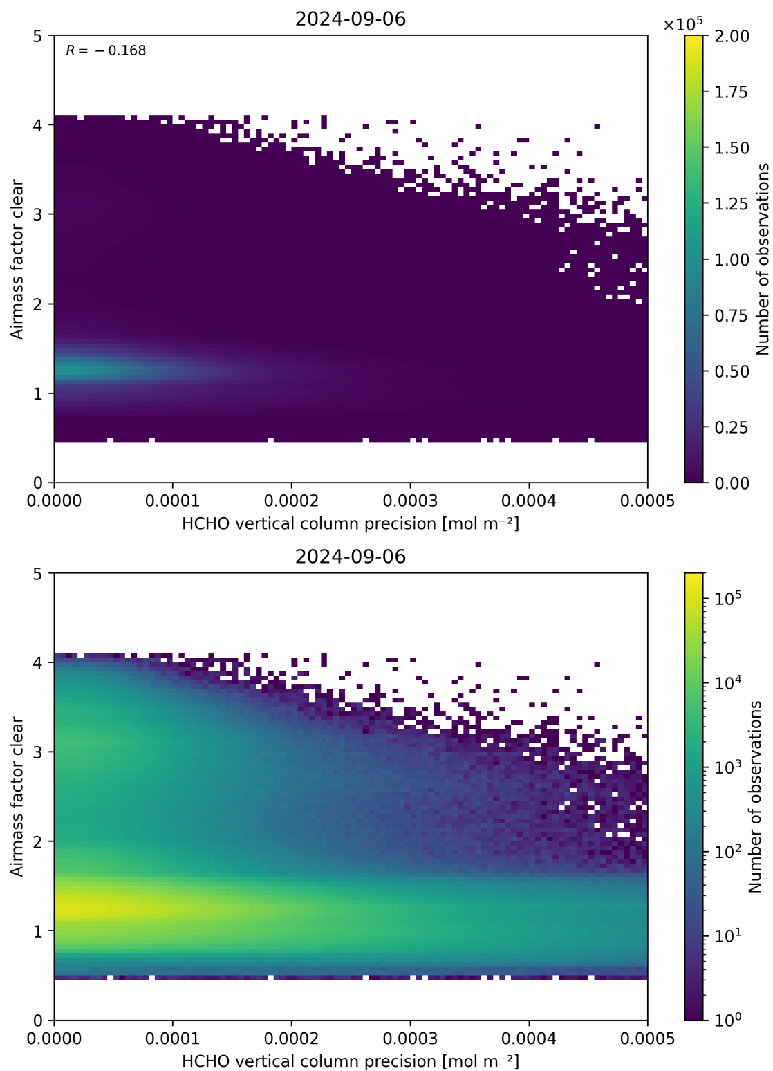
Figure 139: Scatter density plot of “HCHO vertical column precision” against “Airmass factor clear” for 2024-09-06 to 2024-09-07.
