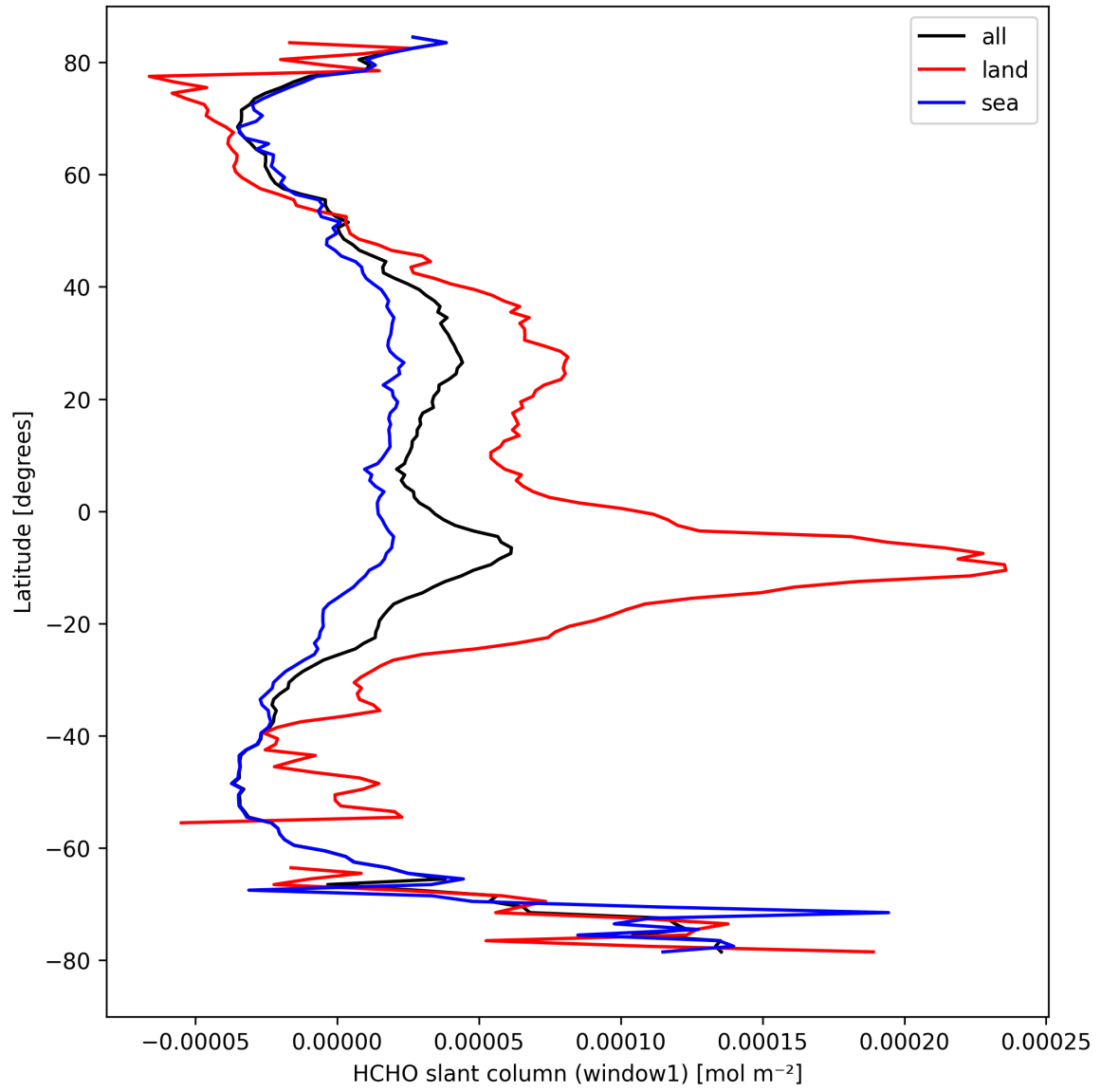
Figure 24: Zonal average of “HCHO slant column (window1)” for 2024-09-06 to 2024-09-07.
