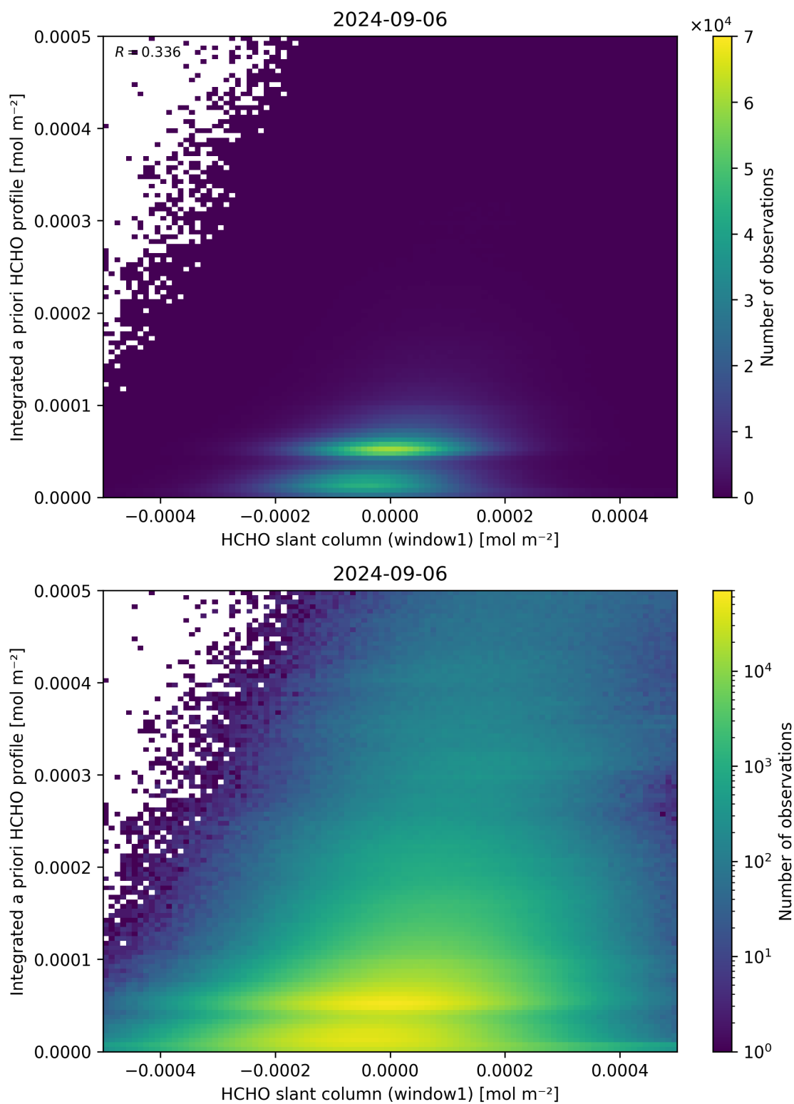
Figure 87: Scatter density plot of “HCHO slant column (window1)” against “Integrated a priori HCHO profile” for 2024-09-06 to 2024-09-07.
