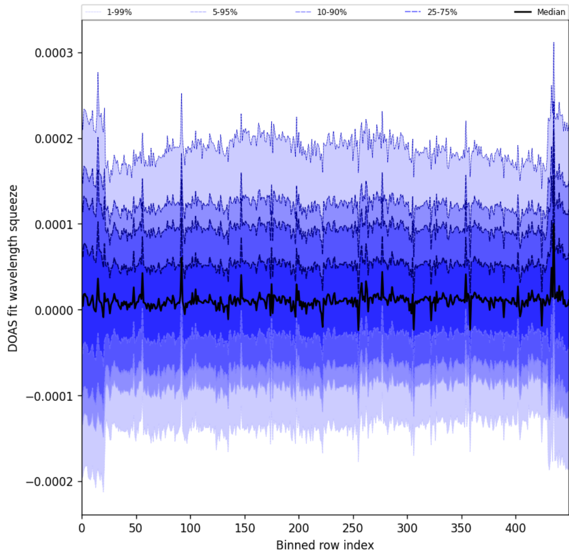
Figure 59: Along track statistics of “DOAS fit wavelength squeeze” for 2024-09-06 to 2024-09-07
