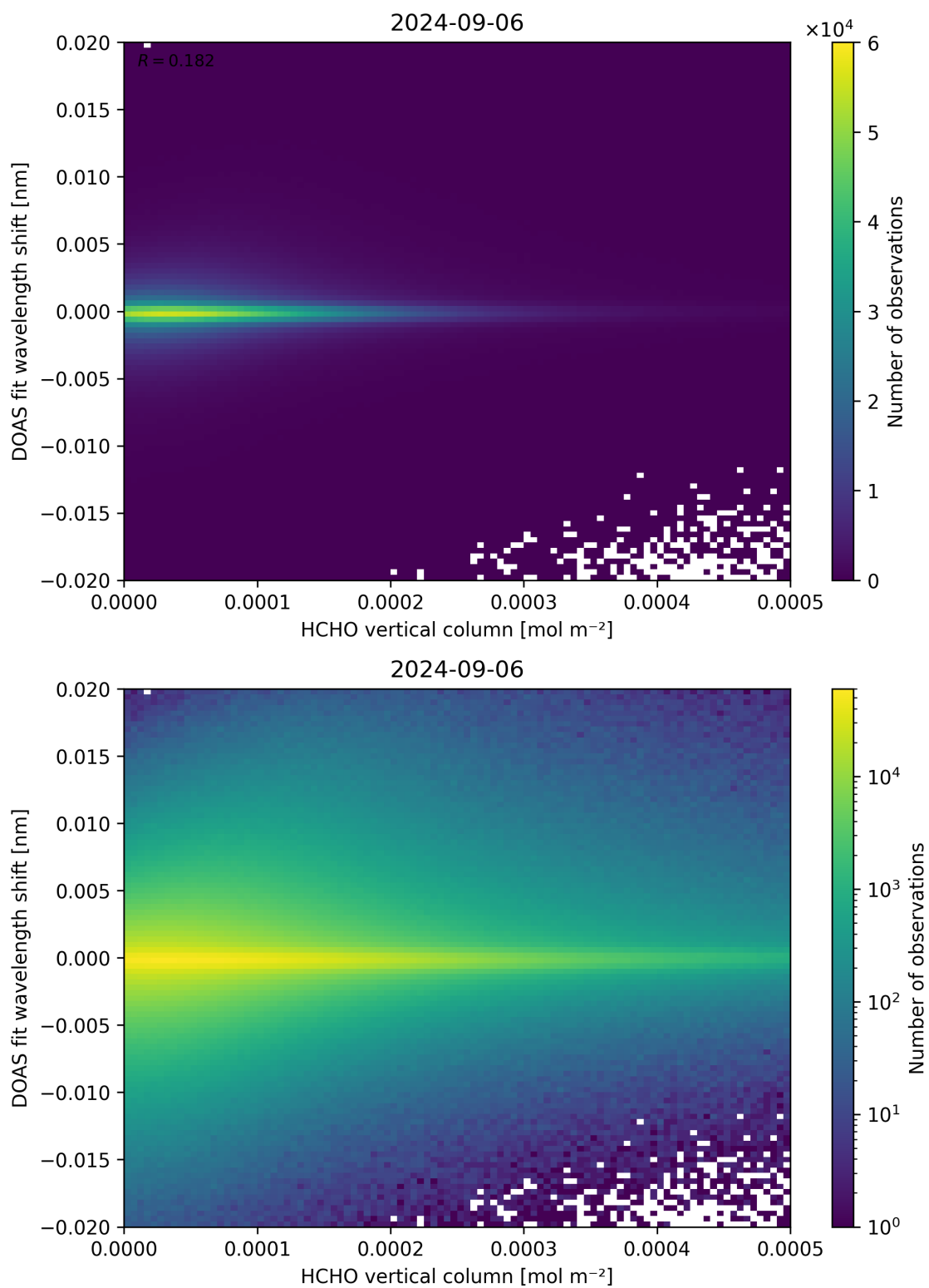
Figure 124: Scatter density plot of “HCHO vertical column” against “DOAS fit wavelength shift” for 2024-09-06 to 2024-09-07.
