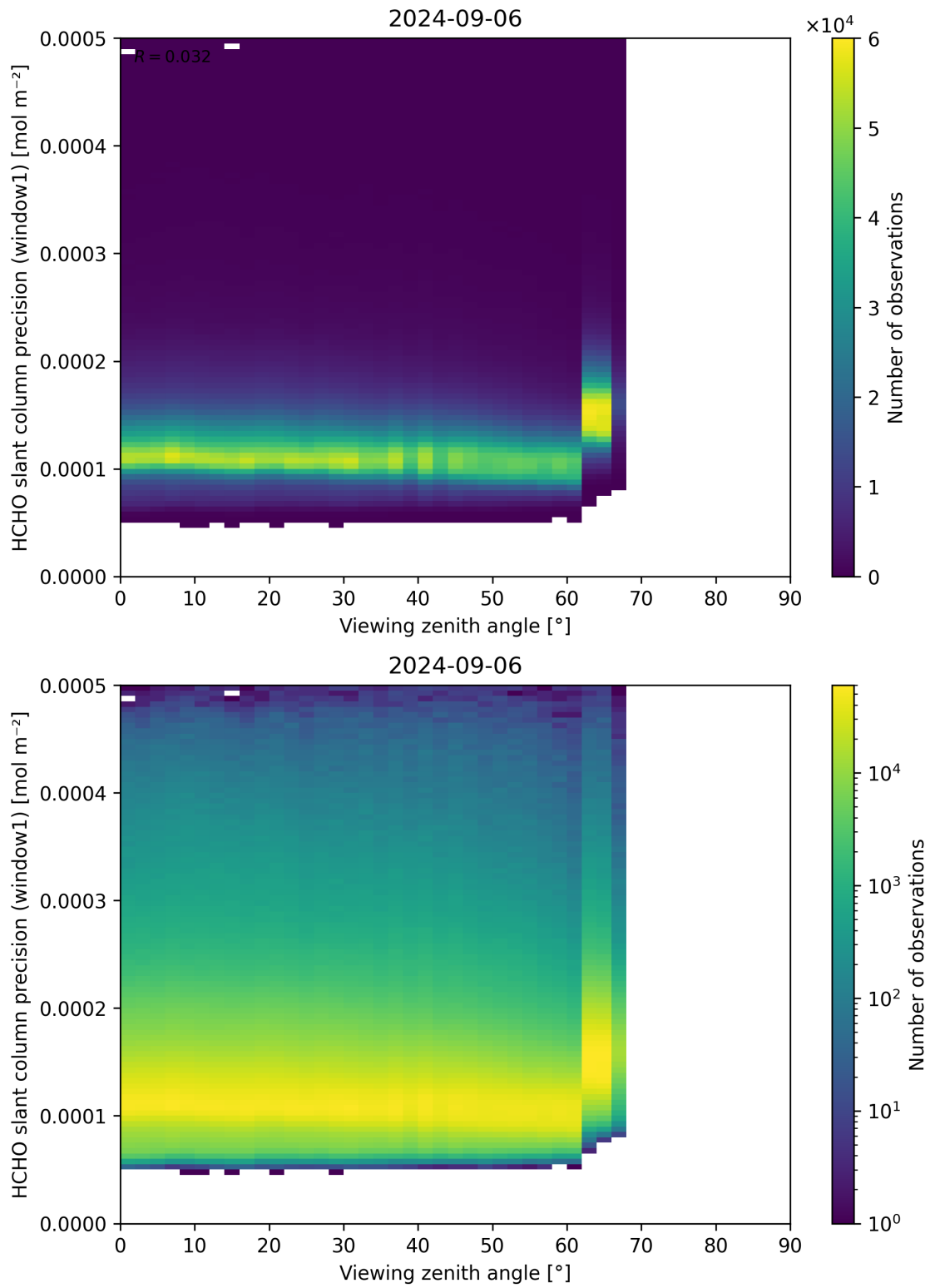
Figure 189: Scatter density plot of “Viewing zenith angle” against “HCHO slant column precision (window1)” for 2024-09-06 to 2024-09-07.
