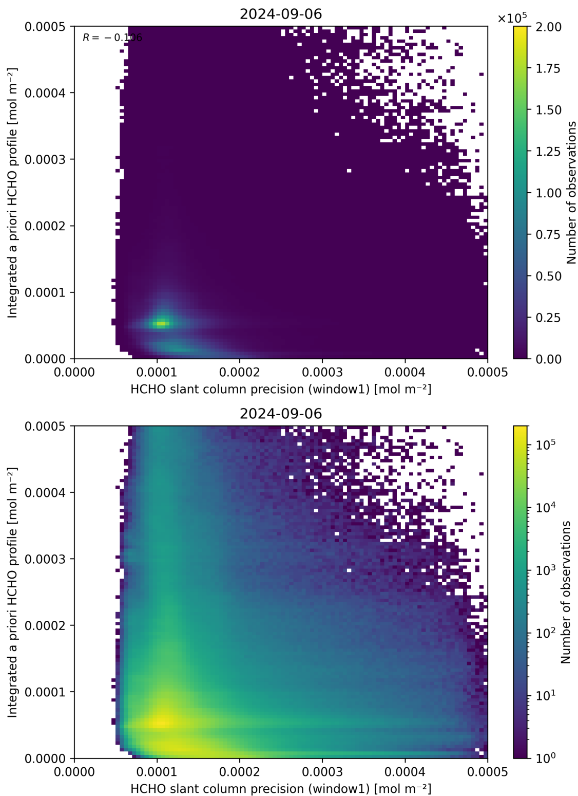
Figure 96: Scatter density plot of “HCHO slant column precision (window1)” against “Integrated a priori HCHO profile” for 2024-09-06 to 2024-09-07.
