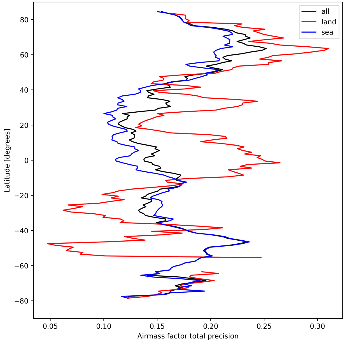
Figure 27: Zonal average of “Airmass factor total precision” for 2024-09-06 to 2024-09-07.
