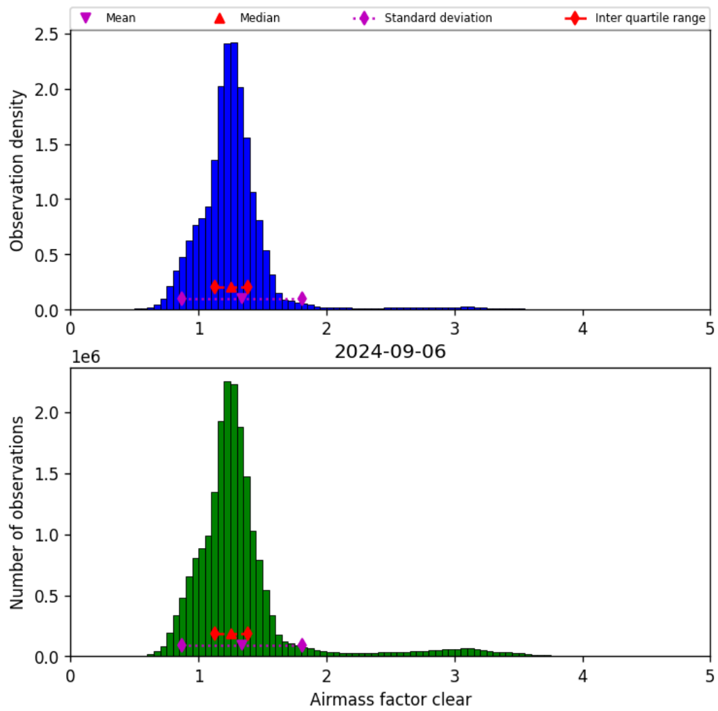
Figure 42: Histogram of “Airmass factor clear” for 2024-09-06 to 2024-09-07
