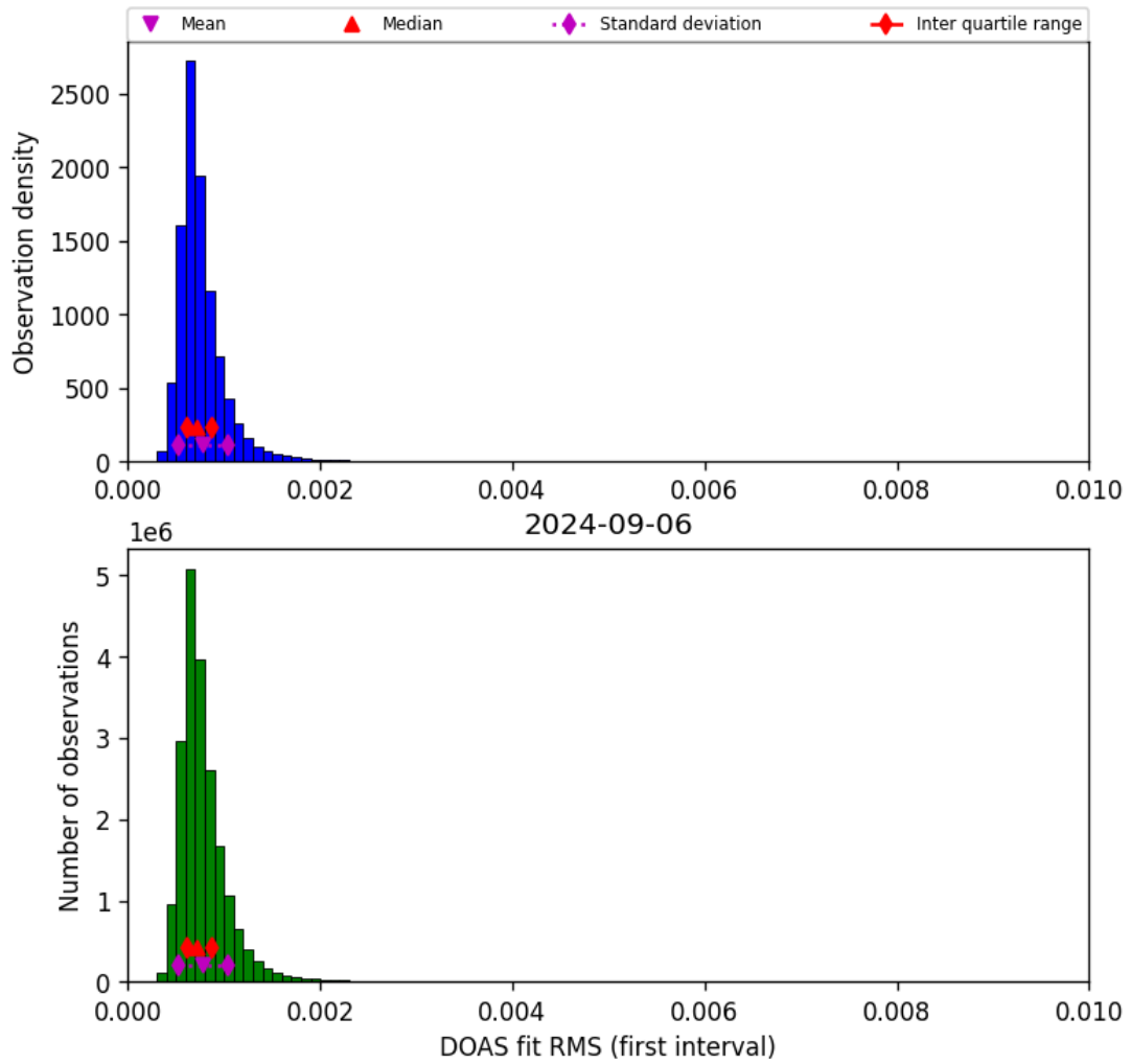
Figure 46: Histogram of “DOAS fit RMS (first interval)” for 2024-09-06 to 2024-09-07
