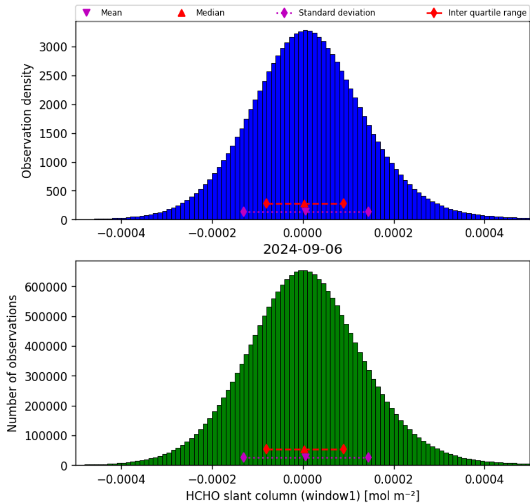
Figure 38: Histogram of “HCHO slant column (window1)” for 2024-09-06 to 2024-09-07
