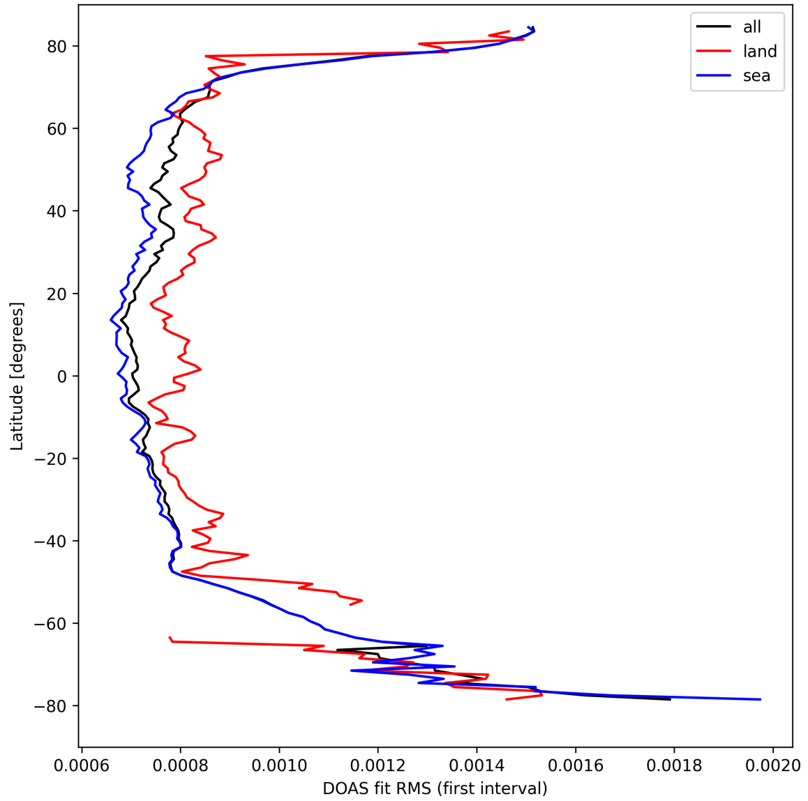
Figure 32: Zonal average of “DOAS fit RMS (first interval)” for 2024-09-06 to 2024-09-07.
