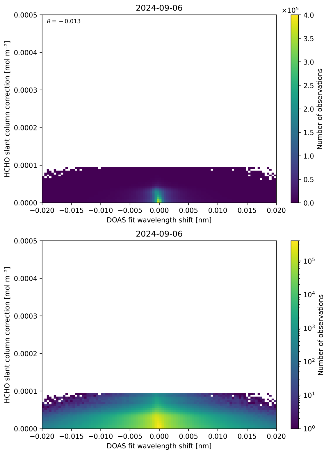
Figure 67: Scatter density plot of “DOAS fit wavelength shift” against “HCHO slant column correction” for 2024-09-06 to 2024-09-07.
