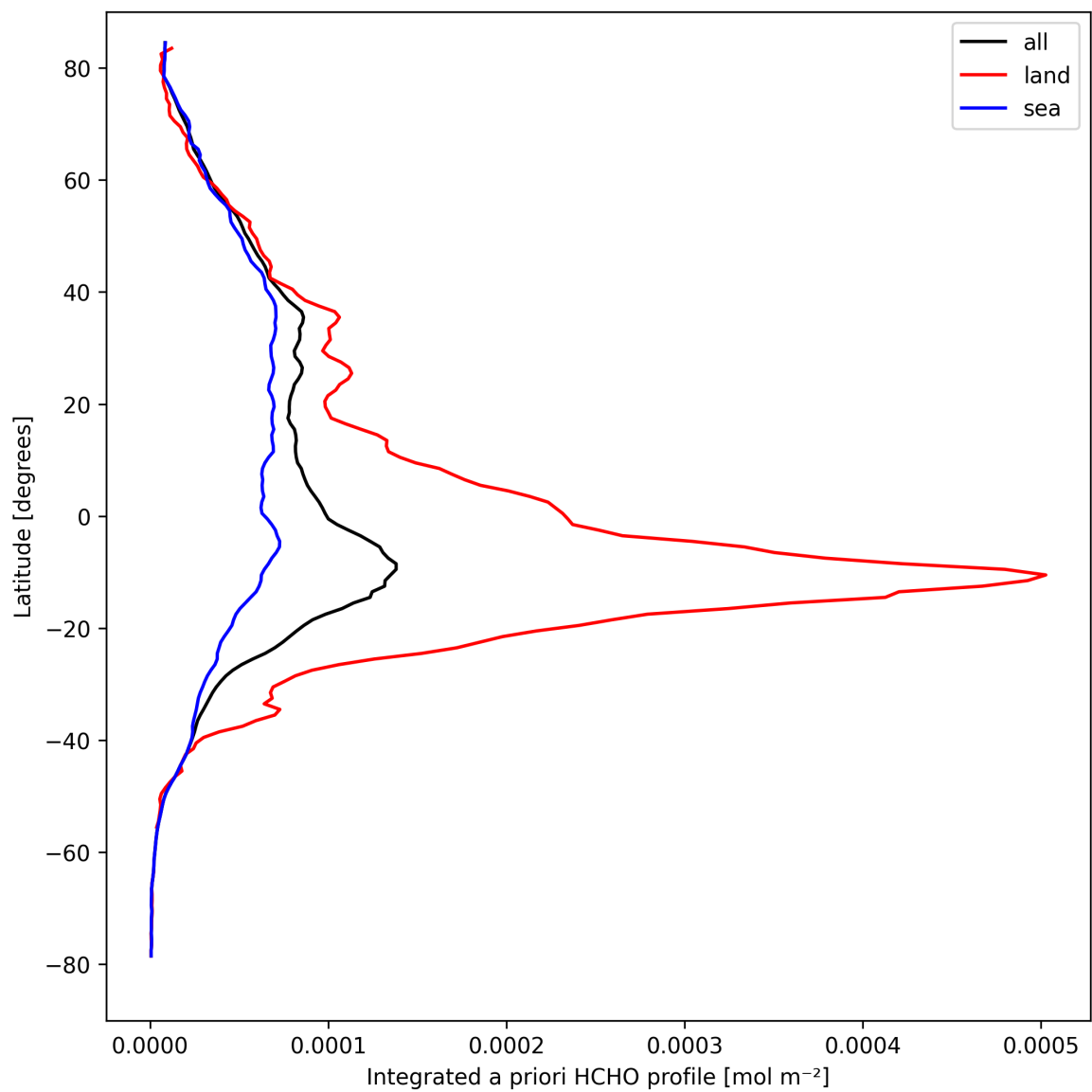
Figure 29: Zonal average of “Integrated a priori HCHO profile” for 2024-09-06 to 2024-09-07.
