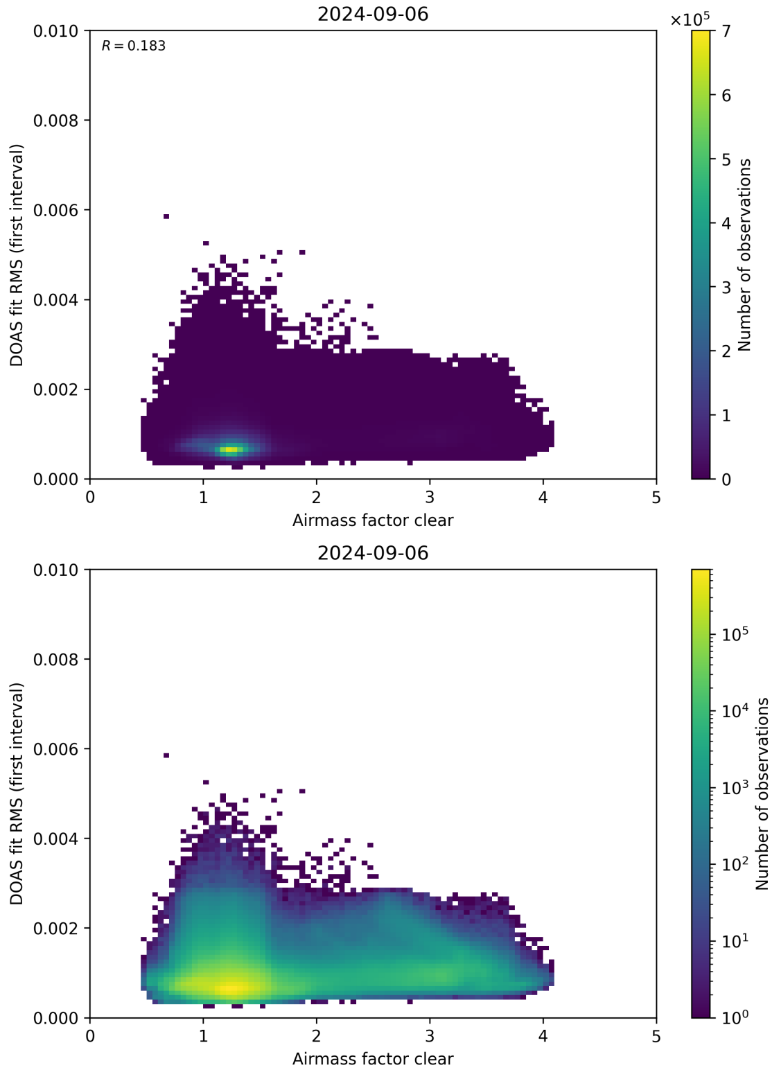
Figure 71: Scatter density plot of “Airmass factor clear” against “DOAS fit RMS (first interval)” for 2024-09-06 to 2024-09-07.
