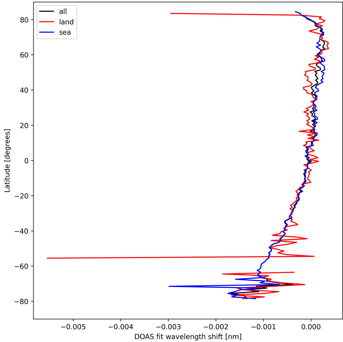
Figure 30: Zonal average of "DOAS fit wavelength shift" for 2024-09-06 to 2024-09-07.
