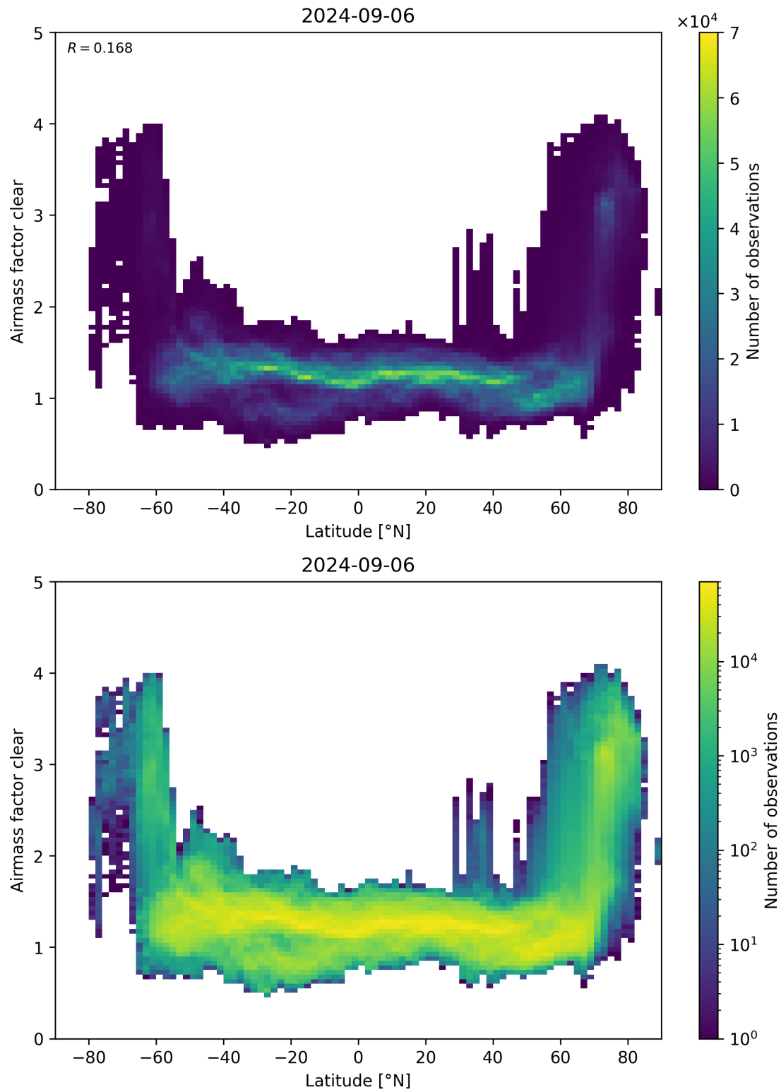
Figure 156: Scatter density plot of “Latitude” against “Airmass factor clear” for 2024-09-06 to 2024-09-07.
