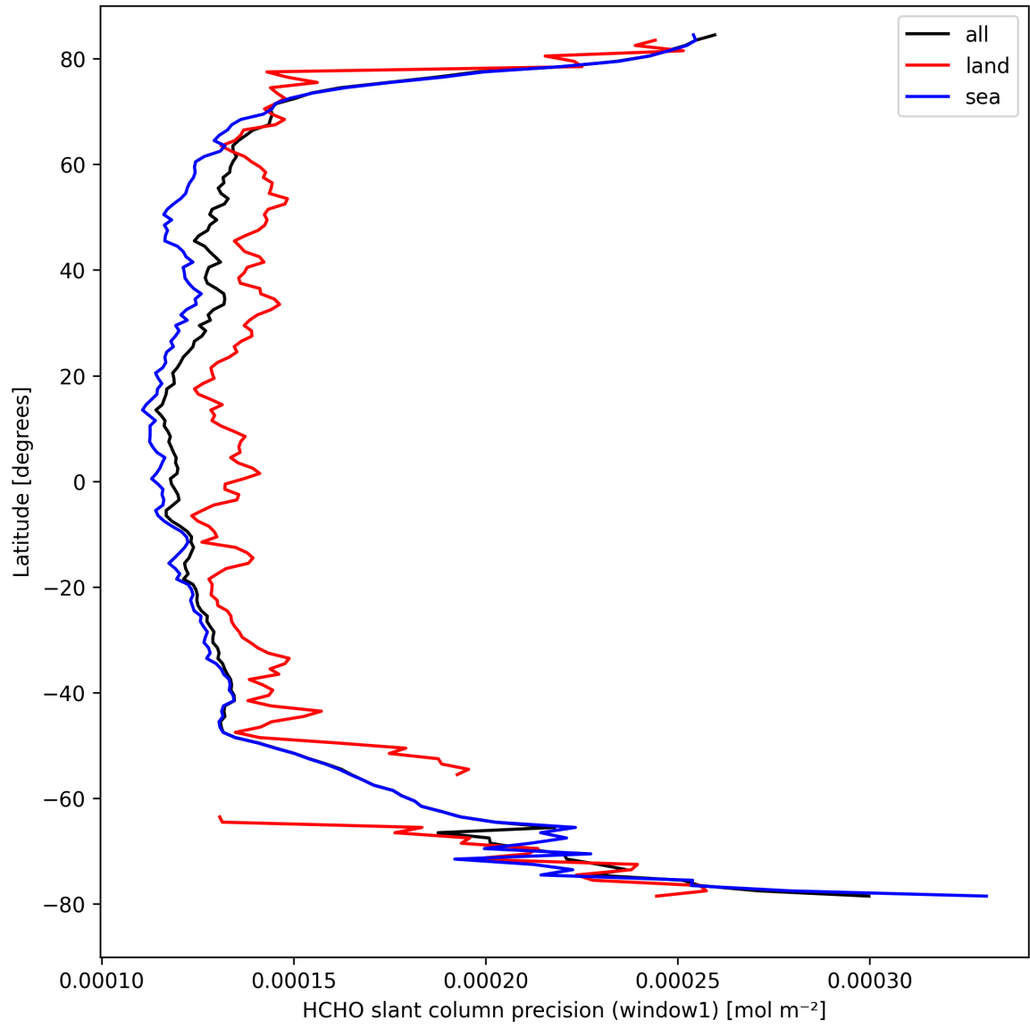
Figure 25: Zonal average of “HCHO slant column precision (window1)” for 2024-09-06 to 2024-09-07.
