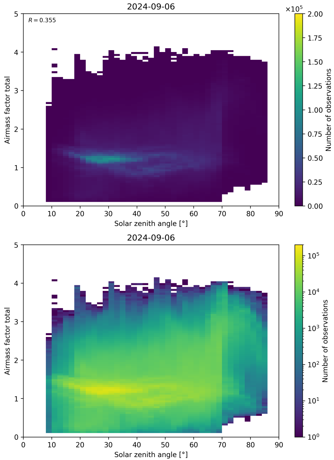
Figure 175: Scatter density plot of “Solar zenith angle” against “Airmass factor total” for 2024-09-06 to 2024-09-07.
