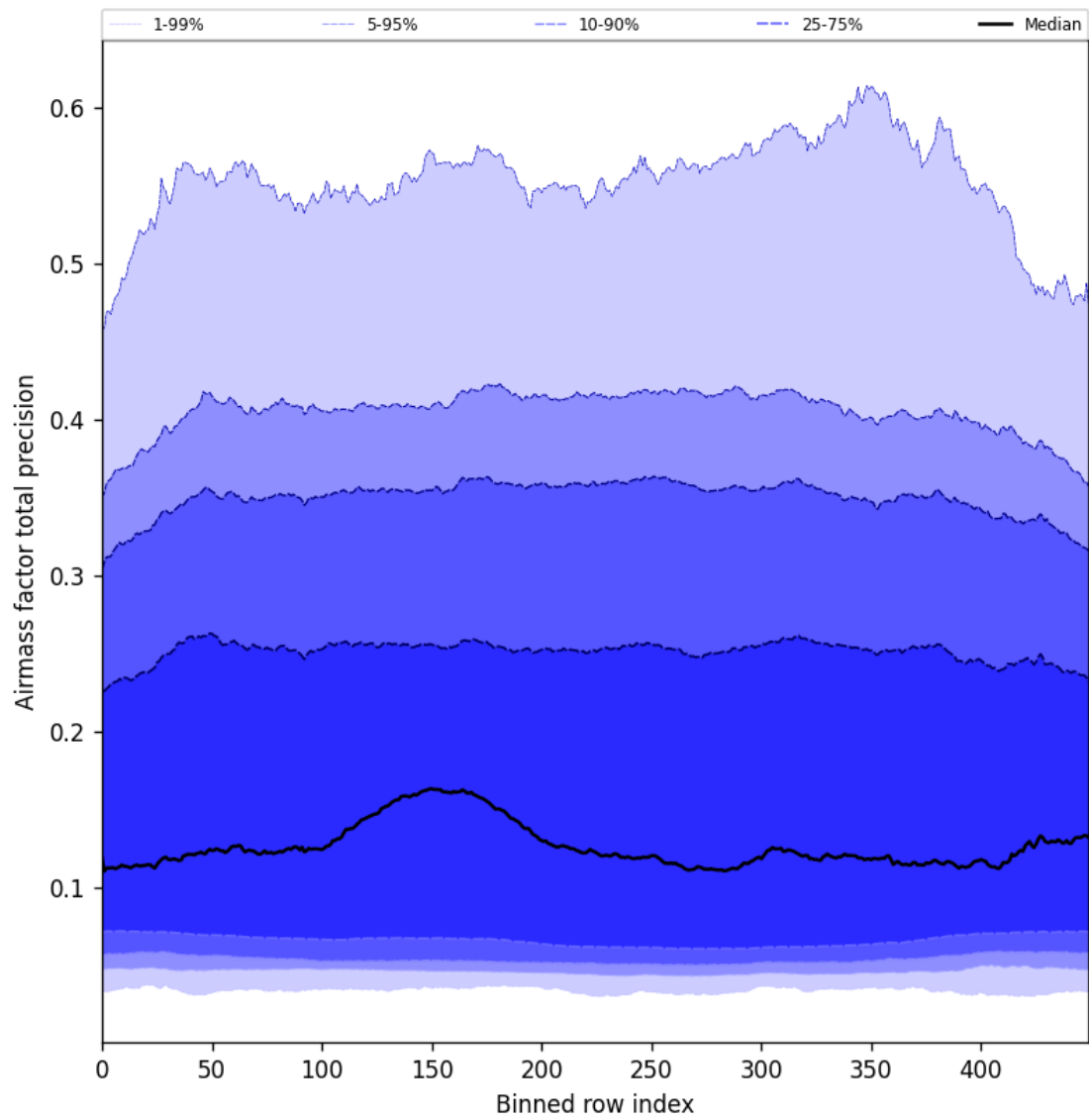
Figure 55: Along track statistics of “Airmass factor total precision” for 2024-09-06 to 2024-09-07
