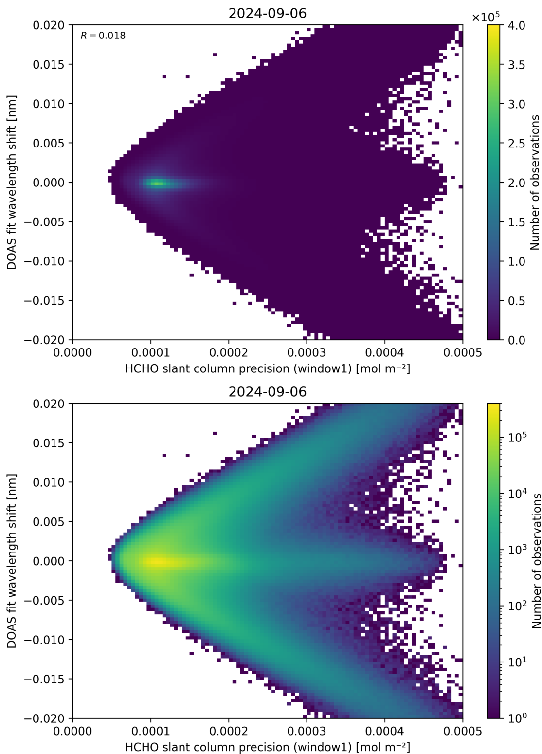
Figure 89: Scatter density plot of “HCHO slant column precision (window1)” against “DOAS fit wavelength shift” for 2024-09-06 to 2024-09-07.
