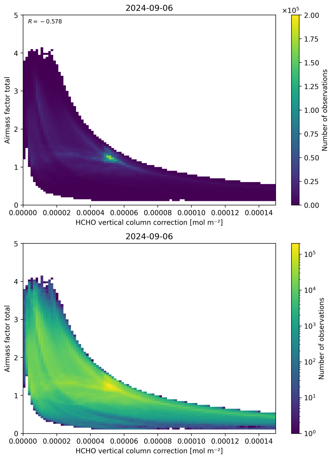
Figure 120: Scatter density plot of “HCHO vertical column correction” against “Airmass factor total” for 2024-09-06 to 2024-09-07.
