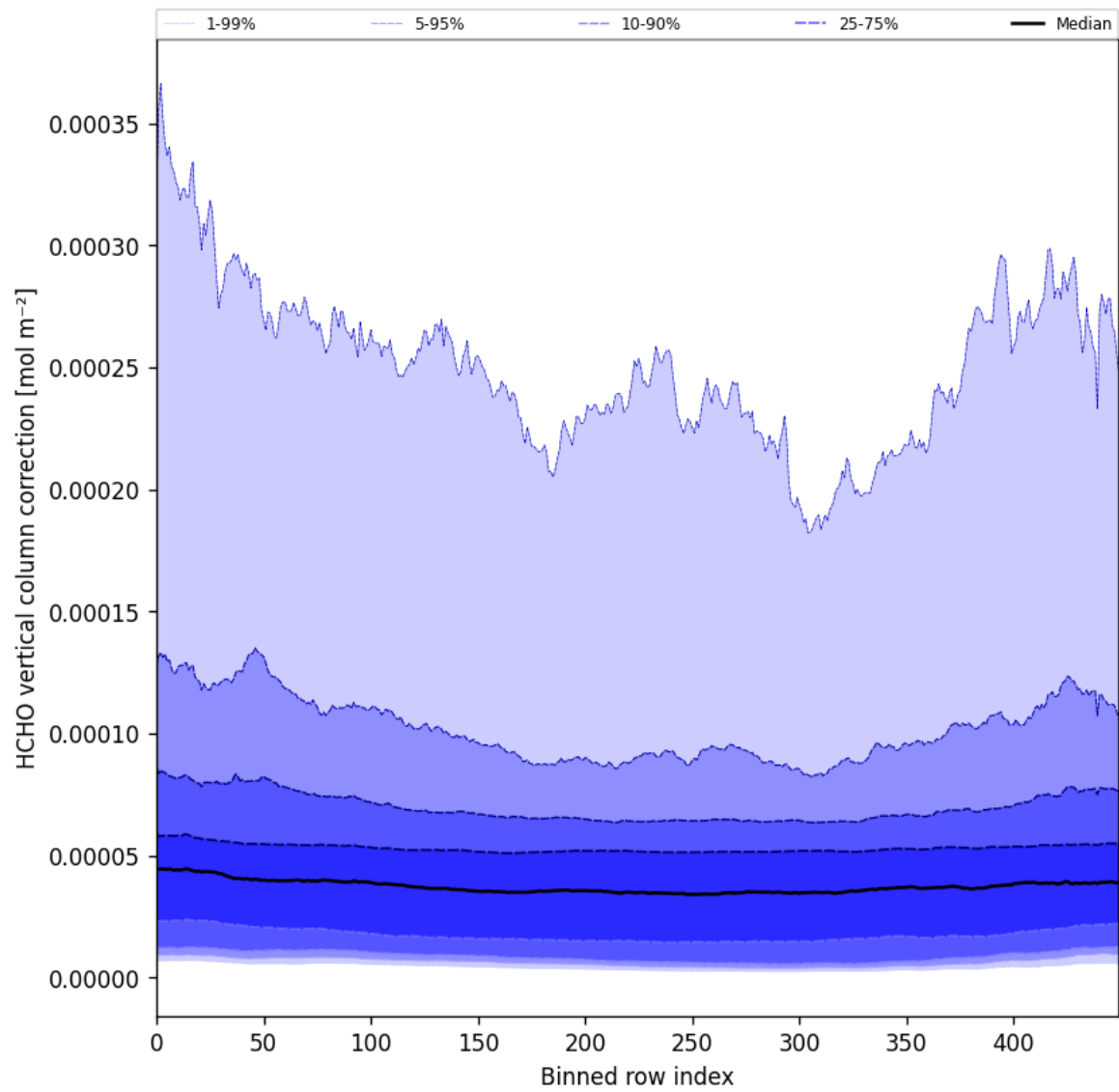
Figure 51: Along track statistics of “HCHO vertical column correction” for 2024-09-06 to 2024-09-07
