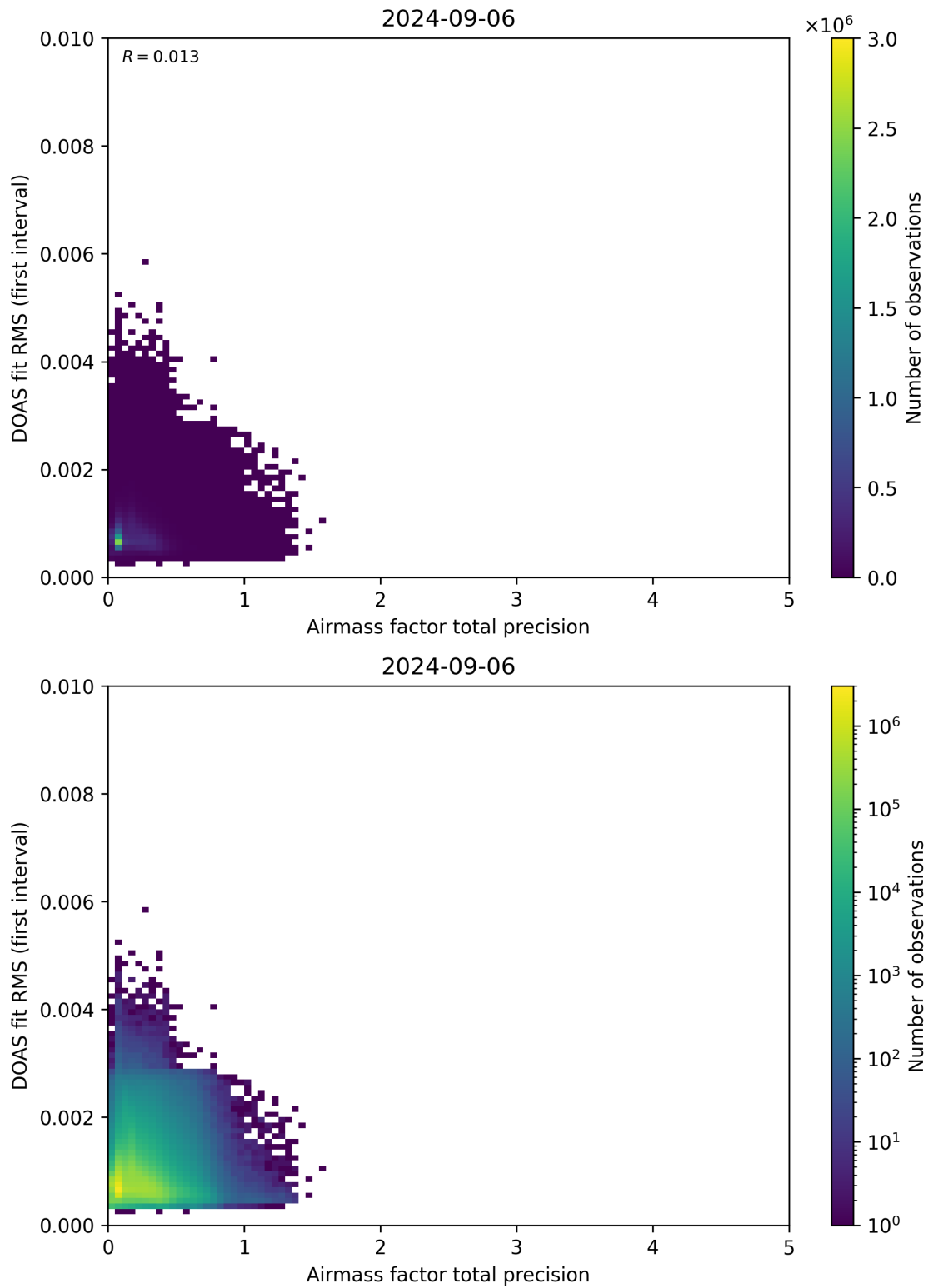
Figure 105: Scatter density plot of “Airmass factor total precision” against “DOAS fit RMS (first interval)” for 2024-09-06 to 2024-09-07.
