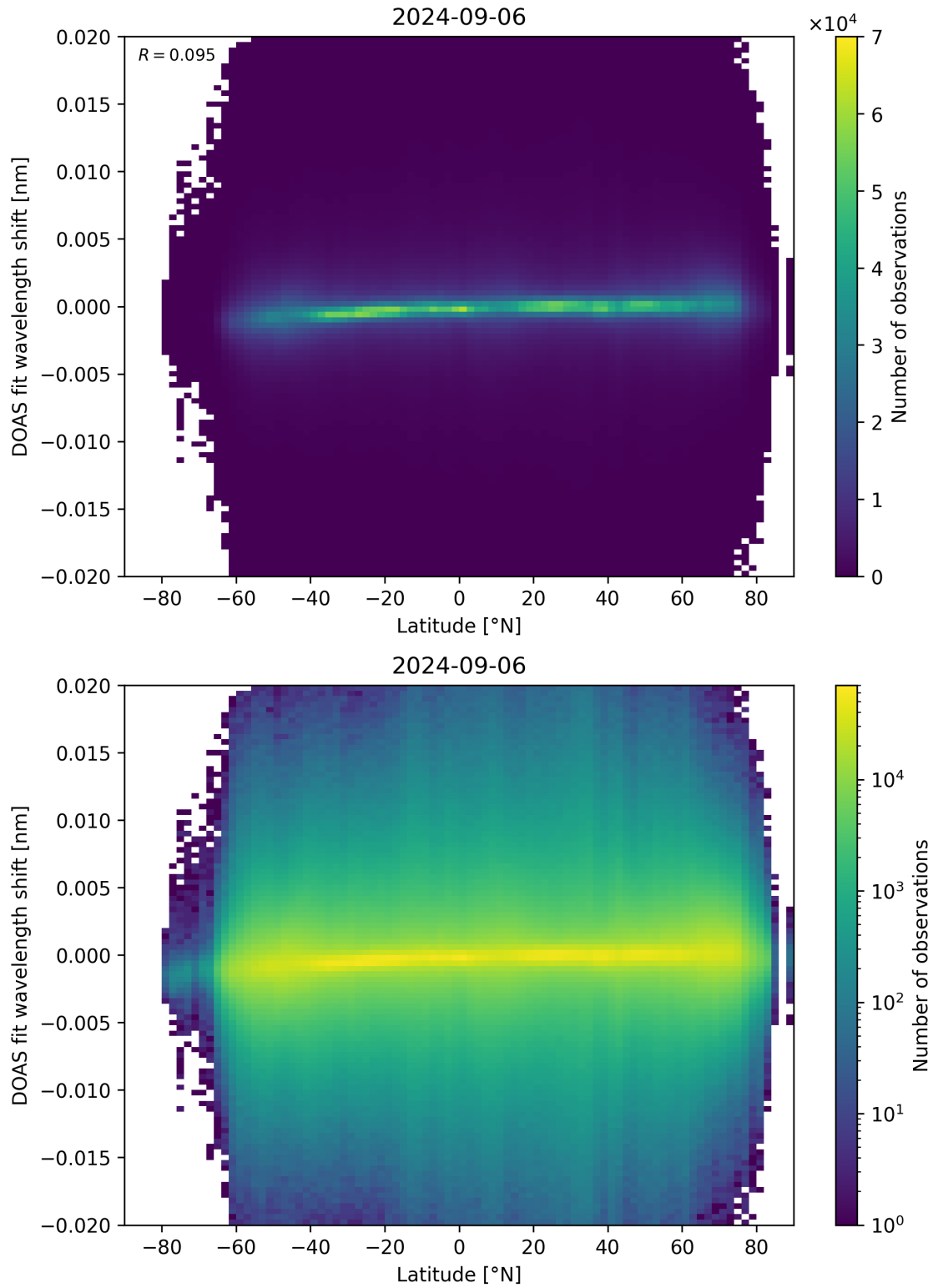
Figure 154: Scatter density plot of “Latitude” against “DOAS fit wavelength shift” for 2024-09-06 to 2024-09-07.
