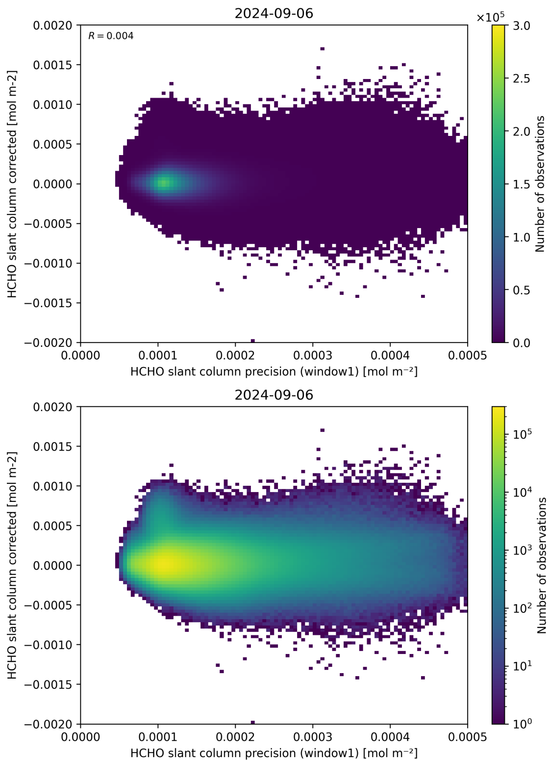
Figure 92: Scatter density plot of “HCHO slant column precision (window1)” against “HCHO slant column corrected” for 2024-09-06 to 2024-09-07.
