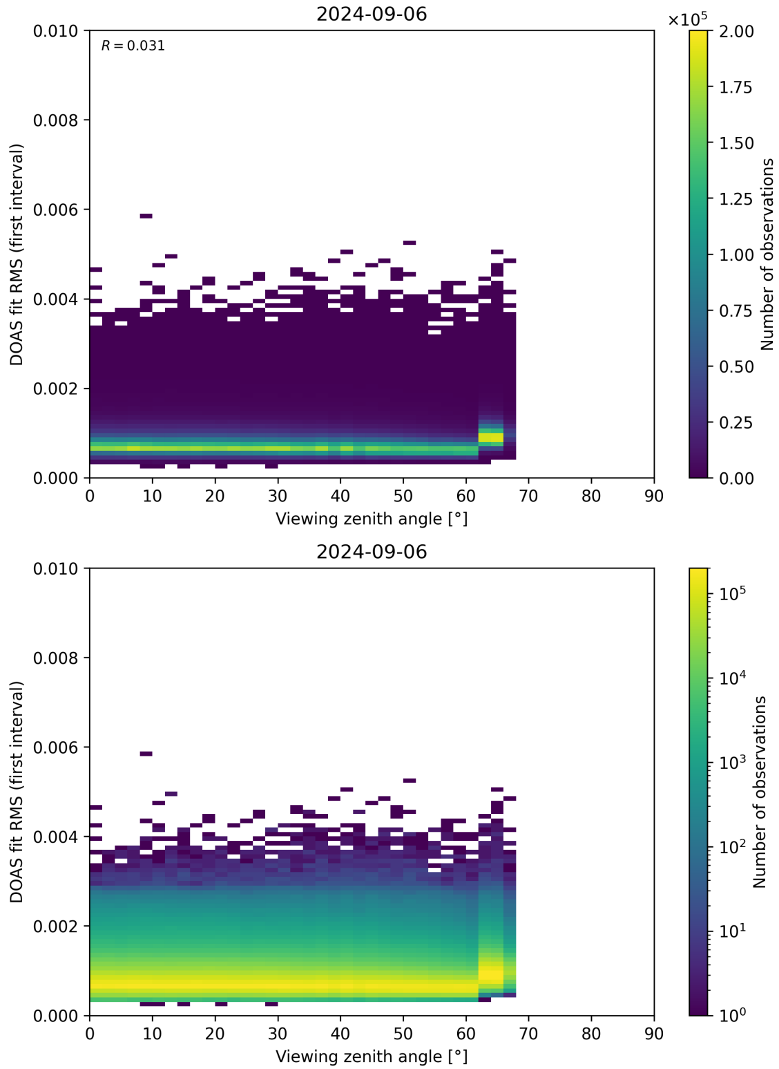
Figure 182: Scatter density plot of “Viewing zenith angle” against “DOAS fit RMS (first interval)” for 2024-09-06 to 2024-09-07.
