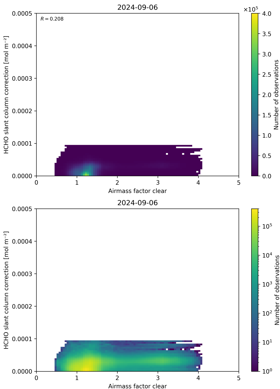
Figure 75: Scatter density plot of “Airmass factor clear” against “HCHO slant column correction” for 2024-09-06 to 2024-09-07.
