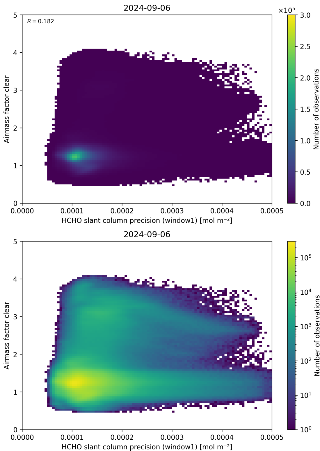
Figure 91: Scatter density plot of “HCHO slant column precision (window1)” against “Airmass factor clear” for 2024-09-06 to 2024-09-07.
