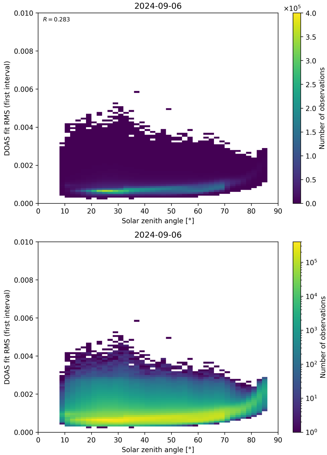
Figure 167: Scatter density plot of “Solar zenith angle” against “DOAS fit RMS (first interval)” for 2024-09-06 to 2024-09-07.
