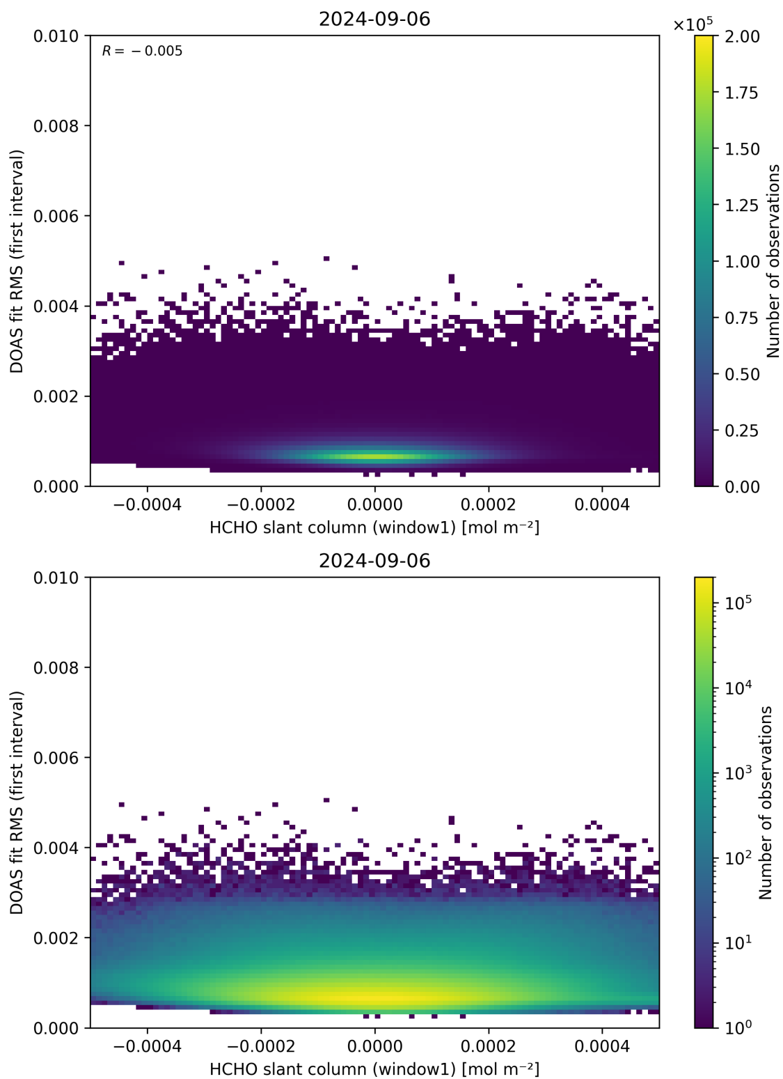
Figure 78: Scatter density plot of “HCHO slant column (window1)” against “DOAS fit RMS (first interval)” for 2024-09-06 to 2024-09-07.
