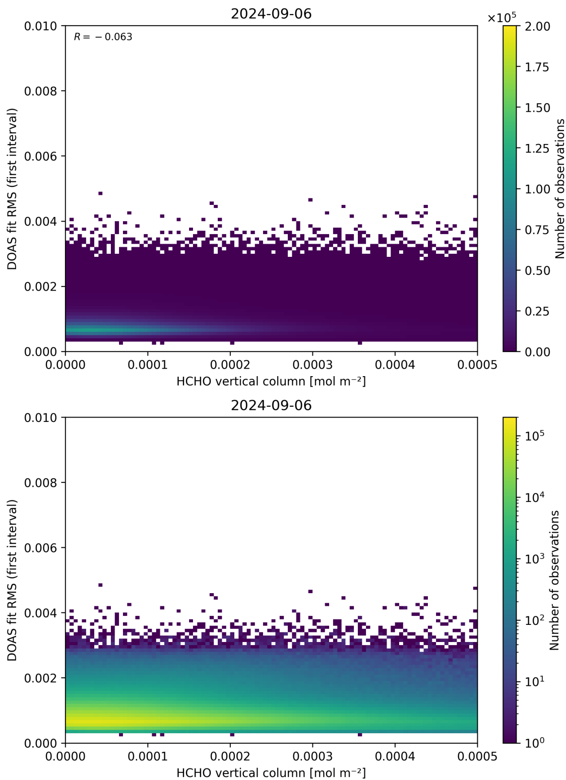
Figure 123: Scatter density plot of “HCHO vertical column” against “DOAS fit RMS (first interval)” for 2024-09-06 to 2024-09-07.
