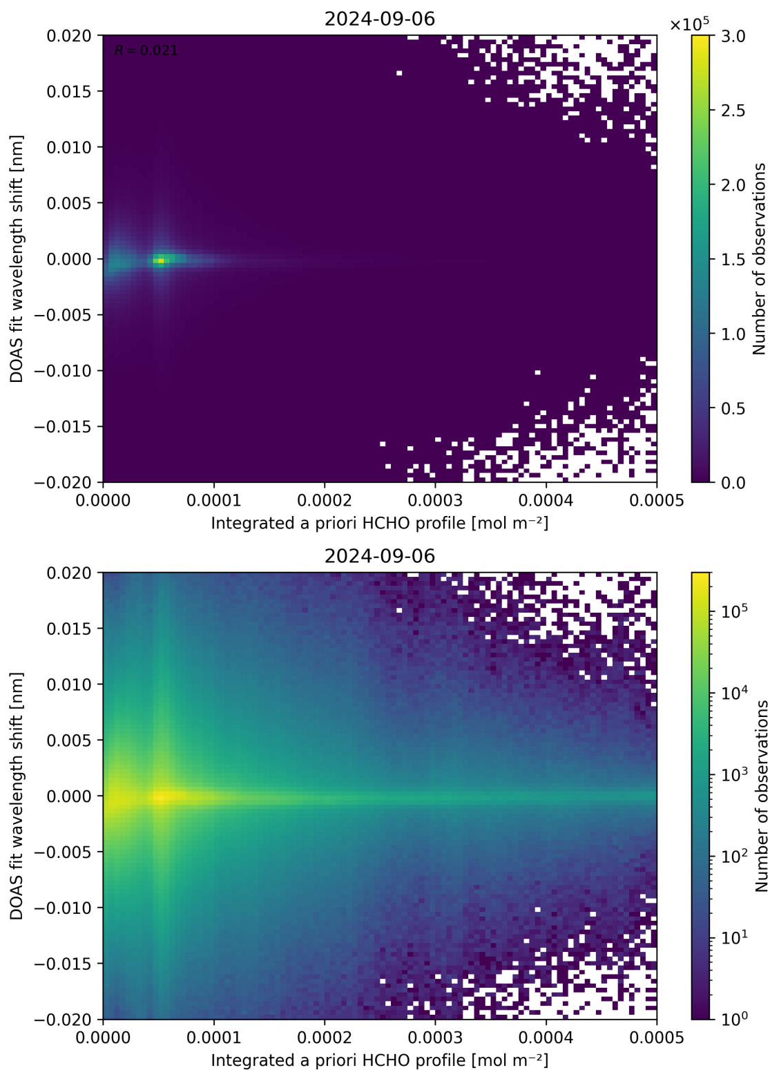
Figure 149: Scatter density plot of “Integrated a priori HCHO profile” against “DOAS fit wavelength shift” for 2024-09-06 to 2024-09-07.
