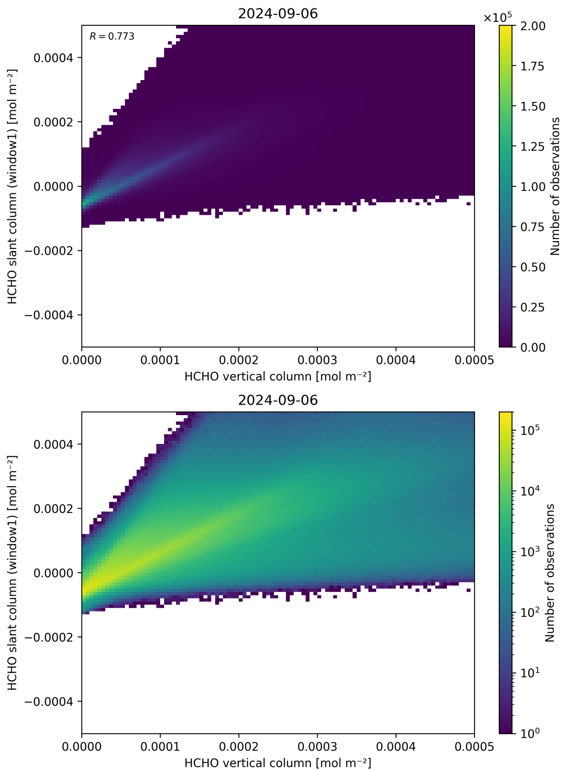
Figure 129: Scatter density plot of “HCHO vertical column” against “HCHO slant column (window1)” for 2024-09-06 to 2024-09-07.
