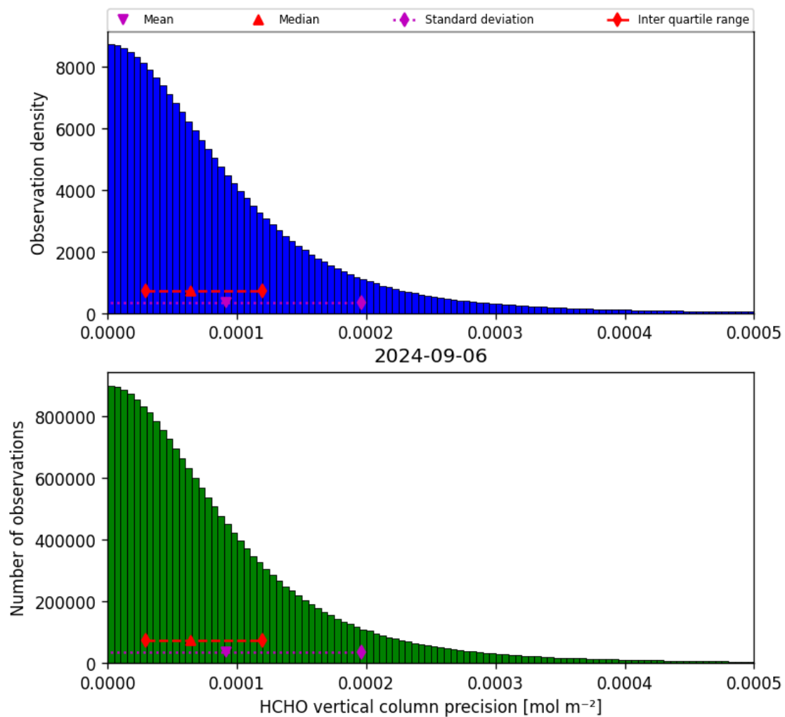
Figure 36: Histogram of “HCHO vertical column precision” for 2024-09-06 to 2024-09-07
