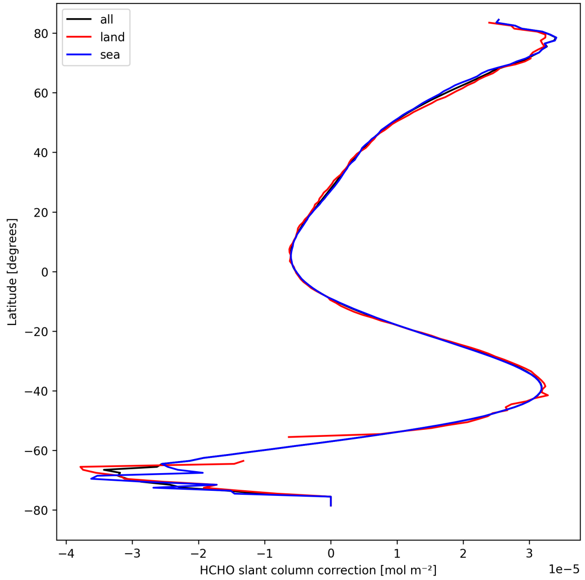
Figure 33: Zonal average of “HCHO slant column correction” for 2024-09-06 to 2024-09-07.
