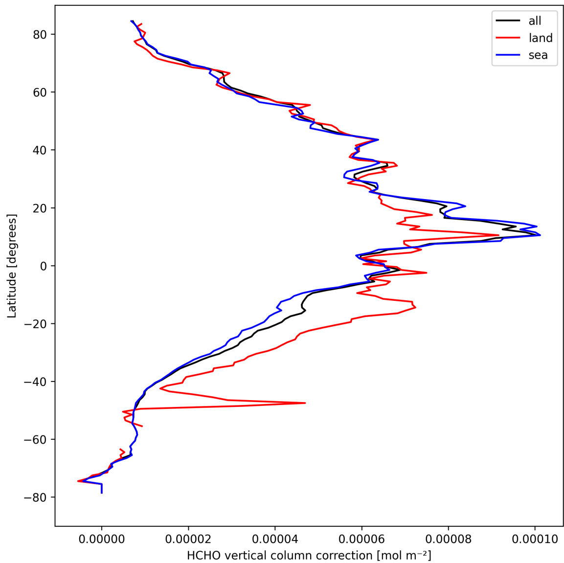
Figure 23: Zonal average of “HCHO vertical column correction” for 2024-09-06 to 2024-09-07.
