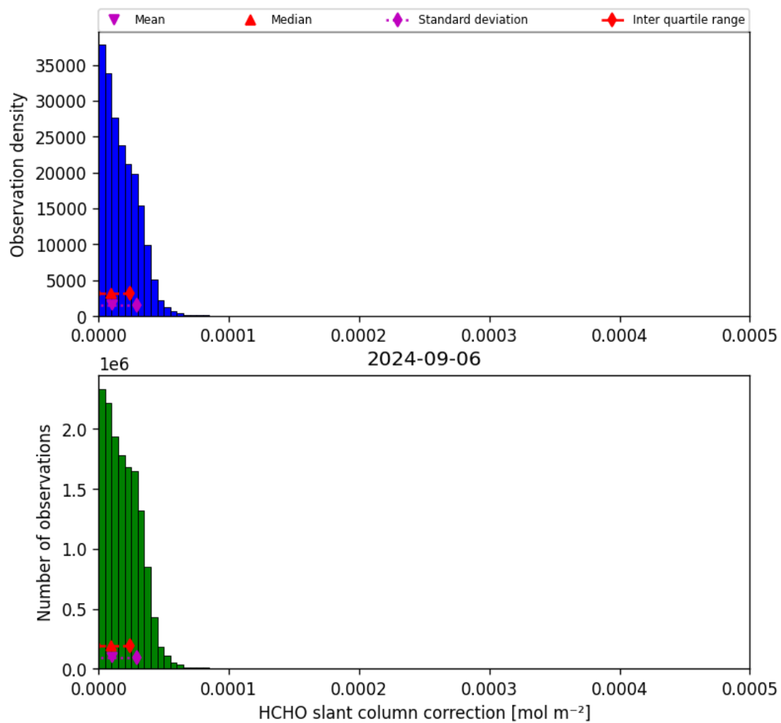
Figure 47: Histogram of “HCHO slant column correction” for 2024-09-06 to 2024-09-07
