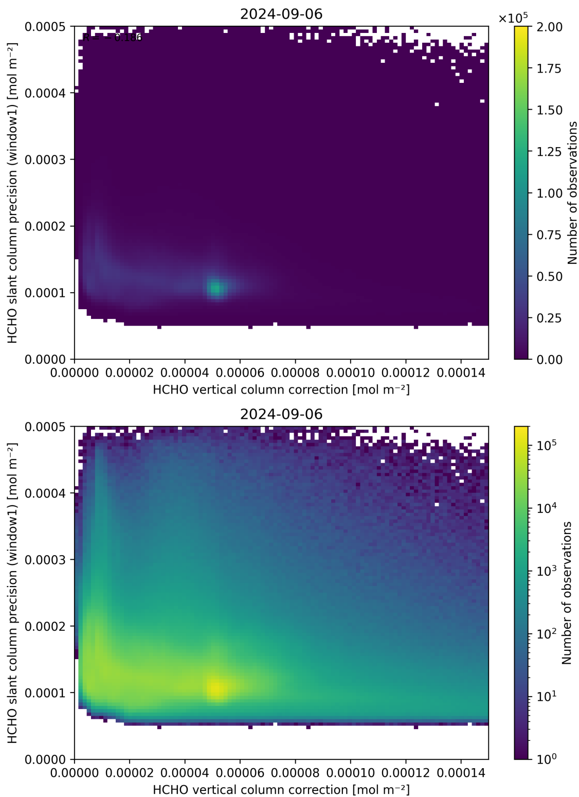
Figure 119: Scatter density plot of “HCHO vertical column correction” against “HCHO slant column precision (window1)” for 2024-09-06 to 2024-09-07.
