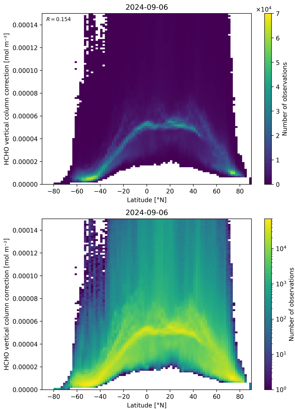
Figure 164: Scatter density plot of “Latitude” against “HCHO vertical column correction” for 2024-09-06 to 2024-09-07.
