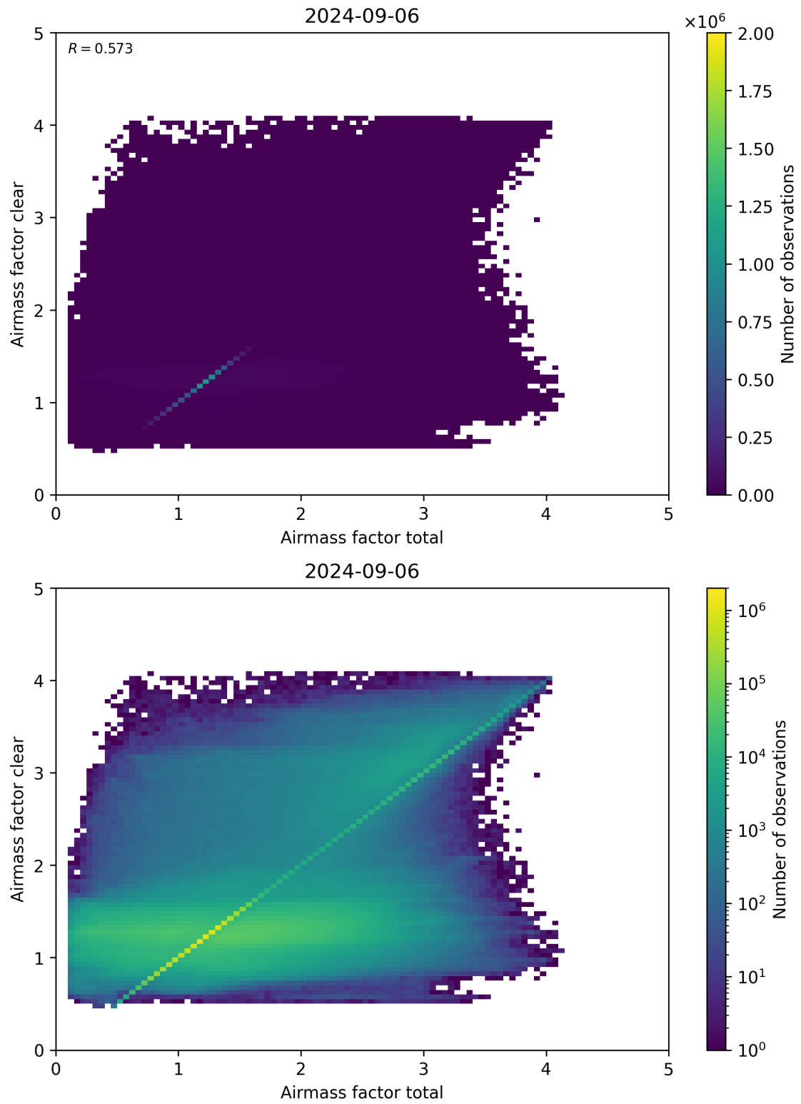
Figure 100: Scatter density plot of “Airmass factor total” against “Airmass factor clear” for 2024-09-06 to 2024-09-07.
