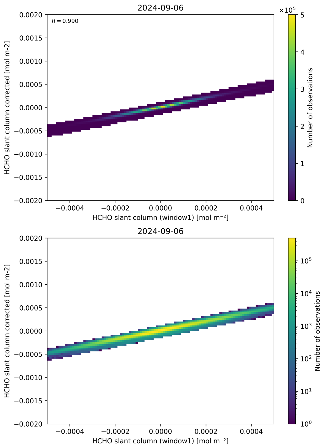
Figure 82: Scatter density plot of “HCHO slant column (window1)” against “HCHO slant column corrected” for 2024-09-06 to 2024-09-07.
