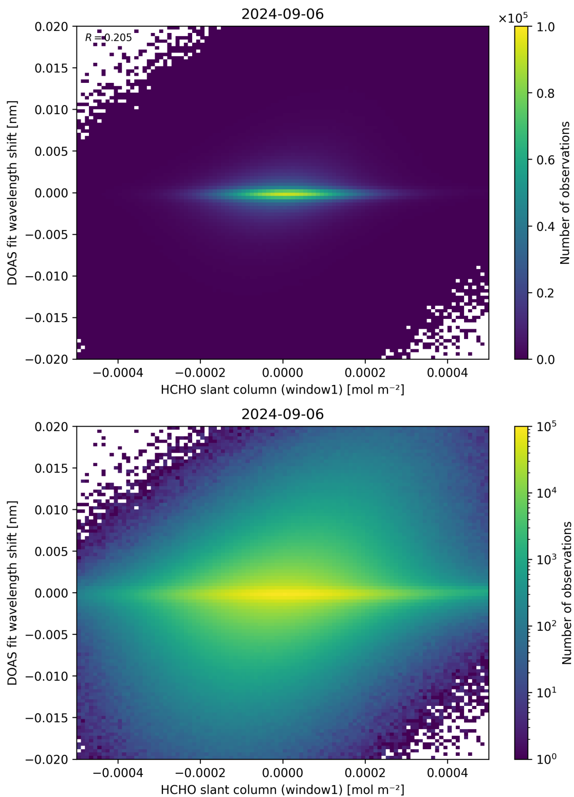
Figure 79: Scatter density plot of “HCHO slant column (window1)” against “DOAS fit wavelength shift” for 2024-09-06 to 2024-09-07.
