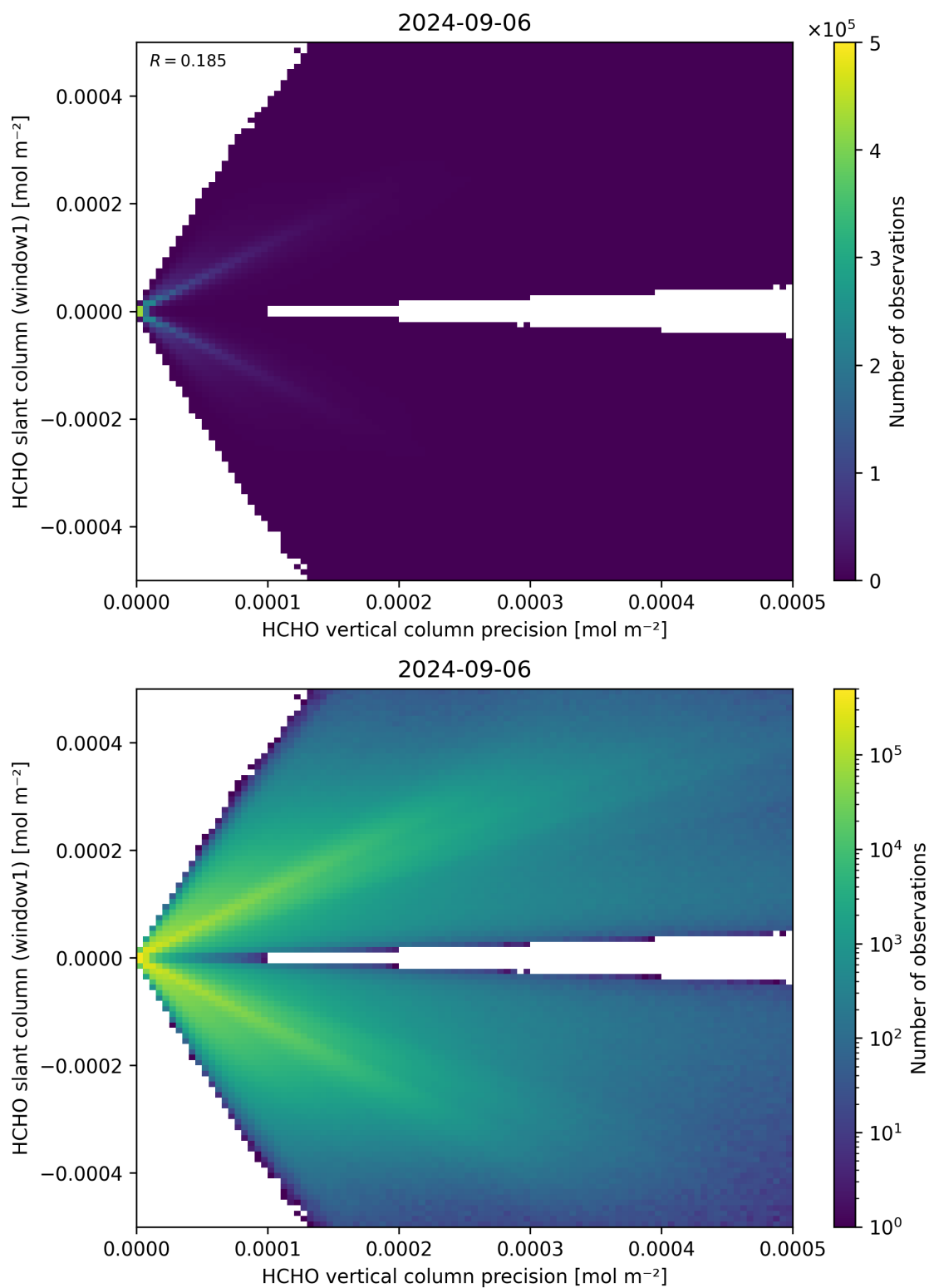
Figure 142: Scatter density plot of “HCHO vertical column precision” against “HCHO slant column (window1)” for 2024-09-06 to 2024-09-07.
