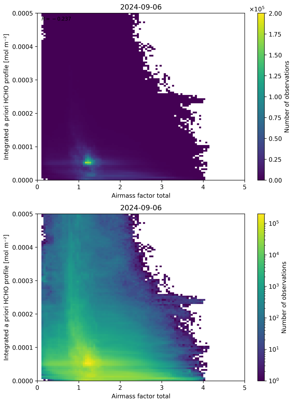
Figure 104: Scatter density plot of “Airmass factor total” against “Integrated a priori HCHO profile” for 2024-09-06 to 2024-09-07.
