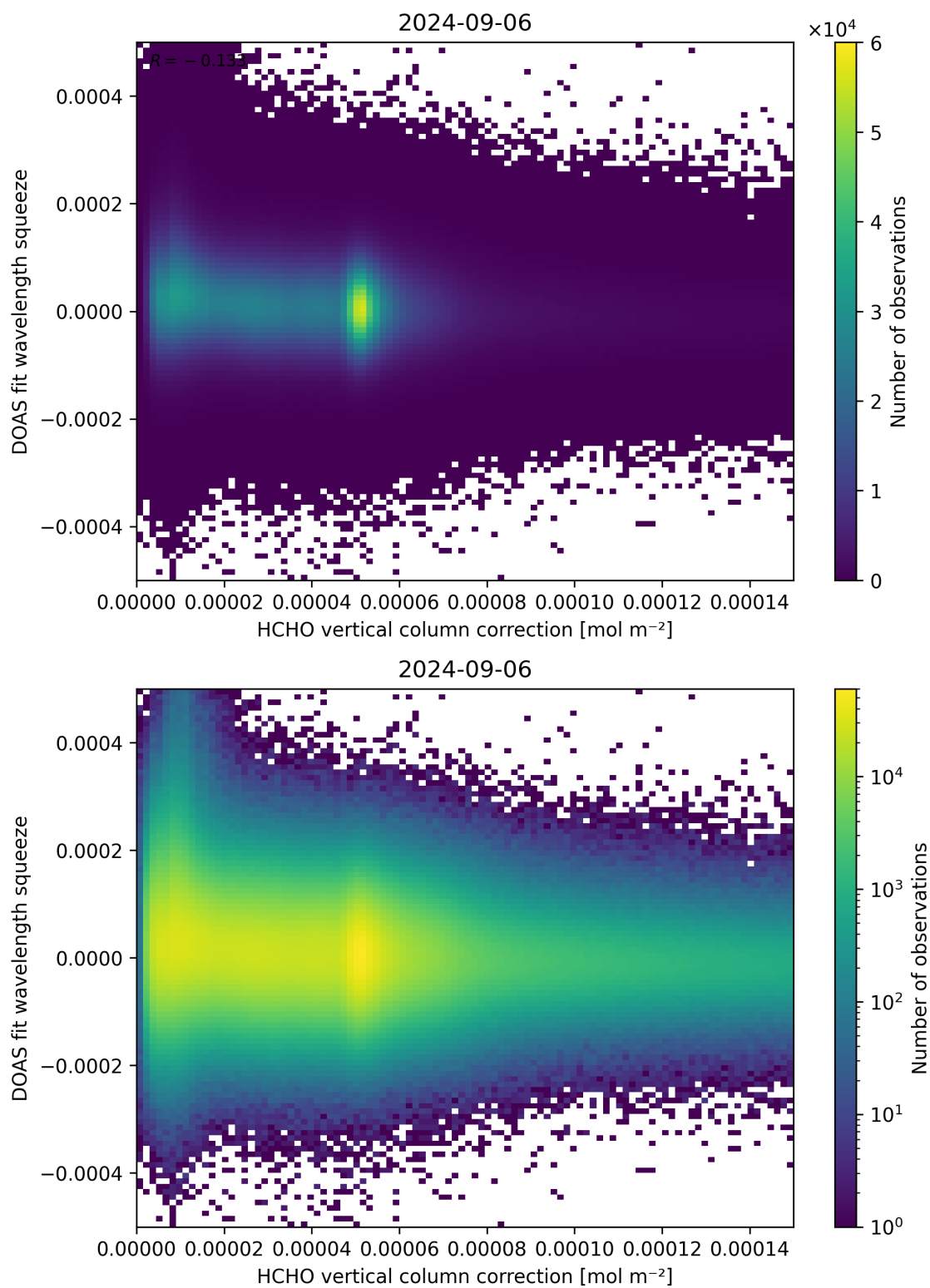
Figure 114: Scatter density plot of “HCHO vertical column correction” against “DOAS fit wavelength squeeze” for 2024-09-06 to 2024-09-07.
