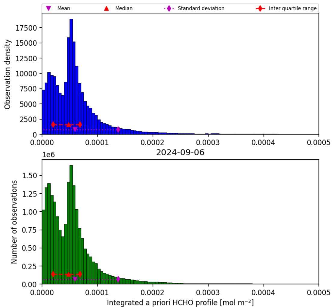
Figure 43: Histogram of “Integrated a priori HCHO profile” for 2024-09-06 to 2024-09-07
