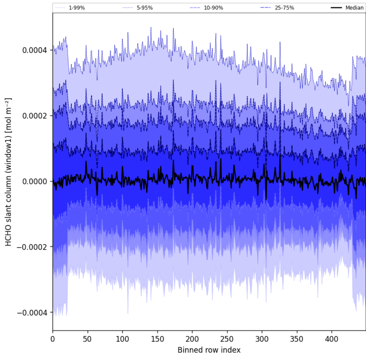
Figure 52: Along track statistics of “HCHO slant column (window1)” for 2024-09-06 to 2024-09-07
