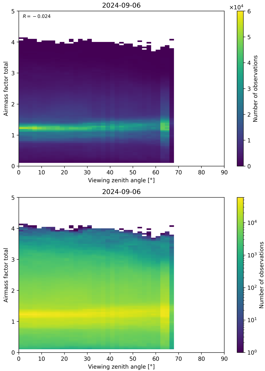
Figure 190: Scatter density plot of “Viewing zenith angle” against “Airmass factor total” for 2024-09-06 to 2024-09-07.
