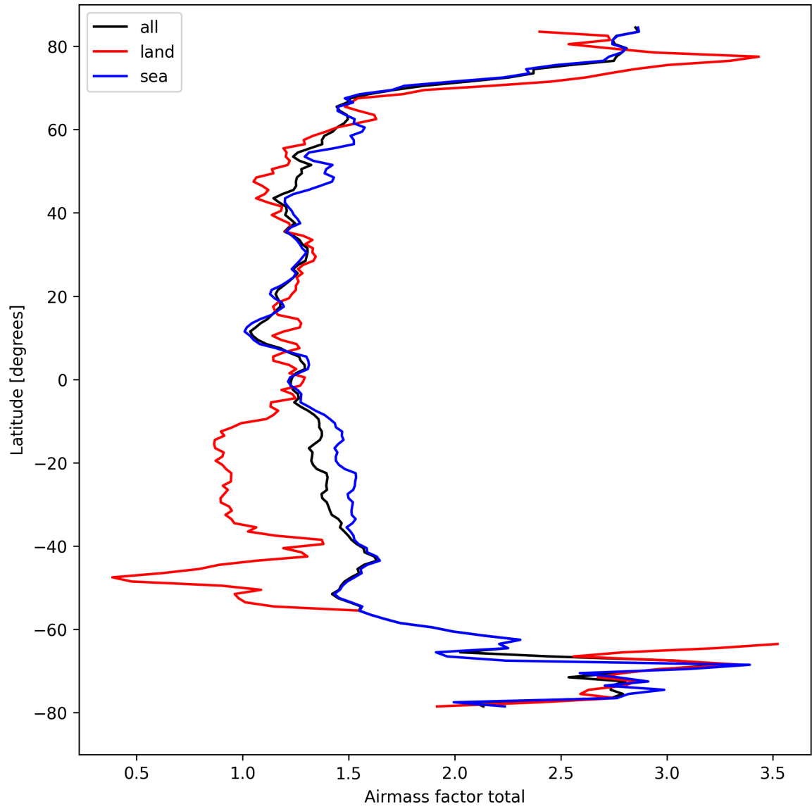
Figure 26: Zonal average of “Airmass factor total” for 2024-09-06 to 2024-09-07.
