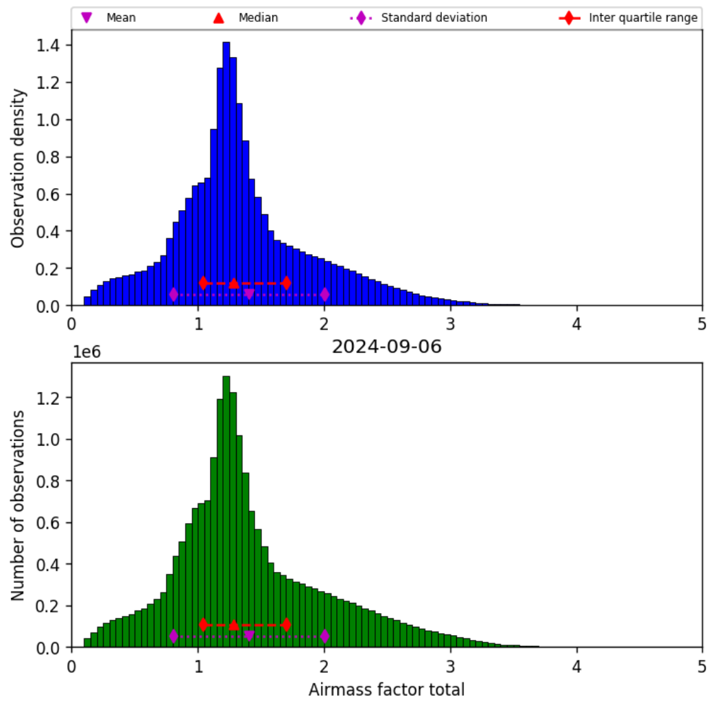
Figure 40: Histogram of “Airmass factor total” for 2024-09-06 to 2024-09-07
