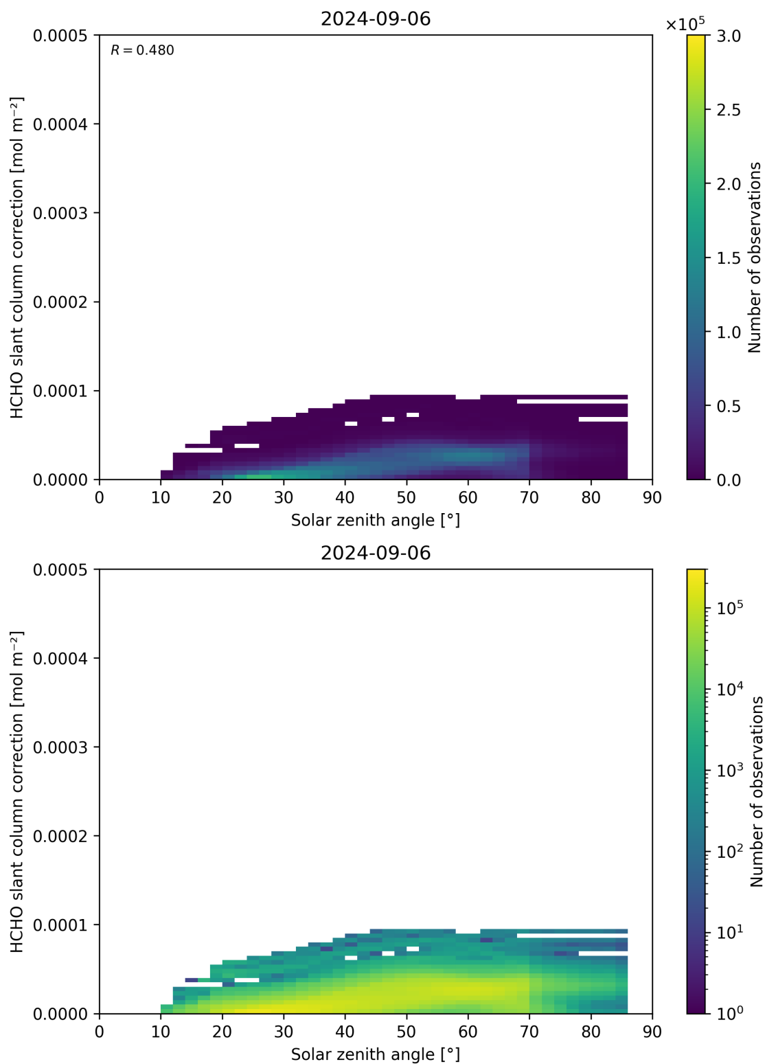
Figure 172: Scatter density plot of “Solar zenith angle” against “HCHO slant column correction” for 2024-09-06 to 2024-09-07.
