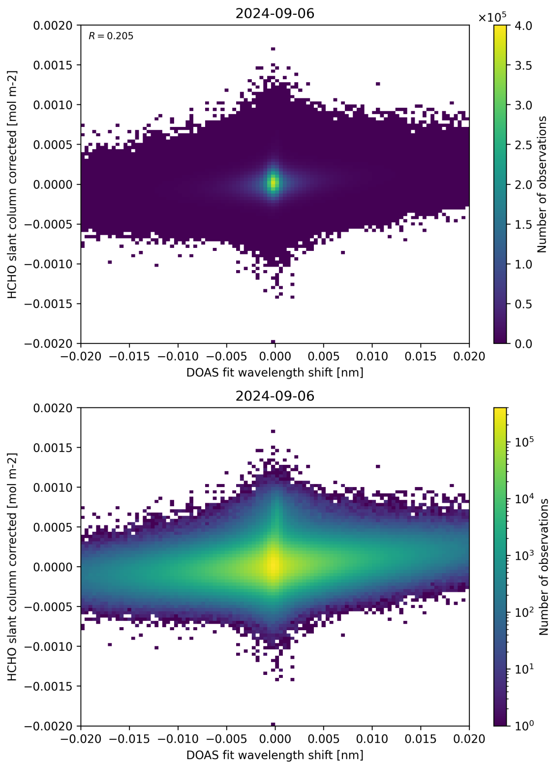
Figure 66: Scatter density plot of “DOAS fit wavelength shift” against “HCHO slant column corrected” for 2024-09-06 to 2024-09-07.
