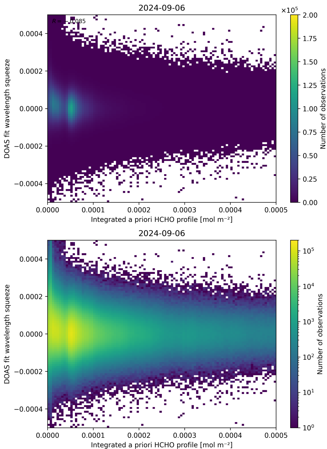
Figure 150: Scatter density plot of “Integrated a priori HCHO profile” against “DOAS fit wavelength squeeze” for 2024-09-06 to 2024-09-07.
