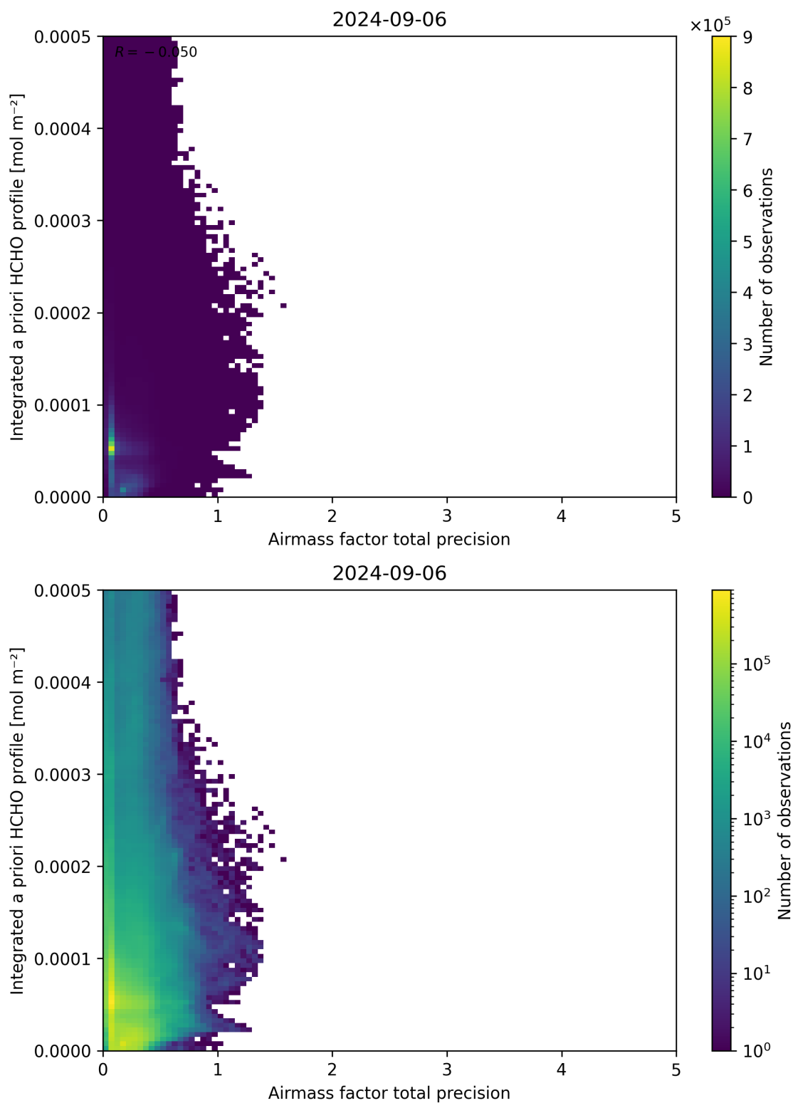
Figure 111: Scatter density plot of “Airmass factor total precision” against “Integrated a priori HCHO profile” for 2024-09-06 to 2024-09-07.
