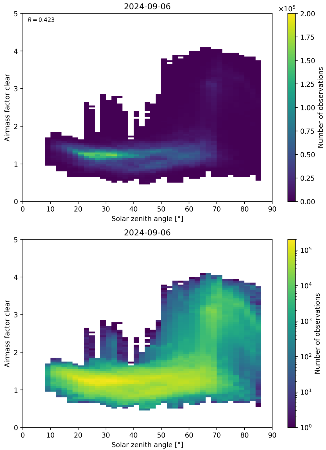
Figure 170: Scatter density plot of “Solar zenith angle” against “Airmass factor clear” for 2024-09-06 to 2024-09-07.
