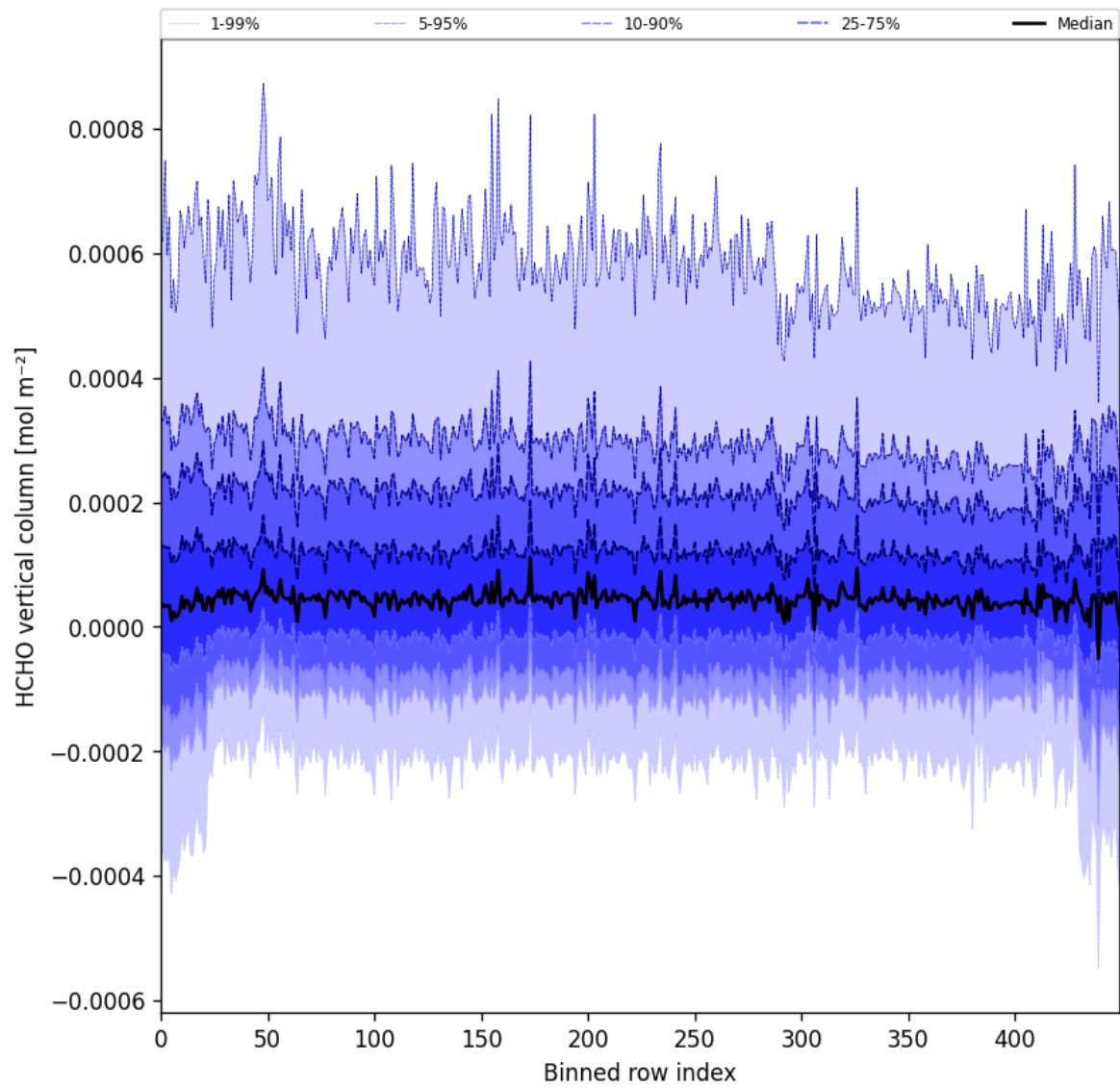
Figure 49: Along track statistics of “HCHO vertical column” for 2024-09-06 to 2024-09-07
