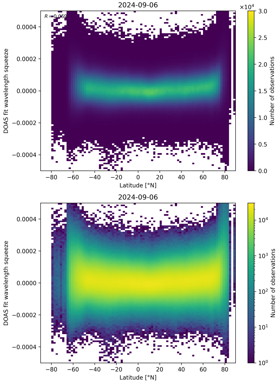
Figure 155: Scatter density plot of “Latitude” against “DOAS fit wavelength squeeze” for 2024-09-06 to 2024-09-07.
