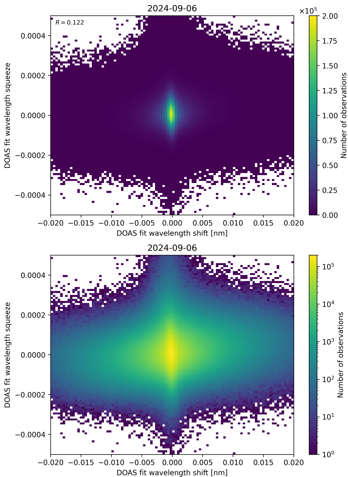
Figure 65: Scatter density plot of “DOAS fit wavelength shift” against “DOAS fit wavelength squeeze” for 2024-09-06 to 2024-09-07.
