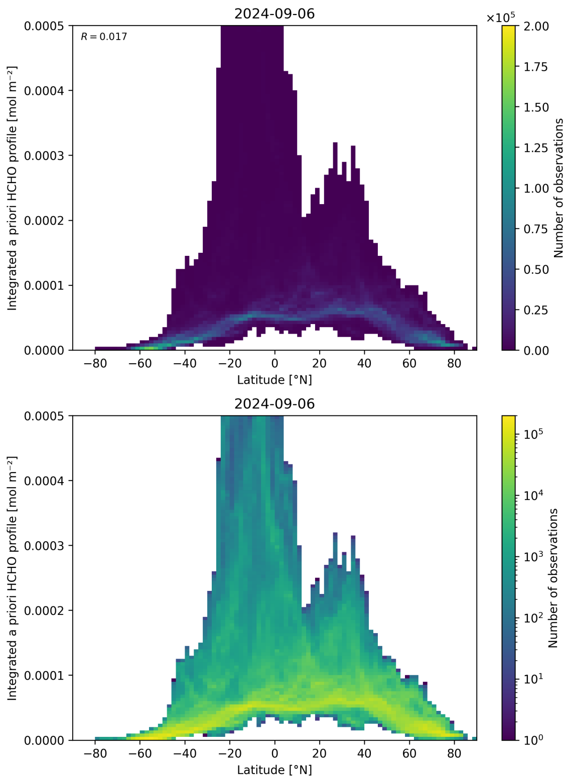
Figure 166: Scatter density plot of “Latitude” against “Integrated a priori HCHO profile” for 2024-09-06 to 2024-09-07.
