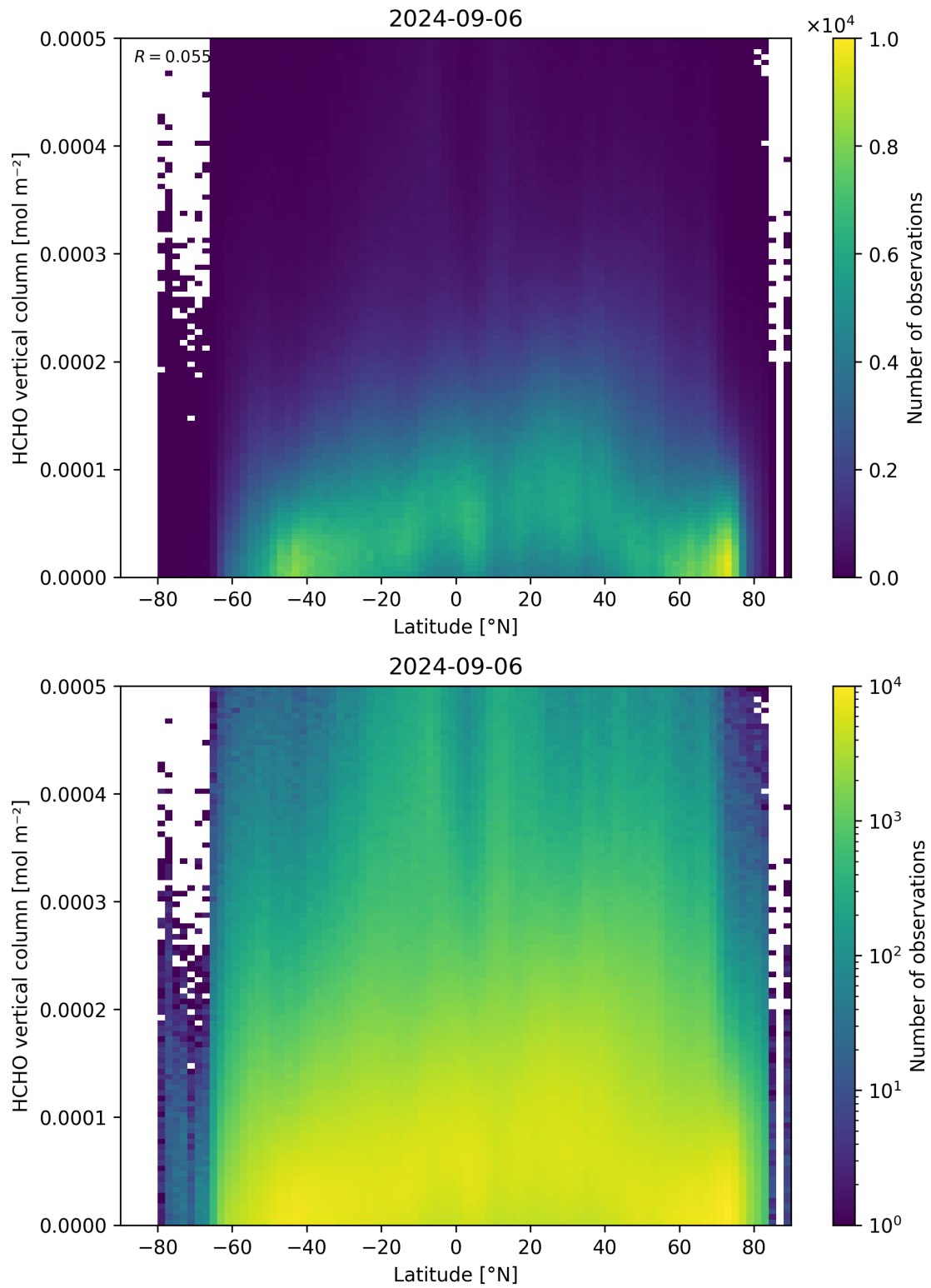
Figure 163: Scatter density plot of “Latitude” against “HCHO vertical column” for 2024-09-06 to 2024-09-07.
