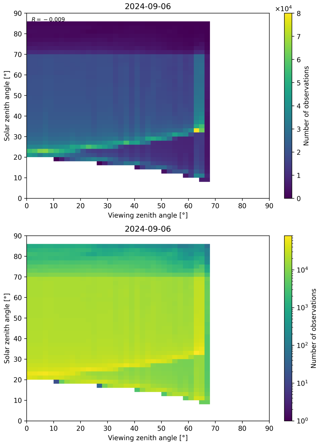
Figure 197: Scatter density plot of “Viewing zenith angle” against “Solar zenith angle” for 2024-09-06 to 2024-09-07.
